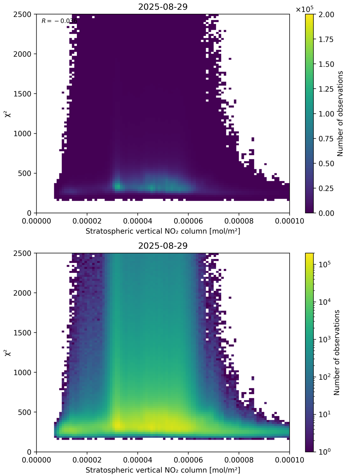
Figure 97: Scatter density plot of “Stratospheric vertical NO 2 column” against “ \chi^2 ” for 2025-08-28 to 2025-08-30.
