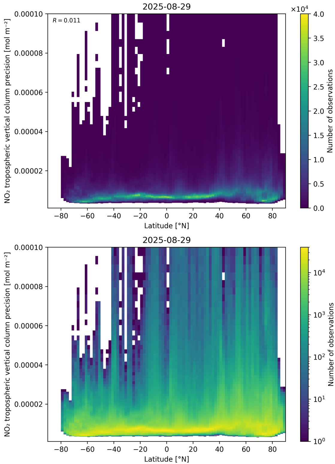
Figure 93: Scatter density plot of “Latitude” against “NO 2 tropospheric vertical column precision” for 2025-08-28 to 2025-08-30.
