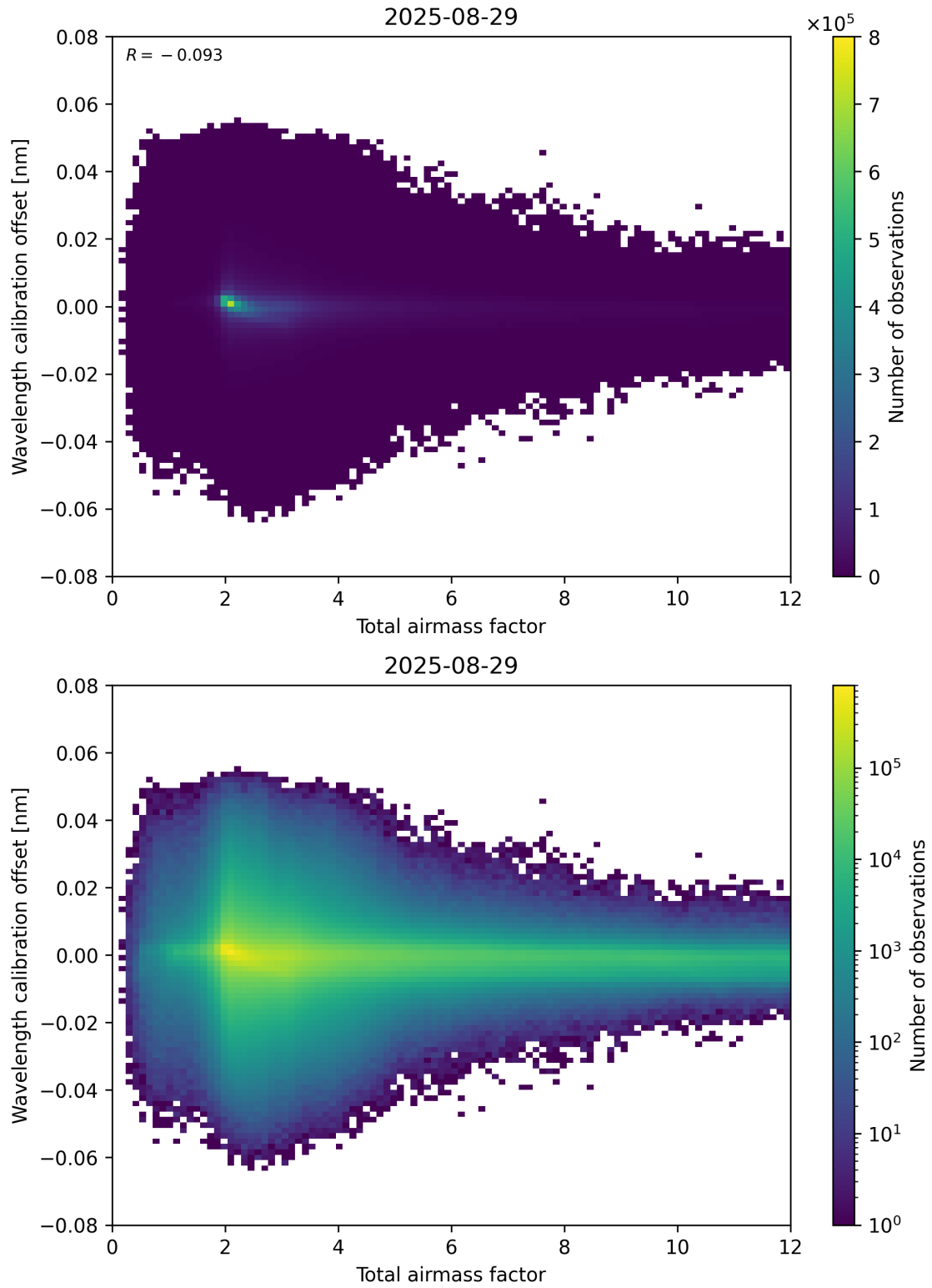
Figure 70: Scatter density plot of “Total airmass factor” against “Wavelength calibration offset” for 2025-08-28 to 2025-08-30.
