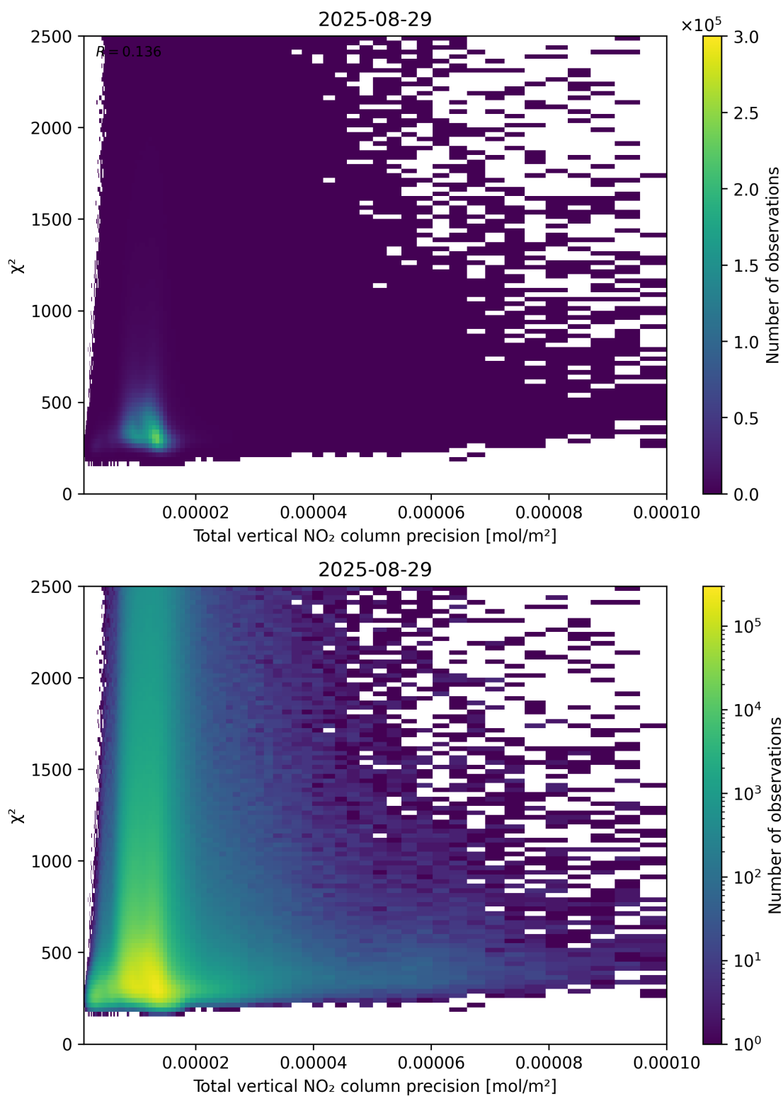
Figure 116: Scatter density plot of “Total vertical NO 2 column precision” against “ \chi^2 ” for 2025-08-28 to 2025-08-30.
