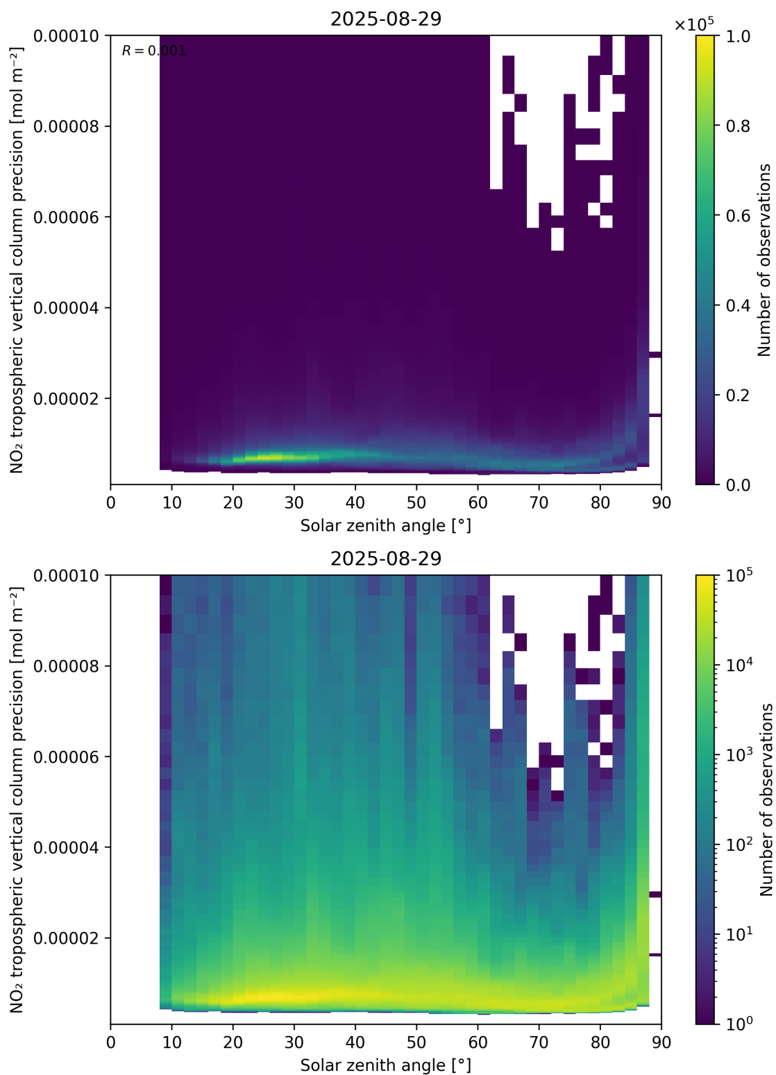
Figure 156: Scatter density plot of “Solar zenith angle” against “NO 2 tropospheric vertical column precision” for 2025-08-28 to 2025-08-30.
