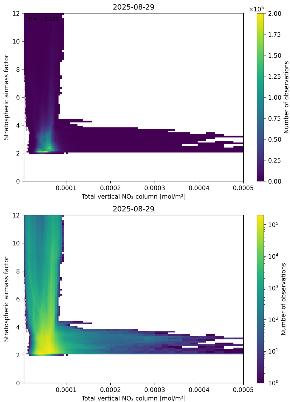
Figure 110: Scatter density plot of “Total vertical NO 2 column” against “Stratospheric airmass factor” for 2025-08-28 to 2025-08-30.
