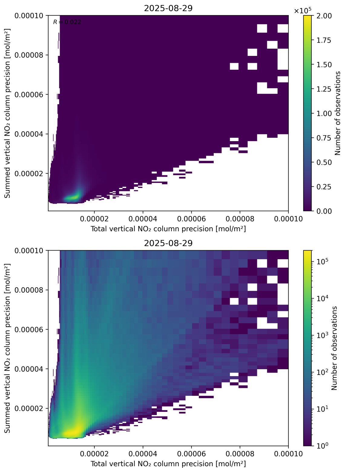
Figure 118: Scatter density plot of “Total vertical NO 2 column precision” against “Summed vertical NO 2 column precision” for 2025-08-28 to 2025-08-30.
