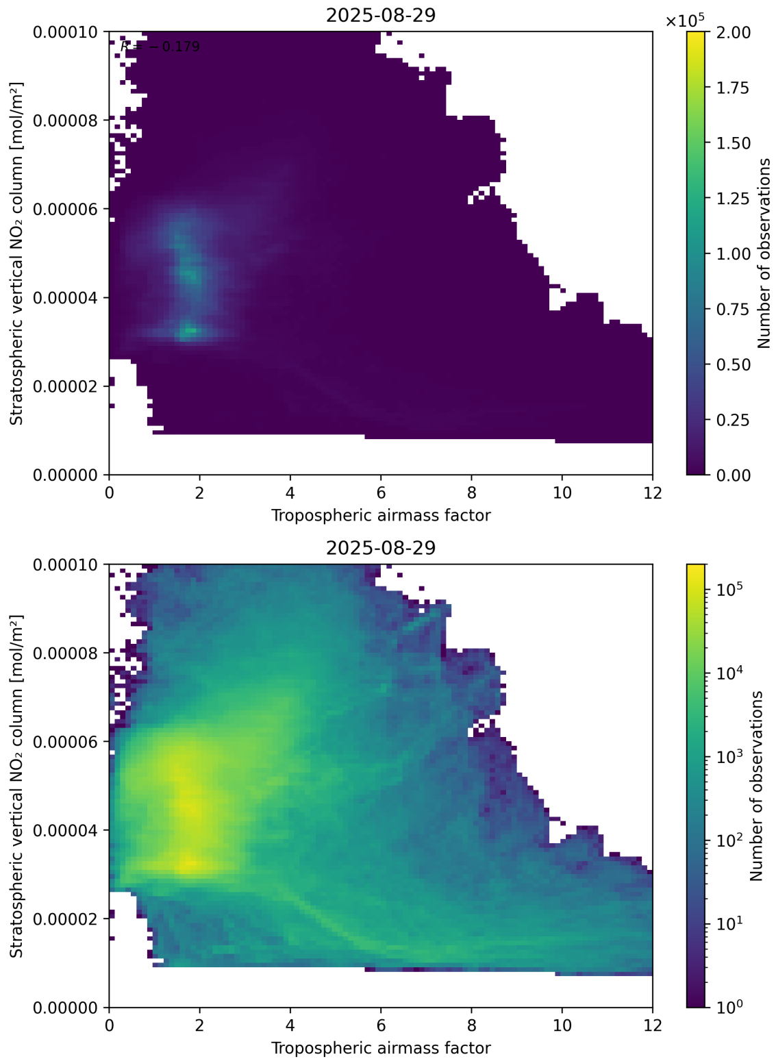
Figure 74: Scatter density plot of “Tropospheric airmass factor” against “Stratospheric vertical NO 2 column” for 2025-08-28 to 2025-08-30.
