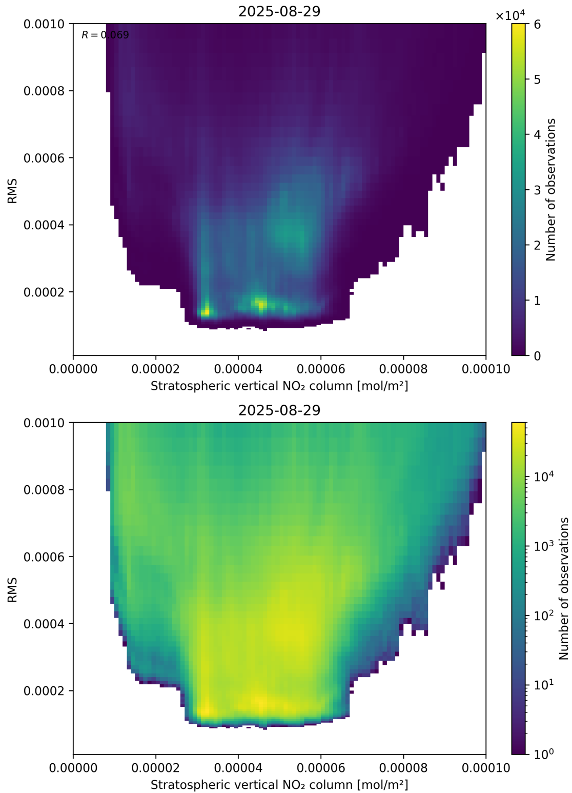
Figure 102: Scatter density plot of “Stratospheric vertical NO 2 column” against “RMS” for 2025-08-28 to 2025-08-30.
