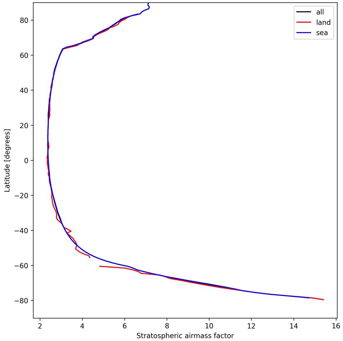
Figure 27: Zonal average of “Stratospheric airmass factor” for 2025-08-28 to 2025-08-30.
