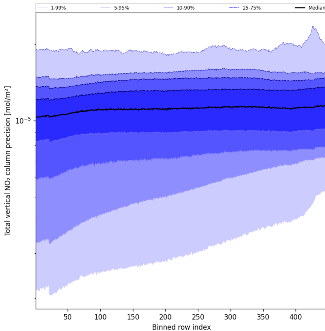
Figure 56: Along track statistics of “Total vertical NO 2 column precision” for 2025-08-28 to 2025-08-30
