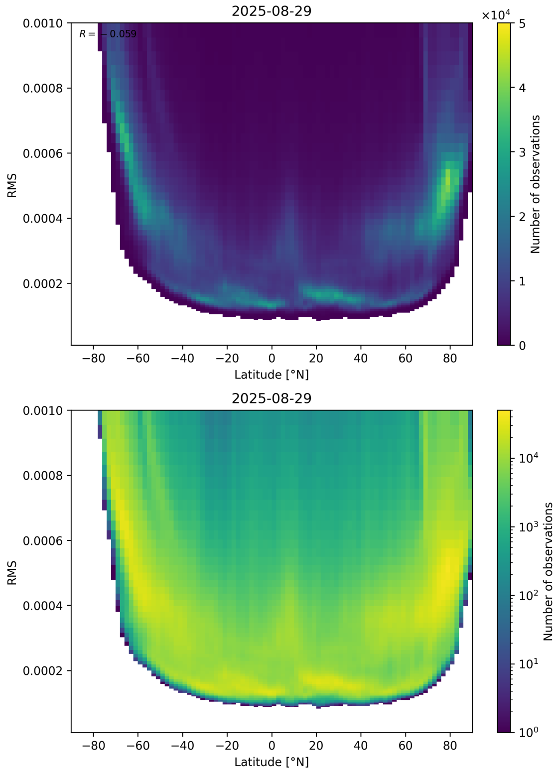
Figure 94: Scatter density plot of “Latitude” against “RMS” for 2025-08-28 to 2025-08-30.
