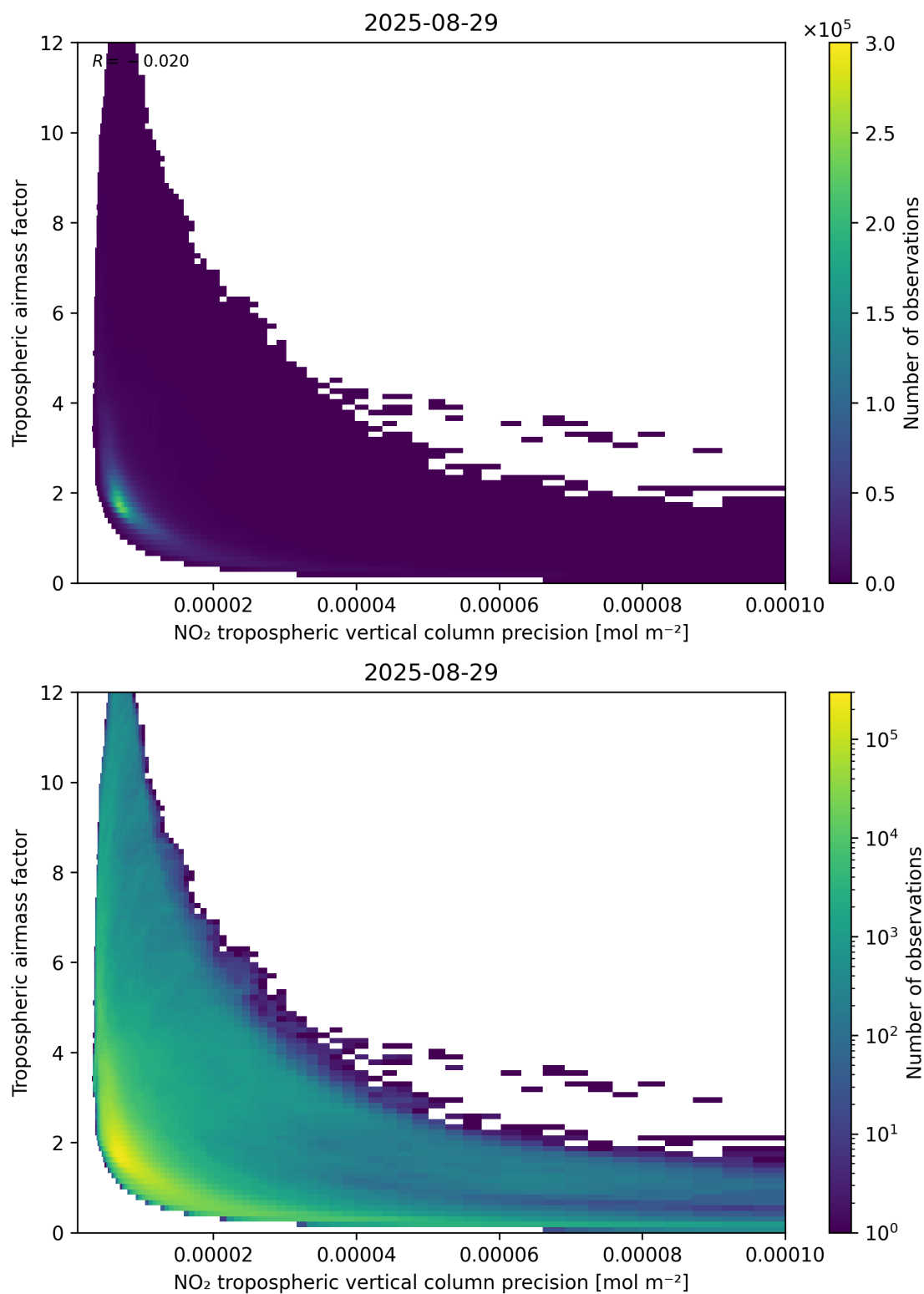
Figure 133: Scatter density plot of “NO 2 tropospheric vertical column precision” against “Tropospheric air mass factor” for 2025-08-28 to 2025-08-30.
