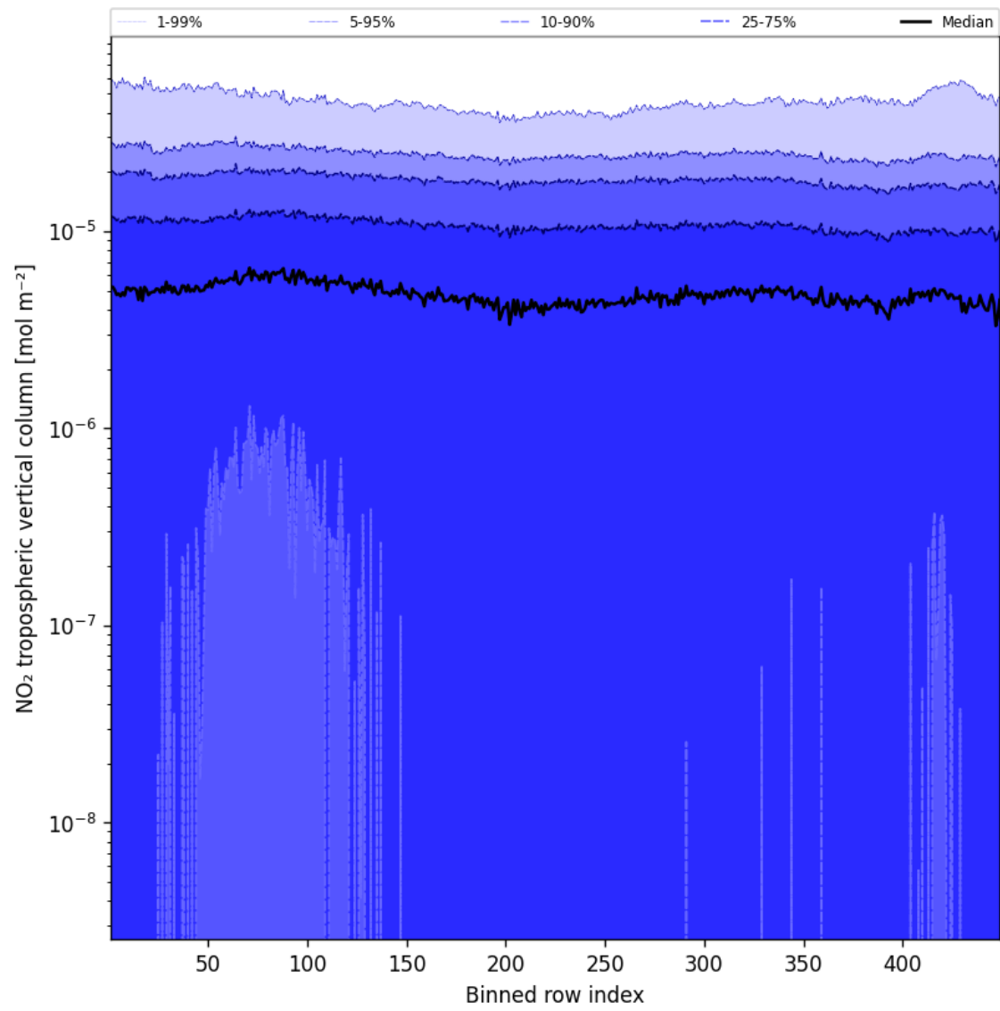
Figure 46: Along track statistics of “NO 2 tropospheric vertical column” for 2025-08-28 to 2025-08-30
