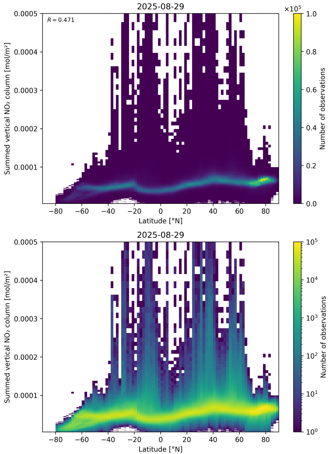
Figure 88: Scatter density plot of “Latitude” against “Summed vertical NO 2 column” for 2025-08-28 to 2025-08-30.
