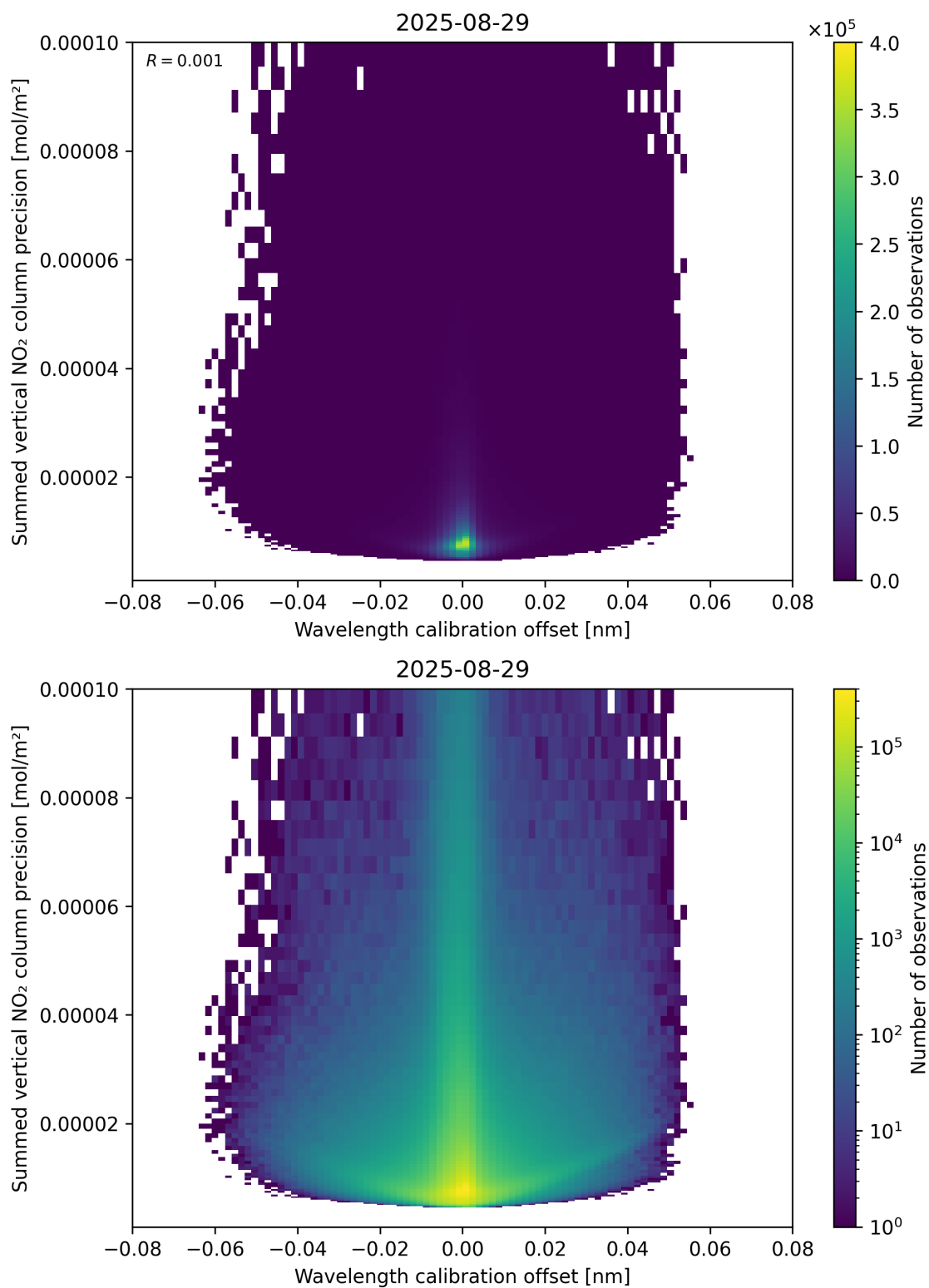
Figure 178: Scatter density plot of “Wavelength calibration offset” against “Summed vertical NO 2 column precision” for 2025-08-28 to 2025-08-30.
