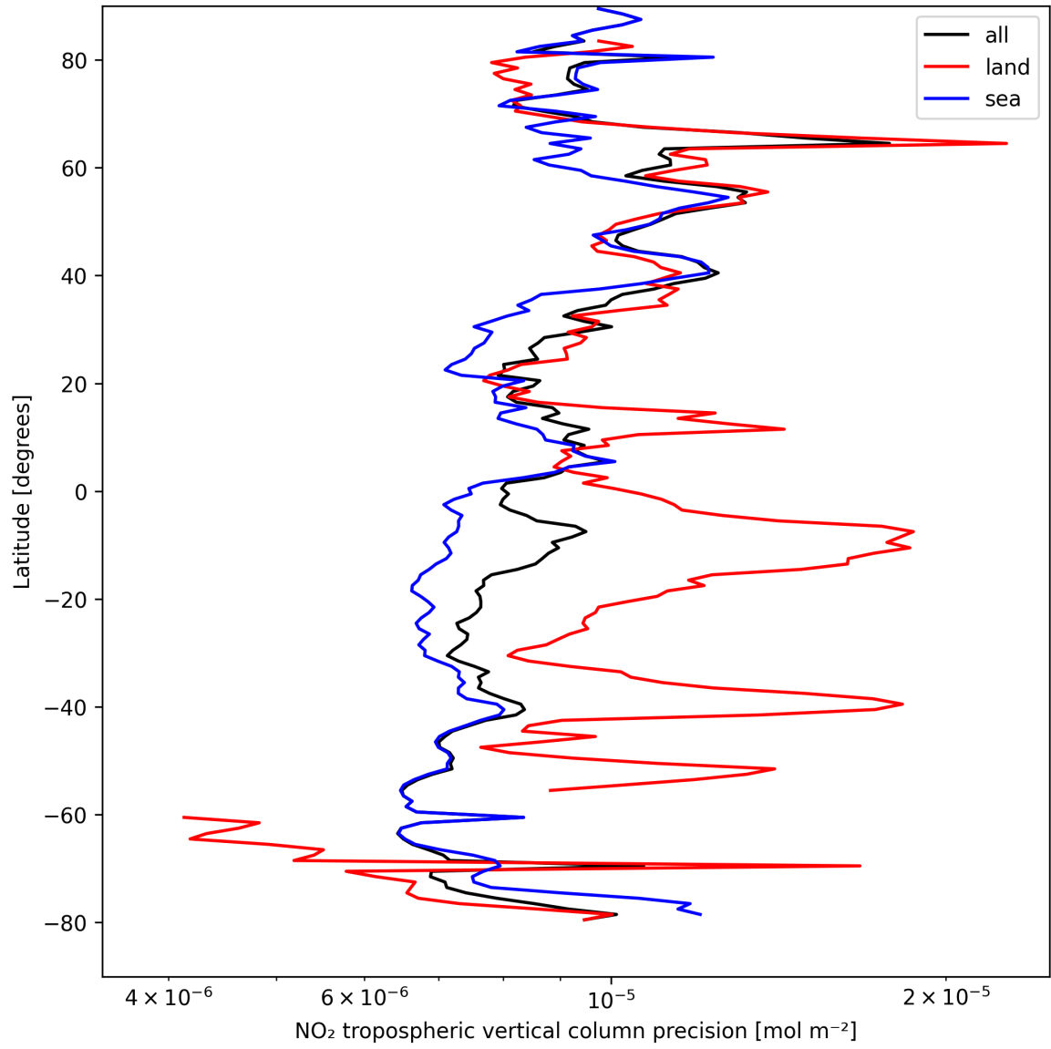
Figure 13: Zonal average of “NO 2 tropospheric vertical column precision” for 2025-08-28 to 2025-08-30.
