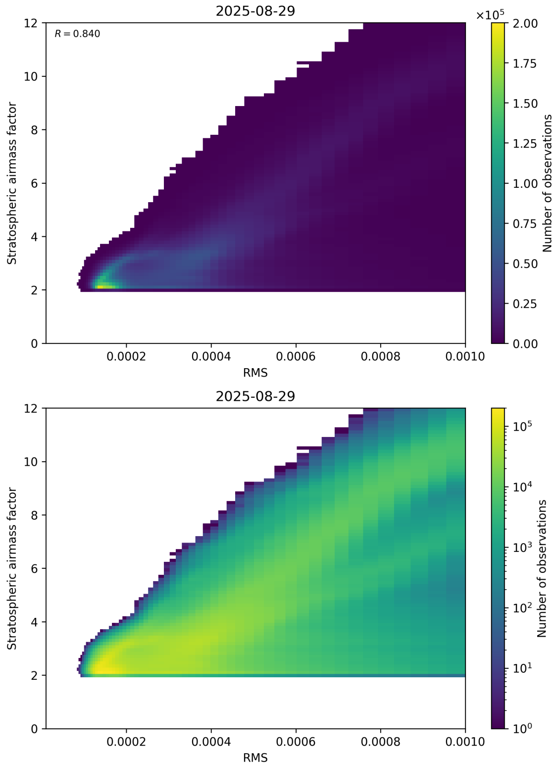
Figure 144: Scatter density plot of “RMS” against “Stratospheric airmass factor” for 2025-08-28 to 2025-08-30.
