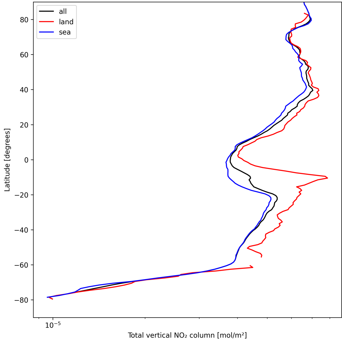
Figure 21: Zonal average of “Total vertical NO 2 column” for 2025-08-28 to 2025-08-30.
