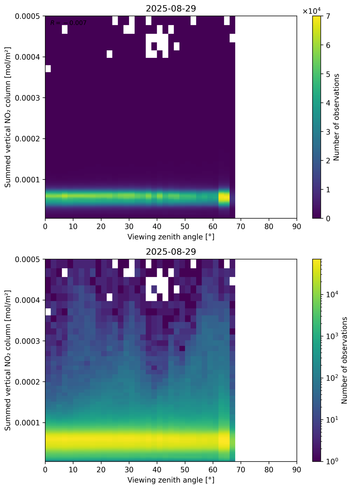
Figure 165: Scatter density plot of “Viewing zenith angle” against “Summed vertical NO 2 column” for 2025-08-28 to 2025-08-30.
