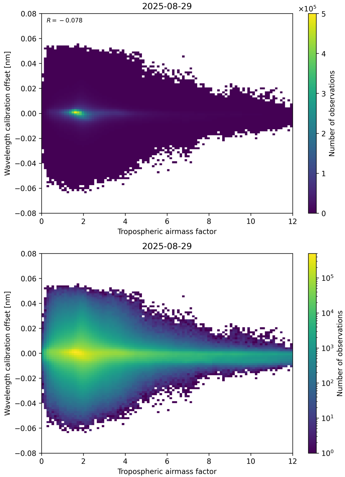
Figure 80: Scatter density plot of “Tropospheric airmass factor” against “Wavelength calibration offset” for 2025-08-28 to 2025-08-30.
