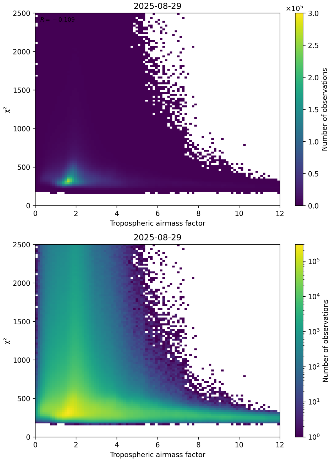
Figure 73: Scatter density plot of “Tropospheric airmass factor” against “ \chi^2 ” for 2025-08-28 to 2025-08-30.
