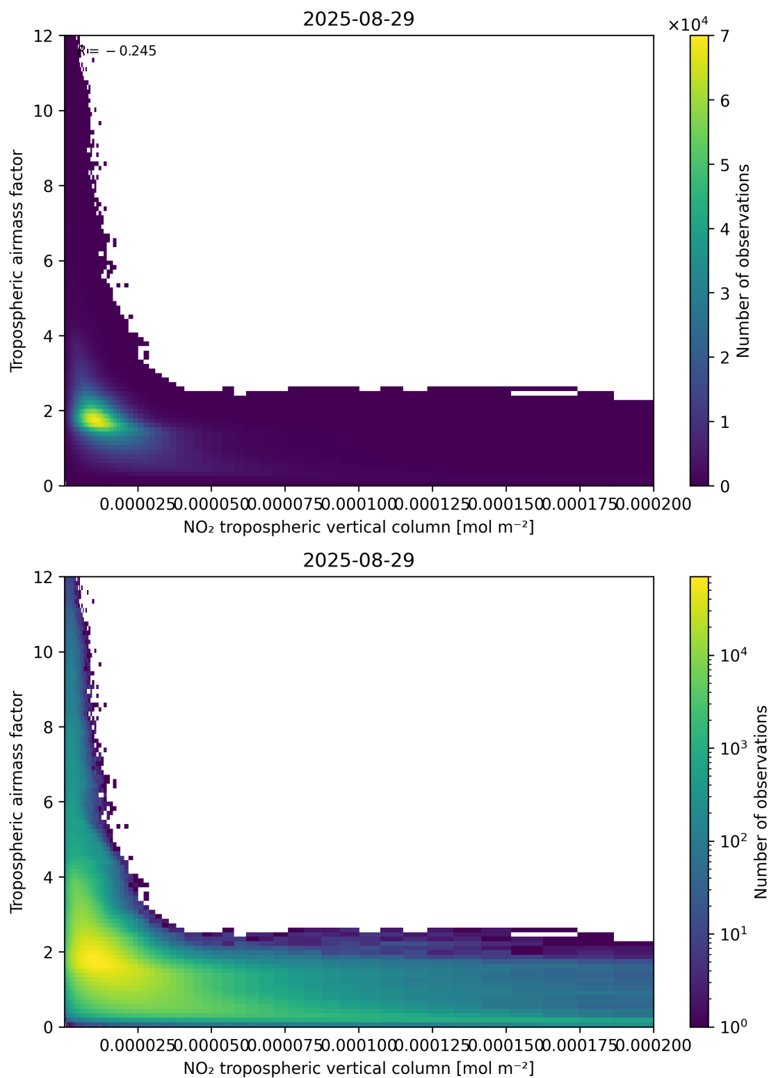
Figure 123: Scatter density plot of “NO 2 tropospheric vertical column” against “Tropospheric airmass factor” for 2025-08-28 to 2025-08-30.
