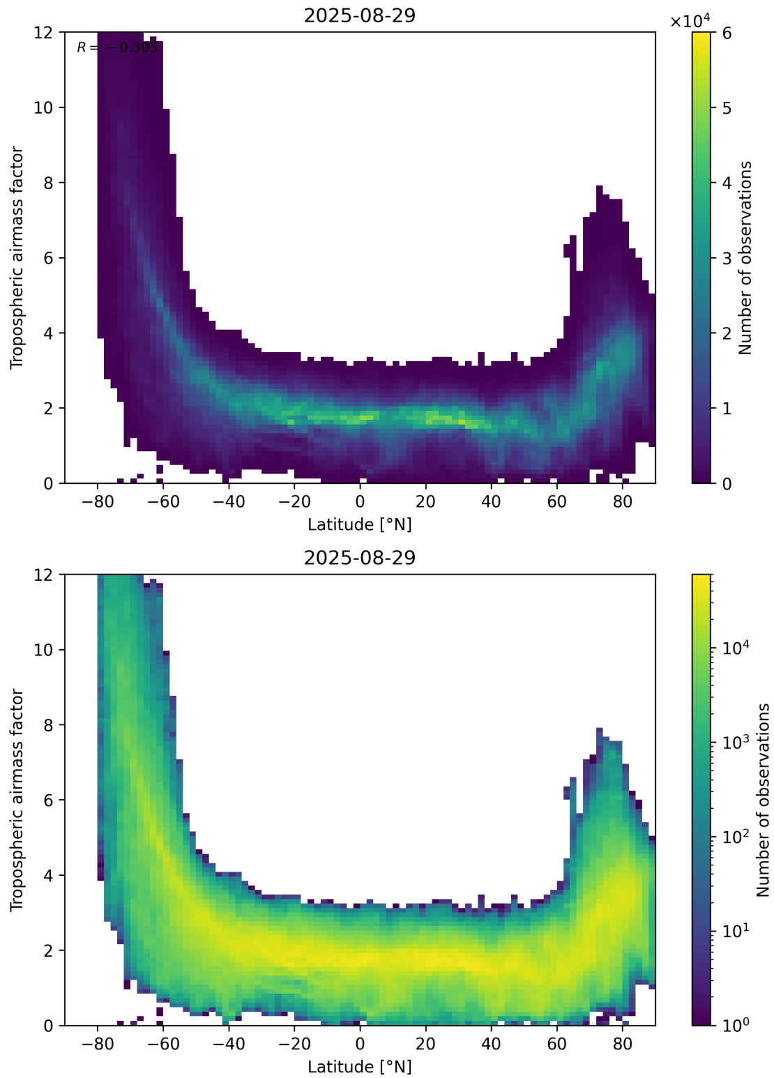
Figure 85: Scatter density plot of “Latitude” against “Tropospheric airmass factor” for 2025-08-28 to 2025-08-30.
