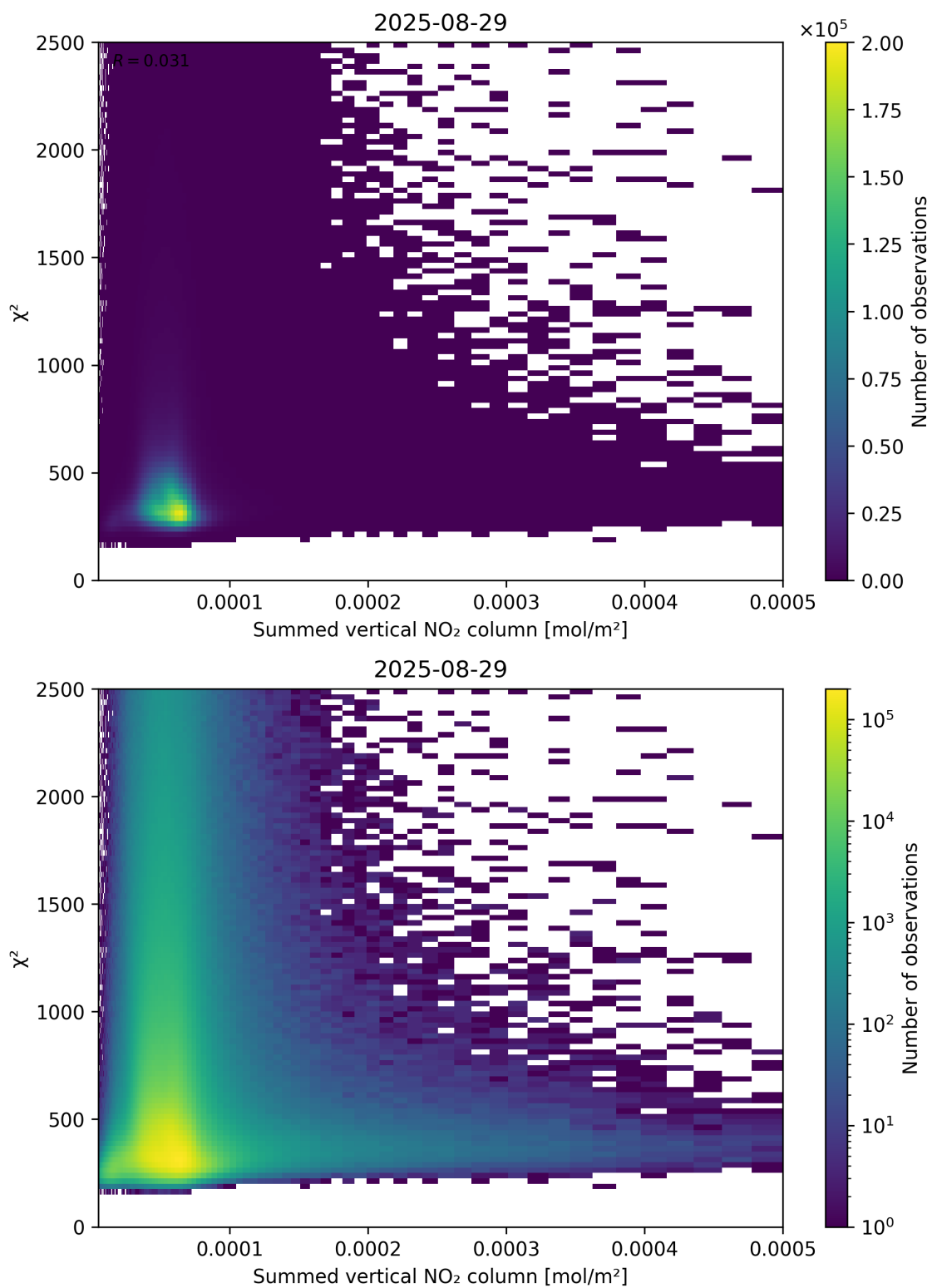
Figure 104: Scatter density plot of “Summed vertical NO 2 column” against “ \chi^2 ” for 2025-08-28 to 2025-08-30.
