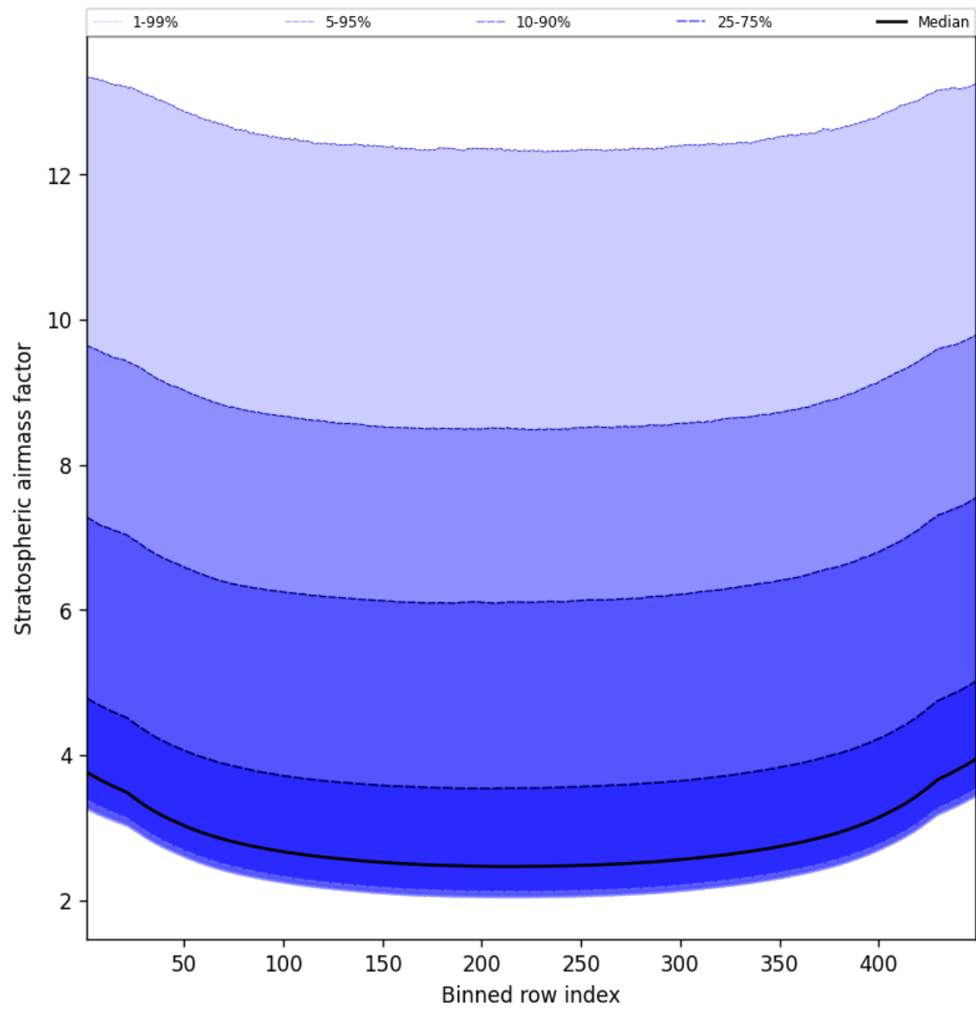
Figure 61: Along track statistics of “Stratospheric airmass factor” for 2025-08-28 to 2025-08-30
