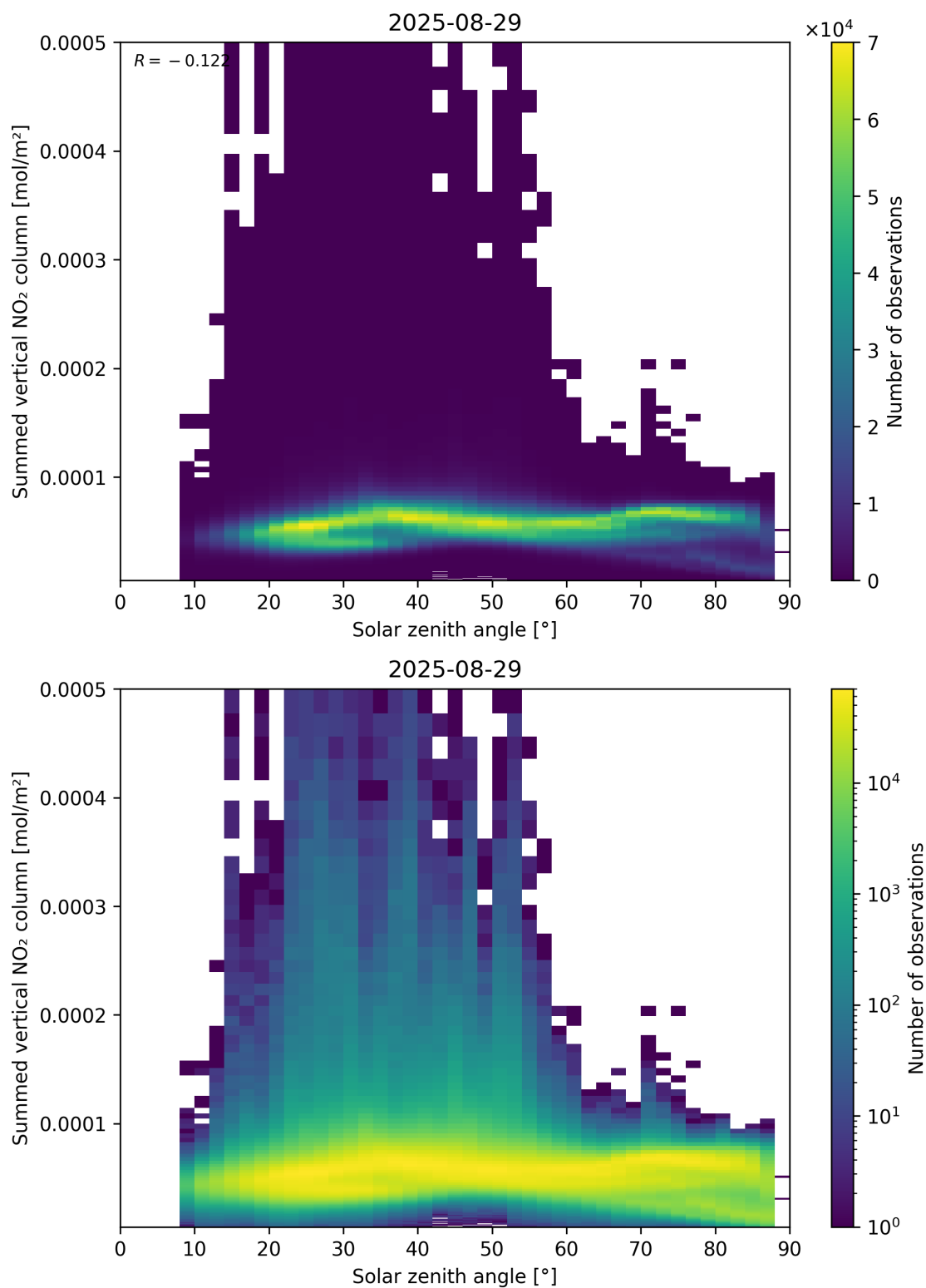
Figure 151: Scatter density plot of “Solar zenith angle” against “Summed vertical NO 2 column” for 2025-08-28 to 2025-08-30.
