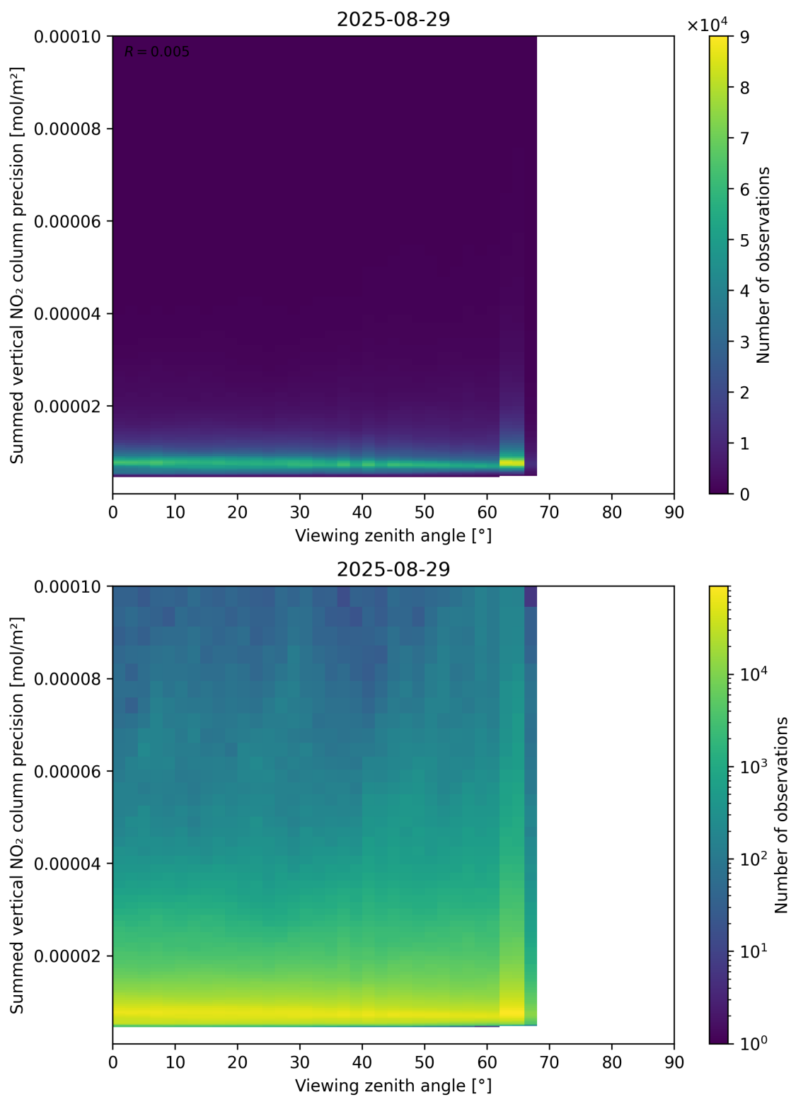
Figure 166: Scatter density plot of “Viewing zenith angle” against “Summed vertical NO 2 column precision” for 2025-08-28 to 2025-08-30.
