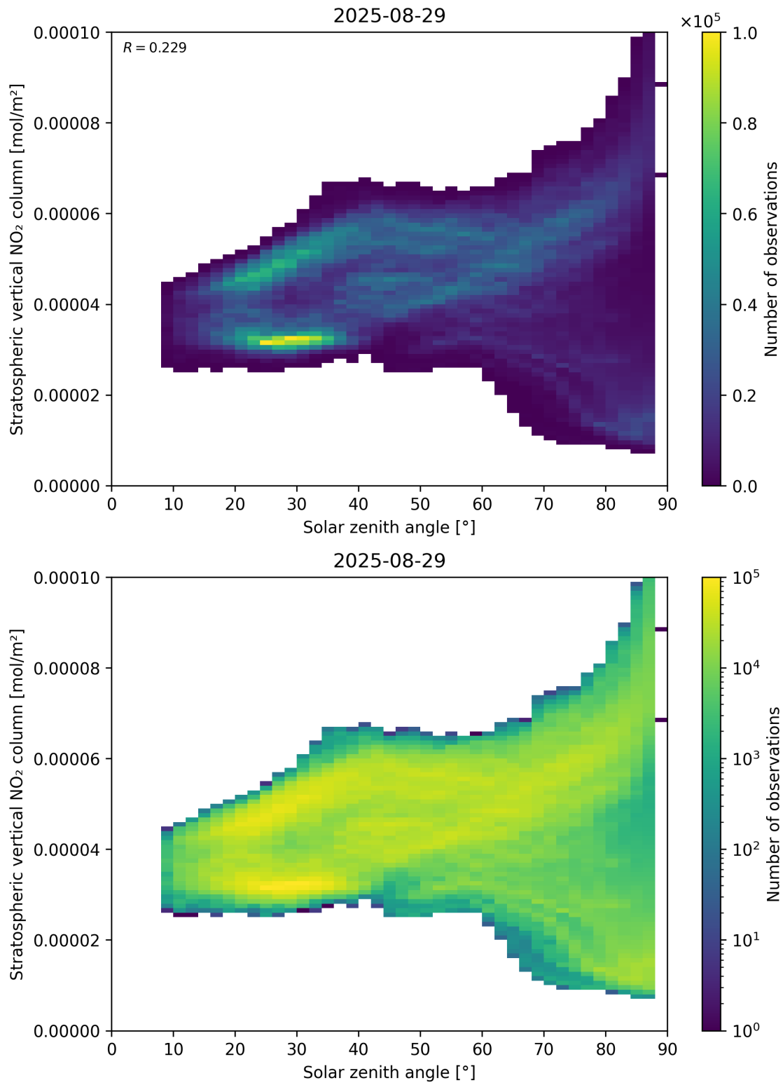
Figure 150: Scatter density plot of “Solar zenith angle” against “Stratospheric vertical NO 2 column” for 2025-08-28 to 2025-08-30.
