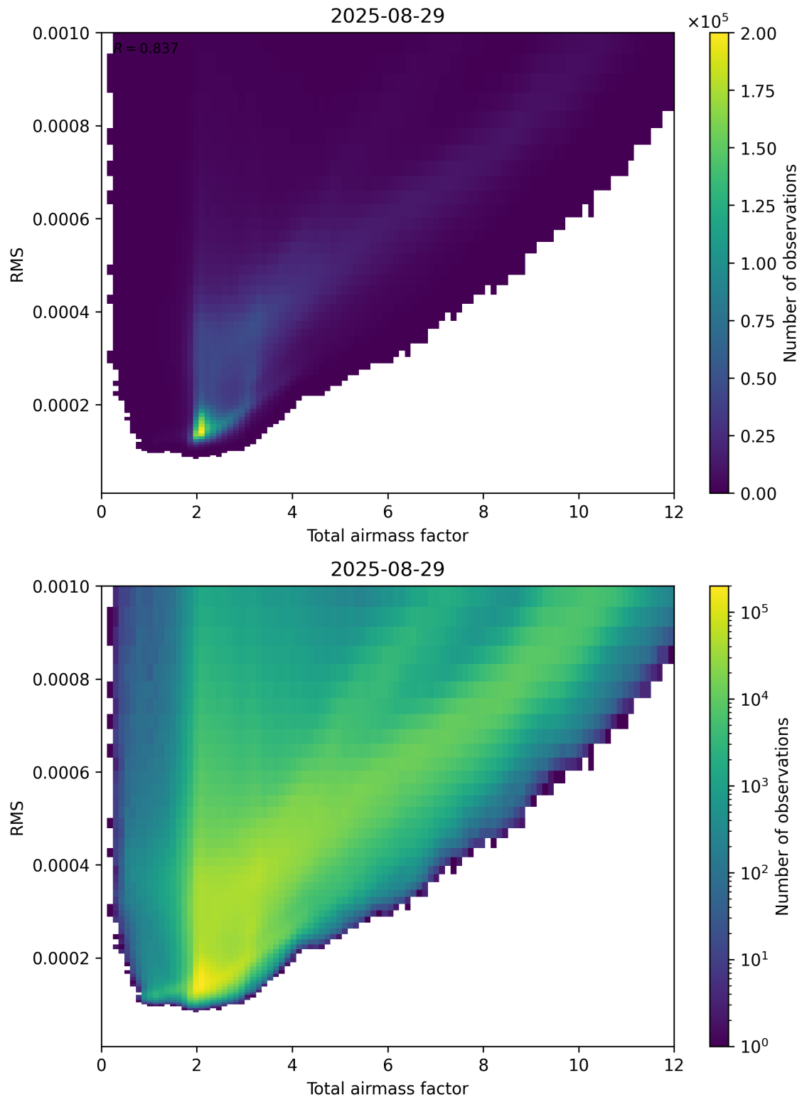
Figure 69: Scatter density plot of “Total airmass factor” against “RMS” for 2025-08-28 to 2025-08-30.
