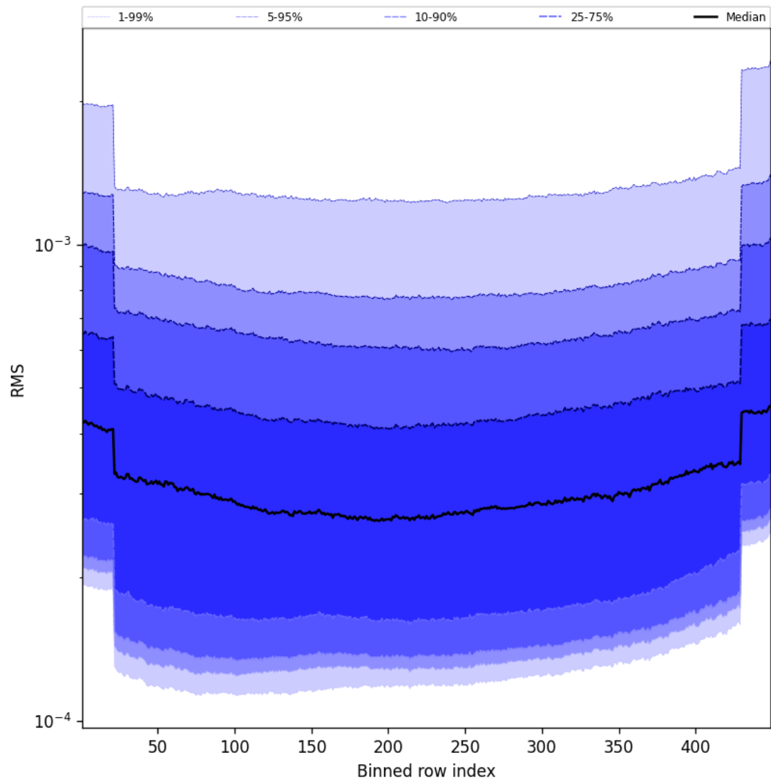
Figure 60: Along track statistics of “RMS” for 2025-08-28 to 2025-08-30
