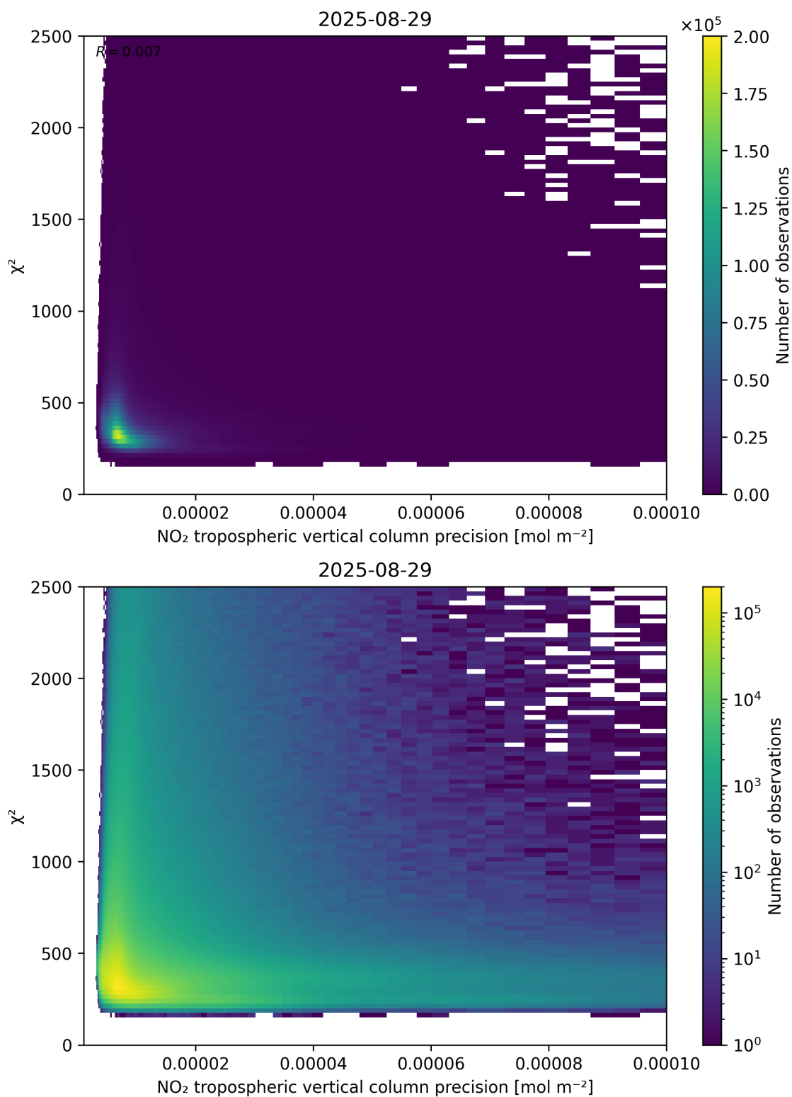
Figure 134: Scatter density plot of “NO 2 tropospheric vertical column precision” against “ \chi^2 ” for 2025-08-28 to 2025-08-30.
