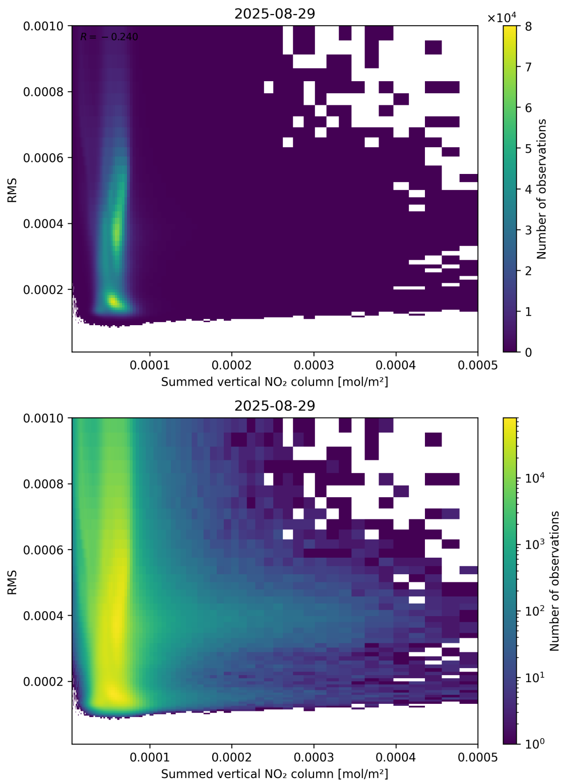
Figure 109: Scatter density plot of “Summed vertical NO 2 column” against “RMS” for 2025-08-28 to 2025-08-30.
