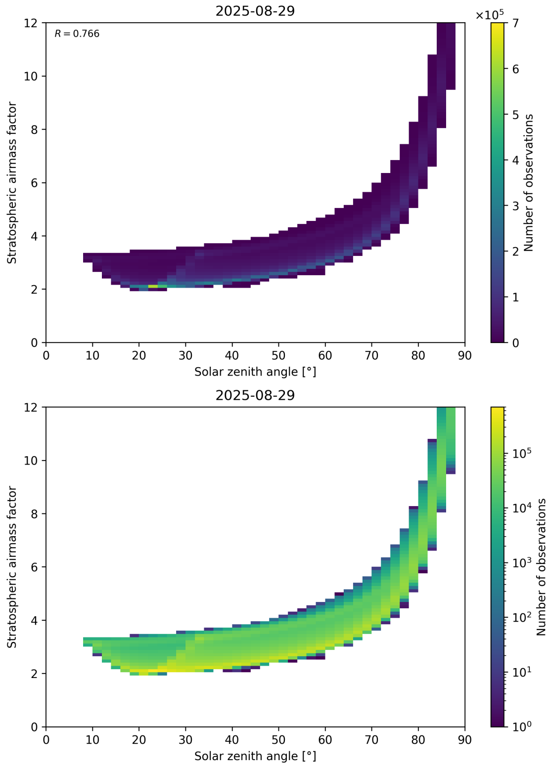
Figure 145: Scatter density plot of “Solar zenith angle” against “Stratospheric airmass factor” for 2025-08-28 to 2025-08-30.
