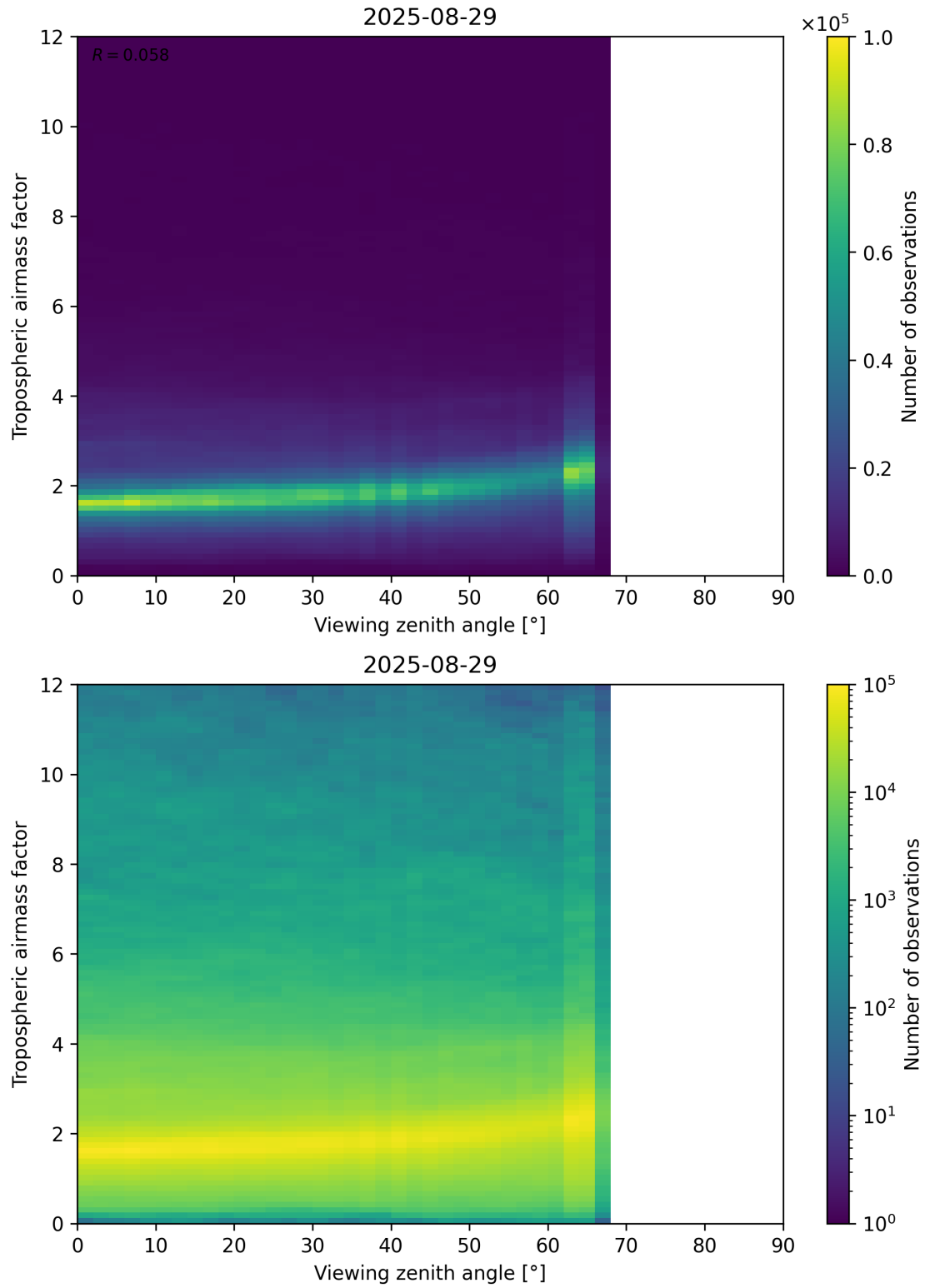
Figure 161: Scatter density plot of “Viewing zenith angle” against “Tropospheric airmass factor” for 2025-08-28 to 2025-08-30.
