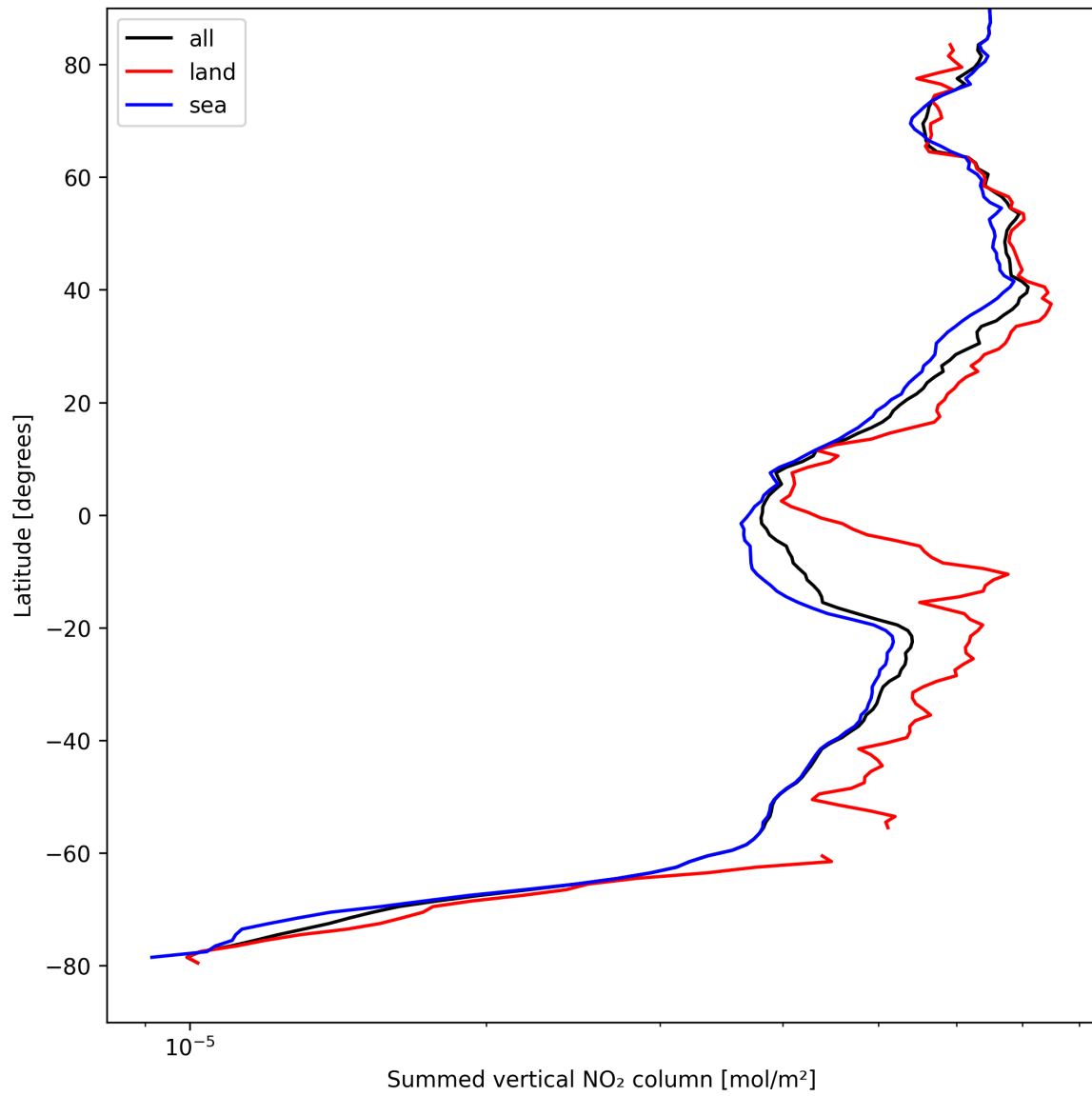
Figure 23: Zonal average of “Summed vertical NO 2 column” for 2025-08-28 to 2025-08-30.
