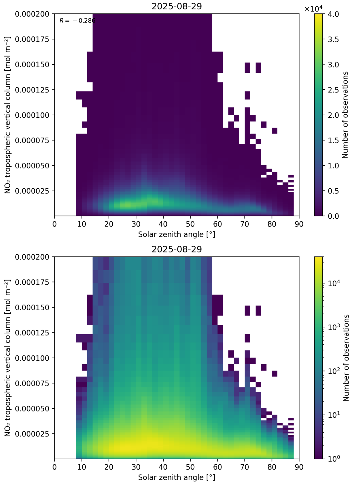
Figure 155: Scatter density plot of “Solar zenith angle” against “NO 2 tropospheric vertical column” for 2025-08-28 to 2025-08-30.
