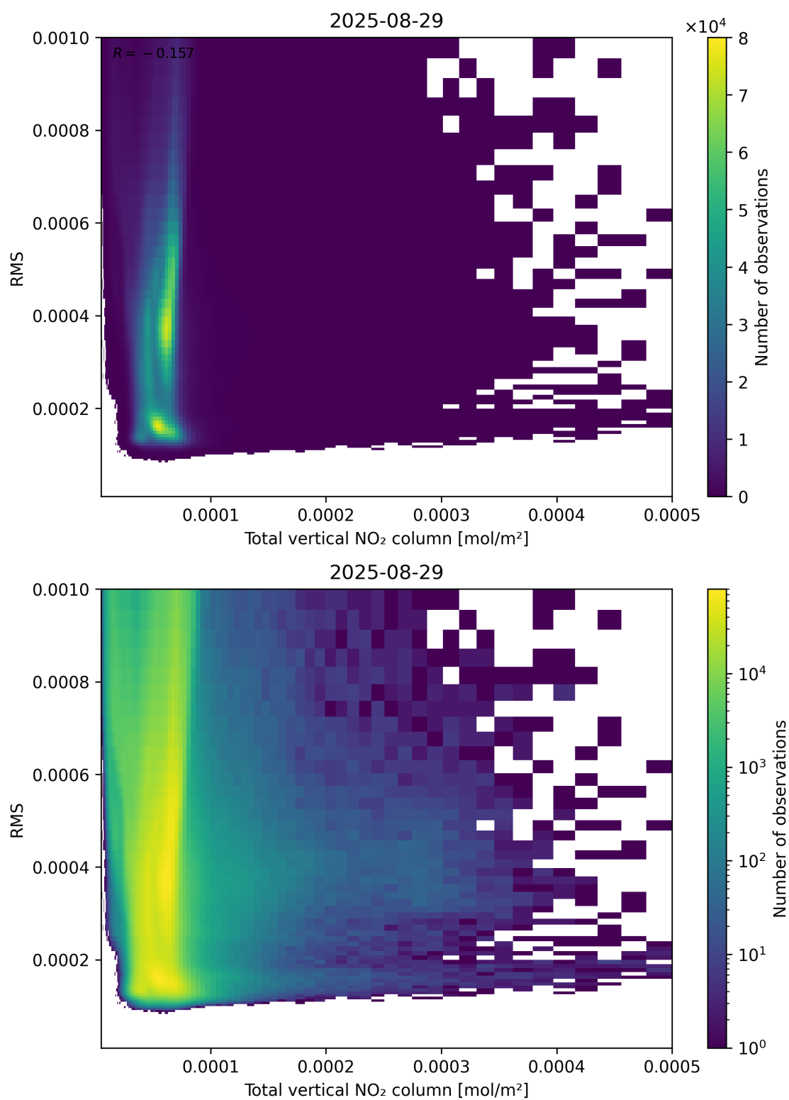
Figure 120: Scatter density plot of “Total vertical NO 2 column” against “RMS” for 2025-08-28 to 2025-08-30.
