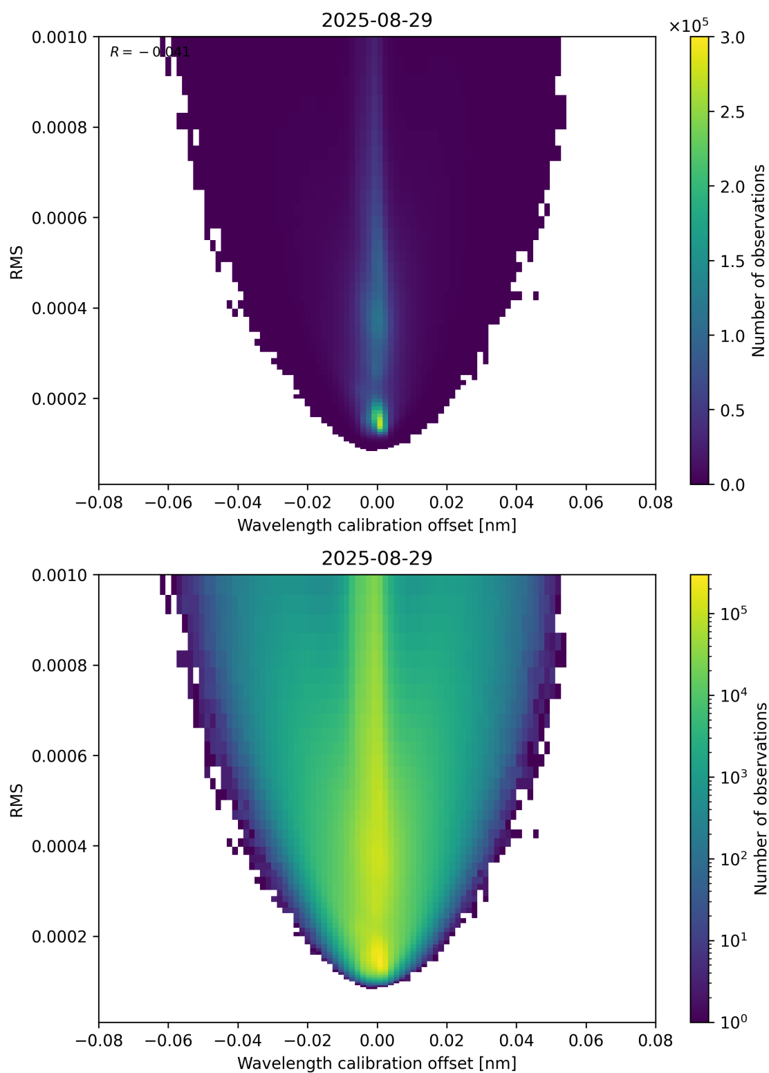
Figure 181: Scatter density plot of “Wavelength calibration offset” against “RMS” for 2025-08-28 to 2025-08-30.
