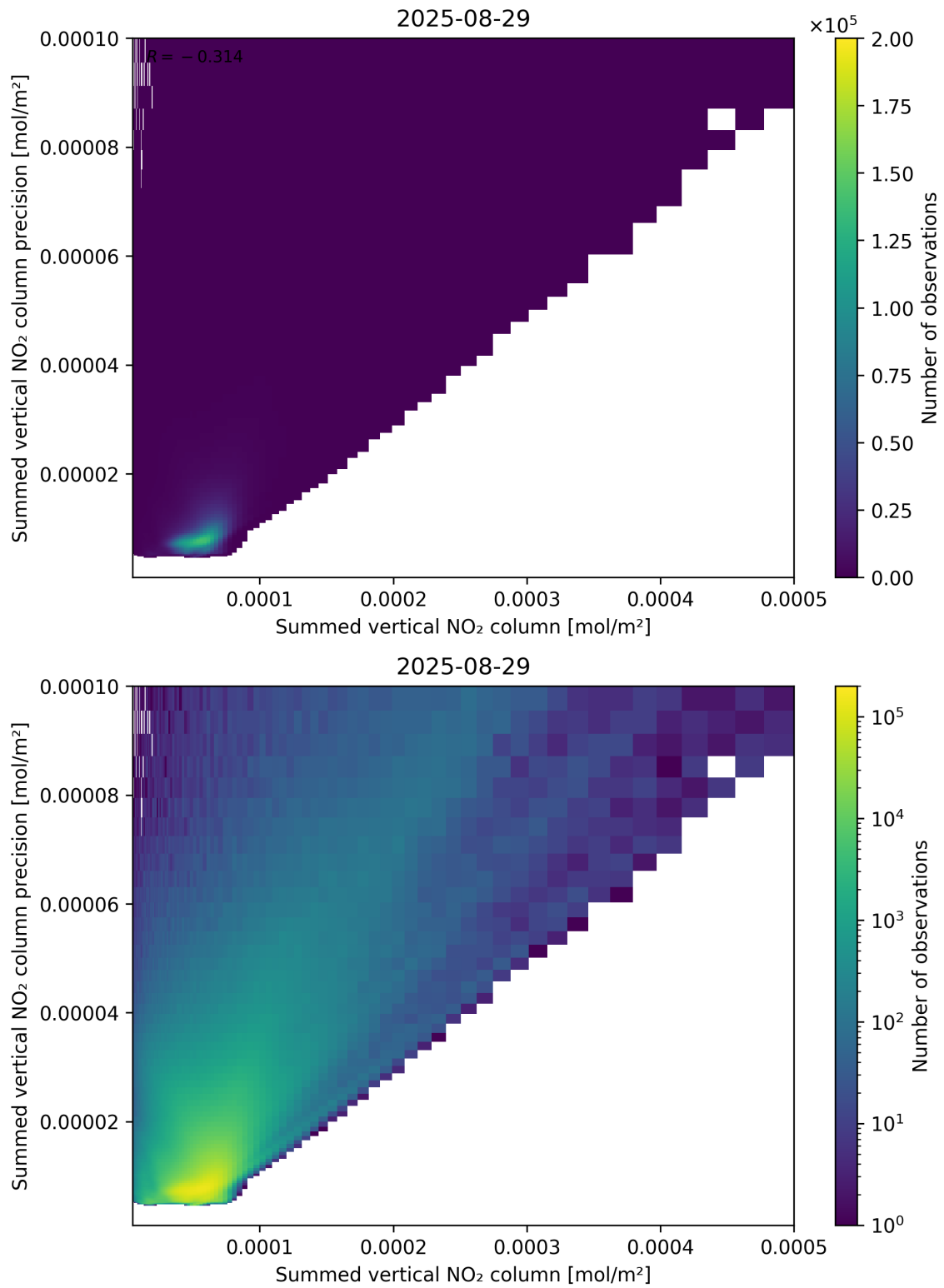
Figure 105: Scatter density plot of “Summed vertical NO 2 column” against “Summed vertical NO 2 column precision” for 2025-08-28 to 2025-08-30.
