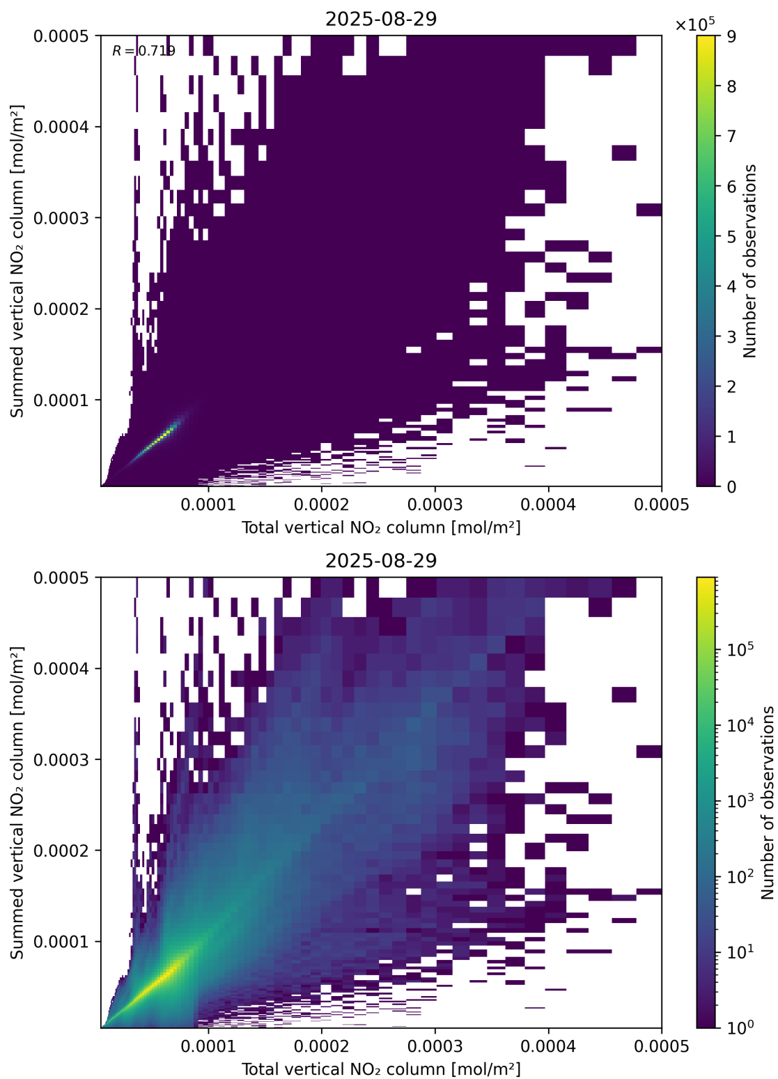
Figure 112: Scatter density plot of “Total vertical NO 2 column” against “Summed vertical NO 2 column” for 2025-08-28 to 2025-08-30.
