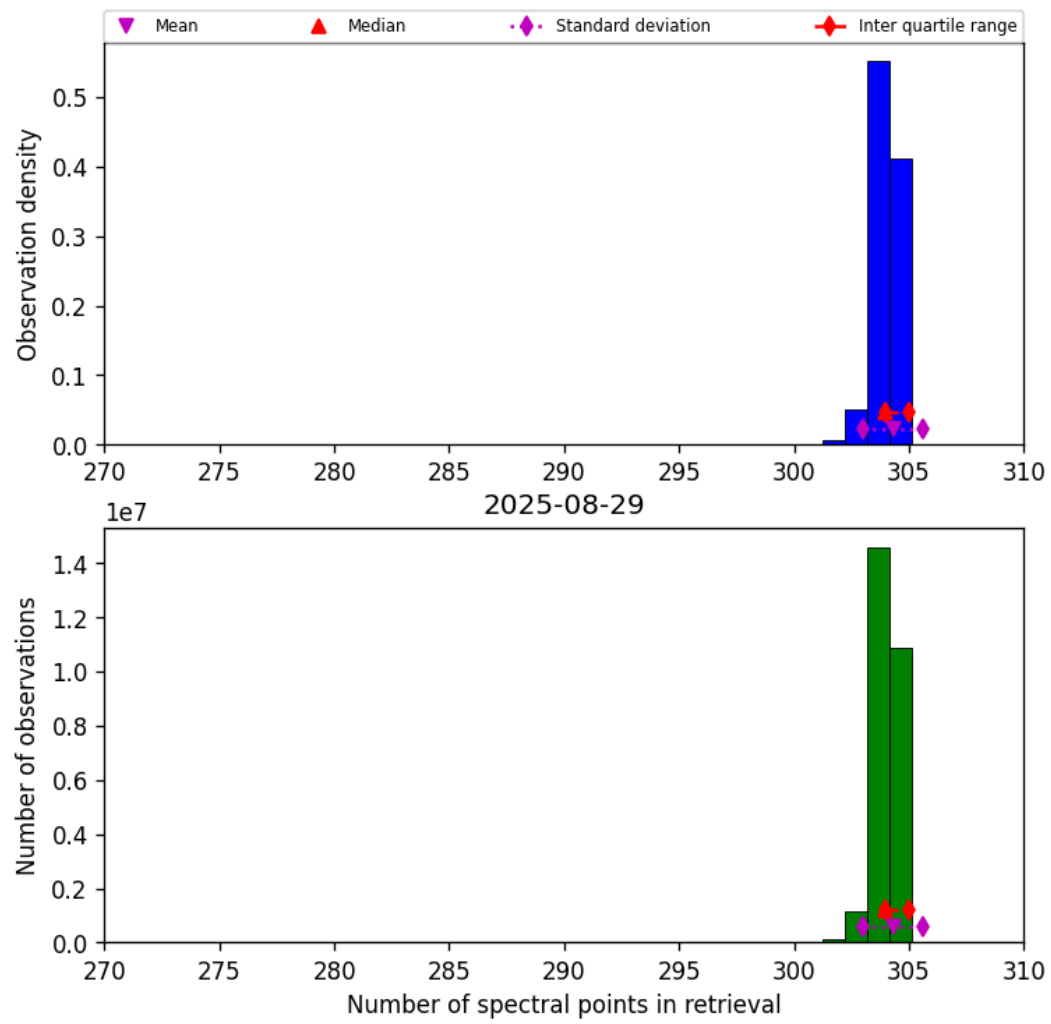
Figure 33: Histogram of “Number of spectral points in retrieval” for 2025-08-28 to 2025-08-30
