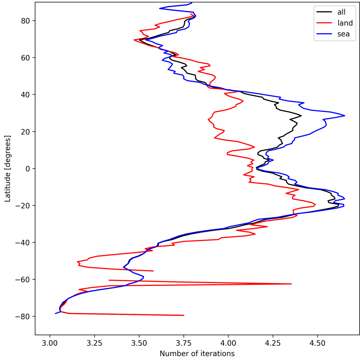
Figure 17: Zonal average of “Number of iterations” for 2025-08-28 to 2025-08-30.
