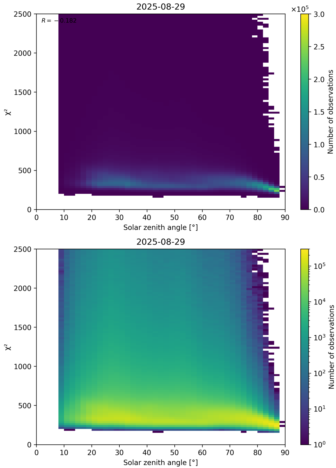
Figure 148: Scatter density plot of “Solar zenith angle” against “ \chi^2 ” for 2025-08-28 to 2025-08-30.
