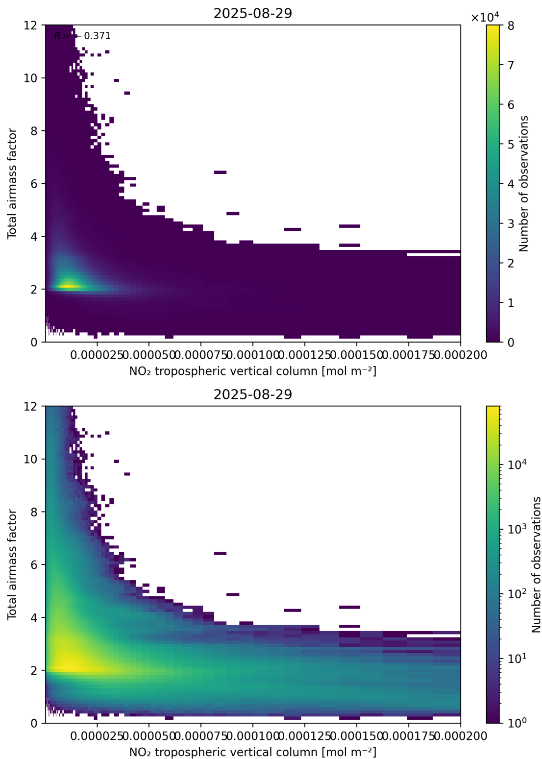
Figure 122: Scatter density plot of “NO 2 tropospheric vertical column” against “Total air mass factor” for 2025-08-28 to 2025-08-30.
