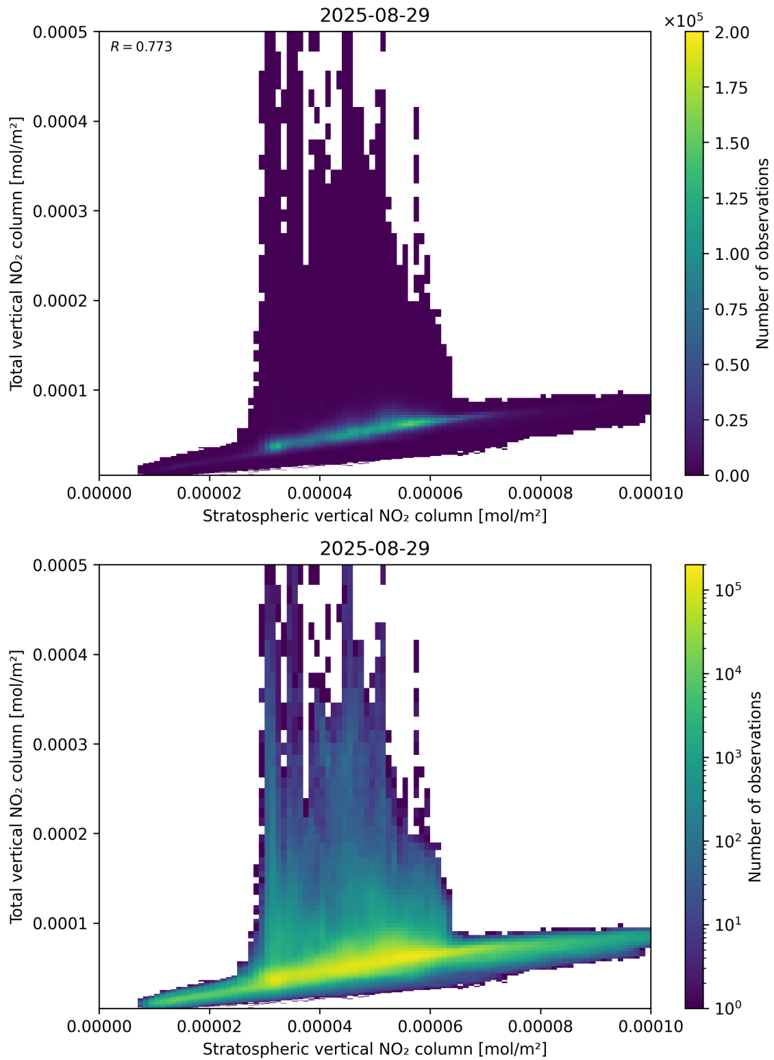
Figure 100: Scatter density plot of “Stratospheric vertical NO 2 column” against “Total vertical NO 2 column” for 2025-08-28 to 2025-08-30.
