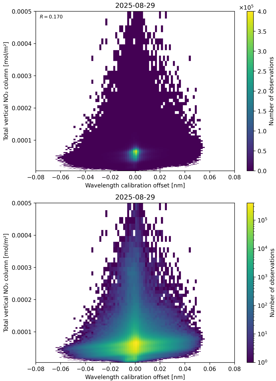
Figure 179: Scatter density plot of “Wavelength calibration offset” against “Total vertical NO 2 column” for 2025-08-28 to 2025-08-30.
