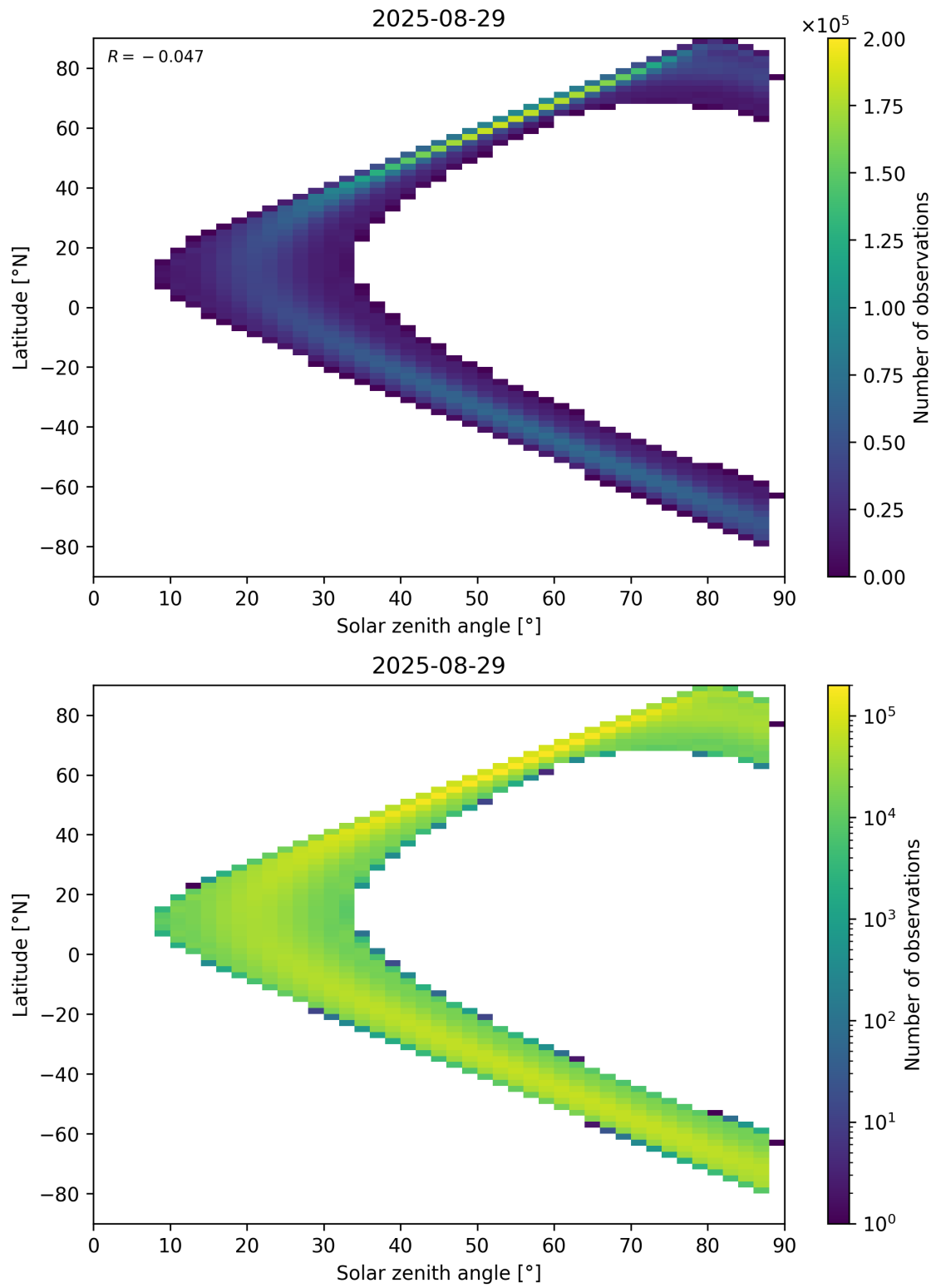
Figure 149: Scatter density plot of “Solar zenith angle” against “Latitude” for 2025-08-28 to 2025-08-30.
