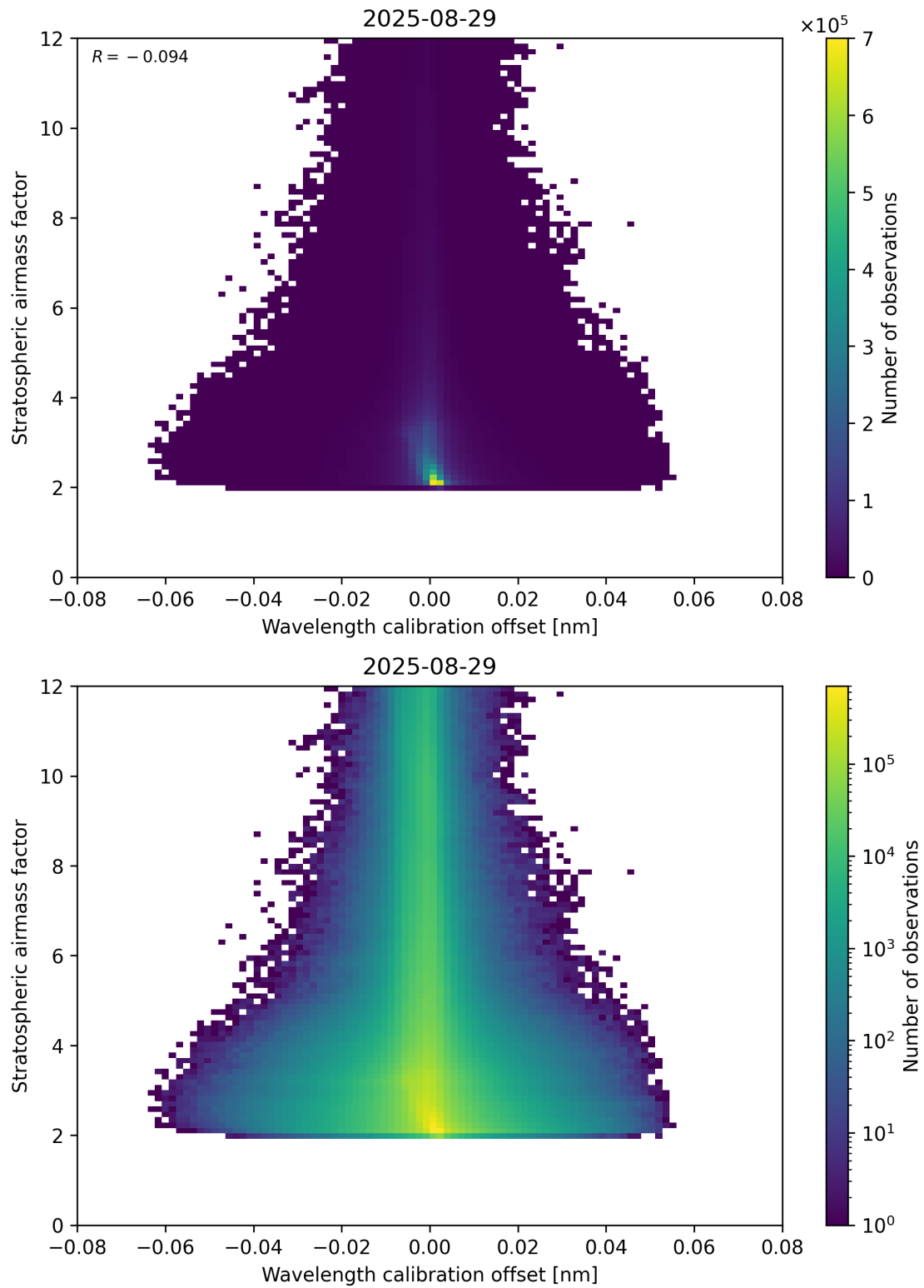
Figure 174: Scatter density plot of “Wavelength calibration offset” against “Stratospheric airmass factor” for 2025-08-28 to 2025-08-30.
