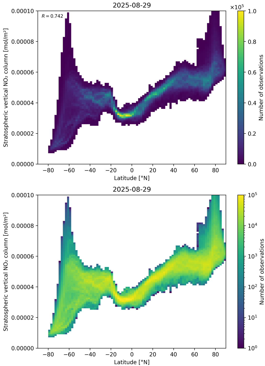
Figure 87: Scatter density plot of “Latitude” against “Stratospheric vertical NO 2 column” for 2025-08-28 to 2025-08-30.
