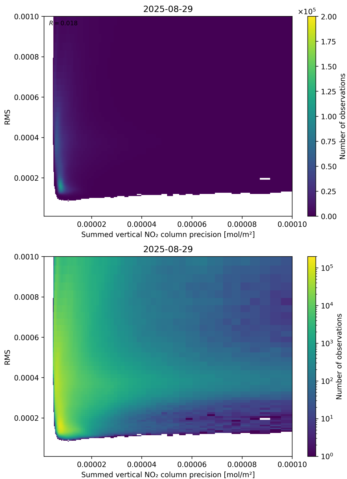
Figure 108: Scatter density plot of “Summed vertical NO 2 column precision” against “RMS” for 2025-08-28 to 2025-08-30.
