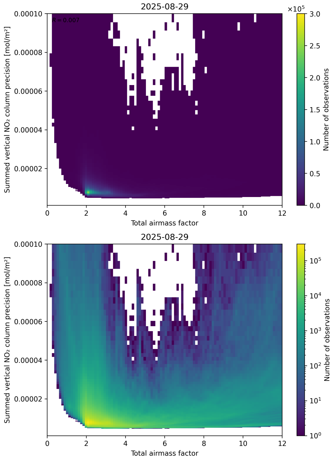
Figure 66: Scatter density plot of “Total airmass factor” against “Summed vertical NO 2 column precision” for 2025-08-28 to 2025-08-30.
