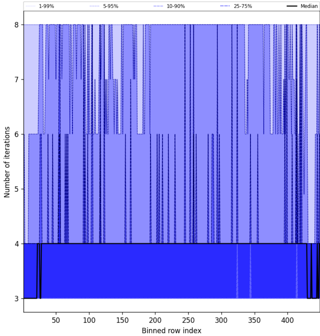
Figure 51: Along track statistics of “Number of iterations” for 2025-08-28 to 2025-08-30
