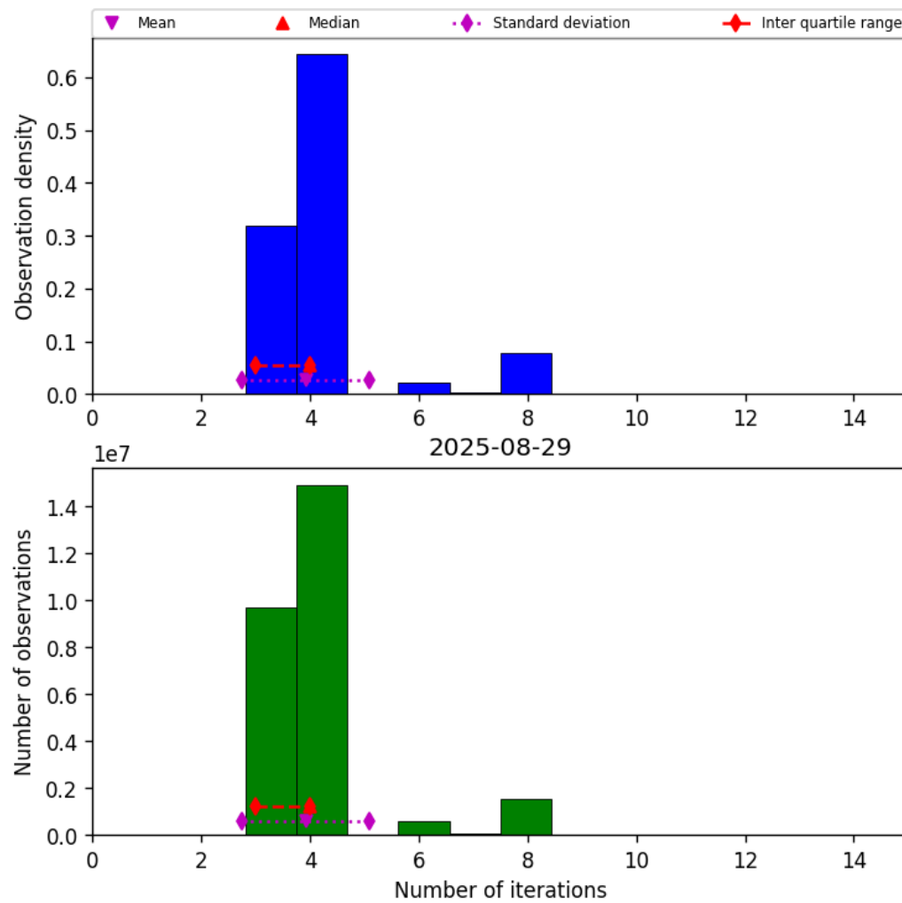
Figure 34: Histogram of “Number of iterations” for 2025-08-28 to 2025-08-30
