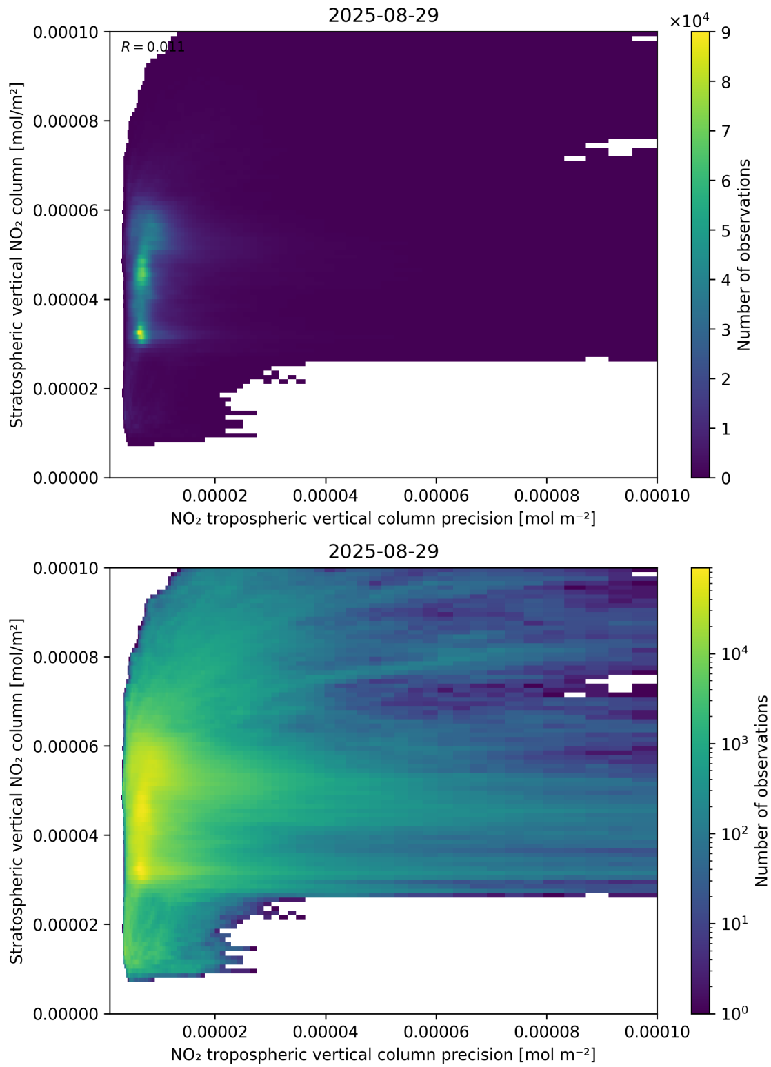
Figure 135: Scatter density plot of “NO 2 tropospheric vertical column precision” against “Stratospheric vertical NO 2 column” for 2025-08-28 to 2025-08-30.
