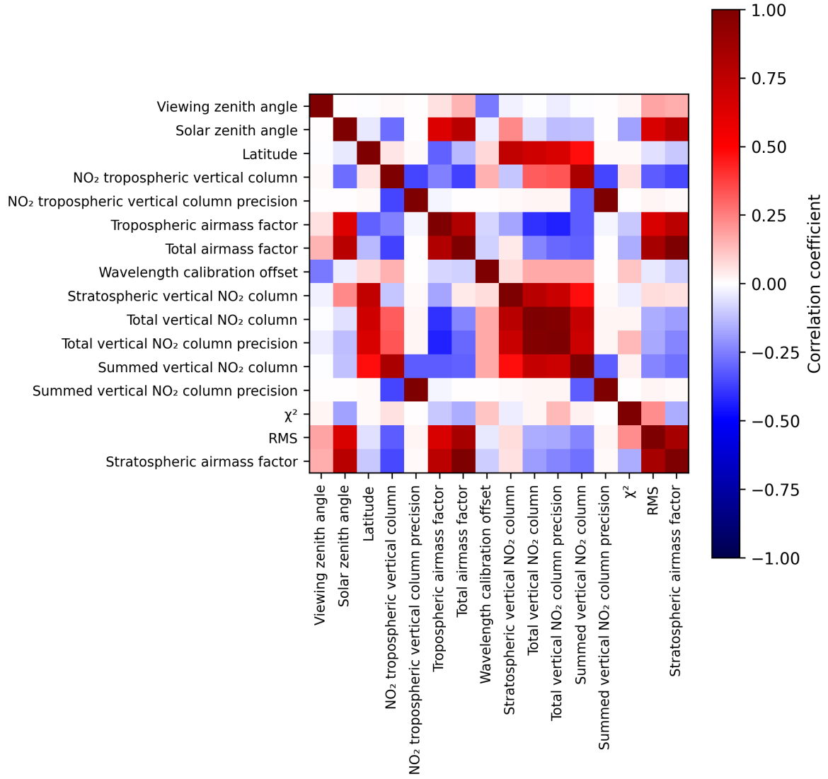
Figure 2: Map of correlation matrix for 2025-08-28 to 2025-08-30.
