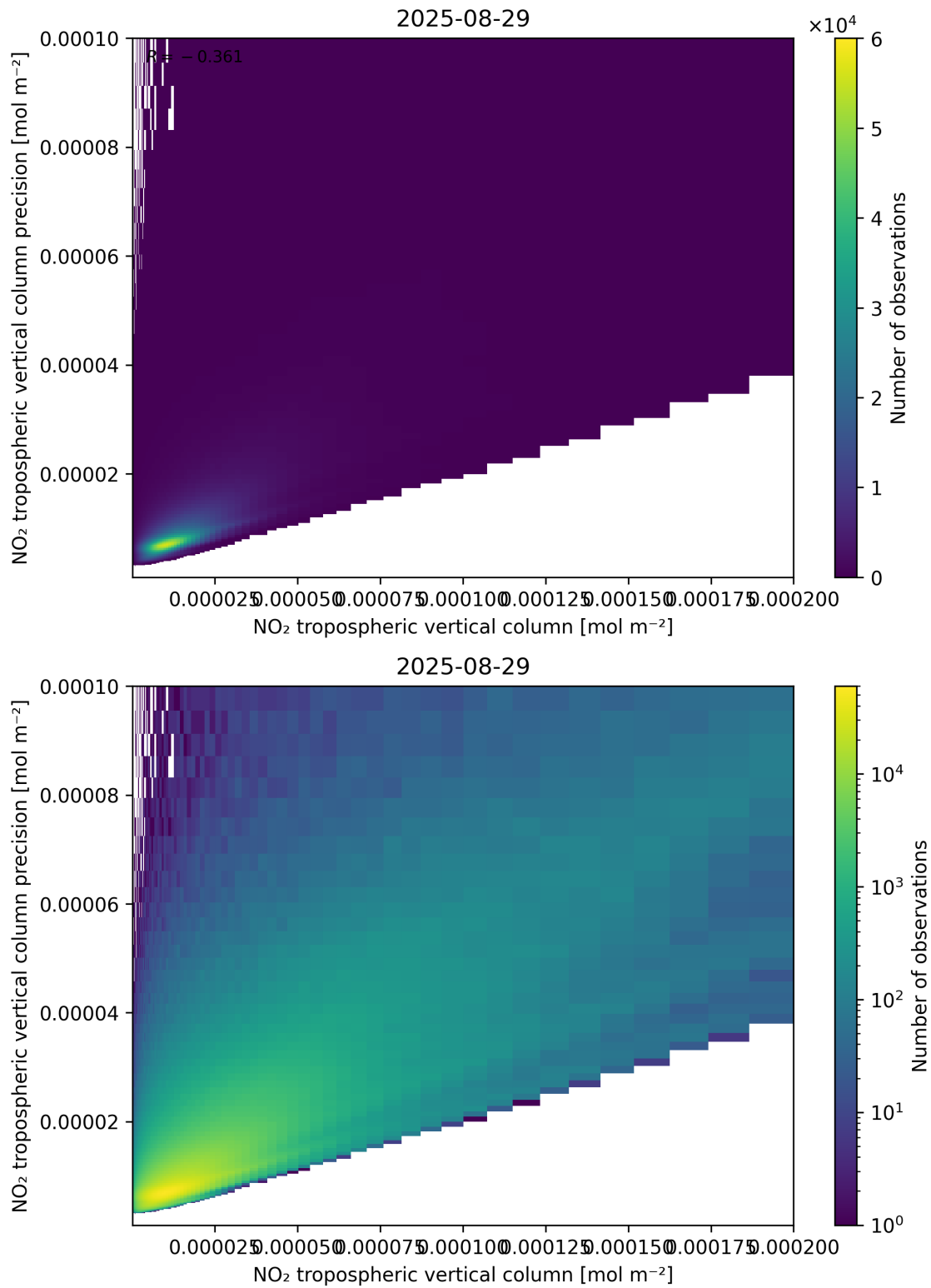
Figure 130: Scatter density plot of “NO 2 tropospheric vertical column” against “NO 2 tropospheric vertical column precision” for 2025-08-28 to 2025-08-30.
