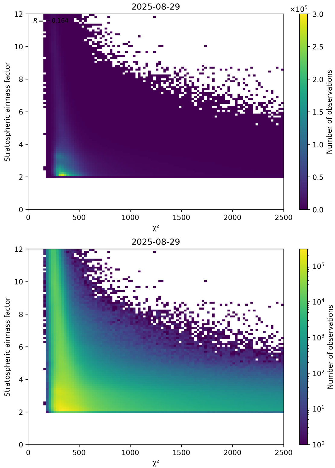
Figure 81: Scatter density plot of “ \chi^2 ” against “Stratospheric airmass factor” for 2025-08-28 to 2025-08-30.
