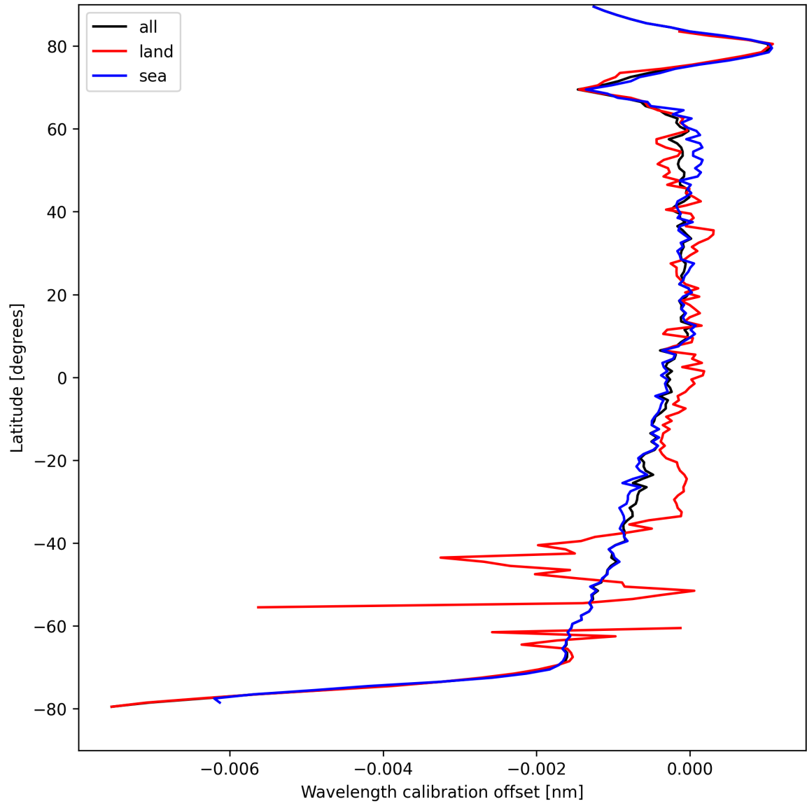
Figure 18: Zonal average of “Wavelength calibration offset” for 2025-08-28 to 2025-08-30.
