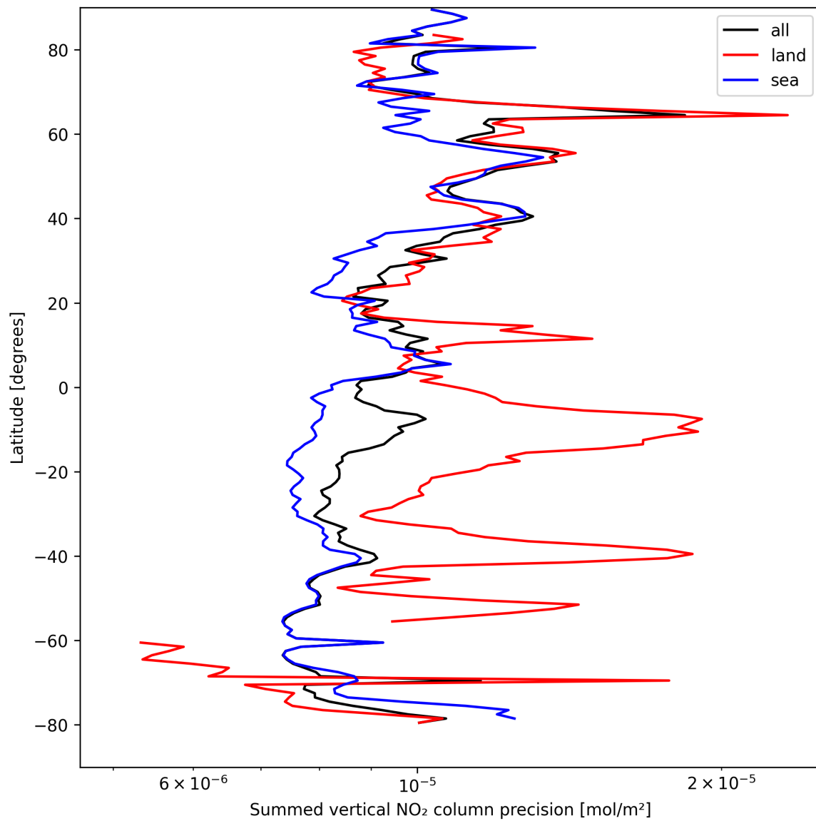
Figure 24: Zonal average of “Summed vertical NO 2 column precision” for 2025-08-28 to 2025-08-30.
