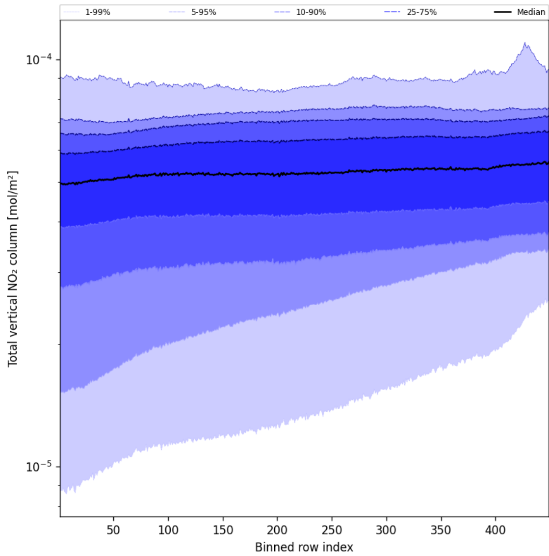
Figure 55: Along track statistics of “Total vertical NO 2 column” for 2025-08-28 to 2025-08-30
