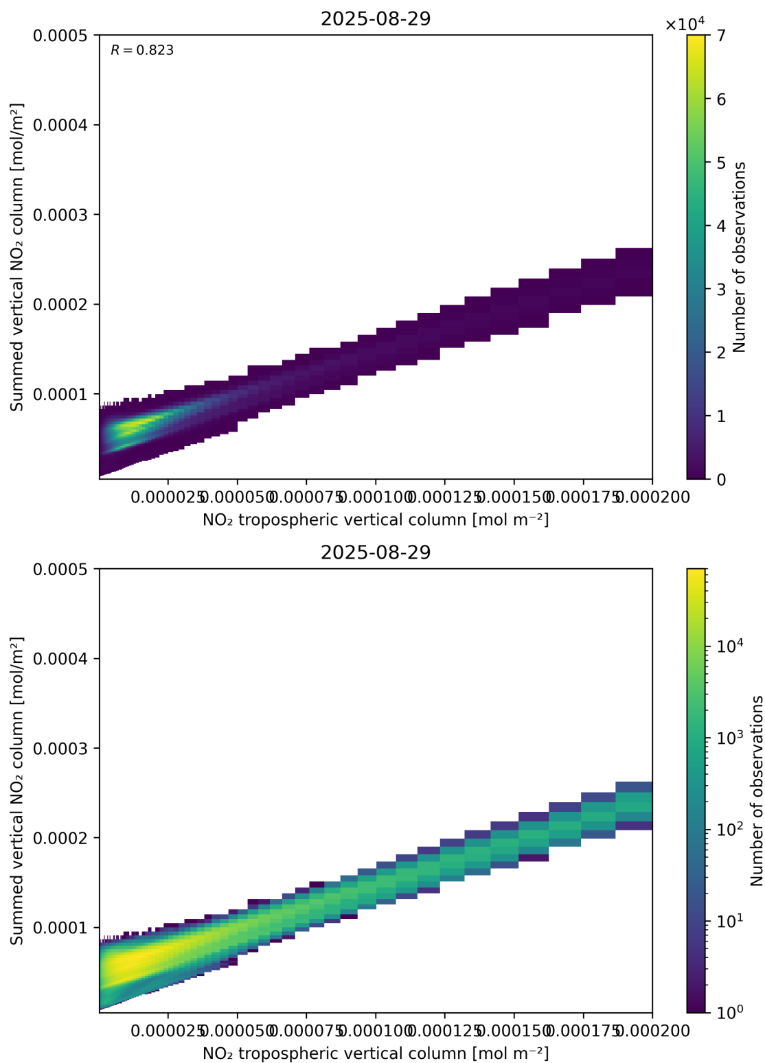
Figure 126: Scatter density plot of “NO 2 tropospheric vertical column” against “Summed vertical NO 2 column” for 2025-08-28 to 2025-08-30.
