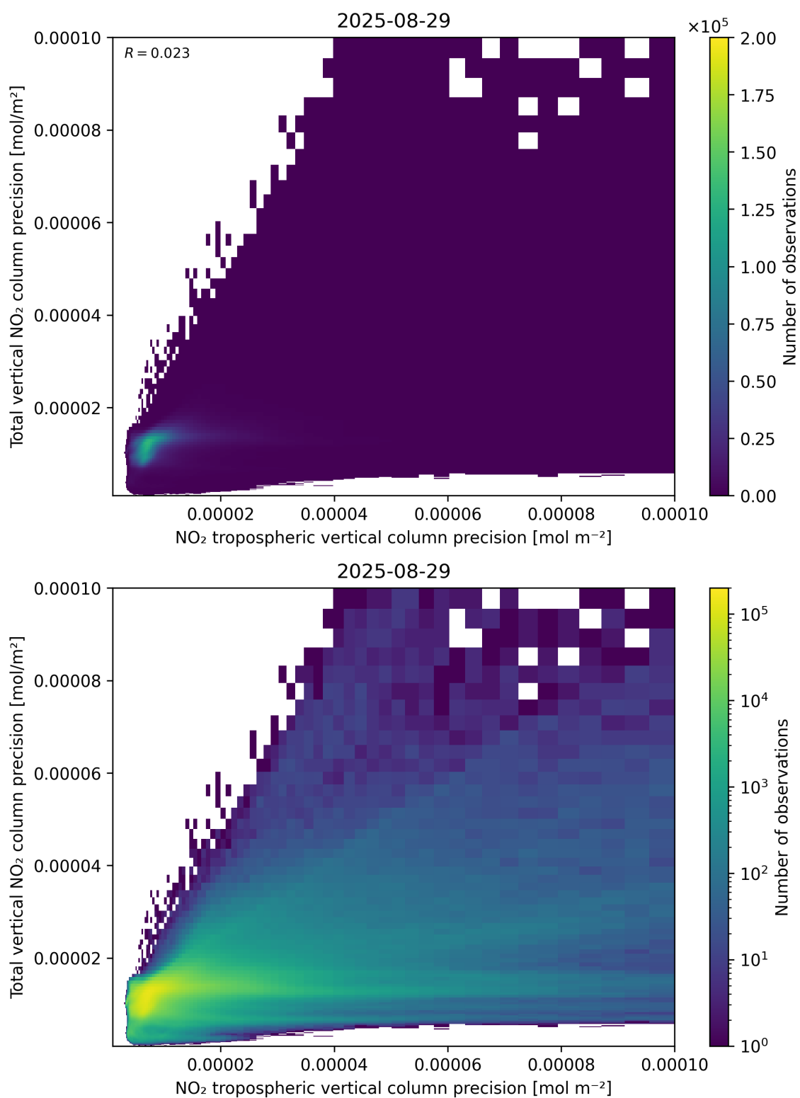
Figure 139: Scatter density plot of “NO 2 tropospheric vertical column precision” against “Total vertical NO 2 column precision” for 2025-08-28 to 2025-08-30.
