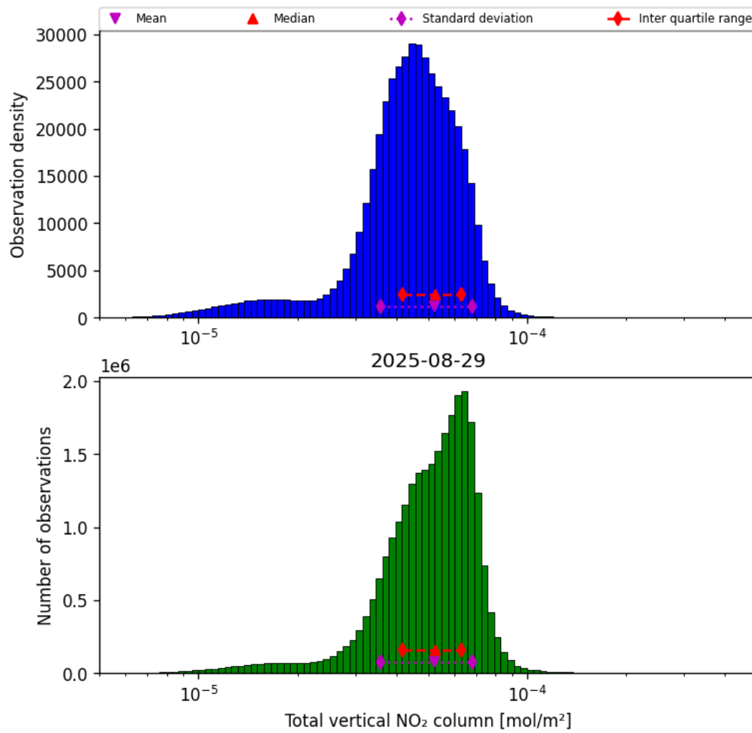
Figure 38: Histogram of “Total vertical NO 2 column” for 2025-08-28 to 2025-08-30
