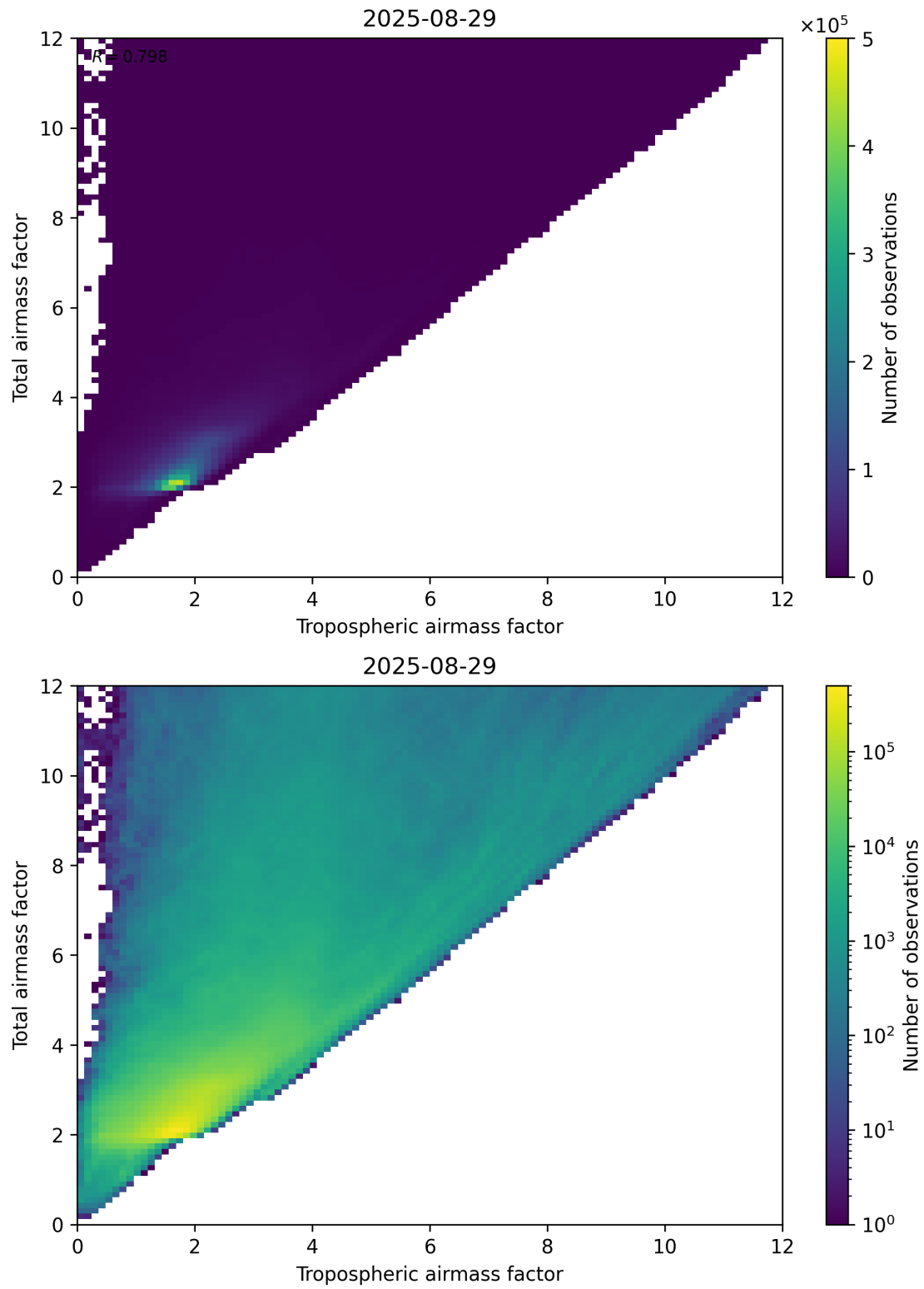
Figure 72: Scatter density plot of “Tropospheric airmass factor” against “Total airmass factor” for 2025-08-28 to 2025-08-30.
