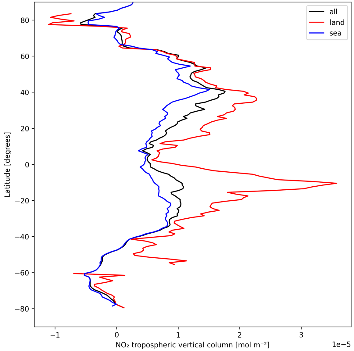
Figure 12: Zonal average of “NO 2 tropospheric vertical column” for 2025-08-28 to 2025-08-30.
