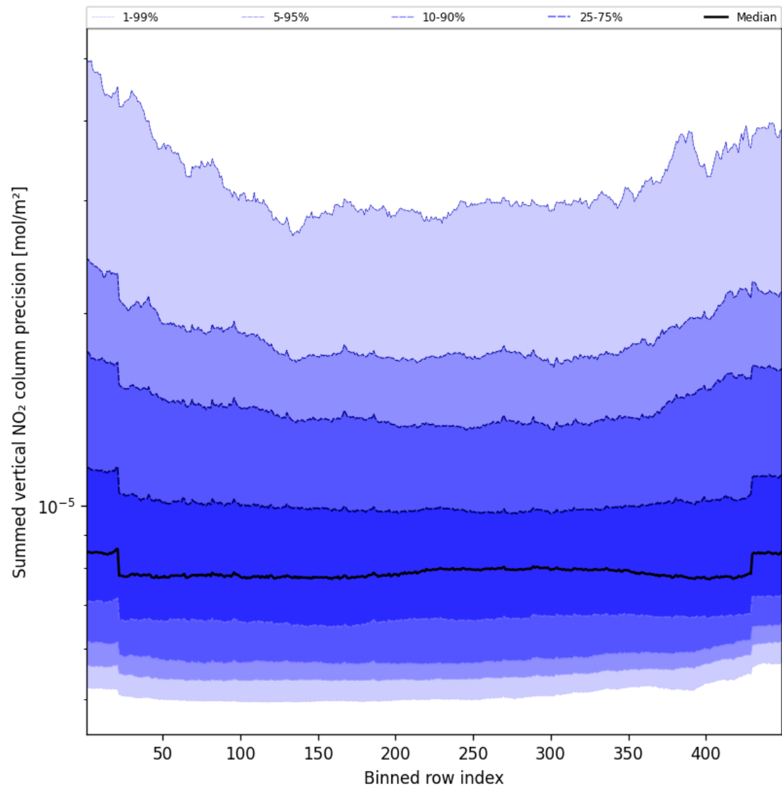
Figure 58: Along track statistics of “Summed vertical NO 2 column precision” for 2025-08-28 to 2025-08-30
