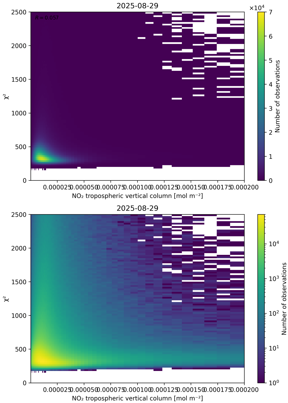
Figure 124: Scatter density plot of “NO 2 tropospheric vertical column” against “ \chi^2 ” for 2025-08-28 to 2025-08-30.
