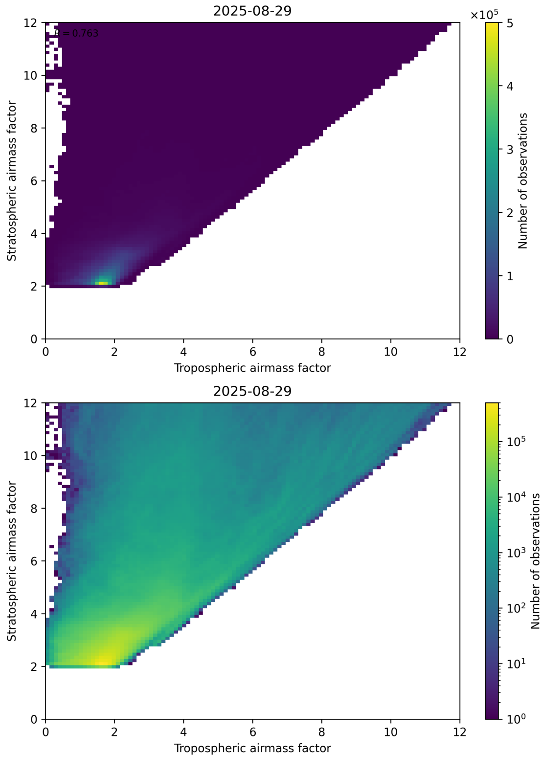
Figure 71: Scatter density plot of “Tropospheric airmass factor” against “Stratospheric airmass factor” for 2025-08-28 to 2025-08-30.
