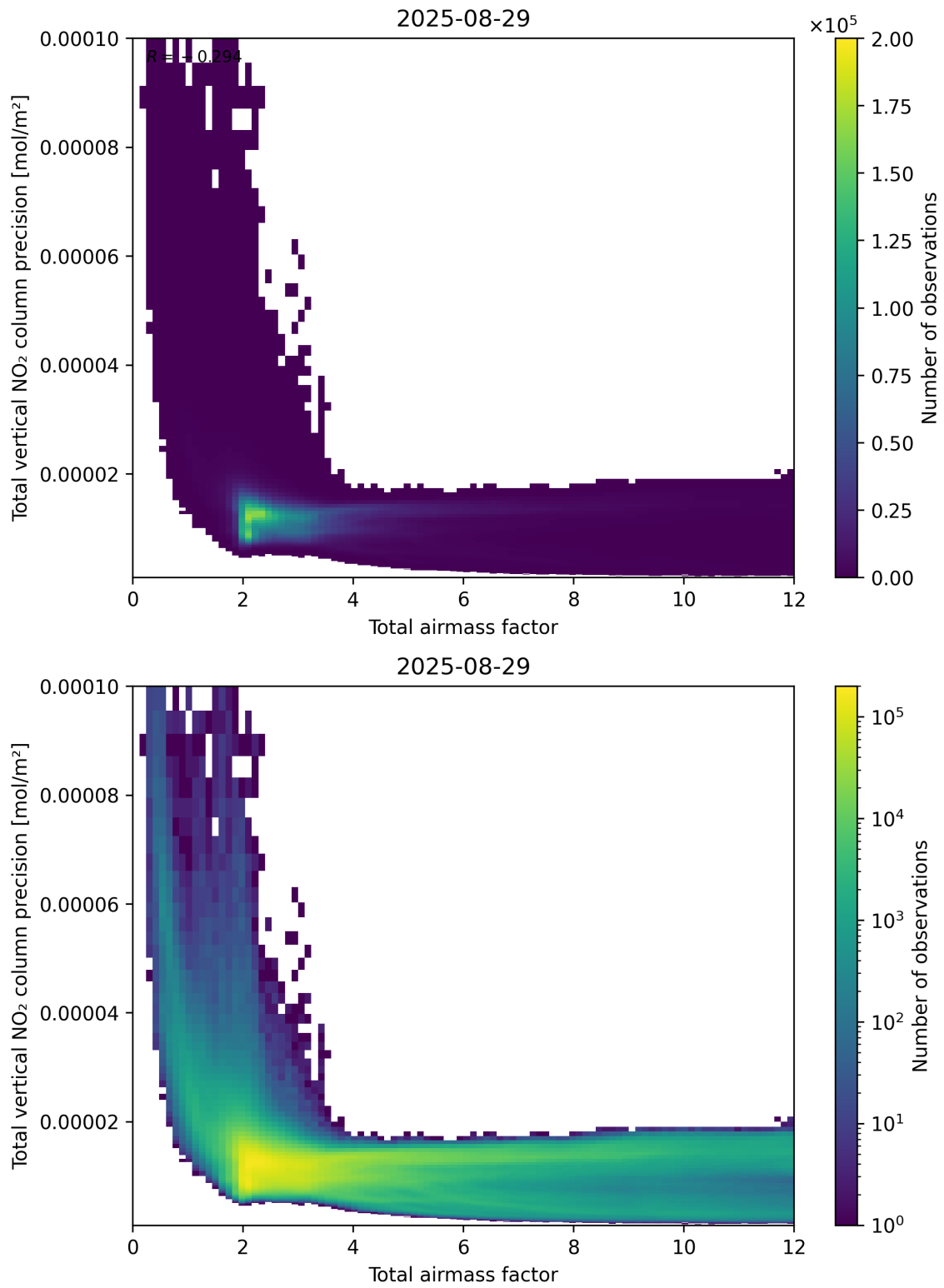
Figure 68: Scatter density plot of “Total airmass factor” against “Total vertical NO 2 column precision” for 2025-08-28 to 2025-08-30.
