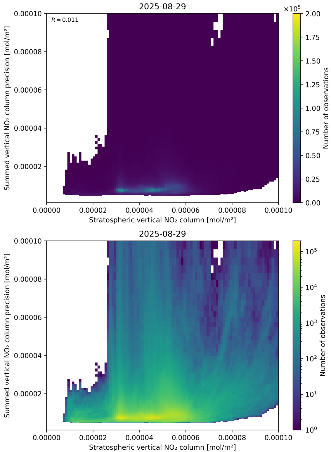
Figure 99: Scatter density plot of “Stratospheric vertical NO 2 column” against “Summed vertical NO 2 column precision” for 2025-08-28 to 2025-08-30.
