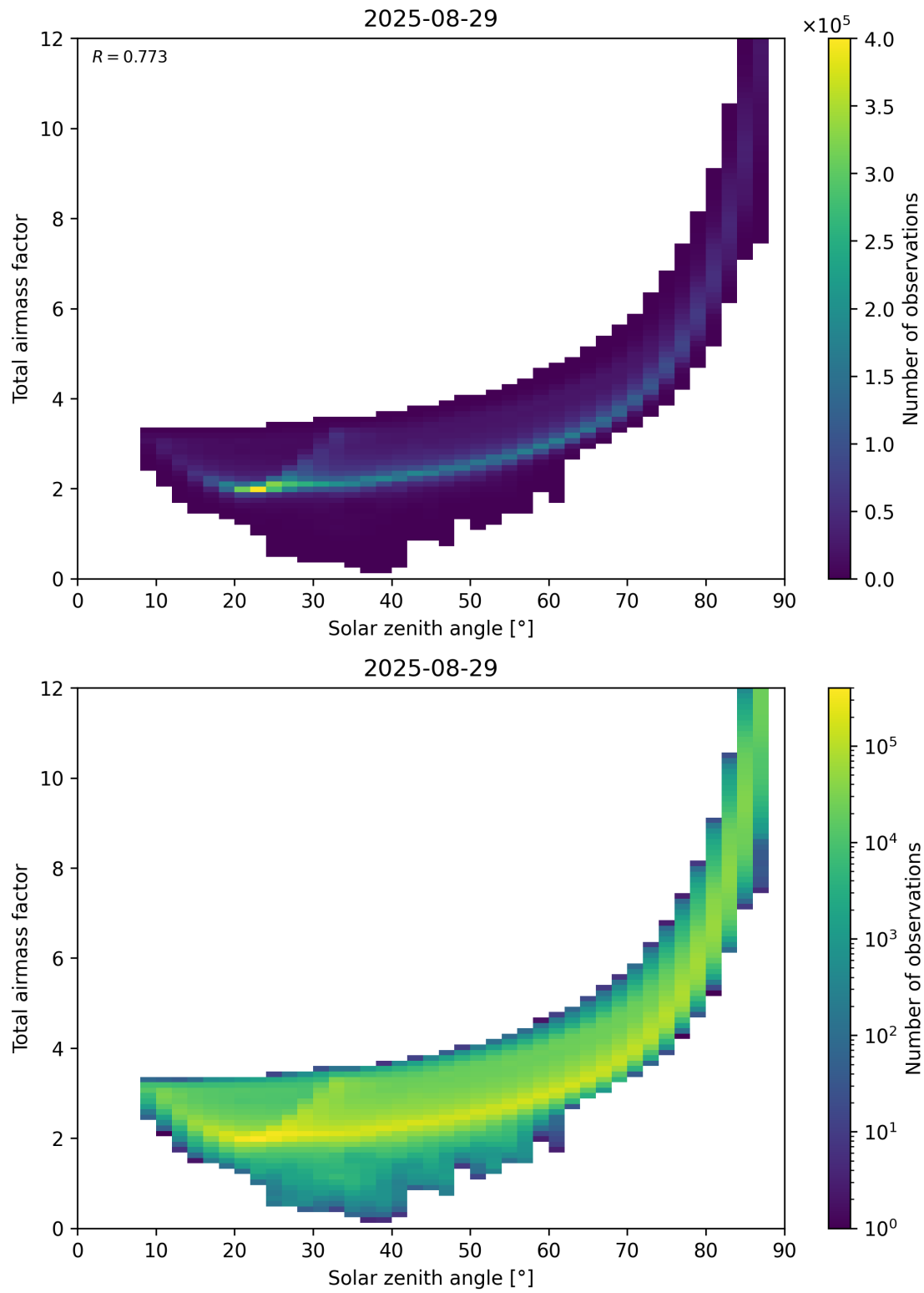
Figure 146: Scatter density plot of “Solar zenith angle” against “Total air mass factor” for 2025-08-28 to 2025-08-30.
