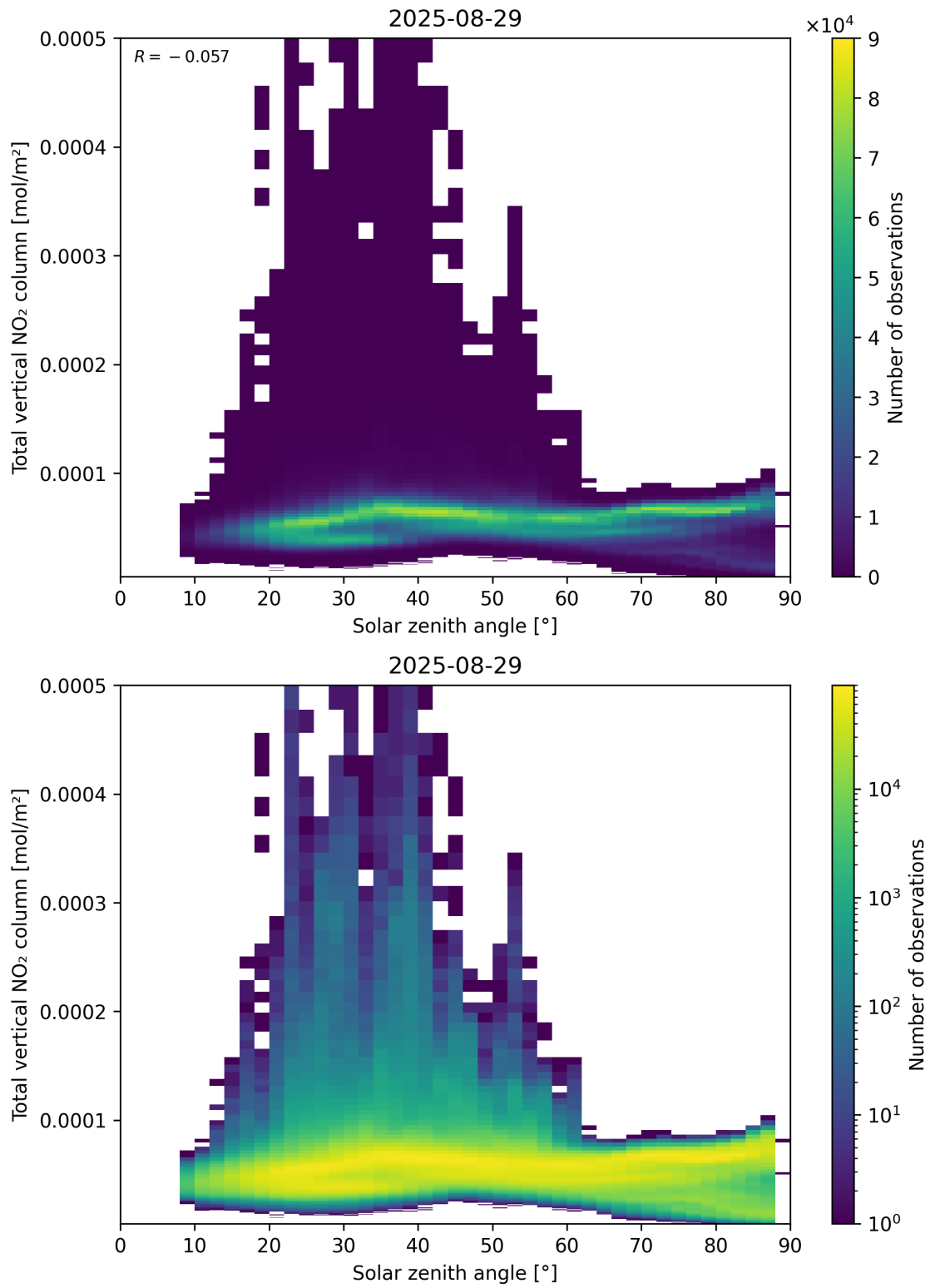
Figure 153: Scatter density plot of “Solar zenith angle” against “Total vertical NO 2 column” for 2025-08-28 to 2025-08-30.
