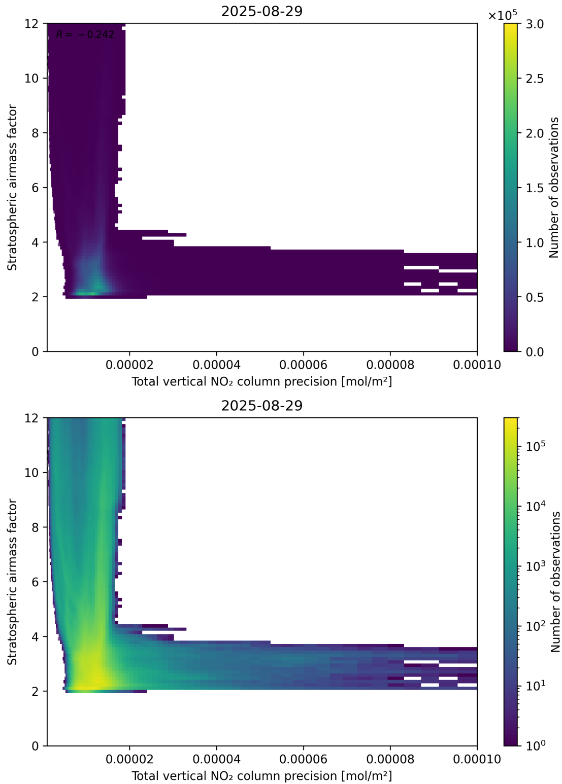
Figure 115: Scatter density plot of “Total vertical NO 2 column precision” against “Stratospheric air mass factor” for 2025-08-28 to 2025-08-30.
