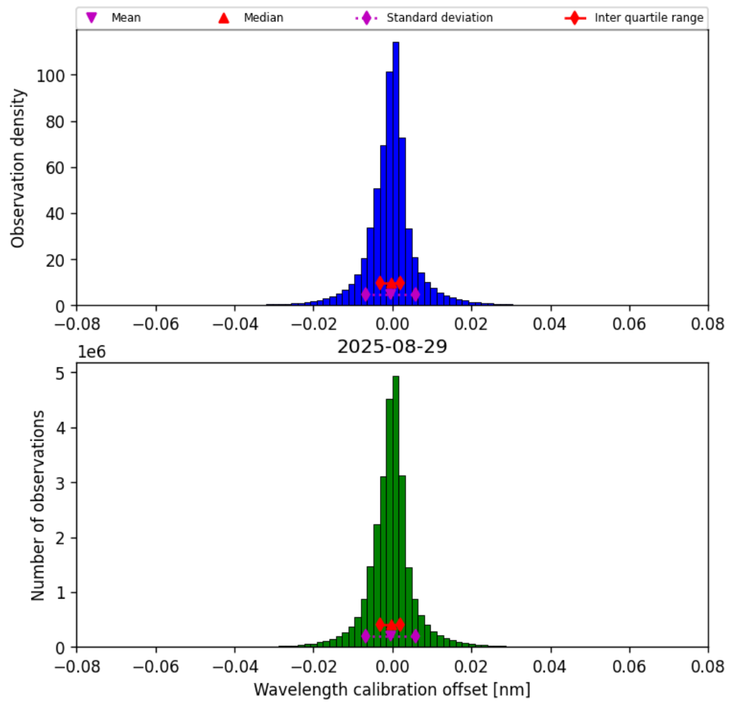
Figure 35: Histogram of “Wavelength calibration offset” for 2025-08-28 to 2025-08-30
