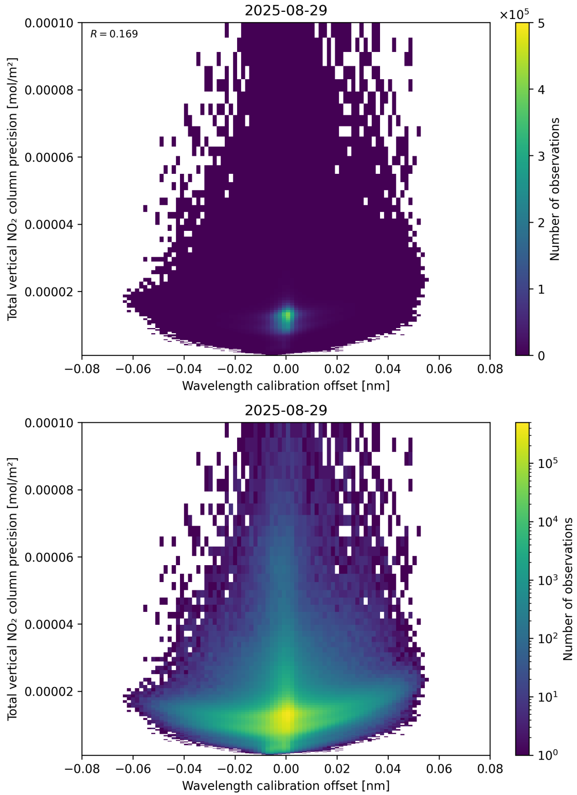
Figure 180: Scatter density plot of “Wavelength calibration offset” against “Total vertical NO 2 column precision” for 2025-08-28 to 2025-08-30.
