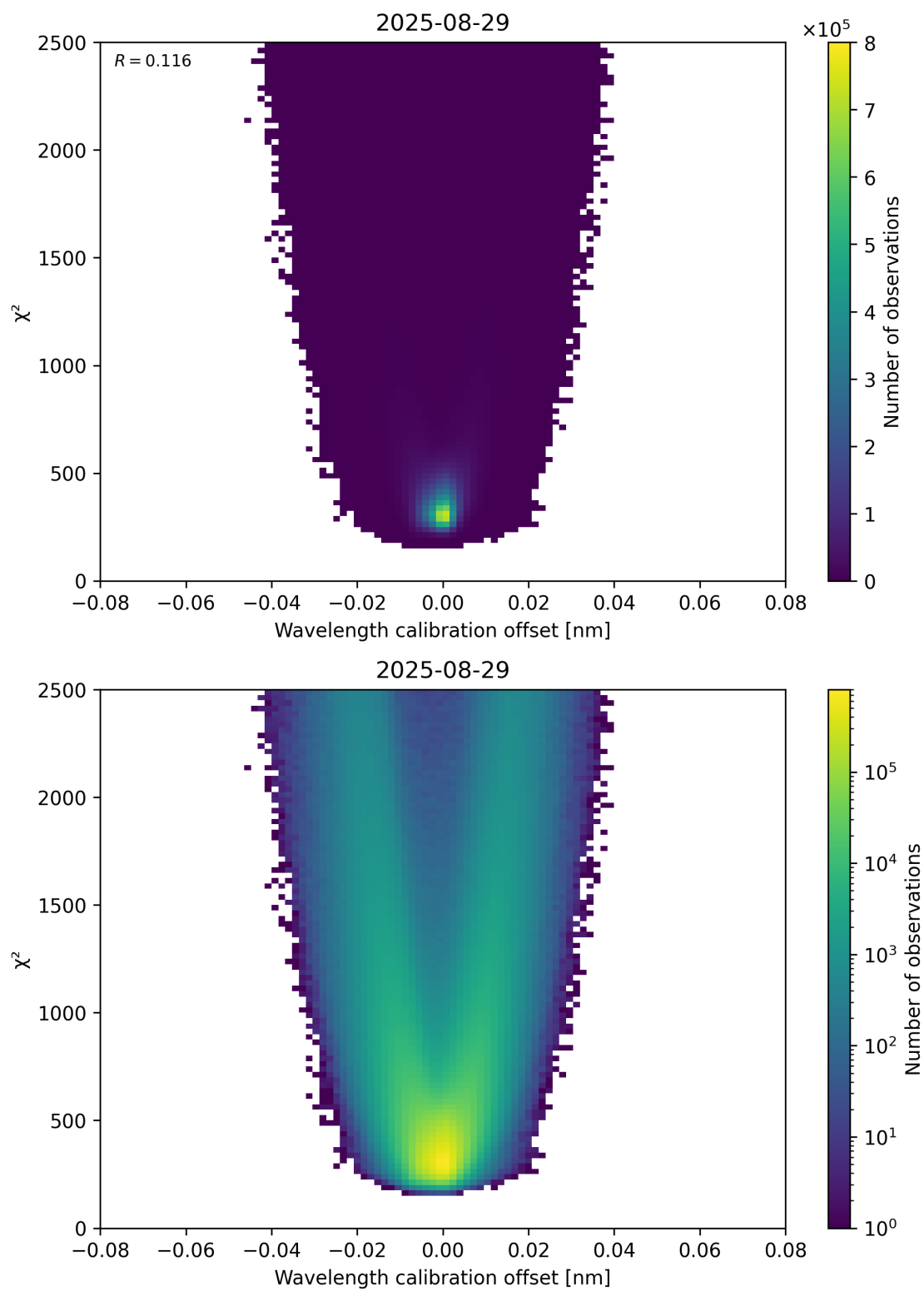
Figure 175: Scatter density plot of “Wavelength calibration offset” against “ \chi^2 ” for 2025-08-28 to 2025-08-30.
