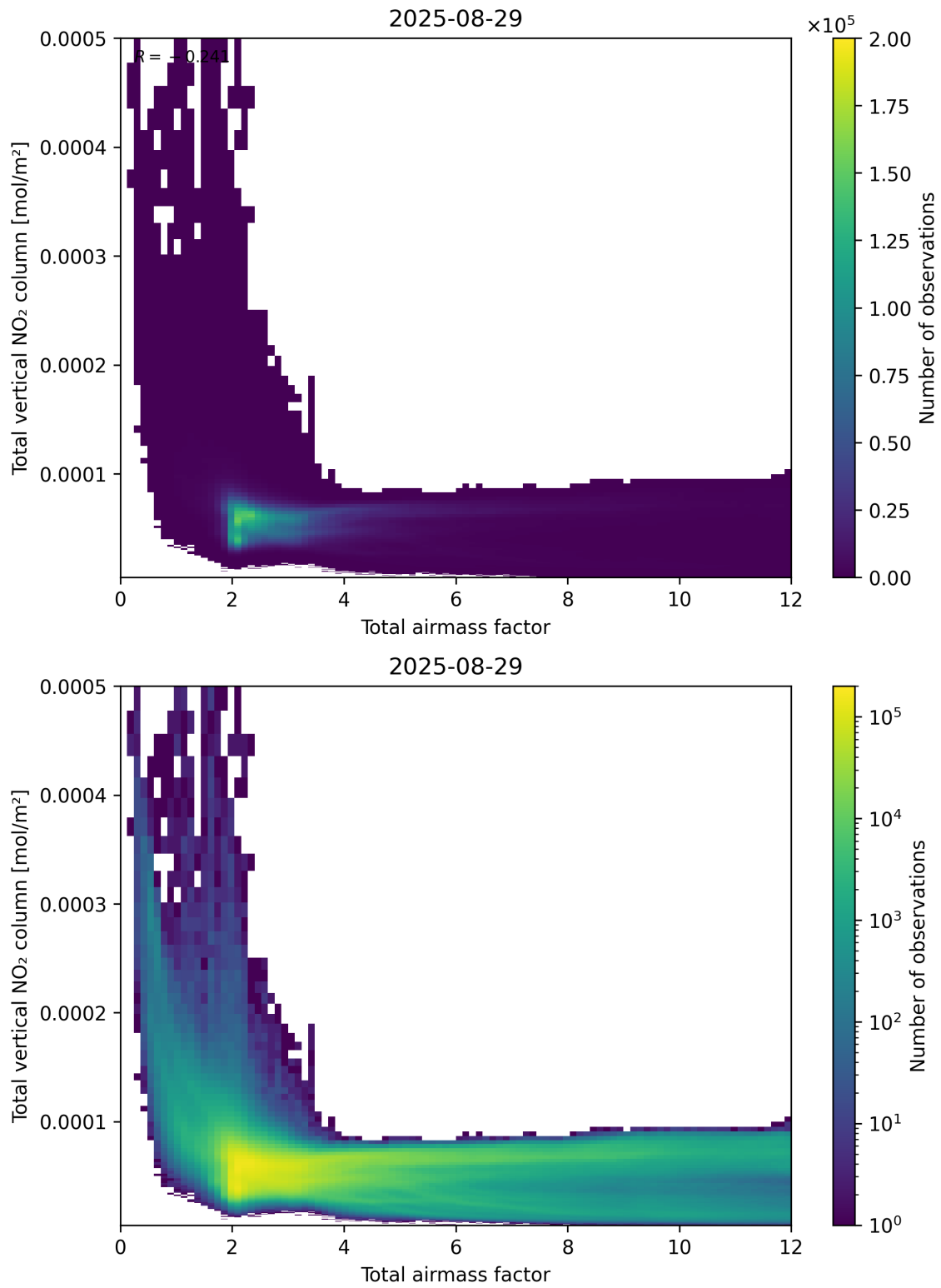
Figure 67: Scatter density plot of “Total airmass factor” against “Total vertical NO 2 column” for 2025-08-28 to 2025-08-30.
