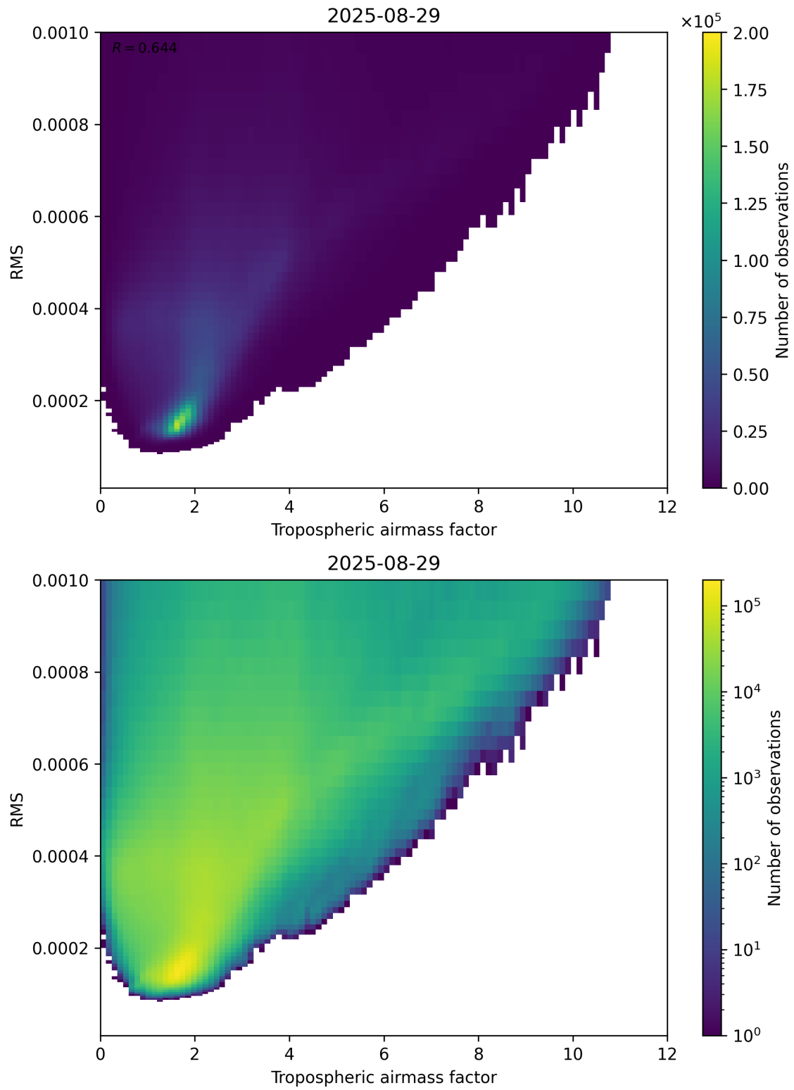
Figure 79: Scatter density plot of “Tropospheric airmass factor” against “RMS” for 2025-08-28 to 2025-08-30.
