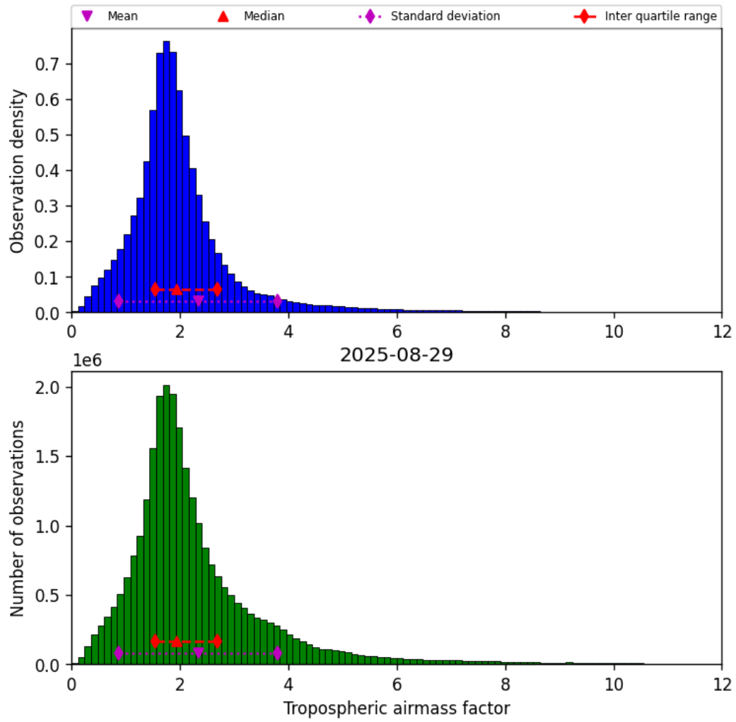
Figure 31: Histogram of “Tropospheric airmass factor” for 2025-08-28 to 2025-08-30
