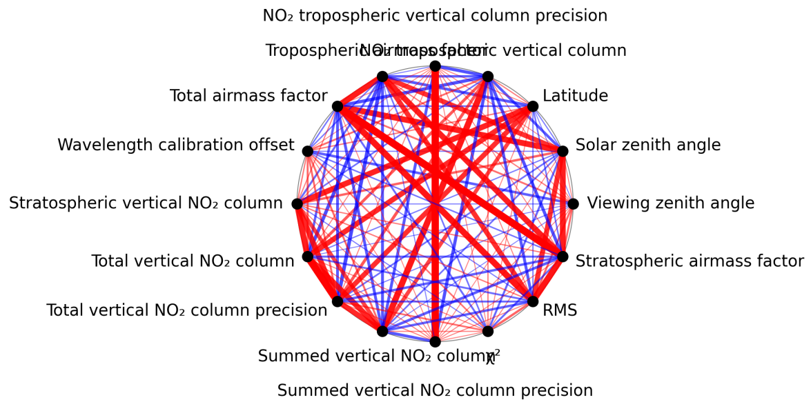
Figure 1: Map of correlation graph for 2025-08-28 to 2025-08-30.
