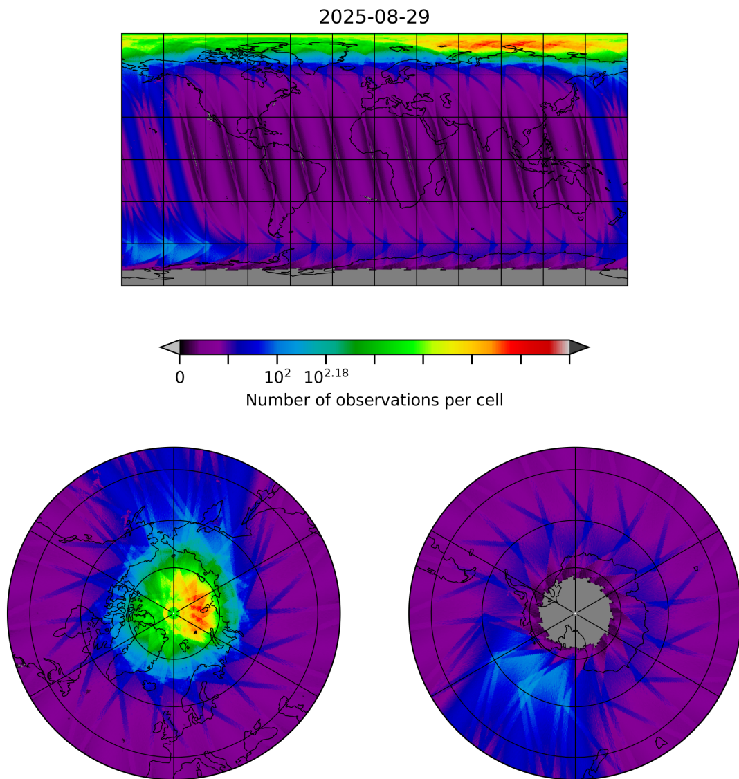
Figure 10: Map of the number of observations for 2025-08-28 to 2025-08-30
