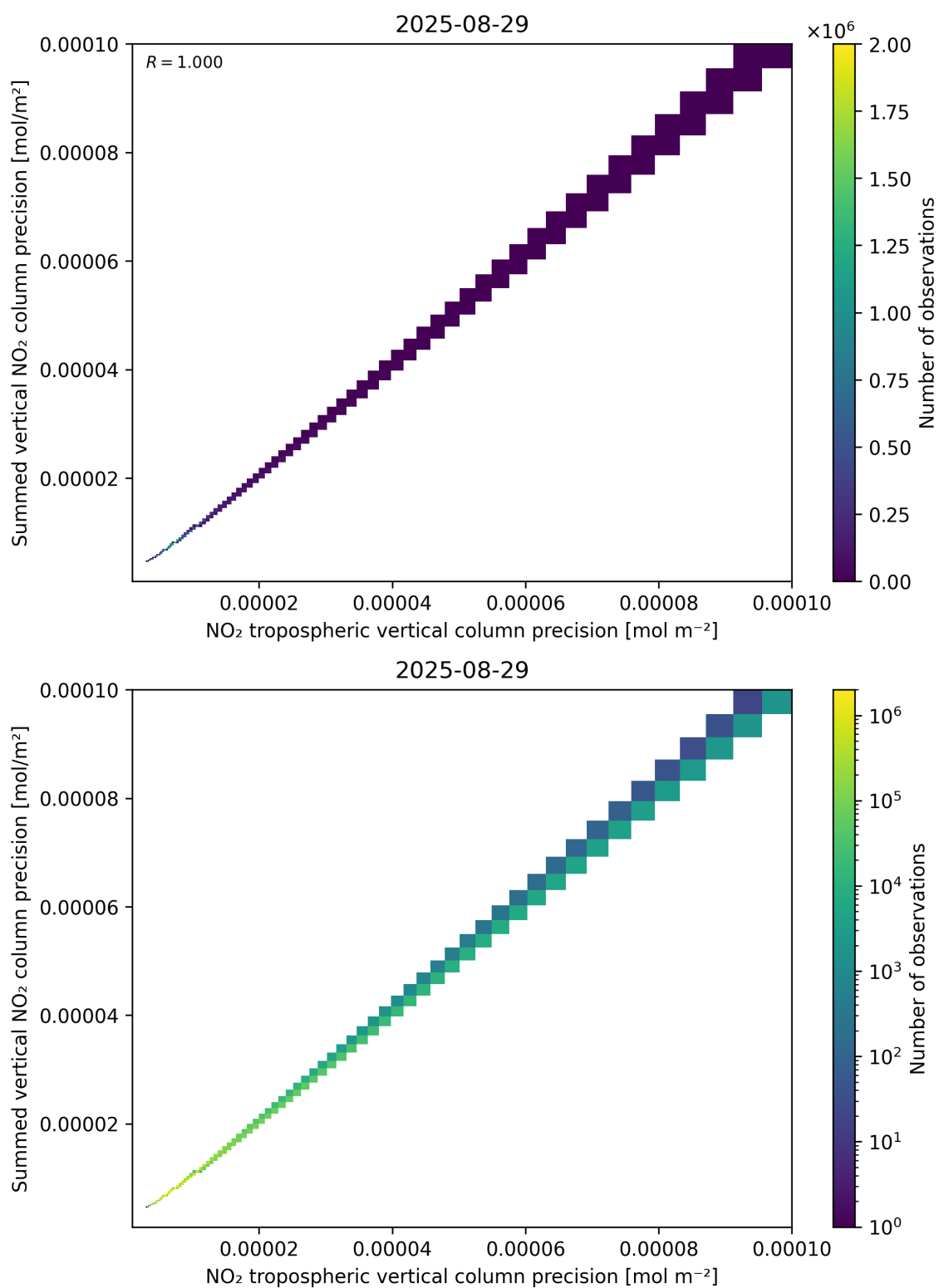
Figure 137: Scatter density plot of “NO 2 tropospheric vertical column precision” against “Summed vertical NO 2 column precision” for 2025-08-28 to 2025-08-30.
