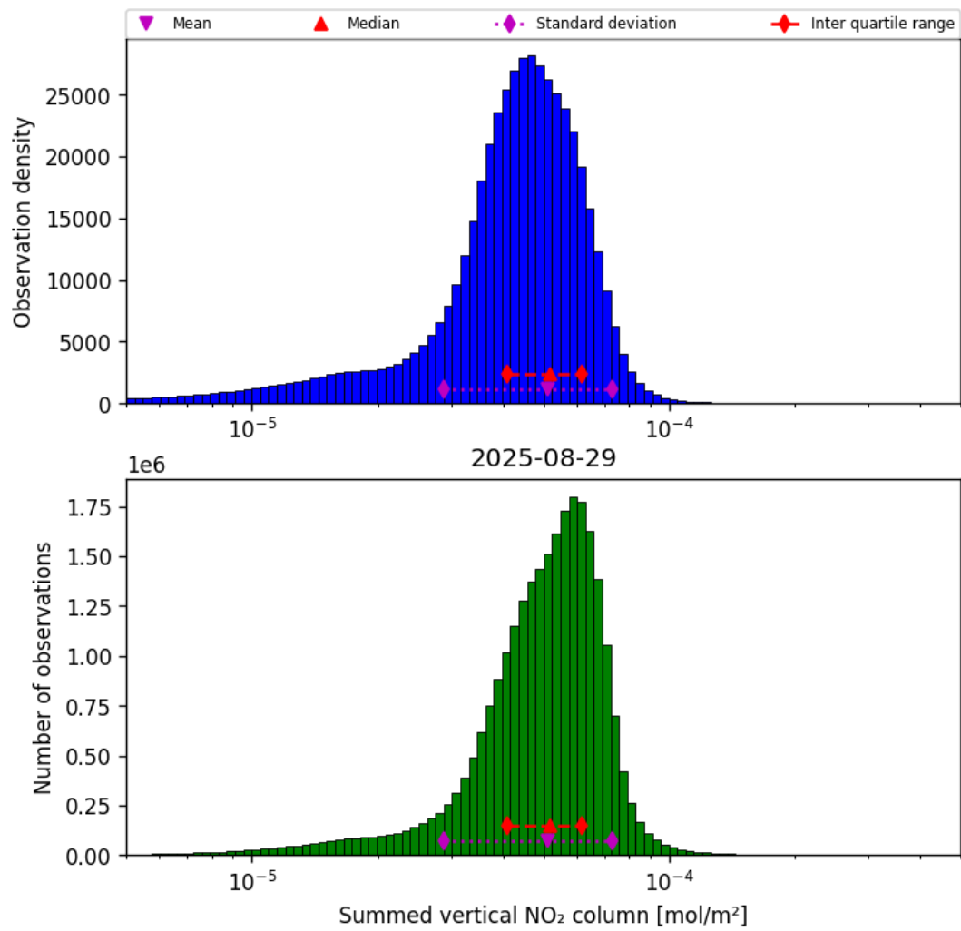
Figure 40: Histogram of “Summed vertical NO 2 column” for 2025-08-28 to 2025-08-30
