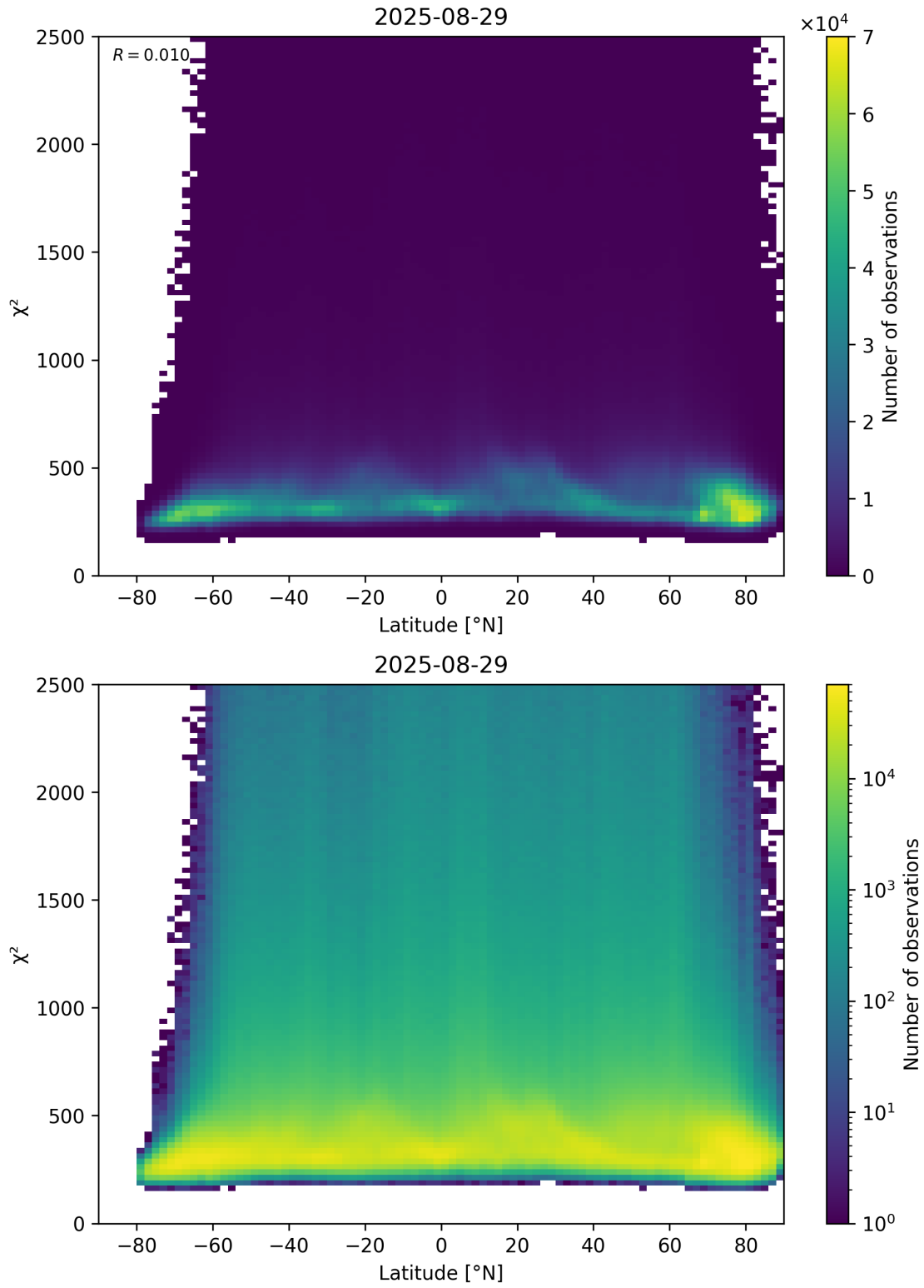
Figure 86: Scatter density plot of “Latitude” against “ \chi^2 ” for 2025-08-28 to 2025-08-30.
