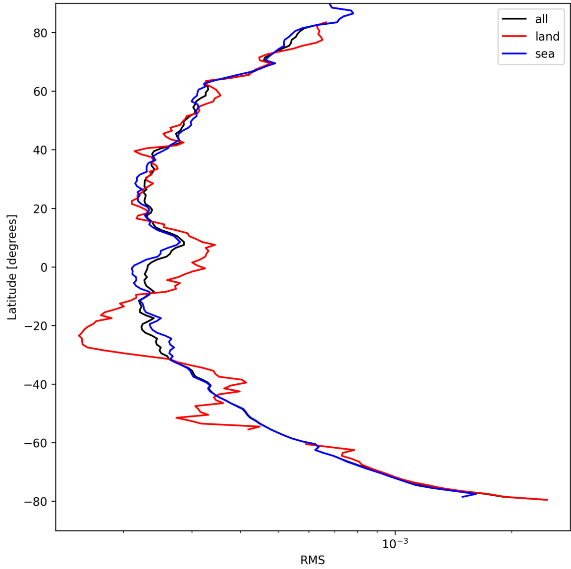
Figure 26: Zonal average of “RMS” for 2025-08-28 to 2025-08-30.
