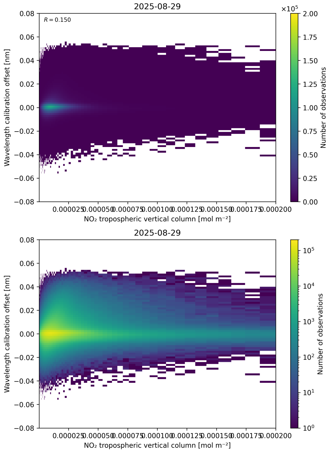
Figure 143: Scatter density plot of “NO 2 tropospheric vertical column” against “Wavelength calibration offset” for 2025-08-28 to 2025-08-30.
