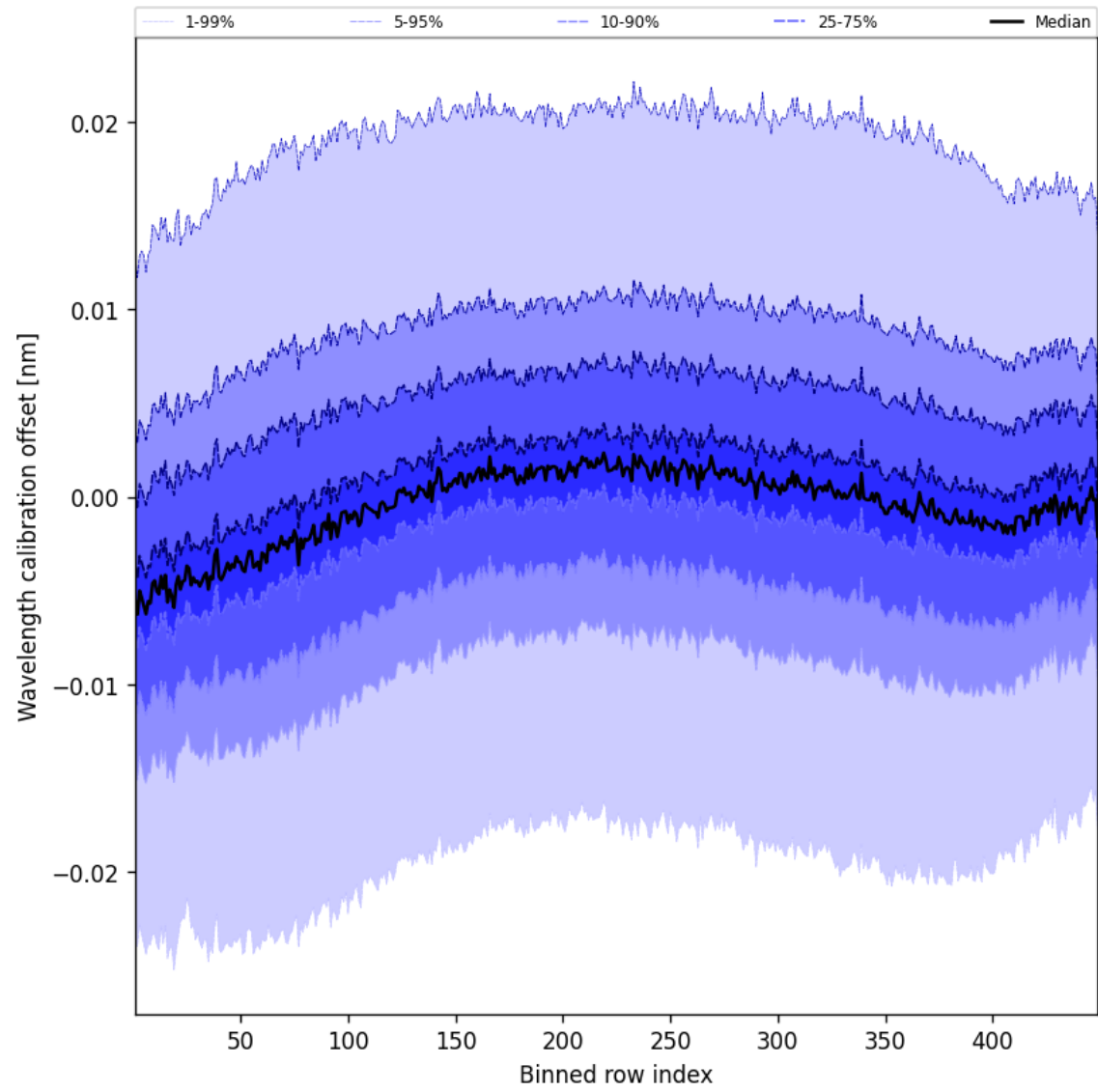
Figure 52: Along track statistics of “Wavelength calibration offset” for 2025-08-28 to 2025-08-30
