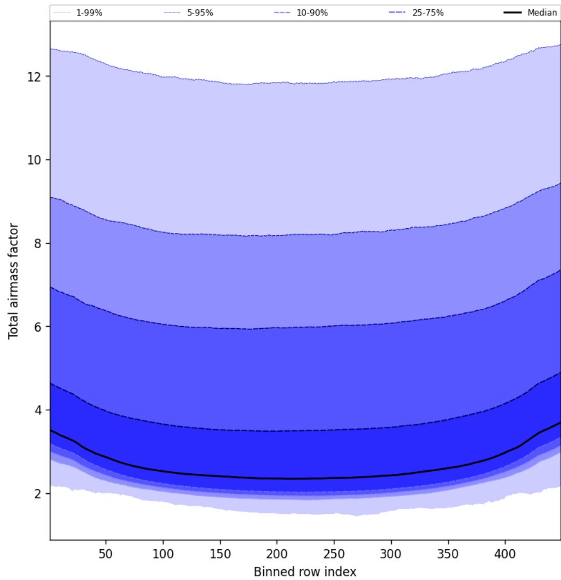
Figure 49: Along track statistics of “Total airmass factor” for 2025-08-28 to 2025-08-30
