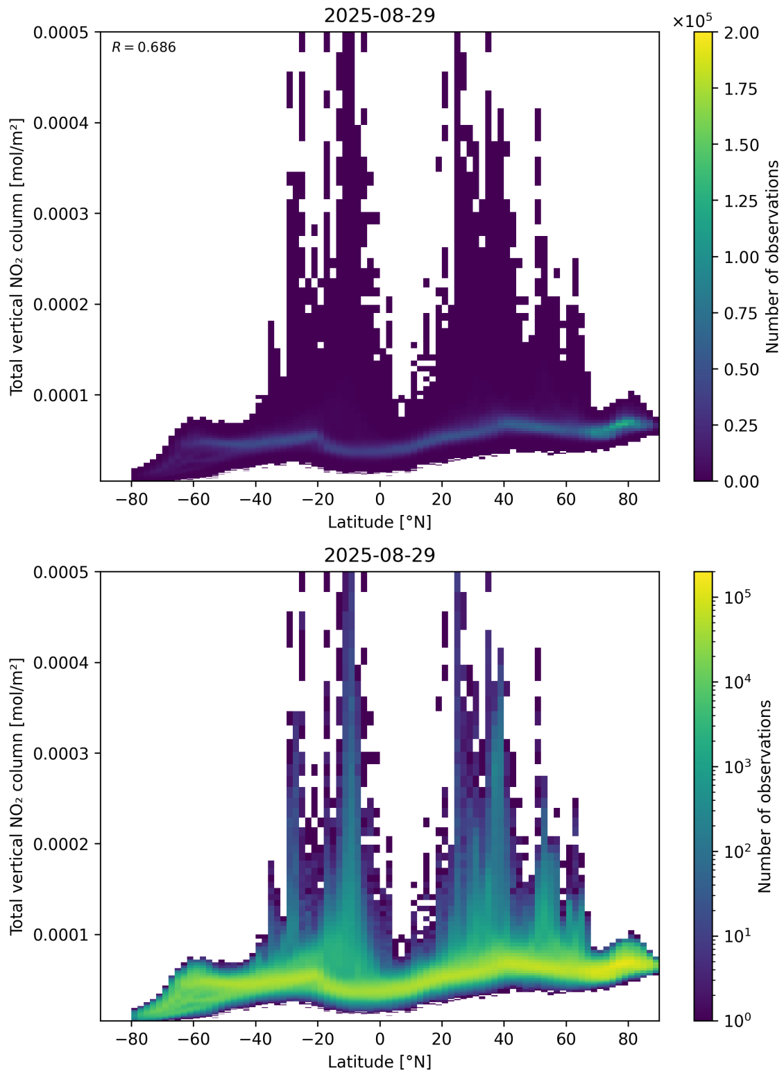
Figure 90: Scatter density plot of “Latitude” against “Total vertical NO 2 column” for 2025-08-28 to 2025-08-30.
