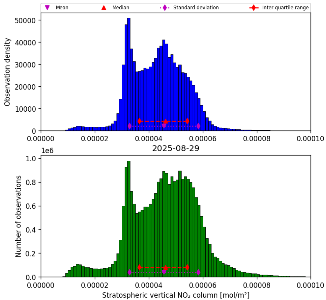
Figure 36: Histogram of “Stratospheric vertical NO 2 column” for 2025-08-28 to 2025-08-30
