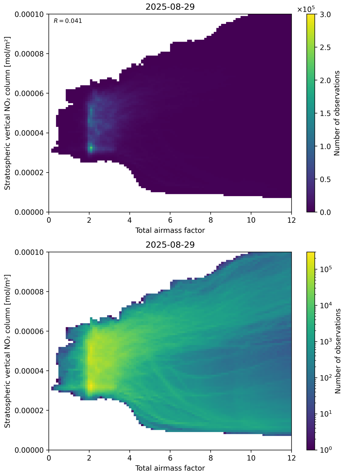
Figure 64: Scatter density plot of “Total airmass factor” against “Stratospheric vertical \text{NO}_2 column” for 2025-08-28 to 2025-08-30.
