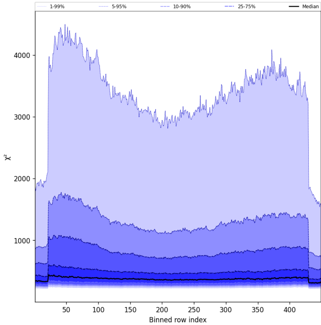
Figure 59: Along track statistics of “ \chi^2 ” for 2025-08-28 to 2025-08-30
