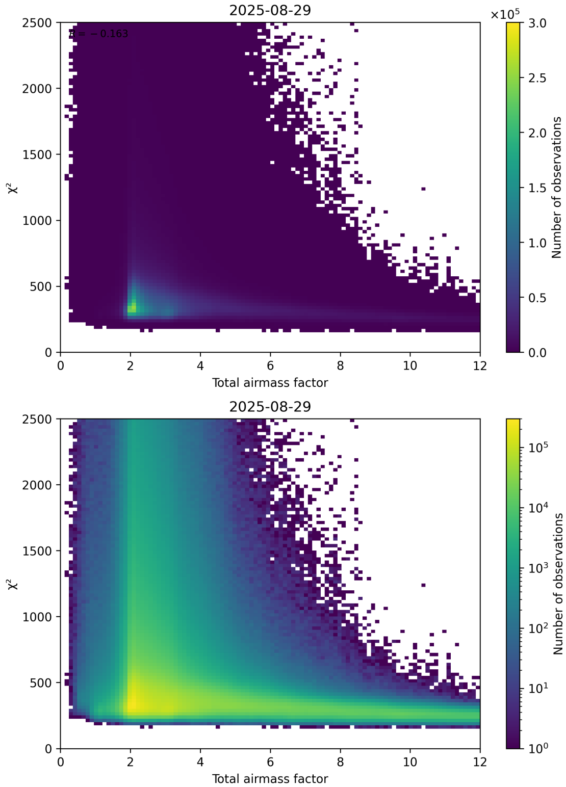
Figure 63: Scatter density plot of “Total airmass factor” against “ \chi^2 ” for 2025-08-28 to 2025-08-30.
