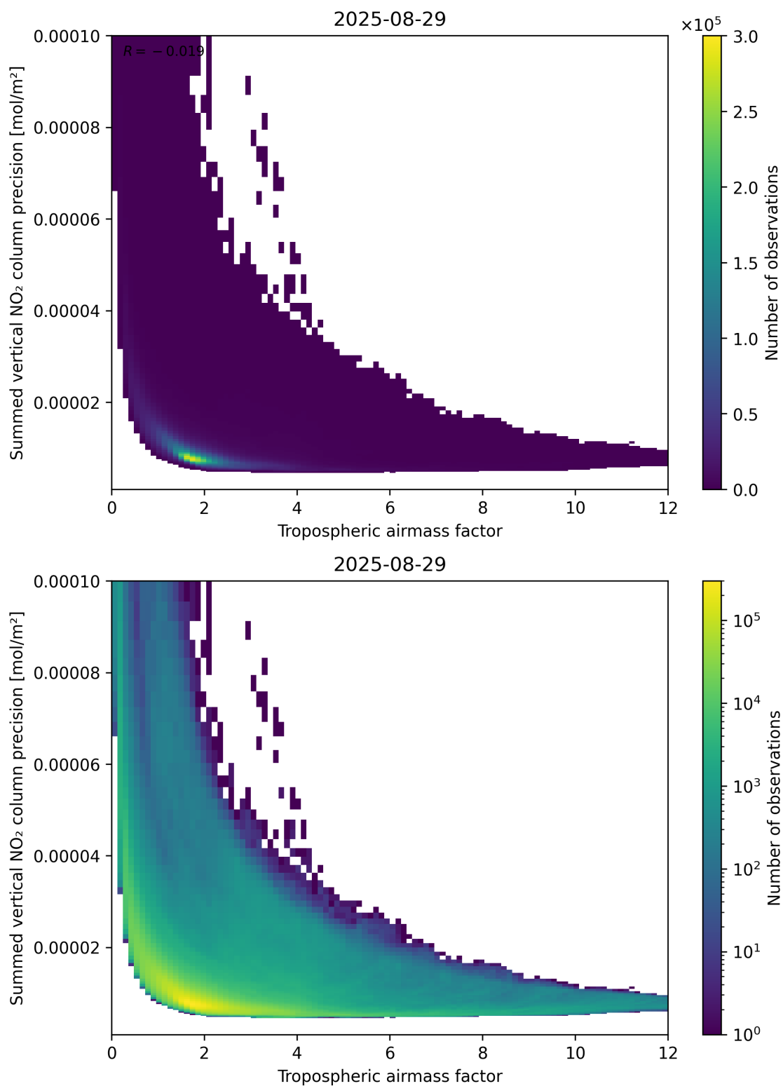
Figure 76: Scatter density plot of “Tropospheric air mass factor” against “Summed vertical NO 2 column precision” for 2025-08-28 to 2025-08-30.
