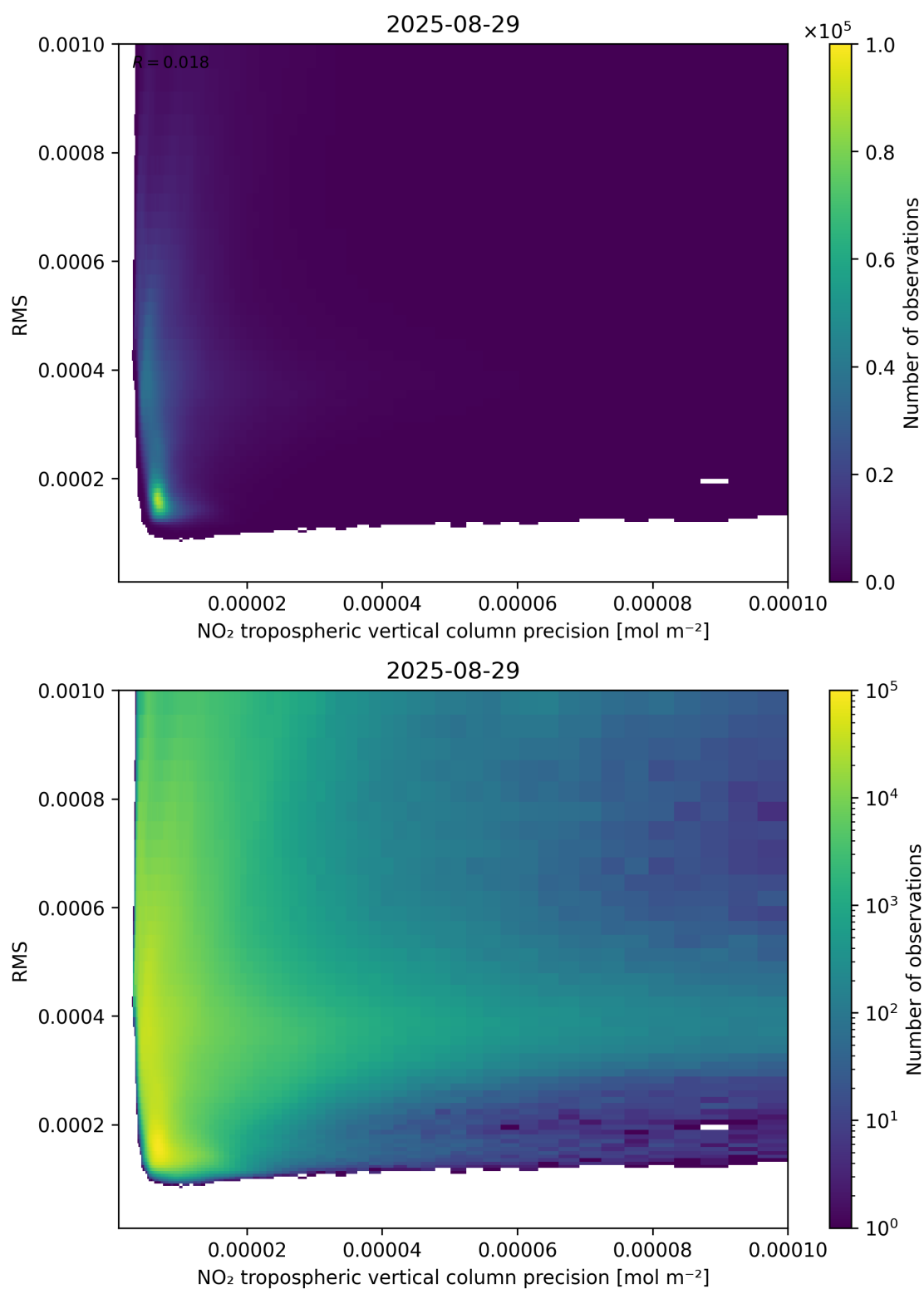
Figure 140: Scatter density plot of “NO 2 tropospheric vertical column precision” against “RMS” for 2025-08-28 to 2025-08-30.
