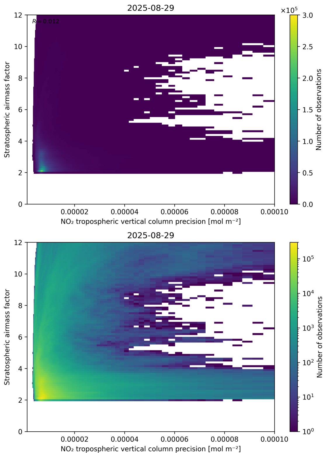
Figure 131: Scatter density plot of “NO 2 tropospheric vertical column precision” against “Stratospheric airmass factor” for 2025-08-28 to 2025-08-30.
