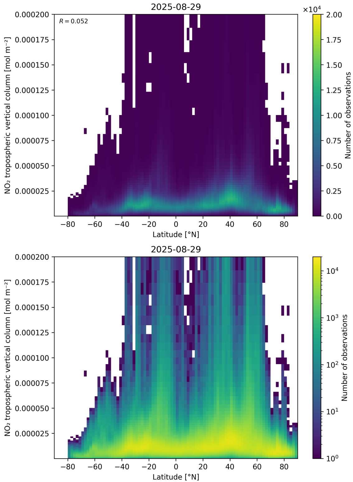
Figure 92: Scatter density plot of “Latitude” against “NO 2 tropospheric vertical column” for 2025-08-28 to 2025-08-30.
