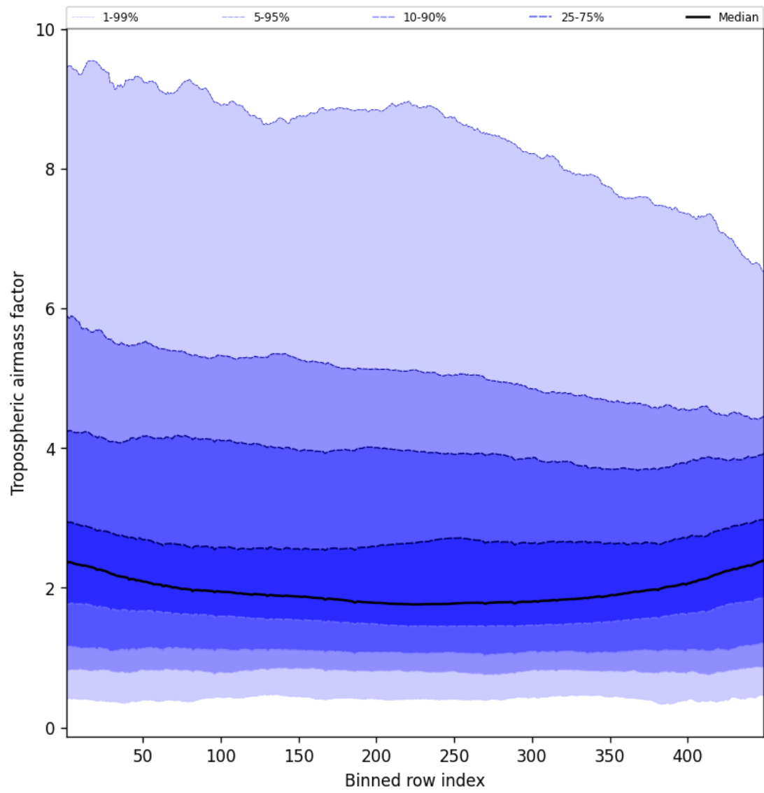
Figure 48: Along track statistics of “Tropospheric air mass factor” for 2025-08-28 to 2025-08-30
