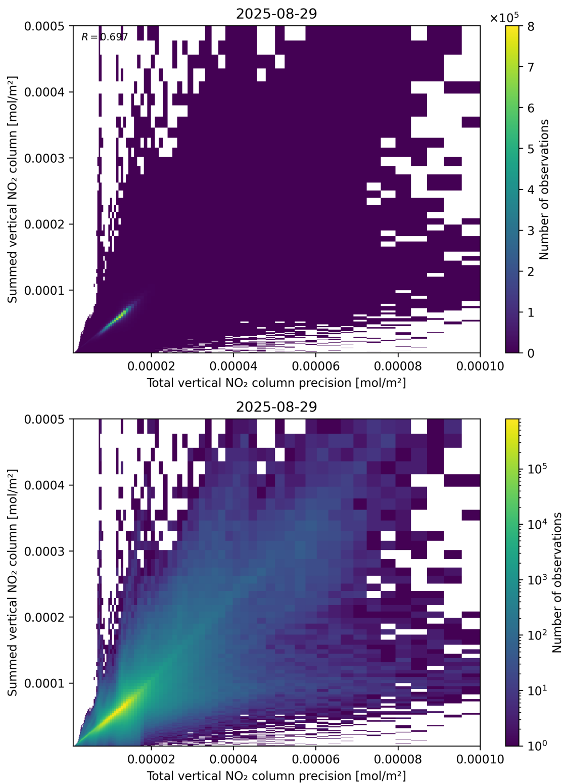
Figure 117: Scatter density plot of “Total vertical NO 2 column precision” against “Summed vertical NO 2 column” for 2025-08-28 to 2025-08-30.
