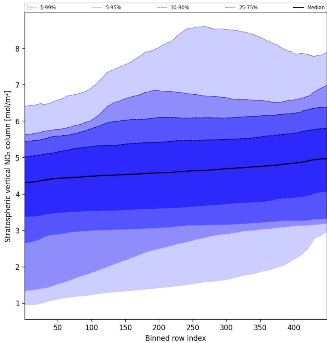
Figure 53: Along track statistics of “Stratospheric vertical NO 2 column” for 2025-08-28 to 2025-08-30
