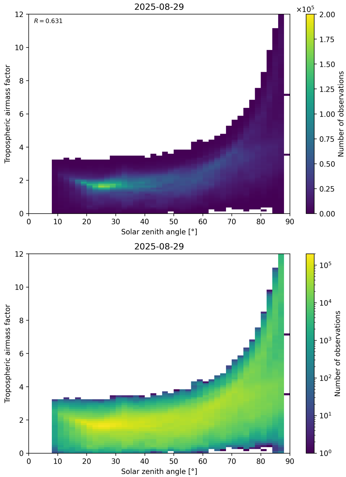
Figure 147: Scatter density plot of “Solar zenith angle” against “Tropospheric airmass factor” for 2025-08-28 to 2025-08-30.
