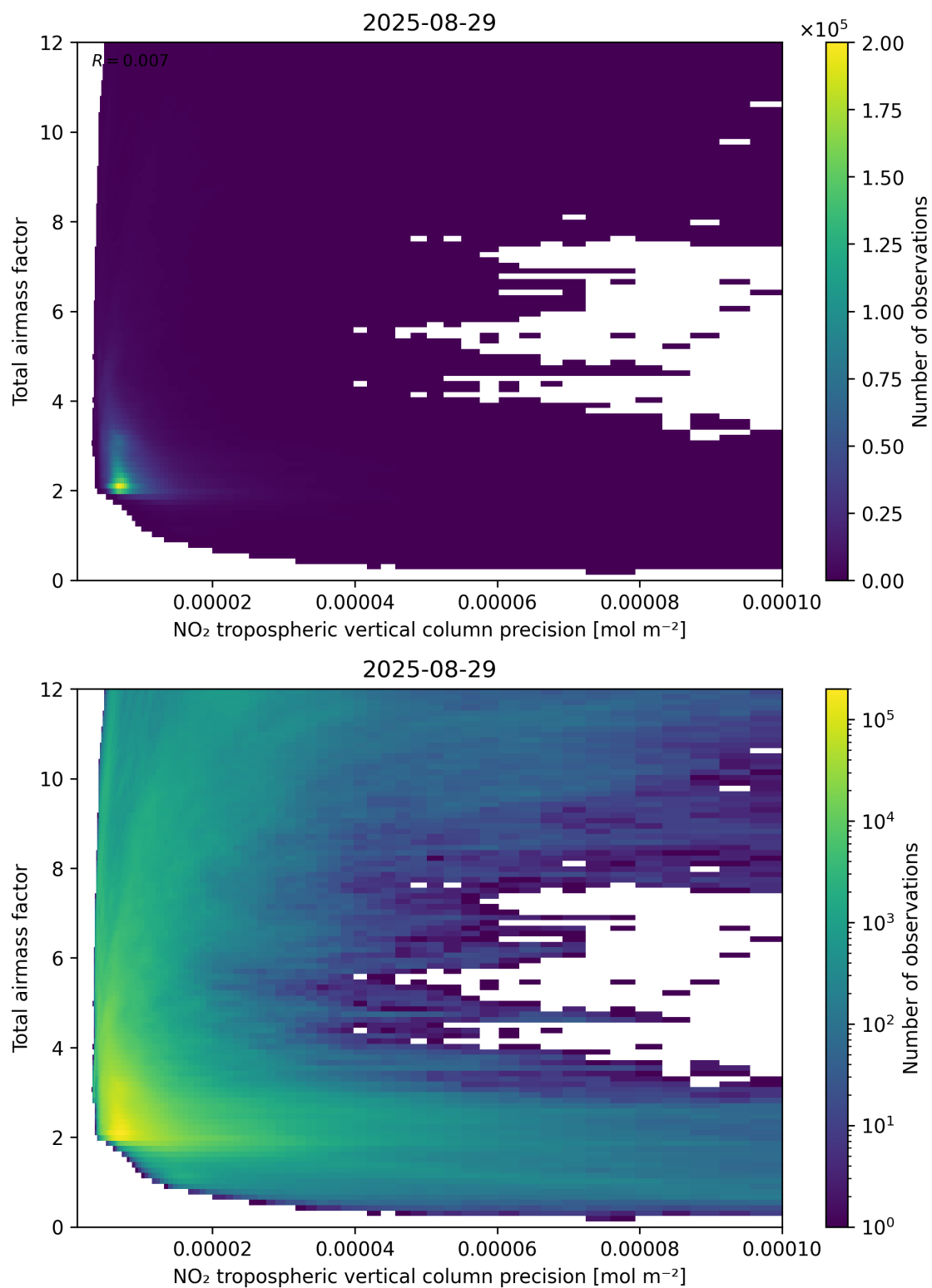
Figure 132: Scatter density plot of “NO 2 tropospheric vertical column precision” against “Total air mass factor” for 2025-08-28 to 2025-08-30.
