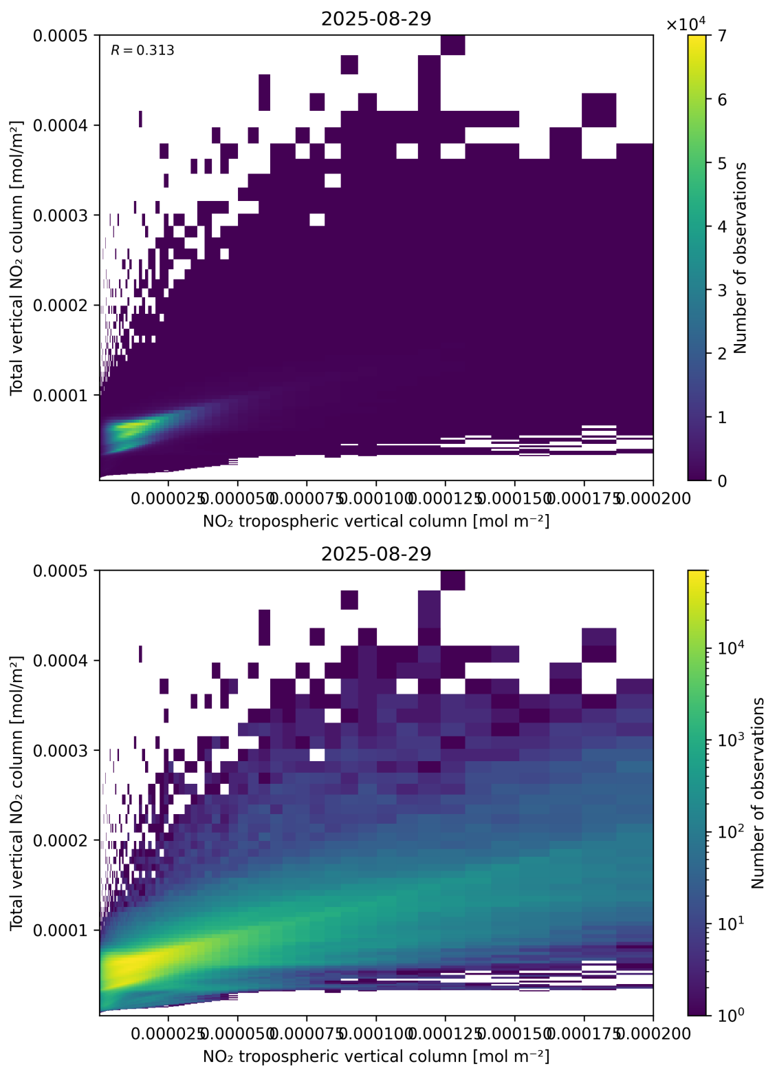
Figure 128: Scatter density plot of “NO 2 tropospheric vertical column” against “Total vertical NO 2 column” for 2025-08-28 to 2025-08-30.
