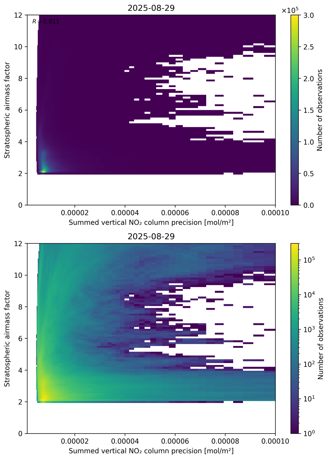
Figure 106: Scatter density plot of “Summed vertical NO 2 column precision” against “Stratospheric airmass factor” for 2025-08-28 to 2025-08-30.
