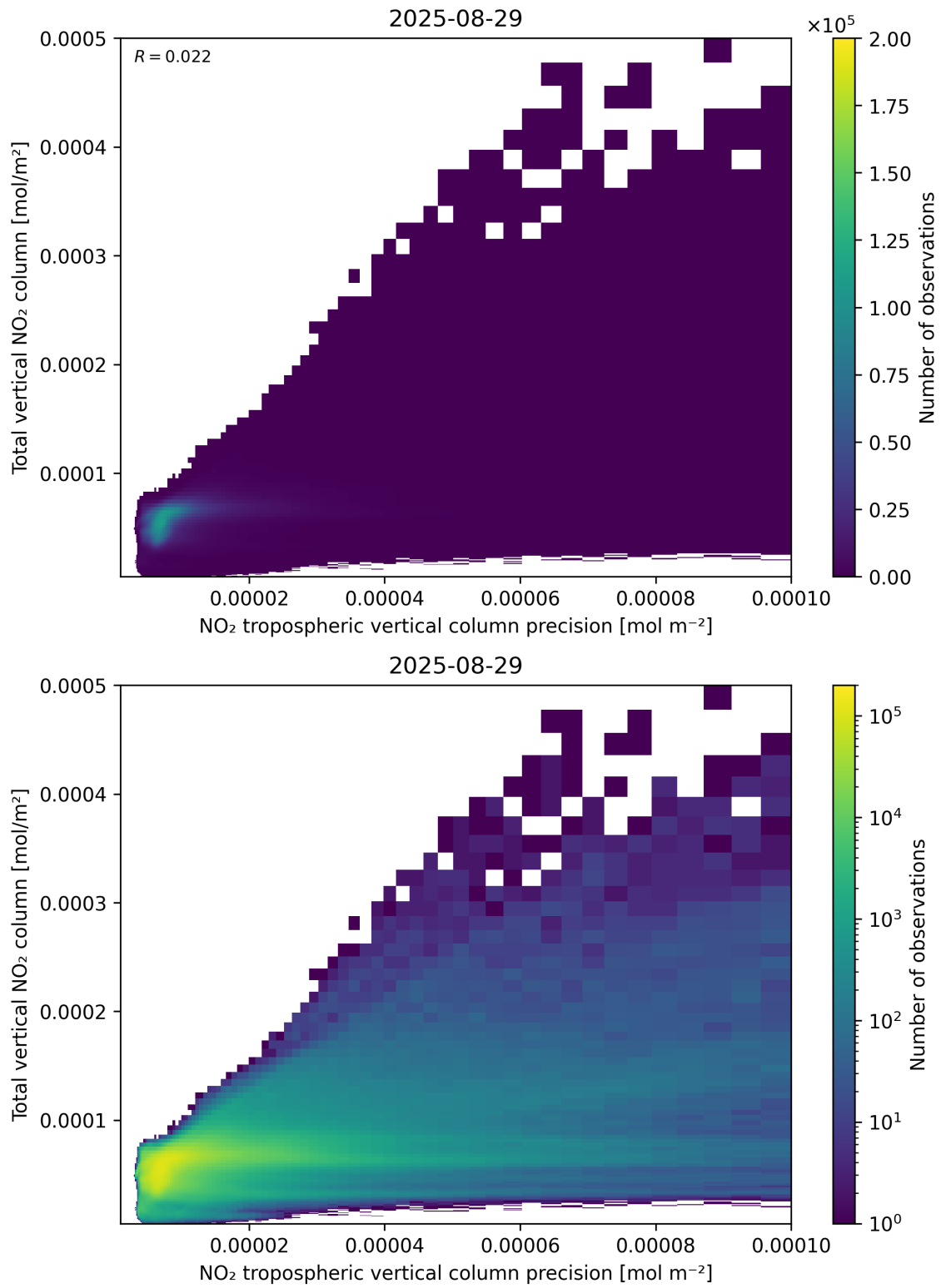
Figure 138: Scatter density plot of “NO 2 tropospheric vertical column precision” against “Total vertical NO 2 column” for 2025-08-28 to 2025-08-30.
