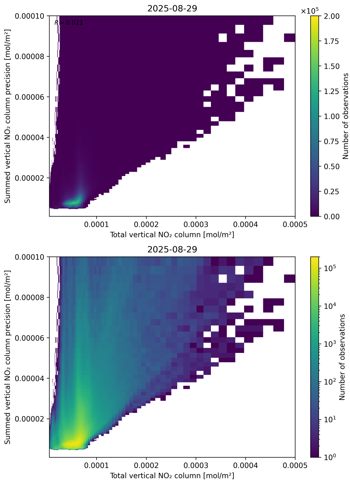
Figure 113: Scatter density plot of “Total vertical NO 2 column” against “Summed vertical NO 2 column precision” for 2025-08-28 to 2025-08-30.
