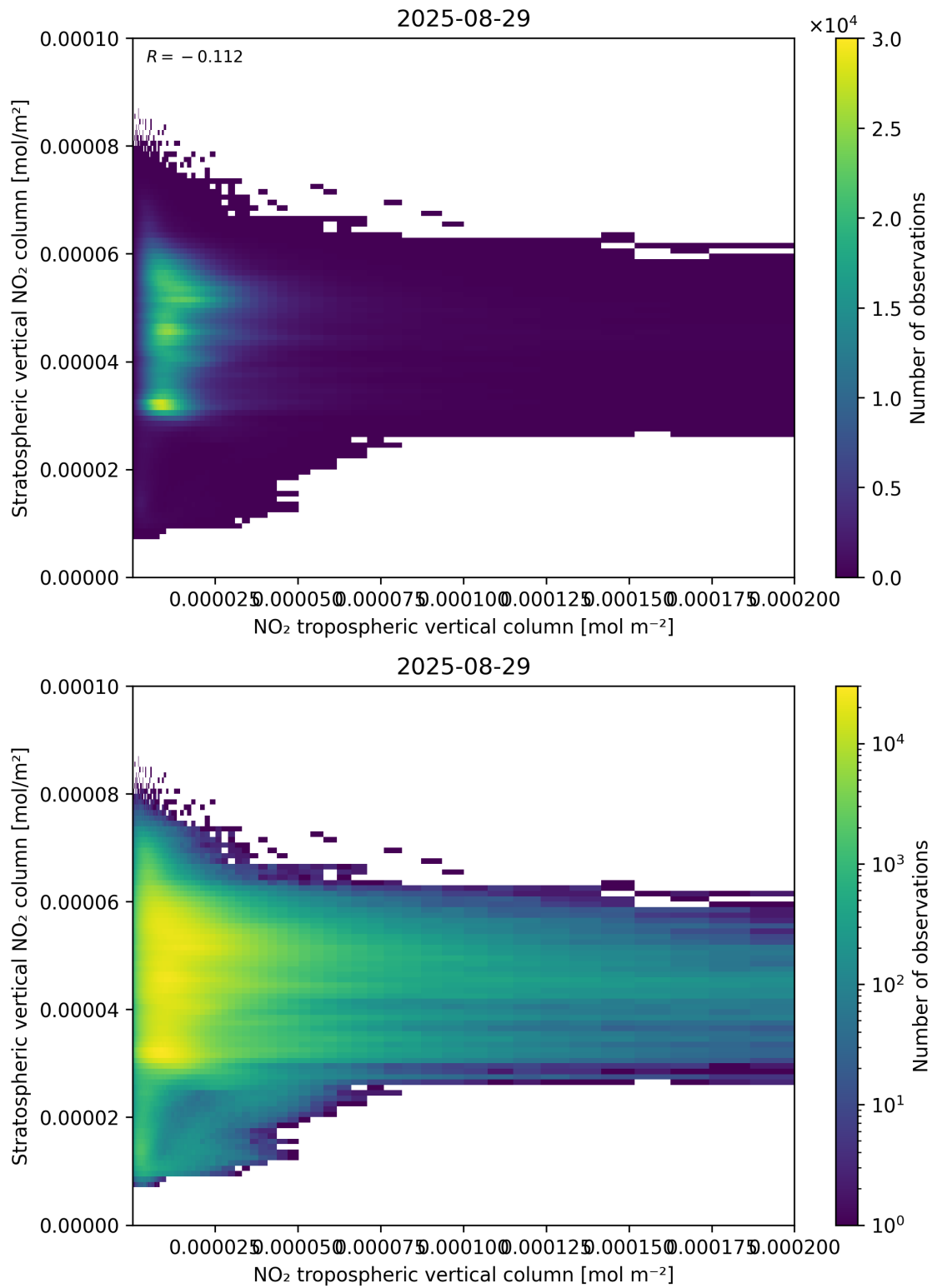
Figure 125: Scatter density plot of “NO 2 tropospheric vertical column” against “Stratospheric vertical NO 2 column” for 2025-08-28 to 2025-08-30.
