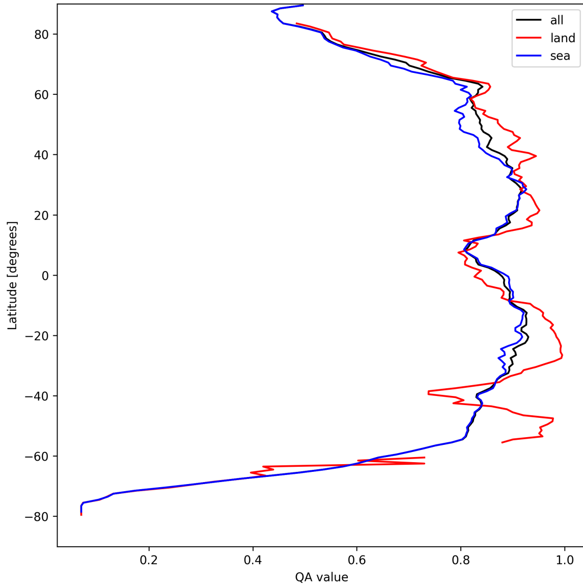
Figure 11: Zonal average of “QA value” for 2025-08-28 to 2025-08-30.
