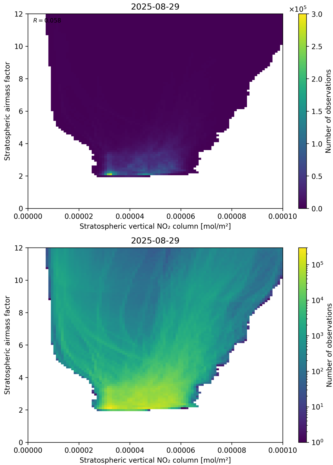
Figure 96: Scatter density plot of “Stratospheric vertical NO 2 column” against “Stratospheric airmass factor” for 2025-08-28 to 2025-08-30.
