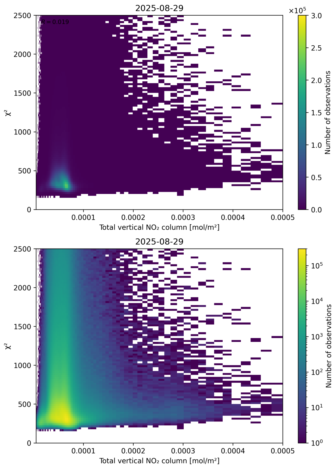
Figure 111: Scatter density plot of “Total vertical NO 2 column” against “ \chi^2 ” for 2025-08-28 to 2025-08-30.
