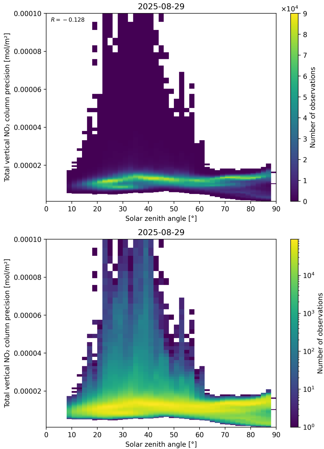
Figure 154: Scatter density plot of “Solar zenith angle” against “Total vertical NO 2 column precision” for 2025-08-28 to 2025-08-30.
