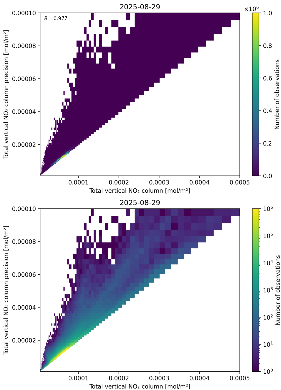
Figure 114: Scatter density plot of “Total vertical NO 2 column” against “Total vertical NO 2 column precision” for 2025-08-28 to 2025-08-30.
