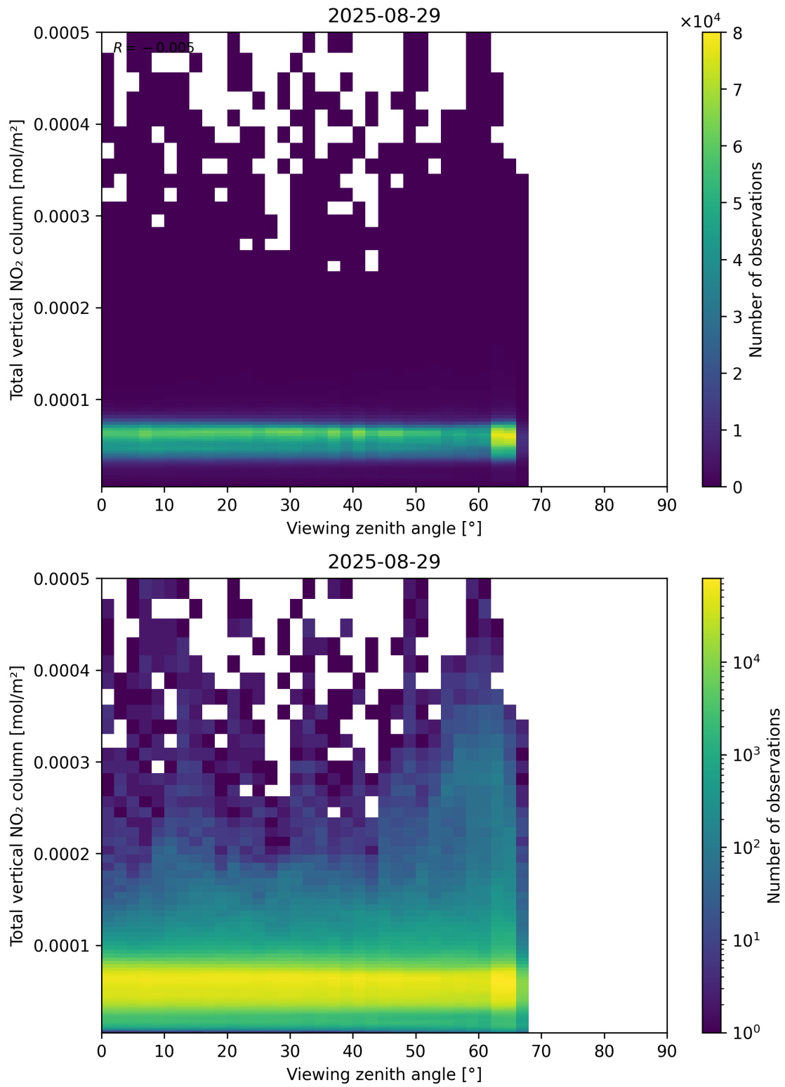
Figure 167: Scatter density plot of “Viewing zenith angle” against “Total vertical NO 2 column” for 2025-08-28 to 2025-08-30.
