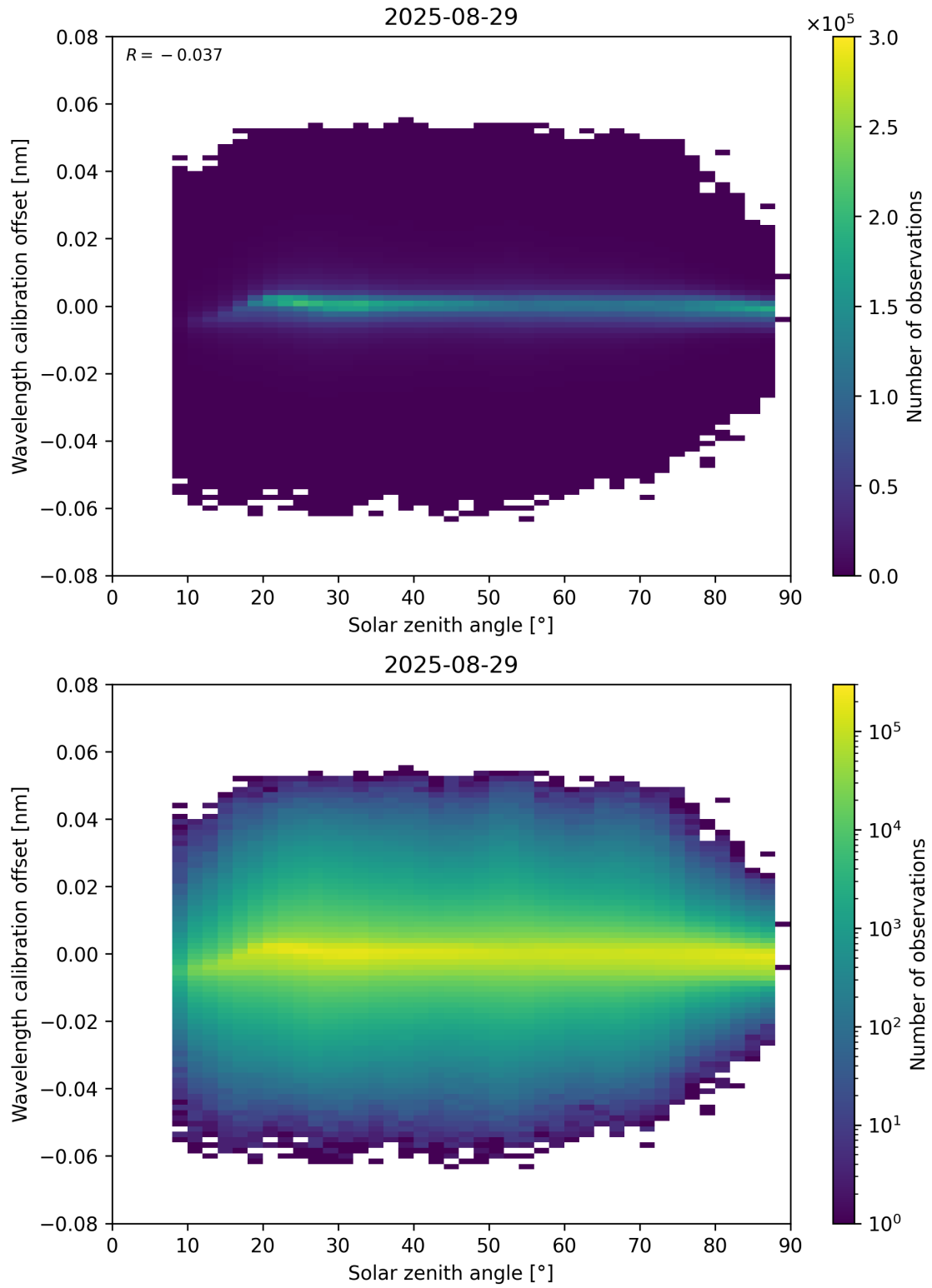
Figure 158: Scatter density plot of “Solar zenith angle” against “Wavelength calibration offset” for 2025-08-28 to 2025-08-30.
