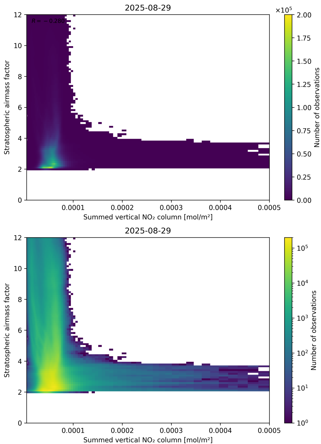
Figure 103: Scatter density plot of “Summed vertical NO 2 column” against “Stratospheric airmass factor” for 2025-08-28 to 2025-08-30.
