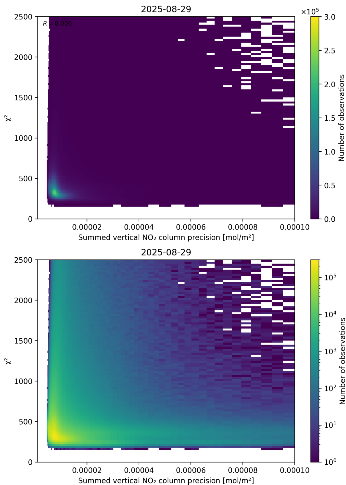
Figure 107: Scatter density plot of “Summed vertical NO 2 column precision” against “ \chi^2 ” for 2025-08-28 to 2025-08-30.
