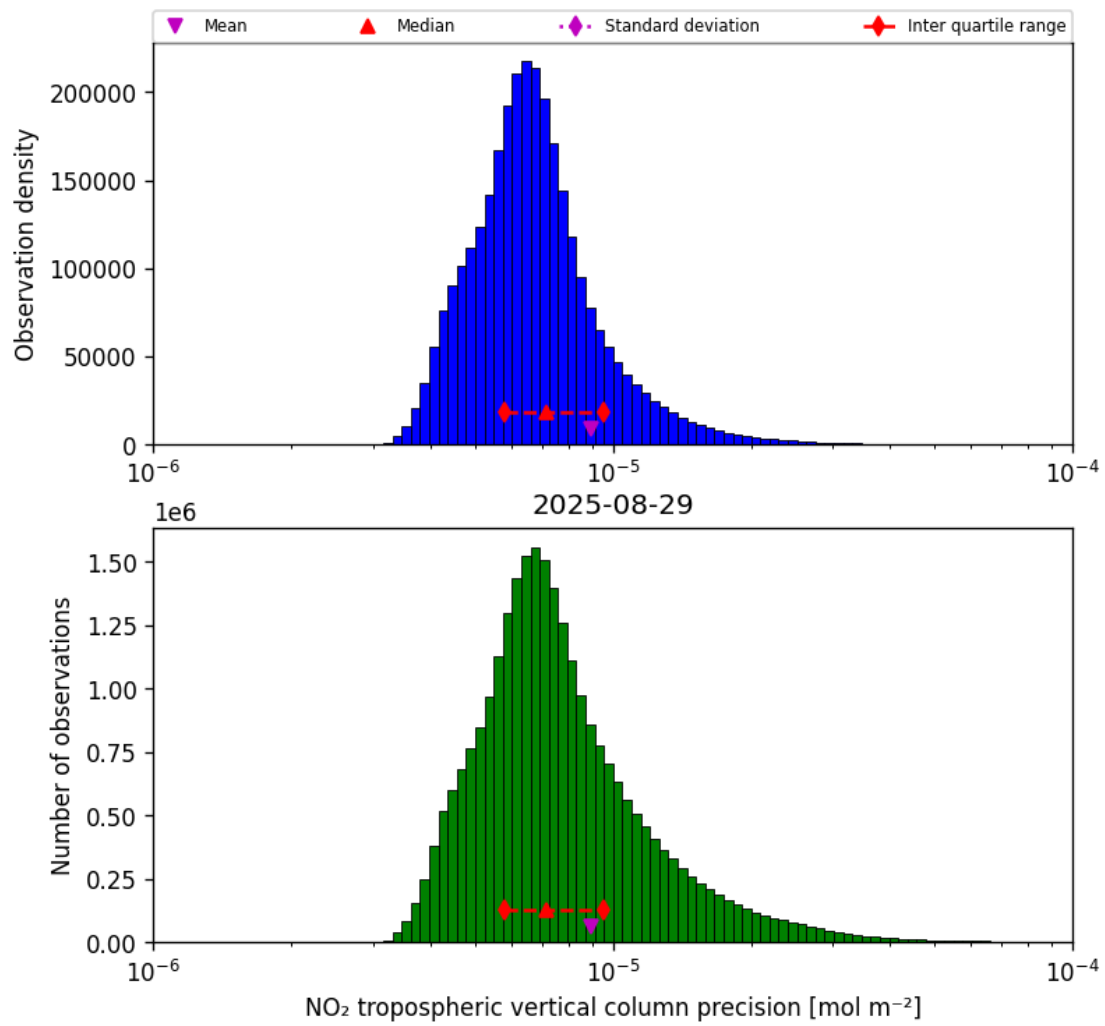
Figure 30: Histogram of “NO 2 tropospheric vertical column precision” for 2025-08-28 to 2025-08-30
