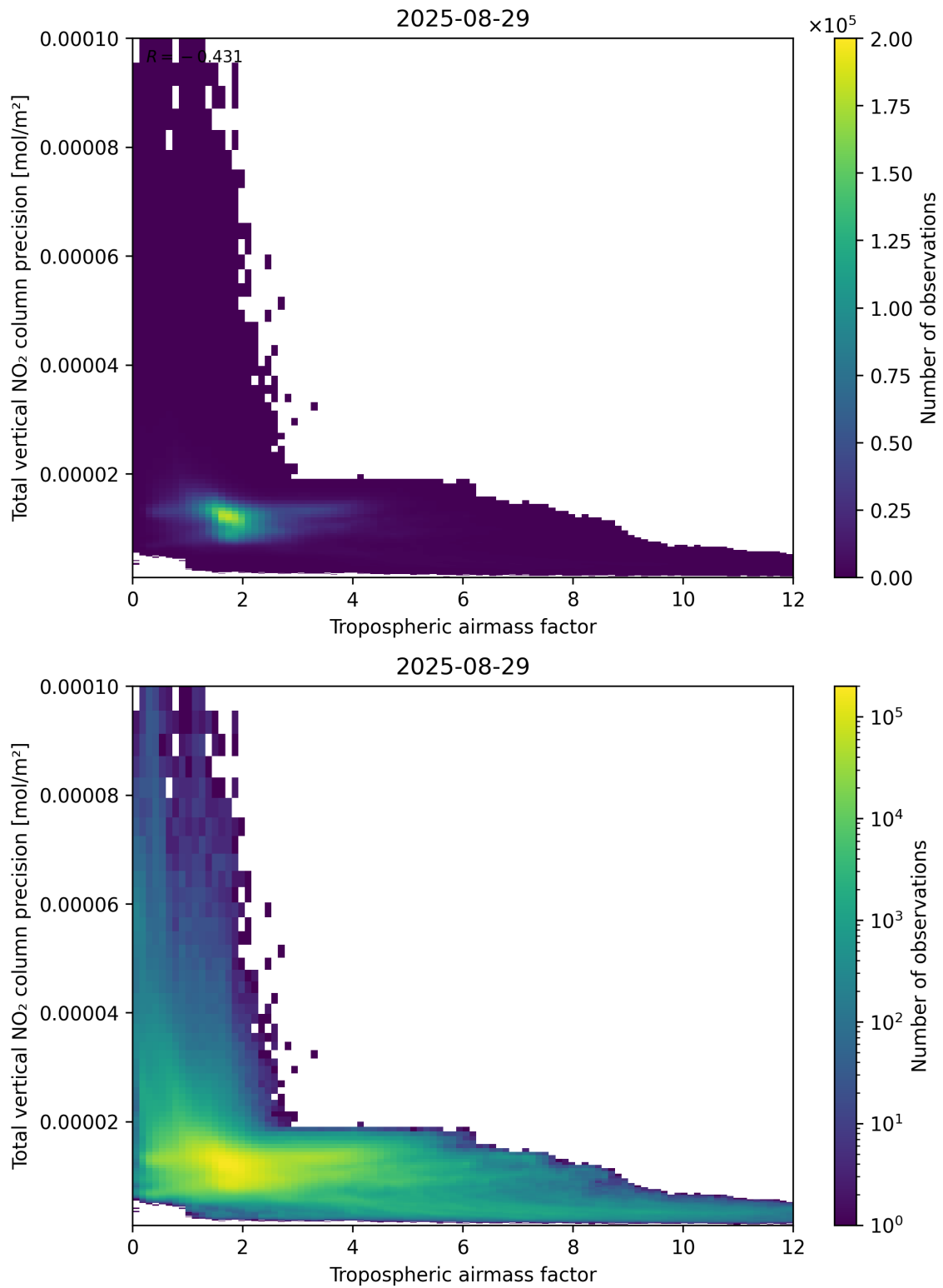
Figure 78: Scatter density plot of “Tropospheric airmass factor” against “Total vertical NO 2 column precision” for 2025-08-28 to 2025-08-30.
