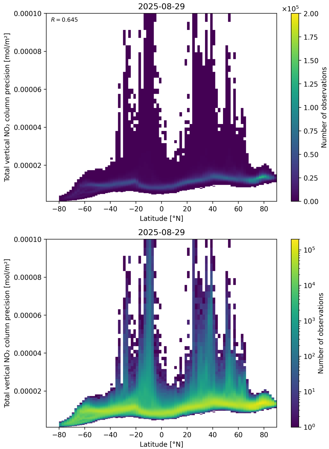
Figure 91: Scatter density plot of “Latitude” against “Total vertical NO 2 column precision” for 2025-08-28 to 2025-08-30.
