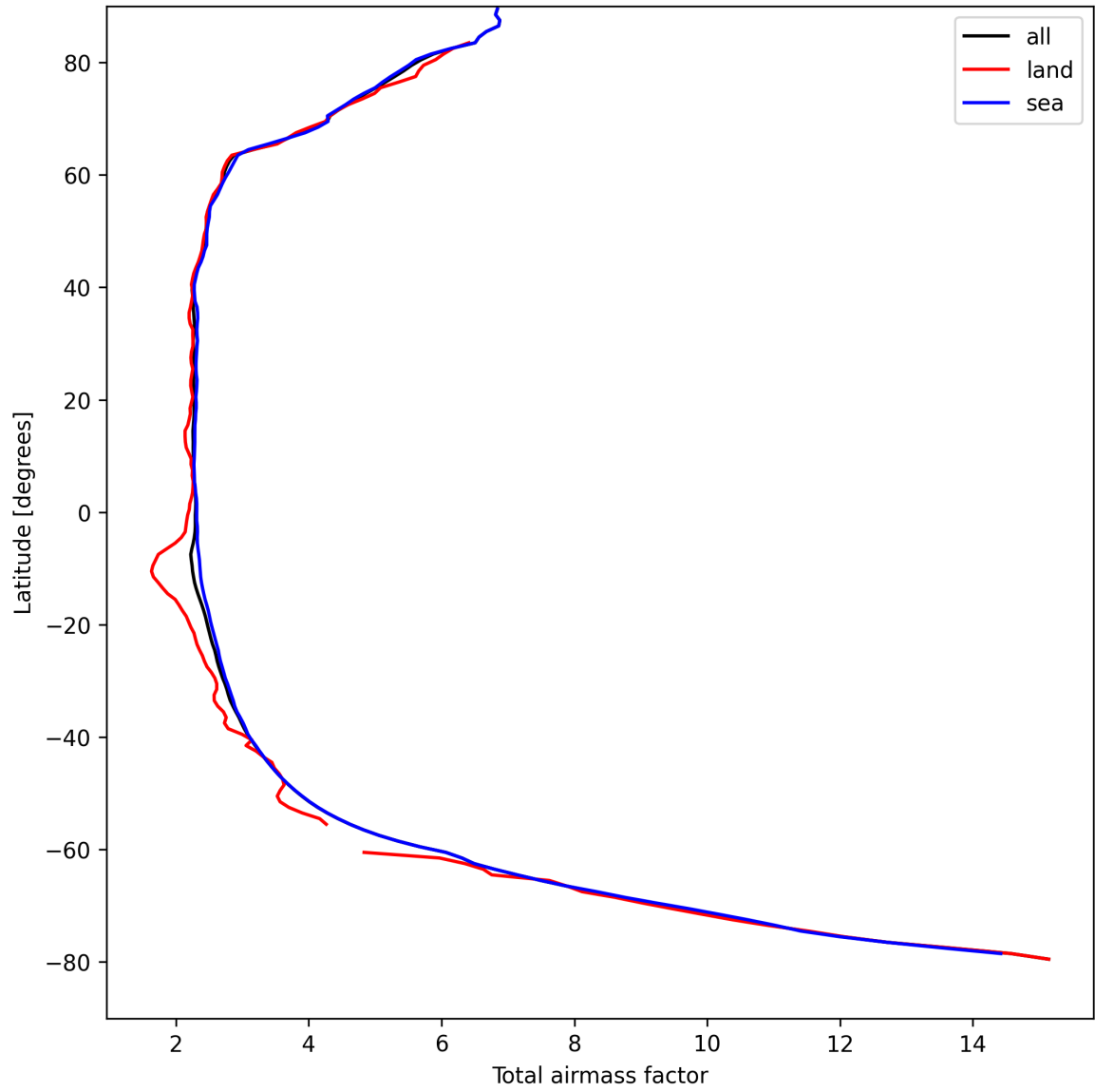
Figure 15: Zonal average of “Total airmass factor” for 2025-08-28 to 2025-08-30.
