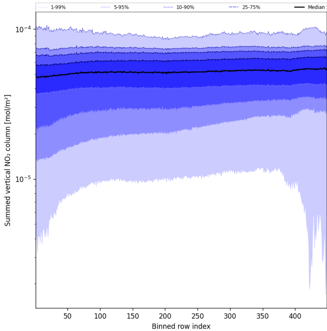
Figure 57: Along track statistics of “Summed vertical NO 2 column” for 2025-08-28 to 2025-08-30
