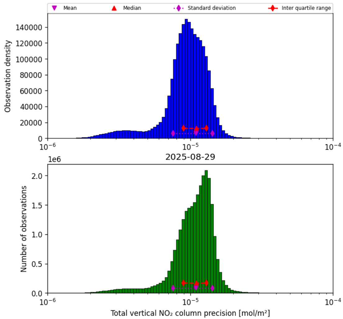
Figure 39: Histogram of “Total vertical NO 2 column precision” for 2025-08-28 to 2025-08-30
