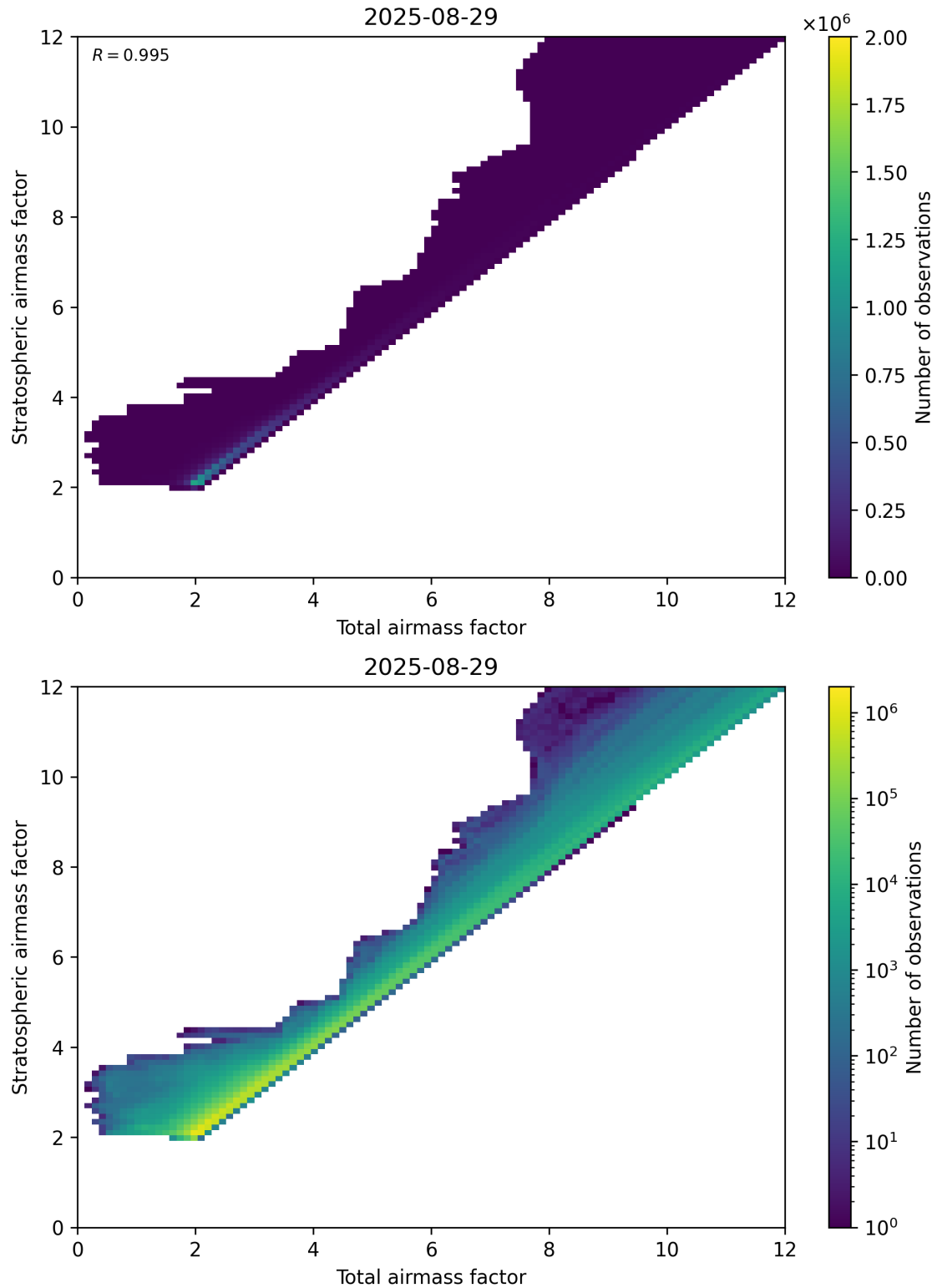
Figure 62: Scatter density plot of “Total airmass factor” against “Stratospheric airmass factor” for 2025-08-28 to 2025-08-30.
