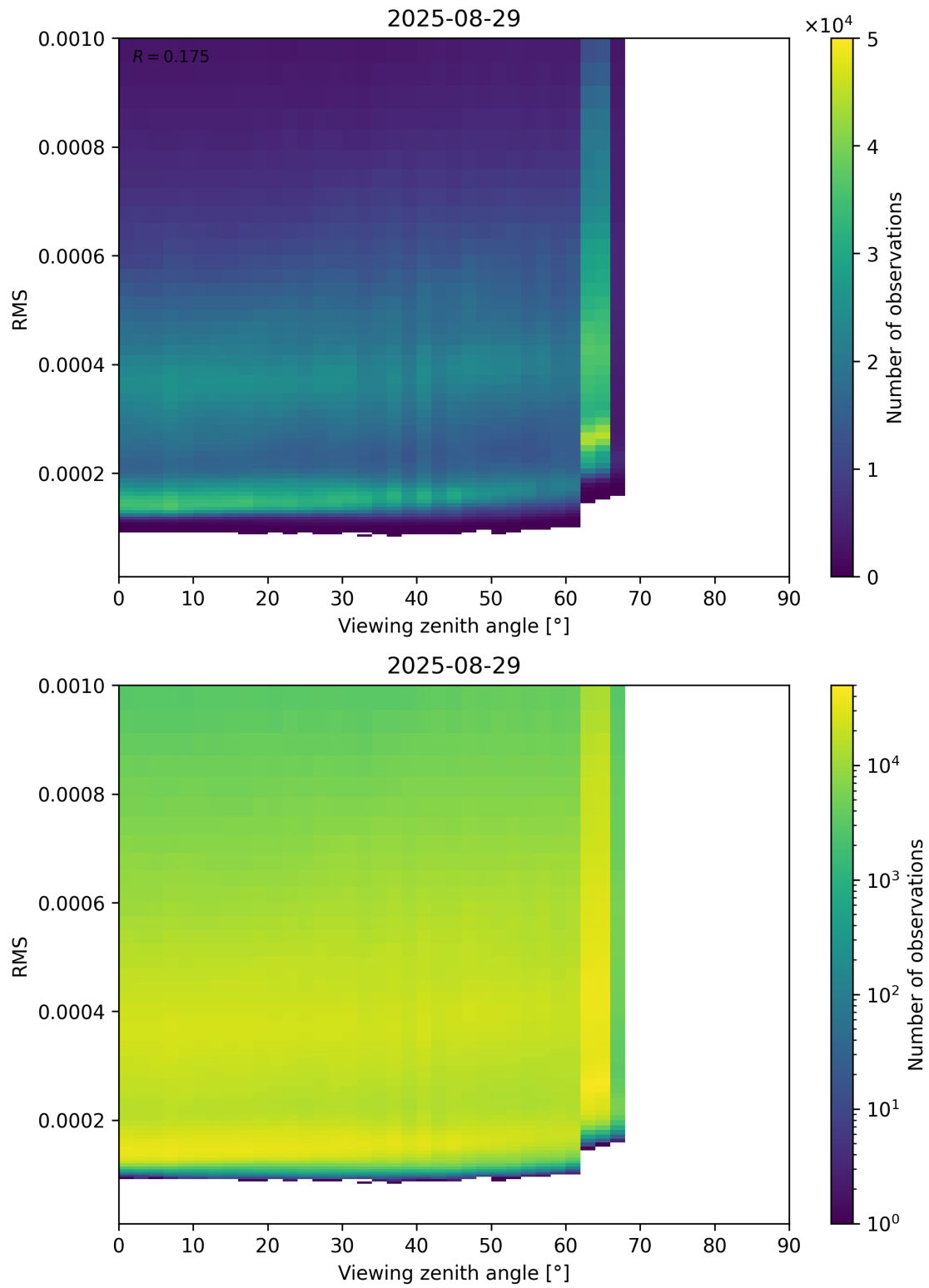
Figure 171: Scatter density plot of “Viewing zenith angle” against “RMS” for 2025-08-28 to 2025-08-30.
