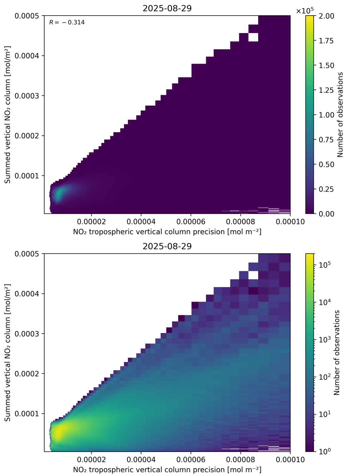
Figure 136: Scatter density plot of “NO 2 tropospheric vertical column precision” against “Summed vertical NO 2 column” for 2025-08-28 to 2025-08-30.
