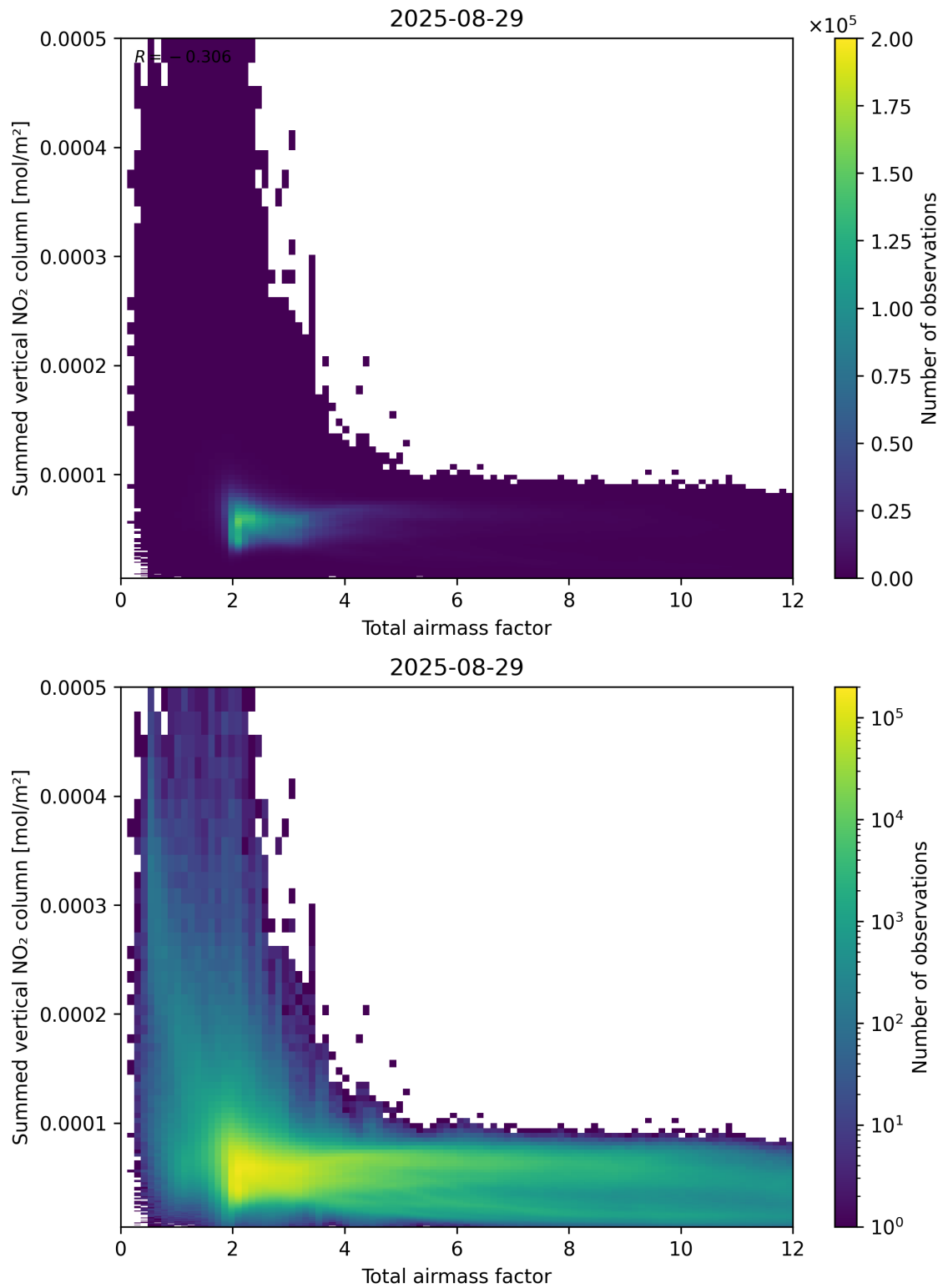
Figure 65: Scatter density plot of “Total airmass factor” against “Summed vertical NO 2 column” for 2025-08-28 to 2025-08-30.
