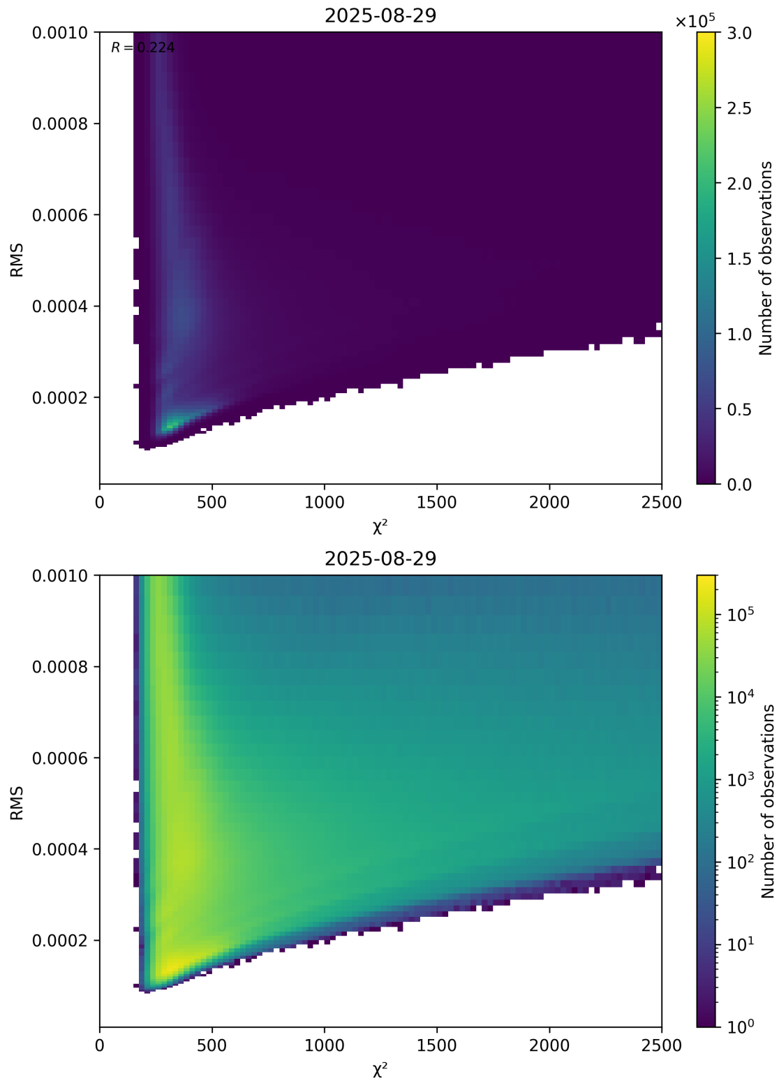
Figure 82: Scatter density plot of “ \chi^2 ” against “RMS” for 2025-08-28 to 2025-08-30.
