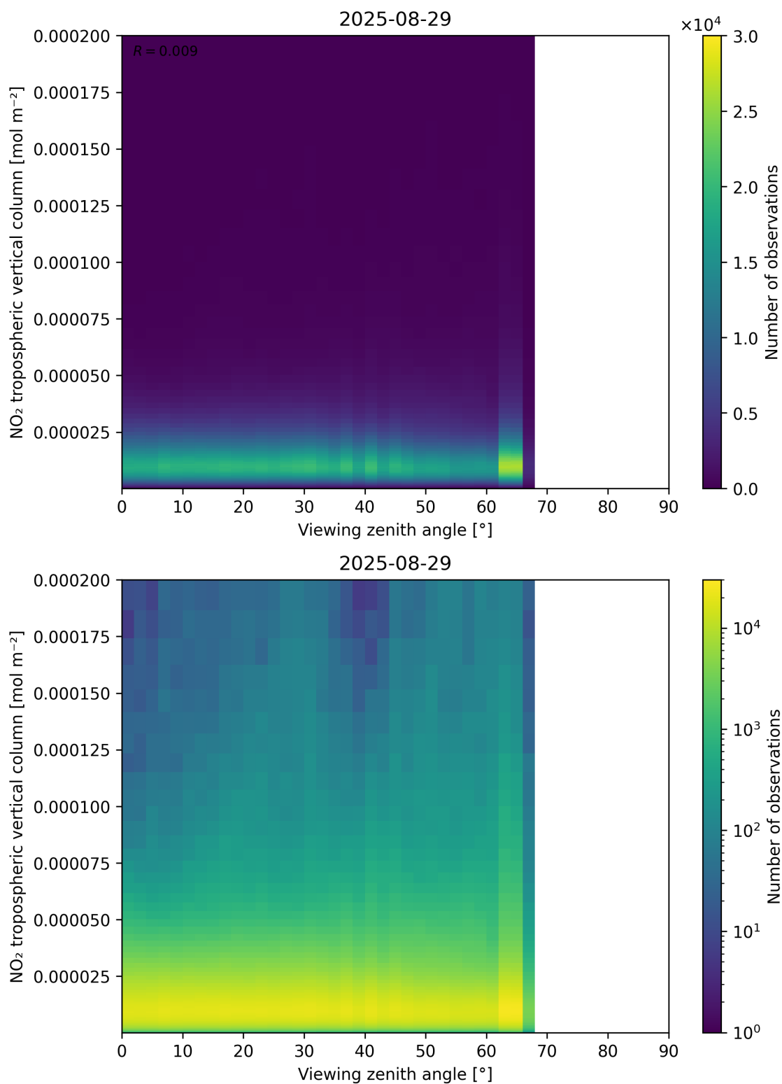
Figure 169: Scatter density plot of “Viewing zenith angle” against “NO 2 tropospheric vertical column” for 2025-08-28 to 2025-08-30.
