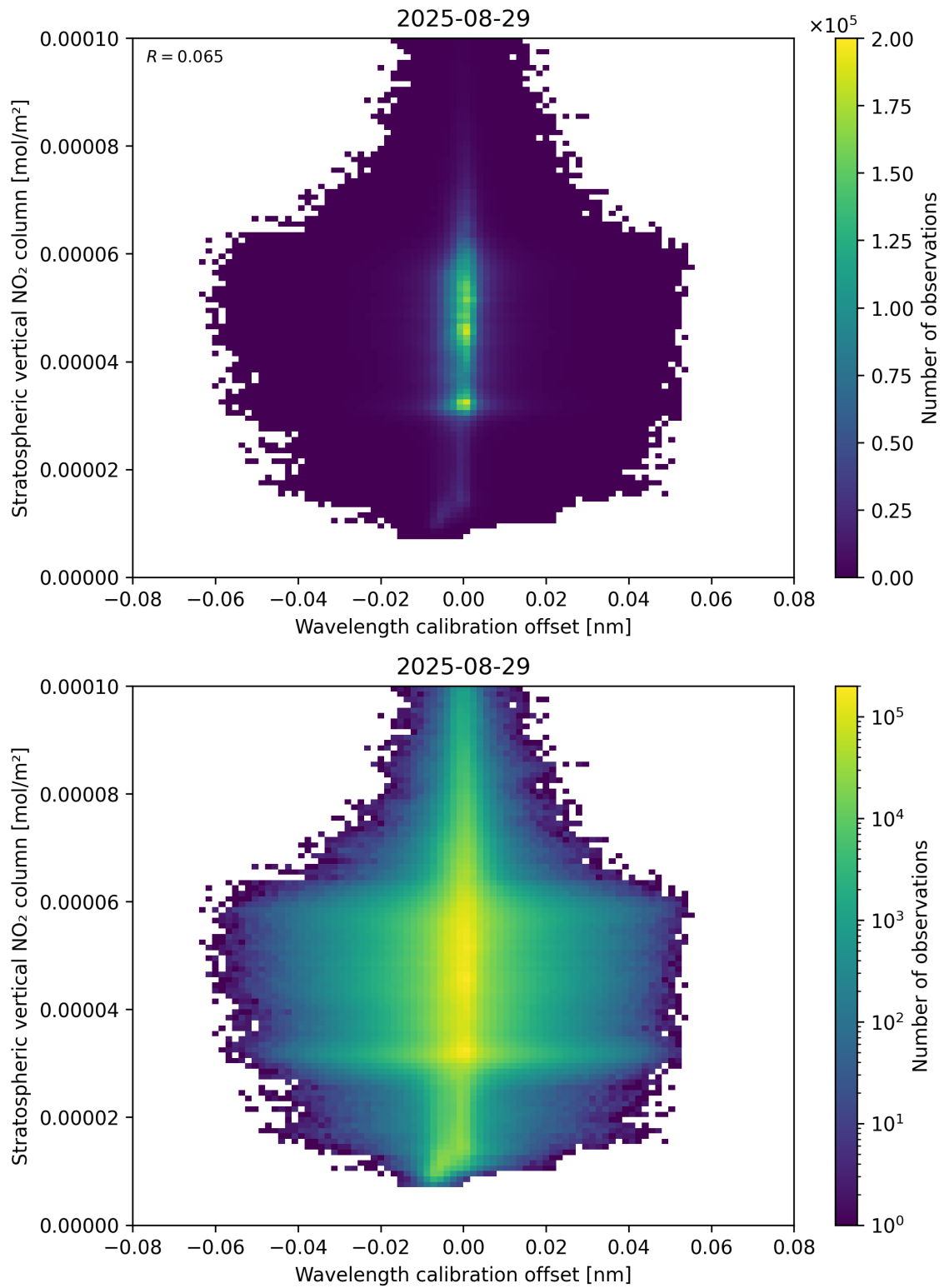
Figure 176: Scatter density plot of “Wavelength calibration offset” against “Stratospheric vertical NO 2 column” for 2025-08-28 to 2025-08-30.
