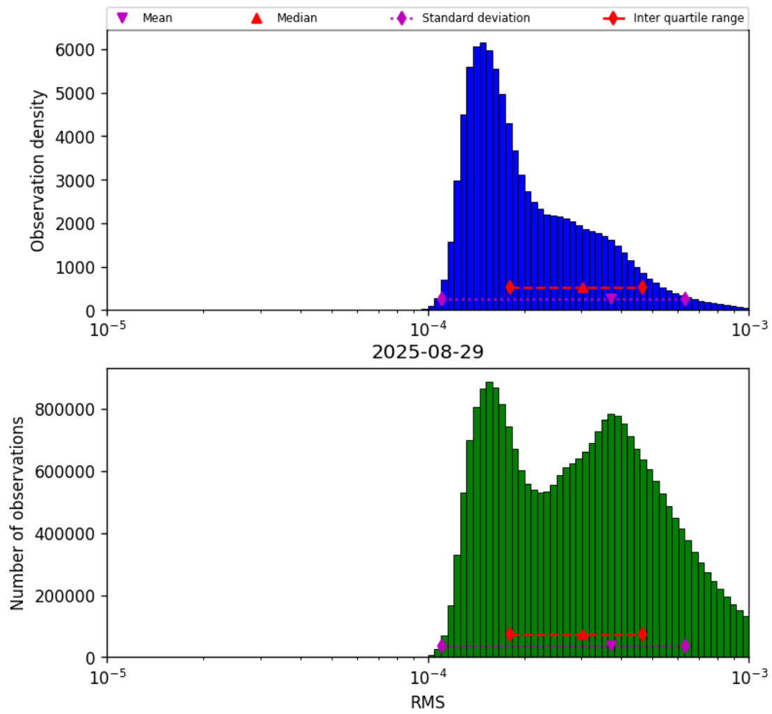
Figure 43: Histogram of “RMS” for 2025-08-28 to 2025-08-30
