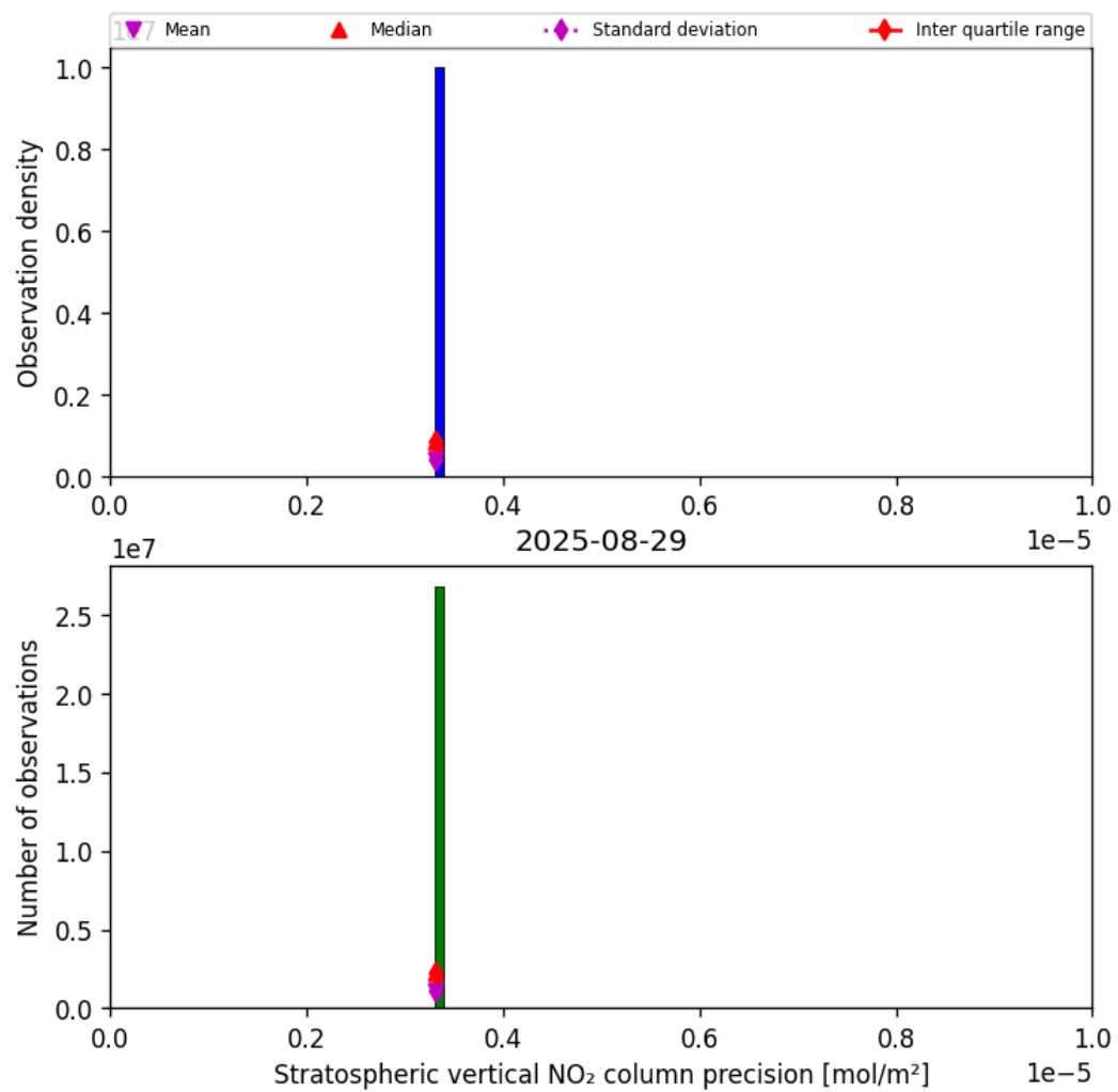
Figure 37: Histogram of “Stratospheric vertical NO 2 column precision” for 2025-08-28 to 2025-08-30
