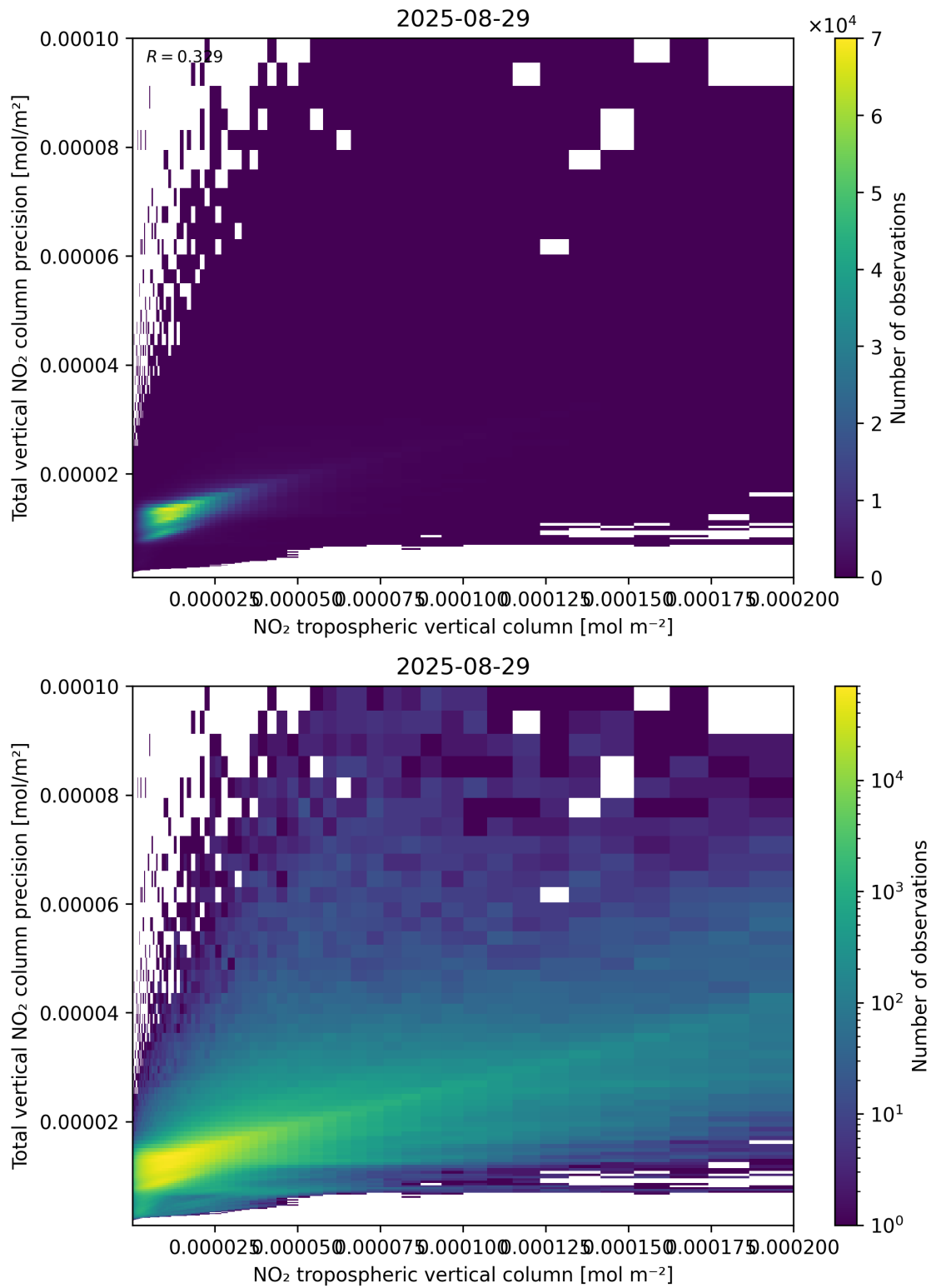
Figure 129: Scatter density plot of “NO 2 tropospheric vertical column” against “Total vertical NO 2 column precision” for 2025-08-28 to 2025-08-30.
