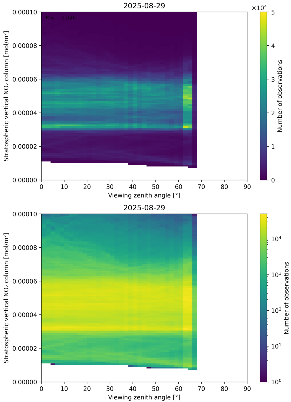
Figure 164: Scatter density plot of “Viewing zenith angle” against “Stratospheric vertical NO 2 column” for 2025-08-28 to 2025-08-30.
