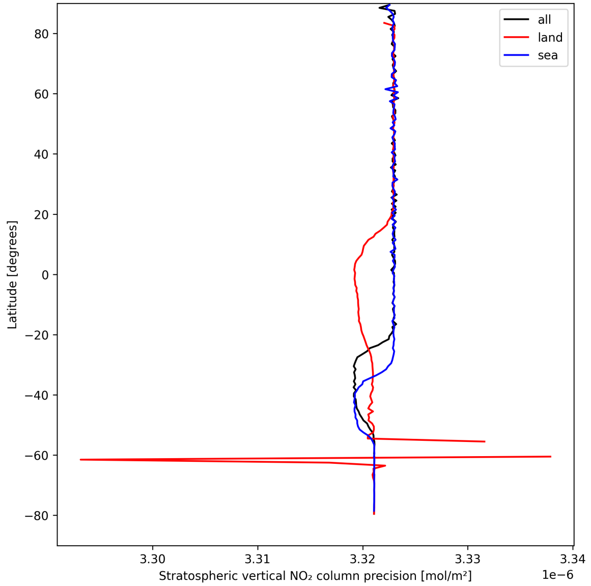
Figure 20: Zonal average of “Stratospheric vertical NO 2 column precision” for 2025-08-28 to 2025-08-30.
