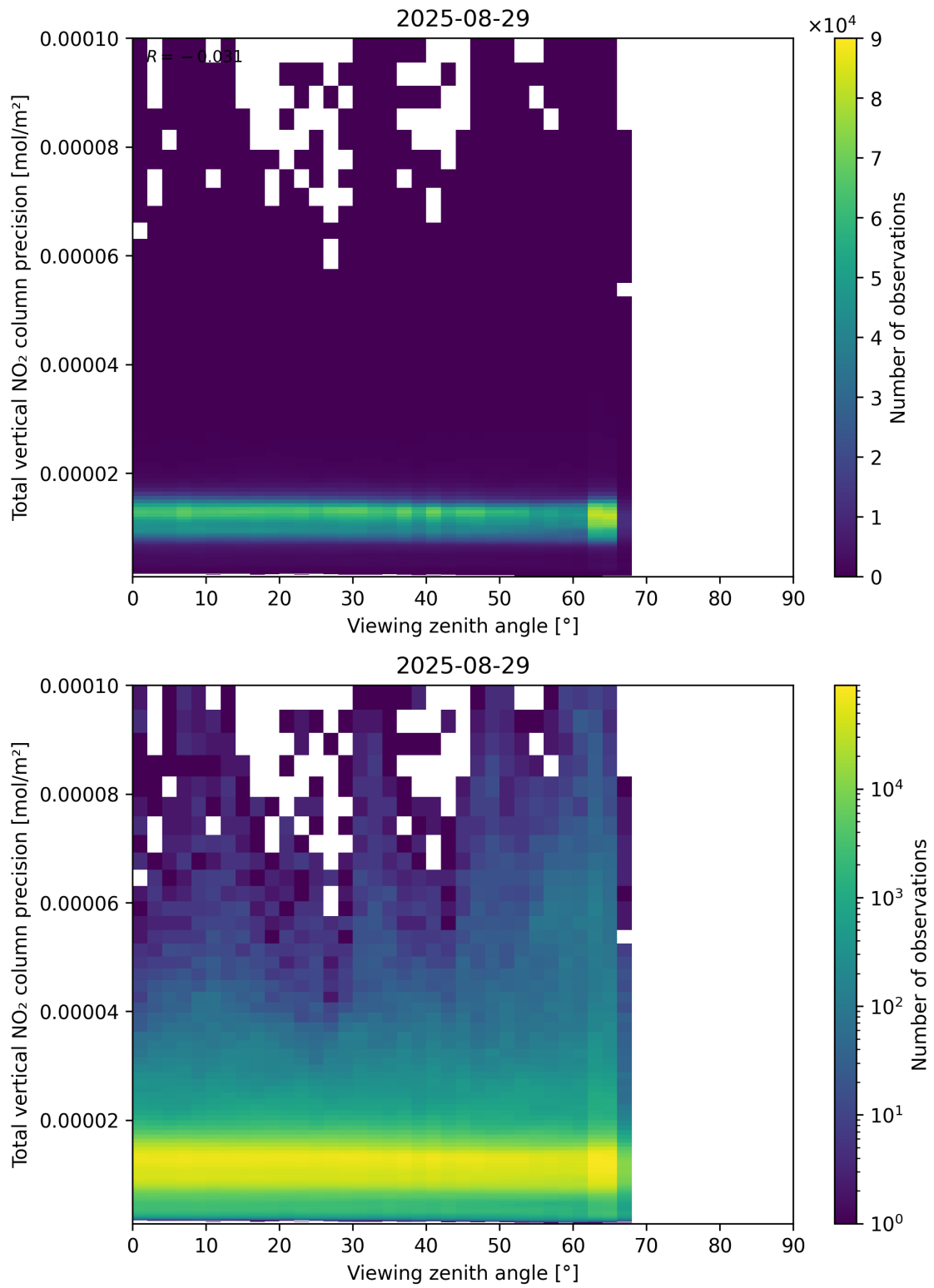
Figure 168: Scatter density plot of “Viewing zenith angle” against “Total vertical NO 2 column precision” for 2025-08-28 to 2025-08-30.
