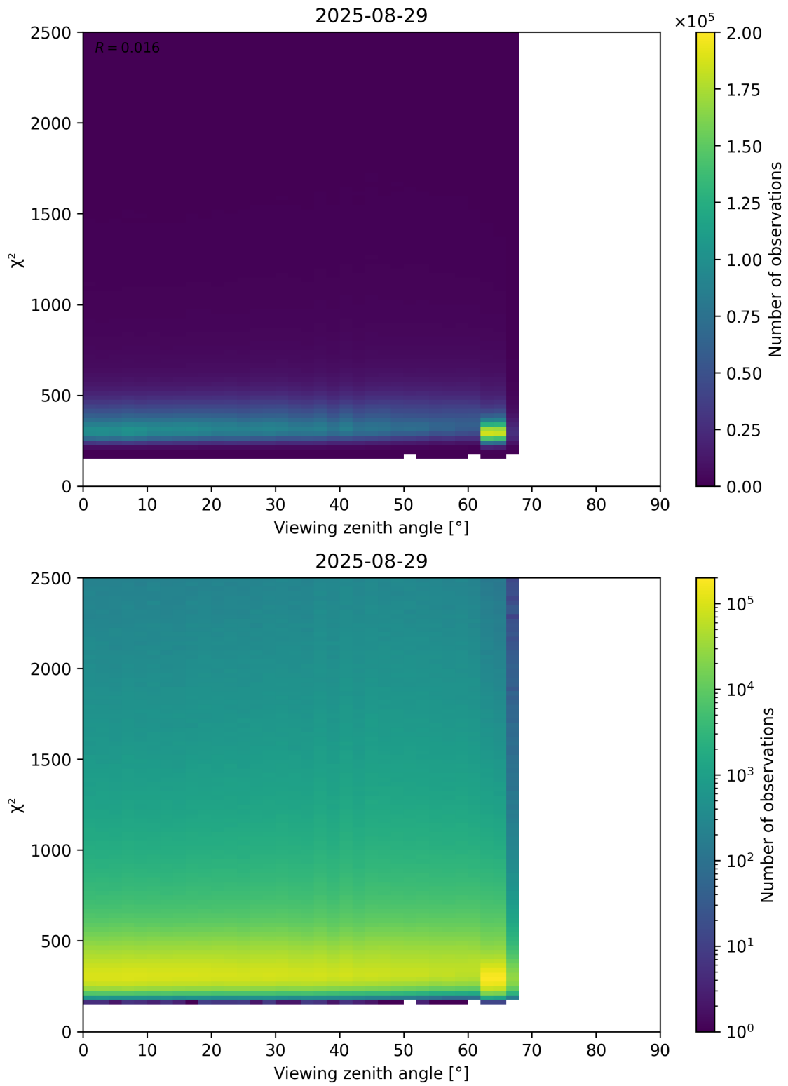
Figure 162: Scatter density plot of “Viewing zenith angle” against “ \chi^2 ” for 2025-08-28 to 2025-08-30.
