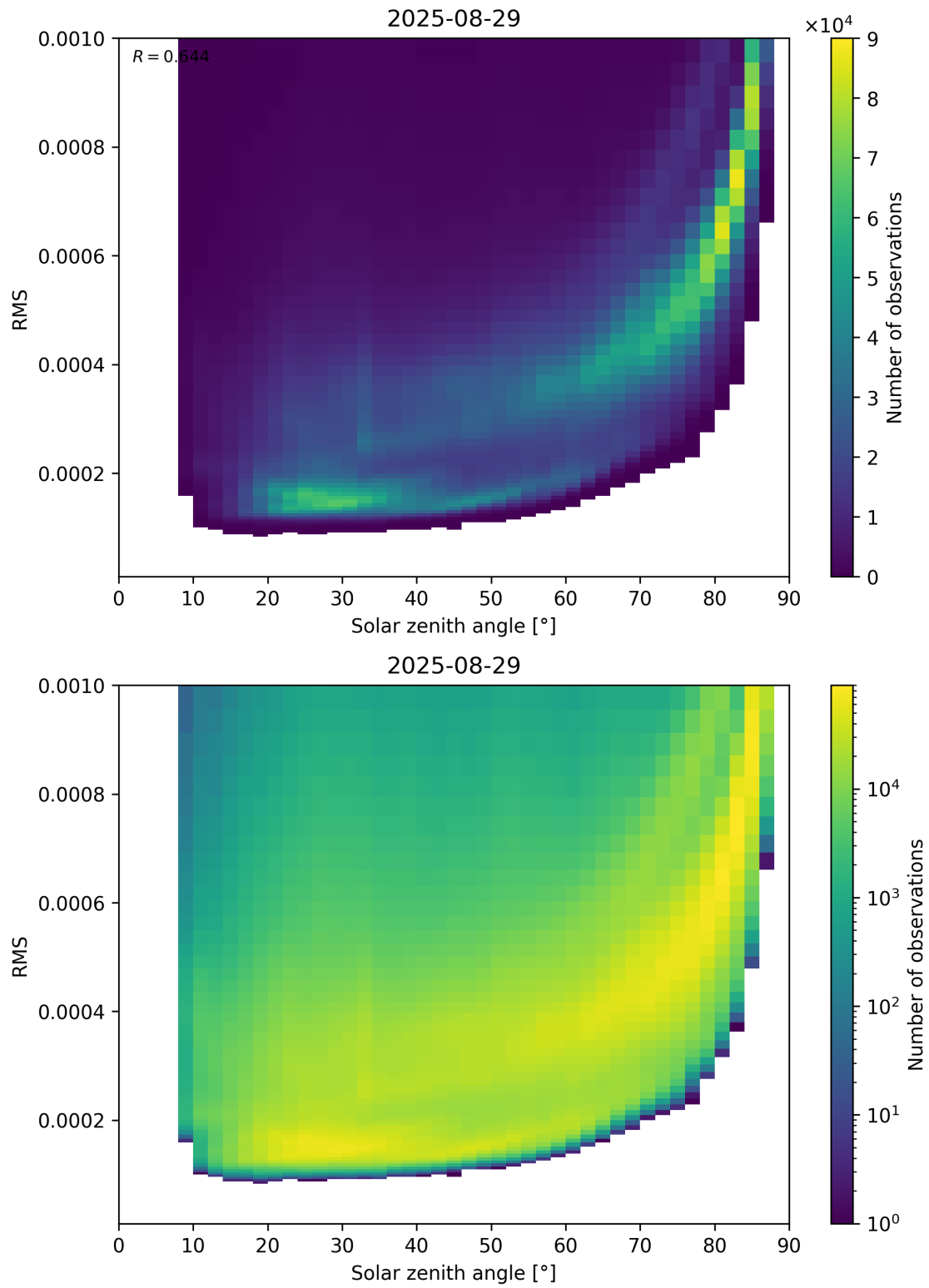
Figure 157: Scatter density plot of “Solar zenith angle” against “RMS” for 2025-08-28 to 2025-08-30.
