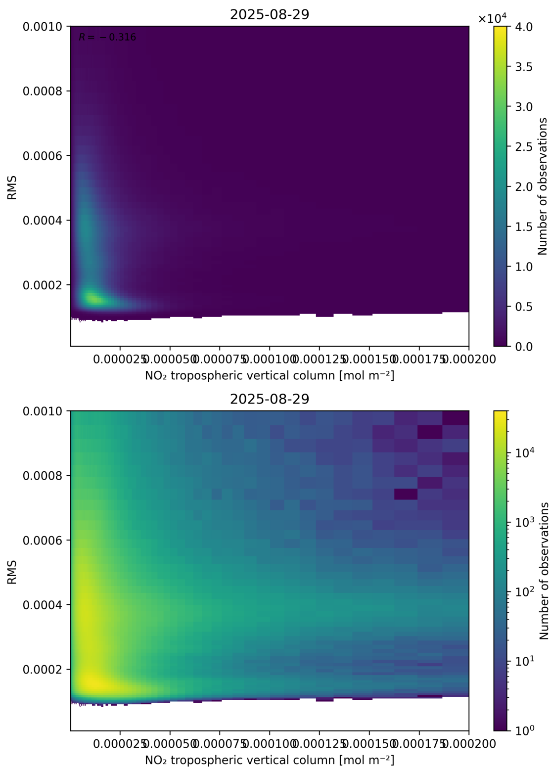
Figure 142: Scatter density plot of “NO 2 tropospheric vertical column” against “RMS” for 2025-08-28 to 2025-08-30.
