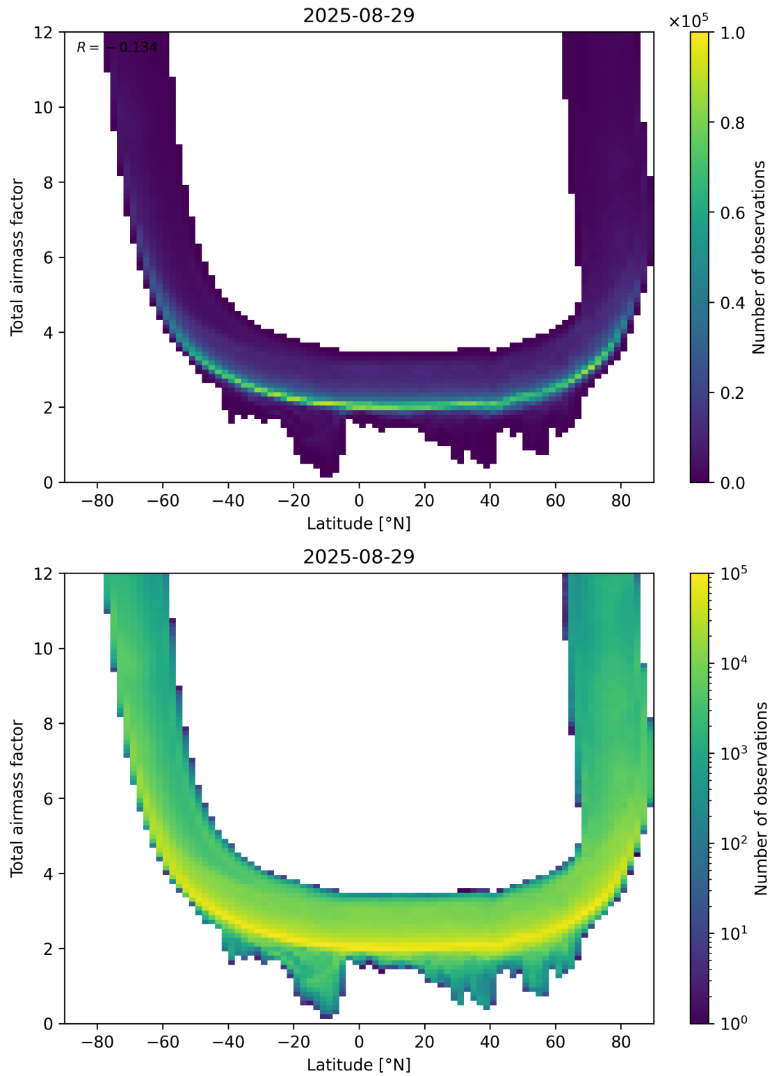
Figure 84: Scatter density plot of “Latitude” against “Total airmass factor” for 2025-08-28 to 2025-08-30.
