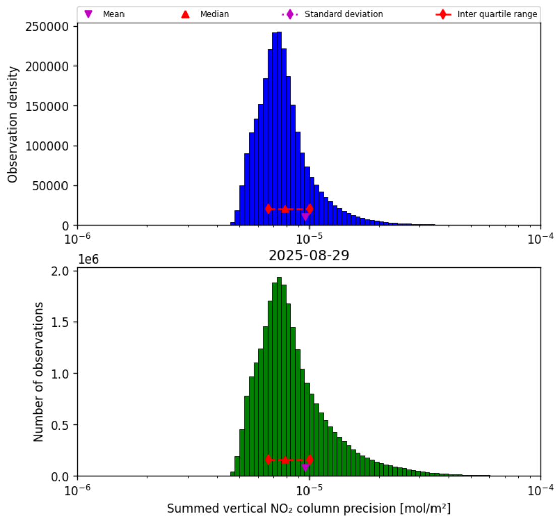
Figure 41: Histogram of “Summed vertical NO 2 column precision” for 2025-08-28 to 2025-08-30
