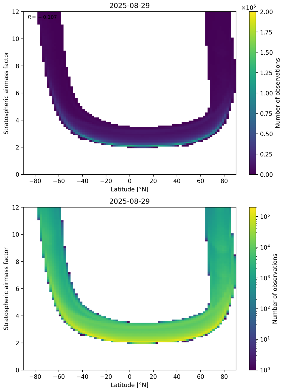
Figure 83: Scatter density plot of “Latitude” against “Stratospheric air mass factor” for 2025-08-28 to 2025-08-30.
