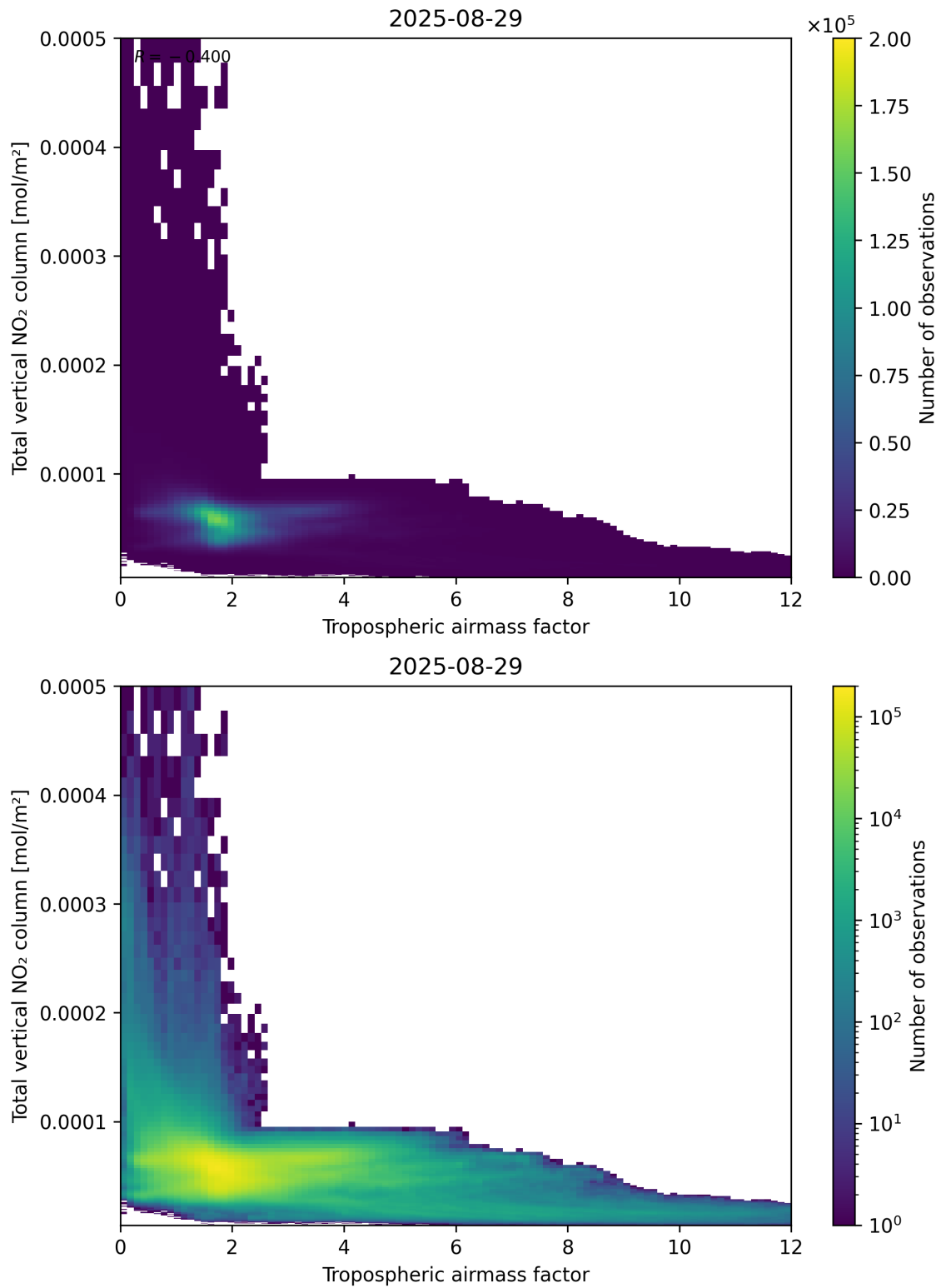
Figure 77: Scatter density plot of “Tropospheric airmass factor” against “Total vertical NO 2 column” for 2025-08-28 to 2025-08-30.
