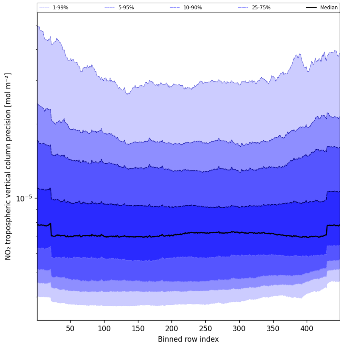
Figure 47: Along track statistics of “NO 2 tropospheric vertical column precision” for 2025-08-28 to 2025-08-30
