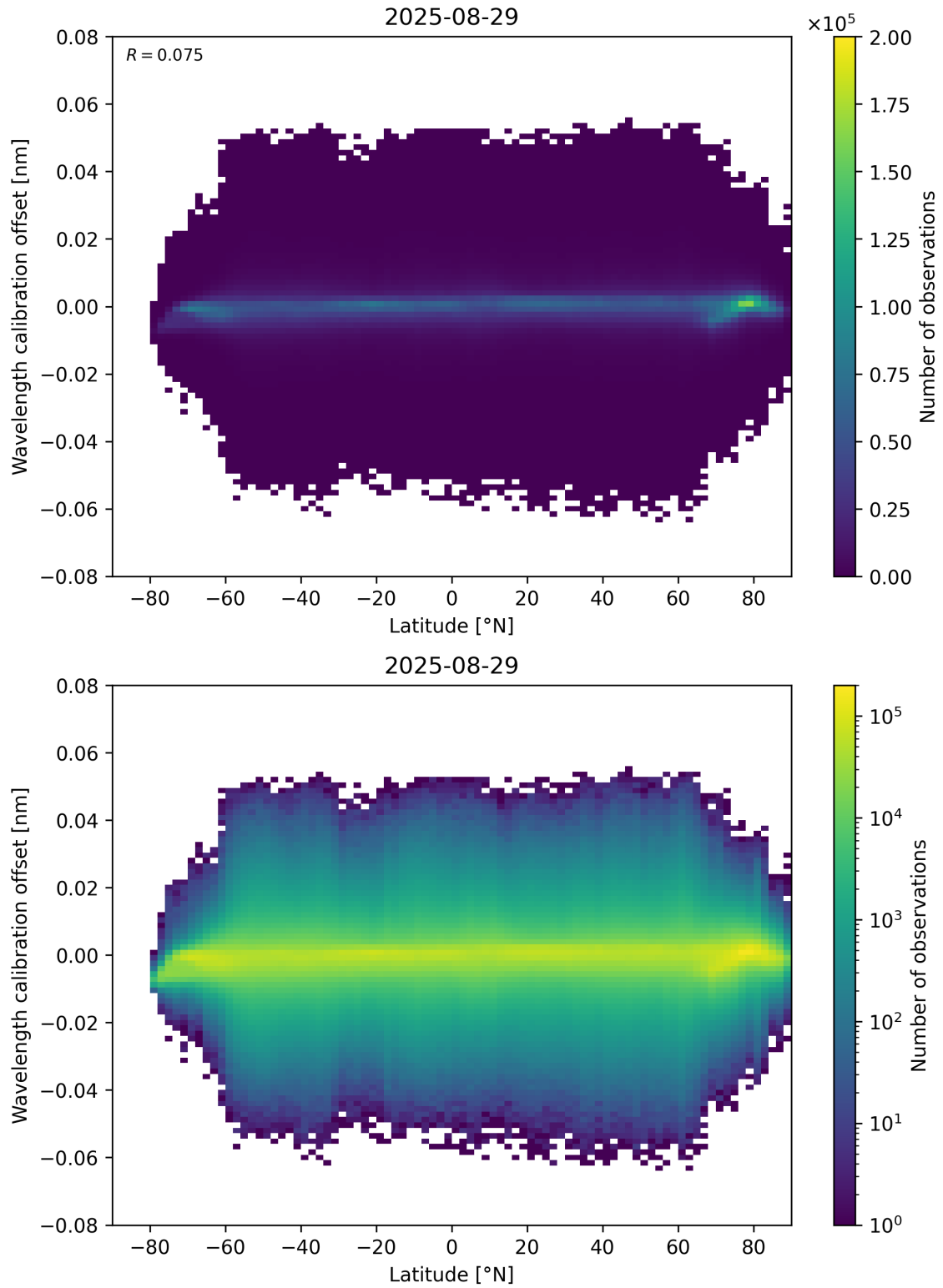
Figure 95: Scatter density plot of “Latitude” against “Wavelength calibration offset” for 2025-08-28 to 2025-08-30.
