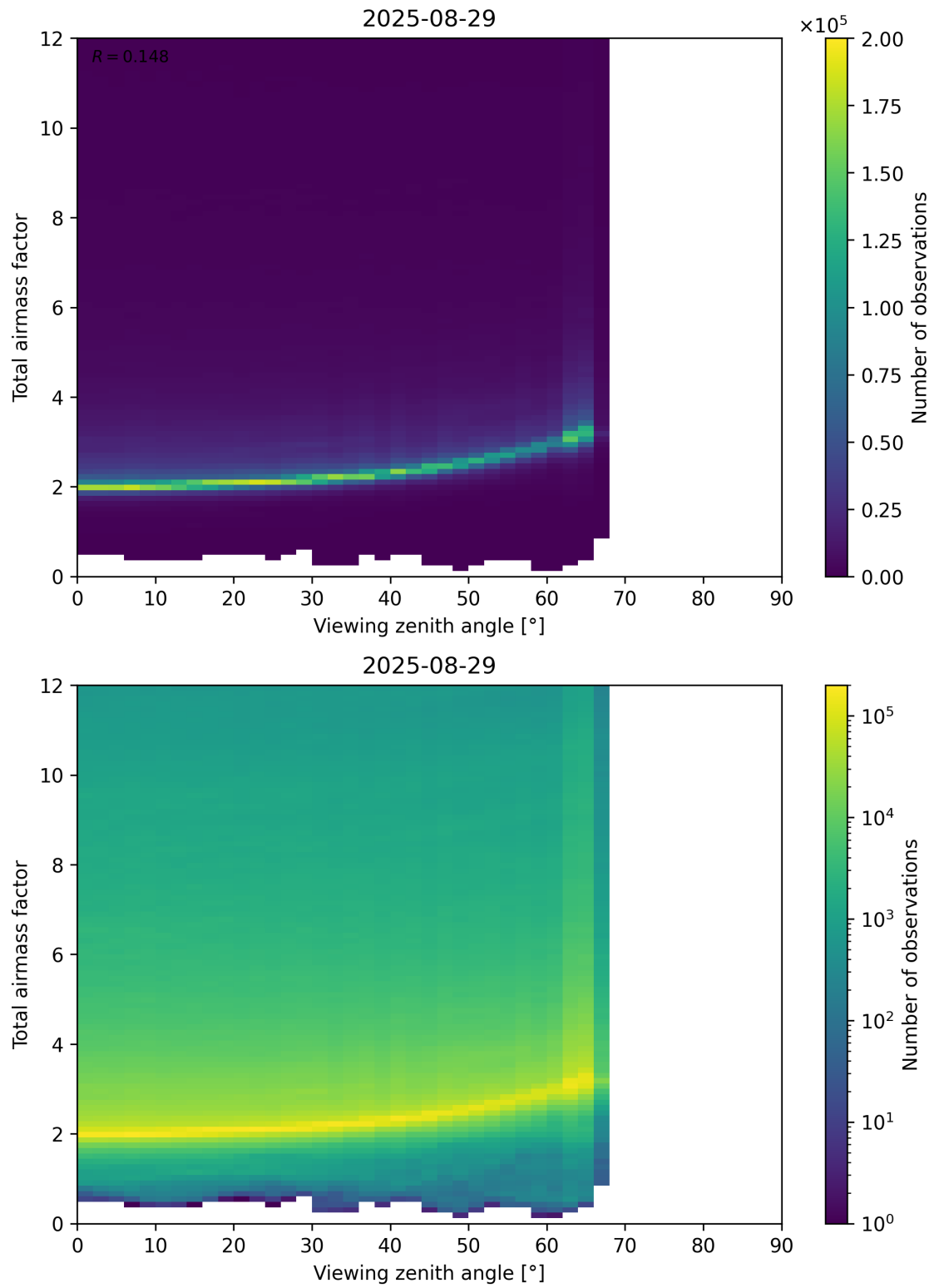
Figure 160: Scatter density plot of “Viewing zenith angle” against “Total airmass factor” for 2025-08-28 to 2025-08-30.
