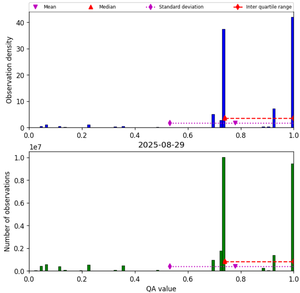
Figure 28: Histogram of “QA value” for 2025-08-28 to 2025-08-30
