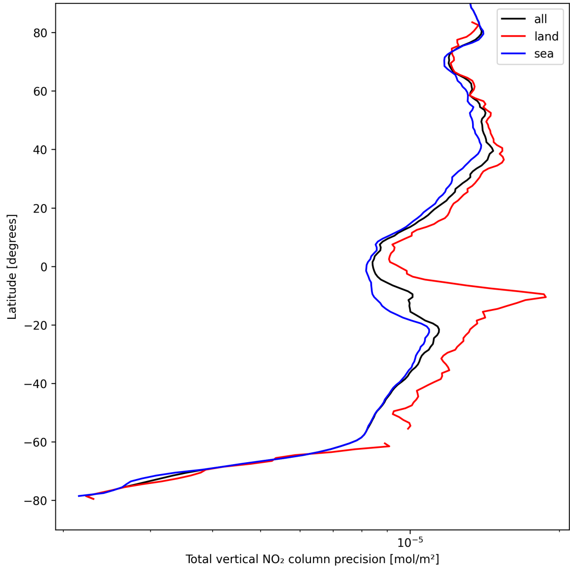
Figure 22: Zonal average of “Total vertical NO 2 column precision” for 2025-08-28 to 2025-08-30.
