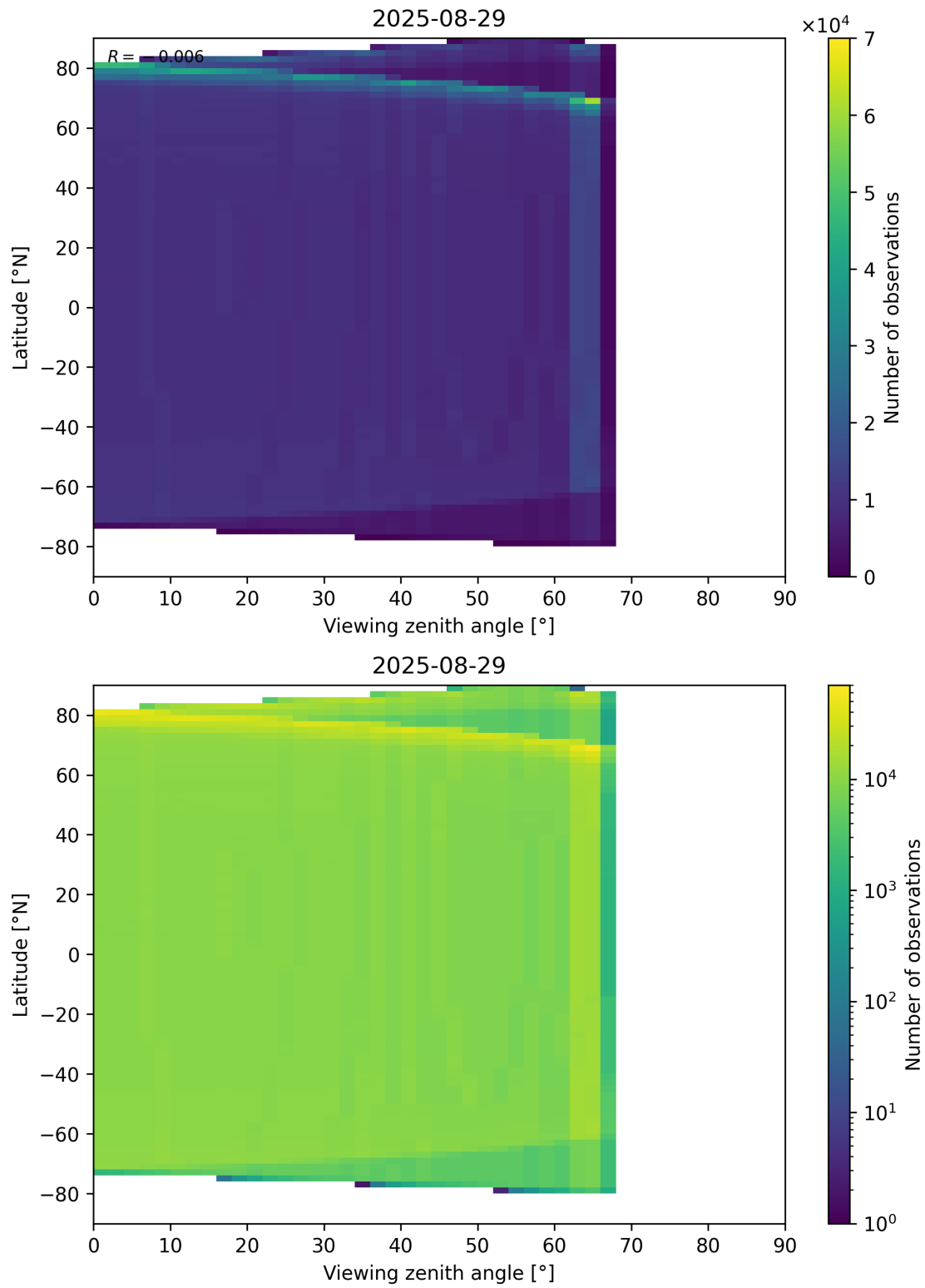
Figure 163: Scatter density plot of “Viewing zenith angle” against “Latitude” for 2025-08-28 to 2025-08-30.
