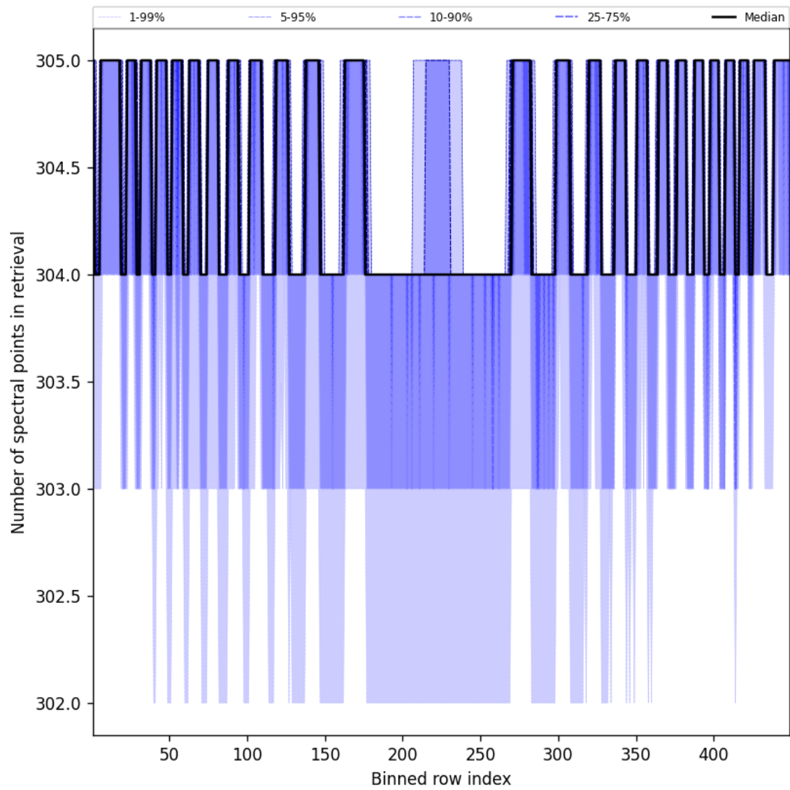
Figure 50: Along track statistics of “Number of spectral points in retrieval” for 2025-08-28 to 2025-08-30
