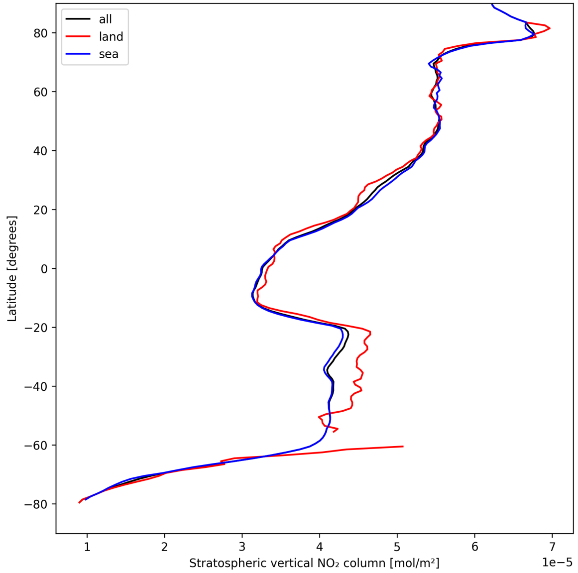
Figure 19: Zonal average of “Stratospheric vertical NO 2 column” for 2025-08-28 to 2025-08-30.
