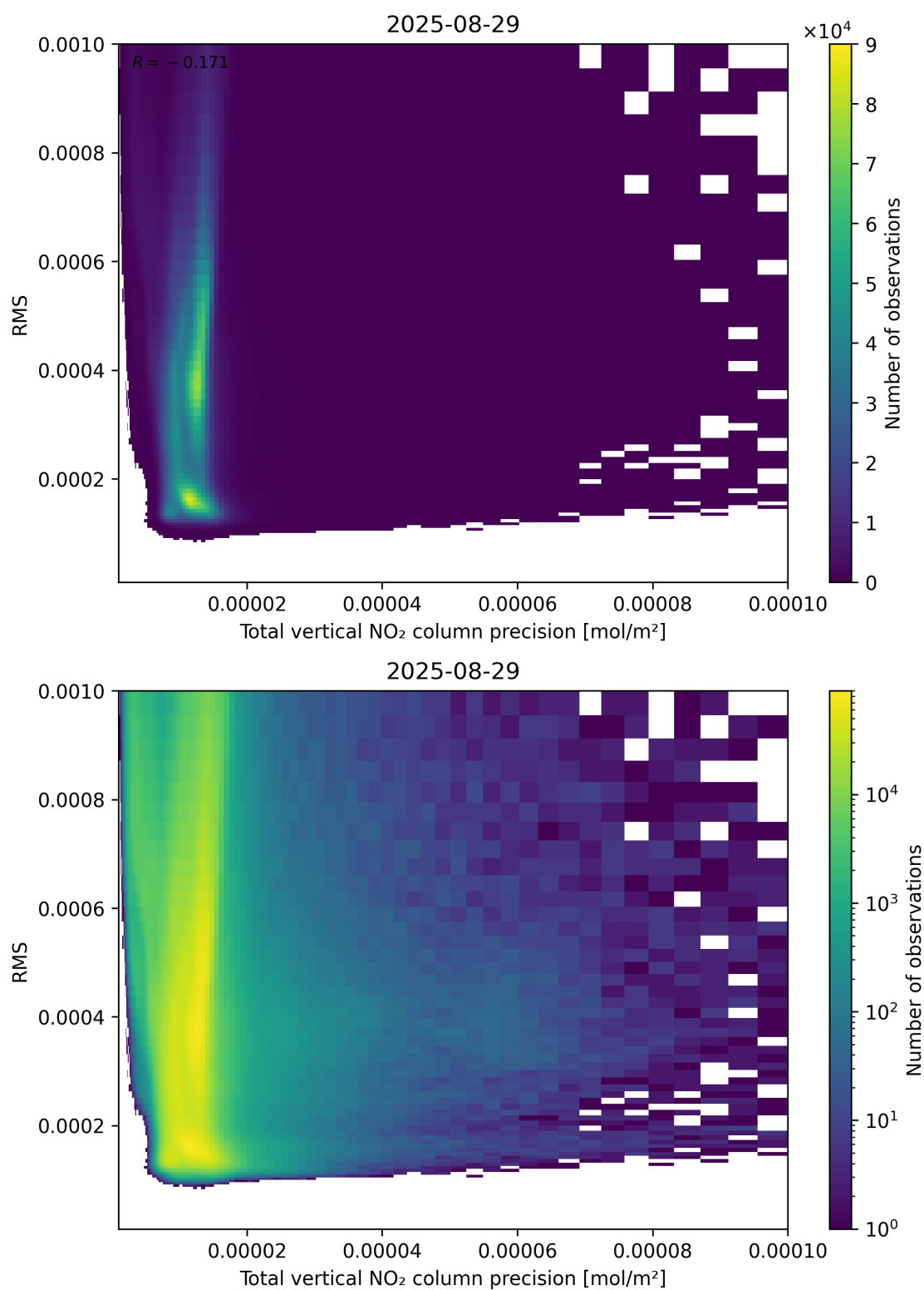
Figure 119: Scatter density plot of “Total vertical NO 2 column precision” against “RMS” for 2025-08-28 to 2025-08-30.
