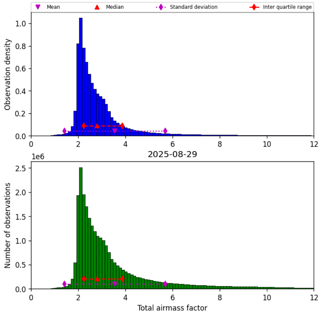
Figure 32: Histogram of “Total airmass factor” for 2025-08-28 to 2025-08-30
