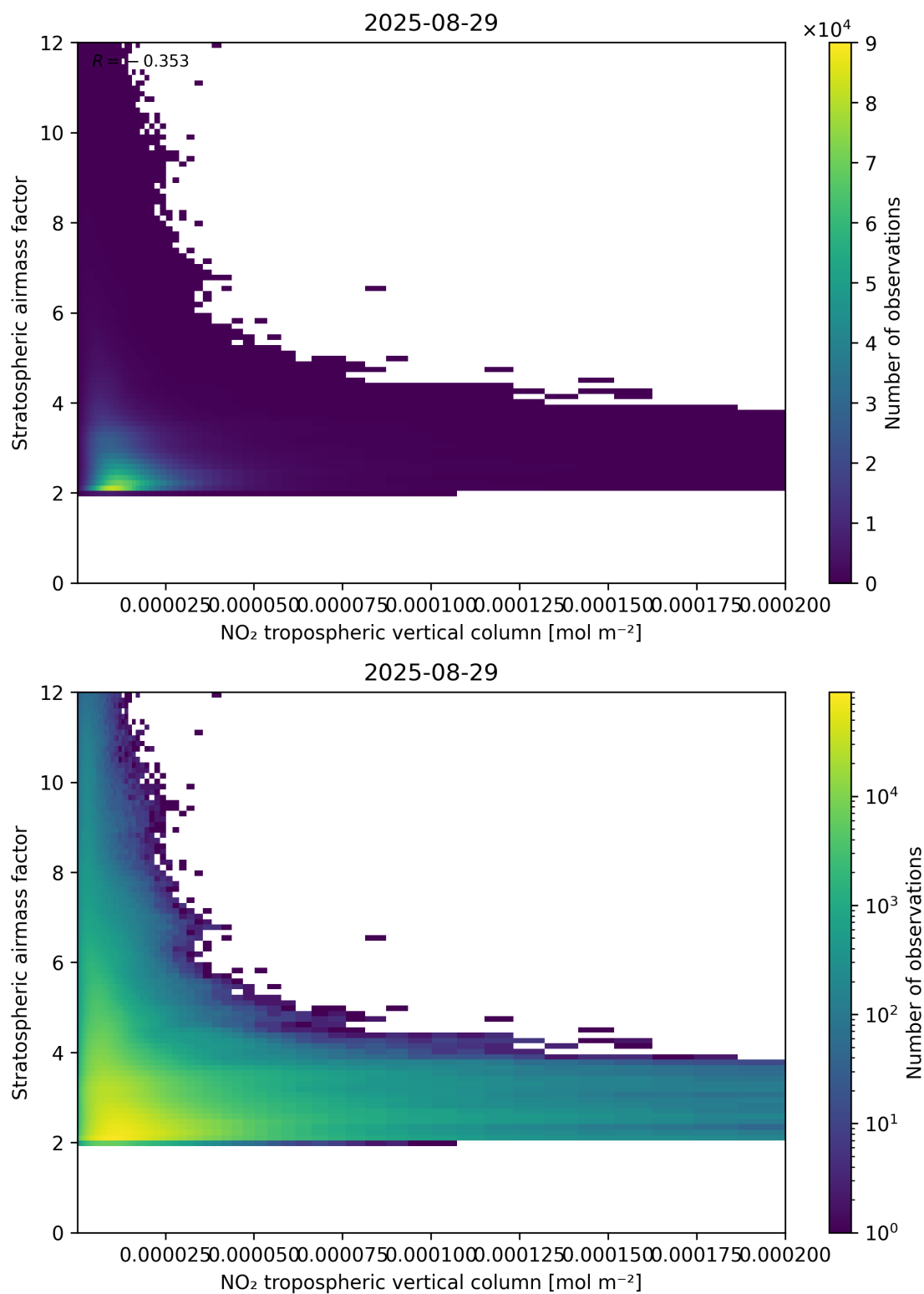
Figure 121: Scatter density plot of “NO 2 tropospheric vertical column” against “Stratospheric airmass factor” for 2025-08-28 to 2025-08-30.
