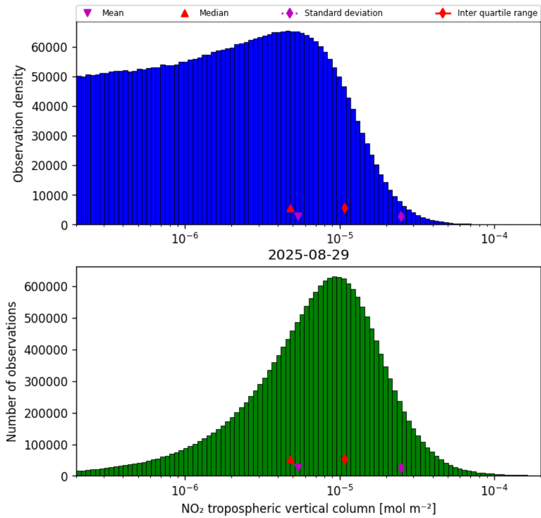
Figure 29: Histogram of “NO 2 tropospheric vertical column” for 2025-08-28 to 2025-08-30
