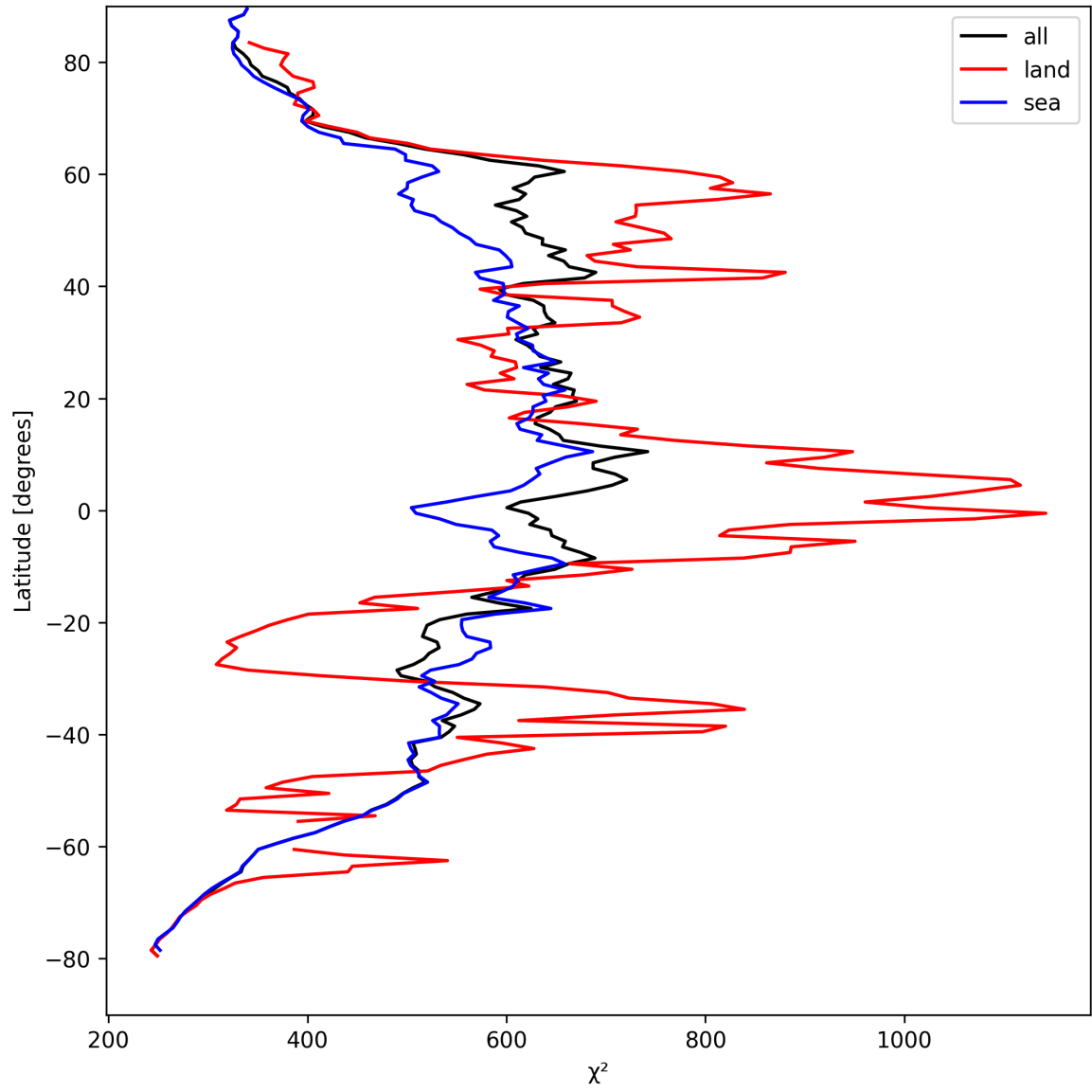
Figure 25: Zonal average of “ \chi^2 ” for 2025-08-28 to 2025-08-30.
