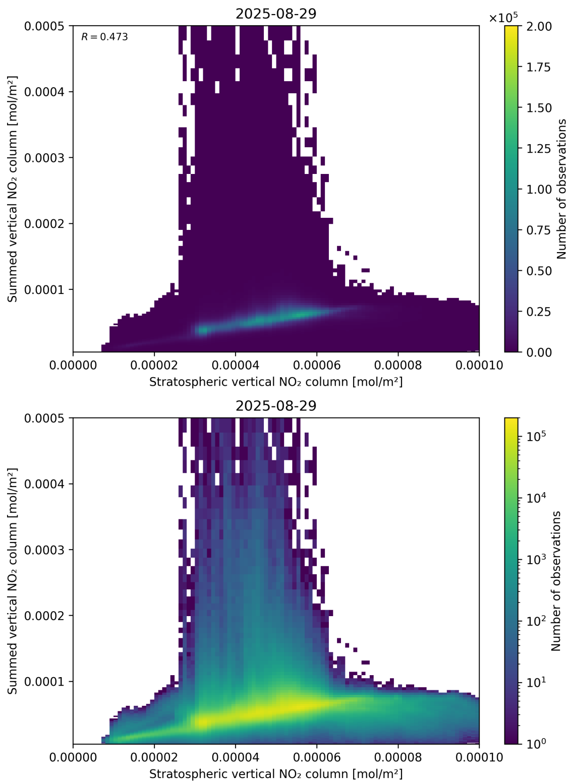
Figure 98: Scatter density plot of “Stratospheric vertical NO 2 column” against “Summed vertical NO 2 column” for 2025-08-28 to 2025-08-30.
