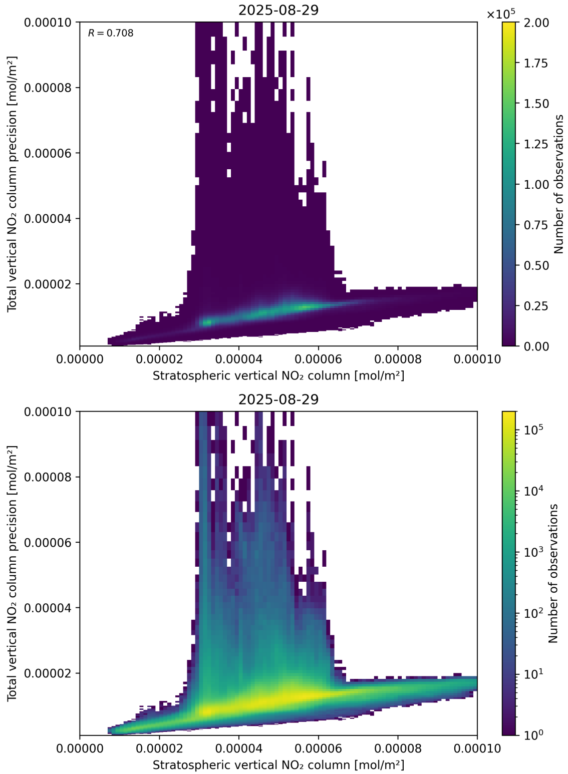
Figure 101: Scatter density plot of “Stratospheric vertical NO 2 column” against “Total vertical NO 2 column precision” for 2025-08-28 to 2025-08-30.
