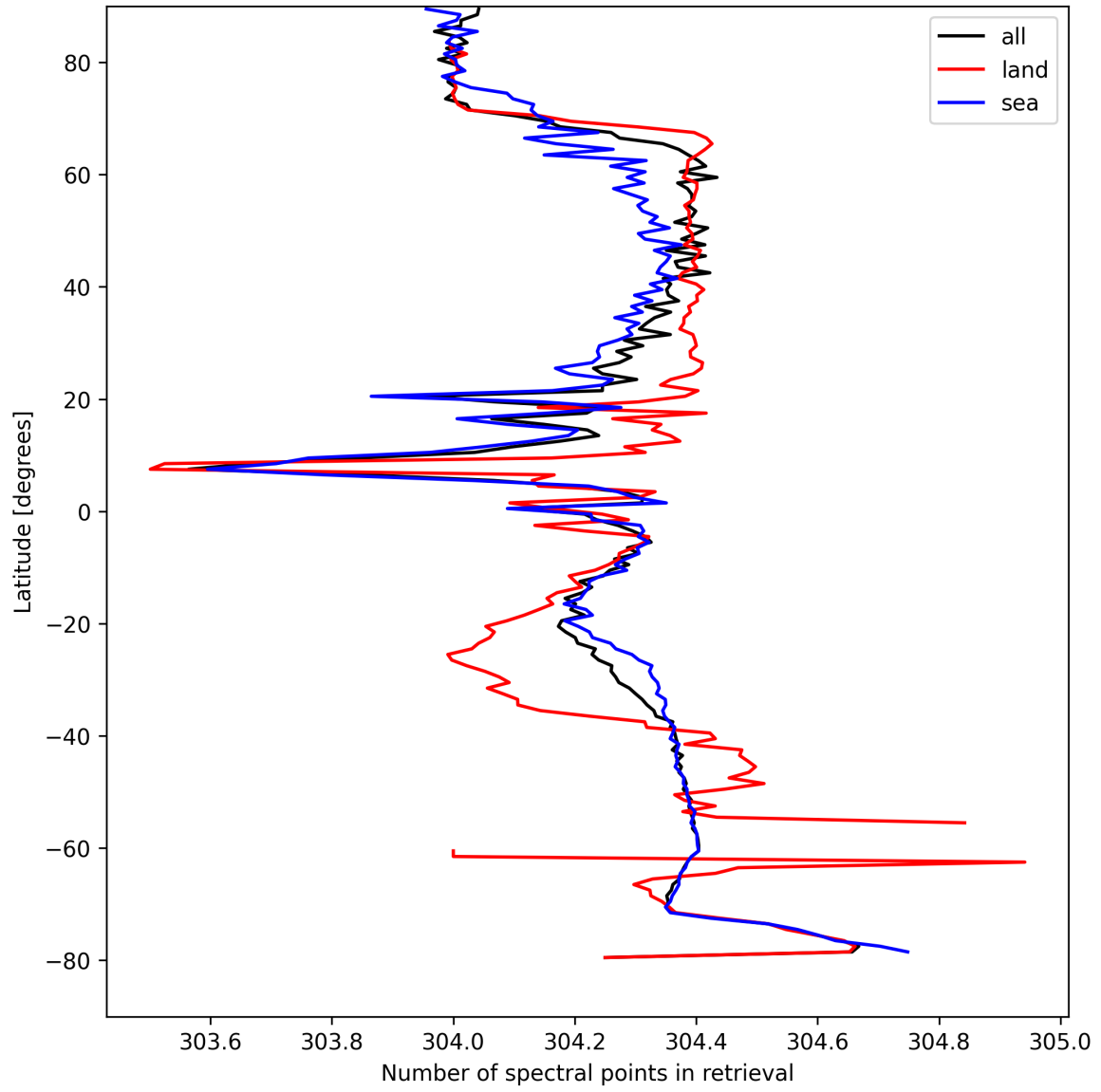
Figure 16: Zonal average of “Number of spectral points in retrieval” for 2025-08-28 to 2025-08-30.
