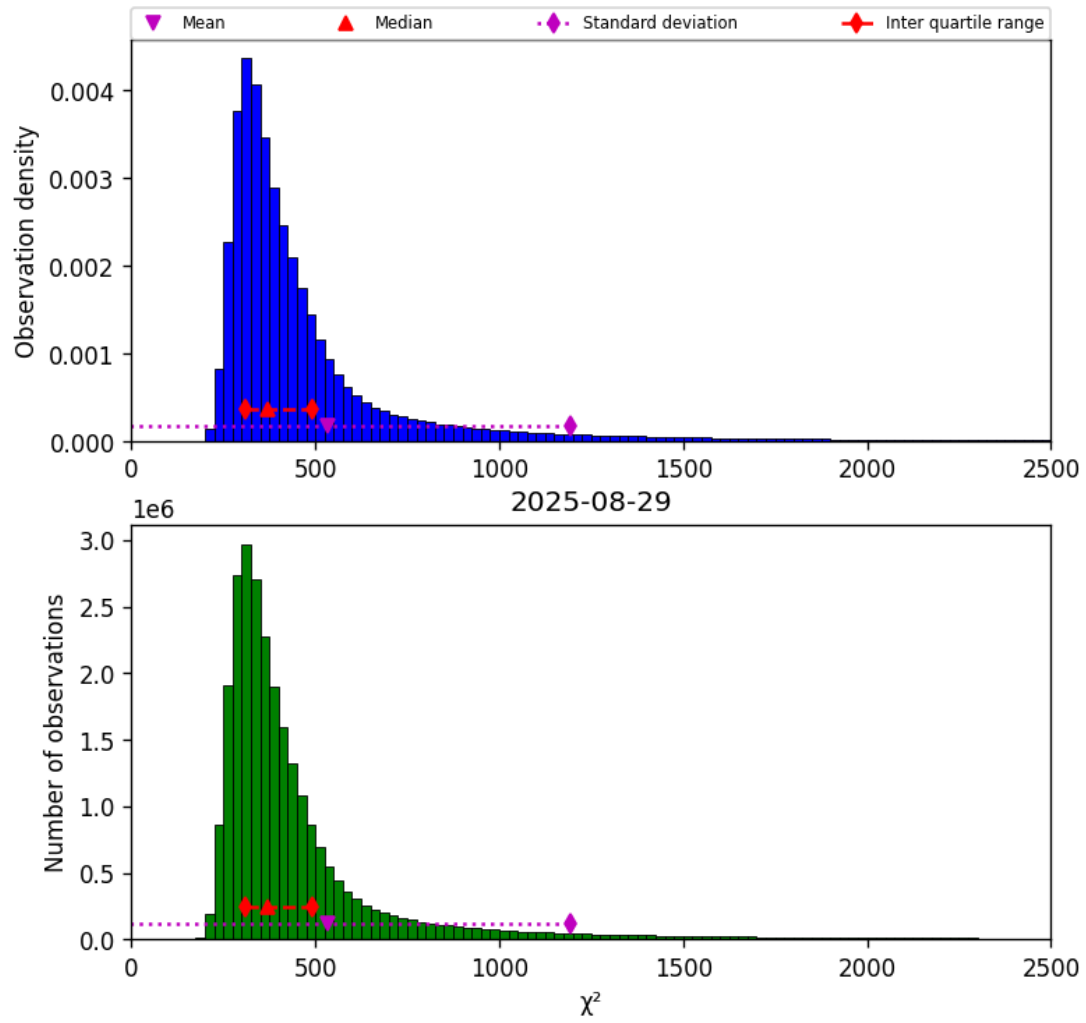
Figure 42: Histogram of “ \chi^2 ” for 2025-08-28 to 2025-08-30
