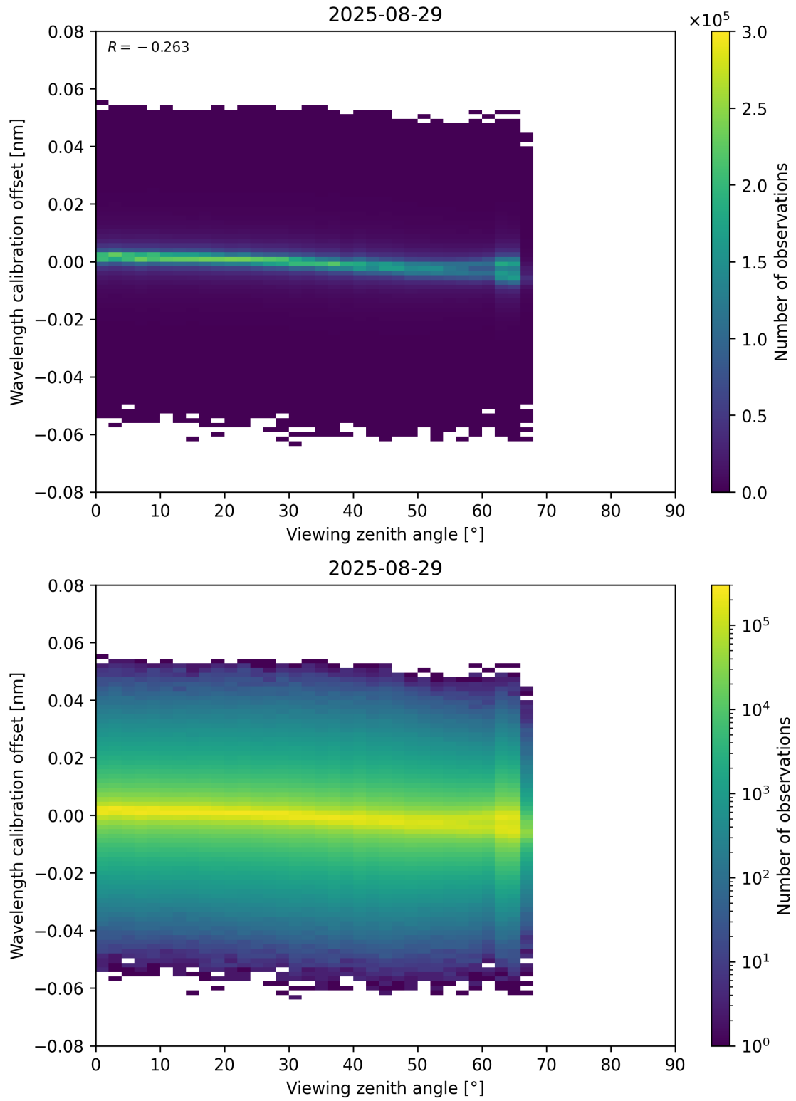
Figure 173: Scatter density plot of “Viewing zenith angle” against “Wavelength calibration offset” for 2025-08-28 to 2025-08-30.
