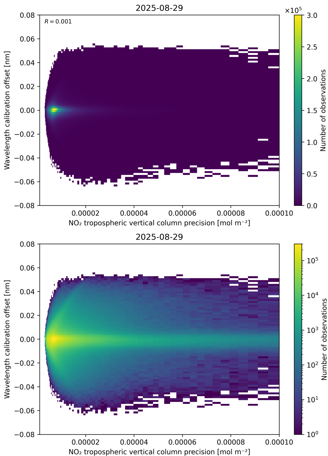
Figure 141: Scatter density plot of “NO 2 tropospheric vertical column precision” against “Wavelength calibration offset” for 2025-08-28 to 2025-08-30.
