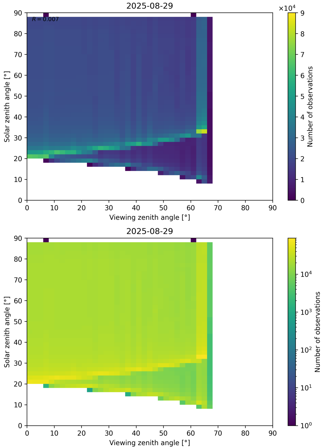
Figure 172: Scatter density plot of “Viewing zenith angle” against “Solar zenith angle” for 2025-08-28 to 2025-08-30.
