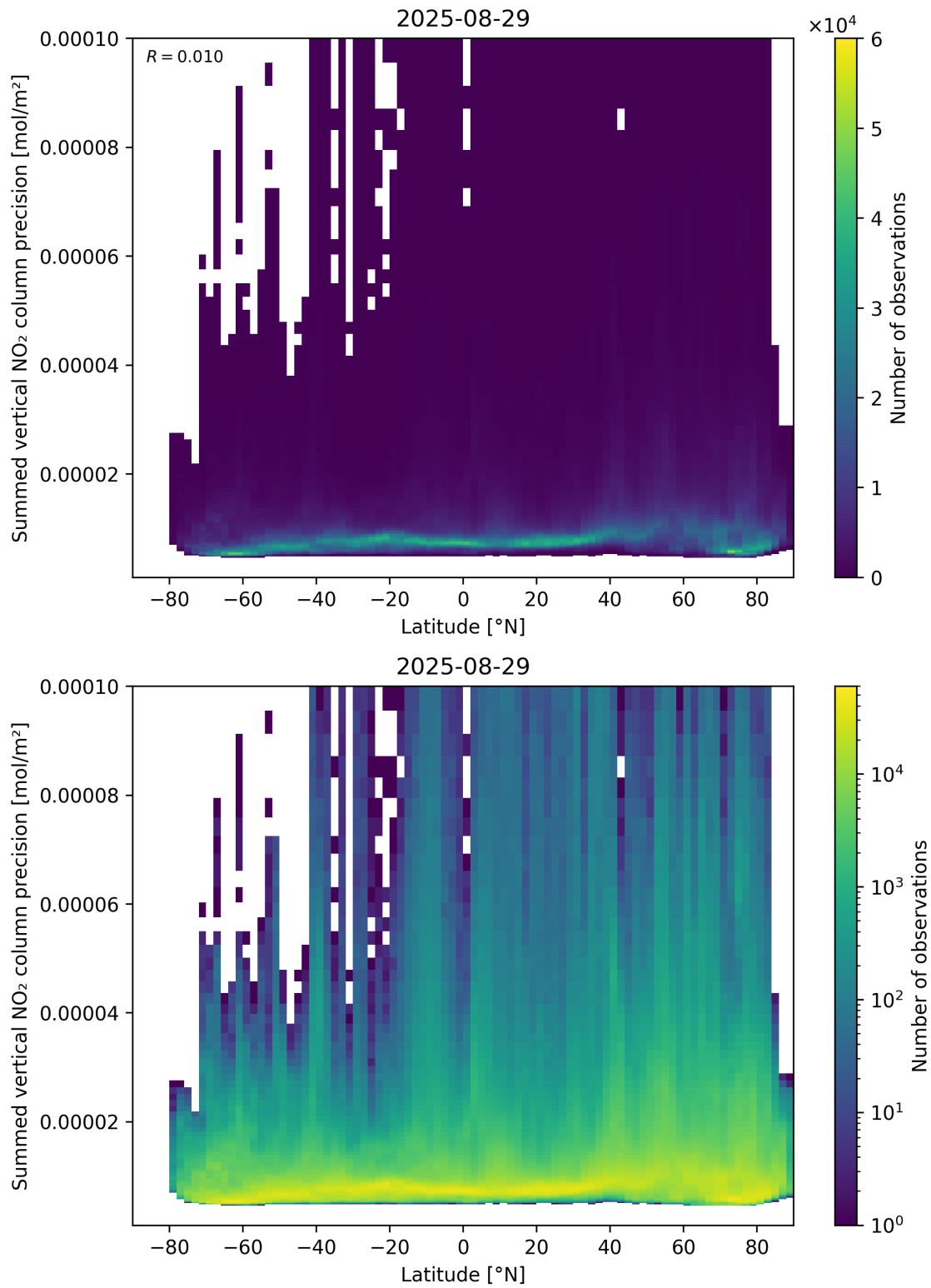
Figure 89: Scatter density plot of “Latitude” against “Summed vertical NO 2 column precision” for 2025-08-28 to 2025-08-30.
