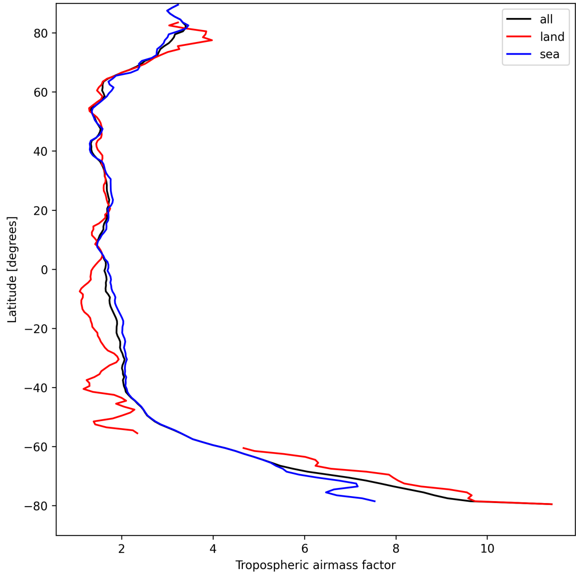
Figure 14: Zonal average of “Tropospheric airmass factor” for 2025-08-28 to 2025-08-30.
