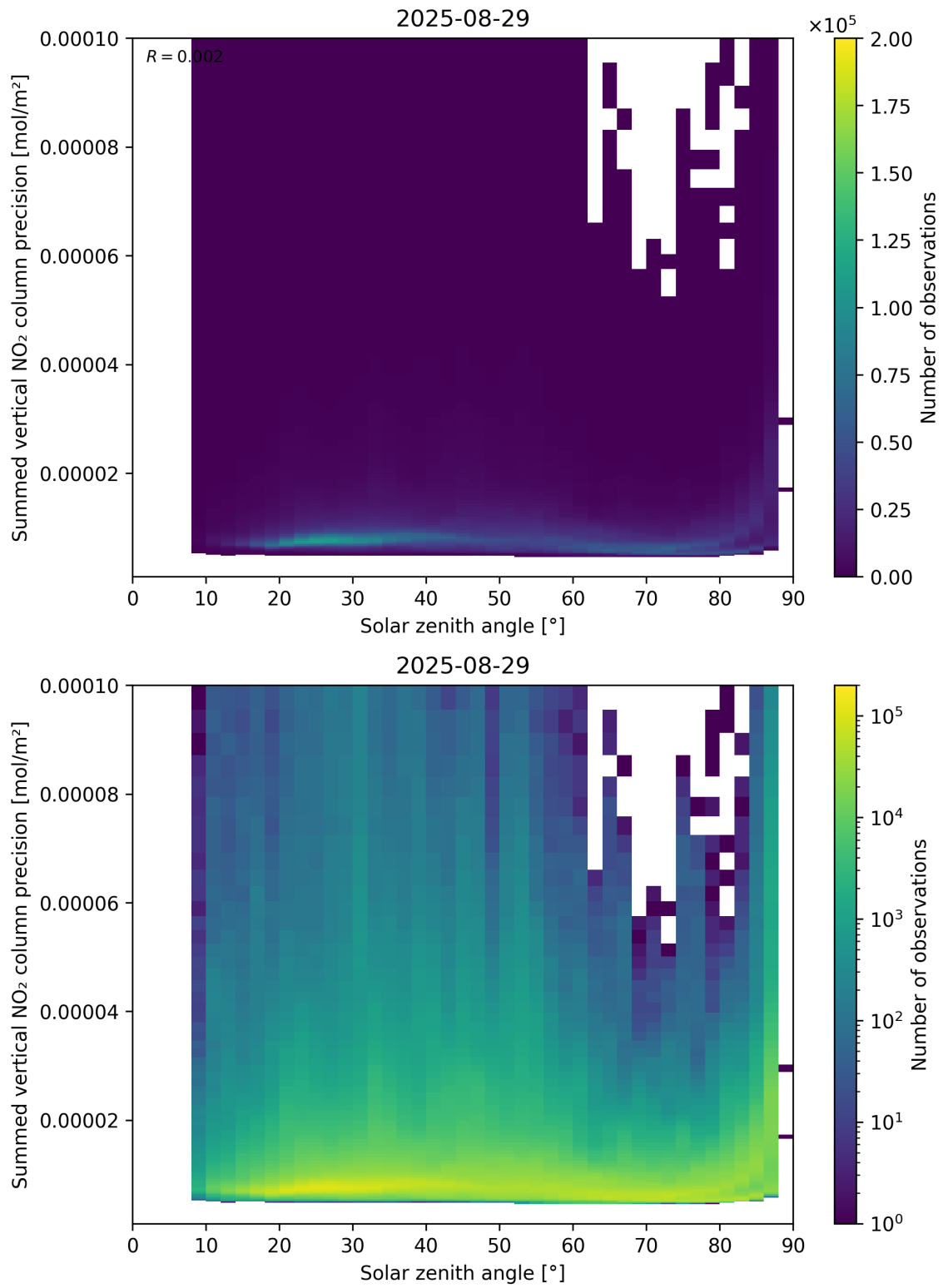
Figure 152: Scatter density plot of “Solar zenith angle” against “Summed vertical NO 2 column precision” for 2025-08-28 to 2025-08-30.
