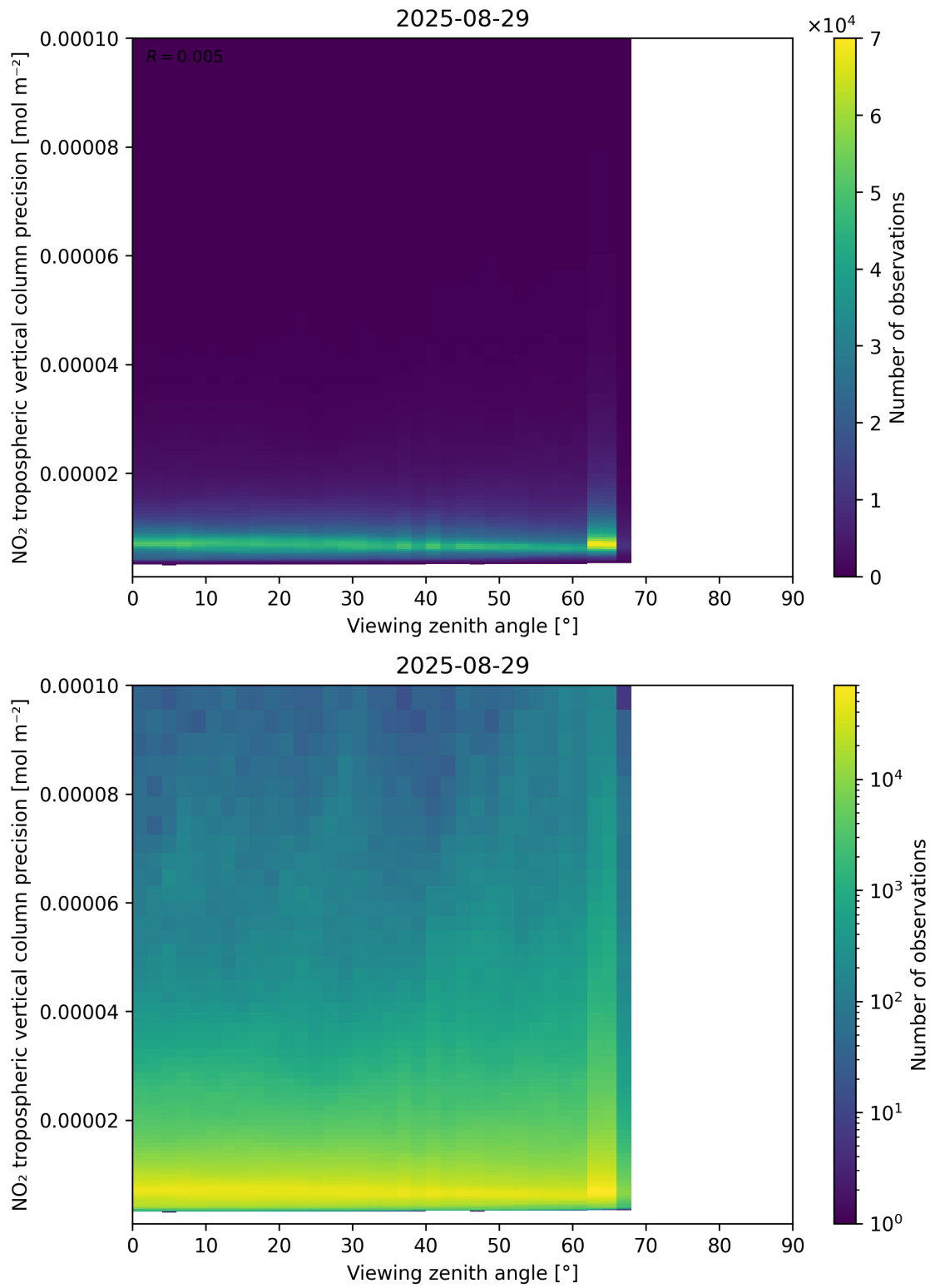
Figure 170: Scatter density plot of “Viewing zenith angle” against “NO 2 tropospheric vertical column precision” for 2025-08-28 to 2025-08-30.
