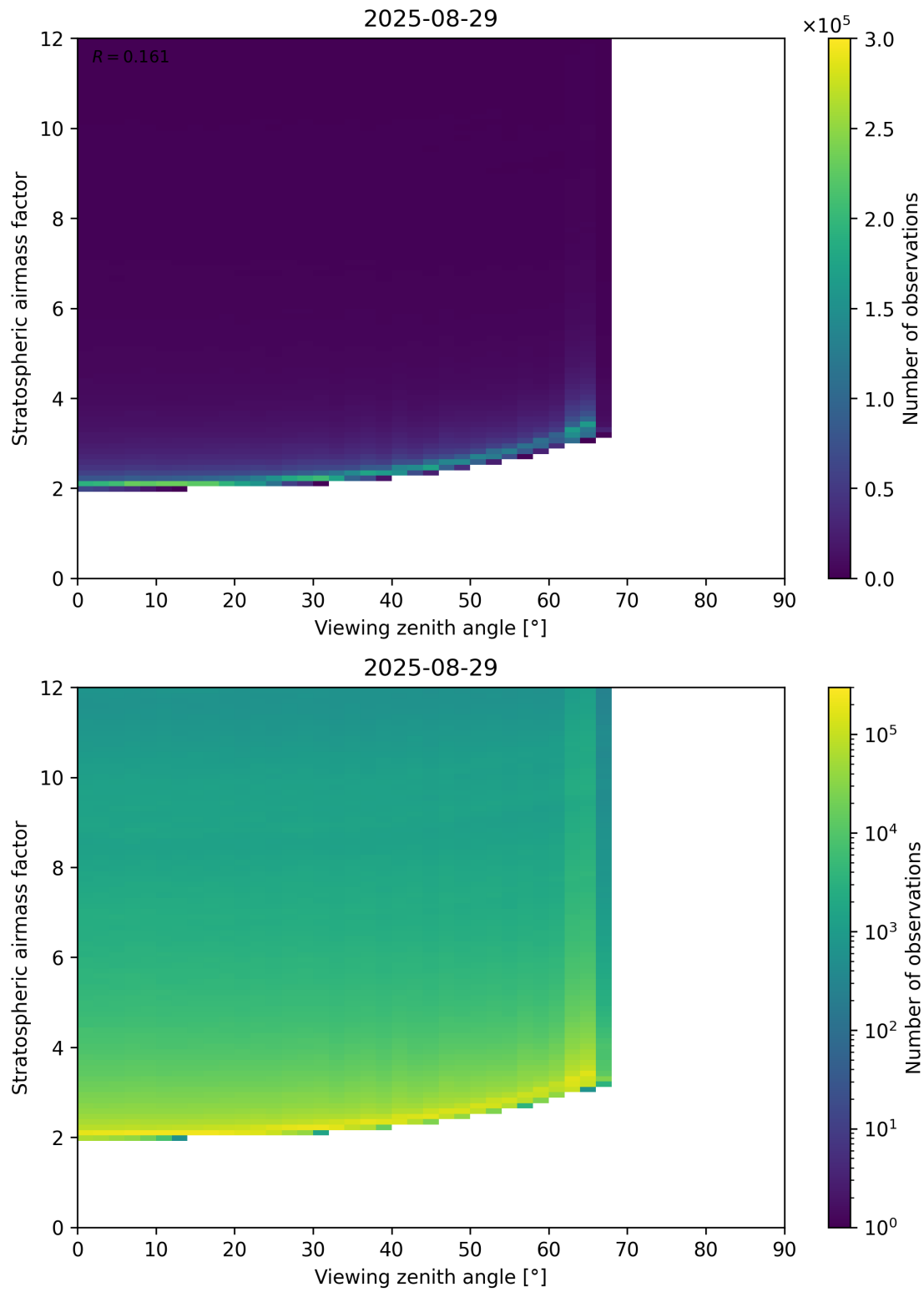
Figure 159: Scatter density plot of “Viewing zenith angle” against “Stratospheric airmass factor” for 2025-08-28 to 2025-08-30.
