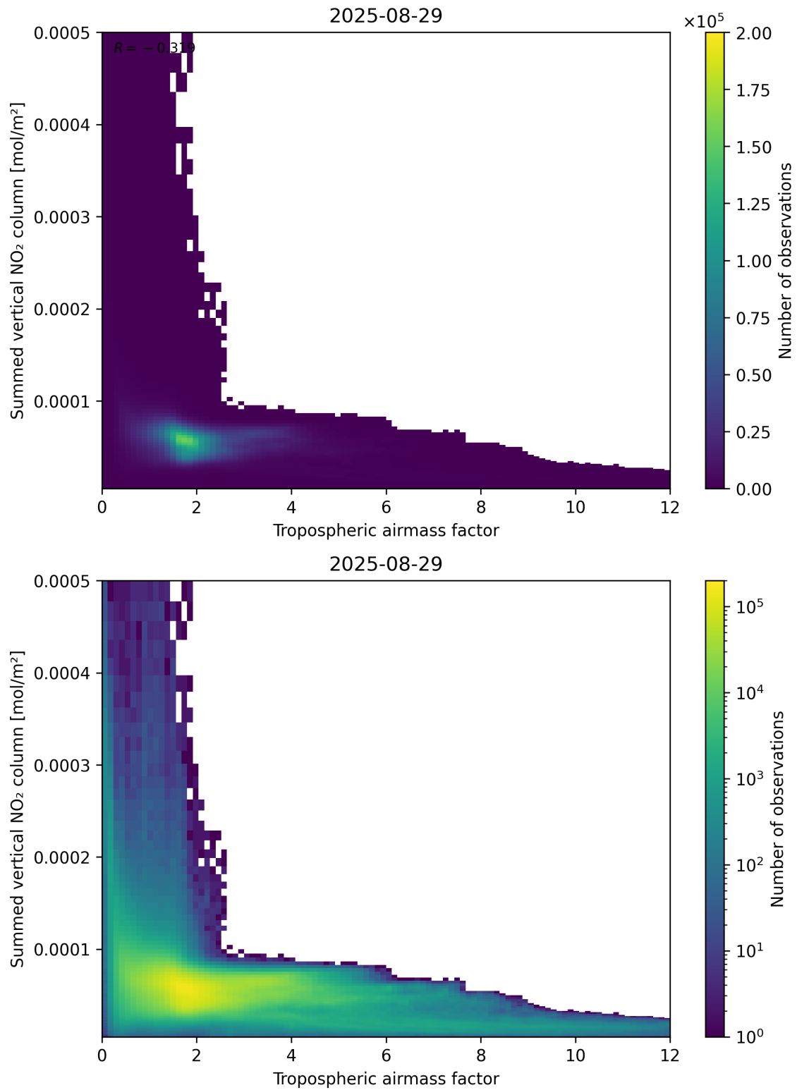
Figure 75: Scatter density plot of “Tropospheric air mass factor” against “Summed vertical NO 2 column” for 2025-08-28 to 2025-08-30.
