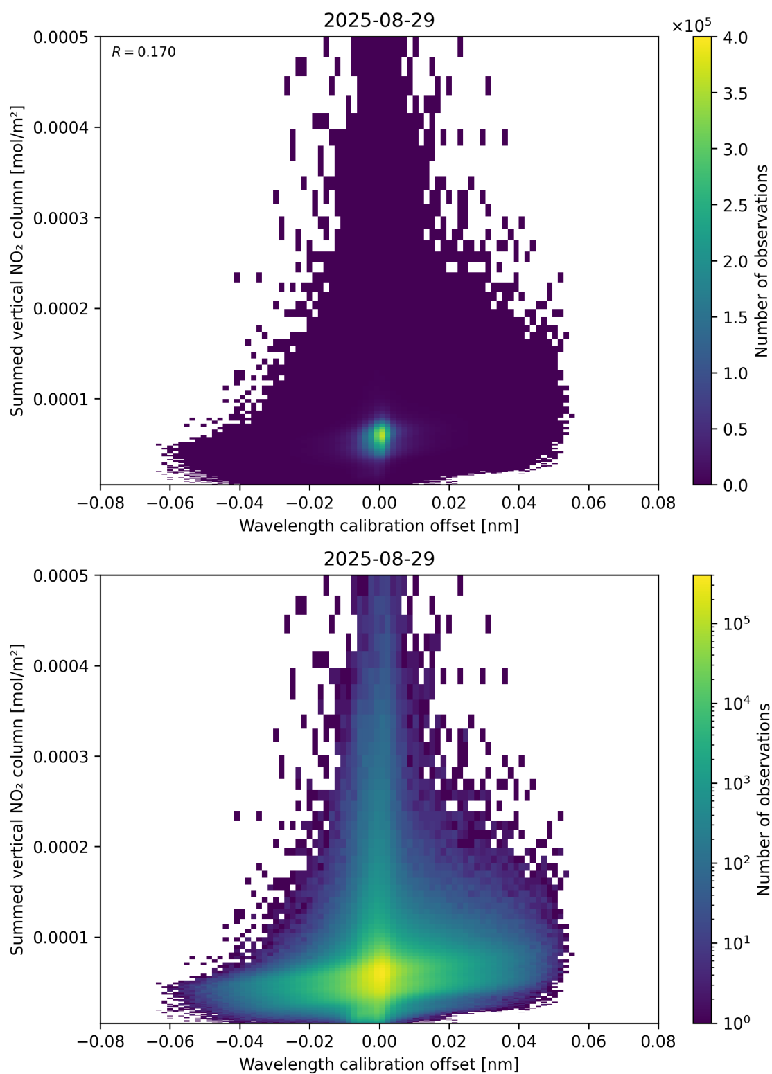
Figure 177: Scatter density plot of “Wavelength calibration offset” against “Summed vertical NO 2 column” for 2025-08-28 to 2025-08-30.
