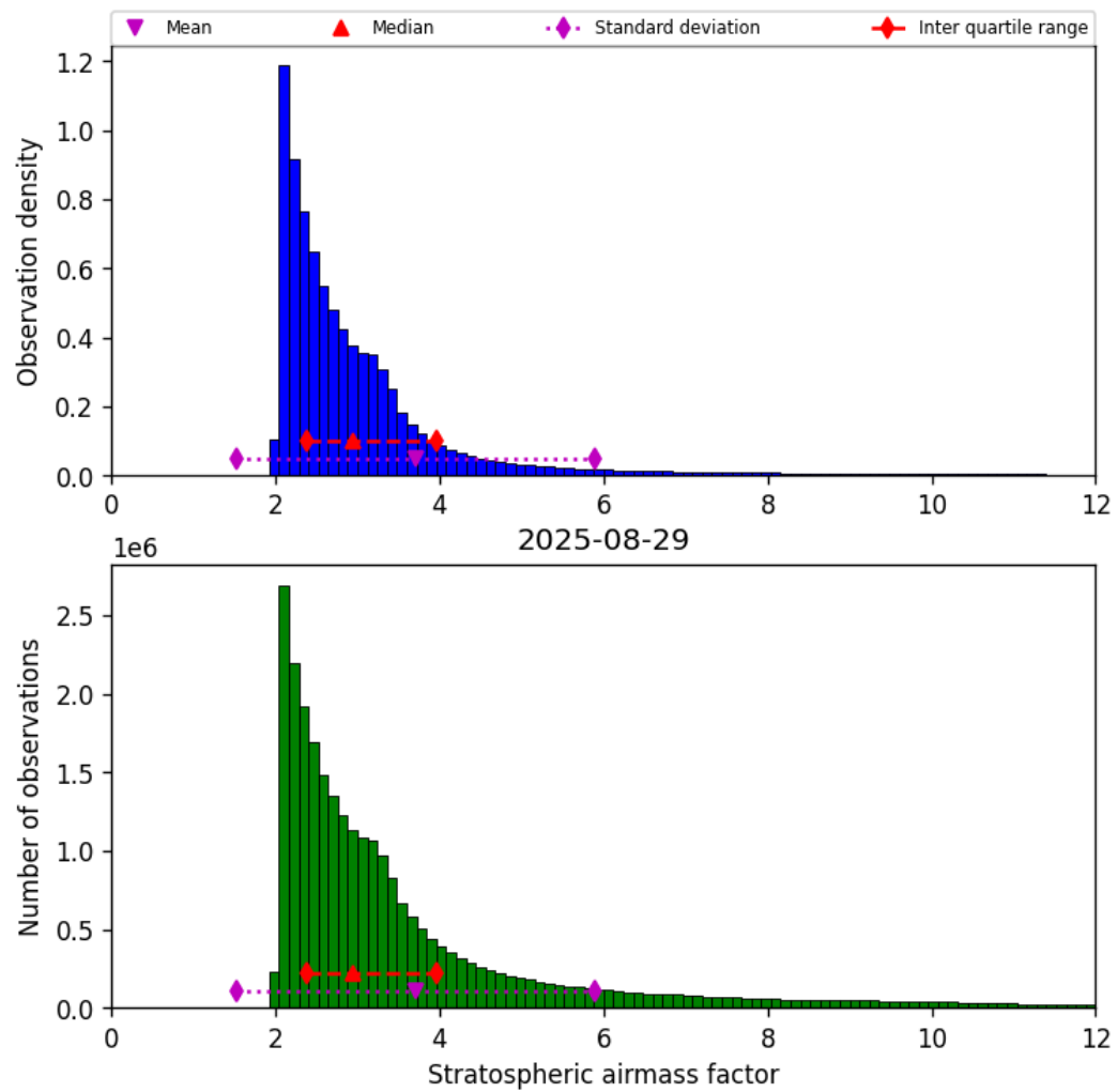
Figure 44: Histogram of “Stratospheric airmass factor” for 2025-08-28 to 2025-08-30
