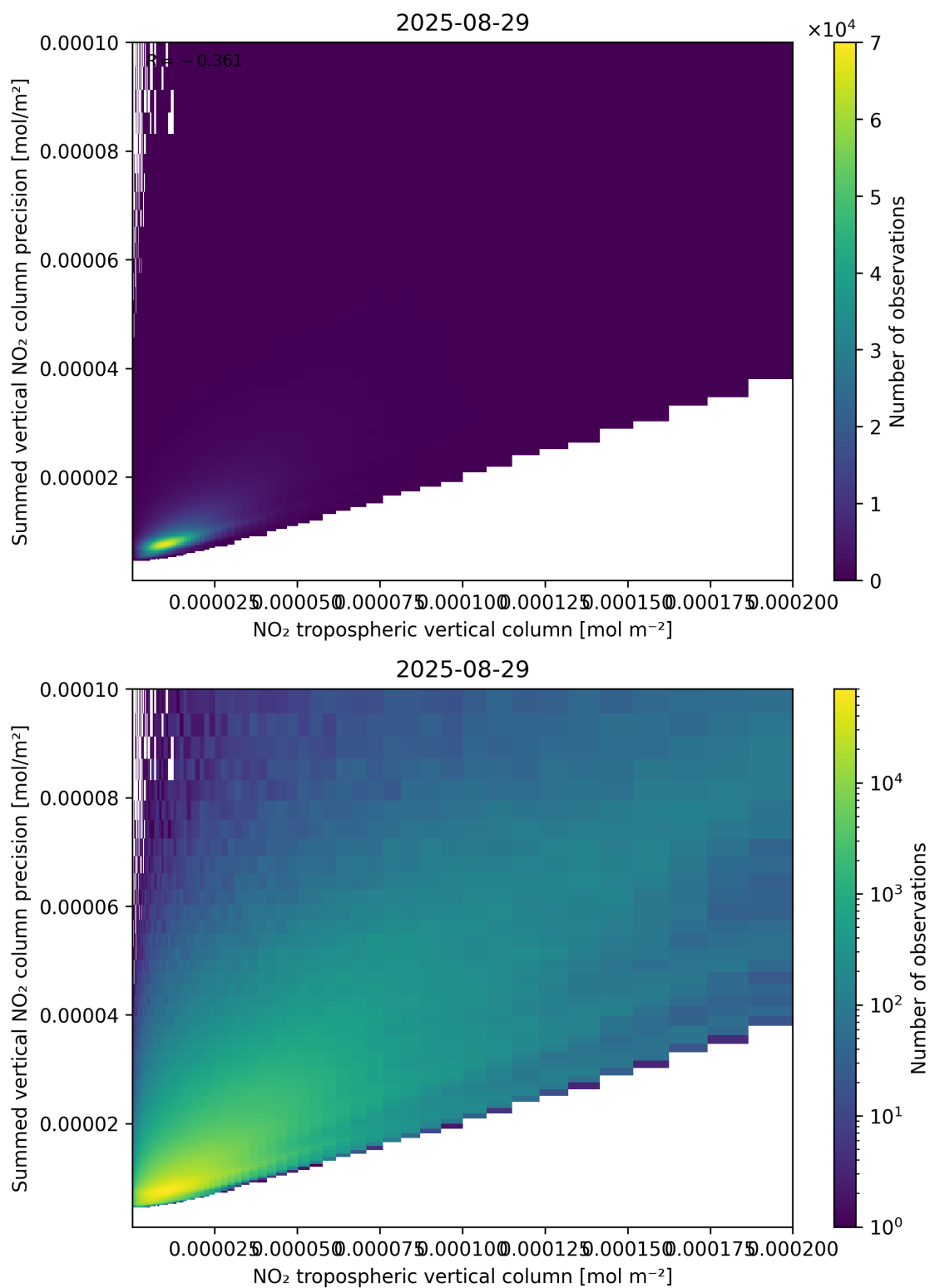
Figure 127: Scatter density plot of “NO 2 tropospheric vertical column” against “Summed vertical NO 2 column precision” for 2025-08-28 to 2025-08-30.
