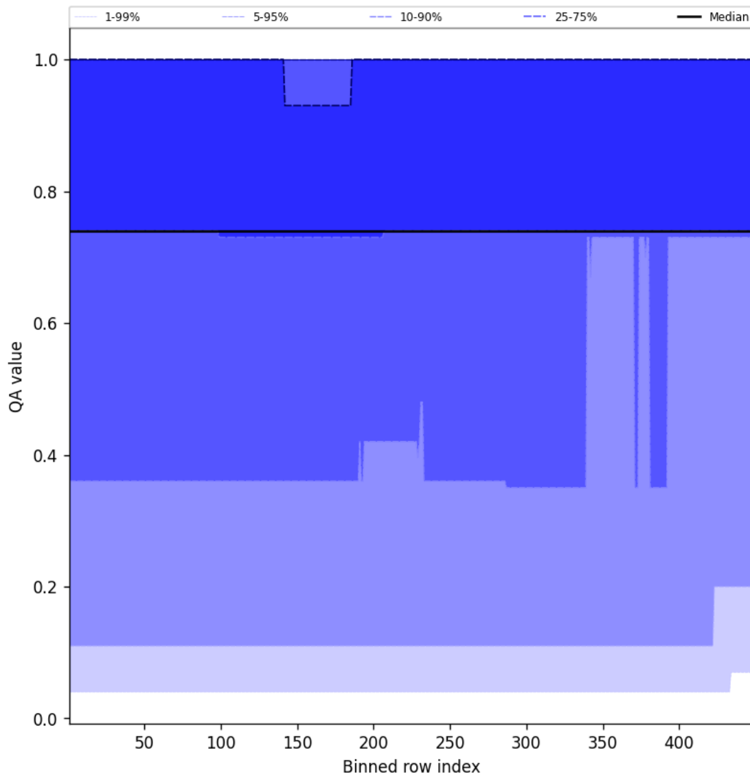
Figure 45: Along track statistics of “QA value” for 2025-08-28 to 2025-08-30
