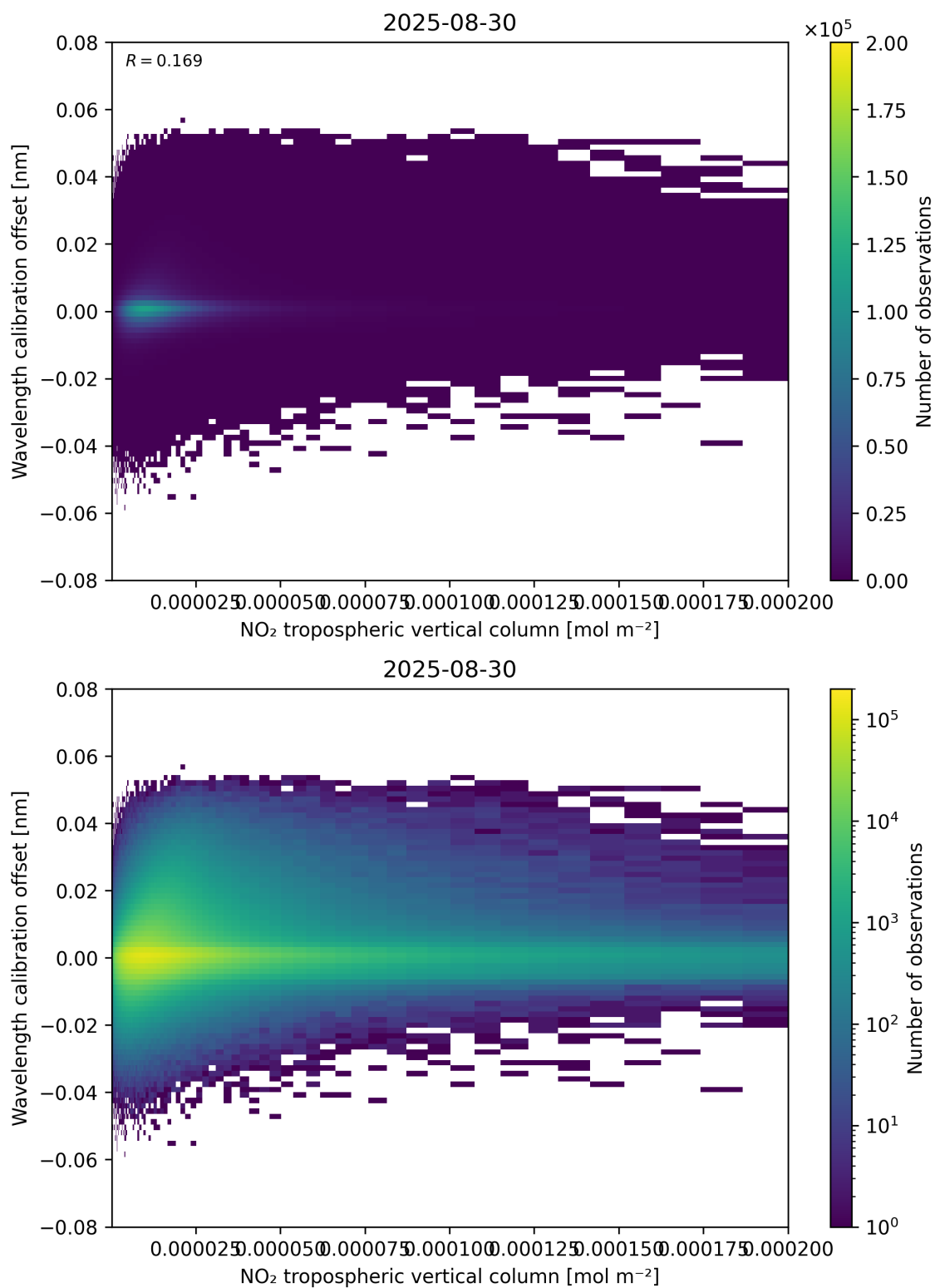
Figure 143: Scatter density plot of “NO 2 tropospheric vertical column” against “Wavelength calibration offset” for 2025-08-30 to 2025-08-31.
