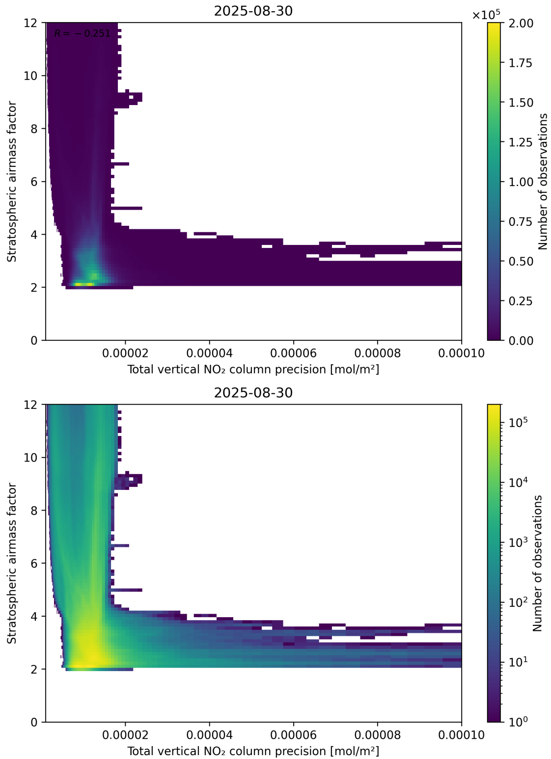
Figure 115: Scatter density plot of “Total vertical NO 2 column precision” against “Stratospheric air mass factor” for 2025-08-30 to 2025-08-31.
