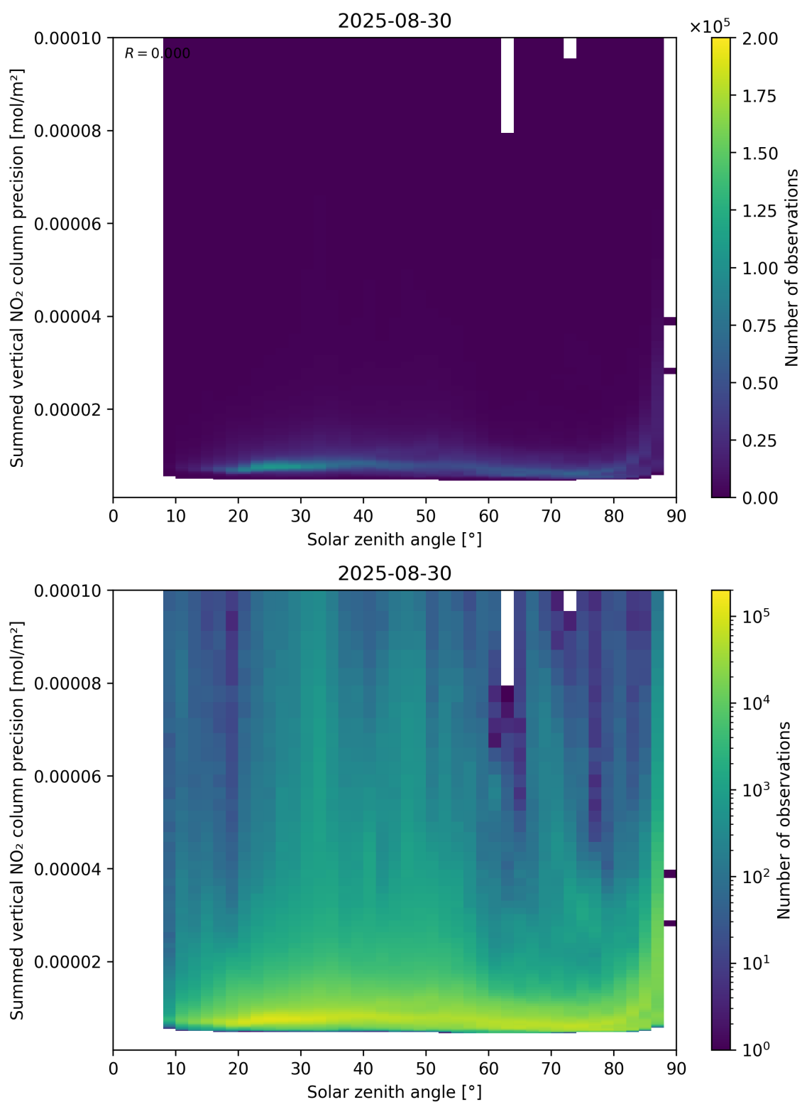
Figure 152: Scatter density plot of “Solar zenith angle” against “Summed vertical NO 2 column precision” for 2025-08-30 to 2025-08-31.
