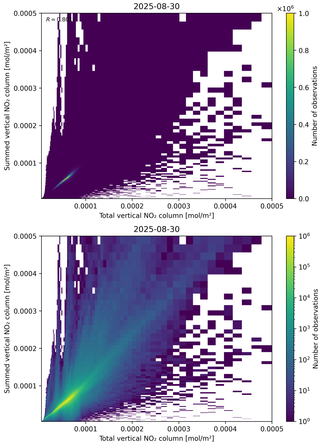
Figure 112: Scatter density plot of “Total vertical NO 2 column” against “Summed vertical NO 2 column” for 2025-08-30 to 2025-08-31.
