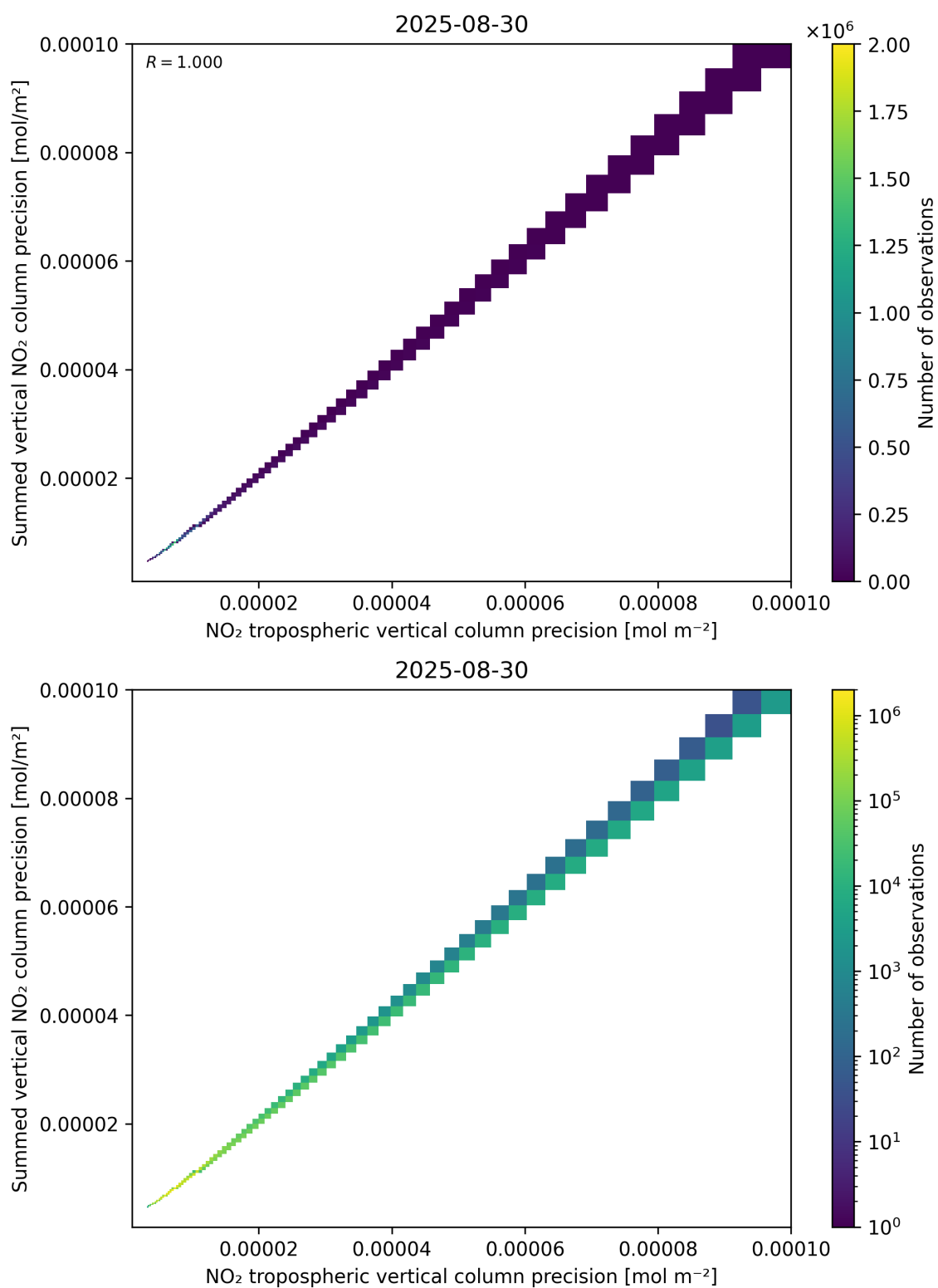
Figure 137: Scatter density plot of “NO 2 tropospheric vertical column precision” against “Summed vertical NO 2 column precision” for 2025-08-30 to 2025-08-31.
