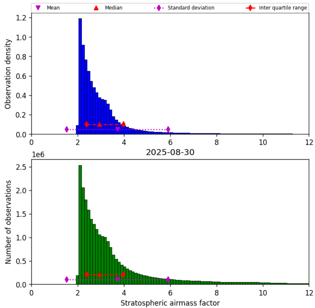
Figure 44: Histogram of “Stratospheric airmass factor” for 2025-08-30 to 2025-08-31
