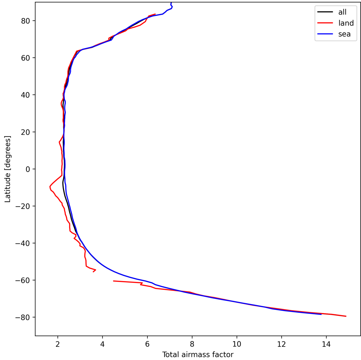
Figure 15: Zonal average of “Total airmass factor” for 2025-08-30 to 2025-08-31.
