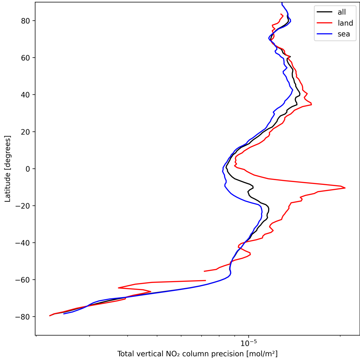
Figure 22: Zonal average of “Total vertical NO 2 column precision” for 2025-08-30 to 2025-08-31.
