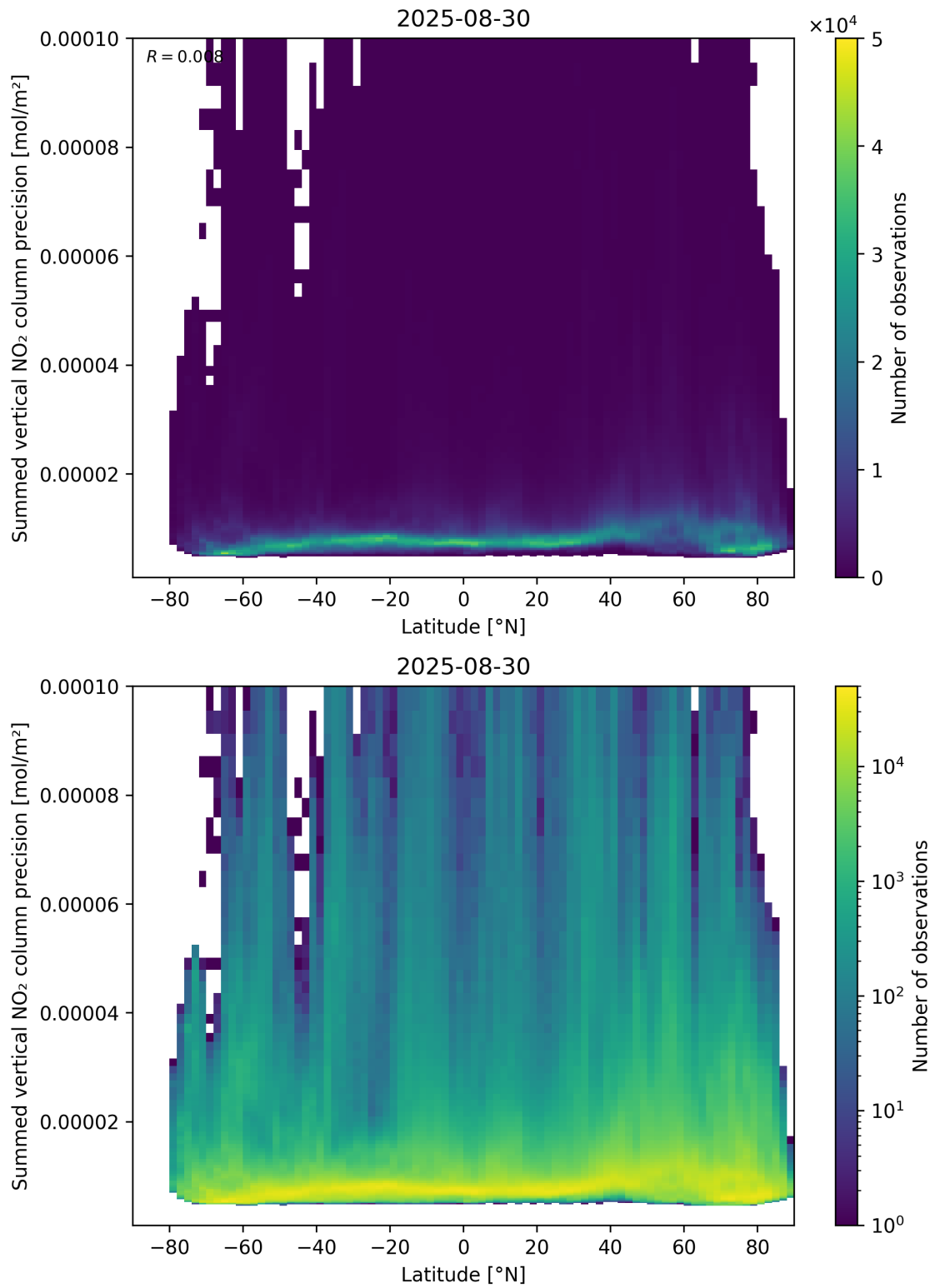
Figure 89: Scatter density plot of “Latitude” against “Summed vertical NO 2 column precision” for 2025-08-30 to 2025-08-31.
