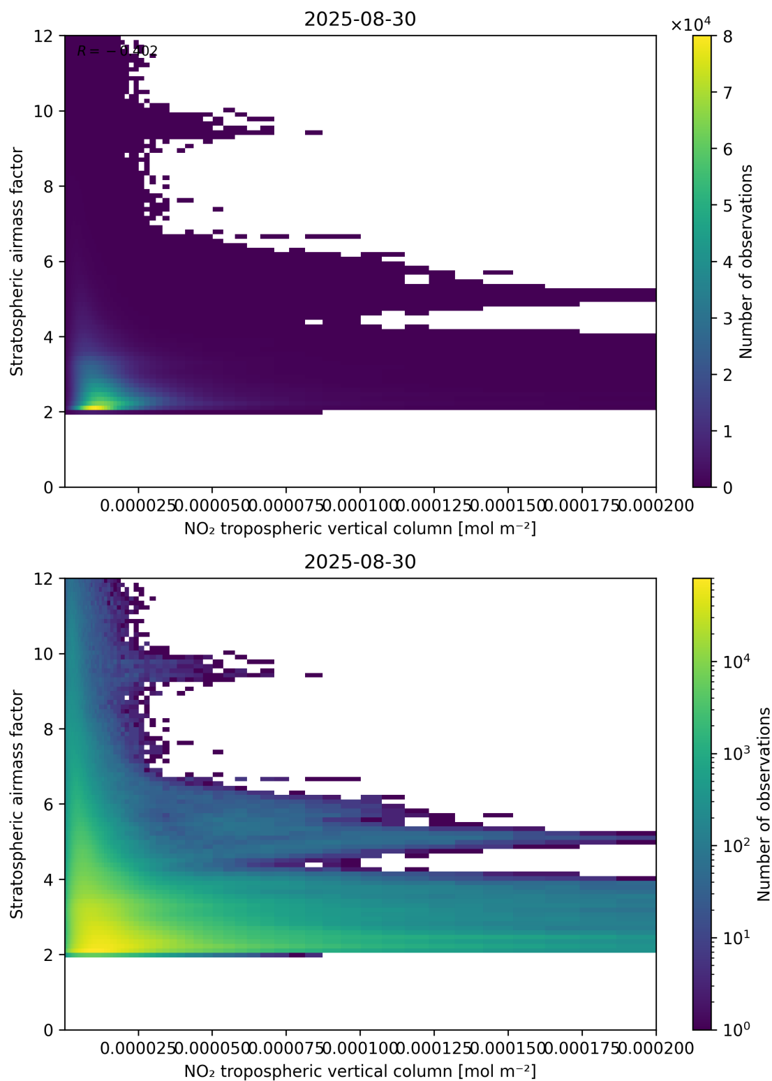
Figure 121: Scatter density plot of “NO 2 tropospheric vertical column” against “Stratospheric air mass factor” for 2025-08-30 to 2025-08-31.
