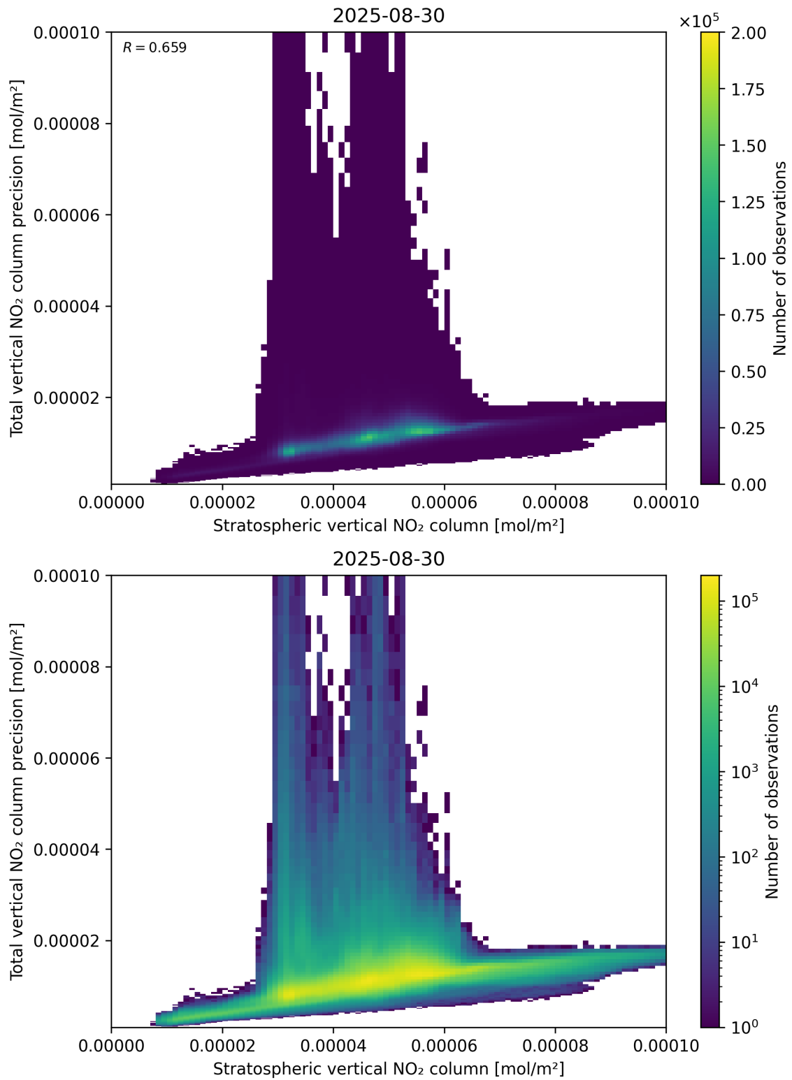
Figure 101: Scatter density plot of “Stratospheric vertical NO 2 column” against “Total vertical NO 2 column precision” for 2025-08-30 to 2025-08-31.
