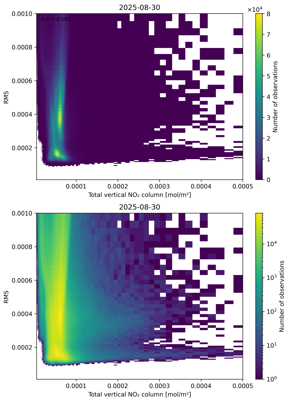
Figure 120: Scatter density plot of “Total vertical NO 2 column” against “RMS” for 2025-08-30 to 2025-08-31.
