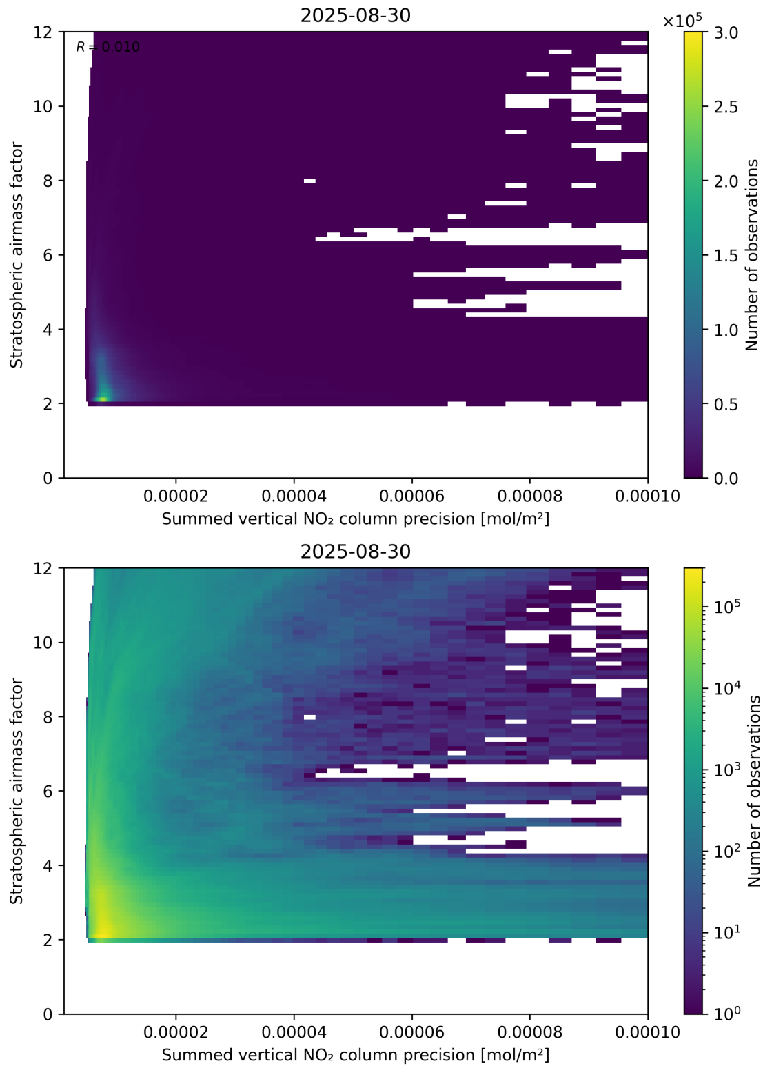
Figure 106: Scatter density plot of “Summed vertical NO 2 column precision” against “Stratospheric airmass factor” for 2025-08-30 to 2025-08-31.
