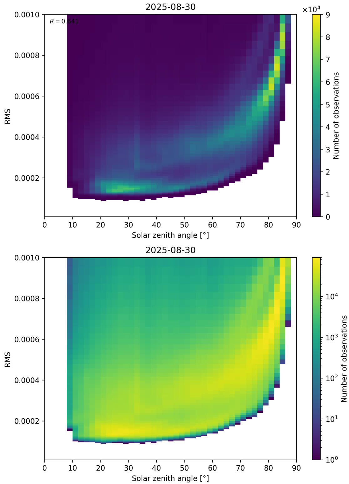
Figure 157: Scatter density plot of “Solar zenith angle” against “RMS” for 2025-08-30 to 2025-08-31.
