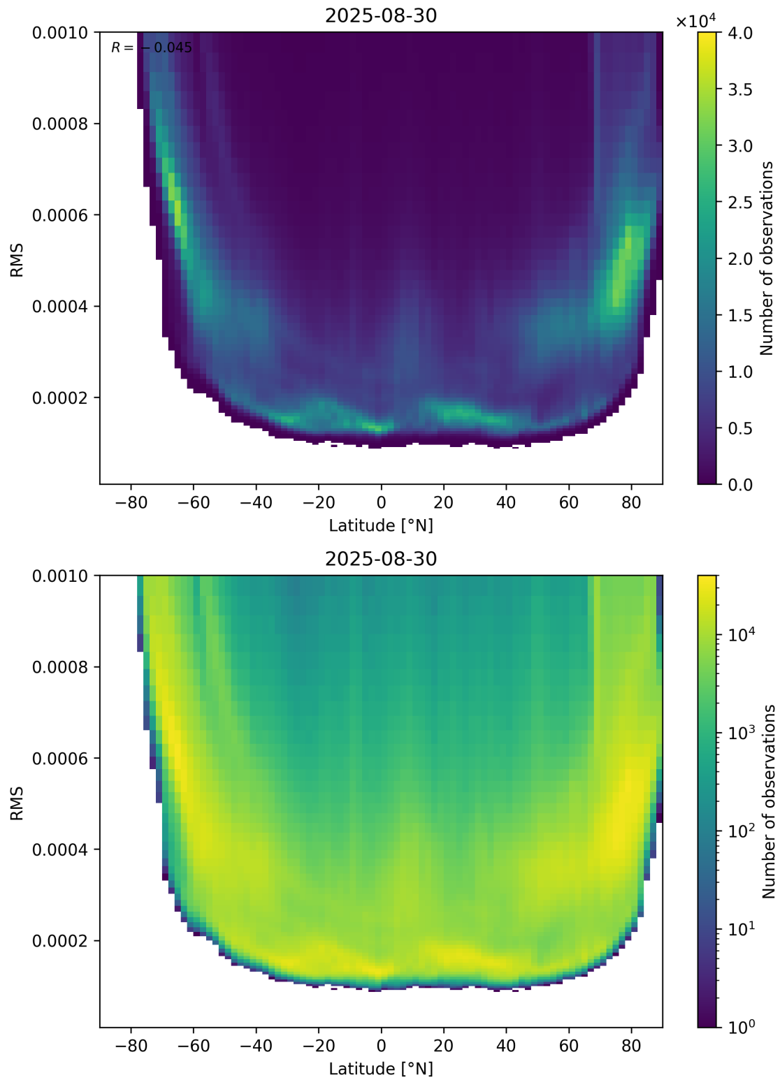
Figure 94: Scatter density plot of “Latitude” against “RMS” for 2025-08-30 to 2025-08-31.
