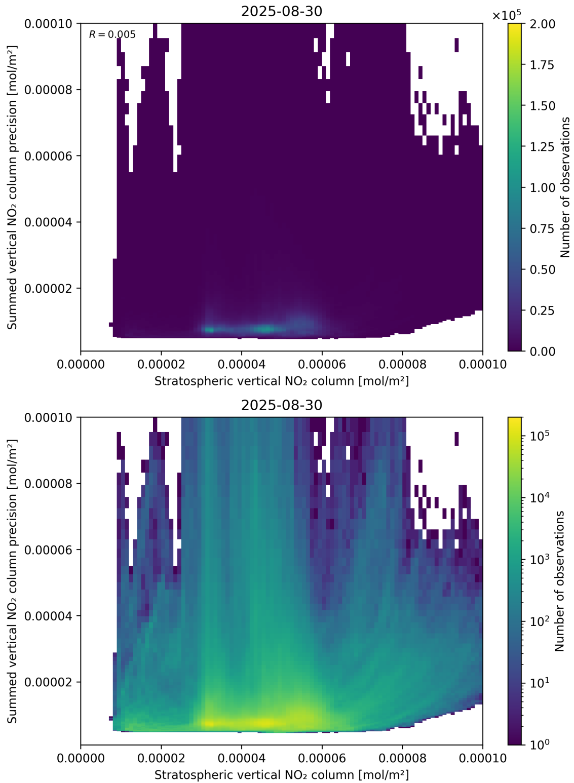
Figure 99: Scatter density plot of “Stratospheric vertical NO 2 column” against “Summed vertical NO 2 column precision” for 2025-08-30 to 2025-08-31.
