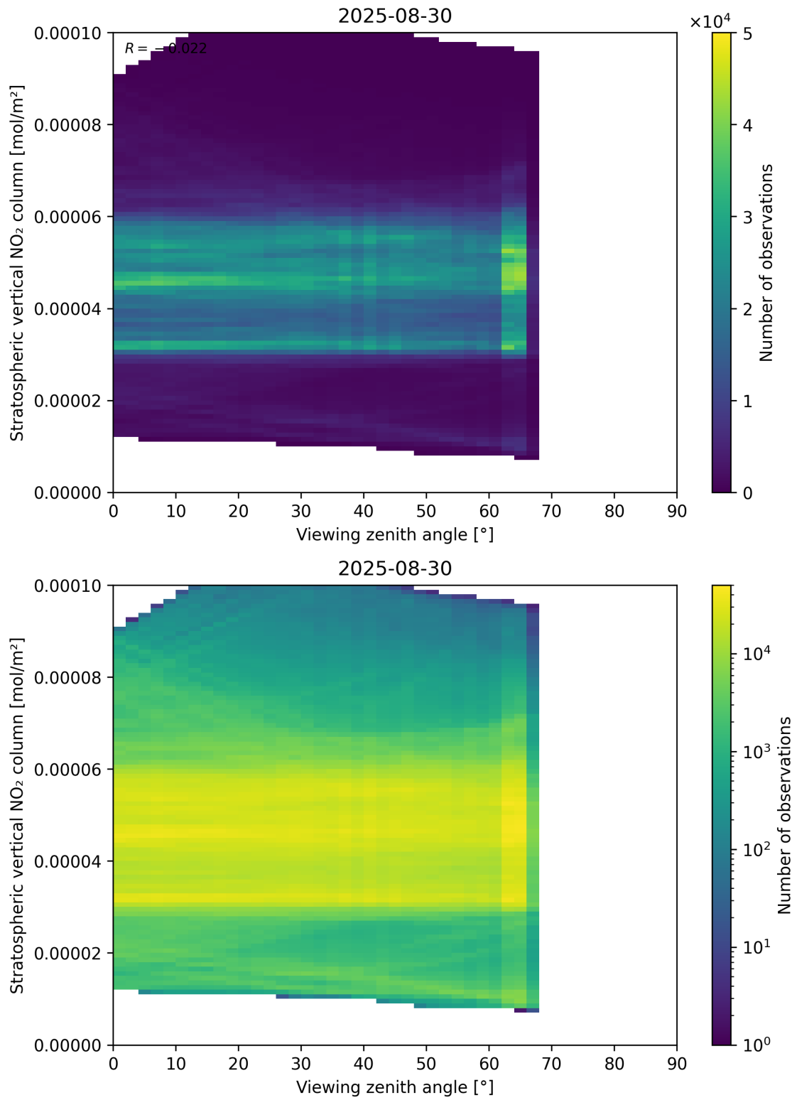
Figure 164: Scatter density plot of “Viewing zenith angle” against “Stratospheric vertical NO 2 column” for 2025-08-30 to 2025-08-31.
