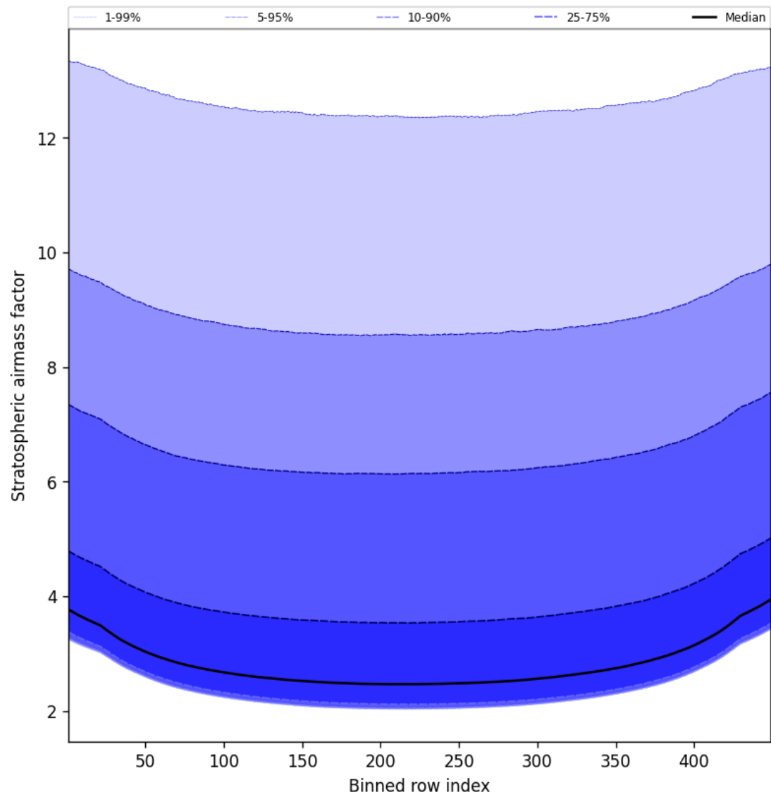
Figure 61: Along track statistics of “Stratospheric airmass factor” for 2025-08-30 to 2025-08-31
