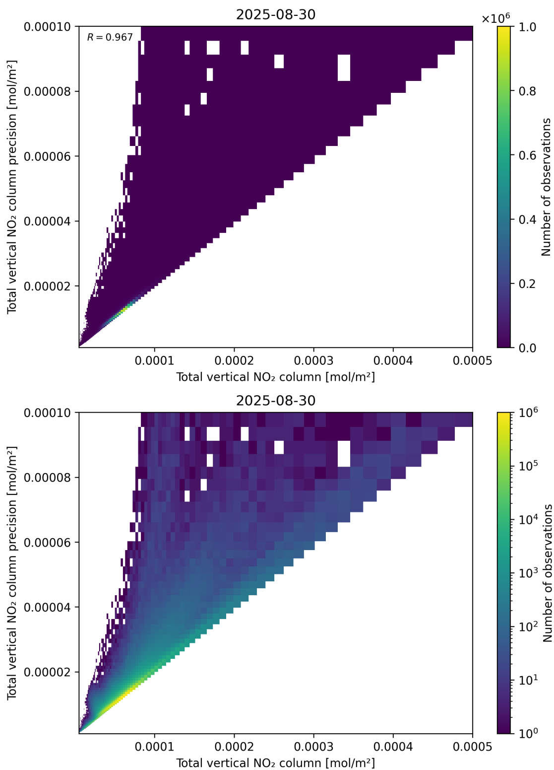
Figure 114: Scatter density plot of “Total vertical NO 2 column” against “Total vertical NO 2 column precision” for 2025-08-30 to 2025-08-31.
