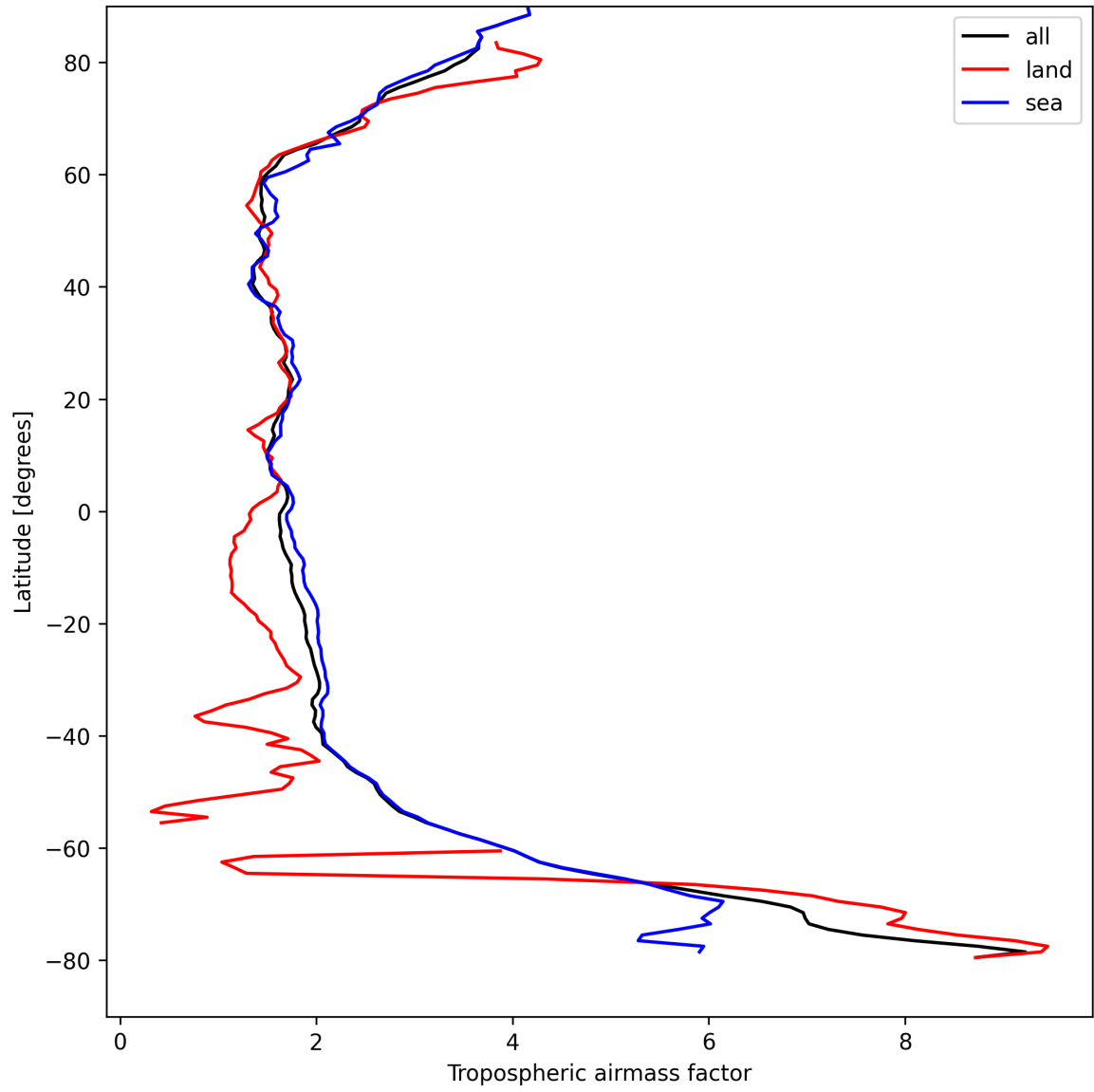
Figure 14: Zonal average of “Tropospheric airmass factor” for 2025-08-30 to 2025-08-31.
