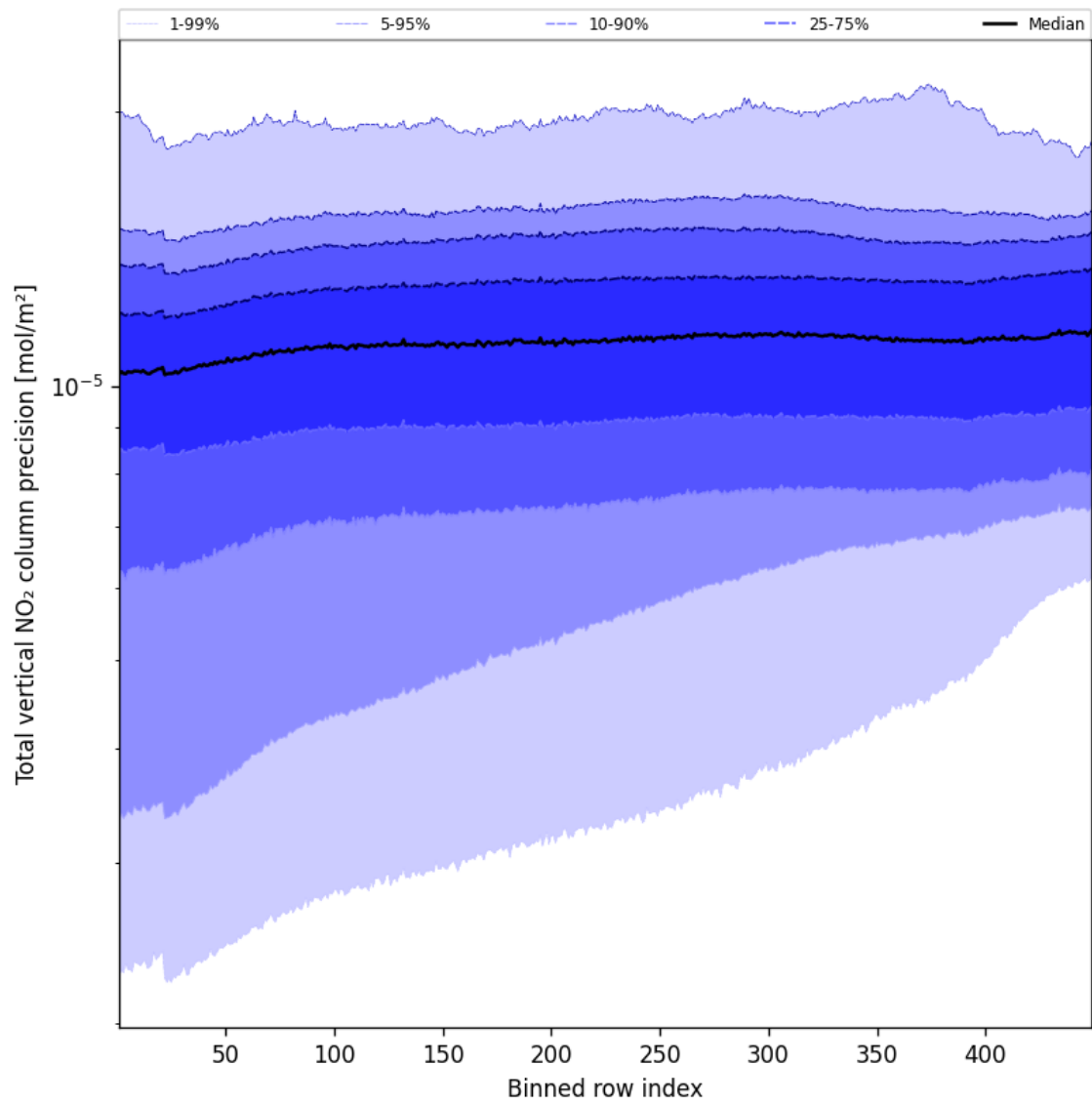
Figure 56: Along track statistics of “Total vertical NO 2 column precision” for 2025-08-30 to 2025-08-31
