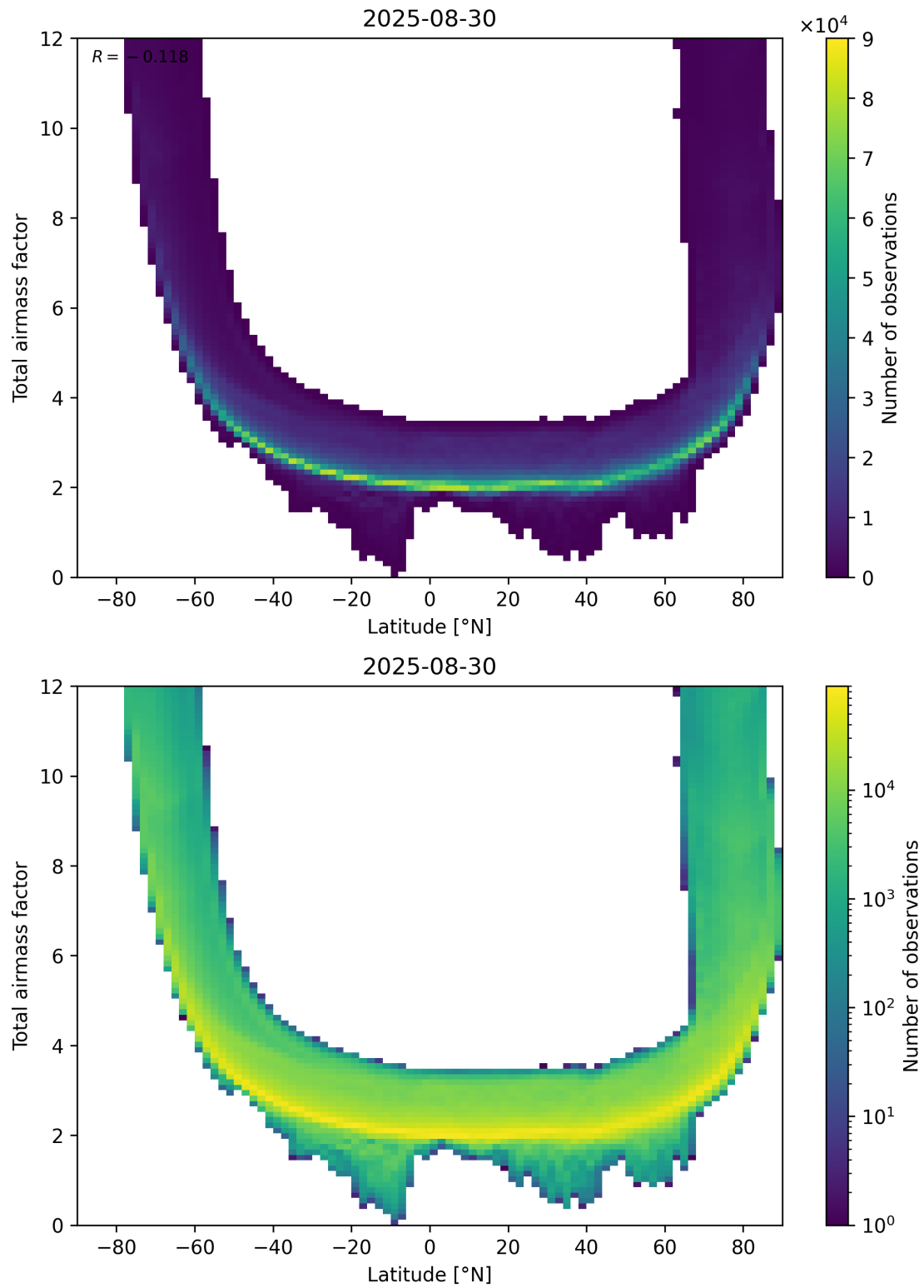
Figure 84: Scatter density plot of “Latitude” against “Total airmass factor” for 2025-08-30 to 2025-08-31.
