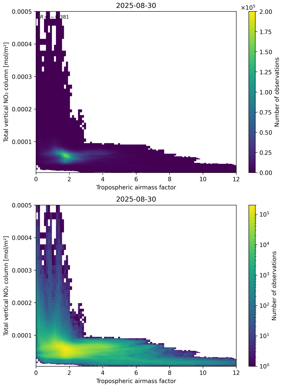
Figure 77: Scatter density plot of “Tropospheric airmass factor” against “Total vertical NO 2 column” for 2025-08-30 to 2025-08-31.
