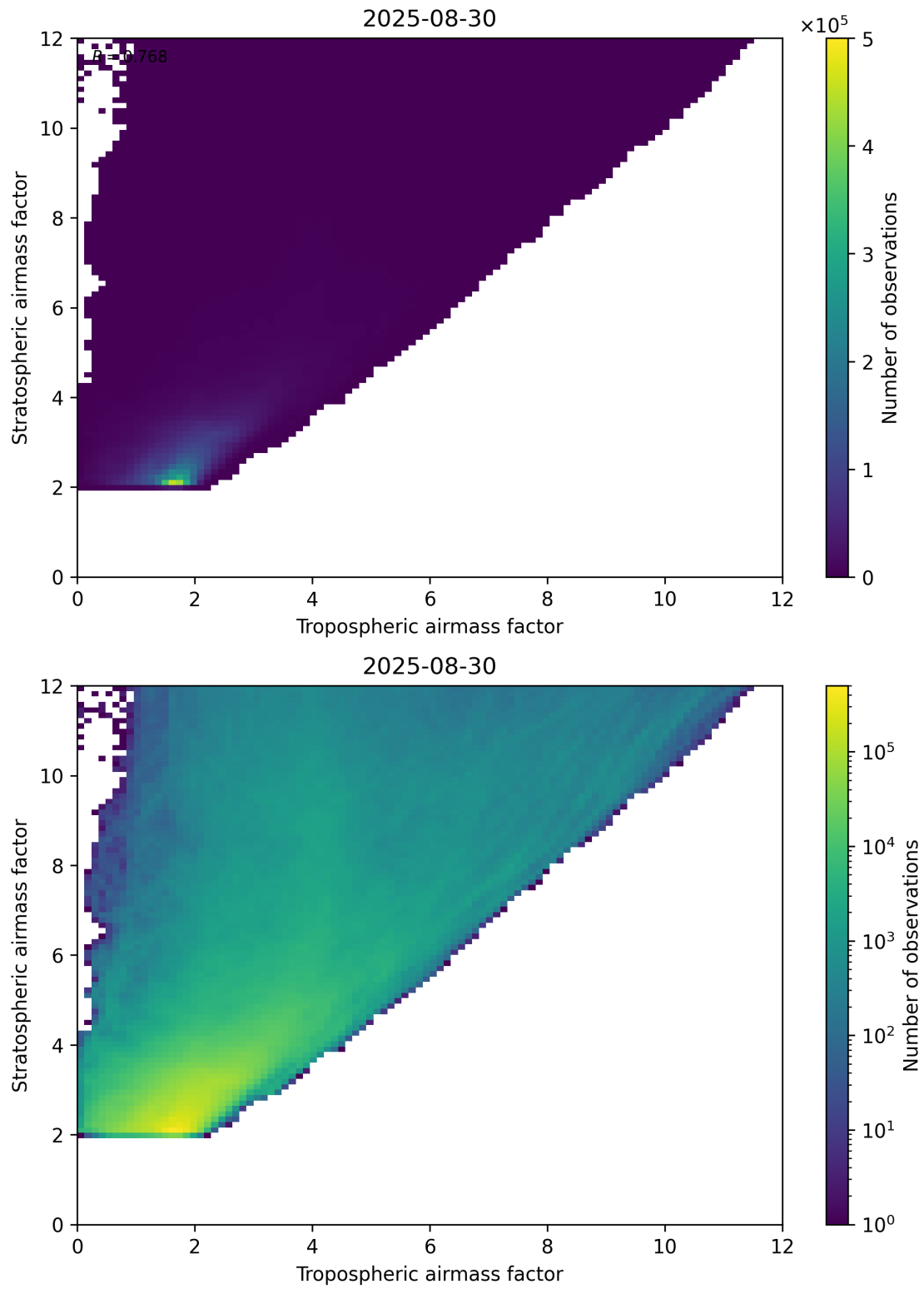
Figure 71: Scatter density plot of “Tropospheric airmass factor” against “Stratospheric airmass factor” for 2025-08-30 to 2025-08-31.
