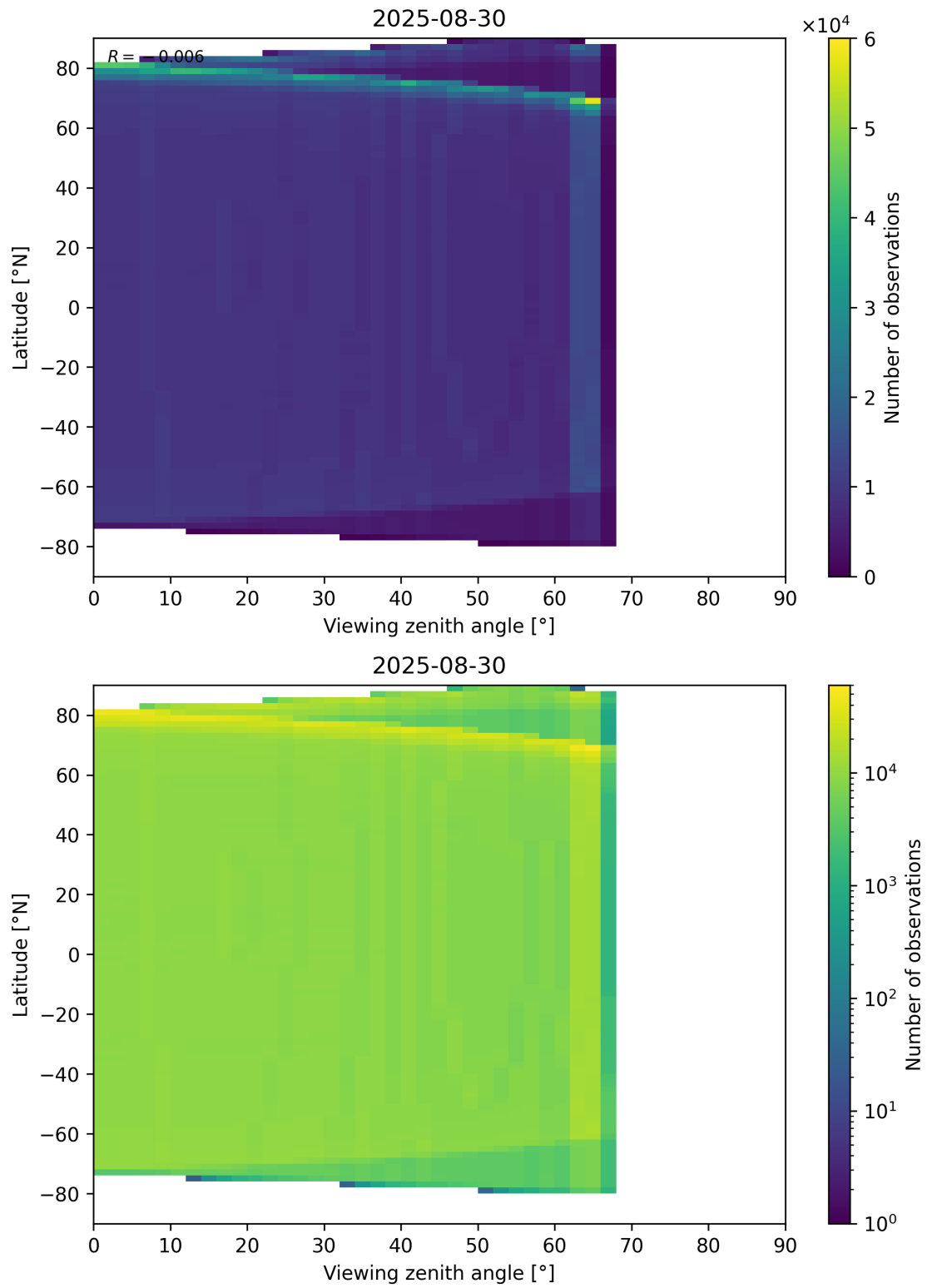
Figure 163: Scatter density plot of “Viewing zenith angle” against “Latitude” for 2025-08-30 to 2025-08-31.
