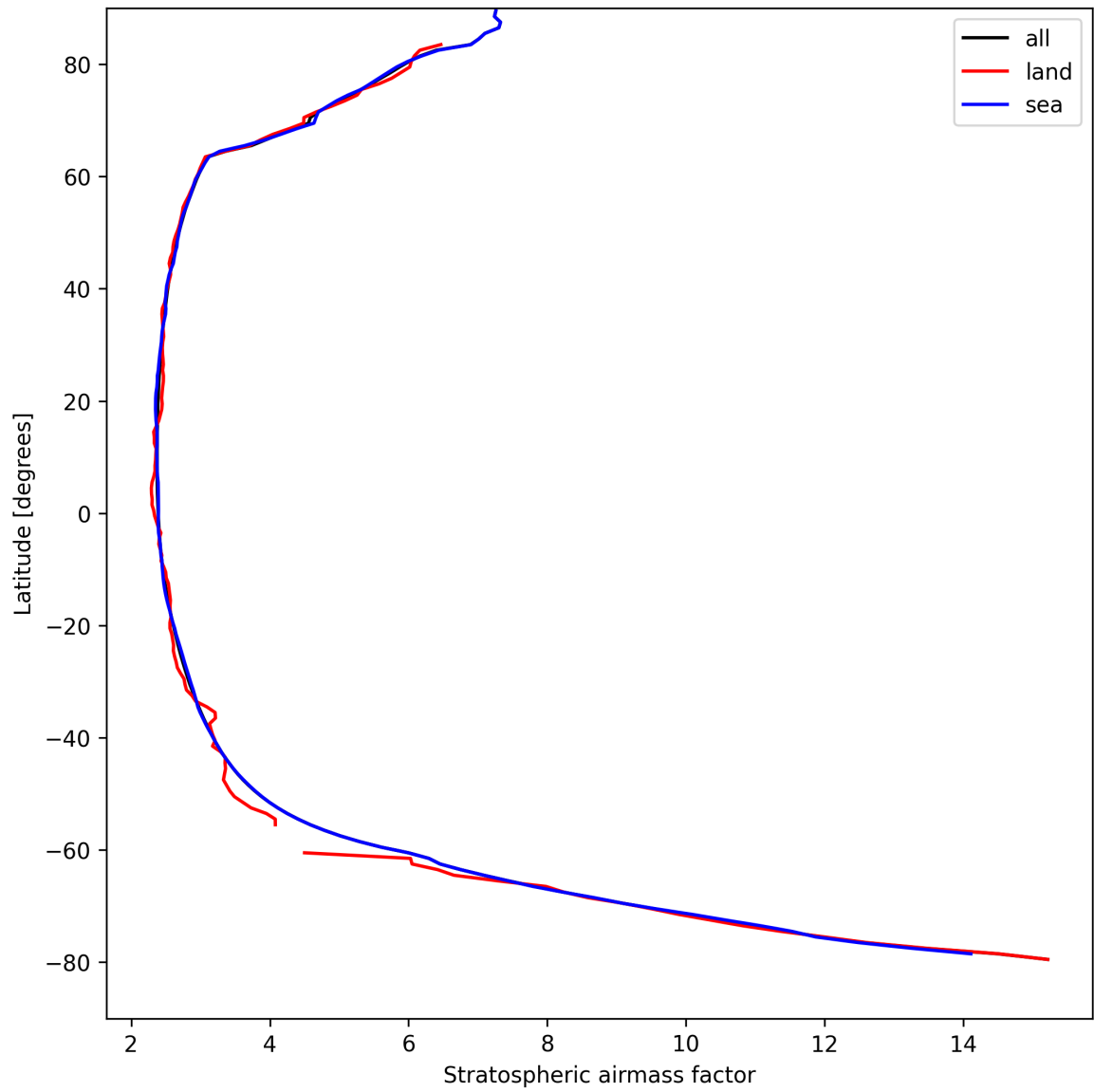
Figure 27: Zonal average of “Stratospheric air mass factor” for 2025-08-30 to 2025-08-31.
