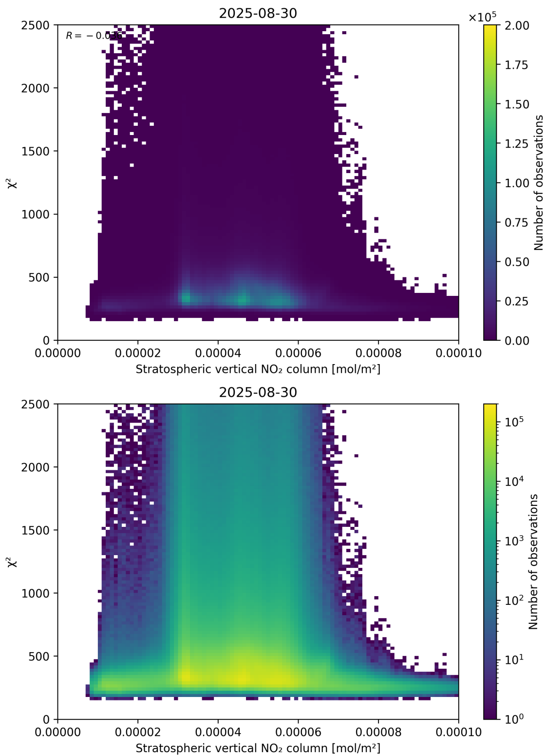
Figure 97: Scatter density plot of “Stratospheric vertical NO 2 column” against “ \chi^2 ” for 2025-08-30 to 2025-08-31.
