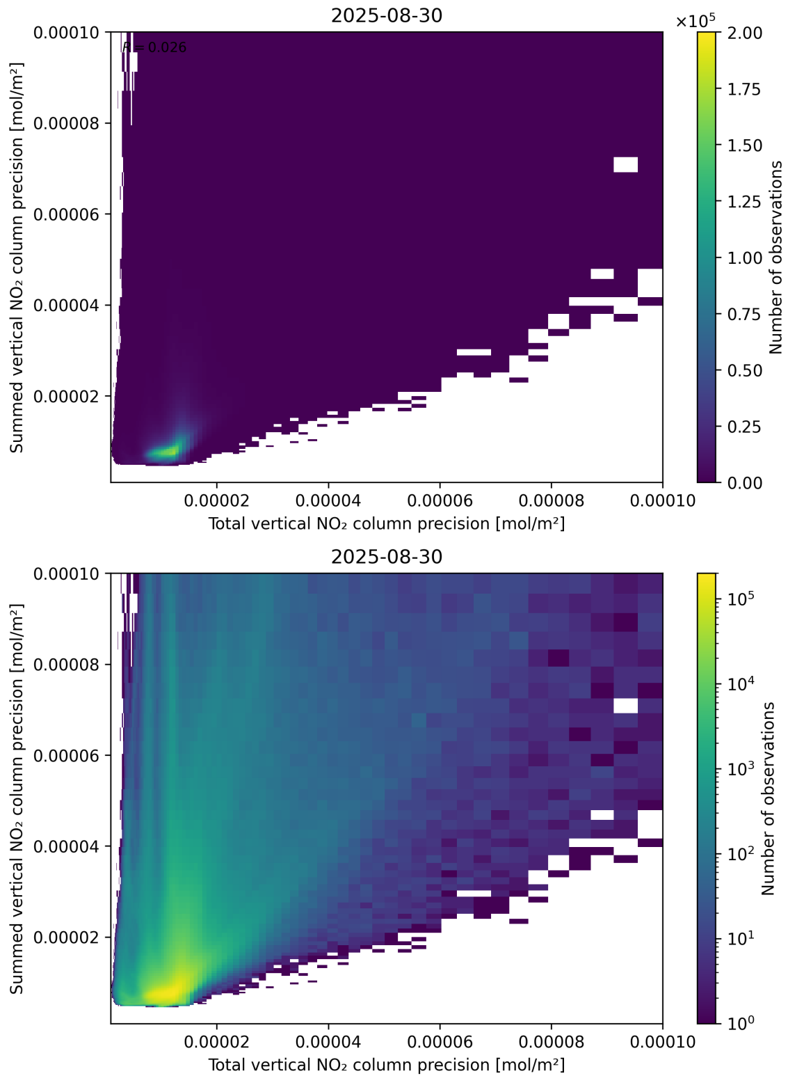
Figure 118: Scatter density plot of “Total vertical NO 2 column precision” against “Summed vertical NO 2 column precision” for 2025-08-30 to 2025-08-31.
