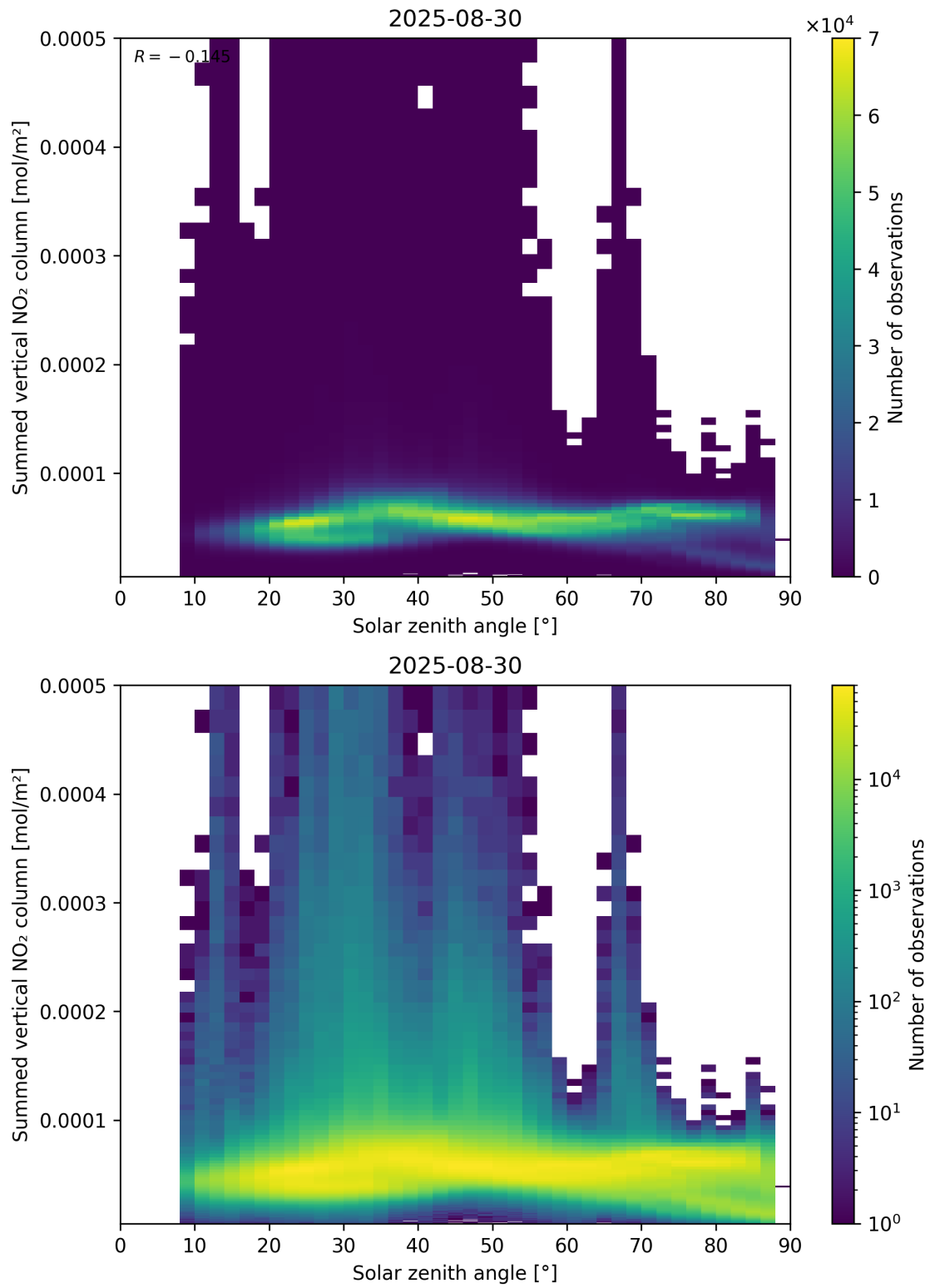
Figure 151: Scatter density plot of “Solar zenith angle” against “Summed vertical NO 2 column” for 2025-08-30 to 2025-08-31.
