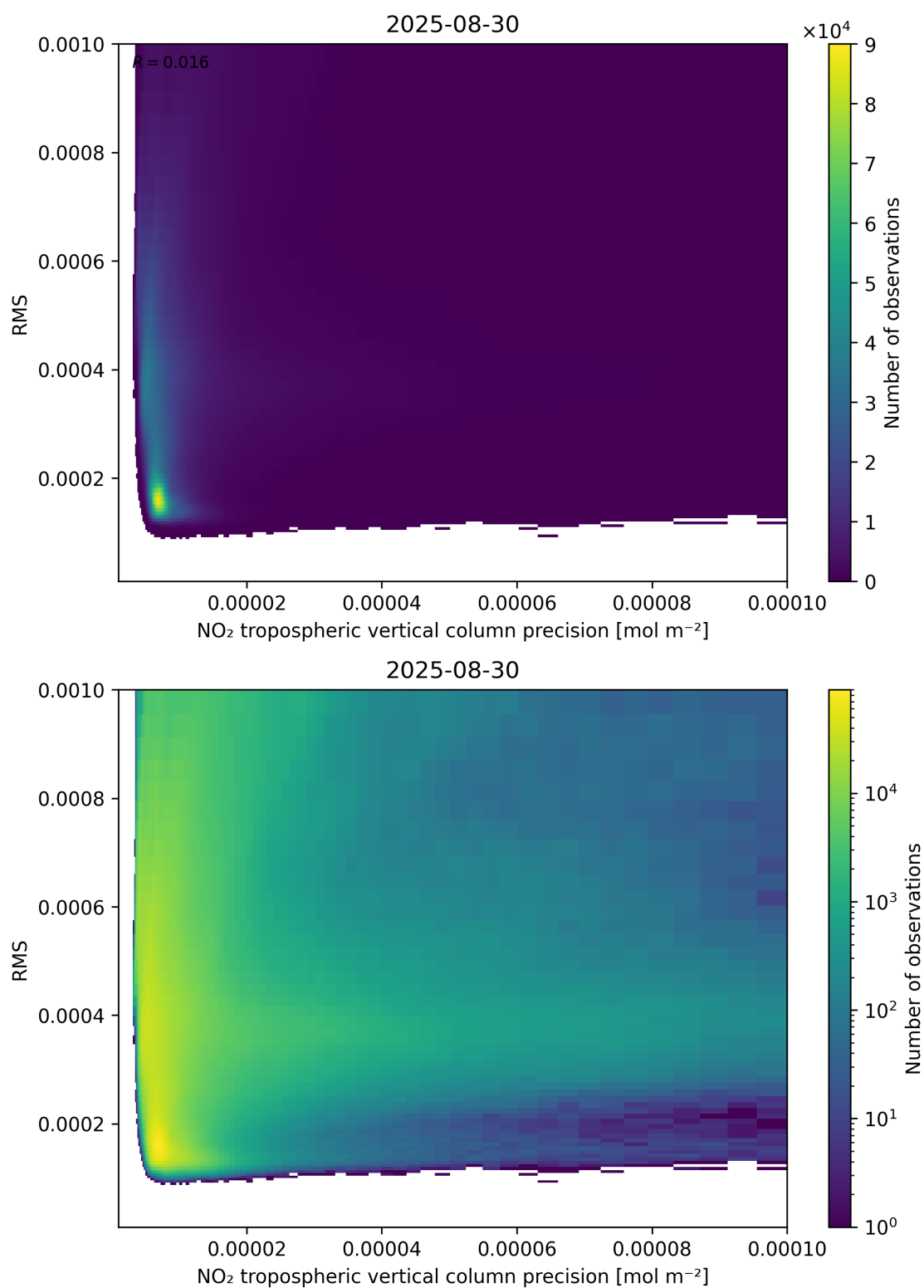
Figure 140: Scatter density plot of “NO 2 tropospheric vertical column precision” against “RMS” for 2025-08-30 to 2025-08-31.
