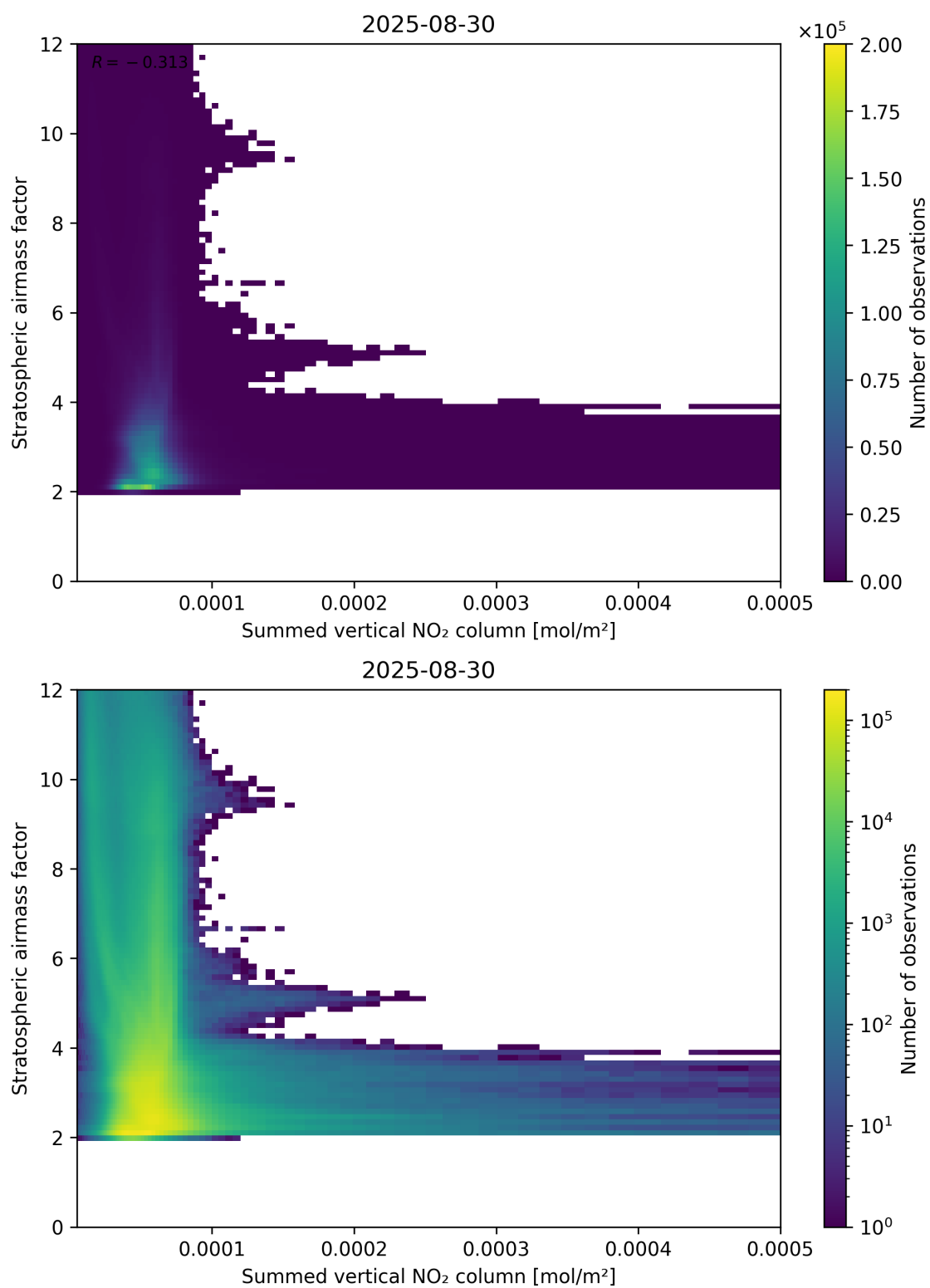
Figure 103: Scatter density plot of “Summed vertical NO 2 column” against “Stratospheric airmass factor” for 2025-08-30 to 2025-08-31.
