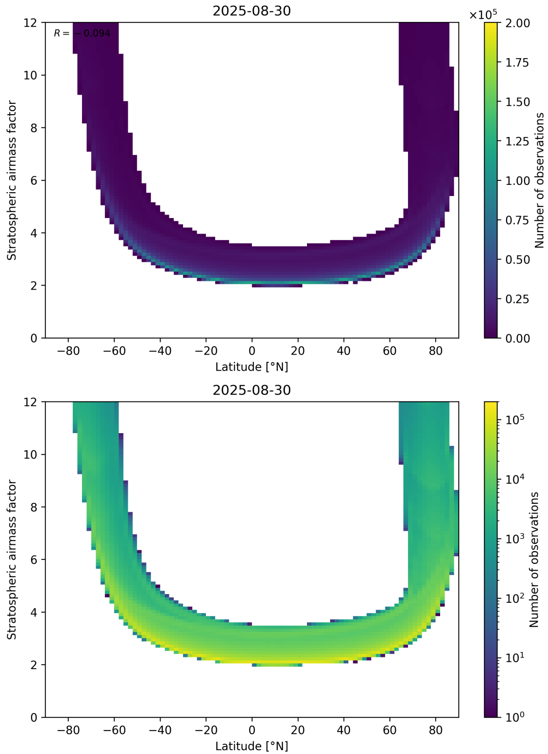
Figure 83: Scatter density plot of “Latitude” against “Stratospheric air mass factor” for 2025-08-30 to 2025-08-31.
