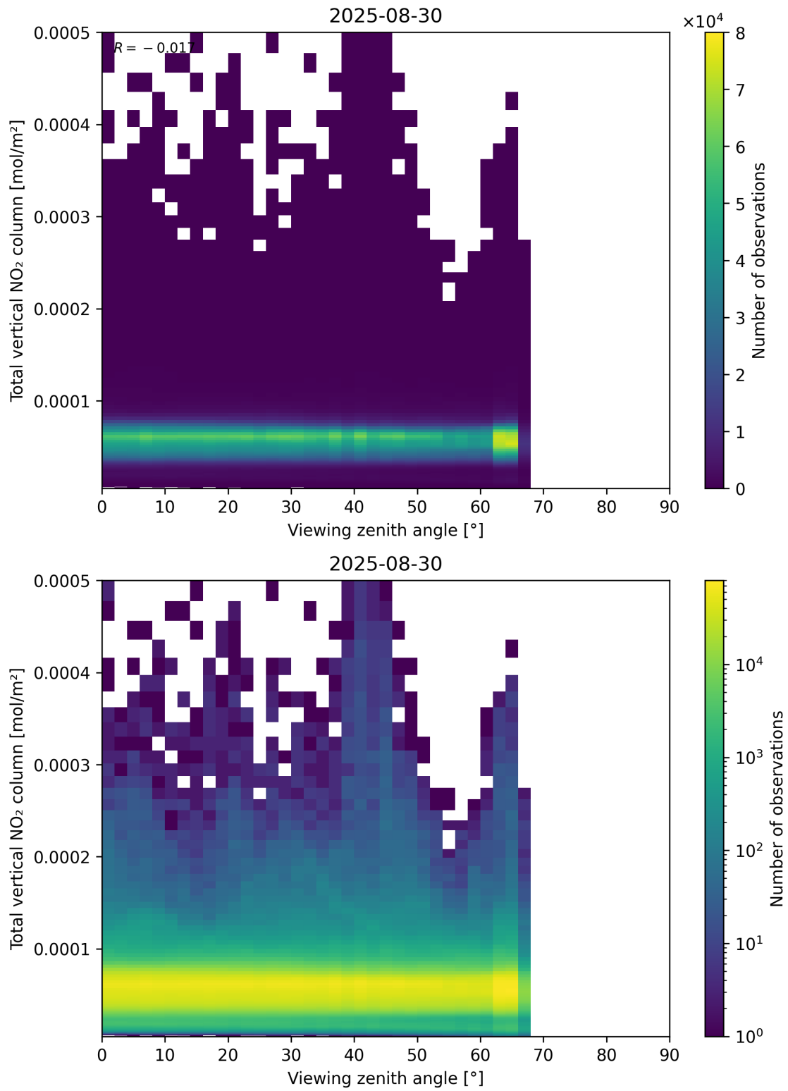
Figure 167: Scatter density plot of “Viewing zenith angle” against “Total vertical NO 2 column” for 2025-08-30 to 2025-08-31.
