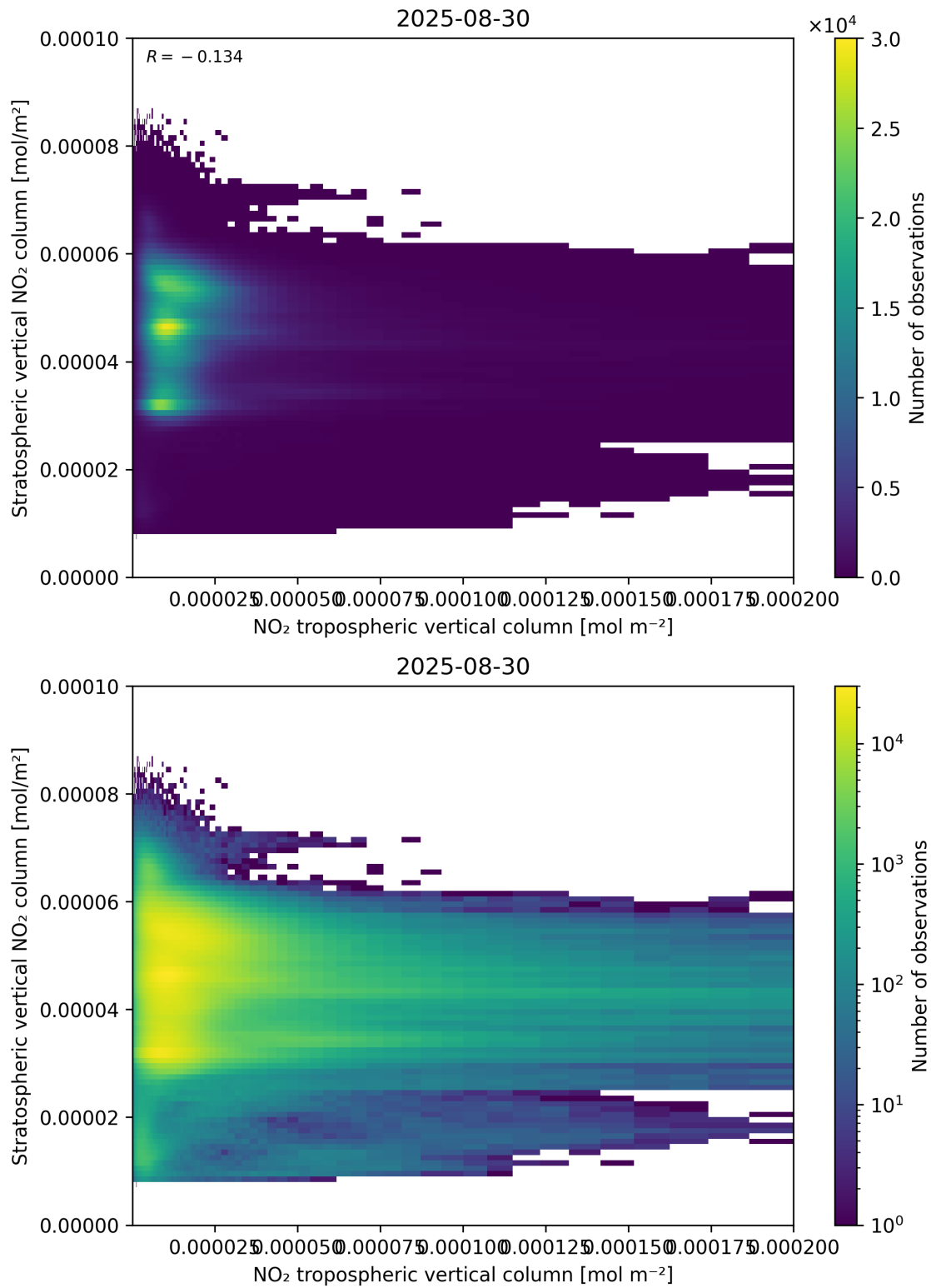
Figure 125: Scatter density plot of “NO 2 tropospheric vertical column” against “Stratospheric vertical NO 2 column” for 2025-08-30 to 2025-08-31.
