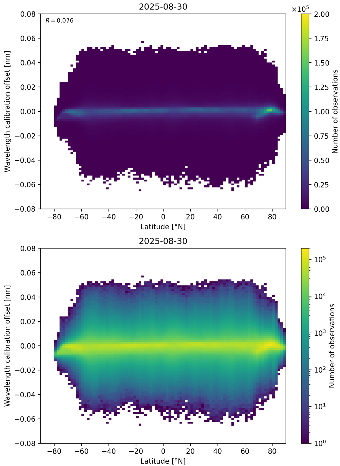
Figure 95: Scatter density plot of “Latitude” against “Wavelength calibration offset” for 2025-08-30 to 2025-08-31.
