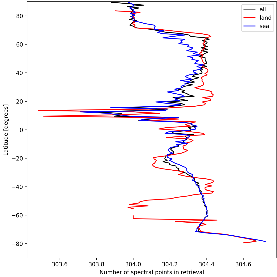
Figure 16: Zonal average of “Number of spectral points in retrieval” for 2025-08-30 to 2025-08-31.
