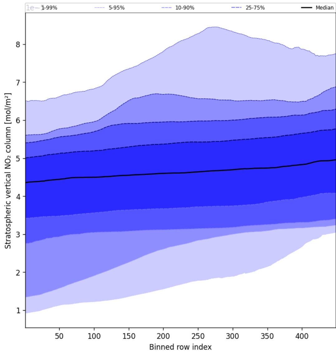
Figure 53: Along track statistics of “Stratospheric vertical NO 2 column” for 2025-08-30 to 2025-08-31
