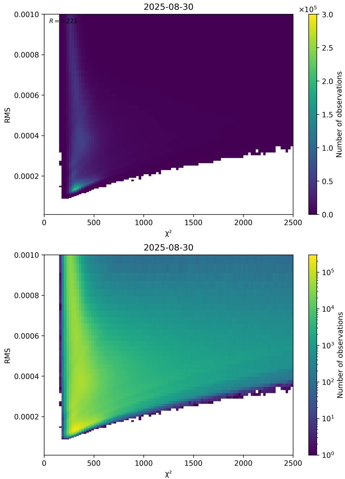
Figure 82: Scatter density plot of “ \chi^2 ” against “RMS” for 2025-08-30 to 2025-08-31.
