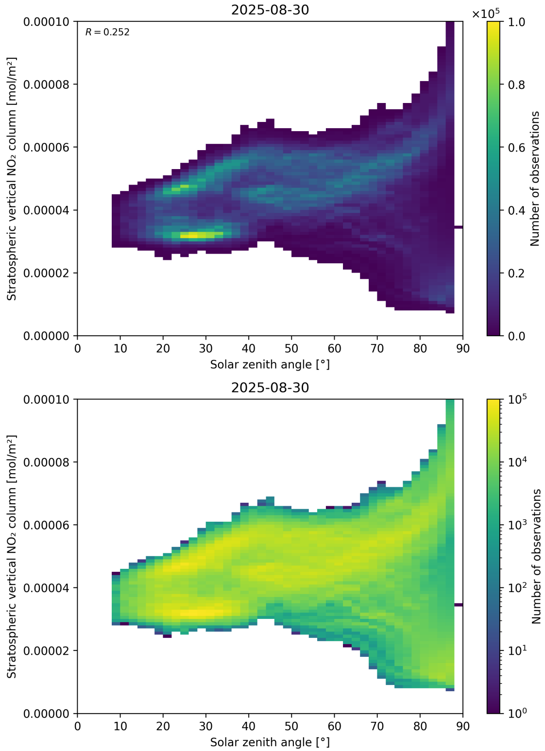
Figure 150: Scatter density plot of “Solar zenith angle” against “Stratospheric vertical NO 2 column” for 2025-08-30 to 2025-08-31.
