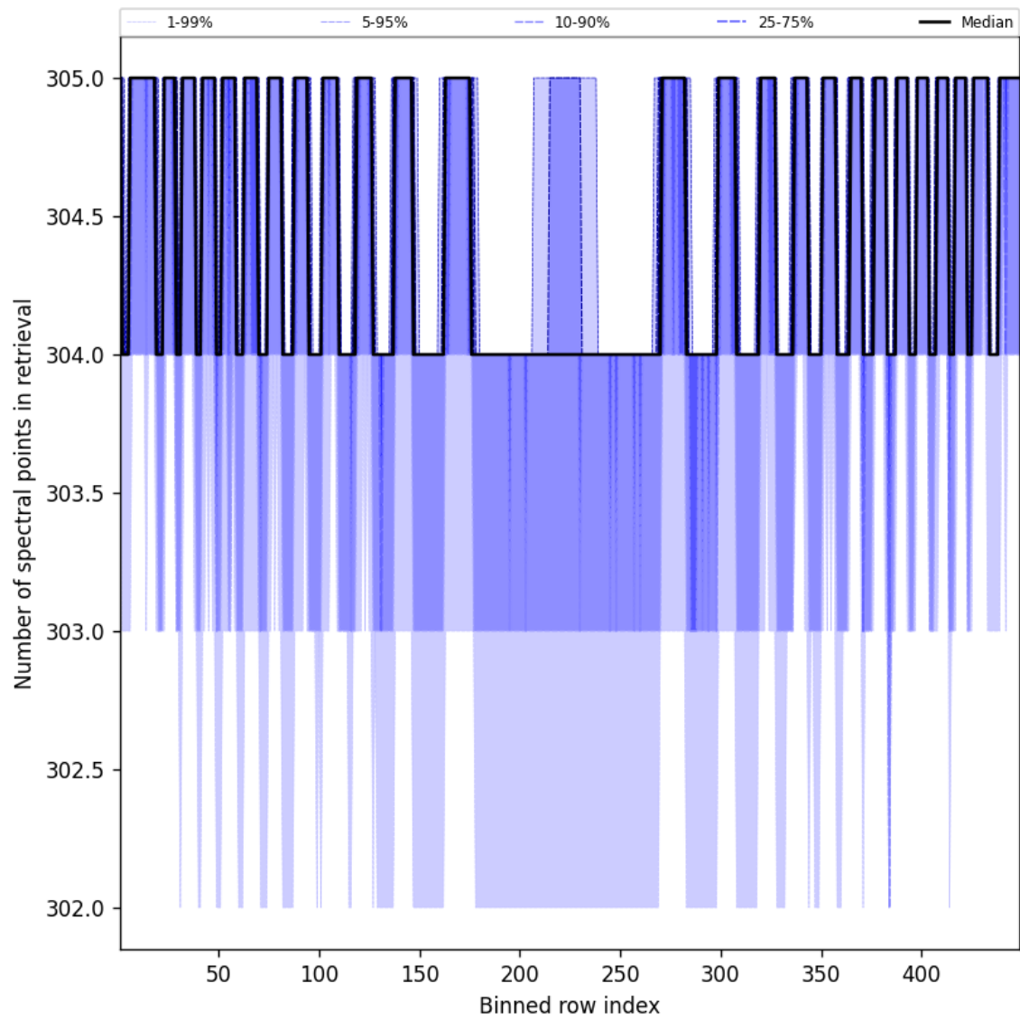
Figure 50: Along track statistics of “Number of spectral points in retrieval” for 2025-08-30 to 2025-08-31
