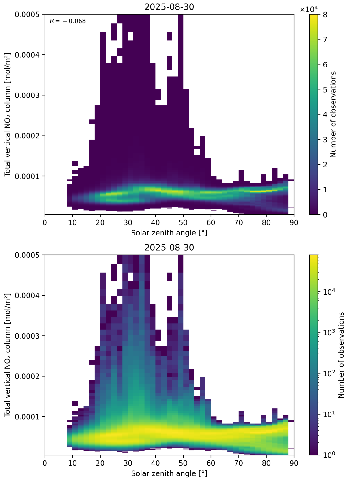
Figure 153: Scatter density plot of “Solar zenith angle” against “Total vertical NO 2 column” for 2025-08-30 to 2025-08-31.
