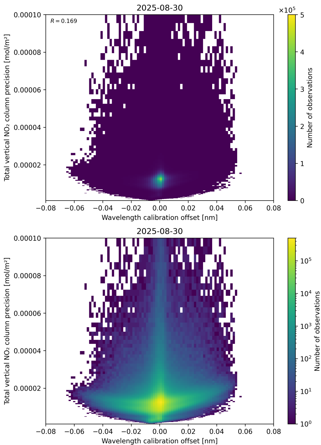
Figure 180: Scatter density plot of “Wavelength calibration offset” against “Total vertical NO 2 column precision” for 2025-08-30 to 2025-08-31.
