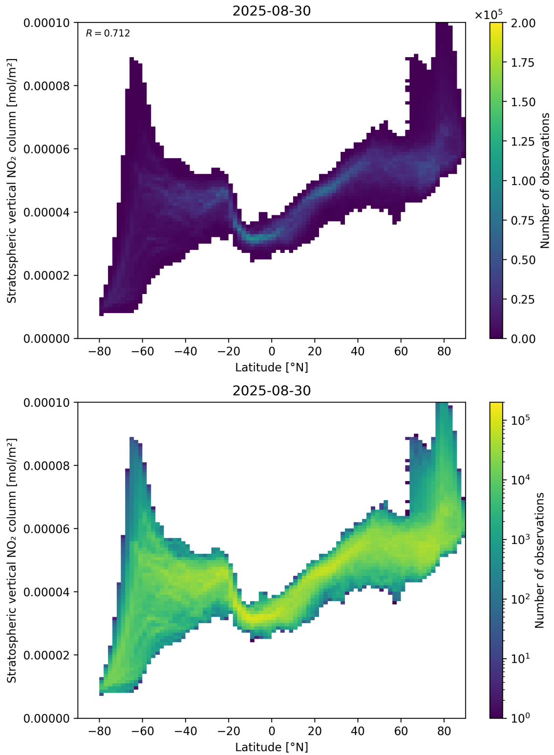
Figure 87: Scatter density plot of “Latitude” against “Stratospheric vertical \text{NO}_2 column” for 2025-08-30 to 2025-08-31.
