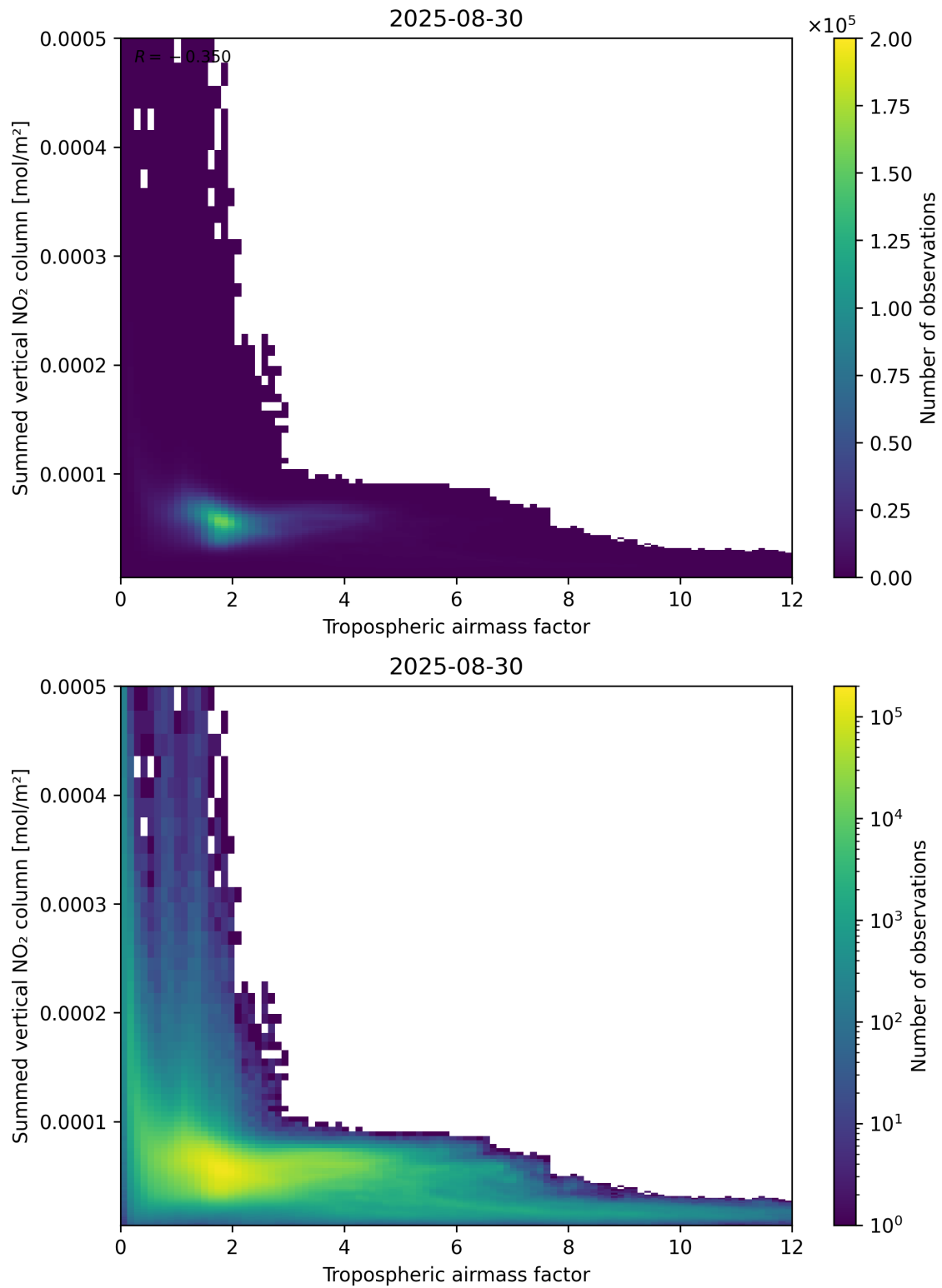
Figure 75: Scatter density plot of “Tropospheric airmass factor” against “Summed vertical NO 2 column” for 2025-08-30 to 2025-08-31.
