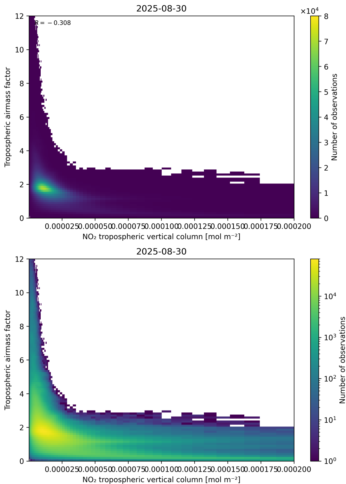
Figure 123: Scatter density plot of “NO 2 tropospheric vertical column” against “Tropospheric air mass factor” for 2025-08-30 to 2025-08-31.
