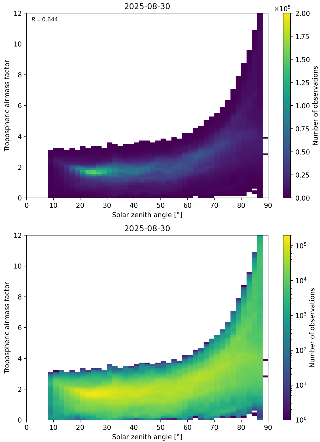
Figure 147: Scatter density plot of “Solar zenith angle” against “Tropospheric airmass factor” for 2025-08-30 to 2025-08-31.
