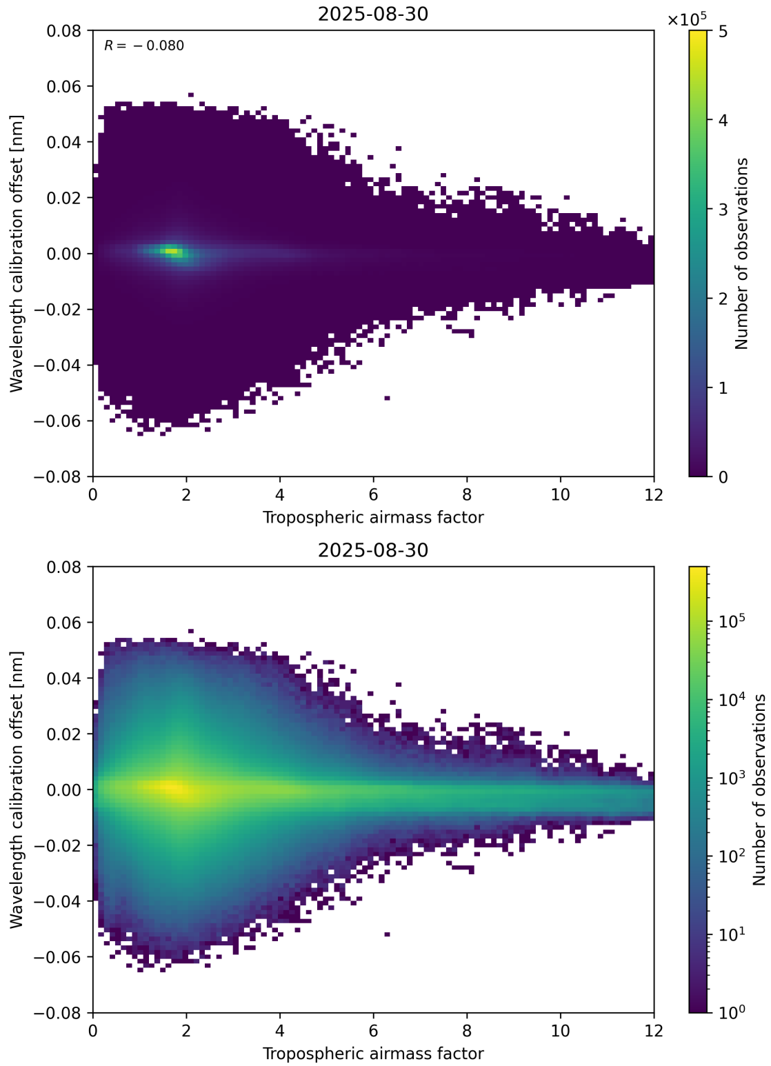
Figure 80: Scatter density plot of “Tropospheric airmass factor” against “Wavelength calibration offset” for 2025-08-30 to 2025-08-31.
