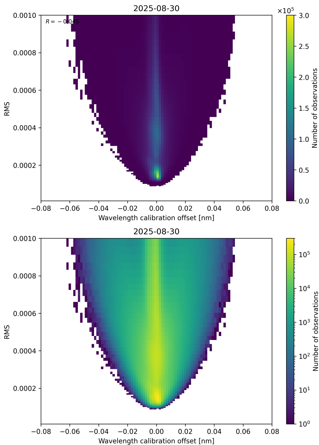
Figure 181: Scatter density plot of “Wavelength calibration offset” against “RMS” for 2025-08-30 to 2025-08-31.
