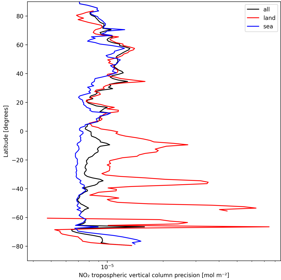
Figure 13: Zonal average of “NO 2 tropospheric vertical column precision” for 2025-08-30 to 2025-08-31.
