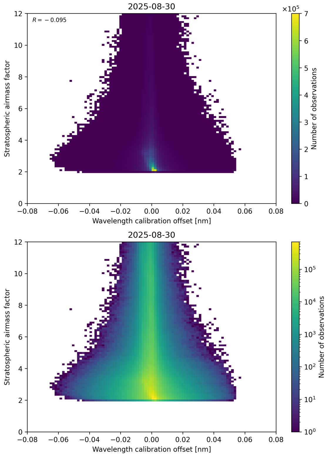
Figure 174: Scatter density plot of “Wavelength calibration offset” against “Stratospheric air mass factor” for 2025-08-30 to 2025-08-31.
