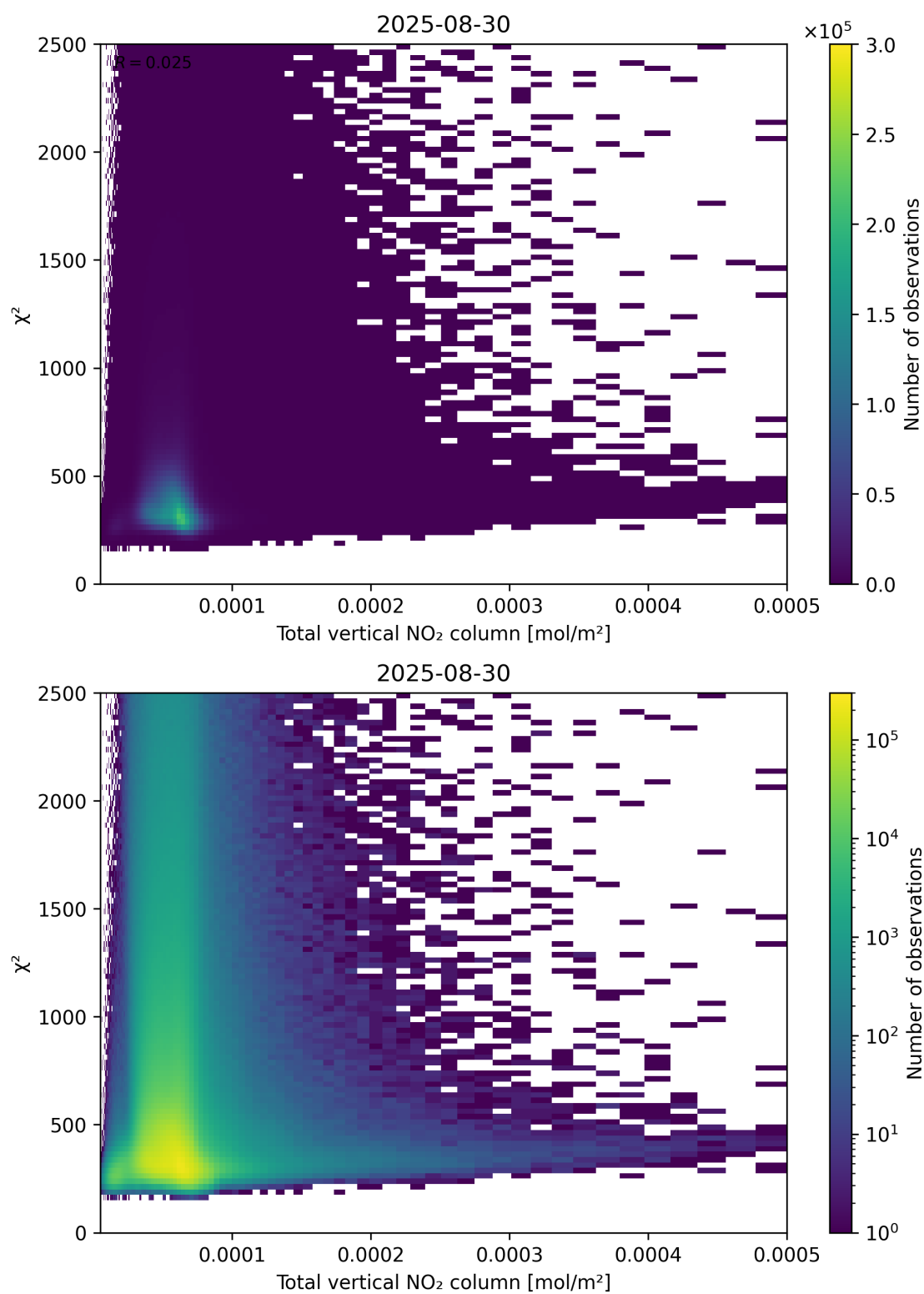
Figure 111: Scatter density plot of “Total vertical NO 2 column” against “ \chi^2 ” for 2025-08-30 to 2025-08-31.
