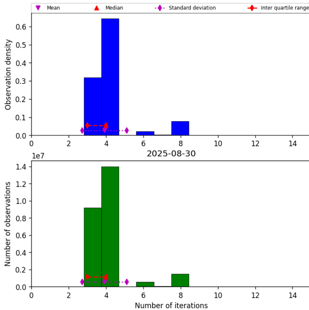
Figure 34: Histogram of “Number of iterations” for 2025-08-30 to 2025-08-31
