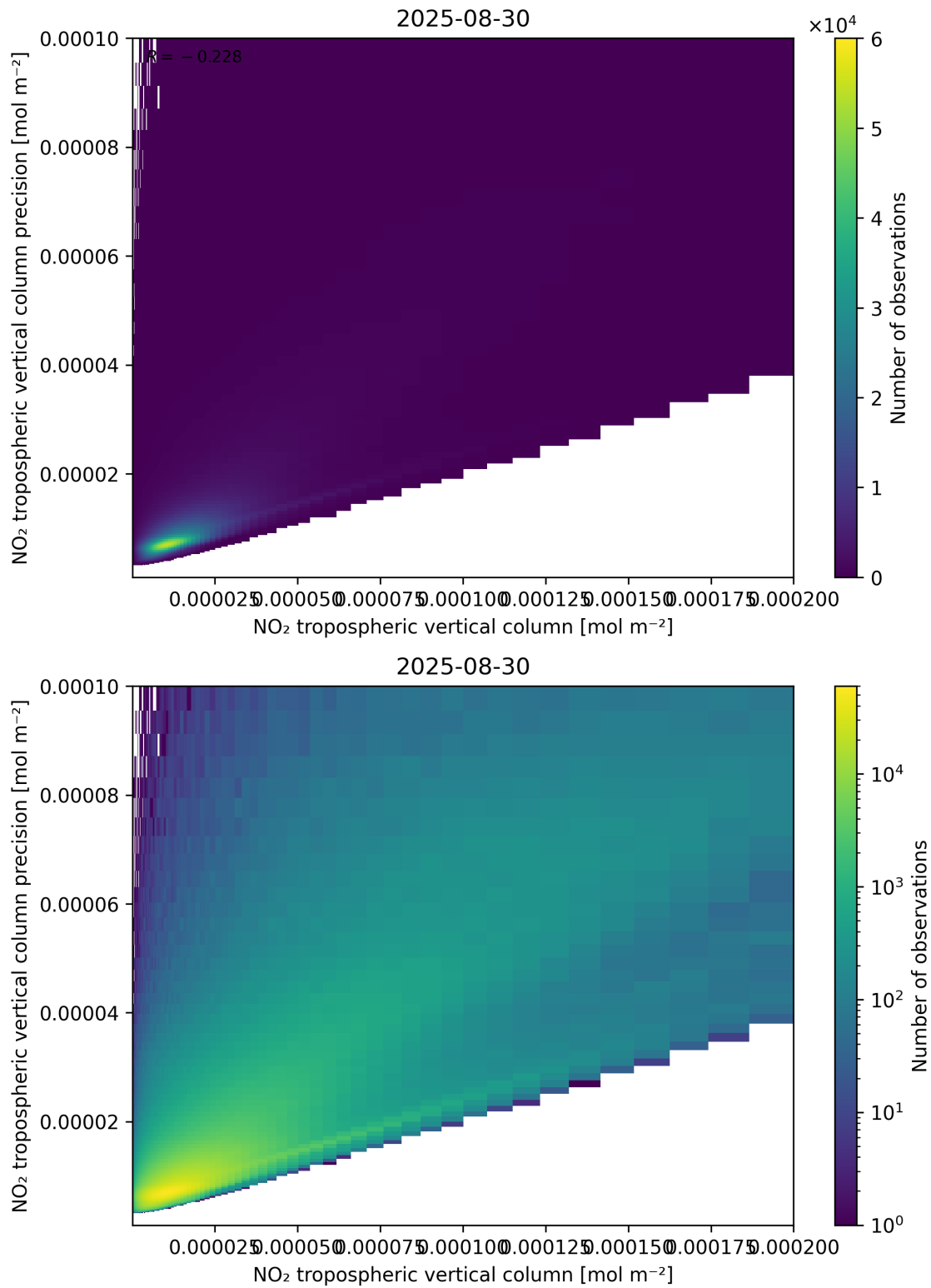
Figure 130: Scatter density plot of “NO 2 tropospheric vertical column” against “NO 2 tropospheric vertical column precision” for 2025-08-30 to 2025-08-31.
