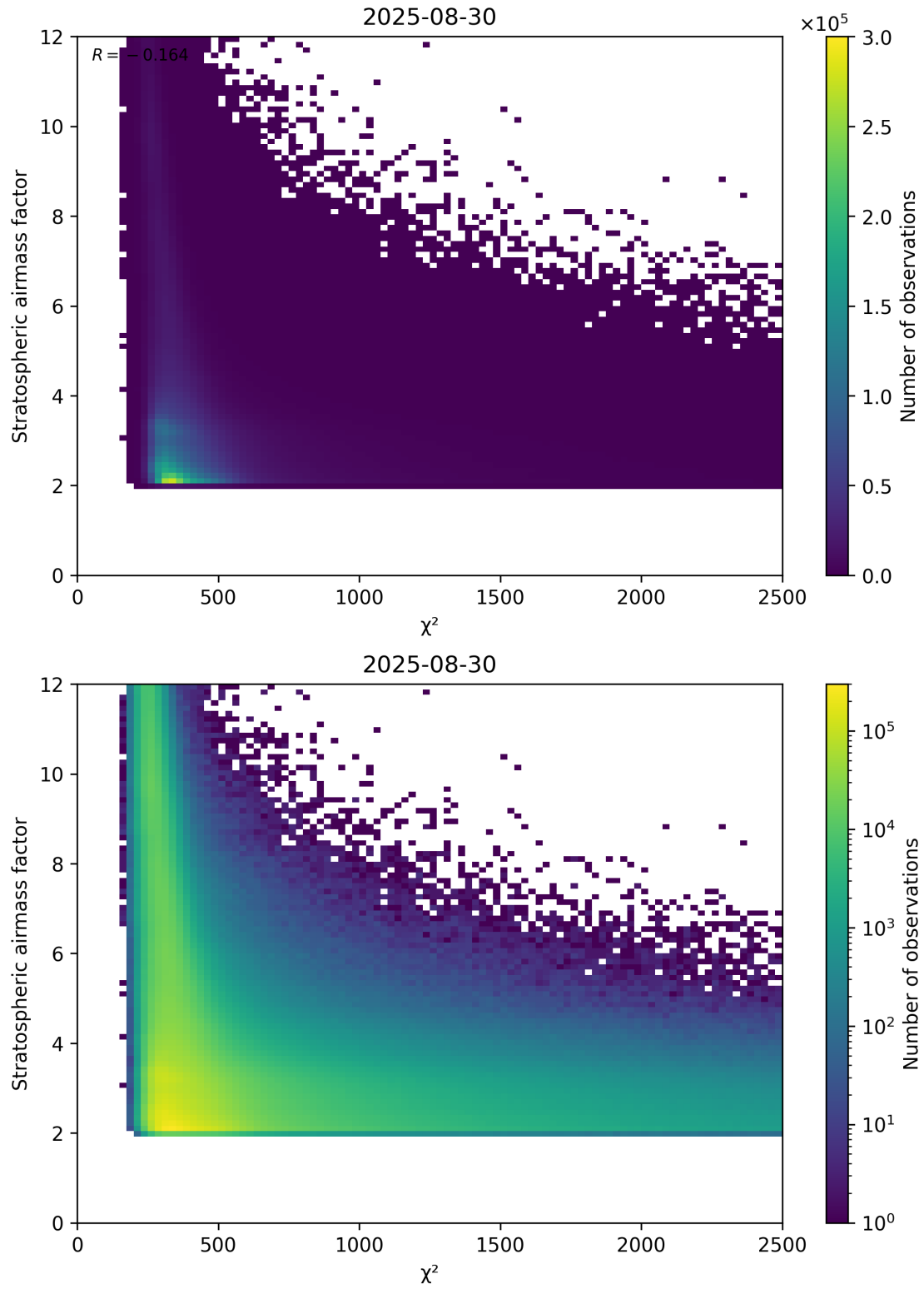
Figure 81: Scatter density plot of “ \chi^2 ” against “Stratospheric airmass factor” for 2025-08-30 to 2025-08-31.
