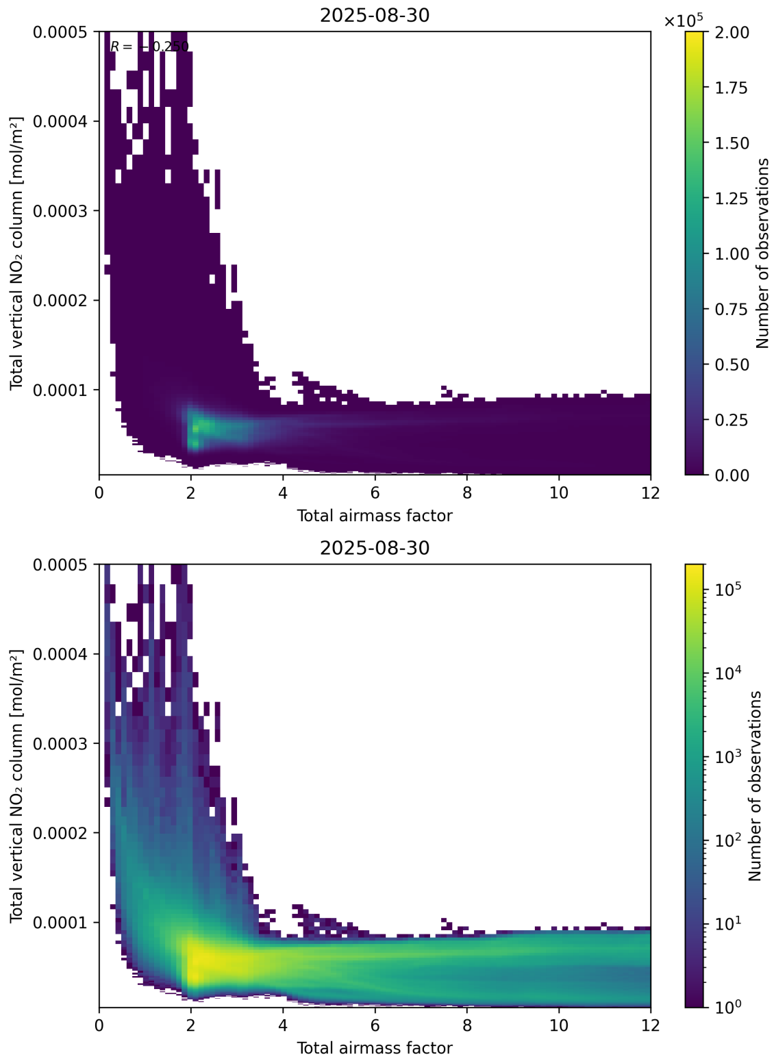
Figure 67: Scatter density plot of “Total air mass factor” against “Total vertical NO 2 column” for 2025-08-30 to 2025-08-31.
