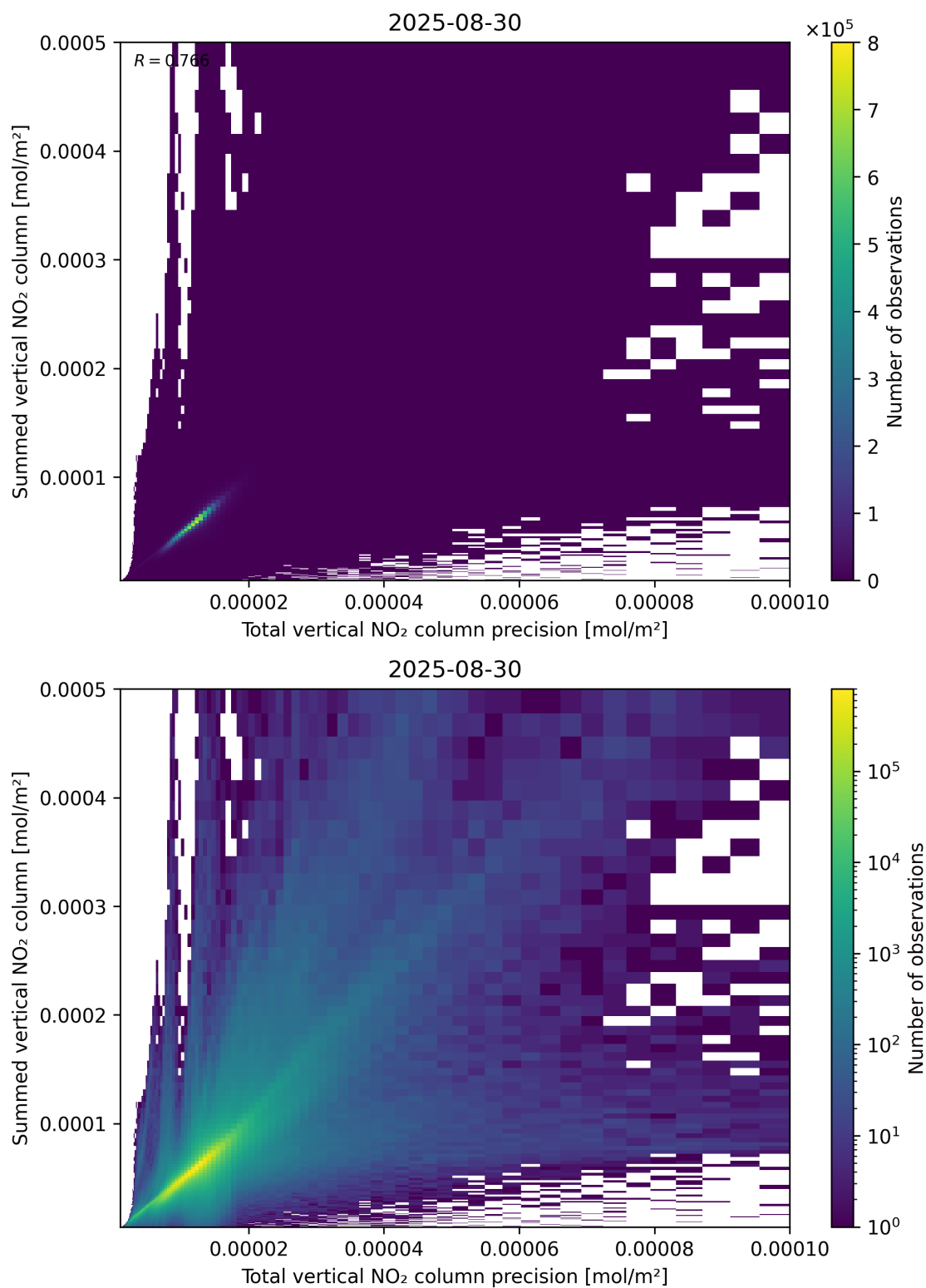
Figure 117: Scatter density plot of “Total vertical NO 2 column precision” against “Summed vertical NO 2 column” for 2025-08-30 to 2025-08-31.
