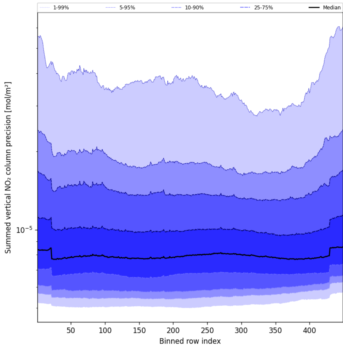
Figure 58: Along track statistics of “Summed vertical NO 2 column precision” for 2025-08-30 to 2025-08-31
