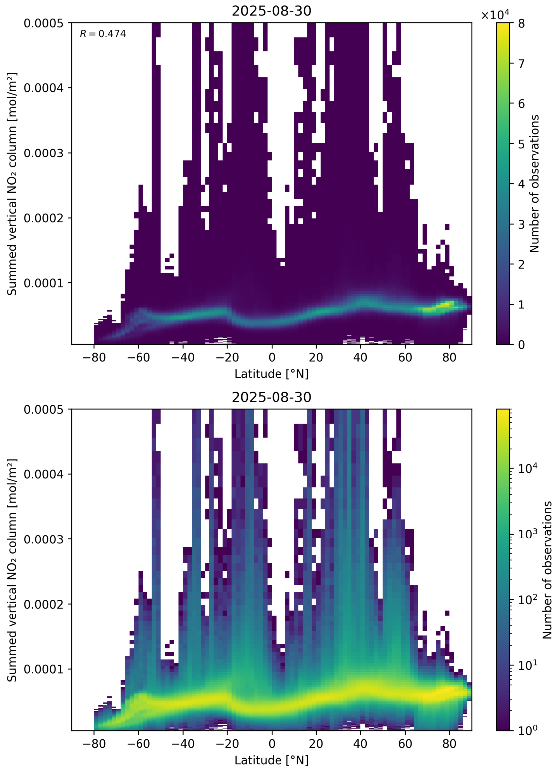
Figure 88: Scatter density plot of “Latitude” against “Summed vertical NO 2 column” for 2025-08-30 to 2025-08-31.
