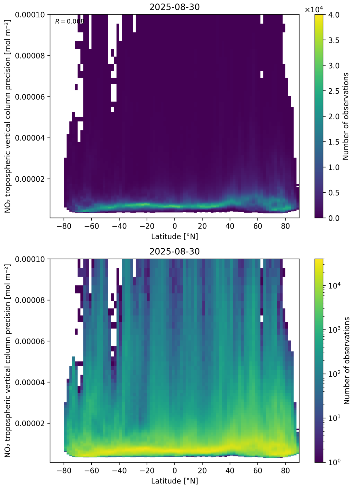
Figure 93: Scatter density plot of “Latitude” against “NO 2 tropospheric vertical column precision” for 2025-08-30 to 2025-08-31.
