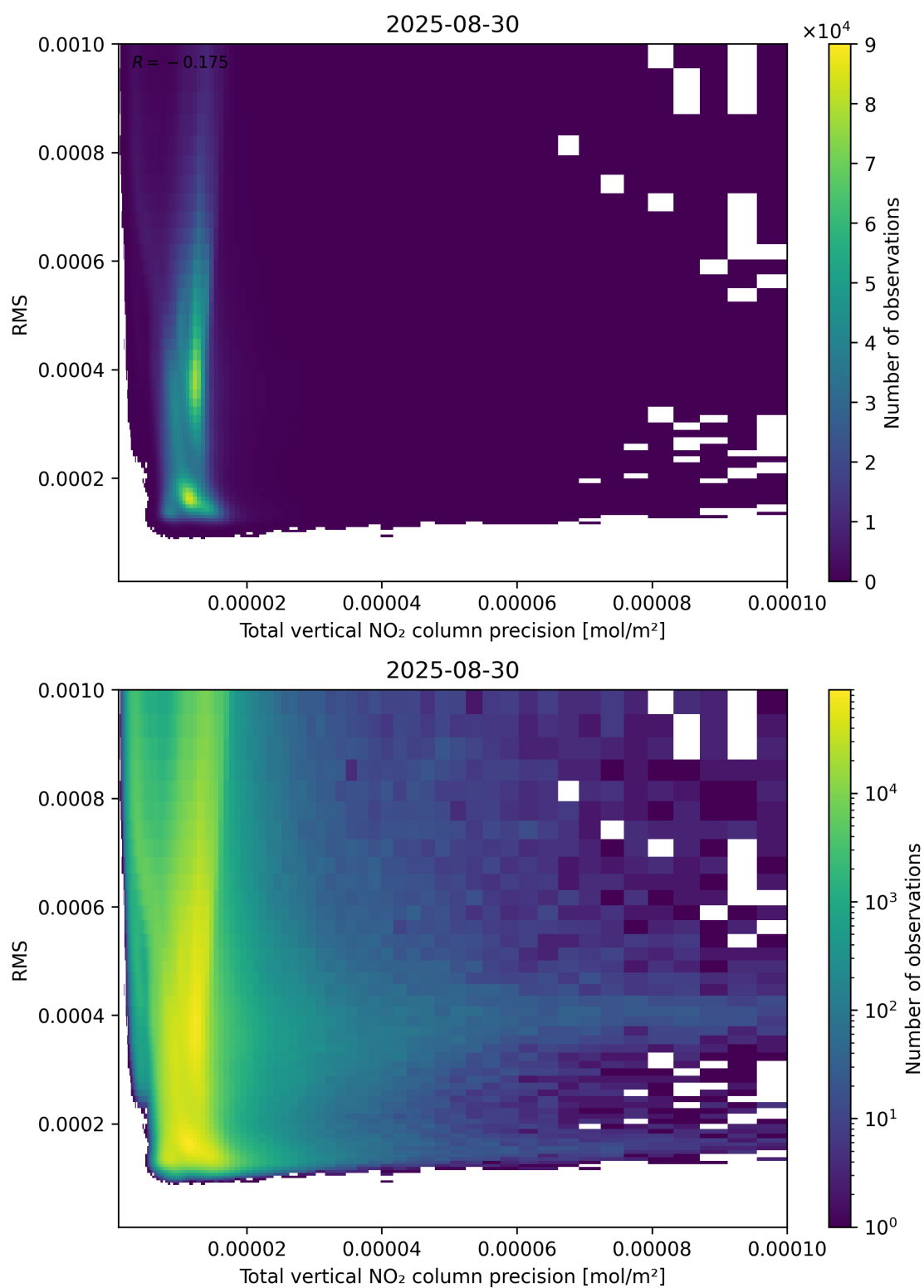
Figure 119: Scatter density plot of “Total vertical NO 2 column precision” against “RMS” for 2025-08-30 to 2025-08-31.
