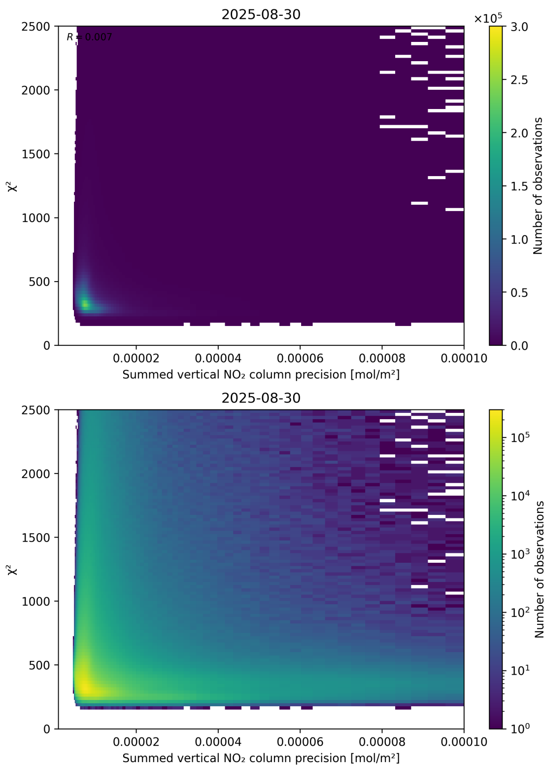
Figure 107: Scatter density plot of “Summed vertical NO 2 column precision” against “ \chi^2 ” for 2025-08-30 to 2025-08-31.
