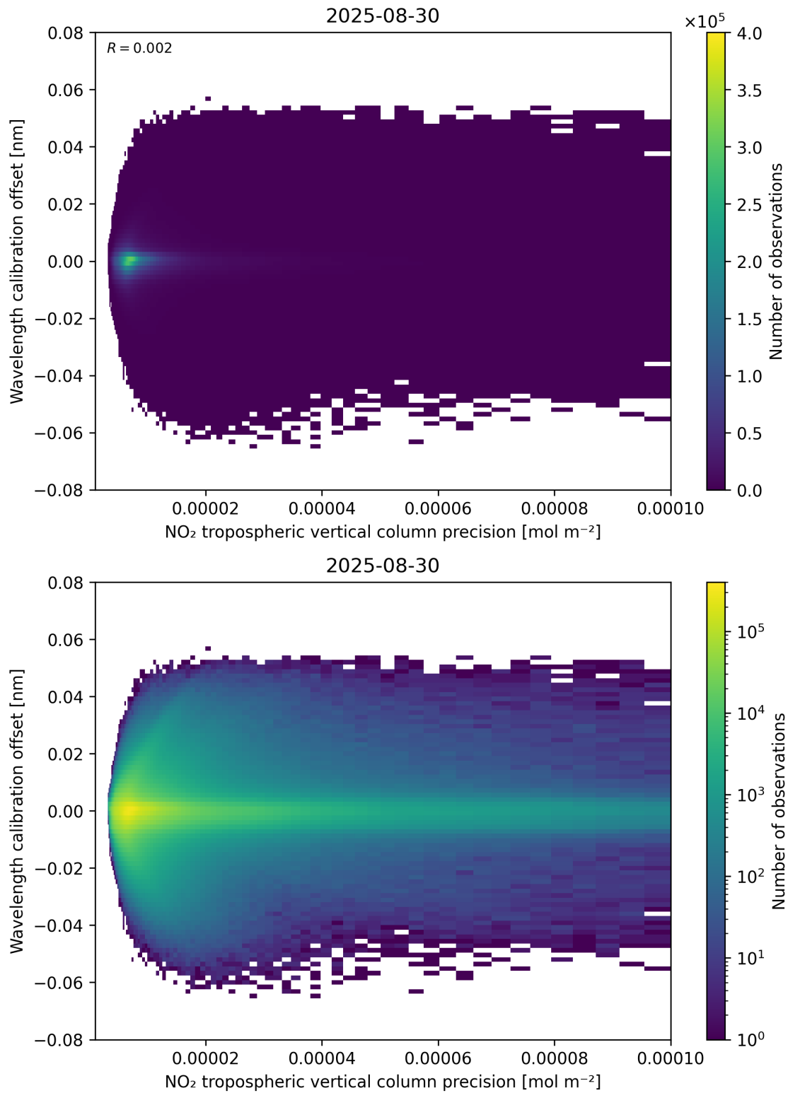
Figure 141: Scatter density plot of “NO 2 tropospheric vertical column precision” against “Wavelength calibration offset” for 2025-08-30 to 2025-08-31.
