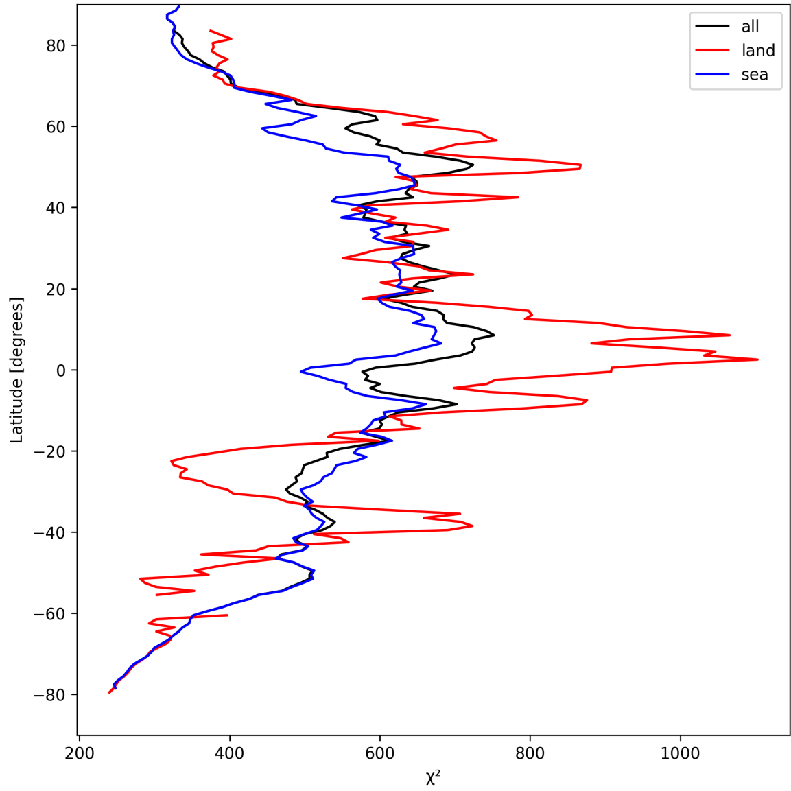
Figure 25: Zonal average of “ \chi^2 ” for 2025-08-30 to 2025-08-31.
