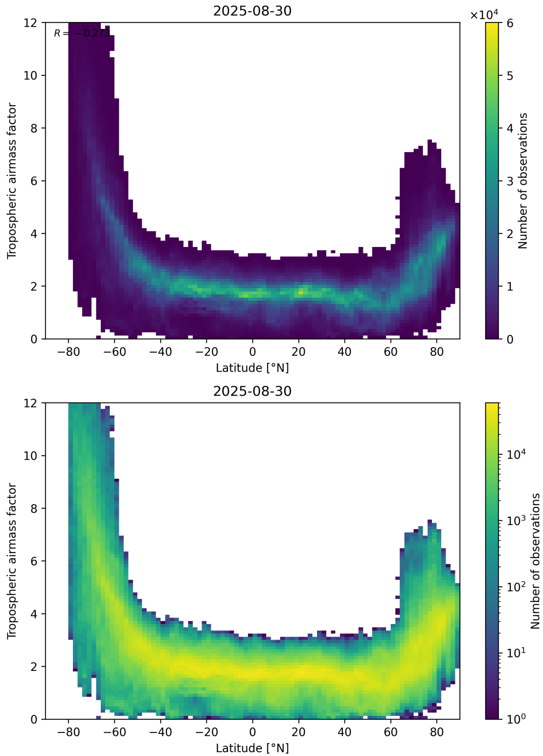
Figure 85: Scatter density plot of “Latitude” against “Tropospheric air mass factor” for 2025-08-30 to 2025-08-31.
