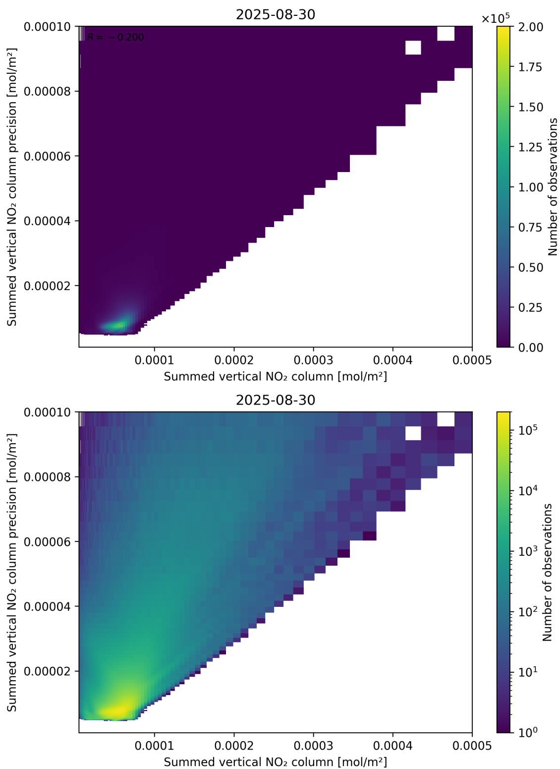
Figure 105: Scatter density plot of “Summed vertical NO 2 column” against “Summed vertical NO 2 column precision” for 2025-08-30 to 2025-08-31.
