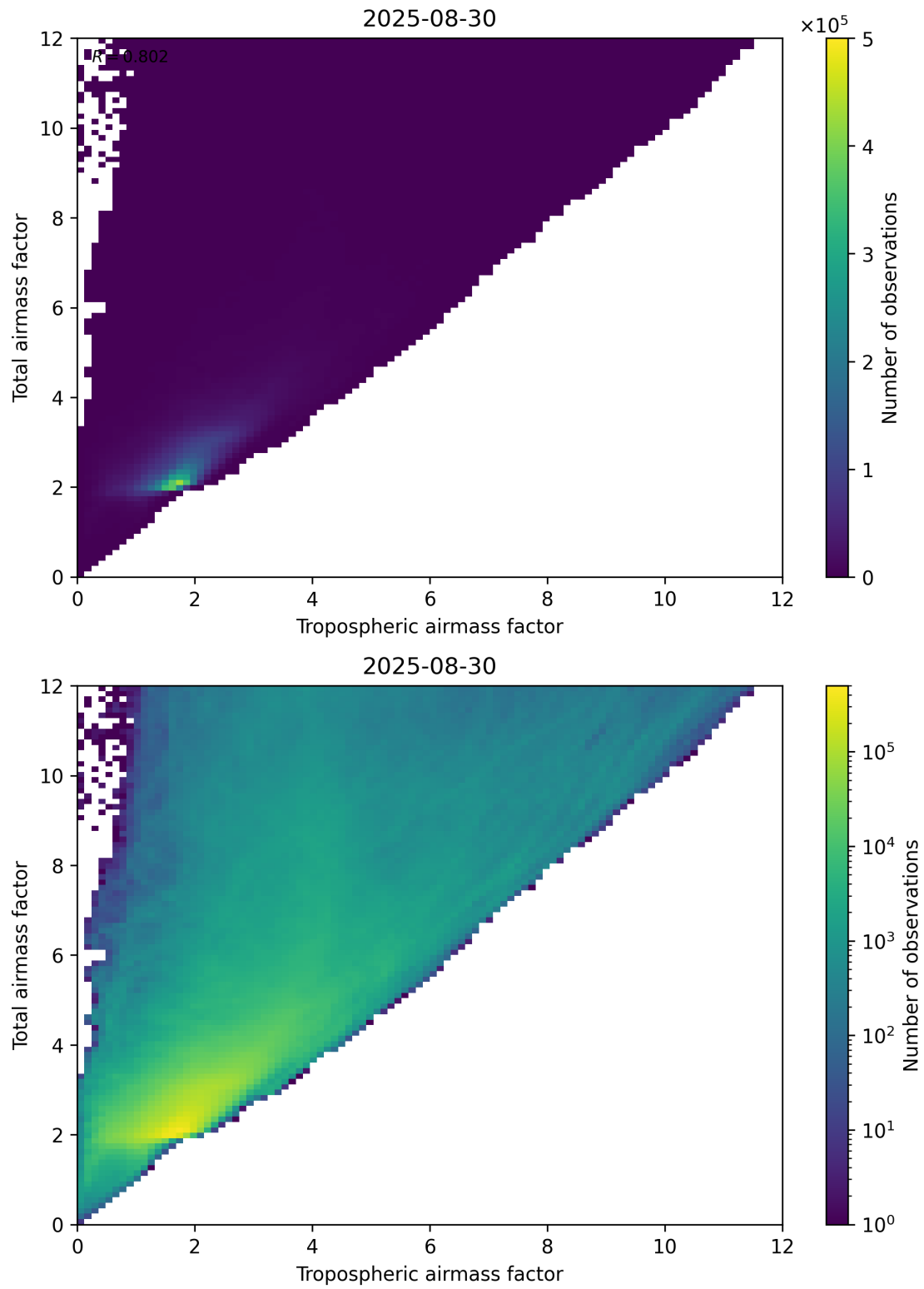
Figure 72: Scatter density plot of “Tropospheric airmass factor” against “Total airmass factor” for 2025-08-30 to 2025-08-31.
