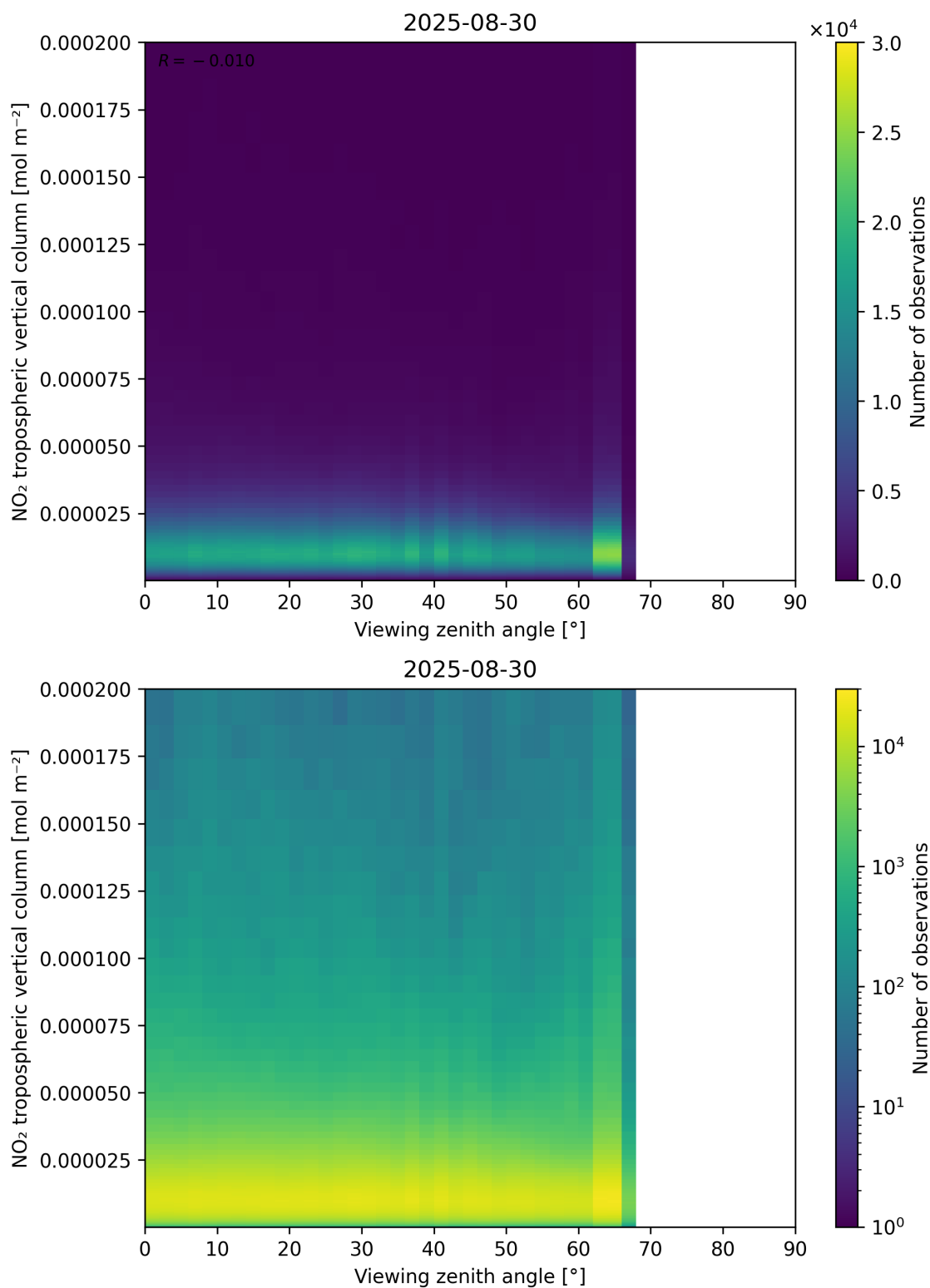
Figure 169: Scatter density plot of “Viewing zenith angle” against “NO 2 tropospheric vertical column” for 2025-08-30 to 2025-08-31.
