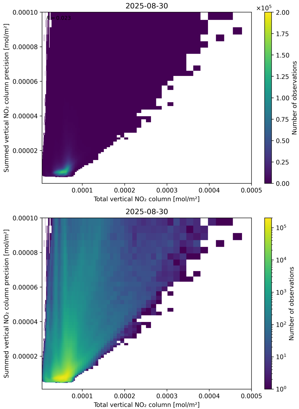
Figure 113: Scatter density plot of “Total vertical NO 2 column” against “Summed vertical NO 2 column precision” for 2025-08-30 to 2025-08-31.
