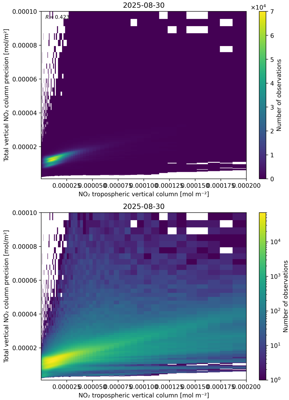
Figure 129: Scatter density plot of “NO 2 tropospheric vertical column” against “Total vertical NO 2 column precision” for 2025-08-30 to 2025-08-31.
