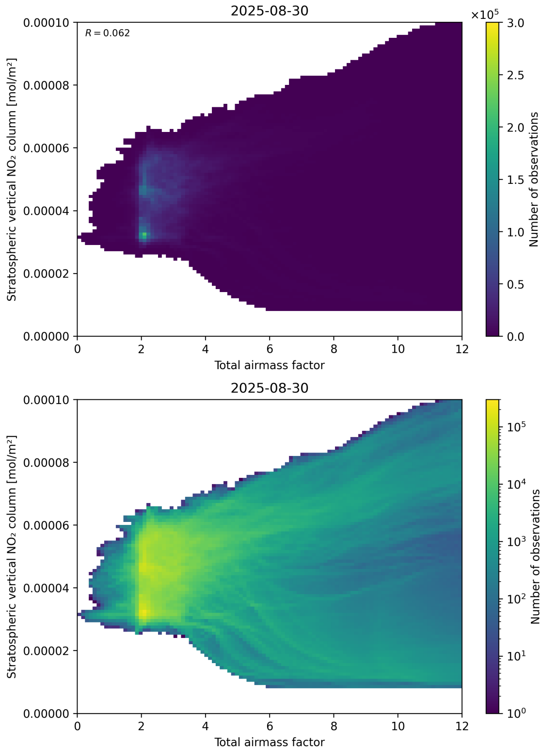
Figure 64: Scatter density plot of “Total airmass factor” against “Stratospheric vertical \text{NO}_2 column” for 2025-08-30 to 2025-08-31.
