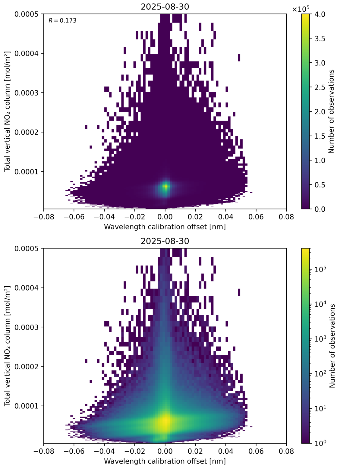
Figure 179: Scatter density plot of “Wavelength calibration offset” against “Total vertical NO 2 column” for 2025-08-30 to 2025-08-31.
