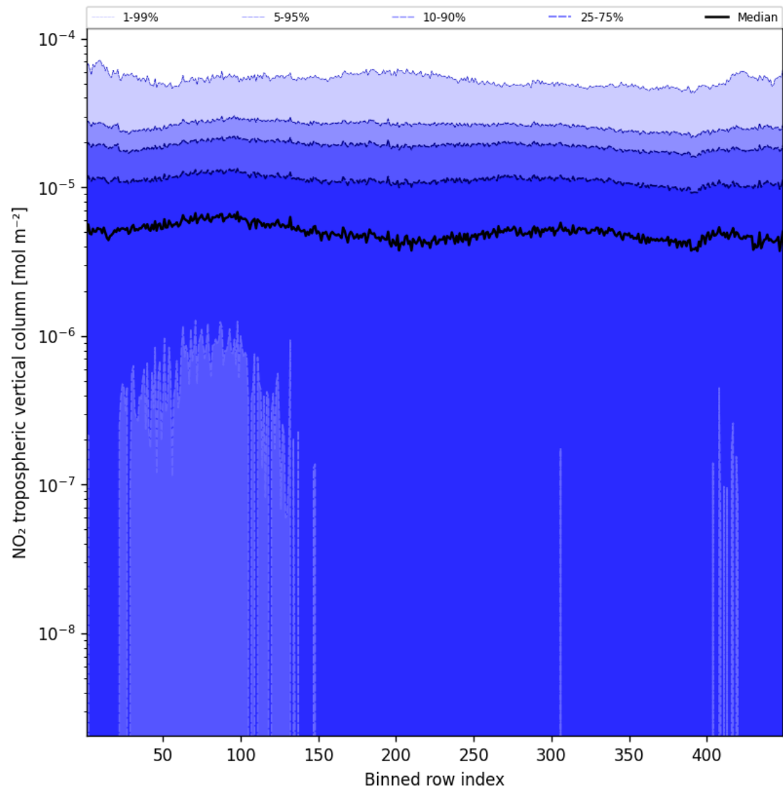
Figure 46: Along track statistics of “NO 2 tropospheric vertical column” for 2025-08-30 to 2025-08-31
