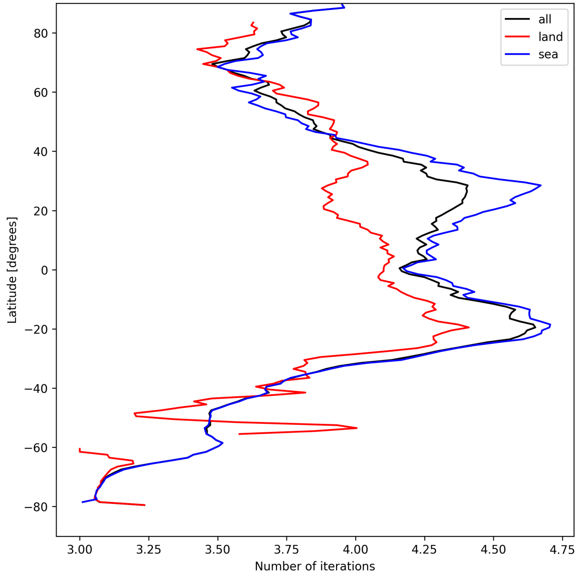
Figure 17: Zonal average of “Number of iterations” for 2025-08-30 to 2025-08-31.
