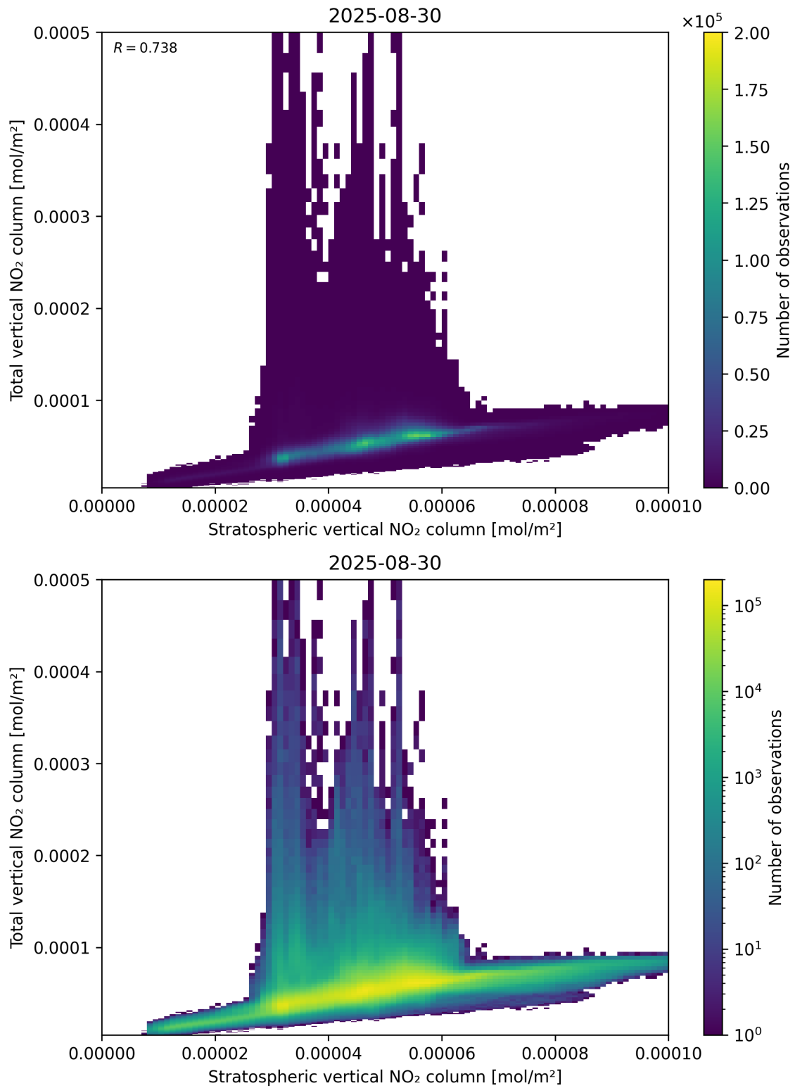
Figure 100: Scatter density plot of “Stratospheric vertical NO 2 column” against “Total vertical NO 2 column” for 2025-08-30 to 2025-08-31.
