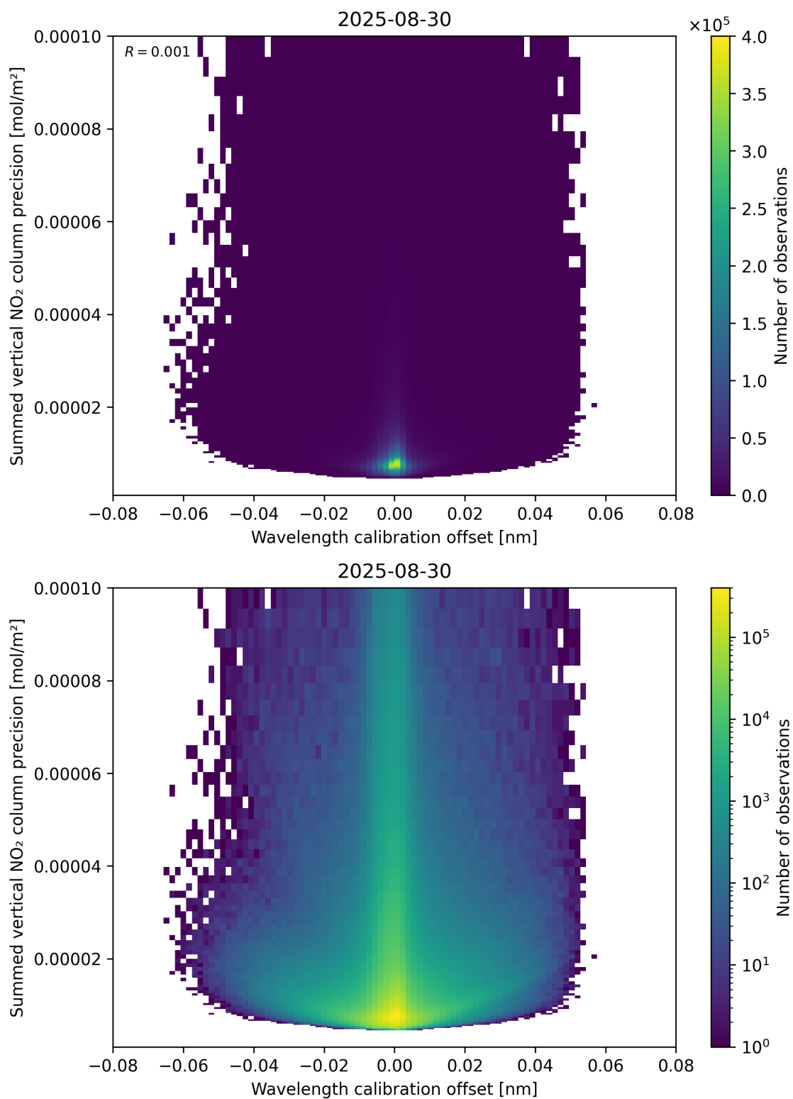
Figure 178: Scatter density plot of “Wavelength calibration offset” against “Summed vertical NO 2 column precision” for 2025-08-30 to 2025-08-31.
