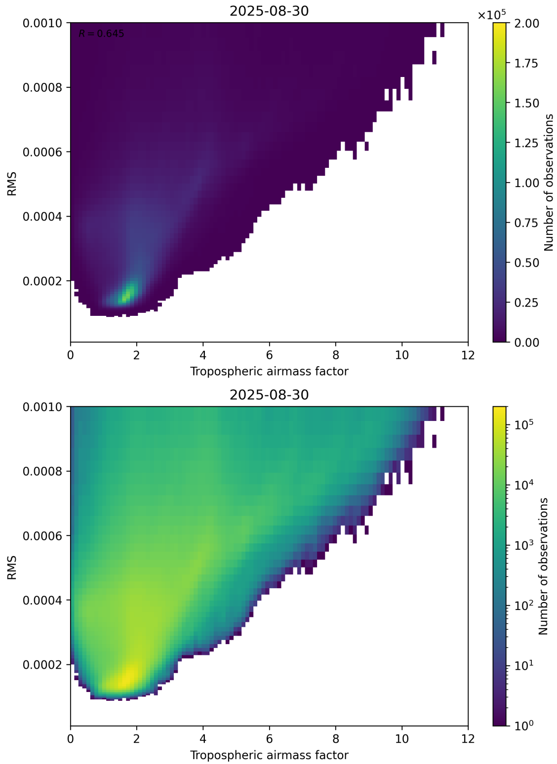
Figure 79: Scatter density plot of “Tropospheric airmass factor” against “RMS” for 2025-08-30 to 2025-08-31.
