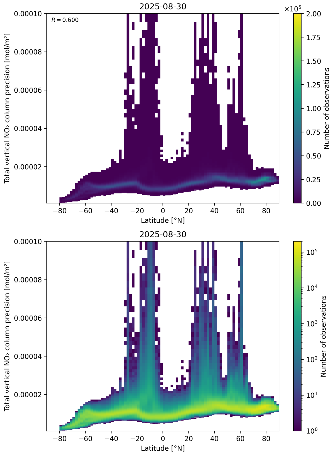
Figure 91: Scatter density plot of “Latitude” against “Total vertical NO 2 column precision” for 2025-08-30 to 2025-08-31.
