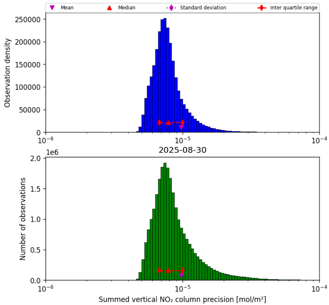
Figure 41: Histogram of "Summed vertical NO 2 column precision" for 2025-08-30 to 2025-08-31
