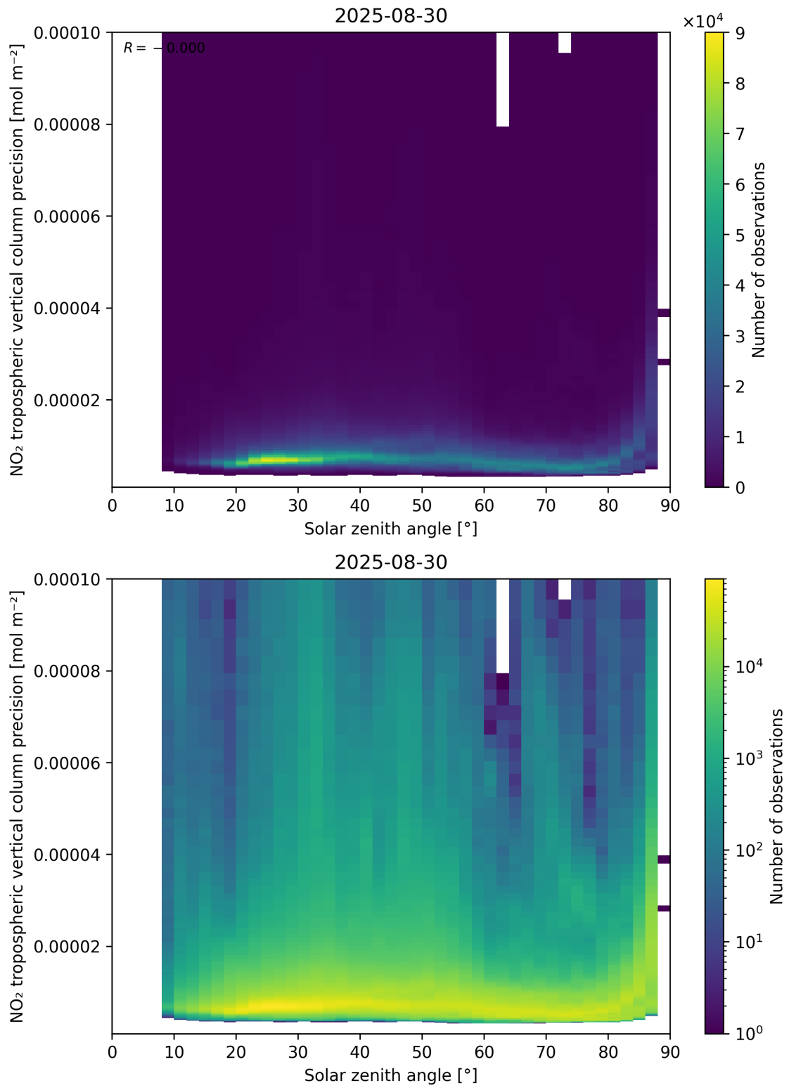
Figure 156: Scatter density plot of “Solar zenith angle” against “NO 2 tropospheric vertical column precision” for 2025-08-30 to 2025-08-31.
