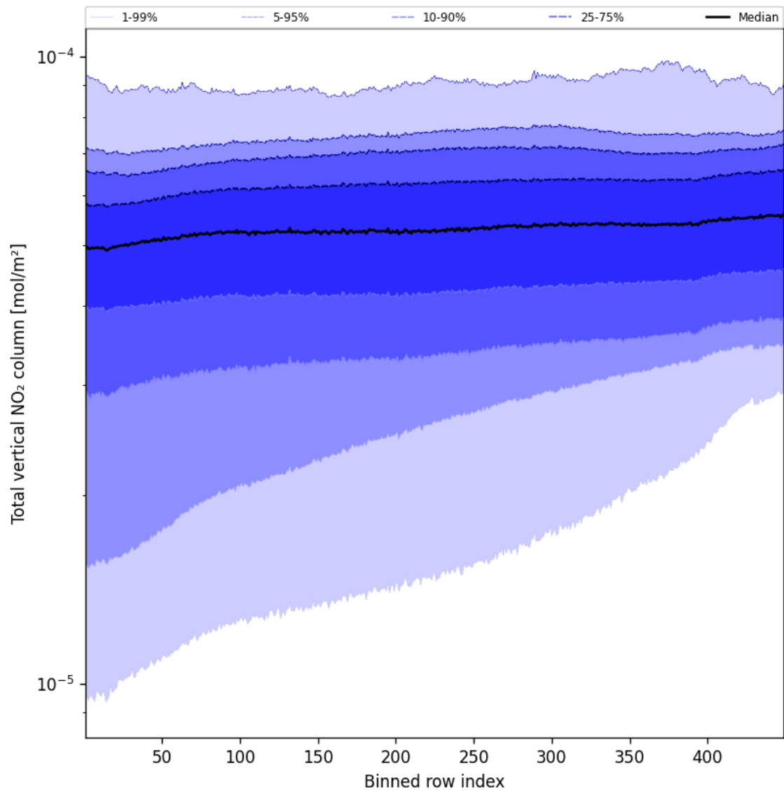
Figure 55: Along track statistics of “Total vertical NO 2 column” for 2025-08-30 to 2025-08-31
