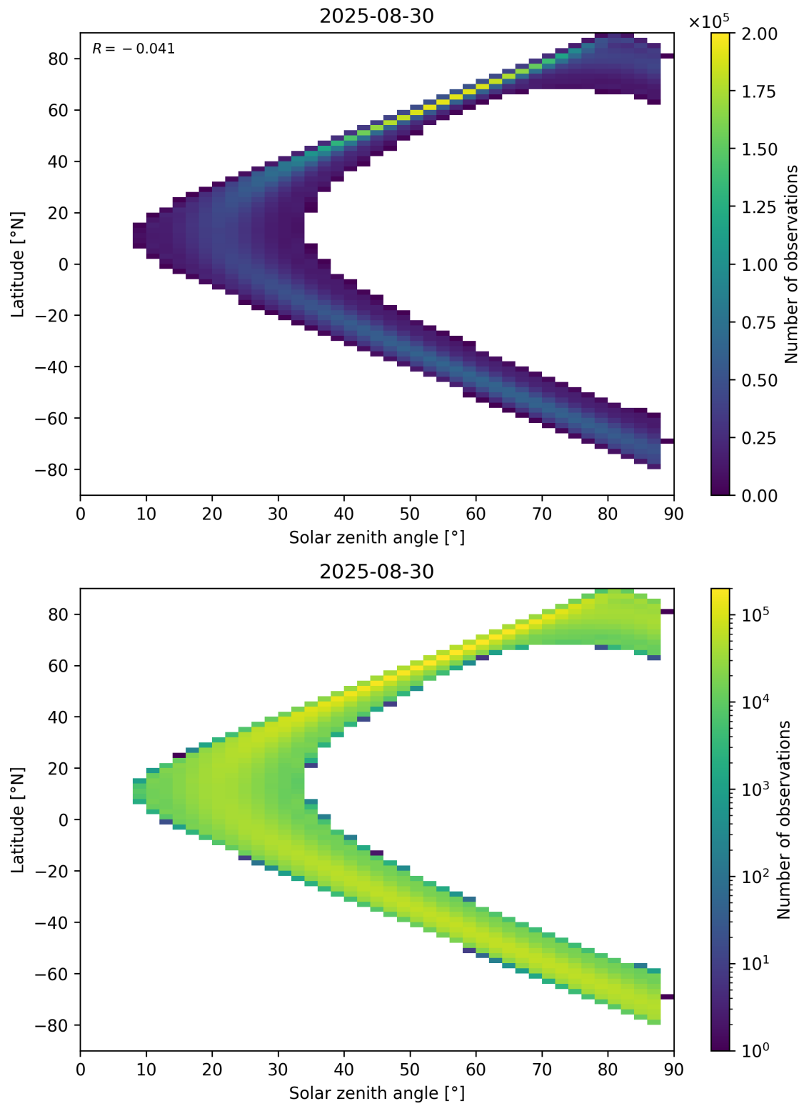
Figure 149: Scatter density plot of “Solar zenith angle” against “Latitude” for 2025-08-30 to 2025-08-31.
