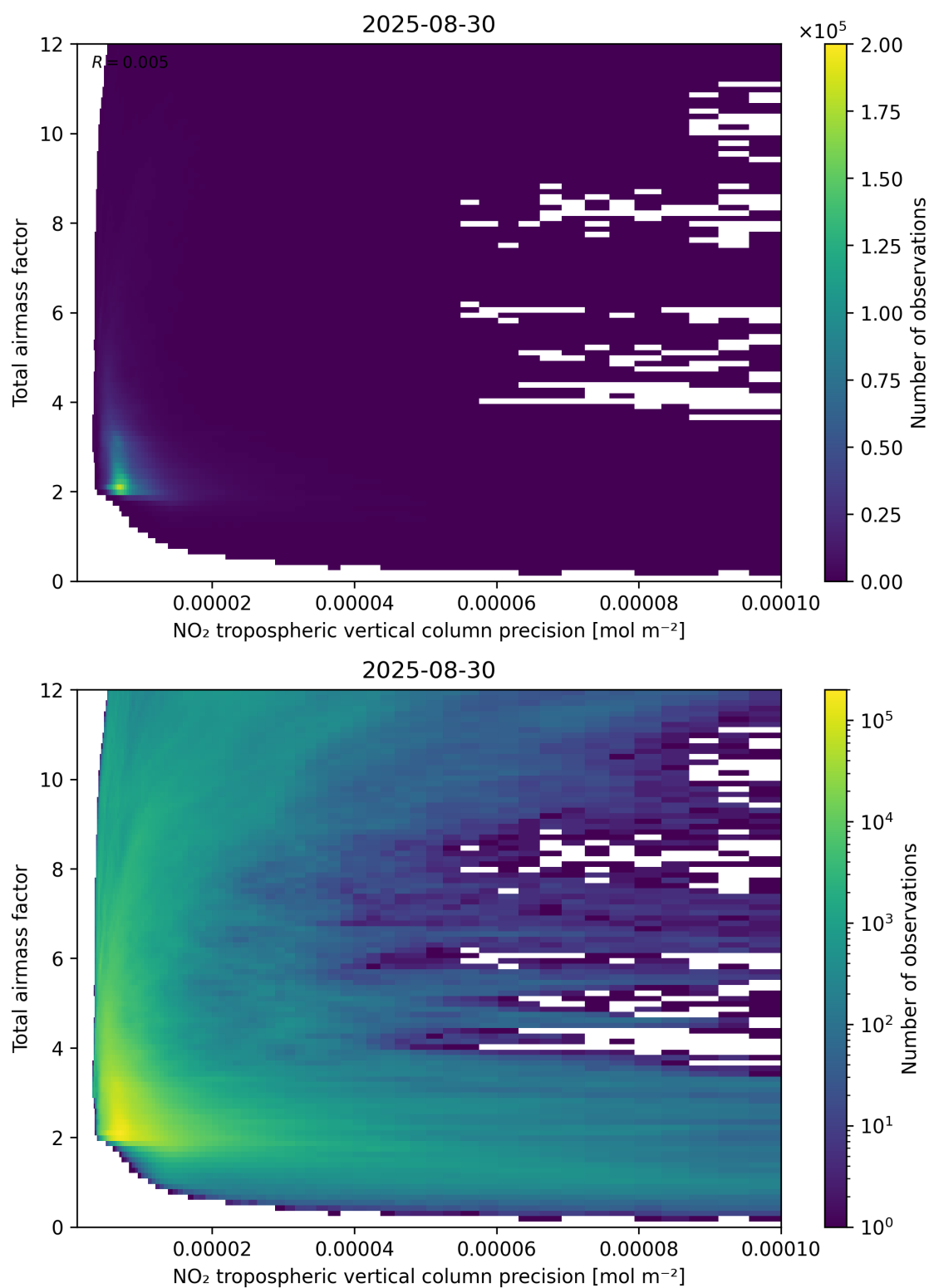
Figure 132: Scatter density plot of “NO 2 tropospheric vertical column precision” against “Total air mass factor” for 2025-08-30 to 2025-08-31.
