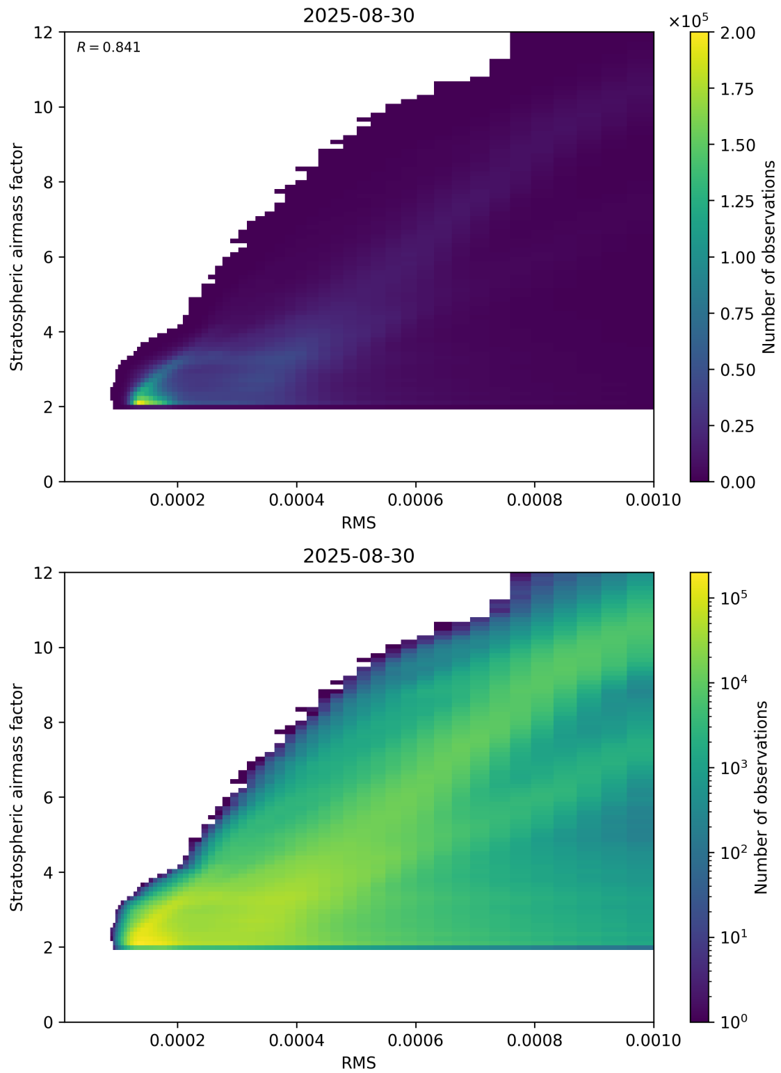
Figure 144: Scatter density plot of “RMS” against “Stratospheric airmass factor” for 2025-08-30 to 2025-08-31.
