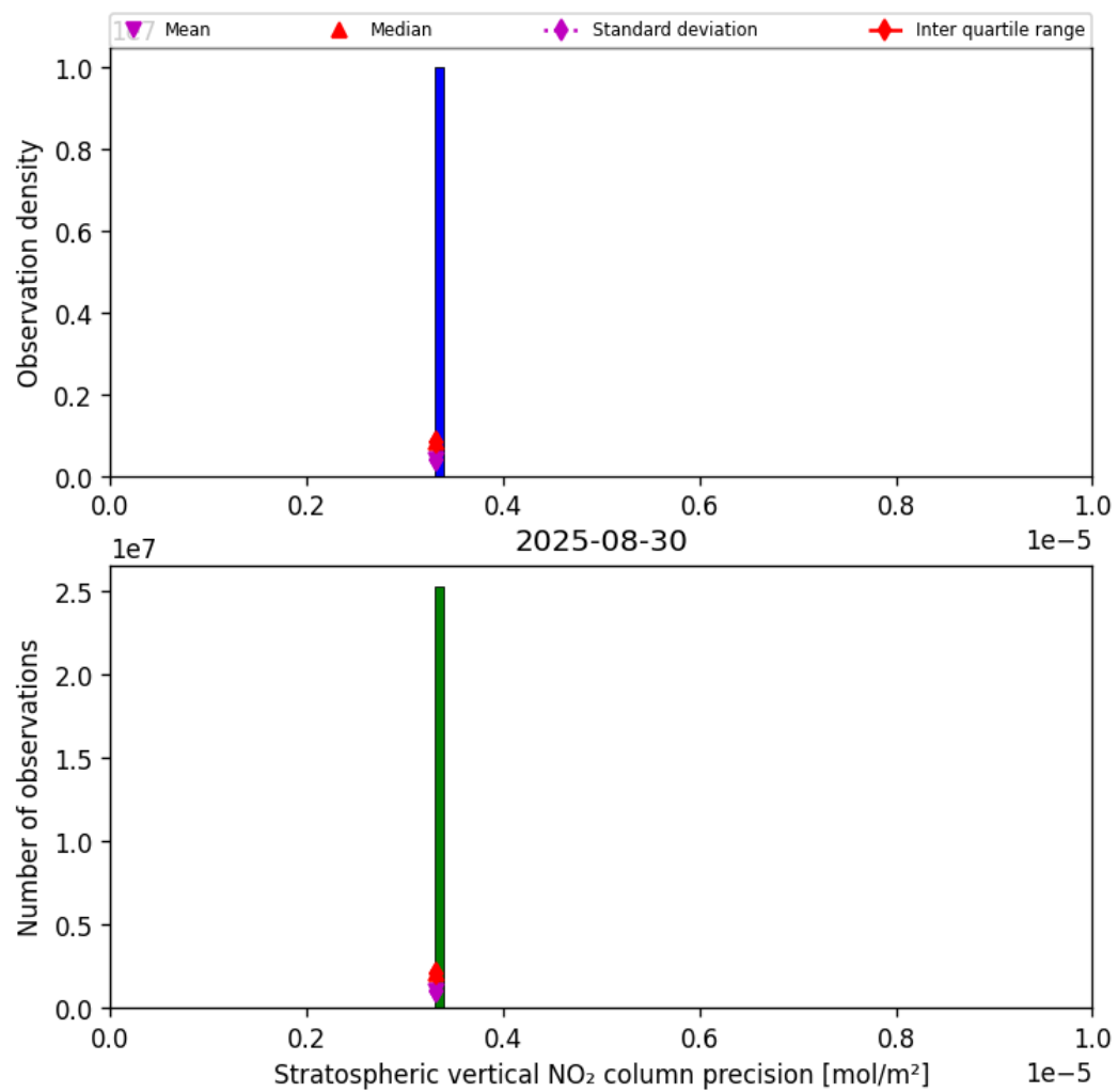
Figure 37: Histogram of “Stratospheric vertical NO 2 column precision” for 2025-08-30 to 2025-08-31
