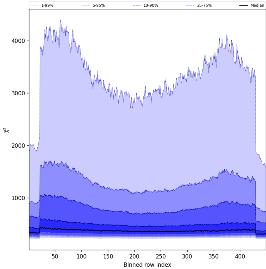
Figure 59: Along track statistics of “ \chi^2 ” for 2025-08-30 to 2025-08-31
