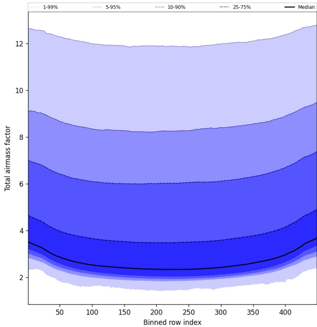
Figure 49: Along track statistics of “Total airmass factor” for 2025-08-30 to 2025-08-31
