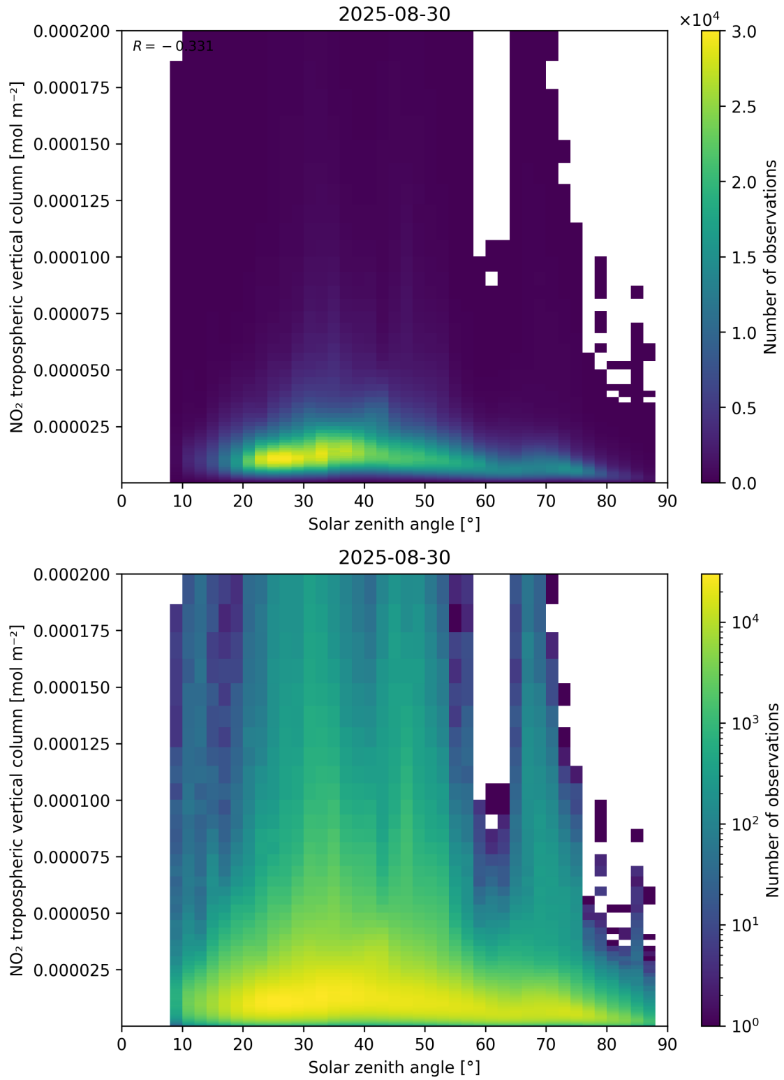
Figure 155: Scatter density plot of “Solar zenith angle” against “NO 2 tropospheric vertical column” for 2025-08-30 to 2025-08-31.
