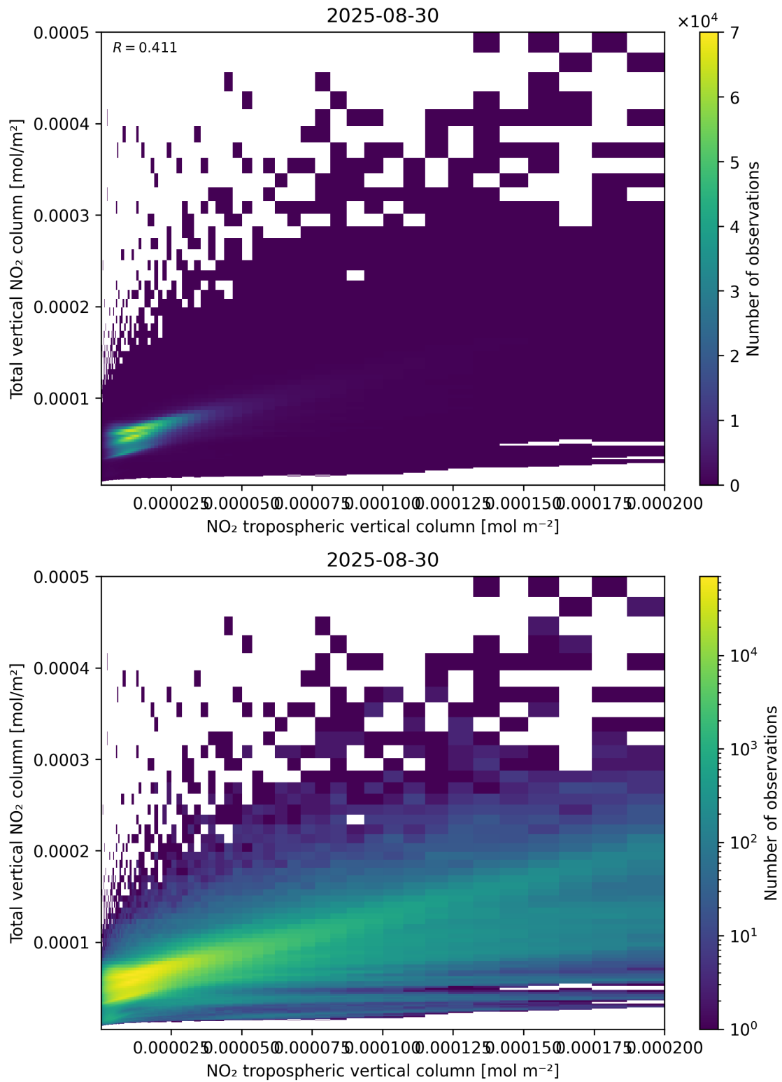
Figure 128: Scatter density plot of “NO 2 tropospheric vertical column” against “Total vertical NO 2 column” for 2025-08-30 to 2025-08-31.
