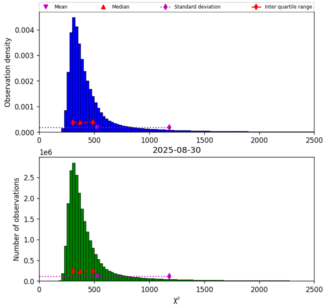
Figure 42: Histogram of " \chi^2 " for 2025-08-30 to 2025-08-31
