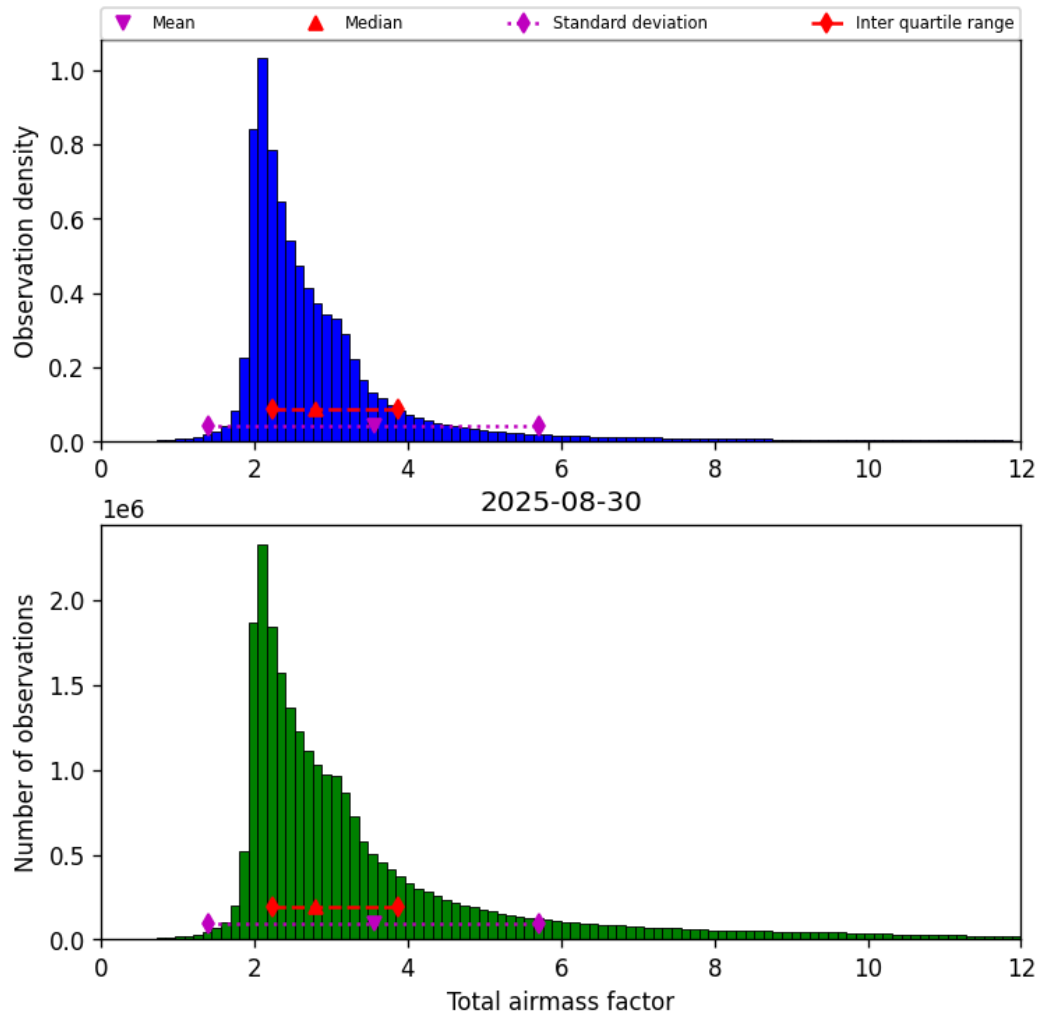
Figure 32: Histogram of “Total airmass factor” for 2025-08-30 to 2025-08-31
