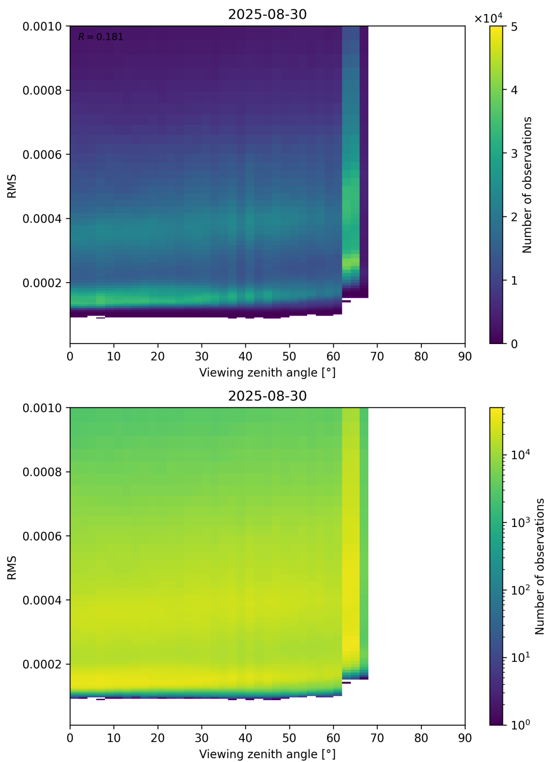
Figure 171: Scatter density plot of “Viewing zenith angle” against “RMS” for 2025-08-30 to 2025-08-31.
