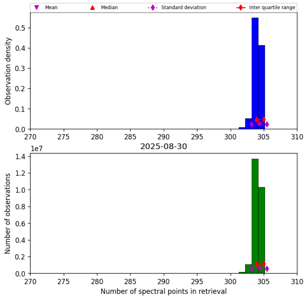
Figure 33: Histogram of “Number of spectral points in retrieval” for 2025-08-30 to 2025-08-31
