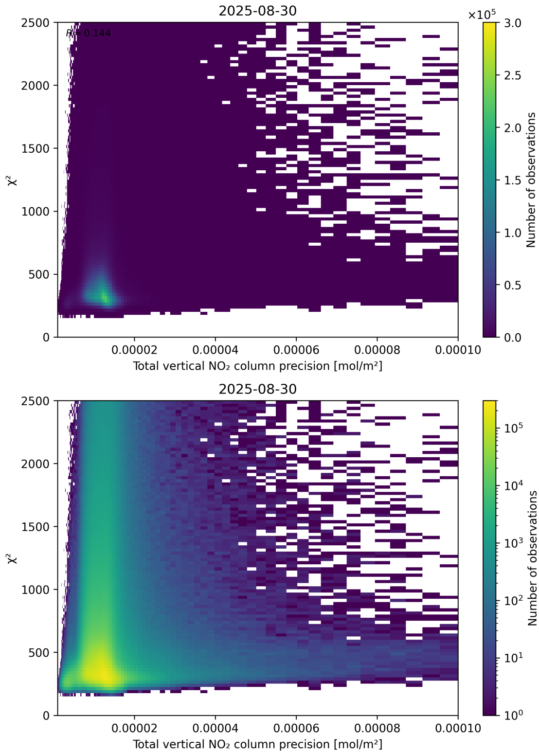
Figure 116: Scatter density plot of “Total vertical NO 2 column precision” against “ \chi^2 ” for 2025-08-30 to 2025-08-31.
