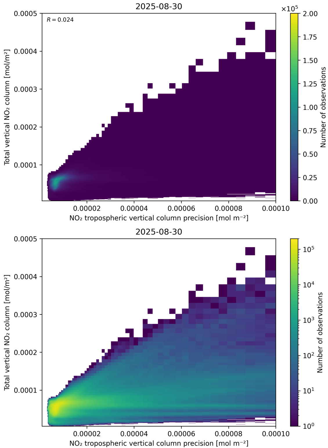
Figure 138: Scatter density plot of “NO 2 tropospheric vertical column precision” against “Total vertical NO 2 column” for 2025-08-30 to 2025-08-31.
