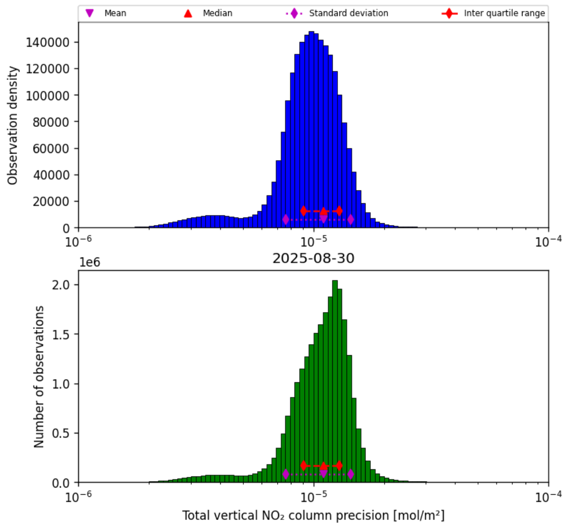
Figure 39: Histogram of “Total vertical NO 2 column precision” for 2025-08-30 to 2025-08-31
