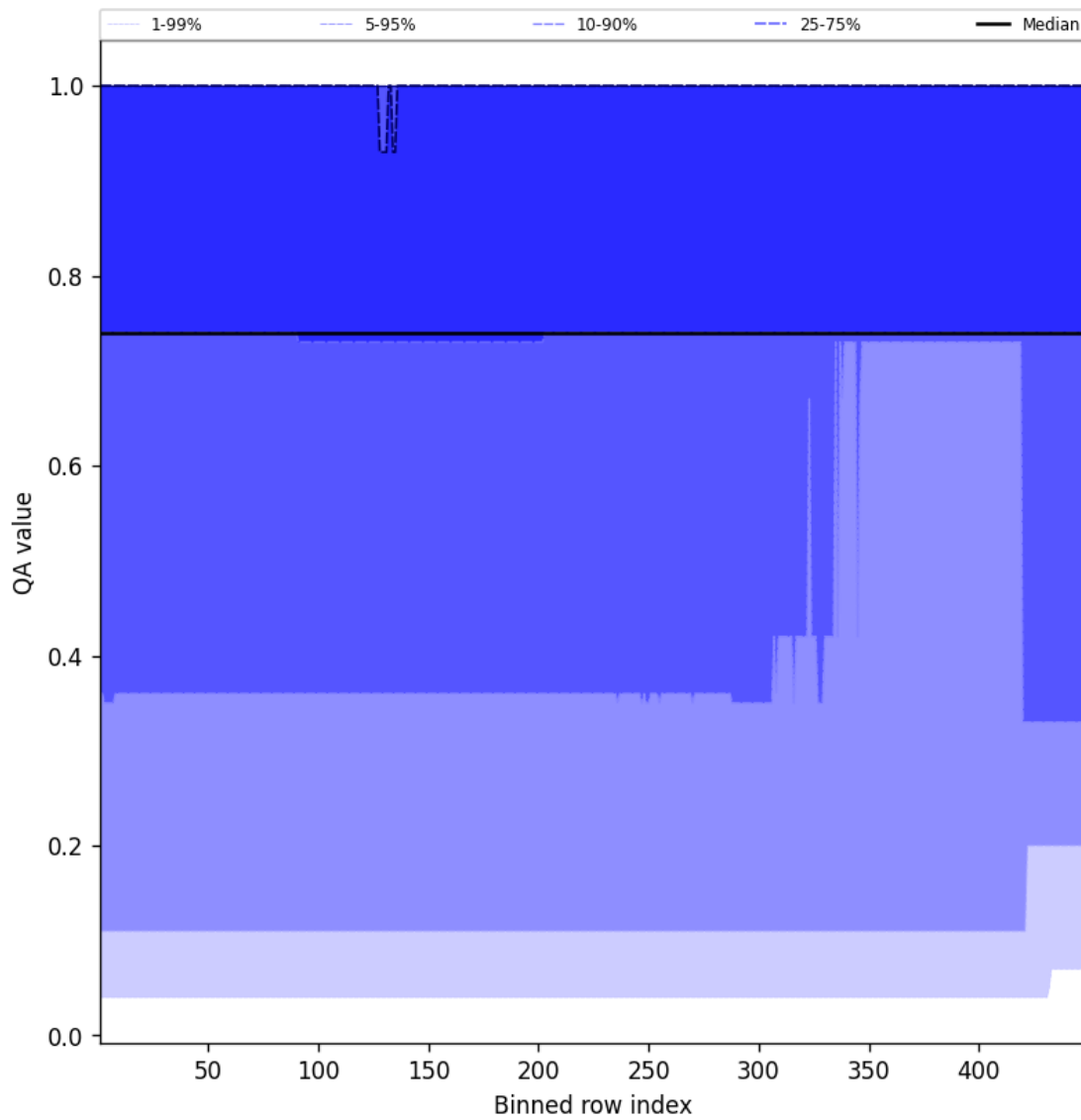
Figure 45: Along track statistics of “QA value” for 2025-08-30 to 2025-08-31
