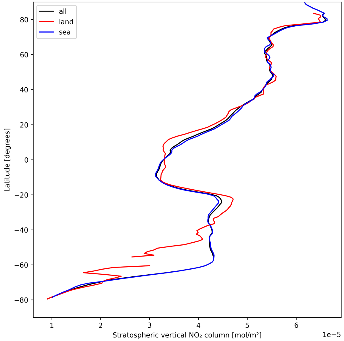
Figure 19: Zonal average of “Stratospheric vertical NO 2 column” for 2025-08-30 to 2025-08-31.
