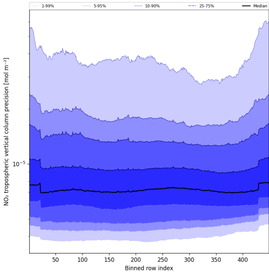
Figure 47: Along track statistics of “NO 2 tropospheric vertical column precision” for 2025-08-30 to 2025-08-31
