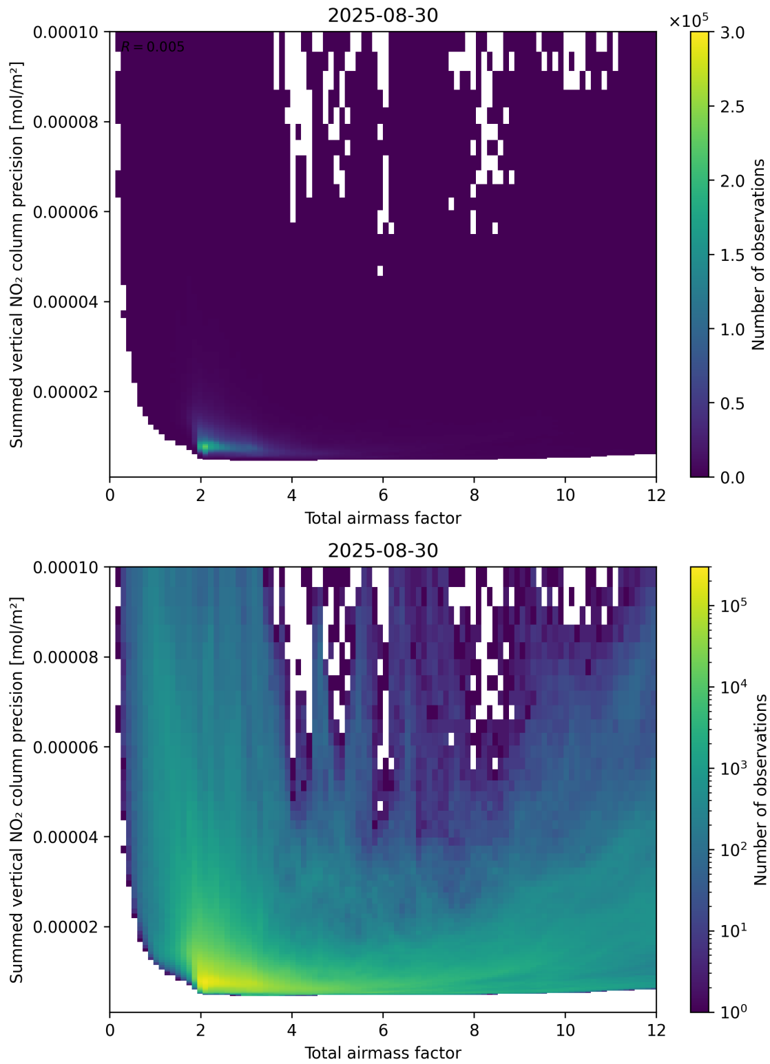
Figure 66: Scatter density plot of “Total airmass factor” against “Summed vertical NO 2 column precision” for 2025-08-30 to 2025-08-31.
