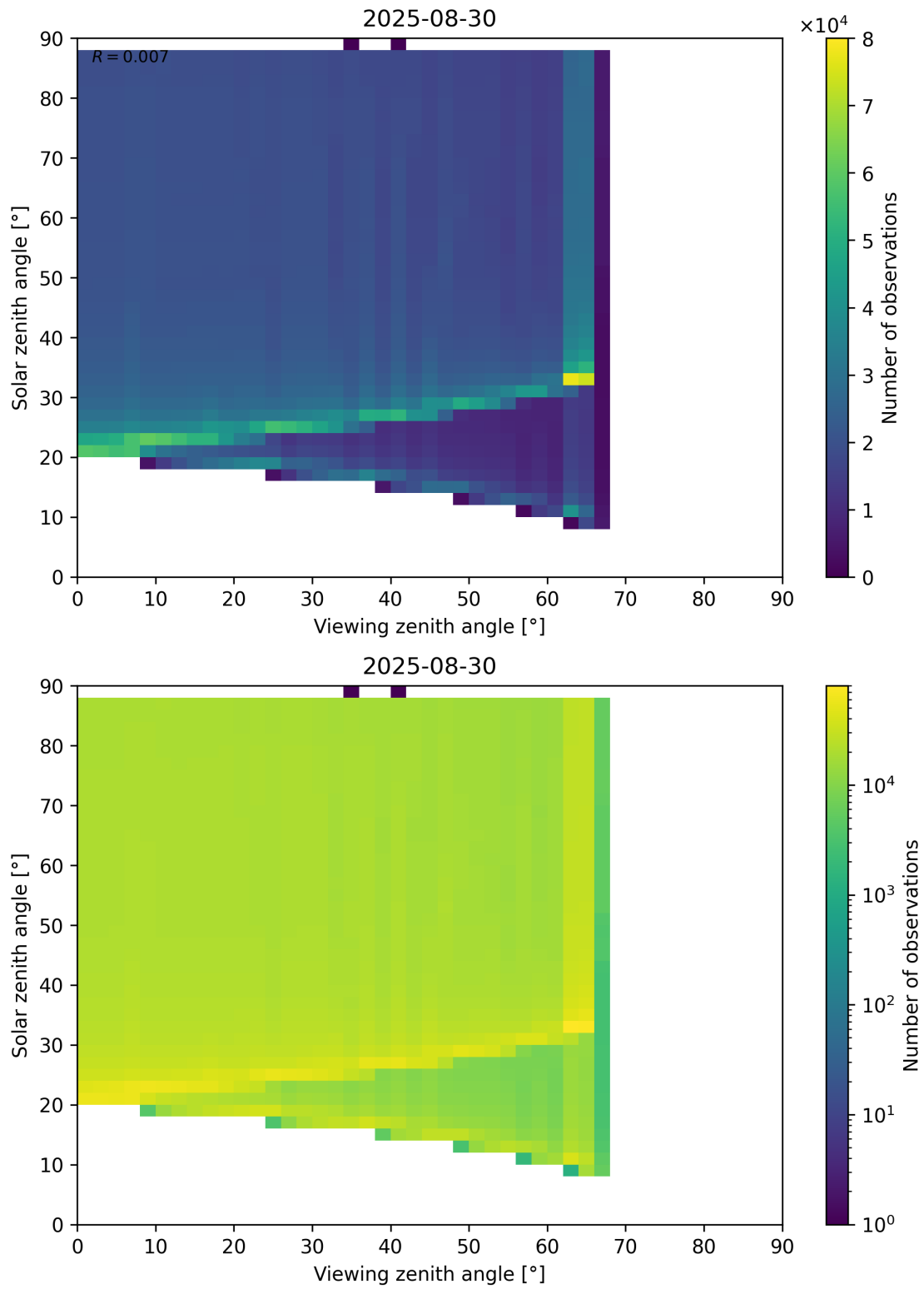
Figure 172: Scatter density plot of “Viewing zenith angle” against “Solar zenith angle” for 2025-08-30 to 2025-08-31.
