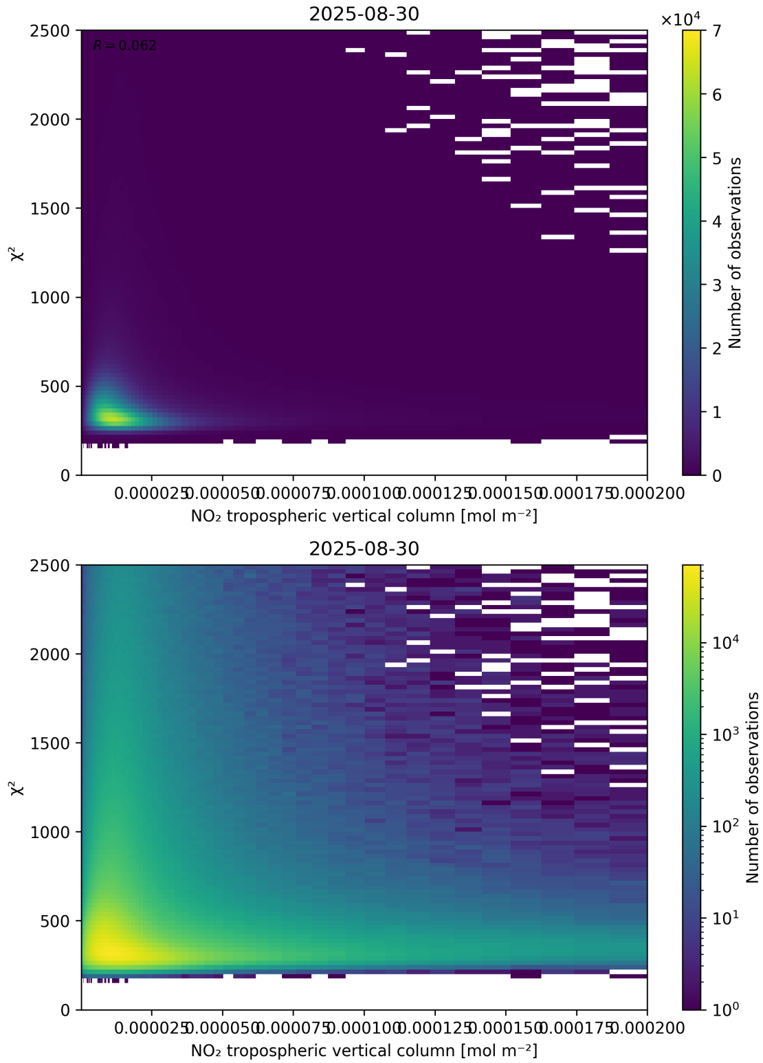
Figure 124: Scatter density plot of “NO 2 tropospheric vertical column” against “ \chi^2 ” for 2025-08-30 to 2025-08-31.
