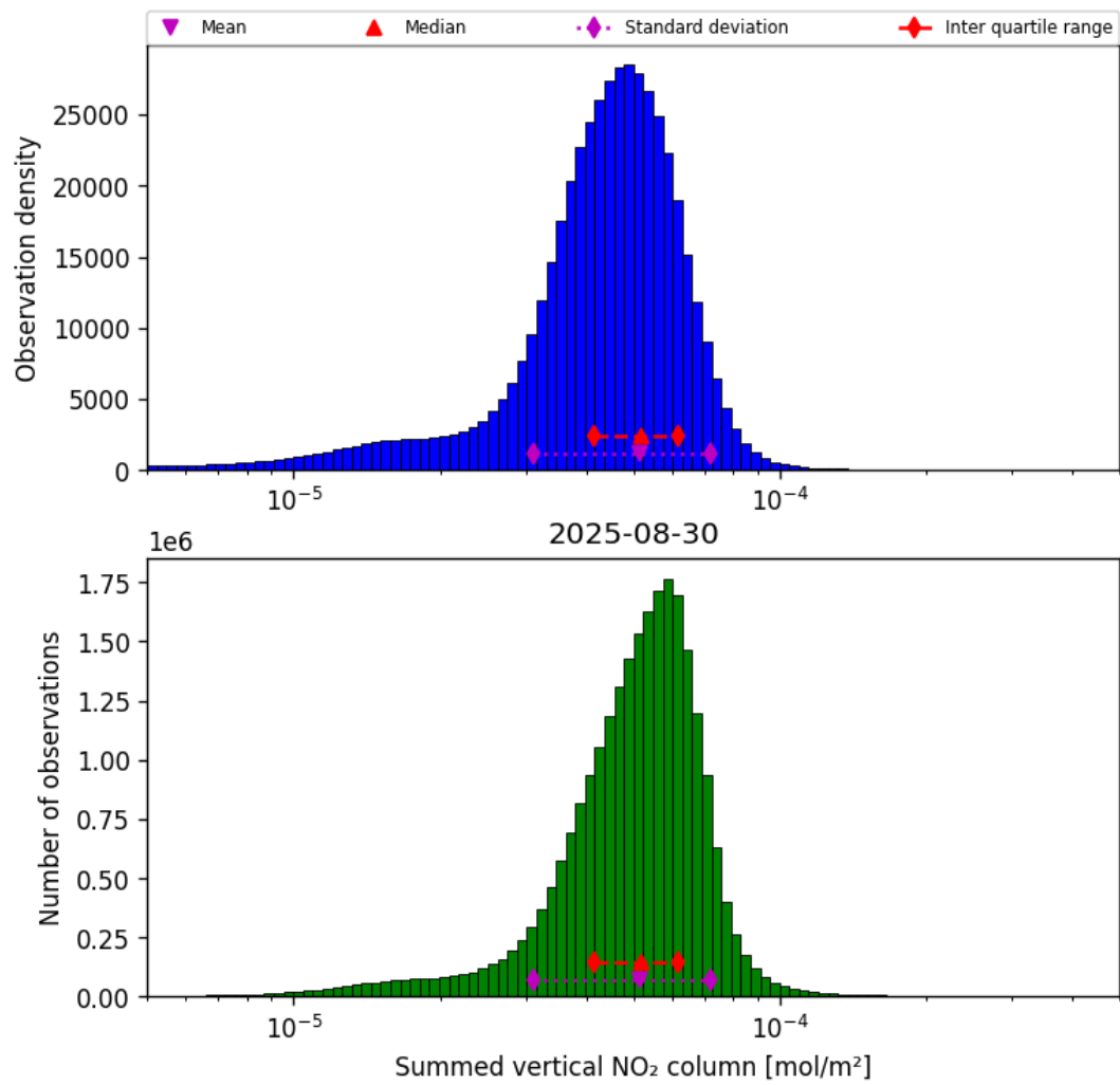
Figure 40: Histogram of “Summed vertical NO 2 column” for 2025-08-30 to 2025-08-31
