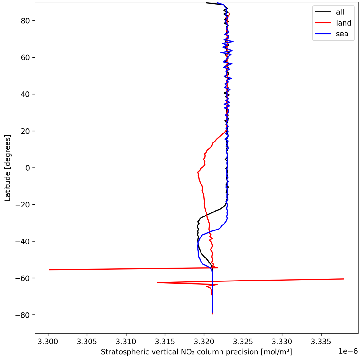
Figure 20: Zonal average of “Stratospheric vertical NO 2 column precision” for 2025-08-30 to 2025-08-31.
