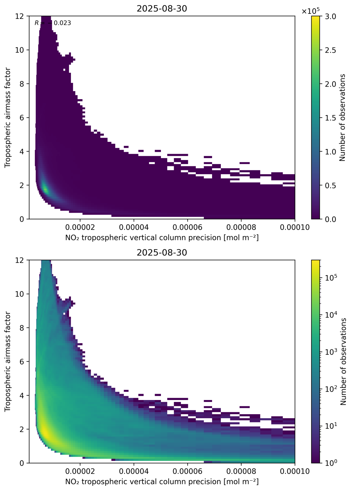
Figure 133: Scatter density plot of “NO 2 tropospheric vertical column precision” against “Tropospheric air mass factor” for 2025-08-30 to 2025-08-31.
