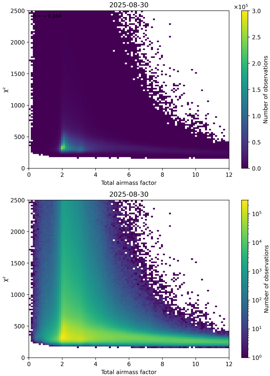
Figure 63: Scatter density plot of “Total airmass factor” against “ \chi^2 ” for 2025-08-30 to 2025-08-31.
