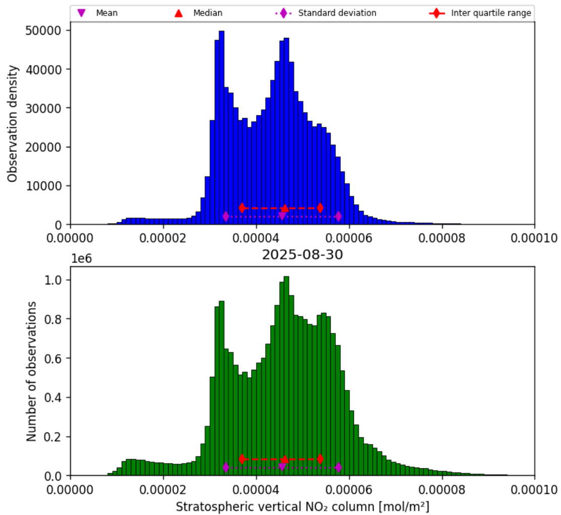
Figure 36: Histogram of “Stratospheric vertical NO 2 column” for 2025-08-30 to 2025-08-31
