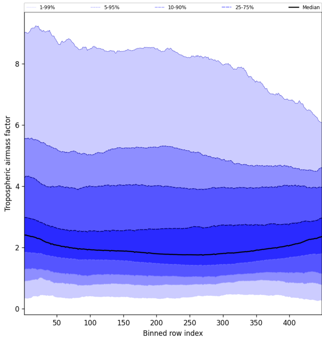
Figure 48: Along track statistics of “Tropospheric airmass factor” for 2025-08-30 to 2025-08-31
