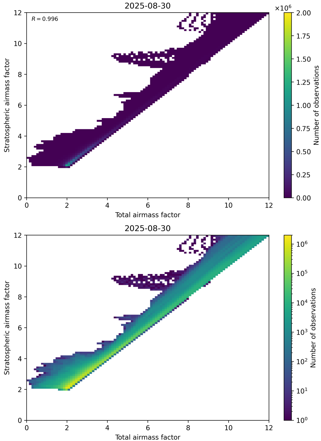
Figure 62: Scatter density plot of “Total airmass factor” against “Stratospheric airmass factor” for 2025-08-30 to 2025-08-31.
