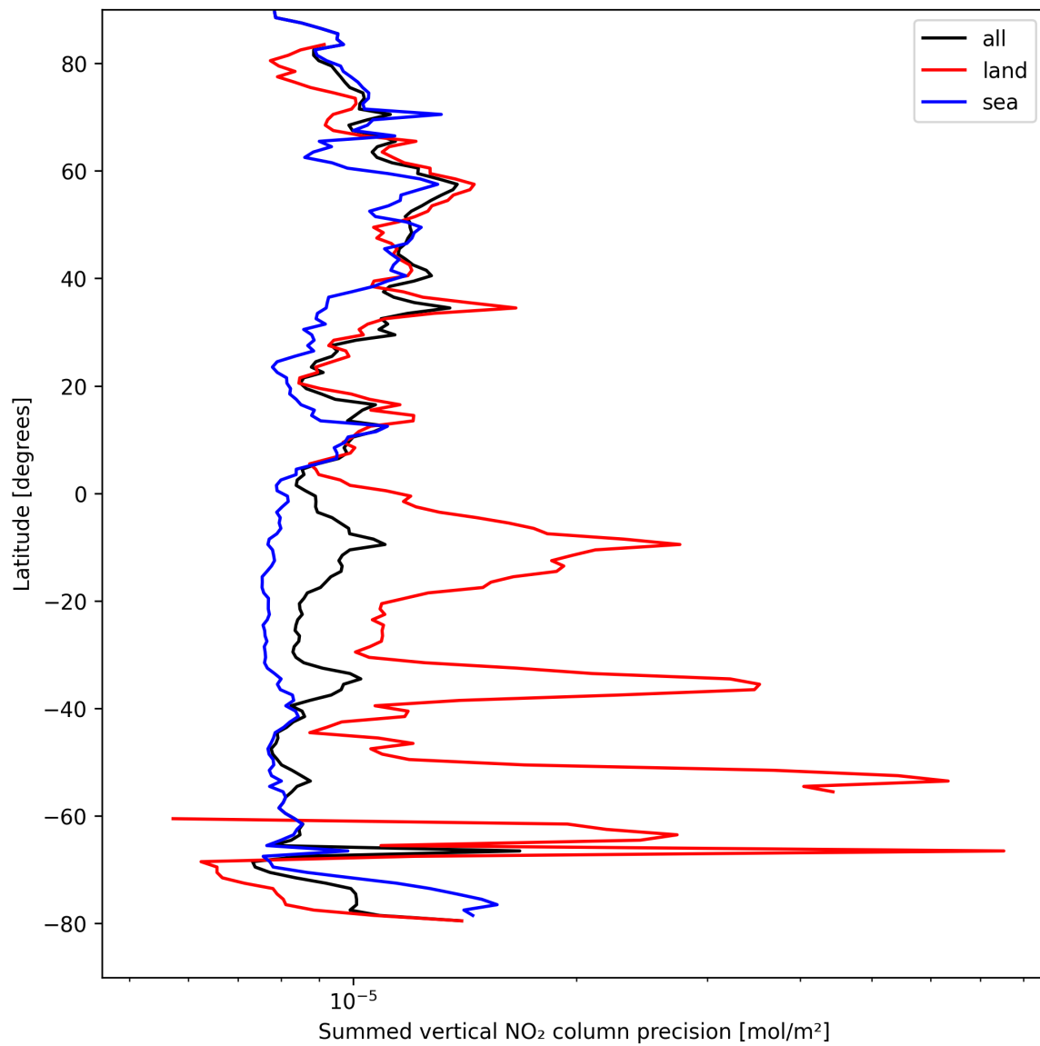
Figure 24: Zonal average of “Summed vertical NO 2 column precision” for 2025-08-30 to 2025-08-31.
