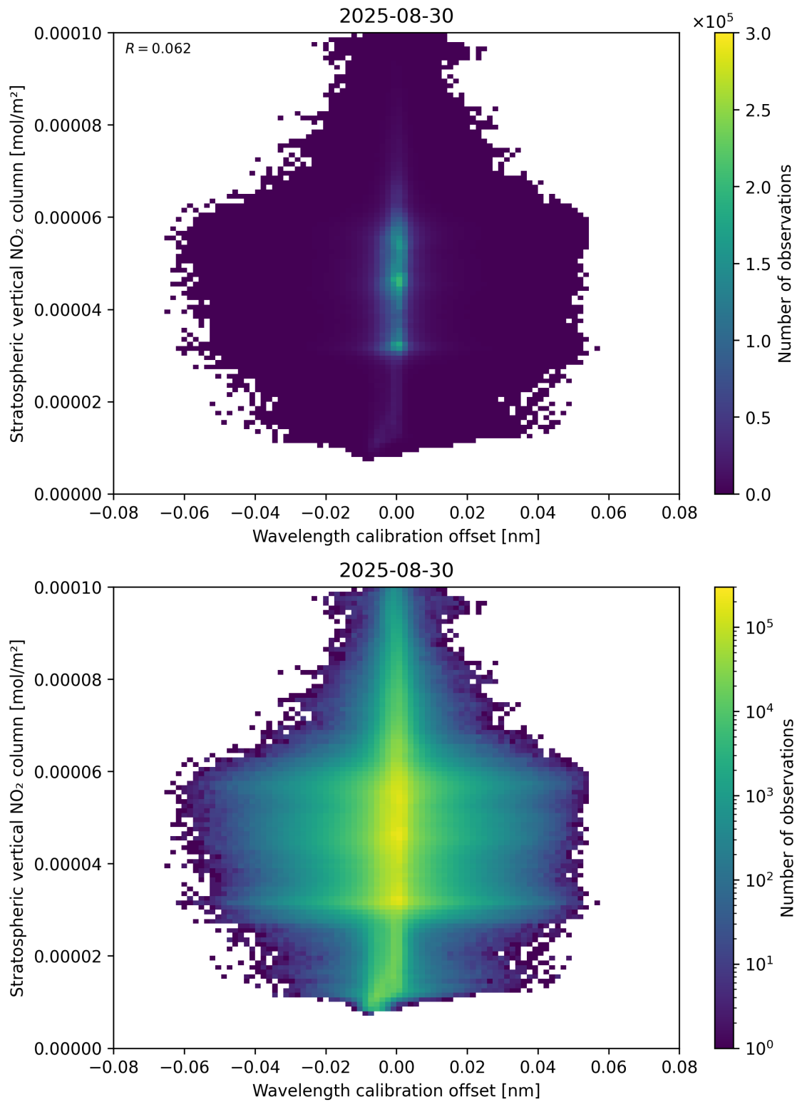
Figure 176: Scatter density plot of “Wavelength calibration offset” against “Stratospheric vertical NO 2 column” for 2025-08-30 to 2025-08-31.
