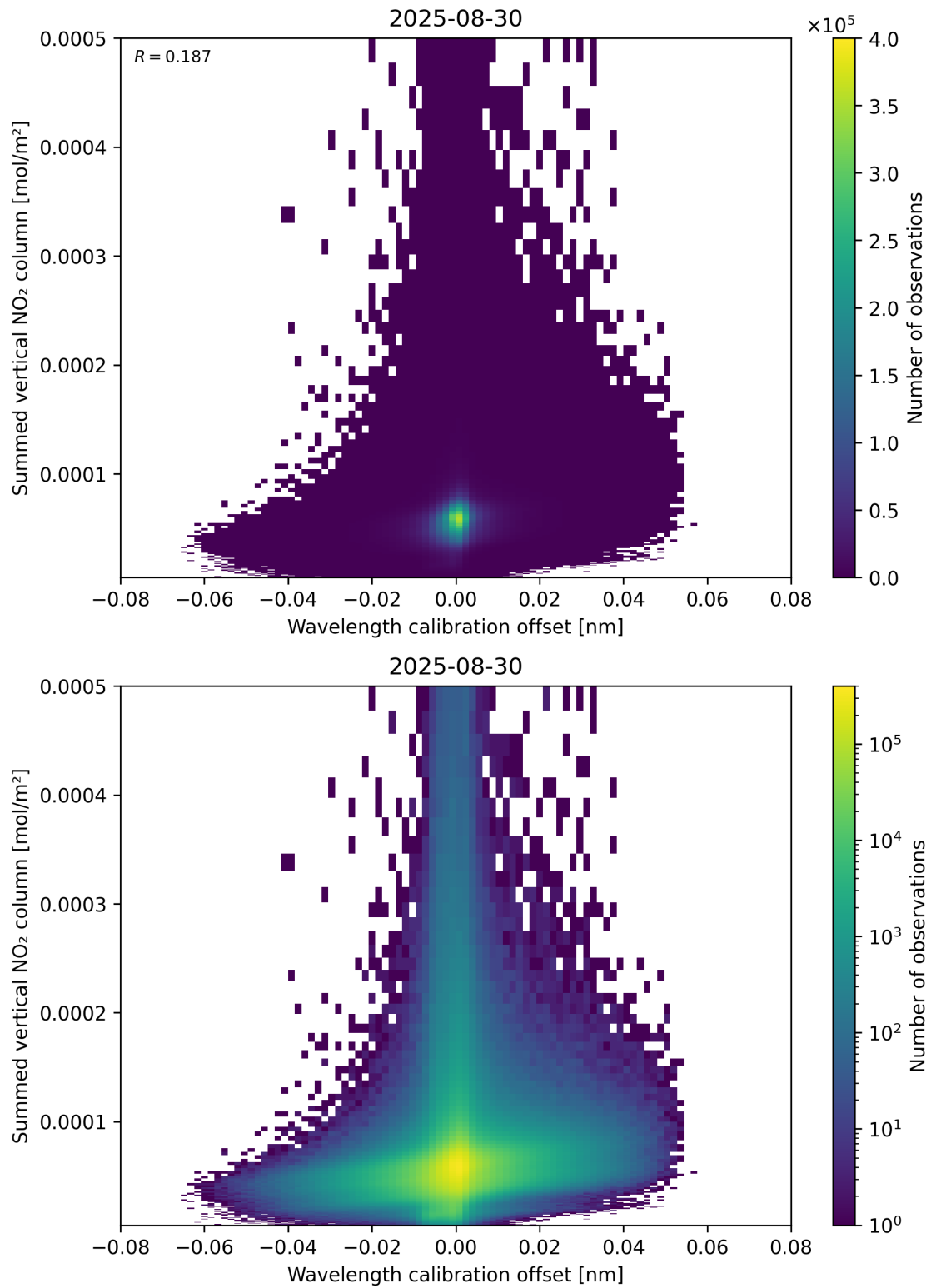
Figure 177: Scatter density plot of “Wavelength calibration offset” against “Summed vertical NO 2 column” for 2025-08-30 to 2025-08-31.
