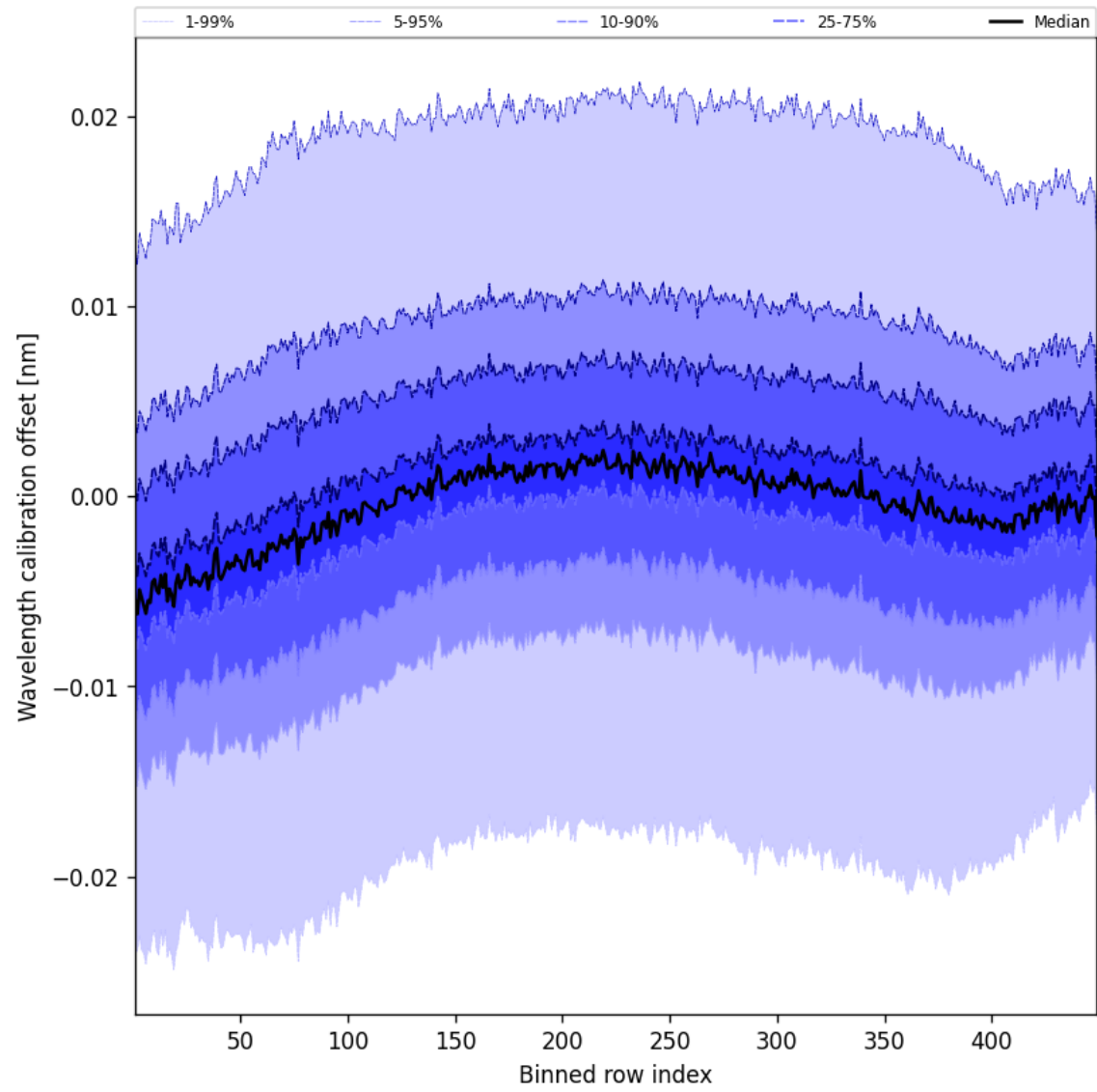
Figure 52: Along track statistics of “Wavelength calibration offset” for 2025-08-30 to 2025-08-31
