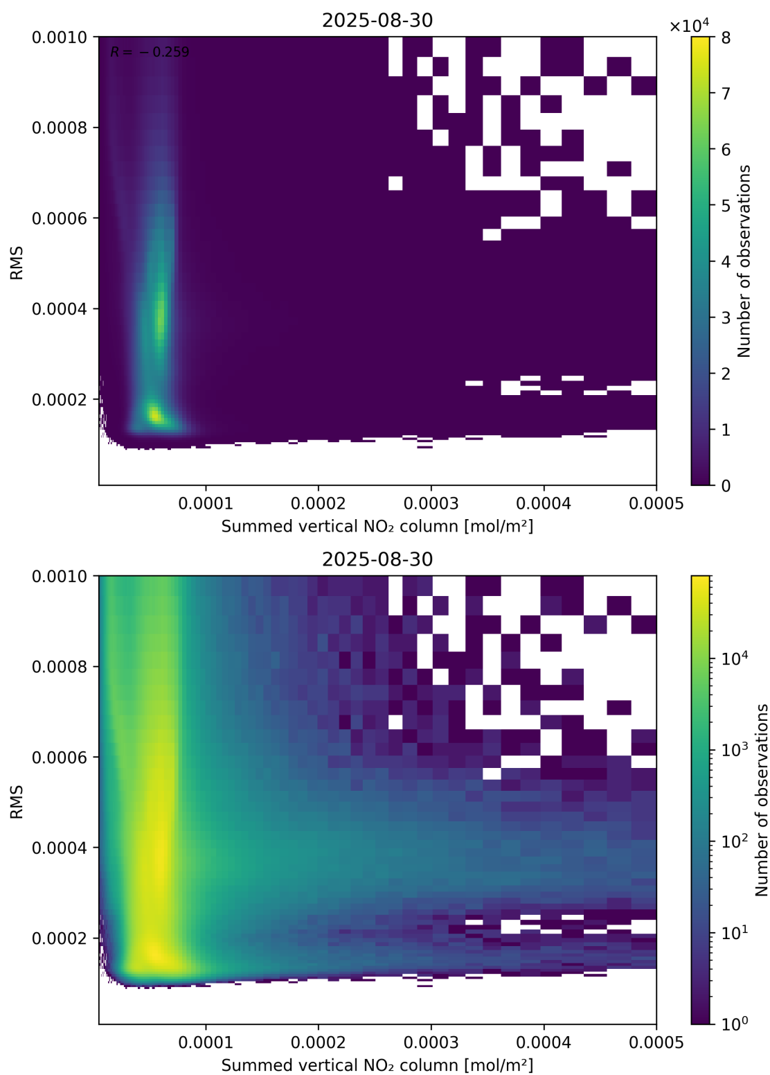
Figure 109: Scatter density plot of “Summed vertical NO 2 column” against “RMS” for 2025-08-30 to 2025-08-31.
