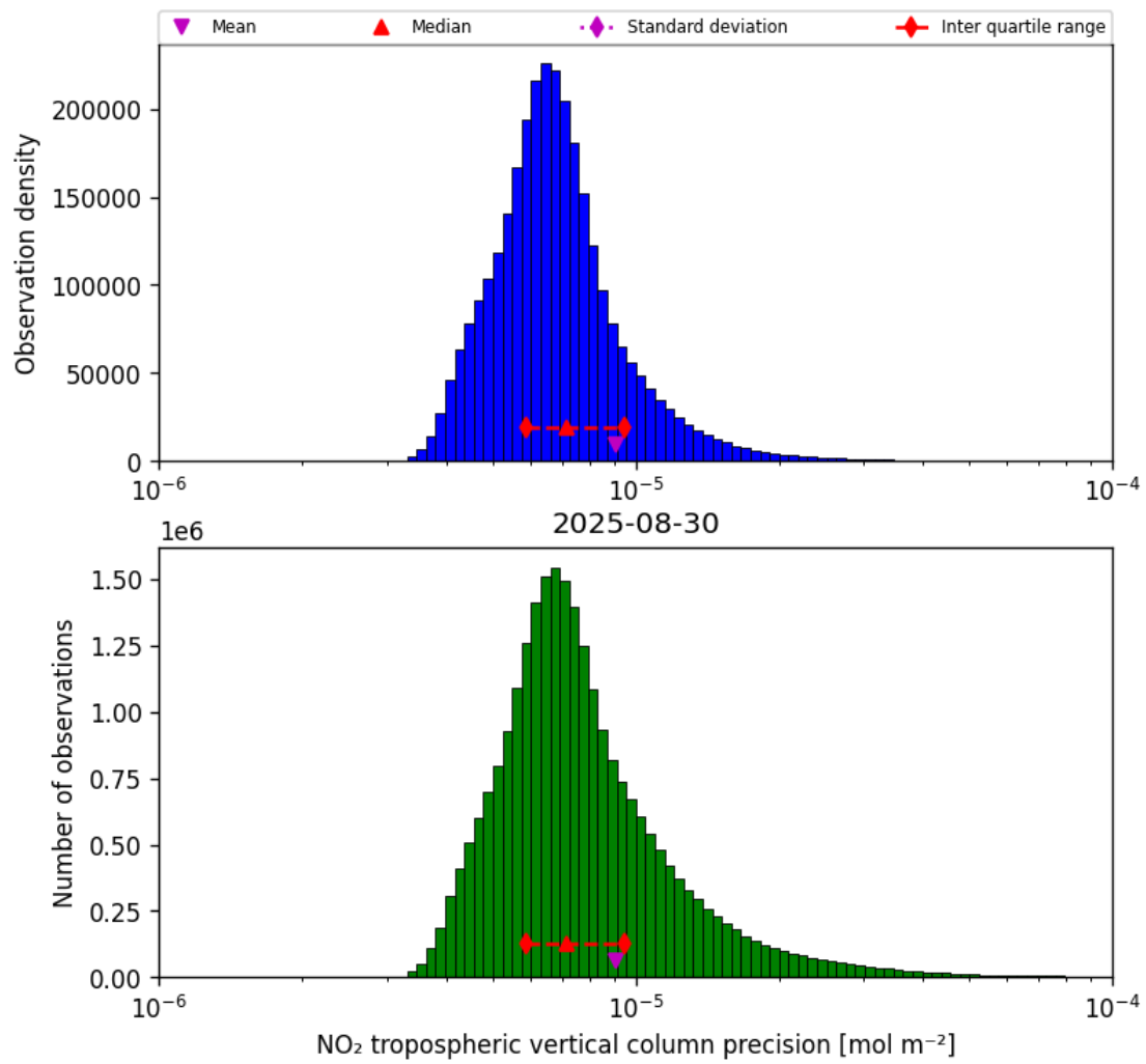
Figure 30: Histogram of “NO 2 tropospheric vertical column precision” for 2025-08-30 to 2025-08-31
