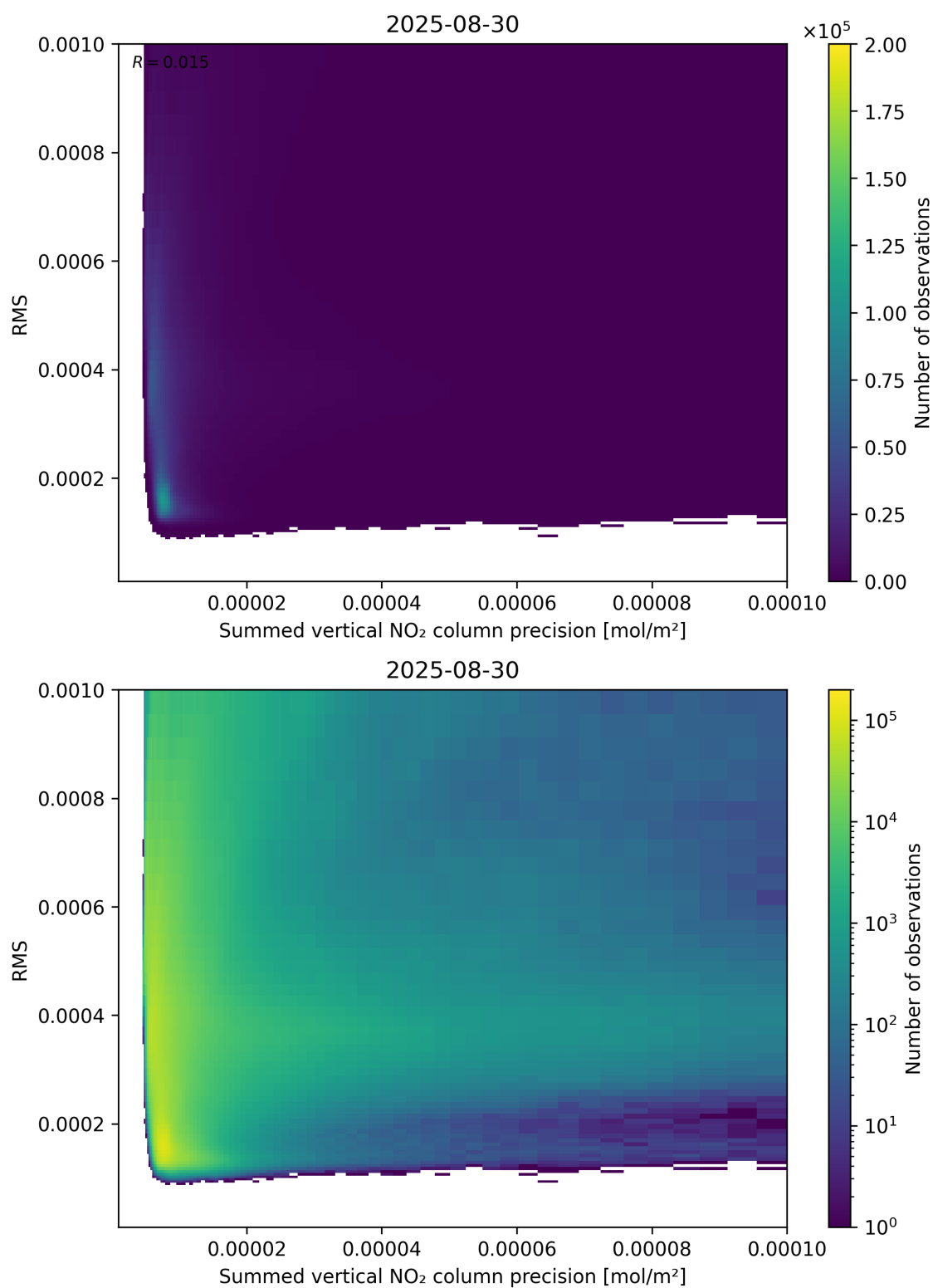
Figure 108: Scatter density plot of “Summed vertical NO 2 column precision” against “RMS” for 2025-08-30 to 2025-08-31.
