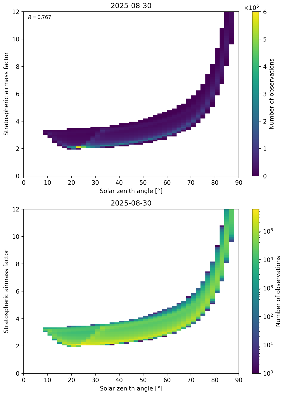
Figure 145: Scatter density plot of “Solar zenith angle” against “Stratospheric airmass factor” for 2025-08-30 to 2025-08-31.
