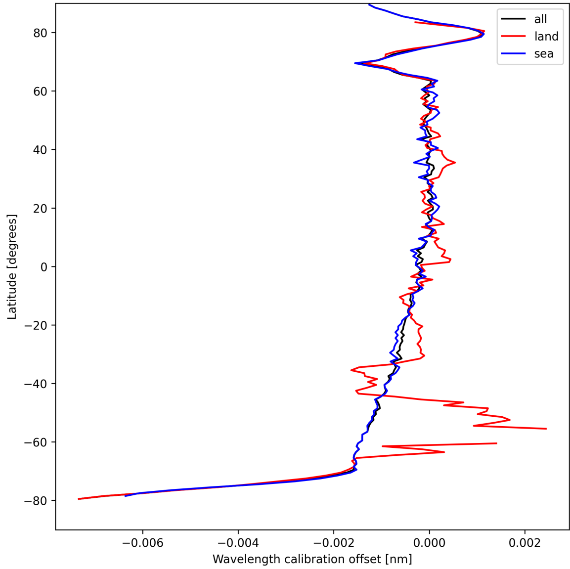
Figure 18: Zonal average of “Wavelength calibration offset” for 2025-08-30 to 2025-08-31.
