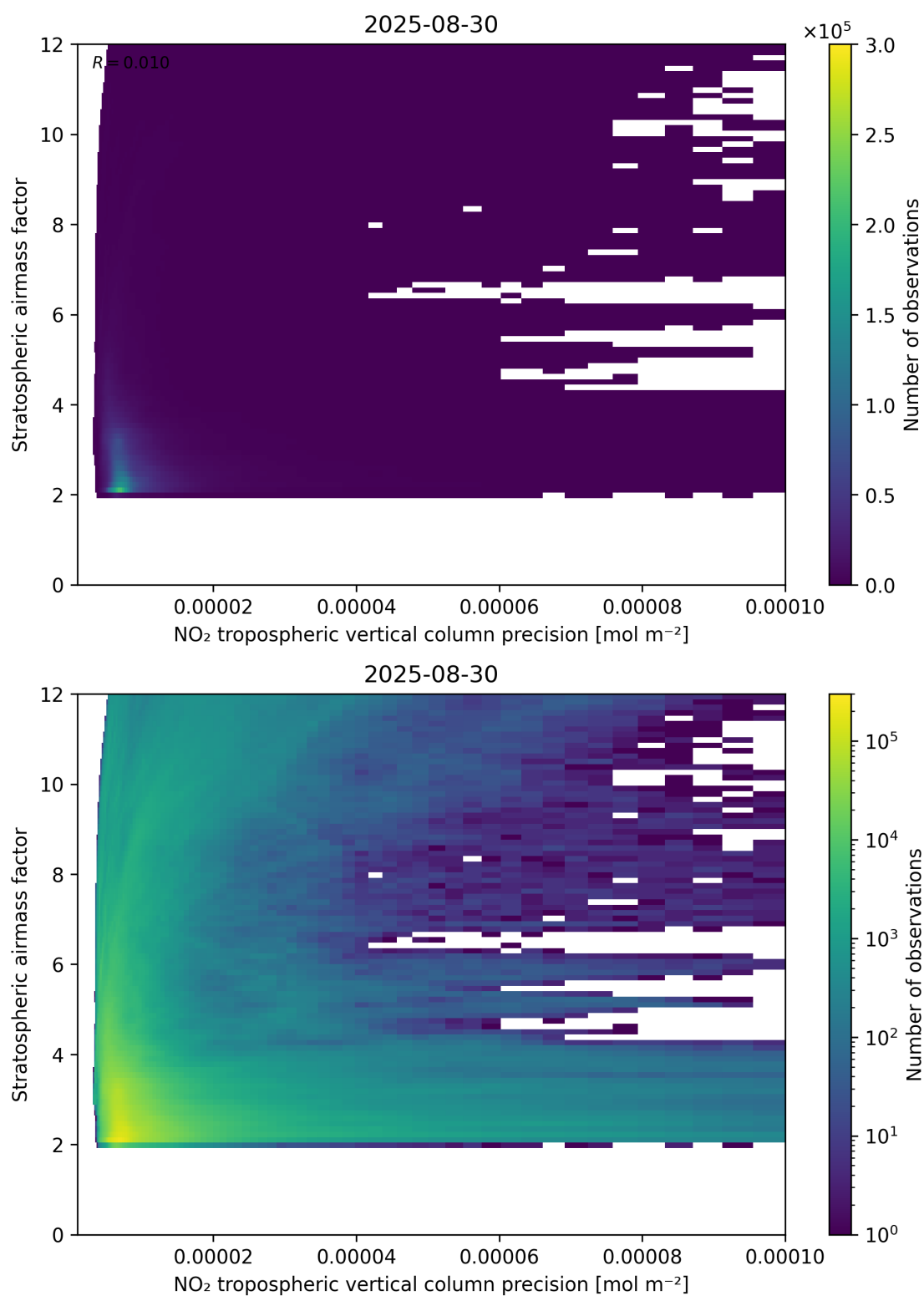
Figure 131: Scatter density plot of “NO 2 tropospheric vertical column precision” against “Stratospheric airmass factor” for 2025-08-30 to 2025-08-31.
