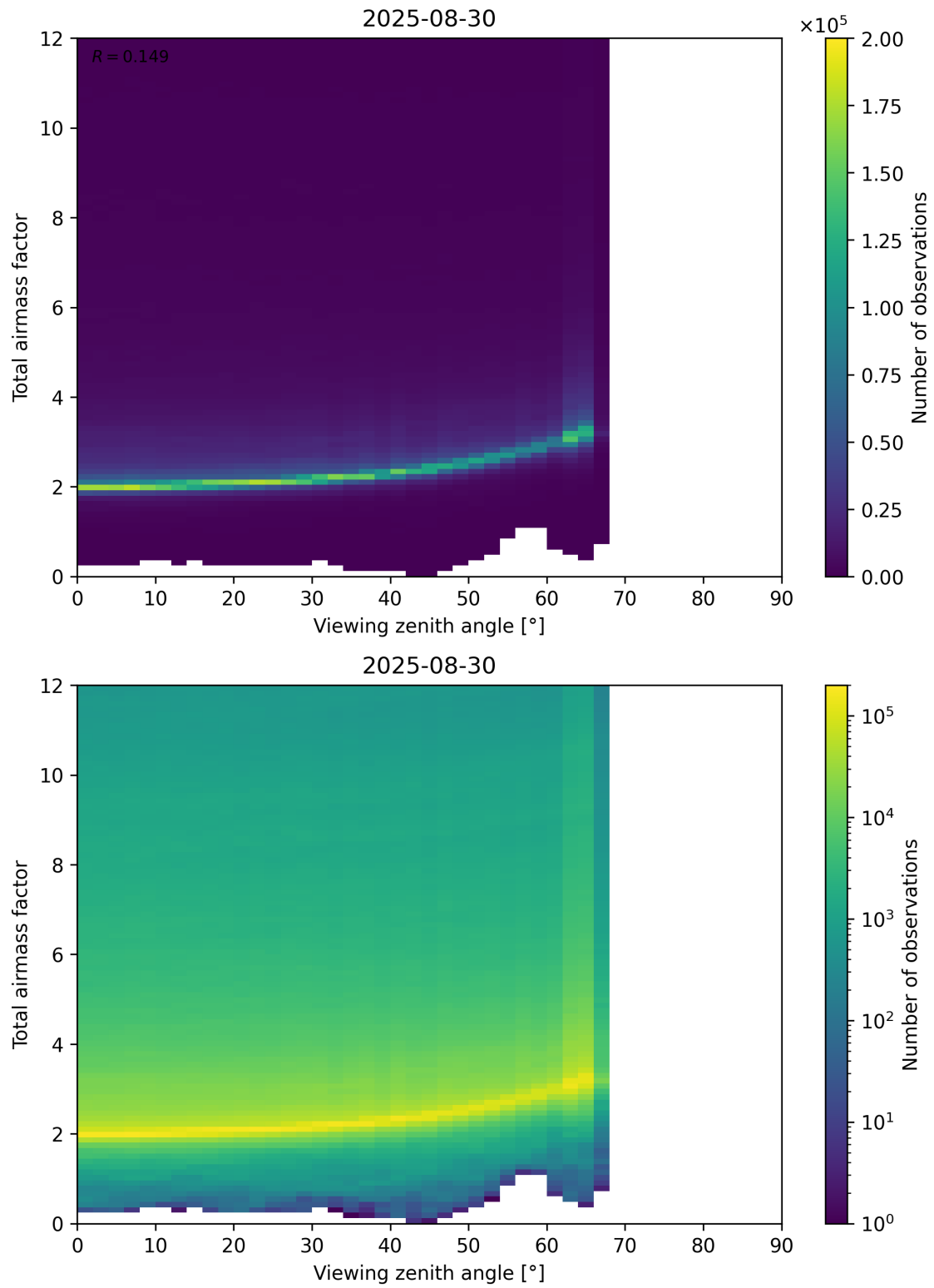
Figure 160: Scatter density plot of “Viewing zenith angle” against “Total airmass factor” for 2025-08-30 to 2025-08-31.
