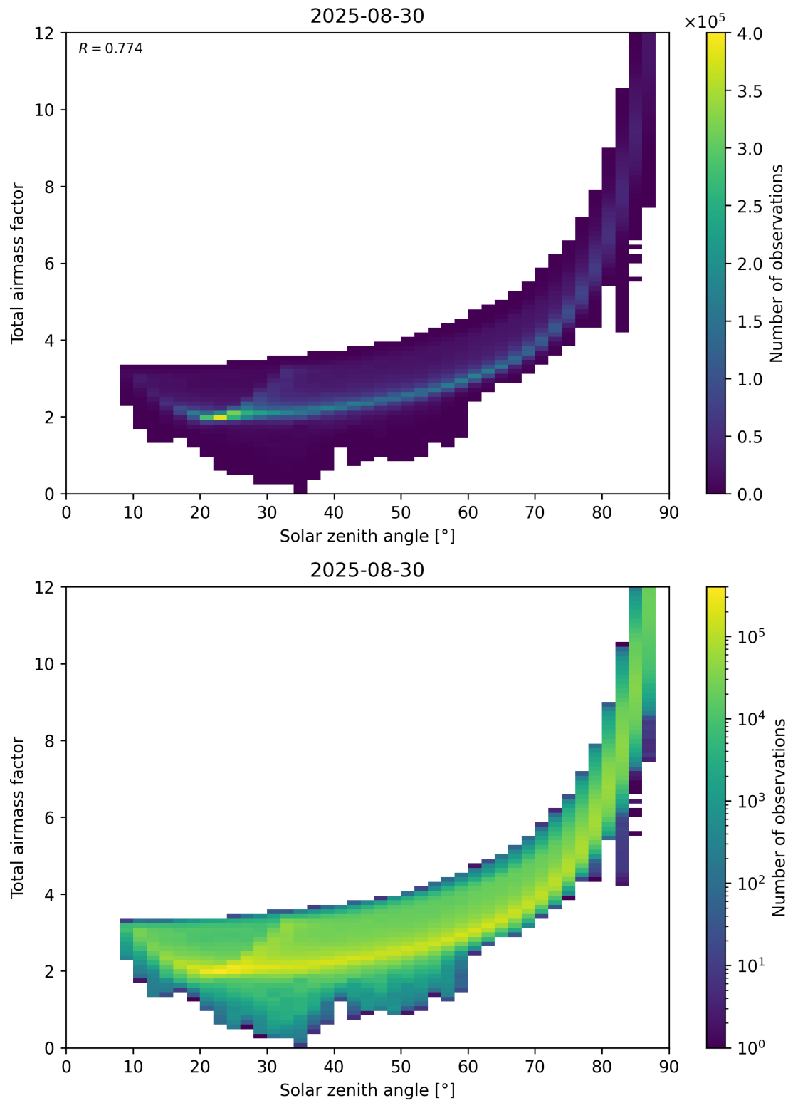
Figure 146: Scatter density plot of “Solar zenith angle” against “Total air mass factor” for 2025-08-30 to 2025-08-31.
