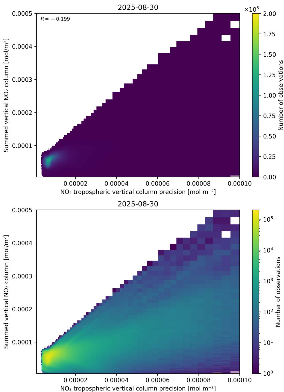
Figure 136: Scatter density plot of “NO 2 tropospheric vertical column precision” against “Summed vertical NO 2 column” for 2025-08-30 to 2025-08-31.
