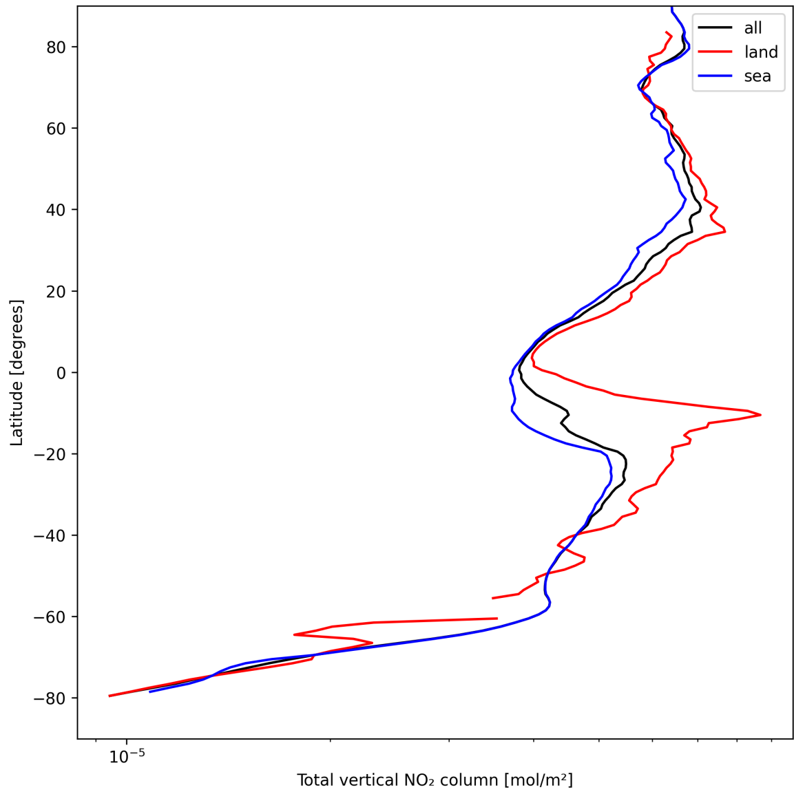
Figure 21: Zonal average of “Total vertical NO 2 column” for 2025-08-30 to 2025-08-31.
