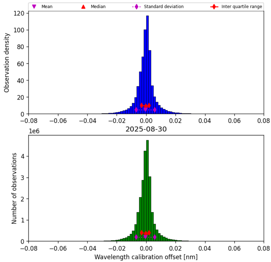
Figure 35: Histogram of “Wavelength calibration offset” for 2025-08-30 to 2025-08-31
