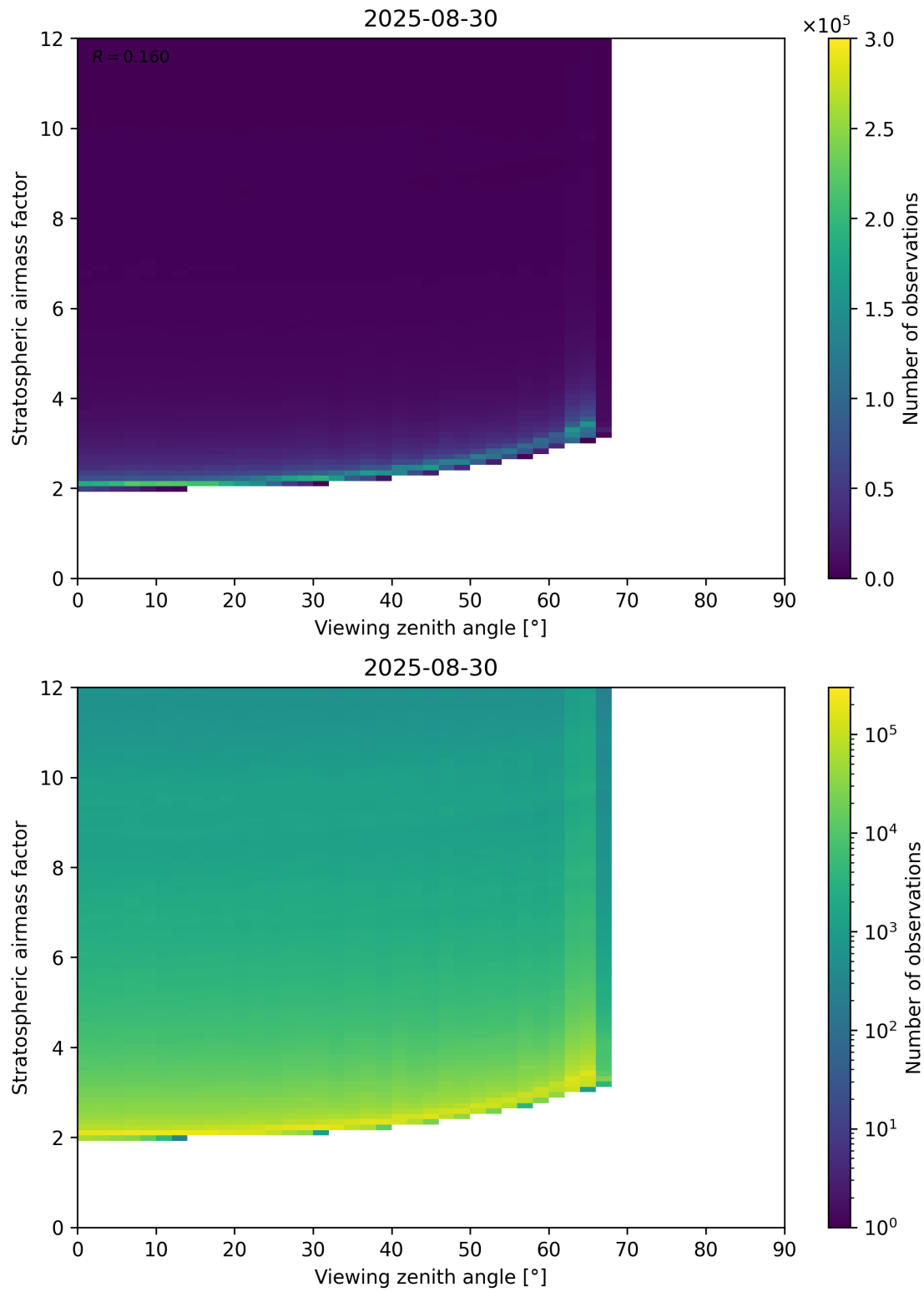
Figure 159: Scatter density plot of “Viewing zenith angle” against “Stratospheric airmass factor” for 2025-08-30 to 2025-08-31.
