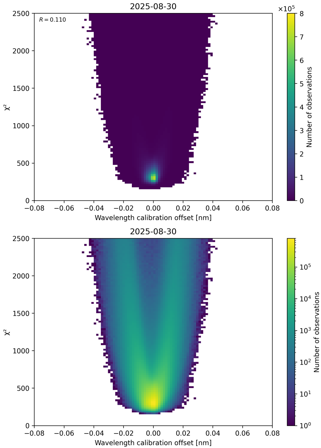
Figure 175: Scatter density plot of “Wavelength calibration offset” against “ \chi^2 ” for 2025-08-30 to 2025-08-31.
