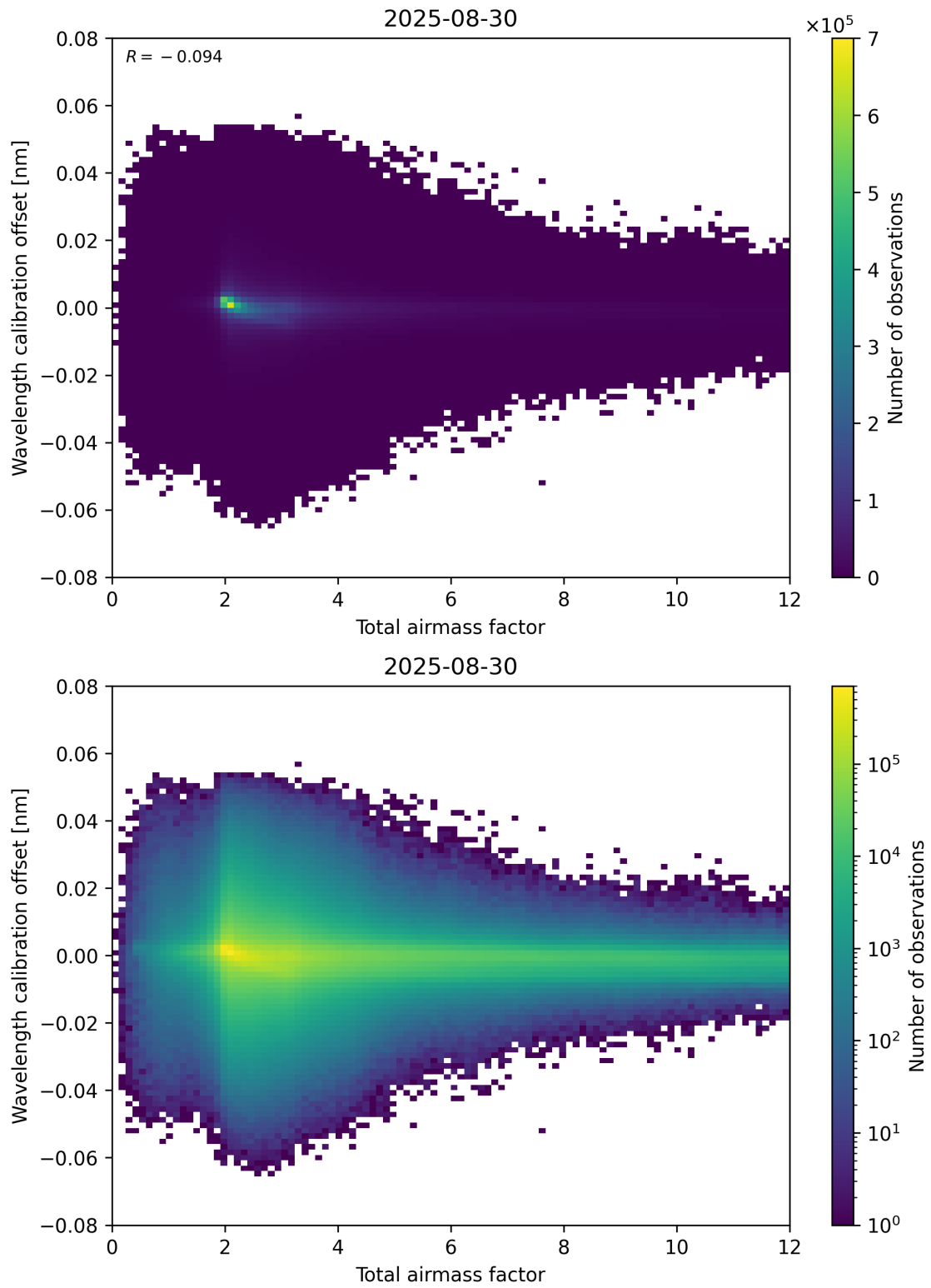
Figure 70: Scatter density plot of “Total airmass factor” against “Wavelength calibration offset” for 2025-08-30 to 2025-08-31.
