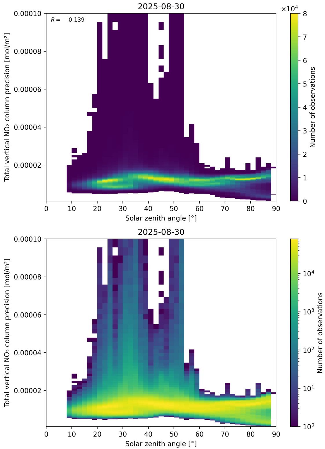
Figure 154: Scatter density plot of “Solar zenith angle” against “Total vertical NO 2 column precision” for 2025-08-30 to 2025-08-31.
