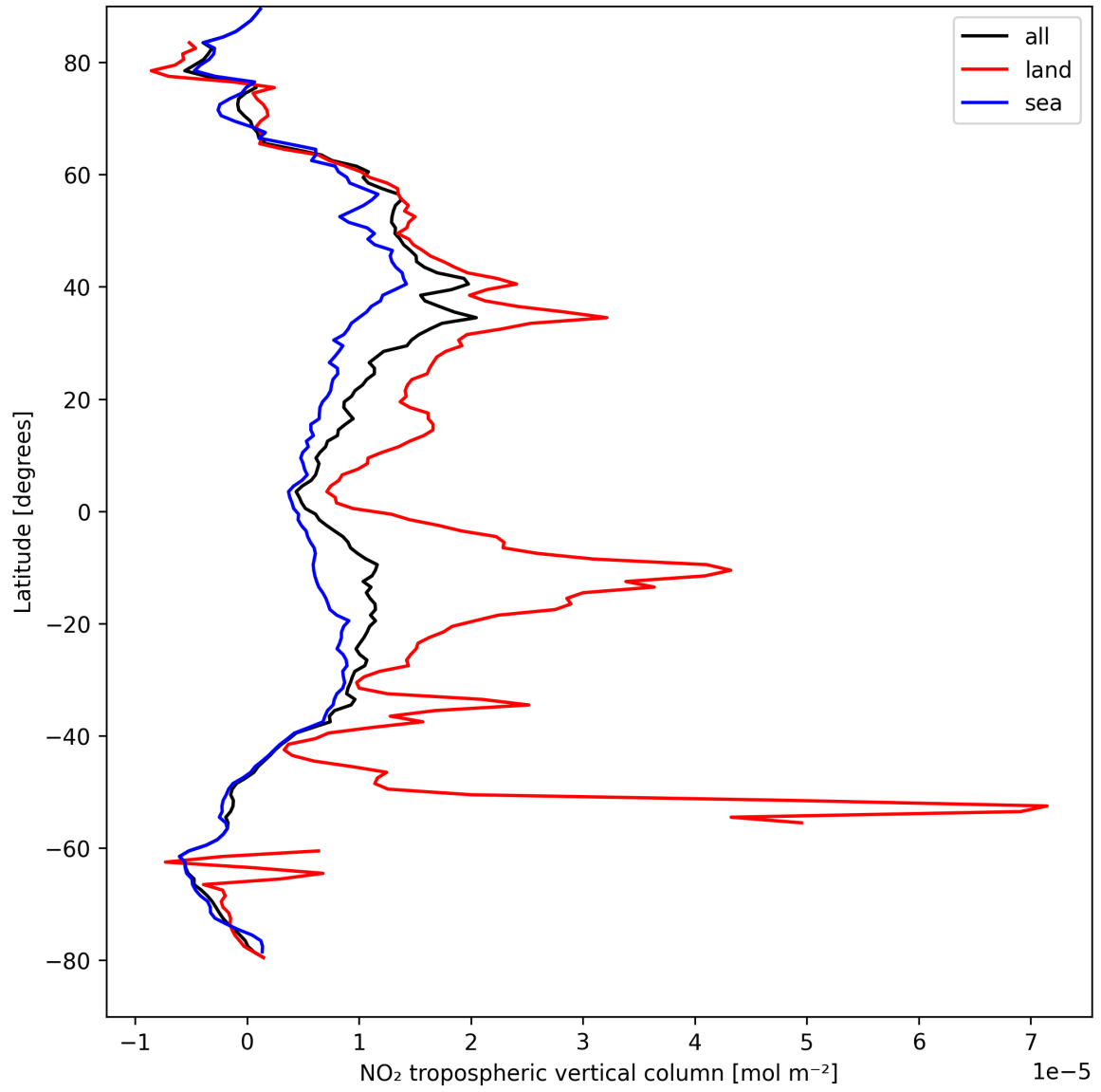
Figure 12: Zonal average of “NO 2 tropospheric vertical column” for 2025-08-30 to 2025-08-31.
