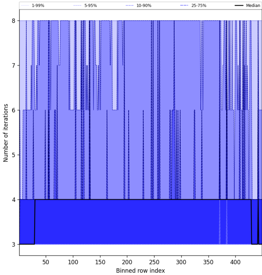
Figure 51: Along track statistics of “Number of iterations” for 2025-08-30 to 2025-08-31
