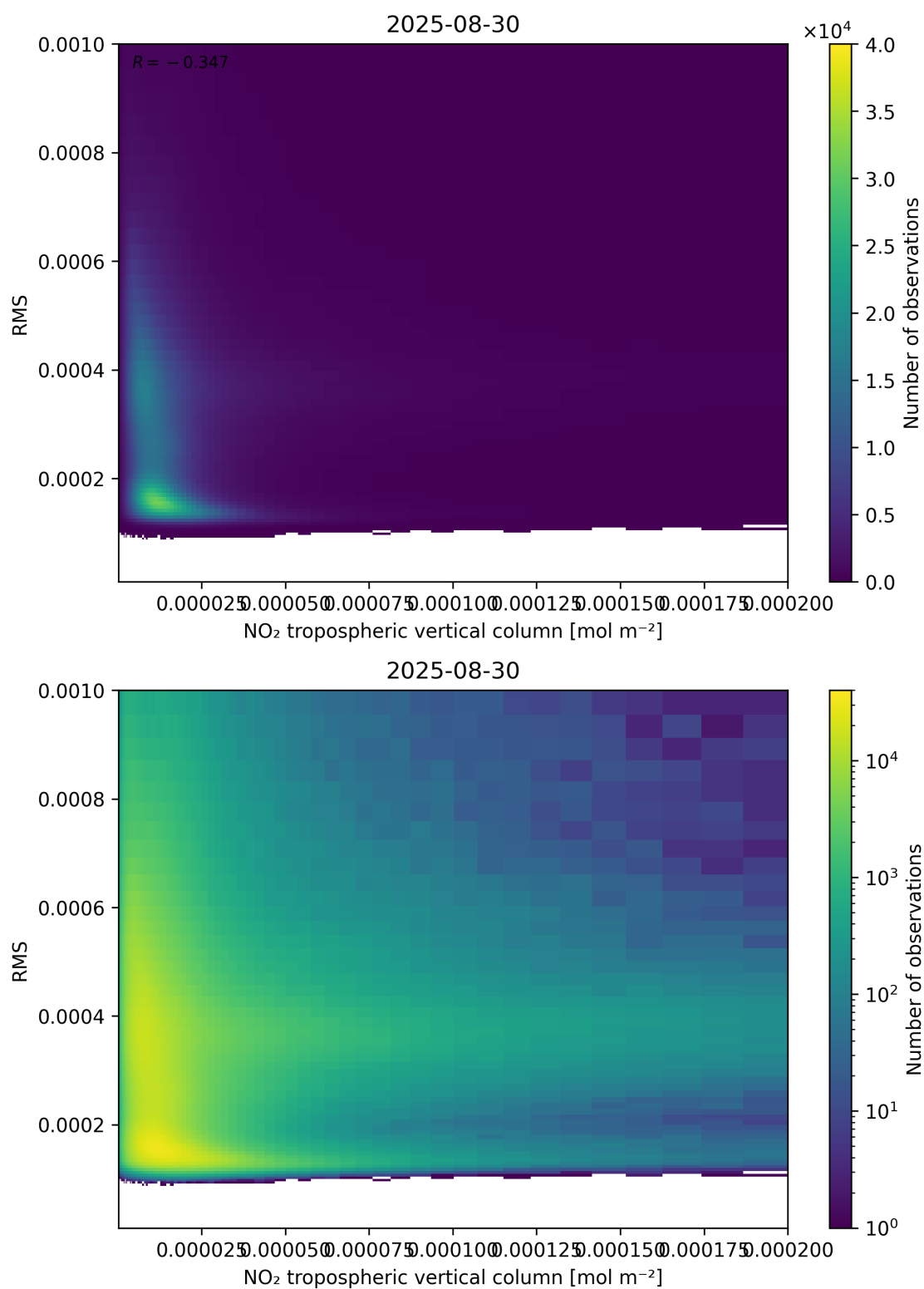
Figure 142: Scatter density plot of “NO 2 tropospheric vertical column” against “RMS” for 2025-08-30 to 2025-08-31.
