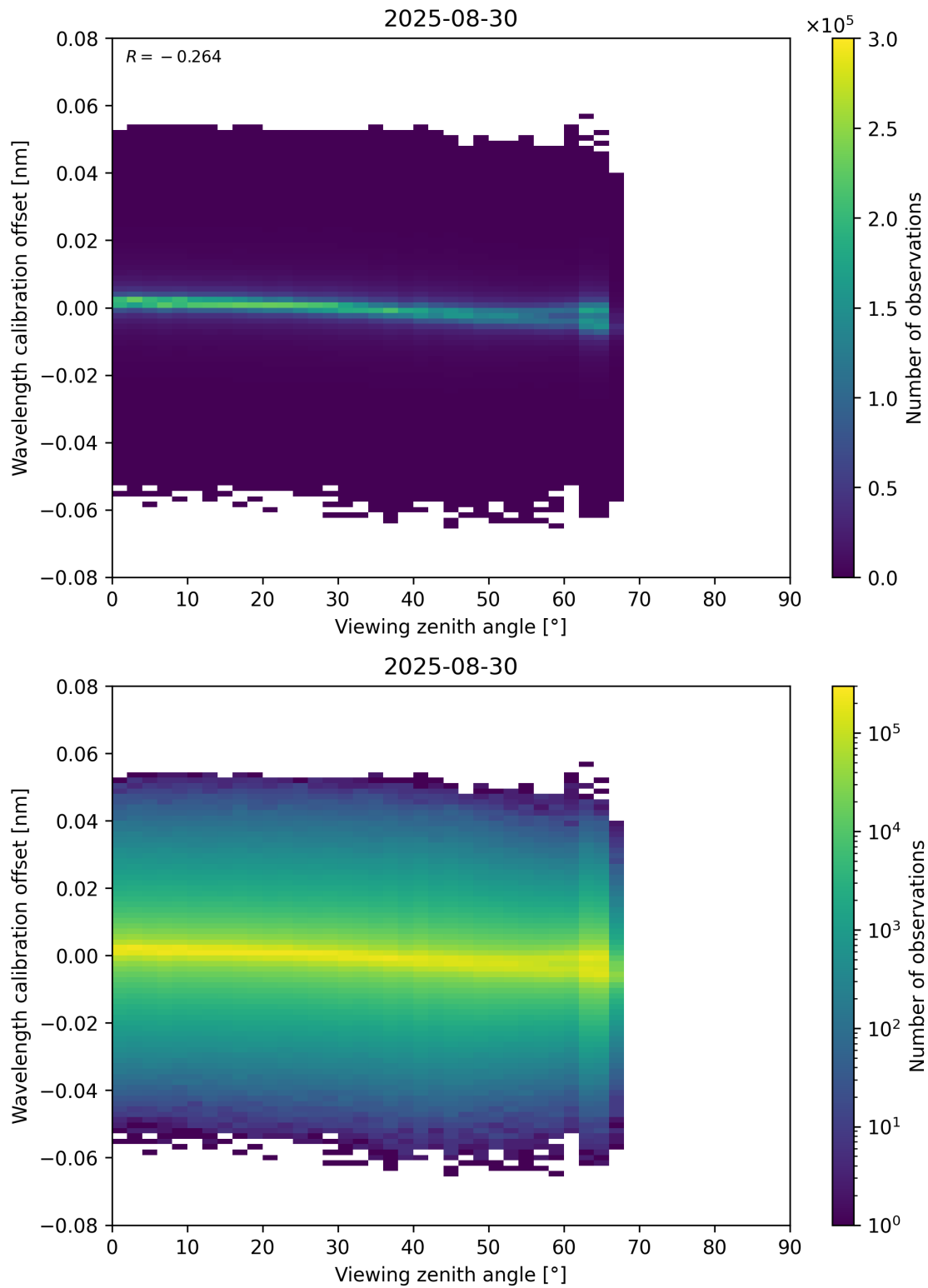
Figure 173: Scatter density plot of “Viewing zenith angle” against “Wavelength calibration offset” for 2025-08-30 to 2025-08-31.
