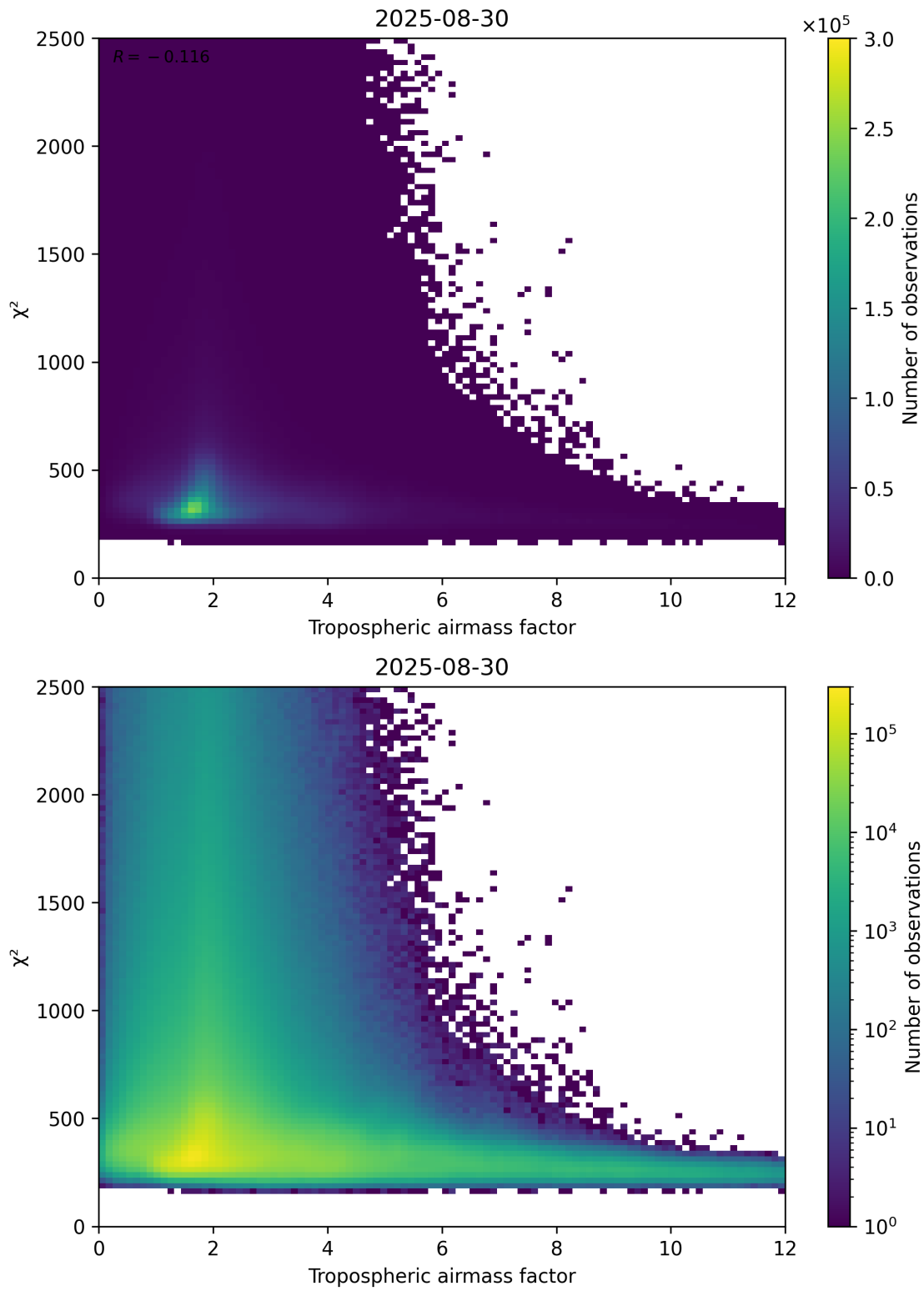
Figure 73: Scatter density plot of “Tropospheric airmass factor” against “ \chi^2 ” for 2025-08-30 to 2025-08-31.
