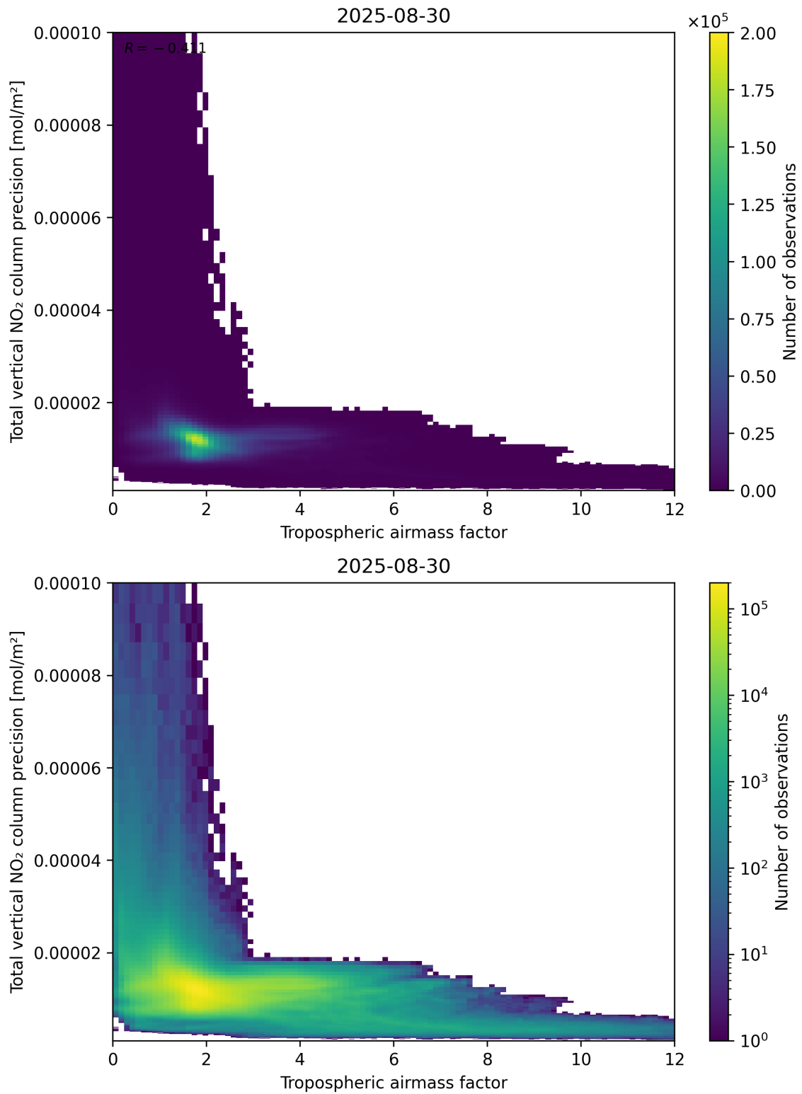
Figure 78: Scatter density plot of “Tropospheric air mass factor” against “Total vertical NO 2 column precision” for 2025-08-30 to 2025-08-31.
