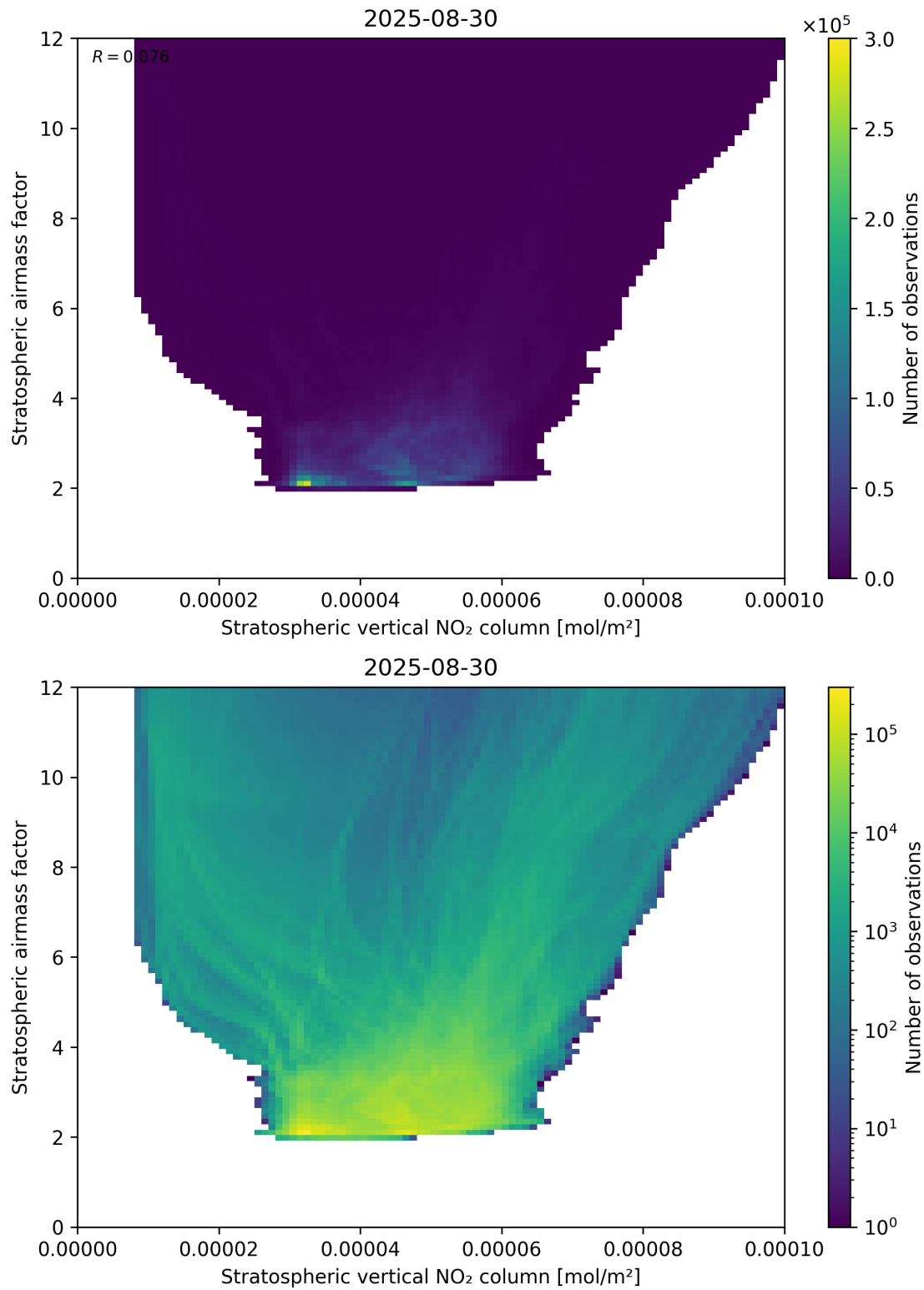
Figure 96: Scatter density plot of “Stratospheric vertical NO 2 column” against “Stratospheric airmass factor” for 2025-08-30 to 2025-08-31.
