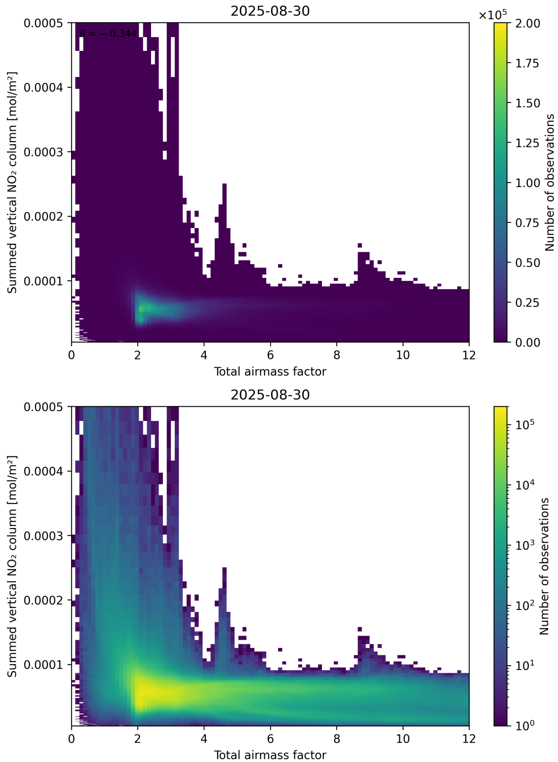
Figure 65: Scatter density plot of “Total airmass factor” against “Summed vertical NO 2 column” for 2025-08-30 to 2025-08-31.
