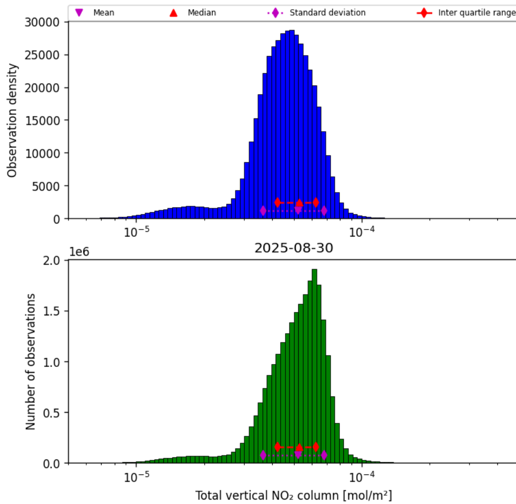
Figure 38: Histogram of “Total vertical NO 2 column” for 2025-08-30 to 2025-08-31
