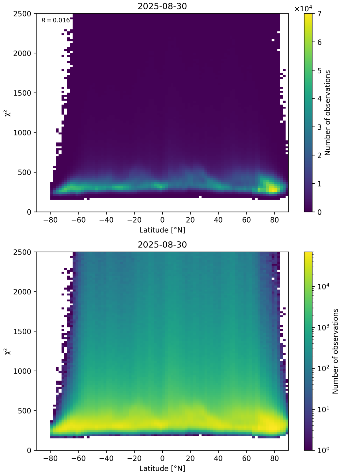
Figure 86: Scatter density plot of “Latitude” against “ \chi^2 ” for 2025-08-30 to 2025-08-31.
