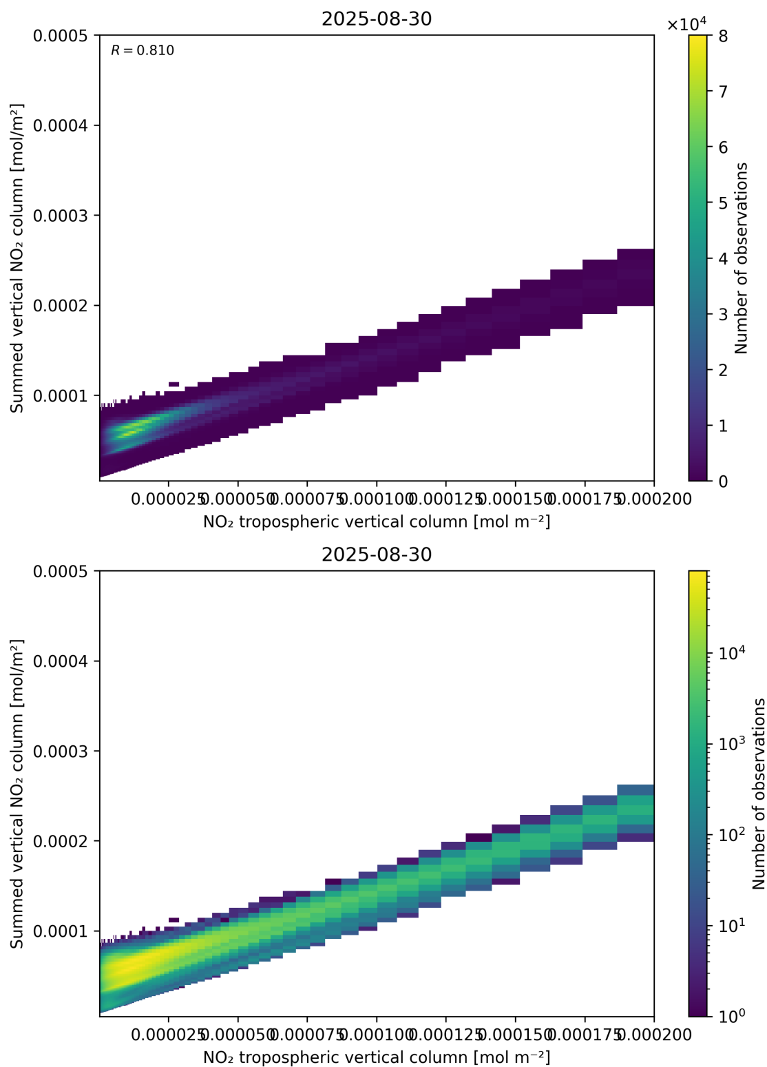
Figure 126: Scatter density plot of “NO 2 tropospheric vertical column” against “Summed vertical NO 2 column” for 2025-08-30 to 2025-08-31.
