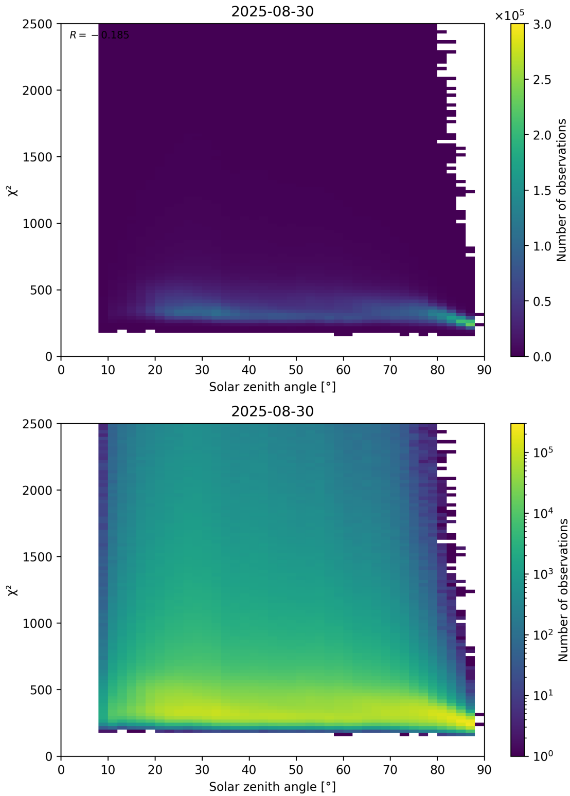
Figure 148: Scatter density plot of “Solar zenith angle” against “ \chi^2 ” for 2025-08-30 to 2025-08-31.
