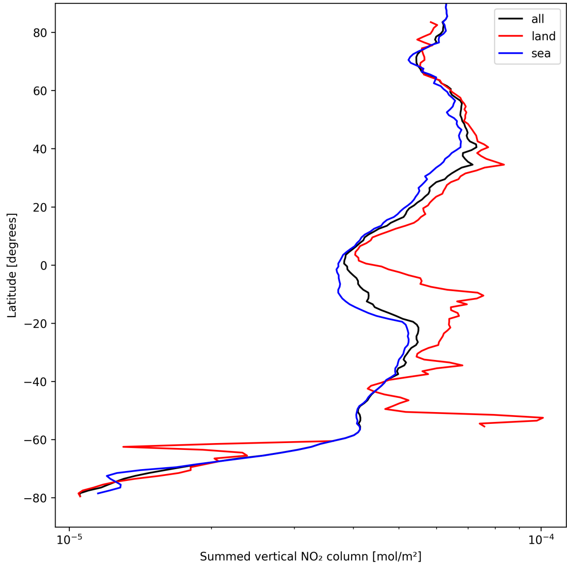
Figure 23: Zonal average of “Summed vertical NO 2 column” for 2025-08-30 to 2025-08-31.
