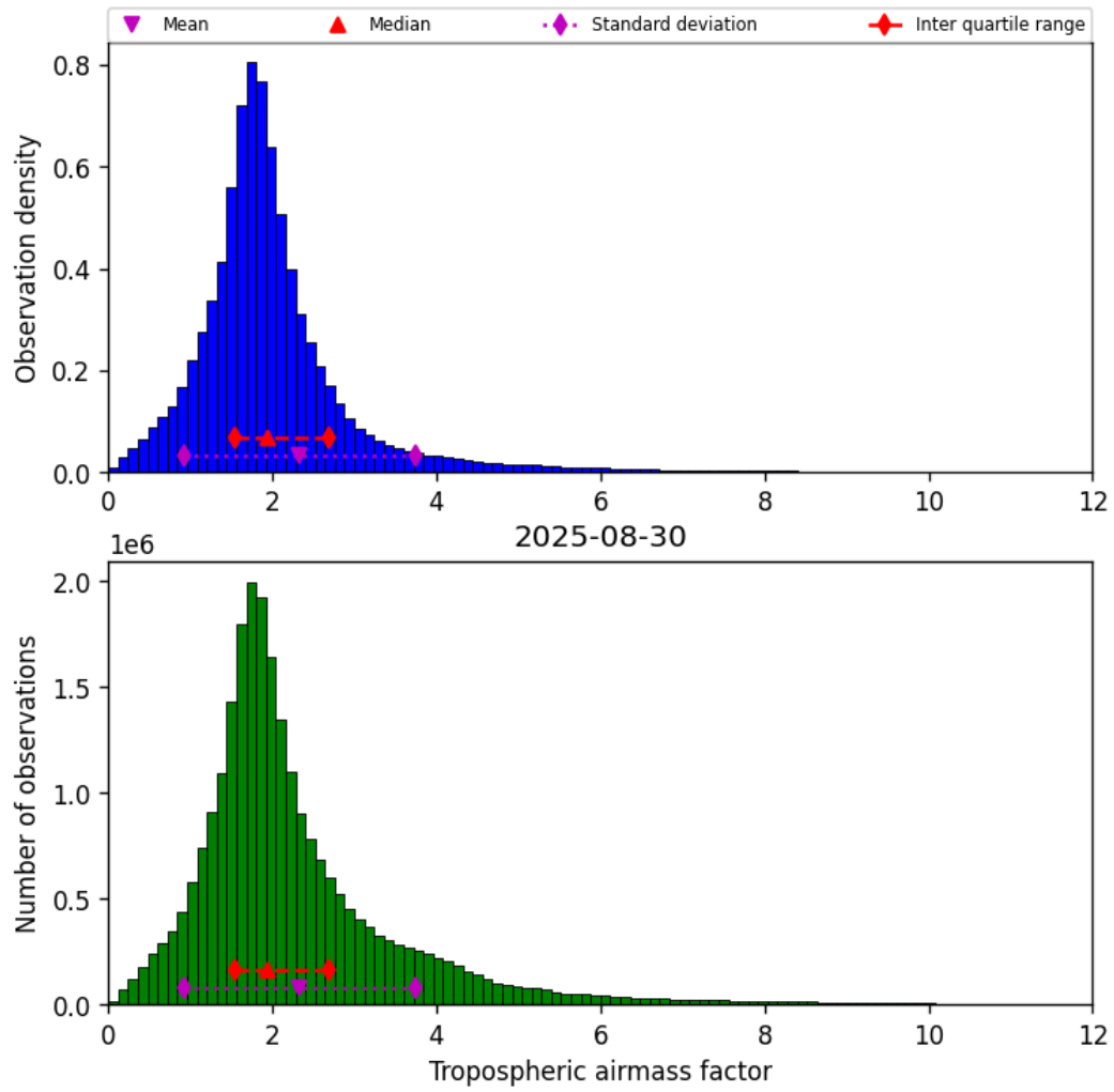
Figure 31: Histogram of “Tropospheric airmass factor” for 2025-08-30 to 2025-08-31
