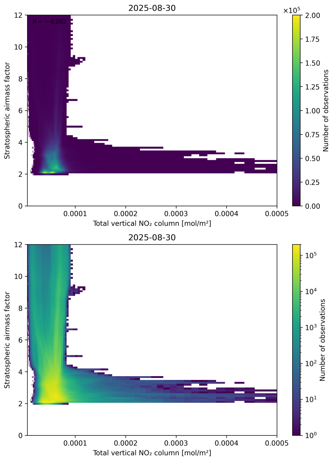
Figure 110: Scatter density plot of “Total vertical NO 2 column” against “Stratospheric airmass factor” for 2025-08-30 to 2025-08-31.
