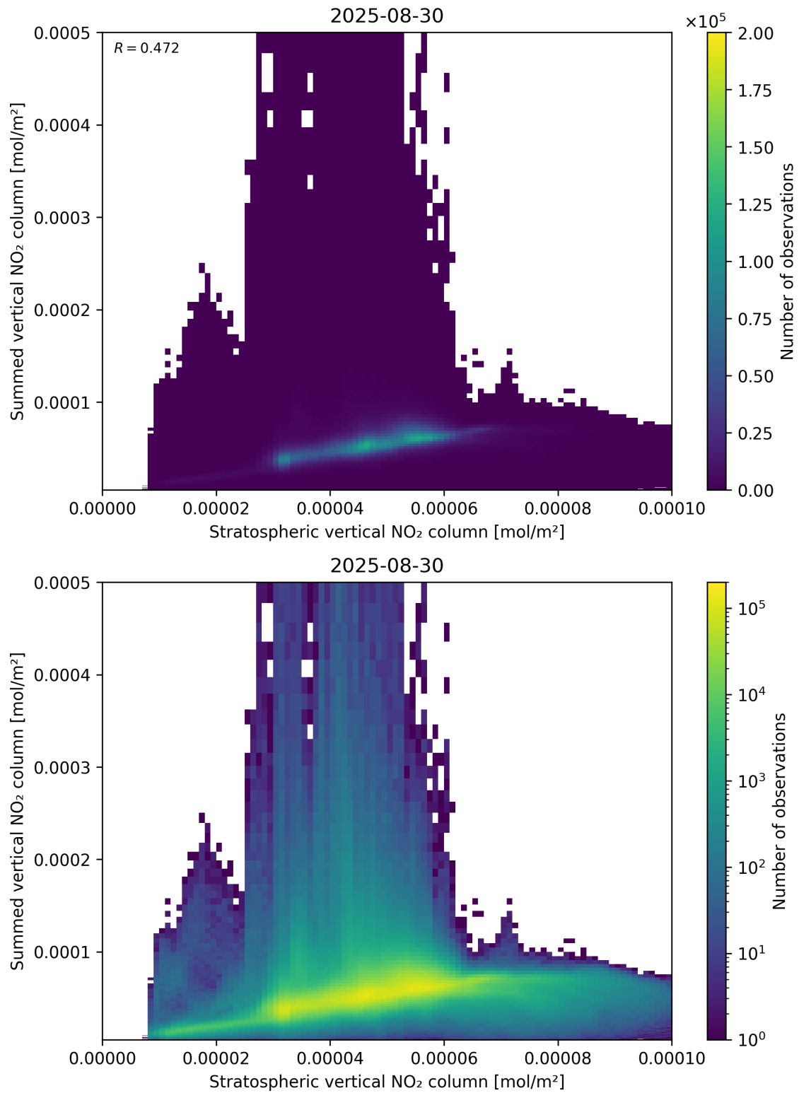
Figure 98: Scatter density plot of “Stratospheric vertical NO 2 column” against “Summed vertical NO 2 column” for 2025-08-30 to 2025-08-31.
