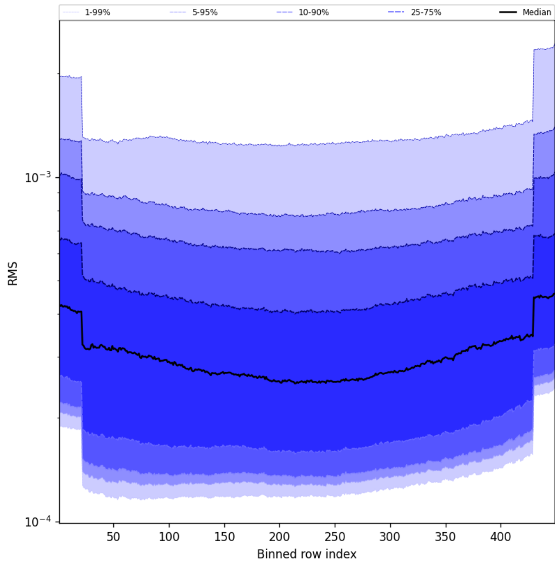
Figure 60: Along track statistics of “RMS” for 2025-08-30 to 2025-08-31
