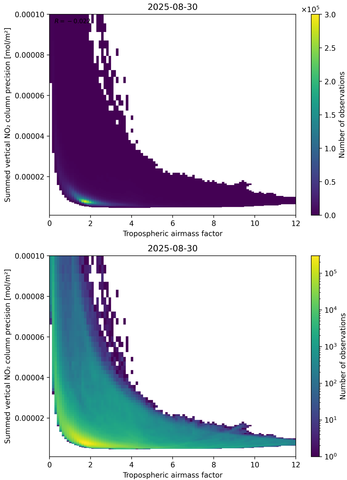
Figure 76: Scatter density plot of “Tropospheric air mass factor” against “Summed vertical NO 2 column precision” for 2025-08-30 to 2025-08-31.
