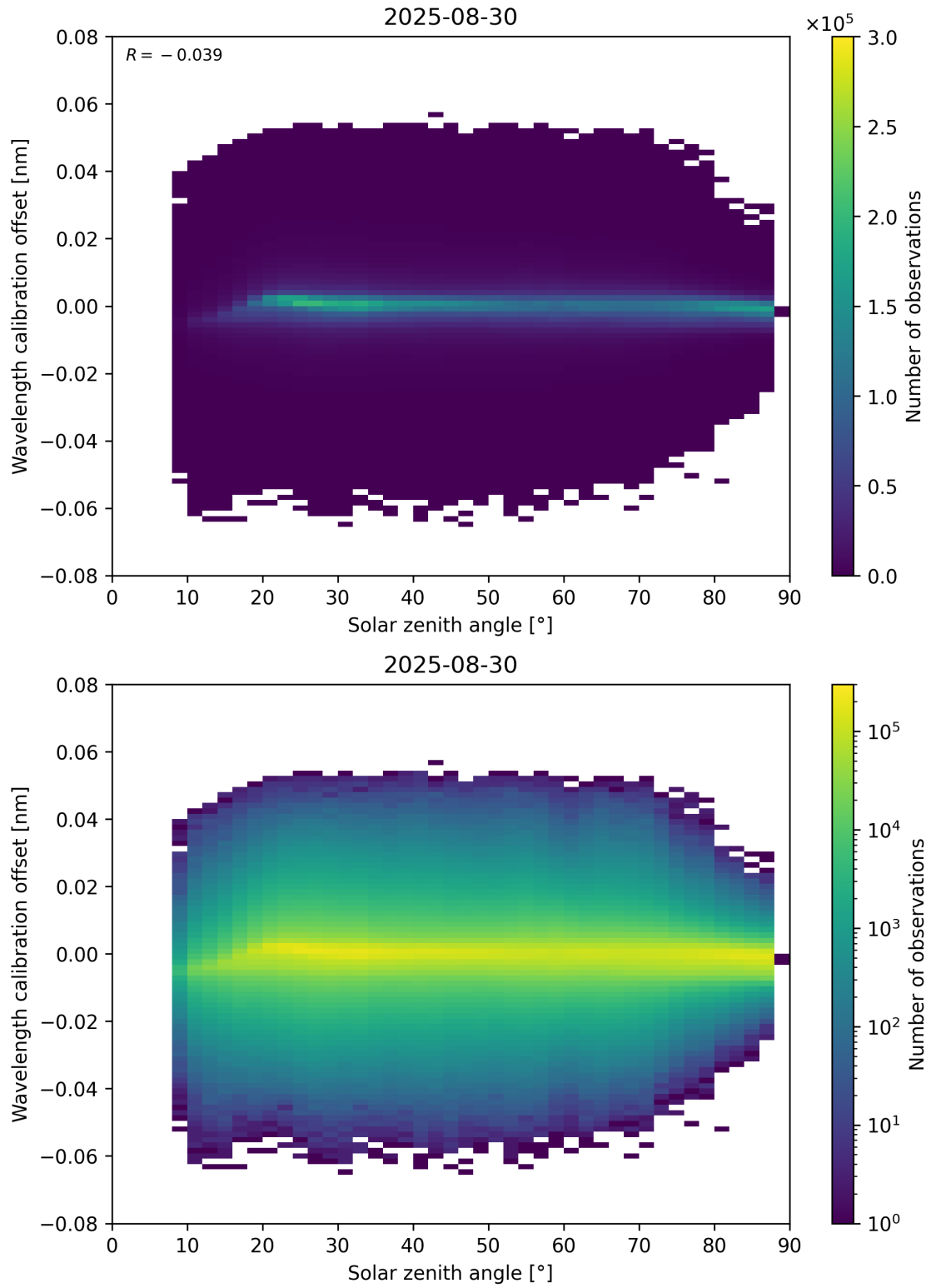
Figure 158: Scatter density plot of “Solar zenith angle” against “Wavelength calibration offset” for 2025-08-30 to 2025-08-31.
