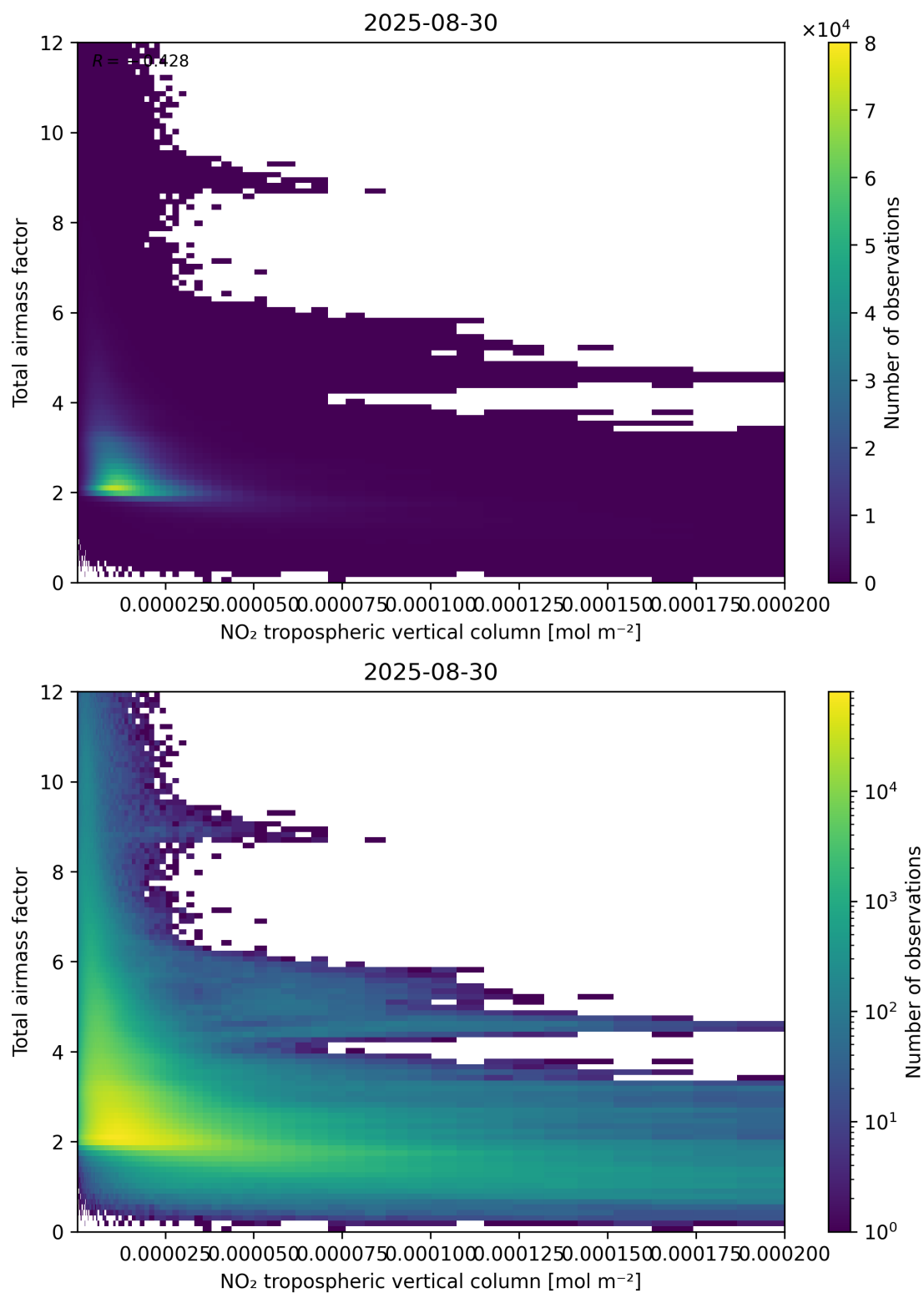
Figure 122: Scatter density plot of “NO 2 tropospheric vertical column” against “Total air mass factor” for 2025-08-30 to 2025-08-31.
