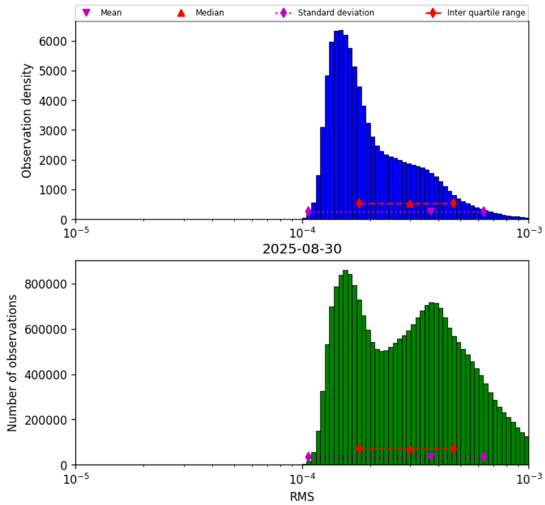
Figure 43: Histogram of “RMS” for 2025-08-30 to 2025-08-31
