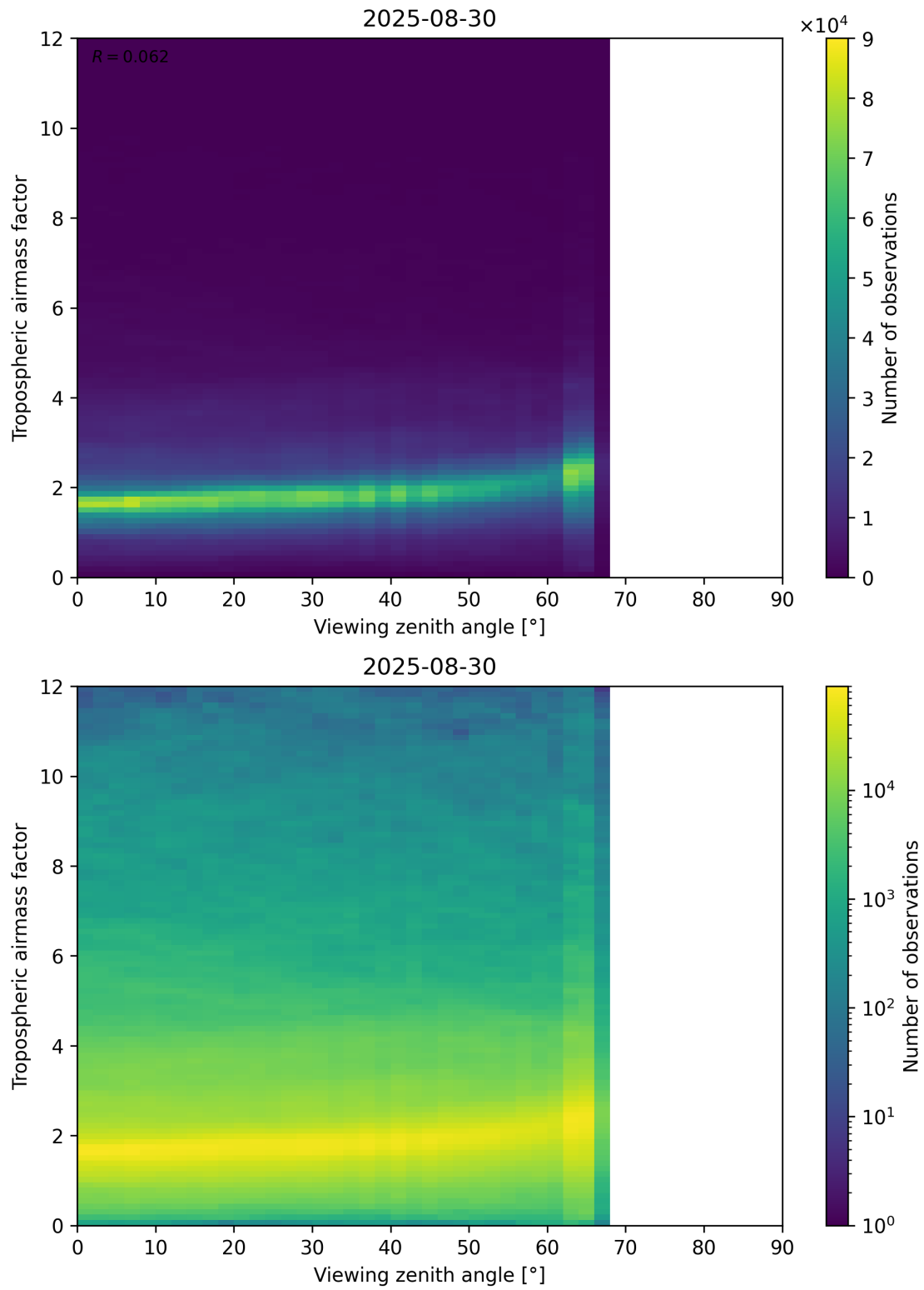
Figure 161: Scatter density plot of “Viewing zenith angle” against “Tropospheric airmass factor” for 2025-08-30 to 2025-08-31.
