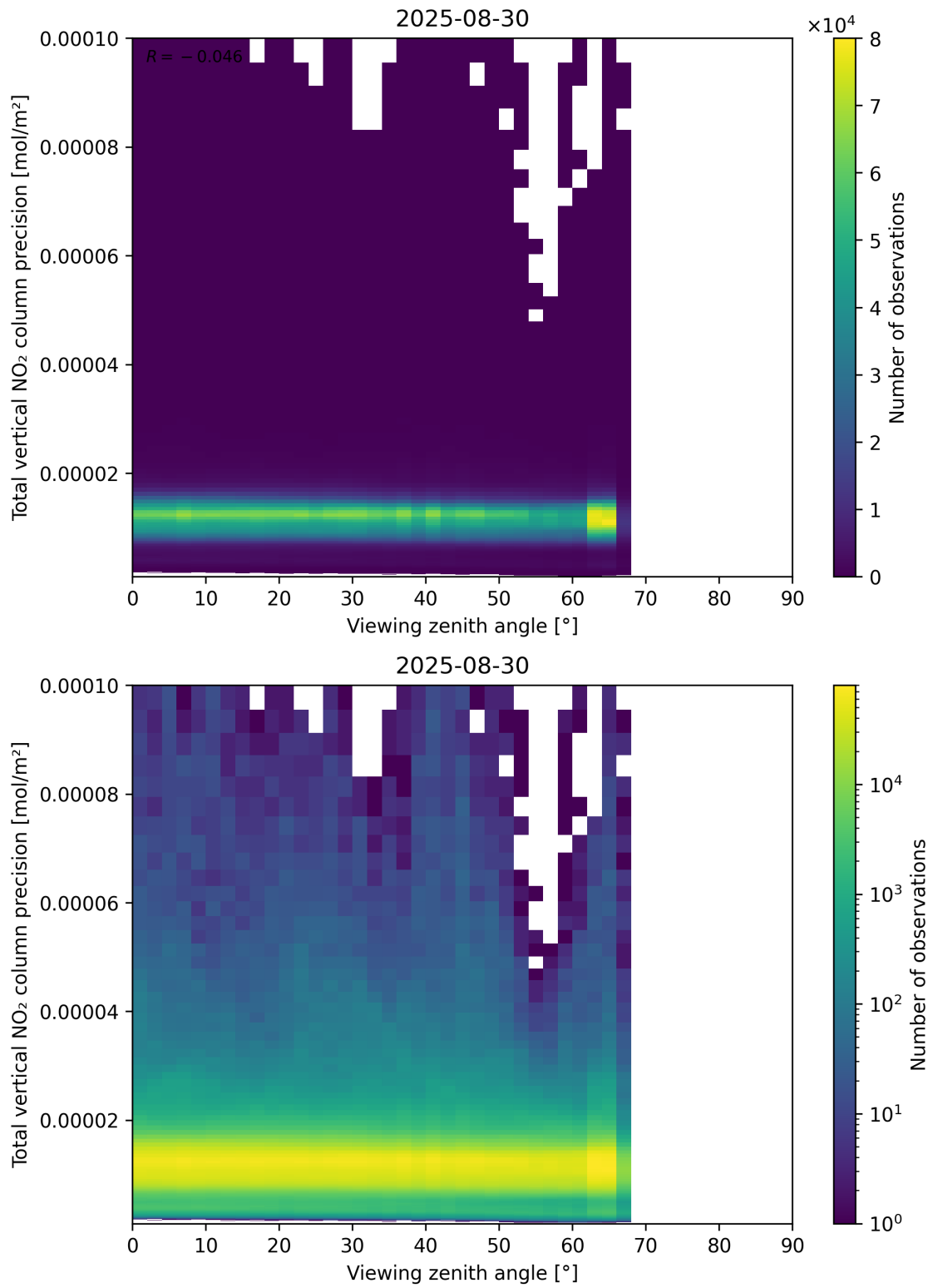
Figure 168: Scatter density plot of “Viewing zenith angle” against “Total vertical NO 2 column precision” for 2025-08-30 to 2025-08-31.
