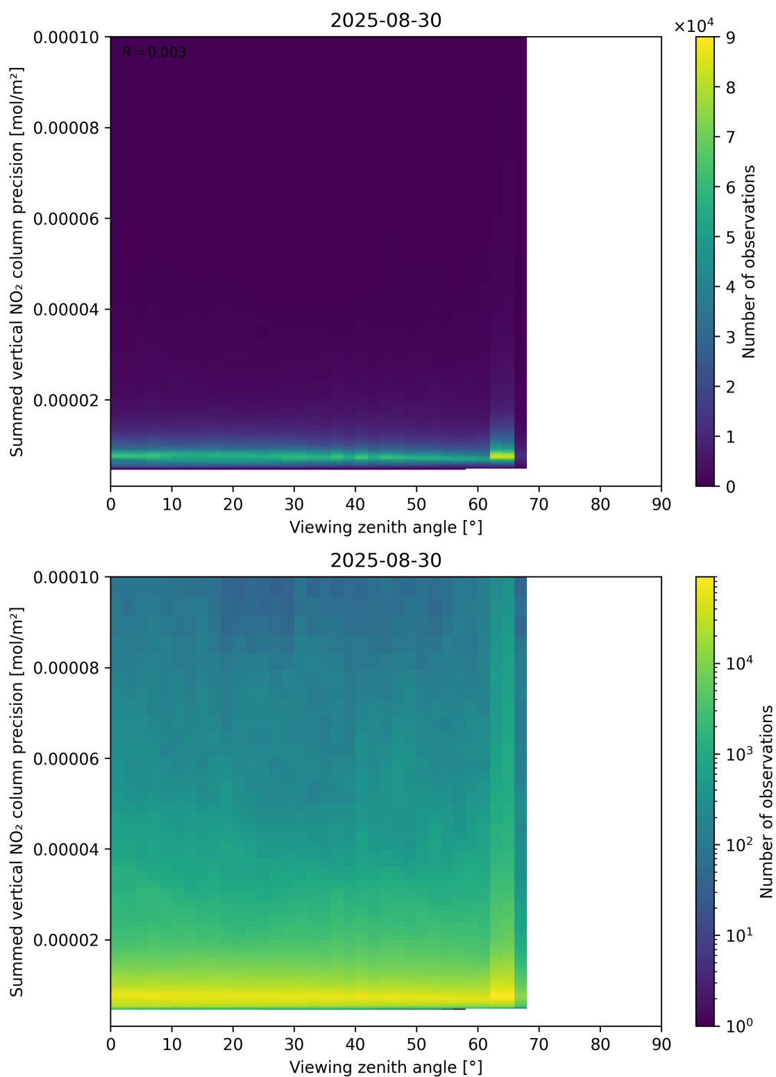
Figure 166: Scatter density plot of “Viewing zenith angle” against “Summed vertical NO 2 column precision” for 2025-08-30 to 2025-08-31.
