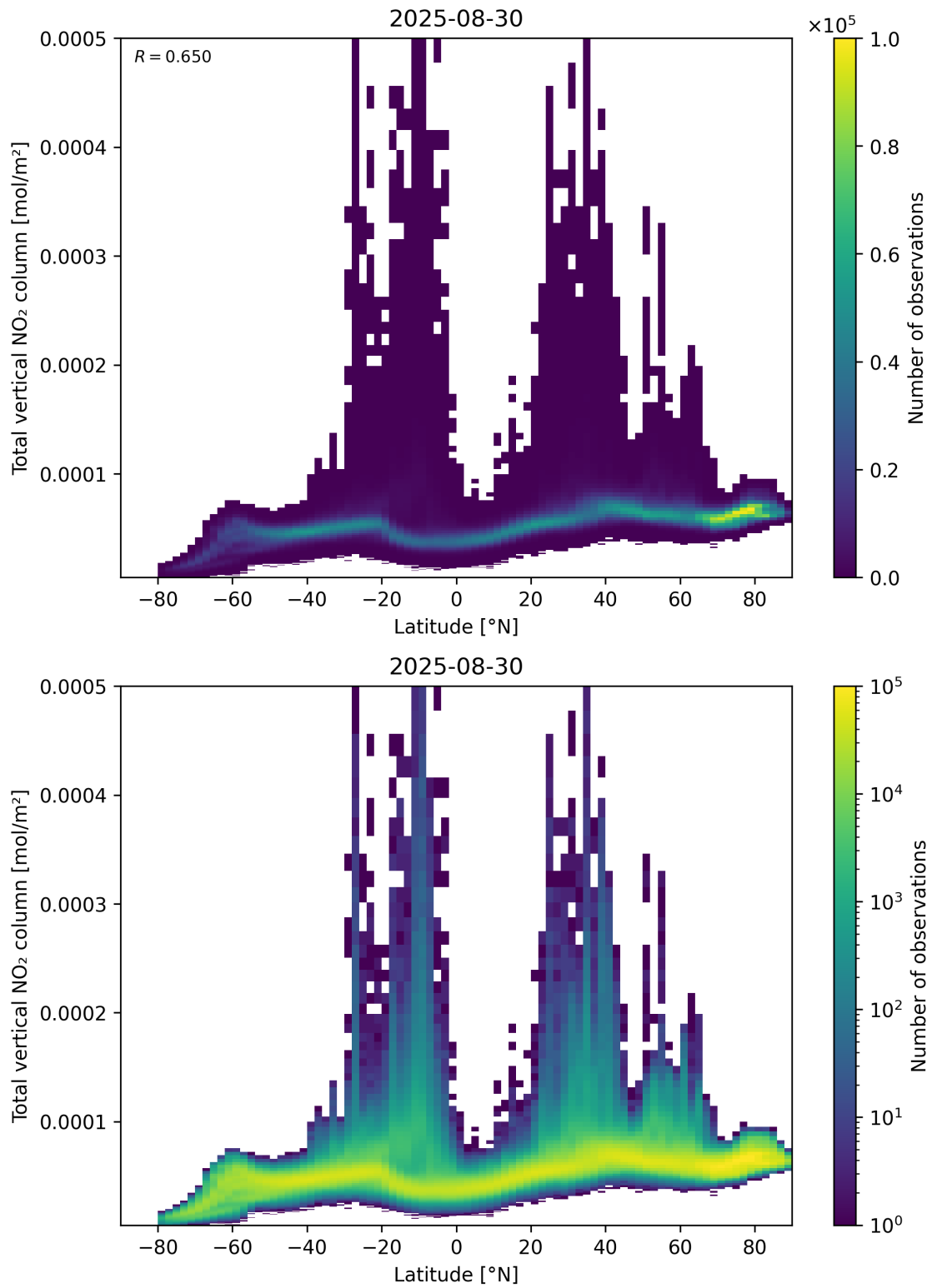
Figure 90: Scatter density plot of “Latitude” against “Total vertical NO 2 column” for 2025-08-30 to 2025-08-31.
