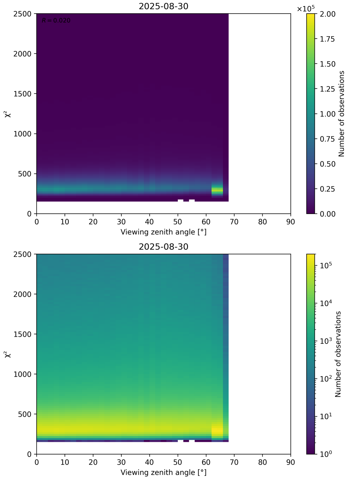
Figure 162: Scatter density plot of “Viewing zenith angle” against “ \chi^2 ” for 2025-08-30 to 2025-08-31.
