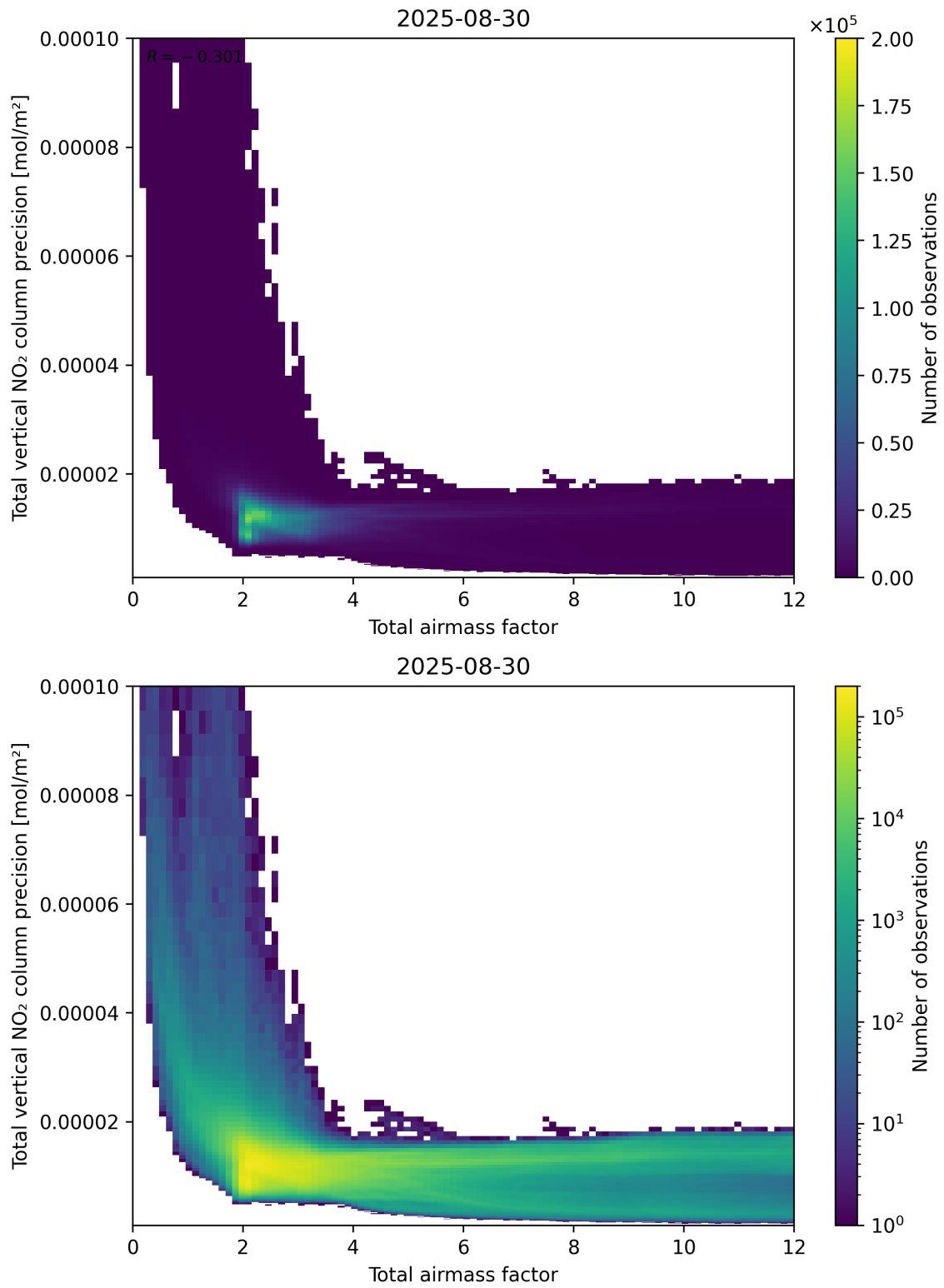
Figure 68: Scatter density plot of “Total airmass factor” against “Total vertical NO 2 column precision” for 2025-08-30 to 2025-08-31.
