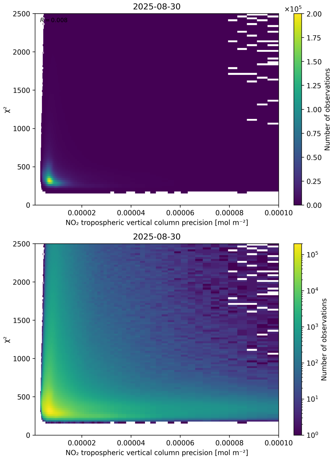
Figure 134: Scatter density plot of “NO 2 tropospheric vertical column precision” against “ \chi^2 ” for 2025-08-30 to 2025-08-31.
