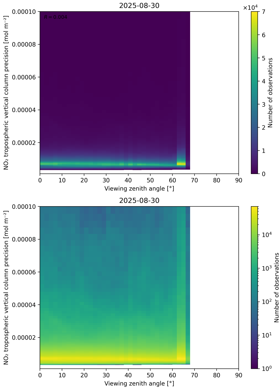
Figure 170: Scatter density plot of “Viewing zenith angle” against “NO 2 tropospheric vertical column precision” for 2025-08-30 to 2025-08-31.
