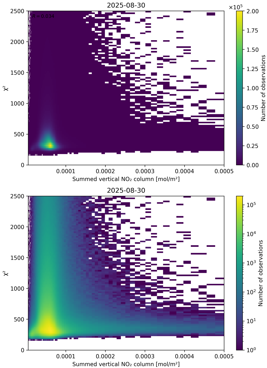
Figure 104: Scatter density plot of “Summed vertical NO 2 column” against “ \chi^2 ” for 2025-08-30 to 2025-08-31.
