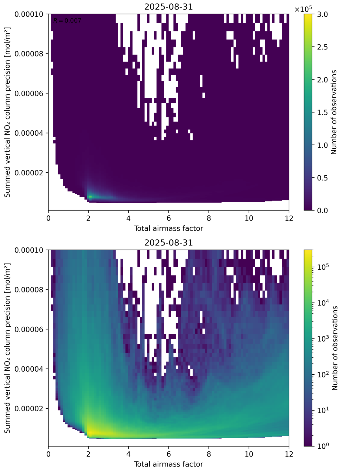
Figure 66: Scatter density plot of “Total airmass factor” against “Summed vertical NO 2 column precision” for 2025-08-30 to 2025-09-01.
