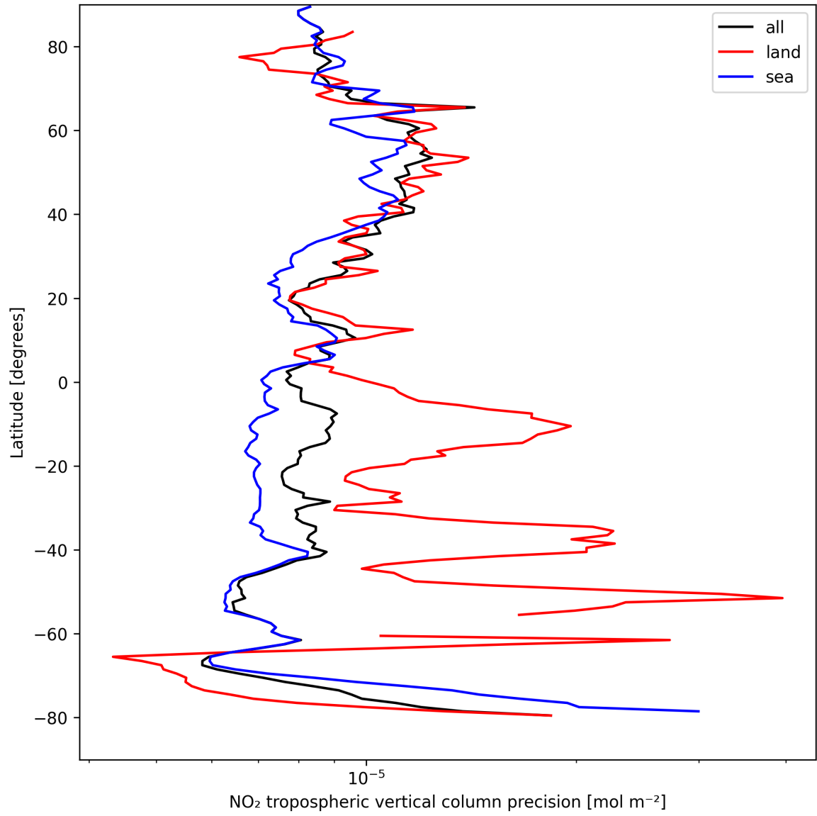
Figure 13: Zonal average of “NO 2 tropospheric vertical column precision” for 2025-08-30 to 2025-09-01.
