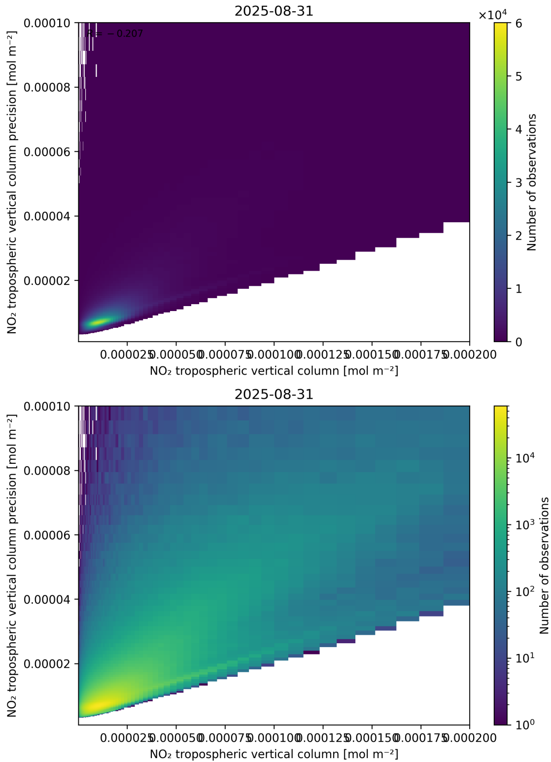
Figure 130: Scatter density plot of “NO 2 tropospheric vertical column” against “NO 2 tropospheric vertical column precision” for 2025-08-30 to 2025-09-01.
