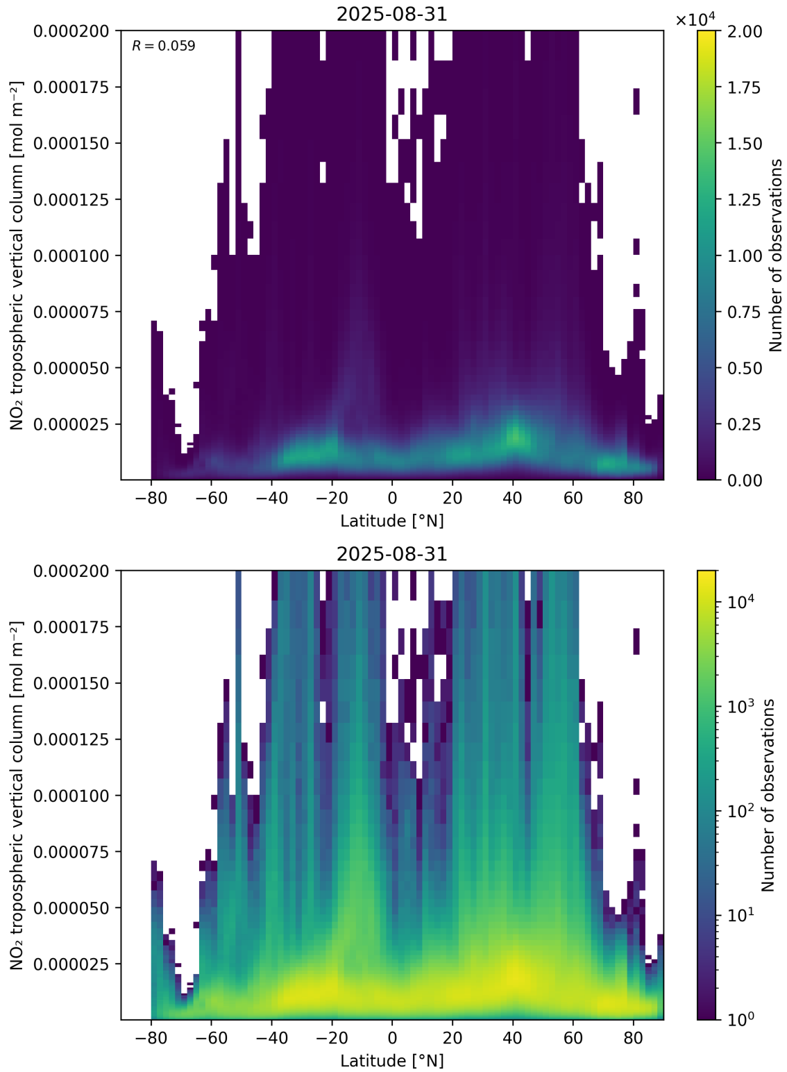
Figure 92: Scatter density plot of “Latitude” against “NO 2 tropospheric vertical column” for 2025-08-30 to 2025-09-01.
