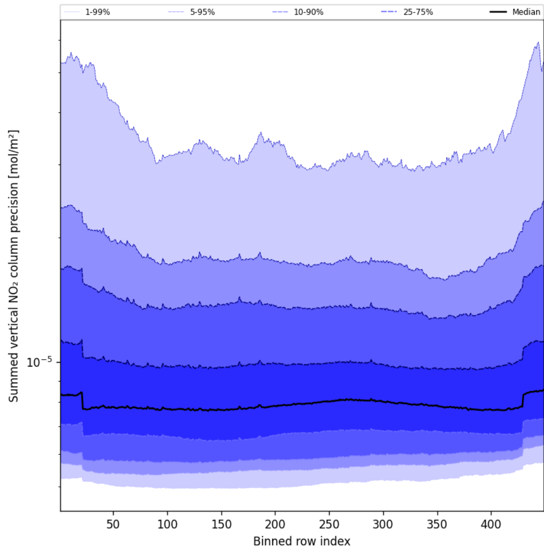
Figure 58: Along track statistics of “Summed vertical NO 2 column precision” for 2025-08-30 to 2025-09-01
