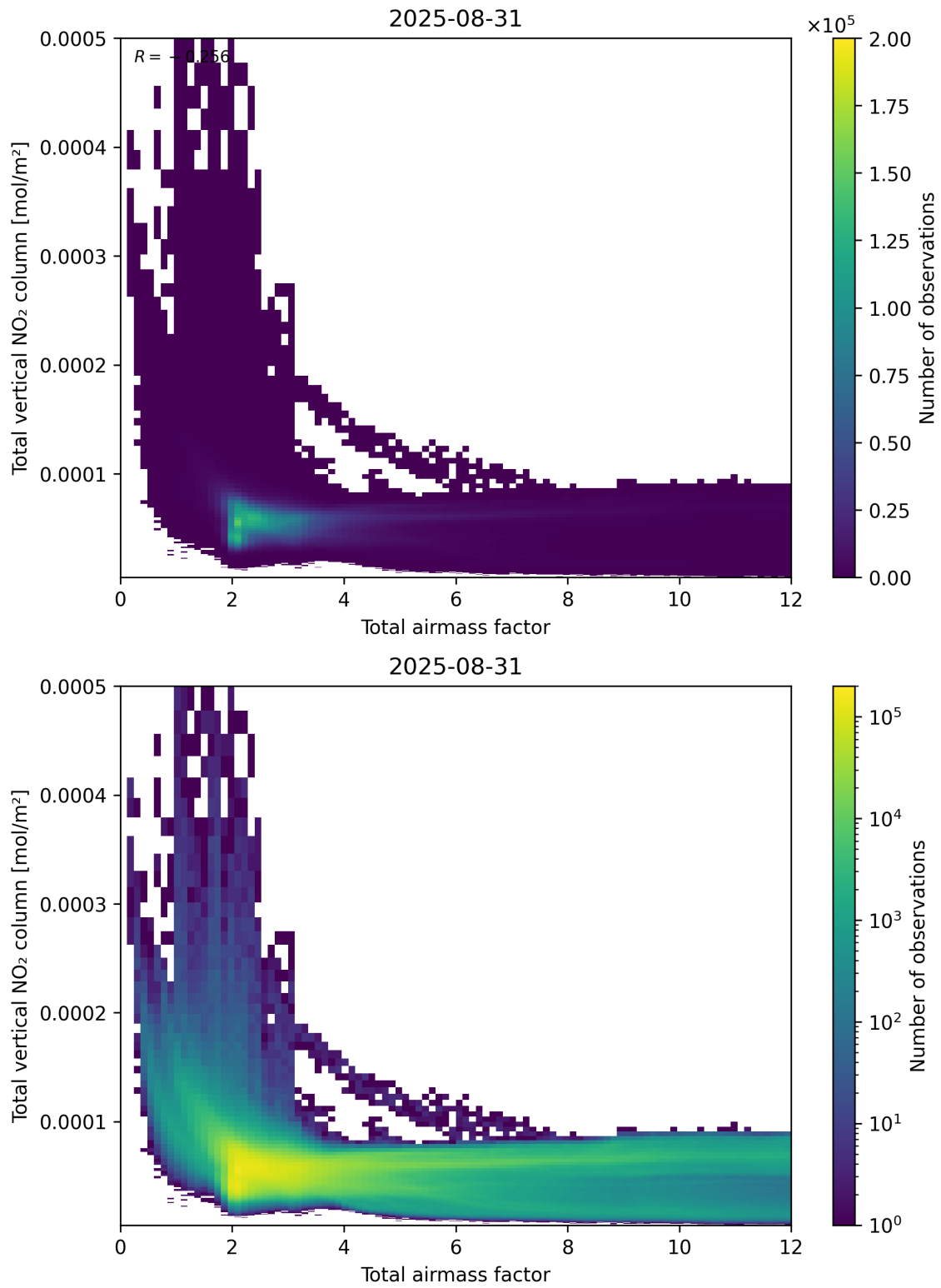
Figure 67: Scatter density plot of “Total airmass factor” against “Total vertical NO 2 column” for 2025-08-30 to 2025-09-01.
