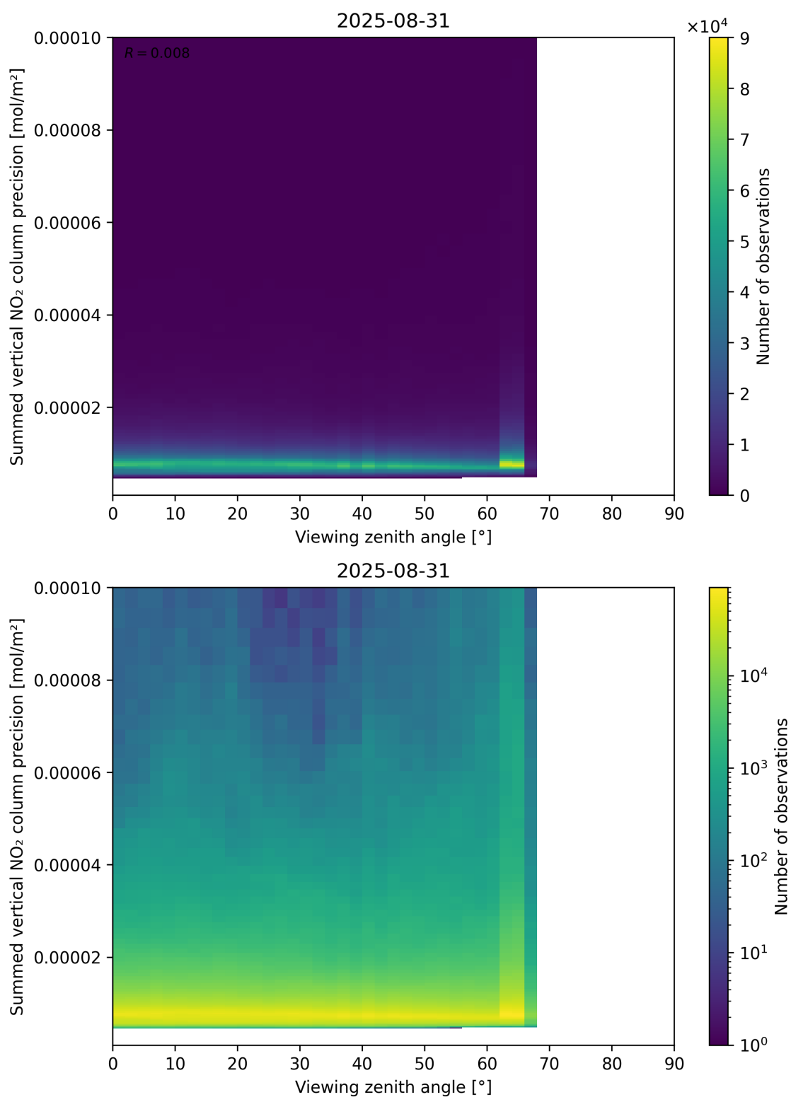
Figure 166: Scatter density plot of “Viewing zenith angle” against “Summed vertical NO 2 column precision” for 2025-08-30 to 2025-09-01.
