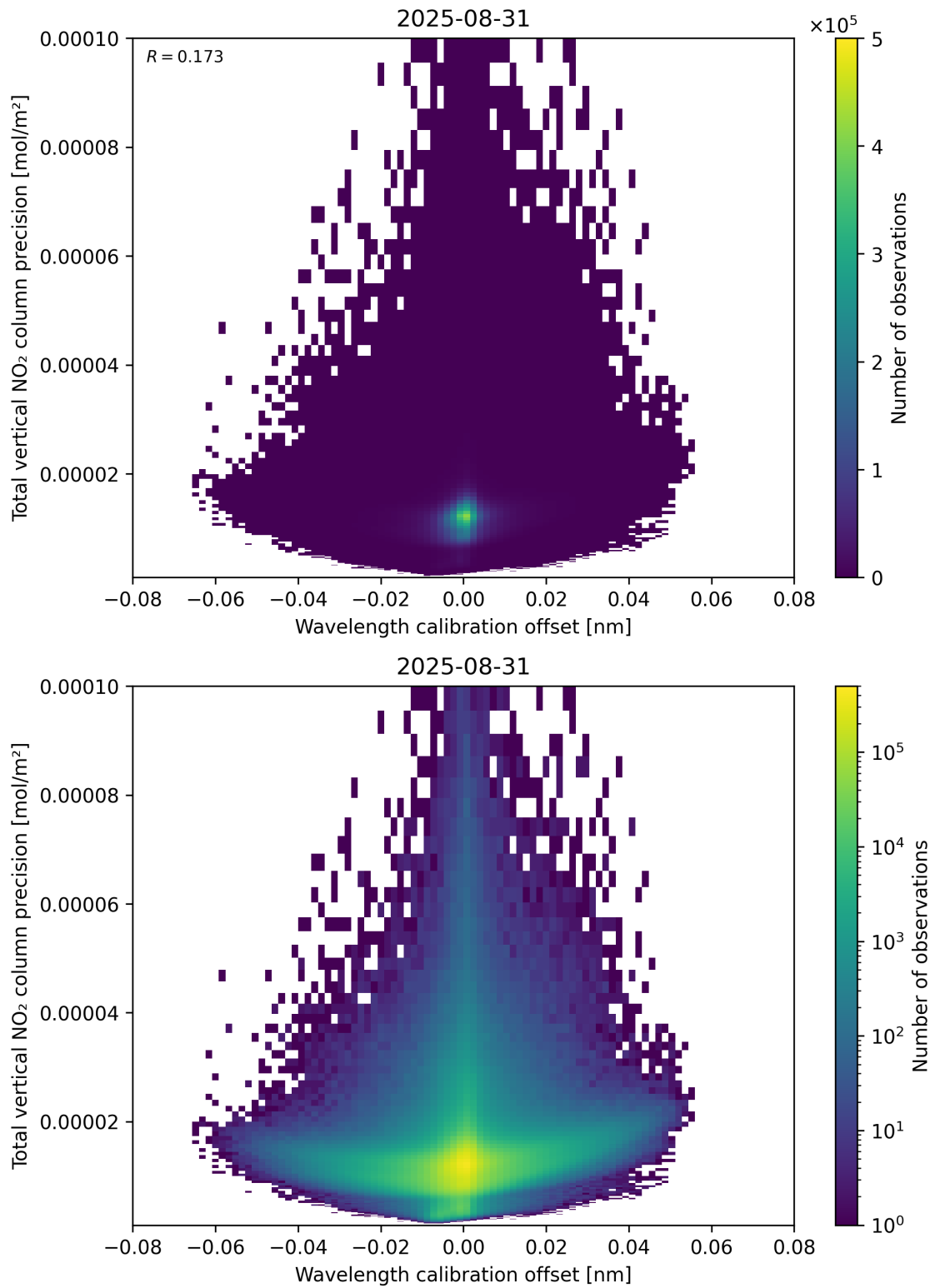
Figure 180: Scatter density plot of “Wavelength calibration offset” against “Total vertical NO 2 column precision” for 2025-08-30 to 2025-09-01.
