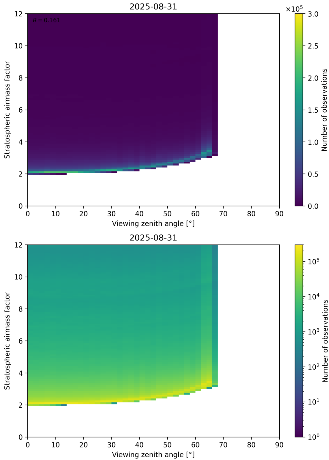
Figure 159: Scatter density plot of “Viewing zenith angle” against “Stratospheric airmass factor” for 2025-08-30 to 2025-09-01.
