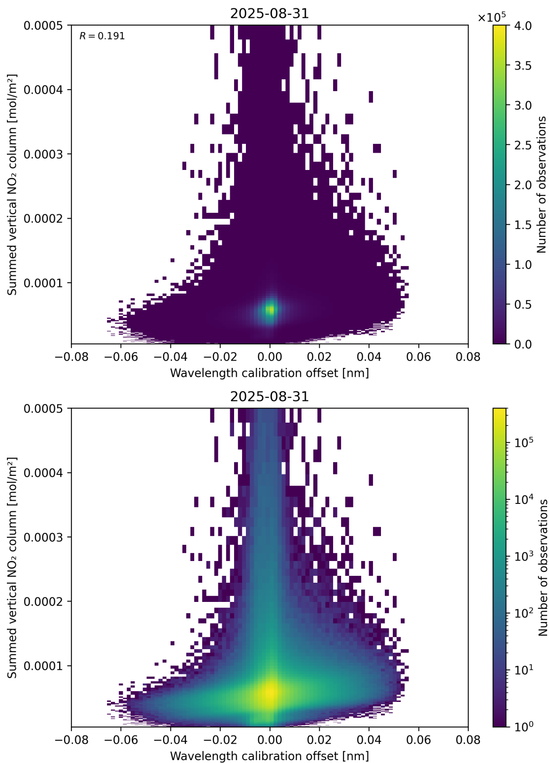
Figure 177: Scatter density plot of “Wavelength calibration offset” against “Summed vertical NO 2 column” for 2025-08-30 to 2025-09-01.
