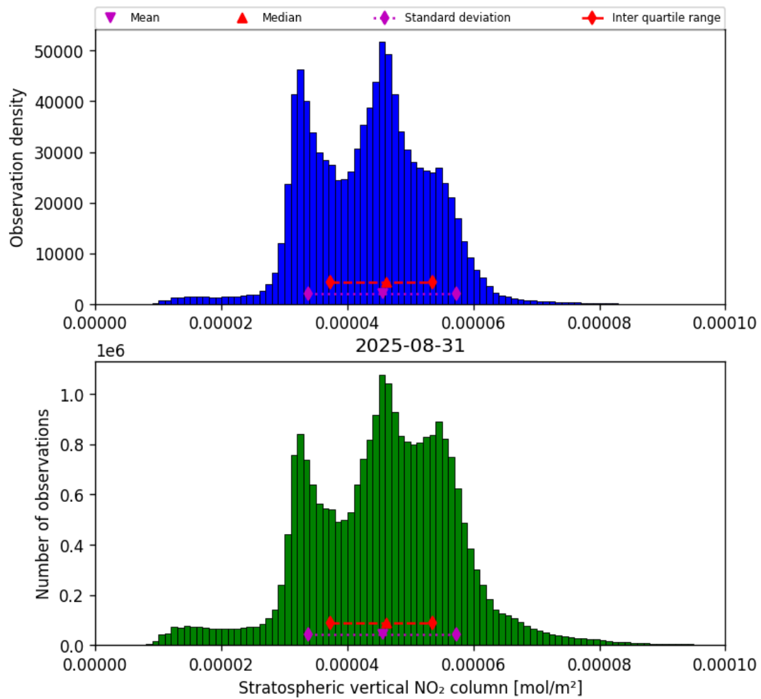
Figure 36: Histogram of “Stratospheric vertical NO 2 column” for 2025-08-30 to 2025-09-01
