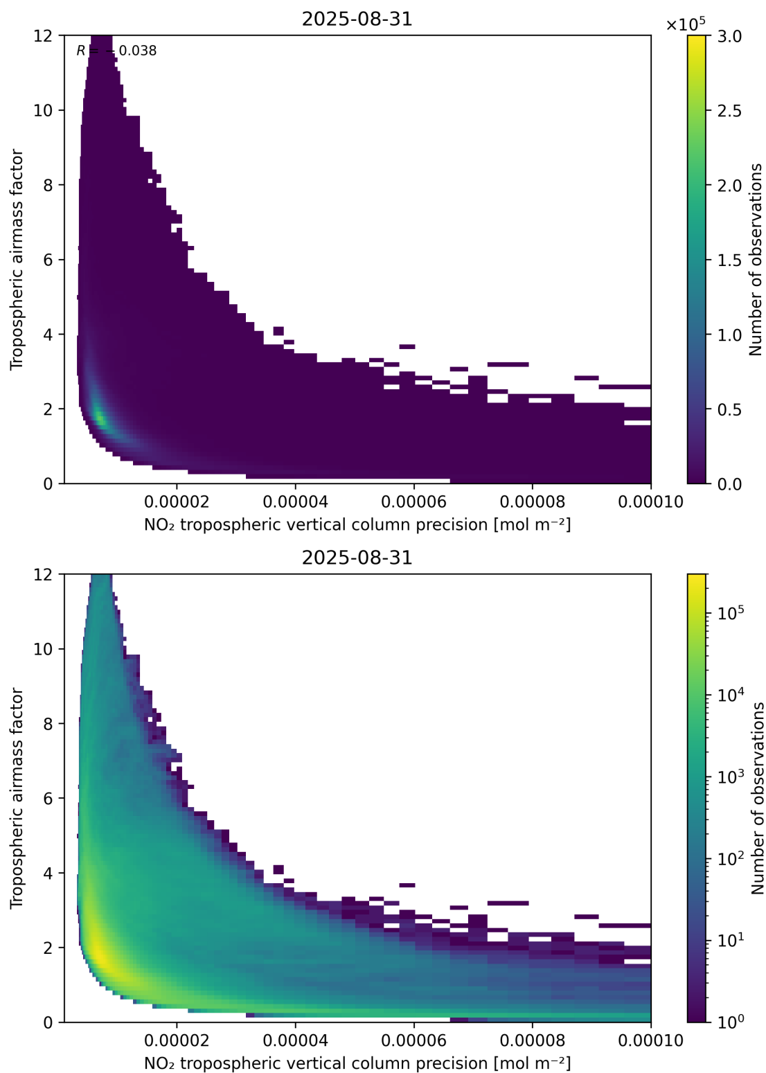
Figure 133: Scatter density plot of “NO 2 tropospheric vertical column precision” against “Tropospheric airmass factor” for 2025-08-30 to 2025-09-01.
