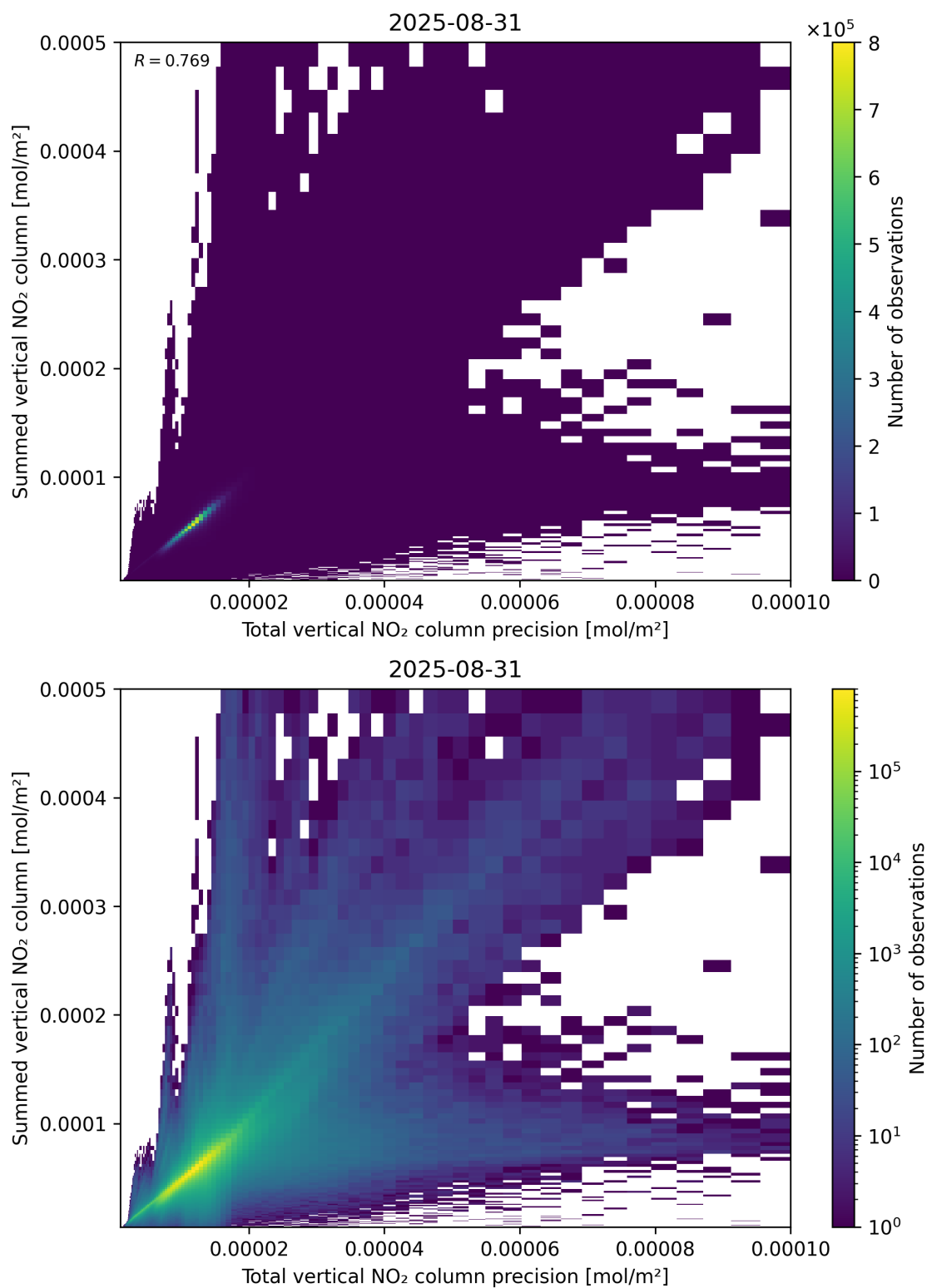
Figure 117: Scatter density plot of “Total vertical NO 2 column precision” against “Summed vertical NO 2 column” for 2025-08-30 to 2025-09-01.
