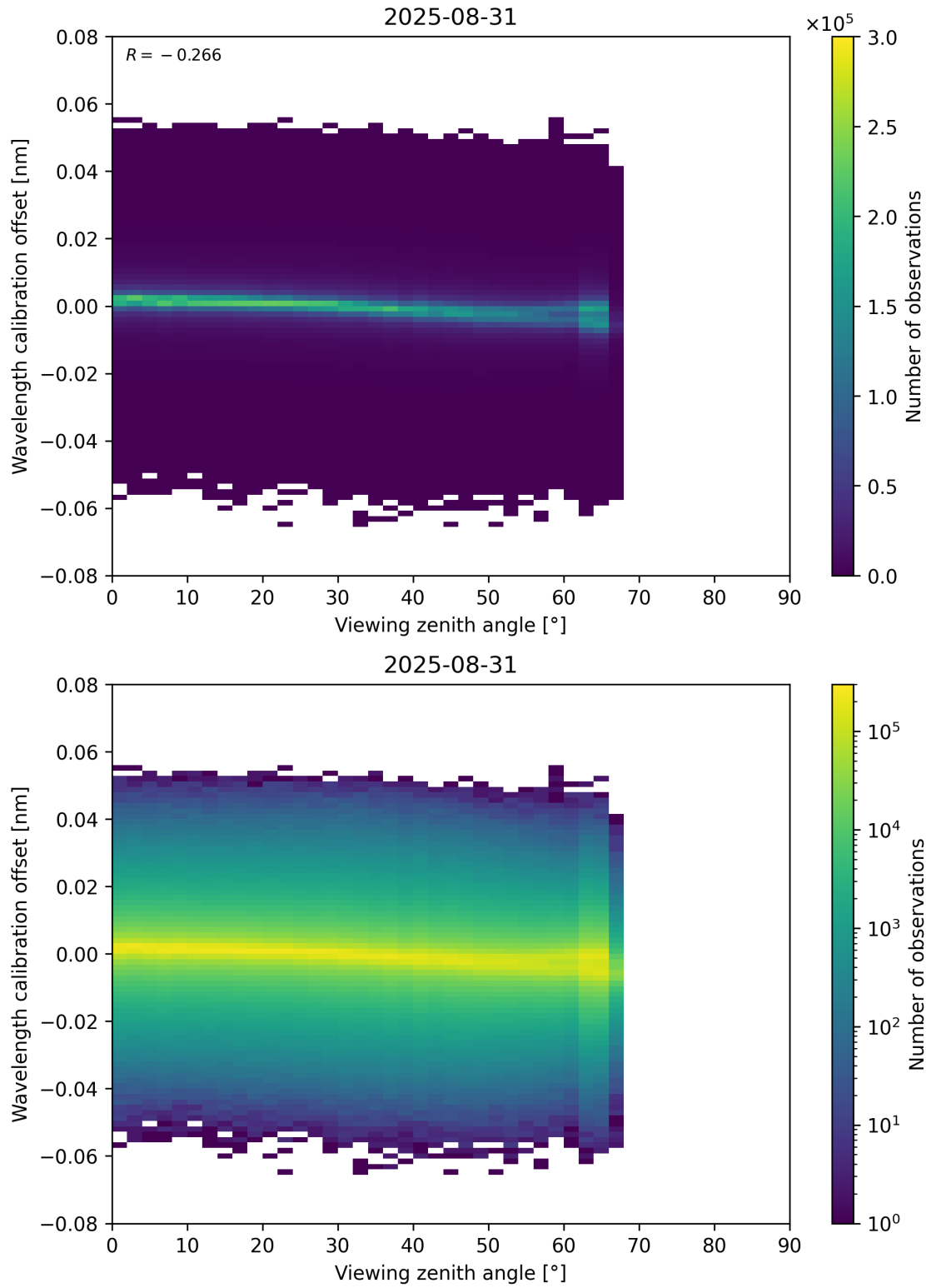
Figure 173: Scatter density plot of “Viewing zenith angle” against “Wavelength calibration offset” for 2025-08-30 to 2025-09-01.
