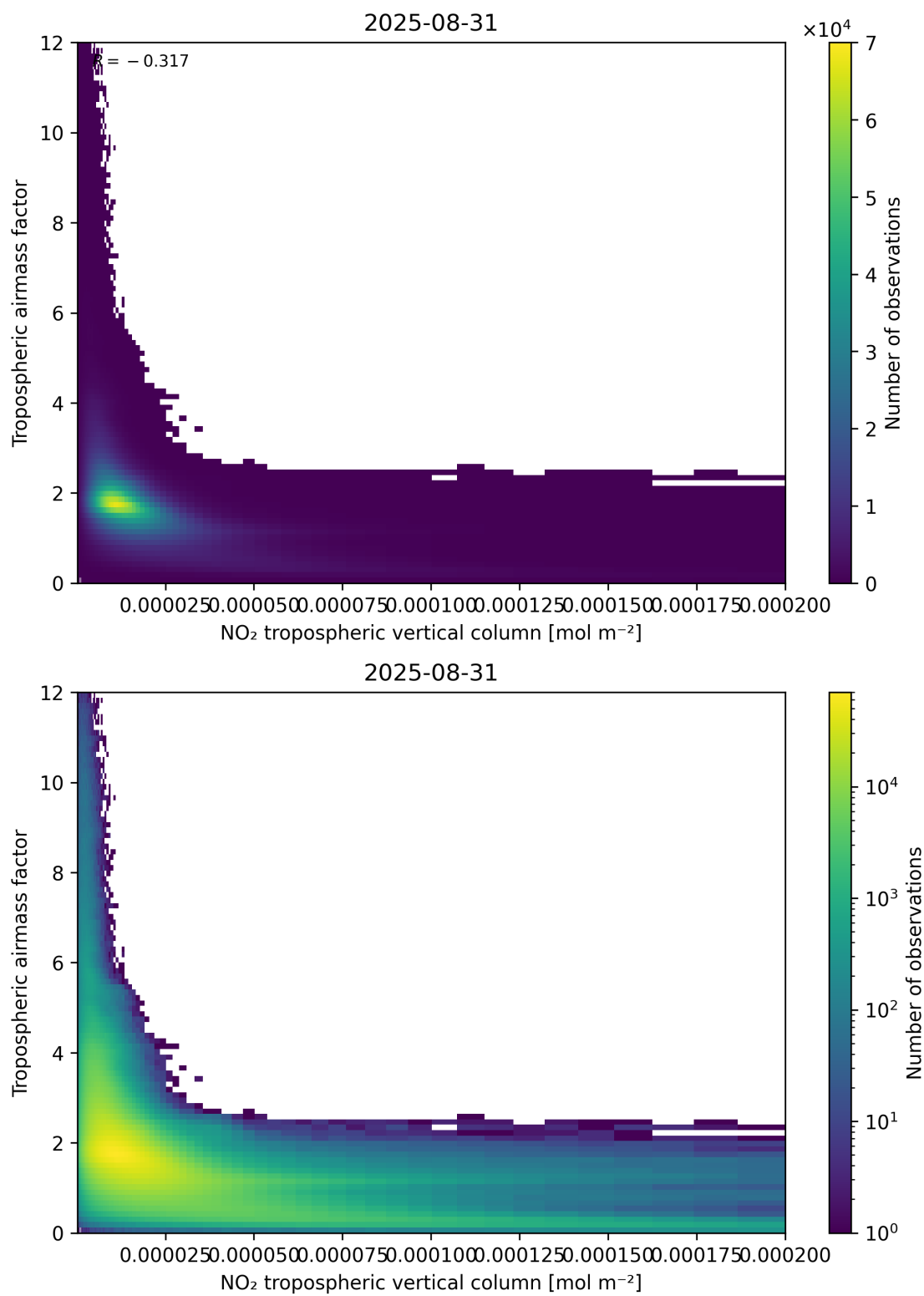
Figure 123: Scatter density plot of “NO 2 tropospheric vertical column” against “Tropospheric air mass factor” for 2025-08-30 to 2025-09-01.
