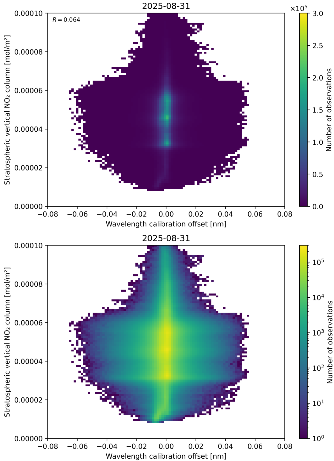
Figure 176: Scatter density plot of “Wavelength calibration offset” against “Stratospheric vertical NO 2 column” for 2025-08-30 to 2025-09-01.
