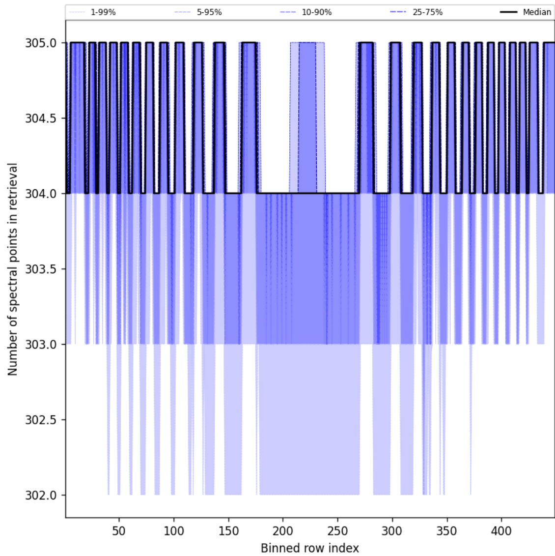
Figure 50: Along track statistics of “Number of spectral points in retrieval” for 2025-08-30 to 2025-09-01
