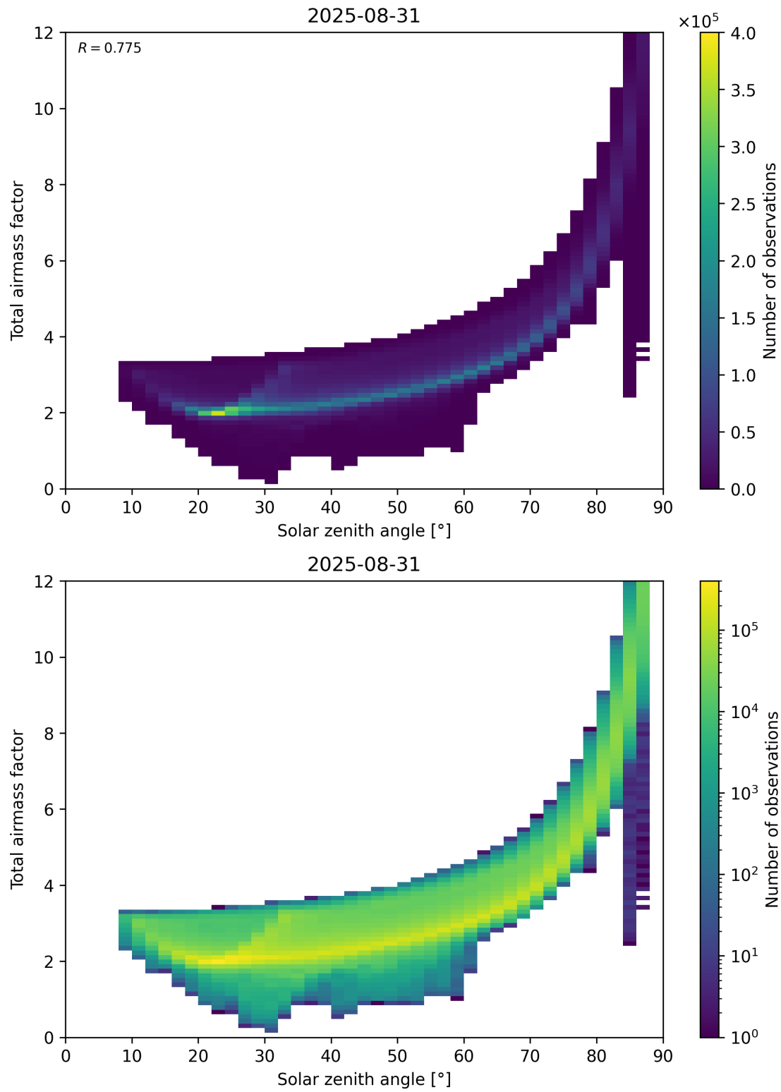
Figure 146: Scatter density plot of “Solar zenith angle” against “Total air mass factor” for 2025-08-30 to 2025-09-01.
