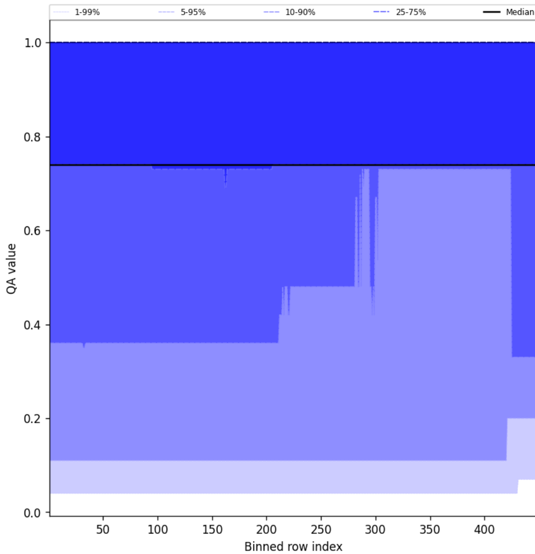
Figure 45: Along track statistics of “QA value” for 2025-08-30 to 2025-09-01
