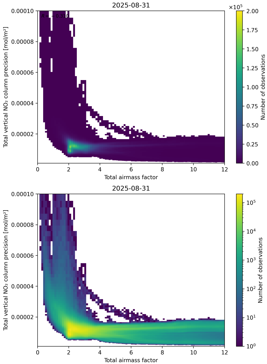
Figure 68: Scatter density plot of “Total airmass factor” against “Total vertical NO 2 column precision” for 2025-08-30 to 2025-09-01.
