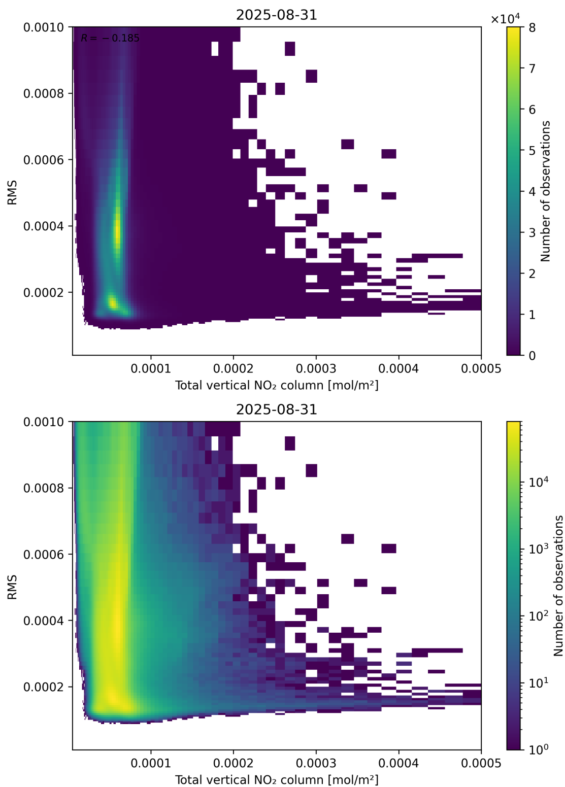
Figure 120: Scatter density plot of “Total vertical NO 2 column” against “RMS” for 2025-08-30 to 2025-09-01.
