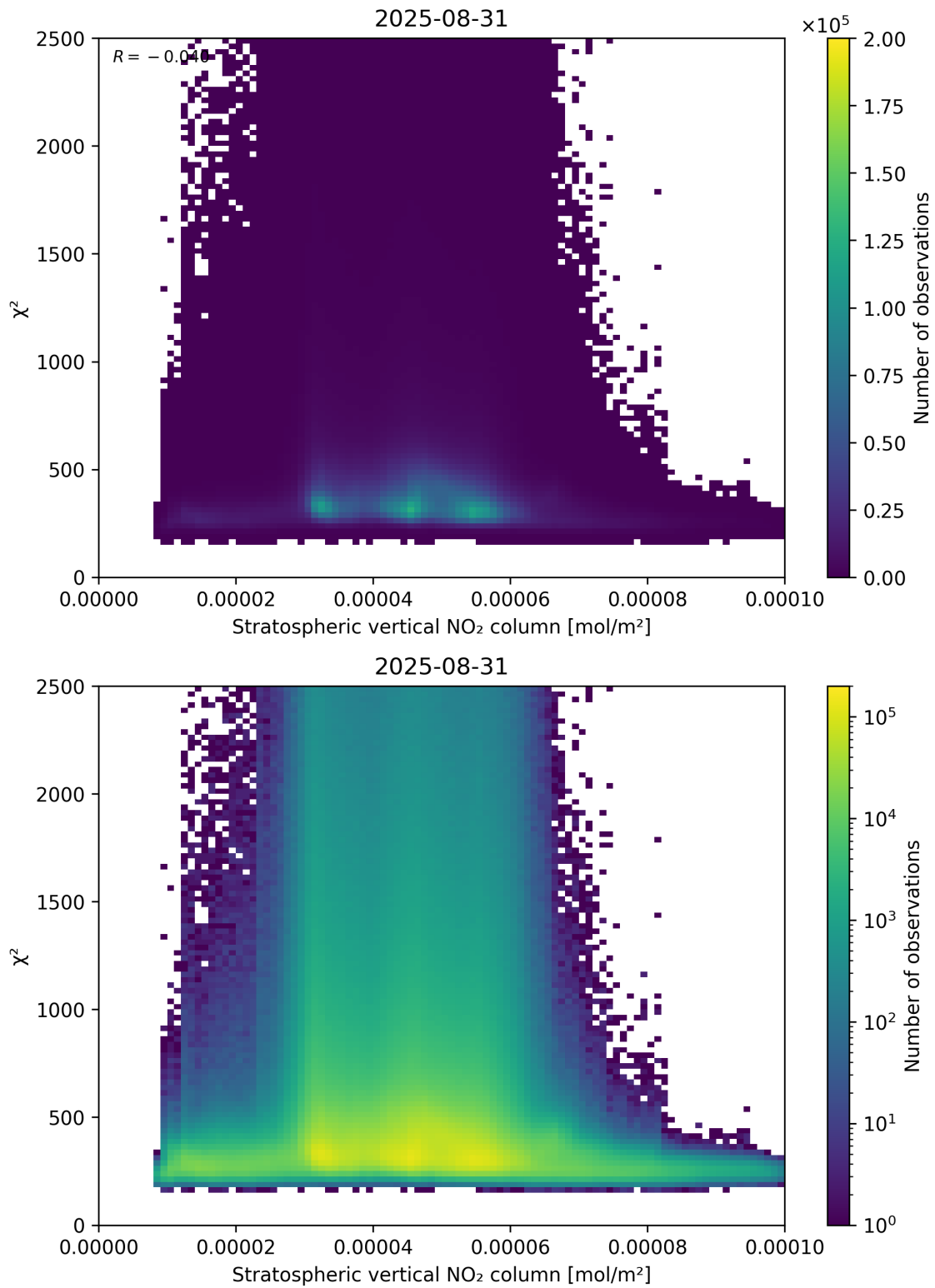
Figure 97: Scatter density plot of “Stratospheric vertical NO 2 column” against “ \chi^2 ” for 2025-08-30 to 2025-09-01.
