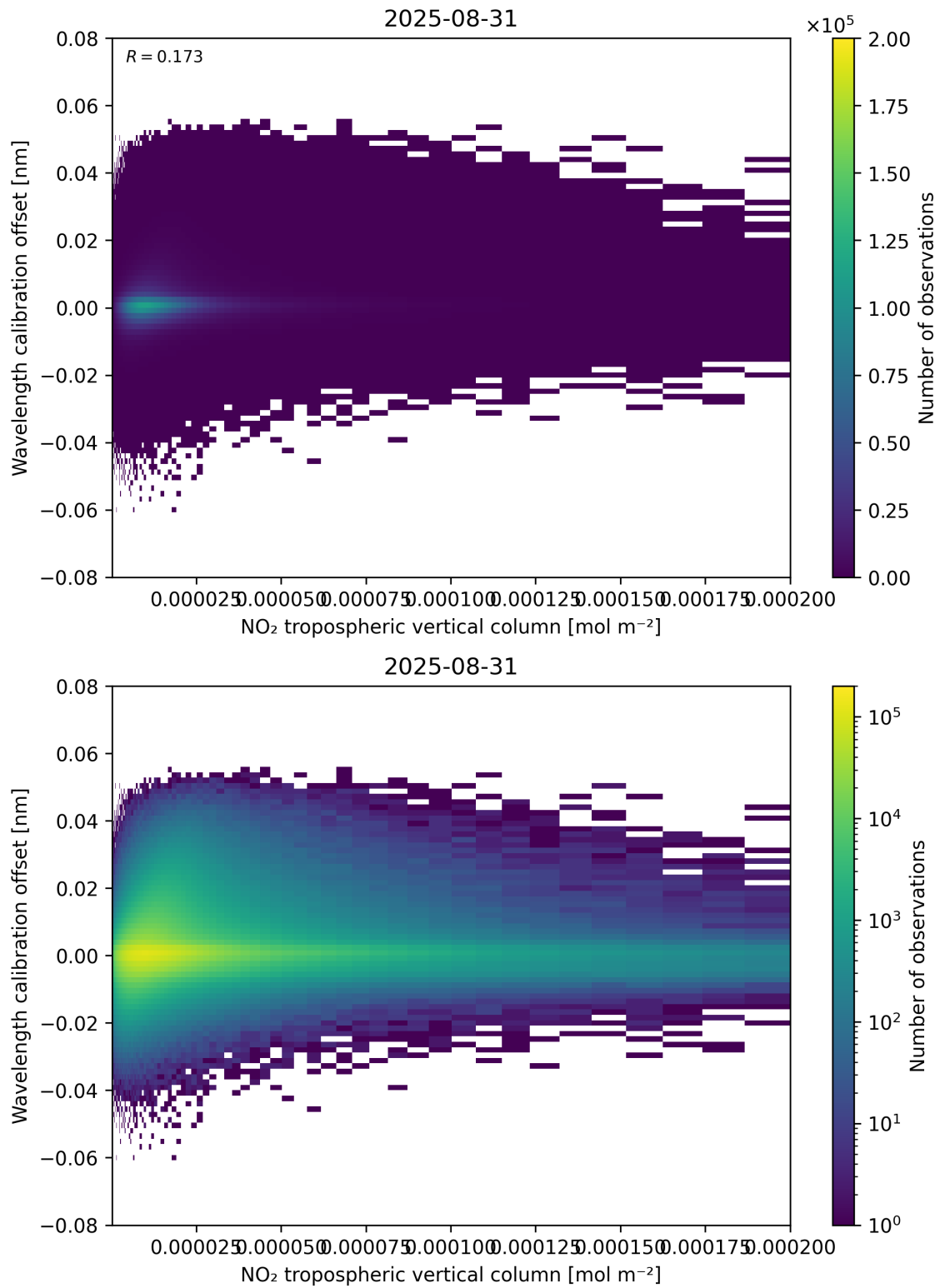
Figure 143: Scatter density plot of “NO 2 tropospheric vertical column” against “Wavelength calibration offset” for 2025-08-30 to 2025-09-01.
