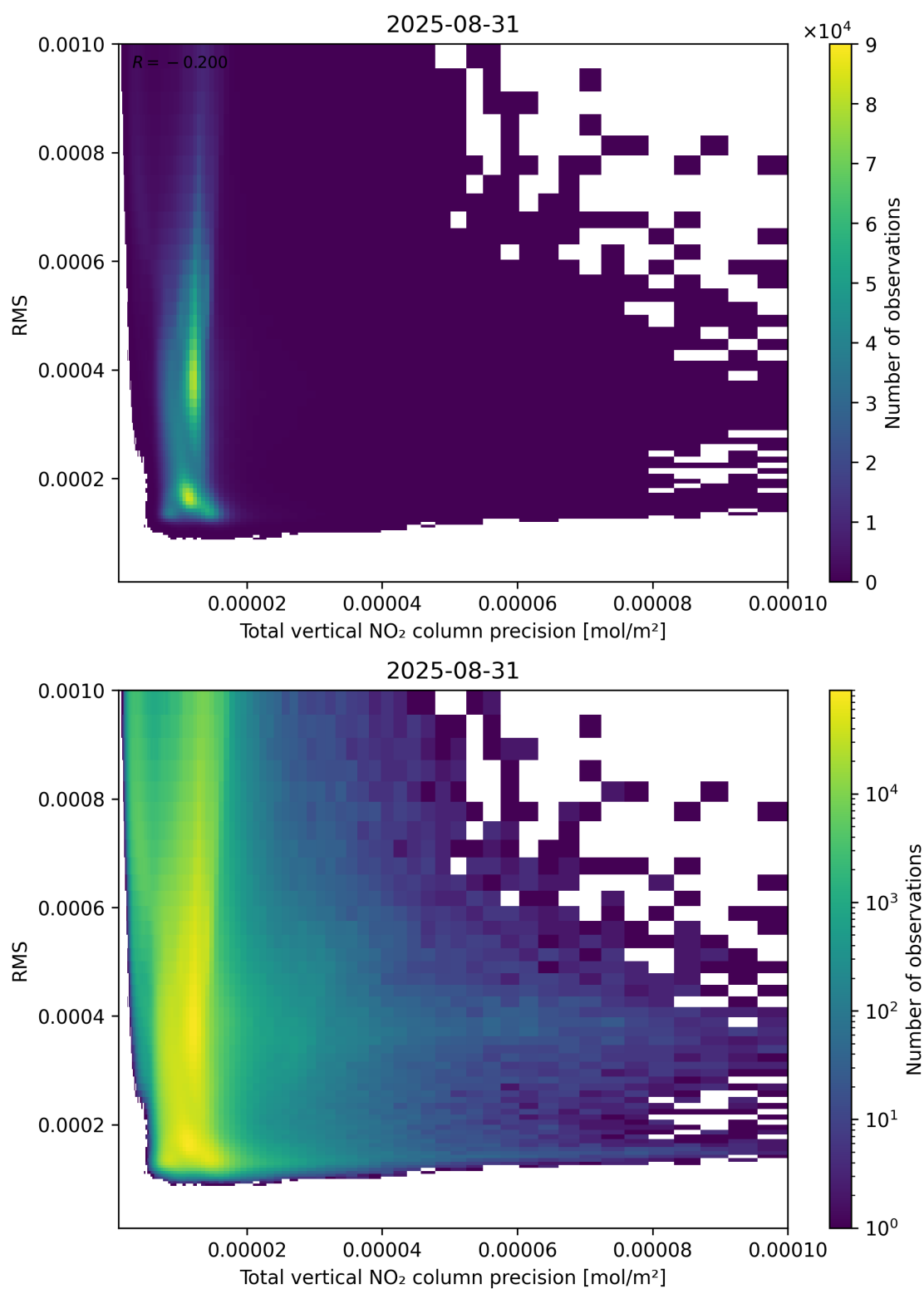
Figure 119: Scatter density plot of “Total vertical NO 2 column precision” against “RMS” for 2025-08-30 to 2025-09-01.
