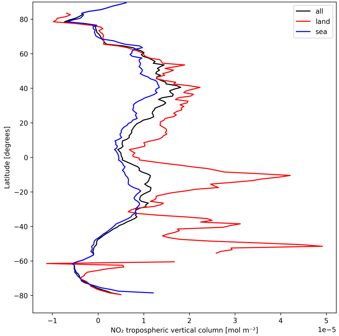
Figure 12: Zonal average of “NO 2 tropospheric vertical column” for 2025-08-30 to 2025-09-01.
