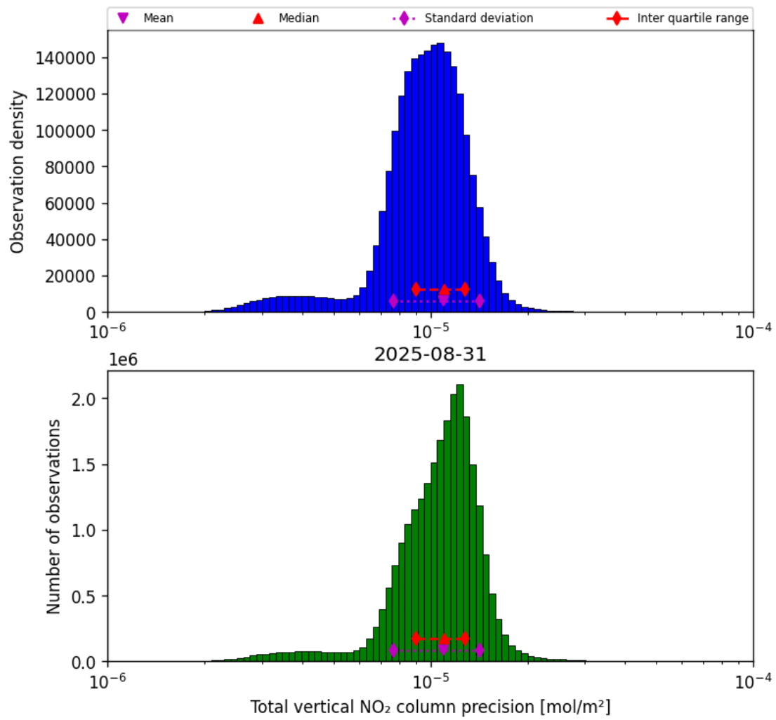
Figure 39: Histogram of “Total vertical NO 2 column precision” for 2025-08-30 to 2025-09-01
