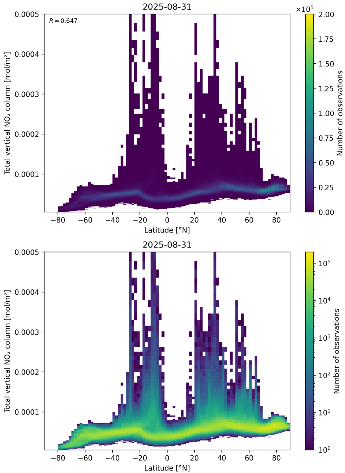
Figure 90: Scatter density plot of “Latitude” against “Total vertical NO 2 column” for 2025-08-30 to 2025-09-01.
