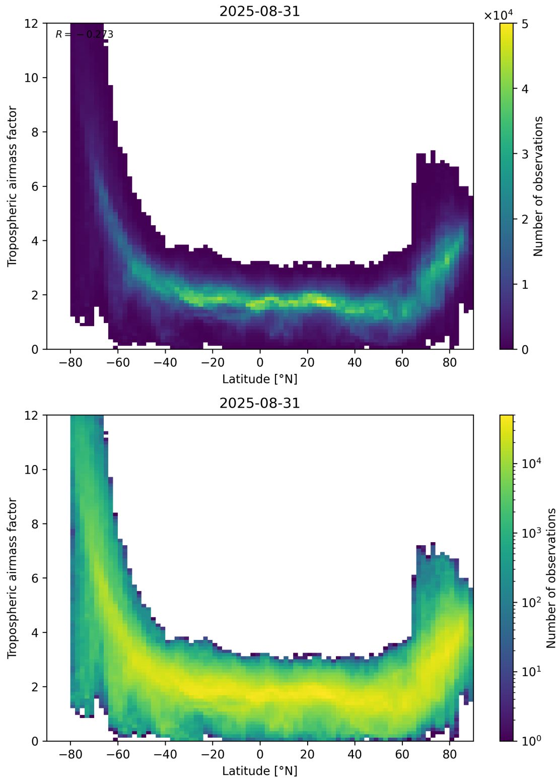
Figure 85: Scatter density plot of “Latitude” against “Tropospheric airmass factor” for 2025-08-30 to 2025-09-01.
