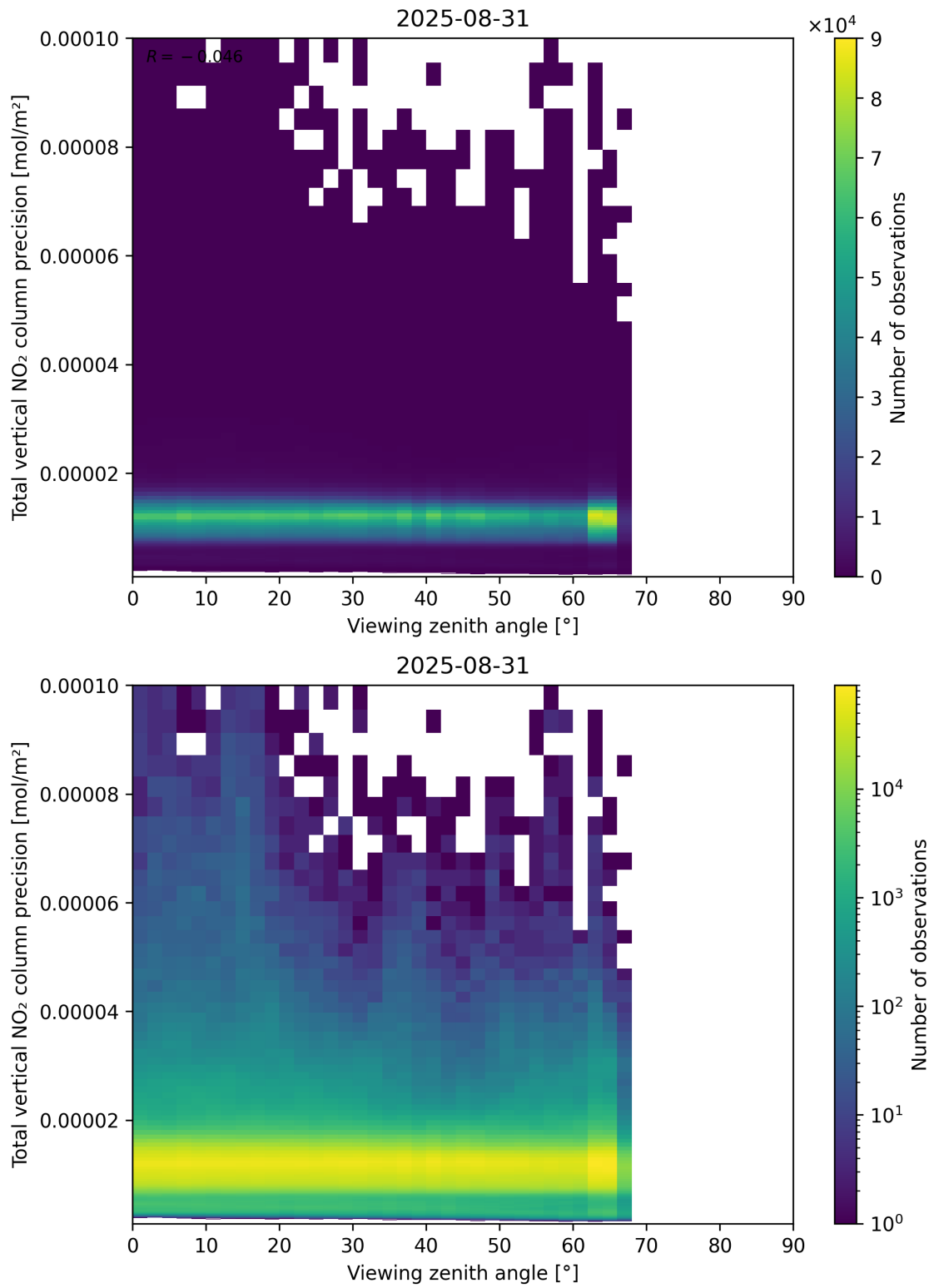
Figure 168: Scatter density plot of “Viewing zenith angle” against “Total vertical NO 2 column precision” for 2025-08-30 to 2025-09-01.
