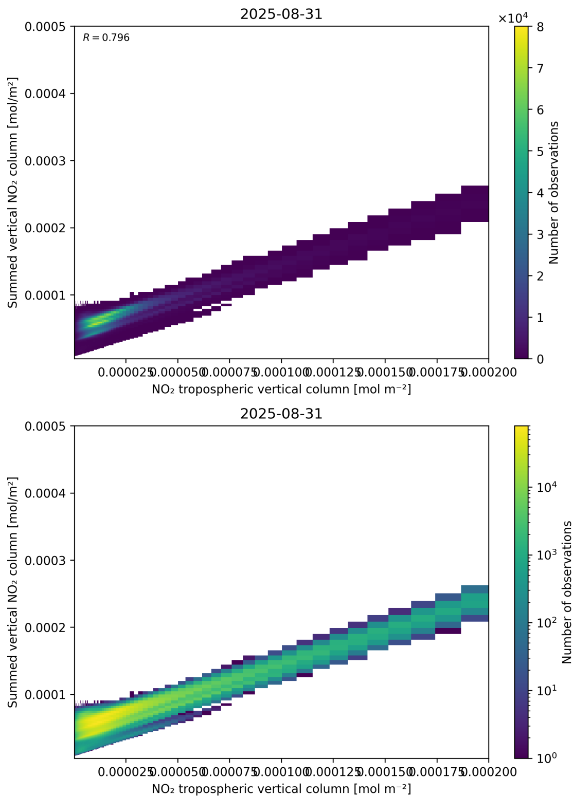
Figure 126: Scatter density plot of “NO 2 tropospheric vertical column” against “Summed vertical NO 2 column” for 2025-08-30 to 2025-09-01.
