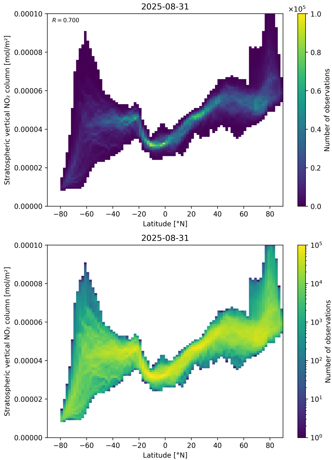
Figure 87: Scatter density plot of “Latitude” against “Stratospheric vertical \text{NO}_2 column” for 2025-08-30 to 2025-09-01.
