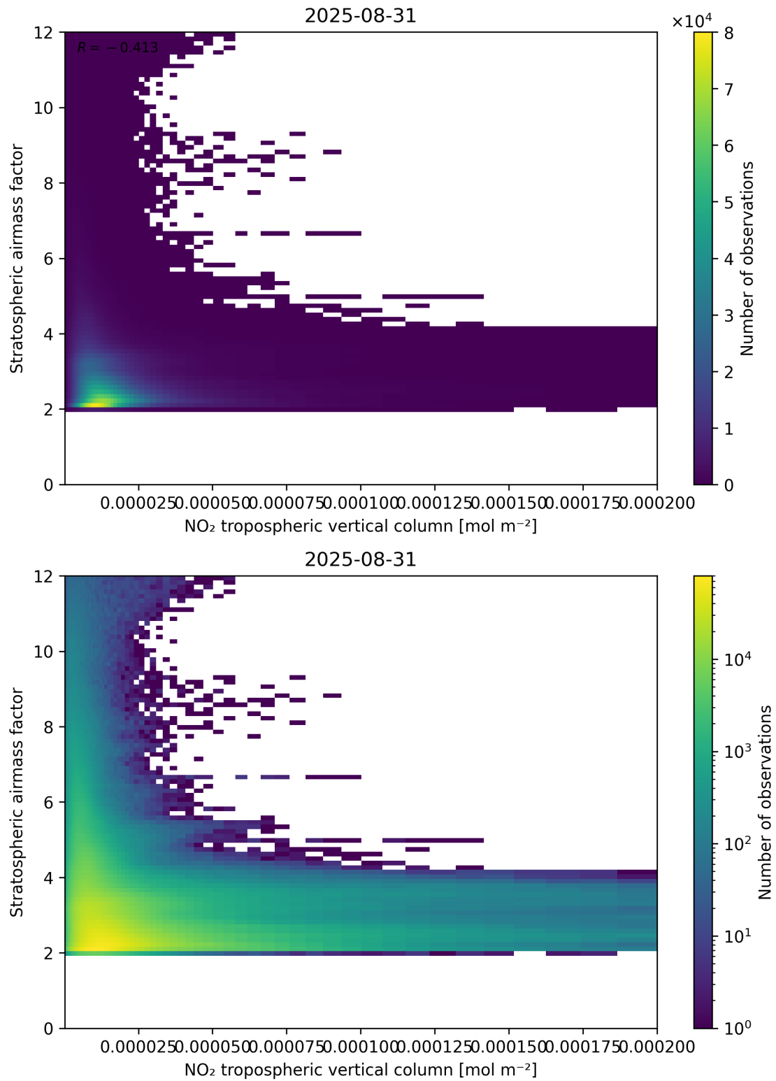
Figure 121: Scatter density plot of “NO 2 tropospheric vertical column” against “Stratospheric air mass factor” for 2025-08-30 to 2025-09-01.
