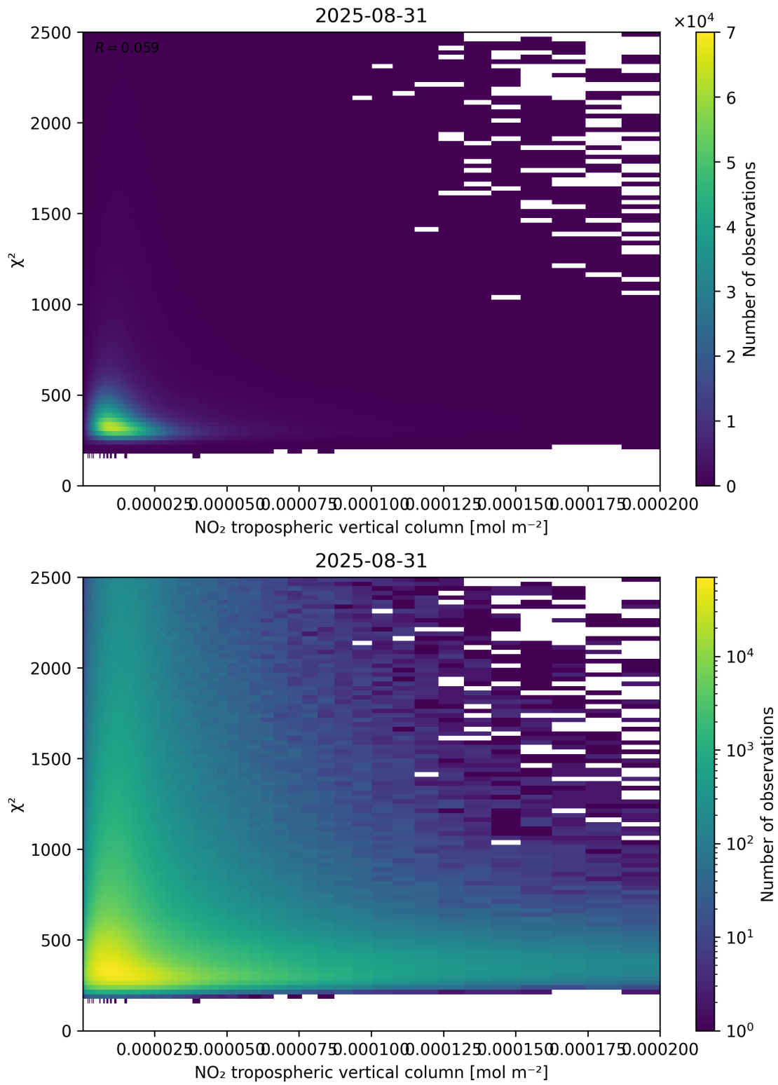
Figure 124: Scatter density plot of “NO 2 tropospheric vertical column” against “ \chi^2 ” for 2025-08-30 to 2025-09-01.
