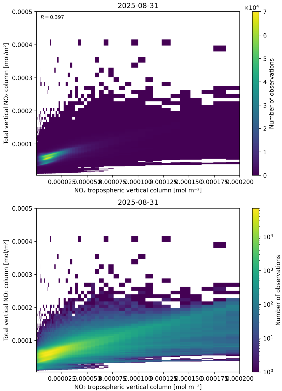
Figure 128: Scatter density plot of “NO 2 tropospheric vertical column” against “Total vertical NO 2 column” for 2025-08-30 to 2025-09-01.
