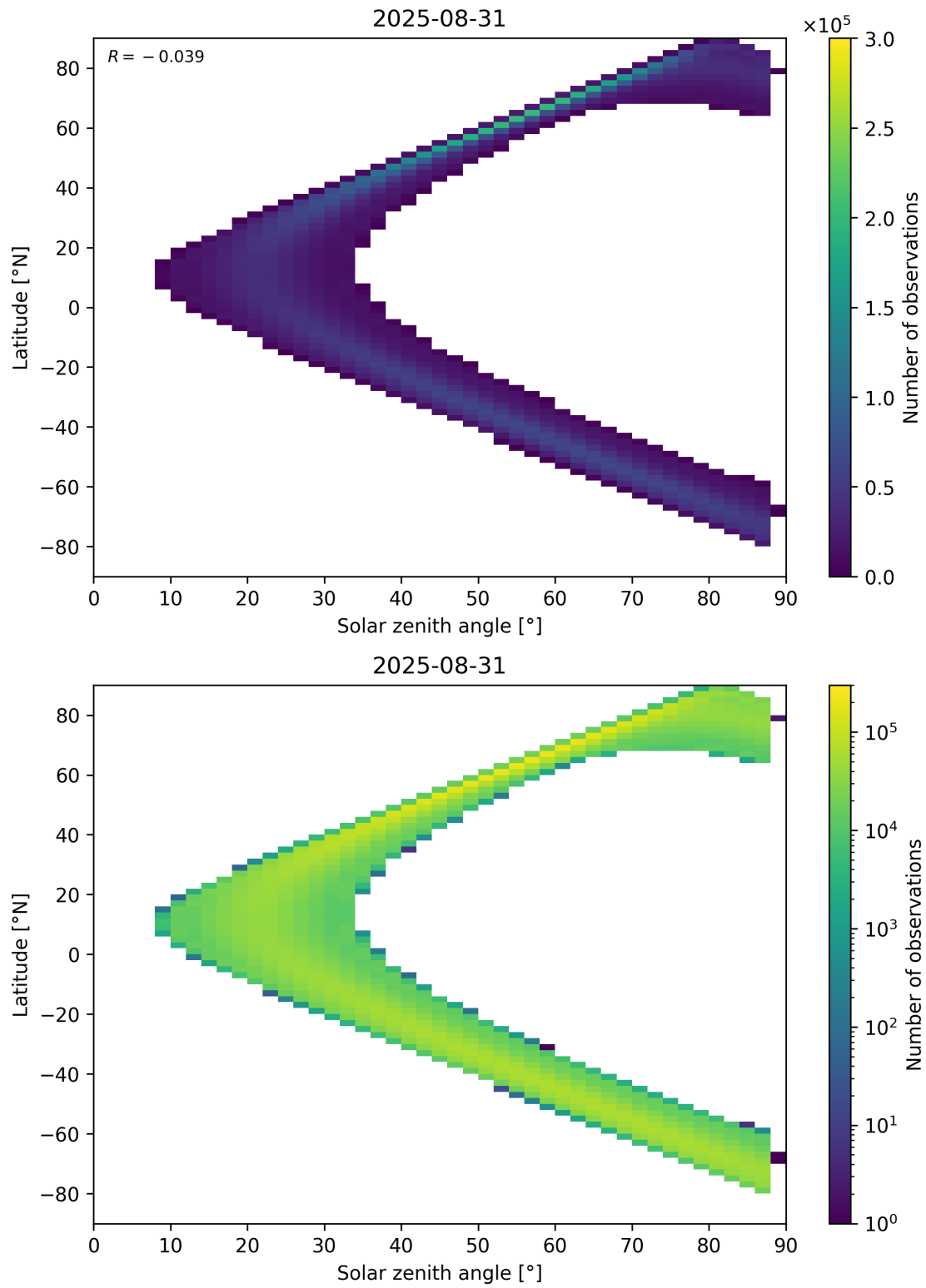
Figure 149: Scatter density plot of “Solar zenith angle” against “Latitude” for 2025-08-30 to 2025-09-01.
