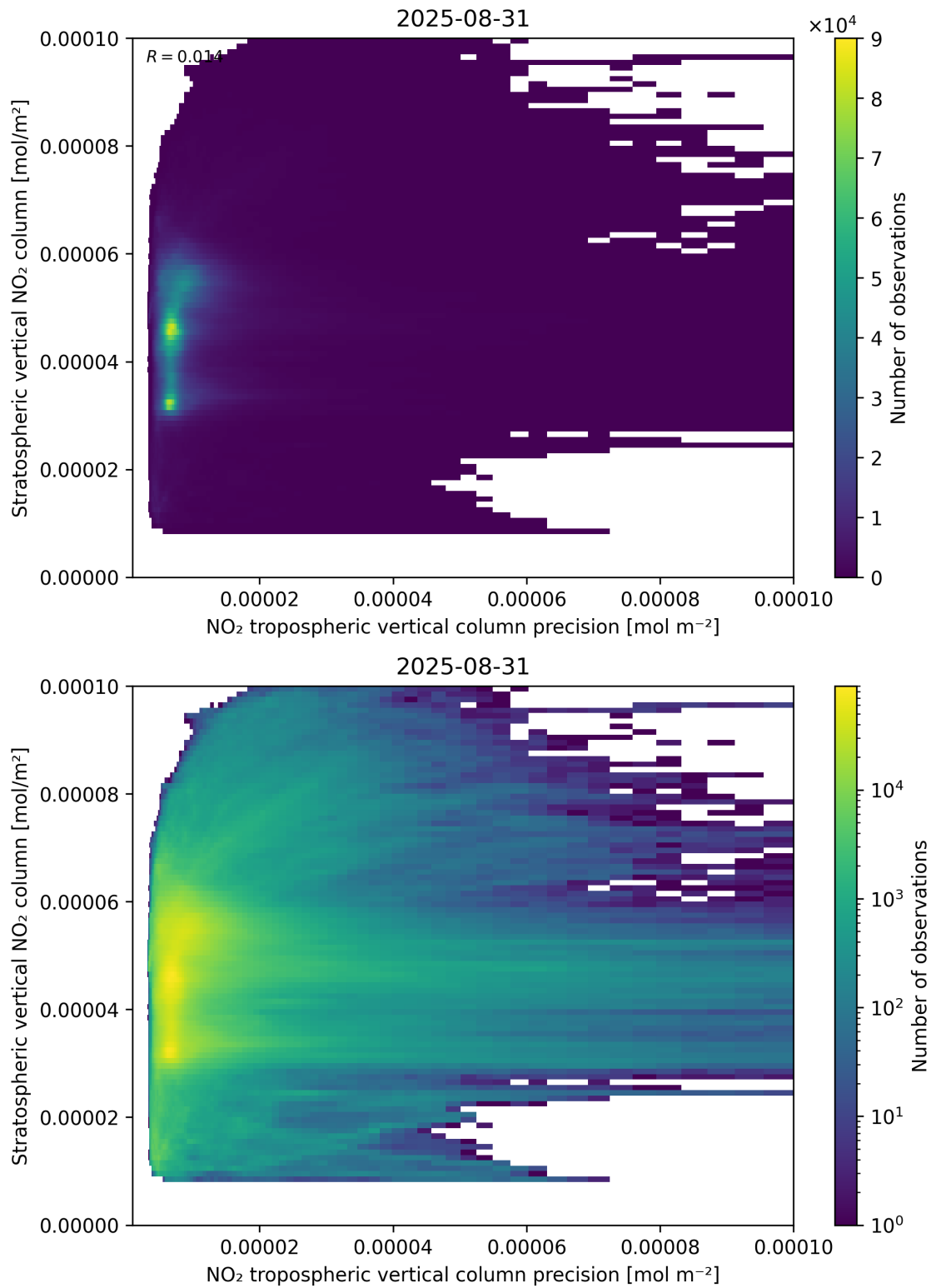
Figure 135: Scatter density plot of “NO 2 tropospheric vertical column precision” against “Stratospheric vertical NO 2 column” for 2025-08-30 to 2025-09-01.
