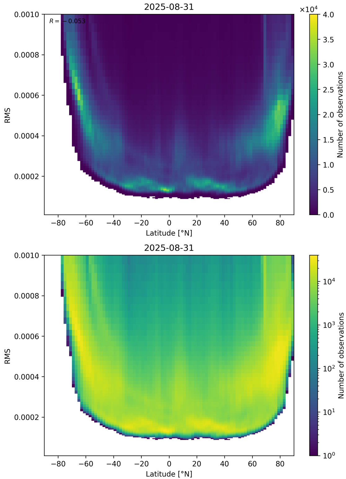
Figure 94: Scatter density plot of “Latitude” against “RMS” for 2025-08-30 to 2025-09-01.
