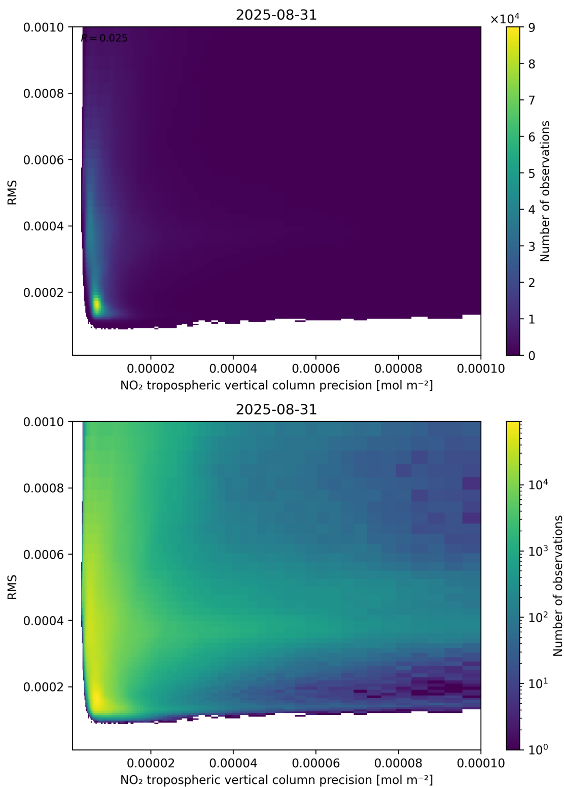
Figure 140: Scatter density plot of “NO 2 tropospheric vertical column precision” against “RMS” for 2025-08-30 to 2025-09-01.
