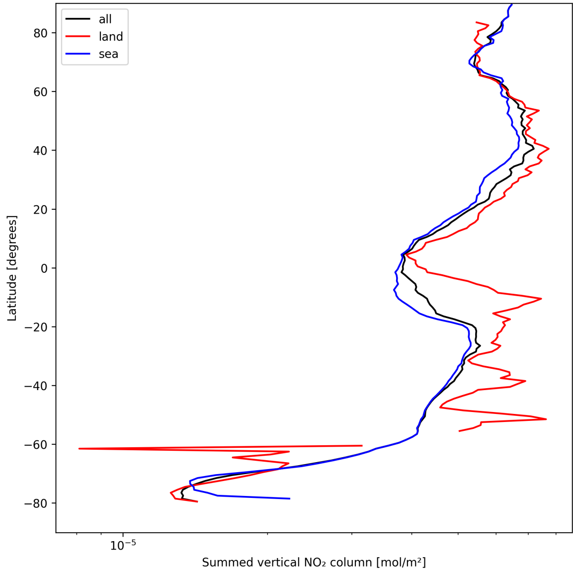
Figure 23: Zonal average of “Summed vertical NO 2 column” for 2025-08-30 to 2025-09-01.
