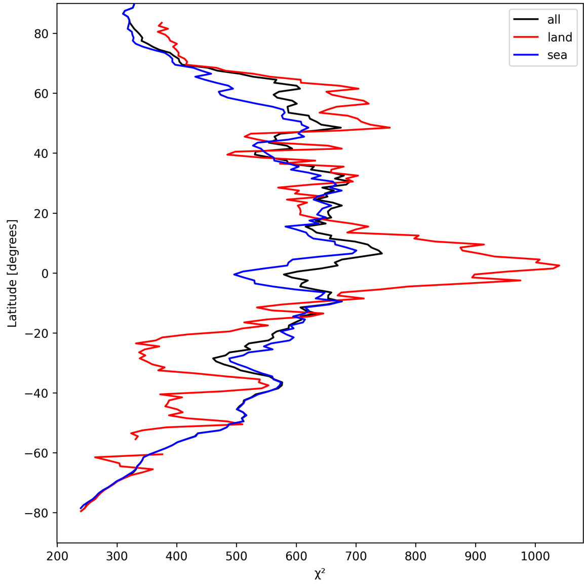
Figure 25: Zonal average of “ \chi^2 ” for 2025-08-30 to 2025-09-01.
