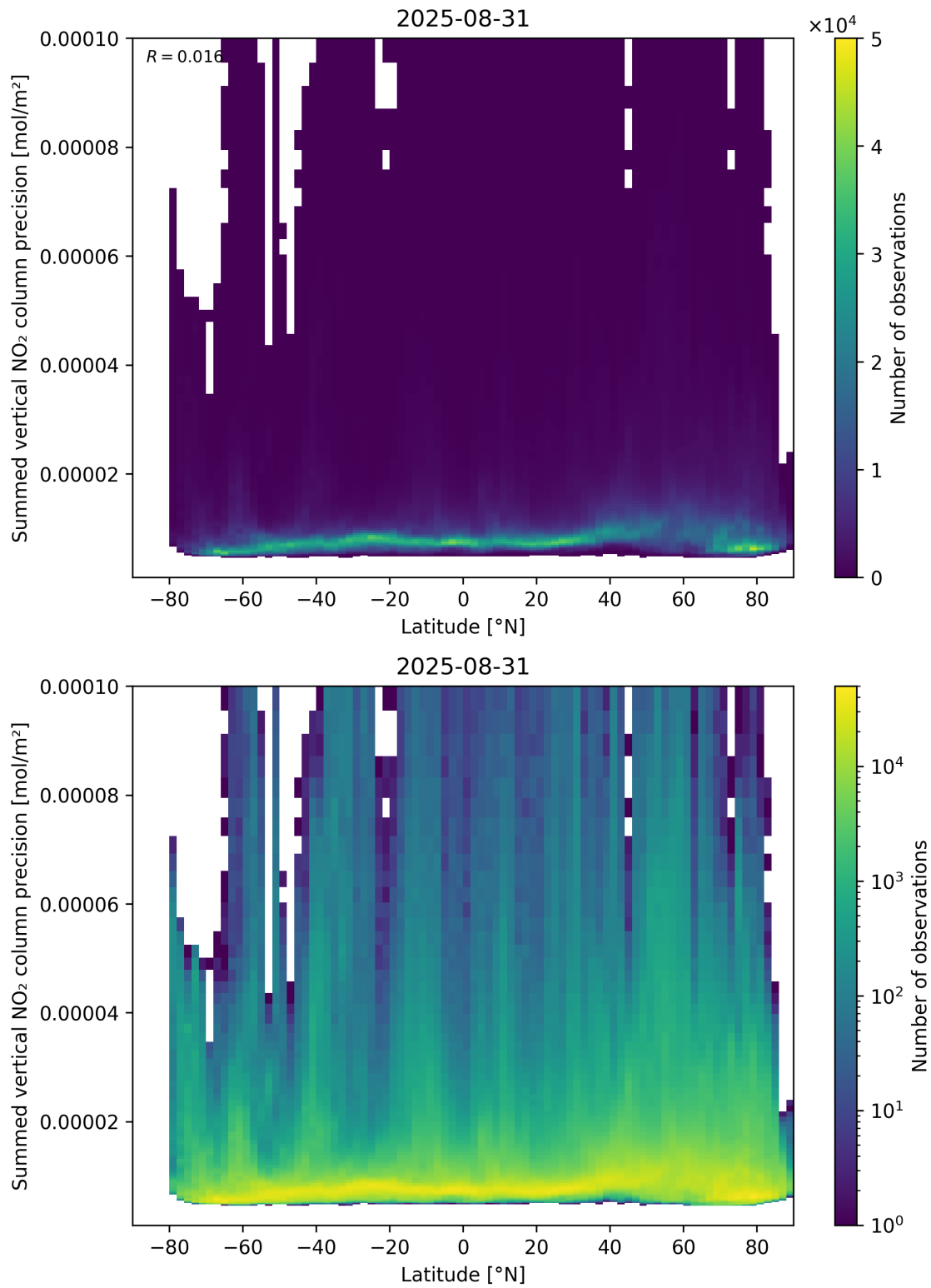
Figure 89: Scatter density plot of “Latitude” against “Summed vertical NO 2 column precision” for 2025-08-30 to 2025-09-01.
