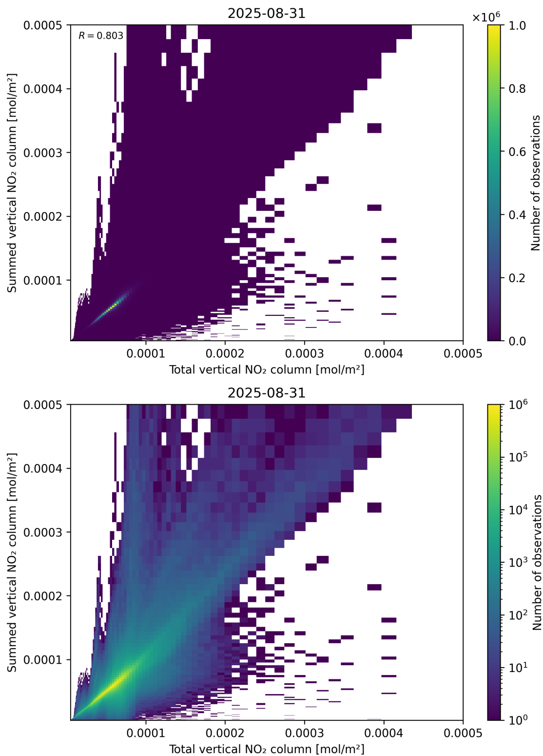
Figure 112: Scatter density plot of “Total vertical NO 2 column” against “Summed vertical NO 2 column” for 2025-08-30 to 2025-09-01.
