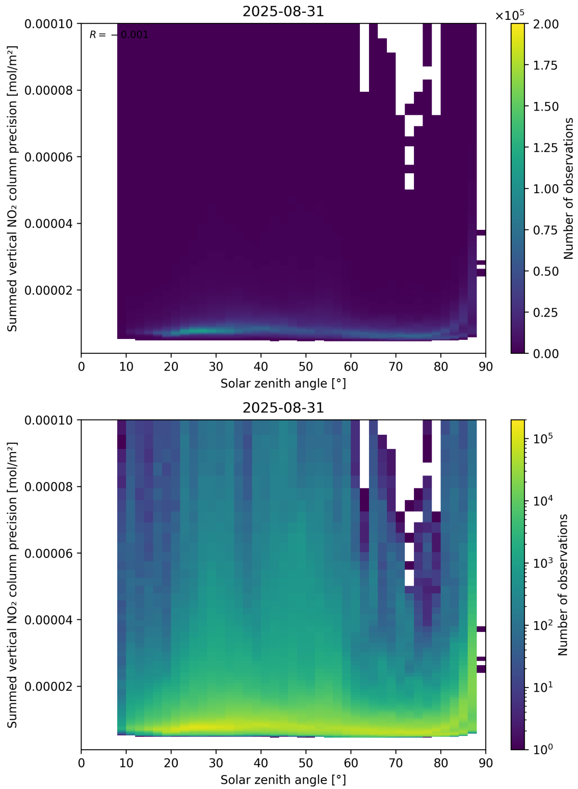
Figure 152: Scatter density plot of “Solar zenith angle” against “Summed vertical NO 2 column precision” for 2025-08-30 to 2025-09-01.
