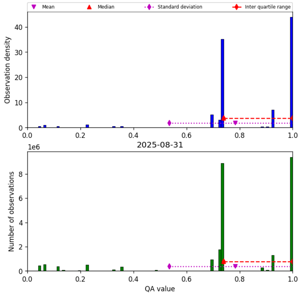
Figure 28: Histogram of “QA value” for 2025-08-30 to 2025-09-01
