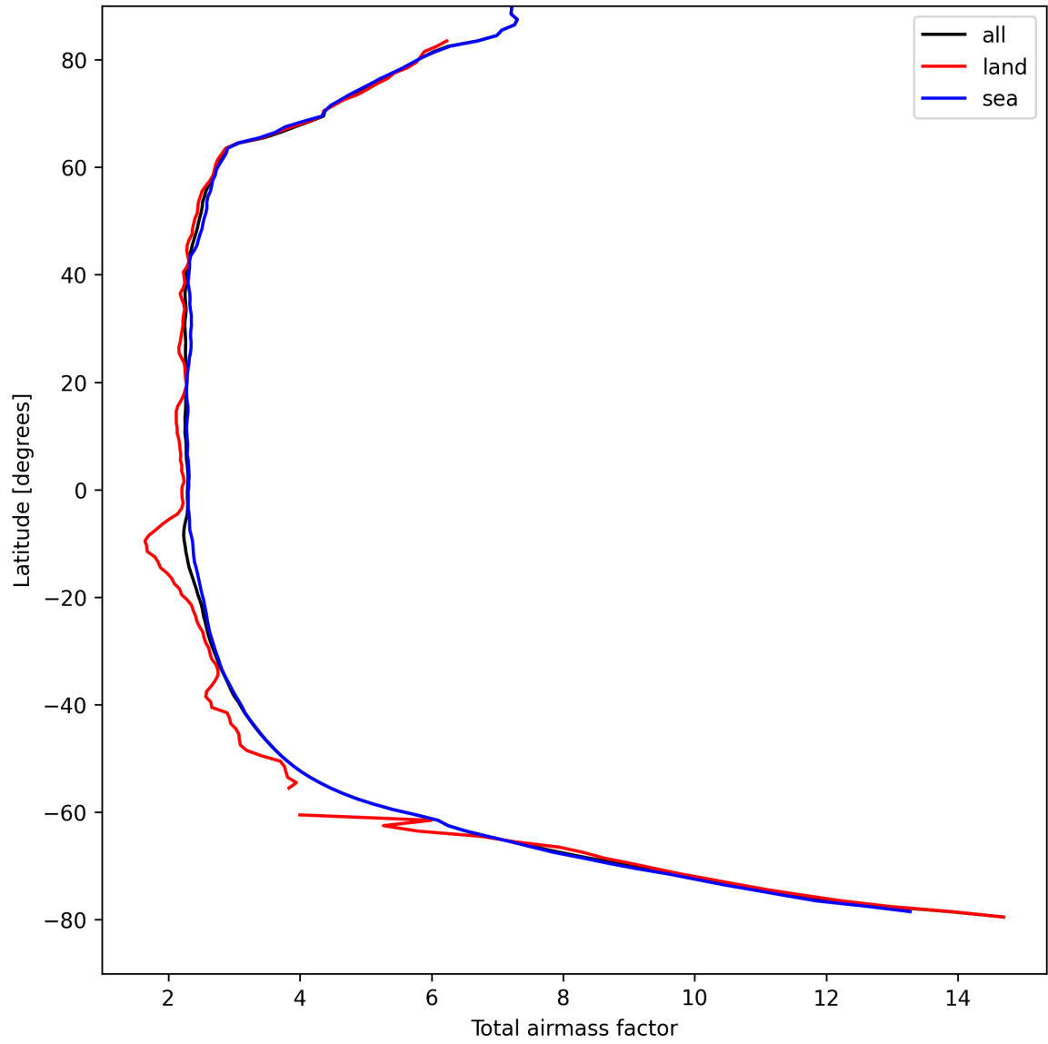
Figure 15: Zonal average of “Total airmass factor” for 2025-08-30 to 2025-09-01.
