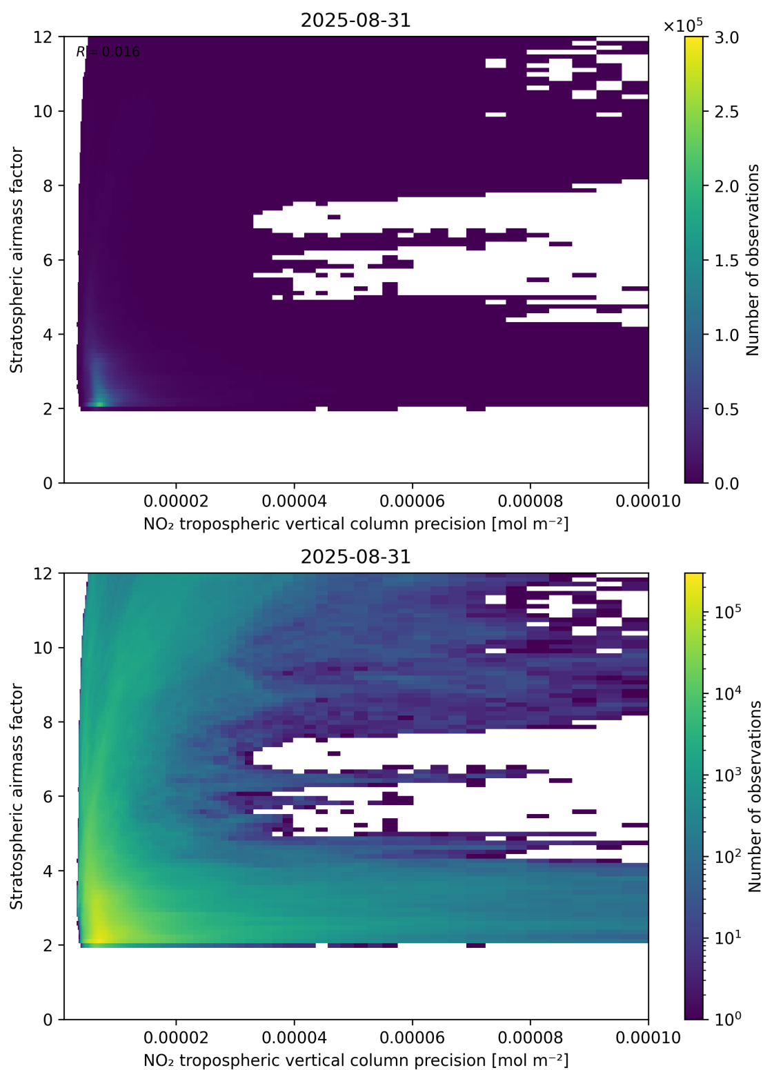
Figure 131: Scatter density plot of “NO 2 tropospheric vertical column precision” against “Stratospheric airmass factor” for 2025-08-30 to 2025-09-01.
