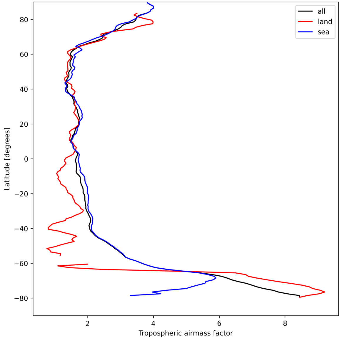
Figure 14: Zonal average of “Tropospheric airmass factor” for 2025-08-30 to 2025-09-01.
