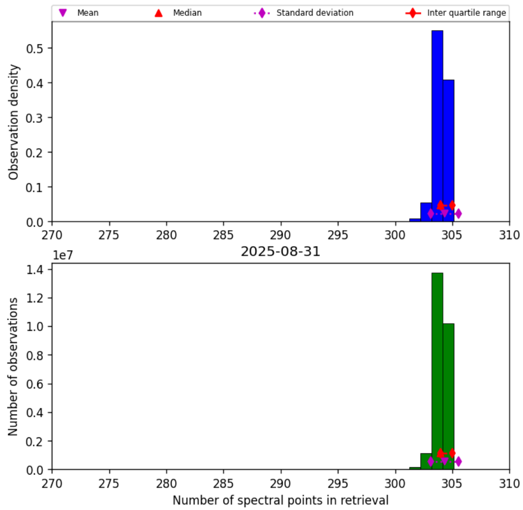
Figure 33: Histogram of “Number of spectral points in retrieval” for 2025-08-30 to 2025-09-01
