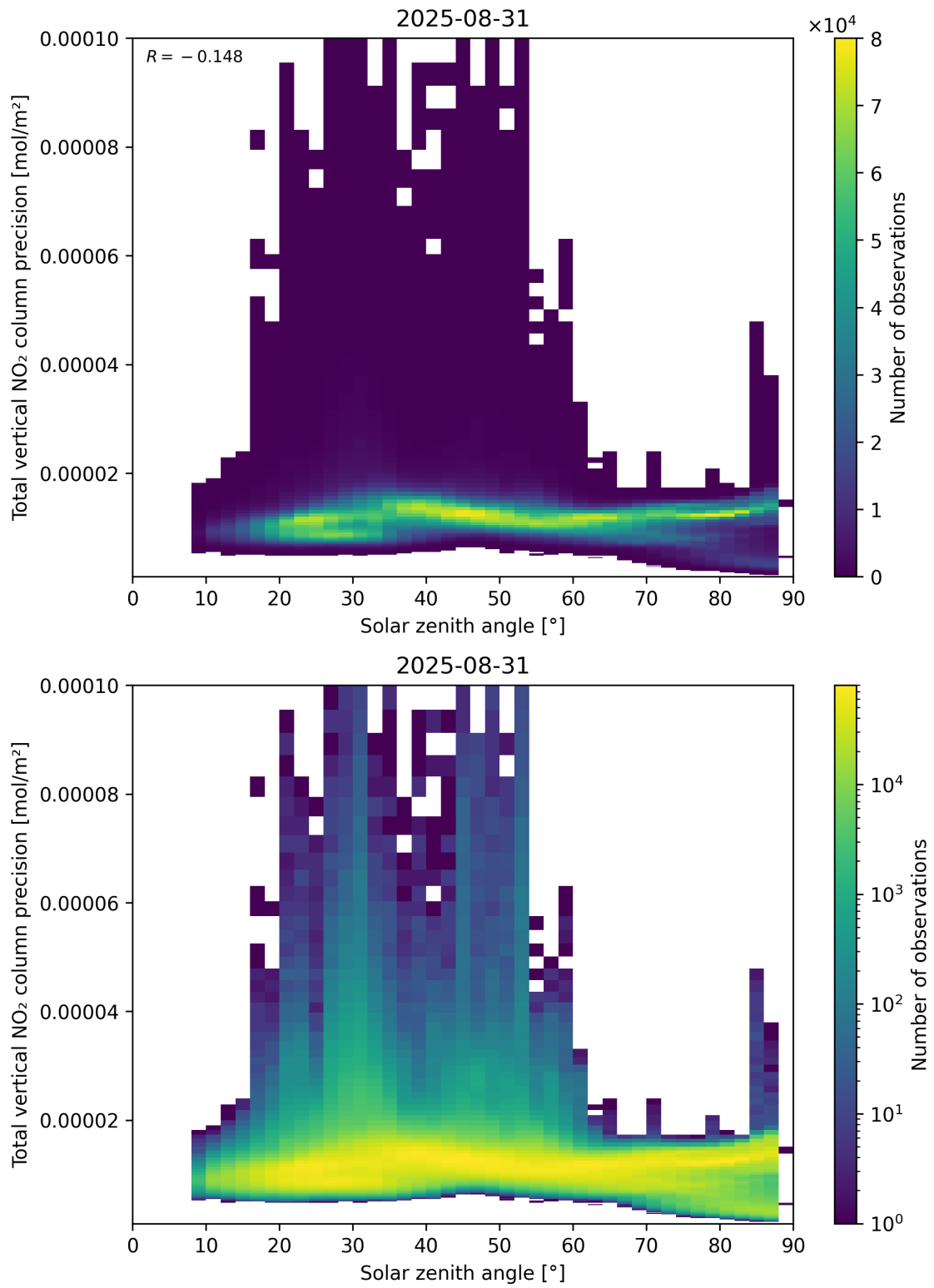
Figure 154: Scatter density plot of “Solar zenith angle” against “Total vertical NO 2 column precision” for 2025-08-30 to 2025-09-01.
