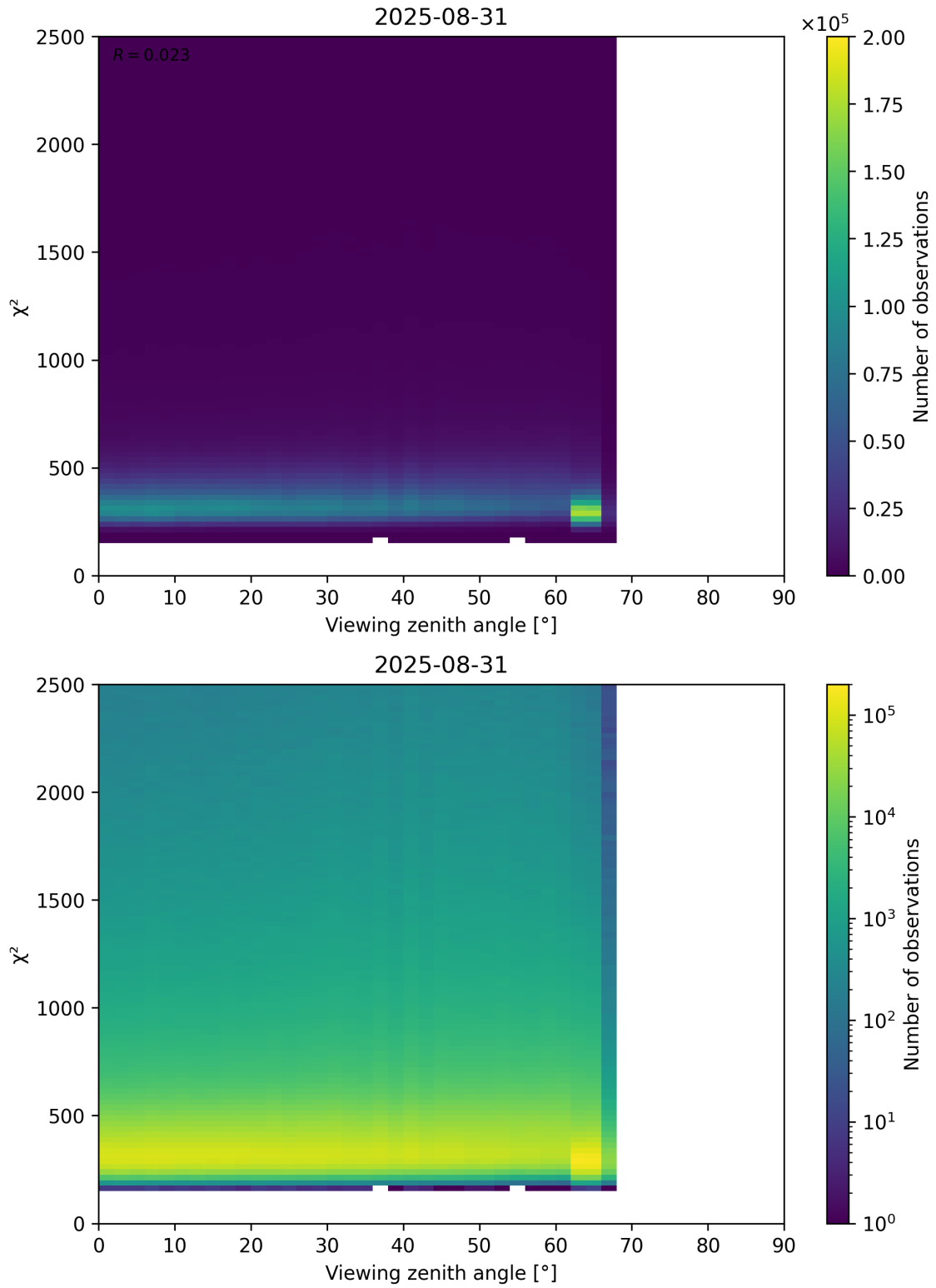
Figure 162: Scatter density plot of “Viewing zenith angle” against “ \chi^2 ” for 2025-08-30 to 2025-09-01.
