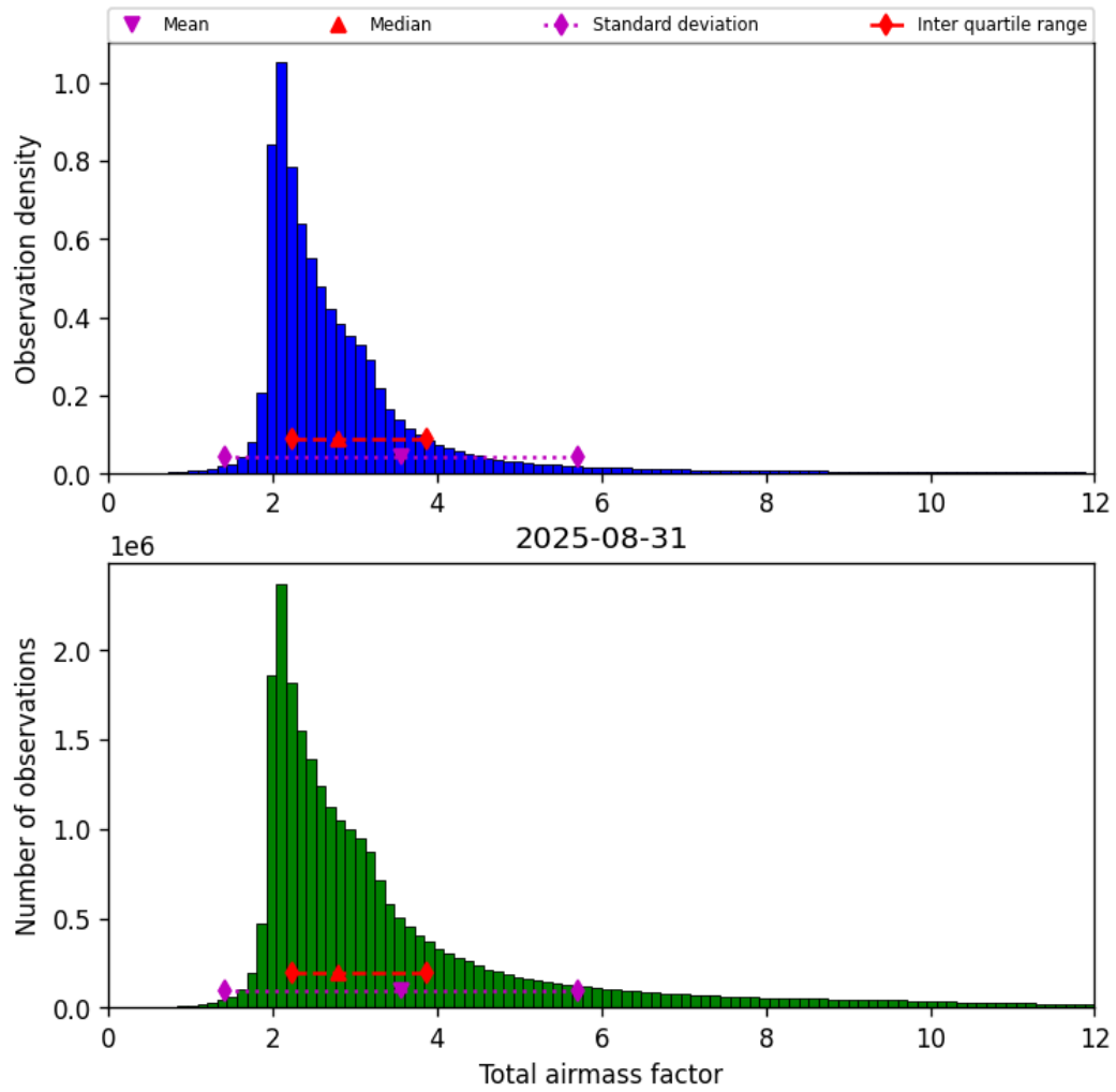
Figure 32: Histogram of “Total airmass factor” for 2025-08-30 to 2025-09-01
