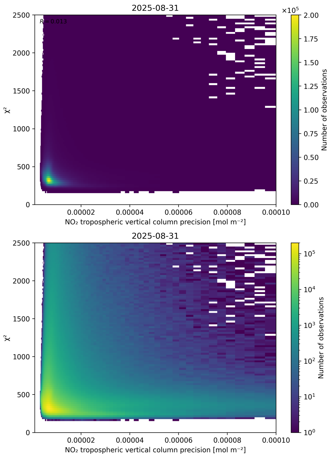
Figure 134: Scatter density plot of “NO 2 tropospheric vertical column precision” against “ \chi^2 ” for 2025-08-30 to 2025-09-01.
