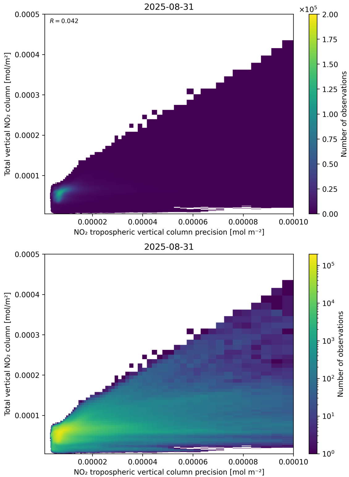
Figure 138: Scatter density plot of “NO 2 tropospheric vertical column precision” against “Total vertical NO 2 column” for 2025-08-30 to 2025-09-01.
