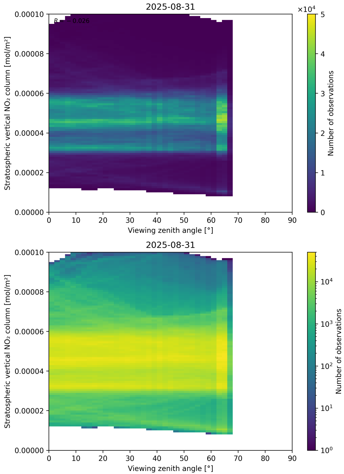
Figure 164: Scatter density plot of “Viewing zenith angle” against “Stratospheric vertical NO 2 column” for 2025-08-30 to 2025-09-01.
