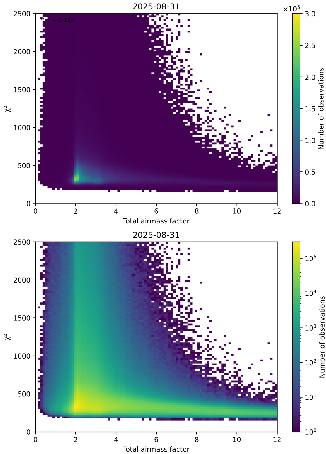
Figure 63: Scatter density plot of “Total airmass factor” against “ \chi^2 ” for 2025-08-30 to 2025-09-01.
