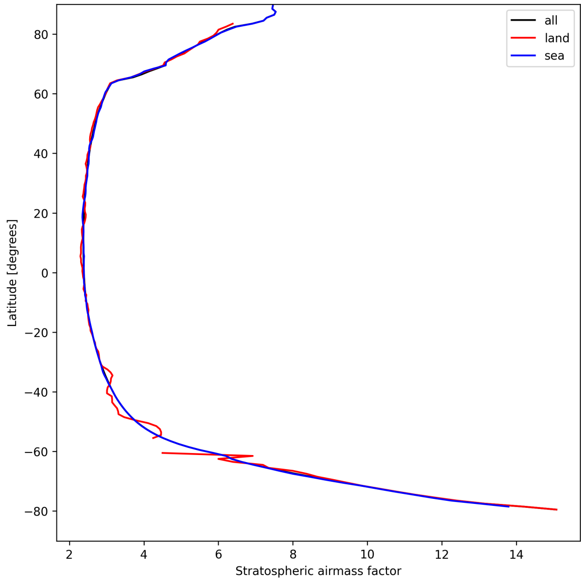
Figure 27: Zonal average of “Stratospheric airmass factor” for 2025-08-30 to 2025-09-01.
