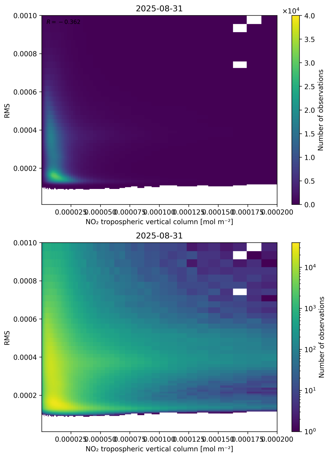
Figure 142: Scatter density plot of “NO 2 tropospheric vertical column” against “RMS” for 2025-08-30 to 2025-09-01.
