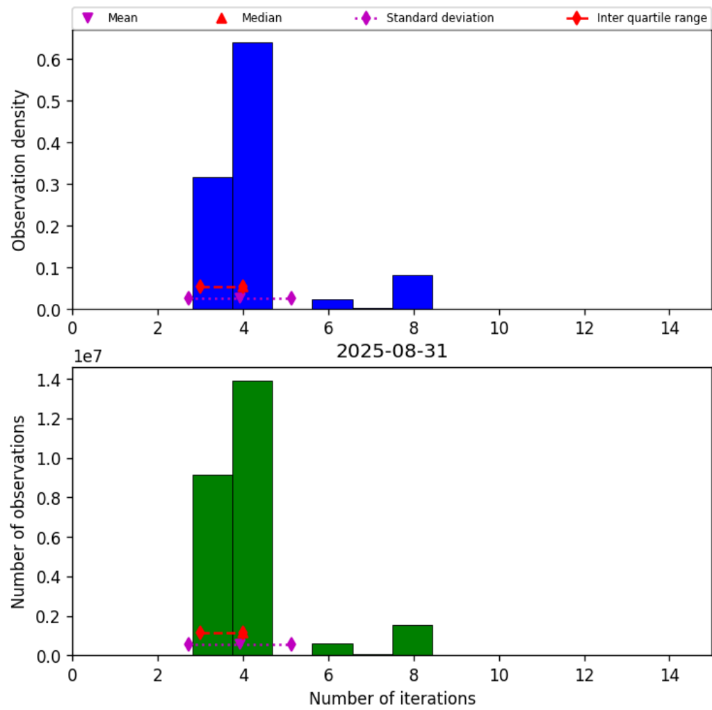
Figure 34: Histogram of “Number of iterations” for 2025-08-30 to 2025-09-01
