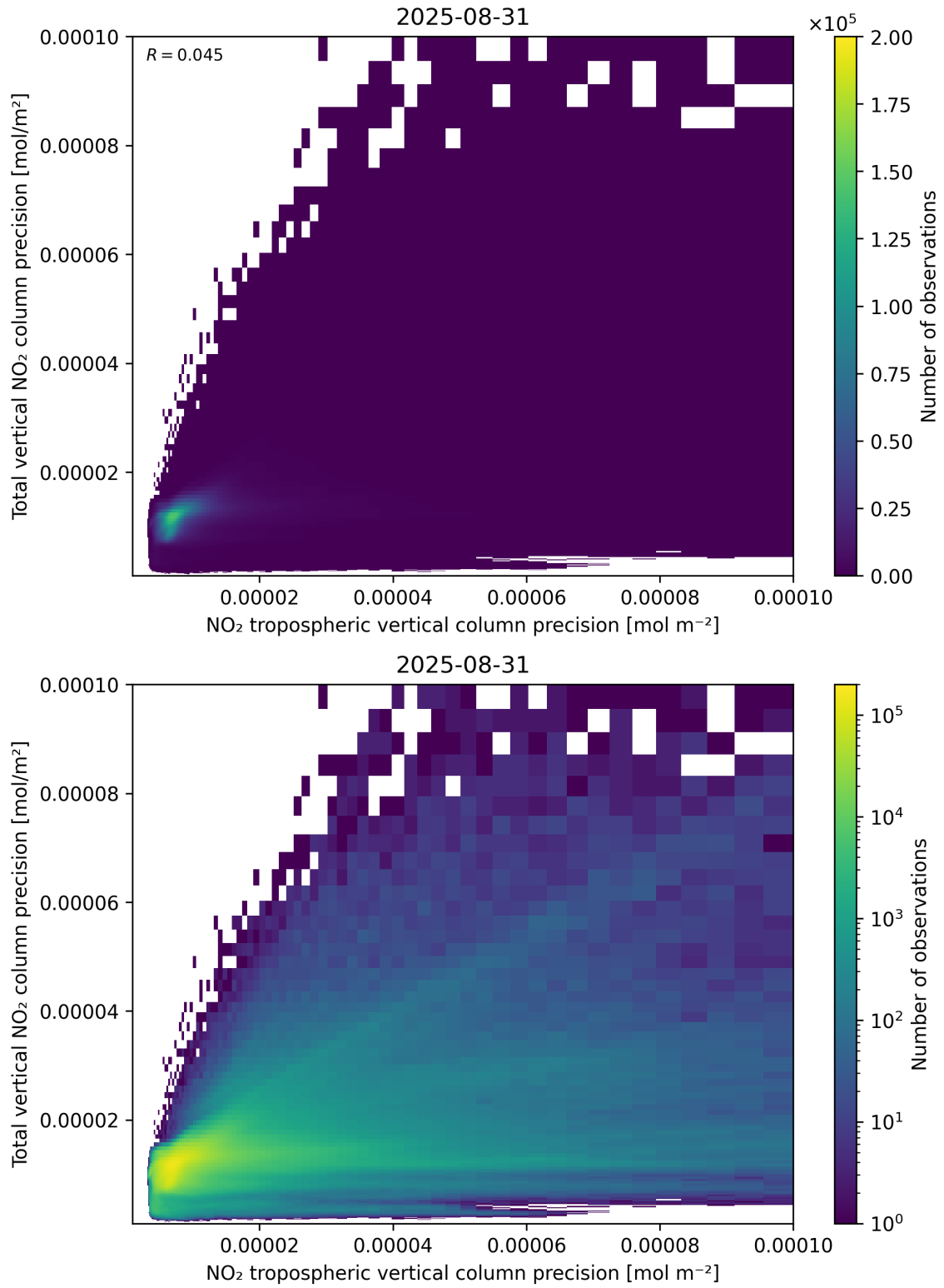
Figure 139: Scatter density plot of “NO 2 tropospheric vertical column precision” against “Total vertical NO 2 column precision” for 2025-08-30 to 2025-09-01.
