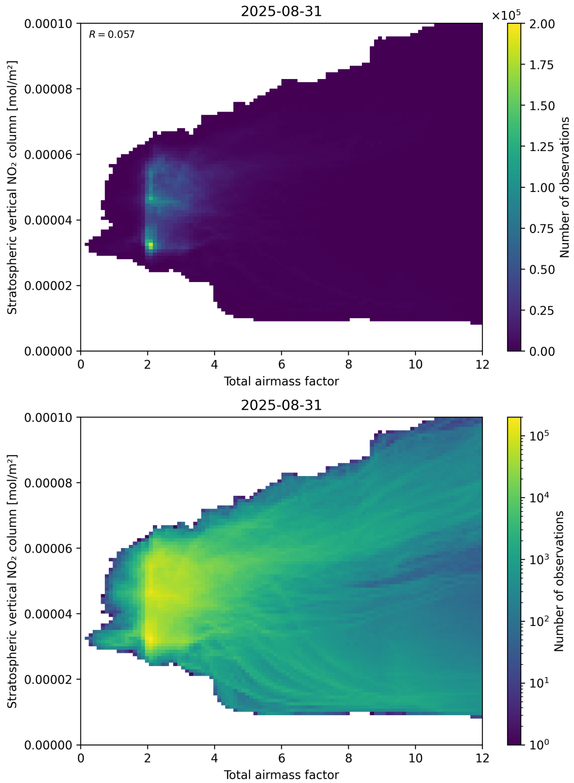
Figure 64: Scatter density plot of “Total airmass factor” against “Stratospheric vertical \text{NO}_2 column” for 2025-08-30 to 2025-09-01.
