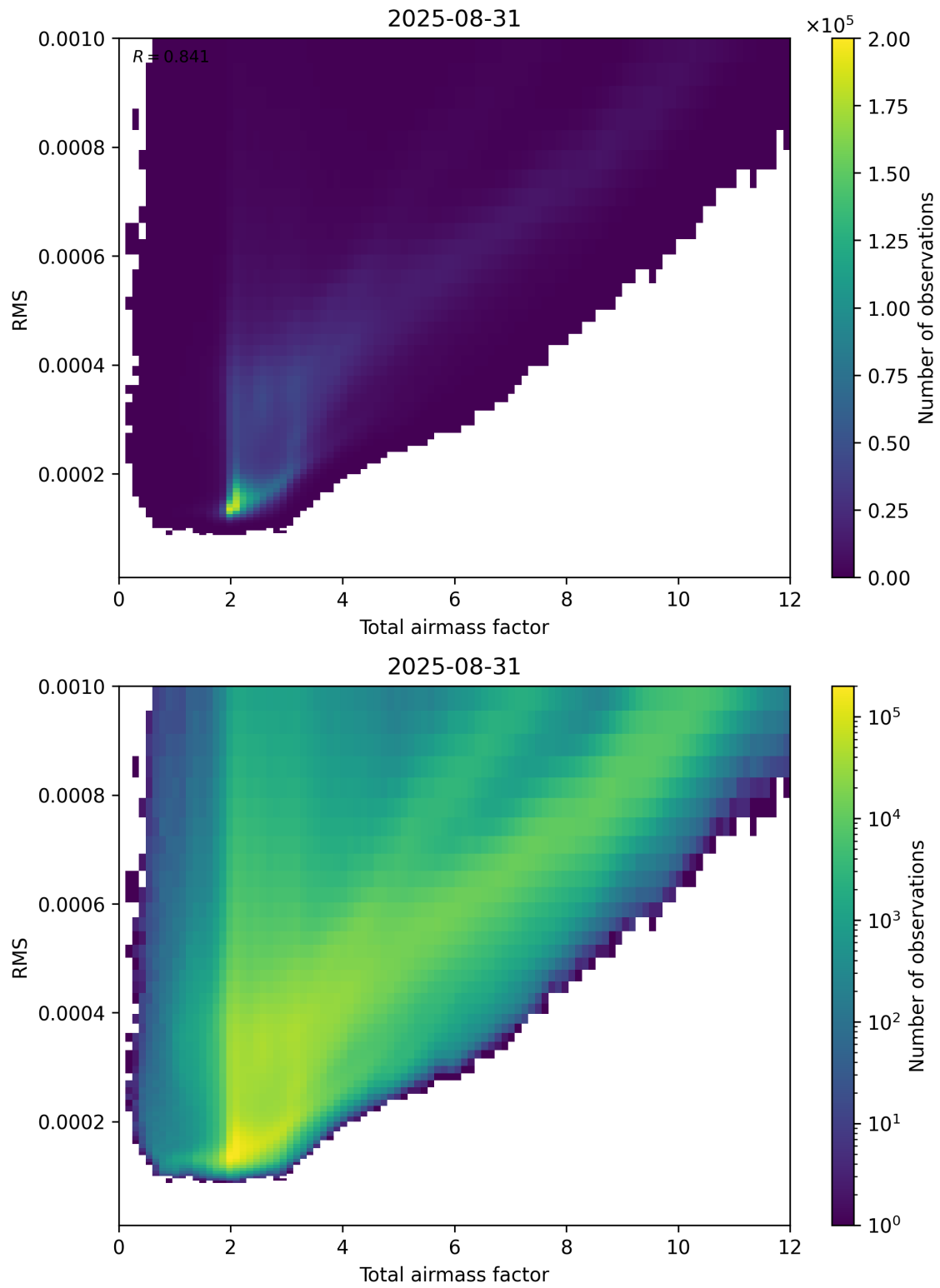
Figure 69: Scatter density plot of “Total airmass factor” against “RMS” for 2025-08-30 to 2025-09-01.
