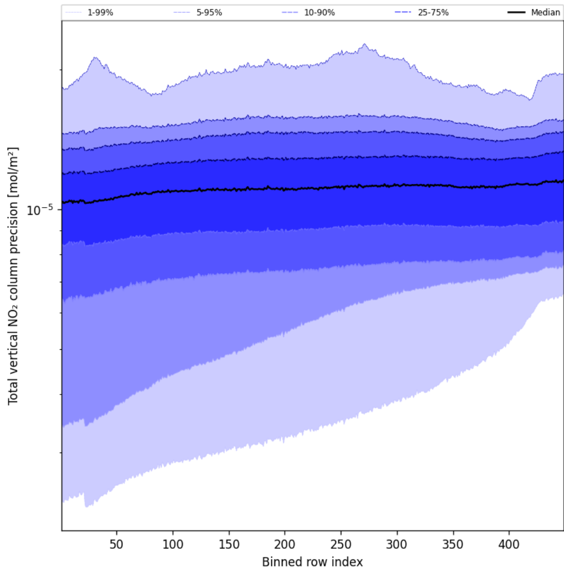
Figure 56: Along track statistics of “Total vertical NO 2 column precision” for 2025-08-30 to 2025-09-01
