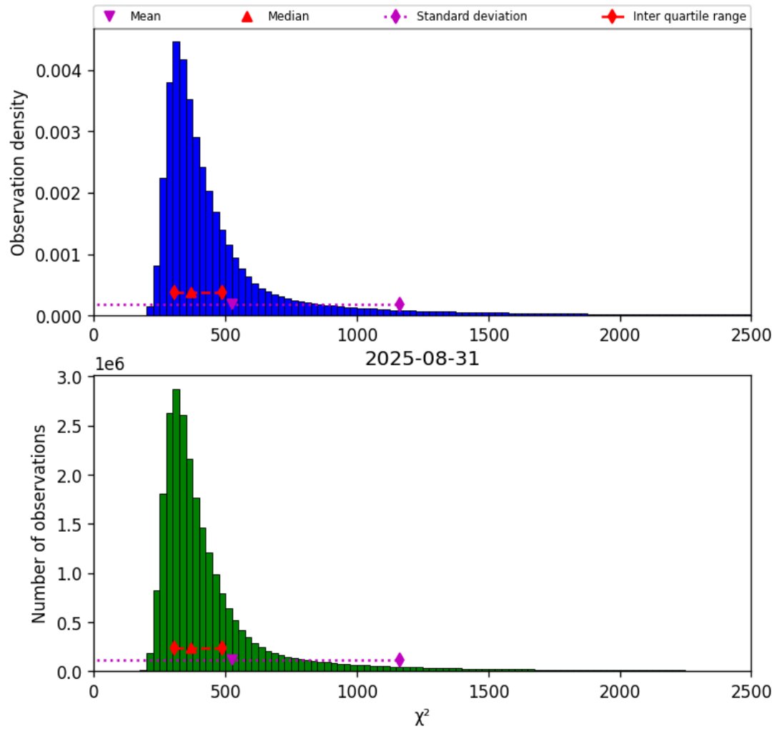
Figure 42: Histogram of “ \chi^2 ” for 2025-08-30 to 2025-09-01
