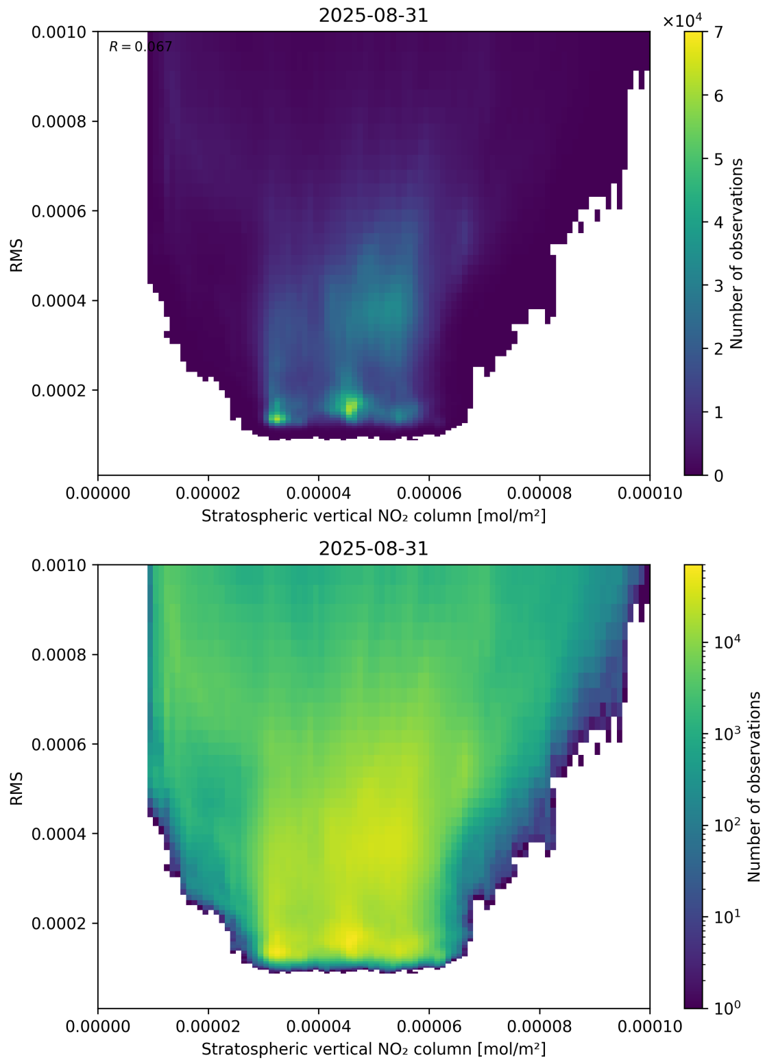
Figure 102: Scatter density plot of “Stratospheric vertical NO 2 column” against “RMS” for 2025-08-30 to 2025-09-01.
