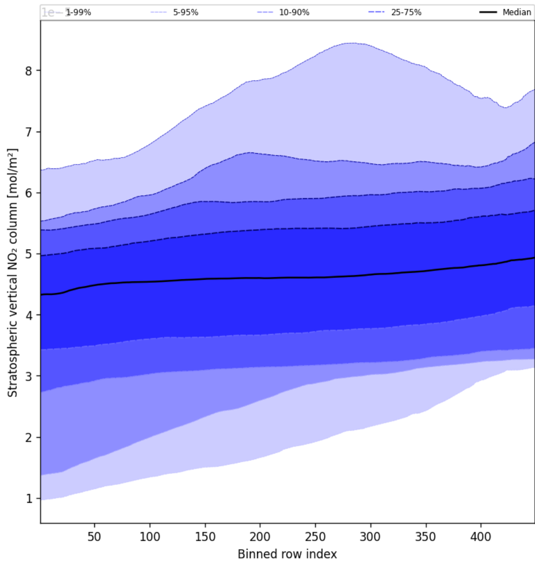
Figure 53: Along track statistics of “Stratospheric vertical NO 2 column” for 2025-08-30 to 2025-09-01
