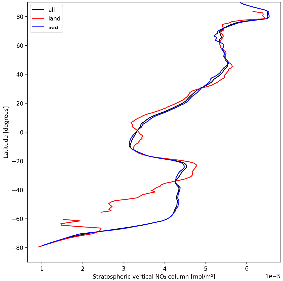
Figure 19: Zonal average of “Stratospheric vertical NO 2 column” for 2025-08-30 to 2025-09-01.
