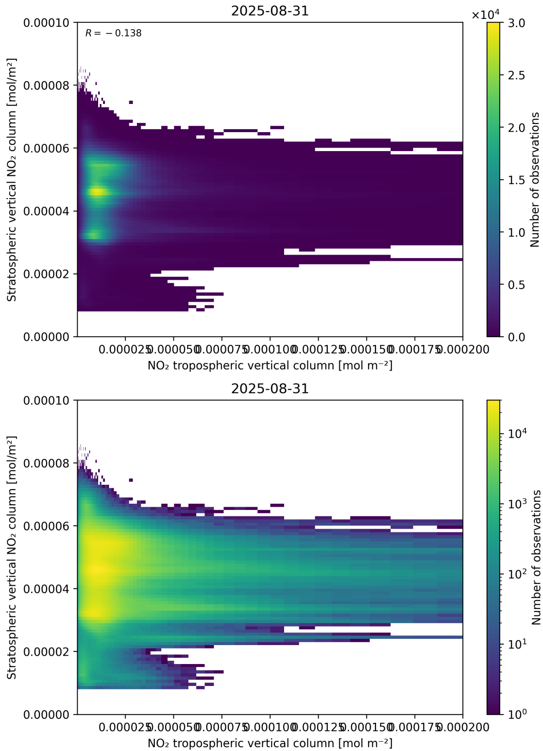
Figure 125: Scatter density plot of “NO 2 tropospheric vertical column” against “Stratospheric vertical NO 2 column” for 2025-08-30 to 2025-09-01.
