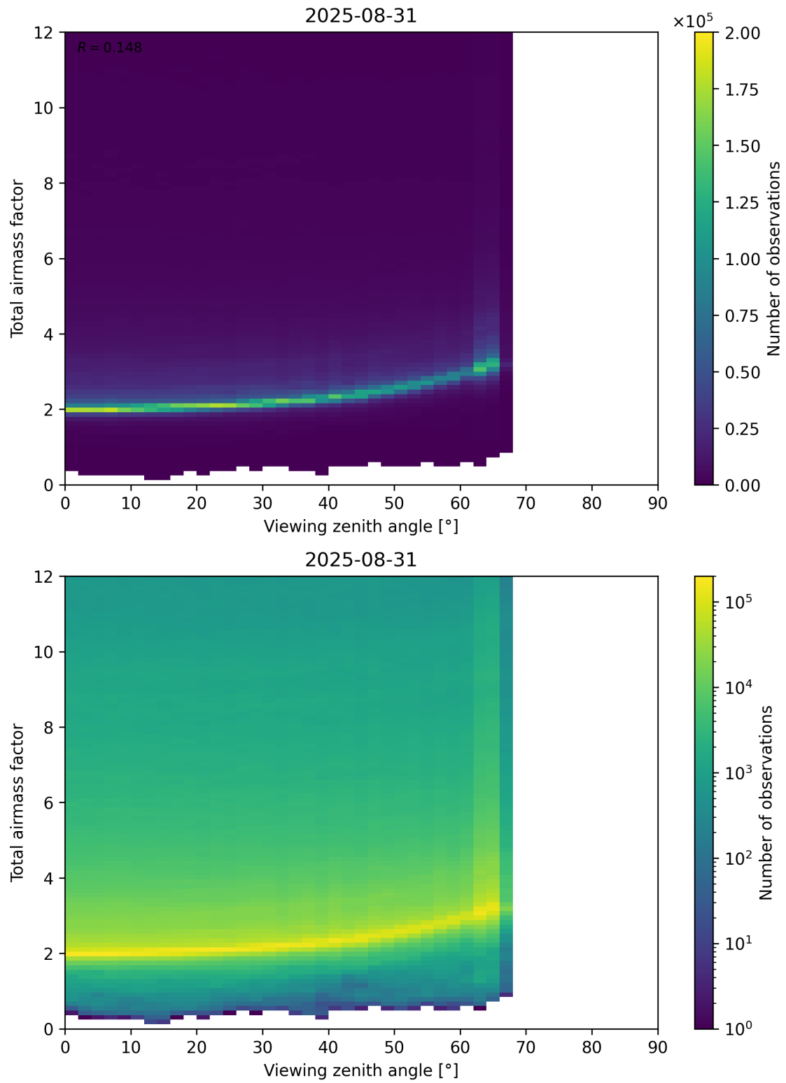
Figure 160: Scatter density plot of “Viewing zenith angle” against “Total airmass factor” for 2025-08-30 to 2025-09-01.
