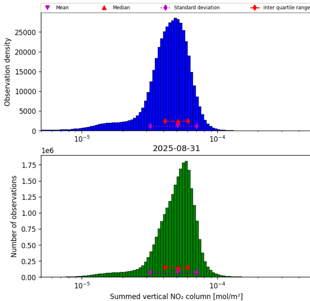
Figure 40: Histogram of “Summed vertical NO 2 column” for 2025-08-30 to 2025-09-01
