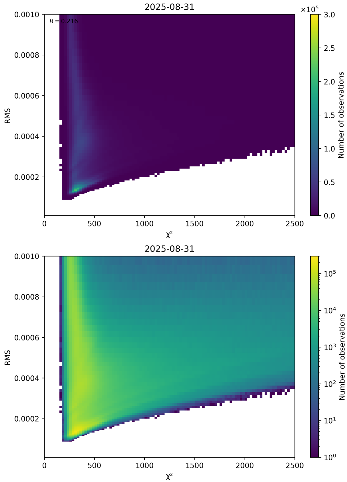
Figure 82: Scatter density plot of “ \chi^2 ” against “RMS” for 2025-08-30 to 2025-09-01.
