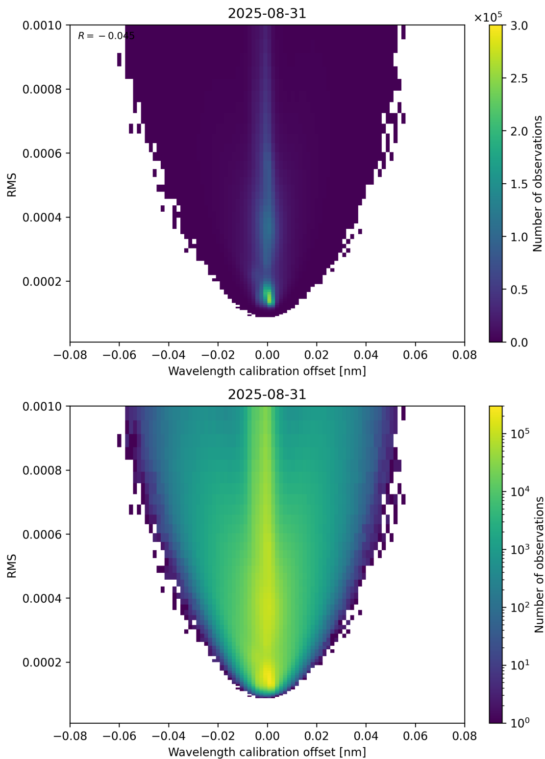
Figure 181: Scatter density plot of “Wavelength calibration offset” against “RMS” for 2025-08-30 to 2025-09-01.
