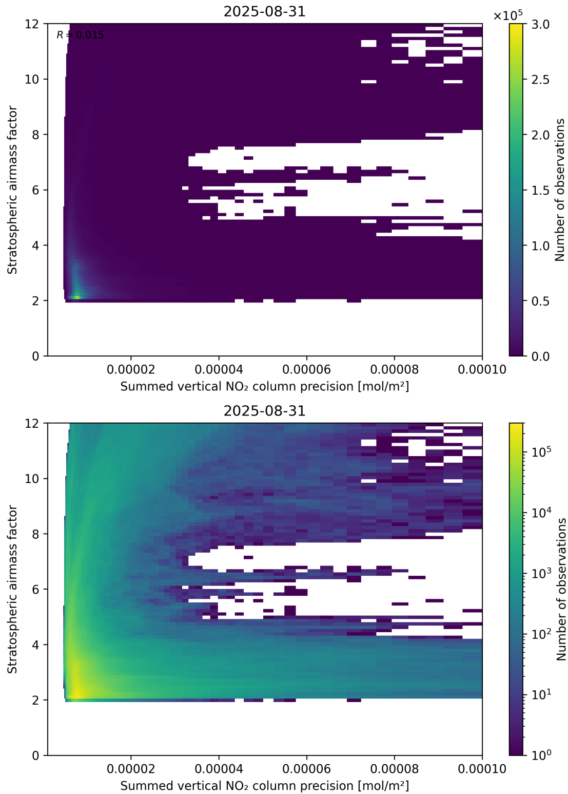
Figure 106: Scatter density plot of “Summed vertical NO 2 column precision” against “Stratospheric airmass factor” for 2025-08-30 to 2025-09-01.
