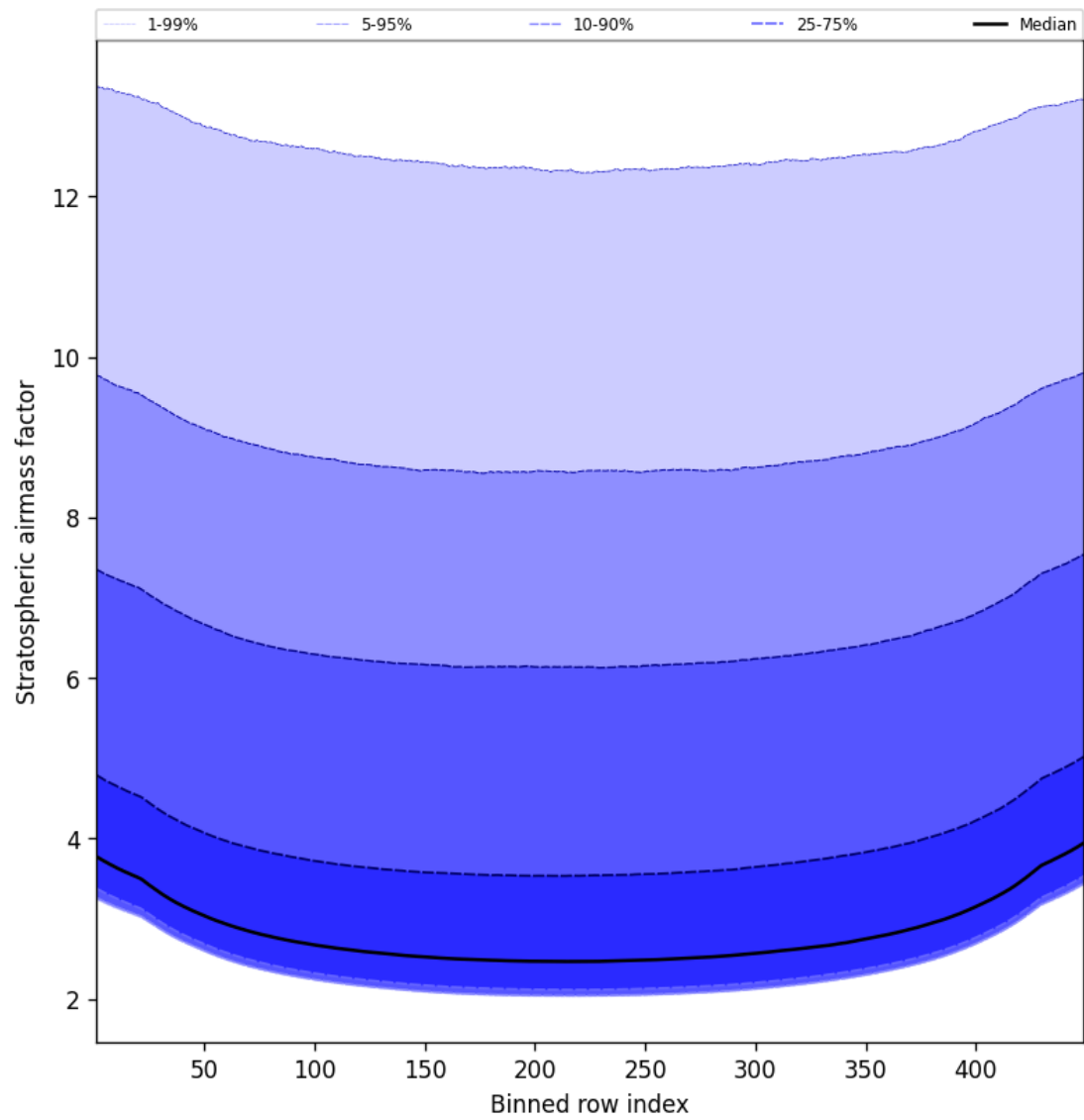
Figure 61: Along track statistics of “Stratospheric air mass factor” for 2025-08-30 to 2025-09-01
