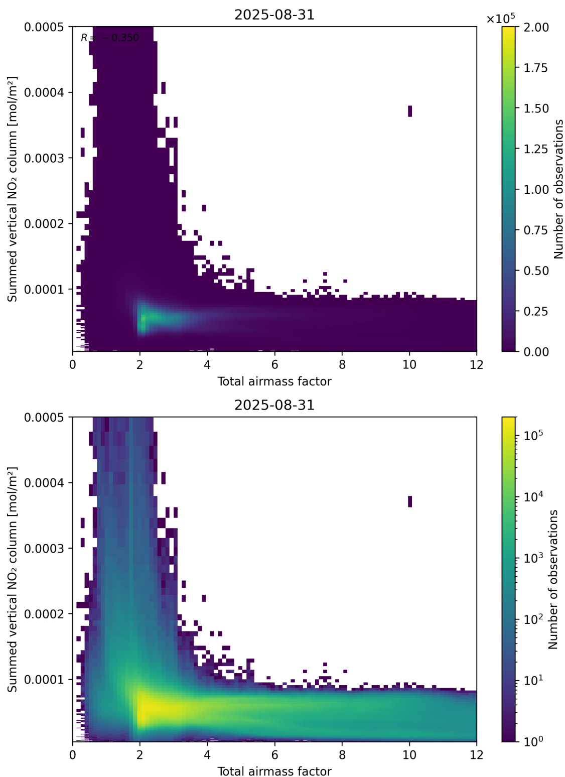
Figure 65: Scatter density plot of “Total airmass factor” against “Summed vertical NO 2 column” for 2025-08-30 to 2025-09-01.
