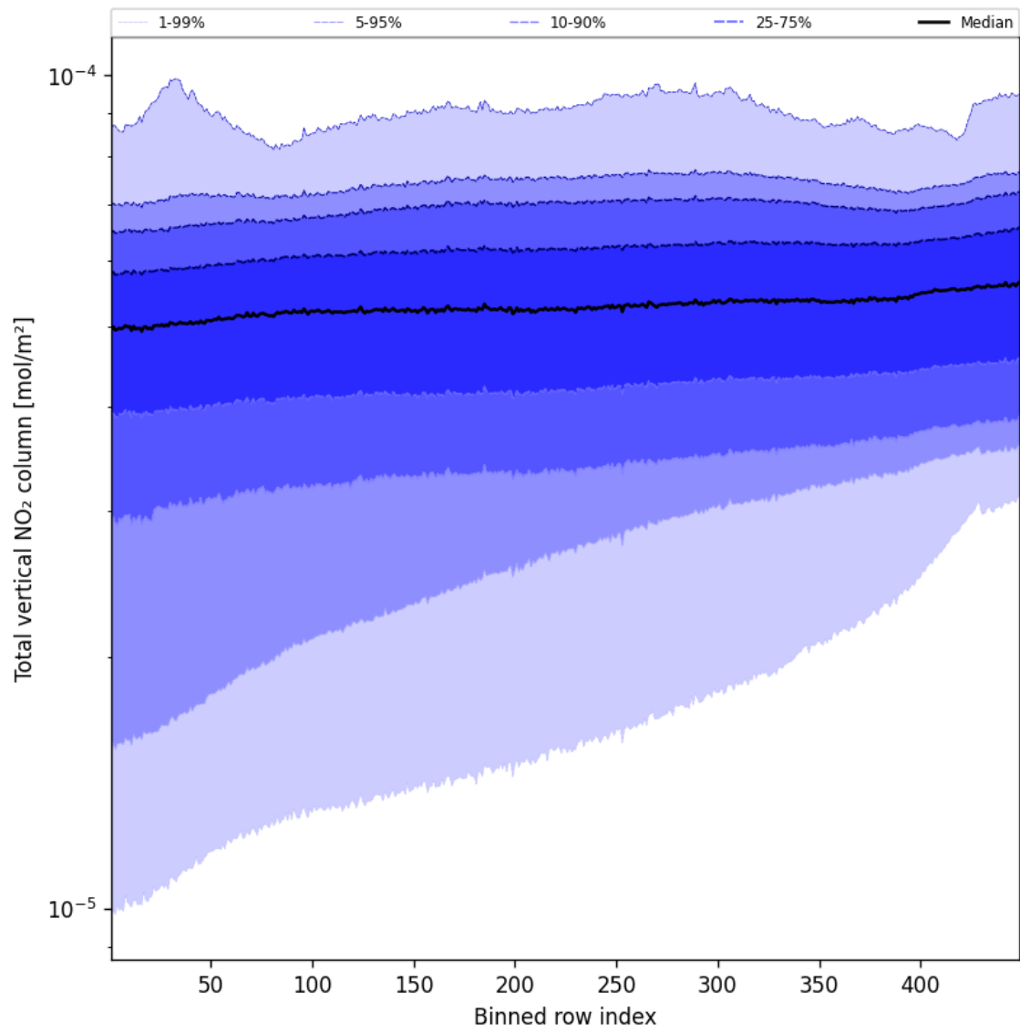
Figure 55: Along track statistics of “Total vertical NO 2 column” for 2025-08-30 to 2025-09-01
