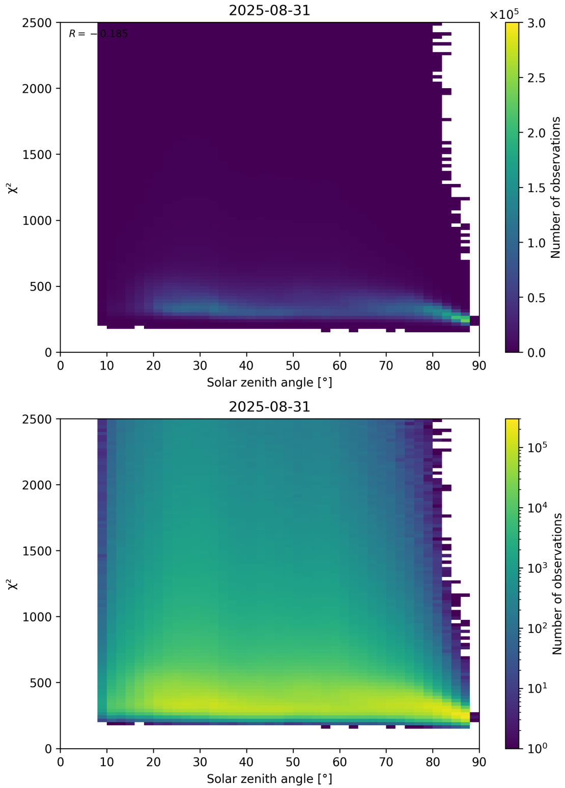
Figure 148: Scatter density plot of “Solar zenith angle” against “ \chi^2 ” for 2025-08-30 to 2025-09-01.
