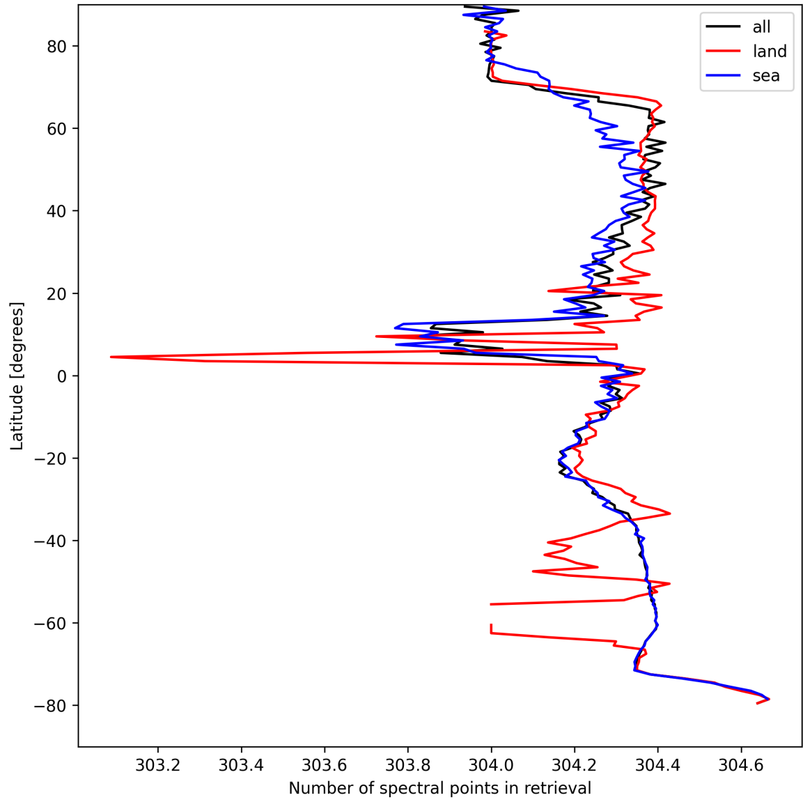
Figure 16: Zonal average of “Number of spectral points in retrieval” for 2025-08-30 to 2025-09-01.
