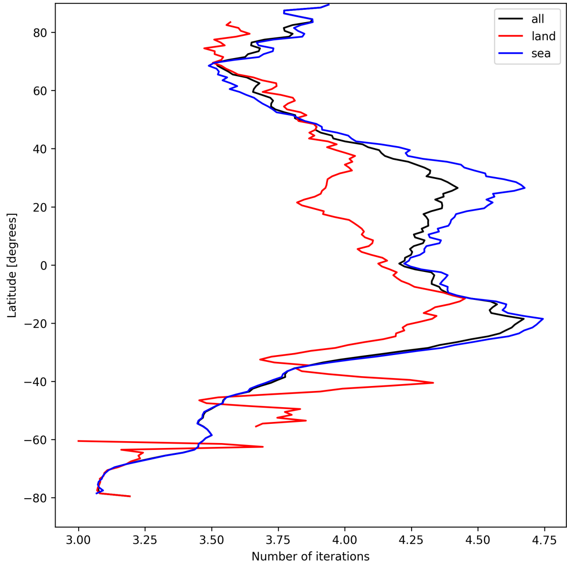
Figure 17: Zonal average of “Number of iterations” for 2025-08-30 to 2025-09-01.
