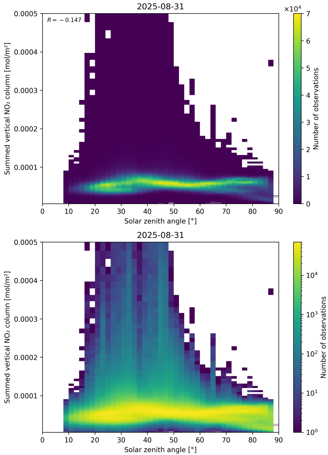
Figure 151: Scatter density plot of “Solar zenith angle” against “Summed vertical NO 2 column” for 2025-08-30 to 2025-09-01.
