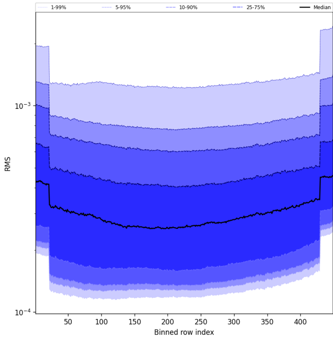
Figure 60: Along track statistics of “RMS” for 2025-08-30 to 2025-09-01
