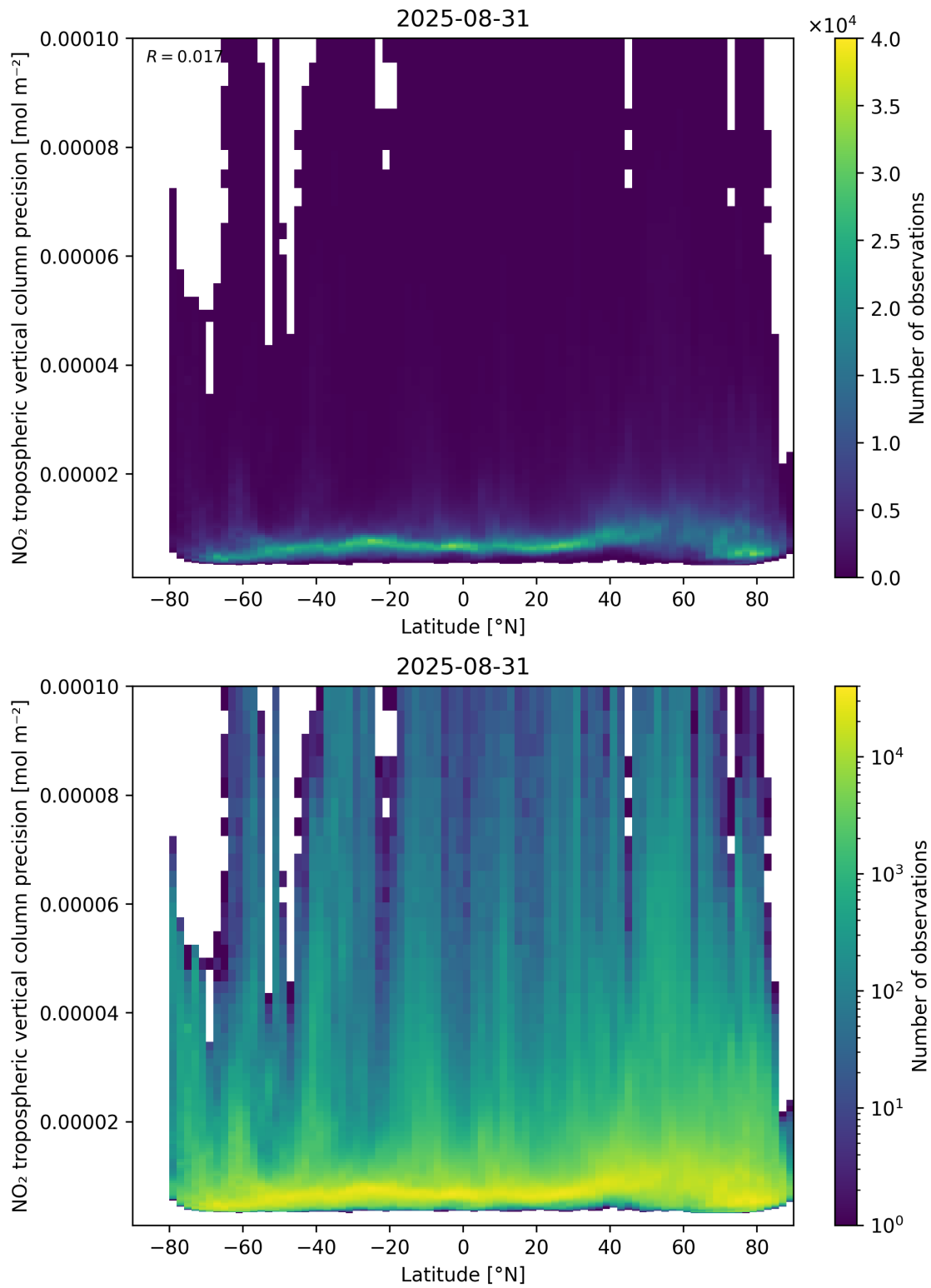
Figure 93: Scatter density plot of “Latitude” against “NO 2 tropospheric vertical column precision” for 2025-08-30 to 2025-09-01.
