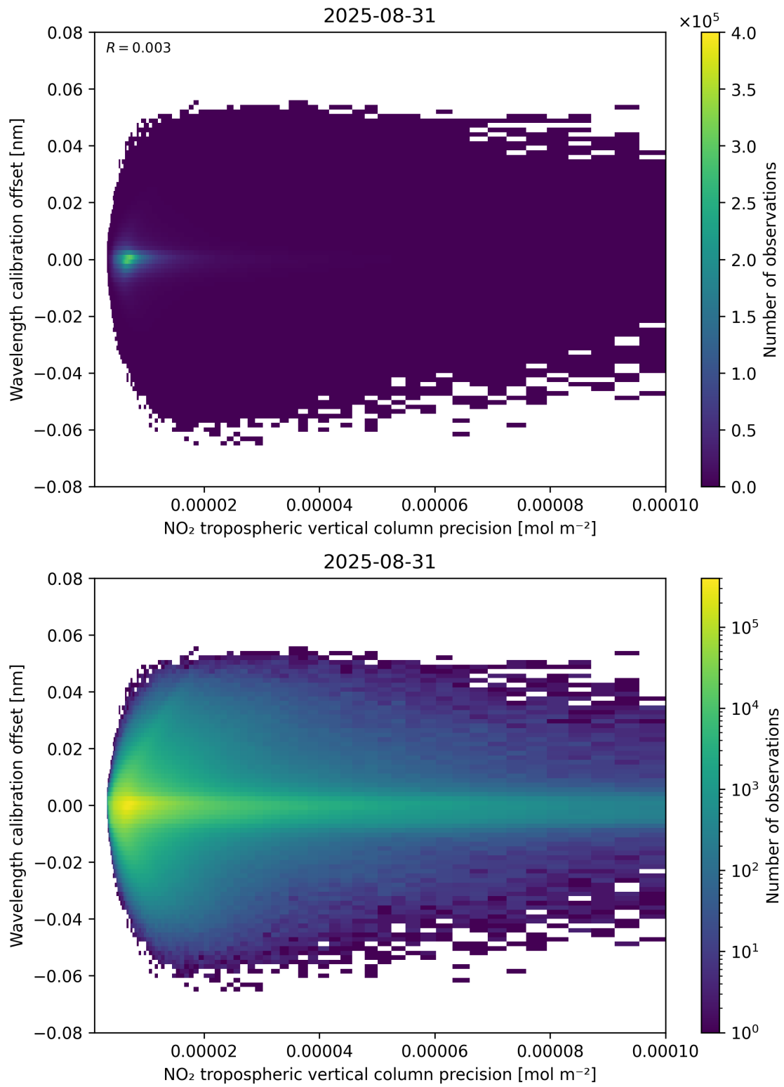
Figure 141: Scatter density plot of “NO 2 tropospheric vertical column precision” against “Wavelength calibration offset” for 2025-08-30 to 2025-09-01.
