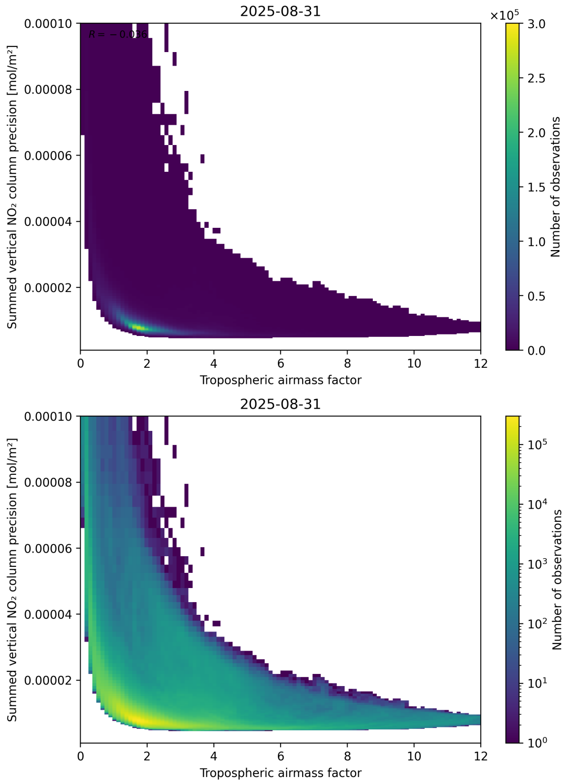
Figure 76: Scatter density plot of “Tropospheric air mass factor” against “Summed vertical NO 2 column precision” for 2025-08-30 to 2025-09-01.
