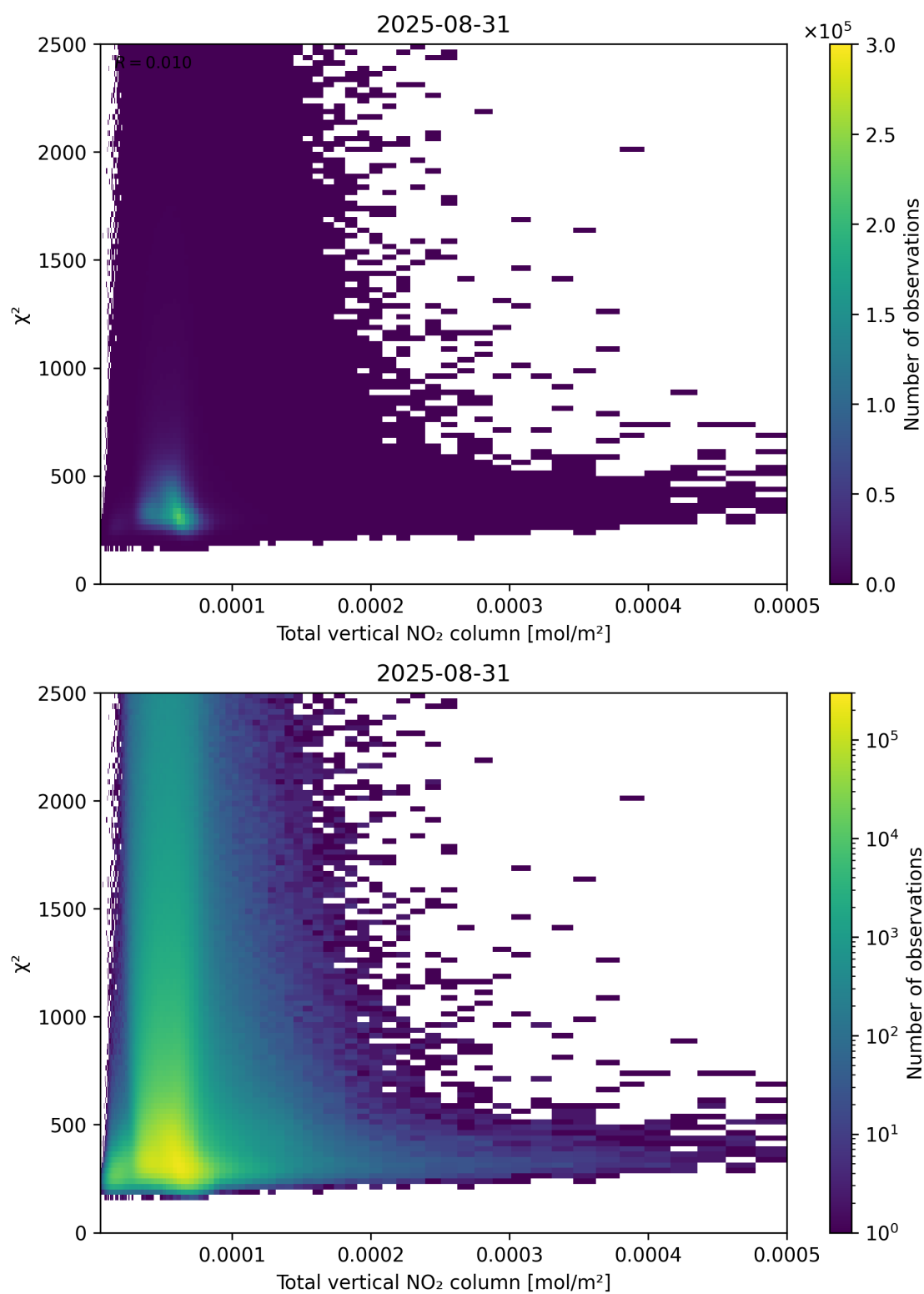
Figure 111: Scatter density plot of “Total vertical NO 2 column” against “ \chi^2 ” for 2025-08-30 to 2025-09-01.
