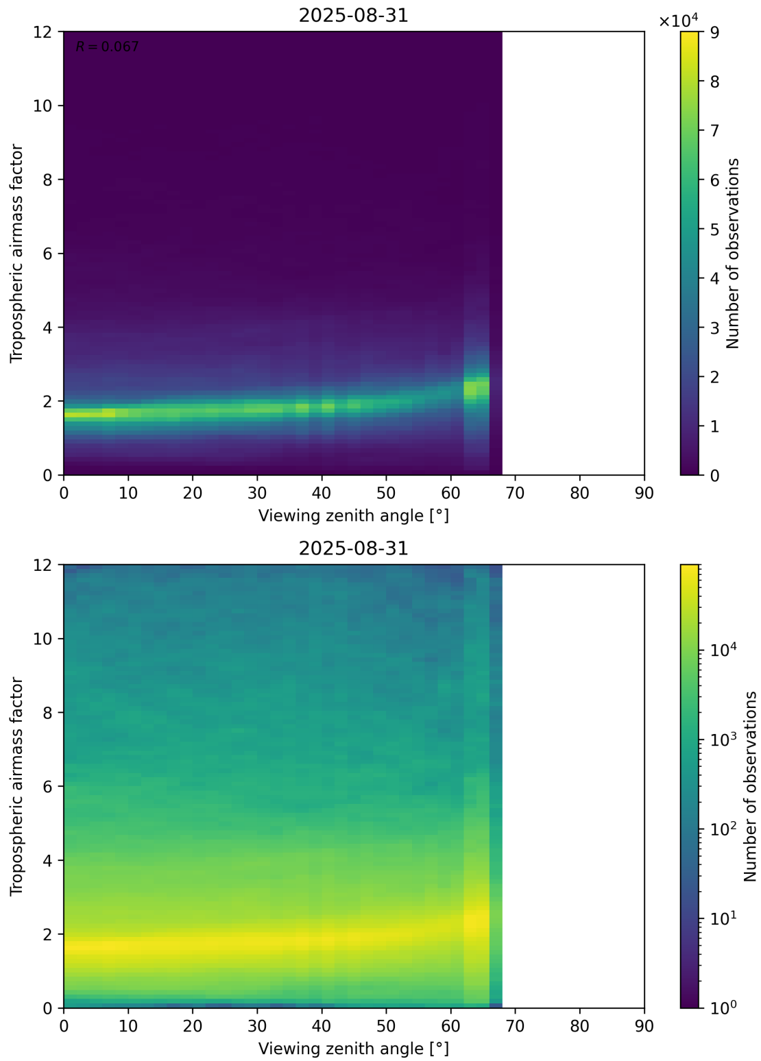
Figure 161: Scatter density plot of “Viewing zenith angle” against “Tropospheric airmass factor” for 2025-08-30 to 2025-09-01.
