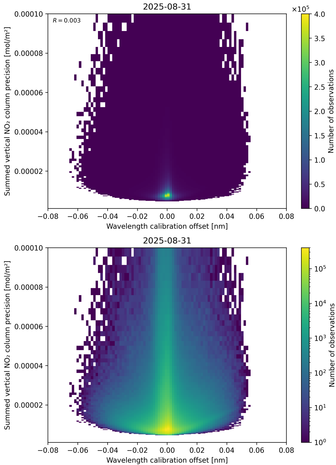
Figure 178: Scatter density plot of “Wavelength calibration offset” against “Summed vertical NO 2 column precision” for 2025-08-30 to 2025-09-01.
