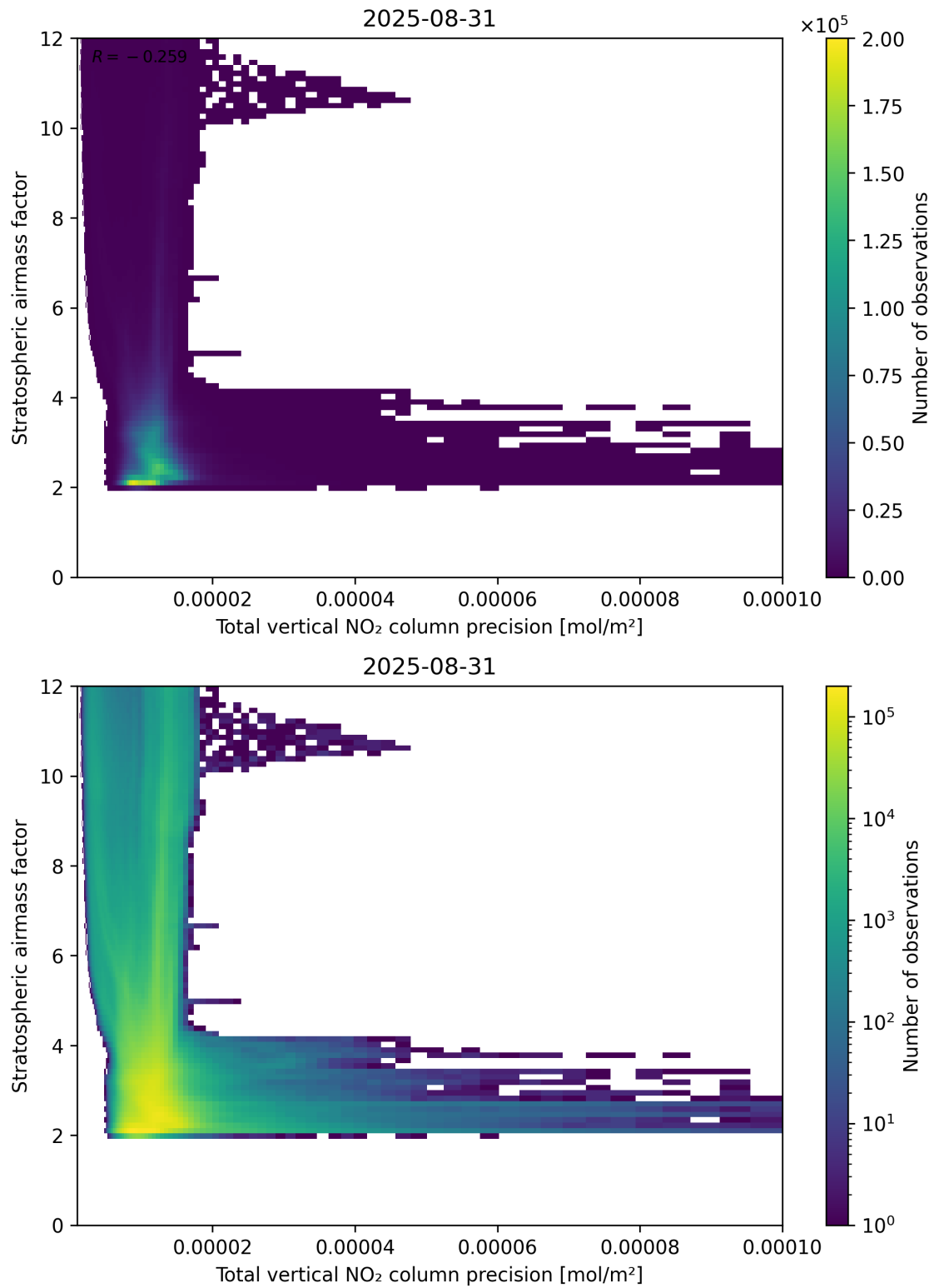
Figure 115: Scatter density plot of “Total vertical NO 2 column precision” against “Stratospheric air mass factor” for 2025-08-30 to 2025-09-01.
