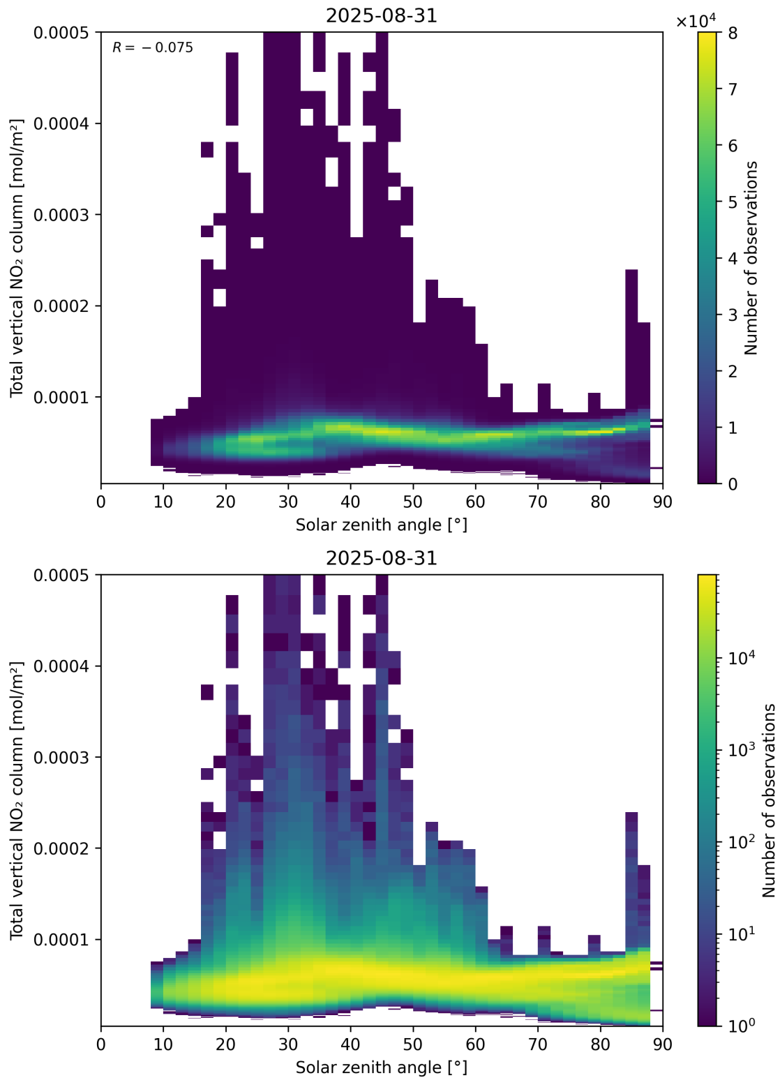
Figure 153: Scatter density plot of “Solar zenith angle” against “Total vertical NO 2 column” for 2025-08-30 to 2025-09-01.
