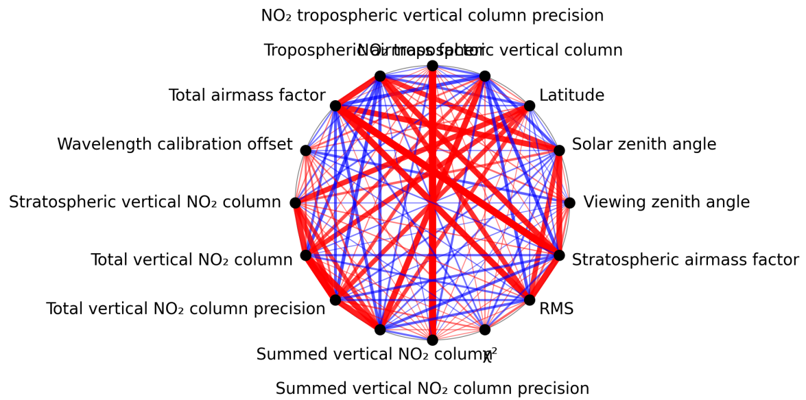
Figure 1: Map of correlation graph for 2025-08-30 to 2025-09-01.
