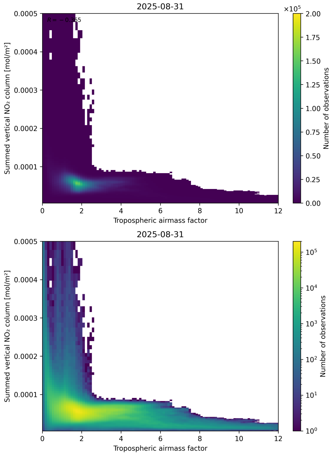
Figure 75: Scatter density plot of “Tropospheric air mass factor” against “Summed vertical NO 2 column” for 2025-08-30 to 2025-09-01.
