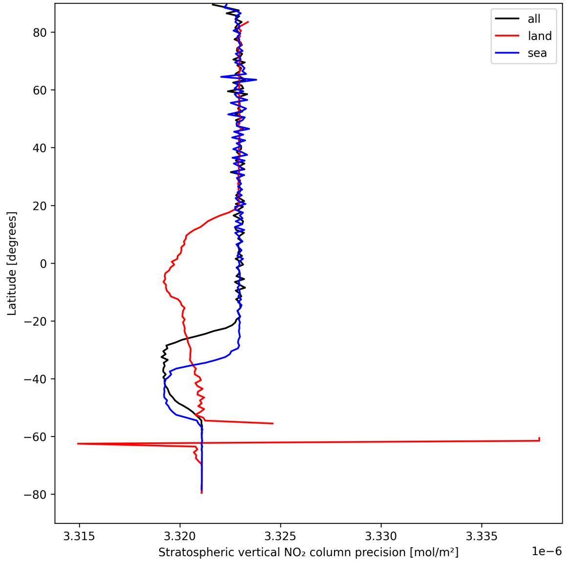
Figure 20: Zonal average of “Stratospheric vertical NO 2 column precision” for 2025-08-30 to 2025-09-01.
