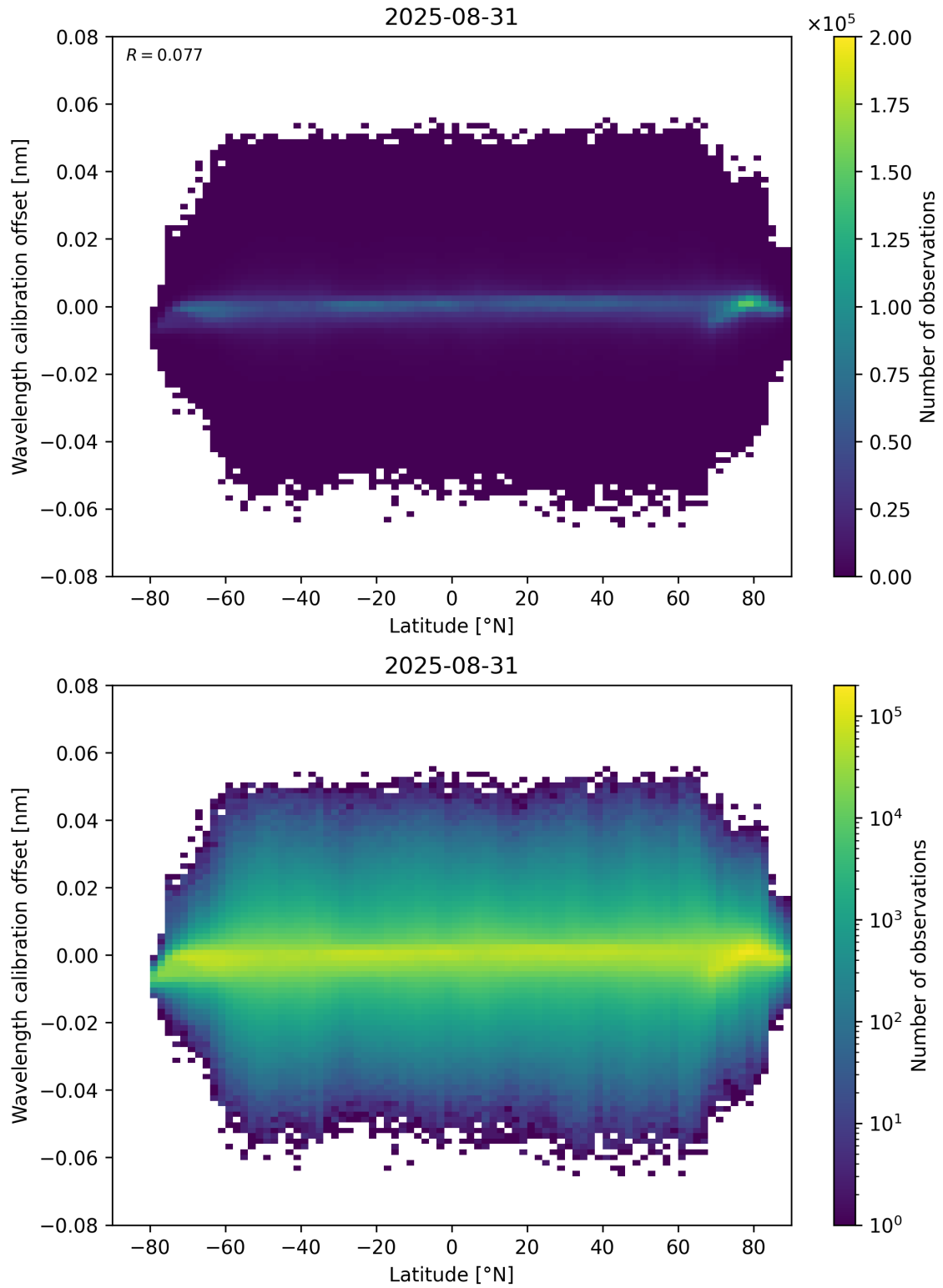
Figure 95: Scatter density plot of “Latitude” against “Wavelength calibration offset” for 2025-08-30 to 2025-09-01.
