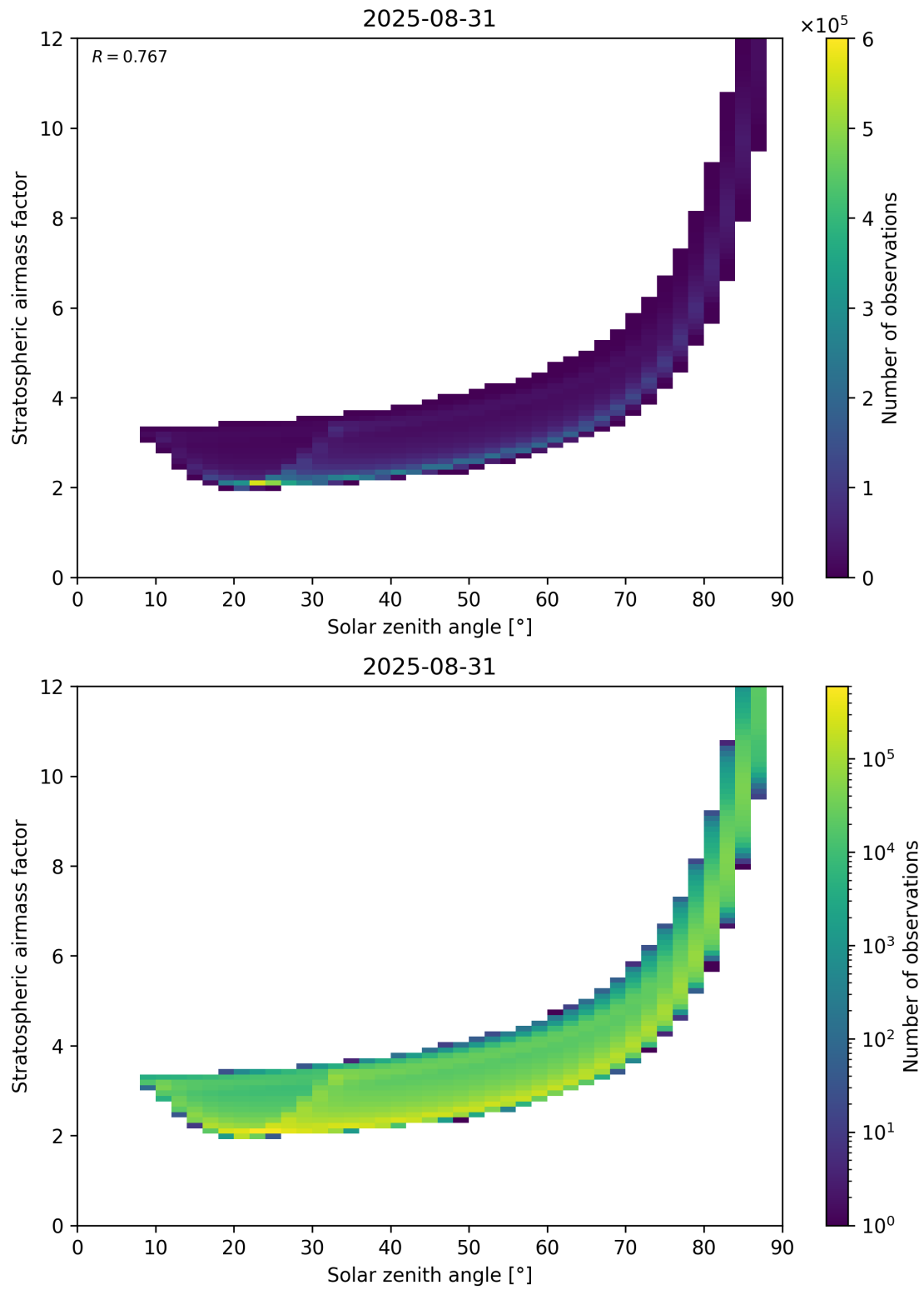
Figure 145: Scatter density plot of “Solar zenith angle” against “Stratospheric airmass factor” for 2025-08-30 to 2025-09-01.
