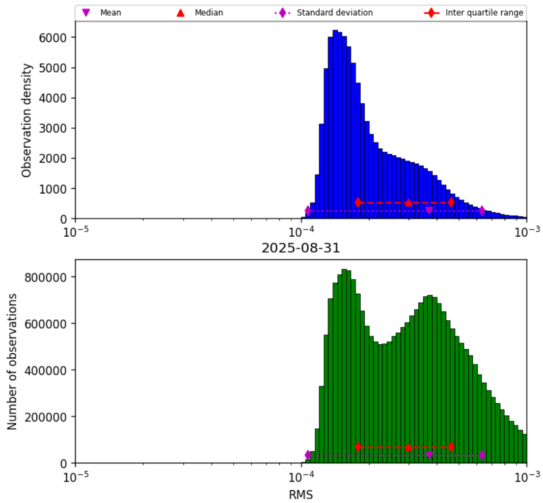
Figure 43: Histogram of “RMS” for 2025-08-30 to 2025-09-01
