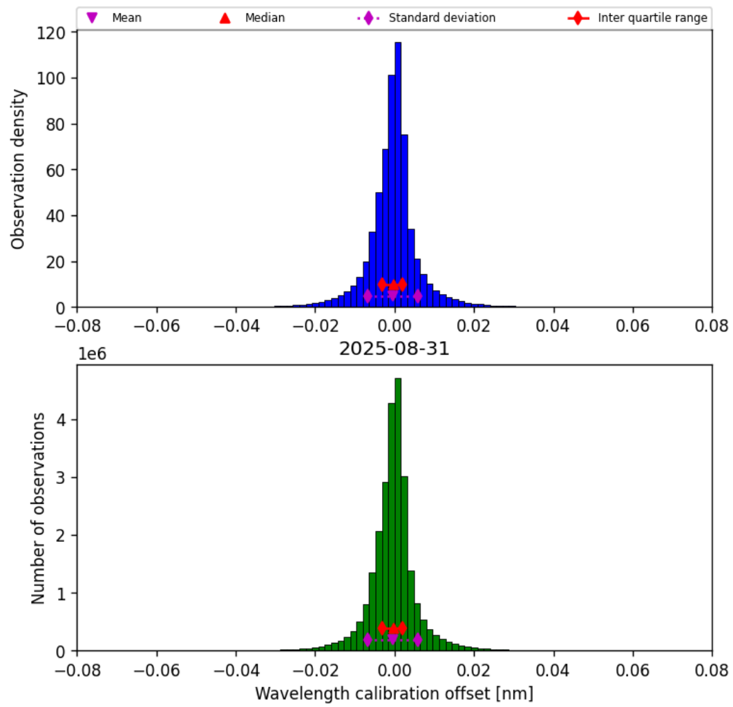
Figure 35: Histogram of “Wavelength calibration offset” for 2025-08-30 to 2025-09-01
