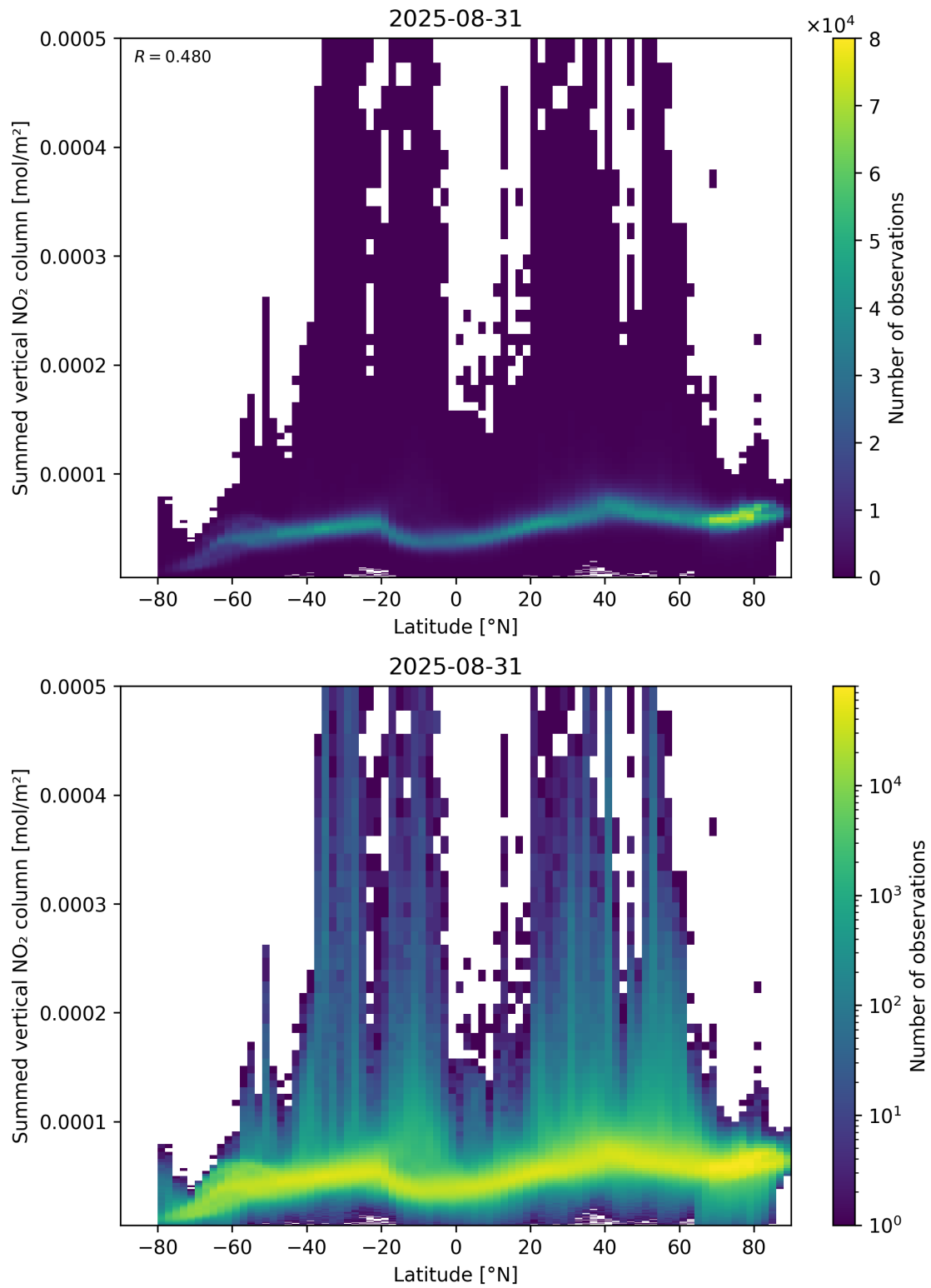
Figure 88: Scatter density plot of “Latitude” against “Summed vertical NO 2 column” for 2025-08-30 to 2025-09-01.
