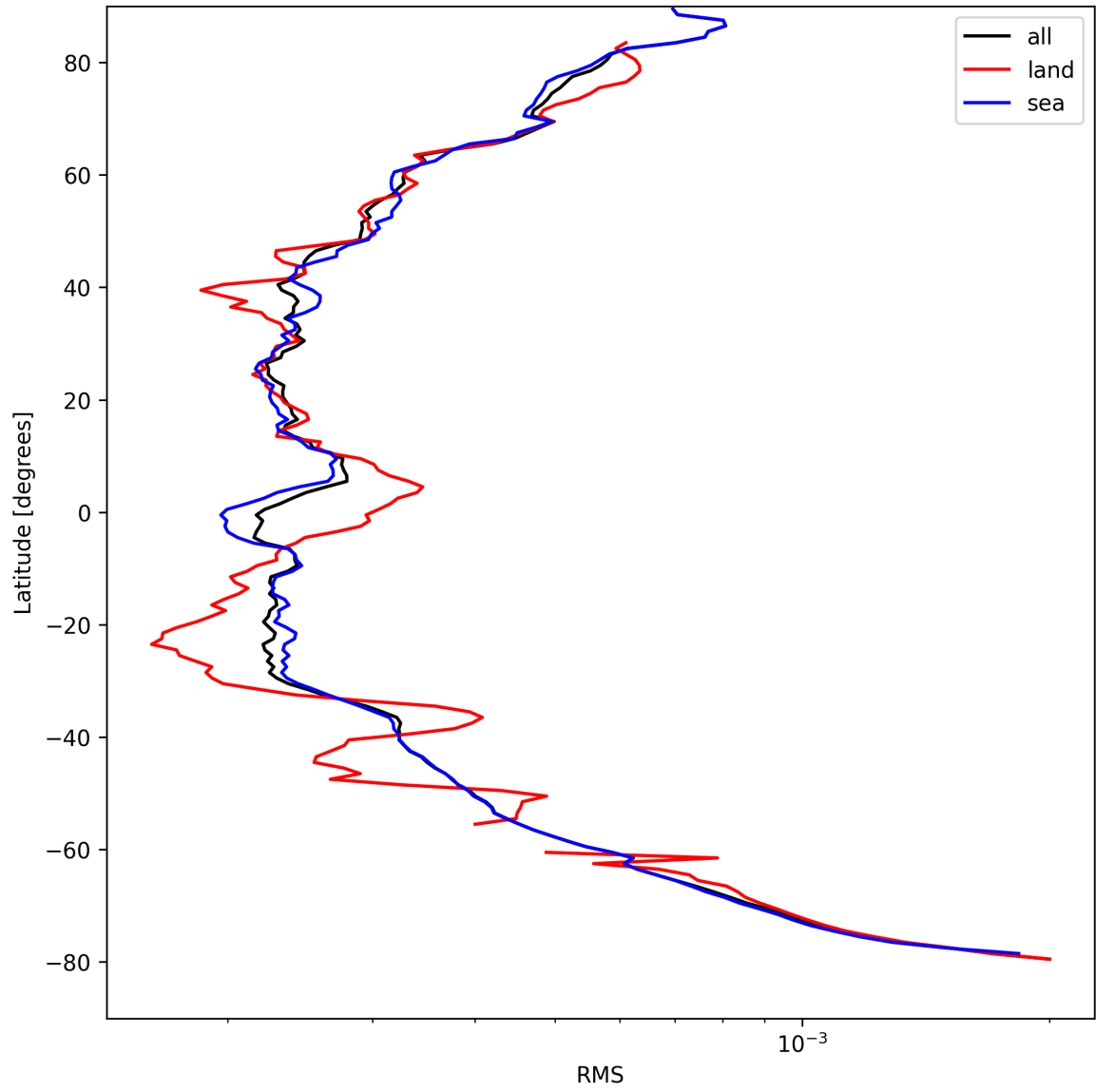
Figure 26: Zonal average of “RMS” for 2025-08-30 to 2025-09-01.
