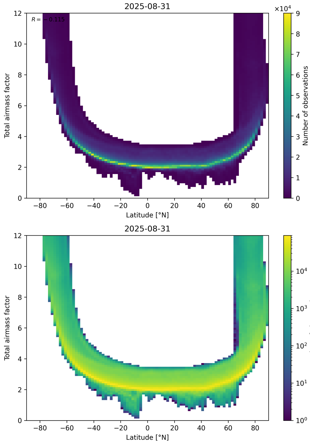
Figure 84: Scatter density plot of “Latitude” against “Total airmass factor” for 2025-08-30 to 2025-09-01.
