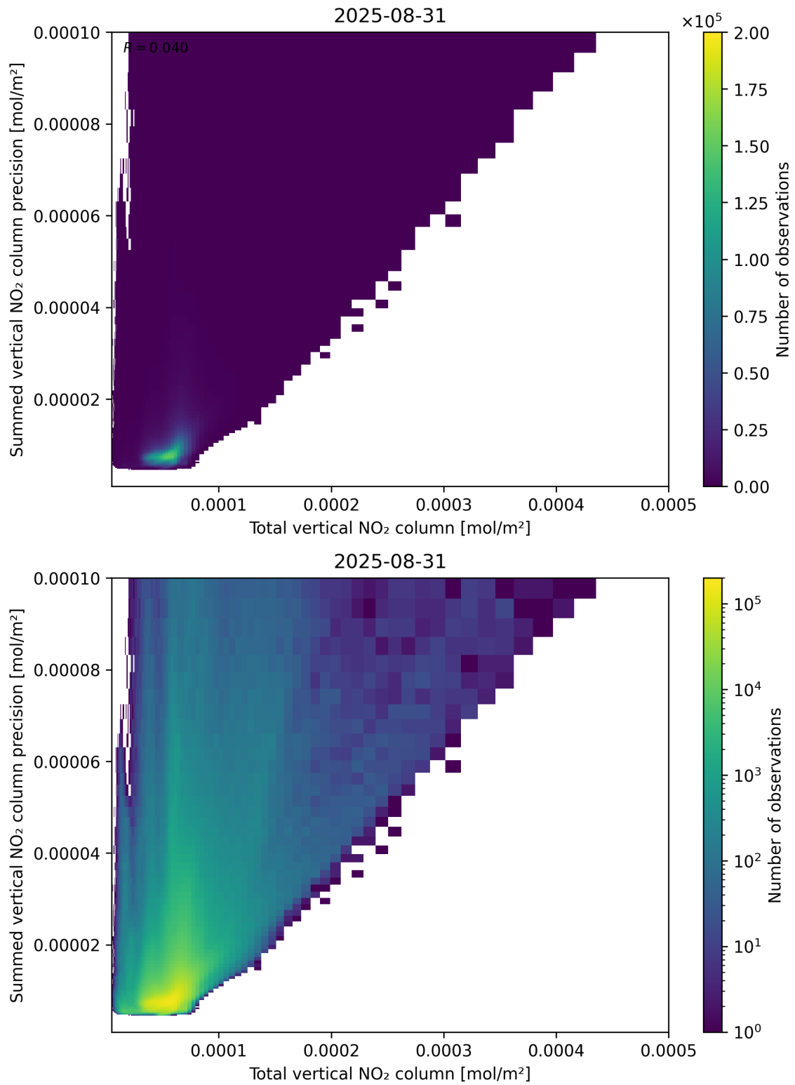
Figure 113: Scatter density plot of “Total vertical NO 2 column” against “Summed vertical NO 2 column precision” for 2025-08-30 to 2025-09-01.
