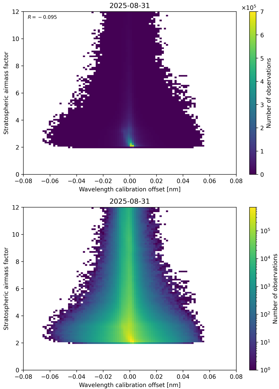
Figure 174: Scatter density plot of “Wavelength calibration offset” against “Stratospheric airmass factor” for 2025-08-30 to 2025-09-01.
