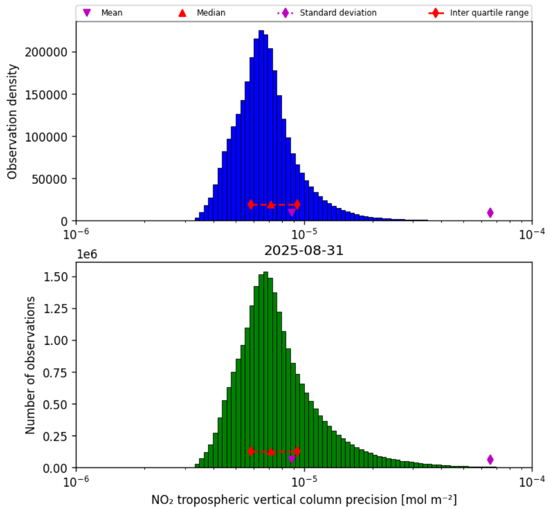
Figure 30: Histogram of “NO 2 tropospheric vertical column precision” for 2025-08-30 to 2025-09-01
