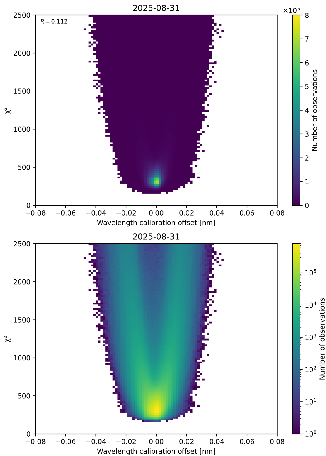
Figure 175: Scatter density plot of “Wavelength calibration offset” against “ \chi^2 ” for 2025-08-30 to 2025-09-01.
