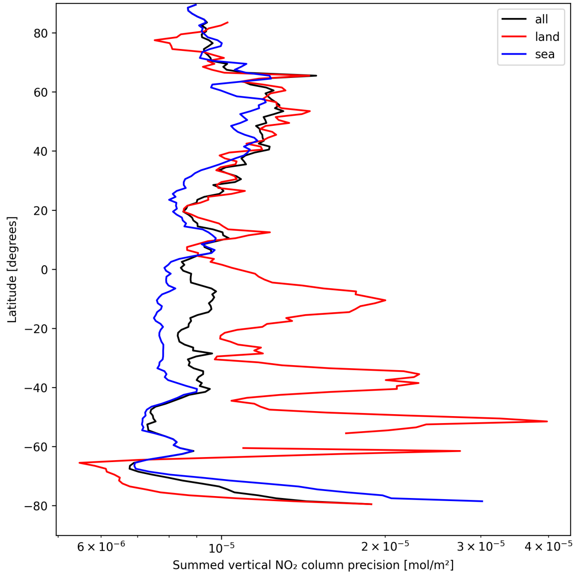
Figure 24: Zonal average of “Summed vertical NO 2 column precision” for 2025-08-30 to 2025-09-01.
