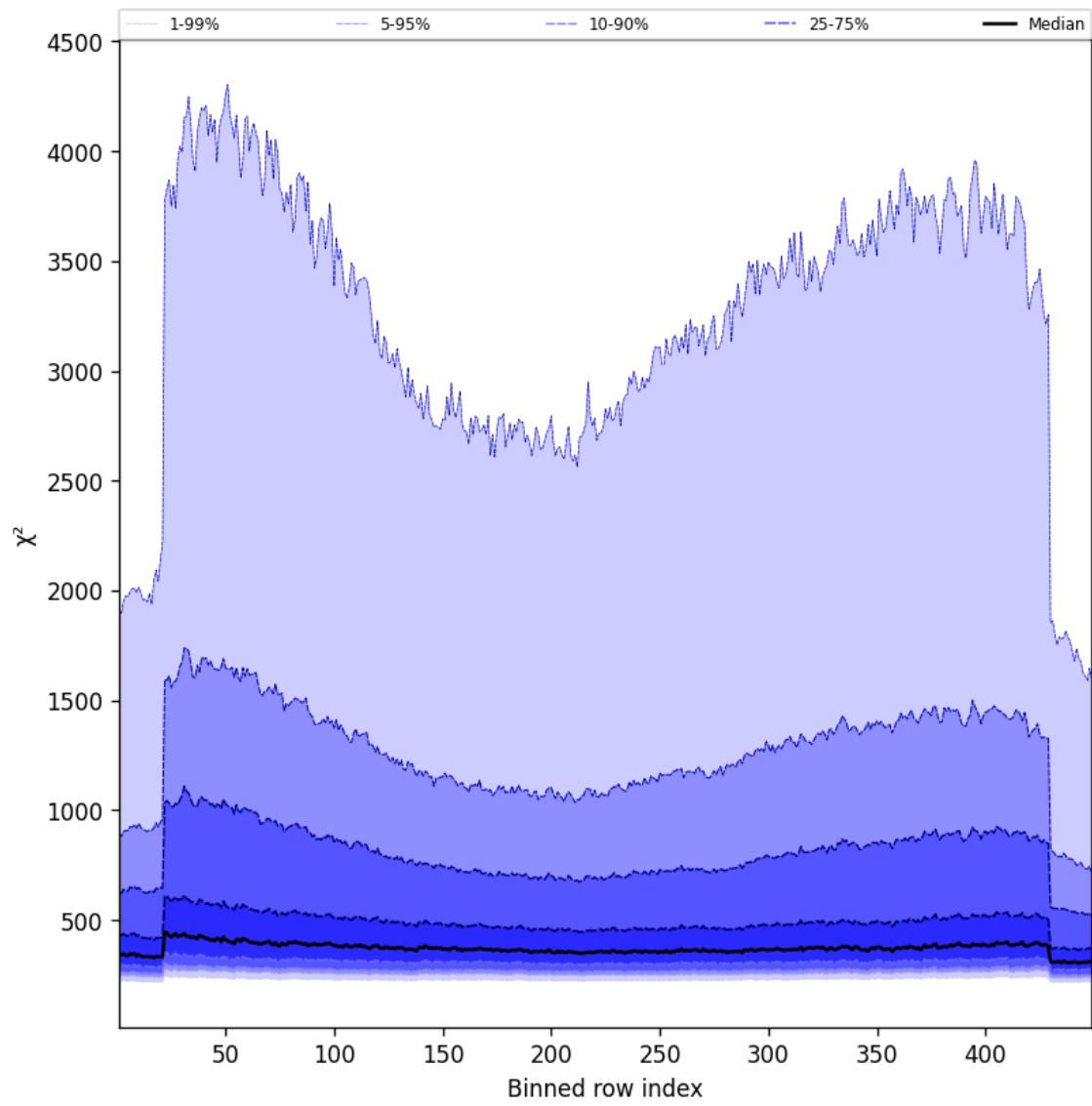
Figure 59: Along track statistics of “ \chi^2 ” for 2025-08-30 to 2025-09-01
