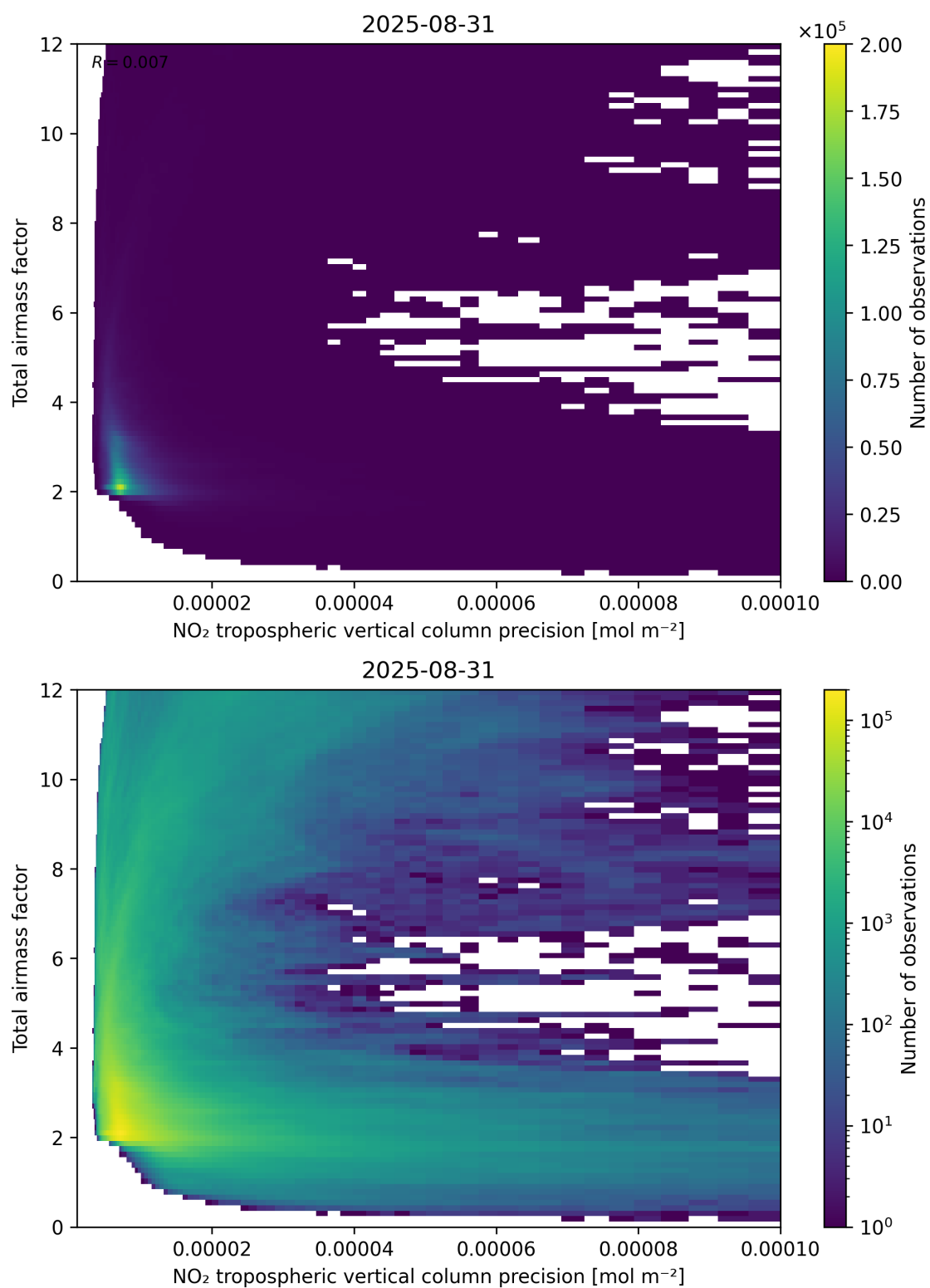
Figure 132: Scatter density plot of “NO 2 tropospheric vertical column precision” against “Total air mass factor” for 2025-08-30 to 2025-09-01.
