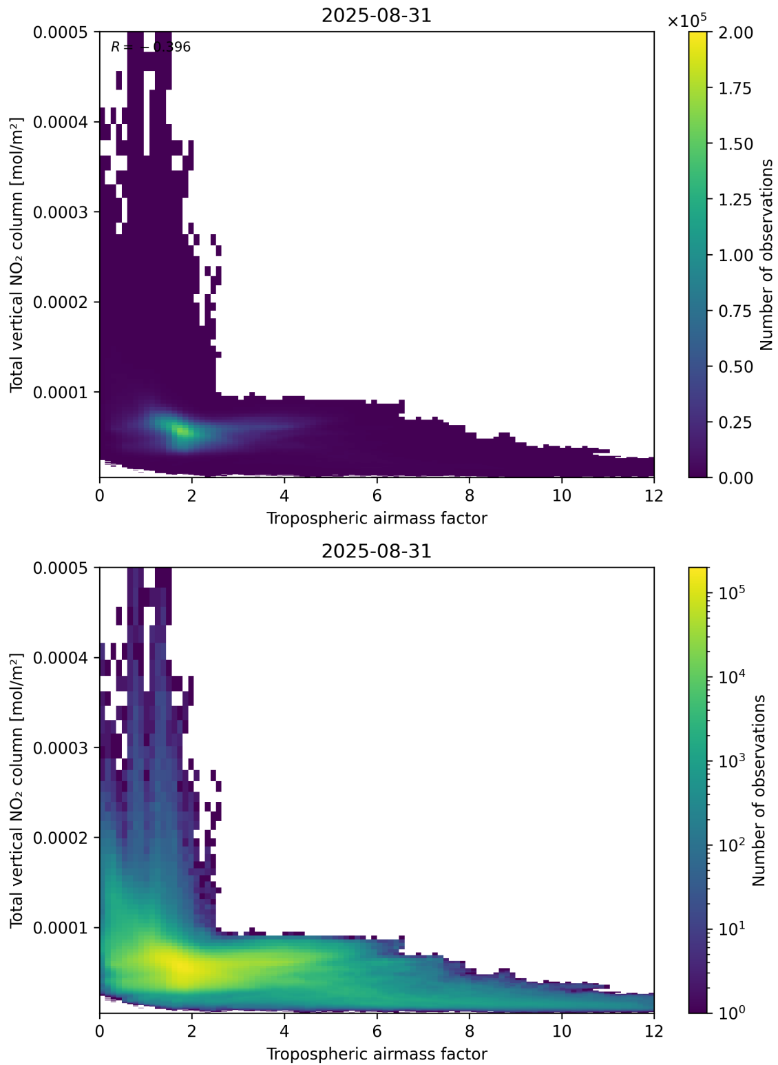
Figure 77: Scatter density plot of “Tropospheric airmass factor” against “Total vertical NO 2 column” for 2025-08-30 to 2025-09-01.
