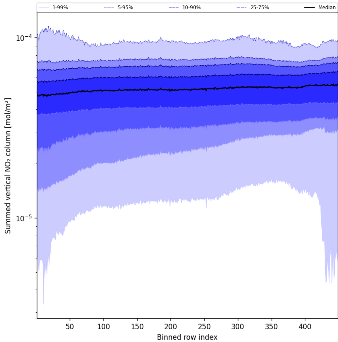
Figure 57: Along track statistics of “Summed vertical NO 2 column” for 2025-08-30 to 2025-09-01
