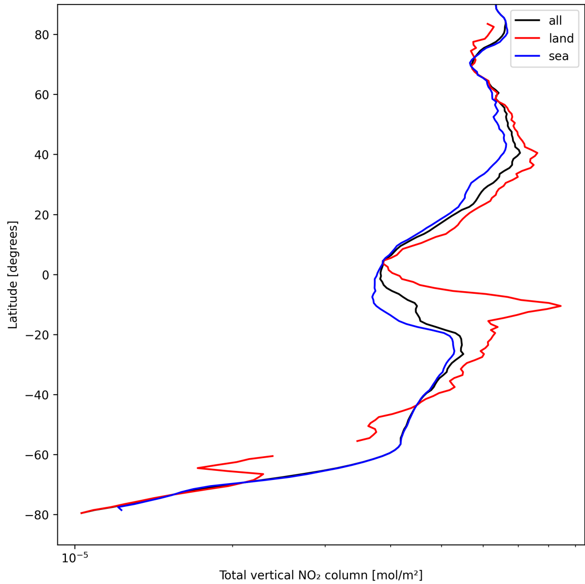
Figure 21: Zonal average of “Total vertical NO 2 column” for 2025-08-30 to 2025-09-01.
