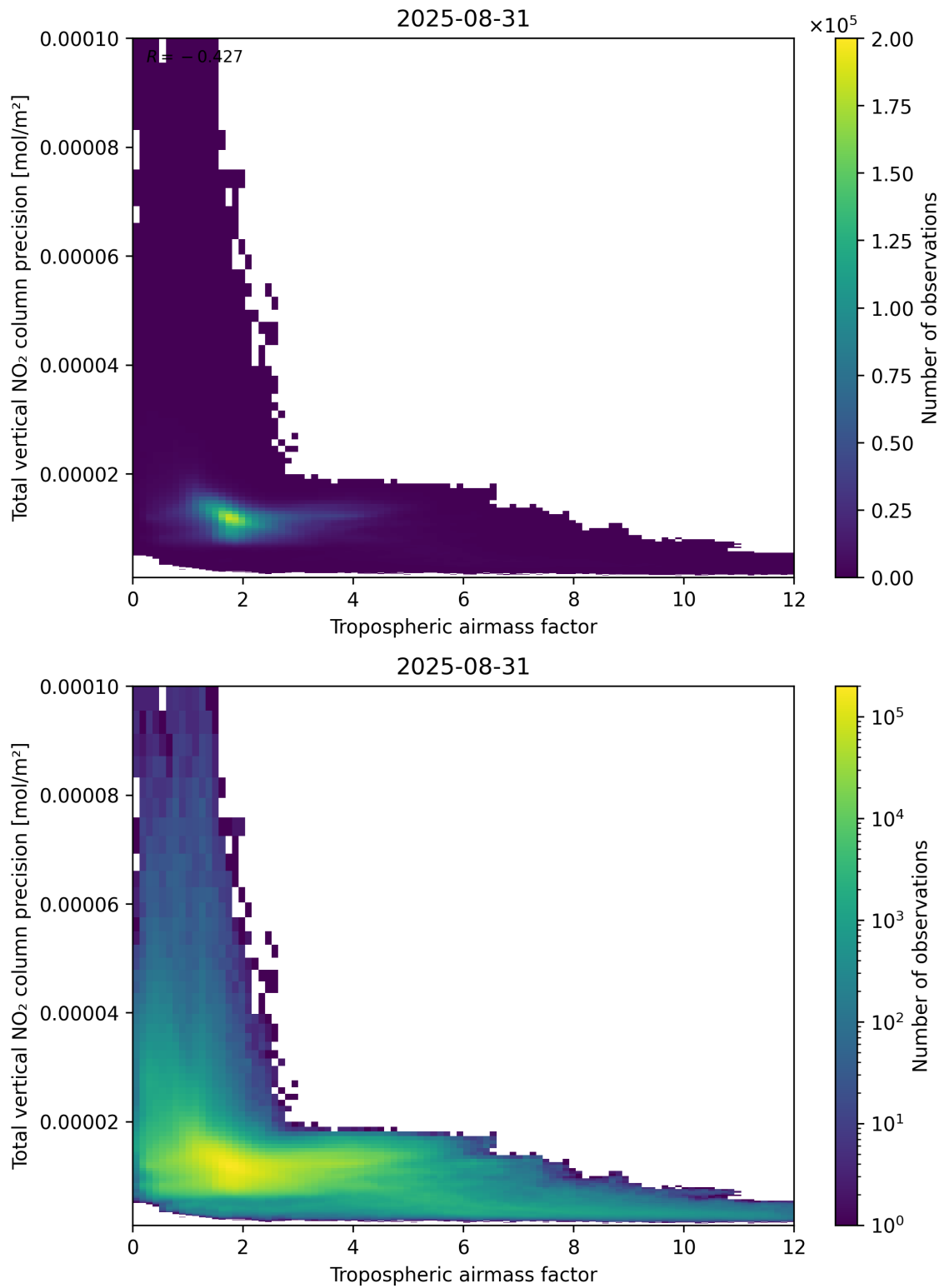
Figure 78: Scatter density plot of “Tropospheric airmass factor” against “Total vertical NO 2 column precision” for 2025-08-30 to 2025-09-01.
