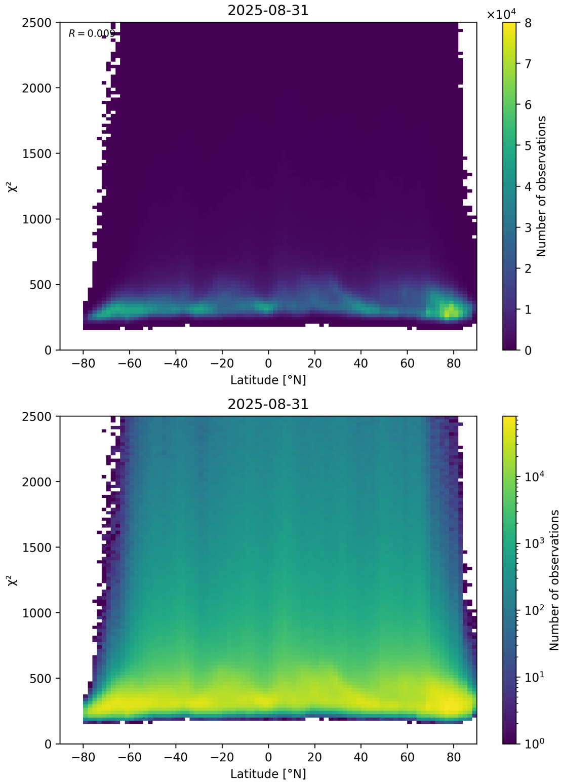
Figure 86: Scatter density plot of “Latitude” against “ \chi^2 ” for 2025-08-30 to 2025-09-01.
