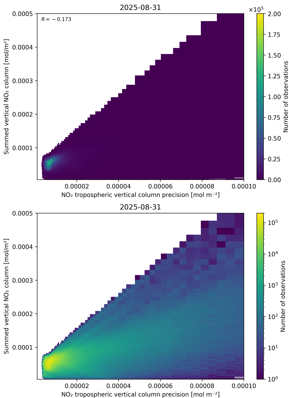
Figure 136: Scatter density plot of “NO 2 tropospheric vertical column precision” against “Summed vertical NO 2 column” for 2025-08-30 to 2025-09-01.
