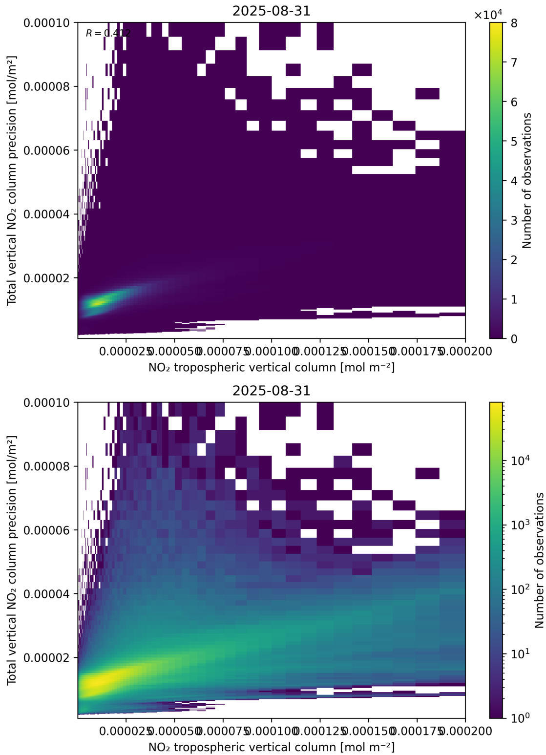
Figure 129: Scatter density plot of “NO 2 tropospheric vertical column” against “Total vertical NO 2 column precision” for 2025-08-30 to 2025-09-01.
