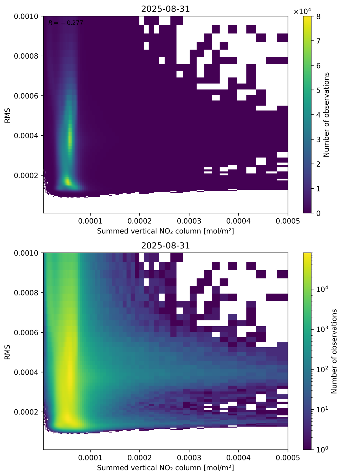
Figure 109: Scatter density plot of “Summed vertical NO 2 column” against “RMS” for 2025-08-30 to 2025-09-01.
