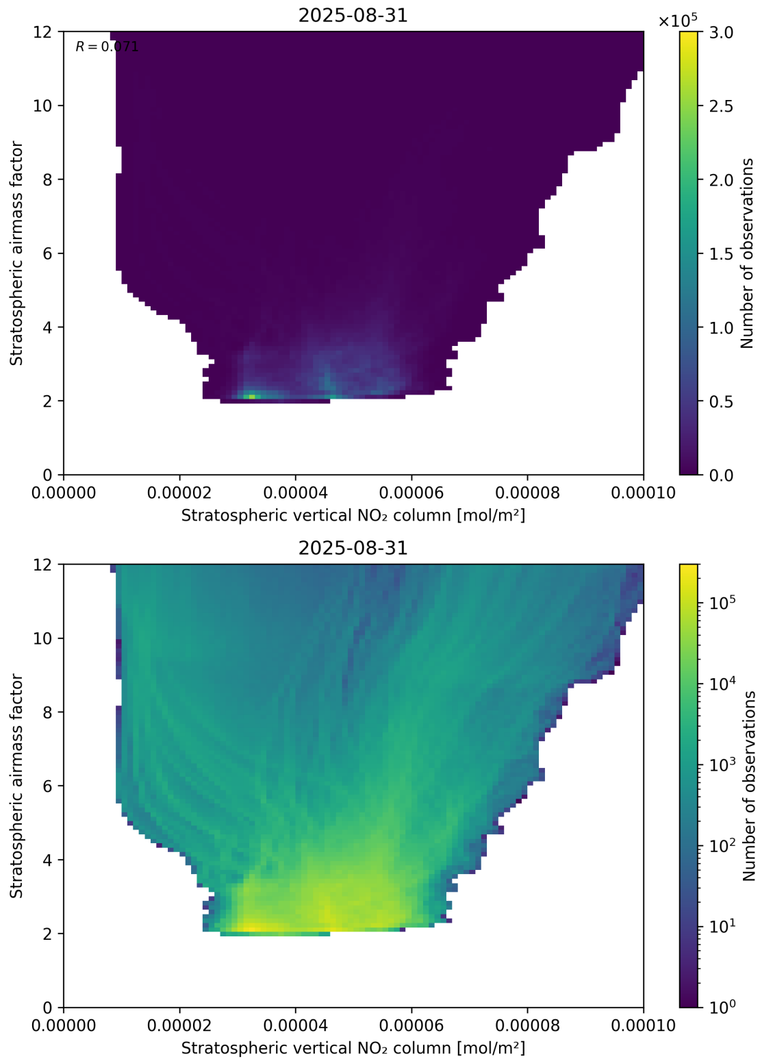
Figure 96: Scatter density plot of “Stratospheric vertical NO 2 column” against “Stratospheric airmass factor” for 2025-08-30 to 2025-09-01.
