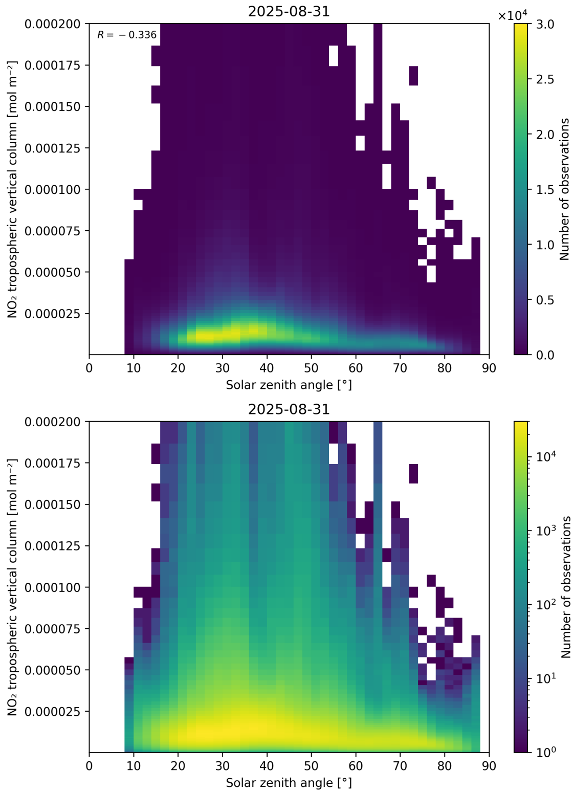
Figure 155: Scatter density plot of “Solar zenith angle” against “NO 2 tropospheric vertical column” for 2025-08-30 to 2025-09-01.
