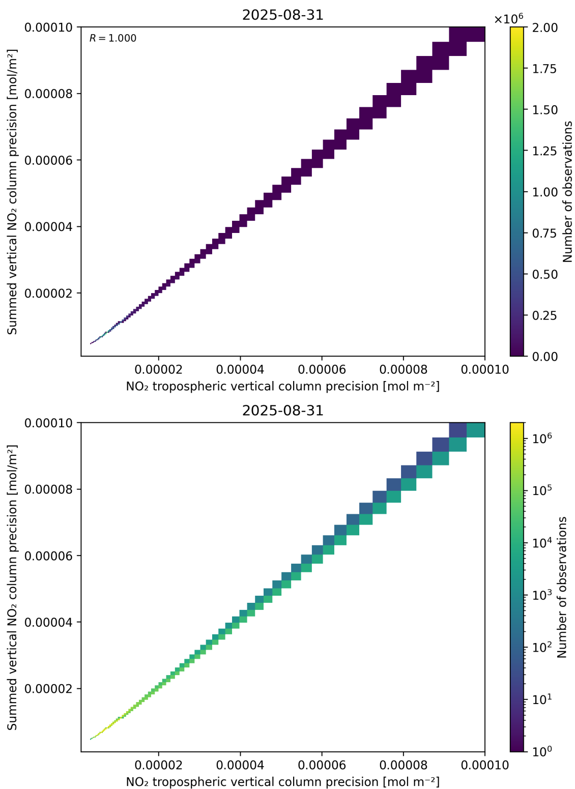
Figure 137: Scatter density plot of “NO 2 tropospheric vertical column precision” against “Summed vertical NO 2 column precision” for 2025-08-30 to 2025-09-01.
