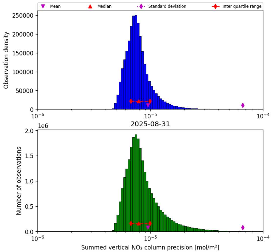
Figure 41: Histogram of "Summed vertical NO 2 column precision" for 2025-08-30 to 2025-09-01
