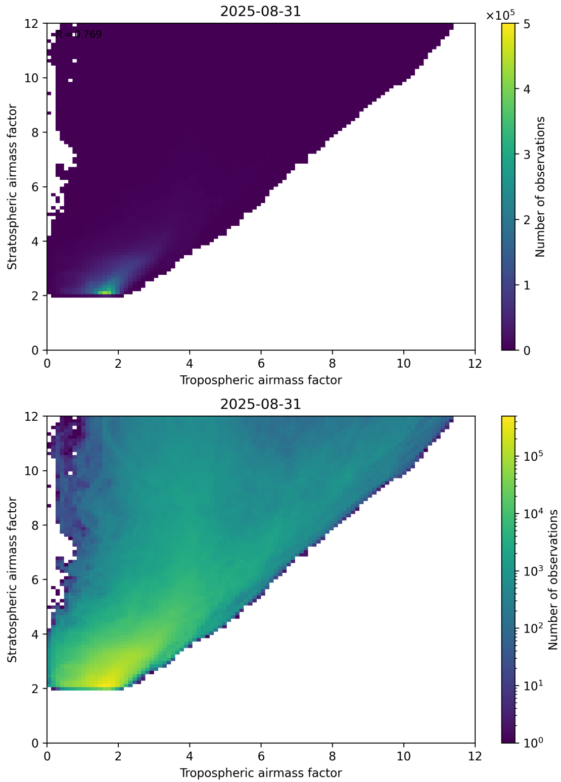
Figure 71: Scatter density plot of “Tropospheric airmass factor” against “Stratospheric airmass factor” for 2025-08-30 to 2025-09-01.
