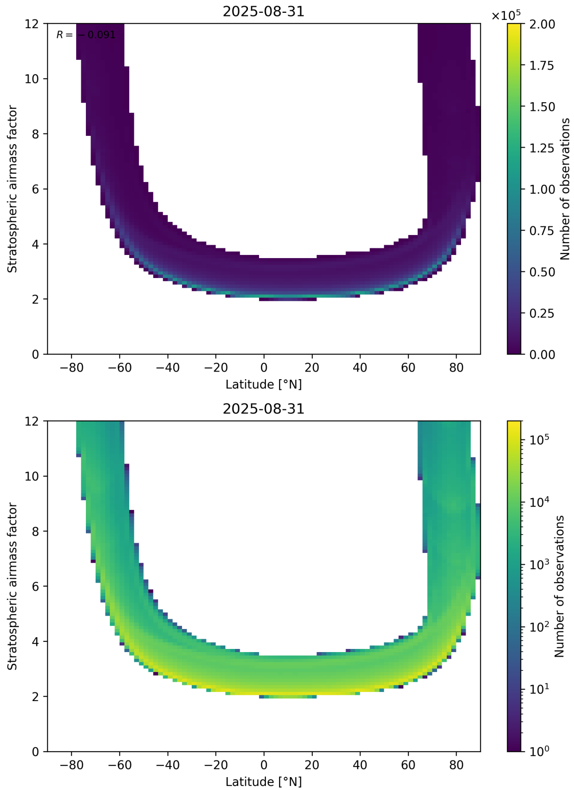
Figure 83: Scatter density plot of “Latitude” against “Stratospheric air mass factor” for 2025-08-30 to 2025-09-01.
