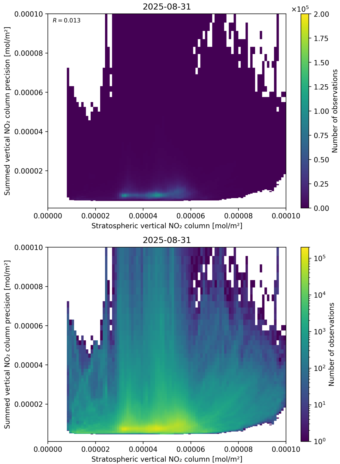
Figure 99: Scatter density plot of “Stratospheric vertical NO 2 column” against “Summed vertical NO 2 column precision” for 2025-08-30 to 2025-09-01.
