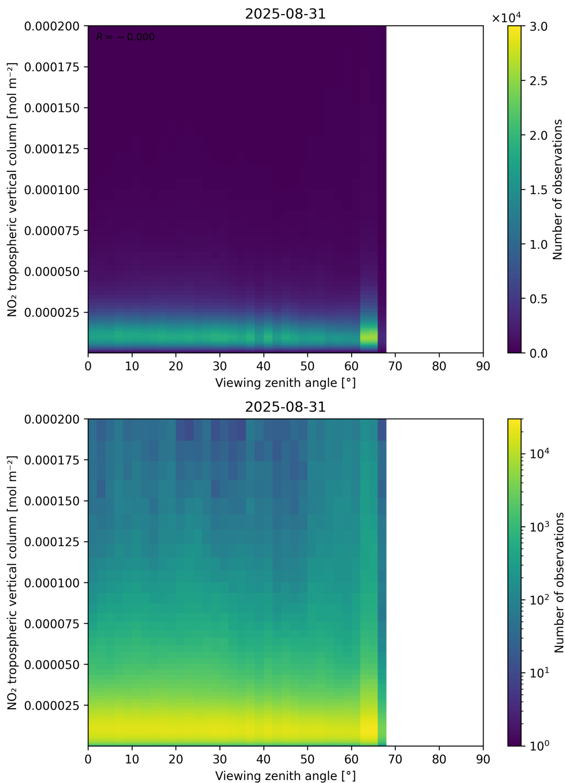
Figure 169: Scatter density plot of “Viewing zenith angle” against “NO 2 tropospheric vertical column” for 2025-08-30 to 2025-09-01.
