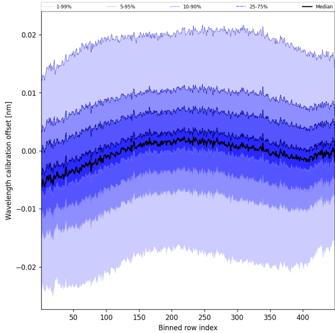
Figure 52: Along track statistics of “Wavelength calibration offset” for 2025-08-30 to 2025-09-01
