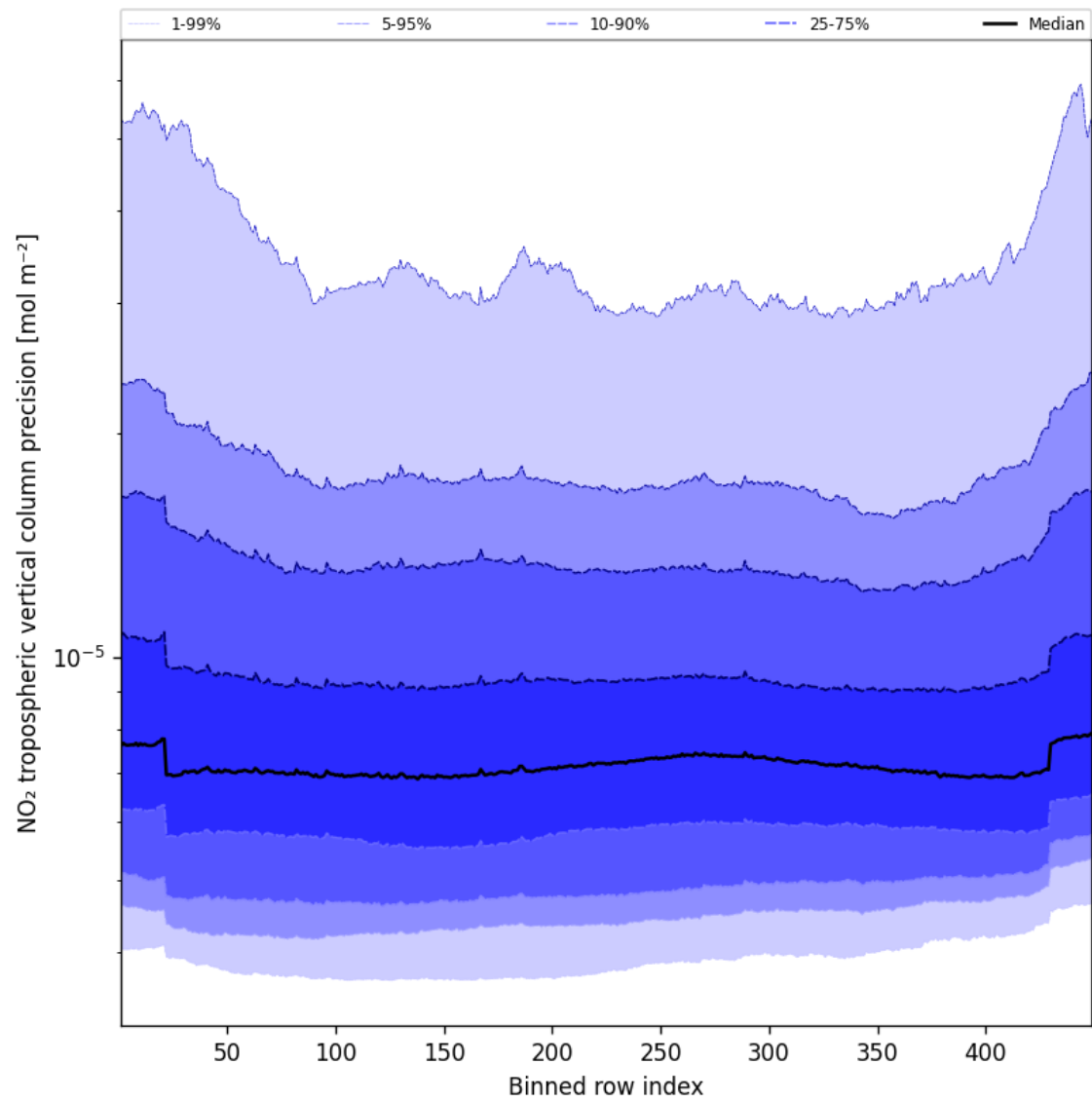
Figure 47: Along track statistics of “NO 2 tropospheric vertical column precision” for 2025-08-30 to 2025-09-01
