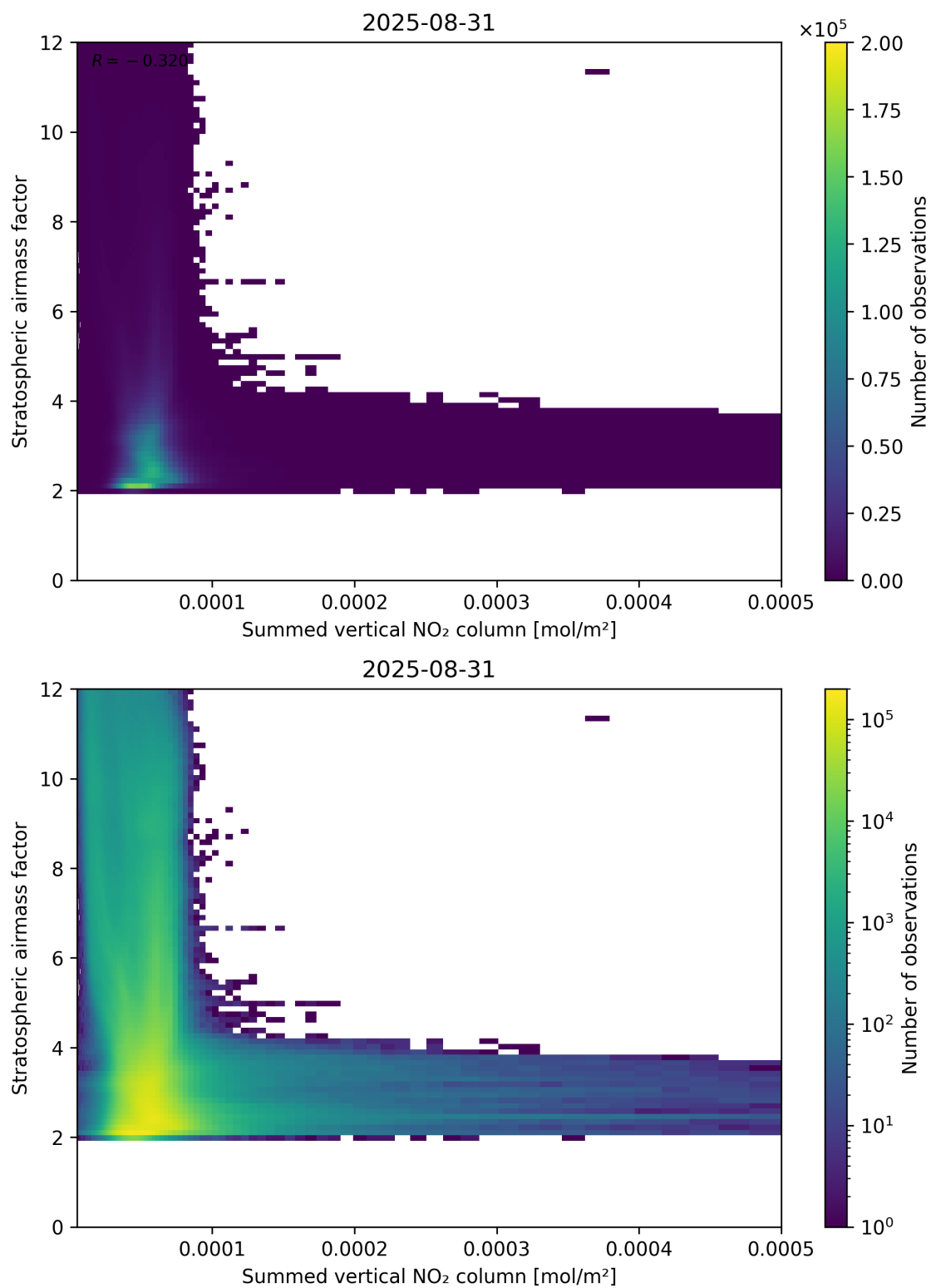
Figure 103: Scatter density plot of “Summed vertical NO 2 column” against “Stratospheric airmass factor” for 2025-08-30 to 2025-09-01.
