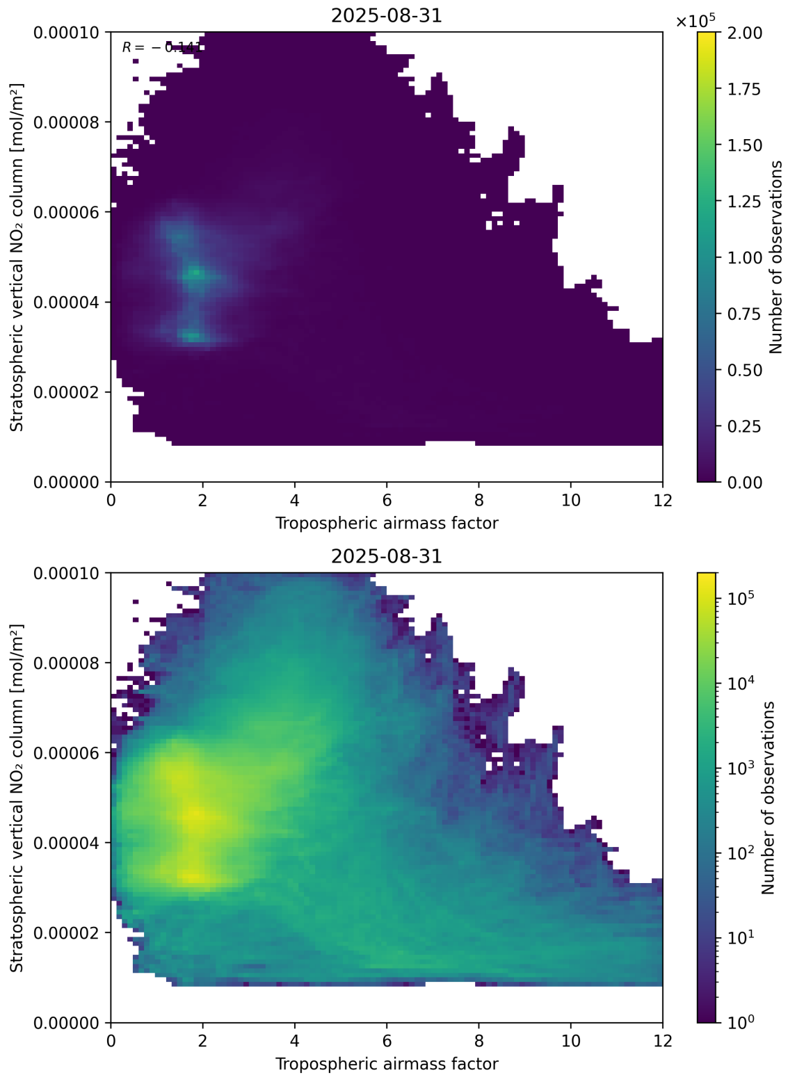
Figure 74: Scatter density plot of “Tropospheric air mass factor” against “Stratospheric vertical NO 2 column” for 2025-08-30 to 2025-09-01.
