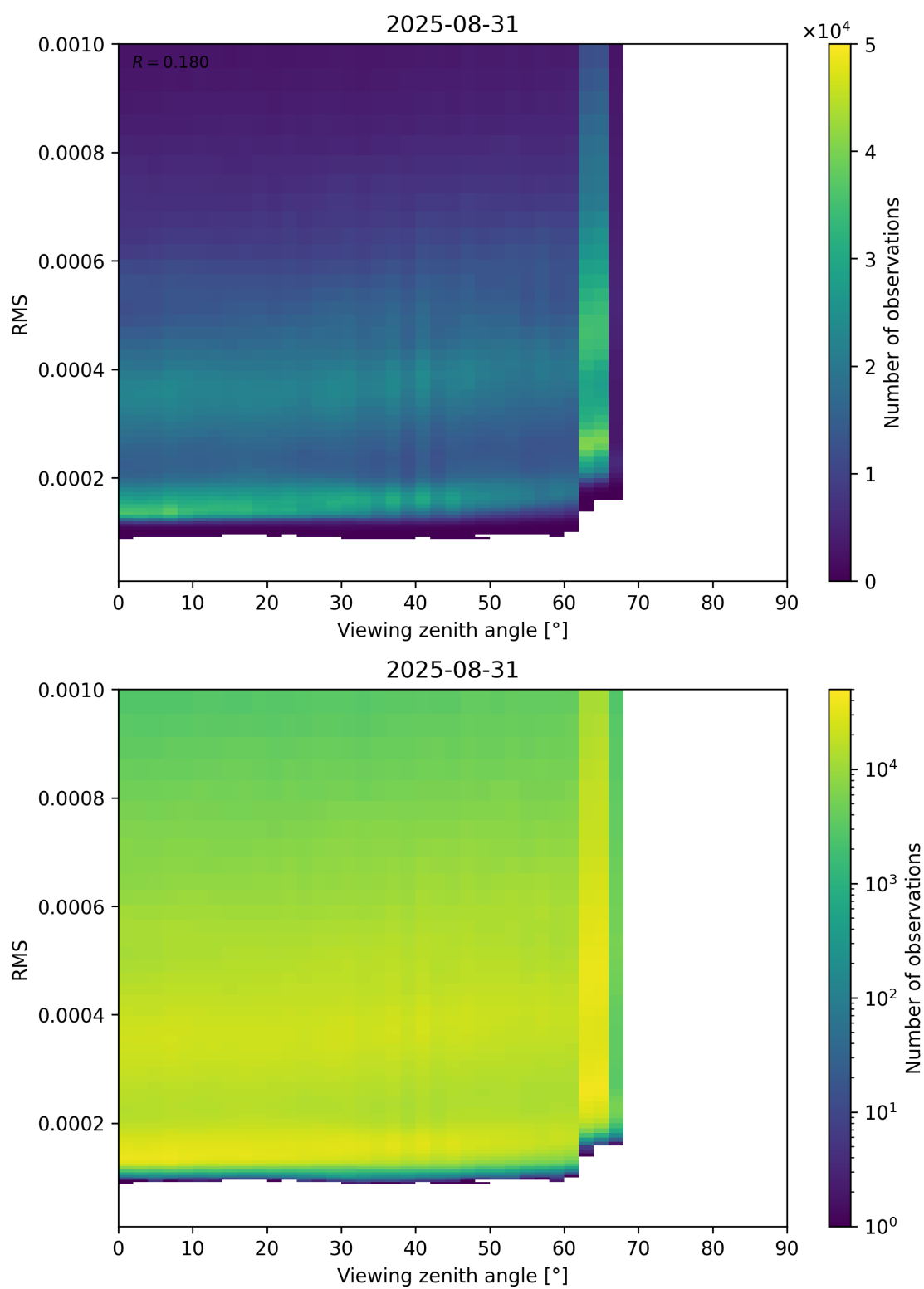
Figure 171: Scatter density plot of “Viewing zenith angle” against “RMS” for 2025-08-30 to 2025-09-01.
