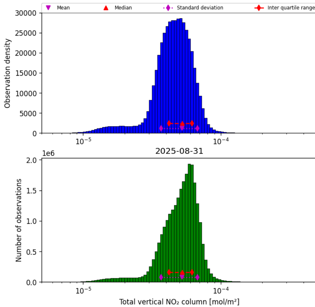
Figure 38: Histogram of “Total vertical NO 2 column” for 2025-08-30 to 2025-09-01
