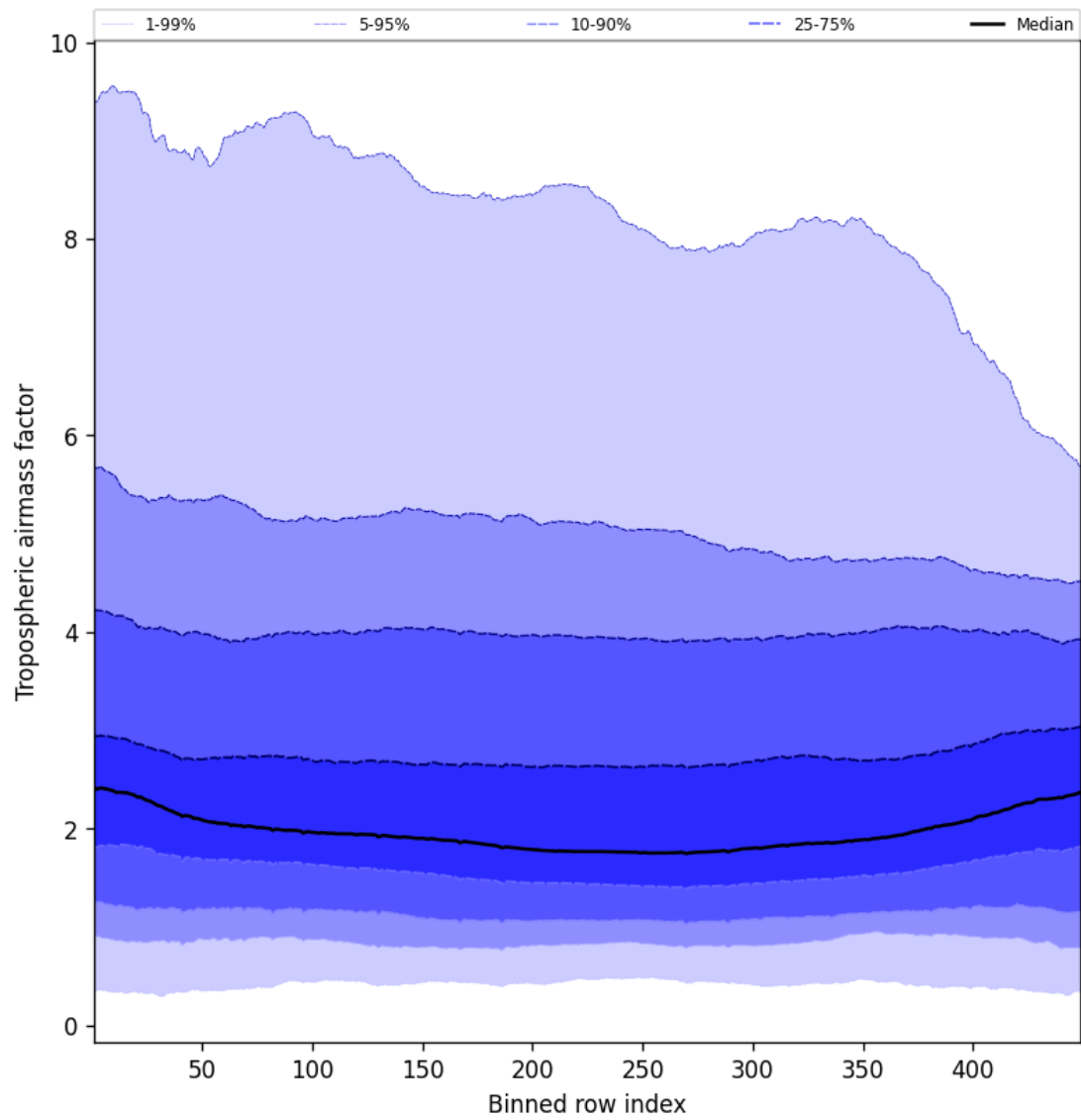
Figure 48: Along track statistics of “Tropospheric air mass factor” for 2025-08-30 to 2025-09-01
