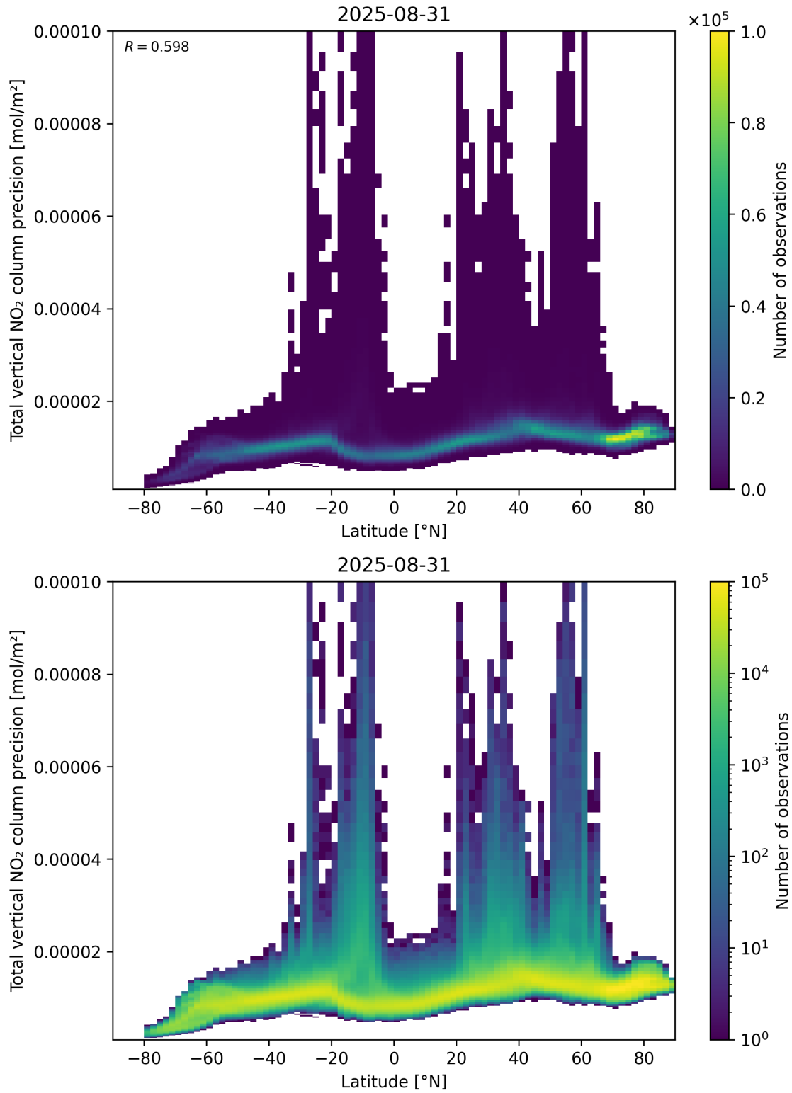
Figure 91: Scatter density plot of “Latitude” against “Total vertical NO 2 column precision” for 2025-08-30 to 2025-09-01.
