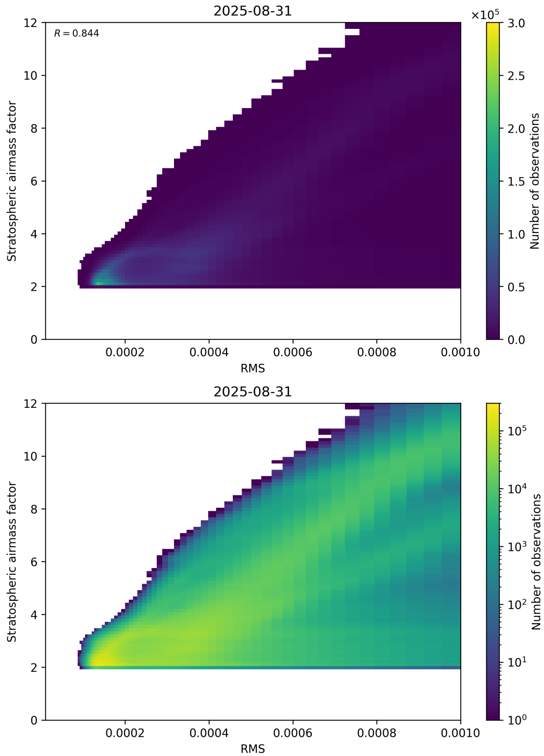
Figure 144: Scatter density plot of “RMS” against “Stratospheric airmass factor” for 2025-08-30 to 2025-09-01.
