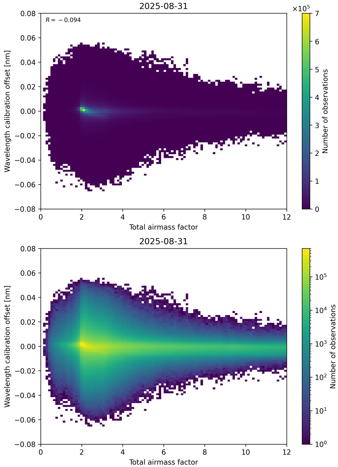
Figure 70: Scatter density plot of “Total airmass factor” against “Wavelength calibration offset” for 2025-08-30 to 2025-09-01.
