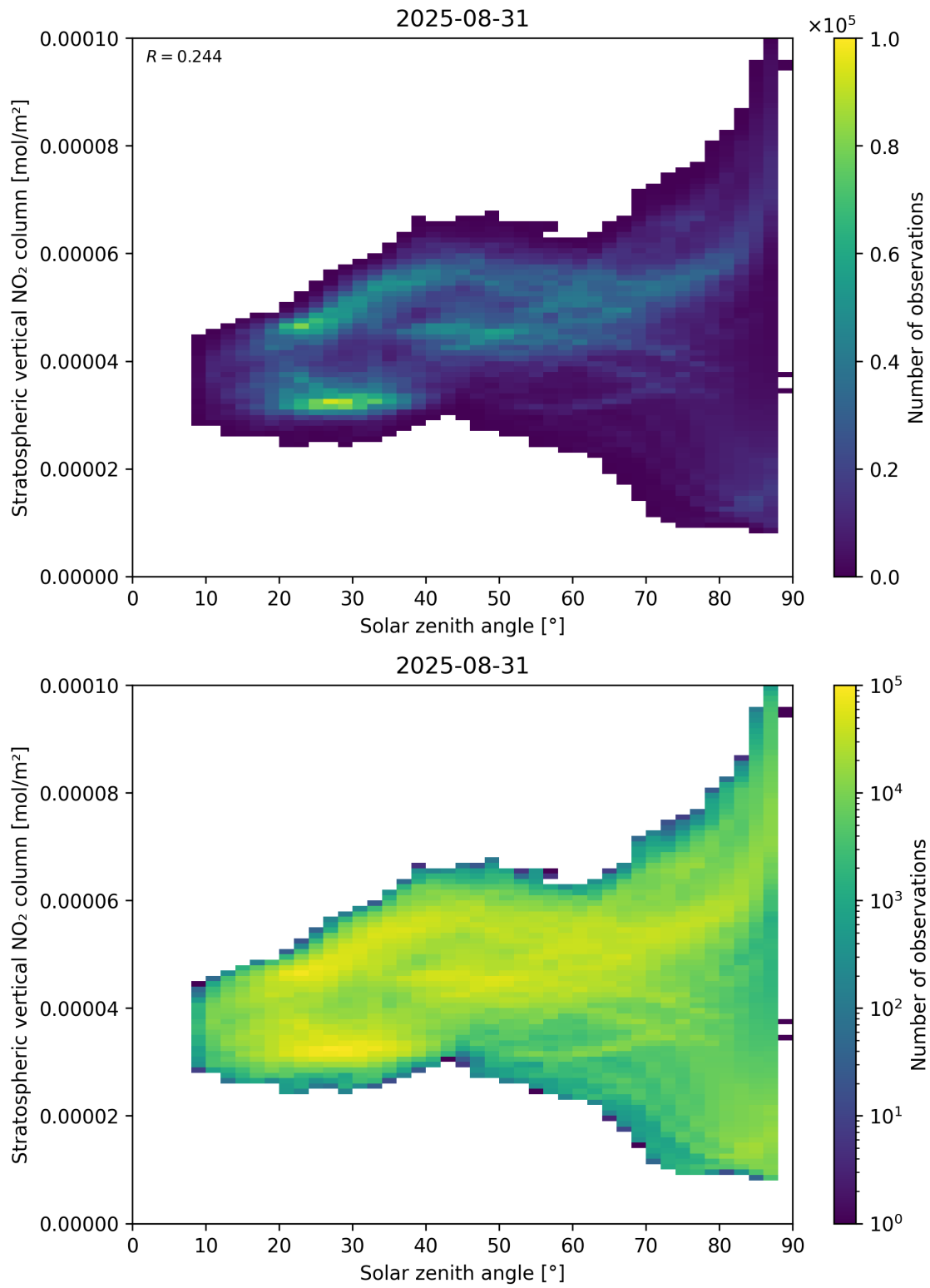
Figure 150: Scatter density plot of “Solar zenith angle” against “Stratospheric vertical NO 2 column” for 2025-08-30 to 2025-09-01.
