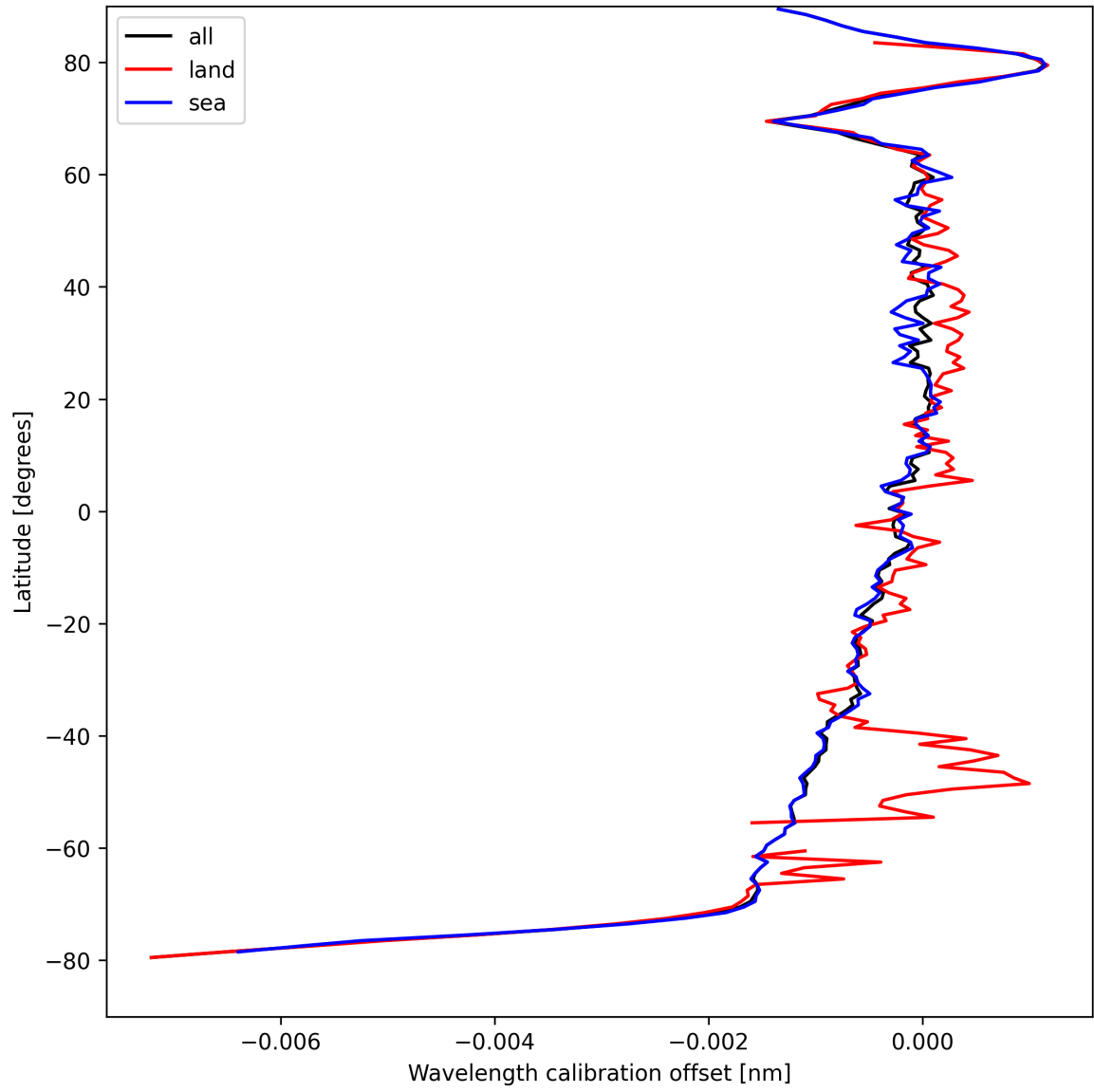
Figure 18: Zonal average of “Wavelength calibration offset” for 2025-08-30 to 2025-09-01.
