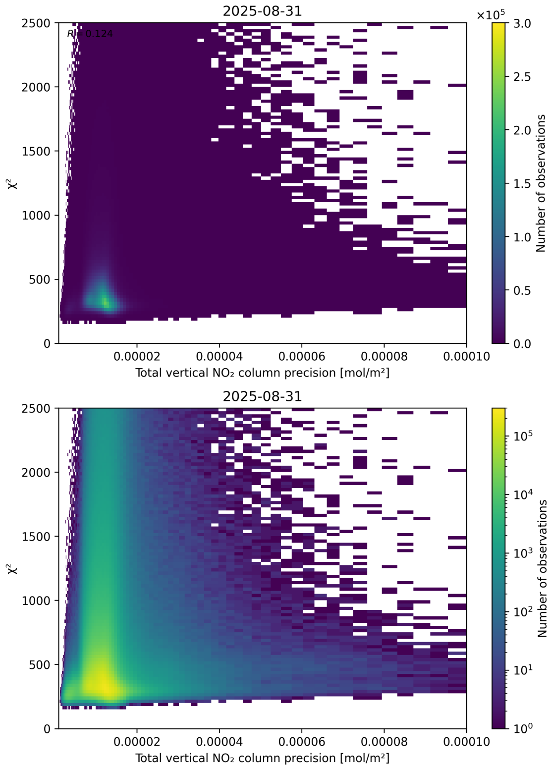
Figure 116: Scatter density plot of “Total vertical NO 2 column precision” against “ \chi^2 ” for 2025-08-30 to 2025-09-01.
