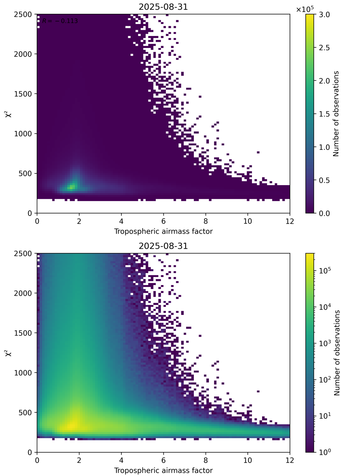
Figure 73: Scatter density plot of “Tropospheric airmass factor” against “ \chi^2 ” for 2025-08-30 to 2025-09-01.
