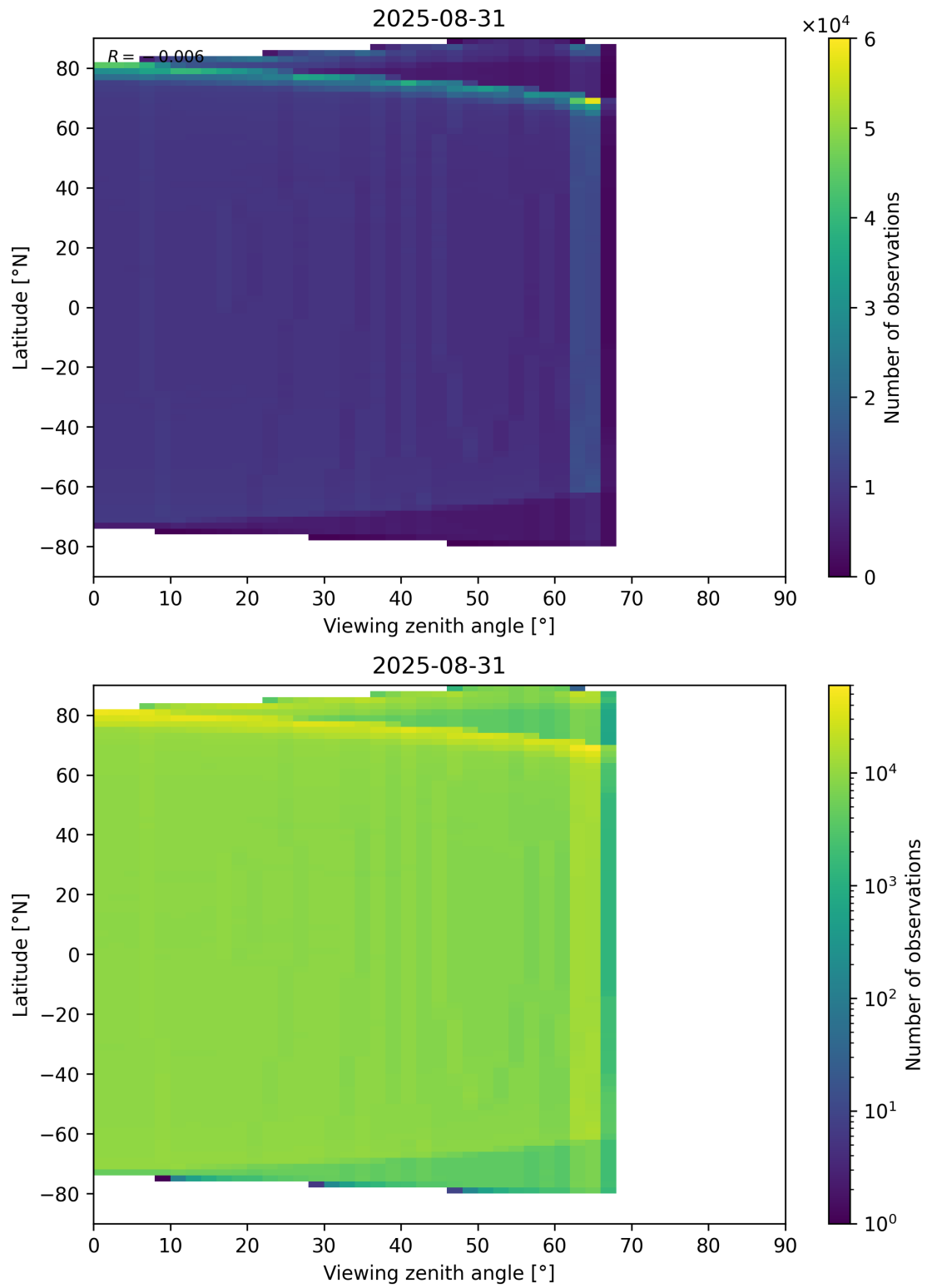
Figure 163: Scatter density plot of “Viewing zenith angle” against “Latitude” for 2025-08-30 to 2025-09-01.
