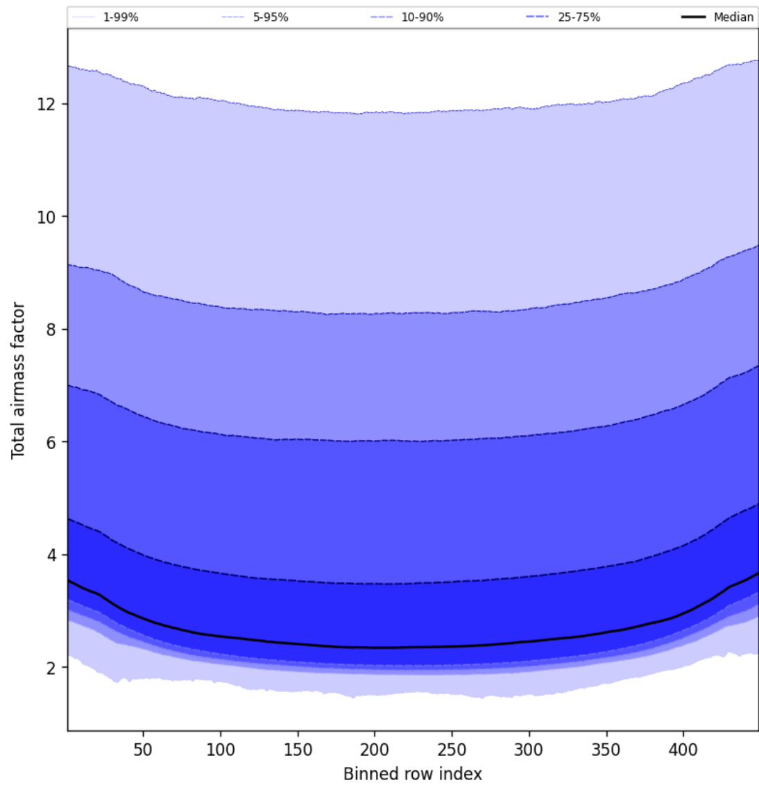
Figure 49: Along track statistics of “Total airmass factor” for 2025-08-30 to 2025-09-01
