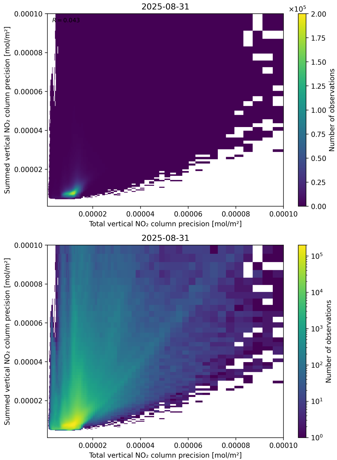
Figure 118: Scatter density plot of “Total vertical NO 2 column precision” against “Summed vertical NO 2 column precision” for 2025-08-30 to 2025-09-01.
