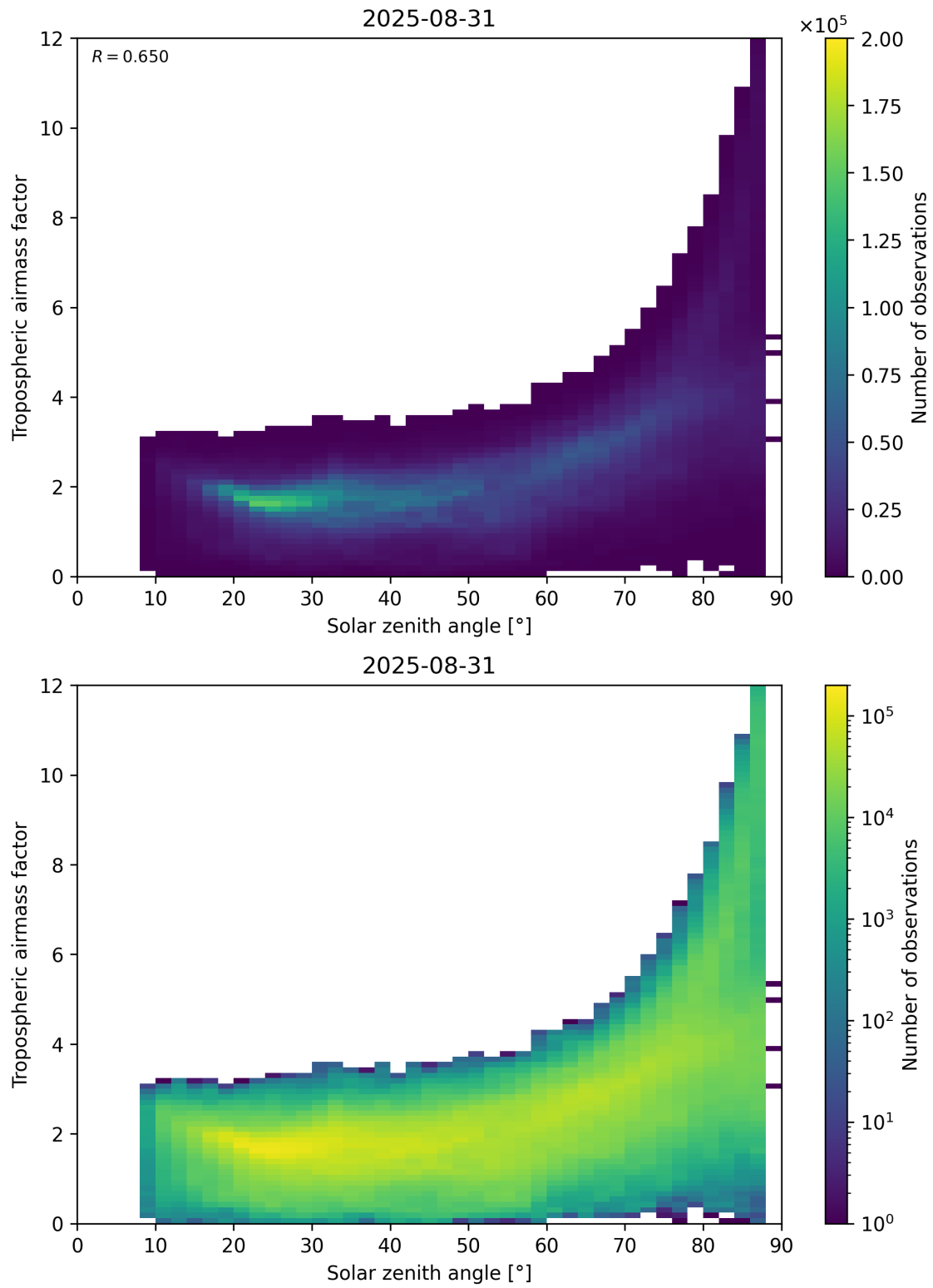
Figure 147: Scatter density plot of “Solar zenith angle” against “Tropospheric airmass factor” for 2025-08-30 to 2025-09-01.
