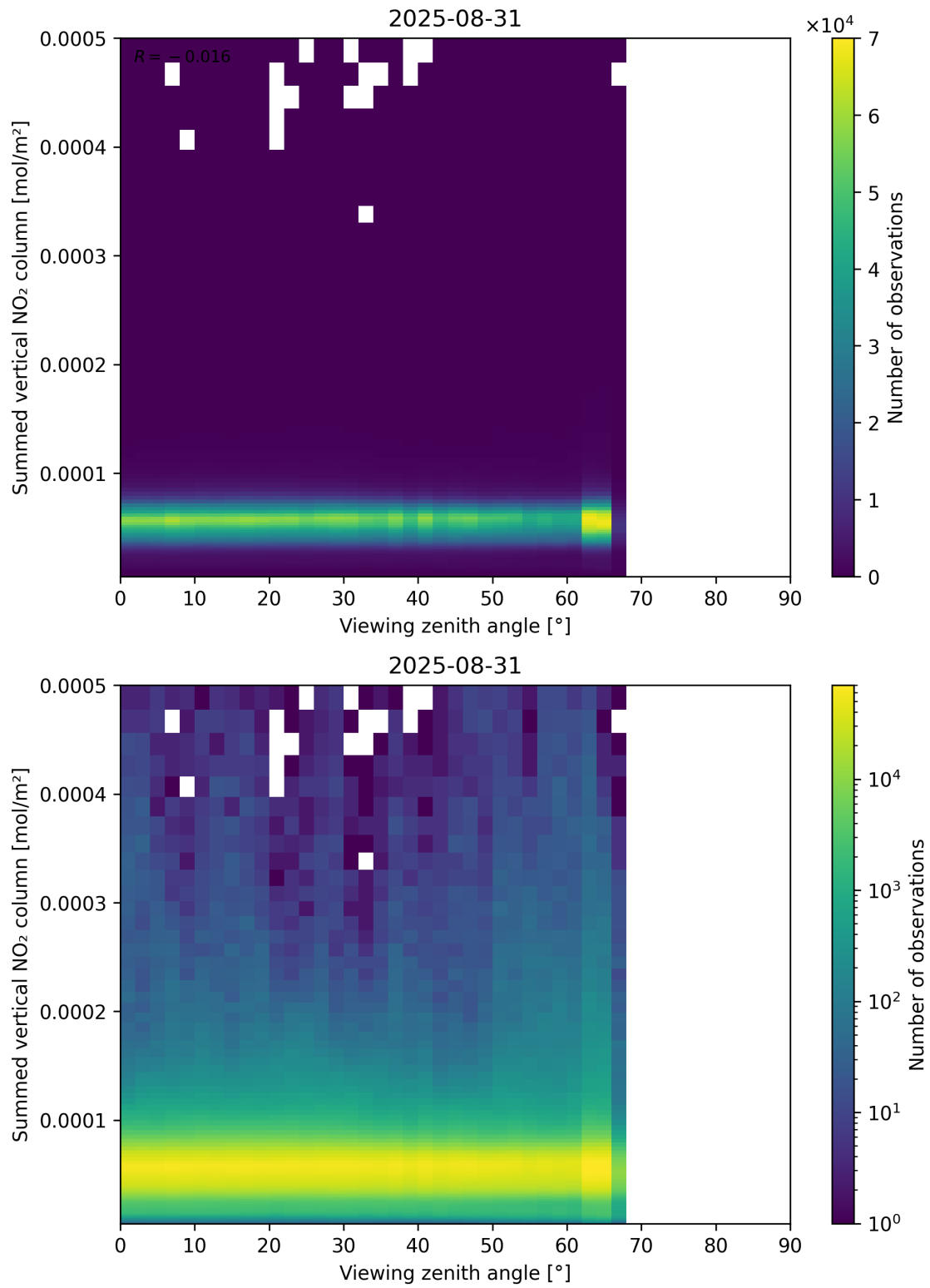
Figure 165: Scatter density plot of “Viewing zenith angle” against “Summed vertical NO 2 column” for 2025-08-30 to 2025-09-01.
