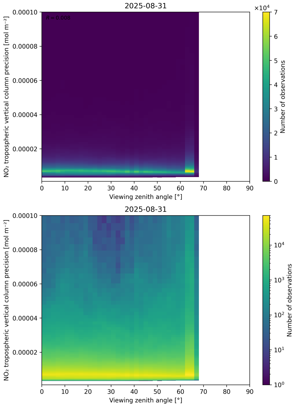
Figure 170: Scatter density plot of “Viewing zenith angle” against “NO 2 tropospheric vertical column precision” for 2025-08-30 to 2025-09-01.
