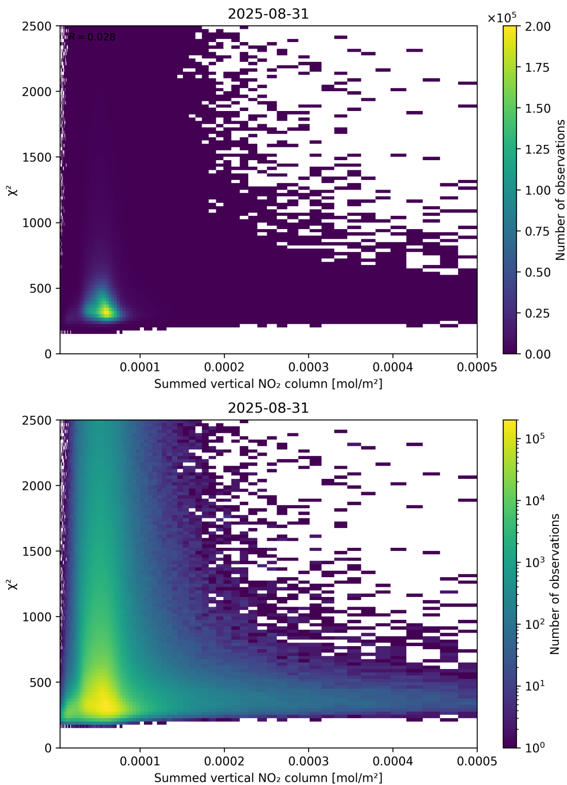
Figure 104: Scatter density plot of “Summed vertical NO 2 column” against “ \chi^2 ” for 2025-08-30 to 2025-09-01.
