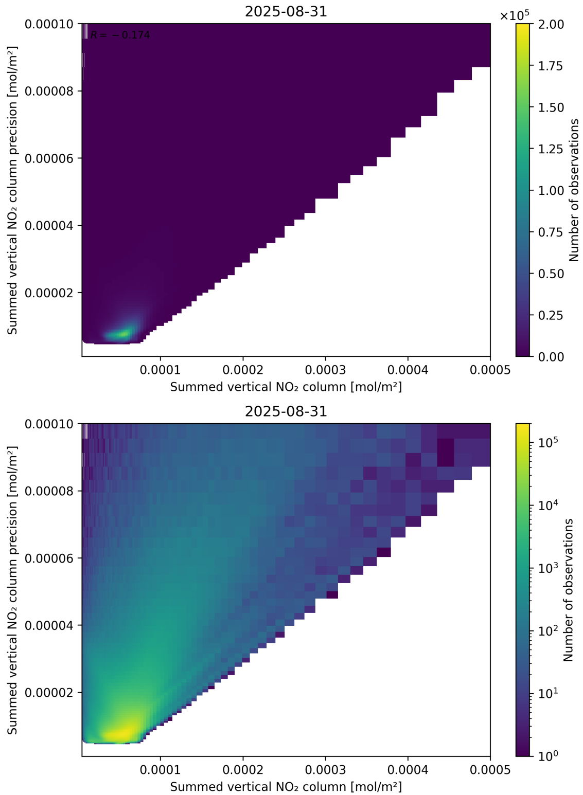
Figure 105: Scatter density plot of “Summed vertical NO 2 column” against “Summed vertical NO 2 column precision” for 2025-08-30 to 2025-09-01.
