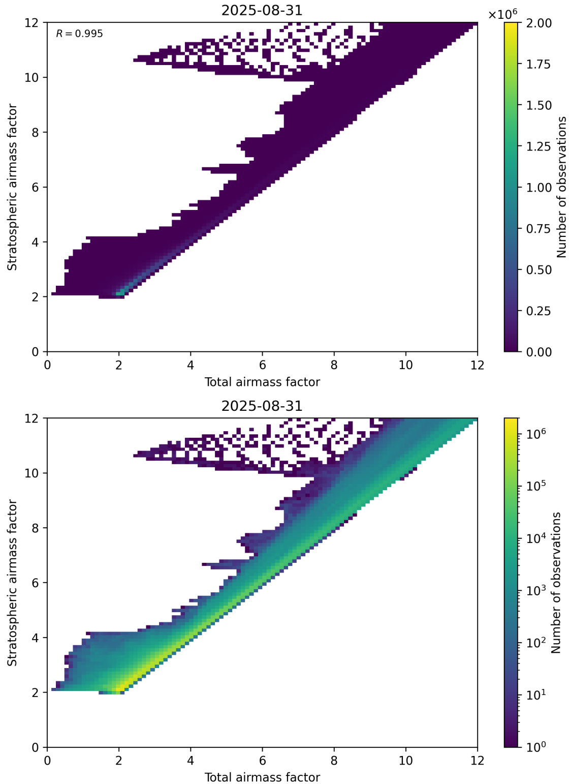
Figure 62: Scatter density plot of “Total airmass factor” against “Stratospheric airmass factor” for 2025-08-30 to 2025-09-01.
