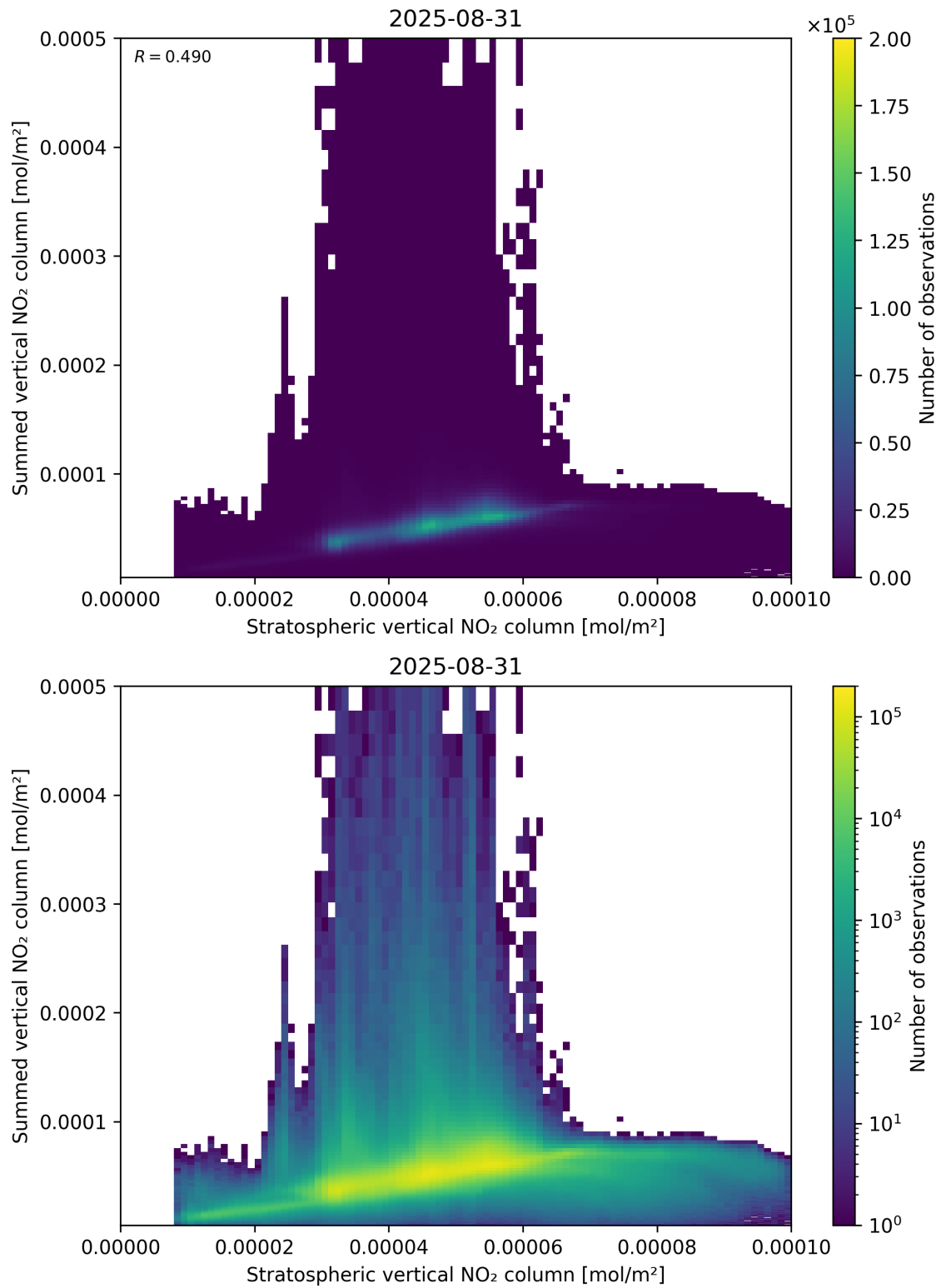
Figure 98: Scatter density plot of “Stratospheric vertical NO 2 column” against “Summed vertical NO 2 column” for 2025-08-30 to 2025-09-01.
