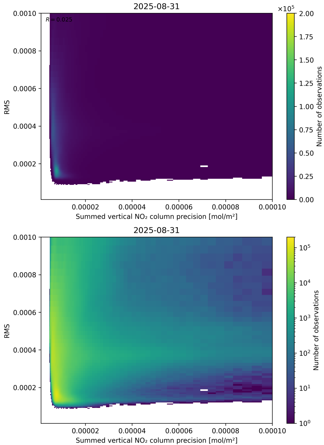
Figure 108: Scatter density plot of “Summed vertical NO 2 column precision” against “RMS” for 2025-08-30 to 2025-09-01.
