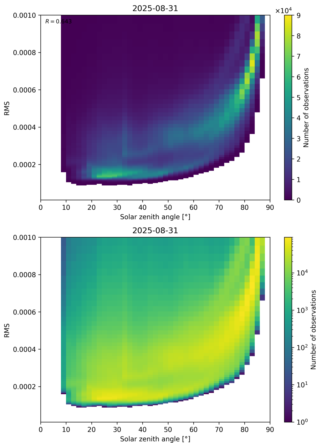
Figure 157: Scatter density plot of “Solar zenith angle” against “RMS” for 2025-08-30 to 2025-09-01.
