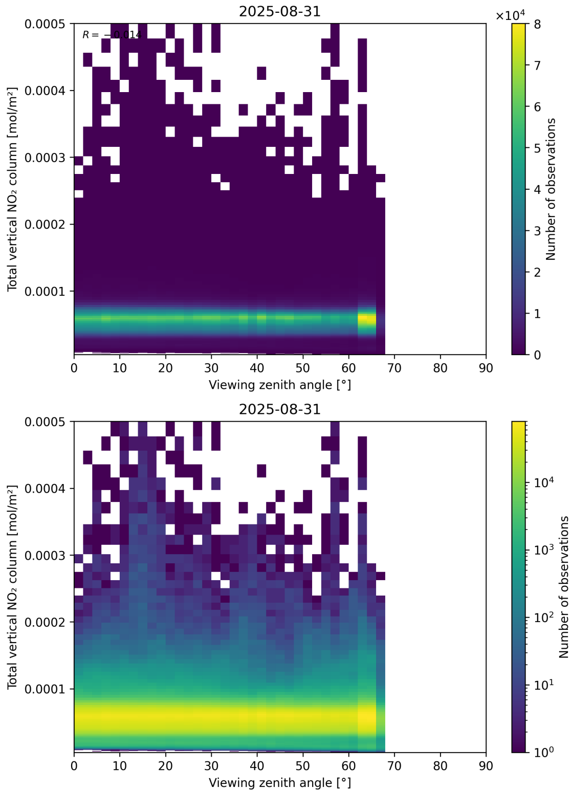
Figure 167: Scatter density plot of “Viewing zenith angle” against “Total vertical NO 2 column” for 2025-08-30 to 2025-09-01.
