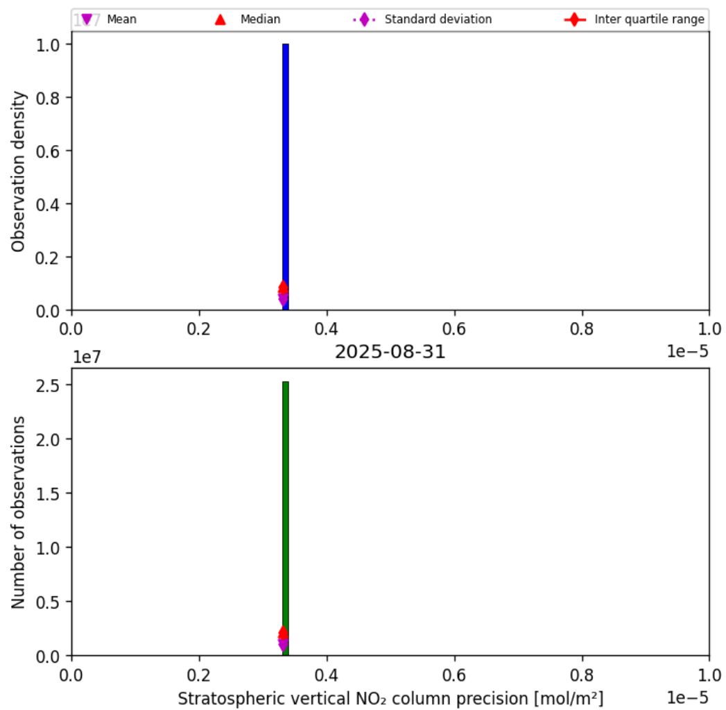
Figure 37: Histogram of “Stratospheric vertical NO 2 column precision” for 2025-08-30 to 2025-09-01
