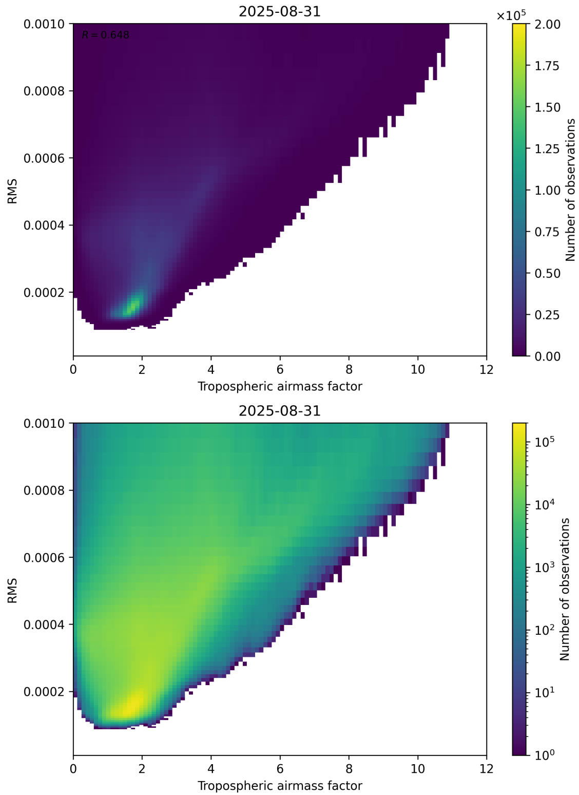
Figure 79: Scatter density plot of “Tropospheric airmass factor” against “RMS” for 2025-08-30 to 2025-09-01.
