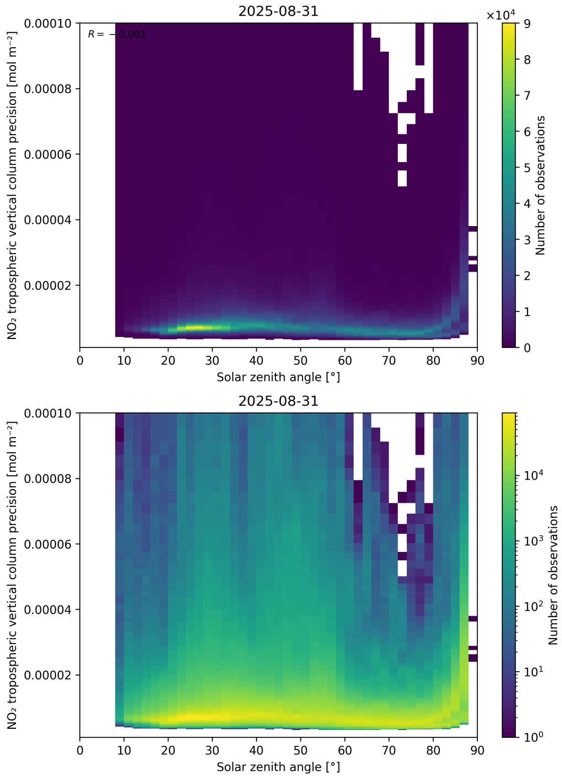
Figure 156: Scatter density plot of “Solar zenith angle” against “NO 2 tropospheric vertical column precision” for 2025-08-30 to 2025-09-01.
