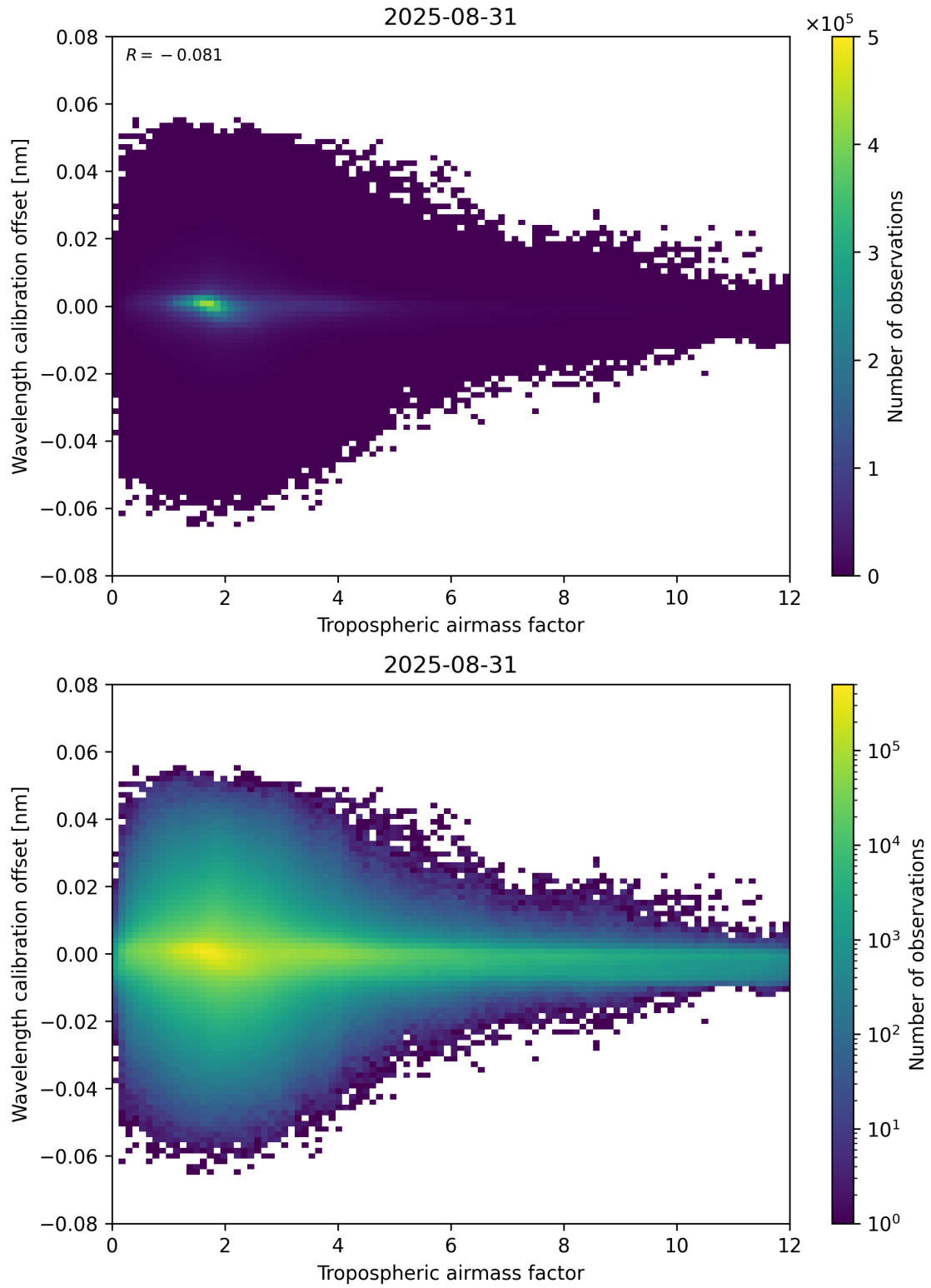
Figure 80: Scatter density plot of “Tropospheric airmass factor” against “Wavelength calibration offset” for 2025-08-30 to 2025-09-01.
