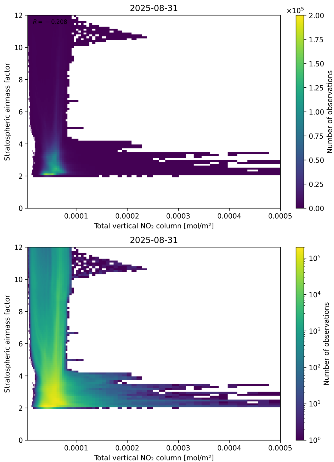
Figure 110: Scatter density plot of “Total vertical NO 2 column” against “Stratospheric airmass factor” for 2025-08-30 to 2025-09-01.
