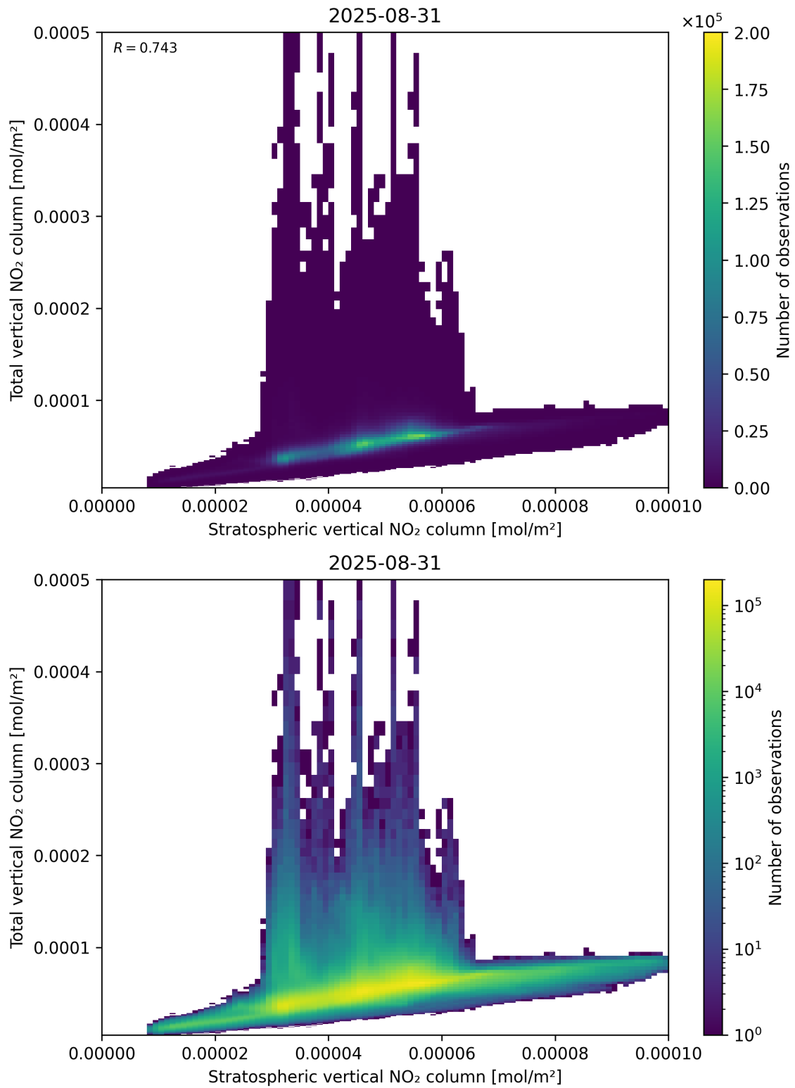
Figure 100: Scatter density plot of “Stratospheric vertical NO 2 column” against “Total vertical NO 2 column” for 2025-08-30 to 2025-09-01.
