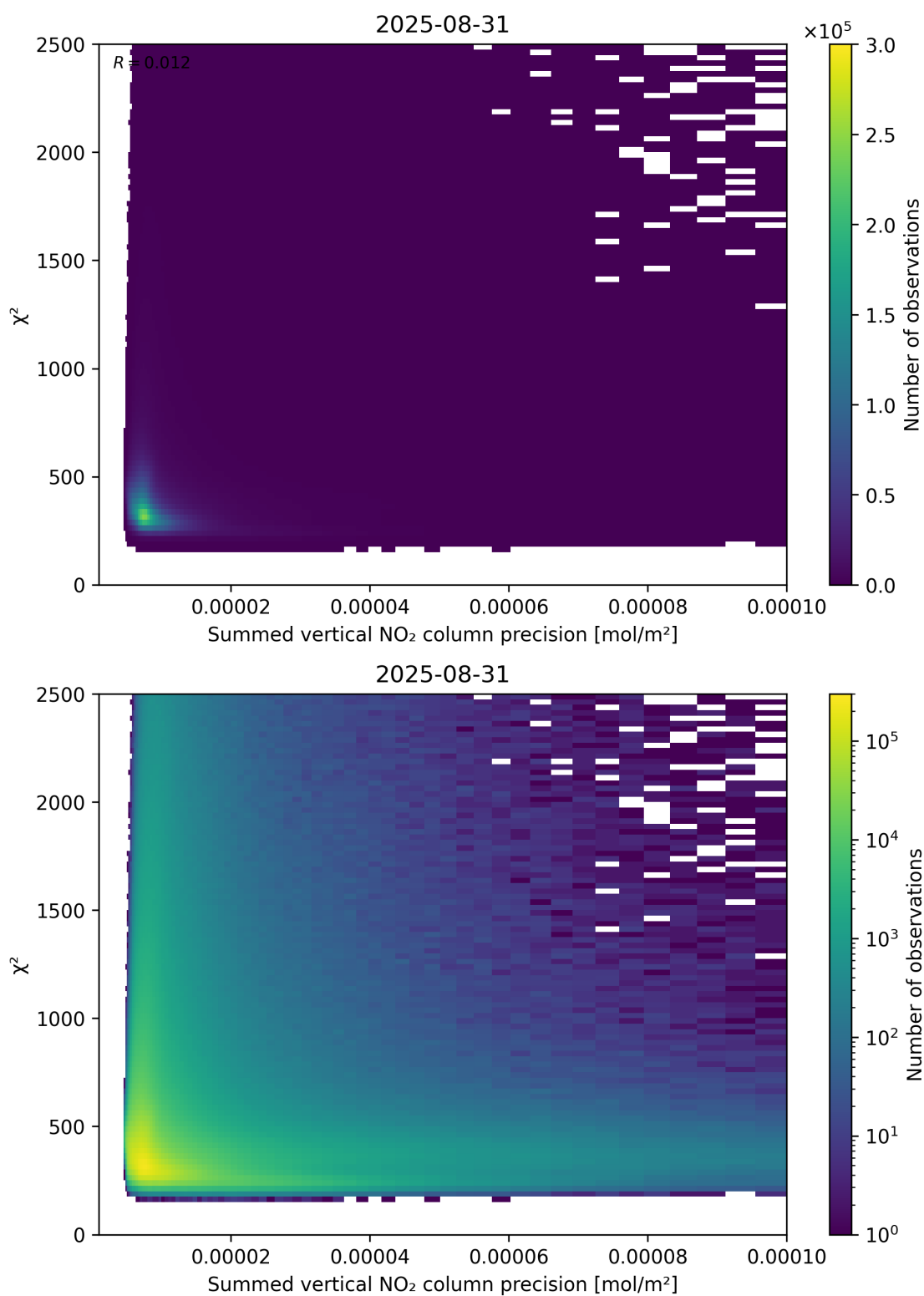
Figure 107: Scatter density plot of “Summed vertical NO 2 column precision” against “ \chi^2 ” for 2025-08-30 to 2025-09-01.
