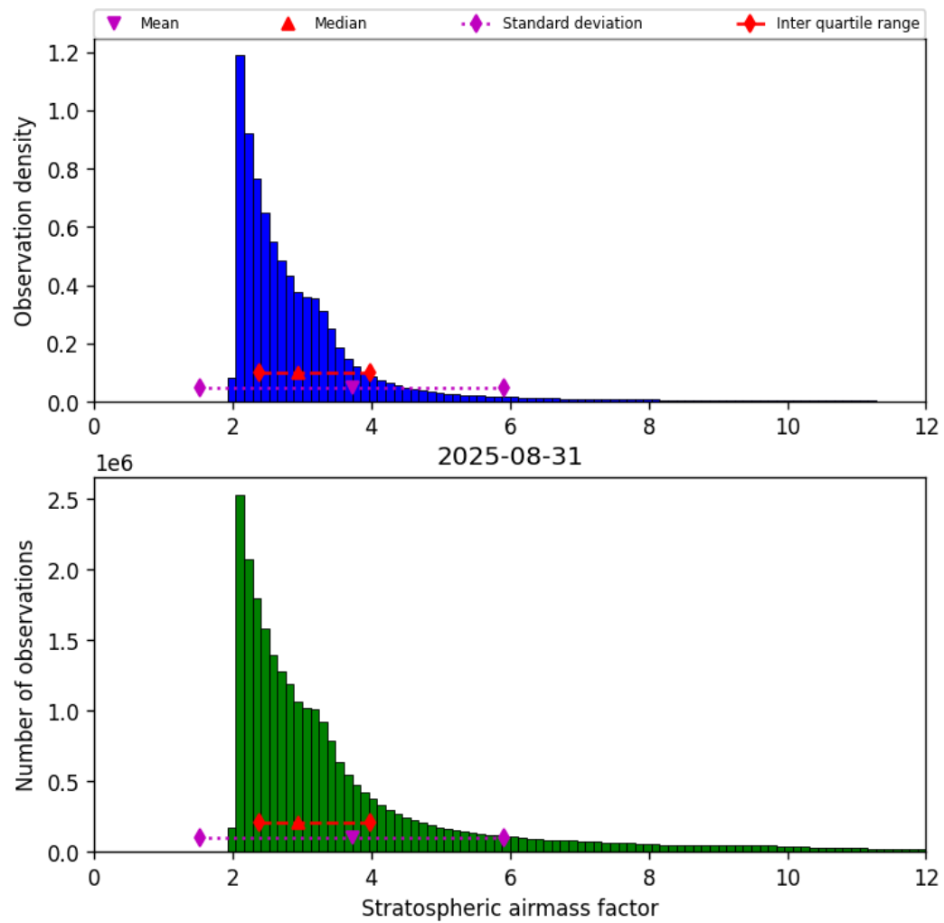
Figure 44: Histogram of “Stratospheric airmass factor” for 2025-08-30 to 2025-09-01
