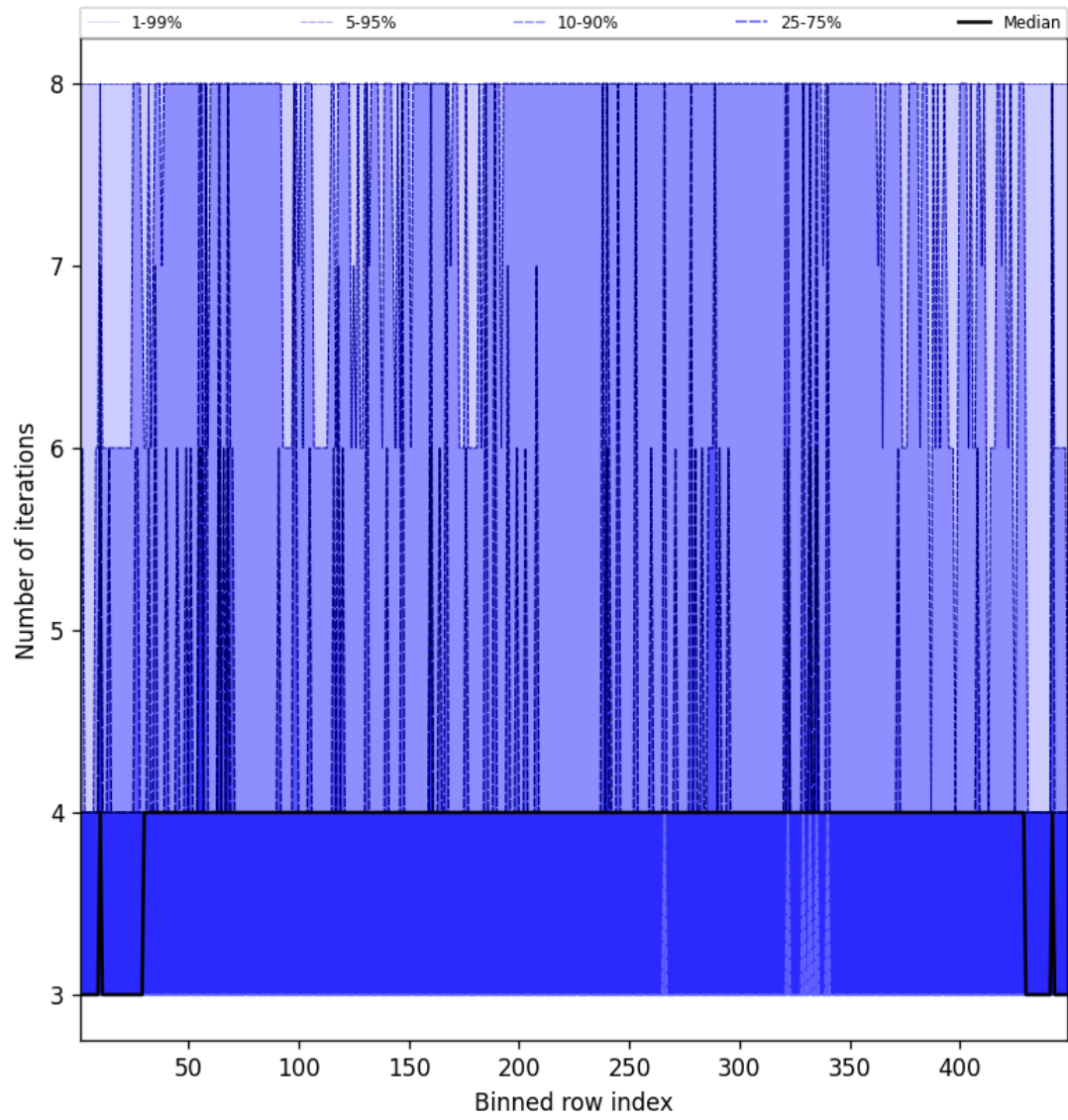
Figure 51: Along track statistics of “Number of iterations” for 2025-08-30 to 2025-09-01
