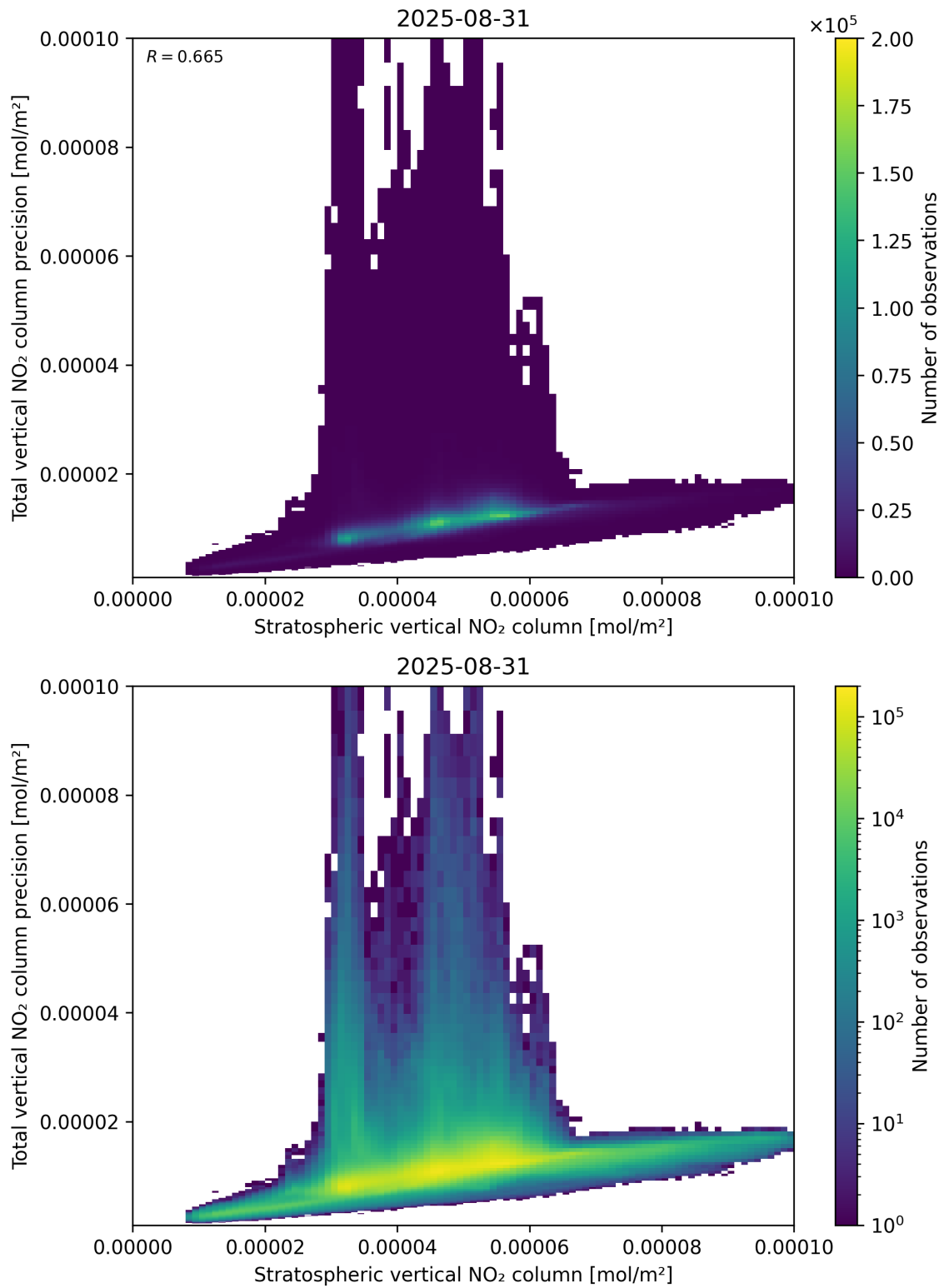
Figure 101: Scatter density plot of “Stratospheric vertical NO 2 column” against “Total vertical NO 2 column precision” for 2025-08-30 to 2025-09-01.
