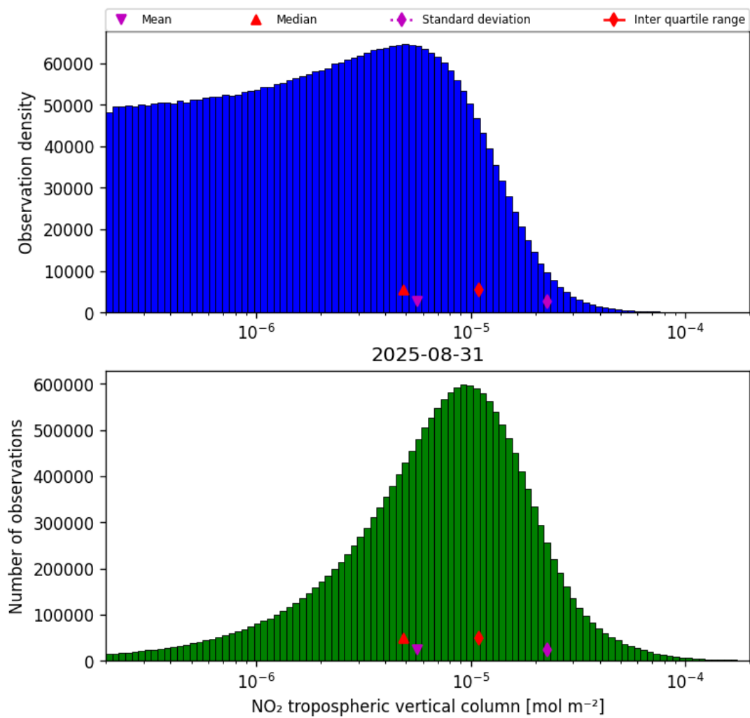
Figure 29: Histogram of “NO 2 tropospheric vertical column” for 2025-08-30 to 2025-09-01
