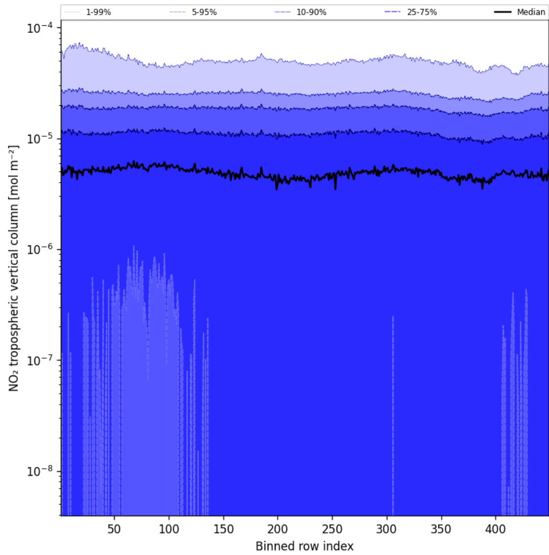
Figure 46: Along track statistics of “NO 2 tropospheric vertical column” for 2025-08-30 to 2025-09-01
