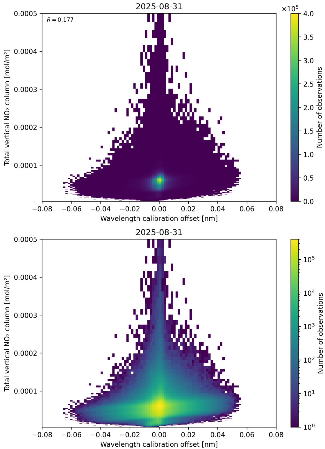
Figure 179: Scatter density plot of “Wavelength calibration offset” against “Total vertical NO 2 column” for 2025-08-30 to 2025-09-01.
