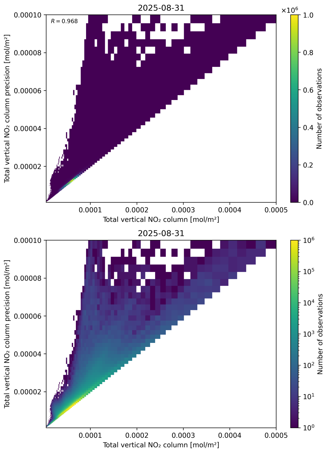
Figure 114: Scatter density plot of “Total vertical NO 2 column” against “Total vertical NO 2 column precision” for 2025-08-30 to 2025-09-01.
