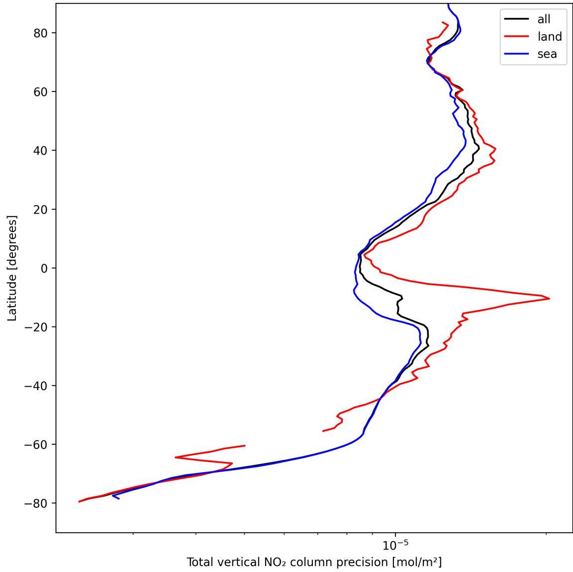
Figure 22: Zonal average of “Total vertical NO 2 column precision” for 2025-08-30 to 2025-09-01.
