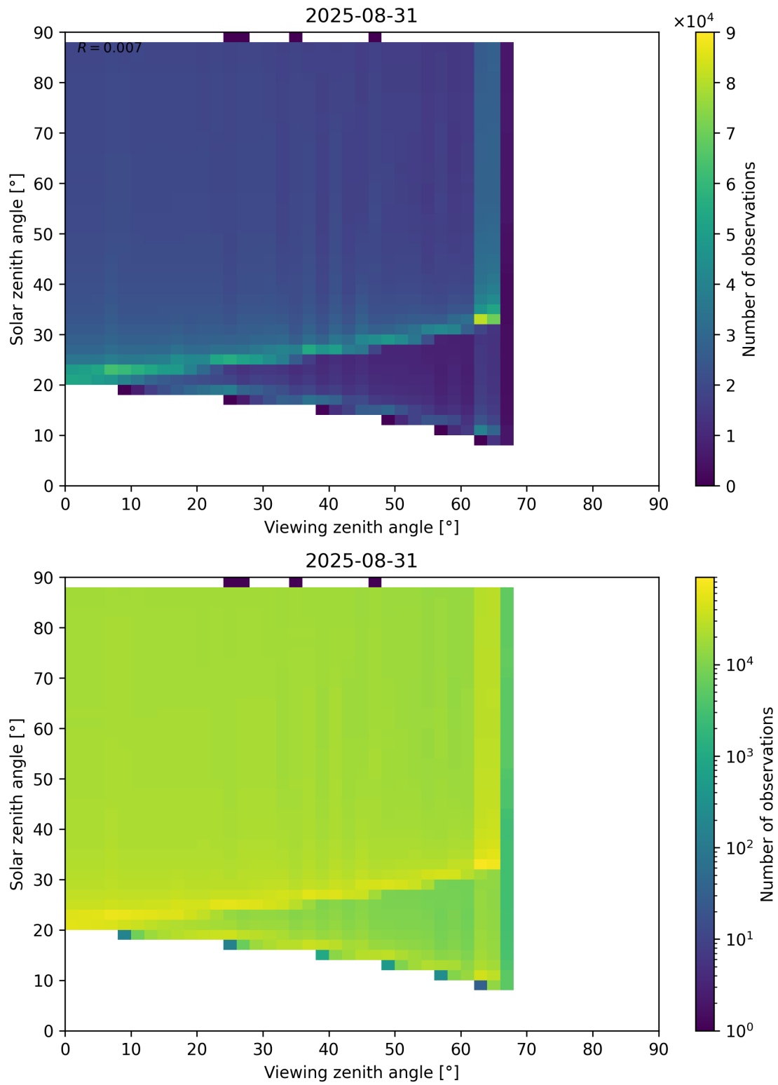
Figure 172: Scatter density plot of “Viewing zenith angle” against “Solar zenith angle” for 2025-08-30 to 2025-09-01.
