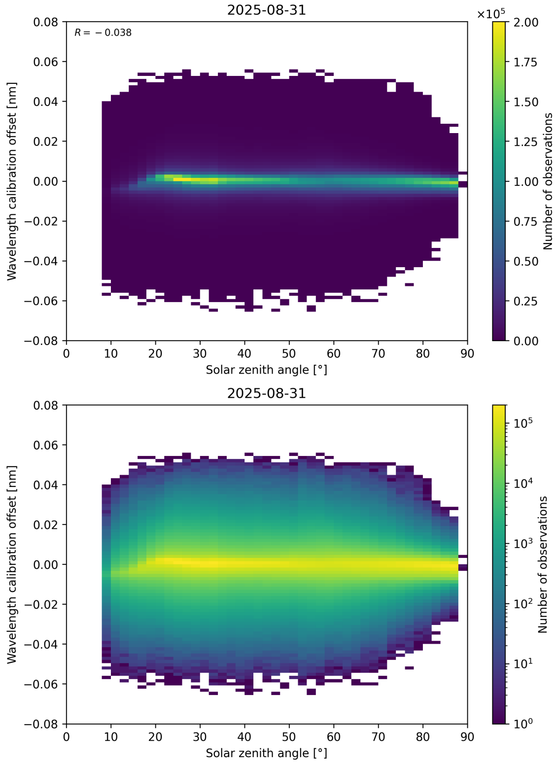
Figure 158: Scatter density plot of “Solar zenith angle” against “Wavelength calibration offset” for 2025-08-30 to 2025-09-01.
