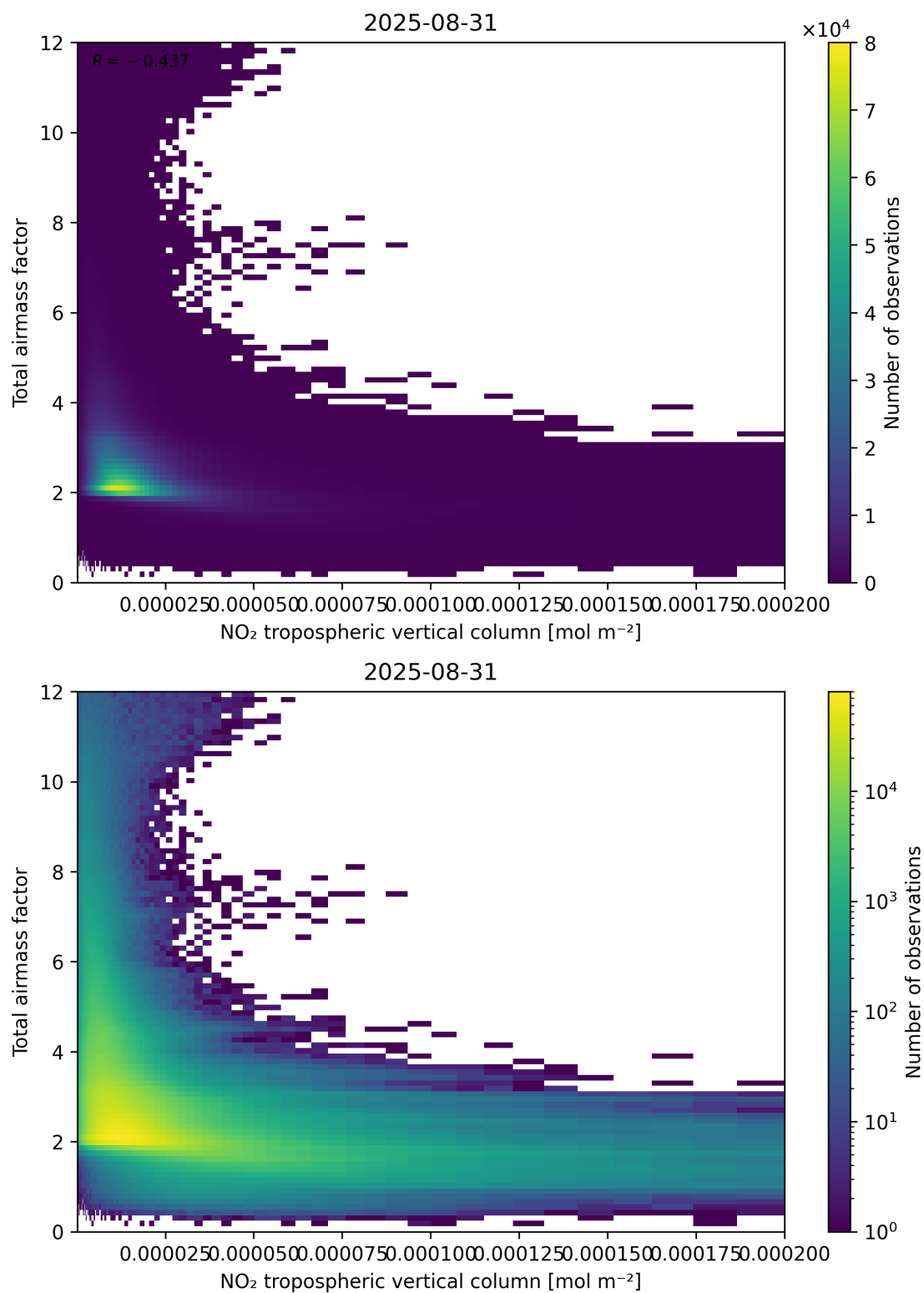
Figure 122: Scatter density plot of “NO 2 tropospheric vertical column” against “Total air mass factor” for 2025-08-30 to 2025-09-01.
