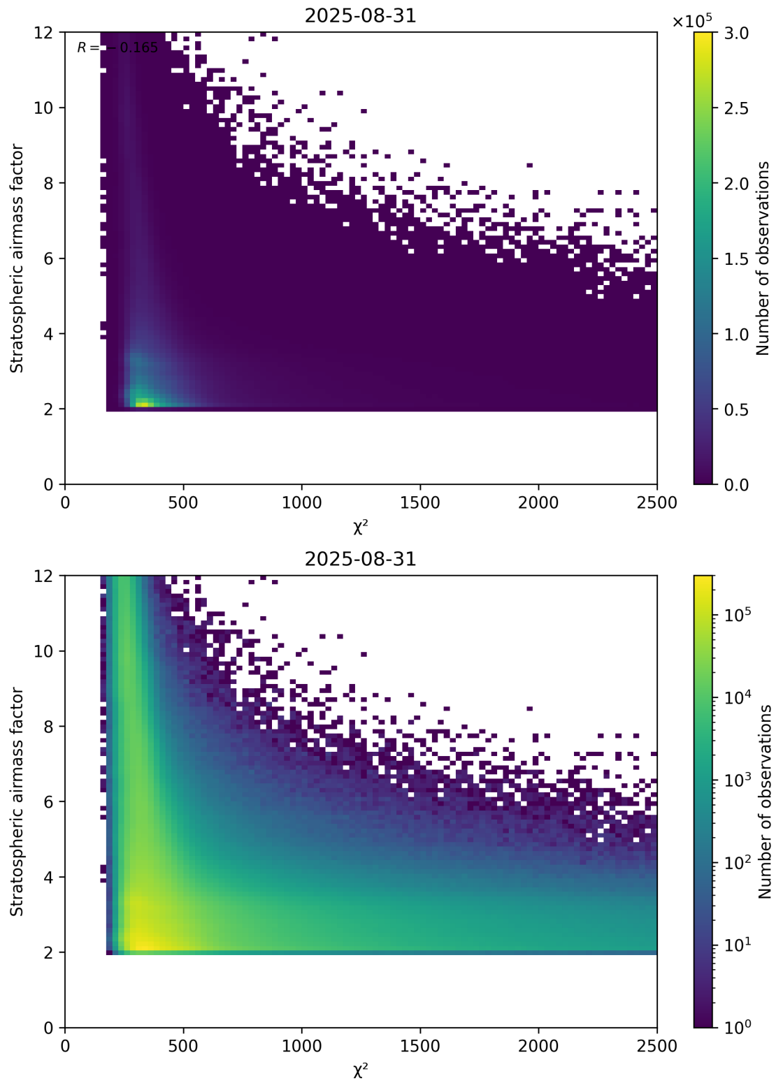
Figure 81: Scatter density plot of “ \chi^2 ” against “Stratospheric airmass factor” for 2025-08-30 to 2025-09-01.
