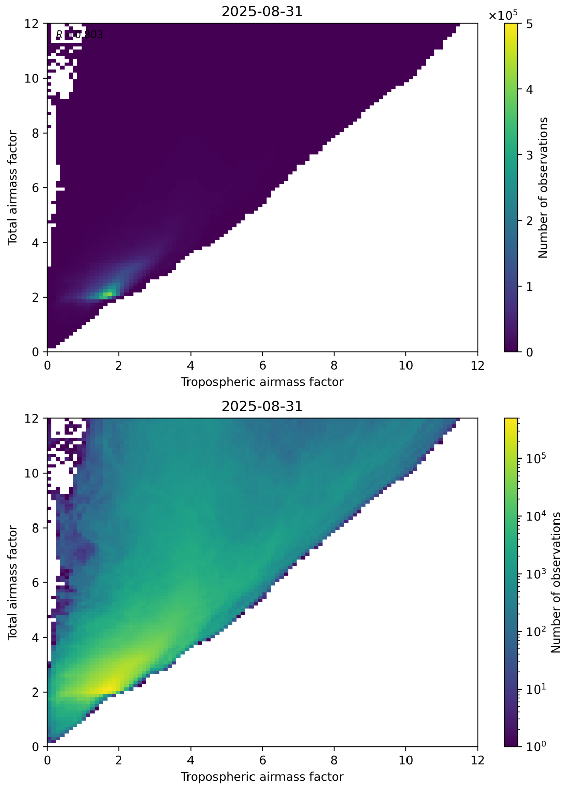
Figure 72: Scatter density plot of “Tropospheric airmass factor” against “Total airmass factor” for 2025-08-30 to 2025-09-01.
