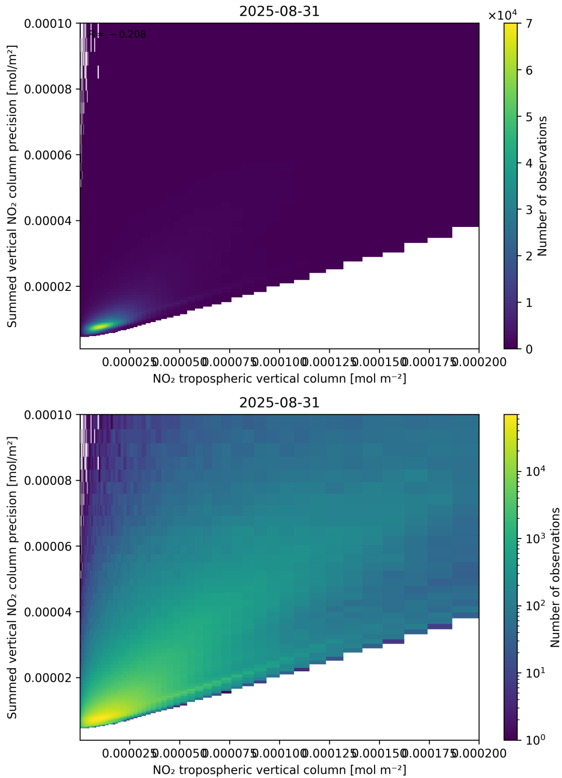
Figure 127: Scatter density plot of “NO 2 tropospheric vertical column” against “Summed vertical NO 2 column precision” for 2025-08-30 to 2025-09-01.
