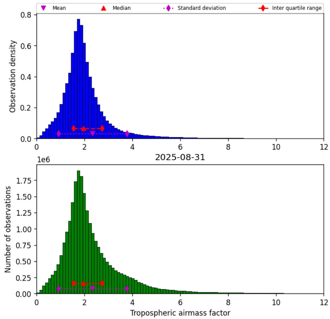
Figure 31: Histogram of “Tropospheric airmass factor” for 2025-08-30 to 2025-09-01
