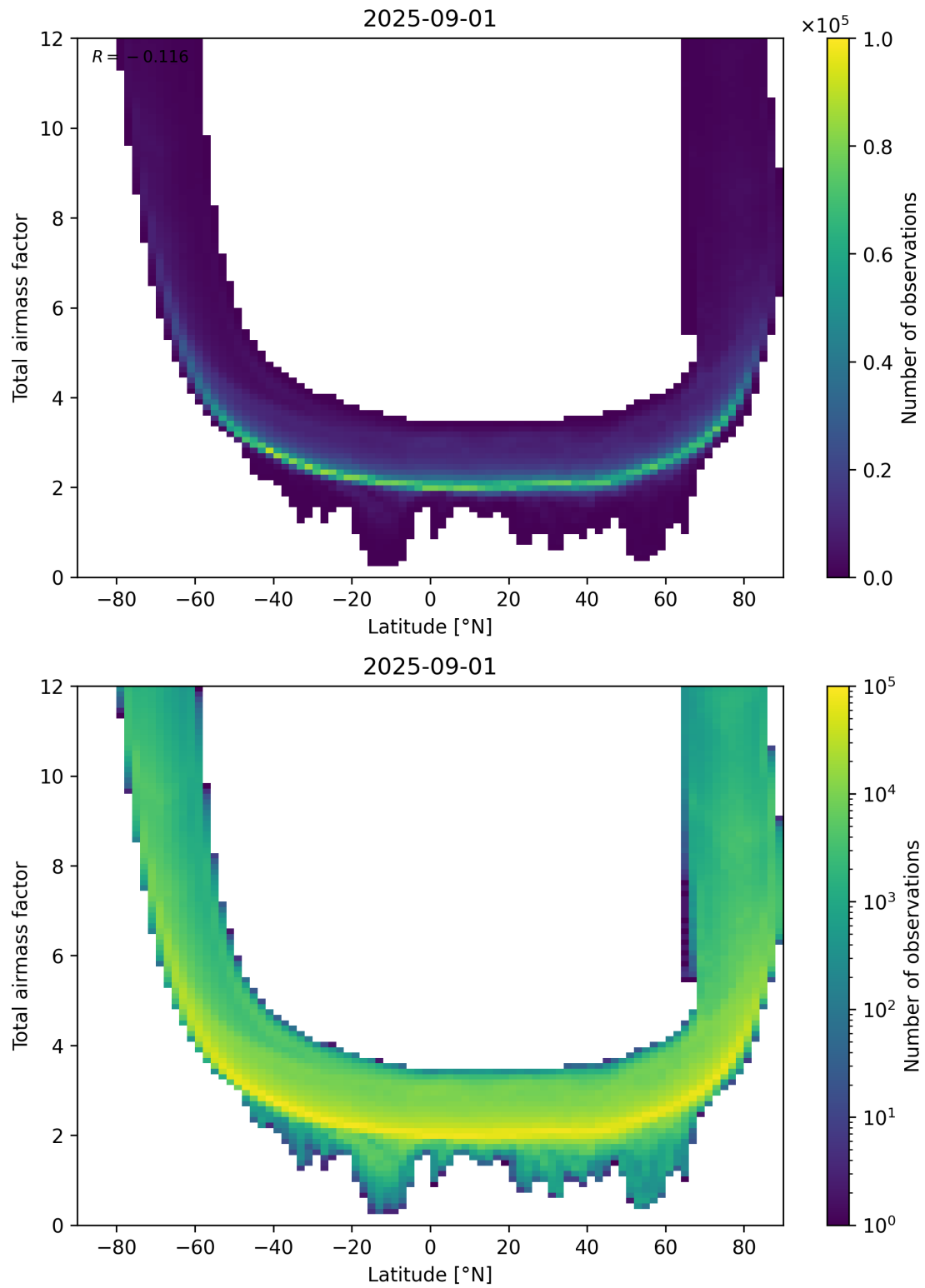
Figure 84: Scatter density plot of “Latitude” against “Total airmass factor” for 2025-08-31 to 2025-09-02.
