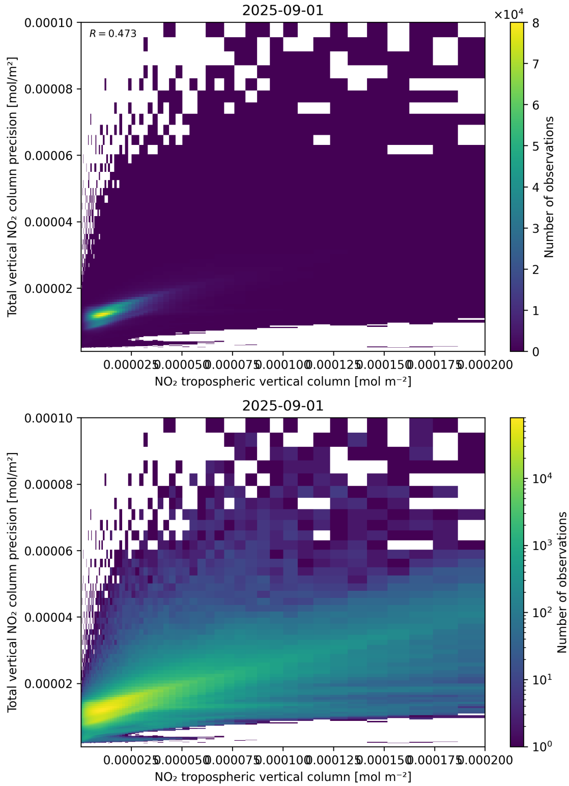
Figure 129: Scatter density plot of “NO 2 tropospheric vertical column” against “Total vertical NO 2 column precision” for 2025-08-31 to 2025-09-02.
