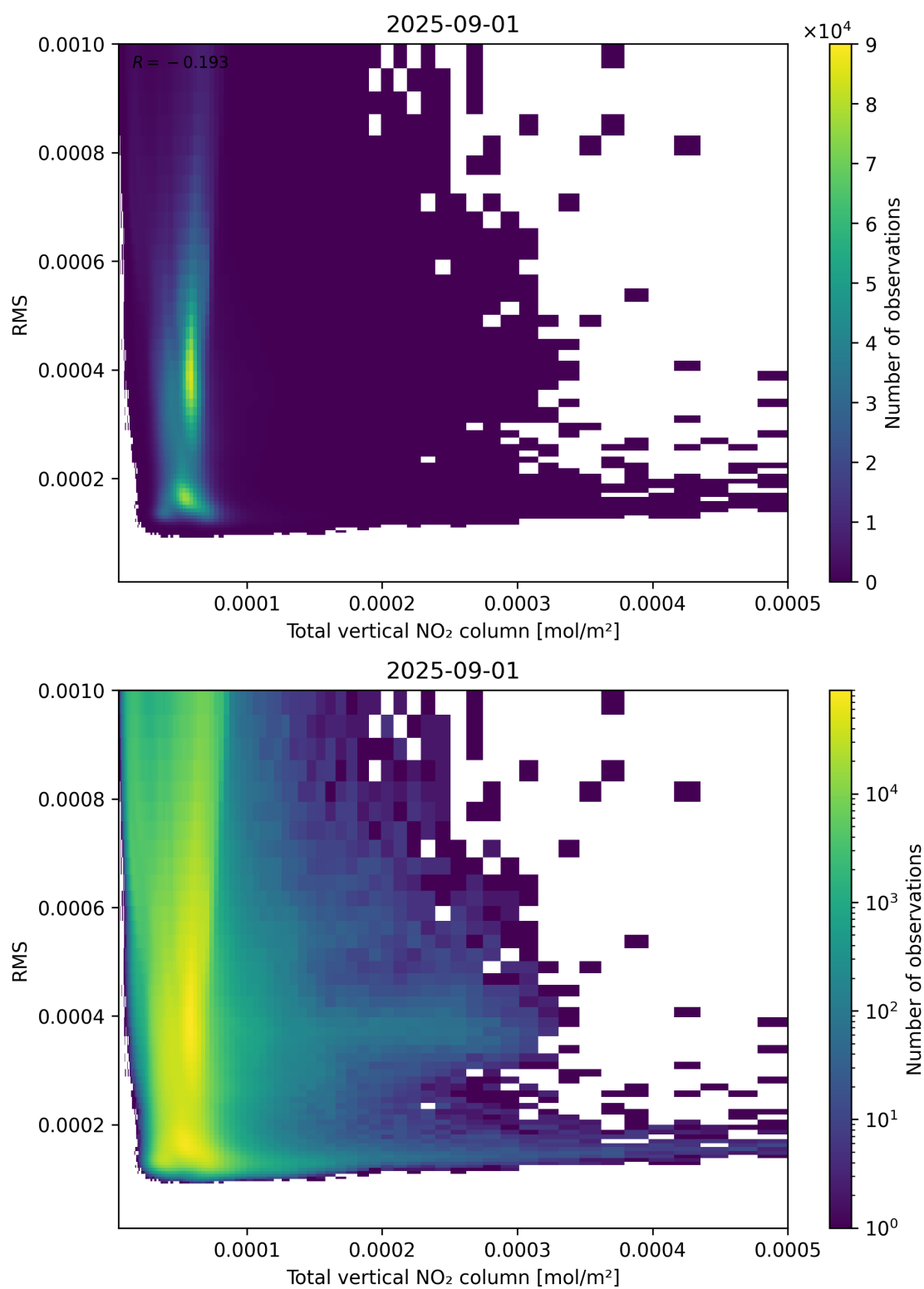
Figure 120: Scatter density plot of “Total vertical NO 2 column” against “RMS” for 2025-08-31 to 2025-09-02.
