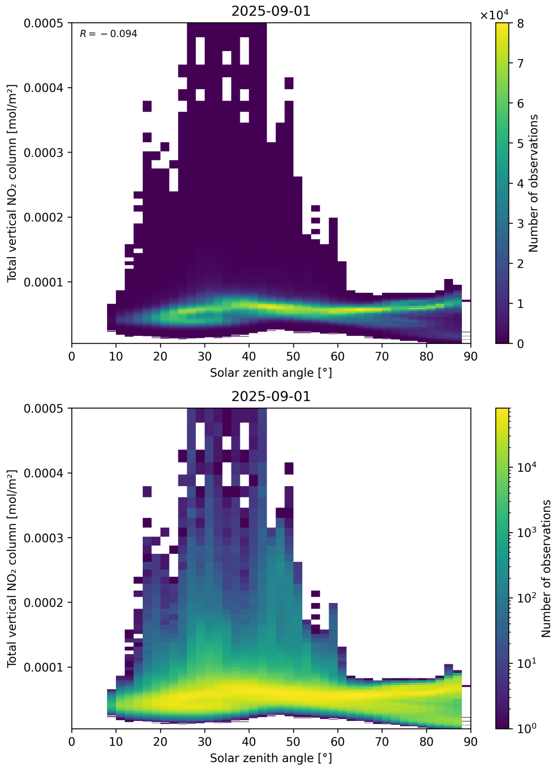
Figure 153: Scatter density plot of “Solar zenith angle” against “Total vertical NO 2 column” for 2025-08-31 to 2025-09-02.
