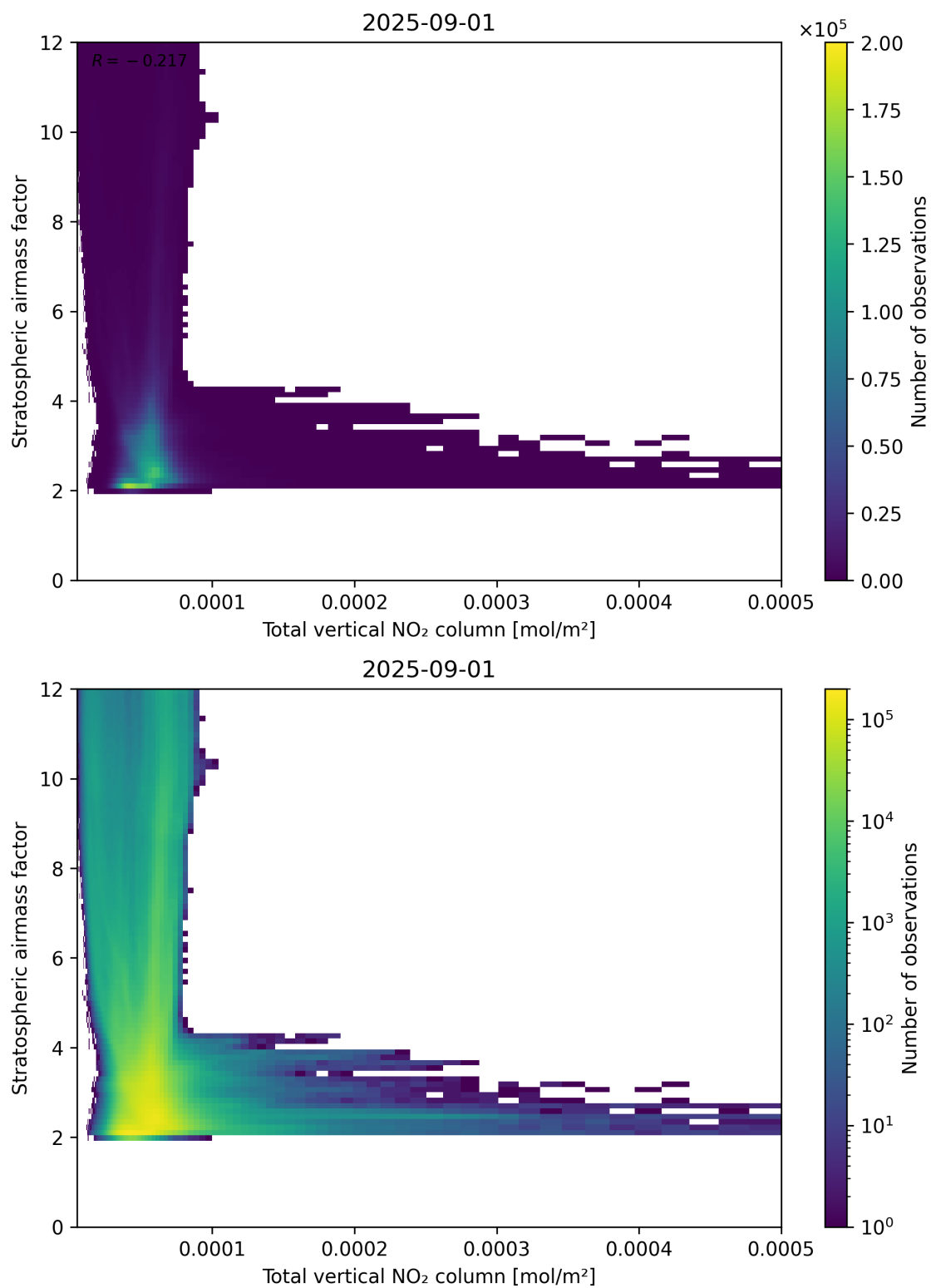
Figure 110: Scatter density plot of “Total vertical NO 2 column” against “Stratospheric airmass factor” for 2025-08-31 to 2025-09-02.
