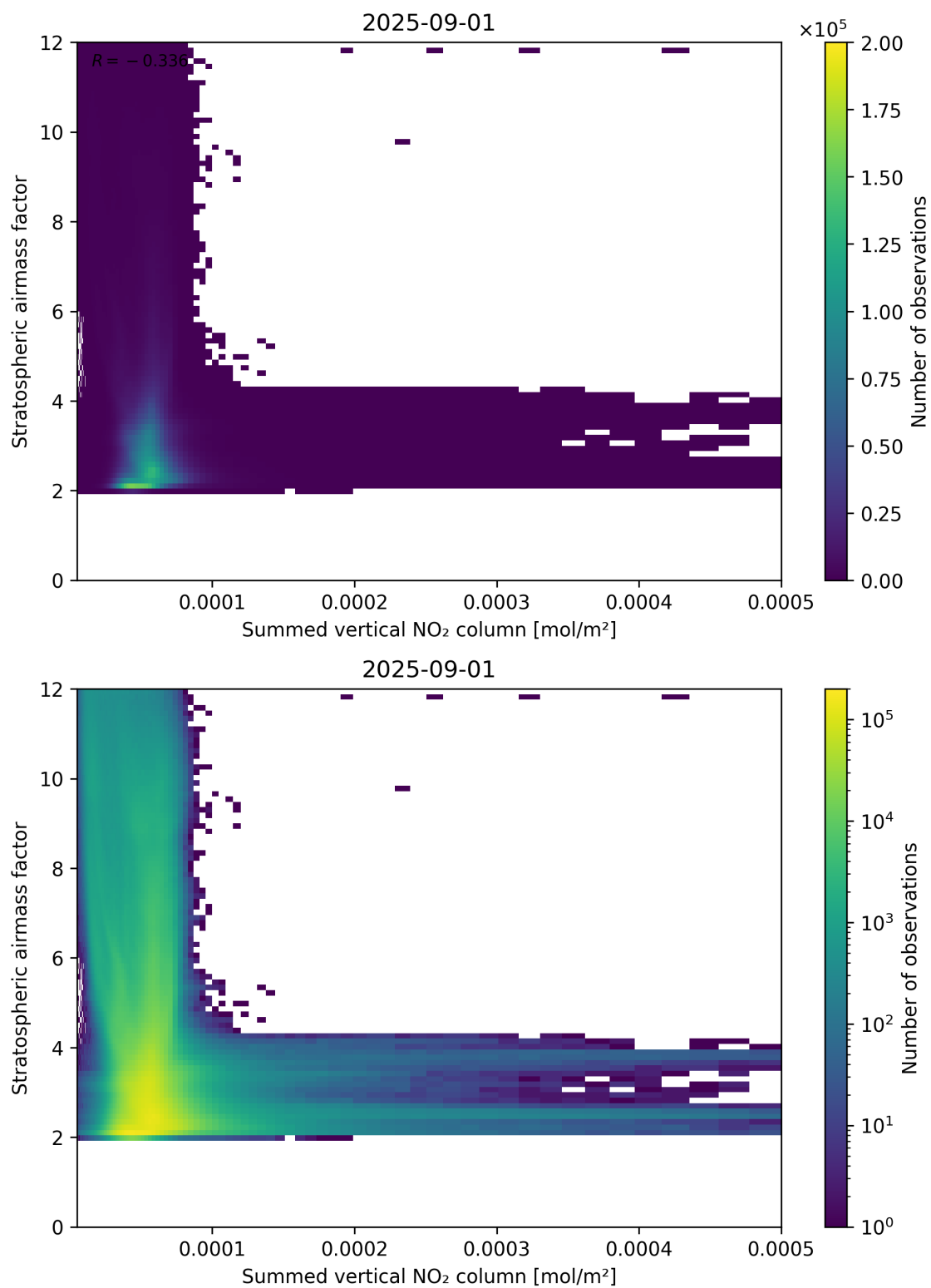
Figure 103: Scatter density plot of “Summed vertical NO 2 column” against “Stratospheric air mass factor” for 2025-08-31 to 2025-09-02.
