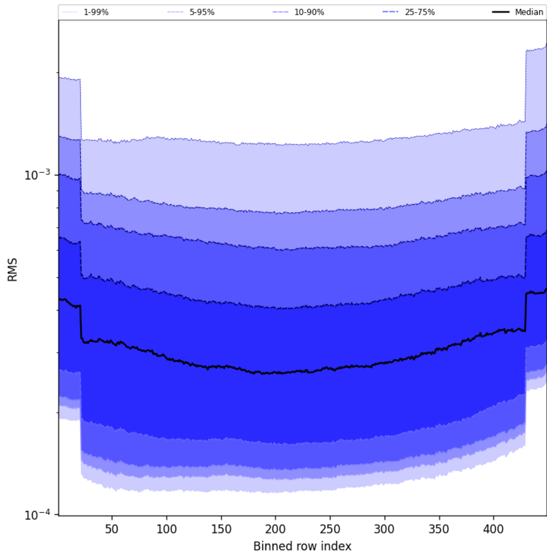
Figure 60: Along track statistics of “RMS” for 2025-08-31 to 2025-09-02
