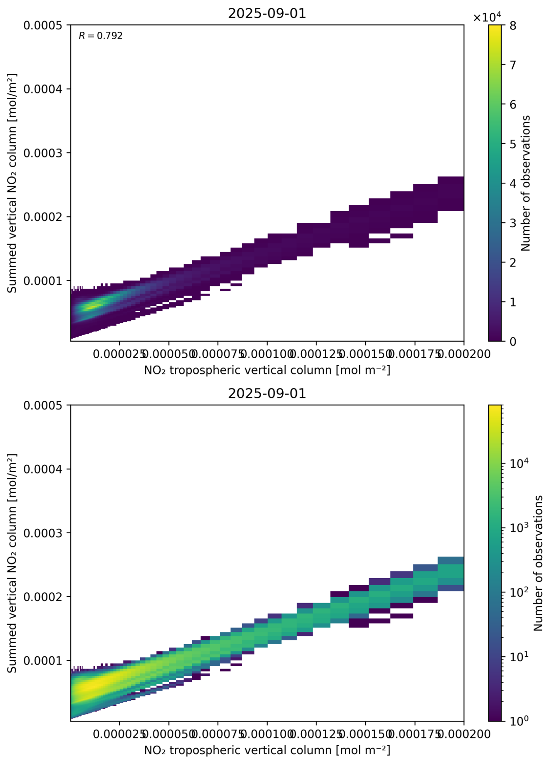
Figure 126: Scatter density plot of “NO 2 tropospheric vertical column” against “Summed vertical NO 2 column” for 2025-08-31 to 2025-09-02.
