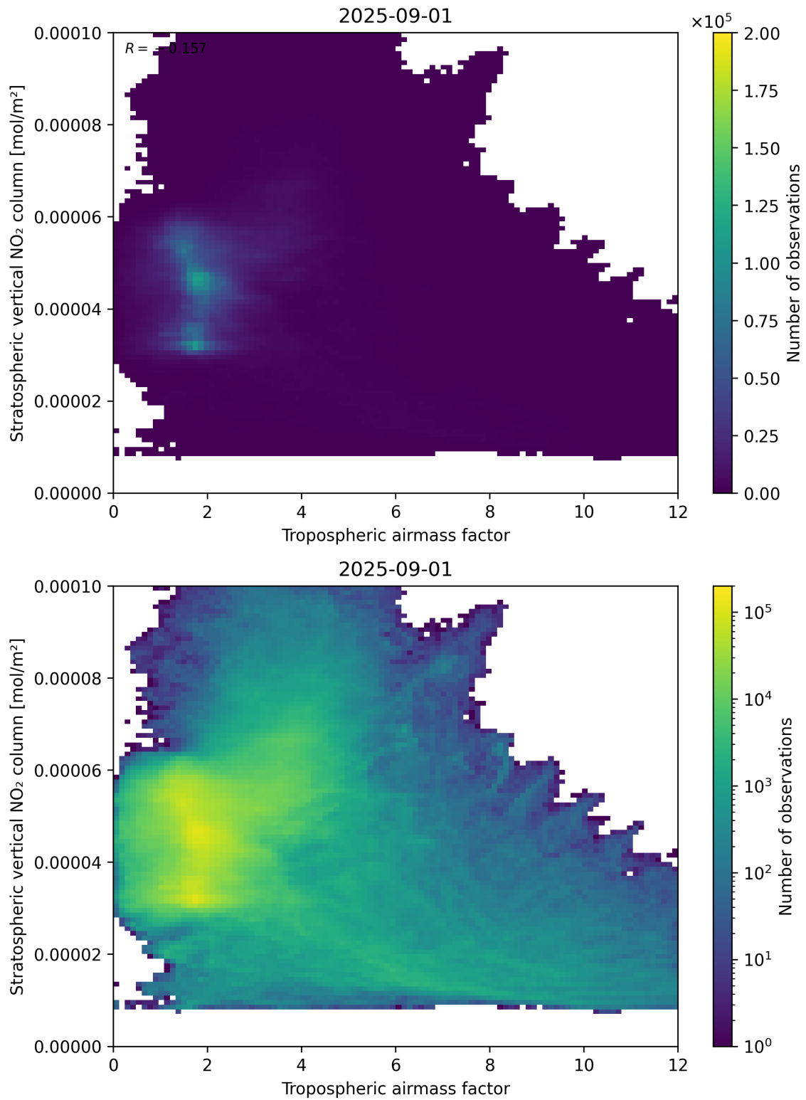
Figure 74: Scatter density plot of “Tropospheric airmass factor” against “Stratospheric vertical NO 2 column” for 2025-08-31 to 2025-09-02.
