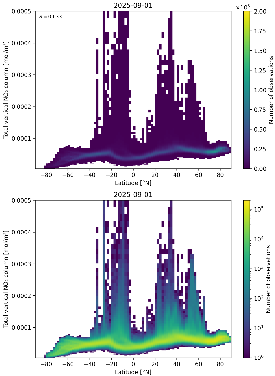
Figure 90: Scatter density plot of “Latitude” against “Total vertical NO 2 column” for 2025-08-31 to 2025-09-02.
