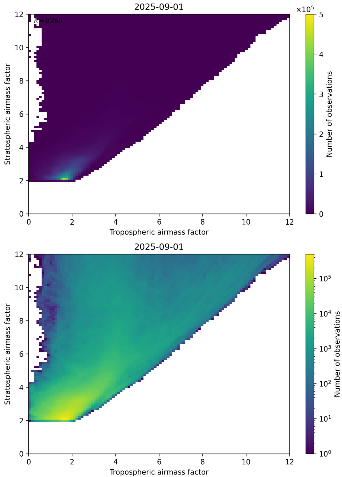
Figure 71: Scatter density plot of “Tropospheric airmass factor” against “Stratospheric airmass factor” for 2025-08-31 to 2025-09-02.
