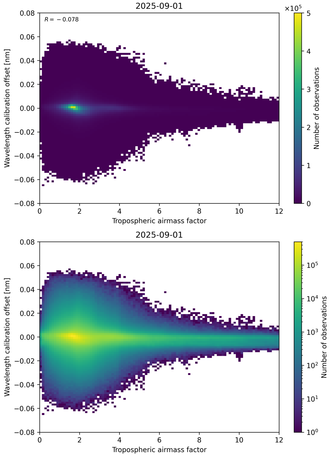
Figure 80: Scatter density plot of “Tropospheric airmass factor” against “Wavelength calibration offset” for 2025-08-31 to 2025-09-02.
