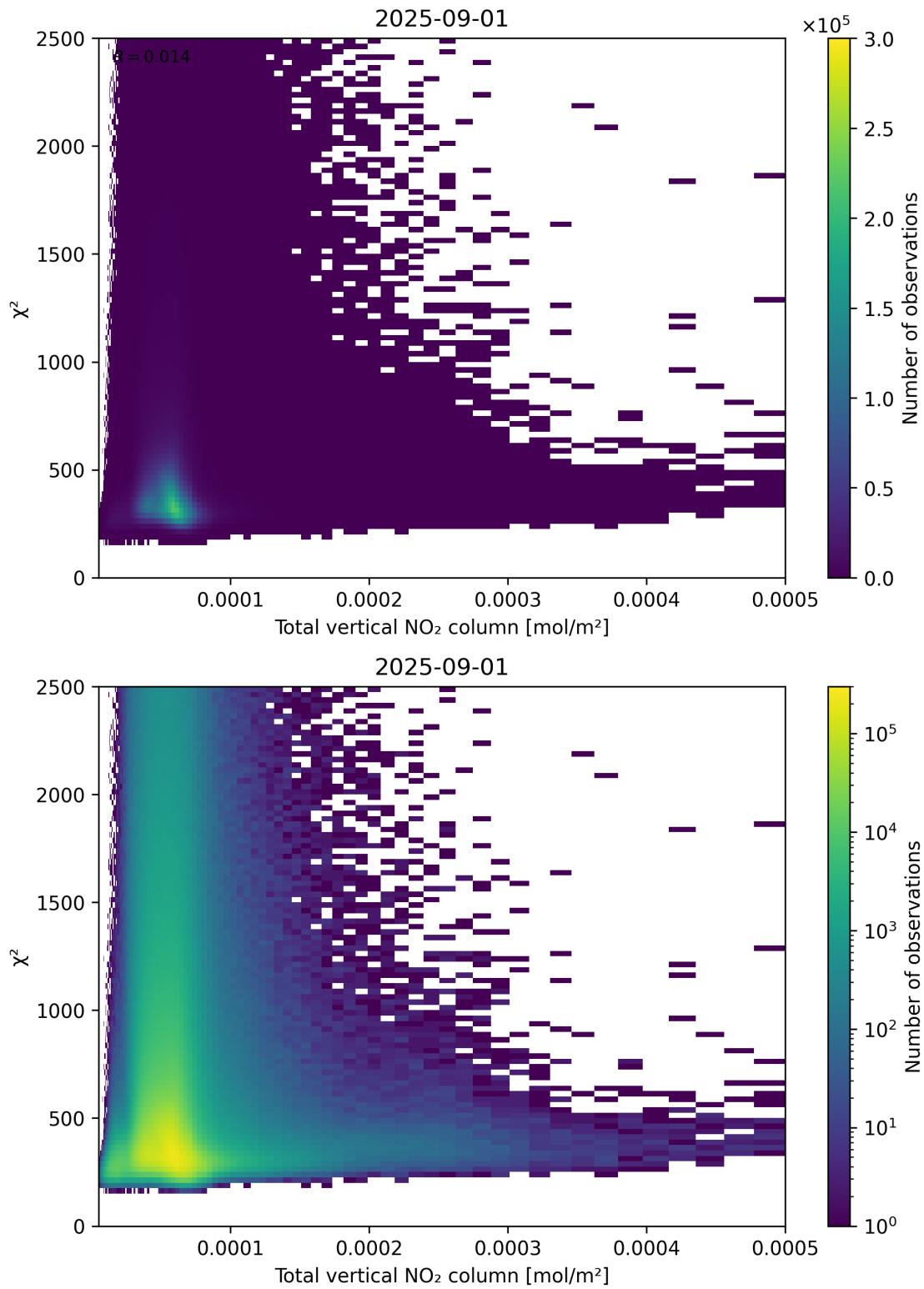
Figure 111: Scatter density plot of “Total vertical NO 2 column” against “ \chi^2 ” for 2025-08-31 to 2025-09-02.
