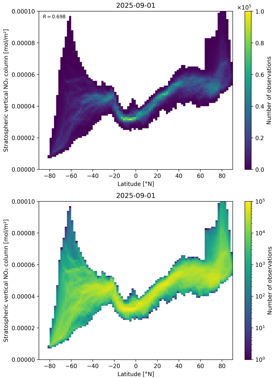
Figure 87: Scatter density plot of “Latitude” against “Stratospheric vertical NO 2 column” for 2025-08-31 to 2025-09-02.
