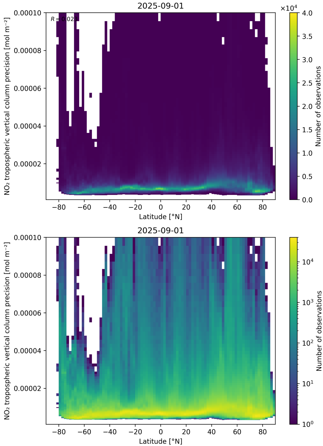
Figure 93: Scatter density plot of “Latitude” against “NO 2 tropospheric vertical column precision” for 2025-08-31 to 2025-09-02.
