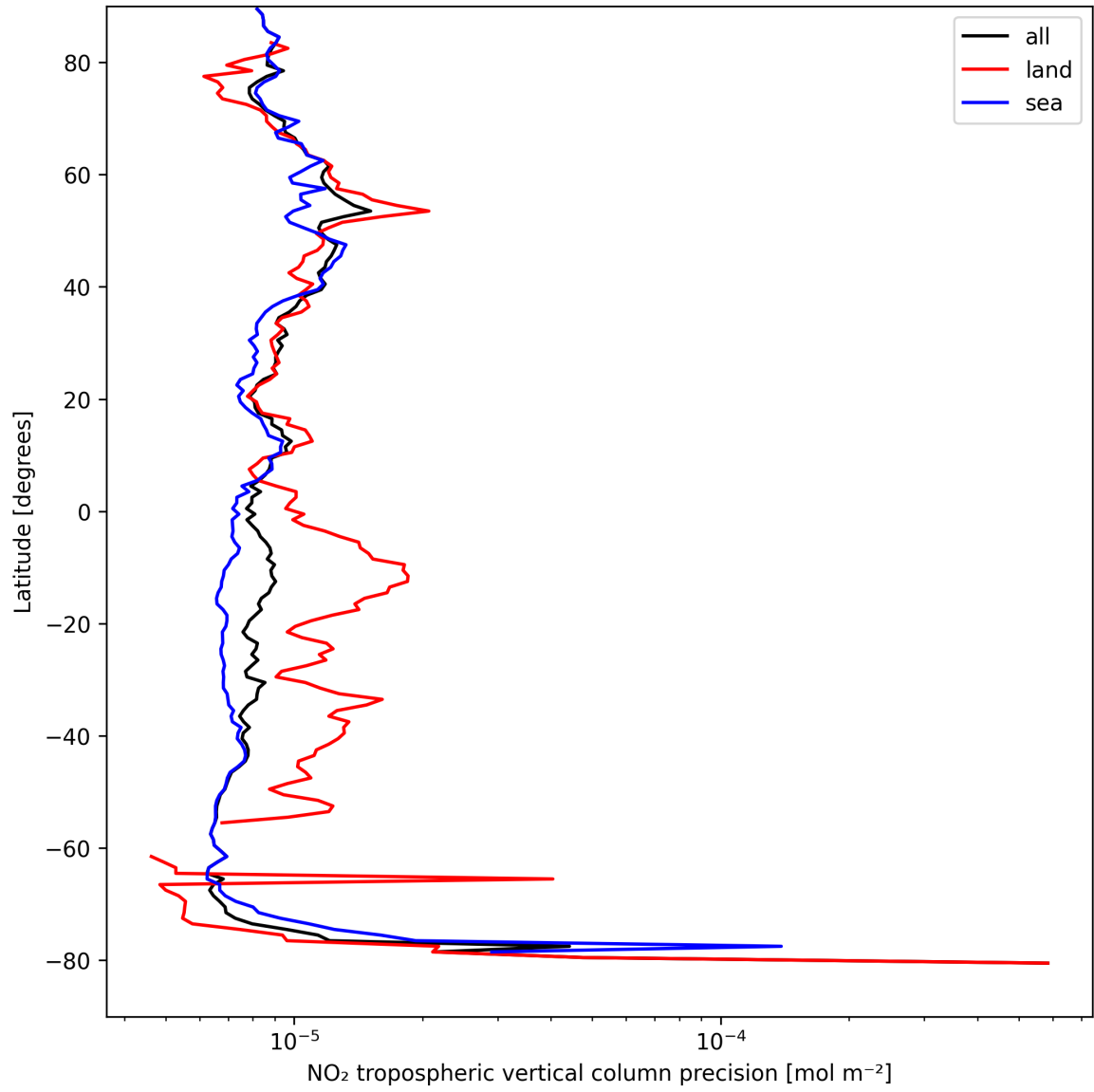
Figure 13: Zonal average of “NO 2 tropospheric vertical column precision” for 2025-08-31 to 2025-09-02.
