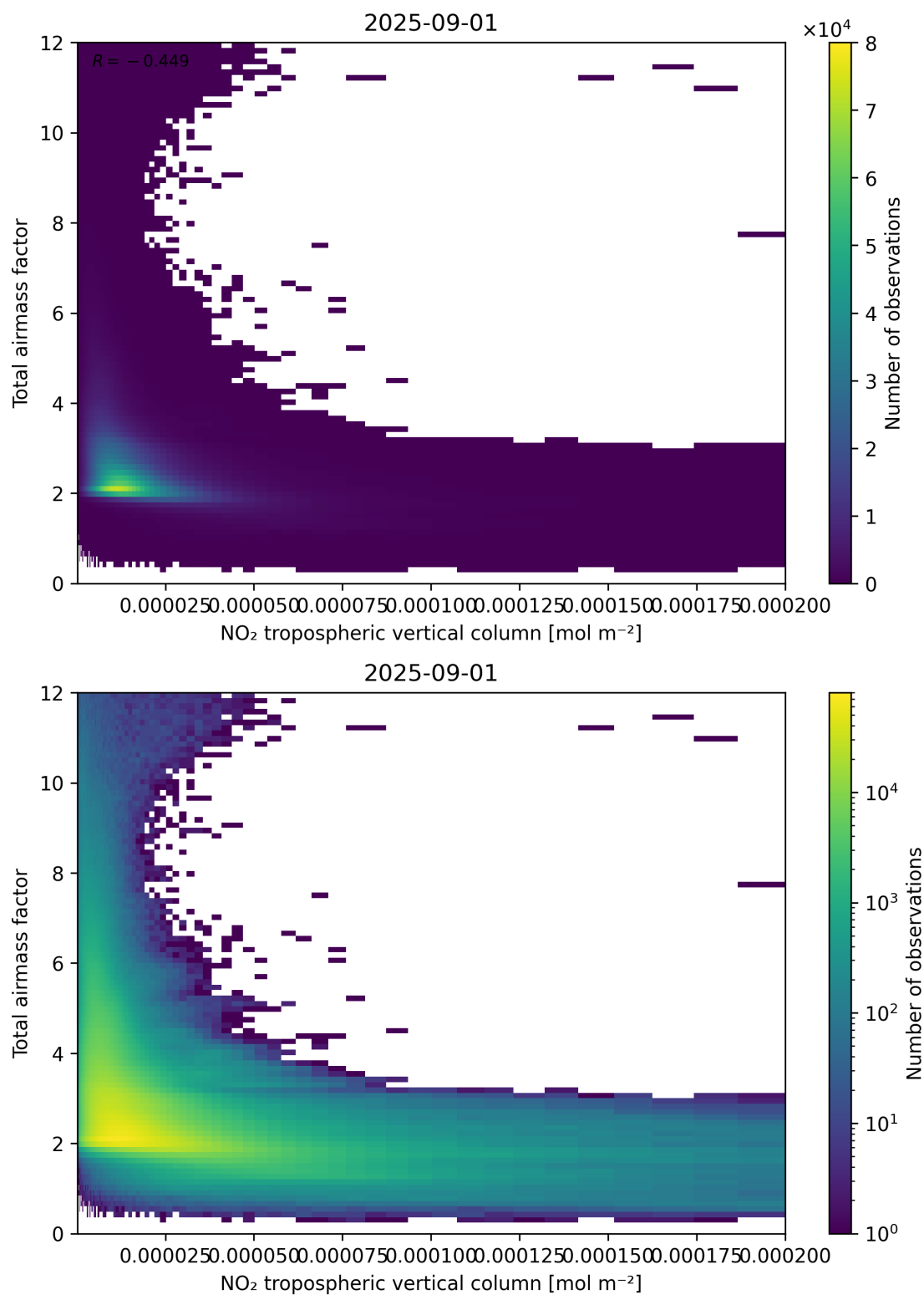
Figure 122: Scatter density plot of “NO 2 tropospheric vertical column” against “Total air mass factor” for 2025-08-31 to 2025-09-02.
