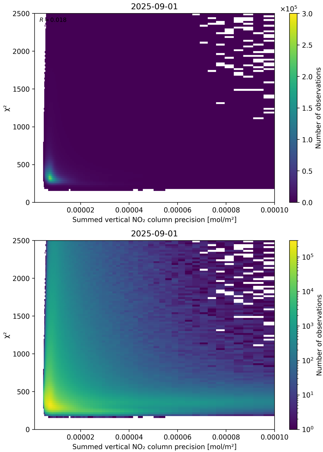
Figure 107: Scatter density plot of “Summed vertical NO 2 column precision” against “ \chi^2 ” for 2025-08-31 to 2025-09-02.
