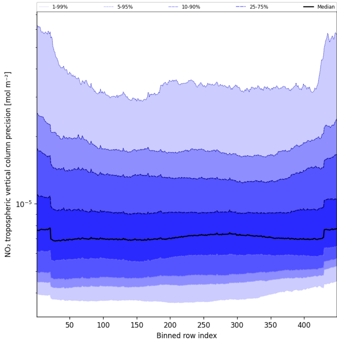
Figure 47: Along track statistics of “NO 2 tropospheric vertical column precision” for 2025-08-31 to 2025-09-02
