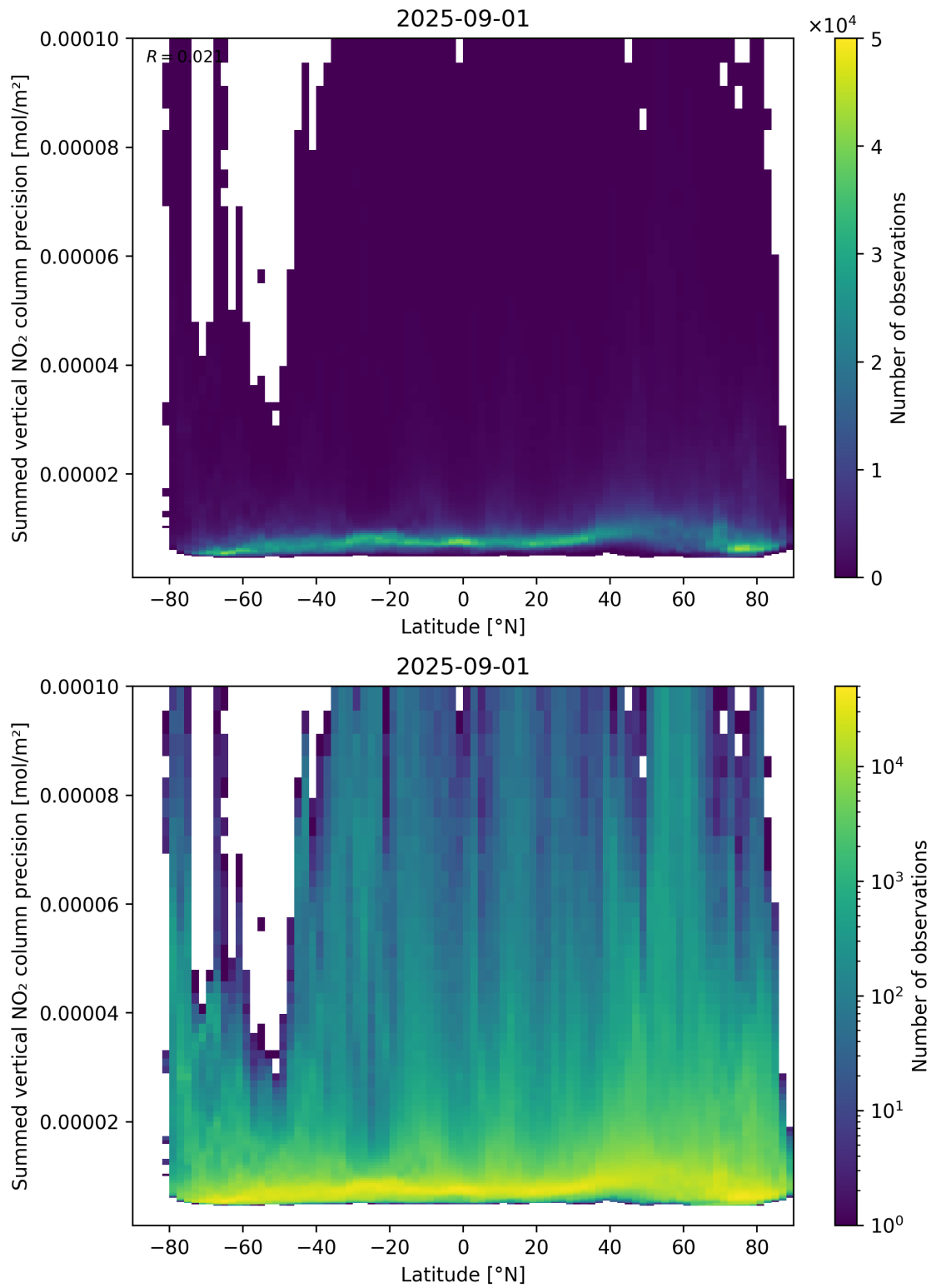
Figure 89: Scatter density plot of “Latitude” against “Summed vertical NO 2 column precision” for 2025-08-31 to 2025-09-02.
