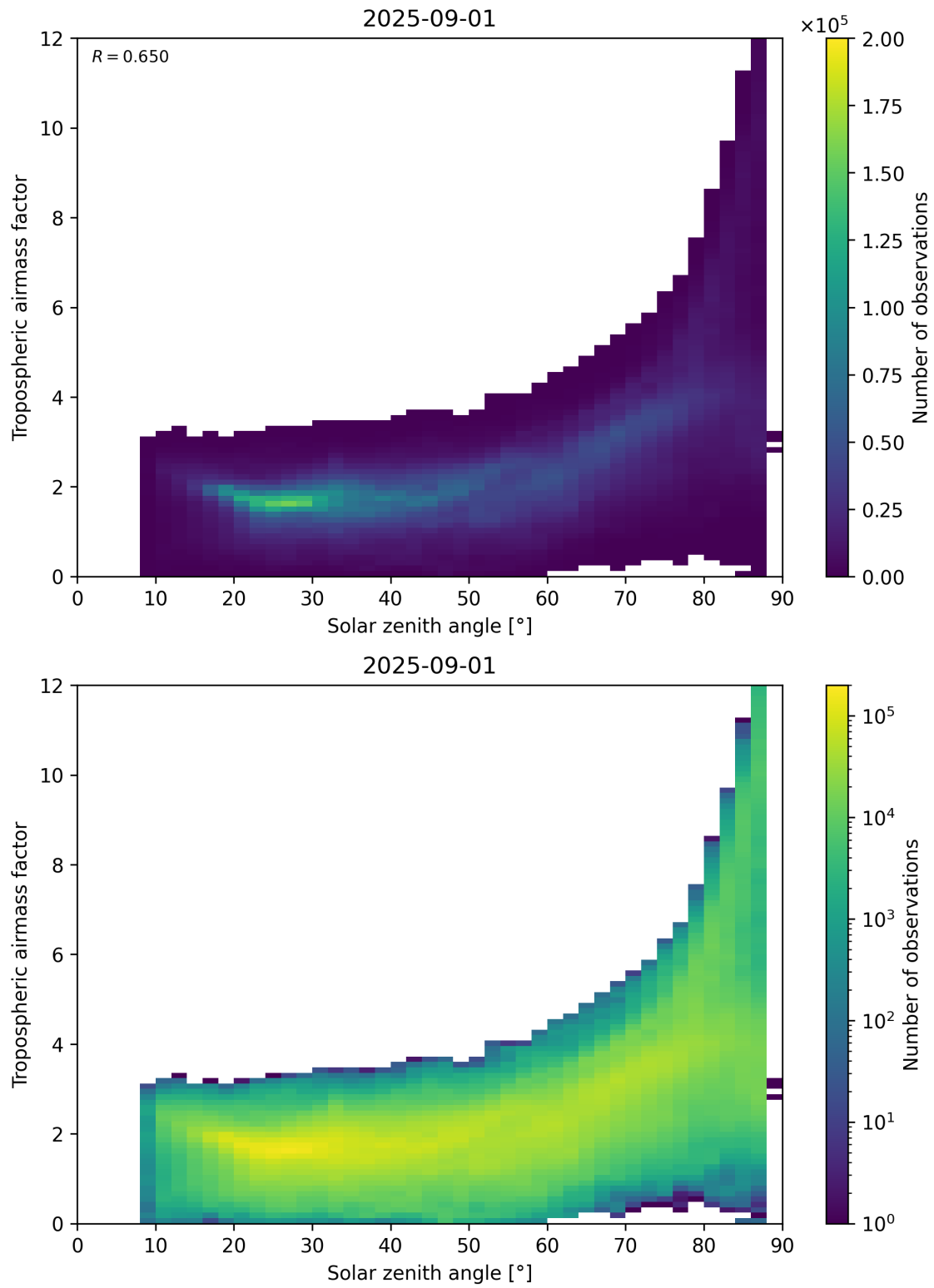
Figure 147: Scatter density plot of “Solar zenith angle” against “Tropospheric airmass factor” for 2025-08-31 to 2025-09-02.
