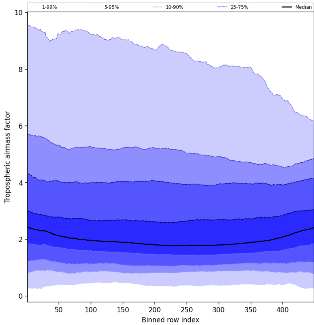
Figure 48: Along track statistics of “Tropospheric airmass factor” for 2025-08-31 to 2025-09-02
