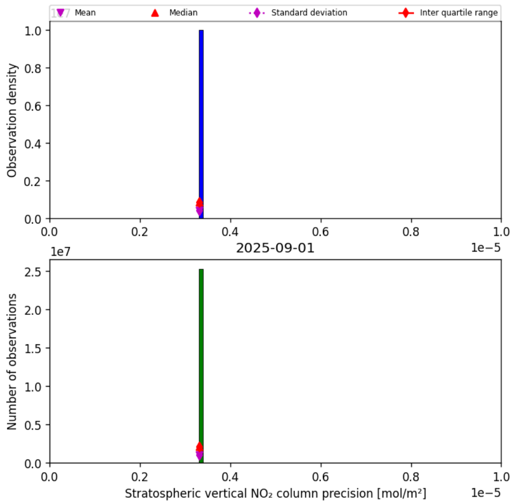
Figure 37: Histogram of “Stratospheric vertical NO 2 column precision” for 2025-08-31 to 2025-09-02
