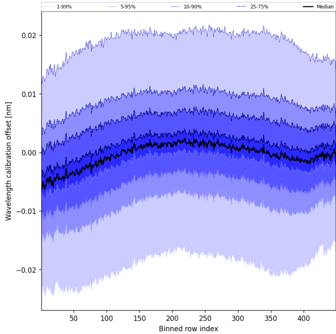
Figure 52: Along track statistics of “Wavelength calibration offset” for 2025-08-31 to 2025-09-02
