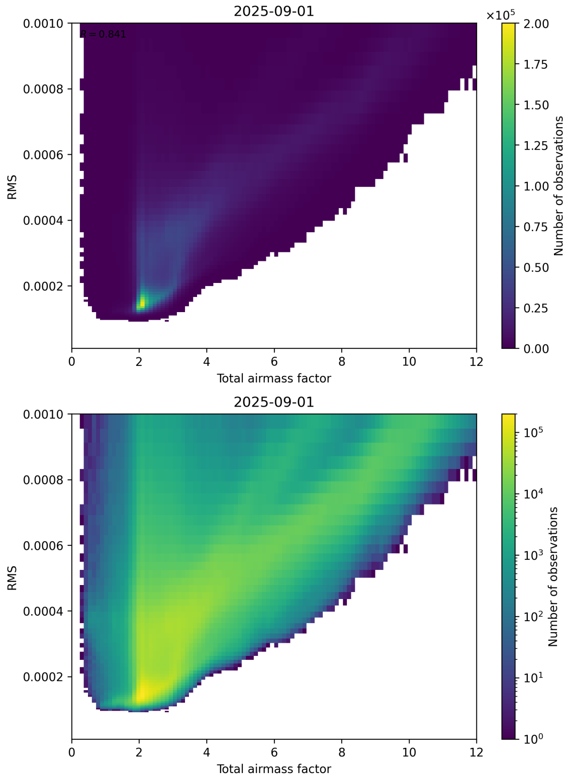
Figure 69: Scatter density plot of “Total airmass factor” against “RMS” for 2025-08-31 to 2025-09-02.
