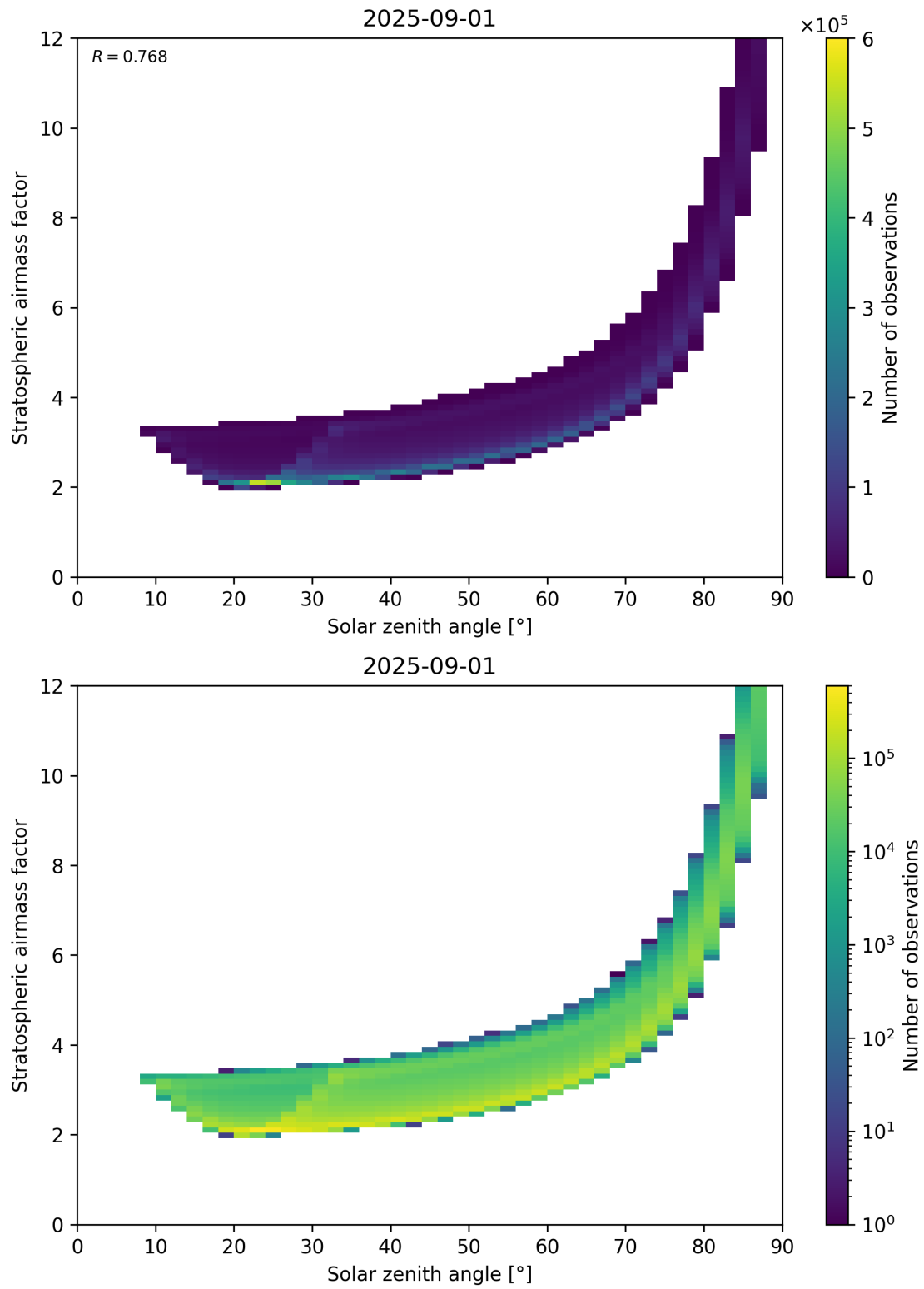
Figure 145: Scatter density plot of “Solar zenith angle” against “Stratospheric airmass factor” for 2025-08-31 to 2025-09-02.
