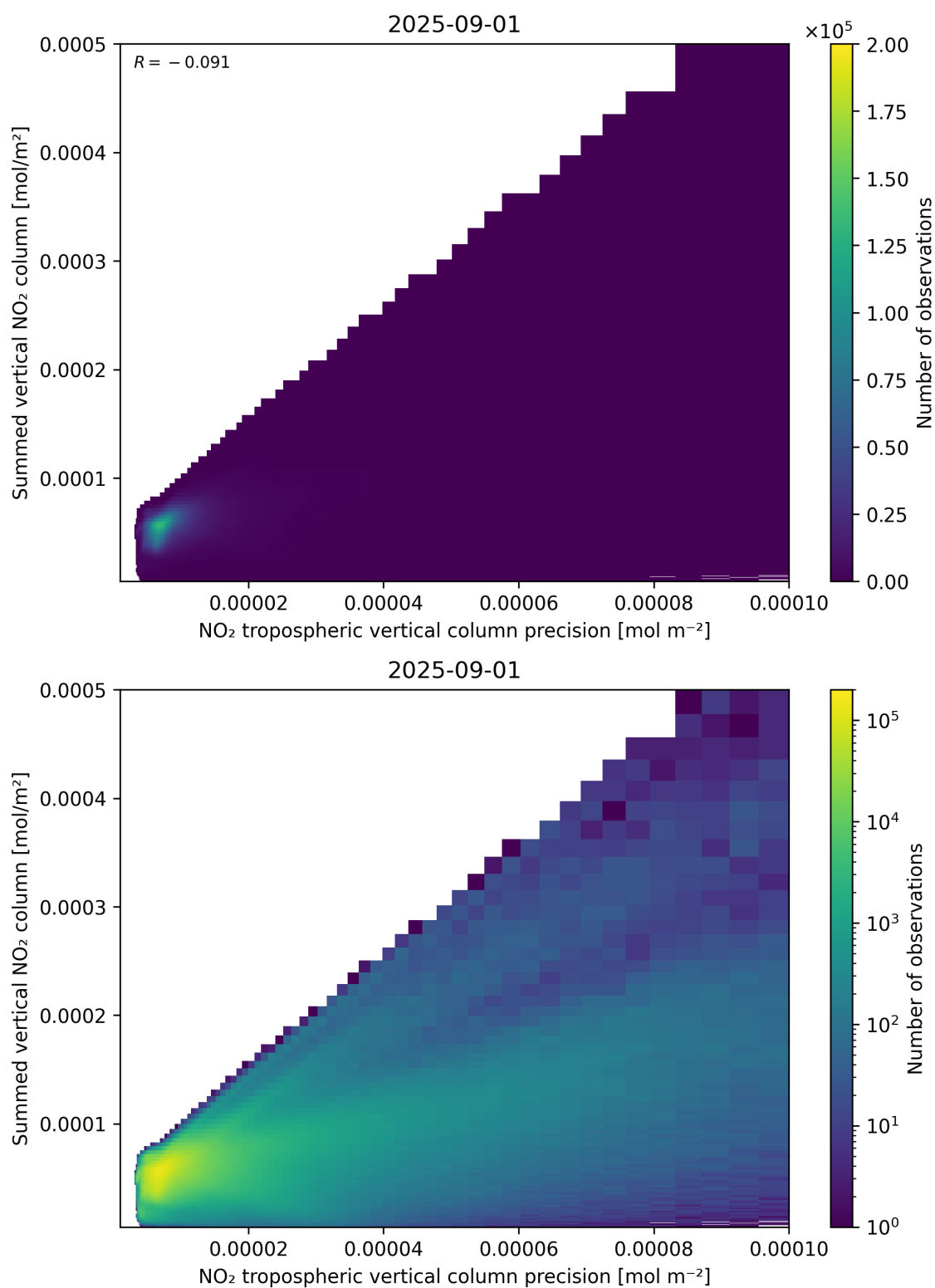
Figure 136: Scatter density plot of “NO 2 tropospheric vertical column precision” against “Summed vertical NO 2 column” for 2025-08-31 to 2025-09-02.
