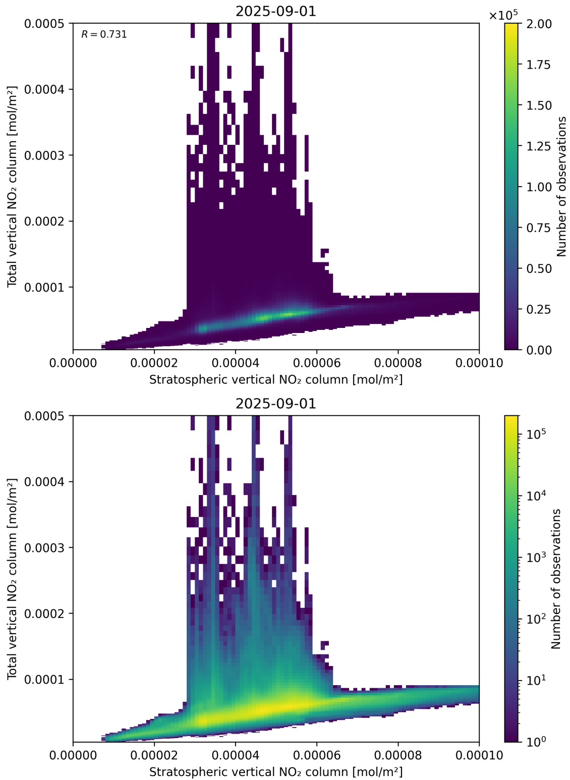
Figure 100: Scatter density plot of “Stratospheric vertical NO 2 column” against “Total vertical NO 2 column” for 2025-08-31 to 2025-09-02.
