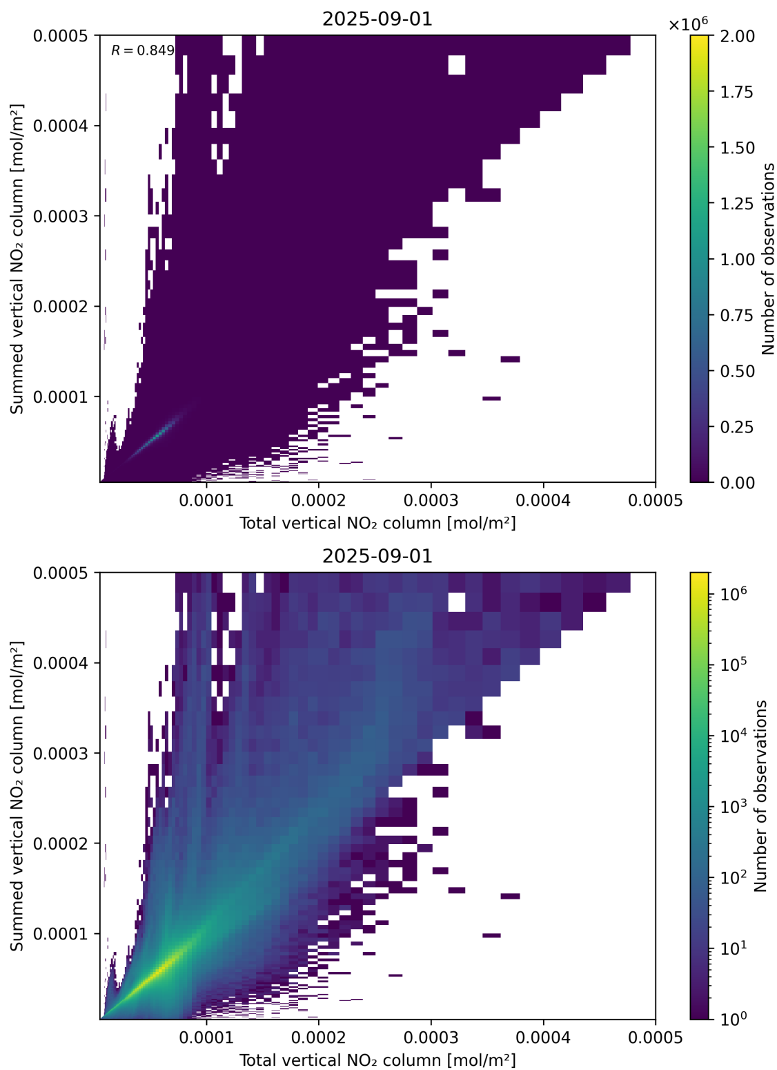
Figure 112: Scatter density plot of “Total vertical NO 2 column” against “Summed vertical NO 2 column” for 2025-08-31 to 2025-09-02.
