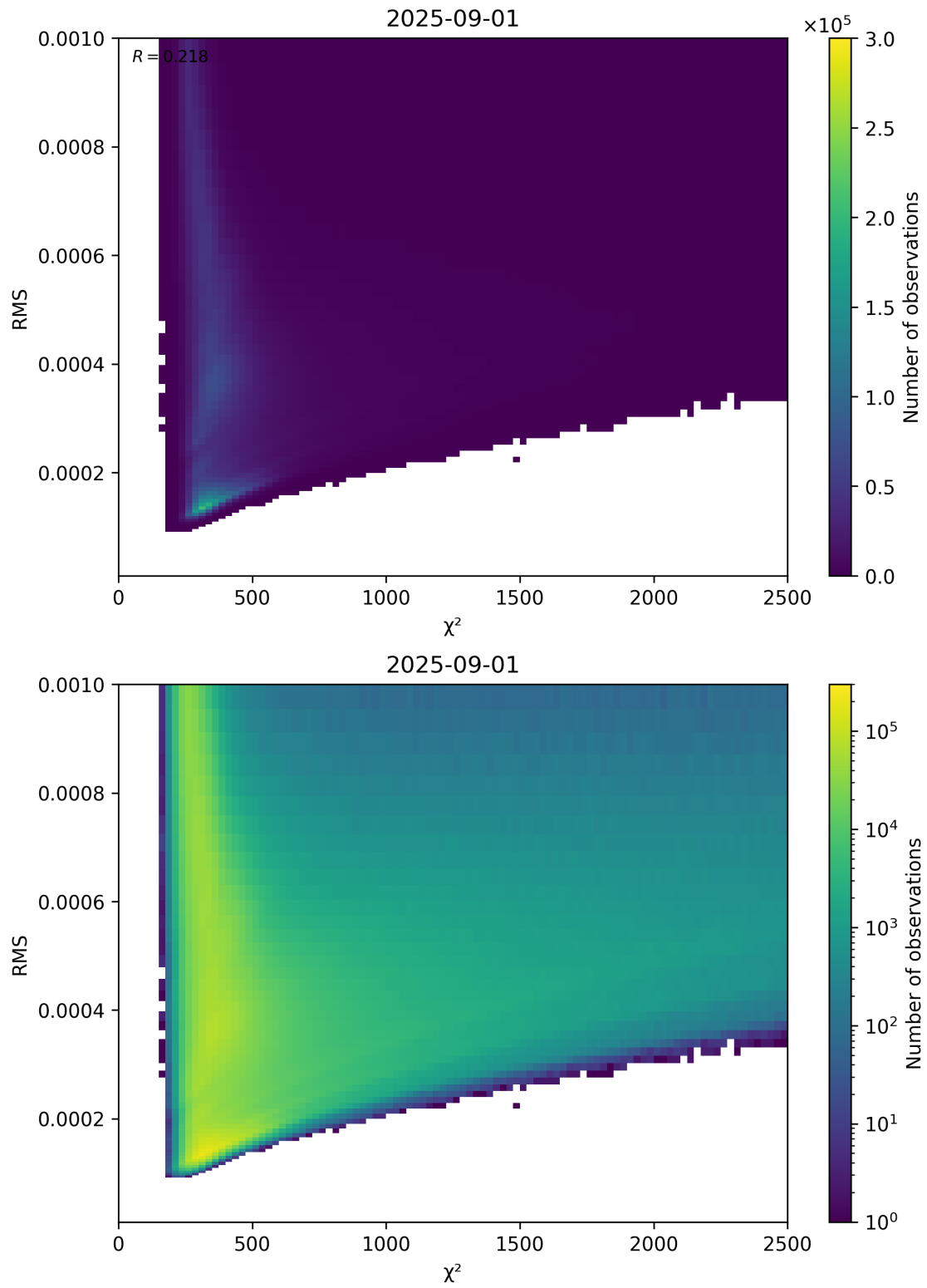
Figure 82: Scatter density plot of “ \chi^2 ” against “RMS” for 2025-08-31 to 2025-09-02.
