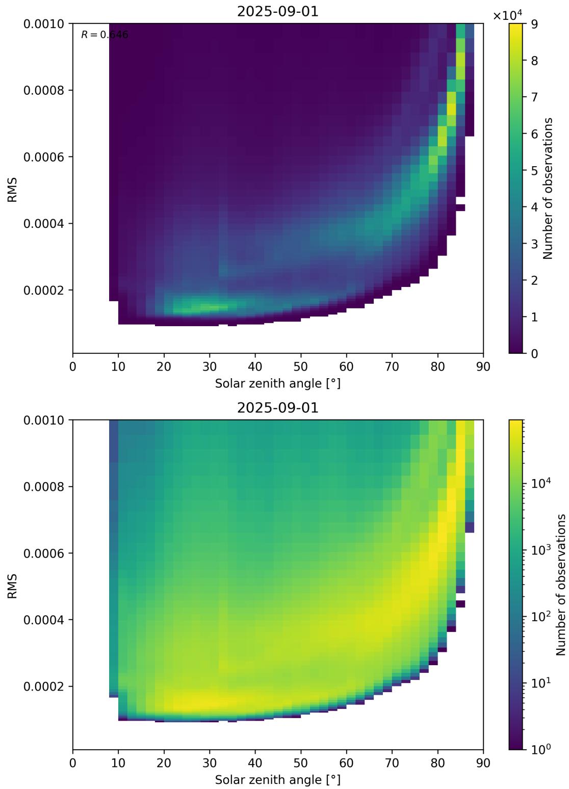
Figure 157: Scatter density plot of “Solar zenith angle” against “RMS” for 2025-08-31 to 2025-09-02.
