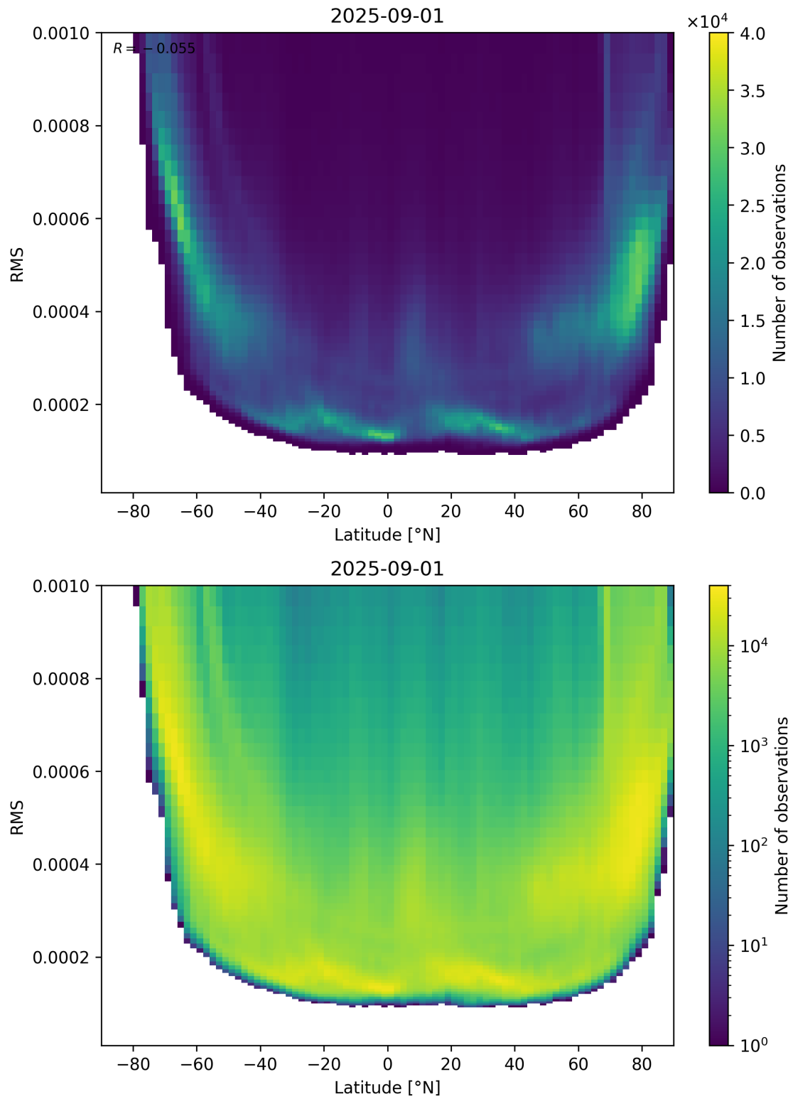
Figure 94: Scatter density plot of “Latitude” against “RMS” for 2025-08-31 to 2025-09-02.
