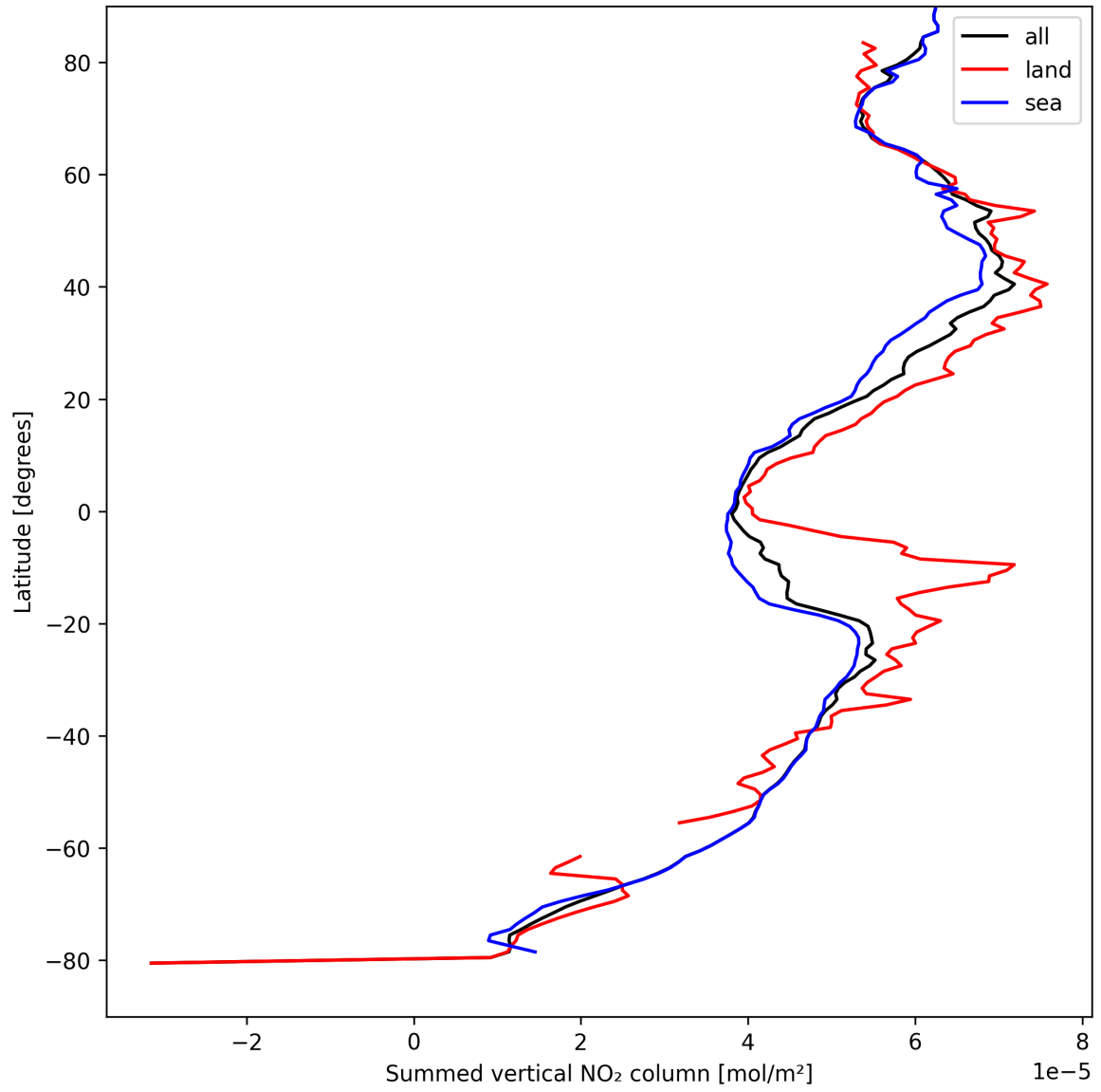
Figure 23: Zonal average of “Summed vertical NO 2 column” for 2025-08-31 to 2025-09-02.
