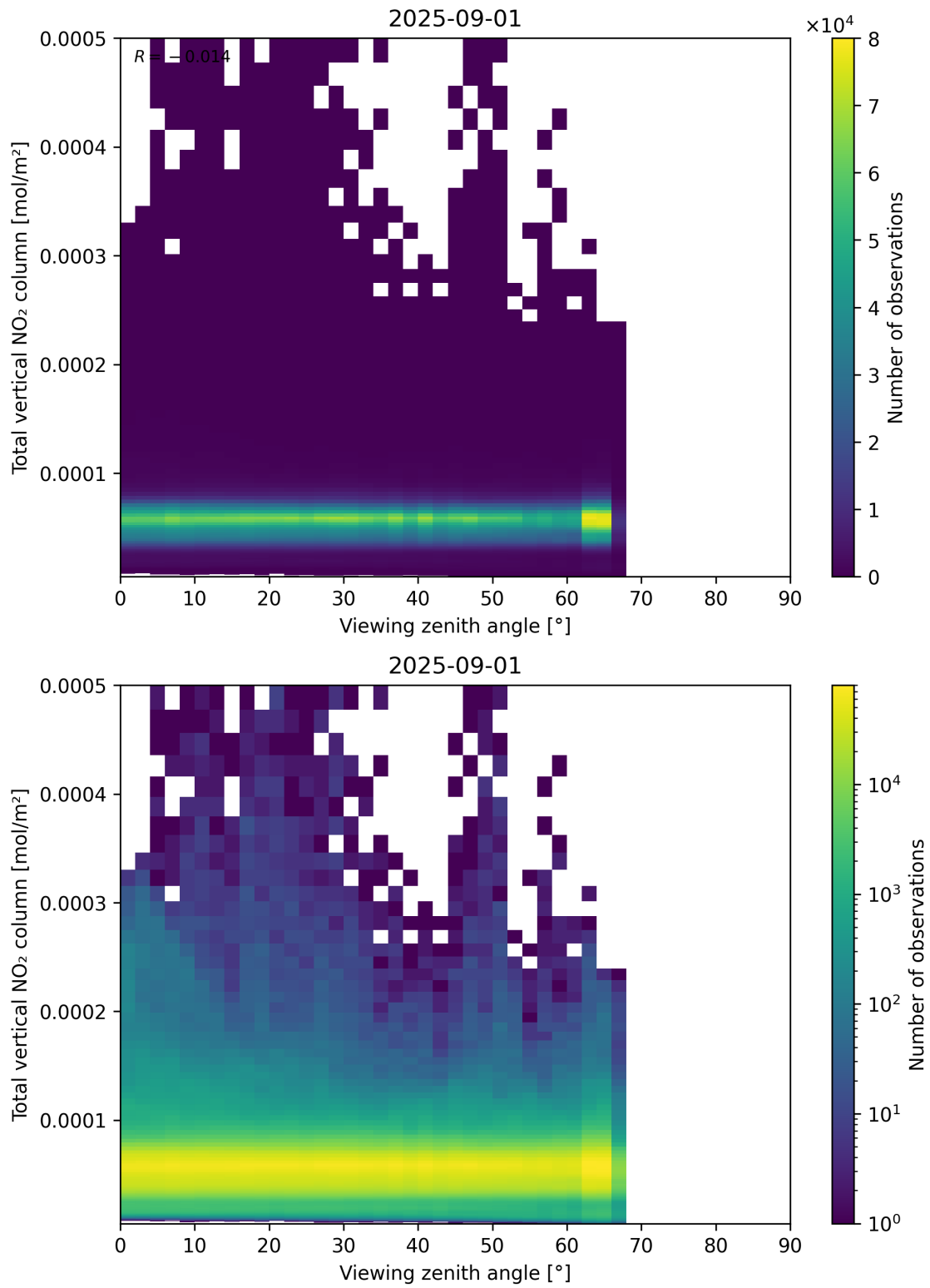
Figure 167: Scatter density plot of “Viewing zenith angle” against “Total vertical NO 2 column” for 2025-08-31 to 2025-09-02.
