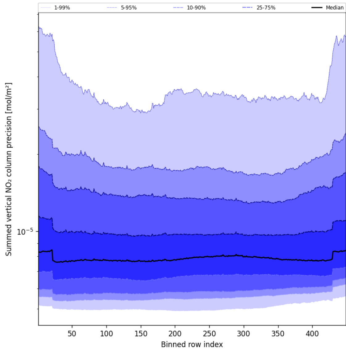
Figure 58: Along track statistics of “Summed vertical NO 2 column precision” for 2025-08-31 to 2025-09-02
