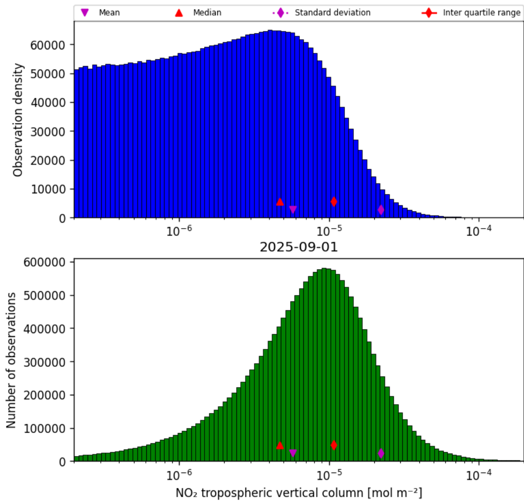
Figure 29: Histogram of “NO 2 tropospheric vertical column” for 2025-08-31 to 2025-09-02
