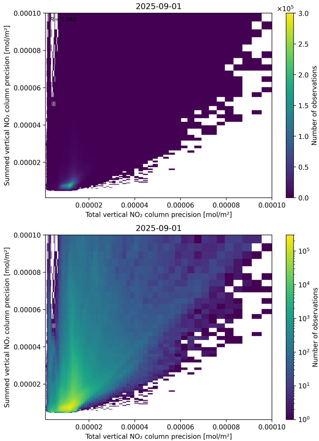
Figure 118: Scatter density plot of “Total vertical NO 2 column precision” against “Summed vertical NO 2 column precision” for 2025-08-31 to 2025-09-02.
