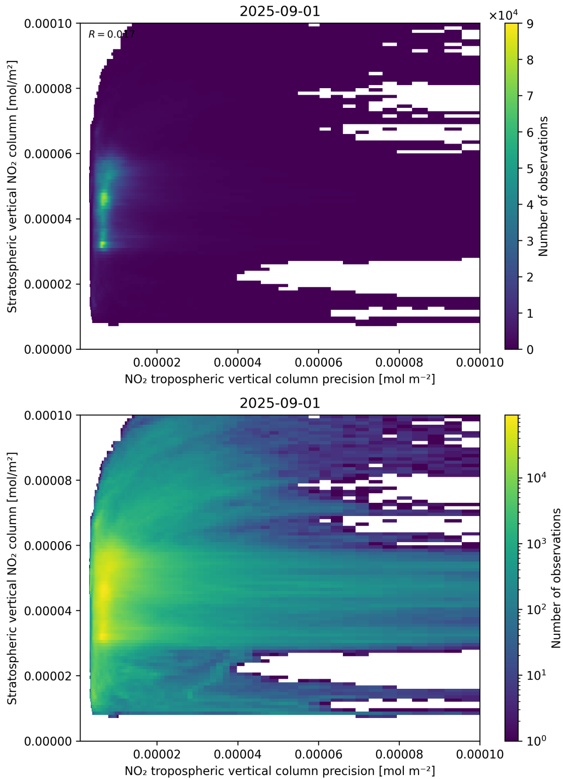
Figure 135: Scatter density plot of “NO 2 tropospheric vertical column precision” against “Stratospheric vertical NO 2 column” for 2025-08-31 to 2025-09-02.
