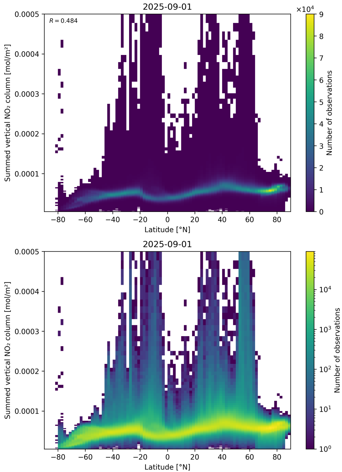
Figure 88: Scatter density plot of “Latitude” against “Summed vertical NO 2 column” for 2025-08-31 to 2025-09-02.
