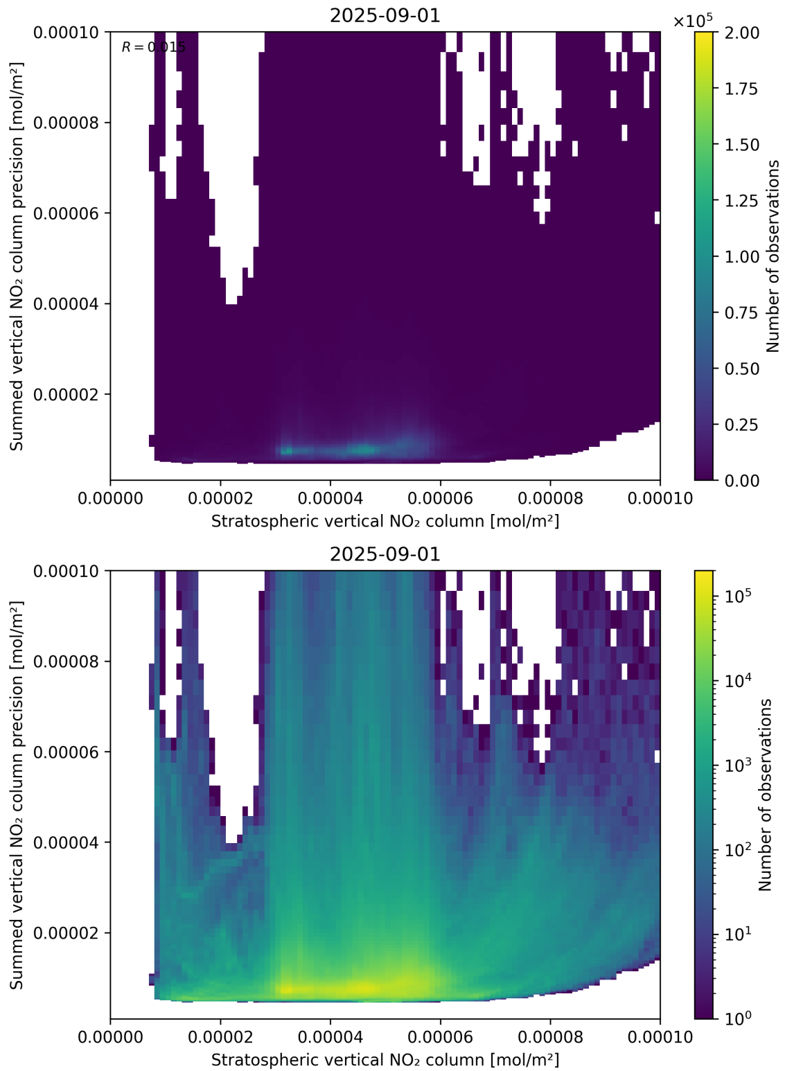
Figure 99: Scatter density plot of “Stratospheric vertical NO 2 column” against “Summed vertical NO 2 column precision” for 2025-08-31 to 2025-09-02.
