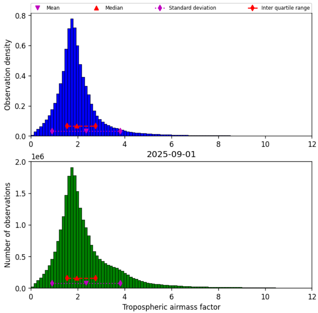
Figure 31: Histogram of “Tropospheric airmass factor” for 2025-08-31 to 2025-09-02
