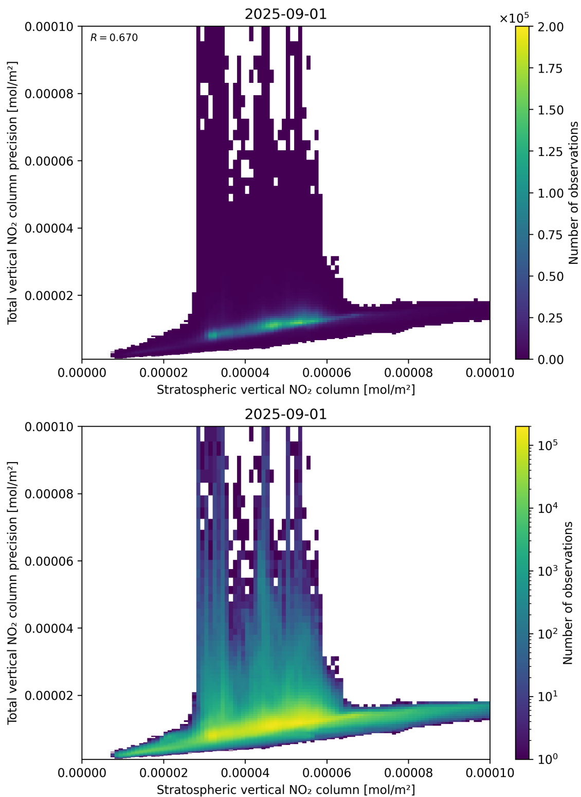
Figure 101: Scatter density plot of “Stratospheric vertical NO 2 column” against “Total vertical NO 2 column precision” for 2025-08-31 to 2025-09-02.
