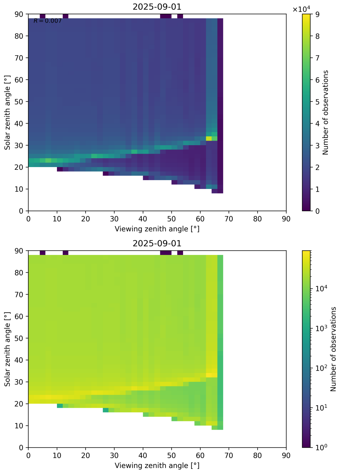
Figure 172: Scatter density plot of “Viewing zenith angle” against “Solar zenith angle” for 2025-08-31 to 2025-09-02.
