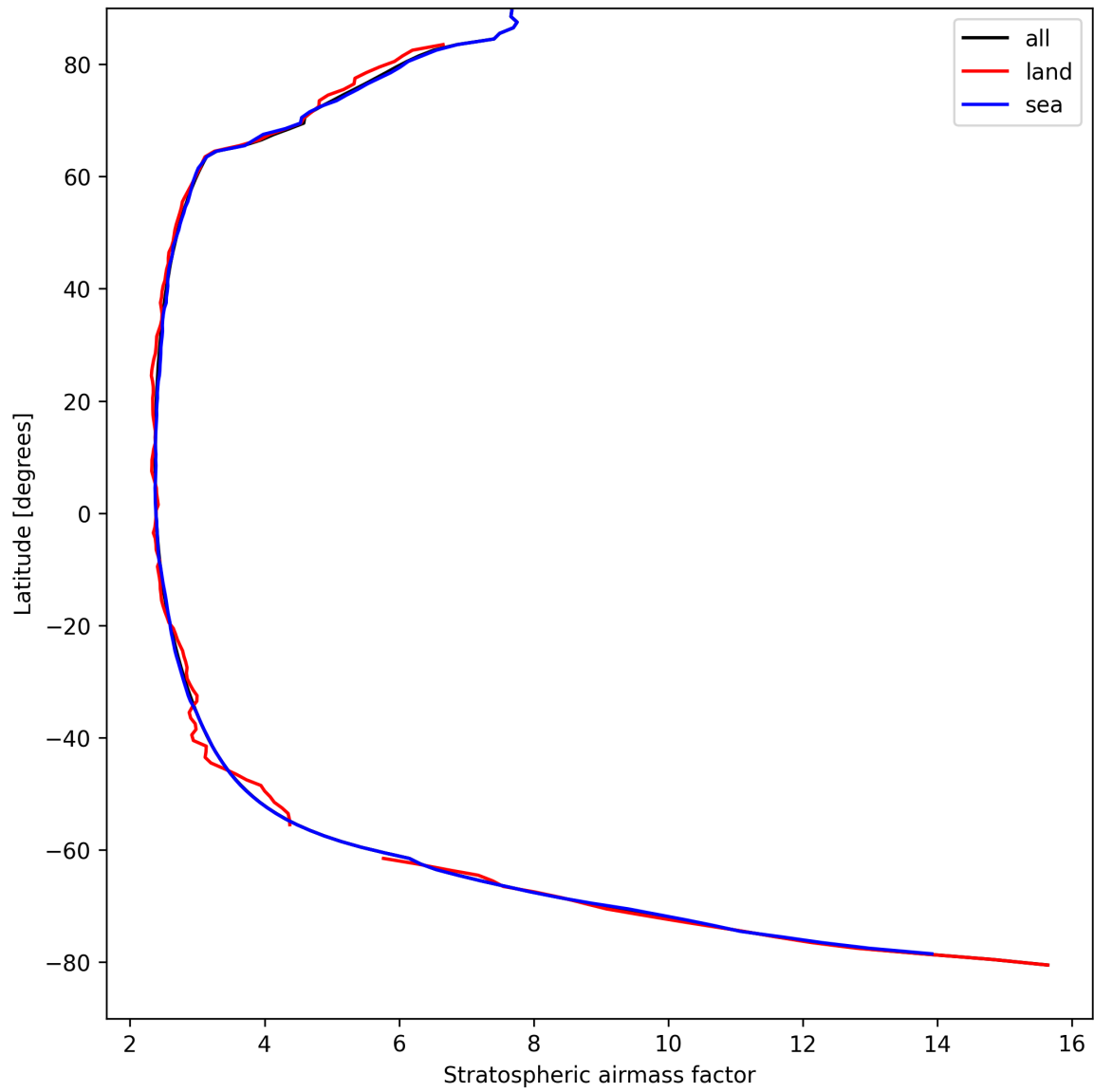
Figure 27: Zonal average of “Stratospheric airmass factor” for 2025-08-31 to 2025-09-02.
