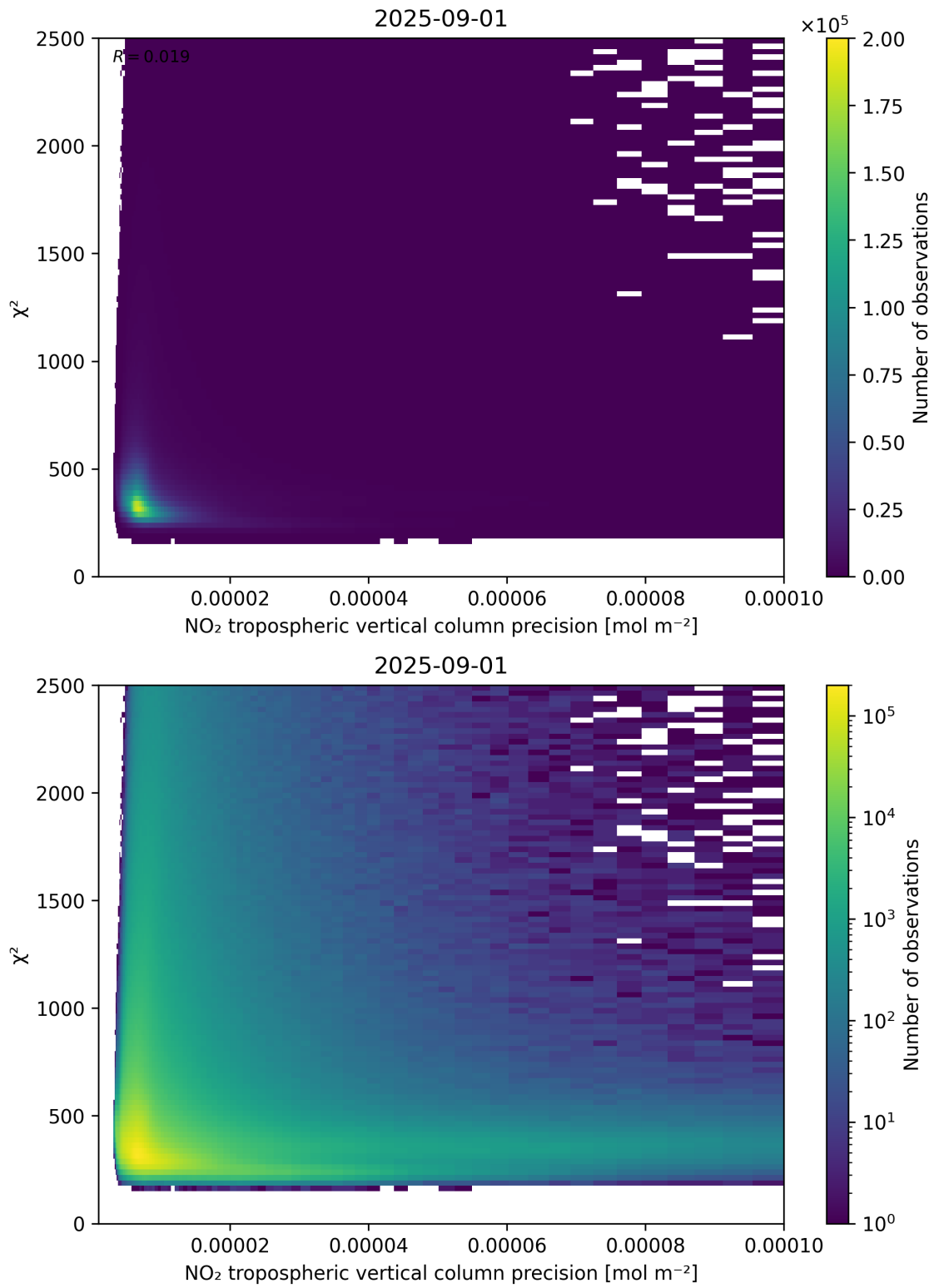
Figure 134: Scatter density plot of “NO 2 tropospheric vertical column precision” against “ \chi^2 ” for 2025-08-31 to 2025-09-02.
