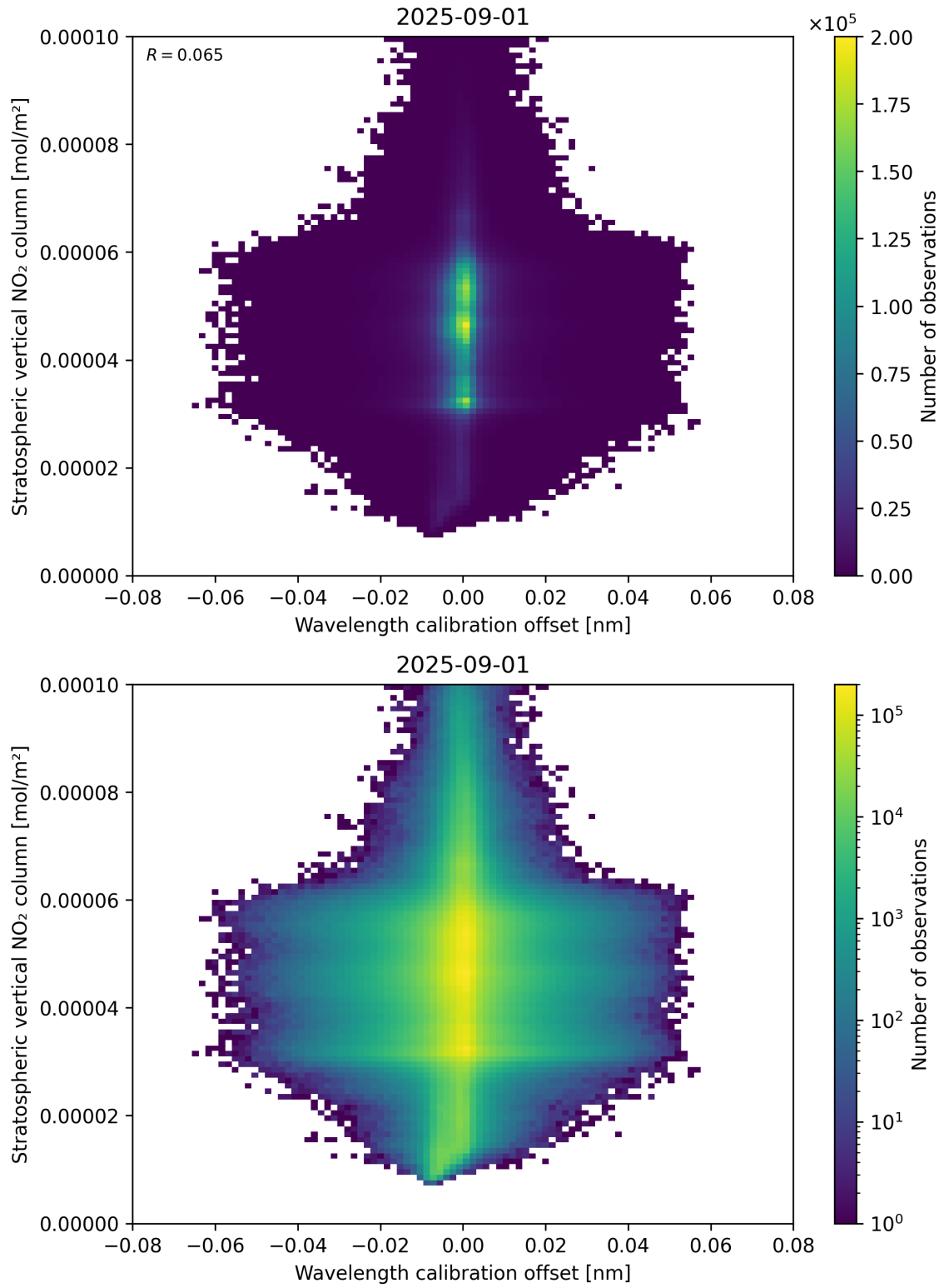
Figure 176: Scatter density plot of “Wavelength calibration offset” against “Stratospheric vertical NO 2 column” for 2025-08-31 to 2025-09-02.
