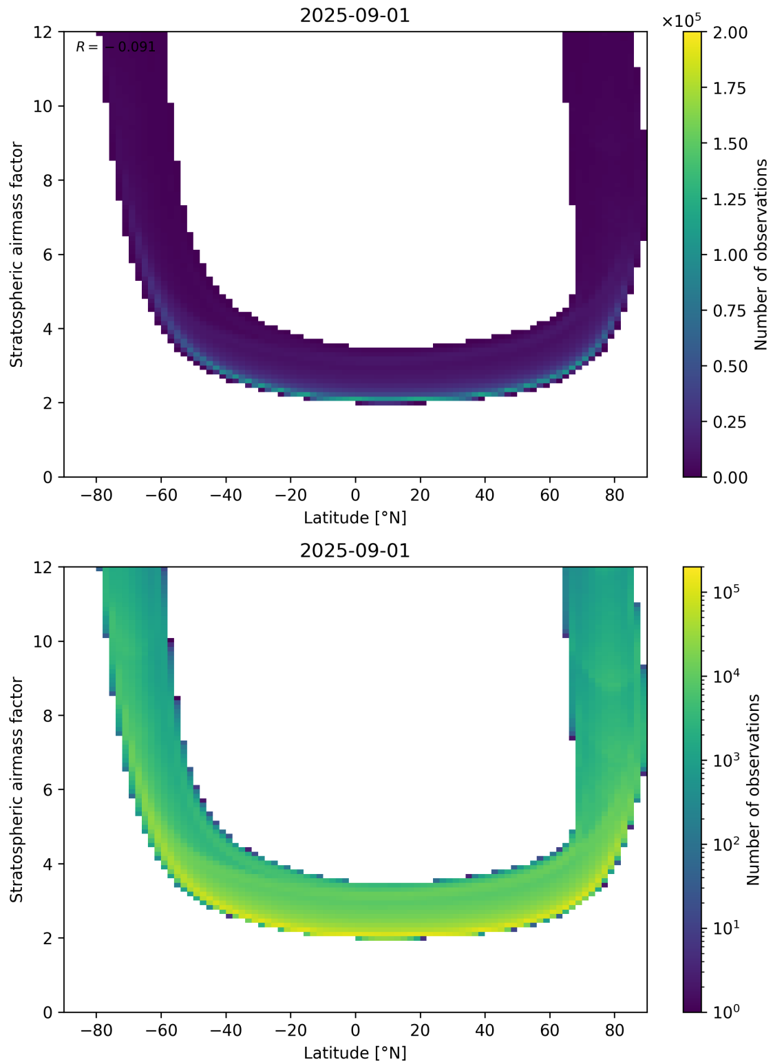
Figure 83: Scatter density plot of “Latitude” against “Stratospheric air mass factor” for 2025-08-31 to 2025-09-02.
