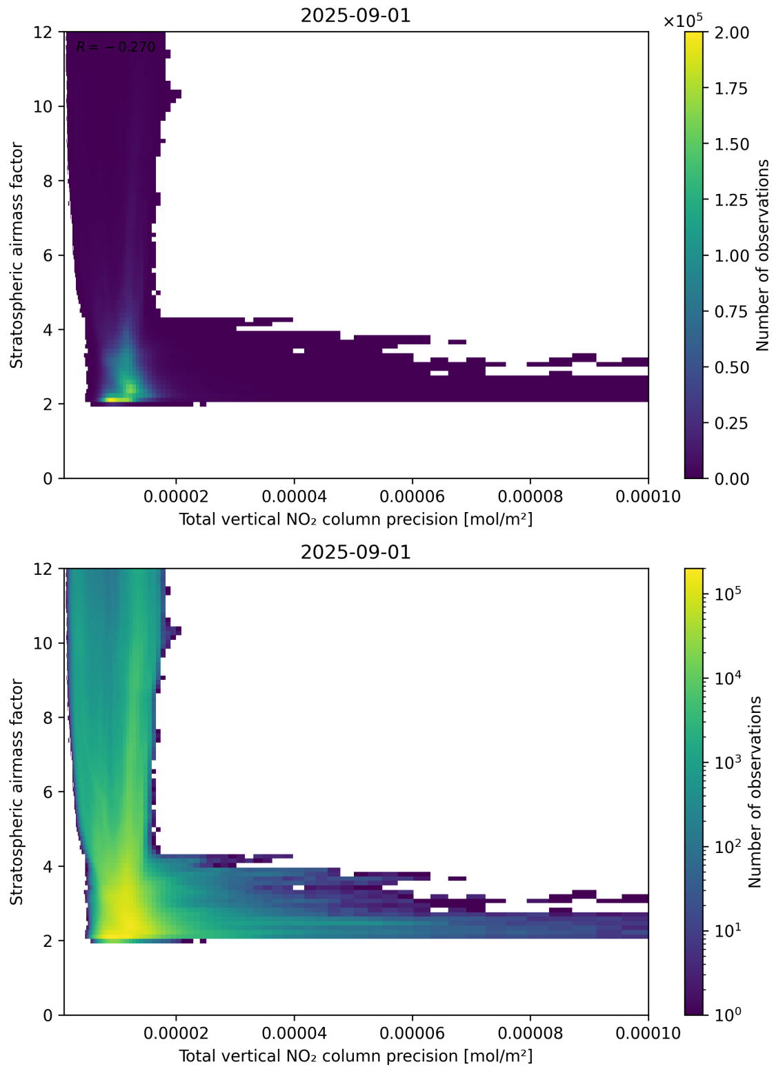
Figure 115: Scatter density plot of “Total vertical NO 2 column precision” against “Stratospheric air mass factor” for 2025-08-31 to 2025-09-02.
