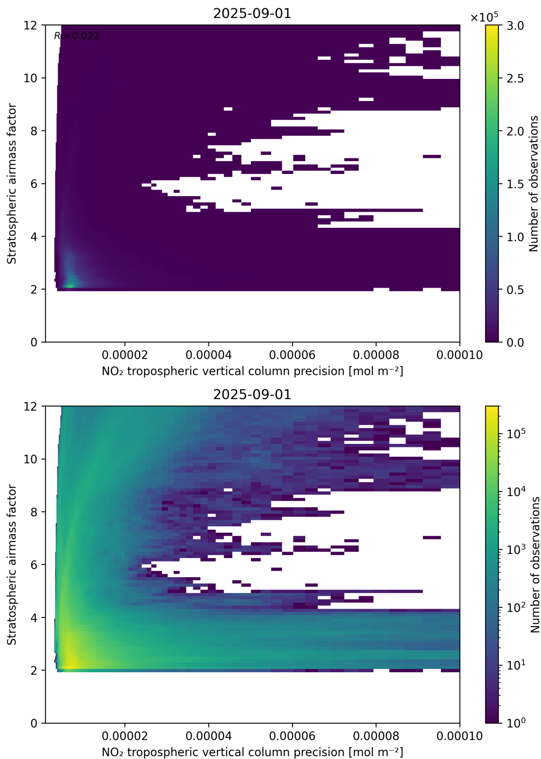
Figure 131: Scatter density plot of “NO 2 tropospheric vertical column precision” against “Stratospheric airmass factor” for 2025-08-31 to 2025-09-02.
