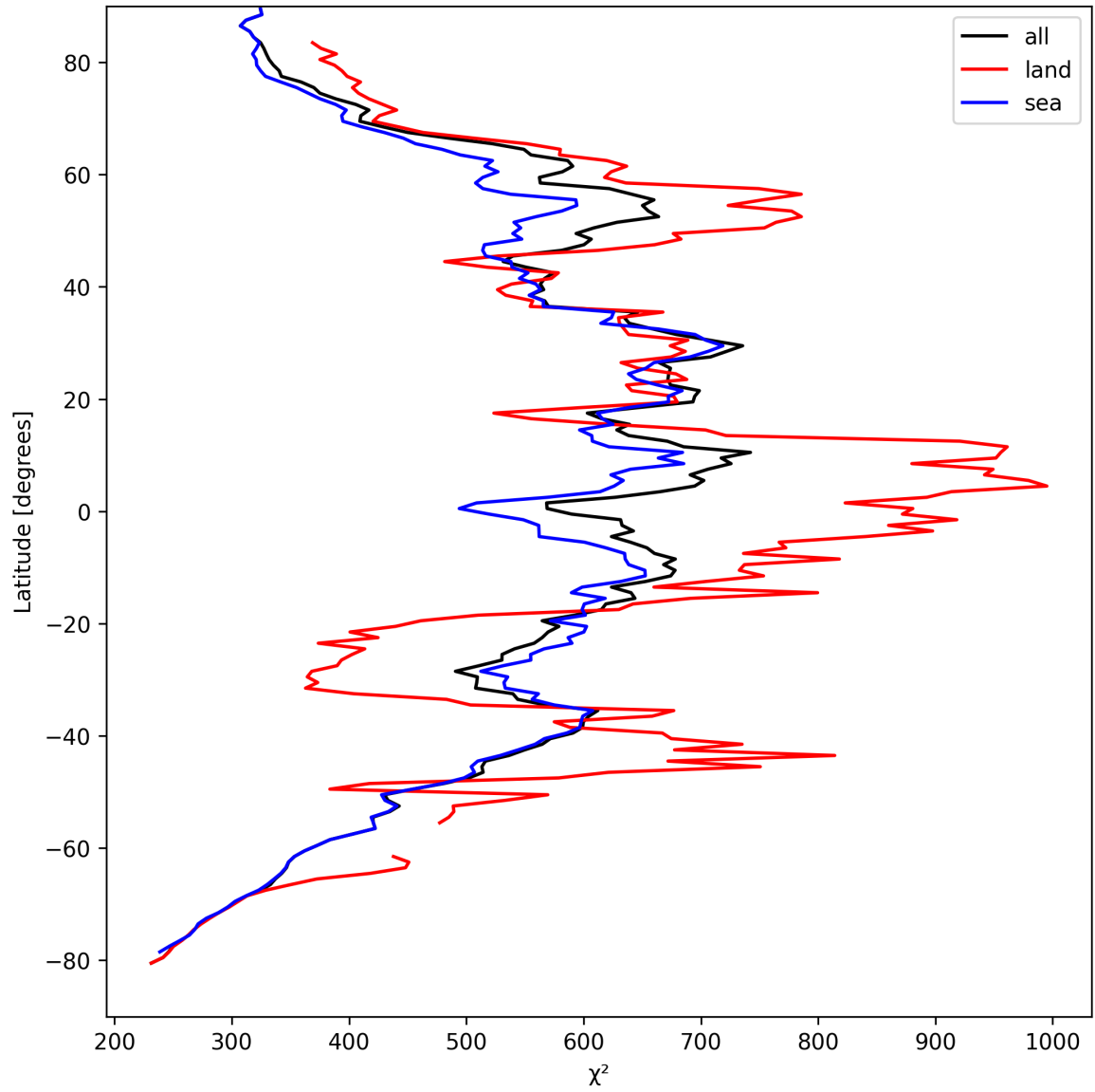
Figure 25: Zonal average of " \chi^2 " for 2025-08-31 to 2025-09-02.
