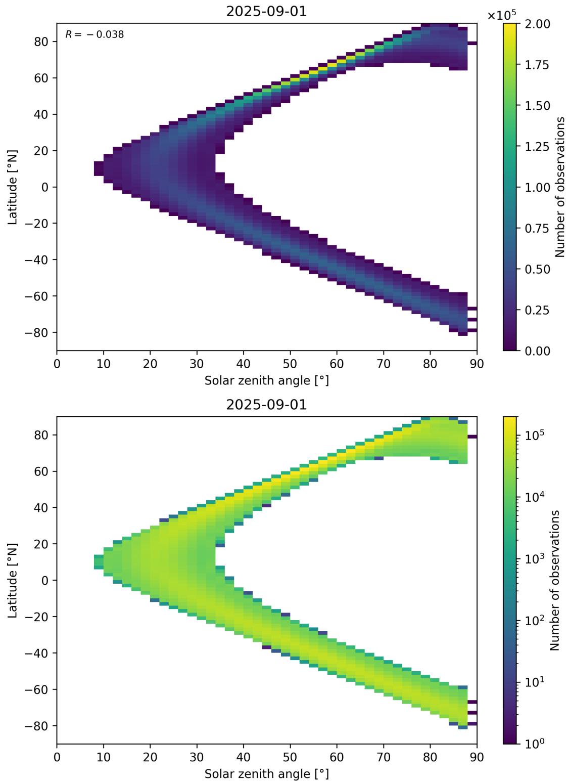
Figure 149: Scatter density plot of “Solar zenith angle” against “Latitude” for 2025-08-31 to 2025-09-02.
