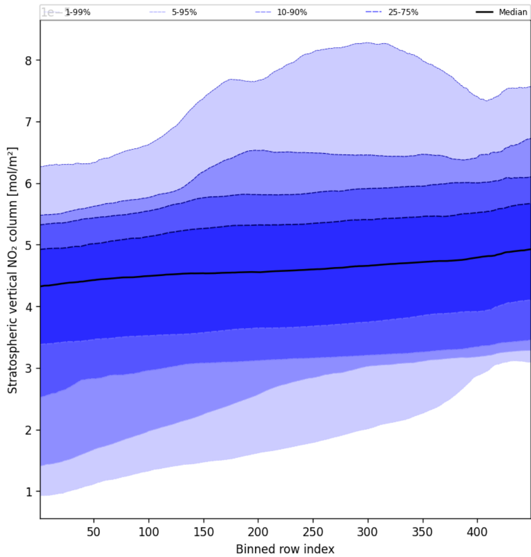
Figure 53: Along track statistics of “Stratospheric vertical NO 2 column” for 2025-08-31 to 2025-09-02
