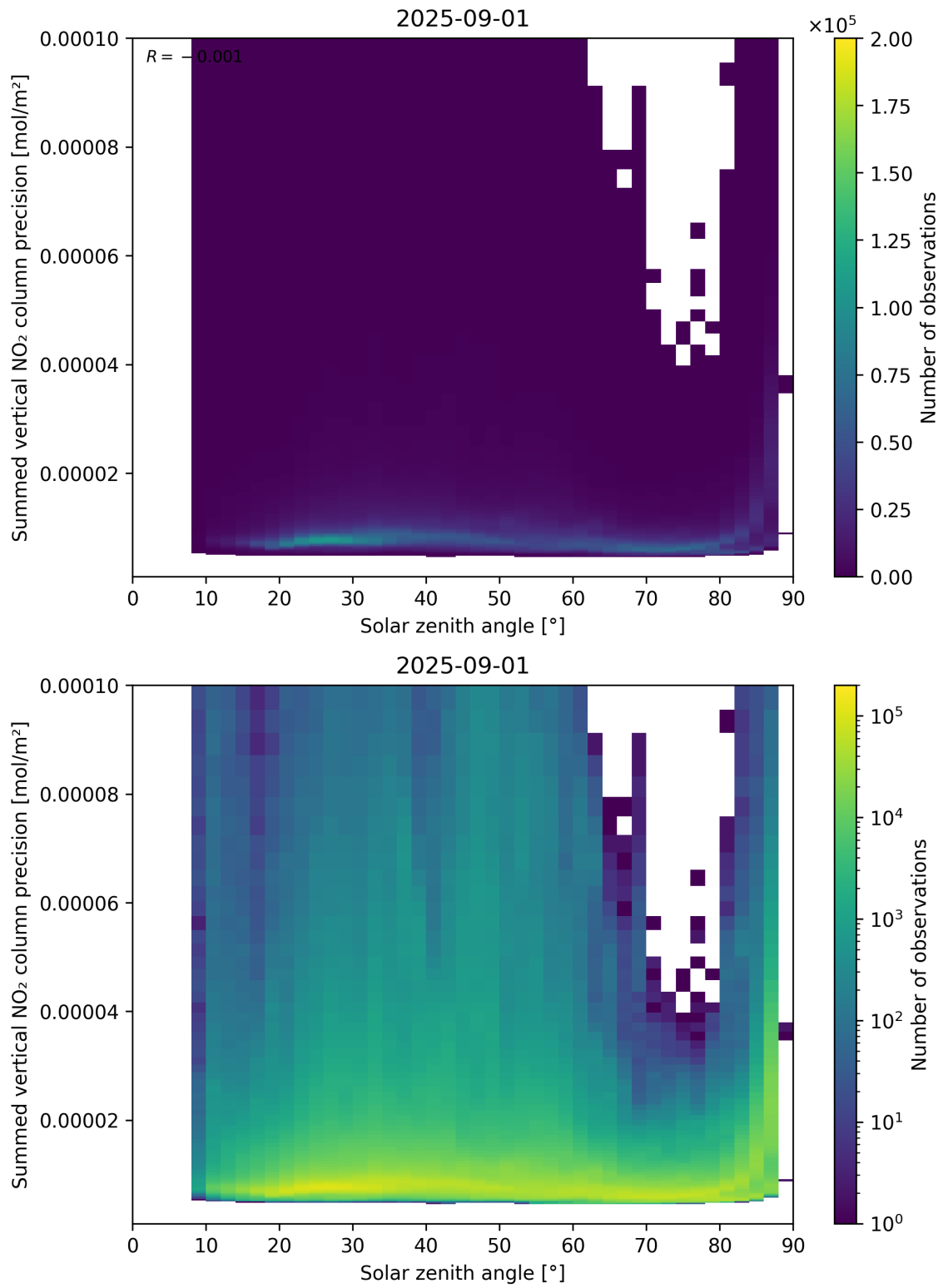
Figure 152: Scatter density plot of “Solar zenith angle” against “Summed vertical NO 2 column precision” for 2025-08-31 to 2025-09-02.
