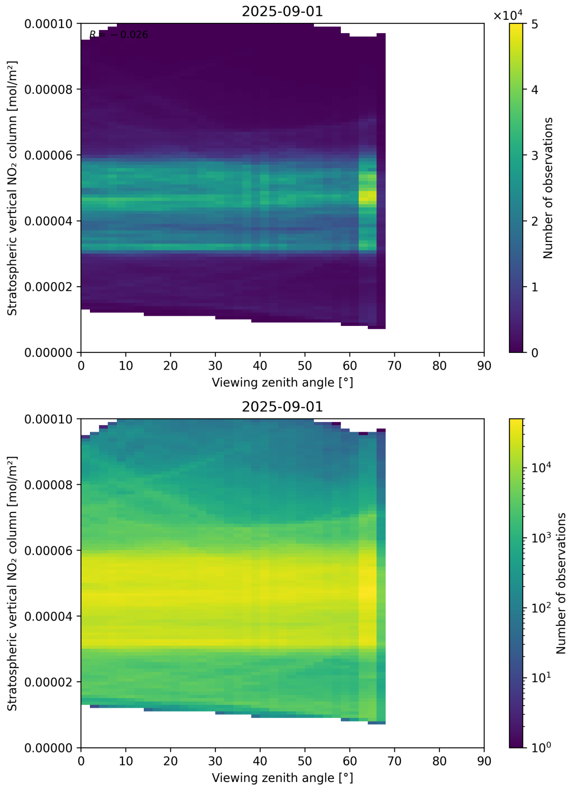
Figure 164: Scatter density plot of “Viewing zenith angle” against “Stratospheric vertical NO 2 column” for 2025-08-31 to 2025-09-02.
