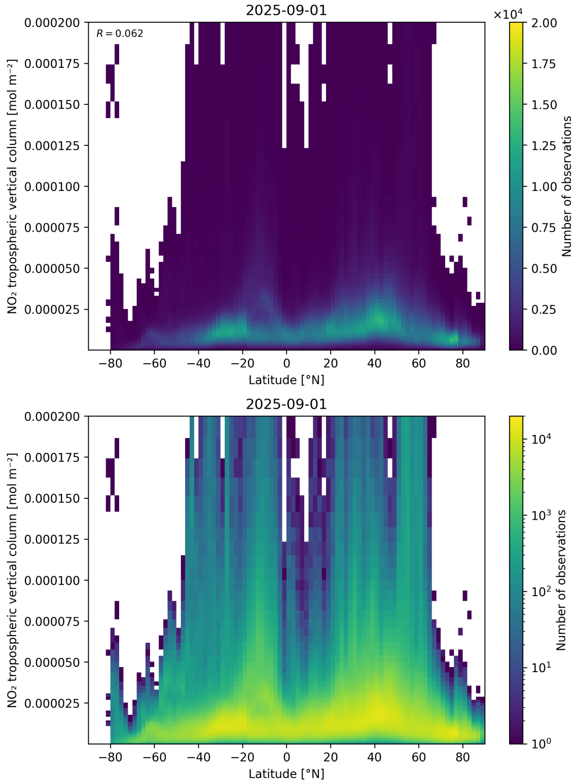
Figure 92: Scatter density plot of “Latitude” against “NO 2 tropospheric vertical column” for 2025-08-31 to 2025-09-02.
