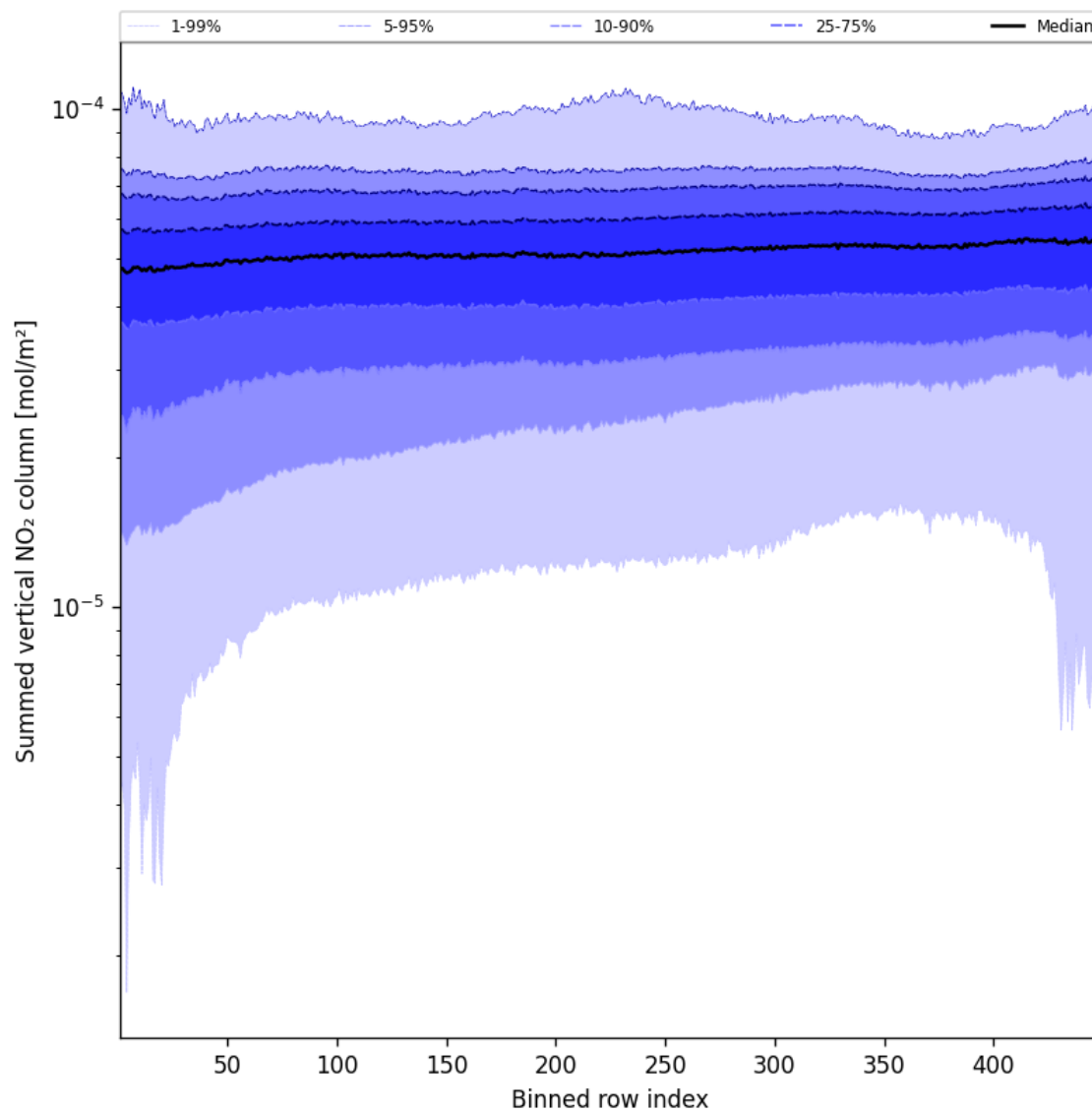
Figure 57: Along track statistics of “Summed vertical NO 2 column” for 2025-08-31 to 2025-09-02
