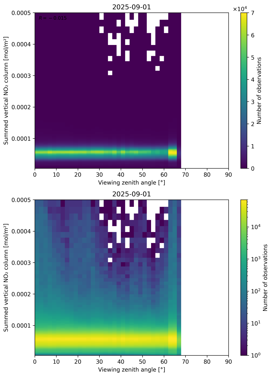
Figure 165: Scatter density plot of “Viewing zenith angle” against “Summed vertical NO 2 column” for 2025-08-31 to 2025-09-02.
