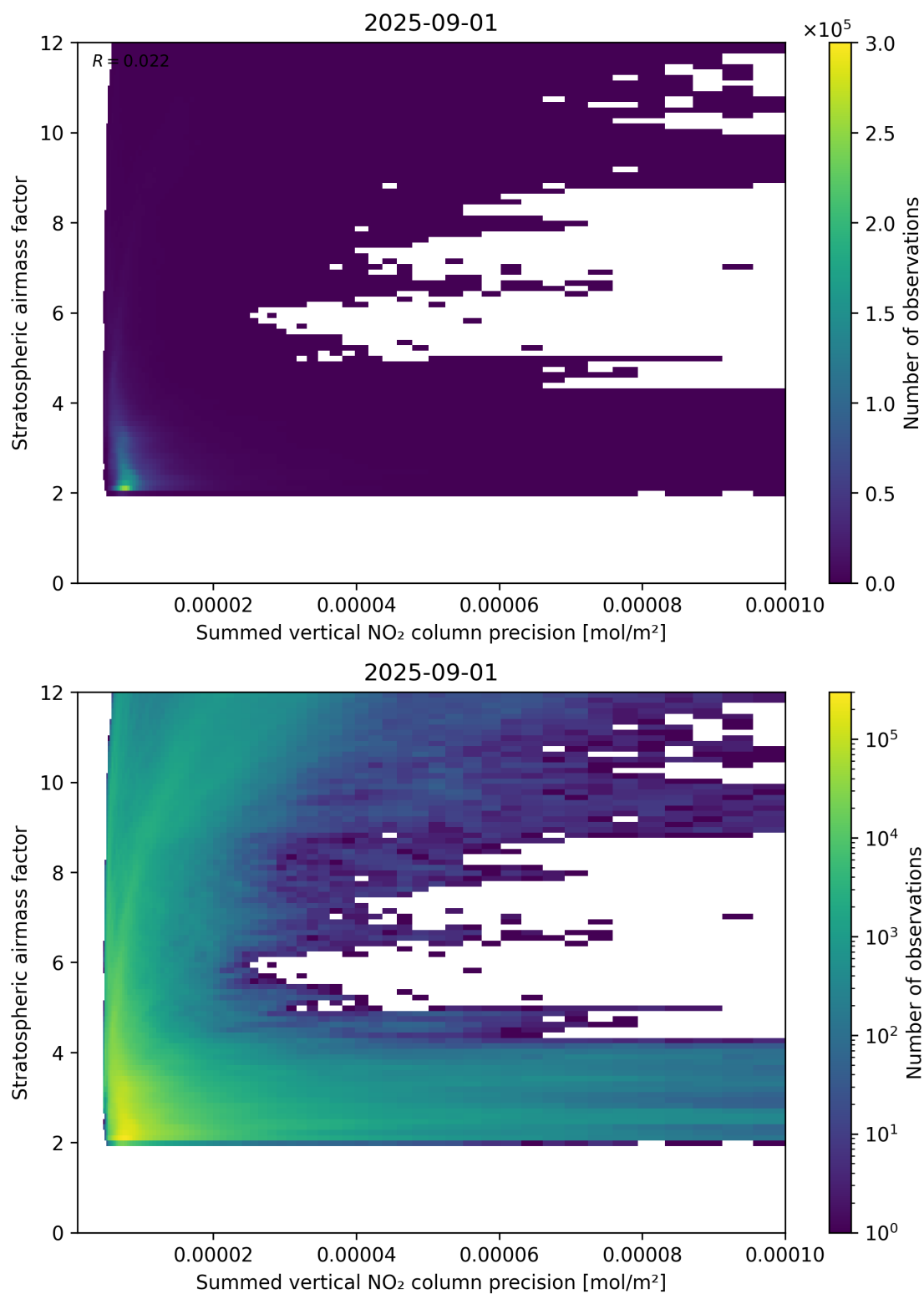
Figure 106: Scatter density plot of “Summed vertical NO 2 column precision” against “Stratospheric airmass factor” for 2025-08-31 to 2025-09-02.
