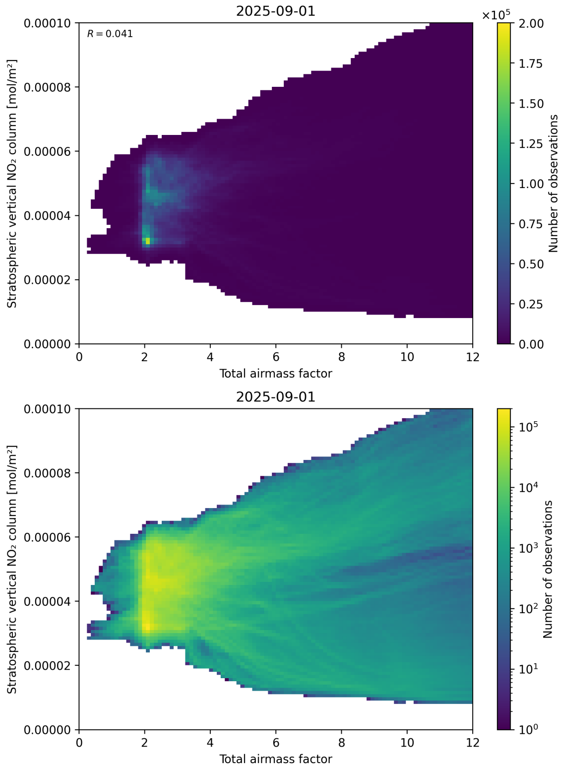
Figure 64: Scatter density plot of “Total airmass factor” against “Stratospheric vertical \text{NO}_2 column” for 2025-08-31 to 2025-09-02.
