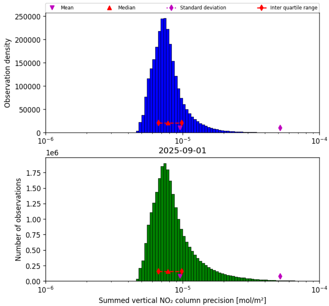
Figure 41: Histogram of "Summed vertical NO 2 column precision" for 2025-08-31 to 2025-09-02
