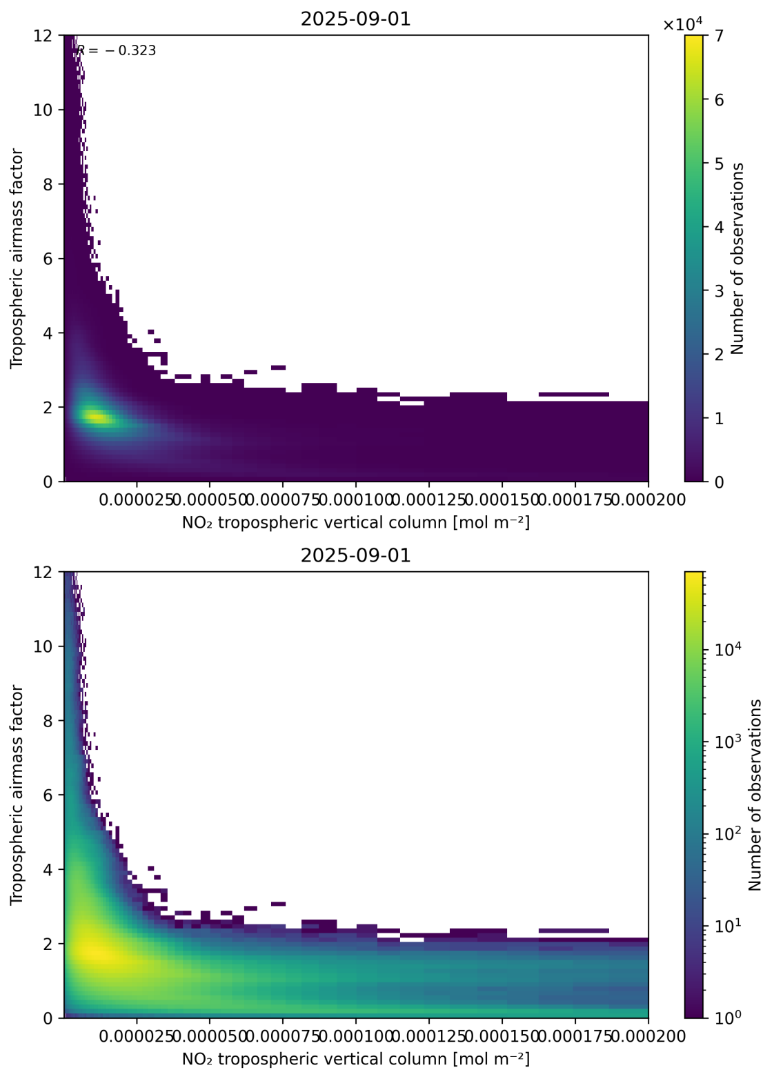
Figure 123: Scatter density plot of “NO 2 tropospheric vertical column” against “Tropospheric air mass factor” for 2025-08-31 to 2025-09-02.
