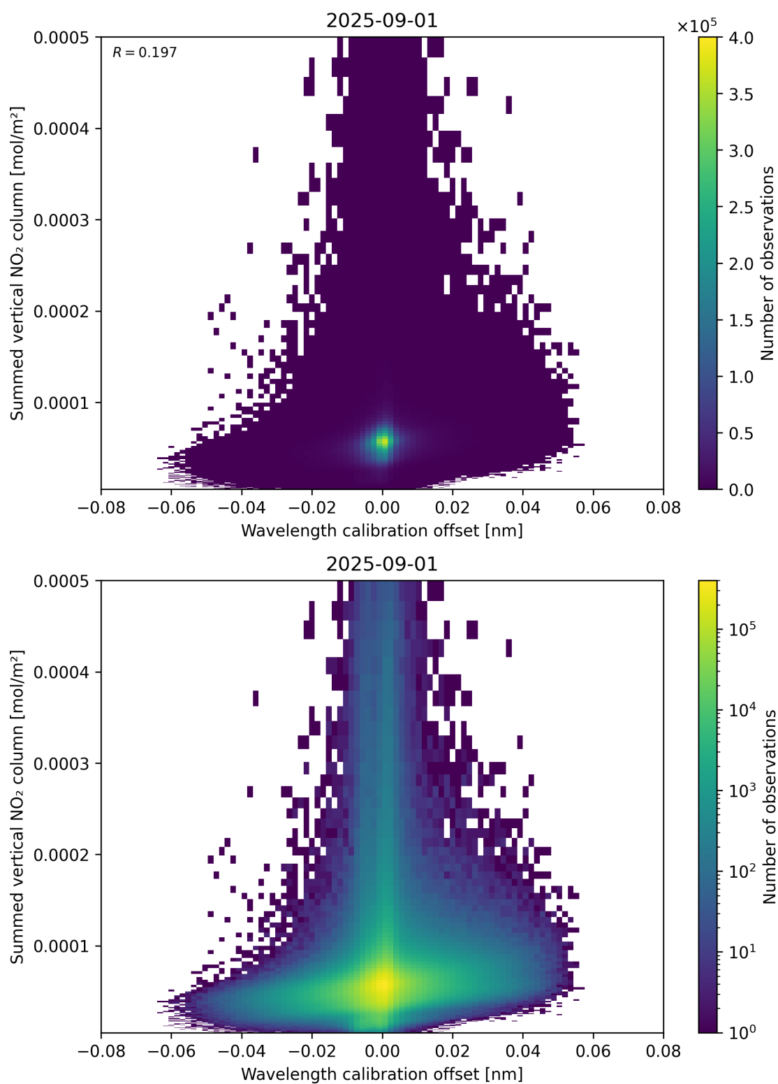
Figure 177: Scatter density plot of “Wavelength calibration offset” against “Summed vertical NO 2 column” for 2025-08-31 to 2025-09-02.
