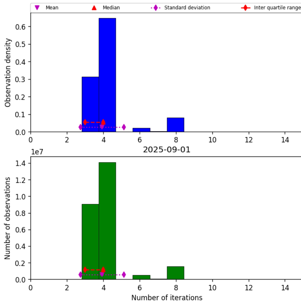
Figure 34: Histogram of “Number of iterations” for 2025-08-31 to 2025-09-02
