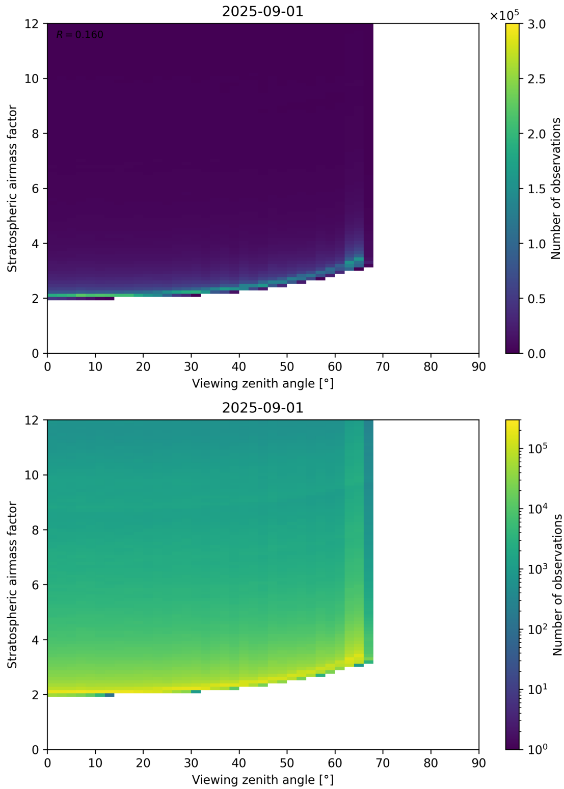
Figure 159: Scatter density plot of “Viewing zenith angle” against “Stratospheric airmass factor” for 2025-08-31 to 2025-09-02.
