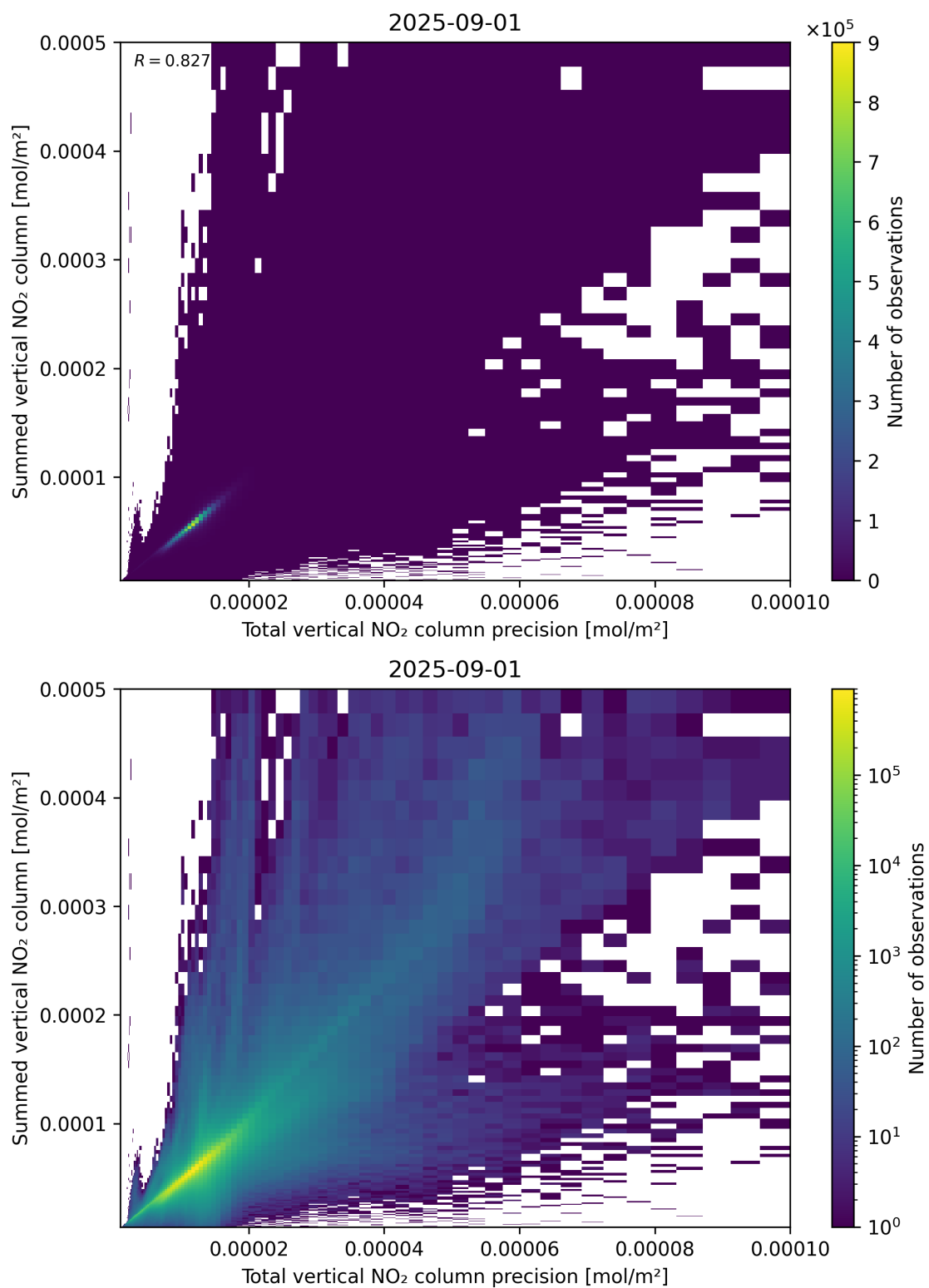
Figure 117: Scatter density plot of “Total vertical NO 2 column precision” against “Summed vertical NO 2 column” for 2025-08-31 to 2025-09-02.
