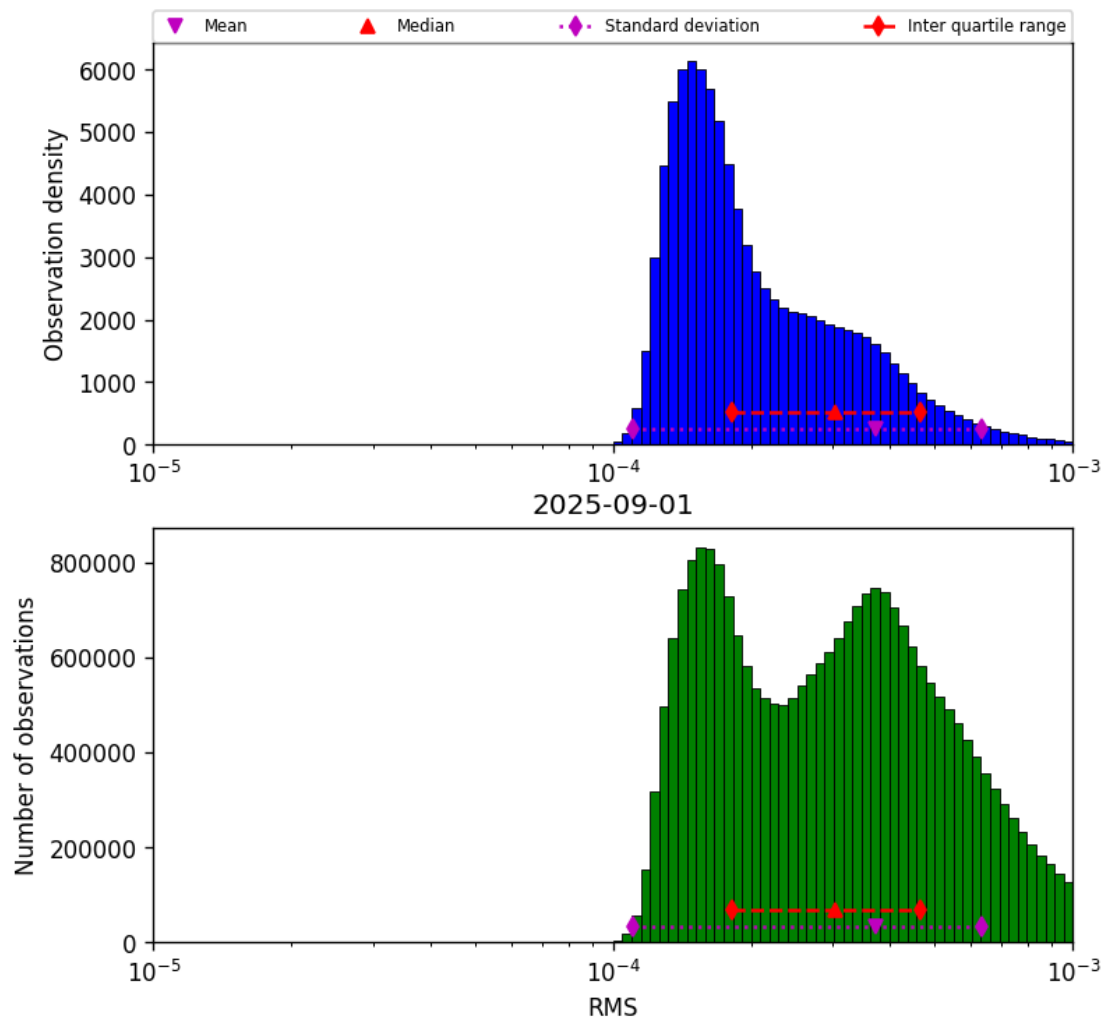
Figure 43: Histogram of “RMS” for 2025-08-31 to 2025-09-02
