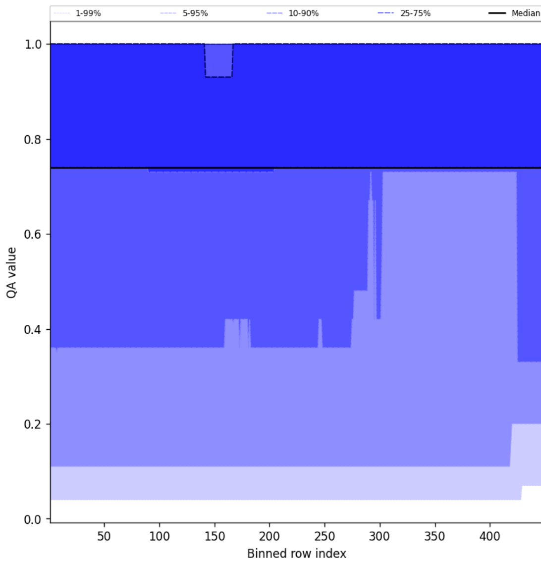
Figure 45: Along track statistics of “QA value” for 2025-08-31 to 2025-09-02
