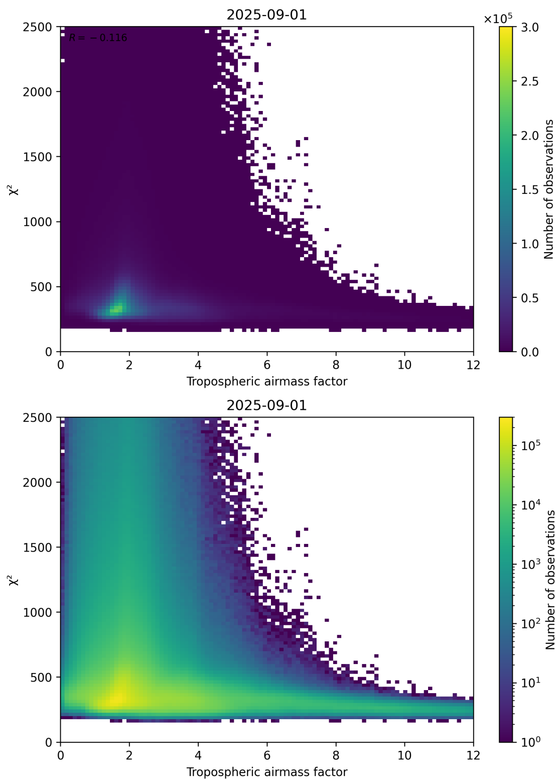
Figure 73: Scatter density plot of “Tropospheric airmass factor” against “ \chi^2 ” for 2025-08-31 to 2025-09-02.
