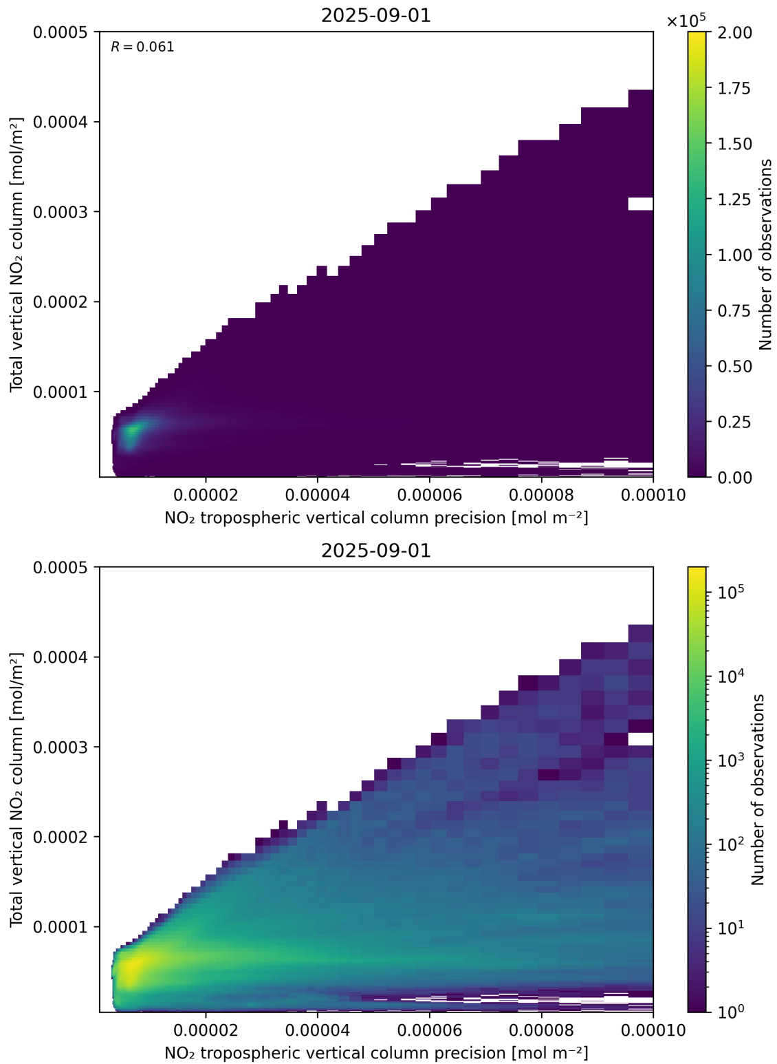
Figure 138: Scatter density plot of “NO 2 tropospheric vertical column precision” against “Total vertical NO 2 column” for 2025-08-31 to 2025-09-02.
