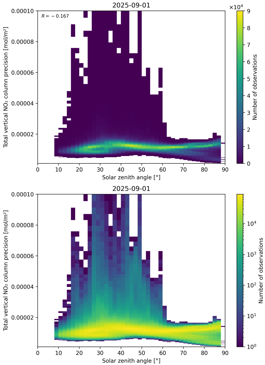
Figure 154: Scatter density plot of “Solar zenith angle” against “Total vertical NO 2 column precision” for 2025-08-31 to 2025-09-02.
