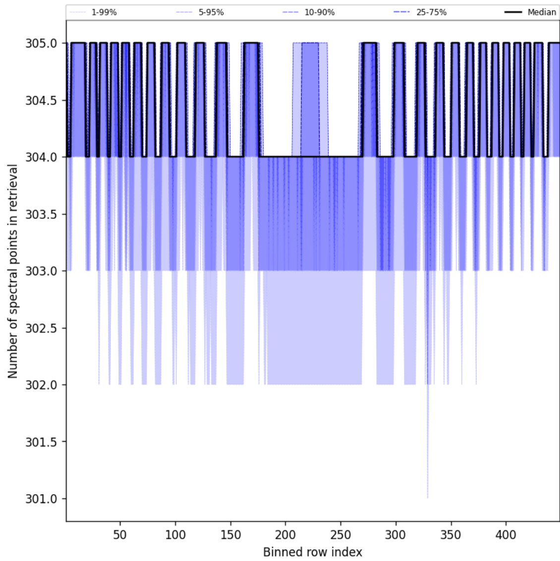
Figure 50: Along track statistics of “Number of spectral points in retrieval” for 2025-08-31 to 2025-09-02
