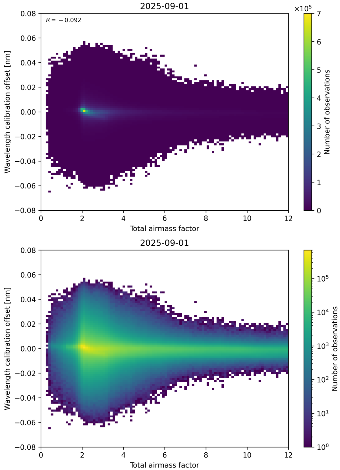
Figure 70: Scatter density plot of “Total airmass factor” against “Wavelength calibration offset” for 2025-08-31 to 2025-09-02.
