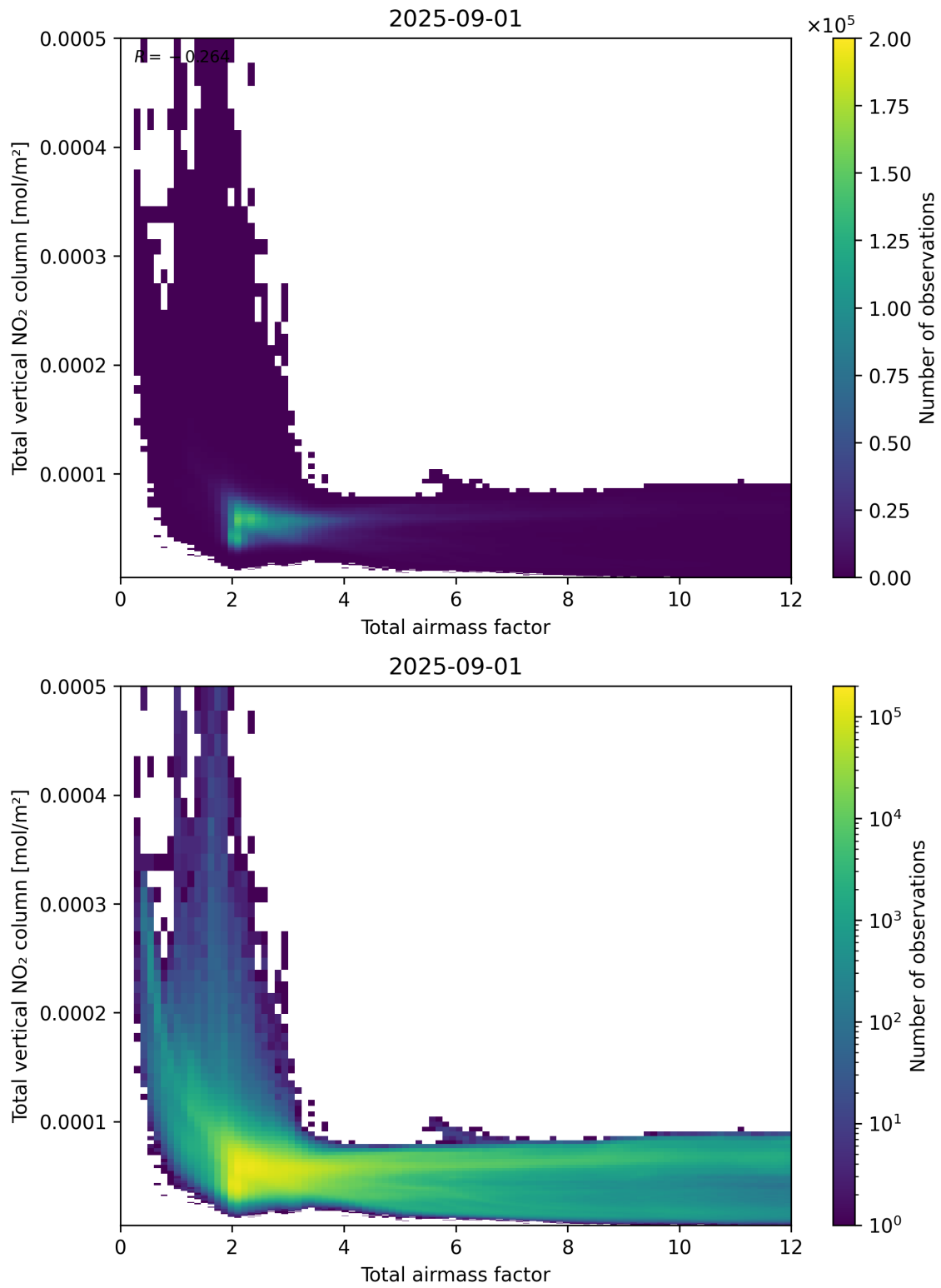
Figure 67: Scatter density plot of “Total airmass factor” against “Total vertical NO 2 column” for 2025-08-31 to 2025-09-02.
