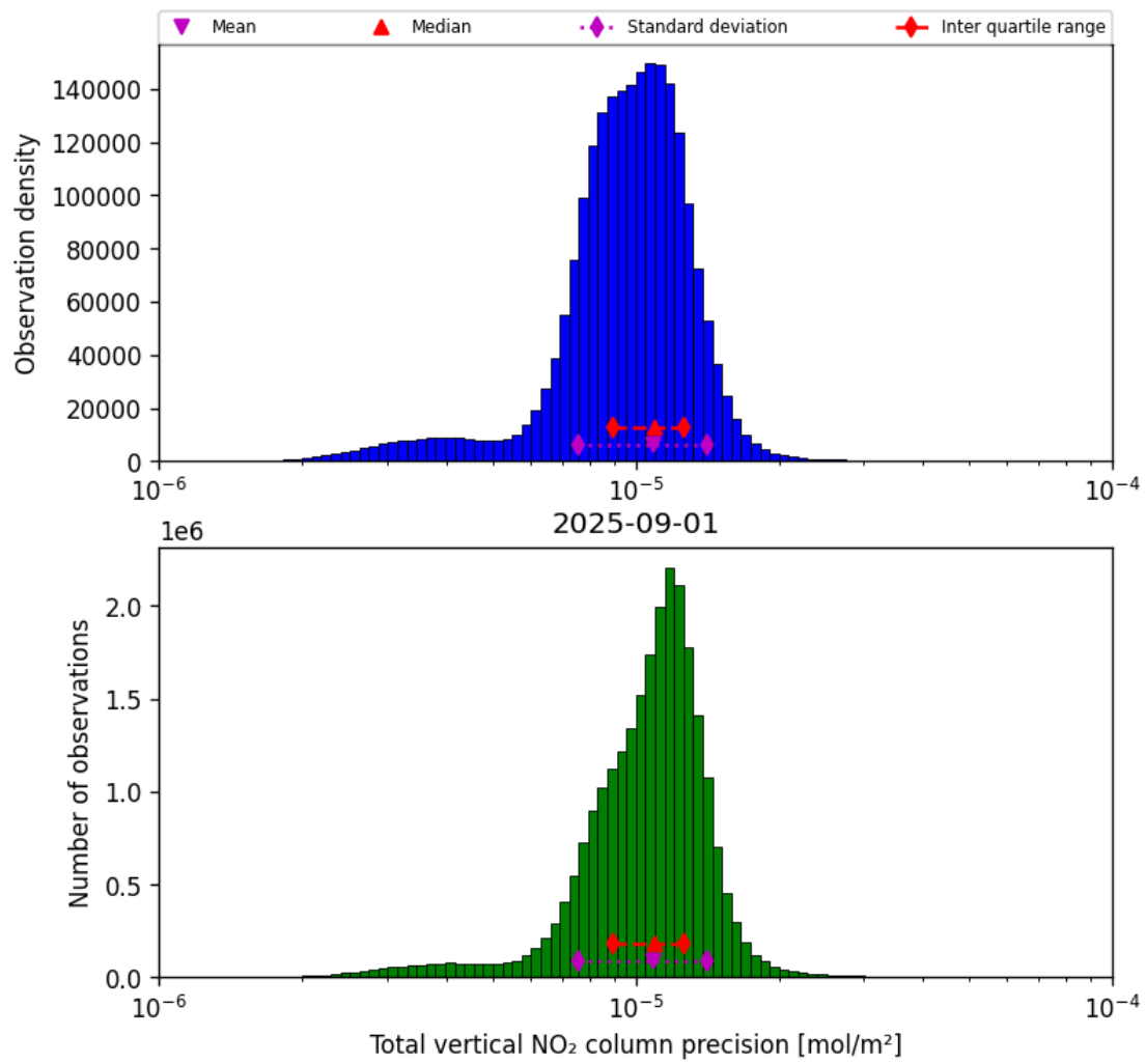
Figure 39: Histogram of “Total vertical NO 2 column precision” for 2025-08-31 to 2025-09-02
