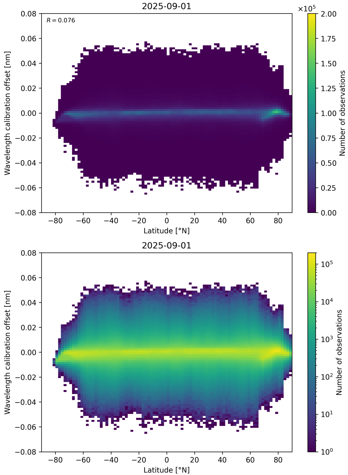
Figure 95: Scatter density plot of “Latitude” against “Wavelength calibration offset” for 2025-08-31 to 2025-09-02.
