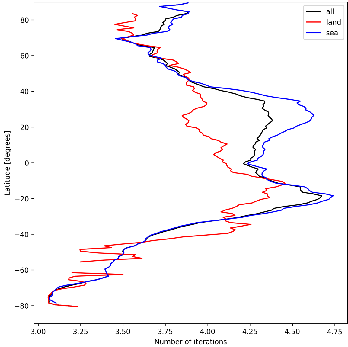
Figure 17: Zonal average of “Number of iterations” for 2025-08-31 to 2025-09-02.
