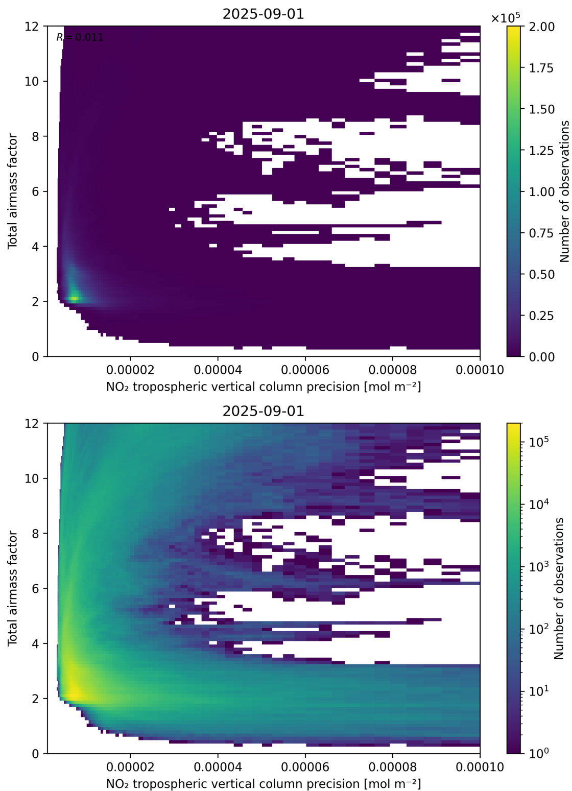
Figure 132: Scatter density plot of “NO 2 tropospheric vertical column precision” against “Total air mass factor” for 2025-08-31 to 2025-09-02.
