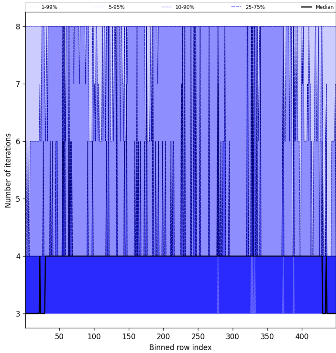
Figure 51: Along track statistics of “Number of iterations” for 2025-08-31 to 2025-09-02
