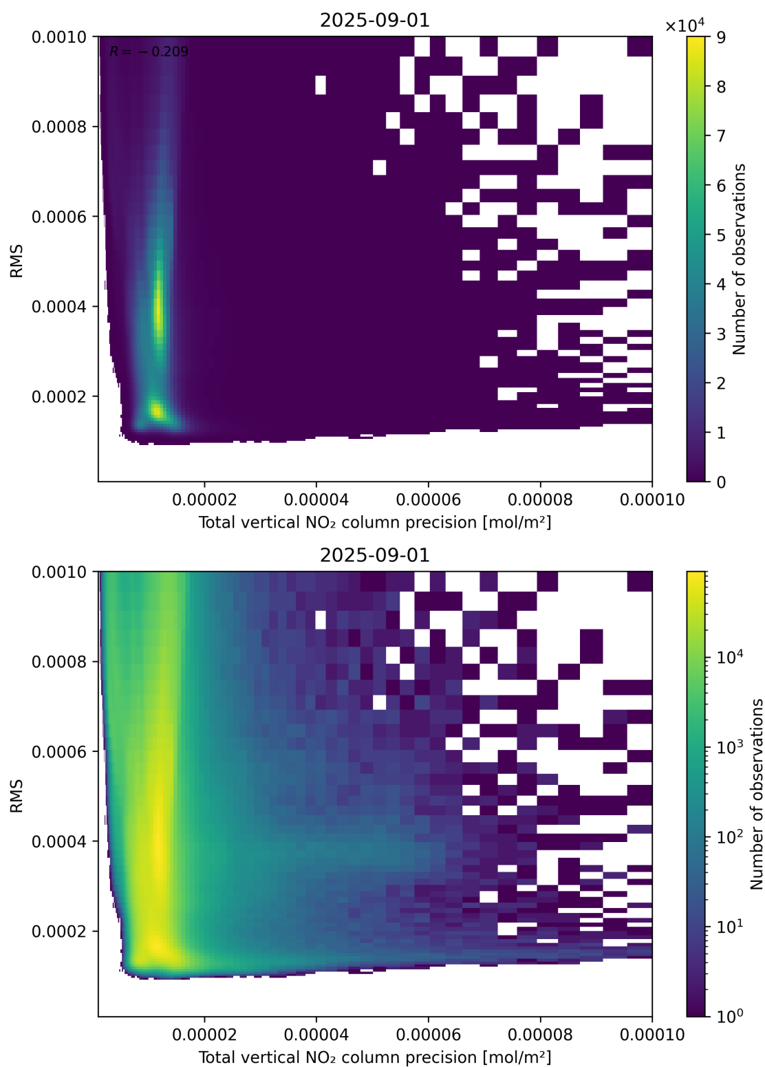
Figure 119: Scatter density plot of “Total vertical NO 2 column precision” against “RMS” for 2025-08-31 to 2025-09-02.
