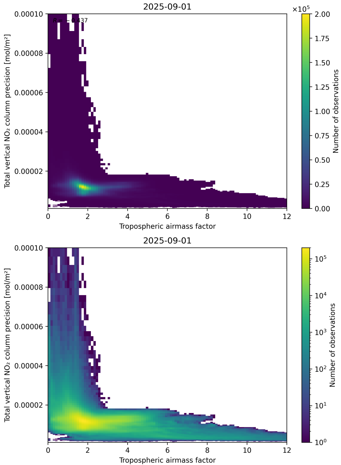
Figure 78: Scatter density plot of “Tropospheric air mass factor” against “Total vertical NO 2 column precision” for 2025-08-31 to 2025-09-02.
