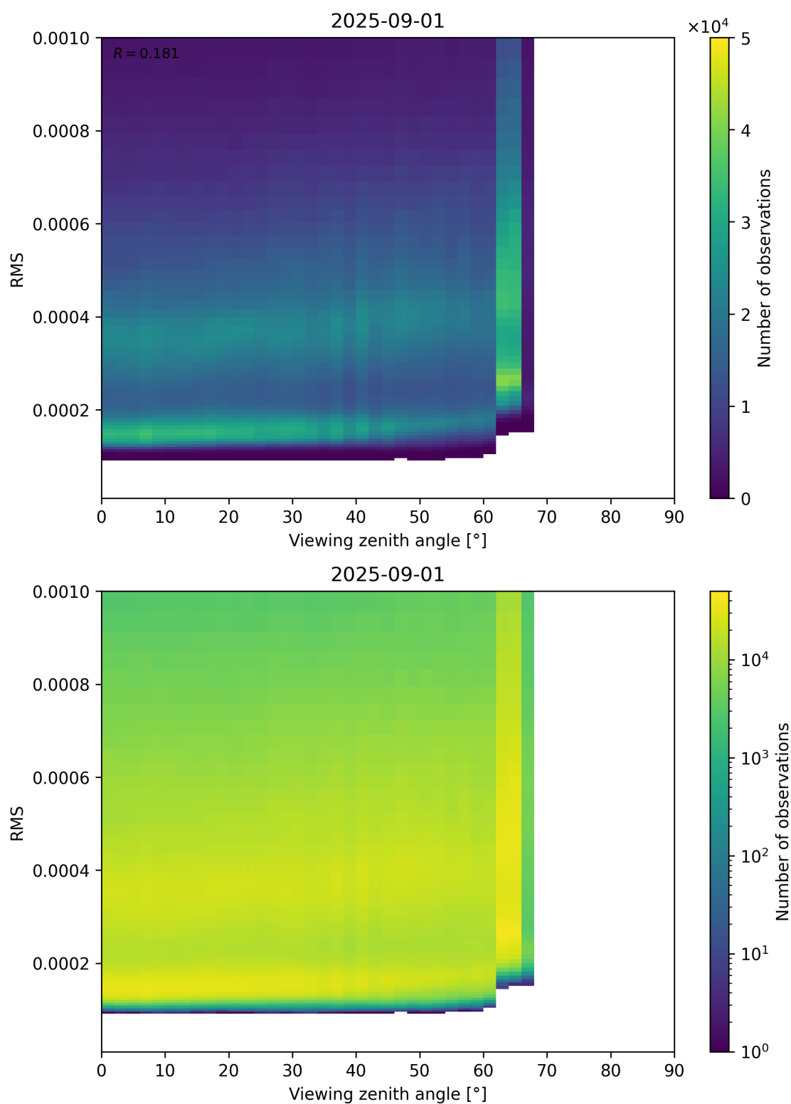
Figure 171: Scatter density plot of “Viewing zenith angle” against “RMS” for 2025-08-31 to 2025-09-02.
