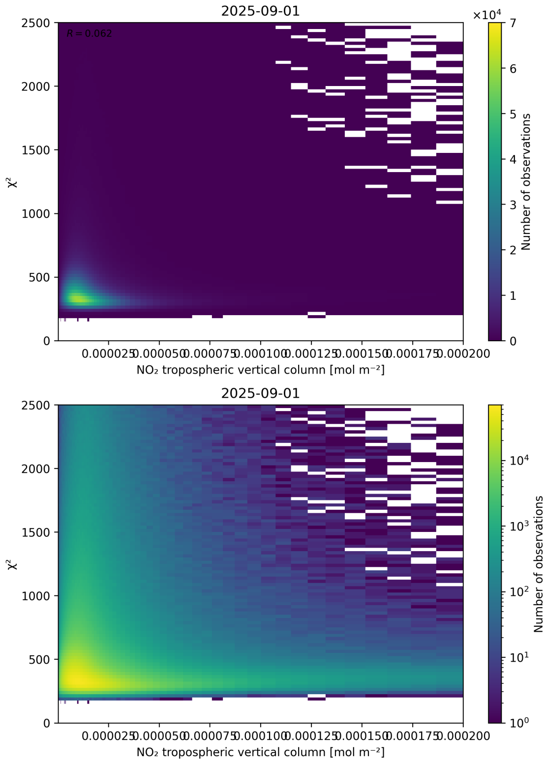
Figure 124: Scatter density plot of “NO 2 tropospheric vertical column” against “ \chi^2 ” for 2025-08-31 to 2025-09-02.
