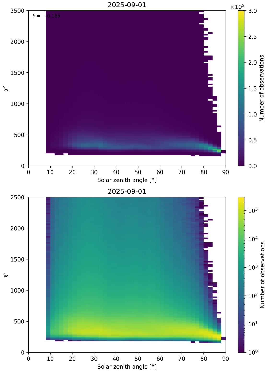
Figure 148: Scatter density plot of “Solar zenith angle” against “ \chi^2 ” for 2025-08-31 to 2025-09-02.
