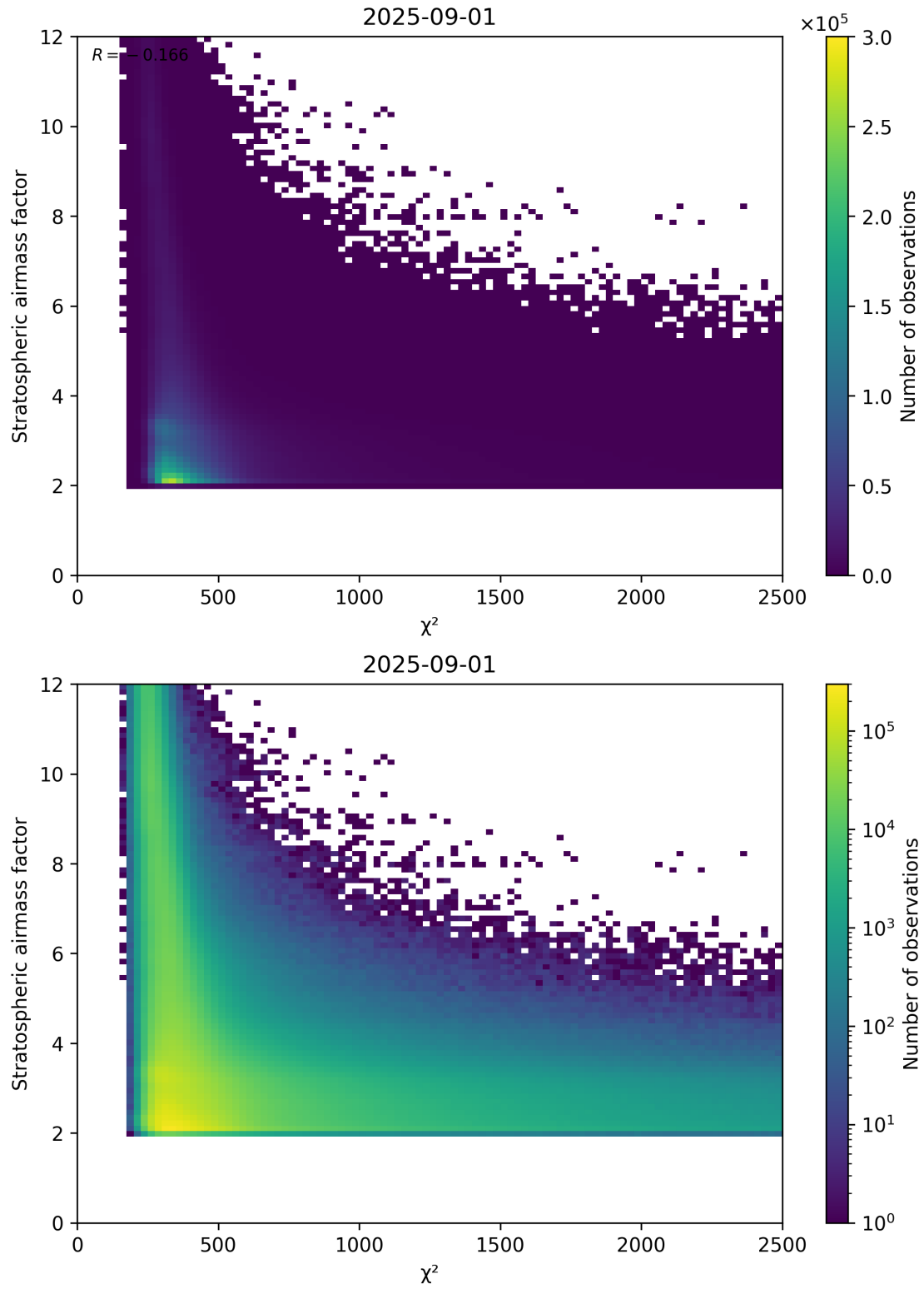
Figure 81: Scatter density plot of “ \chi^2 ” against “Stratospheric airmass factor” for 2025-08-31 to 2025-09-02.
