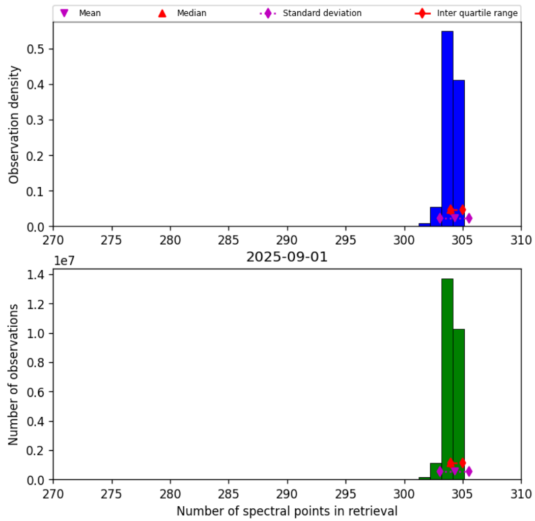
Figure 33: Histogram of “Number of spectral points in retrieval” for 2025-08-31 to 2025-09-02
