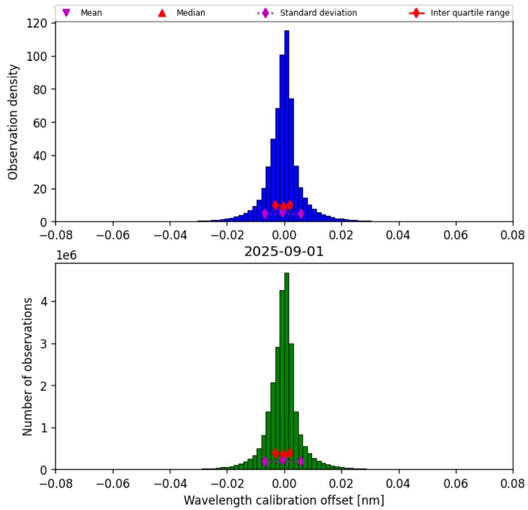
Figure 35: Histogram of “Wavelength calibration offset” for 2025-08-31 to 2025-09-02
