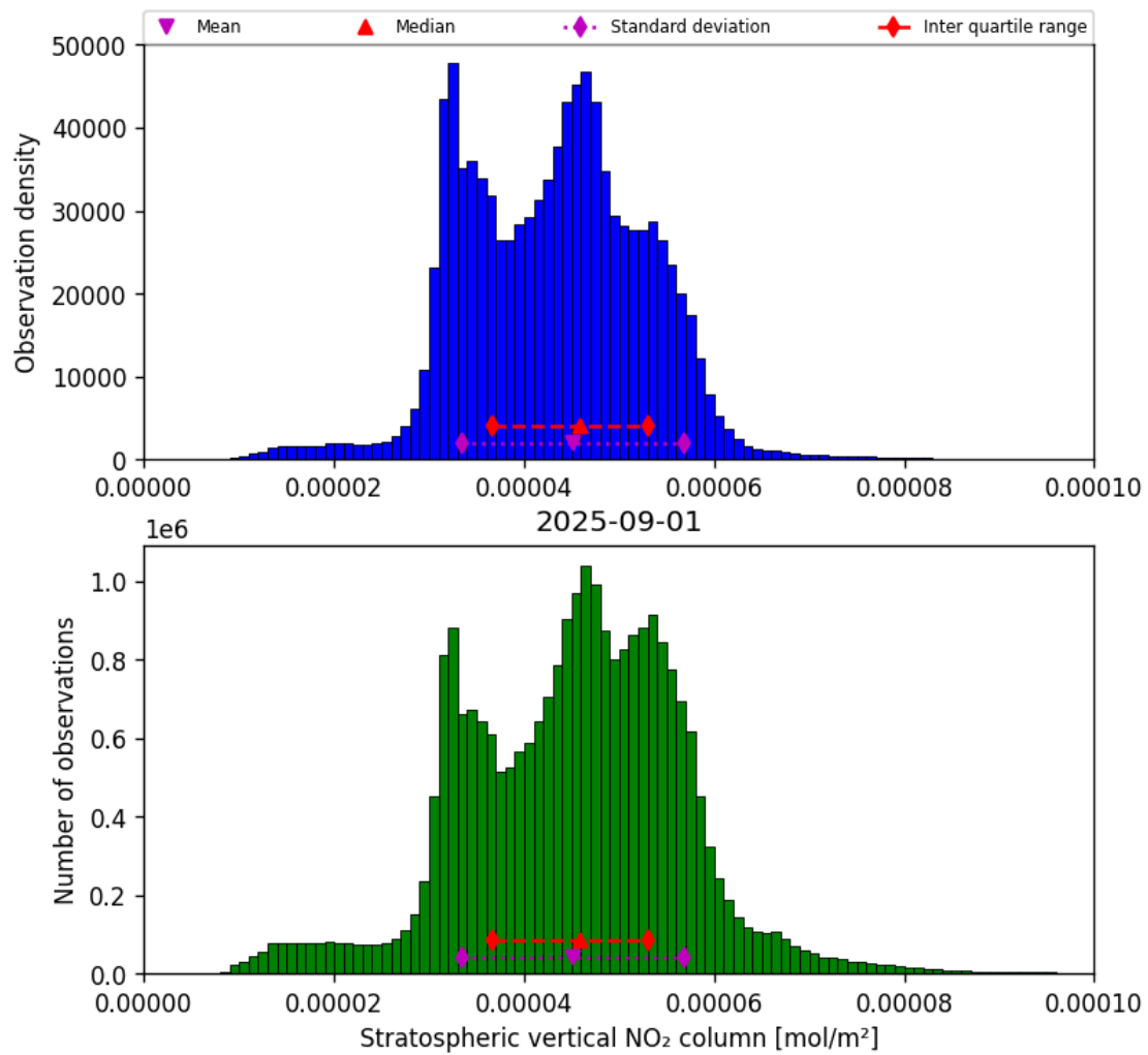
Figure 36: Histogram of “Stratospheric vertical NO 2 column” for 2025-08-31 to 2025-09-02
