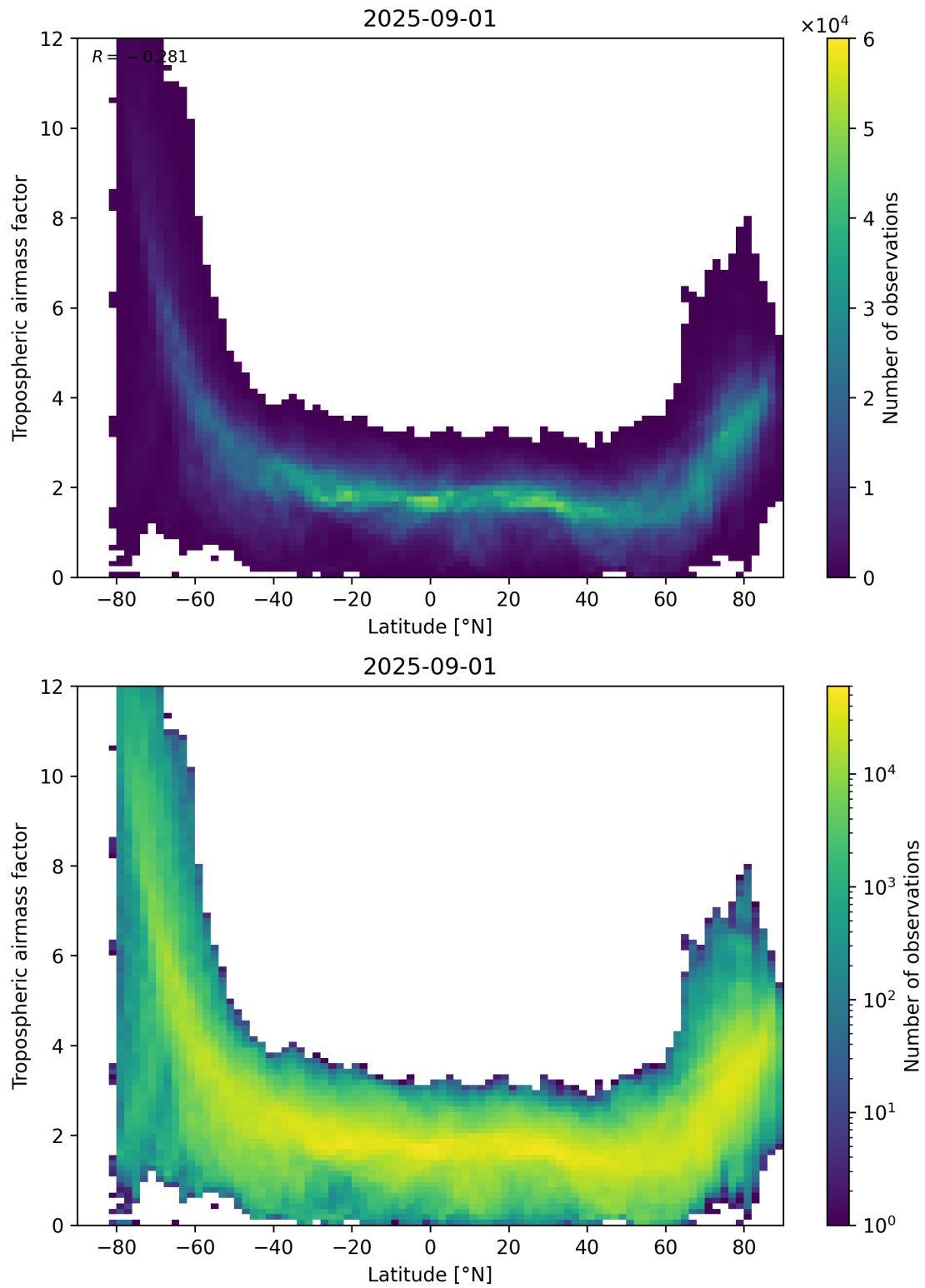
Figure 85: Scatter density plot of “Latitude” against “Tropospheric air mass factor” for 2025-08-31 to 2025-09-02.
