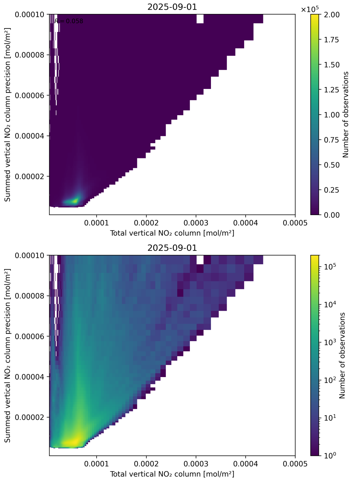
Figure 113: Scatter density plot of “Total vertical NO 2 column” against “Summed vertical NO 2 column precision” for 2025-08-31 to 2025-09-02.
