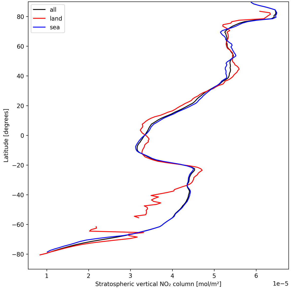
Figure 19: Zonal average of “Stratospheric vertical NO 2 column” for 2025-08-31 to 2025-09-02.
