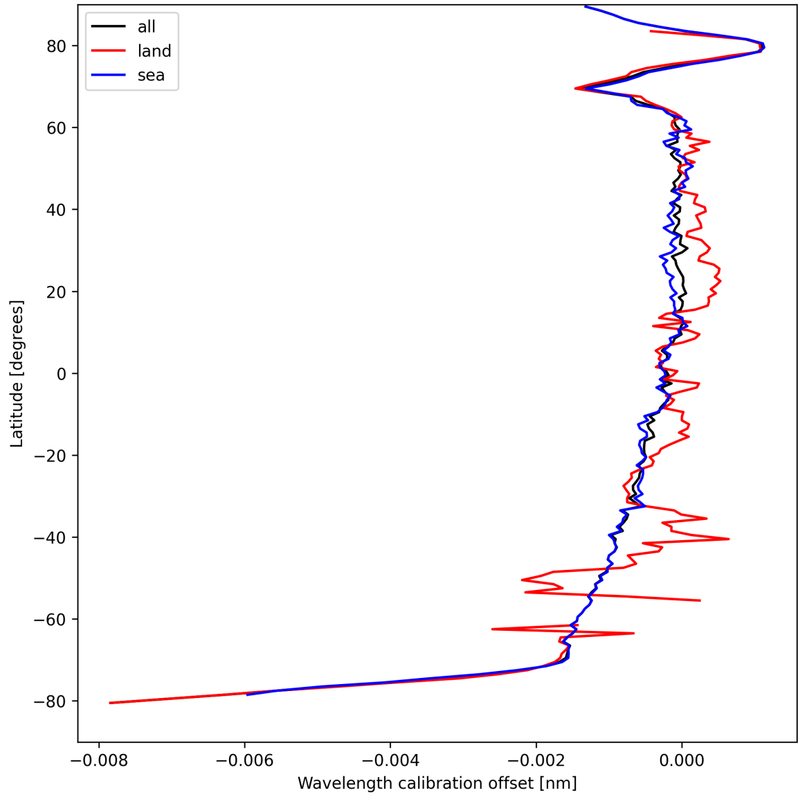
Figure 18: Zonal average of “Wavelength calibration offset” for 2025-08-31 to 2025-09-02.
