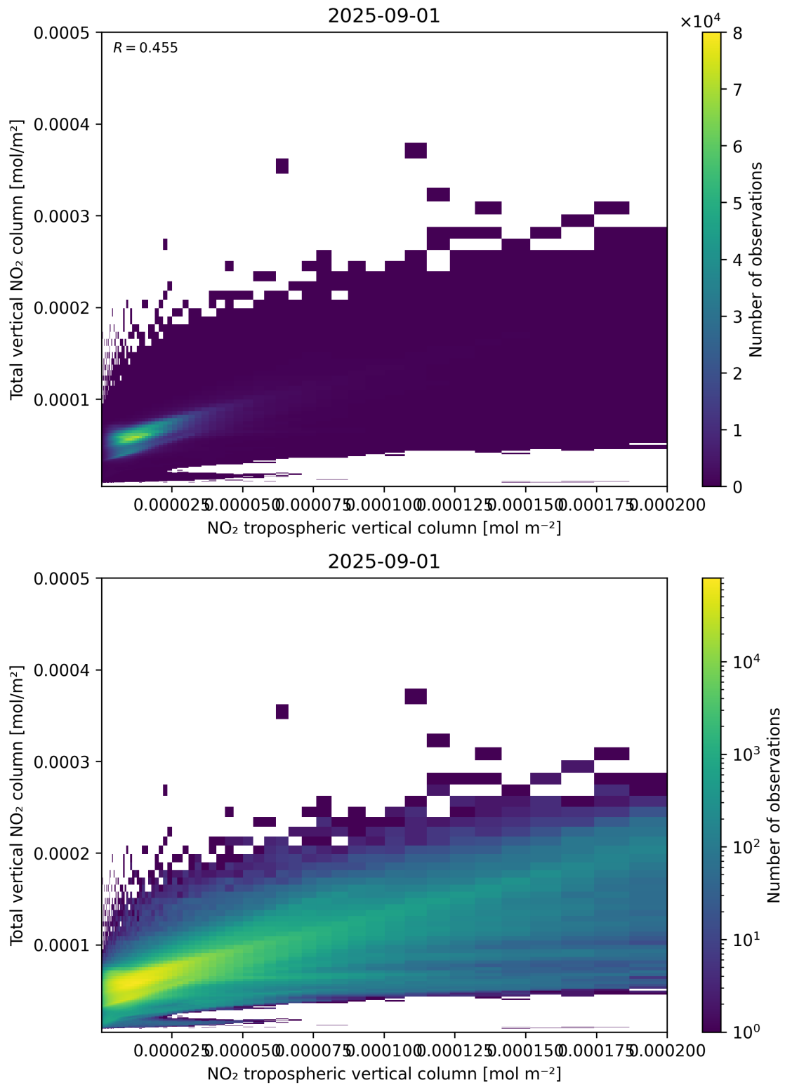
Figure 128: Scatter density plot of “NO 2 tropospheric vertical column” against “Total vertical NO 2 column” for 2025-08-31 to 2025-09-02.
