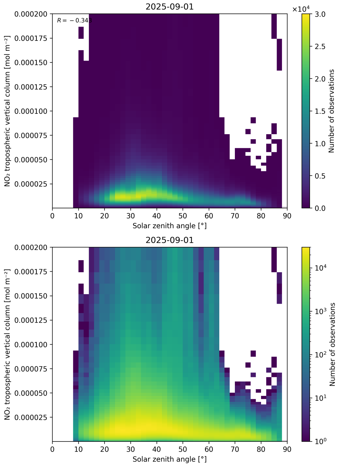
Figure 155: Scatter density plot of “Solar zenith angle” against “NO 2 tropospheric vertical column” for 2025-08-31 to 2025-09-02.
