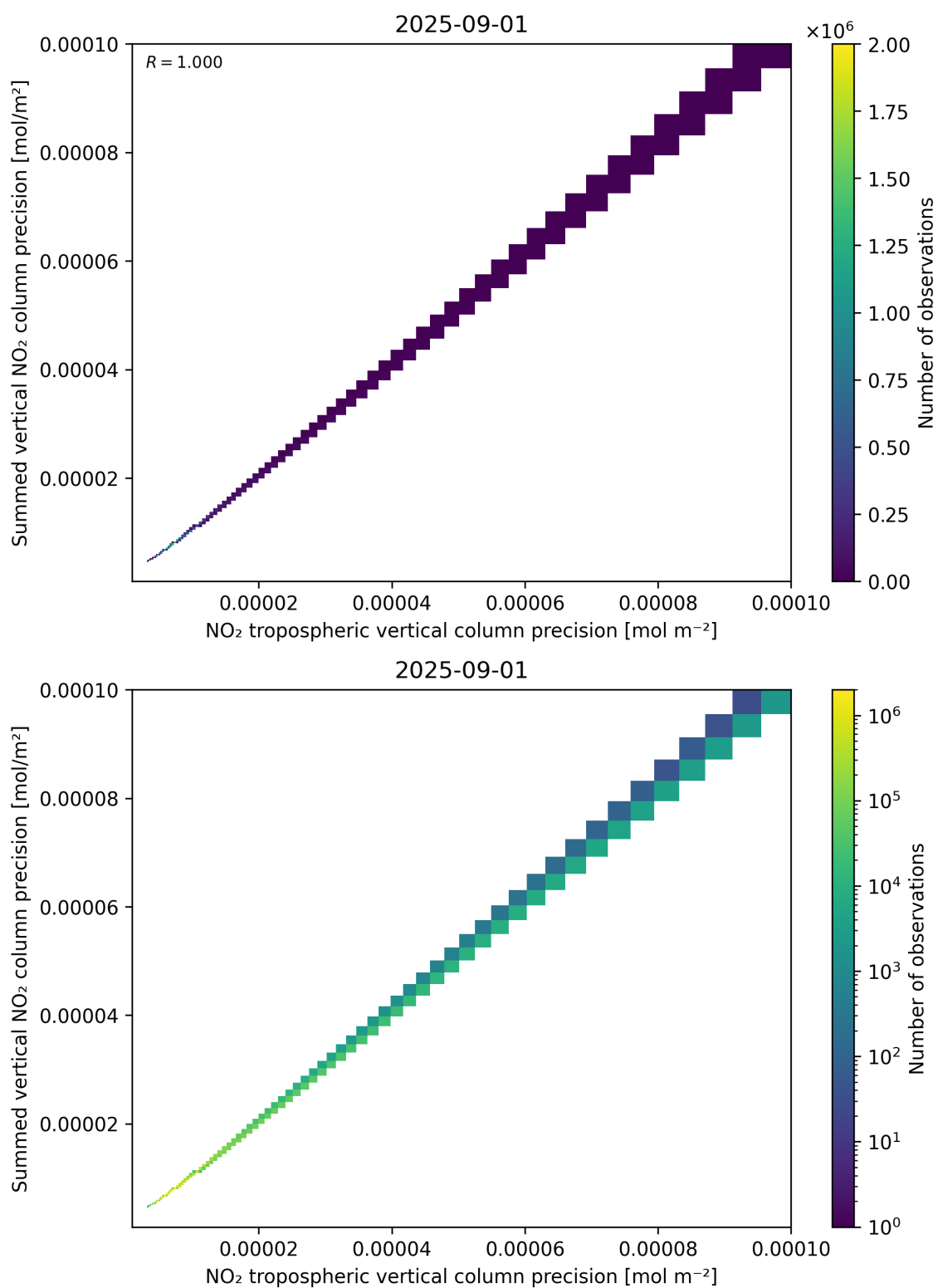
Figure 137: Scatter density plot of “NO 2 tropospheric vertical column precision” against “Summed vertical NO 2 column precision” for 2025-08-31 to 2025-09-02.
