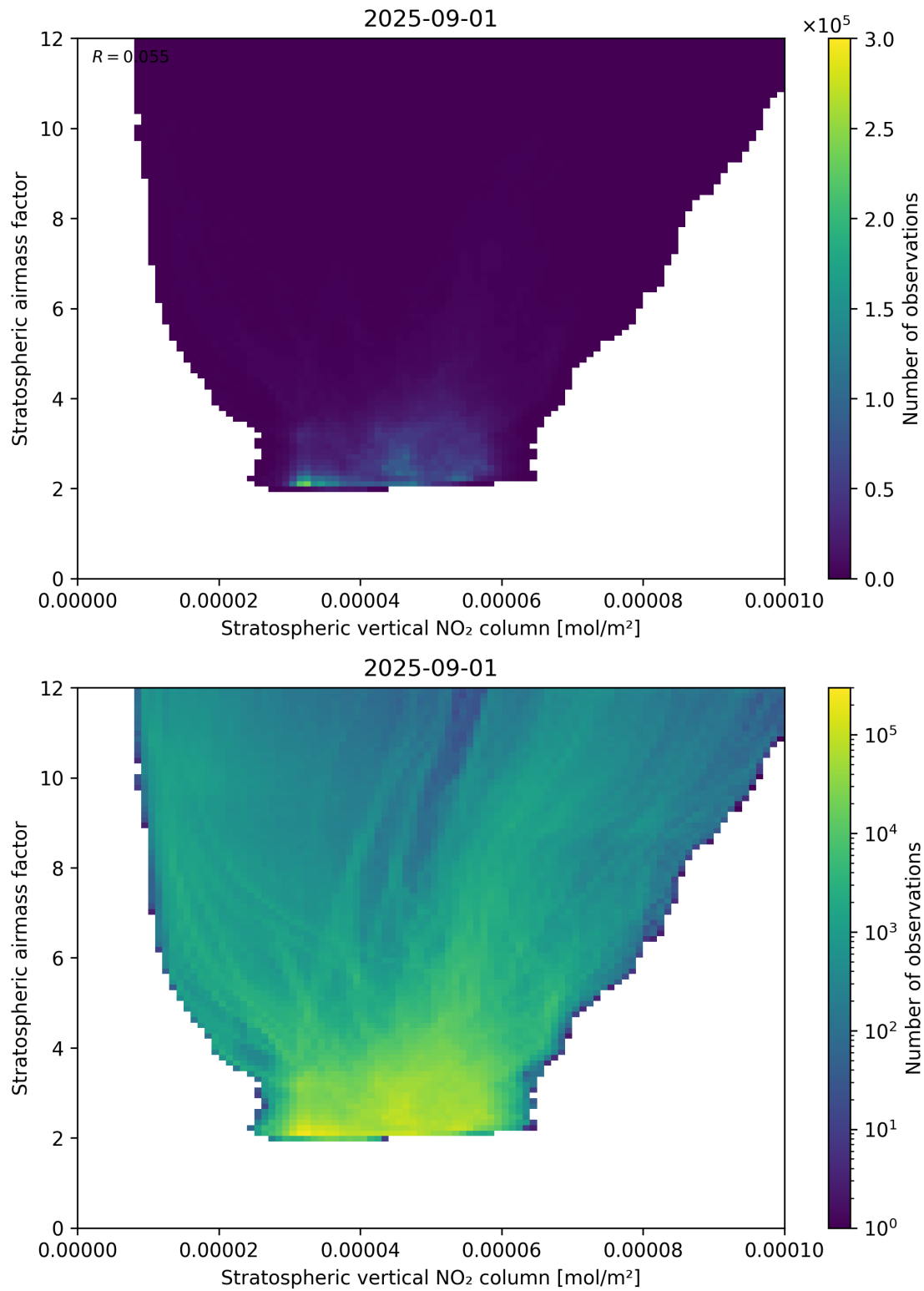
Figure 96: Scatter density plot of “Stratospheric vertical NO 2 column” against “Stratospheric airmass factor” for 2025-08-31 to 2025-09-02.
