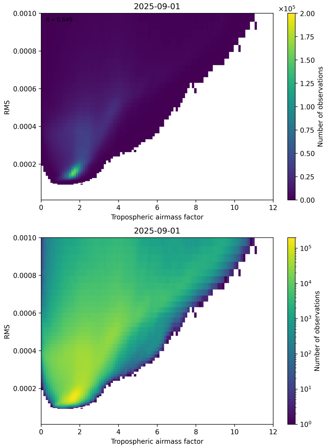
Figure 79: Scatter density plot of “Tropospheric airmass factor” against “RMS” for 2025-08-31 to 2025-09-02.
