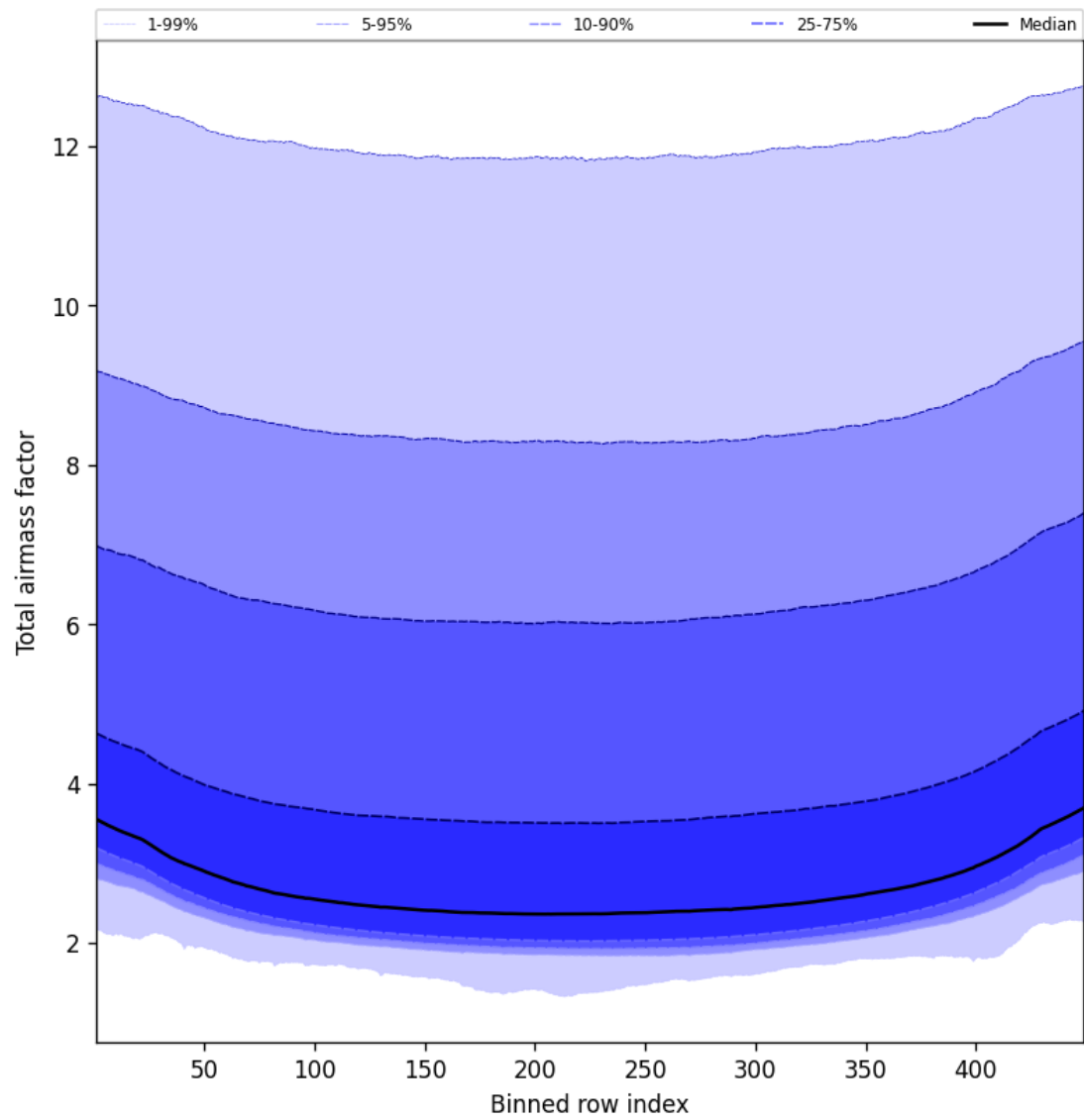
Figure 49: Along track statistics of “Total airmass factor” for 2025-08-31 to 2025-09-02
