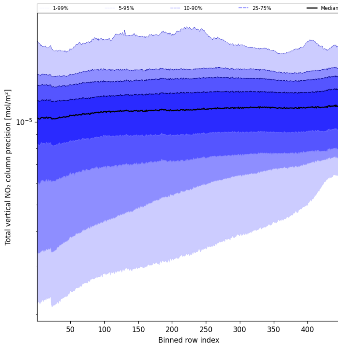
Figure 56: Along track statistics of “Total vertical NO 2 column precision” for 2025-08-31 to 2025-09-02
