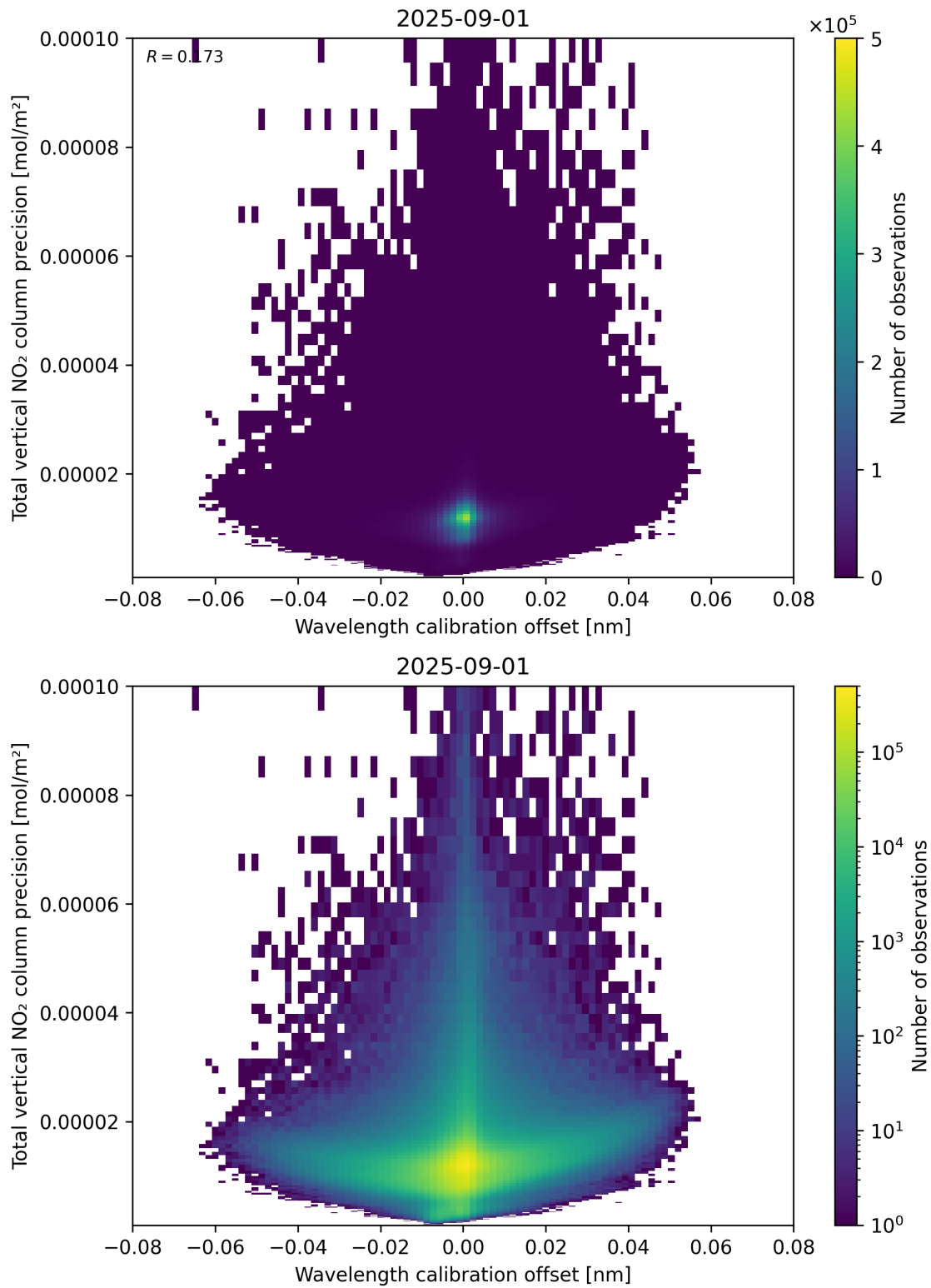
Figure 180: Scatter density plot of “Wavelength calibration offset” against “Total vertical NO 2 column precision” for 2025-08-31 to 2025-09-02.
