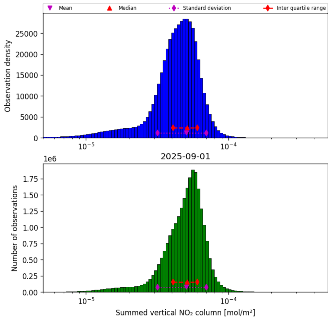
Figure 40: Histogram of "Summed vertical NO 2 column" for 2025-08-31 to 2025-09-02
