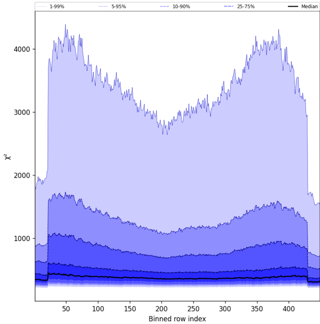
Figure 59: Along track statistics of “ \chi^2 ” for 2025-08-31 to 2025-09-02
