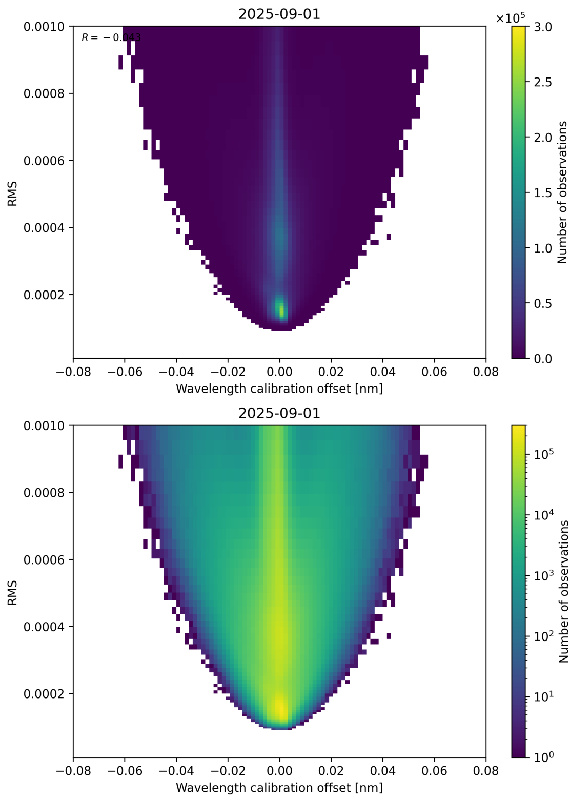
Figure 181: Scatter density plot of “Wavelength calibration offset” against “RMS” for 2025-08-31 to 2025-09-02.
