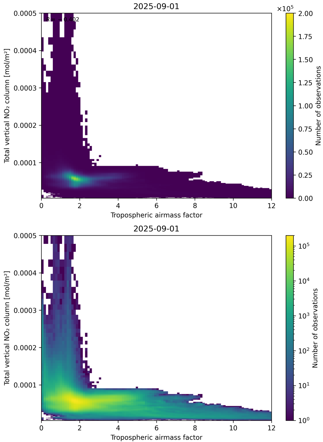
Figure 77: Scatter density plot of “Tropospheric airmass factor” against “Total vertical NO 2 column” for 2025-08-31 to 2025-09-02.
