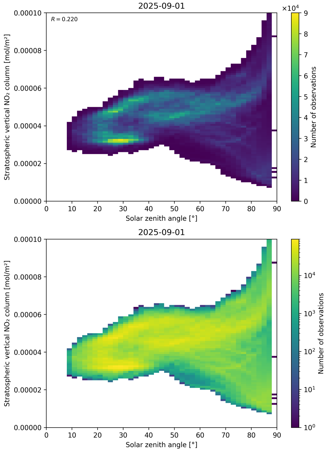
Figure 150: Scatter density plot of “Solar zenith angle” against “Stratospheric vertical NO 2 column” for 2025-08-31 to 2025-09-02.
