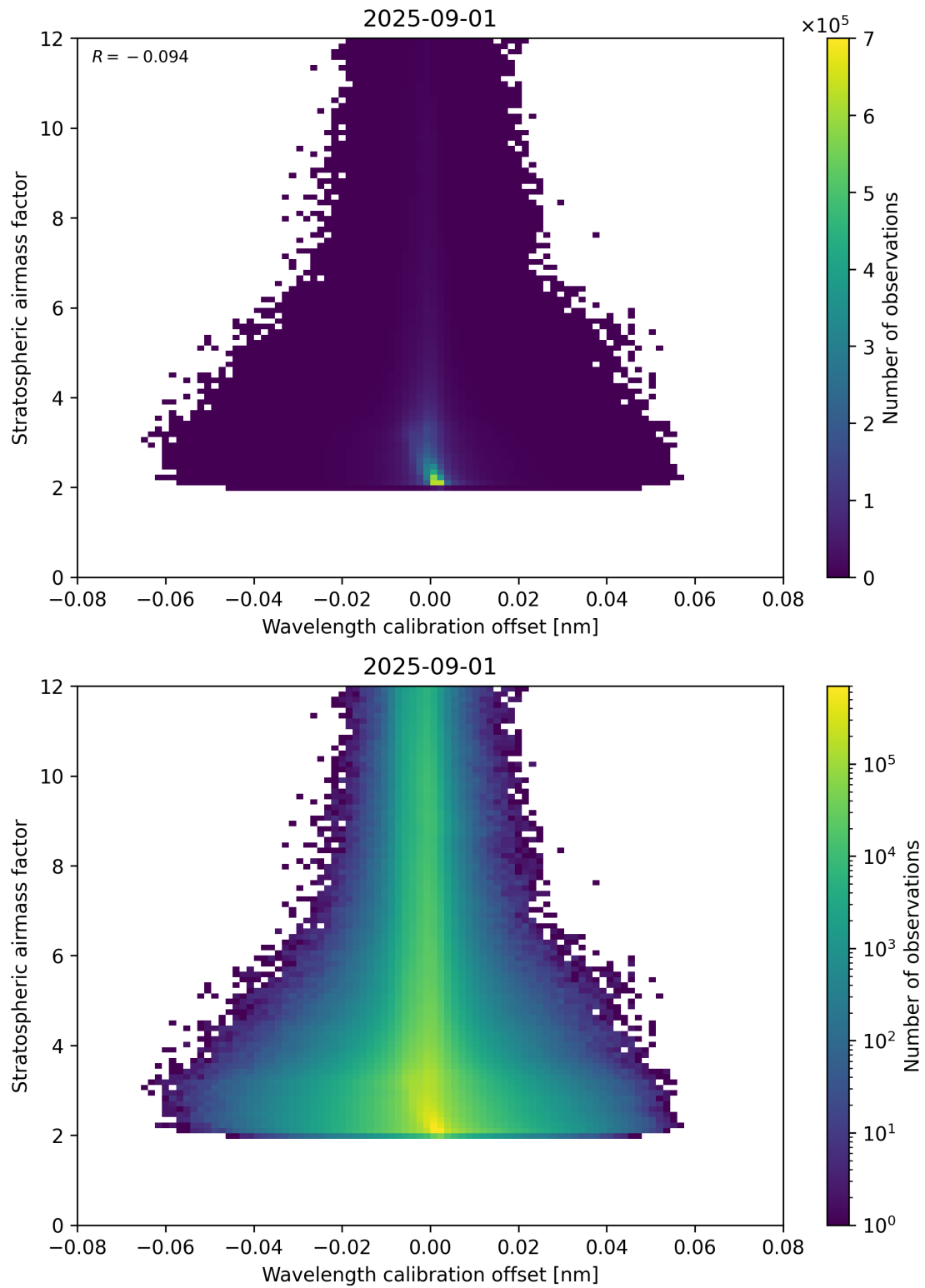
Figure 174: Scatter density plot of “Wavelength calibration offset” against “Stratospheric air mass factor” for 2025-08-31 to 2025-09-02.
