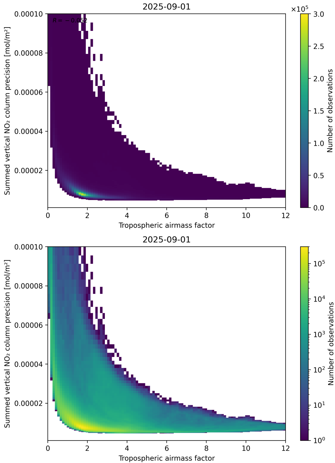
Figure 76: Scatter density plot of “Tropospheric airmass factor” against “Summed vertical NO 2 column precision” for 2025-08-31 to 2025-09-02.
