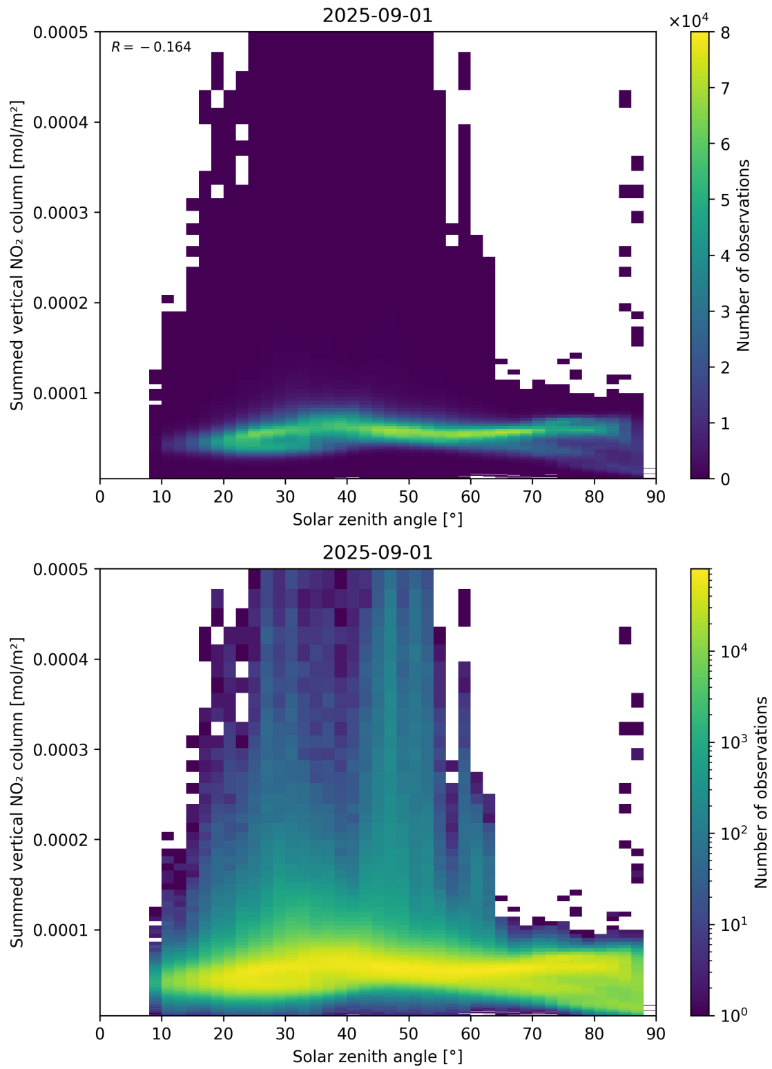
Figure 151: Scatter density plot of “Solar zenith angle” against “Summed vertical NO 2 column” for 2025-08-31 to 2025-09-02.
