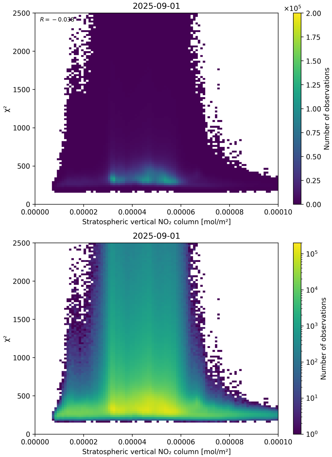
Figure 97: Scatter density plot of “Stratospheric vertical NO 2 column” against “ \chi^2 ” for 2025-08-31 to 2025-09-02.
