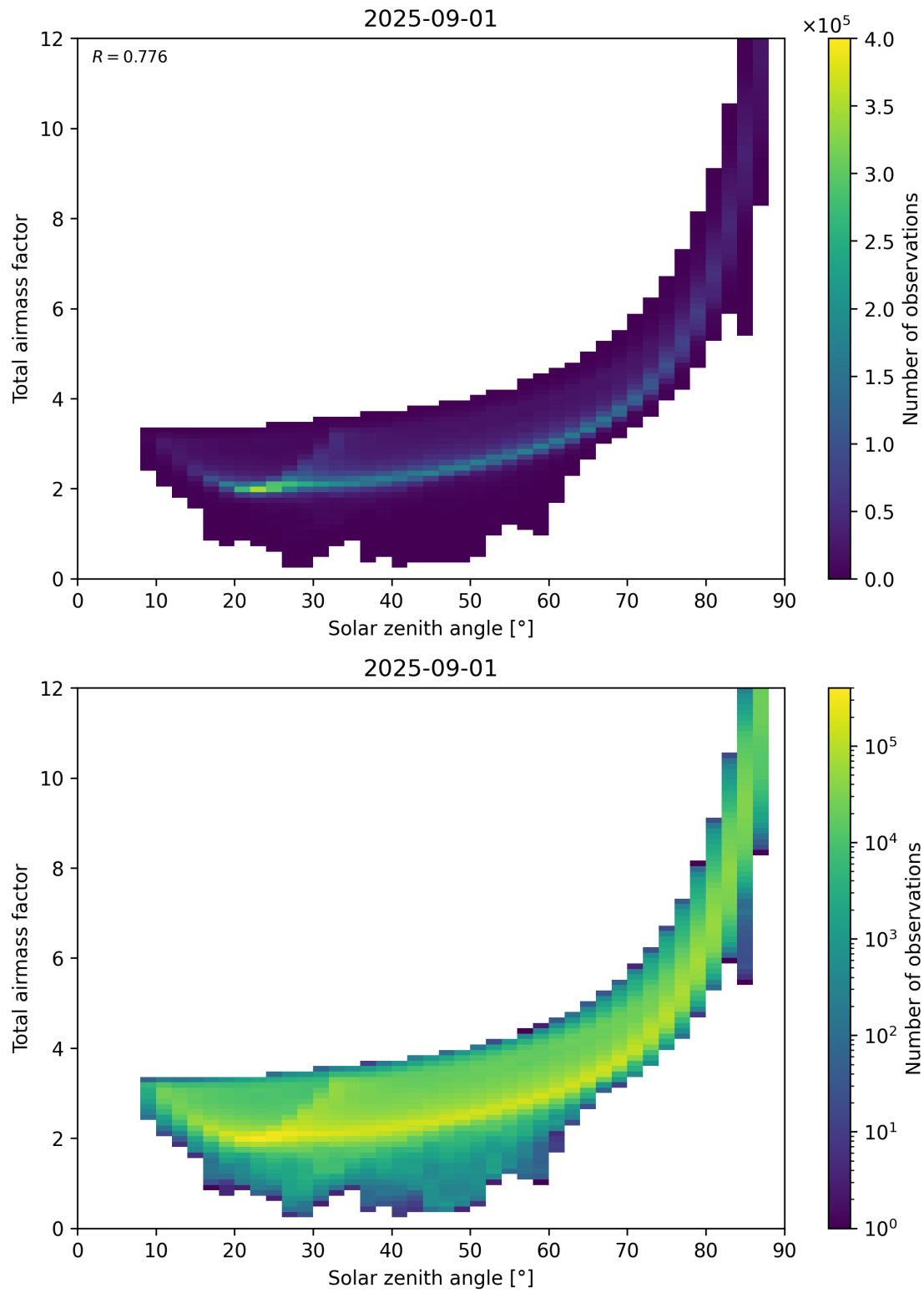
Figure 146: Scatter density plot of “Solar zenith angle” against “Total air mass factor” for 2025-08-31 to 2025-09-02.
