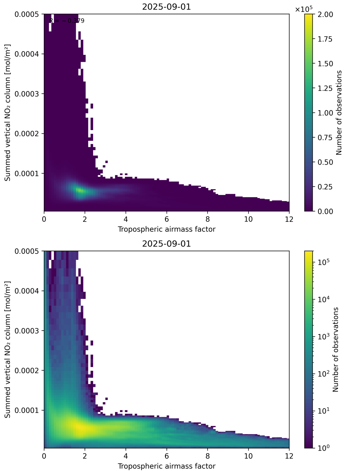
Figure 75: Scatter density plot of “Tropospheric airmass factor” against “Summed vertical NO 2 column” for 2025-08-31 to 2025-09-02.
