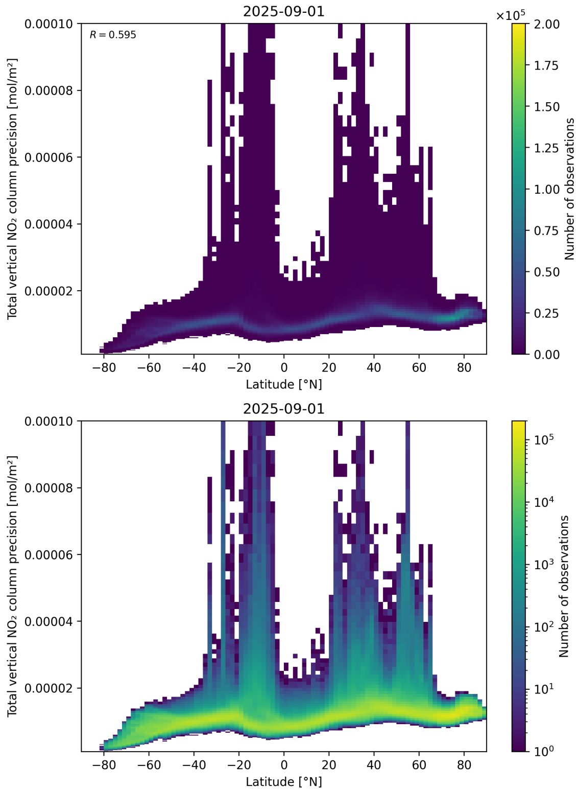
Figure 91: Scatter density plot of “Latitude” against “Total vertical NO 2 column precision” for 2025-08-31 to 2025-09-02.
