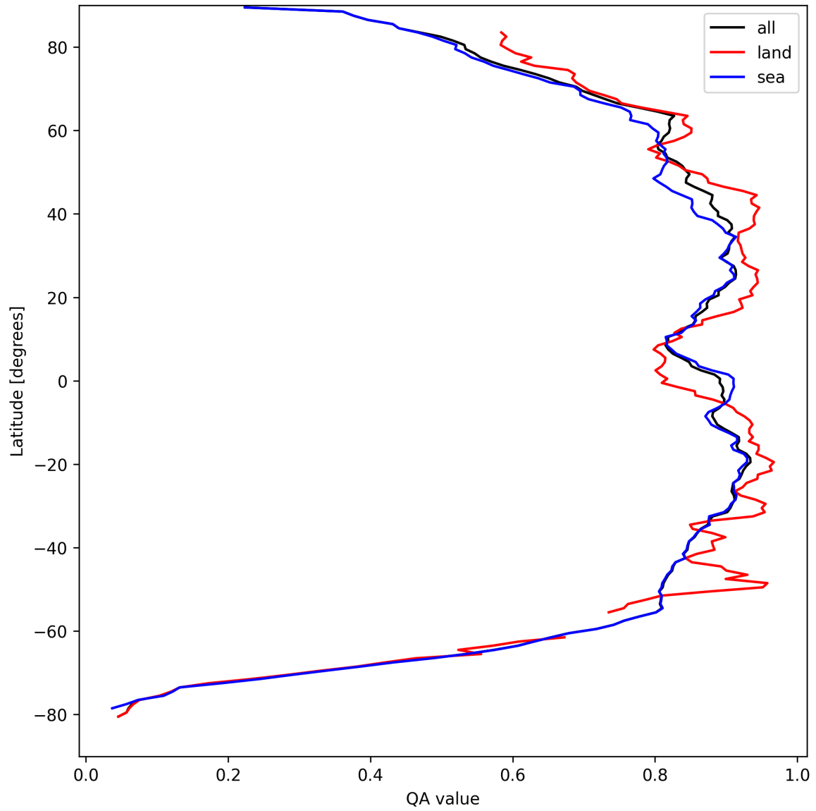
Figure 11: Zonal average of “QA value” for 2025-08-31 to 2025-09-02.
