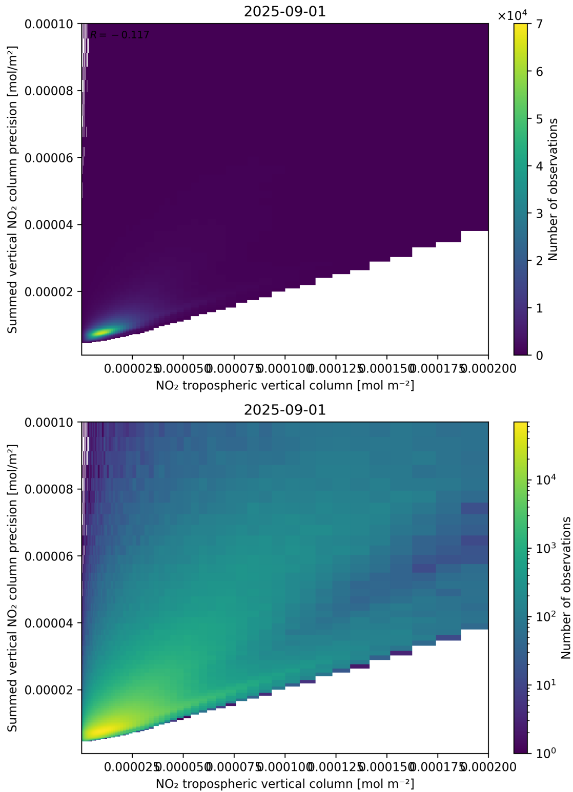
Figure 127: Scatter density plot of “NO 2 tropospheric vertical column” against “Summed vertical NO 2 column precision” for 2025-08-31 to 2025-09-02.
