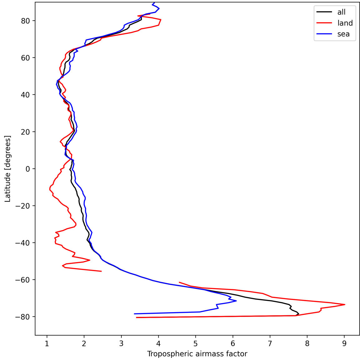
Figure 14: Zonal average of “Tropospheric airmass factor” for 2025-08-31 to 2025-09-02.
