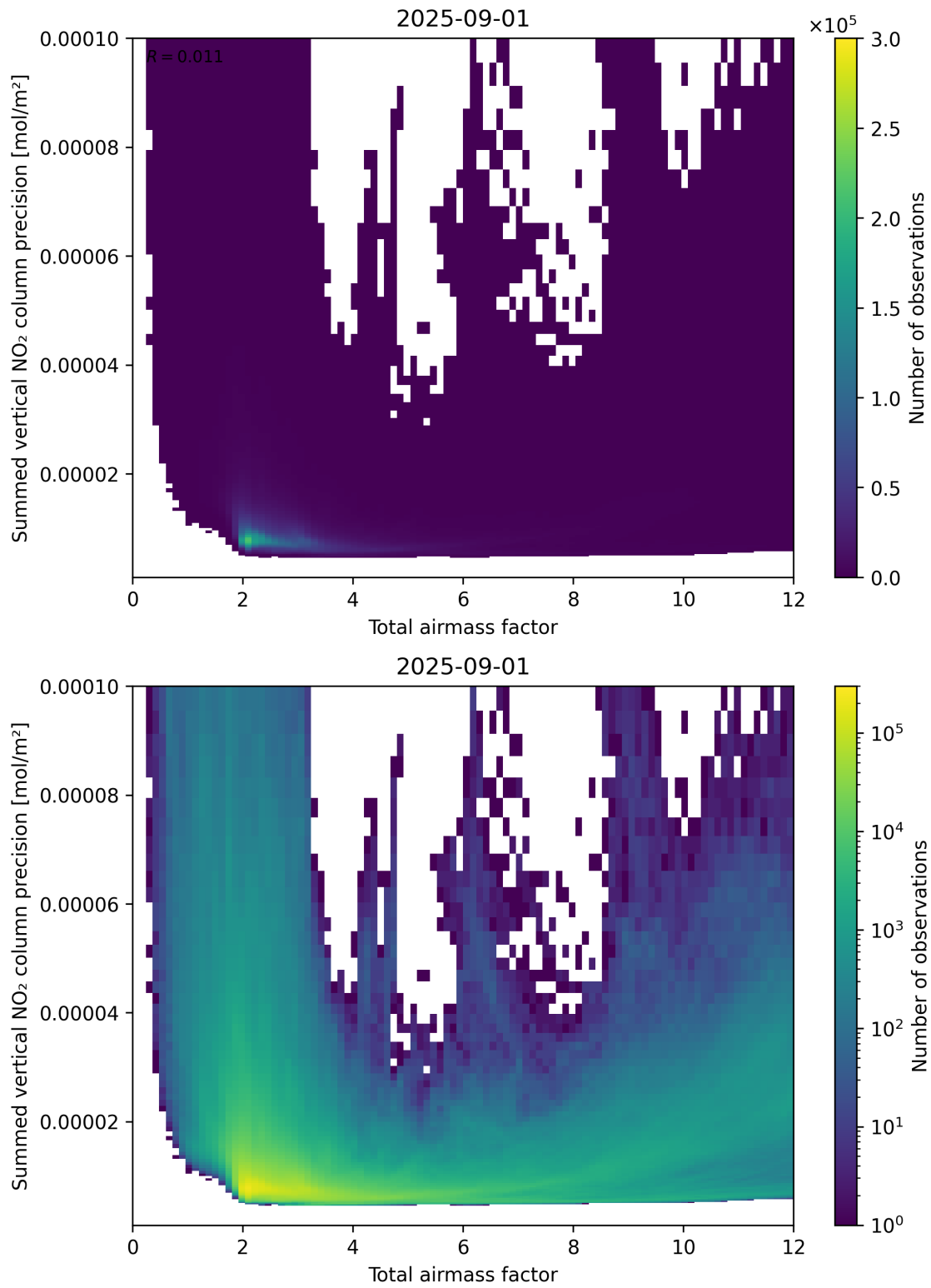
Figure 66: Scatter density plot of “Total airmass factor” against “Summed vertical NO 2 column precision” for 2025-08-31 to 2025-09-02.
