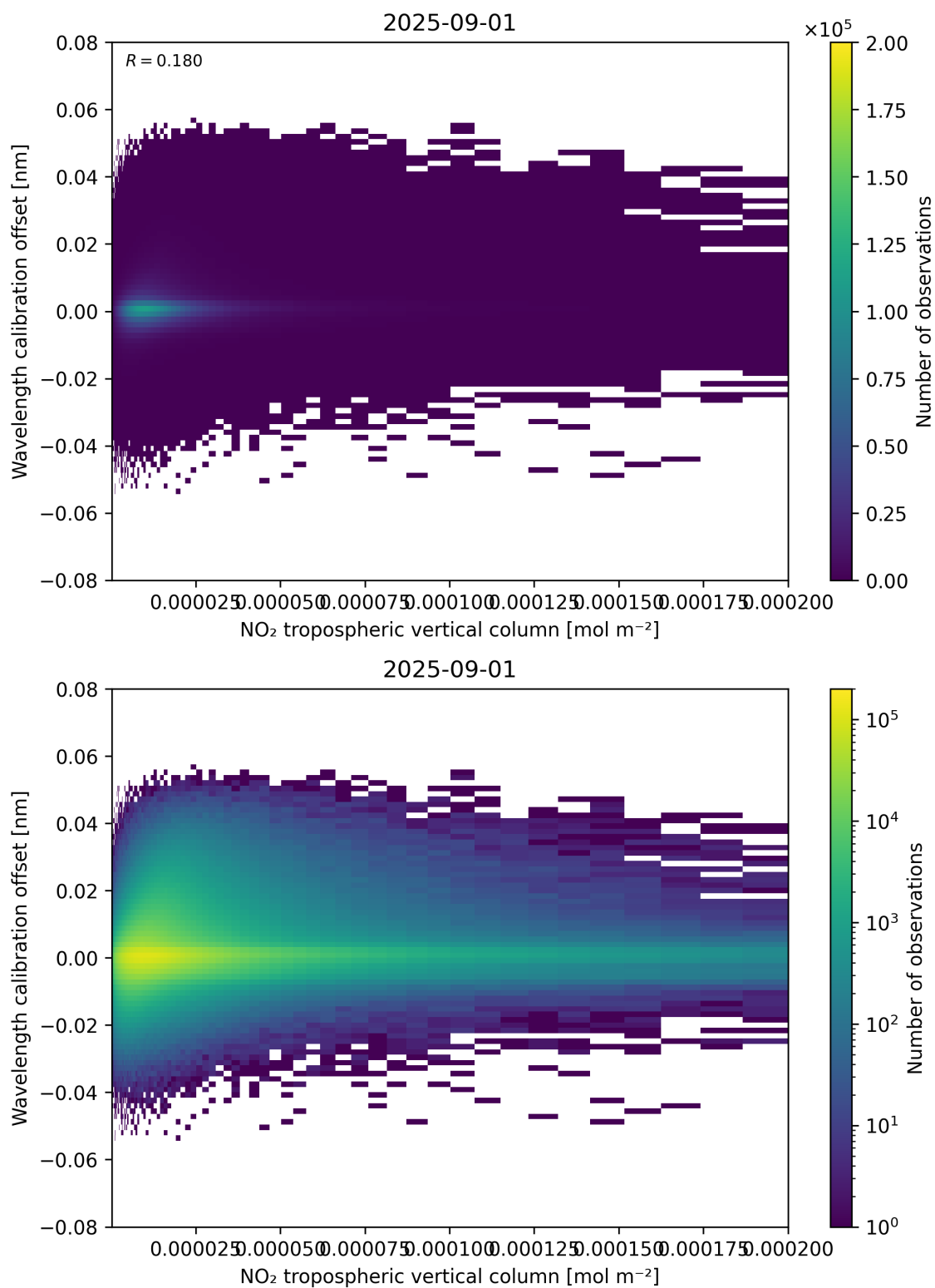
Figure 143: Scatter density plot of “NO 2 tropospheric vertical column” against “Wavelength calibration offset” for 2025-08-31 to 2025-09-02.
