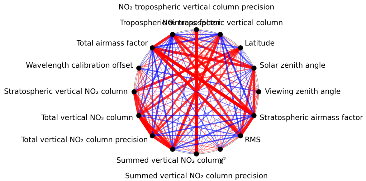
Figure 1: Map of correlation graph for 2025-08-31 to 2025-09-02.
