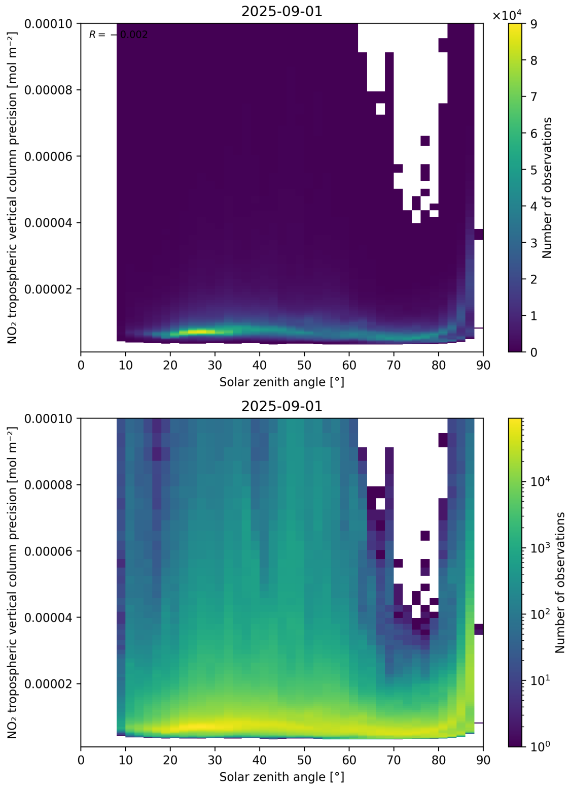
Figure 156: Scatter density plot of “Solar zenith angle” against “NO 2 tropospheric vertical column precision” for 2025-08-31 to 2025-09-02.
