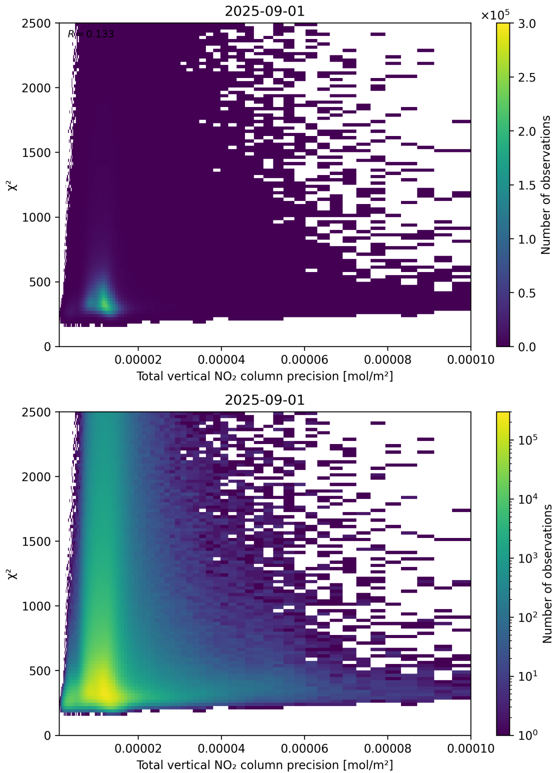
Figure 116: Scatter density plot of “Total vertical NO 2 column precision” against “ \chi^2 ” for 2025-08-31 to 2025-09-02.
