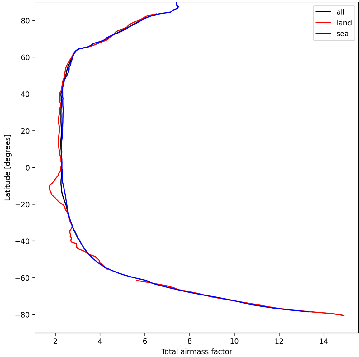
Figure 15: Zonal average of “Total airmass factor” for 2025-08-31 to 2025-09-02.
