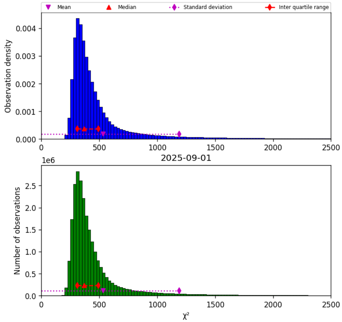
Figure 42: Histogram of “ \chi^2 ” for 2025-08-31 to 2025-09-02
