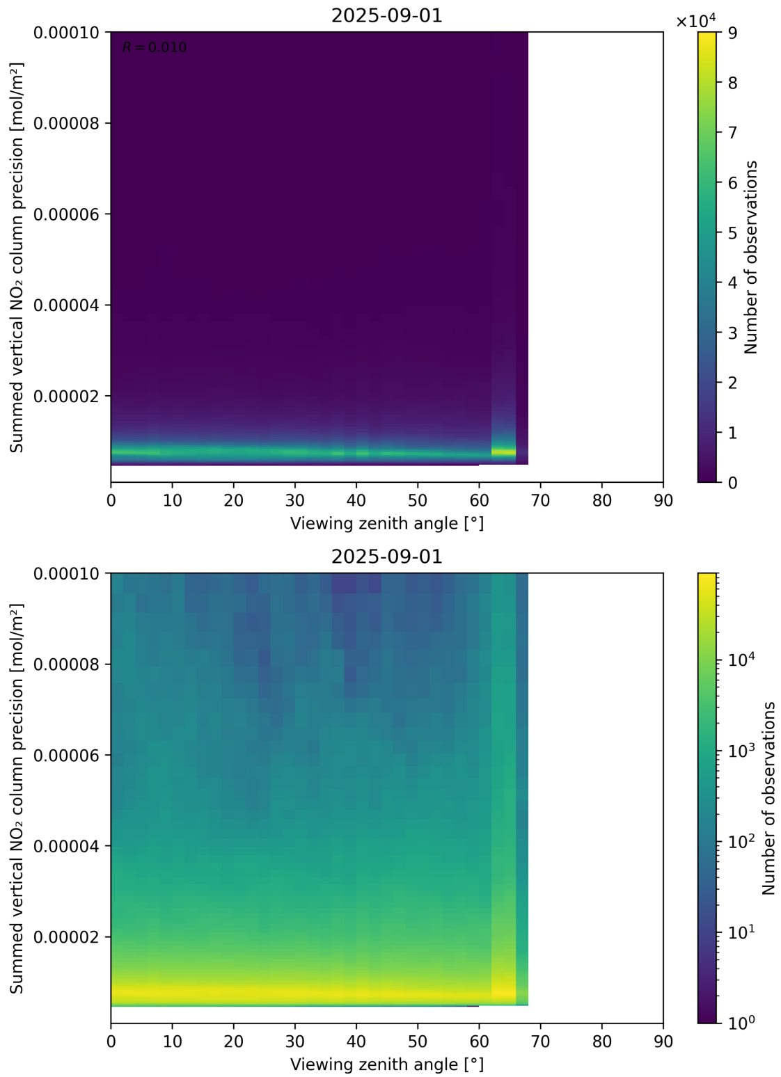
Figure 166: Scatter density plot of “Viewing zenith angle” against “Summed vertical NO 2 column precision” for 2025-08-31 to 2025-09-02.
