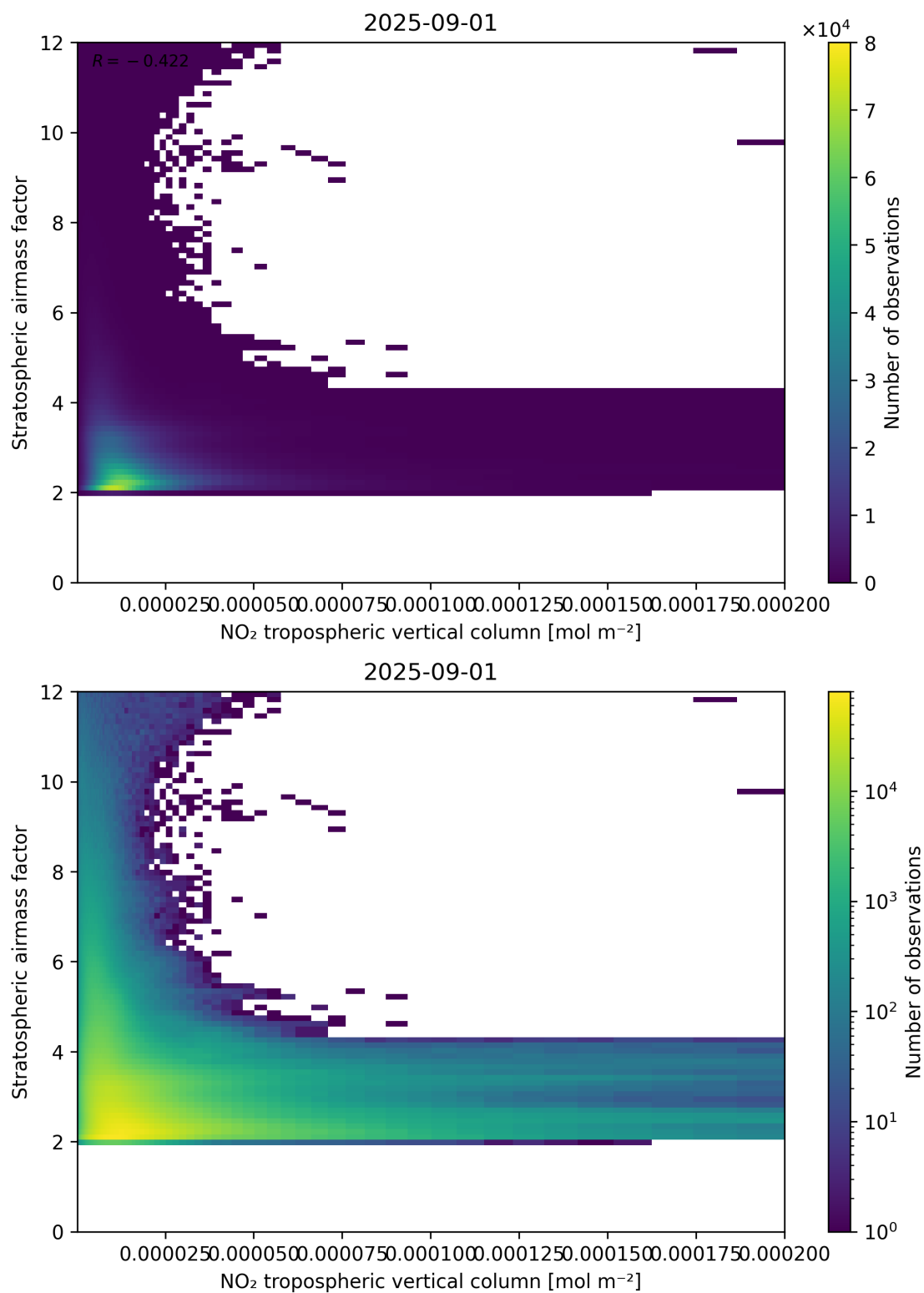
Figure 121: Scatter density plot of “NO 2 tropospheric vertical column” against “Stratospheric airmass factor” for 2025-08-31 to 2025-09-02.
