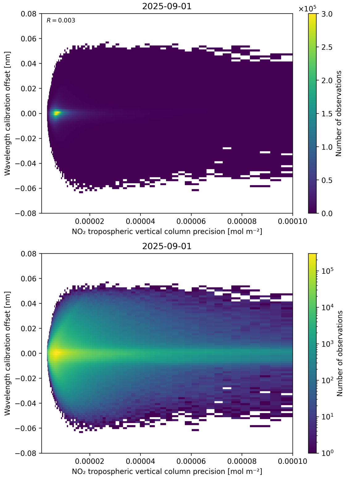
Figure 141: Scatter density plot of “NO 2 tropospheric vertical column precision” against “Wavelength calibration offset” for 2025-08-31 to 2025-09-02.
