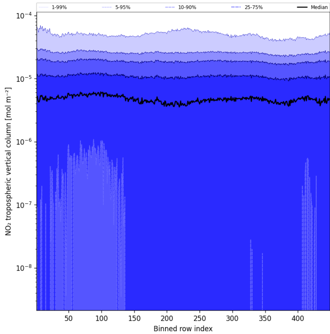
Figure 46: Along track statistics of “NO 2 tropospheric vertical column” for 2025-08-31 to 2025-09-02
