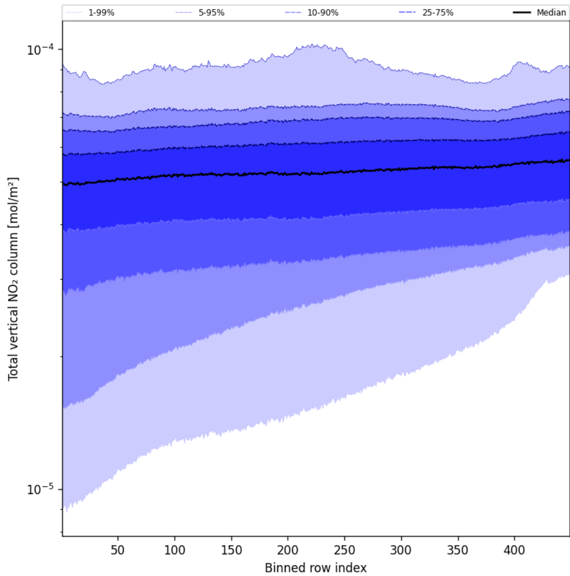
Figure 55: Along track statistics of “Total vertical NO 2 column” for 2025-08-31 to 2025-09-02
