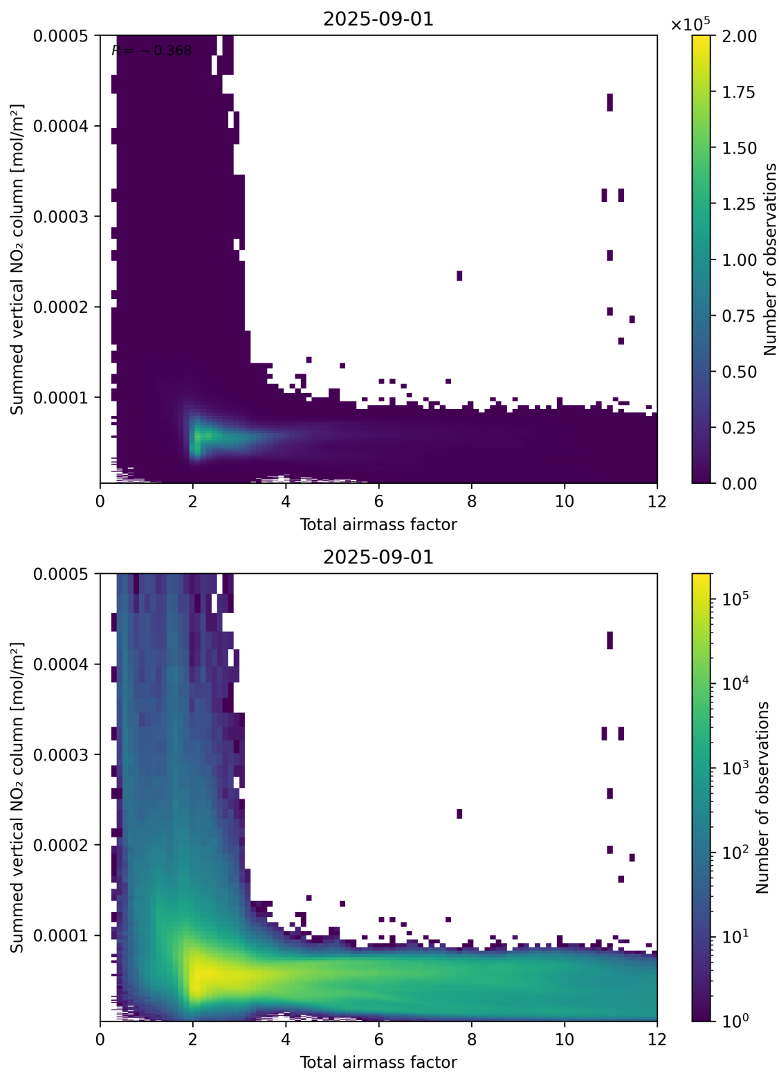
Figure 65: Scatter density plot of “Total airmass factor” against “Summed vertical NO 2 column” for 2025-08-31 to 2025-09-02.
