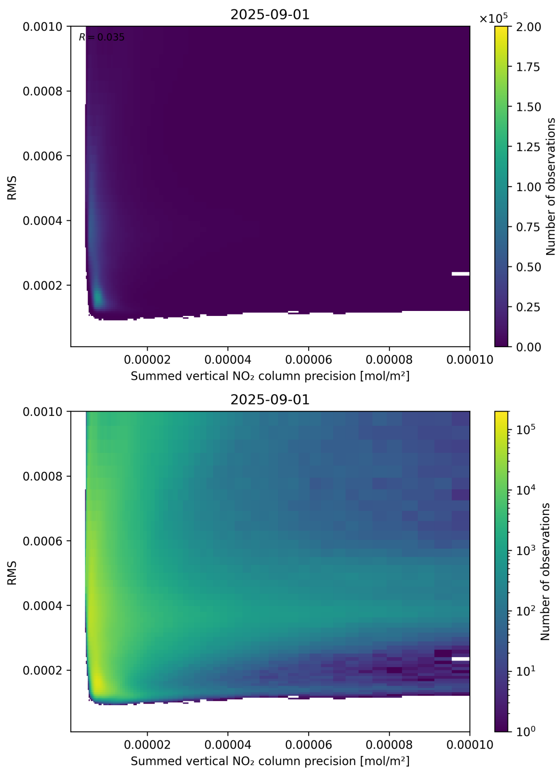
Figure 108: Scatter density plot of “Summed vertical NO 2 column precision” against “RMS” for 2025-08-31 to 2025-09-02.
