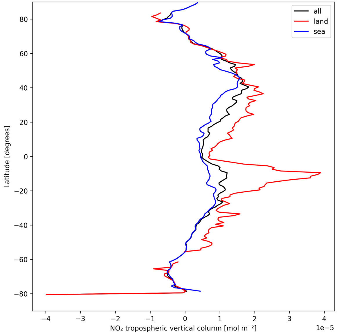
Figure 12: Zonal average of “NO 2 tropospheric vertical column” for 2025-08-31 to 2025-09-02.
