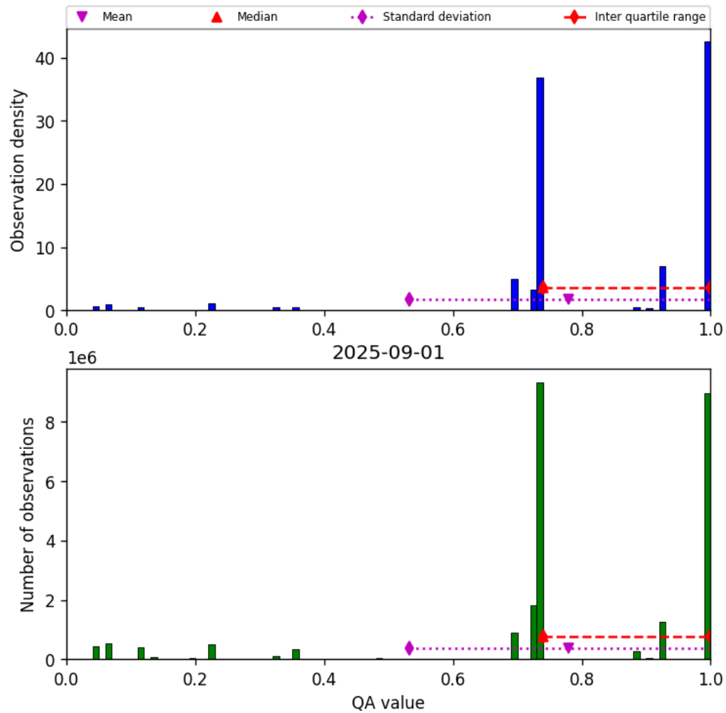
Figure 28: Histogram of “QA value” for 2025-08-31 to 2025-09-02
