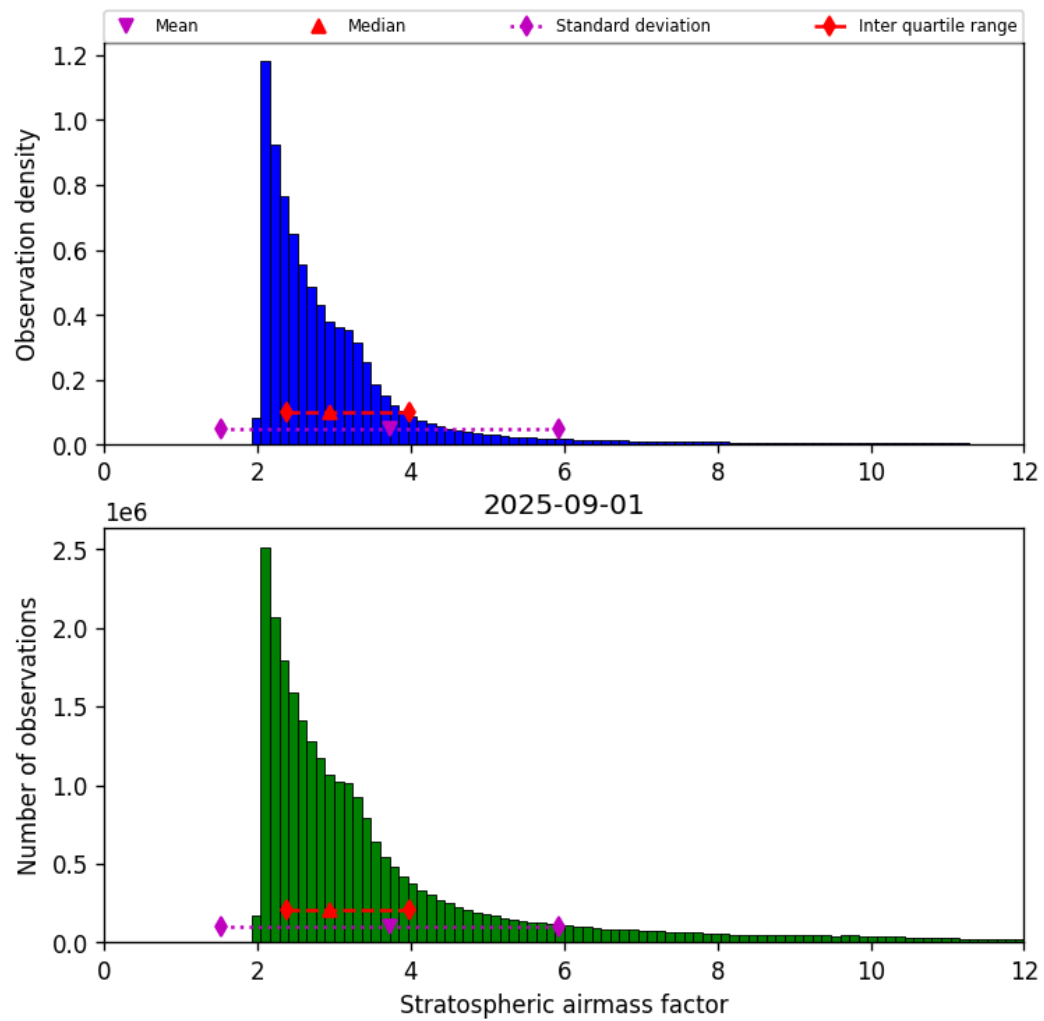
Figure 44: Histogram of “Stratospheric airmass factor” for 2025-08-31 to 2025-09-02
