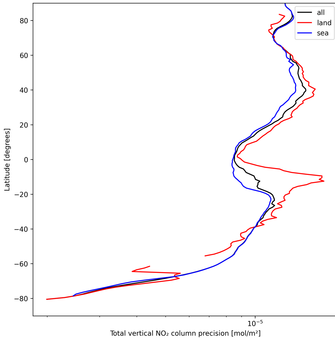
Figure 22: Zonal average of “Total vertical NO 2 column precision” for 2025-08-31 to 2025-09-02.
