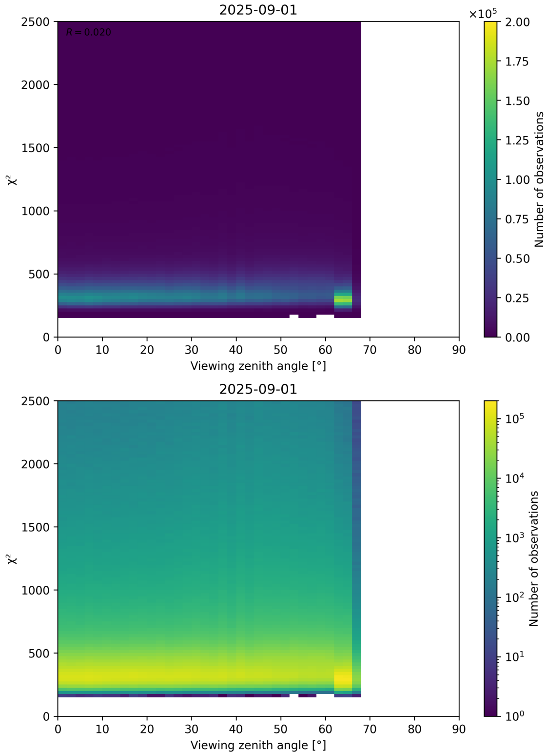
Figure 162: Scatter density plot of “Viewing zenith angle” against “ \chi^2 ” for 2025-08-31 to 2025-09-02.
