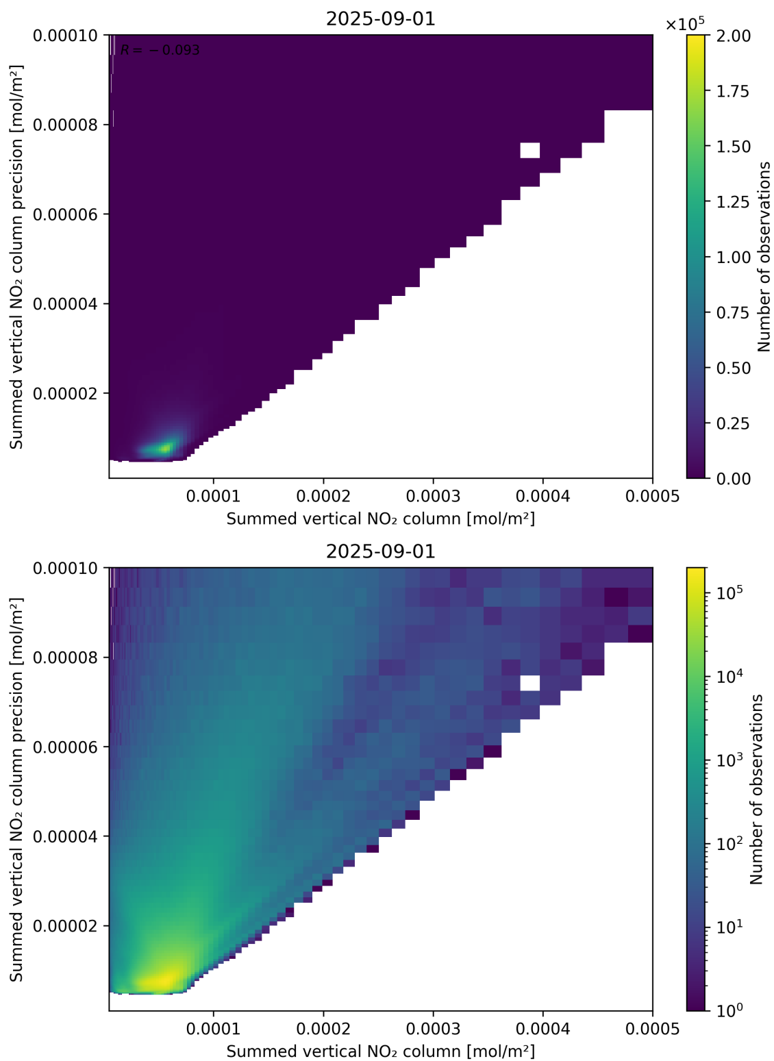
Figure 105: Scatter density plot of “Summed vertical NO 2 column” against “Summed vertical NO 2 column precision” for 2025-08-31 to 2025-09-02.
