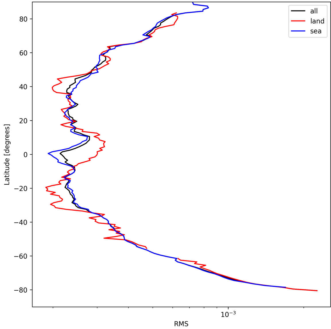
Figure 26: Zonal average of “RMS” for 2025-08-31 to 2025-09-02.
