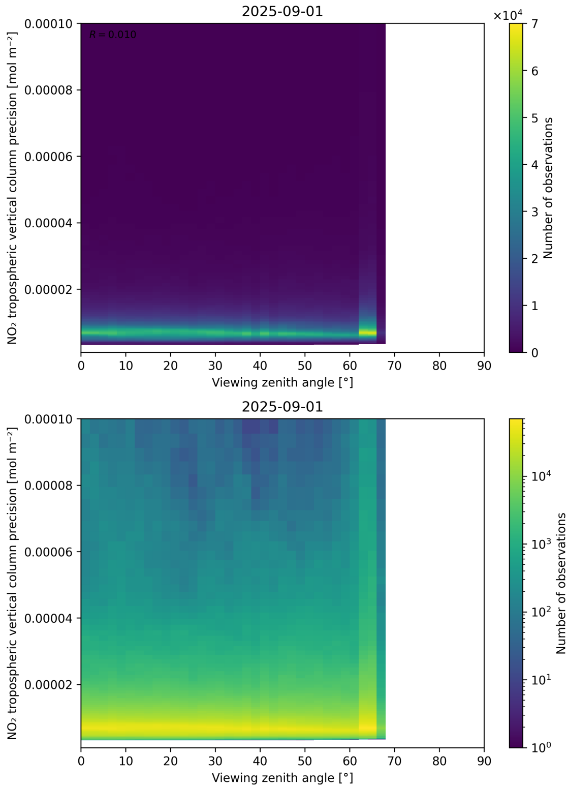
Figure 170: Scatter density plot of “Viewing zenith angle” against “NO 2 tropospheric vertical column precision” for 2025-08-31 to 2025-09-02.
