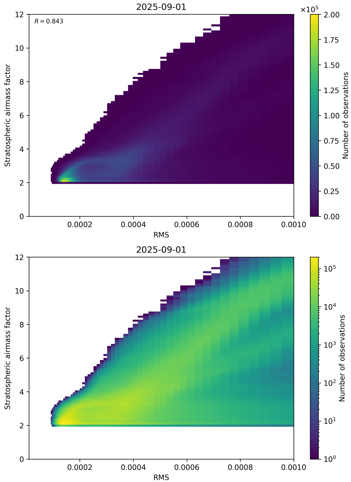
Figure 144: Scatter density plot of “RMS” against “Stratospheric airmass factor” for 2025-08-31 to 2025-09-02.
