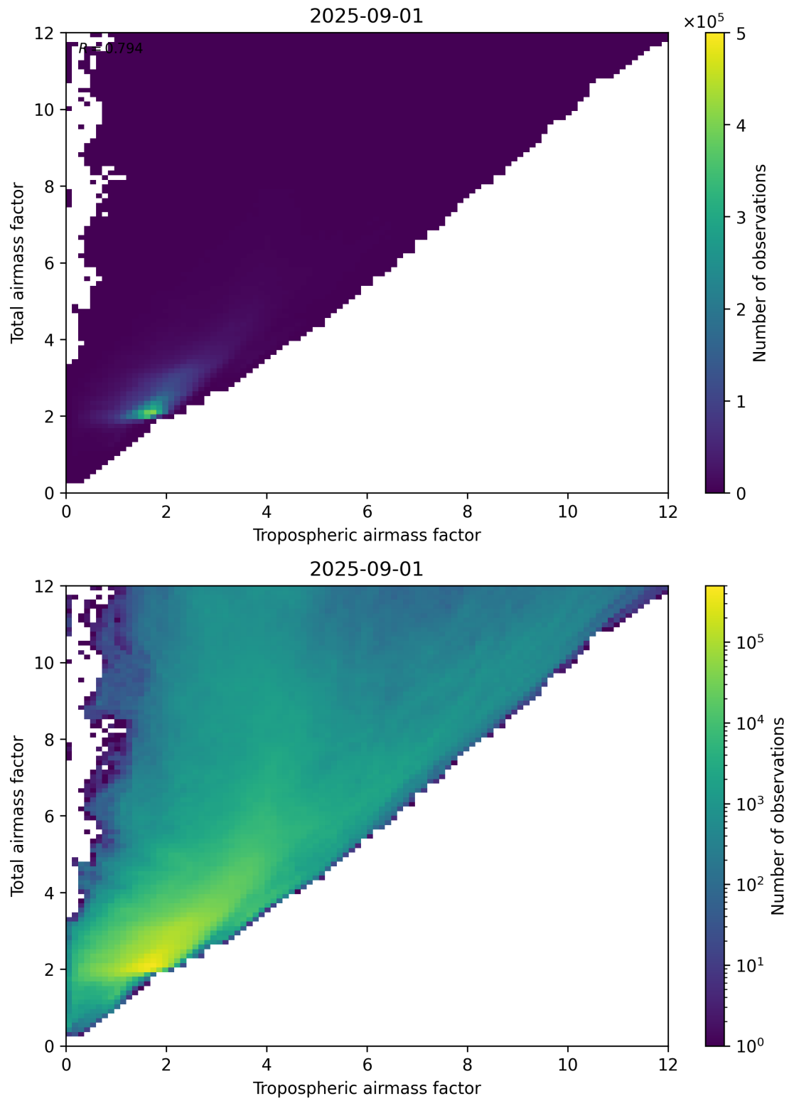
Figure 72: Scatter density plot of “Tropospheric airmass factor” against “Total airmass factor” for 2025-08-31 to 2025-09-02.
