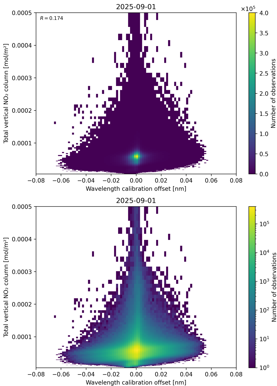
Figure 179: Scatter density plot of “Wavelength calibration offset” against “Total vertical NO 2 column” for 2025-08-31 to 2025-09-02.
