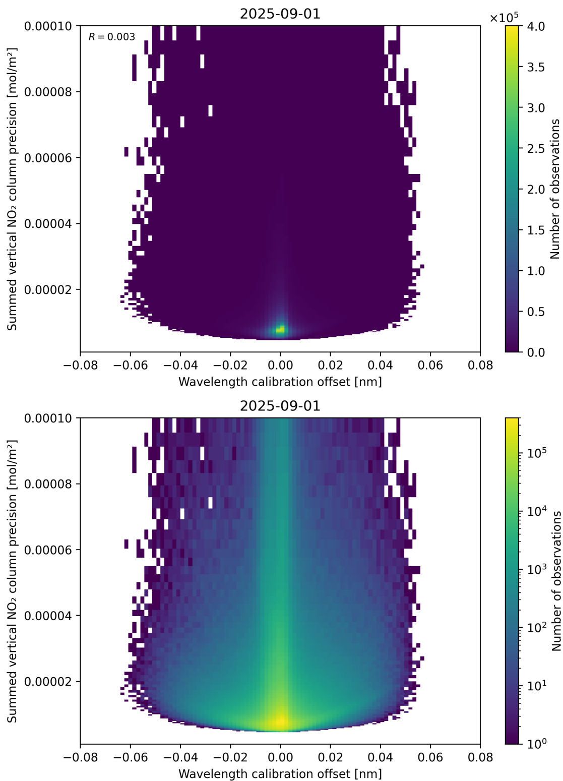
Figure 178: Scatter density plot of “Wavelength calibration offset” against “Summed vertical NO 2 column precision” for 2025-08-31 to 2025-09-02.
