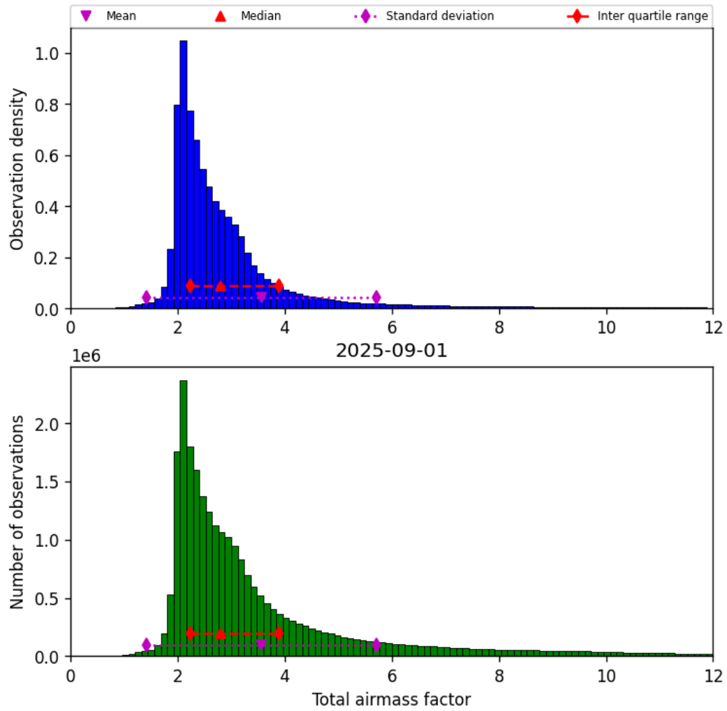
Figure 32: Histogram of “Total airmass factor” for 2025-08-31 to 2025-09-02
