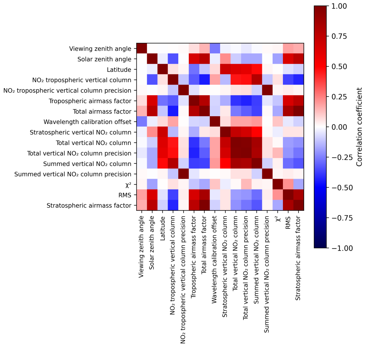
Figure 2: Map of correlation matrix for 2025-08-31 to 2025-09-02.
