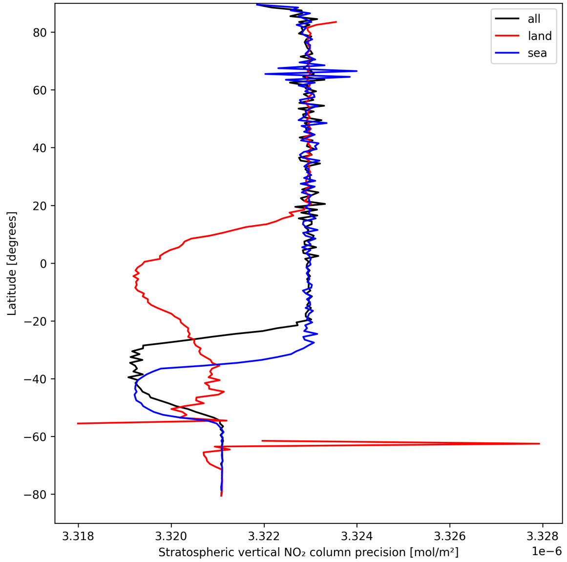
Figure 20: Zonal average of “Stratospheric vertical NO 2 column precision” for 2025-08-31 to 2025-09-02.
