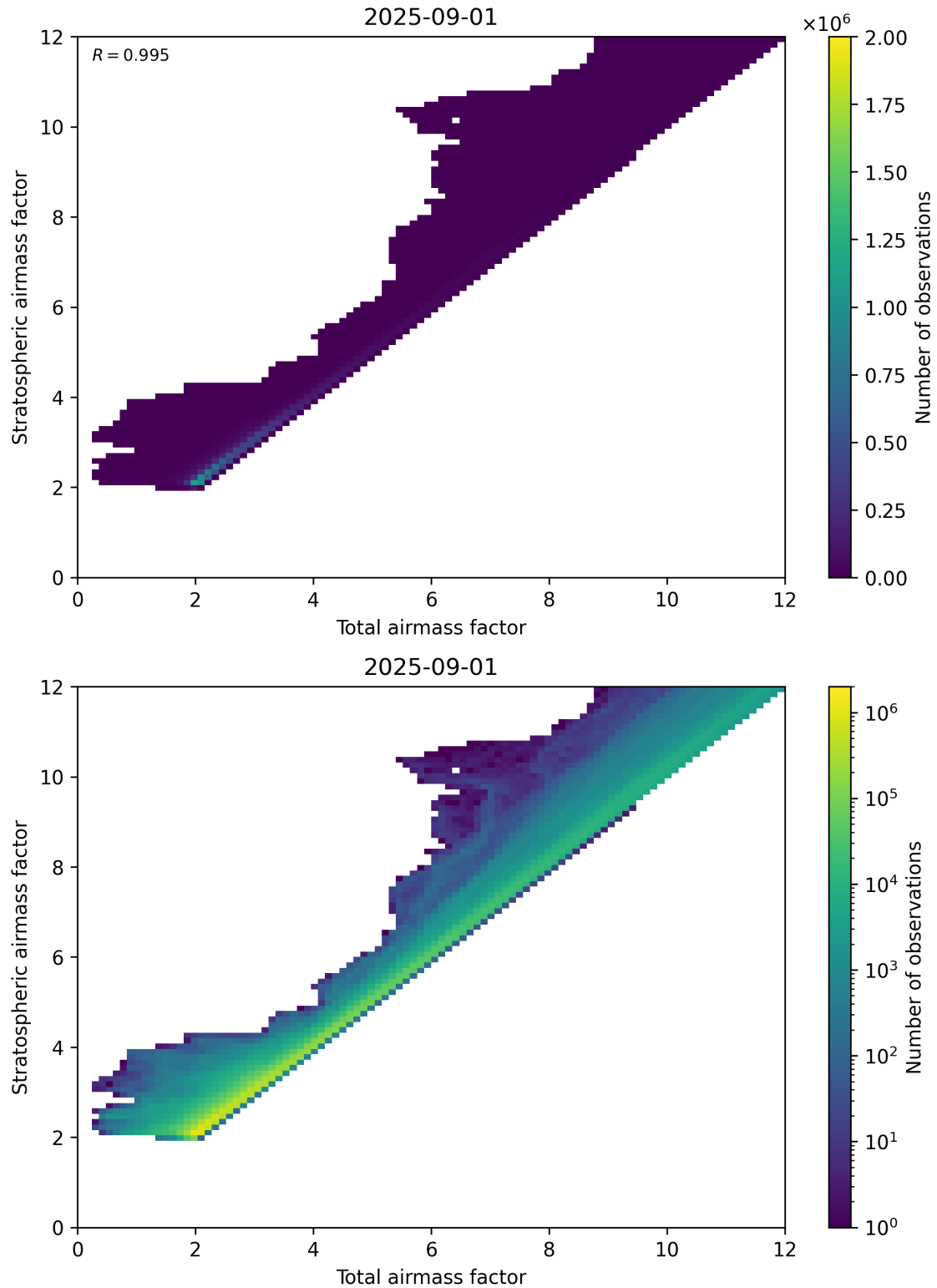
Figure 62: Scatter density plot of “Total airmass factor” against “Stratospheric airmass factor” for 2025-08-31 to 2025-09-02.
