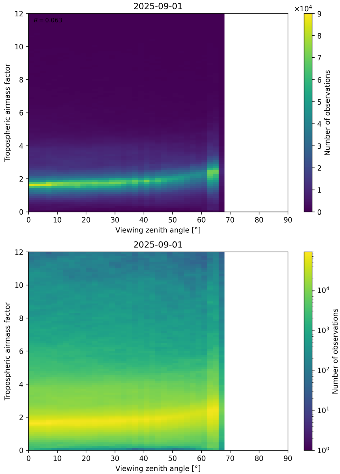
Figure 161: Scatter density plot of “Viewing zenith angle” against “Tropospheric airmass factor” for 2025-08-31 to 2025-09-02.
