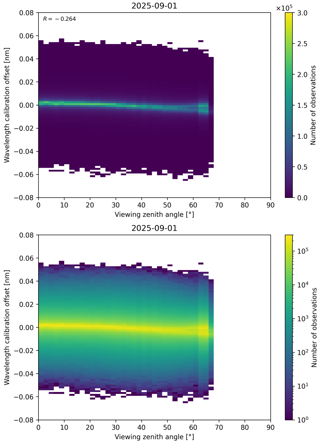
Figure 173: Scatter density plot of “Viewing zenith angle” against “Wavelength calibration offset” for 2025-08-31 to 2025-09-02.
