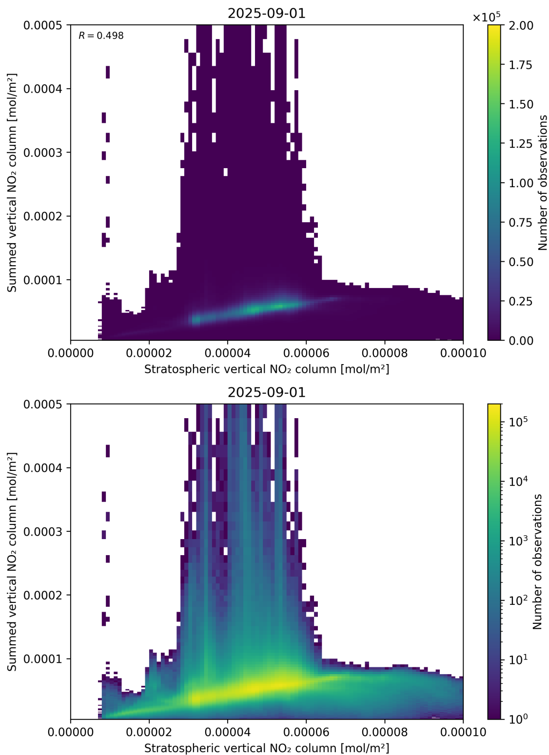
Figure 98: Scatter density plot of “Stratospheric vertical NO 2 column” against “Summed vertical NO 2 column” for 2025-08-31 to 2025-09-02.
