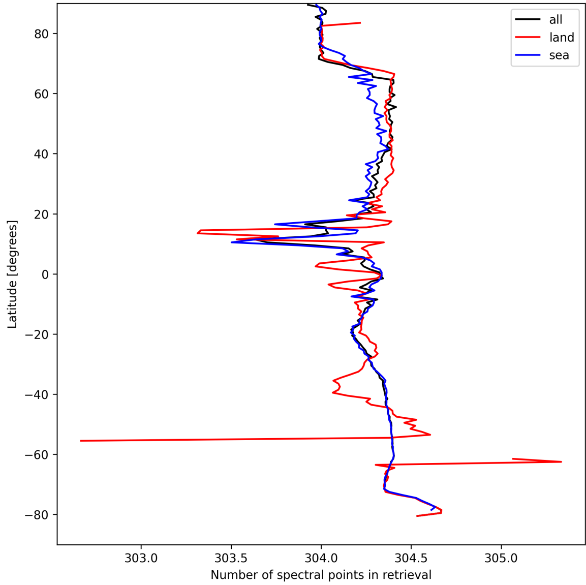
Figure 16: Zonal average of “Number of spectral points in retrieval” for 2025-08-31 to 2025-09-02.
