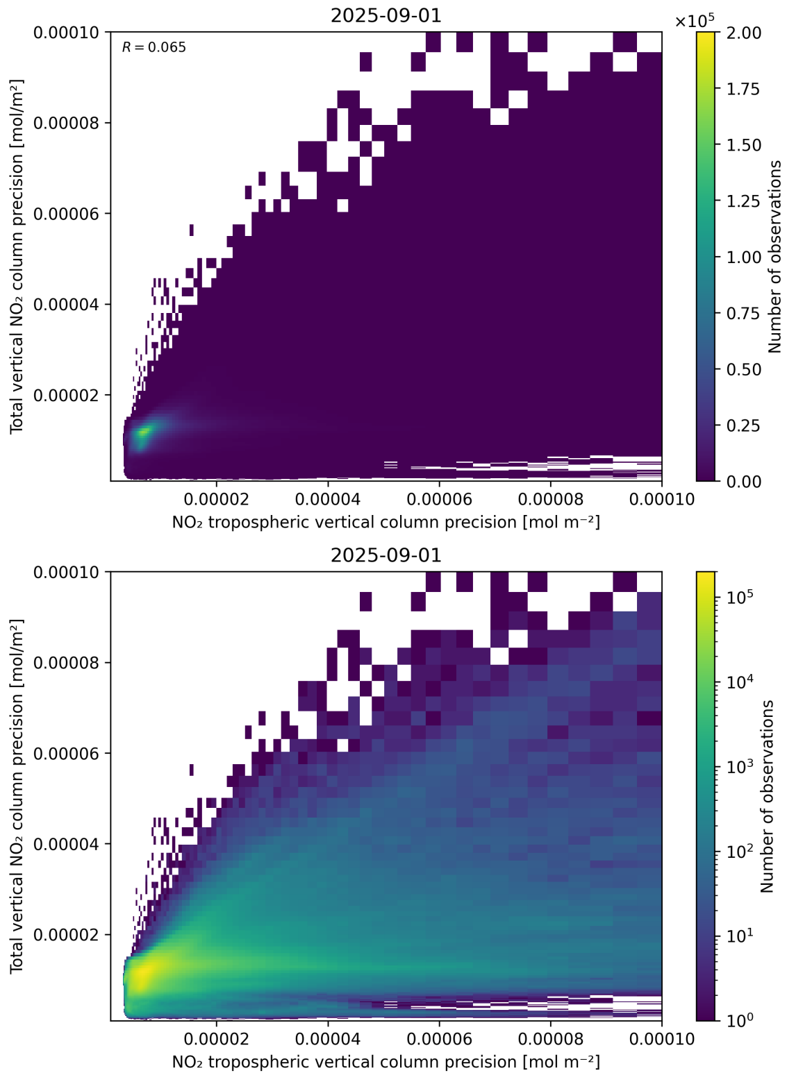
Figure 139: Scatter density plot of “NO 2 tropospheric vertical column precision” against “Total vertical NO 2 column precision” for 2025-08-31 to 2025-09-02.
