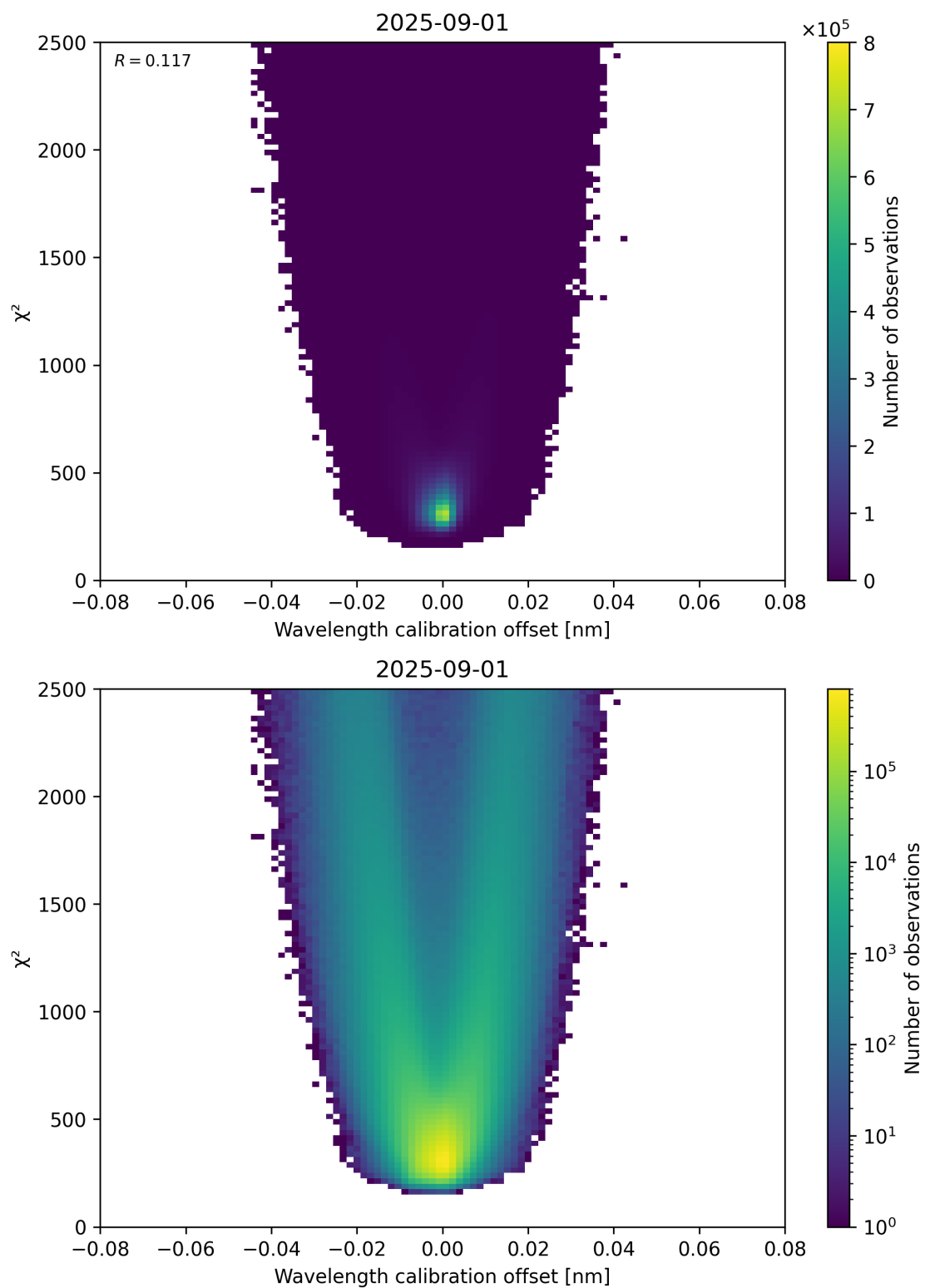
Figure 175: Scatter density plot of “Wavelength calibration offset” against “ \chi^2 ” for 2025-08-31 to 2025-09-02.
