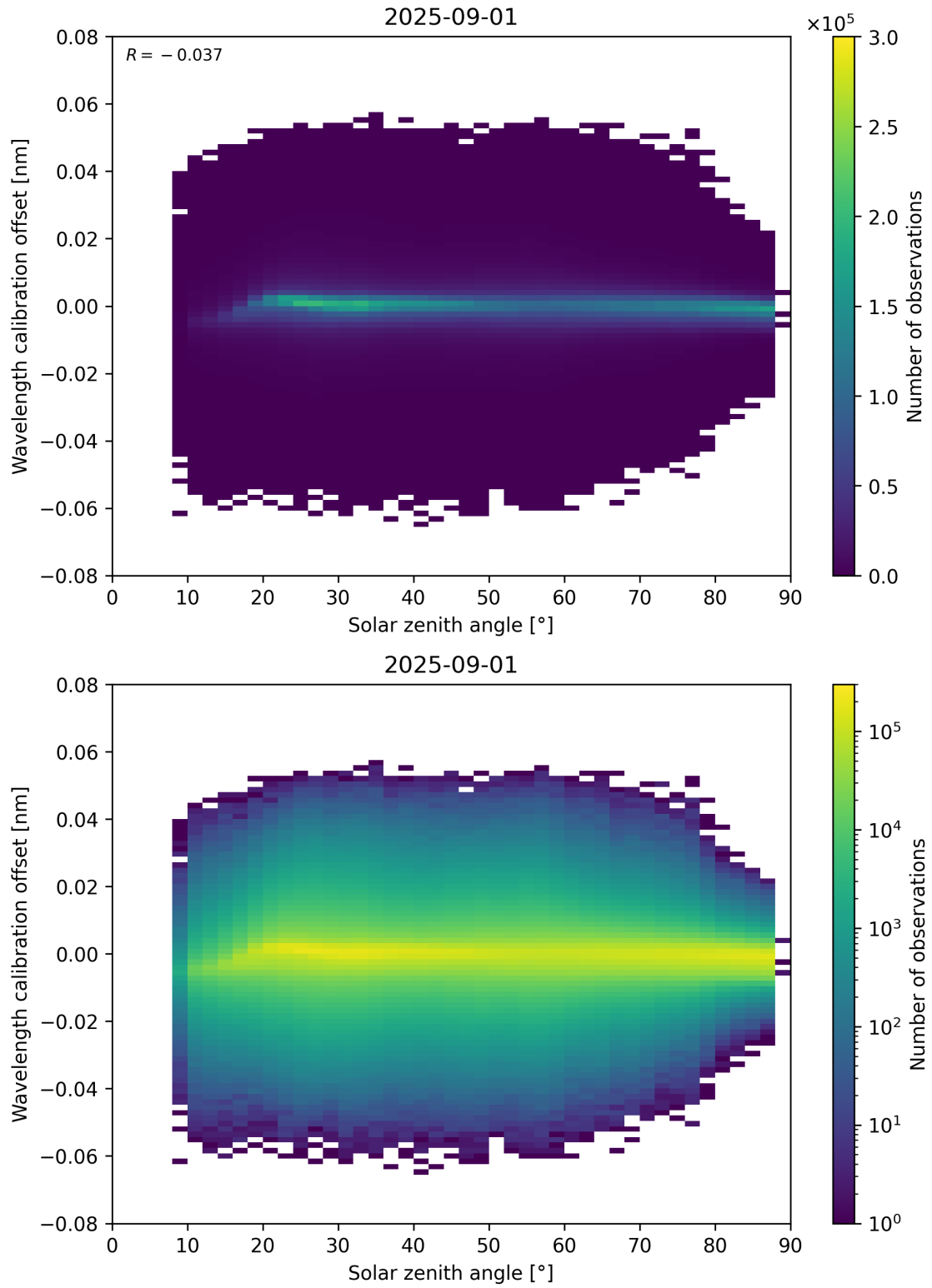
Figure 158: Scatter density plot of “Solar zenith angle” against “Wavelength calibration offset” for 2025-08-31 to 2025-09-02.
