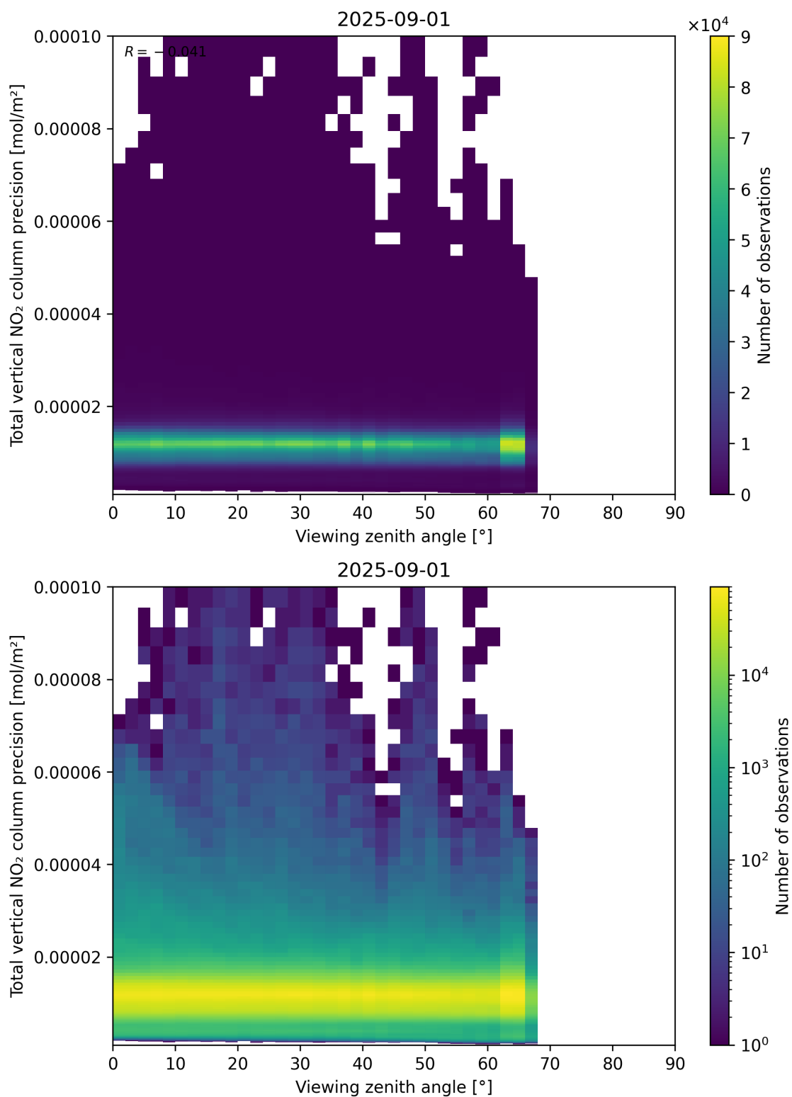
Figure 168: Scatter density plot of “Viewing zenith angle” against “Total vertical NO 2 column precision” for 2025-08-31 to 2025-09-02.
