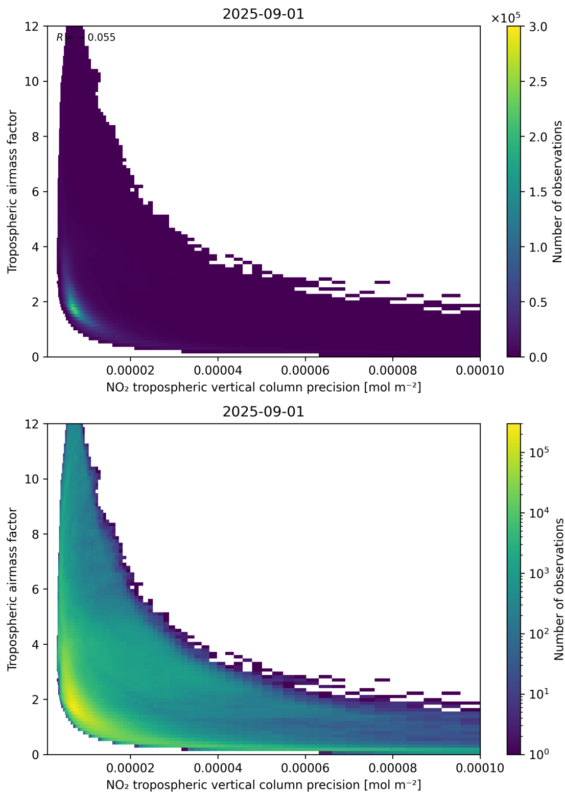
Figure 133: Scatter density plot of “NO 2 tropospheric vertical column precision” against “Tropospheric air mass factor” for 2025-08-31 to 2025-09-02.
