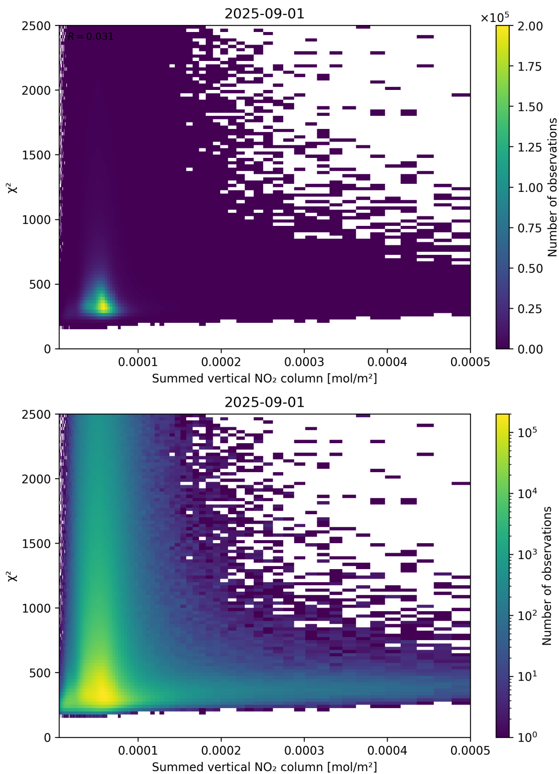
Figure 104: Scatter density plot of “Summed vertical NO 2 column” against “ \chi^2 ” for 2025-08-31 to 2025-09-02.
