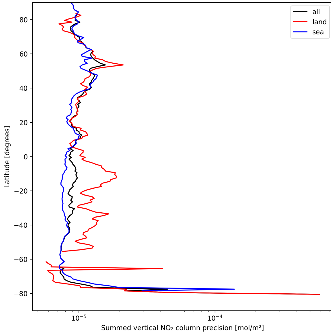
Figure 24: Zonal average of “Summed vertical NO 2 column precision” for 2025-08-31 to 2025-09-02.
