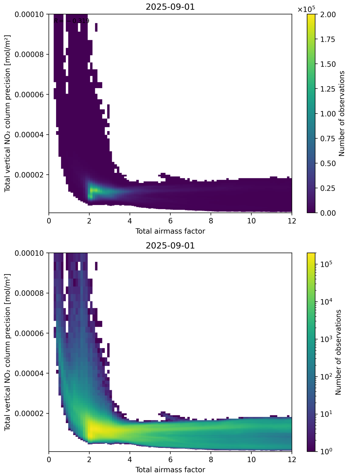
Figure 68: Scatter density plot of “Total airmass factor” against “Total vertical NO 2 column precision” for 2025-08-31 to 2025-09-02.
