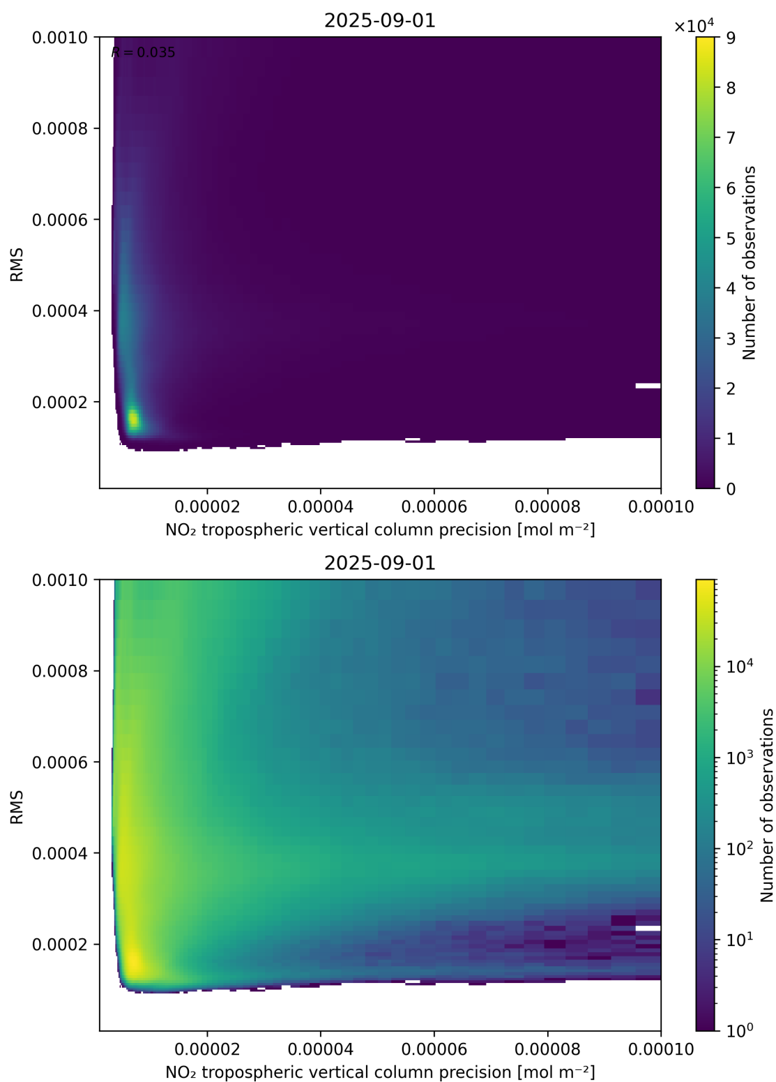
Figure 140: Scatter density plot of “NO 2 tropospheric vertical column precision” against “RMS” for 2025-08-31 to 2025-09-02.
