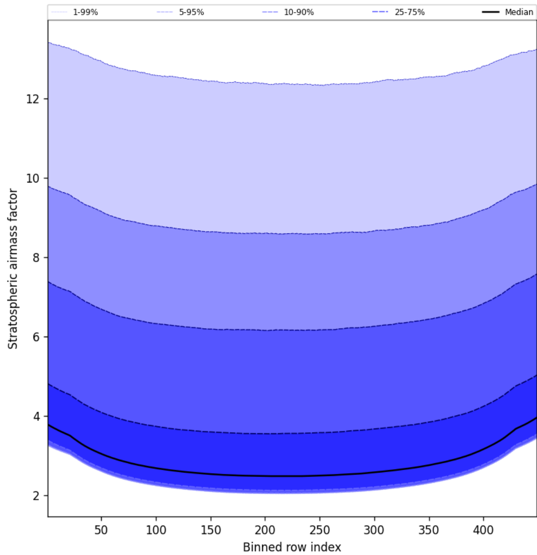
Figure 61: Along track statistics of “Stratospheric airmass factor” for 2025-08-31 to 2025-09-02
