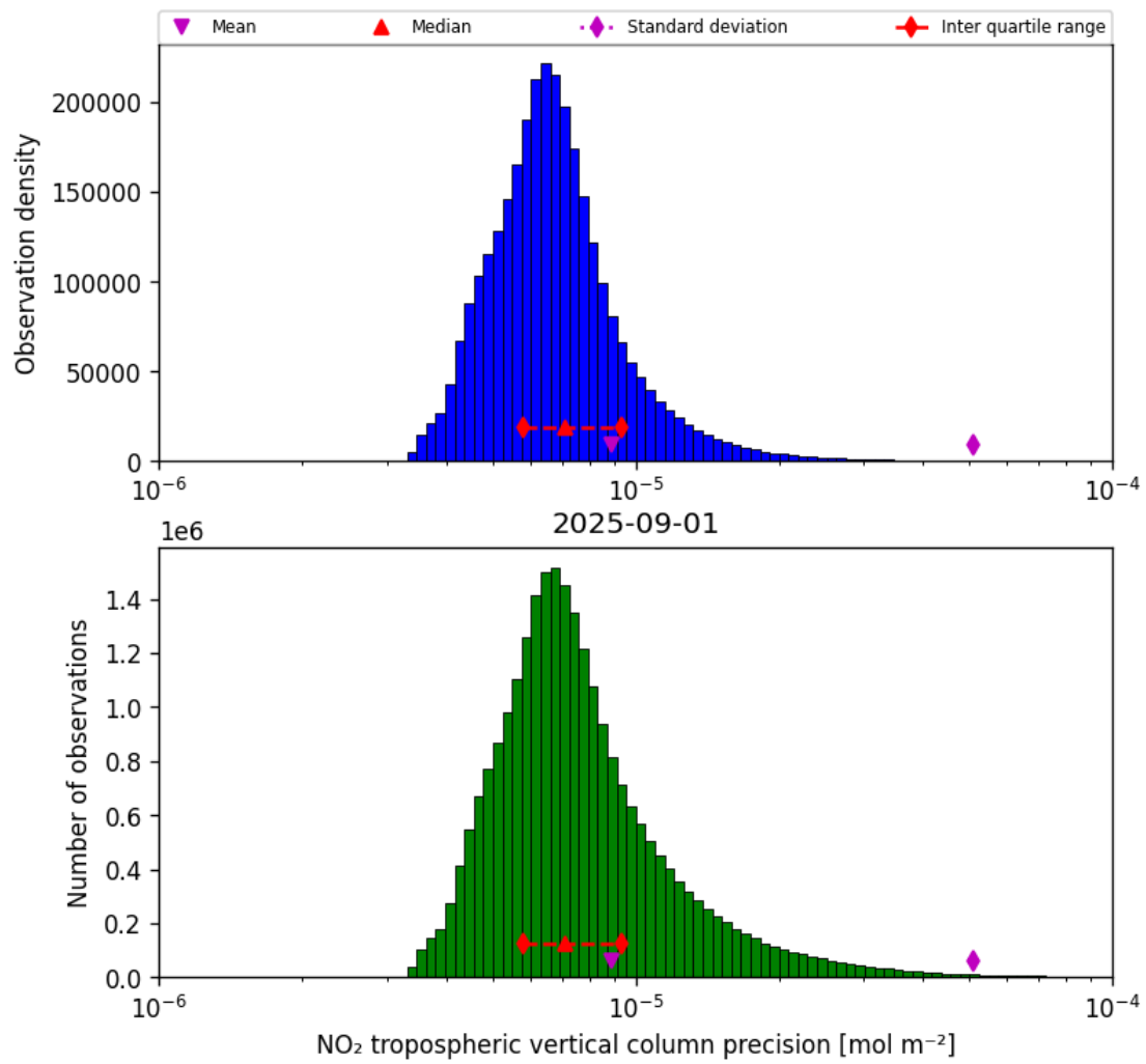
Figure 30: Histogram of “NO 2 tropospheric vertical column precision” for 2025-08-31 to 2025-09-02
