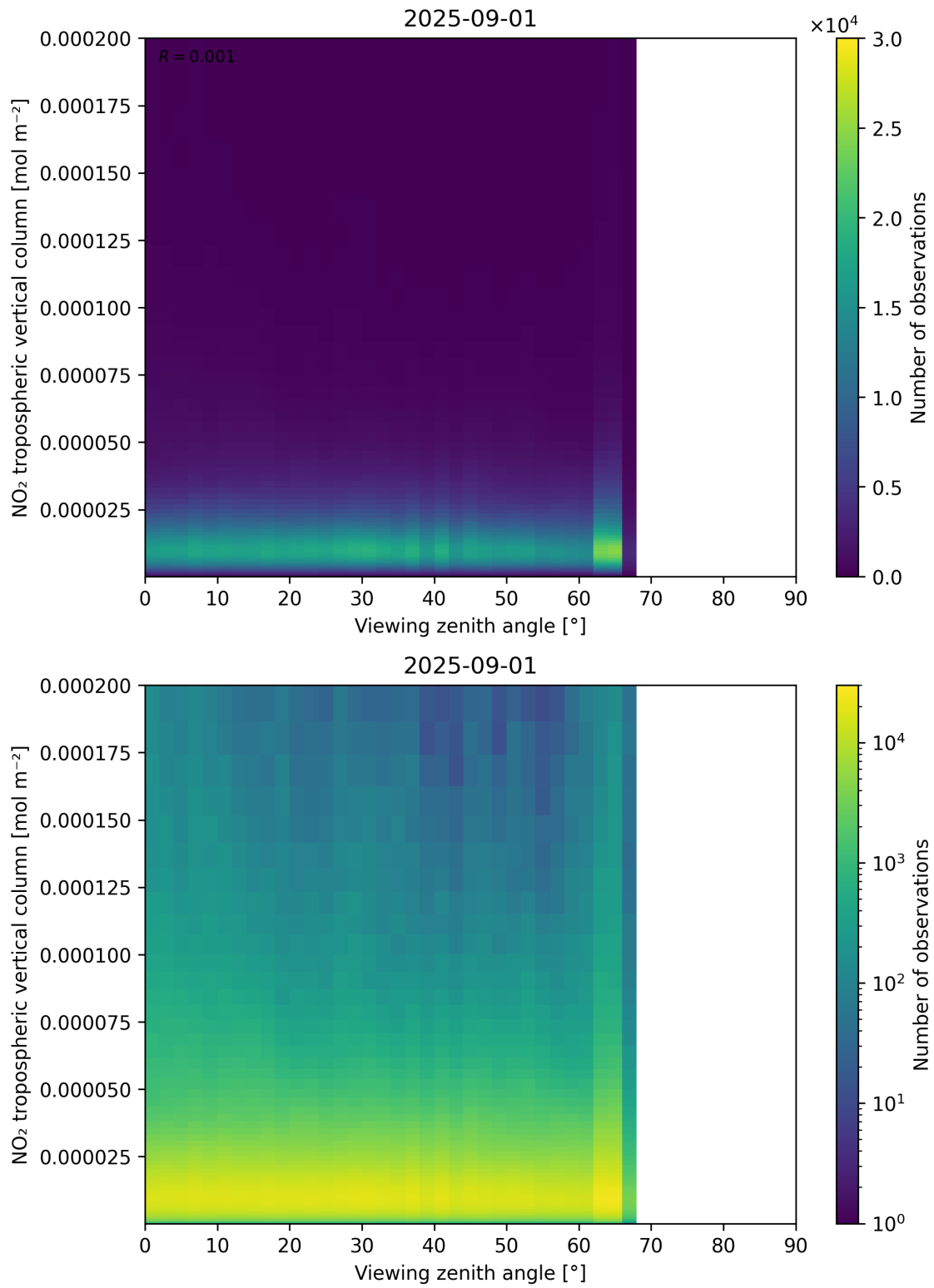
Figure 169: Scatter density plot of “Viewing zenith angle” against “NO 2 tropospheric vertical column” for 2025-08-31 to 2025-09-02.
