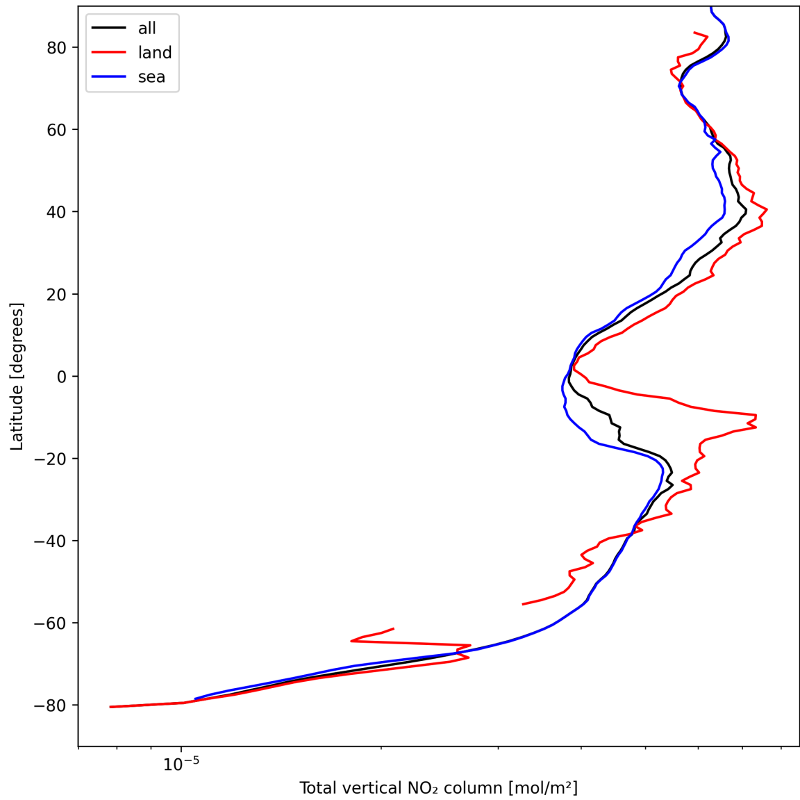
Figure 21: Zonal average of “Total vertical NO 2 column” for 2025-08-31 to 2025-09-02.
