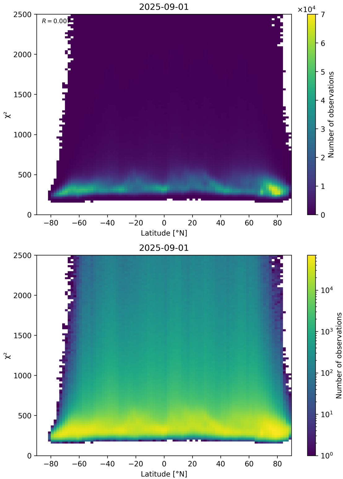
Figure 86: Scatter density plot of “Latitude” against “ \chi^2 ” for 2025-08-31 to 2025-09-02.
