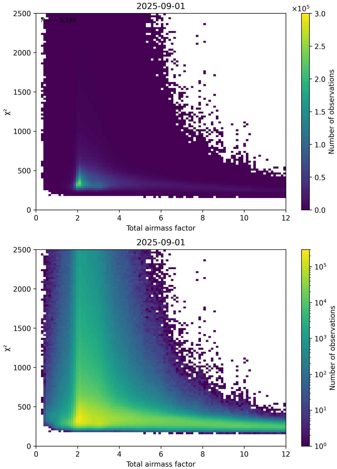
Figure 63: Scatter density plot of “Total airmass factor” against “ \chi^2 ” for 2025-08-31 to 2025-09-02.
