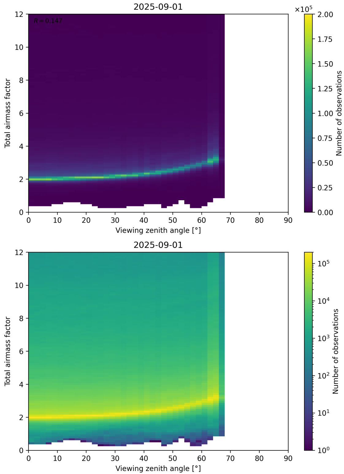
Figure 160: Scatter density plot of “Viewing zenith angle” against “Total airmass factor” for 2025-08-31 to 2025-09-02.
