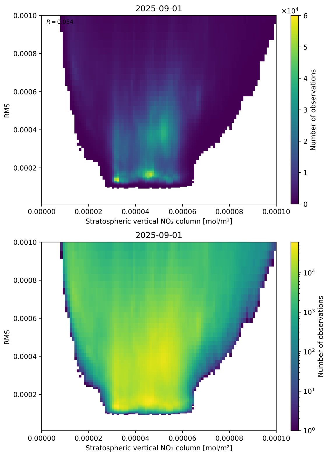
Figure 102: Scatter density plot of “Stratospheric vertical NO 2 column” against “RMS” for 2025-08-31 to 2025-09-02.
