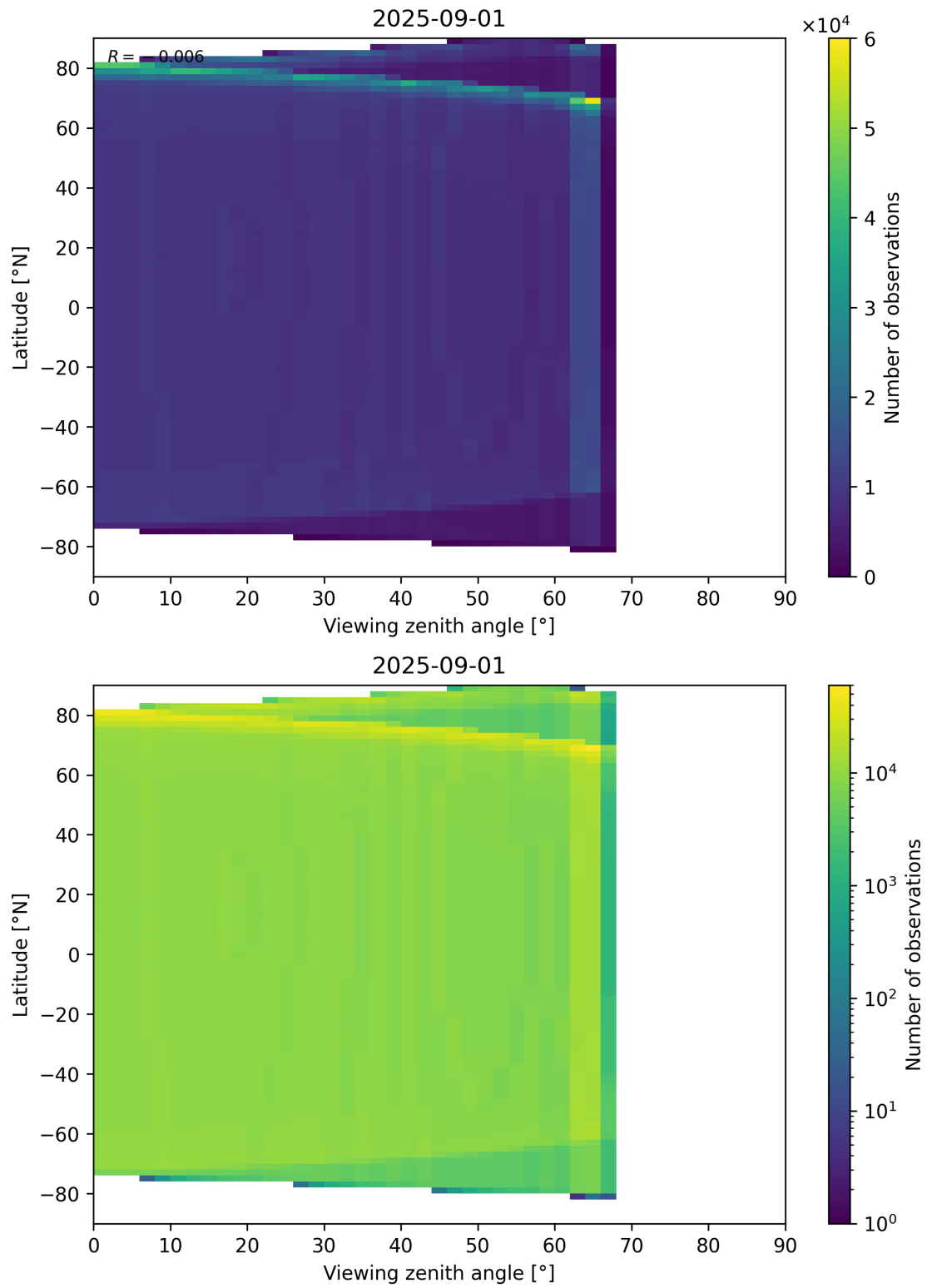
Figure 163: Scatter density plot of “Viewing zenith angle” against “Latitude” for 2025-08-31 to 2025-09-02.
