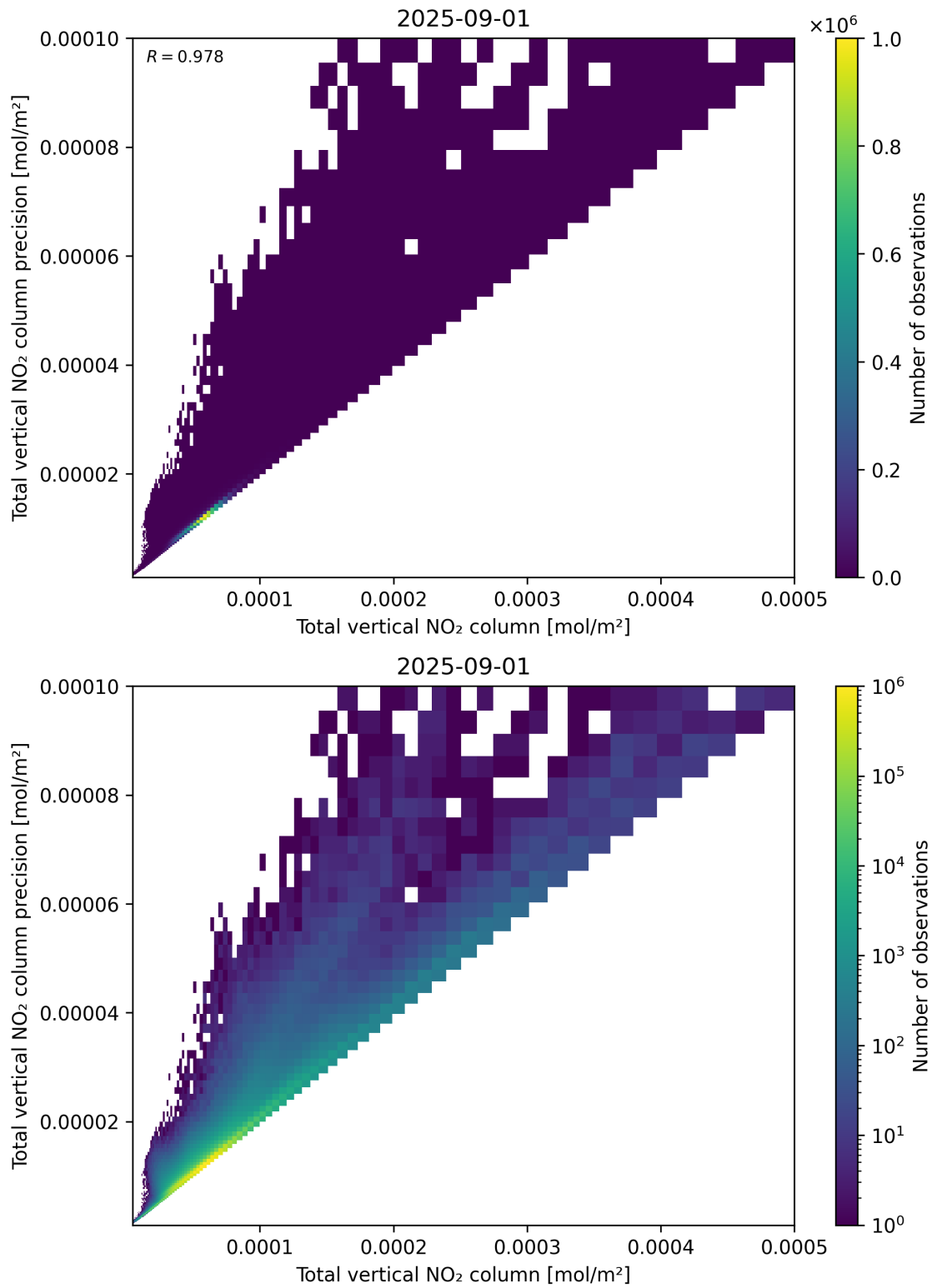
Figure 114: Scatter density plot of “Total vertical NO 2 column” against “Total vertical NO 2 column precision” for 2025-08-31 to 2025-09-02.
