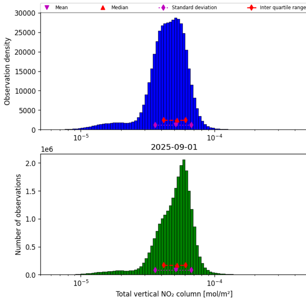
Figure 38: Histogram of “Total vertical NO 2 column” for 2025-08-31 to 2025-09-02
