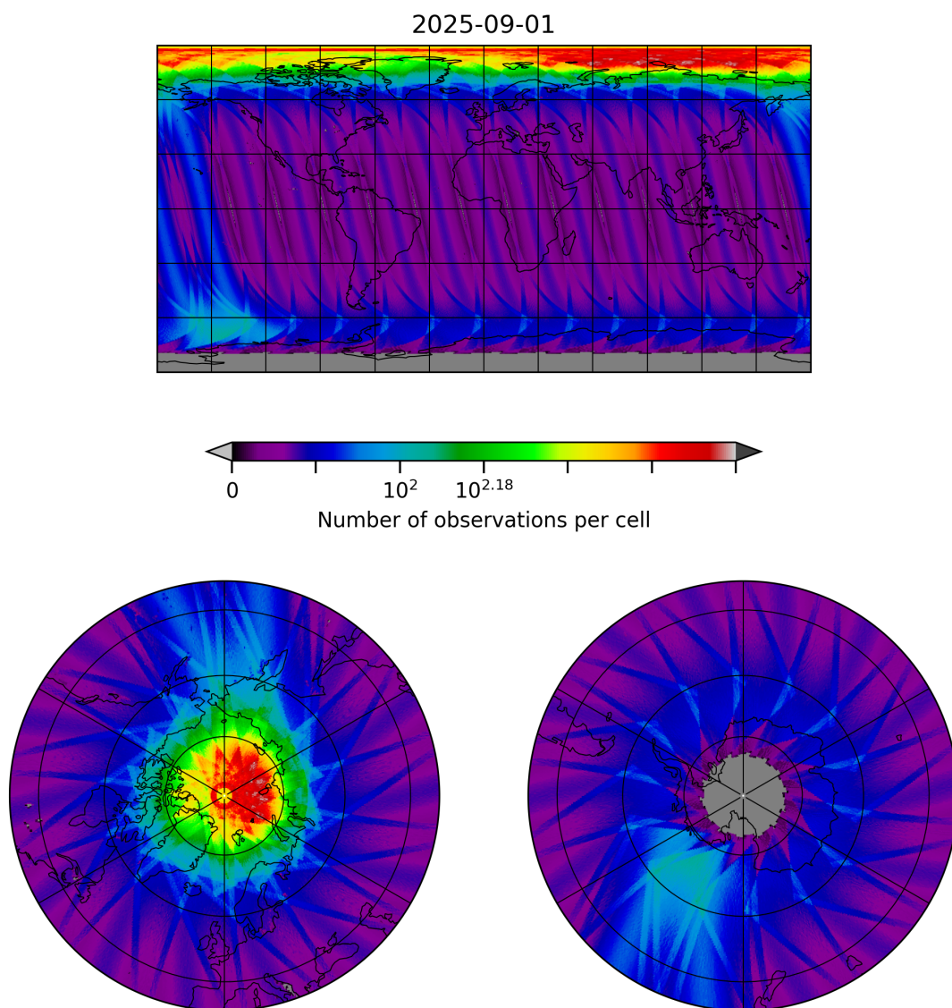
Figure 10: Map of the number of observations for 2025-08-31 to 2025-09-02
