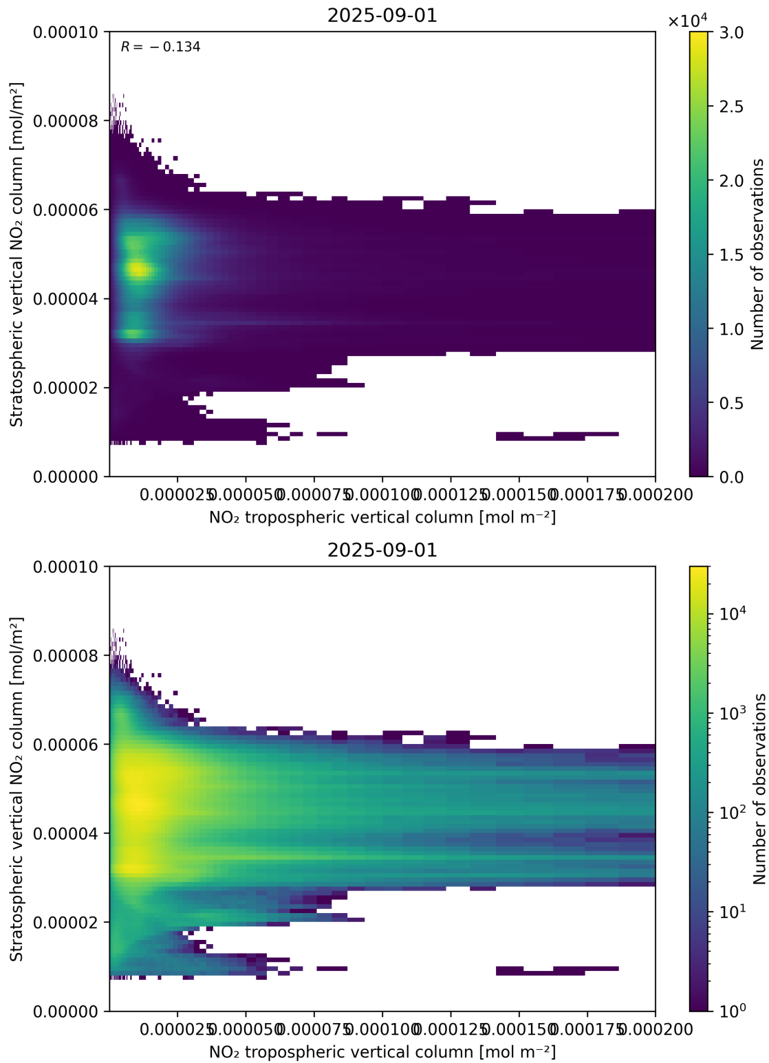
Figure 125: Scatter density plot of “NO 2 tropospheric vertical column” against “Stratospheric vertical NO 2 column” for 2025-08-31 to 2025-09-02.
