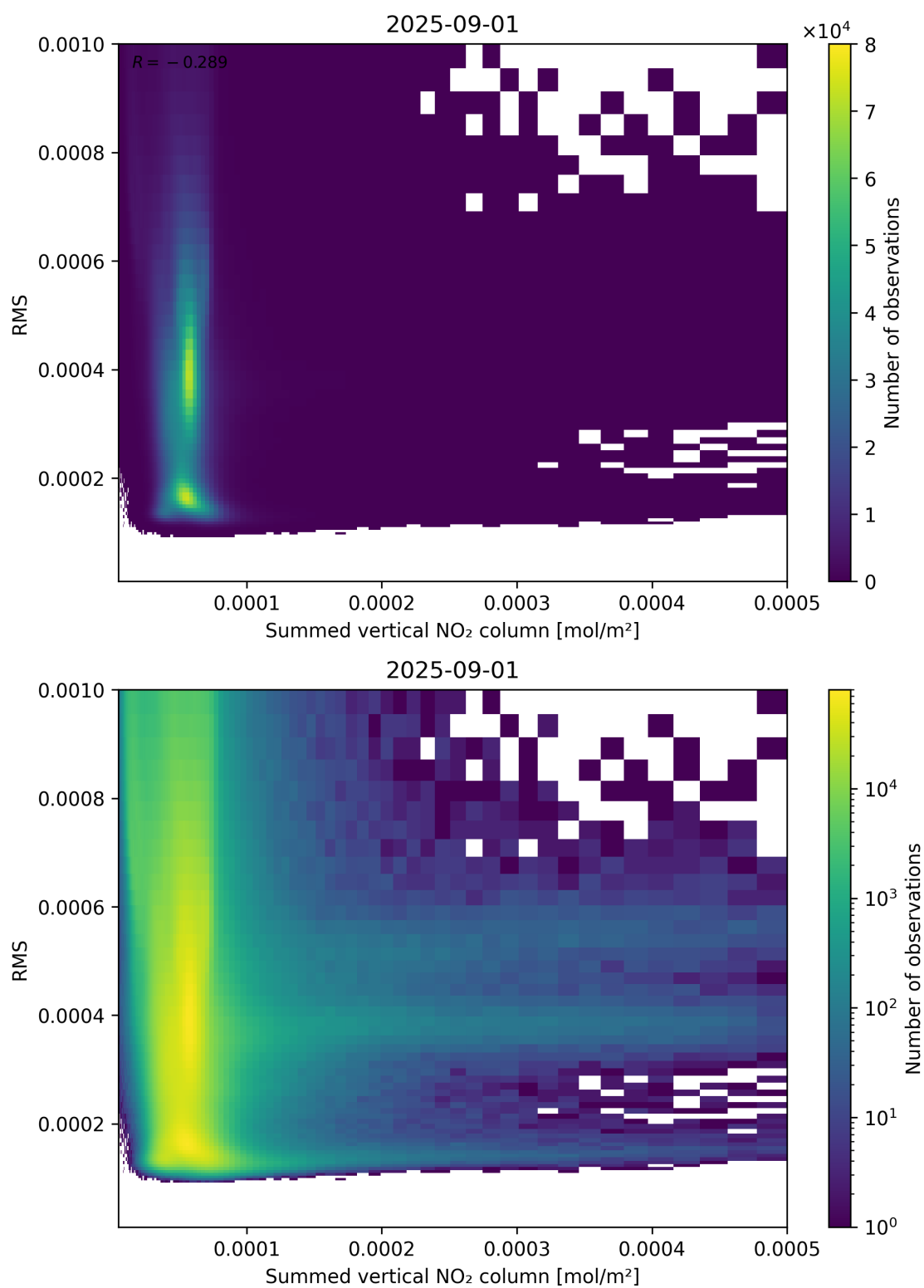
Figure 109: Scatter density plot of “Summed vertical NO 2 column” against “RMS” for 2025-08-31 to 2025-09-02.
