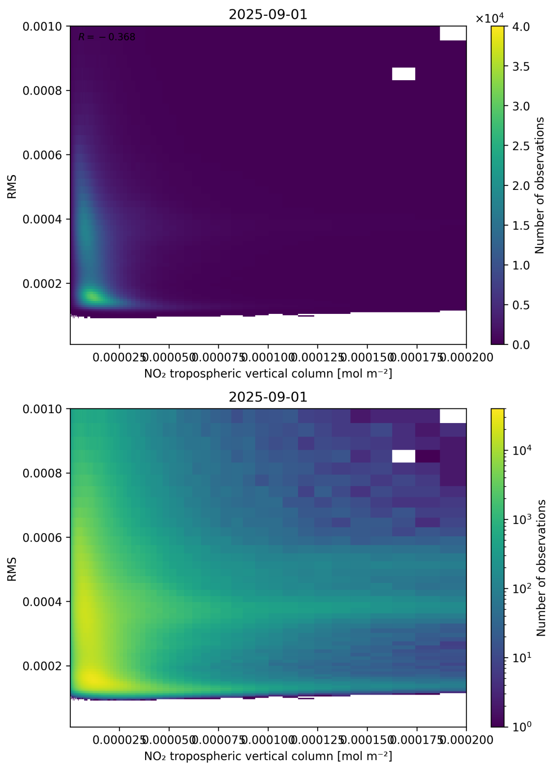
Figure 142: Scatter density plot of “NO 2 tropospheric vertical column” against “RMS” for 2025-08-31 to 2025-09-02.
