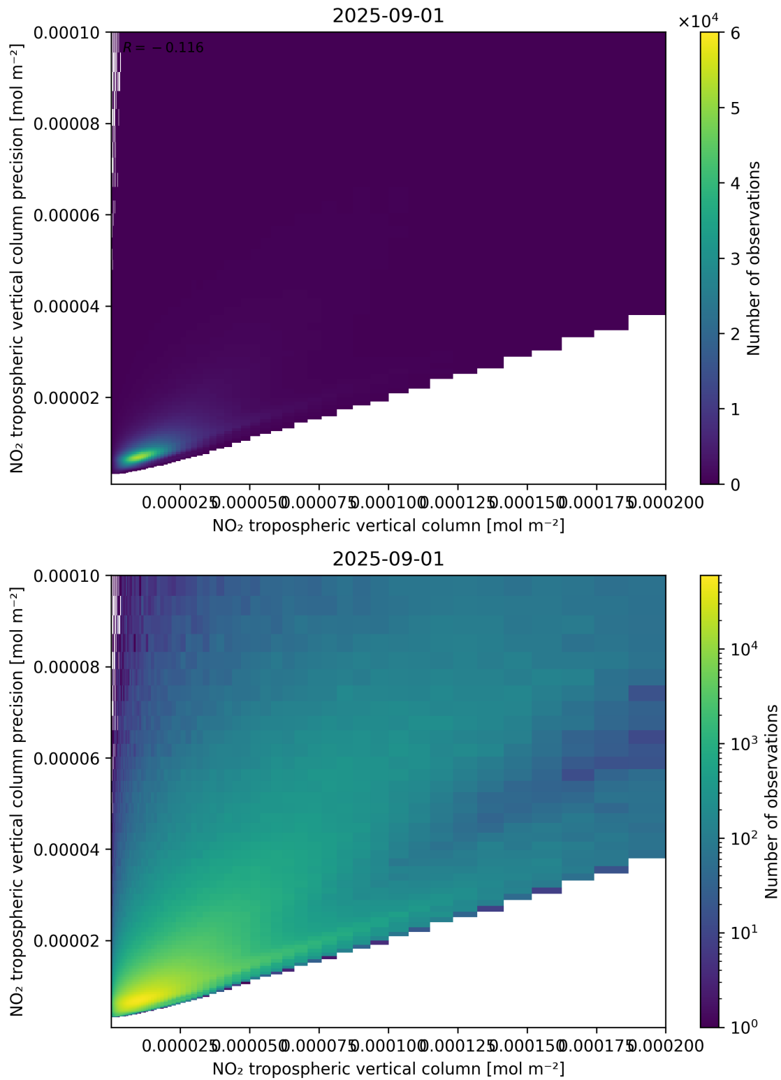
Figure 130: Scatter density plot of “NO 2 tropospheric vertical column” against “NO 2 tropospheric vertical column precision” for 2025-08-31 to 2025-09-02.
