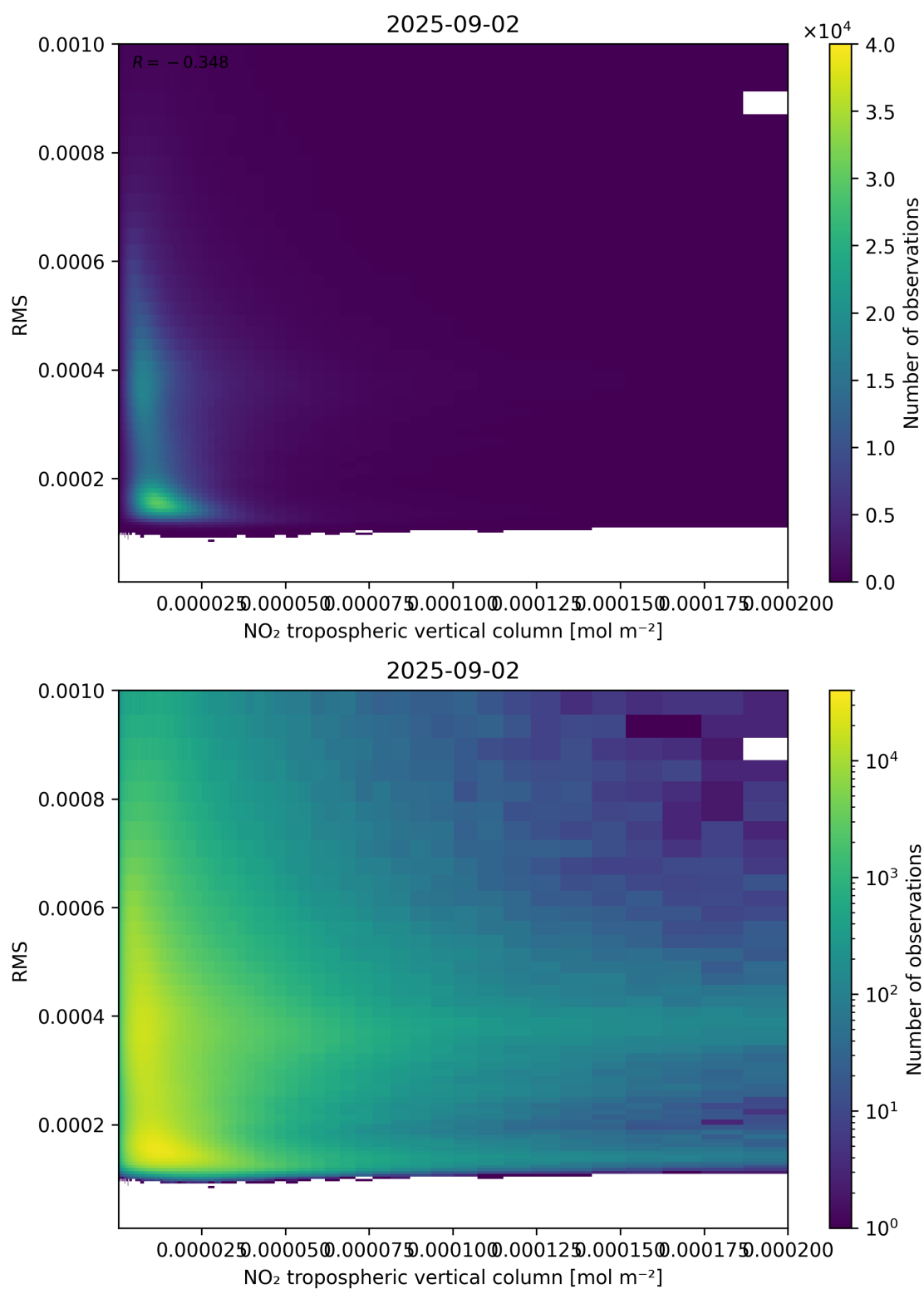
Figure 142: Scatter density plot of “NO 2 tropospheric vertical column” against “RMS” for 2025-09-01 to 2025-09-03.
