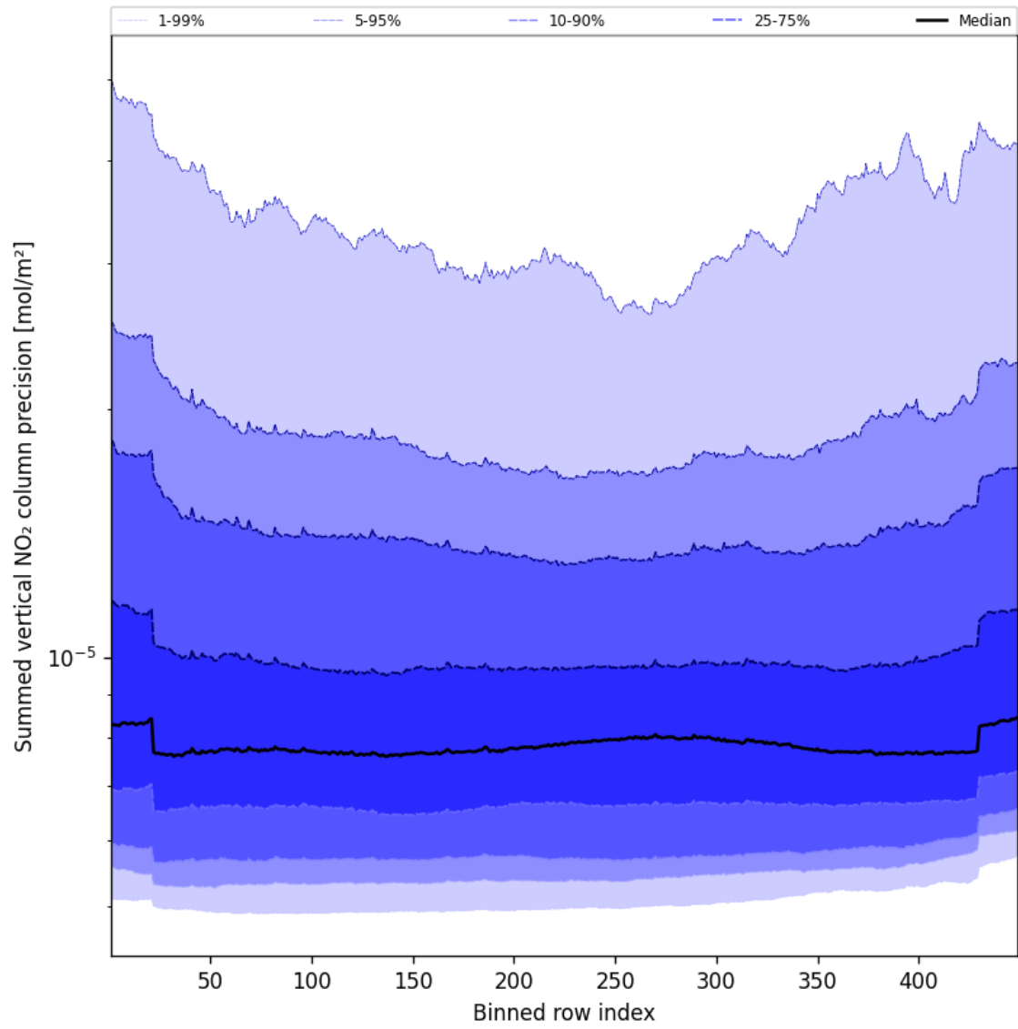
Figure 58: Along track statistics of “Summed vertical NO 2 column precision” for 2025-09-01 to 2025-09-03
