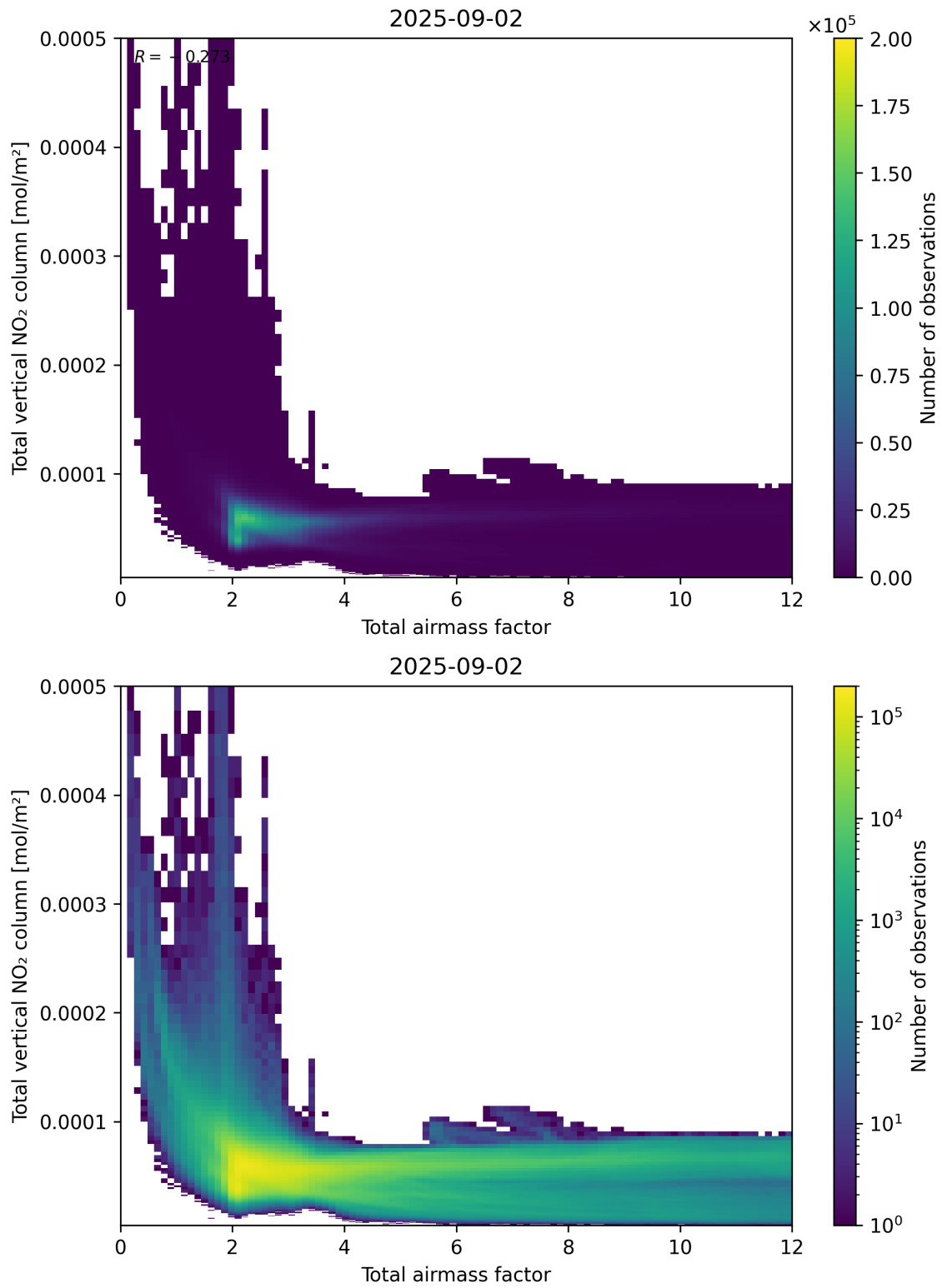
Figure 67: Scatter density plot of “Total airmass factor” against “Total vertical NO 2 column” for 2025-09-01 to 2025-09-03.
