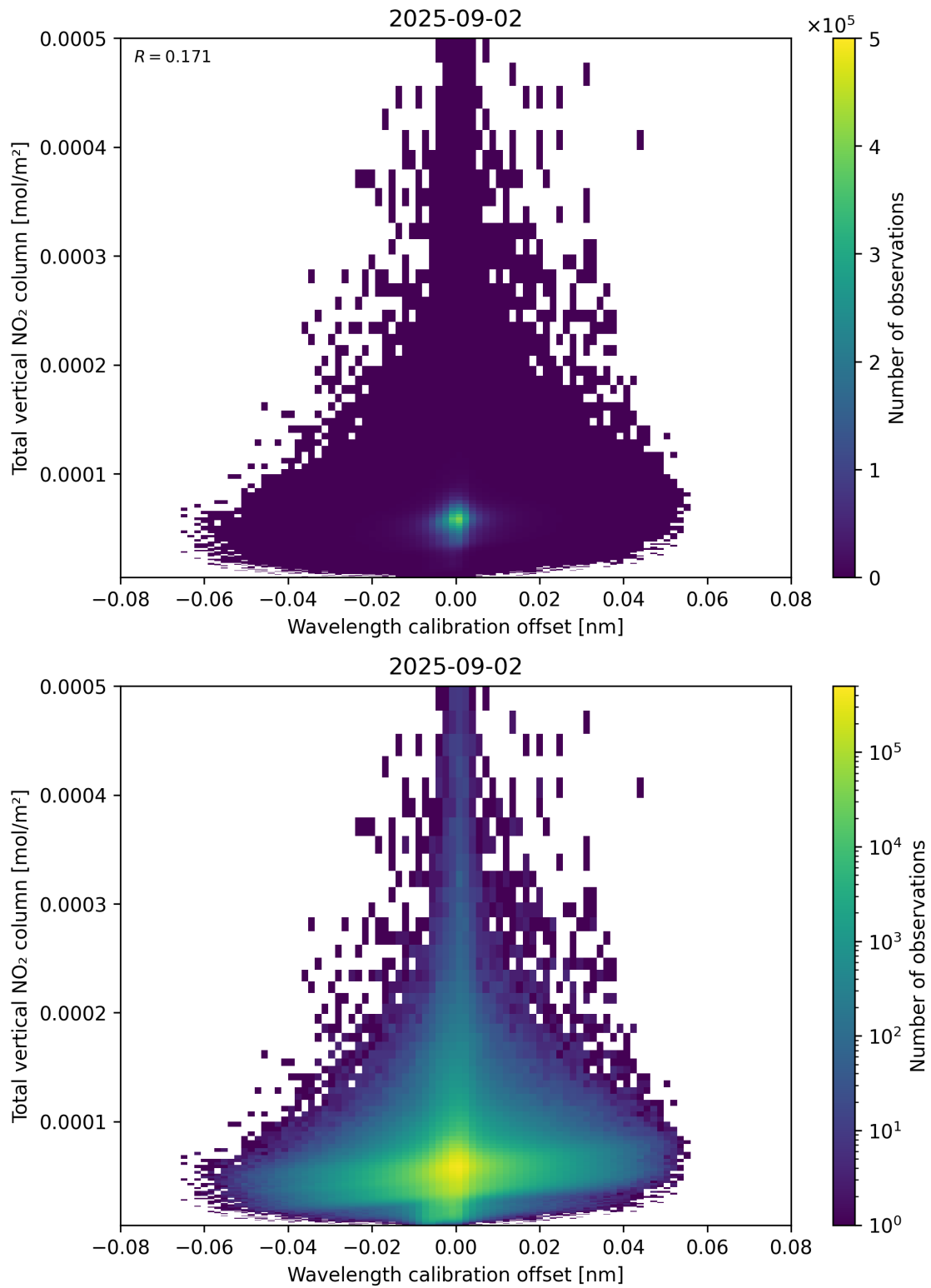
Figure 179: Scatter density plot of “Wavelength calibration offset” against “Total vertical NO 2 column” for 2025-09-01 to 2025-09-03.
