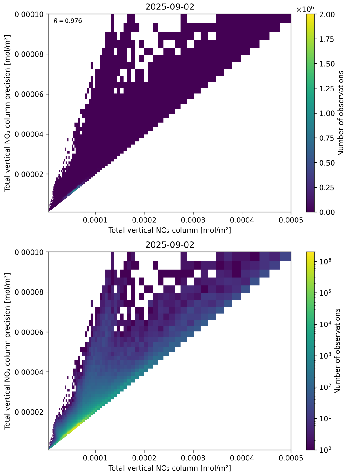
Figure 114: Scatter density plot of “Total vertical NO 2 column” against “Total vertical NO 2 column precision” for 2025-09-01 to 2025-09-03.
