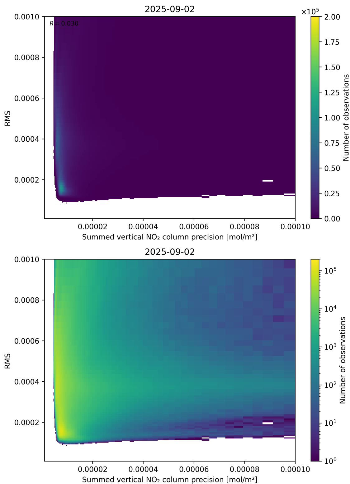
Figure 108: Scatter density plot of “Summed vertical NO 2 column precision” against “RMS” for 2025-09-01 to 2025-09-03.
