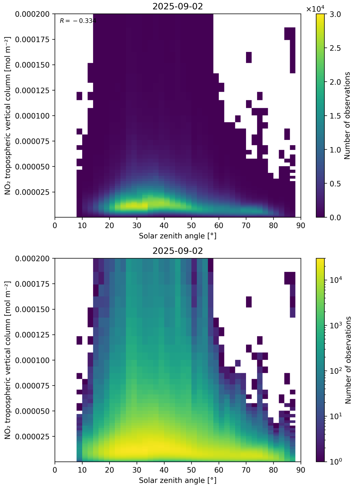
Figure 155: Scatter density plot of “Solar zenith angle” against “NO 2 tropospheric vertical column” for 2025-09-01 to 2025-09-03.
