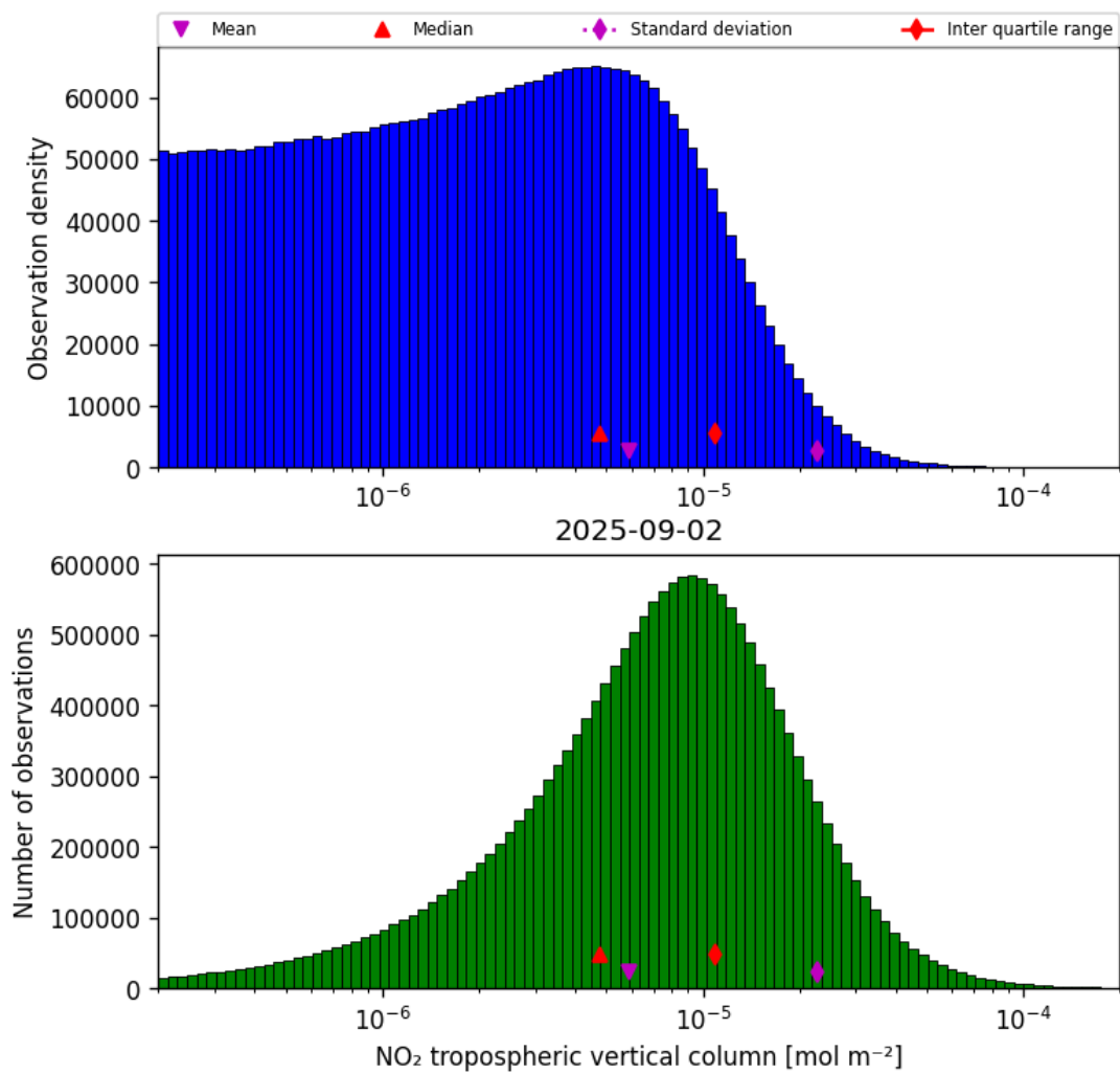
Figure 29: Histogram of “NO 2 tropospheric vertical column” for 2025-09-01 to 2025-09-03
