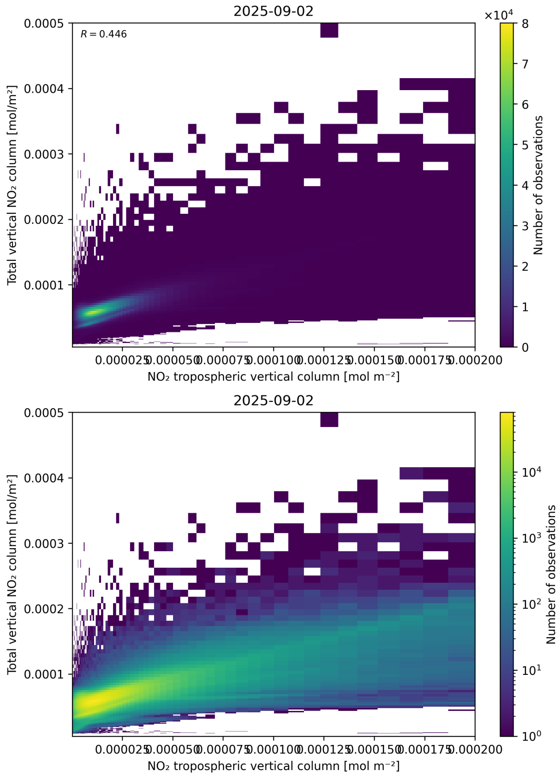
Figure 128: Scatter density plot of “NO 2 tropospheric vertical column” against “Total vertical NO 2 column” for 2025-09-01 to 2025-09-03.
