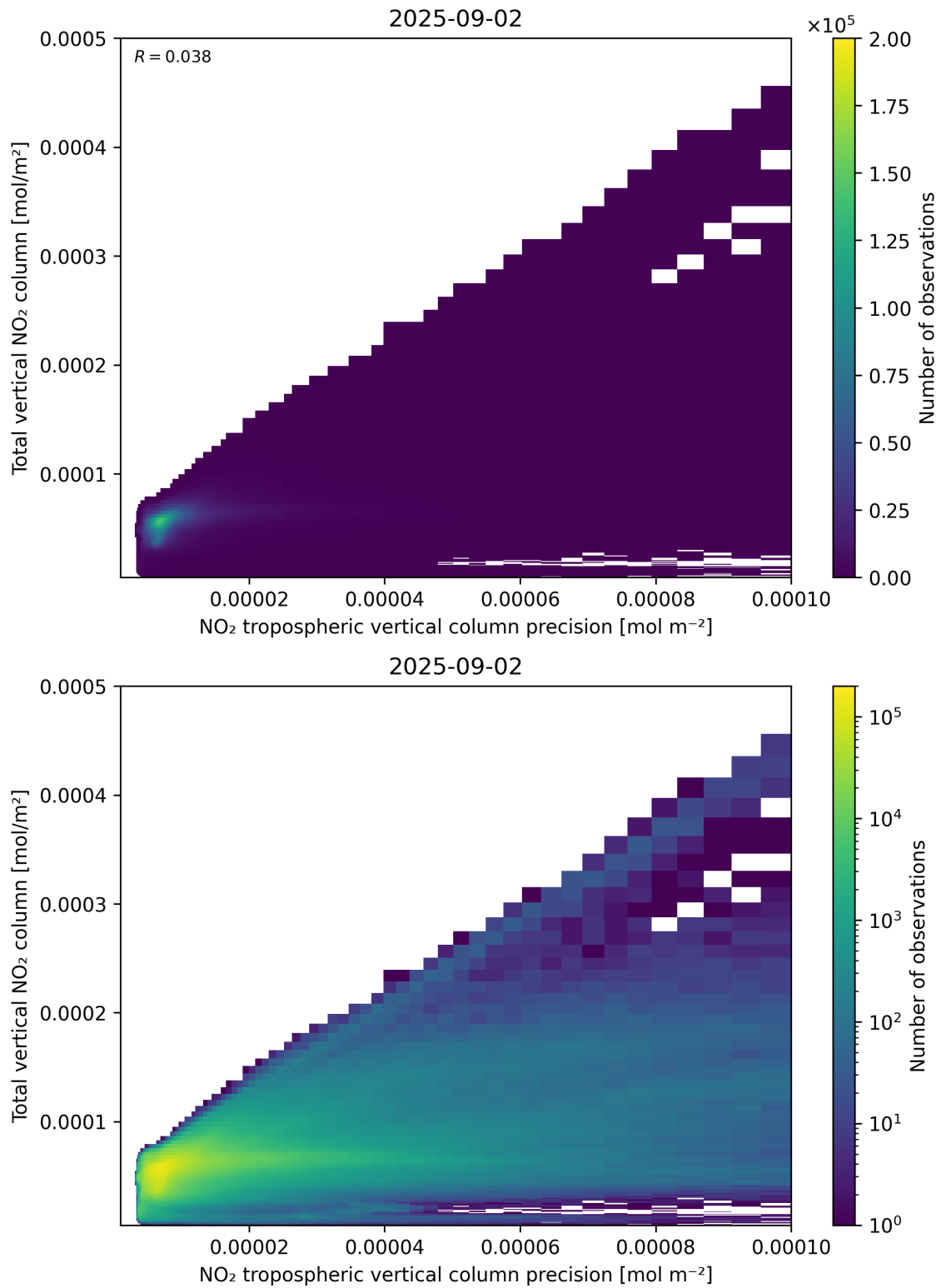
Figure 138: Scatter density plot of “NO 2 tropospheric vertical column precision” against “Total vertical NO 2 column” for 2025-09-01 to 2025-09-03.
