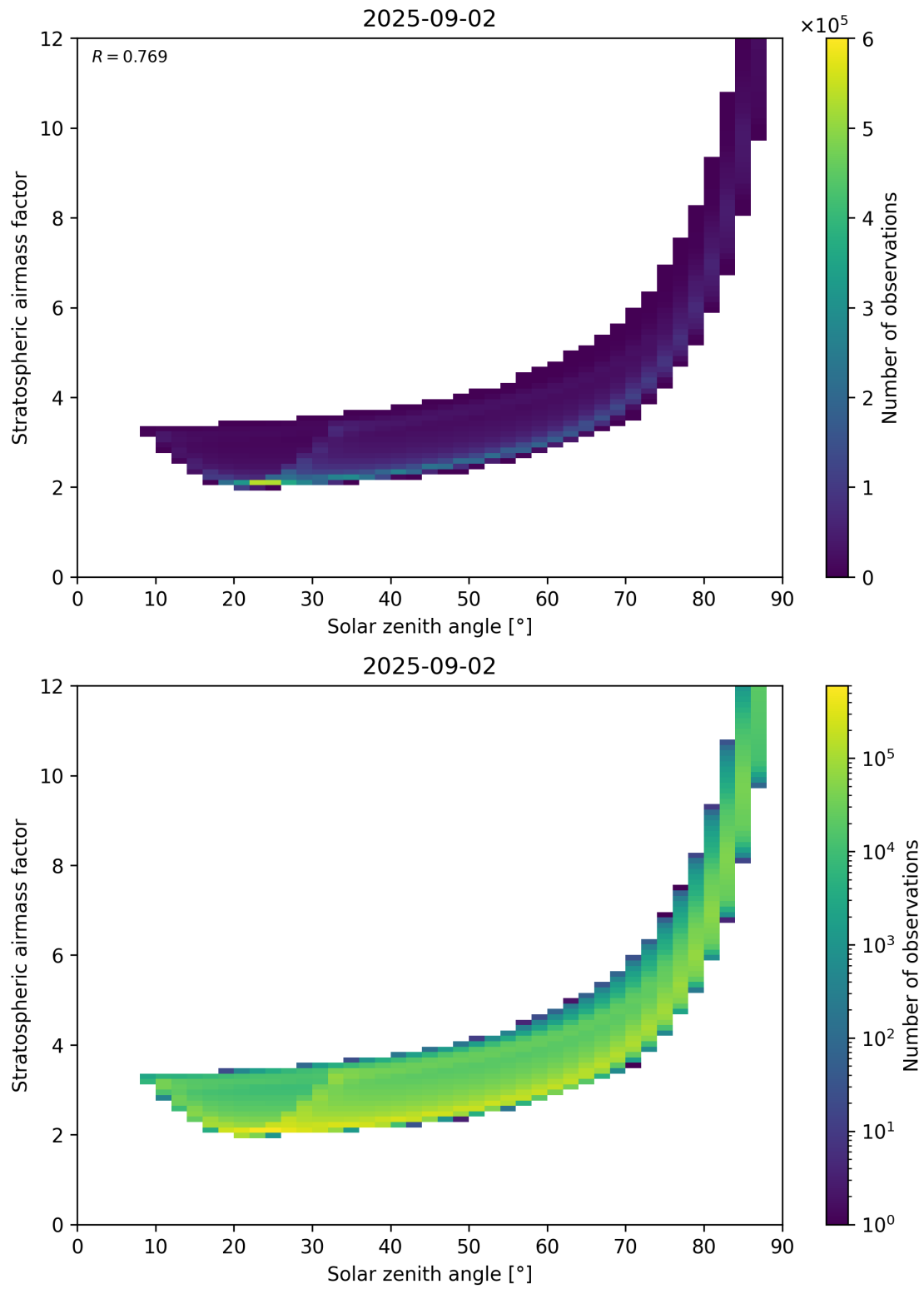
Figure 145: Scatter density plot of “Solar zenith angle” against “Stratospheric airmass factor” for 2025-09-01 to 2025-09-03.
