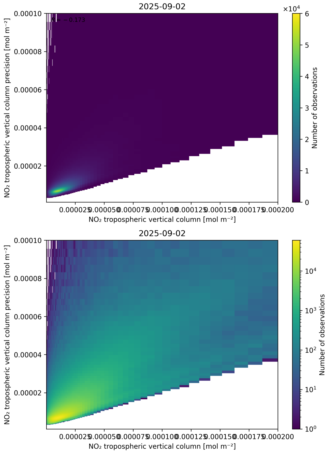
Figure 130: Scatter density plot of “NO 2 tropospheric vertical column” against “NO 2 tropospheric vertical column precision” for 2025-09-01 to 2025-09-03.
