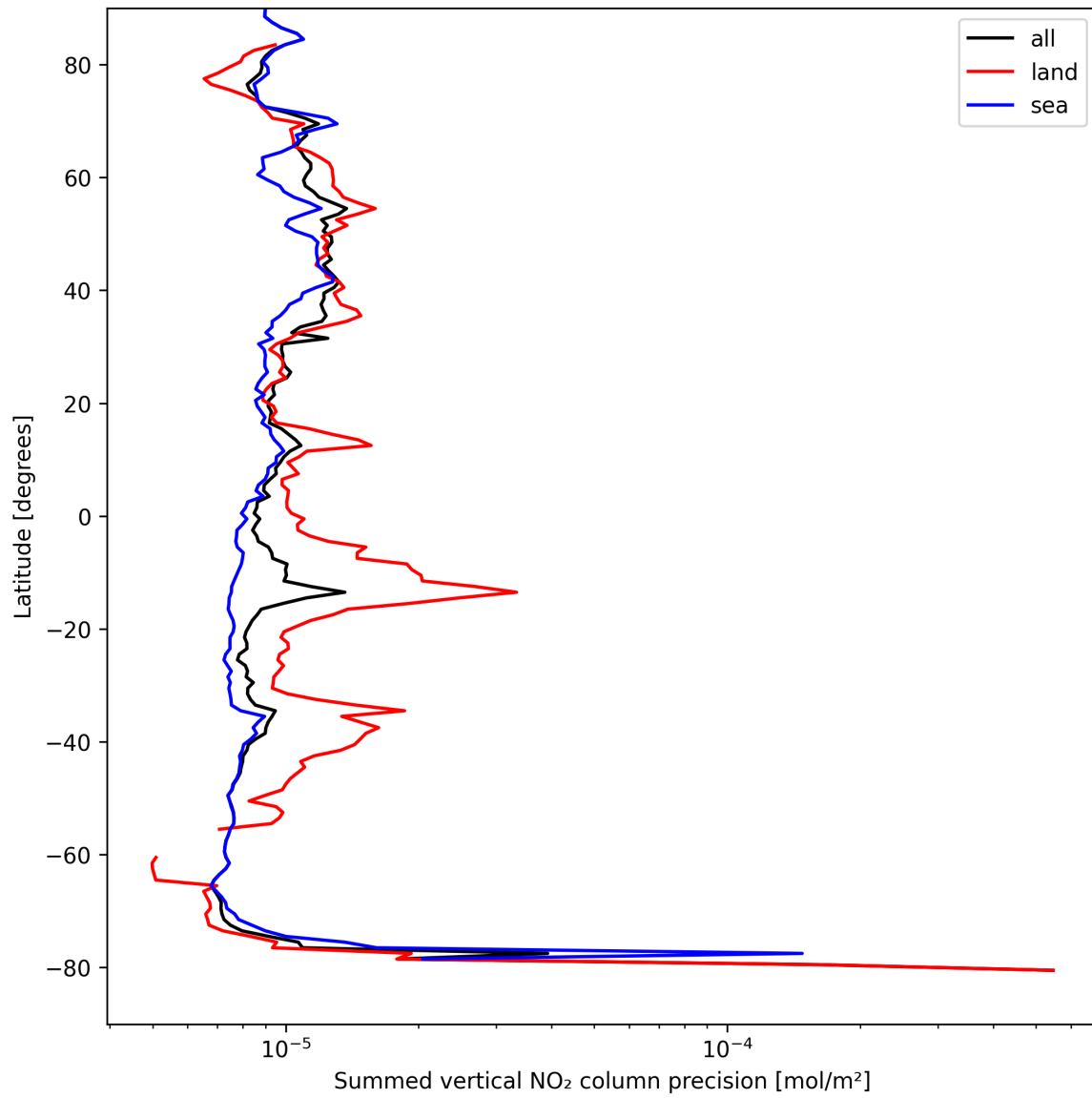
Figure 24: Zonal average of “Summed vertical NO 2 column precision” for 2025-09-01 to 2025-09-03.
