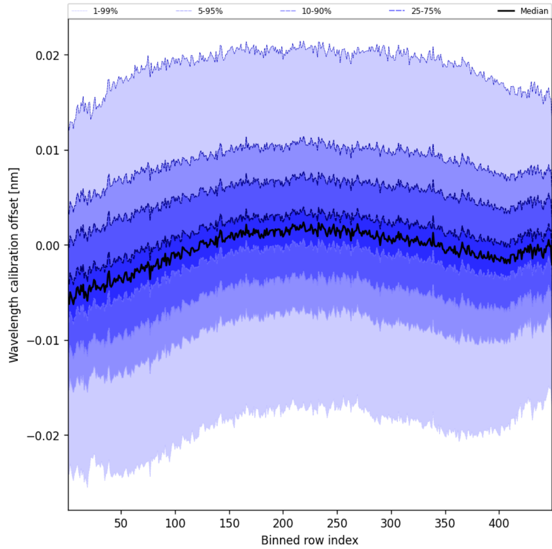
Figure 52: Along track statistics of “Wavelength calibration offset” for 2025-09-01 to 2025-09-03
