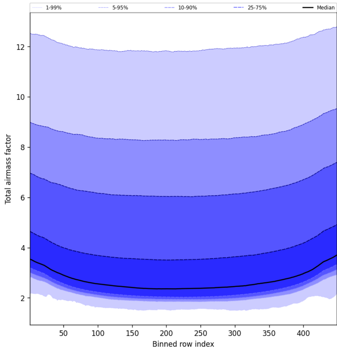
Figure 49: Along track statistics of “Total airmass factor” for 2025-09-01 to 2025-09-03
