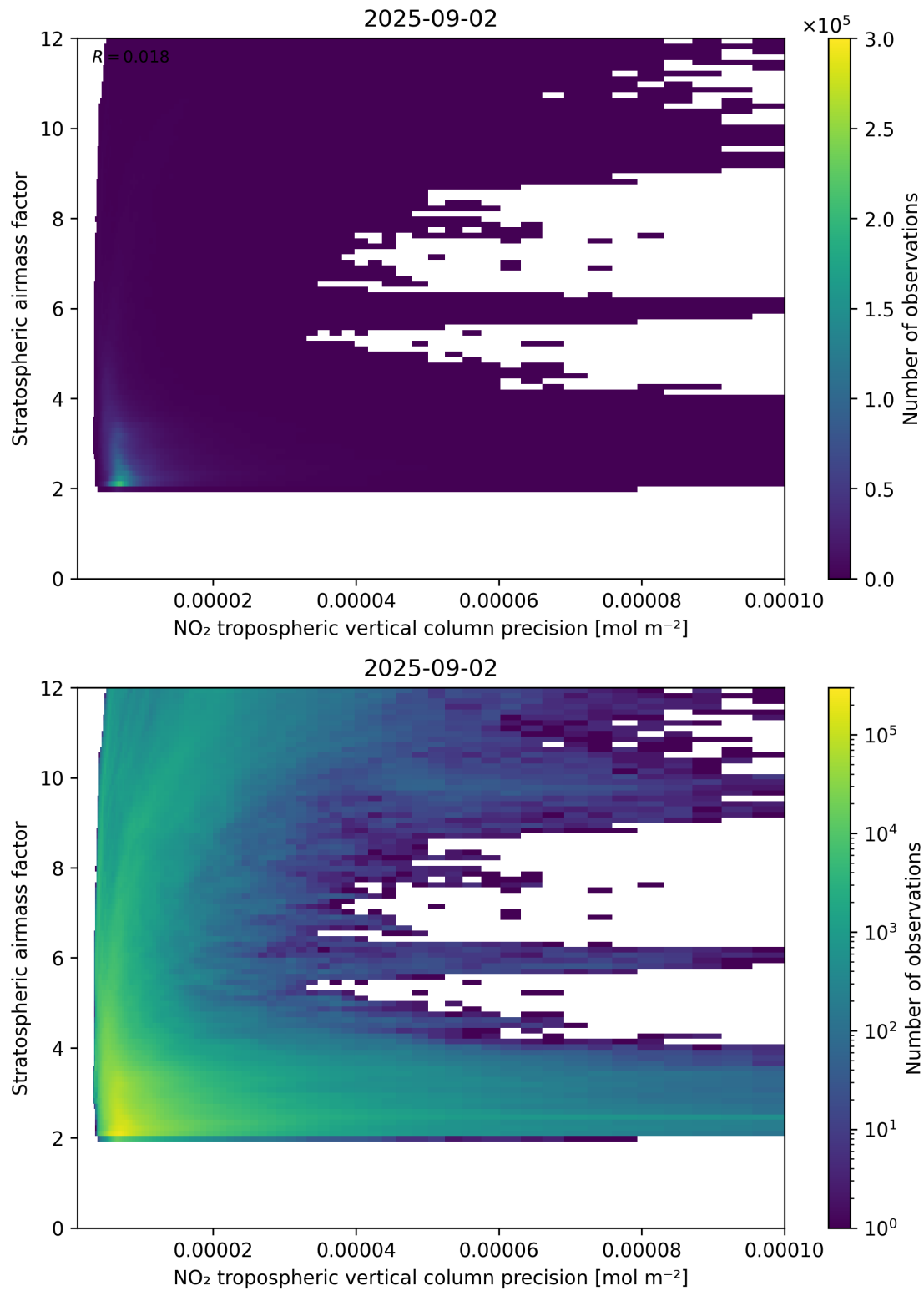
Figure 131: Scatter density plot of “NO 2 tropospheric vertical column precision” against “Stratospheric airmass factor” for 2025-09-01 to 2025-09-03.
