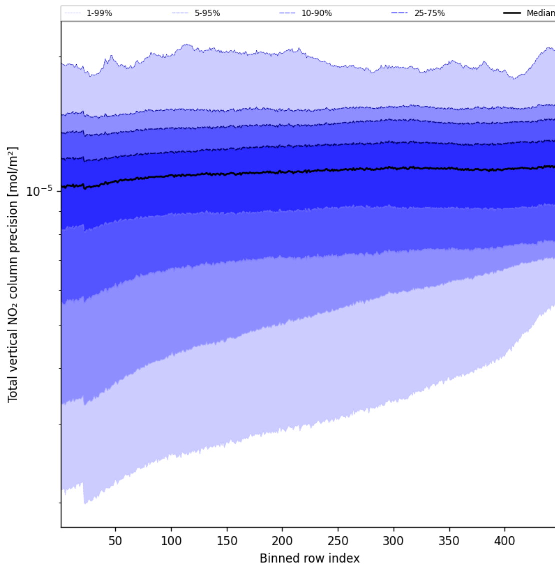
Figure 56: Along track statistics of “Total vertical NO 2 column precision” for 2025-09-01 to 2025-09-03
