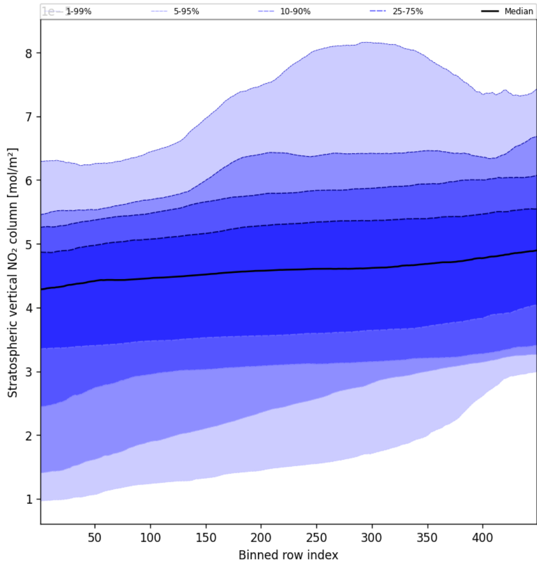
Figure 53: Along track statistics of “Stratospheric vertical NO 2 column” for 2025-09-01 to 2025-09-03
