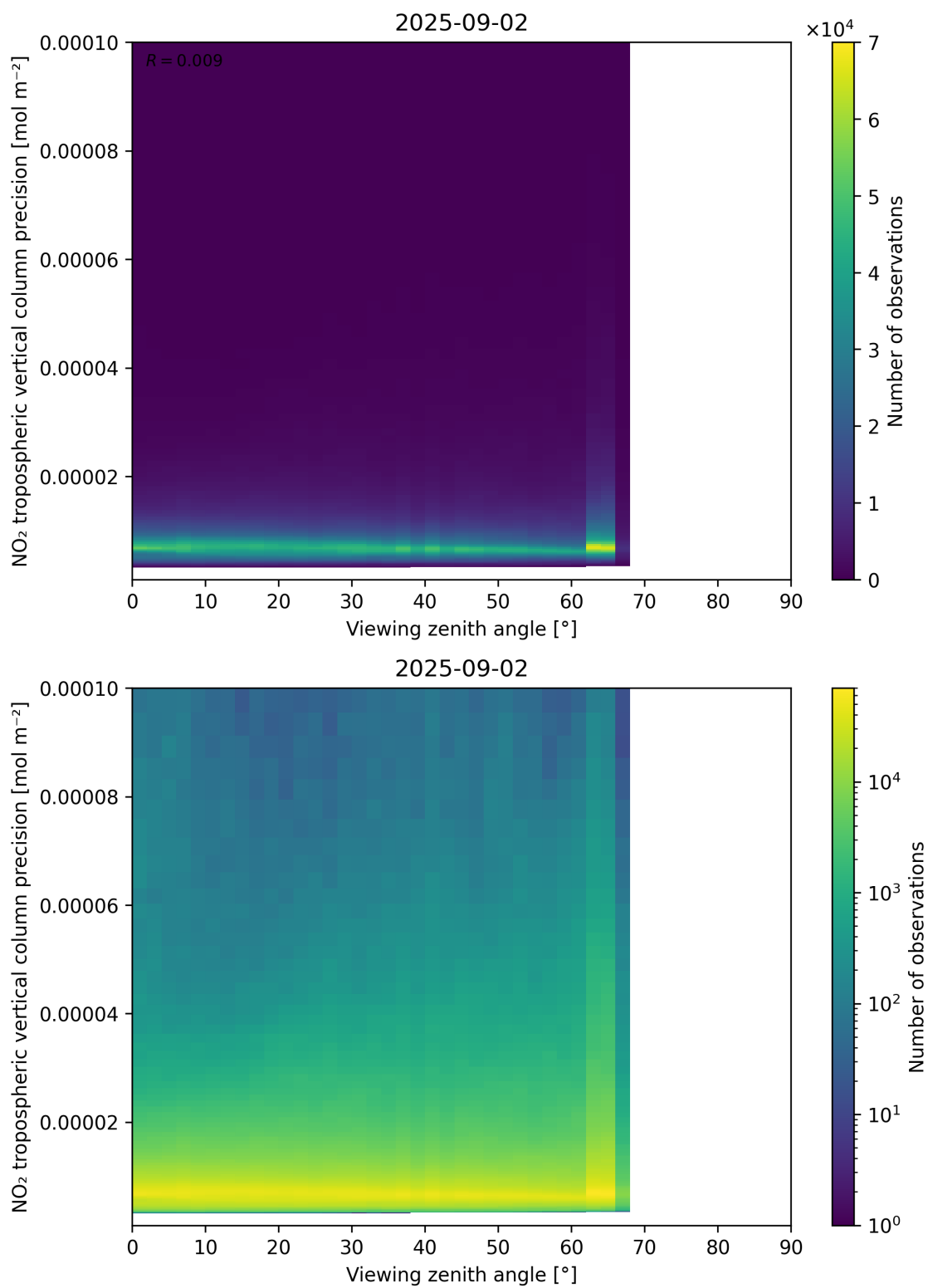
Figure 170: Scatter density plot of “Viewing zenith angle” against “NO 2 tropospheric vertical column precision” for 2025-09-01 to 2025-09-03.
