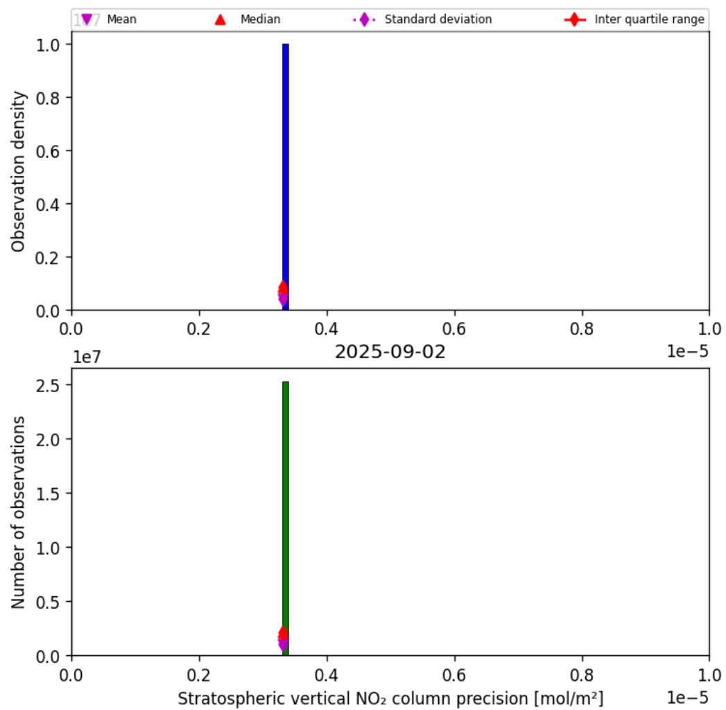
Figure 37: Histogram of “Stratospheric vertical NO 2 column precision” for 2025-09-01 to 2025-09-03
