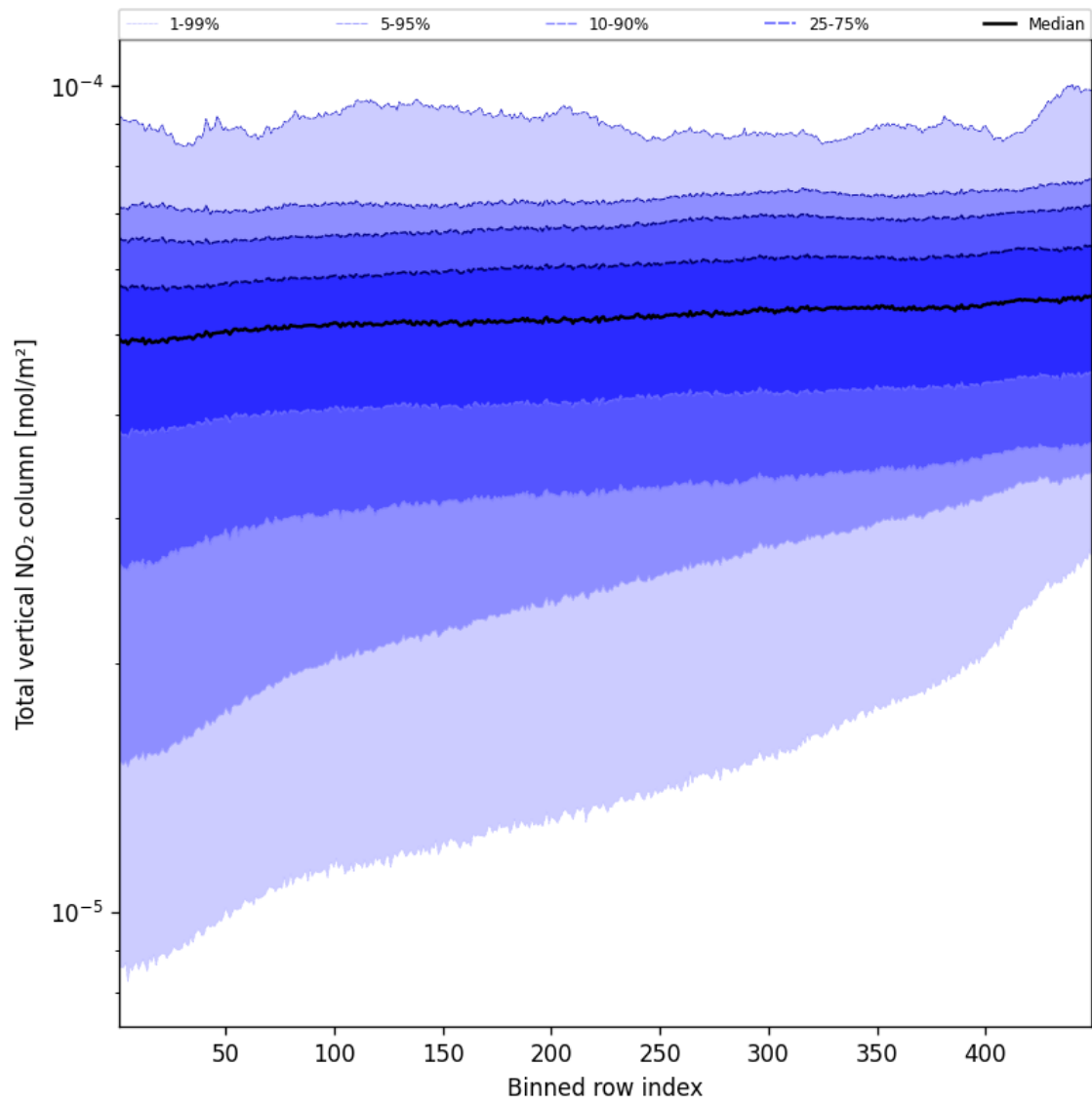
Figure 55: Along track statistics of “Total vertical NO 2 column” for 2025-09-01 to 2025-09-03
