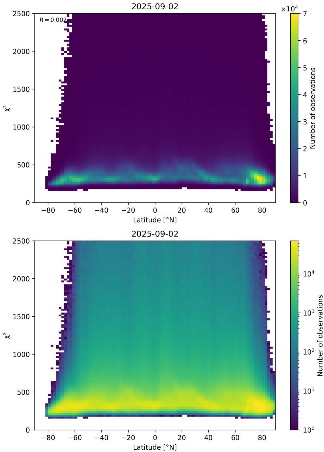
Figure 86: Scatter density plot of “Latitude” against “ \chi^2 ” for 2025-09-01 to 2025-09-03.
