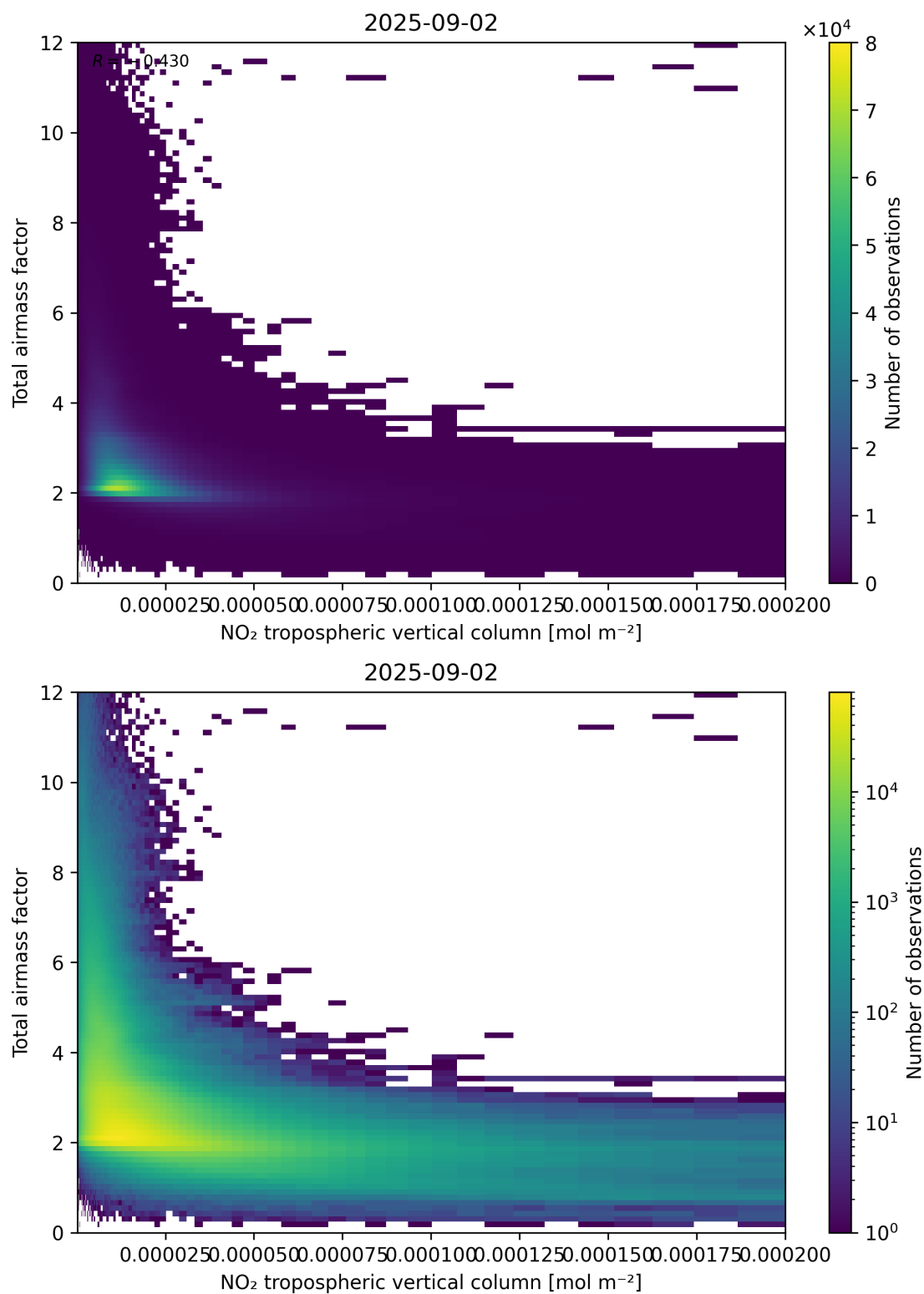
Figure 122: Scatter density plot of “NO 2 tropospheric vertical column” against “Total air mass factor” for 2025-09-01 to 2025-09-03.
