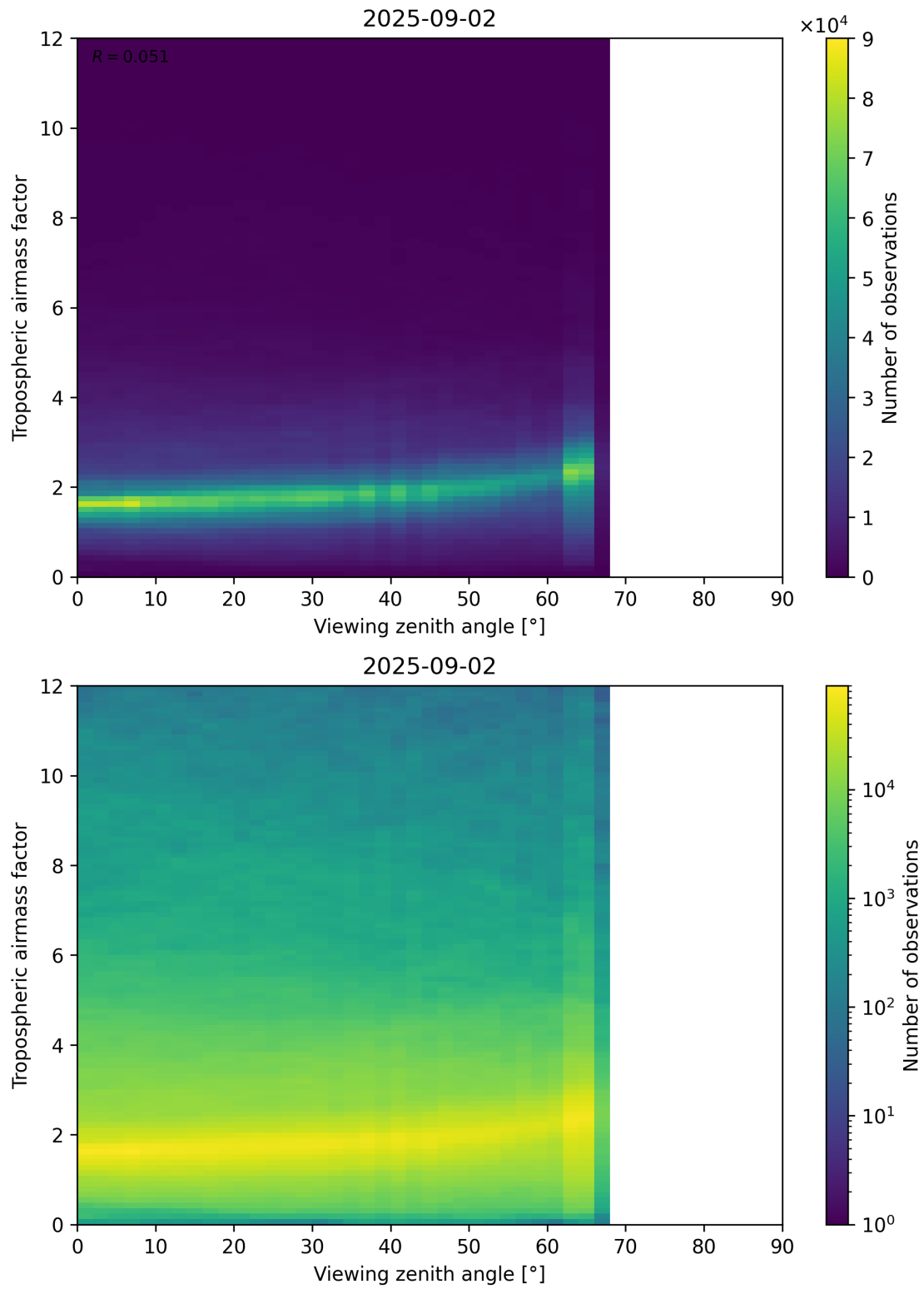
Figure 161: Scatter density plot of “Viewing zenith angle” against “Tropospheric airmass factor” for 2025-09-01 to 2025-09-03.
