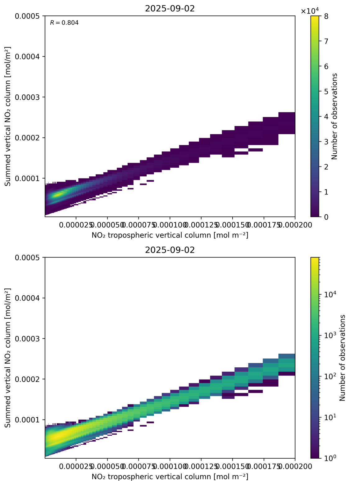
Figure 126: Scatter density plot of “NO 2 tropospheric vertical column” against “Summed vertical NO 2 column” for 2025-09-01 to 2025-09-03.
