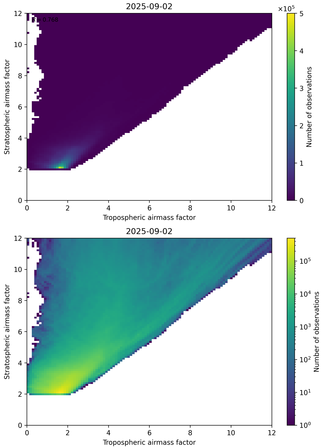
Figure 71: Scatter density plot of “Tropospheric airmass factor” against “Stratospheric airmass factor” for 2025-09-01 to 2025-09-03.
