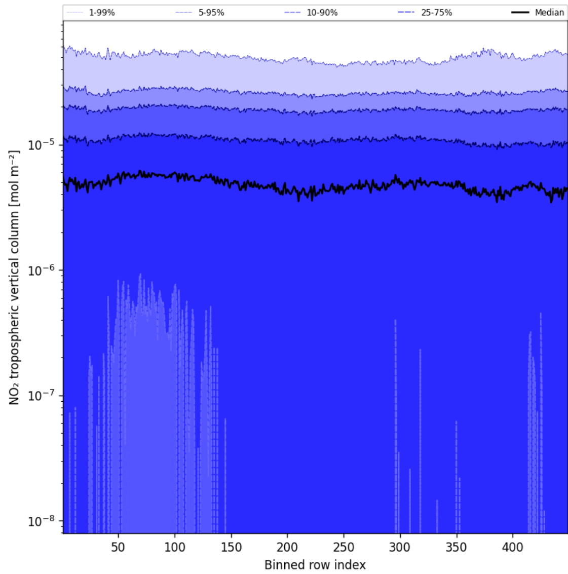
Figure 46: Along track statistics of “NO 2 tropospheric vertical column” for 2025-09-01 to 2025-09-03
