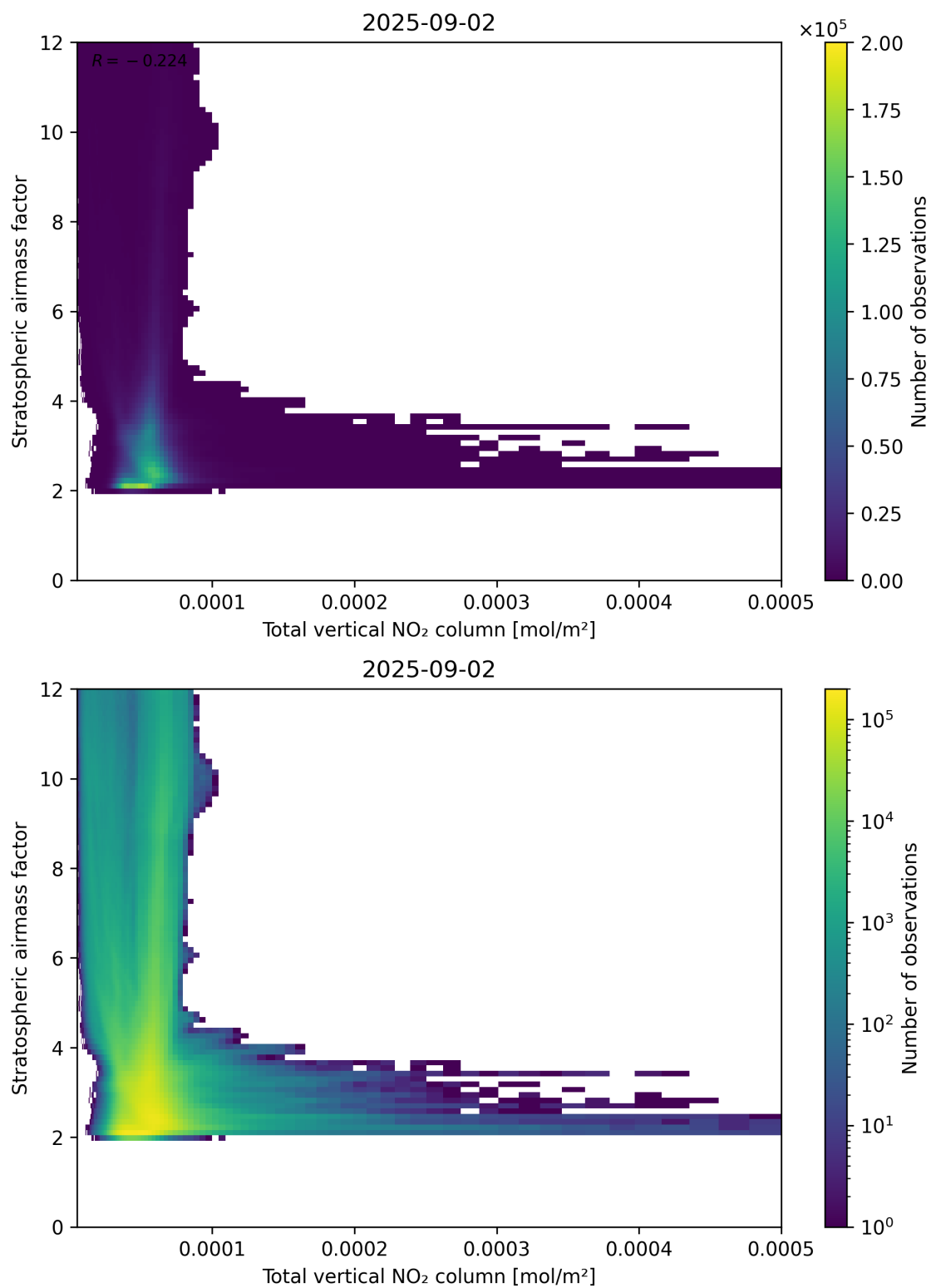
Figure 110: Scatter density plot of “Total vertical NO 2 column” against “Stratospheric airmass factor” for 2025-09-01 to 2025-09-03.
