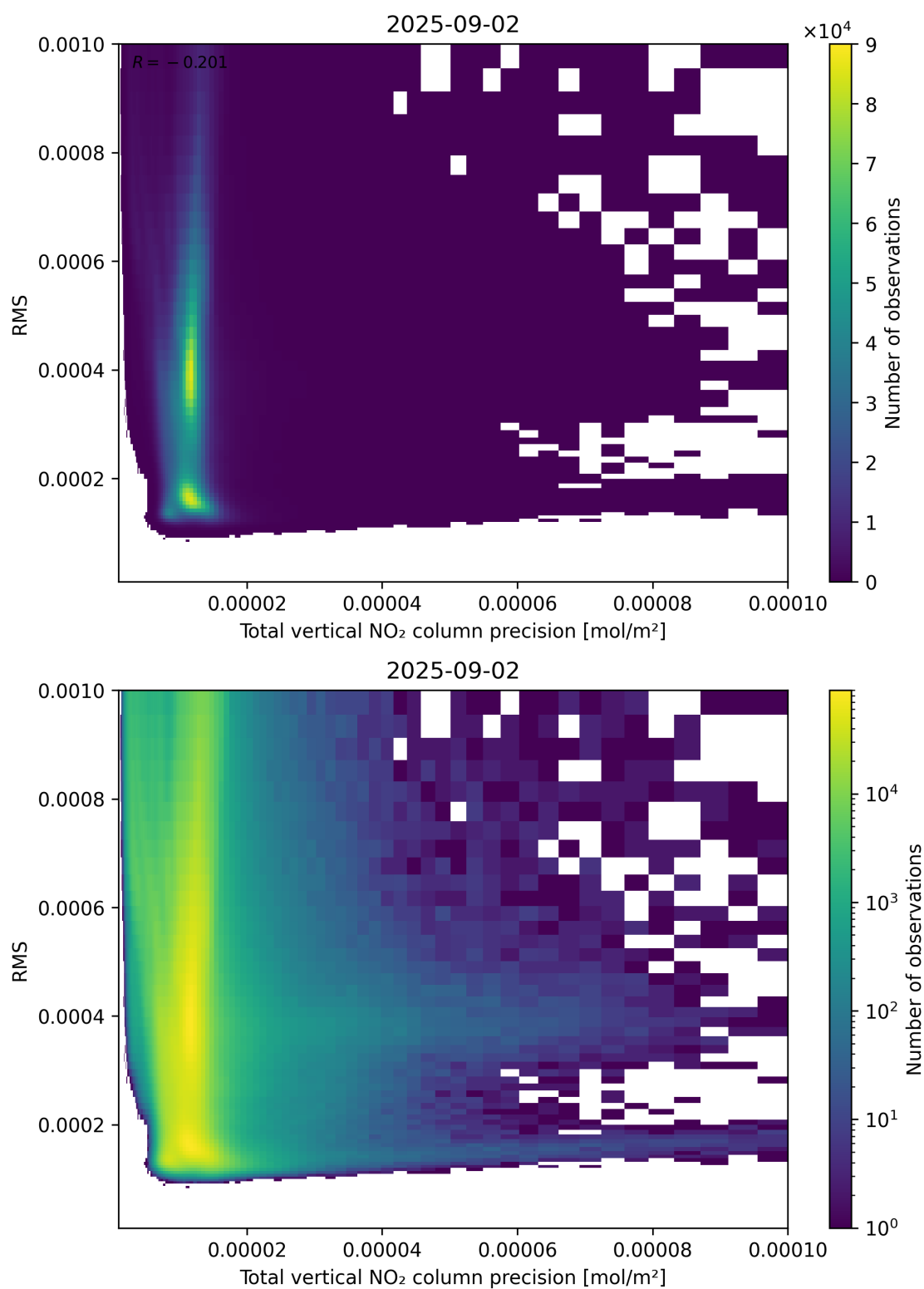
Figure 119: Scatter density plot of “Total vertical NO 2 column precision” against “RMS” for 2025-09-01 to 2025-09-03.
