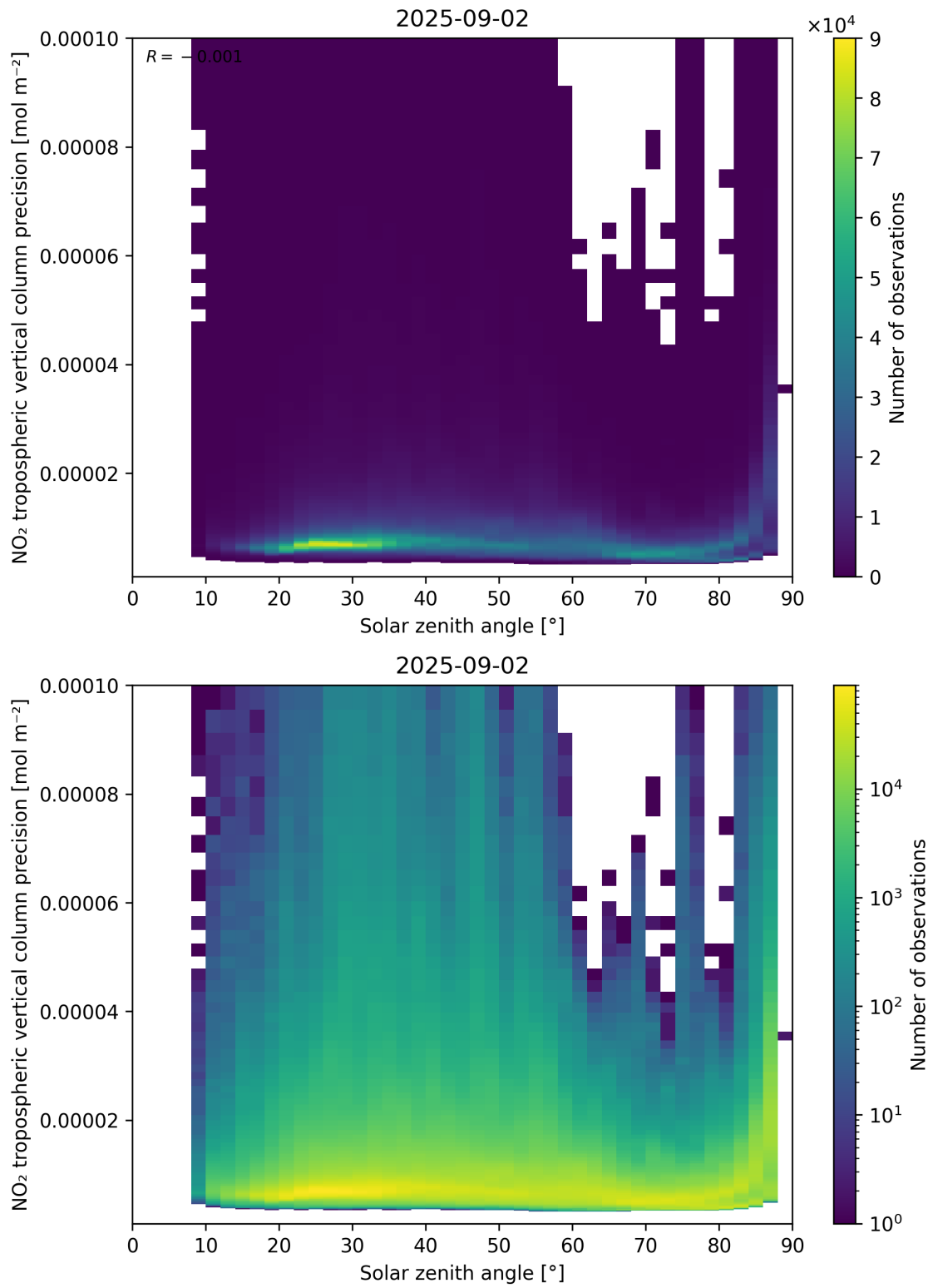
Figure 156: Scatter density plot of “Solar zenith angle” against “NO 2 tropospheric vertical column precision” for 2025-09-01 to 2025-09-03.
