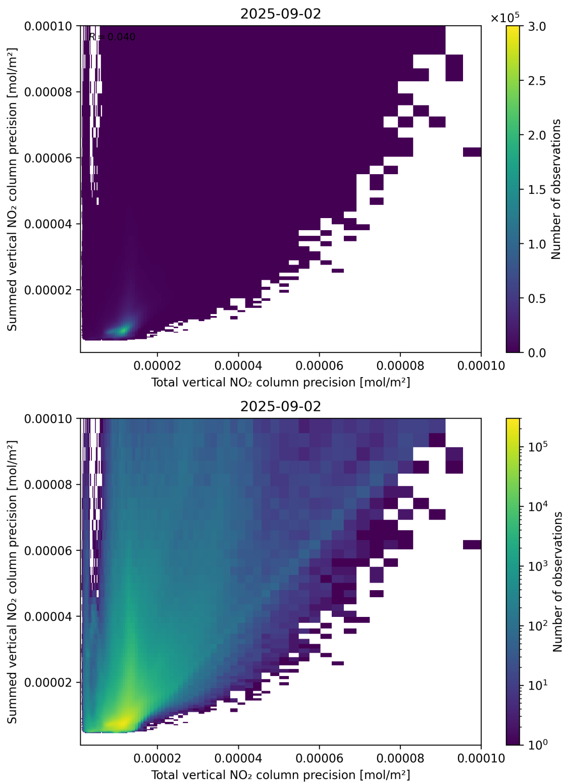
Figure 118: Scatter density plot of “Total vertical NO 2 column precision” against “Summed vertical NO 2 column precision” for 2025-09-01 to 2025-09-03.
