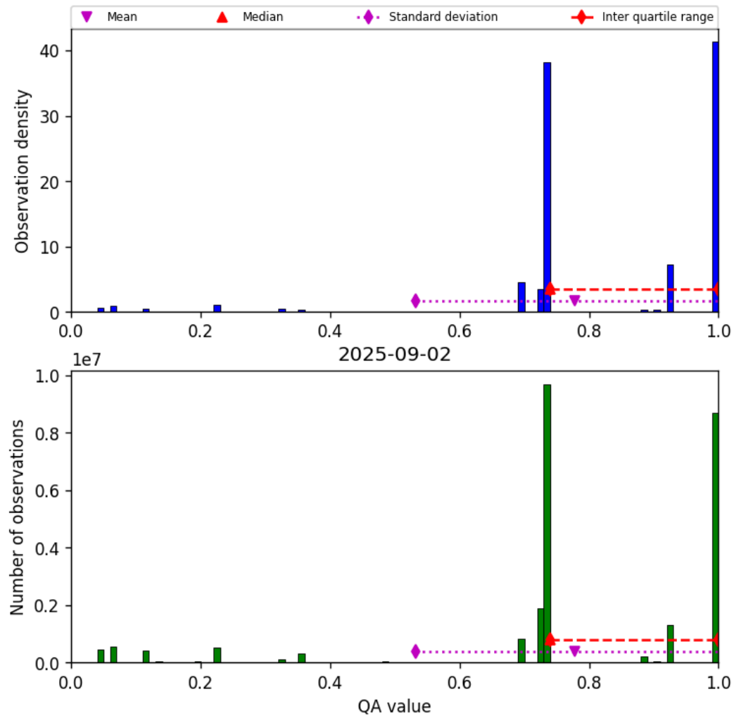
Figure 28: Histogram of “QA value” for 2025-09-01 to 2025-09-03
