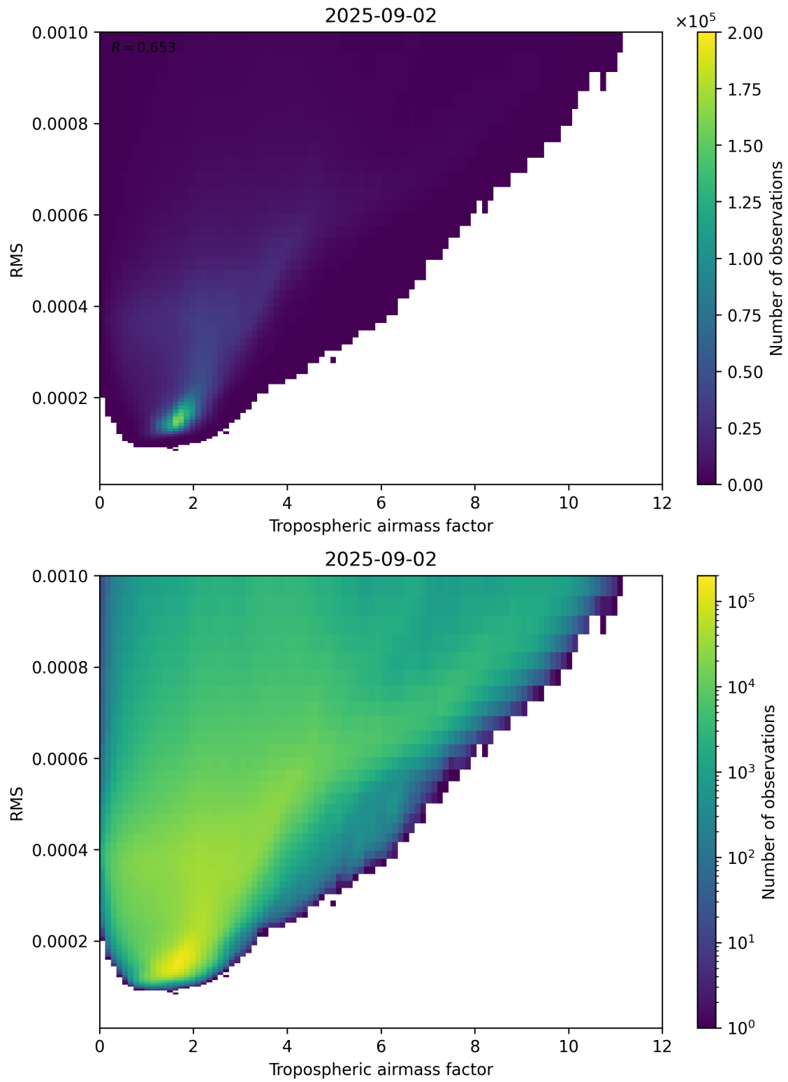
Figure 79: Scatter density plot of “Tropospheric airmass factor” against “RMS” for 2025-09-01 to 2025-09-03.
