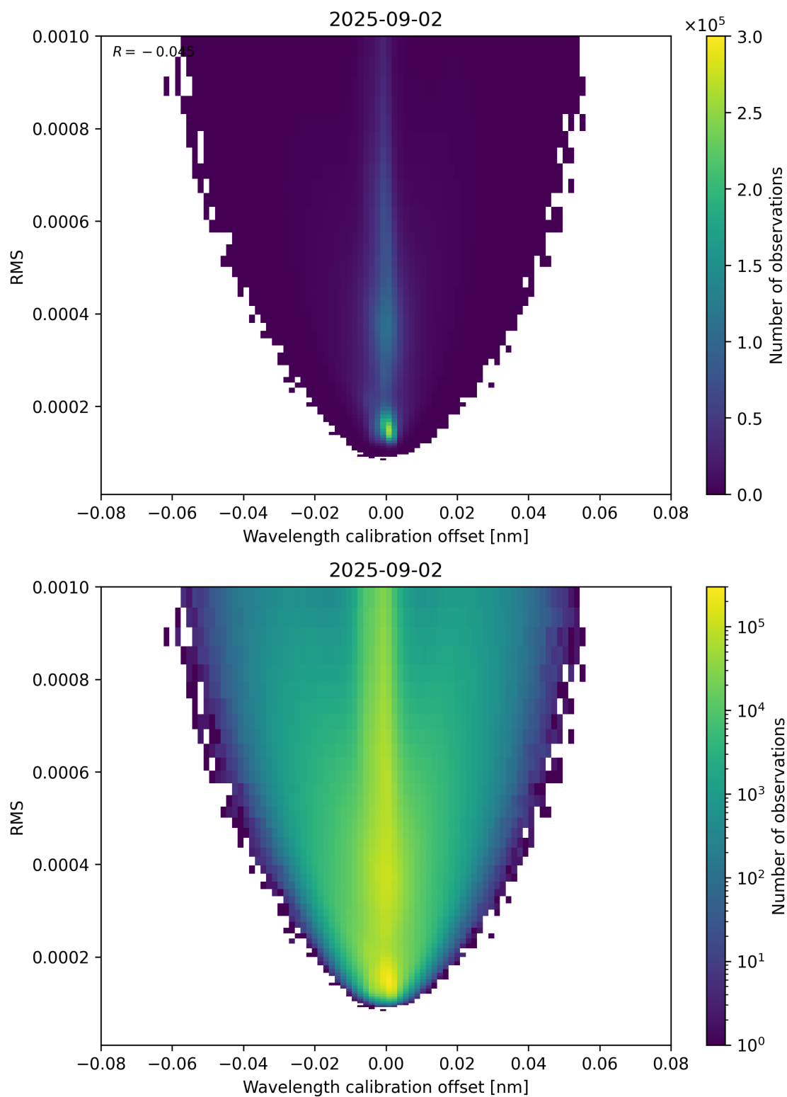
Figure 181: Scatter density plot of “Wavelength calibration offset” against “RMS” for 2025-09-01 to 2025-09-03.
