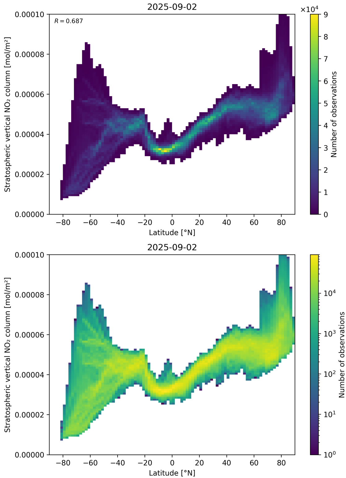
Figure 87: Scatter density plot of “Latitude” against “Stratospheric vertical NO 2 column” for 2025-09-01 to 2025-09-03.
