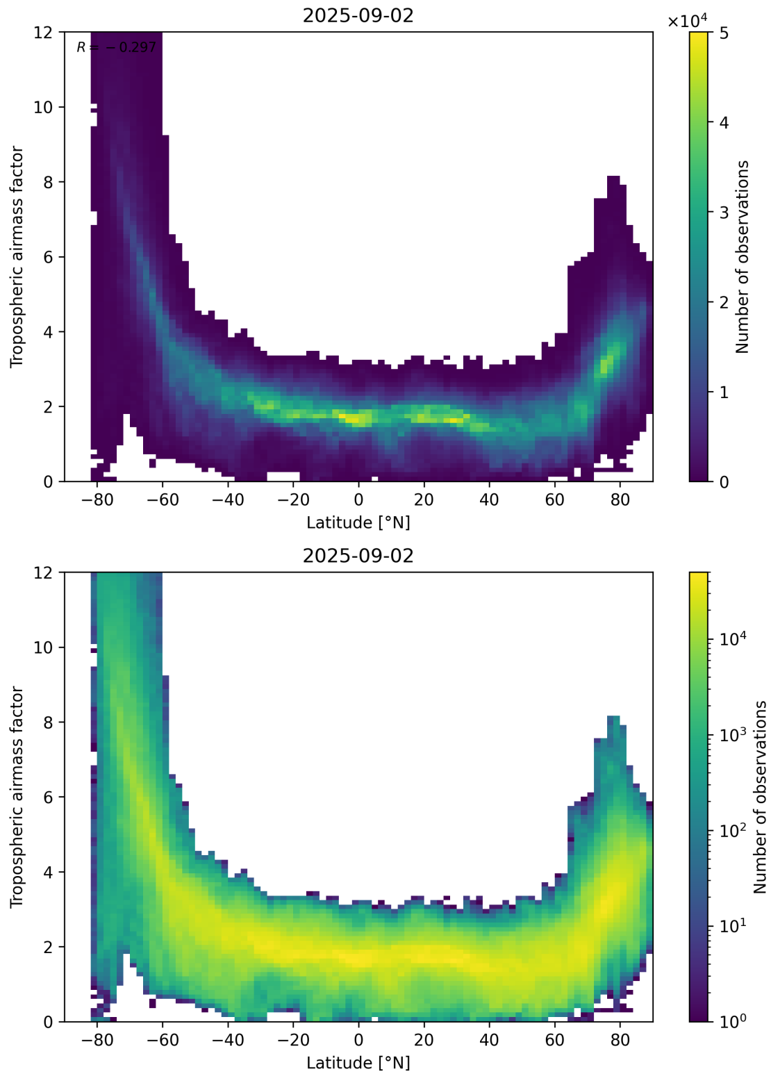
Figure 85: Scatter density plot of “Latitude” against “Tropospheric airmass factor” for 2025-09-01 to 2025-09-03.
