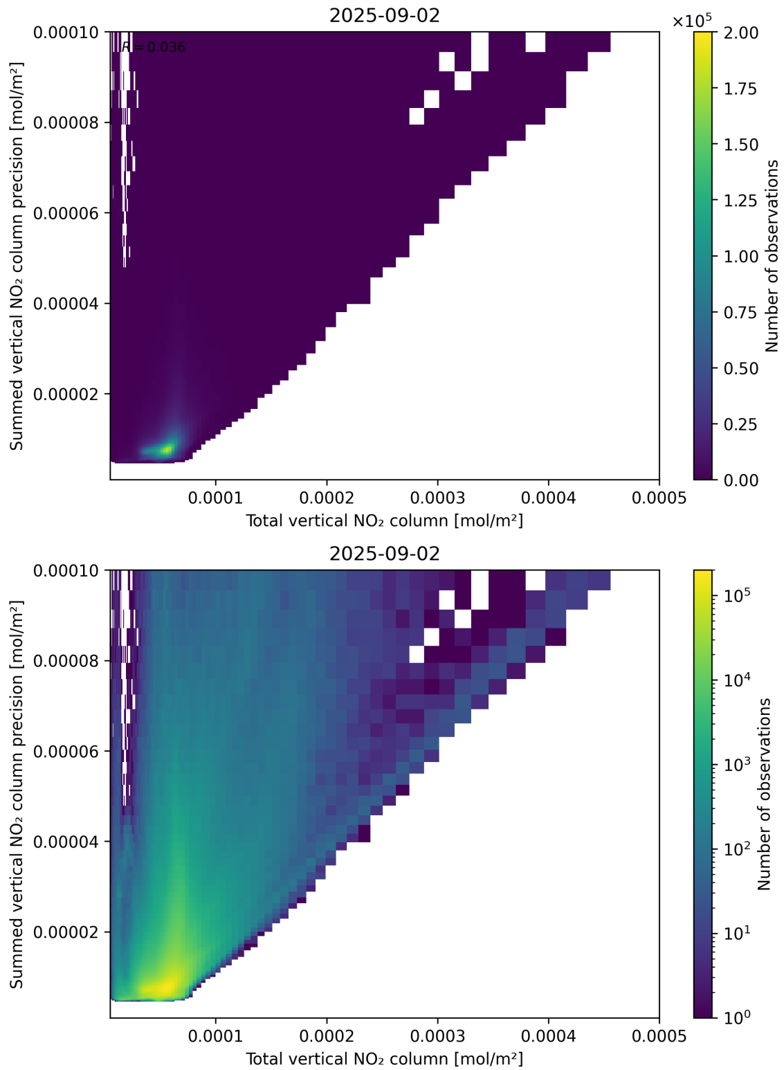
Figure 113: Scatter density plot of “Total vertical NO 2 column” against “Summed vertical NO 2 column precision” for 2025-09-01 to 2025-09-03.
