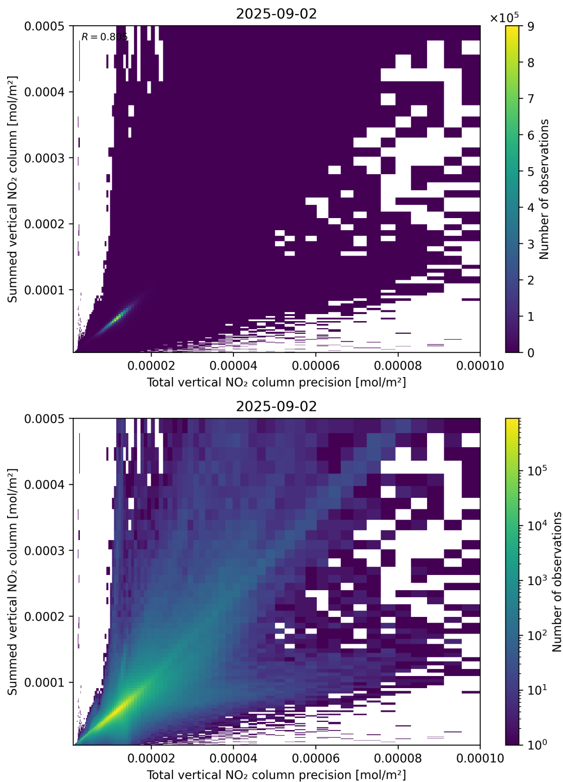
Figure 117: Scatter density plot of “Total vertical NO 2 column precision” against “Summed vertical NO 2 column” for 2025-09-01 to 2025-09-03.
