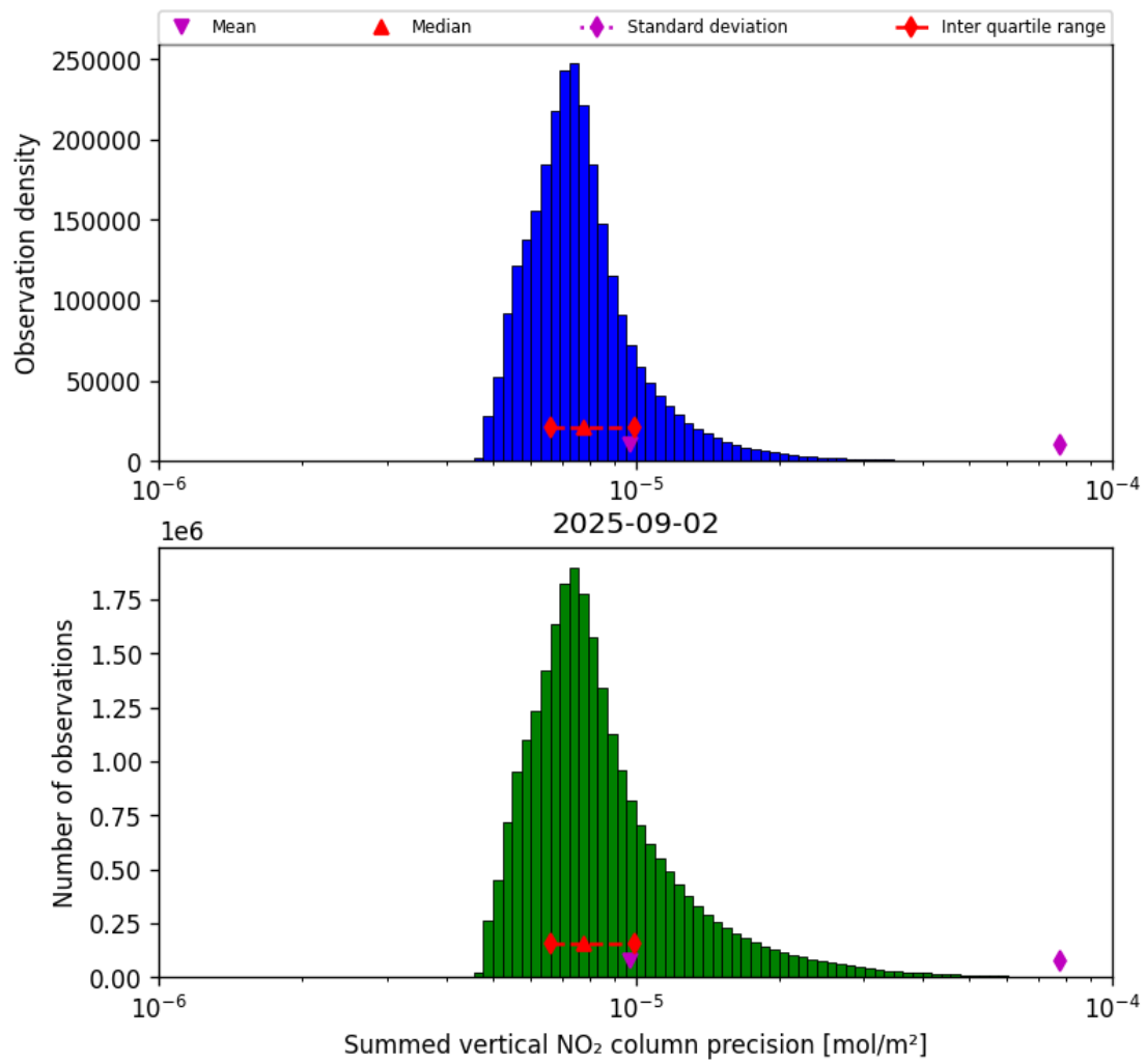
Figure 41: Histogram of “Summed vertical NO 2 column precision” for 2025-09-01 to 2025-09-03
