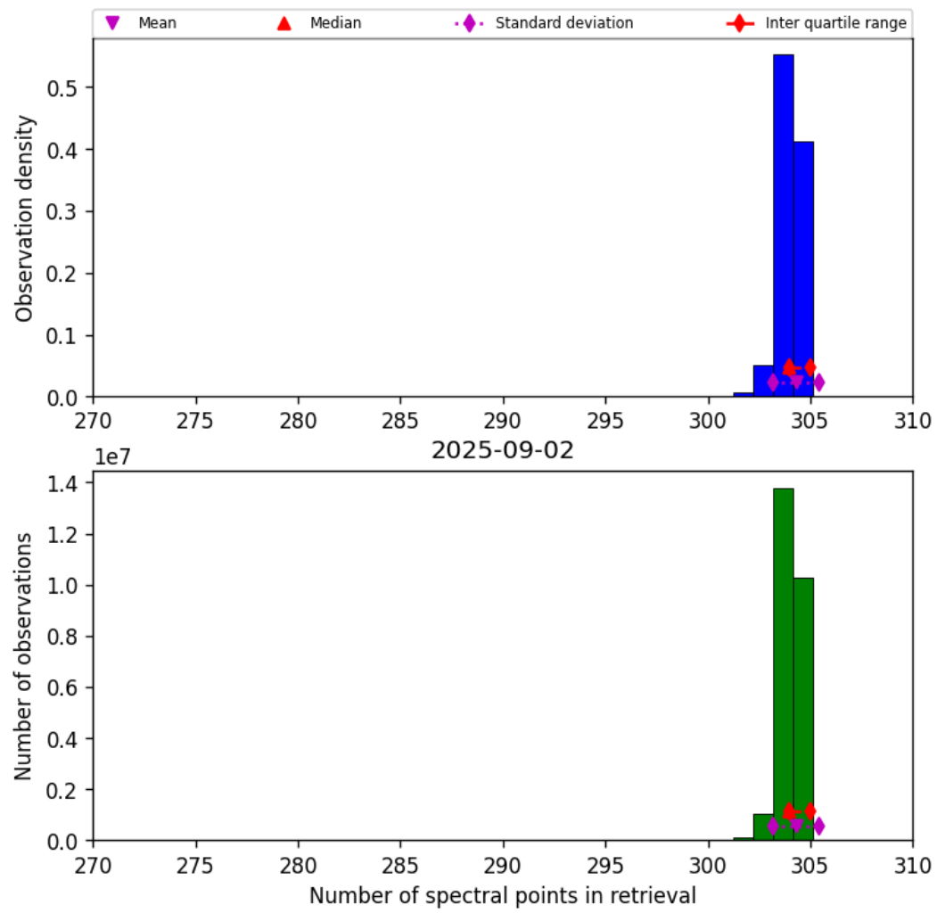
Figure 33: Histogram of “Number of spectral points in retrieval” for 2025-09-01 to 2025-09-03
