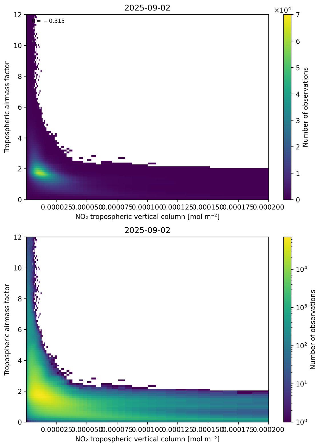
Figure 123: Scatter density plot of “NO 2 tropospheric vertical column” against “Tropospheric air mass factor” for 2025-09-01 to 2025-09-03.
