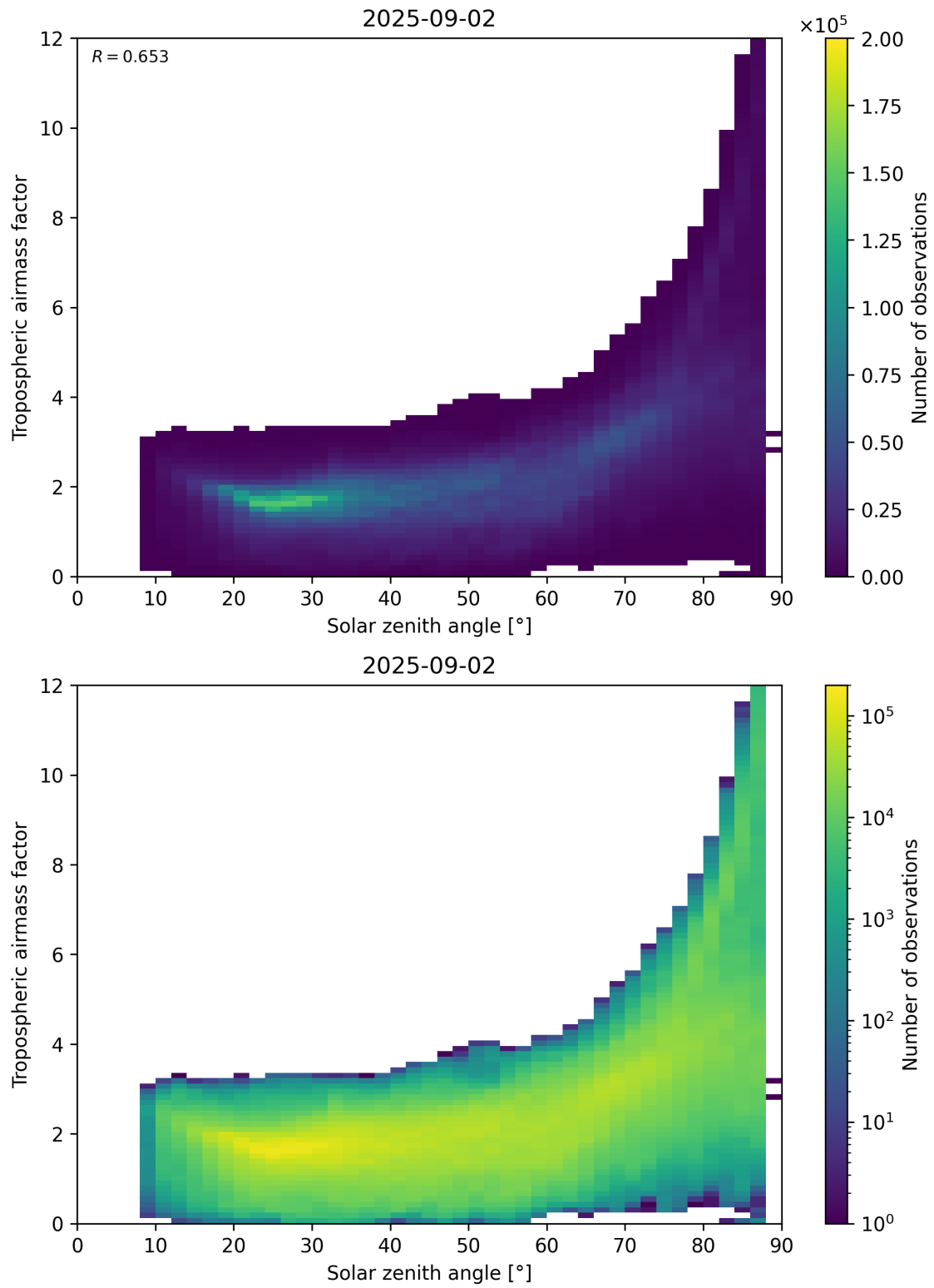
Figure 147: Scatter density plot of “Solar zenith angle” against “Tropospheric airmass factor” for 2025-09-01 to 2025-09-03.
