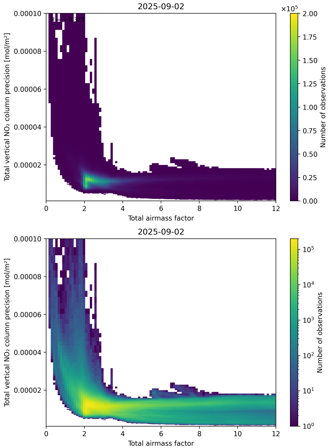
Figure 68: Scatter density plot of “Total airmass factor” against “Total vertical NO 2 column precision” for 2025-09-01 to 2025-09-03.
