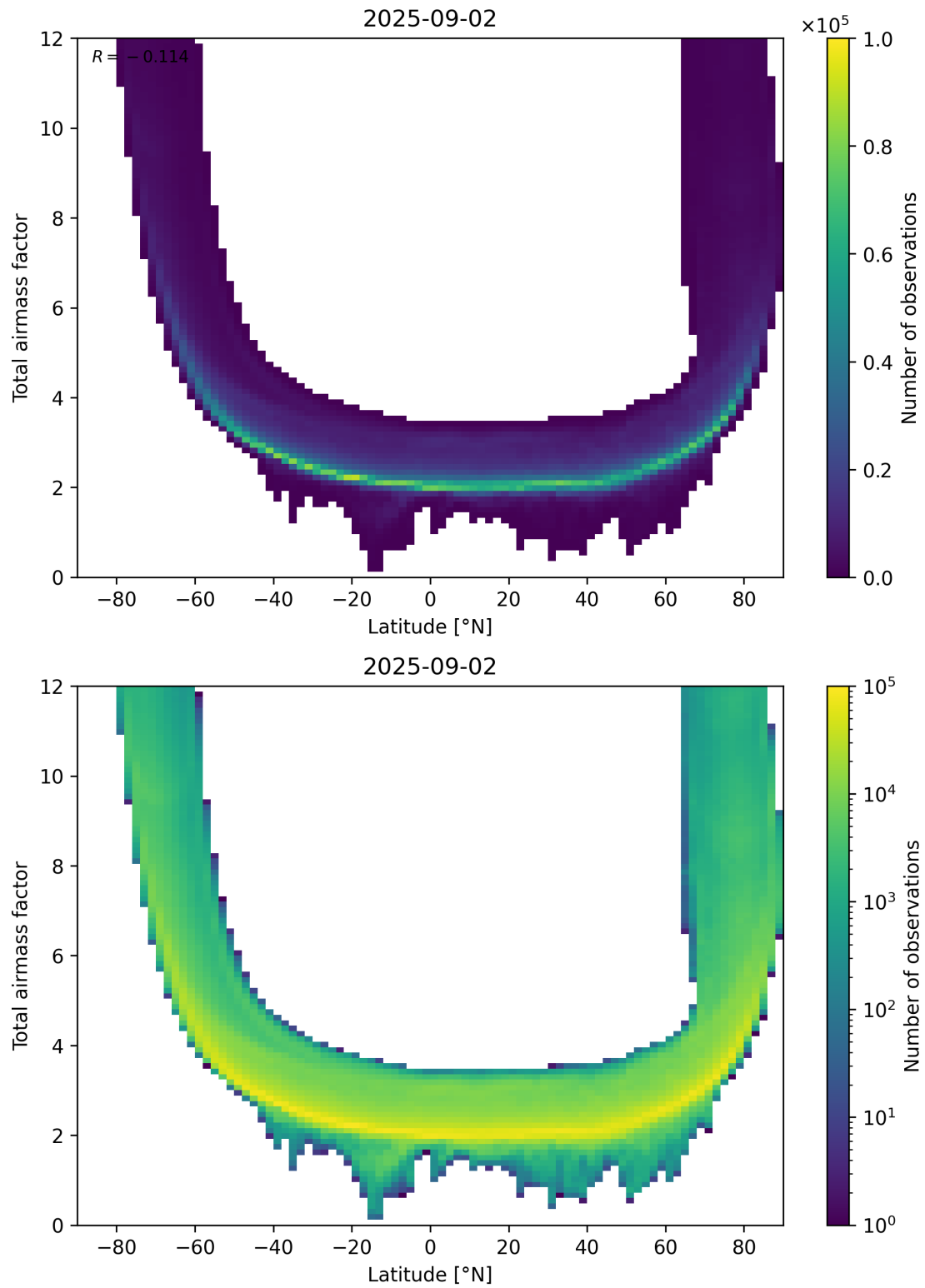
Figure 84: Scatter density plot of “Latitude” against “Total airmass factor” for 2025-09-01 to 2025-09-03.
