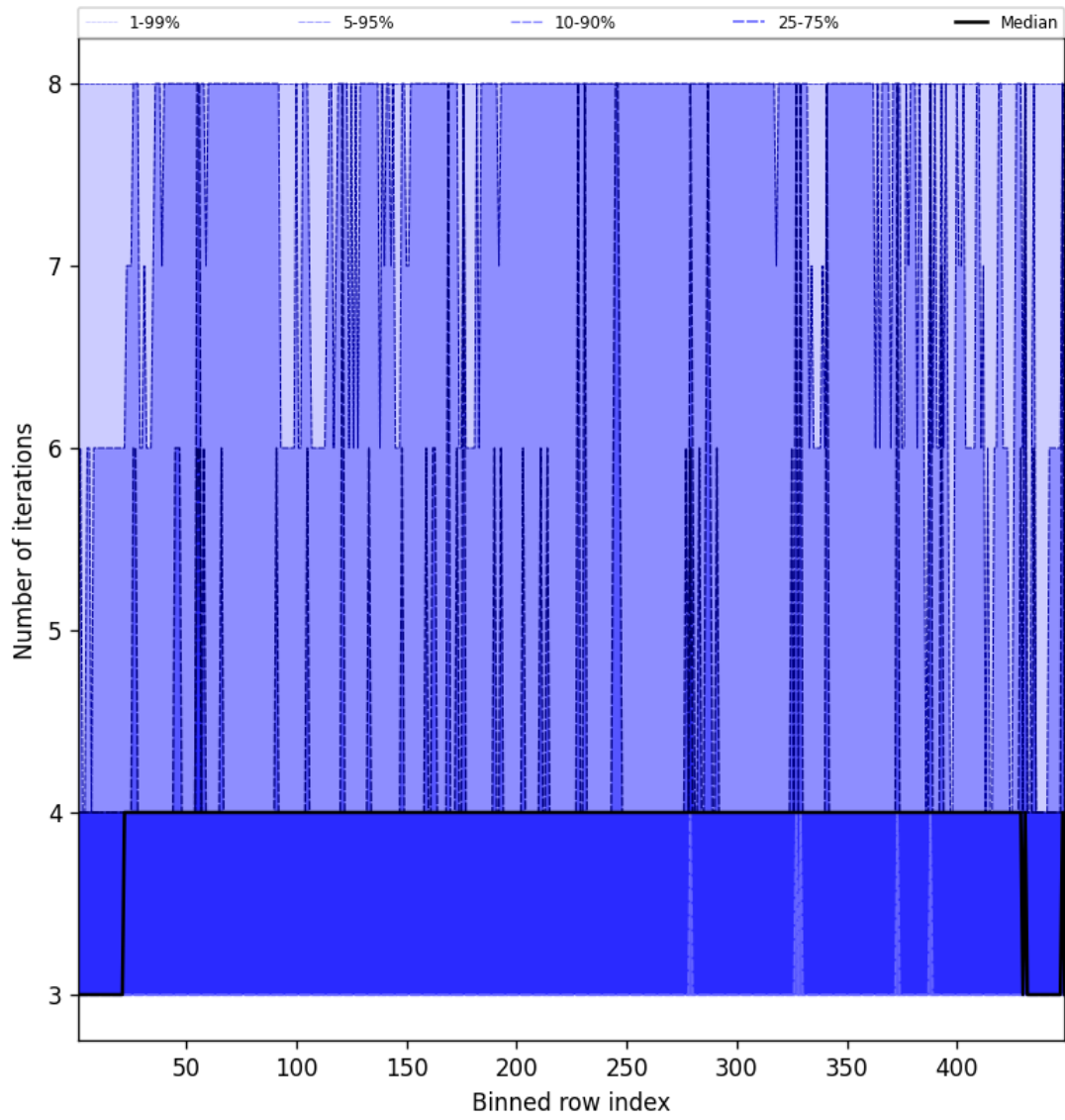
Figure 51: Along track statistics of “Number of iterations” for 2025-09-01 to 2025-09-03
