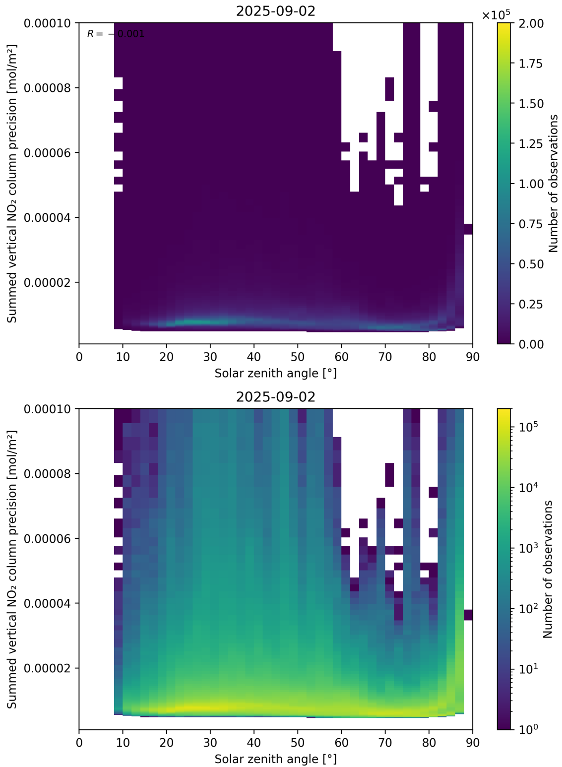
Figure 152: Scatter density plot of “Solar zenith angle” against “Summed vertical NO 2 column precision” for 2025-09-01 to 2025-09-03.
