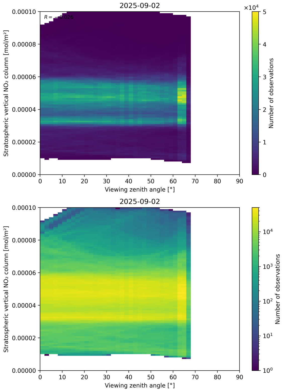
Figure 164: Scatter density plot of “Viewing zenith angle” against “Stratospheric vertical NO 2 column” for 2025-09-01 to 2025-09-03.
