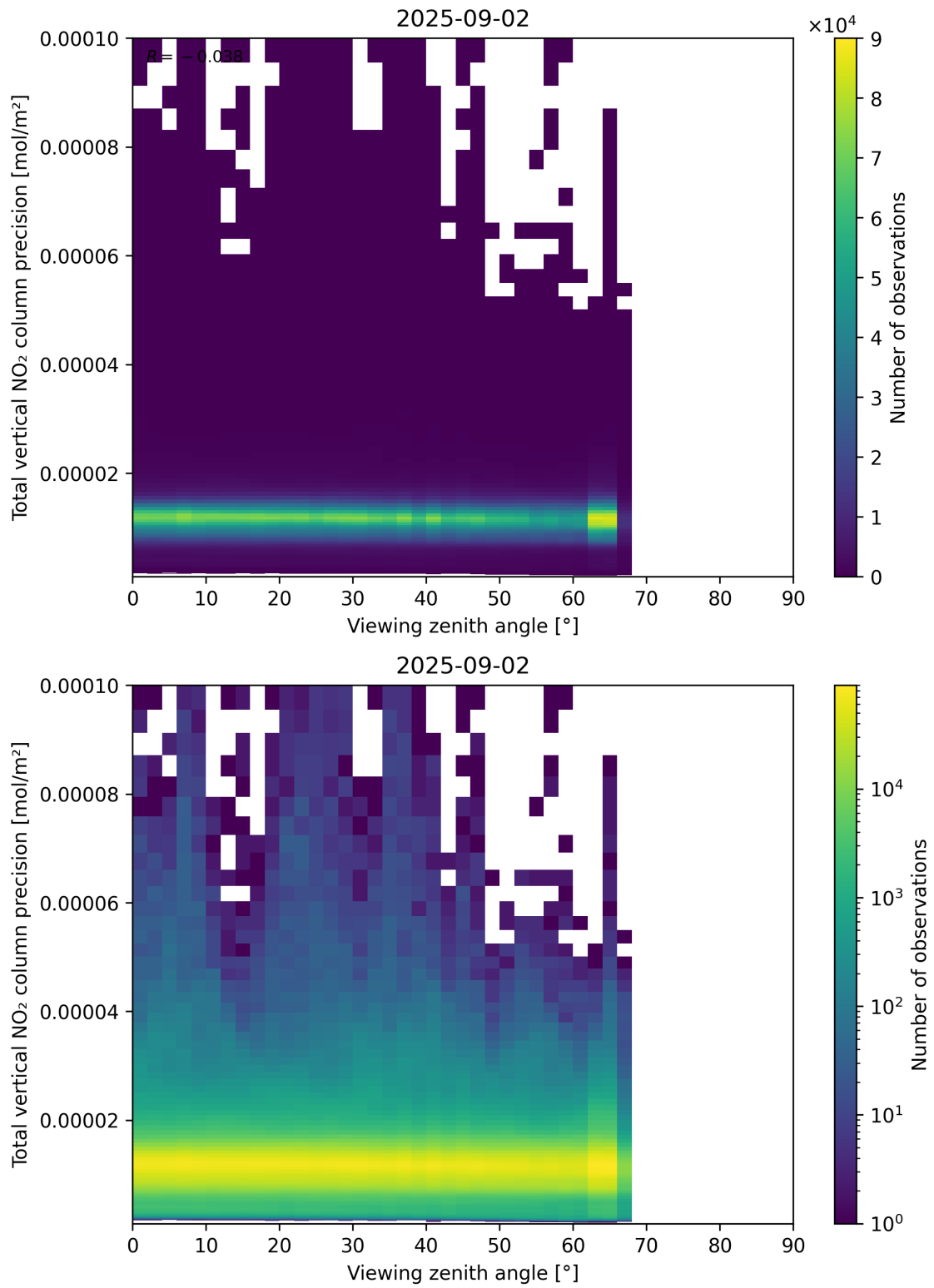
Figure 168: Scatter density plot of “Viewing zenith angle” against “Total vertical NO 2 column precision” for 2025-09-01 to 2025-09-03.
