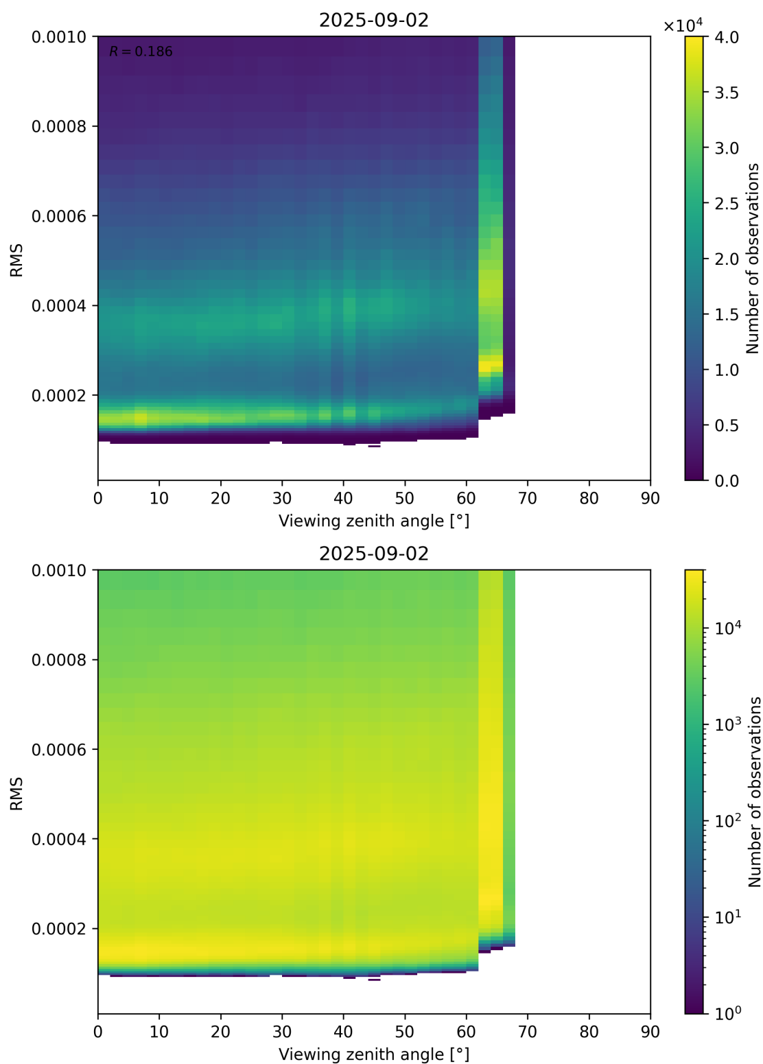
Figure 171: Scatter density plot of “Viewing zenith angle” against “RMS” for 2025-09-01 to 2025-09-03.
