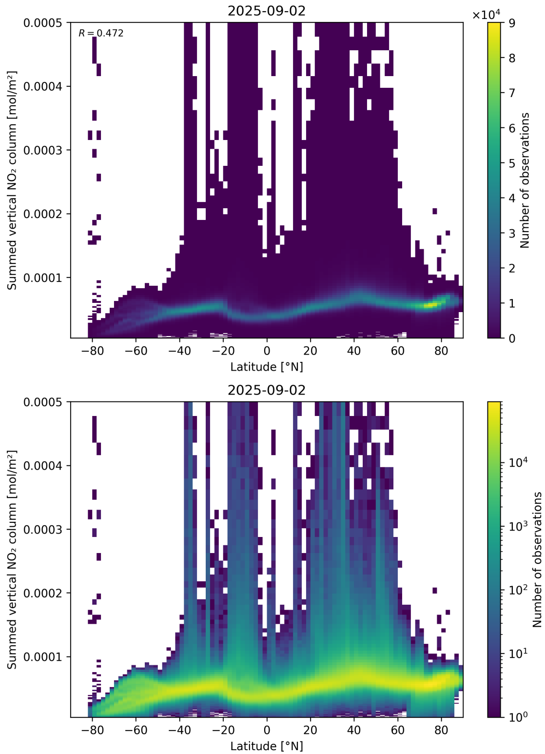
Figure 88: Scatter density plot of “Latitude” against “Summed vertical NO 2 column” for 2025-09-01 to 2025-09-03.
