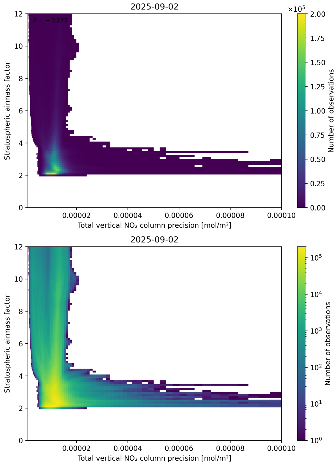
Figure 115: Scatter density plot of “Total vertical NO 2 column precision” against “Stratospheric air mass factor” for 2025-09-01 to 2025-09-03.
