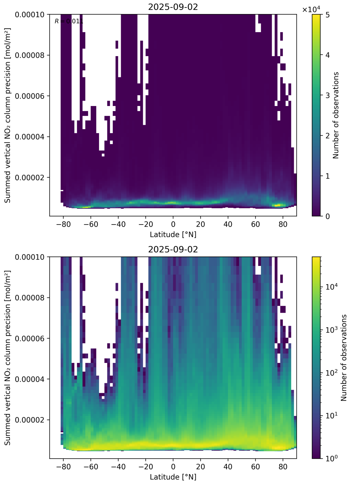
Figure 89: Scatter density plot of “Latitude” against “Summed vertical NO 2 column precision” for 2025-09-01 to 2025-09-03.
