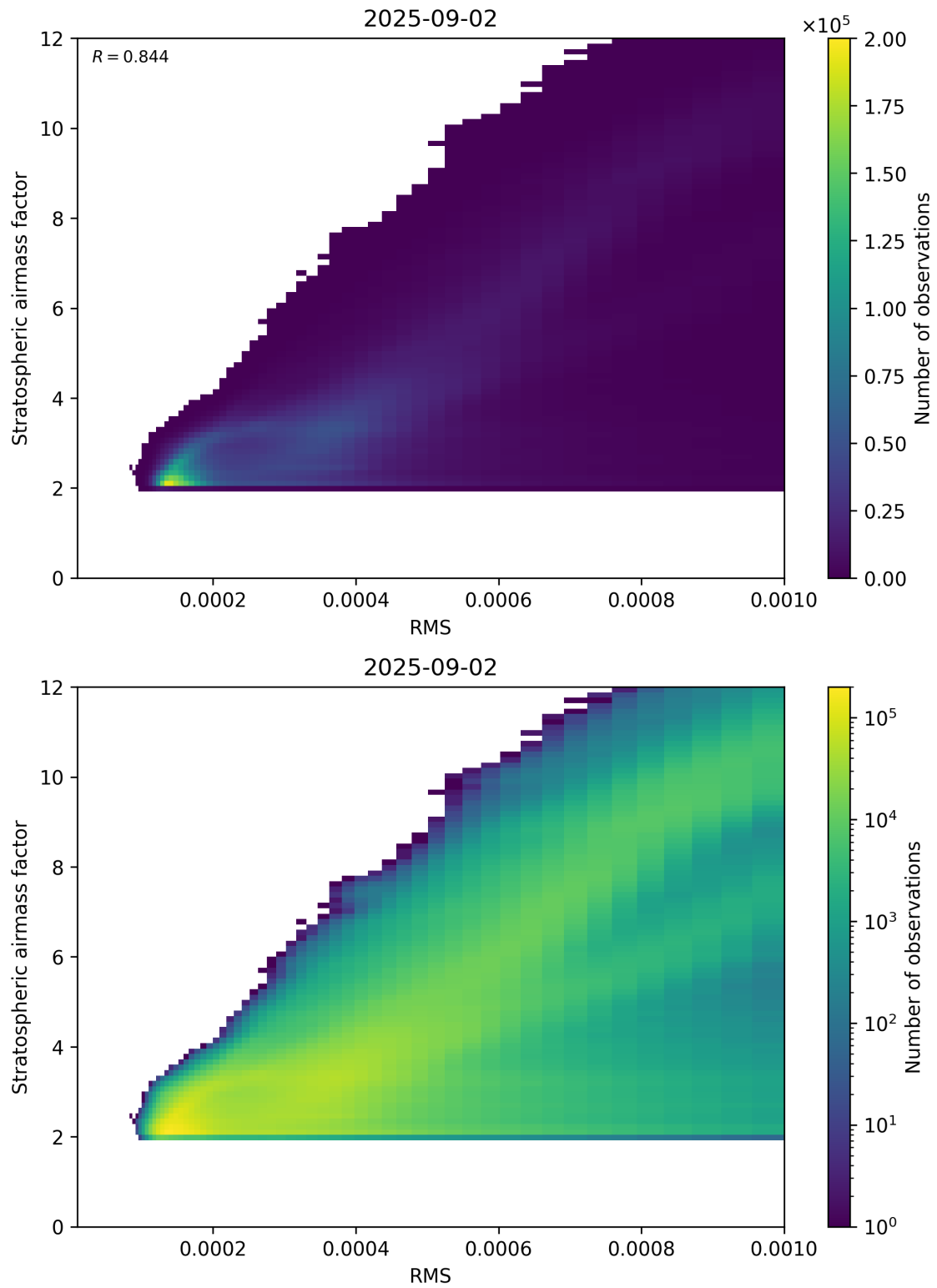
Figure 144: Scatter density plot of “RMS” against “Stratospheric airmass factor” for 2025-09-01 to 2025-09-03.
