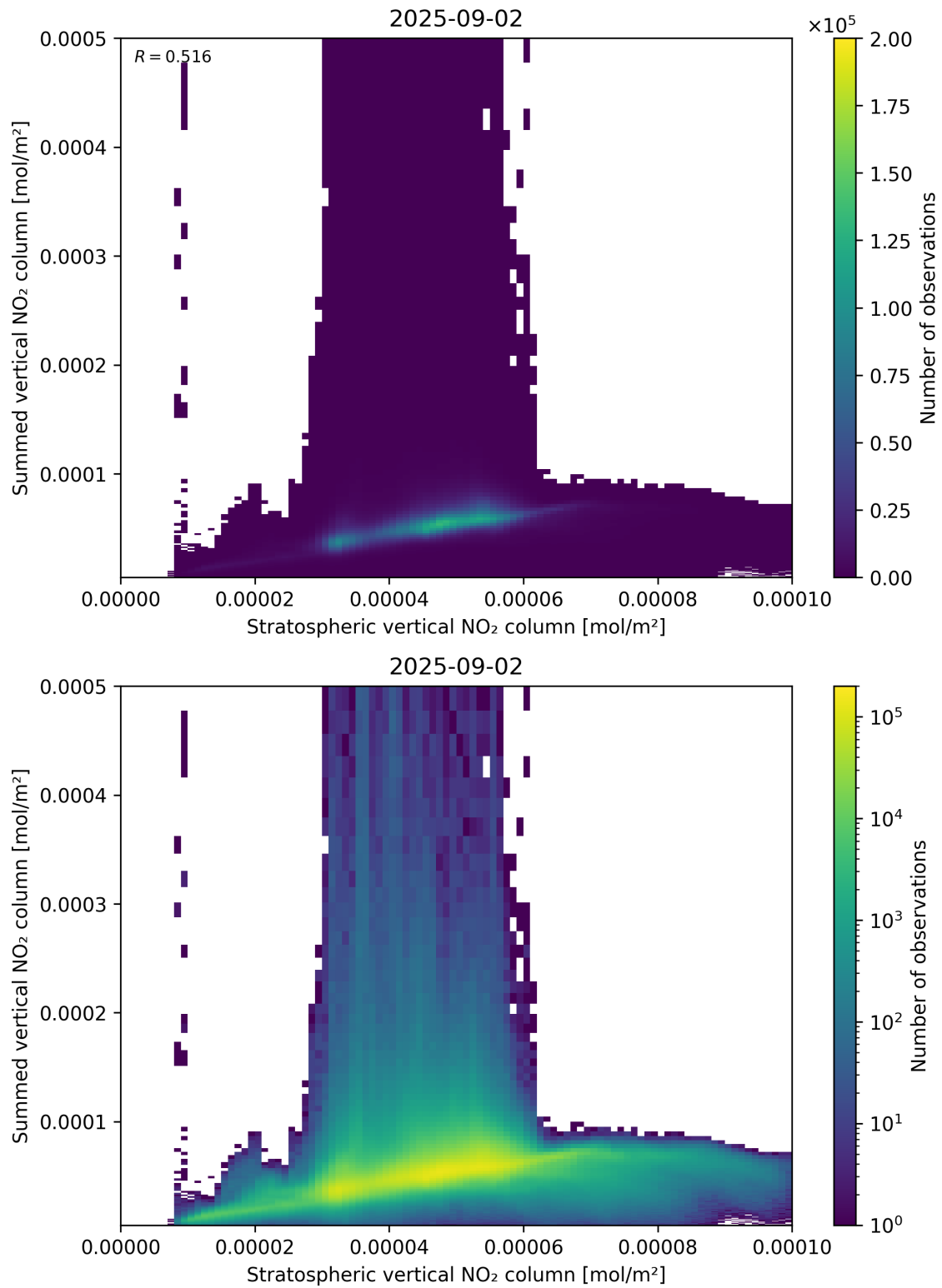
Figure 98: Scatter density plot of “Stratospheric vertical NO 2 column” against “Summed vertical NO 2 column” for 2025-09-01 to 2025-09-03.
