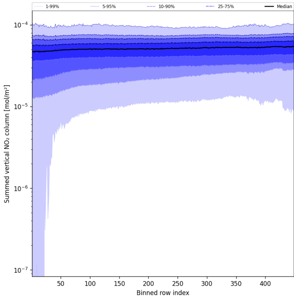
Figure 57: Along track statistics of “Summed vertical NO 2 column” for 2025-09-01 to 2025-09-03
