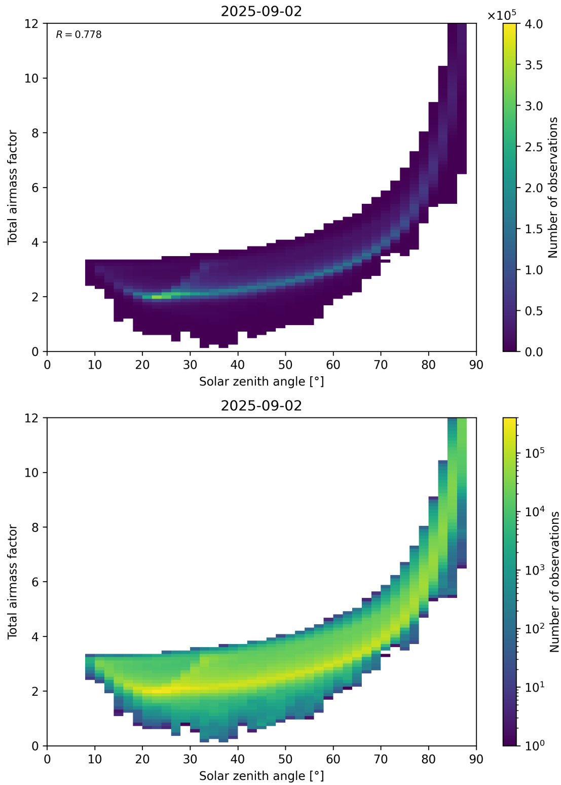
Figure 146: Scatter density plot of “Solar zenith angle” against “Total airmass factor” for 2025-09-01 to 2025-09-03.
