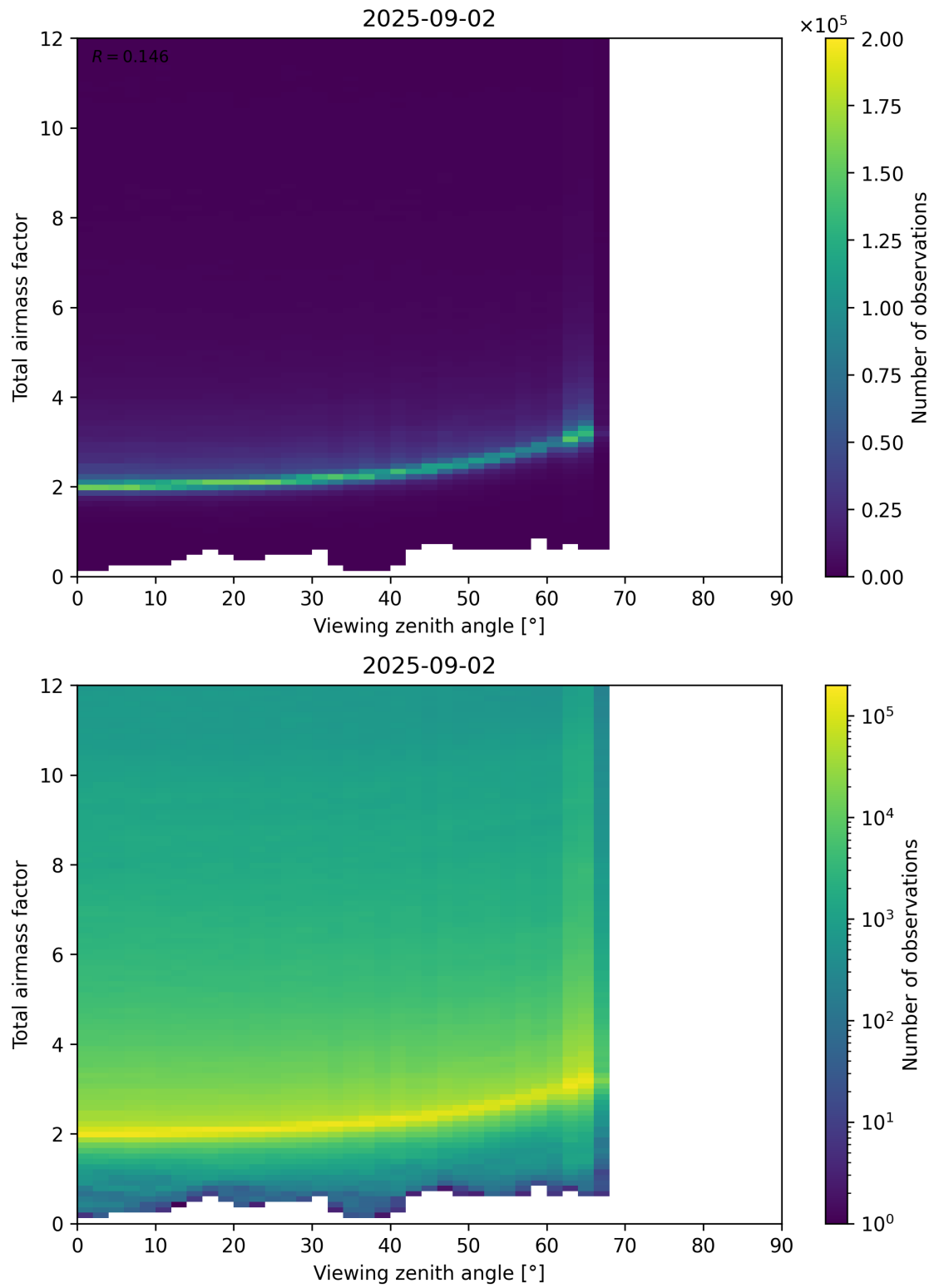
Figure 160: Scatter density plot of “Viewing zenith angle” against “Total airmass factor” for 2025-09-01 to 2025-09-03.
