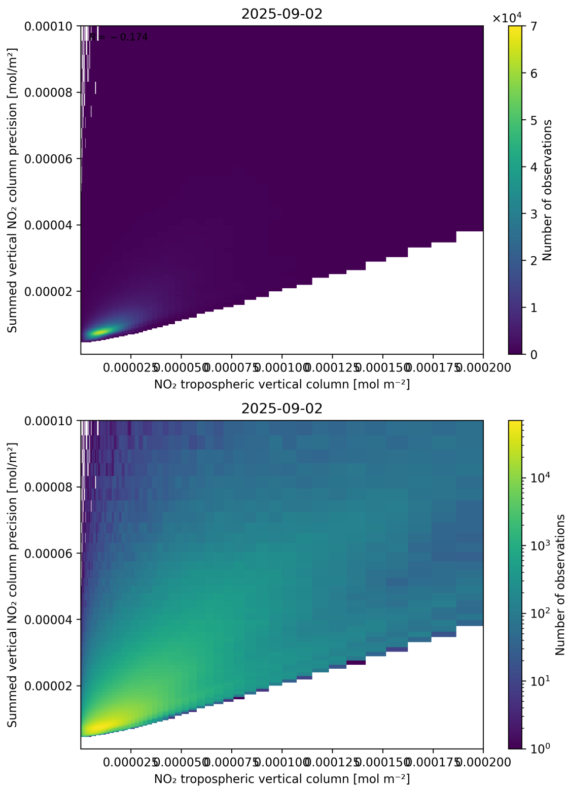
Figure 127: Scatter density plot of “NO 2 tropospheric vertical column” against “Summed vertical NO 2 column precision” for 2025-09-01 to 2025-09-03.
