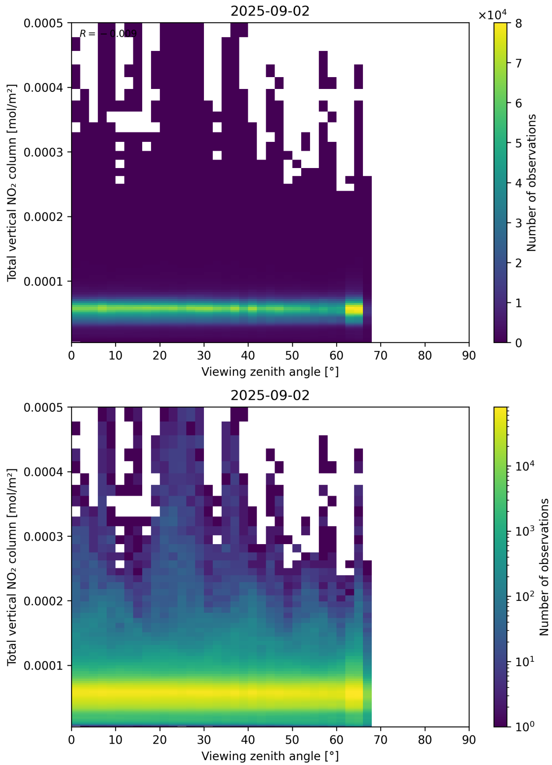
Figure 167: Scatter density plot of “Viewing zenith angle” against “Total vertical NO 2 column” for 2025-09-01 to 2025-09-03.
