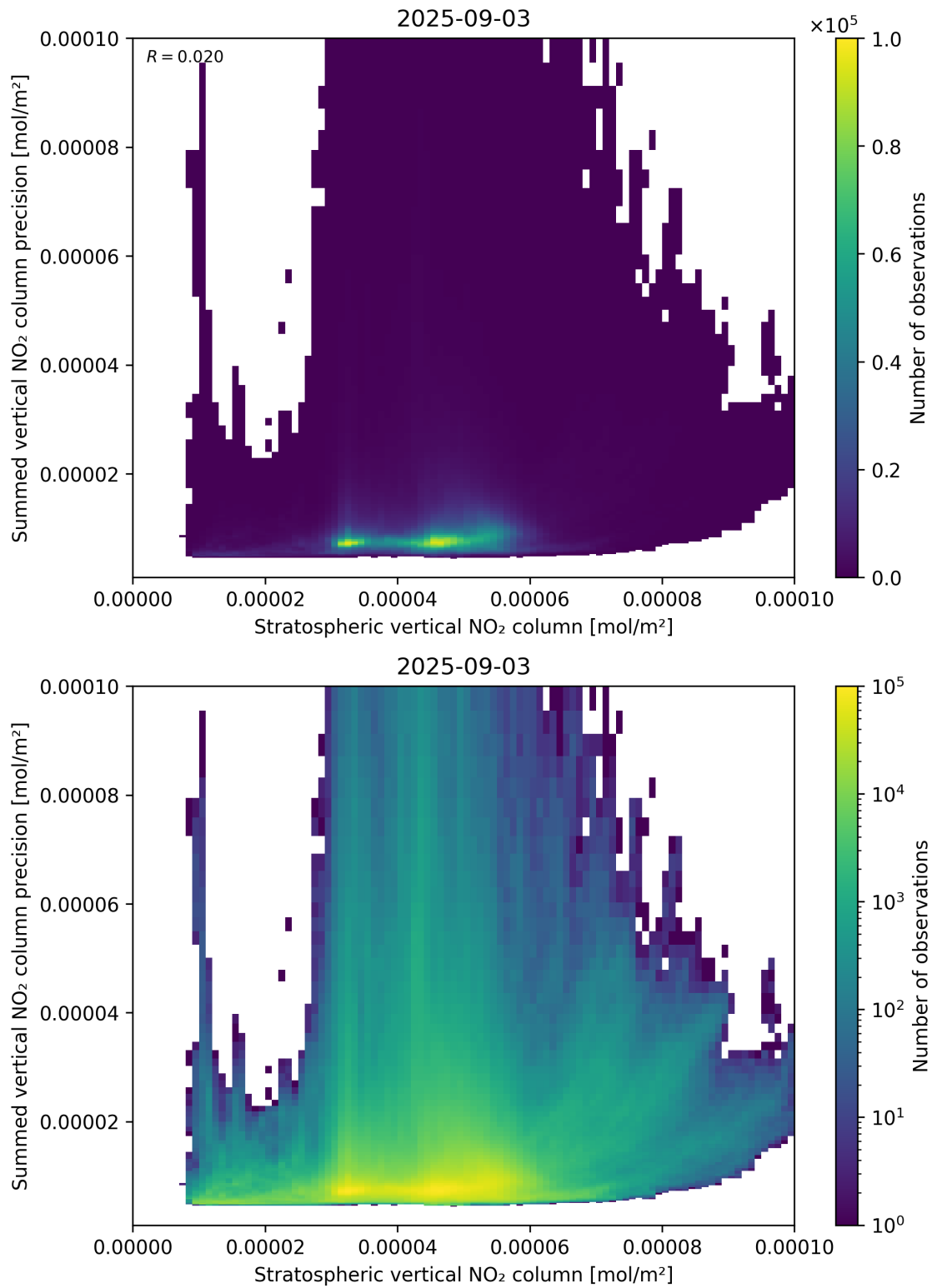
Figure 99: Scatter density plot of “Stratospheric vertical NO 2 column” against “Summed vertical NO 2 column precision” for 2025-09-02 to 2025-09-04.
