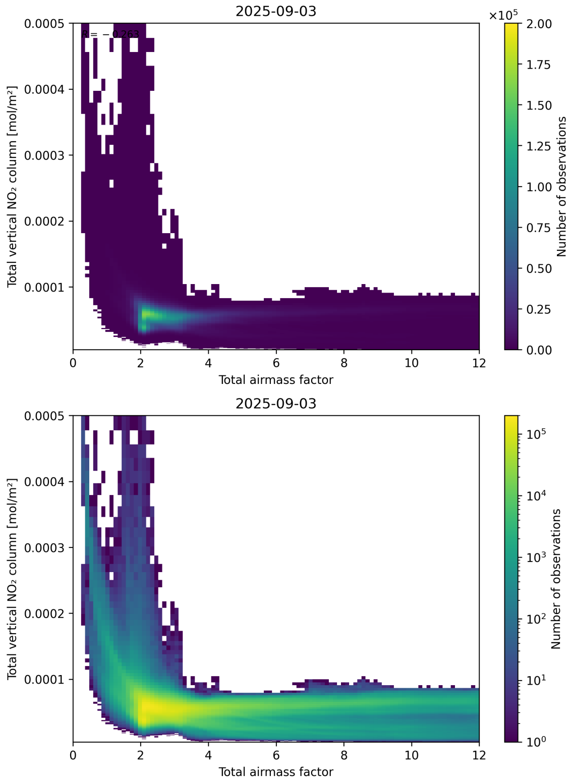
Figure 67: Scatter density plot of “Total airmass factor” against “Total vertical NO 2 column” for 2025-09-02 to 2025-09-04.
