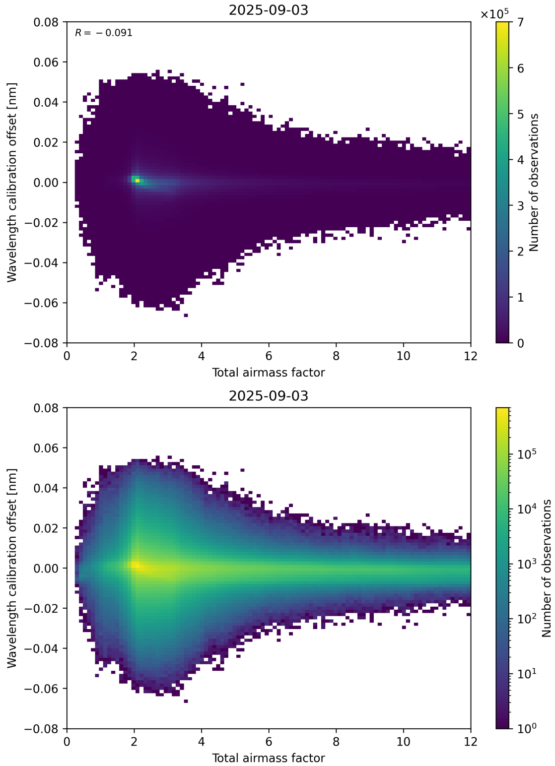
Figure 70: Scatter density plot of “Total airmass factor” against “Wavelength calibration offset” for 2025-09-02 to 2025-09-04.
