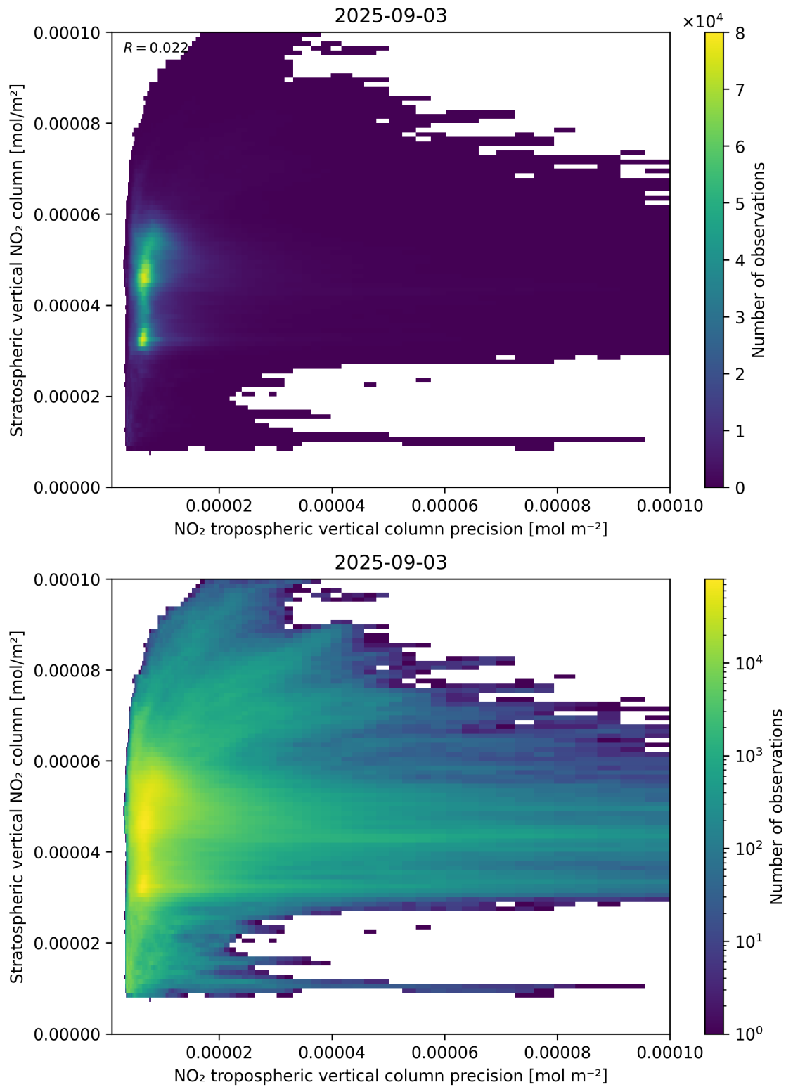
Figure 135: Scatter density plot of “NO 2 tropospheric vertical column precision” against “Stratospheric vertical NO 2 column” for 2025-09-02 to 2025-09-04.
