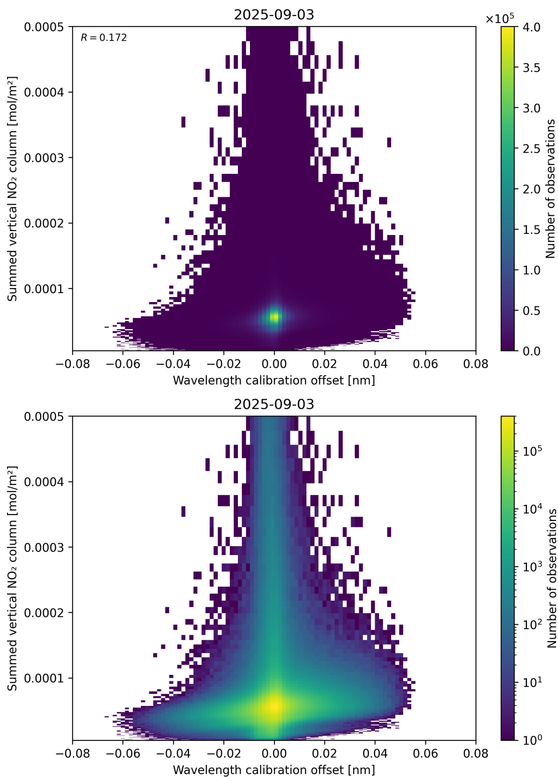
Figure 177: Scatter density plot of “Wavelength calibration offset” against “Summed vertical NO 2 column” for 2025-09-02 to 2025-09-04.
