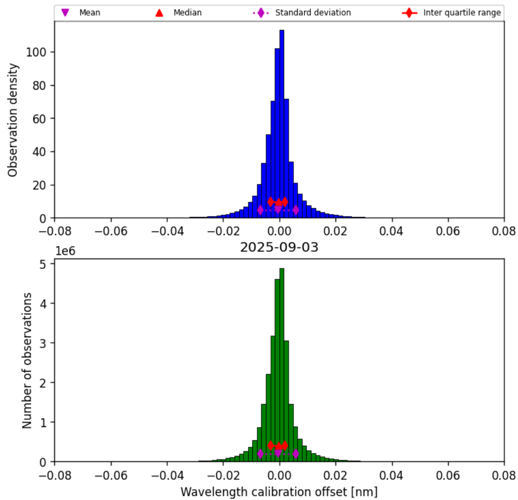
Figure 35: Histogram of “Wavelength calibration offset” for 2025-09-02 to 2025-09-04
