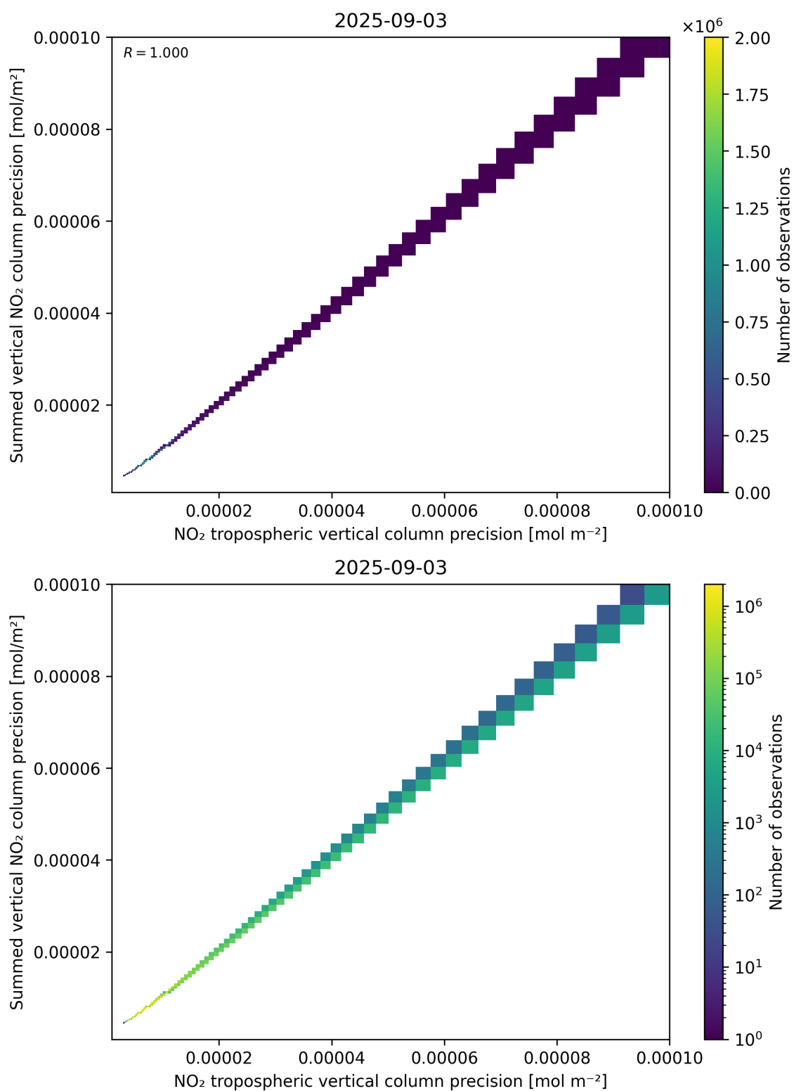
Figure 137: Scatter density plot of “NO 2 tropospheric vertical column precision” against “Summed vertical NO 2 column precision” for 2025-09-02 to 2025-09-04.
