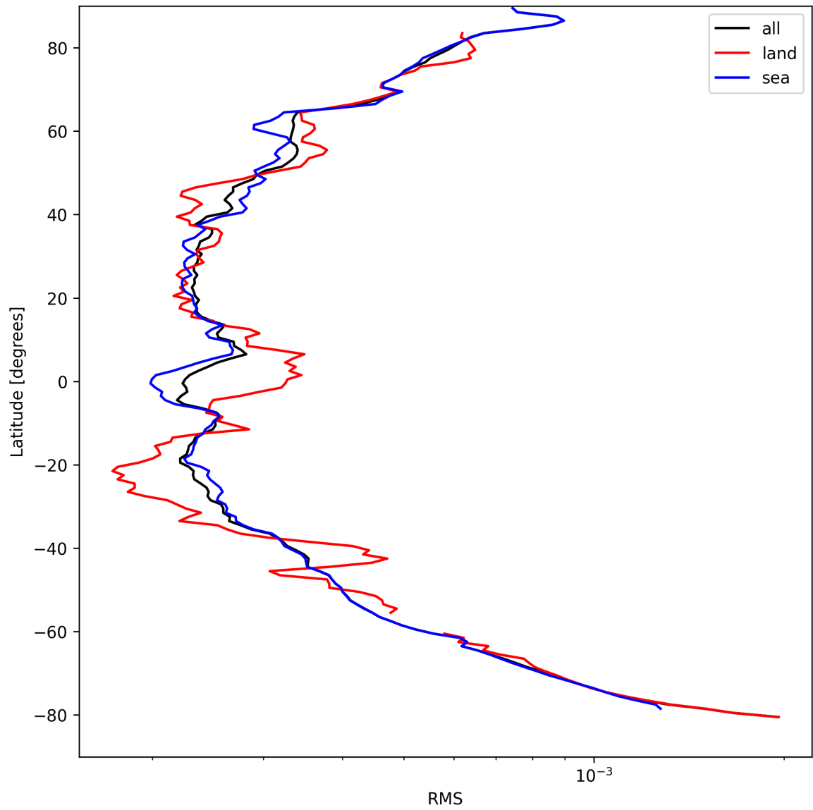
Figure 26: Zonal average of “RMS” for 2025-09-02 to 2025-09-04.
