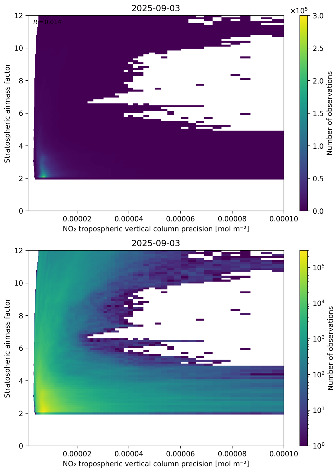
Figure 131: Scatter density plot of “NO 2 tropospheric vertical column precision” against “Stratospheric airmass factor” for 2025-09-02 to 2025-09-04.
