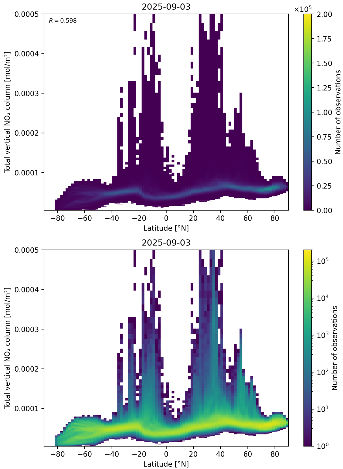
Figure 90: Scatter density plot of “Latitude” against “Total vertical NO 2 column” for 2025-09-02 to 2025-09-04.
