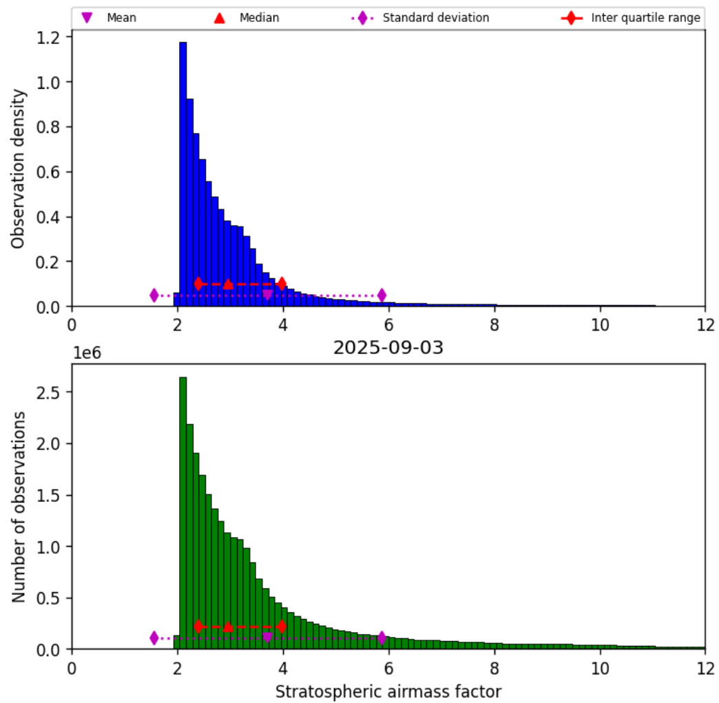
Figure 44: Histogram of “Stratospheric airmass factor” for 2025-09-02 to 2025-09-04
