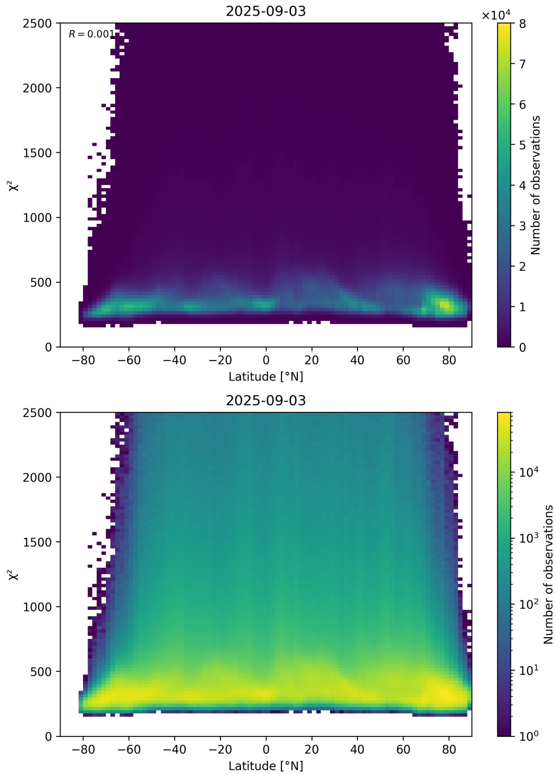
Figure 86: Scatter density plot of “Latitude” against “ \chi^2 ” for 2025-09-02 to 2025-09-04.
