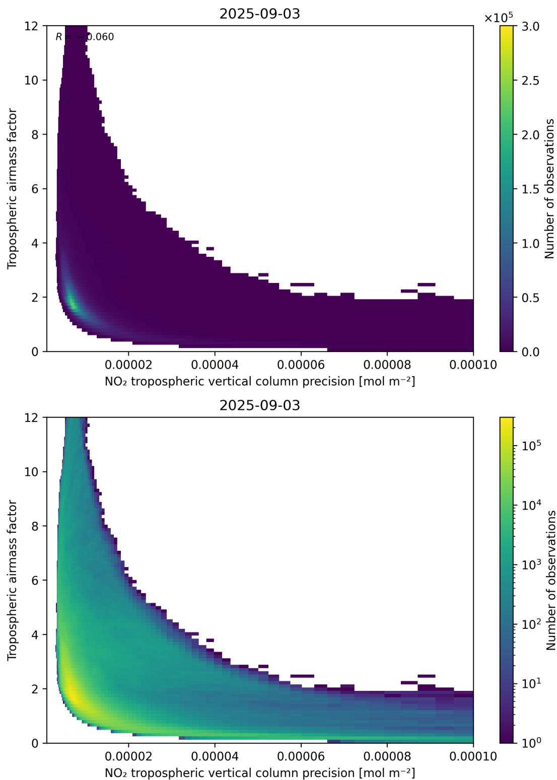
Figure 133: Scatter density plot of “NO 2 tropospheric vertical column precision” against “Tropospheric air mass factor” for 2025-09-02 to 2025-09-04.
