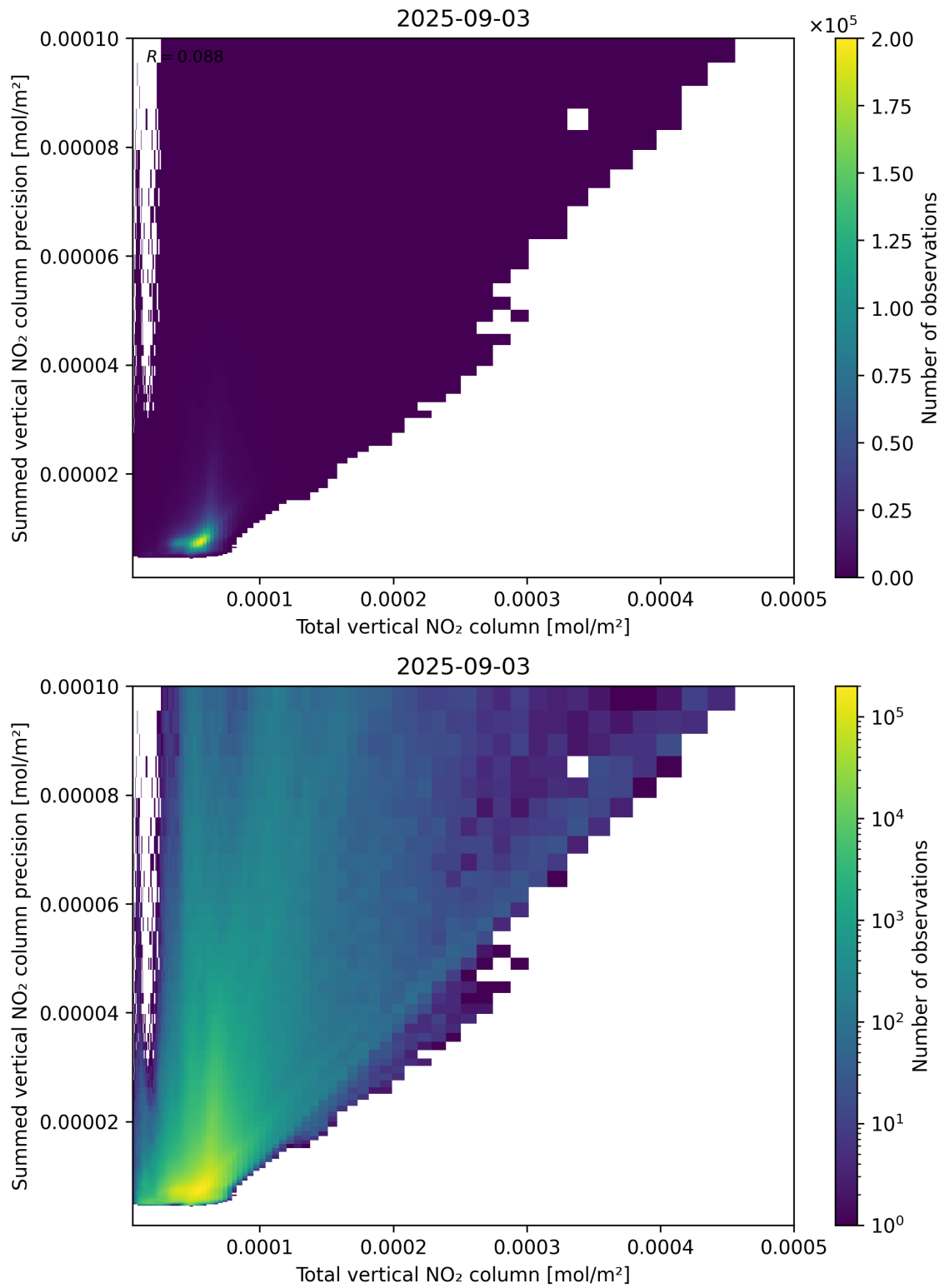
Figure 113: Scatter density plot of “Total vertical NO 2 column” against “Summed vertical NO 2 column precision” for 2025-09-02 to 2025-09-04.
