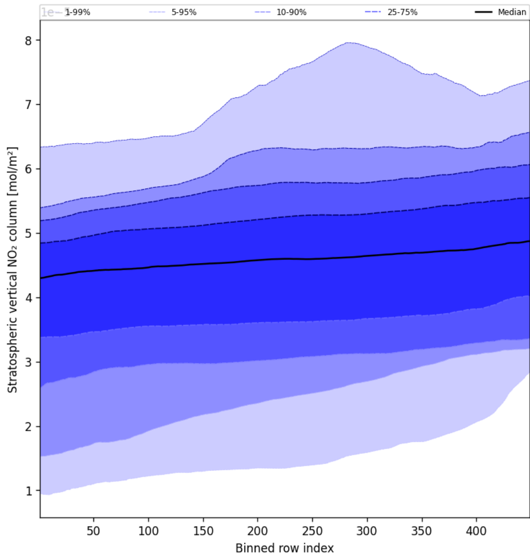
Figure 53: Along track statistics of “Stratospheric vertical NO 2 column” for 2025-09-02 to 2025-09-04
