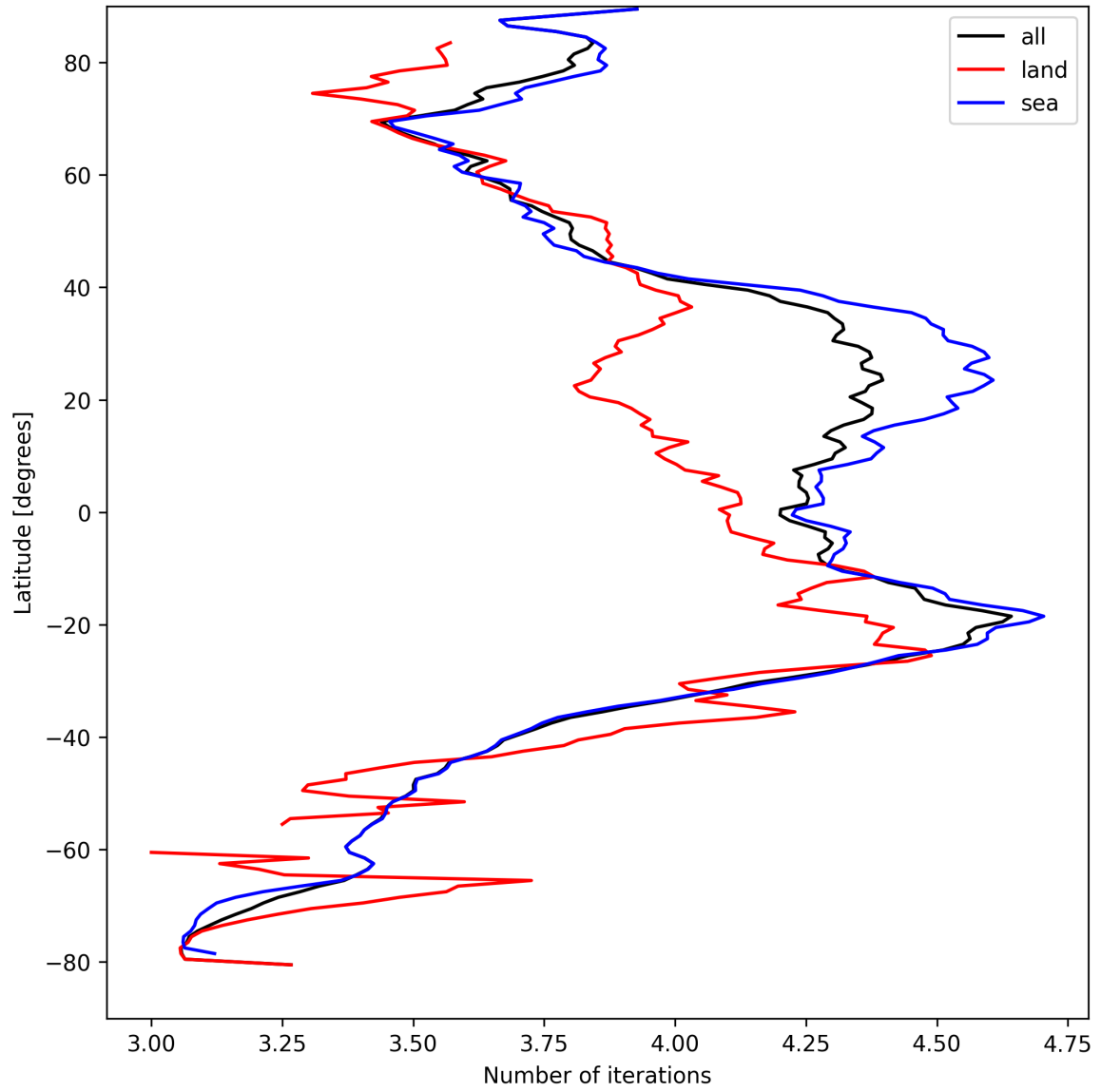
Figure 17: Zonal average of “Number of iterations” for 2025-09-02 to 2025-09-04.
