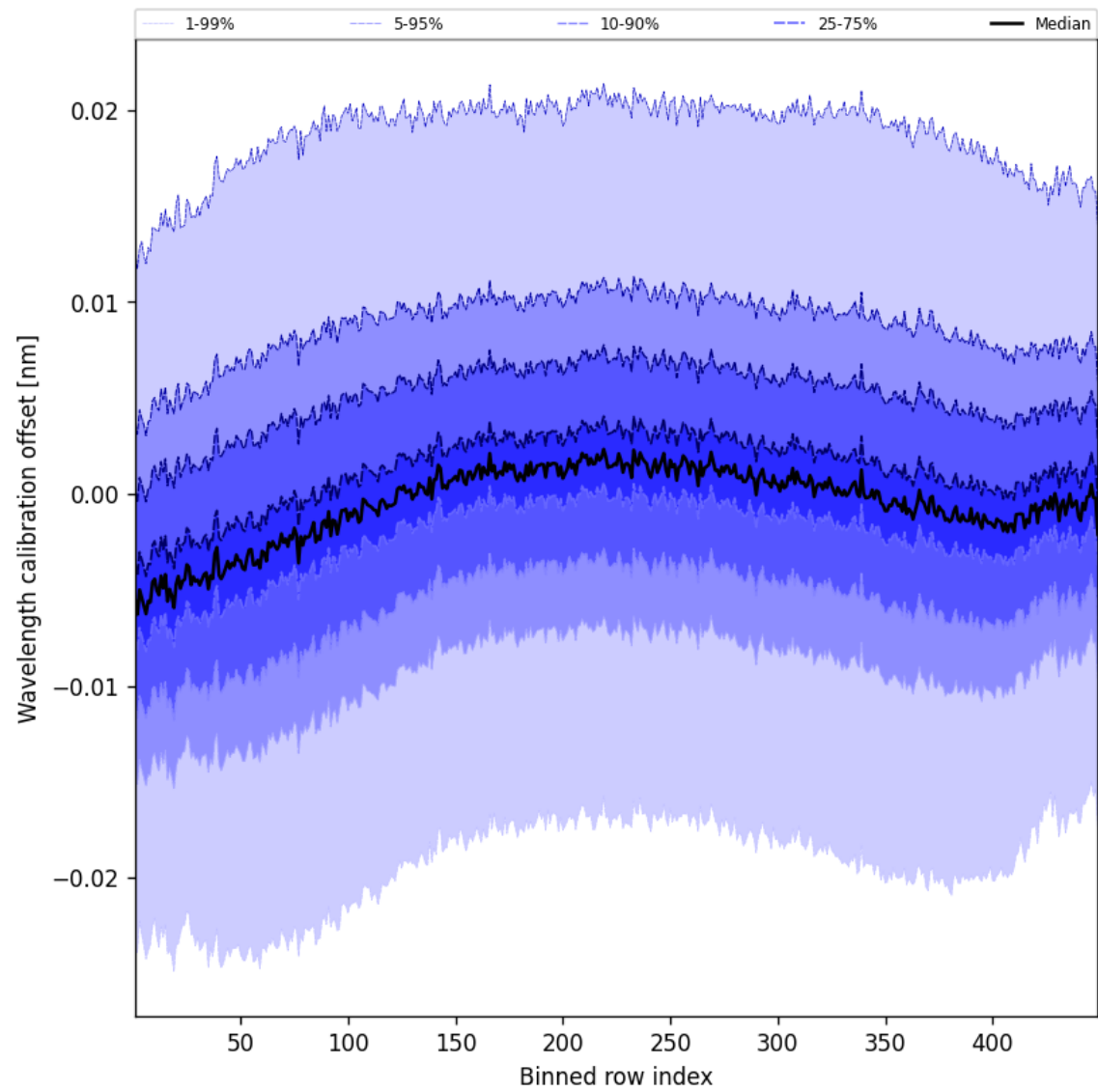
Figure 52: Along track statistics of “Wavelength calibration offset” for 2025-09-02 to 2025-09-04
