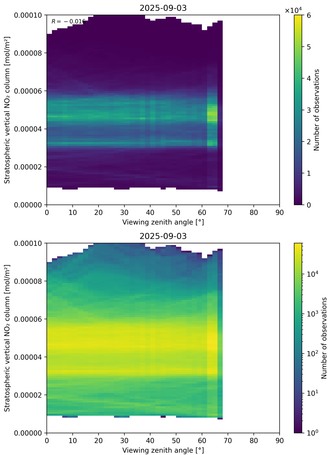
Figure 164: Scatter density plot of “Viewing zenith angle” against “Stratospheric vertical NO 2 column” for 2025-09-02 to 2025-09-04.
