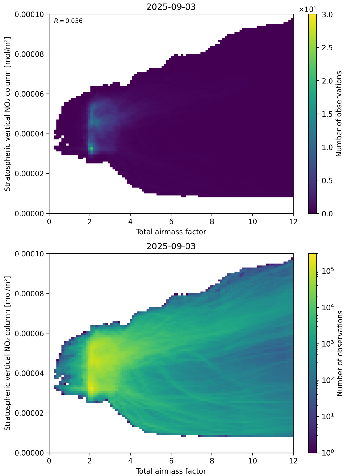
Figure 64: Scatter density plot of “Total airmass factor” against “Stratospheric vertical \text{NO}_2 column” for 2025-09-02 to 2025-09-04.
