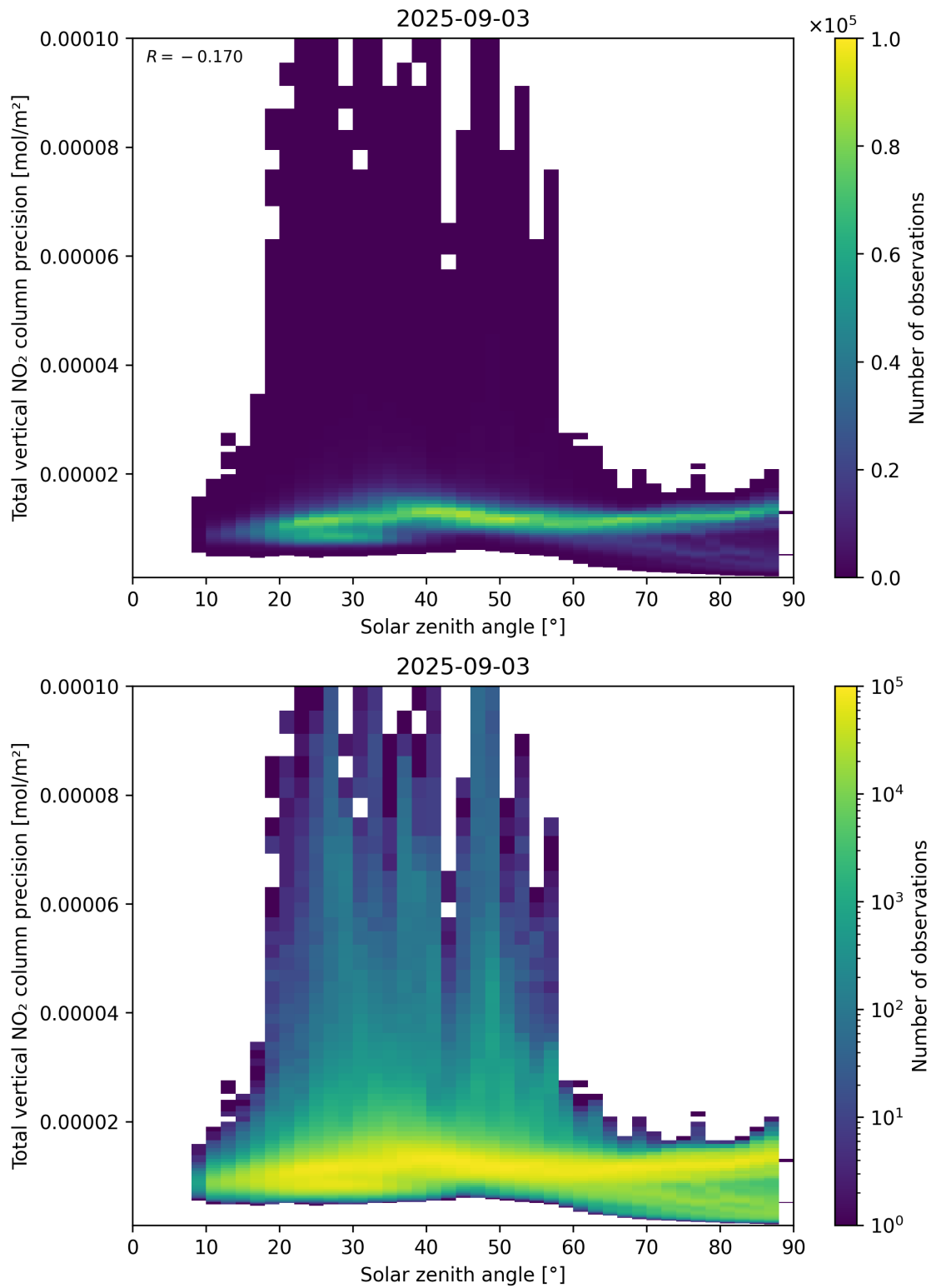
Figure 154: Scatter density plot of “Solar zenith angle” against “Total vertical NO 2 column precision” for 2025-09-02 to 2025-09-04.
