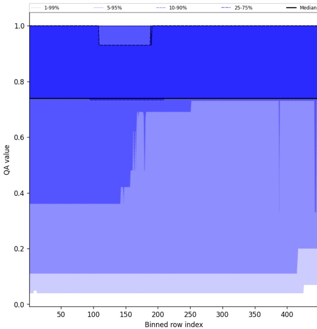
Figure 45: Along track statistics of “QA value” for 2025-09-02 to 2025-09-04
