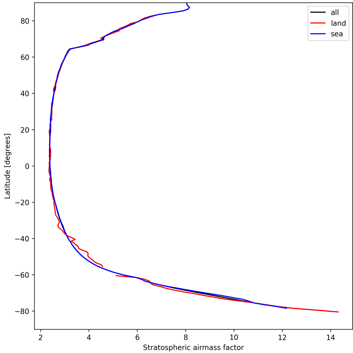
Figure 27: Zonal average of “Stratospheric air mass factor” for 2025-09-02 to 2025-09-04.
