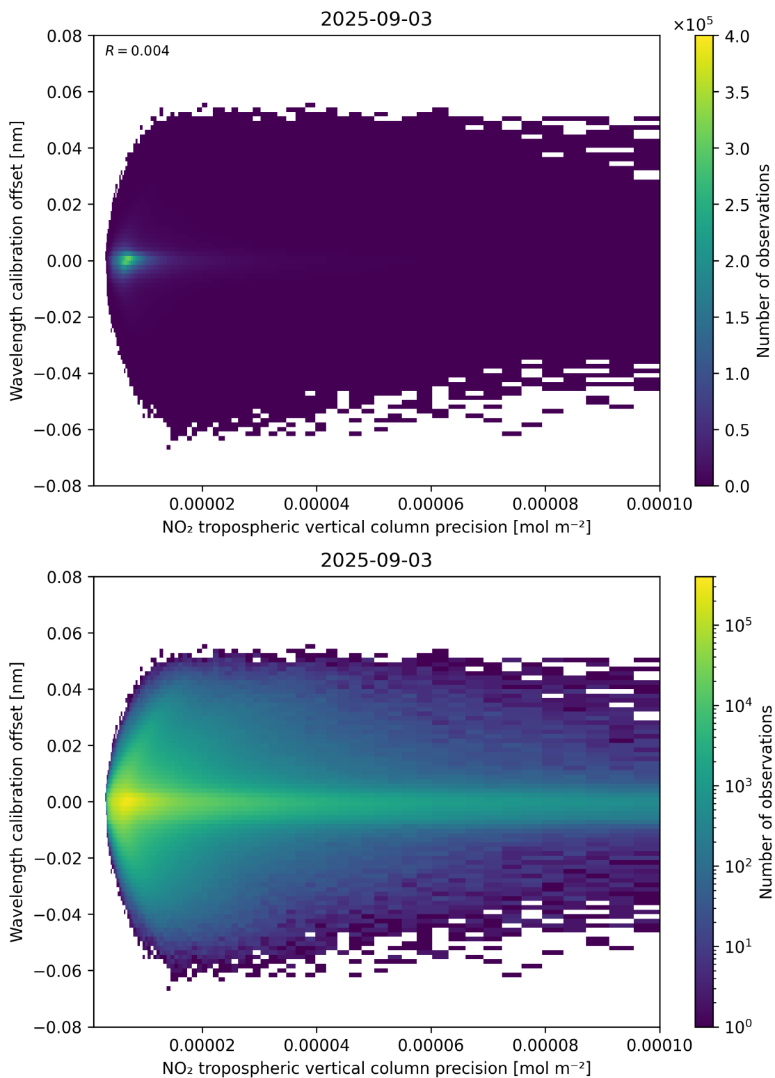
Figure 141: Scatter density plot of “NO 2 tropospheric vertical column precision” against “Wavelength calibration offset” for 2025-09-02 to 2025-09-04.
