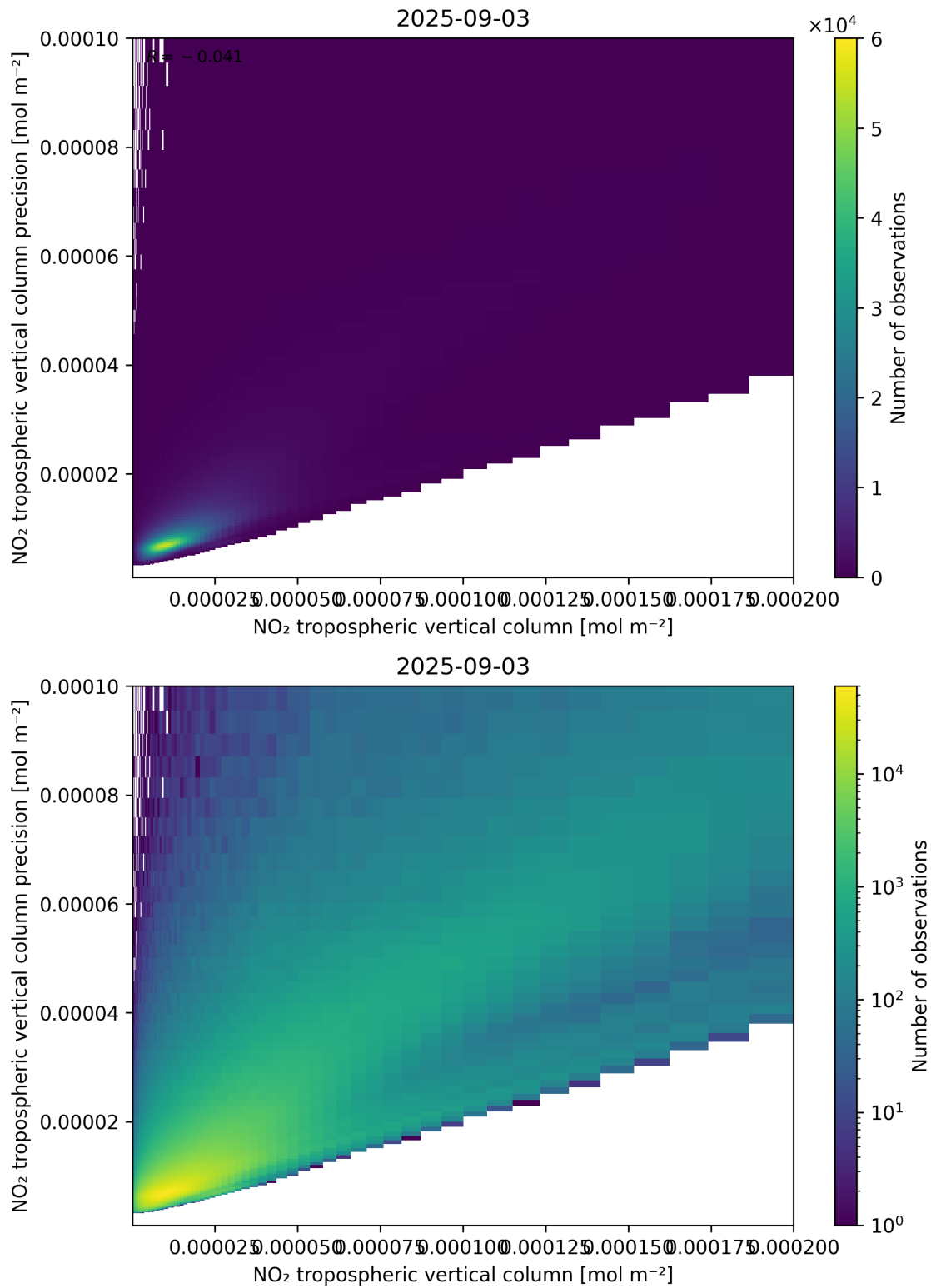
Figure 130: Scatter density plot of “NO 2 tropospheric vertical column” against “NO 2 tropospheric vertical column precision” for 2025-09-02 to 2025-09-04.
