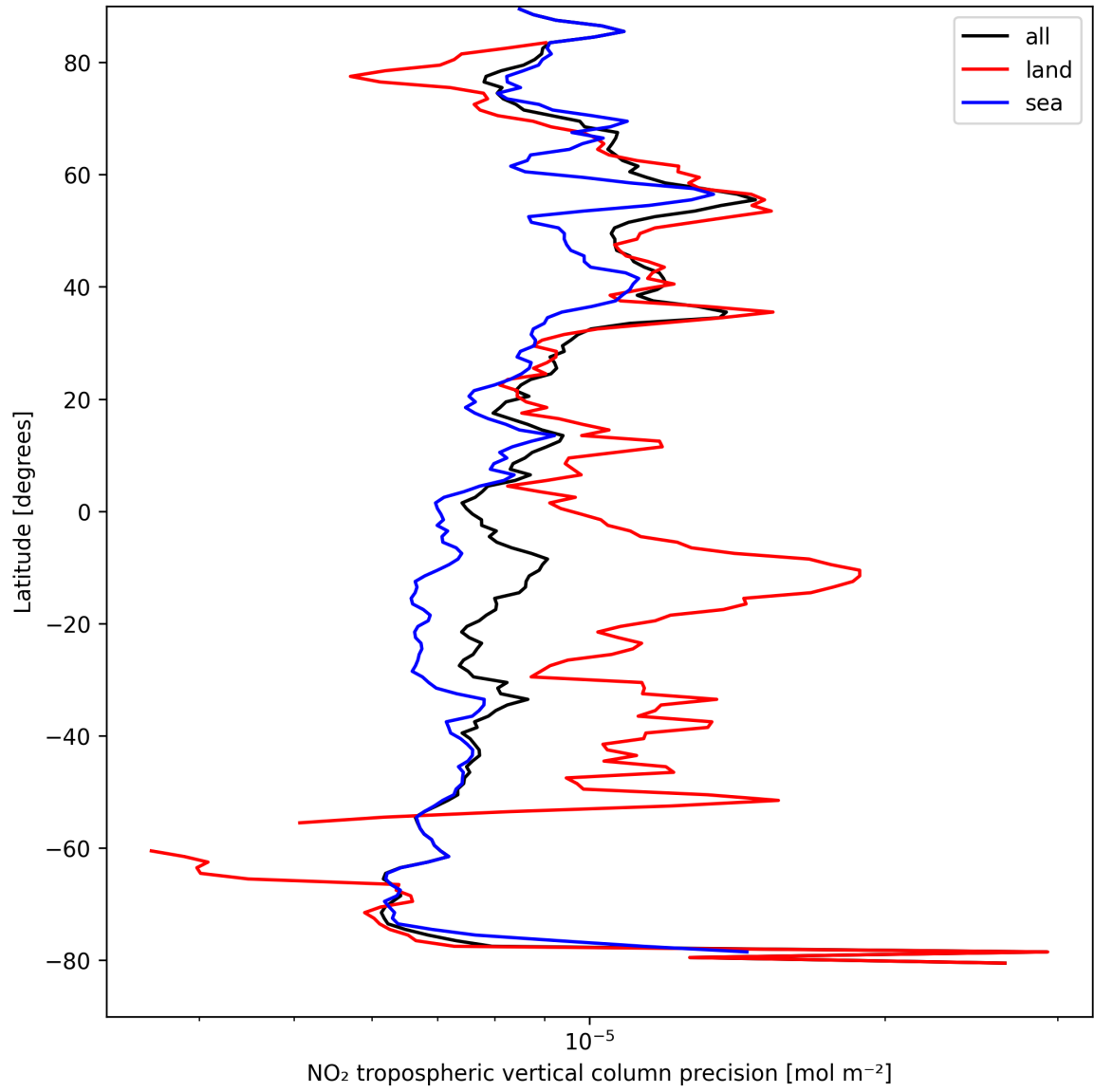
Figure 13: Zonal average of “NO 2 tropospheric vertical column precision” for 2025-09-02 to 2025-09-04.
