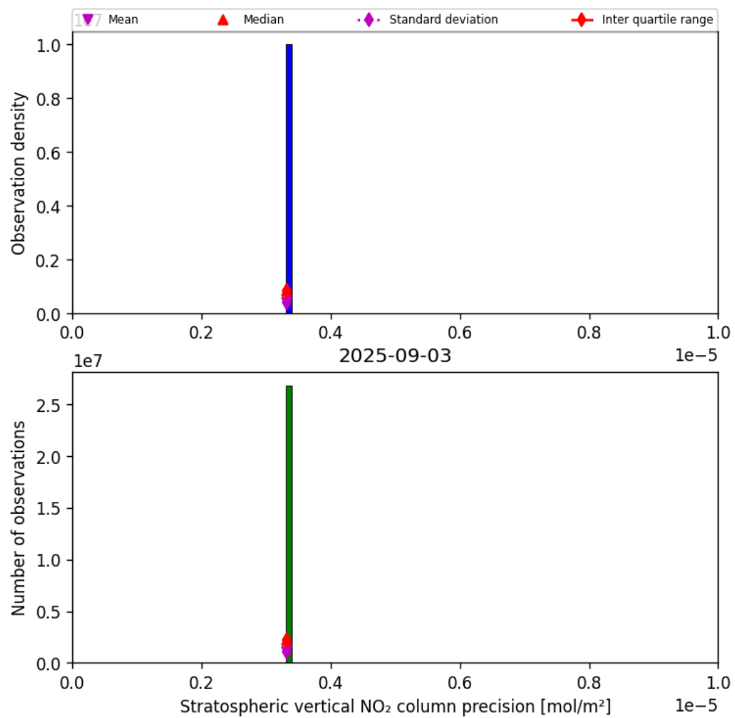
Figure 37: Histogram of “Stratospheric vertical NO 2 column precision” for 2025-09-02 to 2025-09-04
