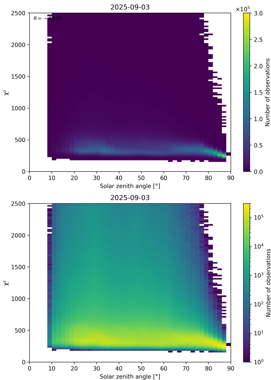
Figure 148: Scatter density plot of “Solar zenith angle” against “ \chi^2 ” for 2025-09-02 to 2025-09-04.
