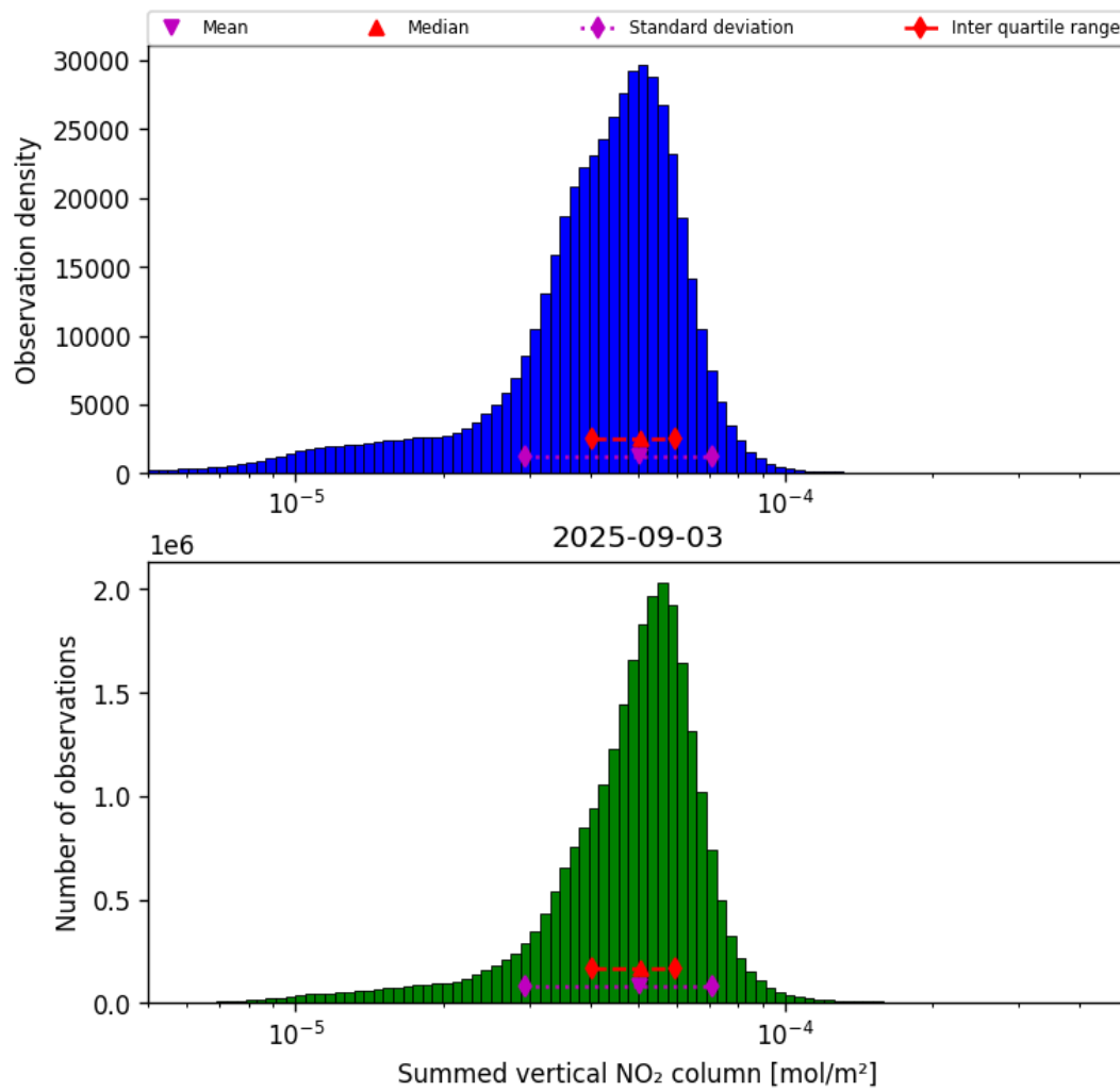
Figure 40: Histogram of "Summed vertical NO 2 column" for 2025-09-02 to 2025-09-04
