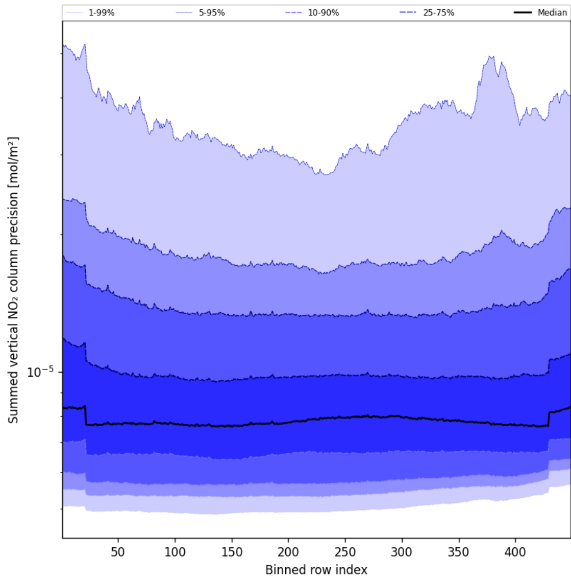
Figure 58: Along track statistics of “Summed vertical NO 2 column precision” for 2025-09-02 to 2025-09-04
