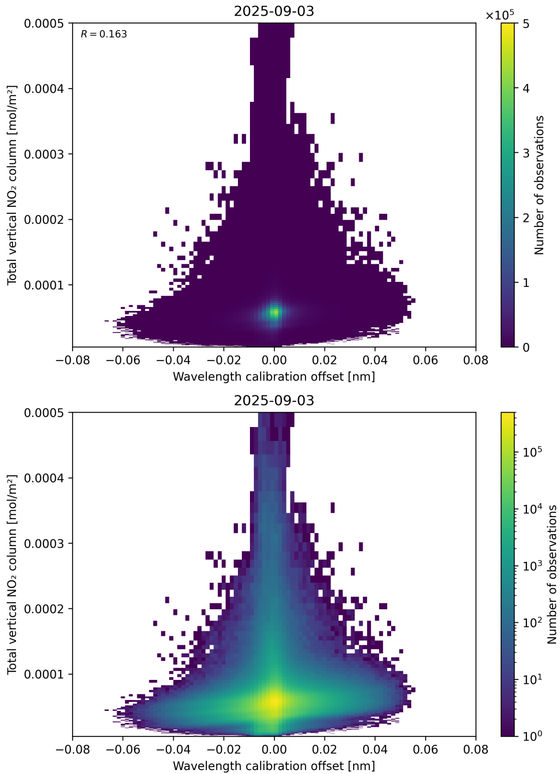
Figure 179: Scatter density plot of “Wavelength calibration offset” against “Total vertical NO 2 column” for 2025-09-02 to 2025-09-04.
