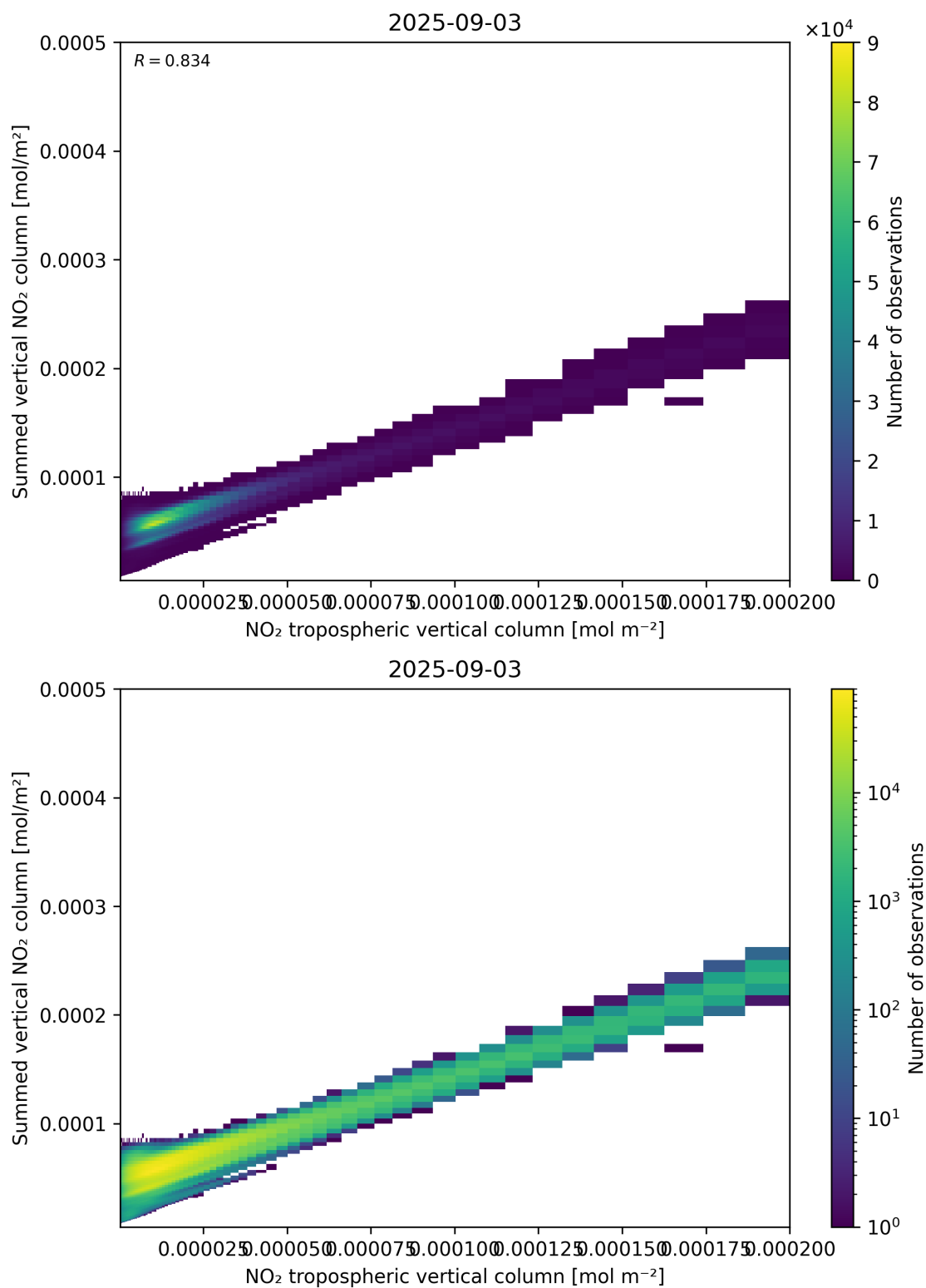
Figure 126: Scatter density plot of “NO 2 tropospheric vertical column” against “Summed vertical NO 2 column” for 2025-09-02 to 2025-09-04.
