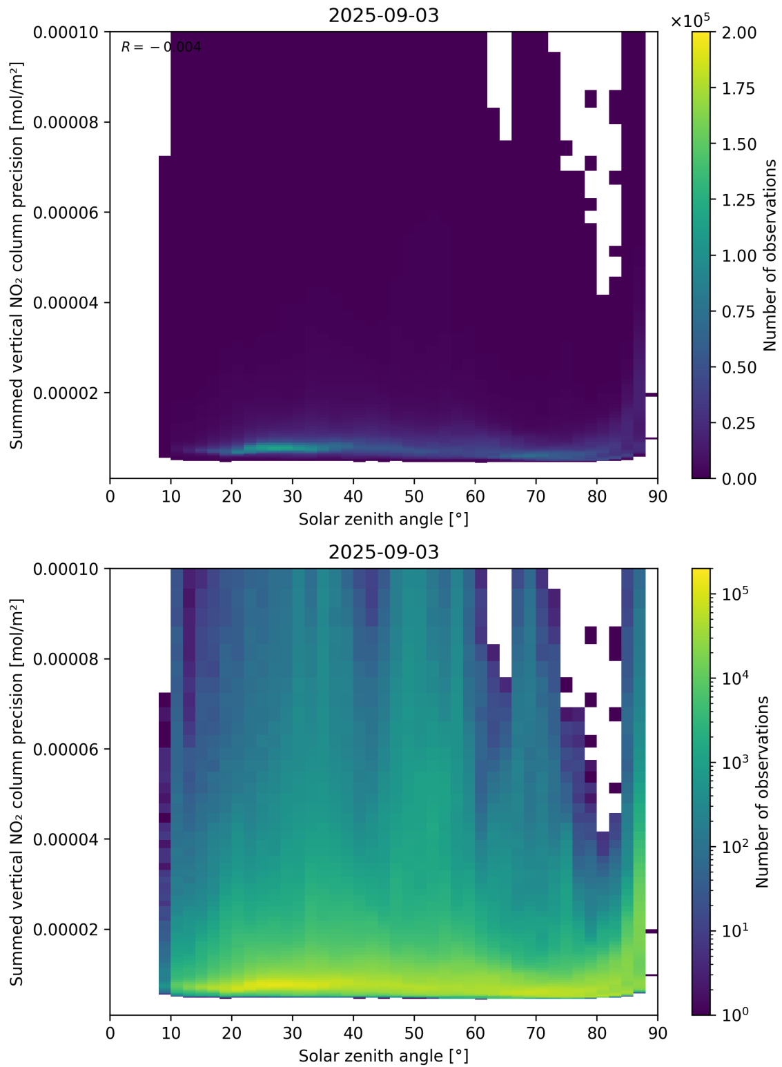
Figure 152: Scatter density plot of “Solar zenith angle” against “Summed vertical NO 2 column precision” for 2025-09-02 to 2025-09-04.
