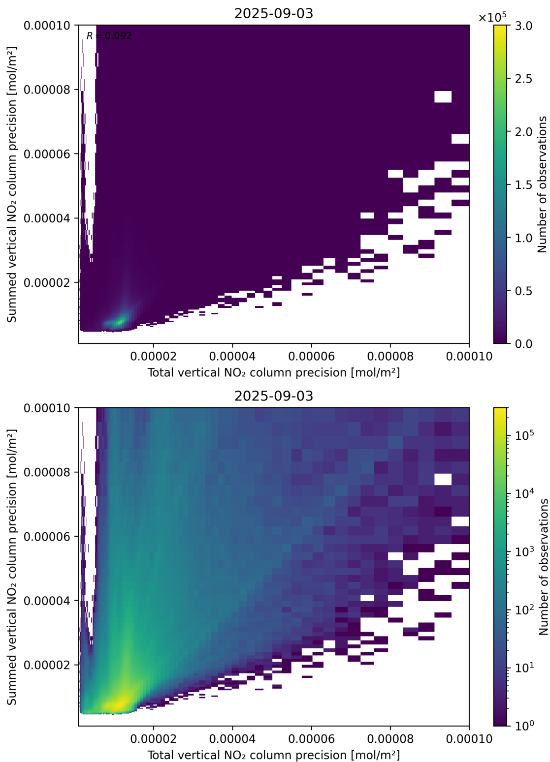
Figure 118: Scatter density plot of “Total vertical NO 2 column precision” against “Summed vertical NO 2 column precision” for 2025-09-02 to 2025-09-04.
