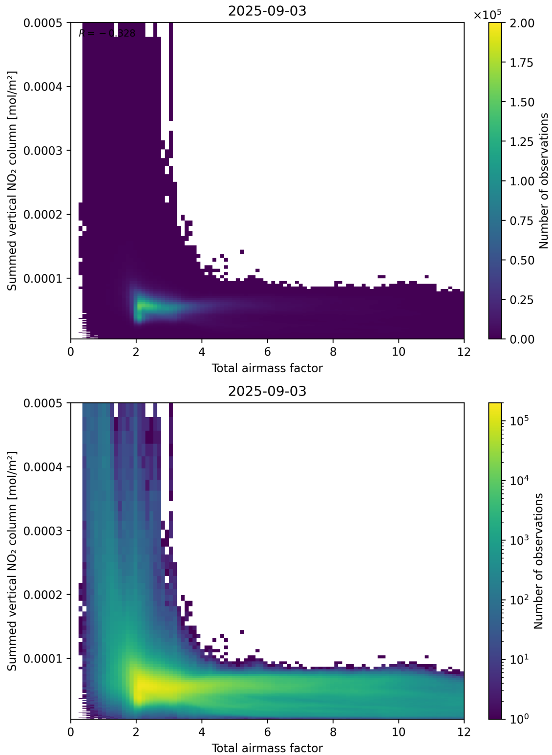
Figure 65: Scatter density plot of “Total airmass factor” against “Summed vertical NO 2 column” for 2025-09-02 to 2025-09-04.
