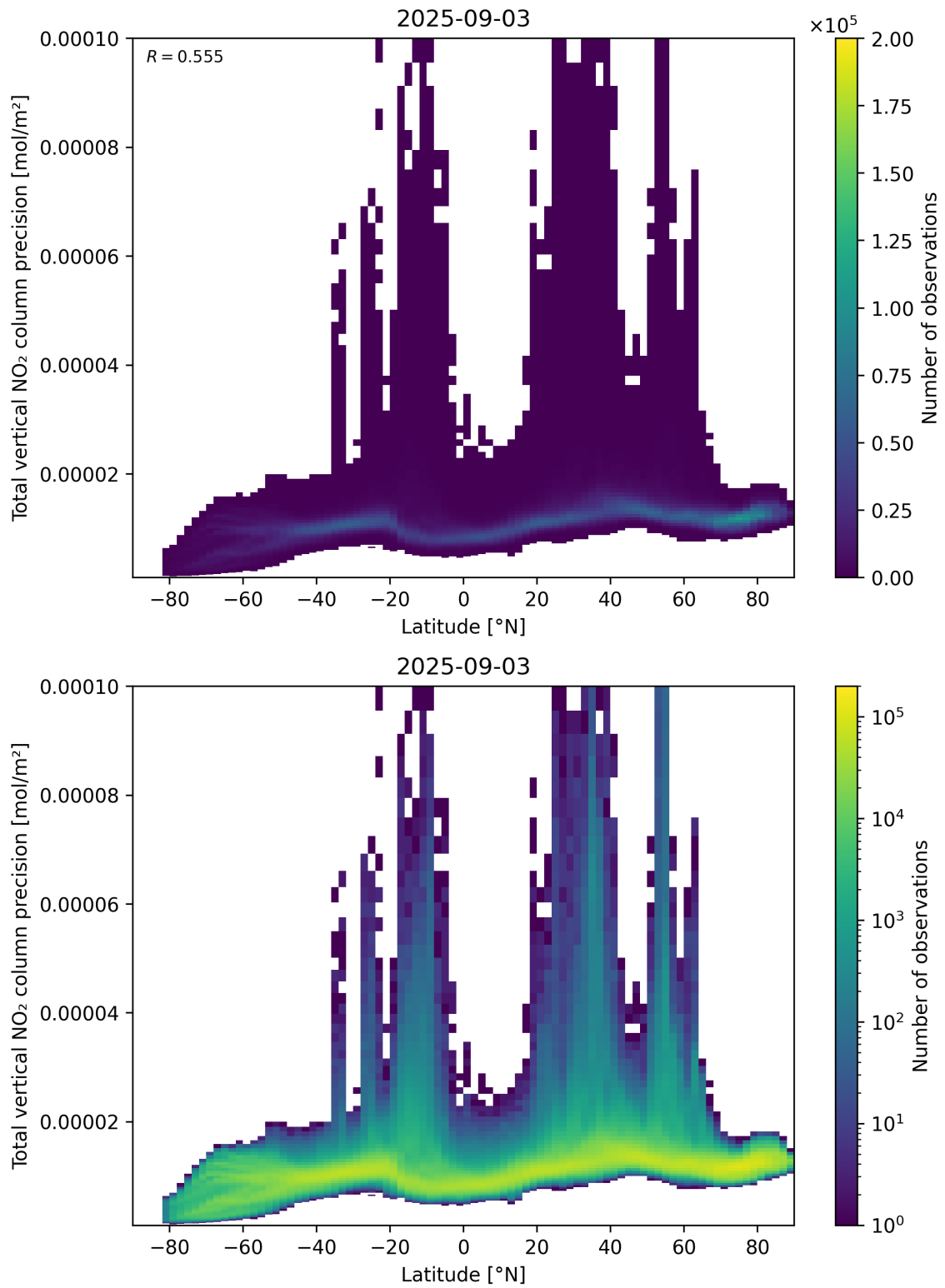
Figure 91: Scatter density plot of “Latitude” against “Total vertical NO 2 column precision” for 2025-09-02 to 2025-09-04.
