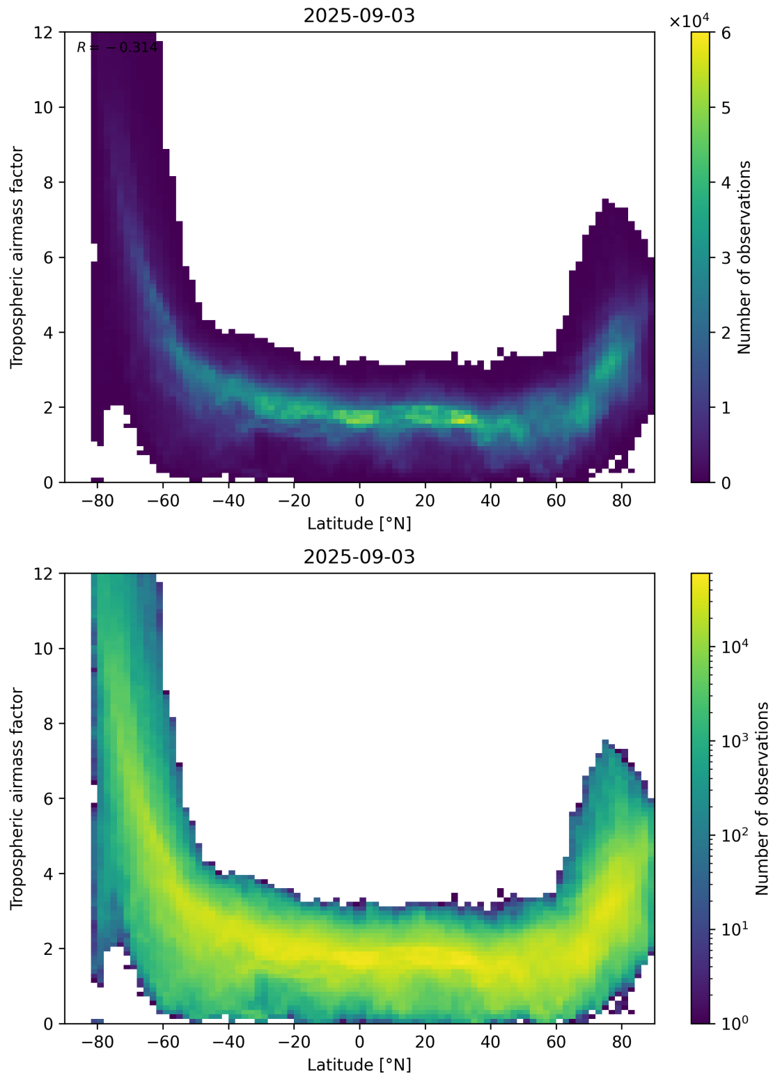
Figure 85: Scatter density plot of “Latitude” against “Tropospheric airmass factor” for 2025-09-02 to 2025-09-04.
