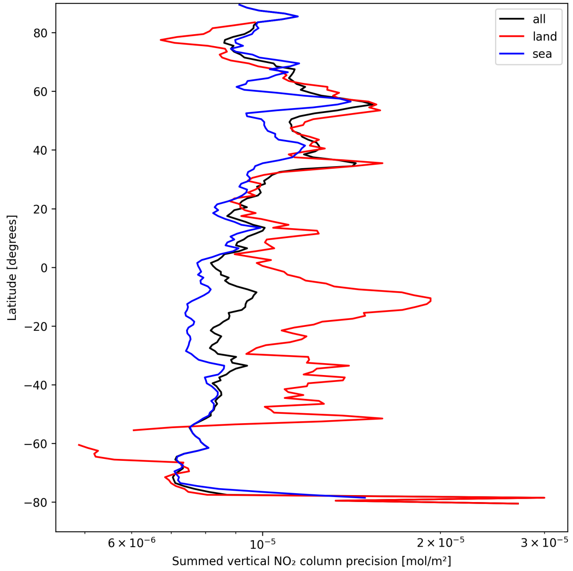
Figure 24: Zonal average of “Summed vertical NO 2 column precision” for 2025-09-02 to 2025-09-04.
