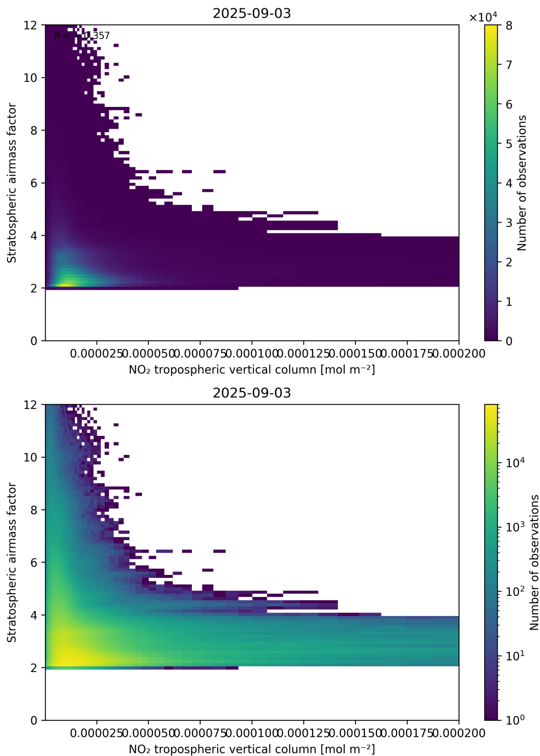
Figure 121: Scatter density plot of “NO 2 tropospheric vertical column” against “Stratospheric air mass factor” for 2025-09-02 to 2025-09-04.
