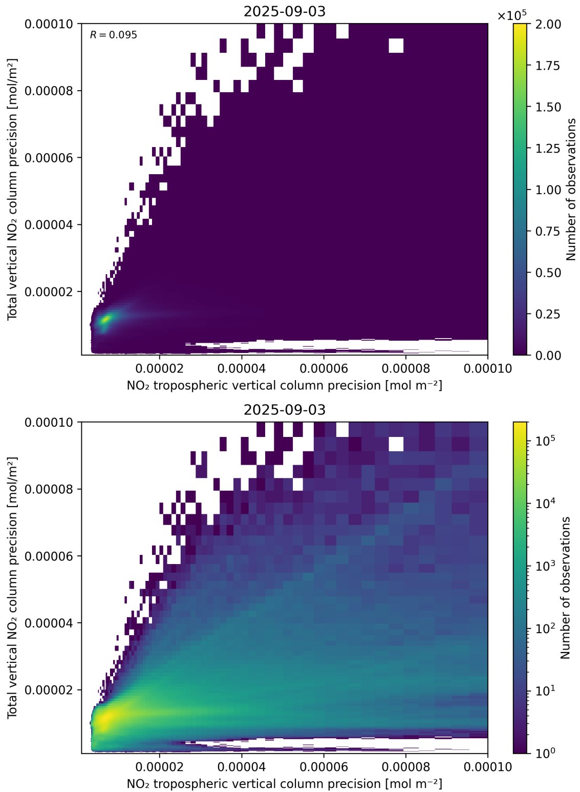
Figure 139: Scatter density plot of “NO 2 tropospheric vertical column precision” against “Total vertical NO 2 column precision” for 2025-09-02 to 2025-09-04.
