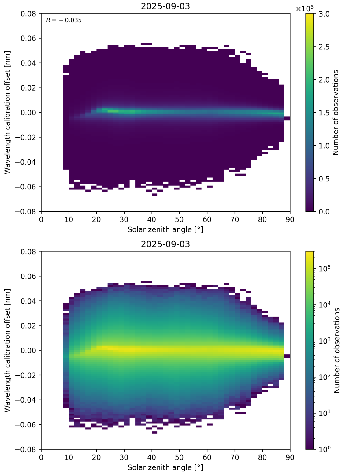
Figure 158: Scatter density plot of “Solar zenith angle” against “Wavelength calibration offset” for 2025-09-02 to 2025-09-04.
