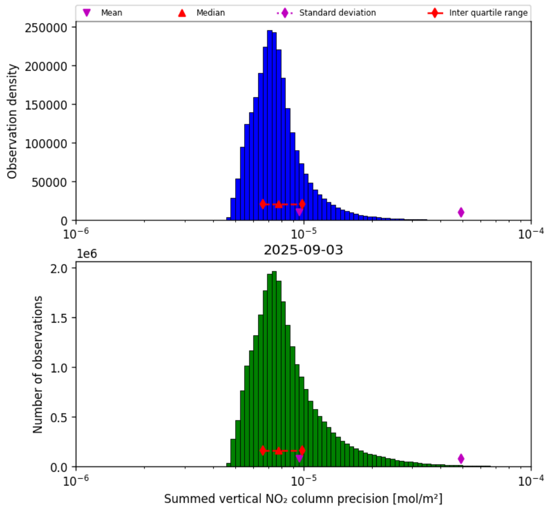
Figure 41: Histogram of "Summed vertical NO 2 column precision" for 2025-09-02 to 2025-09-04
