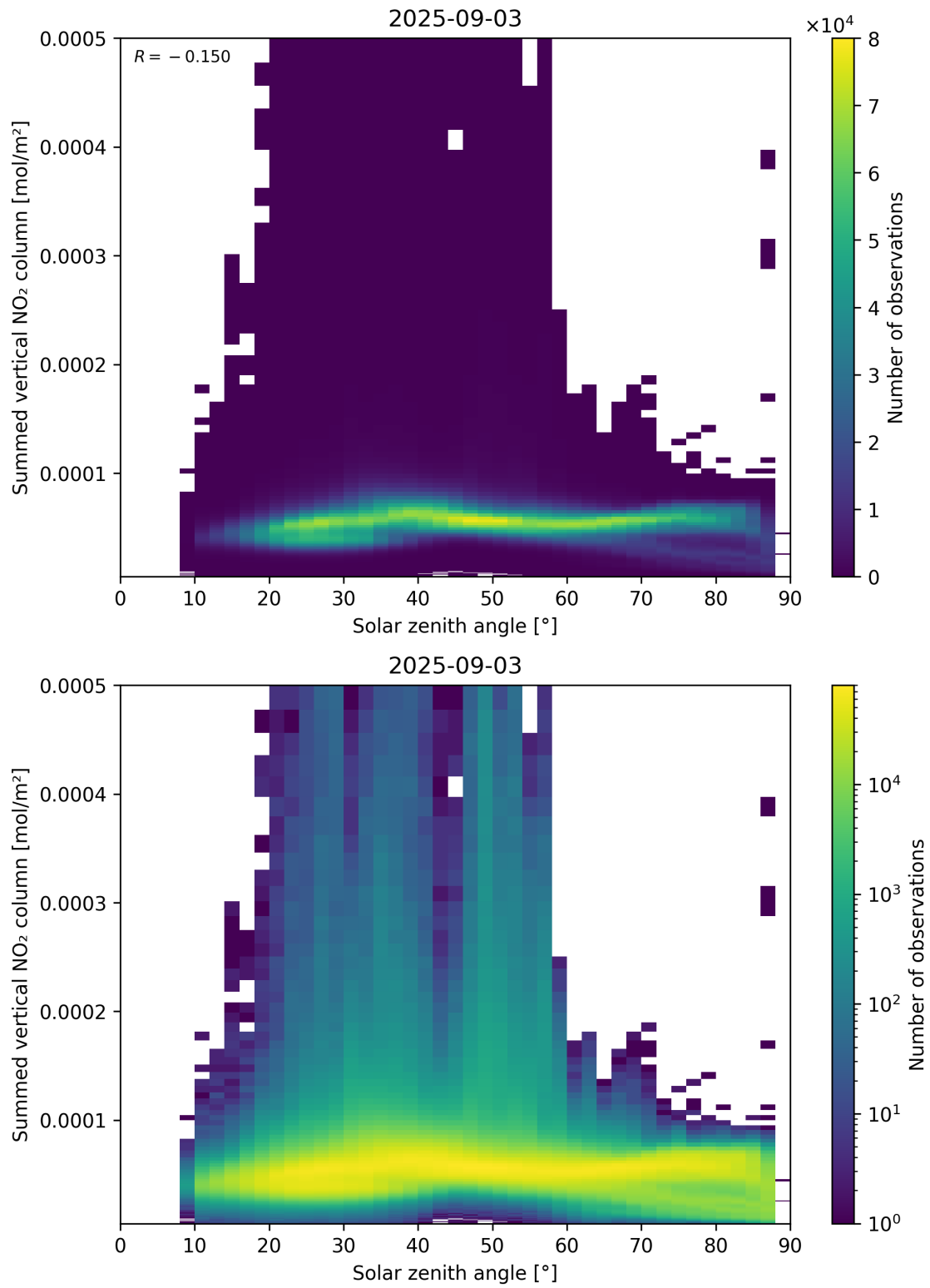
Figure 151: Scatter density plot of “Solar zenith angle” against “Summed vertical NO 2 column” for 2025-09-02 to 2025-09-04.
