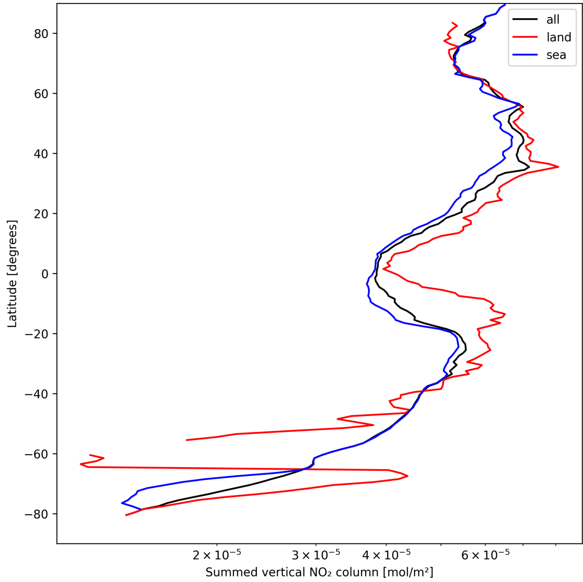
Figure 23: Zonal average of “Summed vertical NO 2 column” for 2025-09-02 to 2025-09-04.
