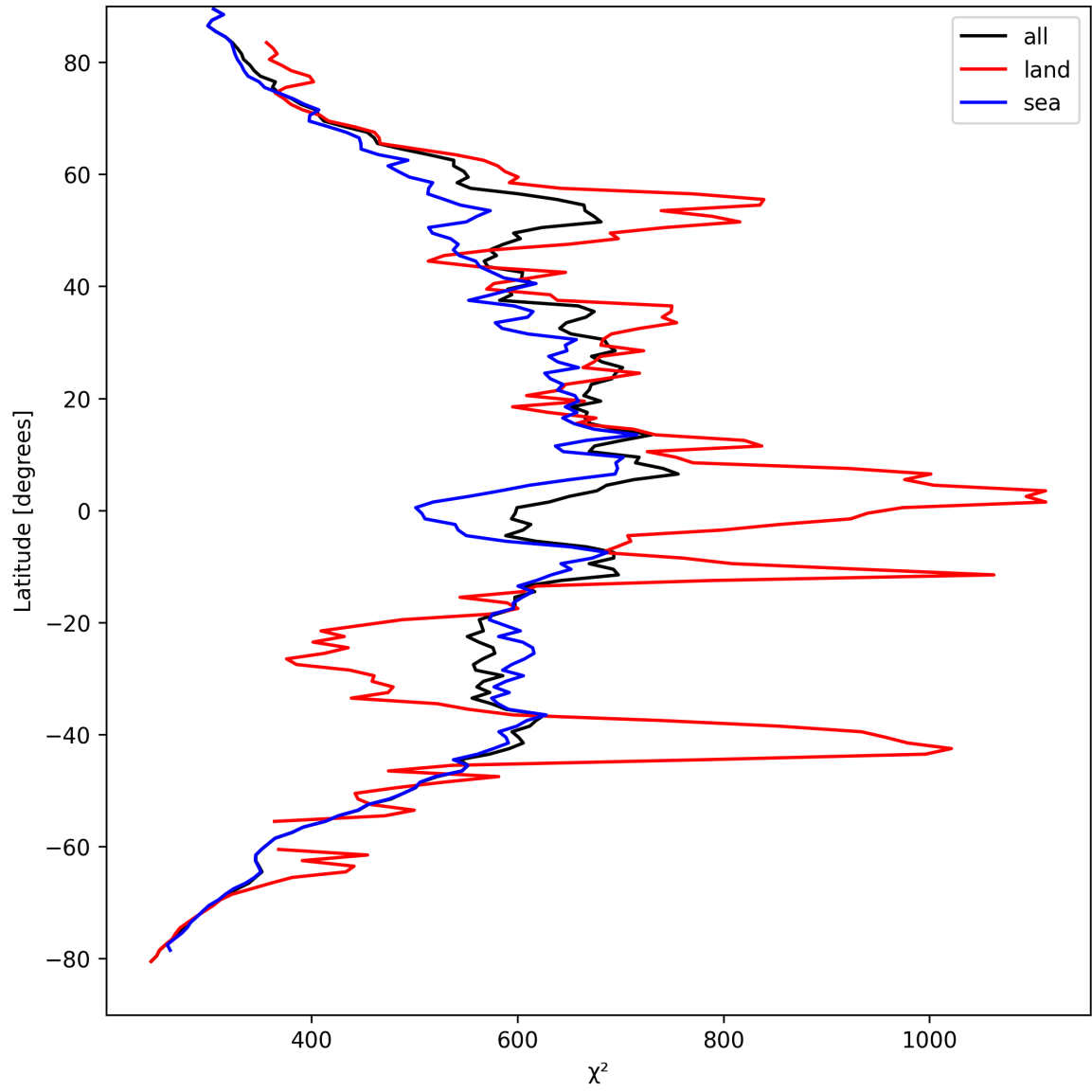
Figure 25: Zonal average of “ \chi^2 ” for 2025-09-02 to 2025-09-04.
