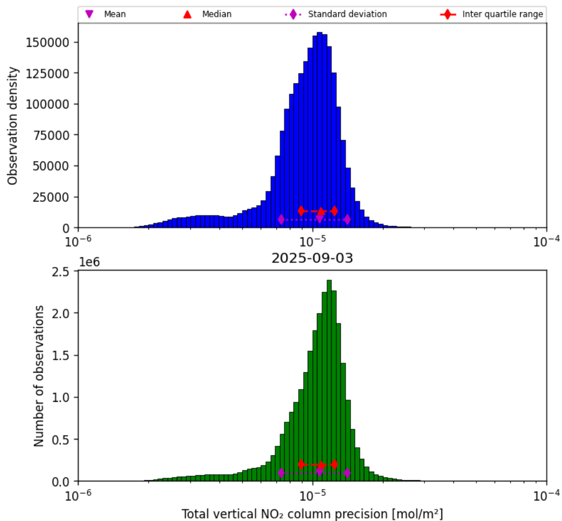
Figure 39: Histogram of “Total vertical NO 2 column precision” for 2025-09-02 to 2025-09-04
