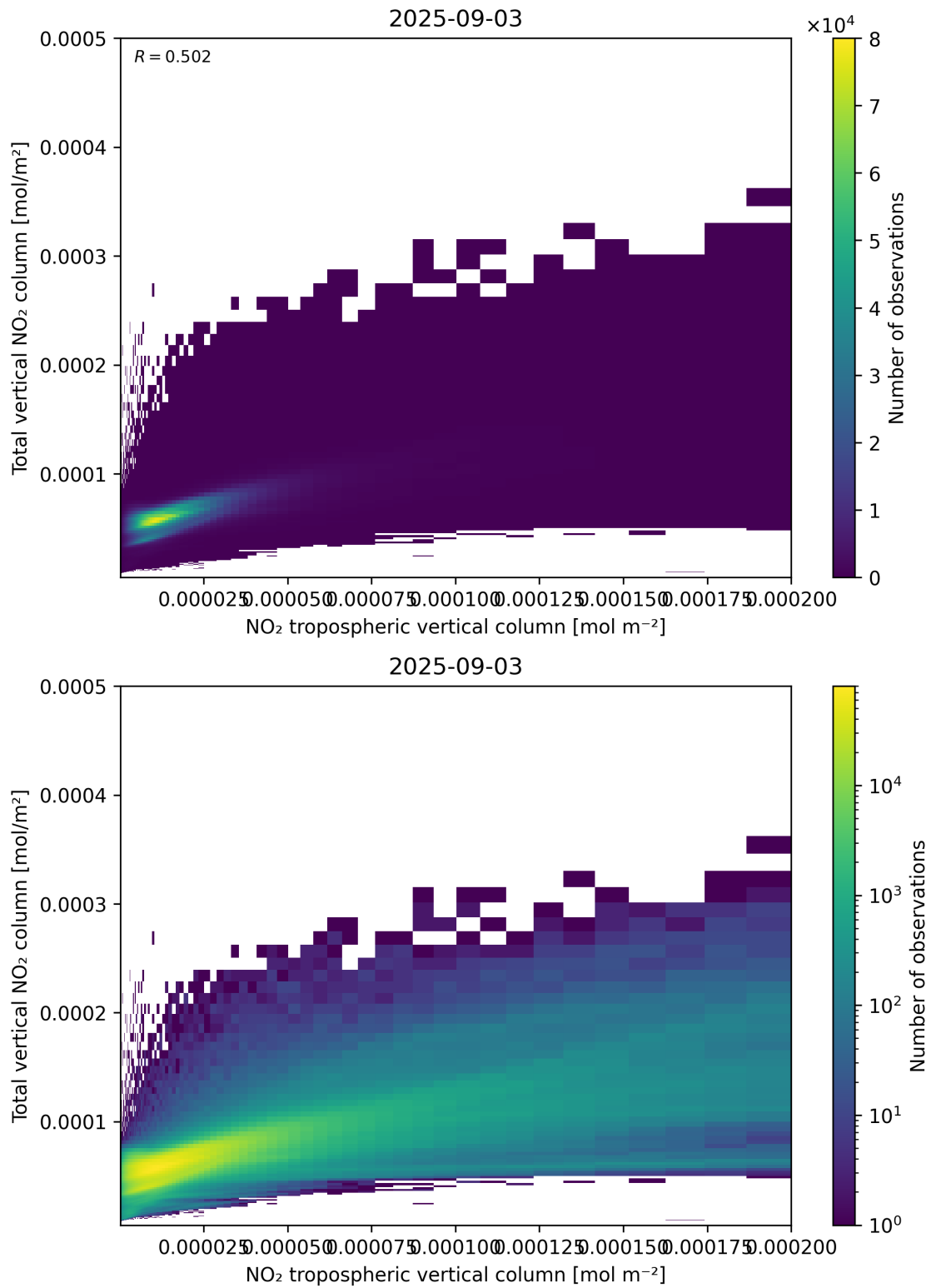
Figure 128: Scatter density plot of “NO 2 tropospheric vertical column” against “Total vertical NO 2 column” for 2025-09-02 to 2025-09-04.
