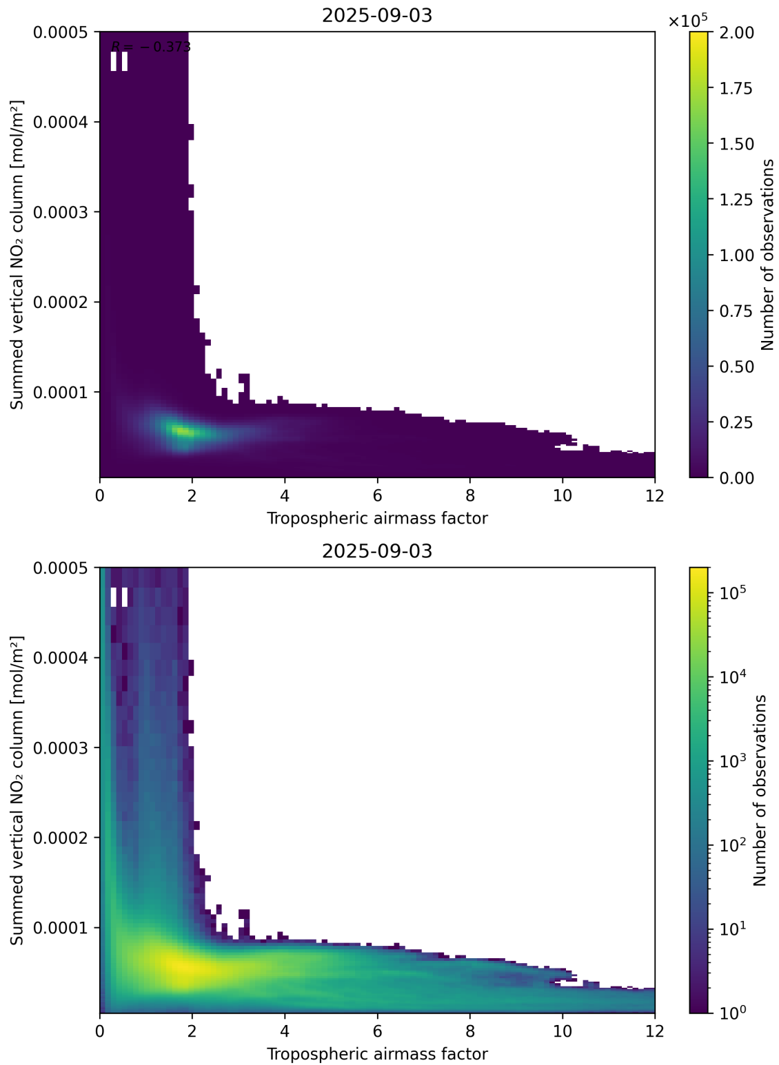
Figure 75: Scatter density plot of “Tropospheric airmass factor” against “Summed vertical NO 2 column” for 2025-09-02 to 2025-09-04.
