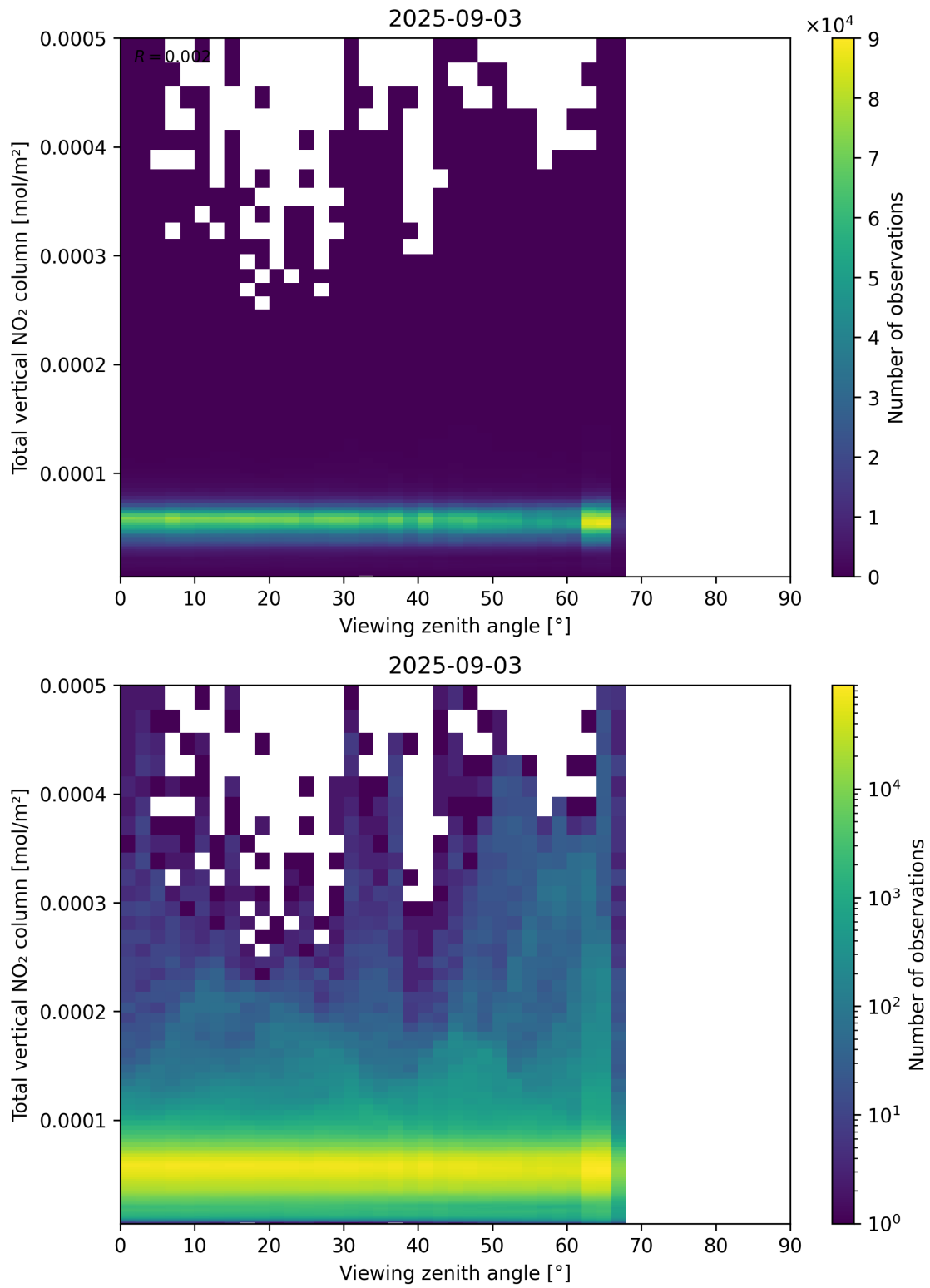
Figure 167: Scatter density plot of “Viewing zenith angle” against “Total vertical NO 2 column” for 2025-09-02 to 2025-09-04.
