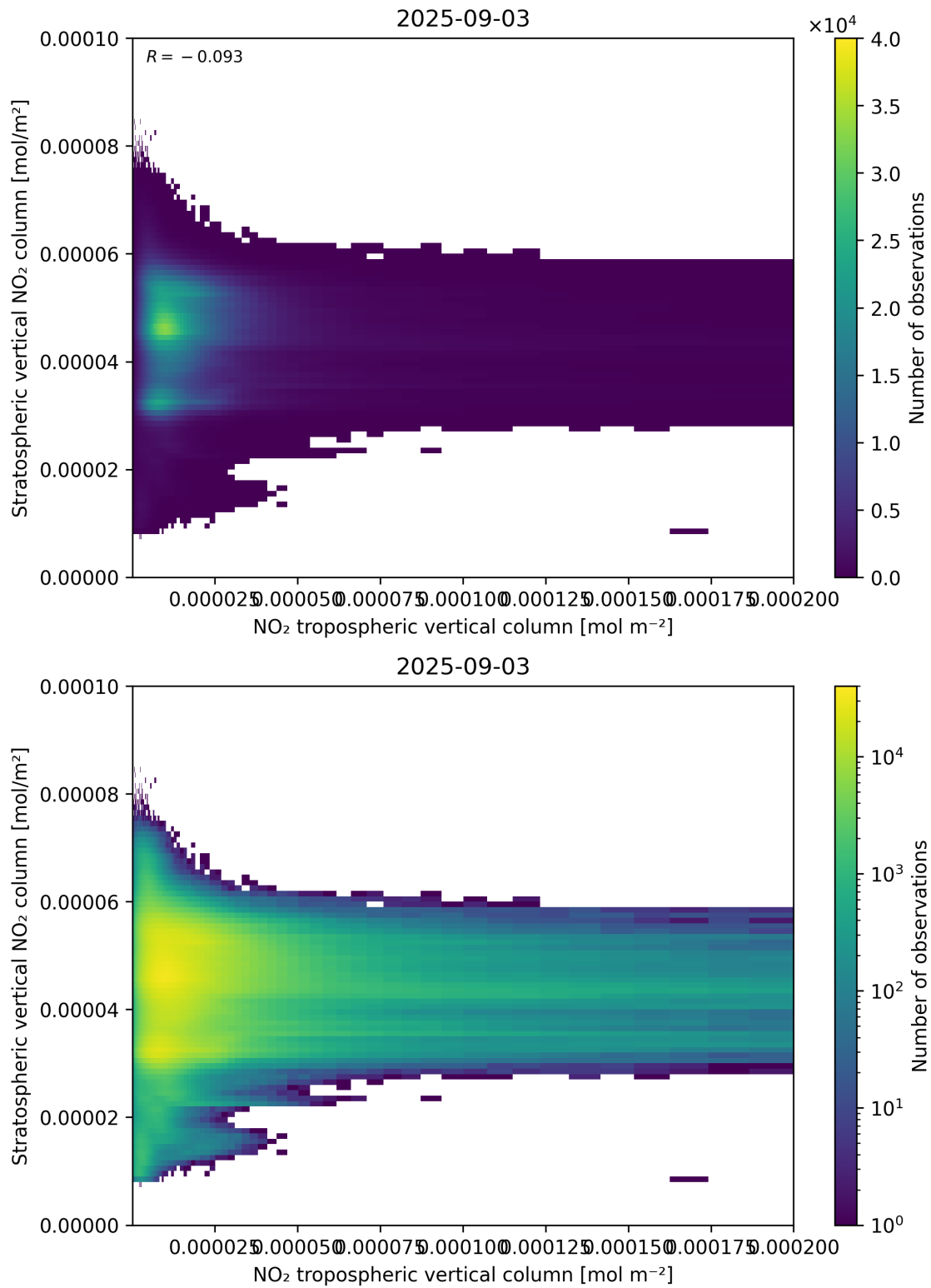
Figure 125: Scatter density plot of “NO 2 tropospheric vertical column” against “Stratospheric vertical NO 2 column” for 2025-09-02 to 2025-09-04.
