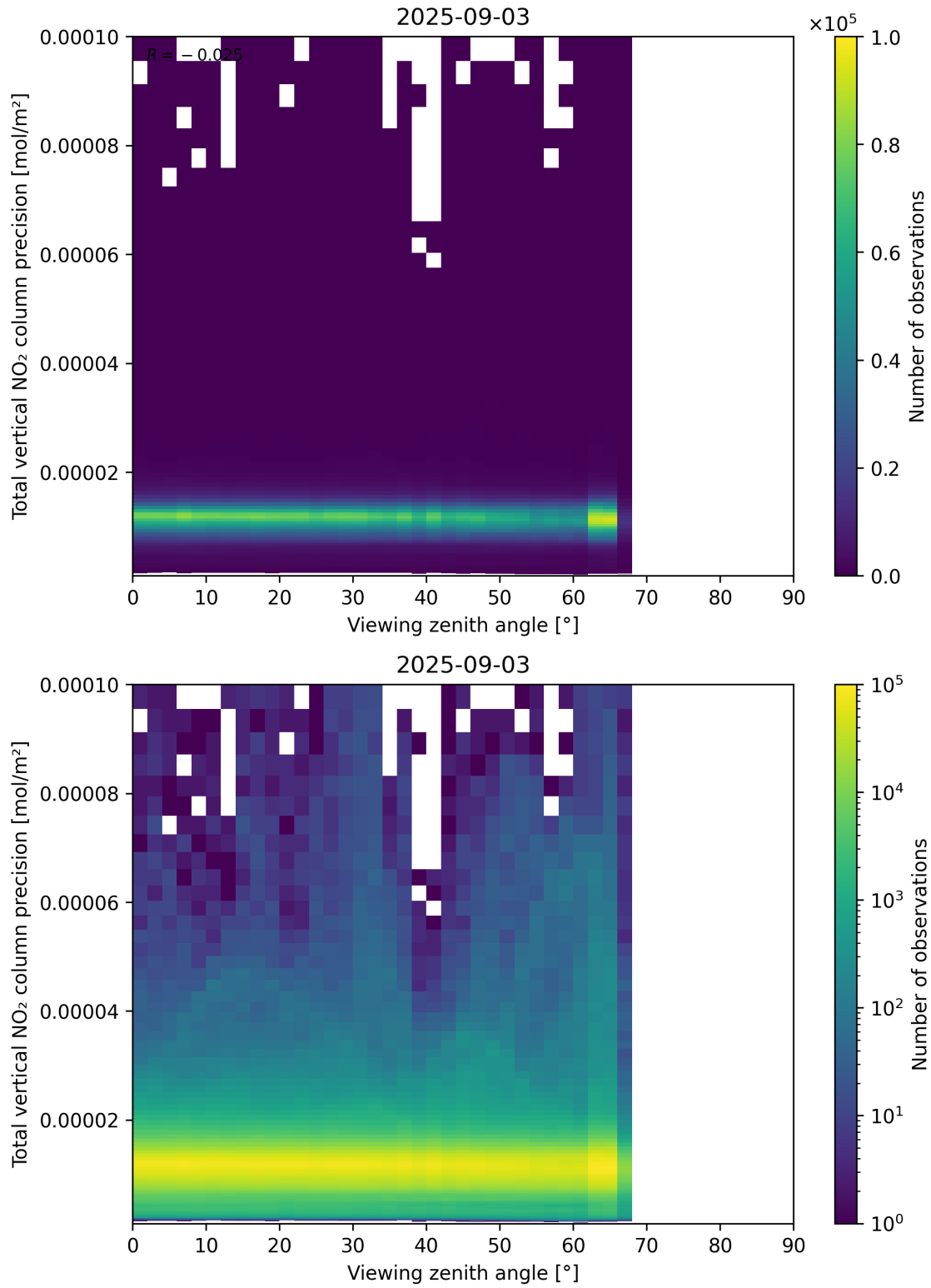
Figure 168: Scatter density plot of “Viewing zenith angle” against “Total vertical NO 2 column precision” for 2025-09-02 to 2025-09-04.
