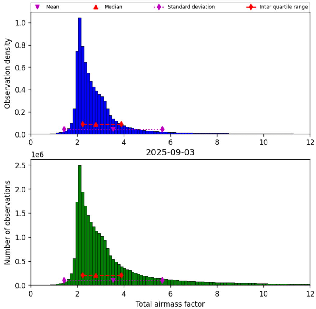
Figure 32: Histogram of “Total airmass factor” for 2025-09-02 to 2025-09-04
