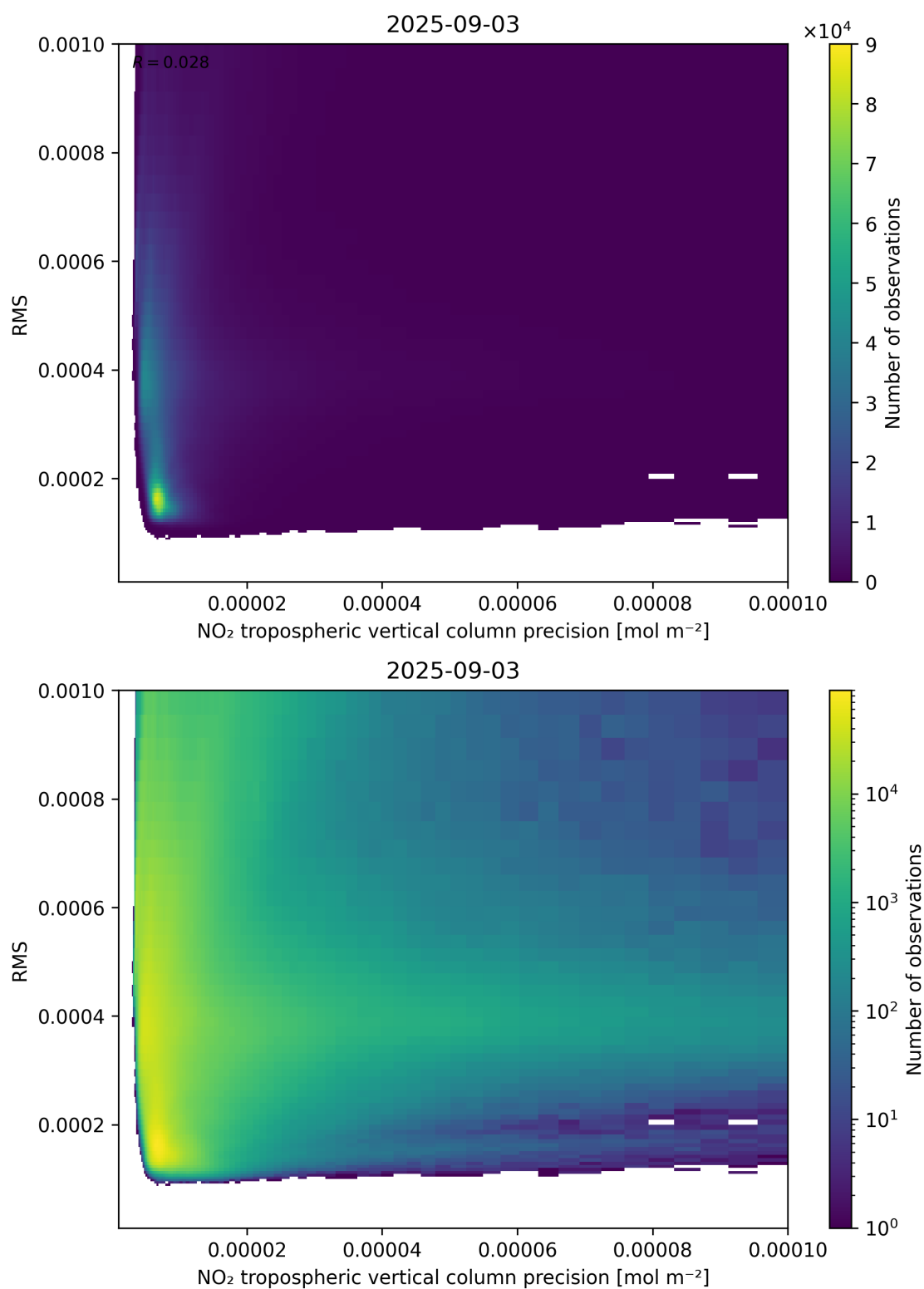
Figure 140: Scatter density plot of “NO 2 tropospheric vertical column precision” against “RMS” for 2025-09-02 to 2025-09-04.
