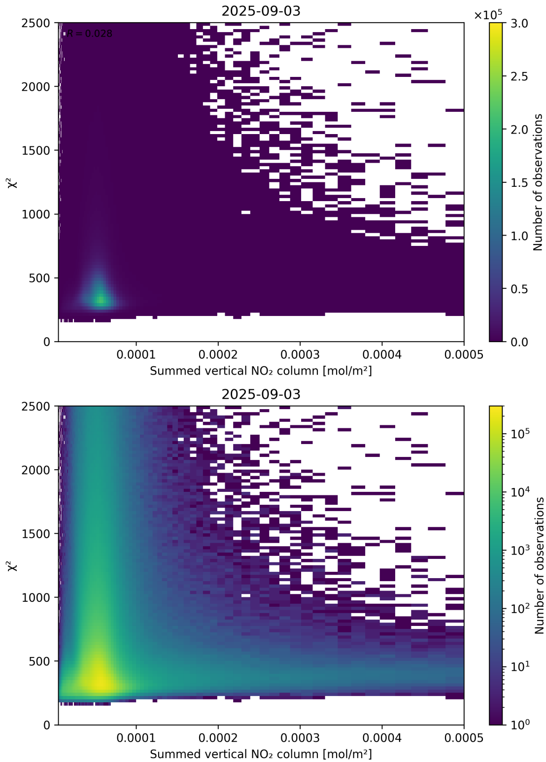
Figure 104: Scatter density plot of “Summed vertical NO 2 column” against “ \chi^2 ” for 2025-09-02 to 2025-09-04.
