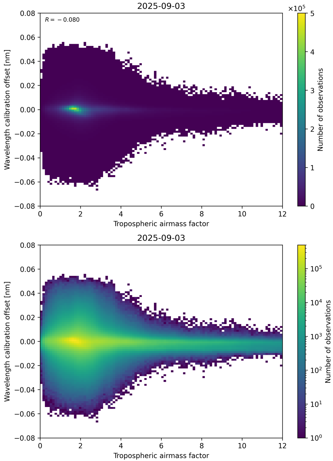
Figure 80: Scatter density plot of “Tropospheric airmass factor” against “Wavelength calibration offset” for 2025-09-02 to 2025-09-04.
