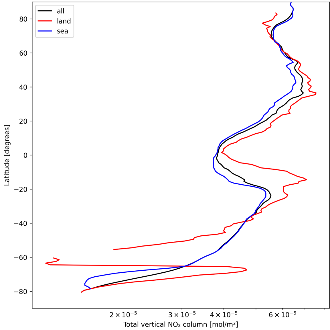
Figure 21: Zonal average of “Total vertical NO 2 column” for 2025-09-02 to 2025-09-04.
