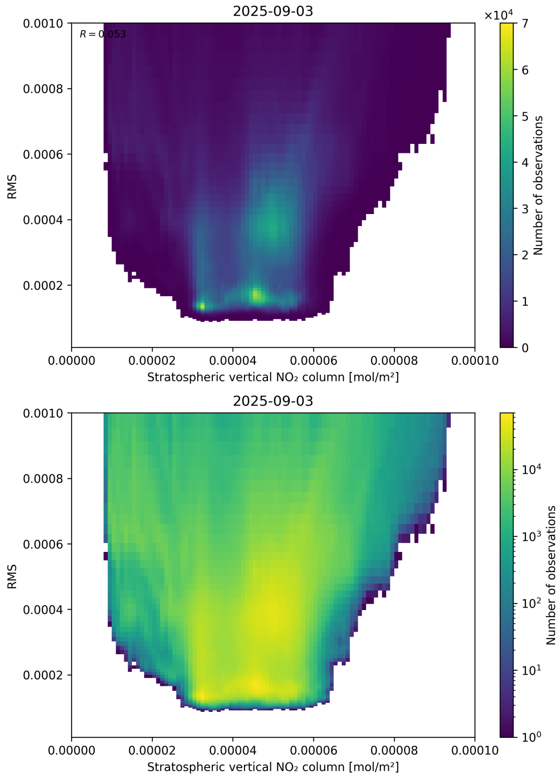
Figure 102: Scatter density plot of “Stratospheric vertical NO 2 column” against “RMS” for 2025-09-02 to 2025-09-04.
