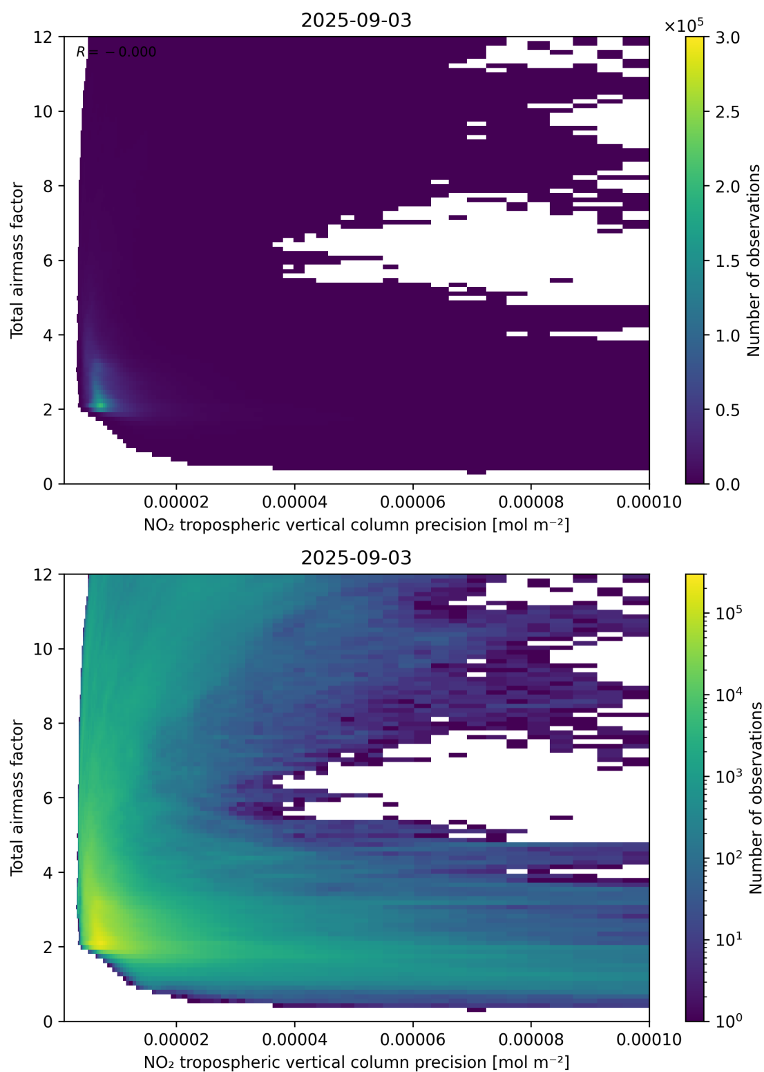
Figure 132: Scatter density plot of “NO 2 tropospheric vertical column precision” against “Total air mass factor” for 2025-09-02 to 2025-09-04.
