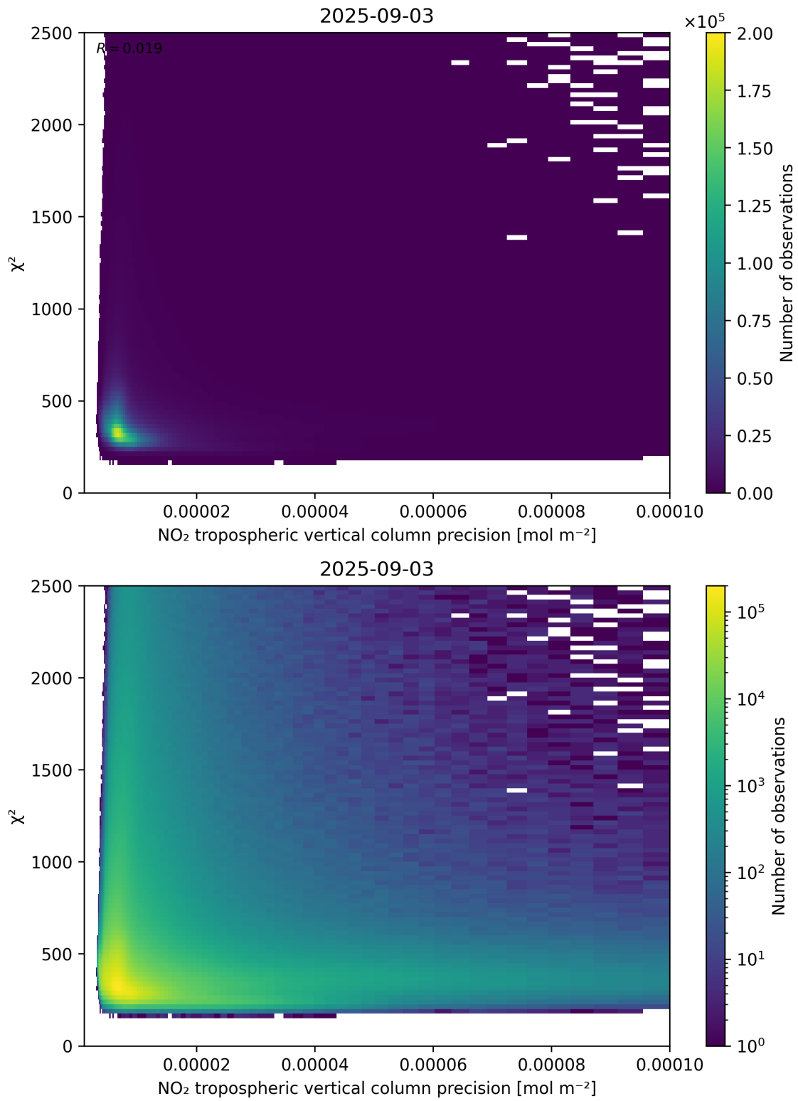
Figure 134: Scatter density plot of “NO 2 tropospheric vertical column precision” against “ \chi^2 ” for 2025-09-02 to 2025-09-04.
