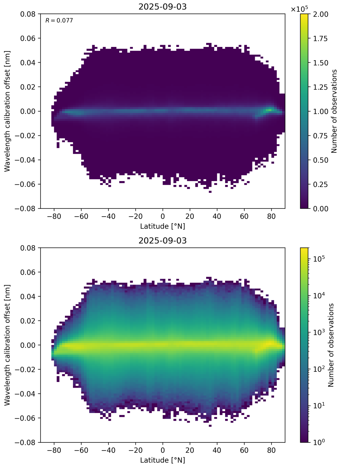
Figure 95: Scatter density plot of “Latitude” against “Wavelength calibration offset” for 2025-09-02 to 2025-09-04.
