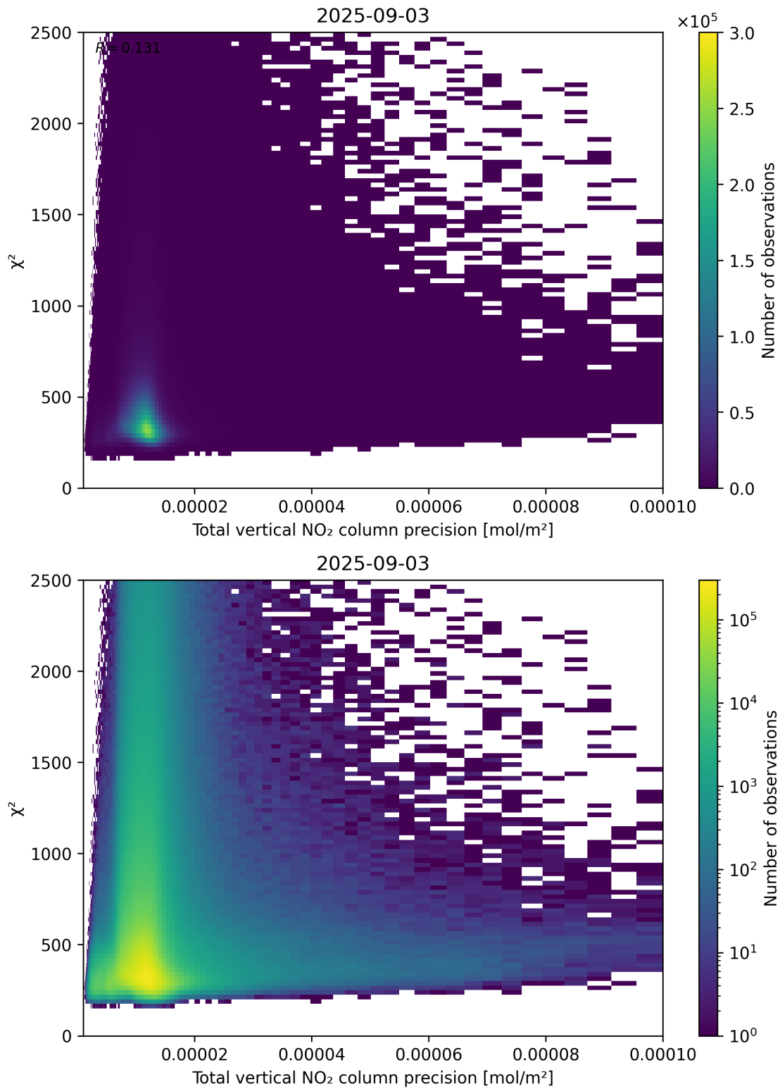
Figure 116: Scatter density plot of “Total vertical NO 2 column precision” against “ \chi^2 ” for 2025-09-02 to 2025-09-04.
