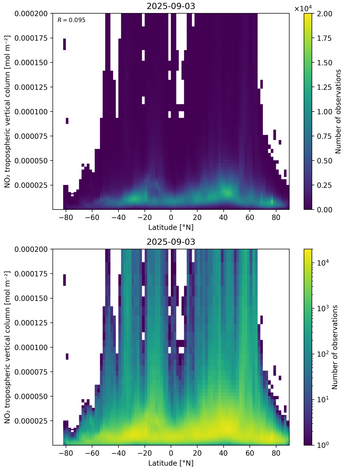
Figure 92: Scatter density plot of “Latitude” against “NO 2 tropospheric vertical column” for 2025-09-02 to 2025-09-04.
