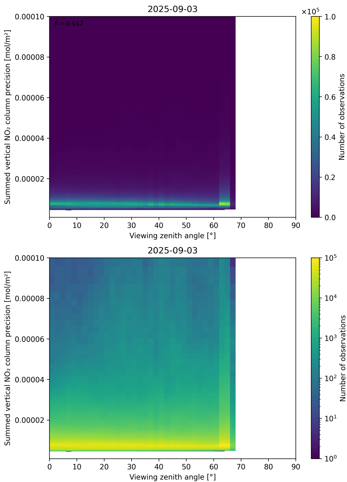
Figure 166: Scatter density plot of “Viewing zenith angle” against “Summed vertical NO 2 column precision” for 2025-09-02 to 2025-09-04.
