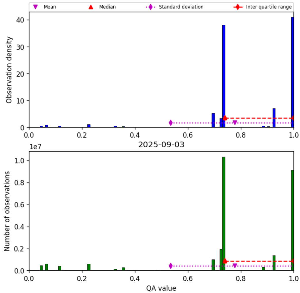
Figure 28: Histogram of “QA value” for 2025-09-02 to 2025-09-04
