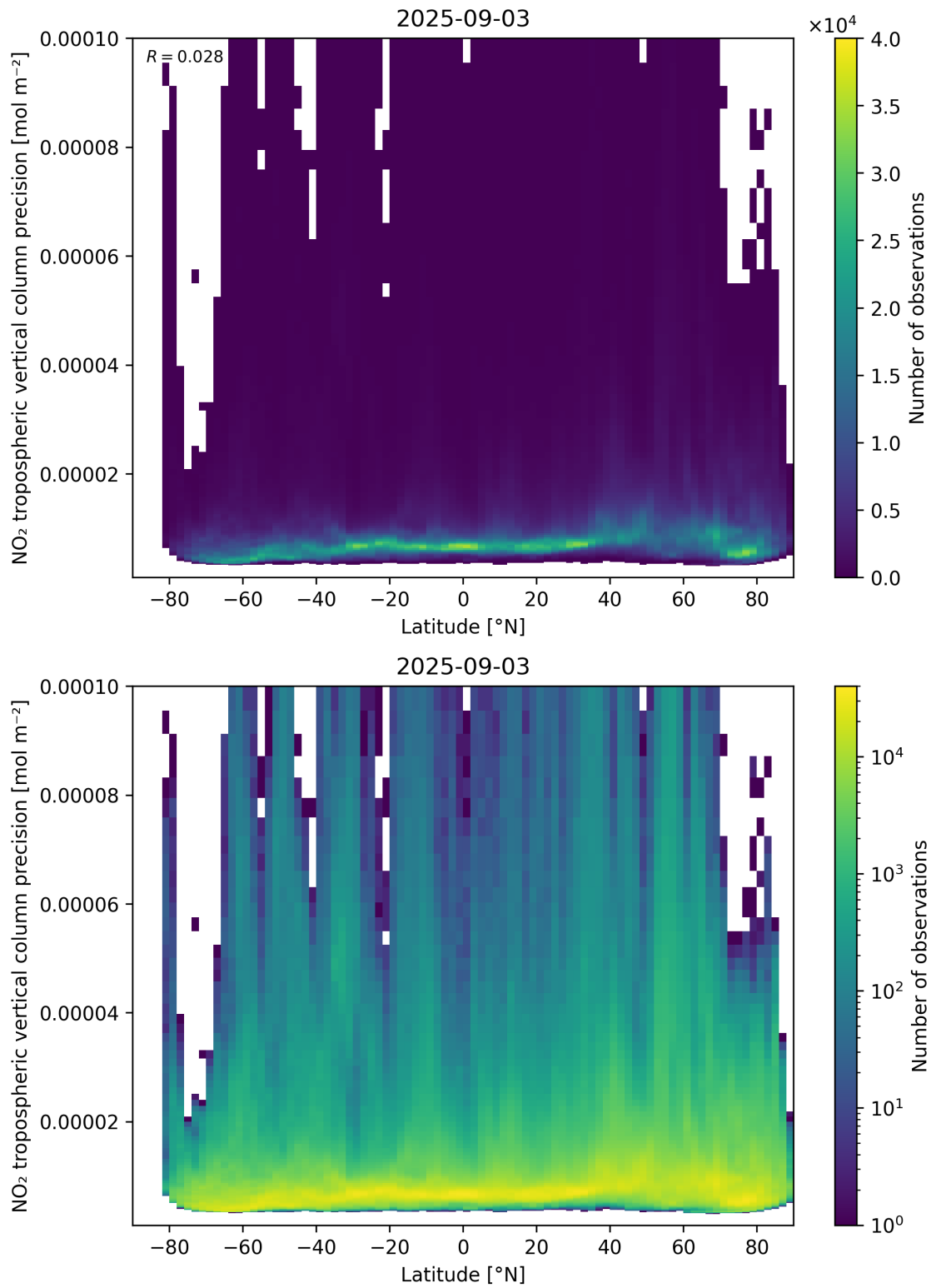
Figure 93: Scatter density plot of “Latitude” against “NO 2 tropospheric vertical column precision” for 2025-09-02 to 2025-09-04.
