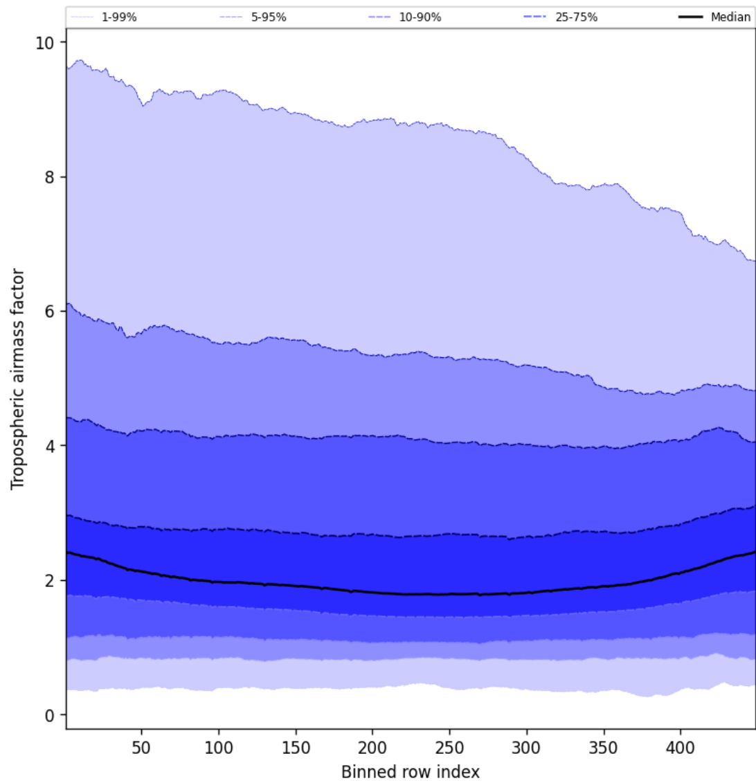
Figure 48: Along track statistics of “Tropospheric air mass factor” for 2025-09-02 to 2025-09-04
