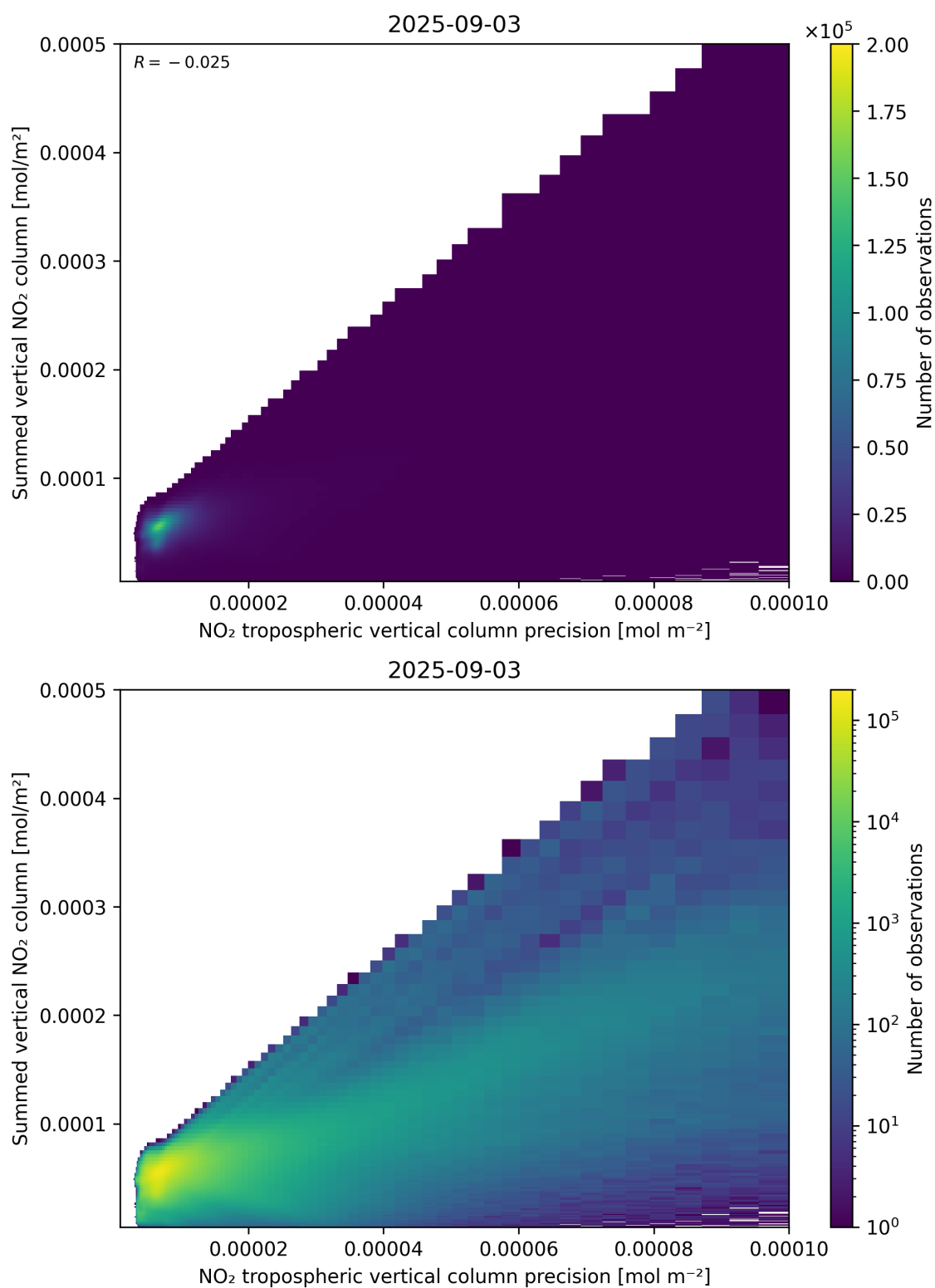
Figure 136: Scatter density plot of “NO 2 tropospheric vertical column precision” against “Summed vertical NO 2 column” for 2025-09-02 to 2025-09-04.
