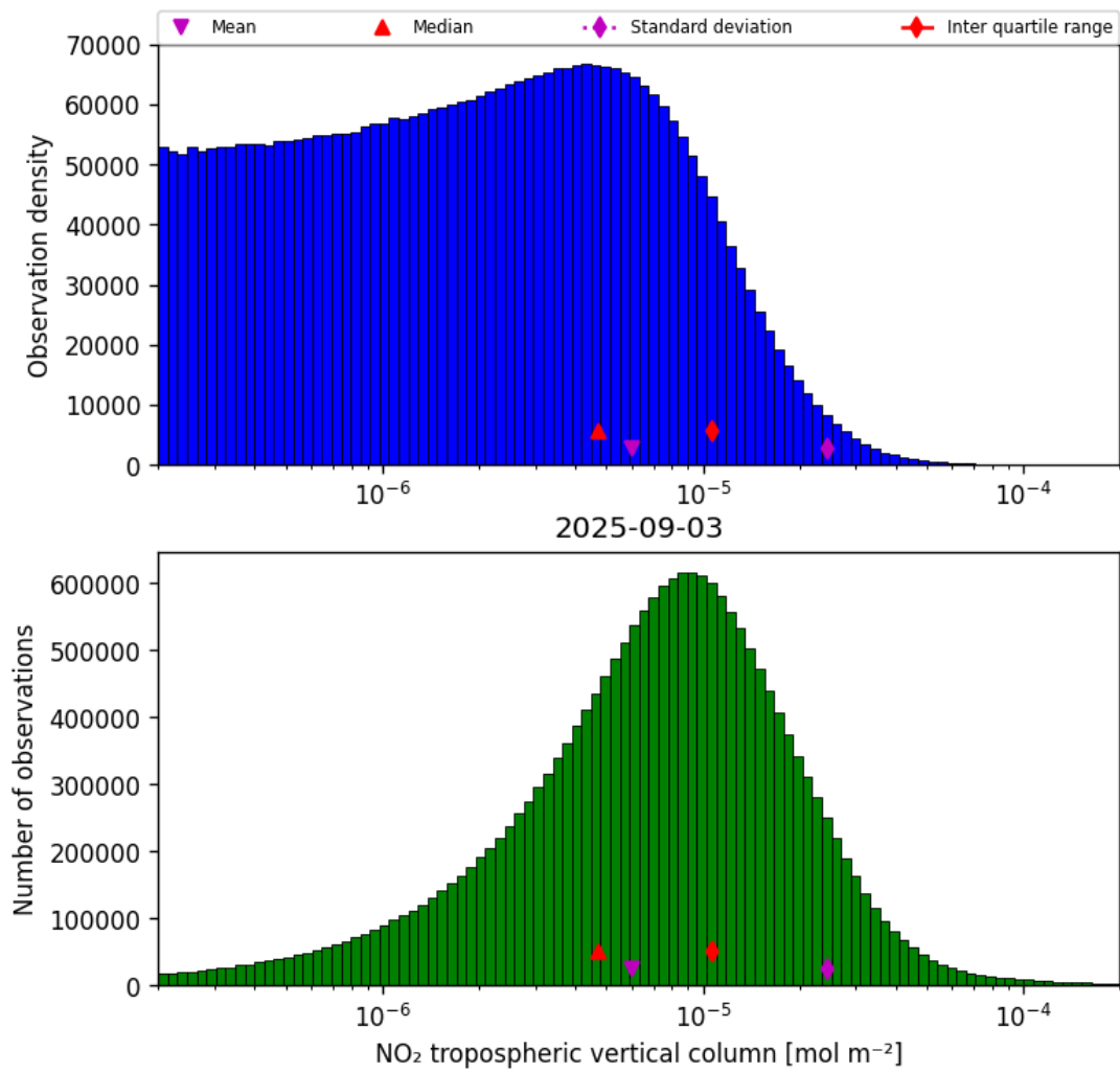
Figure 29: Histogram of “ \text{NO}_2 tropospheric vertical column” for 2025-09-02 to 2025-09-04
