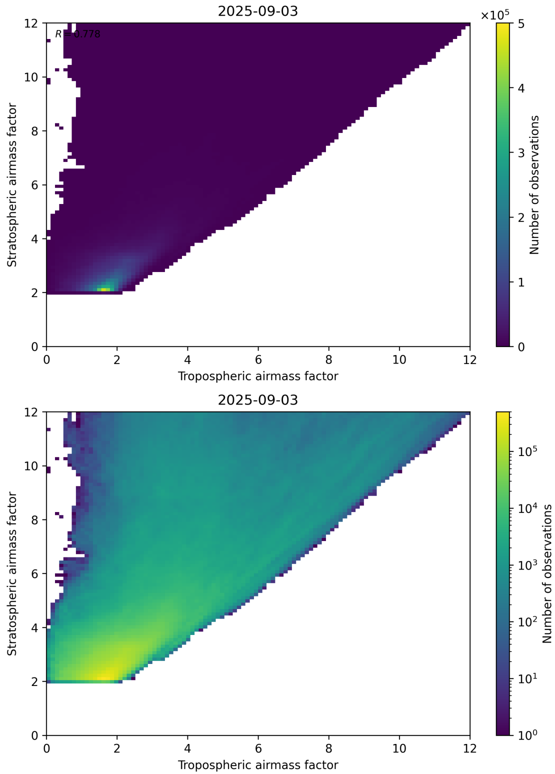
Figure 71: Scatter density plot of “Tropospheric airmass factor” against “Stratospheric airmass factor” for 2025-09-02 to 2025-09-04.
