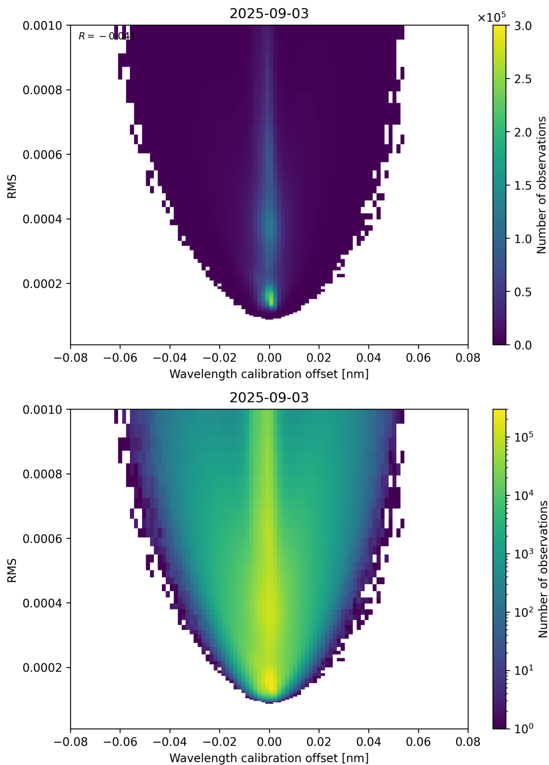
Figure 181: Scatter density plot of “Wavelength calibration offset” against “RMS” for 2025-09-02 to 2025-09-04.
