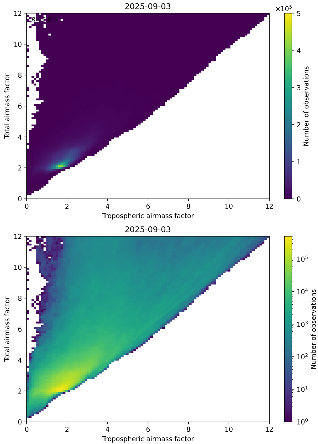
Figure 72: Scatter density plot of “Tropospheric airmass factor” against “Total airmass factor” for 2025-09-02 to 2025-09-04.
