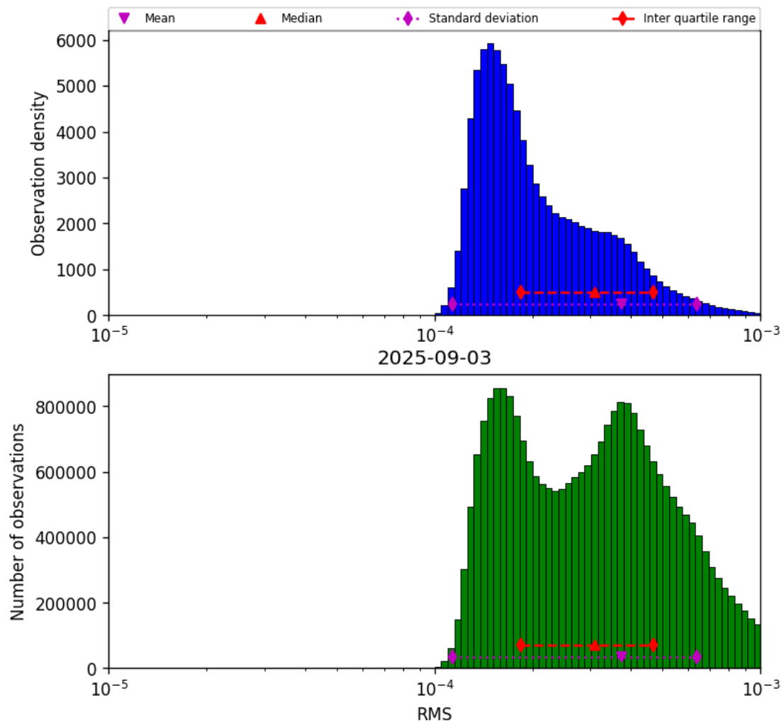
Figure 43: Histogram of “RMS” for 2025-09-02 to 2025-09-04
