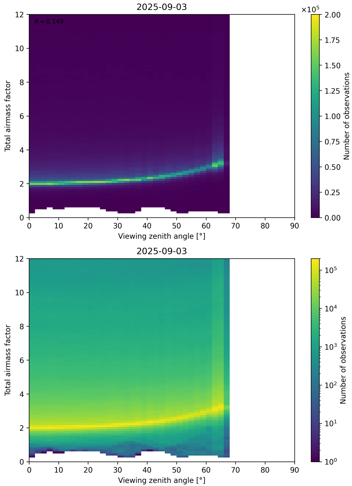
Figure 160: Scatter density plot of “Viewing zenith angle” against “Total airmass factor” for 2025-09-02 to 2025-09-04.
