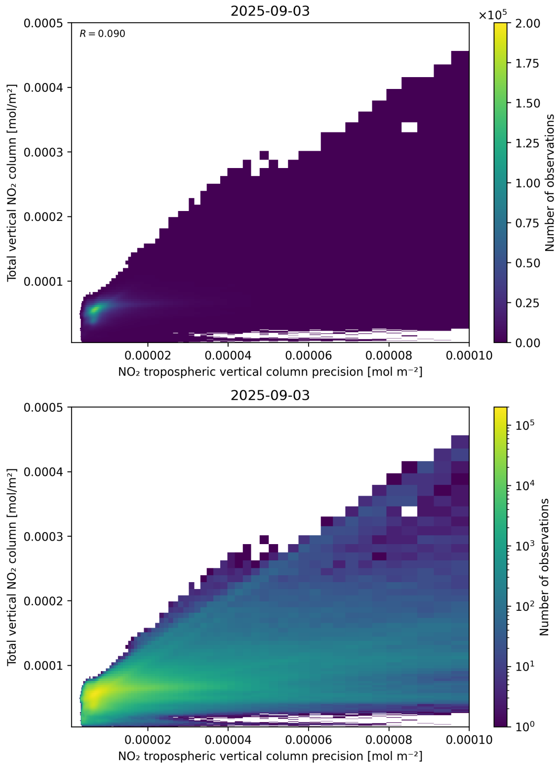
Figure 138: Scatter density plot of “NO 2 tropospheric vertical column precision” against “Total vertical NO 2 column” for 2025-09-02 to 2025-09-04.
