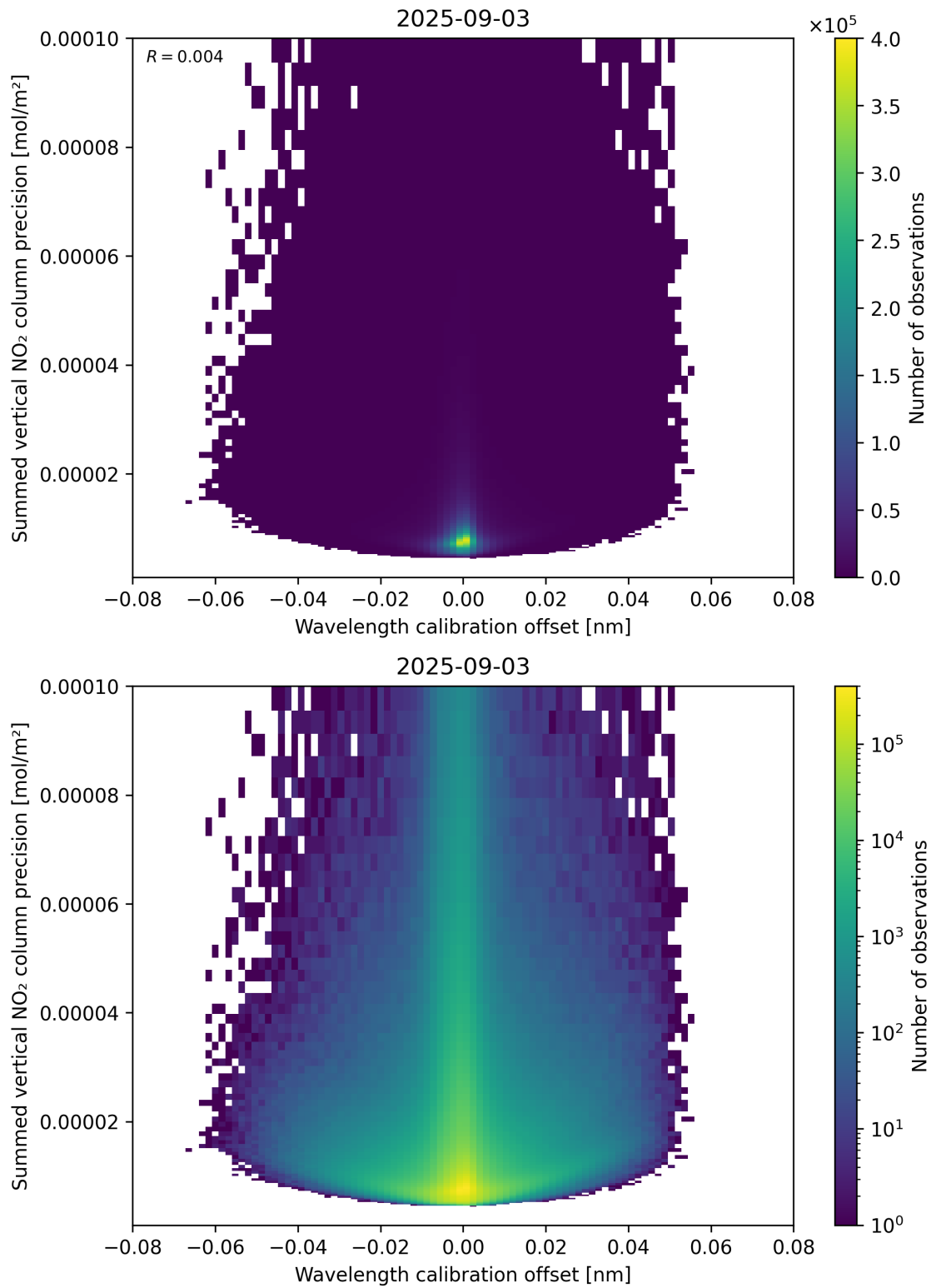
Figure 178: Scatter density plot of “Wavelength calibration offset” against “Summed vertical NO 2 column precision” for 2025-09-02 to 2025-09-04.
