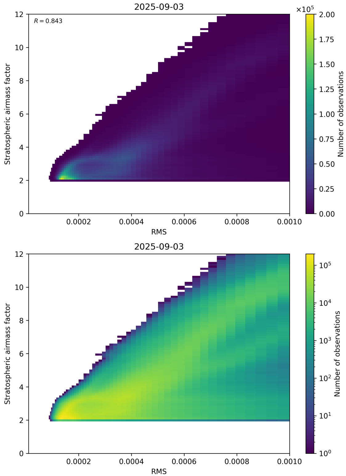
Figure 144: Scatter density plot of “RMS” against “Stratospheric airmass factor” for 2025-09-02 to 2025-09-04.
