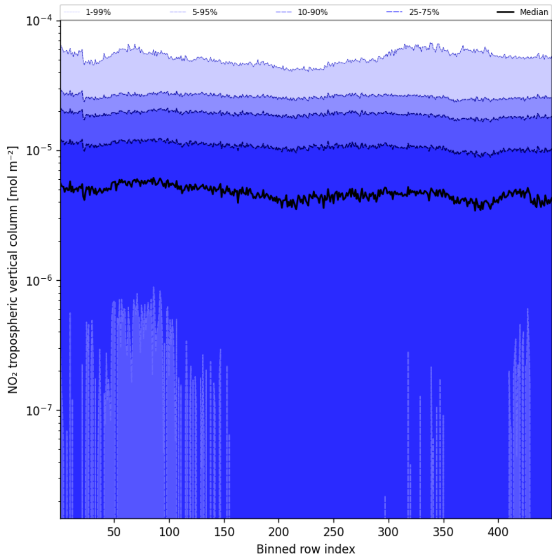
Figure 46: Along track statistics of “NO 2 tropospheric vertical column” for 2025-09-02 to 2025-09-04
