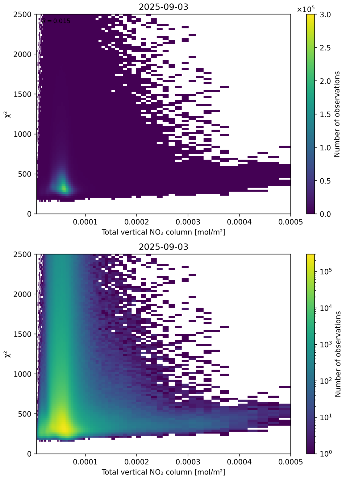
Figure 111: Scatter density plot of “Total vertical NO 2 column” against “ \chi^2 ” for 2025-09-02 to 2025-09-04.
