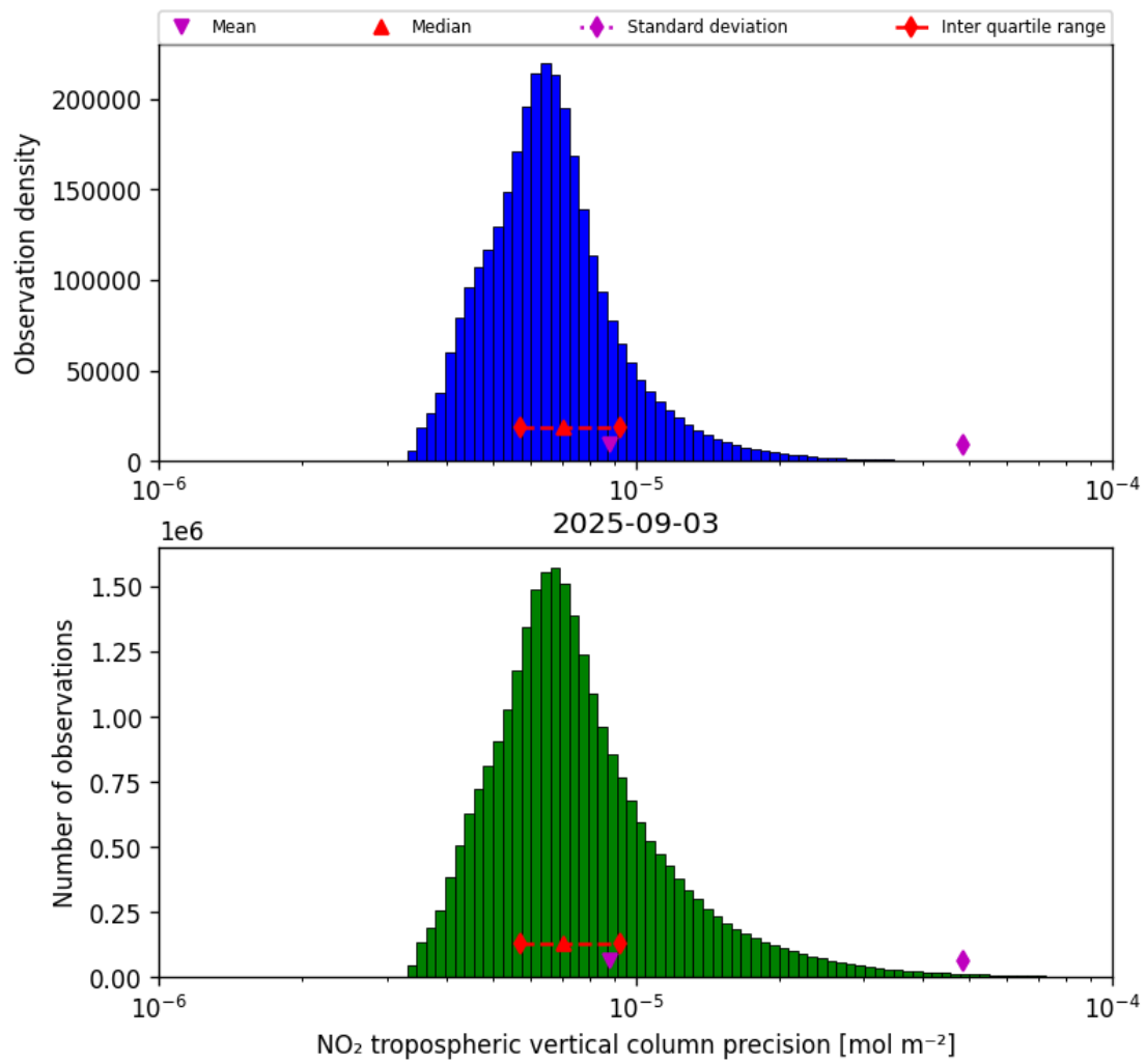
Figure 30: Histogram of “NO 2 tropospheric vertical column precision” for 2025-09-02 to 2025-09-04
