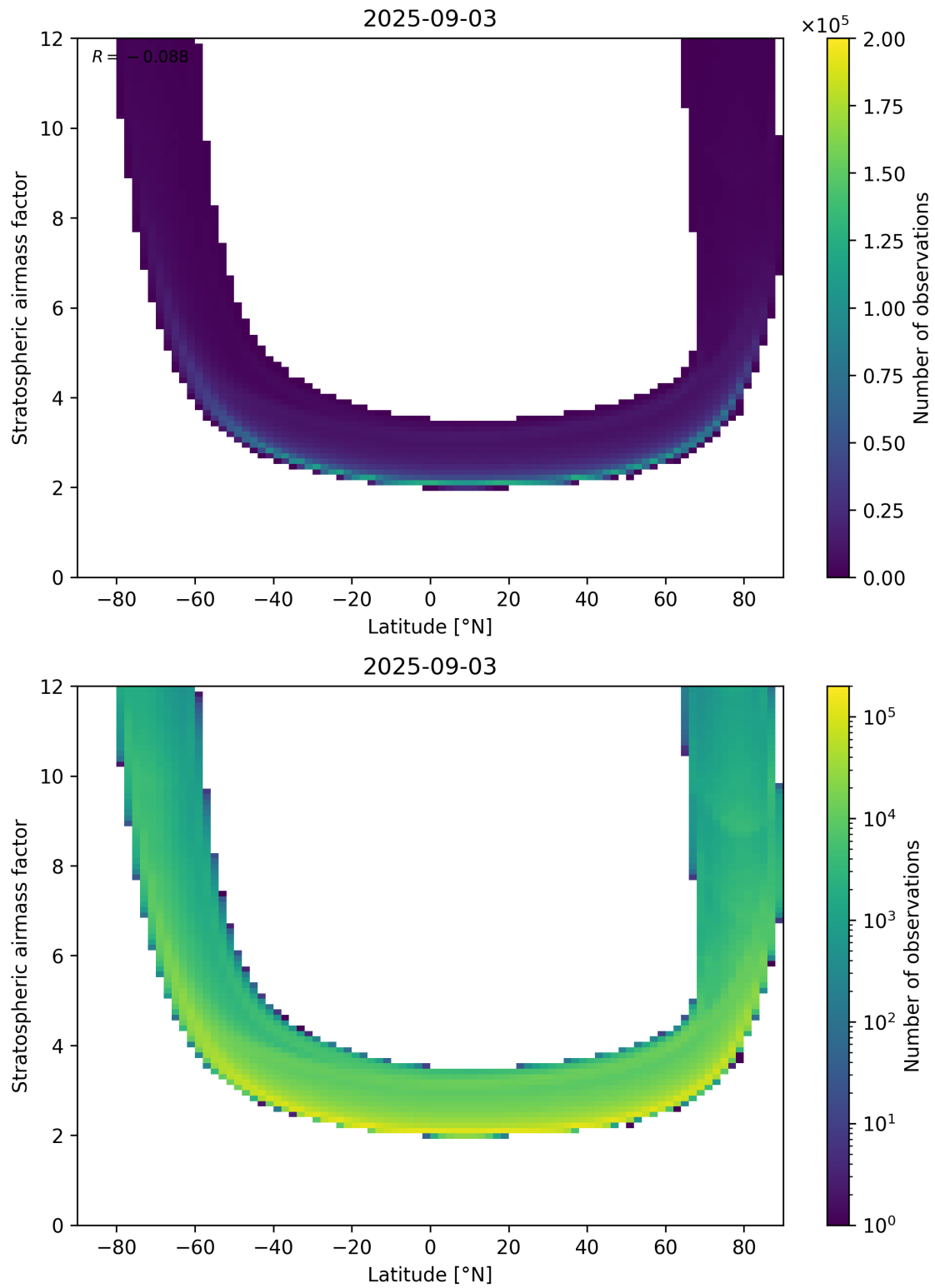
Figure 83: Scatter density plot of “Latitude” against “Stratospheric air mass factor” for 2025-09-02 to 2025-09-04.
