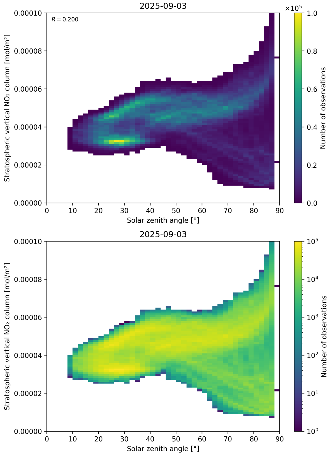
Figure 150: Scatter density plot of “Solar zenith angle” against “Stratospheric vertical NO 2 column” for 2025-09-02 to 2025-09-04.
