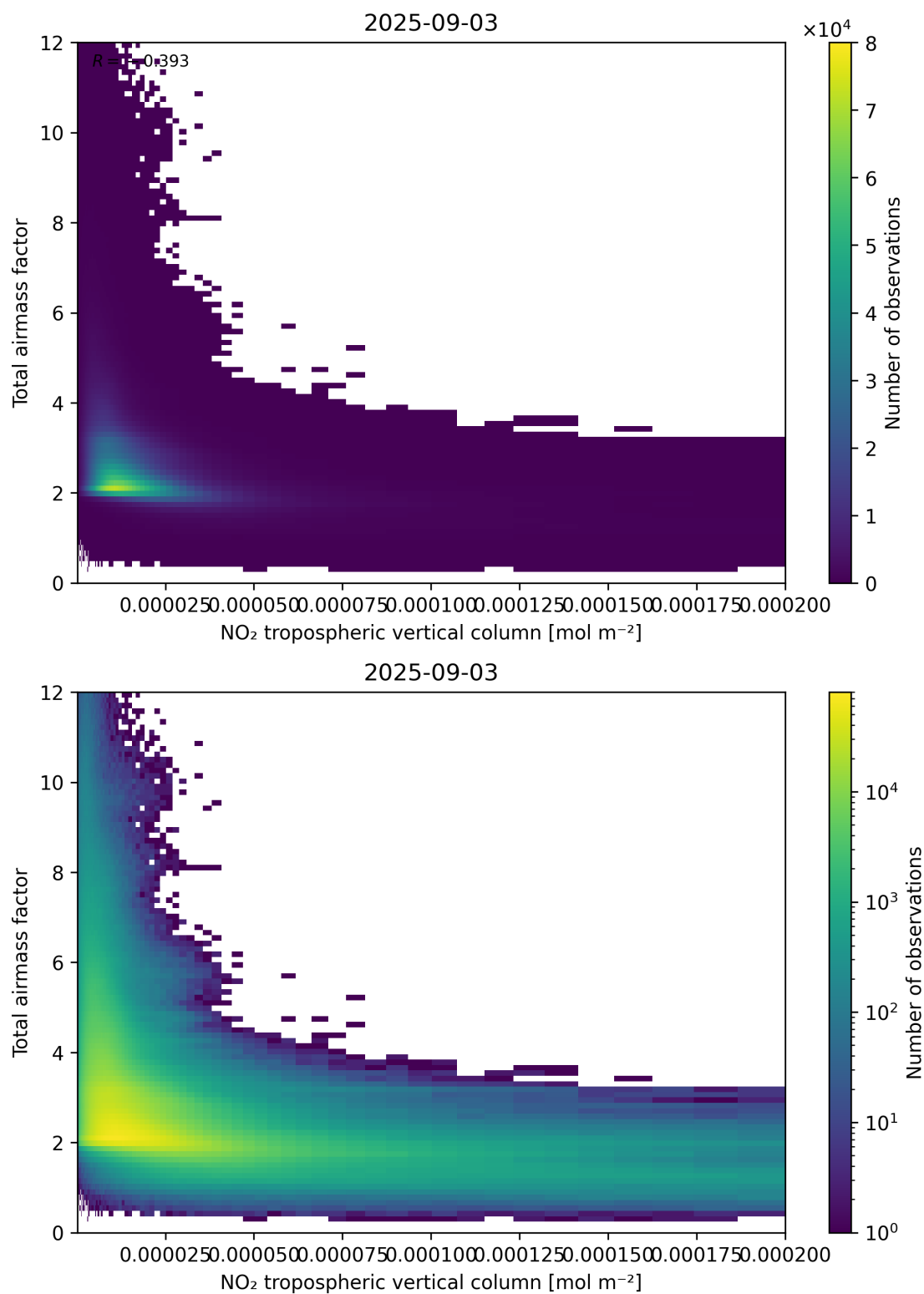
Figure 122: Scatter density plot of “NO 2 tropospheric vertical column” against “Total air mass factor” for 2025-09-02 to 2025-09-04.
