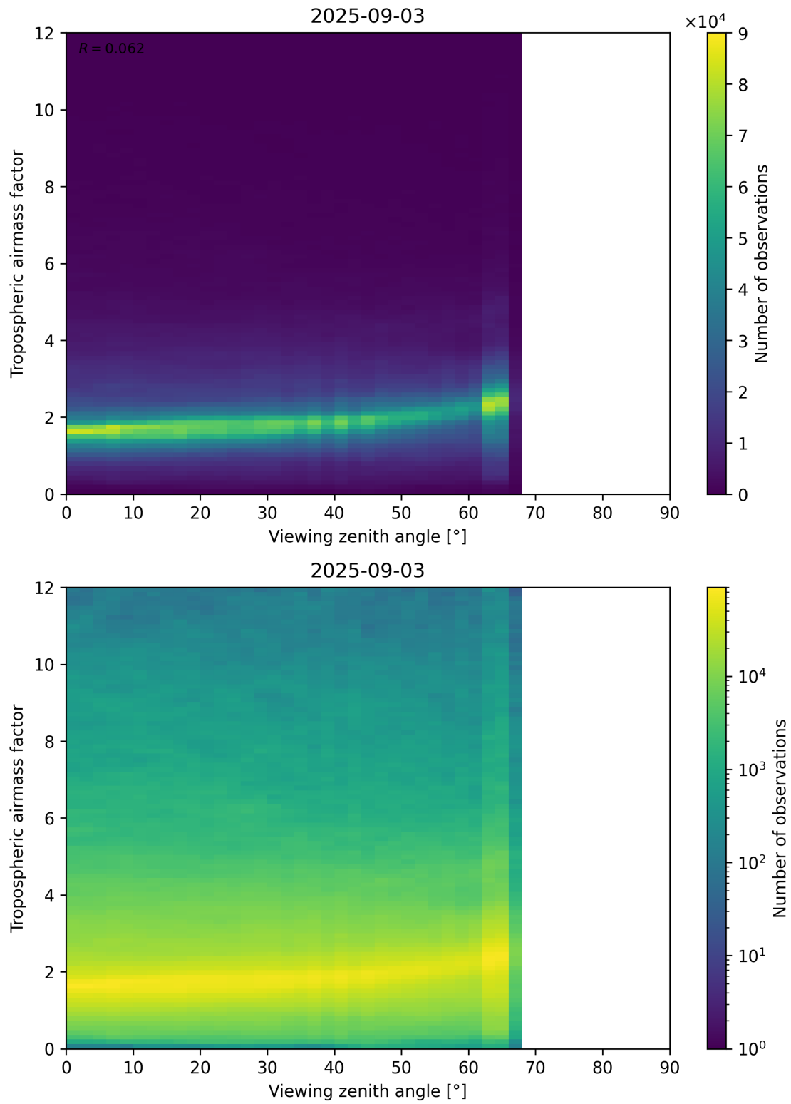
Figure 161: Scatter density plot of “Viewing zenith angle” against “Tropospheric airmass factor” for 2025-09-02 to 2025-09-04.
