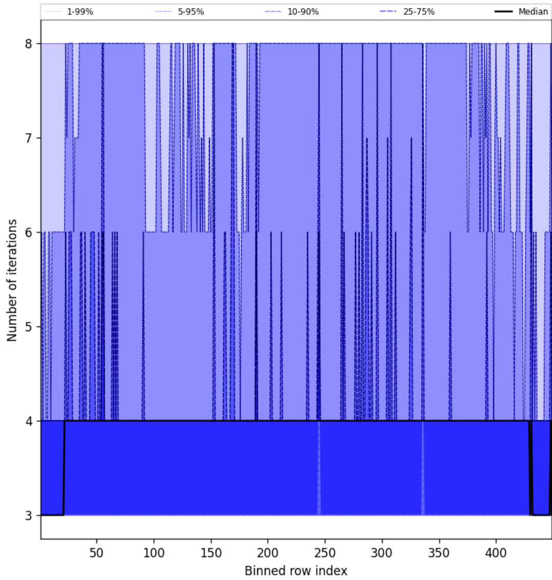
Figure 51: Along track statistics of “Number of iterations” for 2025-09-02 to 2025-09-04
