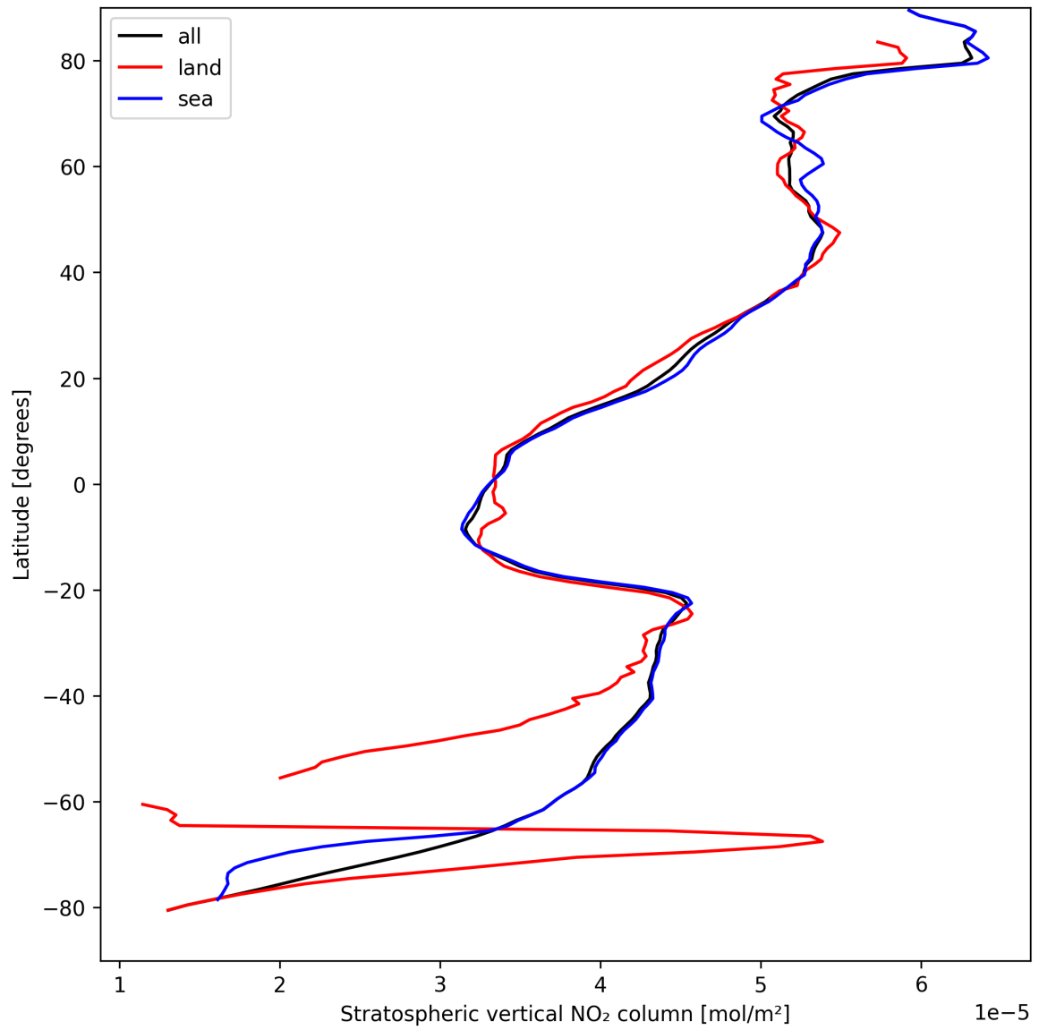
Figure 19: Zonal average of “Stratospheric vertical NO 2 column” for 2025-09-02 to 2025-09-04.
