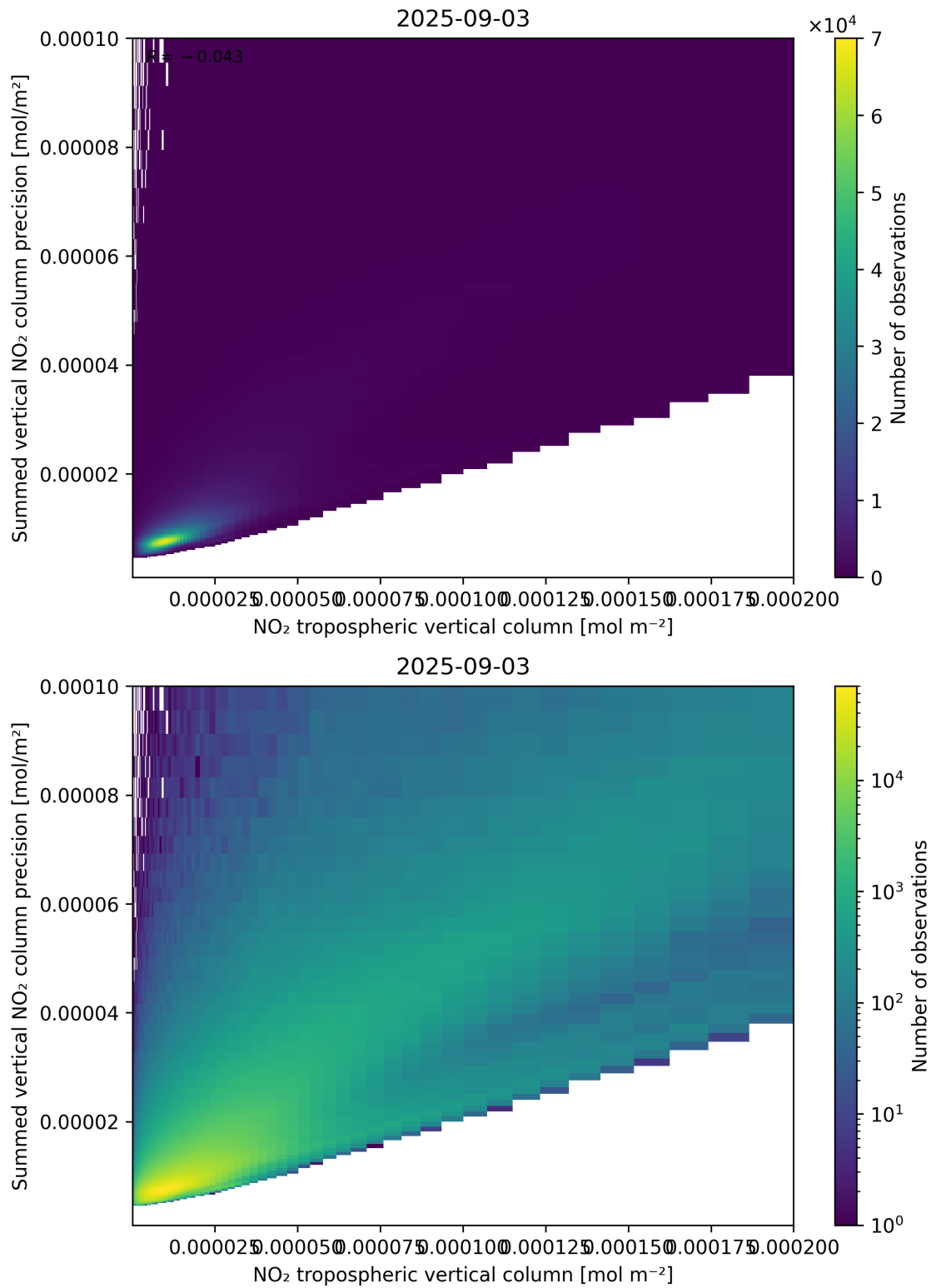
Figure 127: Scatter density plot of “NO 2 tropospheric vertical column” against “Summed vertical NO 2 column precision” for 2025-09-02 to 2025-09-04.
