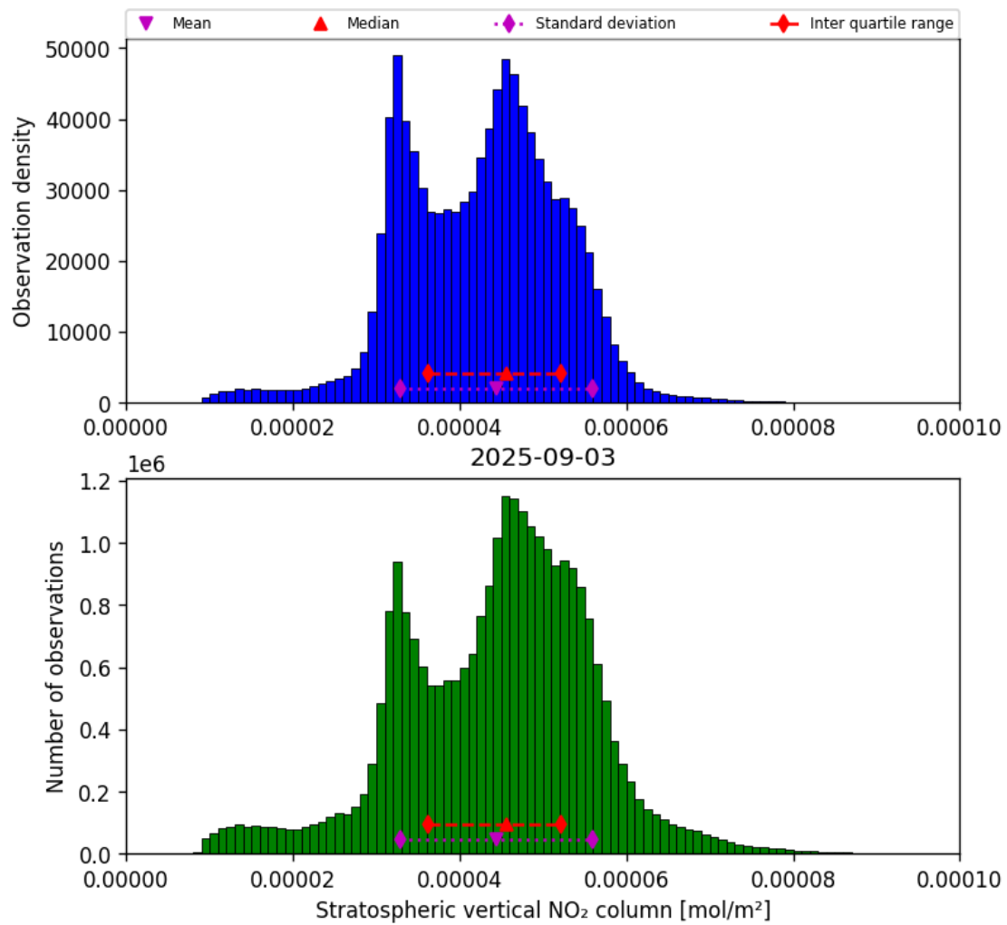
Figure 36: Histogram of “Stratospheric vertical NO 2 column” for 2025-09-02 to 2025-09-04
