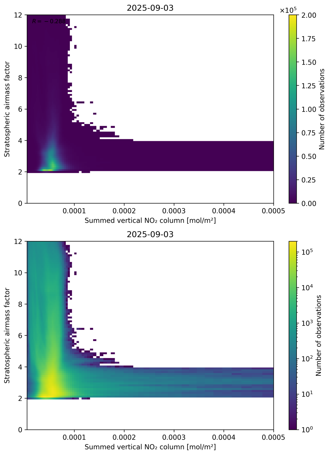
Figure 103: Scatter density plot of “Summed vertical NO 2 column” against “Stratospheric airmass factor” for 2025-09-02 to 2025-09-04.
