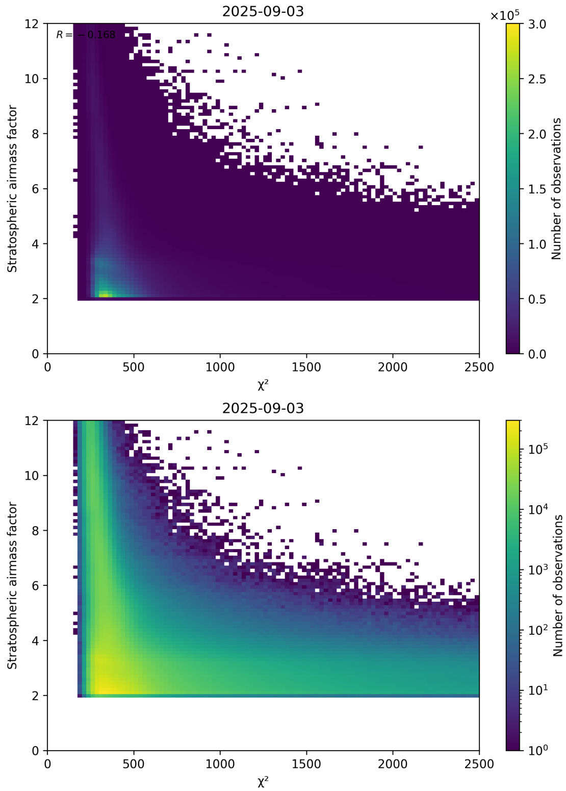
Figure 81: Scatter density plot of “ \chi^2 ” against “Stratospheric airmass factor” for 2025-09-02 to 2025-09-04.
