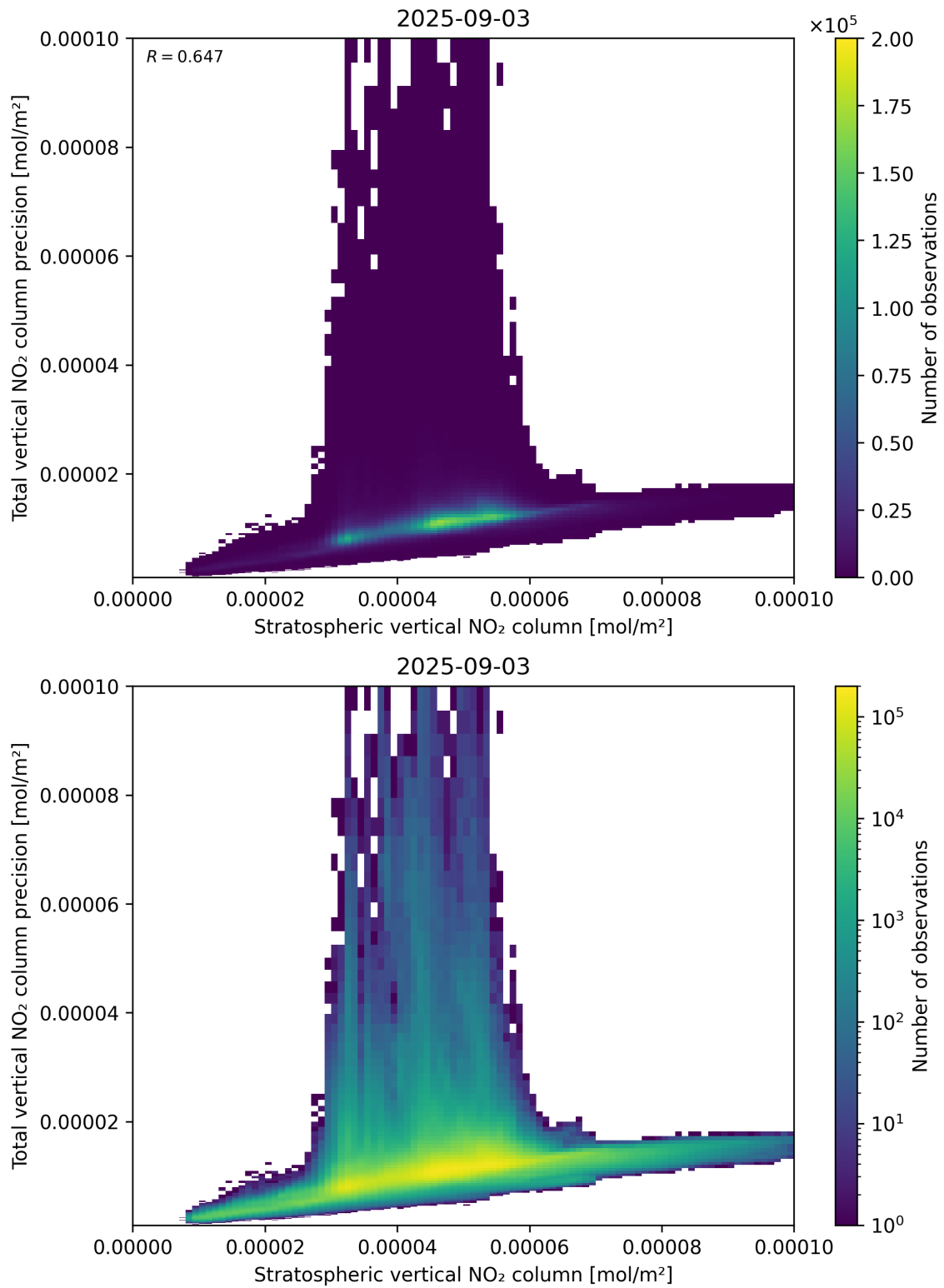
Figure 101: Scatter density plot of “Stratospheric vertical NO 2 column” against “Total vertical NO 2 column precision” for 2025-09-02 to 2025-09-04.
