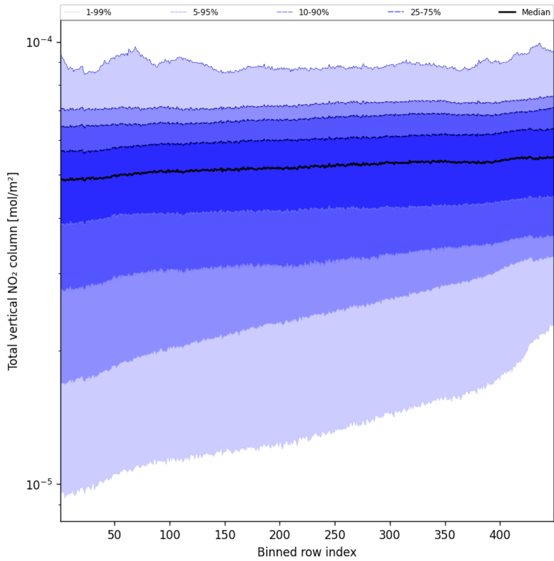
Figure 55: Along track statistics of “Total vertical NO 2 column” for 2025-09-02 to 2025-09-04
