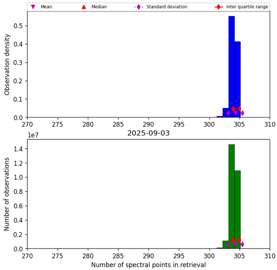
Figure 33: Histogram of “Number of spectral points in retrieval” for 2025-09-02 to 2025-09-04
