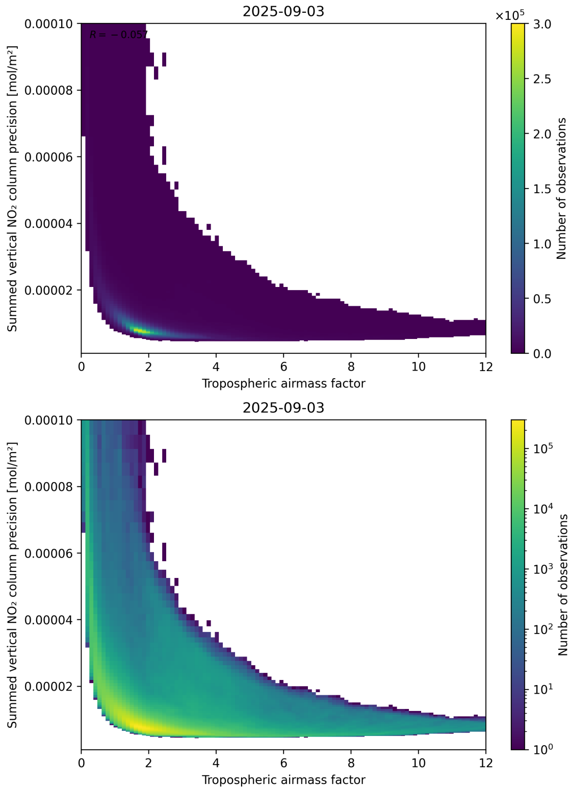
Figure 76: Scatter density plot of “Tropospheric air mass factor” against “Summed vertical NO 2 column precision” for 2025-09-02 to 2025-09-04.
