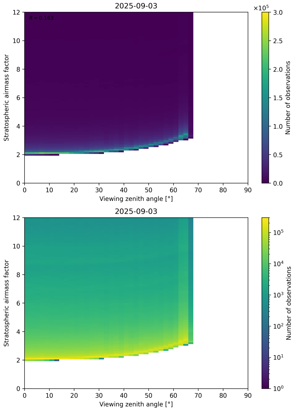
Figure 159: Scatter density plot of “Viewing zenith angle” against “Stratospheric airmass factor” for 2025-09-02 to 2025-09-04.
