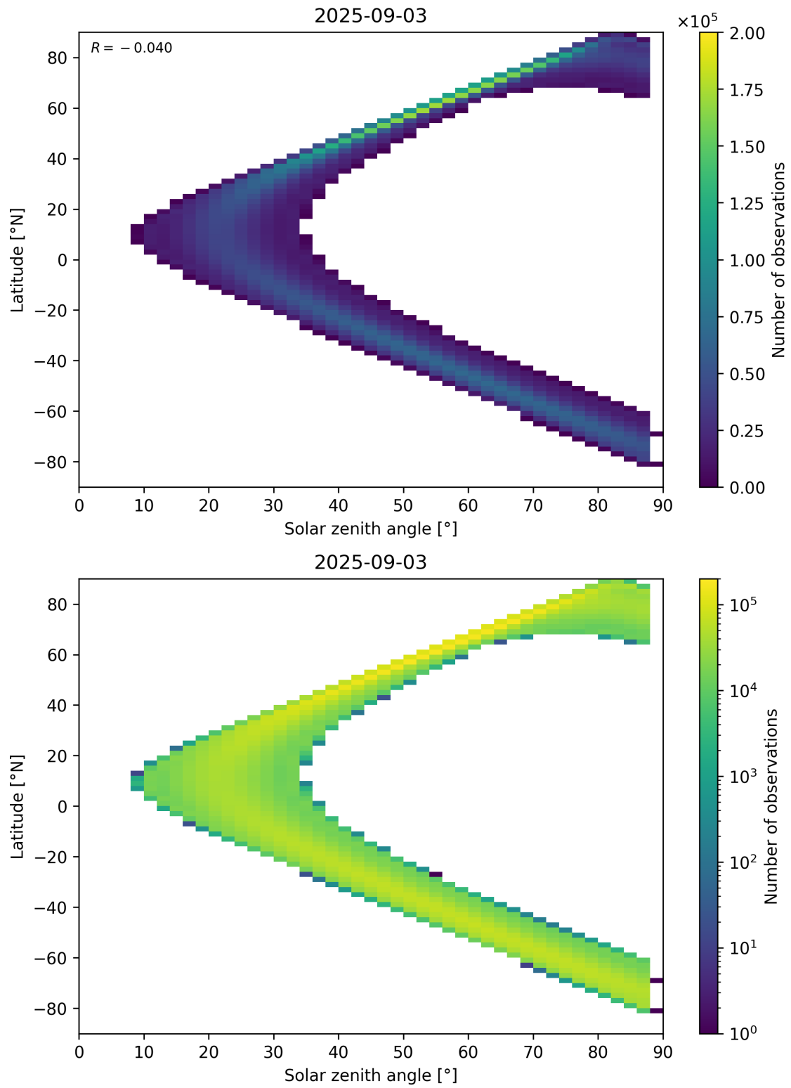
Figure 149: Scatter density plot of “Solar zenith angle” against “Latitude” for 2025-09-02 to 2025-09-04.
