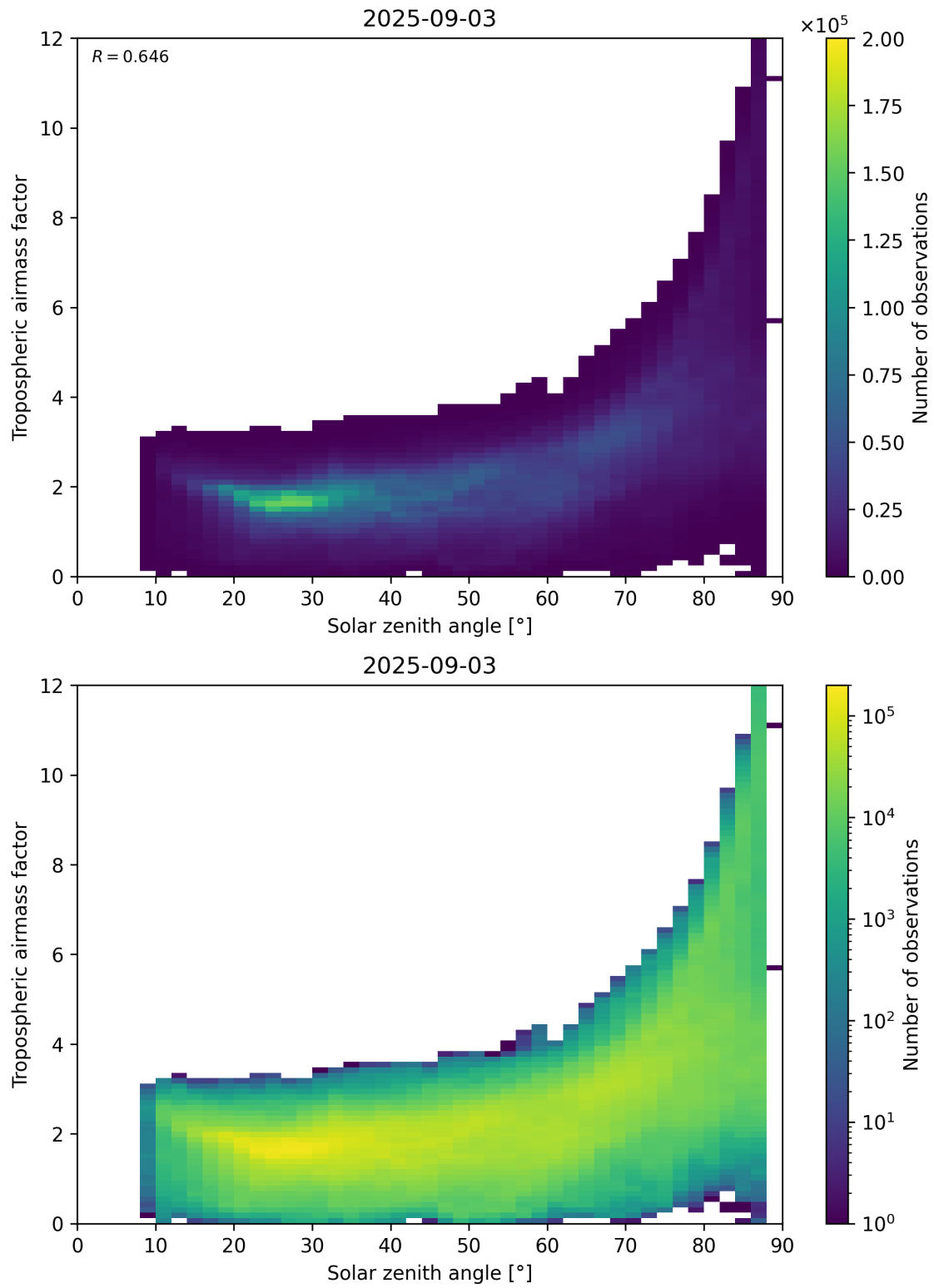
Figure 147: Scatter density plot of “Solar zenith angle” against “Tropospheric airmass factor” for 2025-09-02 to 2025-09-04.
