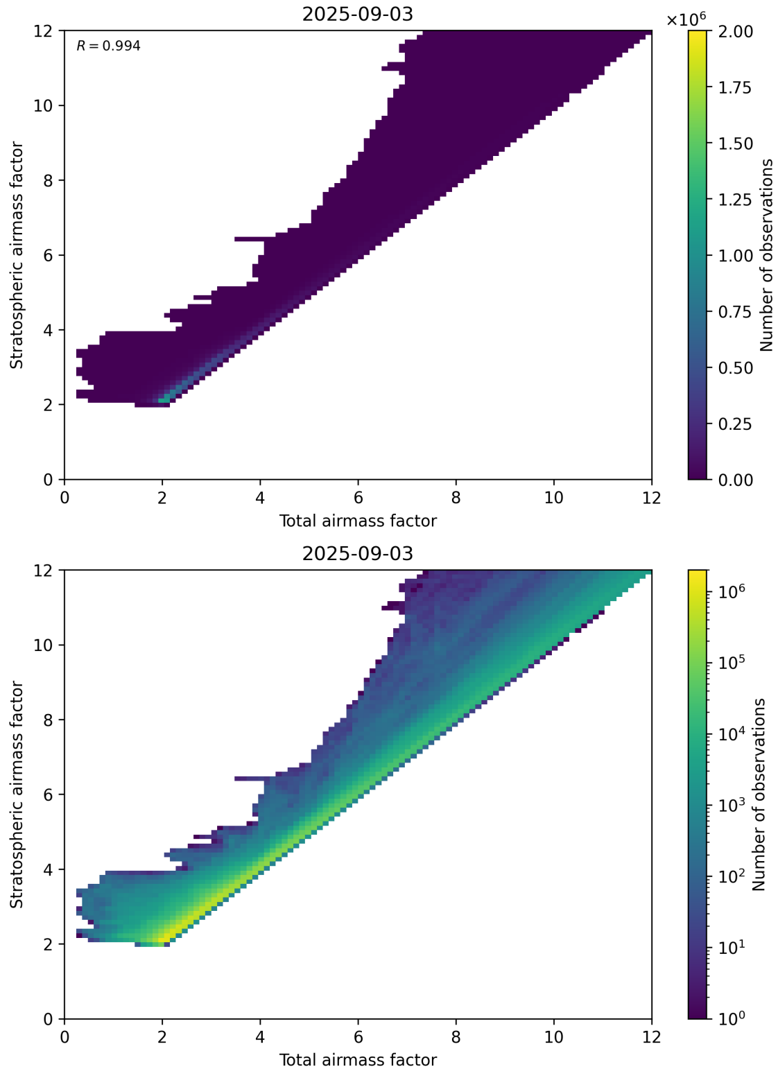
Figure 62: Scatter density plot of “Total airmass factor” against “Stratospheric airmass factor” for 2025-09-02 to 2025-09-04.
