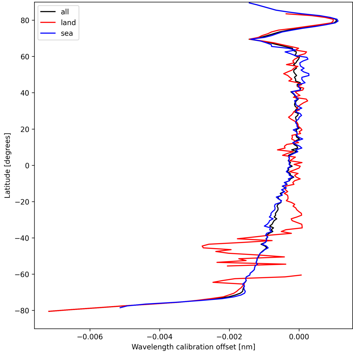
Figure 18: Zonal average of “Wavelength calibration offset” for 2025-09-02 to 2025-09-04.
