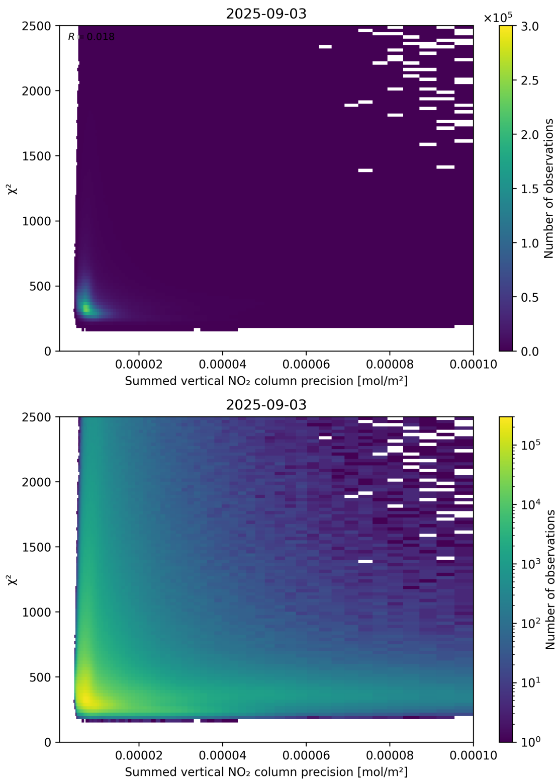
Figure 107: Scatter density plot of “Summed vertical NO 2 column precision” against “ \chi^2 ” for 2025-09-02 to 2025-09-04.
