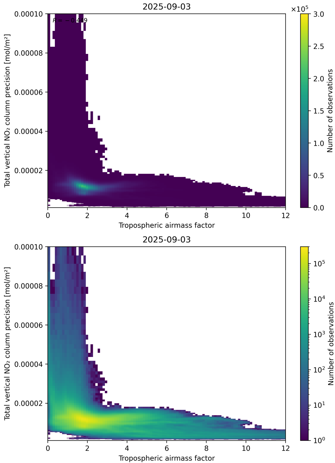
Figure 78: Scatter density plot of “Tropospheric airmass factor” against “Total vertical NO 2 column precision” for 2025-09-02 to 2025-09-04.
