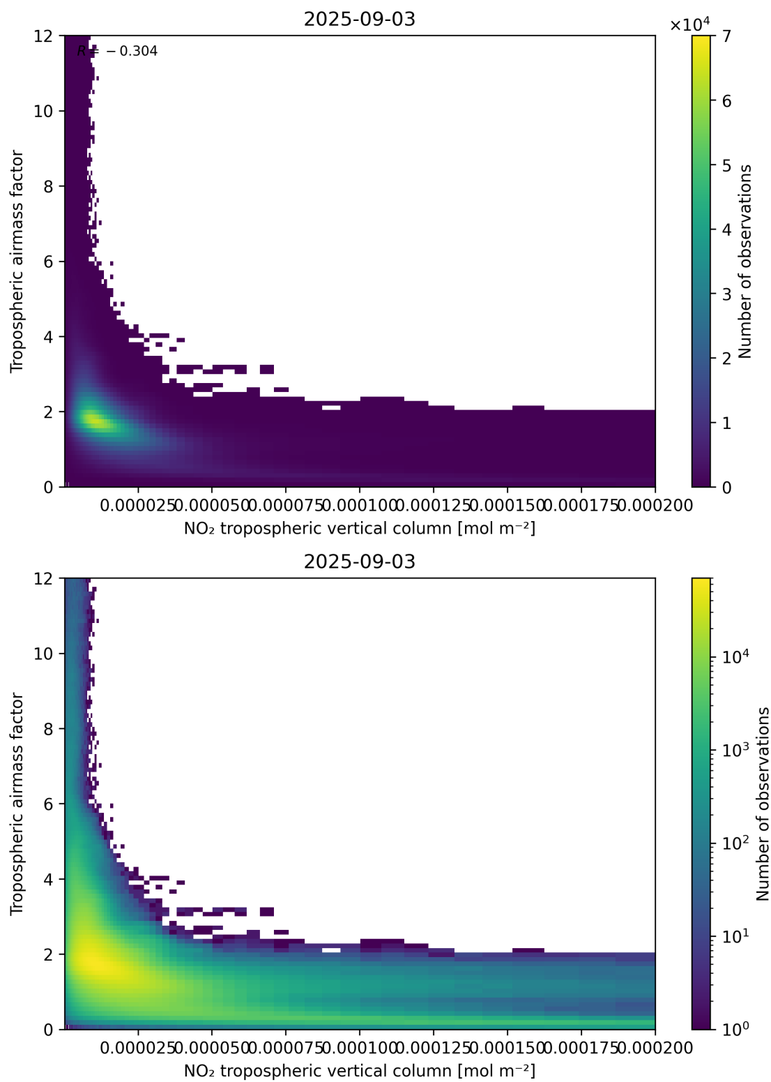
Figure 123: Scatter density plot of “NO 2 tropospheric vertical column” against “Tropospheric air mass factor” for 2025-09-02 to 2025-09-04.
