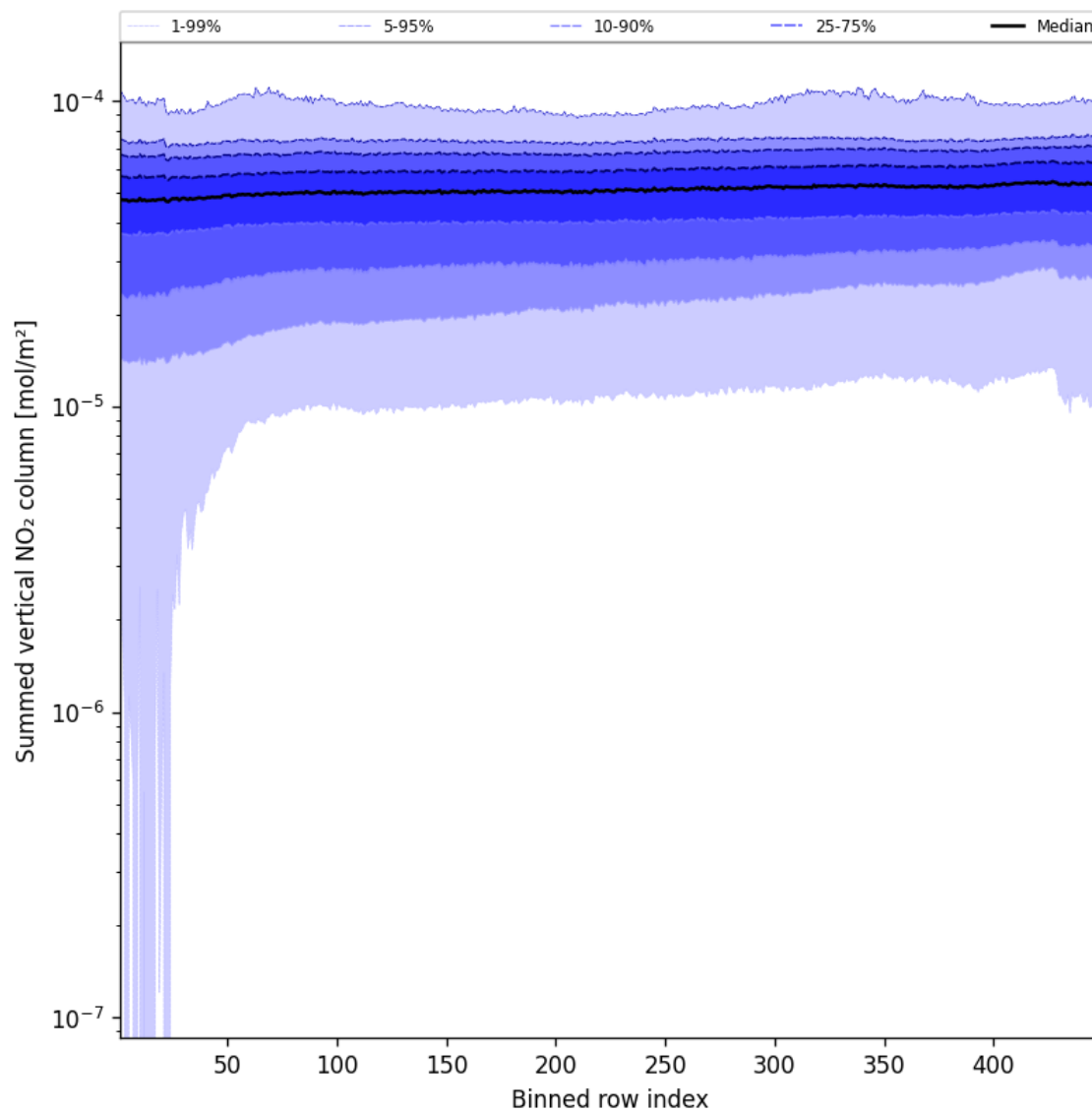
Figure 57: Along track statistics of “Summed vertical NO 2 column” for 2025-09-02 to 2025-09-04
