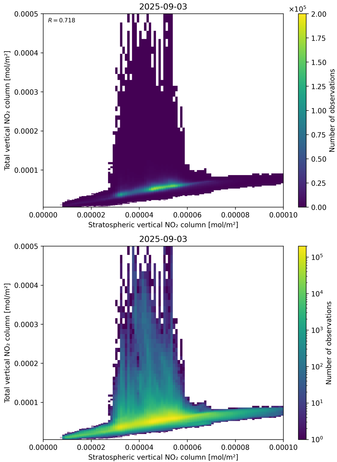
Figure 100: Scatter density plot of “Stratospheric vertical NO 2 column” against “Total vertical NO 2 column” for 2025-09-02 to 2025-09-04.
