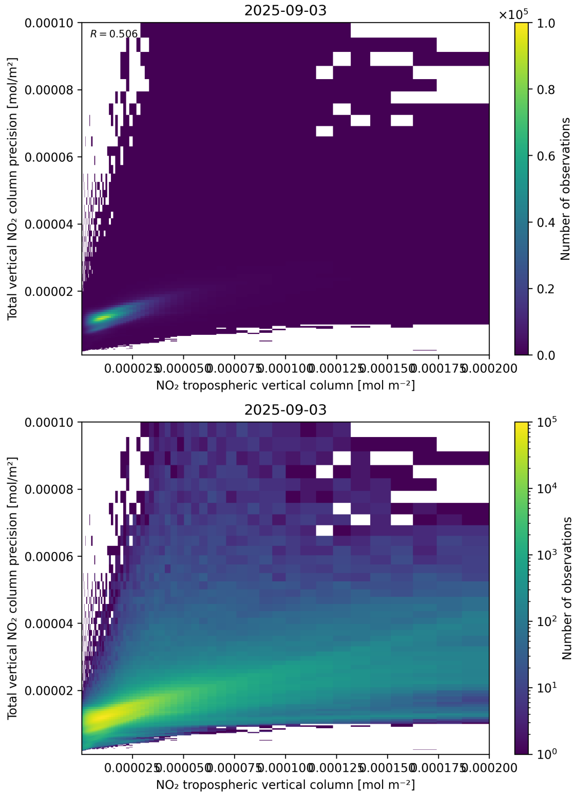
Figure 129: Scatter density plot of “NO 2 tropospheric vertical column” against “Total vertical NO 2 column precision” for 2025-09-02 to 2025-09-04.
