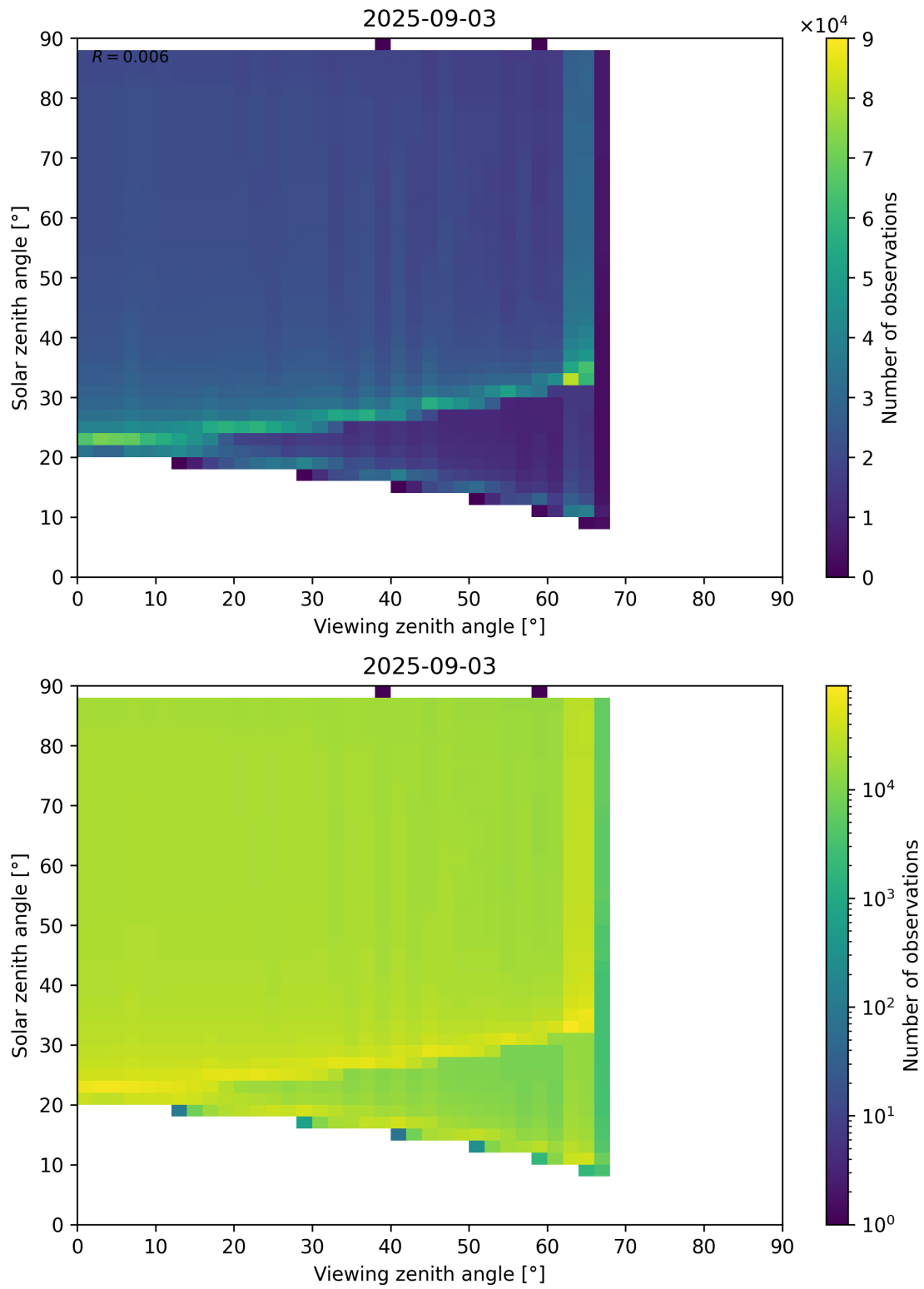
Figure 172: Scatter density plot of “Viewing zenith angle” against “Solar zenith angle” for 2025-09-02 to 2025-09-04.
