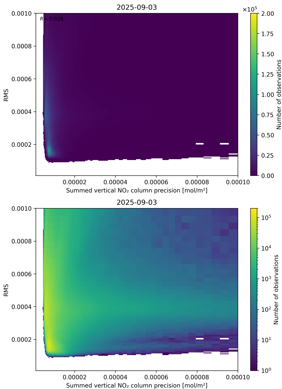
Figure 108: Scatter density plot of “Summed vertical NO 2 column precision” against “RMS” for 2025-09-02 to 2025-09-04.
