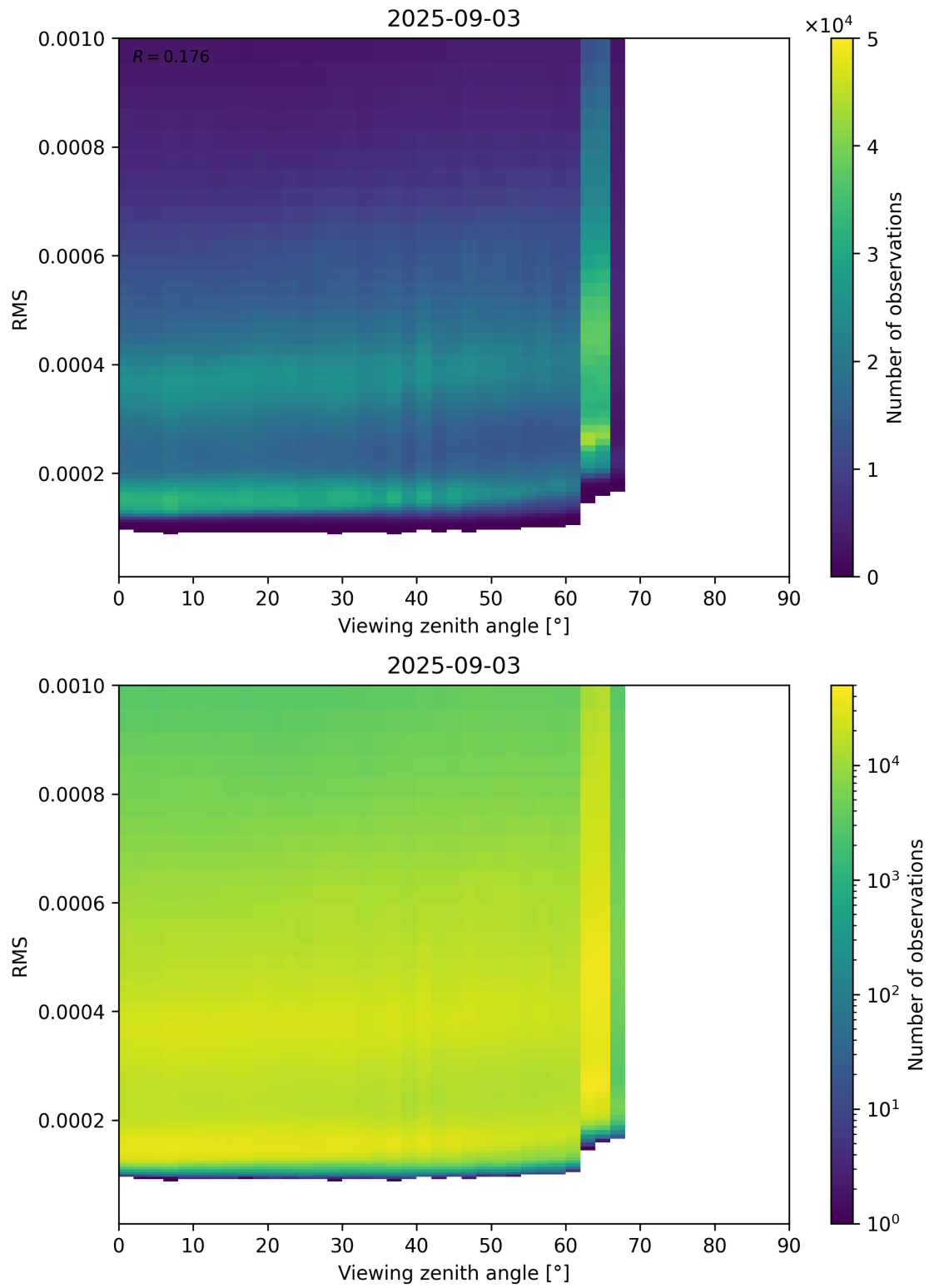
Figure 171: Scatter density plot of “Viewing zenith angle” against “RMS” for 2025-09-02 to 2025-09-04.
