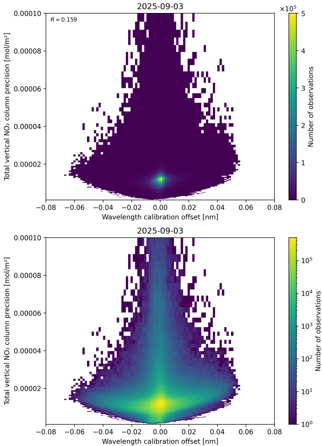
Figure 180: Scatter density plot of “Wavelength calibration offset” against “Total vertical NO 2 column precision” for 2025-09-02 to 2025-09-04.
