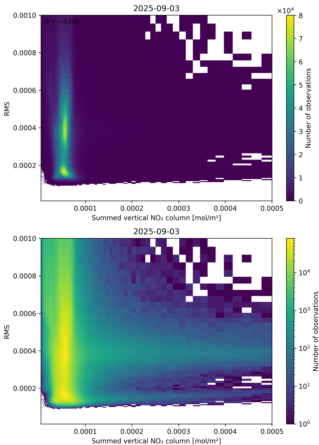
Figure 109: Scatter density plot of “Summed vertical NO 2 column” against “RMS” for 2025-09-02 to 2025-09-04.
