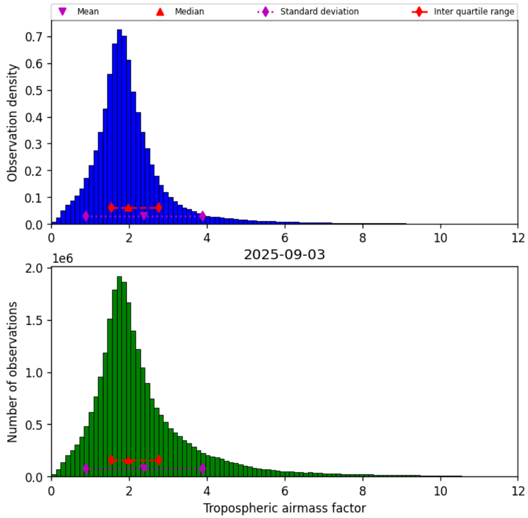
Figure 31: Histogram of “Tropospheric airmass factor” for 2025-09-02 to 2025-09-04
