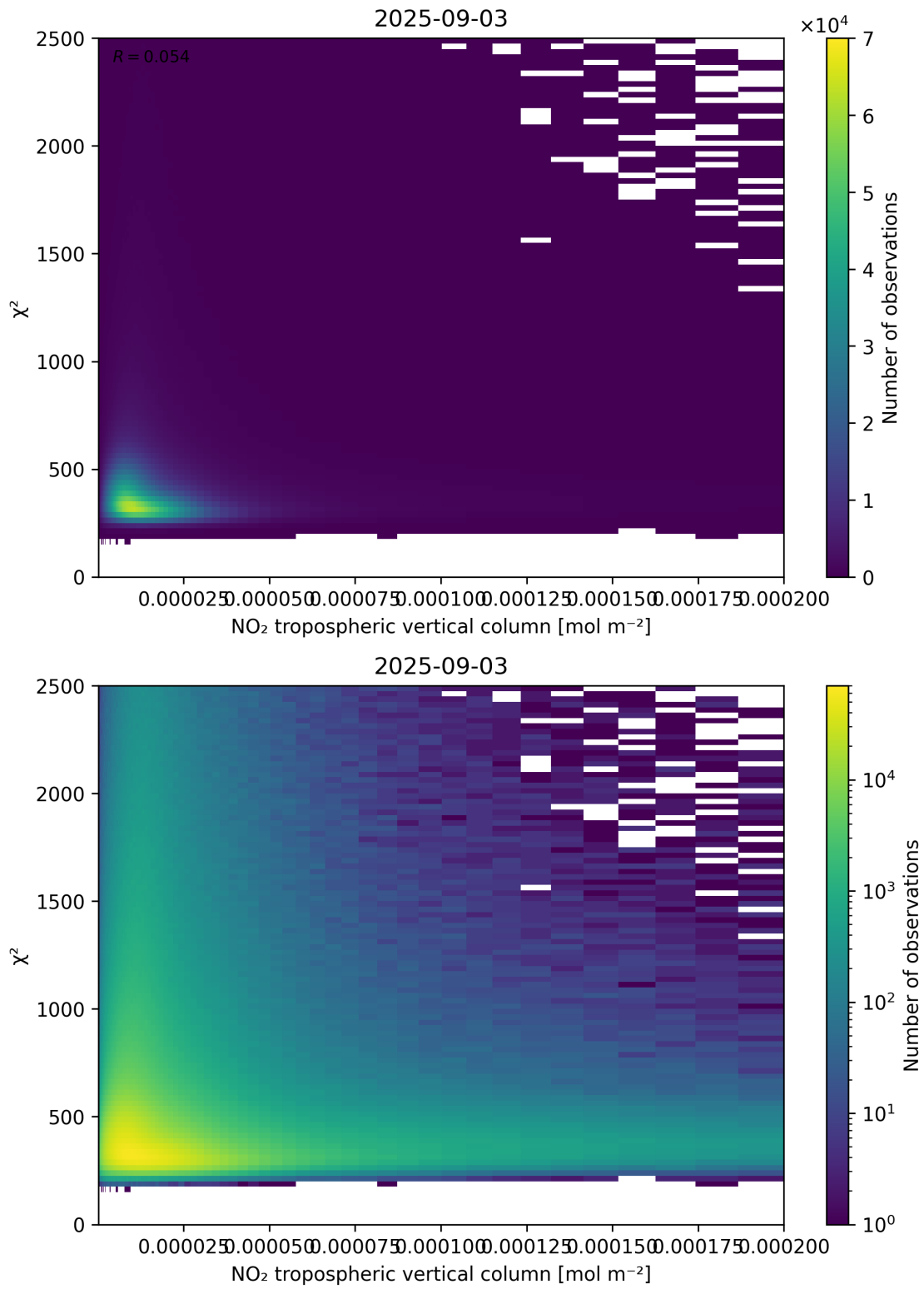
Figure 124: Scatter density plot of “NO 2 tropospheric vertical column” against “ \chi^2 ” for 2025-09-02 to 2025-09-04.
