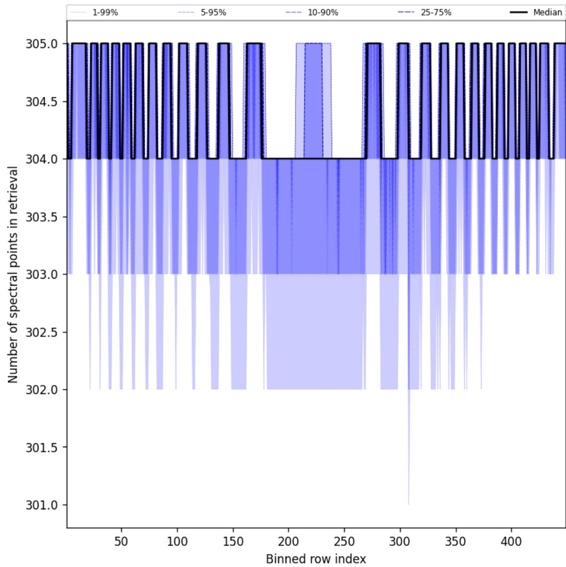
Figure 50: Along track statistics of “Number of spectral points in retrieval” for 2025-09-02 to 2025-09-04
