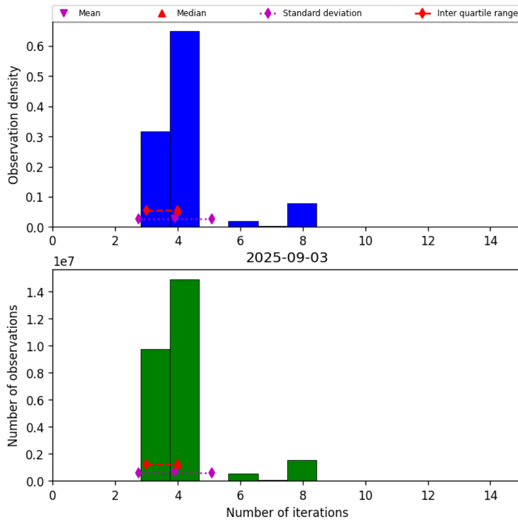
Figure 34: Histogram of “Number of iterations” for 2025-09-02 to 2025-09-04
