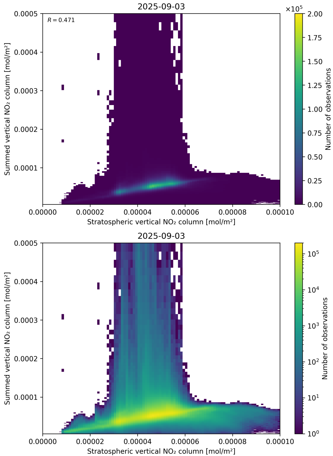
Figure 98: Scatter density plot of “Stratospheric vertical NO 2 column” against “Summed vertical NO 2 column” for 2025-09-02 to 2025-09-04.
