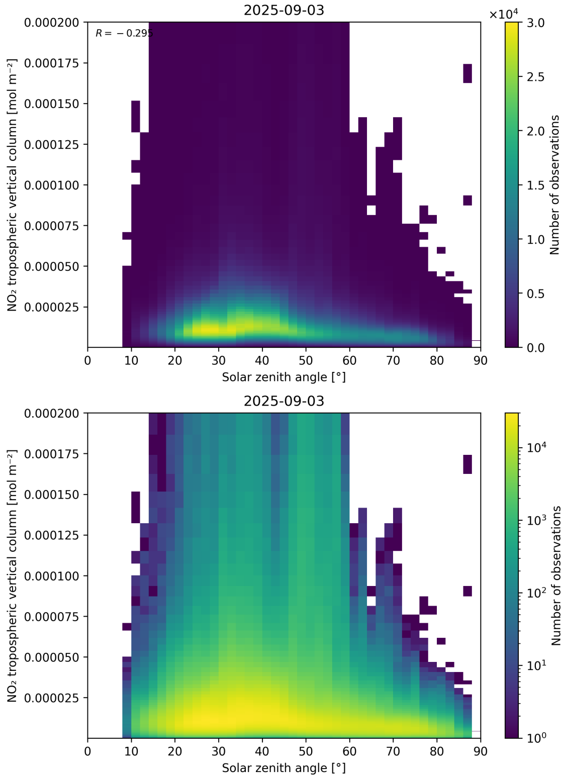
Figure 155: Scatter density plot of “Solar zenith angle” against “NO 2 tropospheric vertical column” for 2025-09-02 to 2025-09-04.
