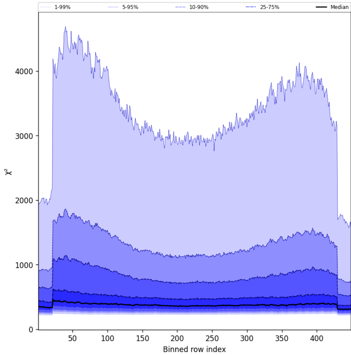
Figure 59: Along track statistics of “ \chi^2 ” for 2025-09-02 to 2025-09-04
