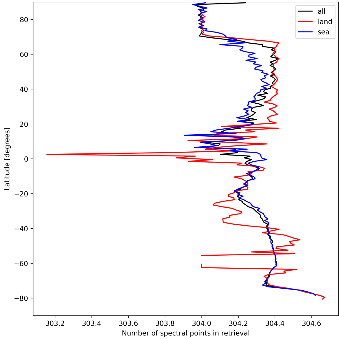
Figure 16: Zonal average of “Number of spectral points in retrieval” for 2025-09-02 to 2025-09-04.
