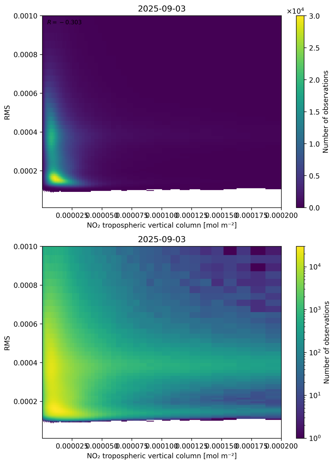
Figure 142: Scatter density plot of “NO 2 tropospheric vertical column” against “RMS” for 2025-09-02 to 2025-09-04.
