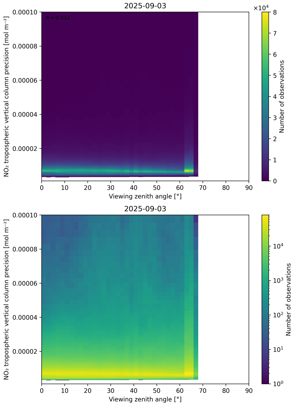
Figure 170: Scatter density plot of “Viewing zenith angle” against “NO 2 tropospheric vertical column precision” for 2025-09-02 to 2025-09-04.
