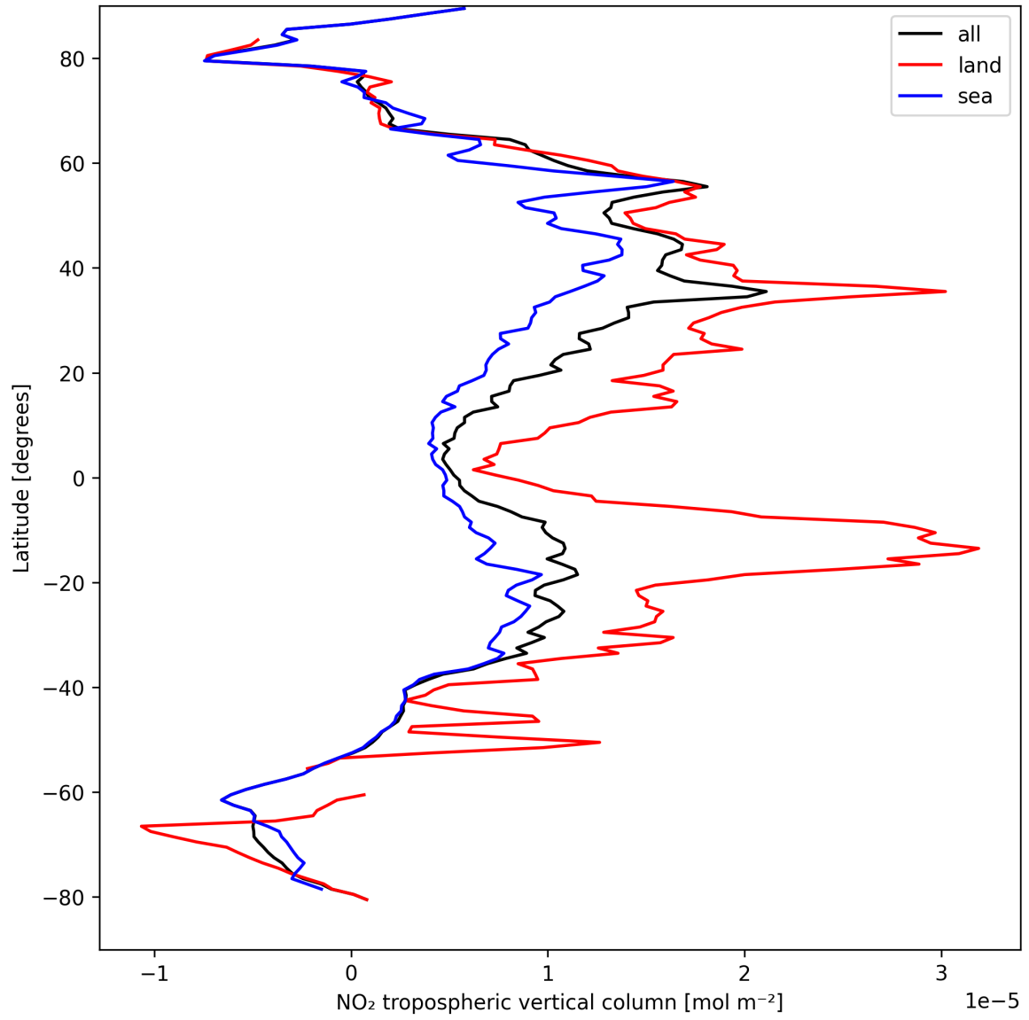
Figure 12: Zonal average of “NO 2 tropospheric vertical column” for 2025-09-02 to 2025-09-04.
