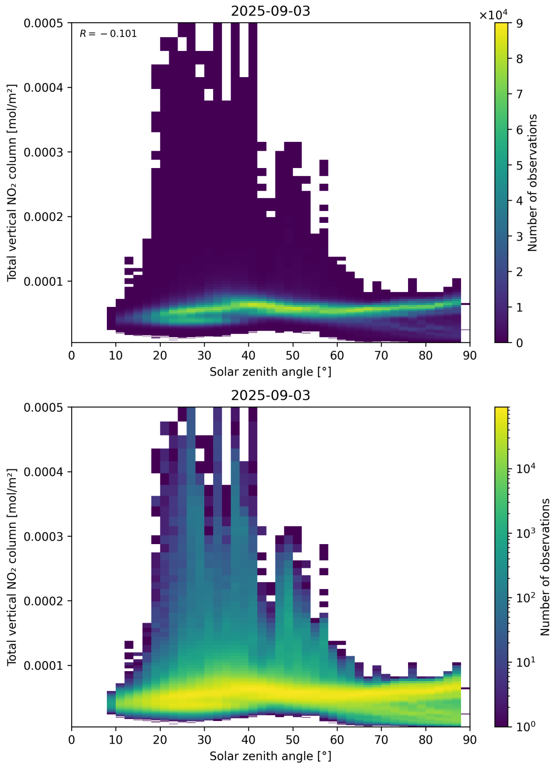
Figure 153: Scatter density plot of “Solar zenith angle” against “Total vertical NO 2 column” for 2025-09-02 to 2025-09-04.
