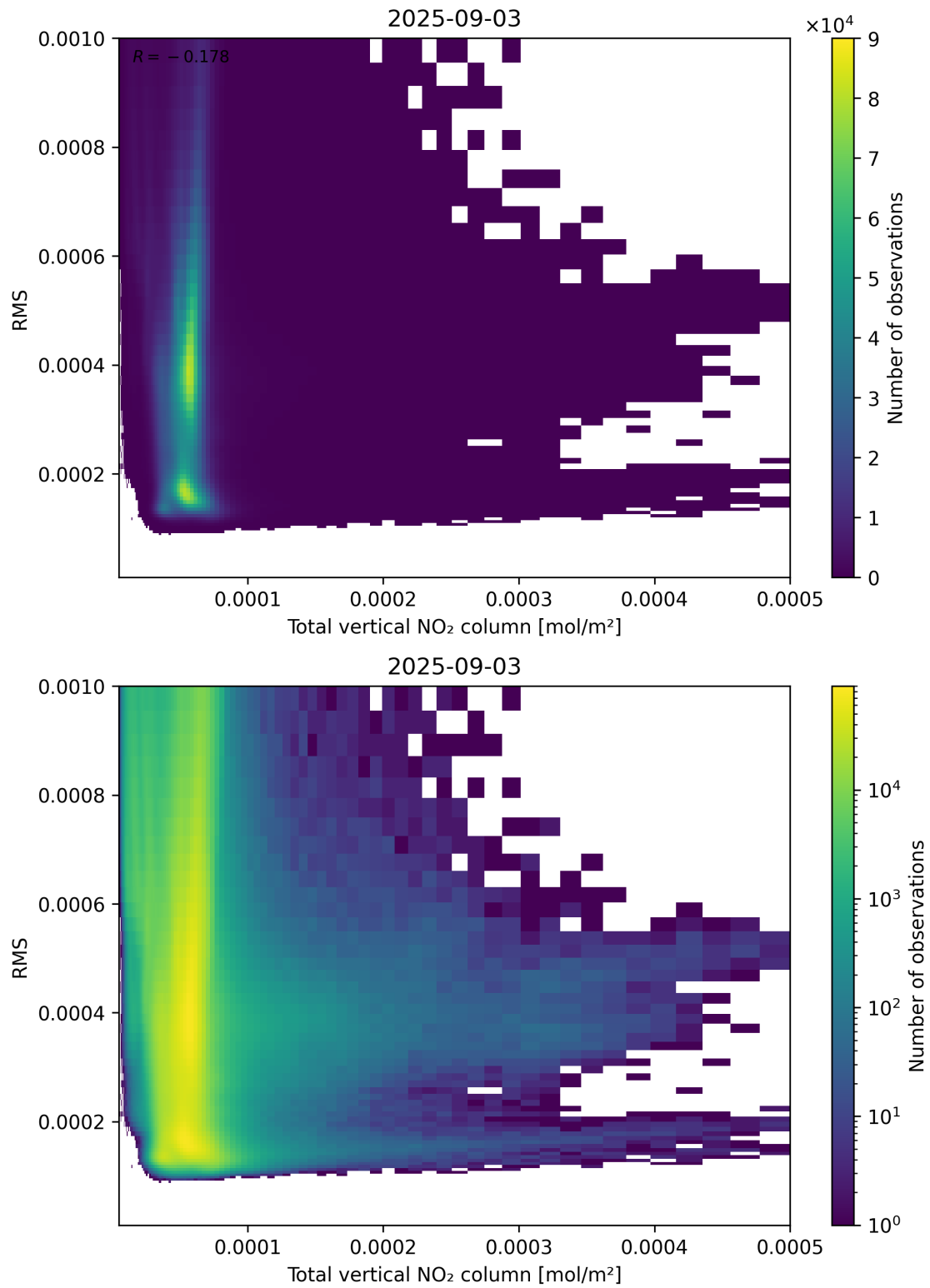
Figure 120: Scatter density plot of “Total vertical NO 2 column” against “RMS” for 2025-09-02 to 2025-09-04.
