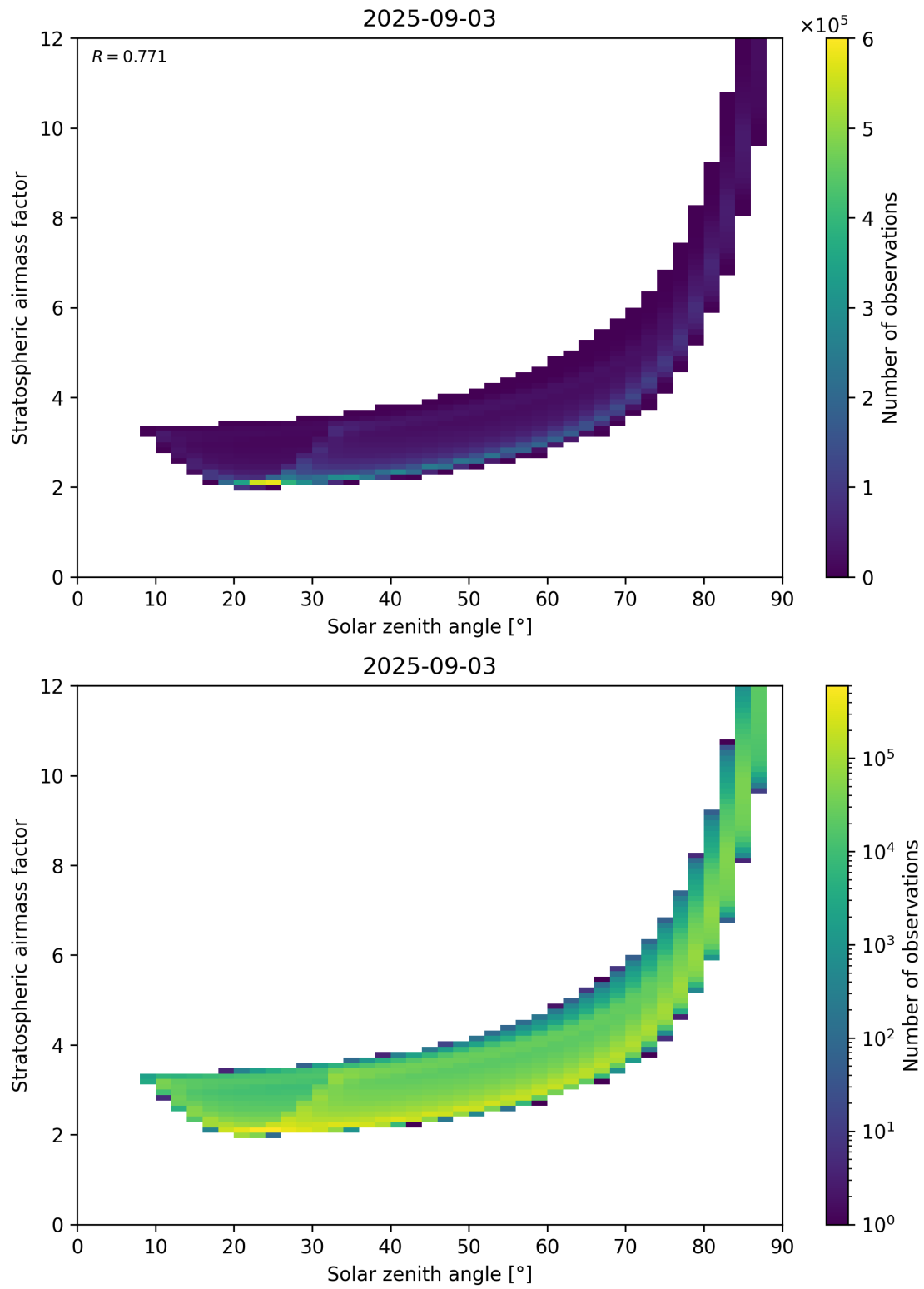
Figure 145: Scatter density plot of “Solar zenith angle” against “Stratospheric airmass factor” for 2025-09-02 to 2025-09-04.
