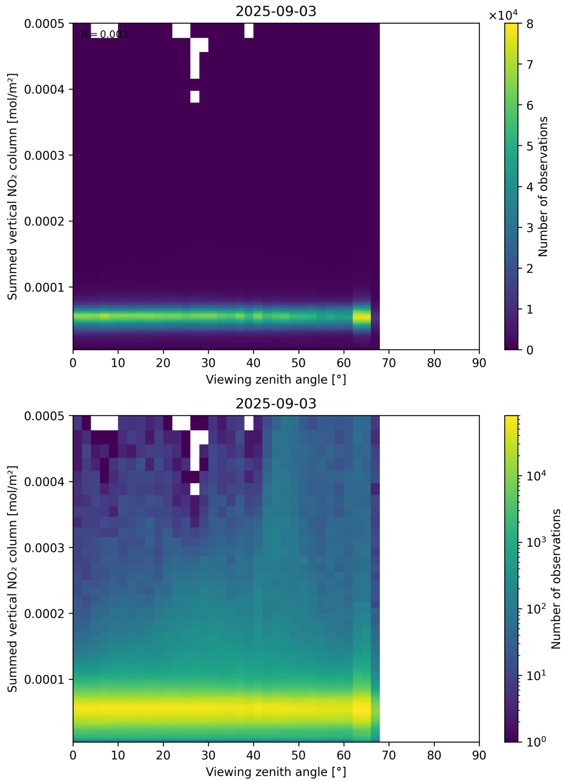
Figure 165: Scatter density plot of “Viewing zenith angle” against “Summed vertical NO 2 column” for 2025-09-02 to 2025-09-04.
