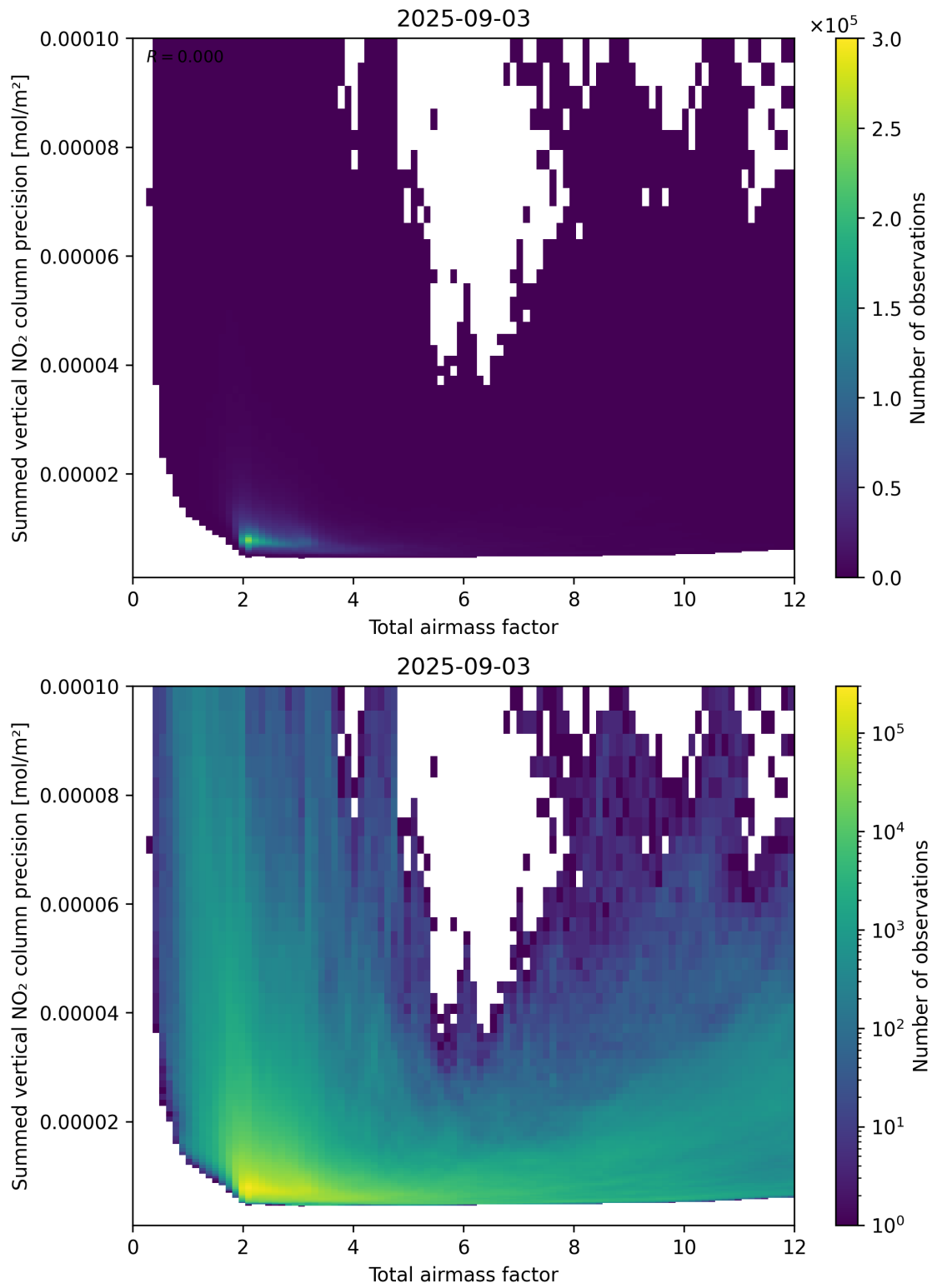
Figure 66: Scatter density plot of “Total airmass factor” against “Summed vertical NO 2 column precision” for 2025-09-02 to 2025-09-04.
