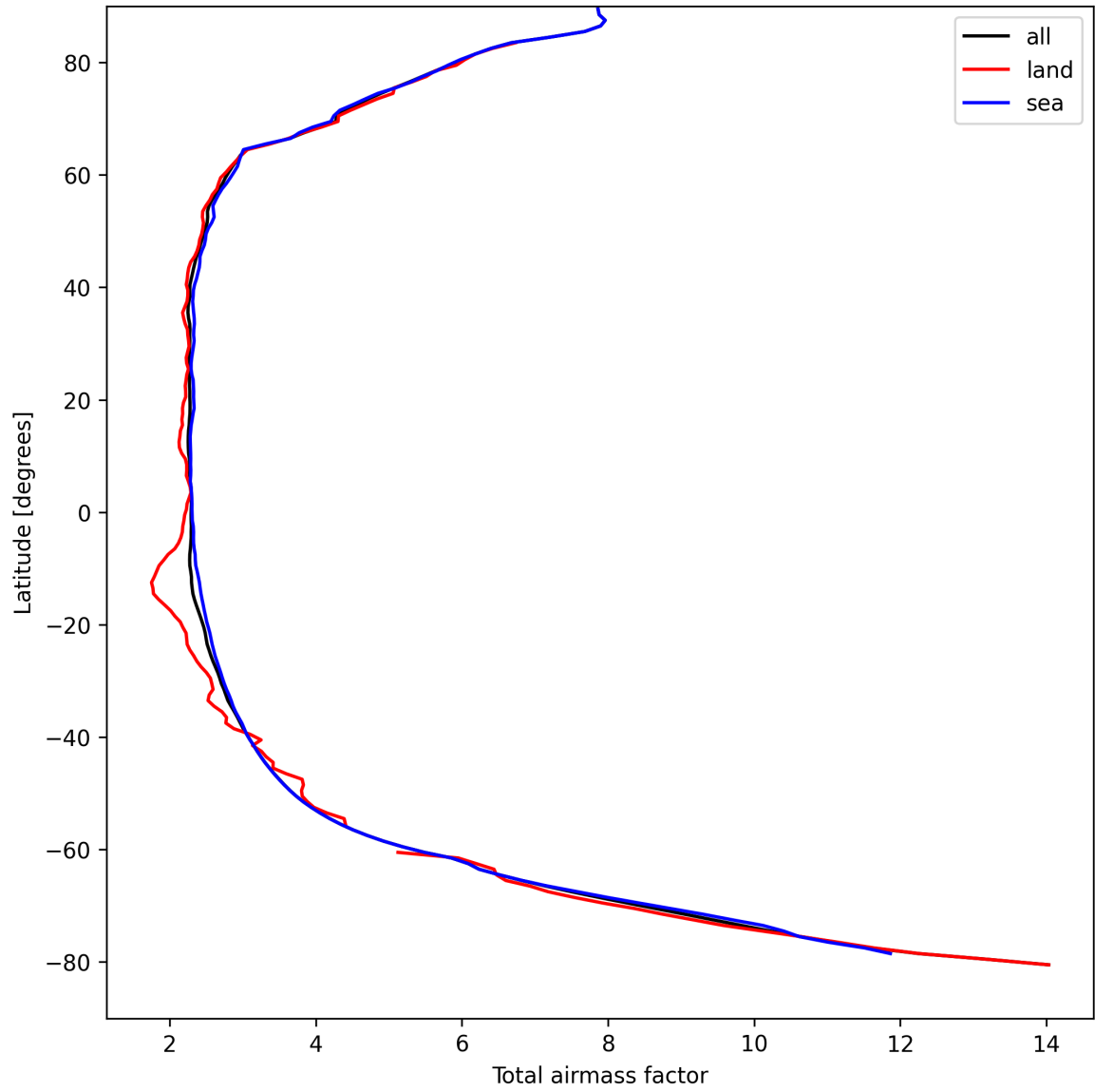
Figure 15: Zonal average of “Total airmass factor” for 2025-09-02 to 2025-09-04.
