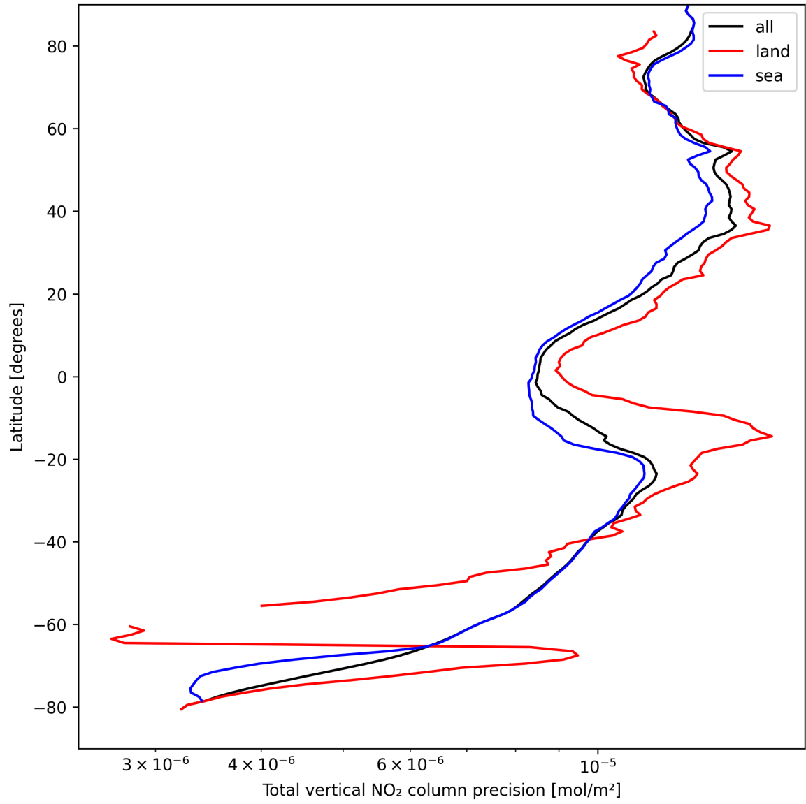
Figure 22: Zonal average of “Total vertical NO 2 column precision” for 2025-09-02 to 2025-09-04.
