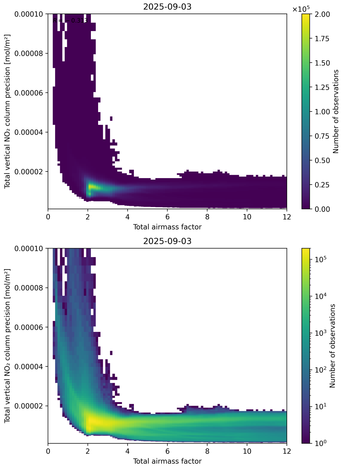
Figure 68: Scatter density plot of “Total airmass factor” against “Total vertical NO 2 column precision” for 2025-09-02 to 2025-09-04.
