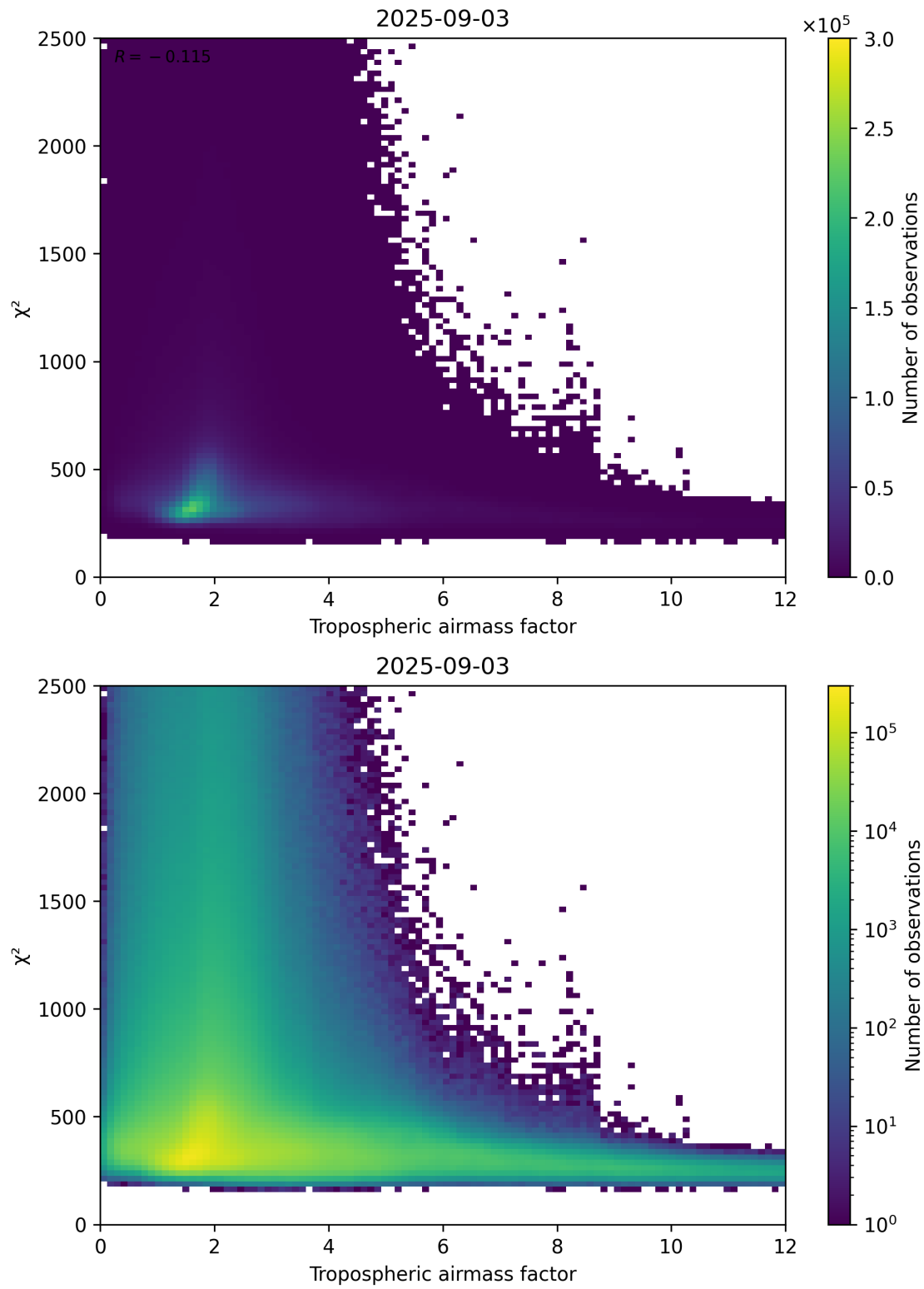
Figure 73: Scatter density plot of “Tropospheric airmass factor” against “ \chi^2 ” for 2025-09-02 to 2025-09-04.
