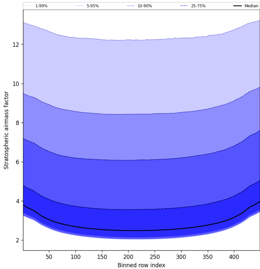
Figure 61: Along track statistics of “Stratospheric airmass factor” for 2025-09-02 to 2025-09-04
