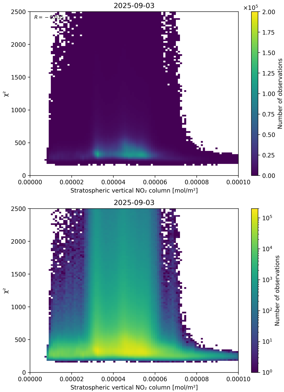
Figure 97: Scatter density plot of “Stratospheric vertical NO 2 column” against “ \chi^2 ” for 2025-09-02 to 2025-09-04.
