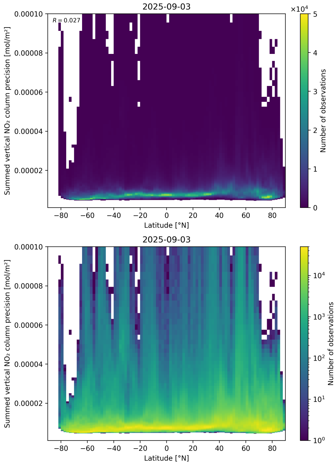
Figure 89: Scatter density plot of “Latitude” against “Summed vertical NO 2 column precision” for 2025-09-02 to 2025-09-04.
