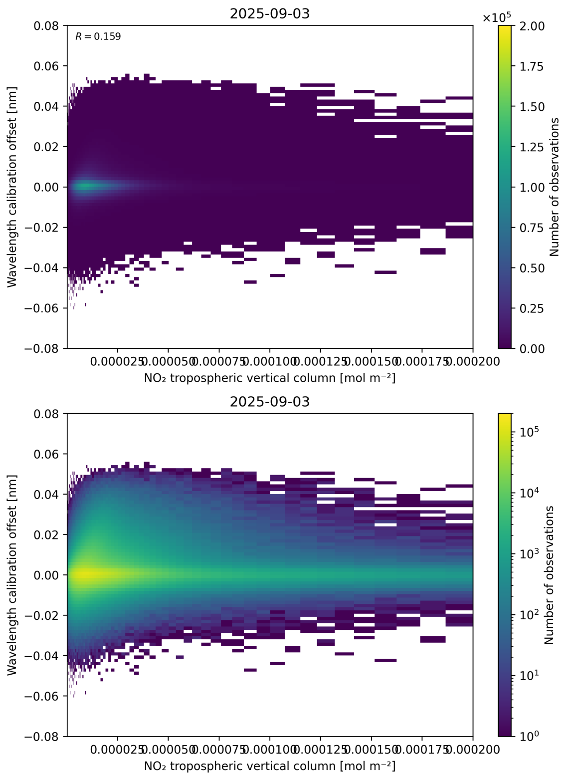
Figure 143: Scatter density plot of “NO 2 tropospheric vertical column” against “Wavelength calibration offset” for 2025-09-02 to 2025-09-04.
