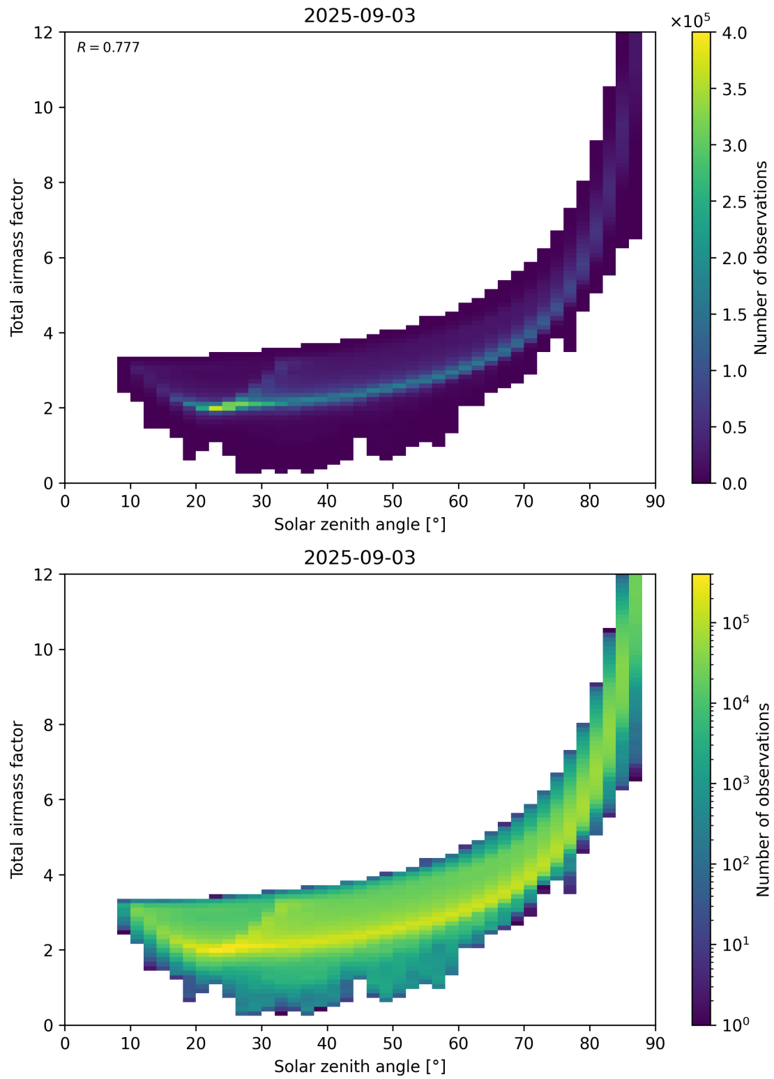
Figure 146: Scatter density plot of “Solar zenith angle” against “Total airmass factor” for 2025-09-02 to 2025-09-04.
