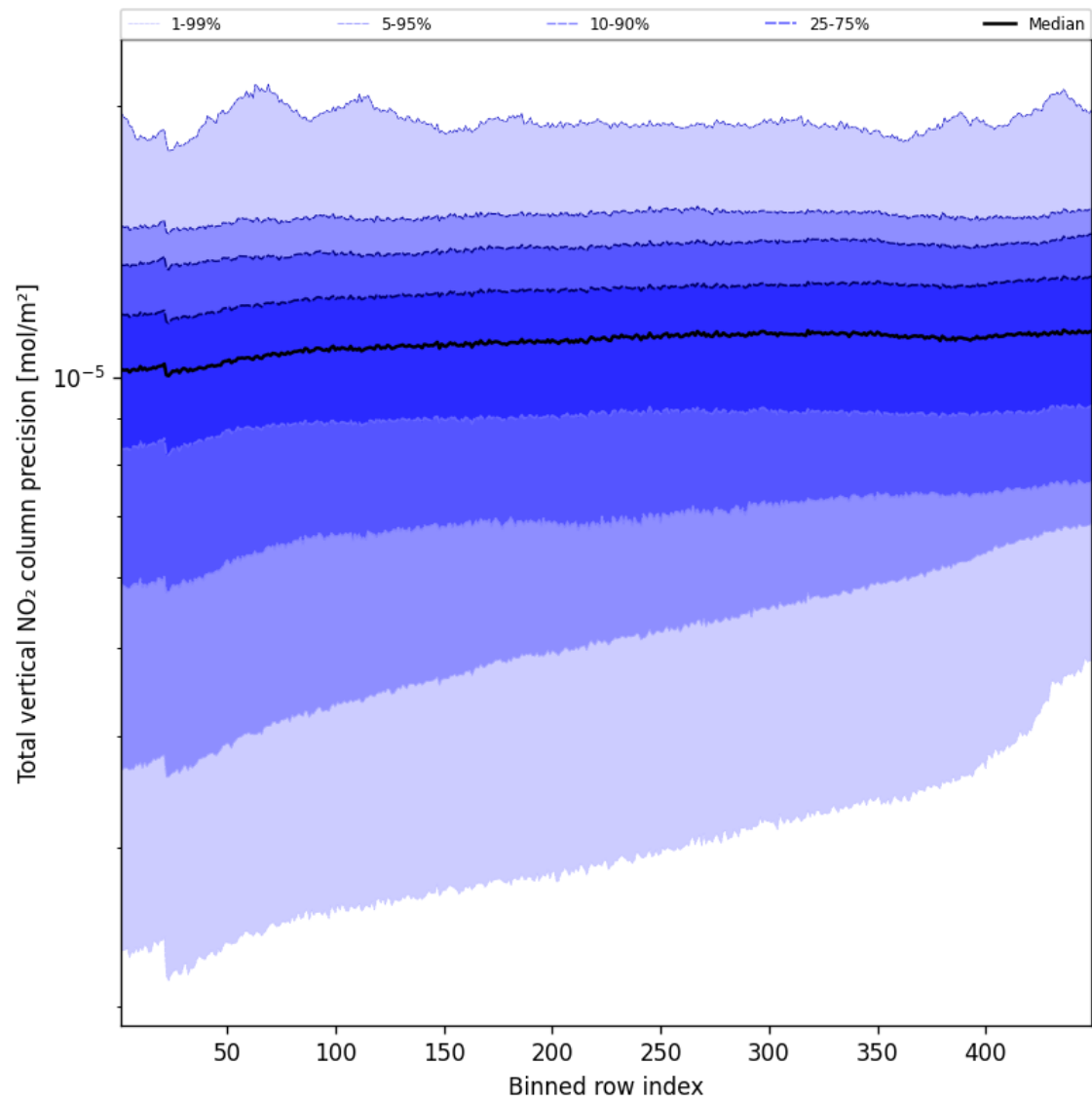
Figure 56: Along track statistics of “Total vertical NO 2 column precision” for 2025-09-02 to 2025-09-04
