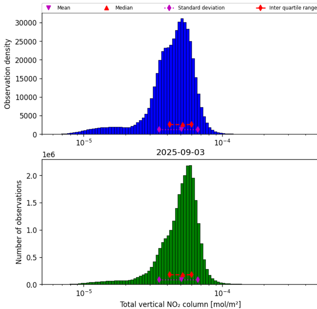
Figure 38: Histogram of “Total vertical NO 2 column” for 2025-09-02 to 2025-09-04
