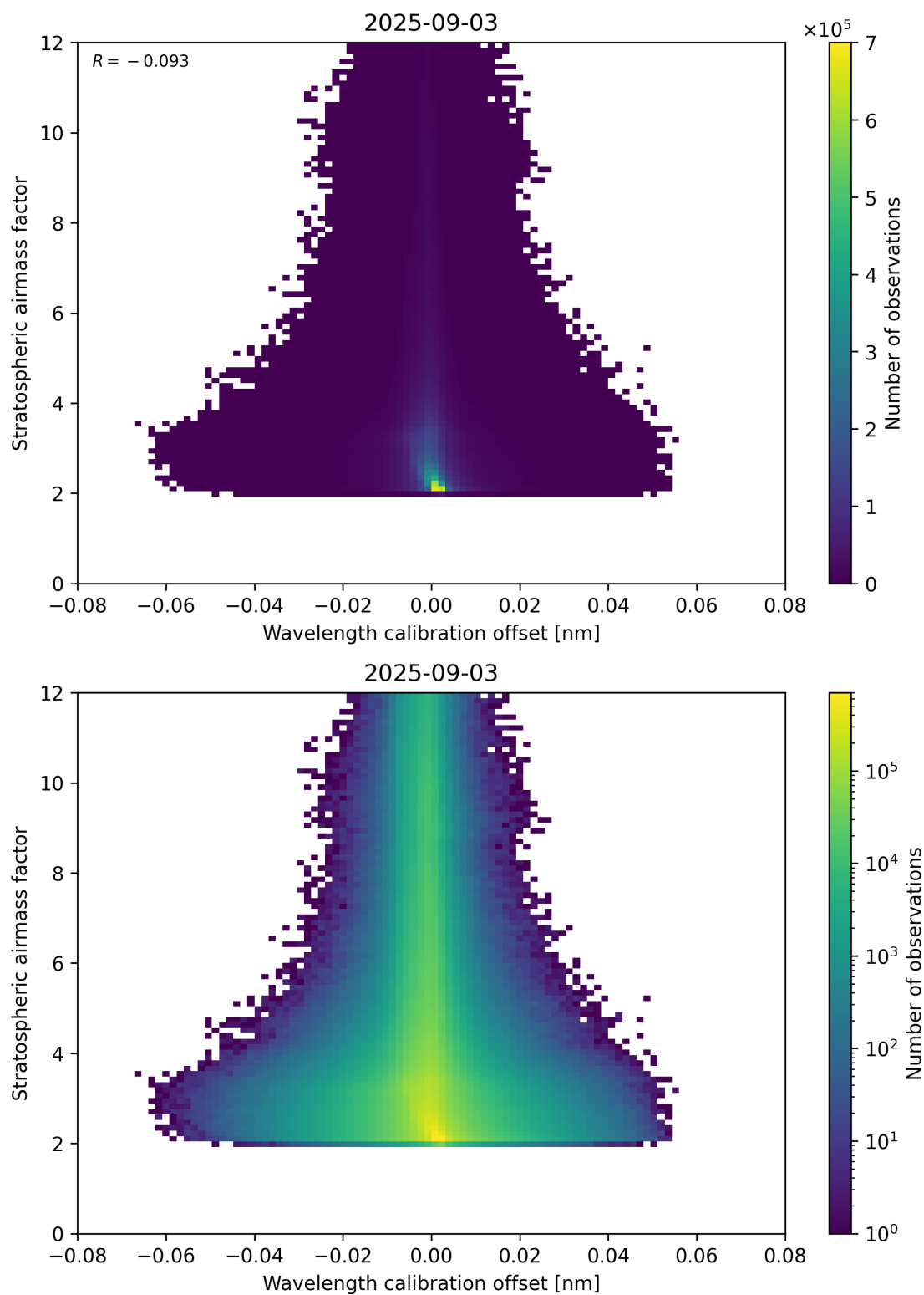
Figure 174: Scatter density plot of “Wavelength calibration offset” against “Stratospheric air mass factor” for 2025-09-02 to 2025-09-04.
