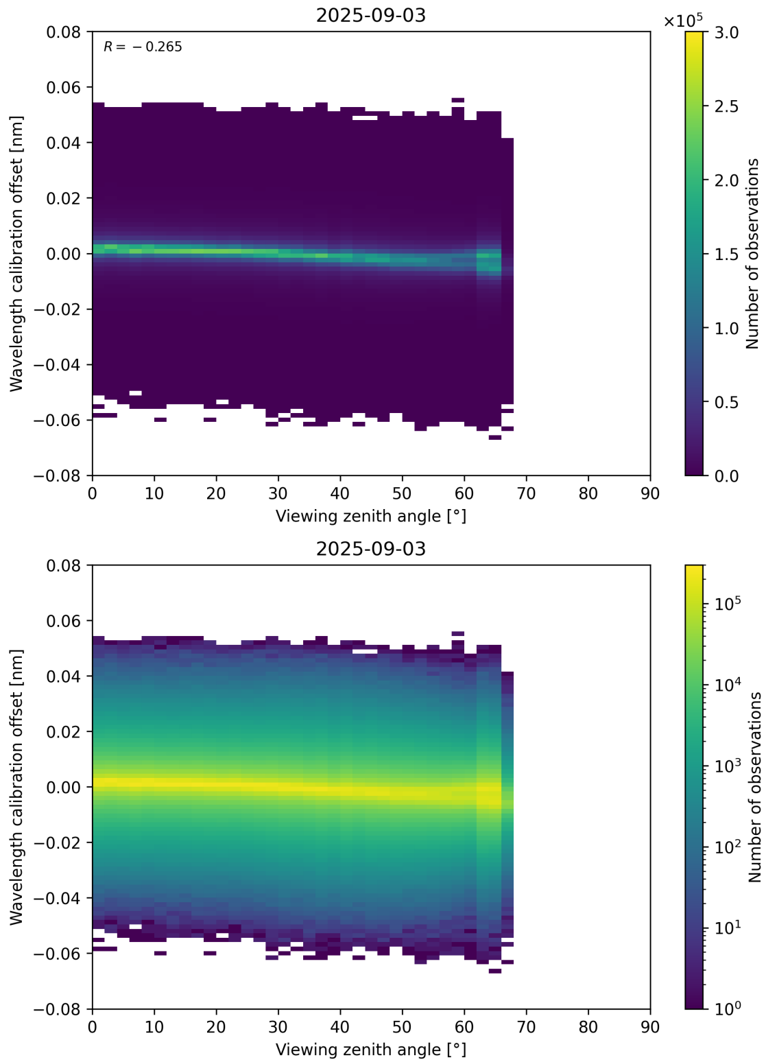
Figure 173: Scatter density plot of “Viewing zenith angle” against “Wavelength calibration offset” for 2025-09-02 to 2025-09-04.
