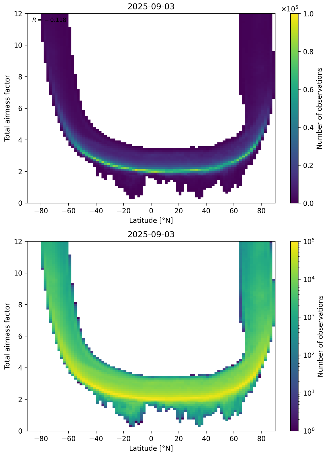
Figure 84: Scatter density plot of “Latitude” against “Total airmass factor” for 2025-09-02 to 2025-09-04.
