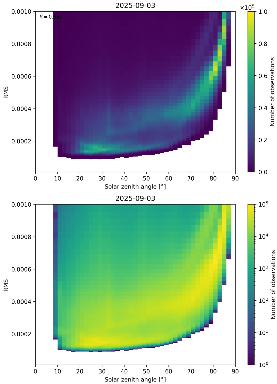
Figure 157: Scatter density plot of “Solar zenith angle” against “RMS” for 2025-09-02 to 2025-09-04.
