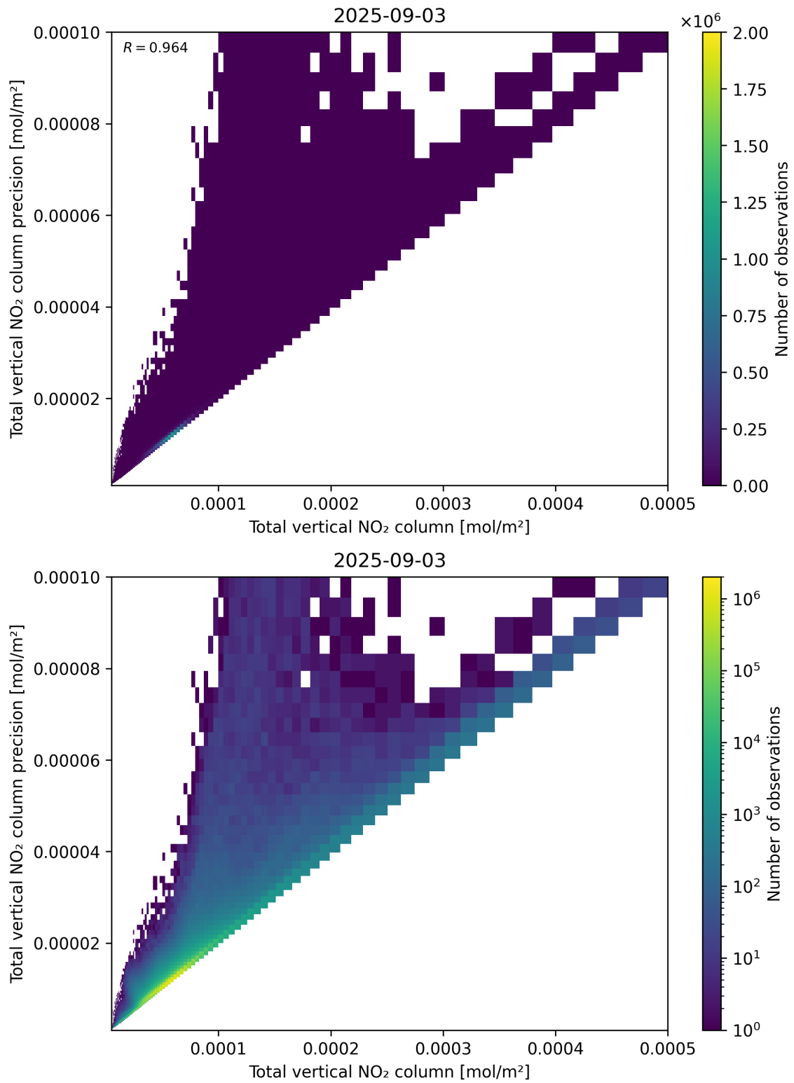
Figure 114: Scatter density plot of “Total vertical NO 2 column” against “Total vertical NO 2 column precision” for 2025-09-02 to 2025-09-04.
