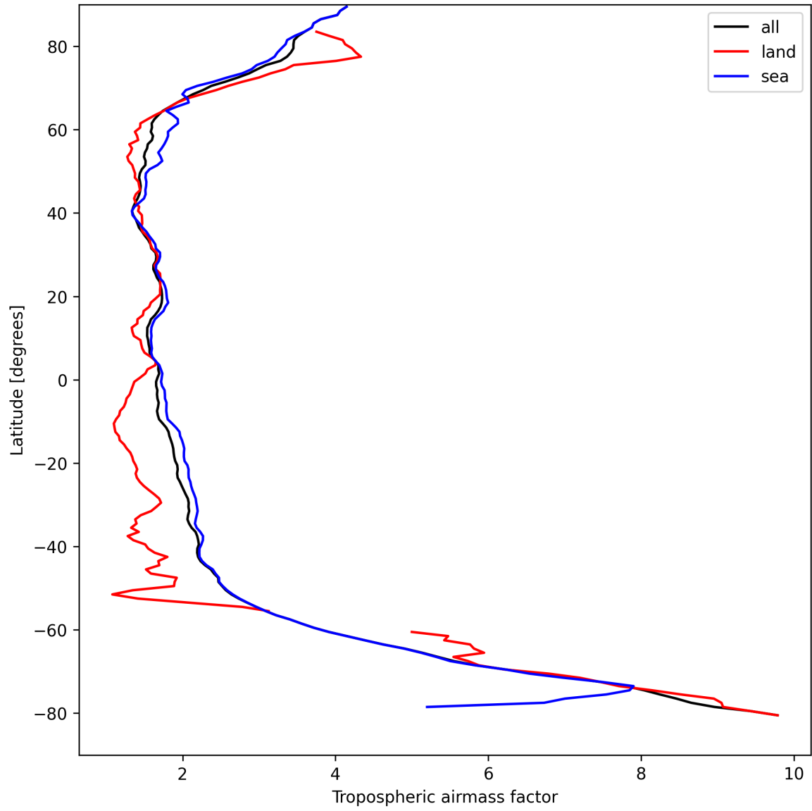
Figure 14: Zonal average of “Tropospheric airmass factor” for 2025-09-02 to 2025-09-04.
