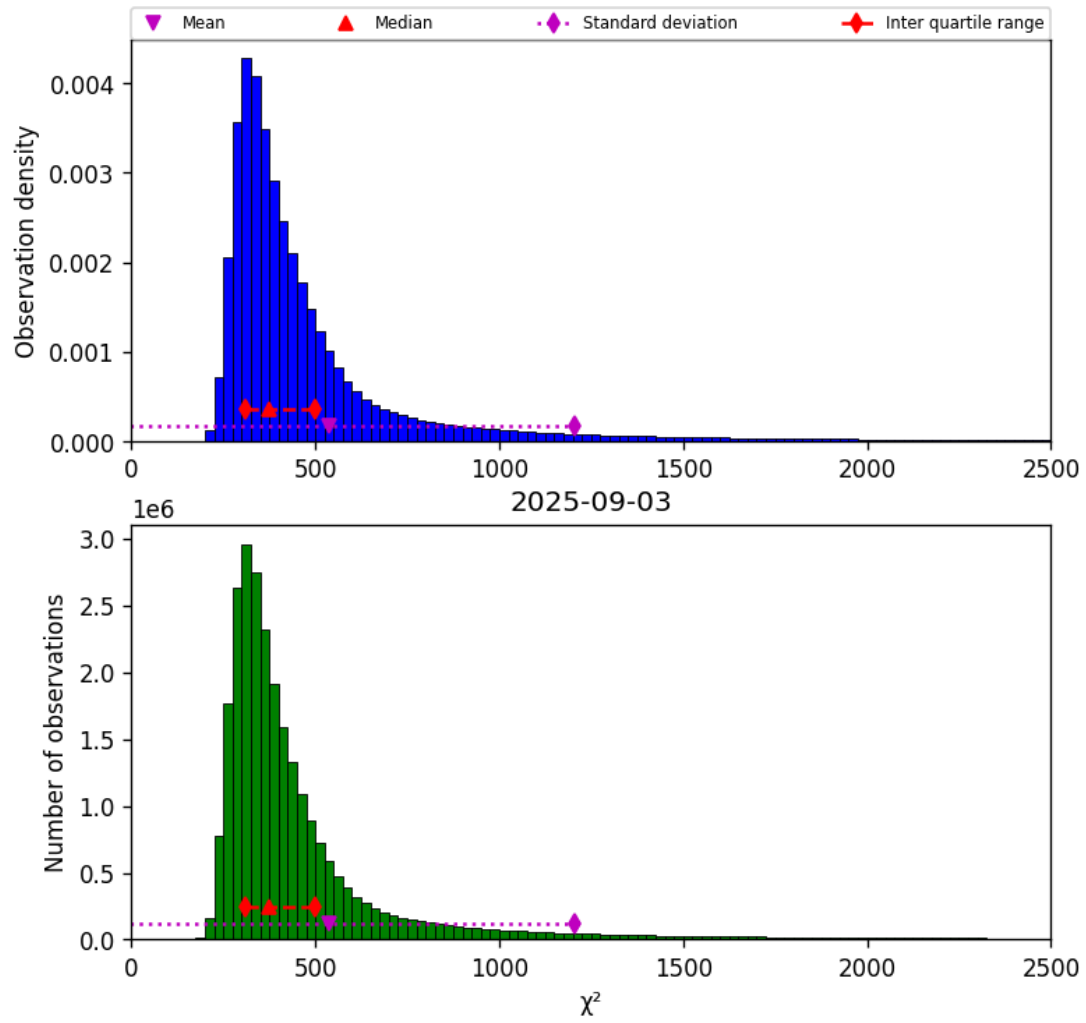
Figure 42: Histogram of “ \chi^2 ” for 2025-09-02 to 2025-09-04
