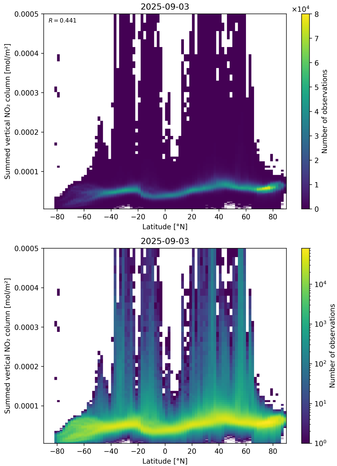
Figure 88: Scatter density plot of “Latitude” against “Summed vertical NO 2 column” for 2025-09-02 to 2025-09-04.
