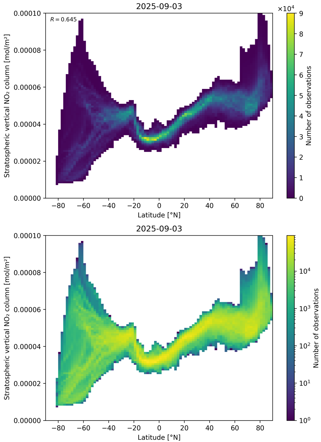
Figure 87: Scatter density plot of “Latitude” against “Stratospheric vertical NO 2 column” for 2025-09-02 to 2025-09-04.
