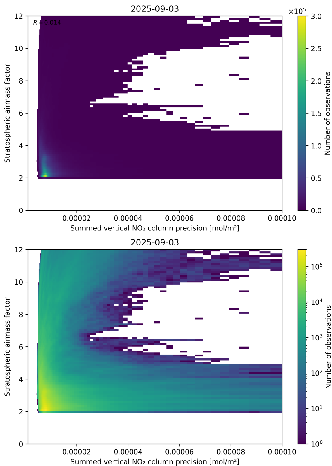
Figure 106: Scatter density plot of “Summed vertical NO 2 column precision” against “Stratospheric airmass factor” for 2025-09-02 to 2025-09-04.
