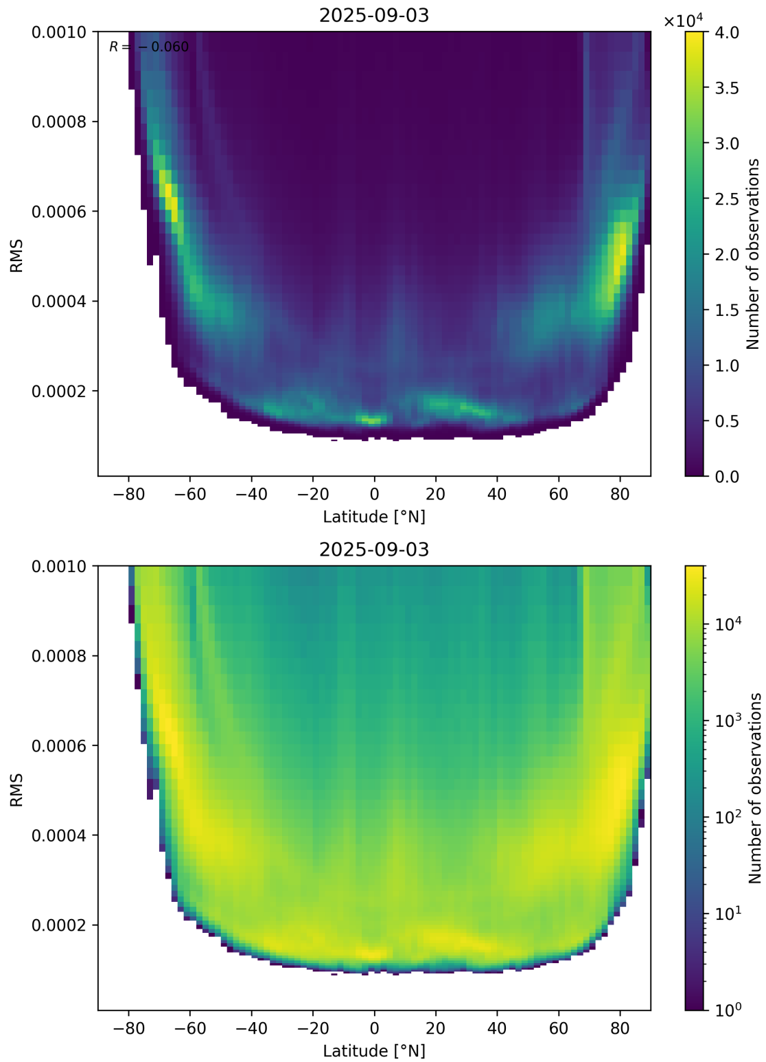
Figure 94: Scatter density plot of “Latitude” against “RMS” for 2025-09-02 to 2025-09-04.
