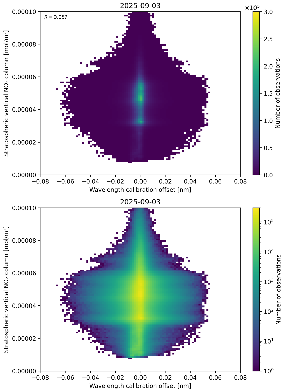
Figure 176: Scatter density plot of “Wavelength calibration offset” against “Stratospheric vertical NO 2 column” for 2025-09-02 to 2025-09-04.
