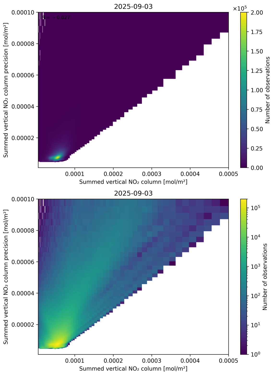
Figure 105: Scatter density plot of “Summed vertical NO 2 column” against “Summed vertical NO 2 column precision” for 2025-09-02 to 2025-09-04.
