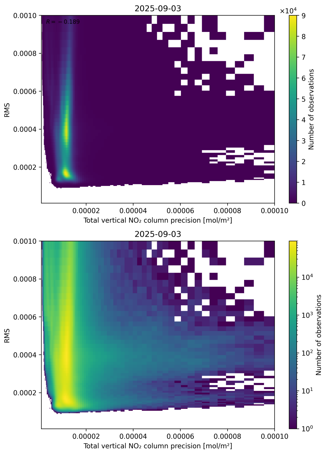
Figure 119: Scatter density plot of “Total vertical NO 2 column precision” against “RMS” for 2025-09-02 to 2025-09-04.
