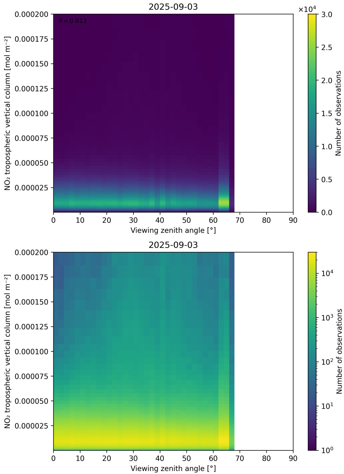
Figure 169: Scatter density plot of “Viewing zenith angle” against “NO 2 tropospheric vertical column” for 2025-09-02 to 2025-09-04.
