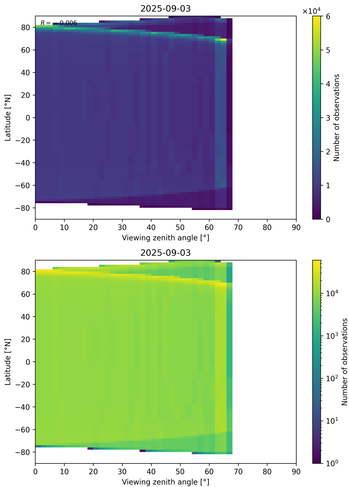
Figure 163: Scatter density plot of “Viewing zenith angle” against “Latitude” for 2025-09-02 to 2025-09-04.
