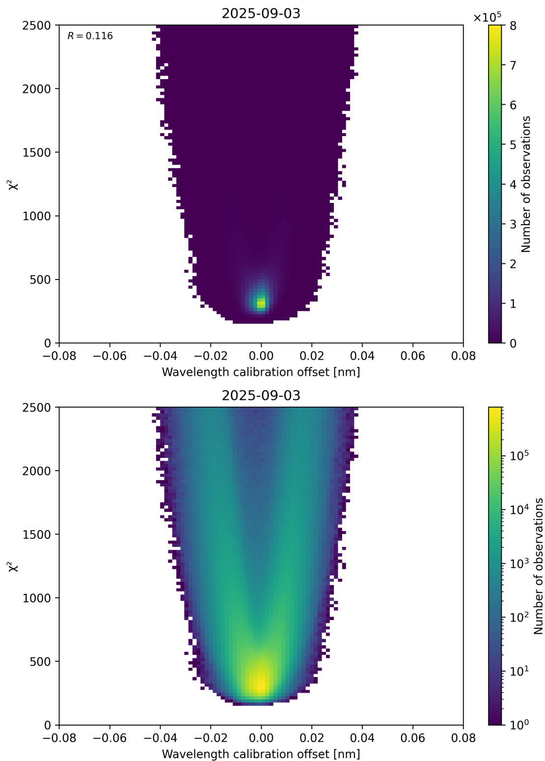
Figure 175: Scatter density plot of “Wavelength calibration offset” against “ \chi^2 ” for 2025-09-02 to 2025-09-04.
