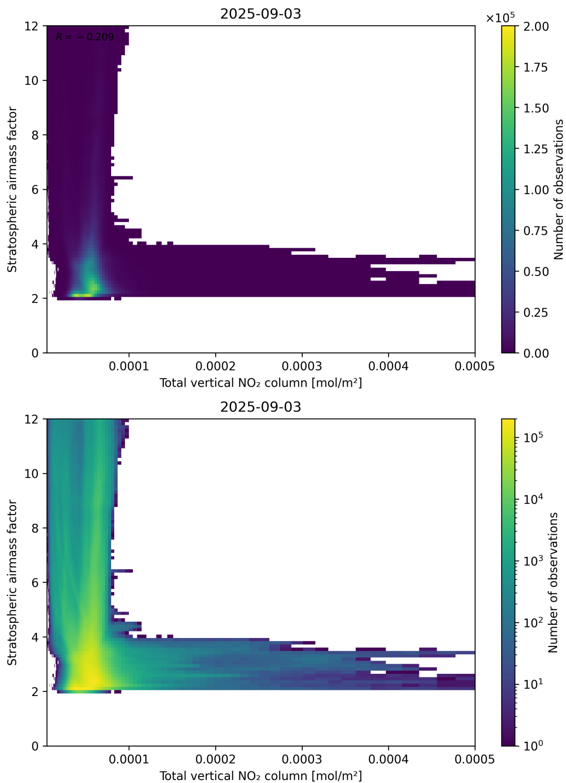
Figure 110: Scatter density plot of “Total vertical NO 2 column” against “Stratospheric airmass factor” for 2025-09-02 to 2025-09-04.
