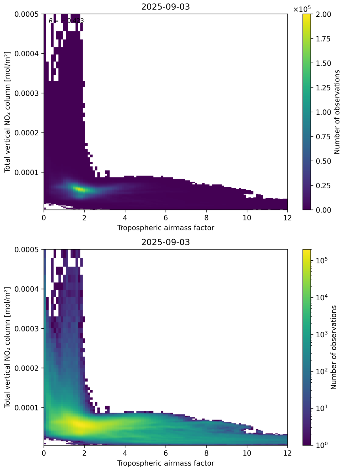
Figure 77: Scatter density plot of “Tropospheric airmass factor” against “Total vertical NO 2 column” for 2025-09-02 to 2025-09-04.
