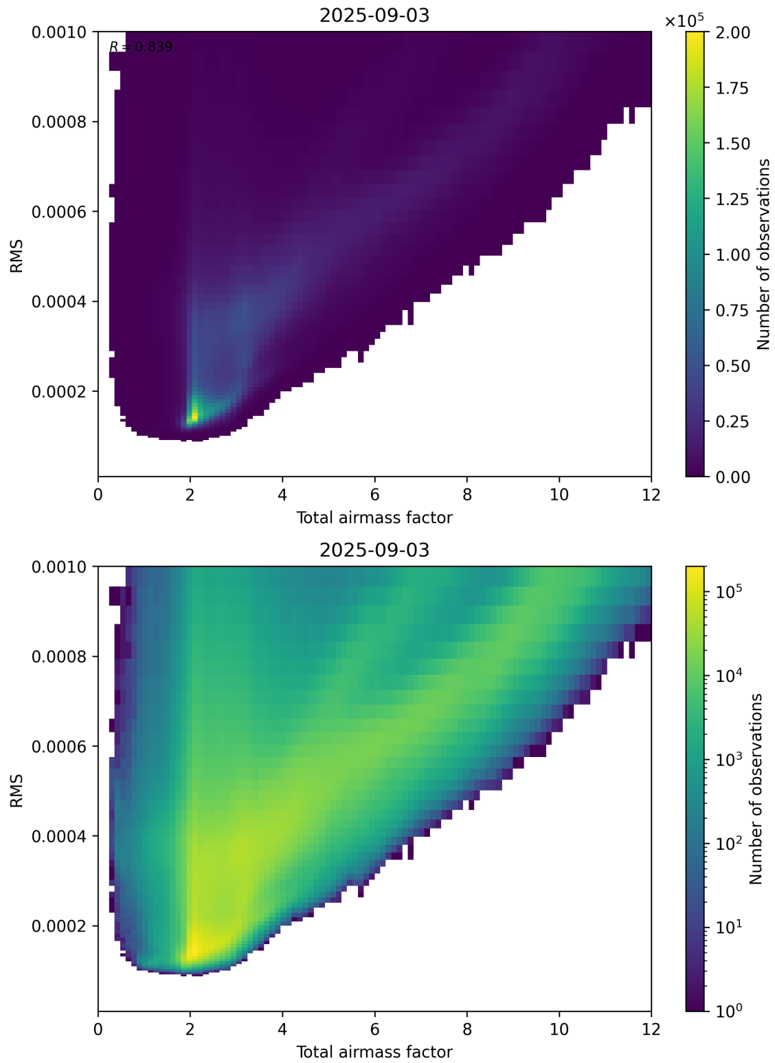
Figure 69: Scatter density plot of “Total airmass factor” against “RMS” for 2025-09-02 to 2025-09-04.
