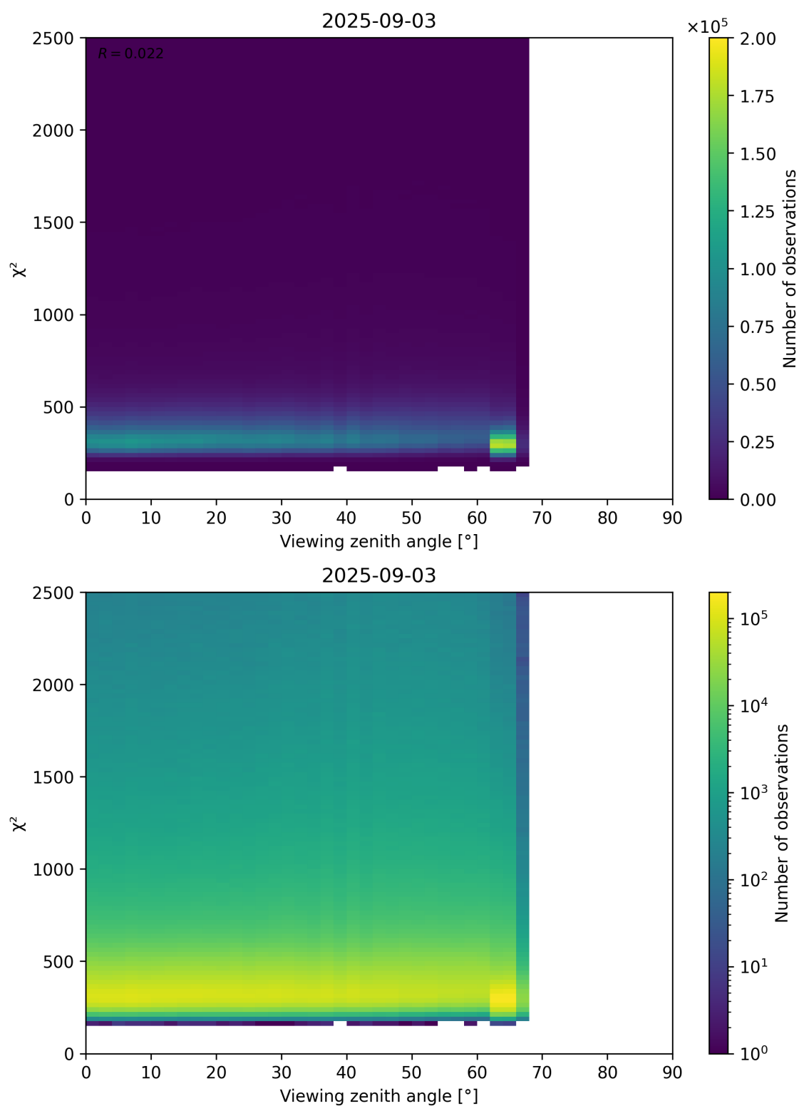
Figure 162: Scatter density plot of “Viewing zenith angle” against “ \chi^2 ” for 2025-09-02 to 2025-09-04.
