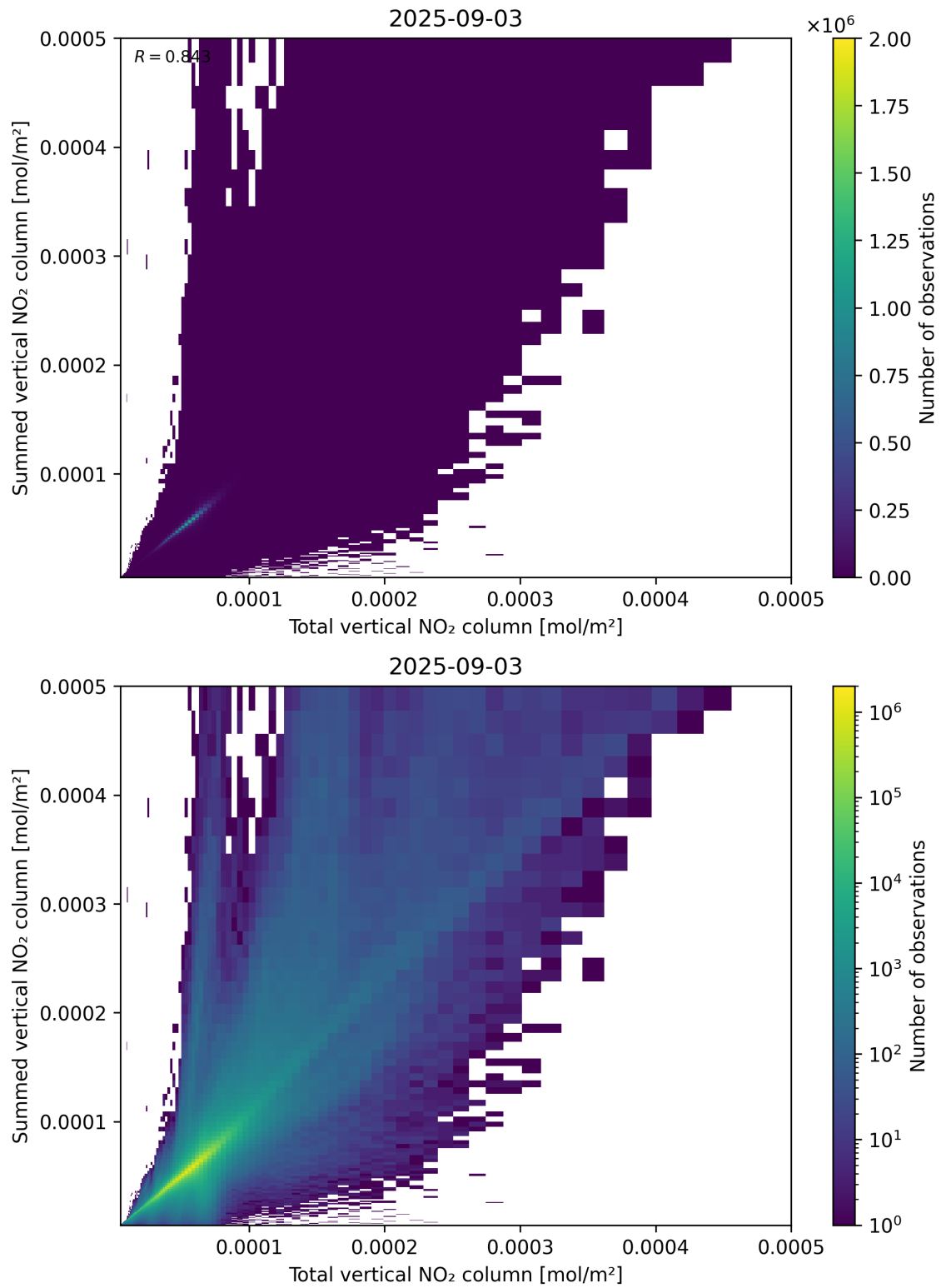
Figure 112: Scatter density plot of “Total vertical NO 2 column” against “Summed vertical NO 2 column” for 2025-09-02 to 2025-09-04.
