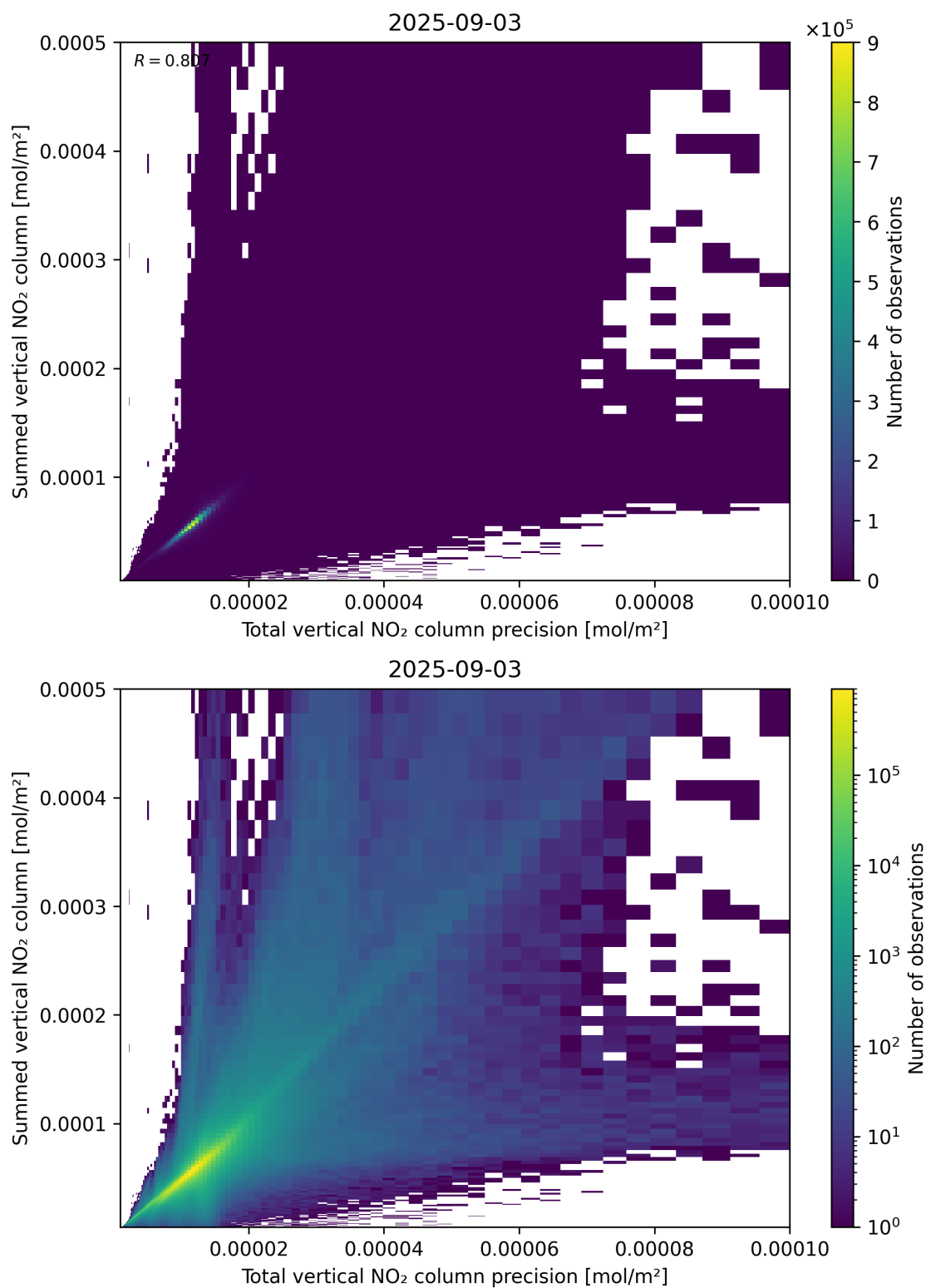
Figure 117: Scatter density plot of “Total vertical NO 2 column precision” against “Summed vertical NO 2 column” for 2025-09-02 to 2025-09-04.
