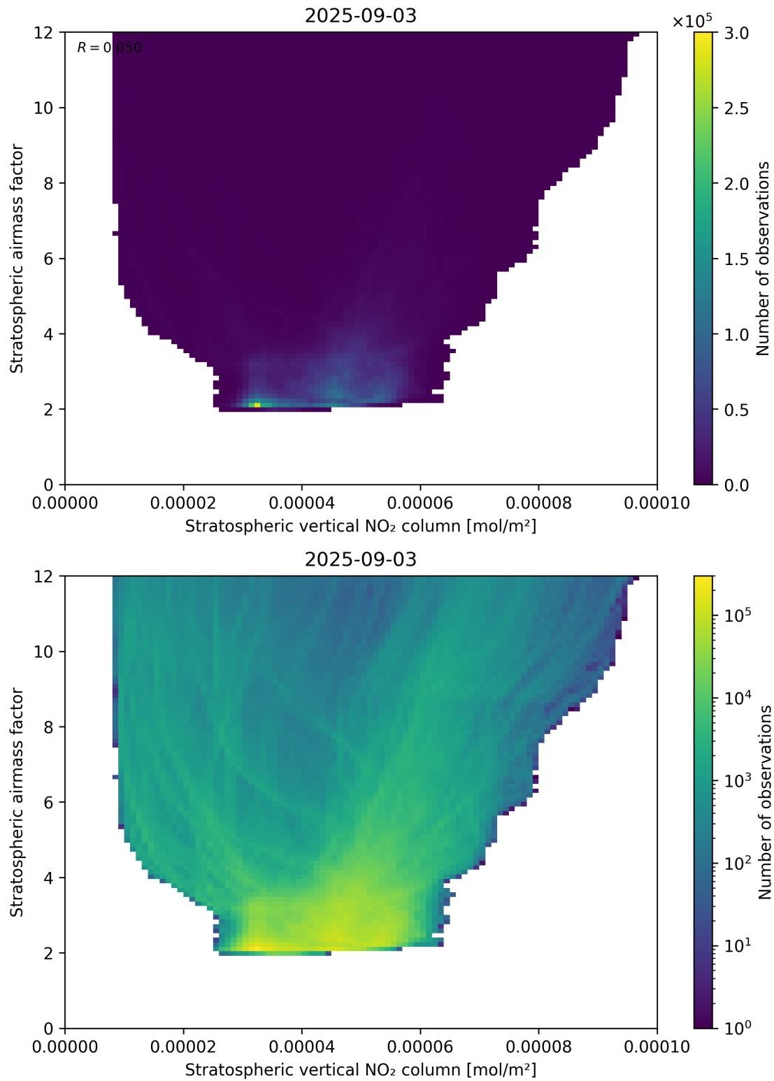
Figure 96: Scatter density plot of “Stratospheric vertical NO 2 column” against “Stratospheric airmass factor” for 2025-09-02 to 2025-09-04.
