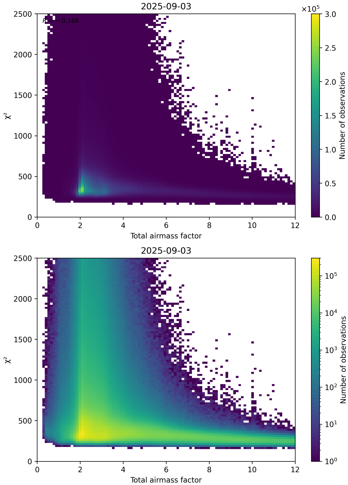
Figure 63: Scatter density plot of “Total airmass factor” against “ \chi^2 ” for 2025-09-02 to 2025-09-04.
