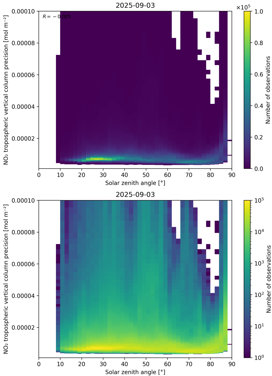
Figure 156: Scatter density plot of “Solar zenith angle” against “NO 2 tropospheric vertical column precision” for 2025-09-02 to 2025-09-04.
