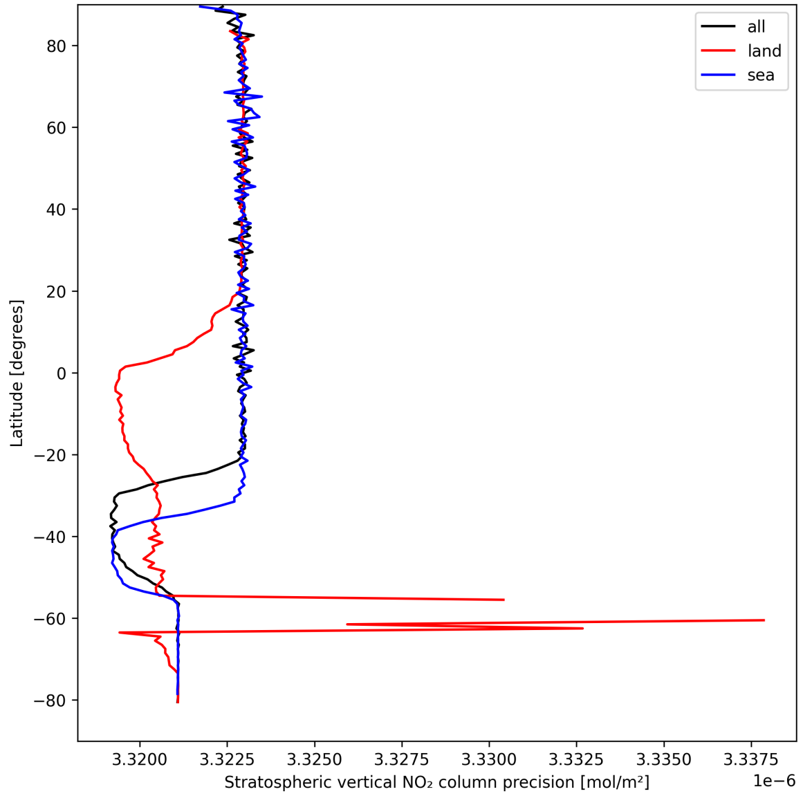
Figure 20: Zonal average of “Stratospheric vertical NO 2 column precision” for 2025-09-02 to 2025-09-04.
