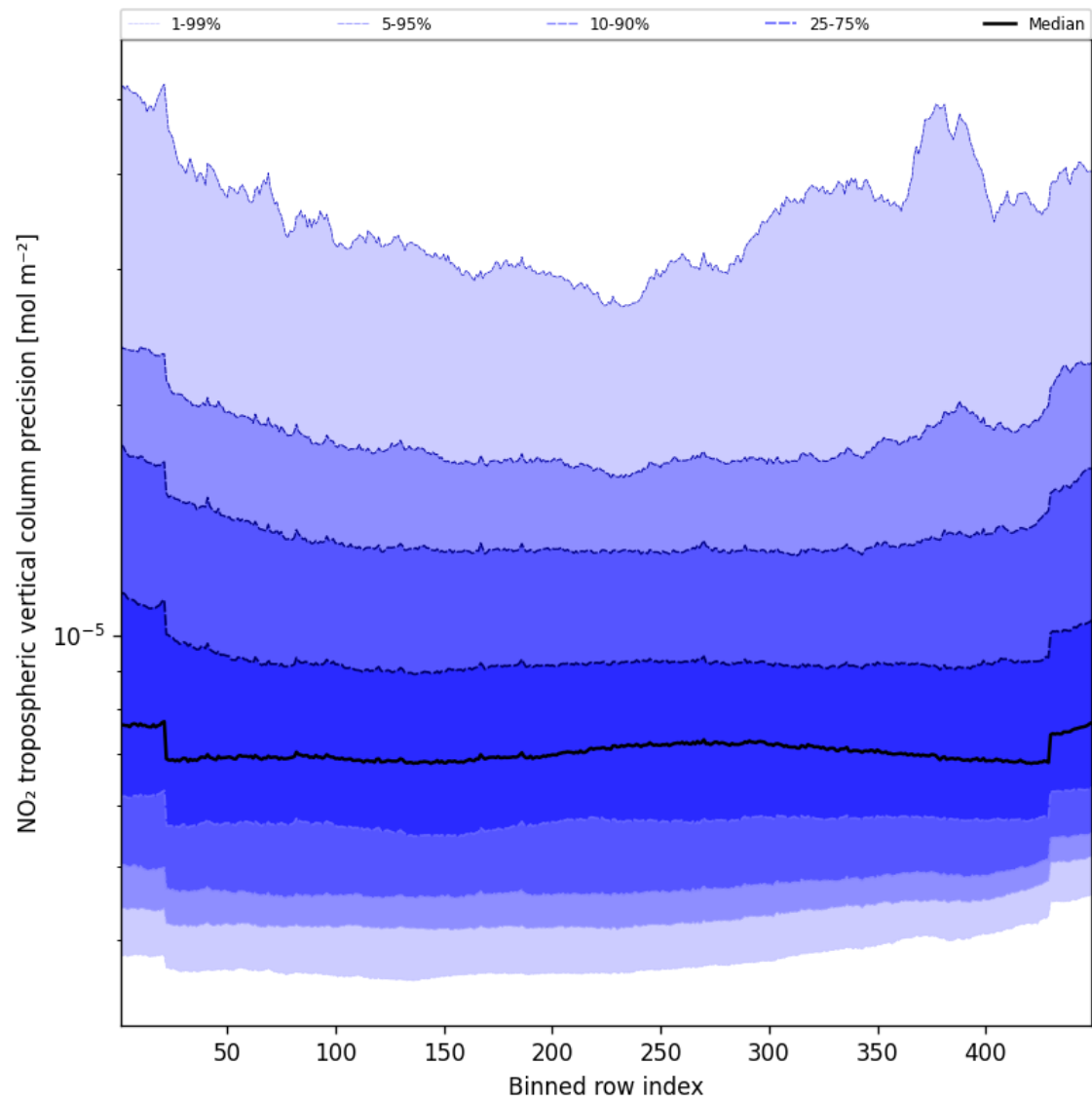
Figure 47: Along track statistics of “NO 2 tropospheric vertical column precision” for 2025-09-02 to 2025-09-04
