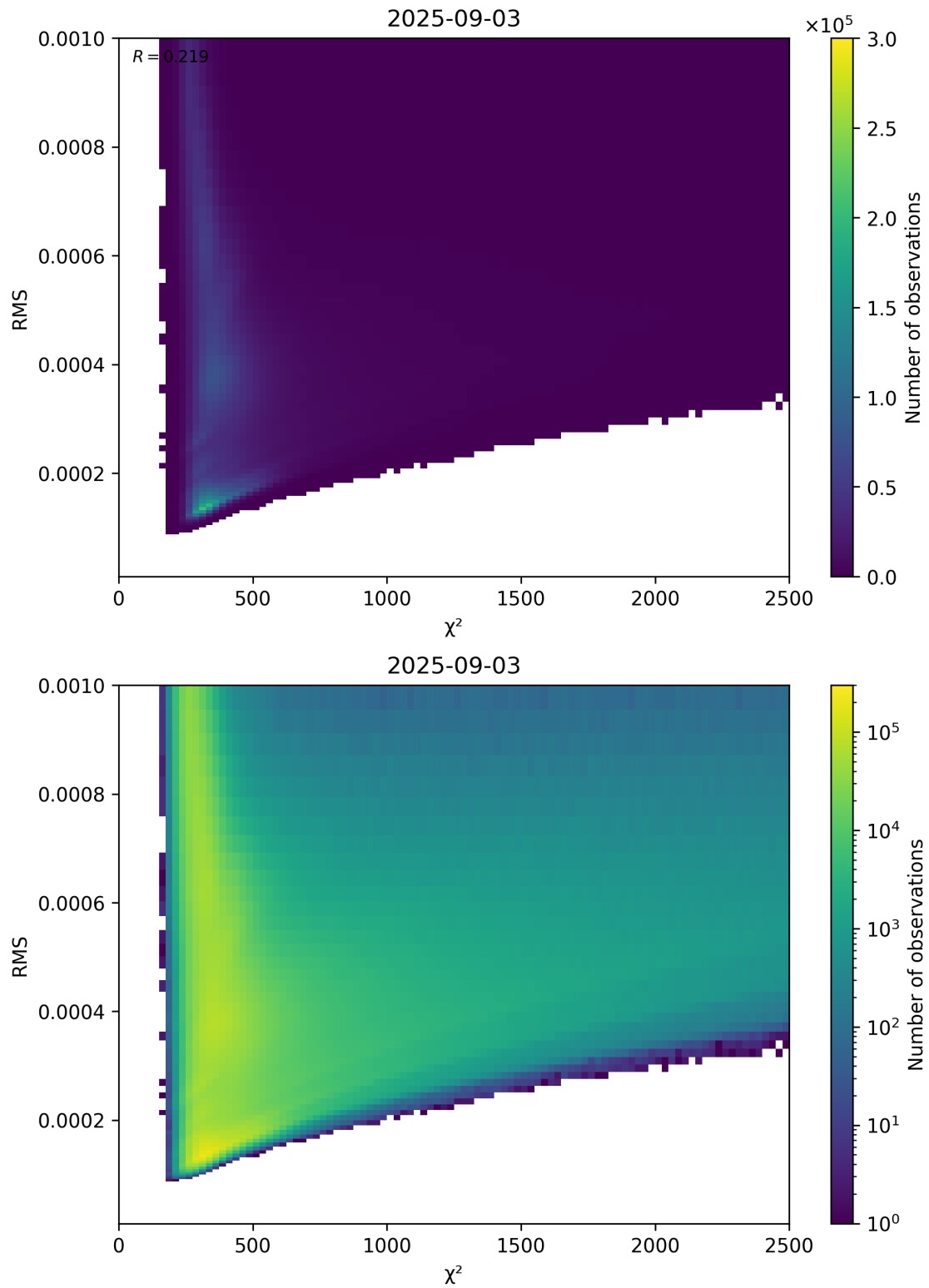
Figure 82: Scatter density plot of “ \chi^2 ” against “RMS” for 2025-09-02 to 2025-09-04.
