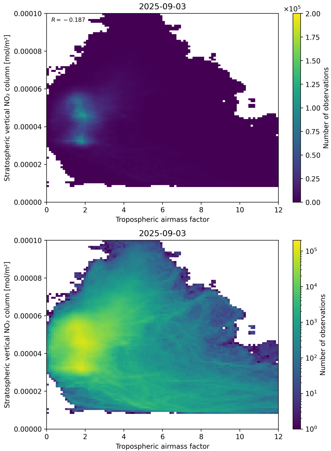
Figure 74: Scatter density plot of “Tropospheric air mass factor” against “Stratospheric vertical NO 2 column” for 2025-09-02 to 2025-09-04.
