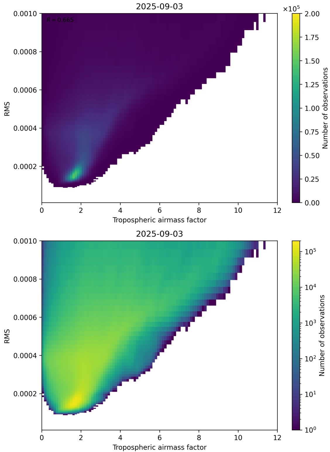
Figure 79: Scatter density plot of “Tropospheric airmass factor” against “RMS” for 2025-09-02 to 2025-09-04.
