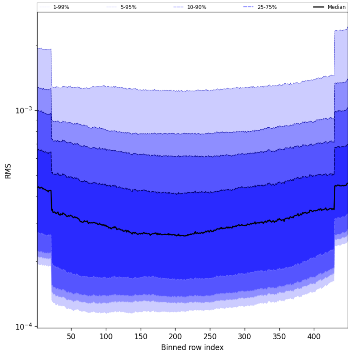
Figure 60: Along track statistics of “RMS” for 2025-09-02 to 2025-09-04
