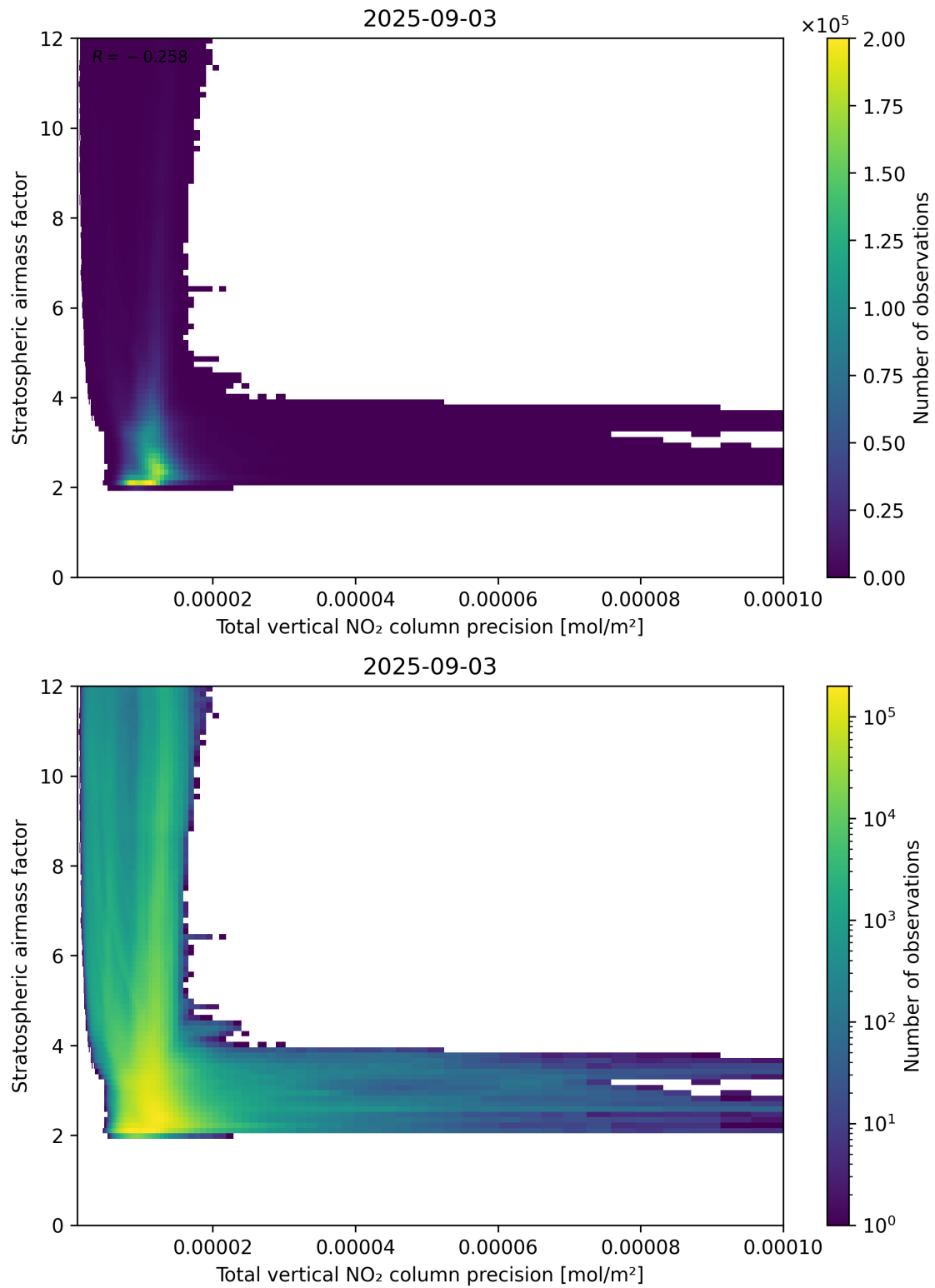
Figure 115: Scatter density plot of “Total vertical NO 2 column precision” against “Stratospheric air mass factor” for 2025-09-02 to 2025-09-04.
