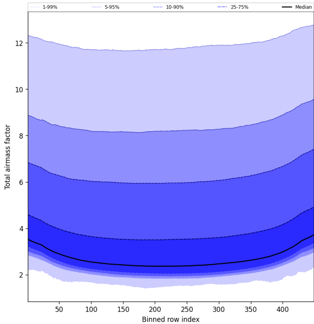
Figure 49: Along track statistics of “Total airmass factor” for 2025-09-02 to 2025-09-04
