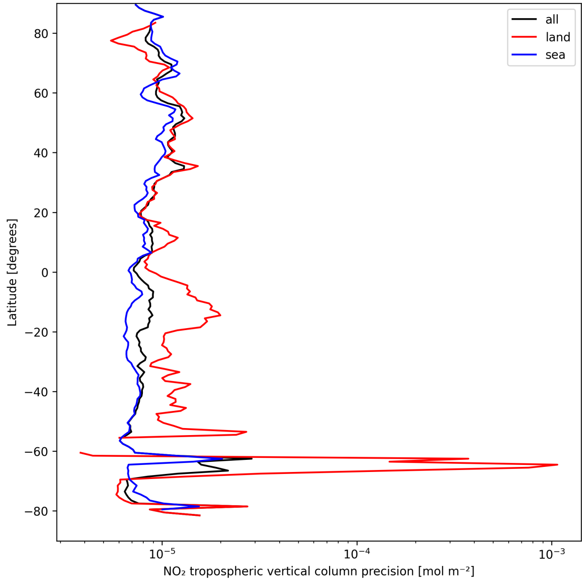
Figure 13: Zonal average of “NO 2 tropospheric vertical column precision” for 2025-09-04 to 2025-09-05.
