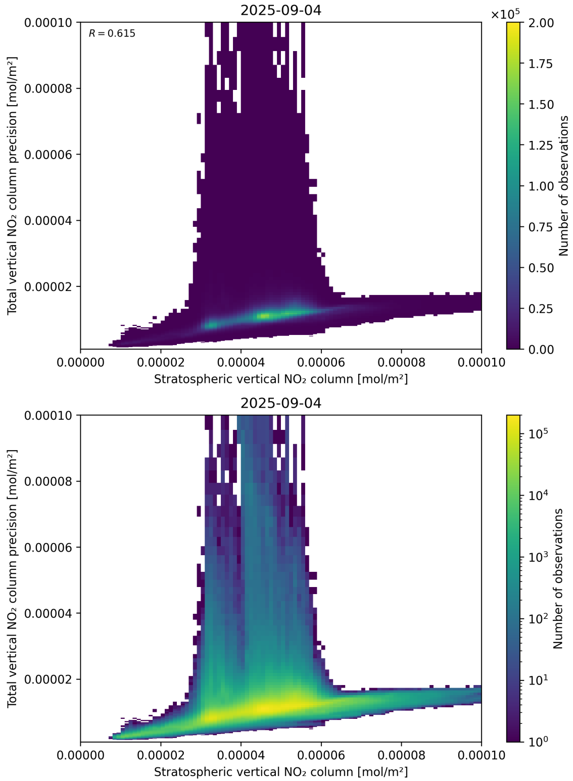
Figure 101: Scatter density plot of “Stratospheric vertical NO 2 column” against “Total vertical NO 2 column precision” for 2025-09-04 to 2025-09-05.
