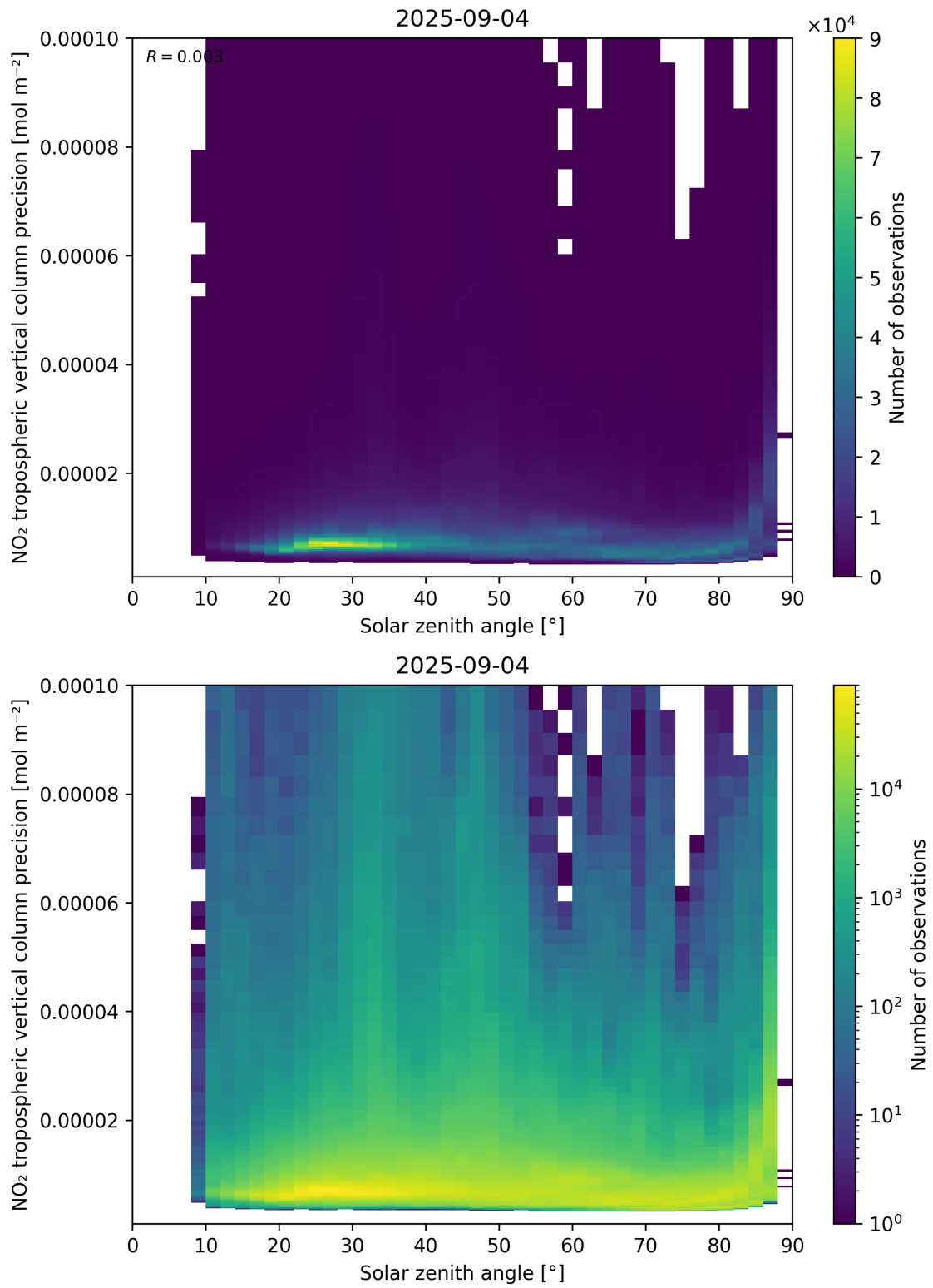
Figure 156: Scatter density plot of “Solar zenith angle” against “NO 2 tropospheric vertical column precision” for 2025-09-04 to 2025-09-05.
