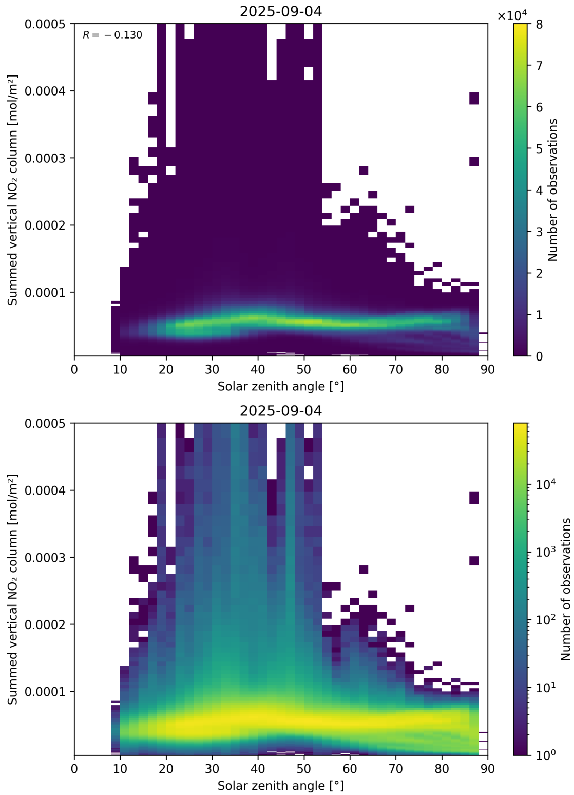
Figure 151: Scatter density plot of “Solar zenith angle” against “Summed vertical NO 2 column” for 2025-09-04 to 2025-09-05.
