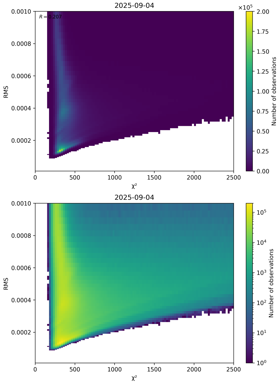
Figure 82: Scatter density plot of “ \chi^2 ” against “RMS” for 2025-09-04 to 2025-09-05.
