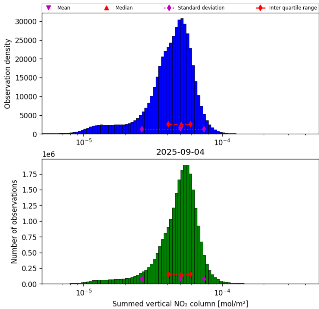
Figure 40: Histogram of “Summed vertical NO 2 column” for 2025-09-04 to 2025-09-05
