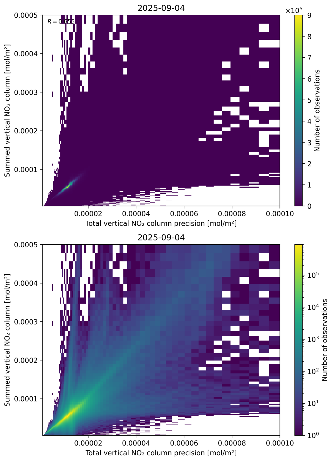
Figure 117: Scatter density plot of “Total vertical NO 2 column precision” against “Summed vertical NO 2 column” for 2025-09-04 to 2025-09-05.
