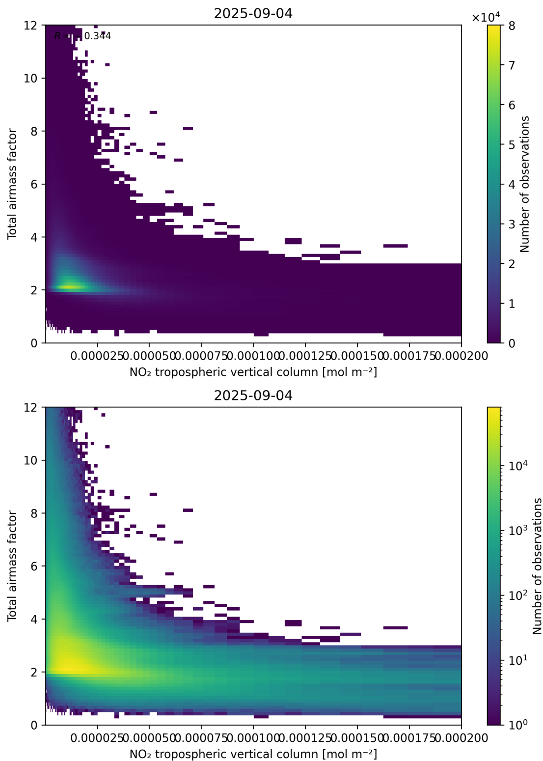
Figure 122: Scatter density plot of “NO 2 tropospheric vertical column” against “Total air mass factor” for 2025-09-04 to 2025-09-05.
