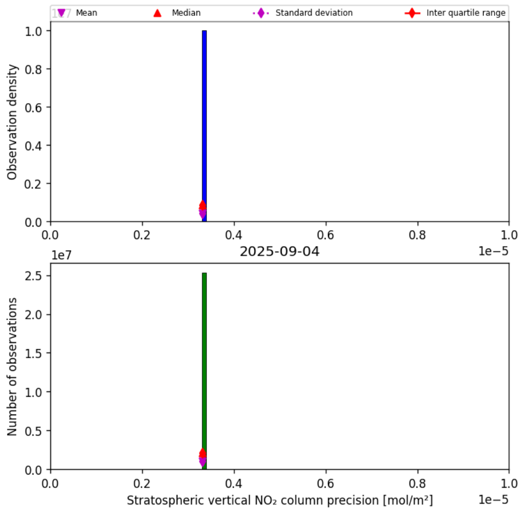
Figure 37: Histogram of “Stratospheric vertical NO 2 column precision” for 2025-09-04 to 2025-09-05
