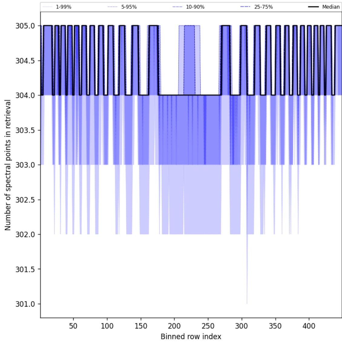
Figure 50: Along track statistics of “Number of spectral points in retrieval” for 2025-09-04 to 2025-09-05
