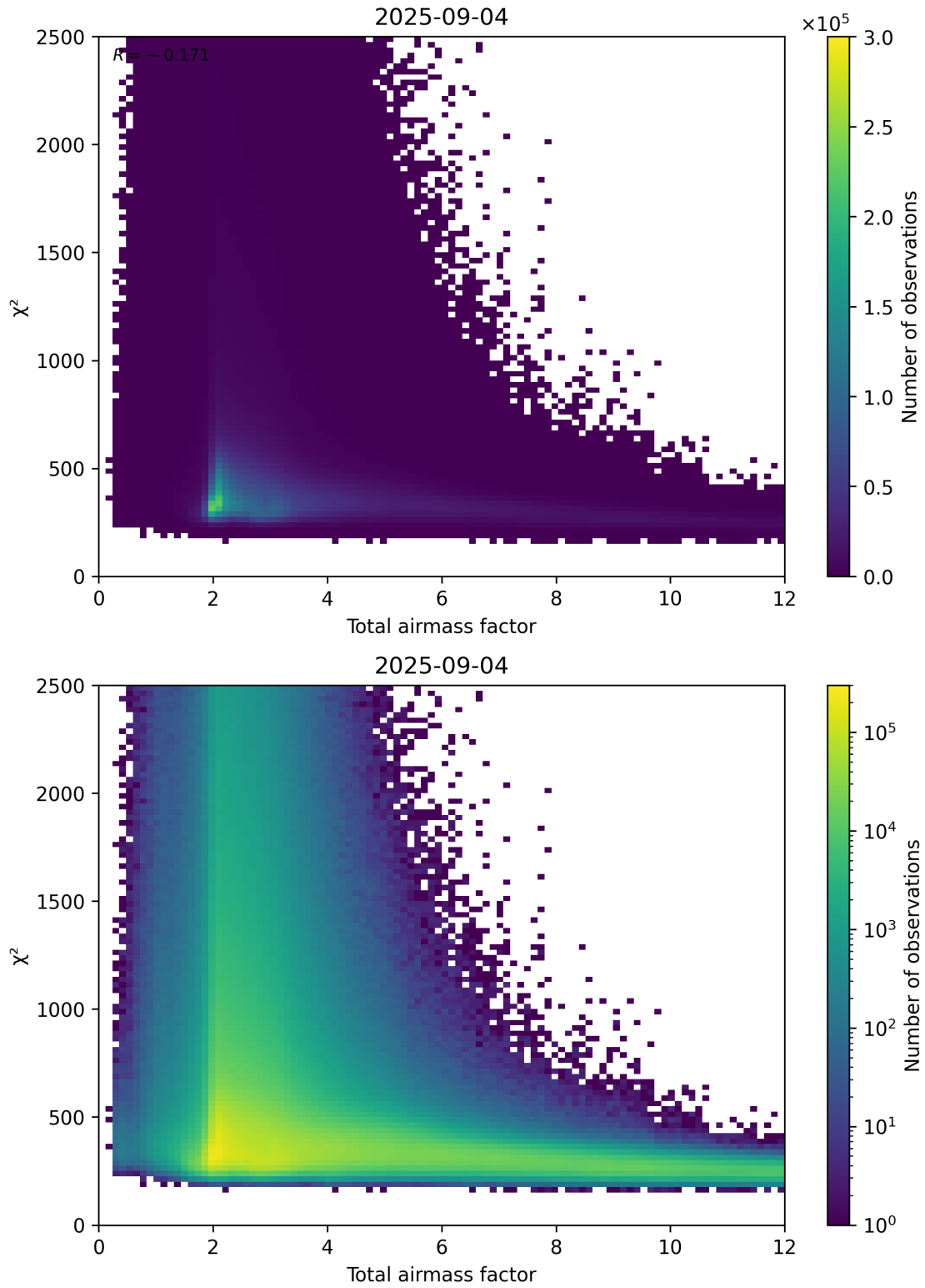
Figure 63: Scatter density plot of “Total airmass factor” against “ \chi^2 ” for 2025-09-04 to 2025-09-05.
