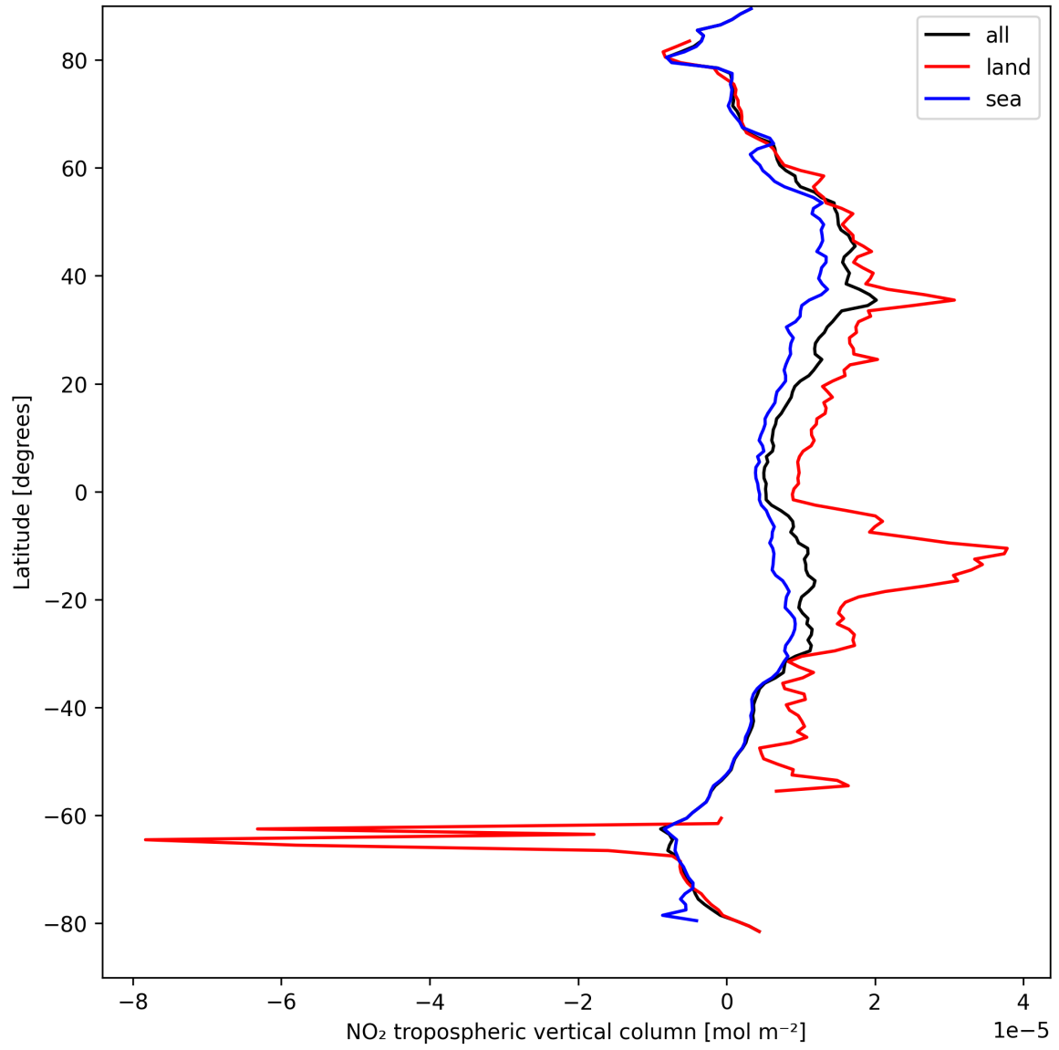
Figure 12: Zonal average of “NO 2 tropospheric vertical column” for 2025-09-04 to 2025-09-05.
