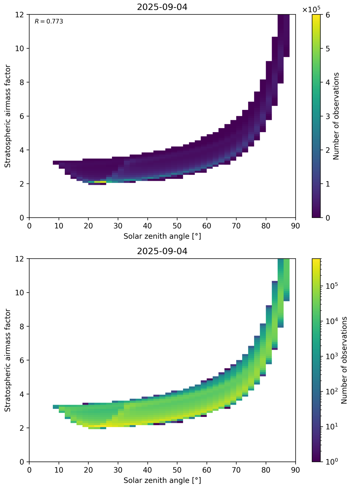
Figure 145: Scatter density plot of “Solar zenith angle” against “Stratospheric airmass factor” for 2025-09-04 to 2025-09-05.
