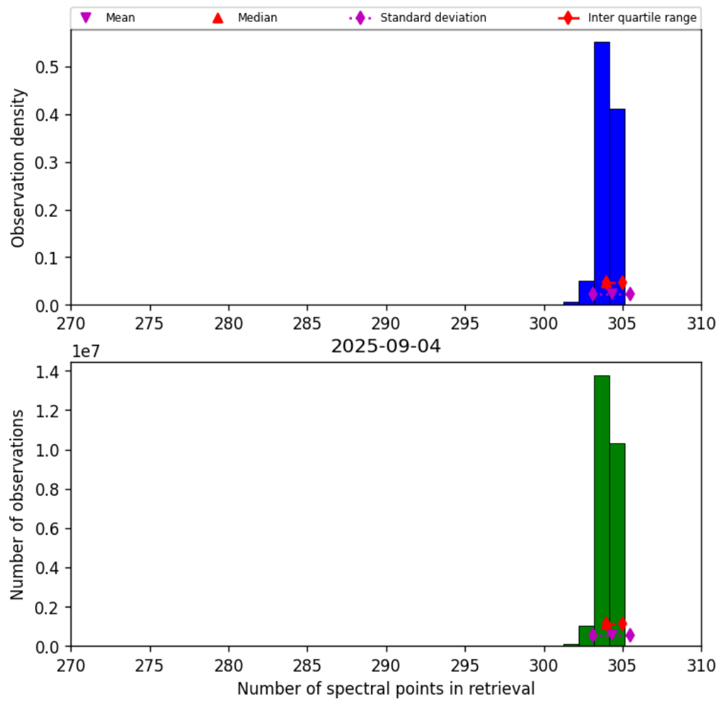
Figure 33: Histogram of “Number of spectral points in retrieval” for 2025-09-04 to 2025-09-05
