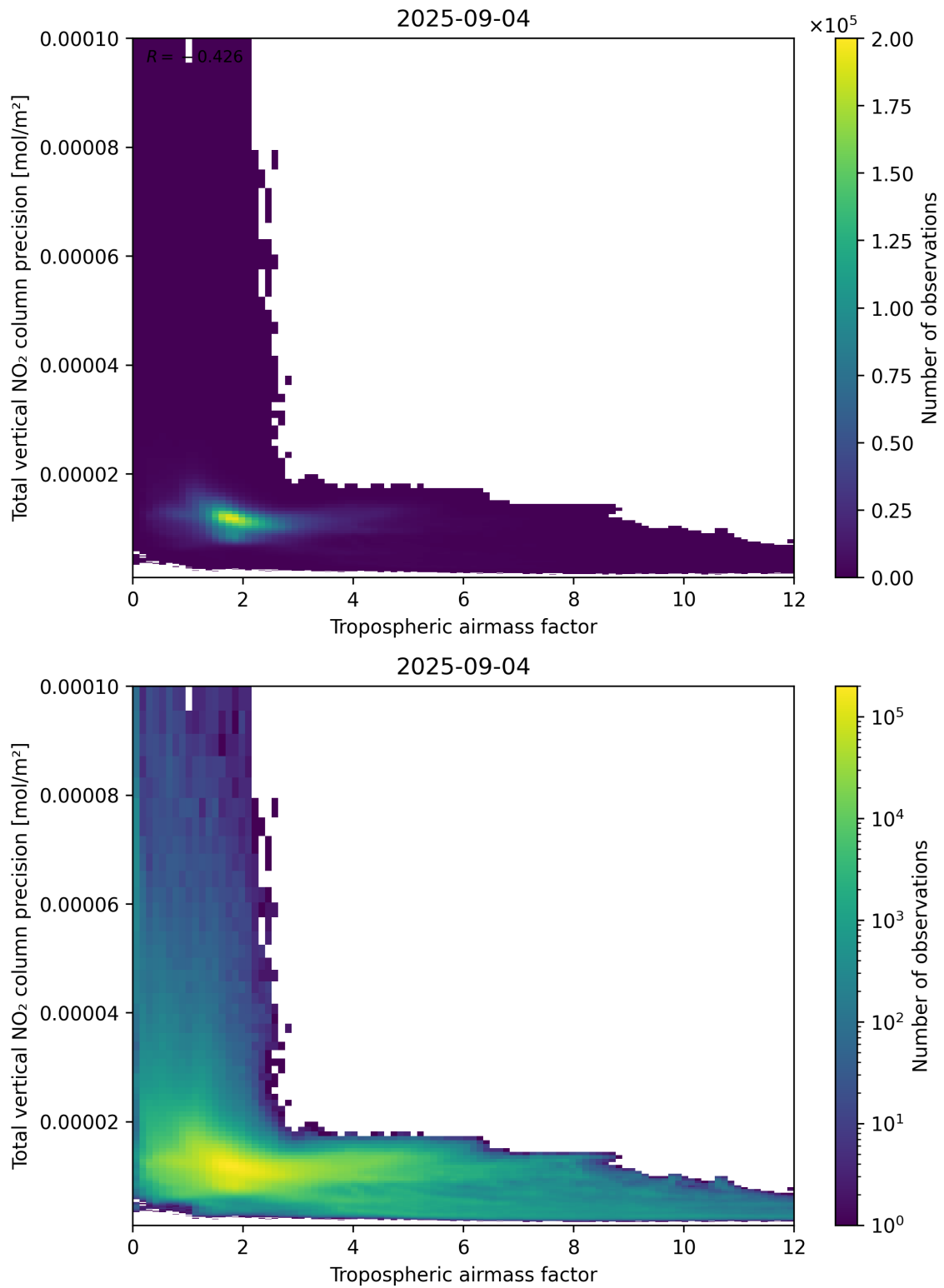
Figure 78: Scatter density plot of “Tropospheric air mass factor” against “Total vertical NO 2 column precision” for 2025-09-04 to 2025-09-05.
