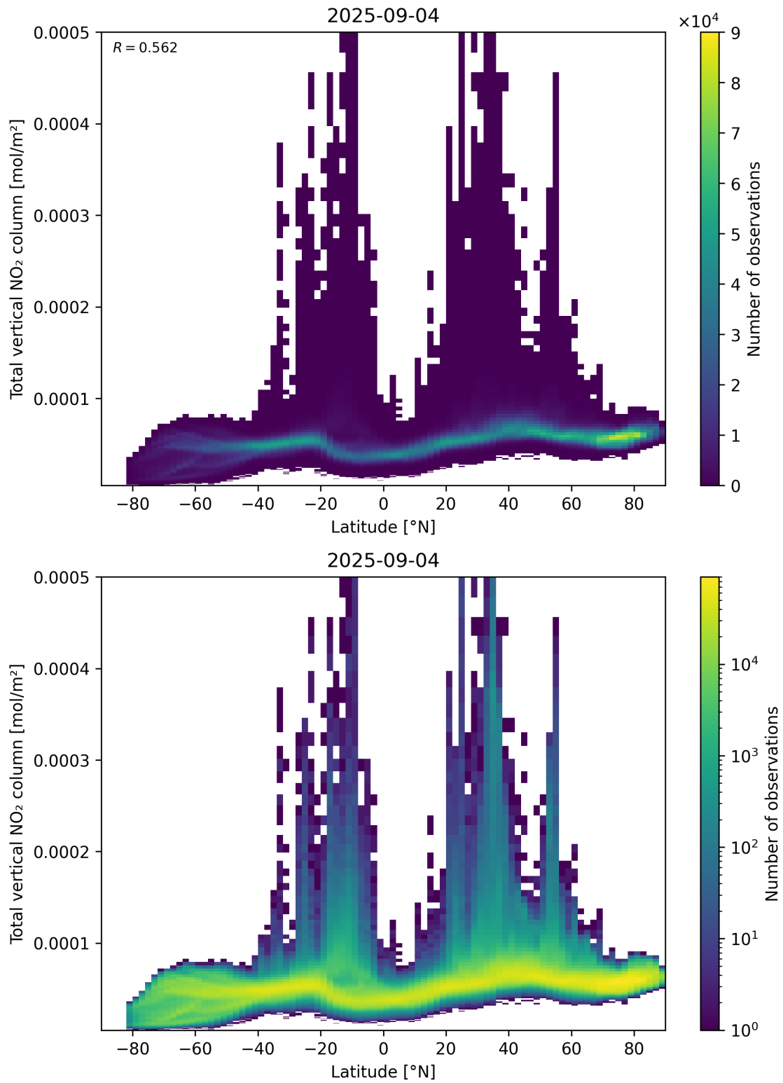
Figure 90: Scatter density plot of “Latitude” against “Total vertical NO 2 column” for 2025-09-04 to 2025-09-05.
