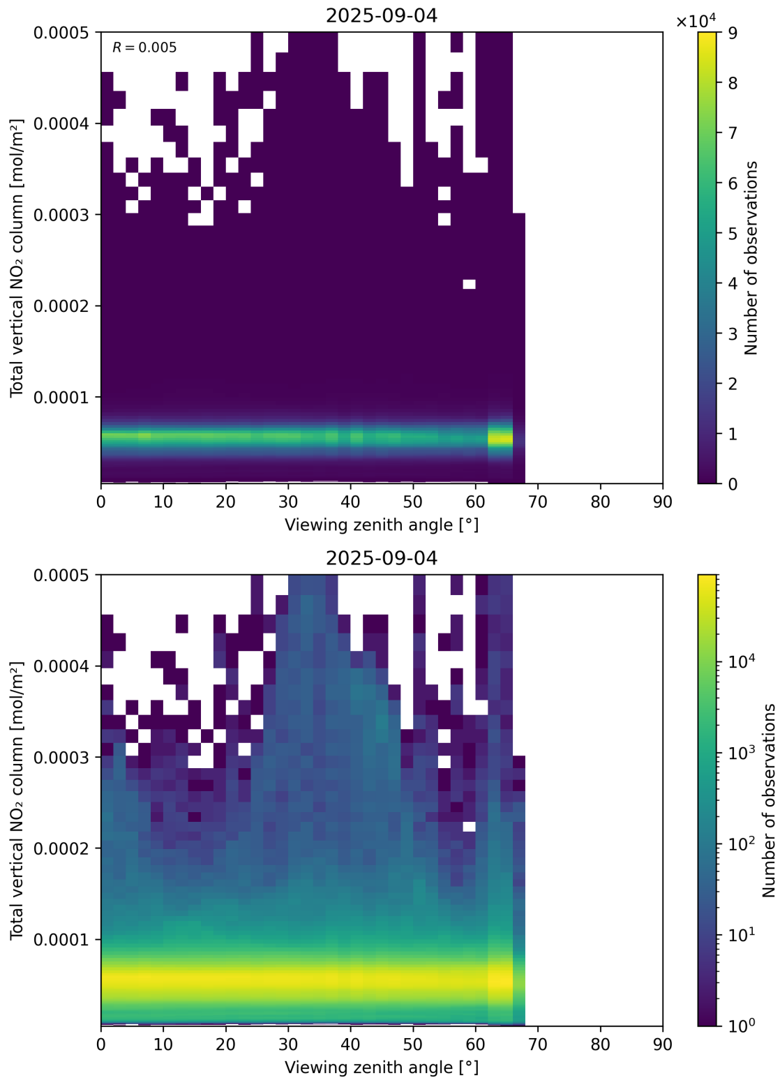
Figure 167: Scatter density plot of “Viewing zenith angle” against “Total vertical NO 2 column” for 2025-09-04 to 2025-09-05.
