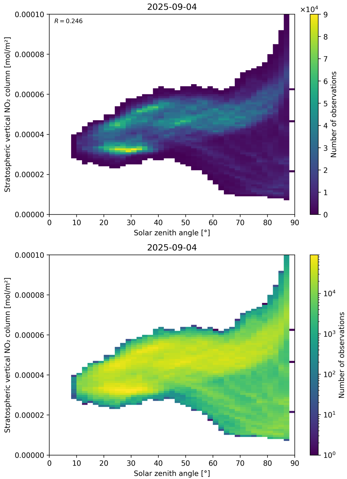
Figure 150: Scatter density plot of “Solar zenith angle” against “Stratospheric vertical NO 2 column” for 2025-09-04 to 2025-09-05.
