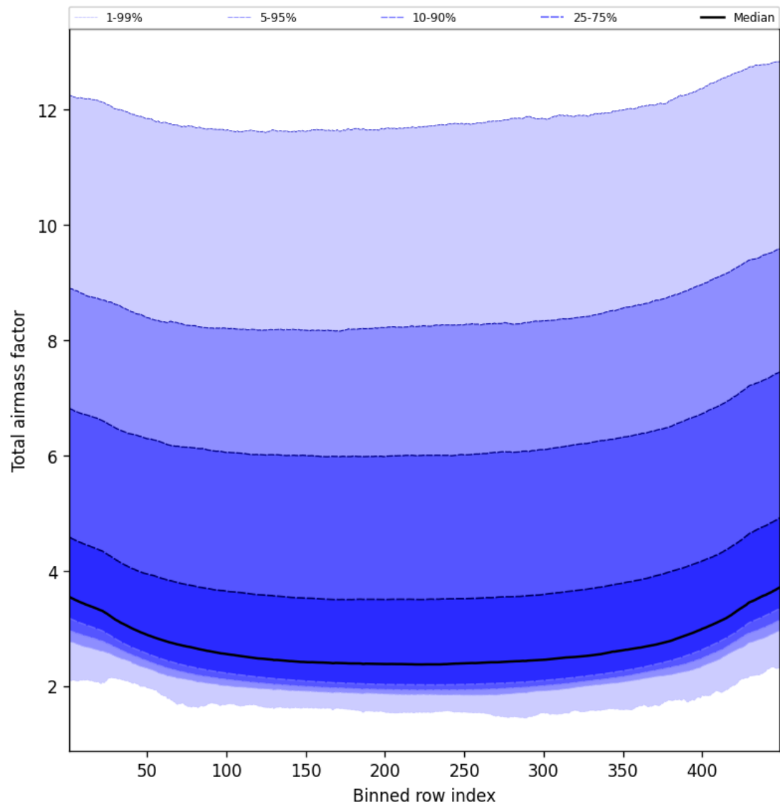
Figure 49: Along track statistics of “Total airmass factor” for 2025-09-04 to 2025-09-05
