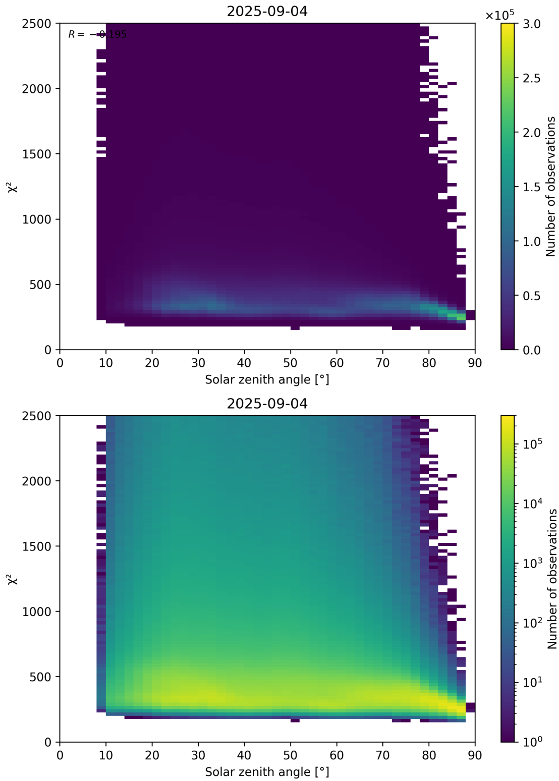
Figure 148: Scatter density plot of “Solar zenith angle” against “ \chi^2 ” for 2025-09-04 to 2025-09-05.
