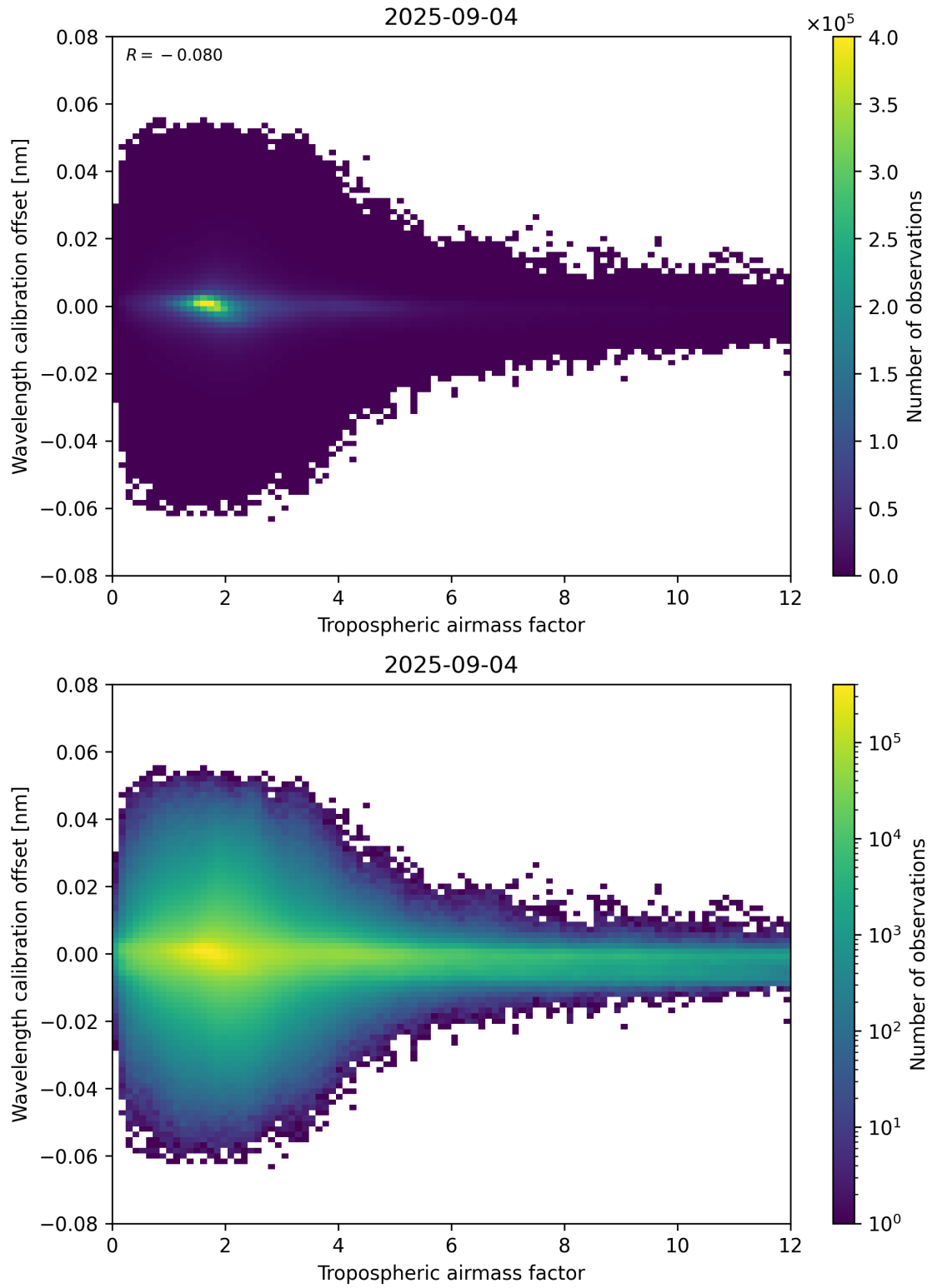
Figure 80: Scatter density plot of “Tropospheric airmass factor” against “Wavelength calibration offset” for 2025-09-04 to 2025-09-05.
