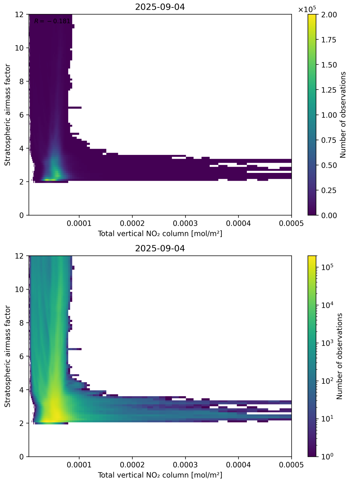
Figure 110: Scatter density plot of “Total vertical NO 2 column” against “Stratospheric airmass factor” for 2025-09-04 to 2025-09-05.
