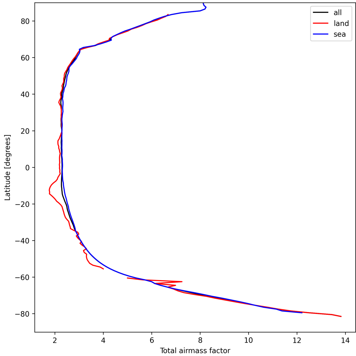
Figure 15: Zonal average of “Total airmass factor” for 2025-09-04 to 2025-09-05.
