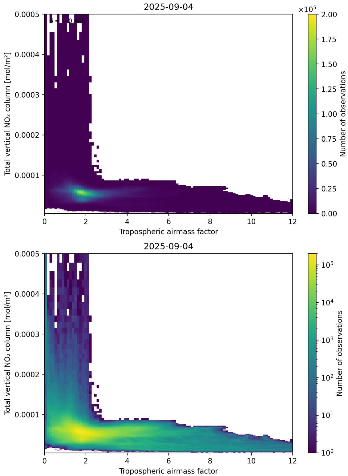
Figure 77: Scatter density plot of “Tropospheric airmass factor” against “Total vertical NO 2 column” for 2025-09-04 to 2025-09-05.
