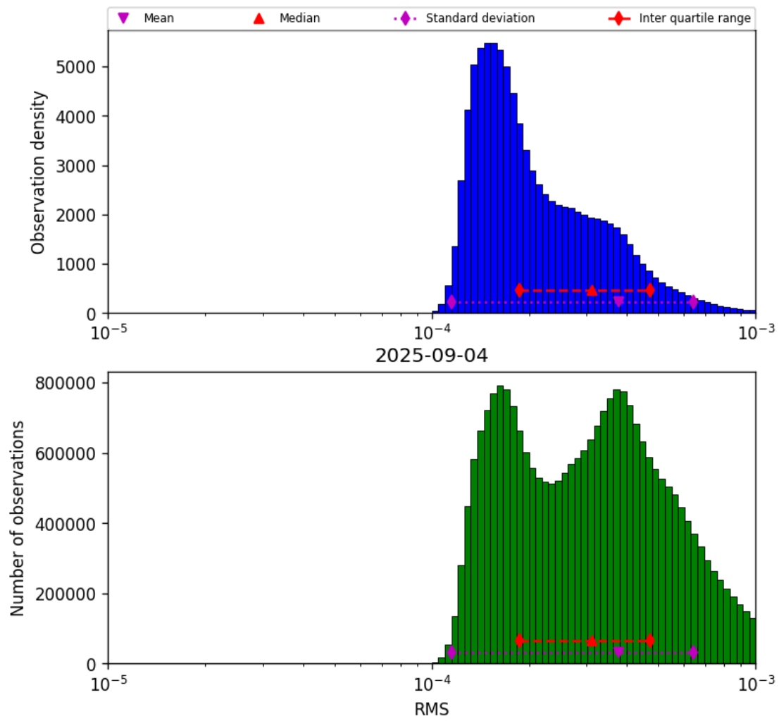
Figure 43: Histogram of “RMS” for 2025-09-04 to 2025-09-05
