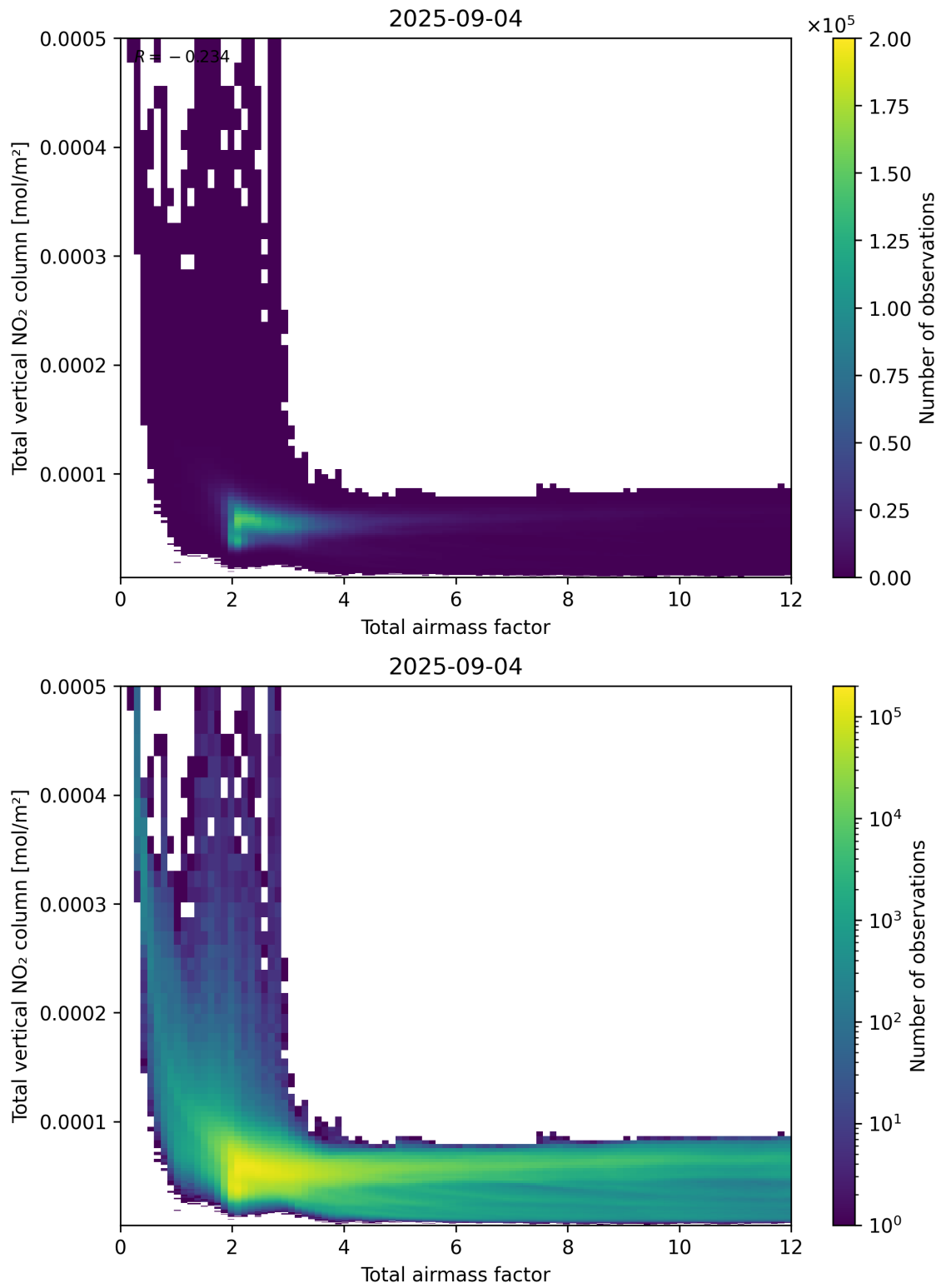
Figure 67: Scatter density plot of “Total air mass factor” against “Total vertical NO 2 column” for 2025-09-04 to 2025-09-05.
