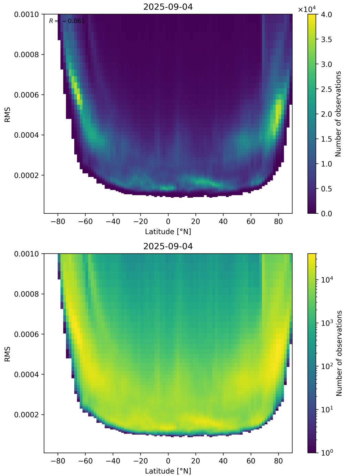
Figure 94: Scatter density plot of “Latitude” against “RMS” for 2025-09-04 to 2025-09-05.
