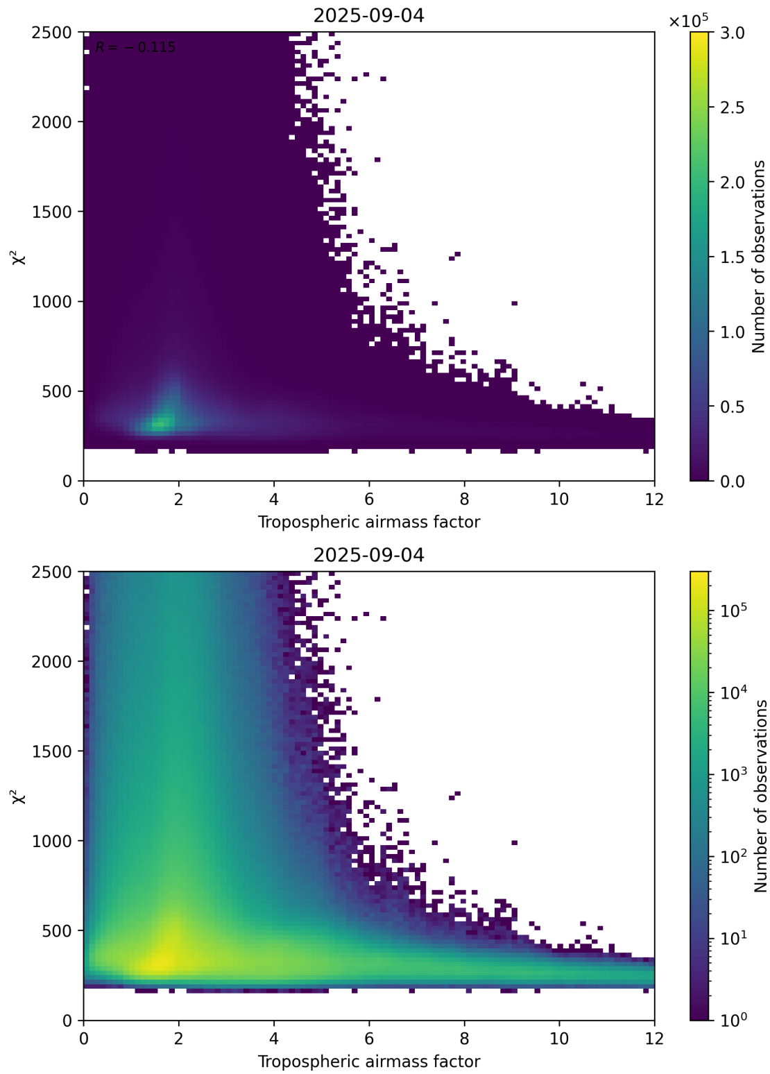
Figure 73: Scatter density plot of “Tropospheric airmass factor” against “ \chi^2 ” for 2025-09-04 to 2025-09-05.
