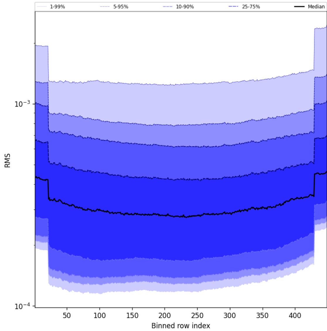
Figure 60: Along track statistics of “RMS” for 2025-09-04 to 2025-09-05
