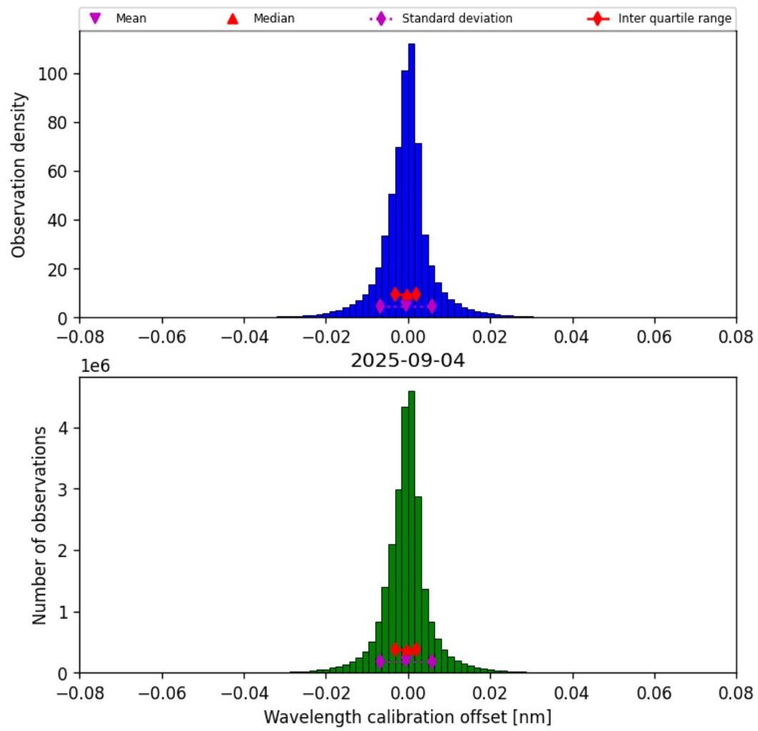
Figure 35: Histogram of “Wavelength calibration offset” for 2025-09-04 to 2025-09-05
