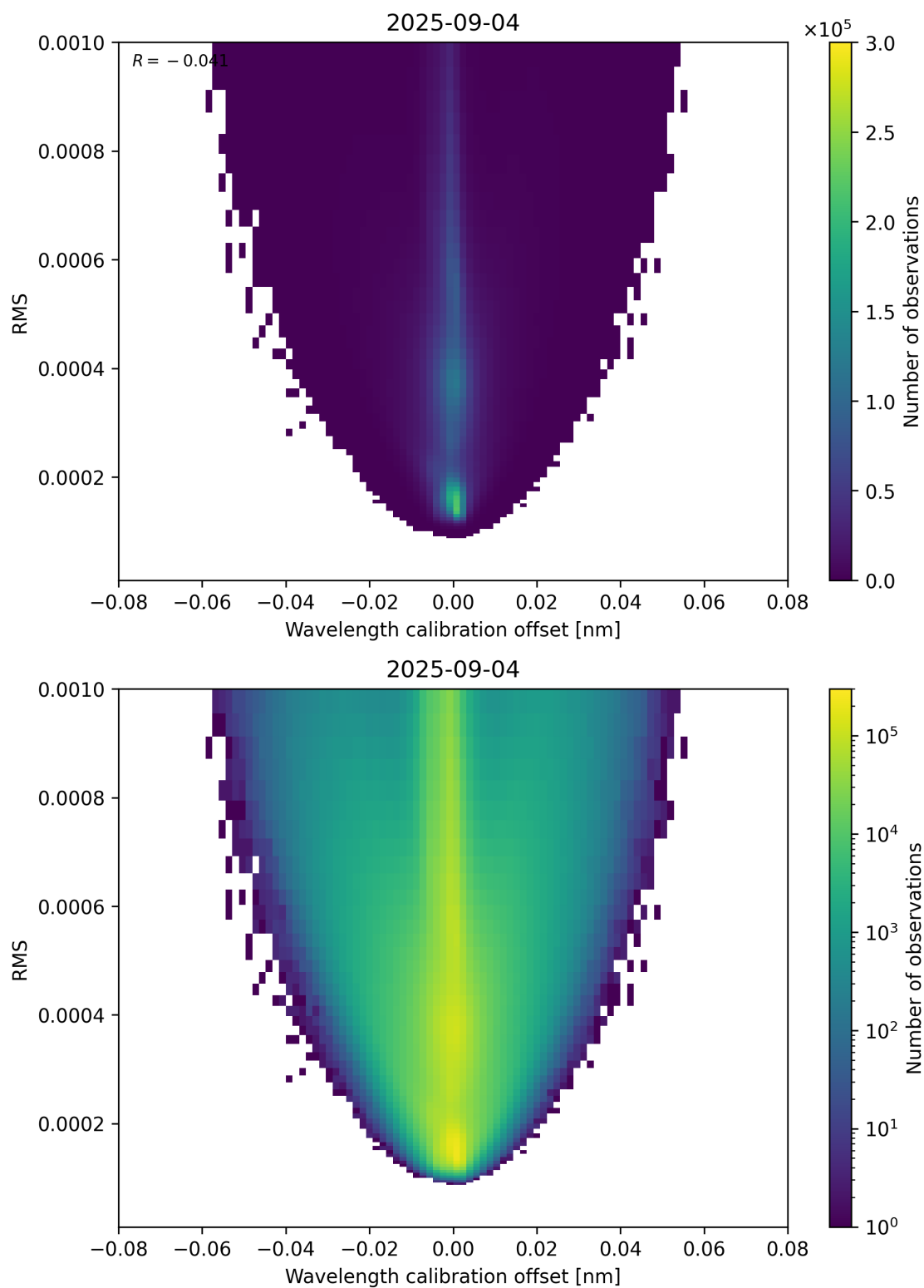
Figure 181: Scatter density plot of “Wavelength calibration offset” against “RMS” for 2025-09-04 to 2025-09-05.
