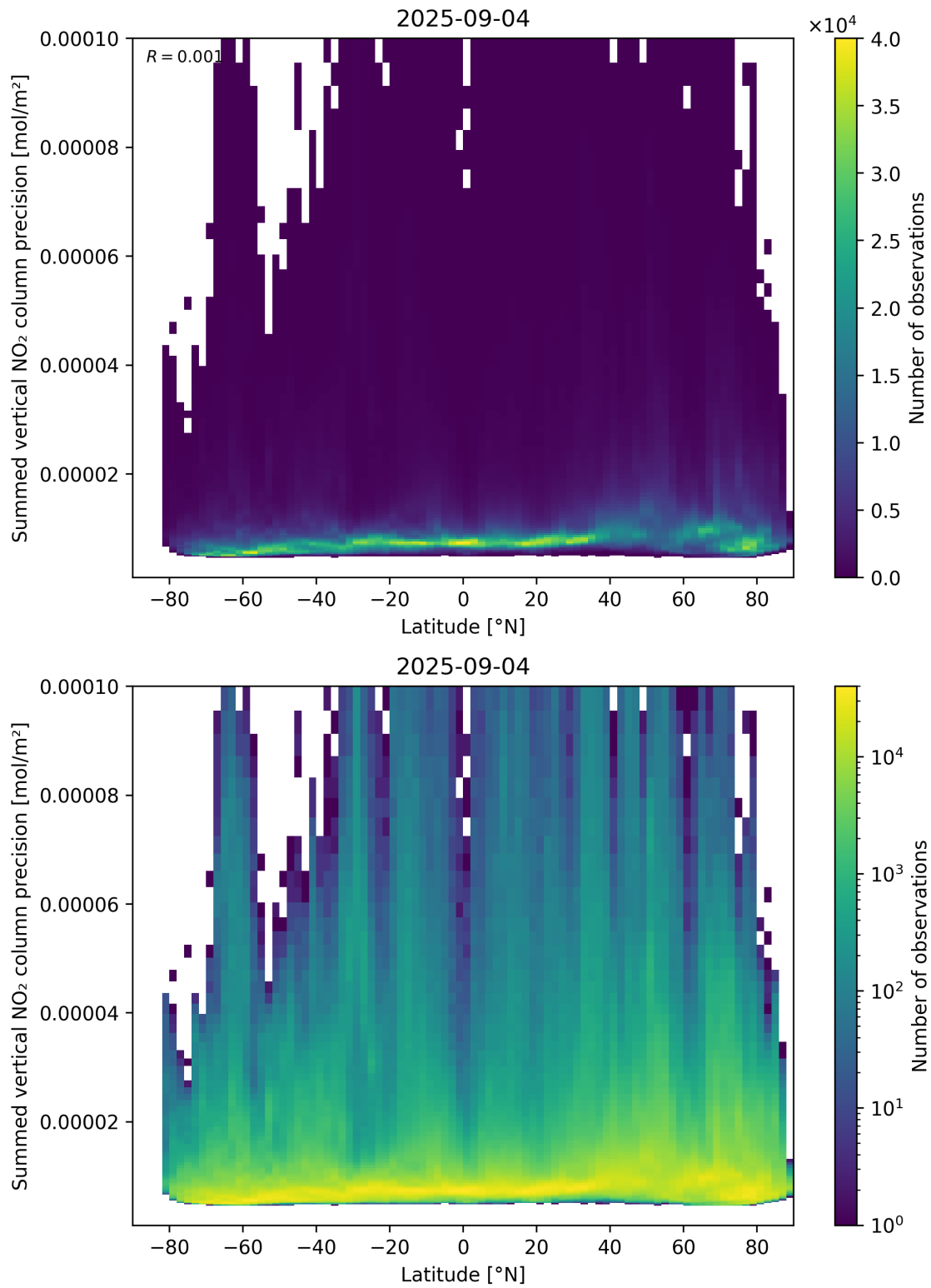
Figure 89: Scatter density plot of “Latitude” against “Summed vertical NO 2 column precision” for 2025-09-04 to 2025-09-05.
