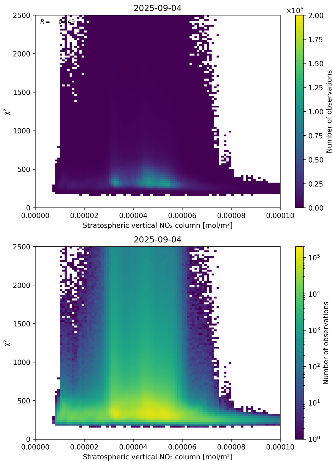
Figure 97: Scatter density plot of “Stratospheric vertical NO 2 column” against “ \chi^2 ” for 2025-09-04 to 2025-09-05.
