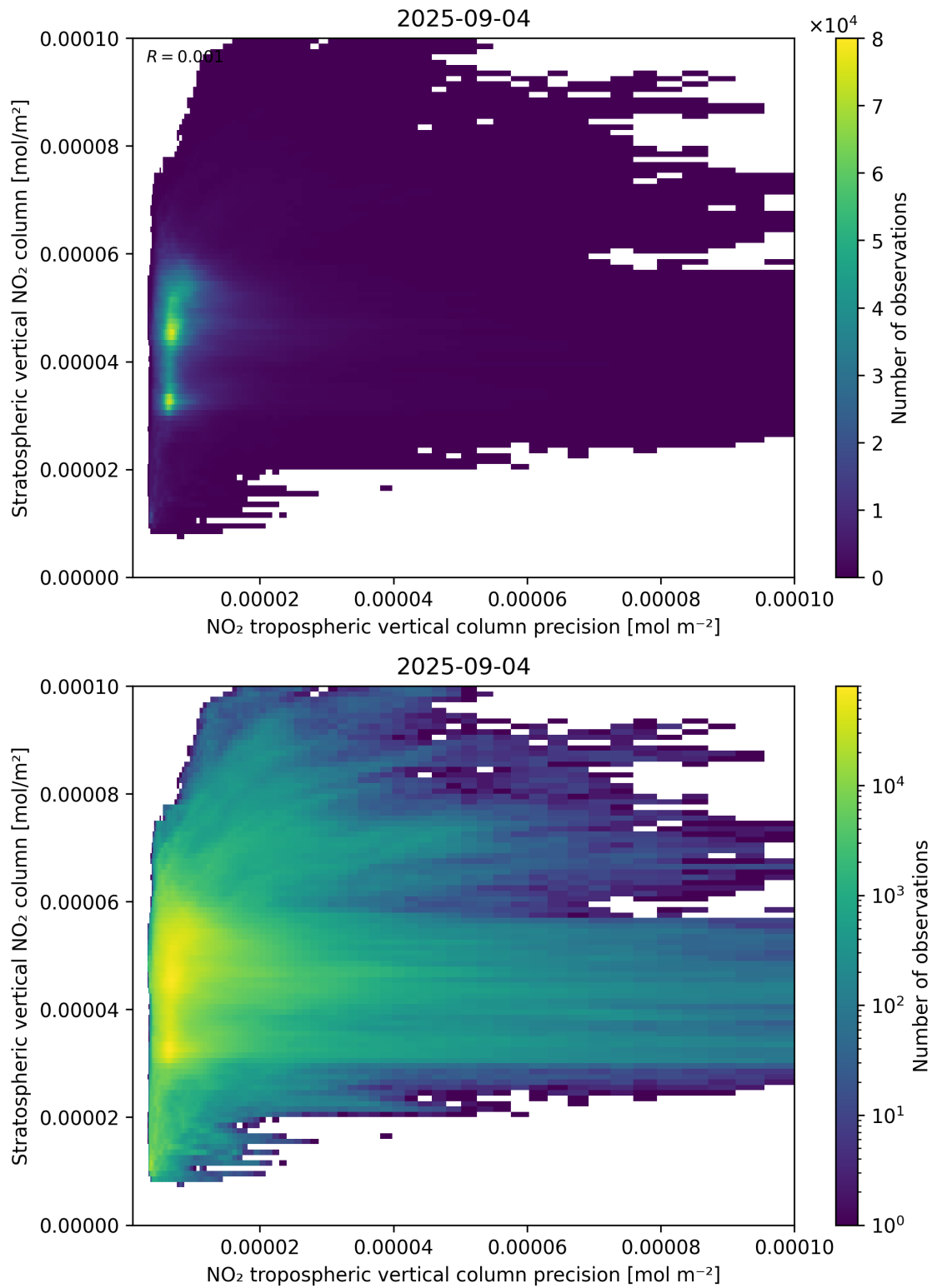
Figure 135: Scatter density plot of “NO 2 tropospheric vertical column precision” against “Stratospheric vertical NO 2 column” for 2025-09-04 to 2025-09-05.
