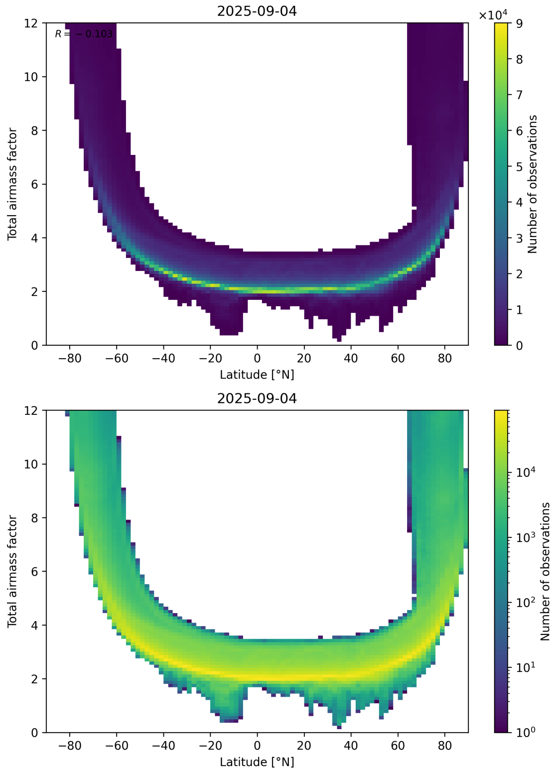
Figure 84: Scatter density plot of “Latitude” against “Total air mass factor” for 2025-09-04 to 2025-09-05.
