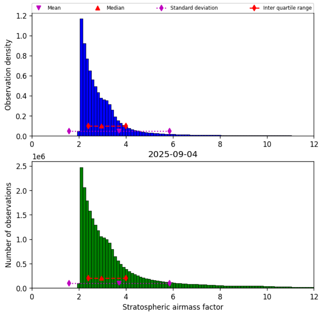
Figure 44: Histogram of “Stratospheric airmass factor” for 2025-09-04 to 2025-09-05
