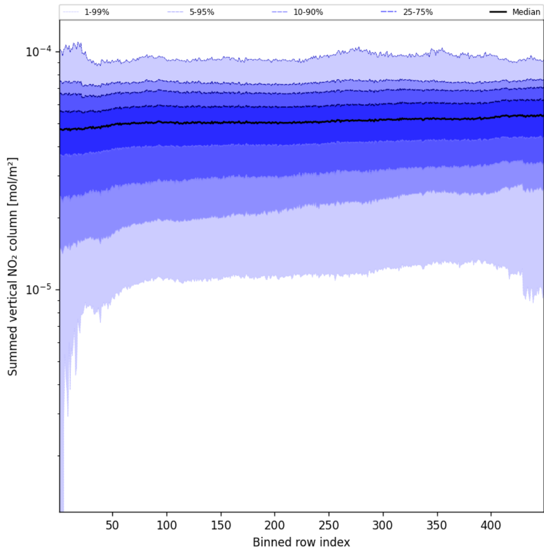
Figure 57: Along track statistics of “Summed vertical NO 2 column” for 2025-09-04 to 2025-09-05
