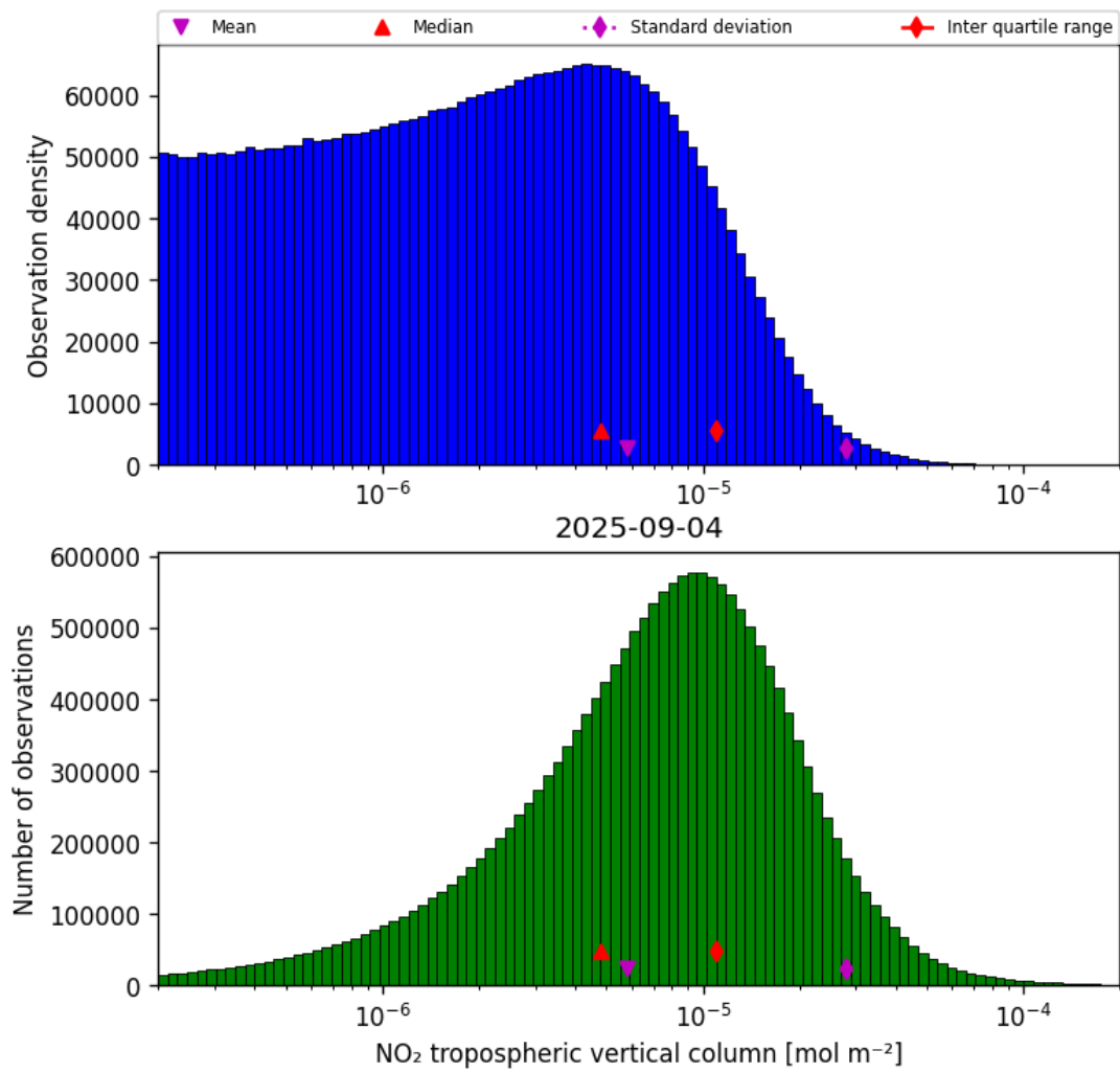
Figure 29: Histogram of “NO 2 tropospheric vertical column” for 2025-09-04 to 2025-09-05
