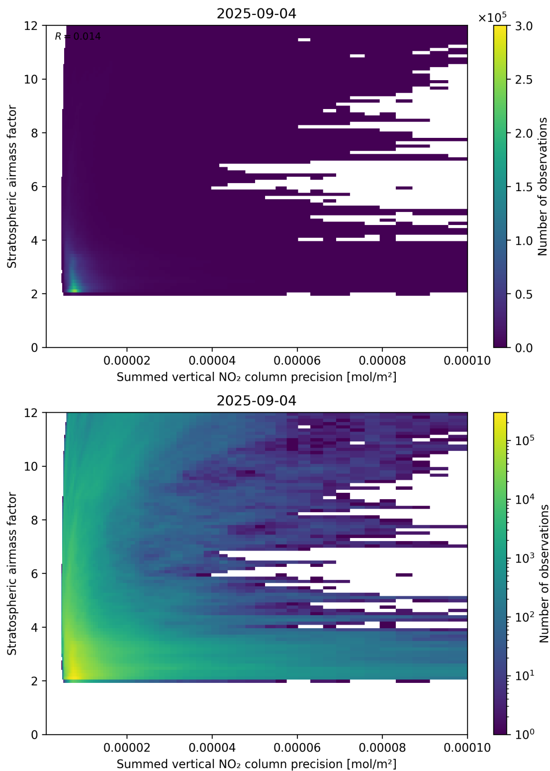
Figure 106: Scatter density plot of “Summed vertical NO 2 column precision” against “Stratospheric airmass factor” for 2025-09-04 to 2025-09-05.
