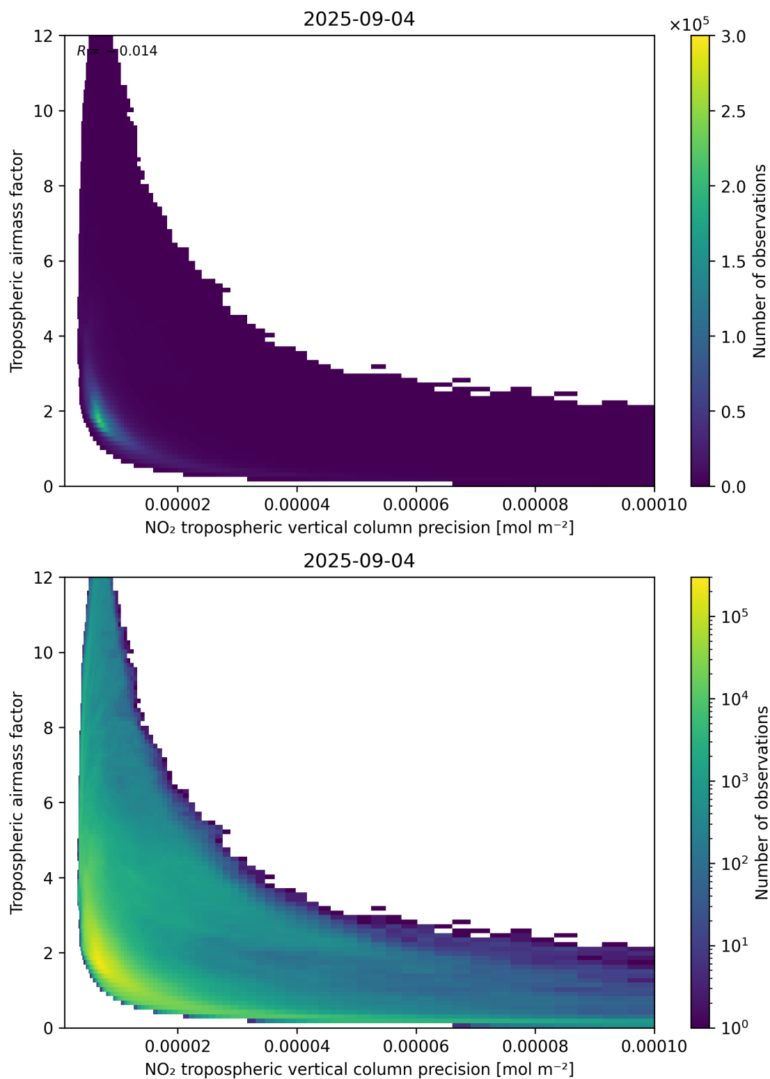
Figure 133: Scatter density plot of “NO 2 tropospheric vertical column precision” against “Tropospheric air mass factor” for 2025-09-04 to 2025-09-05.
