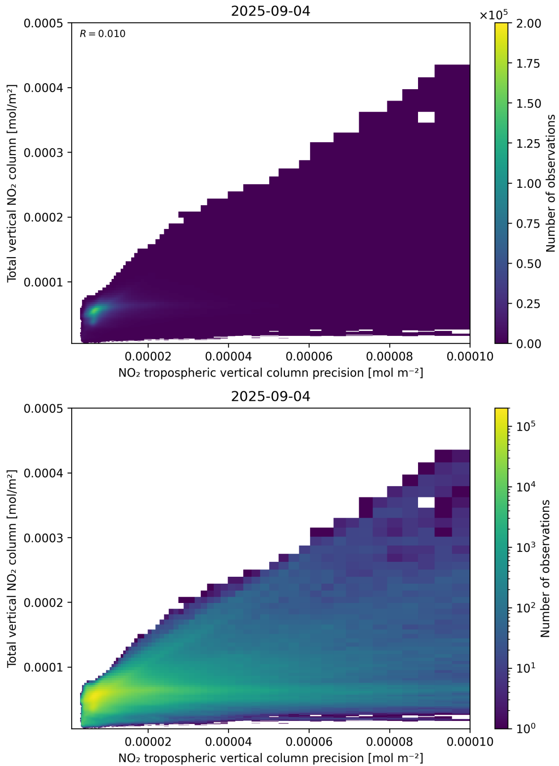
Figure 138: Scatter density plot of “NO 2 tropospheric vertical column precision” against “Total vertical NO 2 column” for 2025-09-04 to 2025-09-05.
