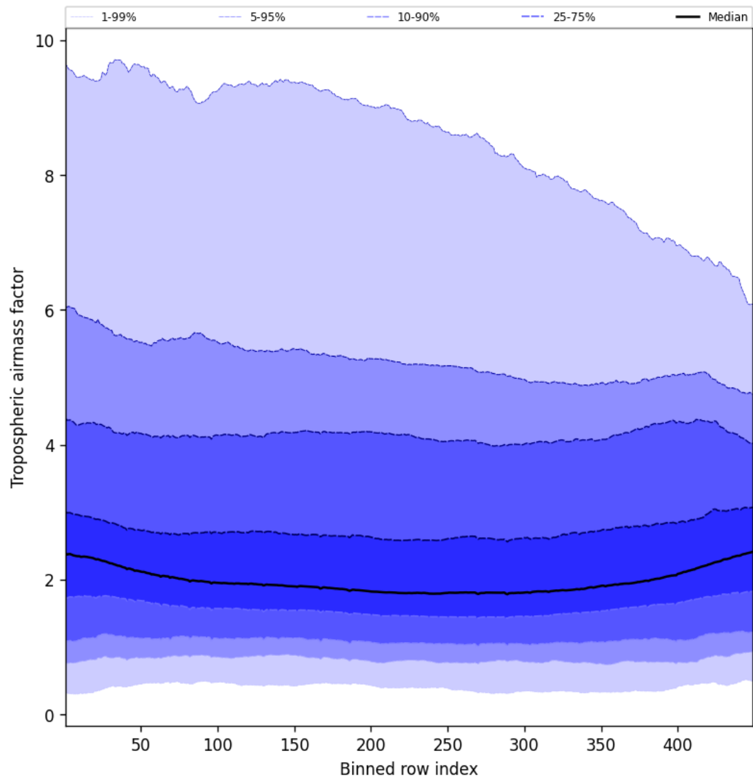
Figure 48: Along track statistics of “Tropospheric air mass factor” for 2025-09-04 to 2025-09-05
