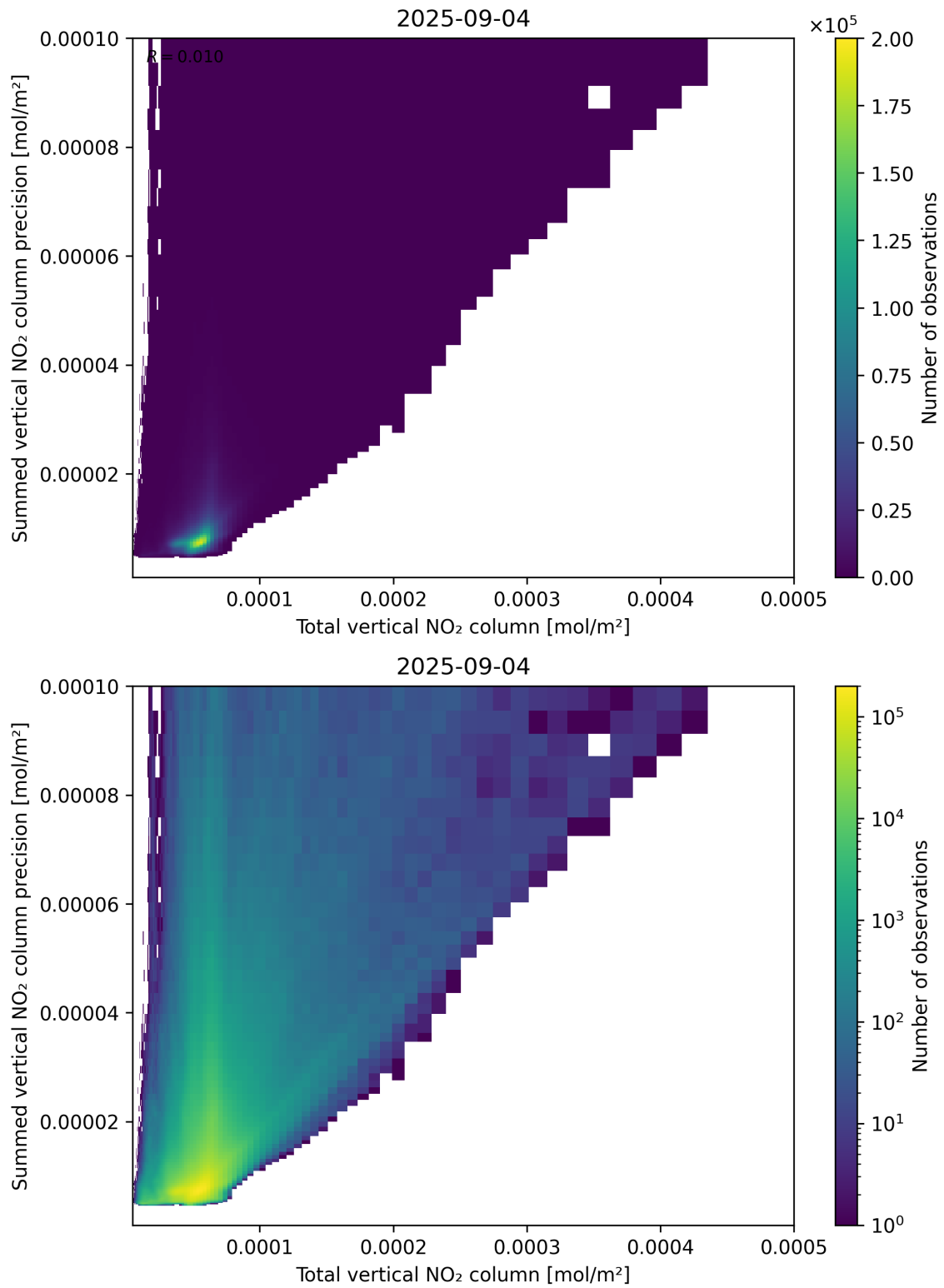
Figure 113: Scatter density plot of “Total vertical NO 2 column” against “Summed vertical NO 2 column precision” for 2025-09-04 to 2025-09-05.
