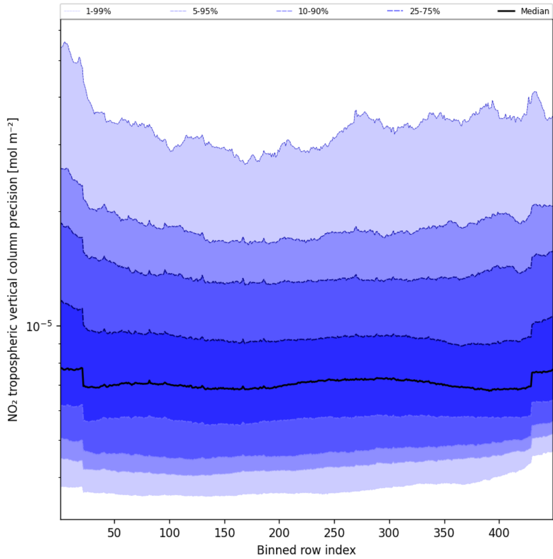
Figure 47: Along track statistics of “NO 2 tropospheric vertical column precision” for 2025-09-04 to 2025-09-05
