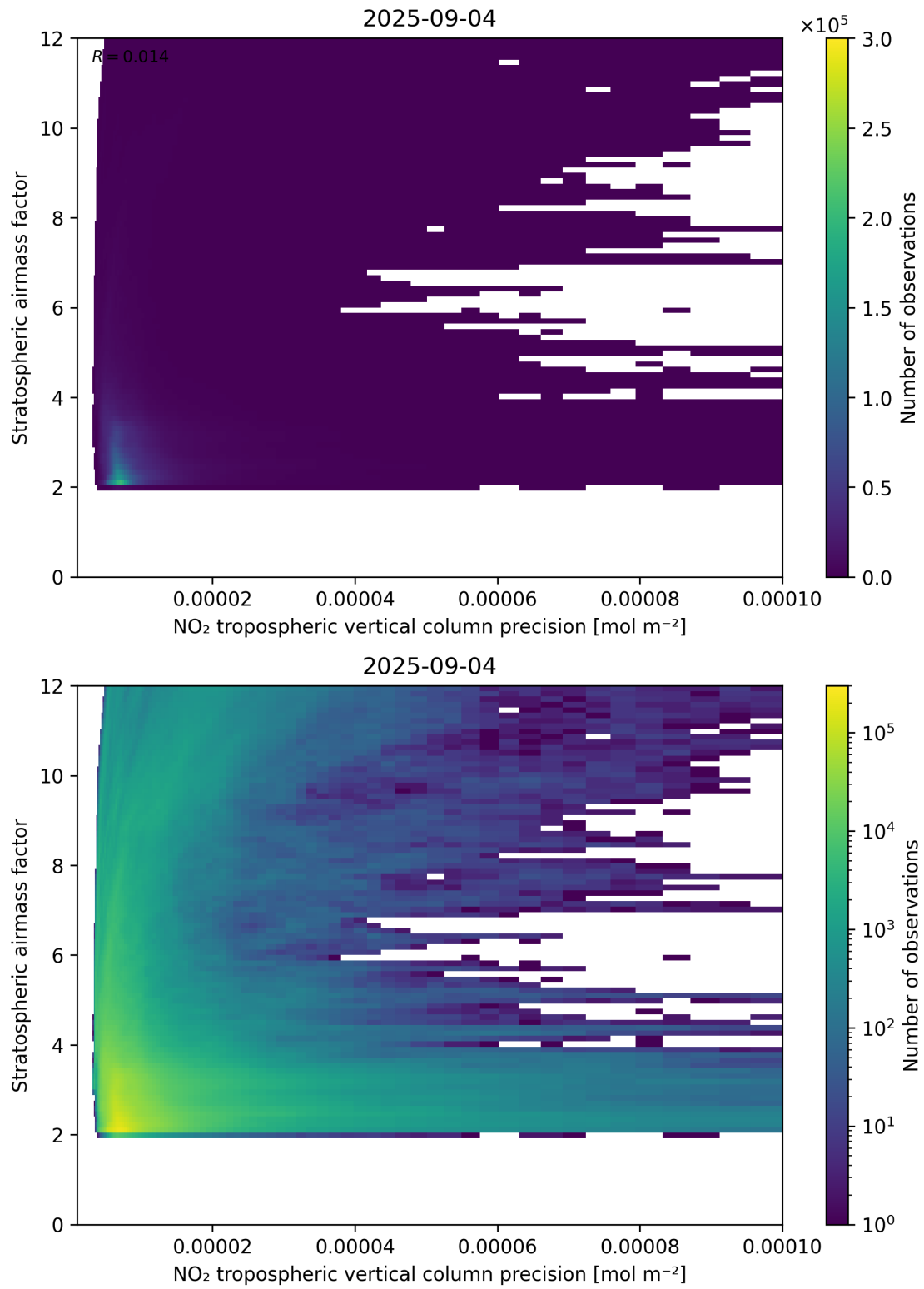
Figure 131: Scatter density plot of “NO 2 tropospheric vertical column precision” against “Stratospheric airmass factor” for 2025-09-04 to 2025-09-05.
