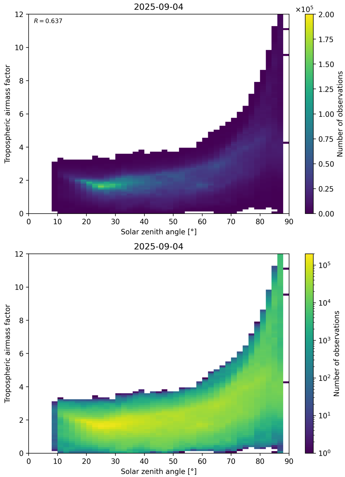
Figure 147: Scatter density plot of “Solar zenith angle” against “Tropospheric airmass factor” for 2025-09-04 to 2025-09-05.
