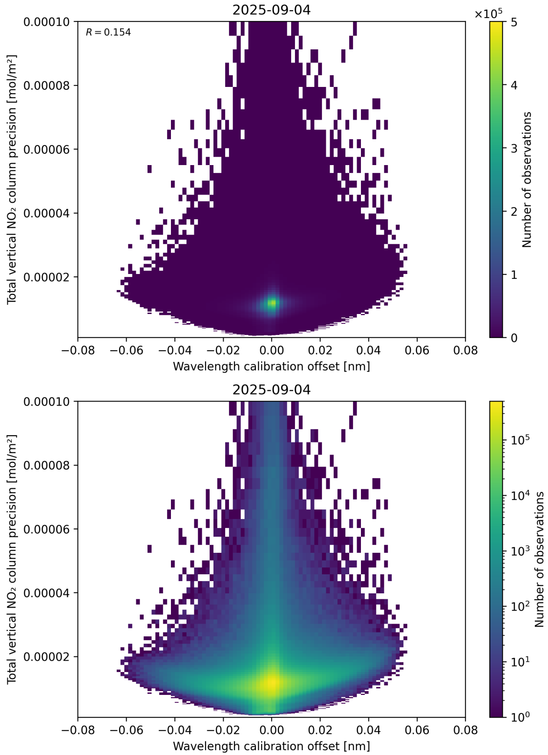
Figure 180: Scatter density plot of “Wavelength calibration offset” against “Total vertical NO 2 column precision” for 2025-09-04 to 2025-09-05.
