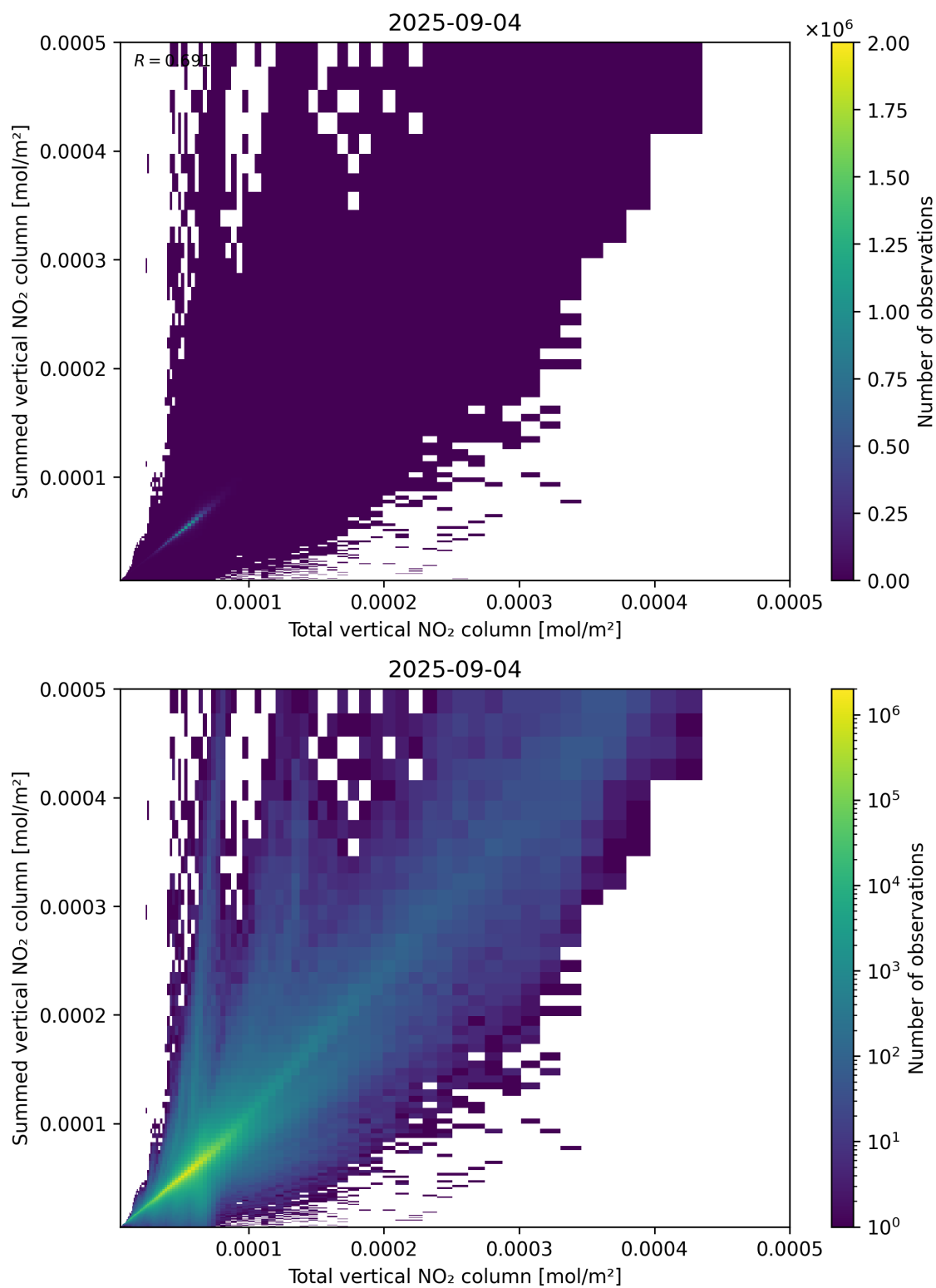
Figure 112: Scatter density plot of “Total vertical NO 2 column” against “Summed vertical NO 2 column” for 2025-09-04 to 2025-09-05.
