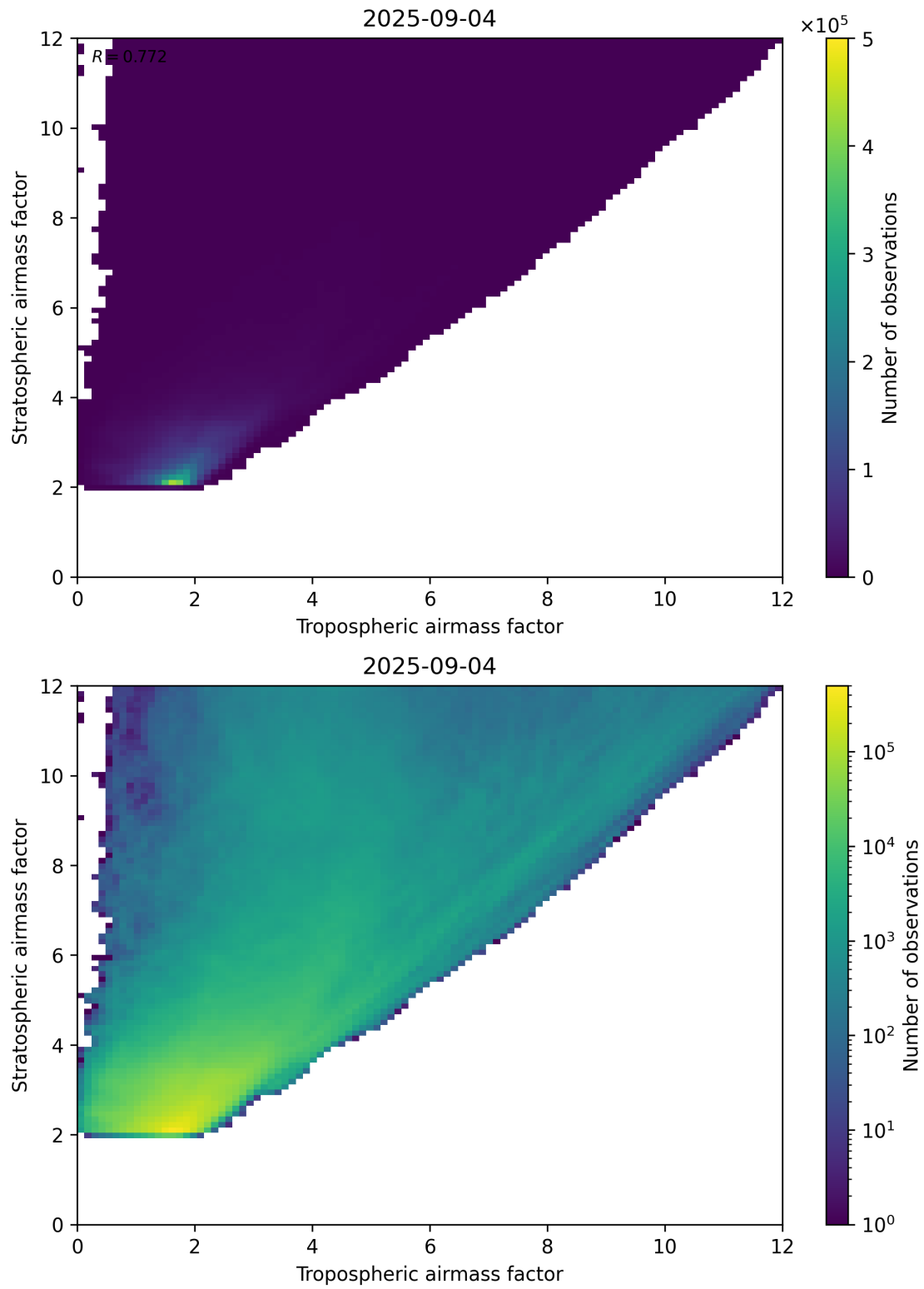
Figure 71: Scatter density plot of “Tropospheric airmass factor” against “Stratospheric airmass factor” for 2025-09-04 to 2025-09-05.
