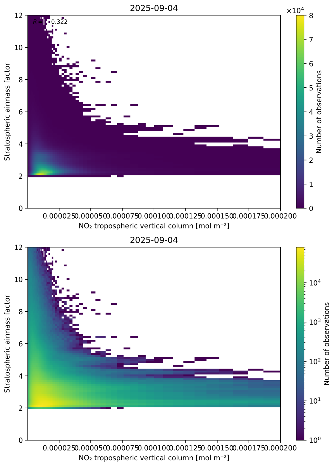
Figure 121: Scatter density plot of “NO 2 tropospheric vertical column” against “Stratospheric airmass factor” for 2025-09-04 to 2025-09-05.
