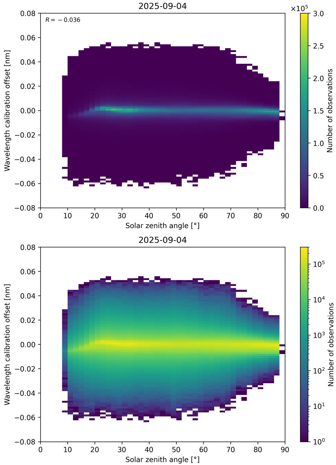
Figure 158: Scatter density plot of “Solar zenith angle” against “Wavelength calibration offset” for 2025-09-04 to 2025-09-05.
