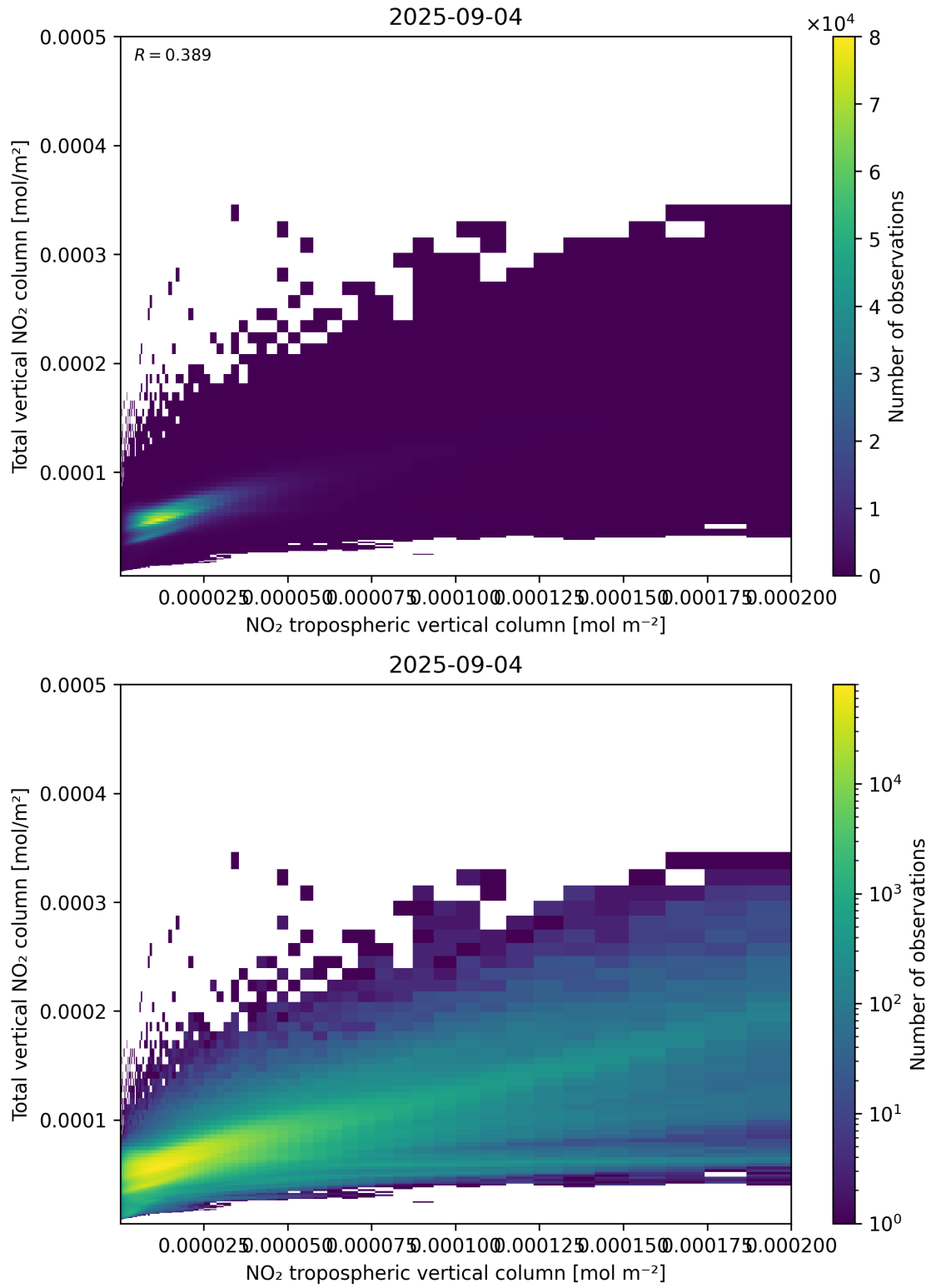
Figure 128: Scatter density plot of “NO 2 tropospheric vertical column” against “Total vertical NO 2 column” for 2025-09-04 to 2025-09-05.
