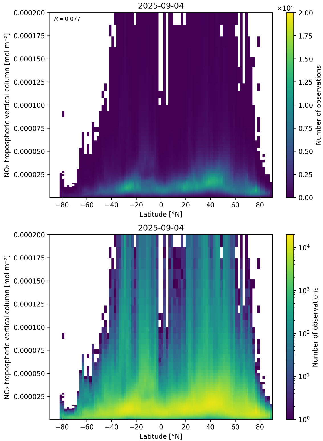
Figure 92: Scatter density plot of “Latitude” against “NO 2 tropospheric vertical column” for 2025-09-04 to 2025-09-05.
