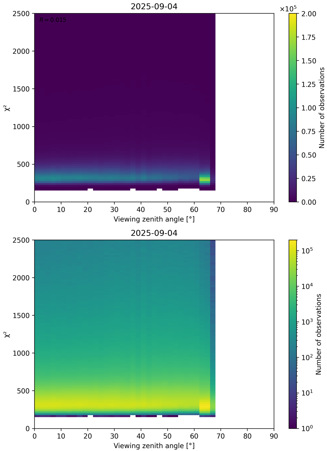
Figure 162: Scatter density plot of “Viewing zenith angle” against “ \chi^2 ” for 2025-09-04 to 2025-09-05.
