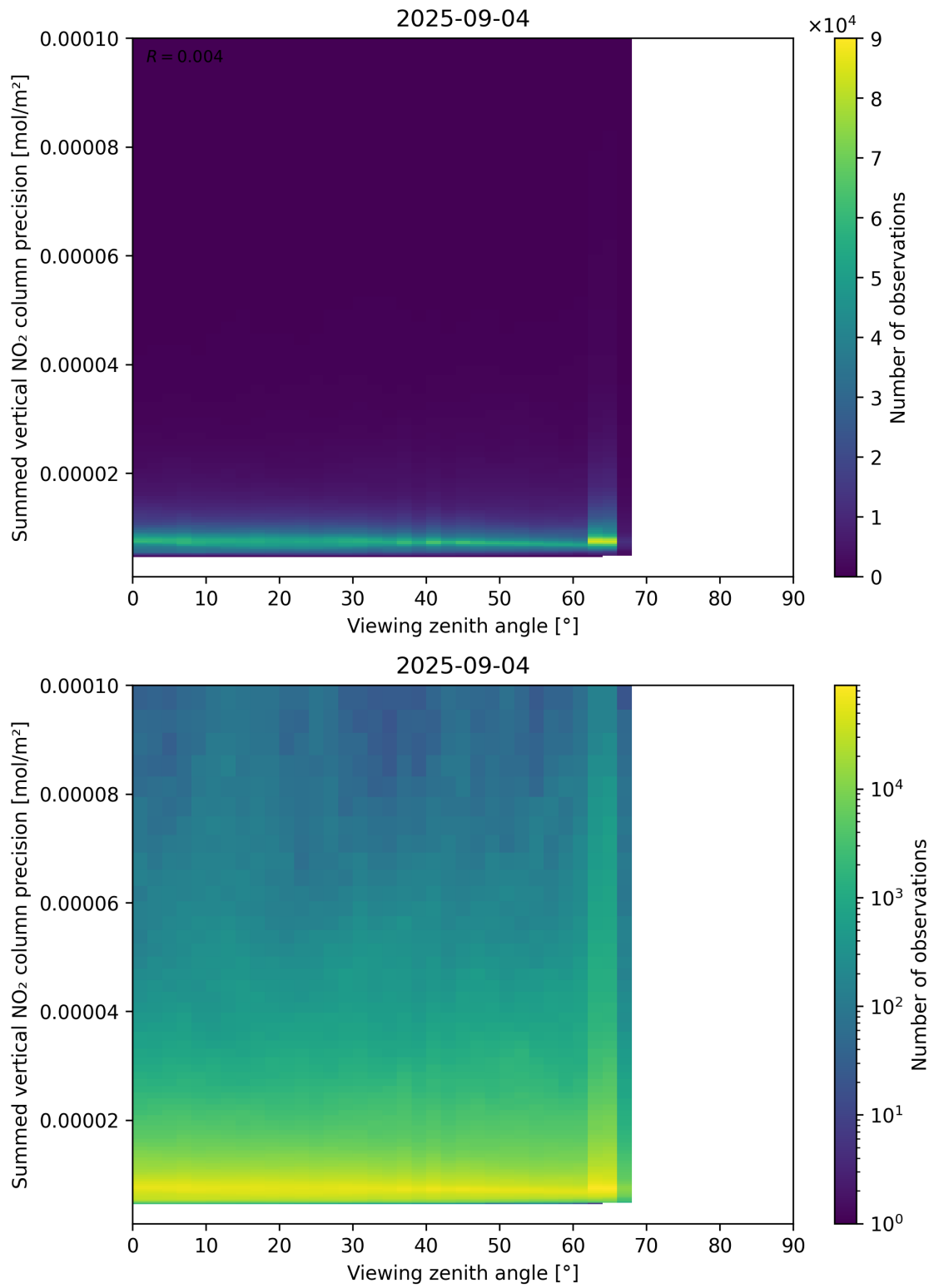
Figure 166: Scatter density plot of “Viewing zenith angle” against “Summed vertical NO 2 column precision” for 2025-09-04 to 2025-09-05.
