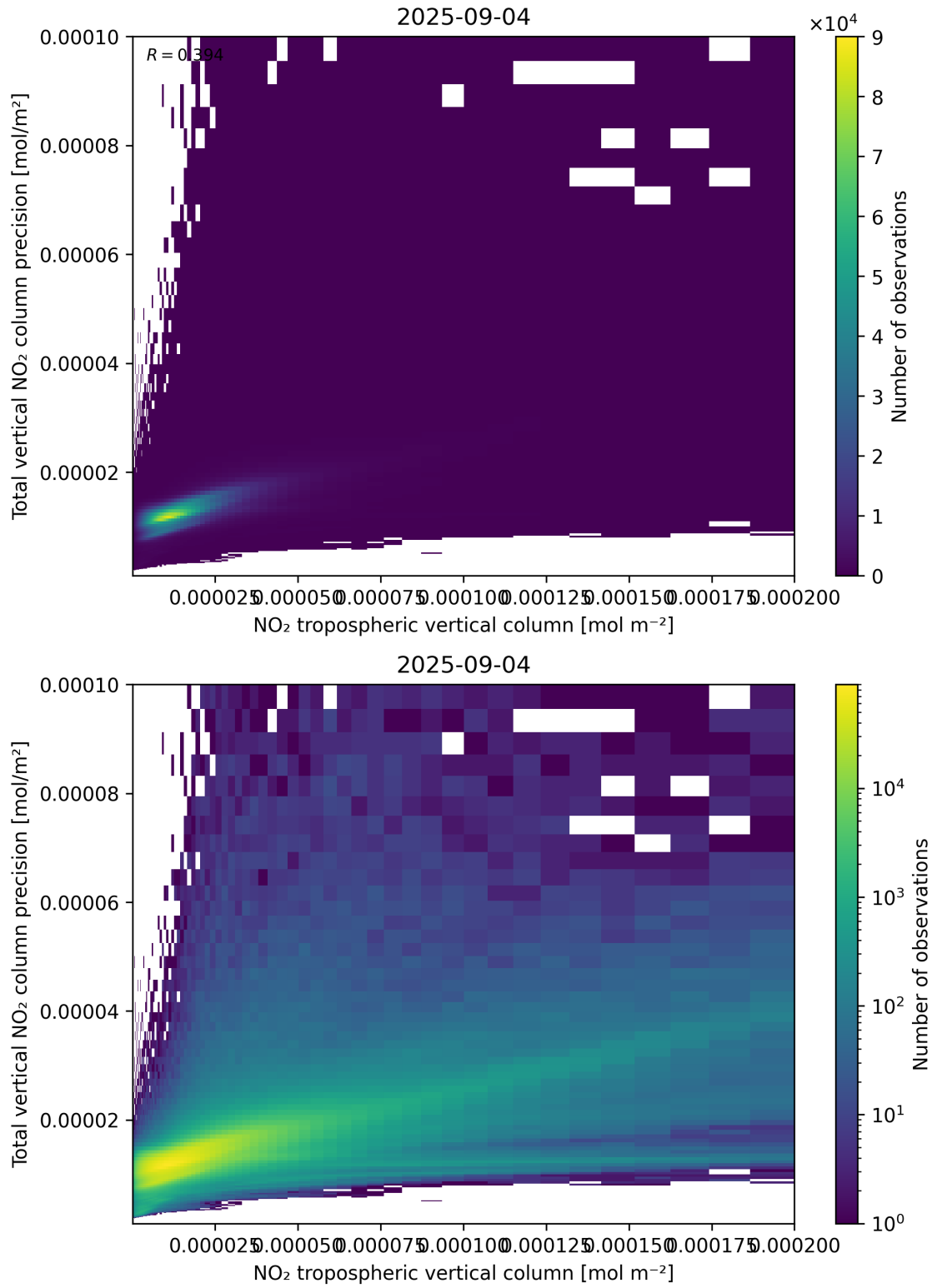
Figure 129: Scatter density plot of “NO 2 tropospheric vertical column” against “Total vertical NO 2 column precision” for 2025-09-04 to 2025-09-05.
