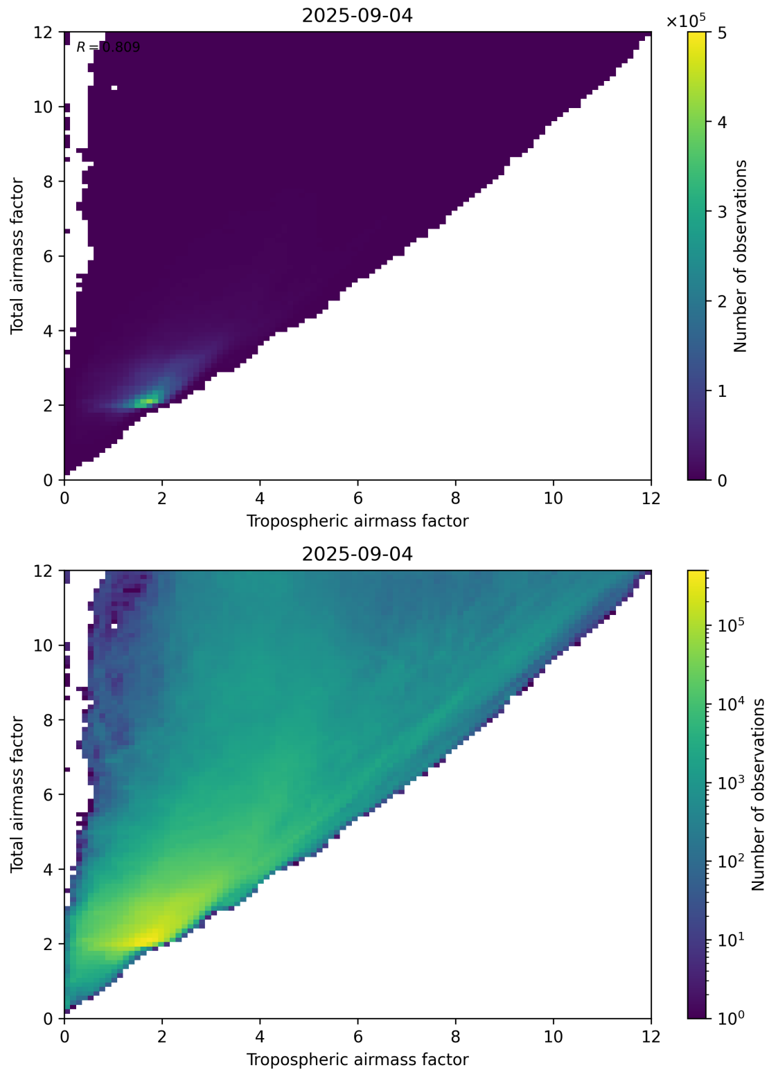
Figure 72: Scatter density plot of “Tropospheric airmass factor” against “Total airmass factor” for 2025-09-04 to 2025-09-05.
