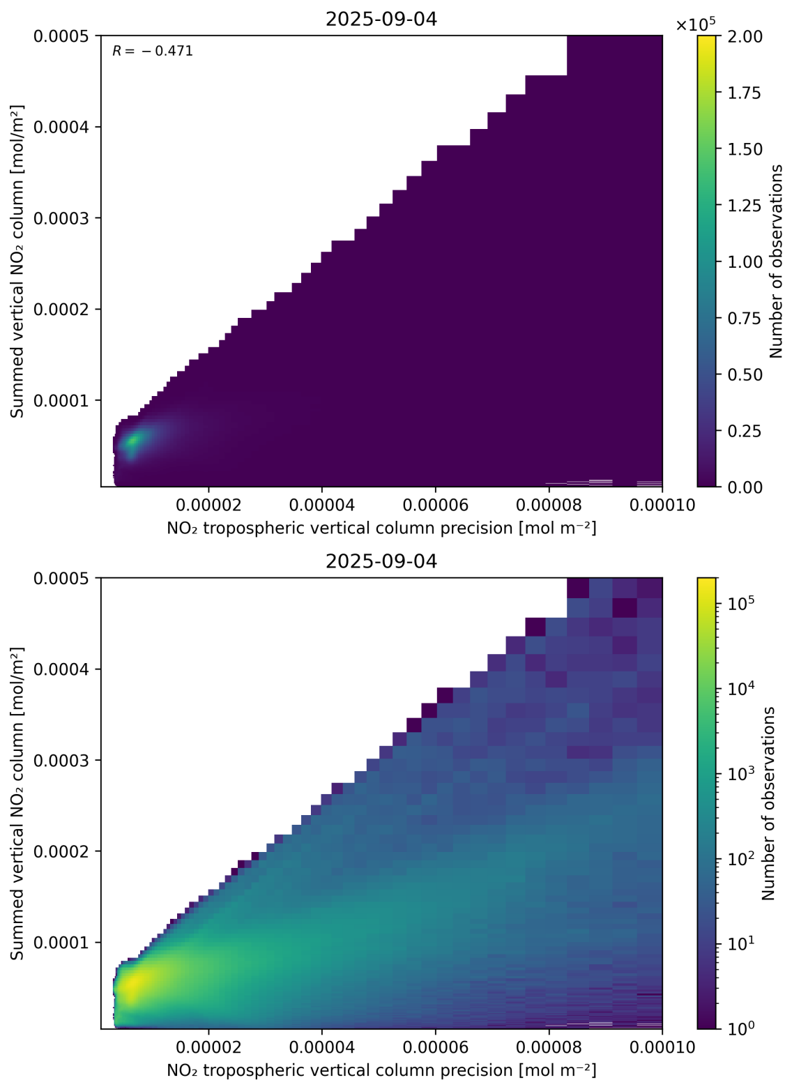
Figure 136: Scatter density plot of “NO 2 tropospheric vertical column precision” against “Summed vertical NO 2 column” for 2025-09-04 to 2025-09-05.
