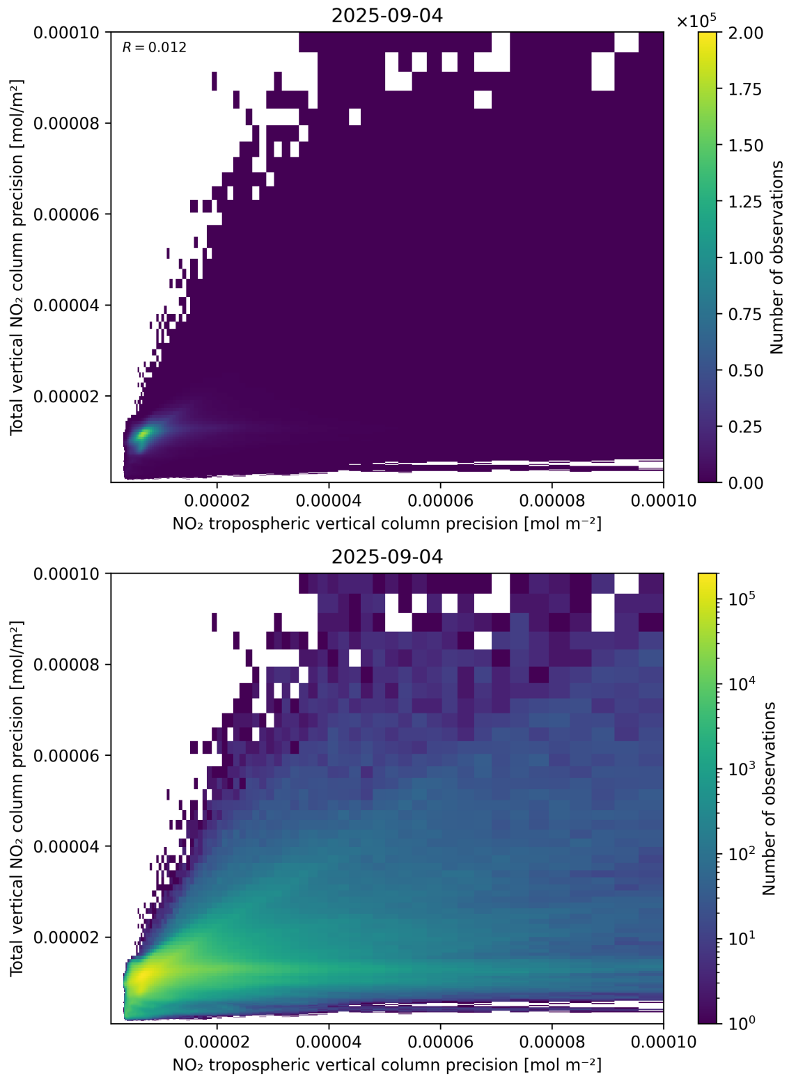
Figure 139: Scatter density plot of “NO 2 tropospheric vertical column precision” against “Total vertical NO 2 column precision” for 2025-09-04 to 2025-09-05.
