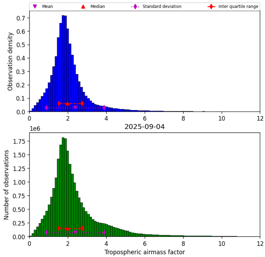
Figure 31: Histogram of “Tropospheric airmass factor” for 2025-09-04 to 2025-09-05
