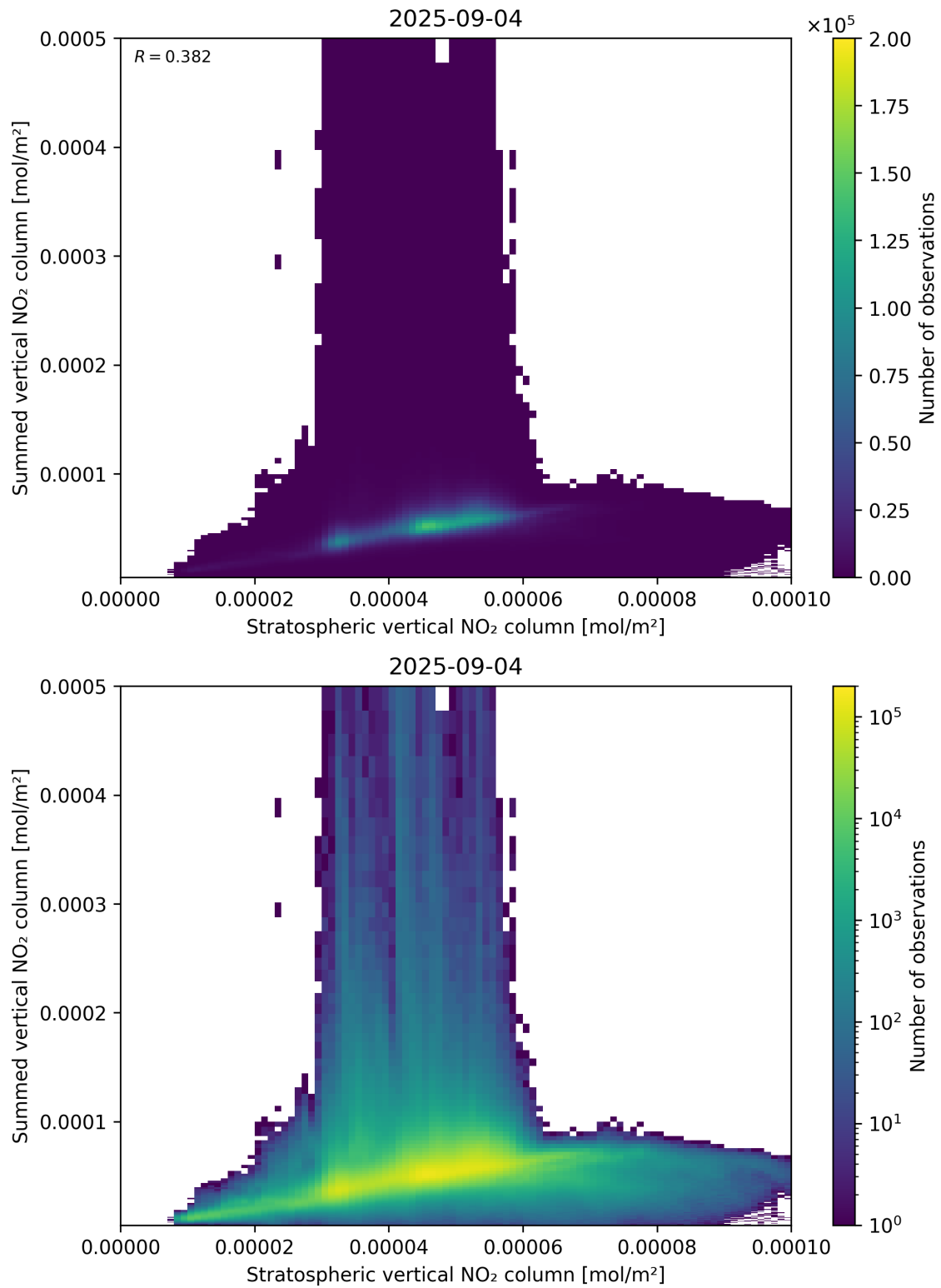
Figure 98: Scatter density plot of “Stratospheric vertical NO 2 column” against “Summed vertical NO 2 column” for 2025-09-04 to 2025-09-05.
