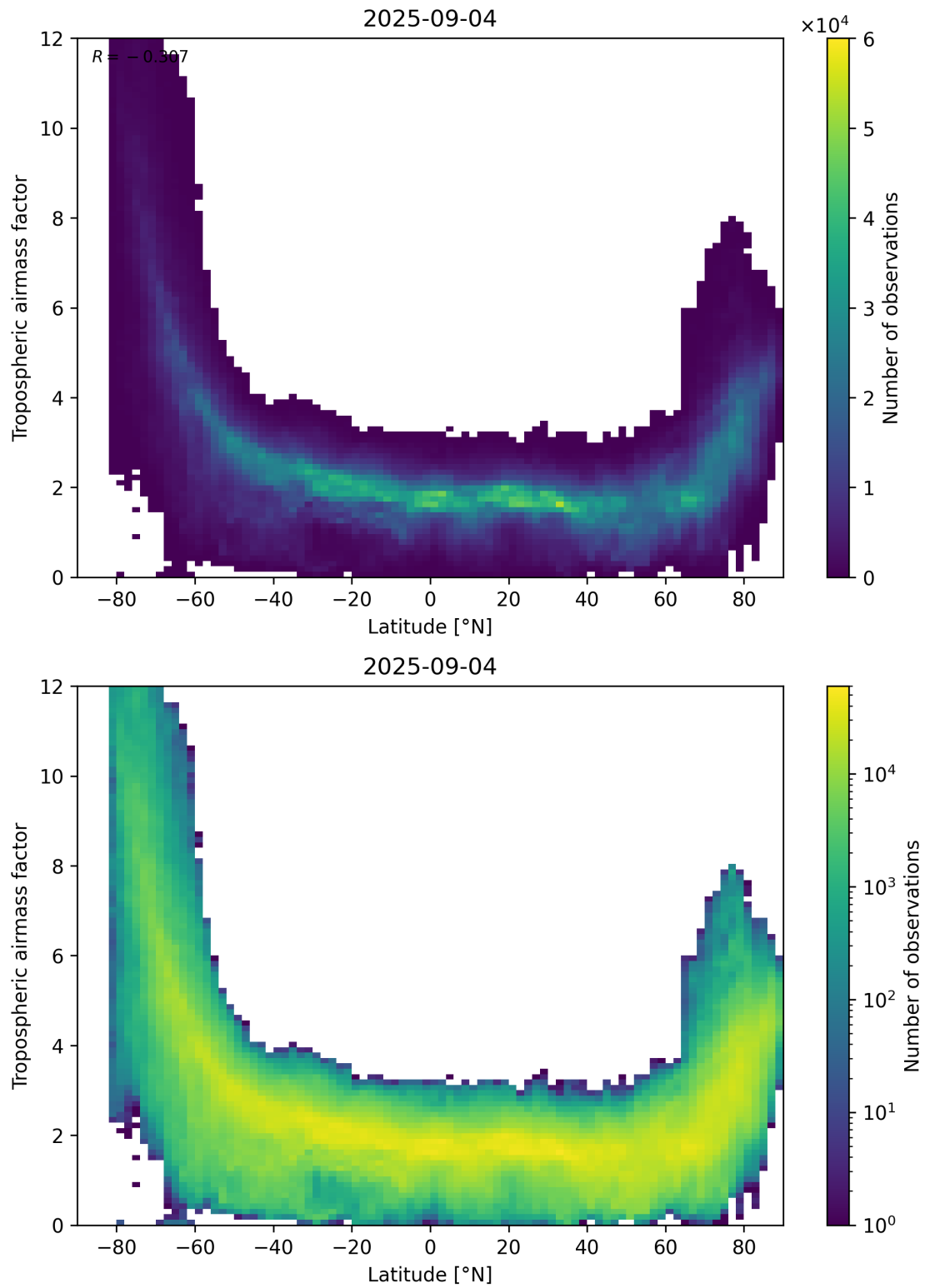
Figure 85: Scatter density plot of “Latitude” against “Tropospheric air mass factor” for 2025-09-04 to 2025-09-05.
