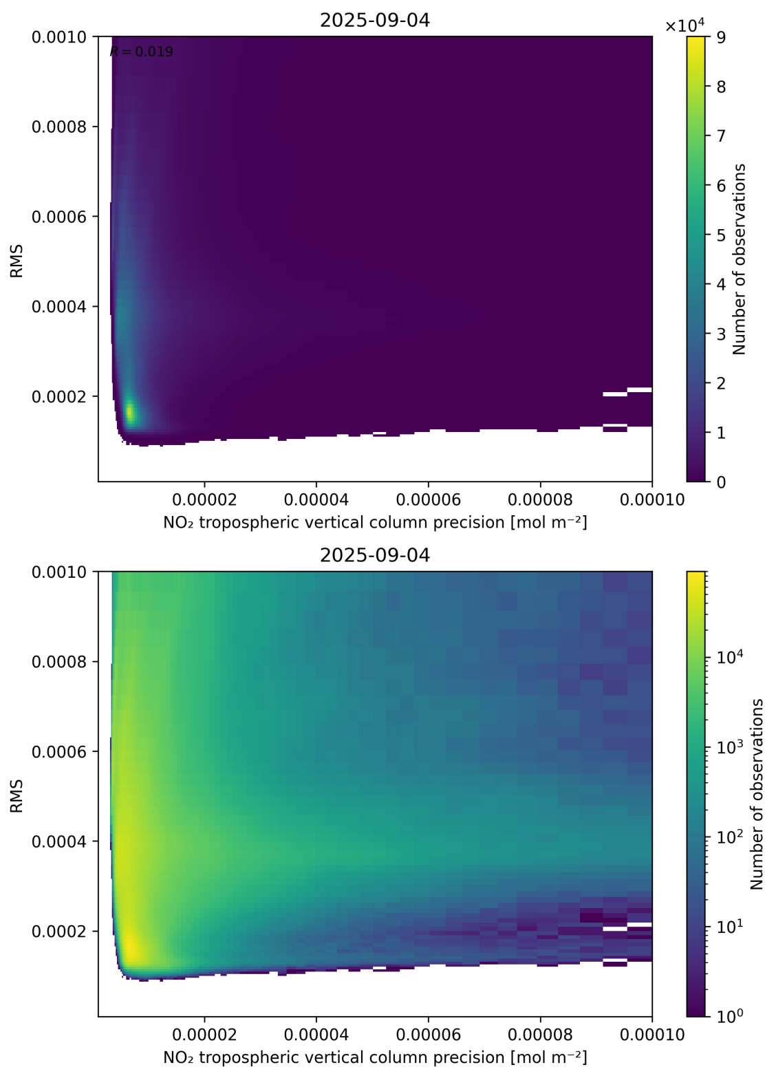
Figure 140: Scatter density plot of “NO 2 tropospheric vertical column precision” against “RMS” for 2025-09-04 to 2025-09-05.
