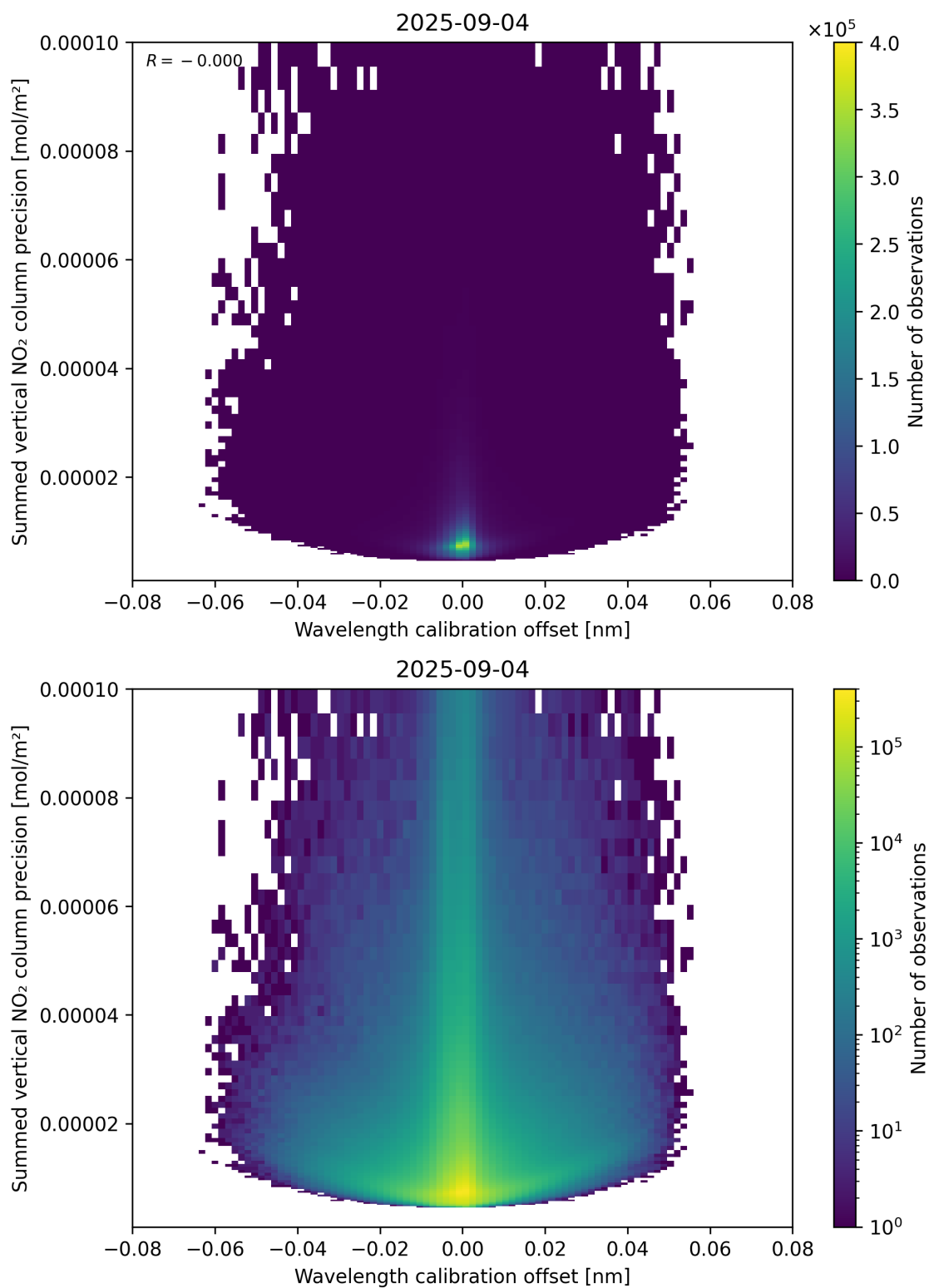
Figure 178: Scatter density plot of “Wavelength calibration offset” against “Summed vertical NO 2 column precision” for 2025-09-04 to 2025-09-05.
