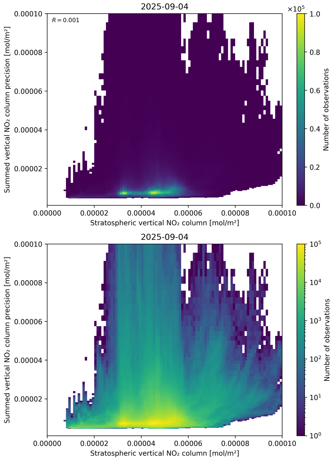
Figure 99: Scatter density plot of “Stratospheric vertical NO 2 column” against “Summed vertical NO 2 column precision” for 2025-09-04 to 2025-09-05.
