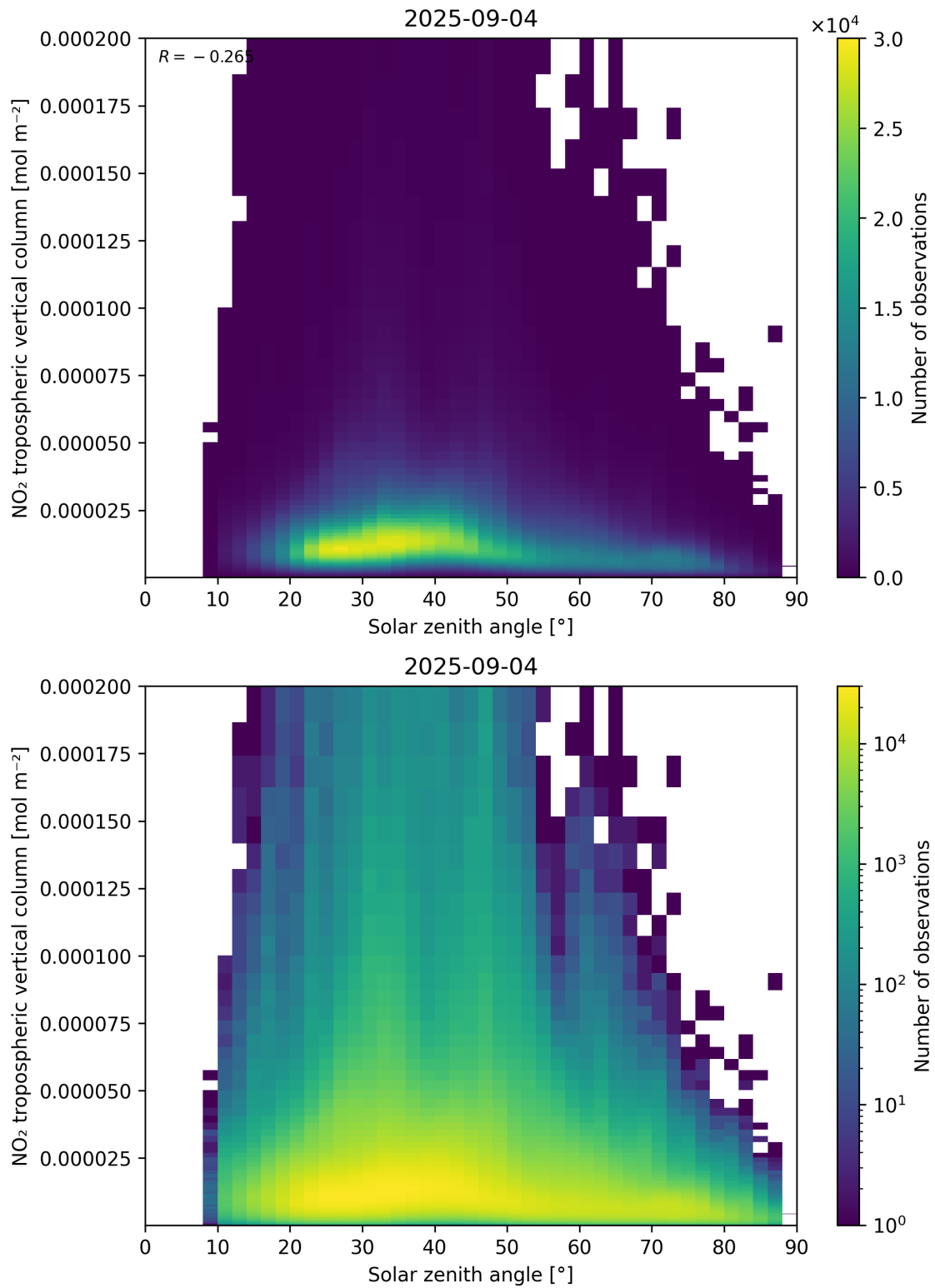
Figure 155: Scatter density plot of “Solar zenith angle” against “NO 2 tropospheric vertical column” for 2025-09-04 to 2025-09-05.
