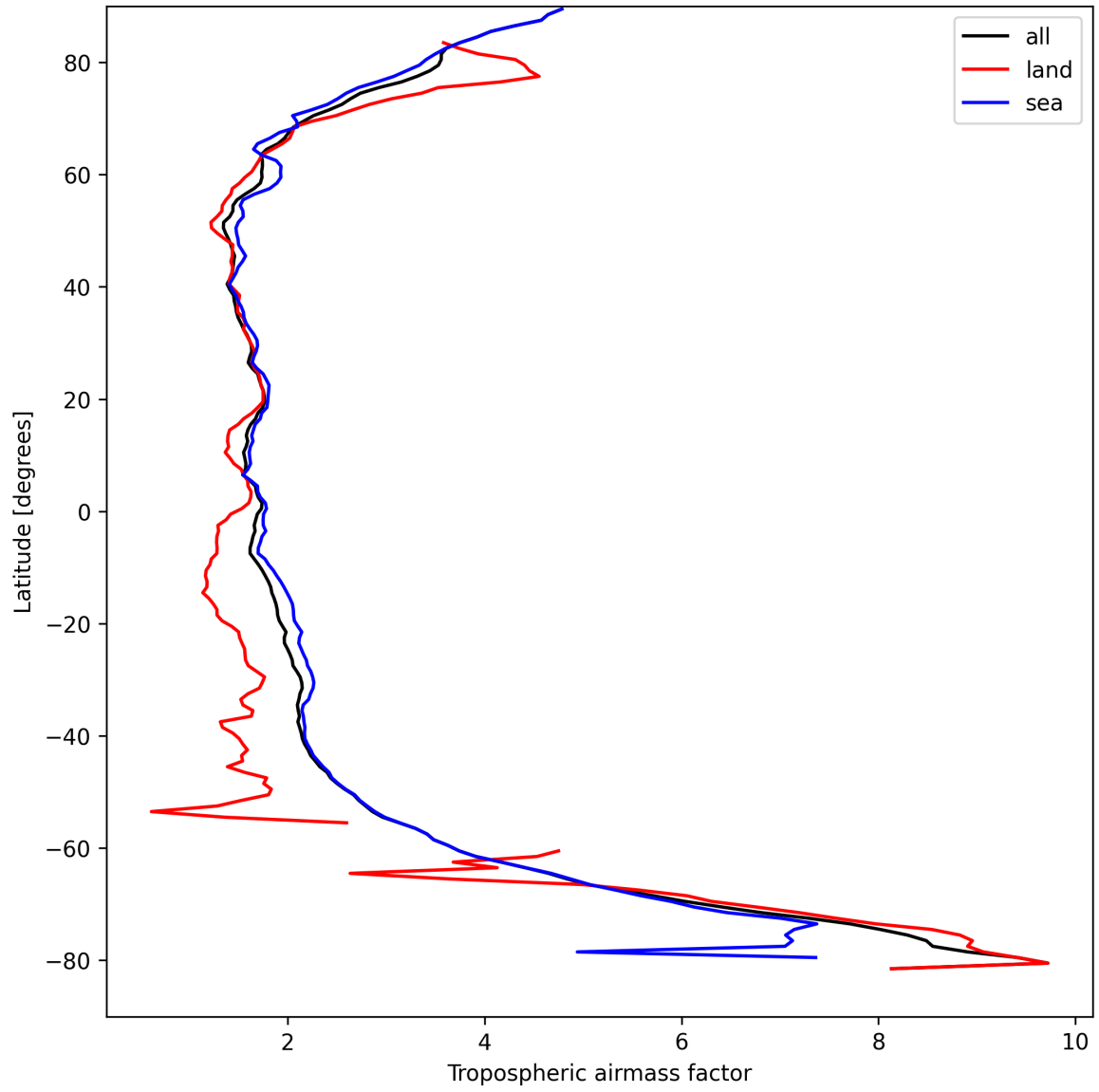
Figure 14: Zonal average of “Tropospheric airmass factor” for 2025-09-04 to 2025-09-05.
