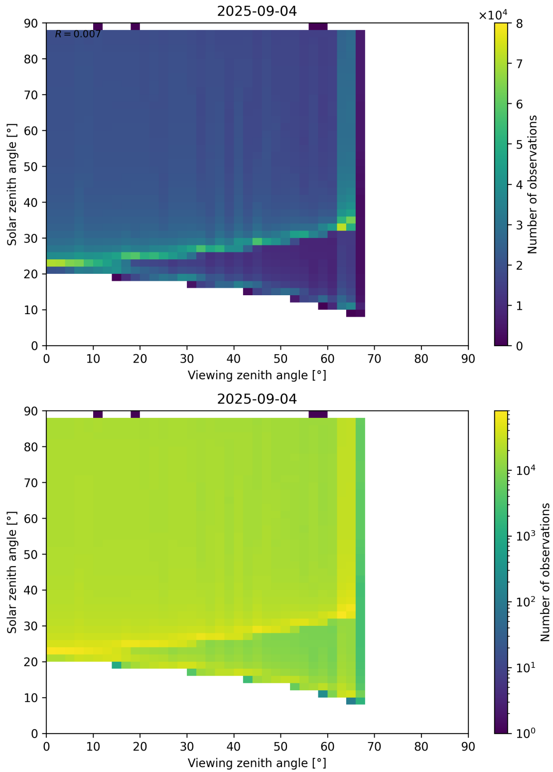
Figure 172: Scatter density plot of “Viewing zenith angle” against “Solar zenith angle” for 2025-09-04 to 2025-09-05.
