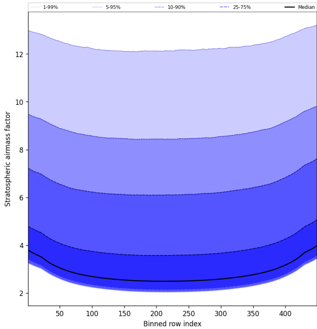
Figure 61: Along track statistics of “Stratospheric air mass factor” for 2025-09-04 to 2025-09-05
