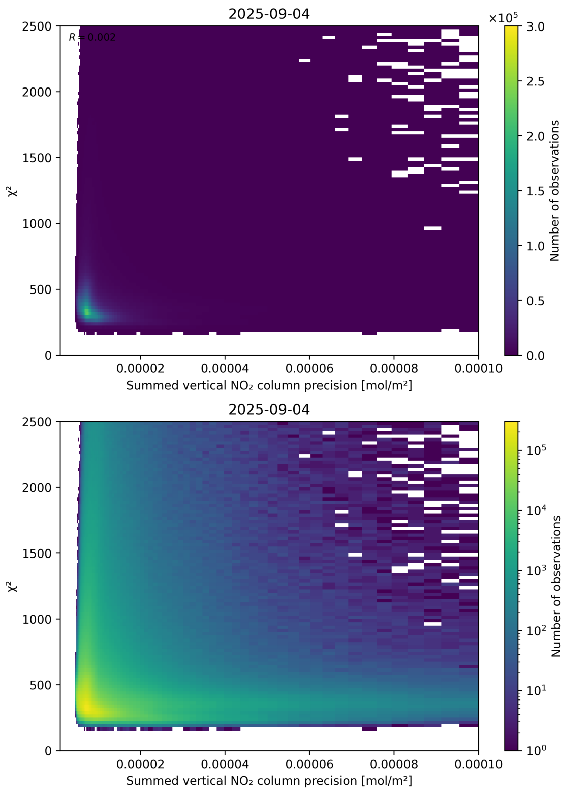
Figure 107: Scatter density plot of “Summed vertical NO 2 column precision” against “ \chi^2 ” for 2025-09-04 to 2025-09-05.
