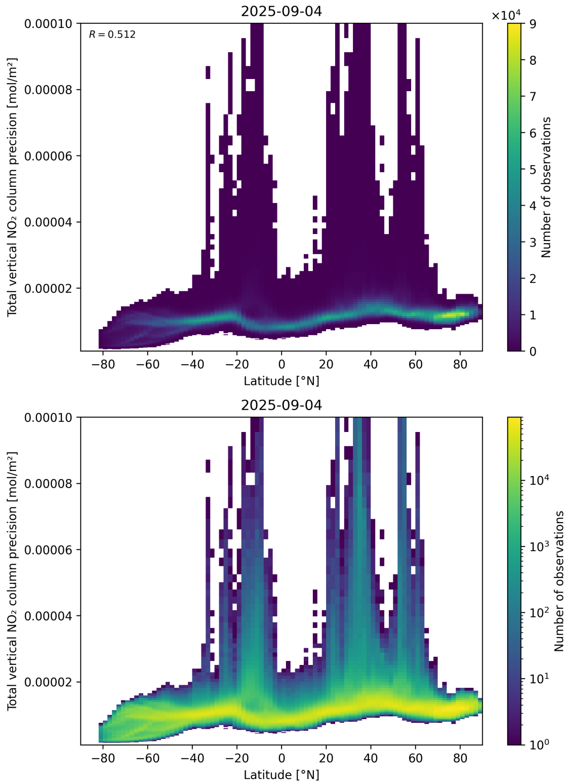
Figure 91: Scatter density plot of “Latitude” against “Total vertical NO 2 column precision” for 2025-09-04 to 2025-09-05.
