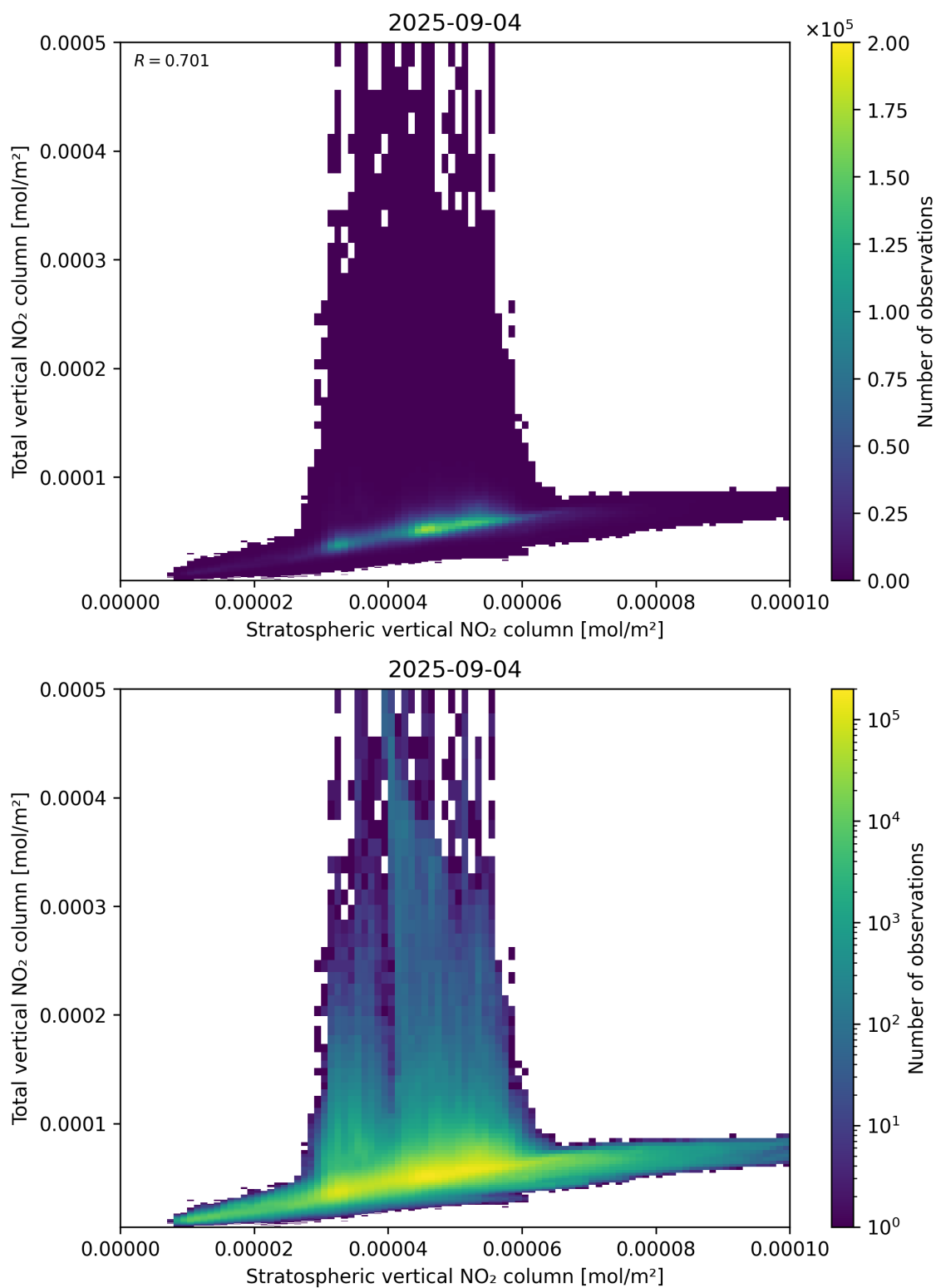
Figure 100: Scatter density plot of “Stratospheric vertical NO 2 column” against “Total vertical NO 2 column” for 2025-09-04 to 2025-09-05.
