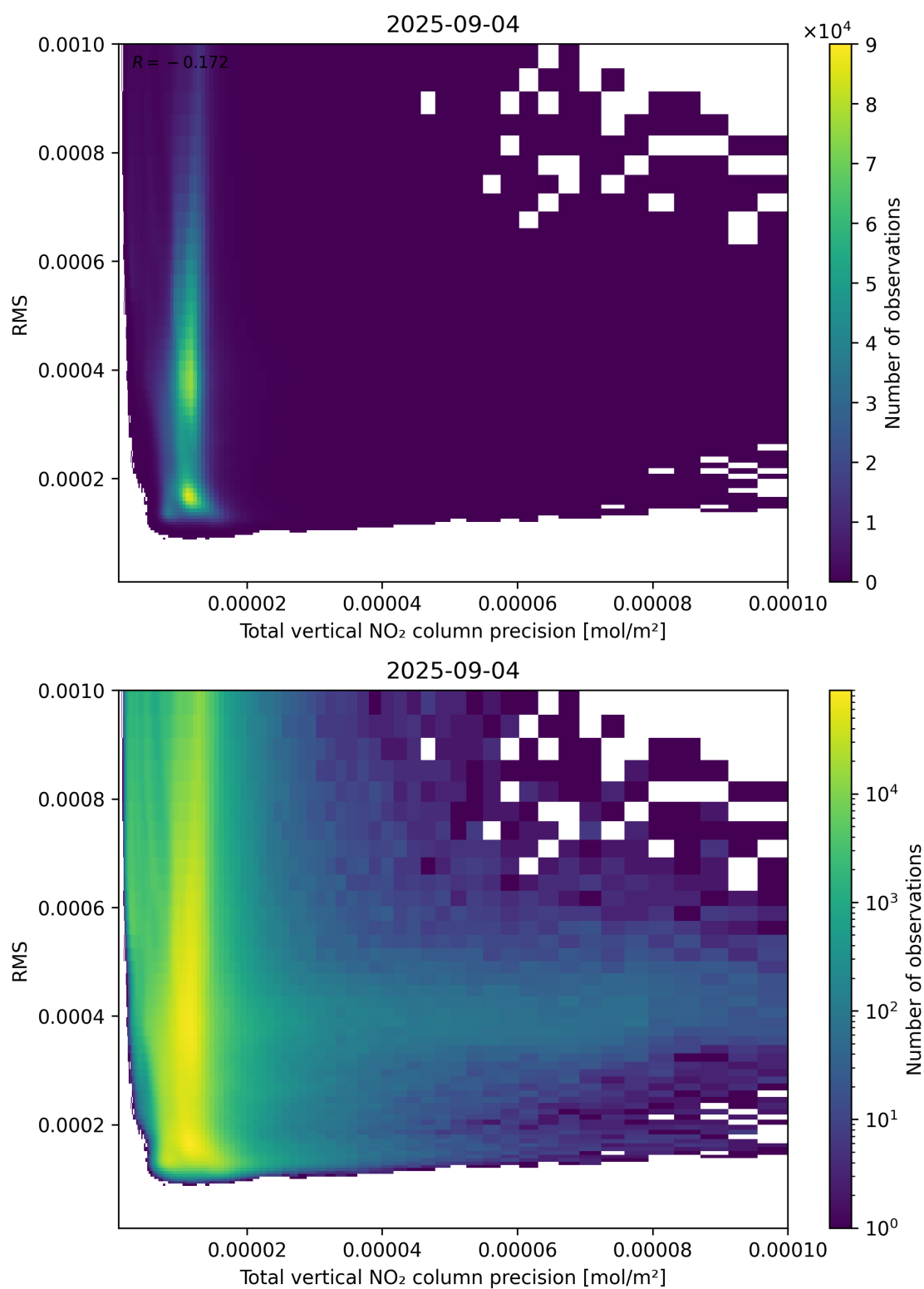
Figure 119: Scatter density plot of “Total vertical NO 2 column precision” against “RMS” for 2025-09-04 to 2025-09-05.
