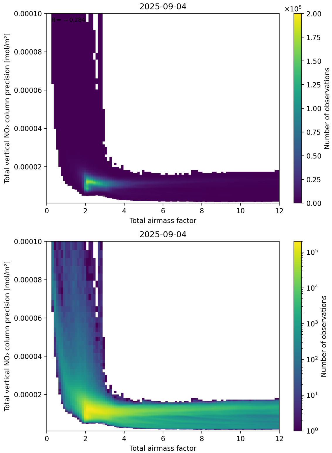
Figure 68: Scatter density plot of “Total airmass factor” against “Total vertical NO 2 column precision” for 2025-09-04 to 2025-09-05.
