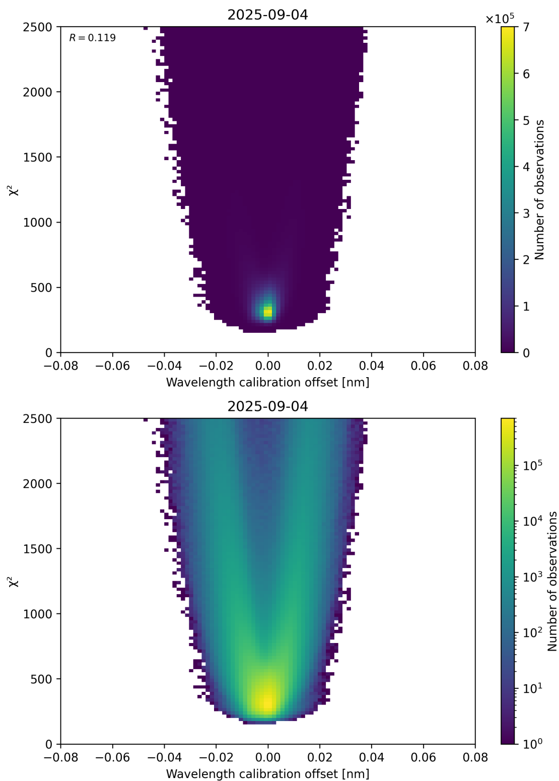
Figure 175: Scatter density plot of “Wavelength calibration offset” against “ \chi^2 ” for 2025-09-04 to 2025-09-05.
