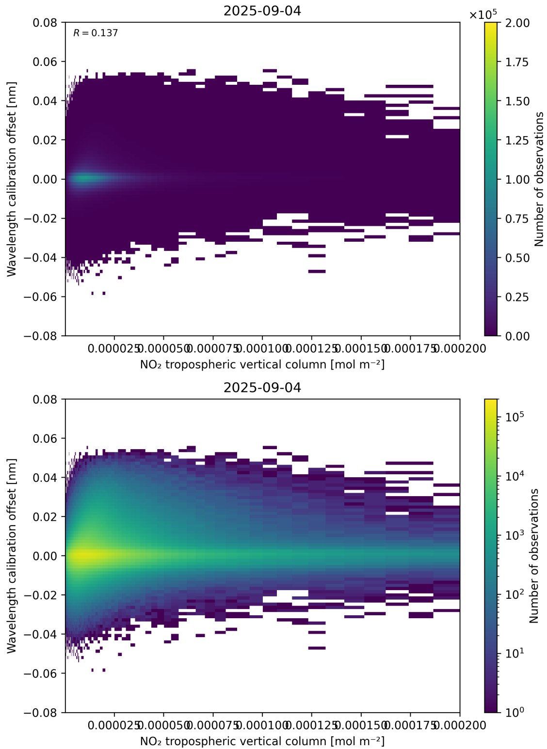
Figure 143: Scatter density plot of “NO 2 tropospheric vertical column” against “Wavelength calibration offset” for 2025-09-04 to 2025-09-05.
