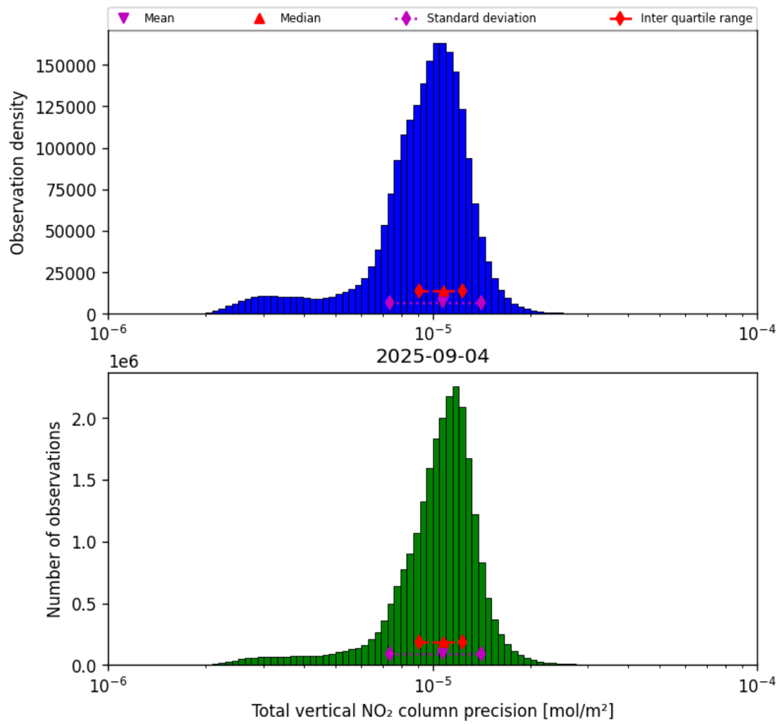
Figure 39: Histogram of “Total vertical NO 2 column precision” for 2025-09-04 to 2025-09-05
