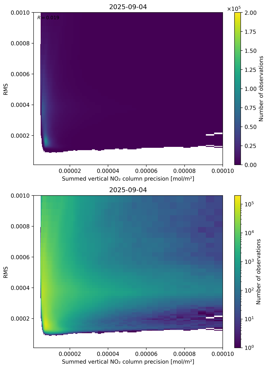
Figure 108: Scatter density plot of “Summed vertical NO 2 column precision” against “RMS” for 2025-09-04 to 2025-09-05.
