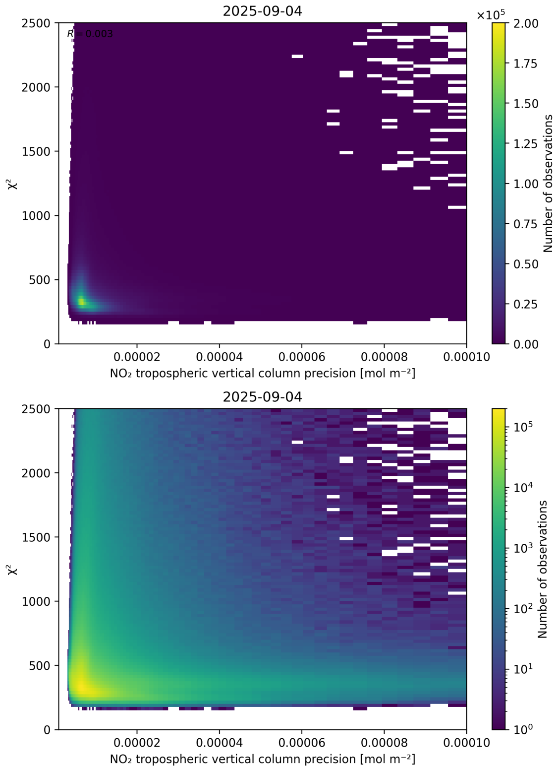
Figure 134: Scatter density plot of “NO 2 tropospheric vertical column precision” against “ \chi^2 ” for 2025-09-04 to 2025-09-05.
