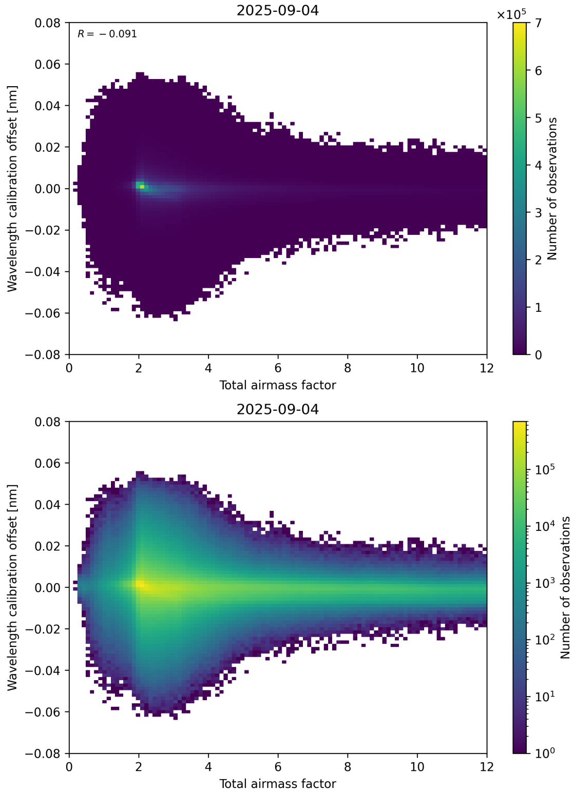
Figure 70: Scatter density plot of “Total airmass factor” against “Wavelength calibration offset” for 2025-09-04 to 2025-09-05.
