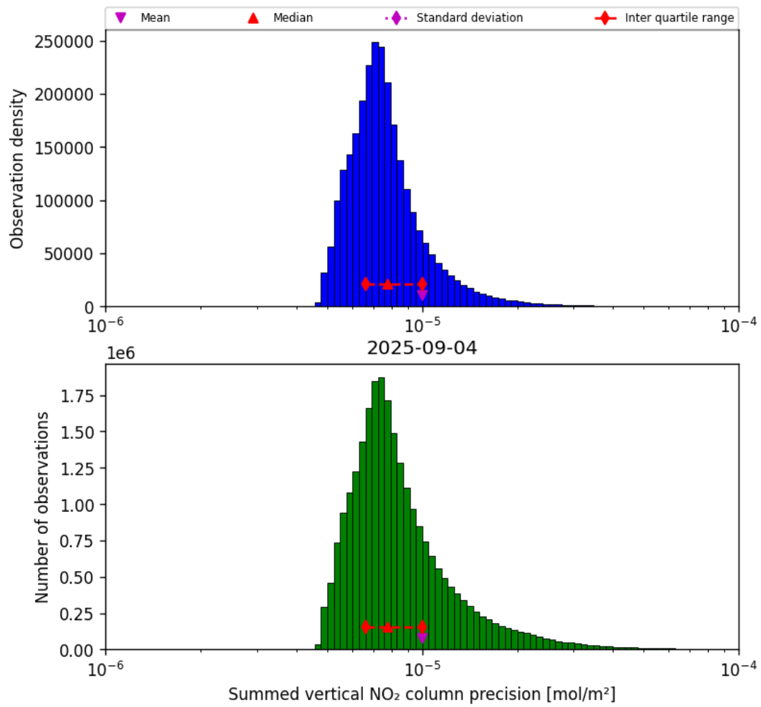
Figure 41: Histogram of “Summed vertical NO 2 column precision” for 2025-09-04 to 2025-09-05
