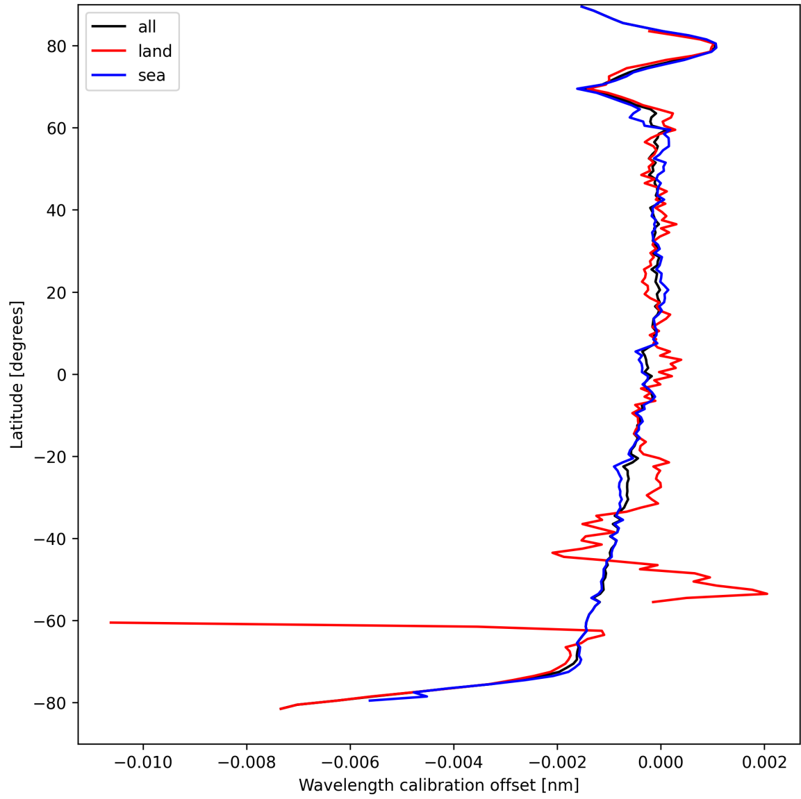
Figure 18: Zonal average of “Wavelength calibration offset” for 2025-09-04 to 2025-09-05.
