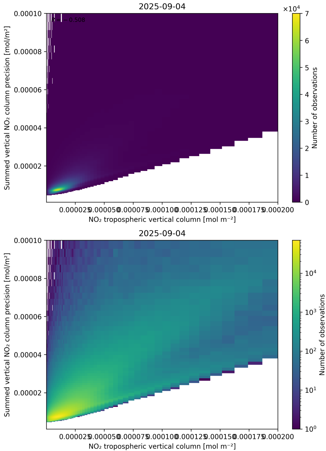
Figure 127: Scatter density plot of “NO 2 tropospheric vertical column” against “Summed vertical NO 2 column precision” for 2025-09-04 to 2025-09-05.
