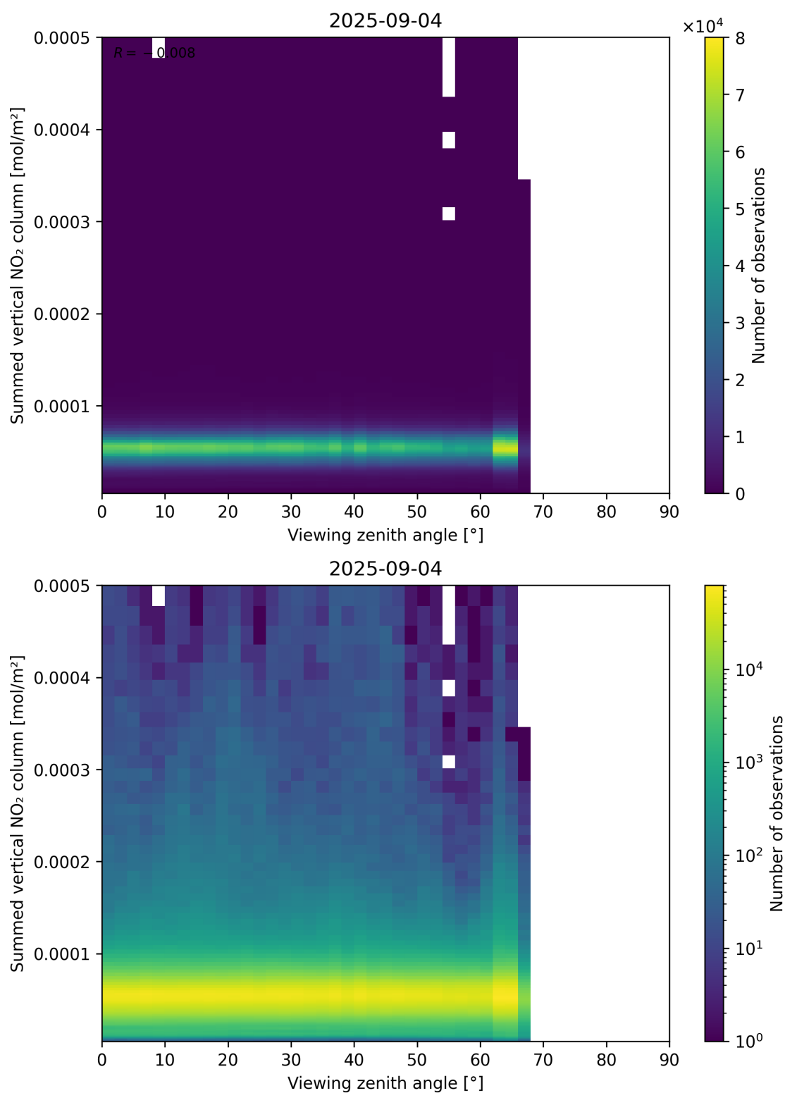
Figure 165: Scatter density plot of “Viewing zenith angle” against “Summed vertical NO 2 column” for 2025-09-04 to 2025-09-05.
