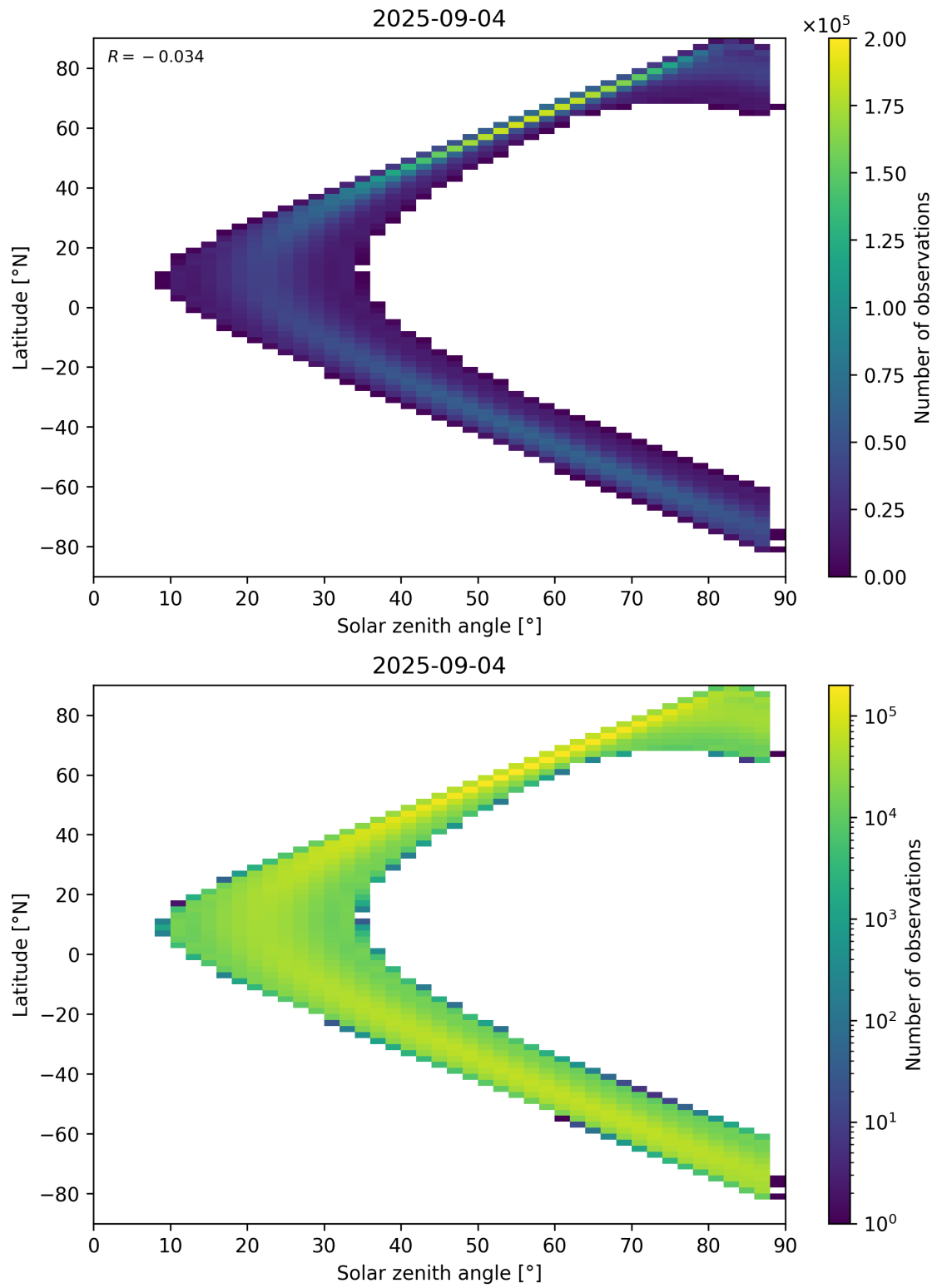
Figure 149: Scatter density plot of “Solar zenith angle” against “Latitude” for 2025-09-04 to 2025-09-05.
