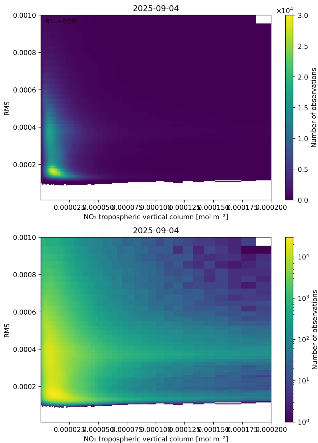
Figure 142: Scatter density plot of “NO 2 tropospheric vertical column” against “RMS” for 2025-09-04 to 2025-09-05.
