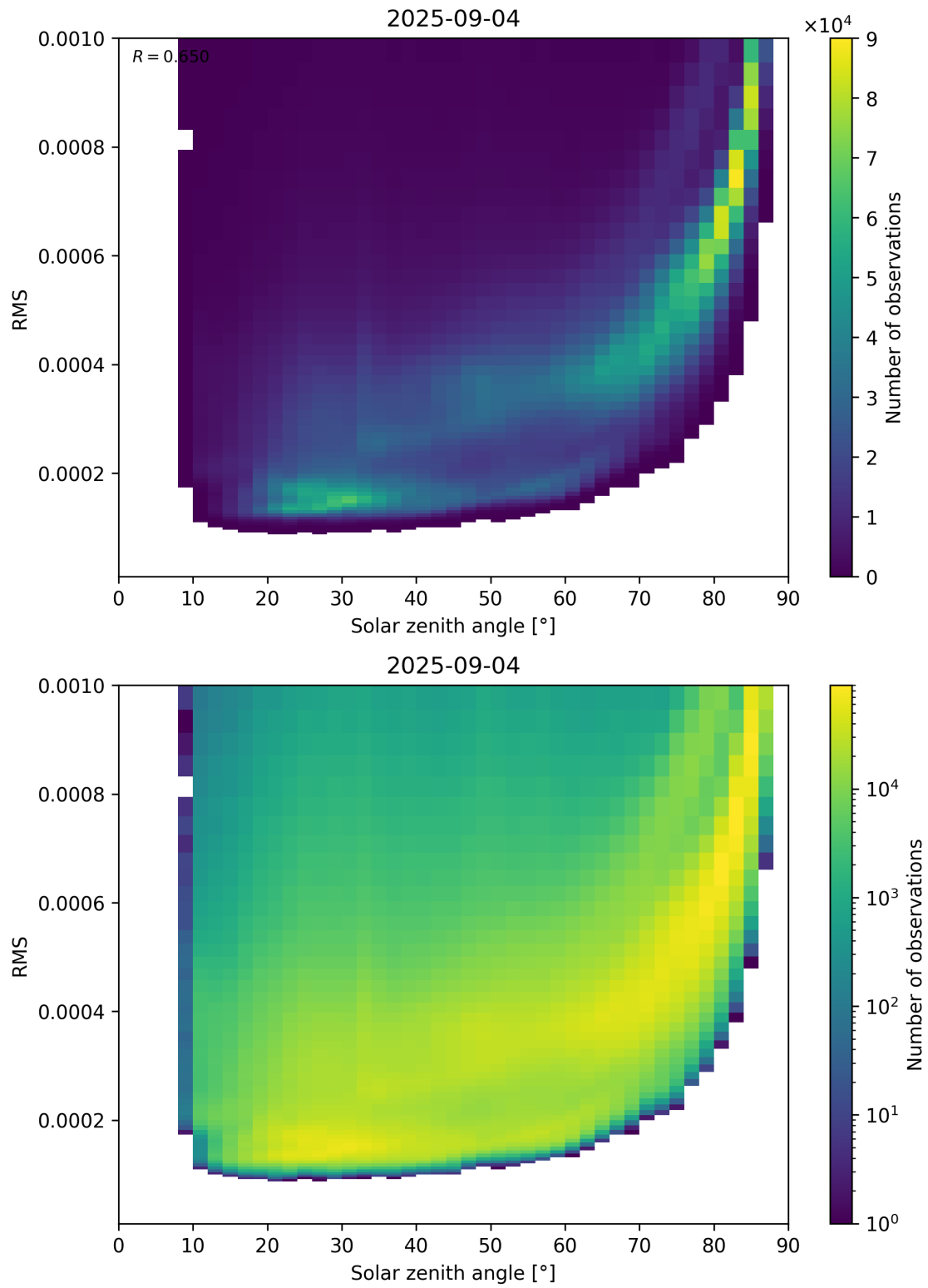
Figure 157: Scatter density plot of “Solar zenith angle” against “RMS” for 2025-09-04 to 2025-09-05.
