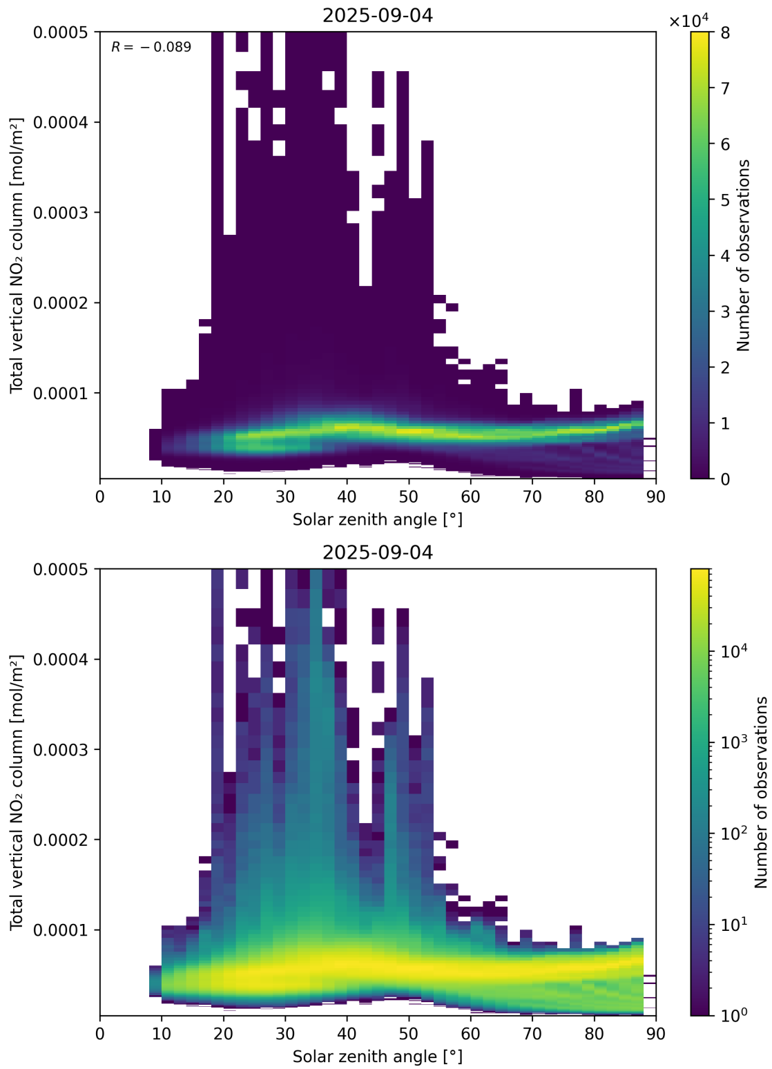
Figure 153: Scatter density plot of “Solar zenith angle” against “Total vertical NO 2 column” for 2025-09-04 to 2025-09-05.
