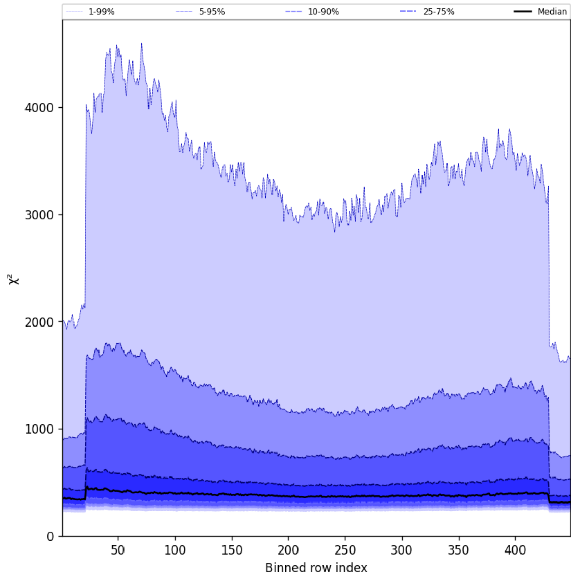
Figure 59: Along track statistics of “ \chi^2 ” for 2025-09-04 to 2025-09-05
