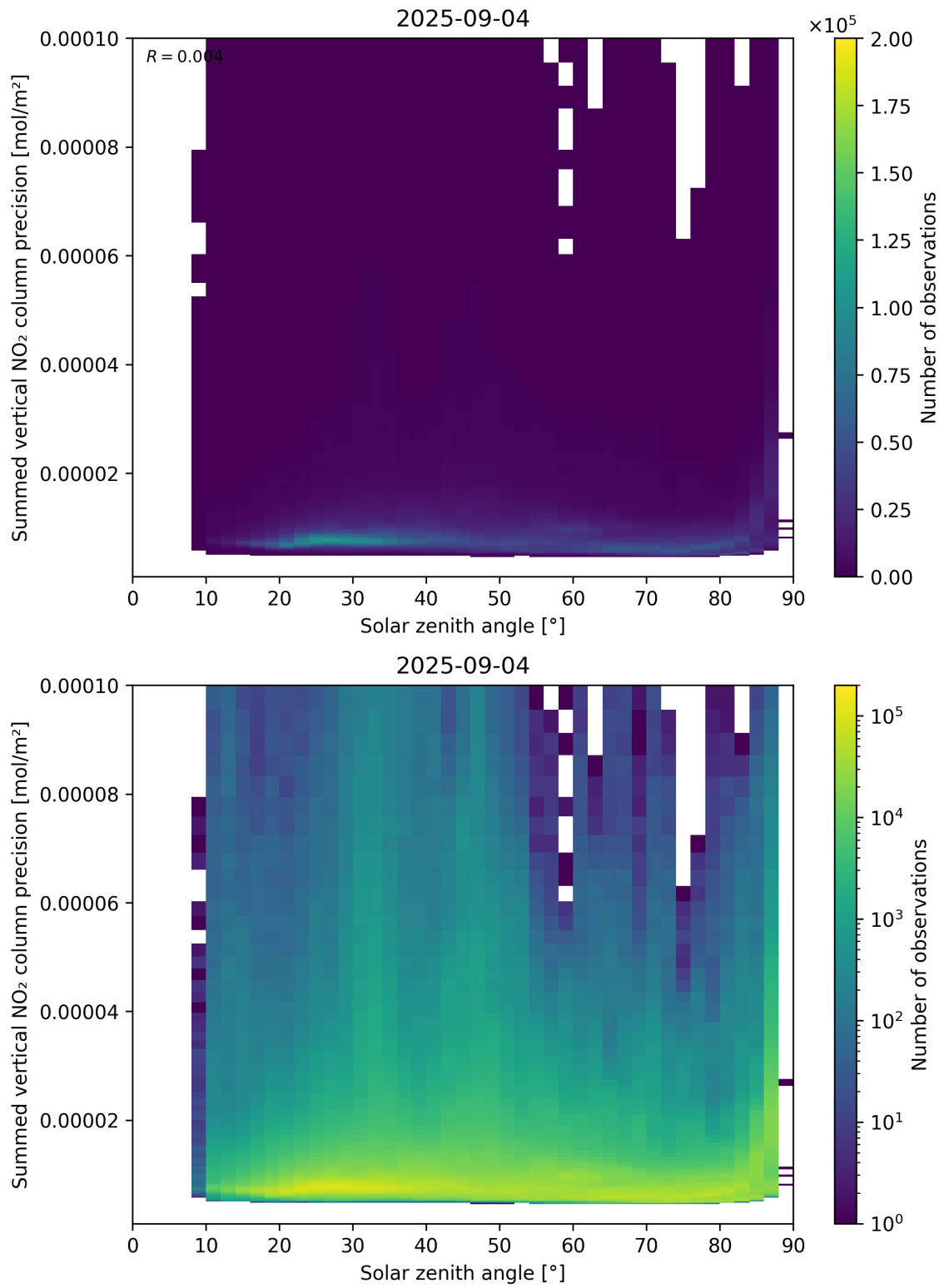
Figure 152: Scatter density plot of “Solar zenith angle” against “Summed vertical NO 2 column precision” for 2025-09-04 to 2025-09-05.
