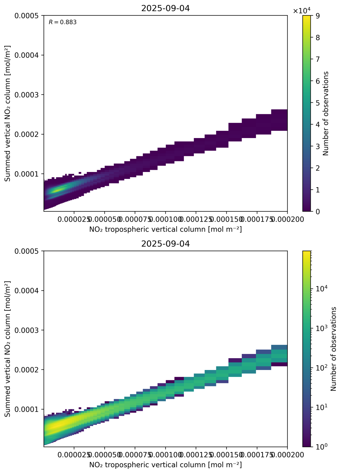
Figure 126: Scatter density plot of “NO 2 tropospheric vertical column” against “Summed vertical NO 2 column” for 2025-09-04 to 2025-09-05.
