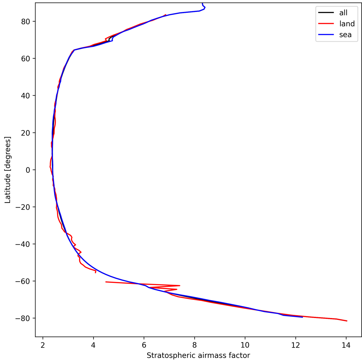
Figure 27: Zonal average of “Stratospheric airmass factor” for 2025-09-04 to 2025-09-05.
