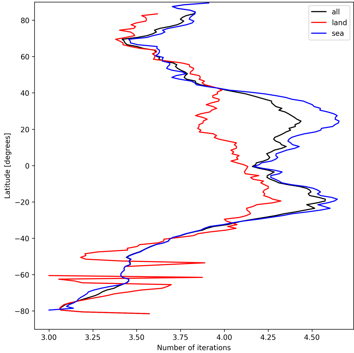
Figure 17: Zonal average of “Number of iterations” for 2025-09-04 to 2025-09-05.
