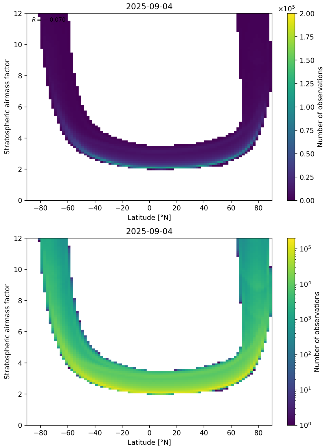
Figure 83: Scatter density plot of “Latitude” against “Stratospheric air mass factor” for 2025-09-04 to 2025-09-05.
