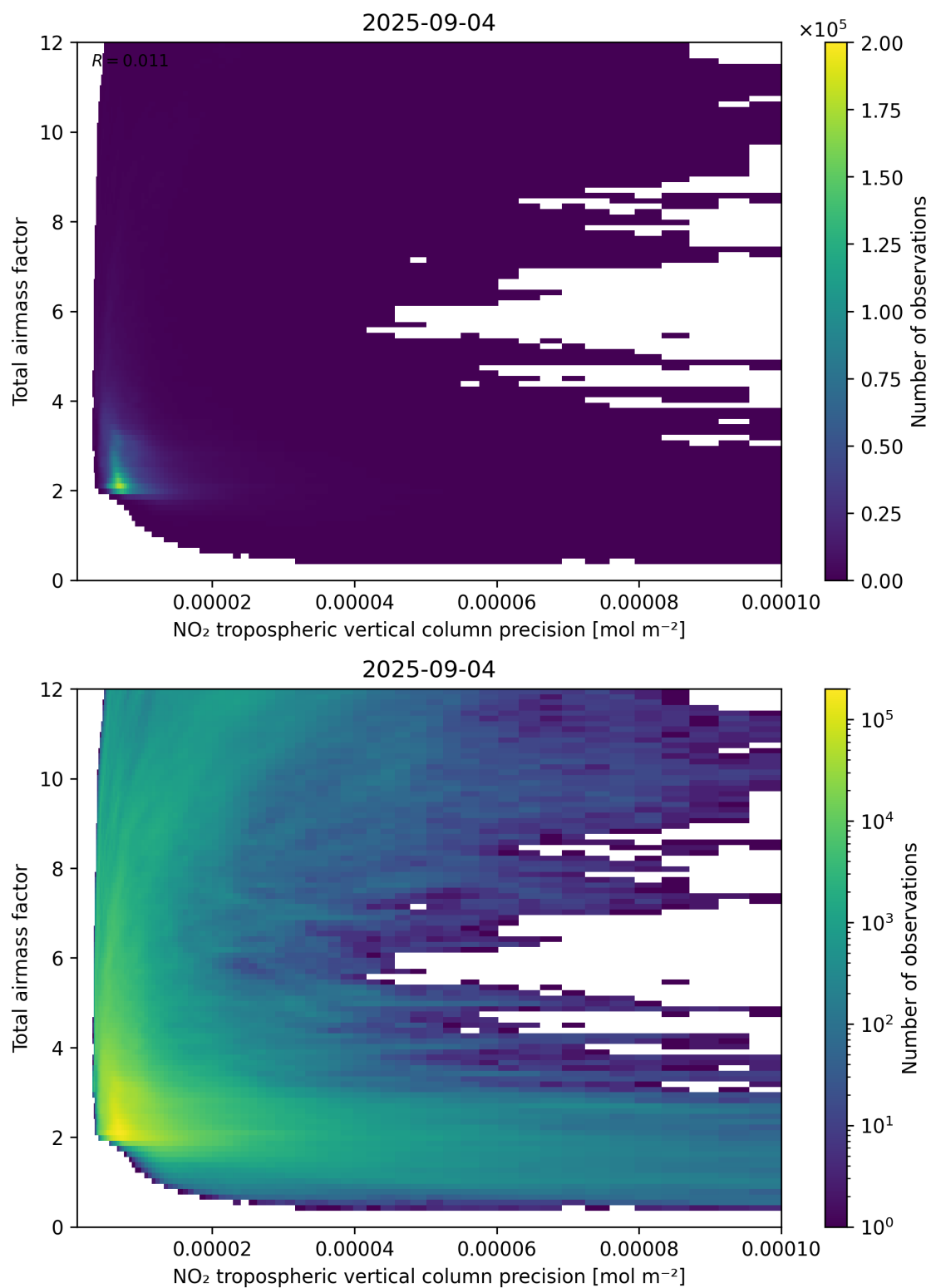
Figure 132: Scatter density plot of “NO 2 tropospheric vertical column precision” against “Total air mass factor” for 2025-09-04 to 2025-09-05.
