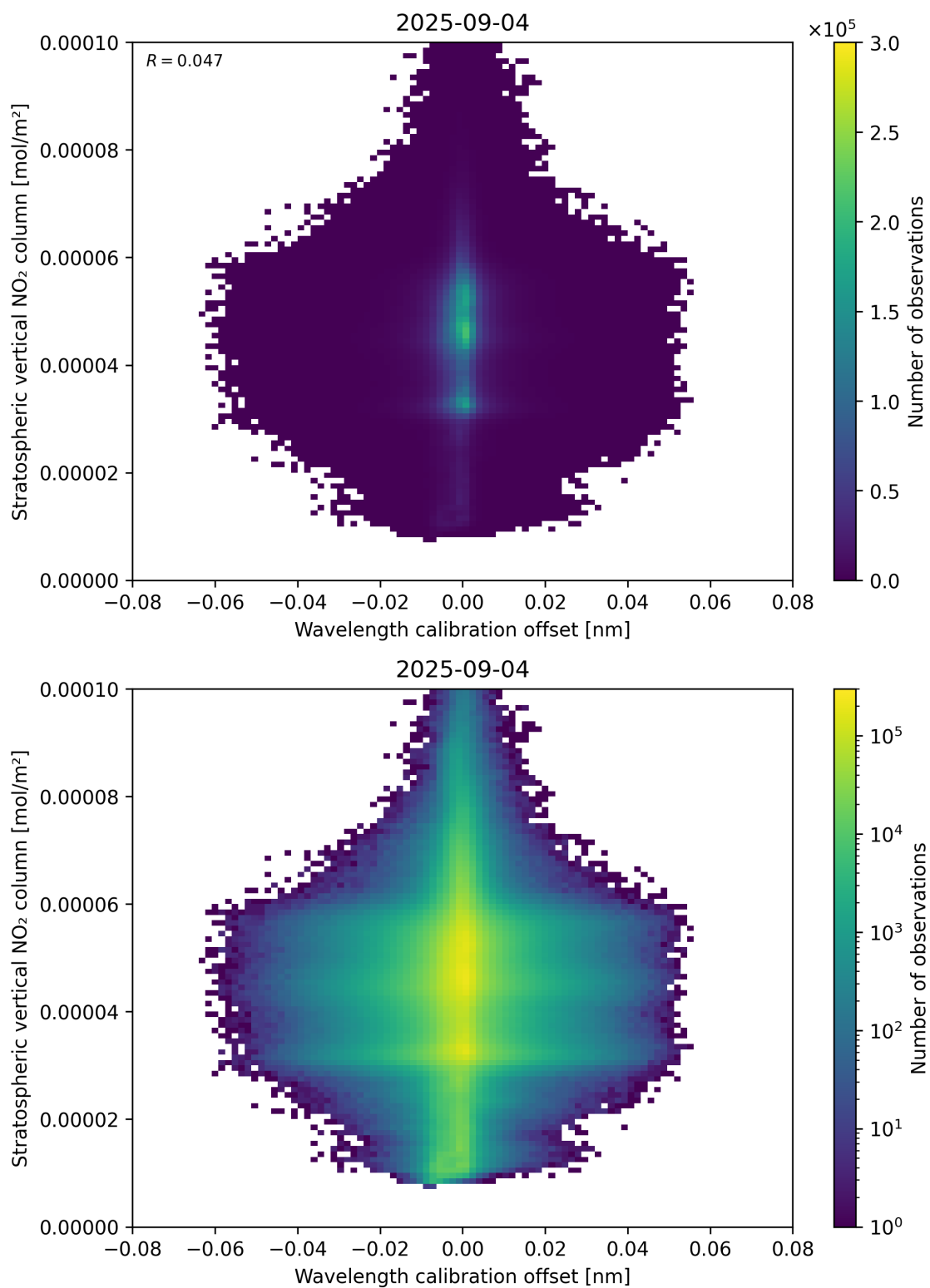
Figure 176: Scatter density plot of “Wavelength calibration offset” against “Stratospheric vertical NO 2 column” for 2025-09-04 to 2025-09-05.
