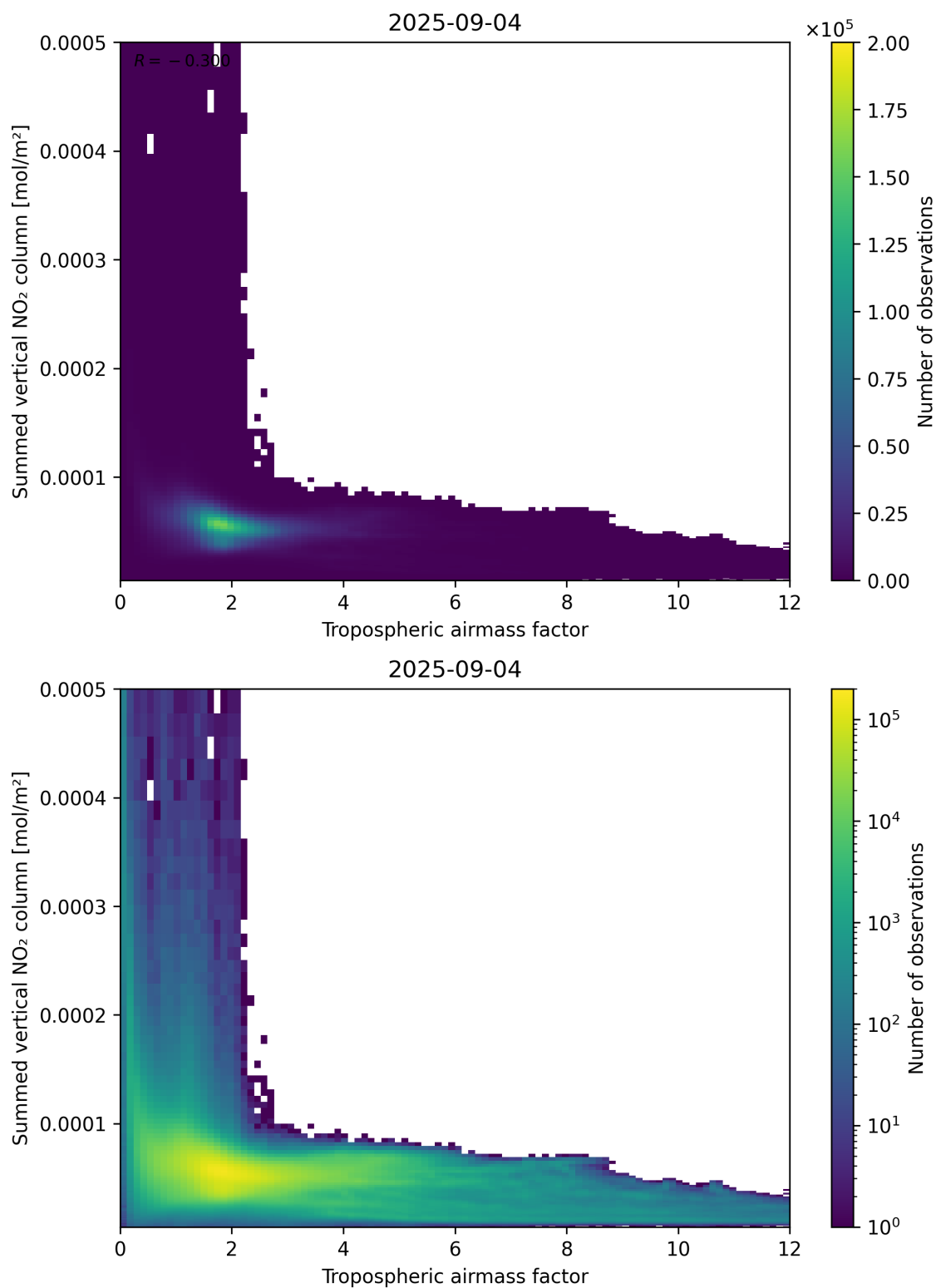
Figure 75: Scatter density plot of “Tropospheric air mass factor” against “Summed vertical NO 2 column” for 2025-09-04 to 2025-09-05.
