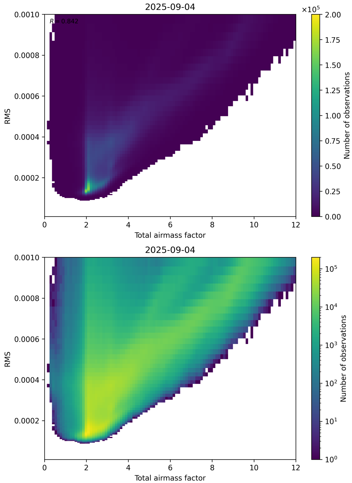
Figure 69: Scatter density plot of “Total airmass factor” against “RMS” for 2025-09-04 to 2025-09-05.
