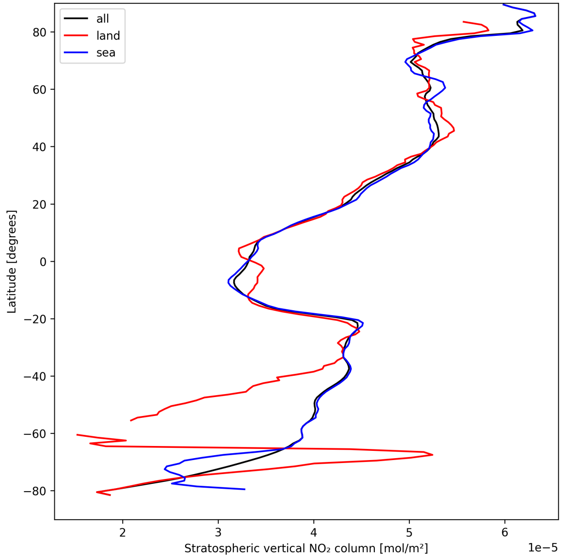
Figure 19: Zonal average of “Stratospheric vertical NO 2 column” for 2025-09-04 to 2025-09-05.
