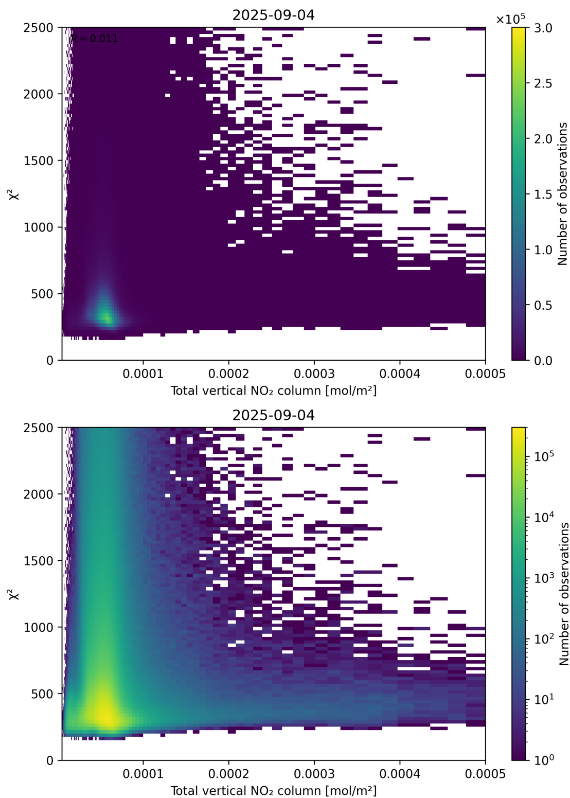
Figure 111: Scatter density plot of “Total vertical NO 2 column” against “ \chi^2 ” for 2025-09-04 to 2025-09-05.
