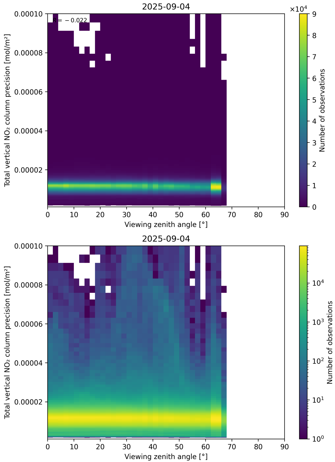
Figure 168: Scatter density plot of “Viewing zenith angle” against “Total vertical NO 2 column precision” for 2025-09-04 to 2025-09-05.
