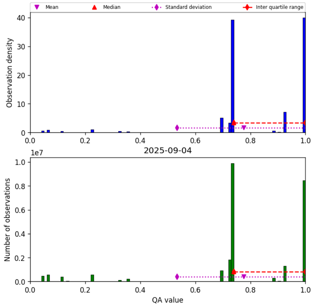
Figure 28: Histogram of “QA value” for 2025-09-04 to 2025-09-05
