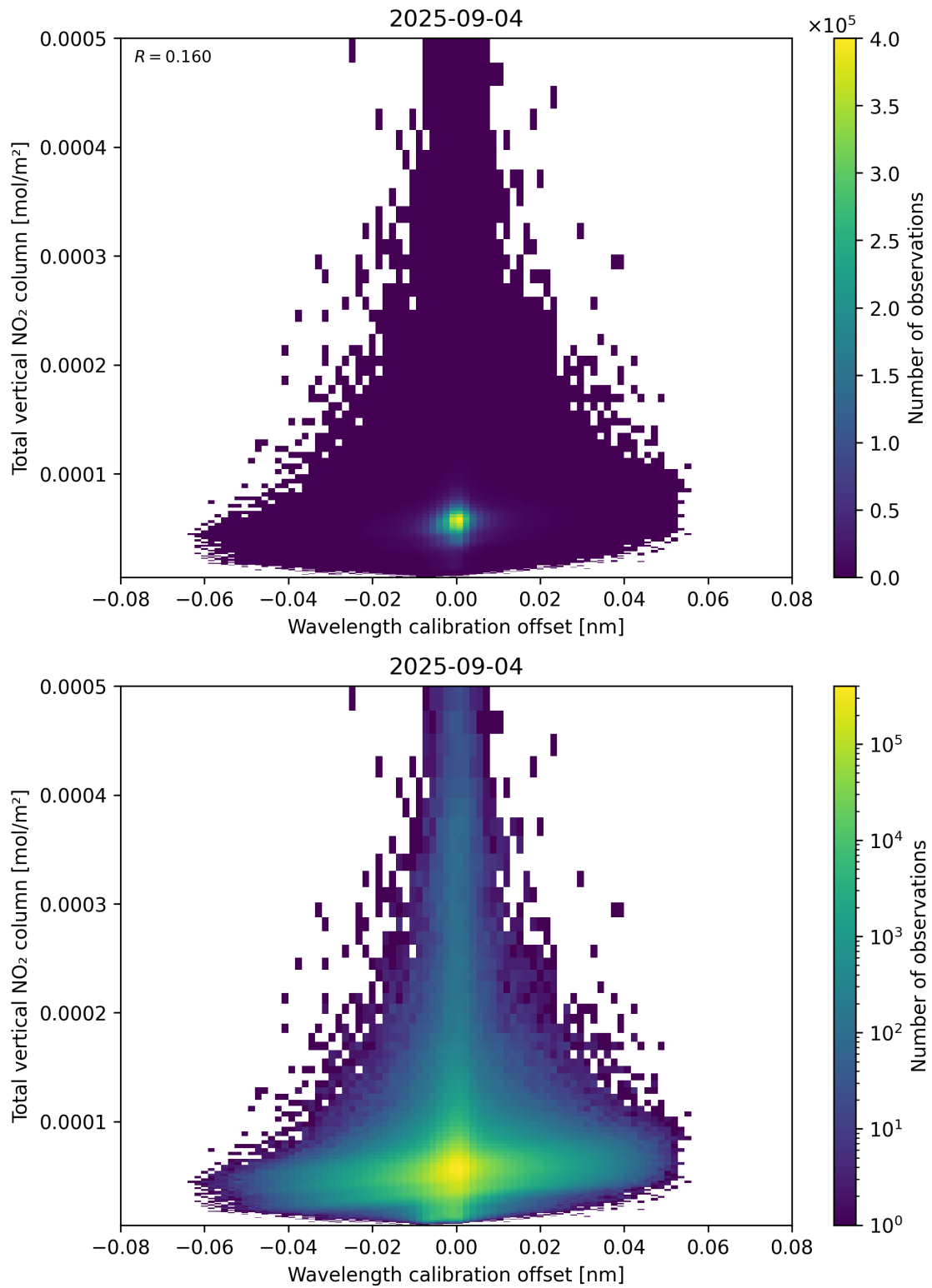
Figure 179: Scatter density plot of “Wavelength calibration offset” against “Total vertical NO 2 column” for 2025-09-04 to 2025-09-05.
