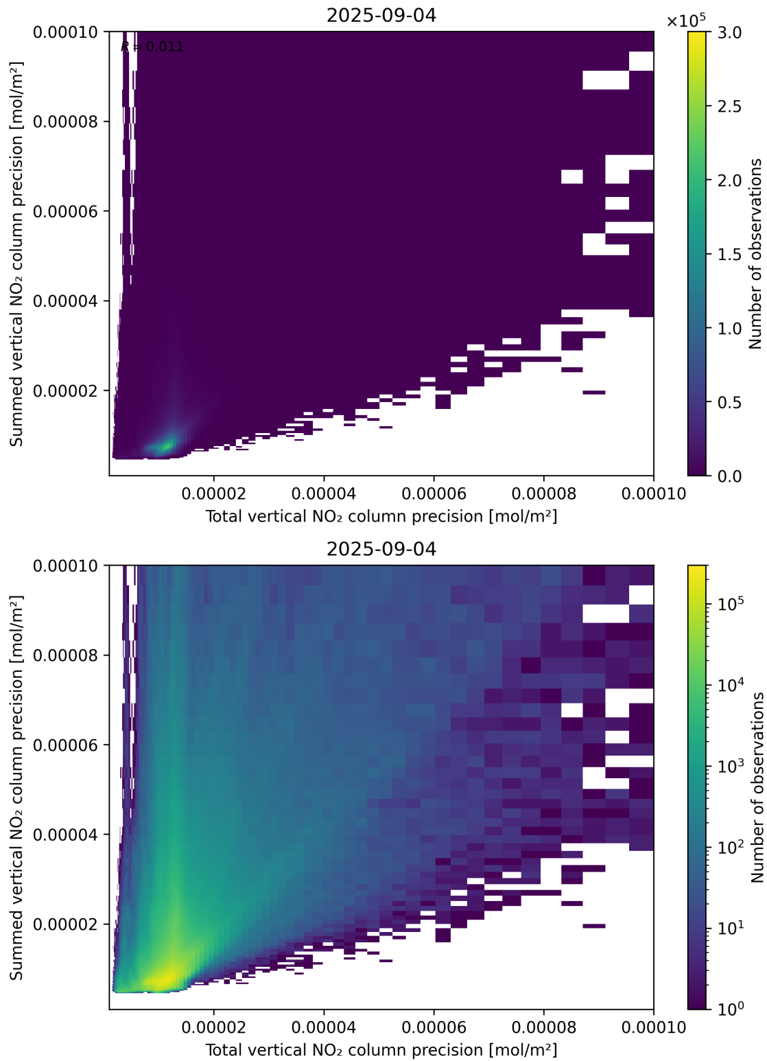
Figure 118: Scatter density plot of “Total vertical NO 2 column precision” against “Summed vertical NO 2 column precision” for 2025-09-04 to 2025-09-05.
