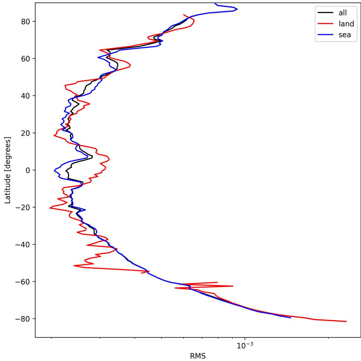
Figure 26: Zonal average of “RMS” for 2025-09-04 to 2025-09-05.
