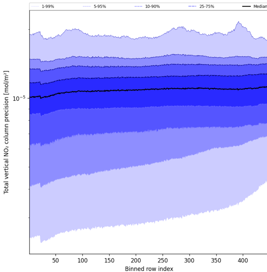
Figure 56: Along track statistics of “Total vertical NO 2 column precision” for 2025-09-04 to 2025-09-05
