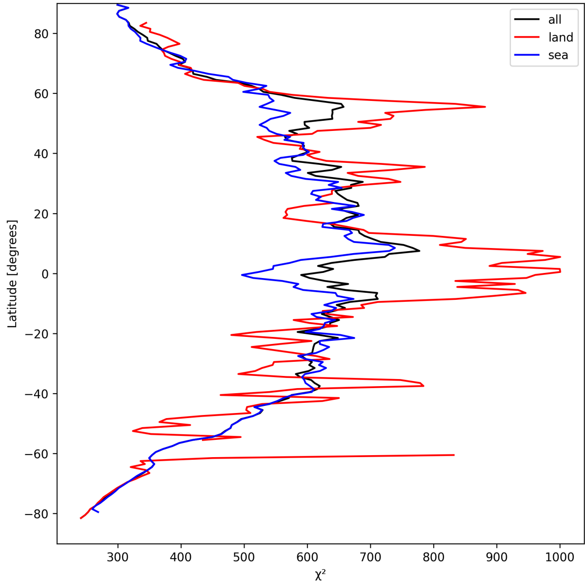
Figure 25: Zonal average of “ \chi^2 ” for 2025-09-04 to 2025-09-05.
