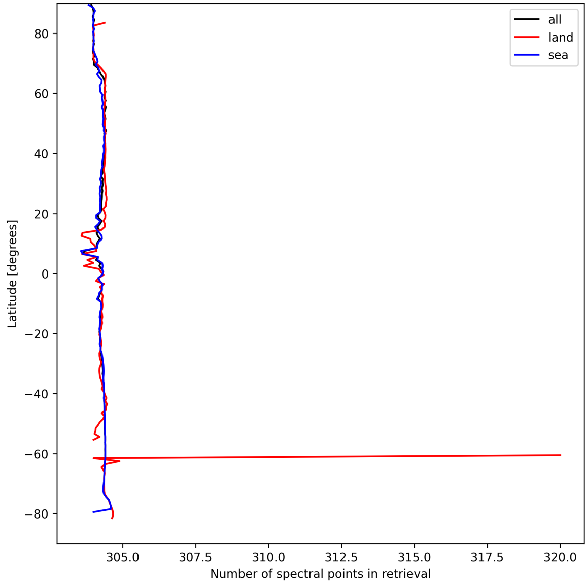
Figure 16: Zonal average of “Number of spectral points in retrieval” for 2025-09-04 to 2025-09-05.
