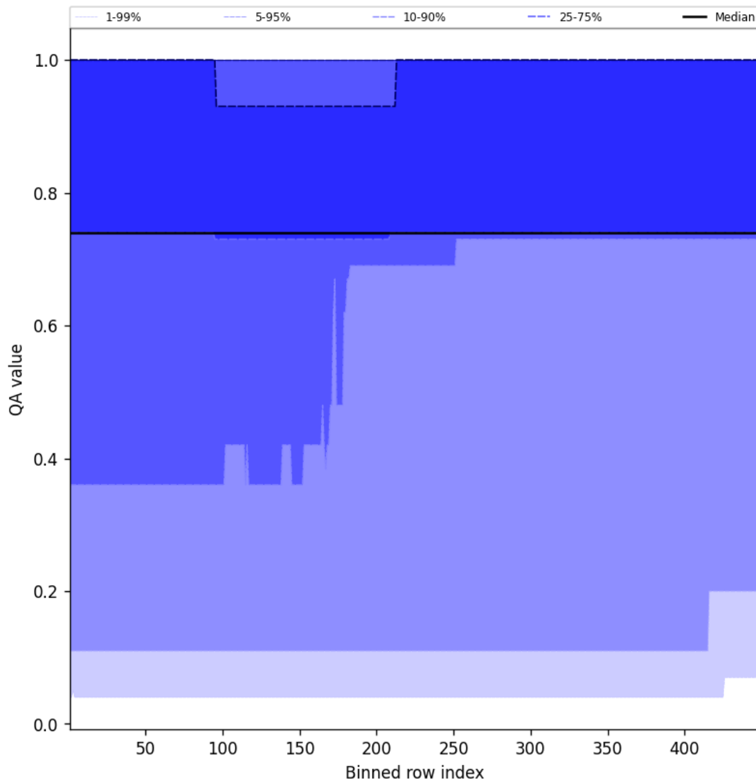
Figure 45: Along track statistics of “QA value” for 2025-09-04 to 2025-09-05
