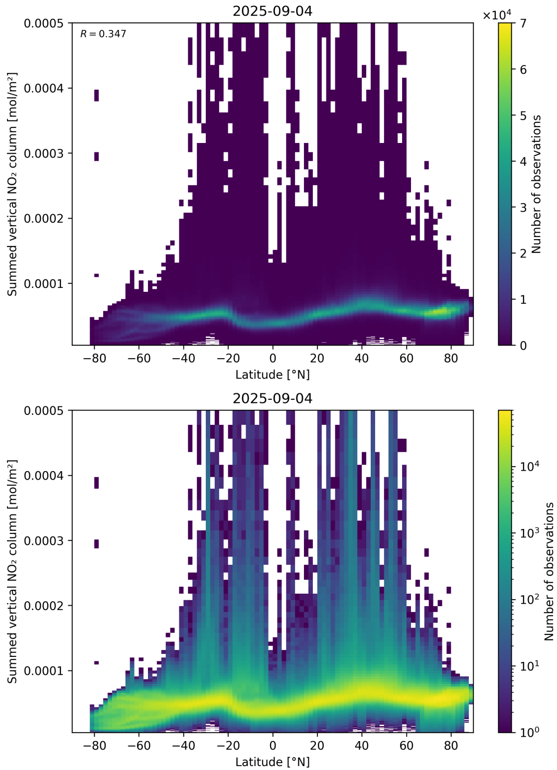
Figure 88: Scatter density plot of “Latitude” against “Summed vertical NO 2 column” for 2025-09-04 to 2025-09-05.
