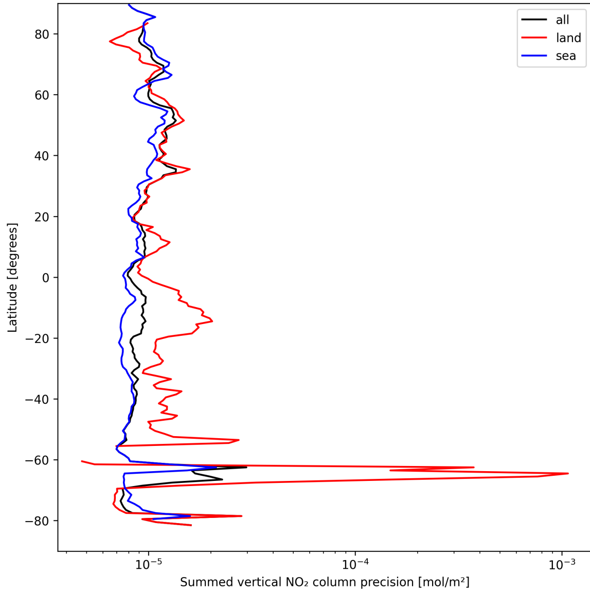
Figure 24: Zonal average of “Summed vertical NO 2 column precision” for 2025-09-04 to 2025-09-05.
