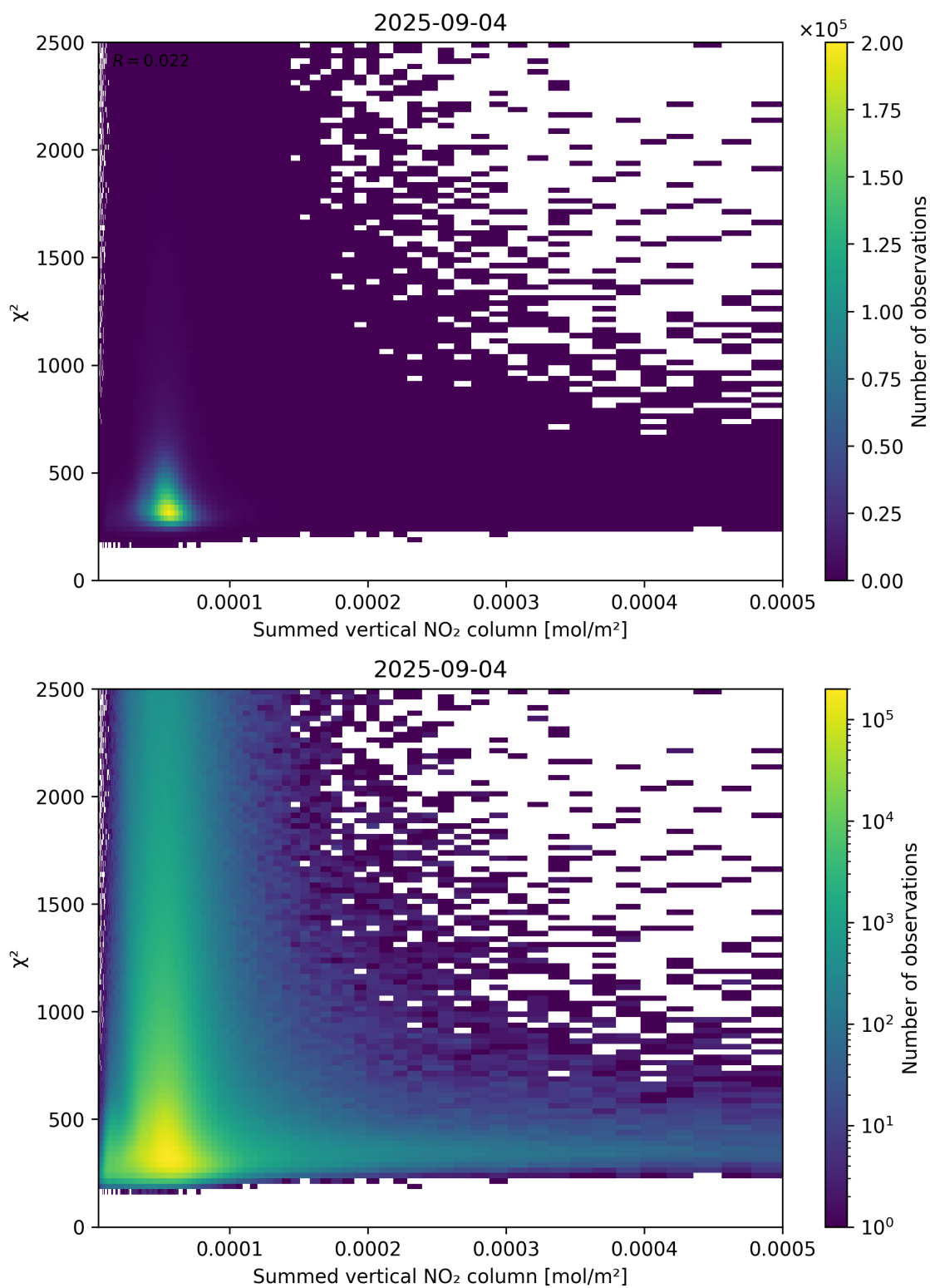
Figure 104: Scatter density plot of “Summed vertical NO 2 column” against “ \chi^2 ” for 2025-09-04 to 2025-09-05.
