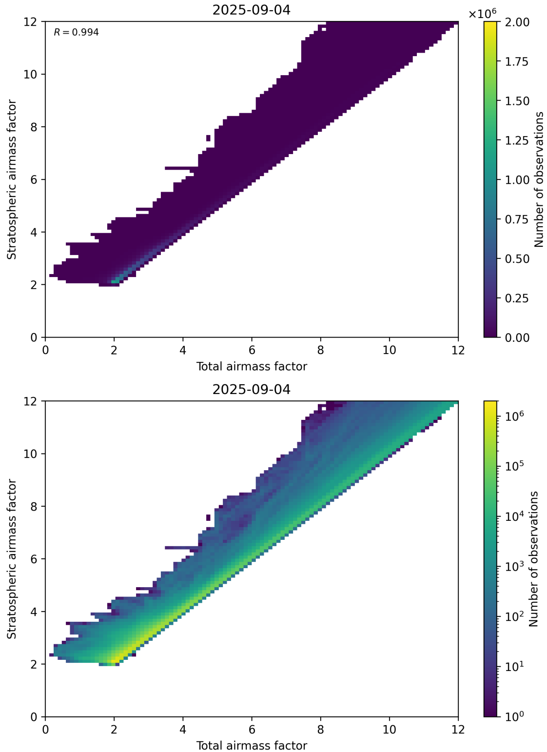
Figure 62: Scatter density plot of “Total airmass factor” against “Stratospheric airmass factor” for 2025-09-04 to 2025-09-05.
