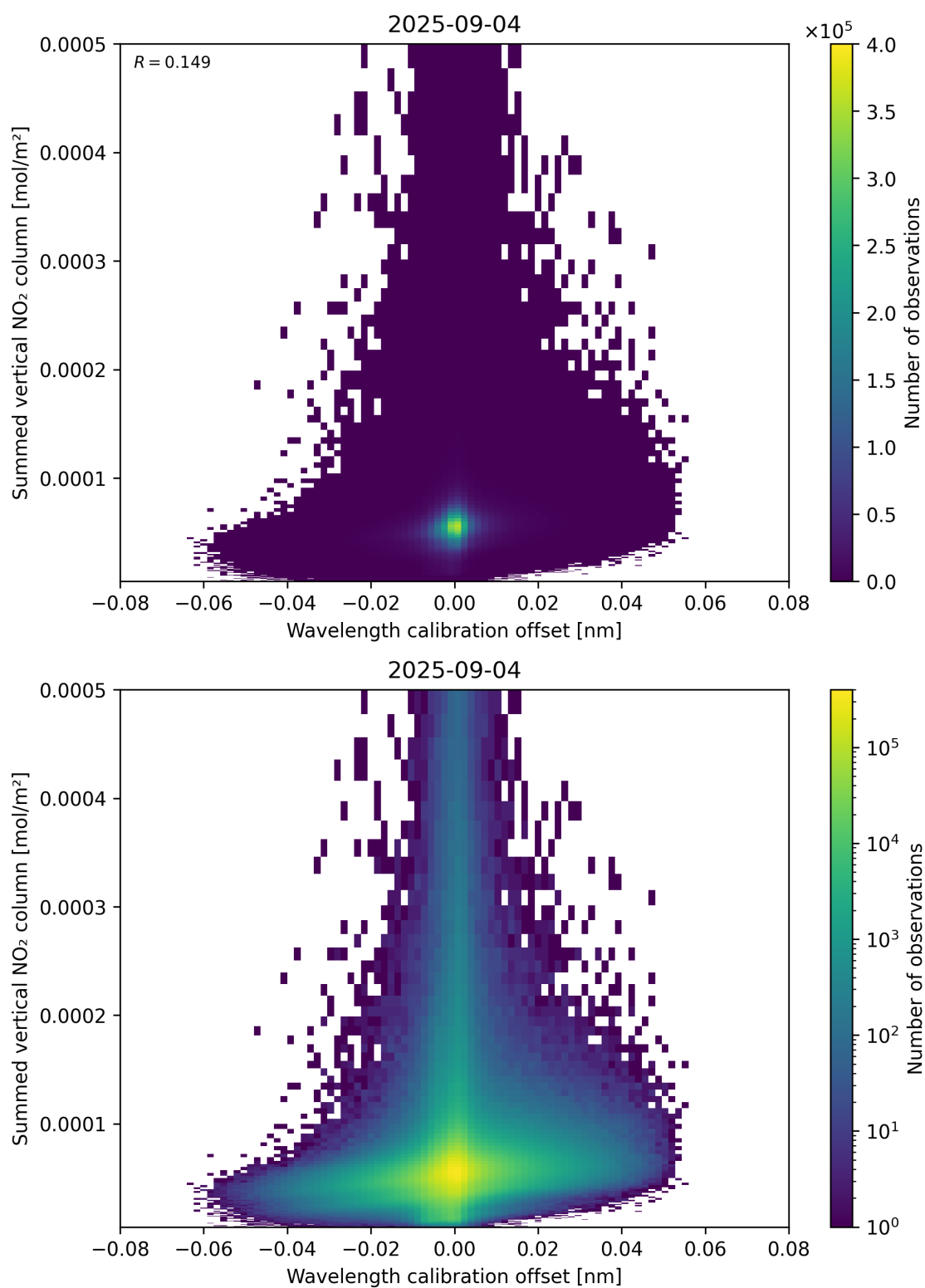
Figure 177: Scatter density plot of “Wavelength calibration offset” against “Summed vertical NO 2 column” for 2025-09-04 to 2025-09-05.
