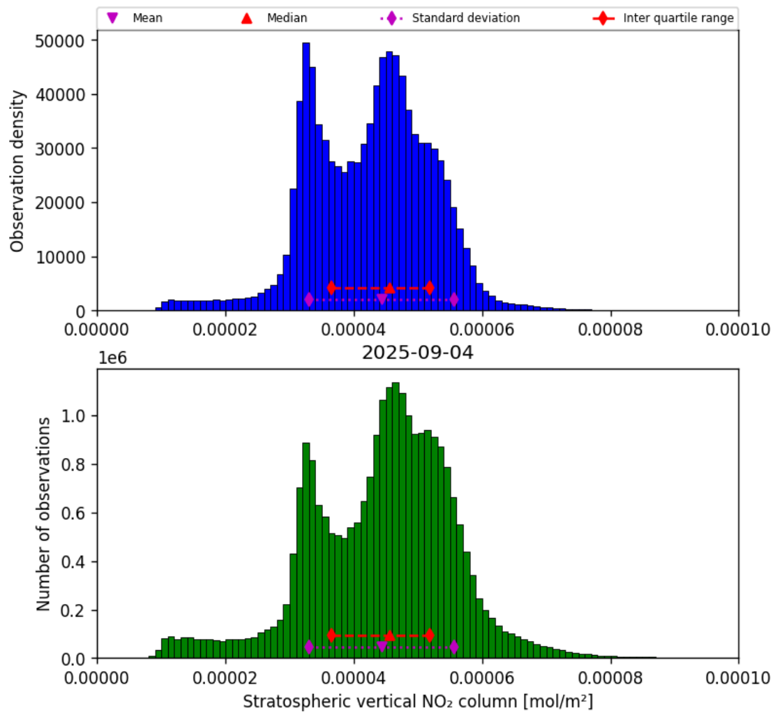
Figure 36: Histogram of “Stratospheric vertical NO 2 column” for 2025-09-04 to 2025-09-05
