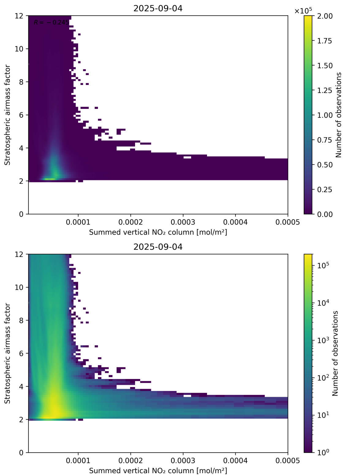
Figure 103: Scatter density plot of “Summed vertical NO 2 column” against “Stratospheric airmass factor” for 2025-09-04 to 2025-09-05.
