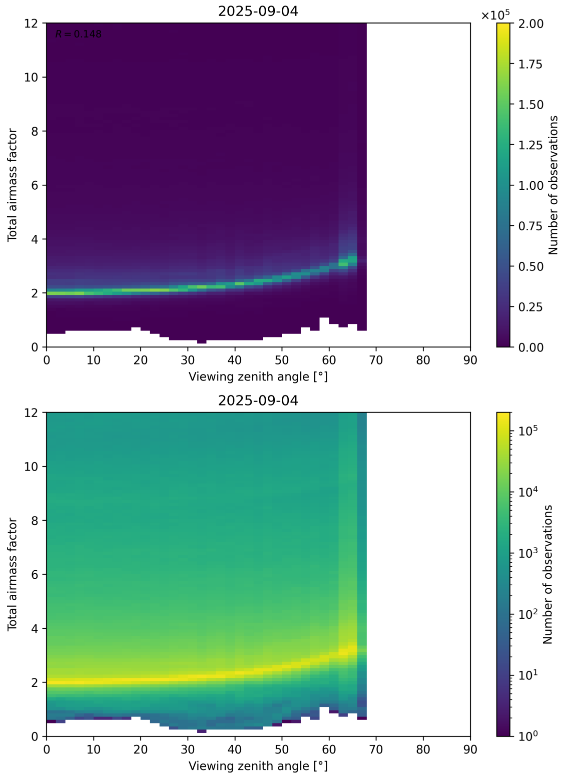
Figure 160: Scatter density plot of “Viewing zenith angle” against “Total airmass factor” for 2025-09-04 to 2025-09-05.
