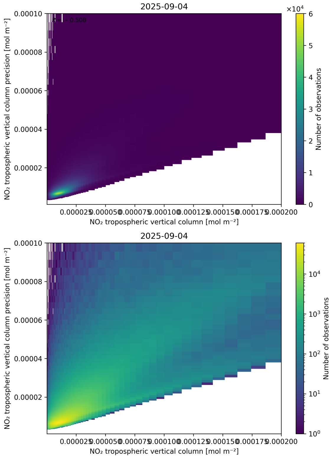
Figure 130: Scatter density plot of “NO 2 tropospheric vertical column” against “NO 2 tropospheric vertical column precision” for 2025-09-04 to 2025-09-05.
