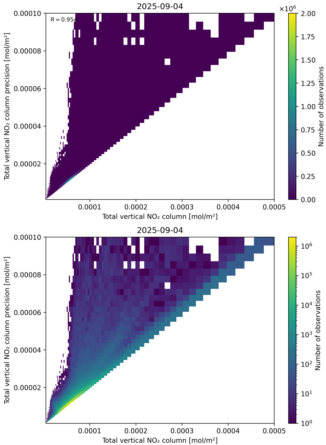
Figure 114: Scatter density plot of “Total vertical NO 2 column” against “Total vertical NO 2 column precision” for 2025-09-04 to 2025-09-05.
