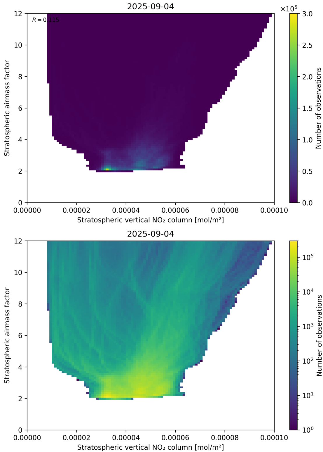
Figure 96: Scatter density plot of “Stratospheric vertical NO 2 column” against “Stratospheric airmass factor” for 2025-09-04 to 2025-09-05.
