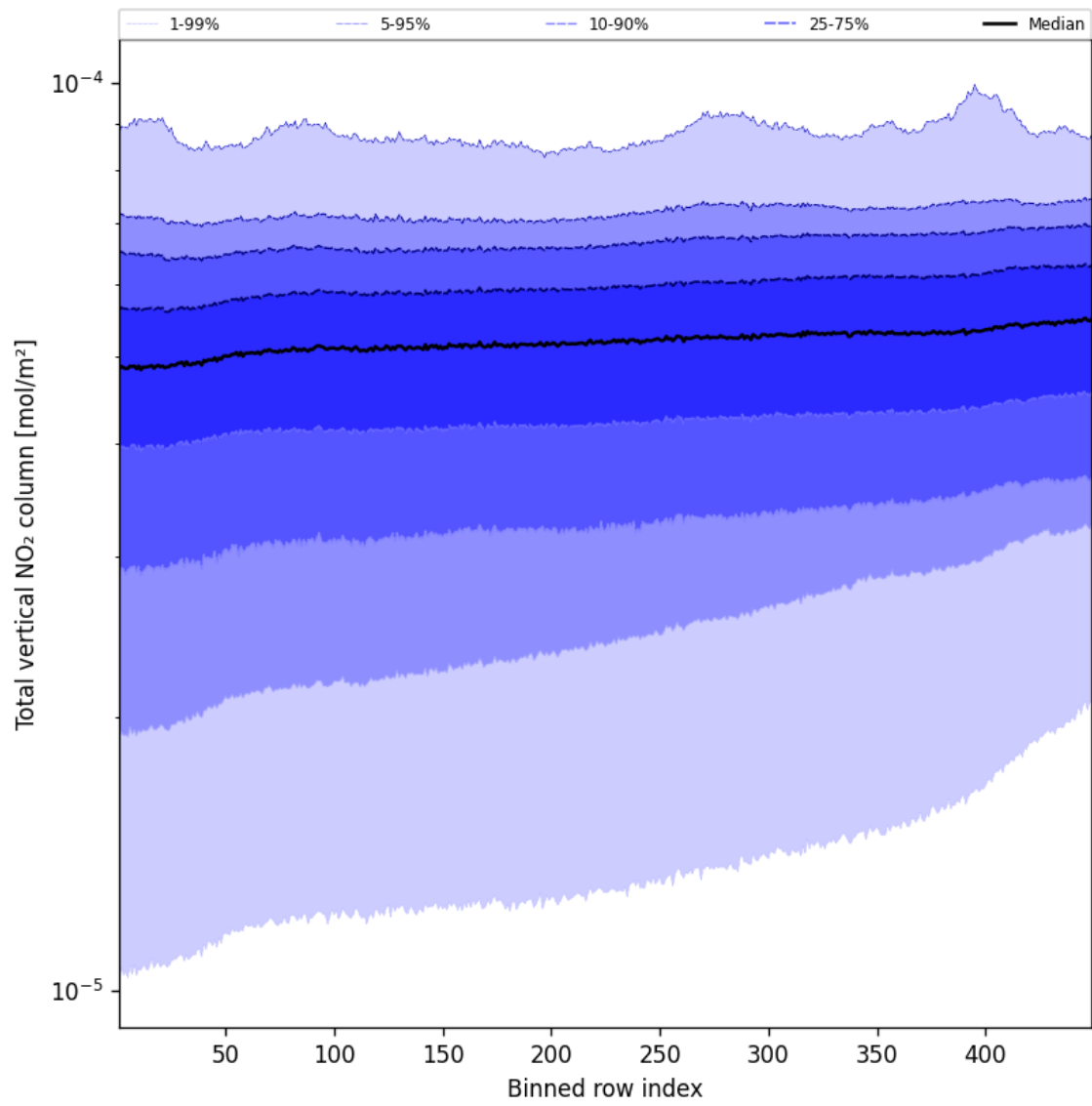
Figure 55: Along track statistics of "Total vertical NO 2 column" for 2025-09-04 to 2025-09-05
