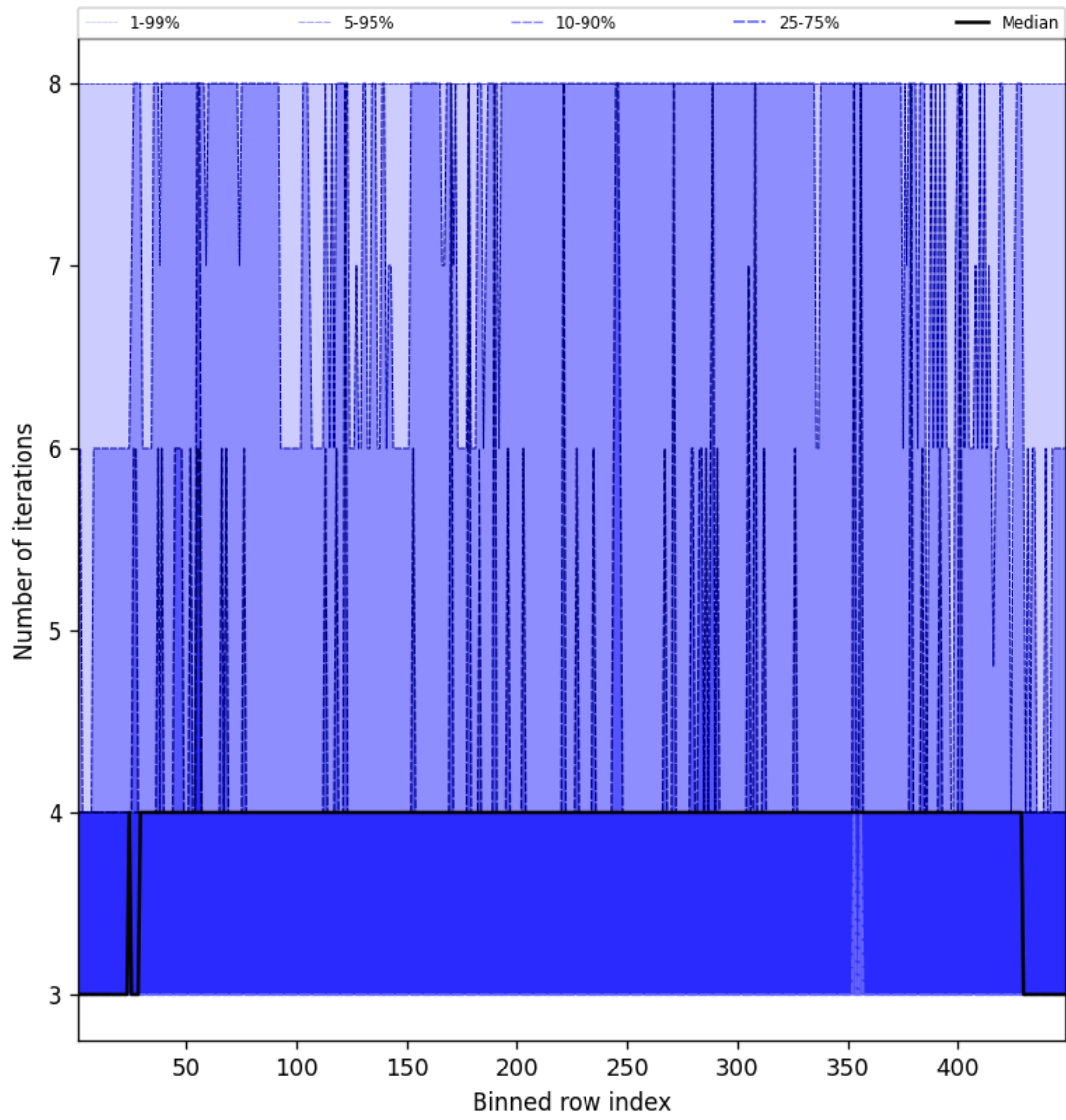
Figure 51: Along track statistics of “Number of iterations” for 2025-09-04 to 2025-09-05
