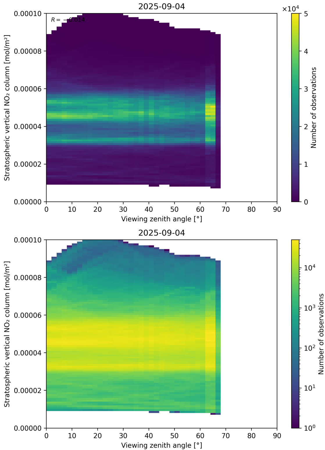
Figure 164: Scatter density plot of “Viewing zenith angle” against “Stratospheric vertical NO 2 column” for 2025-09-04 to 2025-09-05.
