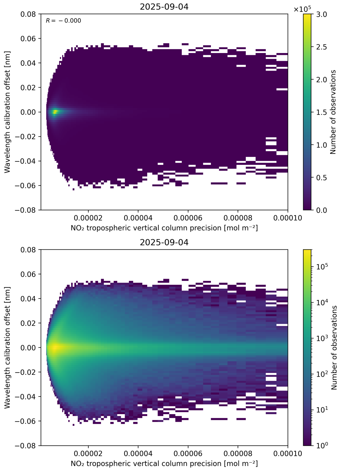
Figure 141: Scatter density plot of “NO 2 tropospheric vertical column precision” against “Wavelength calibration offset” for 2025-09-04 to 2025-09-05.
