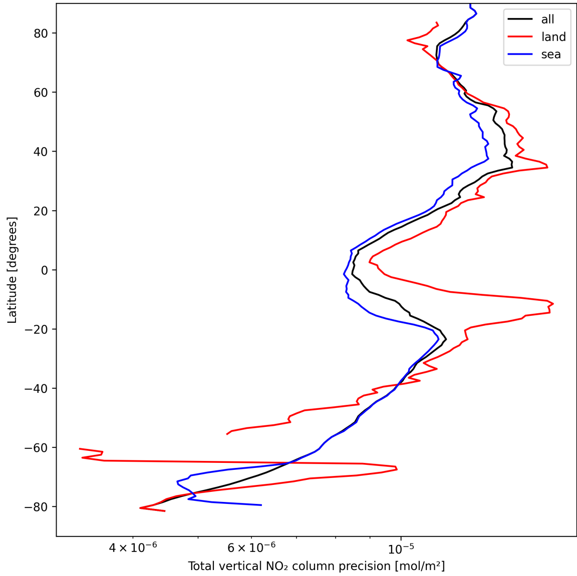
Figure 22: Zonal average of “Total vertical NO 2 column precision” for 2025-09-04 to 2025-09-05.
