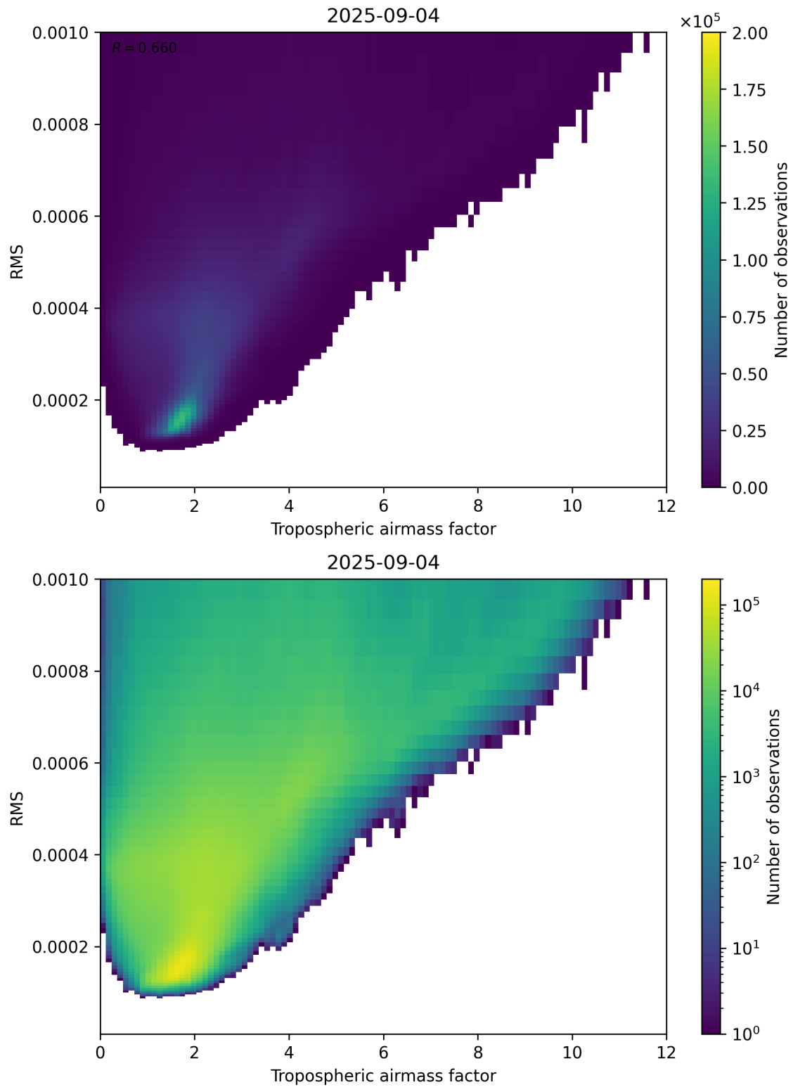
Figure 79: Scatter density plot of “Tropospheric airmass factor” against “RMS” for 2025-09-04 to 2025-09-05.
