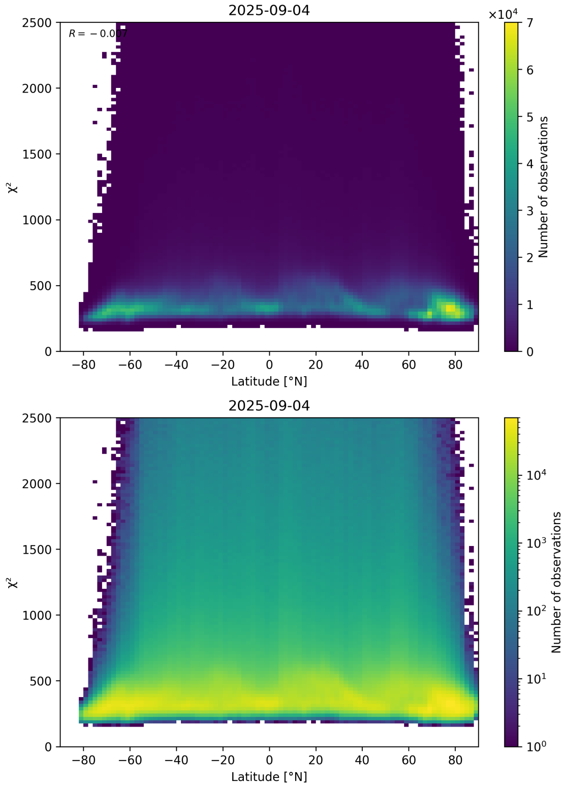
Figure 86: Scatter density plot of “Latitude” against “ \chi^2 ” for 2025-09-04 to 2025-09-05.
