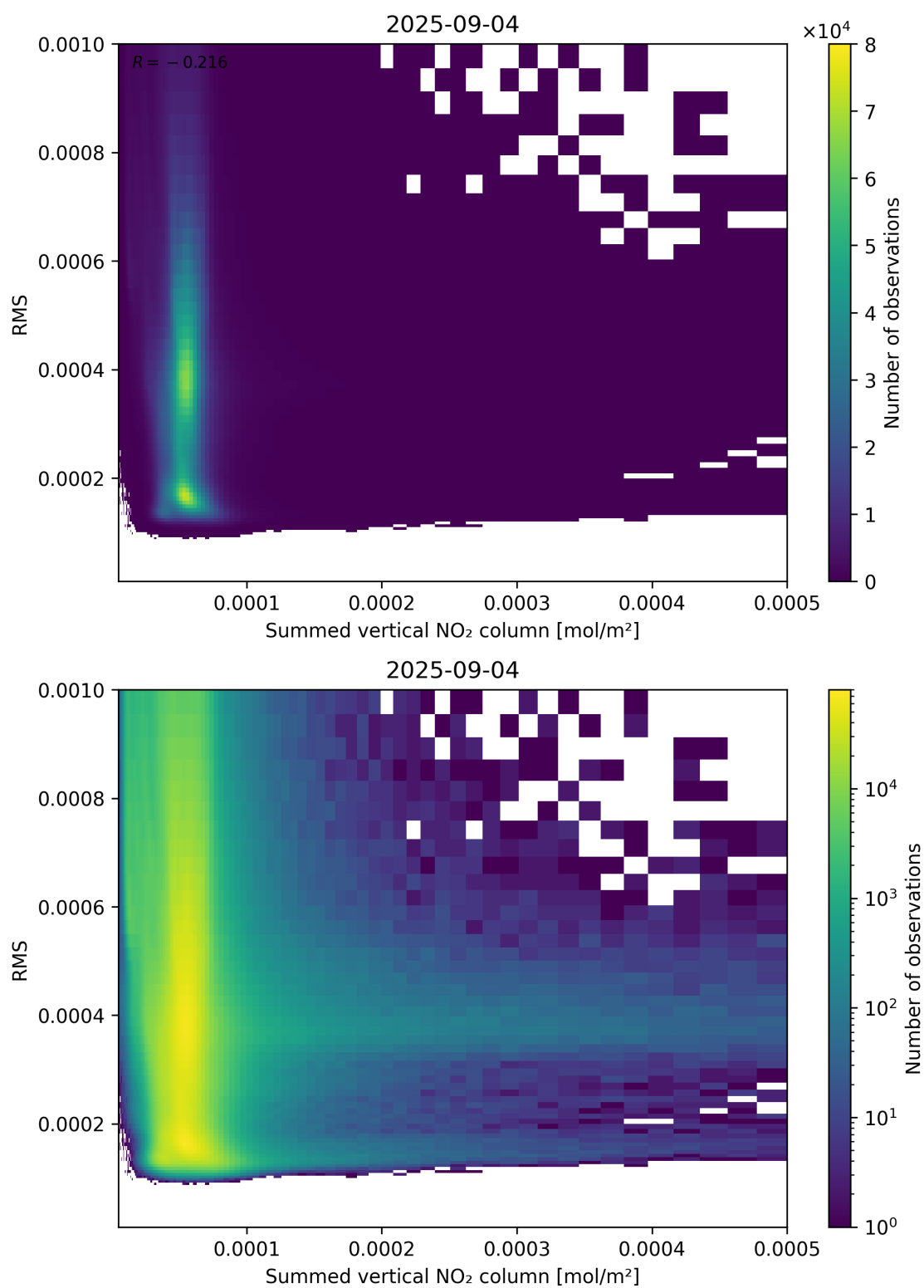
Figure 109: Scatter density plot of “Summed vertical NO 2 column” against “RMS” for 2025-09-04 to 2025-09-05.
