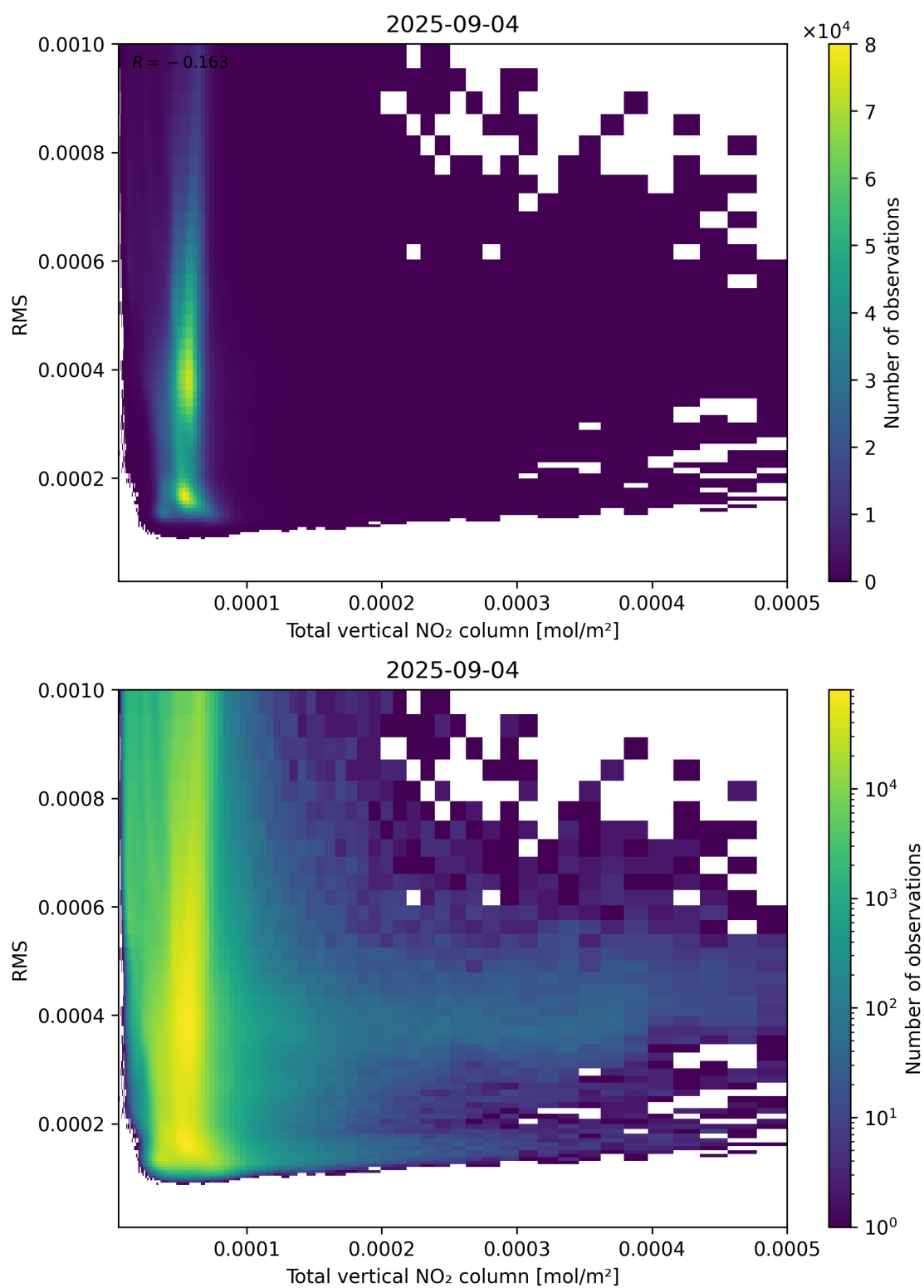
Figure 120: Scatter density plot of “Total vertical NO 2 column” against “RMS” for 2025-09-04 to 2025-09-05.
