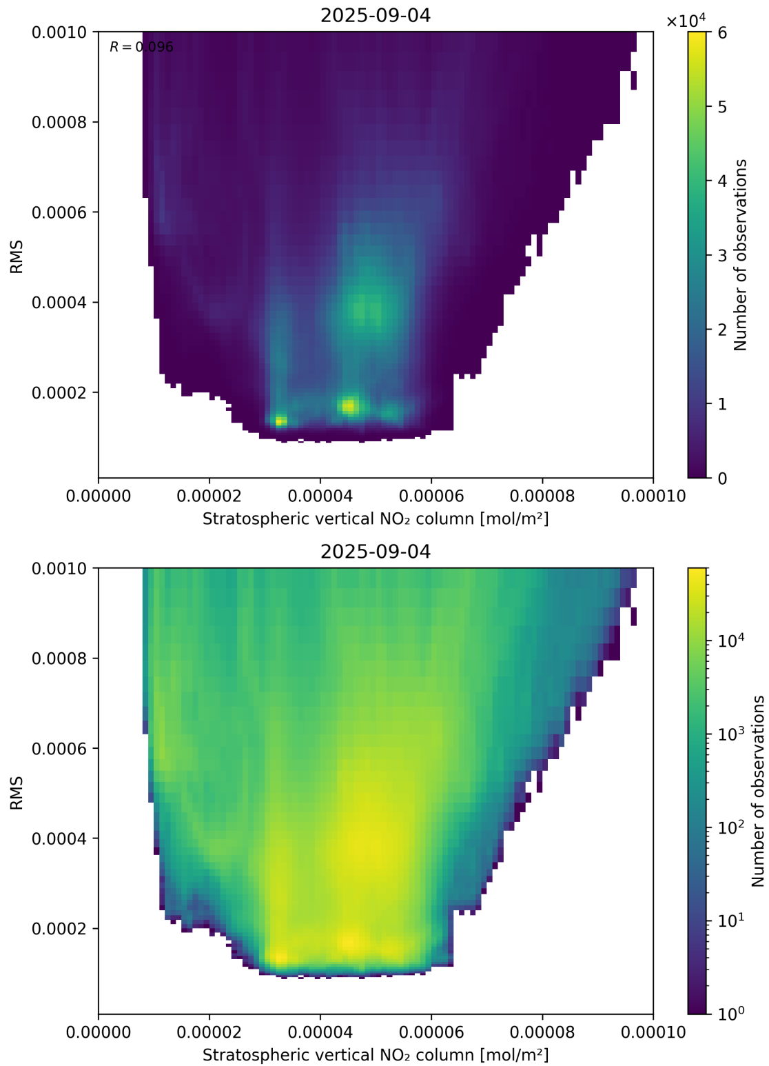
Figure 102: Scatter density plot of “Stratospheric vertical NO 2 column” against “RMS” for 2025-09-04 to 2025-09-05.
