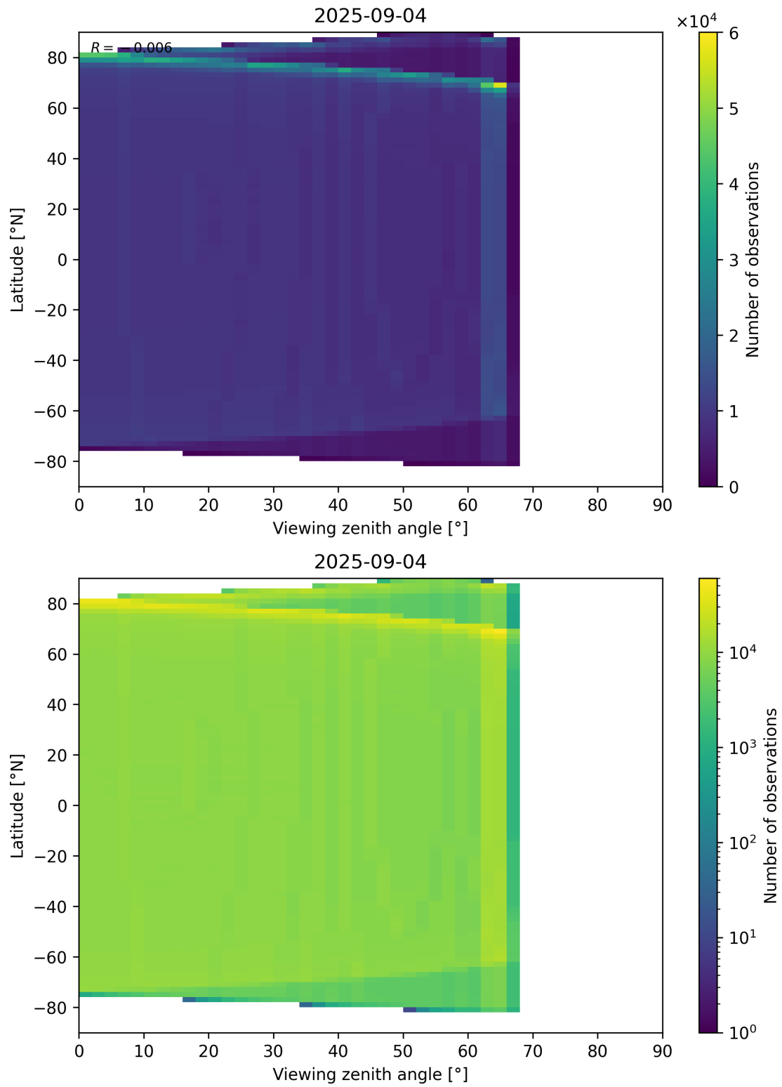
Figure 163: Scatter density plot of “Viewing zenith angle” against “Latitude” for 2025-09-04 to 2025-09-05.
