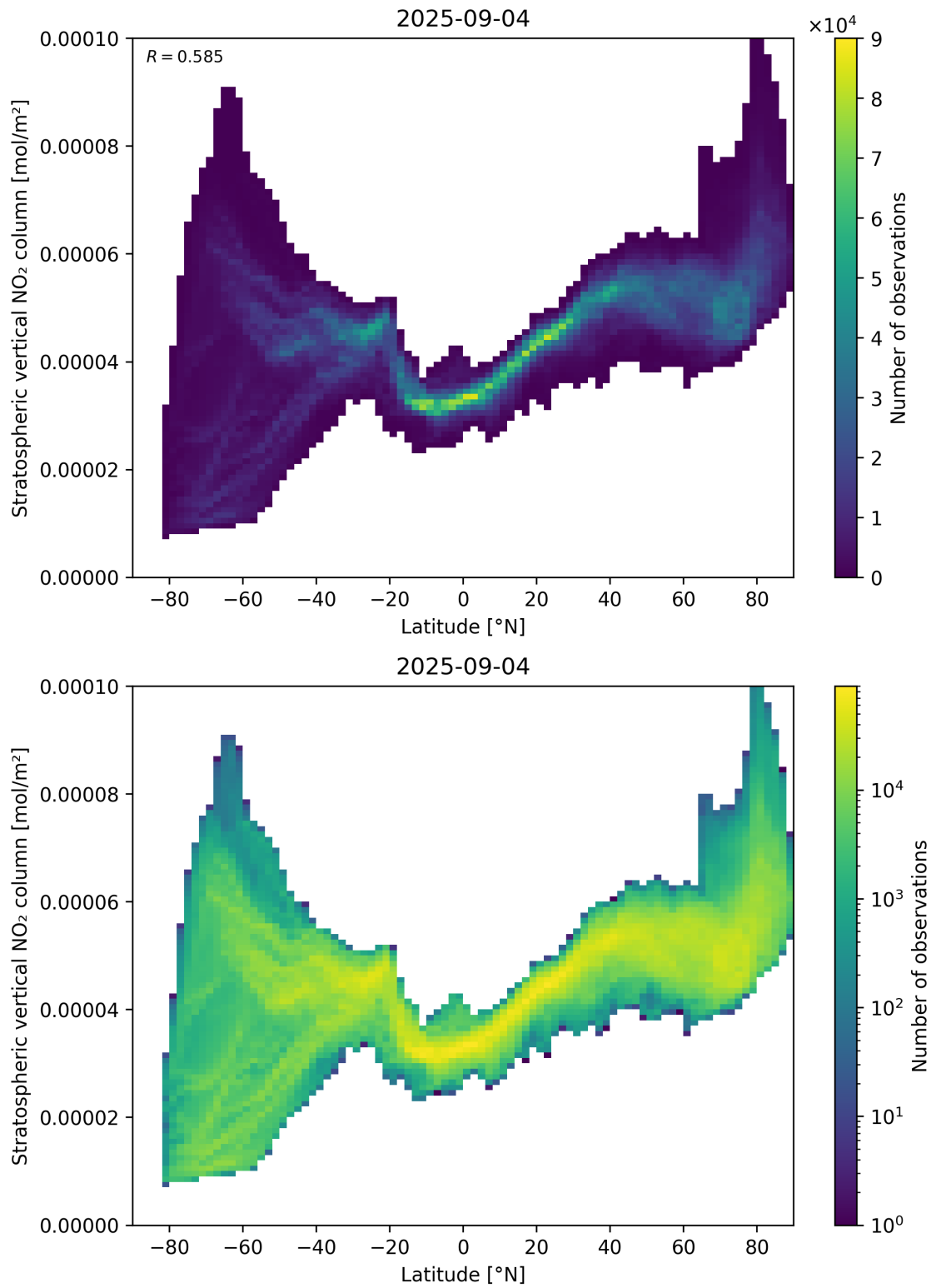
Figure 87: Scatter density plot of “Latitude” against “Stratospheric vertical NO 2 column” for 2025-09-04 to 2025-09-05.
