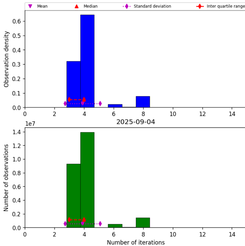
Figure 34: Histogram of “Number of iterations” for 2025-09-04 to 2025-09-05
