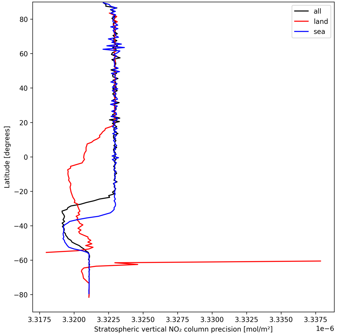
Figure 20: Zonal average of "Stratospheric vertical NO 2 column precision" for 2025-09-04 to 2025-09-05.
