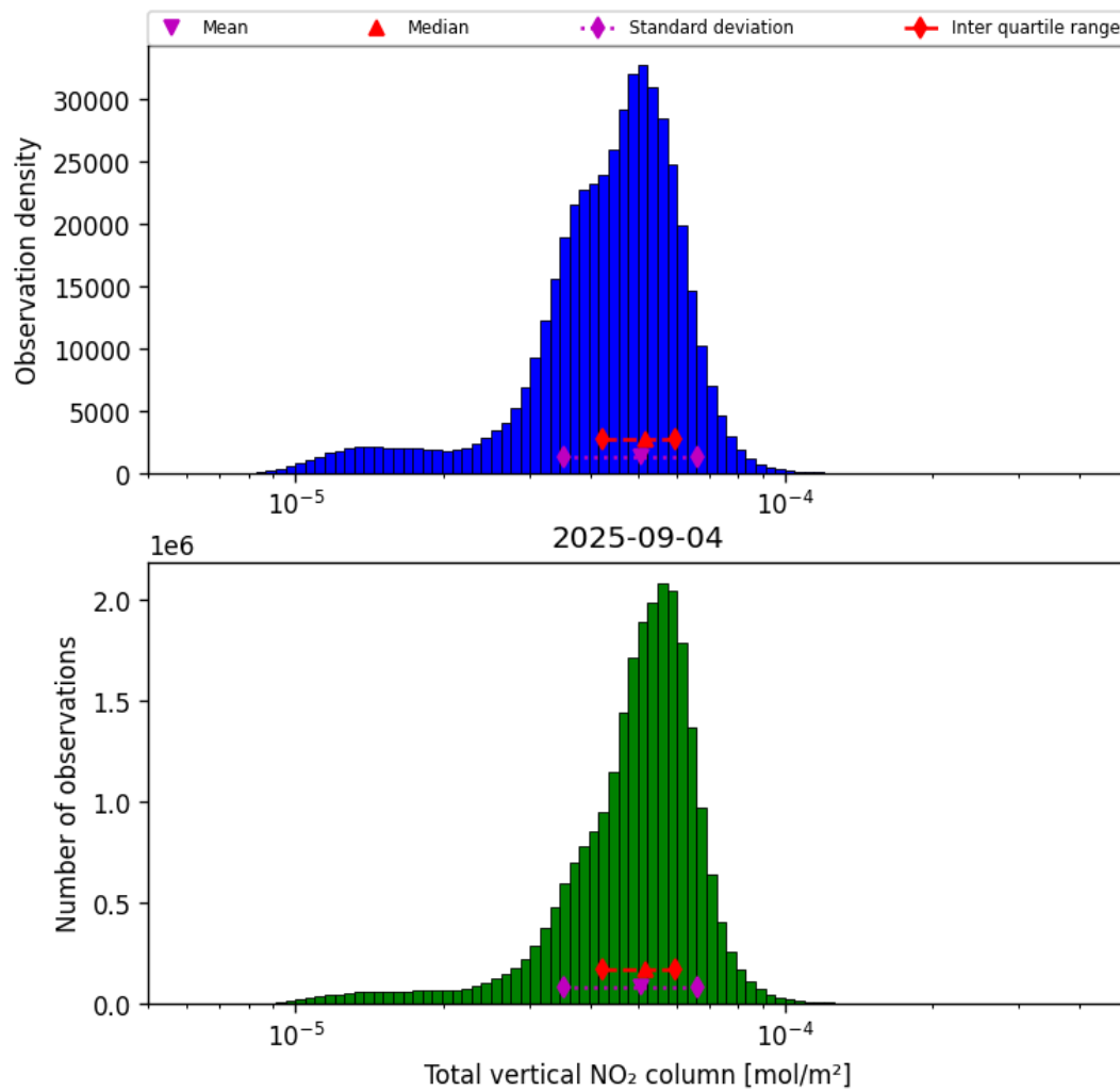
Figure 38: Histogram of “Total vertical NO 2 column” for 2025-09-04 to 2025-09-05
