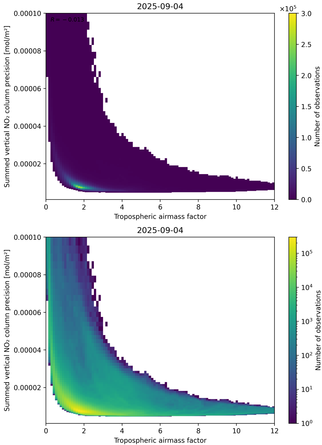
Figure 76: Scatter density plot of “Tropospheric air mass factor” against “Summed vertical NO 2 column precision” for 2025-09-04 to 2025-09-05.
