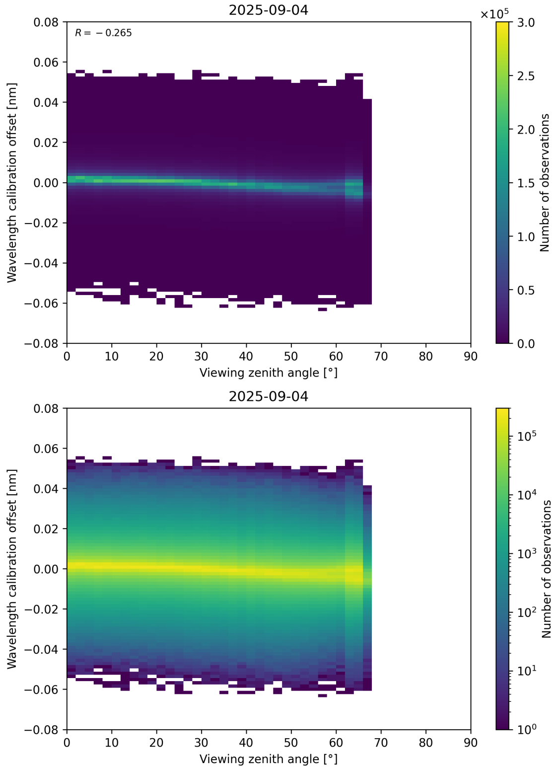
Figure 173: Scatter density plot of “Viewing zenith angle” against “Wavelength calibration offset” for 2025-09-04 to 2025-09-05.
