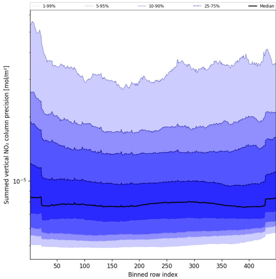
Figure 58: Along track statistics of “Summed vertical NO 2 column precision” for 2025-09-04 to 2025-09-05
