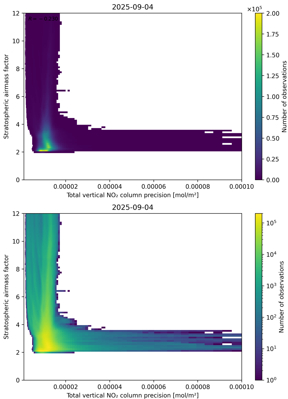
Figure 115: Scatter density plot of “Total vertical NO 2 column precision” against “Stratospheric air mass factor” for 2025-09-04 to 2025-09-05.
