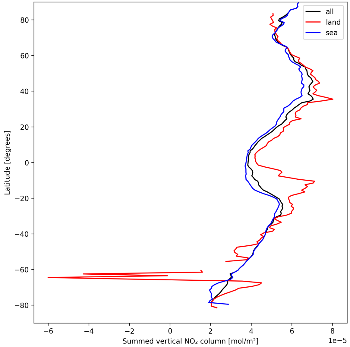
Figure 23: Zonal average of “Summed vertical NO 2 column” for 2025-09-04 to 2025-09-05.
