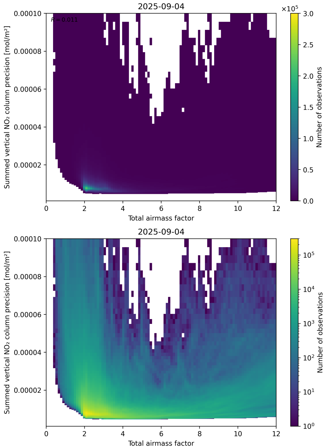
Figure 66: Scatter density plot of “Total airmass factor” against “Summed vertical NO 2 column precision” for 2025-09-04 to 2025-09-05.
