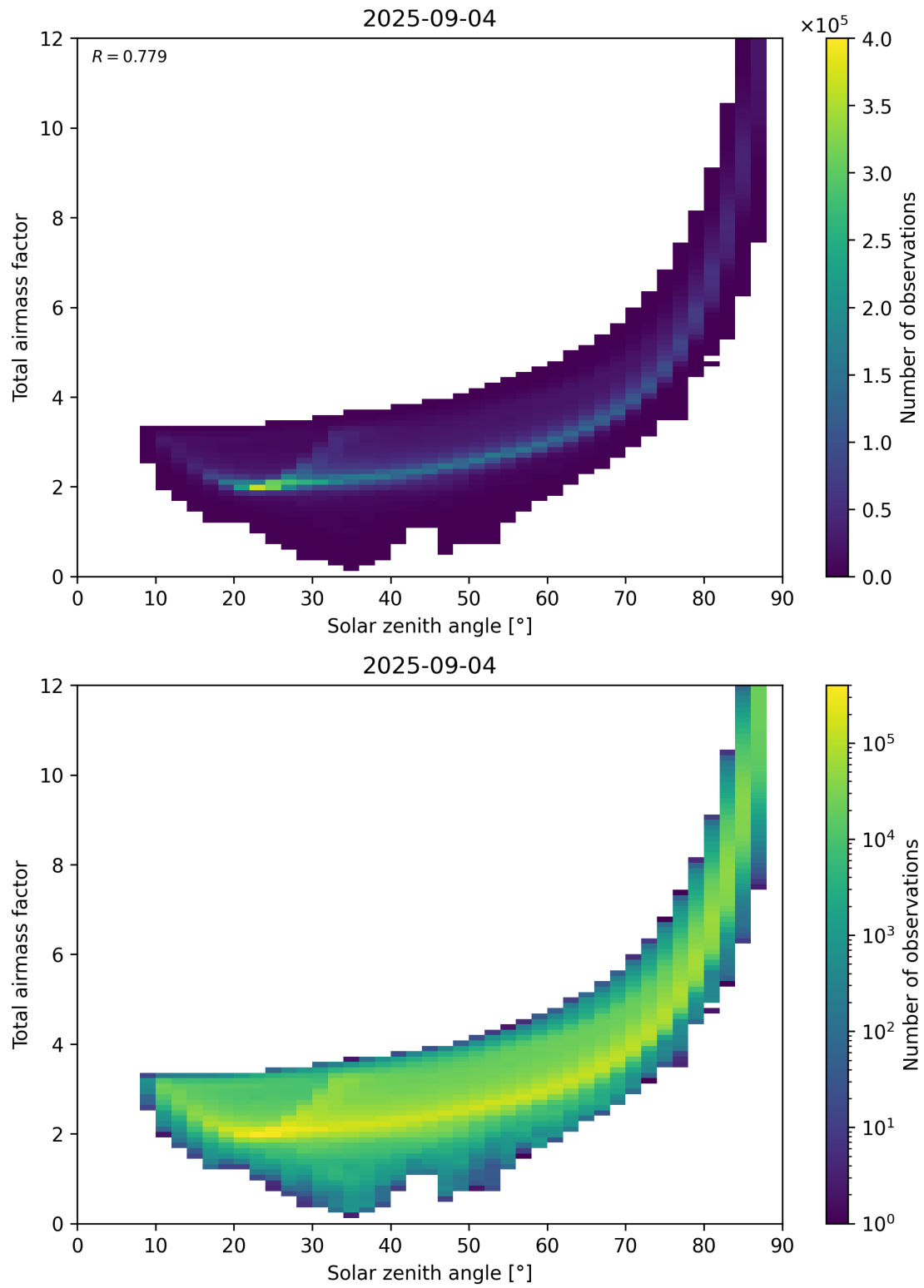
Figure 146: Scatter density plot of “Solar zenith angle” against “Total airmass factor” for 2025-09-04 to 2025-09-05.
