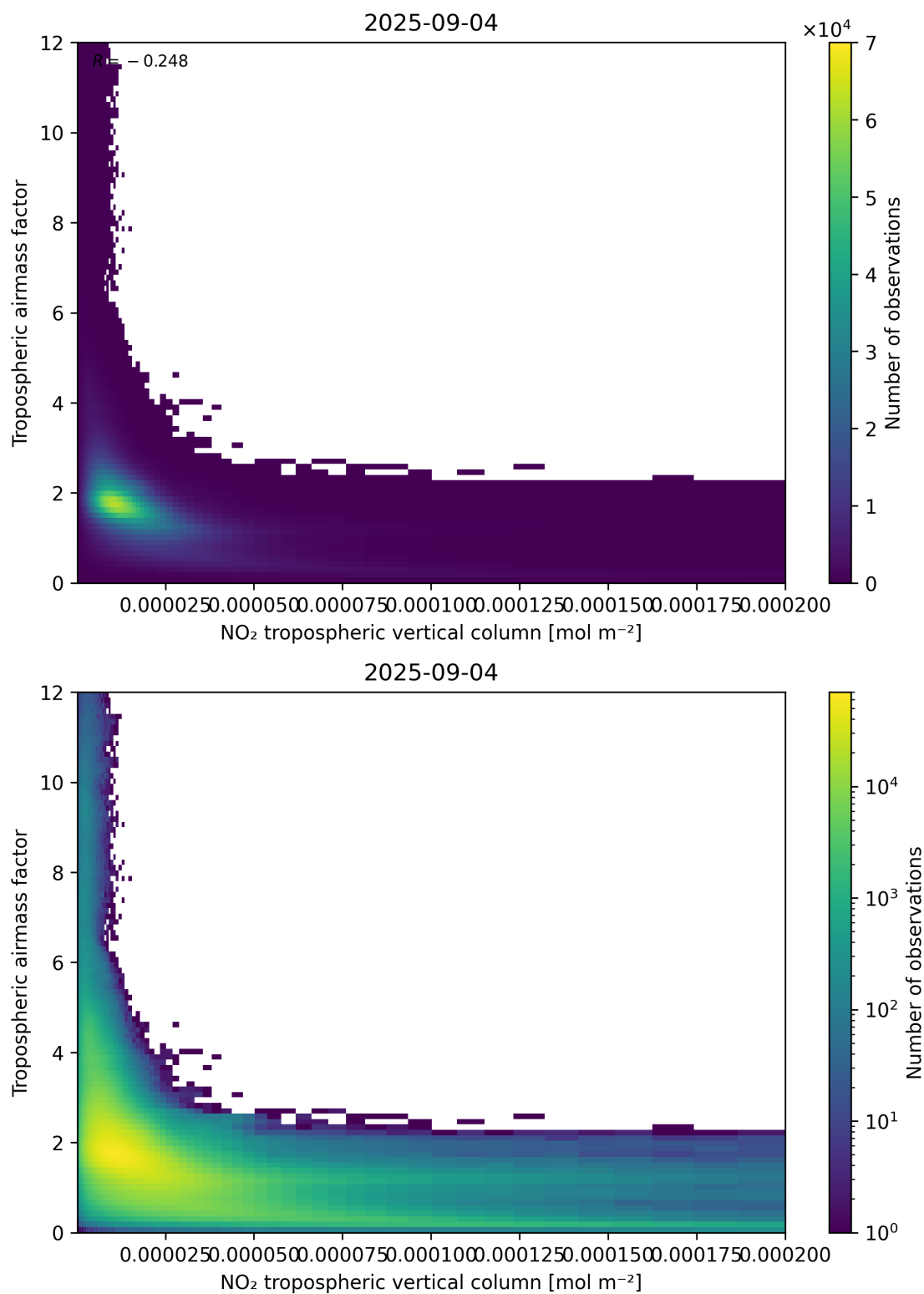
Figure 123: Scatter density plot of “NO 2 tropospheric vertical column” against “Tropospheric air mass factor” for 2025-09-04 to 2025-09-05.
