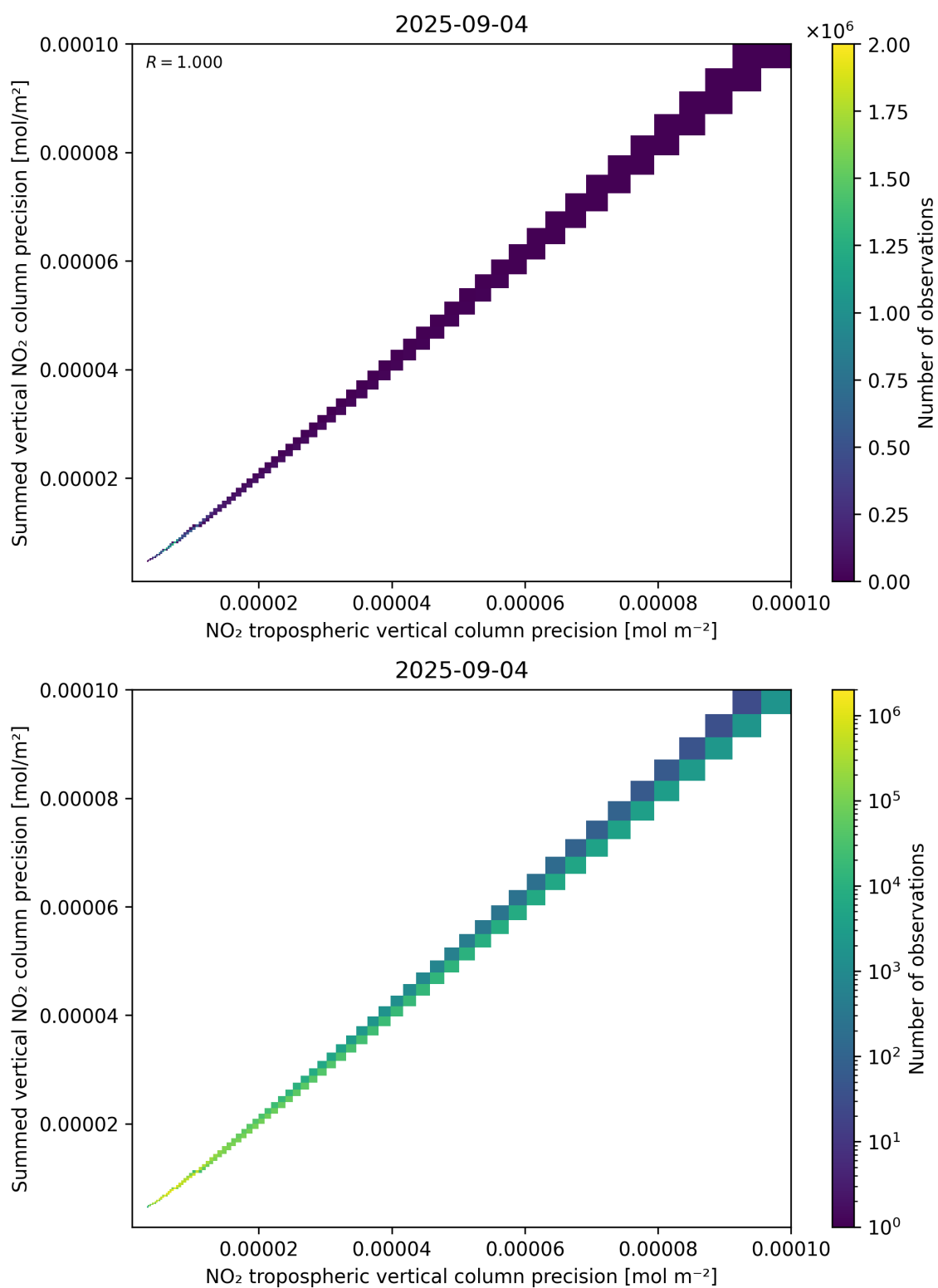
Figure 137: Scatter density plot of “NO 2 tropospheric vertical column precision” against “Summed vertical NO 2 column precision” for 2025-09-04 to 2025-09-05.
