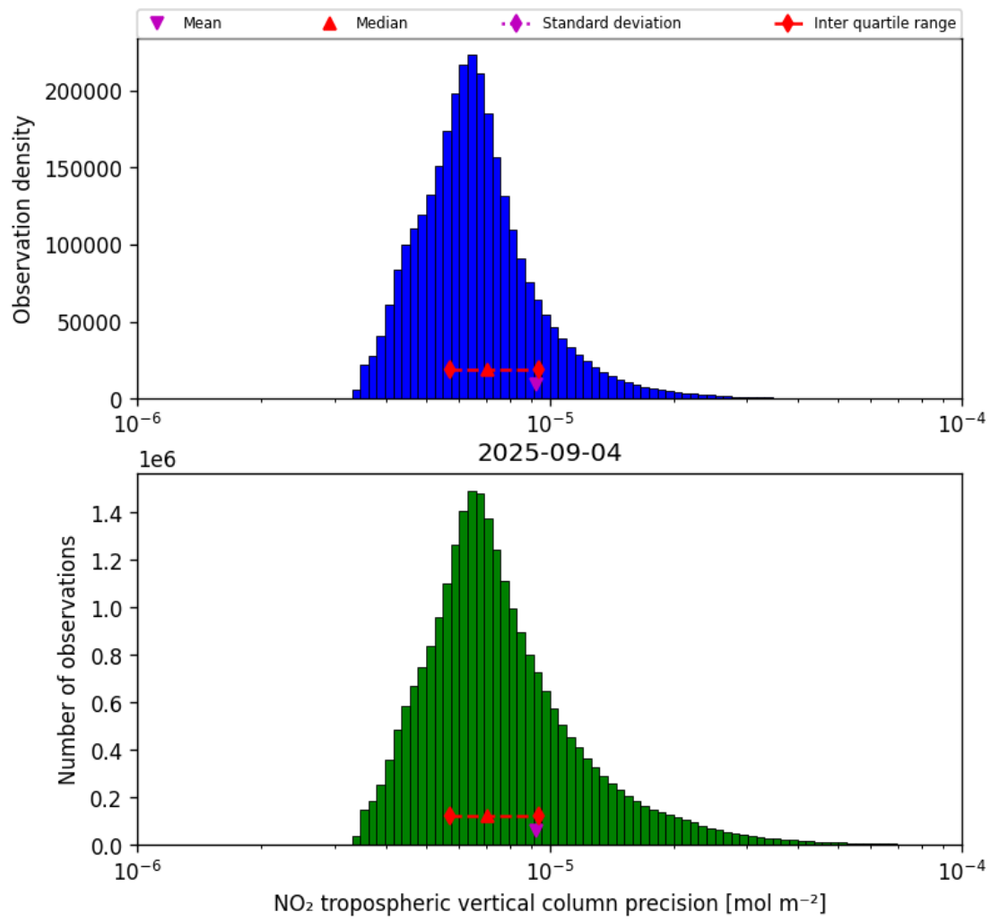
Figure 30: Histogram of “NO 2 tropospheric vertical column precision” for 2025-09-04 to 2025-09-05
