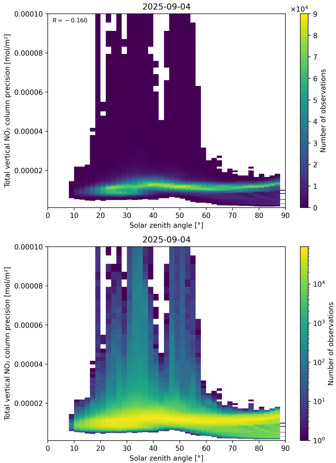
Figure 154: Scatter density plot of “Solar zenith angle” against “Total vertical NO 2 column precision” for 2025-09-04 to 2025-09-05.
