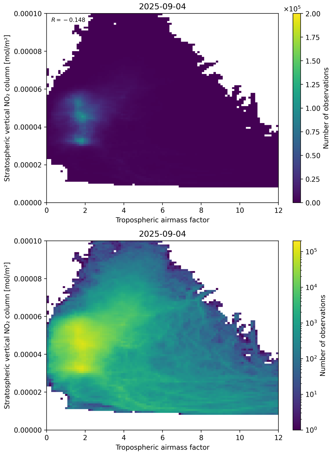
Figure 74: Scatter density plot of “Tropospheric air mass factor” against “Stratospheric vertical NO 2 column” for 2025-09-04 to 2025-09-05.
