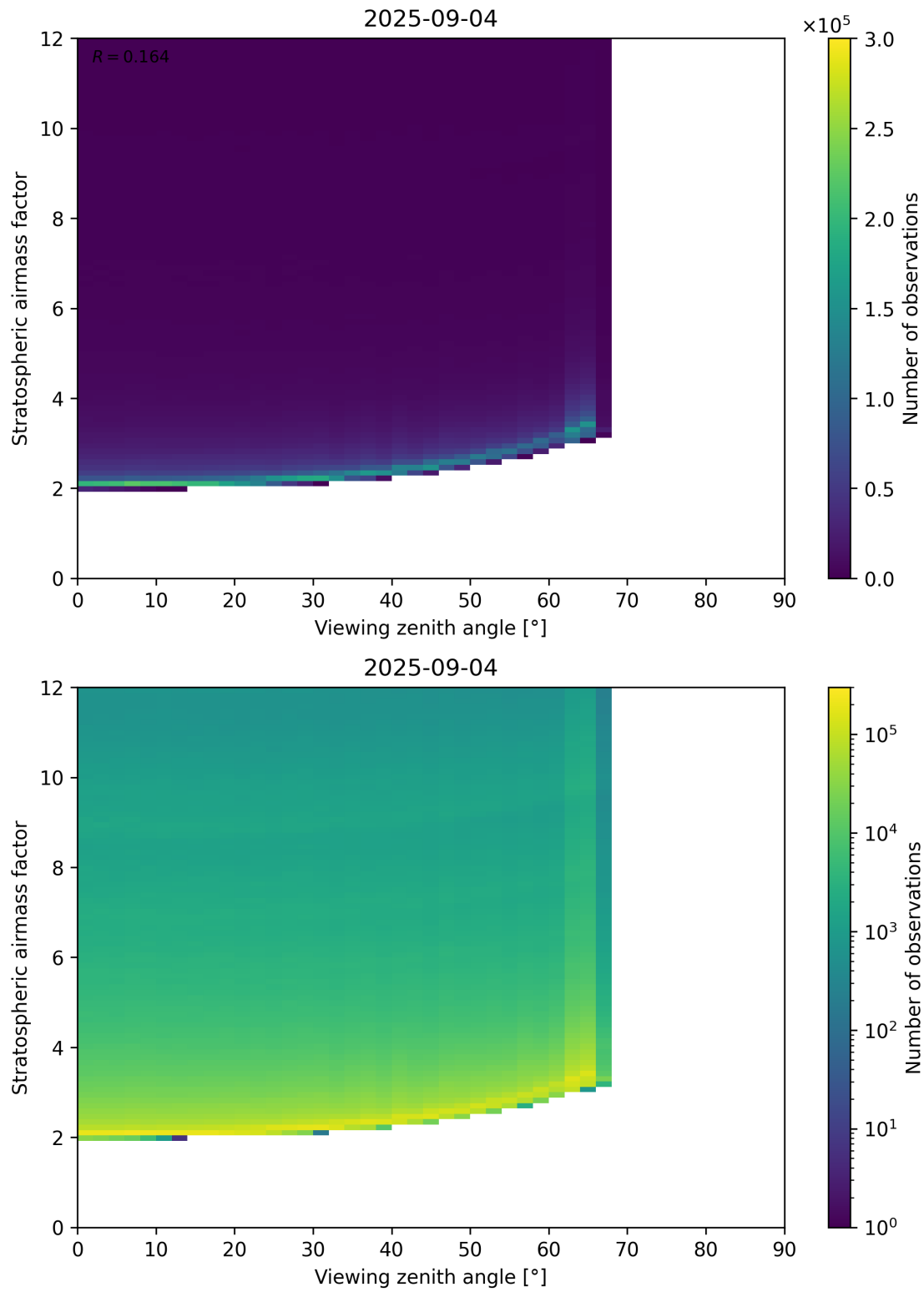
Figure 159: Scatter density plot of “Viewing zenith angle” against “Stratospheric airmass factor” for 2025-09-04 to 2025-09-05.
