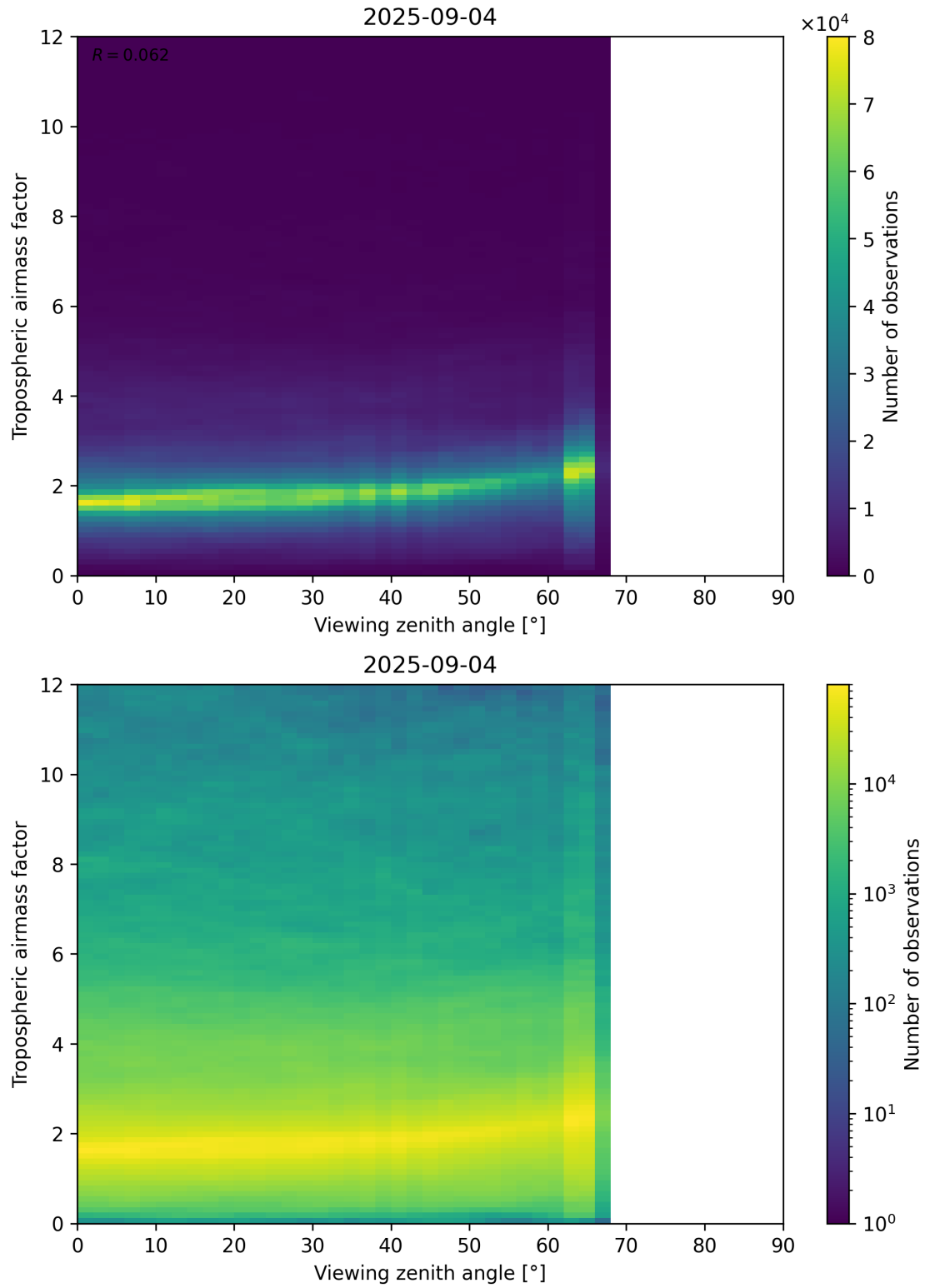
Figure 161: Scatter density plot of “Viewing zenith angle” against “Tropospheric airmass factor” for 2025-09-04 to 2025-09-05.
