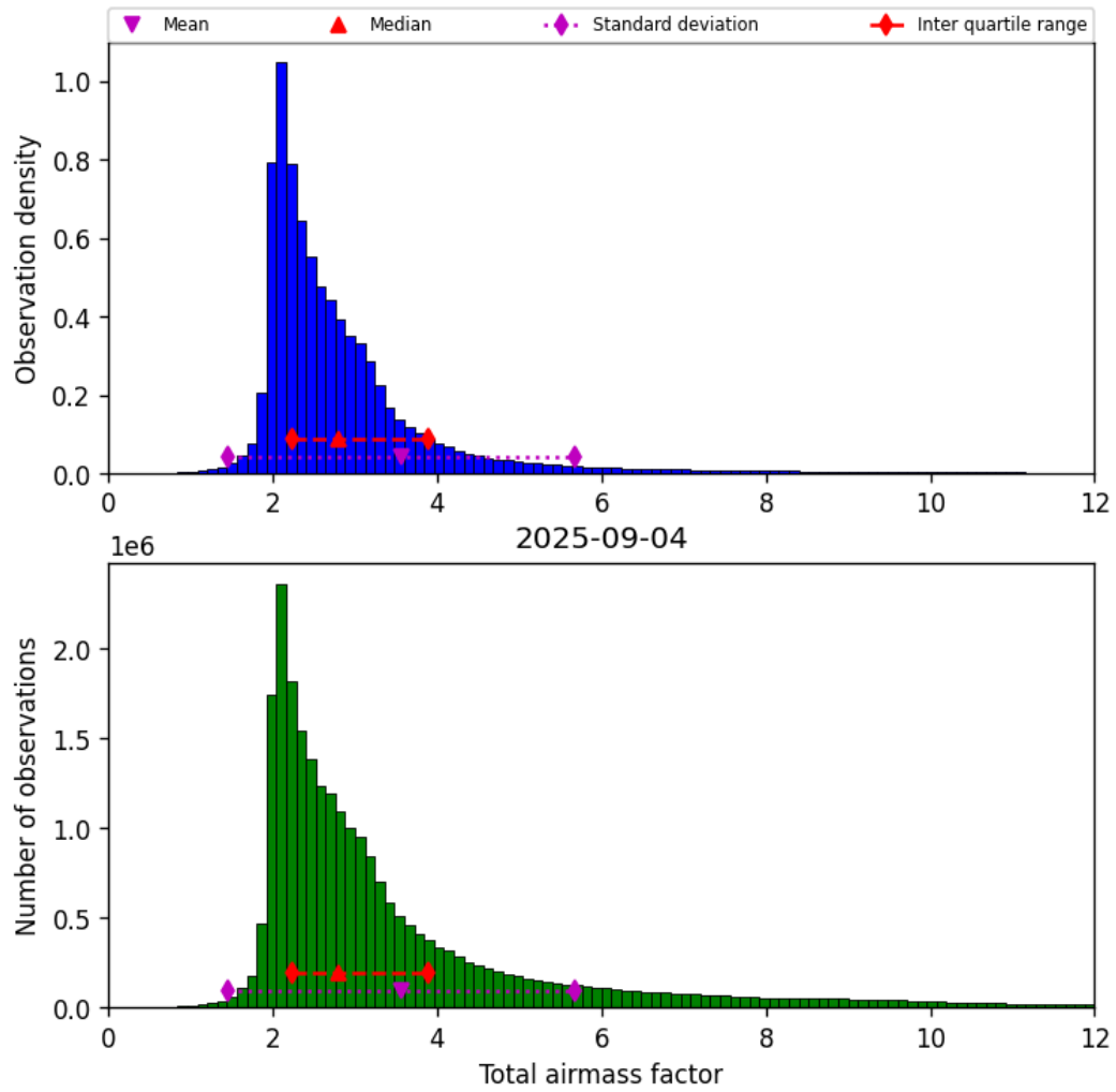
Figure 32: Histogram of “Total airmass factor” for 2025-09-04 to 2025-09-05
