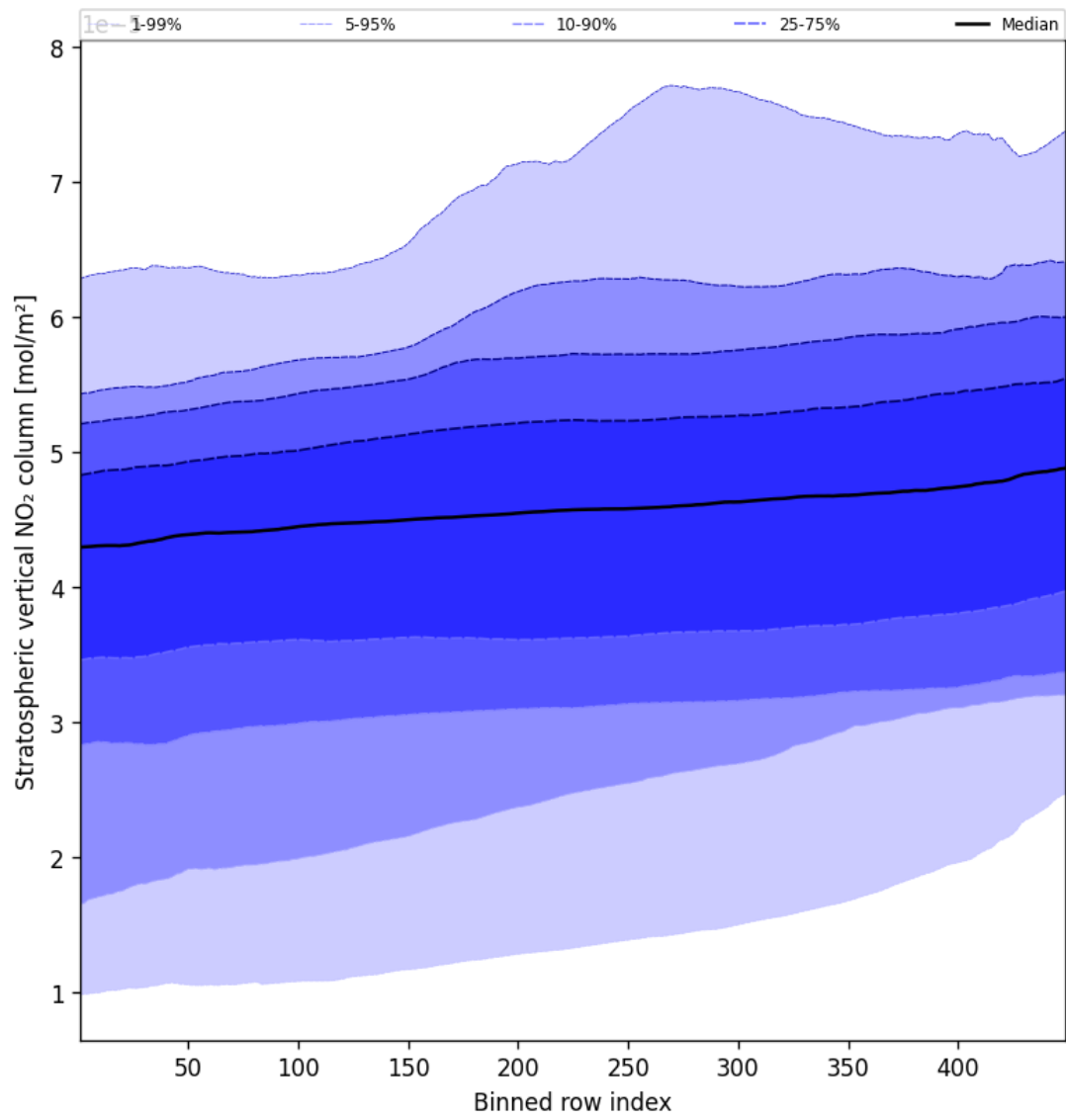
Figure 53: Along track statistics of “Stratospheric vertical NO 2 column” for 2025-09-04 to 2025-09-05
