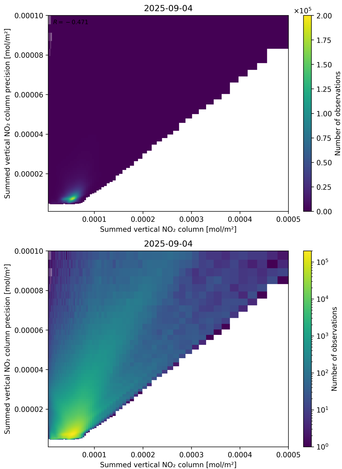
Figure 105: Scatter density plot of “Summed vertical NO 2 column” against “Summed vertical NO 2 column precision” for 2025-09-04 to 2025-09-05.
