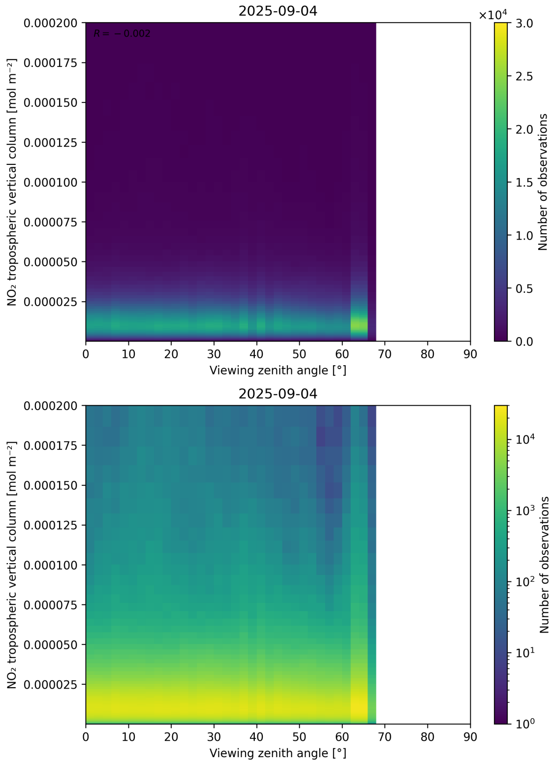
Figure 169: Scatter density plot of “Viewing zenith angle” against “NO 2 tropospheric vertical column” for 2025-09-04 to 2025-09-05.
