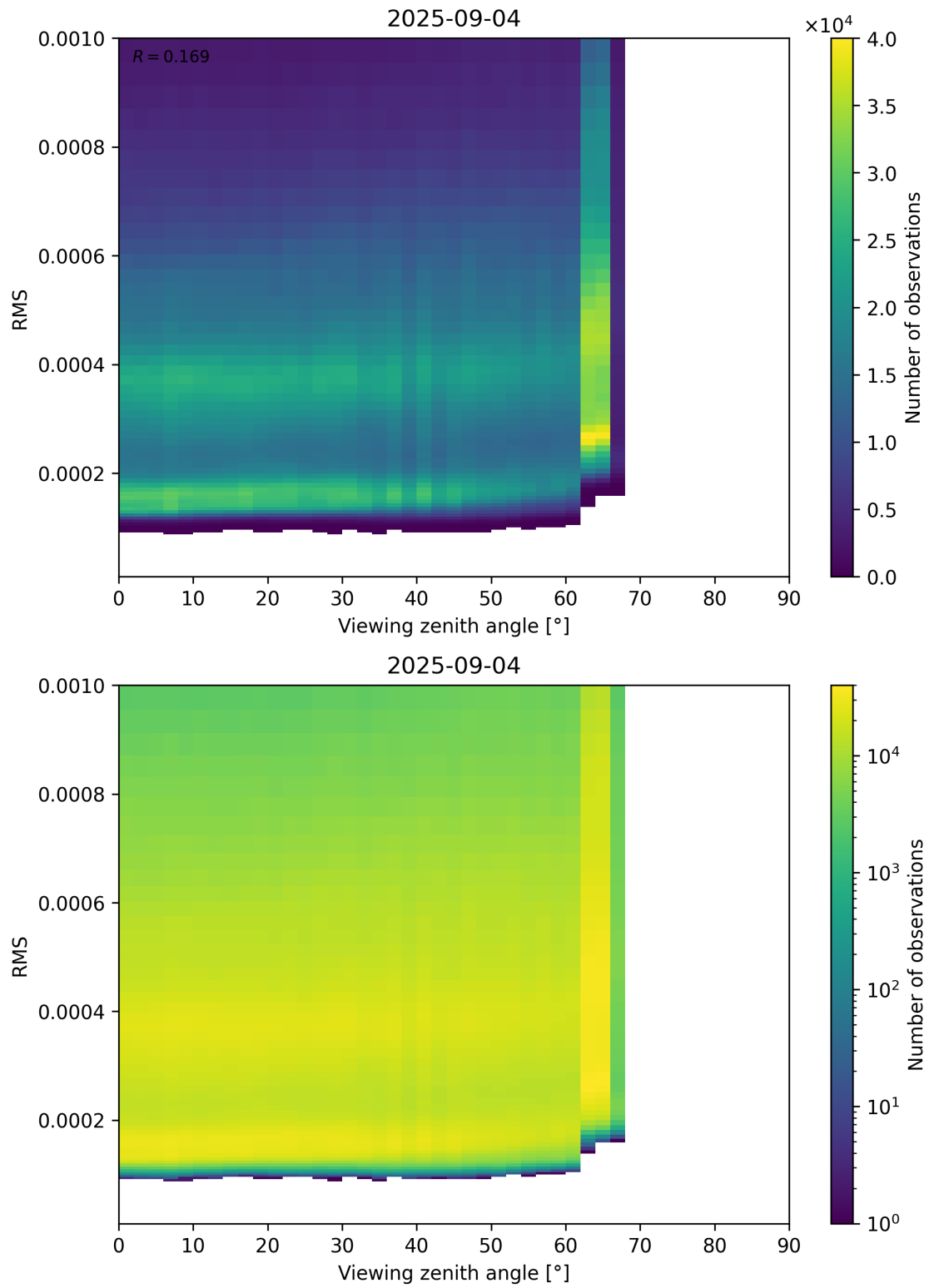
Figure 171: Scatter density plot of “Viewing zenith angle” against “RMS” for 2025-09-04 to 2025-09-05.
