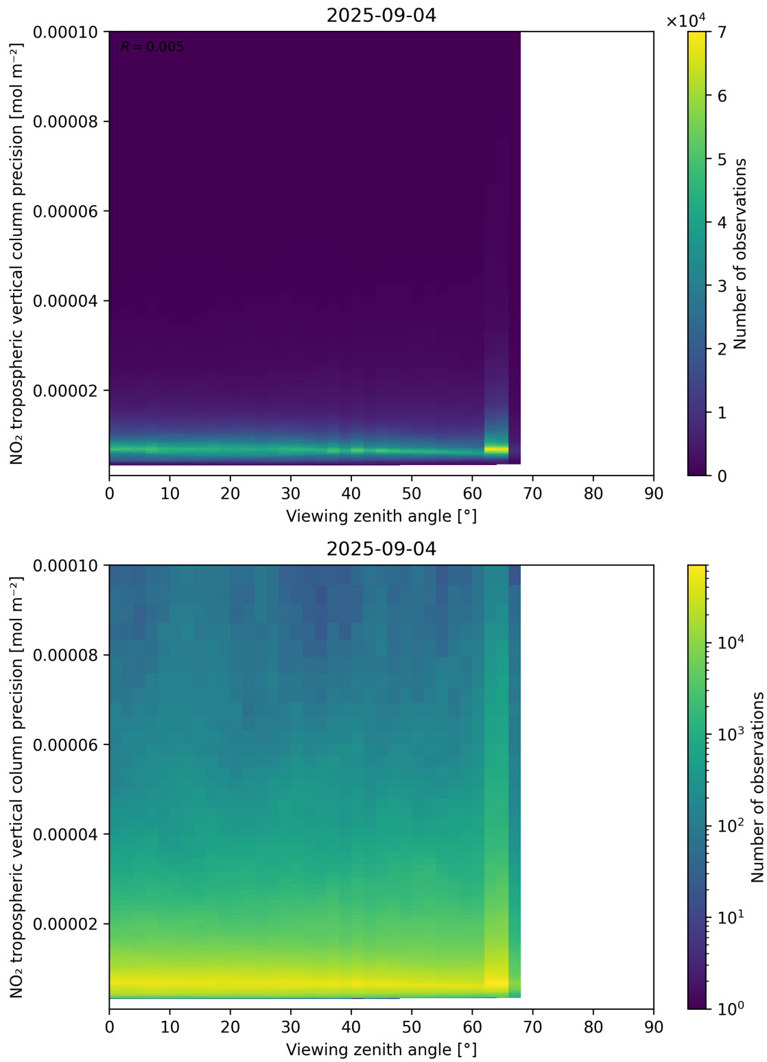
Figure 170: Scatter density plot of “Viewing zenith angle” against “NO 2 tropospheric vertical column precision” for 2025-09-04 to 2025-09-05.
