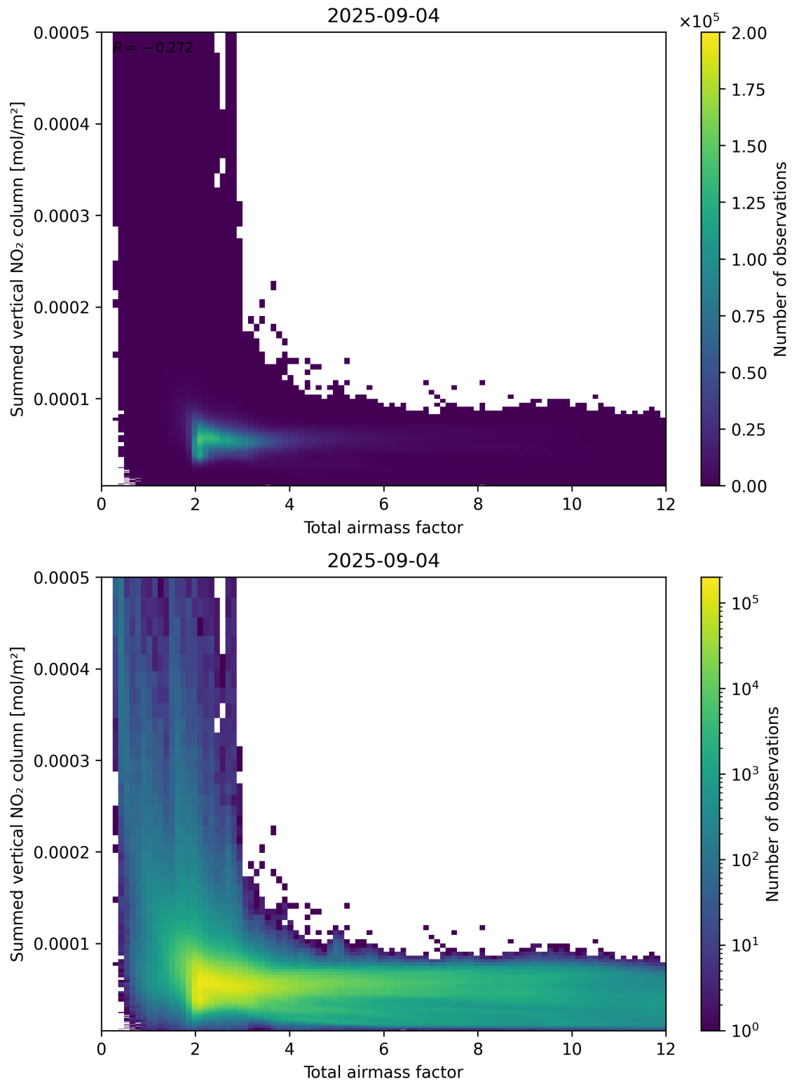
Figure 65: Scatter density plot of “Total airmass factor” against “Summed vertical NO 2 column” for 2025-09-04 to 2025-09-05.
