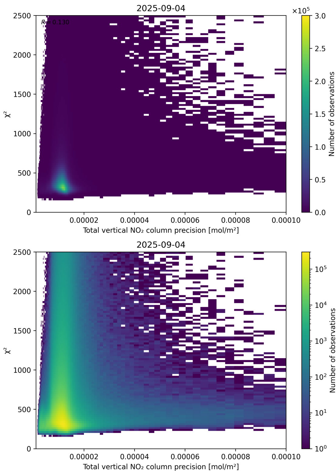
Figure 116: Scatter density plot of “Total vertical NO 2 column precision” against “ \chi^2 ” for 2025-09-04 to 2025-09-05.
