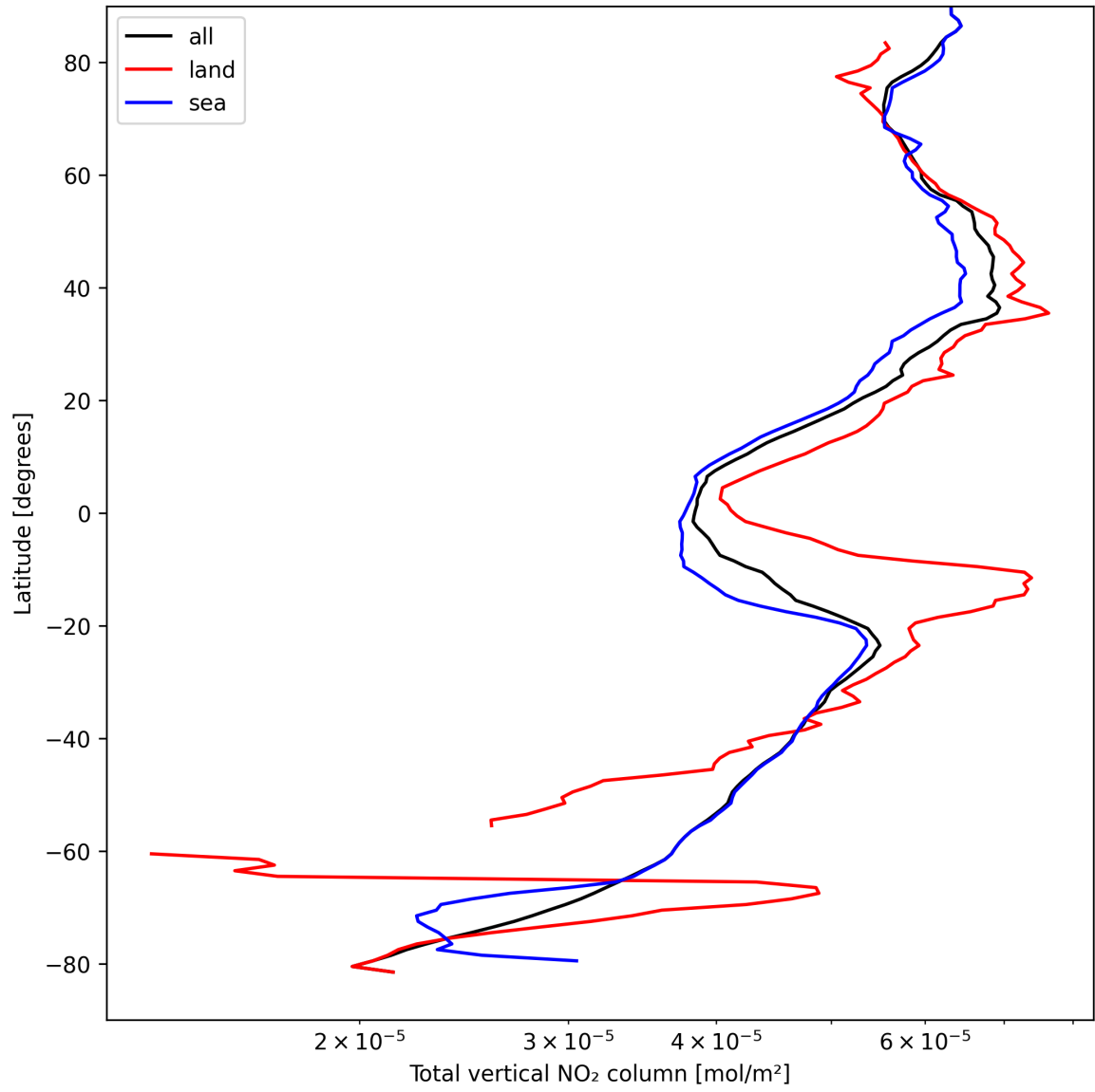
Figure 21: Zonal average of “Total vertical NO 2 column” for 2025-09-04 to 2025-09-05.
