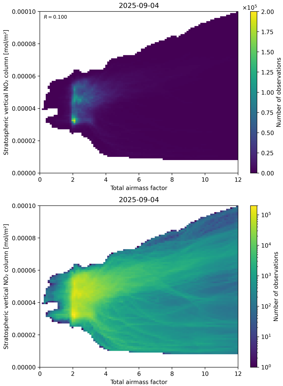
Figure 64: Scatter density plot of “Total airmass factor” against “Stratospheric vertical \text{NO}_2 column” for 2025-09-04 to 2025-09-05.
