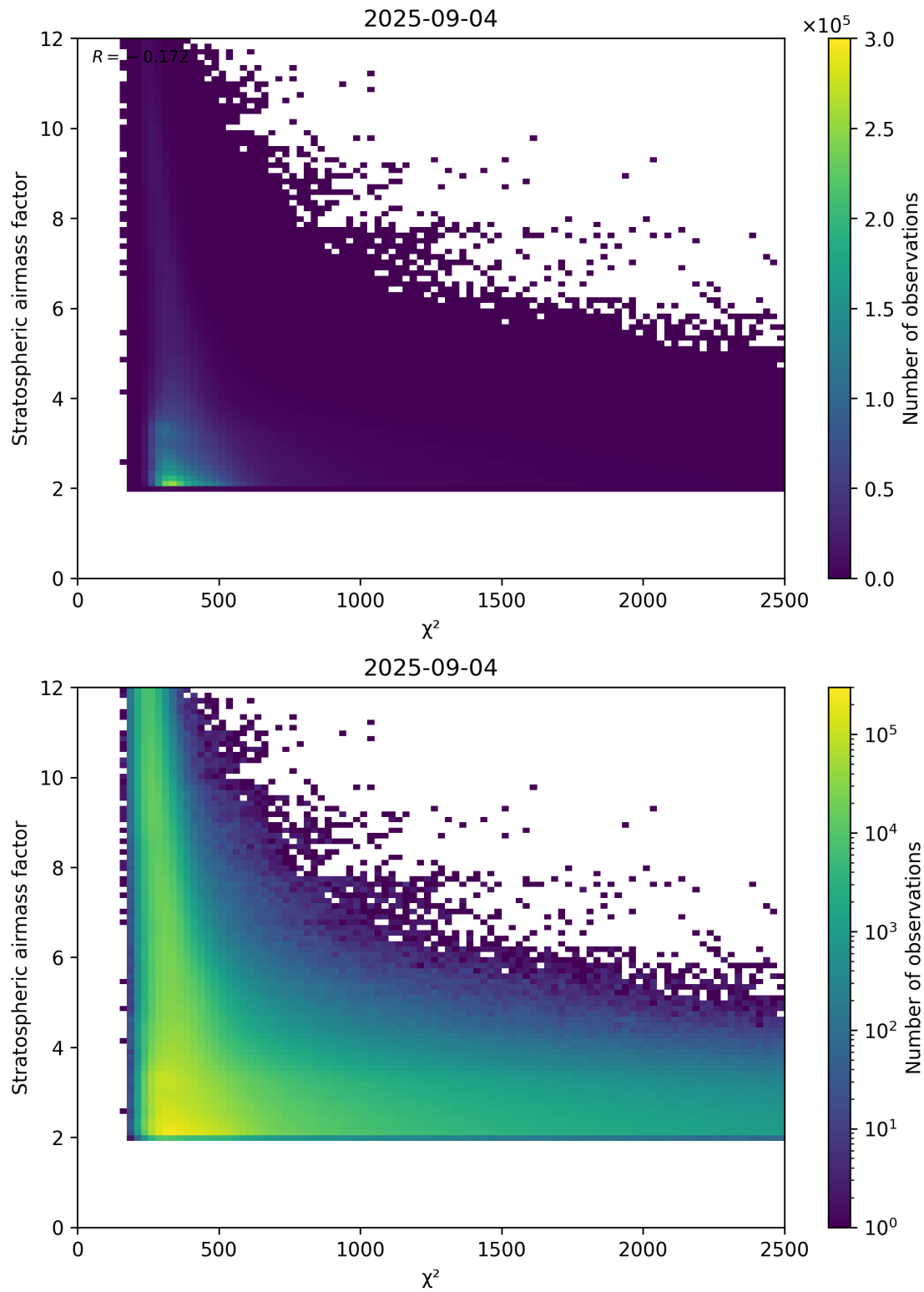
Figure 81: Scatter density plot of “ \chi^2 ” against “Stratospheric airmass factor” for 2025-09-04 to 2025-09-05.
