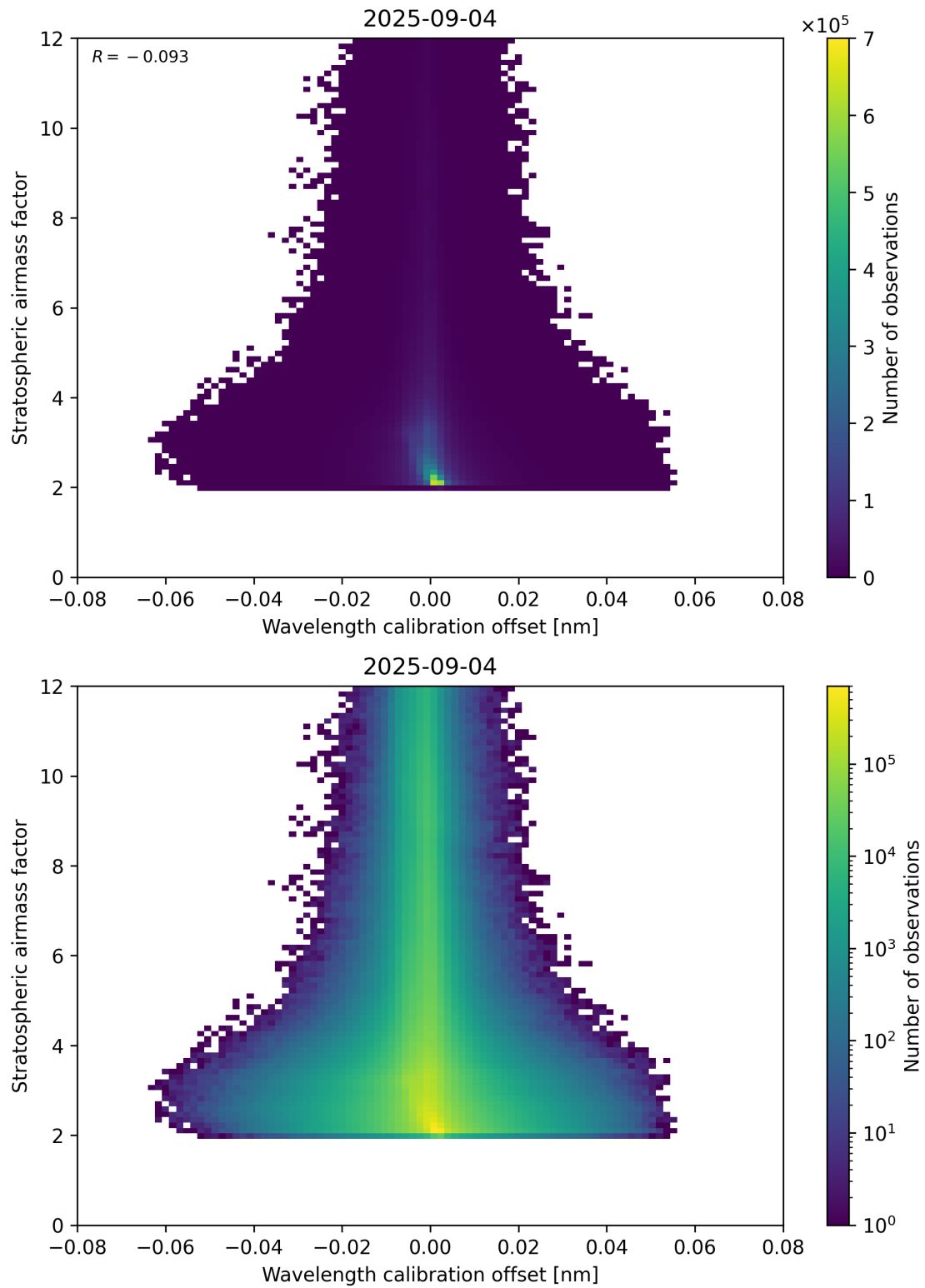
Figure 174: Scatter density plot of “Wavelength calibration offset” against “Stratospheric air mass factor” for 2025-09-04 to 2025-09-05.
