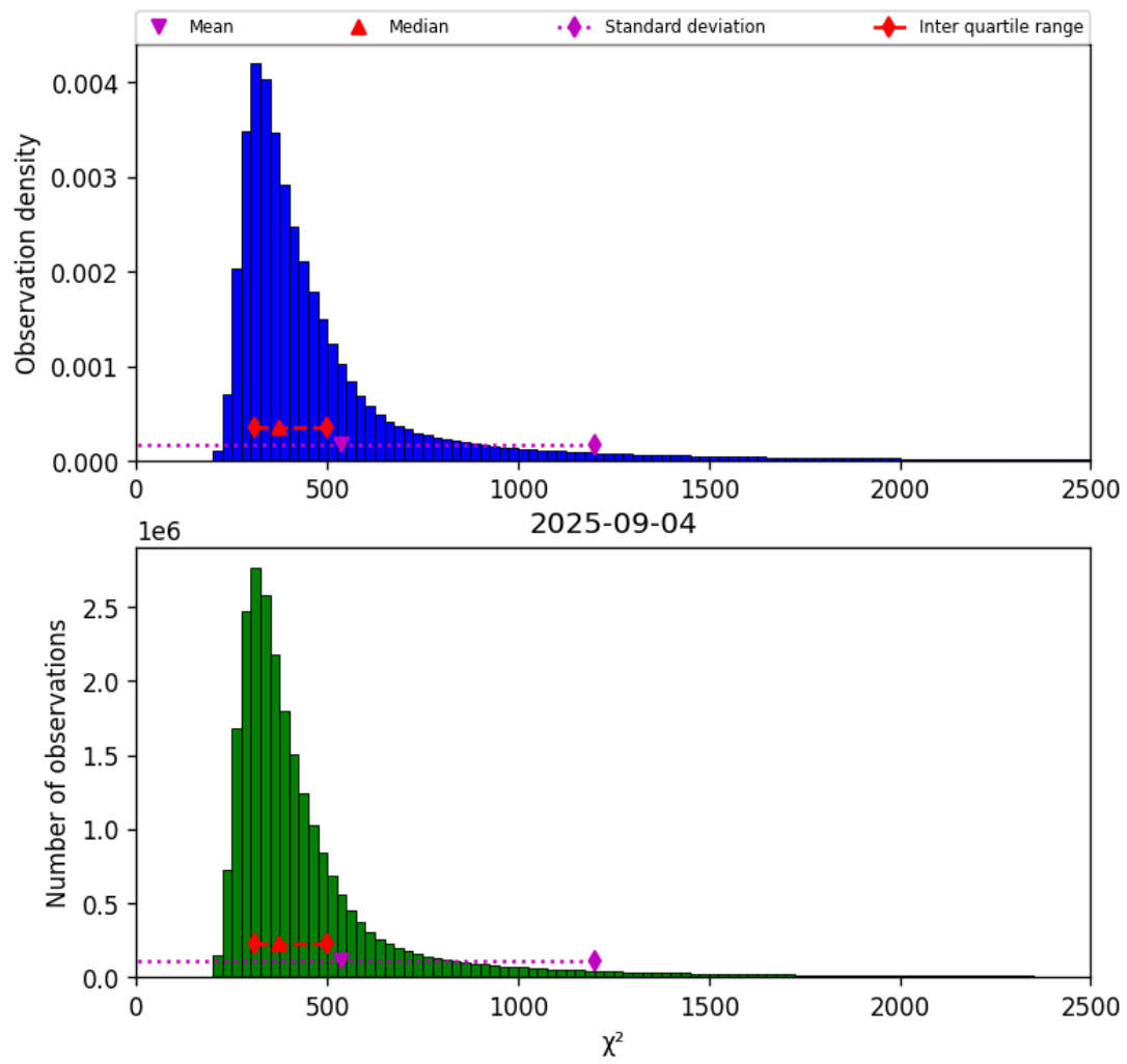
Figure 42: Histogram of “ \chi^2 ” for 2025-09-04 to 2025-09-05
