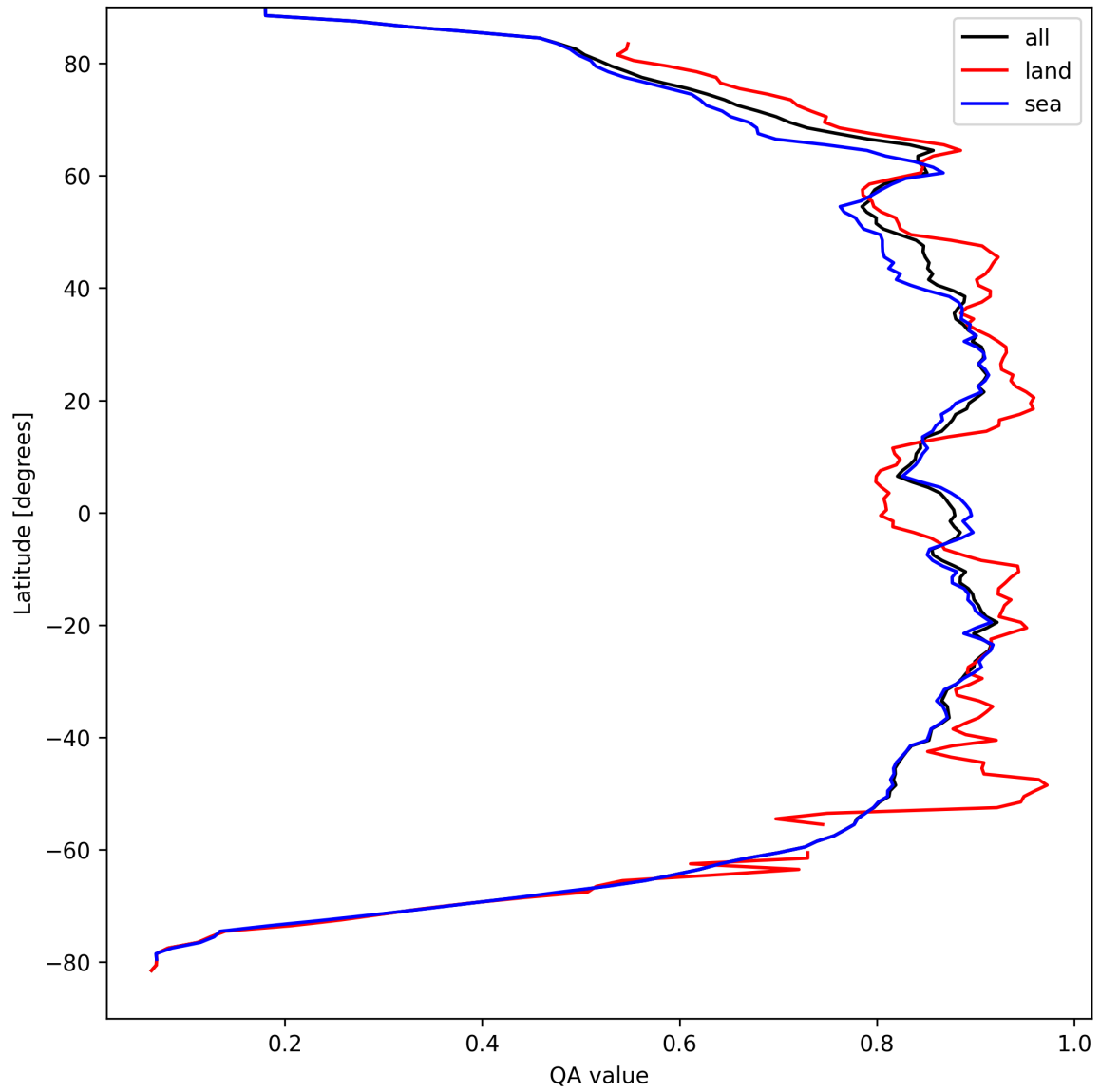
Figure 11: Zonal average of “QA value” for 2025-09-04 to 2025-09-05.
