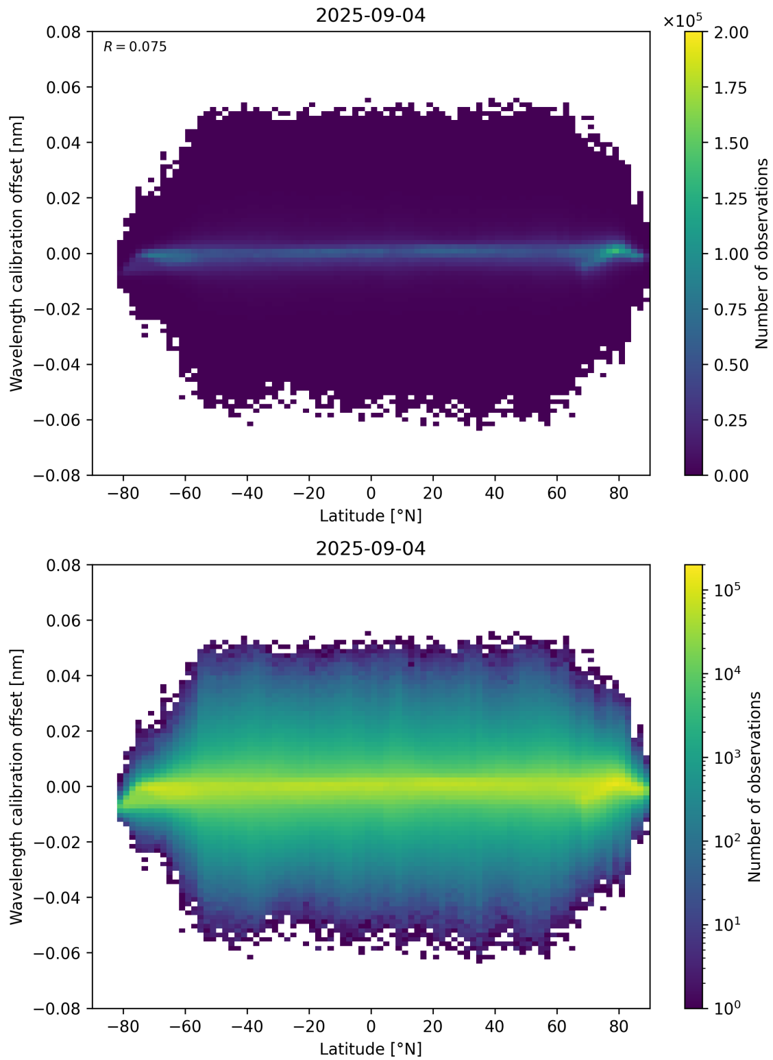
Figure 95: Scatter density plot of “Latitude” against “Wavelength calibration offset” for 2025-09-04 to 2025-09-05.
