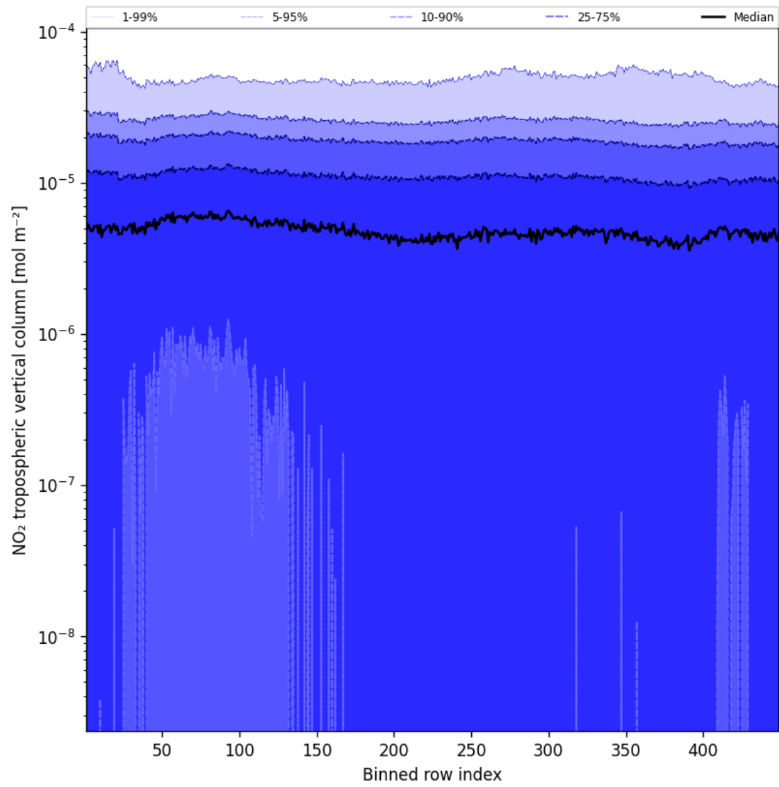
Figure 46: Along track statistics of “ \text{NO}_2 tropospheric vertical column” for 2025-09-04 to 2025-09-05
