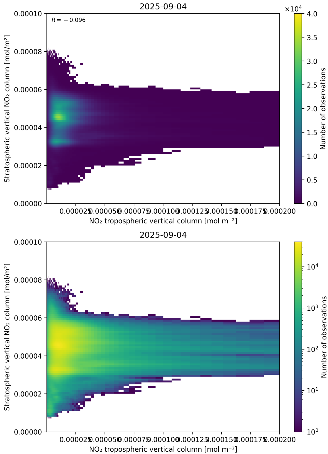
Figure 125: Scatter density plot of “NO 2 tropospheric vertical column” against “Stratospheric vertical NO 2 column” for 2025-09-04 to 2025-09-05.
