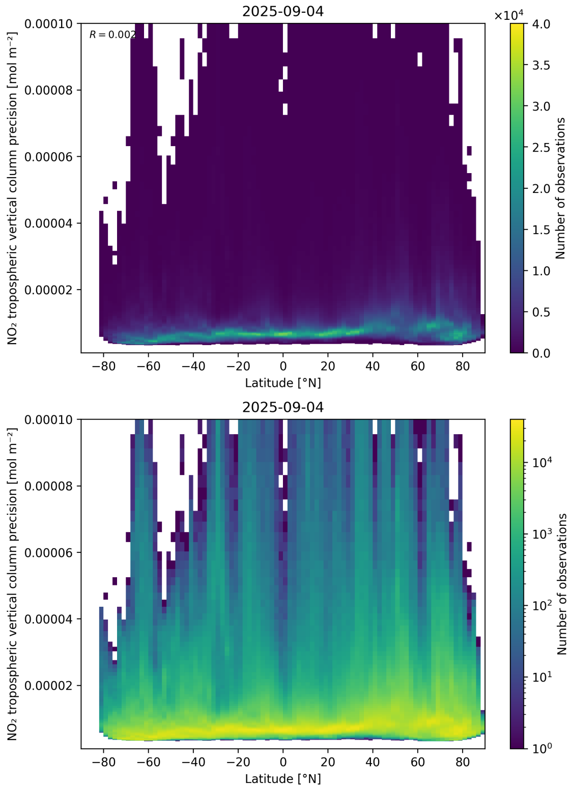
Figure 93: Scatter density plot of “Latitude” against “NO 2 tropospheric vertical column precision” for 2025-09-04 to 2025-09-05.
