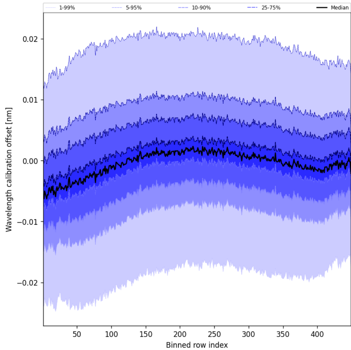
Figure 52: Along track statistics of “Wavelength calibration offset” for 2025-09-04 to 2025-09-05
