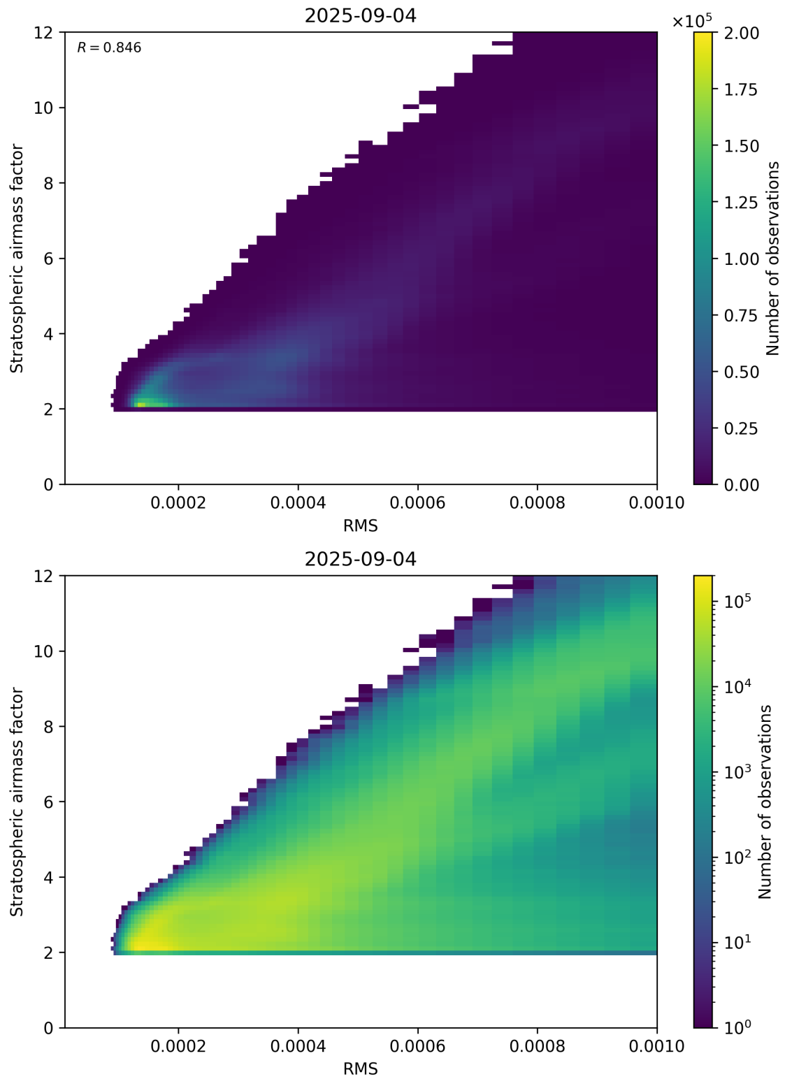
Figure 144: Scatter density plot of “RMS” against “Stratospheric airmass factor” for 2025-09-04 to 2025-09-05.
