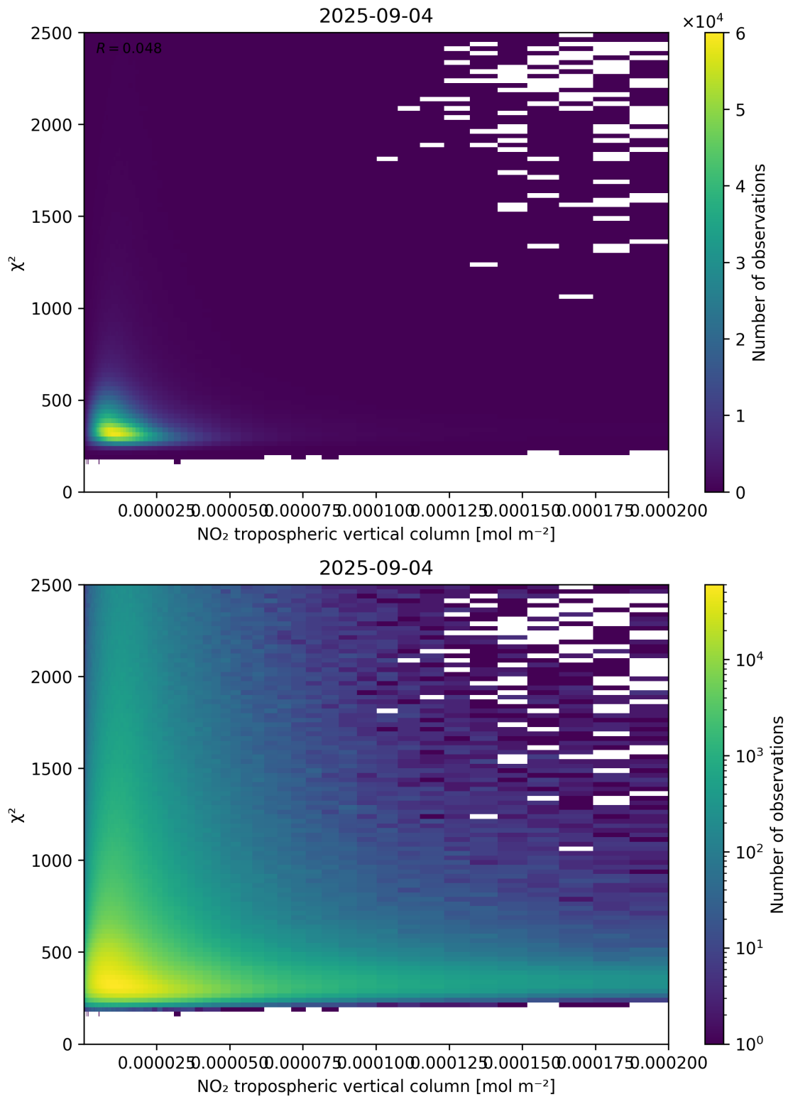
Figure 124: Scatter density plot of “NO 2 tropospheric vertical column” against “ \chi^2 ” for 2025-09-04 to 2025-09-05.
