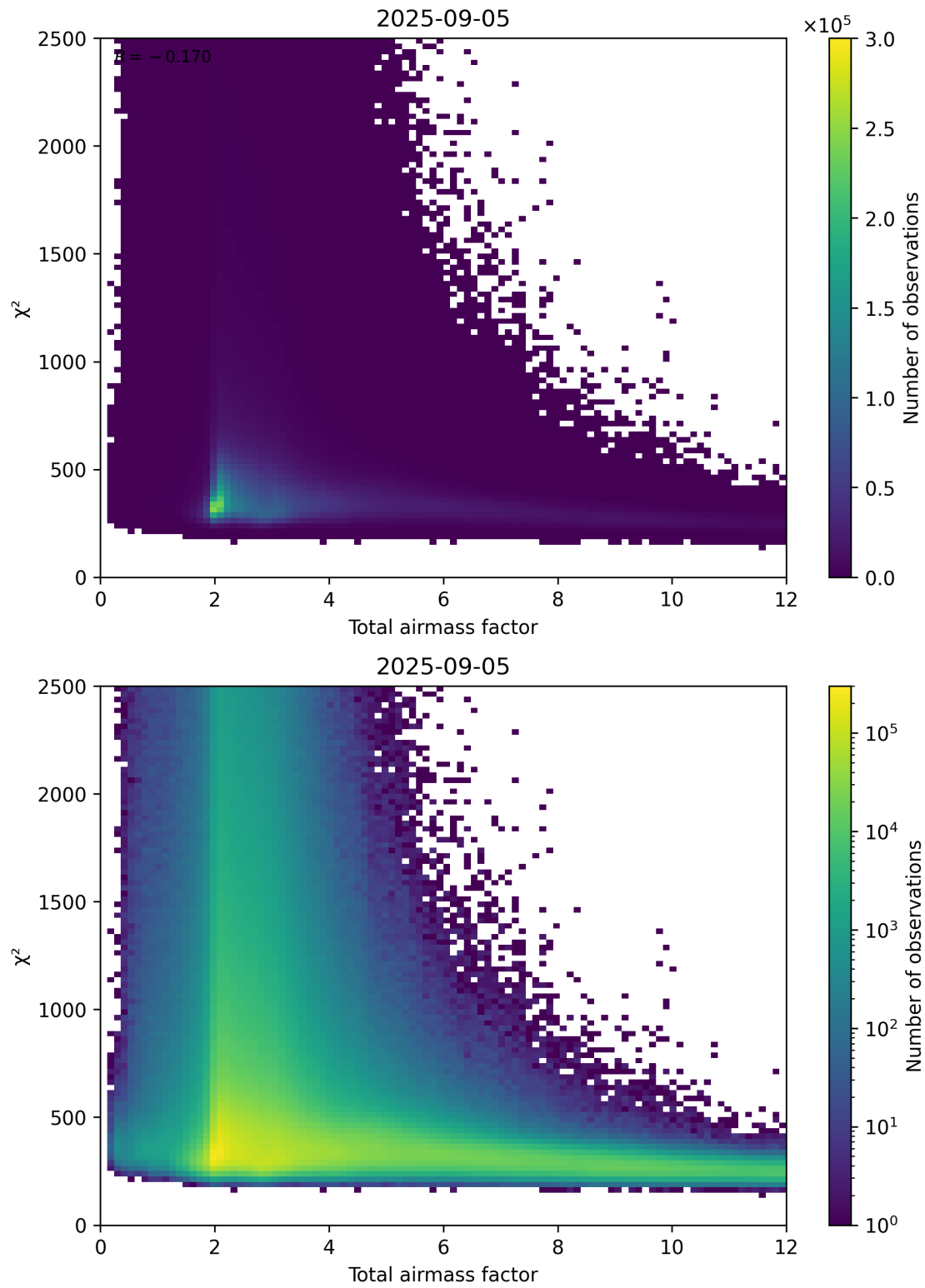
Figure 63: Scatter density plot of “Total airmass factor” against “ \chi^2 ” for 2025-09-04 to 2025-09-06.
