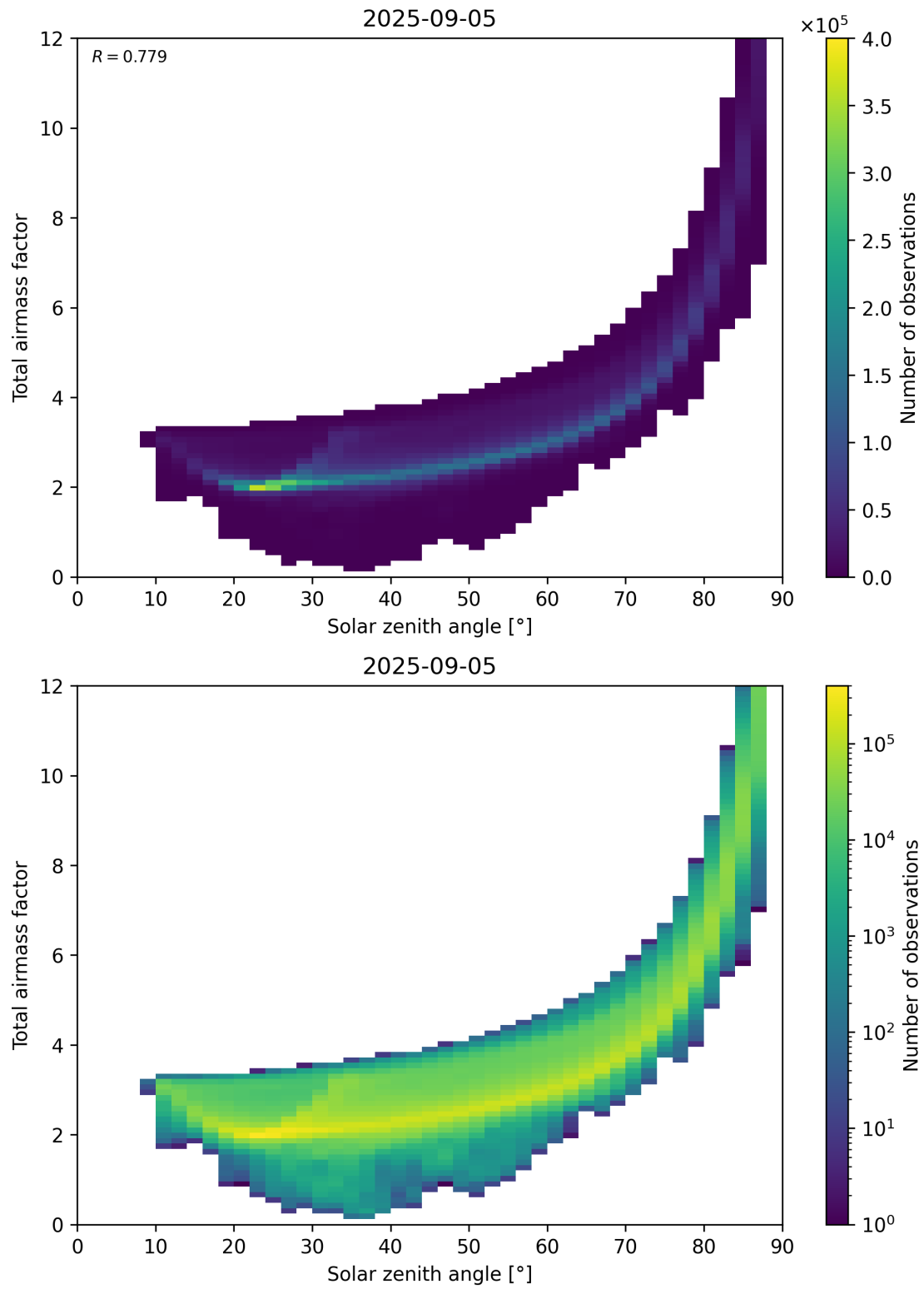
Figure 146: Scatter density plot of “Solar zenith angle” against “Total air mass factor” for 2025-09-04 to 2025-09-06.
