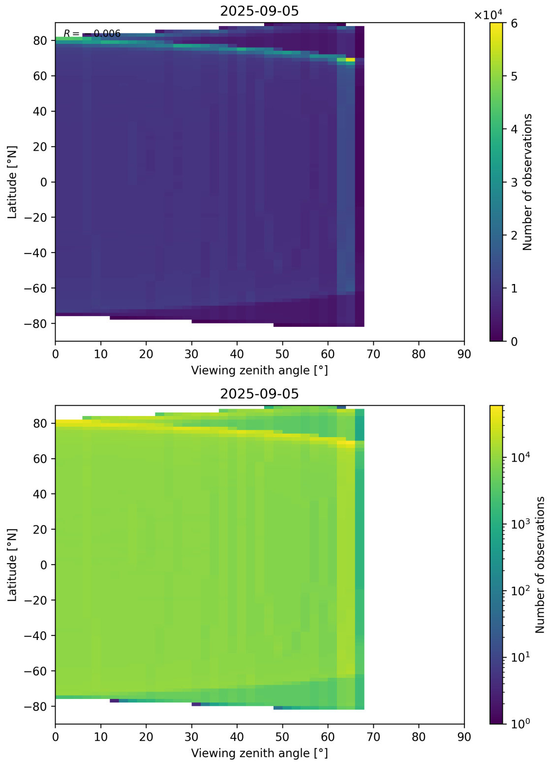
Figure 163: Scatter density plot of “Viewing zenith angle” against “Latitude” for 2025-09-04 to 2025-09-06.
