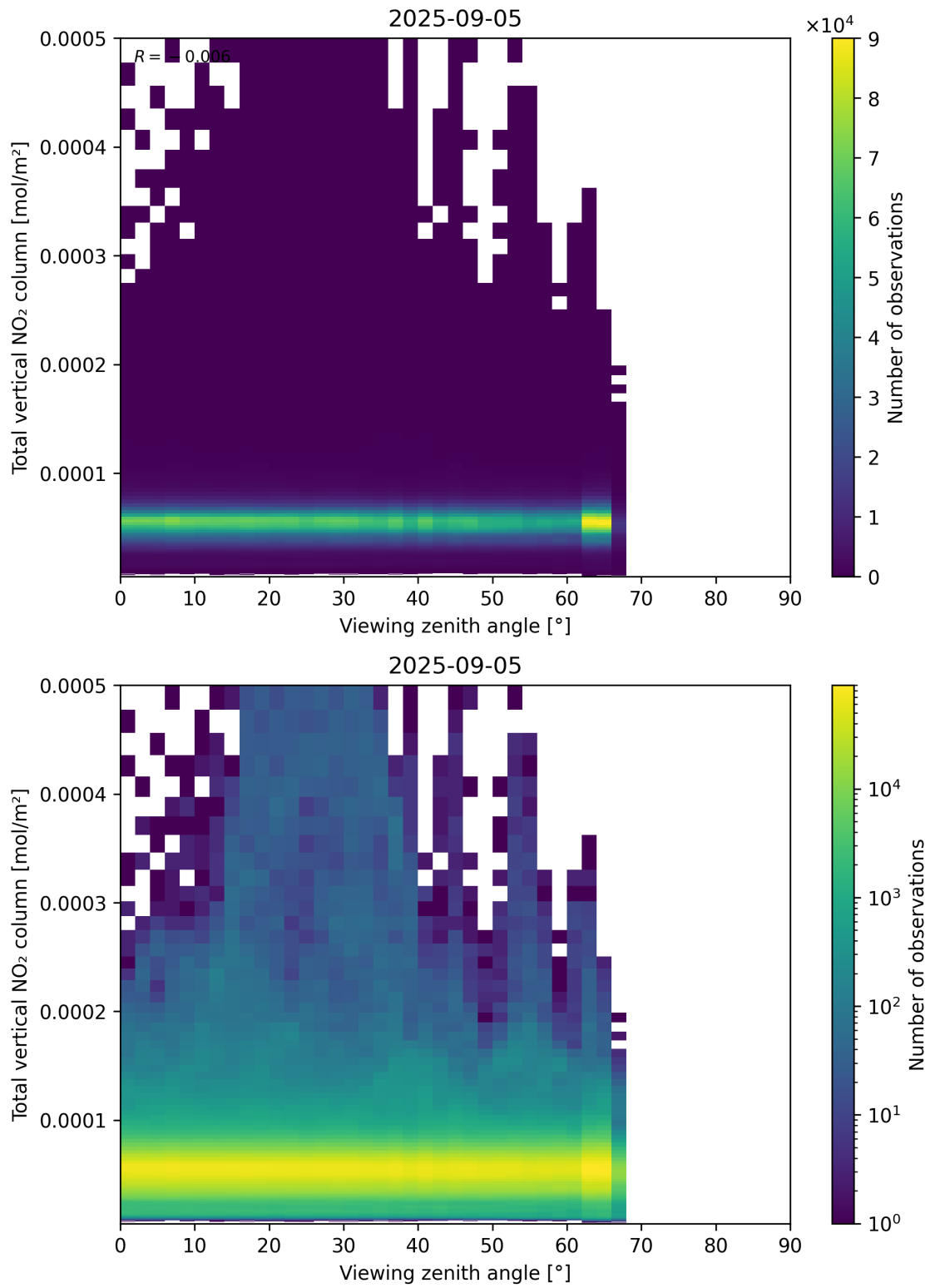
Figure 167: Scatter density plot of “Viewing zenith angle” against “Total vertical NO 2 column” for 2025-09-04 to 2025-09-06.
