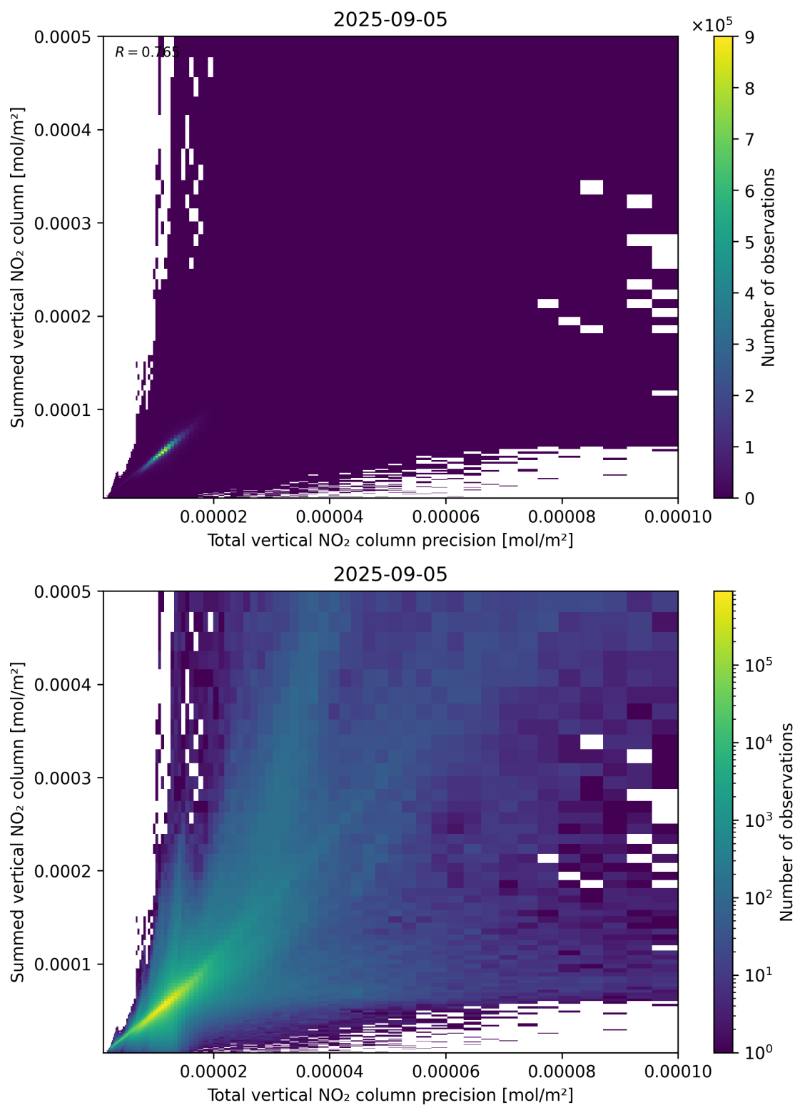
Figure 117: Scatter density plot of “Total vertical NO 2 column precision” against “Summed vertical NO 2 column” for 2025-09-04 to 2025-09-06.
