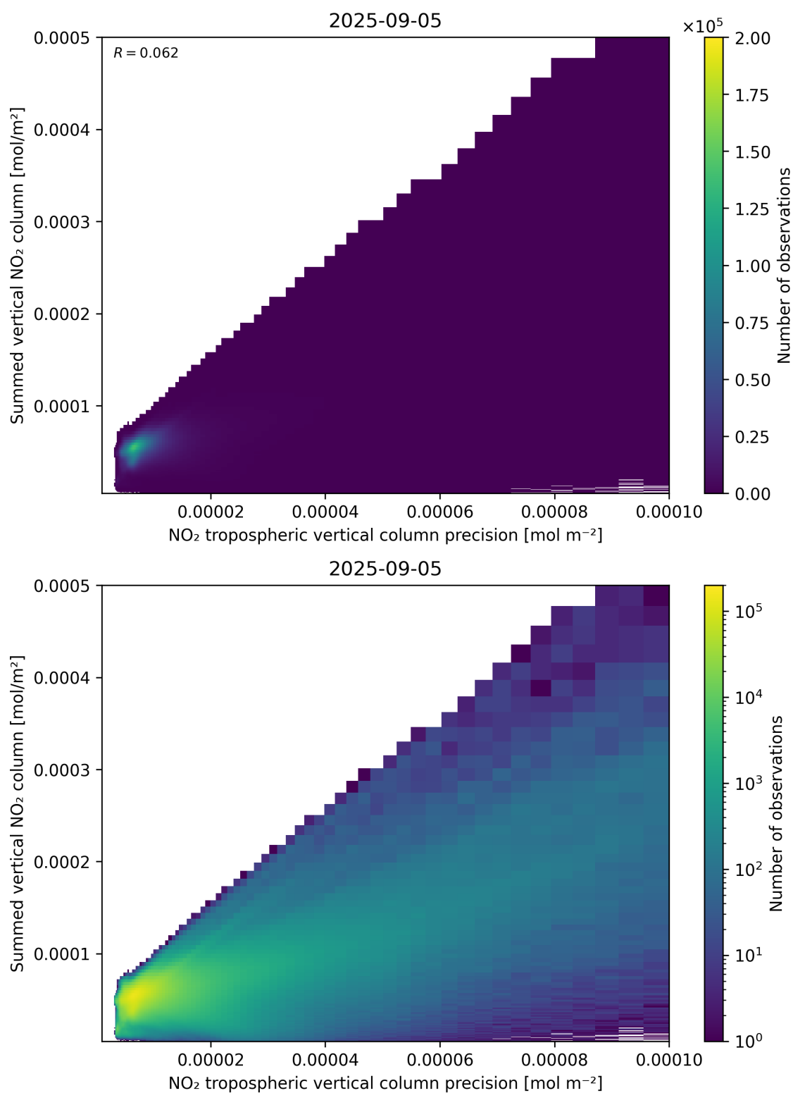
Figure 136: Scatter density plot of “NO 2 tropospheric vertical column precision” against “Summed vertical NO 2 column” for 2025-09-04 to 2025-09-06.
