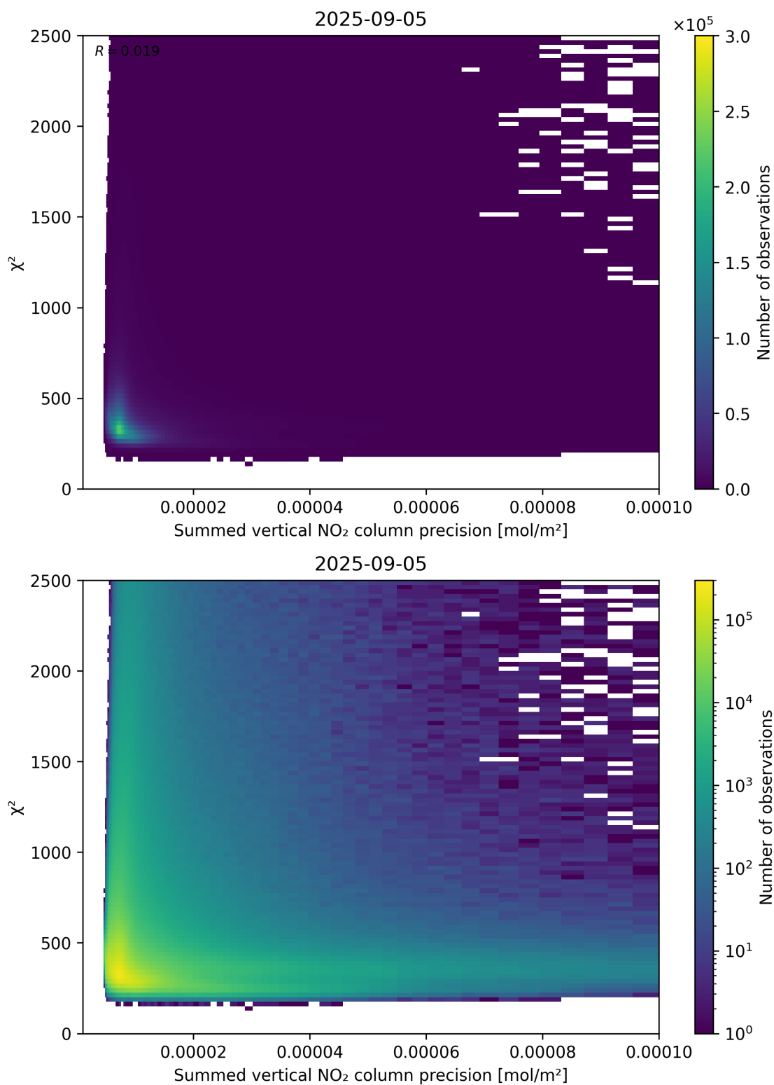
Figure 107: Scatter density plot of “Summed vertical NO 2 column precision” against “ \chi^2 ” for 2025-09-04 to 2025-09-06.
