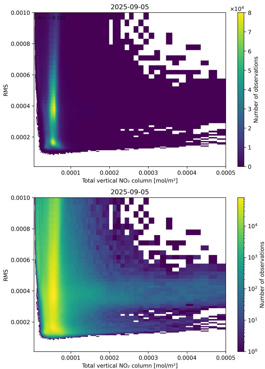
Figure 120: Scatter density plot of “Total vertical NO 2 column” against “RMS” for 2025-09-04 to 2025-09-06.
