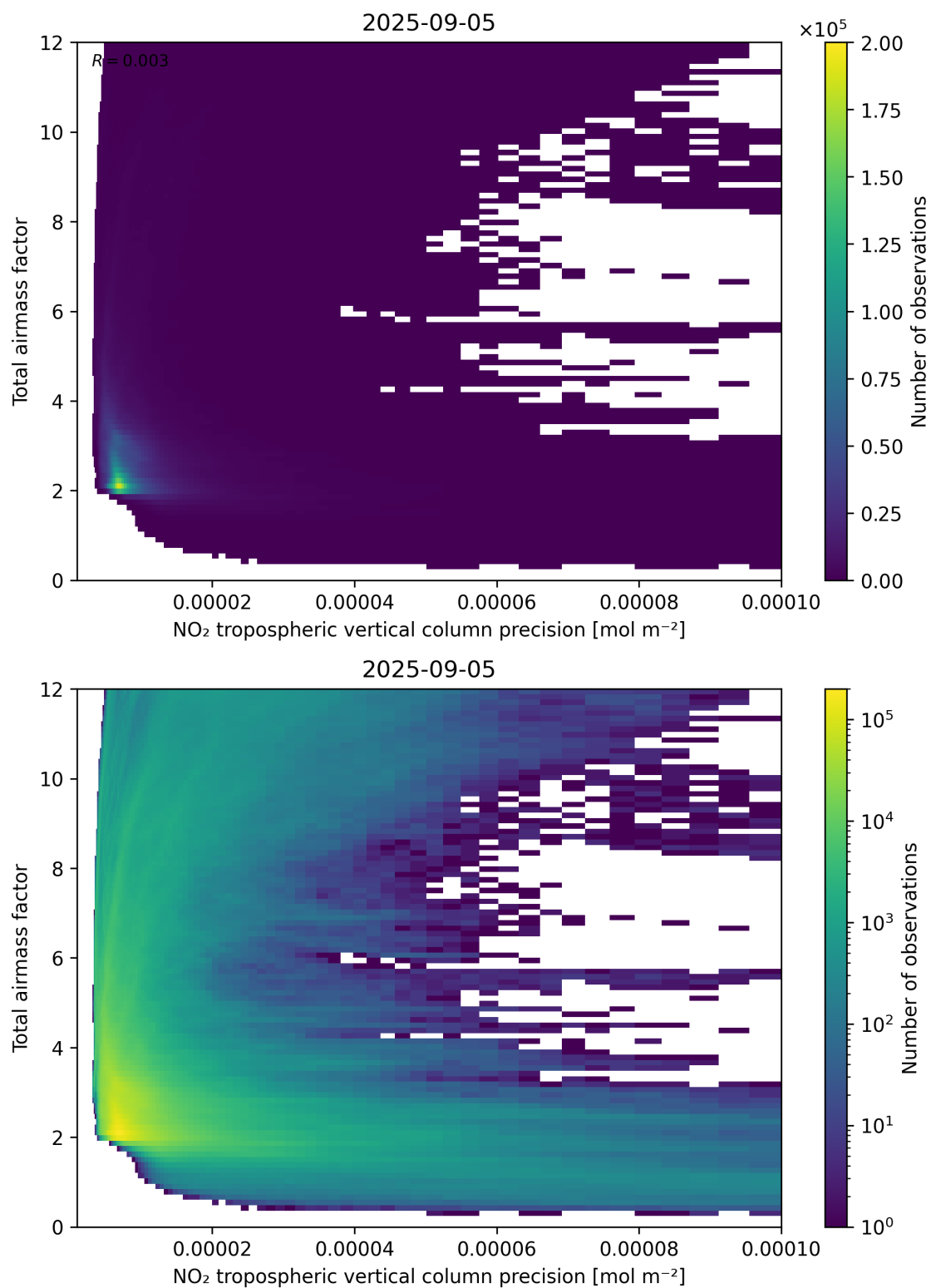
Figure 132: Scatter density plot of “NO 2 tropospheric vertical column precision” against “Total air mass factor” for 2025-09-04 to 2025-09-06.
