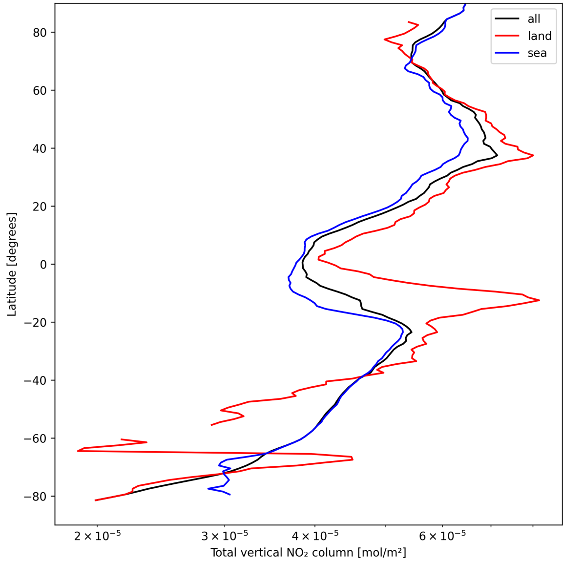
Figure 21: Zonal average of “Total vertical NO 2 column” for 2025-09-04 to 2025-09-06.
