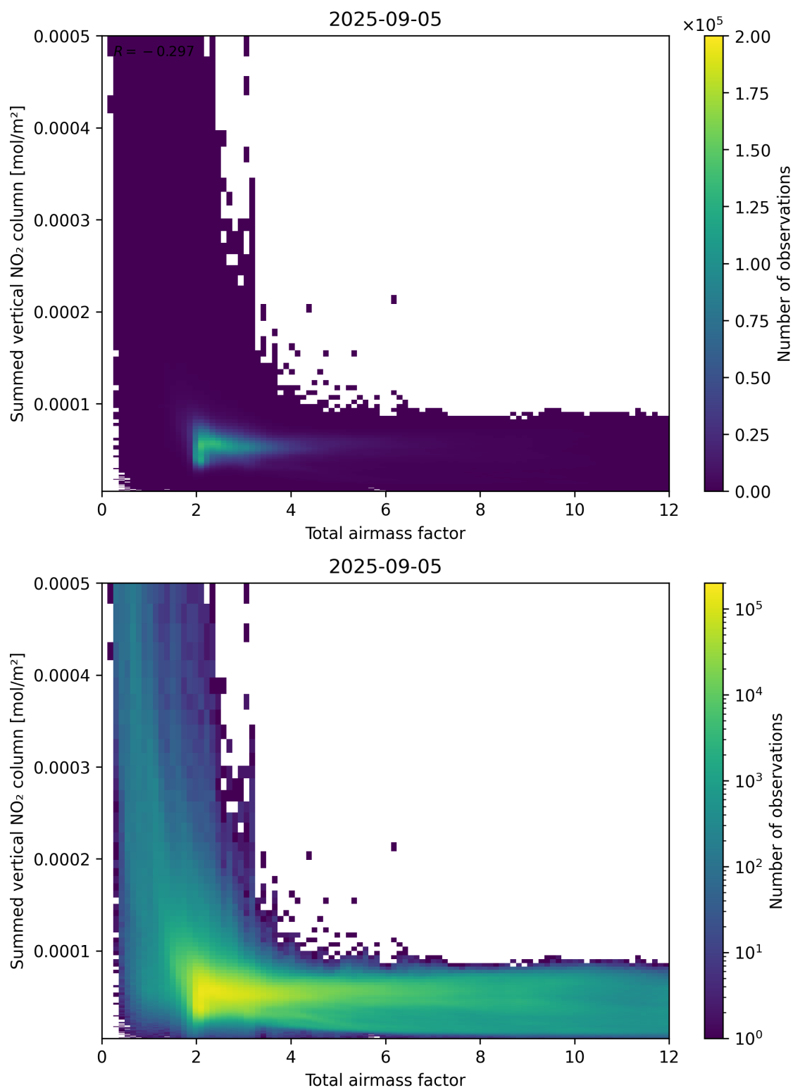
Figure 65: Scatter density plot of “Total airmass factor” against “Summed vertical NO 2 column” for 2025-09-04 to 2025-09-06.
