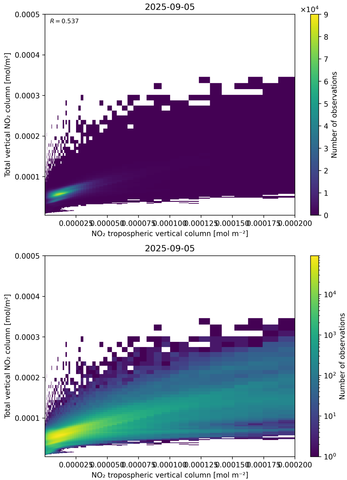
Figure 128: Scatter density plot of “NO 2 tropospheric vertical column” against “Total vertical NO 2 column” for 2025-09-04 to 2025-09-06.
