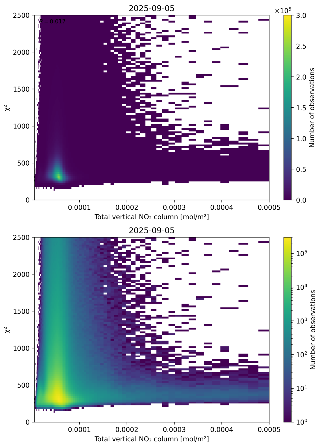
Figure 111: Scatter density plot of “Total vertical NO 2 column” against “ \chi^2 ” for 2025-09-04 to 2025-09-06.
