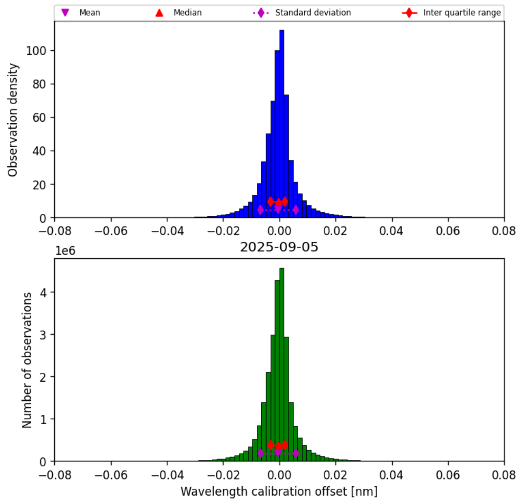
Figure 35: Histogram of “Wavelength calibration offset” for 2025-09-04 to 2025-09-06
