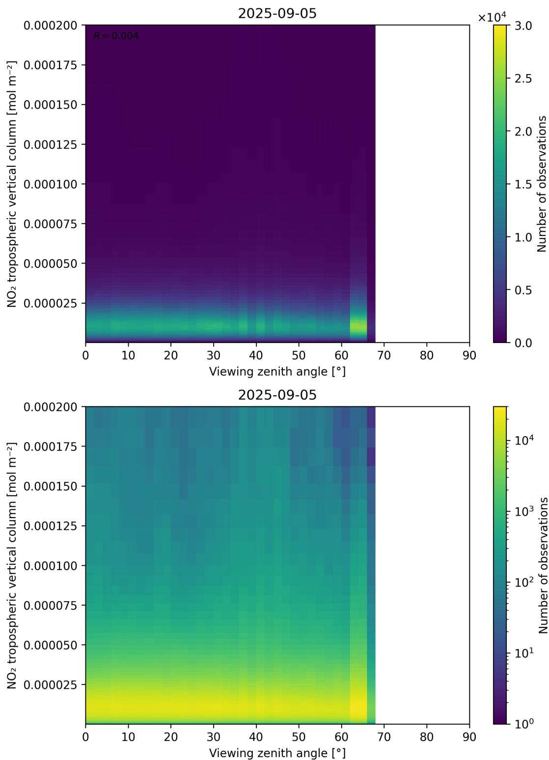
Figure 169: Scatter density plot of “Viewing zenith angle” against “NO 2 tropospheric vertical column” for 2025-09-04 to 2025-09-06.
