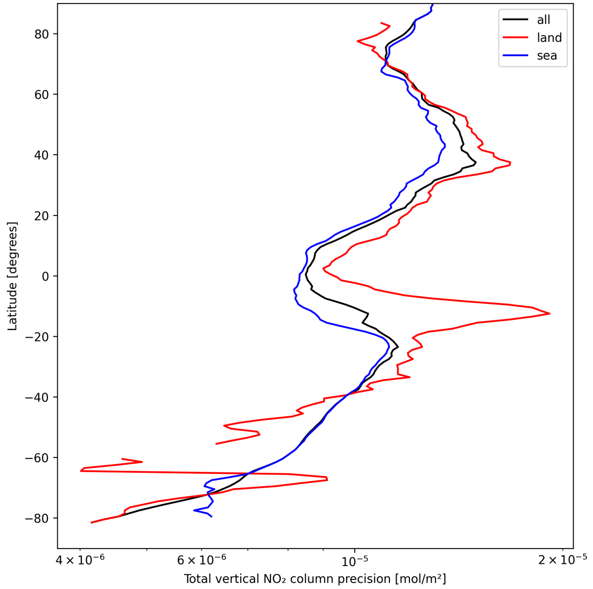
Figure 22: Zonal average of “Total vertical NO 2 column precision” for 2025-09-04 to 2025-09-06.
