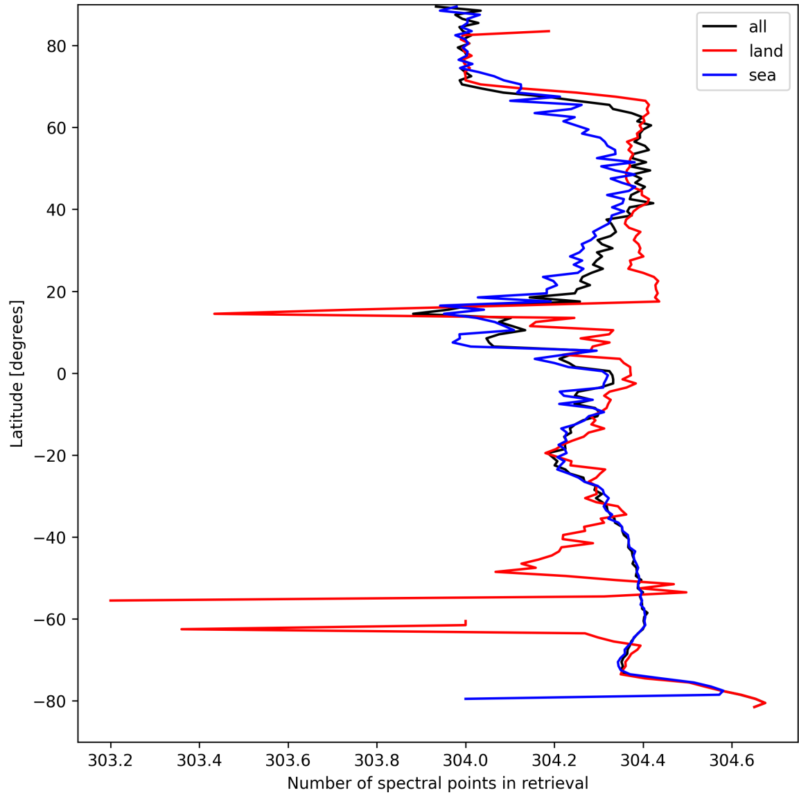
Figure 16: Zonal average of “Number of spectral points in retrieval” for 2025-09-04 to 2025-09-06.
