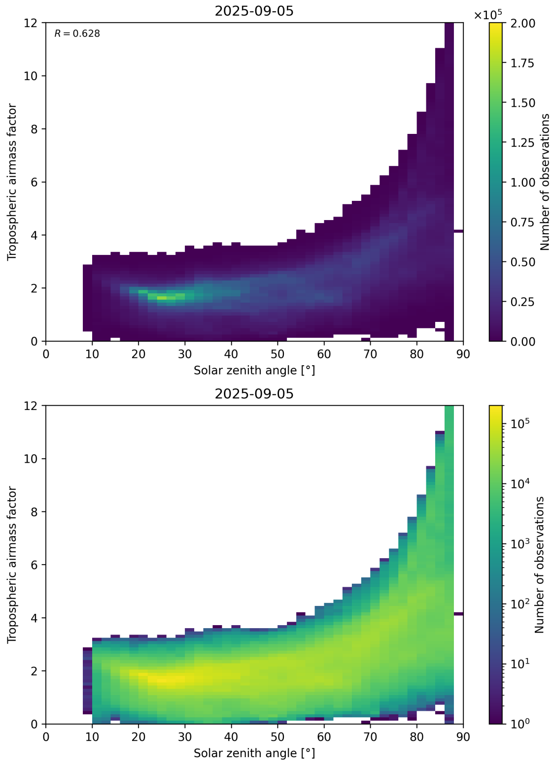
Figure 147: Scatter density plot of “Solar zenith angle” against “Tropospheric airmass factor” for 2025-09-04 to 2025-09-06.
