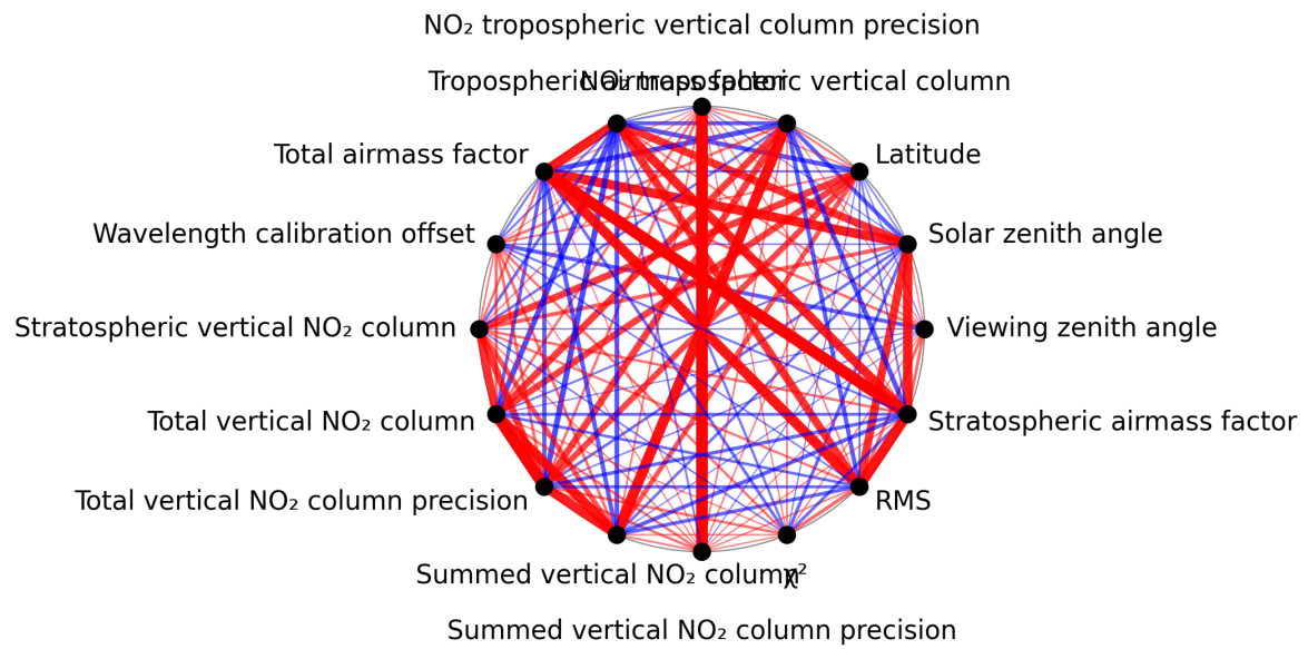
Figure 1: Map of correlation graph for 2025-09-04 to 2025-09-06.
