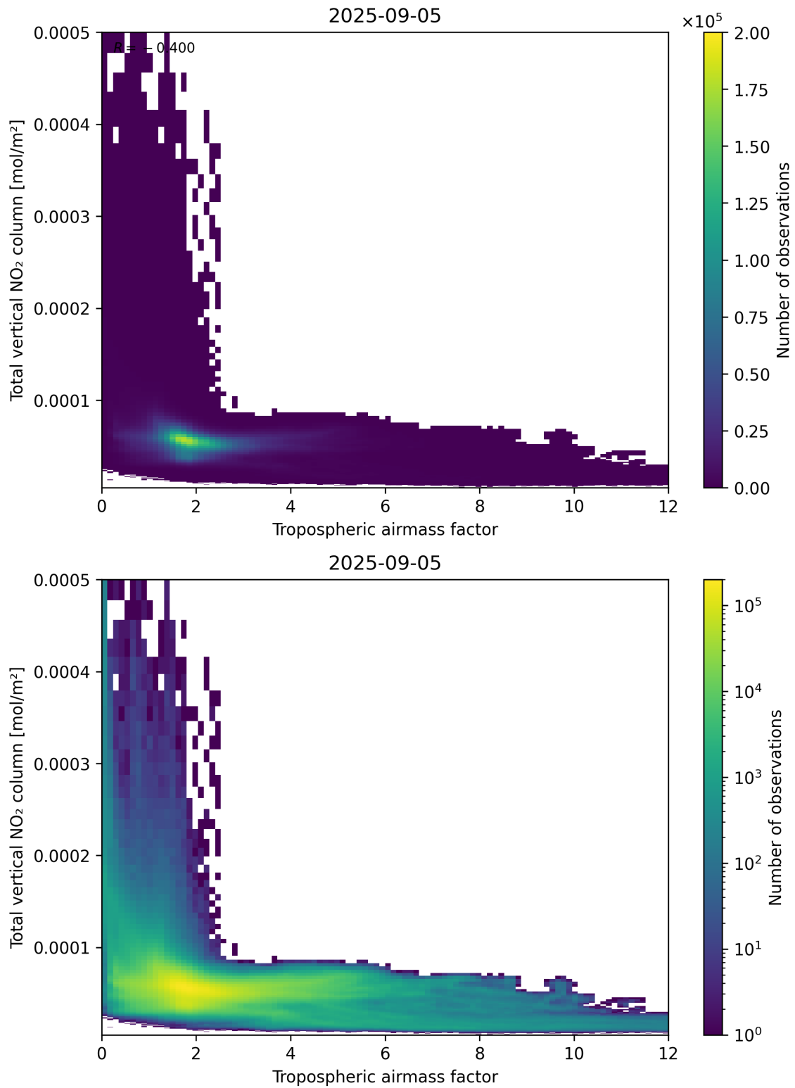
Figure 77: Scatter density plot of “Tropospheric airmass factor” against “Total vertical NO 2 column” for 2025-09-04 to 2025-09-06.
