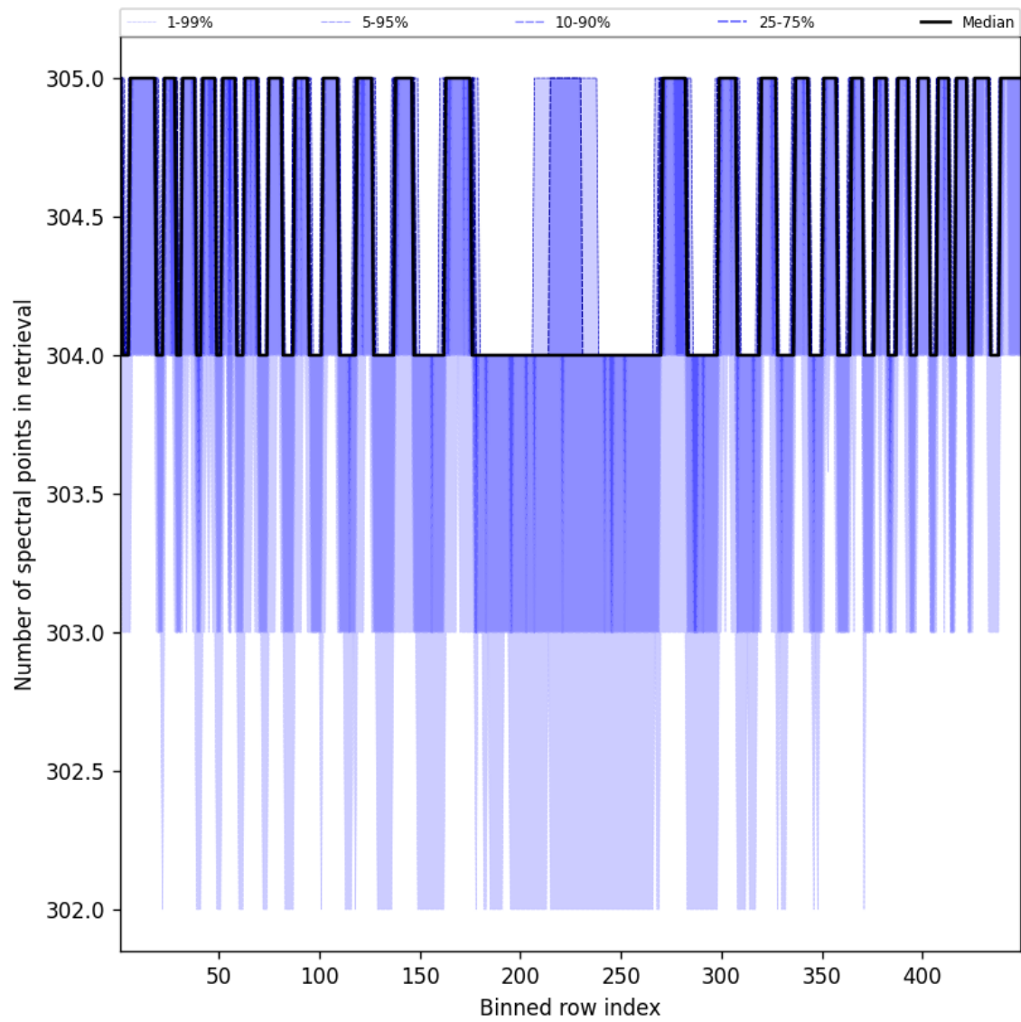
Figure 50: Along track statistics of “Number of spectral points in retrieval” for 2025-09-04 to 2025-09-06
