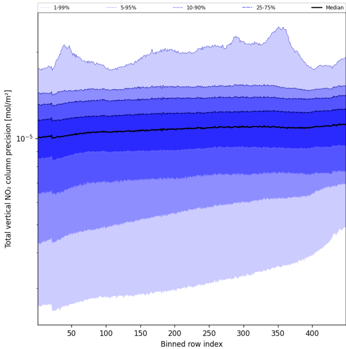
Figure 56: Along track statistics of “Total vertical NO 2 column precision” for 2025-09-04 to 2025-09-06
