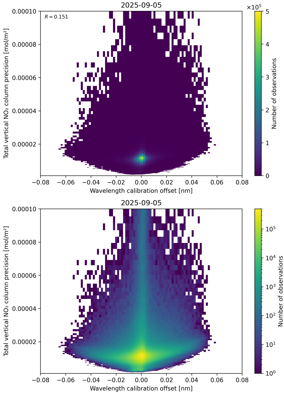
Figure 180: Scatter density plot of “Wavelength calibration offset” against “Total vertical NO 2 column precision” for 2025-09-04 to 2025-09-06.
