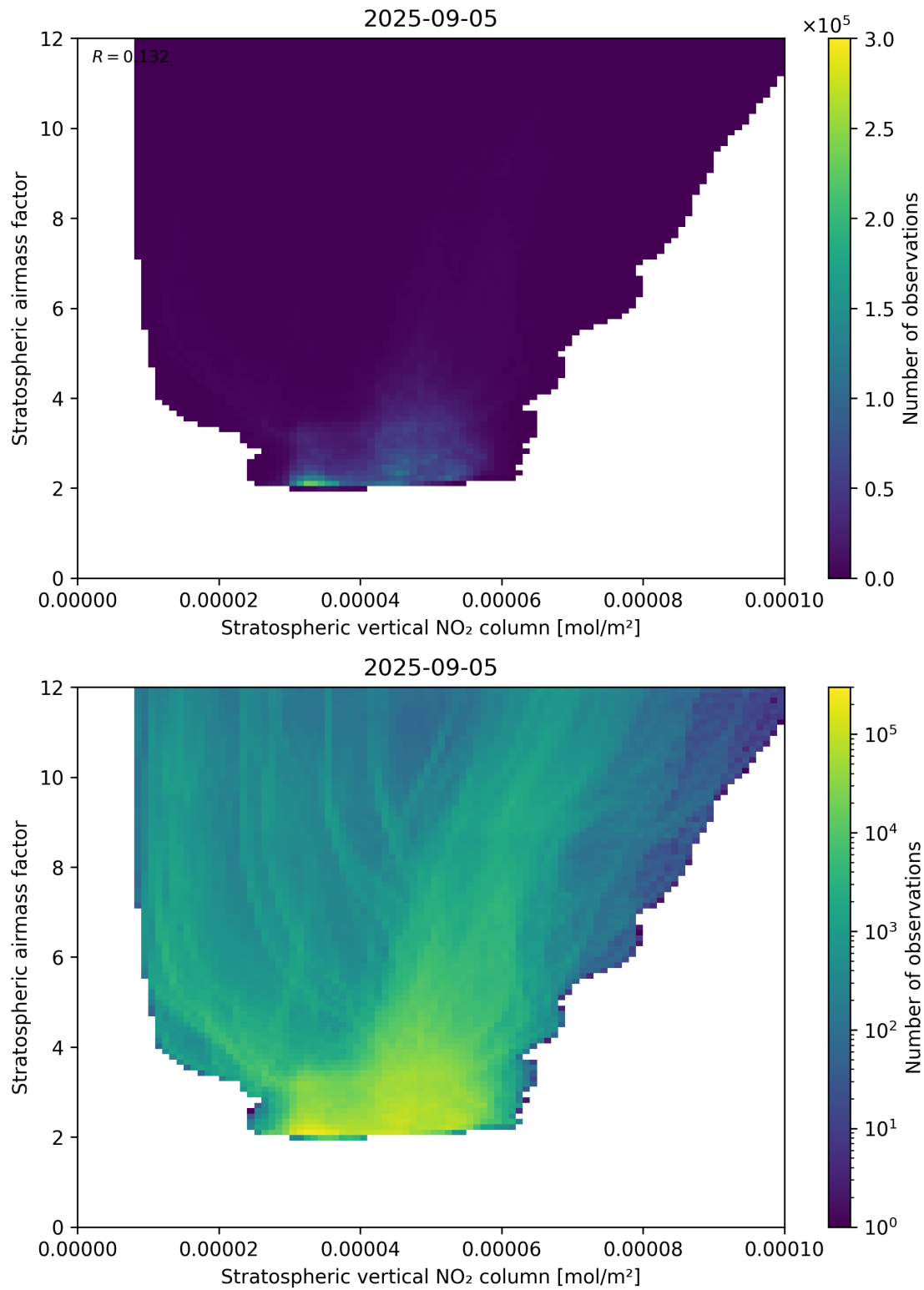
Figure 96: Scatter density plot of “Stratospheric vertical NO 2 column” against “Stratospheric airmass factor” for 2025-09-04 to 2025-09-06.
