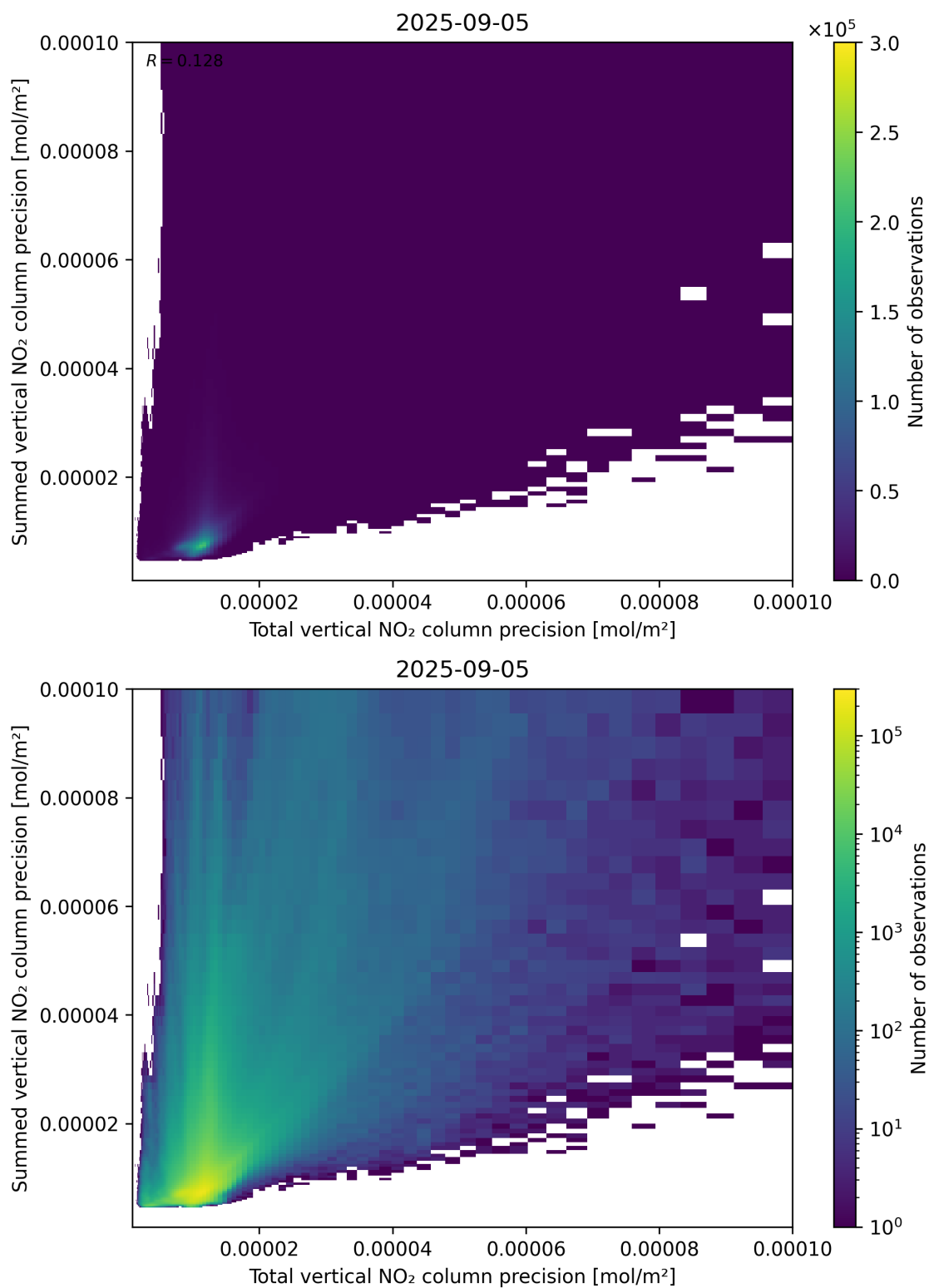
Figure 118: Scatter density plot of “Total vertical NO 2 column precision” against “Summed vertical NO 2 column precision” for 2025-09-04 to 2025-09-06.
