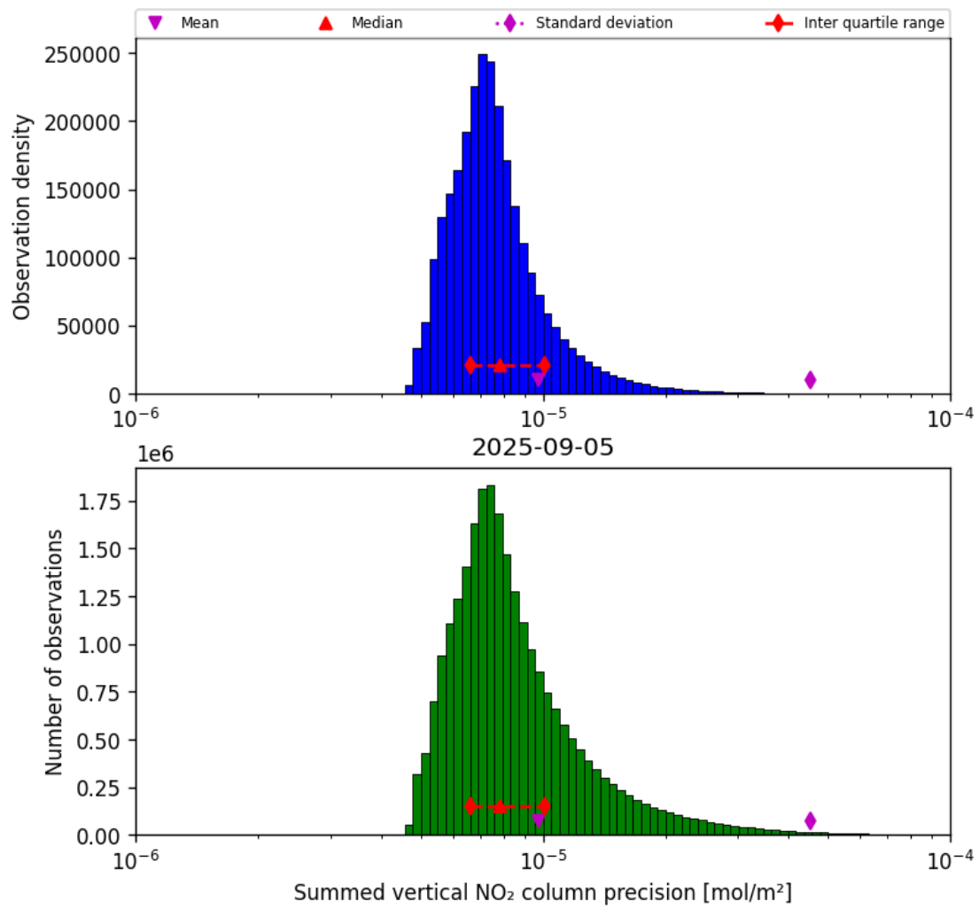
Figure 41: Histogram of “Summed vertical NO 2 column precision” for 2025-09-04 to 2025-09-06
