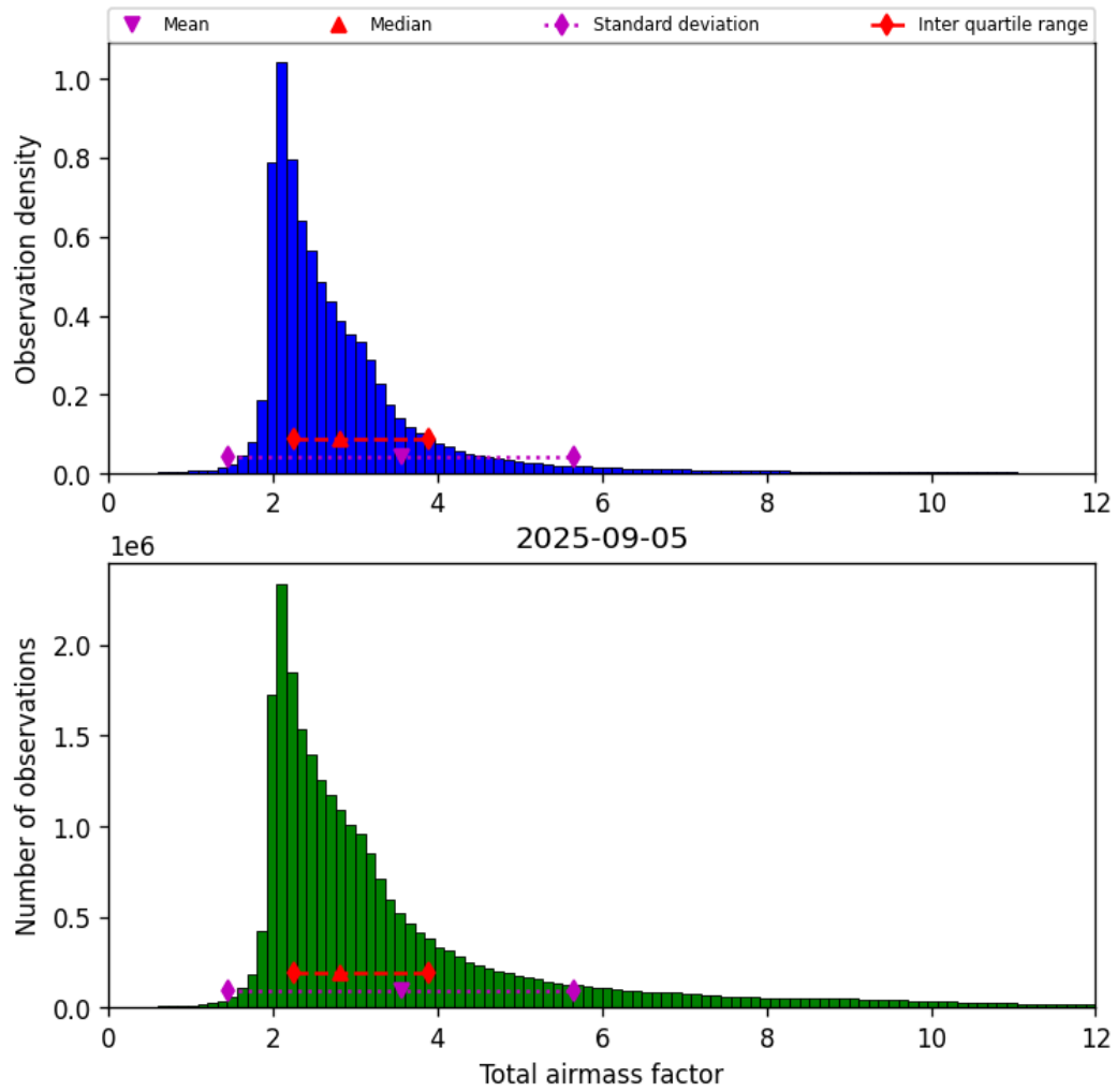
Figure 32: Histogram of “Total airmass factor” for 2025-09-04 to 2025-09-06
