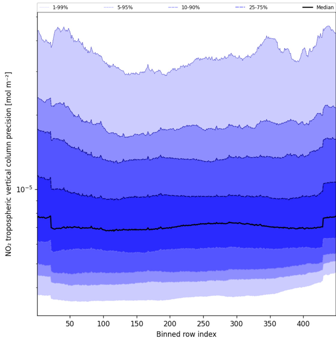
Figure 47: Along track statistics of “NO 2 tropospheric vertical column precision” for 2025-09-04 to 2025-09-06
