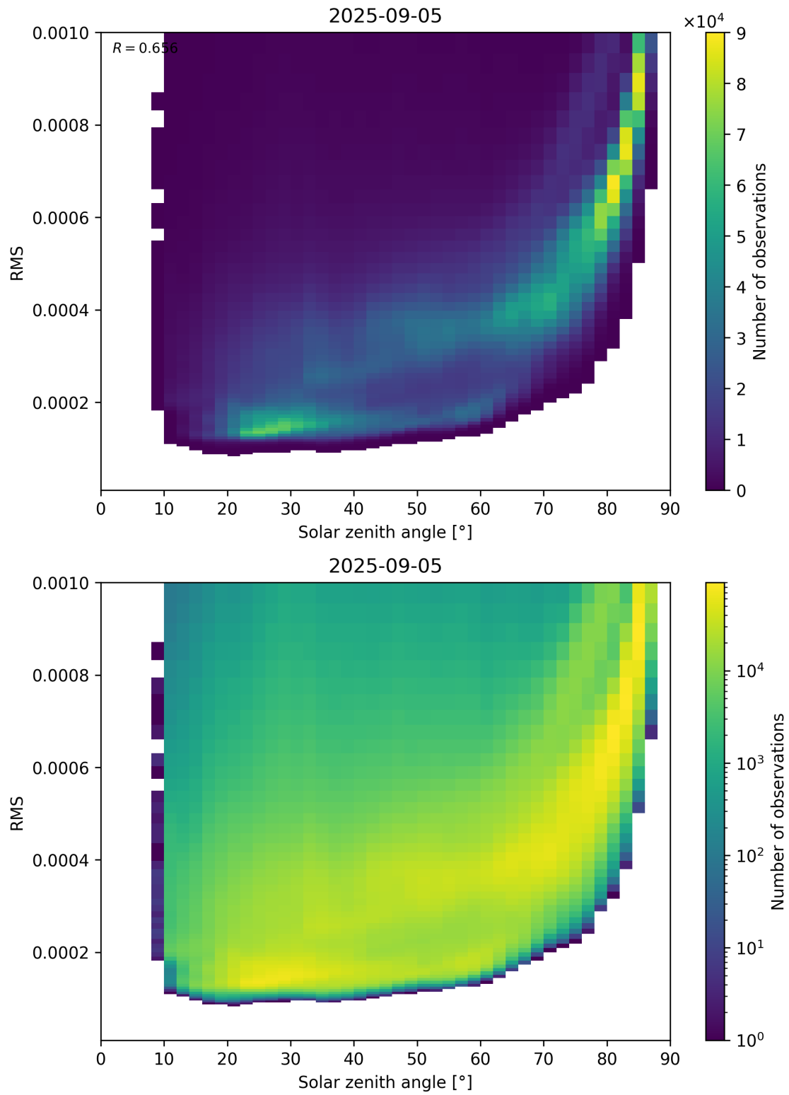
Figure 157: Scatter density plot of “Solar zenith angle” against “RMS” for 2025-09-04 to 2025-09-06.
