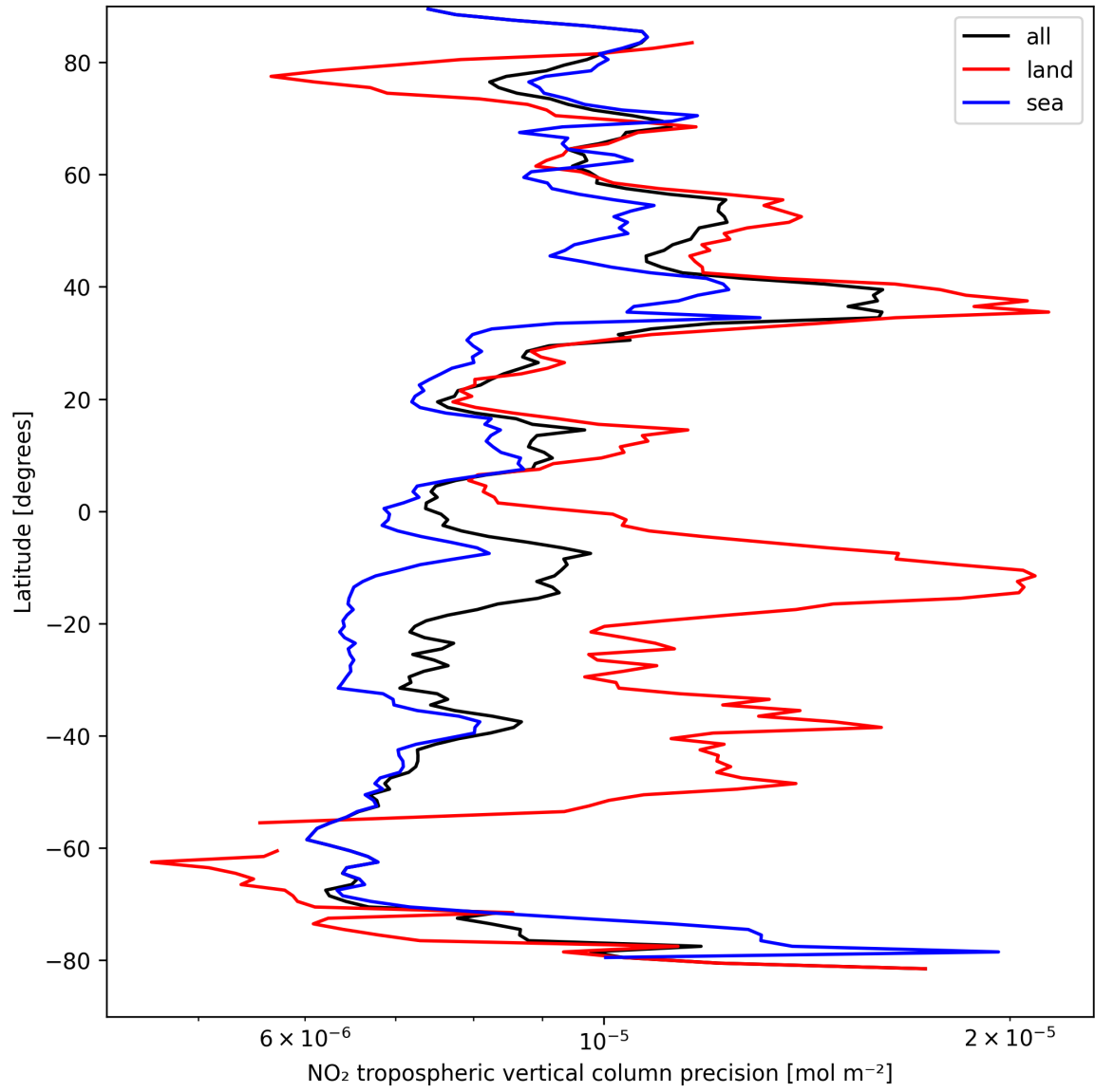
Figure 13: Zonal average of “NO 2 tropospheric vertical column precision” for 2025-09-04 to 2025-09-06.
