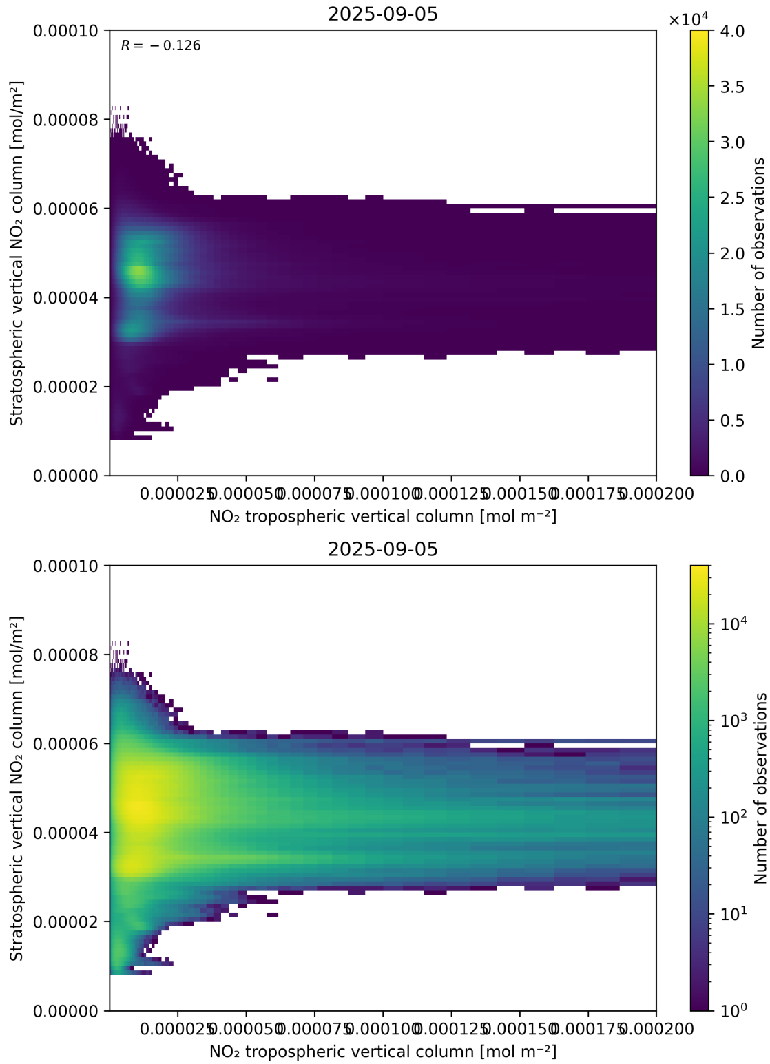
Figure 125: Scatter density plot of “NO 2 tropospheric vertical column” against “Stratospheric vertical NO 2 column” for 2025-09-04 to 2025-09-06.
