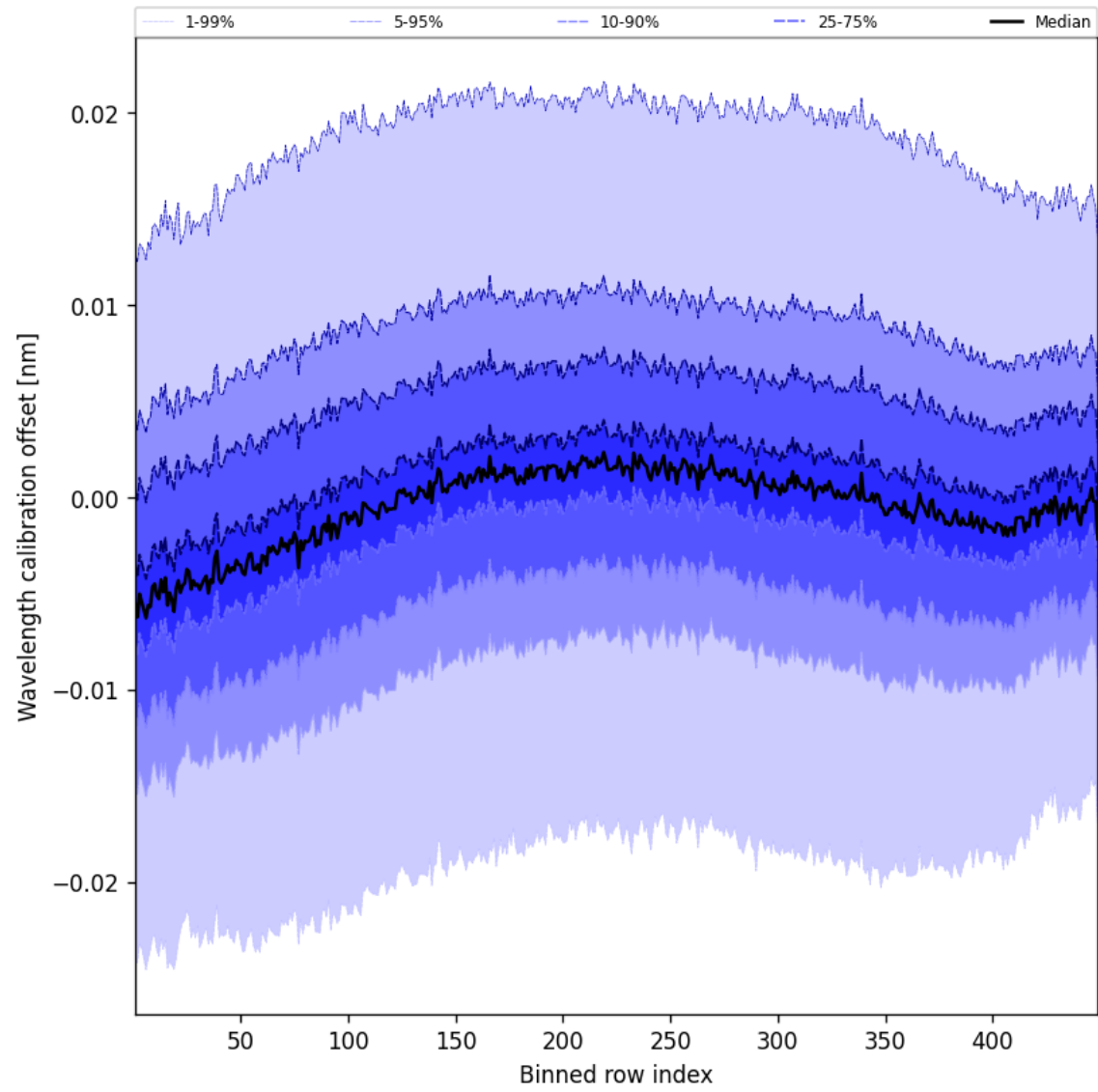
Figure 52: Along track statistics of “Wavelength calibration offset” for 2025-09-04 to 2025-09-06
