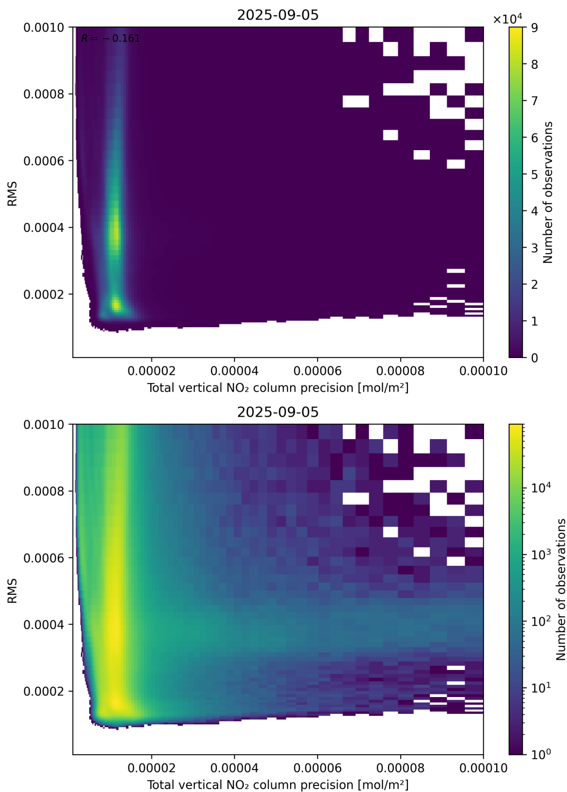
Figure 119: Scatter density plot of “Total vertical NO 2 column precision” against “RMS” for 2025-09-04 to 2025-09-06.
