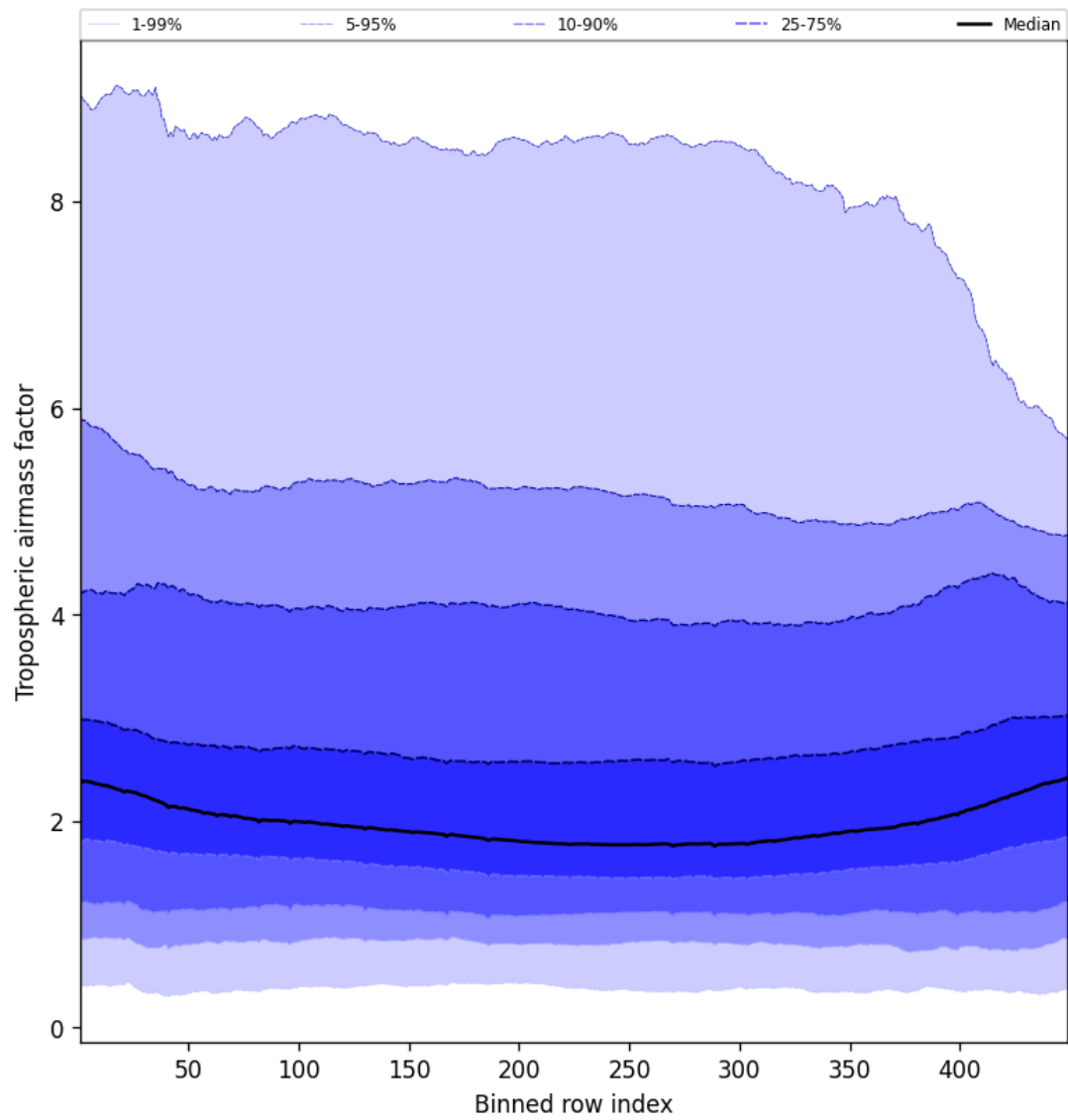
Figure 48: Along track statistics of “Tropospheric air mass factor” for 2025-09-04 to 2025-09-06
