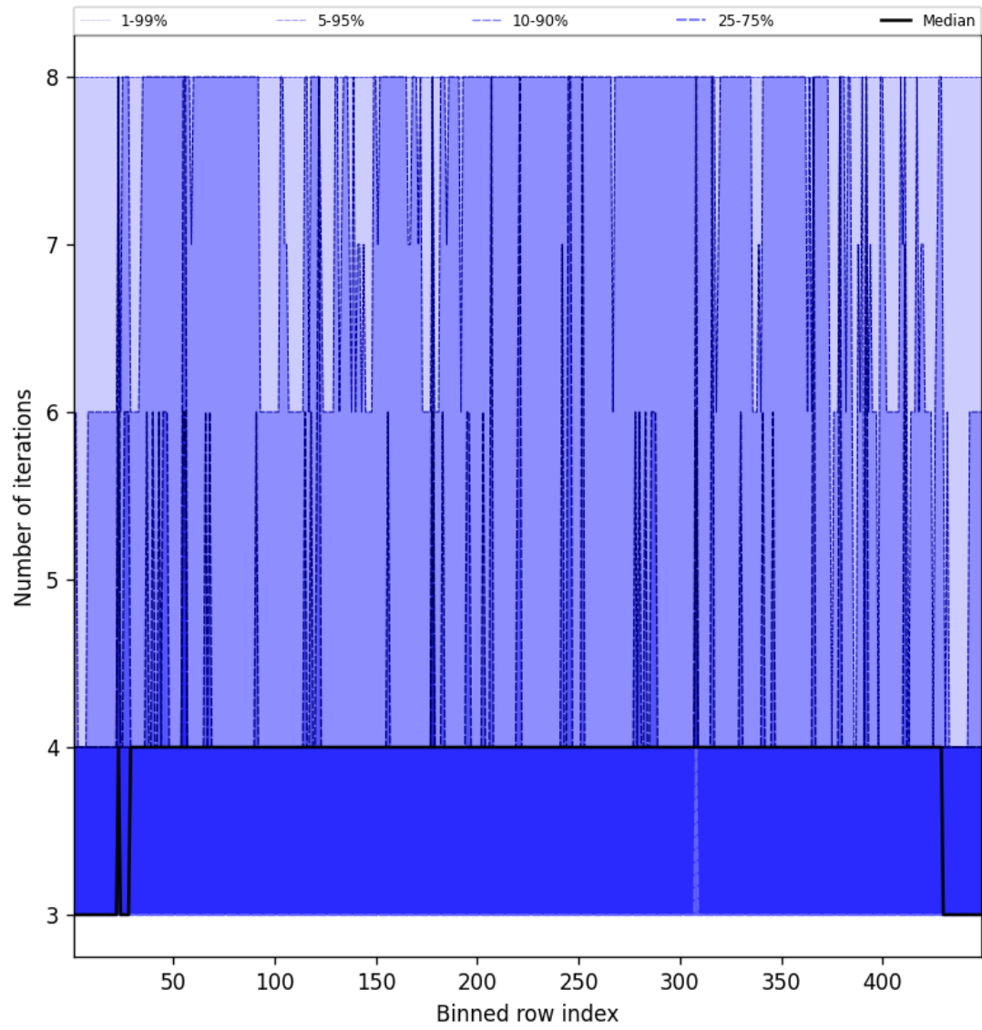
Figure 51: Along track statistics of “Number of iterations” for 2025-09-04 to 2025-09-06
