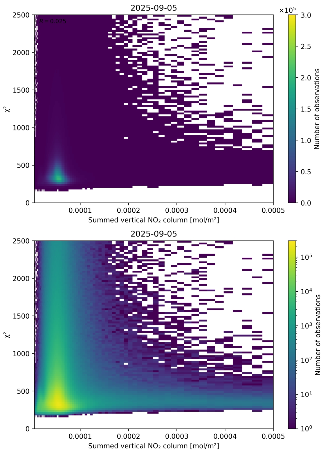
Figure 104: Scatter density plot of “Summed vertical NO 2 column” against “ \chi^2 ” for 2025-09-04 to 2025-09-06.
