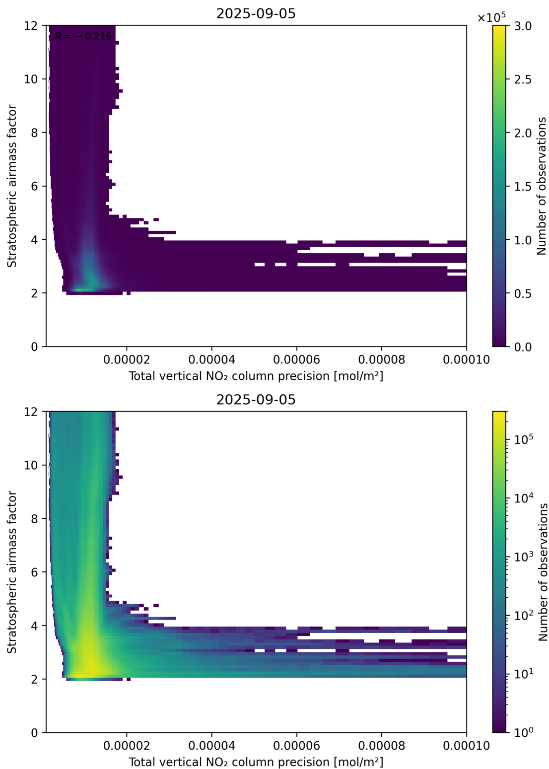
Figure 115: Scatter density plot of “Total vertical NO 2 column precision” against “Stratospheric airmass factor” for 2025-09-04 to 2025-09-06.
