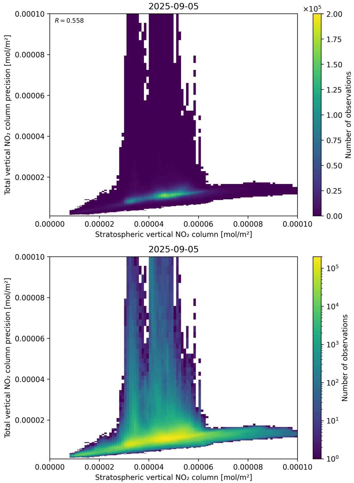
Figure 101: Scatter density plot of “Stratospheric vertical NO 2 column” against “Total vertical NO 2 column precision” for 2025-09-04 to 2025-09-06.
