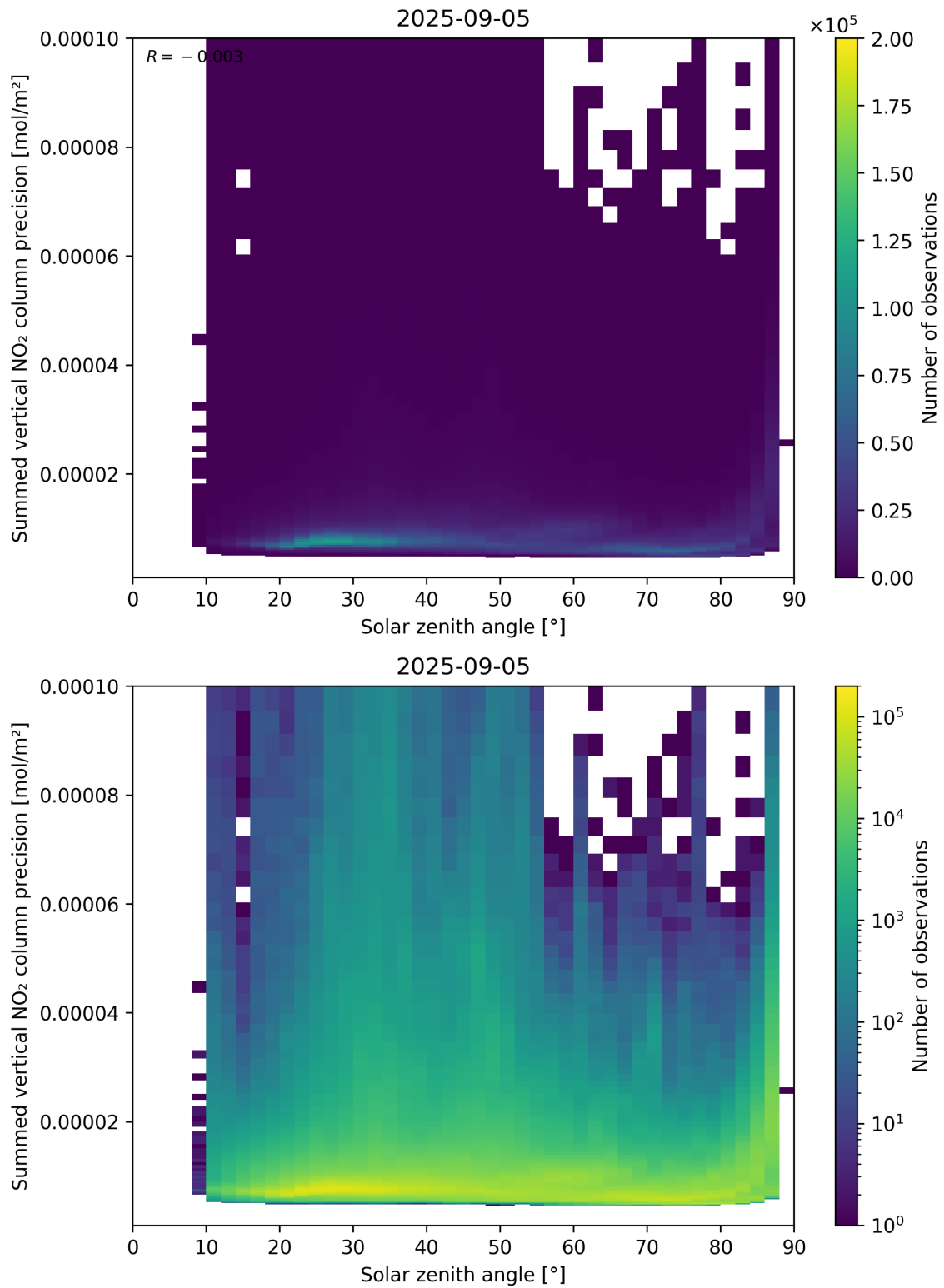
Figure 152: Scatter density plot of “Solar zenith angle” against “Summed vertical NO 2 column precision” for 2025-09-04 to 2025-09-06.
