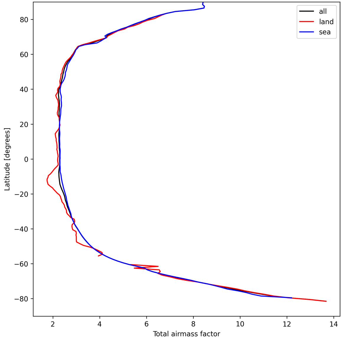
Figure 15: Zonal average of “Total airmass factor” for 2025-09-04 to 2025-09-06.
