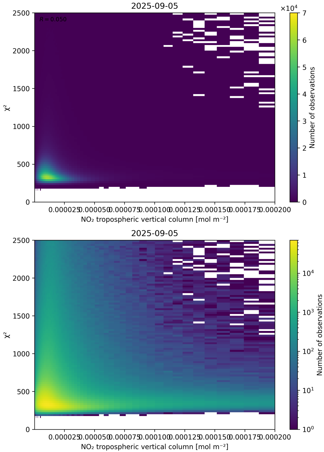
Figure 124: Scatter density plot of “NO 2 tropospheric vertical column” against “ \chi^2 ” for 2025-09-04 to 2025-09-06.
