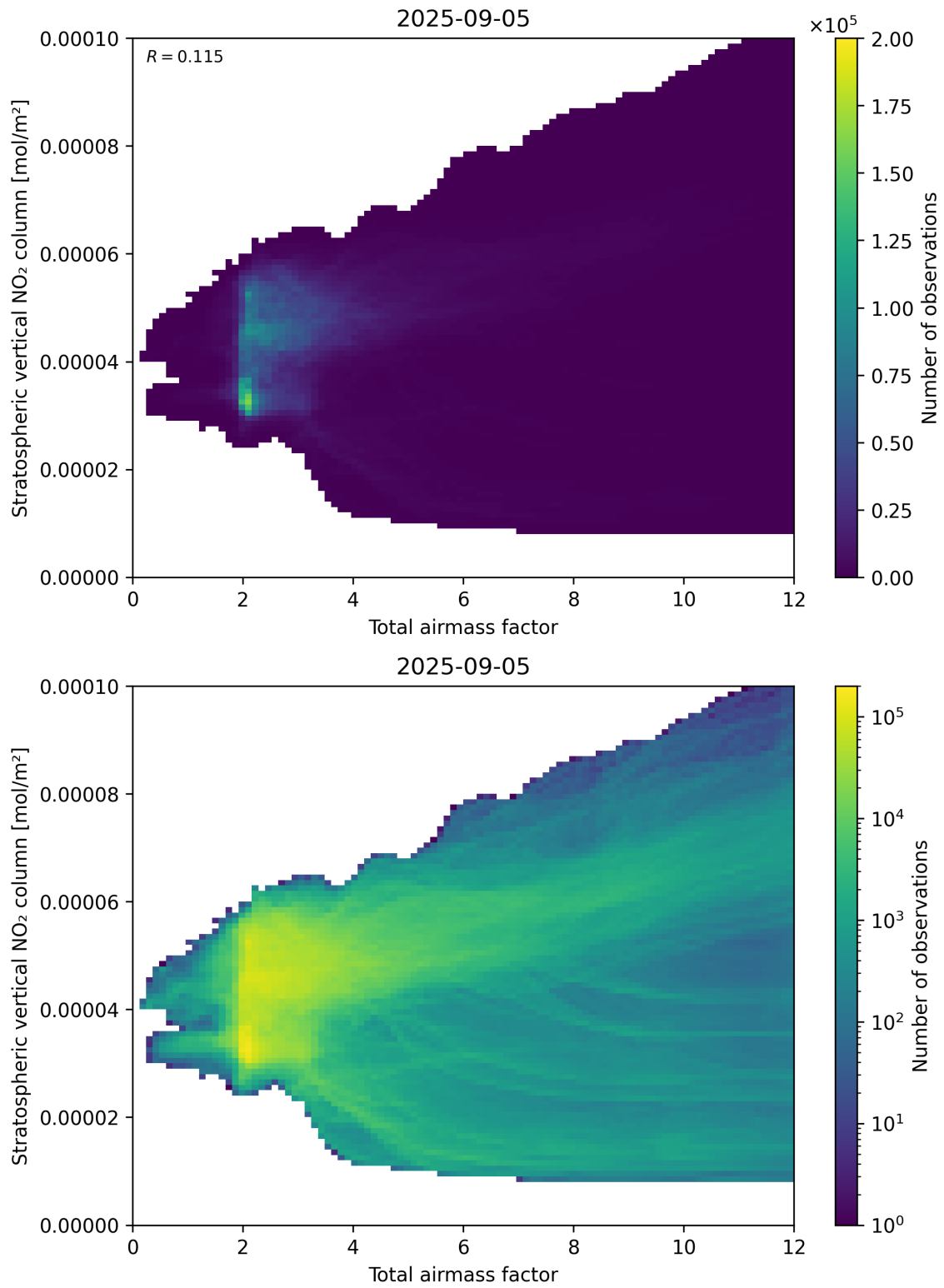
Figure 64: Scatter density plot of “Total airmass factor” against “Stratospheric vertical NO 2 column” for 2025-09-04 to 2025-09-06.
