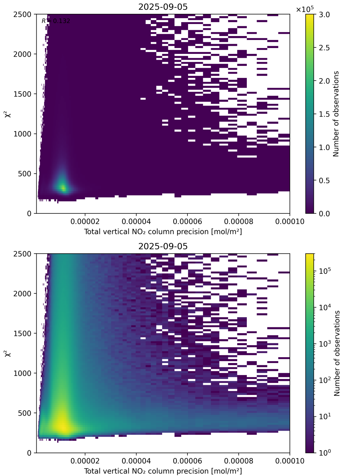
Figure 116: Scatter density plot of “Total vertical NO 2 column precision” against “ \chi^2 ” for 2025-09-04 to 2025-09-06.
