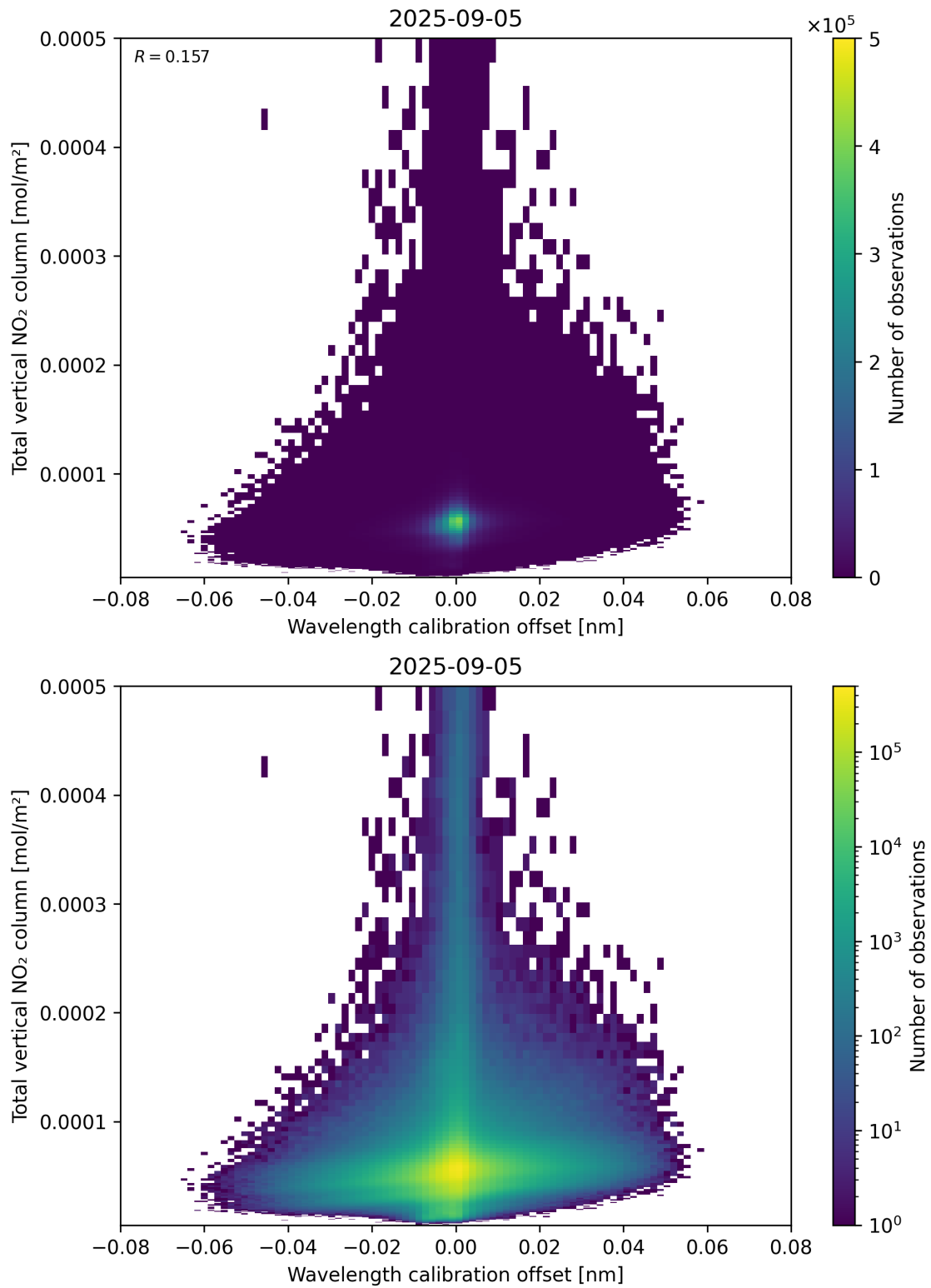
Figure 179: Scatter density plot of “Wavelength calibration offset” against “Total vertical NO 2 column” for 2025-09-04 to 2025-09-06.
