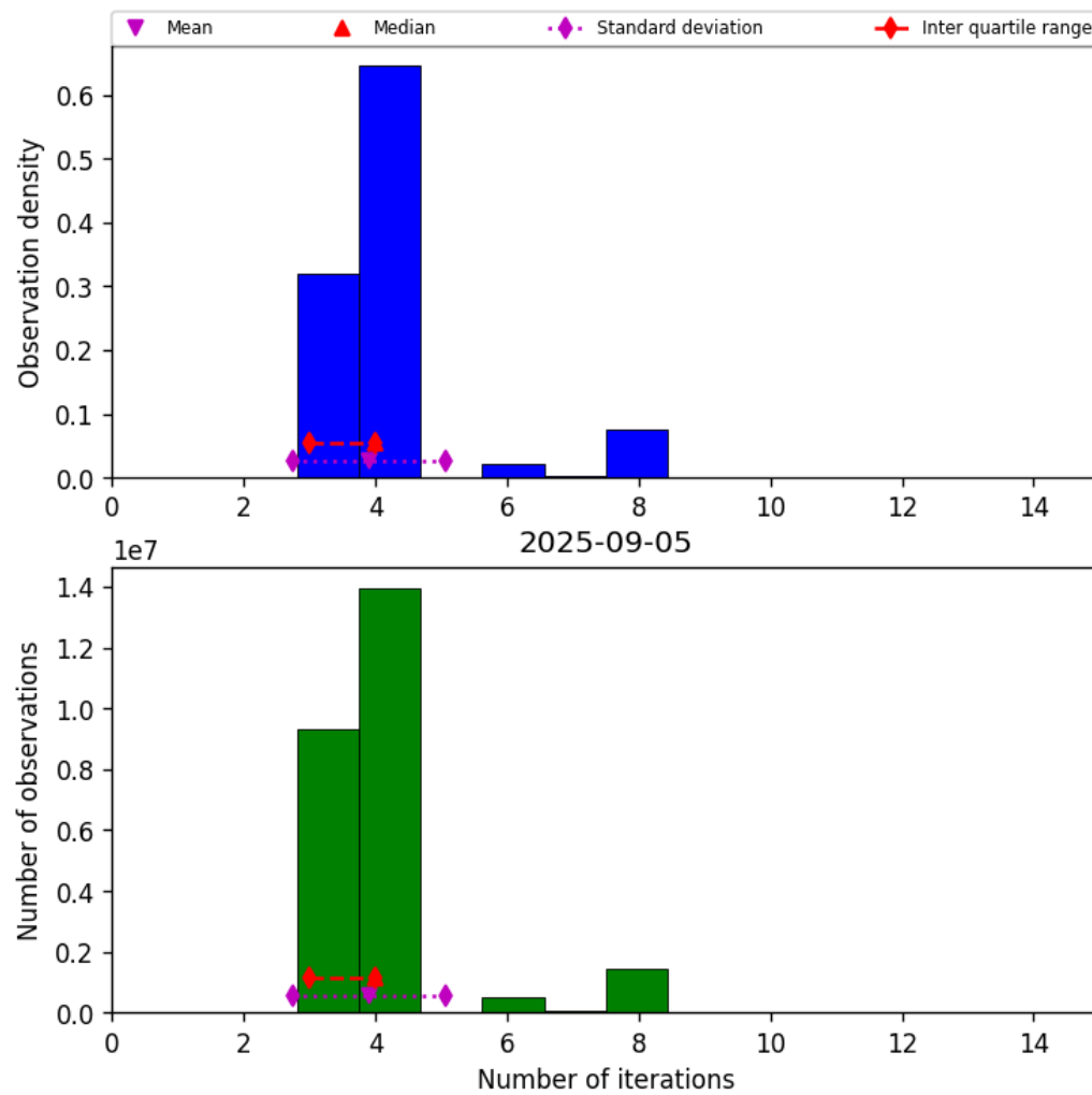
Figure 34: Histogram of “Number of iterations” for 2025-09-04 to 2025-09-06
