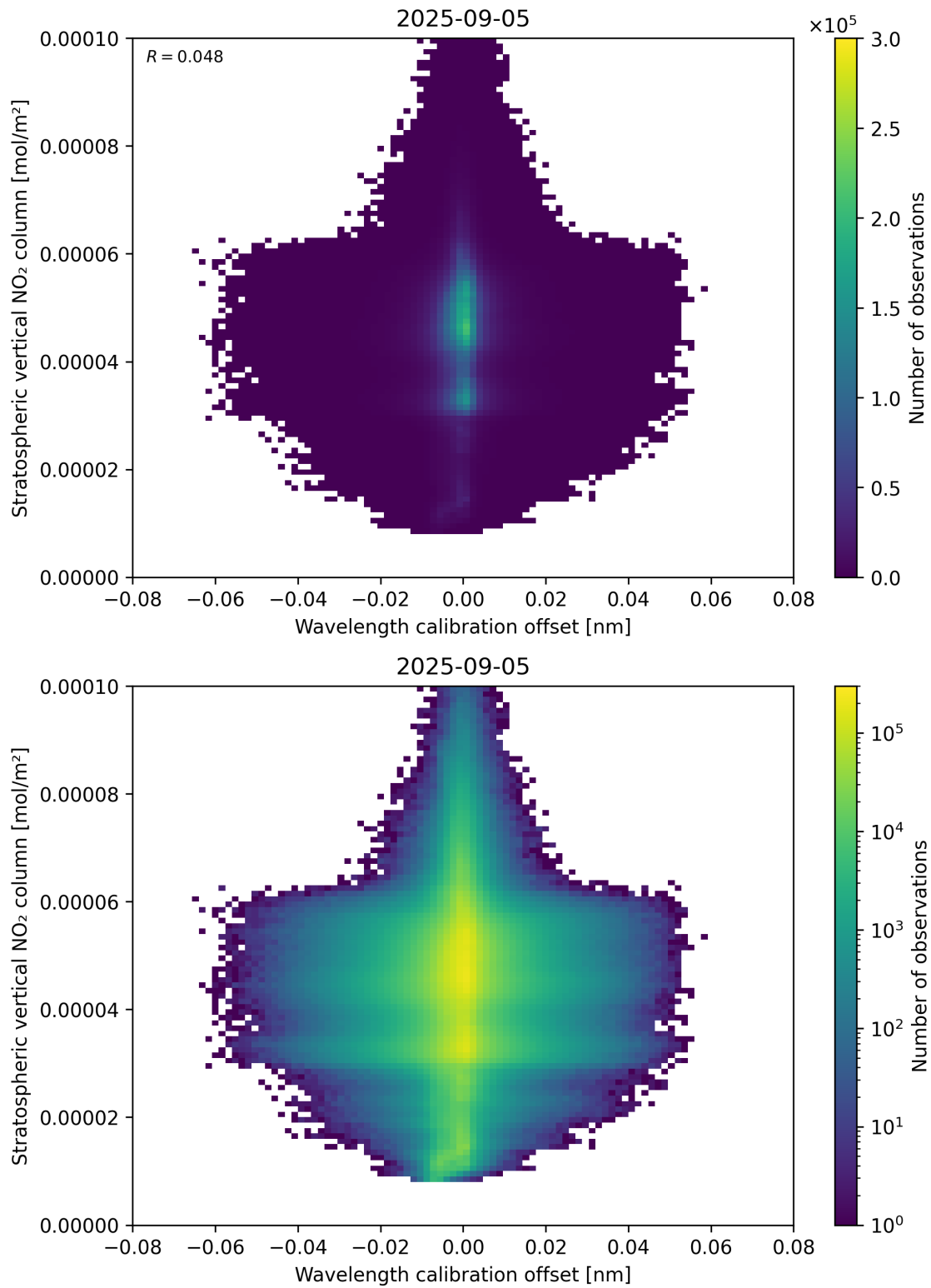
Figure 176: Scatter density plot of “Wavelength calibration offset” against “Stratospheric vertical NO 2 column” for 2025-09-04 to 2025-09-06.
