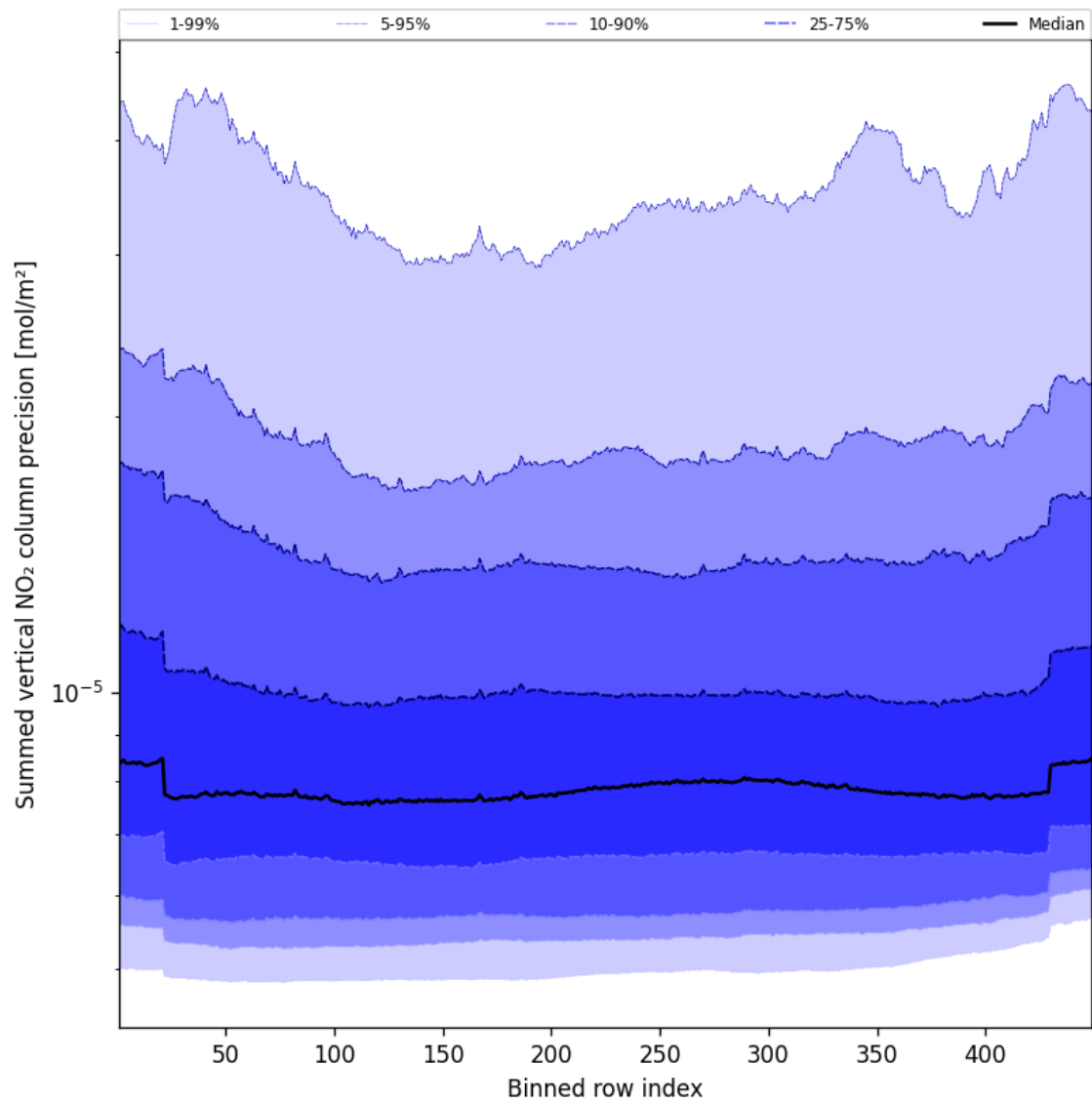
Figure 58: Along track statistics of “Summed vertical NO 2 column precision” for 2025-09-04 to 2025-09-06
