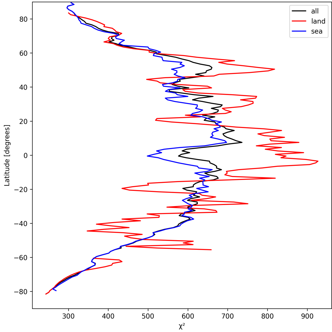
Figure 25: Zonal average of “ \chi^2 ” for 2025-09-04 to 2025-09-06.
