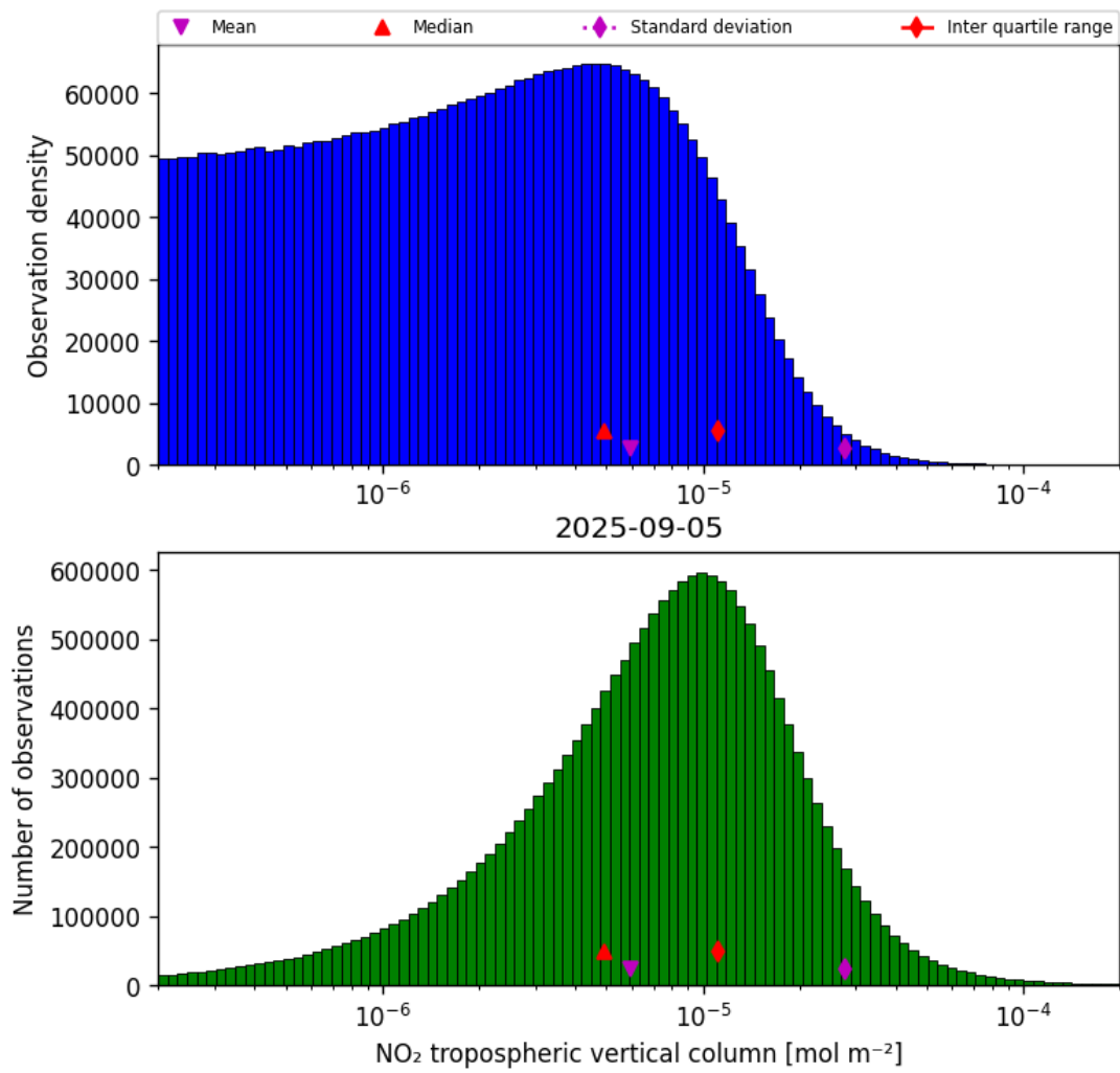
Figure 29: Histogram of “ \text{NO}_2 tropospheric vertical column” for 2025-09-04 to 2025-09-06
