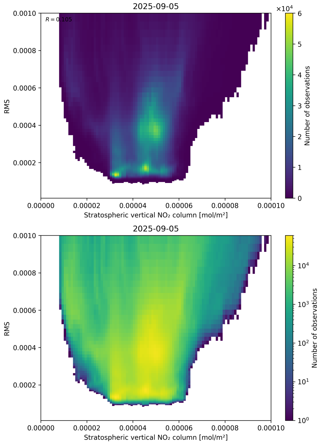
Figure 102: Scatter density plot of “Stratospheric vertical NO 2 column” against “RMS” for 2025-09-04 to 2025-09-06.
