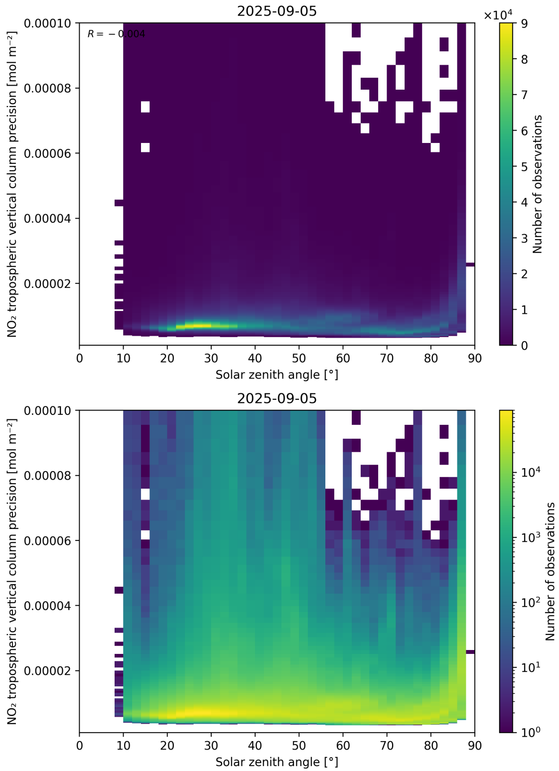
Figure 156: Scatter density plot of “Solar zenith angle” against “NO 2 tropospheric vertical column precision” for 2025-09-04 to 2025-09-06.
