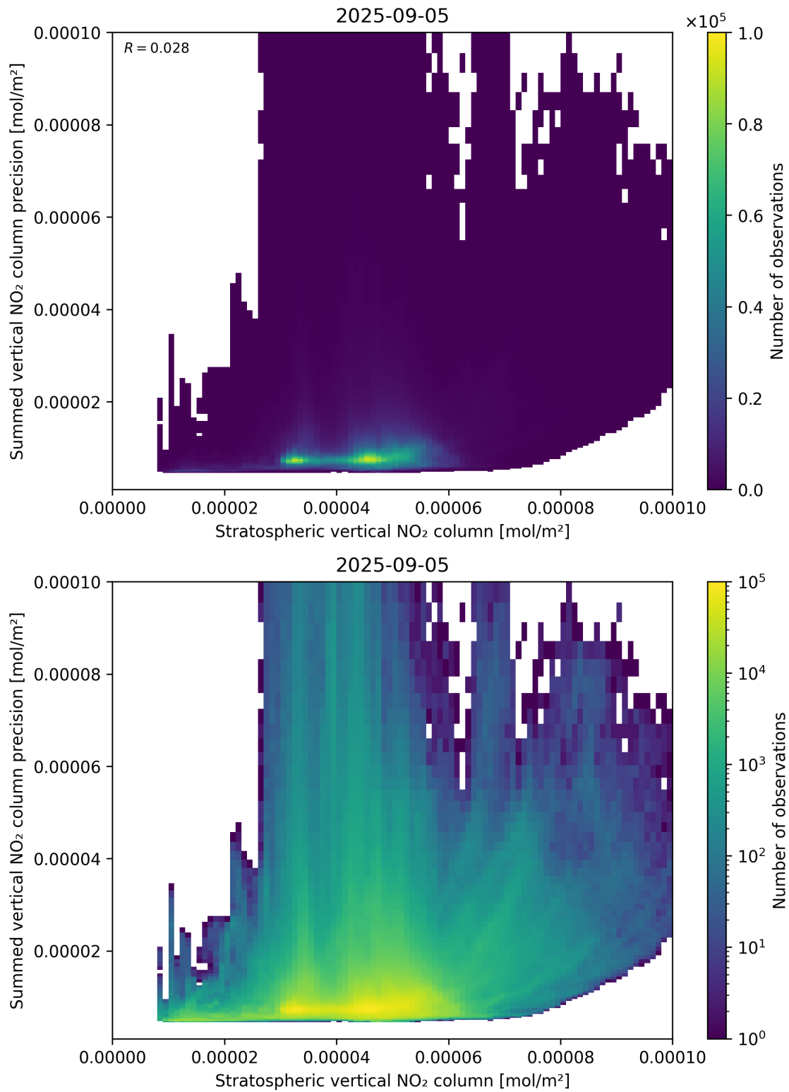
Figure 99: Scatter density plot of “Stratospheric vertical NO 2 column” against “Summed vertical NO 2 column precision” for 2025-09-04 to 2025-09-06.
