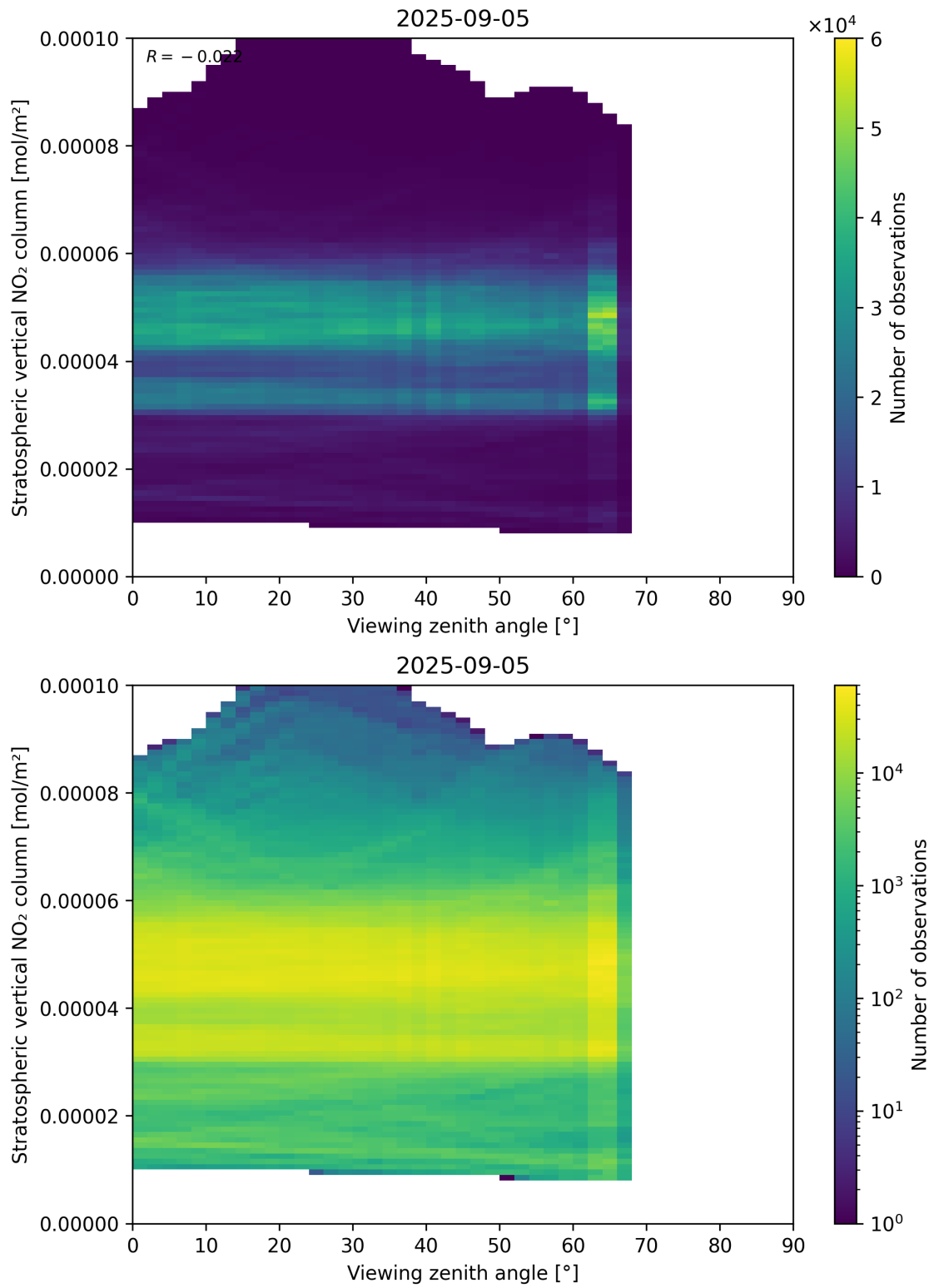
Figure 164: Scatter density plot of “Viewing zenith angle” against “Stratospheric vertical NO 2 column” for 2025-09-04 to 2025-09-06.
