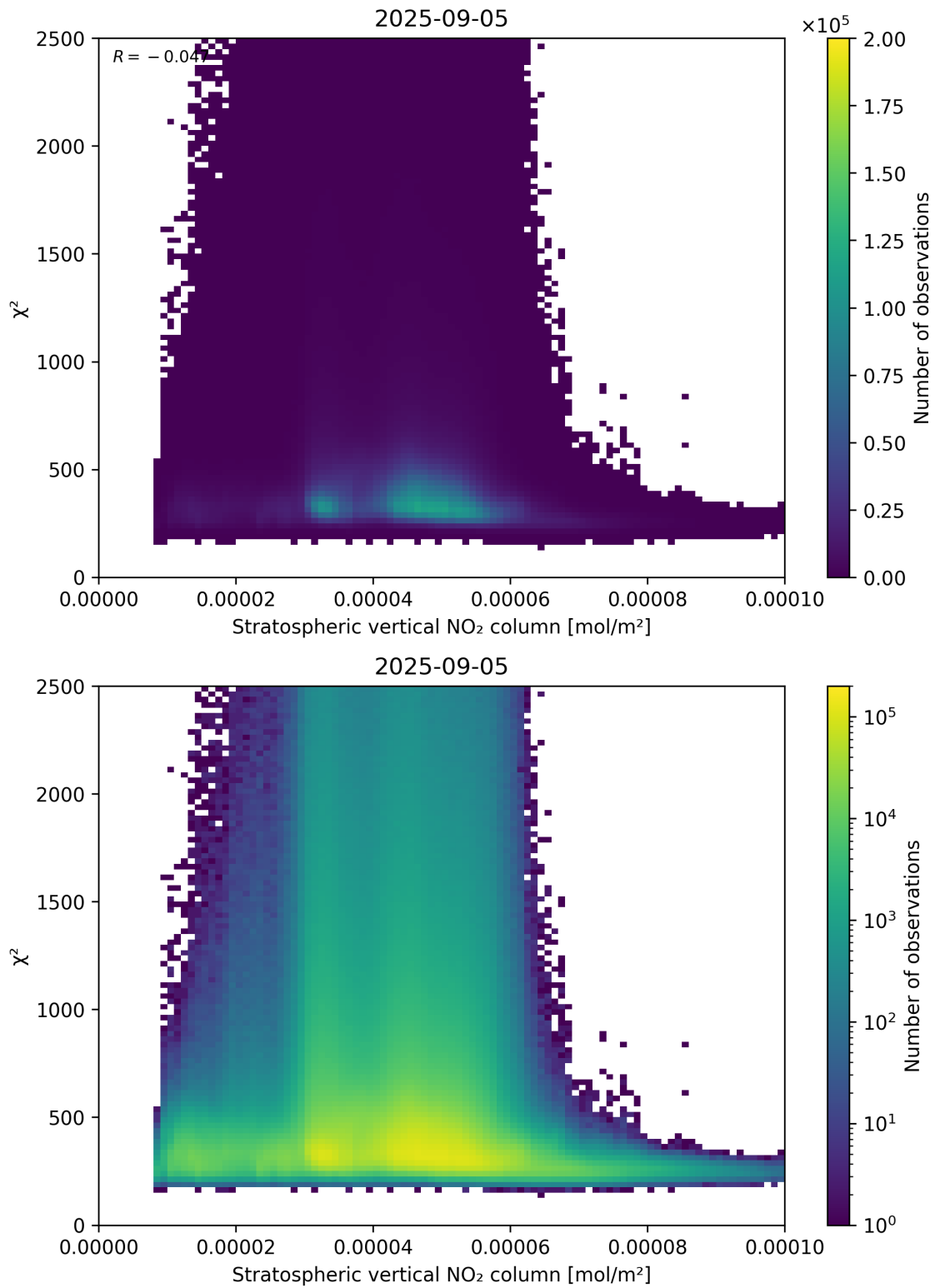
Figure 97: Scatter density plot of “Stratospheric vertical NO 2 column” against “ \chi^2 ” for 2025-09-04 to 2025-09-06.
