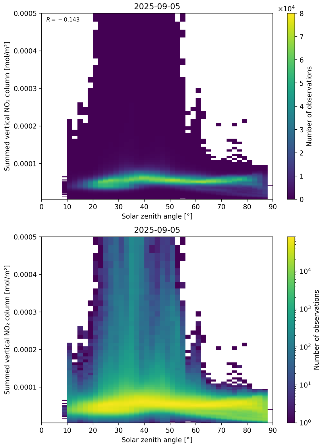
Figure 151: Scatter density plot of “Solar zenith angle” against “Summed vertical NO 2 column” for 2025-09-04 to 2025-09-06.
