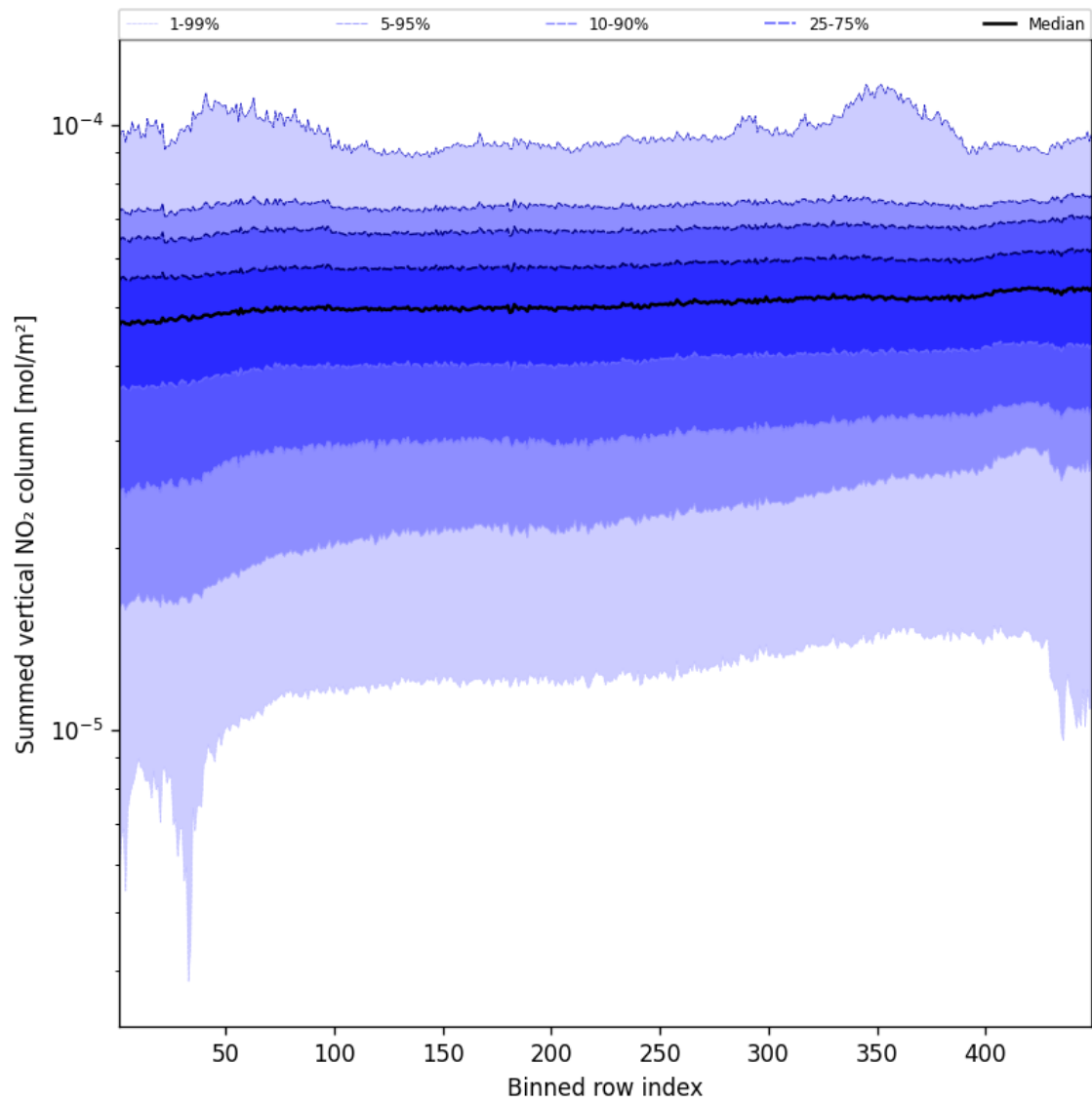
Figure 57: Along track statistics of “Summed vertical NO 2 column” for 2025-09-04 to 2025-09-06
