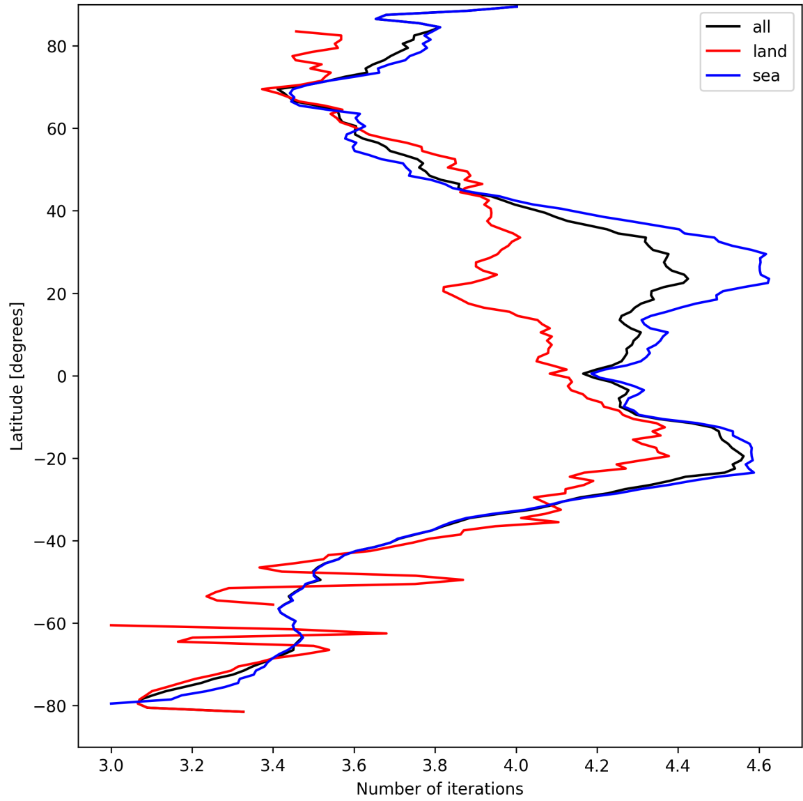
Figure 17: Zonal average of “Number of iterations” for 2025-09-04 to 2025-09-06.
