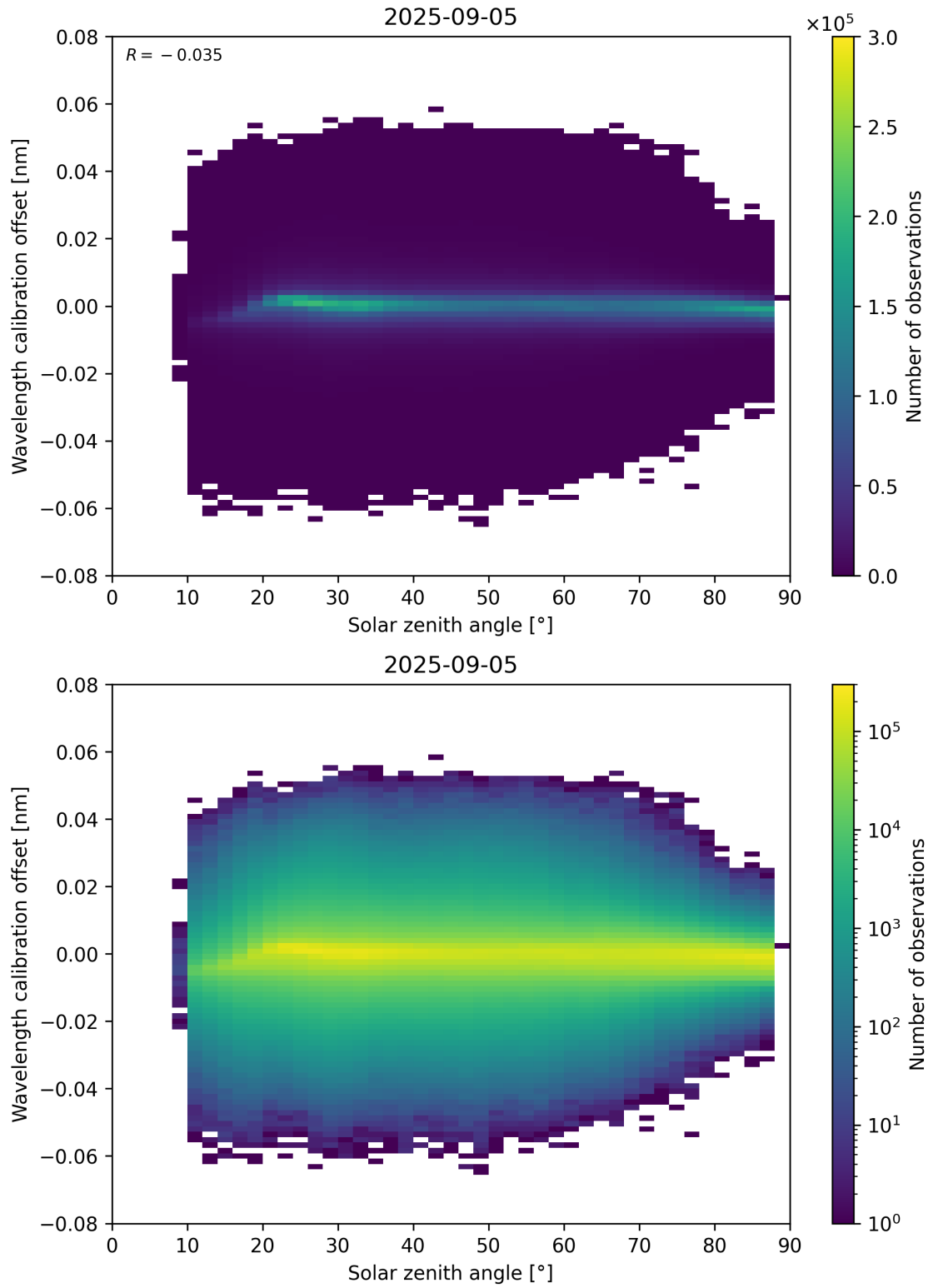
Figure 158: Scatter density plot of “Solar zenith angle” against “Wavelength calibration offset” for 2025-09-04 to 2025-09-06.
