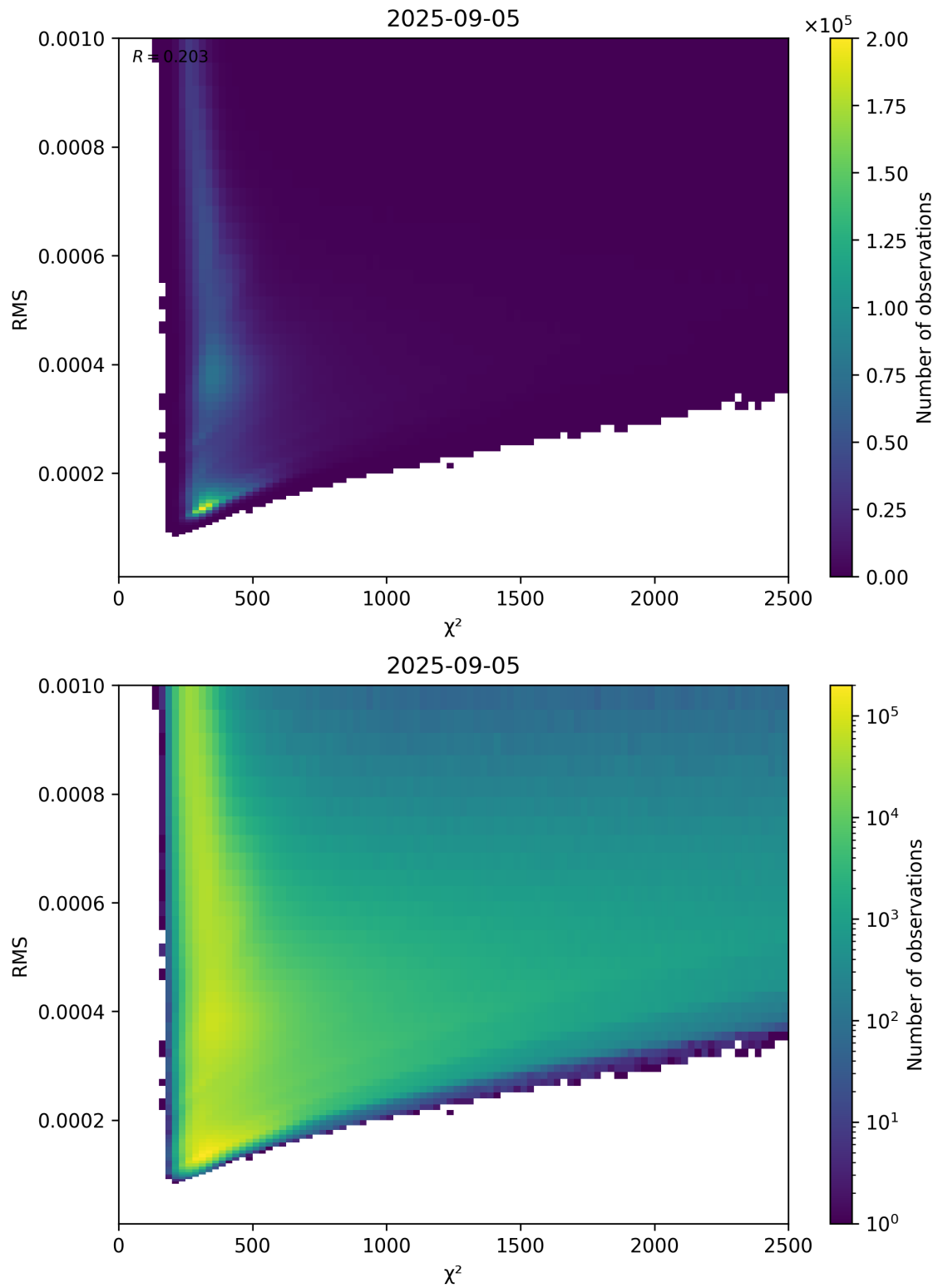
Figure 82: Scatter density plot of “ \chi^2 ” against “RMS” for 2025-09-04 to 2025-09-06.
