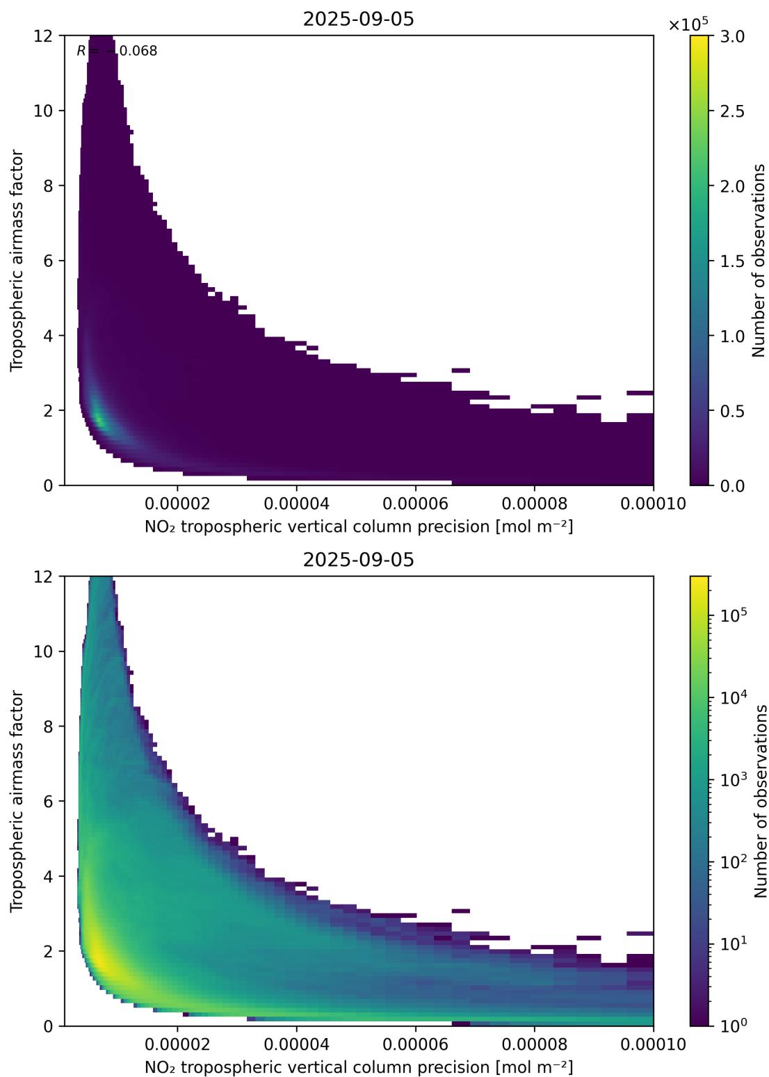
Figure 133: Scatter density plot of “NO 2 tropospheric vertical column precision” against “Tropospheric air mass factor” for 2025-09-04 to 2025-09-06.
