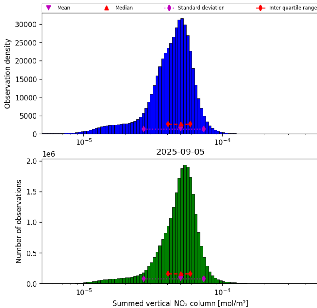
Figure 40: Histogram of “Summed vertical NO 2 column” for 2025-09-04 to 2025-09-06
