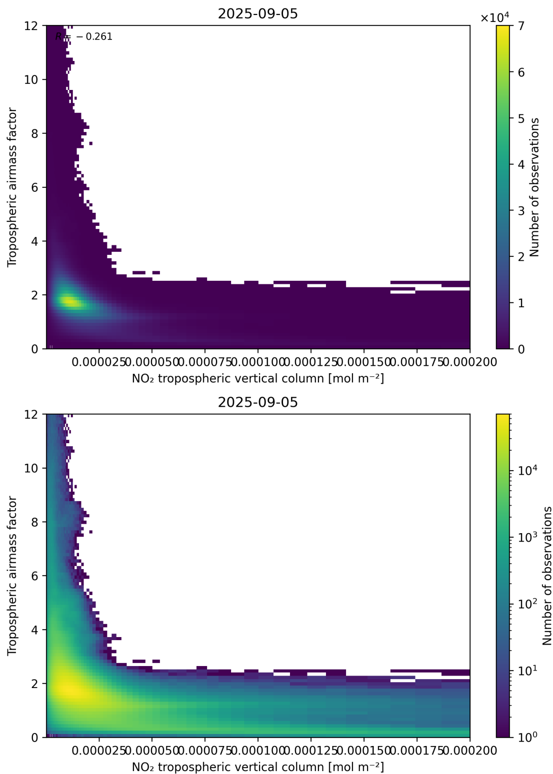
Figure 123: Scatter density plot of “NO 2 tropospheric vertical column” against “Tropospheric air mass factor” for 2025-09-04 to 2025-09-06.
