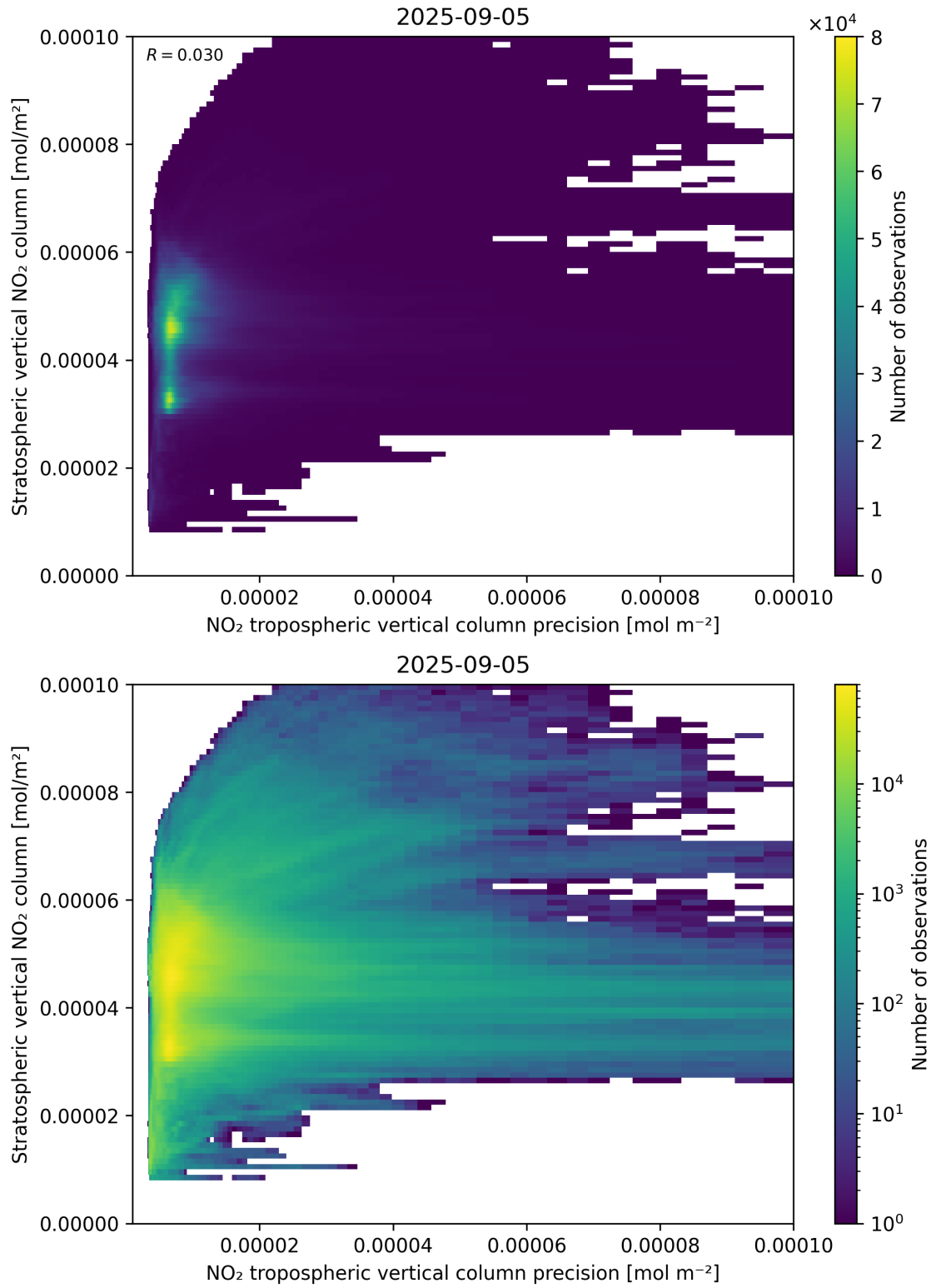
Figure 135: Scatter density plot of “NO 2 tropospheric vertical column precision” against “Stratospheric vertical NO 2 column” for 2025-09-04 to 2025-09-06.
