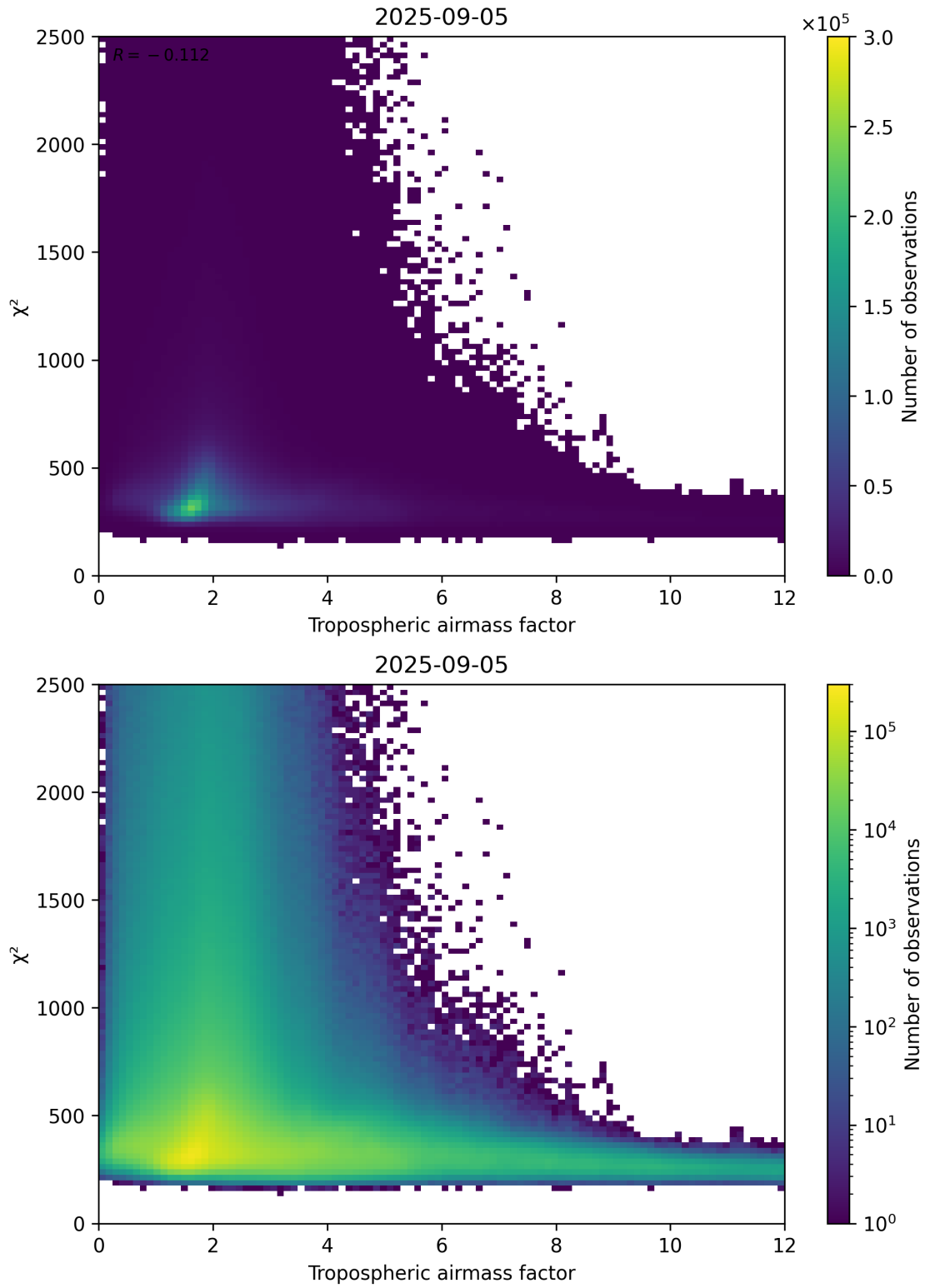
Figure 73: Scatter density plot of “Tropospheric airmass factor” against “ \chi^2 ” for 2025-09-04 to 2025-09-06.
