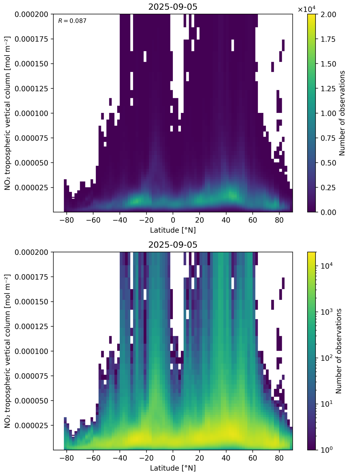
Figure 92: Scatter density plot of “Latitude” against “NO 2 tropospheric vertical column” for 2025-09-04 to 2025-09-06.
