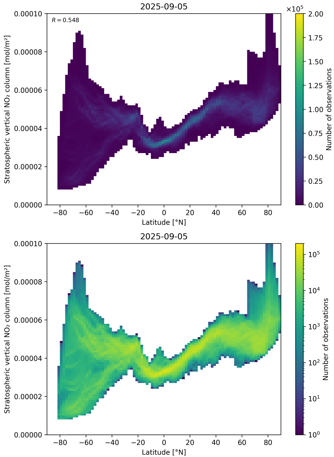
Figure 87: Scatter density plot of “Latitude” against “Stratospheric vertical NO 2 column” for 2025-09-04 to 2025-09-06.
