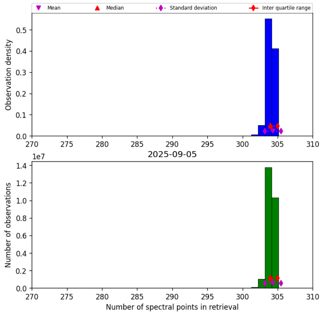
Figure 33: Histogram of “Number of spectral points in retrieval” for 2025-09-04 to 2025-09-06
