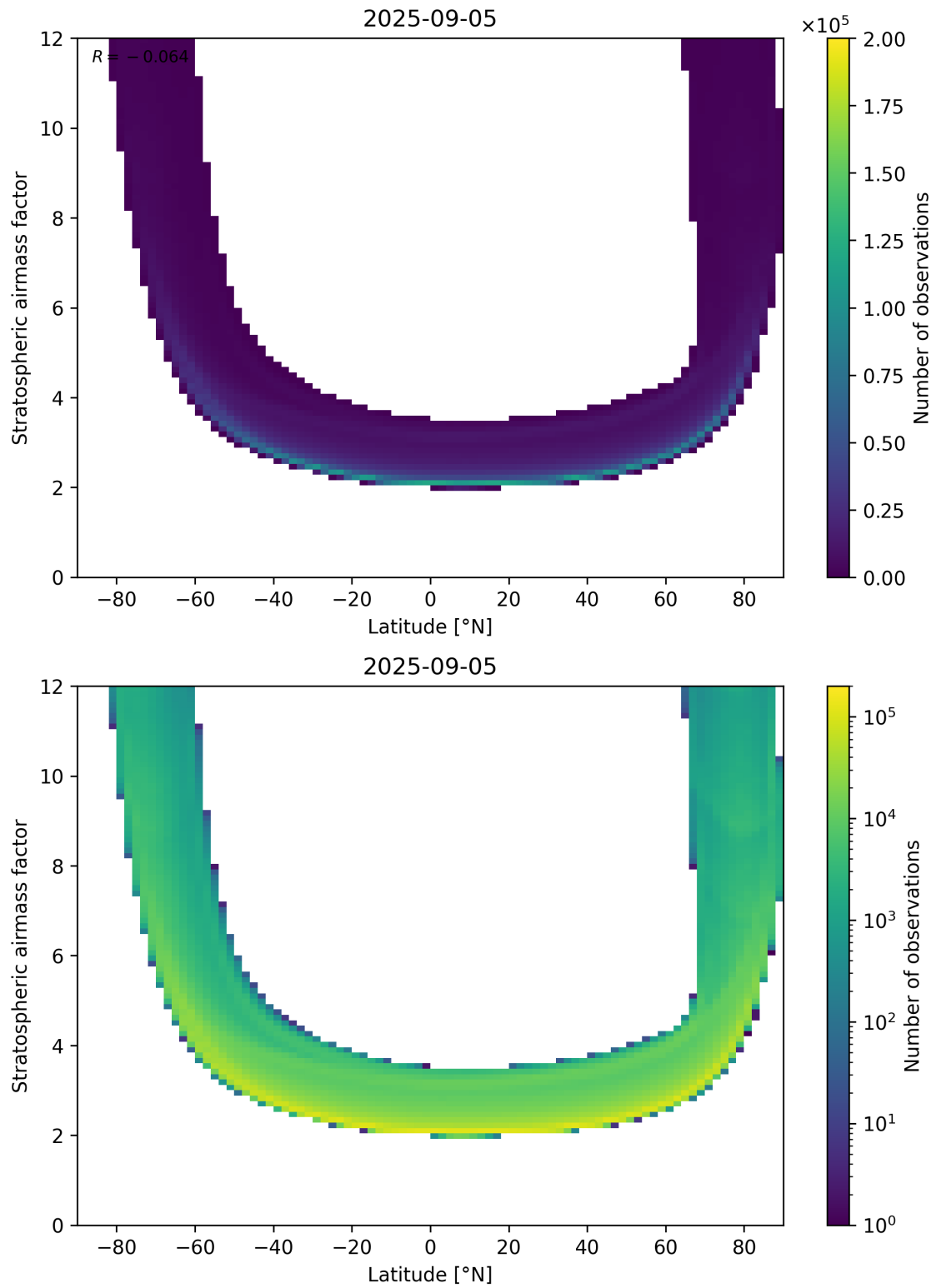
Figure 83: Scatter density plot of “Latitude” against “Stratospheric air mass factor” for 2025-09-04 to 2025-09-06.
