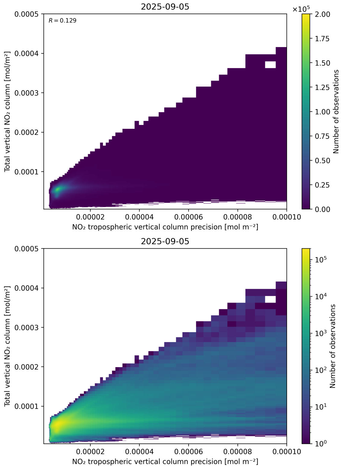
Figure 138: Scatter density plot of “NO 2 tropospheric vertical column precision” against “Total vertical NO 2 column” for 2025-09-04 to 2025-09-06.
