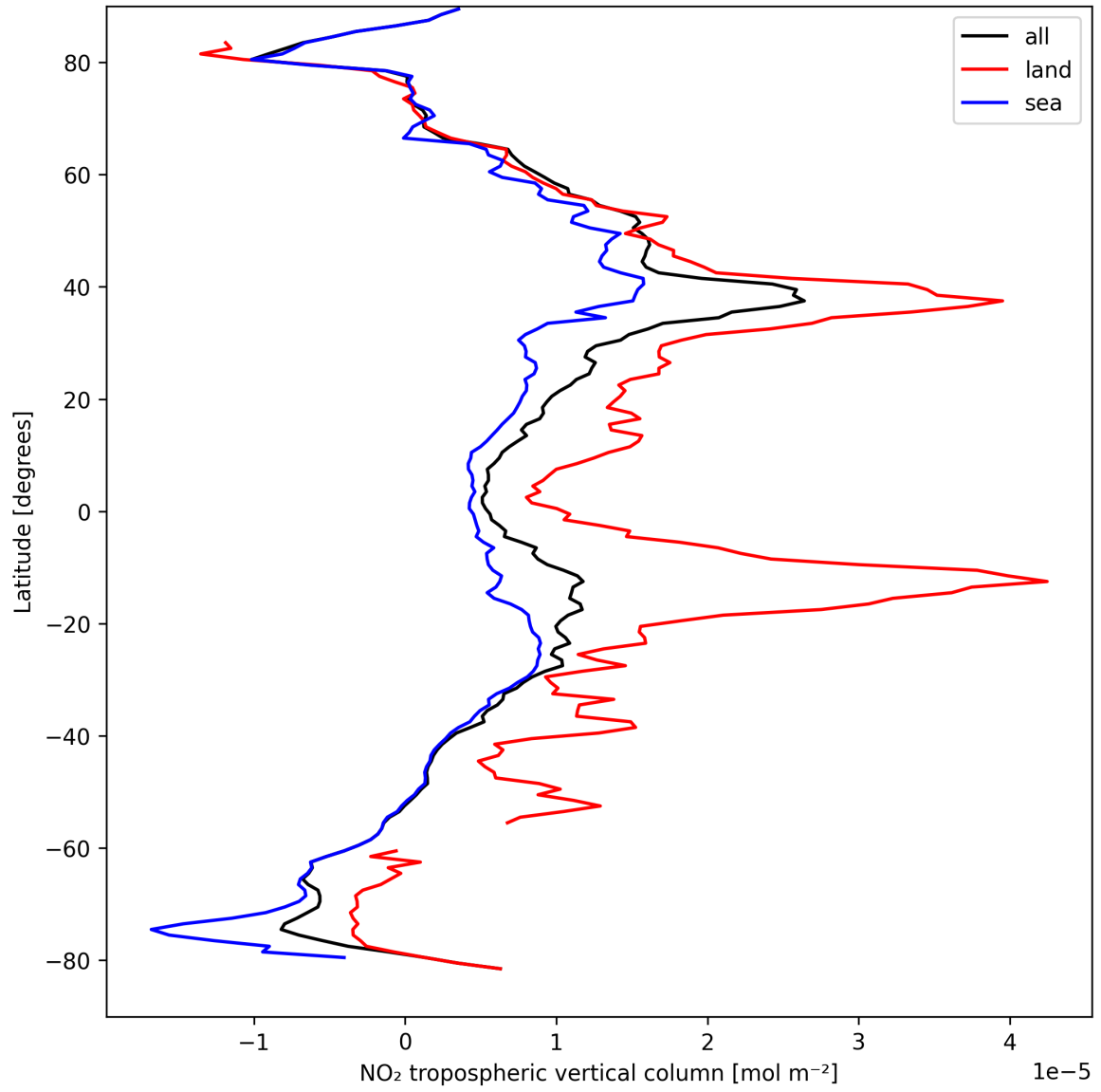
Figure 12: Zonal average of “NO 2 tropospheric vertical column” for 2025-09-04 to 2025-09-06.
