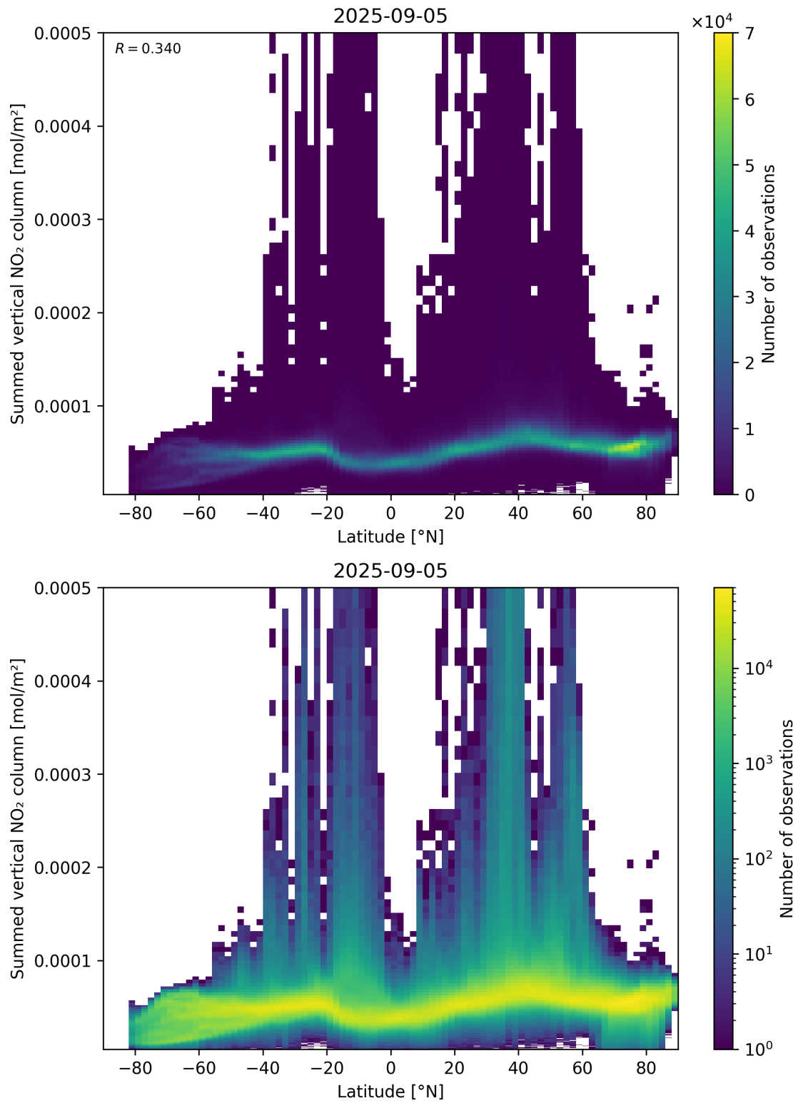
Figure 88: Scatter density plot of “Latitude” against “Summed vertical NO 2 column” for 2025-09-04 to 2025-09-06.
