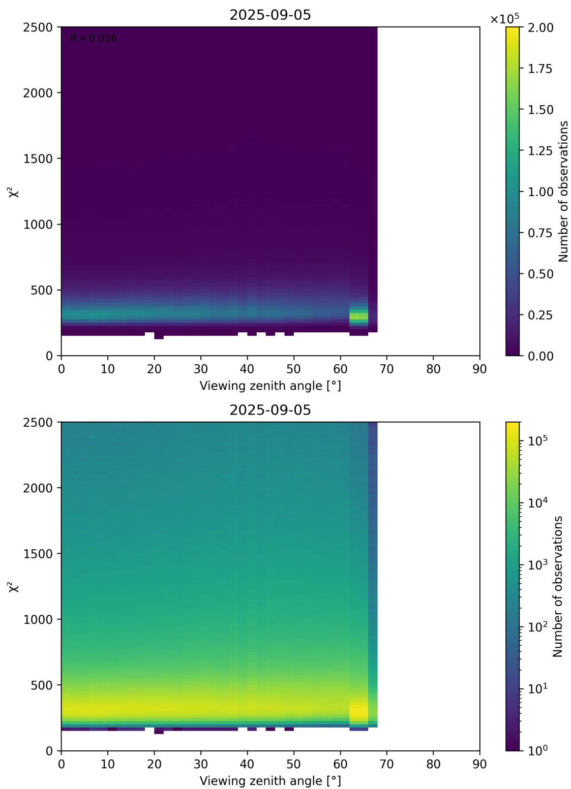
Figure 162: Scatter density plot of “Viewing zenith angle” against “ \chi^2 ” for 2025-09-04 to 2025-09-06.
