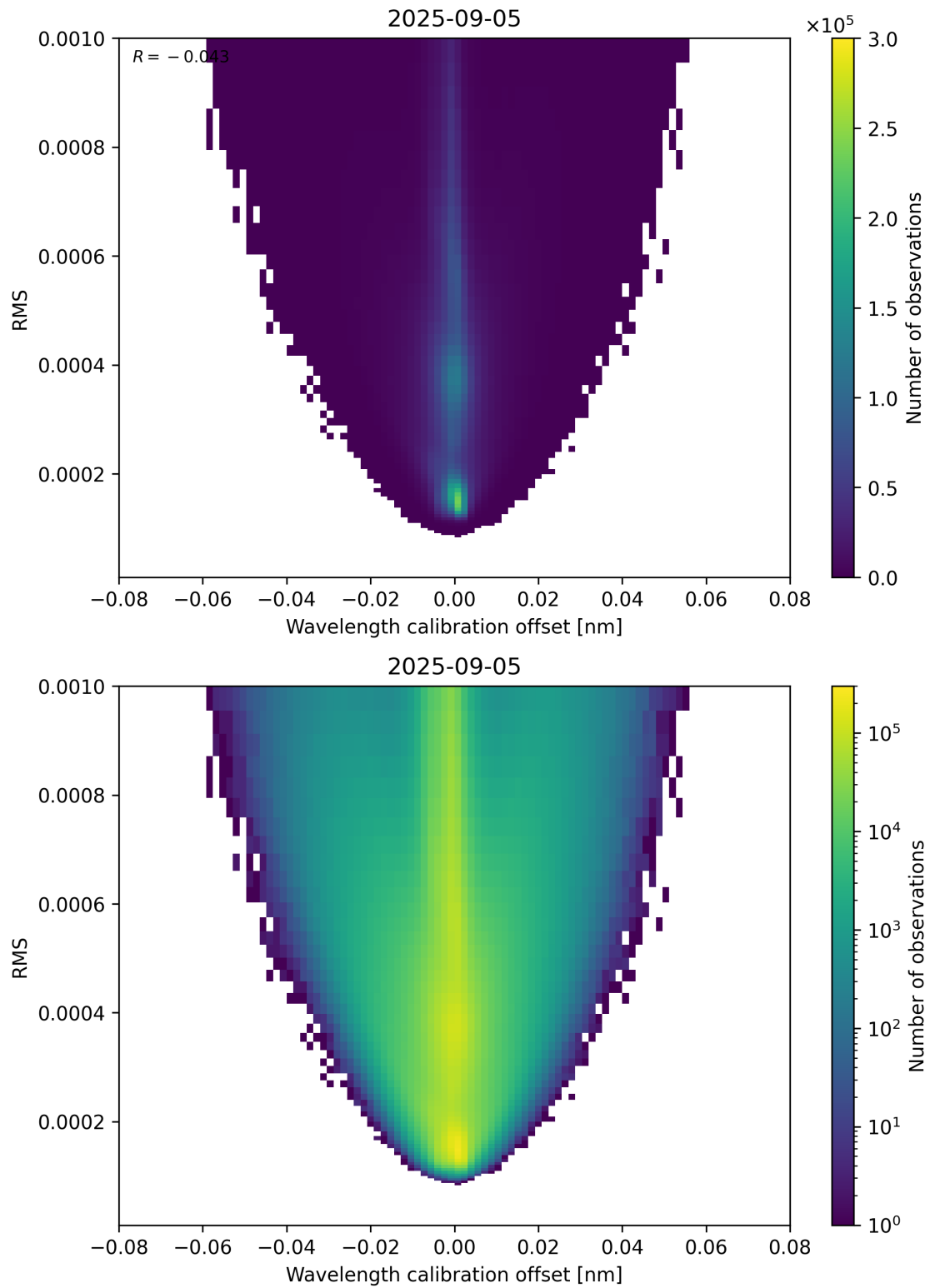
Figure 181: Scatter density plot of “Wavelength calibration offset” against “RMS” for 2025-09-04 to 2025-09-06.
