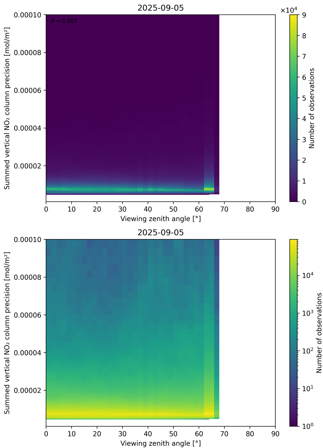
Figure 166: Scatter density plot of “Viewing zenith angle” against “Summed vertical NO 2 column precision” for 2025-09-04 to 2025-09-06.
