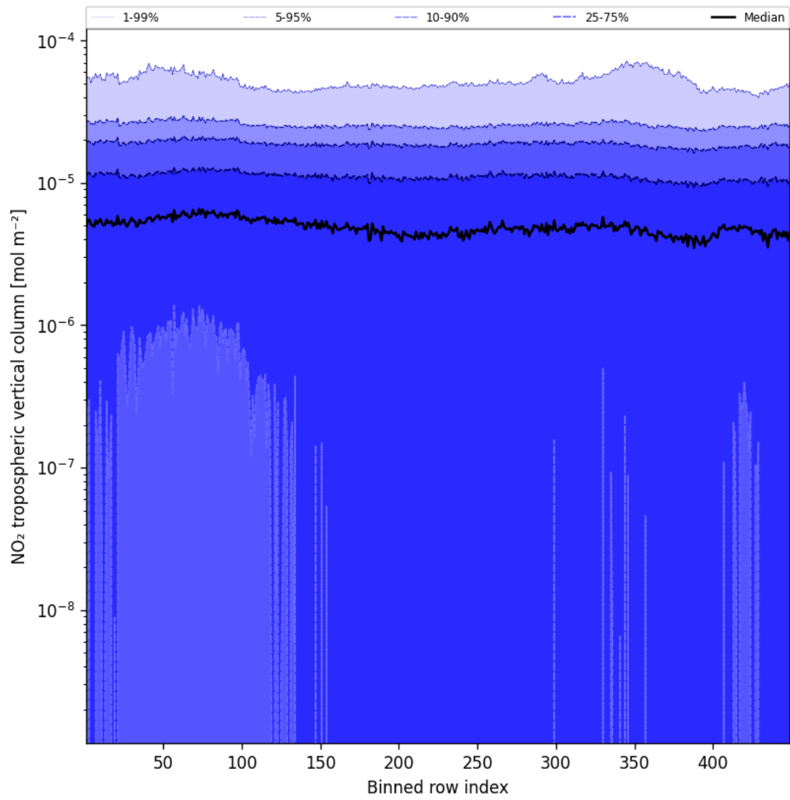
Figure 46: Along track statistics of “NO 2 tropospheric vertical column” for 2025-09-04 to 2025-09-06
