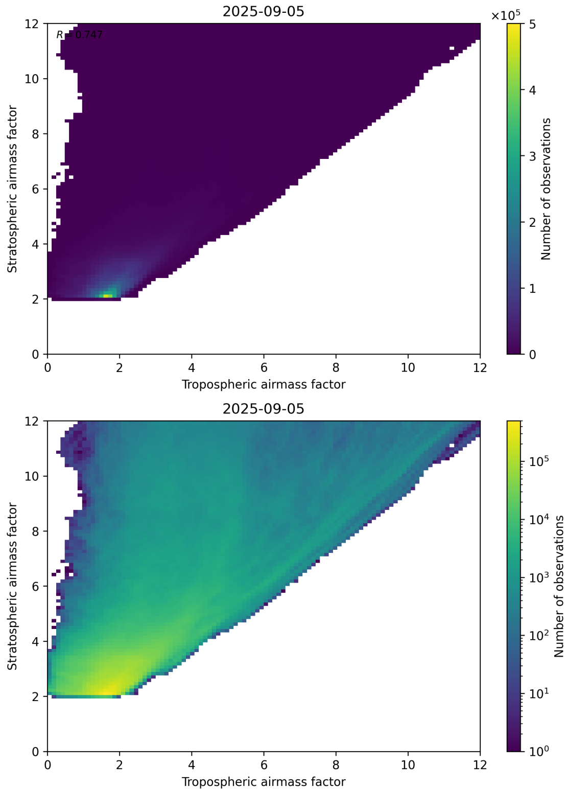
Figure 71: Scatter density plot of “Tropospheric airmass factor” against “Stratospheric airmass factor” for 2025-09-04 to 2025-09-06.
