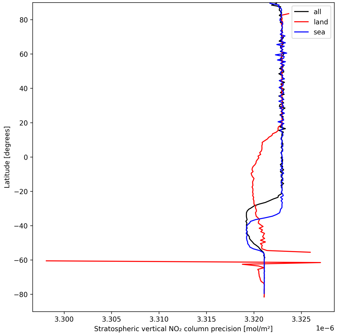
Figure 20: Zonal average of “Stratospheric vertical NO 2 column precision” for 2025-09-04 to 2025-09-06.
