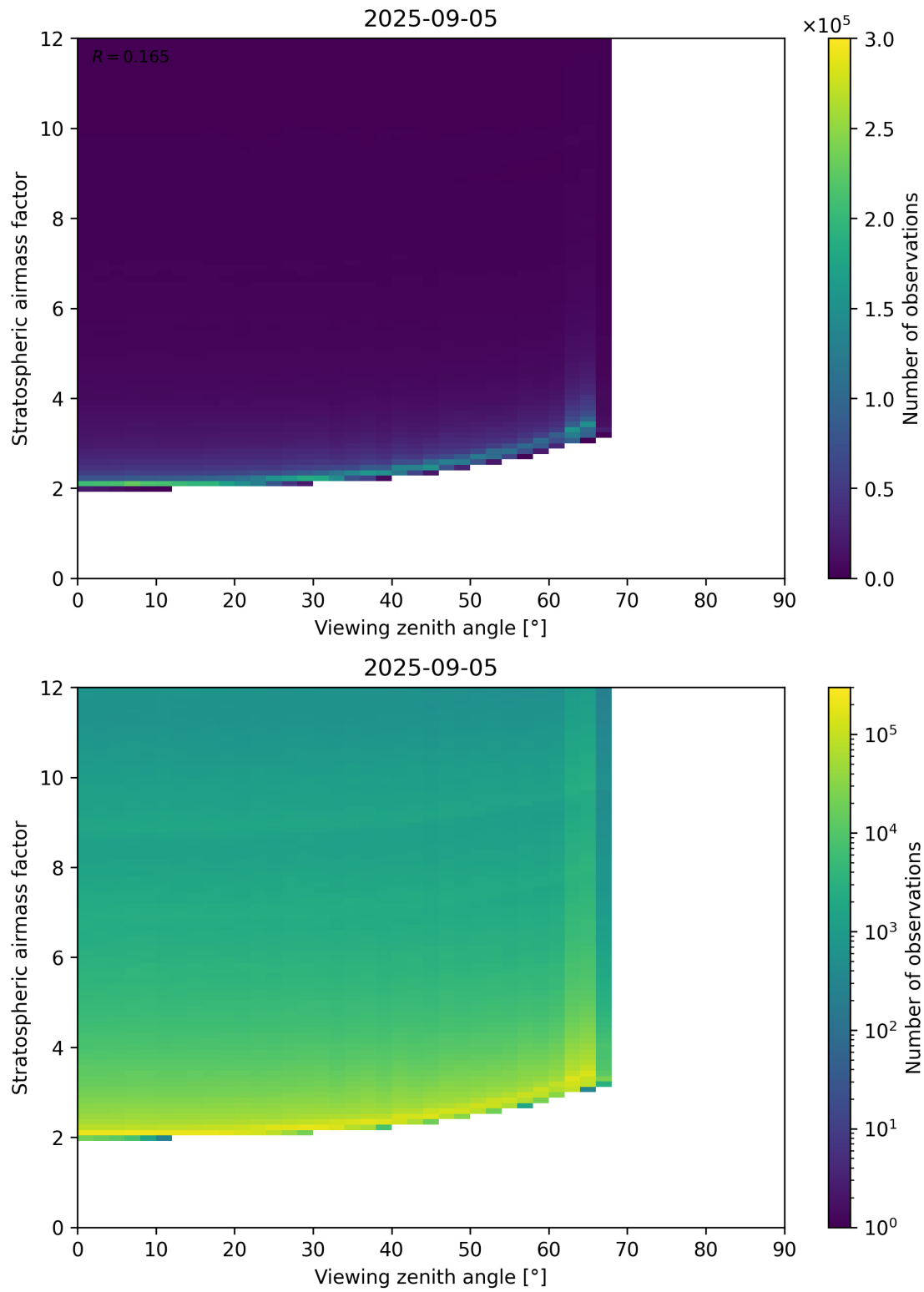
Figure 159: Scatter density plot of “Viewing zenith angle” against “Stratospheric airmass factor” for 2025-09-04 to 2025-09-06.
