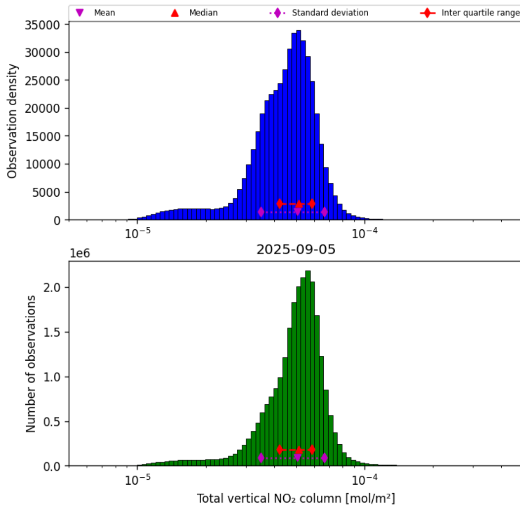
Figure 38: Histogram of “Total vertical NO 2 column” for 2025-09-04 to 2025-09-06
