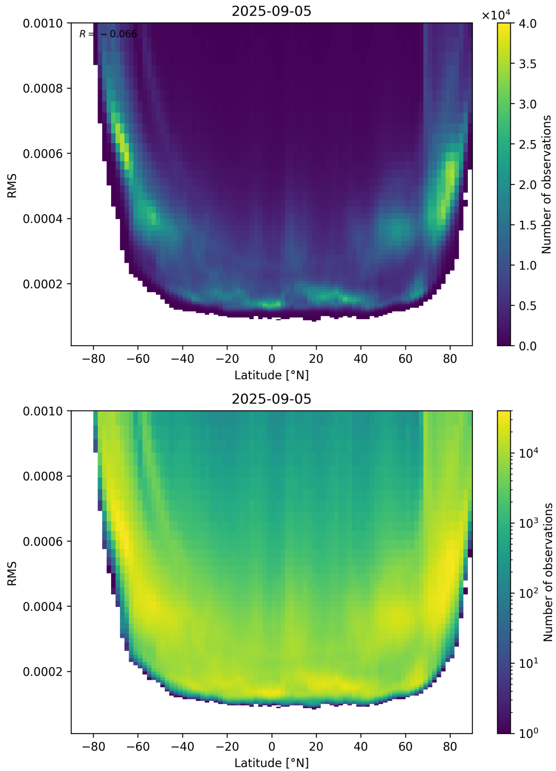
Figure 94: Scatter density plot of “Latitude” against “RMS” for 2025-09-04 to 2025-09-06.
