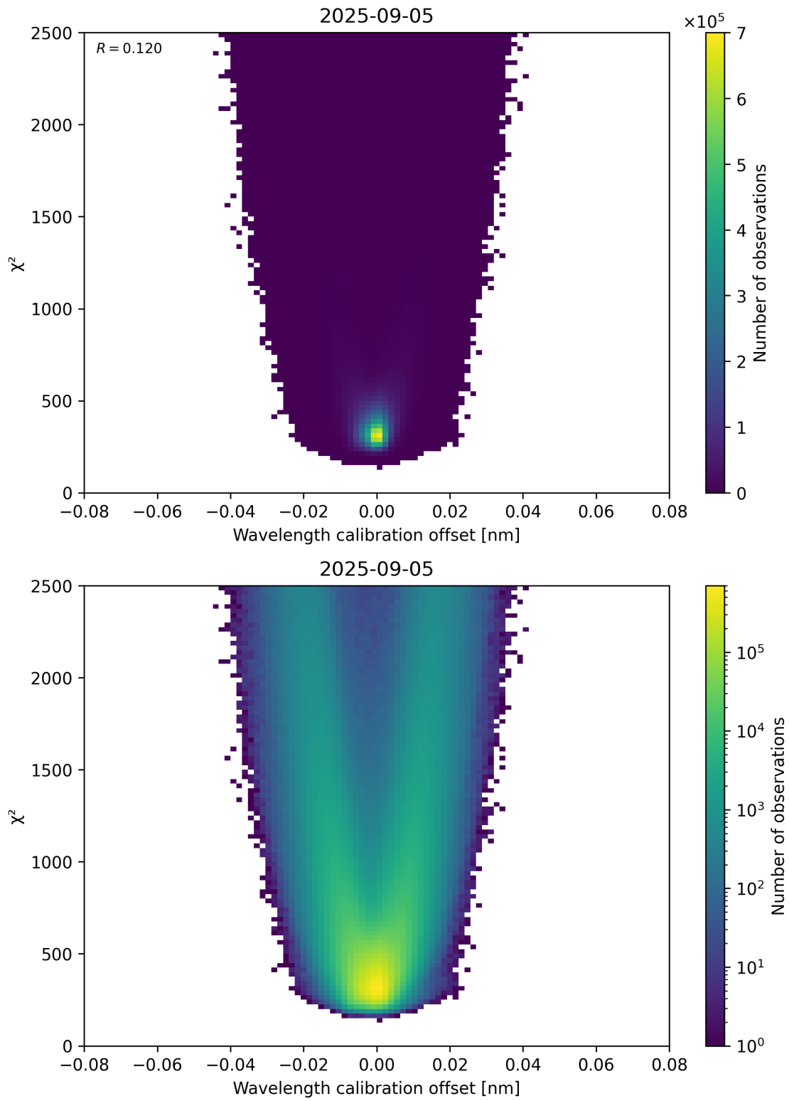
Figure 175: Scatter density plot of “Wavelength calibration offset” against “ \chi^2 ” for 2025-09-04 to 2025-09-06.
