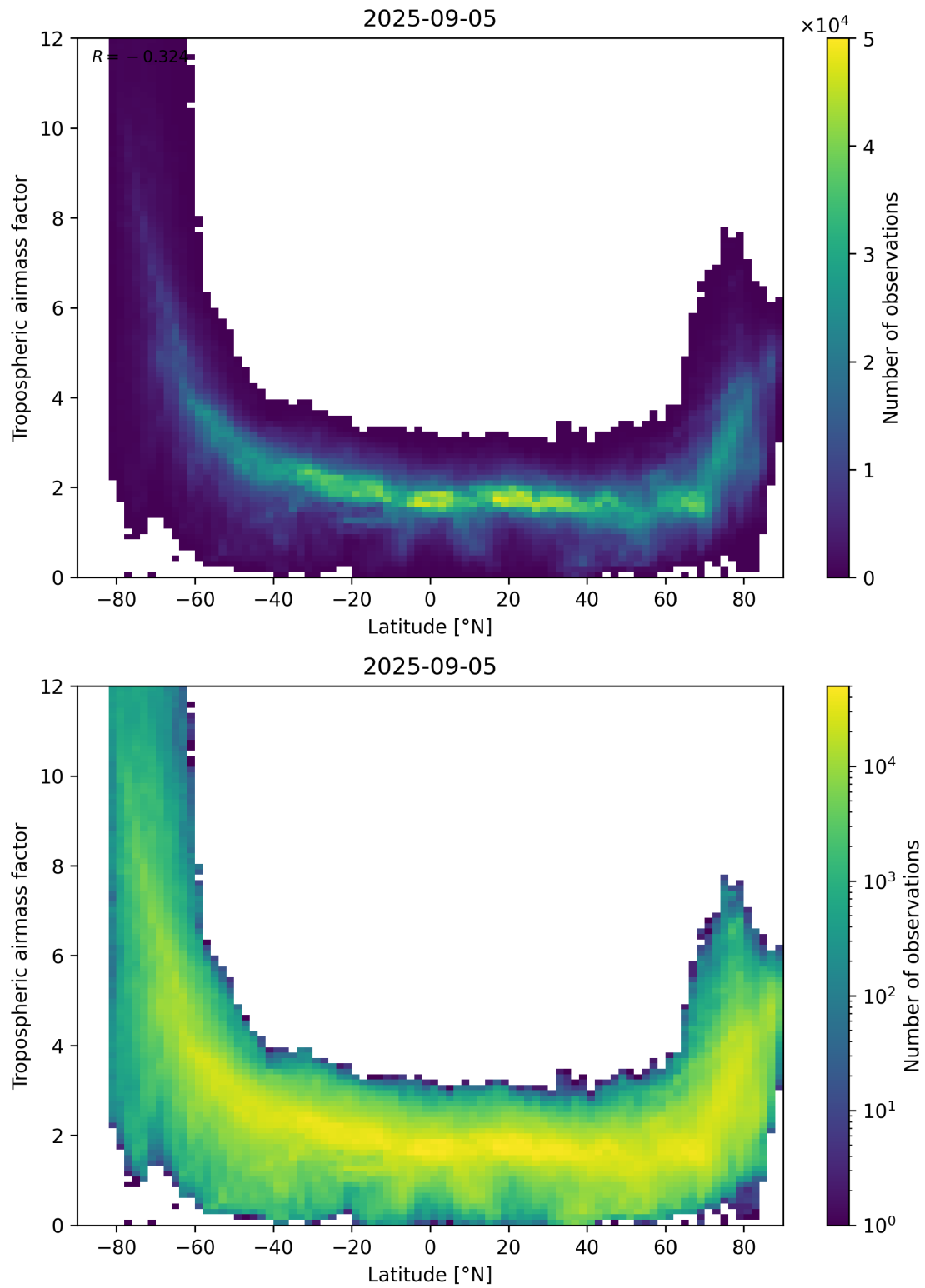
Figure 85: Scatter density plot of “Latitude” against “Tropospheric air mass factor” for 2025-09-04 to 2025-09-06.
