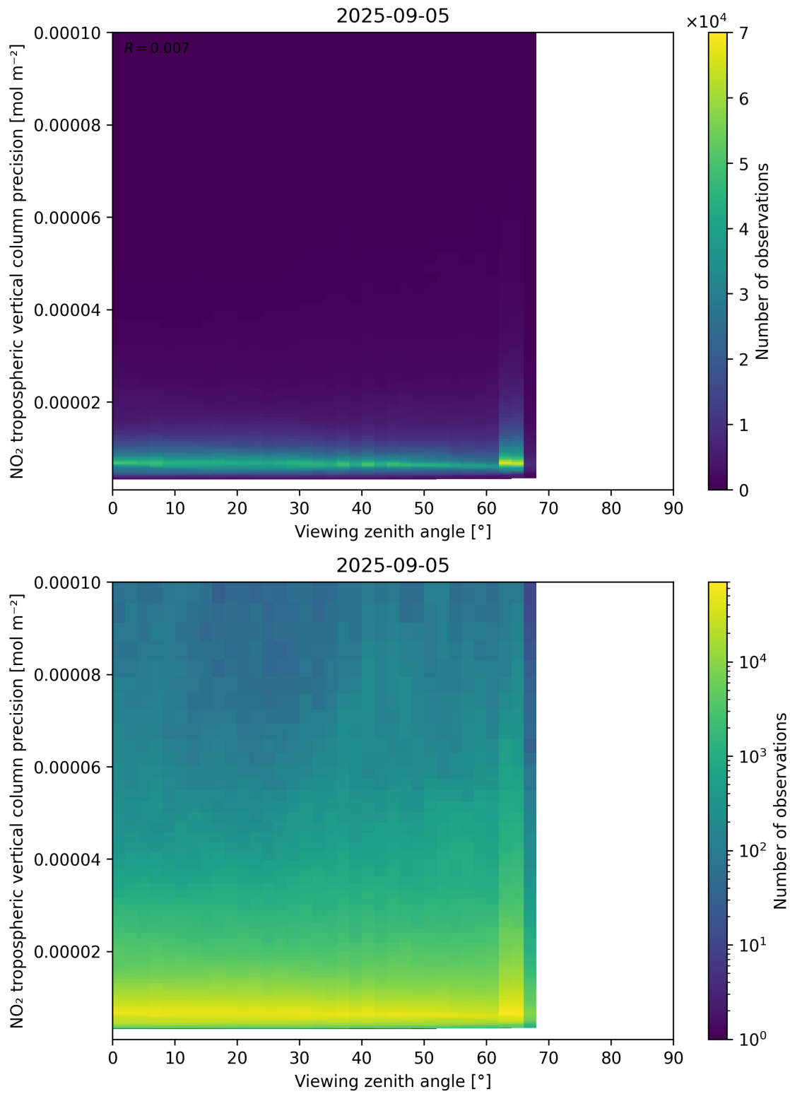
Figure 170: Scatter density plot of “Viewing zenith angle” against “NO 2 tropospheric vertical column precision” for 2025-09-04 to 2025-09-06.
