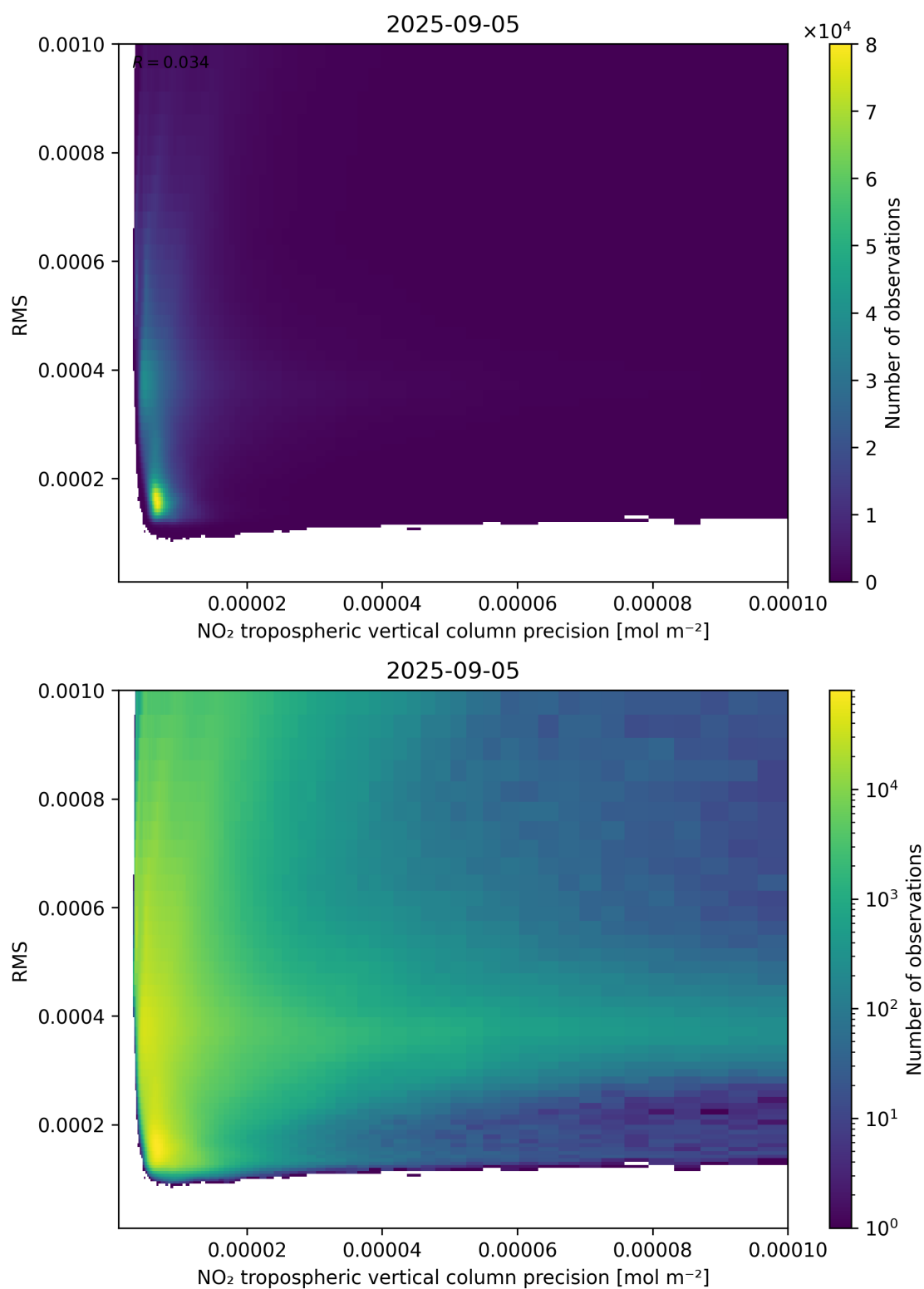
Figure 140: Scatter density plot of “NO 2 tropospheric vertical column precision” against “RMS” for 2025-09-04 to 2025-09-06.
