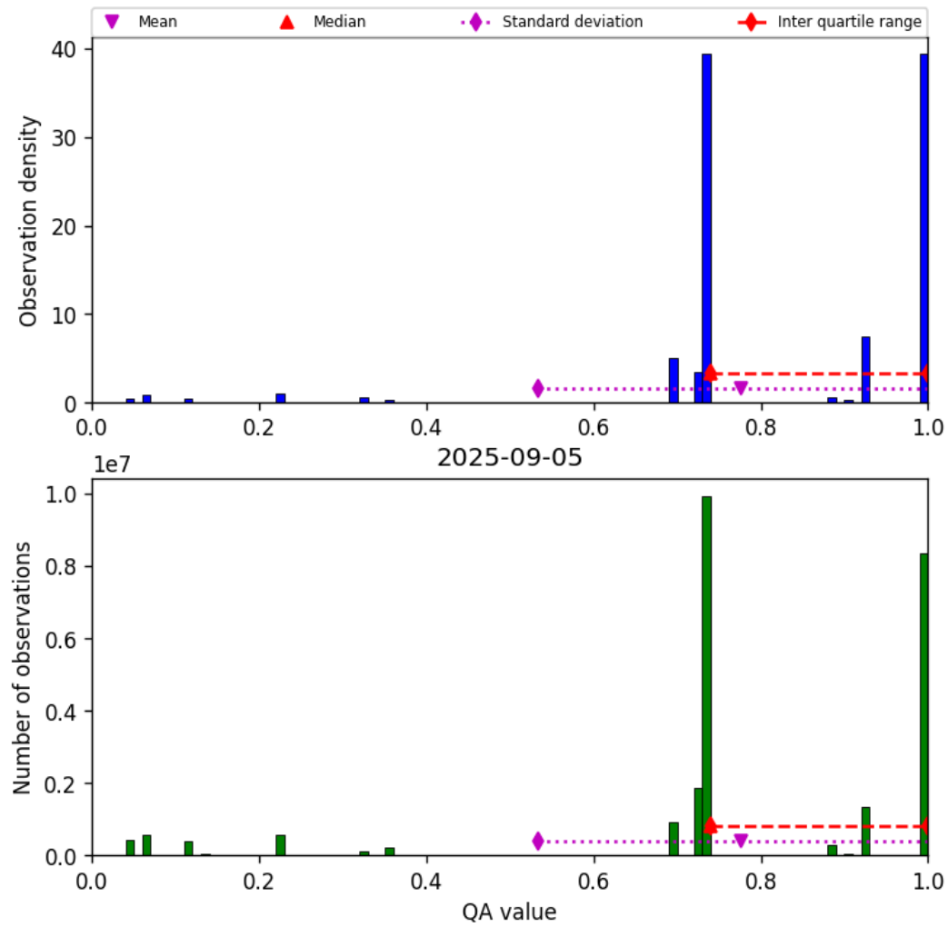
Figure 28: Histogram of “QA value” for 2025-09-04 to 2025-09-06
