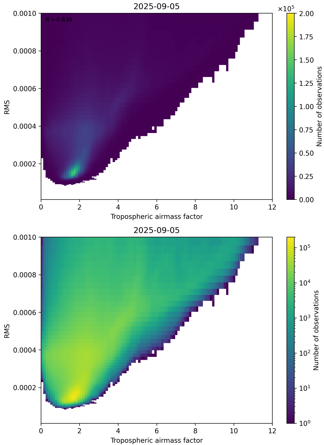
Figure 79: Scatter density plot of “Tropospheric airmass factor” against “RMS” for 2025-09-04 to 2025-09-06.
