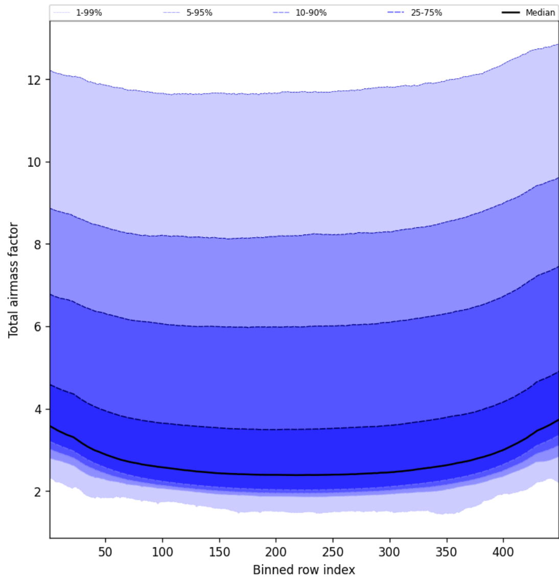
Figure 49: Along track statistics of “Total airmass factor” for 2025-09-04 to 2025-09-06
