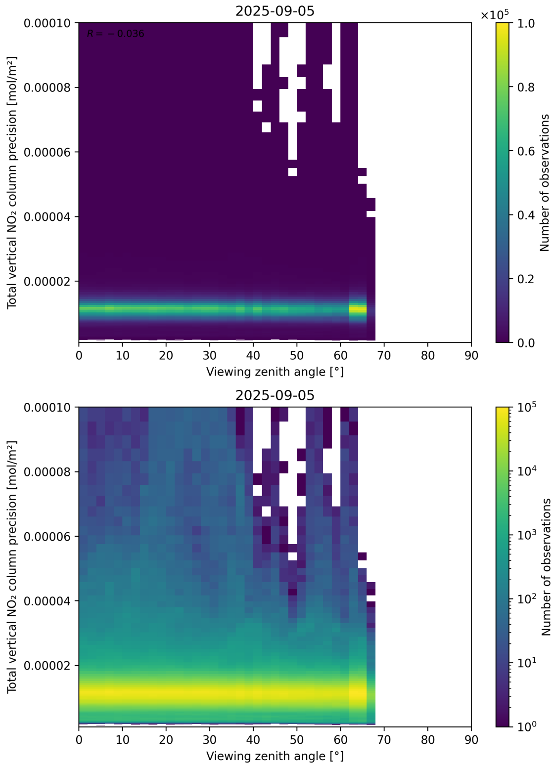
Figure 168: Scatter density plot of “Viewing zenith angle” against “Total vertical NO 2 column precision” for 2025-09-04 to 2025-09-06.
