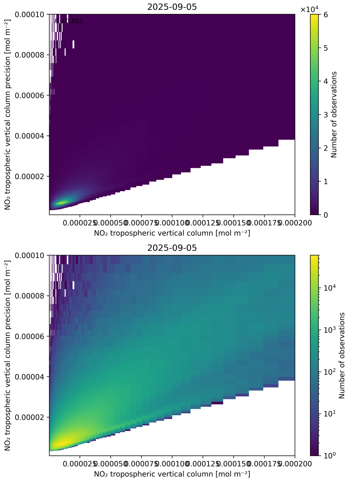
Figure 130: Scatter density plot of “NO 2 tropospheric vertical column” against “NO 2 tropospheric vertical column precision” for 2025-09-04 to 2025-09-06.
