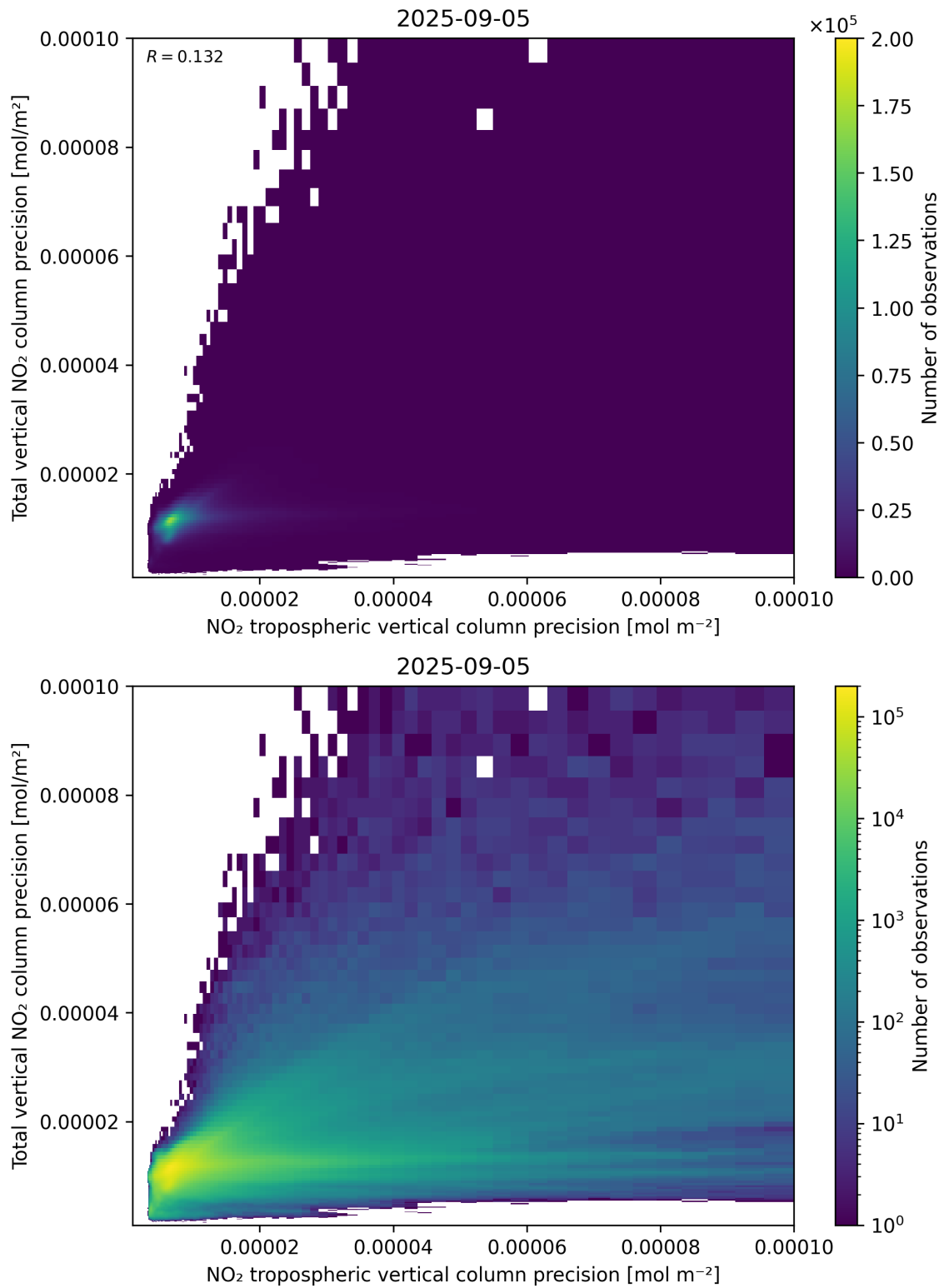
Figure 139: Scatter density plot of “NO 2 tropospheric vertical column precision” against “Total vertical NO 2 column precision” for 2025-09-04 to 2025-09-06.
