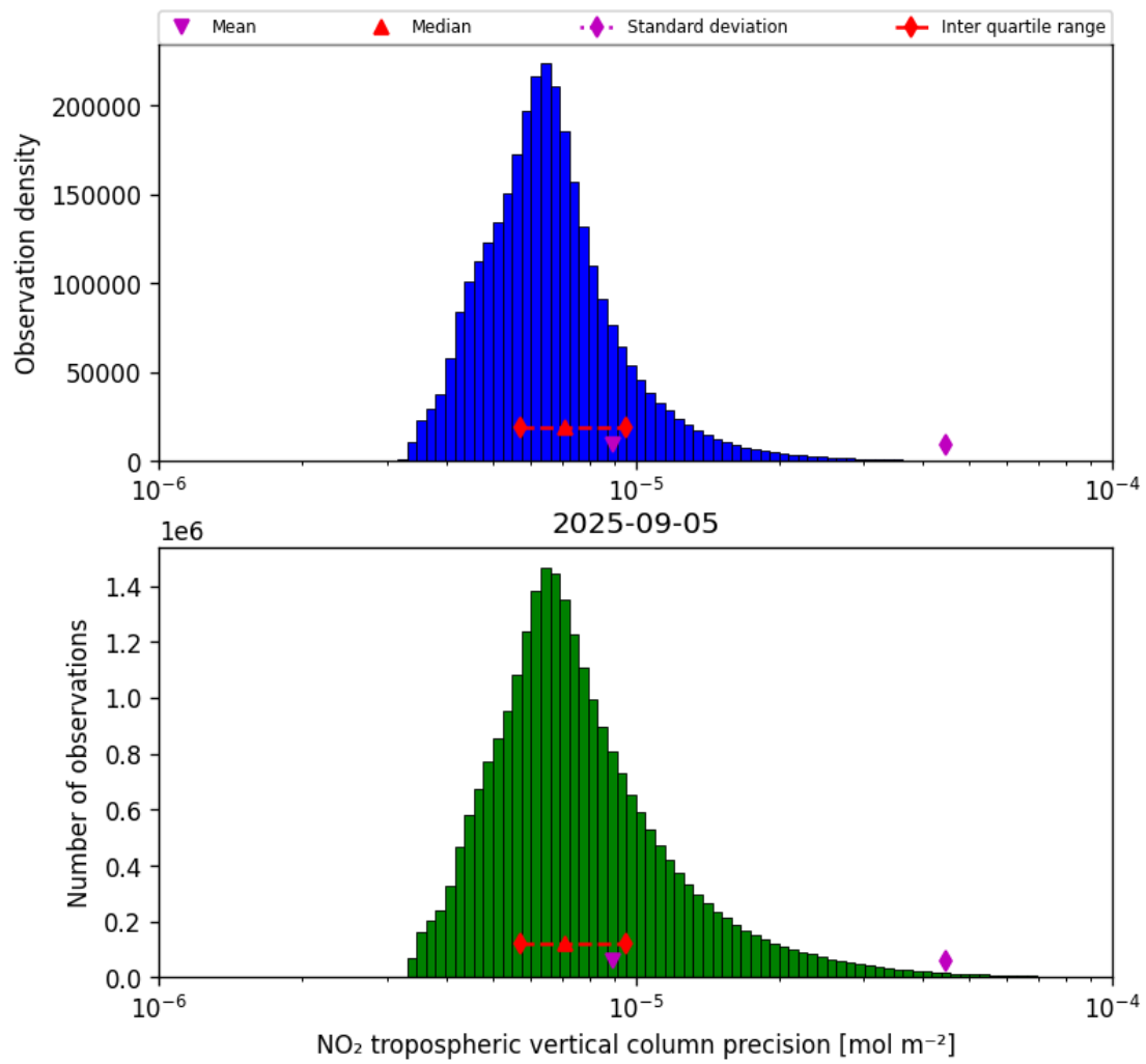
Figure 30: Histogram of “NO 2 tropospheric vertical column precision” for 2025-09-04 to 2025-09-06
