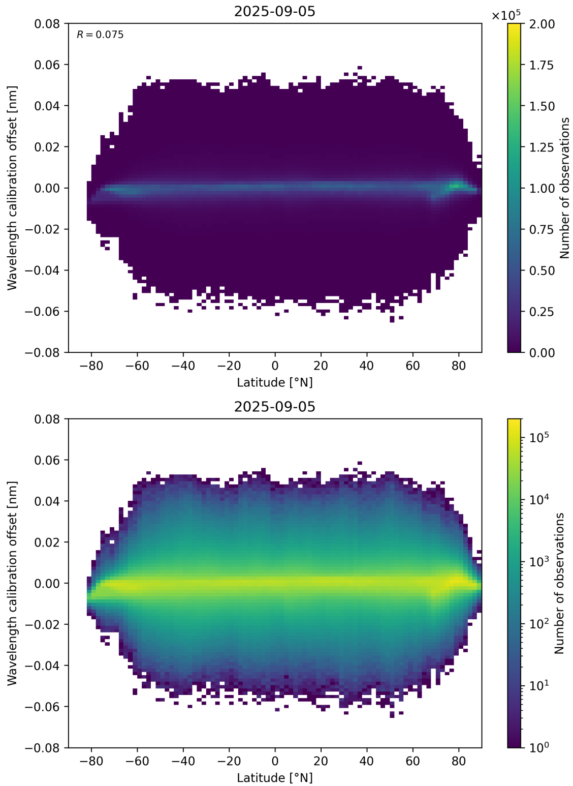
Figure 95: Scatter density plot of “Latitude” against “Wavelength calibration offset” for 2025-09-04 to 2025-09-06.
