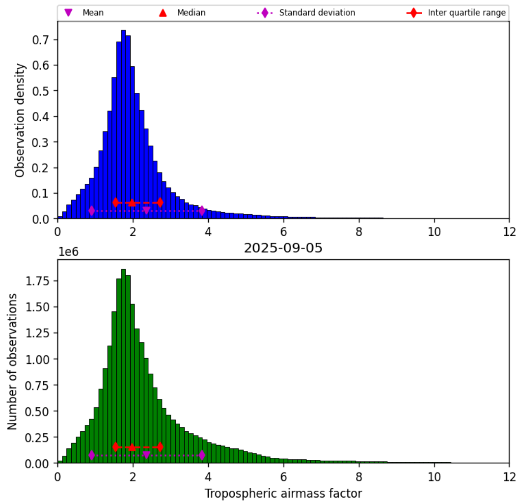
Figure 31: Histogram of “Tropospheric airmass factor” for 2025-09-04 to 2025-09-06
