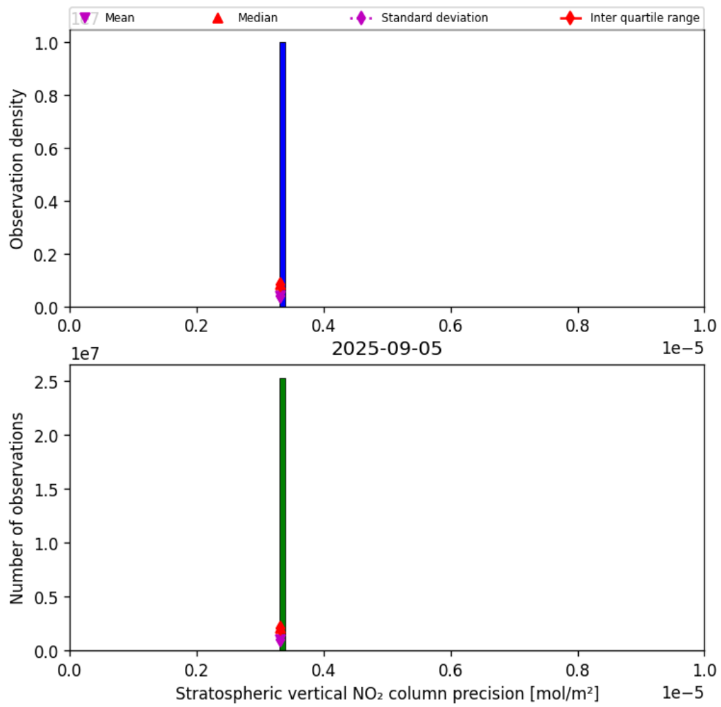
Figure 37: Histogram of “Stratospheric vertical NO 2 column precision” for 2025-09-04 to 2025-09-06
