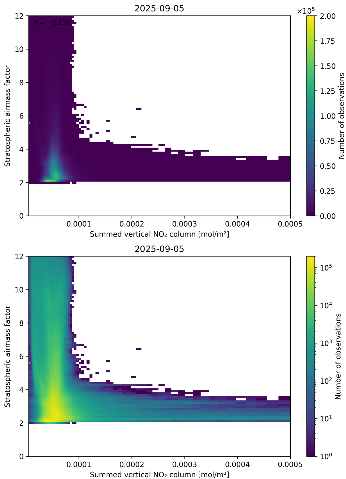
Figure 103: Scatter density plot of “Summed vertical NO 2 column” against “Stratospheric airmass factor” for 2025-09-04 to 2025-09-06.
