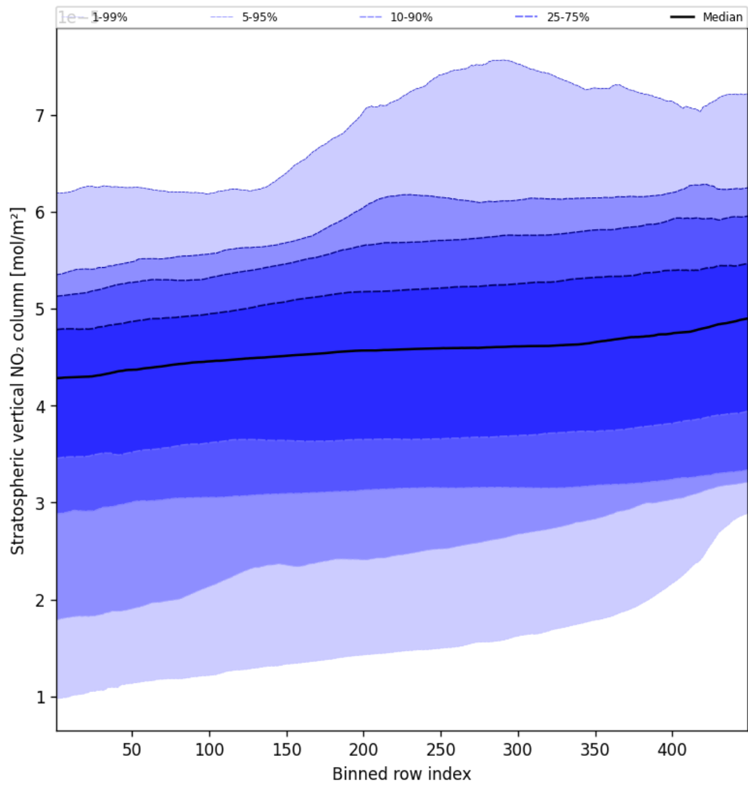
Figure 53: Along track statistics of “Stratospheric vertical NO 2 column” for 2025-09-04 to 2025-09-06
