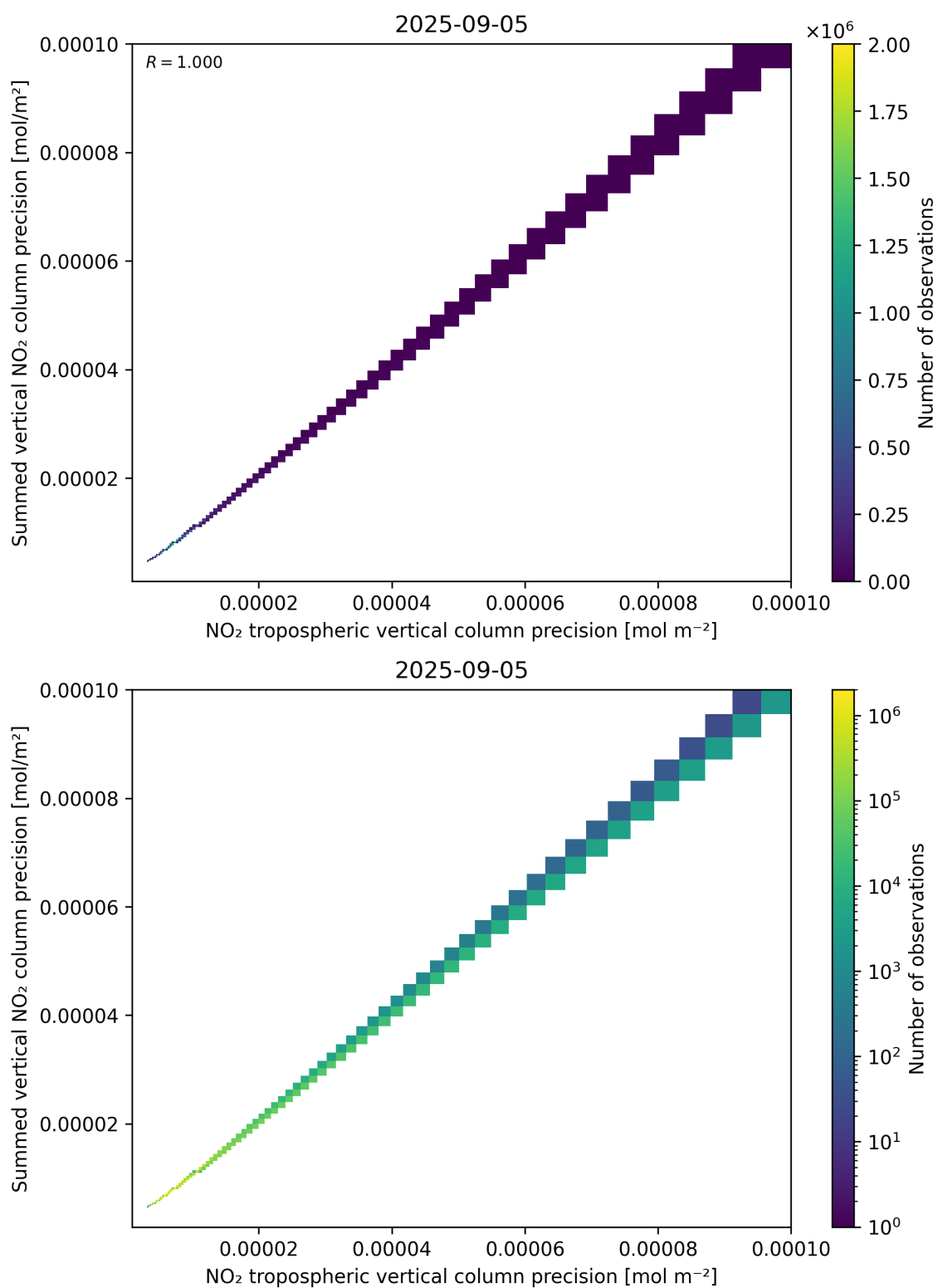
Figure 137: Scatter density plot of “NO 2 tropospheric vertical column precision” against “Summed vertical NO 2 column precision” for 2025-09-04 to 2025-09-06.
