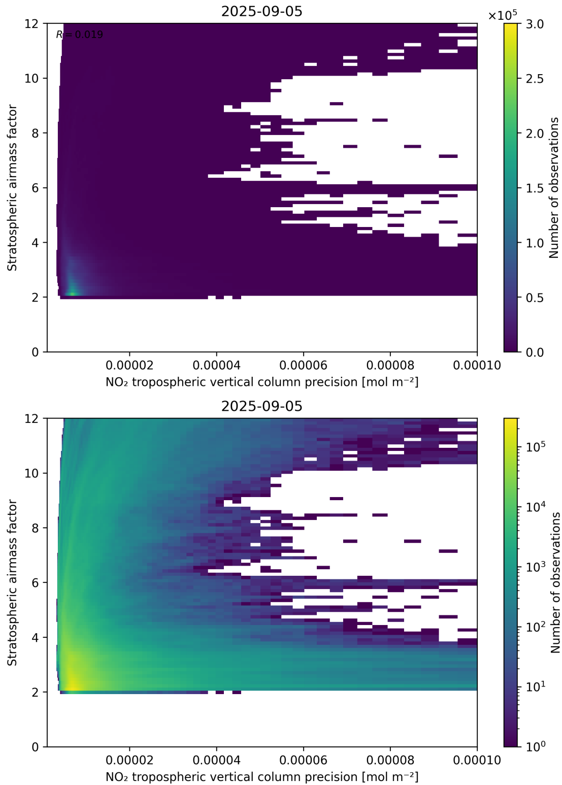
Figure 131: Scatter density plot of “NO 2 tropospheric vertical column precision” against “Stratospheric airmass factor” for 2025-09-04 to 2025-09-06.
