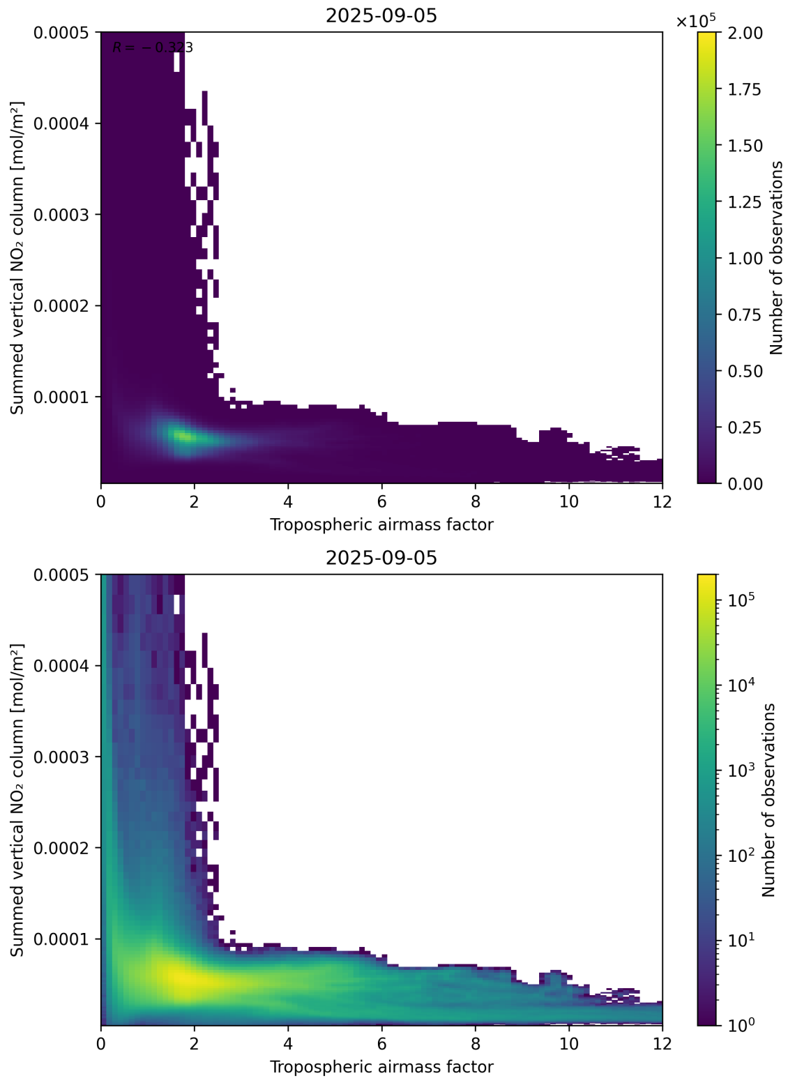
Figure 75: Scatter density plot of “Tropospheric airmass factor” against “Summed vertical NO 2 column” for 2025-09-04 to 2025-09-06.
