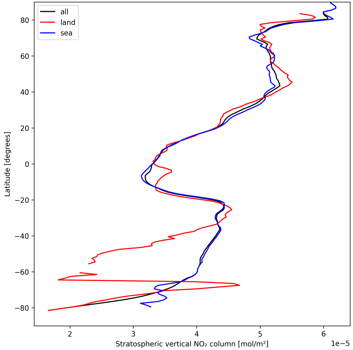
Figure 19: Zonal average of “Stratospheric vertical NO 2 column” for 2025-09-04 to 2025-09-06.
