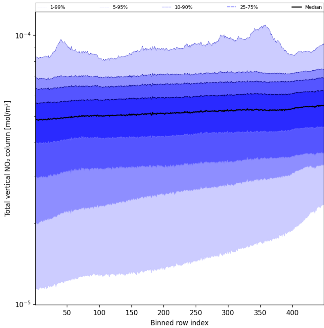
Figure 55: Along track statistics of “Total vertical NO 2 column” for 2025-09-04 to 2025-09-06
