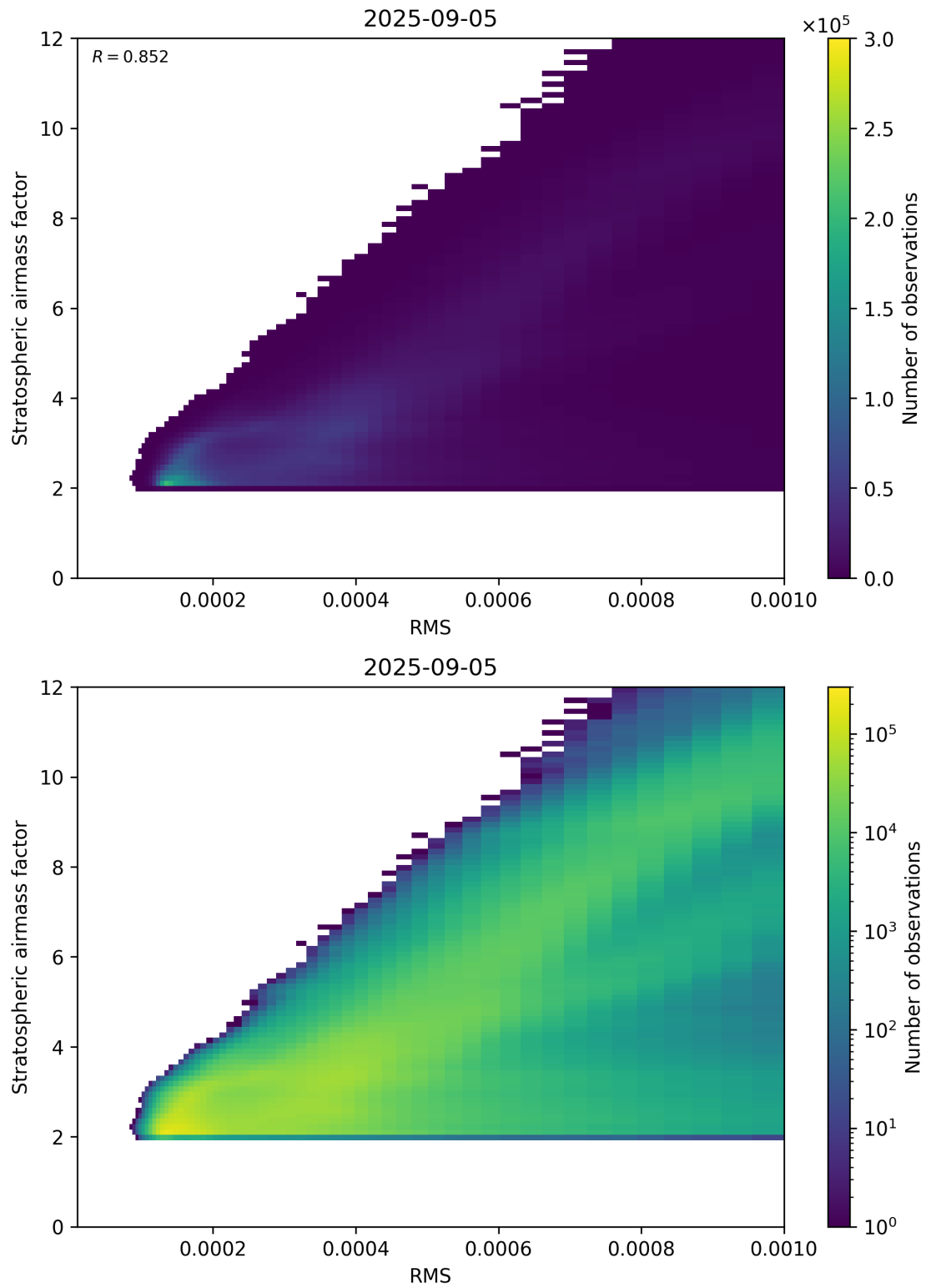
Figure 144: Scatter density plot of “RMS” against “Stratospheric airmass factor” for 2025-09-04 to 2025-09-06.
