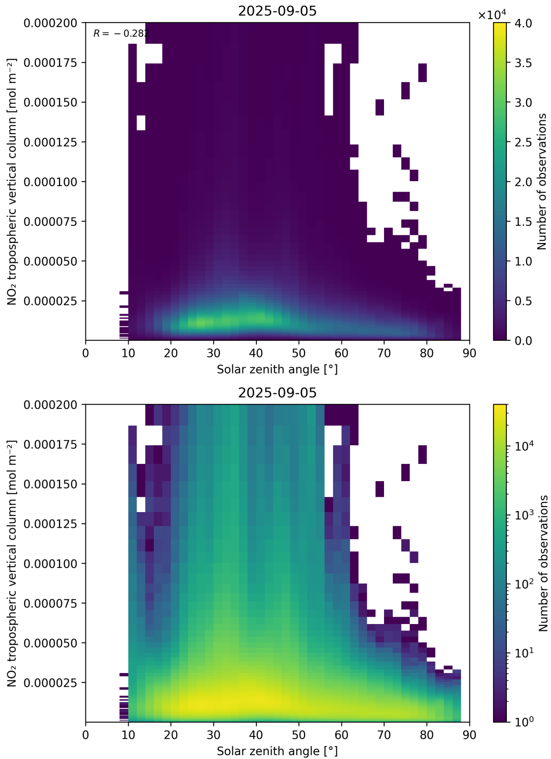
Figure 155: Scatter density plot of “Solar zenith angle” against “NO 2 tropospheric vertical column” for 2025-09-04 to 2025-09-06.
