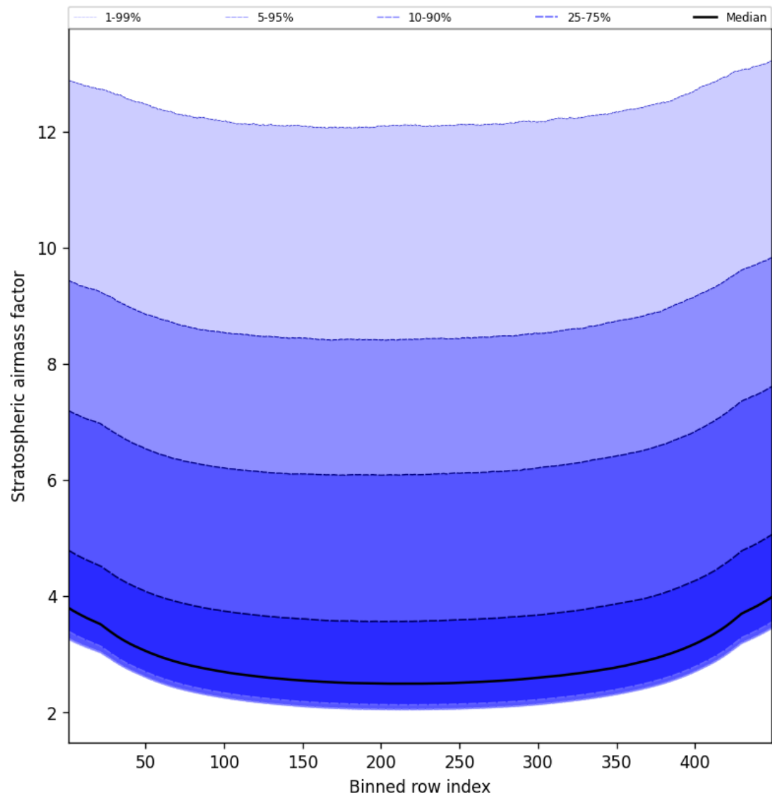
Figure 61: Along track statistics of “Stratospheric airmass factor” for 2025-09-04 to 2025-09-06
