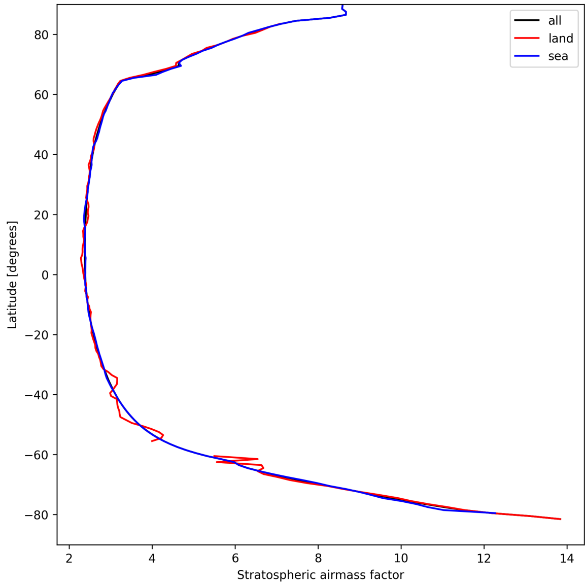
Figure 27: Zonal average of “Stratospheric air mass factor” for 2025-09-04 to 2025-09-06.
