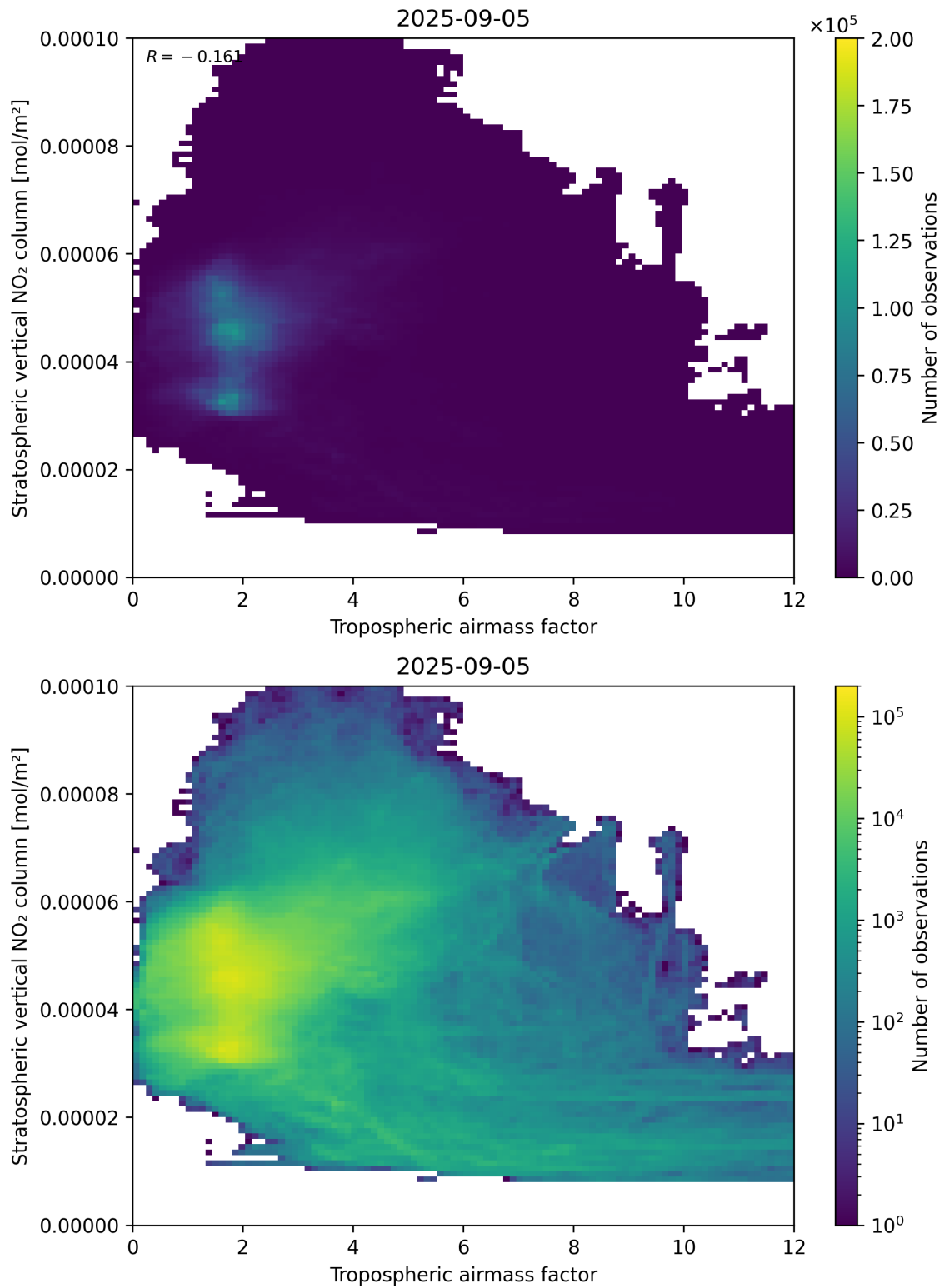
Figure 74: Scatter density plot of “Tropospheric air mass factor” against “Stratospheric vertical NO 2 column” for 2025-09-04 to 2025-09-06.
