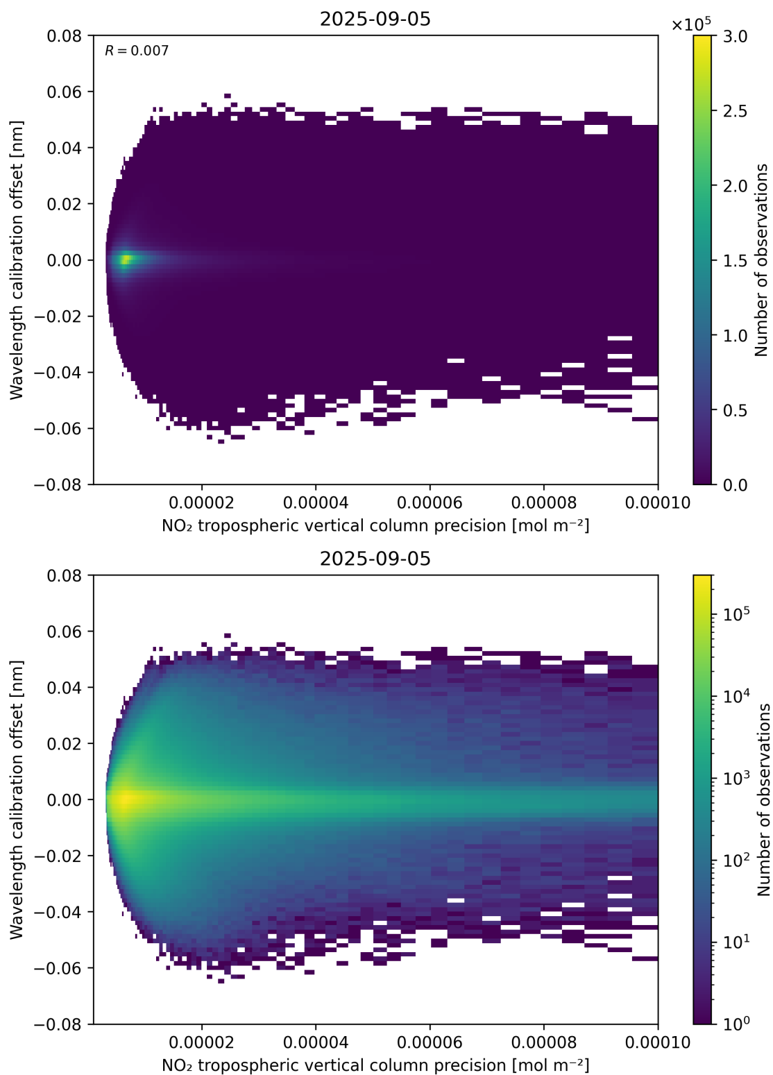
Figure 141: Scatter density plot of “NO 2 tropospheric vertical column precision” against “Wavelength calibration offset” for 2025-09-04 to 2025-09-06.
