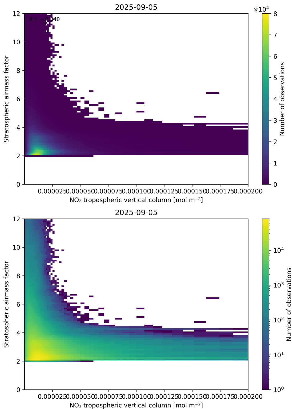
Figure 121: Scatter density plot of “NO 2 tropospheric vertical column” against “Stratospheric air mass factor” for 2025-09-04 to 2025-09-06.
