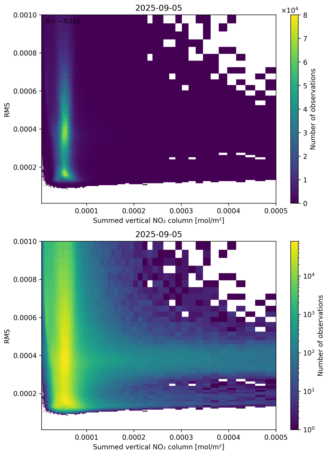
Figure 109: Scatter density plot of “Summed vertical NO 2 column” against “RMS” for 2025-09-04 to 2025-09-06.
