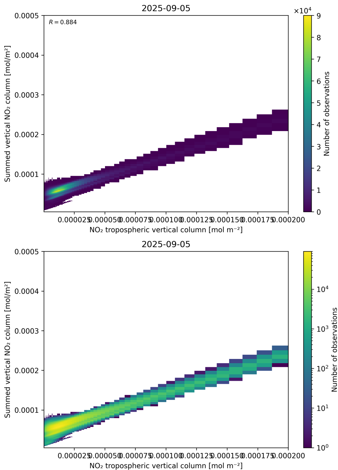
Figure 126: Scatter density plot of “NO 2 tropospheric vertical column” against “Summed vertical NO 2 column” for 2025-09-04 to 2025-09-06.
