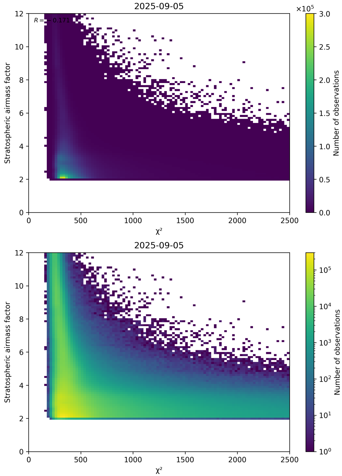
Figure 81: Scatter density plot of “ \chi^2 ” against “Stratospheric airmass factor” for 2025-09-04 to 2025-09-06.
