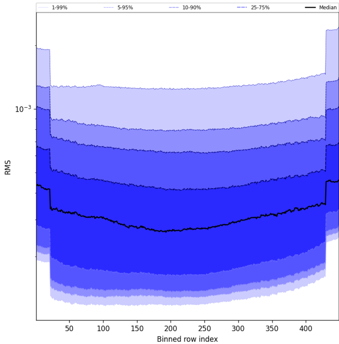
Figure 60: Along track statistics of “RMS” for 2025-09-04 to 2025-09-06
