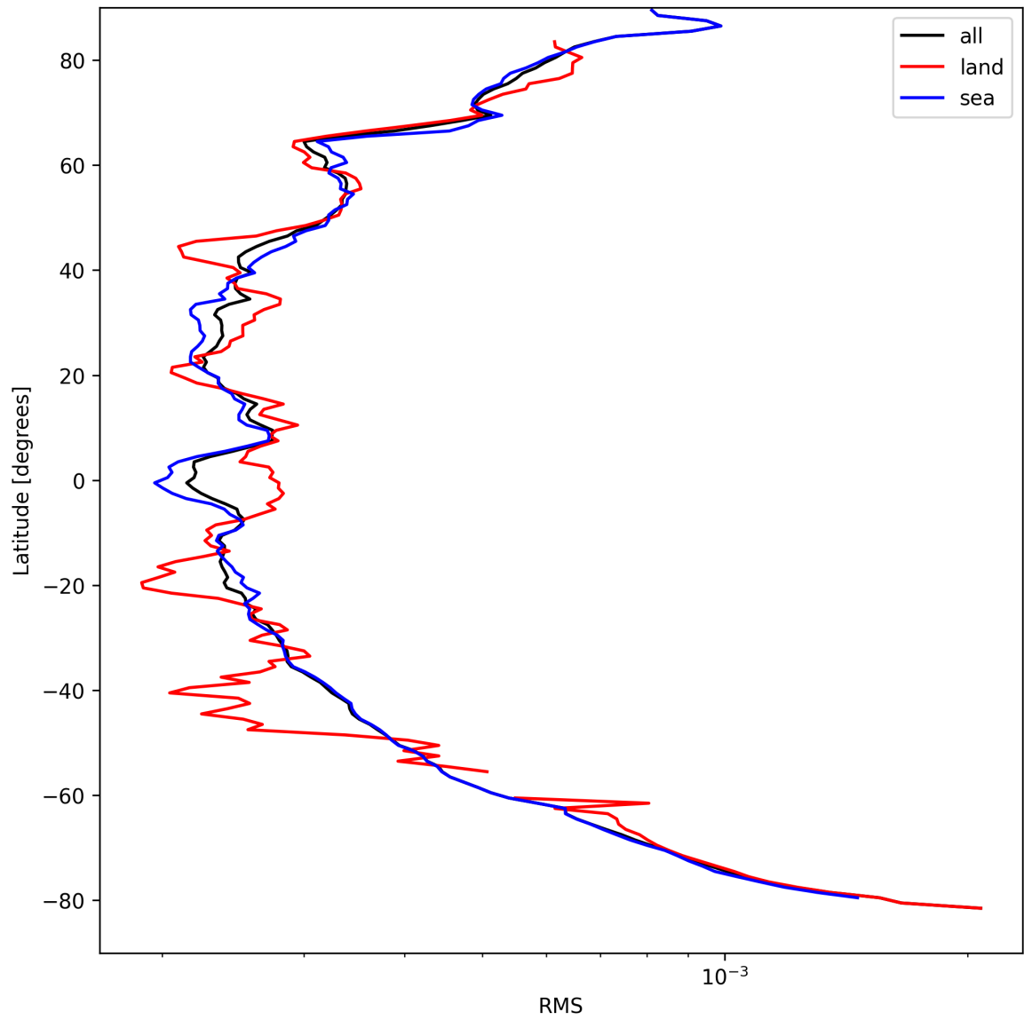
Figure 26: Zonal average of “RMS” for 2025-09-04 to 2025-09-06.
