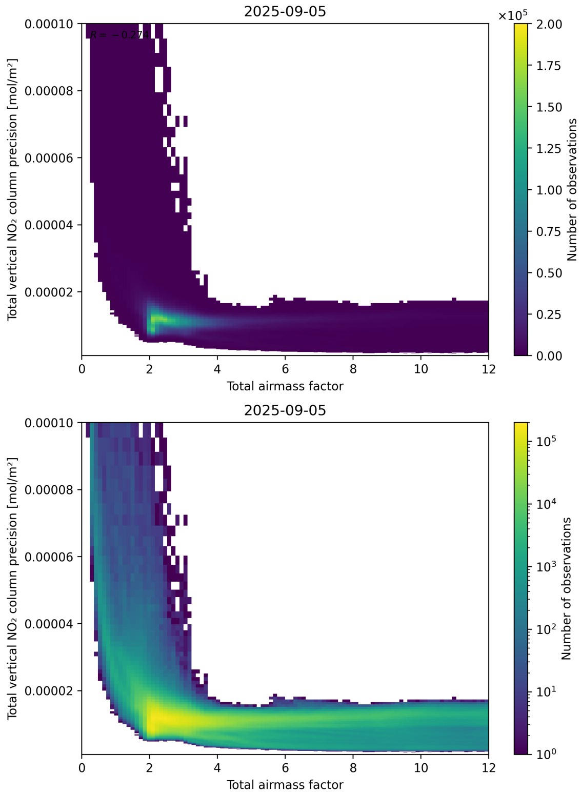
Figure 68: Scatter density plot of “Total airmass factor” against “Total vertical NO 2 column precision” for 2025-09-04 to 2025-09-06.
