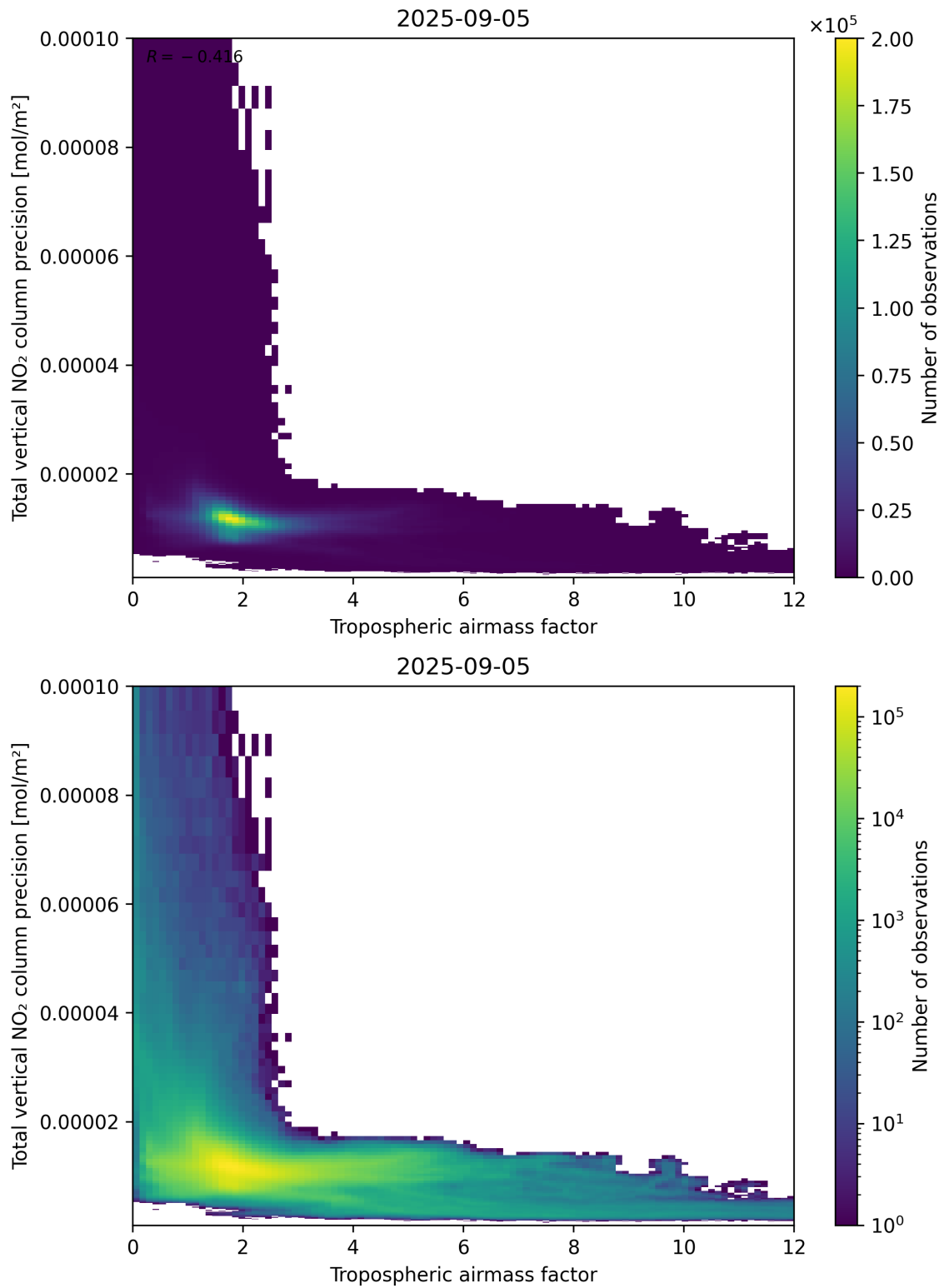
Figure 78: Scatter density plot of “Tropospheric air mass factor” against “Total vertical NO 2 column precision” for 2025-09-04 to 2025-09-06.
