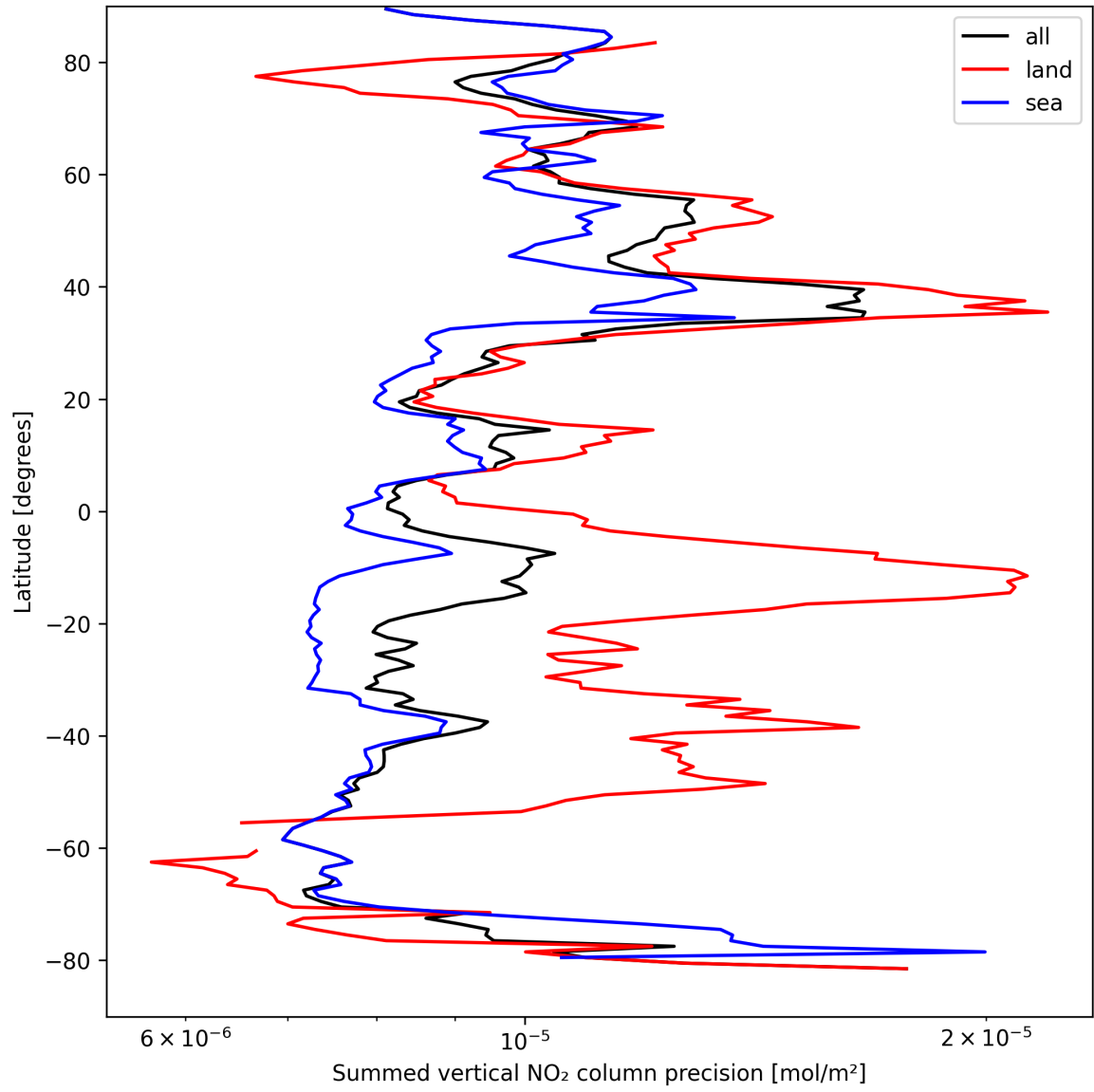
Figure 24: Zonal average of “Summed vertical NO 2 column precision” for 2025-09-04 to 2025-09-06.
