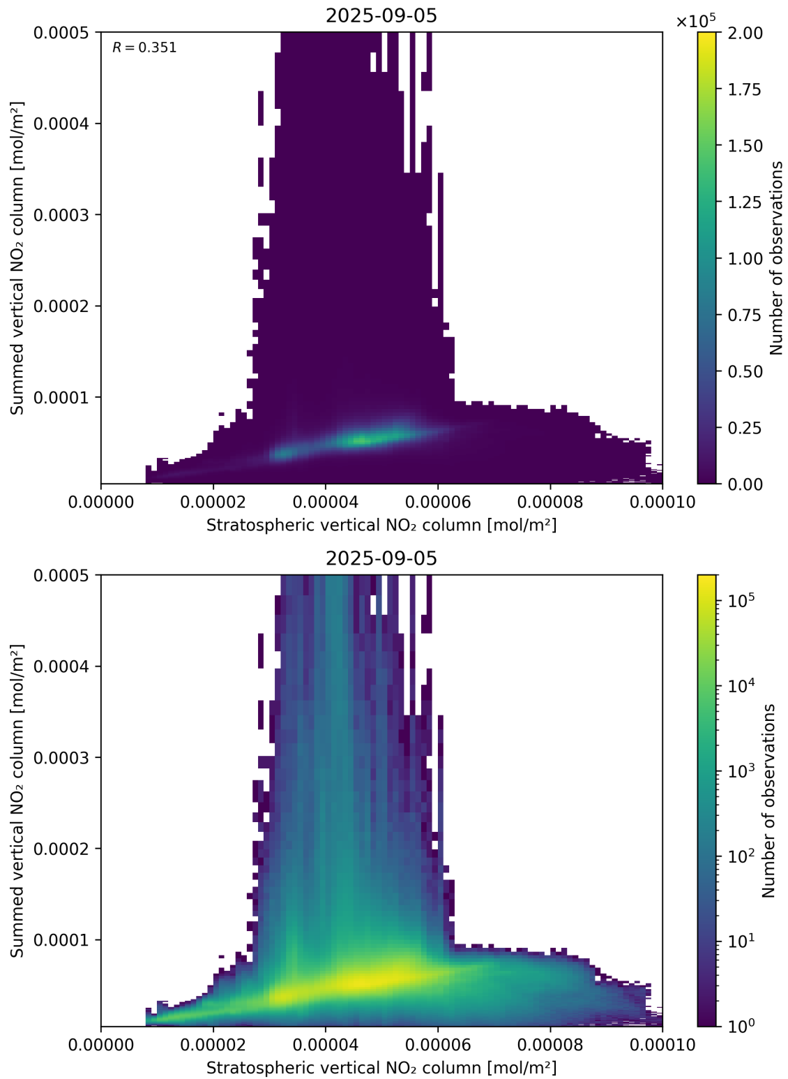
Figure 98: Scatter density plot of “Stratospheric vertical NO 2 column” against “Summed vertical NO 2 column” for 2025-09-04 to 2025-09-06.
