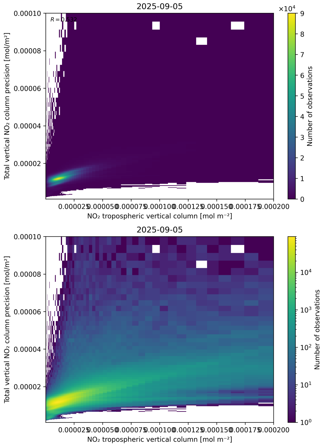
Figure 129: Scatter density plot of “NO 2 tropospheric vertical column” against “Total vertical NO 2 column precision” for 2025-09-04 to 2025-09-06.
