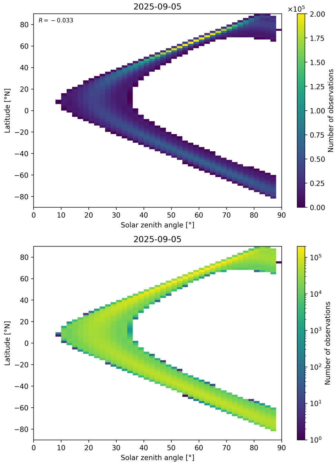
Figure 149: Scatter density plot of “Solar zenith angle” against “Latitude” for 2025-09-04 to 2025-09-06.
