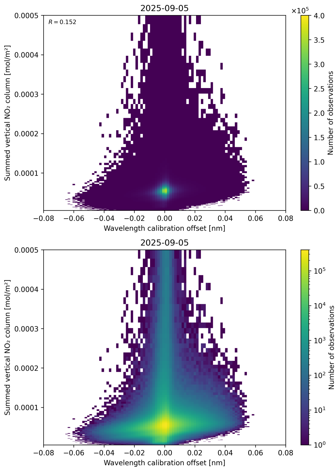
Figure 177: Scatter density plot of “Wavelength calibration offset” against “Summed vertical NO 2 column” for 2025-09-04 to 2025-09-06.
