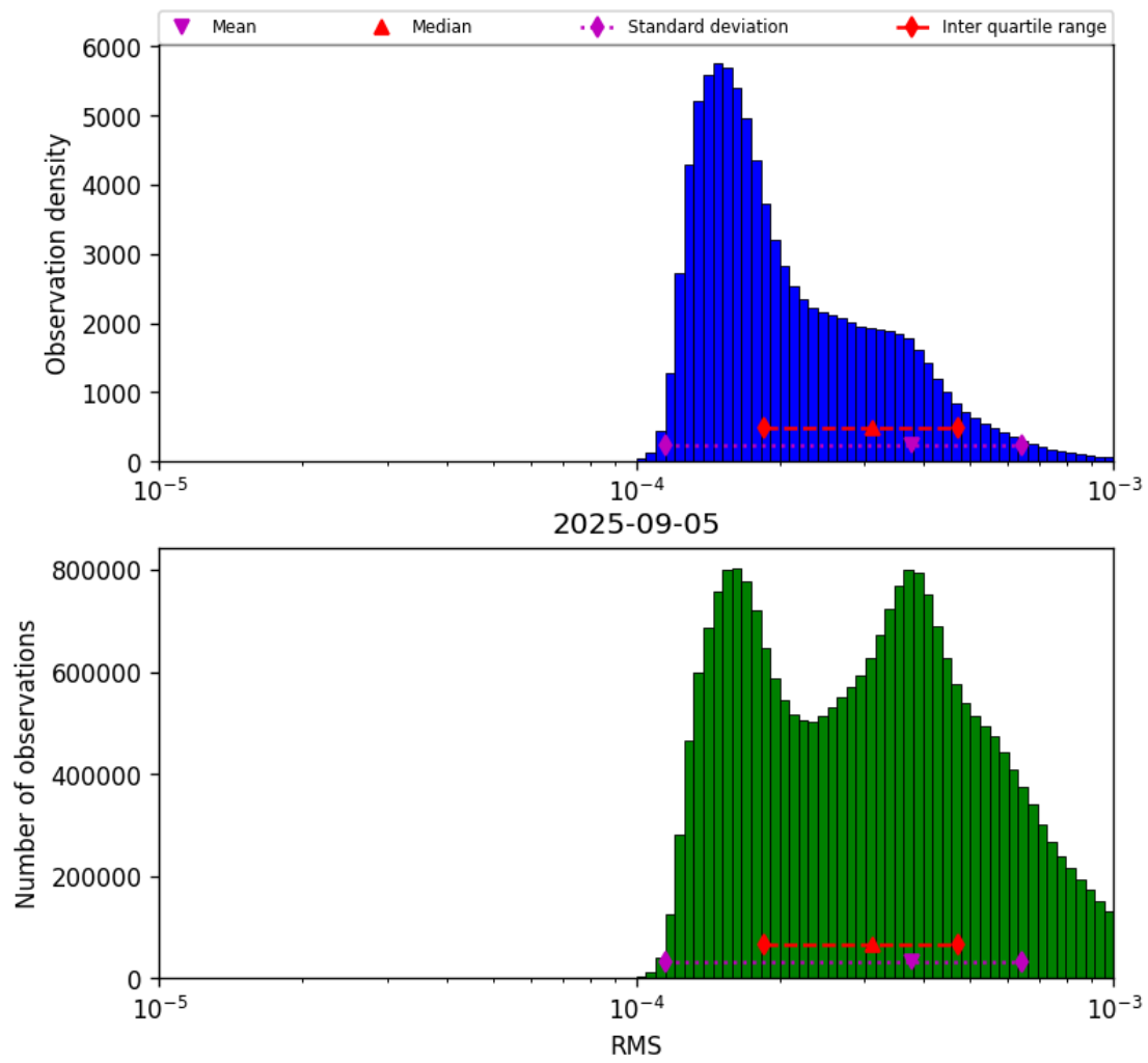
Figure 43: Histogram of “RMS” for 2025-09-04 to 2025-09-06
