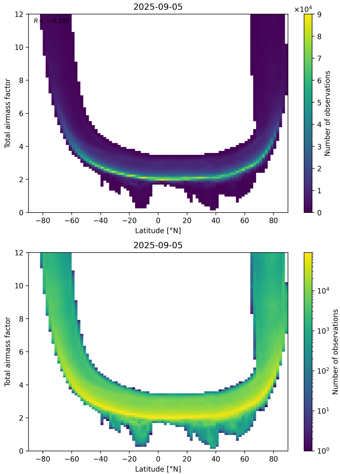
Figure 84: Scatter density plot of “Latitude” against “Total airmass factor” for 2025-09-04 to 2025-09-06.
