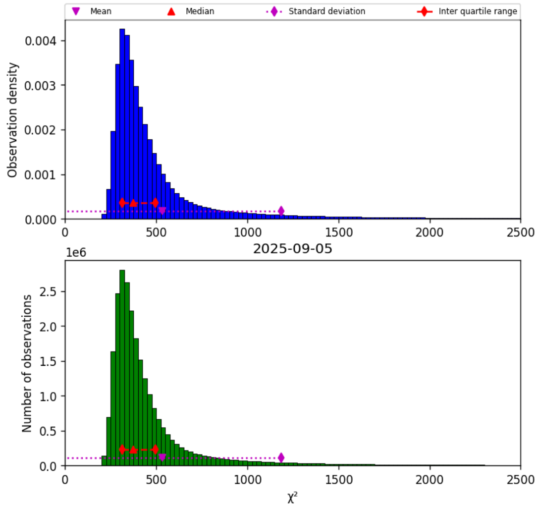
Figure 42: Histogram of “ \chi^2 ” for 2025-09-04 to 2025-09-06
