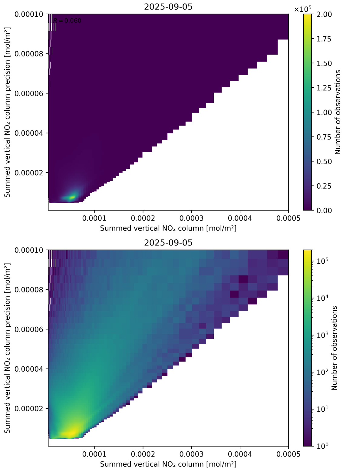
Figure 105: Scatter density plot of “Summed vertical NO 2 column” against “Summed vertical NO 2 column precision” for 2025-09-04 to 2025-09-06.
