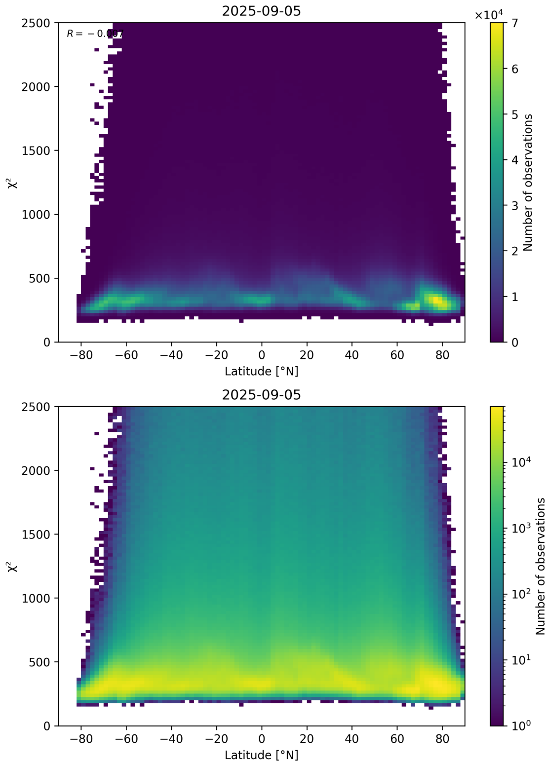
Figure 86: Scatter density plot of “Latitude” against “ \chi^2 ” for 2025-09-04 to 2025-09-06.
