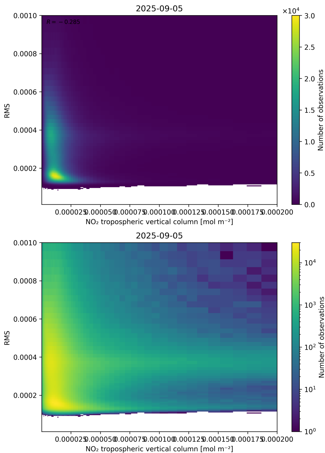
Figure 142: Scatter density plot of “NO 2 tropospheric vertical column” against “RMS” for 2025-09-04 to 2025-09-06.
