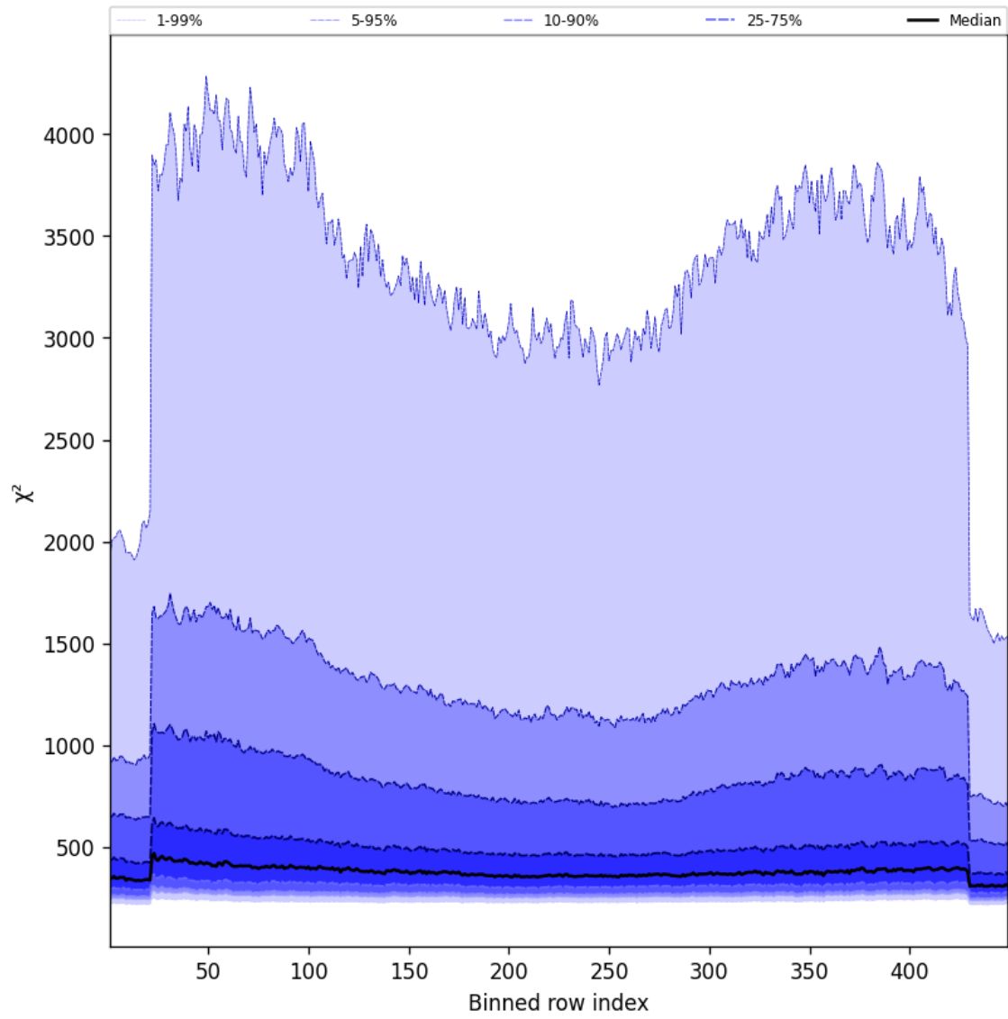
Figure 59: Along track statistics of “ \chi^2 ” for 2025-09-04 to 2025-09-06
