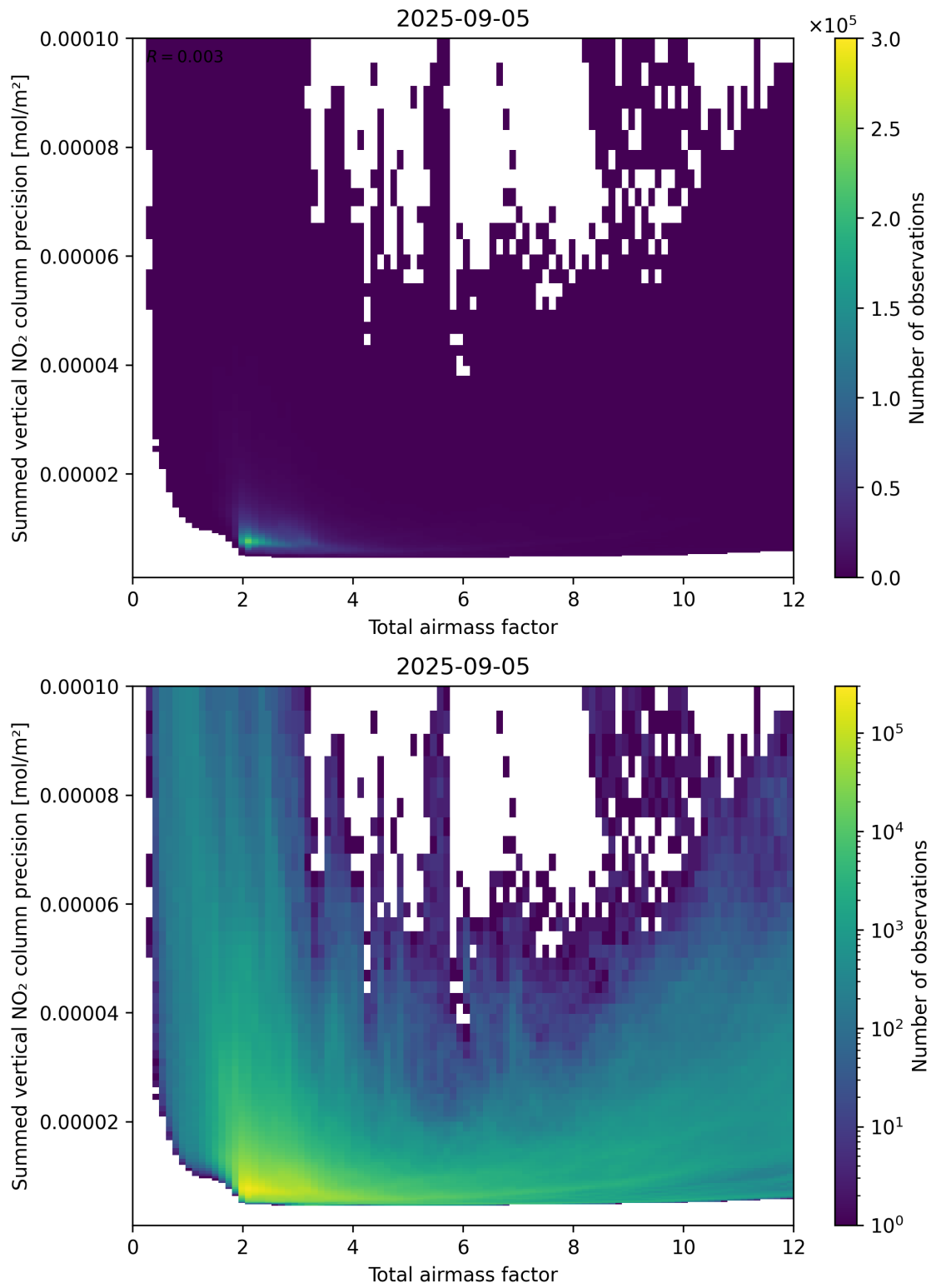
Figure 66: Scatter density plot of “Total airmass factor” against “Summed vertical NO 2 column precision” for 2025-09-04 to 2025-09-06.
