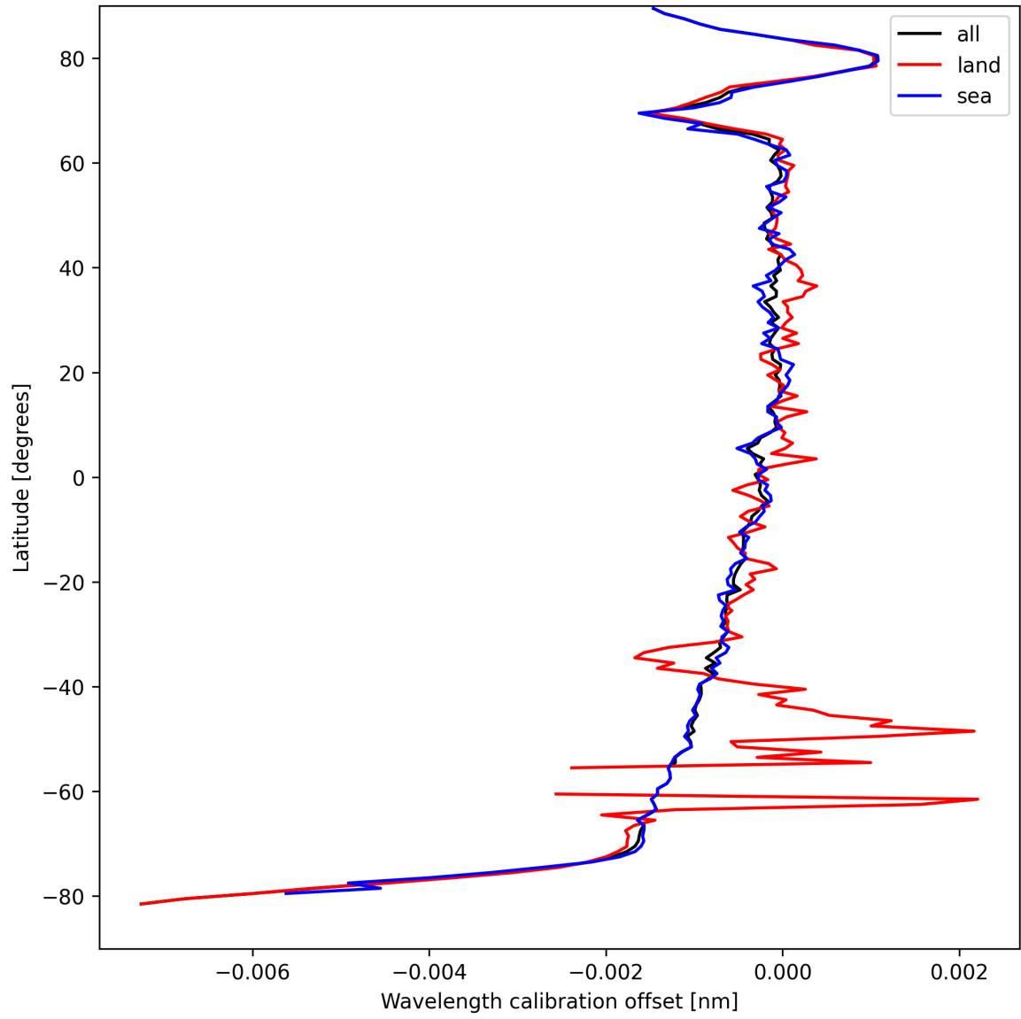
Figure 18: Zonal average of “Wavelength calibration offset” for 2025-09-04 to 2025-09-06.
