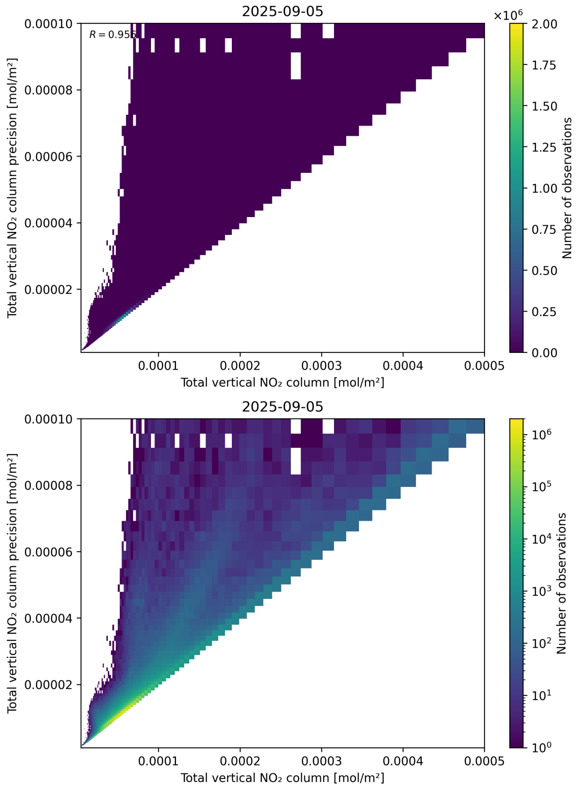
Figure 114: Scatter density plot of “Total vertical NO 2 column” against “Total vertical NO 2 column precision” for 2025-09-04 to 2025-09-06.
