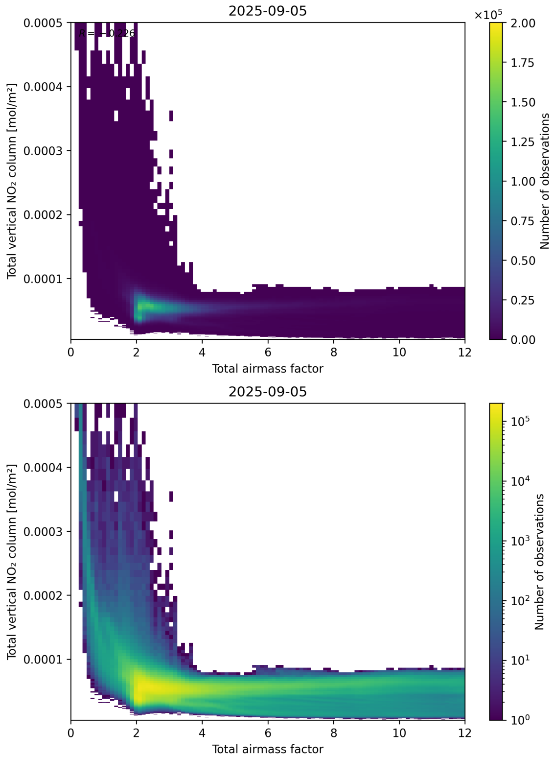
Figure 67: Scatter density plot of “Total air mass factor” against “Total vertical NO 2 column” for 2025-09-04 to 2025-09-06.
