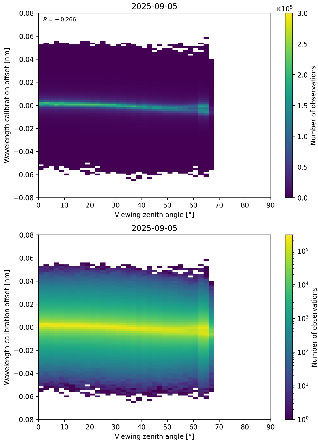
Figure 173: Scatter density plot of “Viewing zenith angle” against “Wavelength calibration offset” for 2025-09-04 to 2025-09-06.
