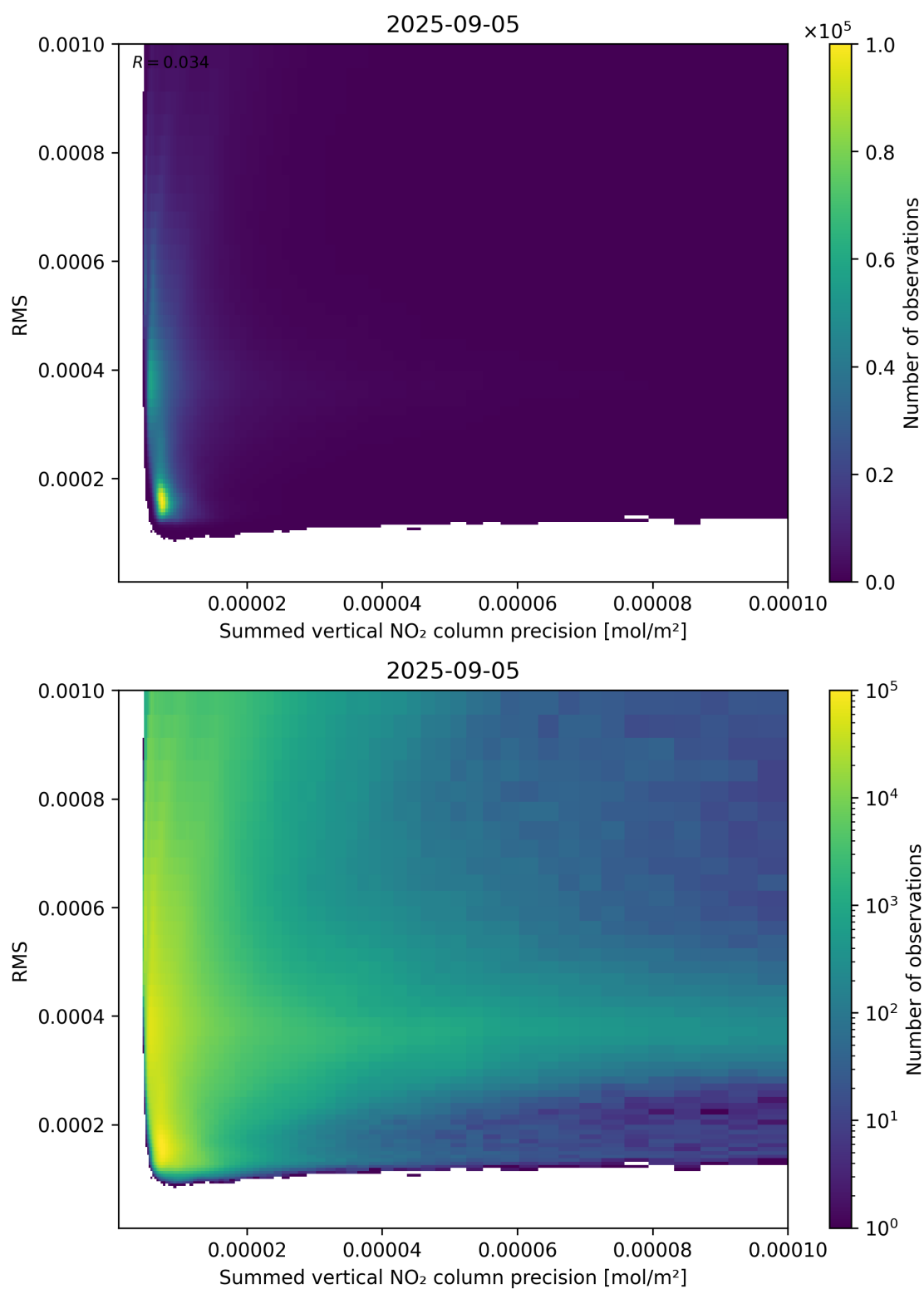
Figure 108: Scatter density plot of “Summed vertical NO 2 column precision” against “RMS” for 2025-09-04 to 2025-09-06.
