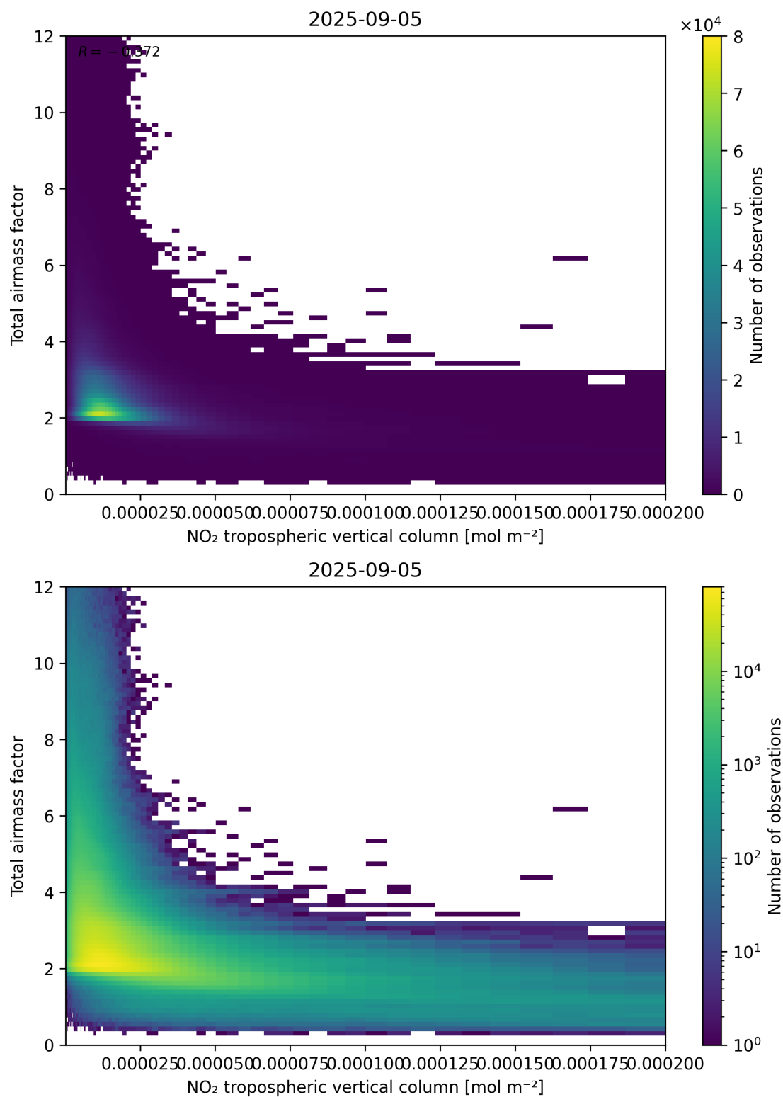
Figure 122: Scatter density plot of “NO 2 tropospheric vertical column” against “Total air mass factor” for 2025-09-04 to 2025-09-06.
