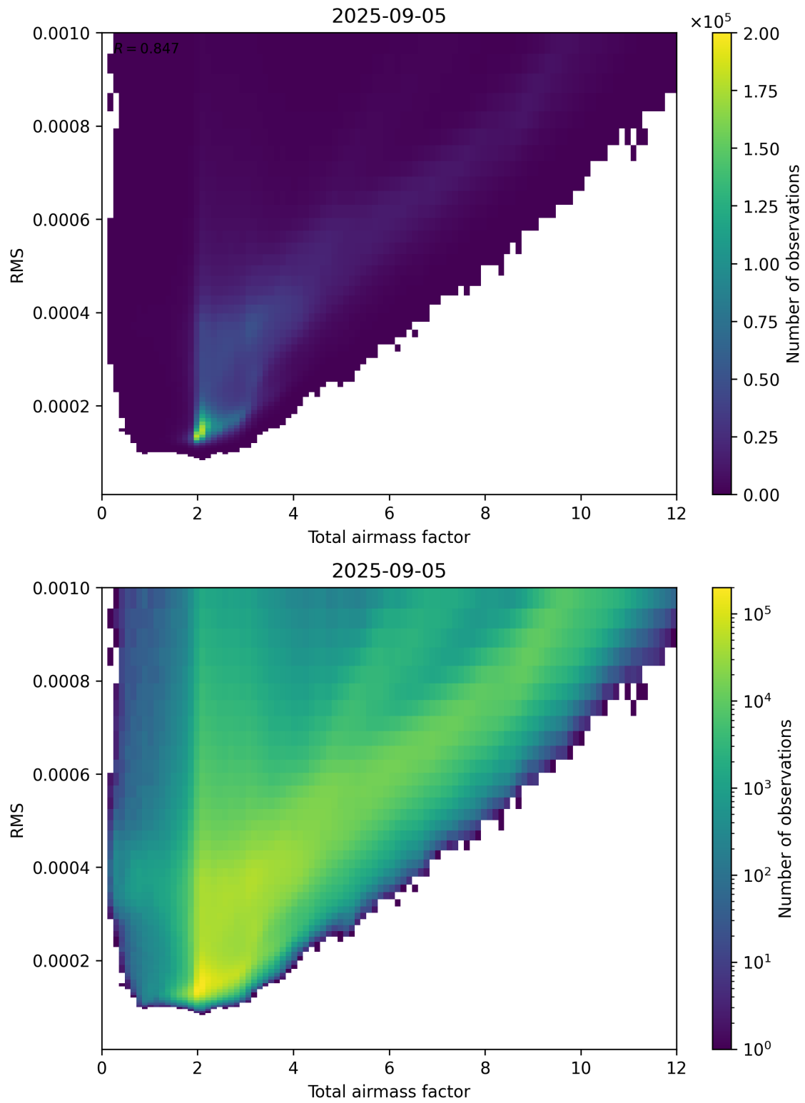
Figure 69: Scatter density plot of “Total airmass factor” against “RMS” for 2025-09-04 to 2025-09-06.
