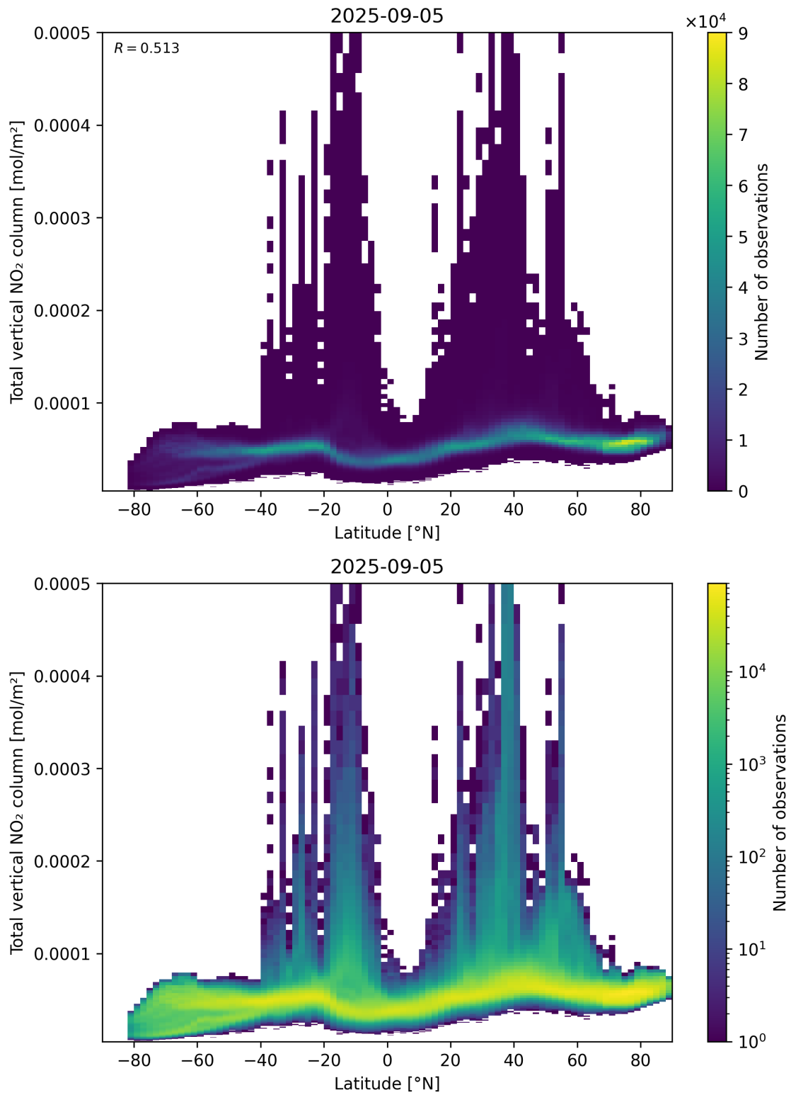
Figure 90: Scatter density plot of “Latitude” against “Total vertical NO 2 column” for 2025-09-04 to 2025-09-06.
