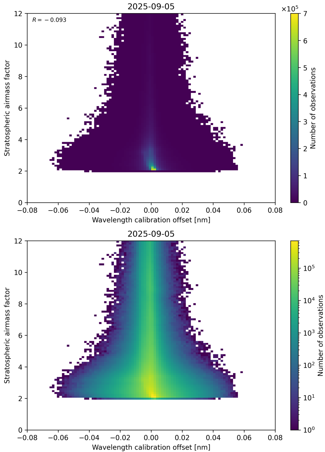
Figure 174: Scatter density plot of “Wavelength calibration offset” against “Stratospheric air mass factor” for 2025-09-04 to 2025-09-06.
