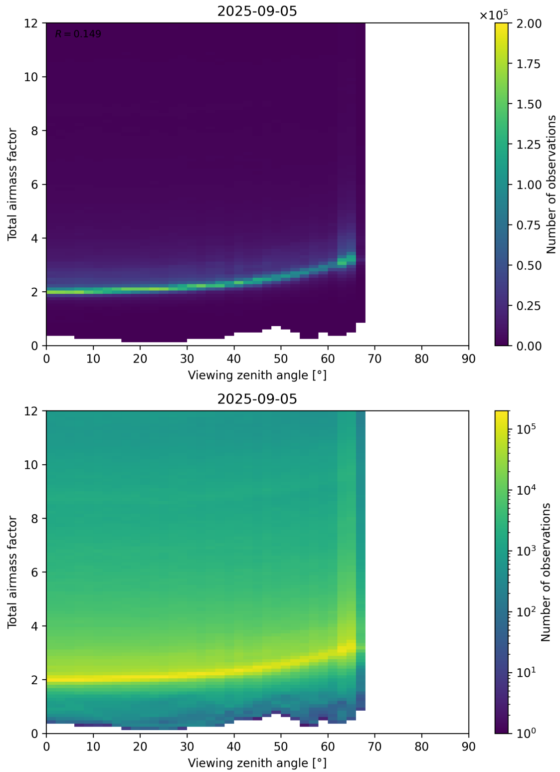
Figure 160: Scatter density plot of “Viewing zenith angle” against “Total airmass factor” for 2025-09-04 to 2025-09-06.
