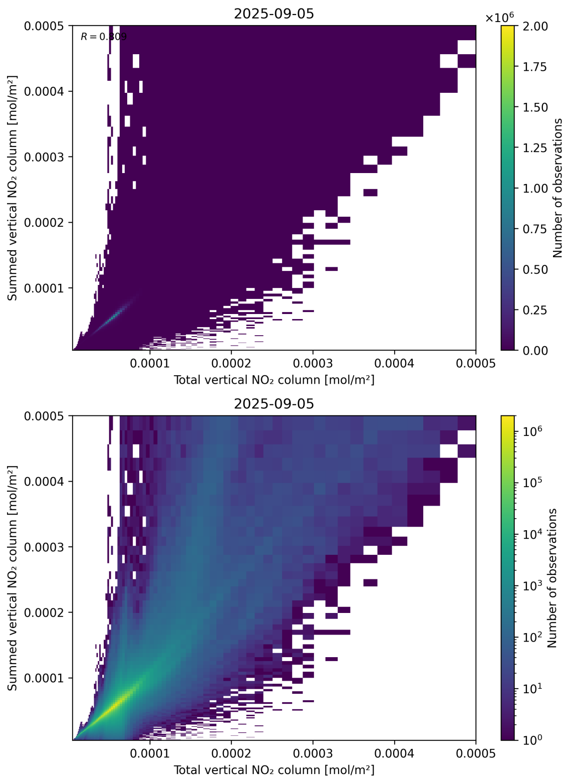
Figure 112: Scatter density plot of “Total vertical NO 2 column” against “Summed vertical NO 2 column” for 2025-09-04 to 2025-09-06.
