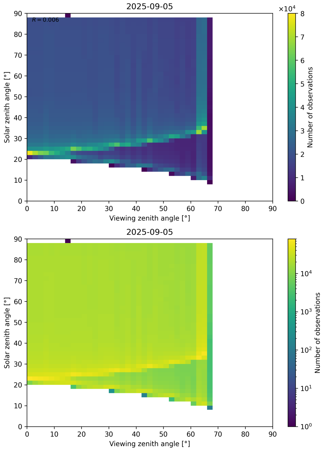
Figure 172: Scatter density plot of “Viewing zenith angle” against “Solar zenith angle” for 2025-09-04 to 2025-09-06.
