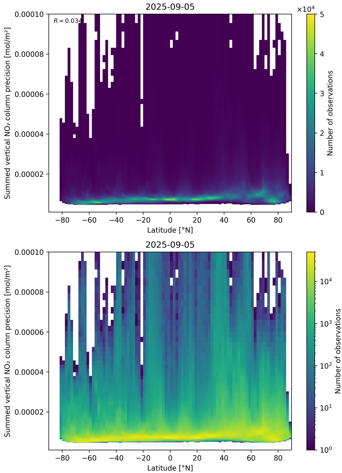
Figure 89: Scatter density plot of “Latitude” against “Summed vertical NO 2 column precision” for 2025-09-04 to 2025-09-06.
