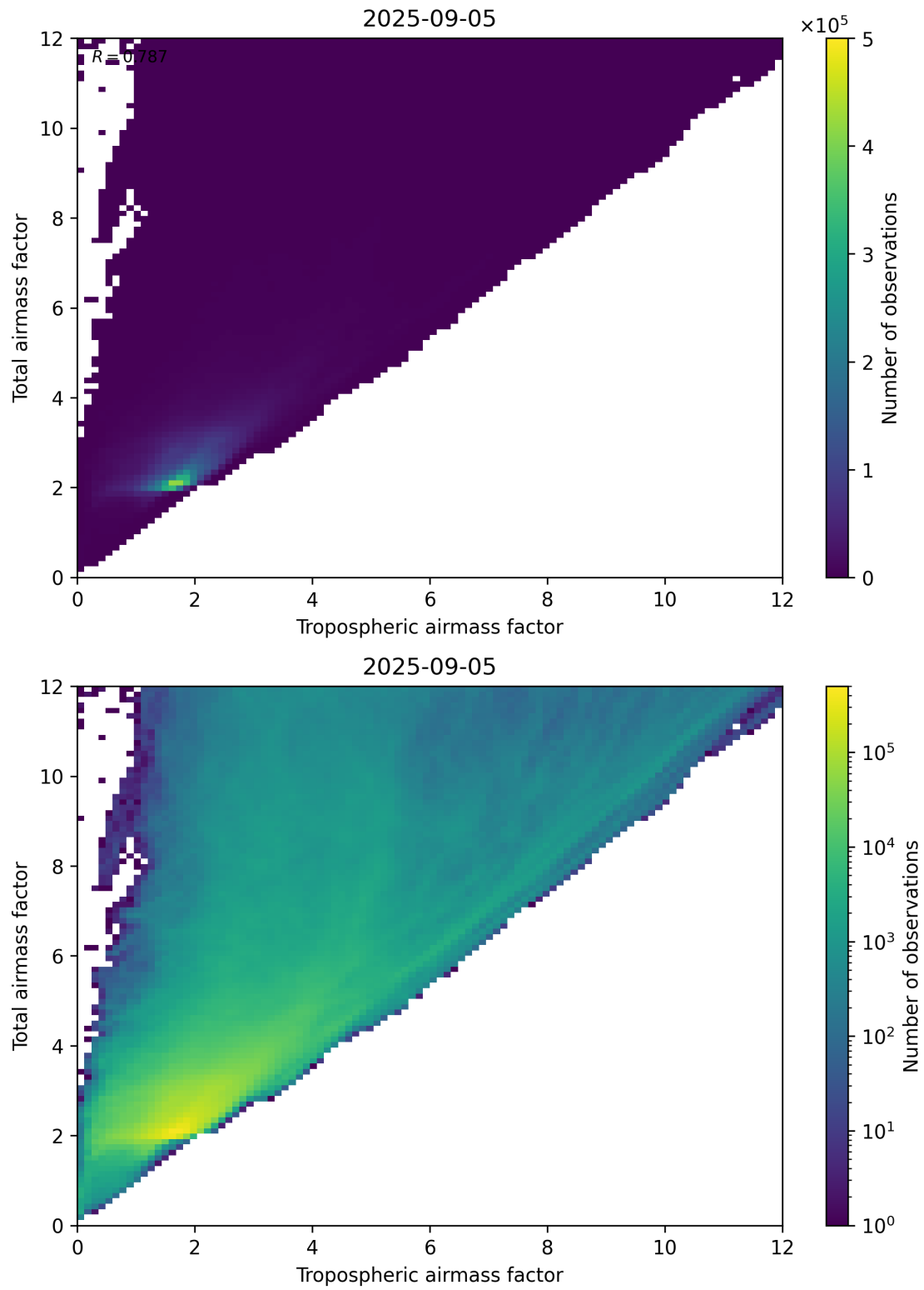
Figure 72: Scatter density plot of “Tropospheric airmass factor” against “Total airmass factor” for 2025-09-04 to 2025-09-06.
