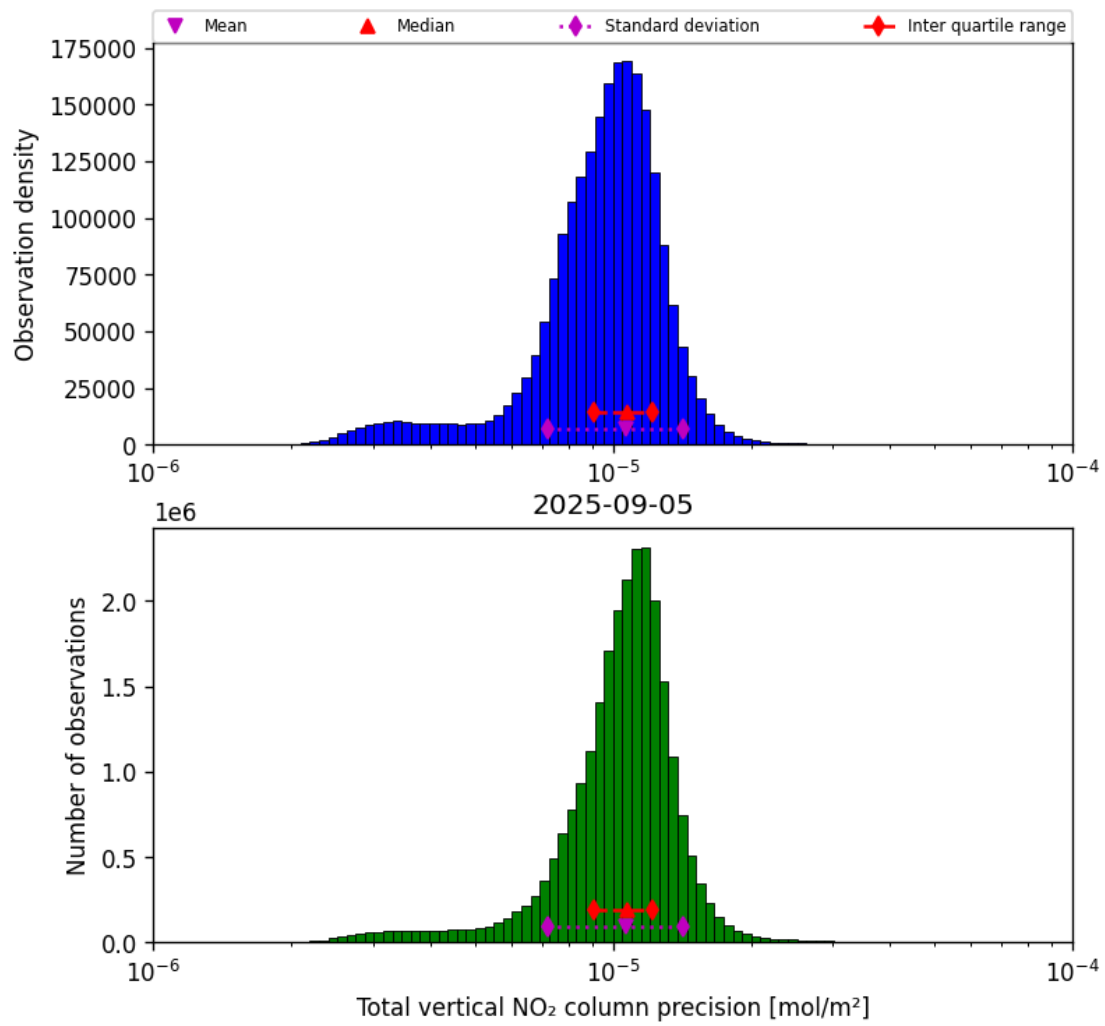
Figure 39: Histogram of “Total vertical NO 2 column precision” for 2025-09-04 to 2025-09-06
