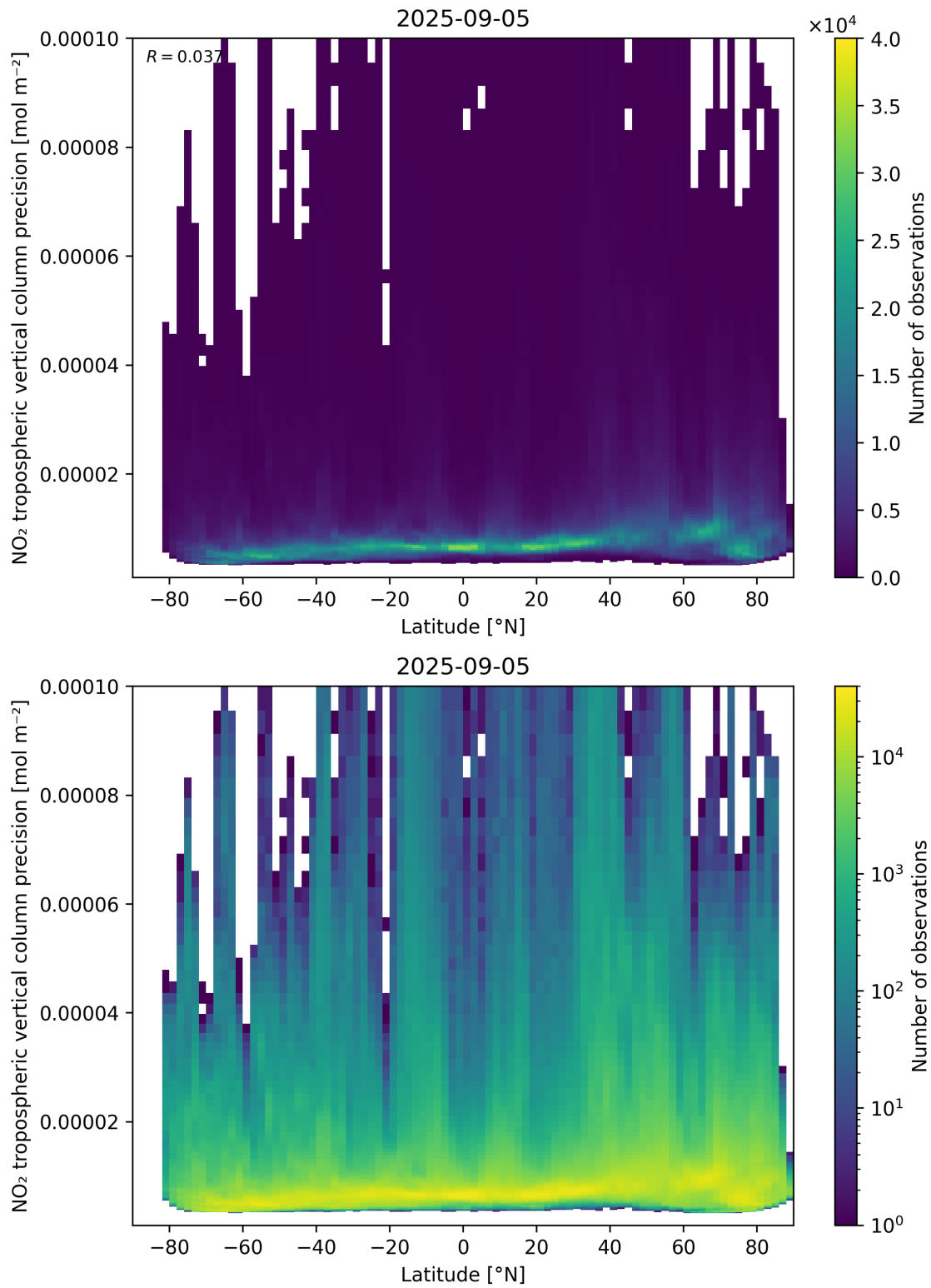
Figure 93: Scatter density plot of “Latitude” against “NO 2 tropospheric vertical column precision” for 2025-09-04 to 2025-09-06.
