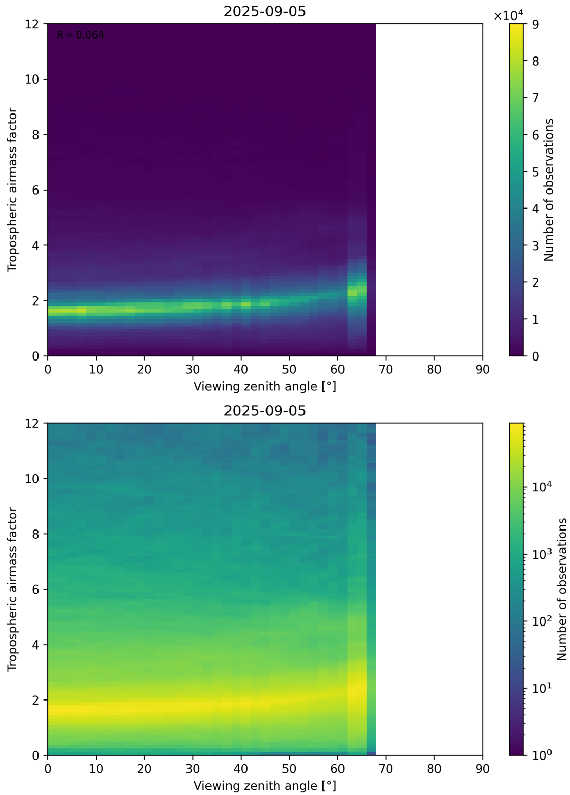
Figure 161: Scatter density plot of “Viewing zenith angle” against “Tropospheric airmass factor” for 2025-09-04 to 2025-09-06.
