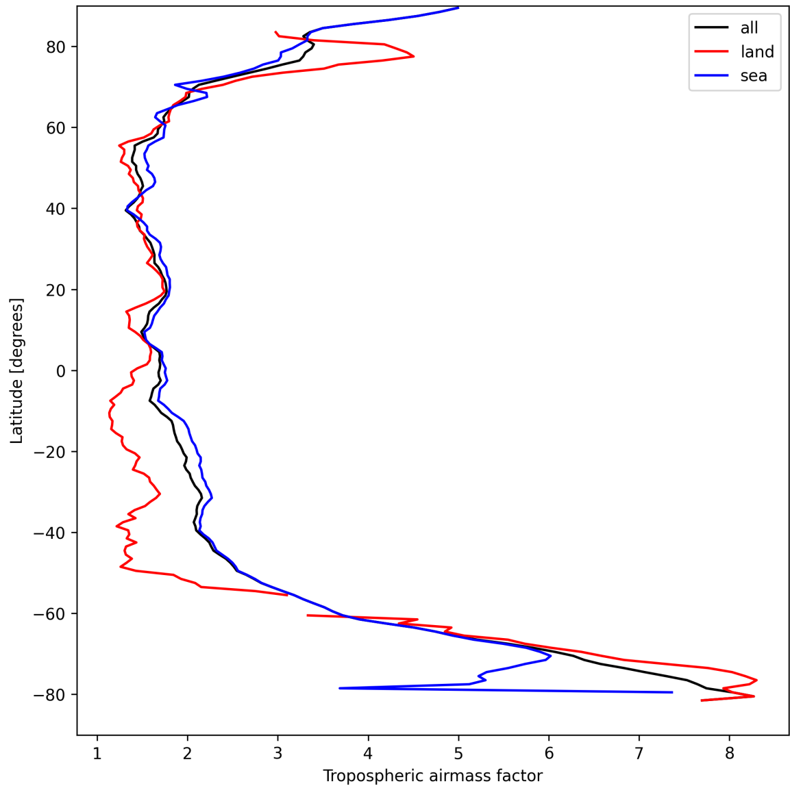
Figure 14: Zonal average of “Tropospheric air mass factor” for 2025-09-04 to 2025-09-06.
