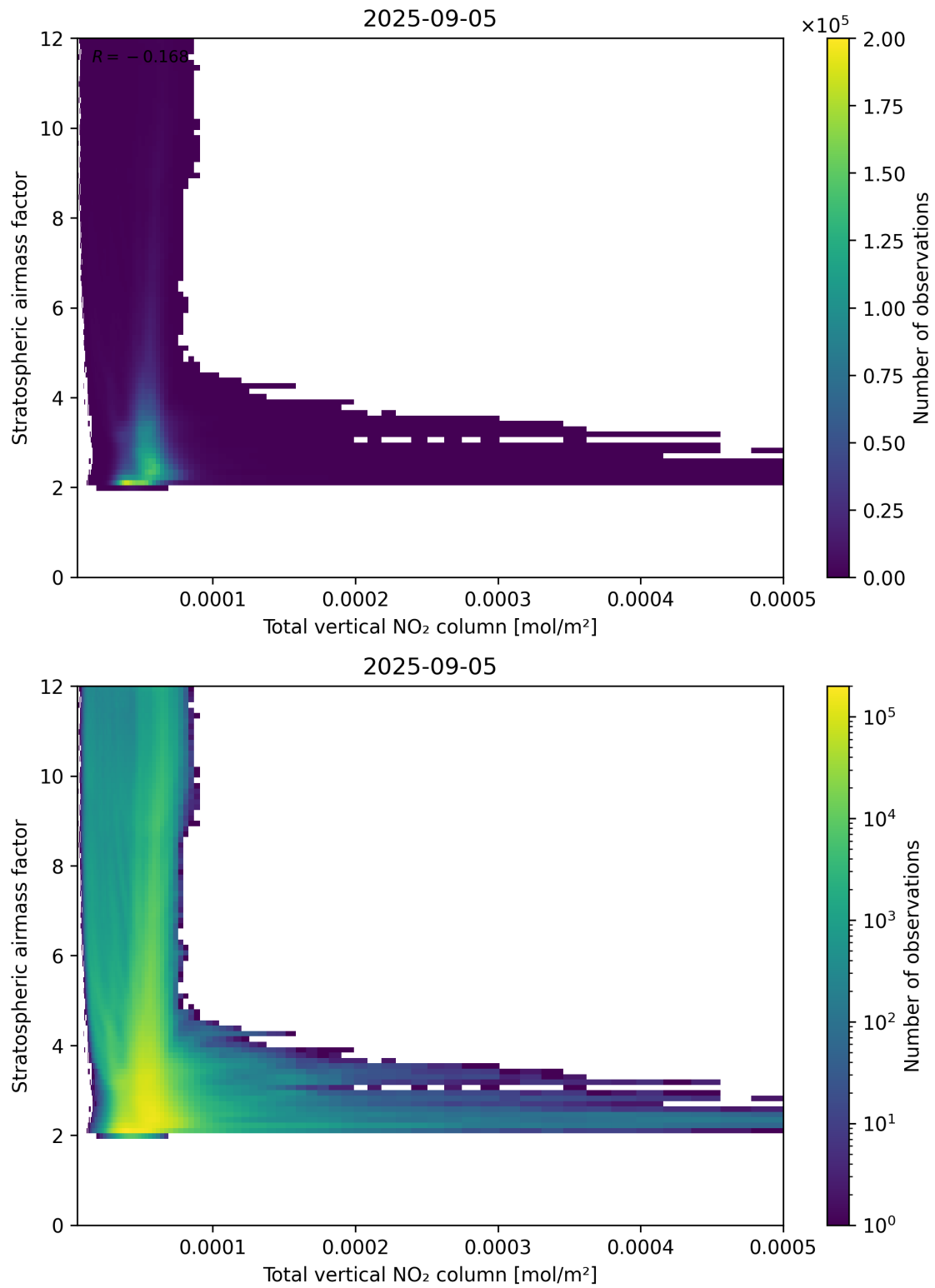
Figure 110: Scatter density plot of “Total vertical NO 2 column” against “Stratospheric airmass factor” for 2025-09-04 to 2025-09-06.
