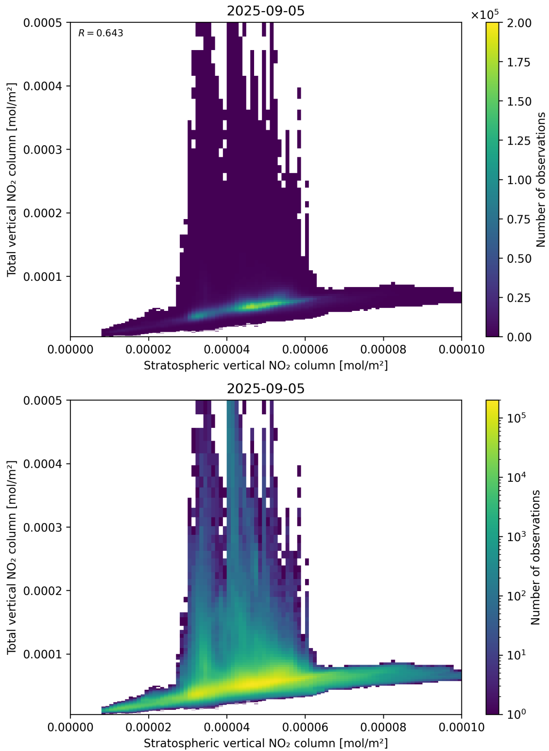
Figure 100: Scatter density plot of “Stratospheric vertical NO 2 column” against “Total vertical NO 2 column” for 2025-09-04 to 2025-09-06.
