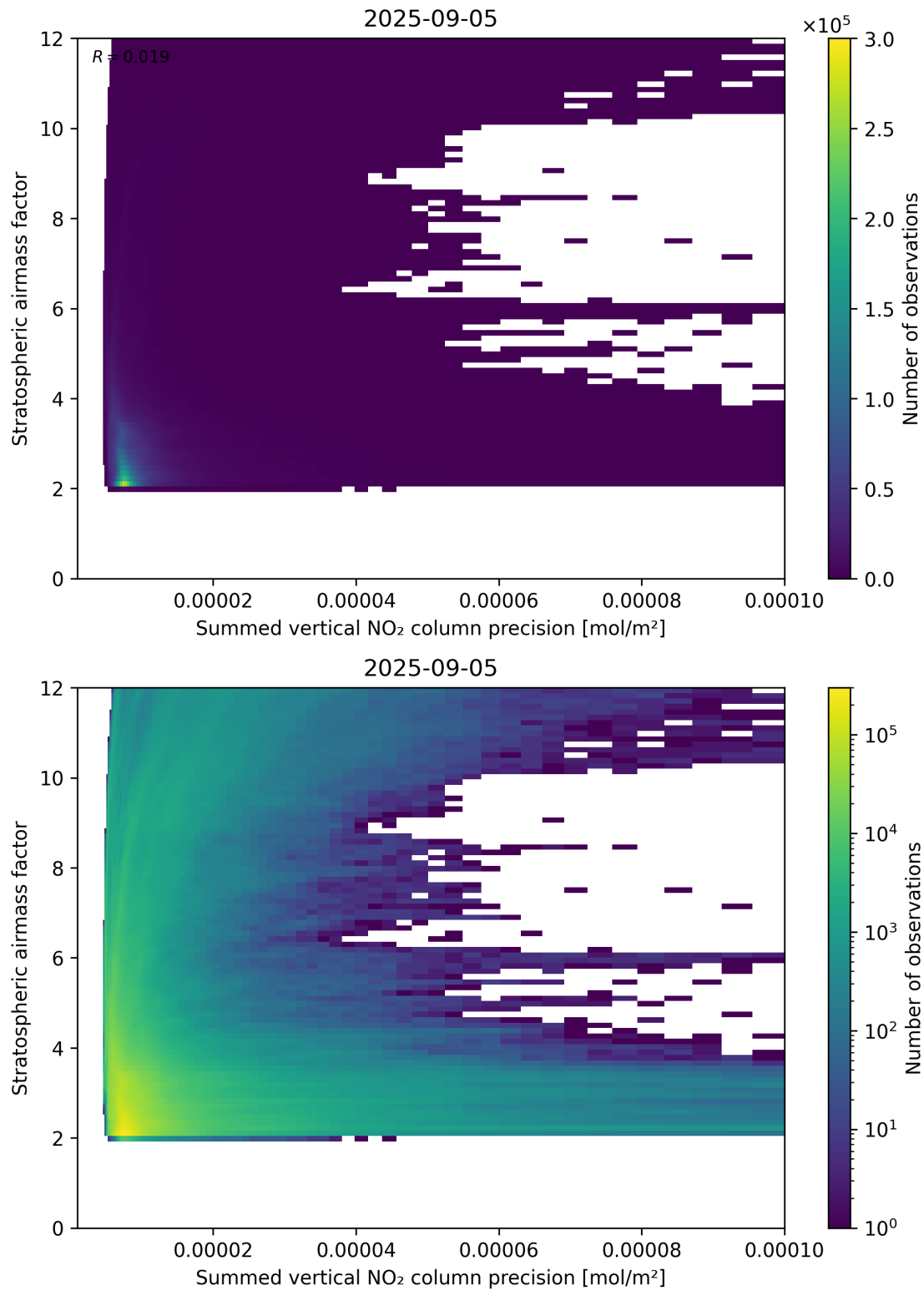
Figure 106: Scatter density plot of “Summed vertical NO 2 column precision” against “Stratospheric airmass factor” for 2025-09-04 to 2025-09-06.
