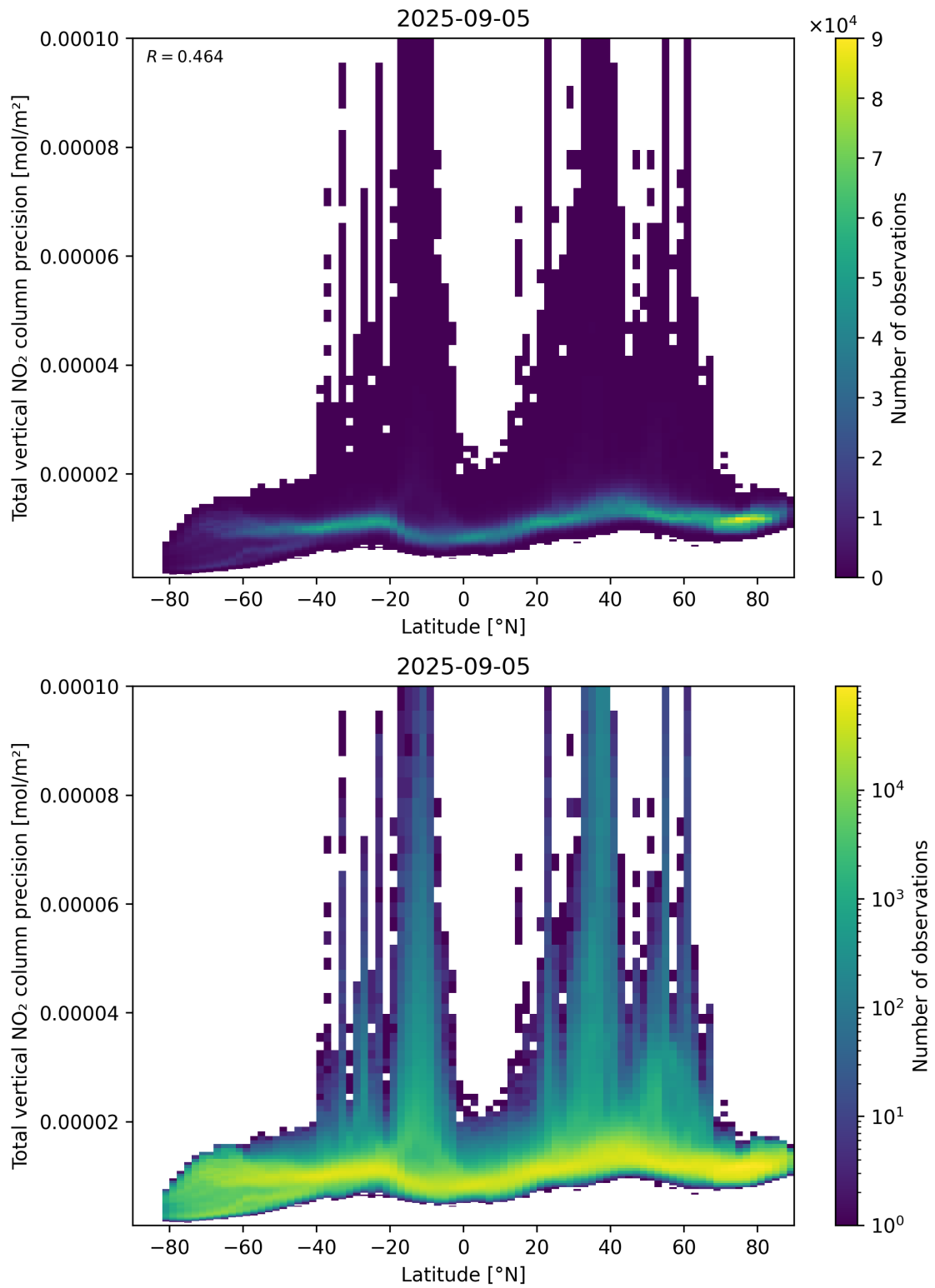
Figure 91: Scatter density plot of “Latitude” against “Total vertical NO 2 column precision” for 2025-09-04 to 2025-09-06.
