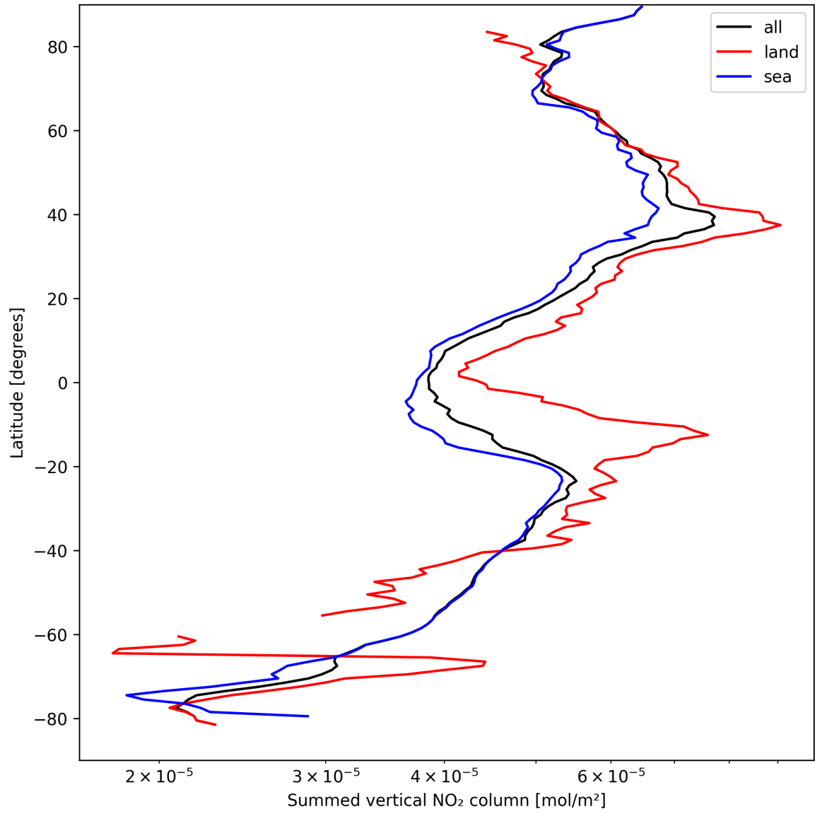
Figure 23: Zonal average of “Summed vertical NO 2 column” for 2025-09-04 to 2025-09-06.
