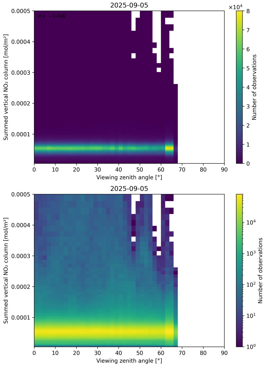
Figure 165: Scatter density plot of “Viewing zenith angle” against “Summed vertical NO 2 column” for 2025-09-04 to 2025-09-06.
