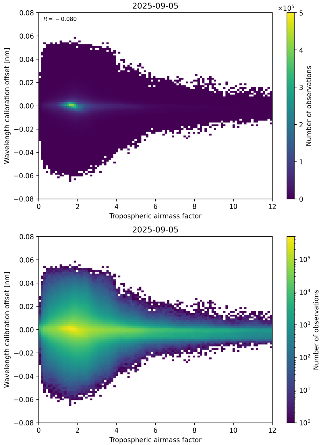
Figure 80: Scatter density plot of “Tropospheric airmass factor” against “Wavelength calibration offset” for 2025-09-04 to 2025-09-06.
