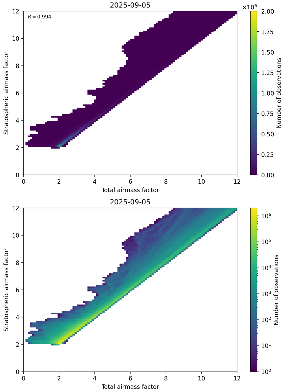
Figure 62: Scatter density plot of “Total airmass factor” against “Stratospheric airmass factor” for 2025-09-04 to 2025-09-06.
