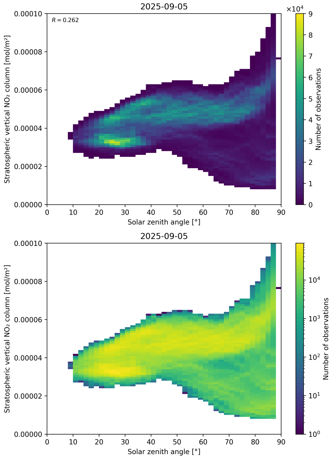
Figure 150: Scatter density plot of “Solar zenith angle” against “Stratospheric vertical NO 2 column” for 2025-09-04 to 2025-09-06.
