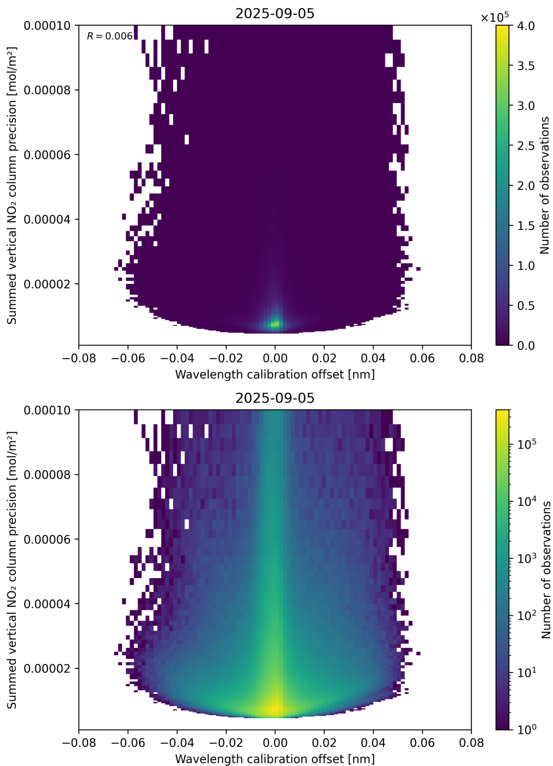
Figure 178: Scatter density plot of “Wavelength calibration offset” against “Summed vertical NO 2 column precision” for 2025-09-04 to 2025-09-06.
