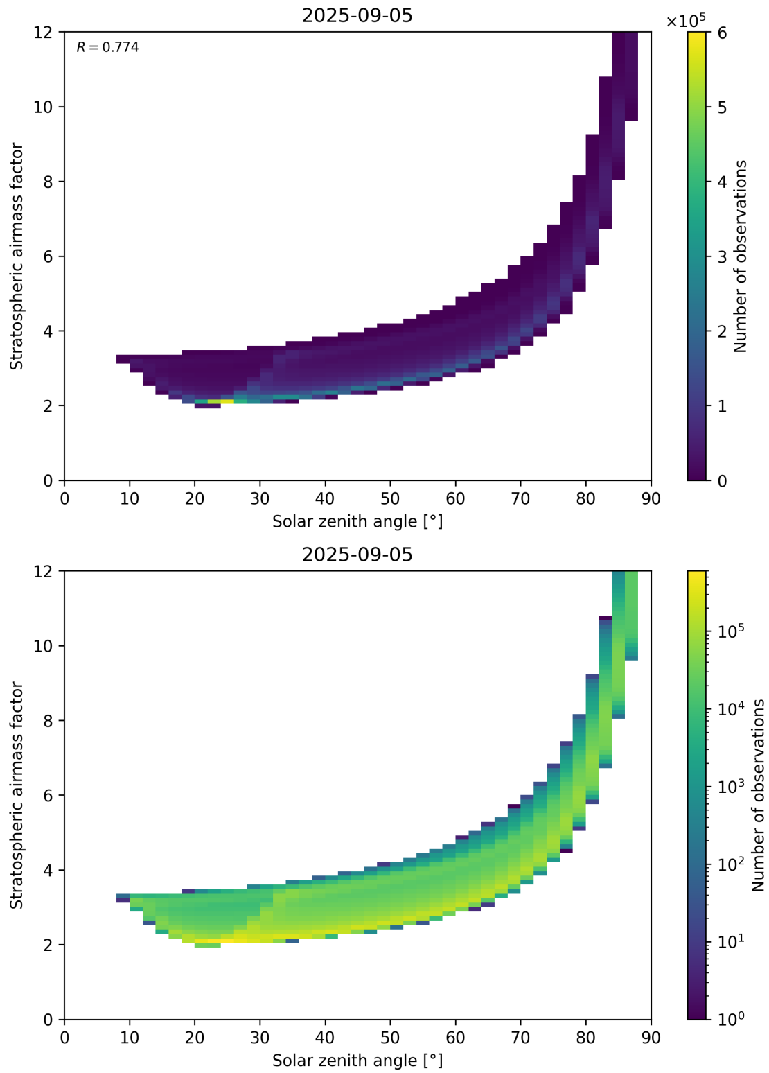
Figure 145: Scatter density plot of “Solar zenith angle” against “Stratospheric airmass factor” for 2025-09-04 to 2025-09-06.
