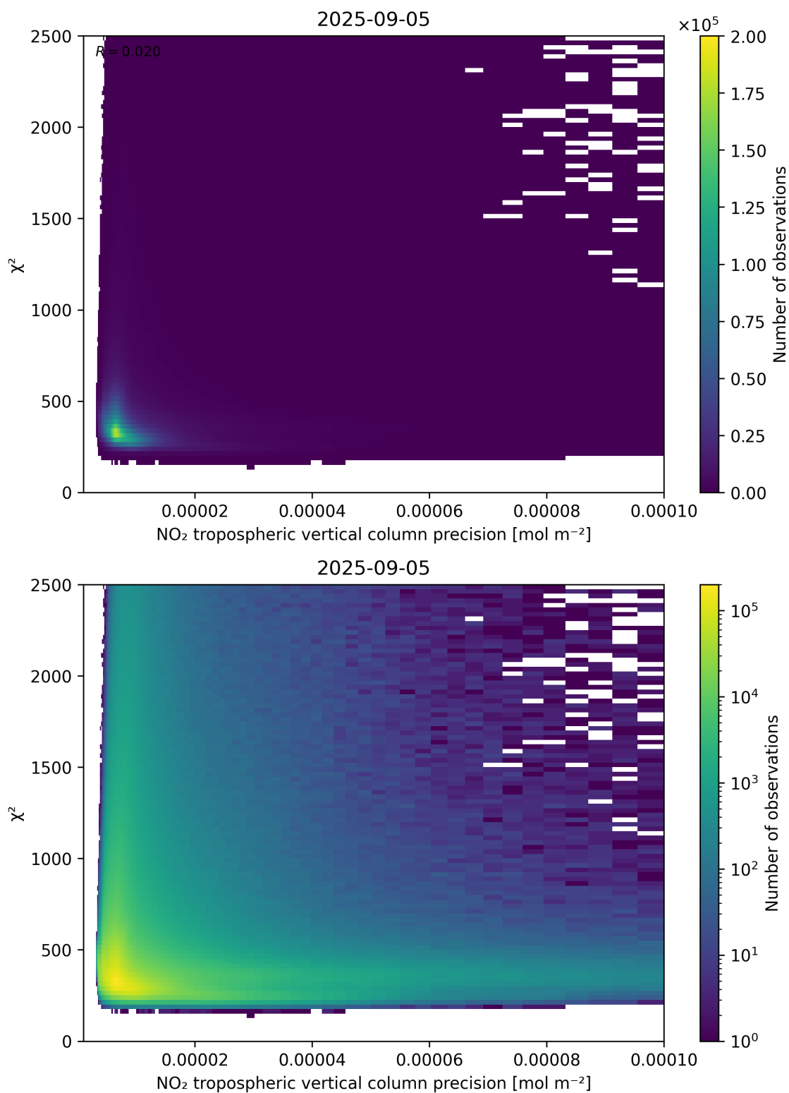
Figure 134: Scatter density plot of “NO 2 tropospheric vertical column precision” against “ \chi^2 ” for 2025-09-04 to 2025-09-06.
