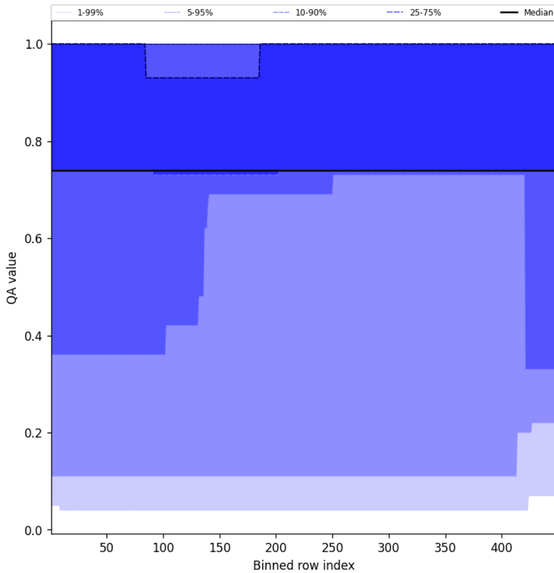
Figure 45: Along track statistics of “QA value” for 2025-09-04 to 2025-09-06
