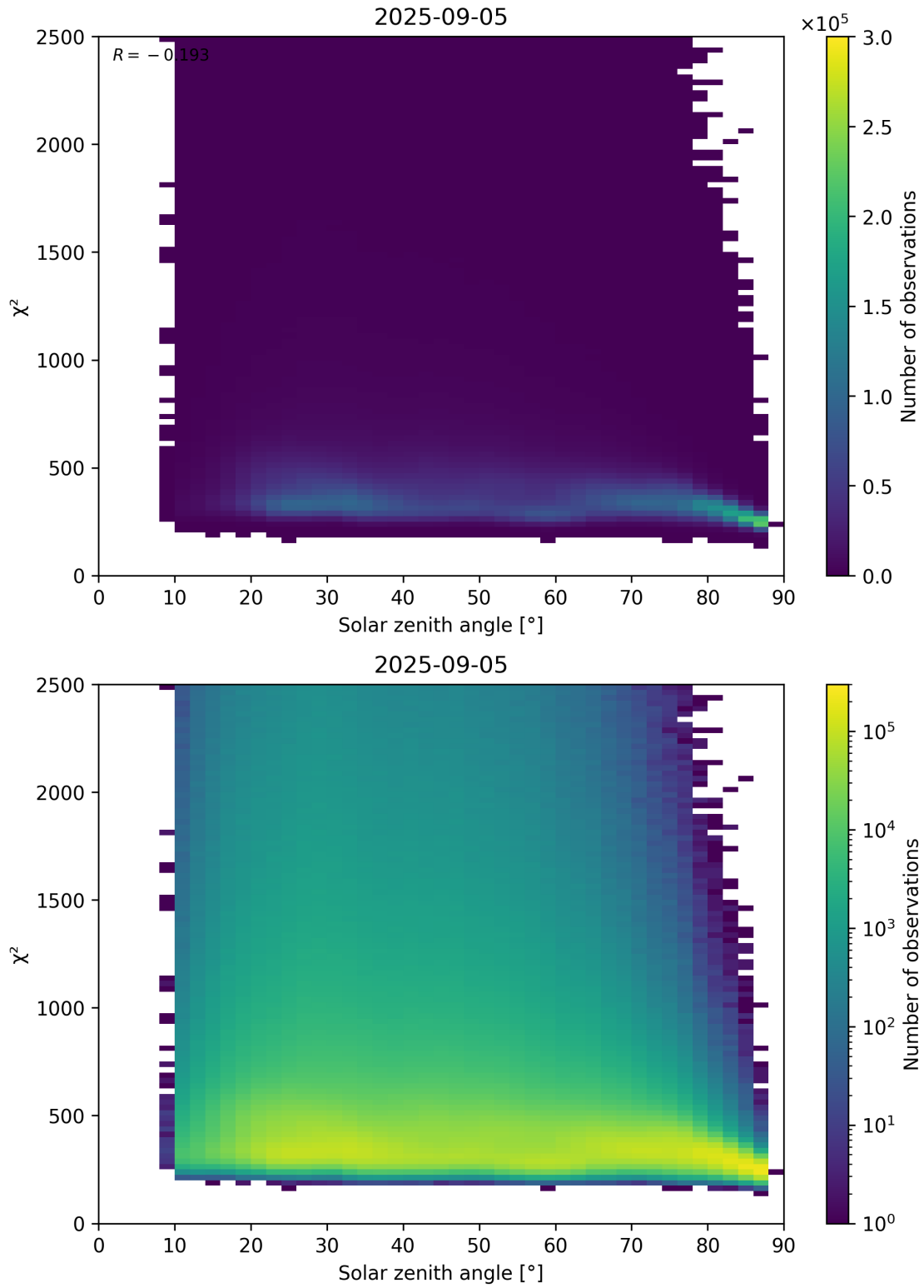
Figure 148: Scatter density plot of “Solar zenith angle” against “ \chi^2 ” for 2025-09-04 to 2025-09-06.
