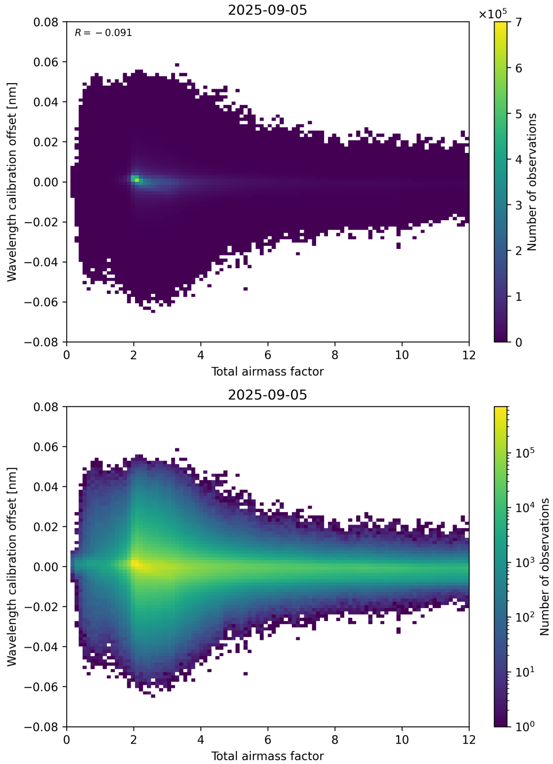
Figure 70: Scatter density plot of “Total airmass factor” against “Wavelength calibration offset” for 2025-09-04 to 2025-09-06.
