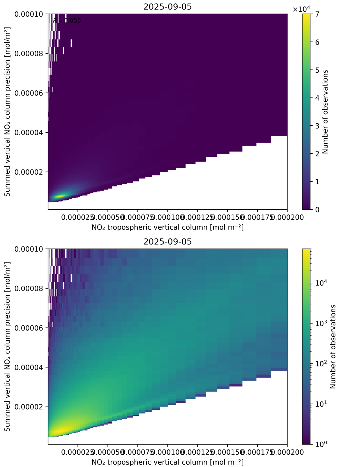
Figure 127: Scatter density plot of “NO 2 tropospheric vertical column” against “Summed vertical NO 2 column precision” for 2025-09-04 to 2025-09-06.
