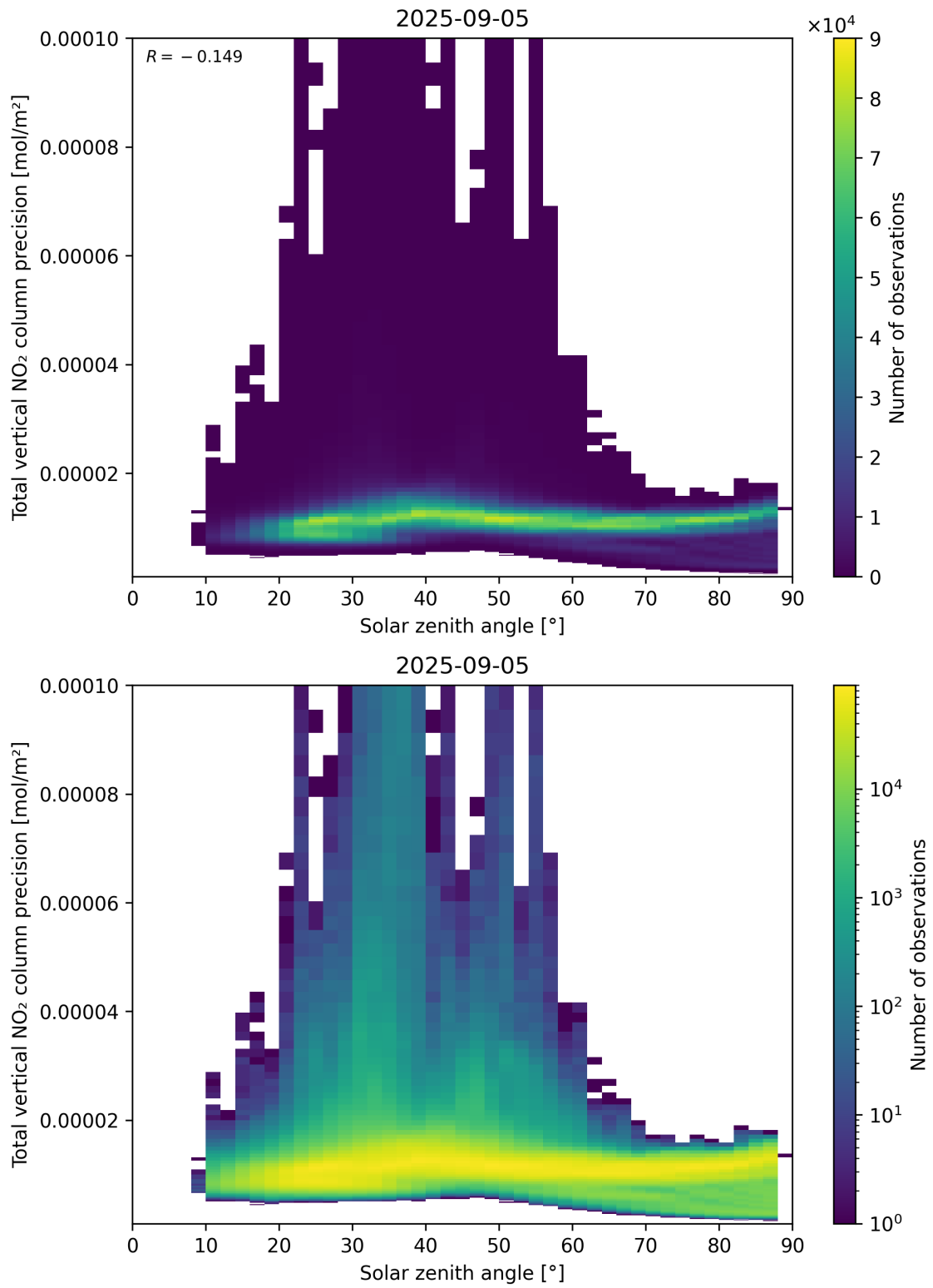
Figure 154: Scatter density plot of “Solar zenith angle” against “Total vertical NO 2 column precision” for 2025-09-04 to 2025-09-06.
