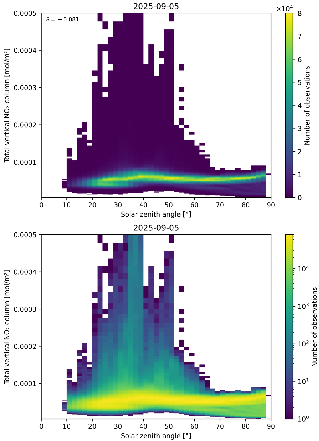
Figure 153: Scatter density plot of “Solar zenith angle” against “Total vertical NO 2 column” for 2025-09-04 to 2025-09-06.
