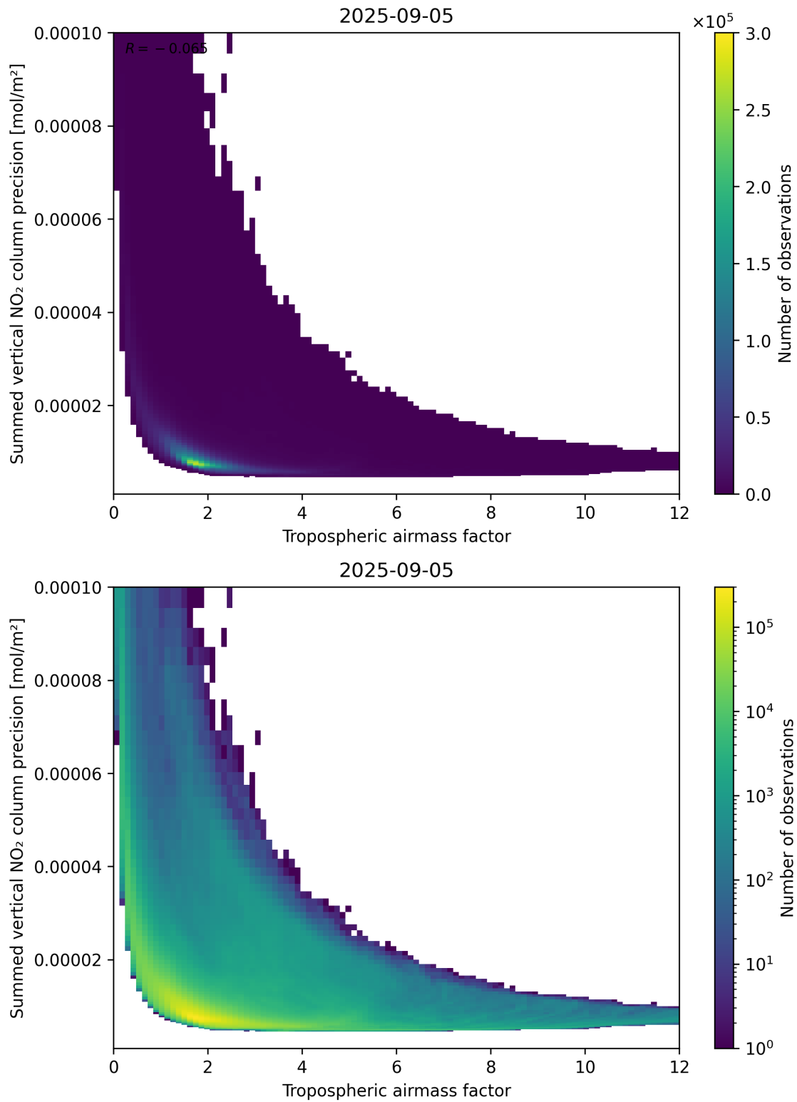
Figure 76: Scatter density plot of “Tropospheric air mass factor” against “Summed vertical NO 2 column precision” for 2025-09-04 to 2025-09-06.
