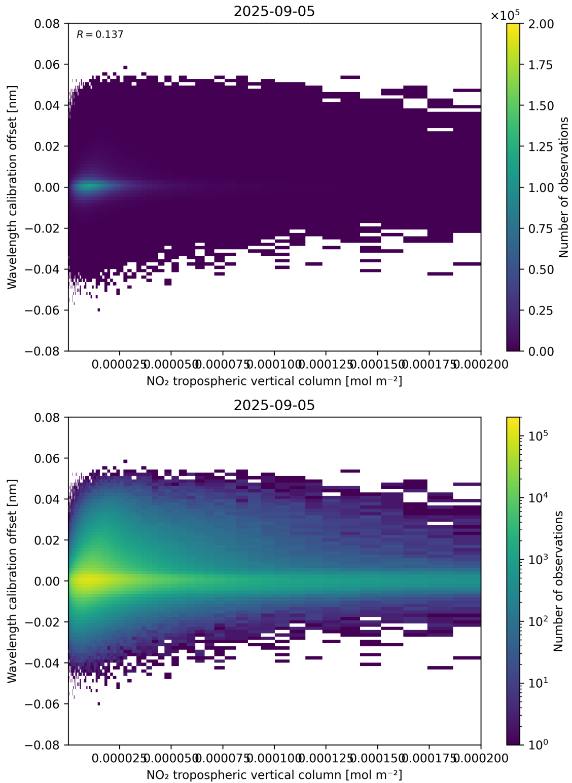
Figure 143: Scatter density plot of “NO 2 tropospheric vertical column” against “Wavelength calibration offset” for 2025-09-04 to 2025-09-06.
