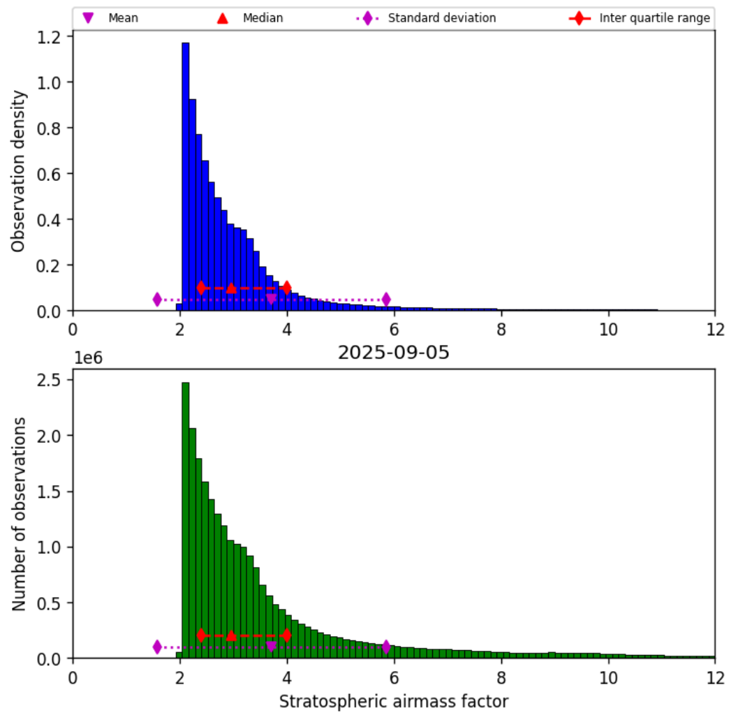
Figure 44: Histogram of “Stratospheric airmass factor” for 2025-09-04 to 2025-09-06
