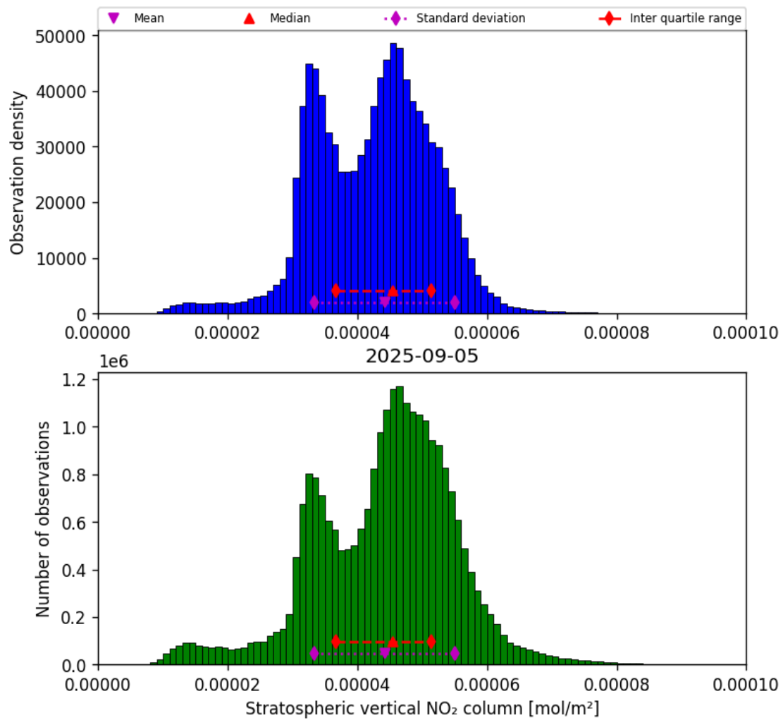
Figure 36: Histogram of “Stratospheric vertical NO 2 column” for 2025-09-04 to 2025-09-06
