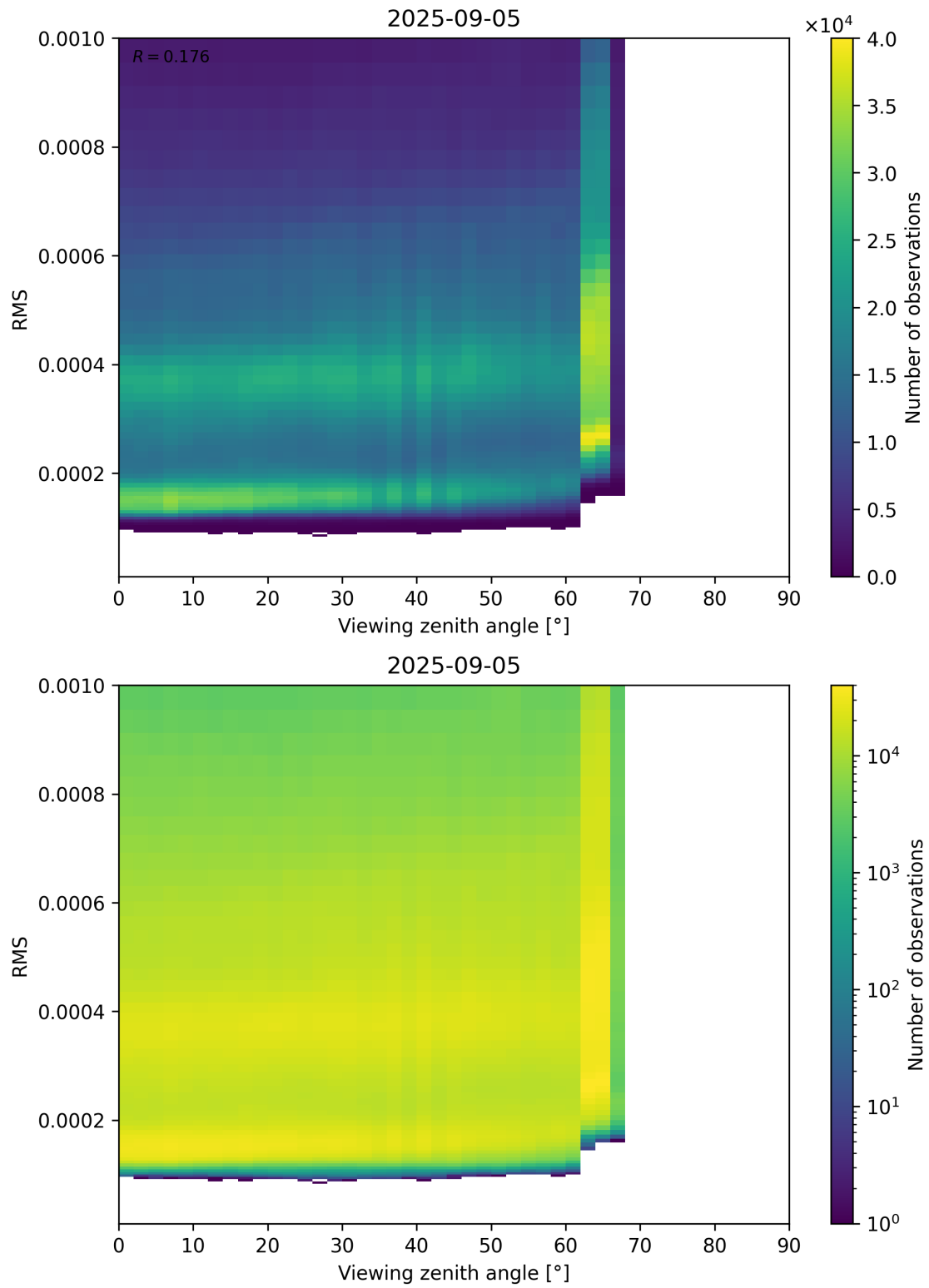
Figure 171: Scatter density plot of “Viewing zenith angle” against “RMS” for 2025-09-04 to 2025-09-06.
