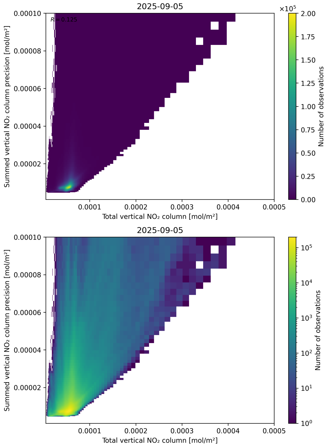
Figure 113: Scatter density plot of “Total vertical NO 2 column” against “Summed vertical NO 2 column precision” for 2025-09-04 to 2025-09-06.
