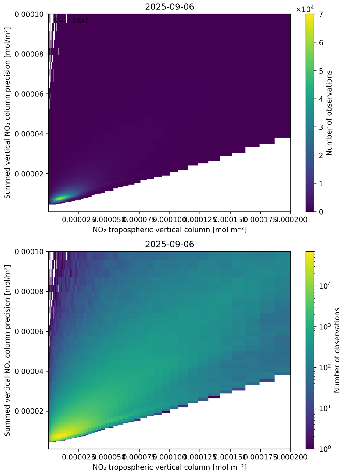
Figure 127: Scatter density plot of “NO 2 tropospheric vertical column” against “Summed vertical NO 2 column precision” for 2025-09-05 to 2025-09-07.
