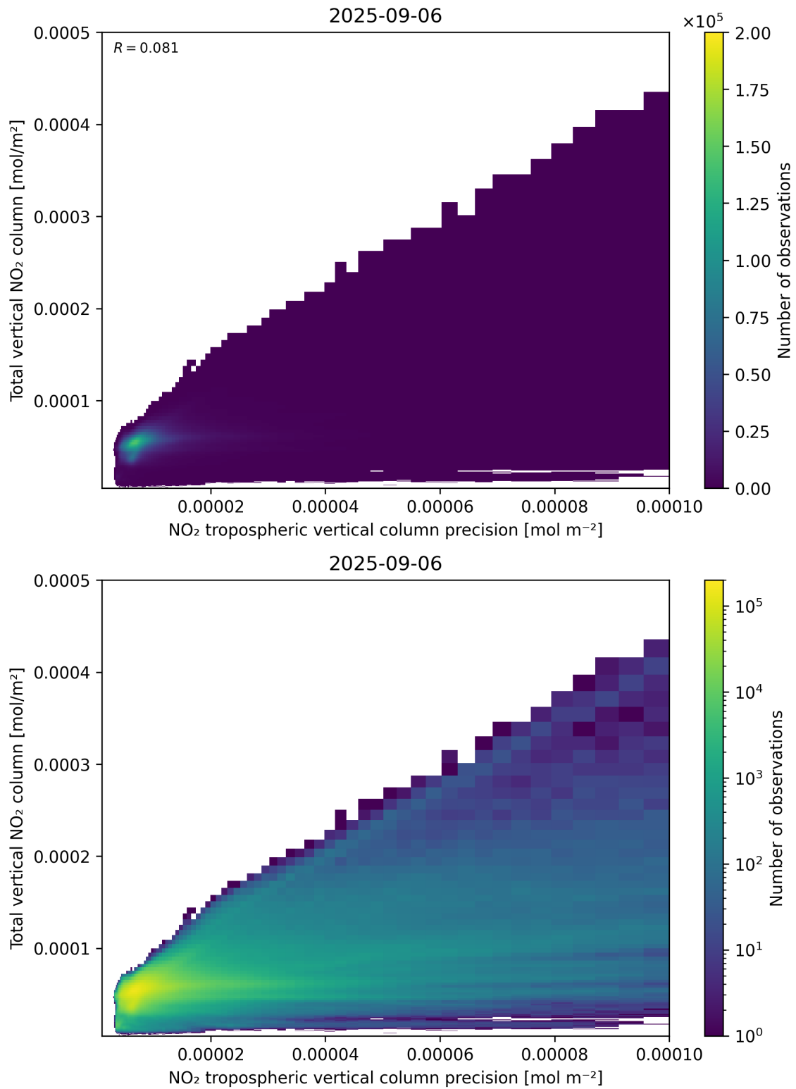
Figure 138: Scatter density plot of “NO 2 tropospheric vertical column precision” against “Total vertical NO 2 column” for 2025-09-05 to 2025-09-07.
