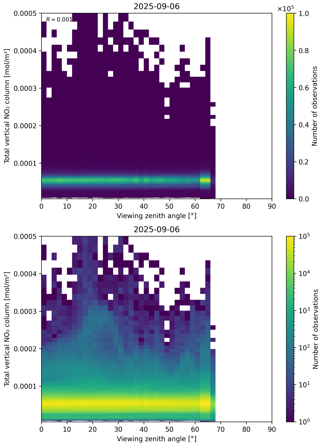
Figure 167: Scatter density plot of “Viewing zenith angle” against “Total vertical NO 2 column” for 2025-09-05 to 2025-09-07.
