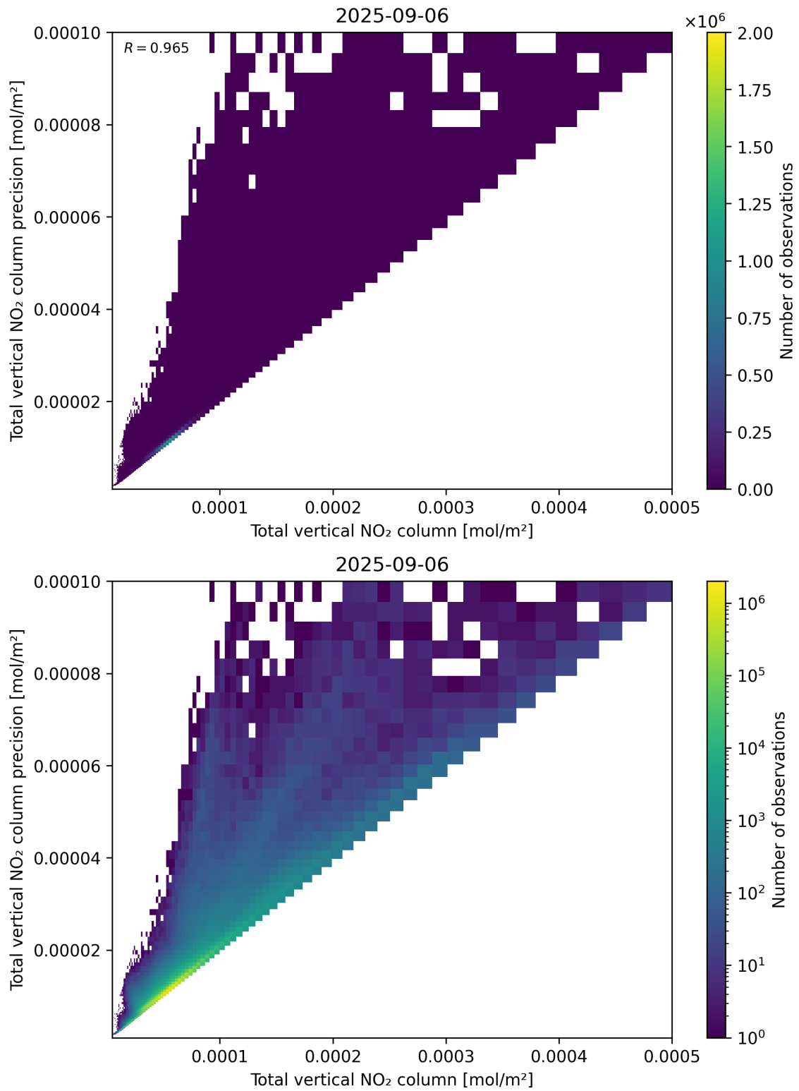
Figure 114: Scatter density plot of “Total vertical NO 2 column” against “Total vertical NO 2 column precision” for 2025-09-05 to 2025-09-07.
