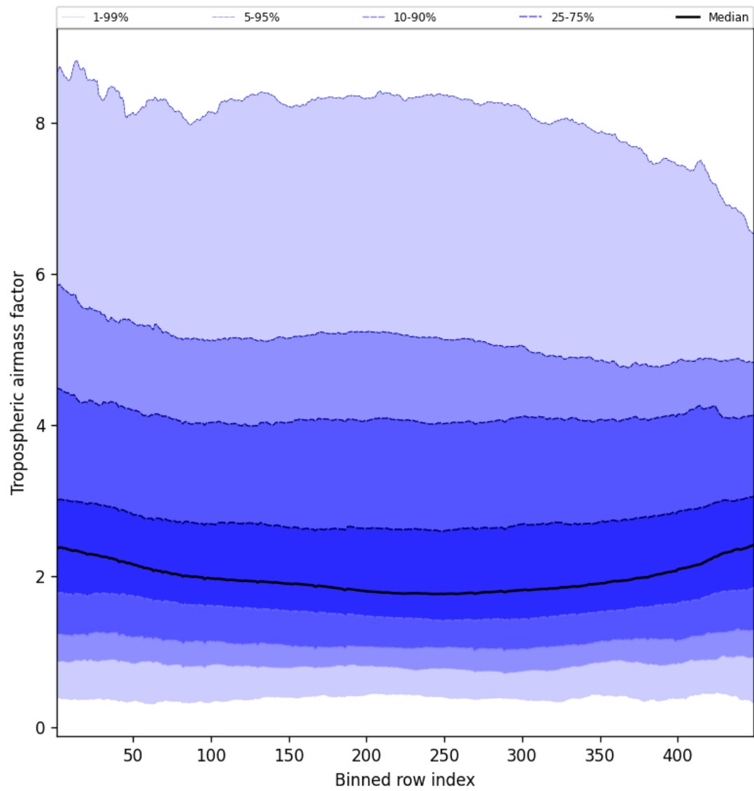
Figure 48: Along track statistics of “Tropospheric airmass factor” for 2025-09-05 to 2025-09-07
