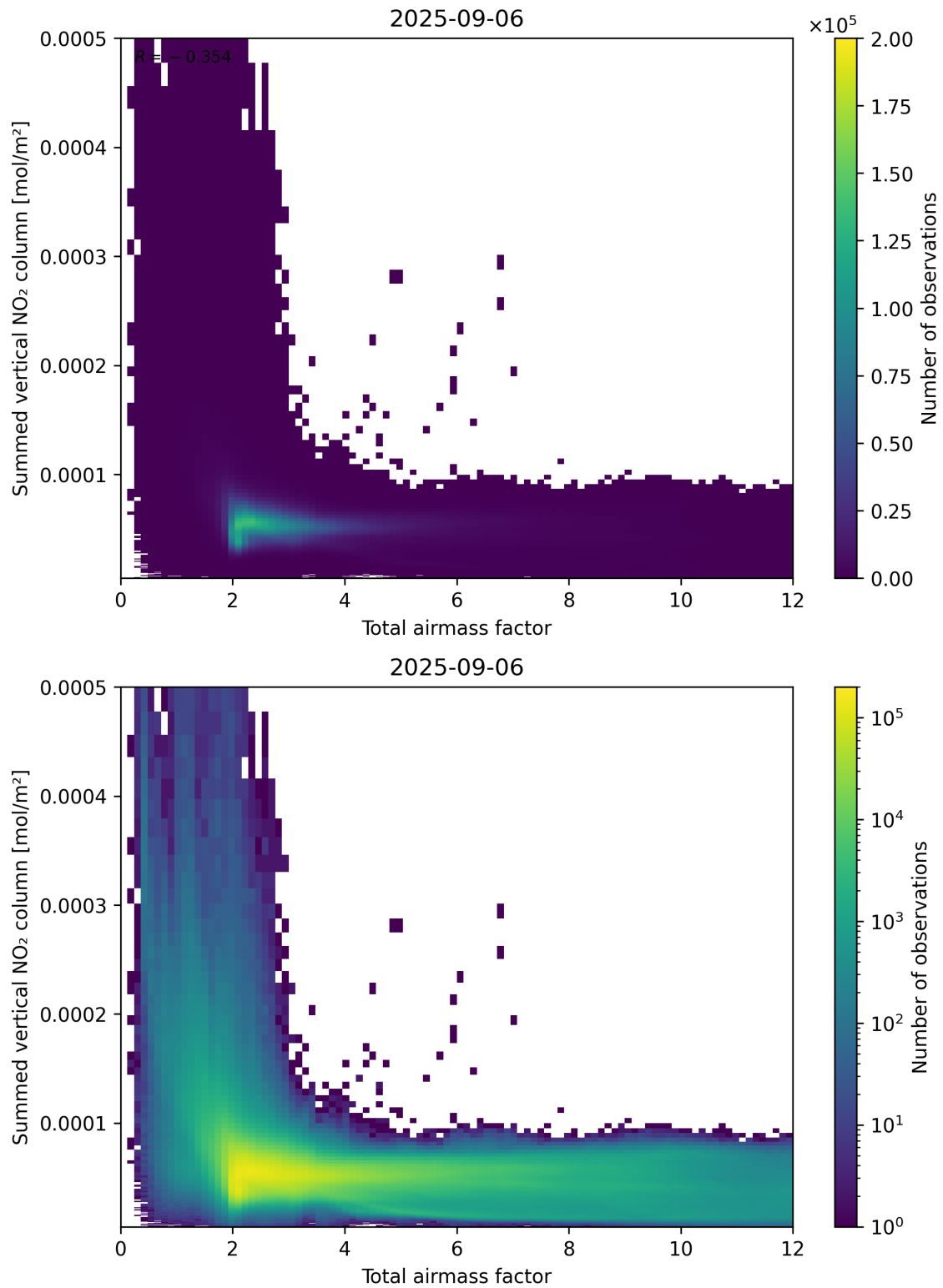
Figure 65: Scatter density plot of “Total airmass factor” against “Summed vertical NO 2 column” for 2025-09-05 to 2025-09-07.
