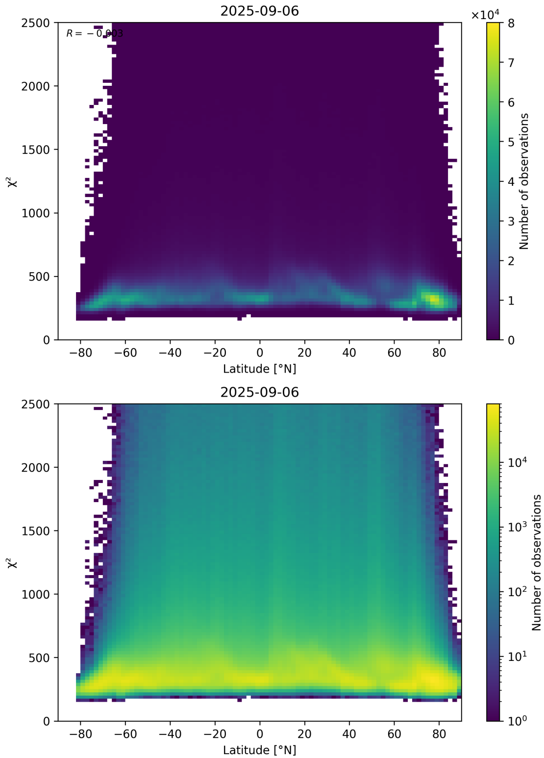
Figure 86: Scatter density plot of “Latitude” against “ \chi^2 ” for 2025-09-05 to 2025-09-07.
