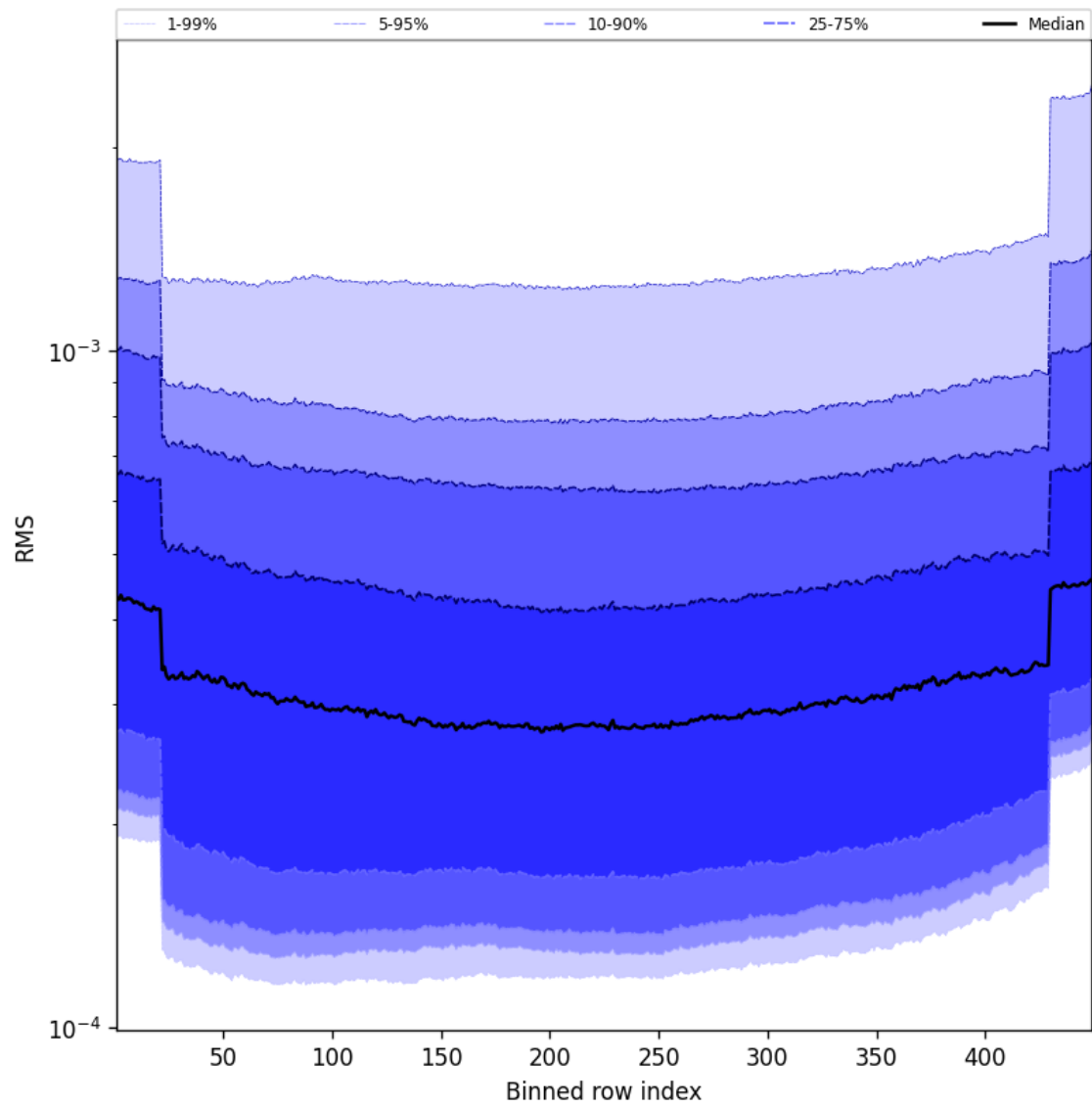
Figure 60: Along track statistics of “RMS” for 2025-09-05 to 2025-09-07
