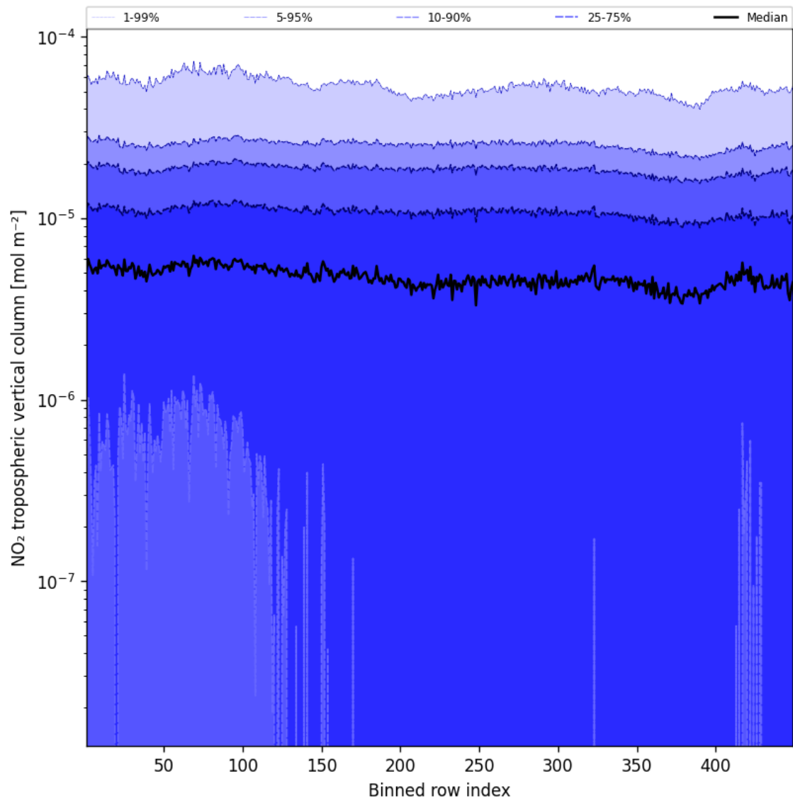
Figure 46: Along track statistics of “NO 2 tropospheric vertical column” for 2025-09-05 to 2025-09-07
