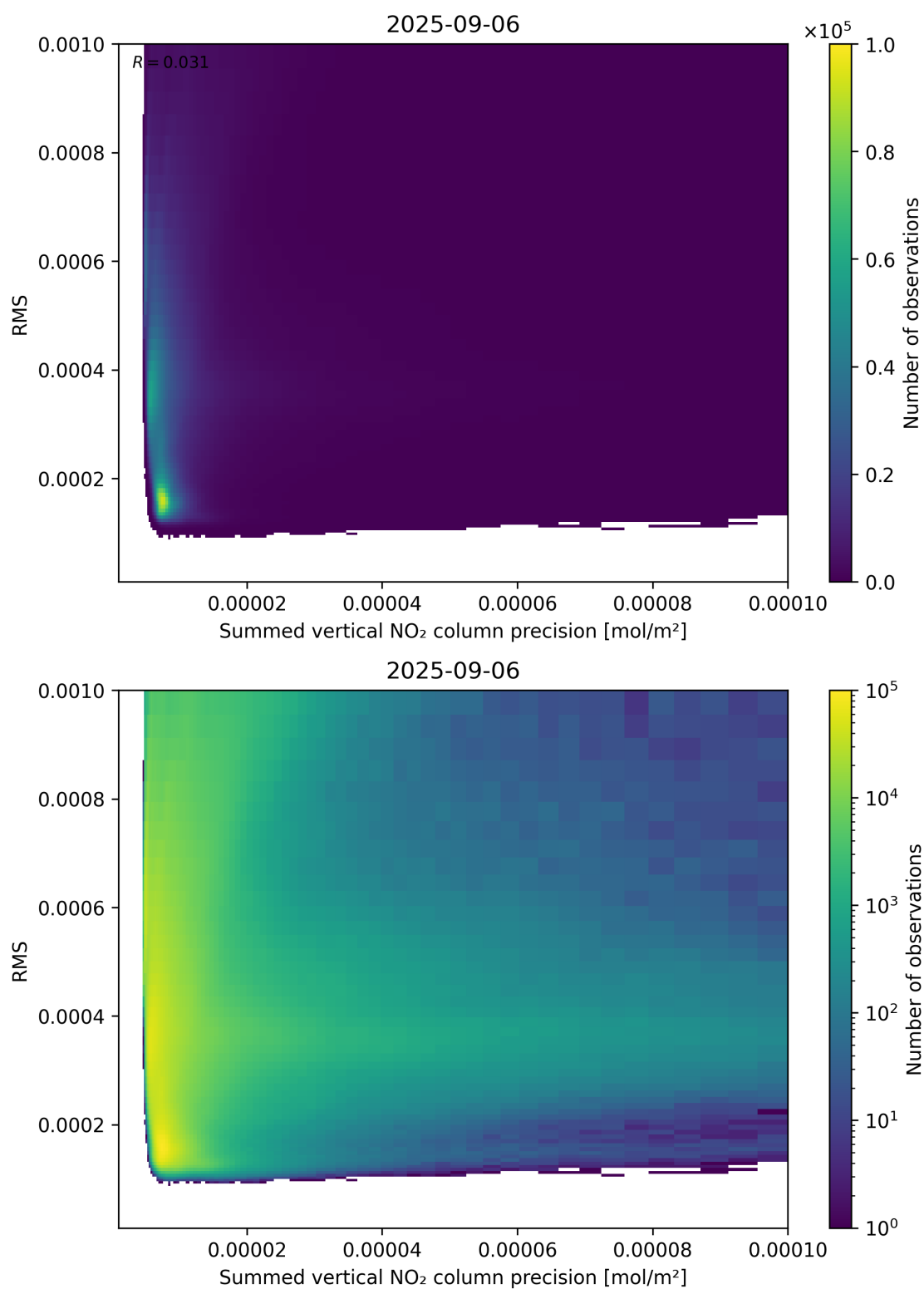
Figure 108: Scatter density plot of “Summed vertical NO 2 column precision” against “RMS” for 2025-09-05 to 2025-09-07.
