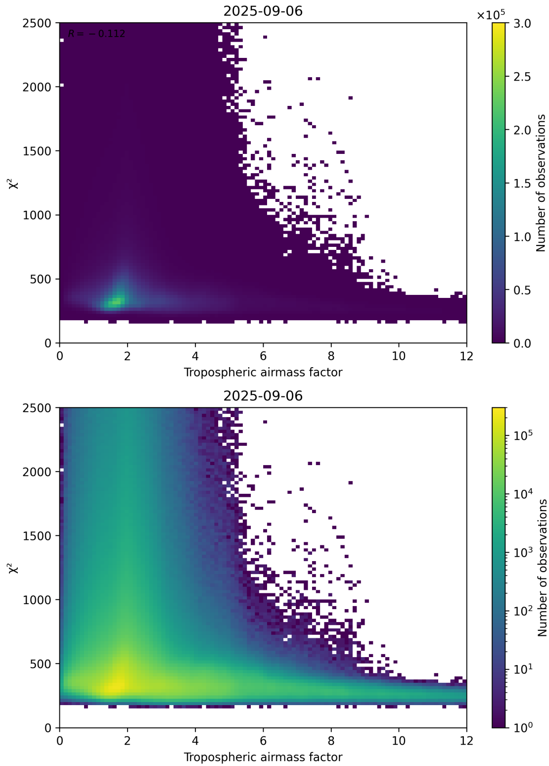
Figure 73: Scatter density plot of “Tropospheric airmass factor” against “ \chi^2 ” for 2025-09-05 to 2025-09-07.
