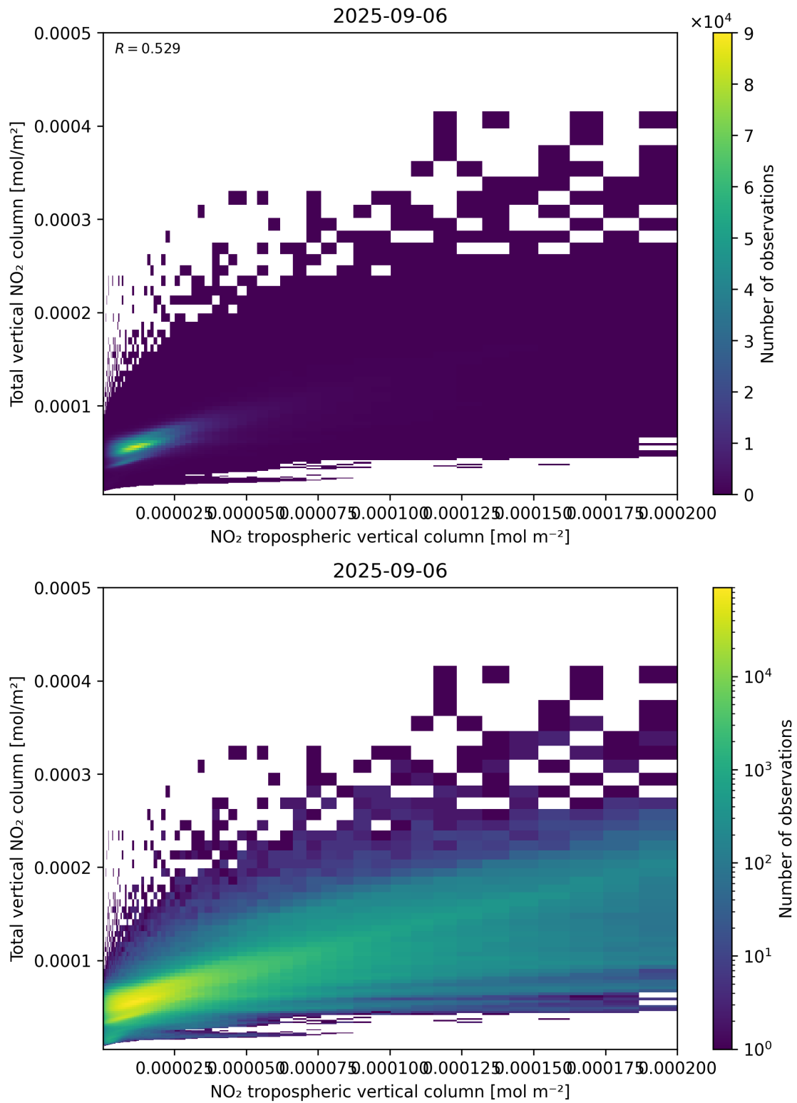
Figure 128: Scatter density plot of “NO 2 tropospheric vertical column” against “Total vertical NO 2 column” for 2025-09-05 to 2025-09-07.
