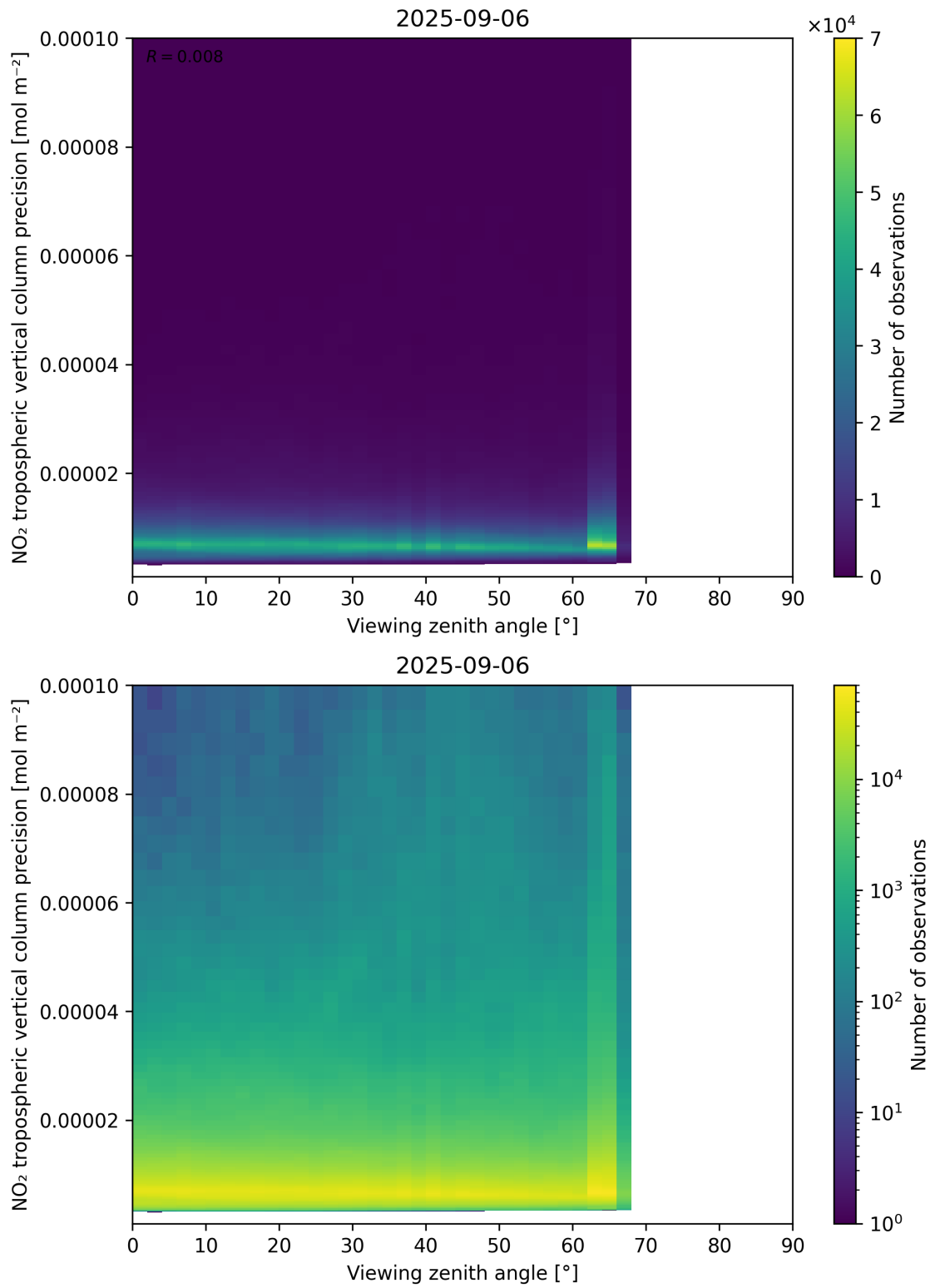
Figure 170: Scatter density plot of “Viewing zenith angle” against “NO 2 tropospheric vertical column precision” for 2025-09-05 to 2025-09-07.
