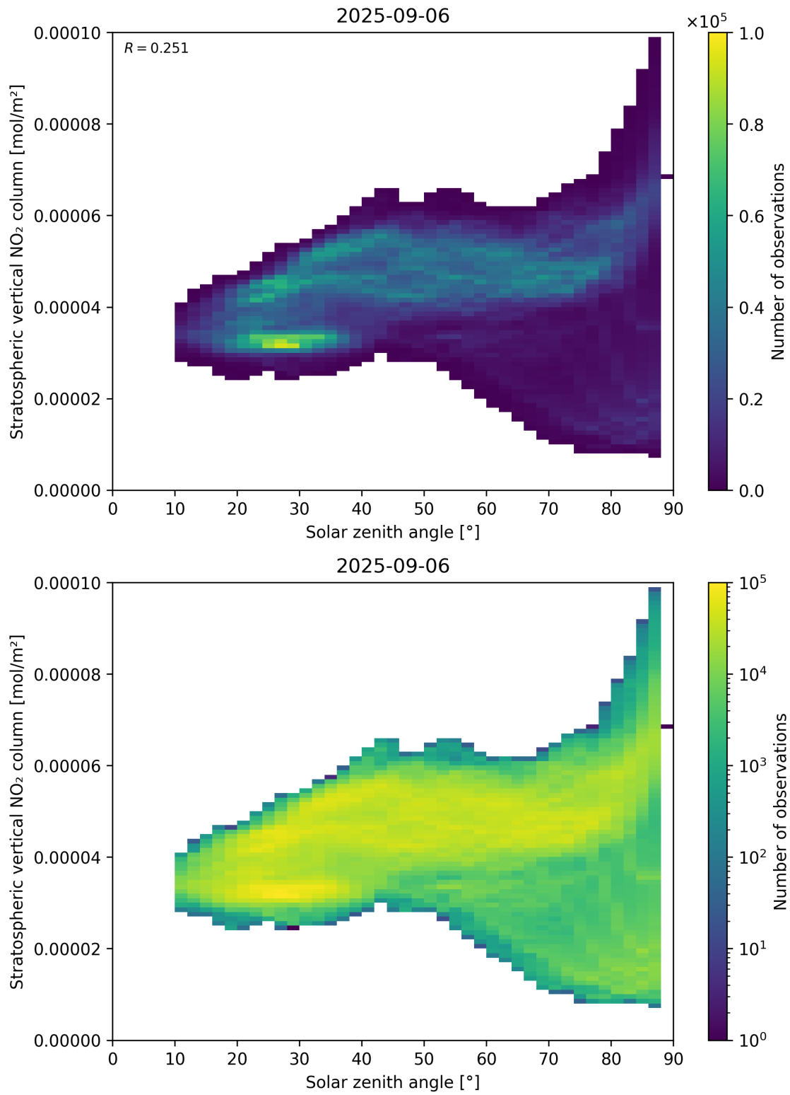
Figure 150: Scatter density plot of “Solar zenith angle” against “Stratospheric vertical NO 2 column” for 2025-09-05 to 2025-09-07.
