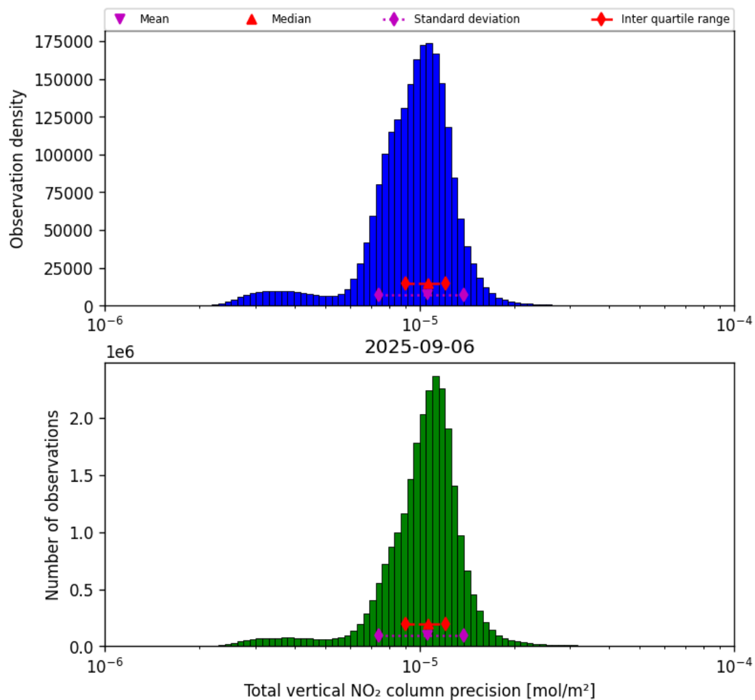
Figure 39: Histogram of “Total vertical NO 2 column precision” for 2025-09-05 to 2025-09-07
