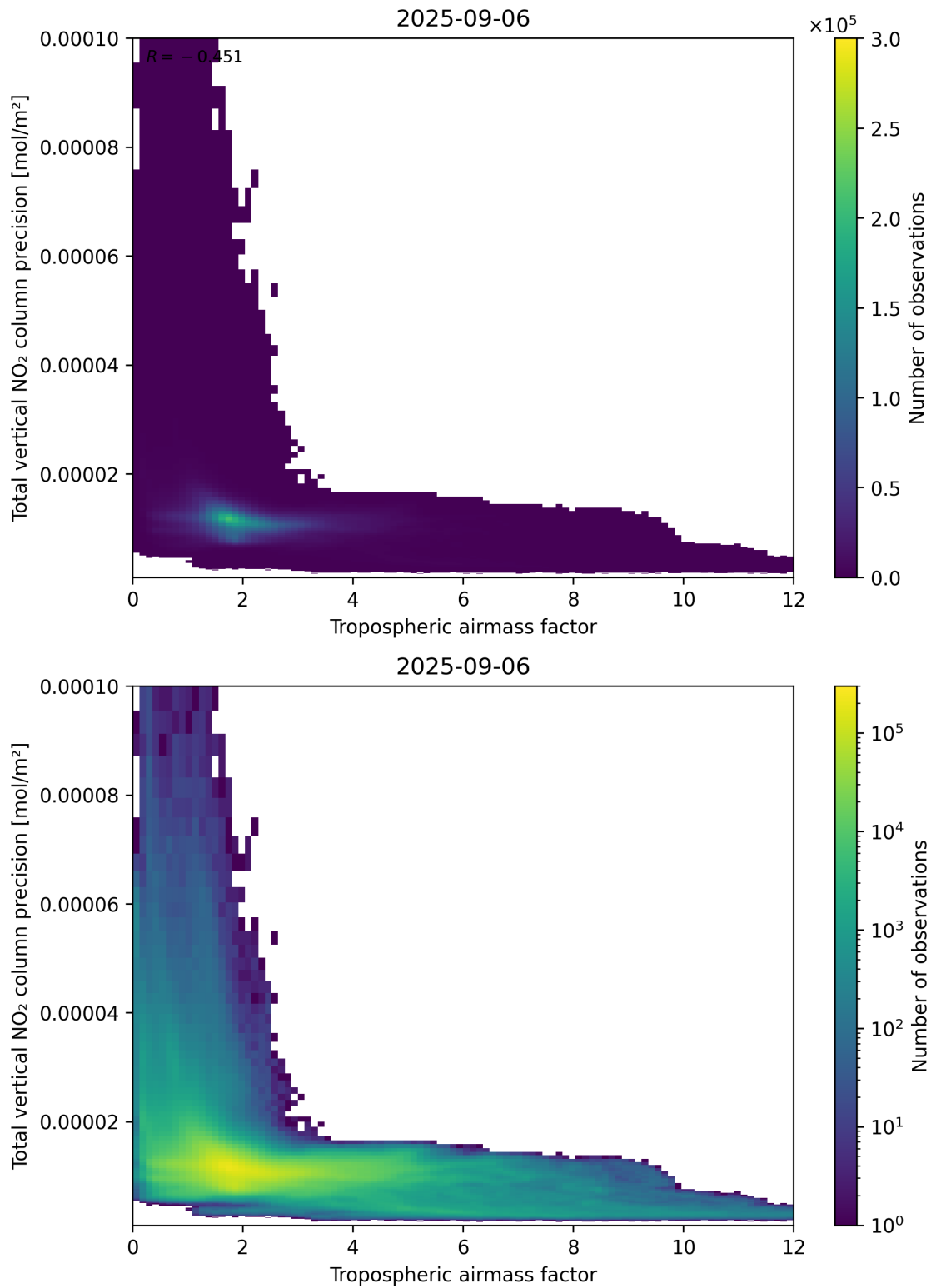
Figure 78: Scatter density plot of “Tropospheric airmass factor” against “Total vertical NO 2 column precision” for 2025-09-05 to 2025-09-07.
