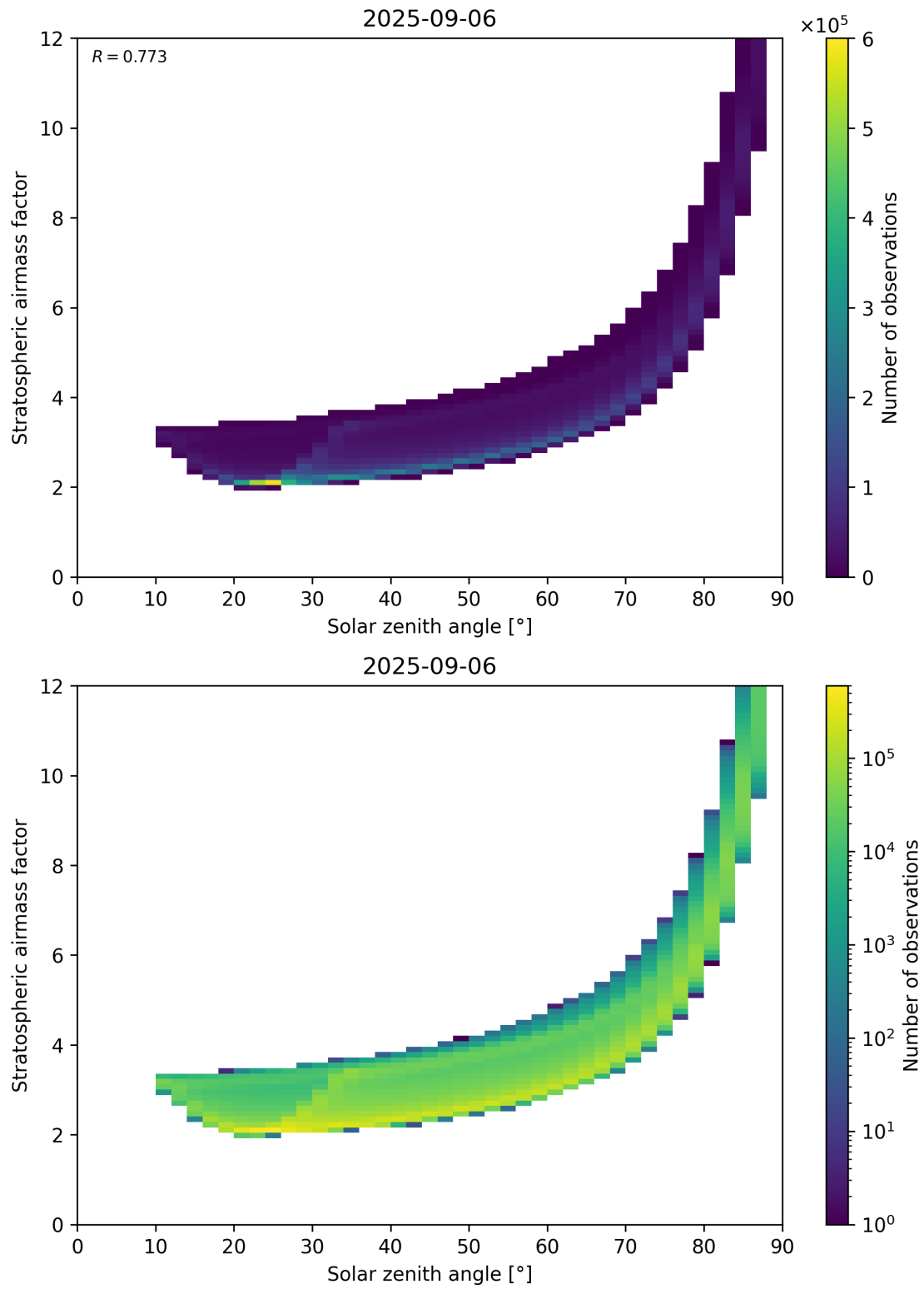
Figure 145: Scatter density plot of “Solar zenith angle” against “Stratospheric airmass factor” for 2025-09-05 to 2025-09-07.
