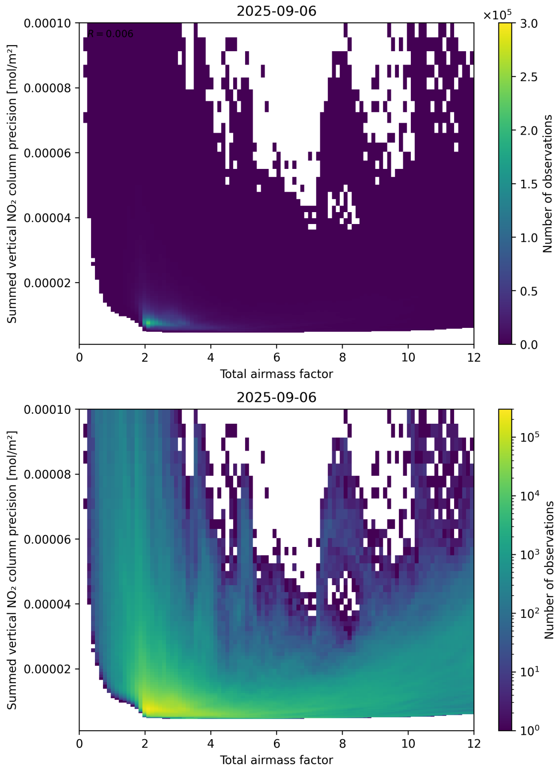
Figure 66: Scatter density plot of “Total airmass factor” against “Summed vertical NO 2 column precision” for 2025-09-05 to 2025-09-07.
