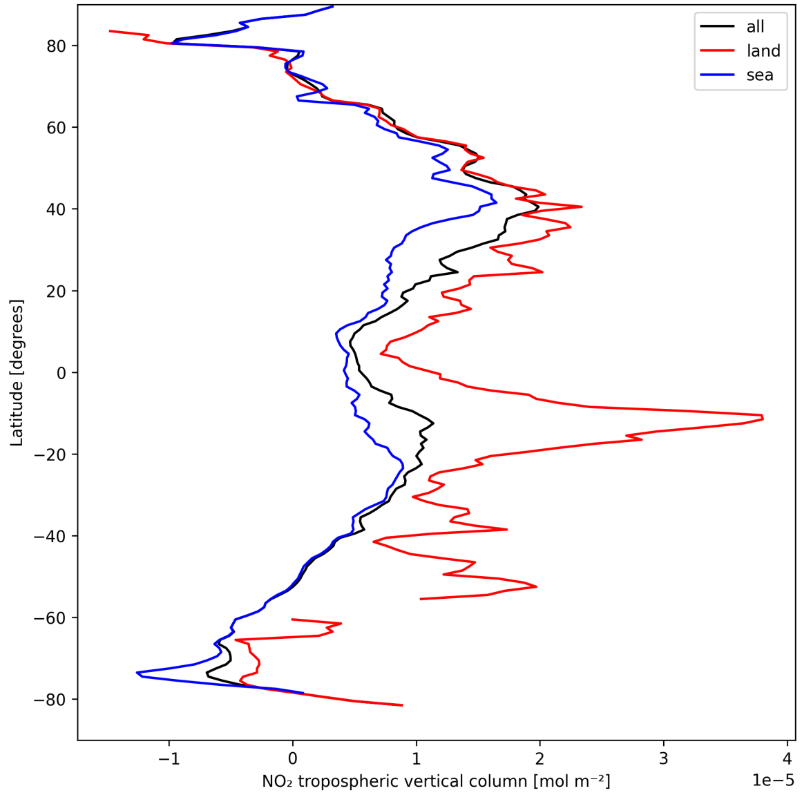
Figure 12: Zonal average of “NO 2 tropospheric vertical column” for 2025-09-05 to 2025-09-07.
