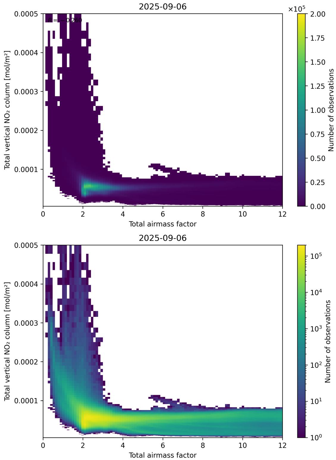
Figure 67: Scatter density plot of “Total airmass factor” against “Total vertical NO 2 column” for 2025-09-05 to 2025-09-07.
