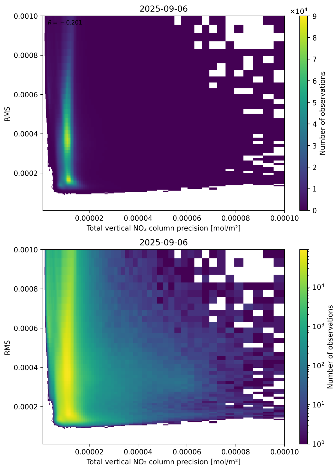
Figure 119: Scatter density plot of “Total vertical NO 2 column precision” against “RMS” for 2025-09-05 to 2025-09-07.
