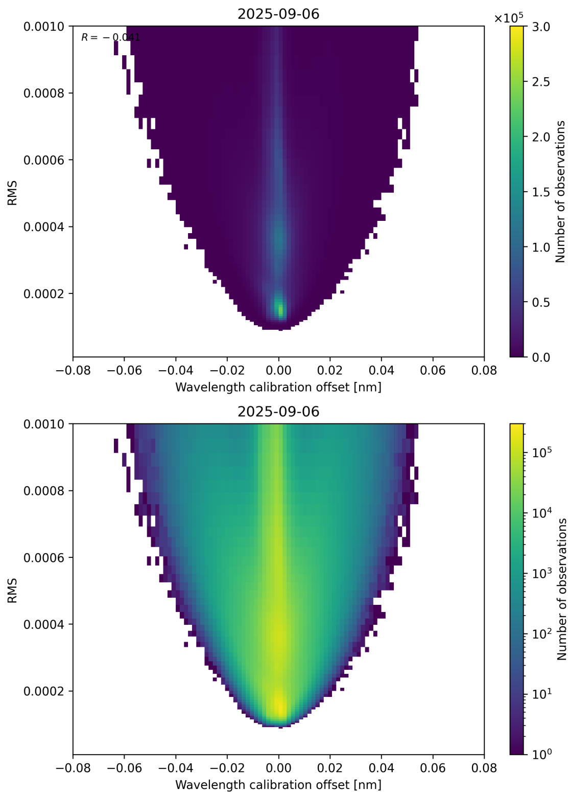
Figure 181: Scatter density plot of “Wavelength calibration offset” against “RMS” for 2025-09-05 to 2025-09-07.
