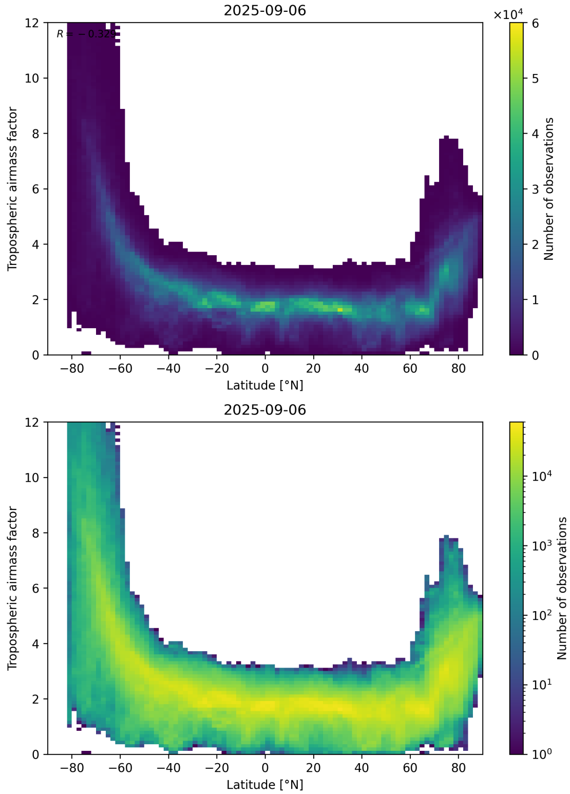
Figure 85: Scatter density plot of “Latitude” against “Tropospheric air mass factor” for 2025-09-05 to 2025-09-07.
