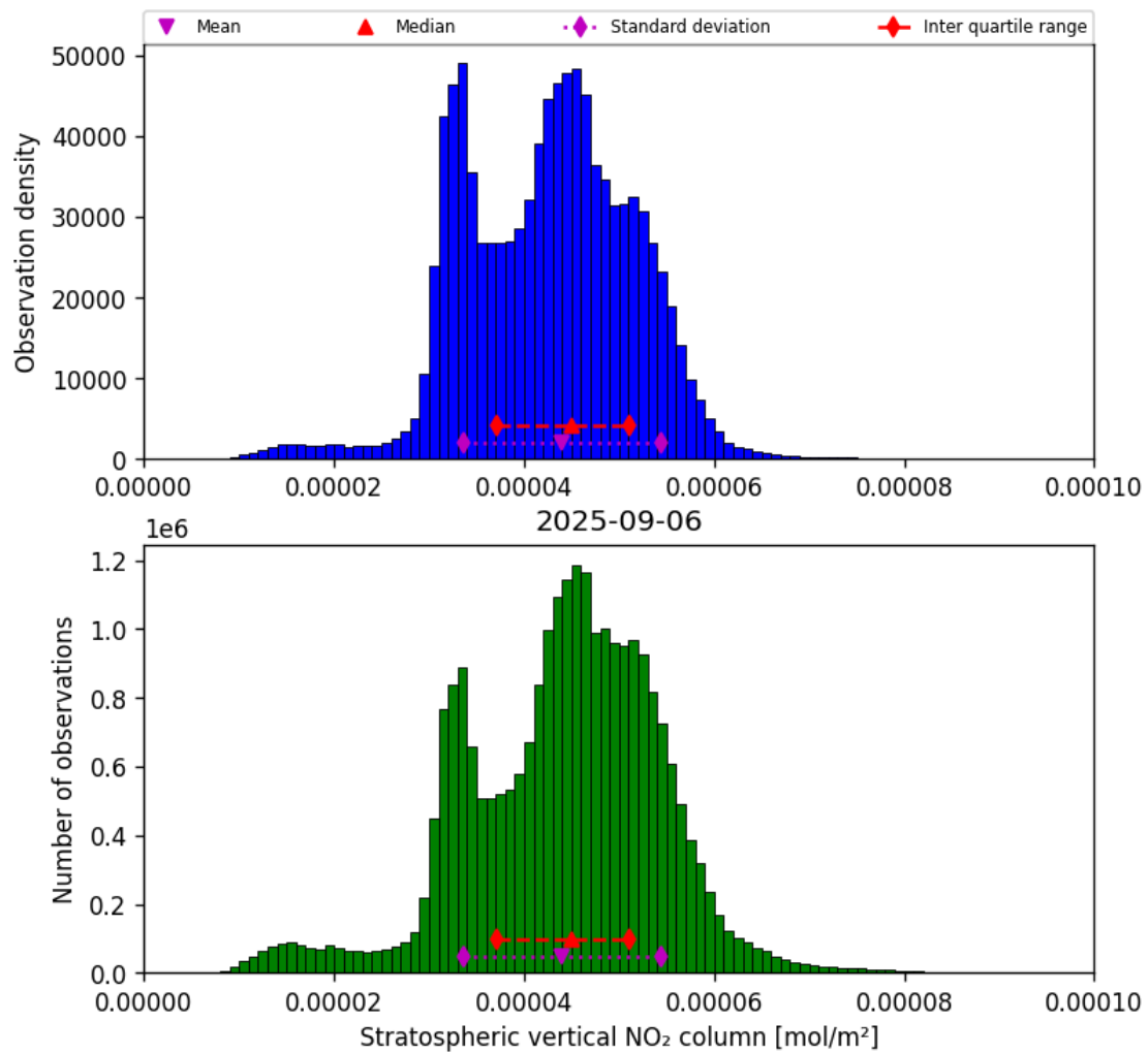
Figure 36: Histogram of “Stratospheric vertical NO 2 column” for 2025-09-05 to 2025-09-07
