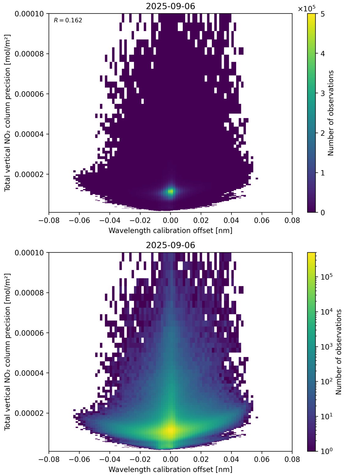
Figure 180: Scatter density plot of “Wavelength calibration offset” against “Total vertical NO 2 column precision” for 2025-09-05 to 2025-09-07.
