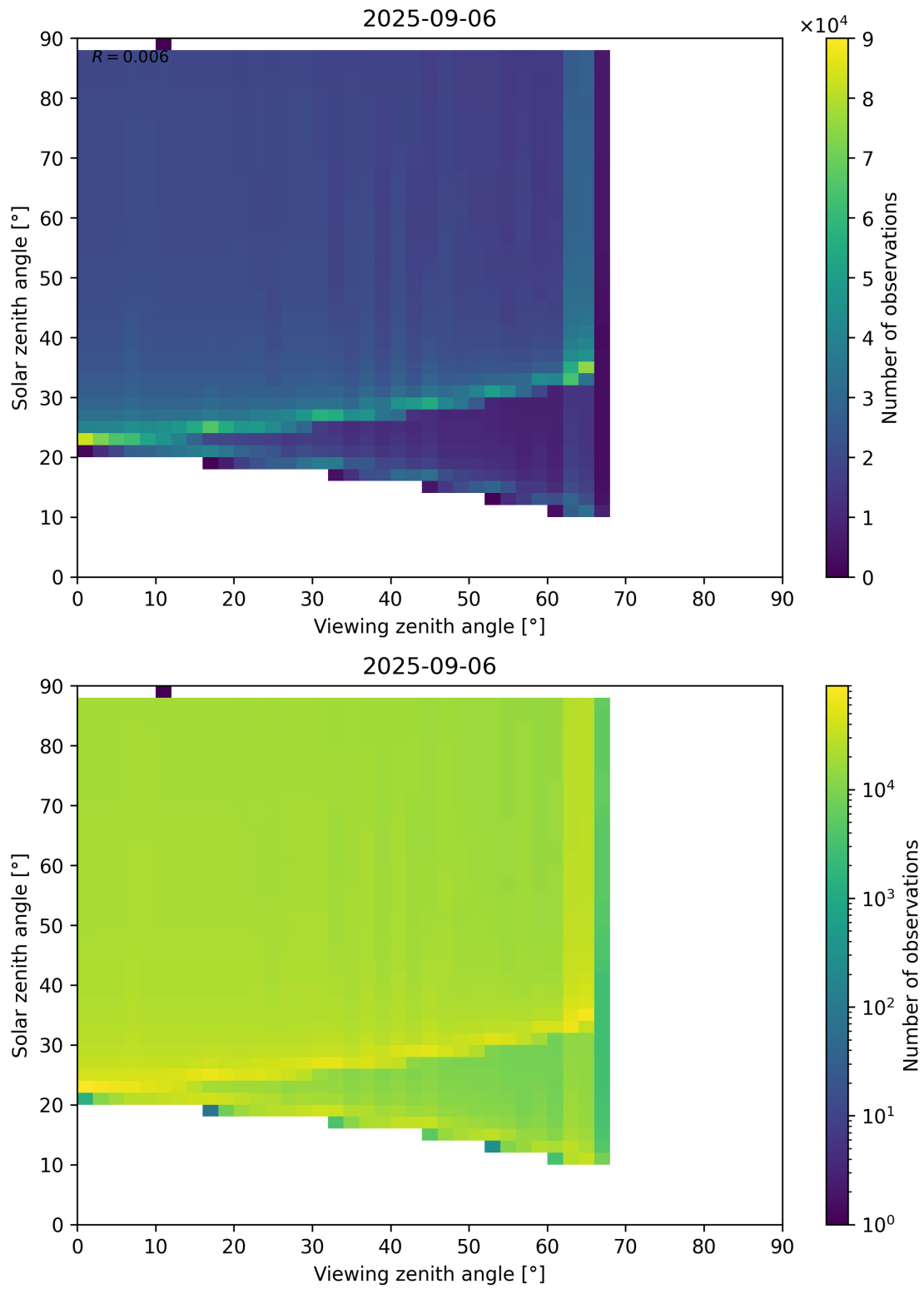
Figure 172: Scatter density plot of “Viewing zenith angle” against “Solar zenith angle” for 2025-09-05 to 2025-09-07.
