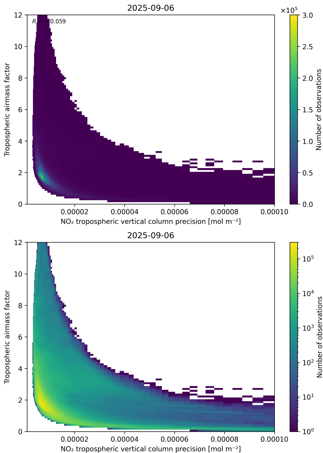
Figure 133: Scatter density plot of “NO 2 tropospheric vertical column precision” against “Tropospheric air mass factor” for 2025-09-05 to 2025-09-07.
