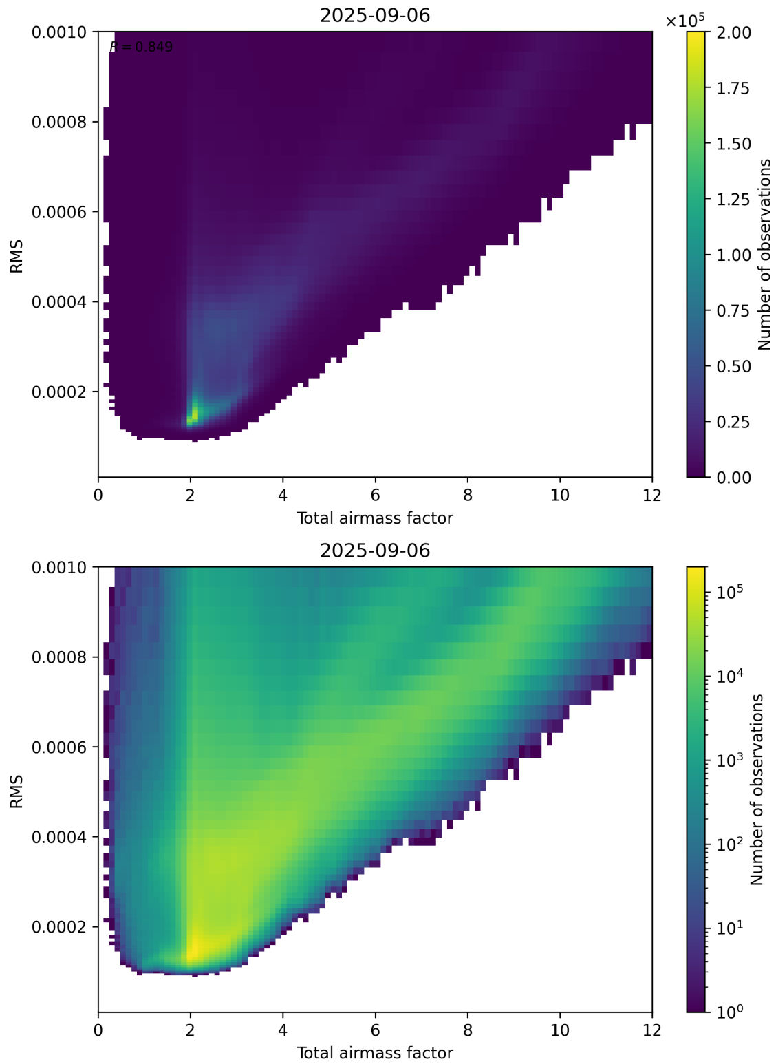
Figure 69: Scatter density plot of “Total airmass factor” against “RMS” for 2025-09-05 to 2025-09-07.
