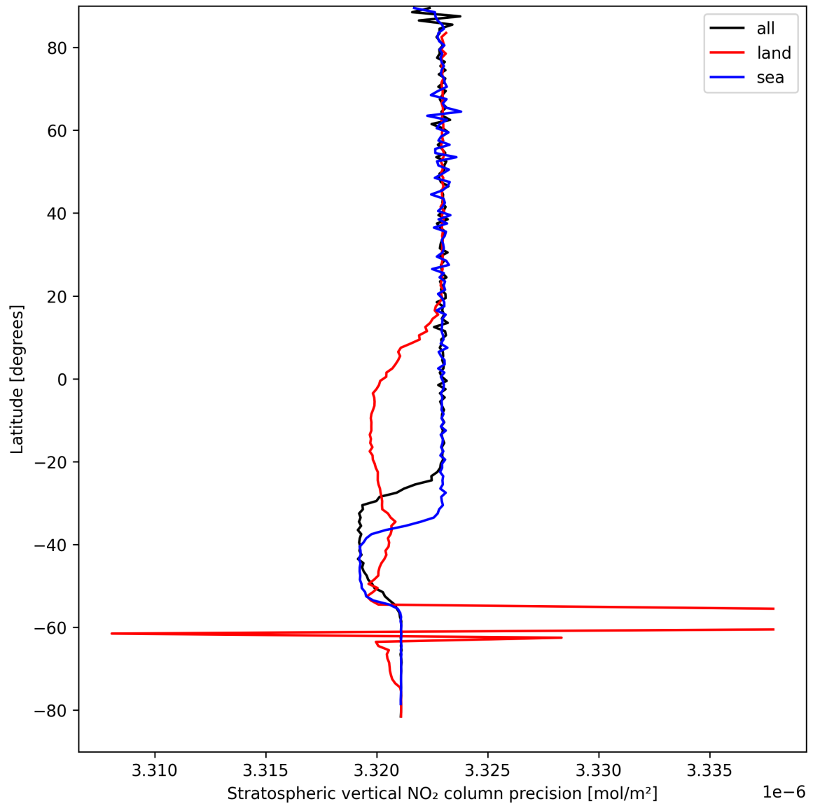
Figure 20: Zonal average of “Stratospheric vertical NO 2 column precision” for 2025-09-05 to 2025-09-07.
