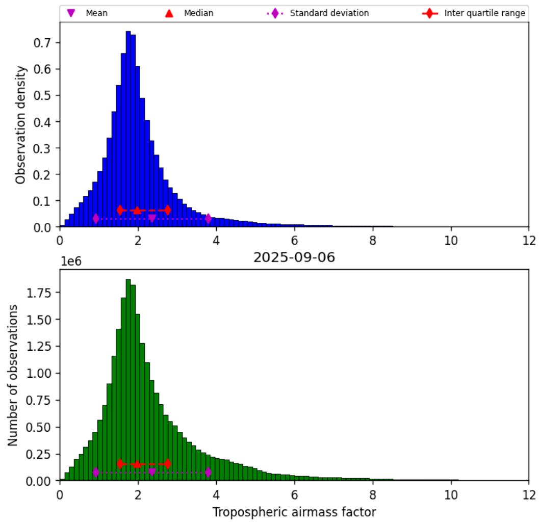
Figure 31: Histogram of “Tropospheric airmass factor” for 2025-09-05 to 2025-09-07
