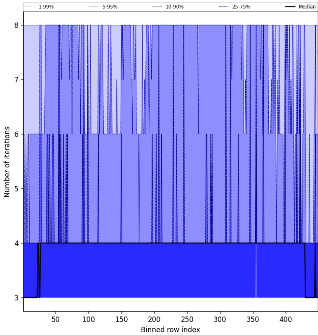
Figure 51: Along track statistics of “Number of iterations” for 2025-09-05 to 2025-09-07
