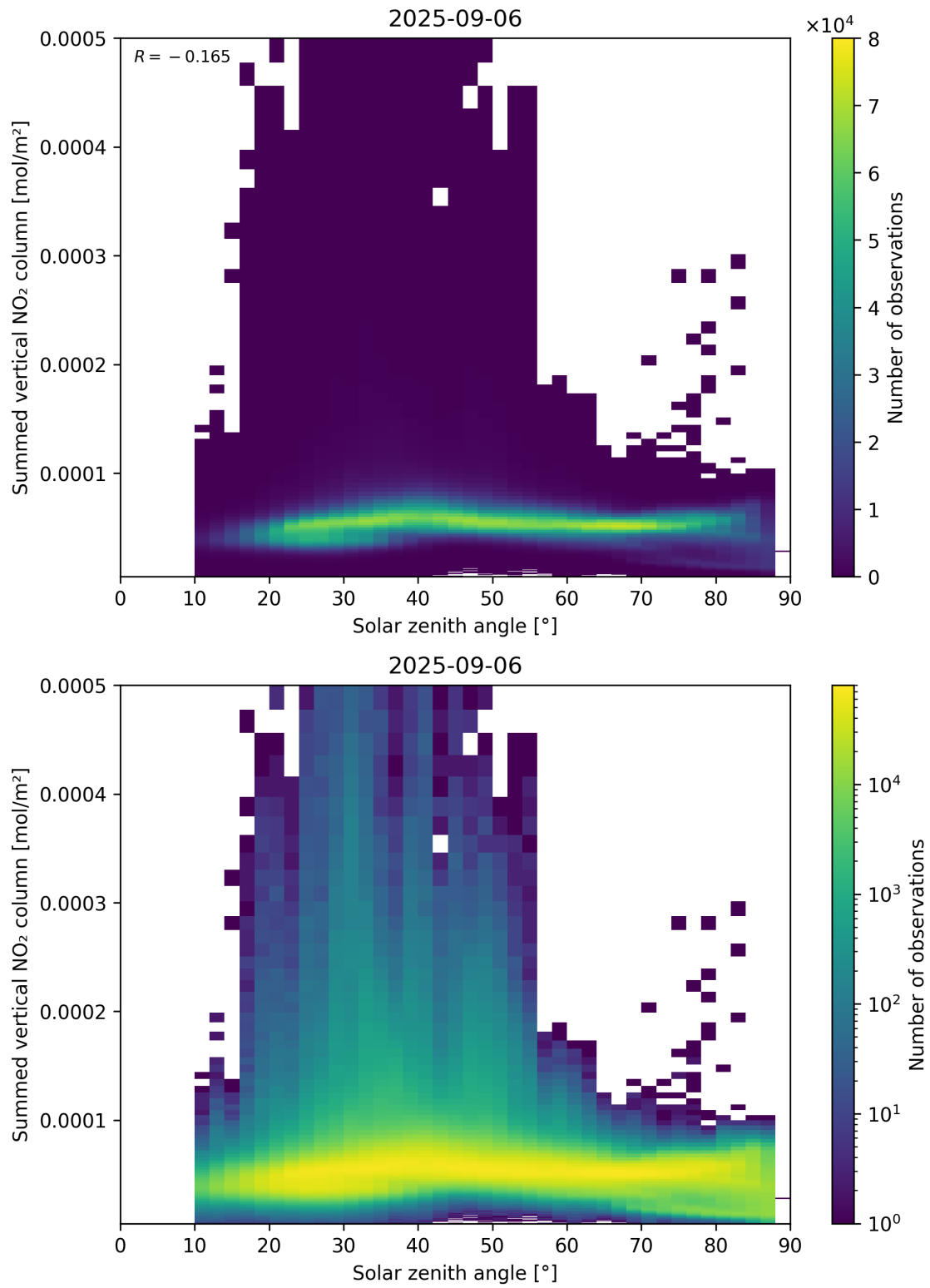
Figure 151: Scatter density plot of “Solar zenith angle” against “Summed vertical NO 2 column” for 2025-09-05 to 2025-09-07.
