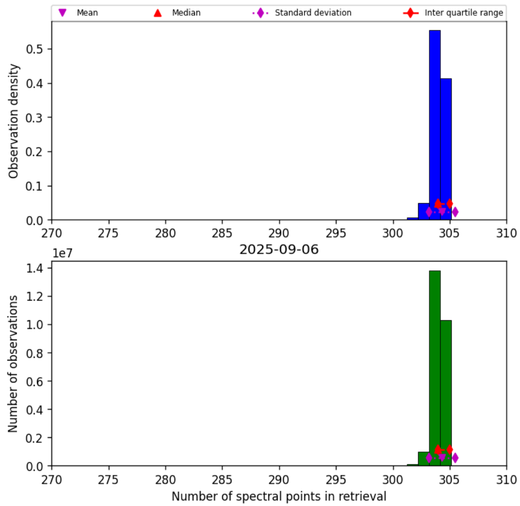
Figure 33: Histogram of “Number of spectral points in retrieval” for 2025-09-05 to 2025-09-07
