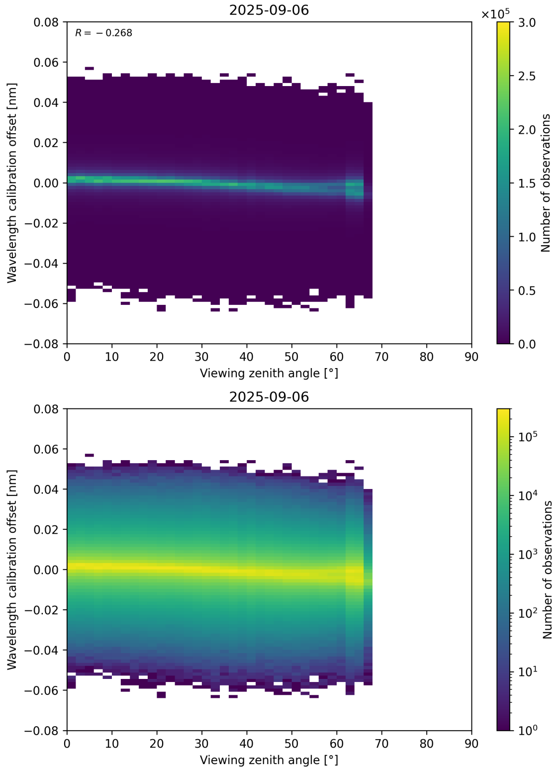
Figure 173: Scatter density plot of “Viewing zenith angle” against “Wavelength calibration offset” for 2025-09-05 to 2025-09-07.
