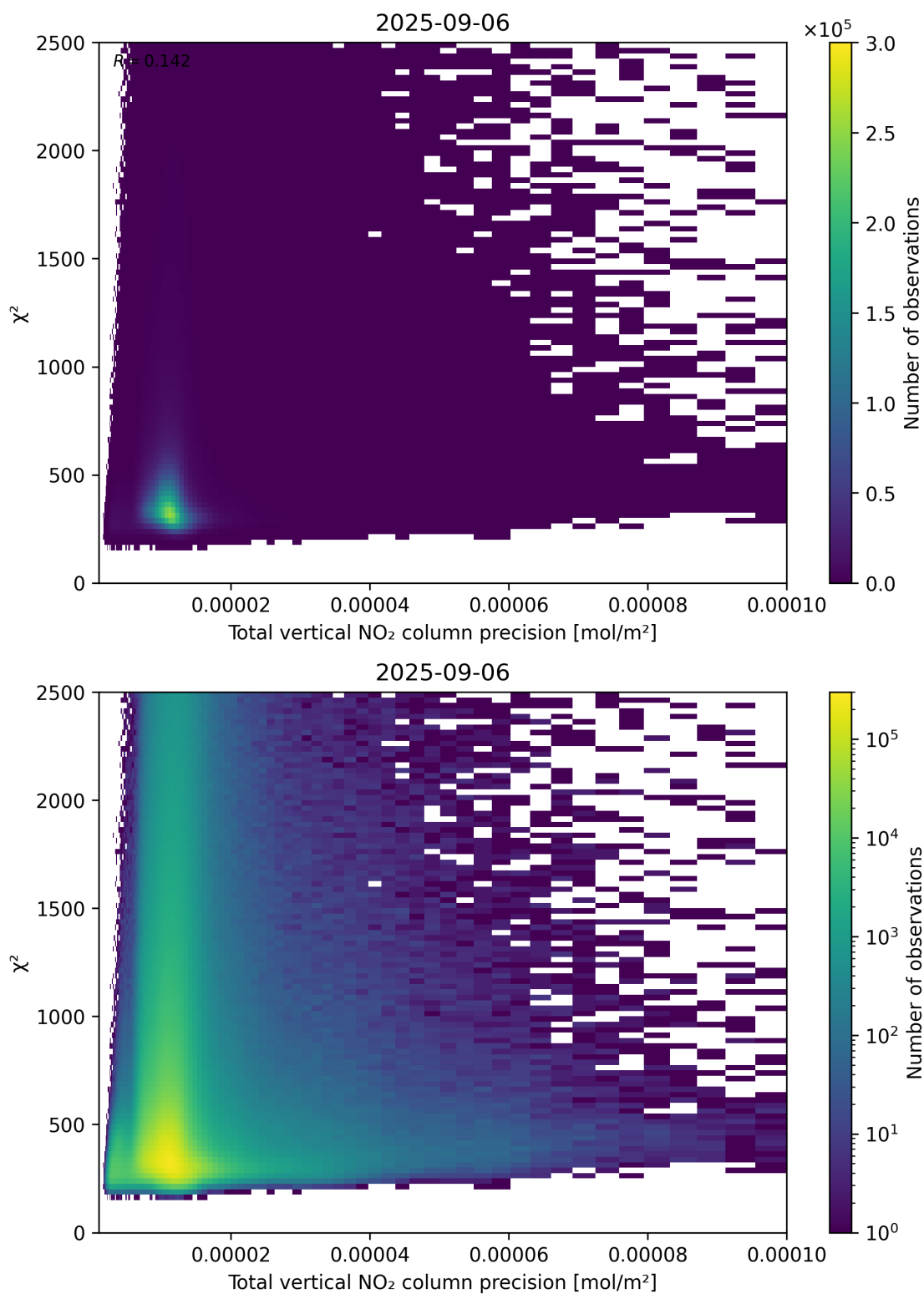
Figure 116: Scatter density plot of “Total vertical NO 2 column precision” against “ \chi^2 ” for 2025-09-05 to 2025-09-07.
