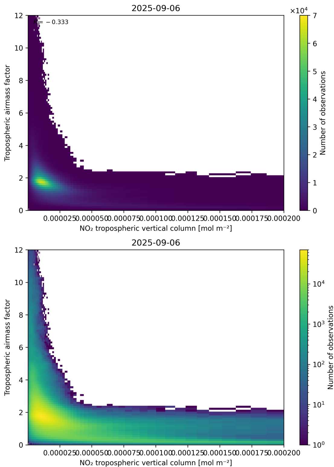
Figure 123: Scatter density plot of “NO 2 tropospheric vertical column” against “Tropospheric air mass factor” for 2025-09-05 to 2025-09-07.
