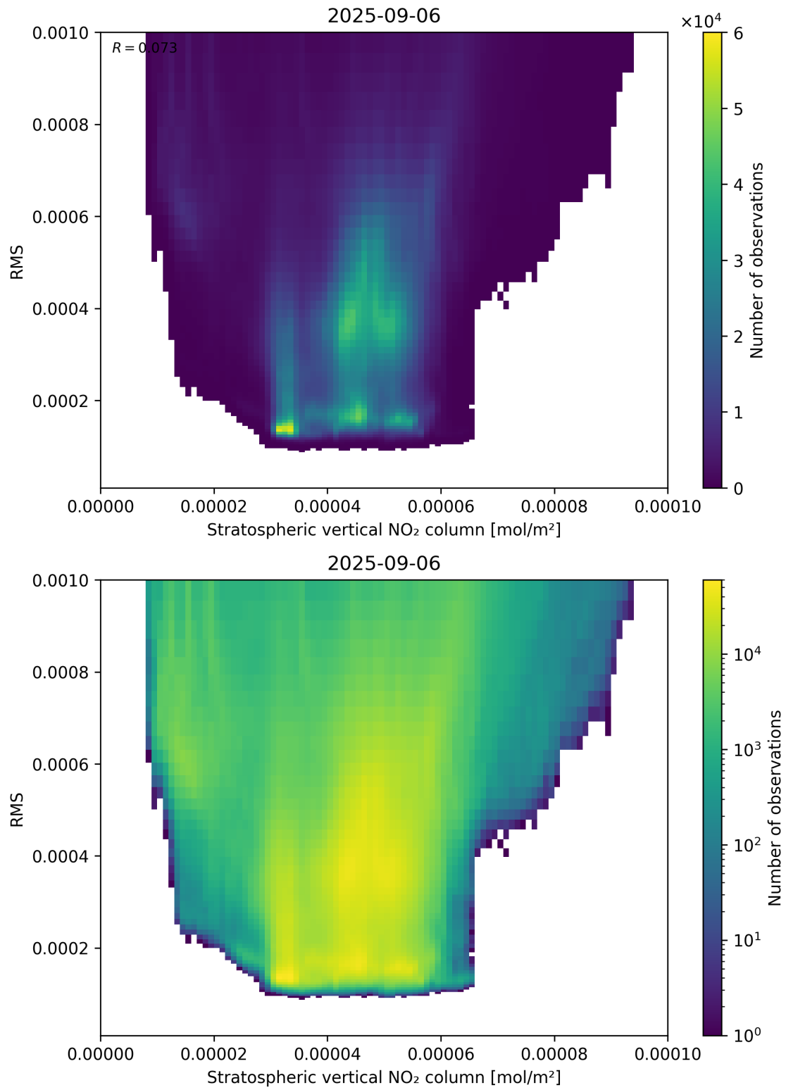
Figure 102: Scatter density plot of “Stratospheric vertical NO 2 column” against “RMS” for 2025-09-05 to 2025-09-07.
