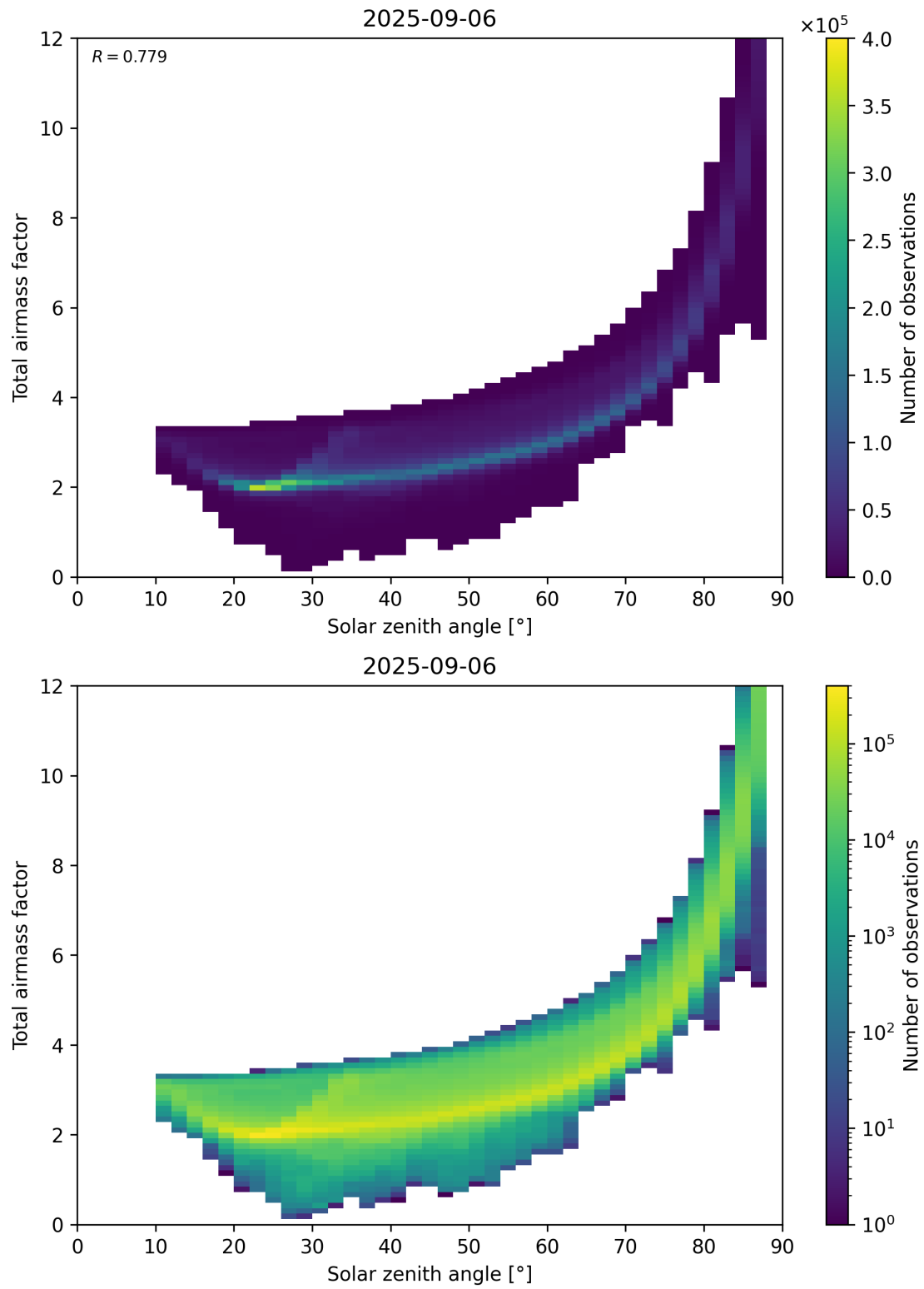
Figure 146: Scatter density plot of “Solar zenith angle” against “Total airmass factor” for 2025-09-05 to 2025-09-07.
