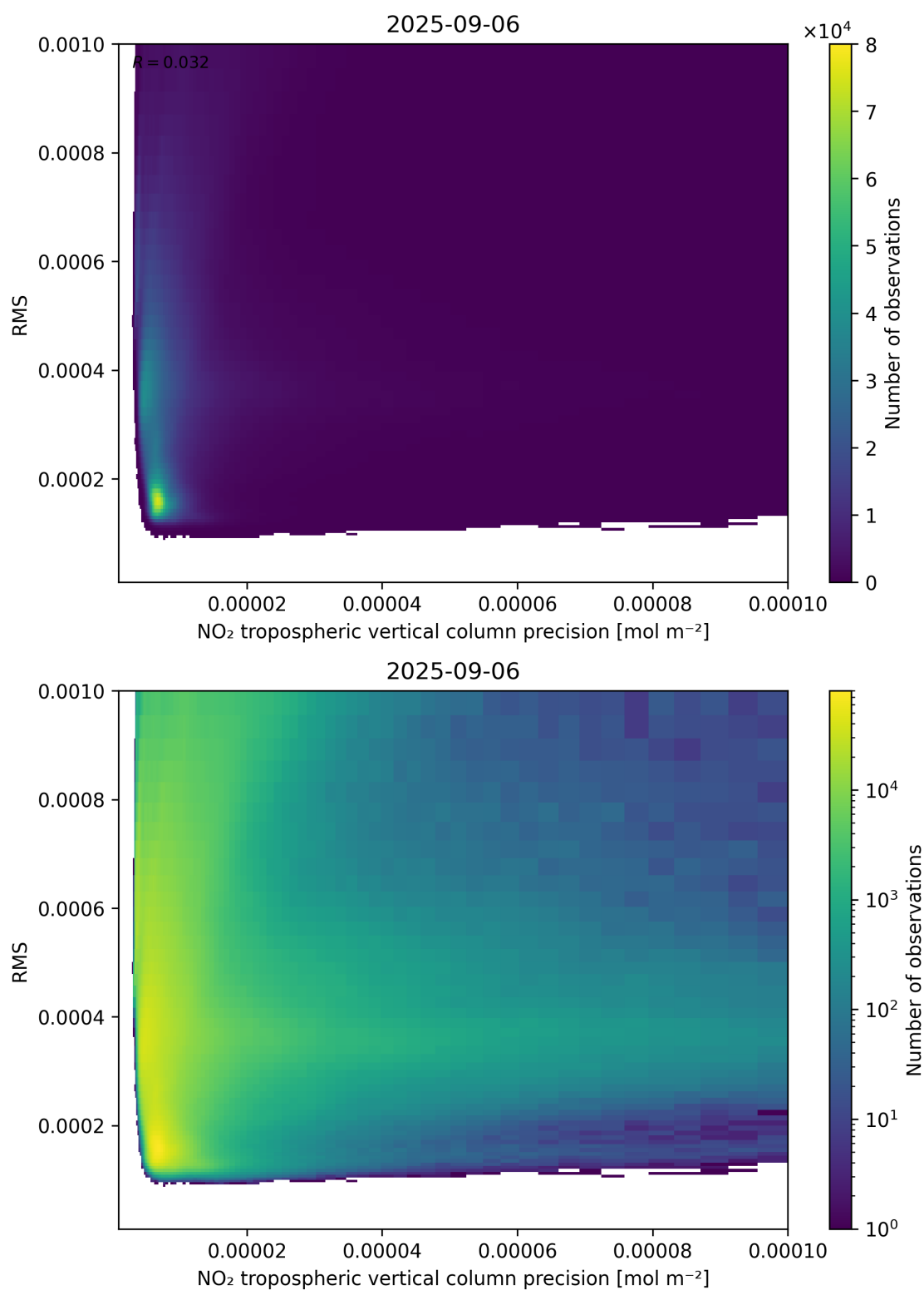
Figure 140: Scatter density plot of “NO 2 tropospheric vertical column precision” against “RMS” for 2025-09-05 to 2025-09-07.
