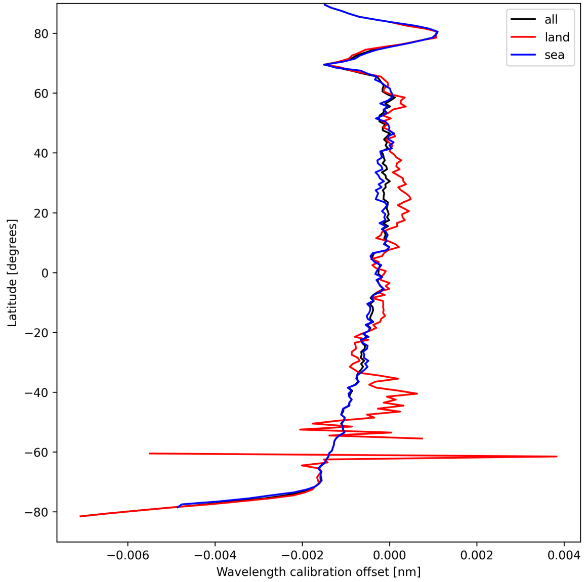
Figure 18: Zonal average of “Wavelength calibration offset” for 2025-09-05 to 2025-09-07.
