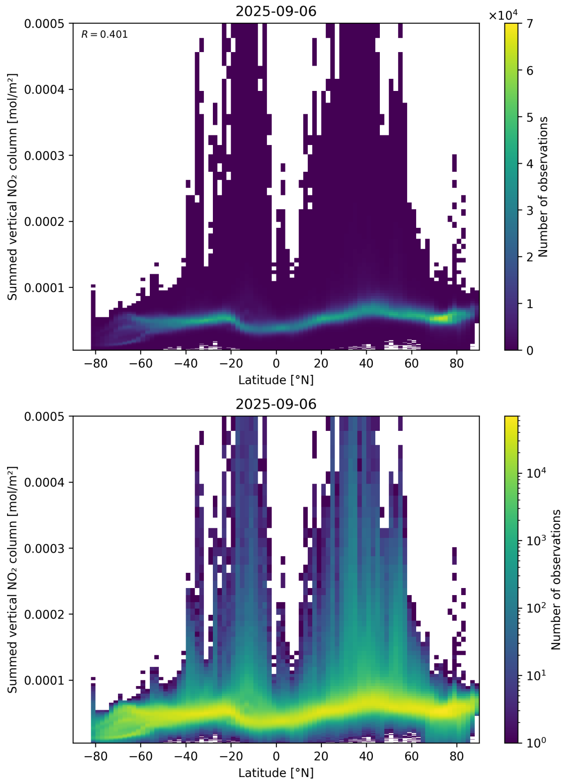
Figure 88: Scatter density plot of “Latitude” against “Summed vertical NO 2 column” for 2025-09-05 to 2025-09-07.
