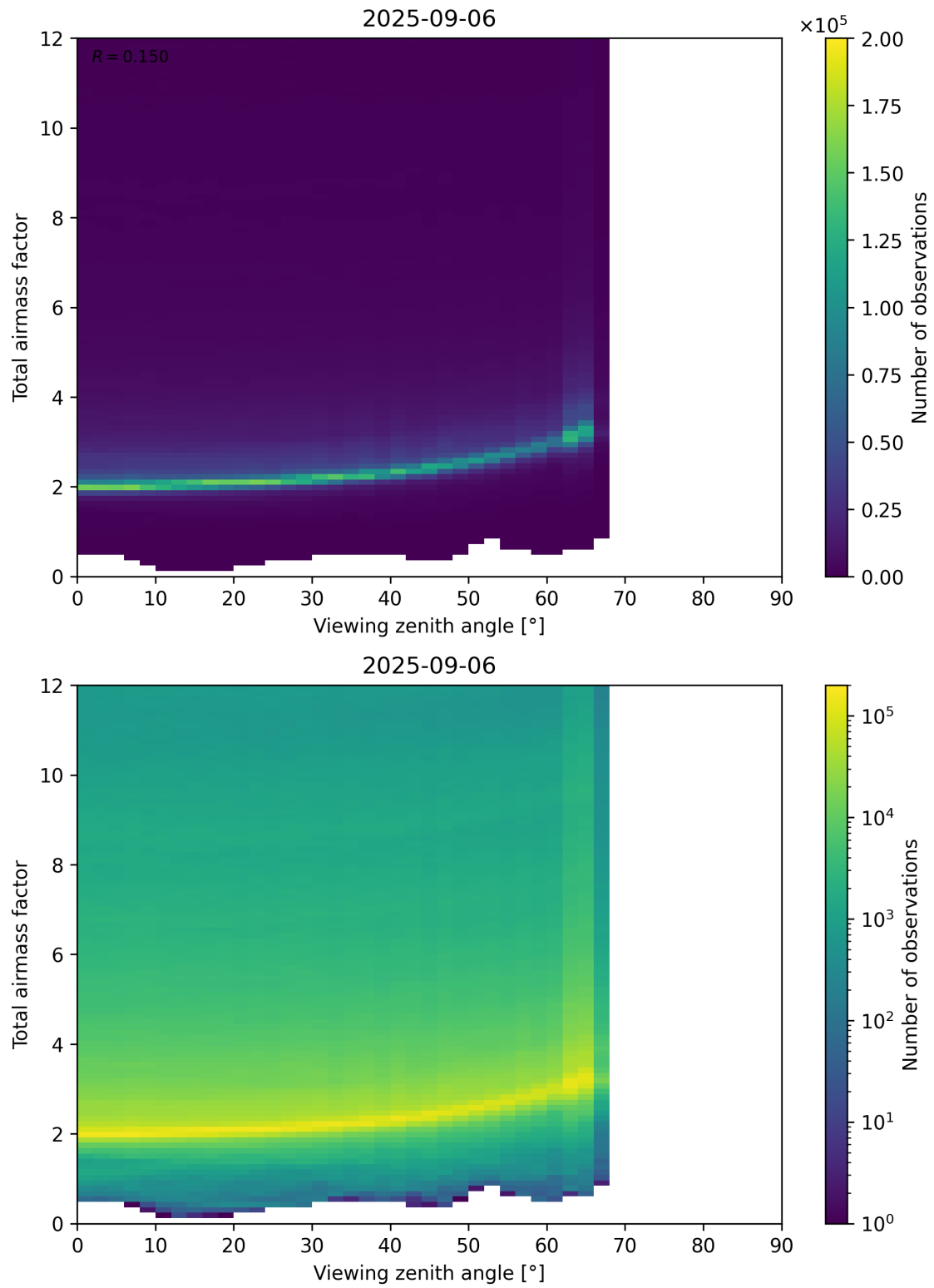
Figure 160: Scatter density plot of “Viewing zenith angle” against “Total airmass factor” for 2025-09-05 to 2025-09-07.
