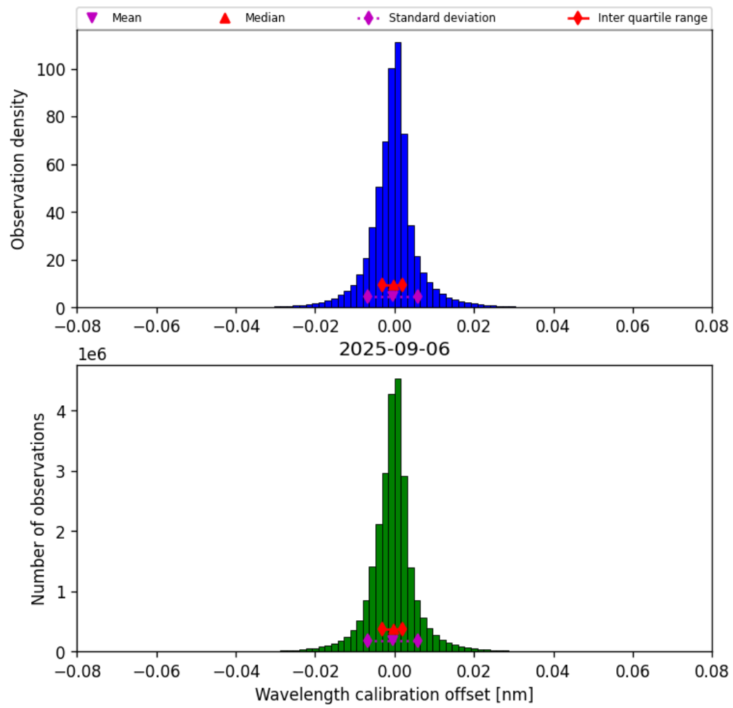
Figure 35: Histogram of “Wavelength calibration offset” for 2025-09-05 to 2025-09-07
