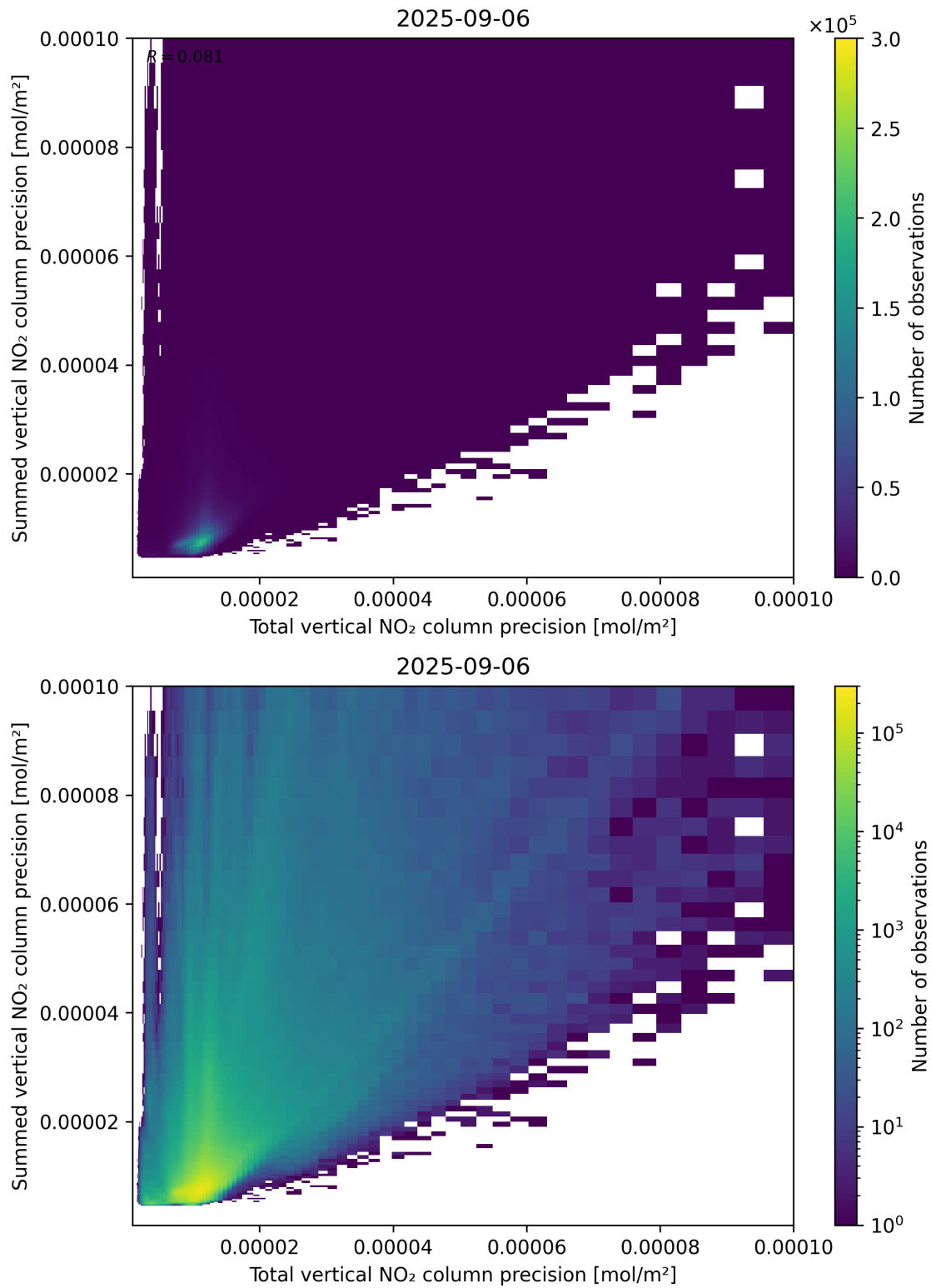
Figure 118: Scatter density plot of “Total vertical NO 2 column precision” against “Summed vertical NO 2 column precision” for 2025-09-05 to 2025-09-07.
