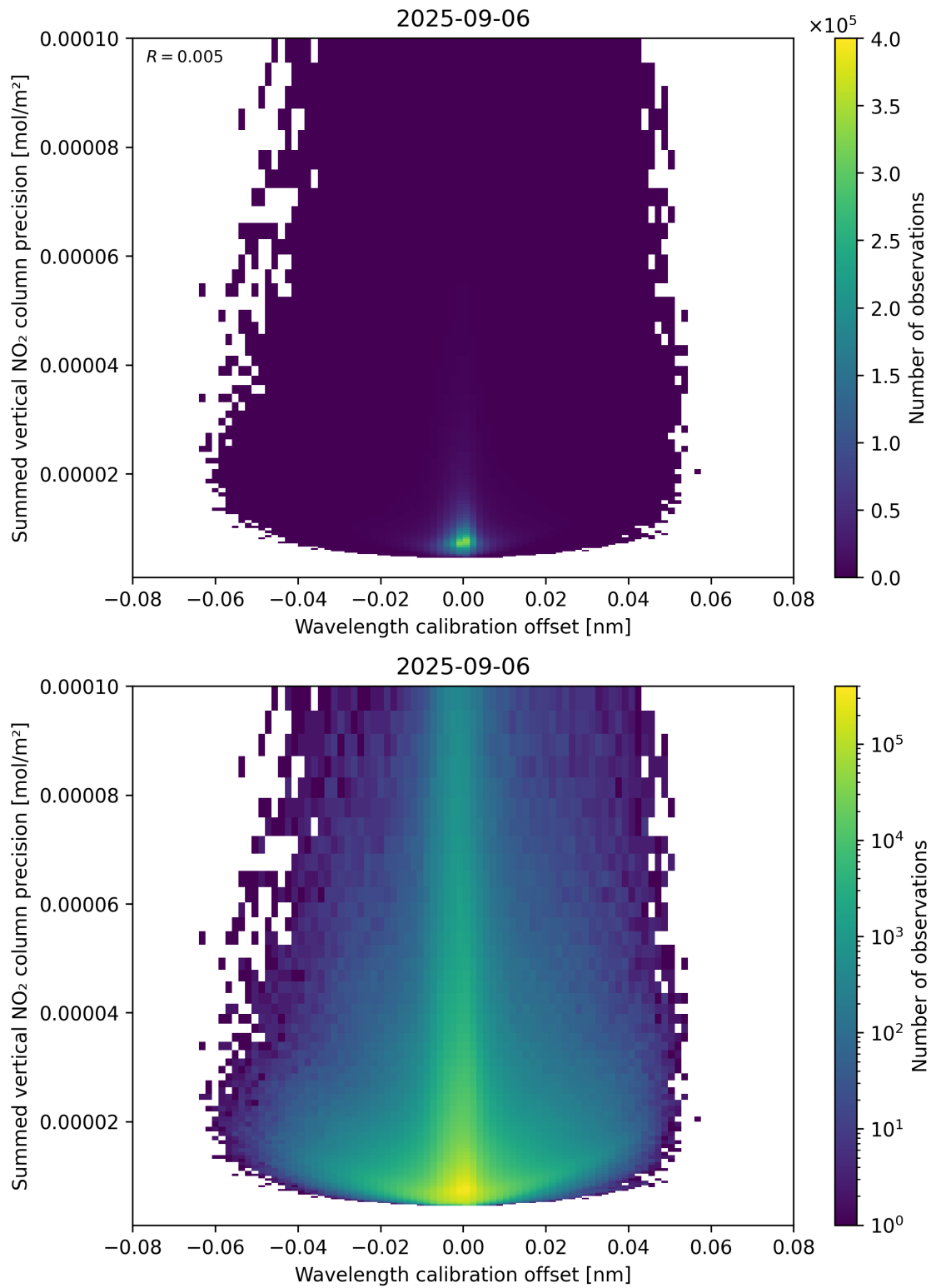
Figure 178: Scatter density plot of “Wavelength calibration offset” against “Summed vertical NO 2 column precision” for 2025-09-05 to 2025-09-07.
