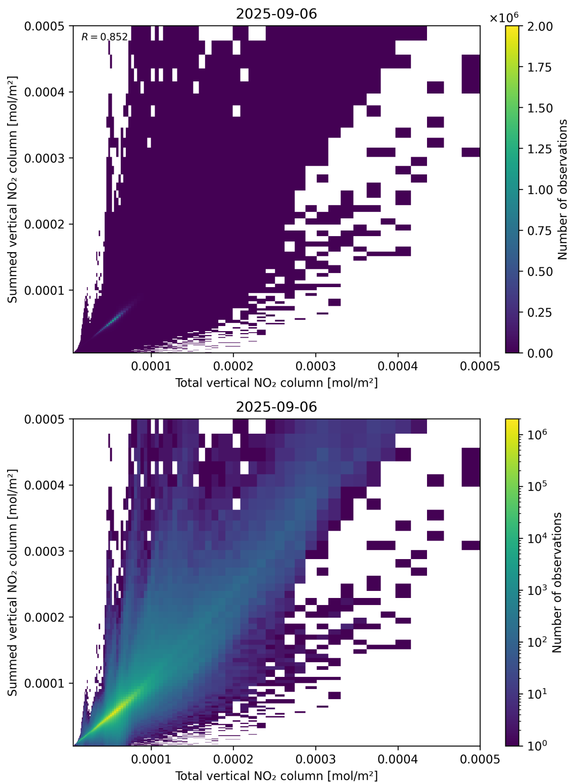
Figure 112: Scatter density plot of “Total vertical NO 2 column” against “Summed vertical NO 2 column” for 2025-09-05 to 2025-09-07.
