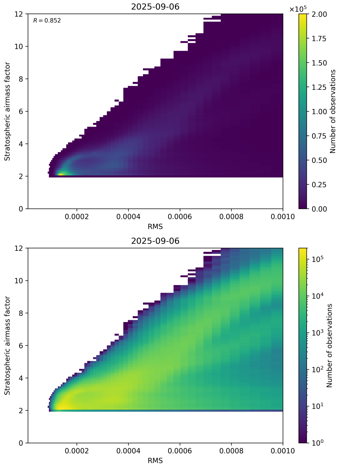
Figure 144: Scatter density plot of “RMS” against “Stratospheric airmass factor” for 2025-09-05 to 2025-09-07.
