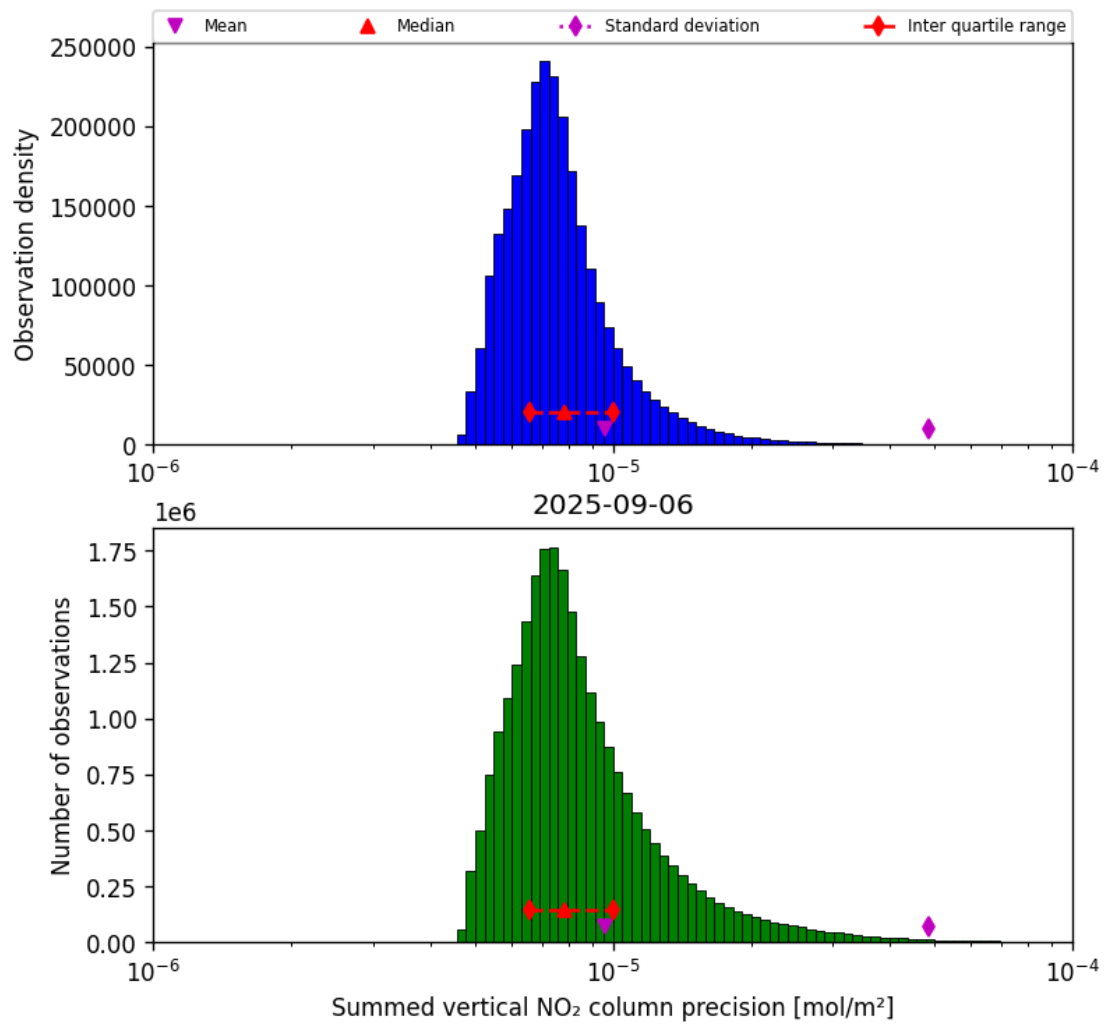
Figure 41: Histogram of "Summed vertical NO 2 column precision" for 2025-09-05 to 2025-09-07
