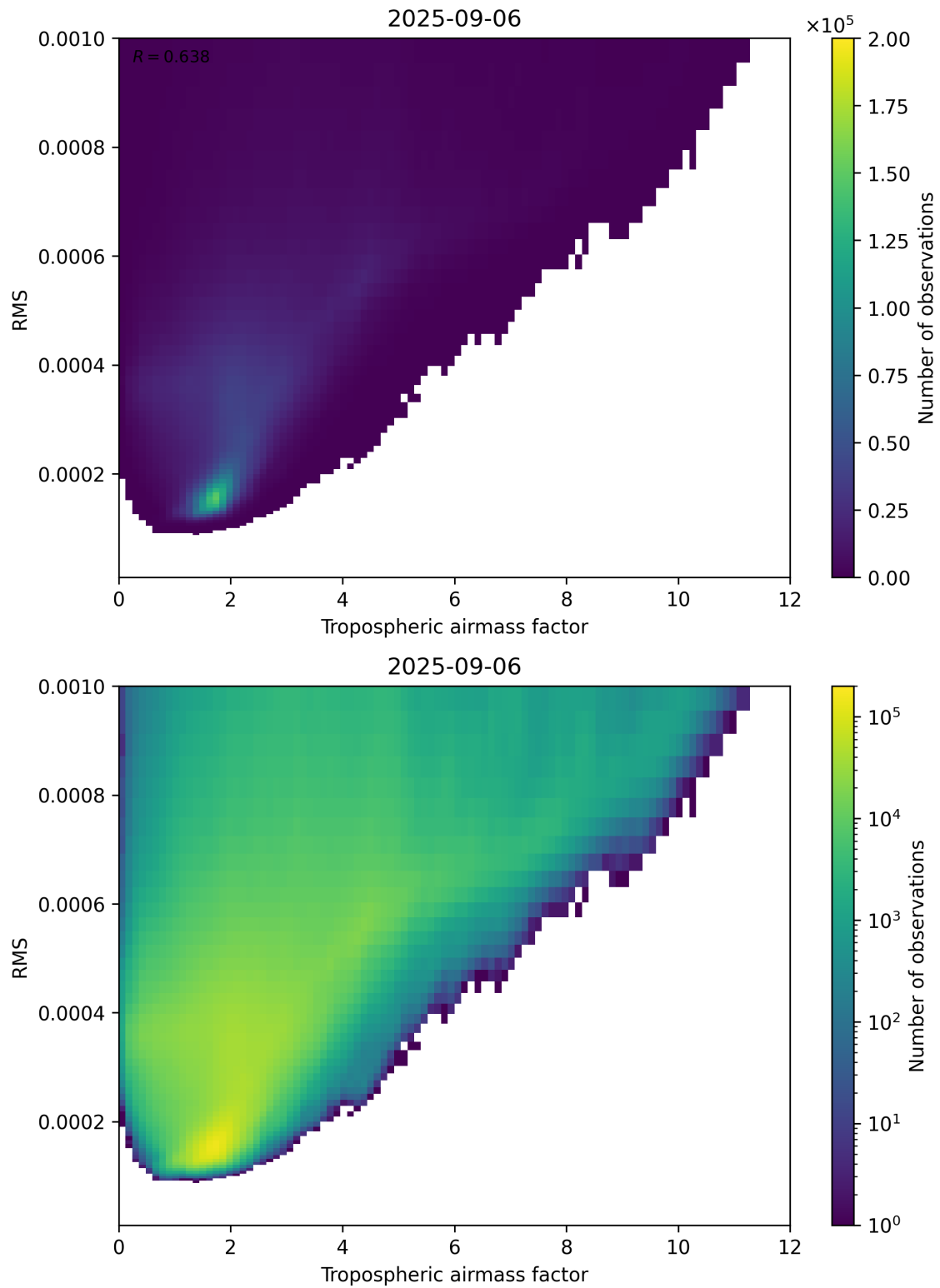
Figure 79: Scatter density plot of “Tropospheric airmass factor” against “RMS” for 2025-09-05 to 2025-09-07.
