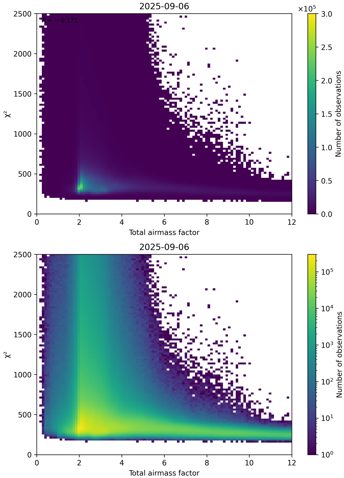
Figure 63: Scatter density plot of “Total airmass factor” against “ \chi^2 ” for 2025-09-05 to 2025-09-07.
