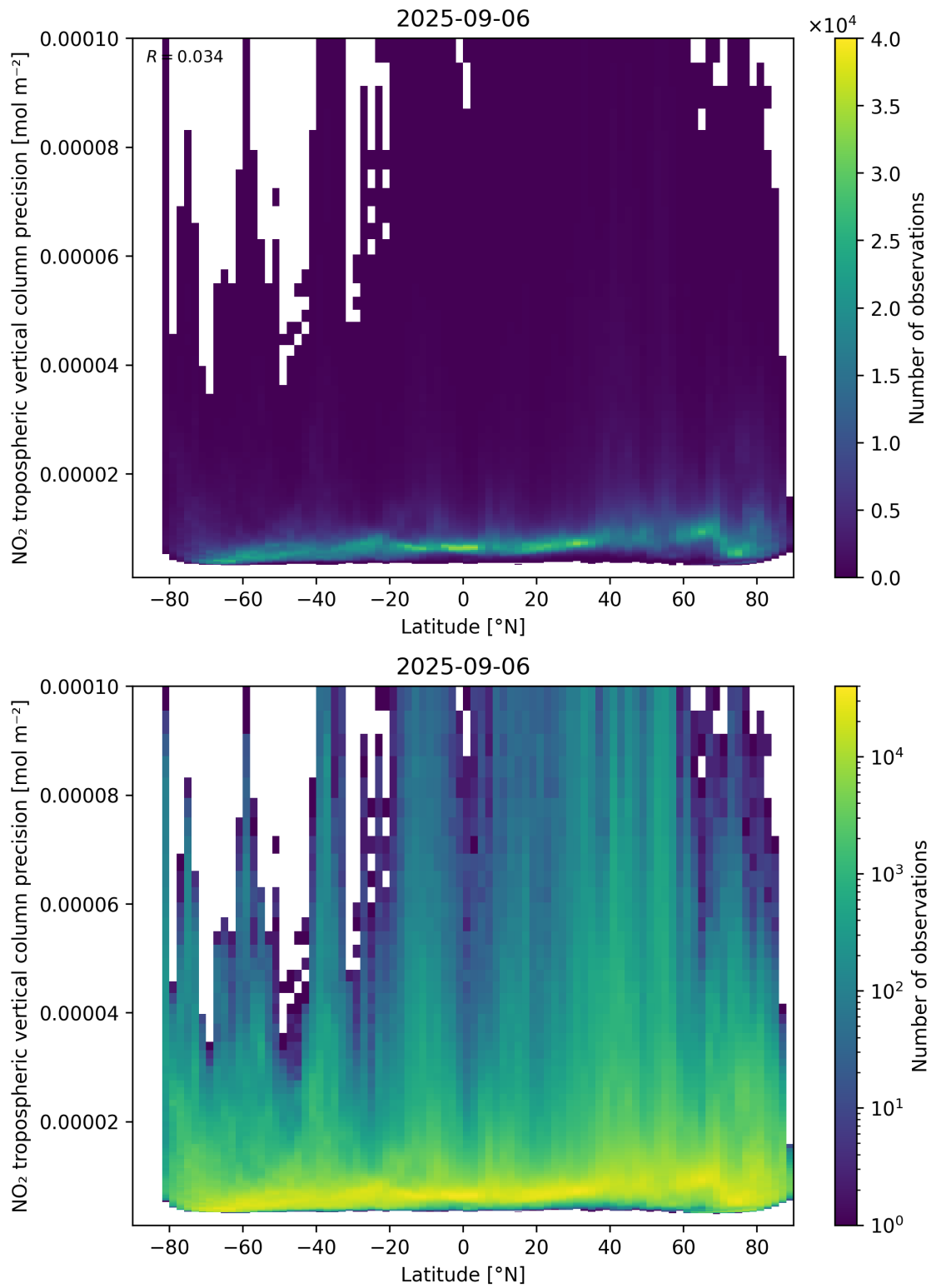
Figure 93: Scatter density plot of “Latitude” against “NO 2 tropospheric vertical column precision” for 2025-09-05 to 2025-09-07.
