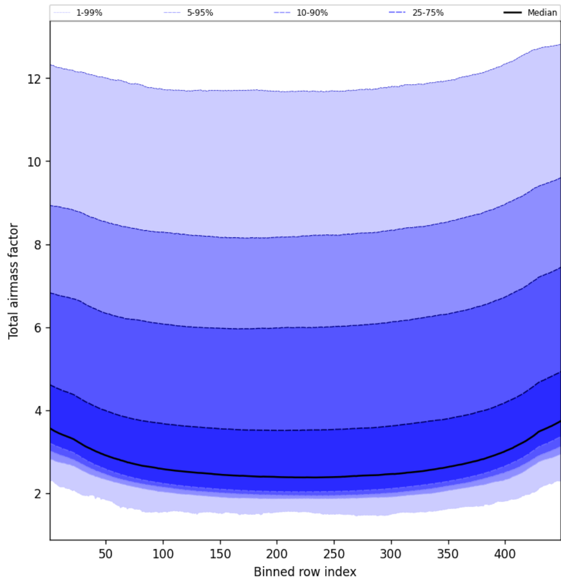
Figure 49: Along track statistics of “Total airmass factor” for 2025-09-05 to 2025-09-07
