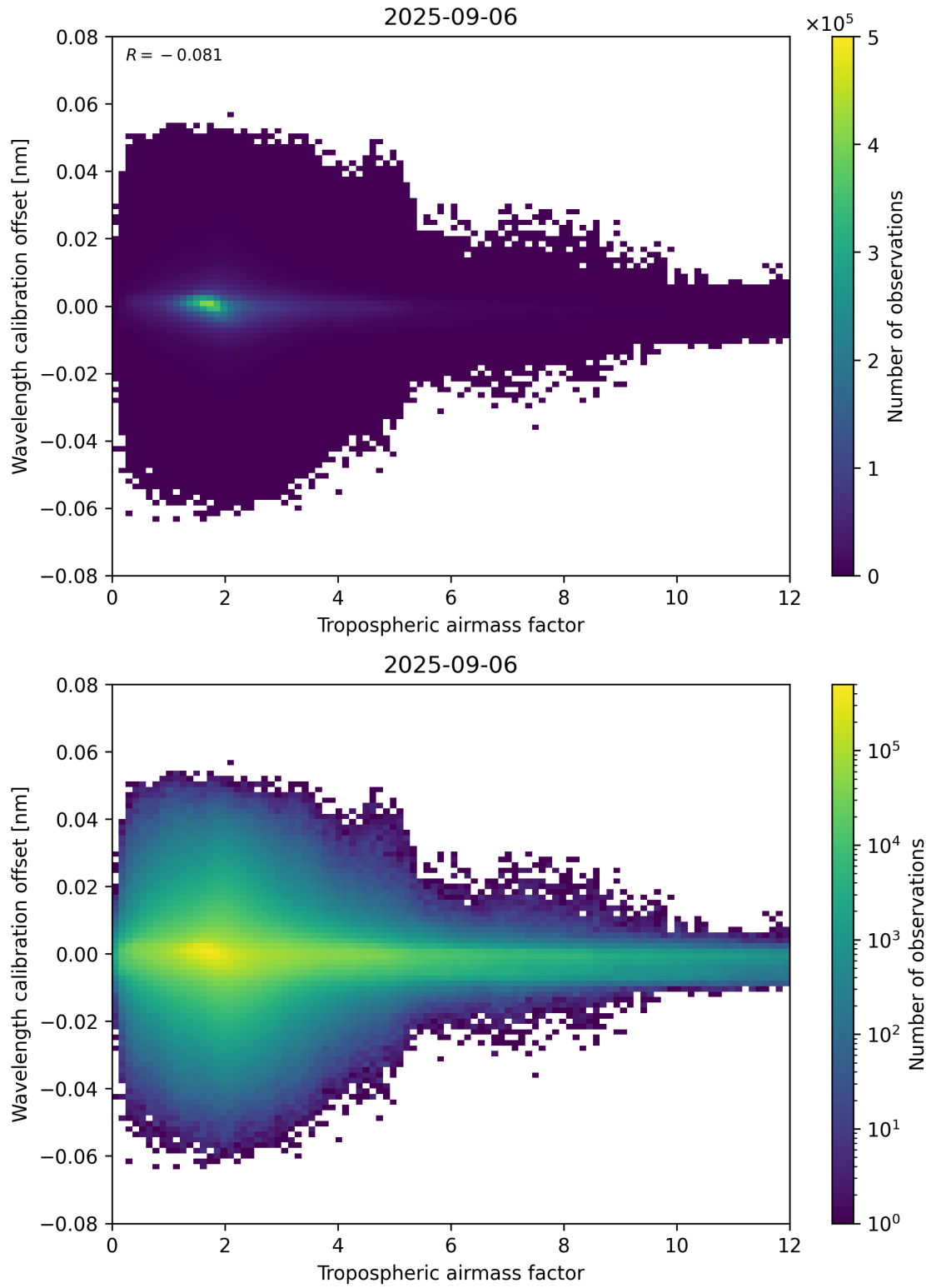
Figure 80: Scatter density plot of “Tropospheric airmass factor” against “Wavelength calibration offset” for 2025-09-05 to 2025-09-07.
