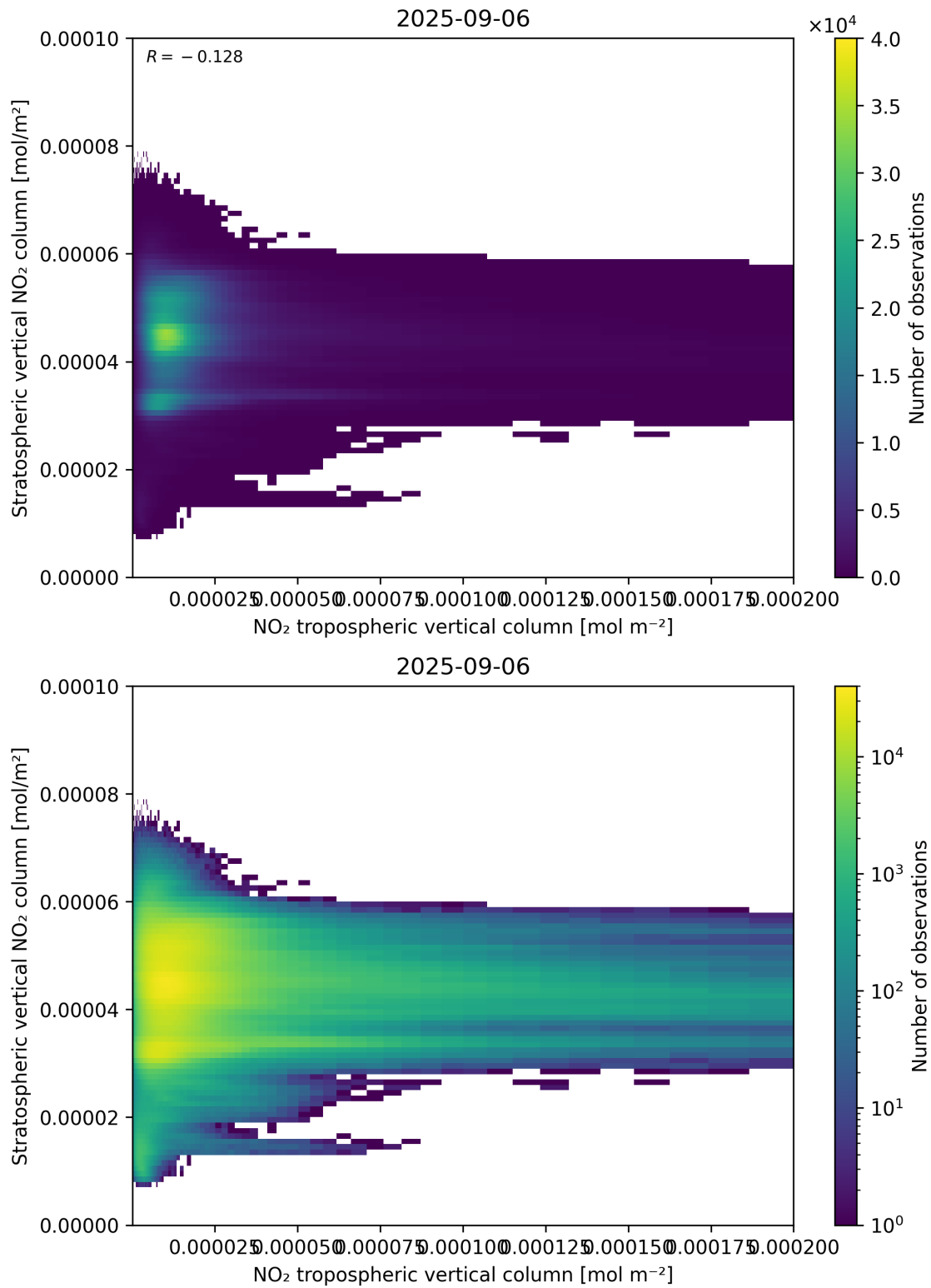
Figure 125: Scatter density plot of “NO 2 tropospheric vertical column” against “Stratospheric vertical NO 2 column” for 2025-09-05 to 2025-09-07.
