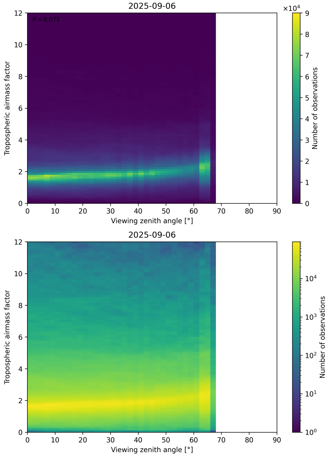
Figure 161: Scatter density plot of “Viewing zenith angle” against “Tropospheric airmass factor” for 2025-09-05 to 2025-09-07.
