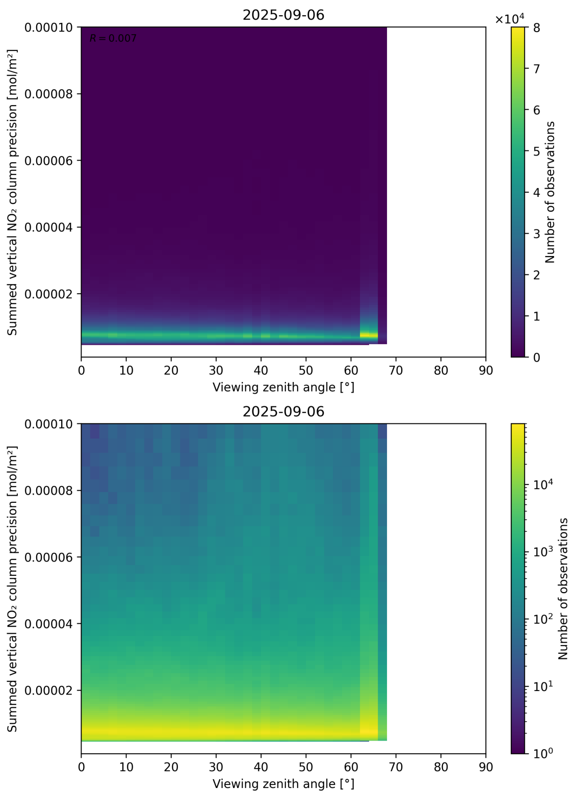
Figure 166: Scatter density plot of “Viewing zenith angle” against “Summed vertical NO 2 column precision” for 2025-09-05 to 2025-09-07.
