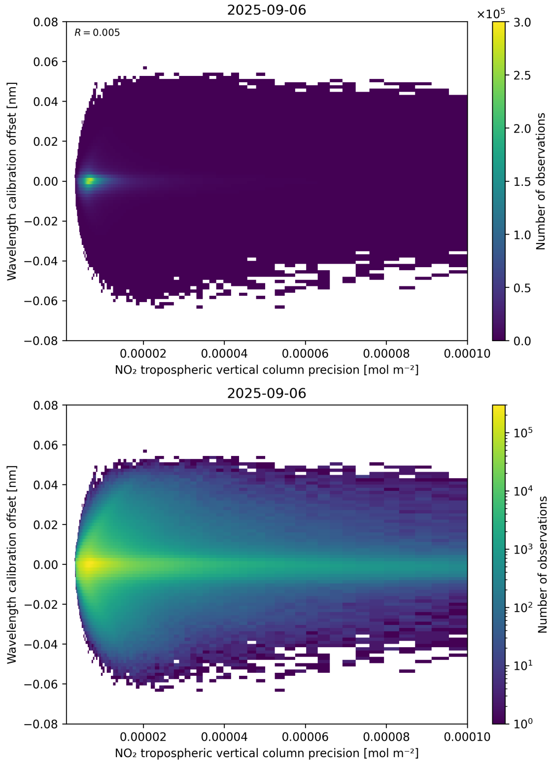
Figure 141: Scatter density plot of “NO 2 tropospheric vertical column precision” against “Wavelength calibration offset” for 2025-09-05 to 2025-09-07.
