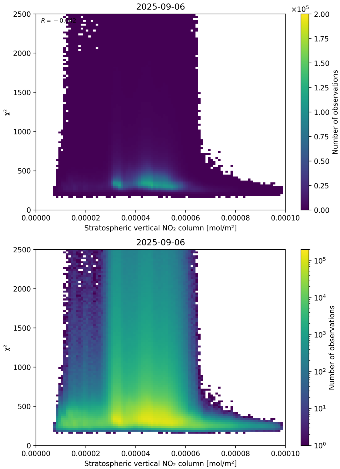
Figure 97: Scatter density plot of “Stratospheric vertical NO 2 column” against “ \chi^2 ” for 2025-09-05 to 2025-09-07.
