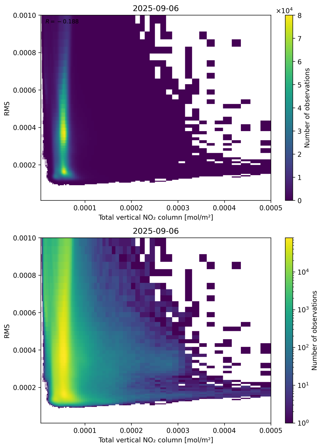
Figure 120: Scatter density plot of “Total vertical NO 2 column” against “RMS” for 2025-09-05 to 2025-09-07.
