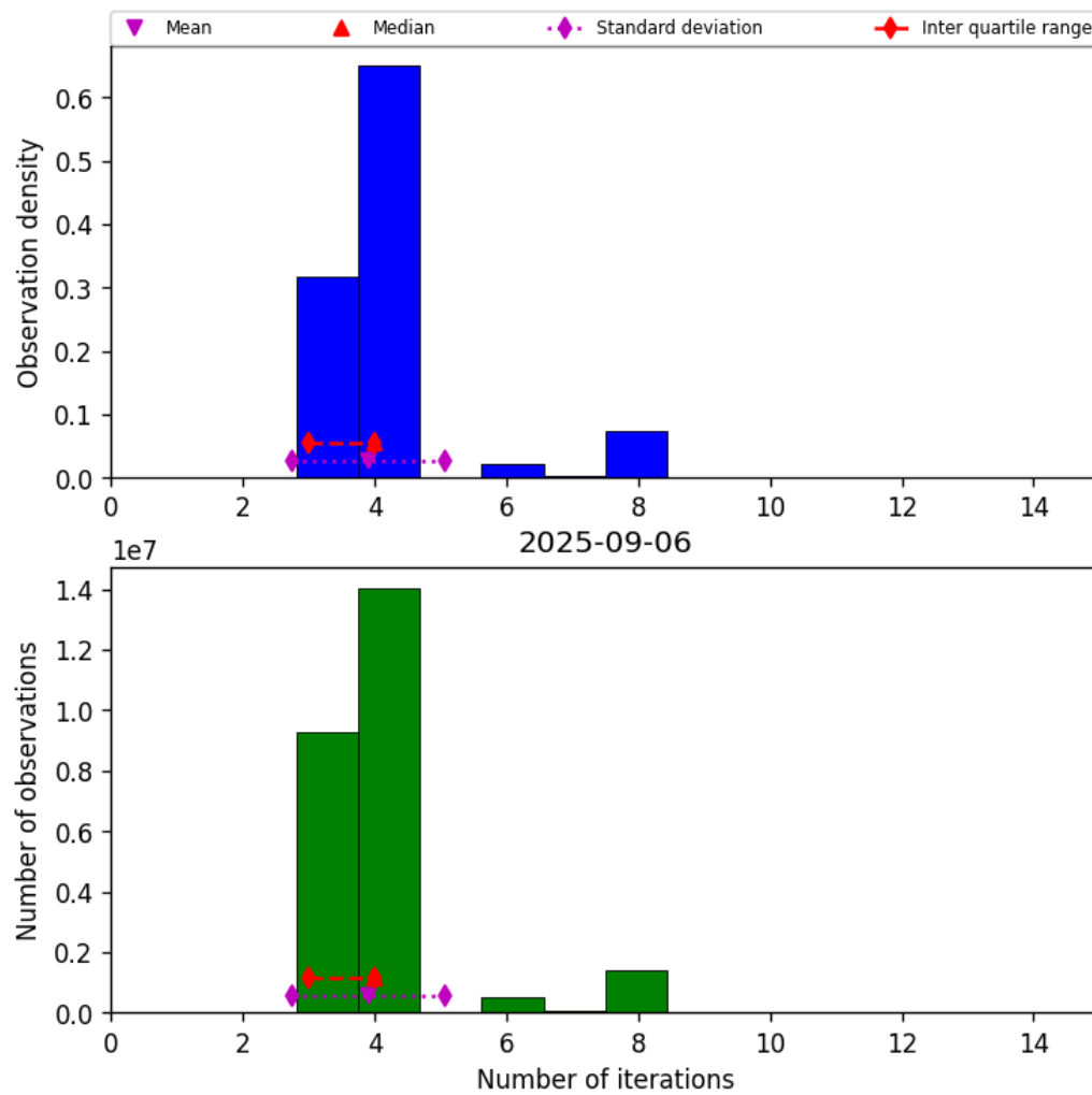
Figure 34: Histogram of “Number of iterations” for 2025-09-05 to 2025-09-07
