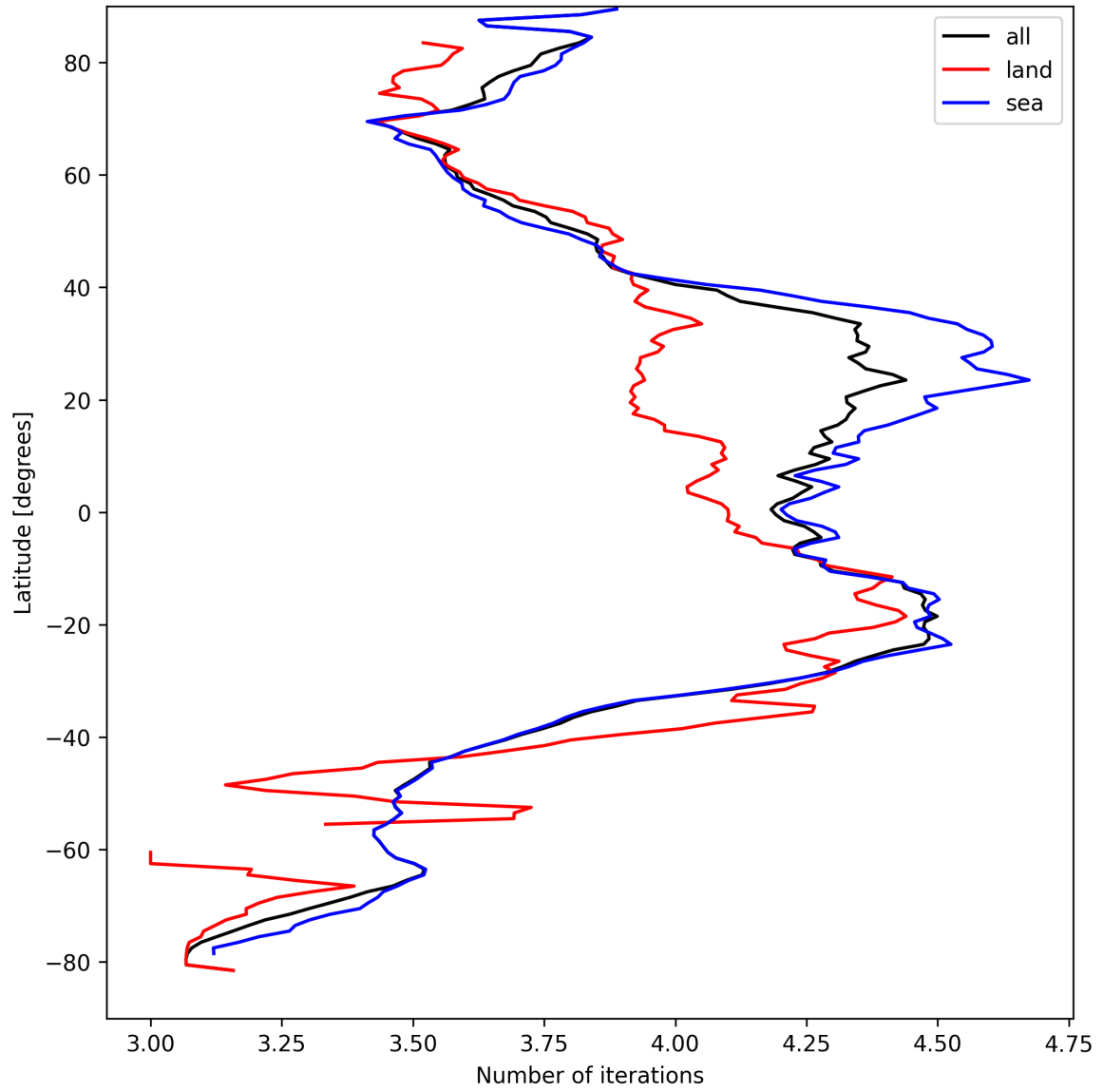
Figure 17: Zonal average of “Number of iterations” for 2025-09-05 to 2025-09-07.
