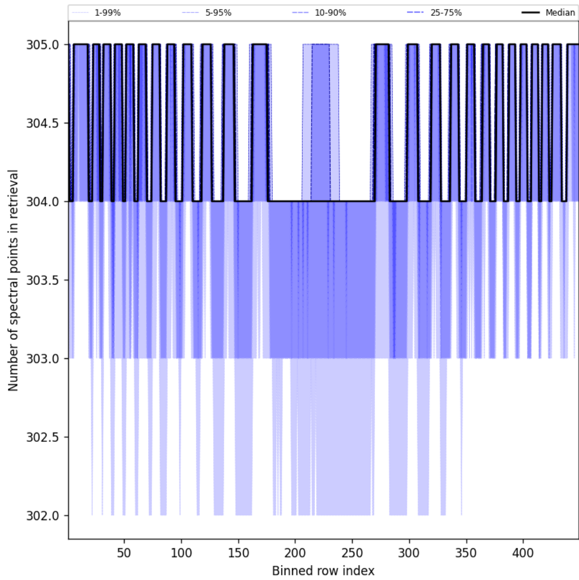
Figure 50: Along track statistics of “Number of spectral points in retrieval” for 2025-09-05 to 2025-09-07
