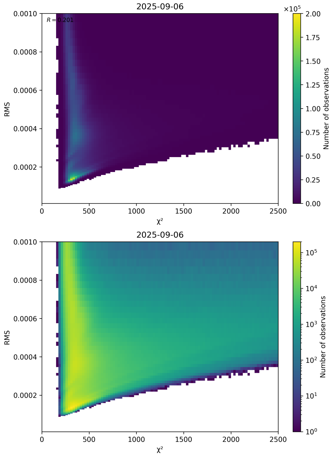
Figure 82: Scatter density plot of “ \chi^2 ” against “RMS” for 2025-09-05 to 2025-09-07.
