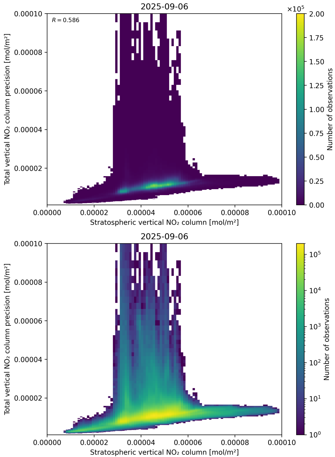
Figure 101: Scatter density plot of “Stratospheric vertical NO 2 column” against “Total vertical NO 2 column precision” for 2025-09-05 to 2025-09-07.
