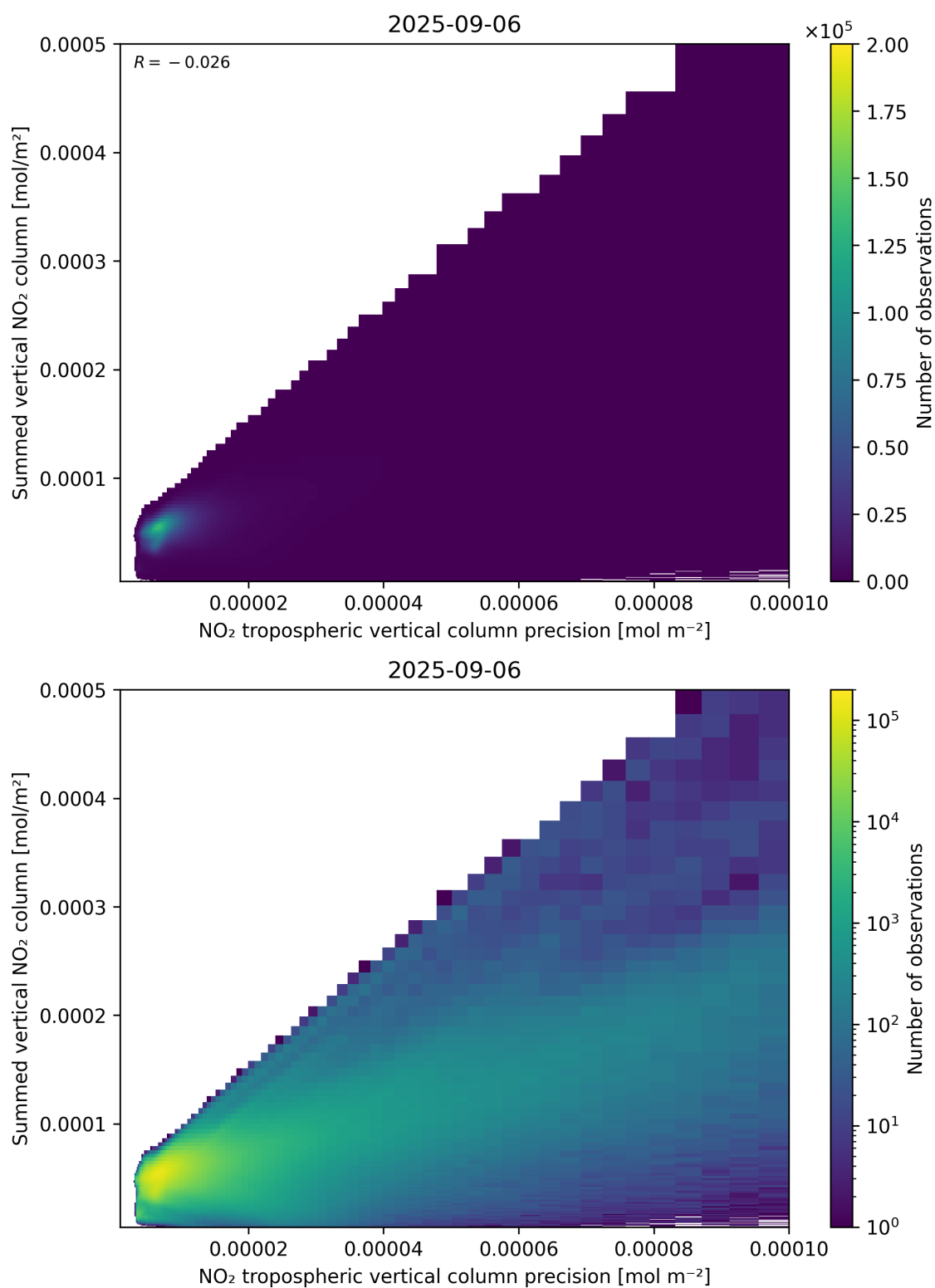
Figure 136: Scatter density plot of “NO 2 tropospheric vertical column precision” against “Summed vertical NO 2 column” for 2025-09-05 to 2025-09-07.
