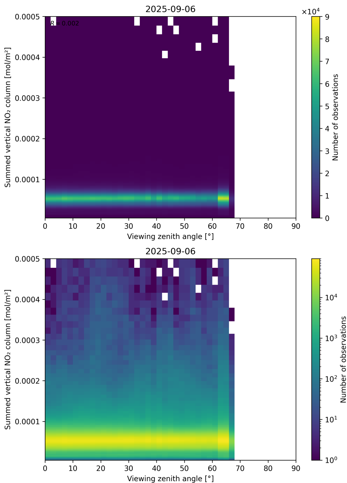
Figure 165: Scatter density plot of “Viewing zenith angle” against “Summed vertical NO 2 column” for 2025-09-05 to 2025-09-07.
