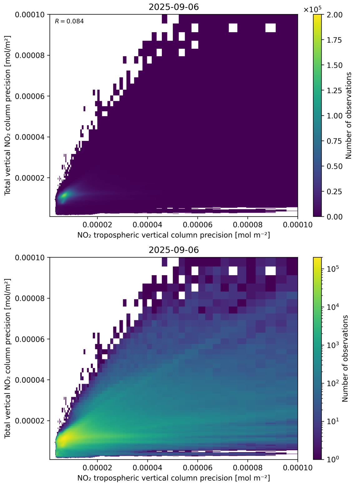
Figure 139: Scatter density plot of “NO 2 tropospheric vertical column precision” against “Total vertical NO 2 column precision” for 2025-09-05 to 2025-09-07.
