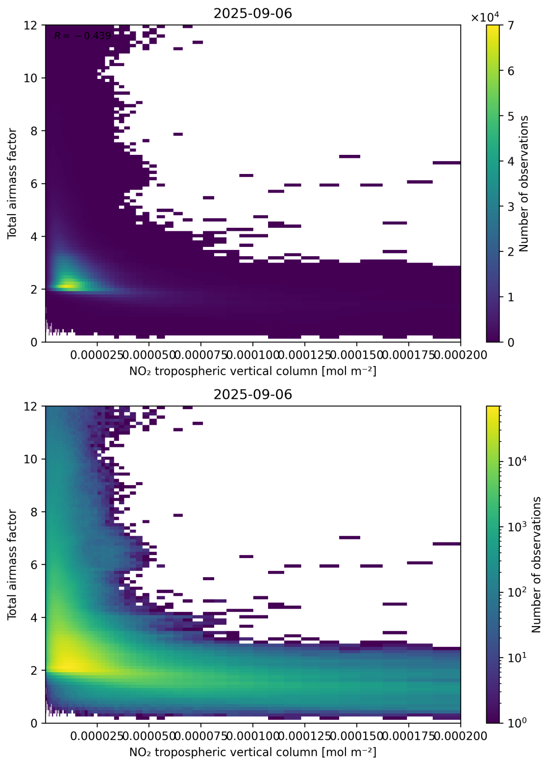
Figure 122: Scatter density plot of “NO 2 tropospheric vertical column” against “Total air mass factor” for 2025-09-05 to 2025-09-07.
