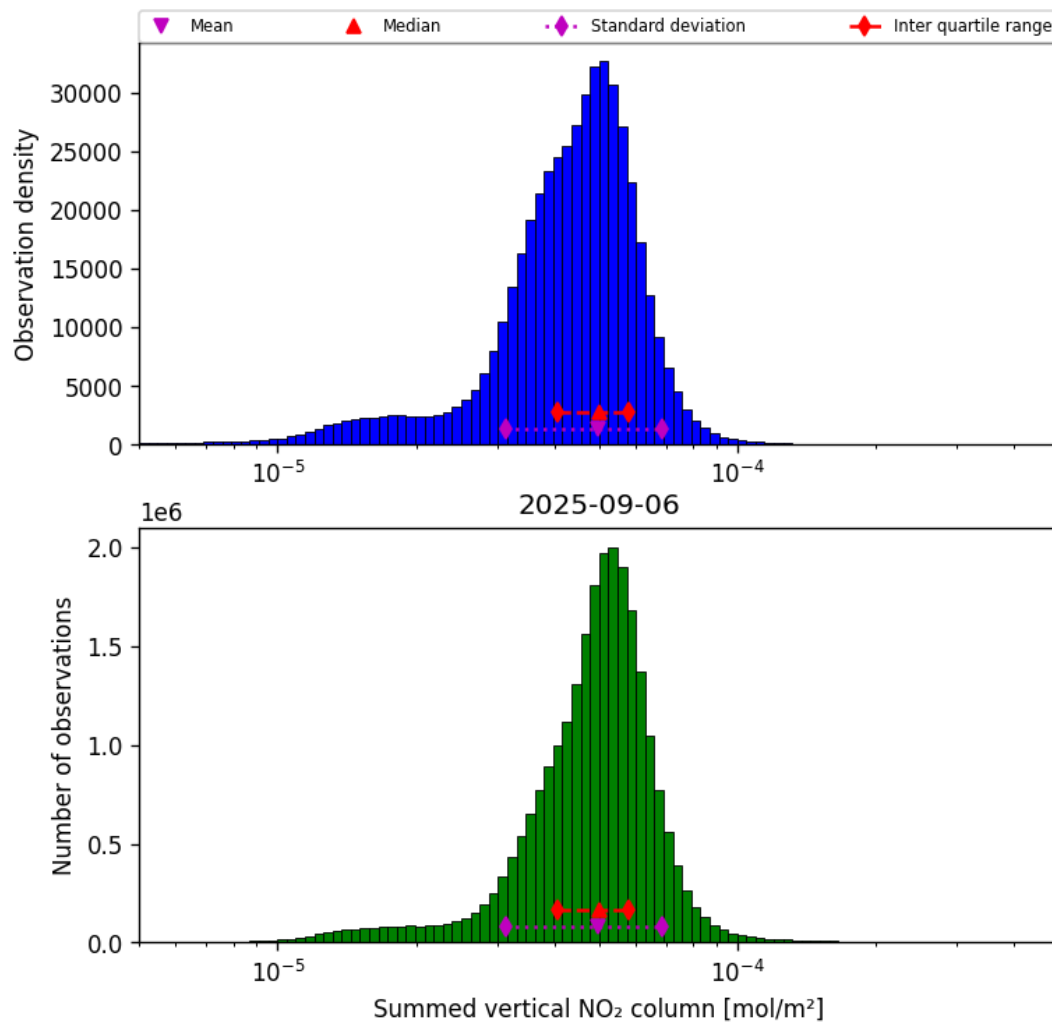
Figure 40: Histogram of “Summed vertical NO 2 column” for 2025-09-05 to 2025-09-07
