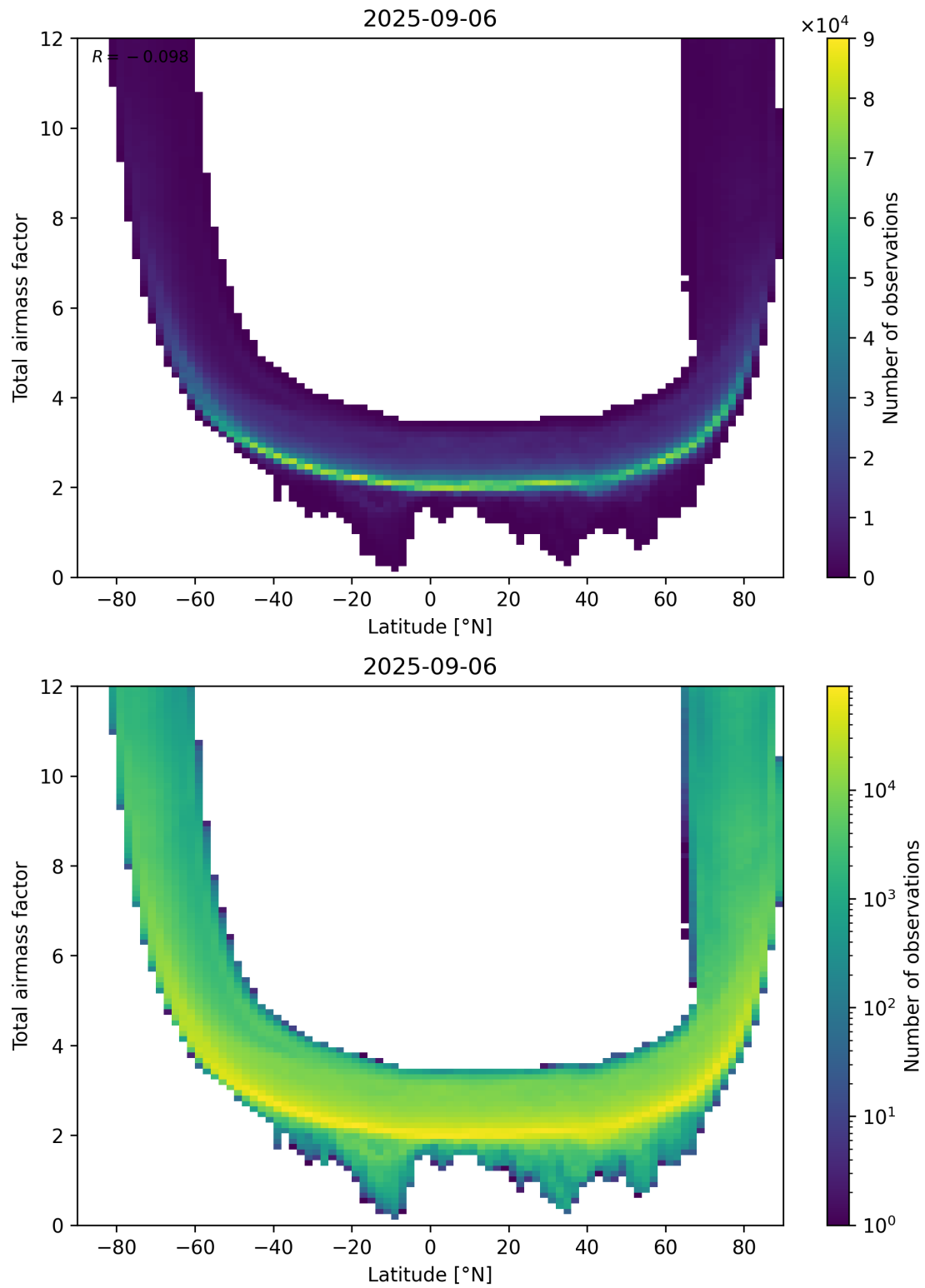
Figure 84: Scatter density plot of “Latitude” against “Total airmass factor” for 2025-09-05 to 2025-09-07.
