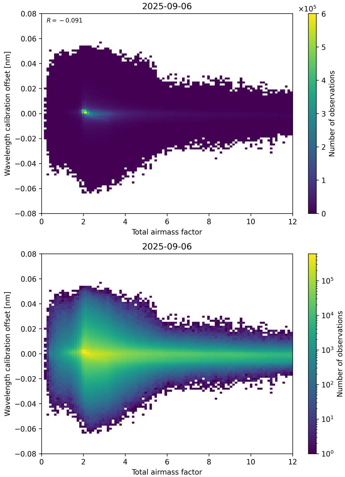
Figure 70: Scatter density plot of “Total airmass factor” against “Wavelength calibration offset” for 2025-09-05 to 2025-09-07.
