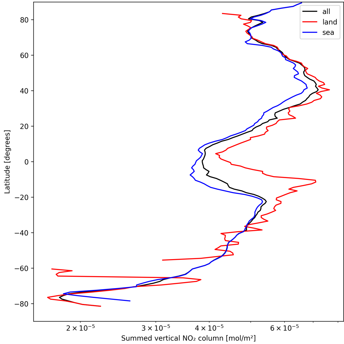
Figure 23: Zonal average of “Summed vertical NO 2 column” for 2025-09-05 to 2025-09-07.
