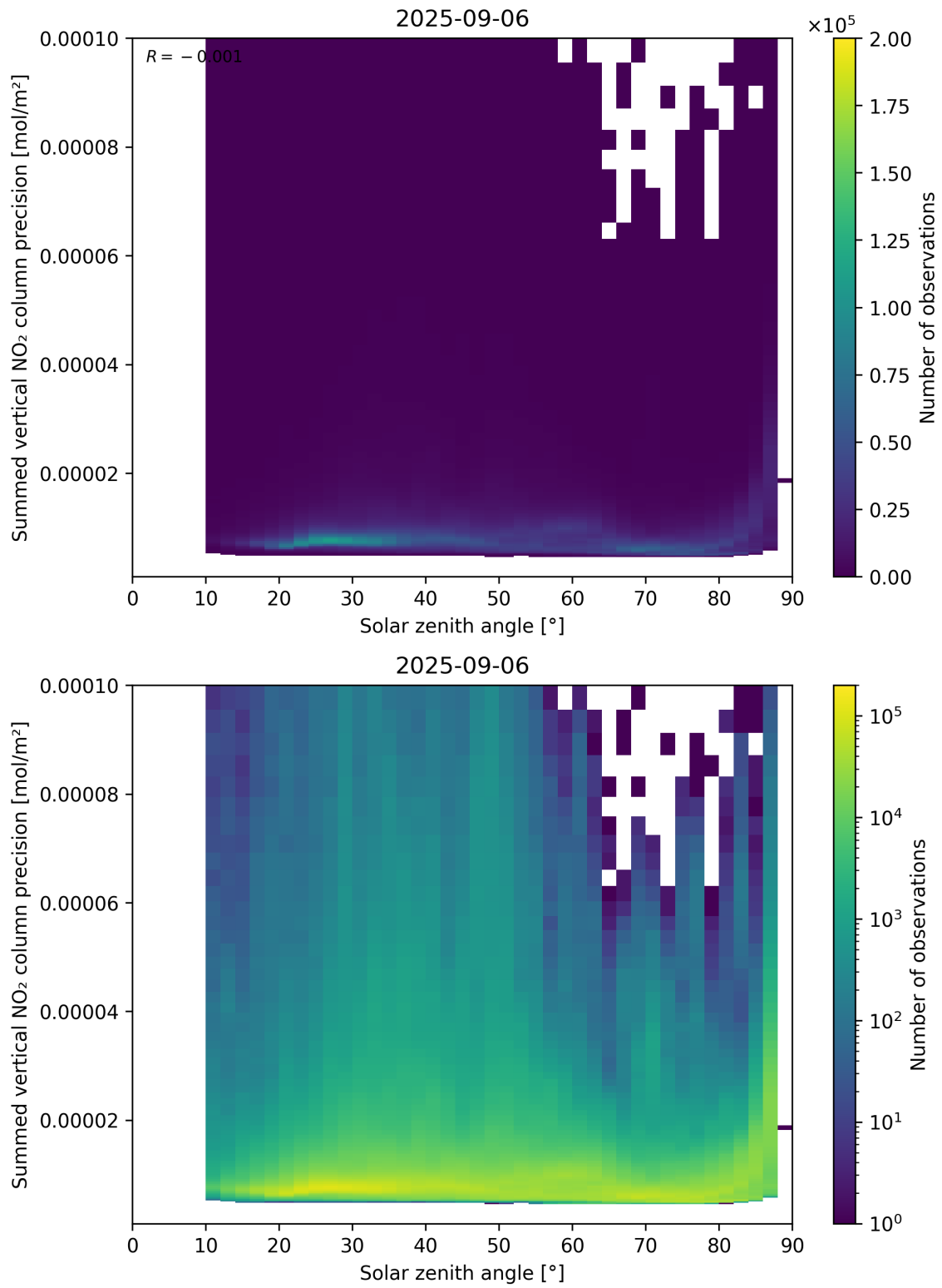
Figure 152: Scatter density plot of “Solar zenith angle” against “Summed vertical NO 2 column precision” for 2025-09-05 to 2025-09-07.
