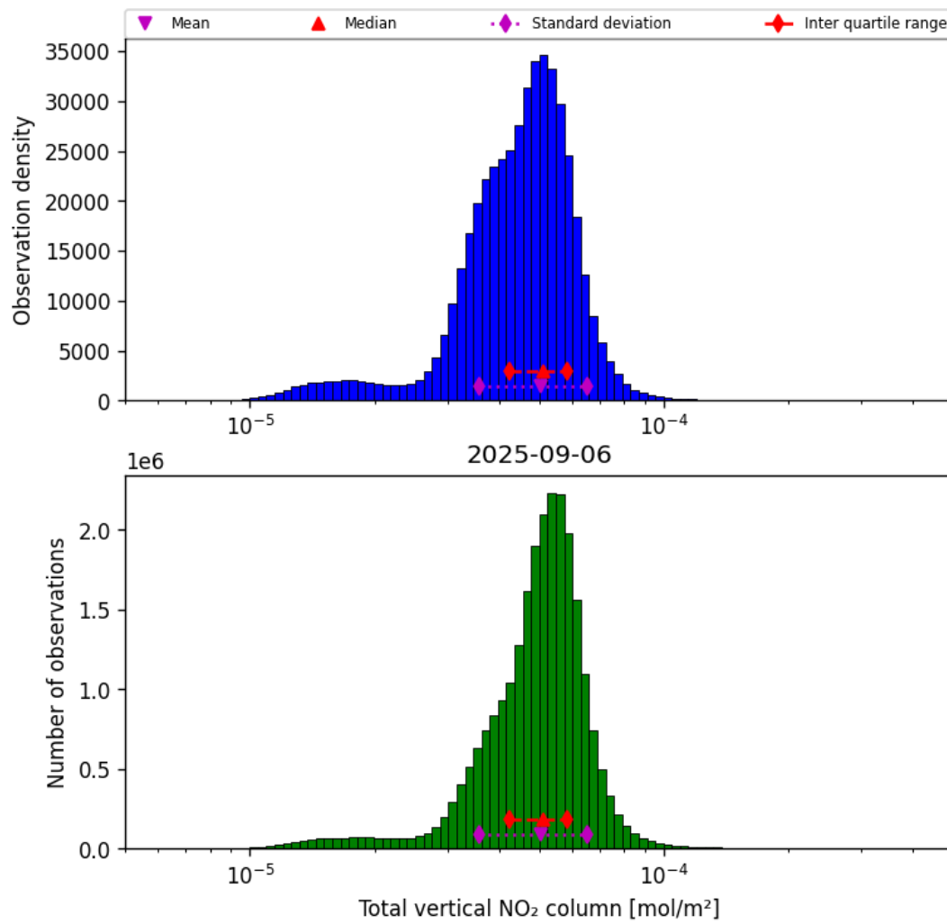
Figure 38: Histogram of “Total vertical NO 2 column” for 2025-09-05 to 2025-09-07
