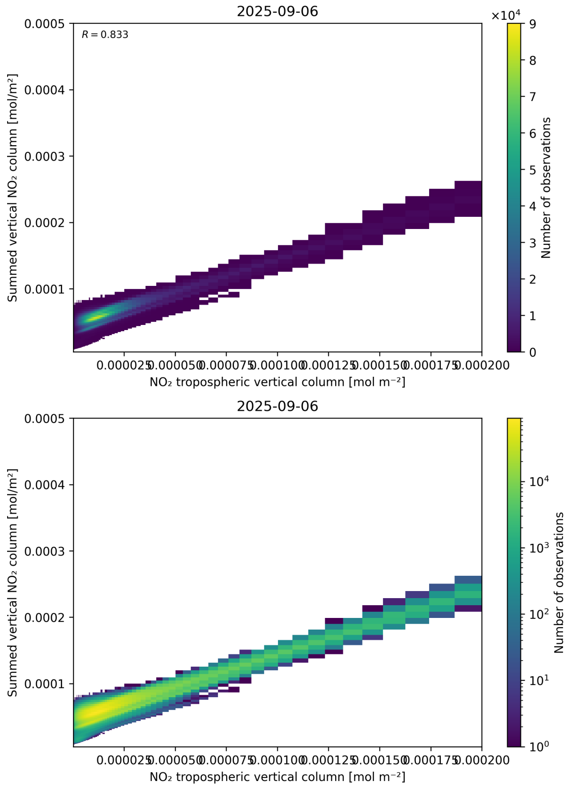
Figure 126: Scatter density plot of “NO 2 tropospheric vertical column” against “Summed vertical NO 2 column” for 2025-09-05 to 2025-09-07.
