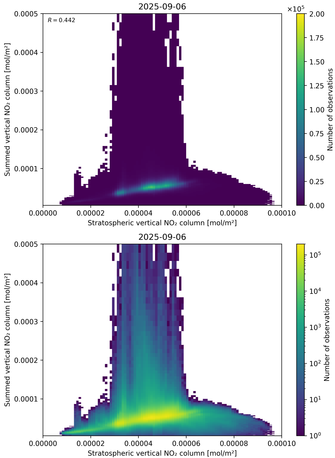
Figure 98: Scatter density plot of “Stratospheric vertical NO 2 column” against “Summed vertical NO 2 column” for 2025-09-05 to 2025-09-07.
