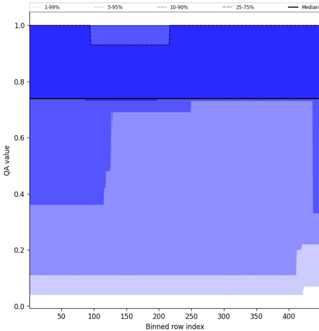
Figure 45: Along track statistics of “QA value” for 2025-09-05 to 2025-09-07
