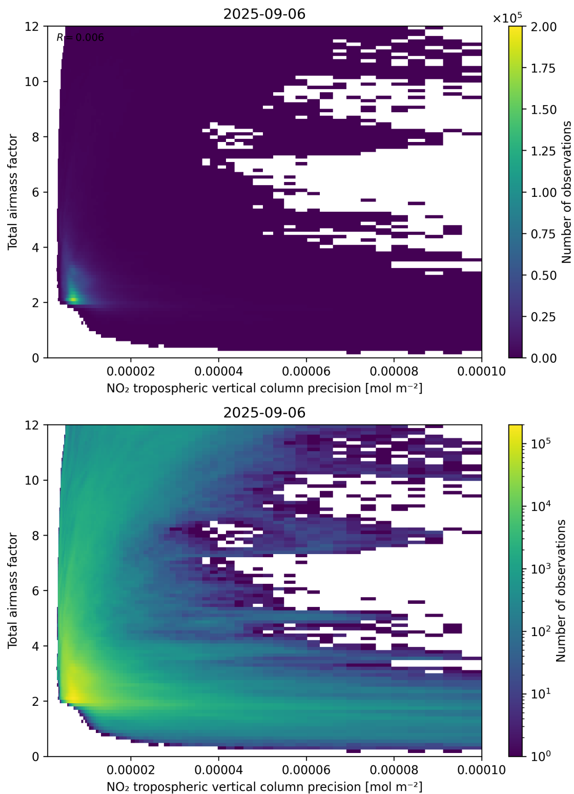
Figure 132: Scatter density plot of “NO 2 tropospheric vertical column precision” against “Total air mass factor” for 2025-09-05 to 2025-09-07.
