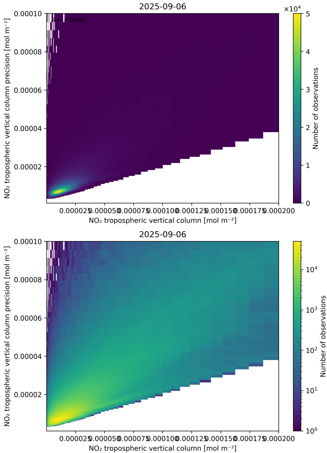
Figure 130: Scatter density plot of “NO 2 tropospheric vertical column” against “NO 2 tropospheric vertical column precision” for 2025-09-05 to 2025-09-07.
