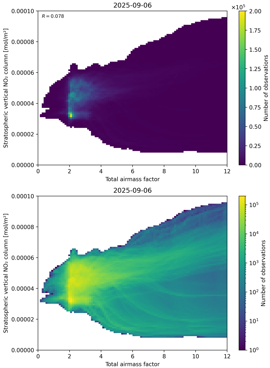
Figure 64: Scatter density plot of “Total airmass factor” against “Stratospheric vertical \text{NO}_2 column” for 2025-09-05 to 2025-09-07.
