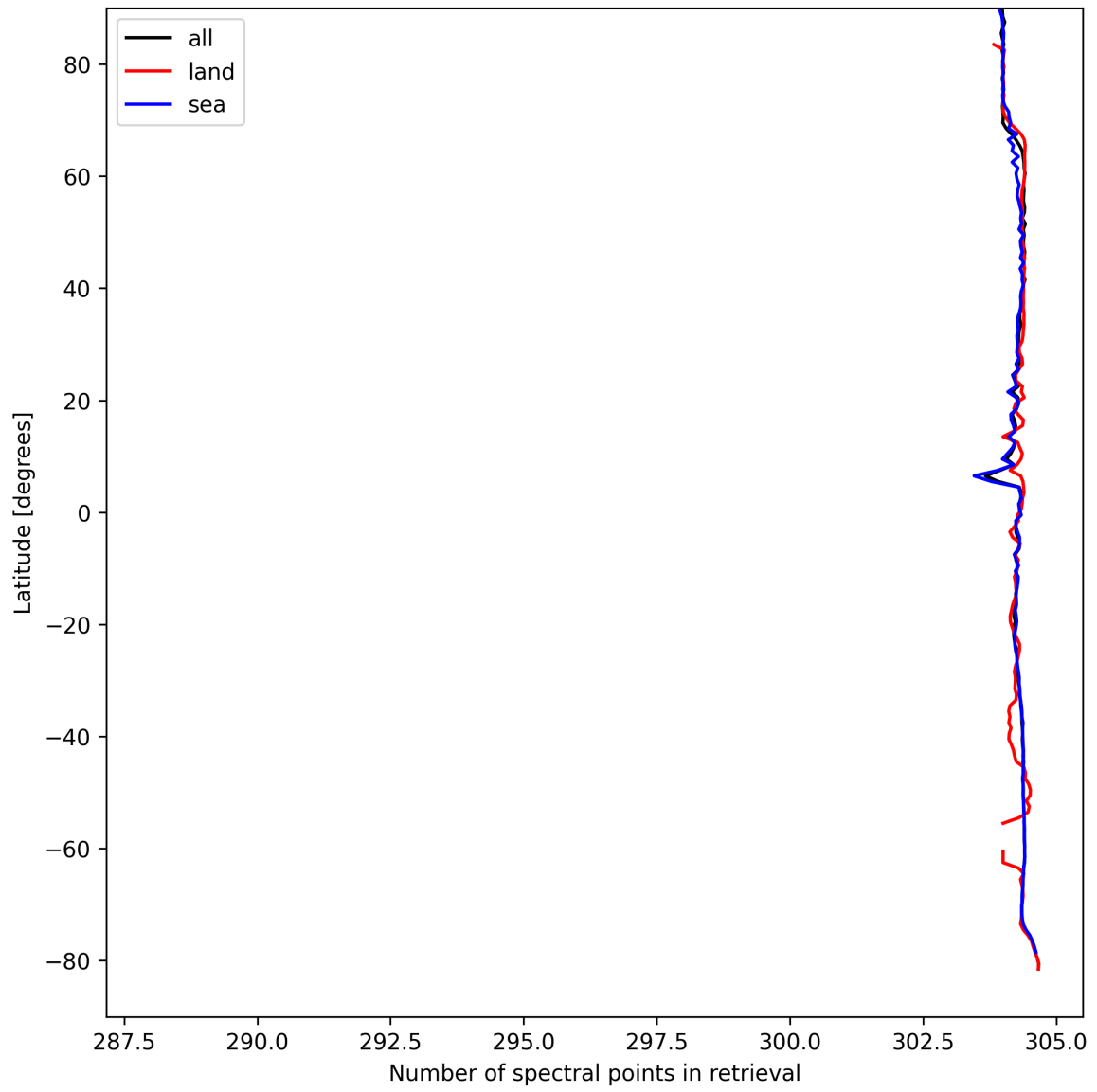
Figure 16: Zonal average of “Number of spectral points in retrieval” for 2025-09-05 to 2025-09-07.
