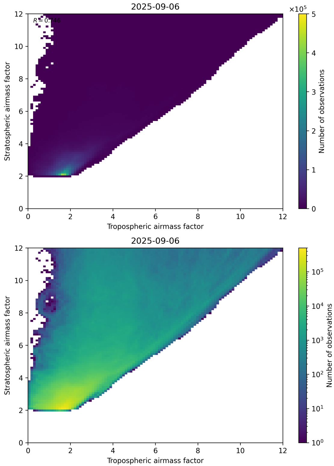
Figure 71: Scatter density plot of “Tropospheric airmass factor” against “Stratospheric airmass factor” for 2025-09-05 to 2025-09-07.
