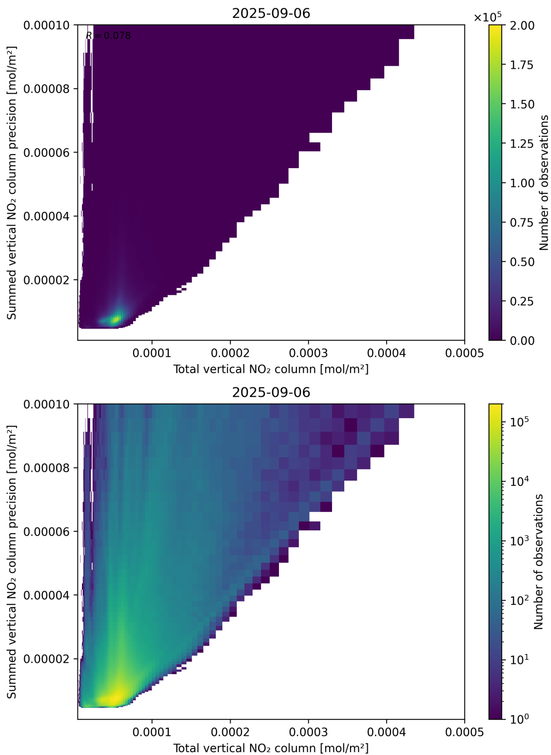
Figure 113: Scatter density plot of “Total vertical NO 2 column” against “Summed vertical NO 2 column precision” for 2025-09-05 to 2025-09-07.
