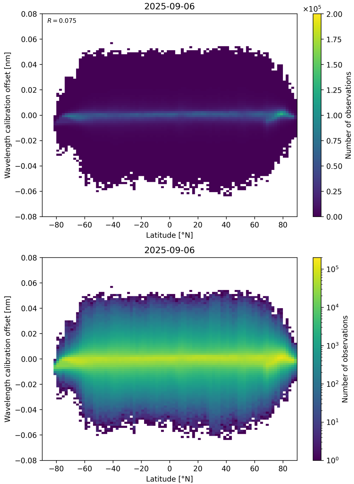
Figure 95: Scatter density plot of “Latitude” against “Wavelength calibration offset” for 2025-09-05 to 2025-09-07.
