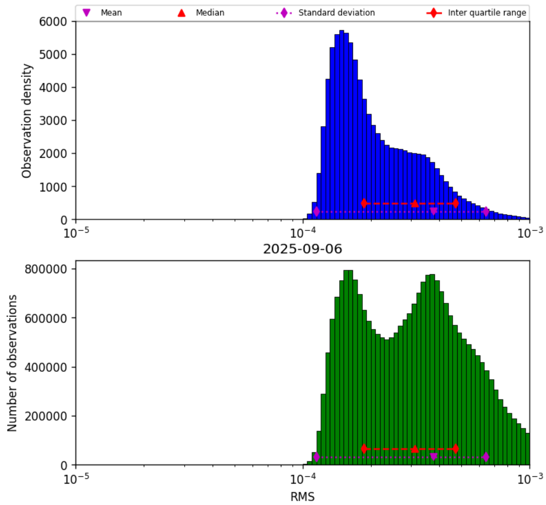
Figure 43: Histogram of “RMS” for 2025-09-05 to 2025-09-07
