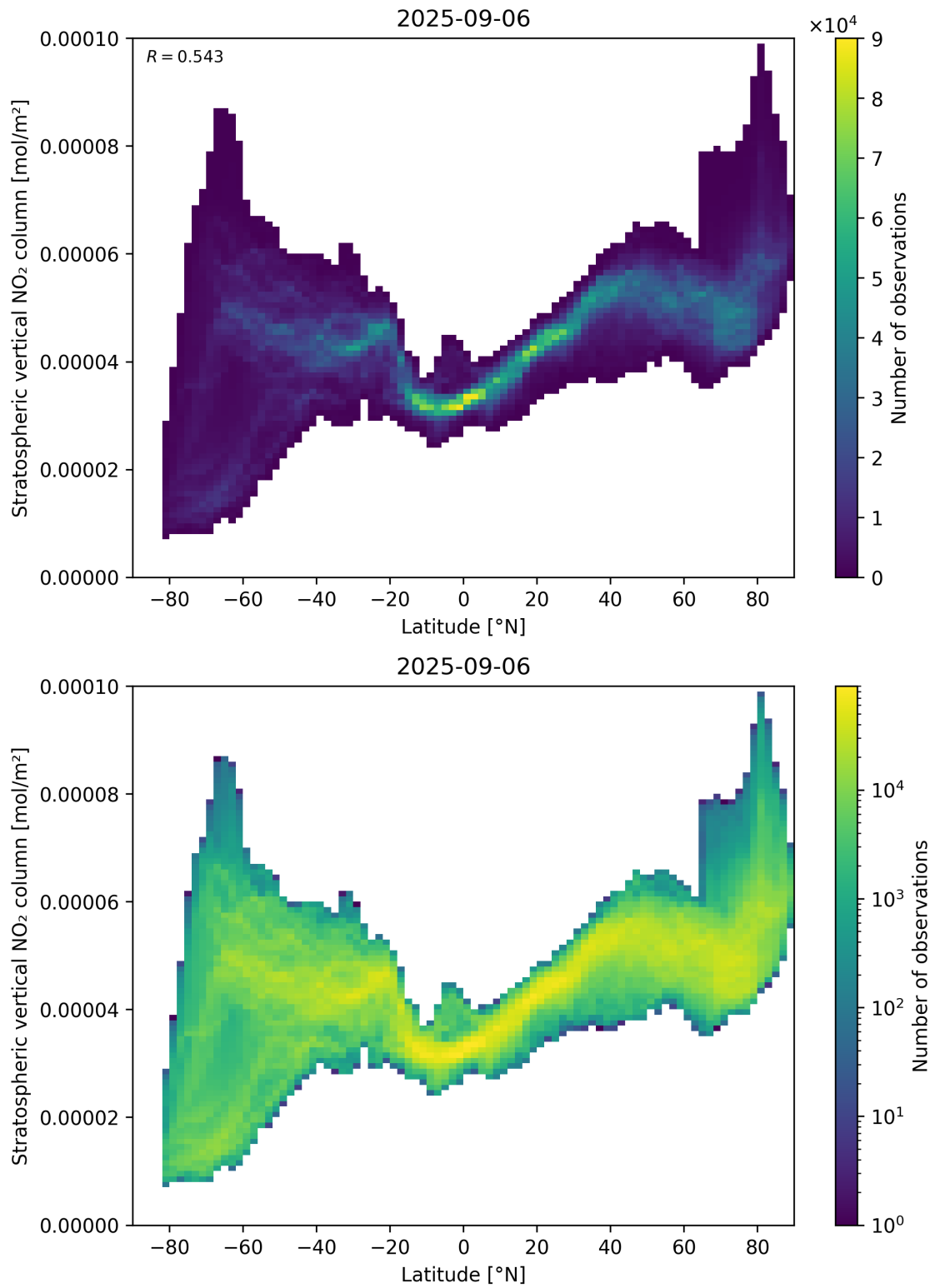
Figure 87: Scatter density plot of “Latitude” against “Stratospheric vertical NO 2 column” for 2025-09-05 to 2025-09-07.
