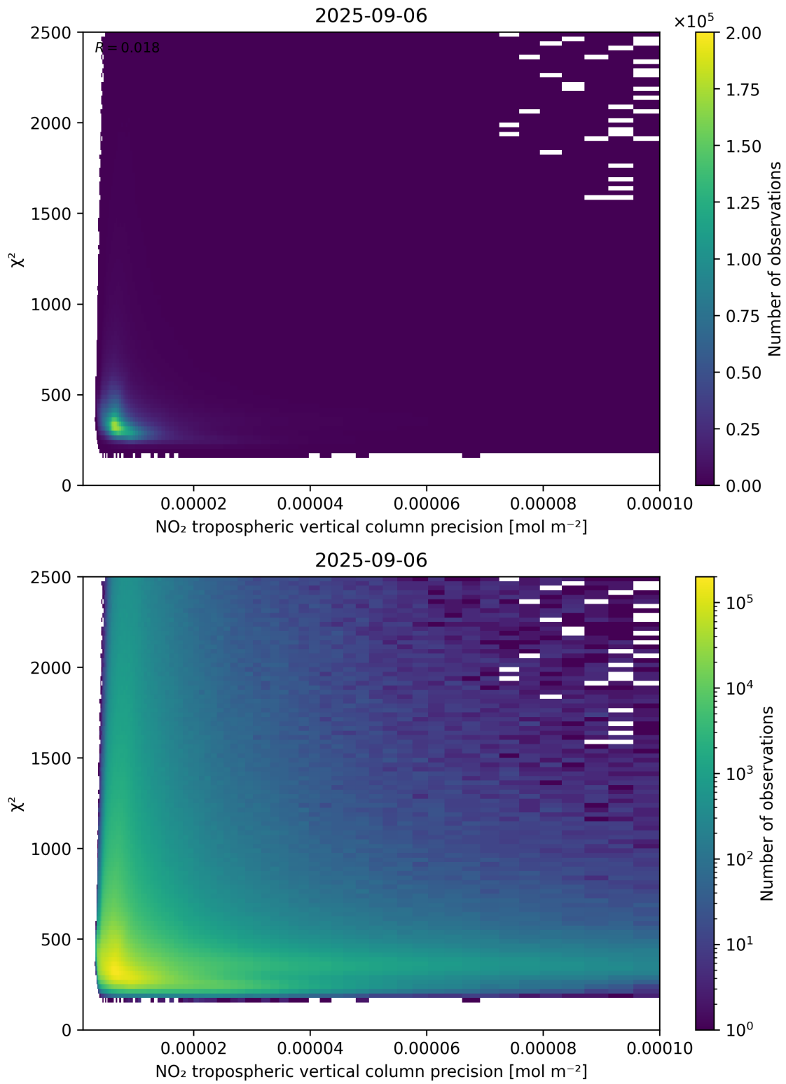
Figure 134: Scatter density plot of “NO 2 tropospheric vertical column precision” against “ \chi^2 ” for 2025-09-05 to 2025-09-07.
