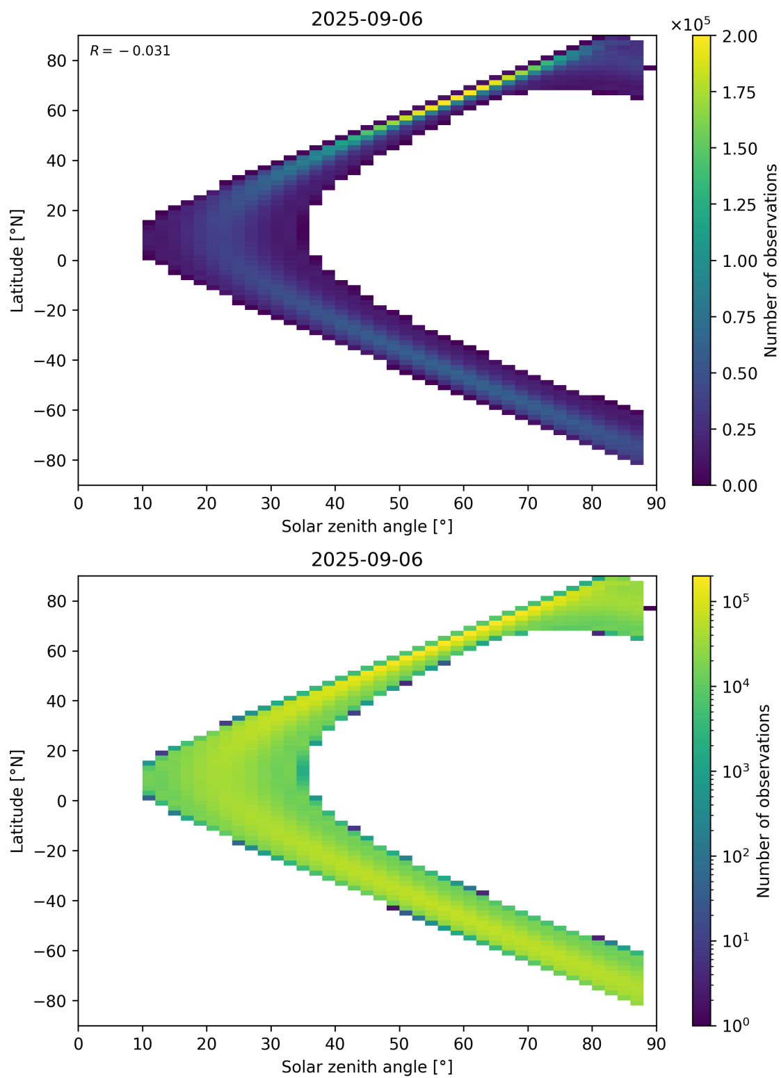
Figure 149: Scatter density plot of “Solar zenith angle” against “Latitude” for 2025-09-05 to 2025-09-07.
