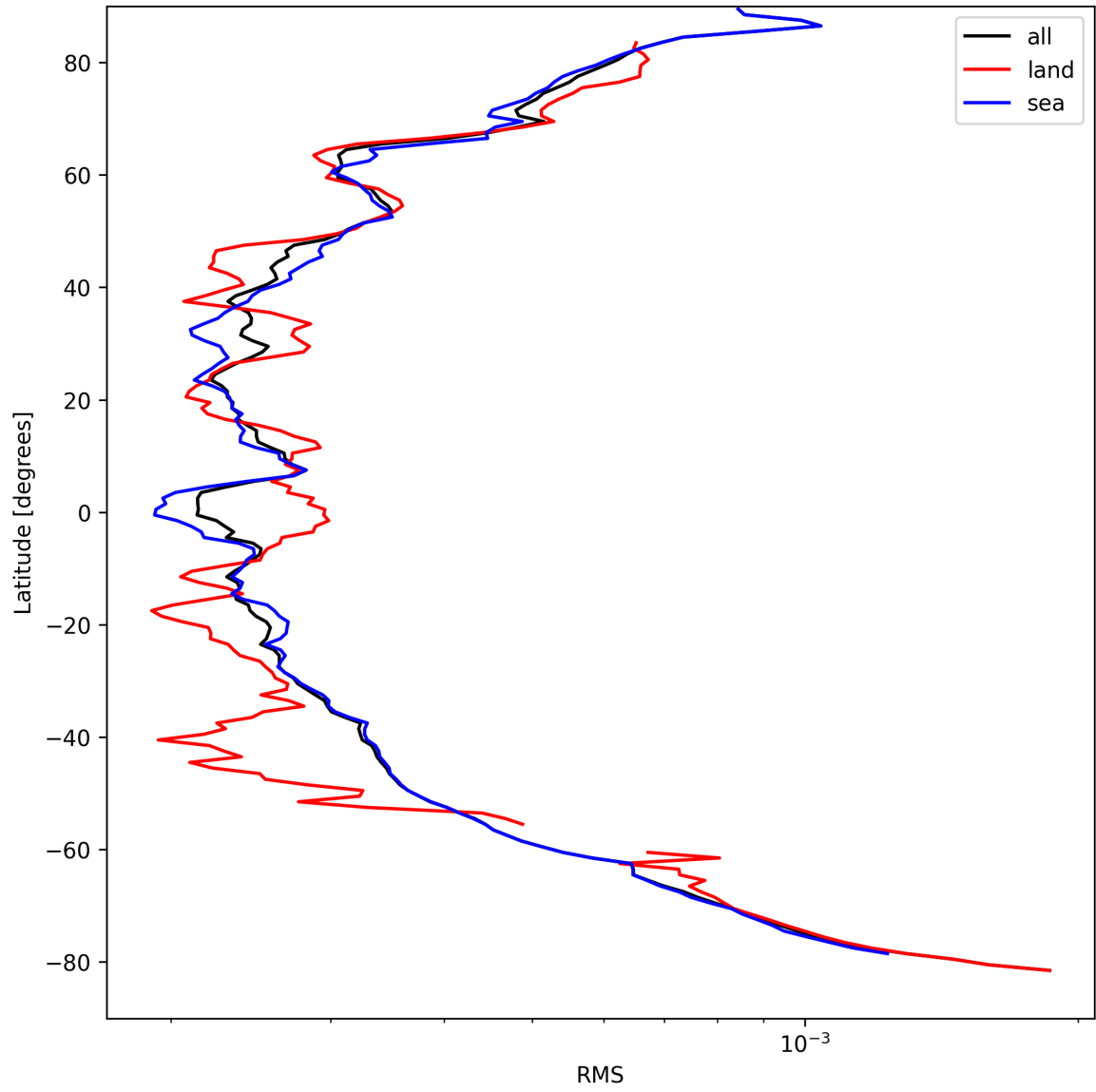
Figure 26: Zonal average of “RMS” for 2025-09-05 to 2025-09-07.
