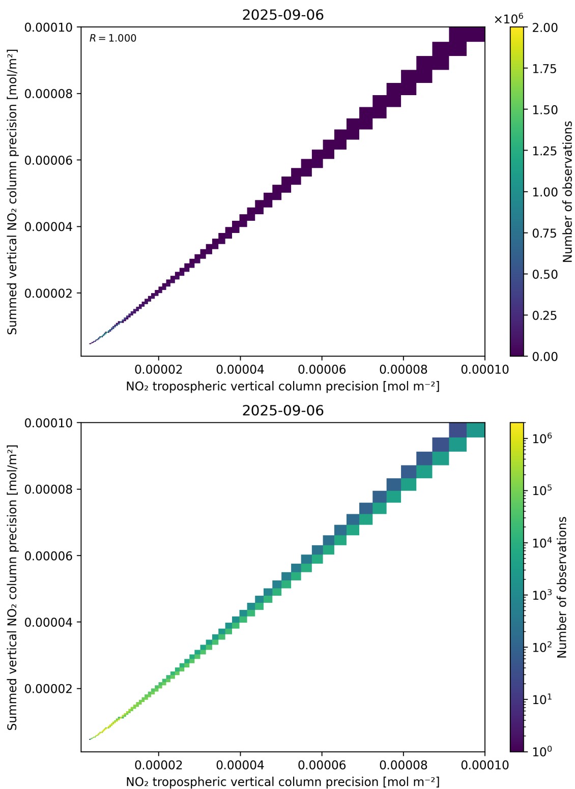
Figure 137: Scatter density plot of “NO 2 tropospheric vertical column precision” against “Summed vertical NO 2 column precision” for 2025-09-05 to 2025-09-07.
