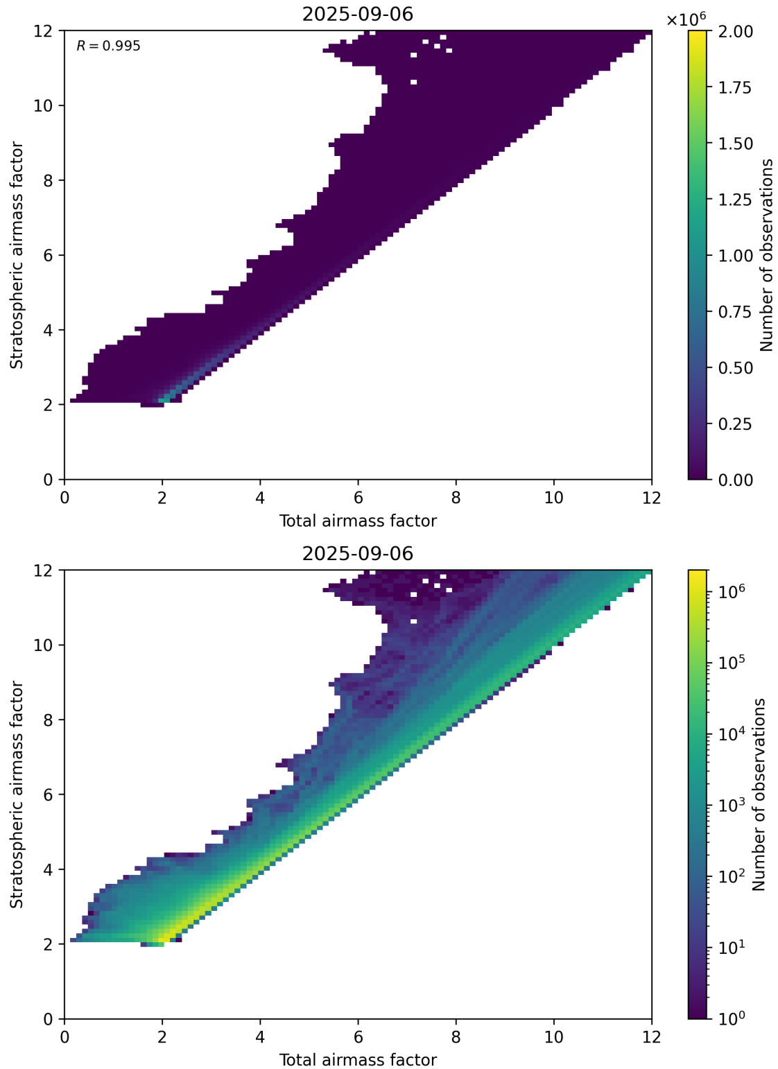
Figure 62: Scatter density plot of “Total airmass factor” against “Stratospheric airmass factor” for 2025-09-05 to 2025-09-07.
