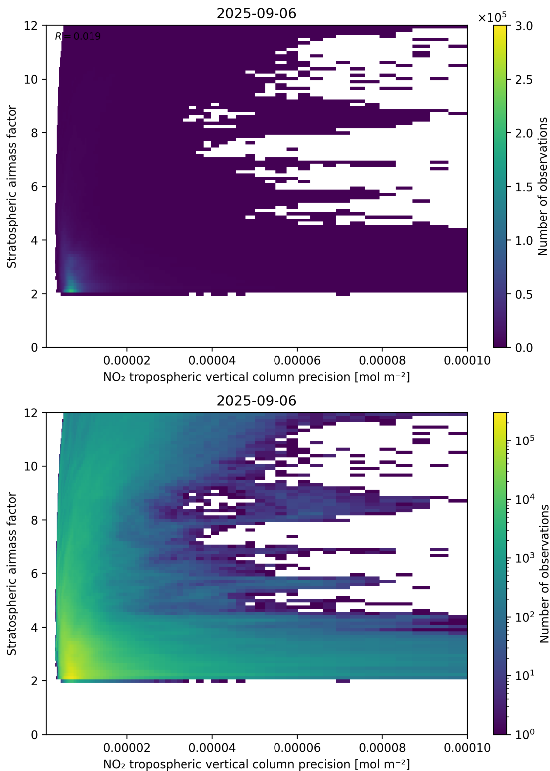
Figure 131: Scatter density plot of “NO 2 tropospheric vertical column precision” against “Stratospheric airmass factor” for 2025-09-05 to 2025-09-07.
