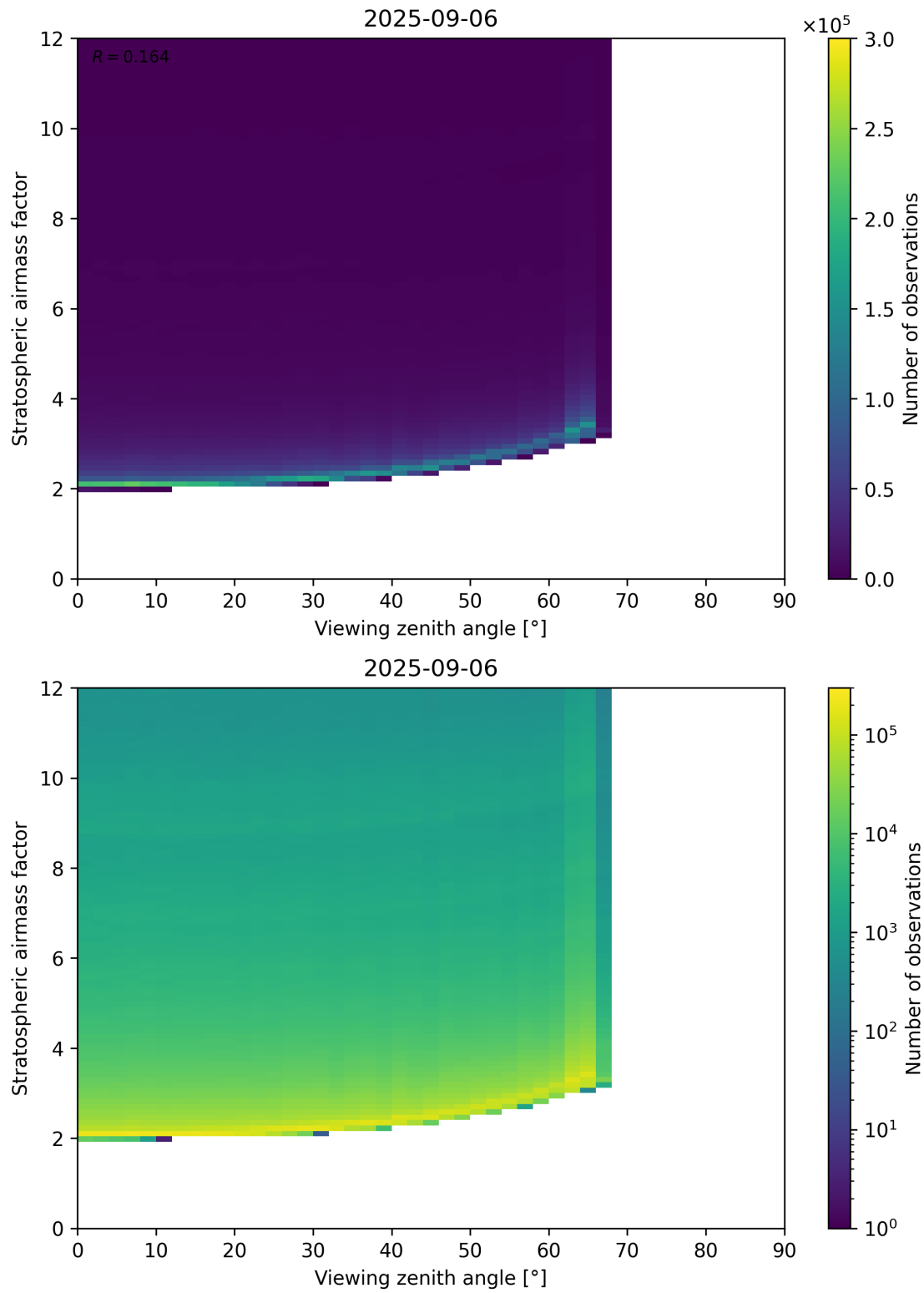
Figure 159: Scatter density plot of “Viewing zenith angle” against “Stratospheric airmass factor” for 2025-09-05 to 2025-09-07.
