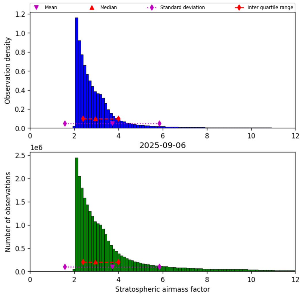
Figure 44: Histogram of “Stratospheric airmass factor” for 2025-09-05 to 2025-09-07
