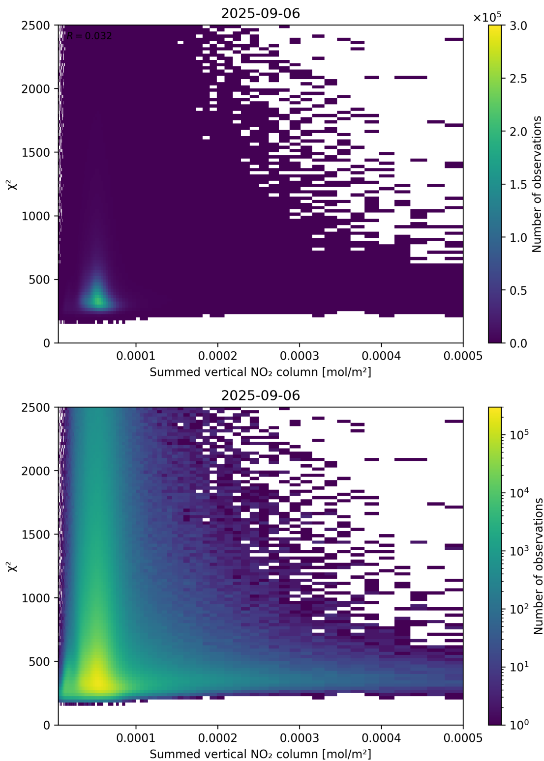
Figure 104: Scatter density plot of “Summed vertical NO 2 column” against “ \chi^2 ” for 2025-09-05 to 2025-09-07.
