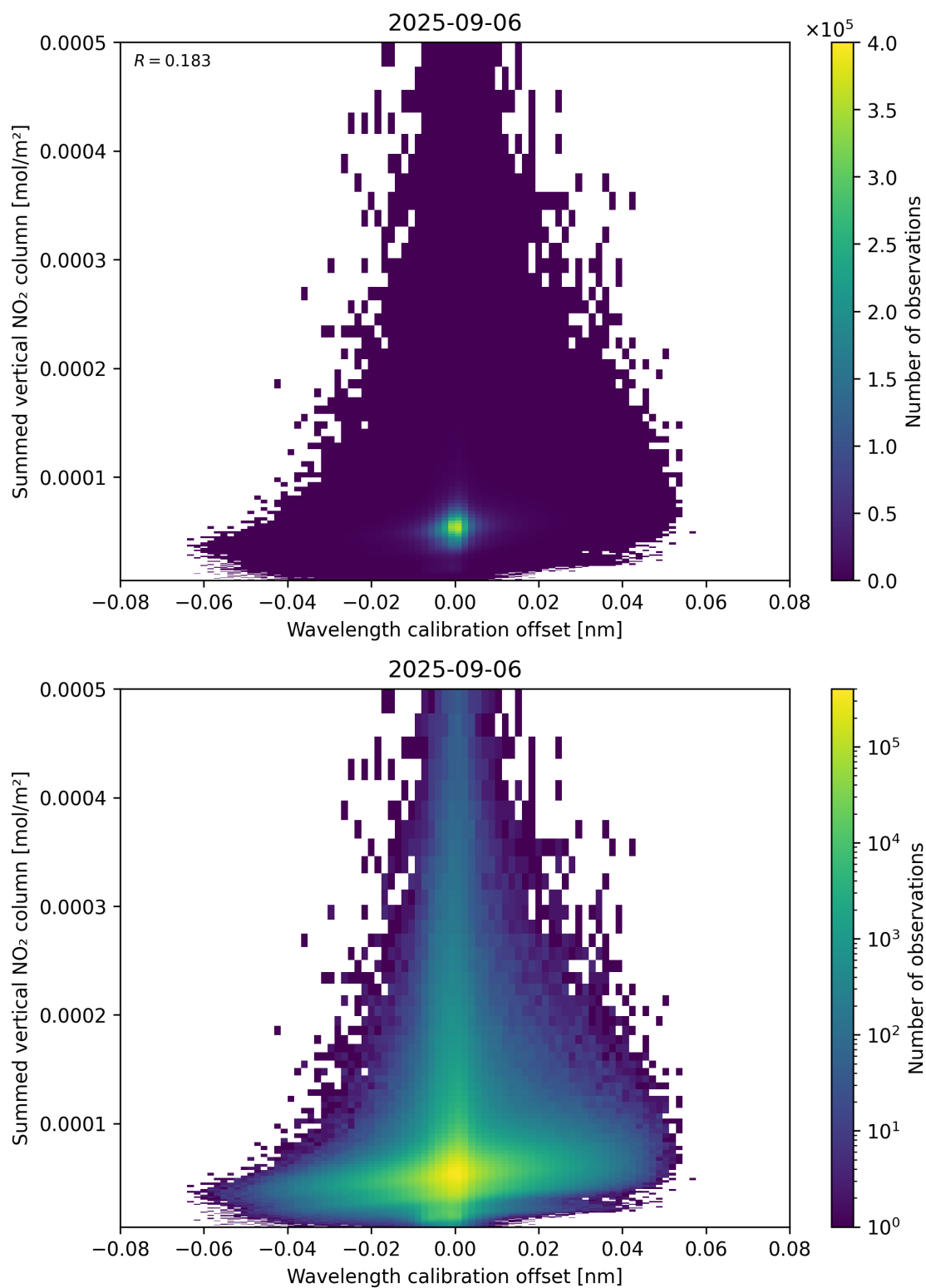
Figure 177: Scatter density plot of “Wavelength calibration offset” against “Summed vertical NO 2 column” for 2025-09-05 to 2025-09-07.
