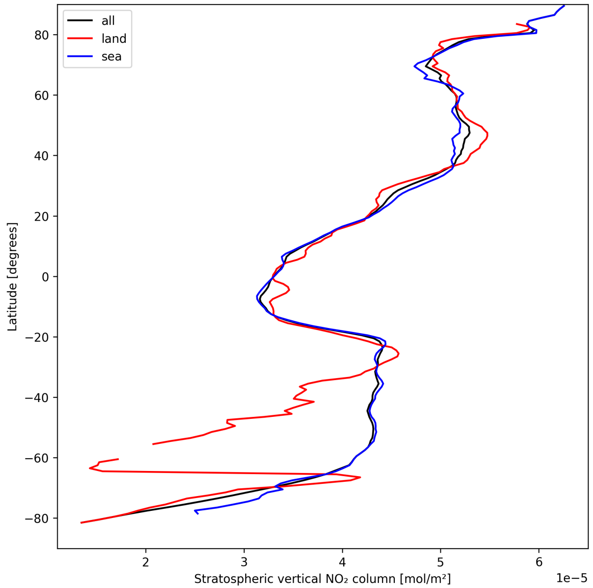
Figure 19: Zonal average of “Stratospheric vertical NO 2 column” for 2025-09-05 to 2025-09-07.
