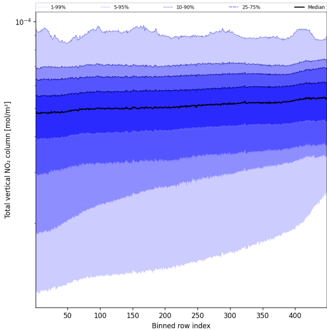
Figure 55: Along track statistics of “Total vertical NO 2 column” for 2025-09-05 to 2025-09-07
