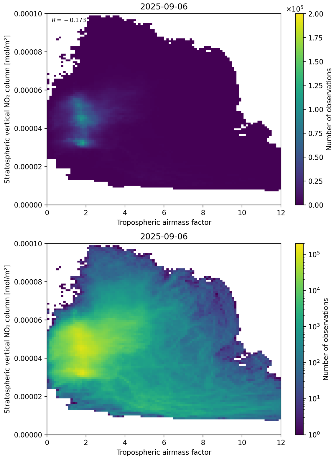
Figure 74: Scatter density plot of “Tropospheric air mass factor” against “Stratospheric vertical NO 2 column” for 2025-09-05 to 2025-09-07.
