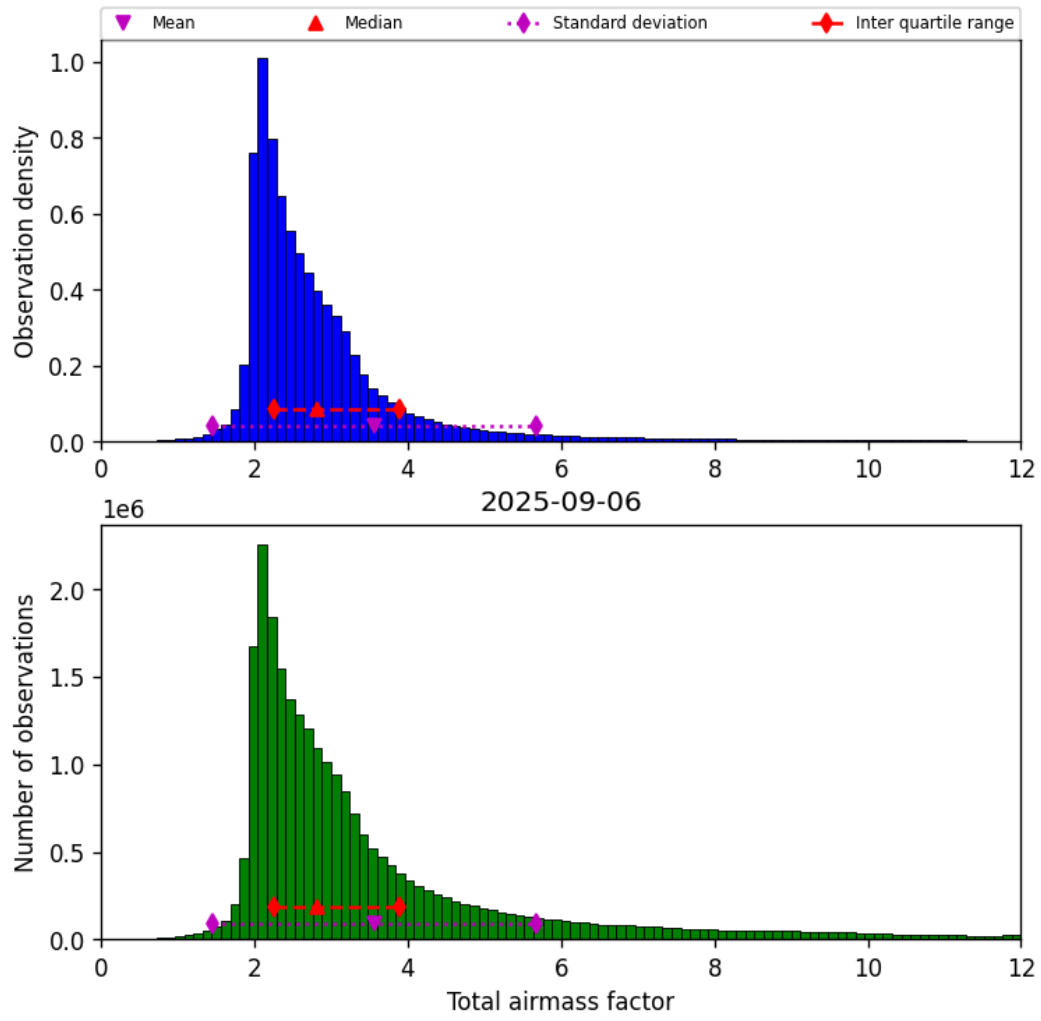
Figure 32: Histogram of “Total airmass factor” for 2025-09-05 to 2025-09-07
