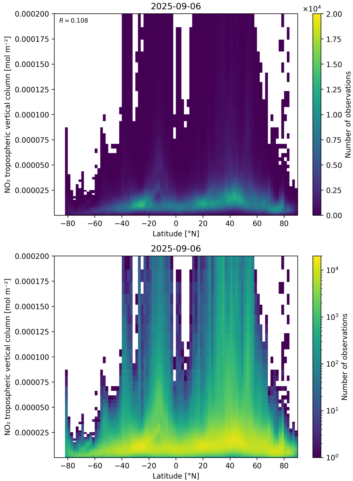
Figure 92: Scatter density plot of “Latitude” against “NO 2 tropospheric vertical column” for 2025-09-05 to 2025-09-07.
