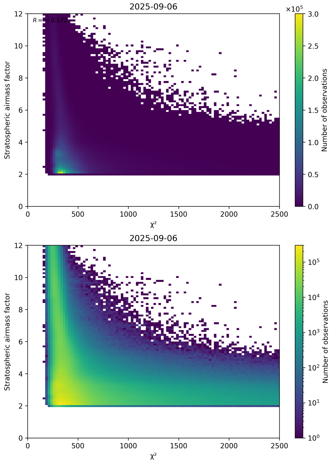
Figure 81: Scatter density plot of “ \chi^2 ” against “Stratospheric airmass factor” for 2025-09-05 to 2025-09-07.
