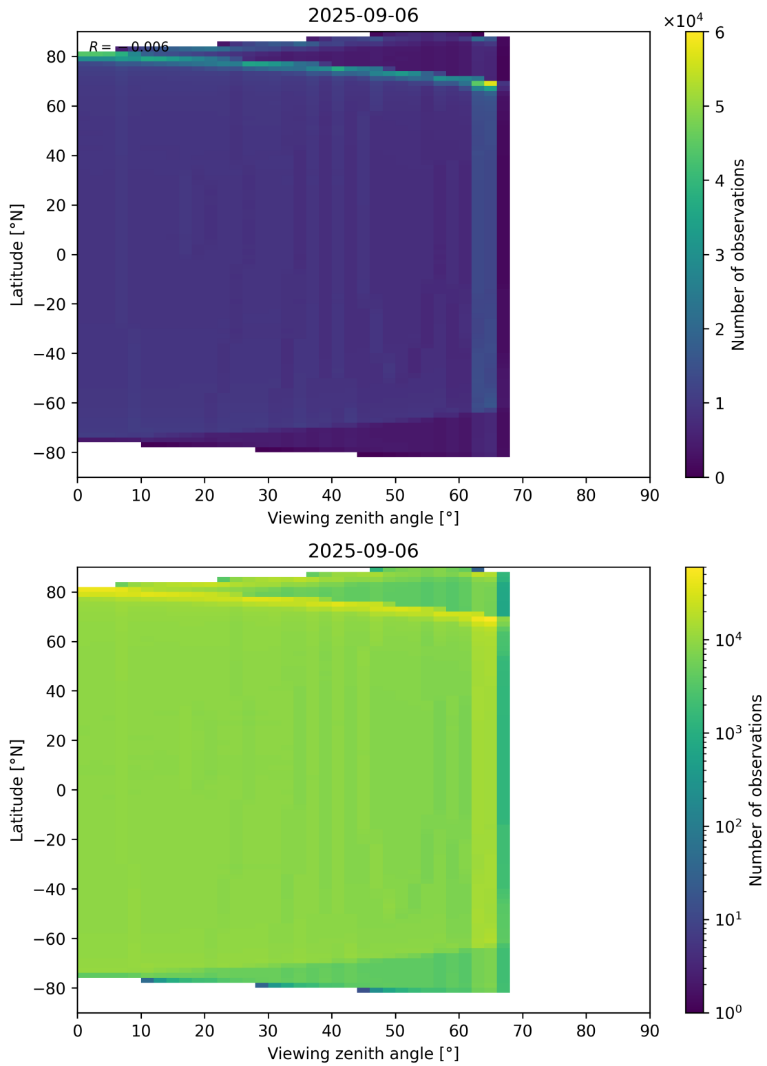
Figure 163: Scatter density plot of “Viewing zenith angle” against “Latitude” for 2025-09-05 to 2025-09-07.
