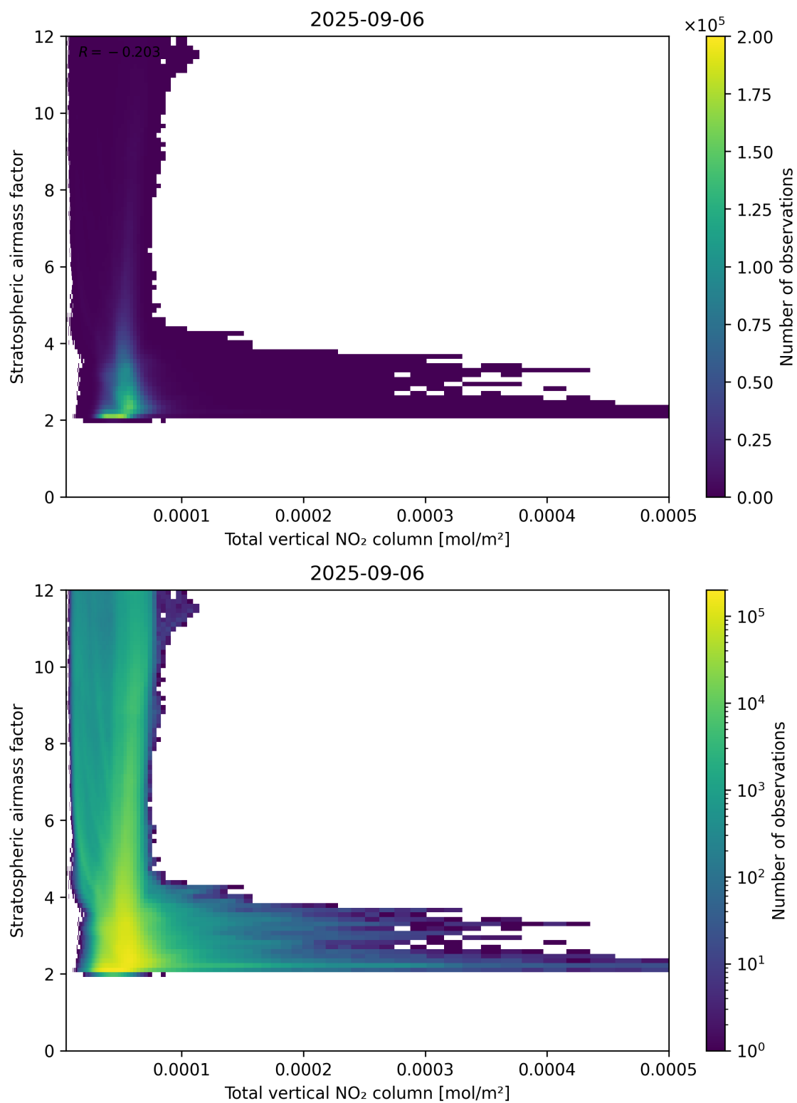
Figure 110: Scatter density plot of “Total vertical NO 2 column” against “Stratospheric airmass factor” for 2025-09-05 to 2025-09-07.
