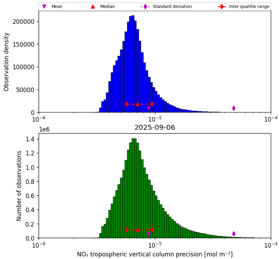
Figure 30: Histogram of “NO 2 tropospheric vertical column precision” for 2025-09-05 to 2025-09-07
