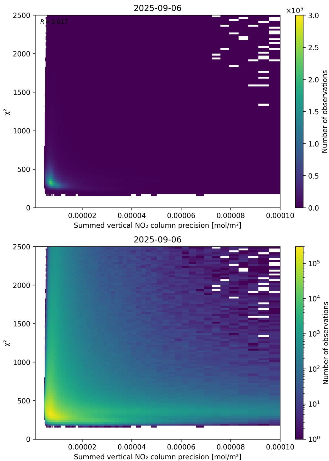
Figure 107: Scatter density plot of “Summed vertical NO 2 column precision” against “ \chi^2 ” for 2025-09-05 to 2025-09-07.
