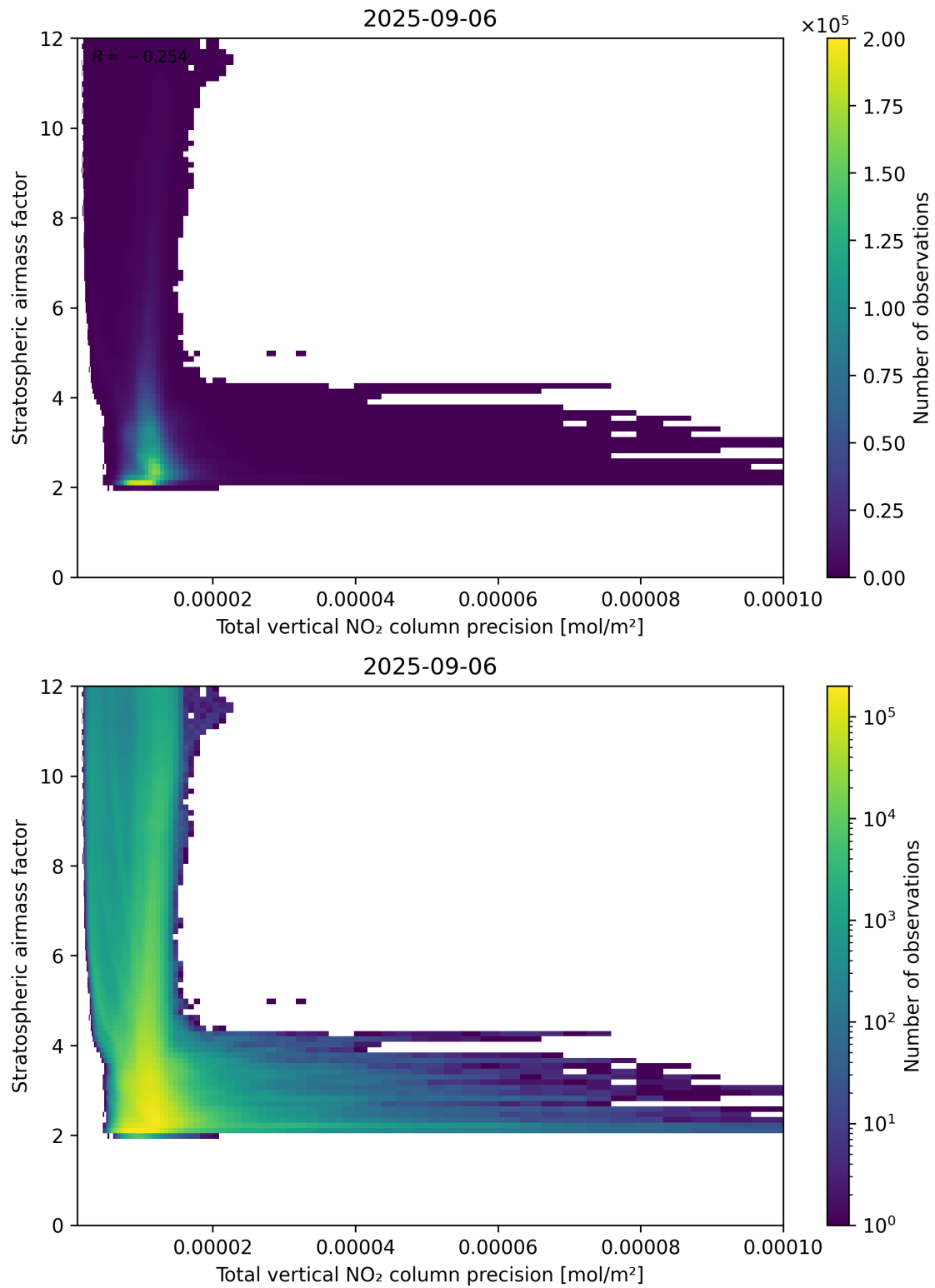
Figure 115: Scatter density plot of “Total vertical NO 2 column precision” against “Stratospheric air mass factor” for 2025-09-05 to 2025-09-07.
