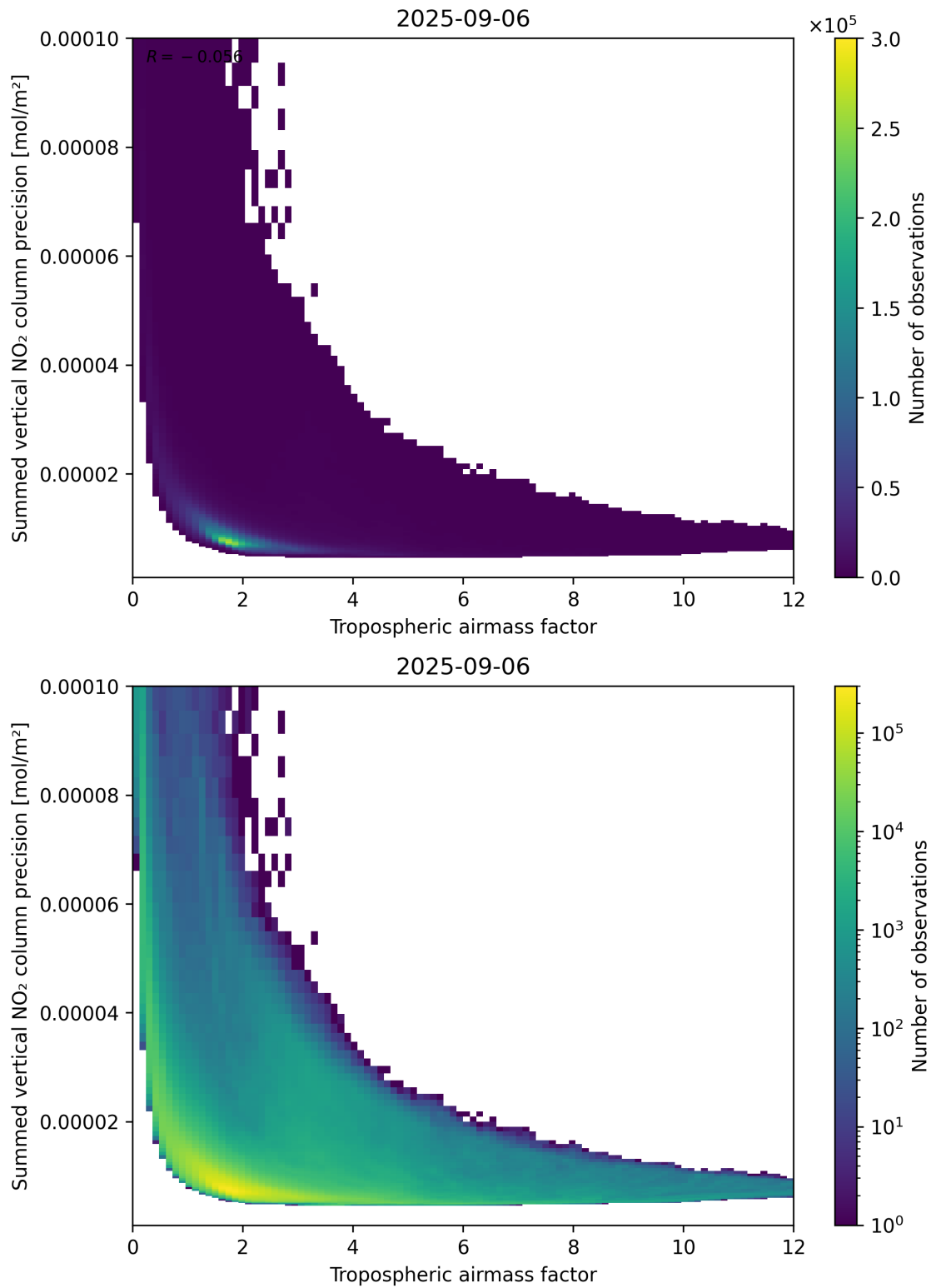
Figure 76: Scatter density plot of “Tropospheric air mass factor” against “Summed vertical NO 2 column precision” for 2025-09-05 to 2025-09-07.
