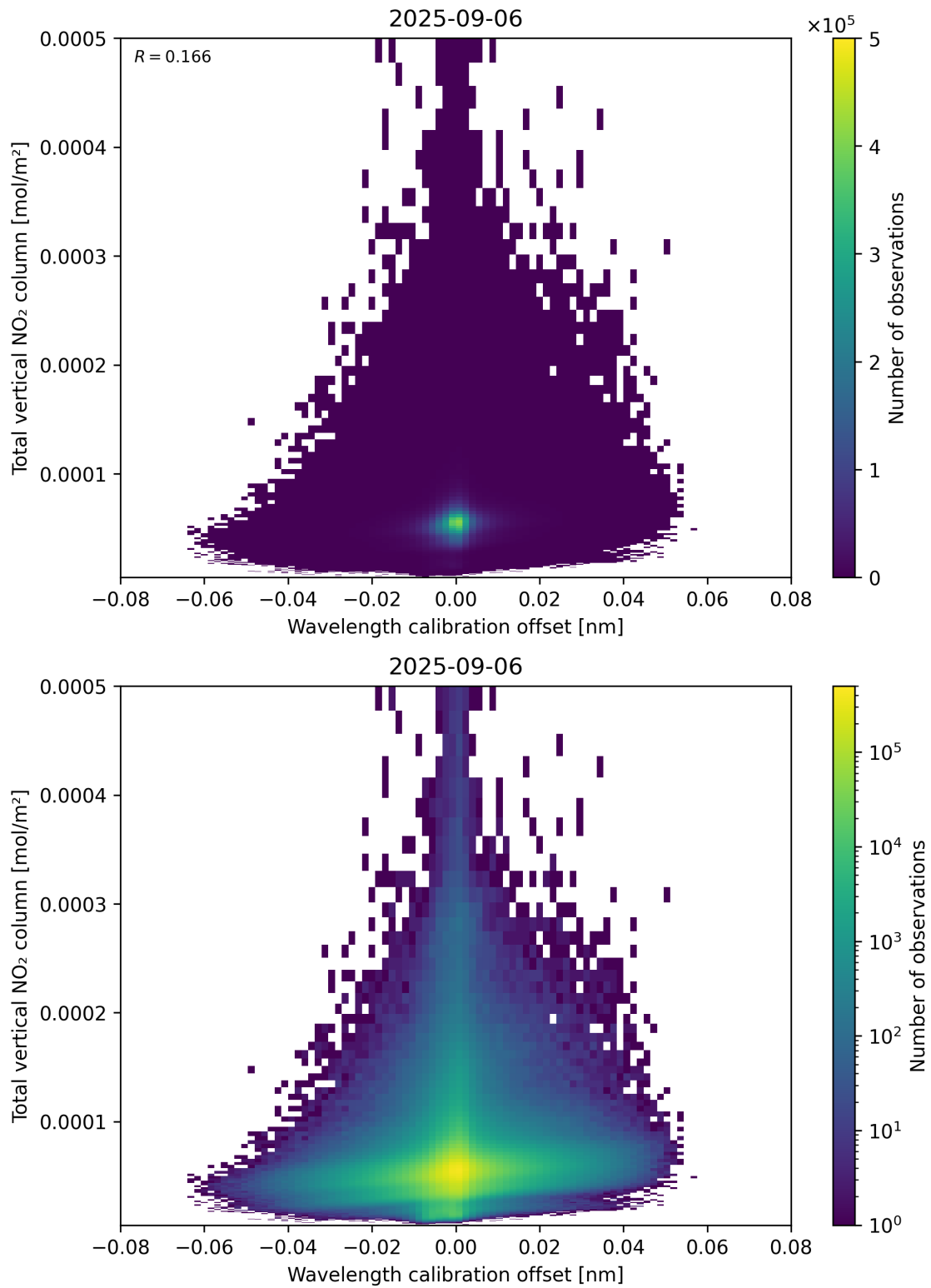
Figure 179: Scatter density plot of “Wavelength calibration offset” against “Total vertical NO 2 column” for 2025-09-05 to 2025-09-07.
