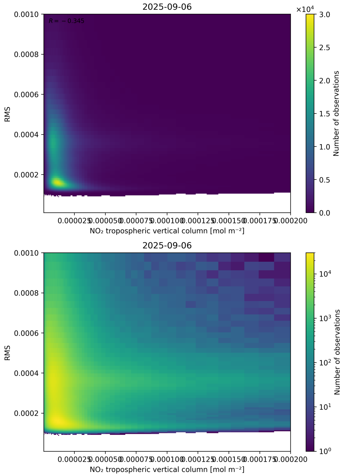
Figure 142: Scatter density plot of “NO 2 tropospheric vertical column” against “RMS” for 2025-09-05 to 2025-09-07.
