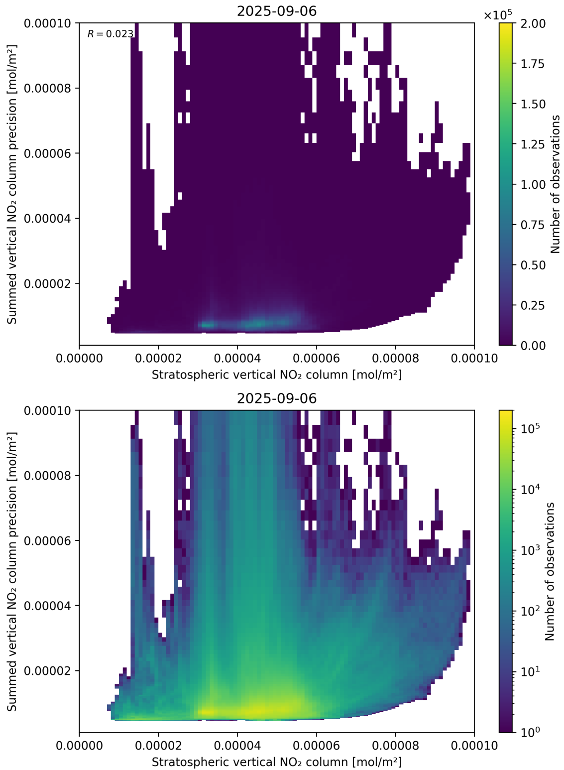
Figure 99: Scatter density plot of “Stratospheric vertical NO 2 column” against “Summed vertical NO 2 column precision” for 2025-09-05 to 2025-09-07.
