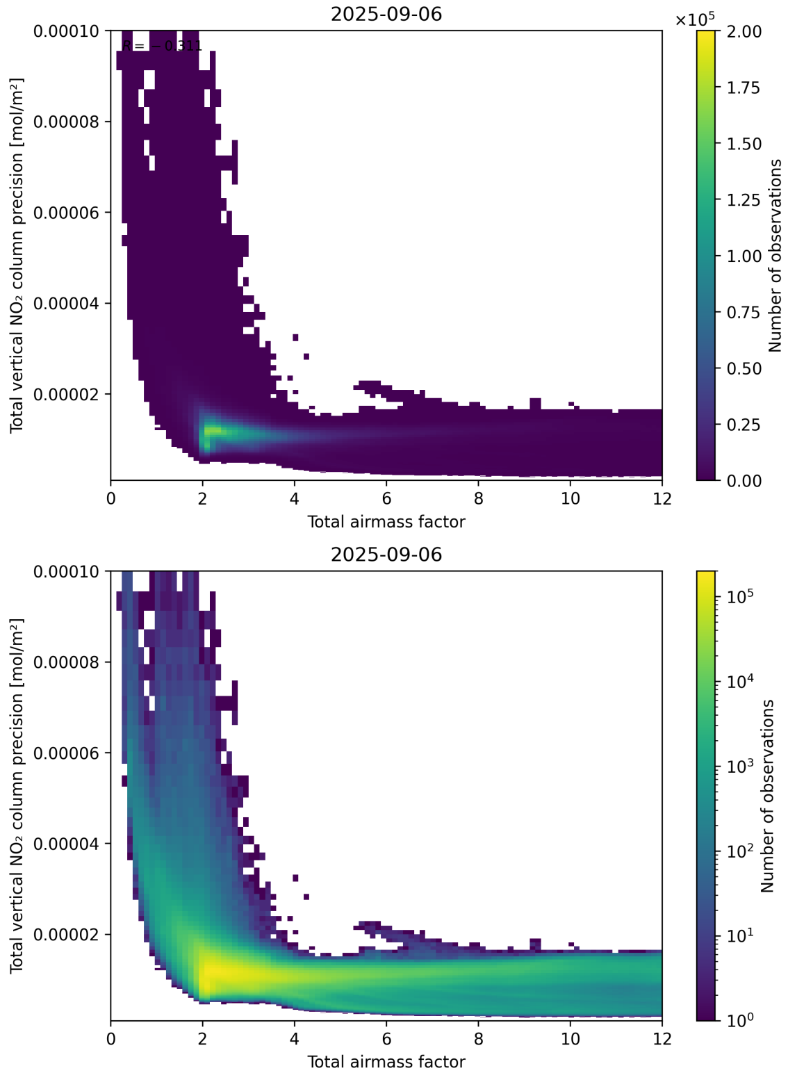
Figure 68: Scatter density plot of “Total airmass factor” against “Total vertical NO 2 column precision” for 2025-09-05 to 2025-09-07.
