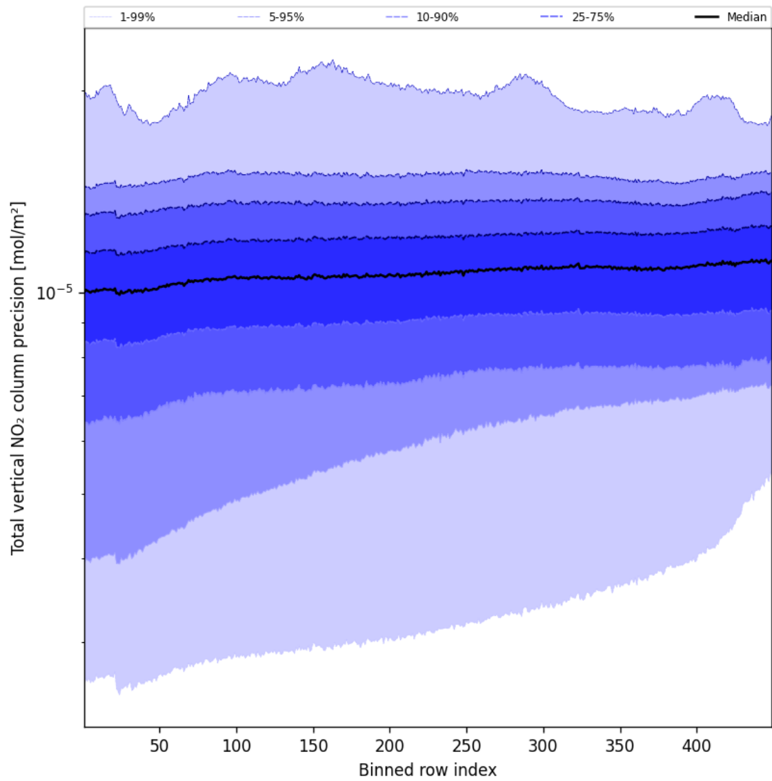
Figure 56: Along track statistics of “Total vertical NO 2 column precision” for 2025-09-05 to 2025-09-07
