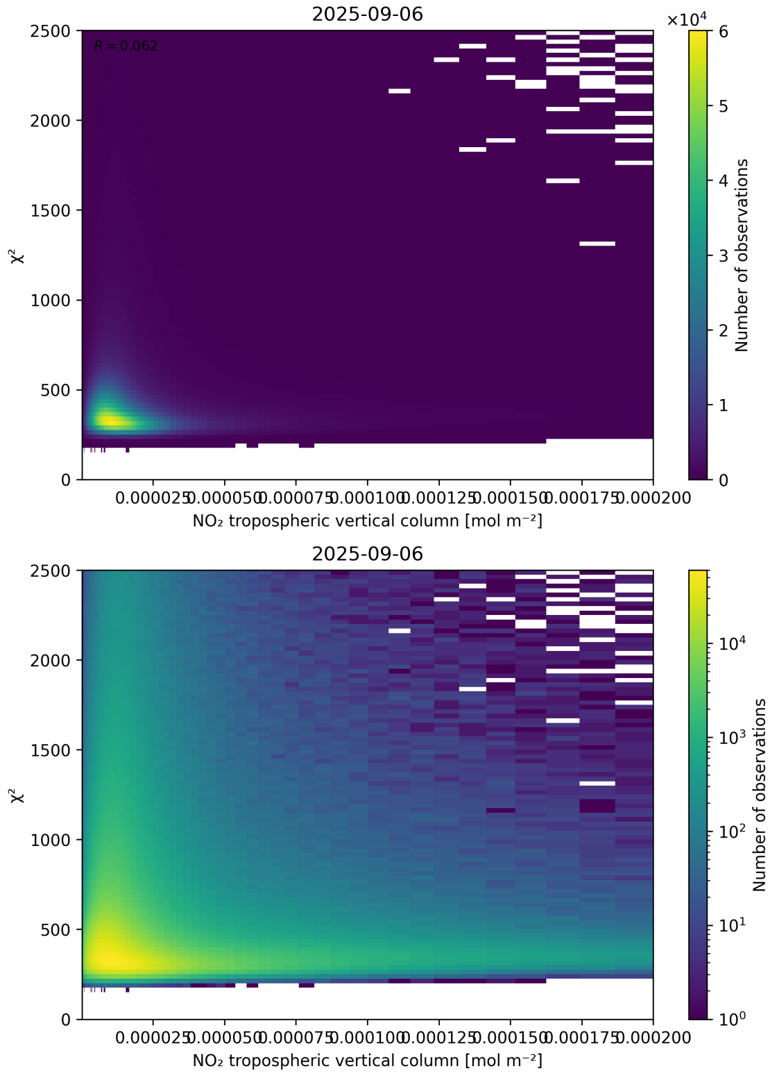
Figure 124: Scatter density plot of “NO 2 tropospheric vertical column” against “ \chi^2 ” for 2025-09-05 to 2025-09-07.
