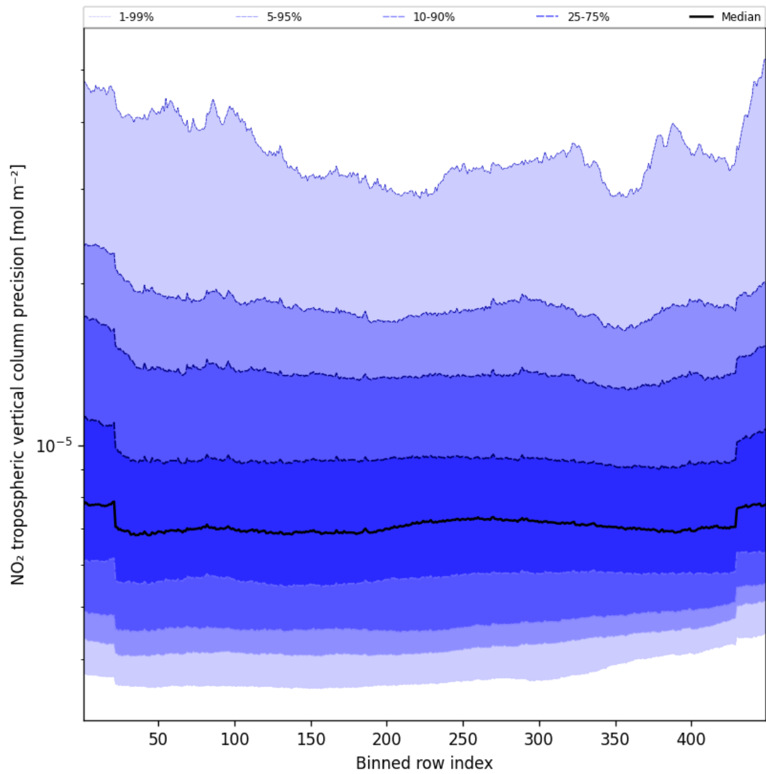
Figure 47: Along track statistics of “NO 2 tropospheric vertical column precision” for 2025-09-05 to 2025-09-07
