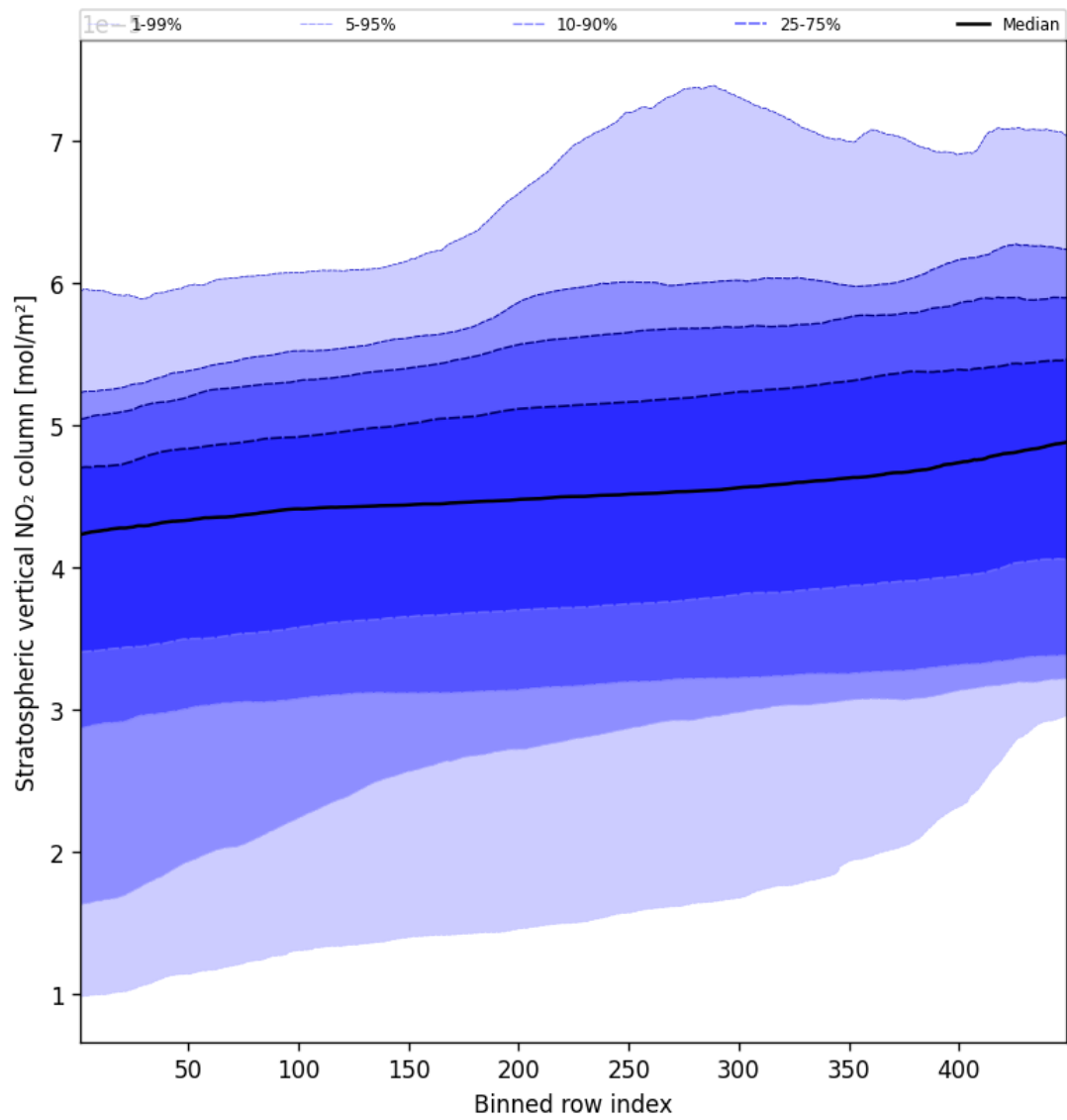
Figure 53: Along track statistics of “Stratospheric vertical NO 2 column” for 2025-09-05 to 2025-09-07
