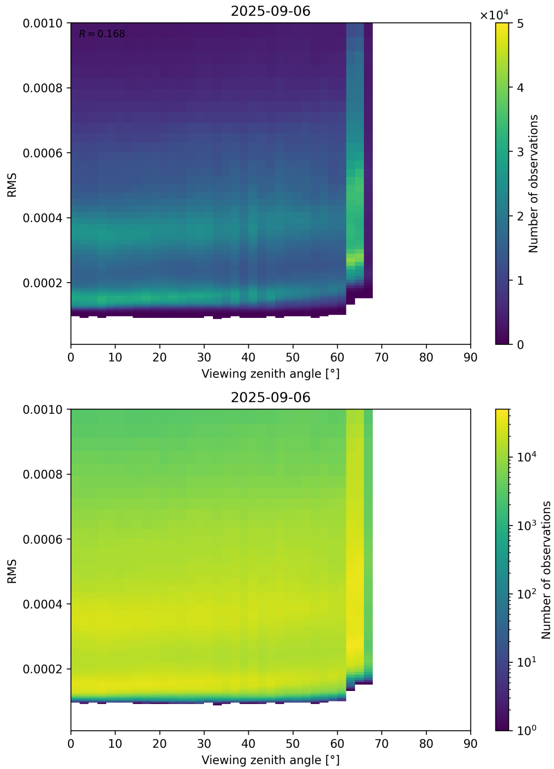
Figure 171: Scatter density plot of “Viewing zenith angle” against “RMS” for 2025-09-05 to 2025-09-07.
