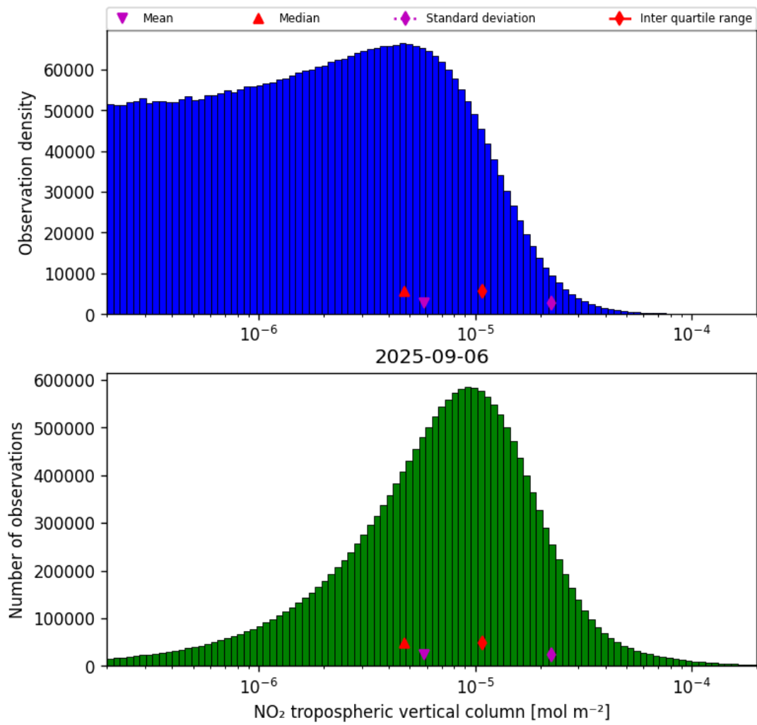
Figure 29: Histogram of “NO 2 tropospheric vertical column” for 2025-09-05 to 2025-09-07
