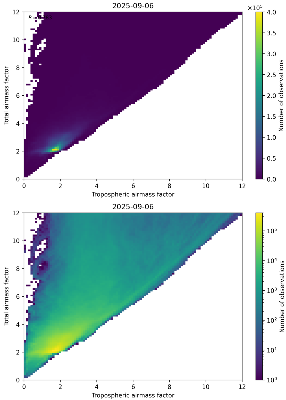
Figure 72: Scatter density plot of “Tropospheric airmass factor” against “Total airmass factor” for 2025-09-05 to 2025-09-07.
