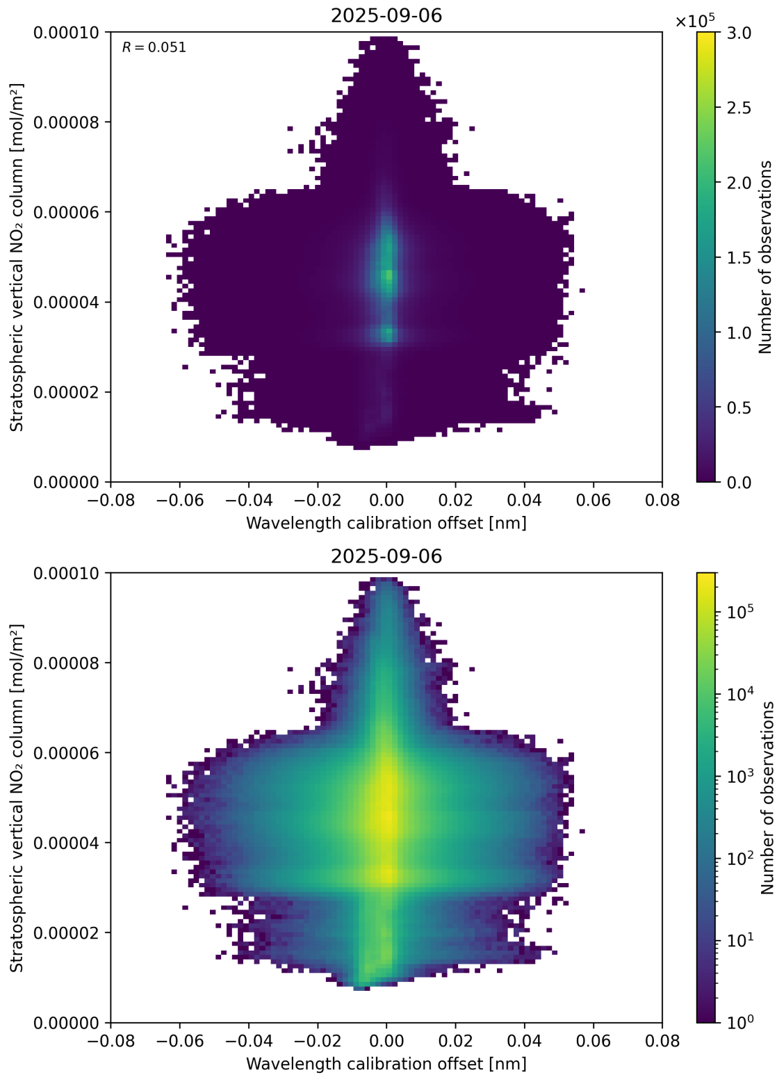
Figure 176: Scatter density plot of “Wavelength calibration offset” against “Stratospheric vertical NO 2 column” for 2025-09-05 to 2025-09-07.
