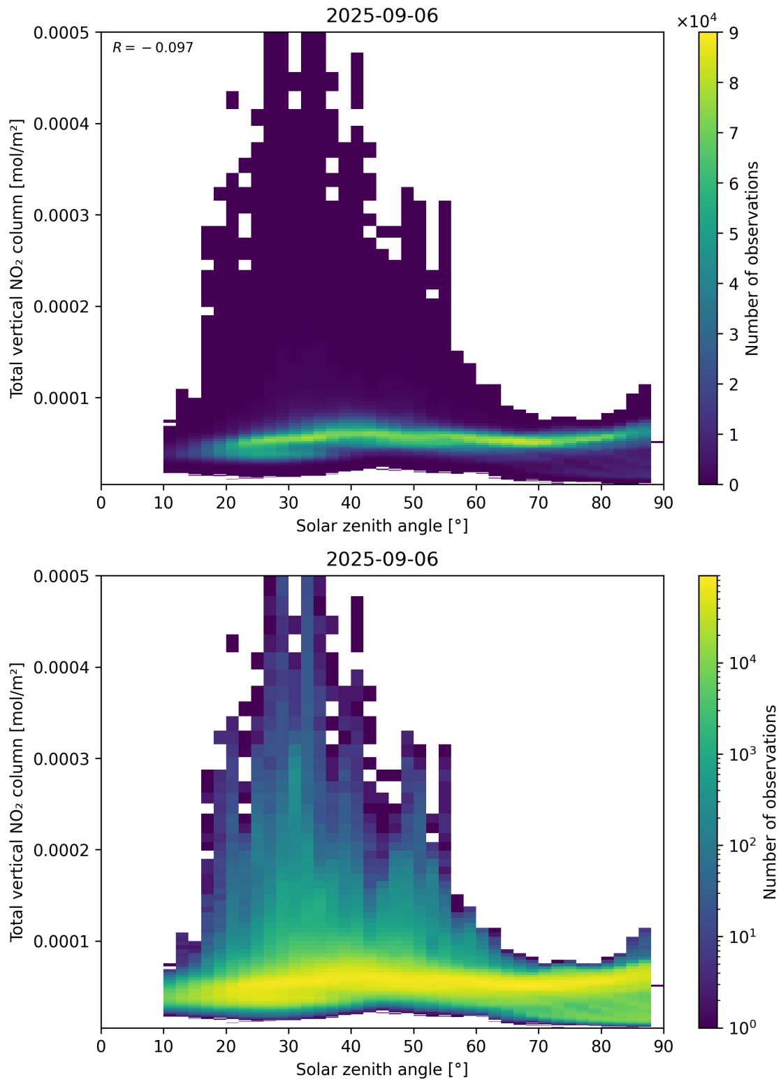
Figure 153: Scatter density plot of “Solar zenith angle” against “Total vertical NO 2 column” for 2025-09-05 to 2025-09-07.
