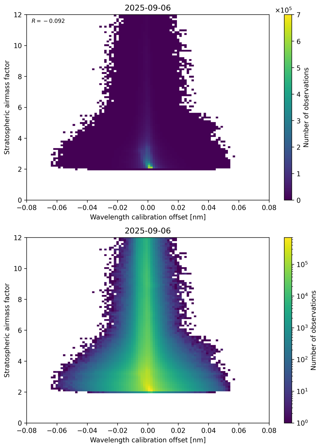
Figure 174: Scatter density plot of “Wavelength calibration offset” against “Stratospheric air mass factor” for 2025-09-05 to 2025-09-07.
