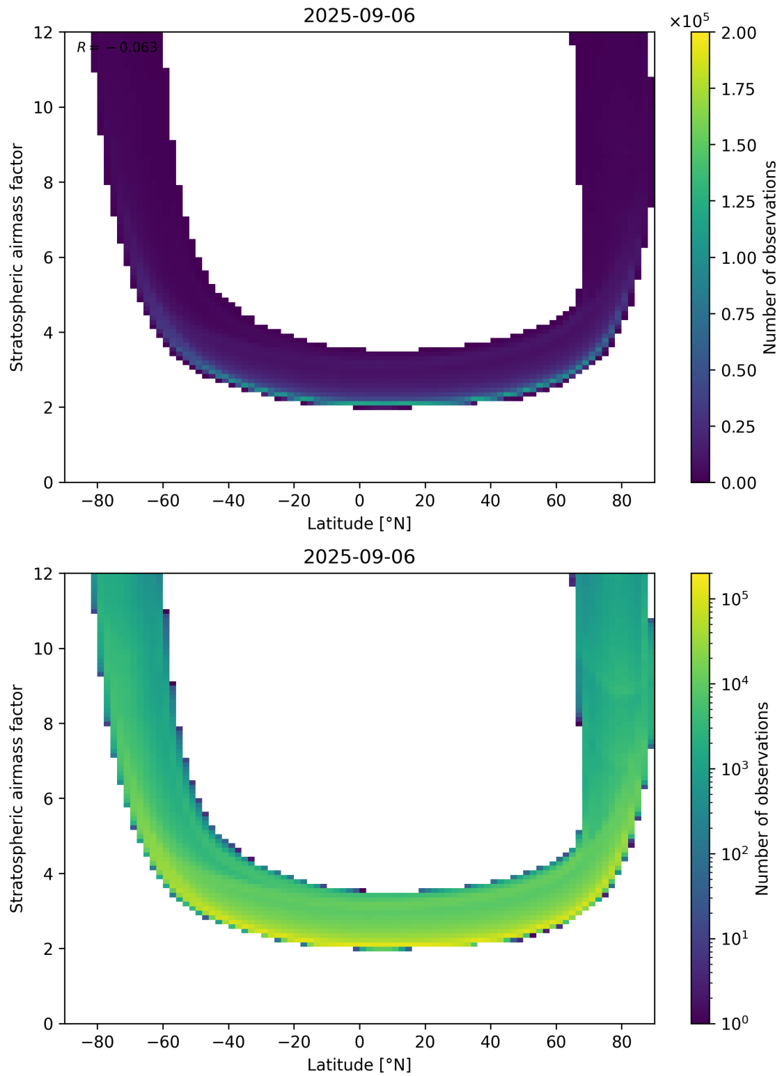
Figure 83: Scatter density plot of “Latitude” against “Stratospheric air mass factor” for 2025-09-05 to 2025-09-07.
