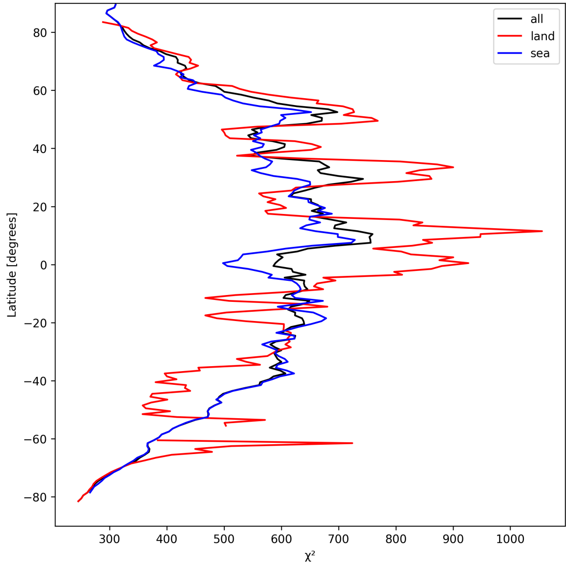
Figure 25: Zonal average of “ \chi^2 ” for 2025-09-05 to 2025-09-07.
