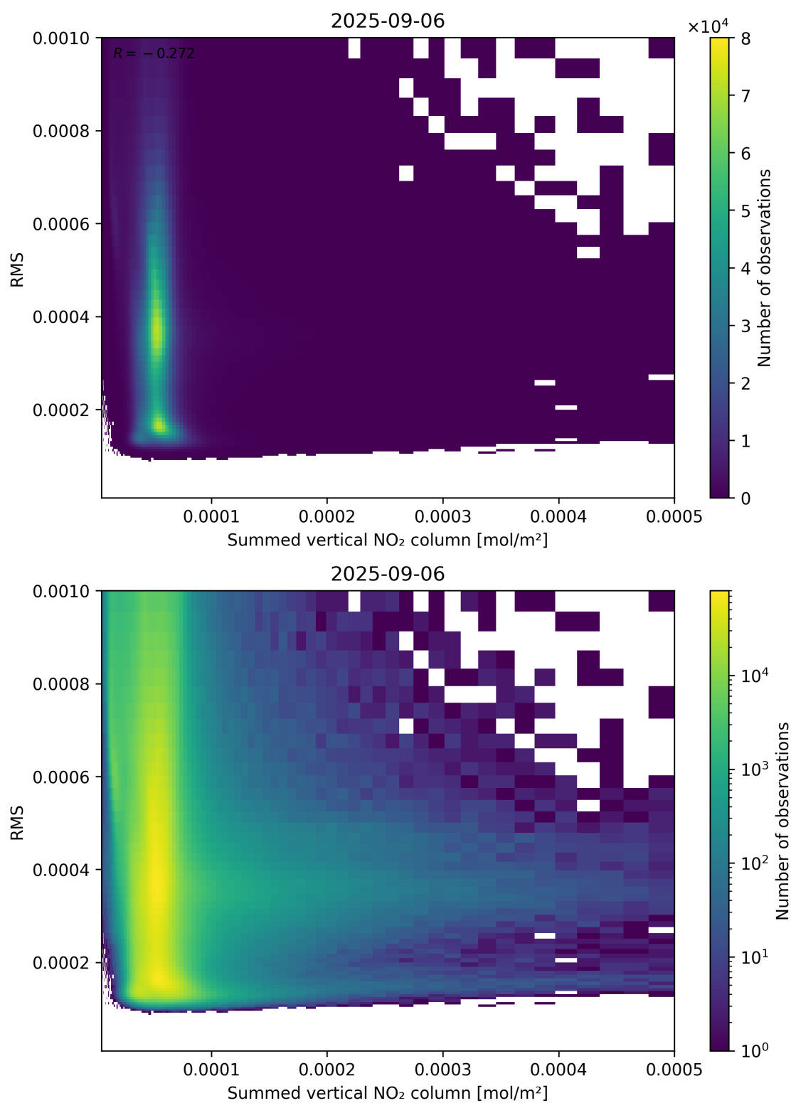
Figure 109: Scatter density plot of “Summed vertical NO 2 column” against “RMS” for 2025-09-05 to 2025-09-07.
