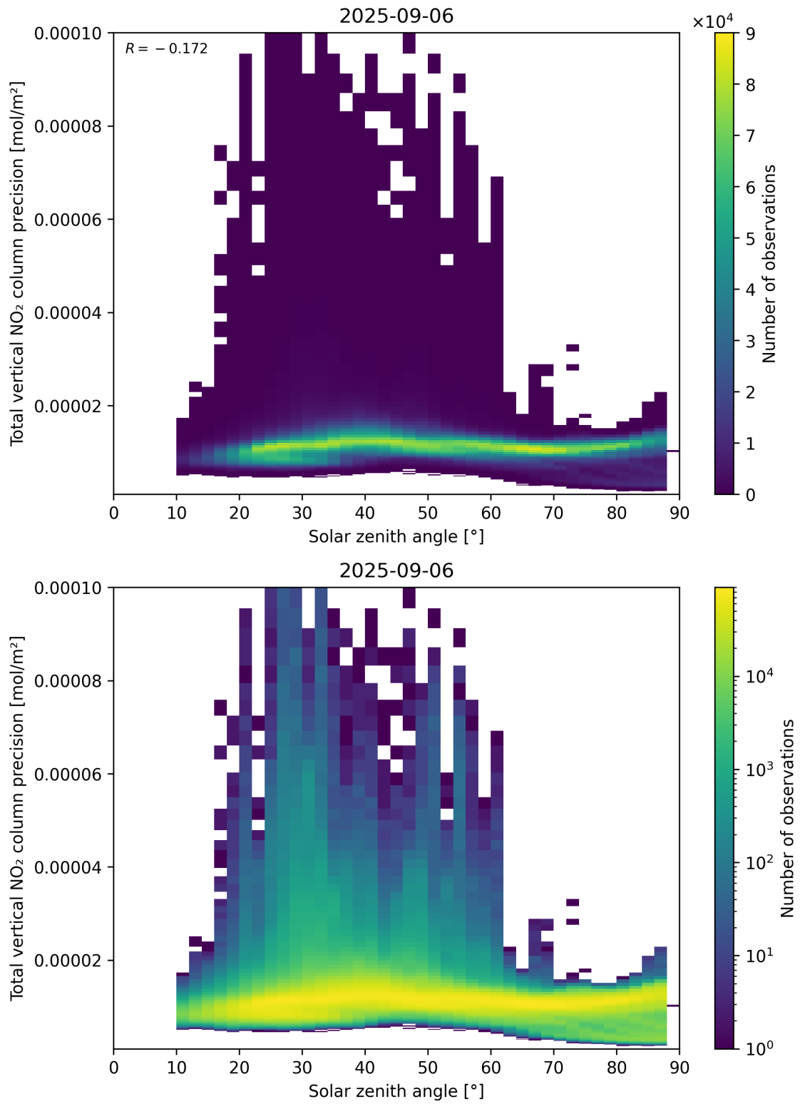
Figure 154: Scatter density plot of “Solar zenith angle” against “Total vertical NO 2 column precision” for 2025-09-05 to 2025-09-07.
