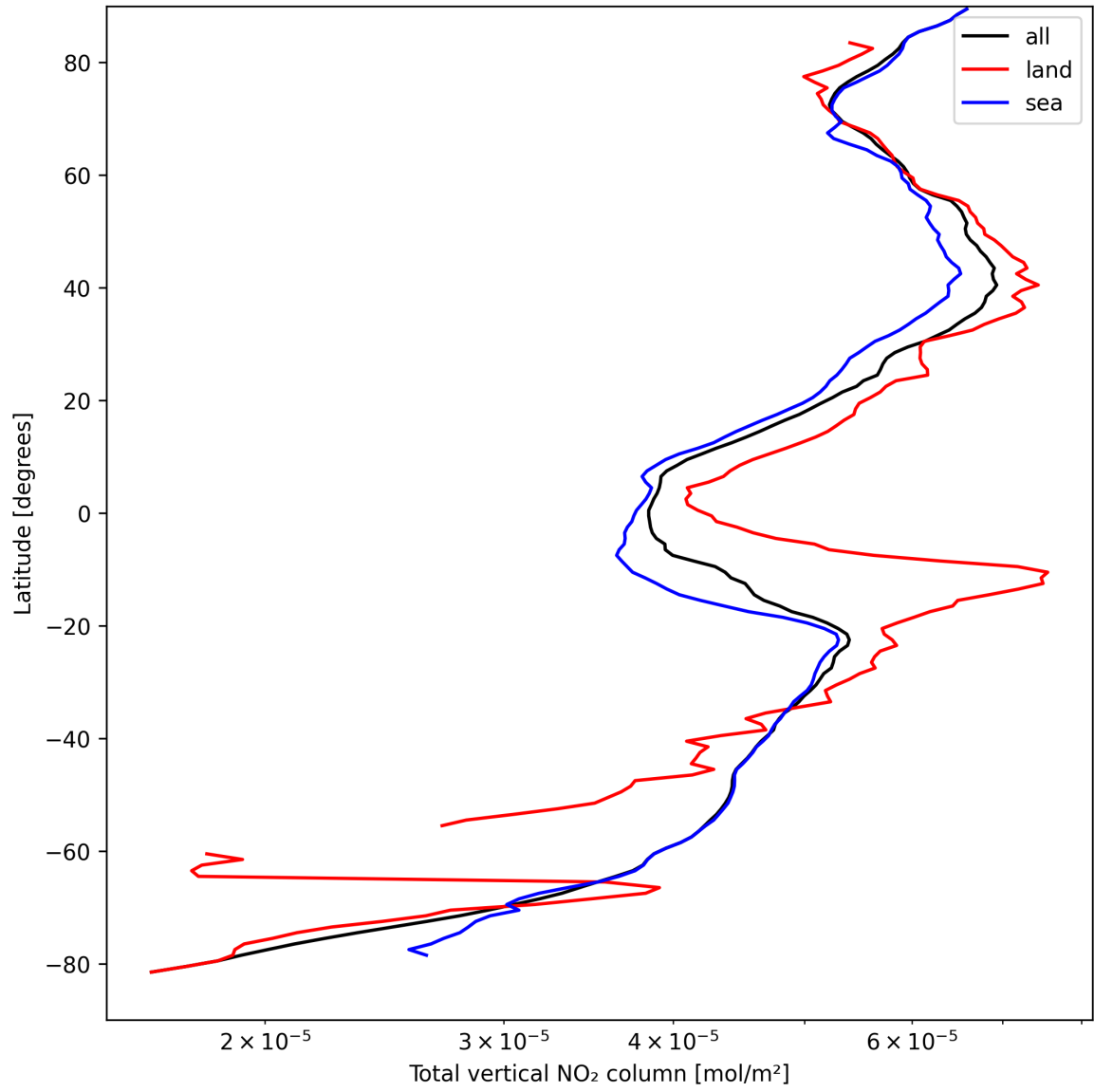
Figure 21: Zonal average of “Total vertical NO 2 column” for 2025-09-05 to 2025-09-07.
