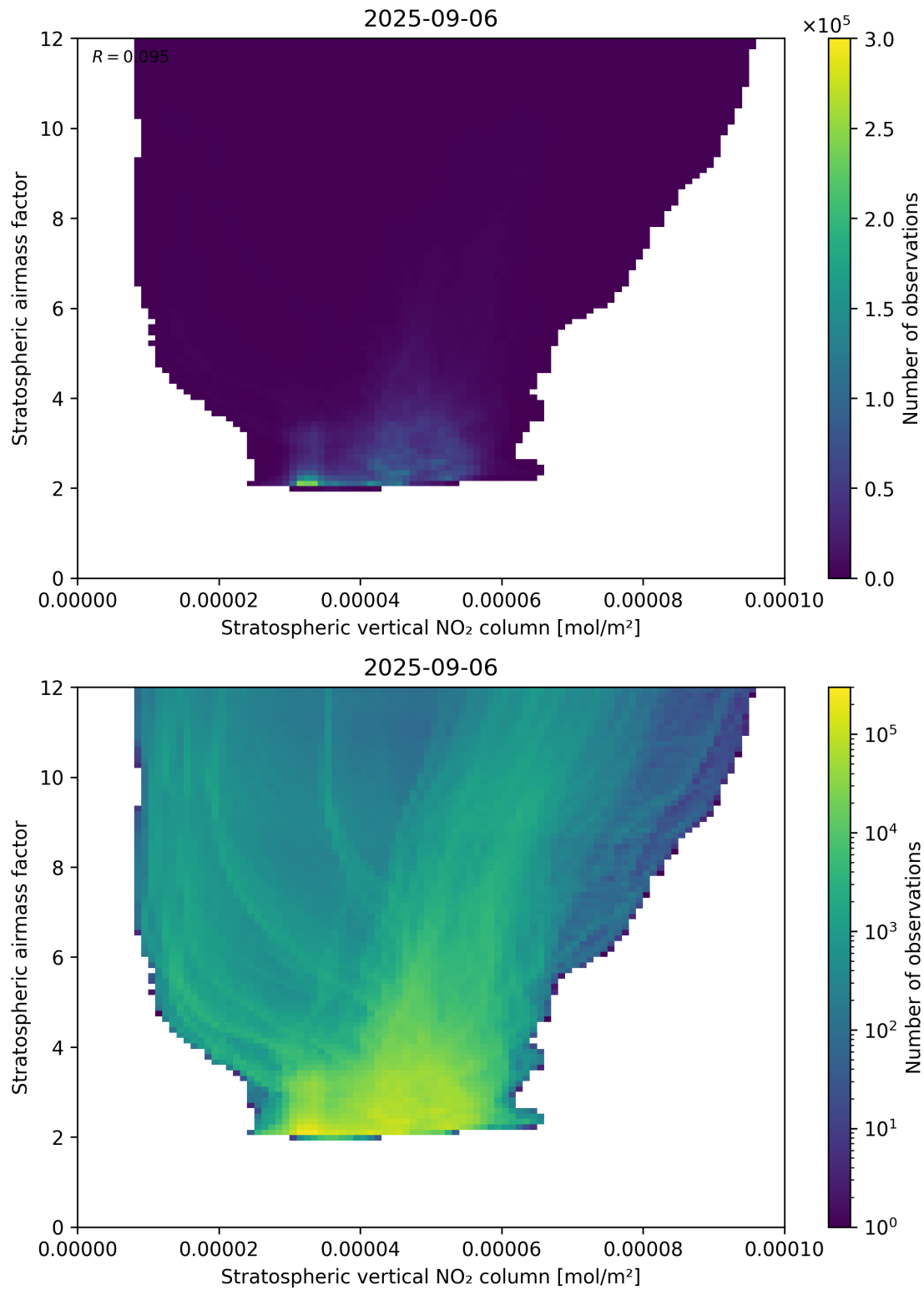
Figure 96: Scatter density plot of “Stratospheric vertical NO 2 column” against “Stratospheric airmass factor” for 2025-09-05 to 2025-09-07.
