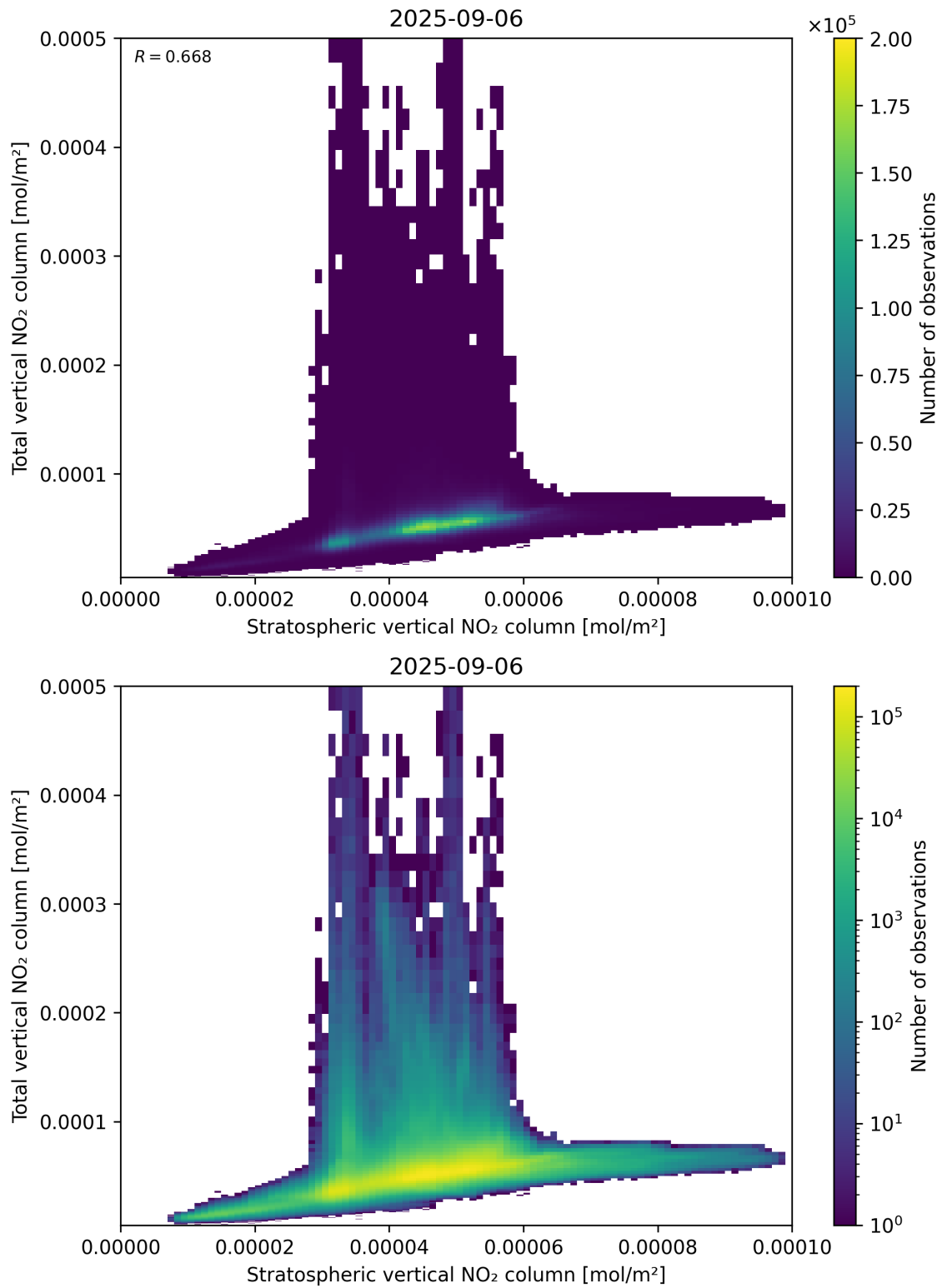
Figure 100: Scatter density plot of “Stratospheric vertical NO 2 column” against “Total vertical NO 2 column” for 2025-09-05 to 2025-09-07.
