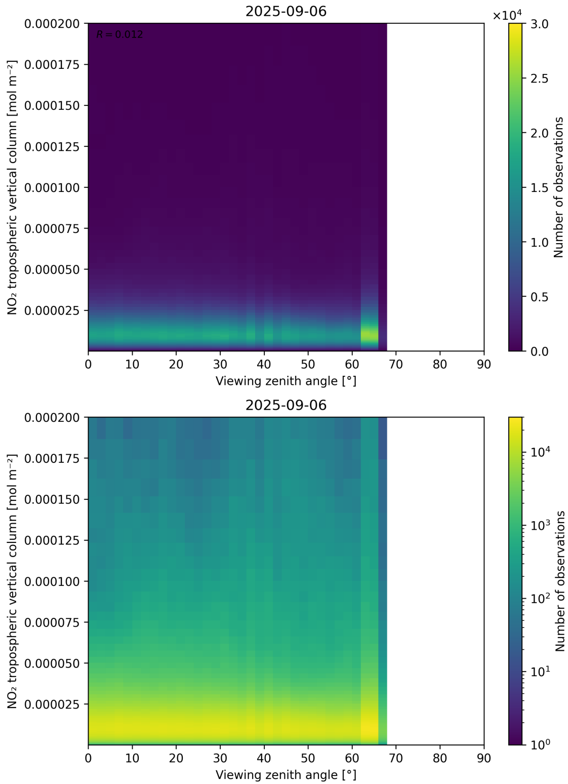
Figure 169: Scatter density plot of “Viewing zenith angle” against “NO 2 tropospheric vertical column” for 2025-09-05 to 2025-09-07.
