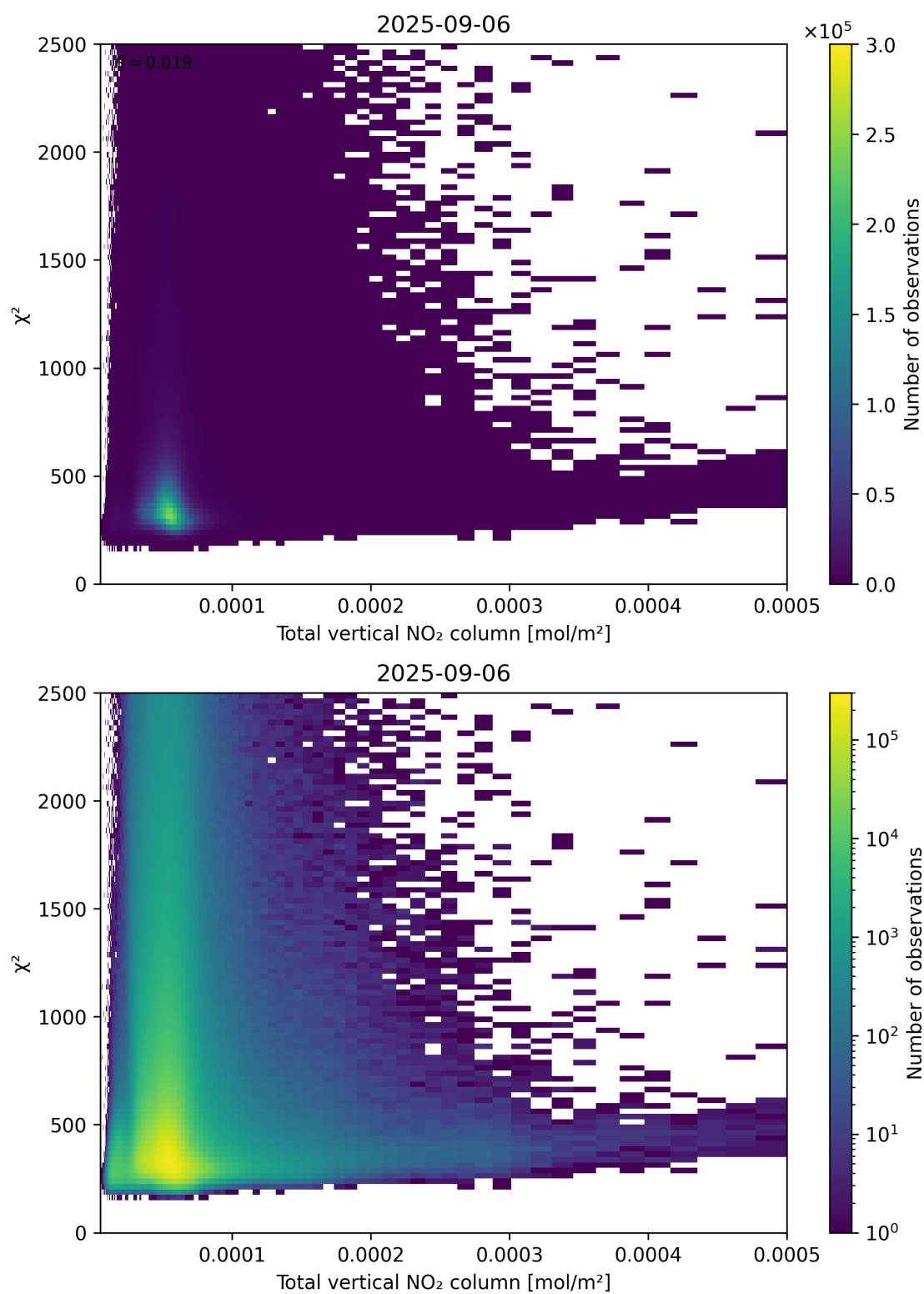
Figure 111: Scatter density plot of “Total vertical NO 2 column” against “ \chi^2 ” for 2025-09-05 to 2025-09-07.
