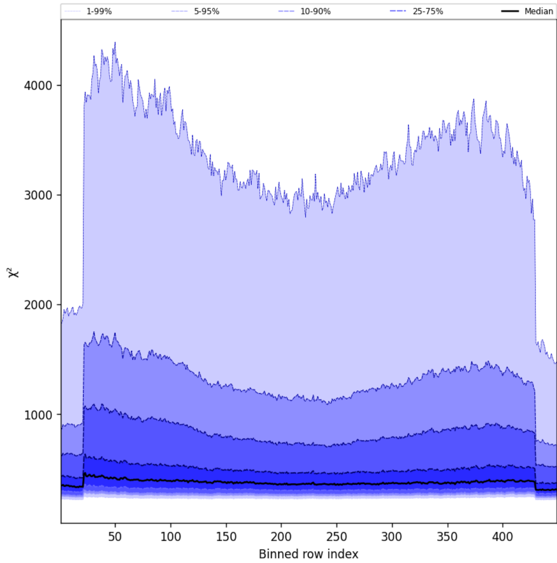
Figure 59: Along track statistics of “ \chi^2 ” for 2025-09-05 to 2025-09-07
