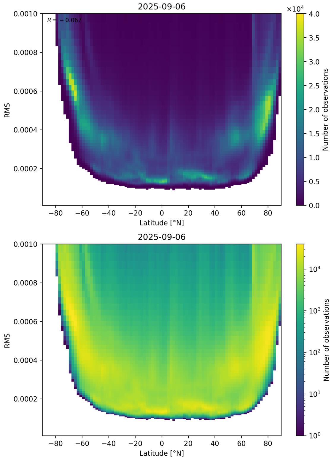
Figure 94: Scatter density plot of “Latitude” against “RMS” for 2025-09-05 to 2025-09-07.
