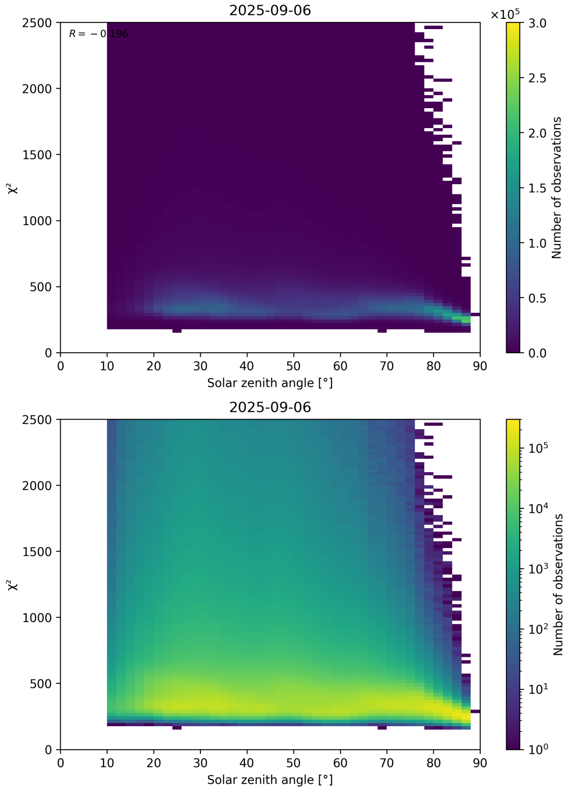
Figure 148: Scatter density plot of “Solar zenith angle” against “ \chi^2 ” for 2025-09-05 to 2025-09-07.
