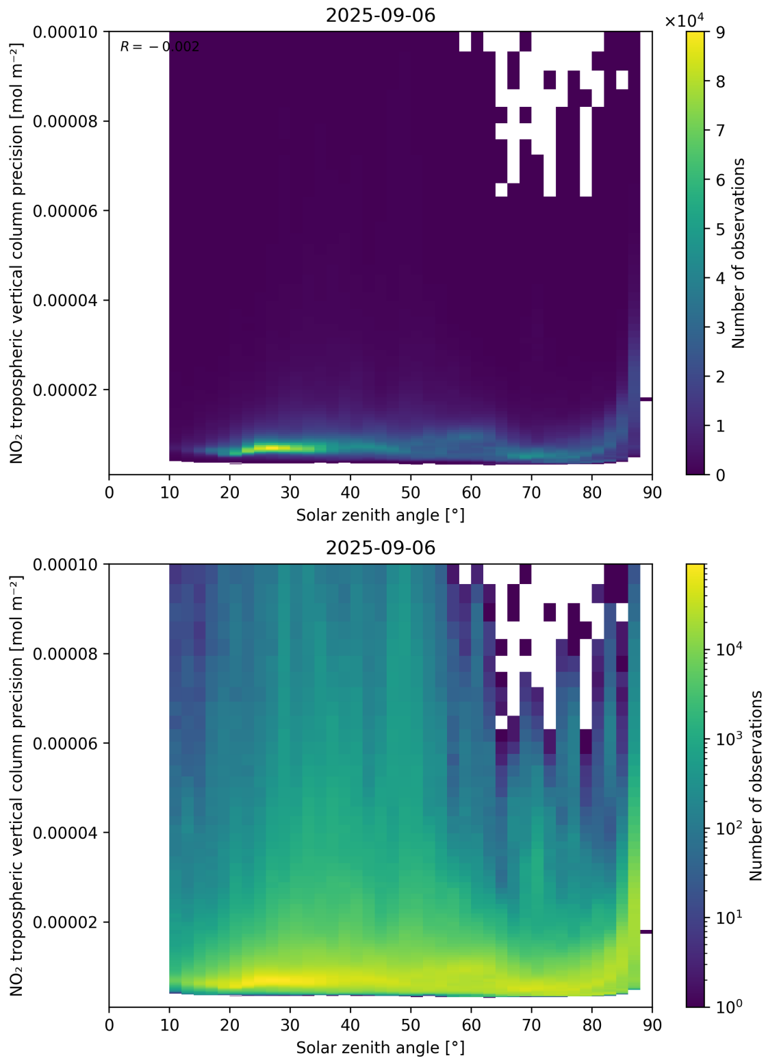
Figure 156: Scatter density plot of “Solar zenith angle” against “NO 2 tropospheric vertical column precision” for 2025-09-05 to 2025-09-07.
