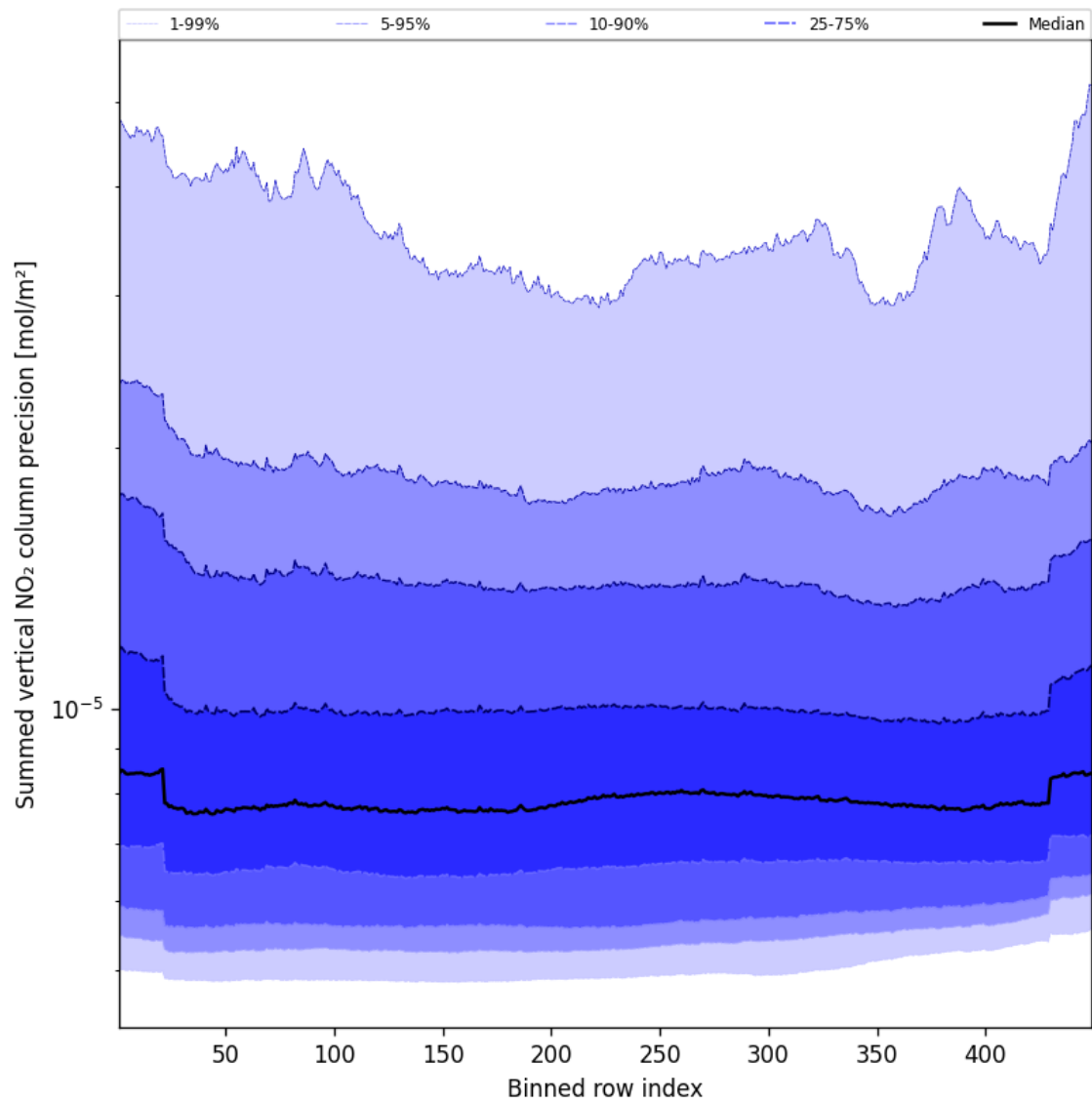
Figure 58: Along track statistics of “Summed vertical NO 2 column precision” for 2025-09-05 to 2025-09-07
