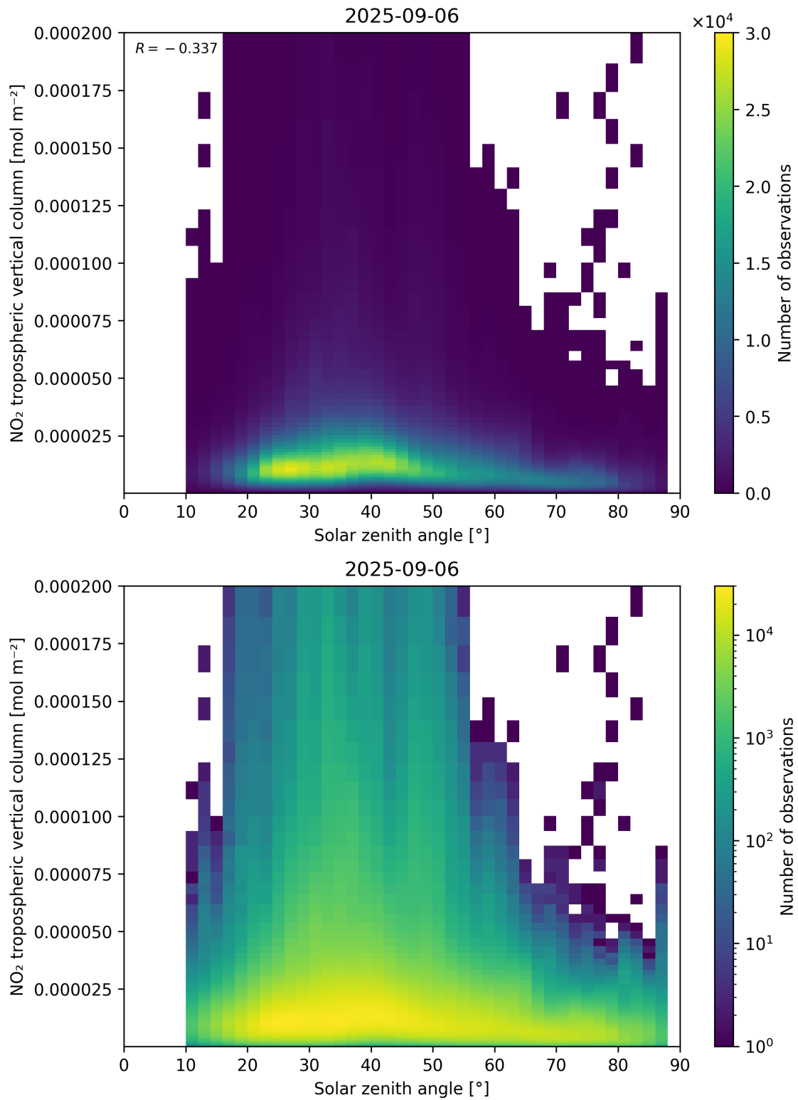
Figure 155: Scatter density plot of “Solar zenith angle” against “NO 2 tropospheric vertical column” for 2025-09-05 to 2025-09-07.
