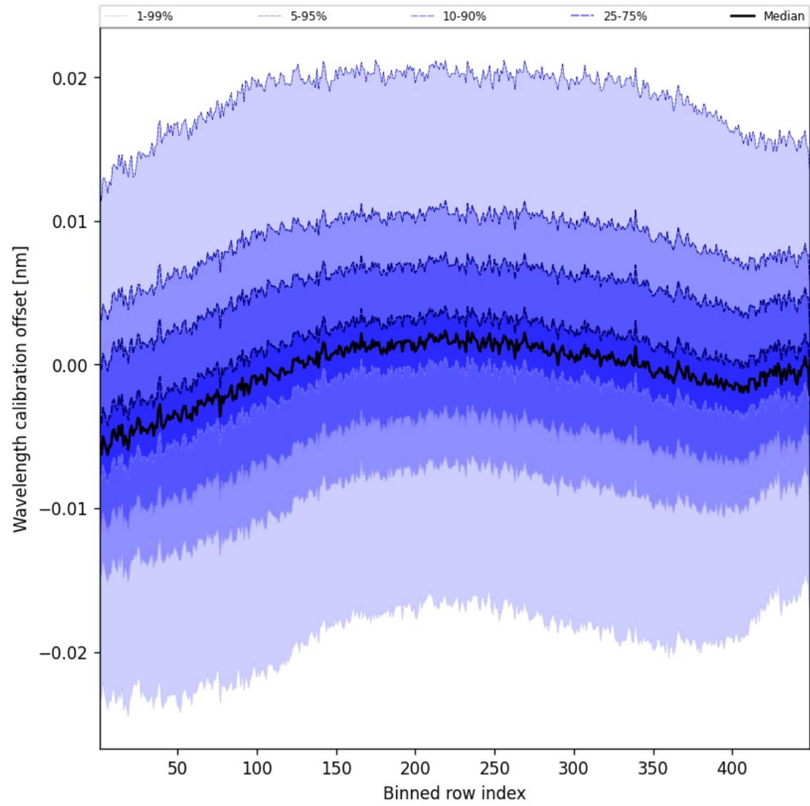
Figure 52: Along track statistics of “Wavelength calibration offset” for 2025-09-05 to 2025-09-07
