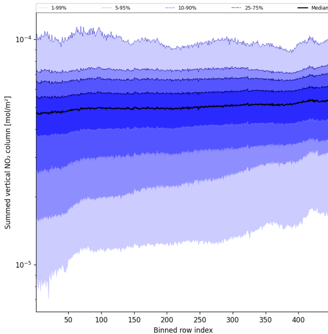
Figure 57: Along track statistics of “Summed vertical NO 2 column” for 2025-09-05 to 2025-09-07
