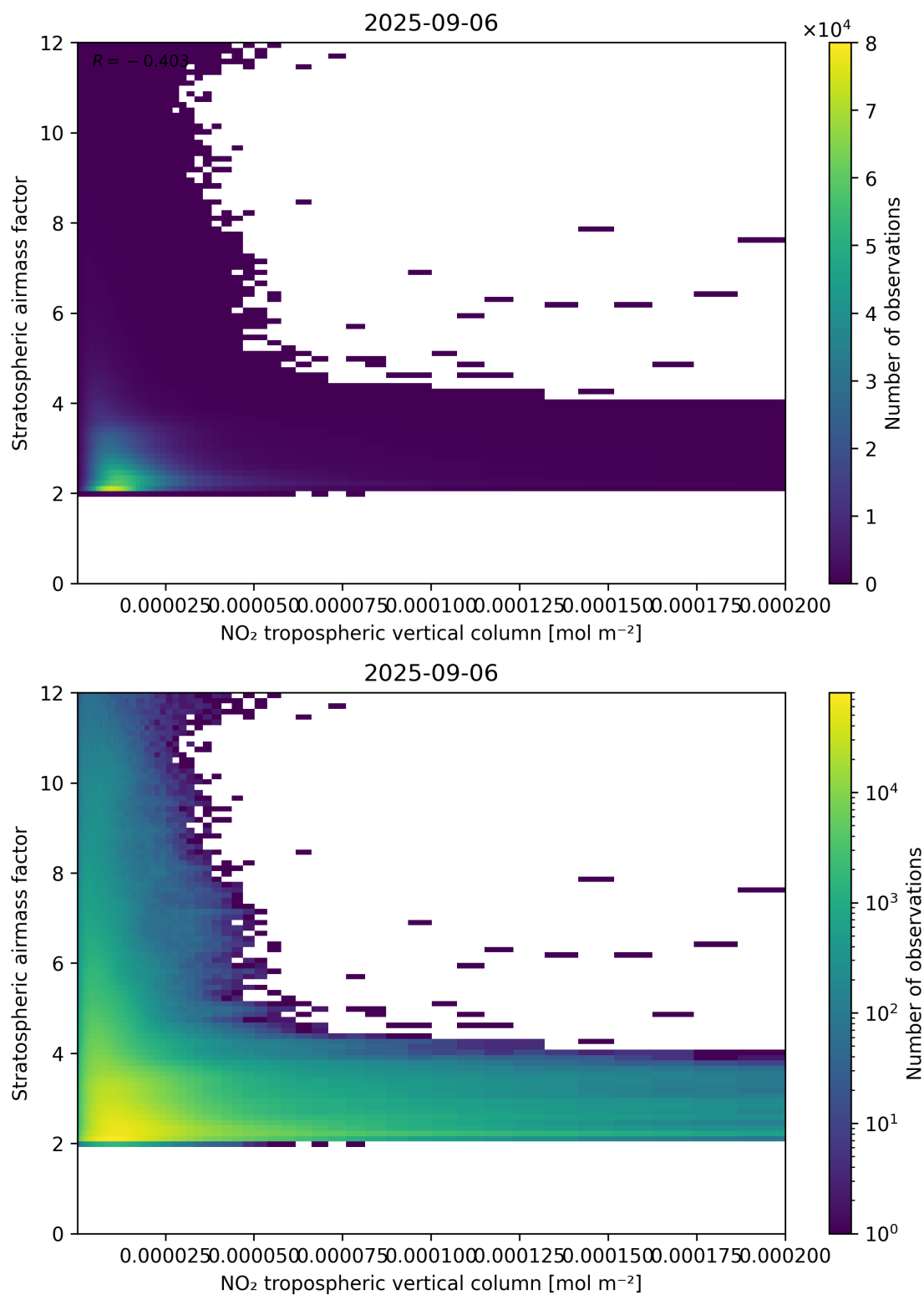
Figure 121: Scatter density plot of “NO 2 tropospheric vertical column” against “Stratospheric air mass factor” for 2025-09-05 to 2025-09-07.
