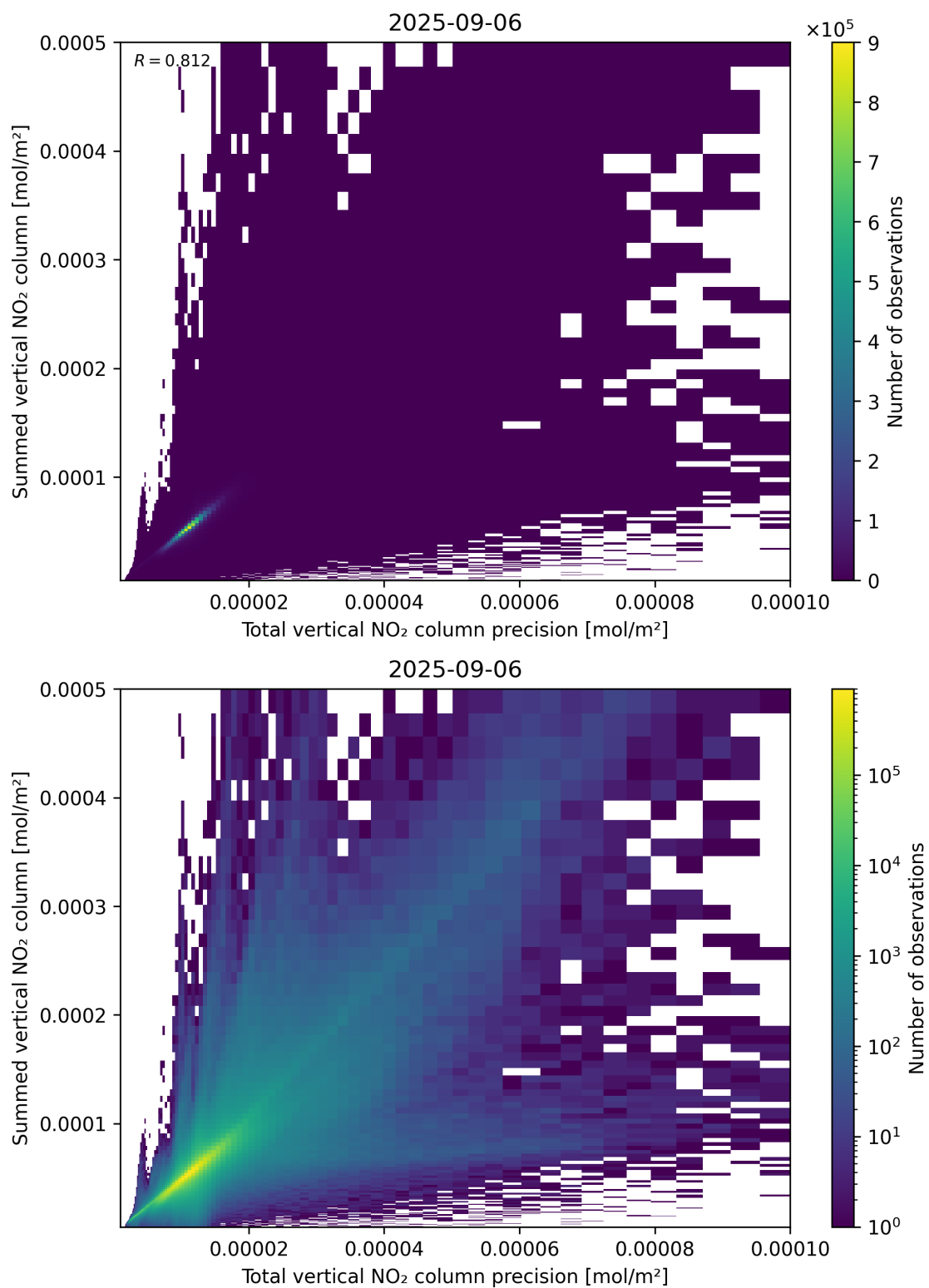
Figure 117: Scatter density plot of “Total vertical NO 2 column precision” against “Summed vertical NO 2 column” for 2025-09-05 to 2025-09-07.
