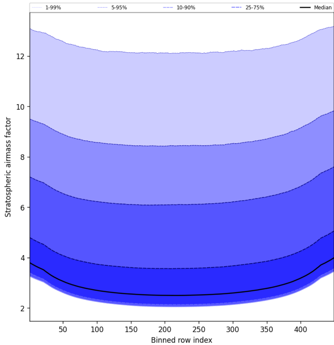
Figure 61: Along track statistics of “Stratospheric airmass factor” for 2025-09-05 to 2025-09-07
