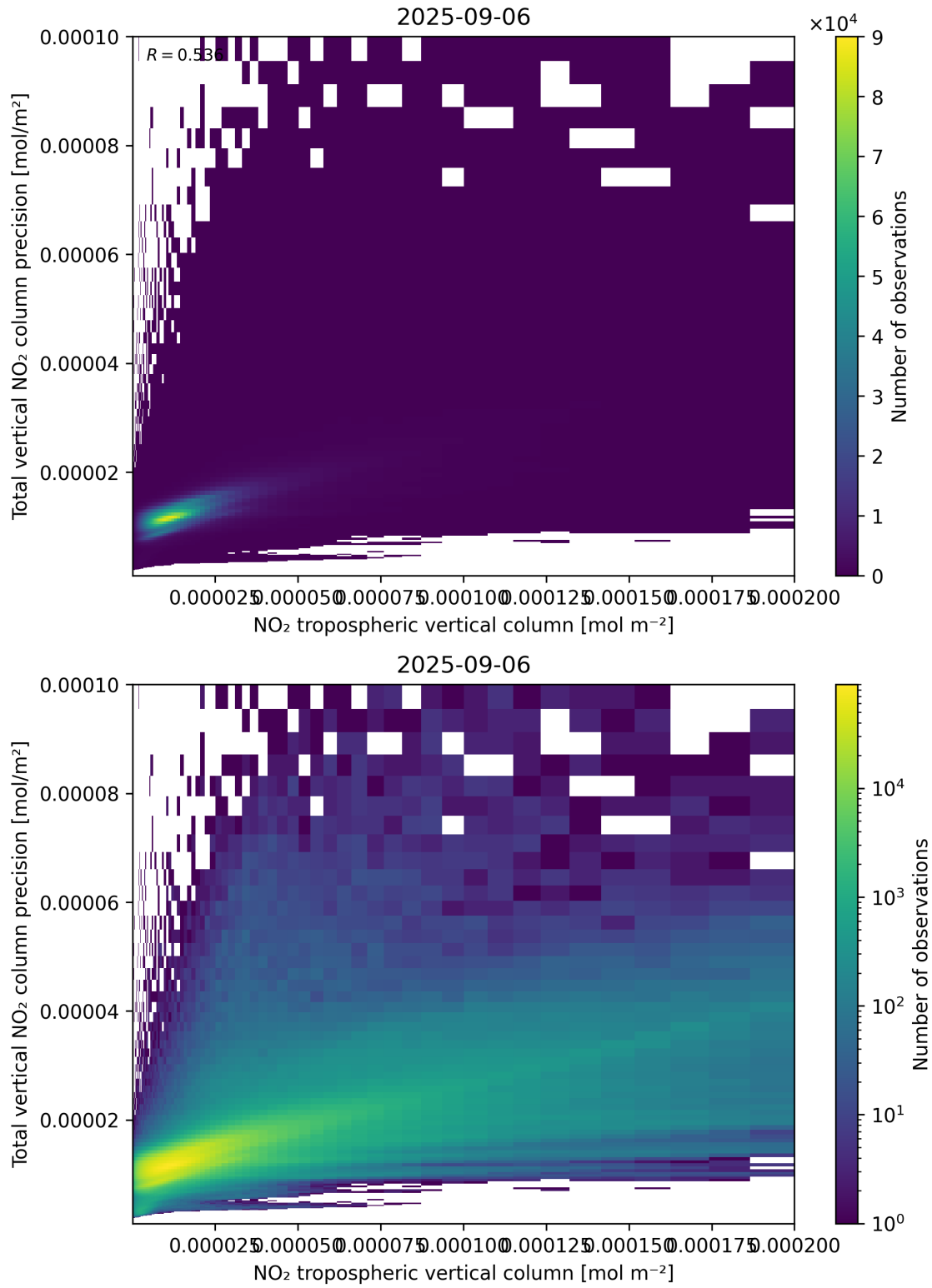
Figure 129: Scatter density plot of “NO 2 tropospheric vertical column” against “Total vertical NO 2 column precision” for 2025-09-05 to 2025-09-07.
