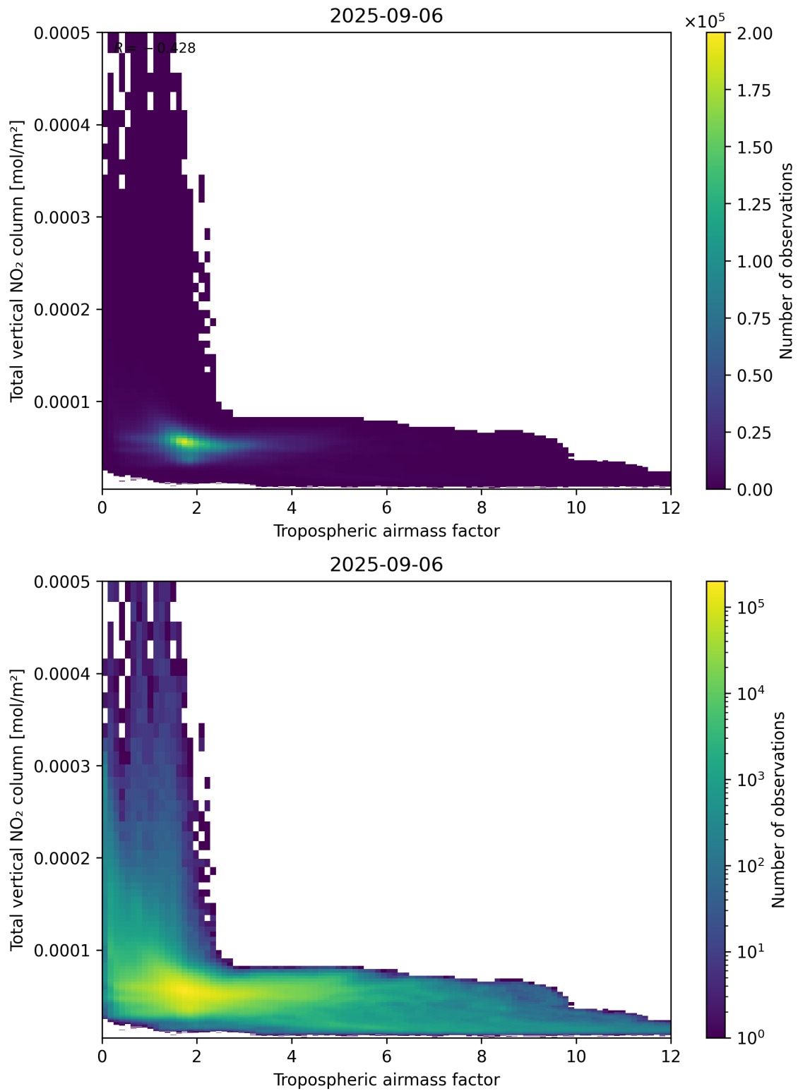
Figure 77: Scatter density plot of “Tropospheric airmass factor” against “Total vertical NO 2 column” for 2025-09-05 to 2025-09-07.
