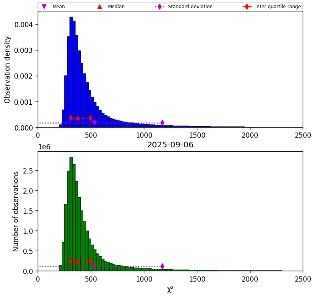
Figure 42: Histogram of “ \chi^2 ” for 2025-09-05 to 2025-09-07
