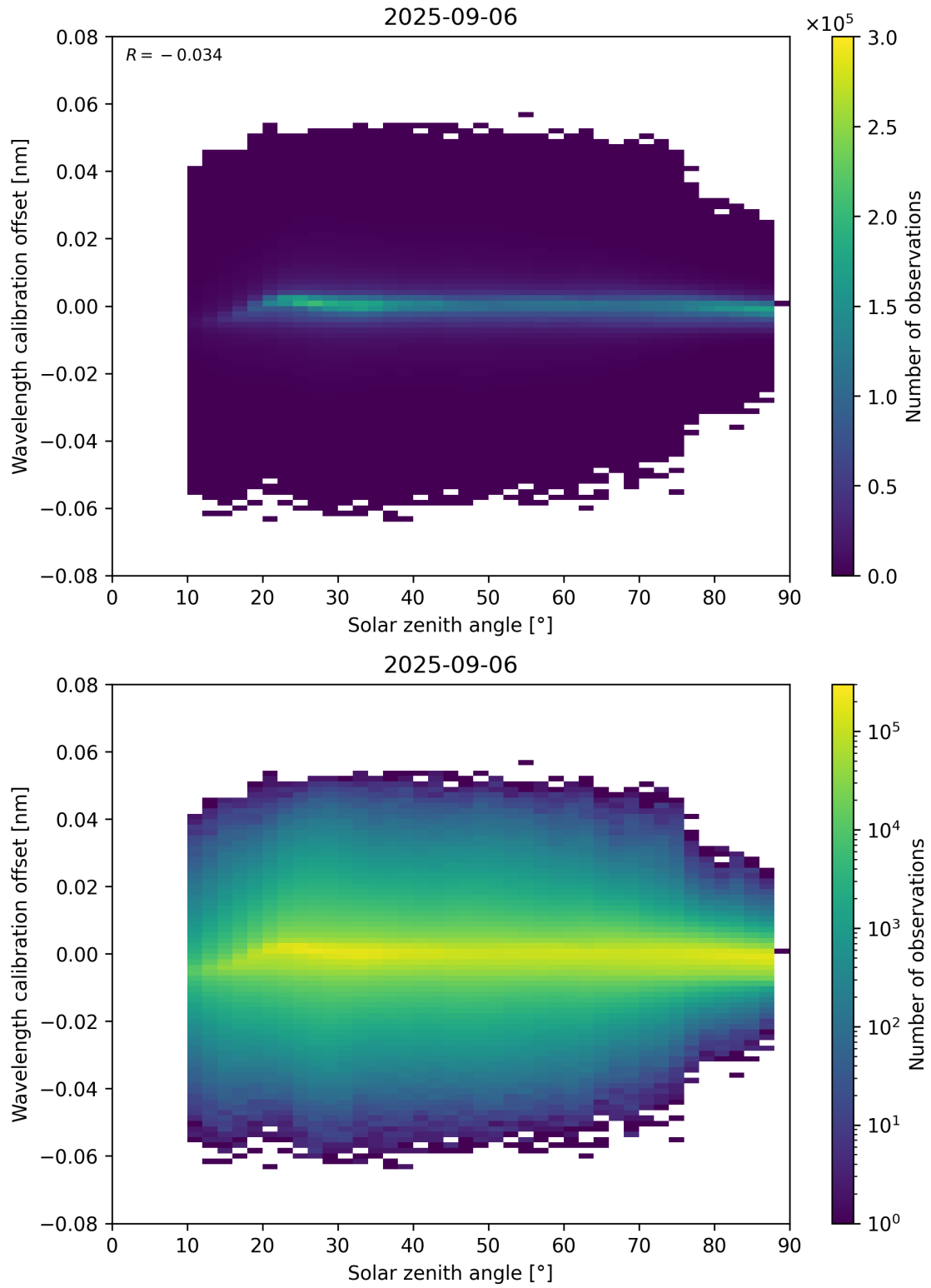
Figure 158: Scatter density plot of “Solar zenith angle” against “Wavelength calibration offset” for 2025-09-05 to 2025-09-07.
