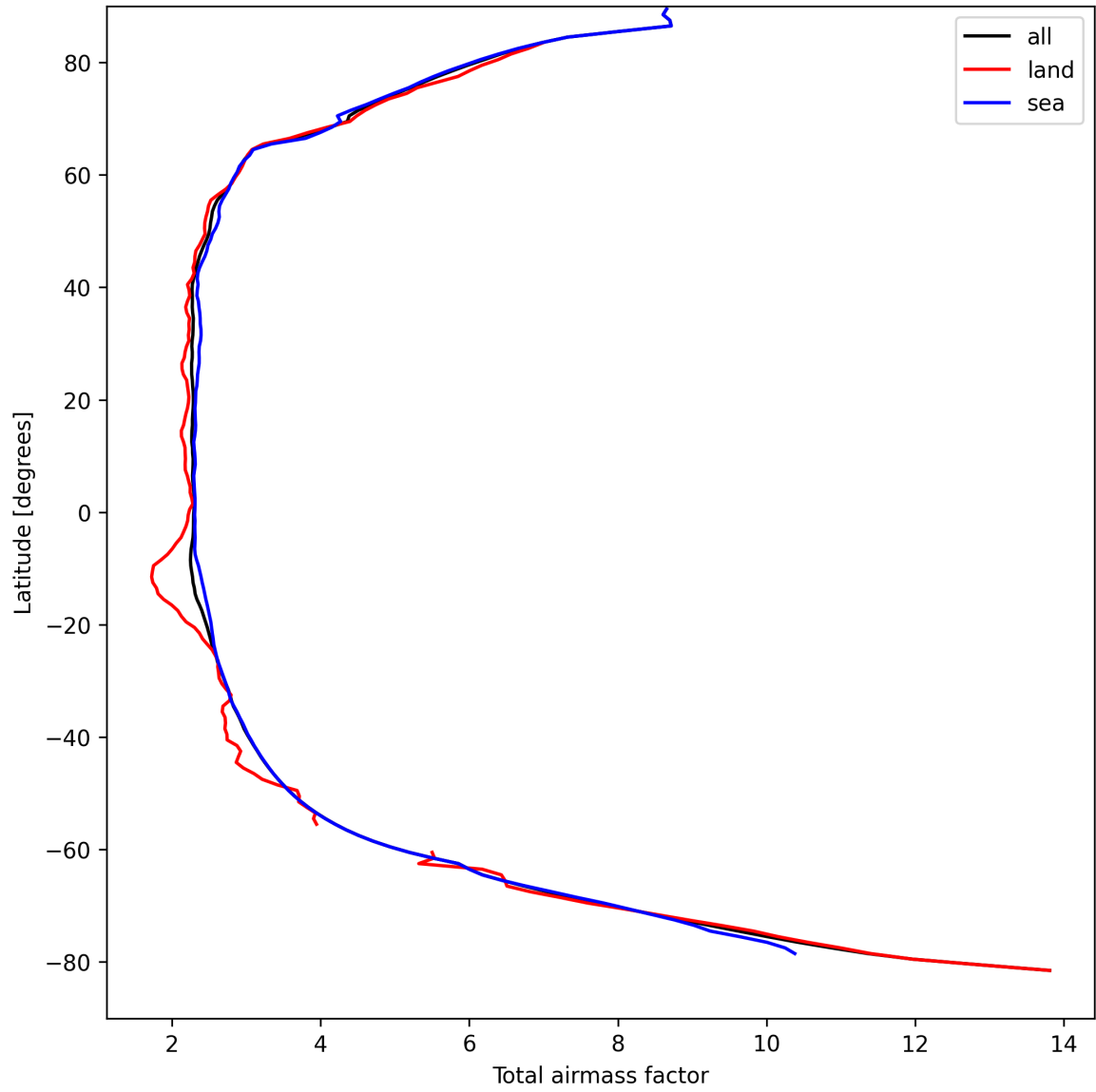
Figure 15: Zonal average of “Total airmass factor” for 2025-09-05 to 2025-09-07.
