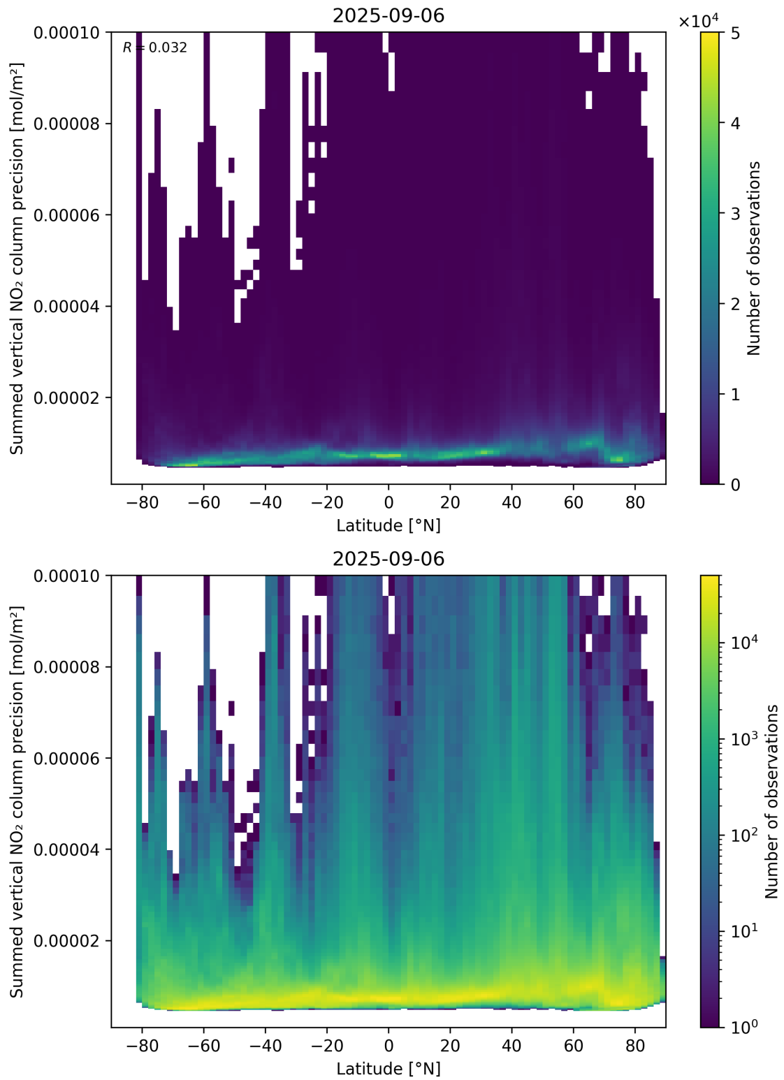
Figure 89: Scatter density plot of “Latitude” against “Summed vertical NO 2 column precision” for 2025-09-05 to 2025-09-07.
