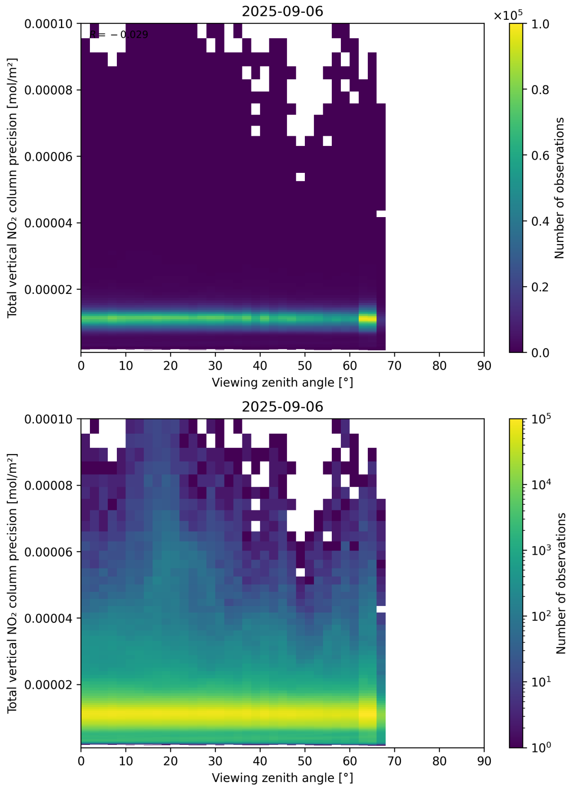
Figure 168: Scatter density plot of “Viewing zenith angle” against “Total vertical NO 2 column precision” for 2025-09-05 to 2025-09-07.
