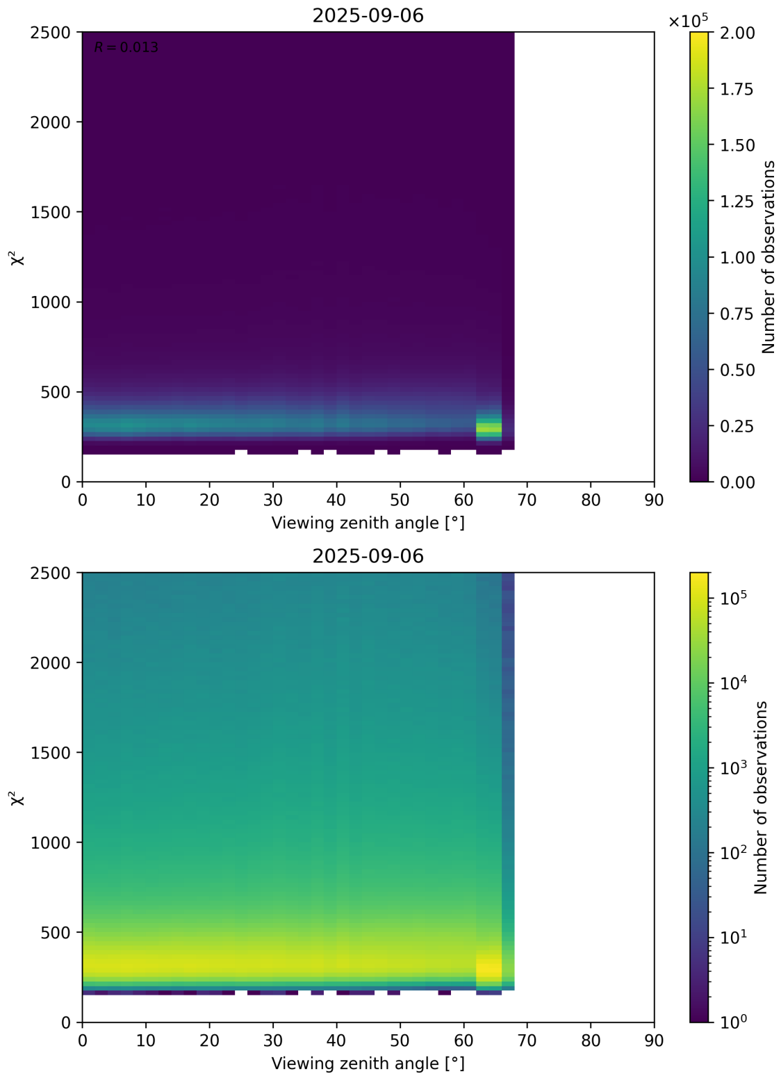
Figure 162: Scatter density plot of “Viewing zenith angle” against “ \chi^2 ” for 2025-09-05 to 2025-09-07.
