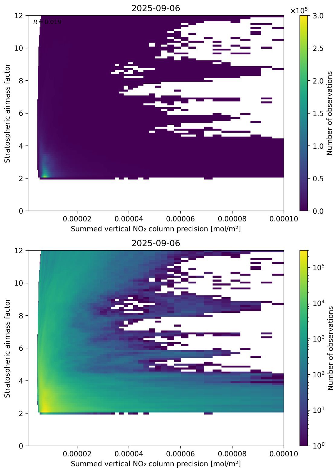
Figure 106: Scatter density plot of “Summed vertical NO 2 column precision” against “Stratospheric airmass factor” for 2025-09-05 to 2025-09-07.
