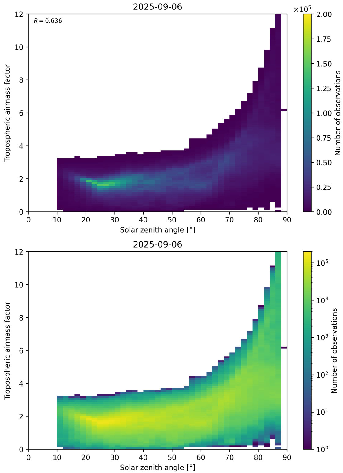
Figure 147: Scatter density plot of “Solar zenith angle” against “Tropospheric airmass factor” for 2025-09-05 to 2025-09-07.
