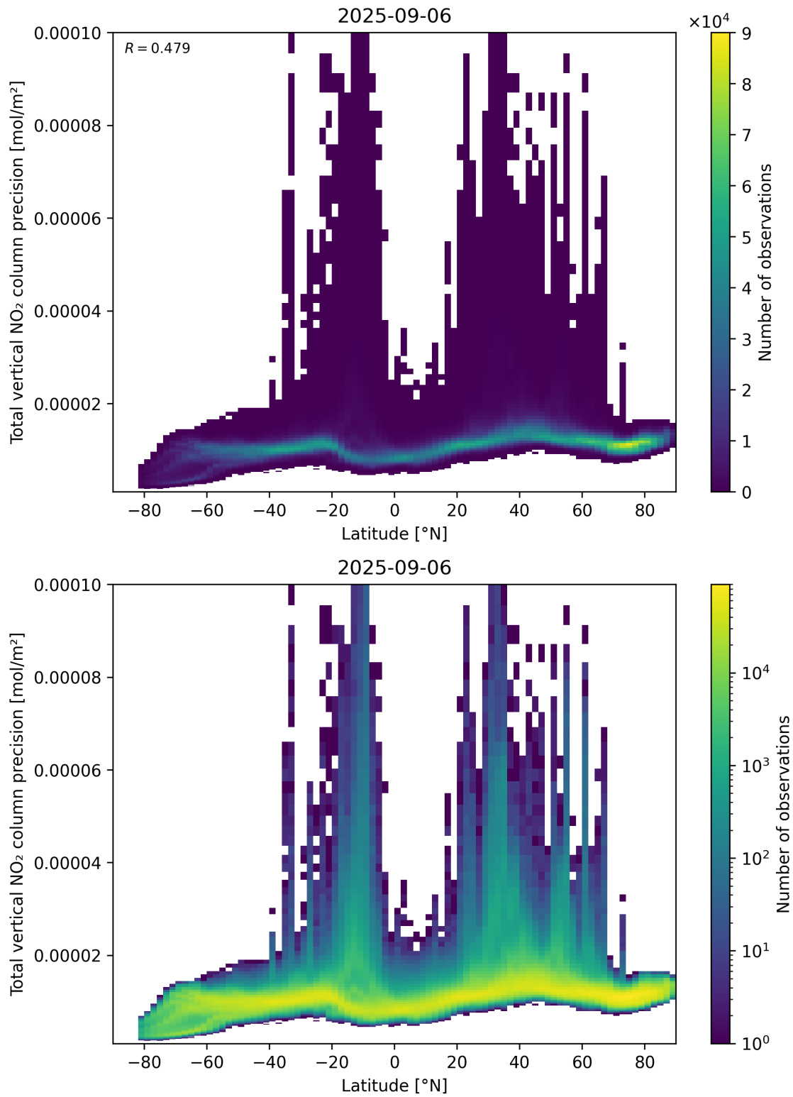
Figure 91: Scatter density plot of “Latitude” against “Total vertical NO 2 column precision” for 2025-09-05 to 2025-09-07.
