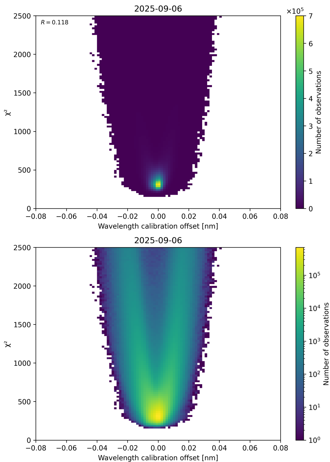
Figure 175: Scatter density plot of “Wavelength calibration offset” against “ \chi^2 ” for 2025-09-05 to 2025-09-07.
