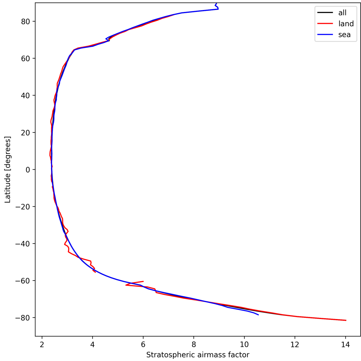
Figure 27: Zonal average of “Stratospheric air mass factor” for 2025-09-05 to 2025-09-07.
