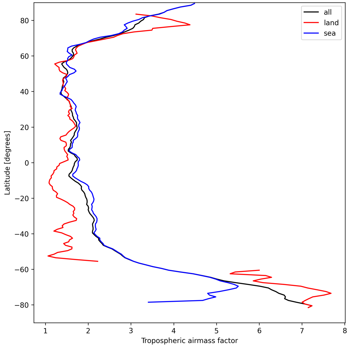
Figure 14: Zonal average of “Tropospheric airmass factor” for 2025-09-05 to 2025-09-07.
