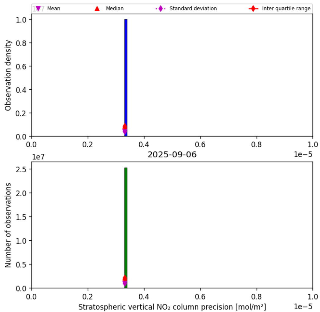
Figure 37: Histogram of “Stratospheric vertical NO 2 column precision” for 2025-09-05 to 2025-09-07
