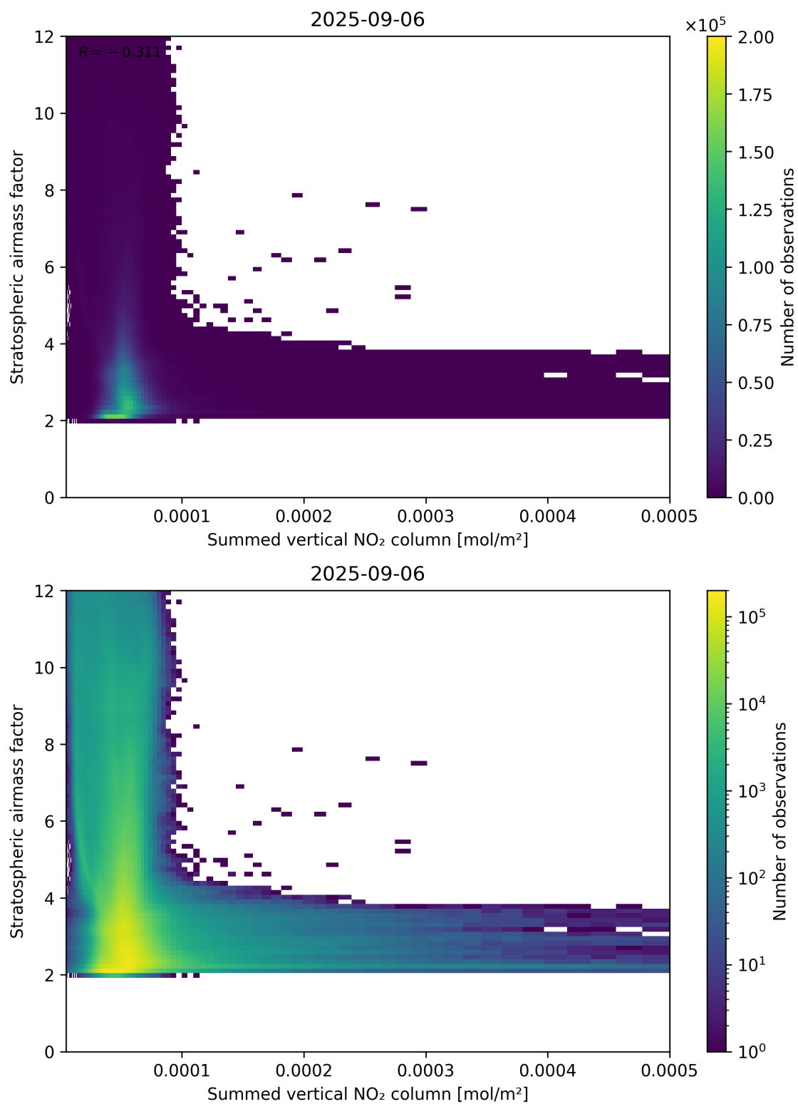
Figure 103: Scatter density plot of “Summed vertical NO 2 column” against “Stratospheric air mass factor” for 2025-09-05 to 2025-09-07.
