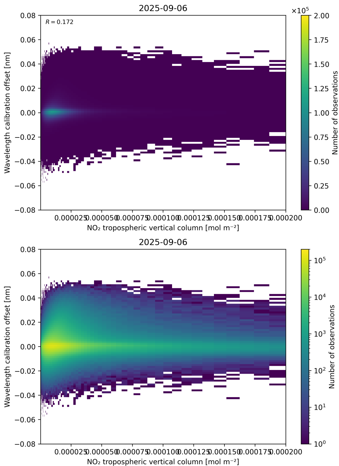
Figure 143: Scatter density plot of “NO 2 tropospheric vertical column” against “Wavelength calibration offset” for 2025-09-05 to 2025-09-07.
