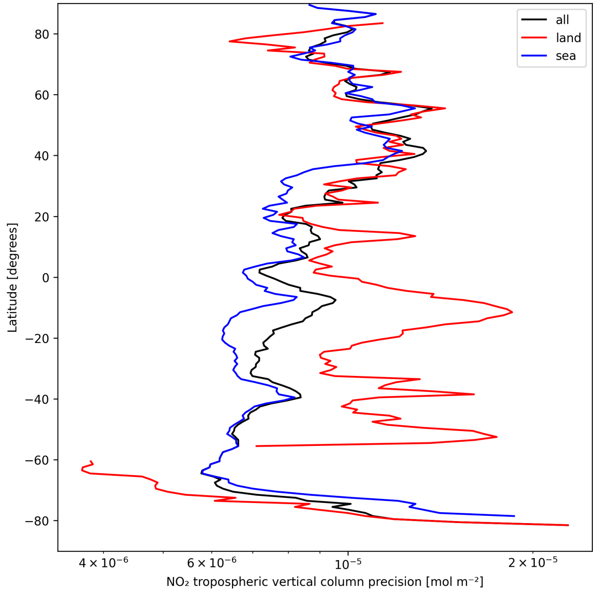
Figure 13: Zonal average of “NO 2 tropospheric vertical column precision” for 2025-09-05 to 2025-09-07.
