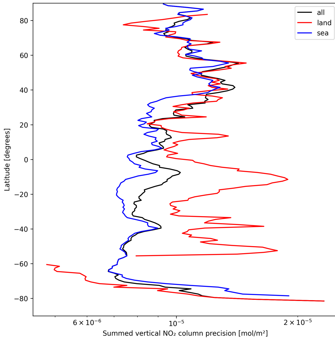
Figure 24: Zonal average of “Summed vertical NO 2 column precision” for 2025-09-05 to 2025-09-07.
