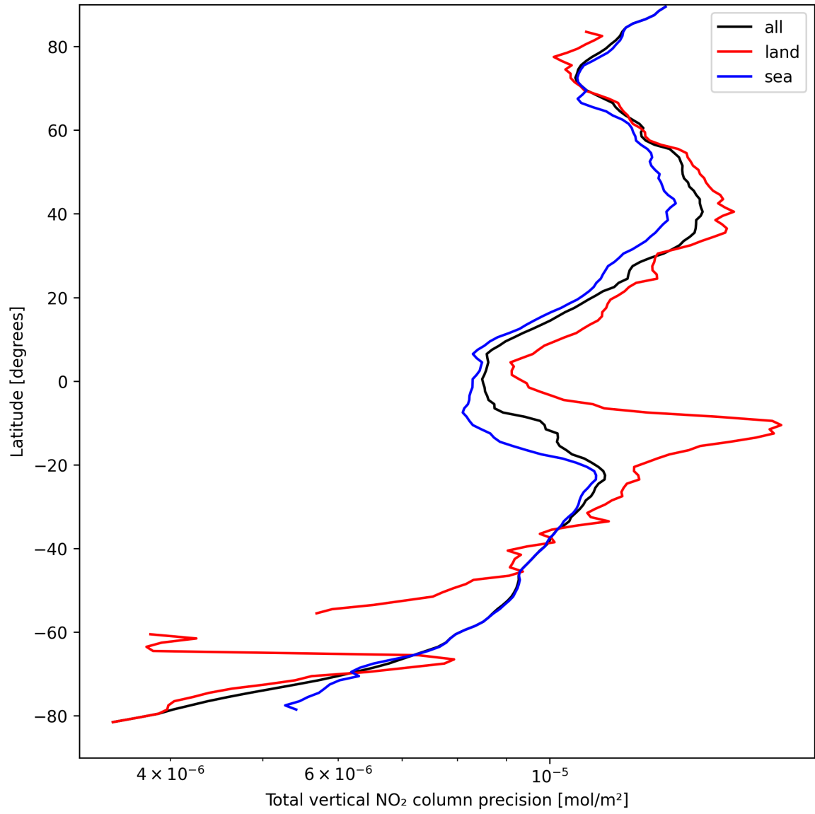
Figure 22: Zonal average of “Total vertical NO 2 column precision” for 2025-09-05 to 2025-09-07.
