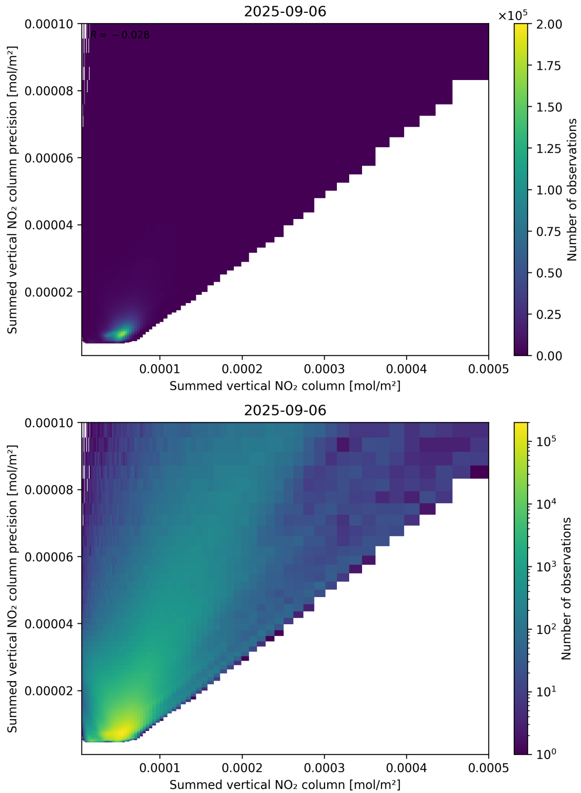
Figure 105: Scatter density plot of “Summed vertical NO 2 column” against “Summed vertical NO 2 column precision” for 2025-09-05 to 2025-09-07.
