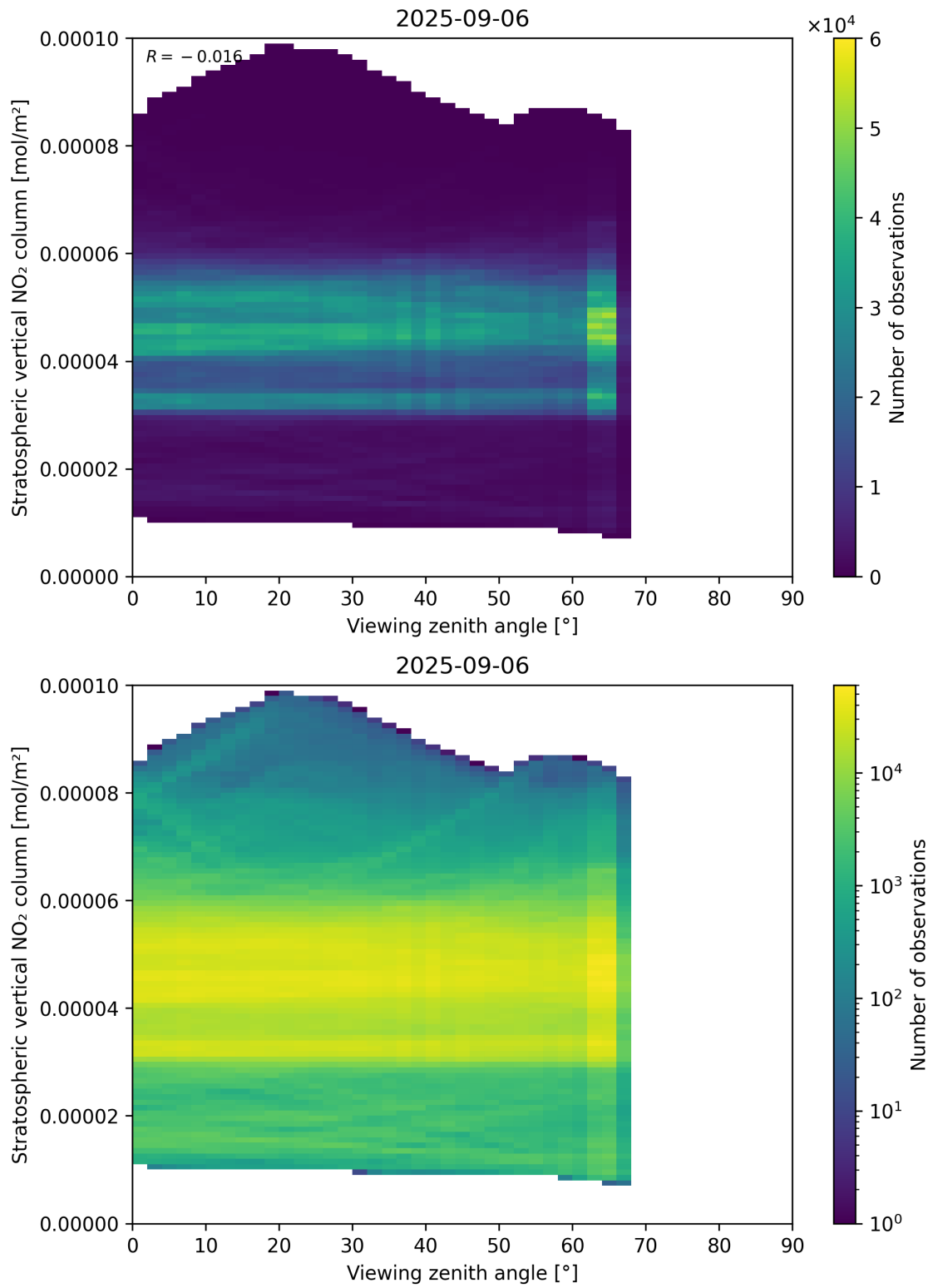
Figure 164: Scatter density plot of “Viewing zenith angle” against “Stratospheric vertical NO 2 column” for 2025-09-05 to 2025-09-07.
