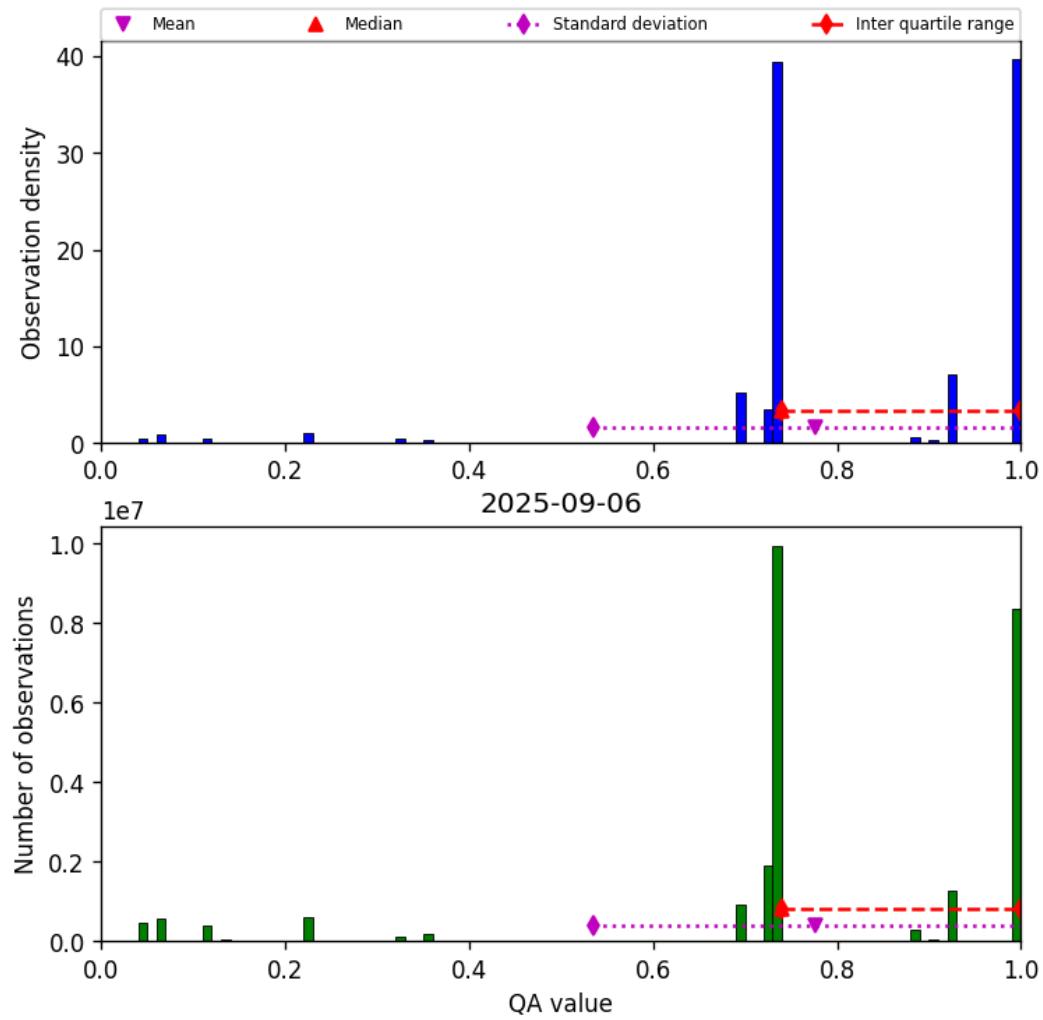
Figure 28: Histogram of “QA value” for 2025-09-05 to 2025-09-07
