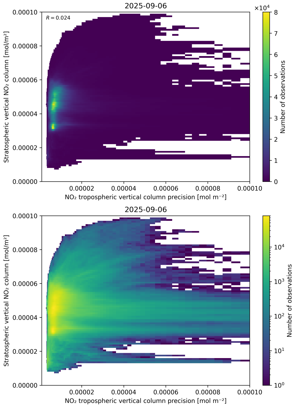
Figure 135: Scatter density plot of “NO 2 tropospheric vertical column precision” against “Stratospheric vertical NO 2 column” for 2025-09-05 to 2025-09-07.
