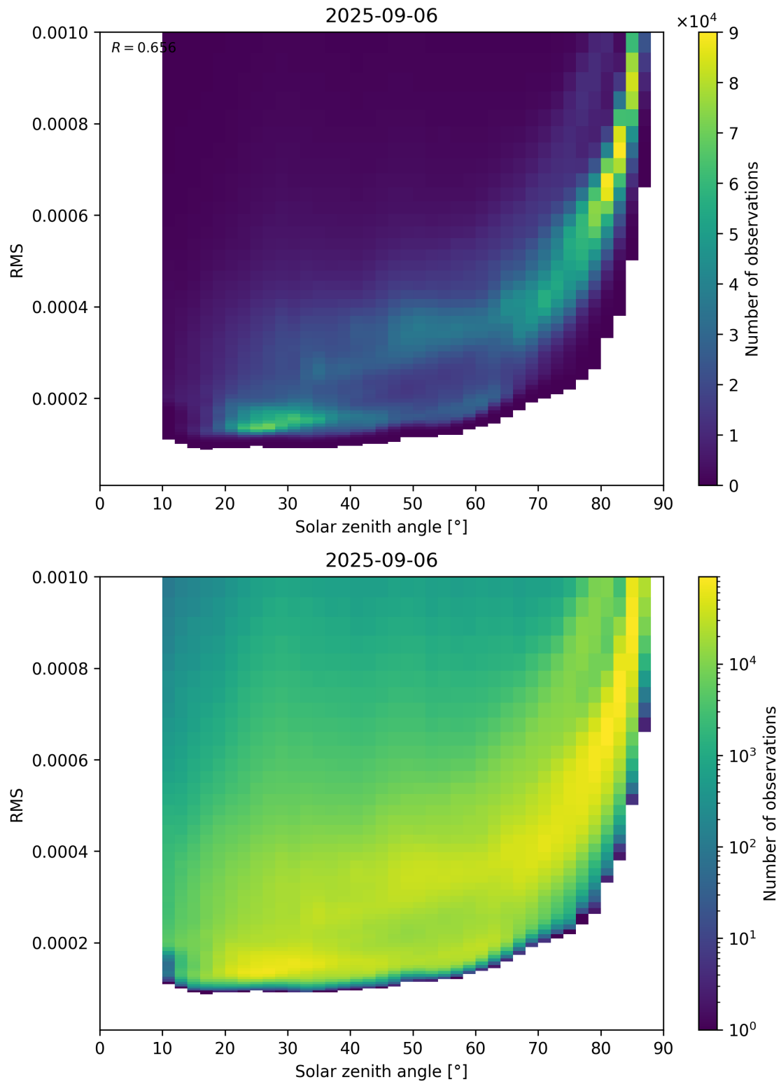
Figure 157: Scatter density plot of “Solar zenith angle” against “RMS” for 2025-09-05 to 2025-09-07.
