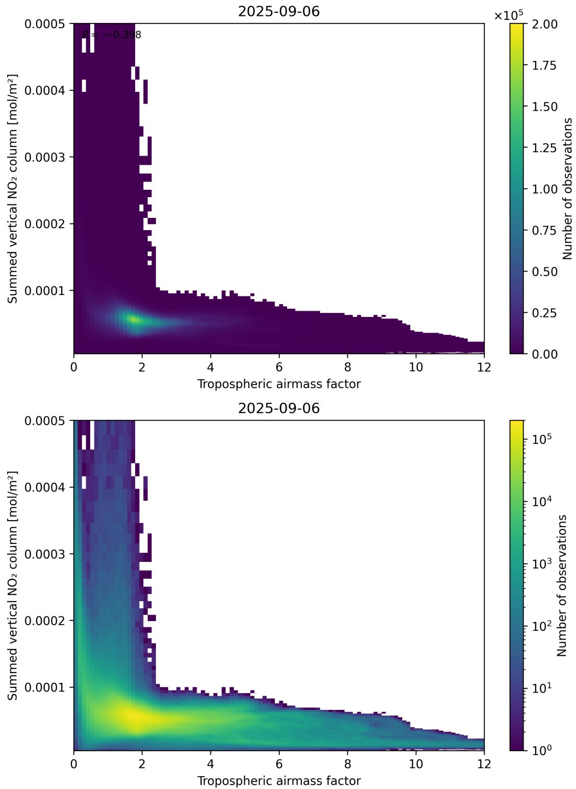
Figure 75: Scatter density plot of “Tropospheric airmass factor” against “Summed vertical NO 2 column” for 2025-09-05 to 2025-09-07.
