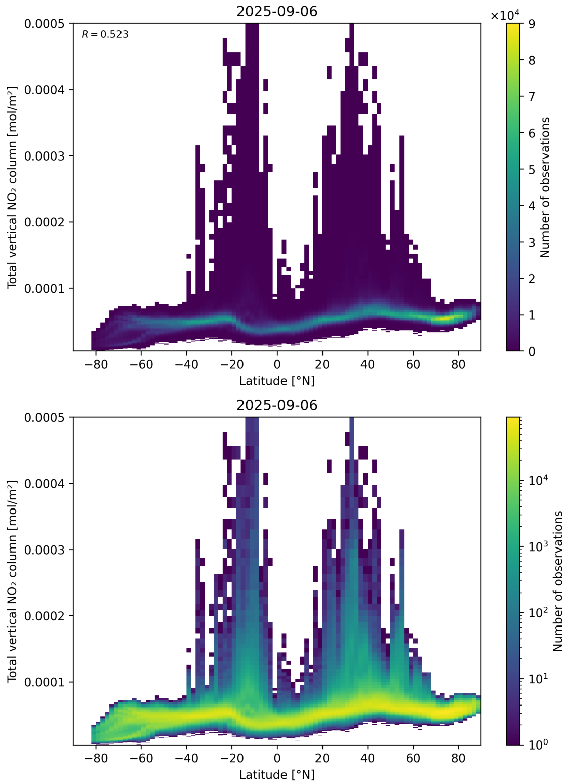
Figure 90: Scatter density plot of “Latitude” against “Total vertical NO 2 column” for 2025-09-05 to 2025-09-07.
