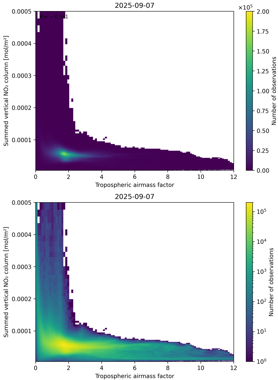
Figure 75: Scatter density plot of “Tropospheric air mass factor” against “Summed vertical NO 2 column” for 2025-09-06 to 2025-09-08.
