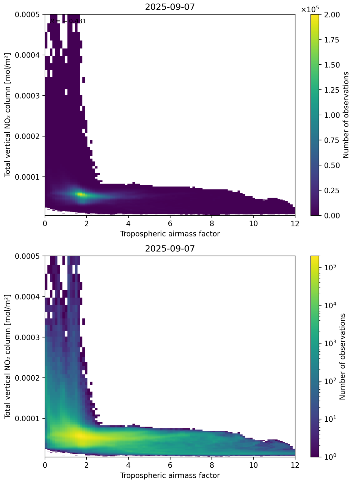
Figure 77: Scatter density plot of “Tropospheric airmass factor” against “Total vertical NO 2 column” for 2025-09-06 to 2025-09-08.
