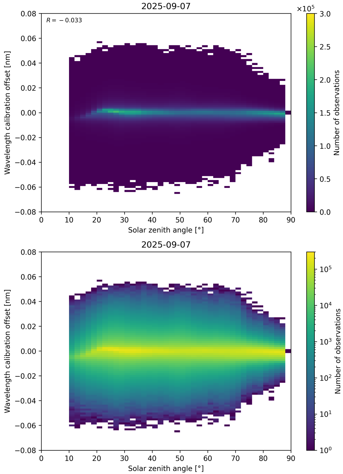
Figure 158: Scatter density plot of “Solar zenith angle” against “Wavelength calibration offset” for 2025-09-06 to 2025-09-08.
