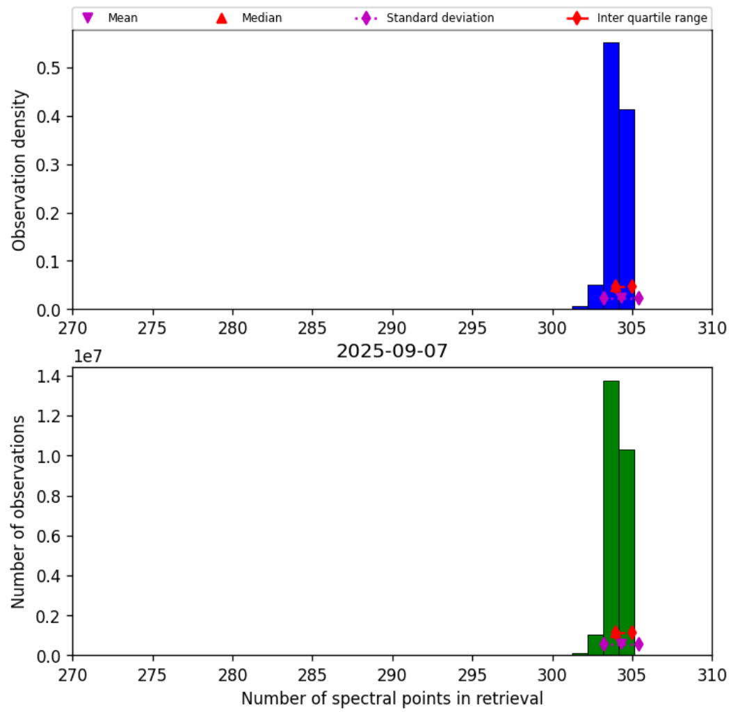
Figure 33: Histogram of “Number of spectral points in retrieval” for 2025-09-06 to 2025-09-08
