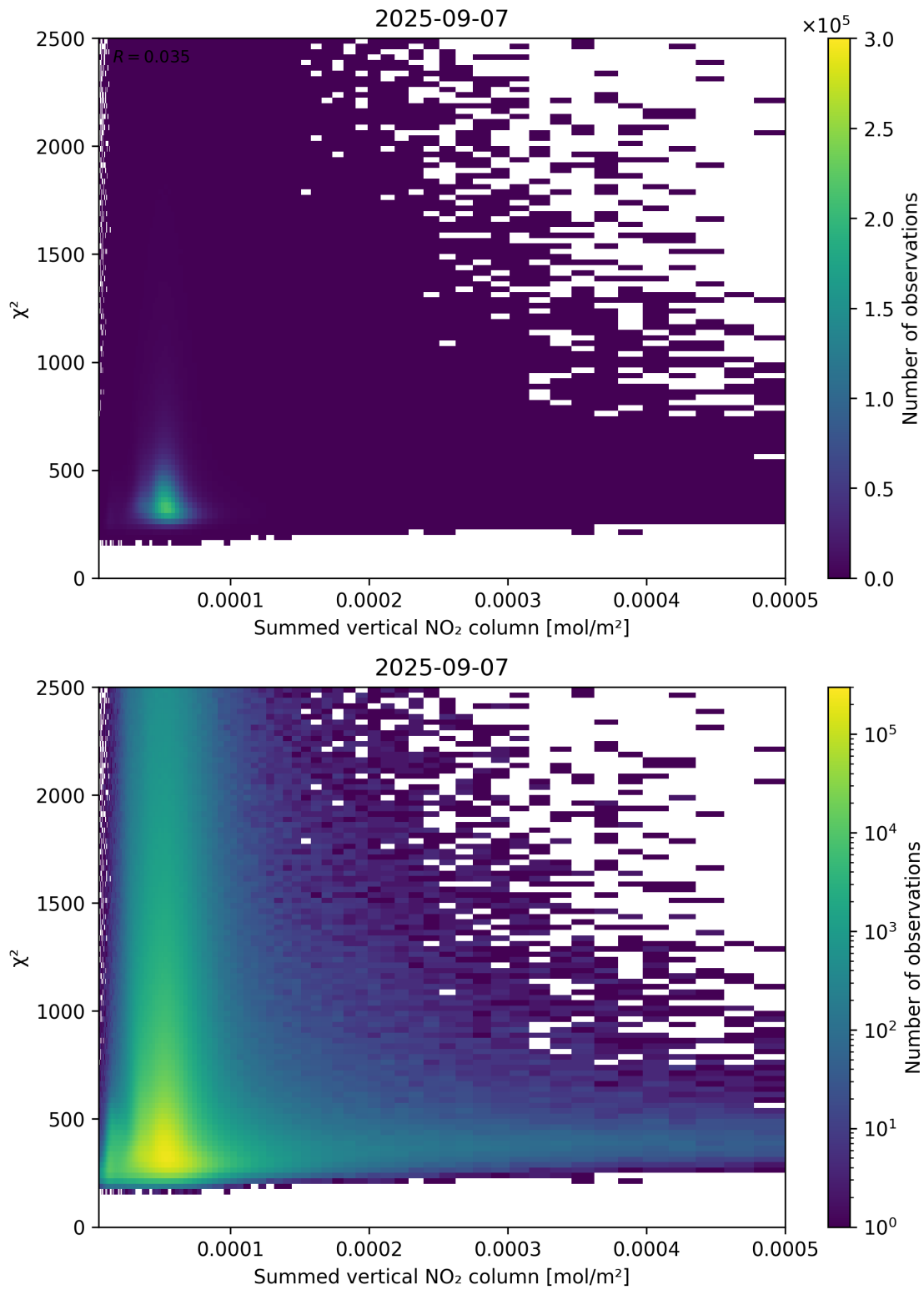
Figure 104: Scatter density plot of “Summed vertical NO 2 column” against “ \chi^2 ” for 2025-09-06 to 2025-09-08.
