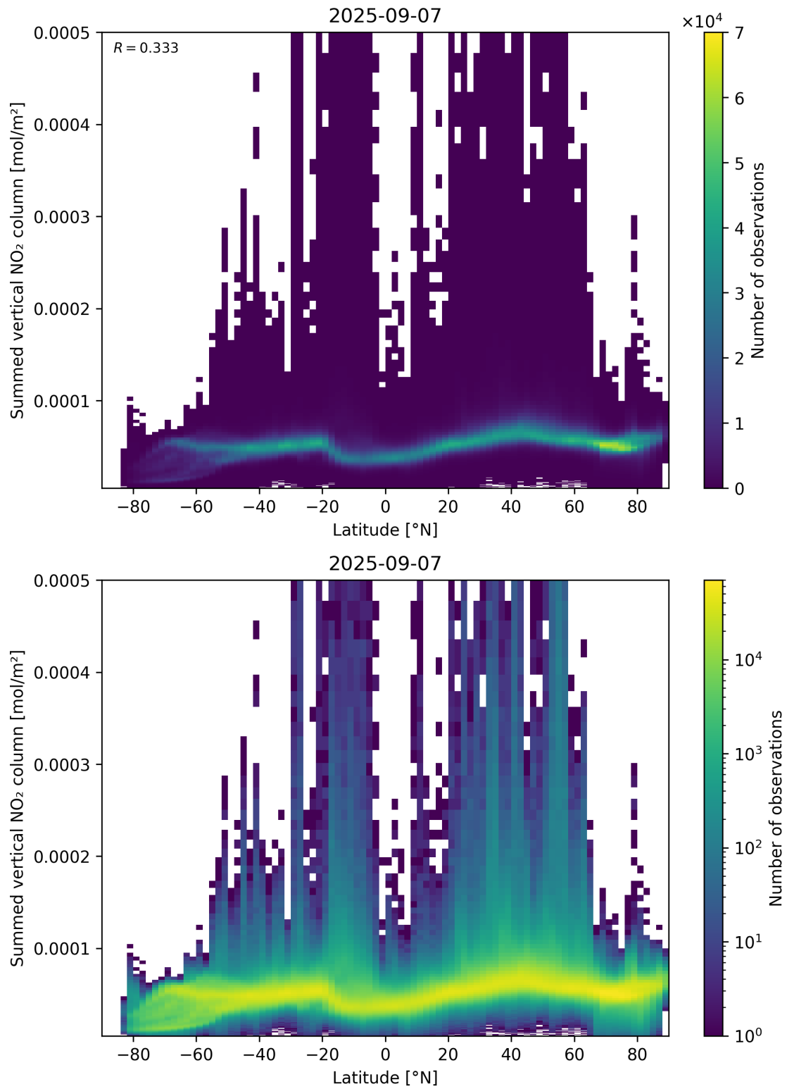
Figure 88: Scatter density plot of “Latitude” against “Summed vertical NO 2 column” for 2025-09-06 to 2025-09-08.
