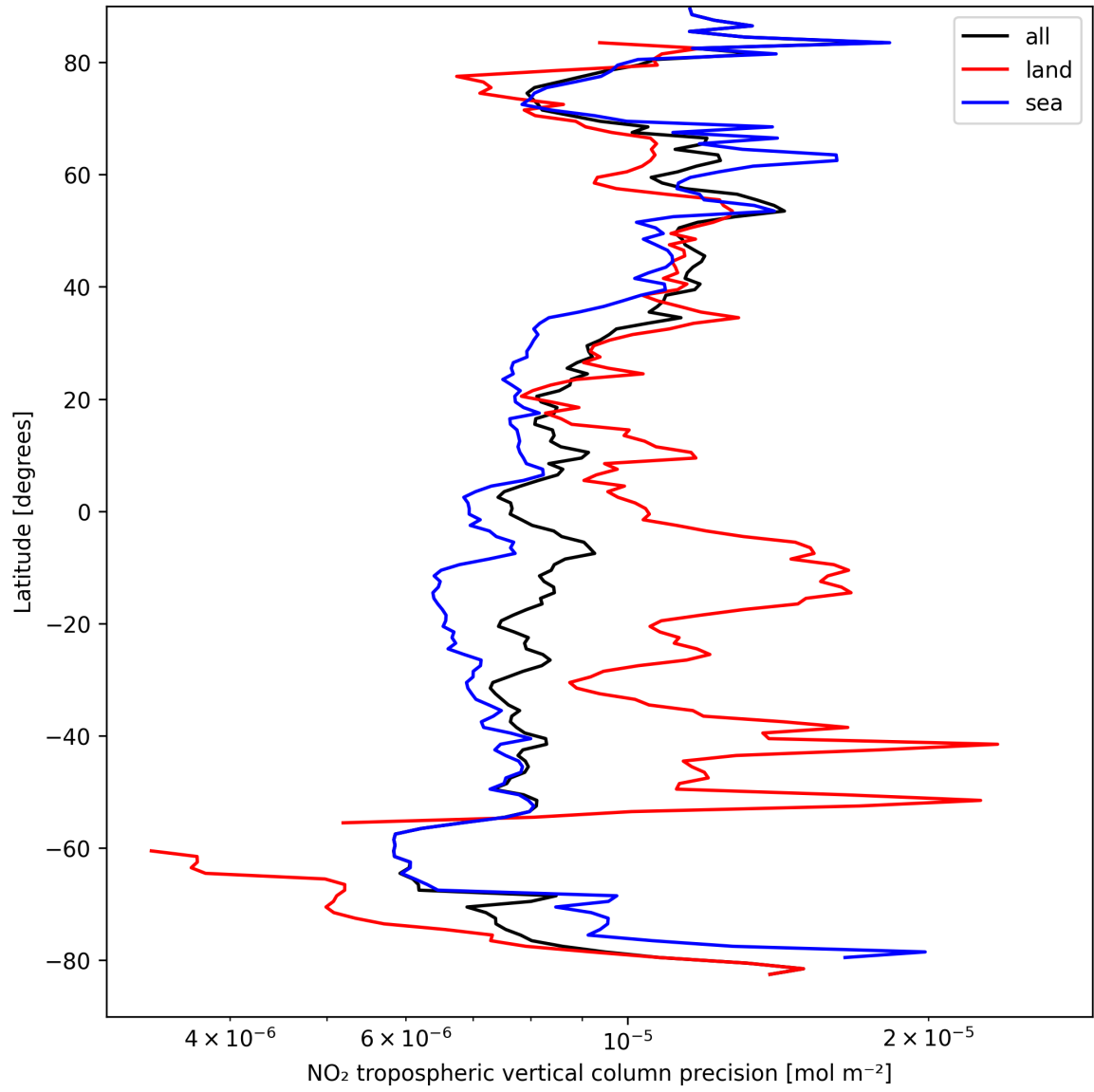
Figure 13: Zonal average of “NO 2 tropospheric vertical column precision” for 2025-09-06 to 2025-09-08.
