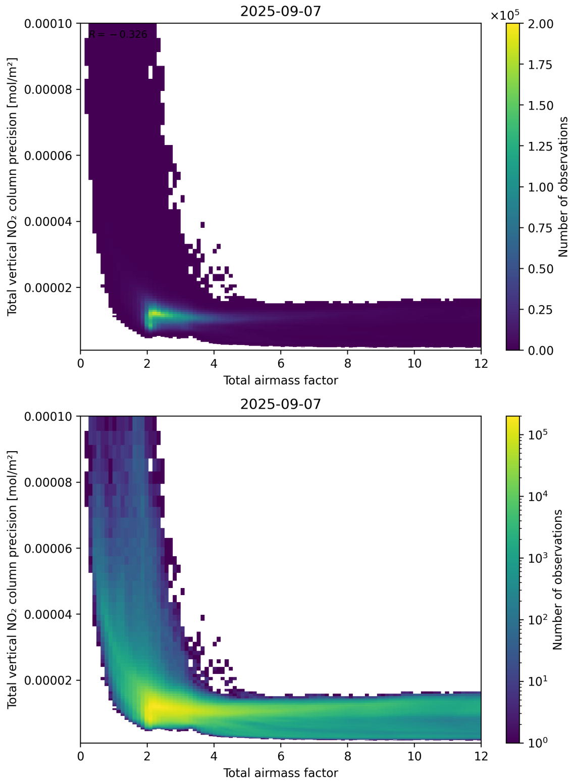
Figure 68: Scatter density plot of “Total airmass factor” against “Total vertical NO 2 column precision” for 2025-09-06 to 2025-09-08.
