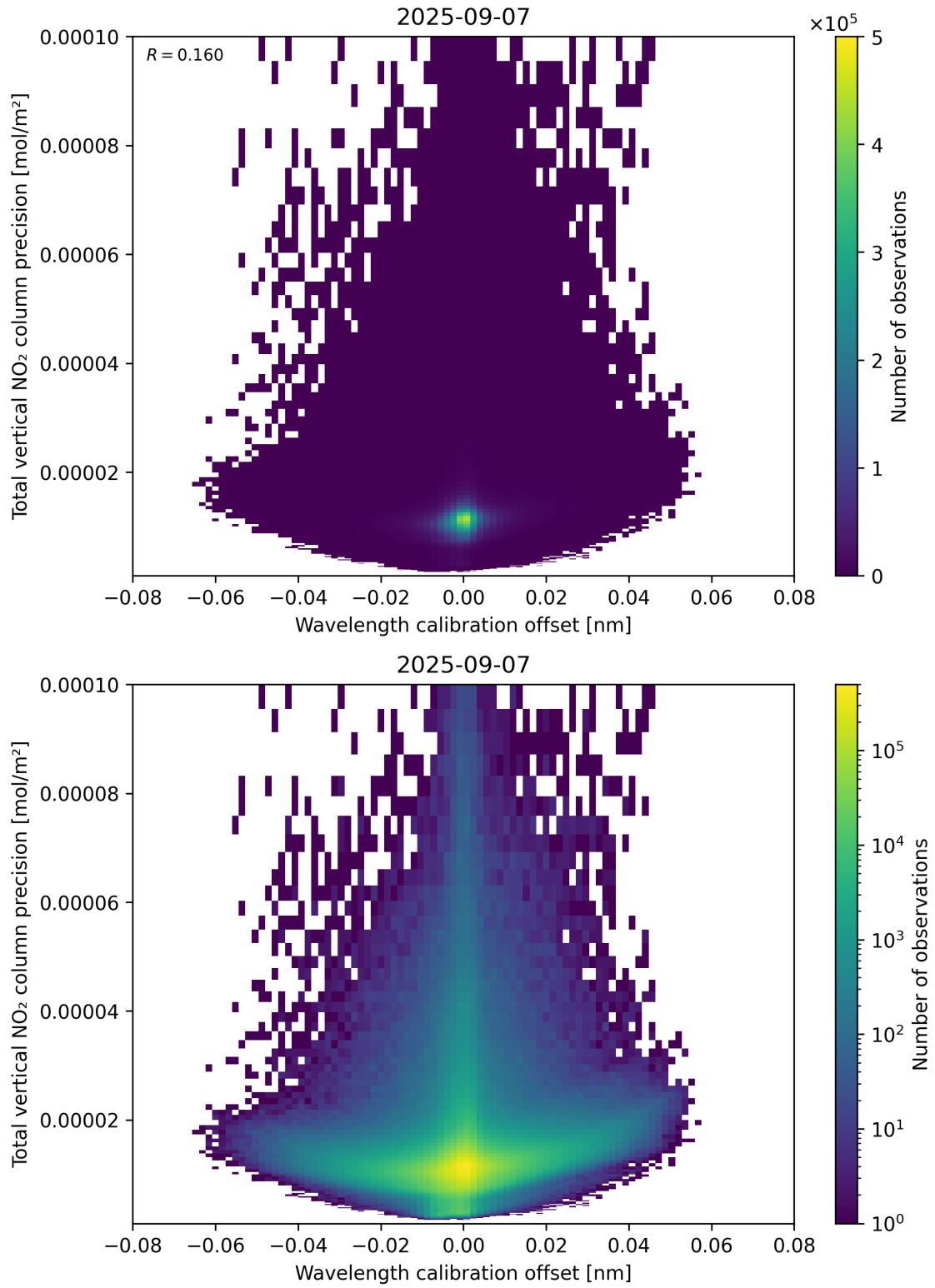
Figure 180: Scatter density plot of “Wavelength calibration offset” against “Total vertical NO 2 column precision” for 2025-09-06 to 2025-09-08.
