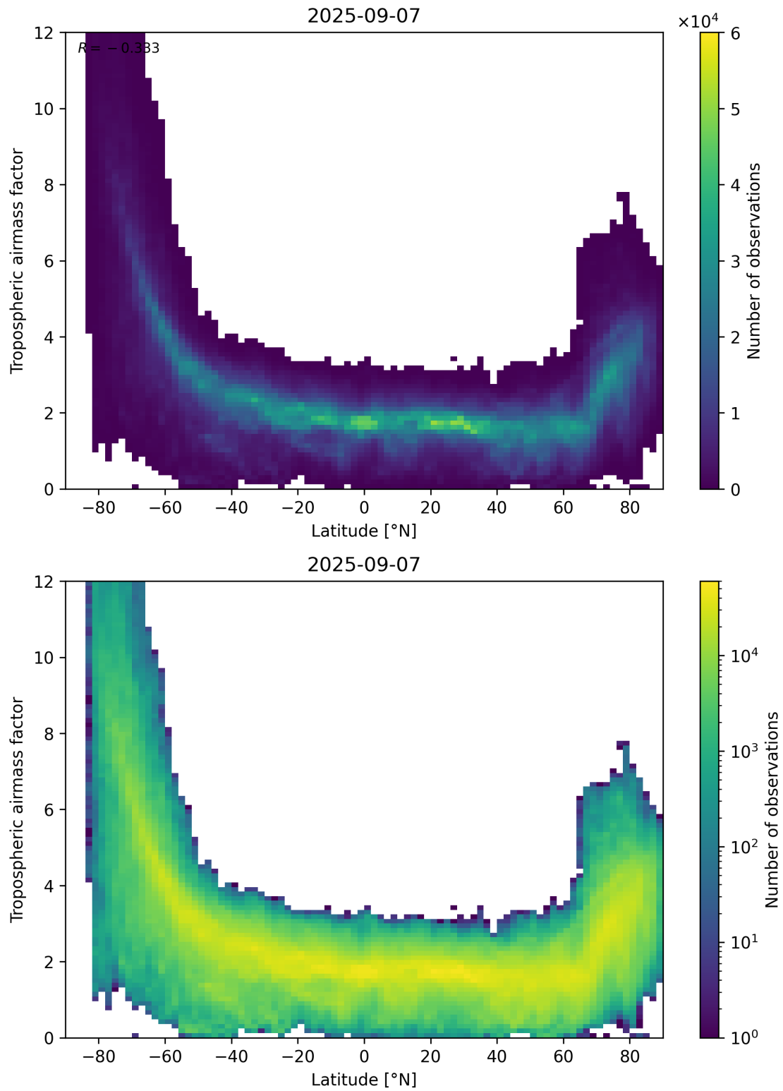
Figure 85: Scatter density plot of “Latitude” against “Tropospheric airmass factor” for 2025-09-06 to 2025-09-08.
