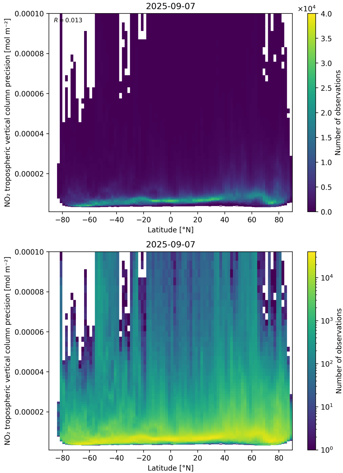
Figure 93: Scatter density plot of “Latitude” against “NO 2 tropospheric vertical column precision” for 2025-09-06 to 2025-09-08.
