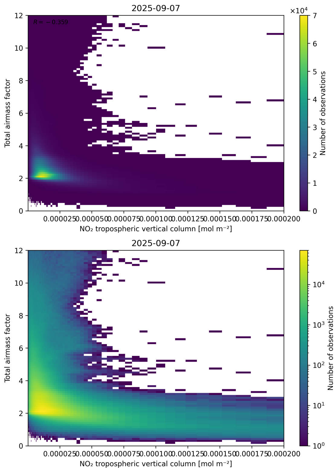
Figure 122: Scatter density plot of “NO 2 tropospheric vertical column” against “Total air mass factor” for 2025-09-06 to 2025-09-08.
