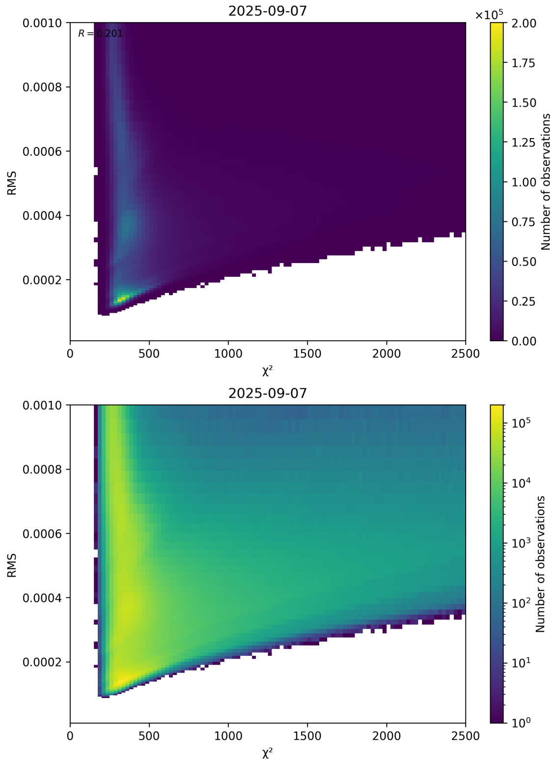
Figure 82: Scatter density plot of “ \chi^2 ” against “RMS” for 2025-09-06 to 2025-09-08.
