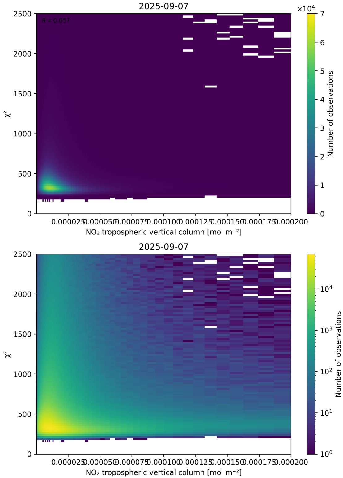
Figure 124: Scatter density plot of “NO 2 tropospheric vertical column” against “ \chi^2 ” for 2025-09-06 to 2025-09-08.
