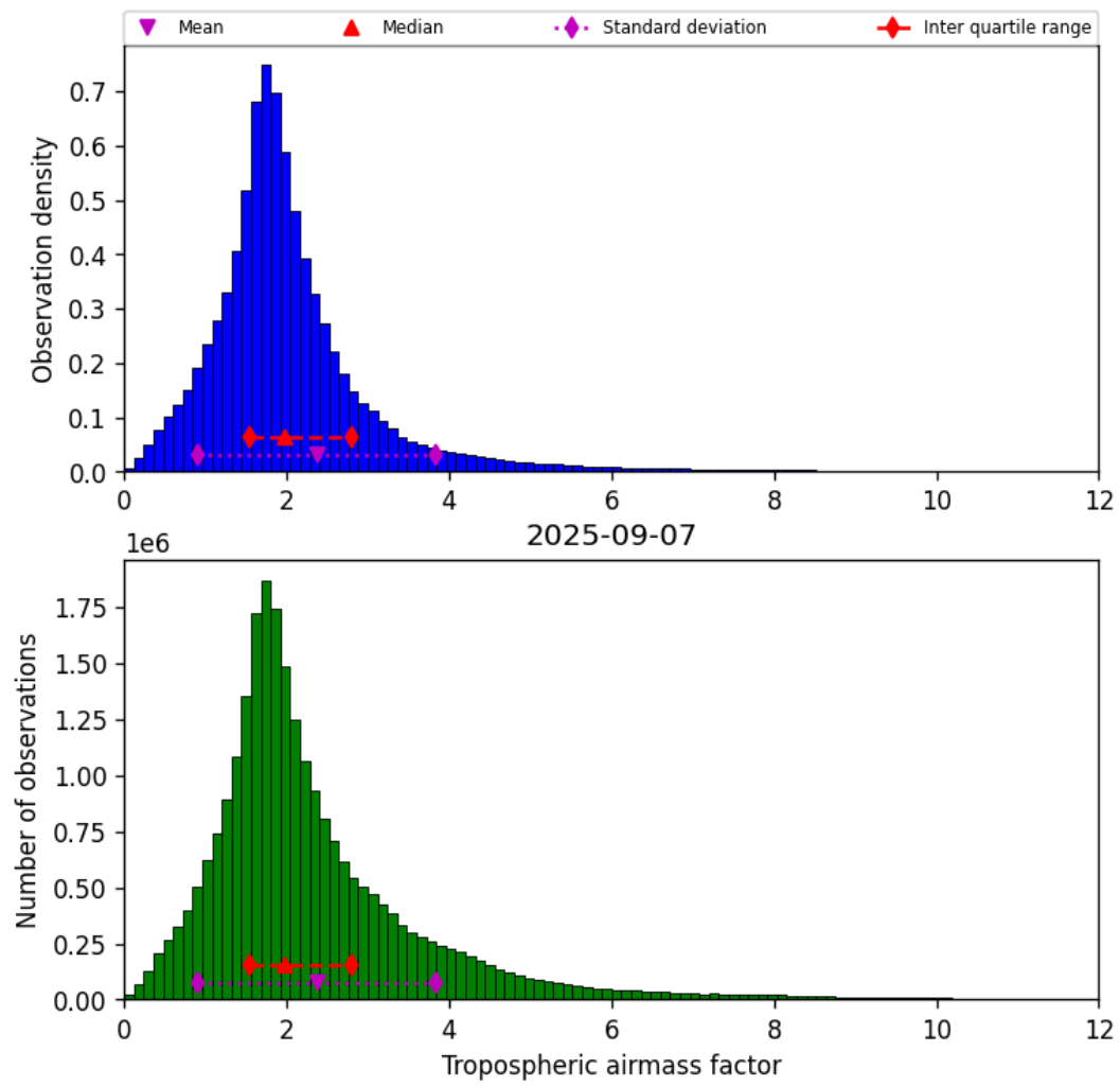
Figure 31: Histogram of “Tropospheric airmass factor” for 2025-09-06 to 2025-09-08
