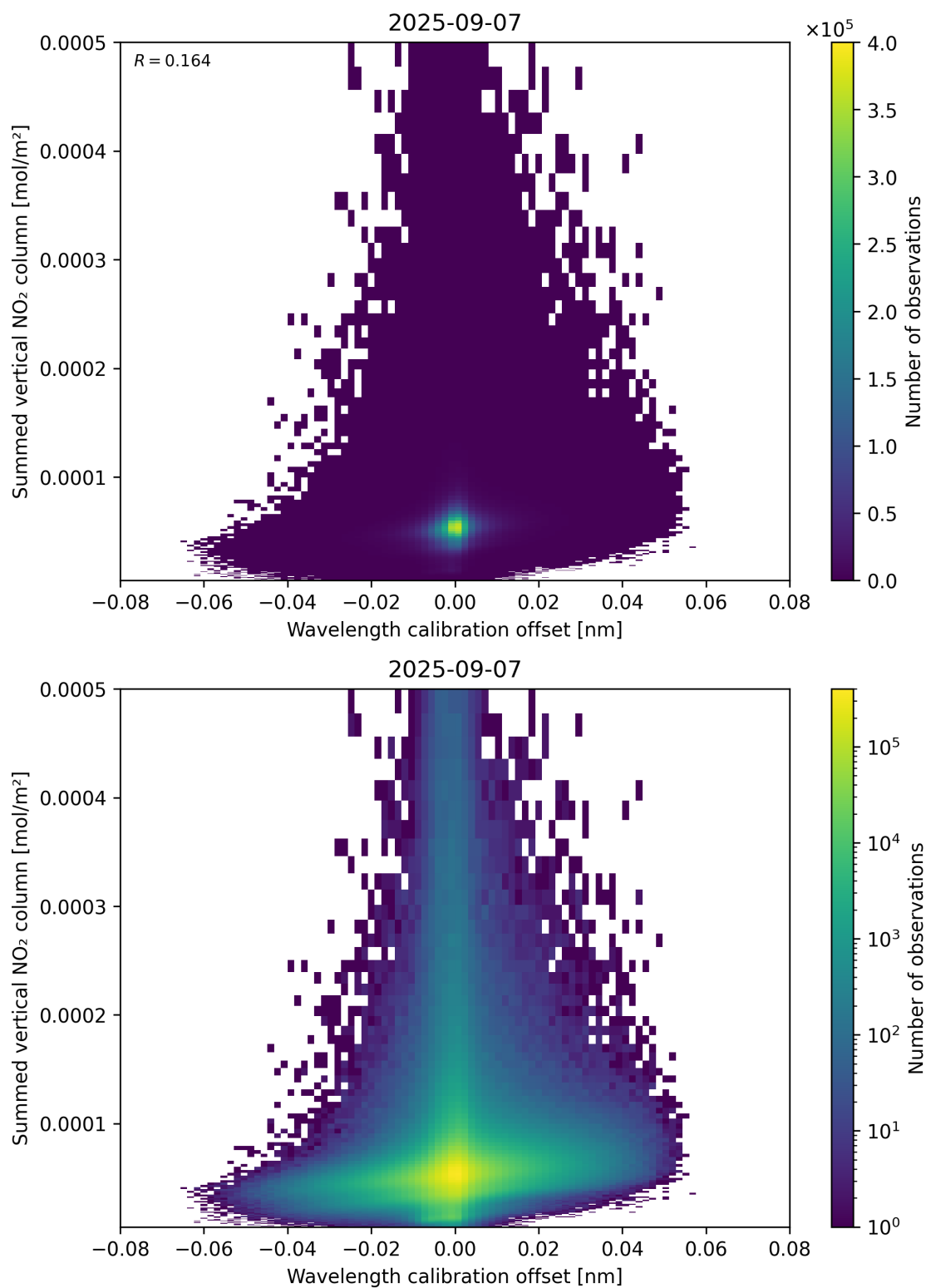
Figure 177: Scatter density plot of “Wavelength calibration offset” against “Summed vertical NO 2 column” for 2025-09-06 to 2025-09-08.
