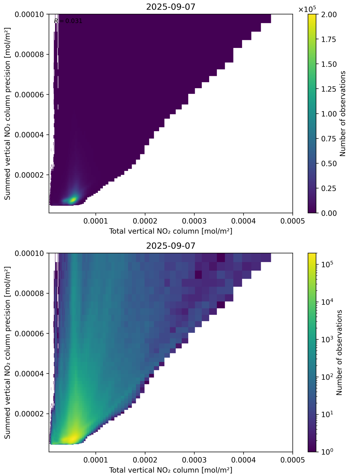
Figure 113: Scatter density plot of “Total vertical NO 2 column” against “Summed vertical NO 2 column precision” for 2025-09-06 to 2025-09-08.
