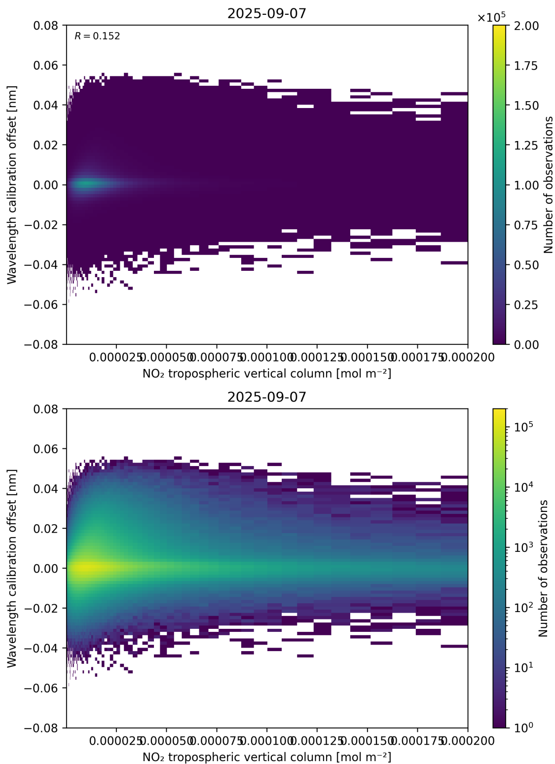
Figure 143: Scatter density plot of “NO 2 tropospheric vertical column” against “Wavelength calibration offset” for 2025-09-06 to 2025-09-08.
