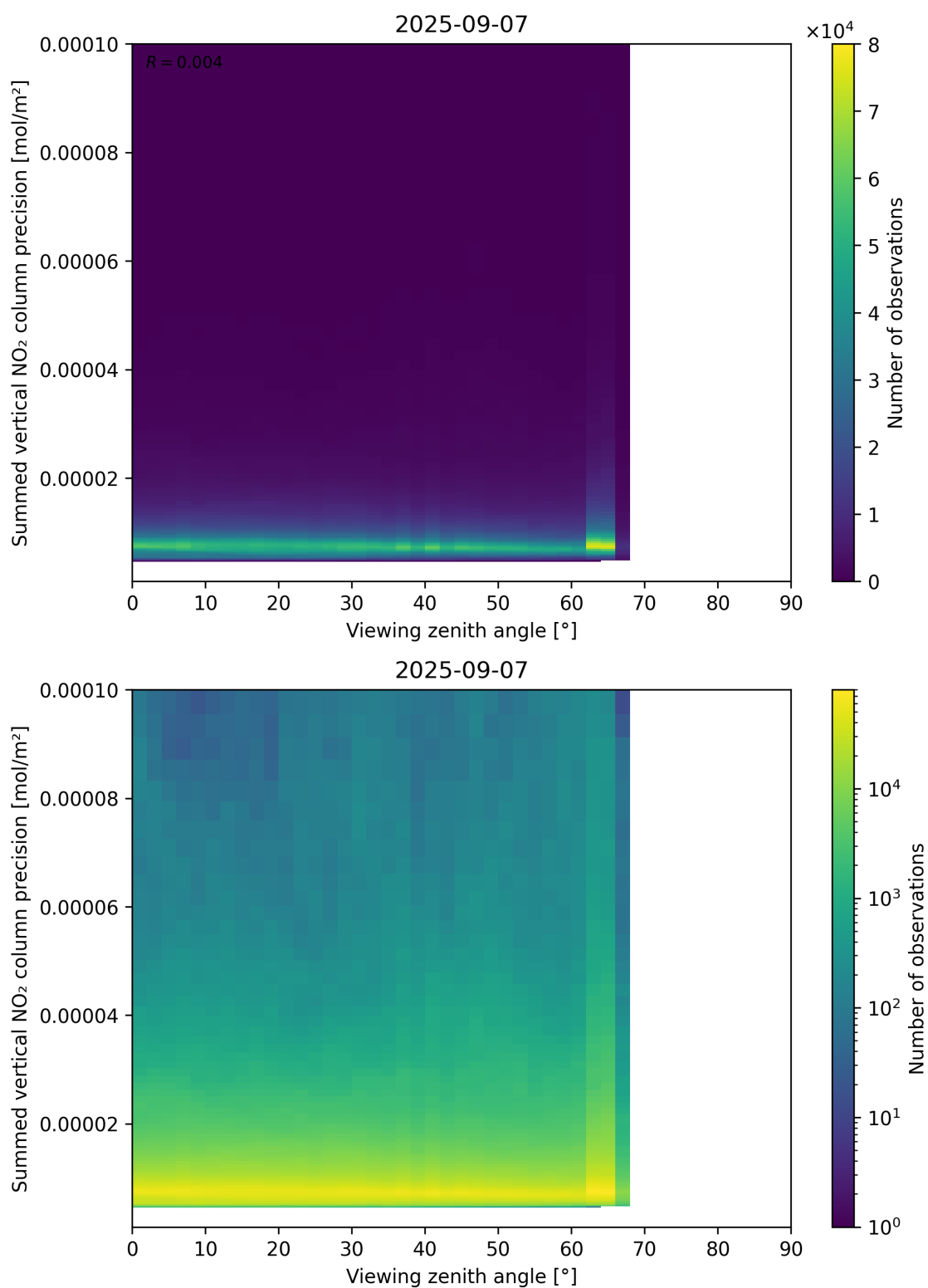
Figure 166: Scatter density plot of “Viewing zenith angle” against “Summed vertical NO 2 column precision” for 2025-09-06 to 2025-09-08.
