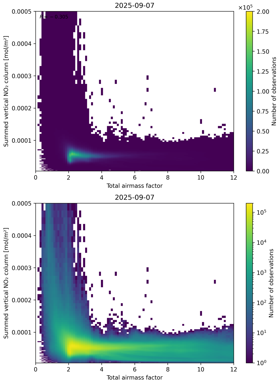
Figure 65: Scatter density plot of “Total airmass factor” against “Summed vertical NO 2 column” for 2025-09-06 to 2025-09-08.
