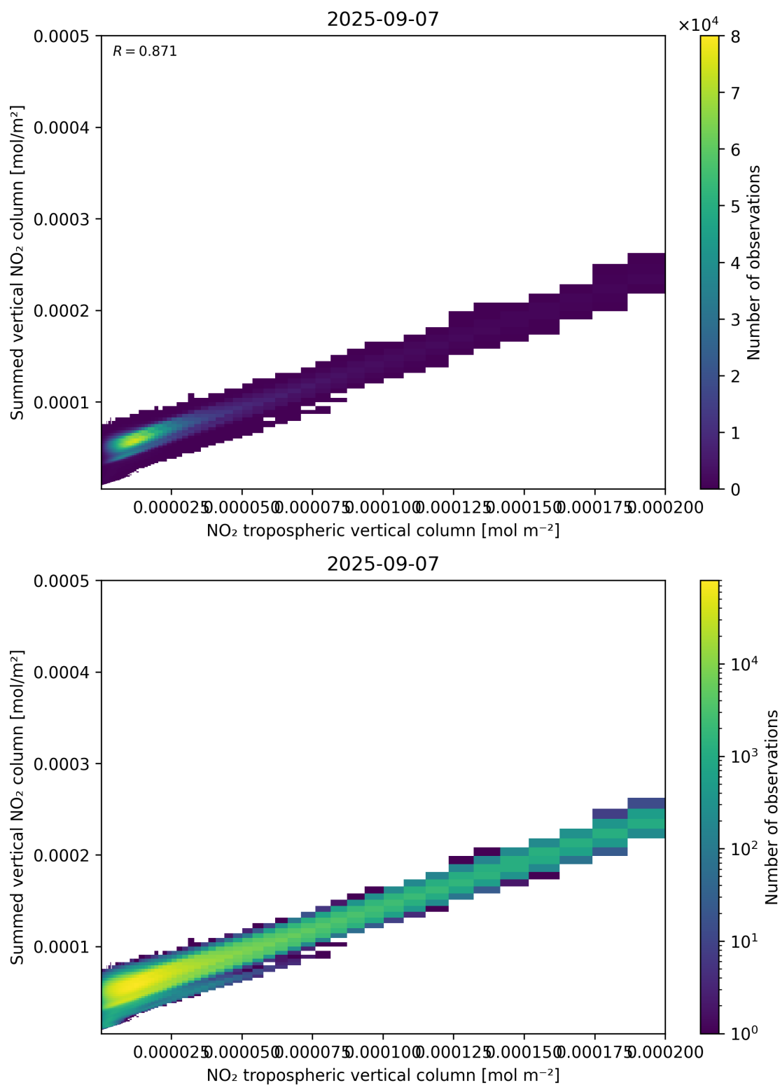
Figure 126: Scatter density plot of “NO 2 tropospheric vertical column” against “Summed vertical NO 2 column” for 2025-09-06 to 2025-09-08.
