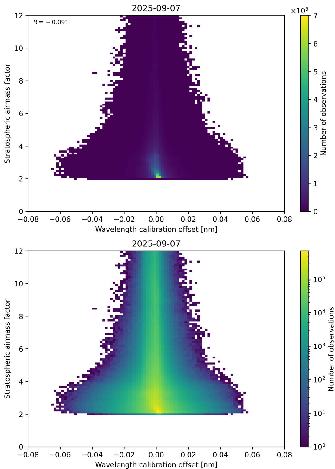
Figure 174: Scatter density plot of “Wavelength calibration offset” against “Stratospheric air mass factor” for 2025-09-06 to 2025-09-08.
