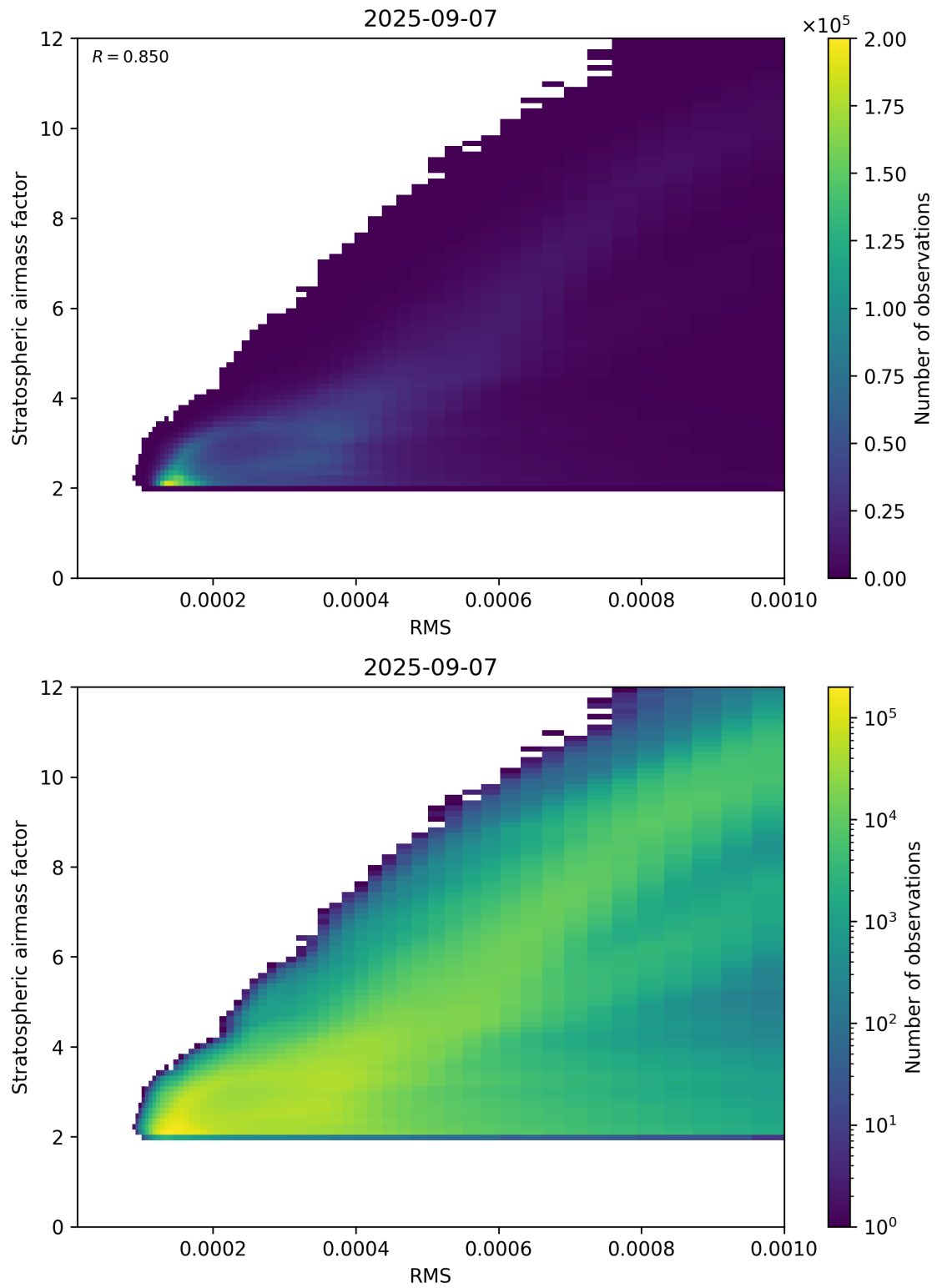
Figure 144: Scatter density plot of “RMS” against “Stratospheric airmass factor” for 2025-09-06 to 2025-09-08.
