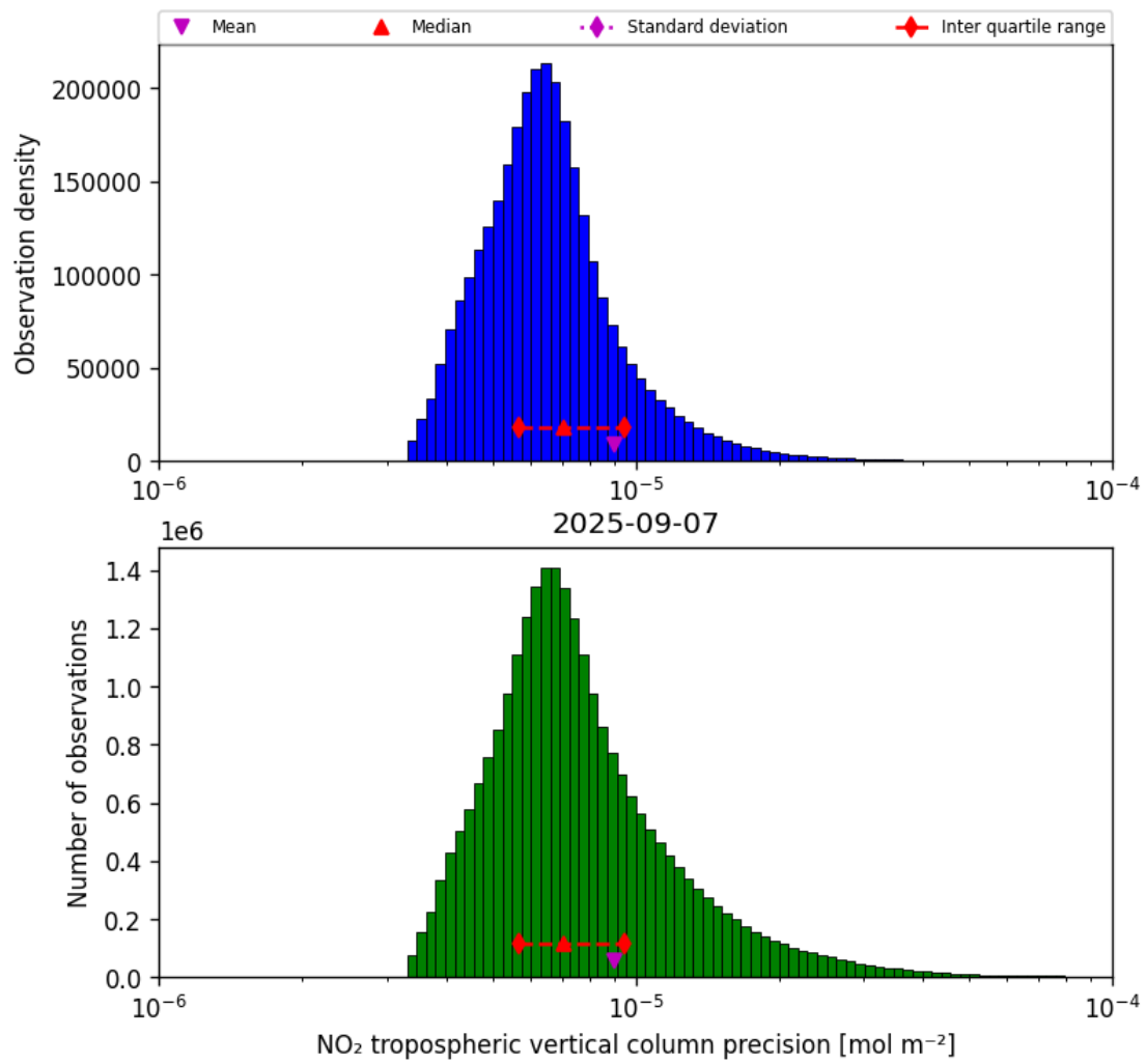
Figure 30: Histogram of “NO 2 tropospheric vertical column precision” for 2025-09-06 to 2025-09-08
