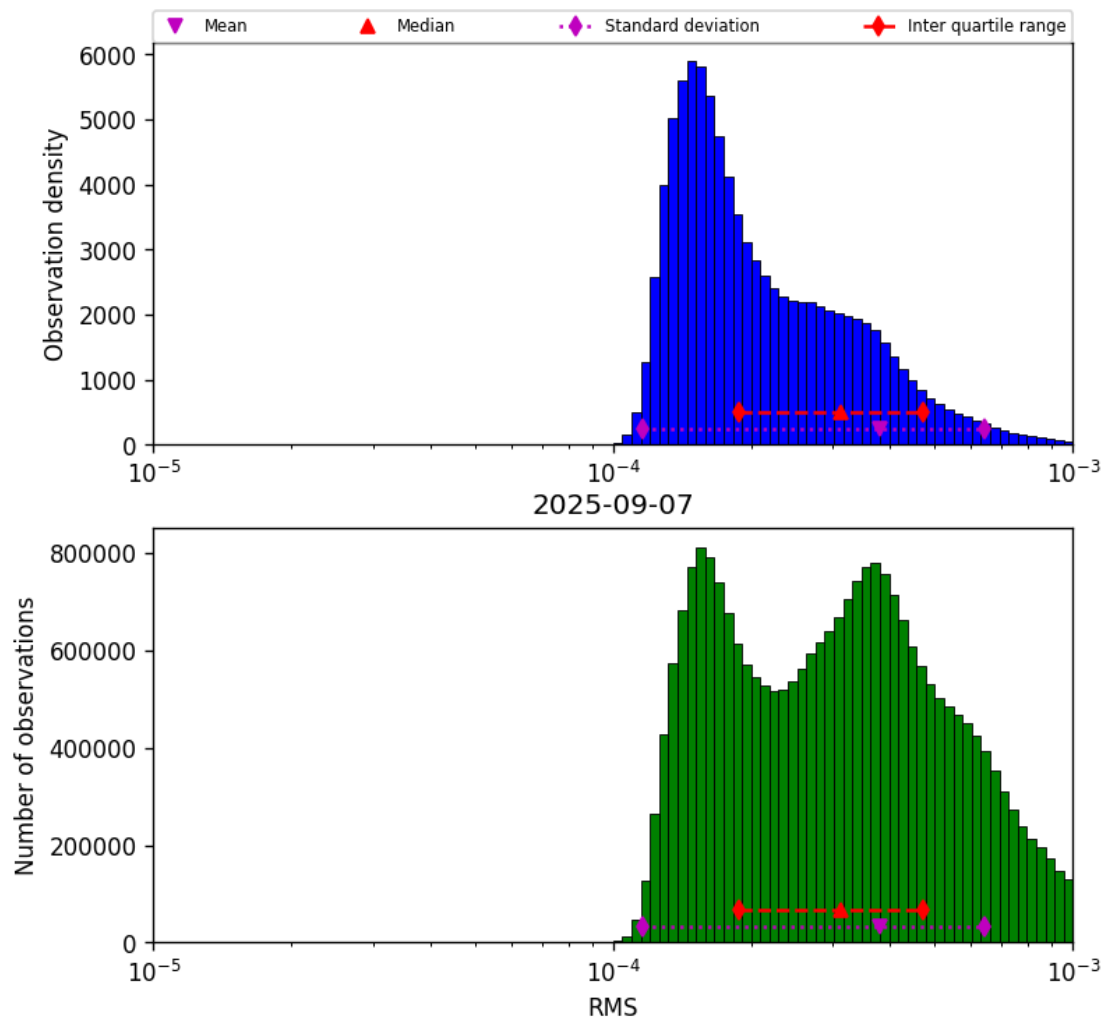
Figure 43: Histogram of “RMS” for 2025-09-06 to 2025-09-08
