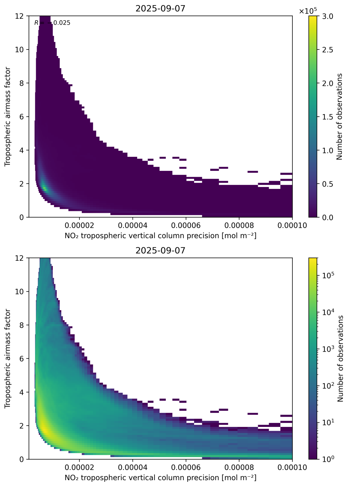
Figure 133: Scatter density plot of “NO 2 tropospheric vertical column precision” against “Tropospheric airmass factor” for 2025-09-06 to 2025-09-08.
