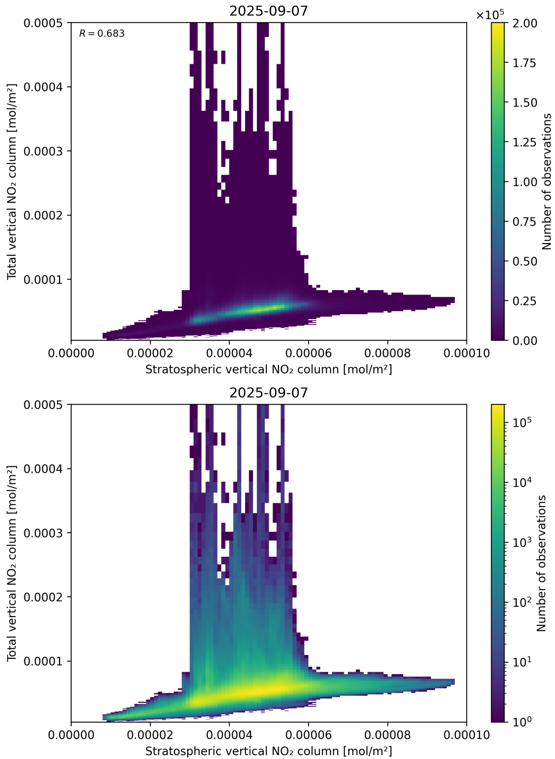
Figure 100: Scatter density plot of “Stratospheric vertical NO 2 column” against “Total vertical NO 2 column” for 2025-09-06 to 2025-09-08.
