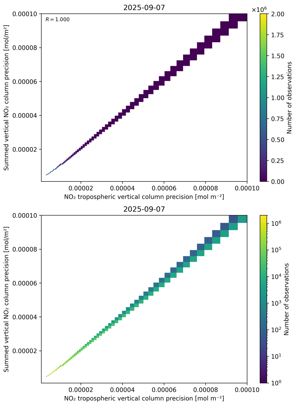
Figure 137: Scatter density plot of “NO 2 tropospheric vertical column precision” against “Summed vertical NO 2 column precision” for 2025-09-06 to 2025-09-08.
