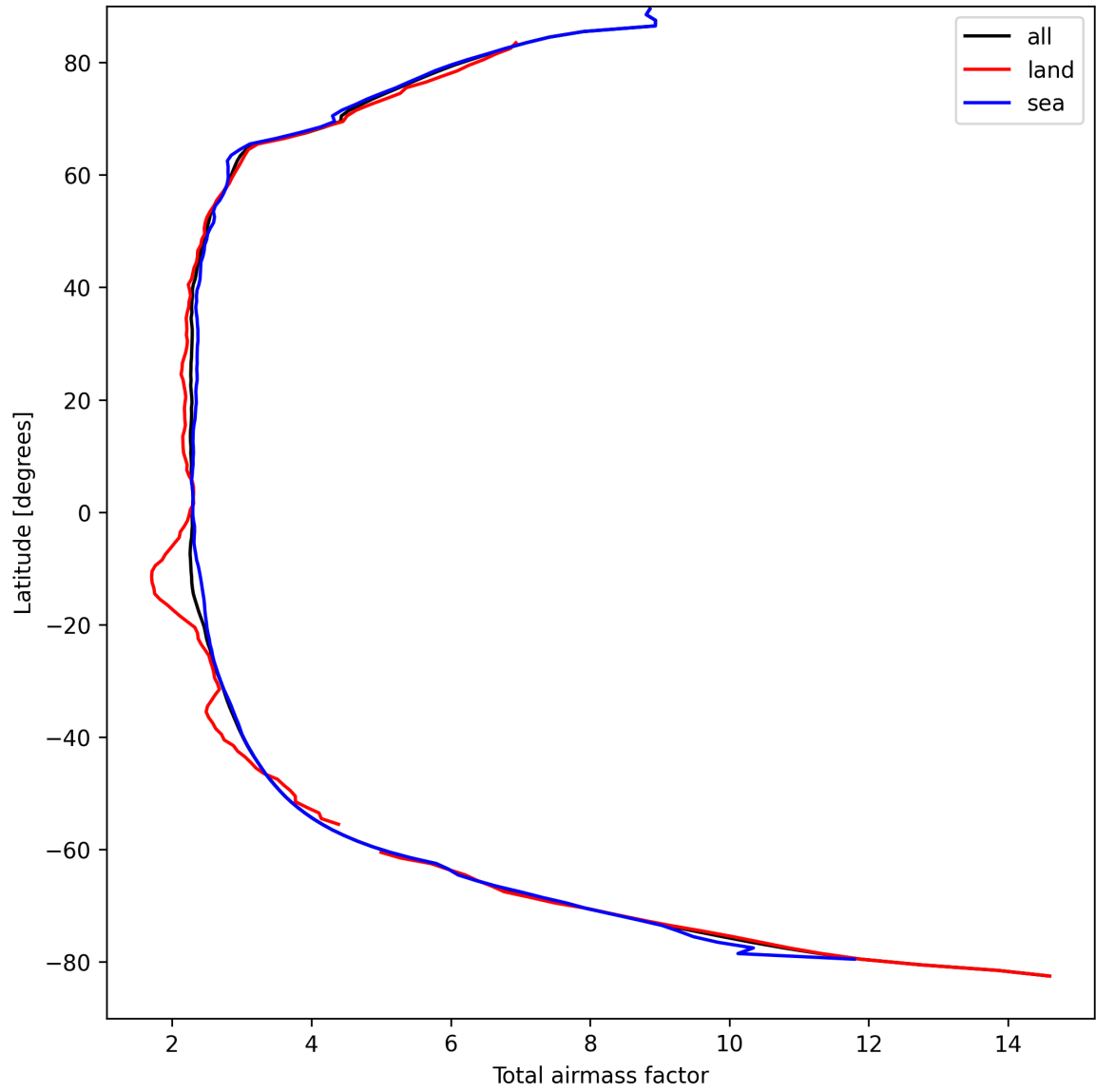
Figure 15: Zonal average of “Total airmass factor” for 2025-09-06 to 2025-09-08.
