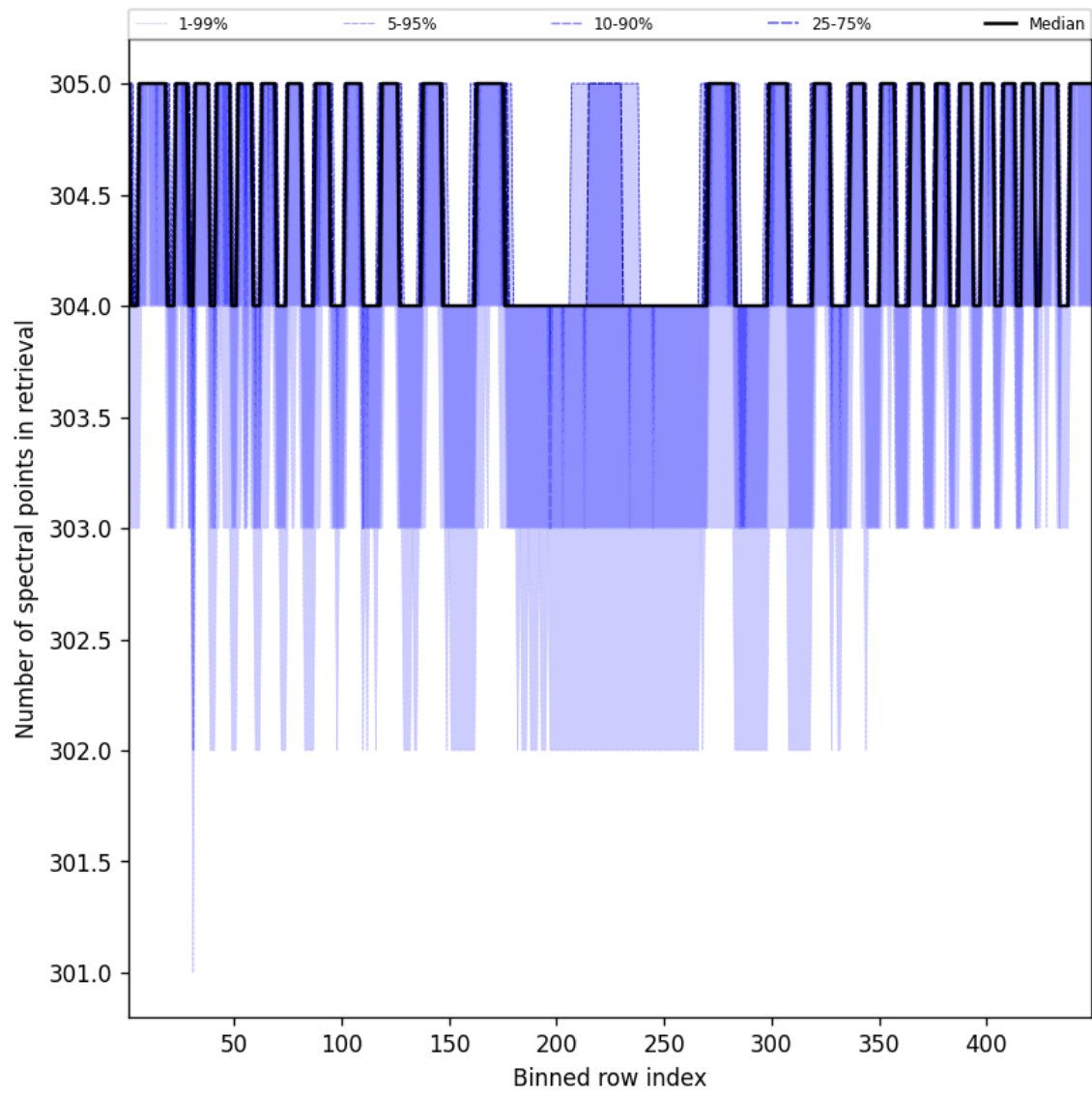
Figure 50: Along track statistics of “Number of spectral points in retrieval” for 2025-09-06 to 2025-09-08
