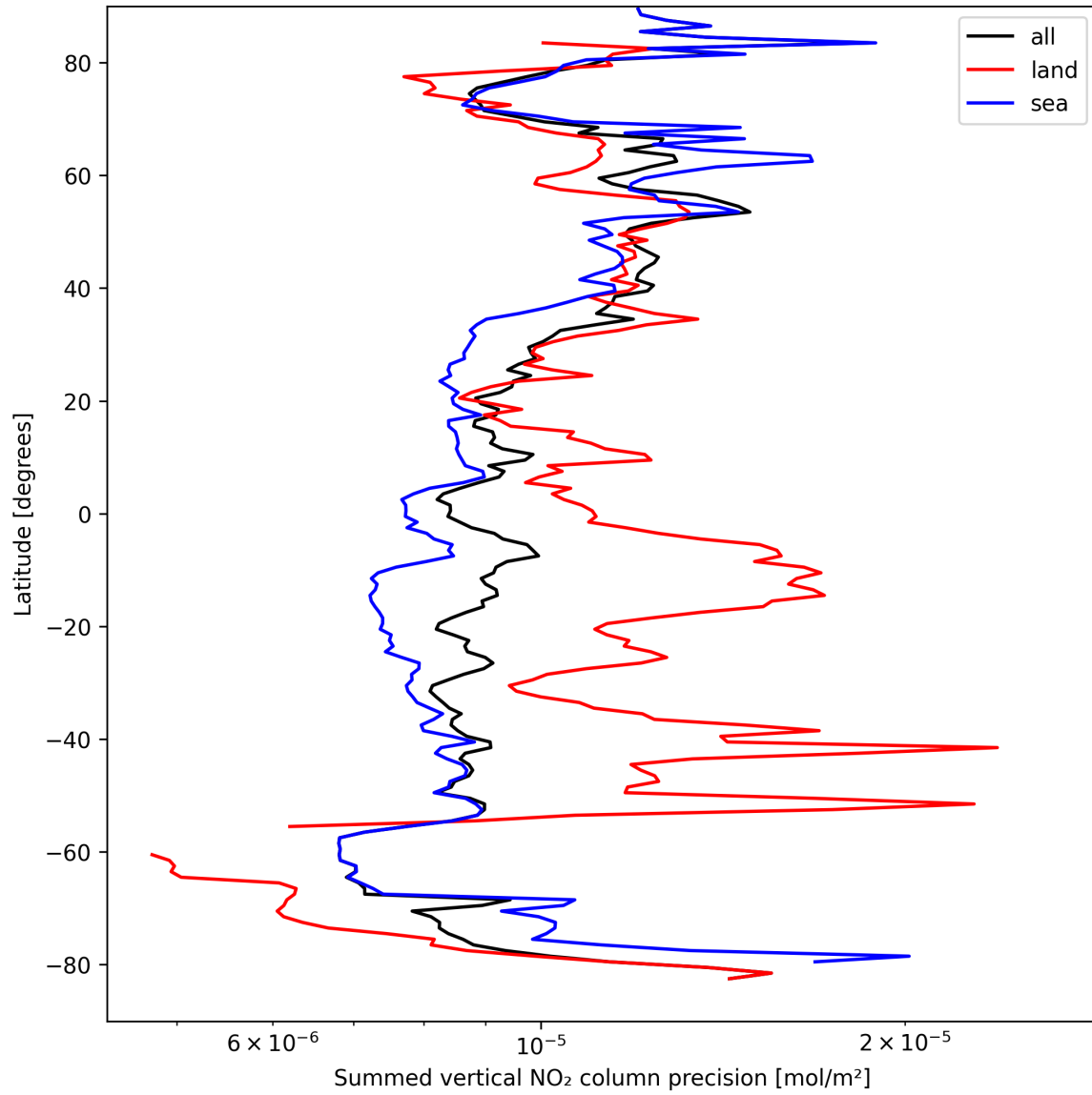
Figure 24: Zonal average of “Summed vertical NO 2 column precision” for 2025-09-06 to 2025-09-08.
