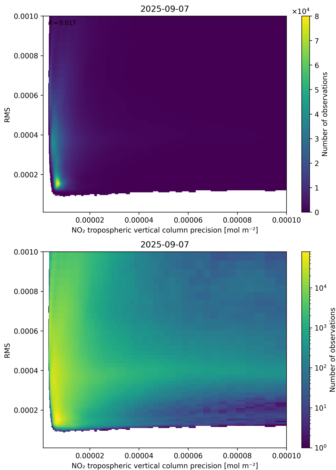
Figure 140: Scatter density plot of “NO 2 tropospheric vertical column precision” against “RMS” for 2025-09-06 to 2025-09-08.
