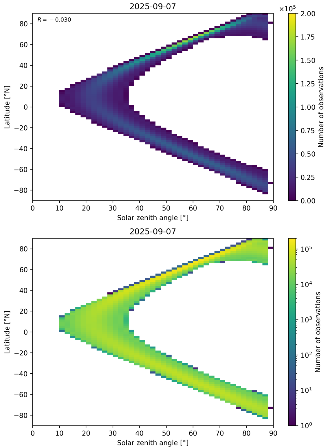
Figure 149: Scatter density plot of “Solar zenith angle” against “Latitude” for 2025-09-06 to 2025-09-08.
