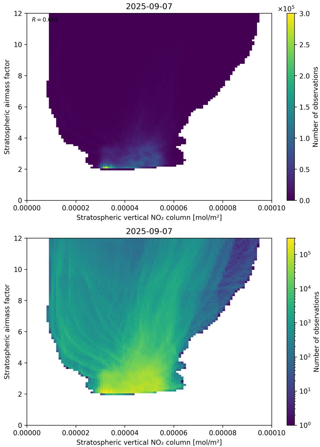
Figure 96: Scatter density plot of “Stratospheric vertical NO 2 column” against “Stratospheric airmass factor” for 2025-09-06 to 2025-09-08.
