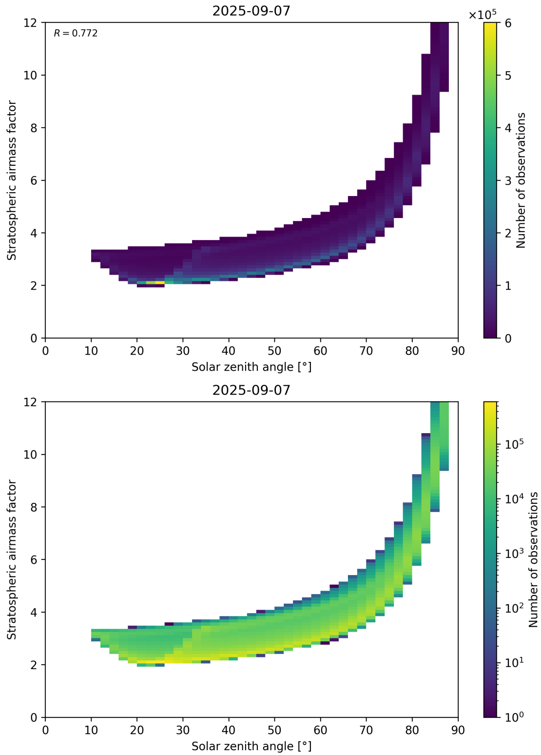
Figure 145: Scatter density plot of “Solar zenith angle” against “Stratospheric airmass factor” for 2025-09-06 to 2025-09-08.
