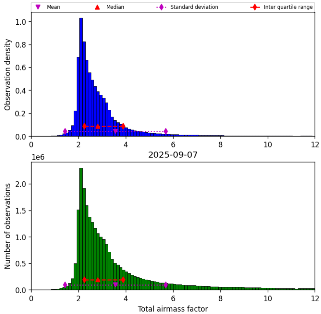
Figure 32: Histogram of “Total airmass factor” for 2025-09-06 to 2025-09-08
