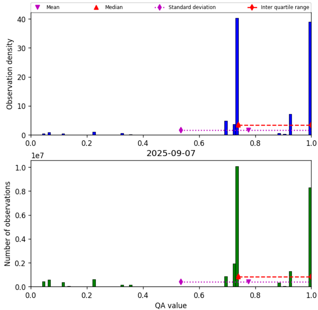
Figure 28: Histogram of “QA value” for 2025-09-06 to 2025-09-08
