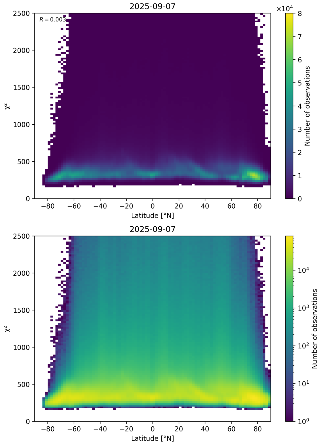
Figure 86: Scatter density plot of “Latitude” against “ \chi^2 ” for 2025-09-06 to 2025-09-08.
