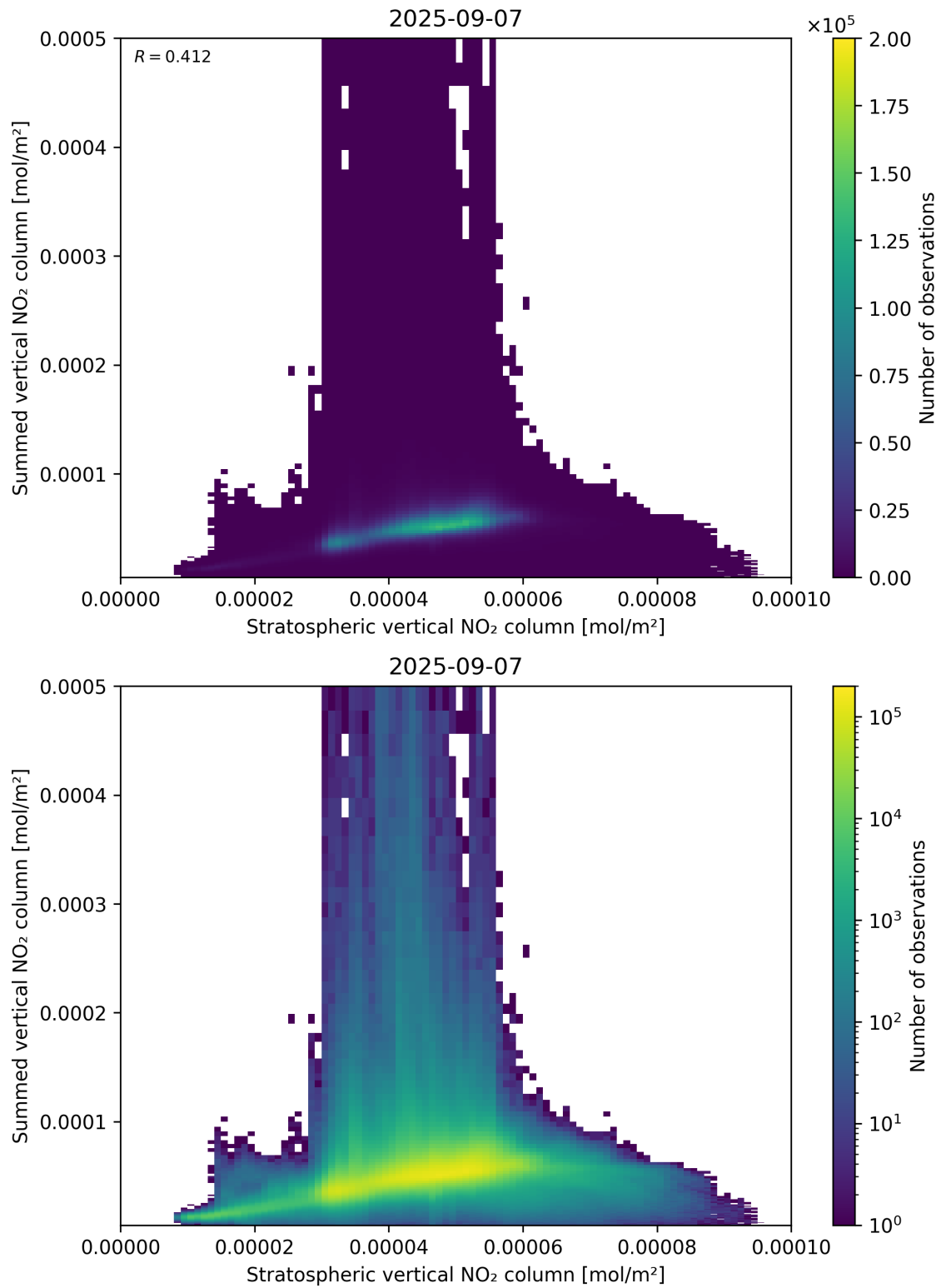
Figure 98: Scatter density plot of “Stratospheric vertical NO 2 column” against “Summed vertical NO 2 column” for 2025-09-06 to 2025-09-08.
