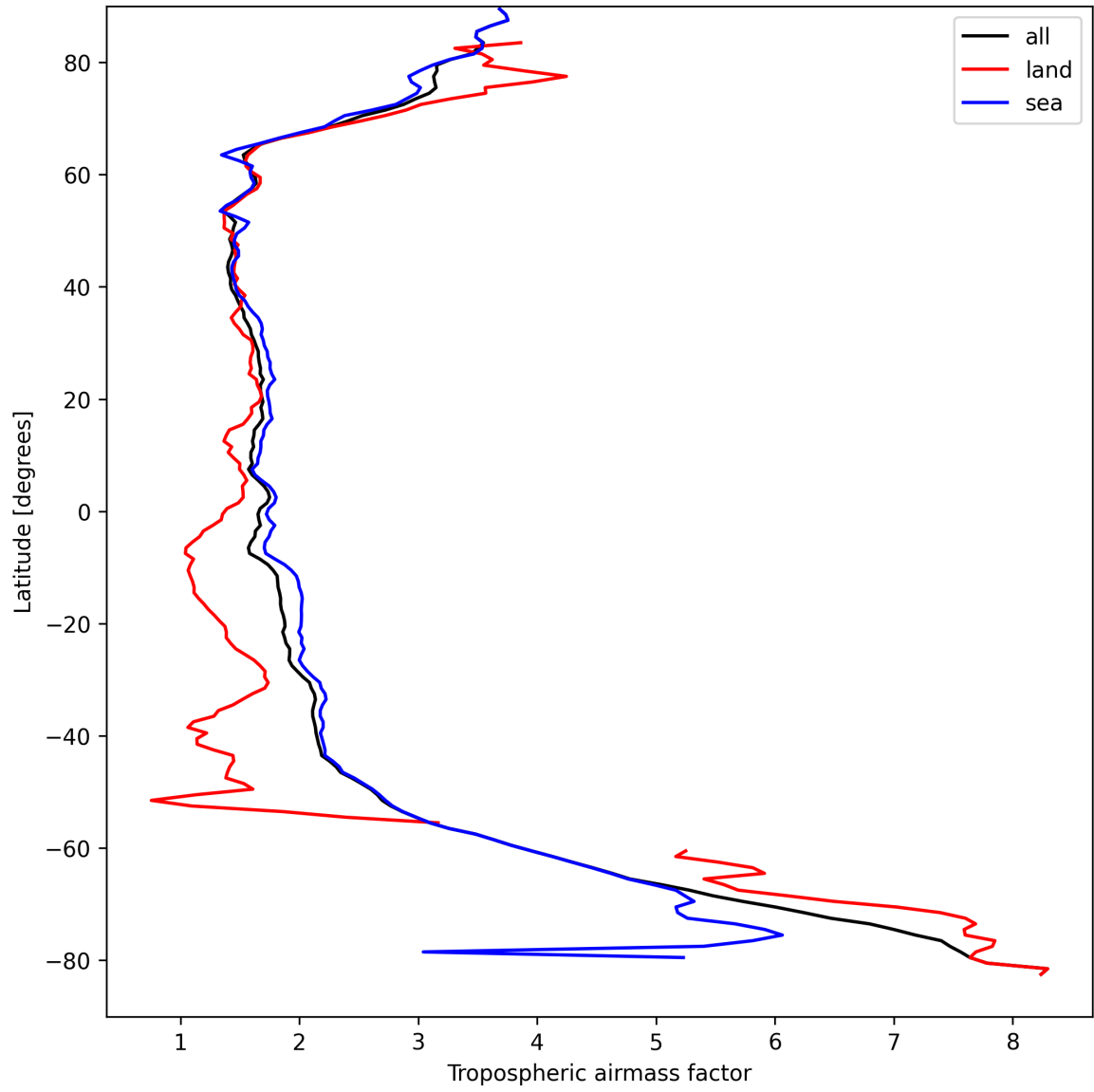
Figure 14: Zonal average of “Tropospheric airmass factor” for 2025-09-06 to 2025-09-08.
