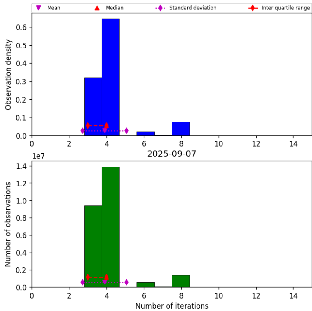
Figure 34: Histogram of “Number of iterations” for 2025-09-06 to 2025-09-08
