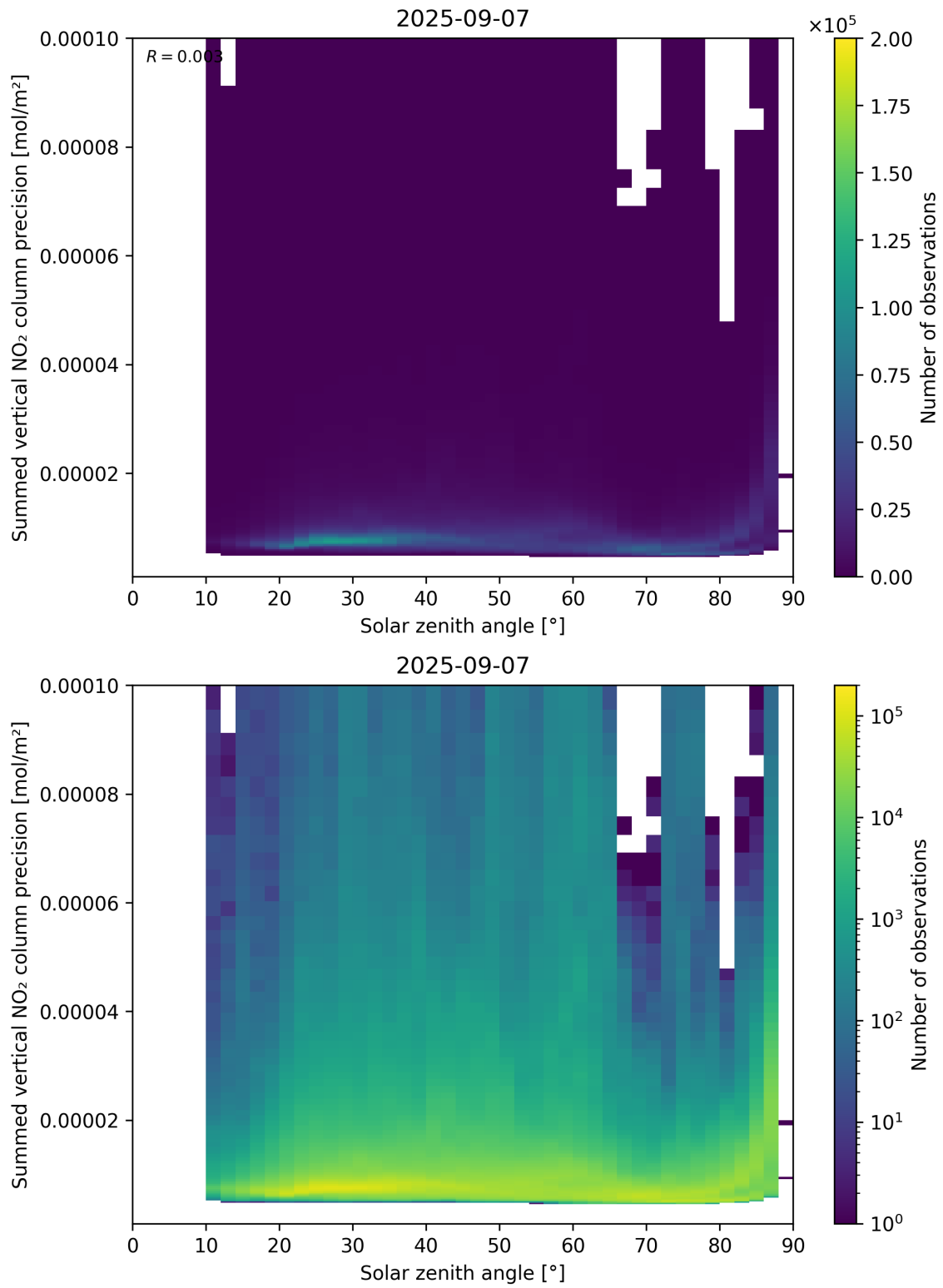
Figure 152: Scatter density plot of “Solar zenith angle” against “Summed vertical NO 2 column precision” for 2025-09-06 to 2025-09-08.
