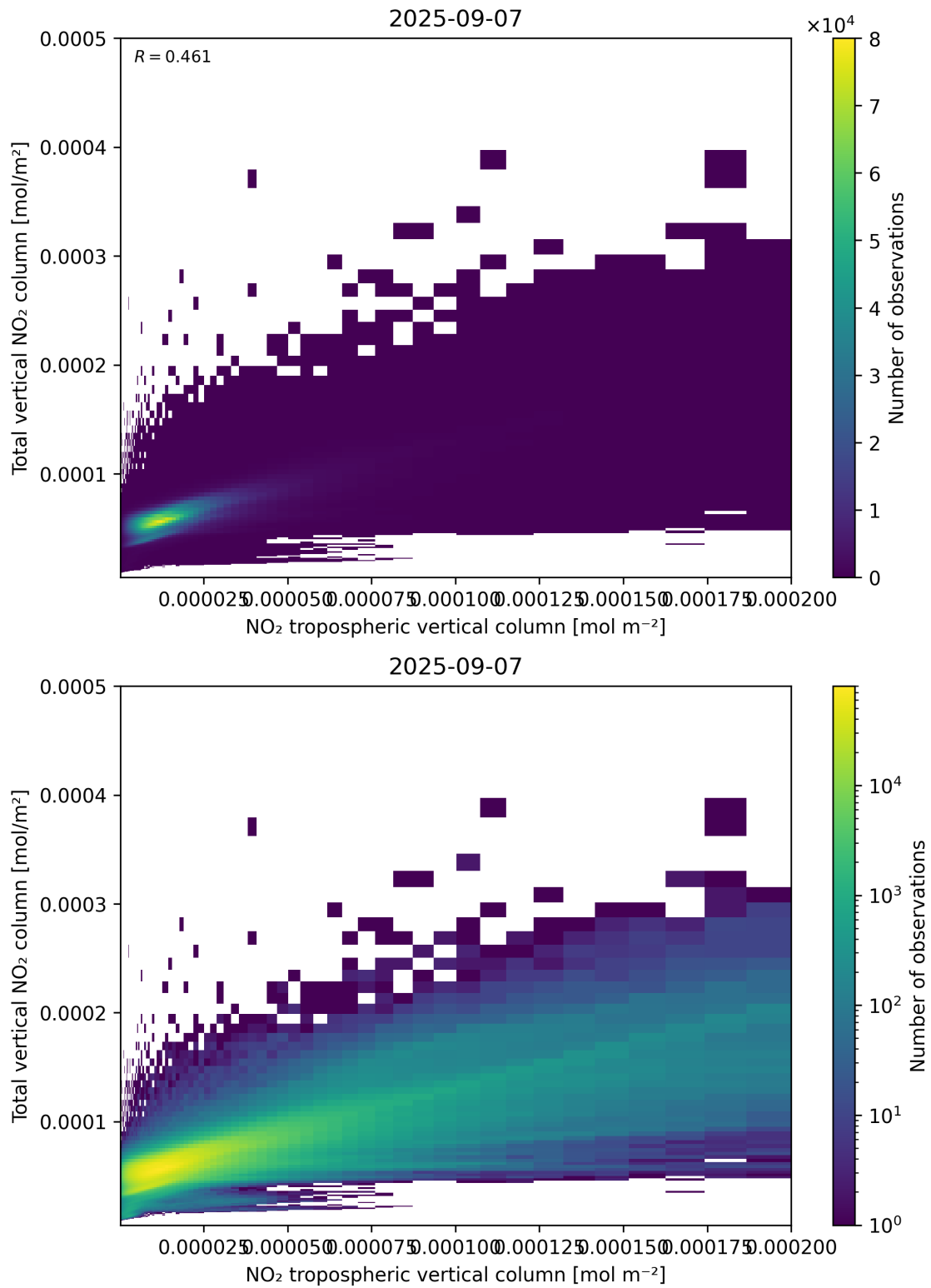
Figure 128: Scatter density plot of “NO 2 tropospheric vertical column” against “Total vertical NO 2 column” for 2025-09-06 to 2025-09-08.
