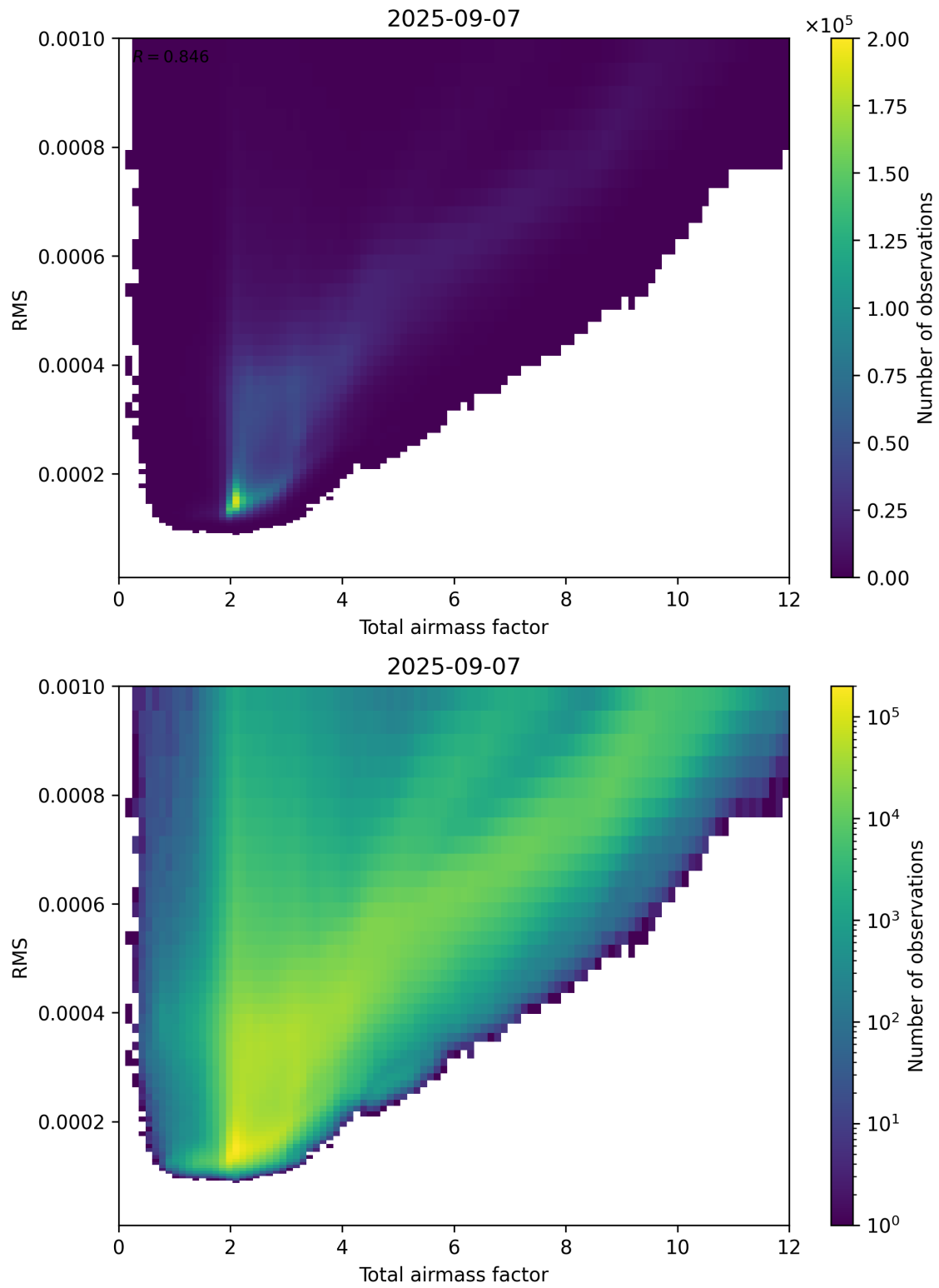
Figure 69: Scatter density plot of “Total airmass factor” against “RMS” for 2025-09-06 to 2025-09-08.
