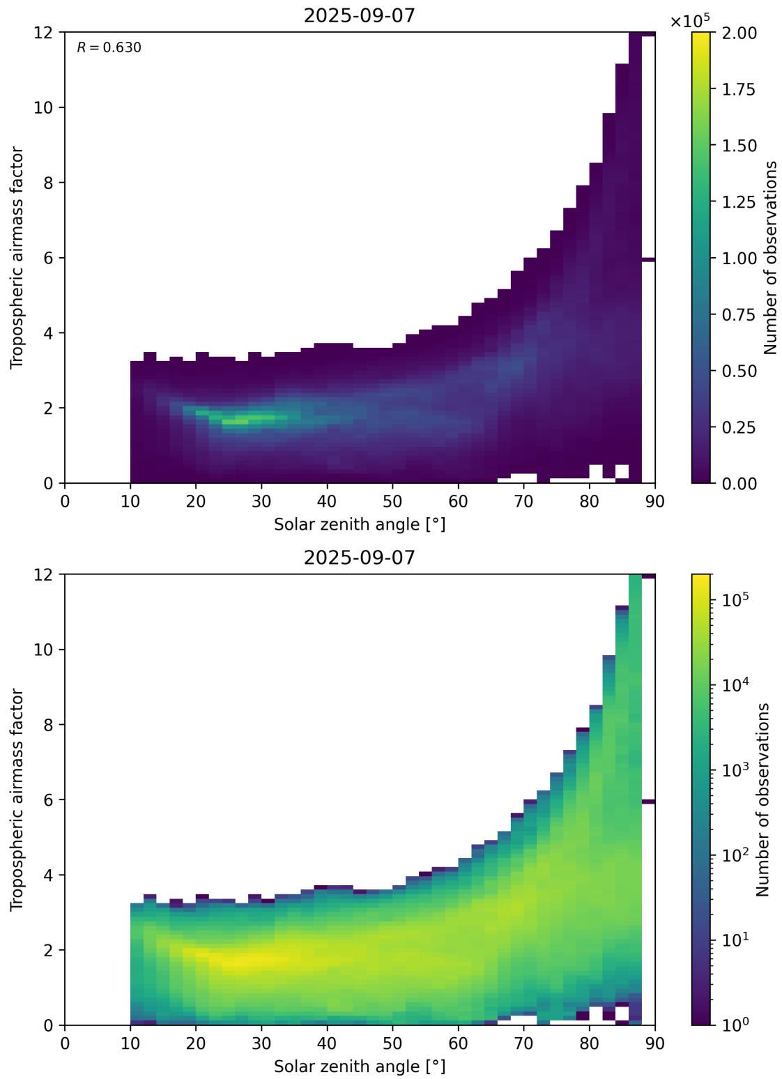
Figure 147: Scatter density plot of “Solar zenith angle” against “Tropospheric airmass factor” for 2025-09-06 to 2025-09-08.
