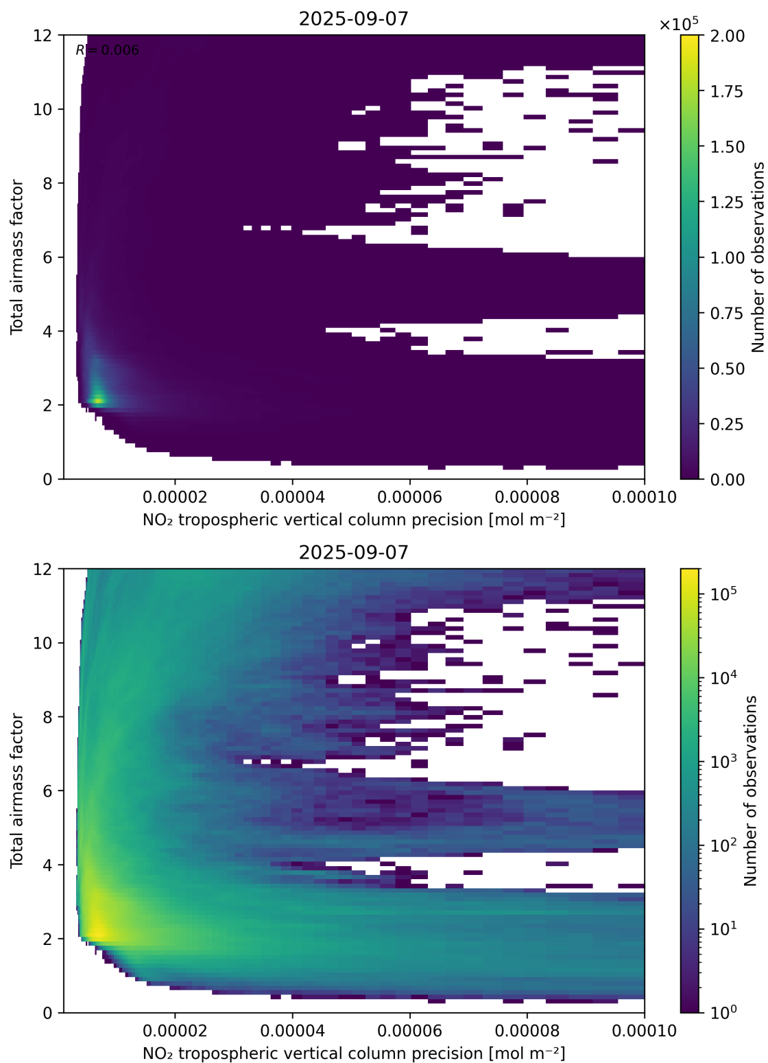
Figure 132: Scatter density plot of “NO 2 tropospheric vertical column precision” against “Total air mass factor” for 2025-09-06 to 2025-09-08.
