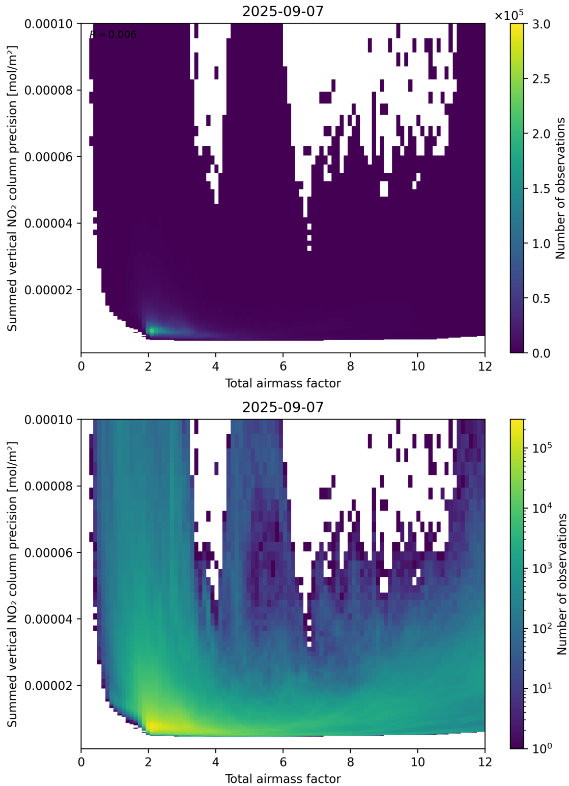
Figure 66: Scatter density plot of “Total airmass factor” against “Summed vertical NO 2 column precision” for 2025-09-06 to 2025-09-08.
