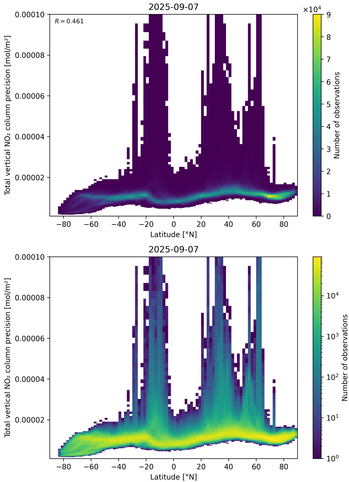
Figure 91: Scatter density plot of “Latitude” against “Total vertical NO 2 column precision” for 2025-09-06 to 2025-09-08.
