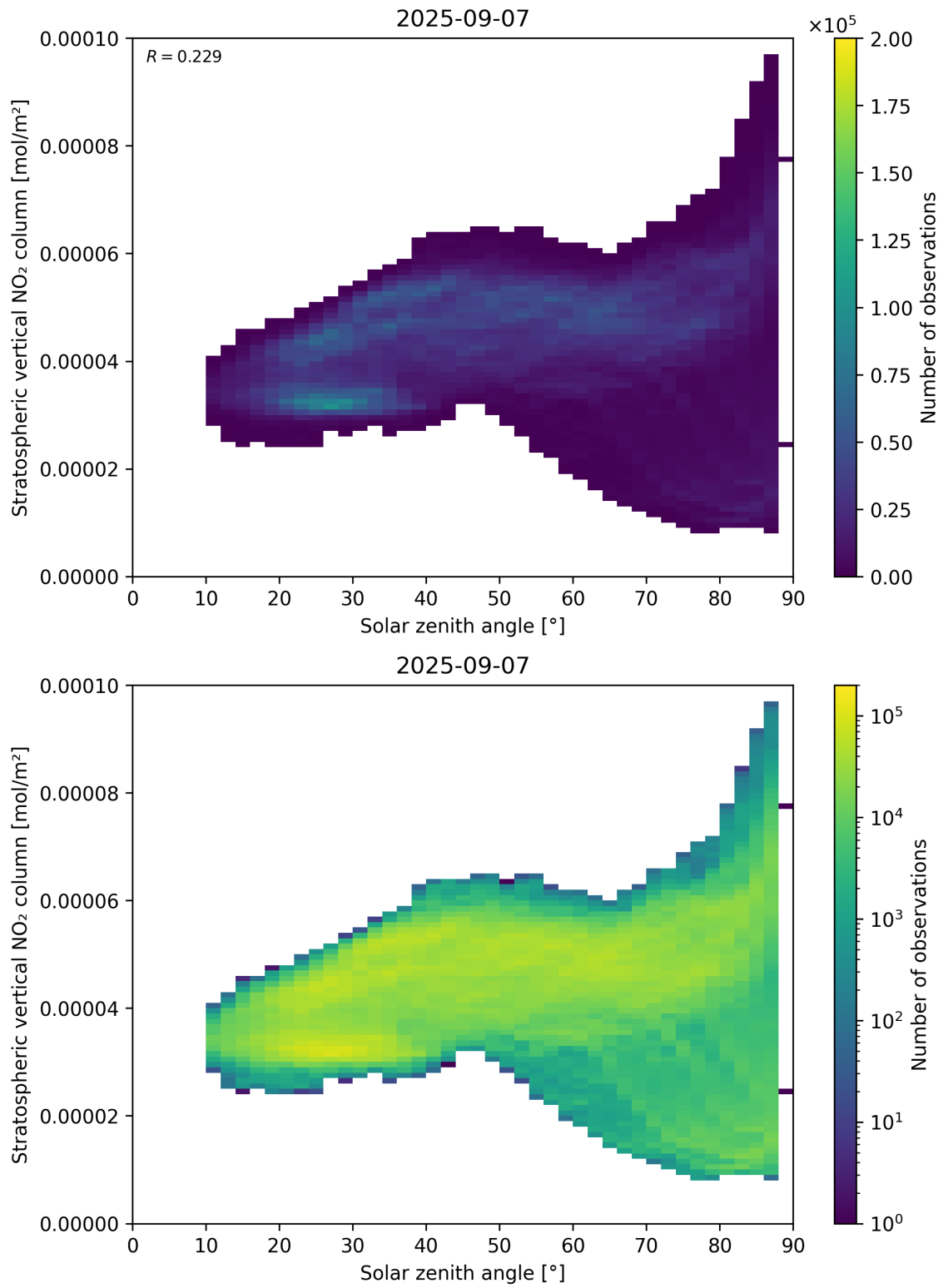
Figure 150: Scatter density plot of “Solar zenith angle” against “Stratospheric vertical NO 2 column” for 2025-09-06 to 2025-09-08.
