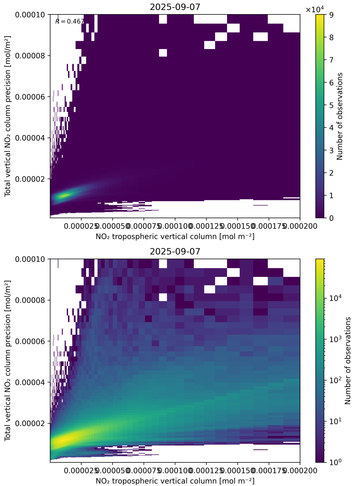
Figure 129: Scatter density plot of “NO 2 tropospheric vertical column” against “Total vertical NO 2 column precision” for 2025-09-06 to 2025-09-08.
