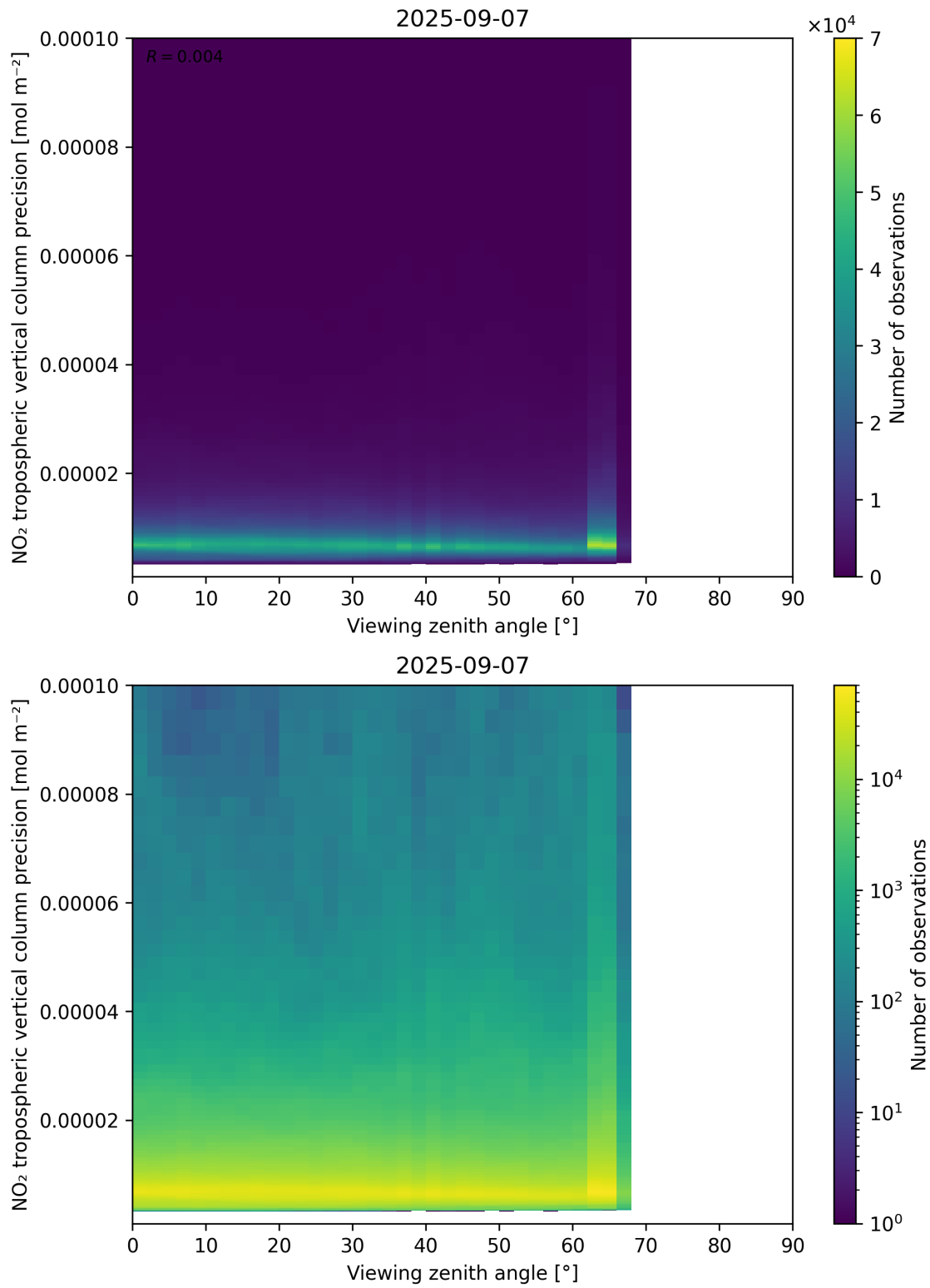
Figure 170: Scatter density plot of “Viewing zenith angle” against “NO 2 tropospheric vertical column precision” for 2025-09-06 to 2025-09-08.
