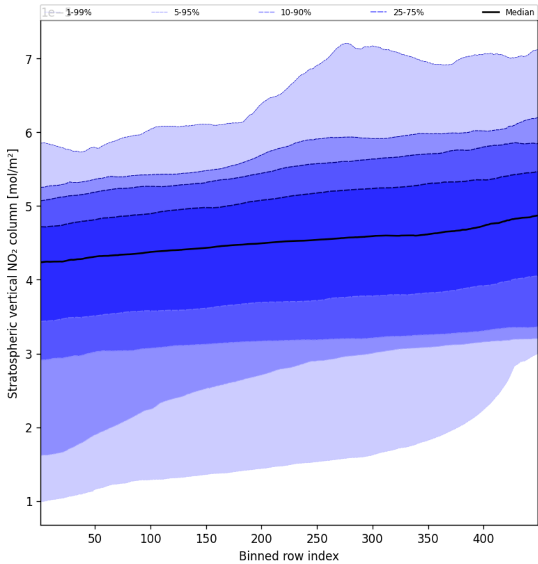
Figure 53: Along track statistics of “Stratospheric vertical NO 2 column” for 2025-09-06 to 2025-09-08
