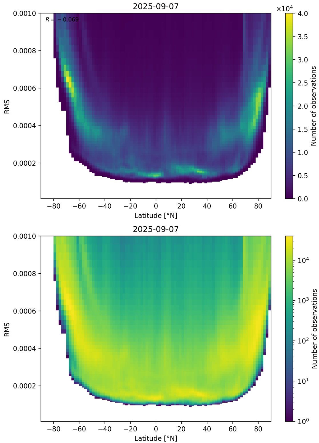
Figure 94: Scatter density plot of “Latitude” against “RMS” for 2025-09-06 to 2025-09-08.
