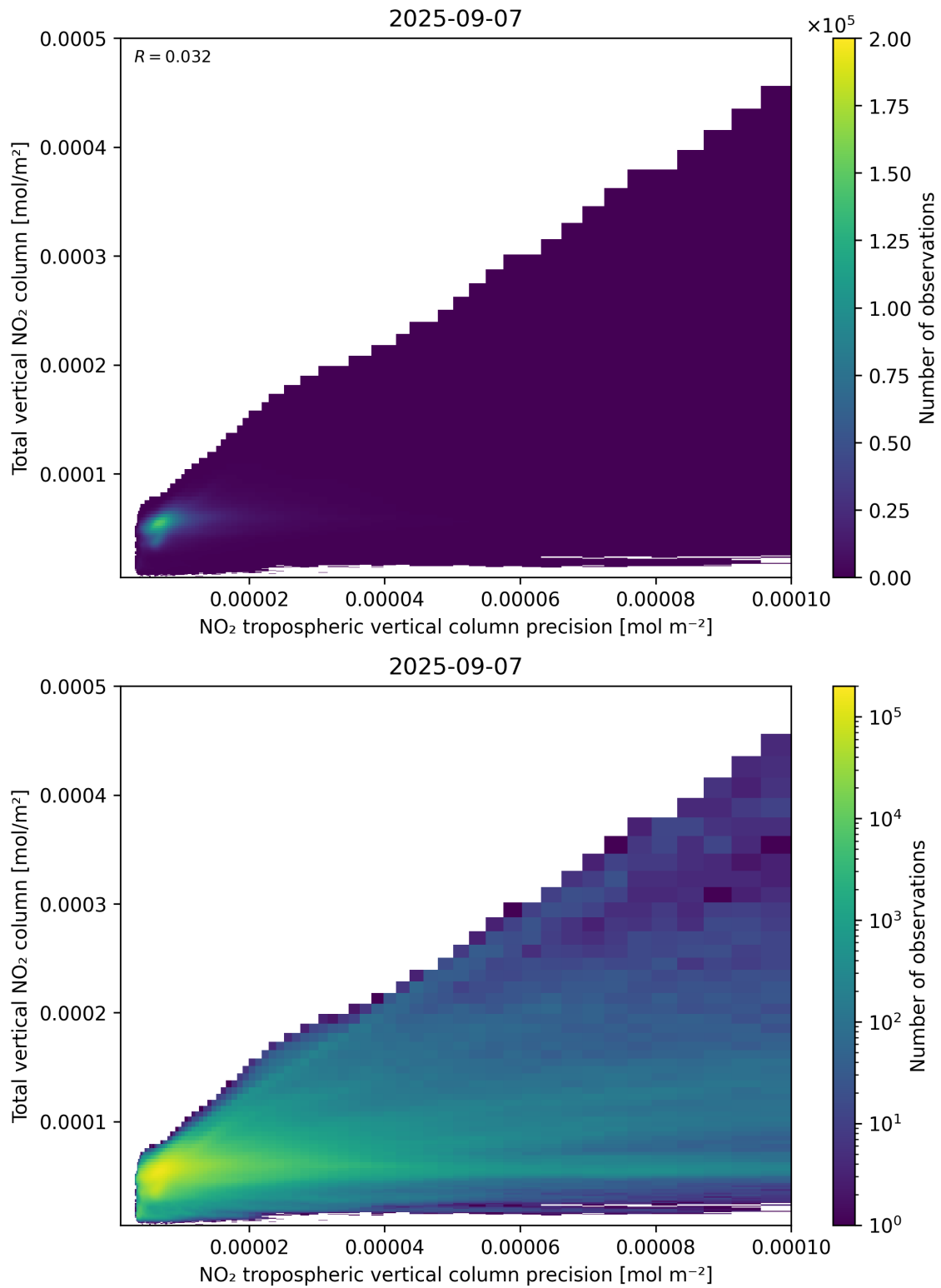
Figure 138: Scatter density plot of “NO 2 tropospheric vertical column precision” against “Total vertical NO 2 column” for 2025-09-06 to 2025-09-08.
