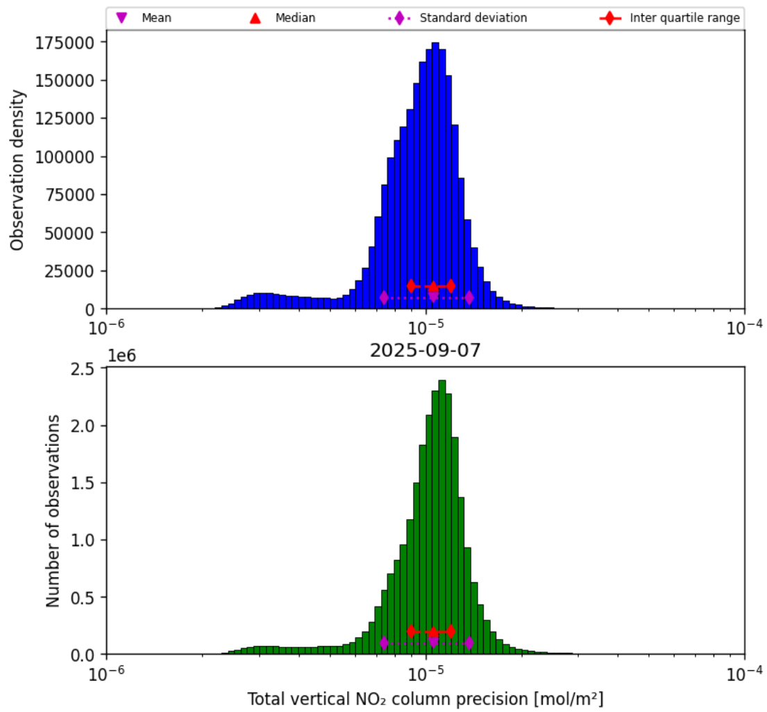
Figure 39: Histogram of "Total vertical NO 2 column precision" for 2025-09-06 to 2025-09-08
