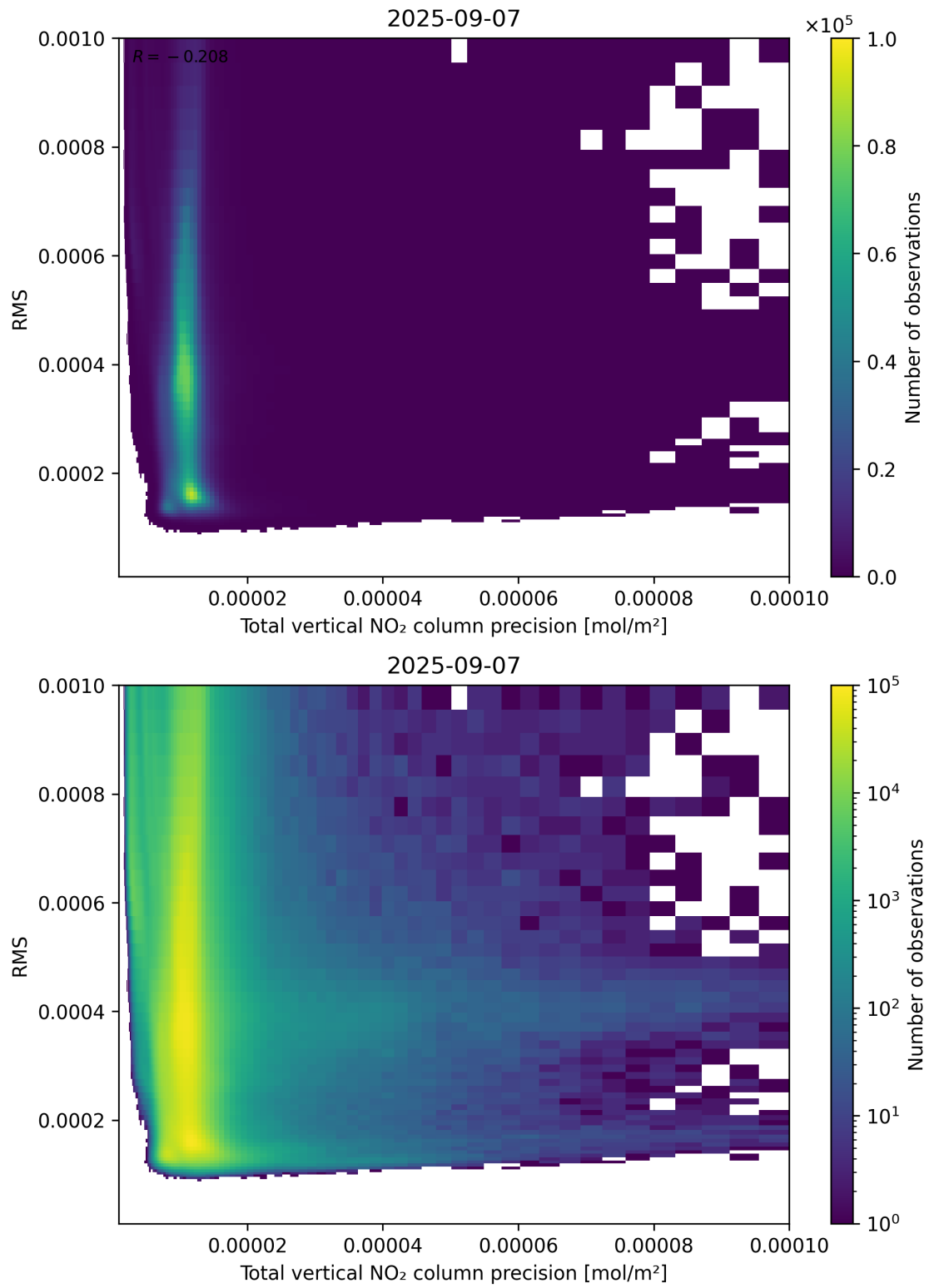
Figure 119: Scatter density plot of “Total vertical NO 2 column precision” against “RMS” for 2025-09-06 to 2025-09-08.
