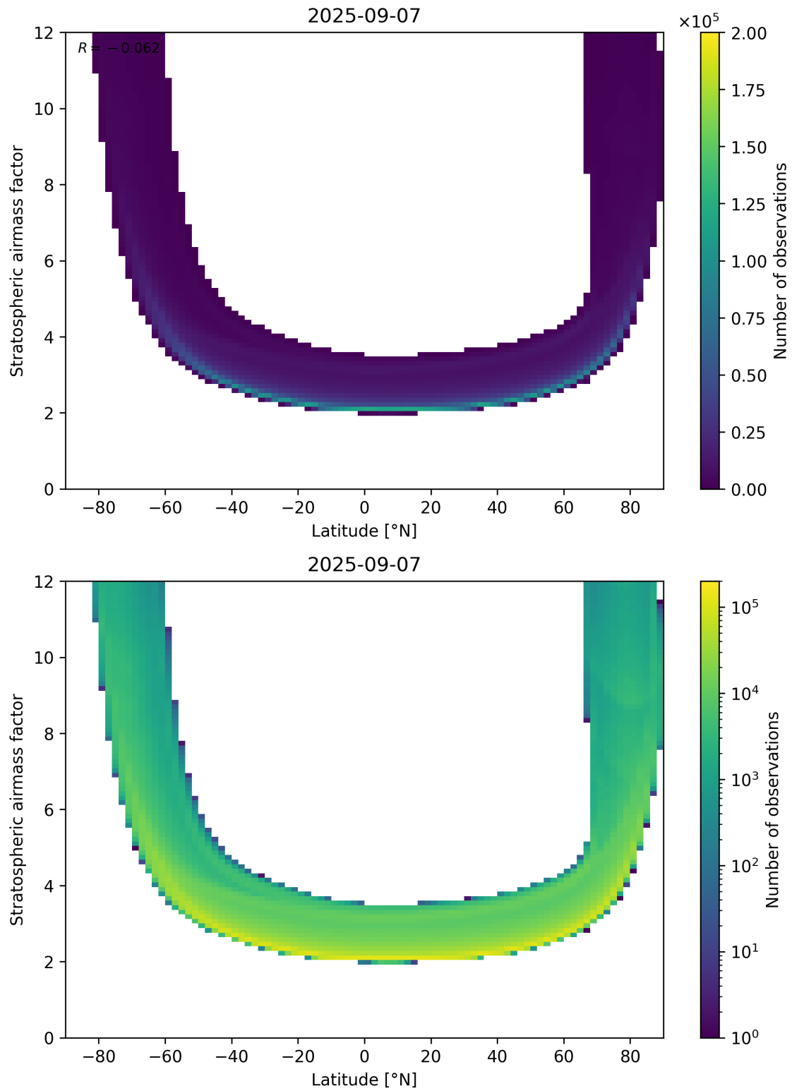
Figure 83: Scatter density plot of “Latitude” against “Stratospheric airmass factor” for 2025-09-06 to 2025-09-08.
