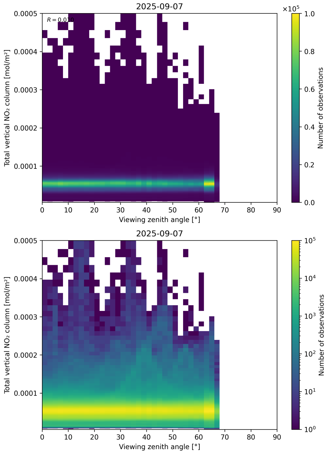
Figure 167: Scatter density plot of “Viewing zenith angle” against “Total vertical NO 2 column” for 2025-09-06 to 2025-09-08.
