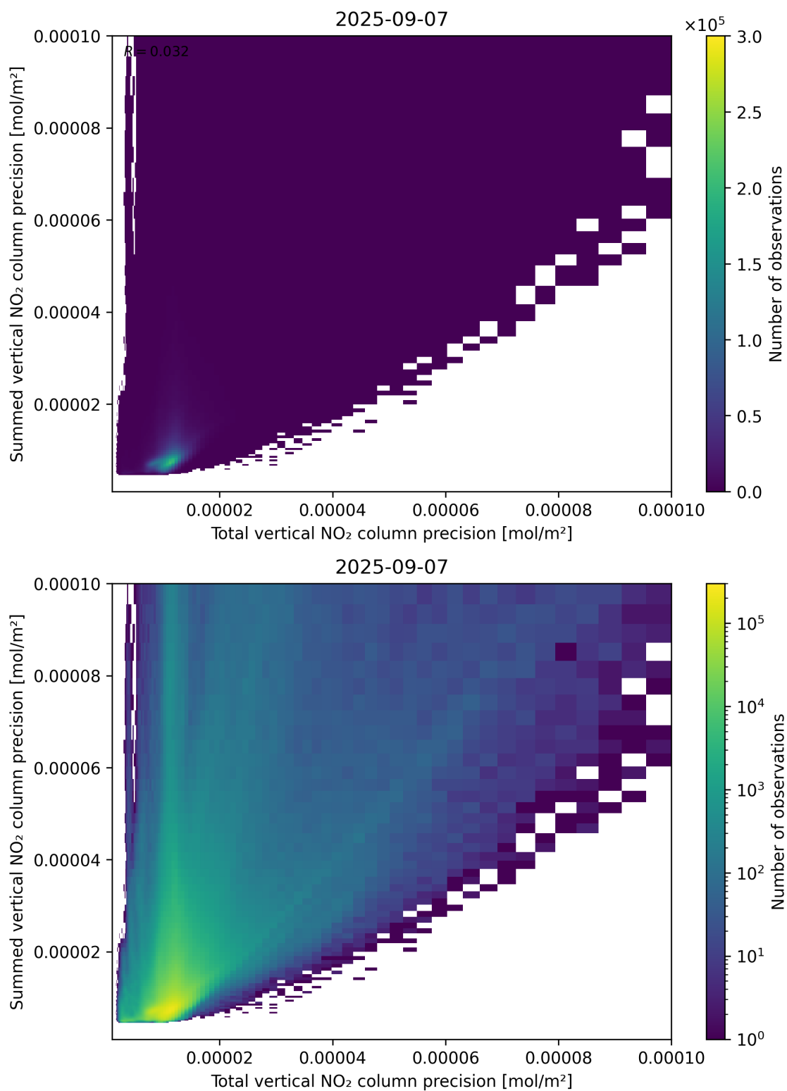
Figure 118: Scatter density plot of “Total vertical NO 2 column precision” against “Summed vertical NO 2 column precision” for 2025-09-06 to 2025-09-08.
