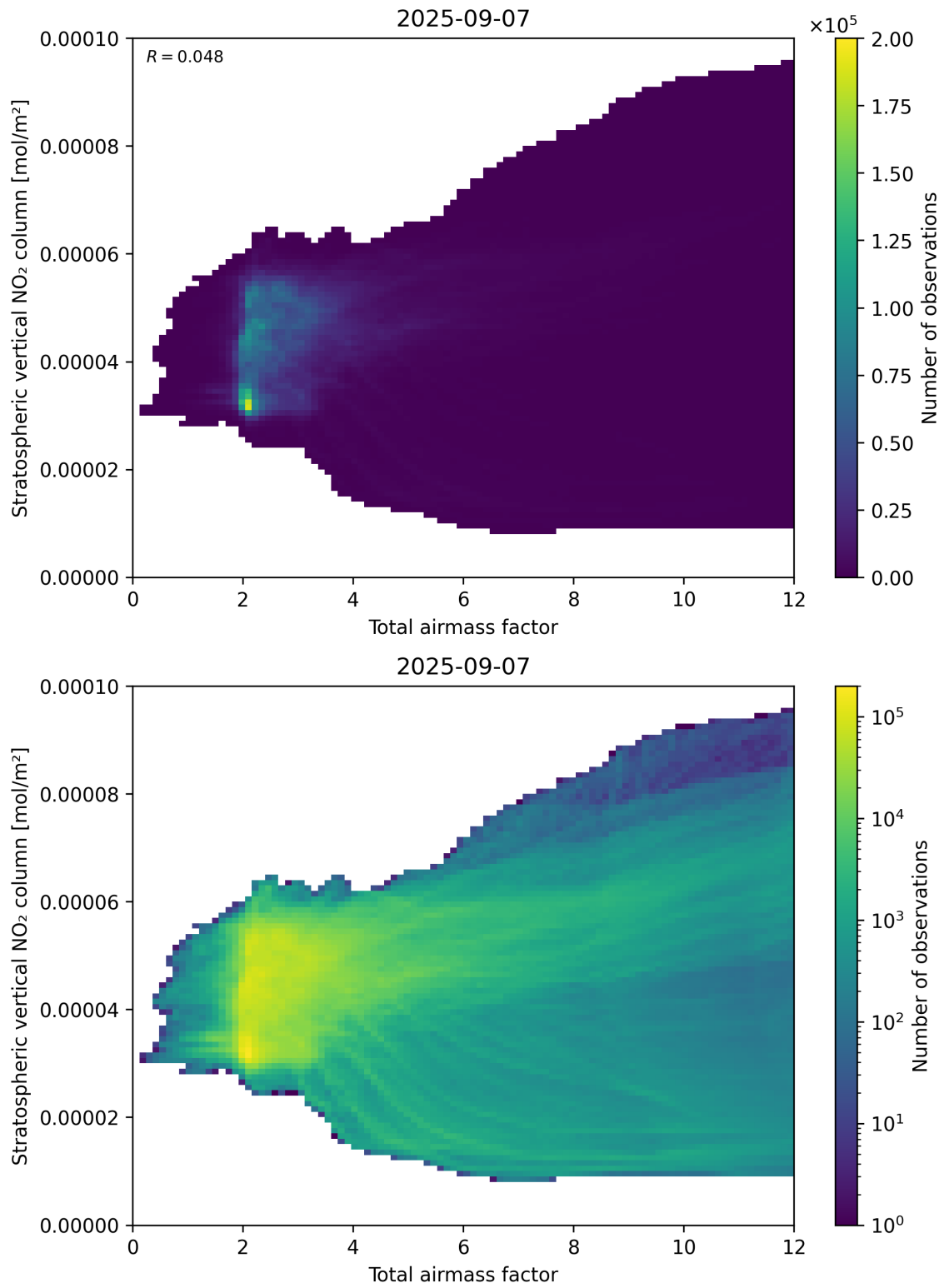
Figure 64: Scatter density plot of “Total airmass factor” against “Stratospheric vertical \text{NO}_2 column” for 2025-09-06 to 2025-09-08.
