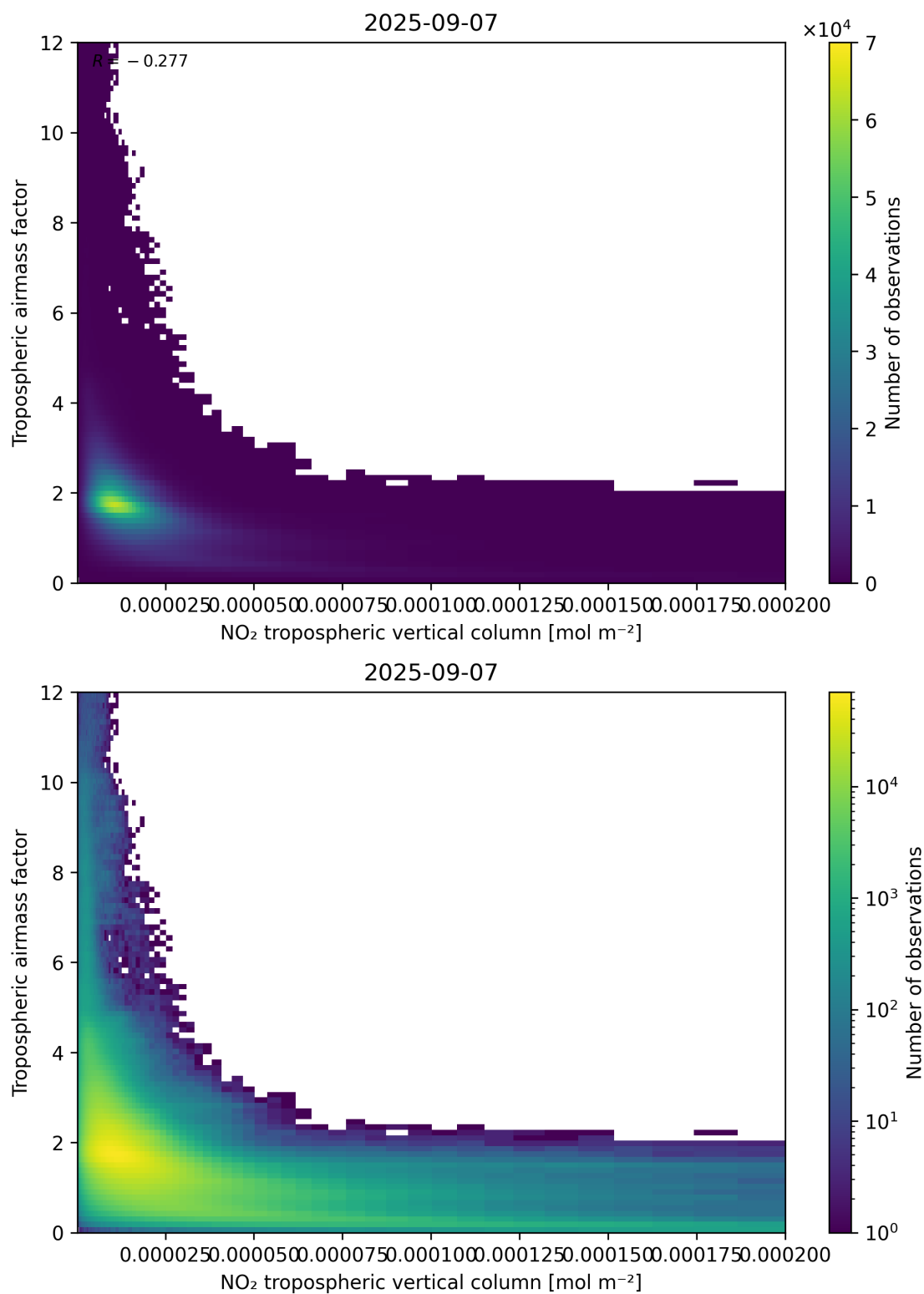
Figure 123: Scatter density plot of “NO 2 tropospheric vertical column” against “Tropospheric air mass factor” for 2025-09-06 to 2025-09-08.
