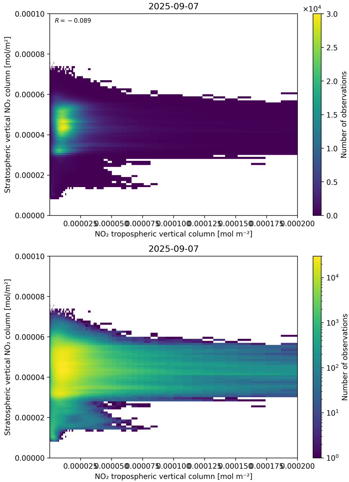
Figure 125: Scatter density plot of “NO 2 tropospheric vertical column” against “Stratospheric vertical NO 2 column” for 2025-09-06 to 2025-09-08.
