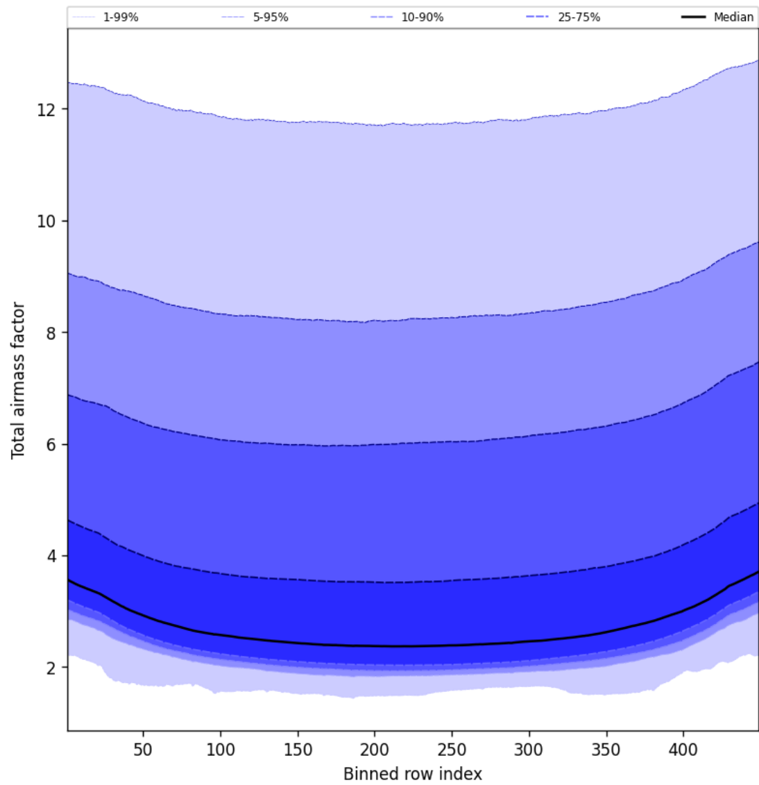
Figure 49: Along track statistics of “Total airmass factor” for 2025-09-06 to 2025-09-08
