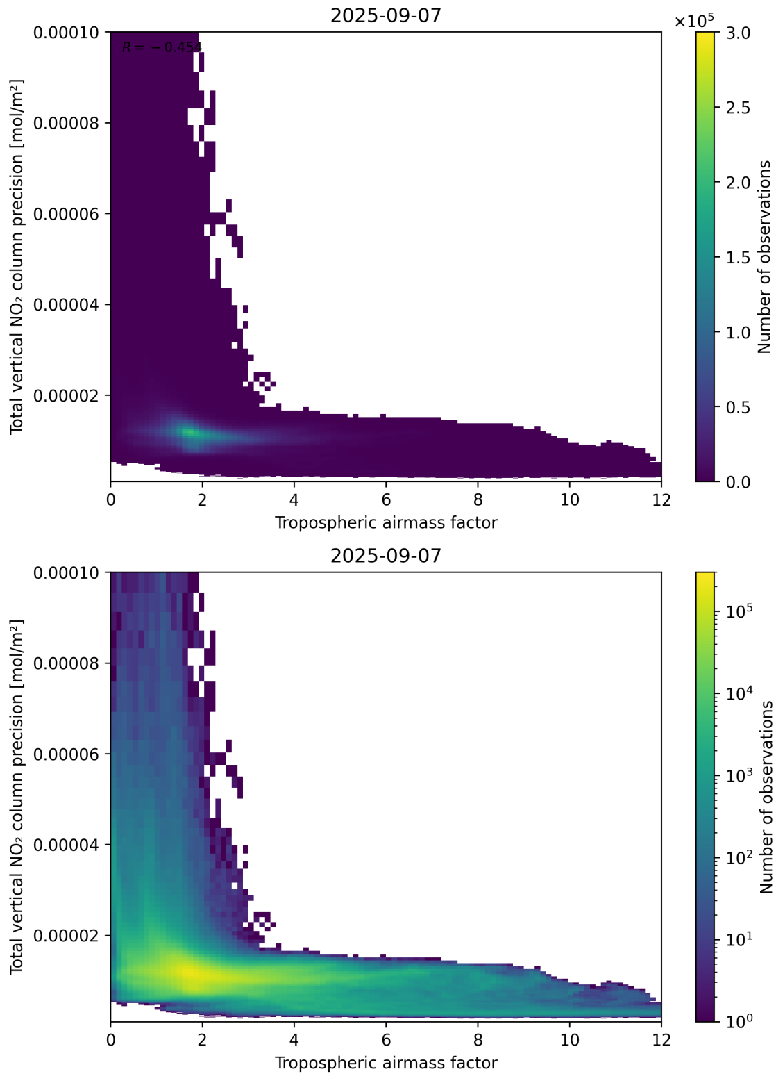
Figure 78: Scatter density plot of “Tropospheric air mass factor” against “Total vertical NO 2 column precision” for 2025-09-06 to 2025-09-08.
