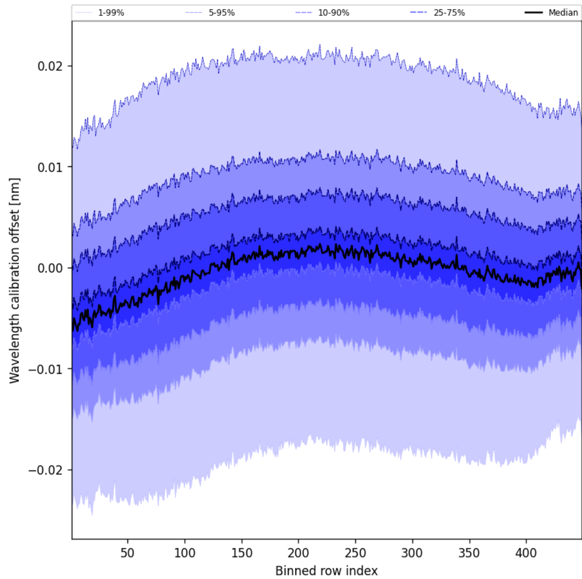
Figure 52: Along track statistics of “Wavelength calibration offset” for 2025-09-06 to 2025-09-08
