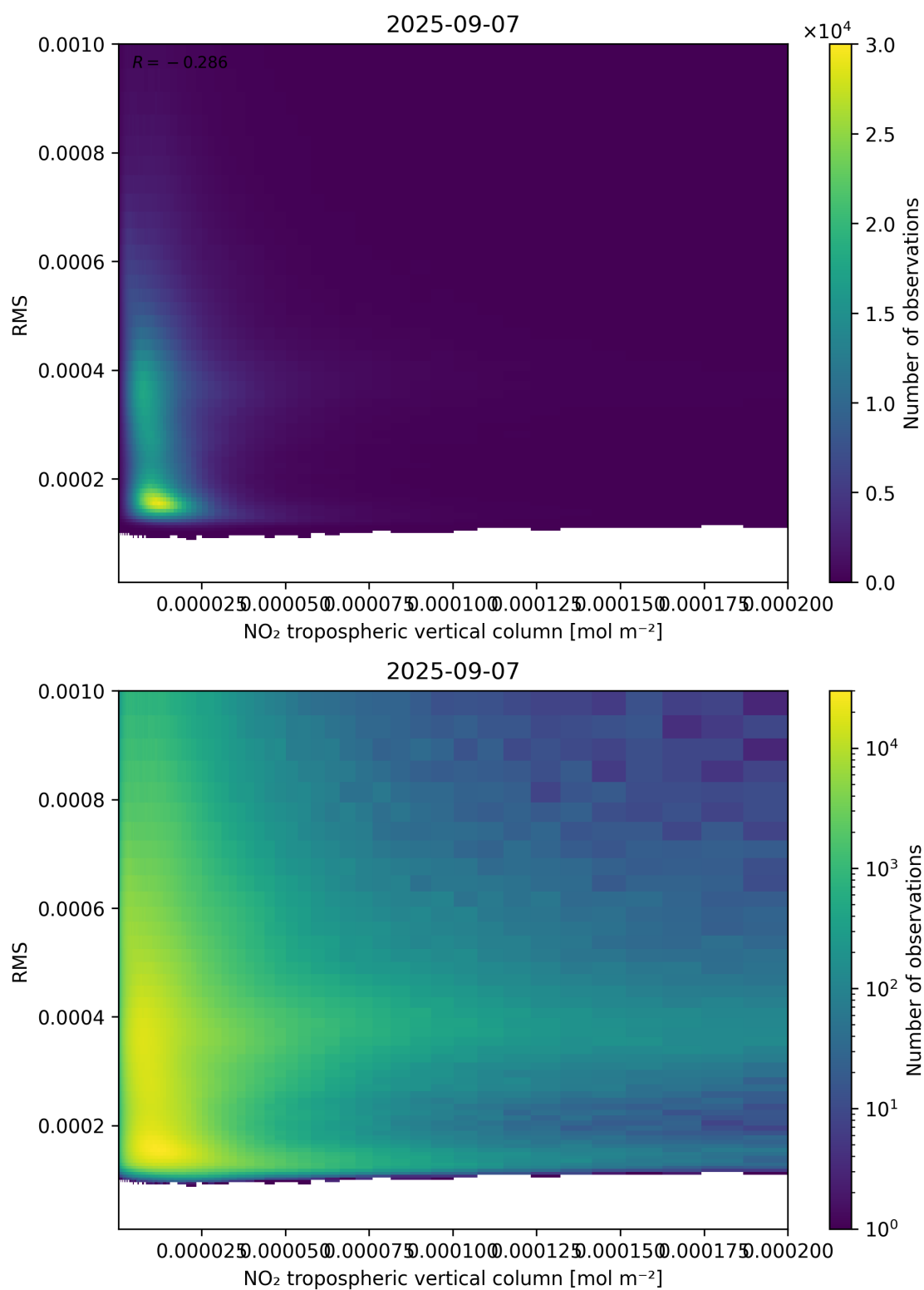
Figure 142: Scatter density plot of “NO 2 tropospheric vertical column” against “RMS” for 2025-09-06 to 2025-09-08.
