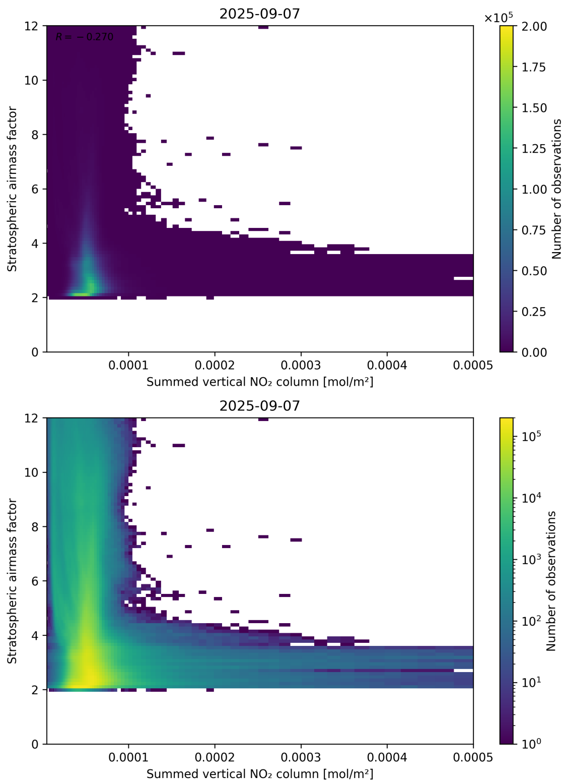
Figure 103: Scatter density plot of “Summed vertical NO 2 column” against “Stratospheric airmass factor” for 2025-09-06 to 2025-09-08.
