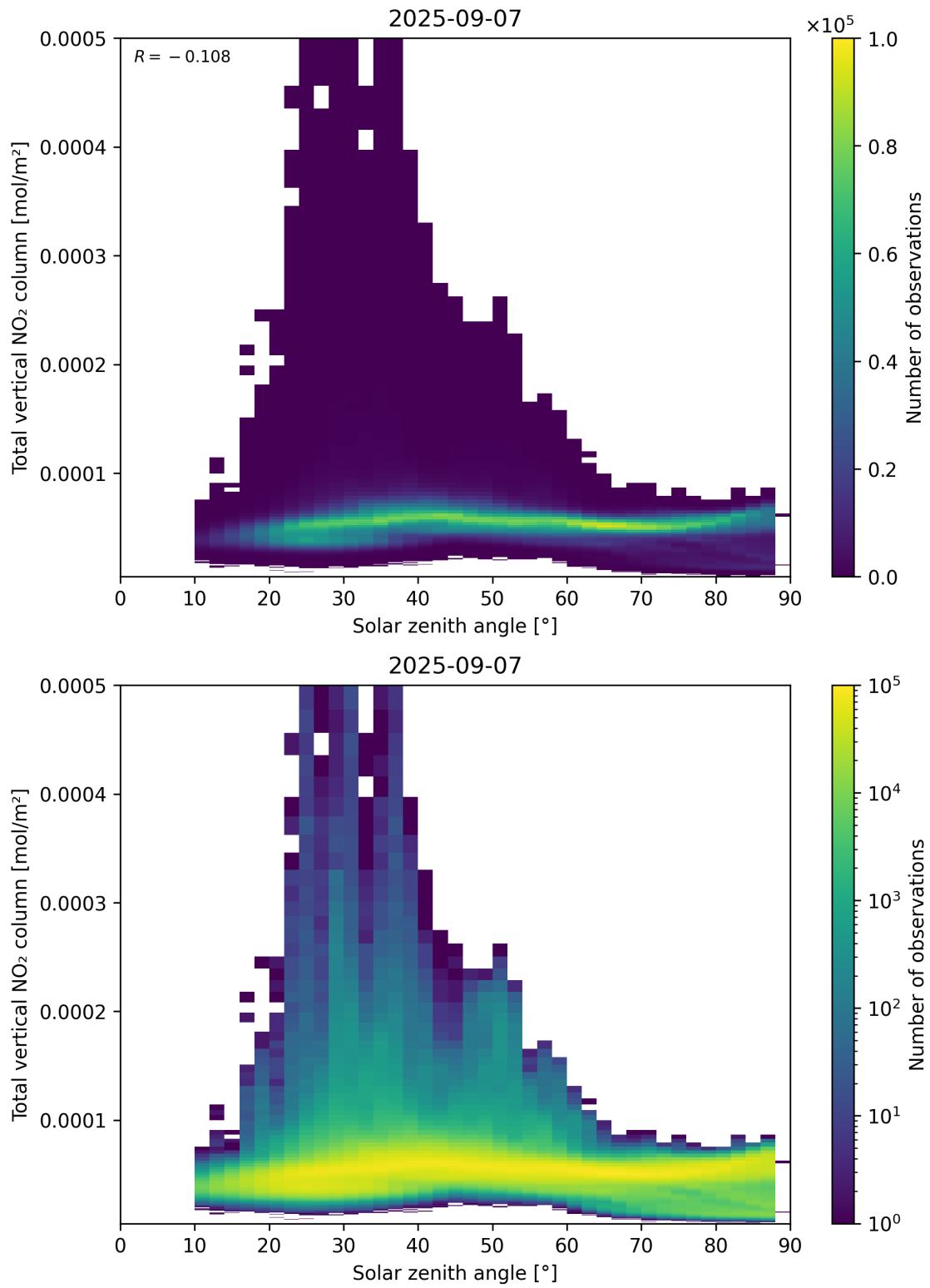
Figure 153: Scatter density plot of “Solar zenith angle” against “Total vertical NO 2 column” for 2025-09-06 to 2025-09-08.
