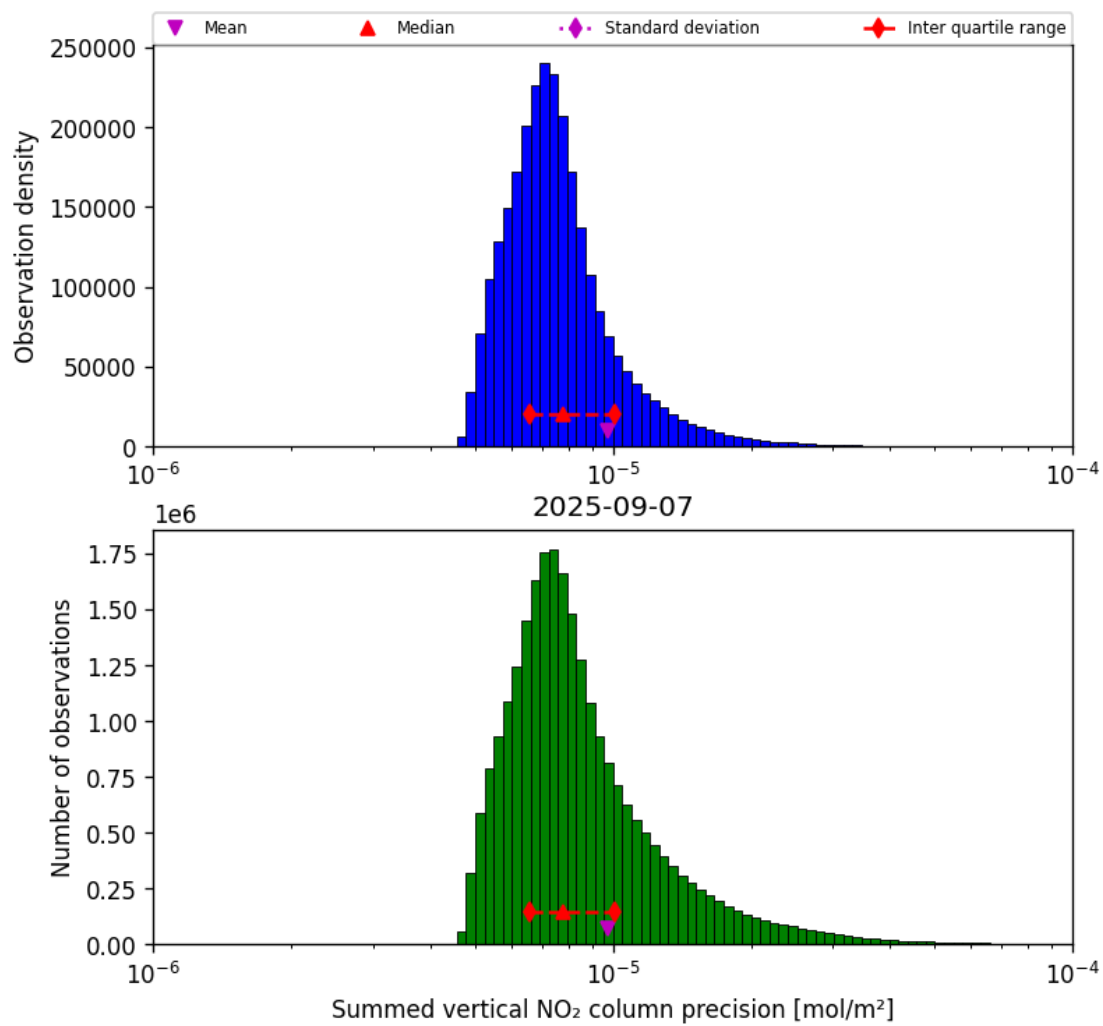
Figure 41: Histogram of "Summed vertical NO 2 column precision" for 2025-09-06 to 2025-09-08
