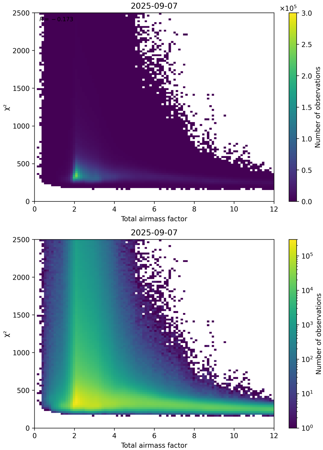
Figure 63: Scatter density plot of “Total airmass factor” against “ \chi^2 ” for 2025-09-06 to 2025-09-08.
