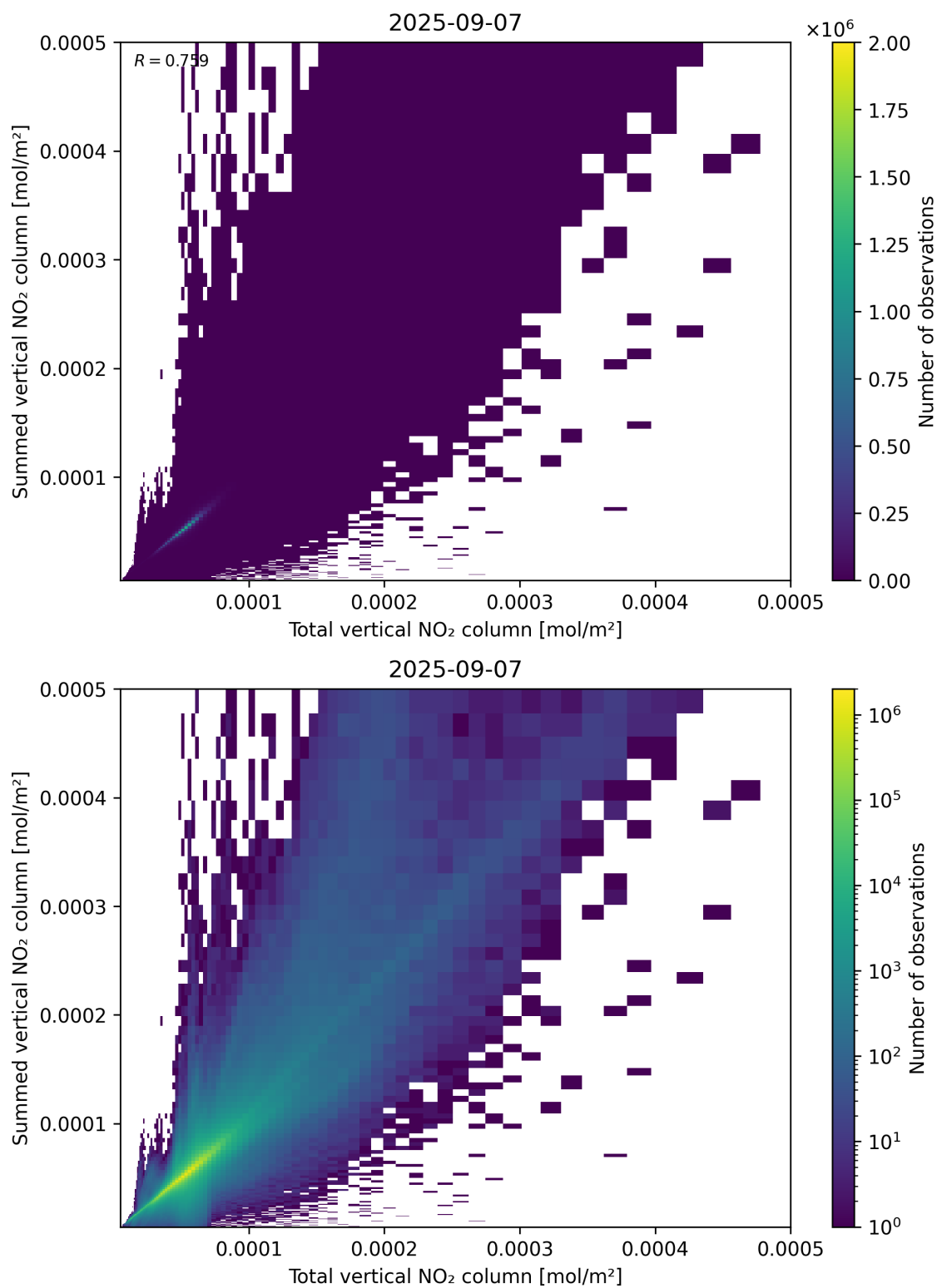
Figure 112: Scatter density plot of “Total vertical NO 2 column” against “Summed vertical NO 2 column” for 2025-09-06 to 2025-09-08.
