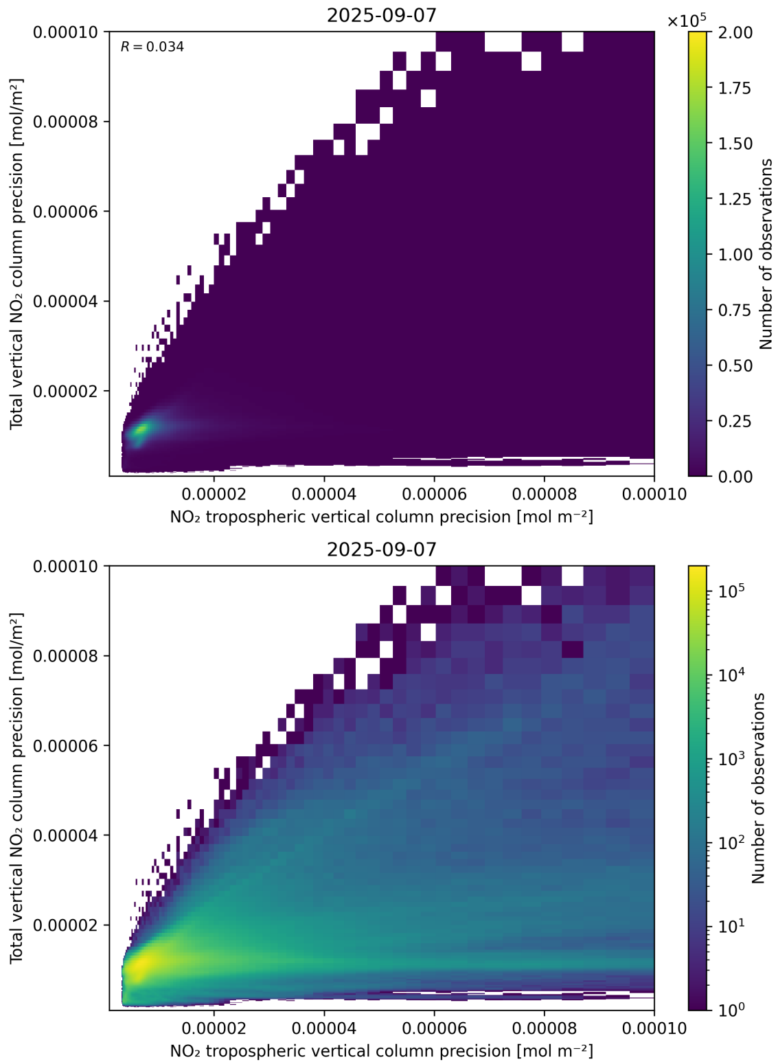
Figure 139: Scatter density plot of “NO 2 tropospheric vertical column precision” against “Total vertical NO 2 column precision” for 2025-09-06 to 2025-09-08.
