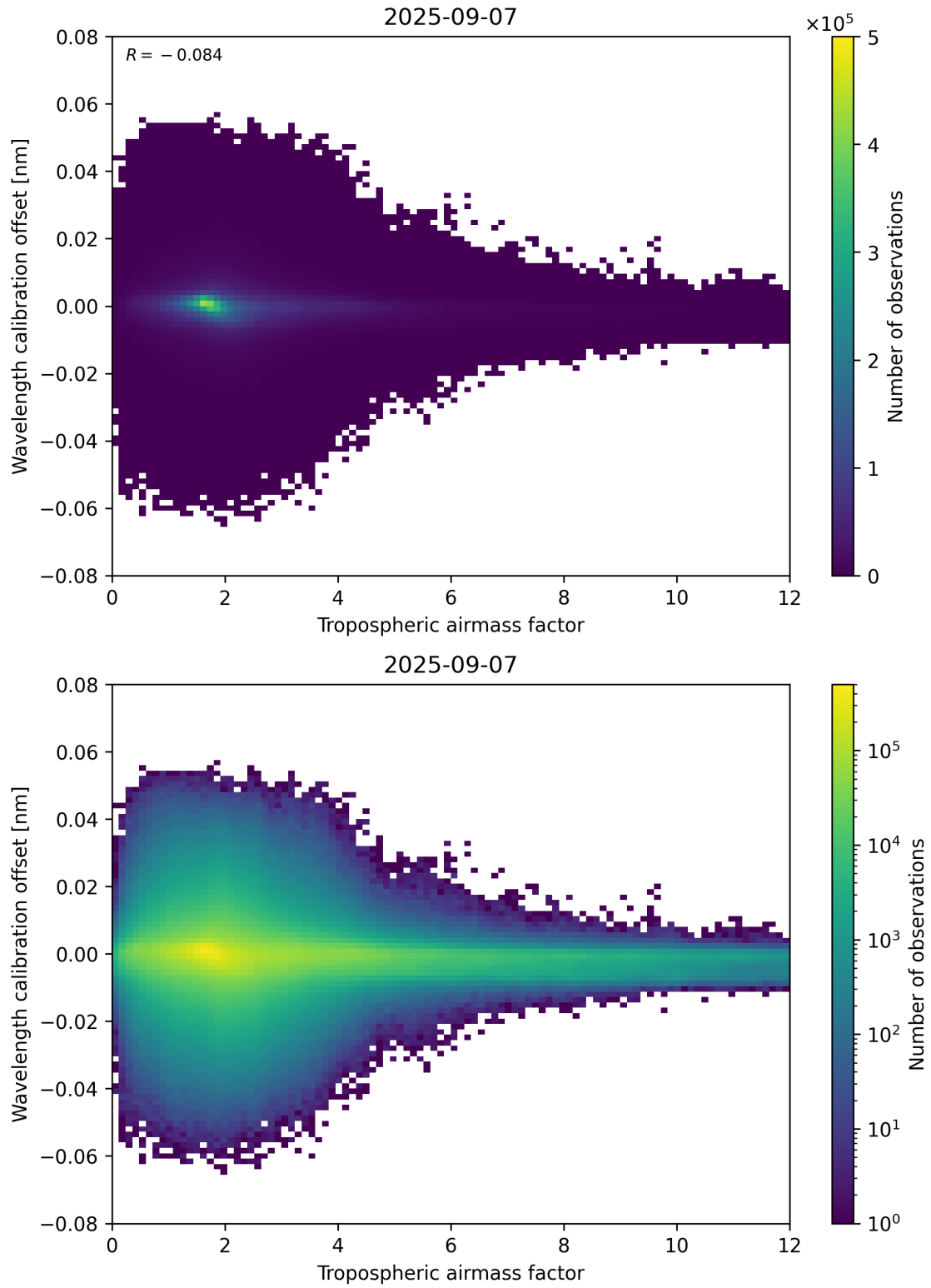
Figure 80: Scatter density plot of “Tropospheric airmass factor” against “Wavelength calibration offset” for 2025-09-06 to 2025-09-08.
