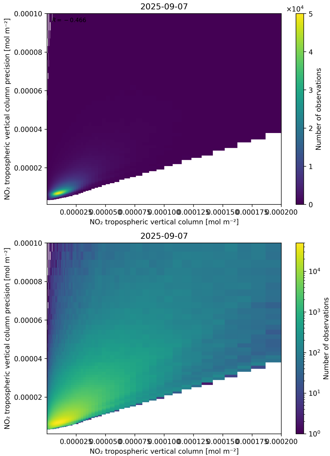
Figure 130: Scatter density plot of “NO 2 tropospheric vertical column” against “NO 2 tropospheric vertical column precision” for 2025-09-06 to 2025-09-08.
