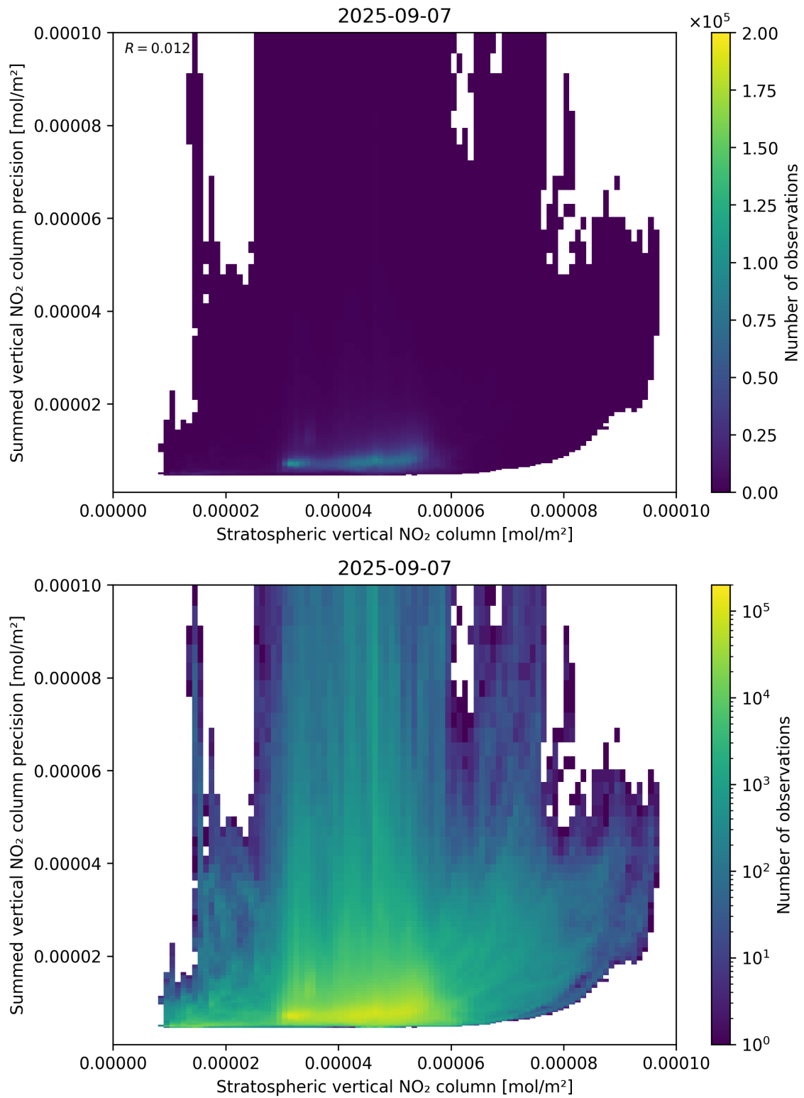
Figure 99: Scatter density plot of “Stratospheric vertical NO 2 column” against “Summed vertical NO 2 column precision” for 2025-09-06 to 2025-09-08.
