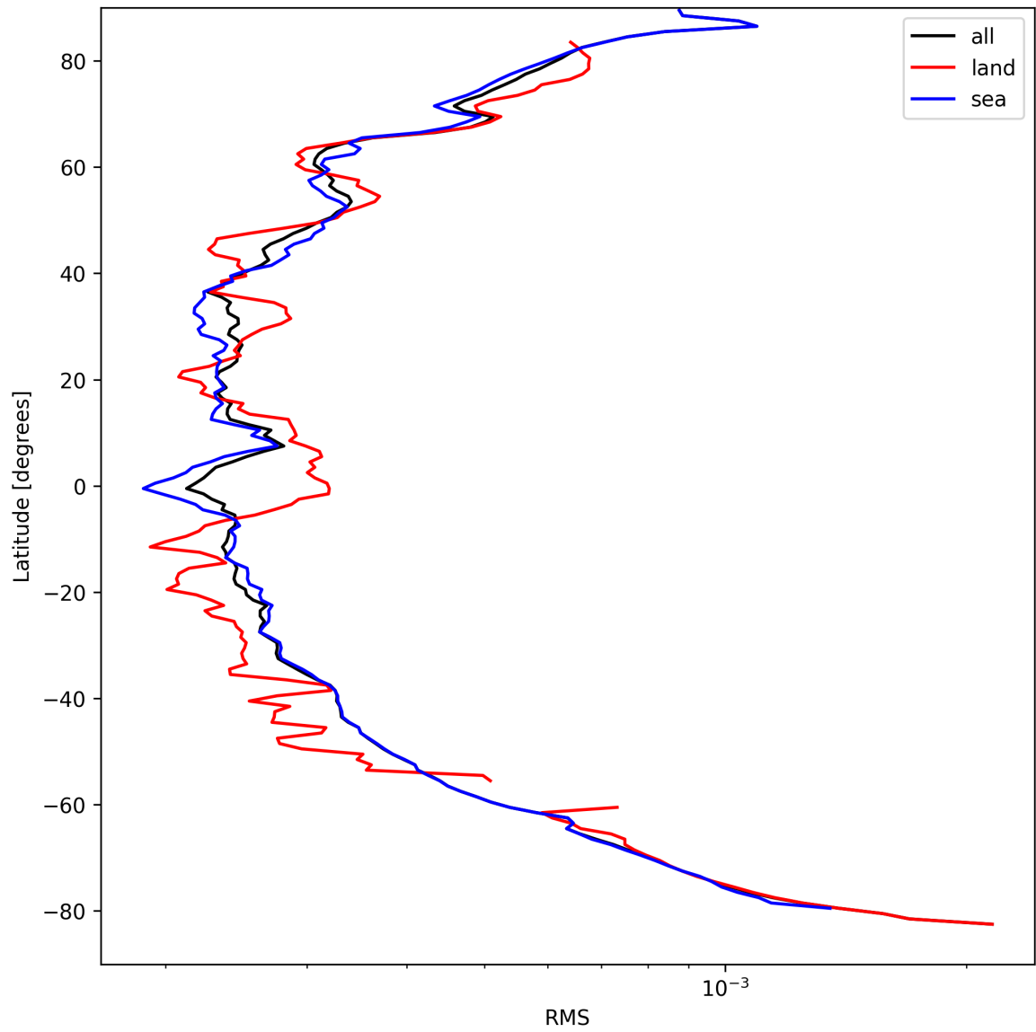
Figure 26: Zonal average of “RMS” for 2025-09-06 to 2025-09-08.
