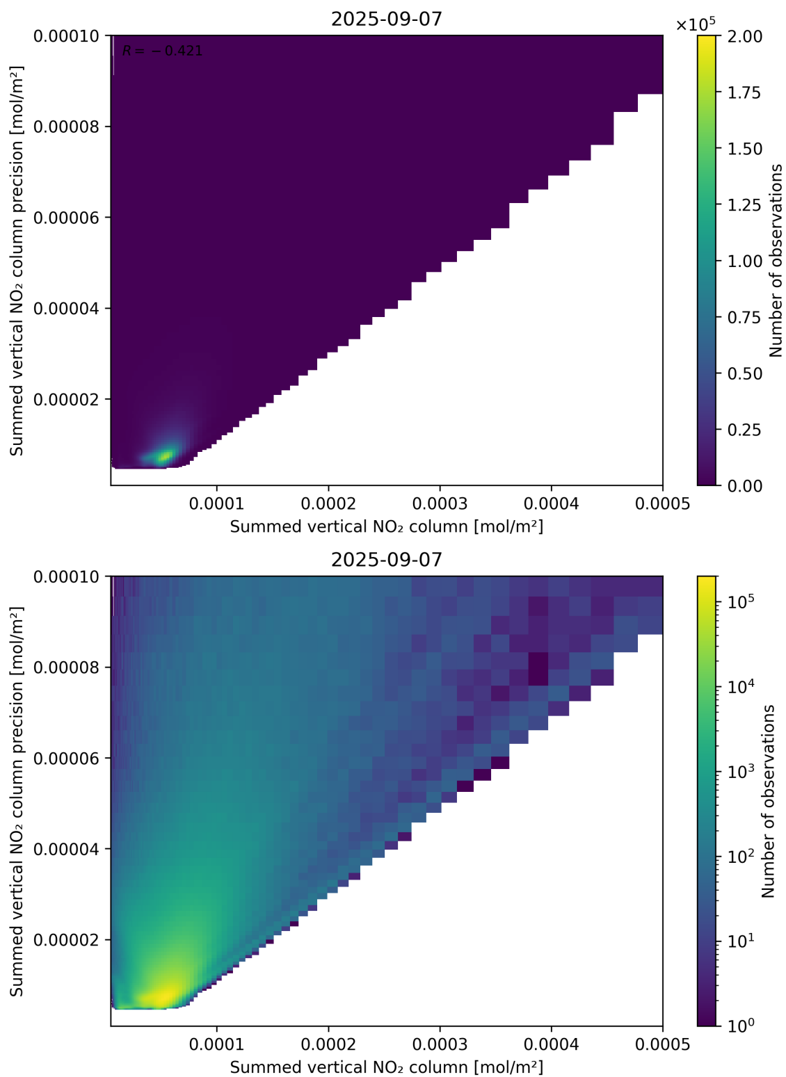
Figure 105: Scatter density plot of “Summed vertical NO 2 column” against “Summed vertical NO 2 column precision” for 2025-09-06 to 2025-09-08.
