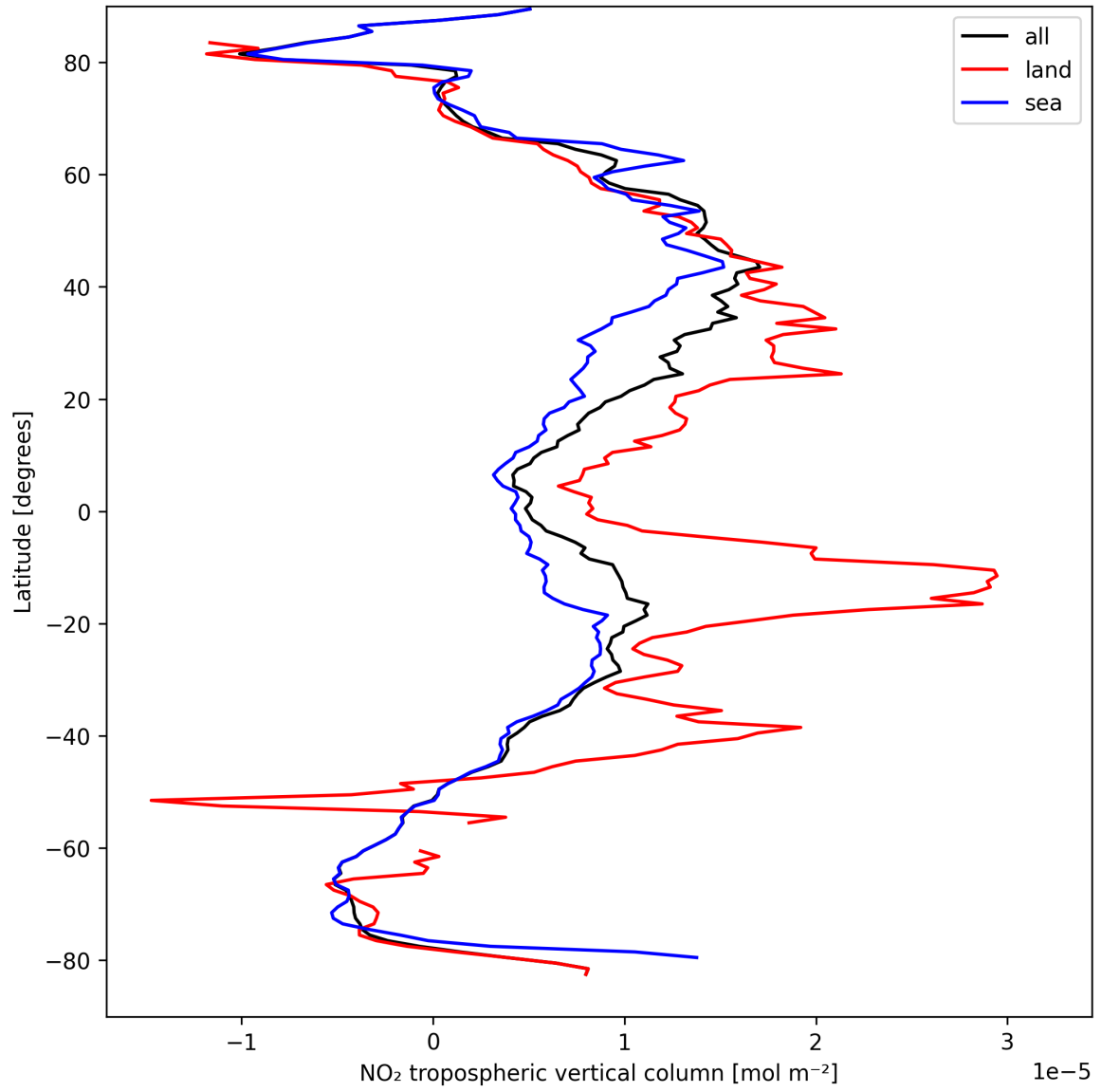
Figure 12: Zonal average of “NO 2 tropospheric vertical column” for 2025-09-06 to 2025-09-08.
