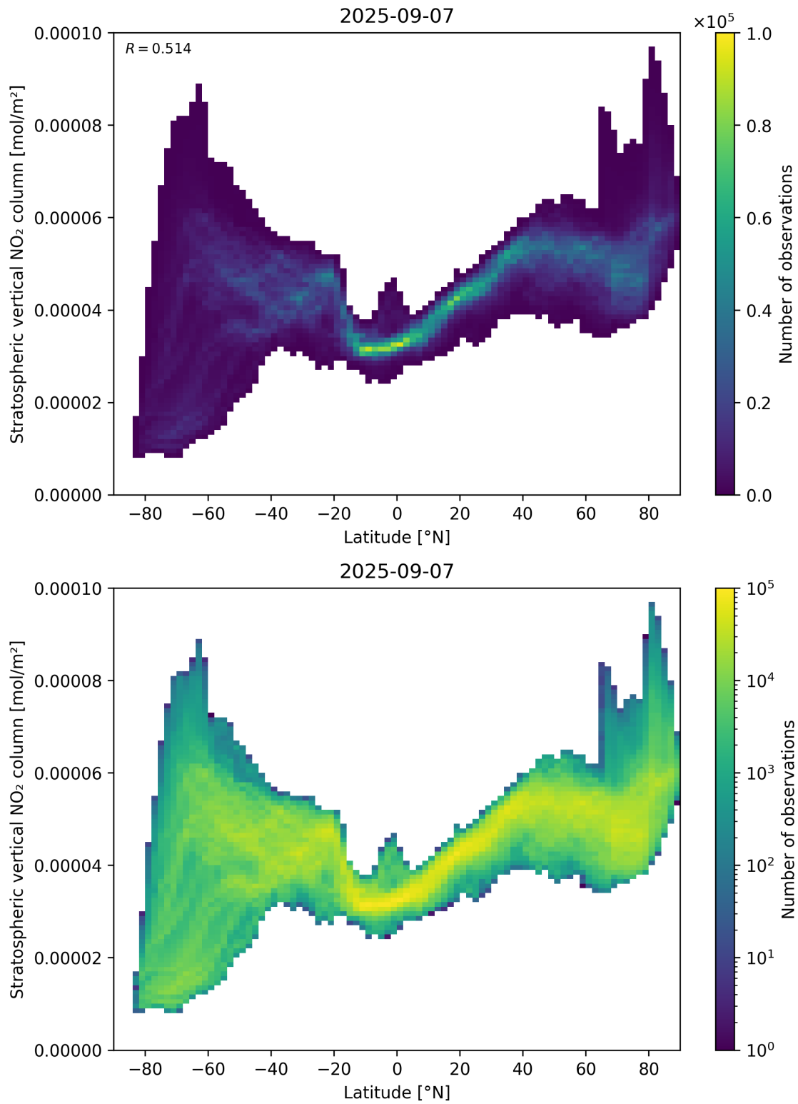
Figure 87: Scatter density plot of “Latitude” against “Stratospheric vertical NO 2 column” for 2025-09-06 to 2025-09-08.
