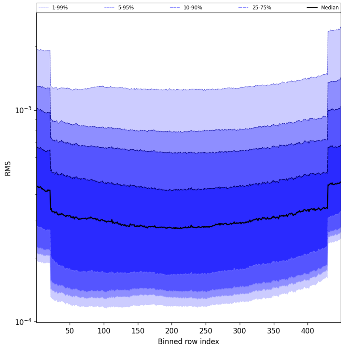
Figure 60: Along track statistics of “RMS” for 2025-09-06 to 2025-09-08
