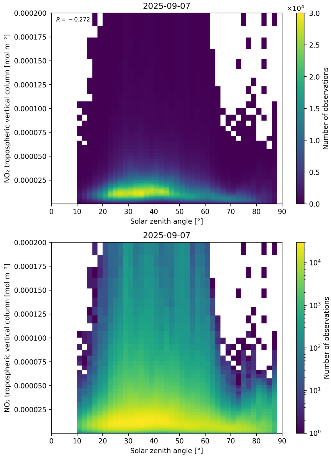
Figure 155: Scatter density plot of “Solar zenith angle” against “NO 2 tropospheric vertical column” for 2025-09-06 to 2025-09-08.
