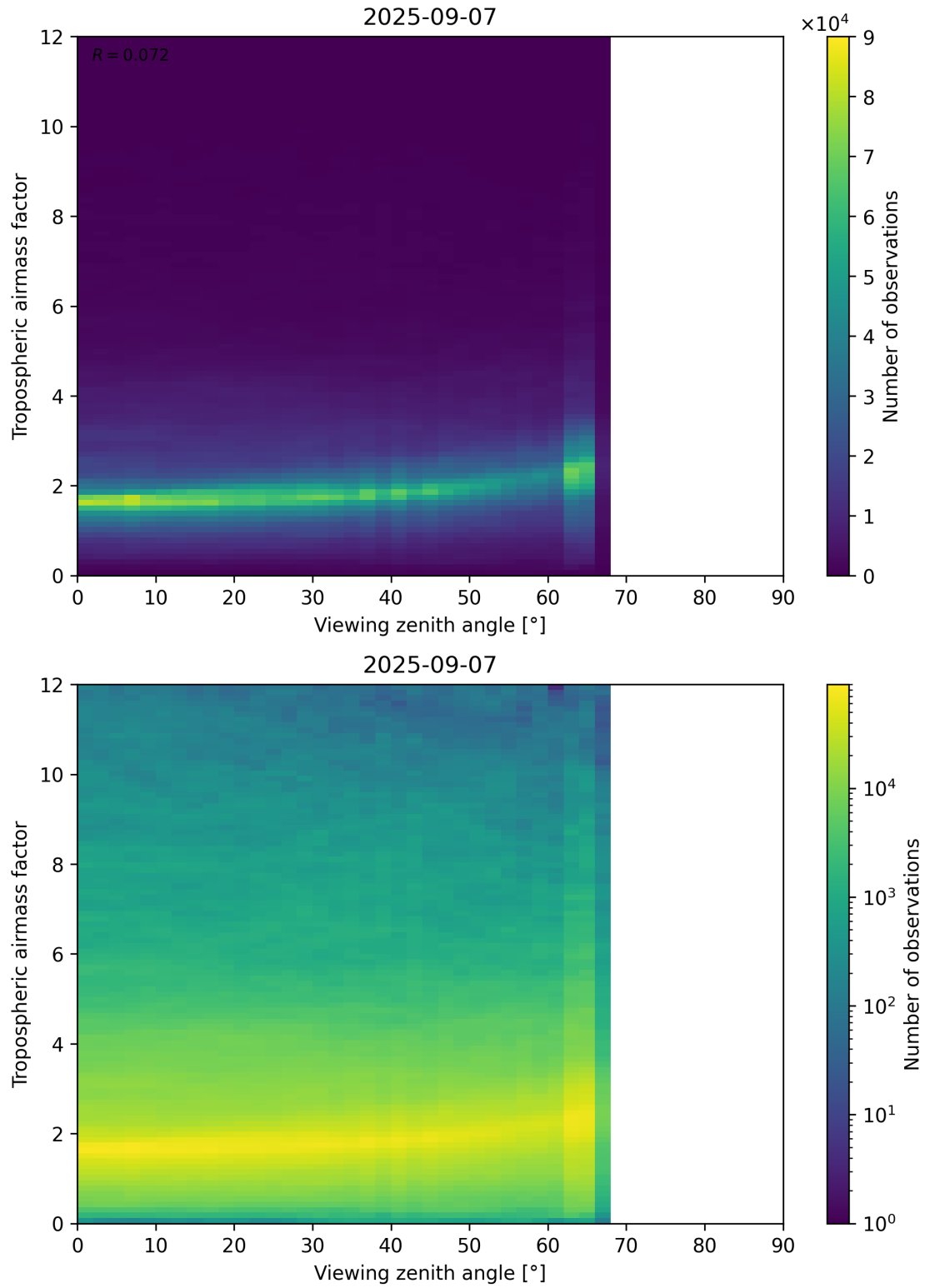
Figure 161: Scatter density plot of “Viewing zenith angle” against “Tropospheric airmass factor” for 2025-09-06 to 2025-09-08.
