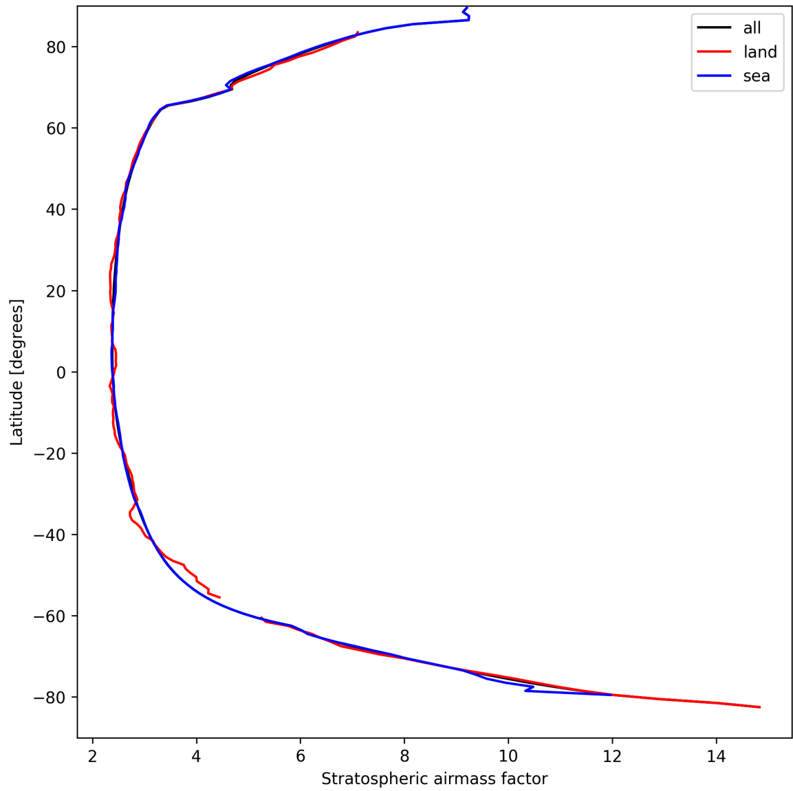
Figure 27: Zonal average of “Stratospheric air mass factor” for 2025-09-06 to 2025-09-08.
