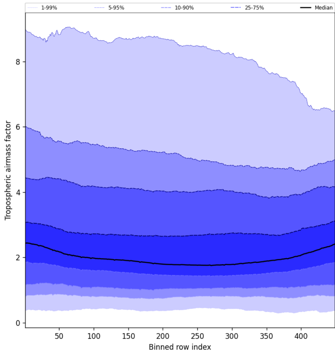
Figure 48: Along track statistics of “Tropospheric air mass factor” for 2025-09-06 to 2025-09-08
