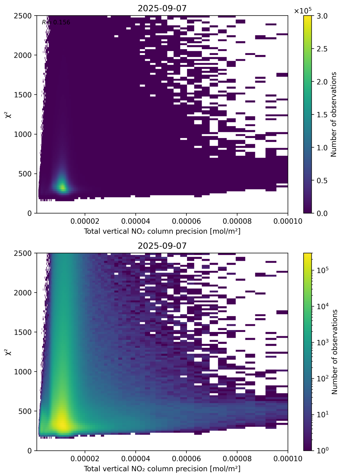
Figure 116: Scatter density plot of “Total vertical NO 2 column precision” against “ \chi^2 ” for 2025-09-06 to 2025-09-08.
