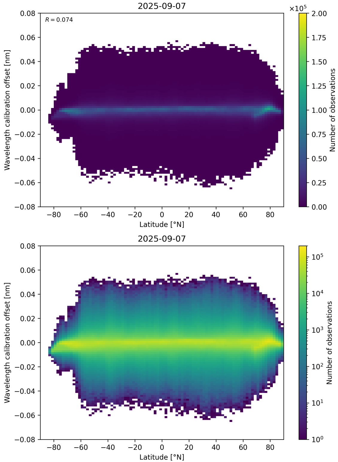
Figure 95: Scatter density plot of “Latitude” against “Wavelength calibration offset” for 2025-09-06 to 2025-09-08.
