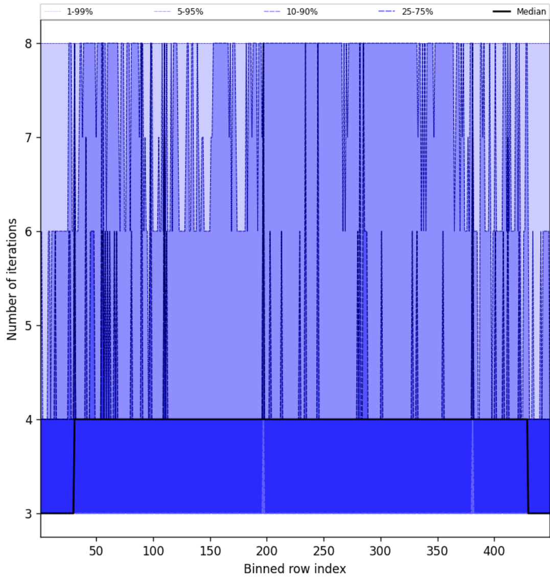
Figure 51: Along track statistics of “Number of iterations” for 2025-09-06 to 2025-09-08
