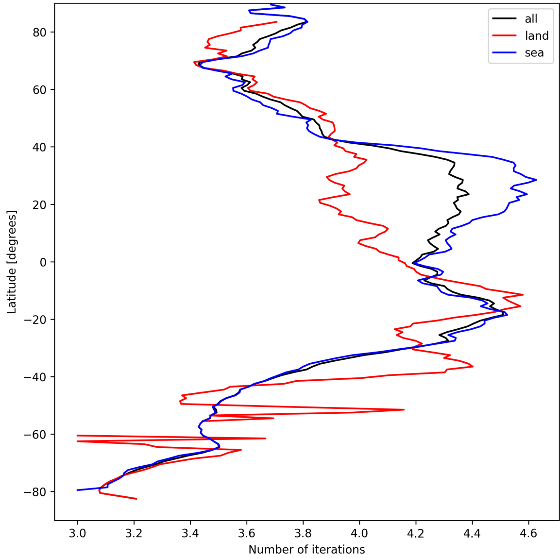
Figure 17: Zonal average of “Number of iterations” for 2025-09-06 to 2025-09-08.
