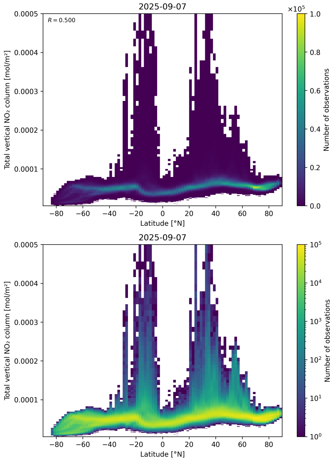
Figure 90: Scatter density plot of “Latitude” against “Total vertical NO 2 column” for 2025-09-06 to 2025-09-08.
