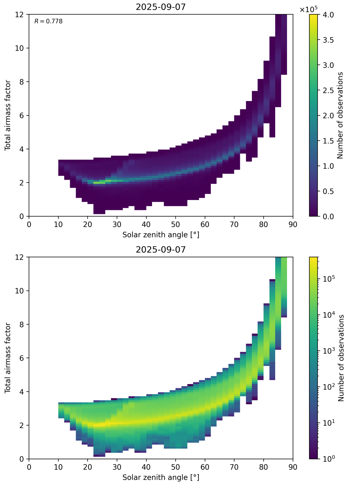
Figure 146: Scatter density plot of “Solar zenith angle” against “Total air mass factor” for 2025-09-06 to 2025-09-08.
