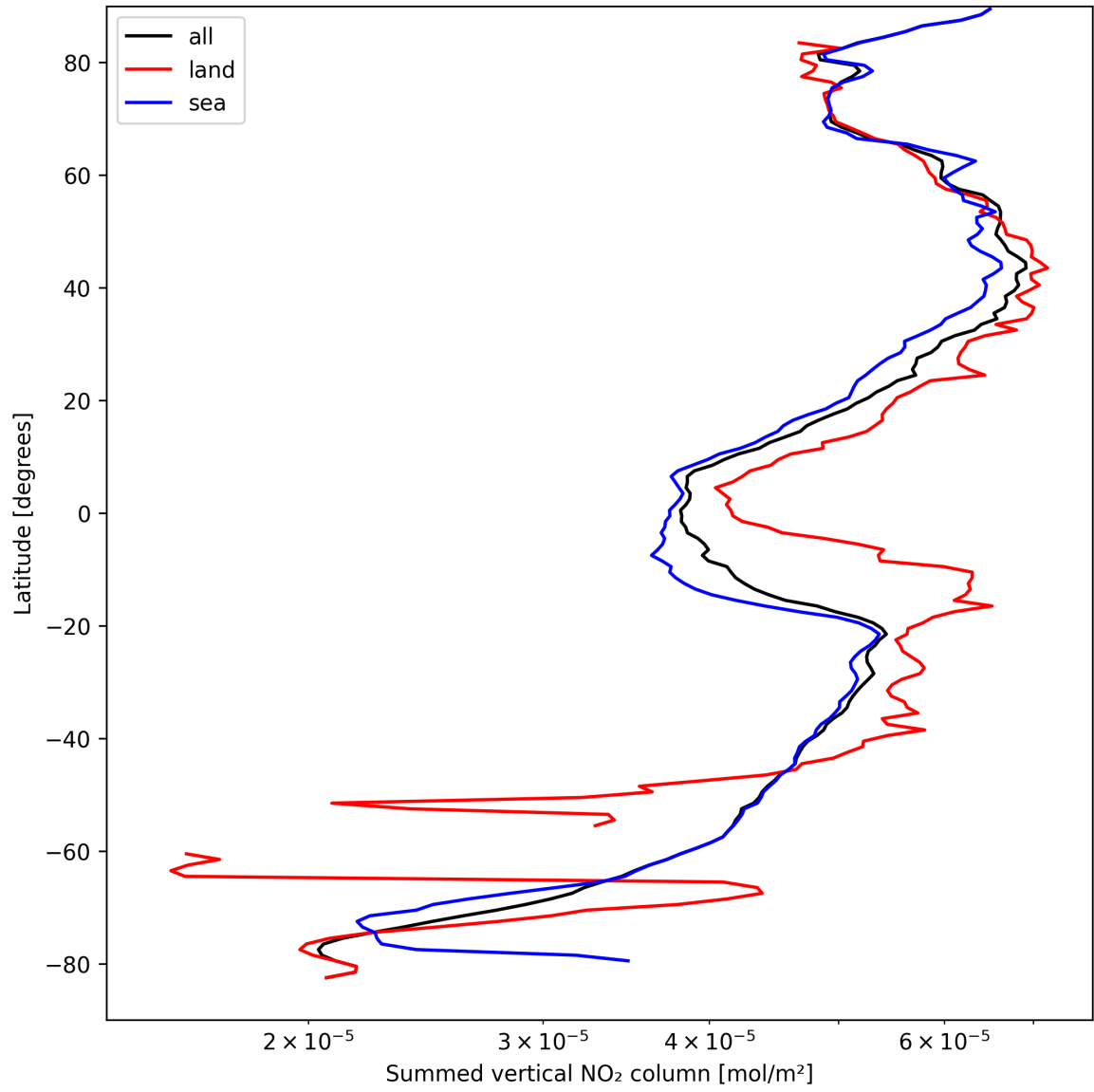
Figure 23: Zonal average of “Summed vertical NO 2 column” for 2025-09-06 to 2025-09-08.
