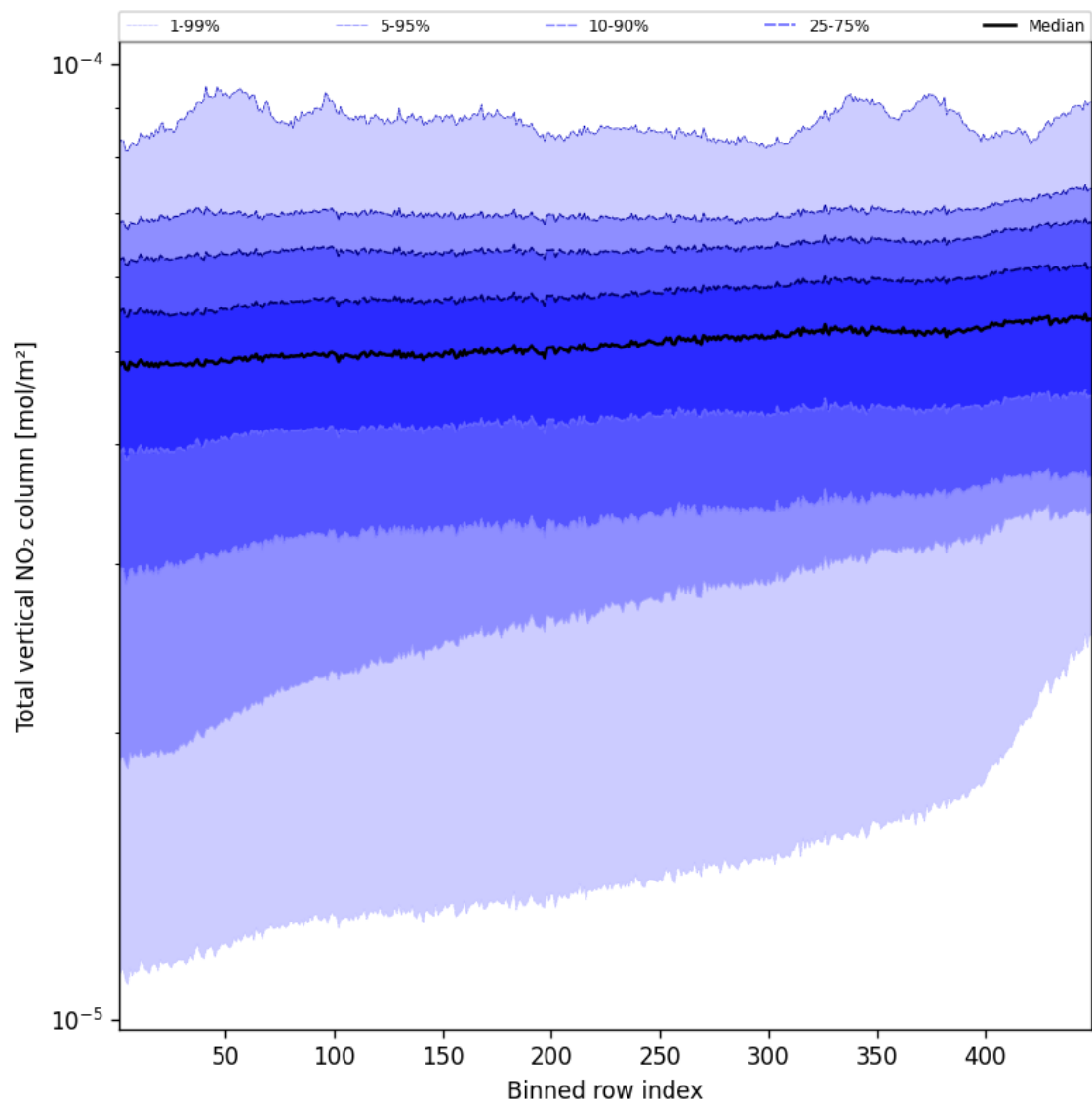
Figure 55: Along track statistics of “Total vertical NO 2 column” for 2025-09-06 to 2025-09-08
