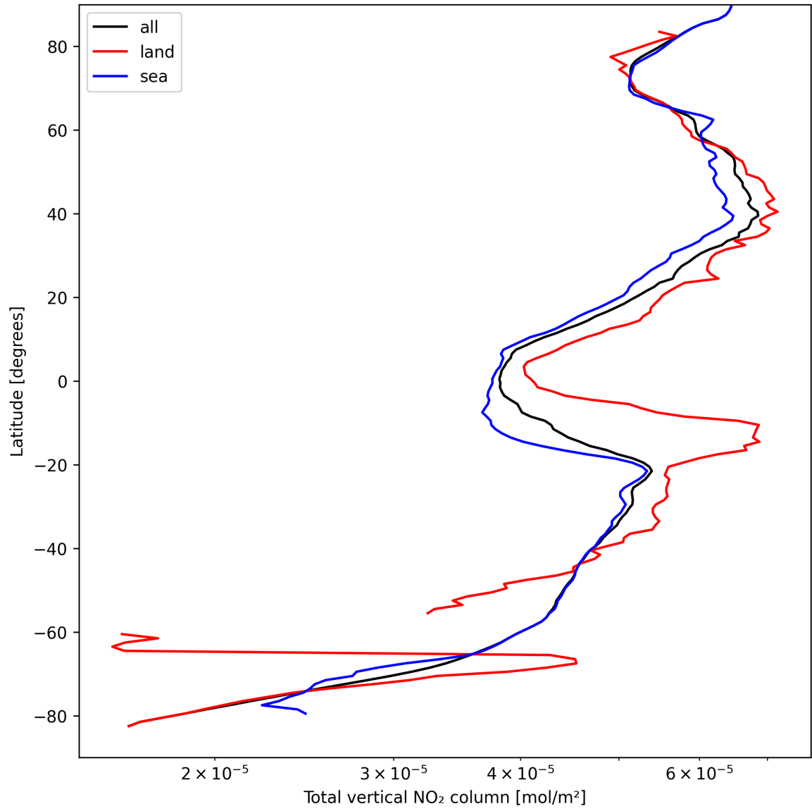
Figure 21: Zonal average of “Total vertical NO 2 column” for 2025-09-06 to 2025-09-08.
