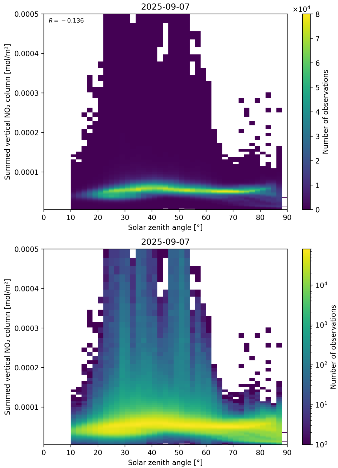
Figure 151: Scatter density plot of “Solar zenith angle” against “Summed vertical NO 2 column” for 2025-09-06 to 2025-09-08.
