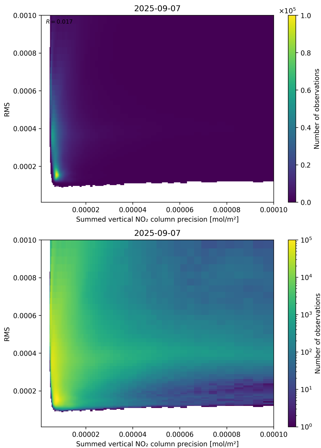
Figure 108: Scatter density plot of “Summed vertical NO 2 column precision” against “RMS” for 2025-09-06 to 2025-09-08.
