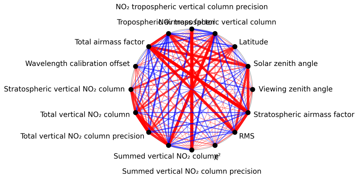
Figure 1: Map of correlation graph for 2025-09-06 to 2025-09-08.
