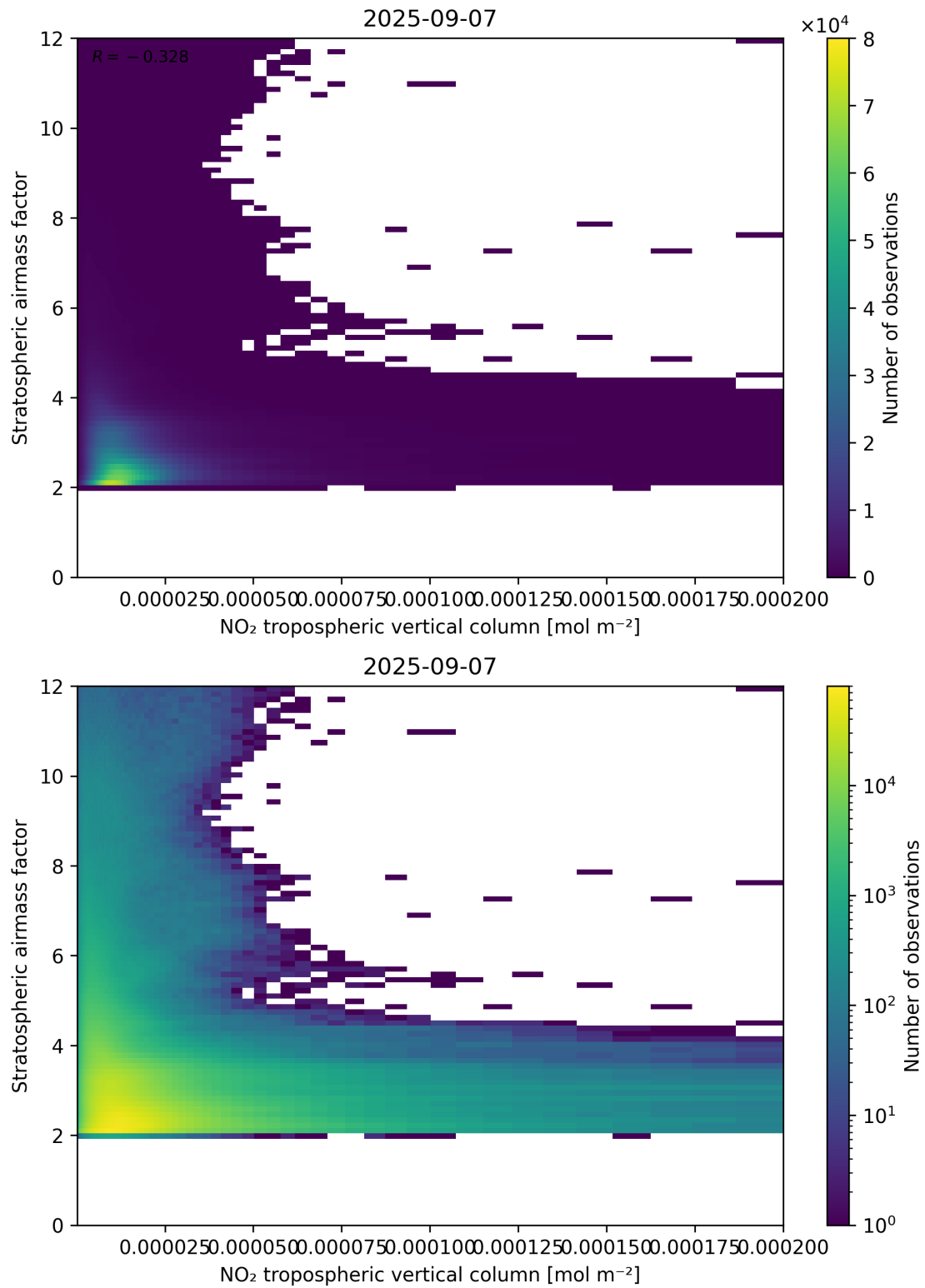
Figure 121: Scatter density plot of “NO 2 tropospheric vertical column” against “Stratospheric air mass factor” for 2025-09-06 to 2025-09-08.
