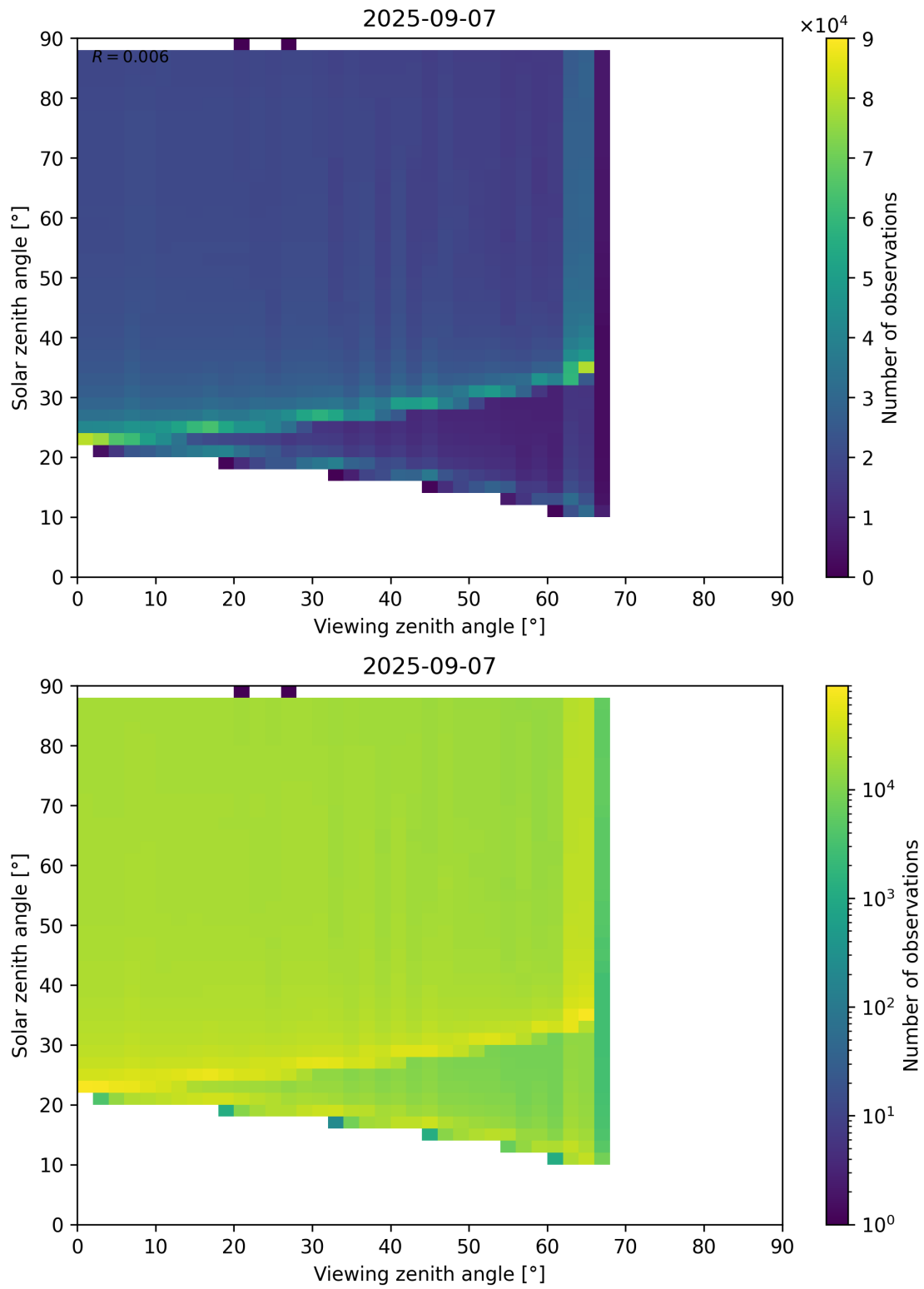
Figure 172: Scatter density plot of “Viewing zenith angle” against “Solar zenith angle” for 2025-09-06 to 2025-09-08.
