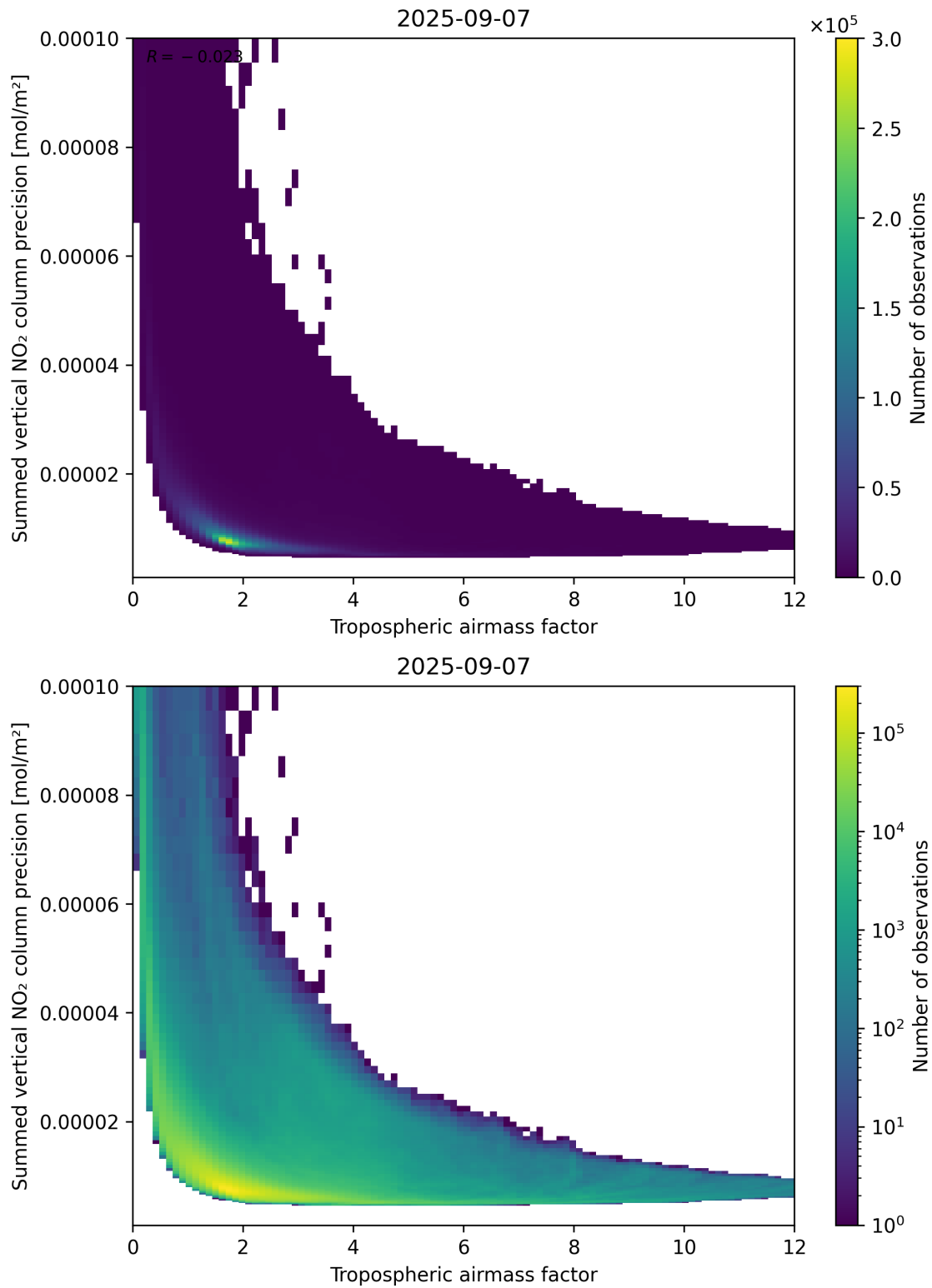
Figure 76: Scatter density plot of “Tropospheric air mass factor” against “Summed vertical NO 2 column precision” for 2025-09-06 to 2025-09-08.
