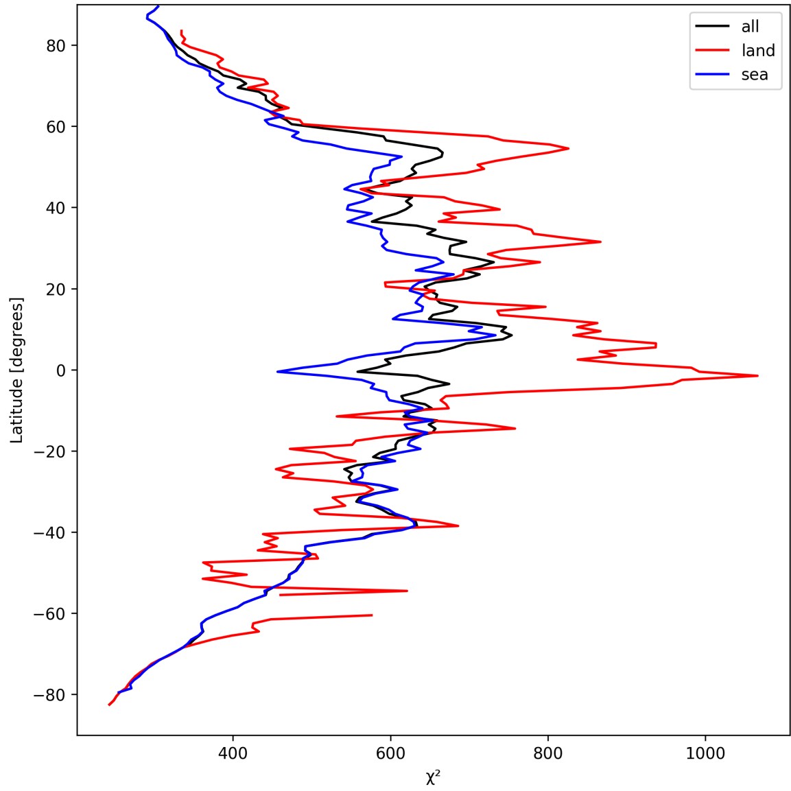
Figure 25: Zonal average of “ \chi^2 ” for 2025-09-06 to 2025-09-08.
