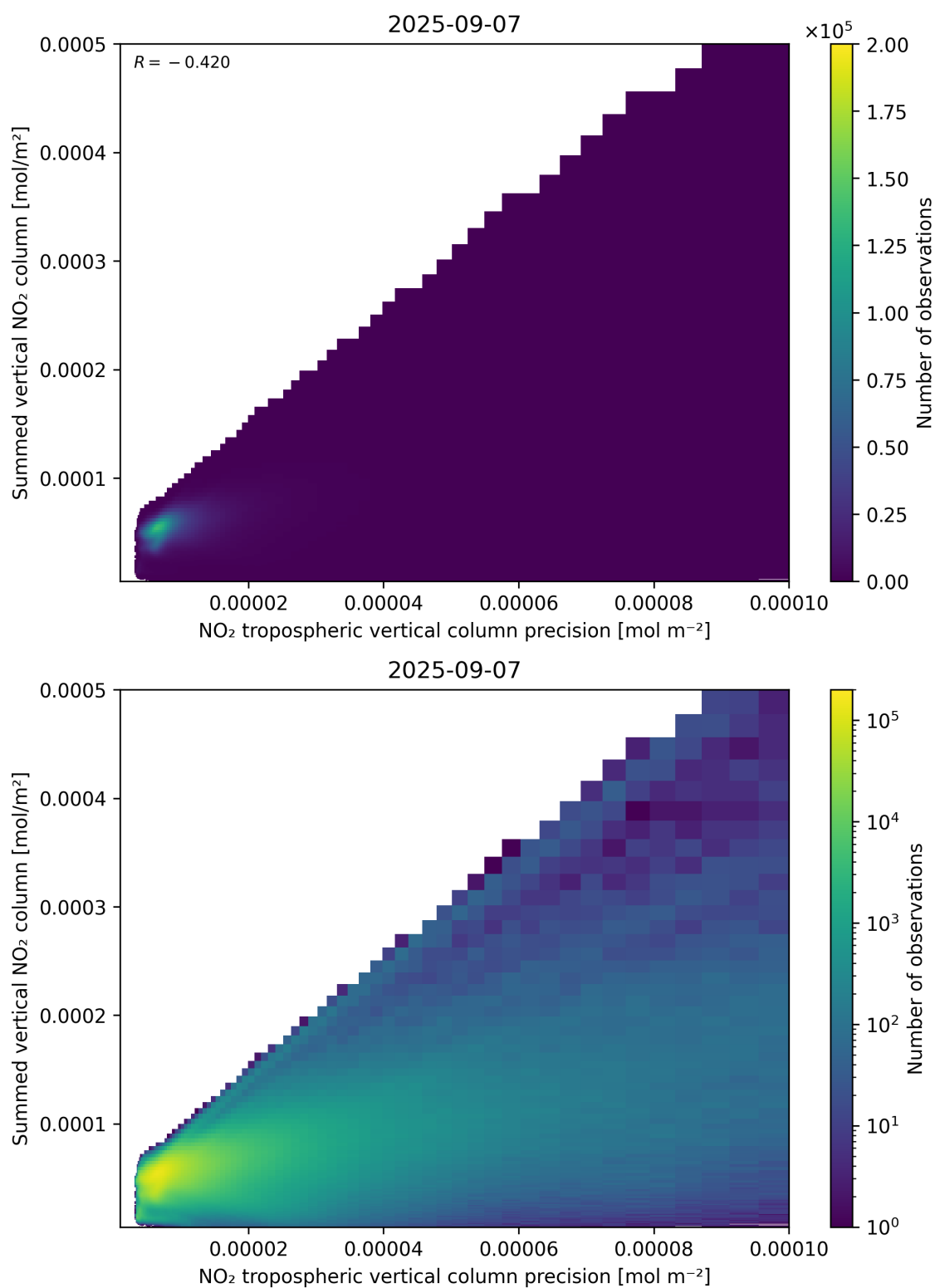
Figure 136: Scatter density plot of “NO 2 tropospheric vertical column precision” against “Summed vertical NO 2 column” for 2025-09-06 to 2025-09-08.
