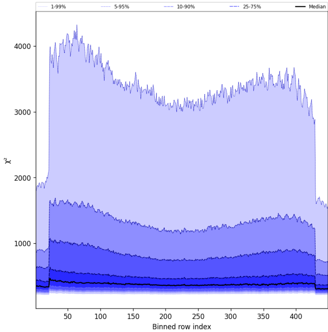
Figure 59: Along track statistics of “ \chi^2 ” for 2025-09-06 to 2025-09-08
