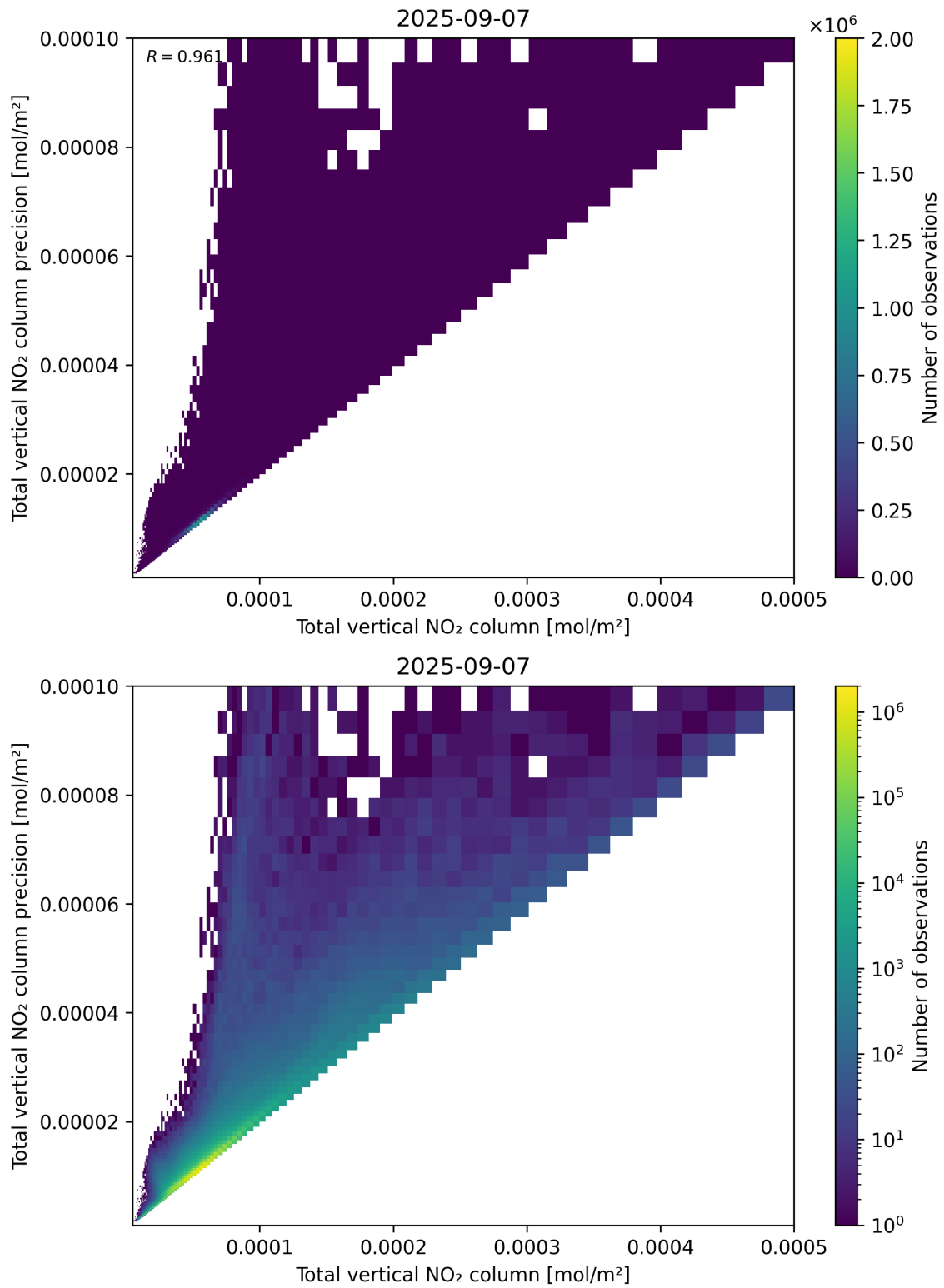
Figure 114: Scatter density plot of “Total vertical NO 2 column” against “Total vertical NO 2 column precision” for 2025-09-06 to 2025-09-08.
