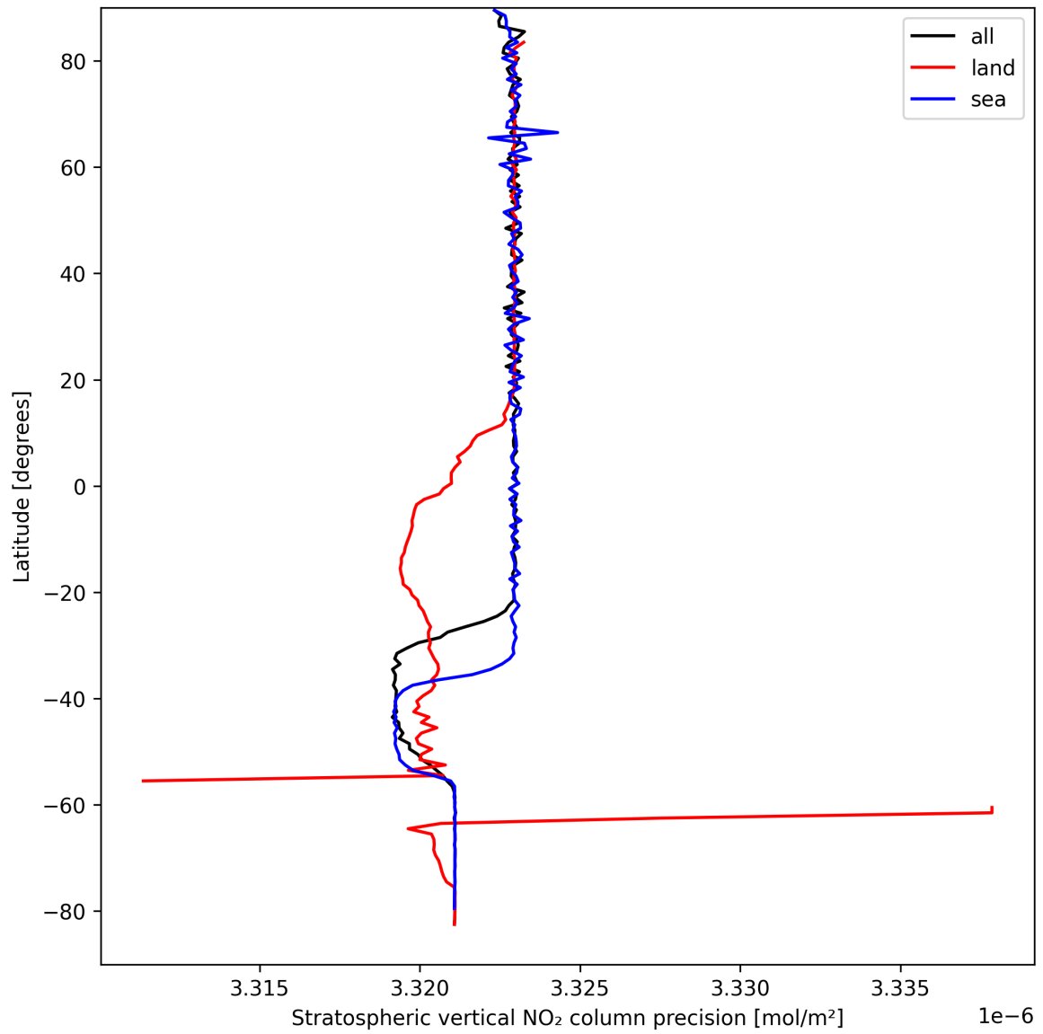
Figure 20: Zonal average of “Stratospheric vertical NO 2 column precision” for 2025-09-06 to 2025-09-08.
