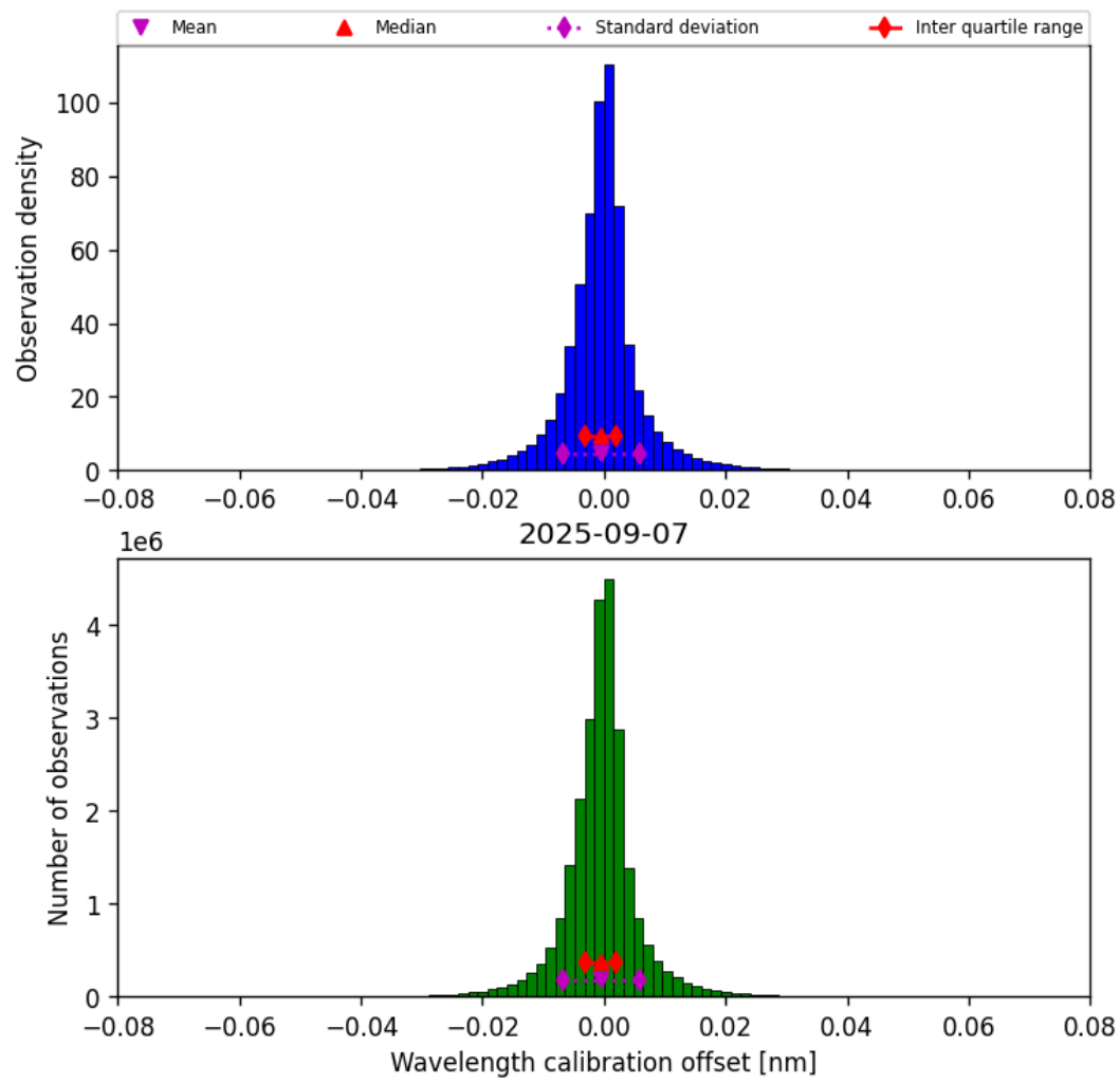
Figure 35: Histogram of “Wavelength calibration offset” for 2025-09-06 to 2025-09-08
