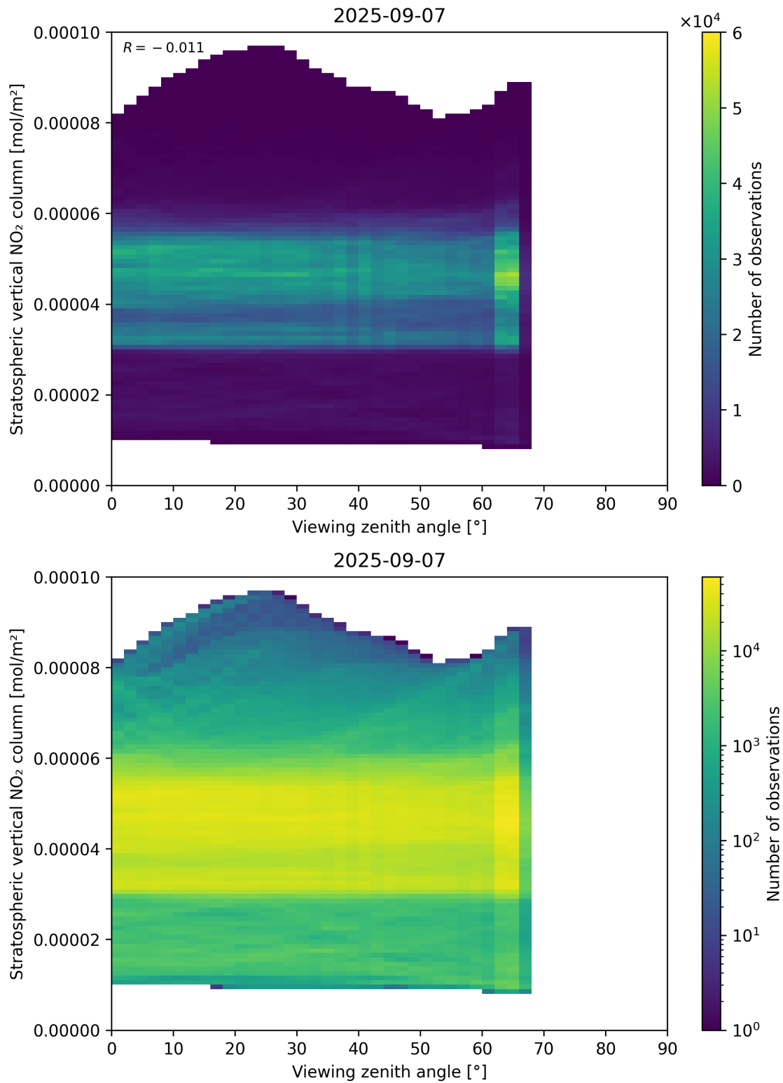
Figure 164: Scatter density plot of “Viewing zenith angle” against “Stratospheric vertical NO 2 column” for 2025-09-06 to 2025-09-08.
