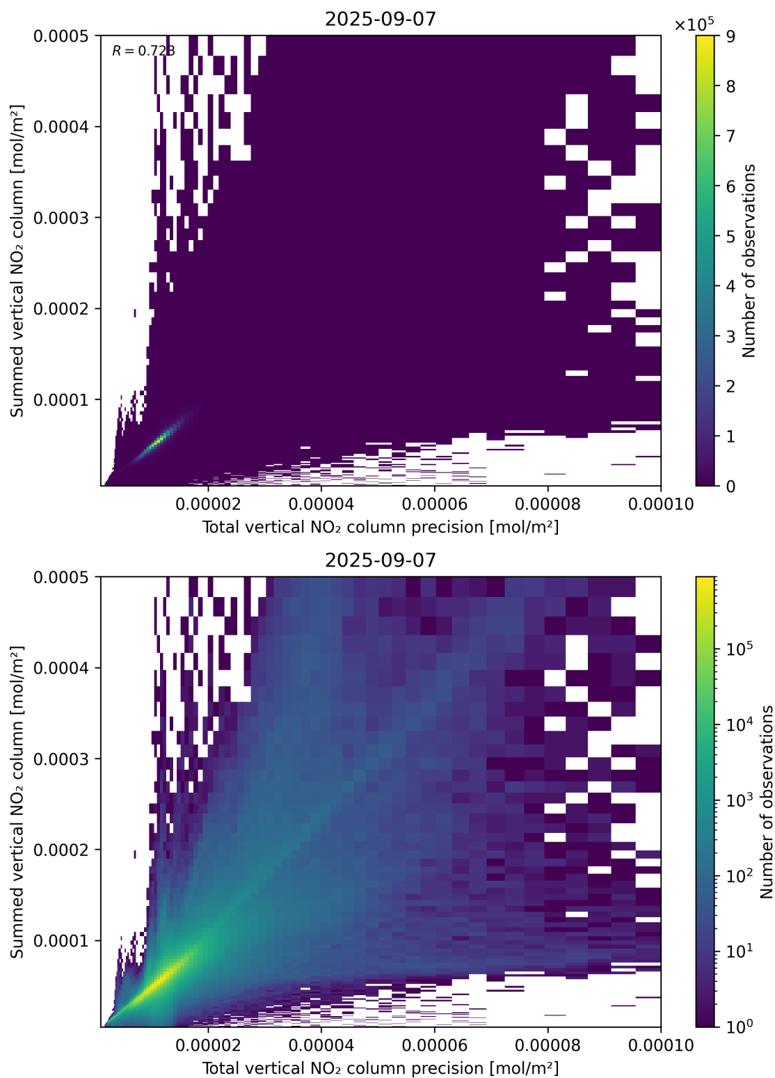
Figure 117: Scatter density plot of “Total vertical NO 2 column precision” against “Summed vertical NO 2 column” for 2025-09-06 to 2025-09-08.
