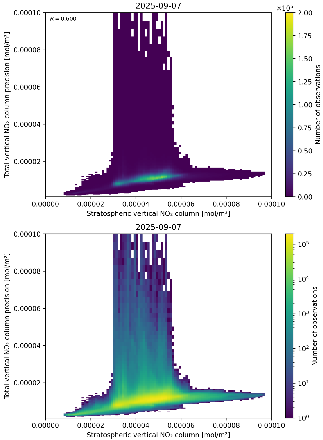
Figure 101: Scatter density plot of “Stratospheric vertical NO 2 column” against “Total vertical NO 2 column precision” for 2025-09-06 to 2025-09-08.
