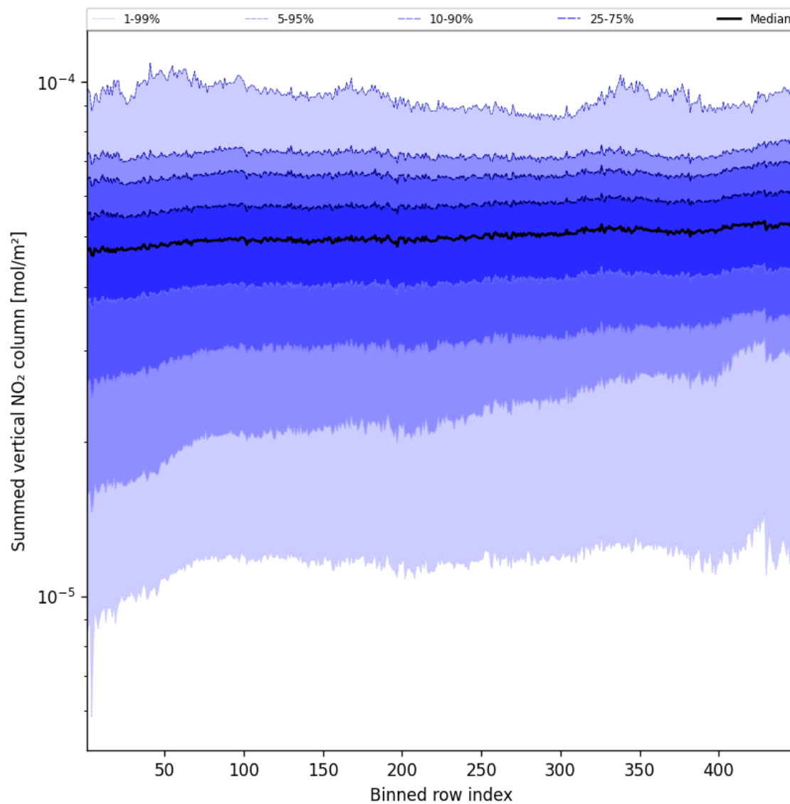
Figure 57: Along track statistics of “Summed vertical NO 2 column” for 2025-09-06 to 2025-09-08
