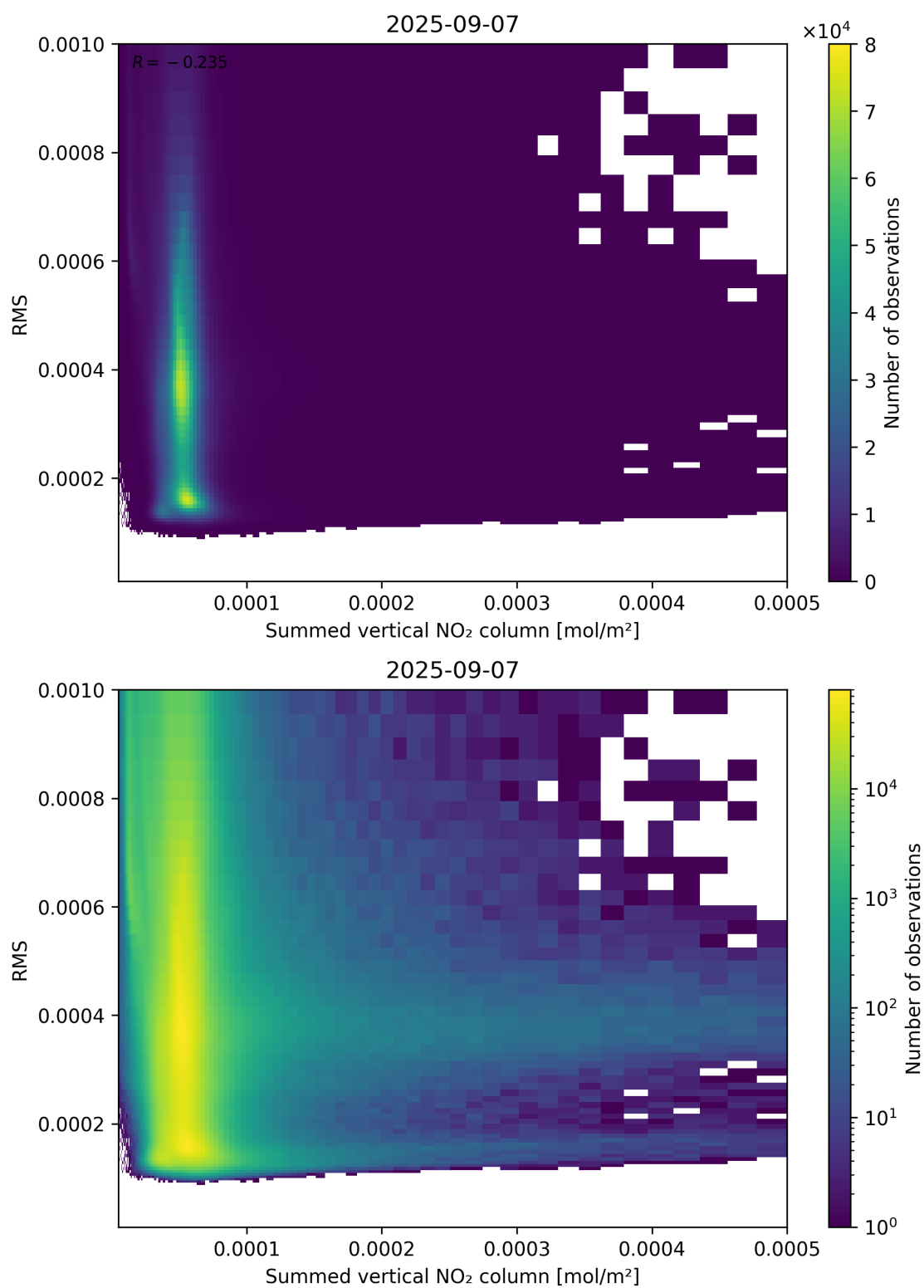
Figure 109: Scatter density plot of “Summed vertical NO 2 column” against “RMS” for 2025-09-06 to 2025-09-08.
