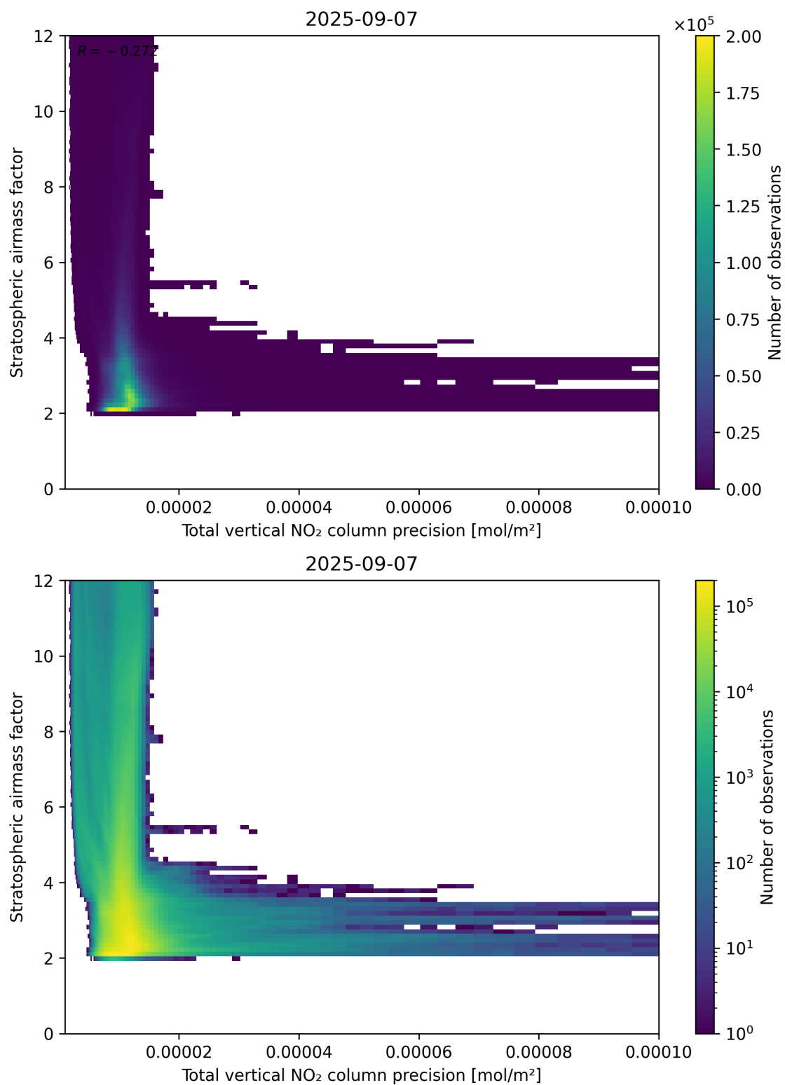
Figure 115: Scatter density plot of “Total vertical NO 2 column precision” against “Stratospheric air mass factor” for 2025-09-06 to 2025-09-08.
