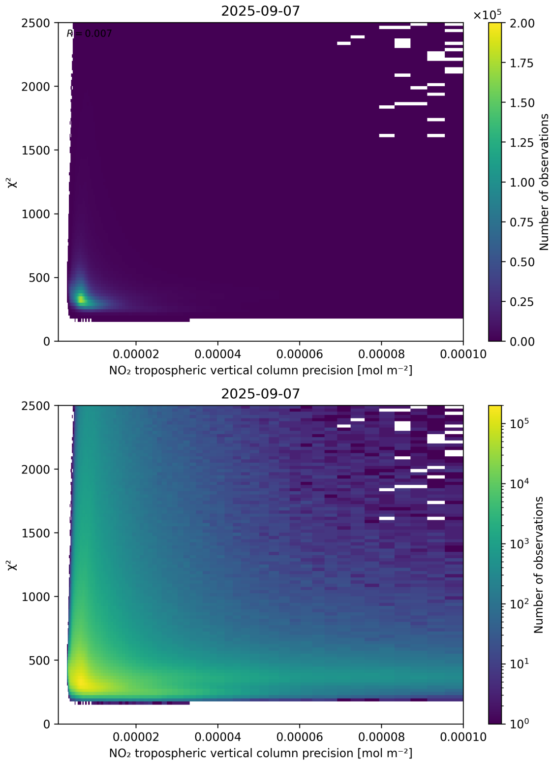
Figure 134: Scatter density plot of “NO 2 tropospheric vertical column precision” against “ \chi^2 ” for 2025-09-06 to 2025-09-08.
