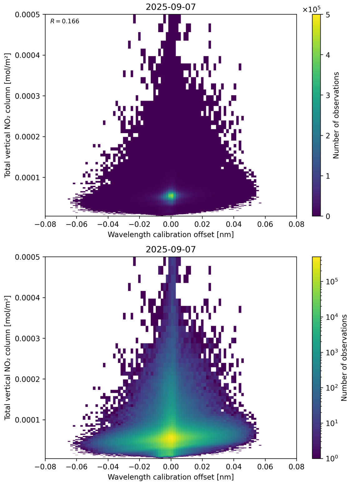
Figure 179: Scatter density plot of “Wavelength calibration offset” against “Total vertical NO 2 column” for 2025-09-06 to 2025-09-08.
