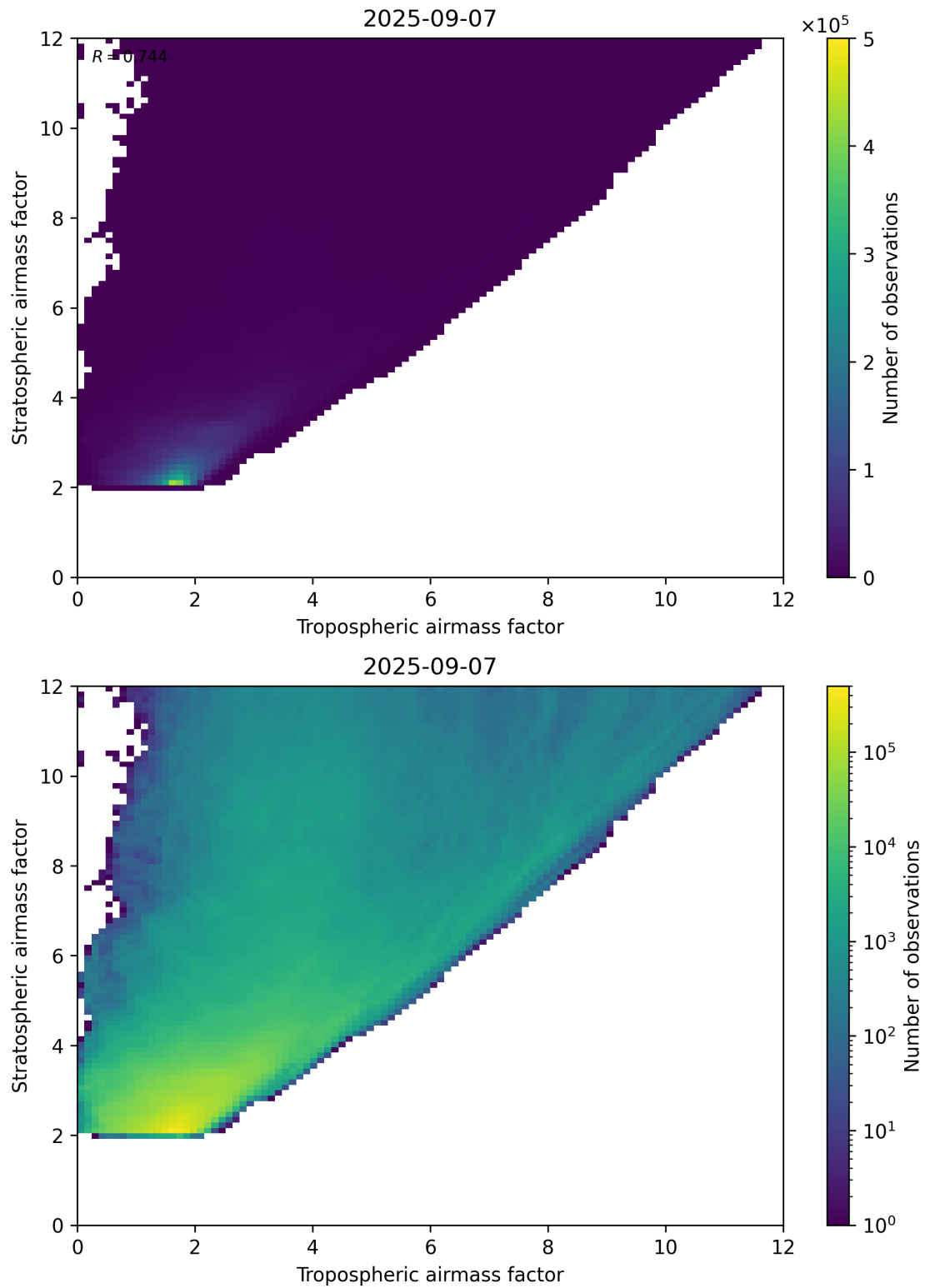
Figure 71: Scatter density plot of “Tropospheric airmass factor” against “Stratospheric airmass factor” for 2025-09-06 to 2025-09-08.
