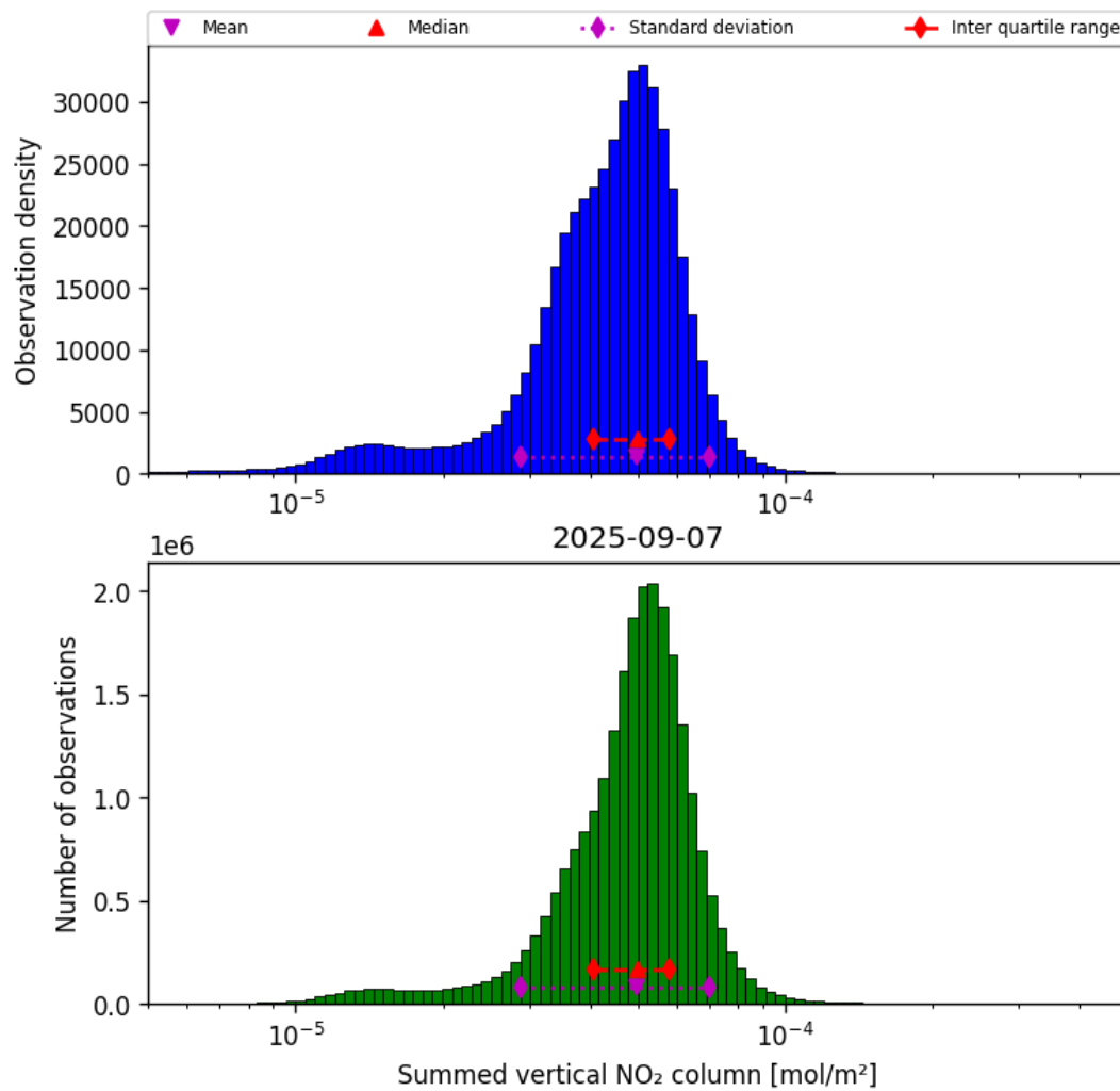
Figure 40: Histogram of “Summed vertical NO 2 column” for 2025-09-06 to 2025-09-08
