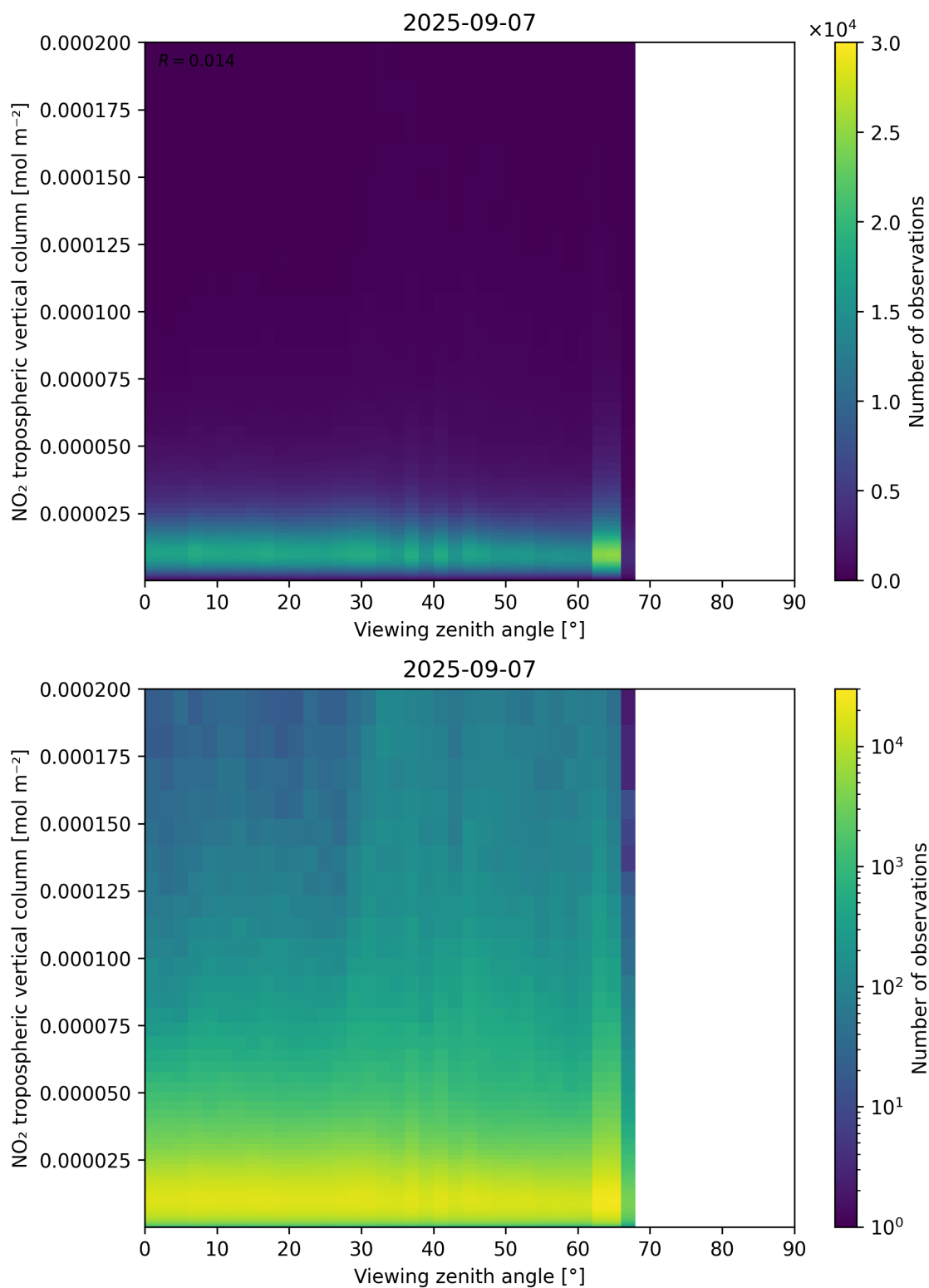
Figure 169: Scatter density plot of “Viewing zenith angle” against “NO 2 tropospheric vertical column” for 2025-09-06 to 2025-09-08.
