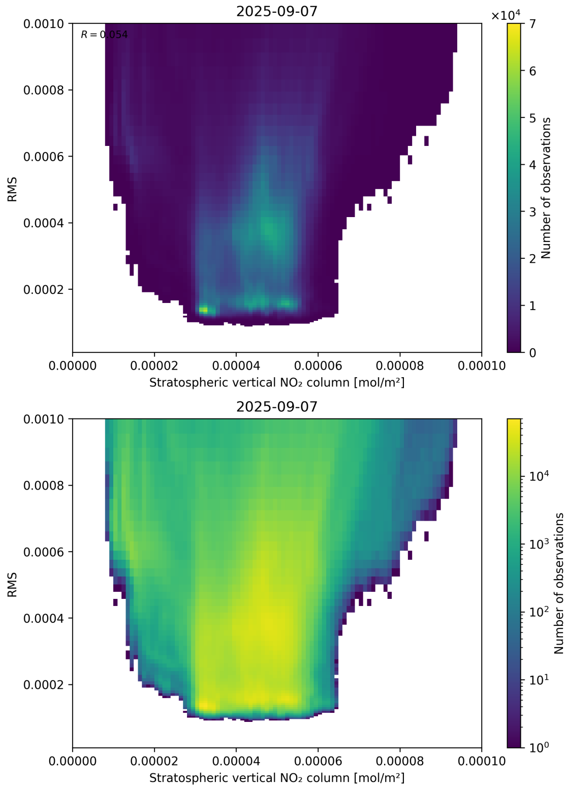
Figure 102: Scatter density plot of “Stratospheric vertical NO 2 column” against “RMS” for 2025-09-06 to 2025-09-08.
