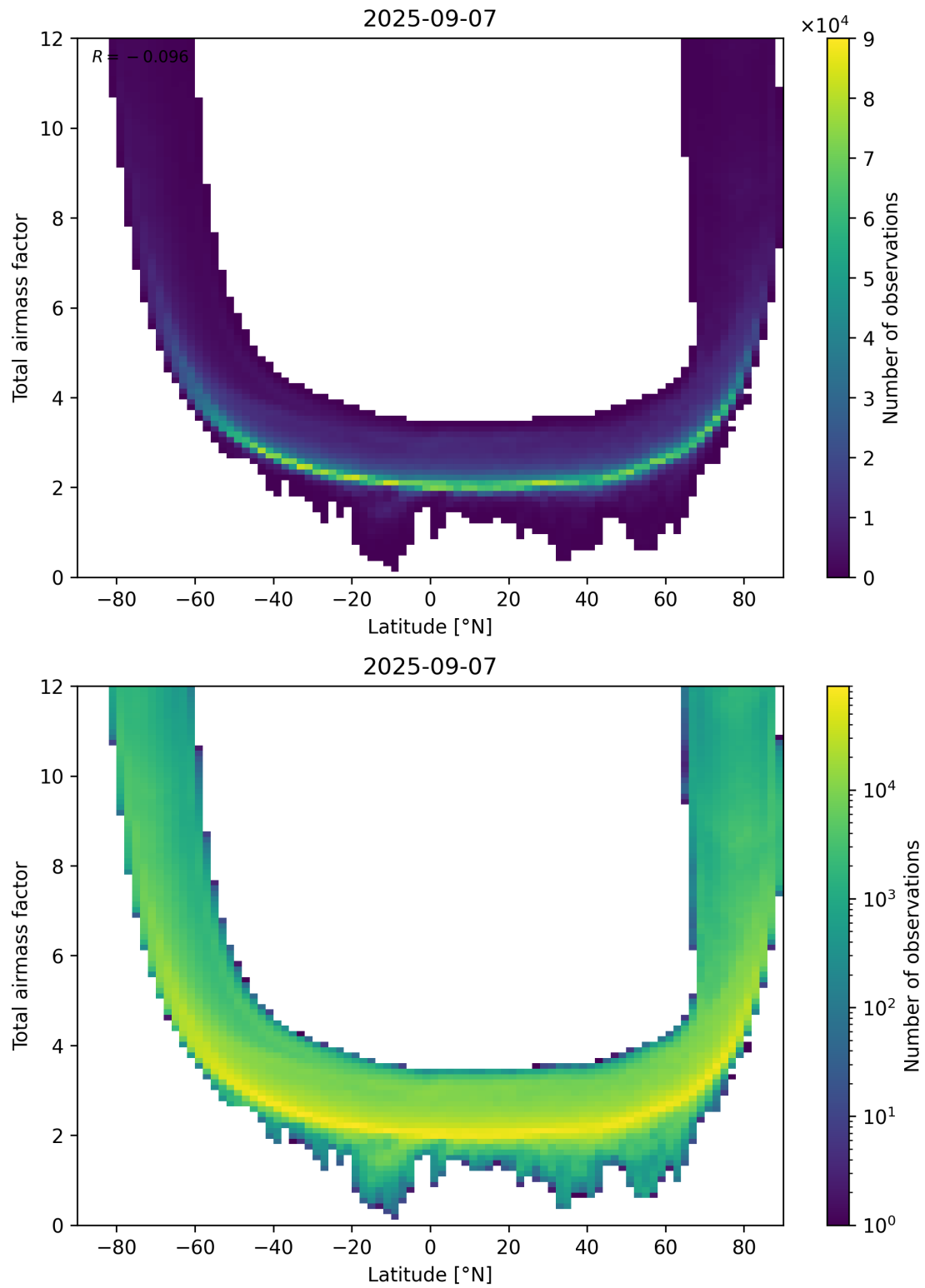
Figure 84: Scatter density plot of “Latitude” against “Total airmass factor” for 2025-09-06 to 2025-09-08.
