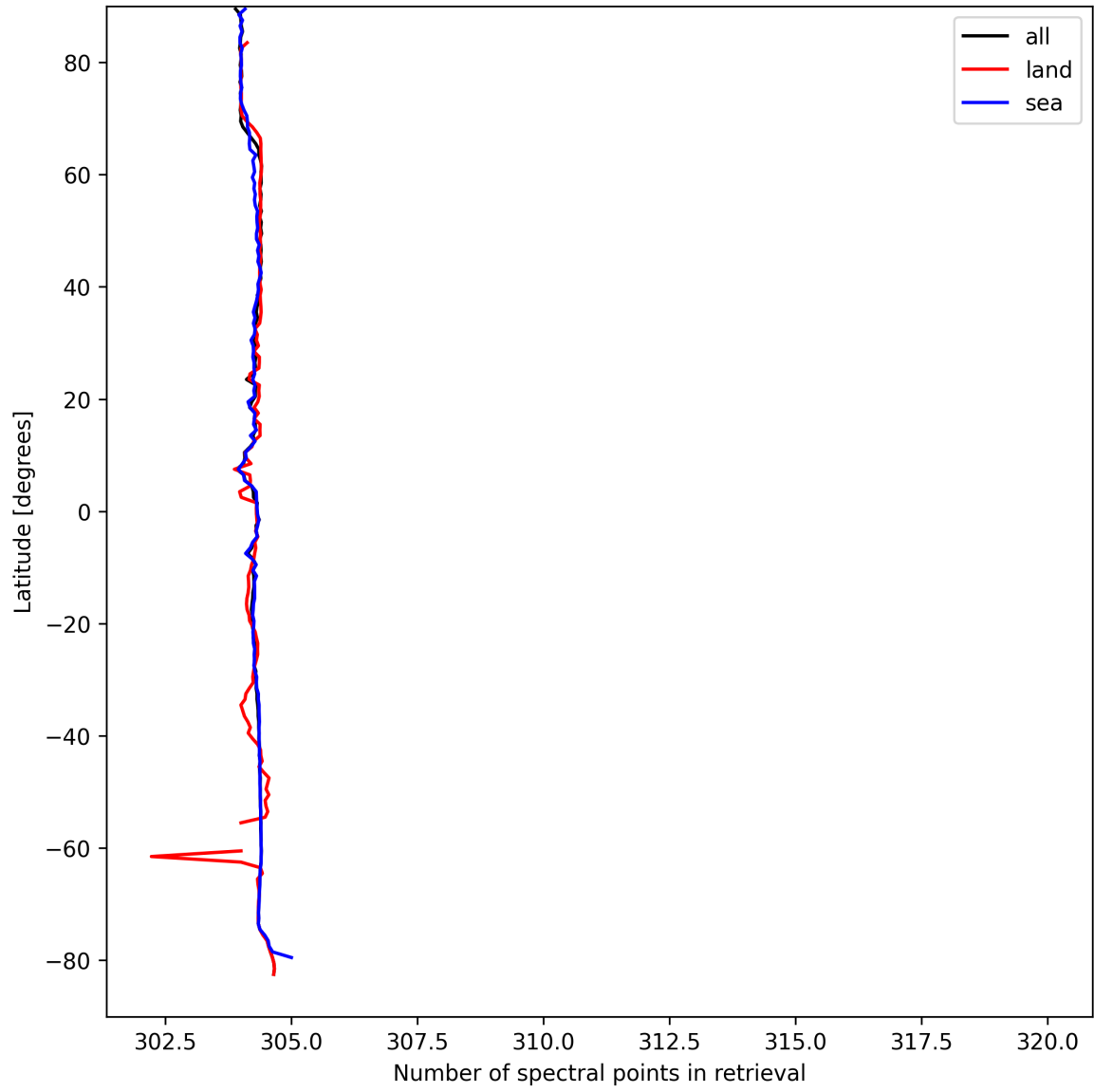
Figure 16: Zonal average of “Number of spectral points in retrieval” for 2025-09-06 to 2025-09-08.
