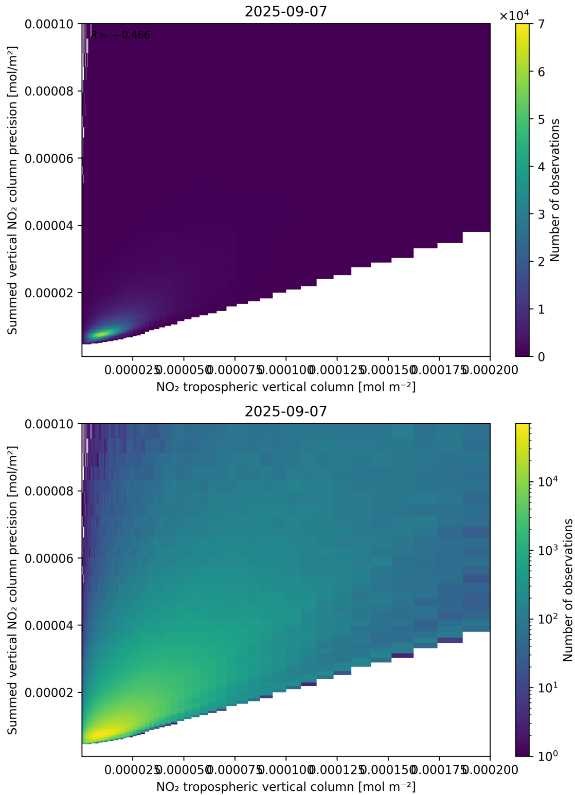
Figure 127: Scatter density plot of “NO 2 tropospheric vertical column” against “Summed vertical NO 2 column precision” for 2025-09-06 to 2025-09-08.
