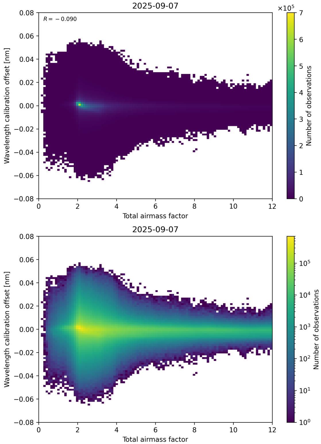
Figure 70: Scatter density plot of “Total airmass factor” against “Wavelength calibration offset” for 2025-09-06 to 2025-09-08.
