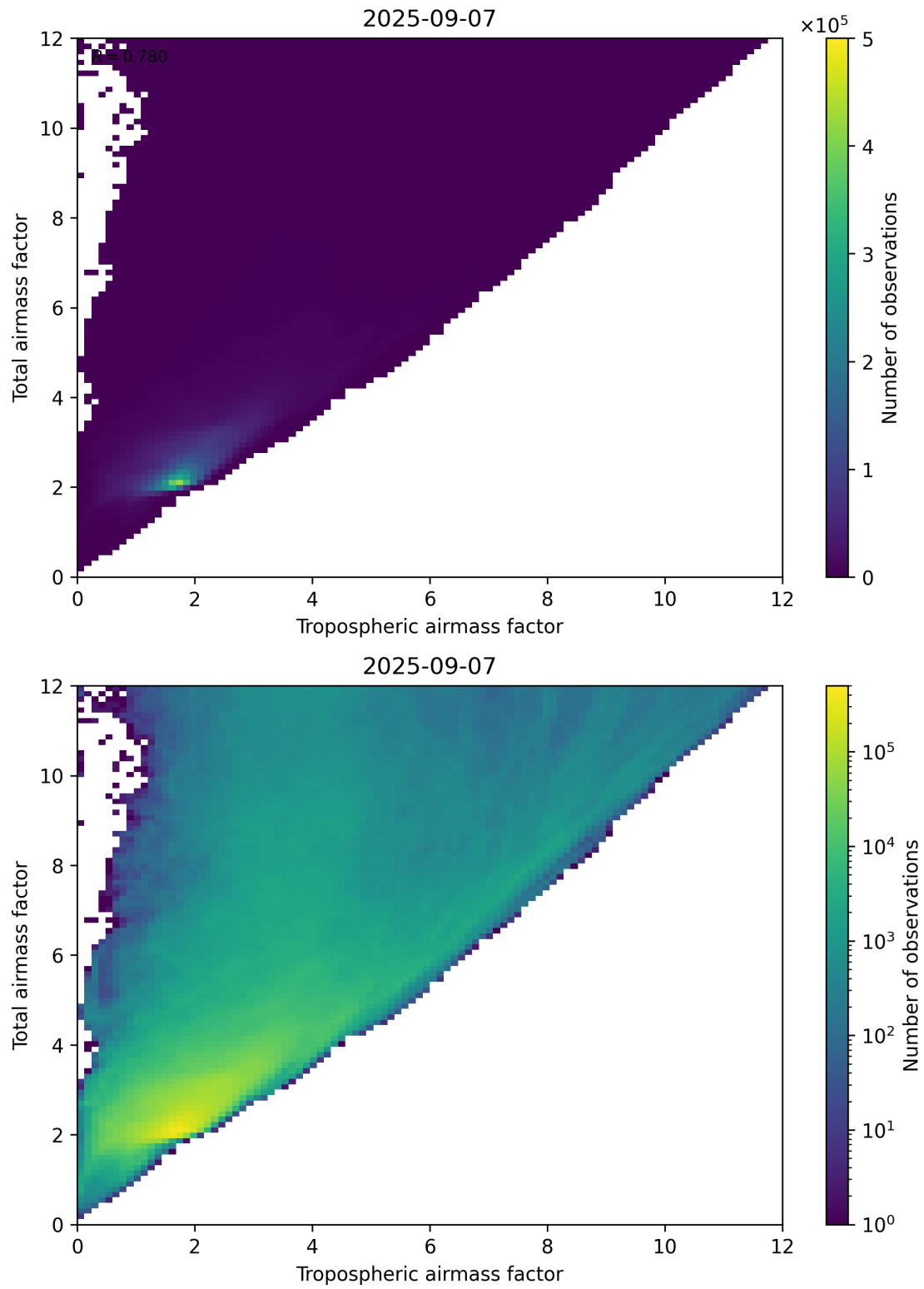
Figure 72: Scatter density plot of “Tropospheric airmass factor” against “Total airmass factor” for 2025-09-06 to 2025-09-08.
