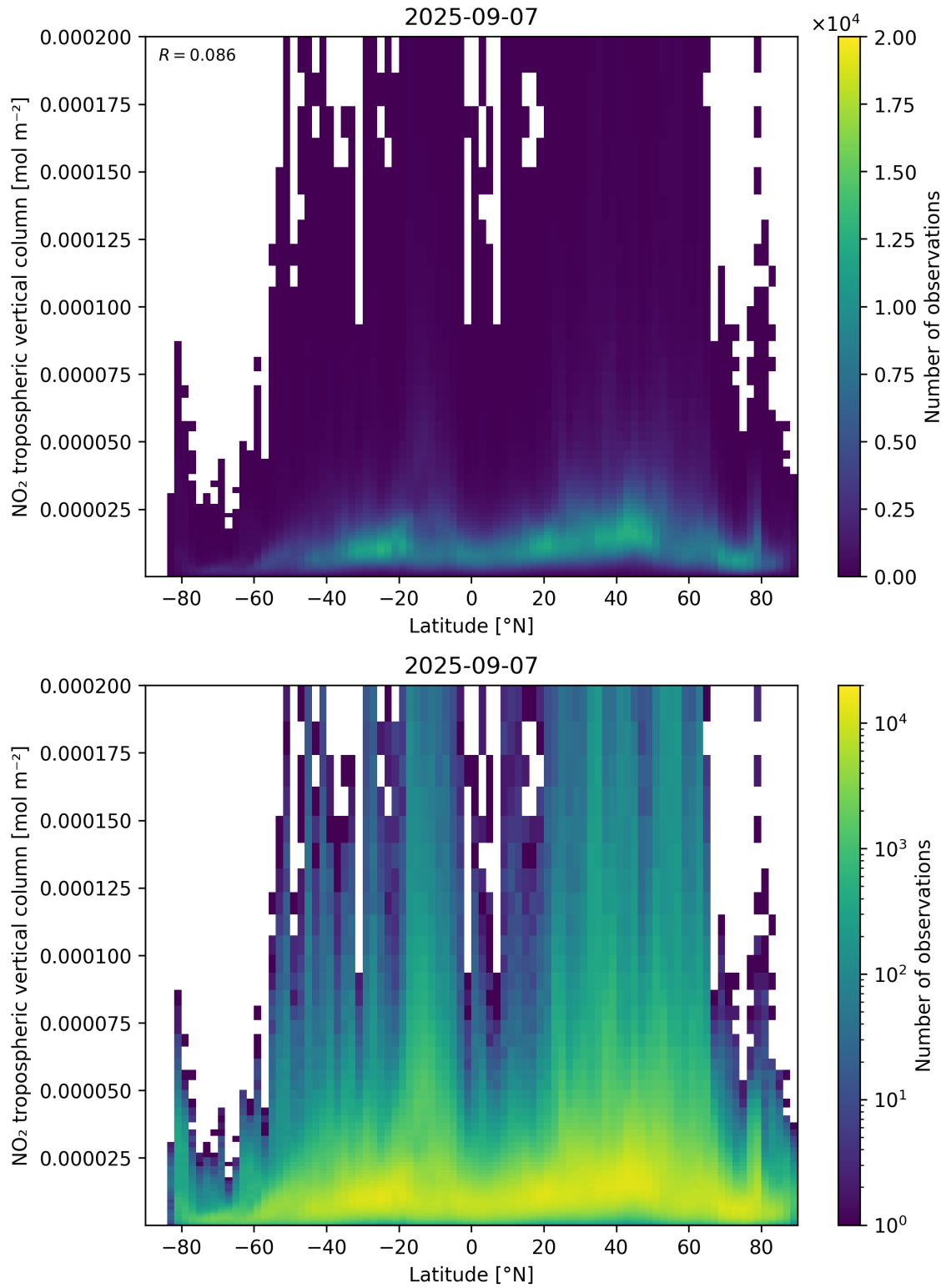
Figure 92: Scatter density plot of “Latitude” against “NO 2 tropospheric vertical column” for 2025-09-06 to 2025-09-08.
