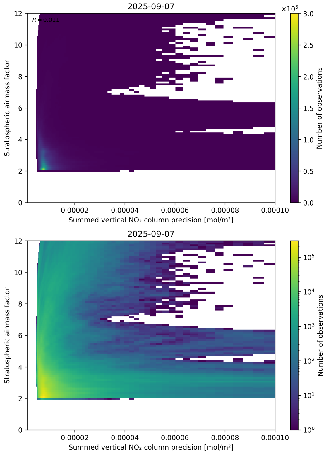
Figure 106: Scatter density plot of “Summed vertical NO 2 column precision” against “Stratospheric airmass factor” for 2025-09-06 to 2025-09-08.
