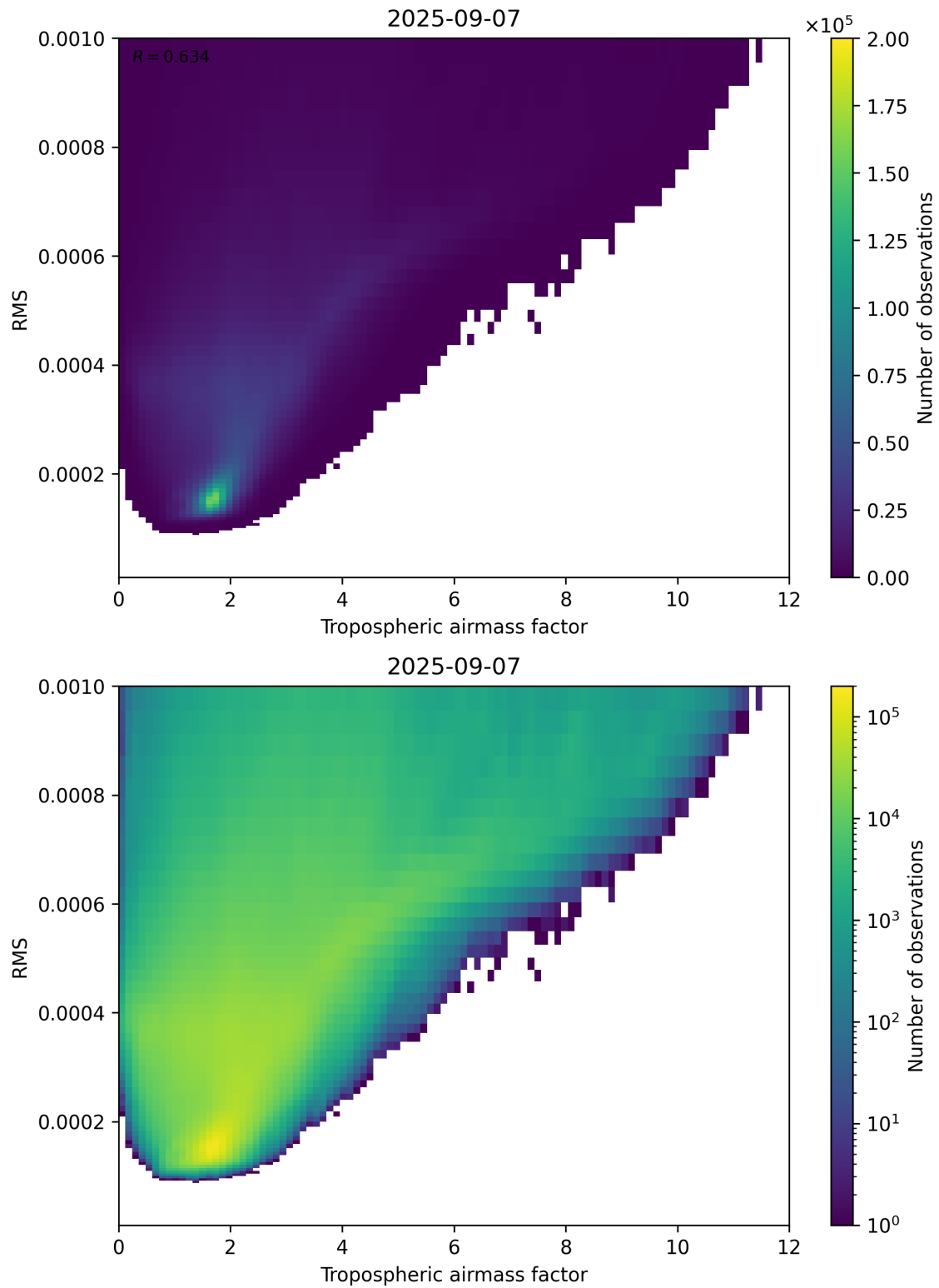
Figure 79: Scatter density plot of “Tropospheric airmass factor” against “RMS” for 2025-09-06 to 2025-09-08.
