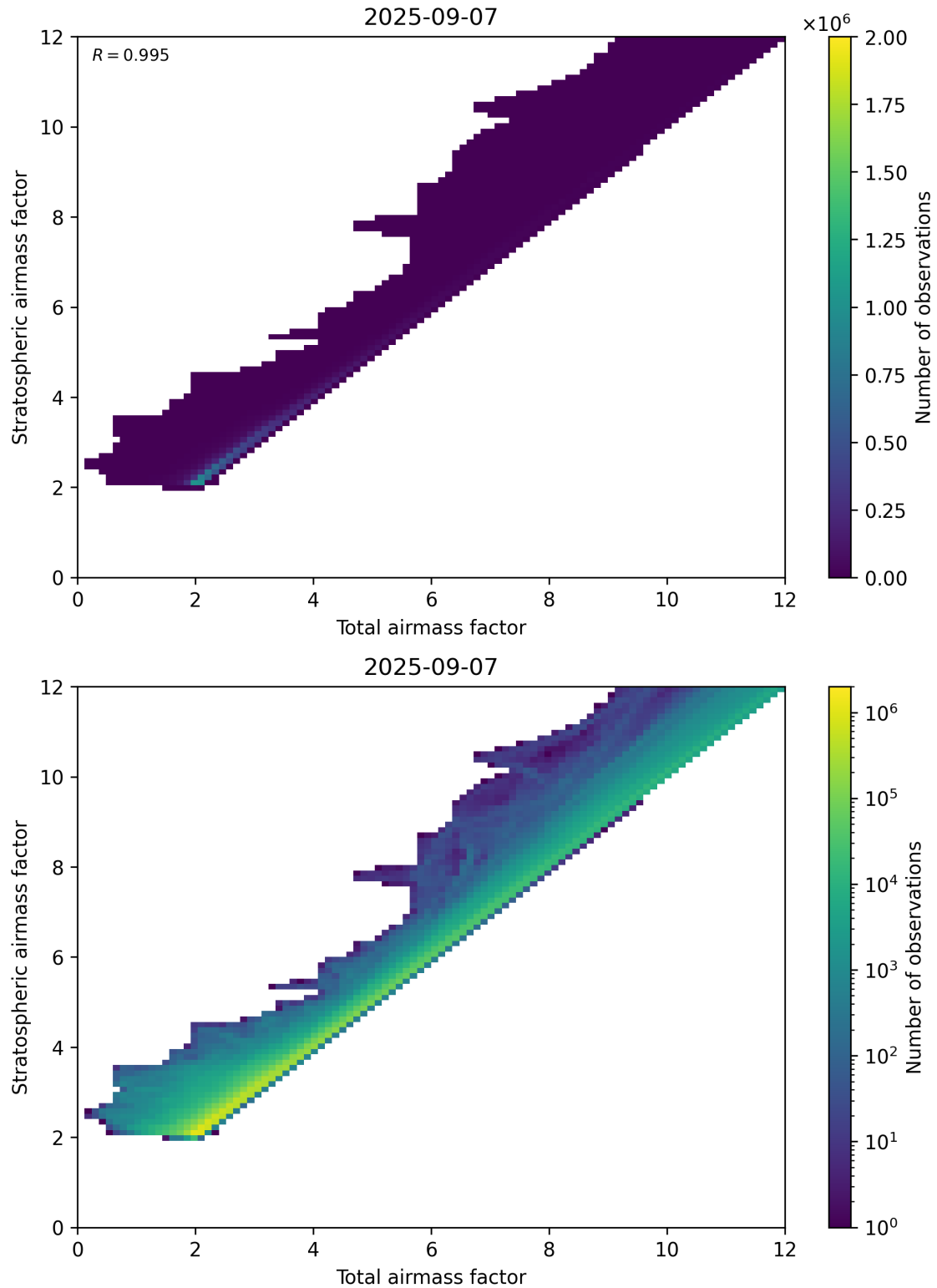
Figure 62: Scatter density plot of “Total airmass factor” against “Stratospheric airmass factor” for 2025-09-06 to 2025-09-08.
