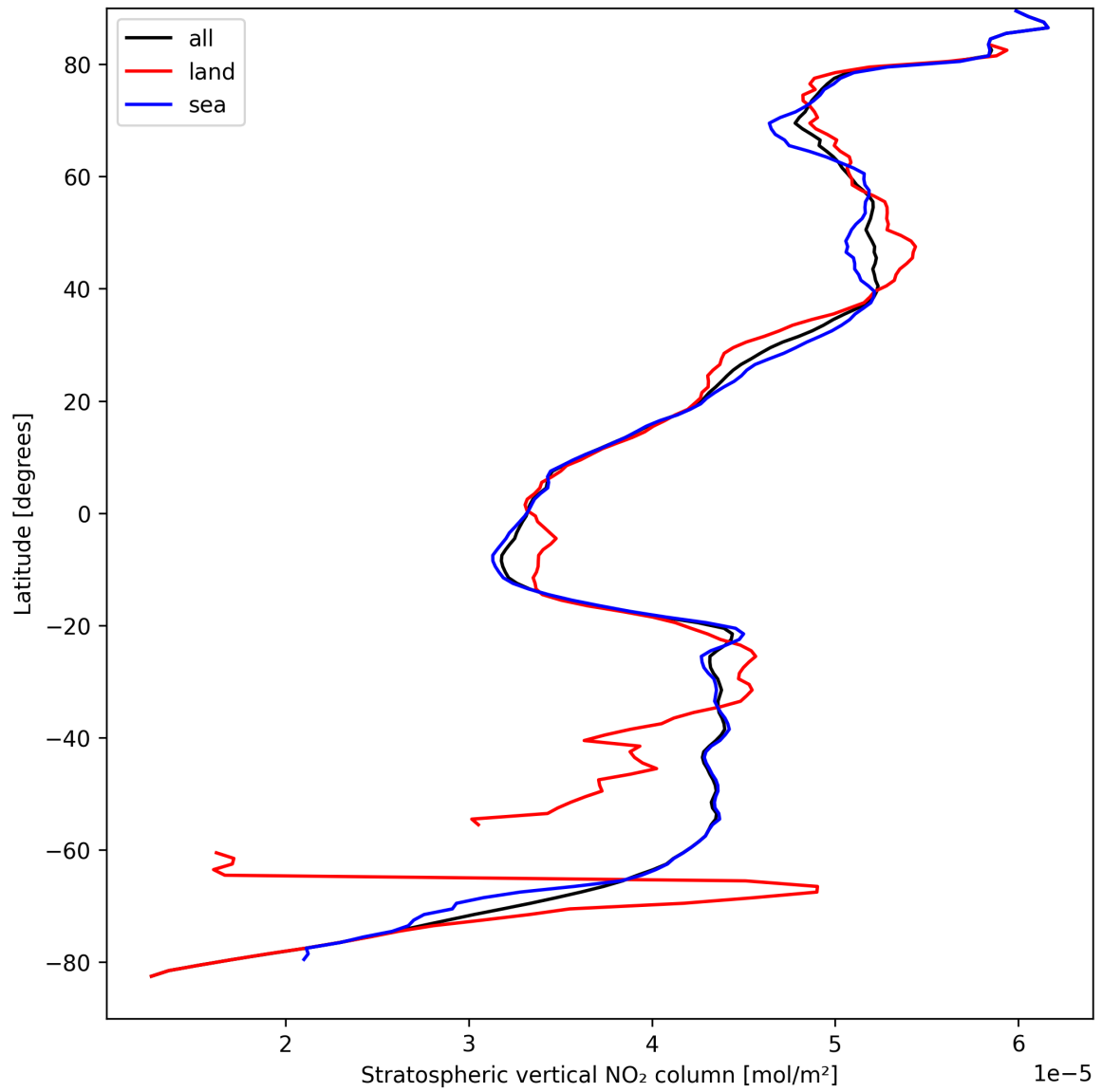
Figure 19: Zonal average of “Stratospheric vertical NO 2 column” for 2025-09-06 to 2025-09-08.
