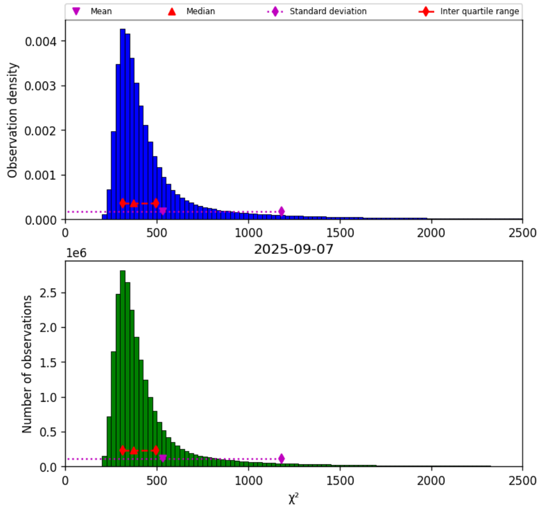
Figure 42: Histogram of “ \chi^2 ” for 2025-09-06 to 2025-09-08
