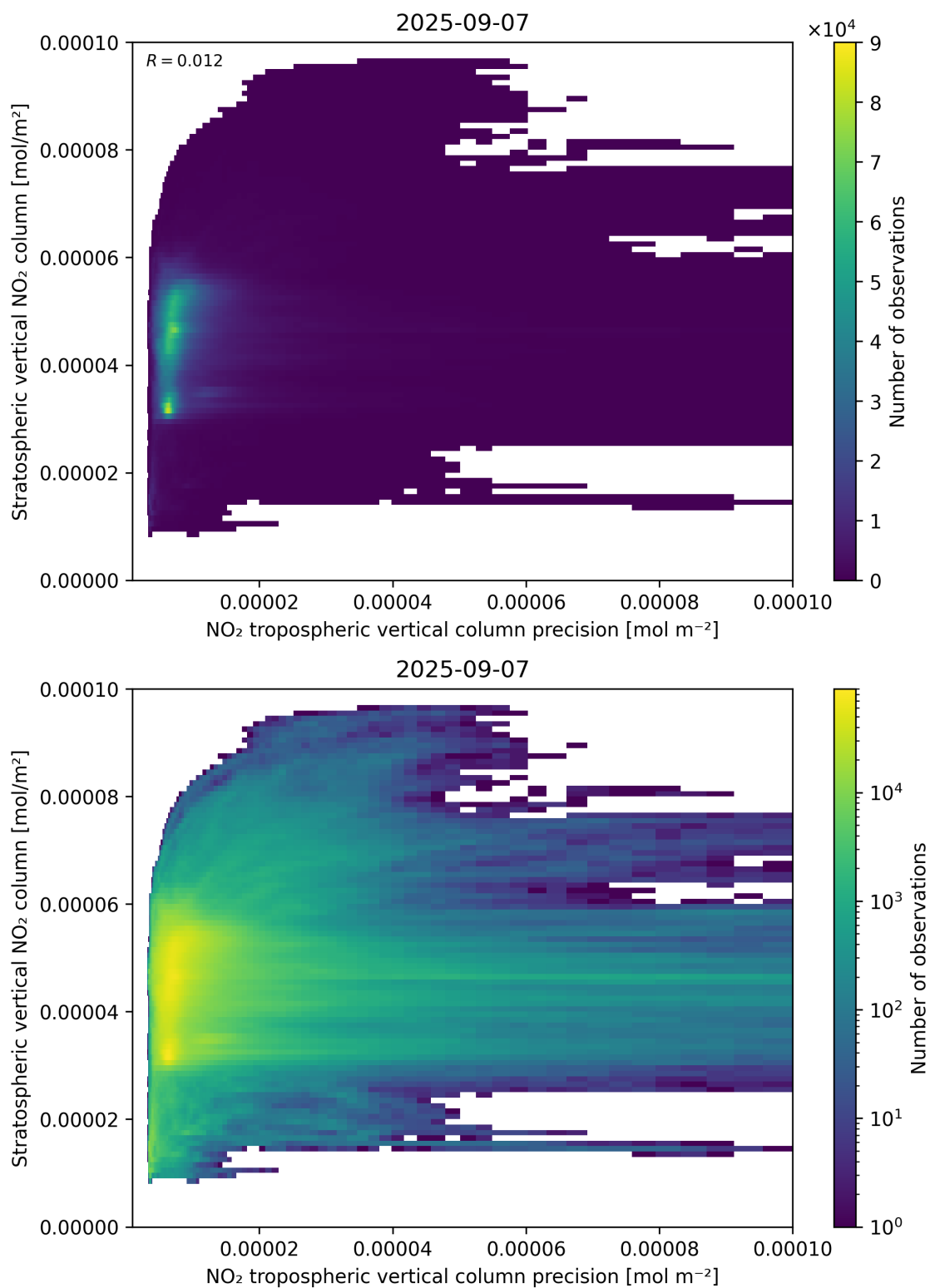
Figure 135: Scatter density plot of “NO 2 tropospheric vertical column precision” against “Stratospheric vertical NO 2 column” for 2025-09-06 to 2025-09-08.
