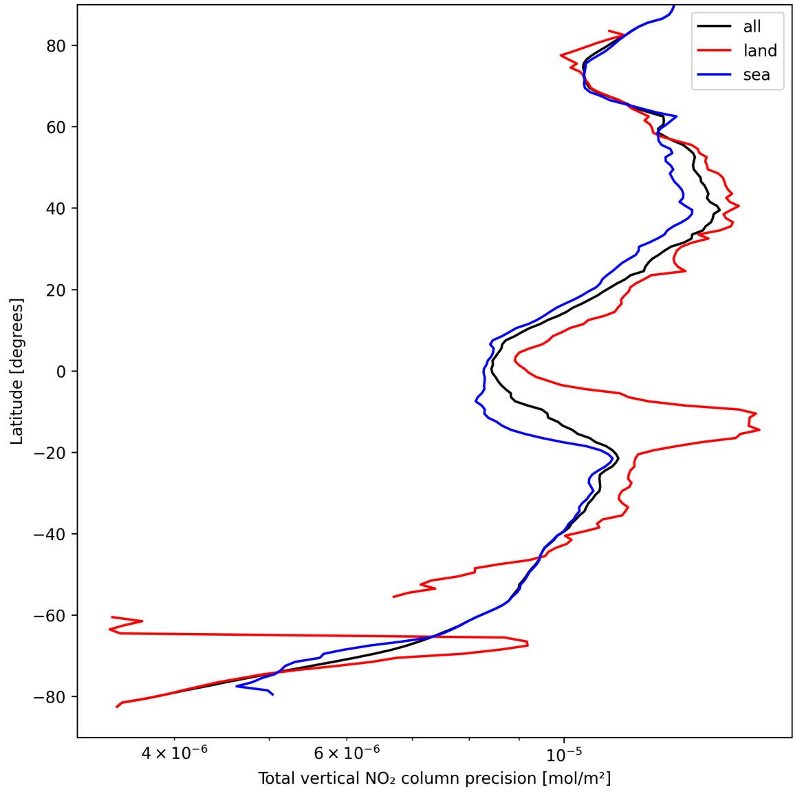
Figure 22: Zonal average of “Total vertical NO 2 column precision” for 2025-09-06 to 2025-09-08.
