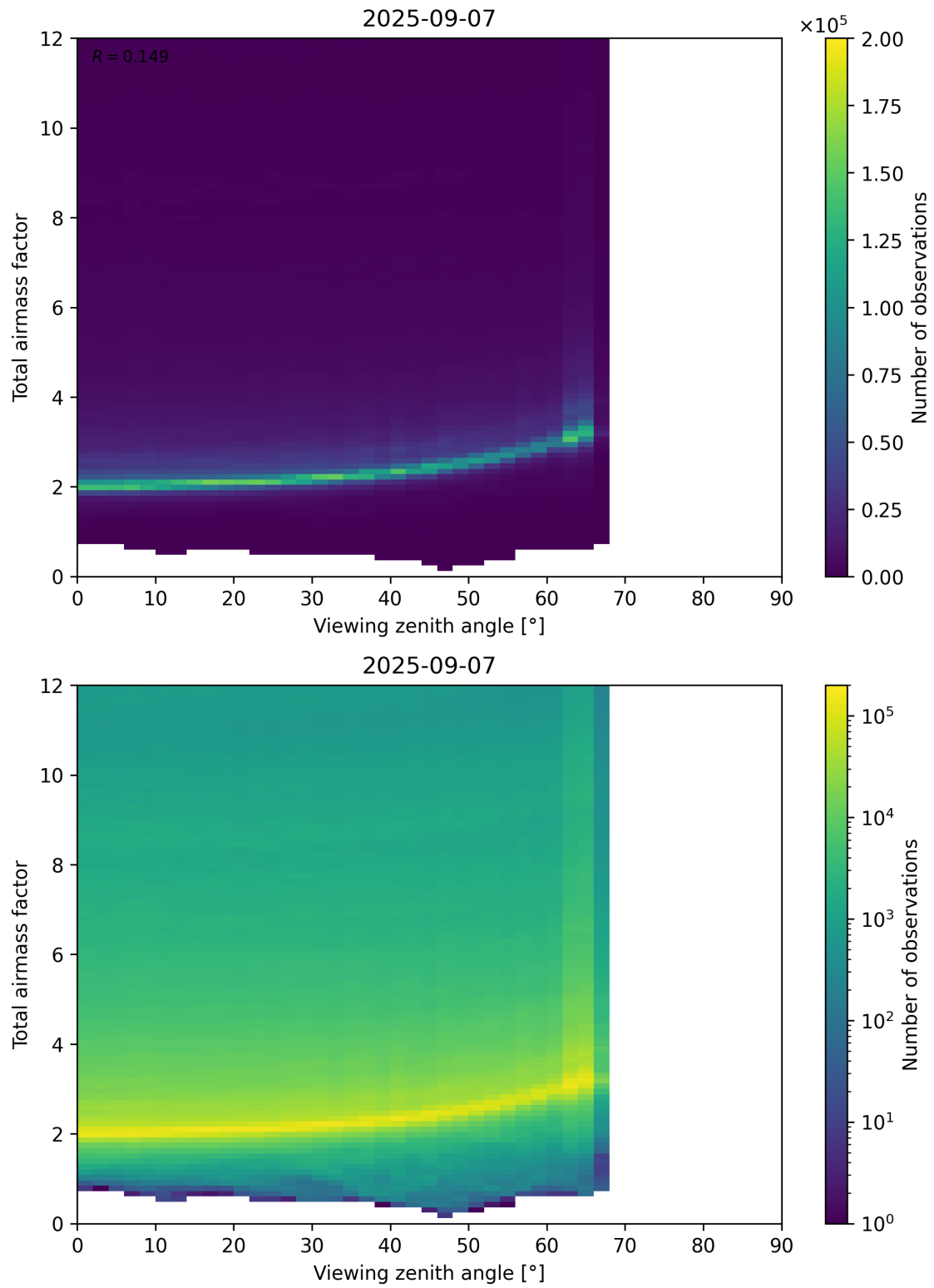
Figure 160: Scatter density plot of “Viewing zenith angle” against “Total airmass factor” for 2025-09-06 to 2025-09-08.
