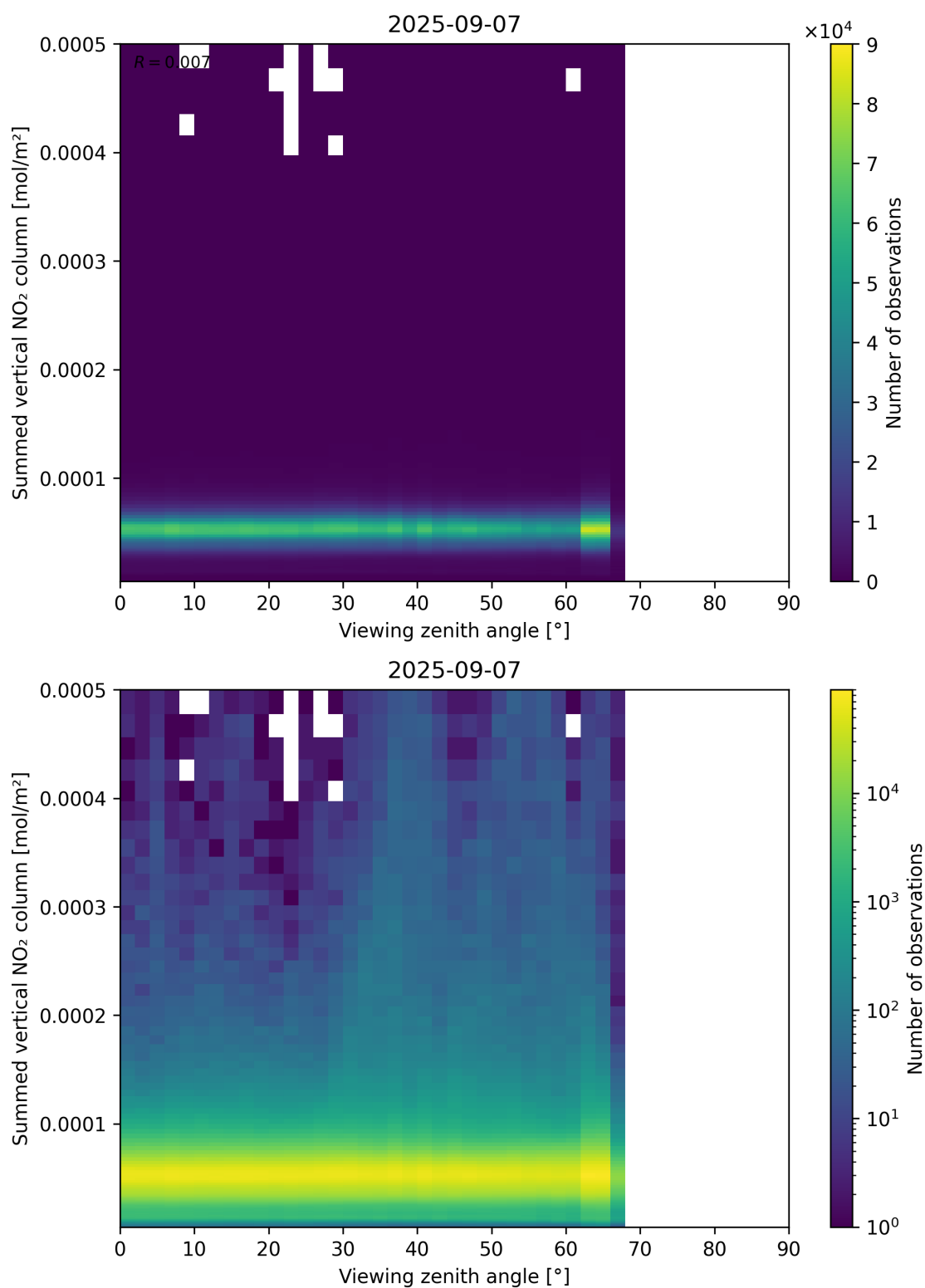
Figure 165: Scatter density plot of “Viewing zenith angle” against “Summed vertical NO 2 column” for 2025-09-06 to 2025-09-08.
