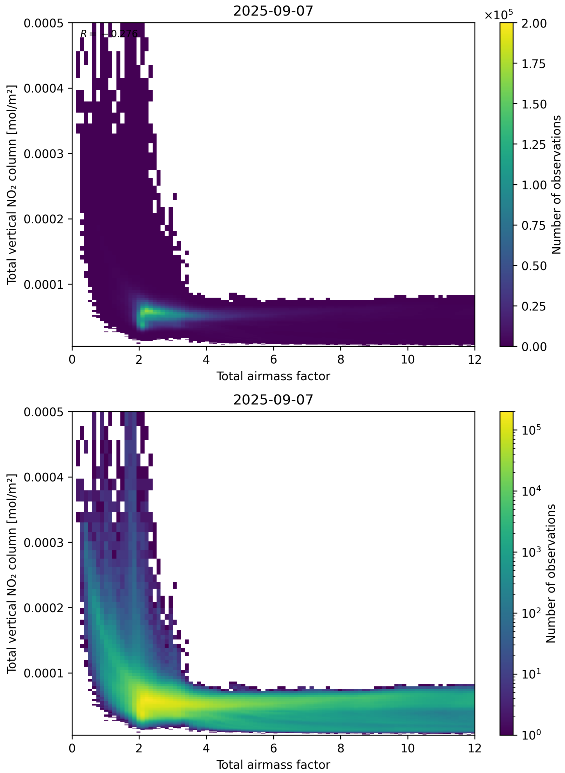
Figure 67: Scatter density plot of “Total airmass factor” against “Total vertical NO 2 column” for 2025-09-06 to 2025-09-08.
