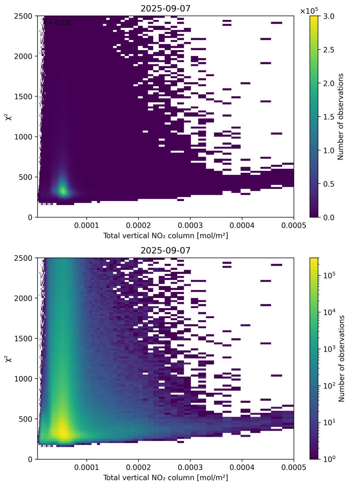
Figure 111: Scatter density plot of “Total vertical NO 2 column” against “ \chi^2 ” for 2025-09-06 to 2025-09-08.
