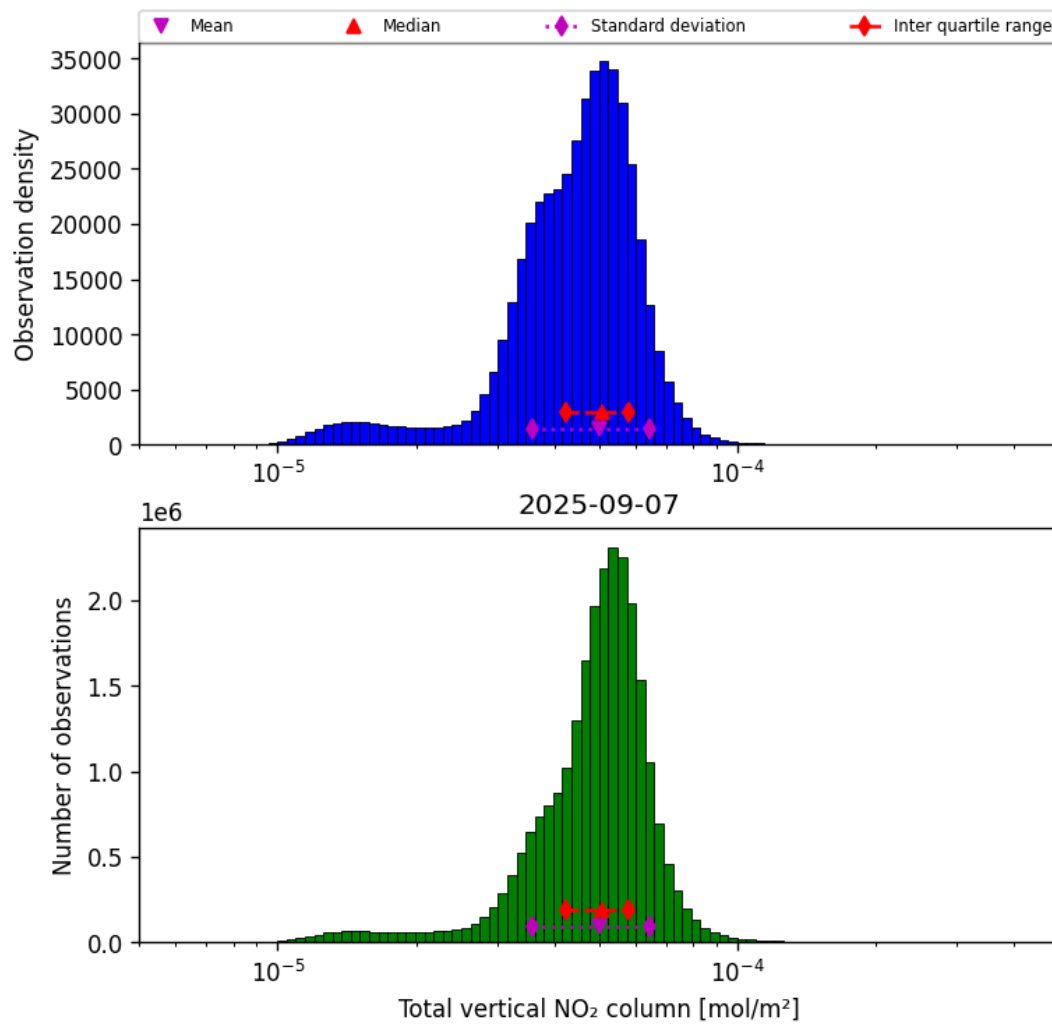
Figure 38: Histogram of “Total vertical NO 2 column” for 2025-09-06 to 2025-09-08
