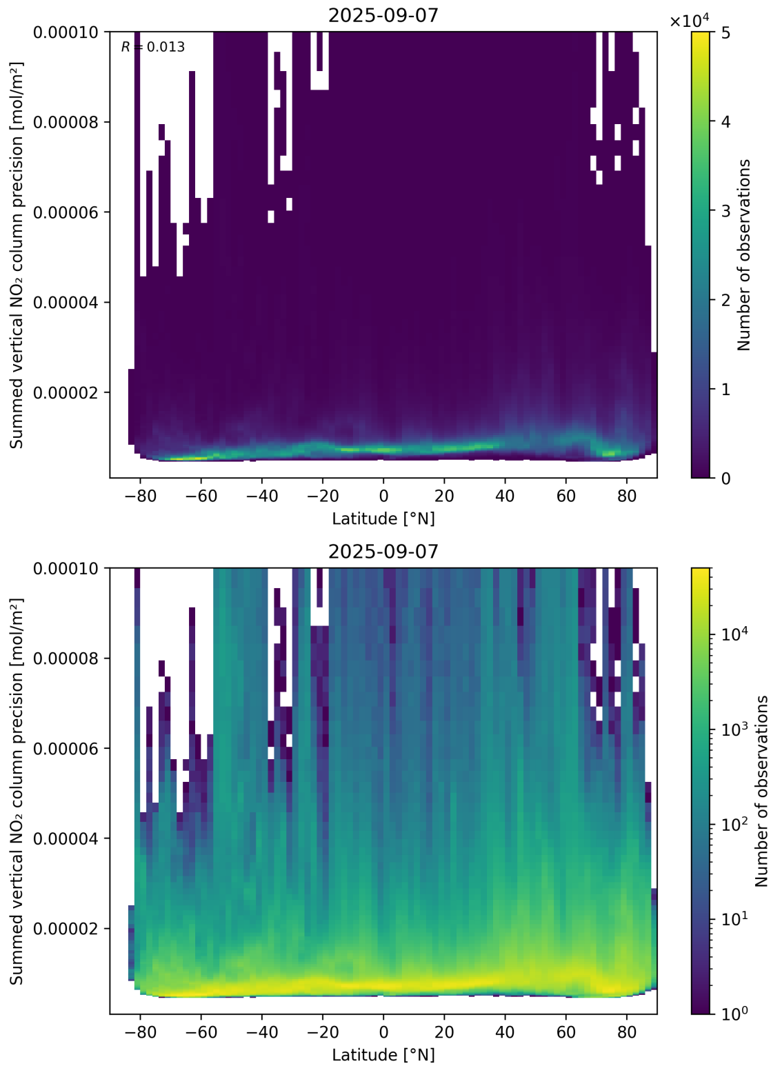
Figure 89: Scatter density plot of “Latitude” against “Summed vertical NO 2 column precision” for 2025-09-06 to 2025-09-08.
