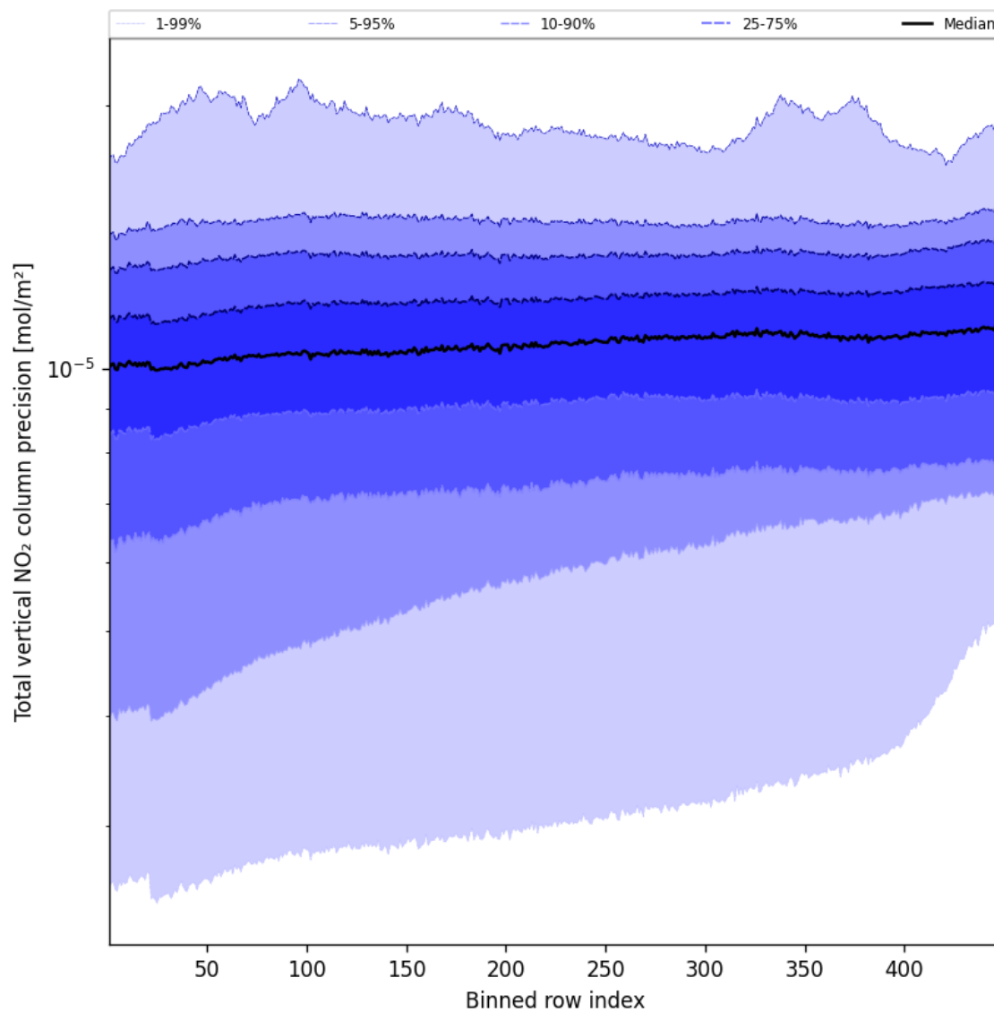
Figure 56: Along track statistics of “Total vertical NO 2 column precision” for 2025-09-06 to 2025-09-08
