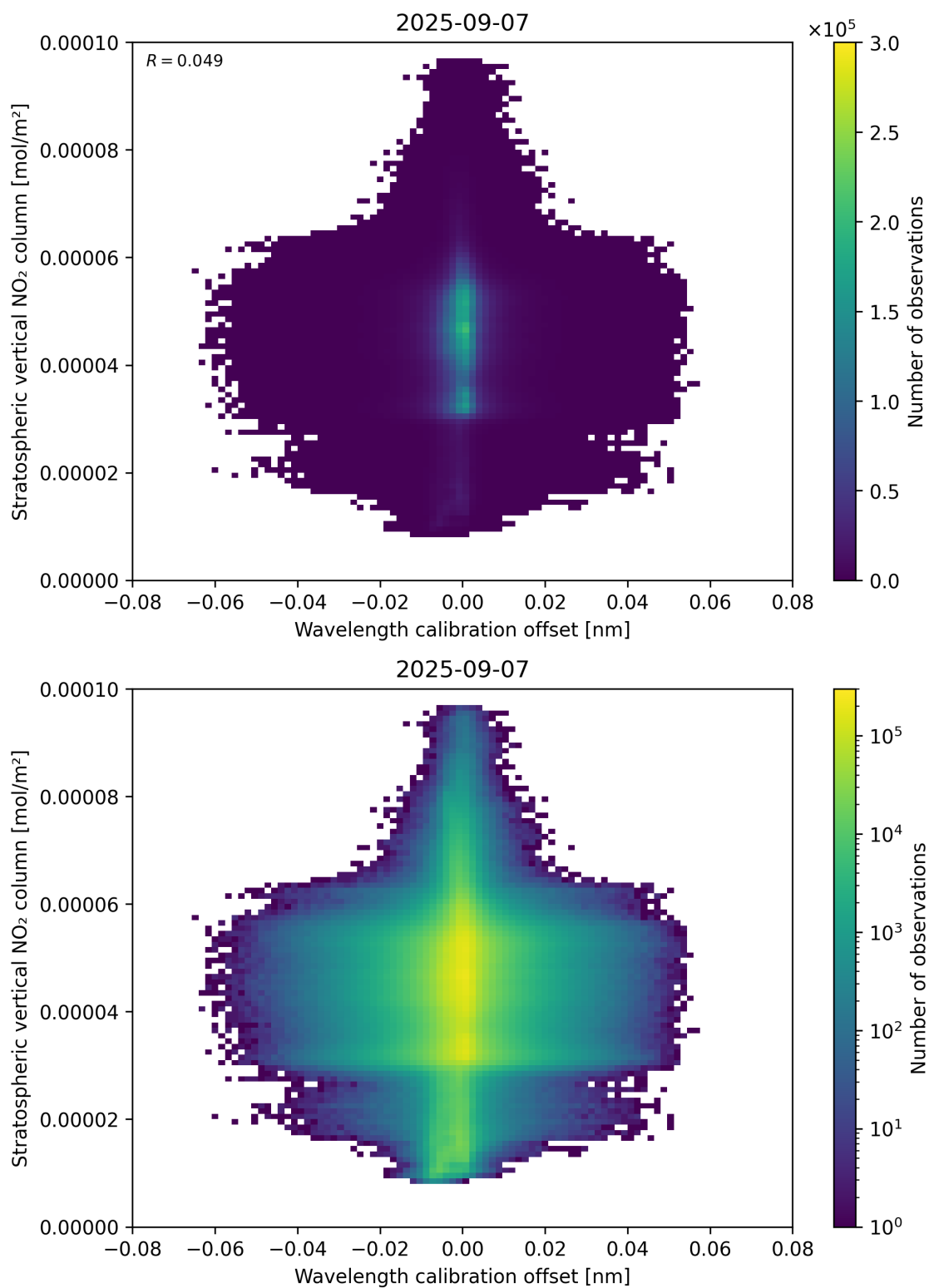
Figure 176: Scatter density plot of “Wavelength calibration offset” against “Stratospheric vertical NO 2 column” for 2025-09-06 to 2025-09-08.
