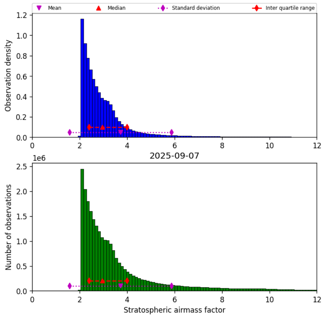
Figure 44: Histogram of “Stratospheric airmass factor” for 2025-09-06 to 2025-09-08
