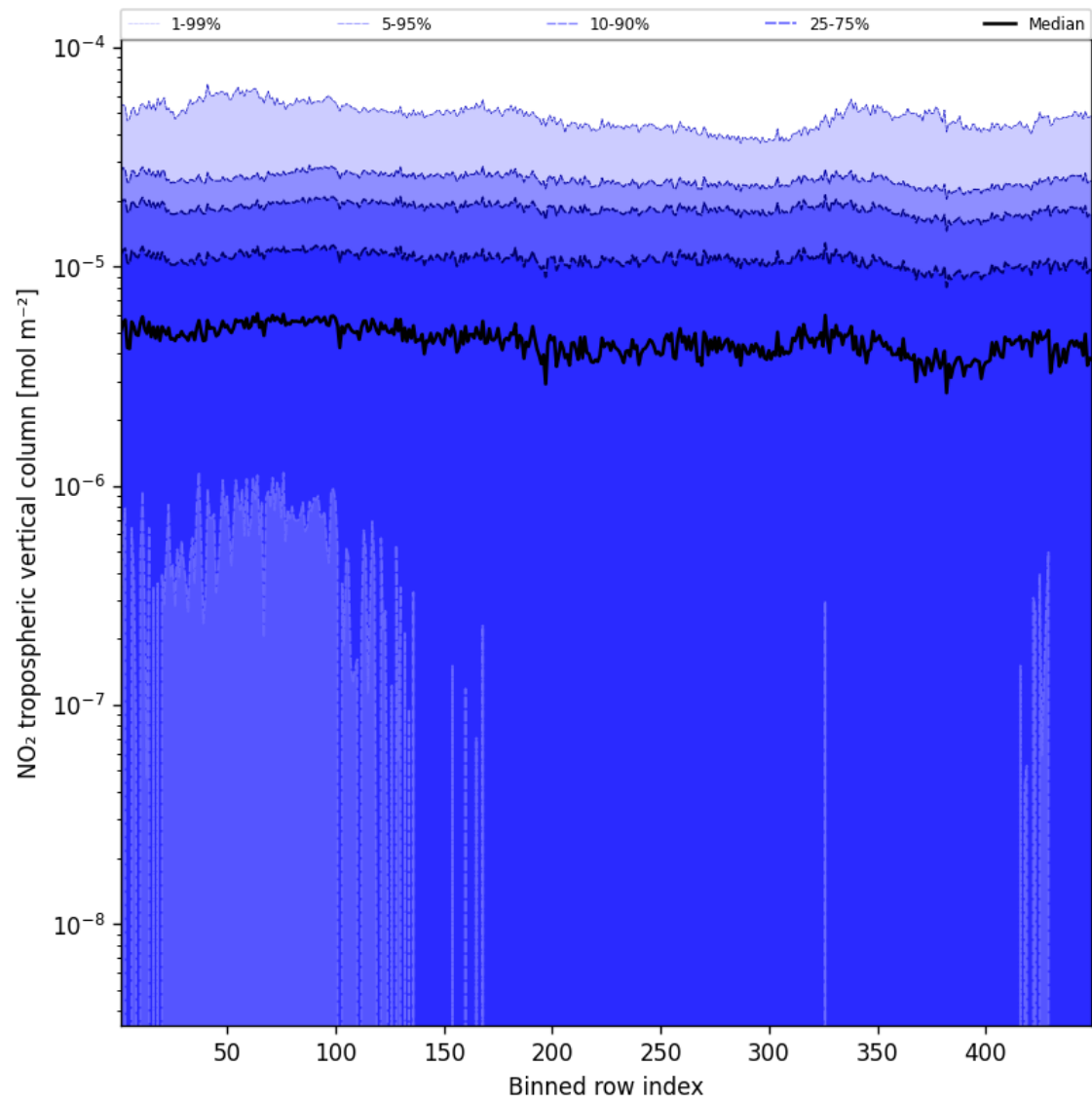
Figure 46: Along track statistics of “NO 2 tropospheric vertical column” for 2025-09-06 to 2025-09-08
