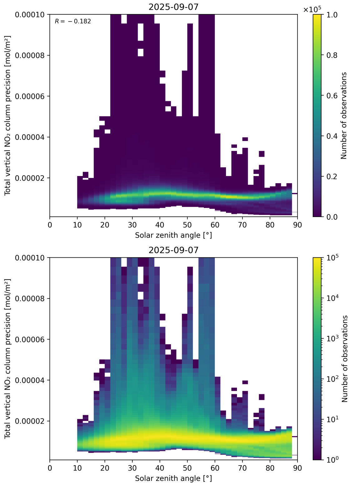
Figure 154: Scatter density plot of “Solar zenith angle” against “Total vertical NO 2 column precision” for 2025-09-06 to 2025-09-08.
