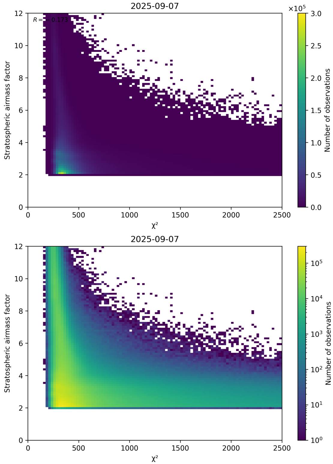
Figure 81: Scatter density plot of “ \chi^2 ” against “Stratospheric airmass factor” for 2025-09-06 to 2025-09-08.
