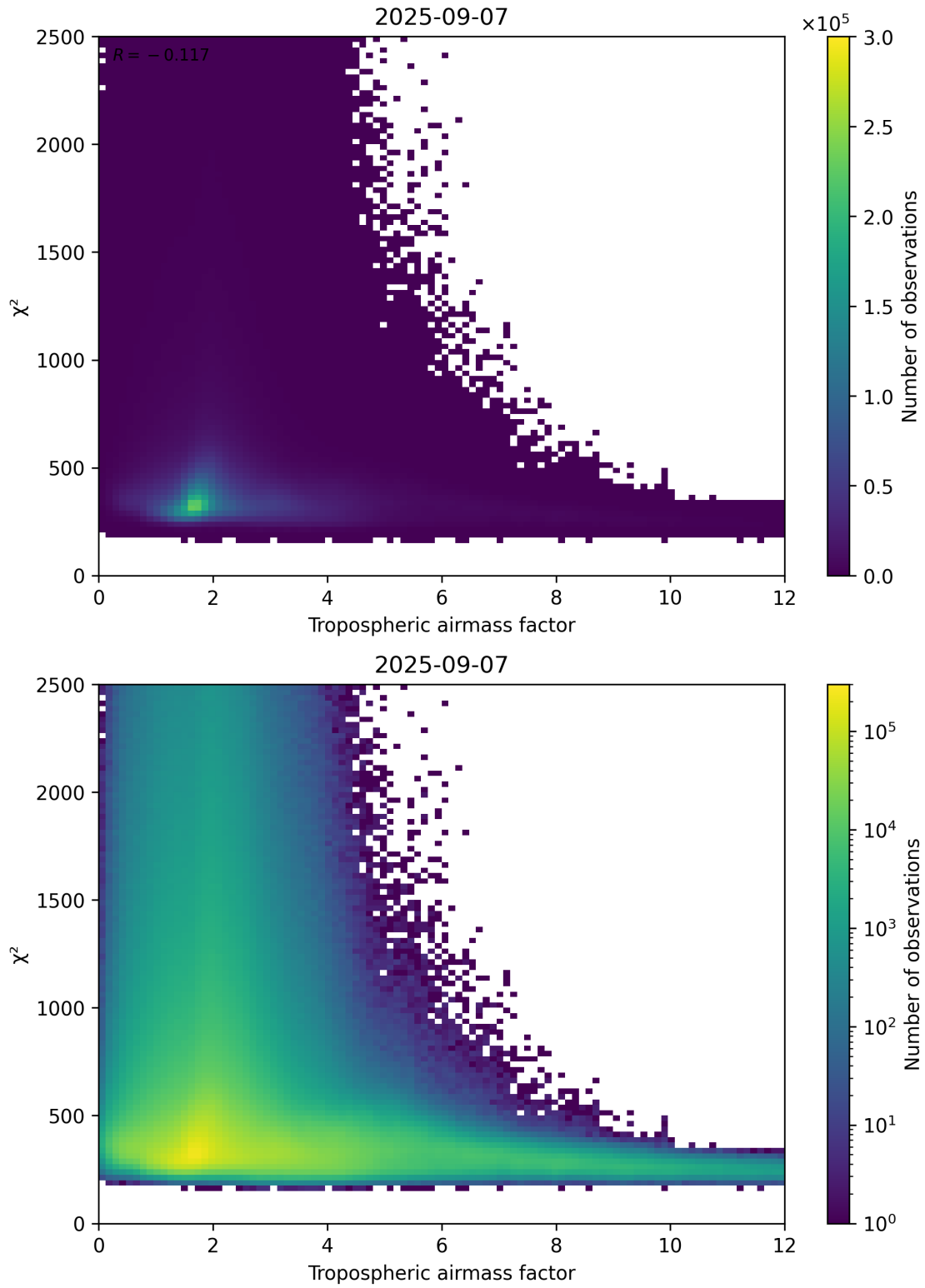
Figure 73: Scatter density plot of “Tropospheric airmass factor” against “ \chi^2 ” for 2025-09-06 to 2025-09-08.
