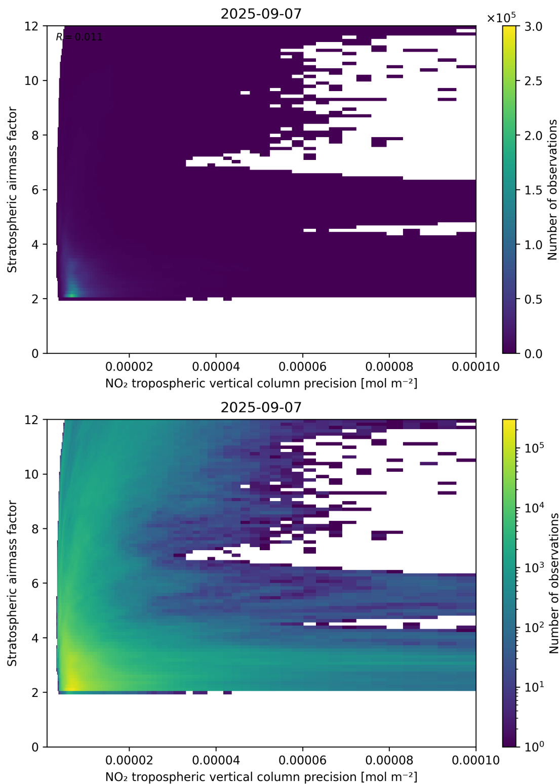
Figure 131: Scatter density plot of “NO 2 tropospheric vertical column precision” against “Stratospheric airmass factor” for 2025-09-06 to 2025-09-08.
