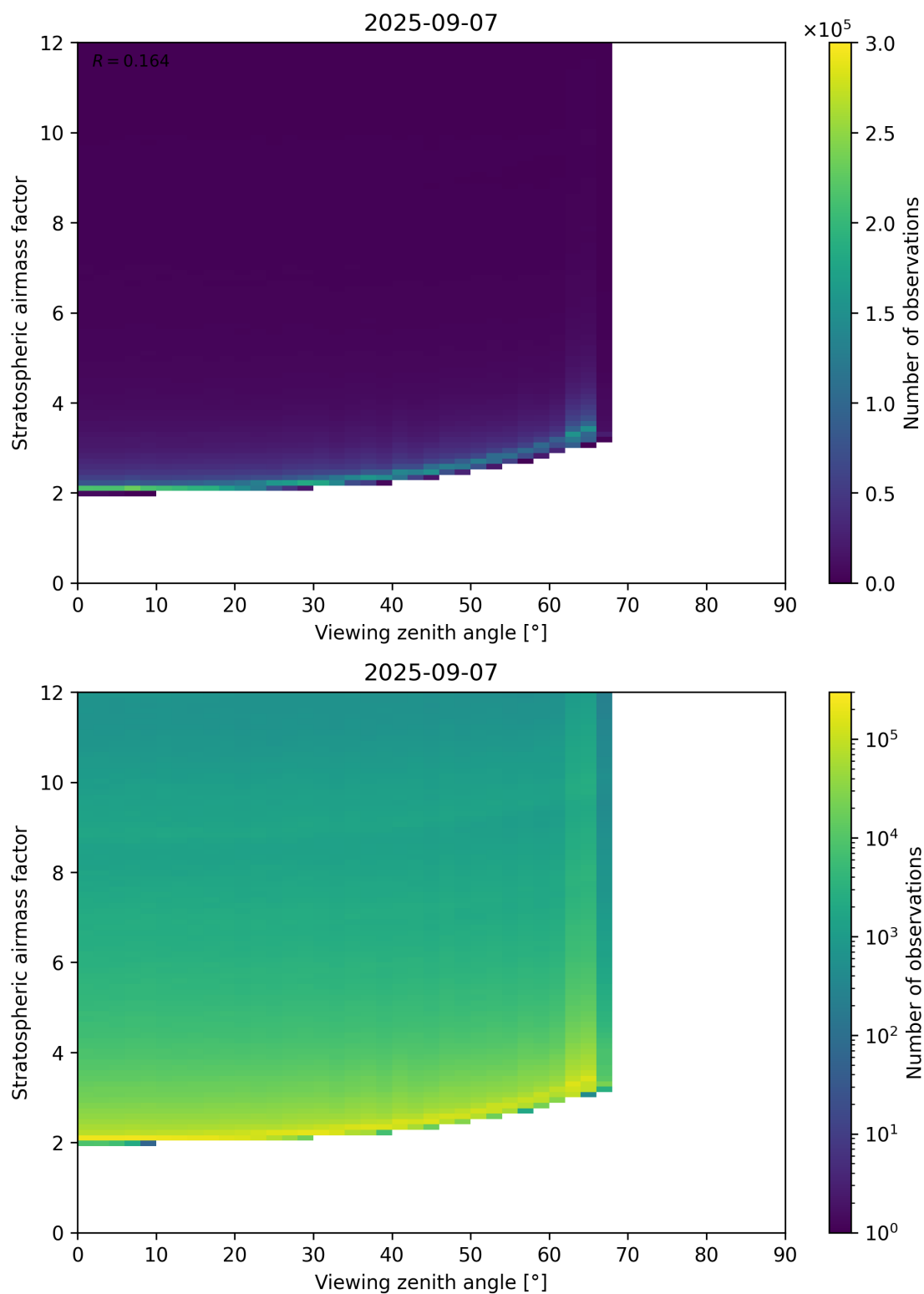
Figure 159: Scatter density plot of “Viewing zenith angle” against “Stratospheric airmass factor” for 2025-09-06 to 2025-09-08.
