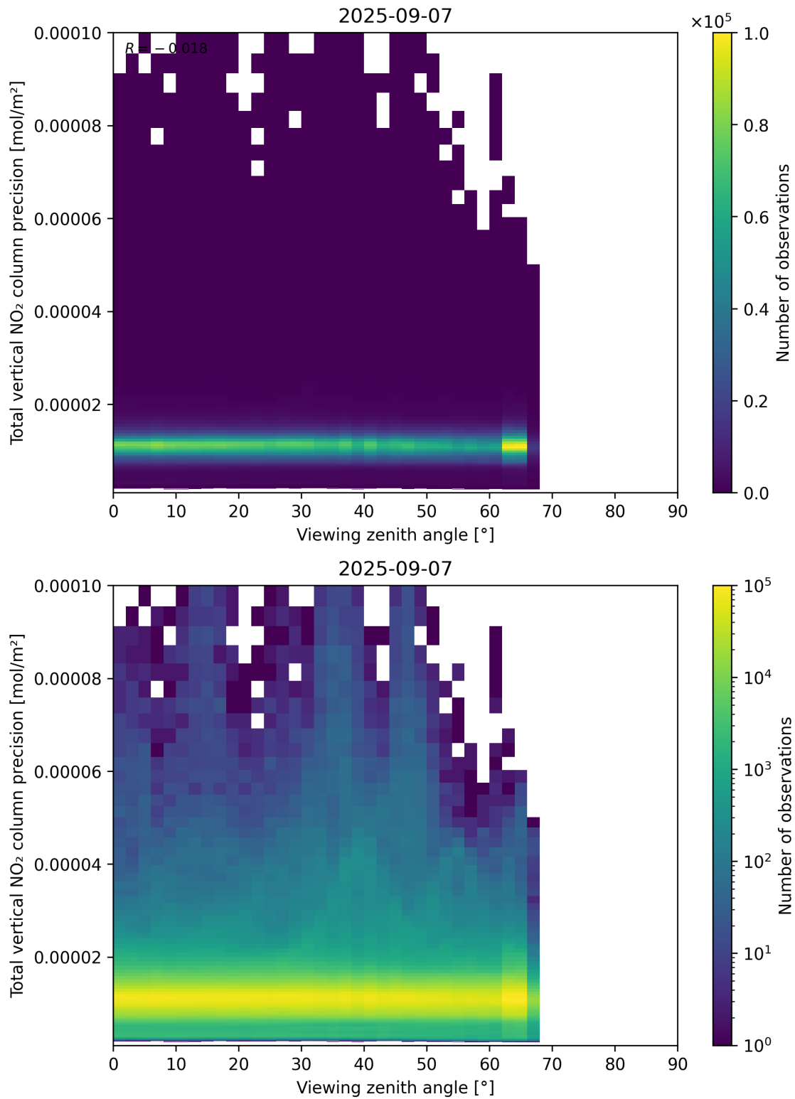
Figure 168: Scatter density plot of “Viewing zenith angle” against “Total vertical NO 2 column precision” for 2025-09-06 to 2025-09-08.
