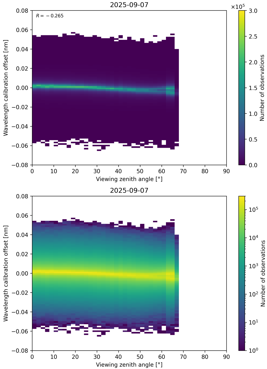
Figure 173: Scatter density plot of “Viewing zenith angle” against “Wavelength calibration offset” for 2025-09-06 to 2025-09-08.
