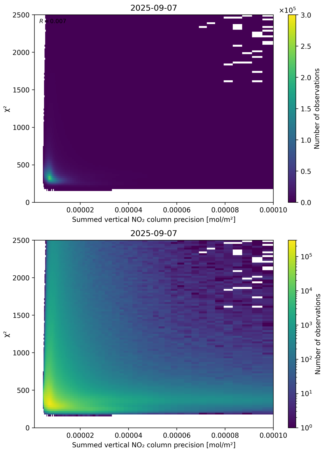
Figure 107: Scatter density plot of “Summed vertical NO 2 column precision” against “ \chi^2 ” for 2025-09-06 to 2025-09-08.
