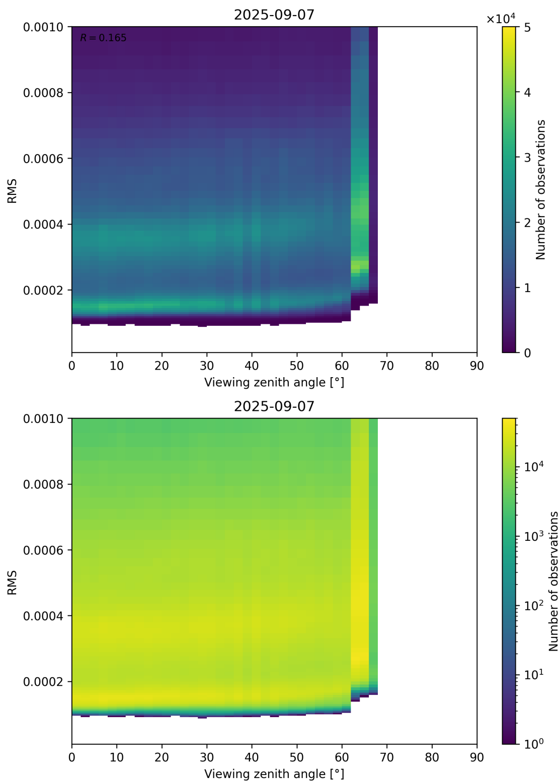
Figure 171: Scatter density plot of “Viewing zenith angle” against “RMS” for 2025-09-06 to 2025-09-08.
