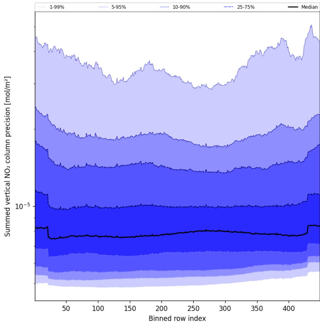
Figure 58: Along track statistics of “Summed vertical NO 2 column precision” for 2025-09-06 to 2025-09-08
