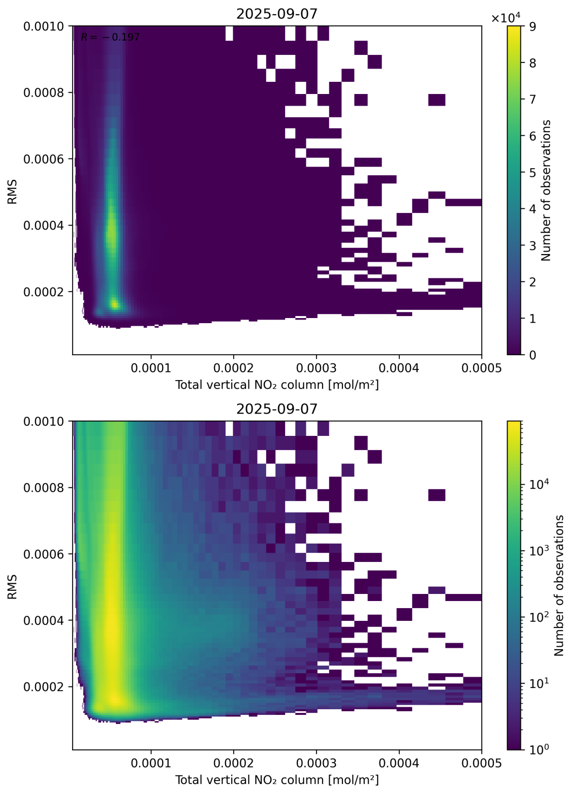
Figure 120: Scatter density plot of “Total vertical NO 2 column” against “RMS” for 2025-09-06 to 2025-09-08.
