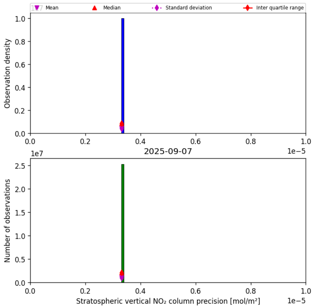
Figure 37: Histogram of “Stratospheric vertical NO 2 column precision” for 2025-09-06 to 2025-09-08
