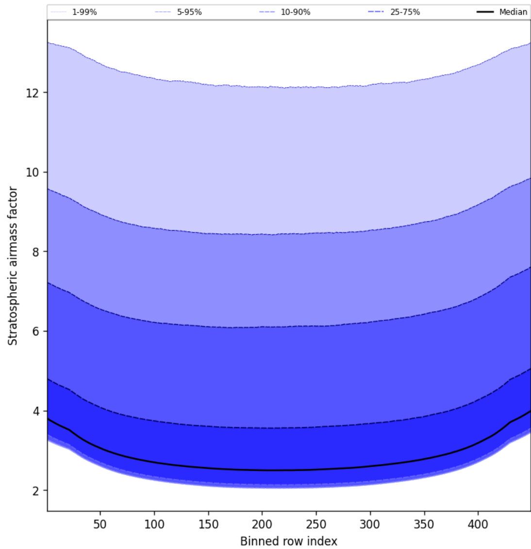
Figure 61: Along track statistics of “Stratospheric airmass factor” for 2025-09-06 to 2025-09-08
