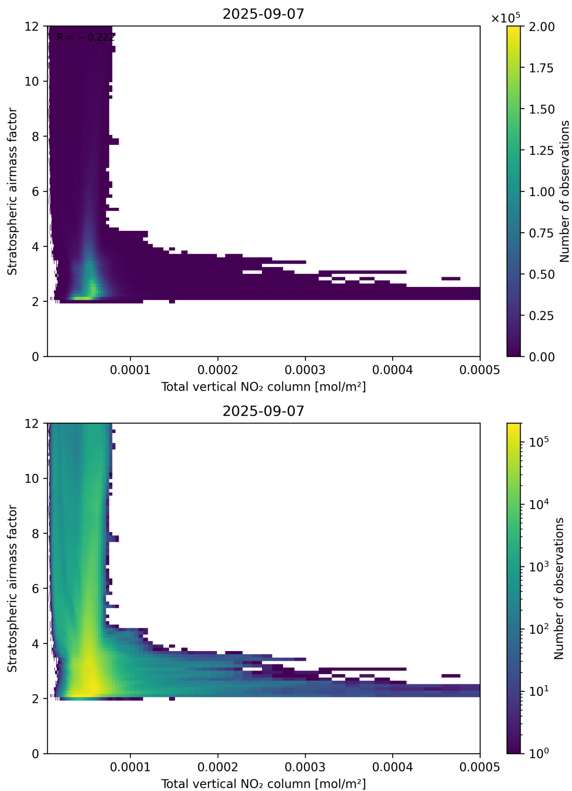
Figure 110: Scatter density plot of “Total vertical NO 2 column” against “Stratospheric airmass factor” for 2025-09-06 to 2025-09-08.
