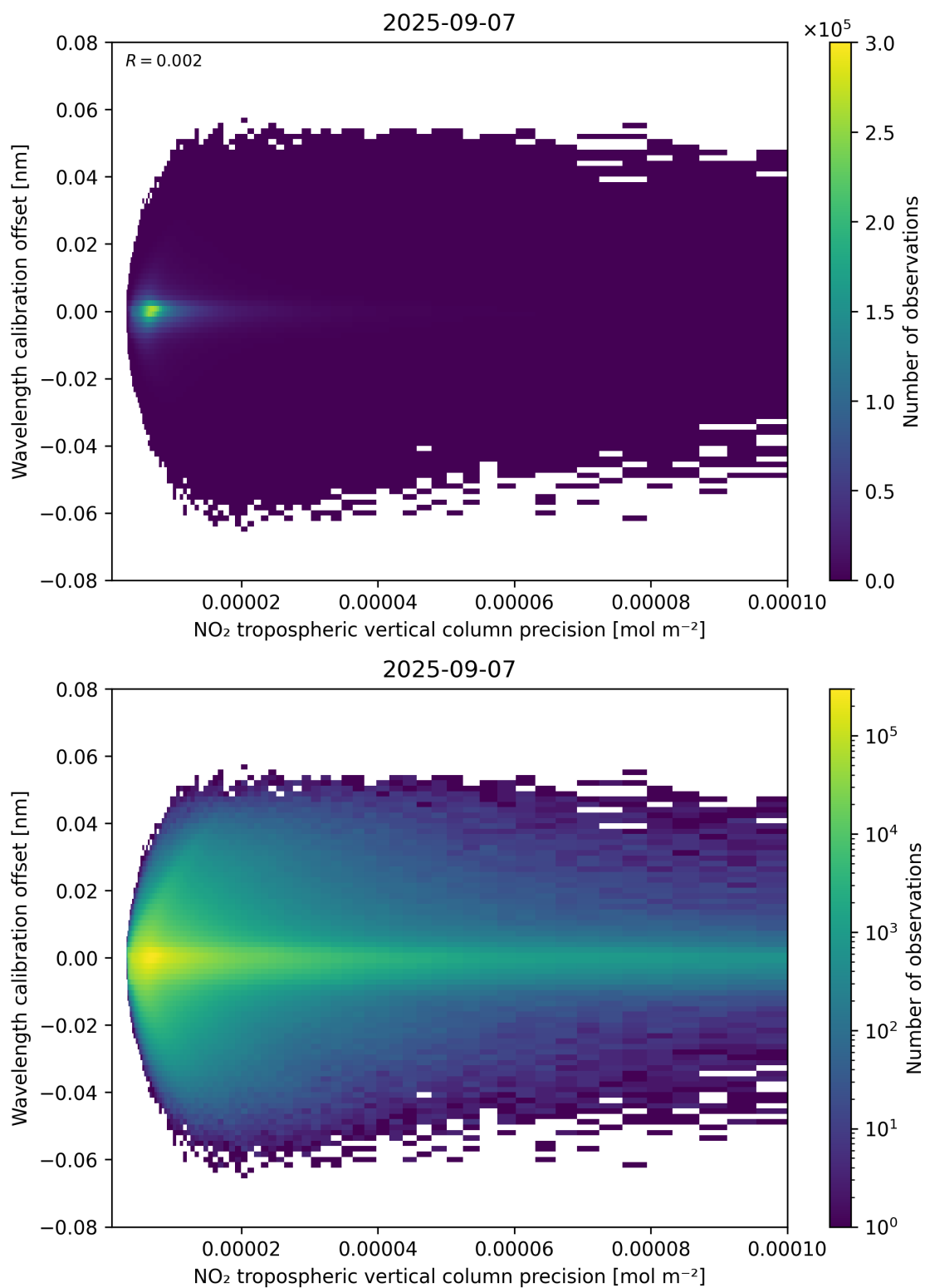
Figure 141: Scatter density plot of “NO 2 tropospheric vertical column precision” against “Wavelength calibration offset” for 2025-09-06 to 2025-09-08.
