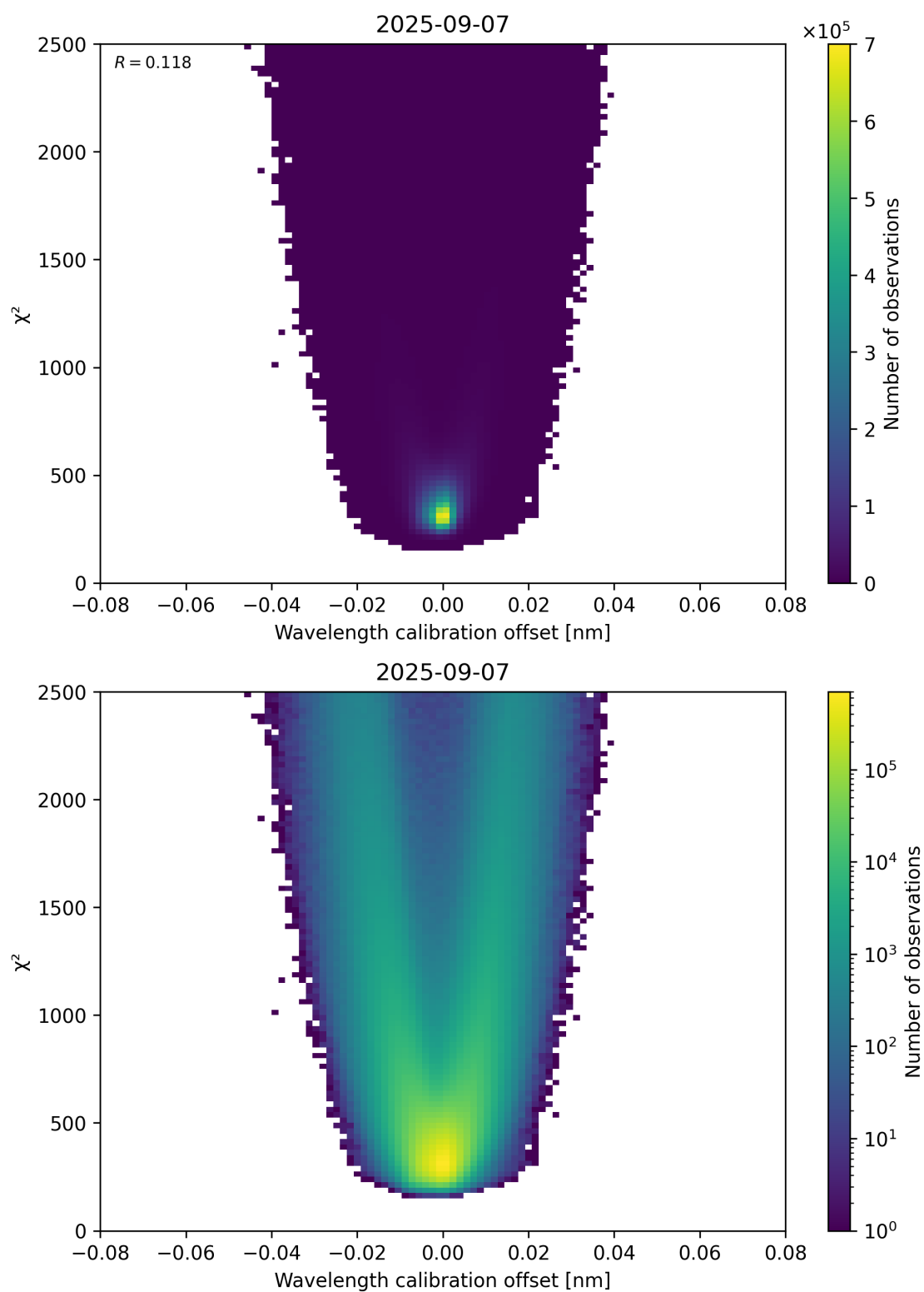
Figure 175: Scatter density plot of “Wavelength calibration offset” against “ \chi^2 ” for 2025-09-06 to 2025-09-08.
