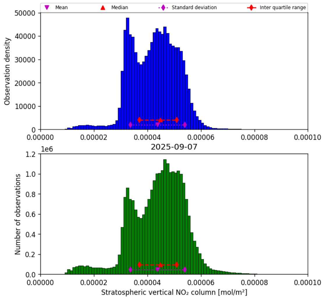
Figure 36: Histogram of “Stratospheric vertical NO 2 column” for 2025-09-06 to 2025-09-08
