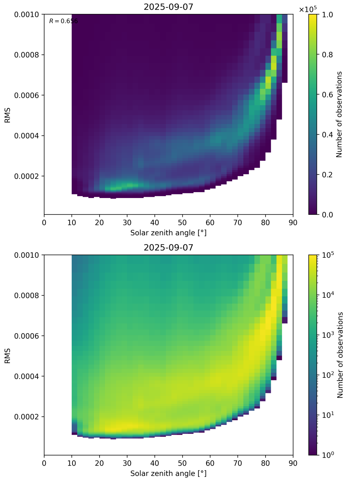
Figure 157: Scatter density plot of “Solar zenith angle” against “RMS” for 2025-09-06 to 2025-09-08.
