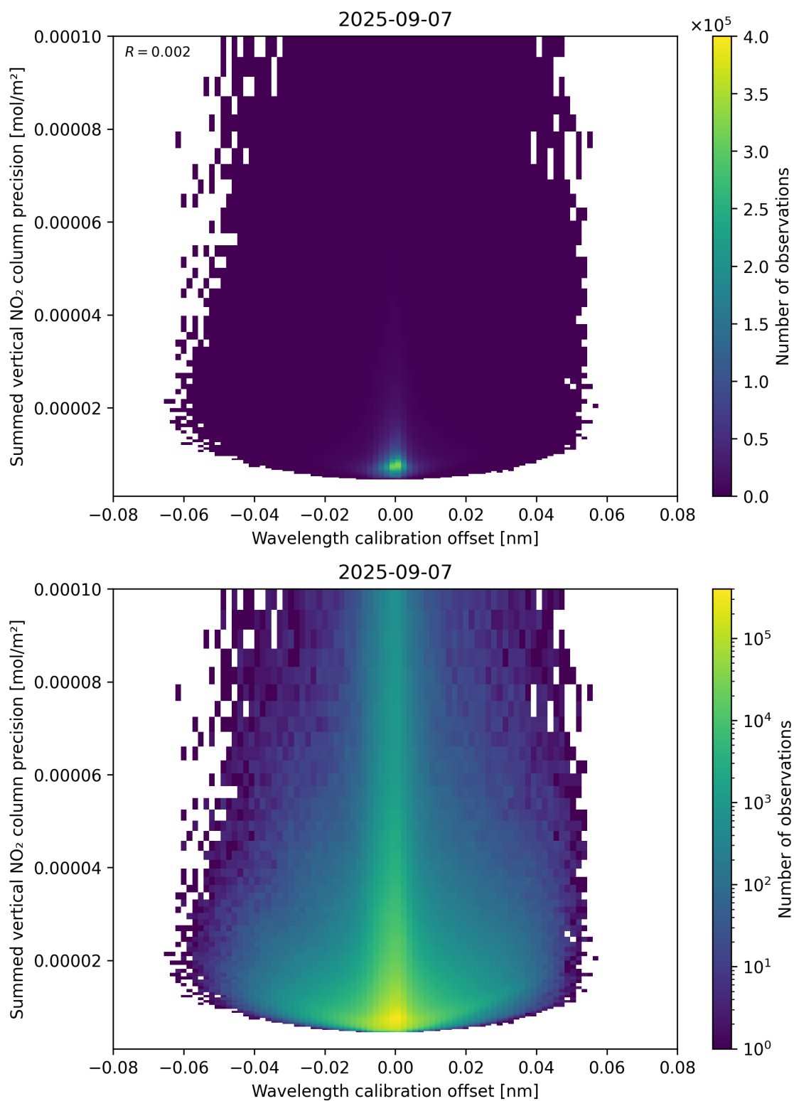
Figure 178: Scatter density plot of “Wavelength calibration offset” against “Summed vertical NO 2 column precision” for 2025-09-06 to 2025-09-08.
