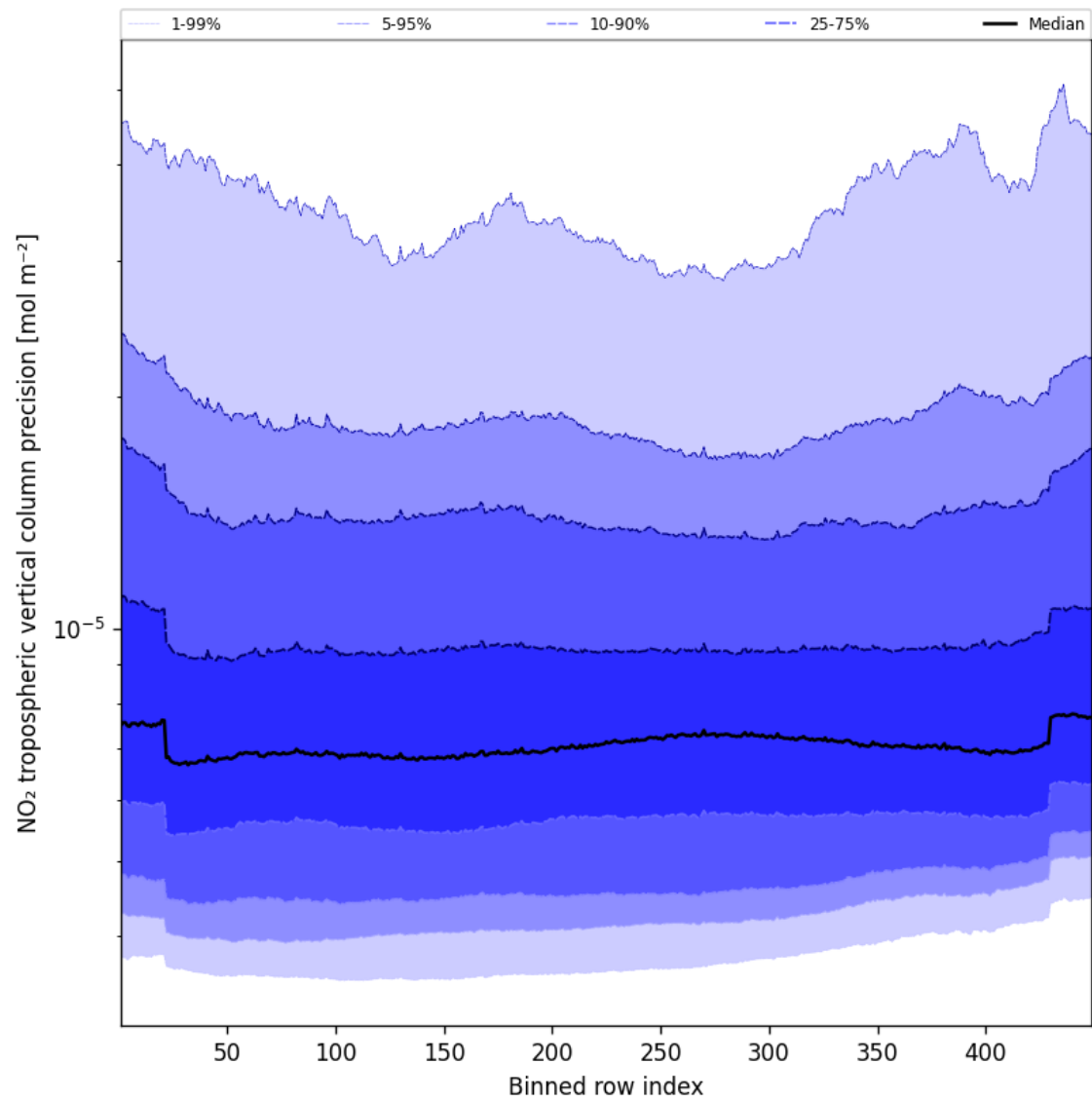
Figure 47: Along track statistics of “NO 2 tropospheric vertical column precision” for 2025-09-06 to 2025-09-08
