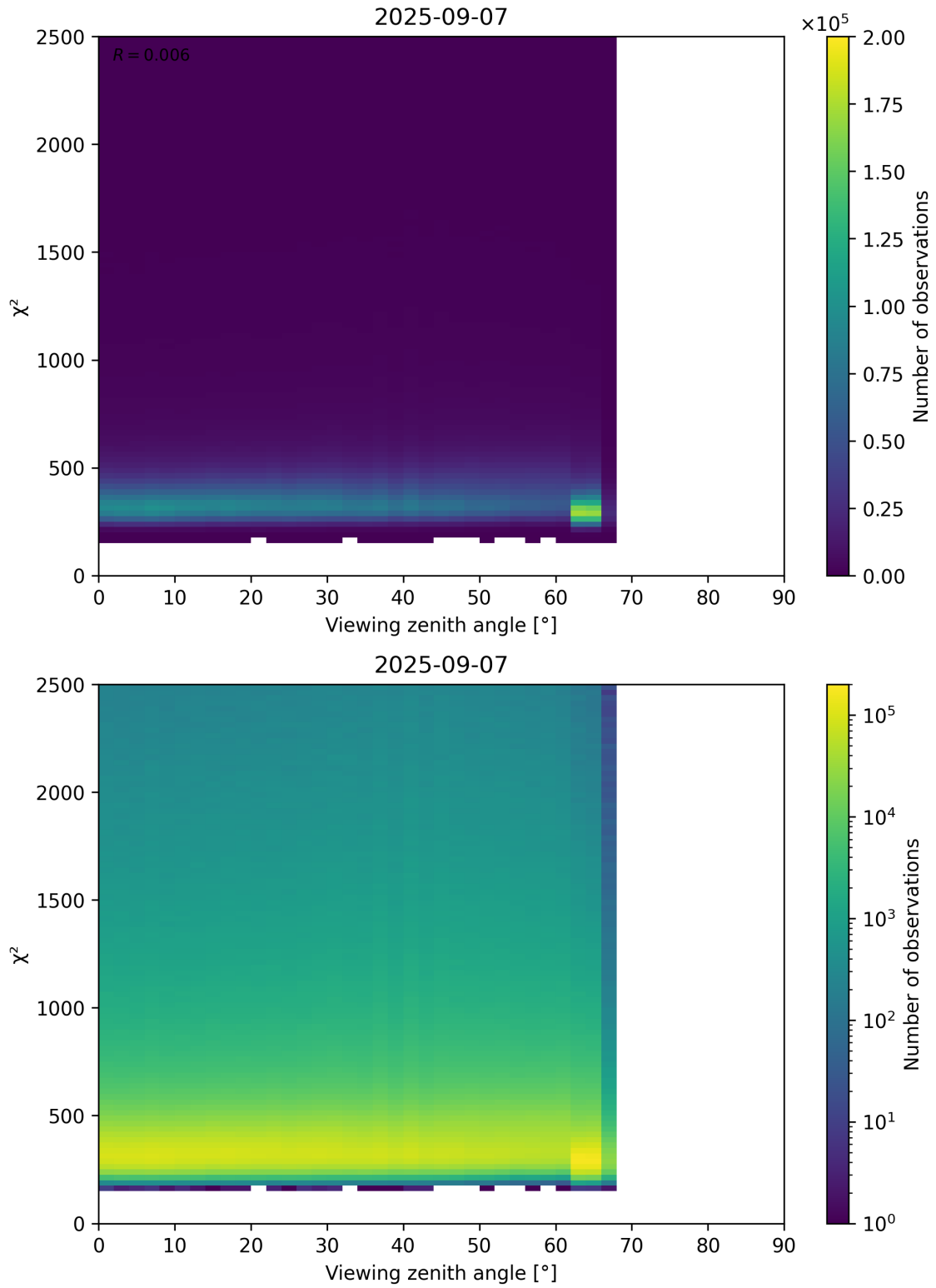
Figure 162: Scatter density plot of “Viewing zenith angle” against “ \chi^2 ” for 2025-09-06 to 2025-09-08.
