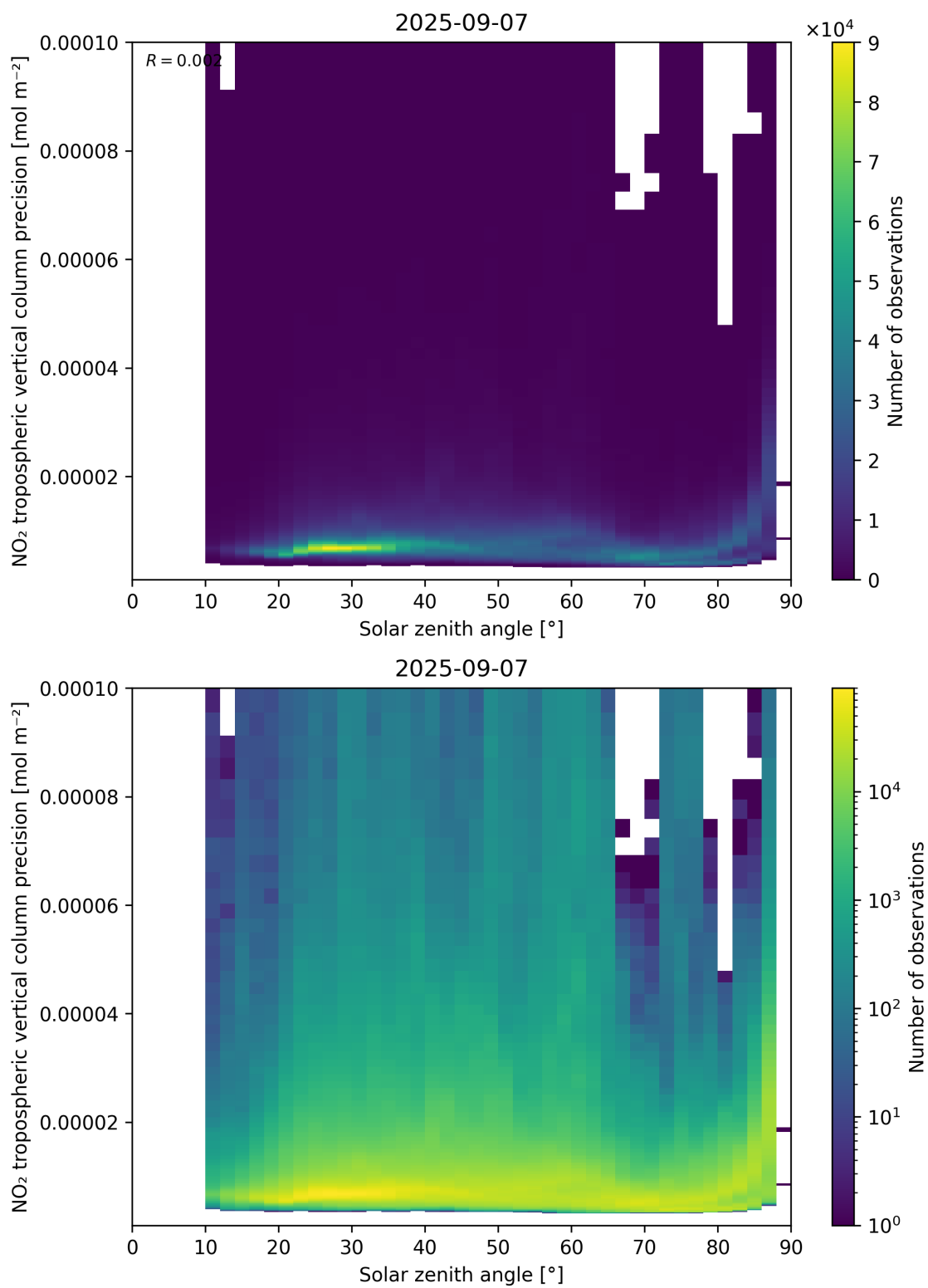
Figure 156: Scatter density plot of “Solar zenith angle” against “NO 2 tropospheric vertical column precision” for 2025-09-06 to 2025-09-08.
