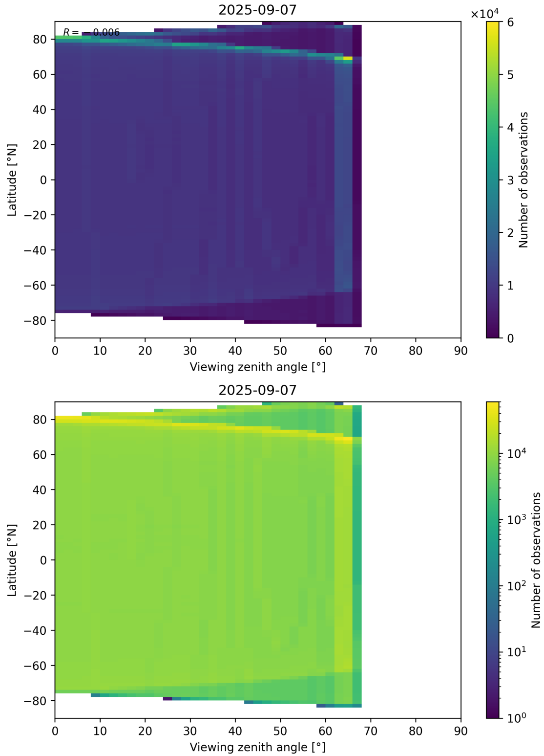
Figure 163: Scatter density plot of “Viewing zenith angle” against “Latitude” for 2025-09-06 to 2025-09-08.
