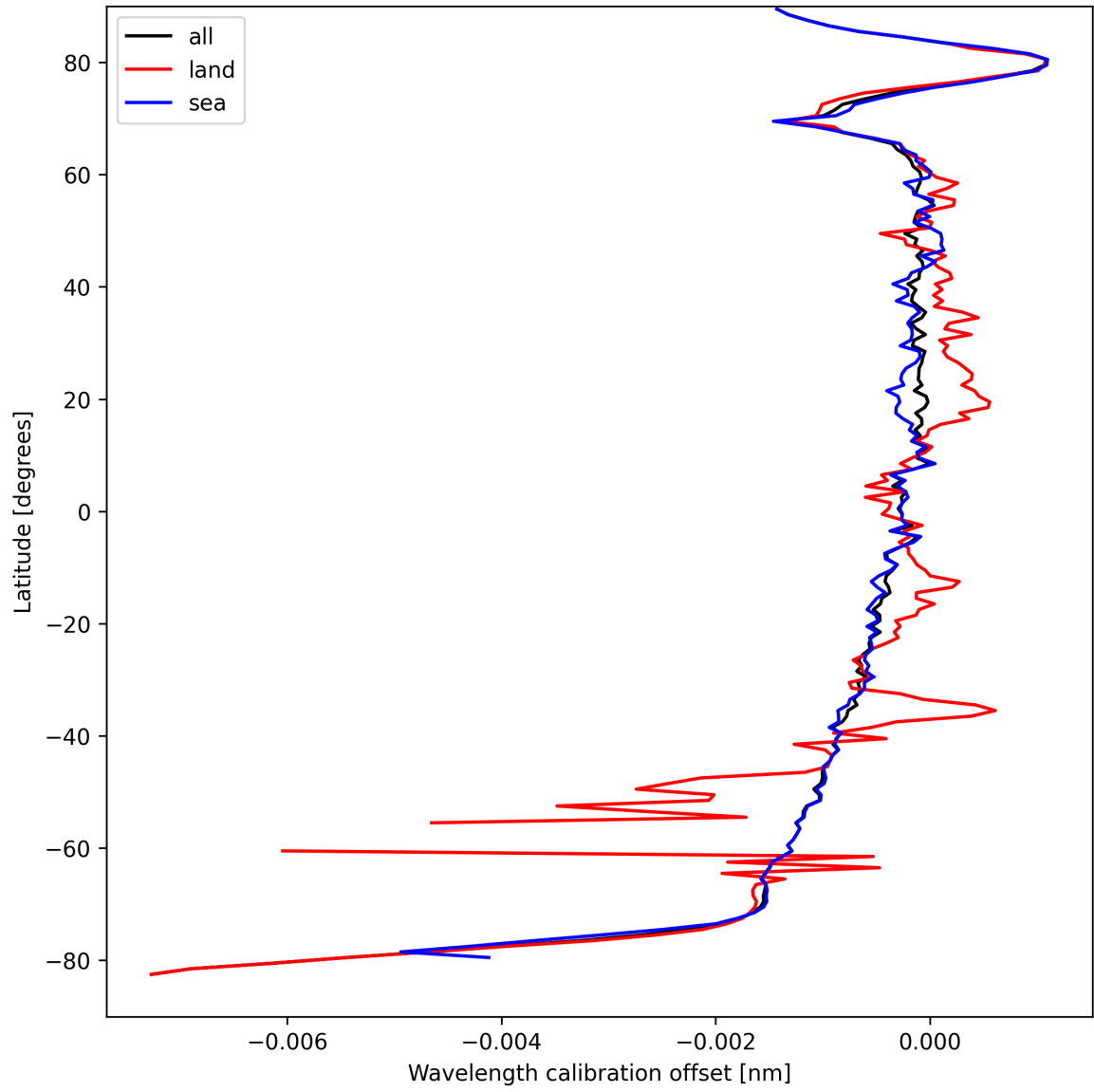
Figure 18: Zonal average of “Wavelength calibration offset” for 2025-09-06 to 2025-09-08.
