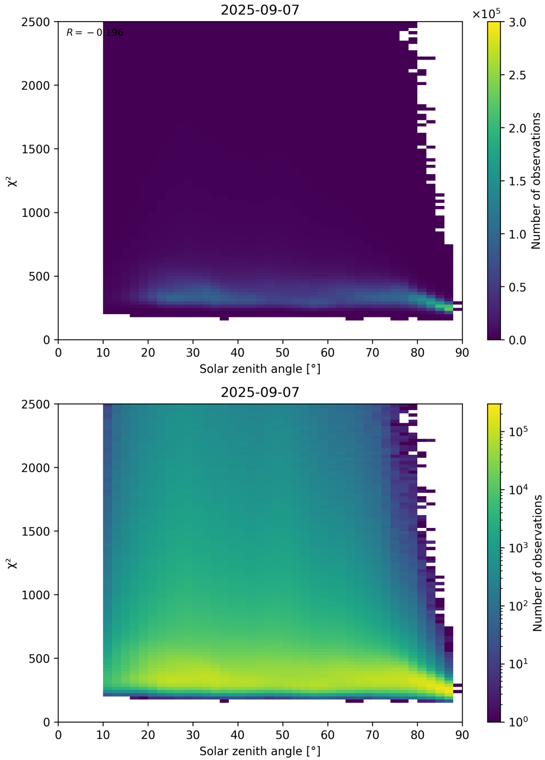
Figure 148: Scatter density plot of “Solar zenith angle” against “ \chi^2 ” for 2025-09-06 to 2025-09-08.
