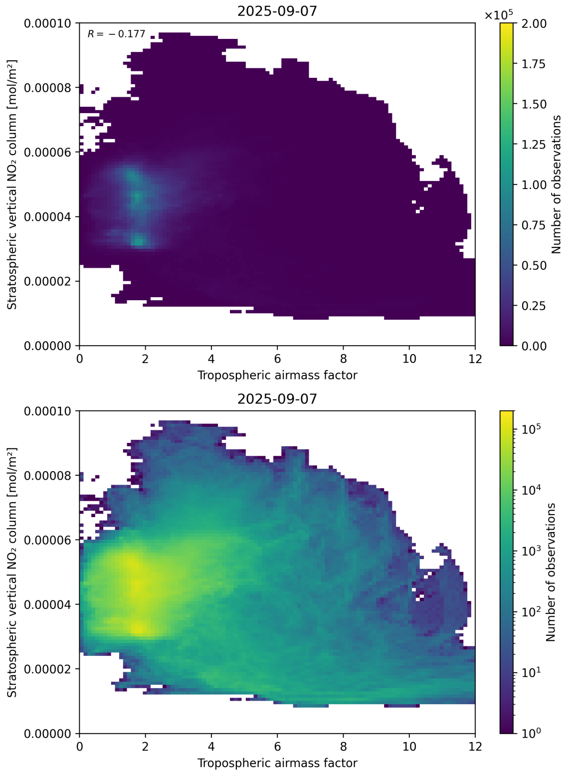
Figure 74: Scatter density plot of “Tropospheric air mass factor” against “Stratospheric vertical NO 2 column” for 2025-09-06 to 2025-09-08.
