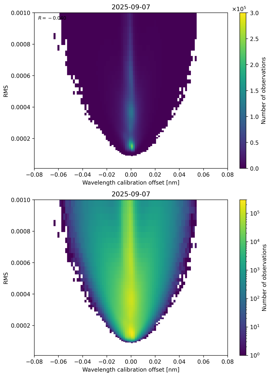
Figure 181: Scatter density plot of “Wavelength calibration offset” against “RMS” for 2025-09-06 to 2025-09-08.
