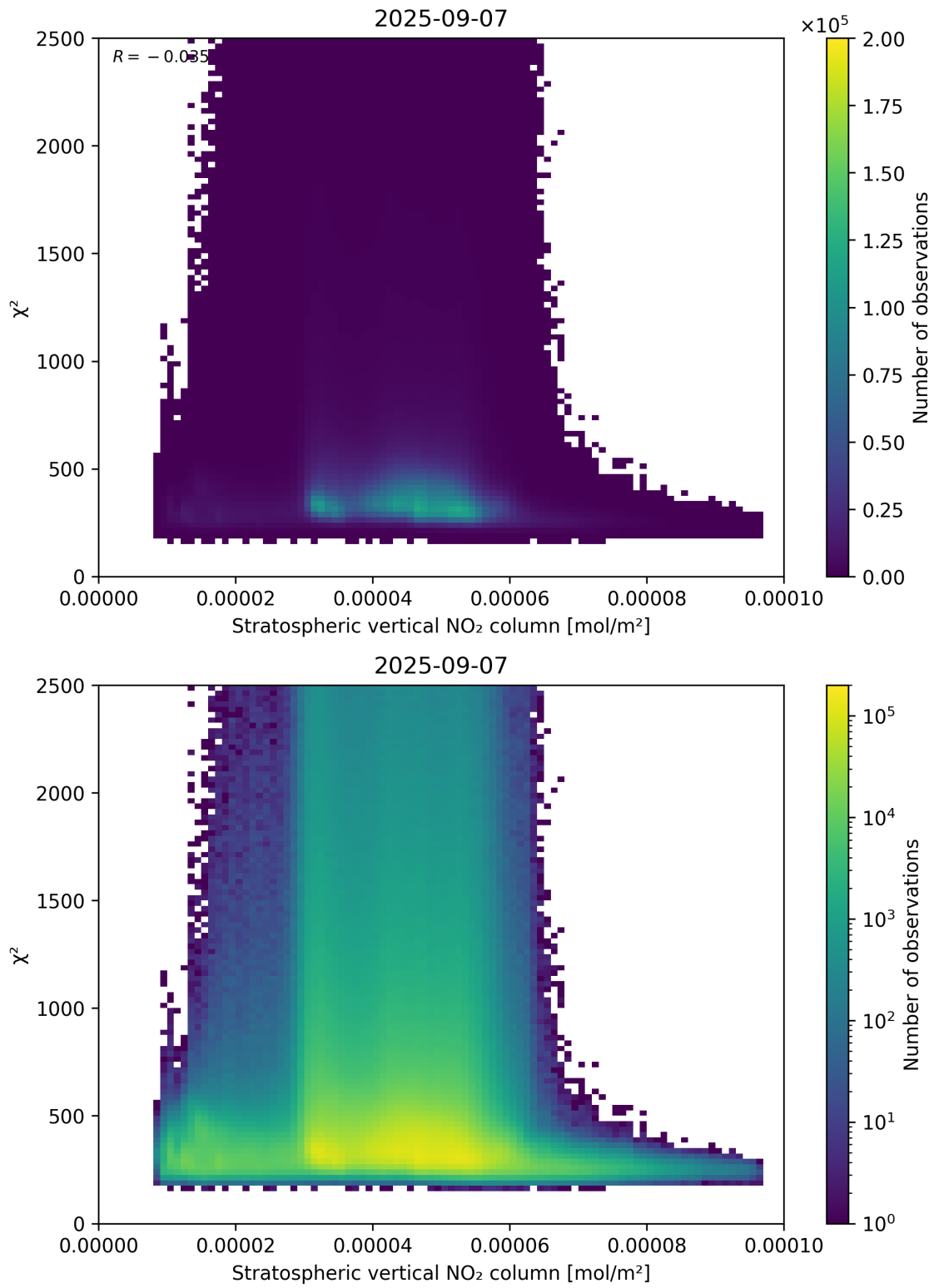
Figure 97: Scatter density plot of “Stratospheric vertical NO 2 column” against “ \chi^2 ” for 2025-09-06 to 2025-09-08.
