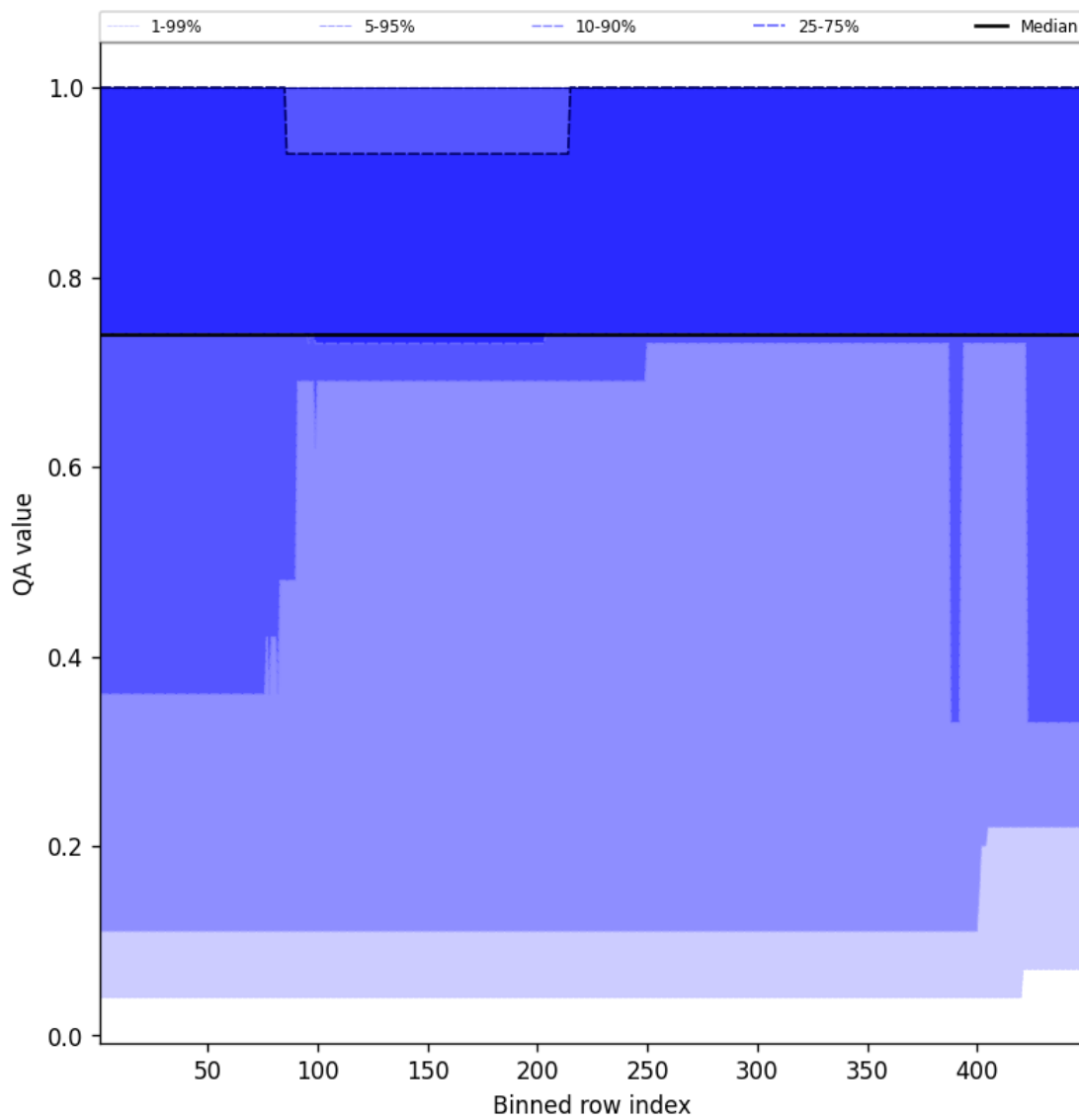
Figure 45: Along track statistics of “QA value” for 2025-09-06 to 2025-09-08
