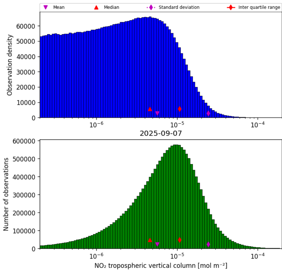
Figure 29: Histogram of “NO 2 tropospheric vertical column” for 2025-09-06 to 2025-09-08
