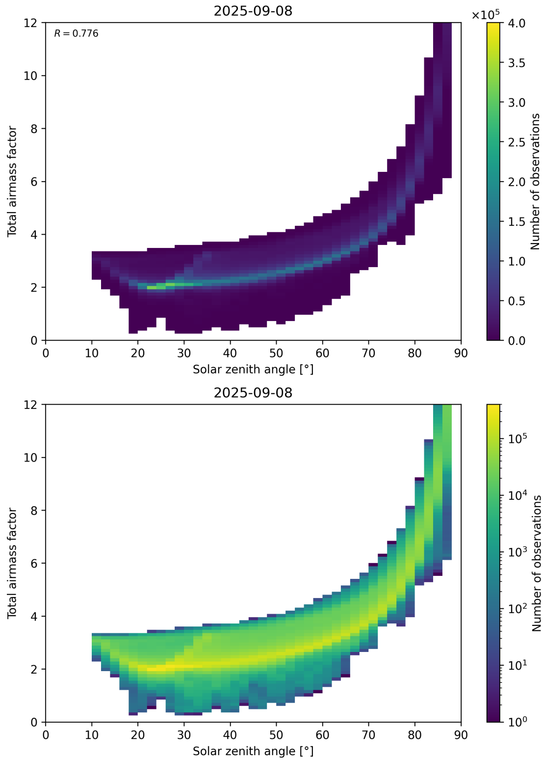
Figure 146: Scatter density plot of “Solar zenith angle” against “Total air mass factor” for 2025-09-07 to 2025-09-09.
