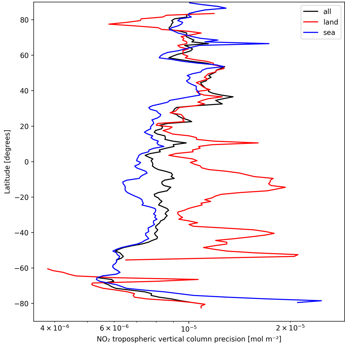
Figure 13: Zonal average of “NO 2 tropospheric vertical column precision” for 2025-09-07 to 2025-09-09.
