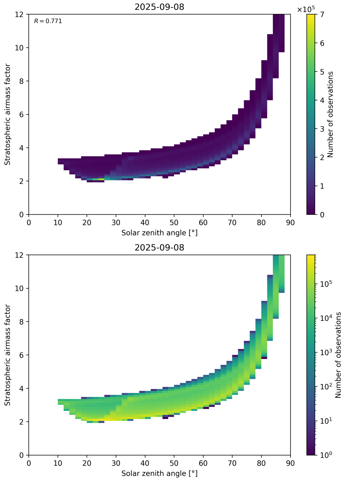
Figure 145: Scatter density plot of “Solar zenith angle” against “Stratospheric airmass factor” for 2025-09-07 to 2025-09-09.
