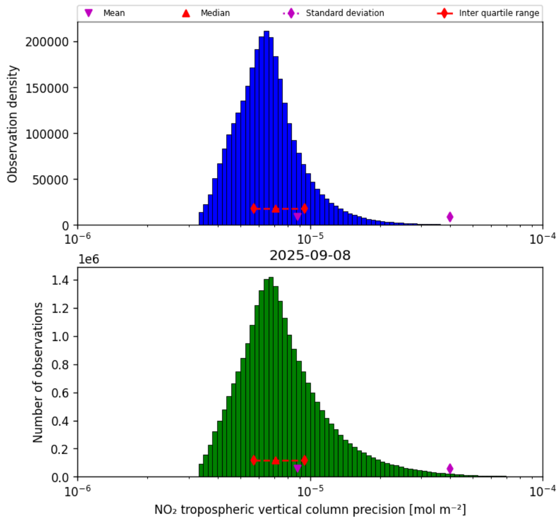
Figure 30: Histogram of “NO 2 tropospheric vertical column precision” for 2025-09-07 to 2025-09-09
