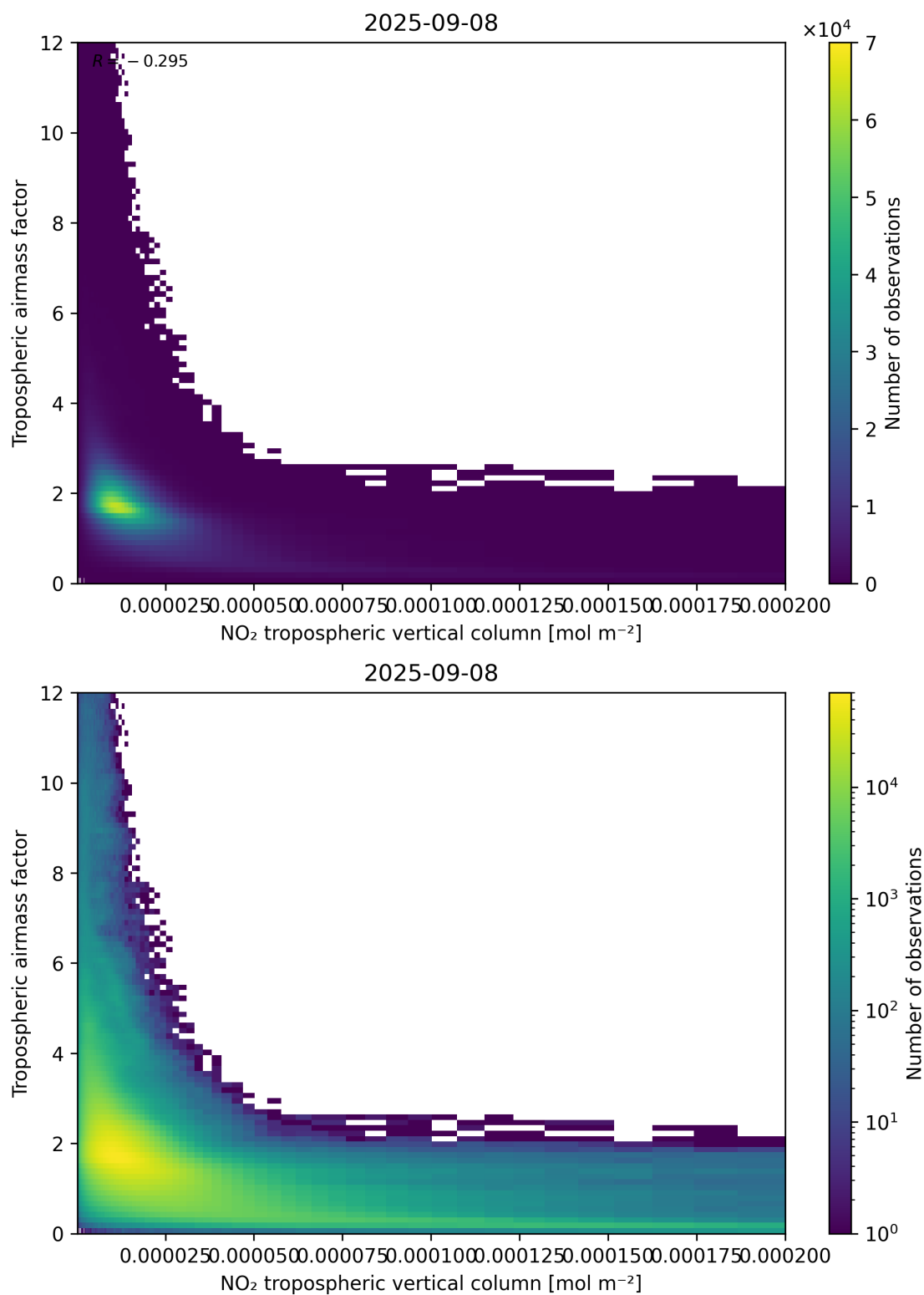
Figure 123: Scatter density plot of “NO 2 tropospheric vertical column” against “Tropospheric air mass factor” for 2025-09-07 to 2025-09-09.
