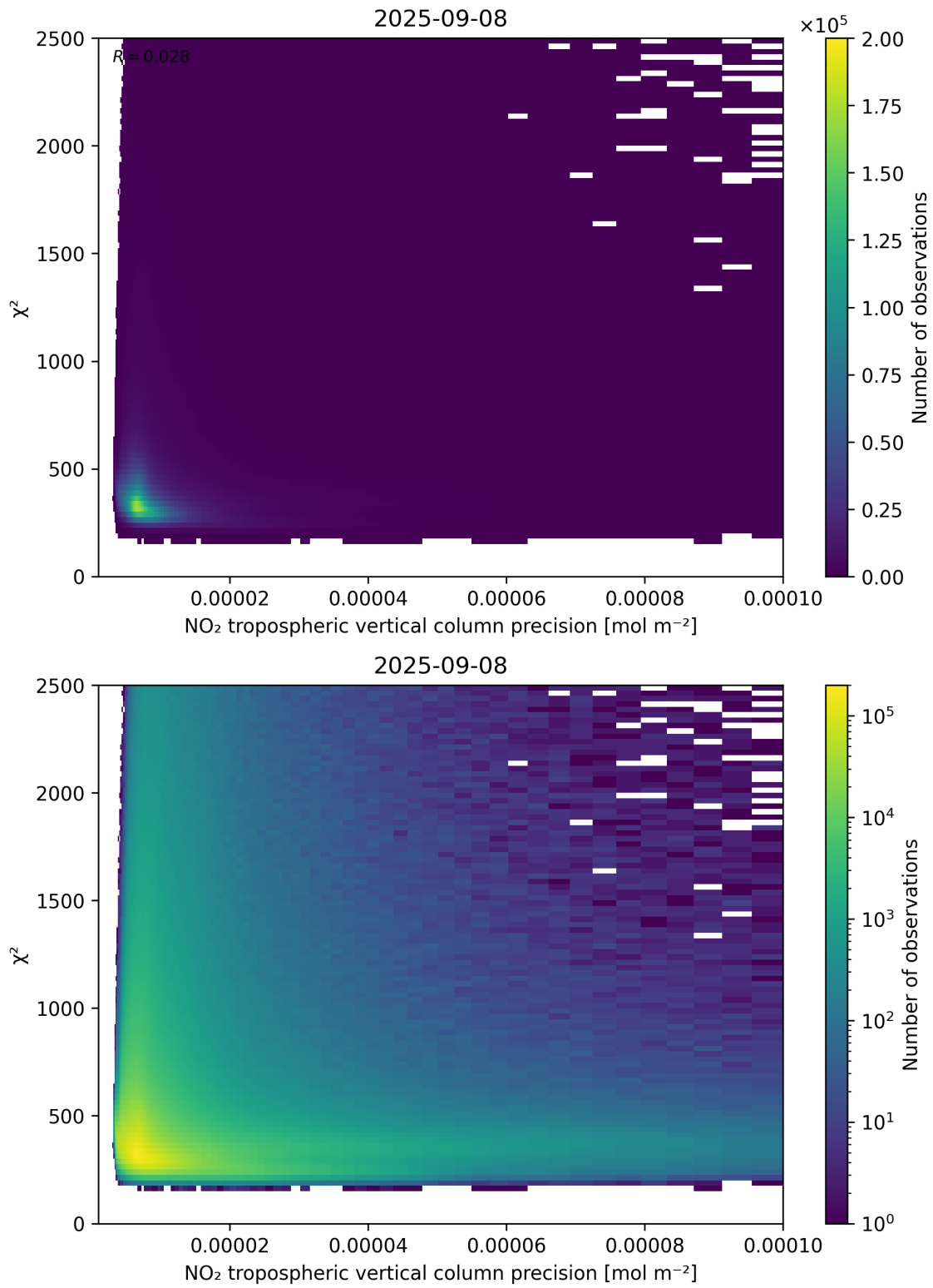
Figure 134: Scatter density plot of “NO 2 tropospheric vertical column precision” against “ \chi^2 ” for 2025-09-07 to 2025-09-09.
