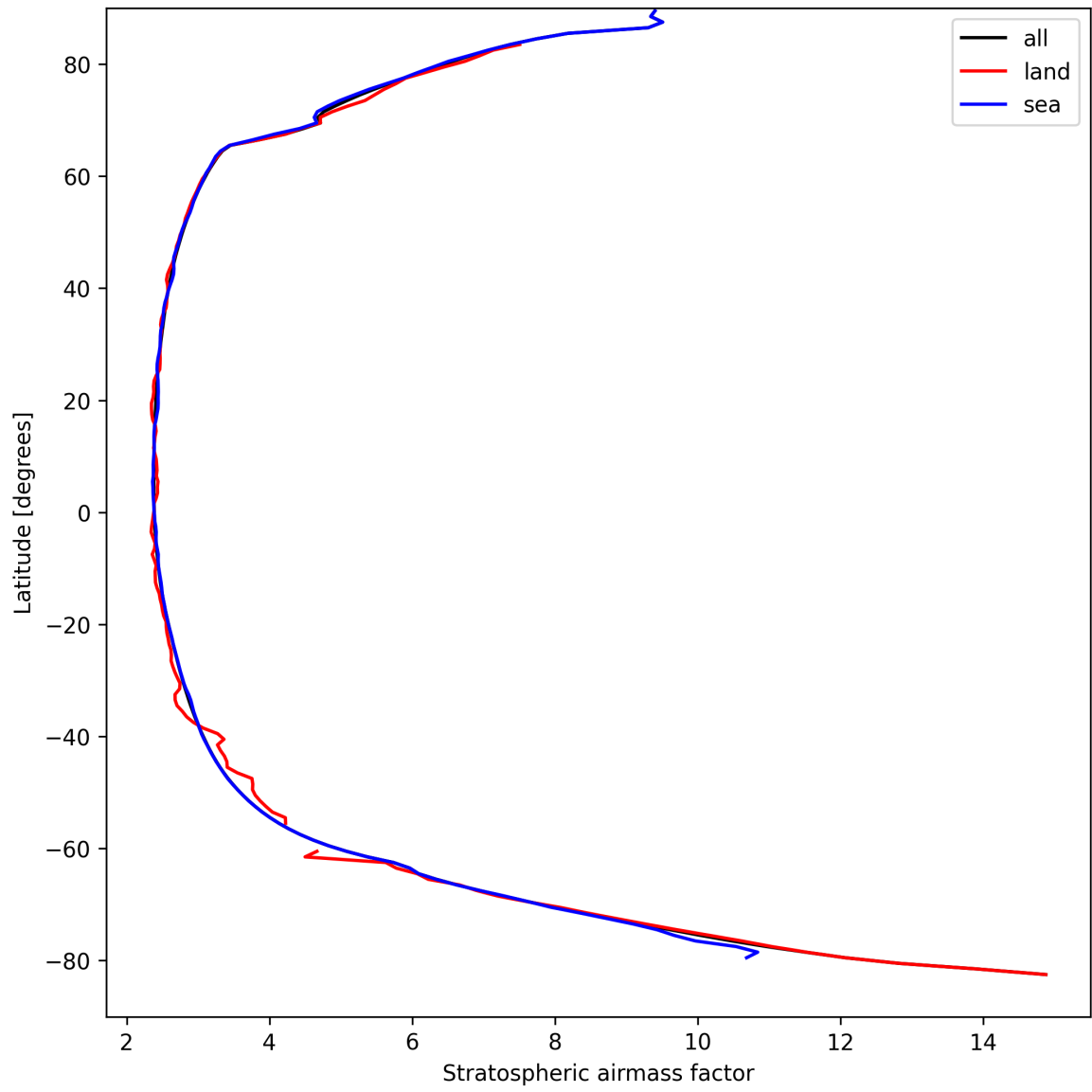
Figure 27: Zonal average of “Stratospheric air mass factor” for 2025-09-07 to 2025-09-09.
