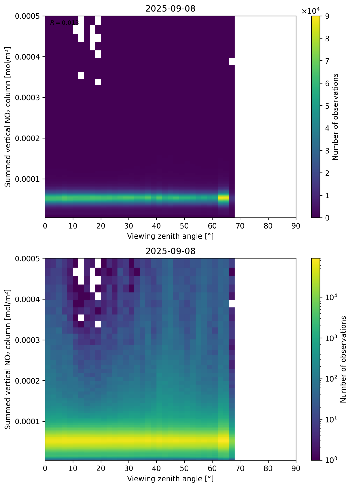
Figure 165: Scatter density plot of “Viewing zenith angle” against “Summed vertical NO 2 column” for 2025-09-07 to 2025-09-09.
