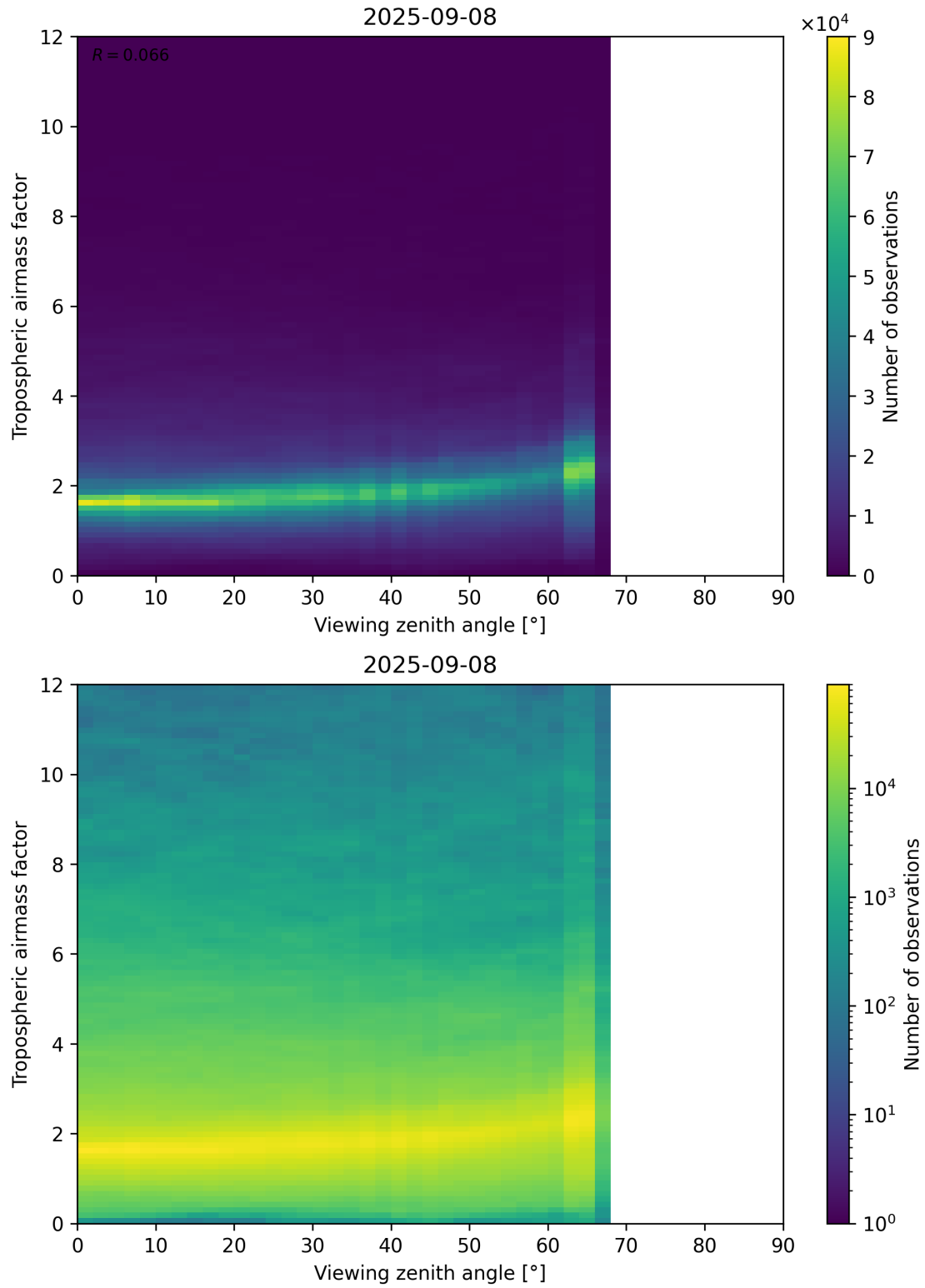
Figure 161: Scatter density plot of “Viewing zenith angle” against “Tropospheric airmass factor” for 2025-09-07 to 2025-09-09.
