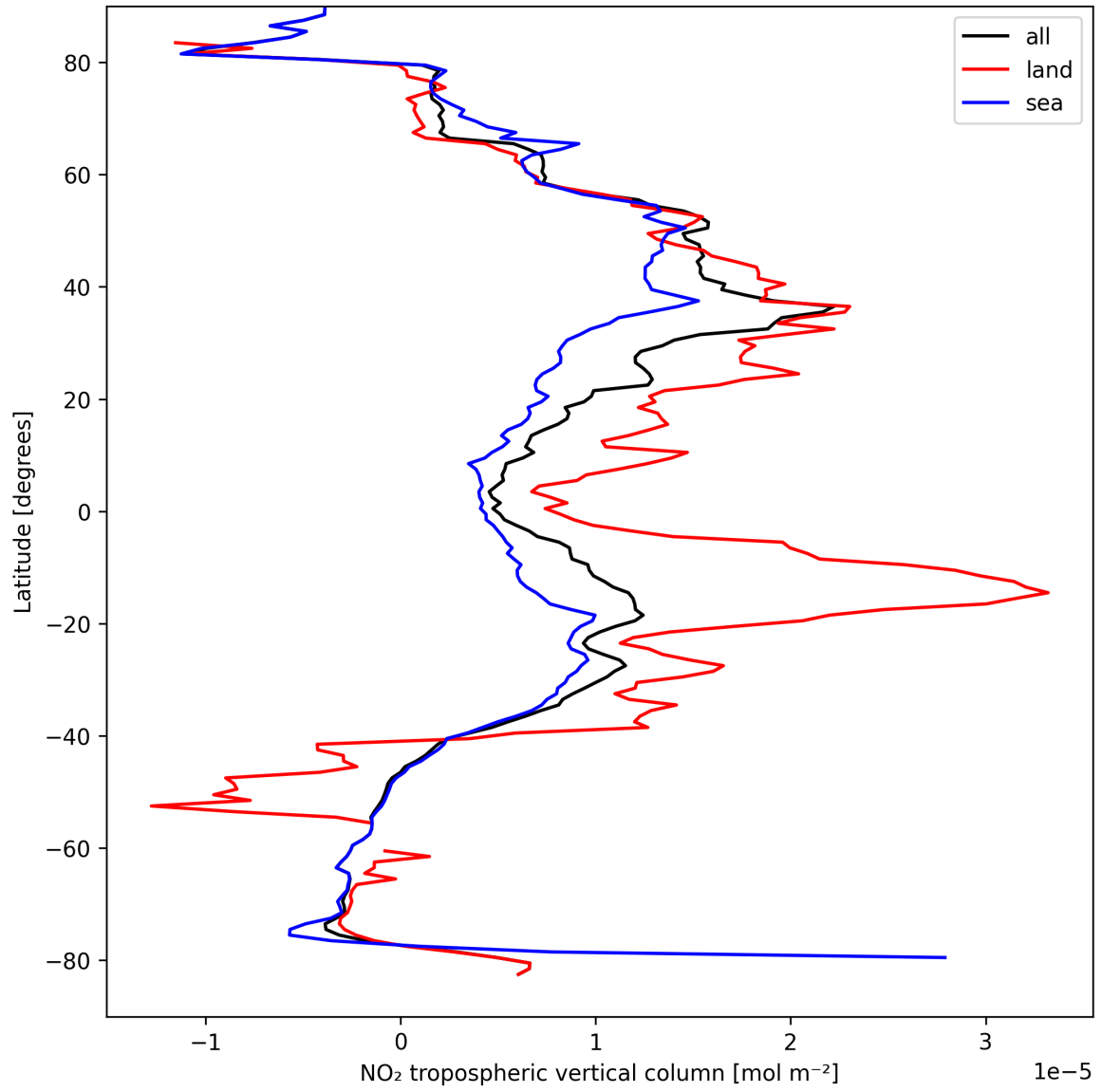
Figure 12: Zonal average of “NO 2 tropospheric vertical column” for 2025-09-07 to 2025-09-09.
