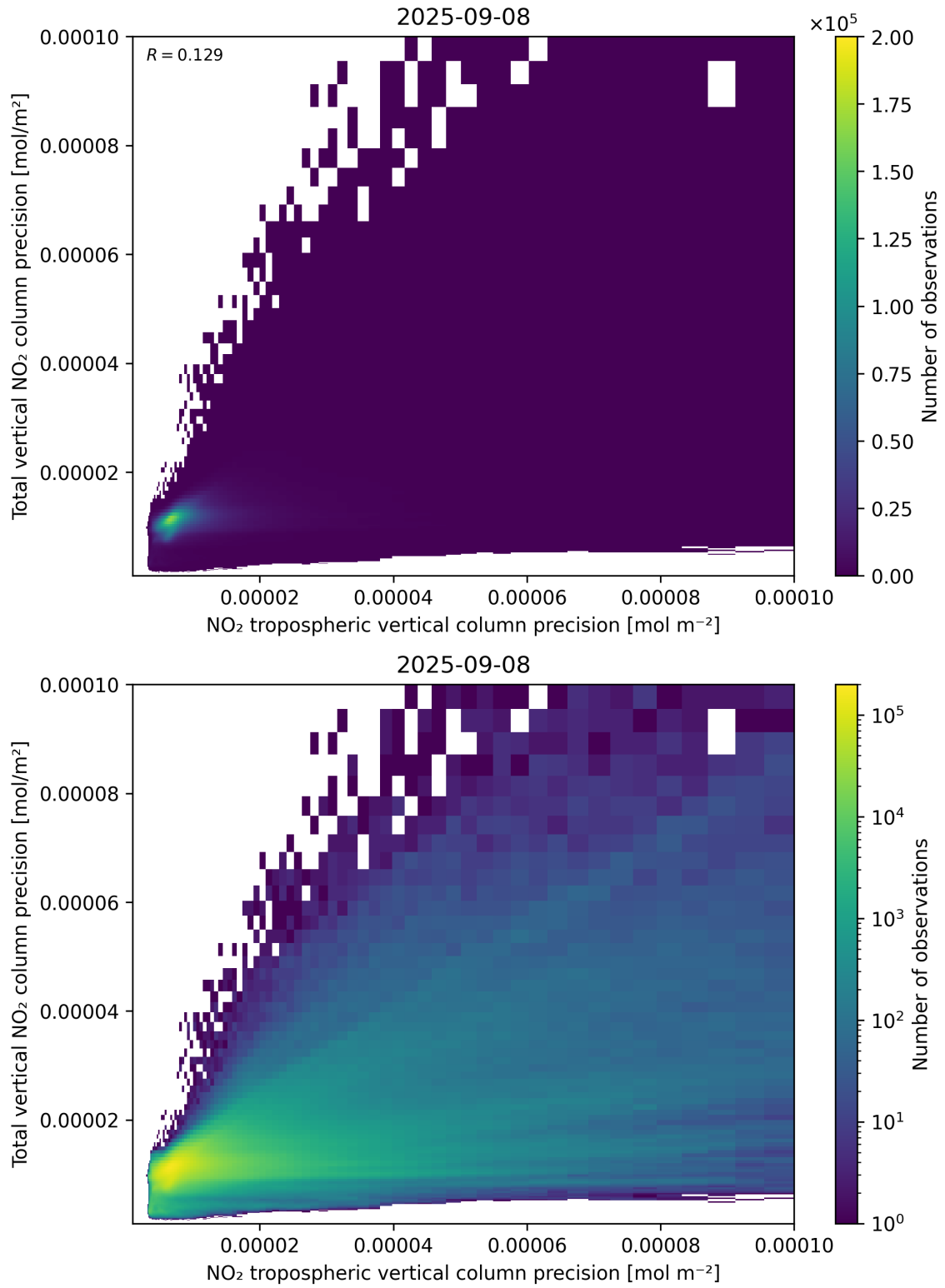
Figure 139: Scatter density plot of “NO 2 tropospheric vertical column precision” against “Total vertical NO 2 column precision” for 2025-09-07 to 2025-09-09.
