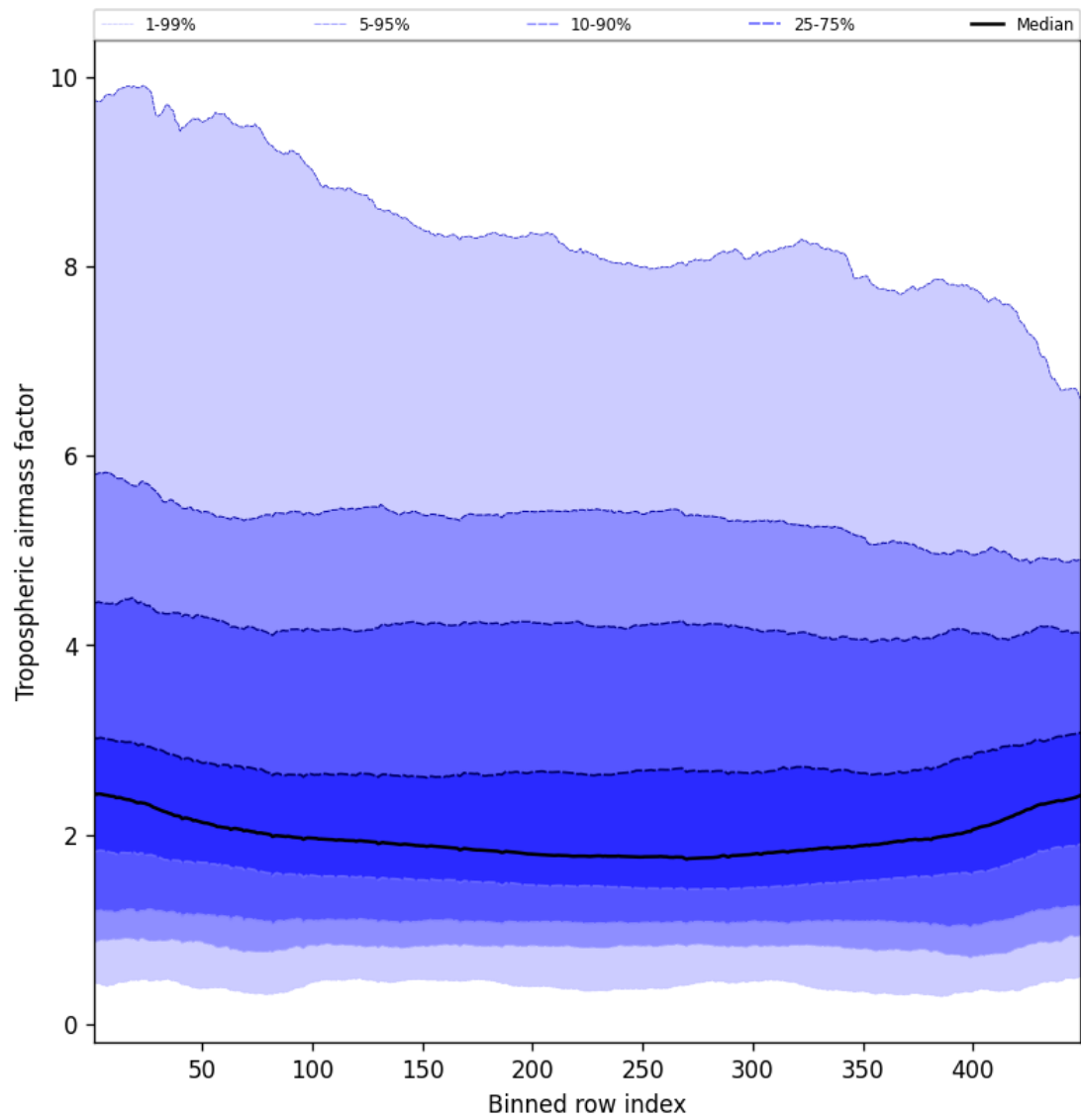
Figure 48: Along track statistics of “Tropospheric air mass factor” for 2025-09-07 to 2025-09-09
