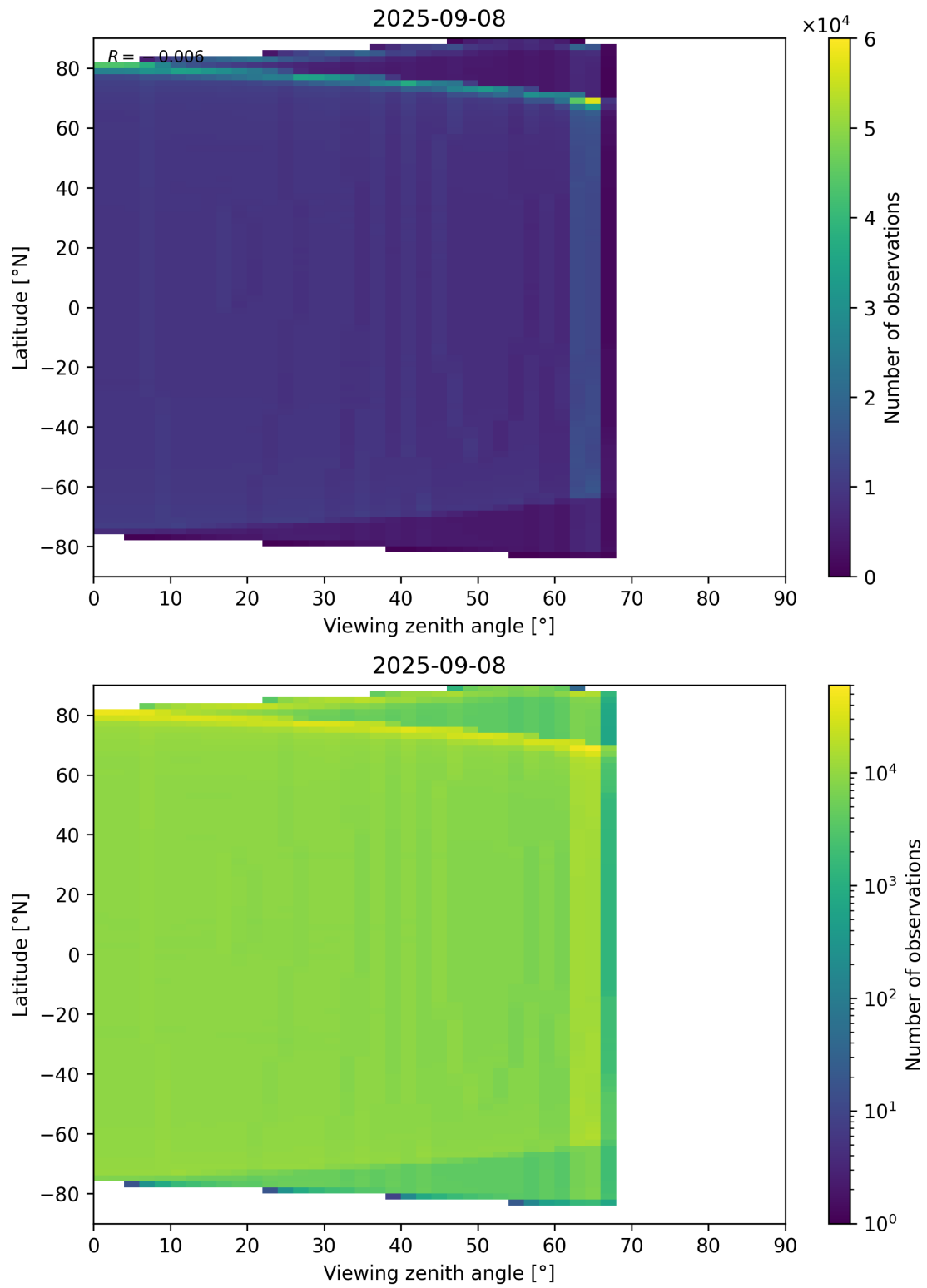
Figure 163: Scatter density plot of “Viewing zenith angle” against “Latitude” for 2025-09-07 to 2025-09-09.
