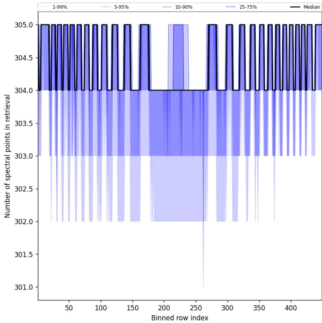
Figure 50: Along track statistics of “Number of spectral points in retrieval” for 2025-09-07 to 2025-09-09
