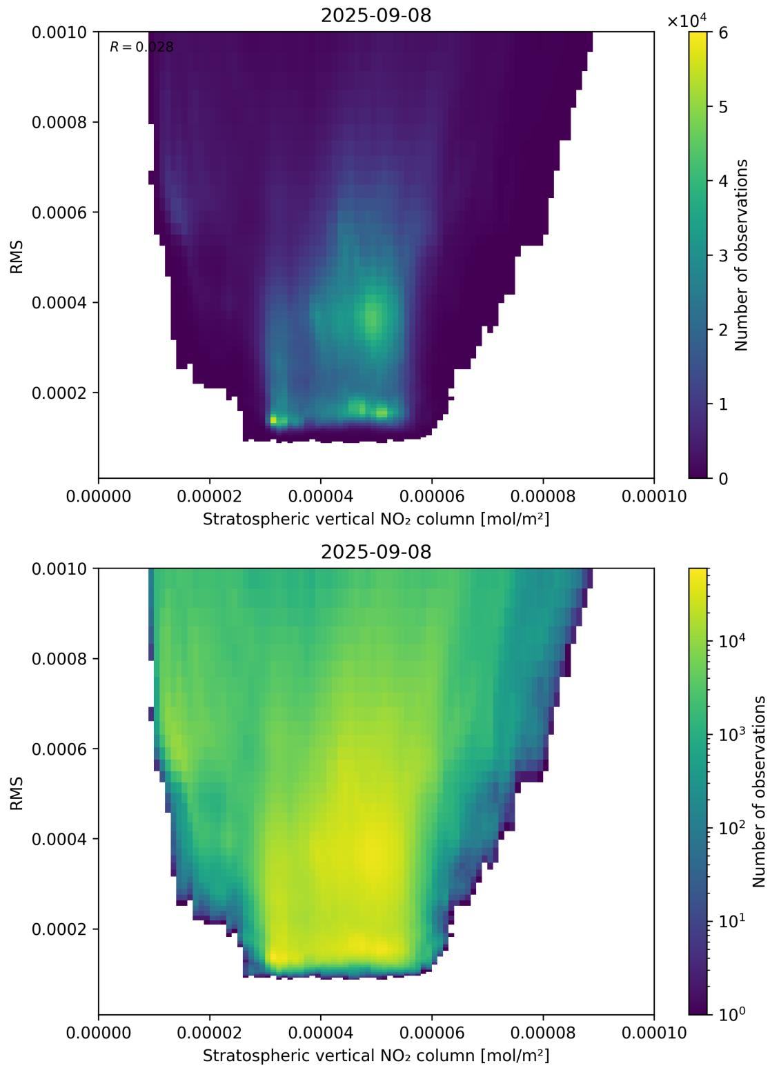
Figure 102: Scatter density plot of “Stratospheric vertical NO 2 column” against “RMS” for 2025-09-07 to 2025-09-09.
