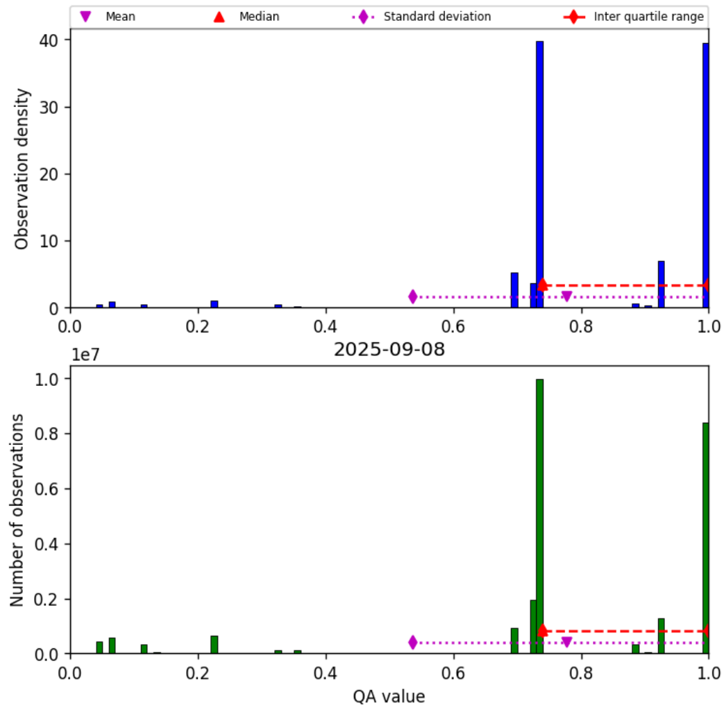
Figure 28: Histogram of “QA value” for 2025-09-07 to 2025-09-09
