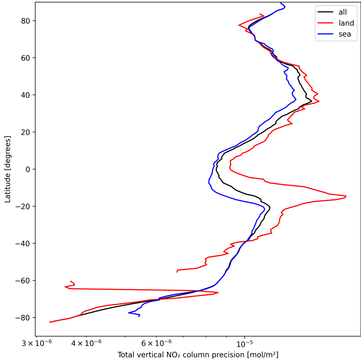
Figure 22: Zonal average of “Total vertical NO 2 column precision” for 2025-09-07 to 2025-09-09.
