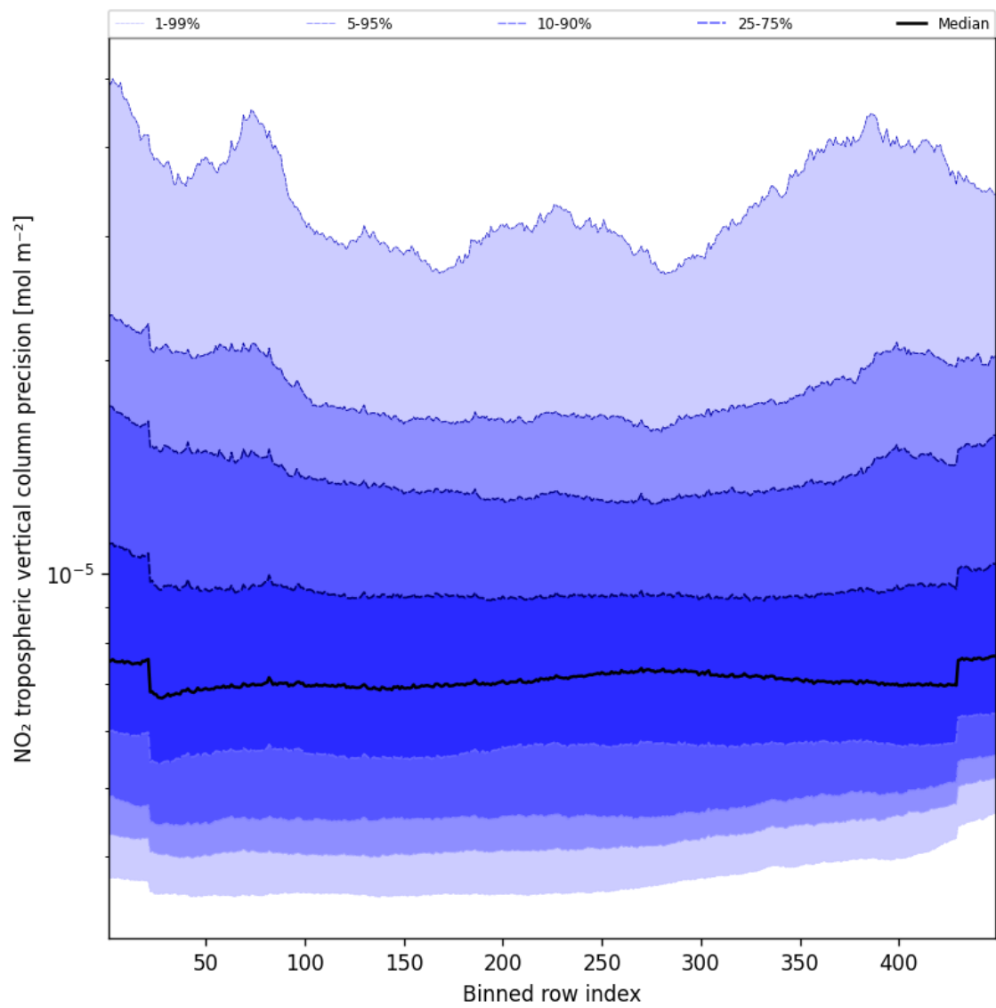
Figure 47: Along track statistics of “NO 2 tropospheric vertical column precision” for 2025-09-07 to 2025-09-09
