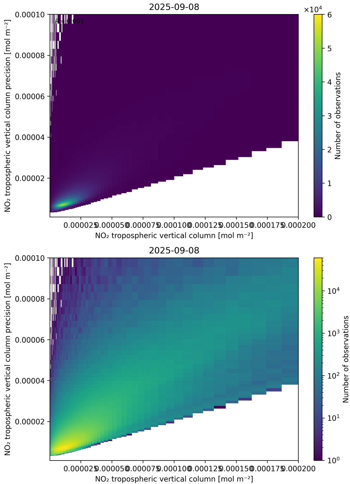
Figure 130: Scatter density plot of “NO 2 tropospheric vertical column” against “NO 2 tropospheric vertical column precision” for 2025-09-07 to 2025-09-09.
