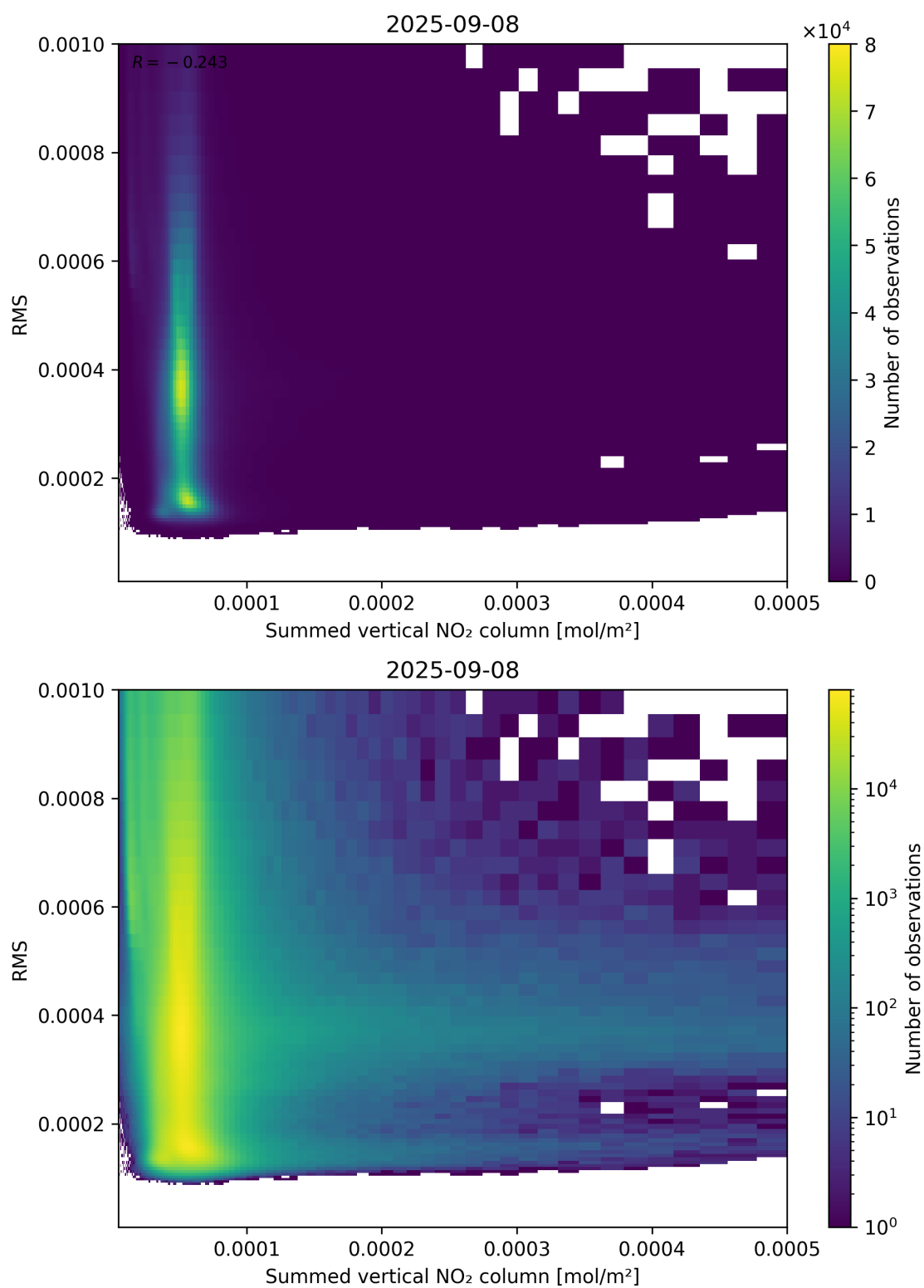
Figure 109: Scatter density plot of “Summed vertical NO 2 column” against “RMS” for 2025-09-07 to 2025-09-09.
