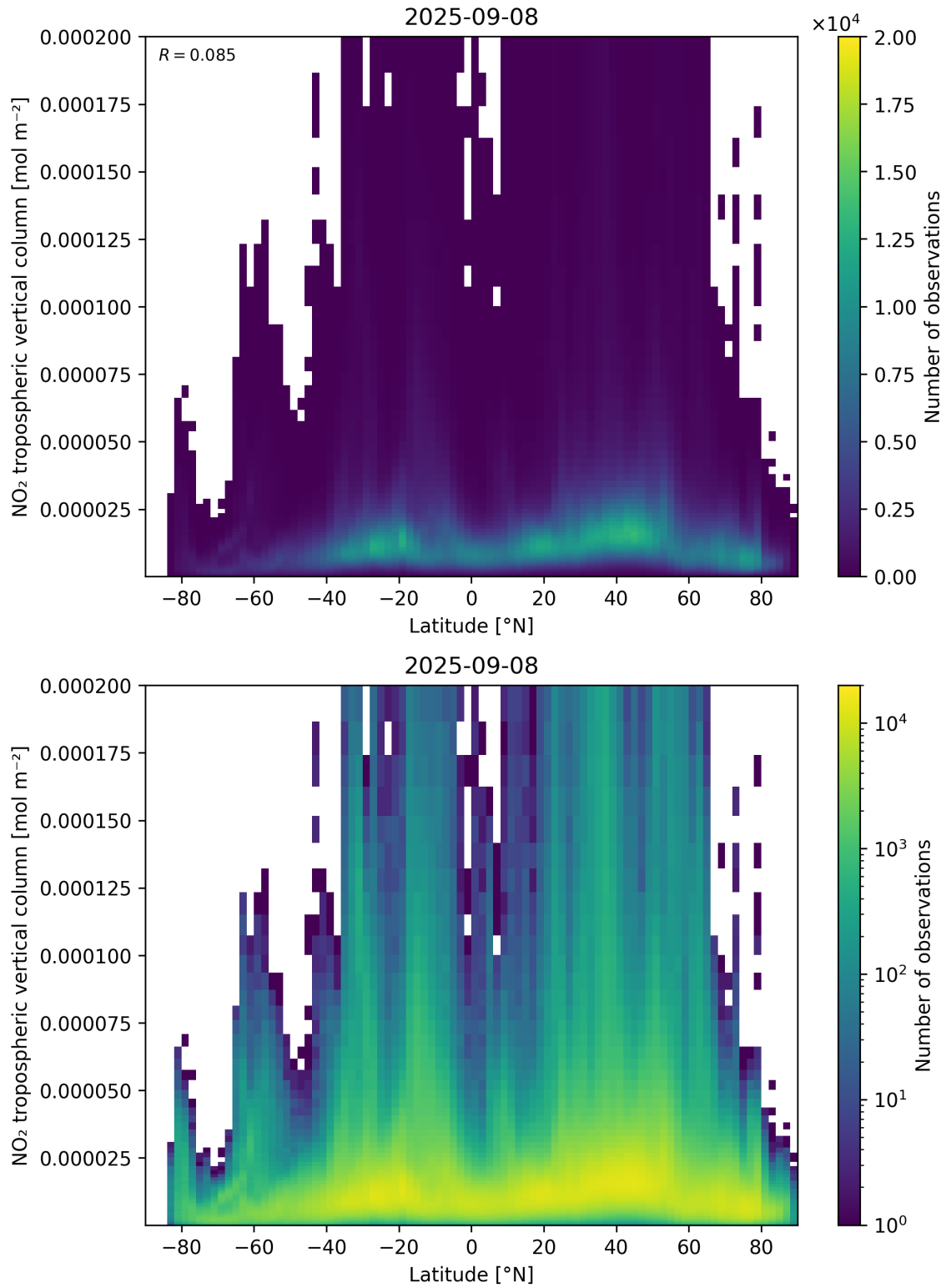
Figure 92: Scatter density plot of “Latitude” against “NO 2 tropospheric vertical column” for 2025-09-07 to 2025-09-09.
