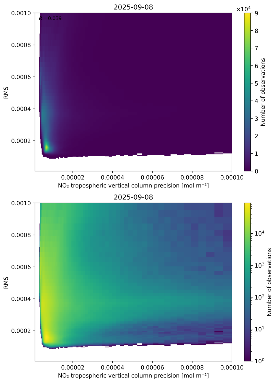
Figure 140: Scatter density plot of “NO 2 tropospheric vertical column precision” against “RMS” for 2025-09-07 to 2025-09-09.
