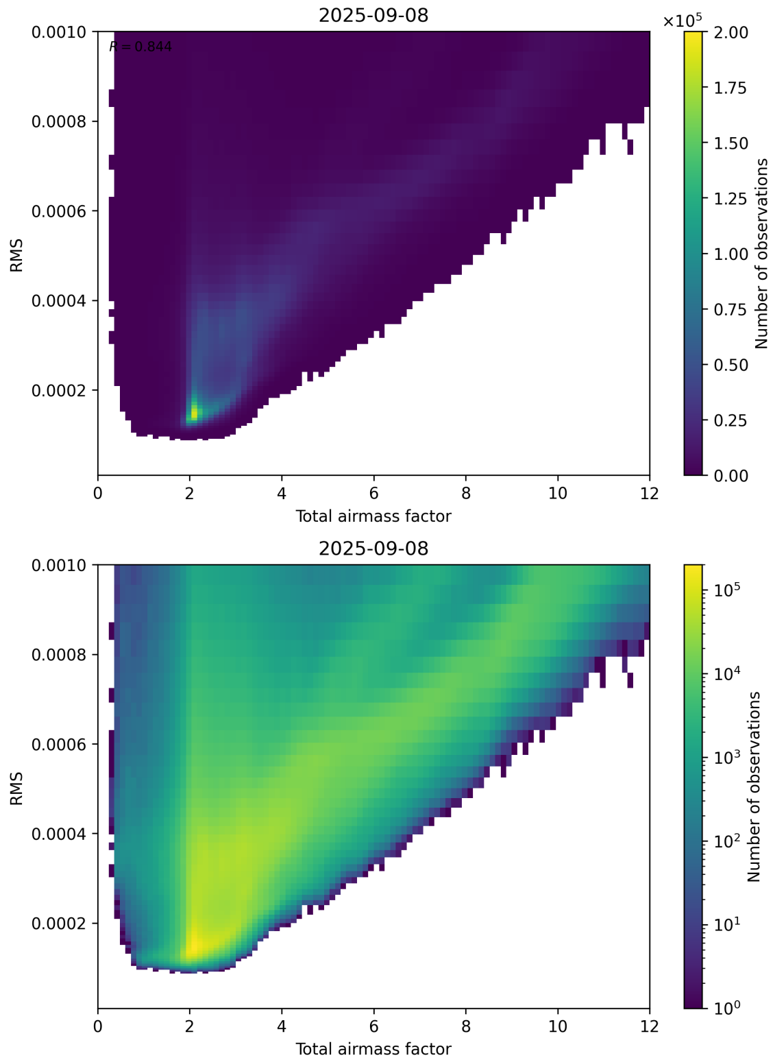
Figure 69: Scatter density plot of “Total airmass factor” against “RMS” for 2025-09-07 to 2025-09-09.
