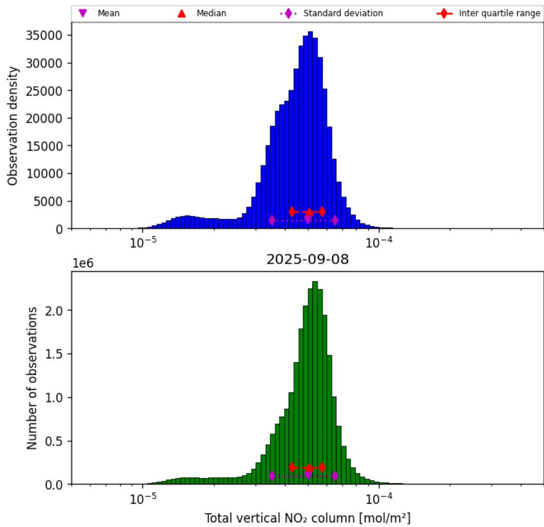
Figure 38: Histogram of “Total vertical NO 2 column” for 2025-09-07 to 2025-09-09
