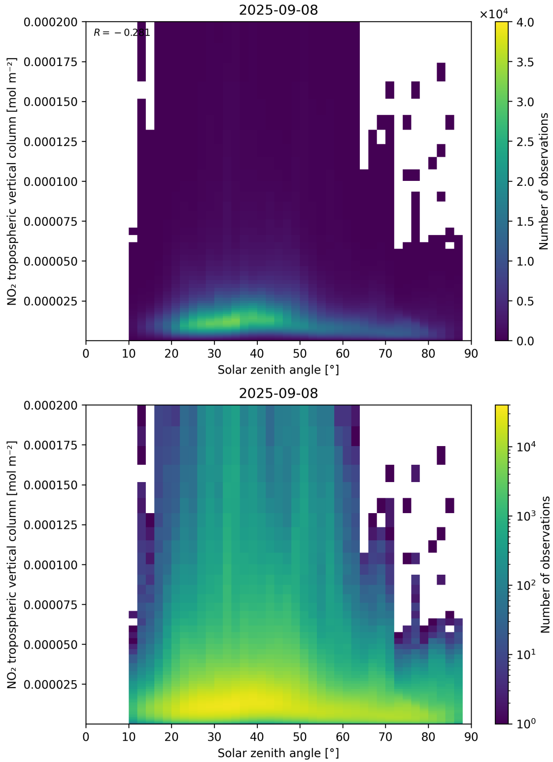
Figure 155: Scatter density plot of “Solar zenith angle” against “NO 2 tropospheric vertical column” for 2025-09-07 to 2025-09-09.
