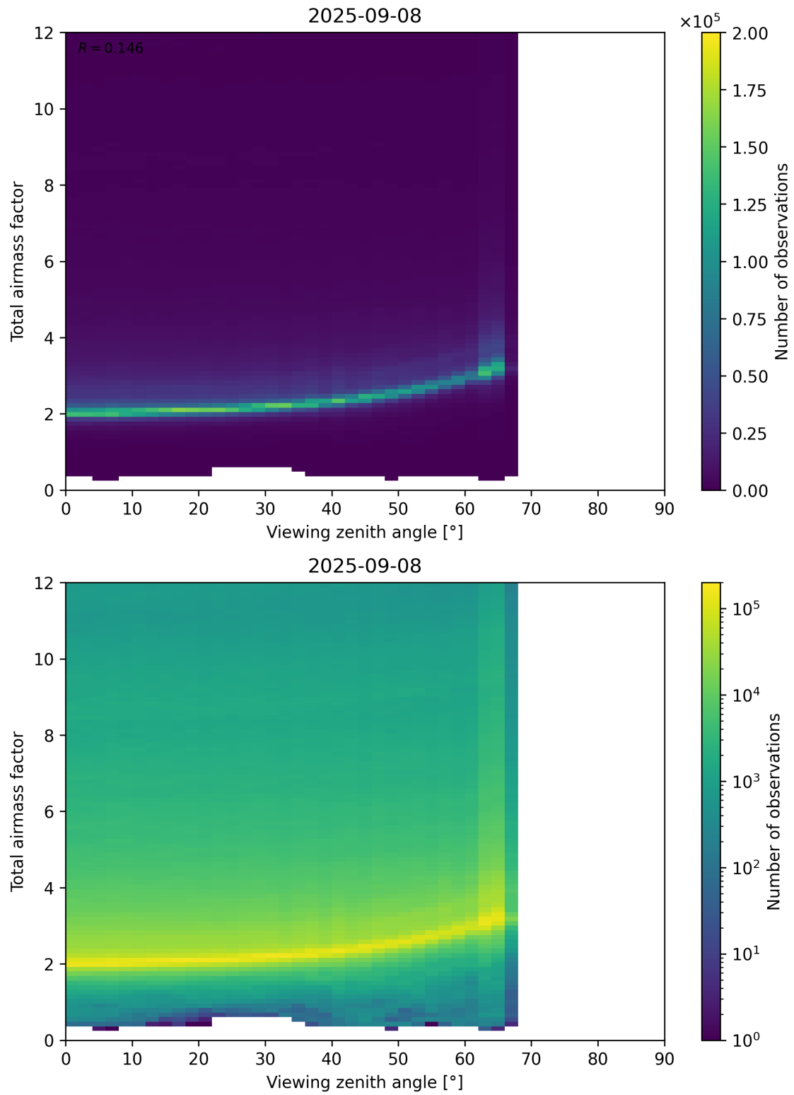
Figure 160: Scatter density plot of “Viewing zenith angle” against “Total airmass factor” for 2025-09-07 to 2025-09-09.
