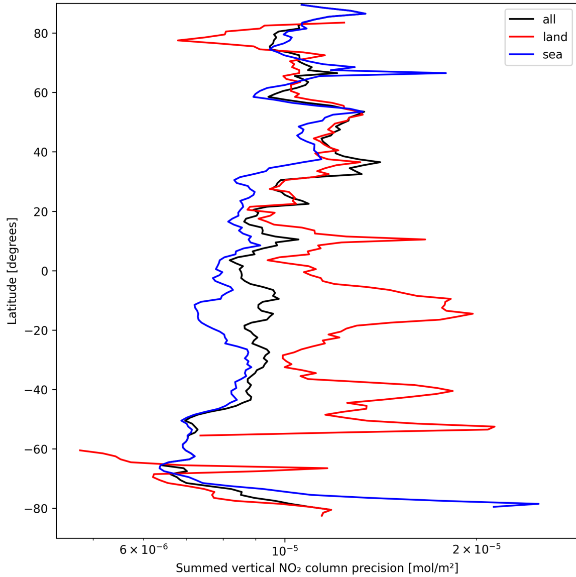
Figure 24: Zonal average of “Summed vertical NO 2 column precision” for 2025-09-07 to 2025-09-09.
