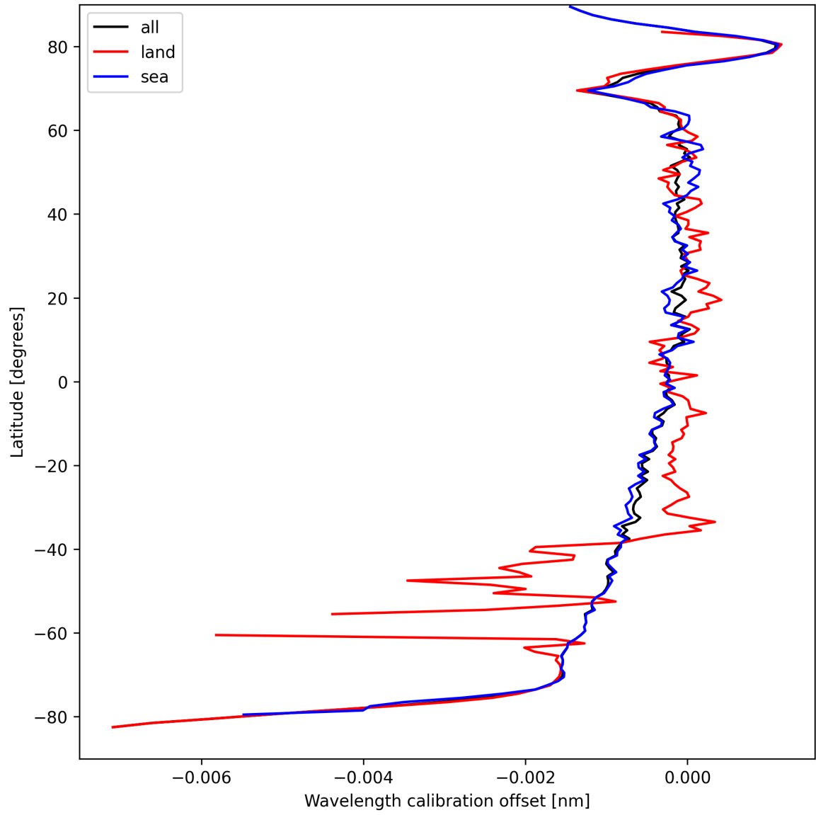
Figure 18: Zonal average of “Wavelength calibration offset” for 2025-09-07 to 2025-09-09.
