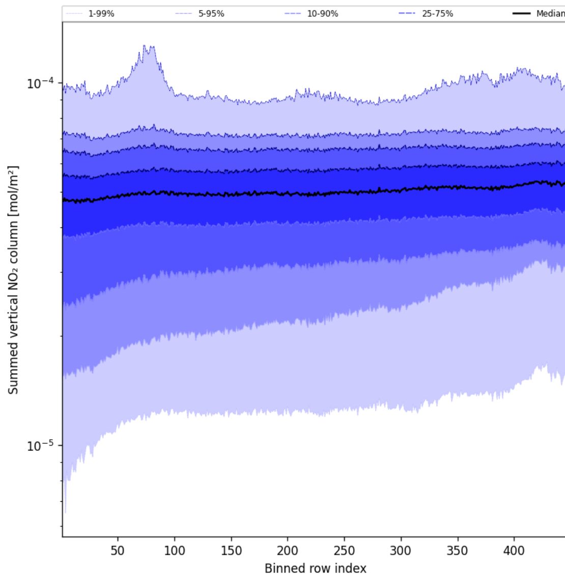
Figure 57: Along track statistics of “Summed vertical NO 2 column” for 2025-09-07 to 2025-09-09
