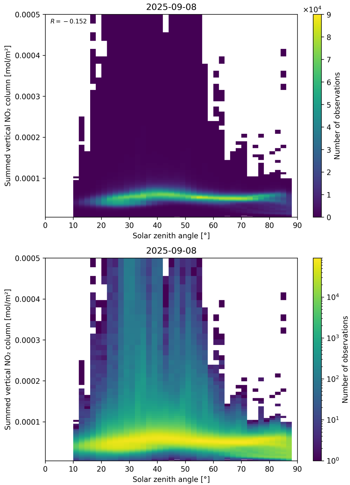
Figure 151: Scatter density plot of “Solar zenith angle” against “Summed vertical NO 2 column” for 2025-09-07 to 2025-09-09.
