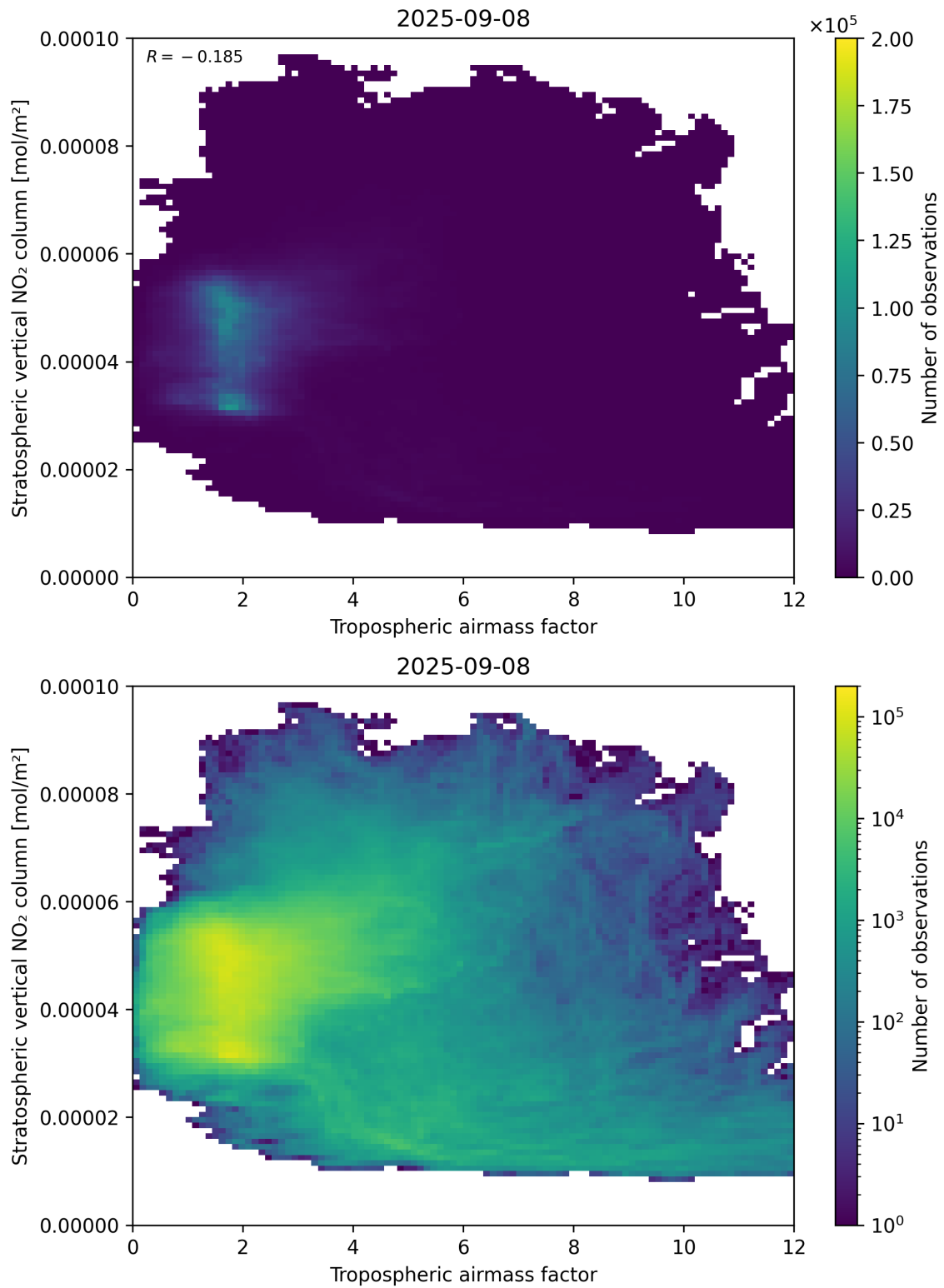
Figure 74: Scatter density plot of “Tropospheric air mass factor” against “Stratospheric vertical NO 2 column” for 2025-09-07 to 2025-09-09.
