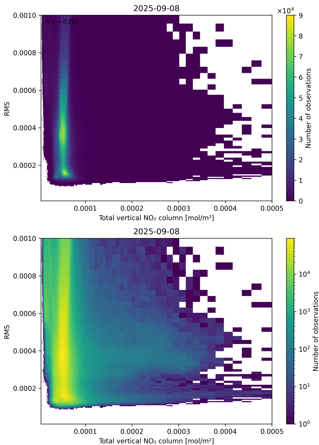
Figure 120: Scatter density plot of “Total vertical NO 2 column” against “RMS” for 2025-09-07 to 2025-09-09.
