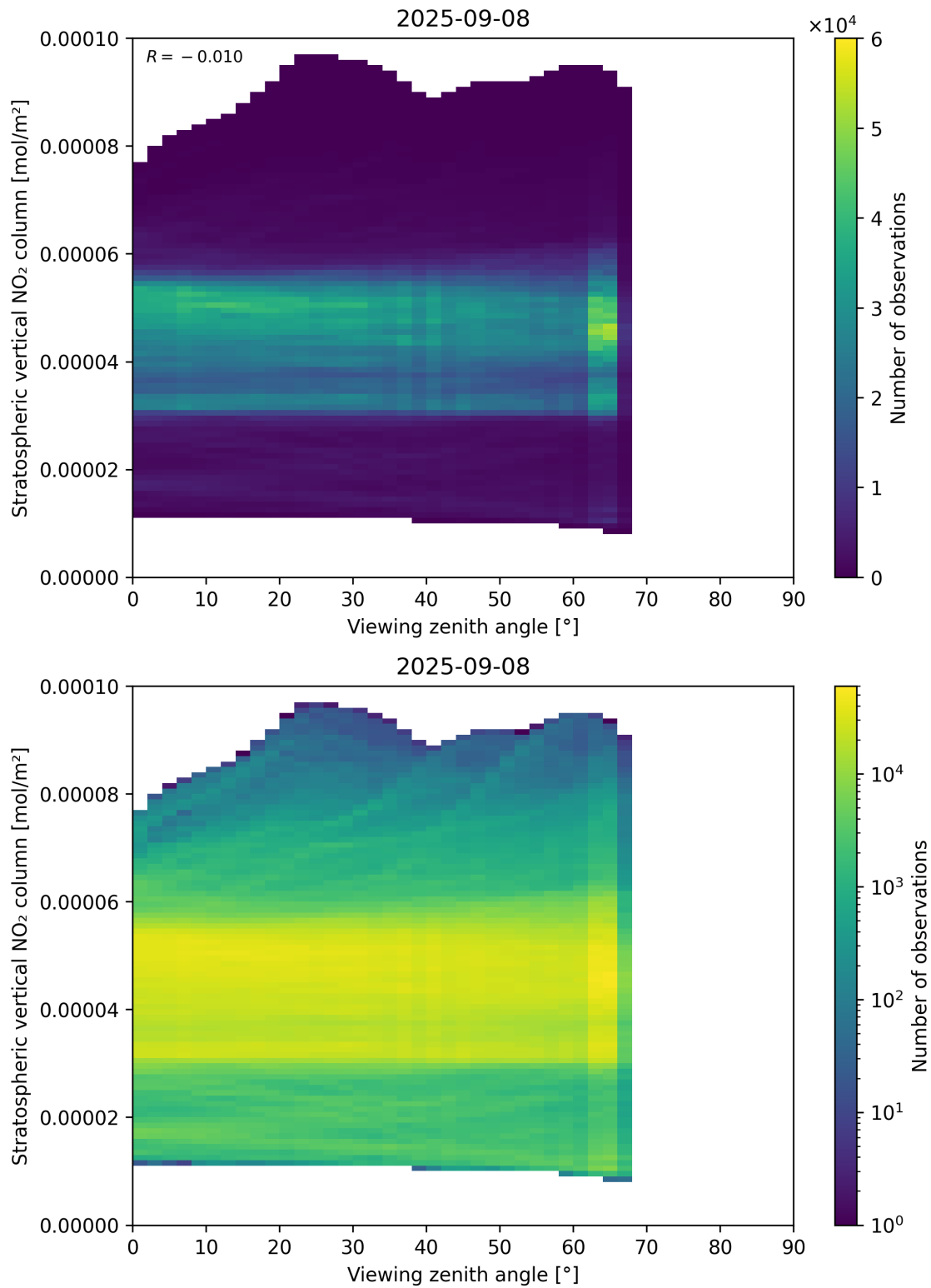
Figure 164: Scatter density plot of “Viewing zenith angle” against “Stratospheric vertical NO 2 column” for 2025-09-07 to 2025-09-09.
