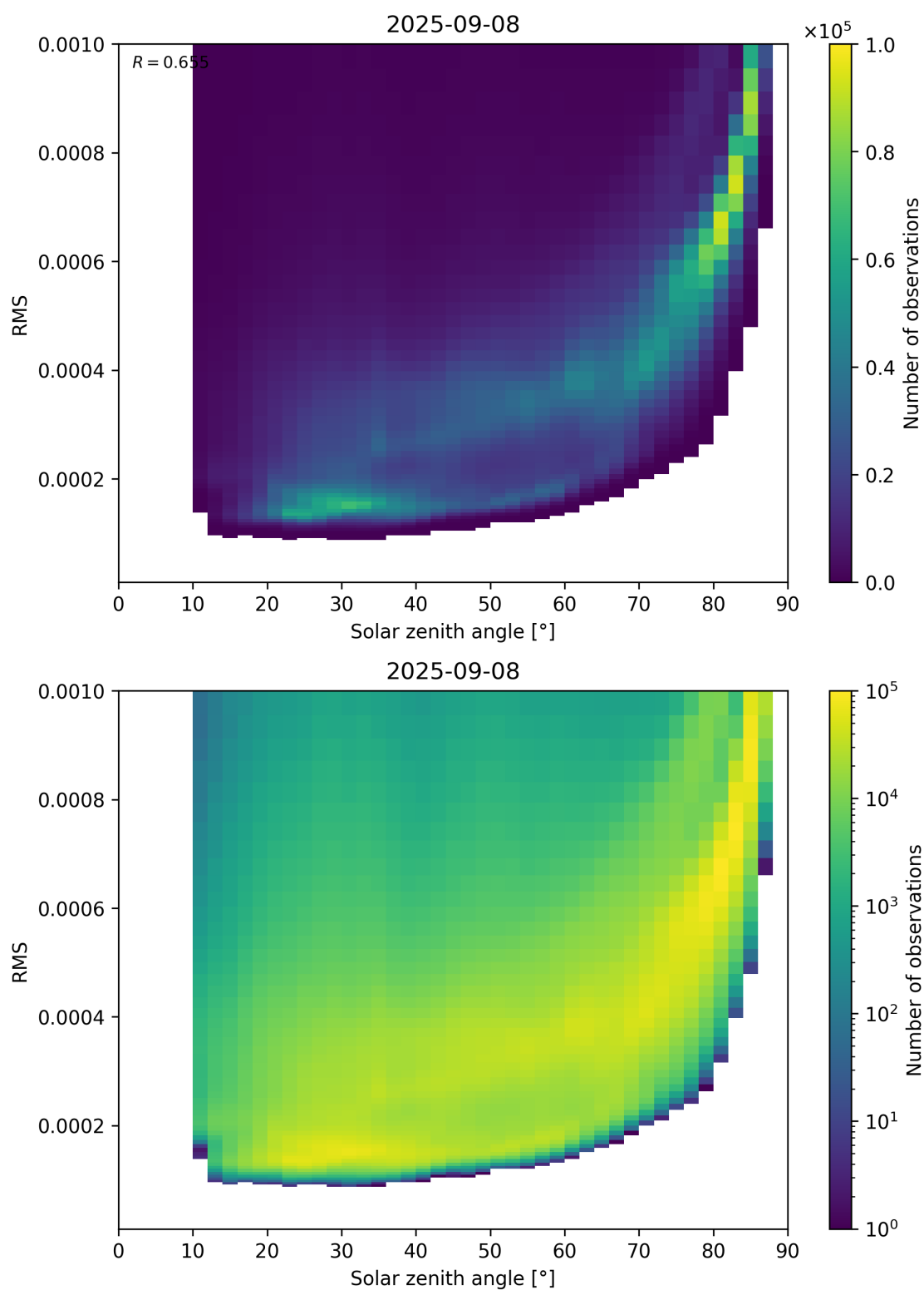
Figure 157: Scatter density plot of “Solar zenith angle” against “RMS” for 2025-09-07 to 2025-09-09.
