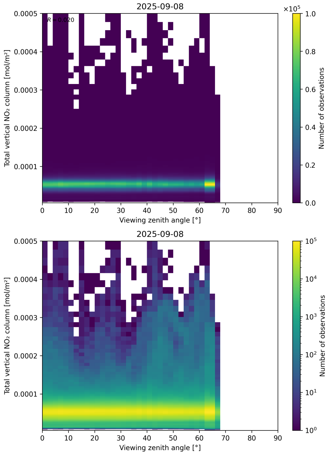
Figure 167: Scatter density plot of “Viewing zenith angle” against “Total vertical NO 2 column” for 2025-09-07 to 2025-09-09.
