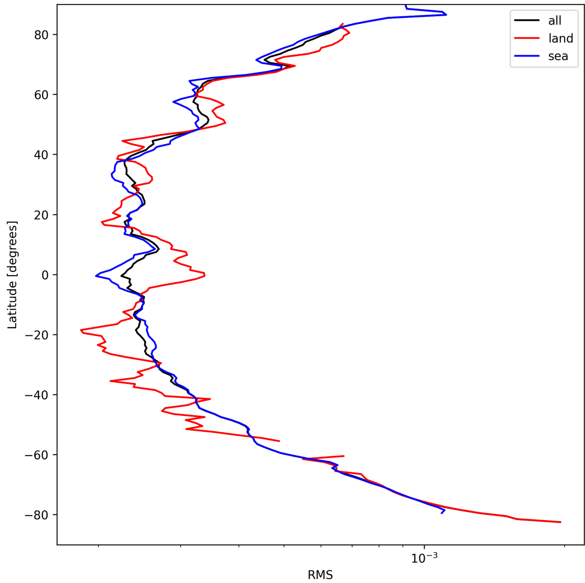
Figure 26: Zonal average of “RMS” for 2025-09-07 to 2025-09-09.
