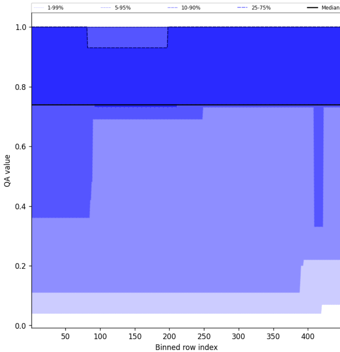
Figure 45: Along track statistics of “QA value” for 2025-09-07 to 2025-09-09
