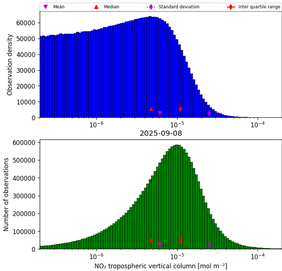
Figure 29: Histogram of “NO 2 tropospheric vertical column” for 2025-09-07 to 2025-09-09
