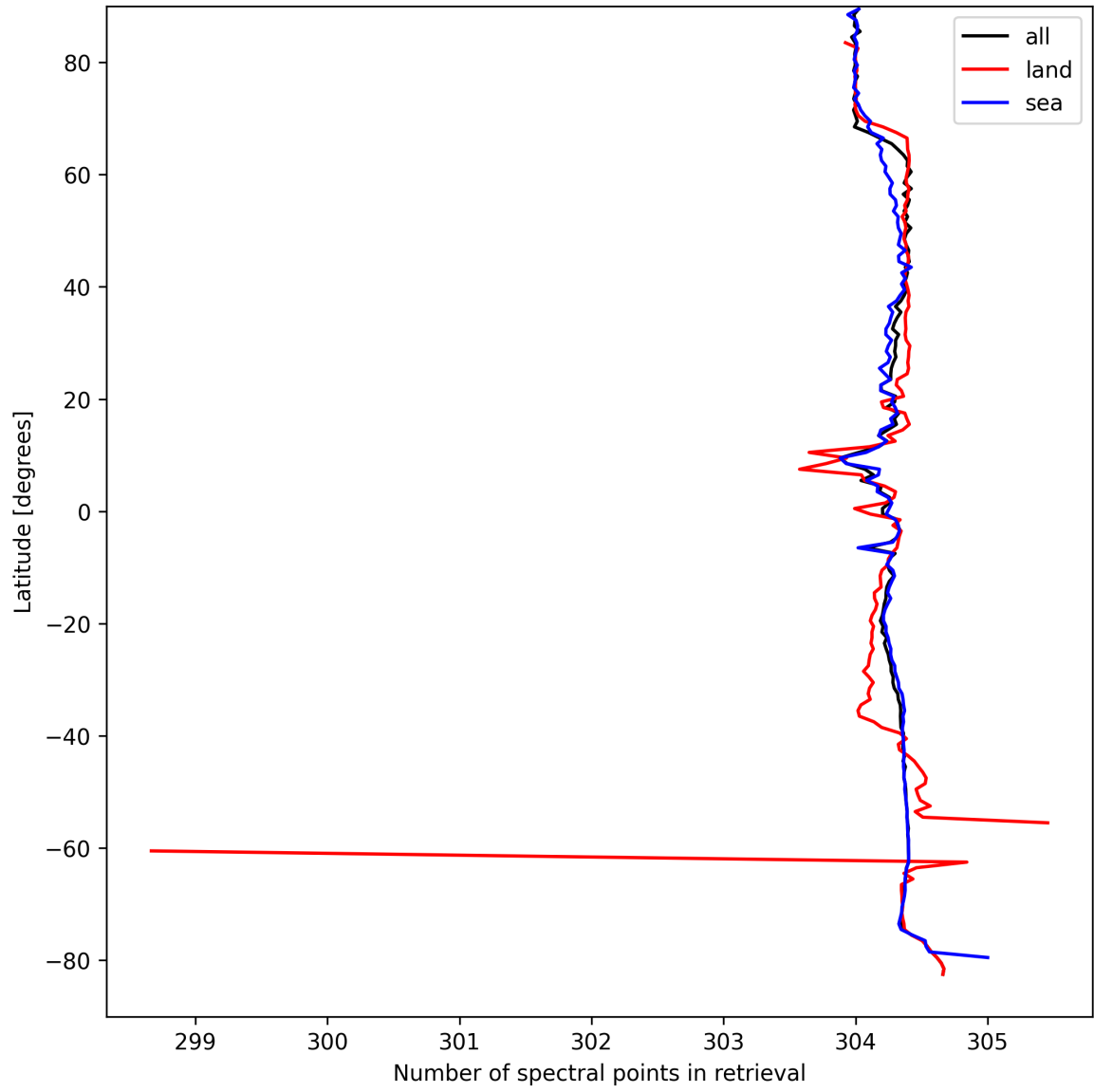
Figure 16: Zonal average of “Number of spectral points in retrieval” for 2025-09-07 to 2025-09-09.
