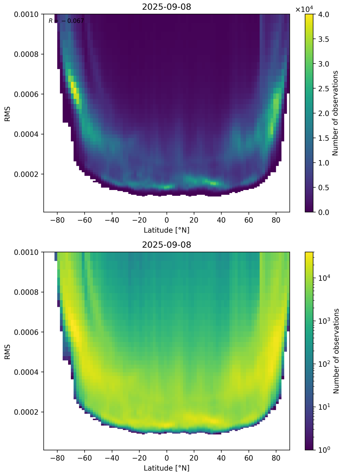
Figure 94: Scatter density plot of “Latitude” against “RMS” for 2025-09-07 to 2025-09-09.
