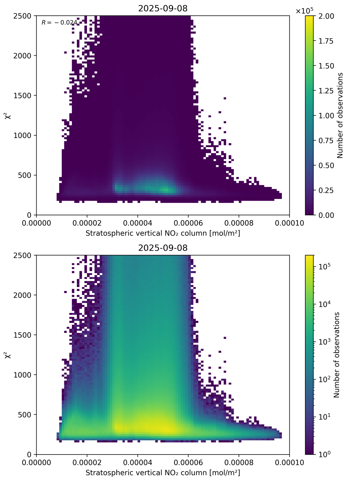
Figure 97: Scatter density plot of “Stratospheric vertical NO 2 column” against “ \chi^2 ” for 2025-09-07 to 2025-09-09.
