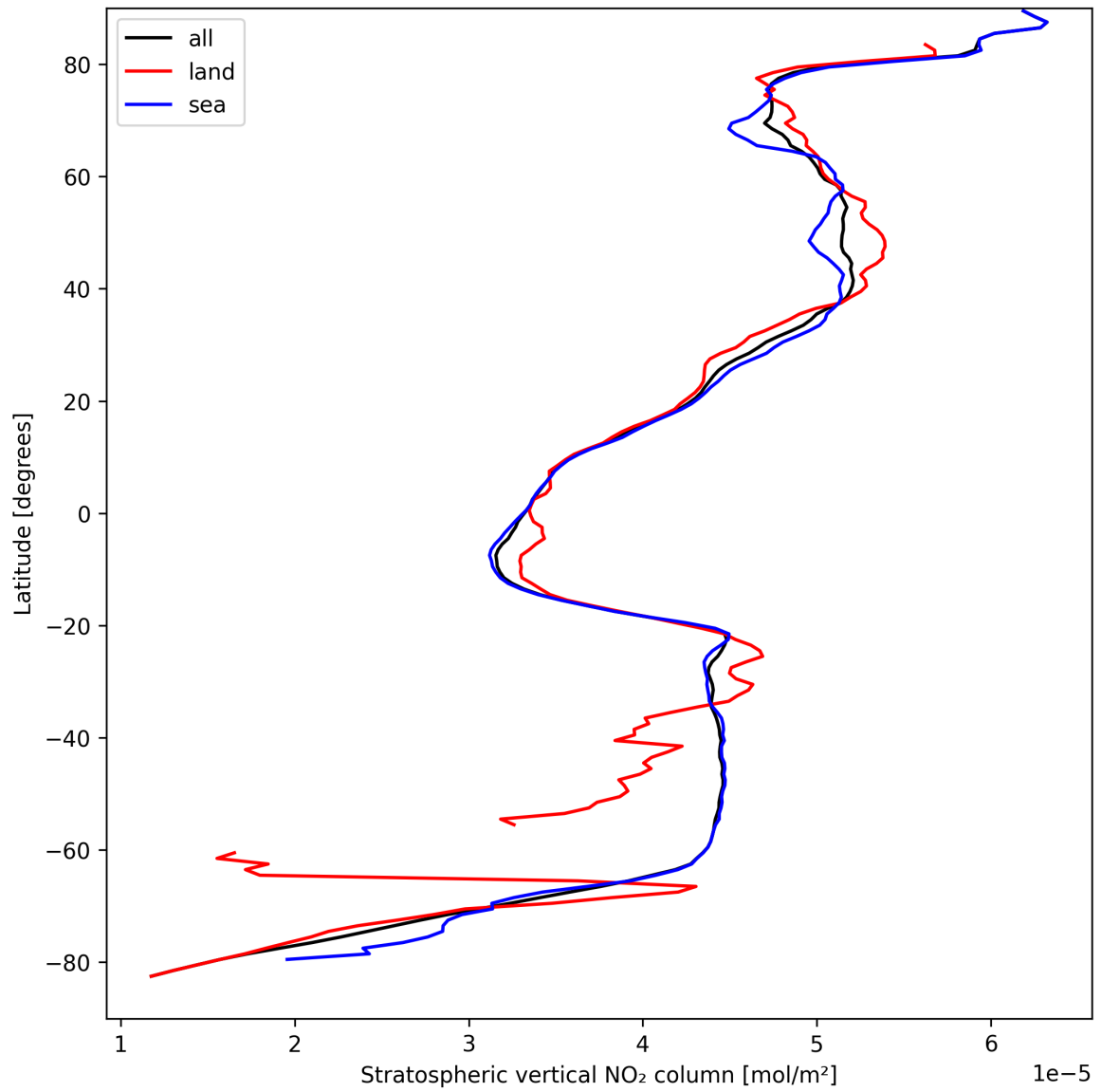
Figure 19: Zonal average of “Stratospheric vertical NO 2 column” for 2025-09-07 to 2025-09-09.
