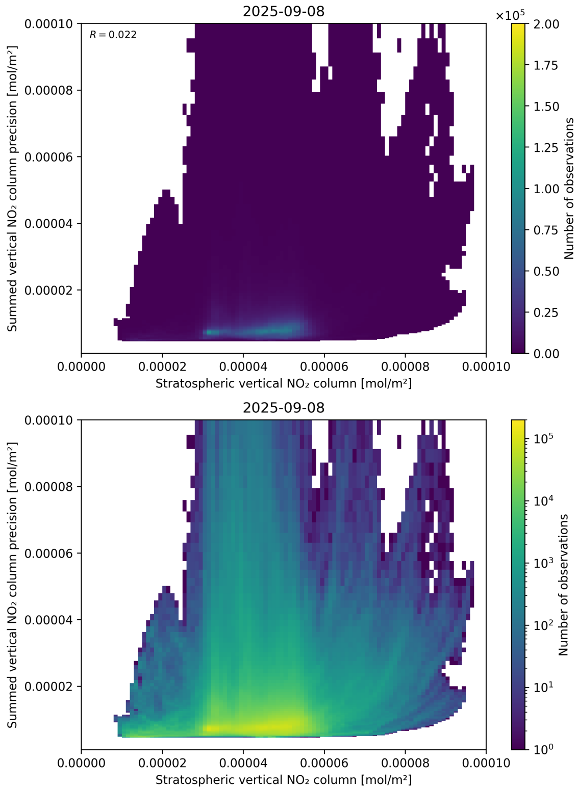
Figure 99: Scatter density plot of “Stratospheric vertical NO 2 column” against “Summed vertical NO 2 column precision” for 2025-09-07 to 2025-09-09.
