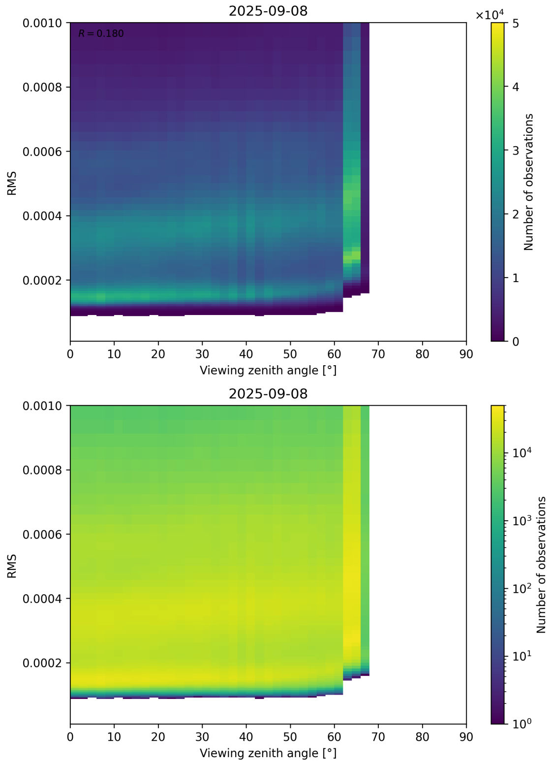
Figure 171: Scatter density plot of “Viewing zenith angle” against “RMS” for 2025-09-07 to 2025-09-09.
