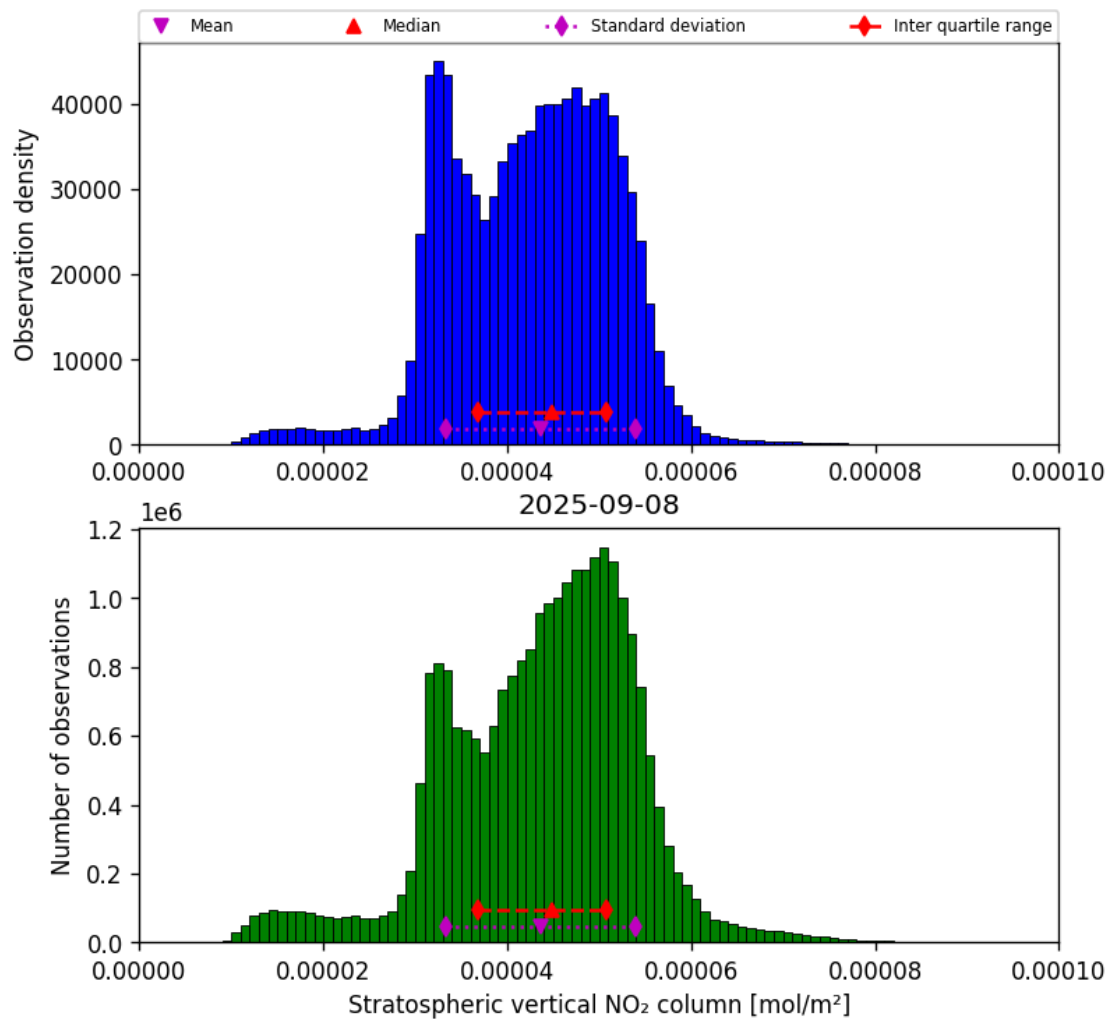
Figure 36: Histogram of “Stratospheric vertical NO 2 column” for 2025-09-07 to 2025-09-09
