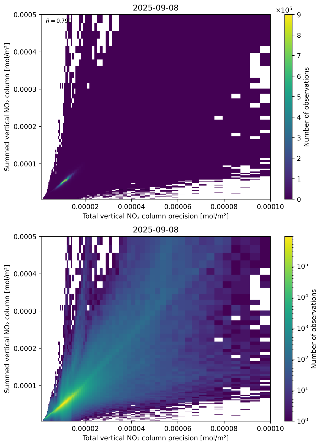
Figure 117: Scatter density plot of “Total vertical NO 2 column precision” against “Summed vertical NO 2 column” for 2025-09-07 to 2025-09-09.
