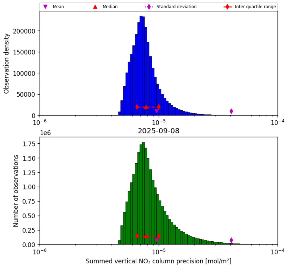
Figure 41: Histogram of “Summed vertical NO 2 column precision” for 2025-09-07 to 2025-09-09
