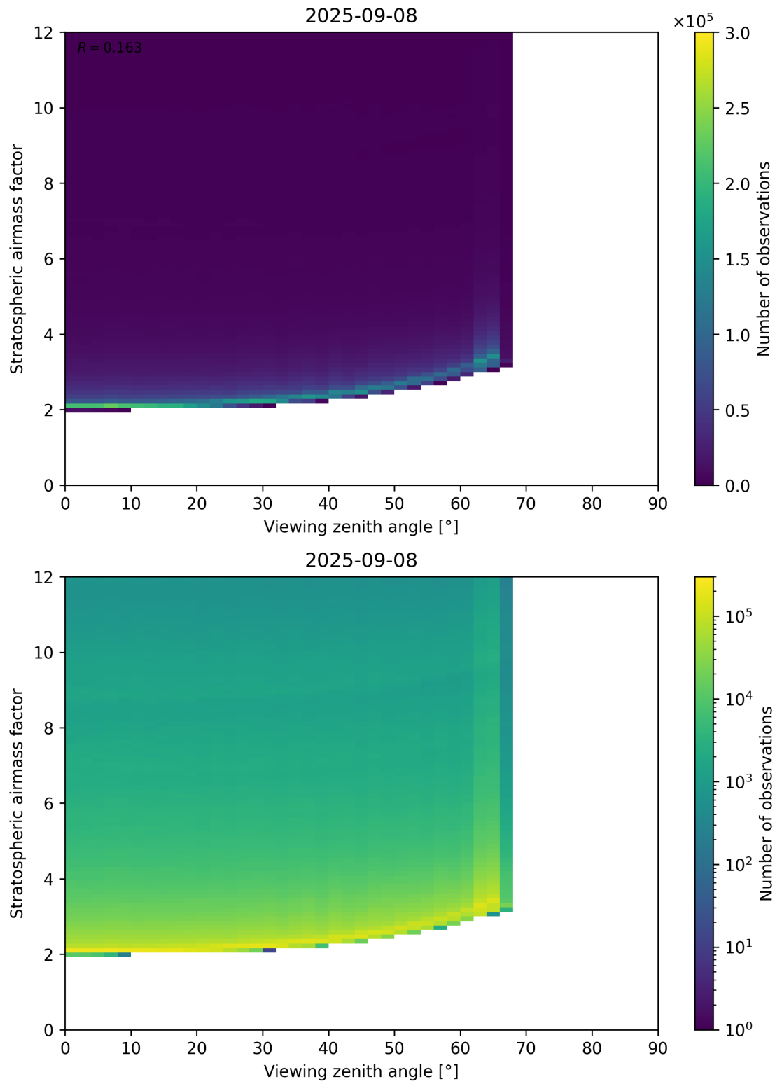
Figure 159: Scatter density plot of “Viewing zenith angle” against “Stratospheric airmass factor” for 2025-09-07 to 2025-09-09.
