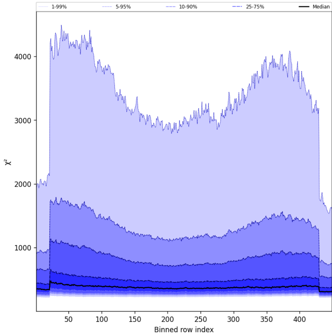
Figure 59: Along track statistics of “ \chi^2 ” for 2025-09-07 to 2025-09-09
