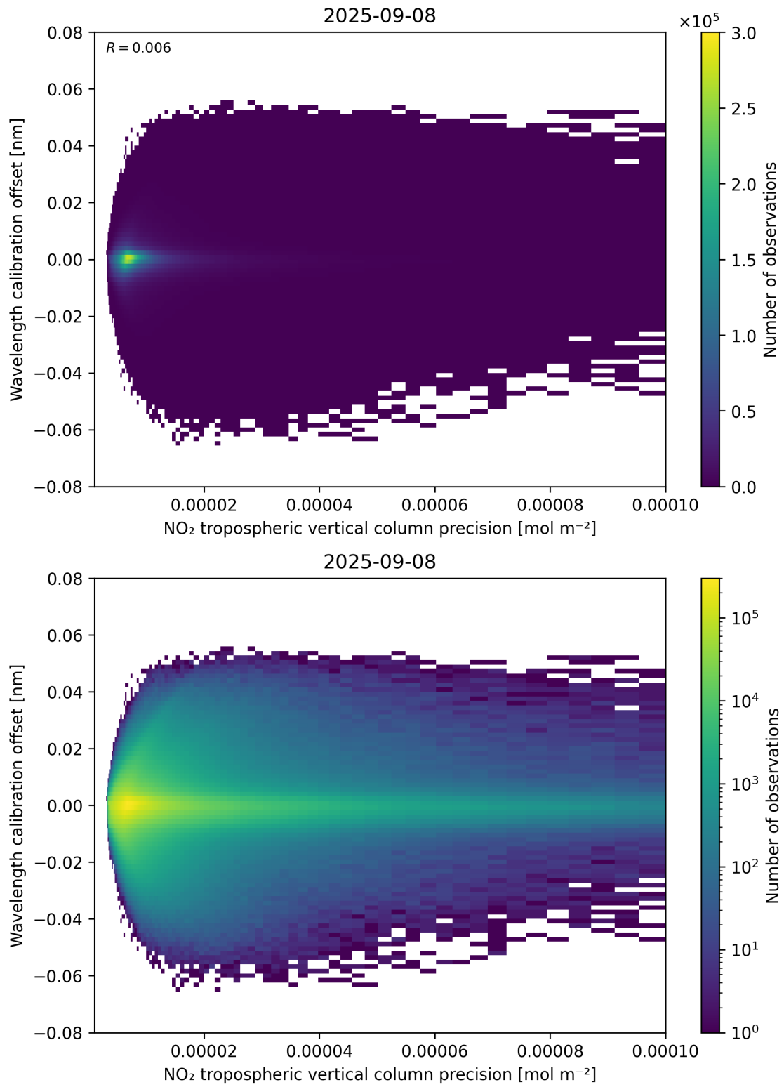
Figure 141: Scatter density plot of “NO 2 tropospheric vertical column precision” against “Wavelength calibration offset” for 2025-09-07 to 2025-09-09.
