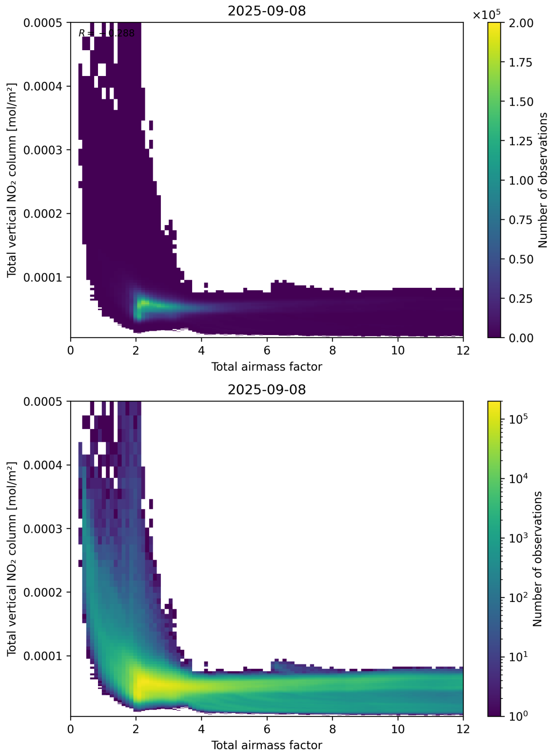
Figure 67: Scatter density plot of “Total airmass factor” against “Total vertical NO 2 column” for 2025-09-07 to 2025-09-09.
