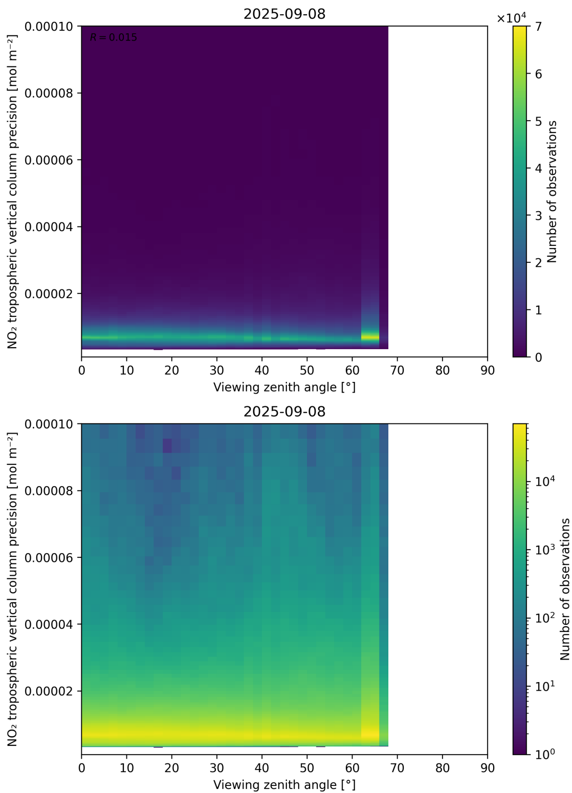
Figure 170: Scatter density plot of “Viewing zenith angle” against “NO 2 tropospheric vertical column precision” for 2025-09-07 to 2025-09-09.
