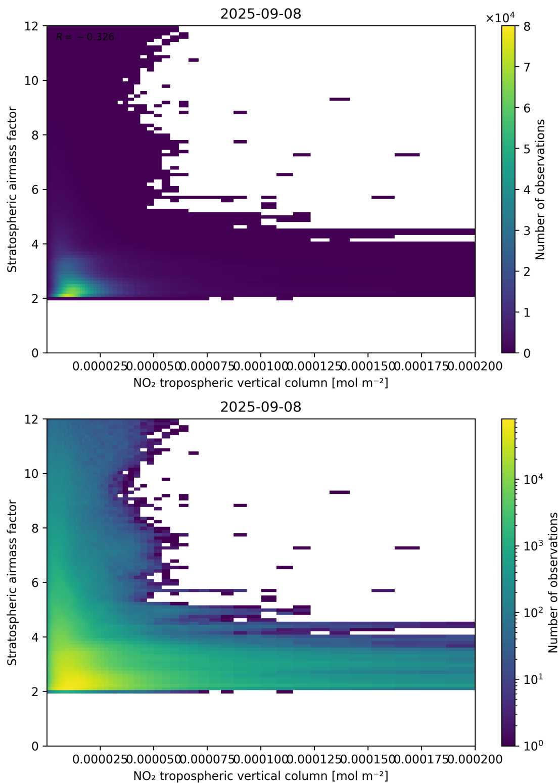
Figure 121: Scatter density plot of “NO 2 tropospheric vertical column” against “Stratospheric air mass factor” for 2025-09-07 to 2025-09-09.
