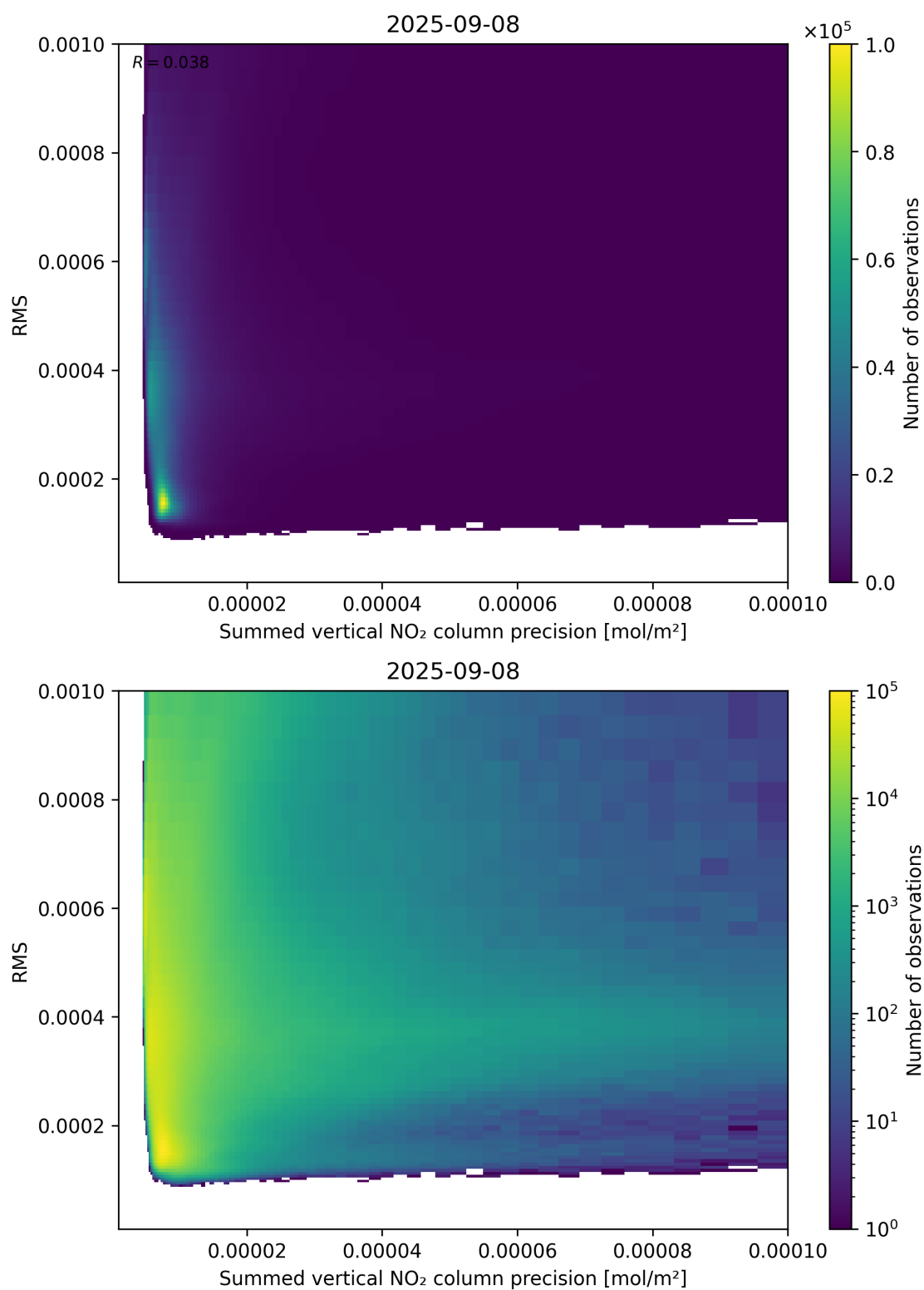
Figure 108: Scatter density plot of “Summed vertical NO 2 column precision” against “RMS” for 2025-09-07 to 2025-09-09.
