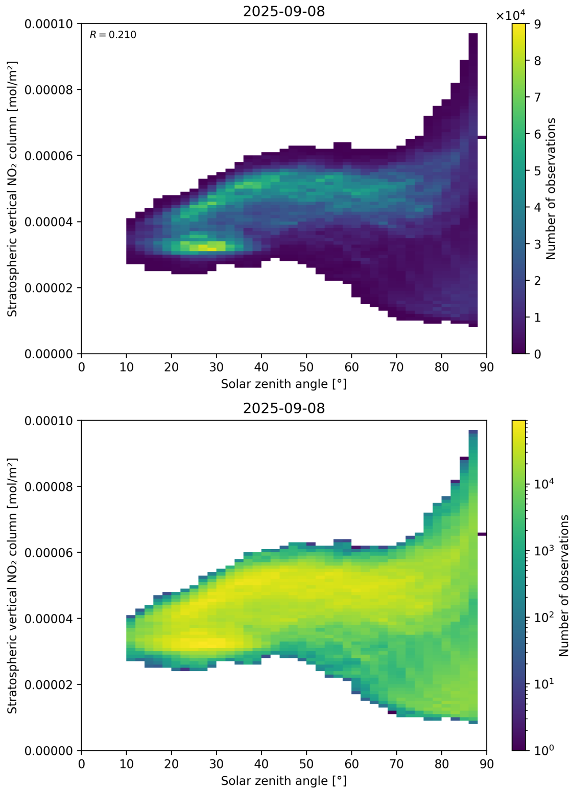
Figure 150: Scatter density plot of “Solar zenith angle” against “Stratospheric vertical NO 2 column” for 2025-09-07 to 2025-09-09.
