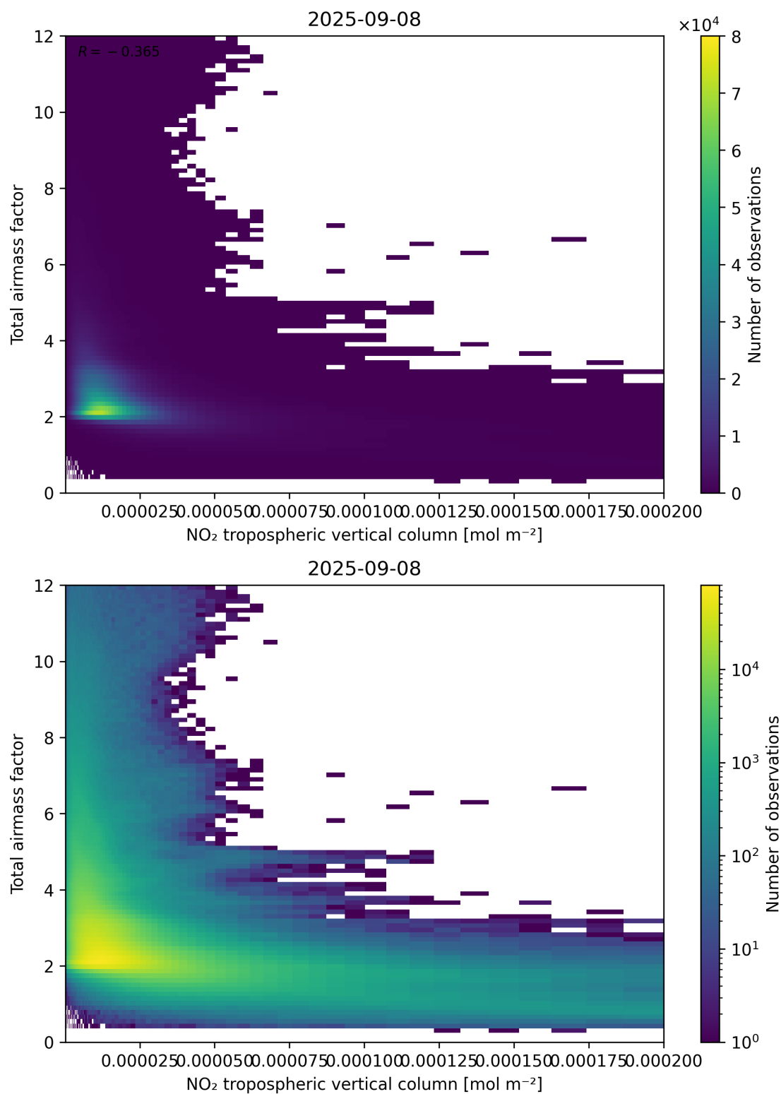
Figure 122: Scatter density plot of “NO 2 tropospheric vertical column” against “Total air mass factor” for 2025-09-07 to 2025-09-09.
