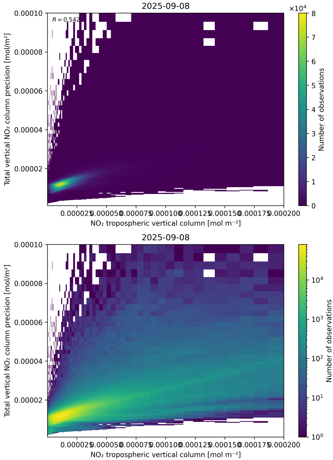
Figure 129: Scatter density plot of “NO 2 tropospheric vertical column” against “Total vertical NO 2 column precision” for 2025-09-07 to 2025-09-09.
