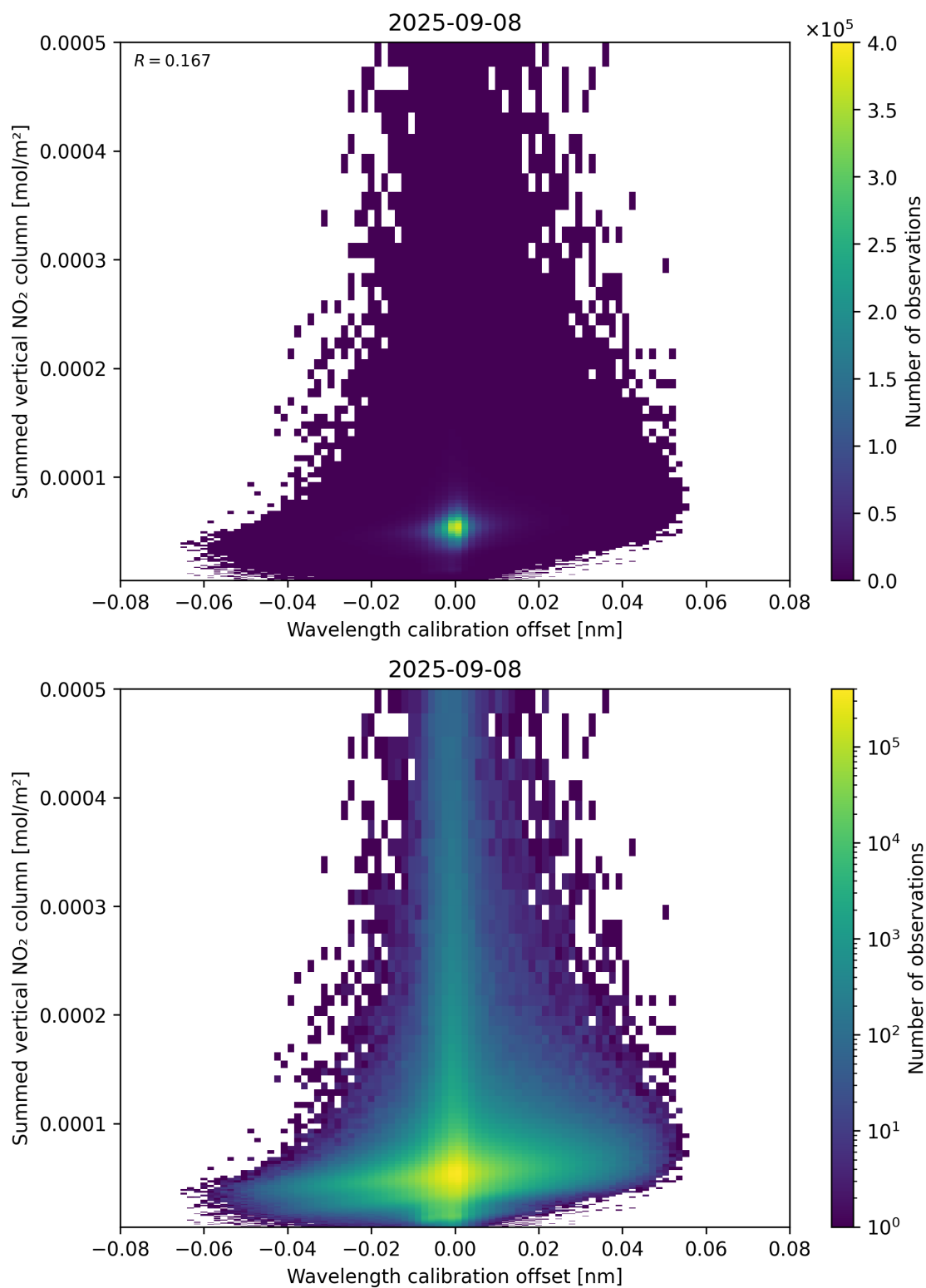
Figure 177: Scatter density plot of “Wavelength calibration offset” against “Summed vertical NO 2 column” for 2025-09-07 to 2025-09-09.
