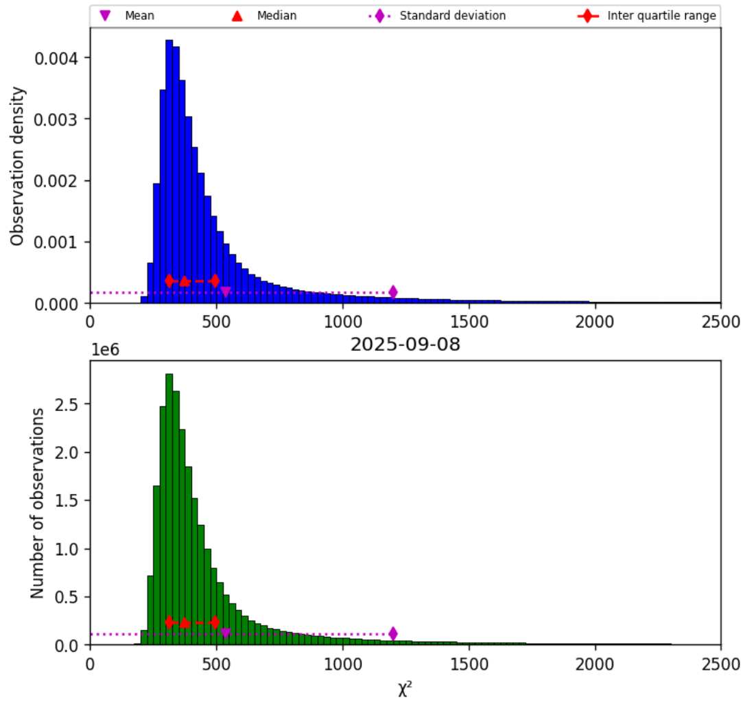
Figure 42: Histogram of “ \chi^2 ” for 2025-09-07 to 2025-09-09
