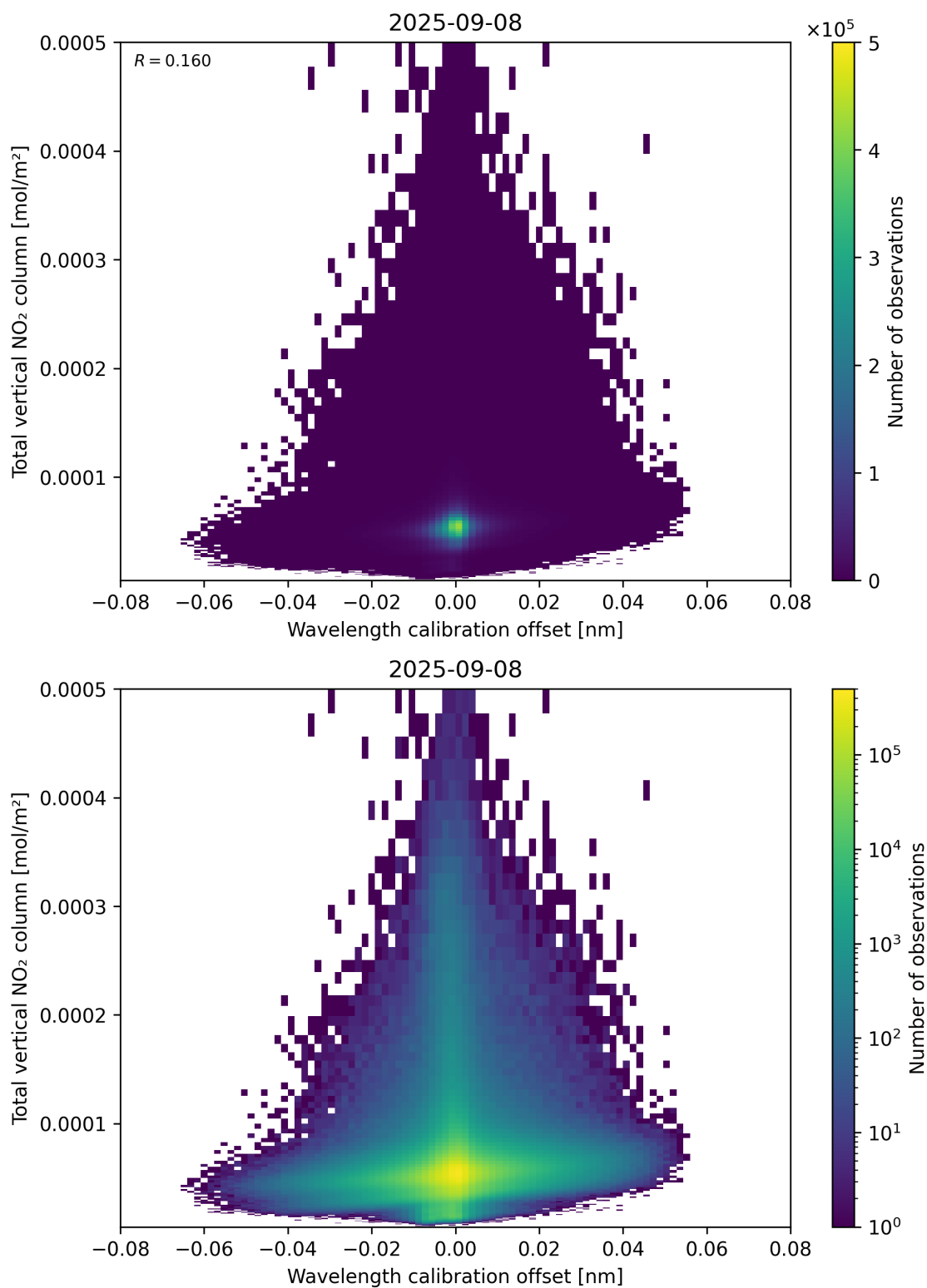
Figure 179: Scatter density plot of “Wavelength calibration offset” against “Total vertical NO 2 column” for 2025-09-07 to 2025-09-09.
