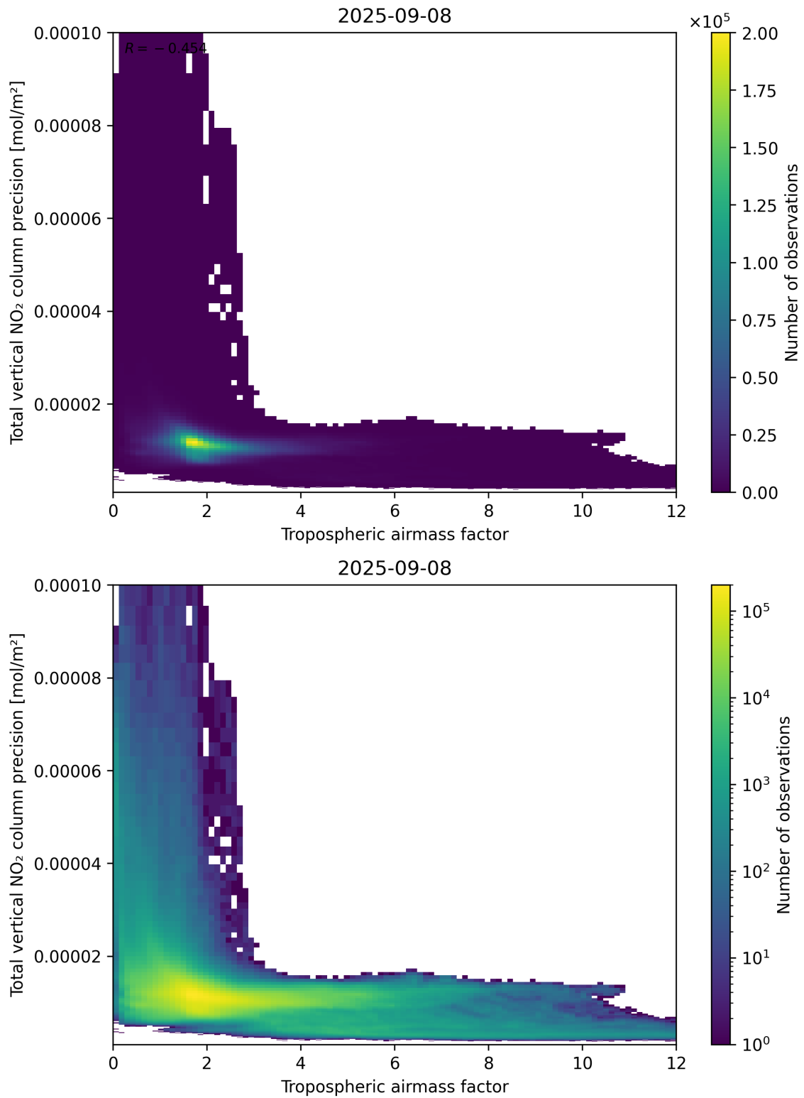
Figure 78: Scatter density plot of “Tropospheric air mass factor” against “Total vertical NO 2 column precision” for 2025-09-07 to 2025-09-09.
