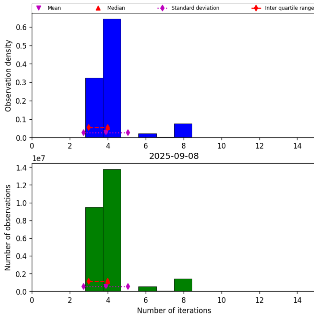
Figure 34: Histogram of “Number of iterations” for 2025-09-07 to 2025-09-09
