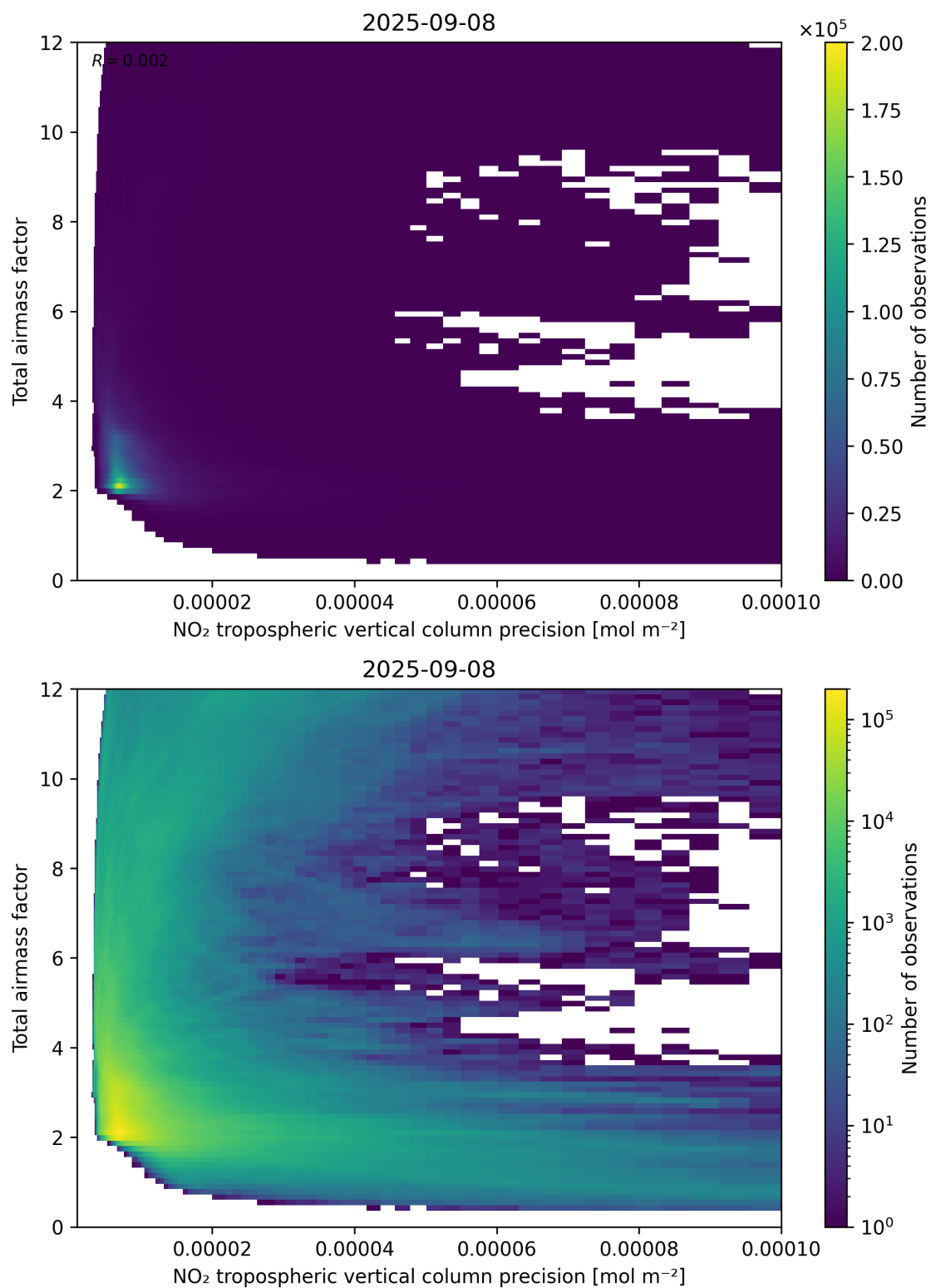
Figure 132: Scatter density plot of “NO 2 tropospheric vertical column precision” against “Total air mass factor” for 2025-09-07 to 2025-09-09.
