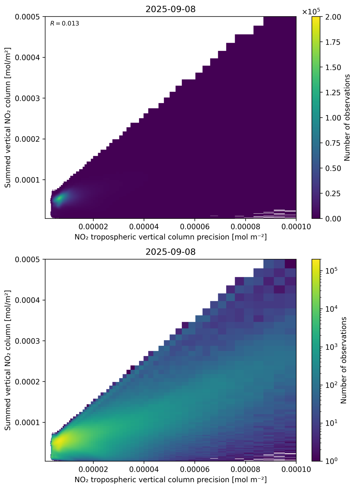
Figure 136: Scatter density plot of “NO 2 tropospheric vertical column precision” against “Summed vertical NO 2 column” for 2025-09-07 to 2025-09-09.
