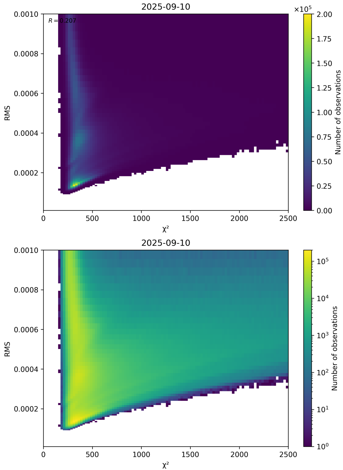
Figure 82: Scatter density plot of “ \chi^2 ” against “RMS” for 2025-09-10 to 2025-09-11.
