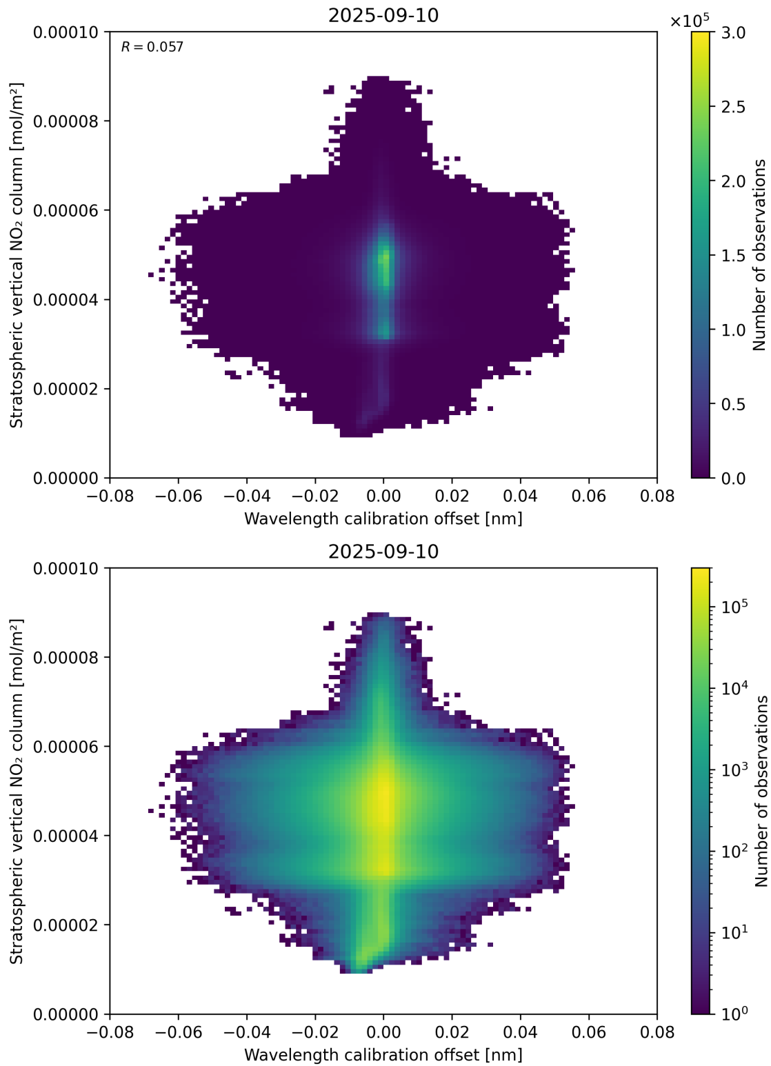
Figure 176: Scatter density plot of “Wavelength calibration offset” against “Stratospheric vertical NO 2 column” for 2025-09-10 to 2025-09-11.
