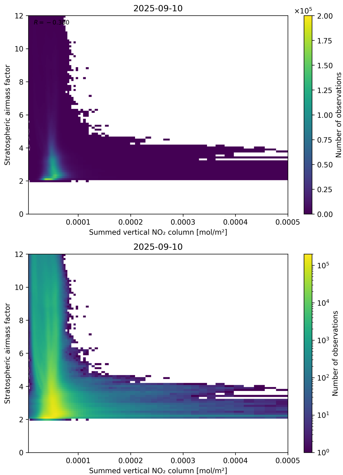
Figure 103: Scatter density plot of “Summed vertical NO 2 column” against “Stratospheric airmass factor” for 2025-09-10 to 2025-09-11.
