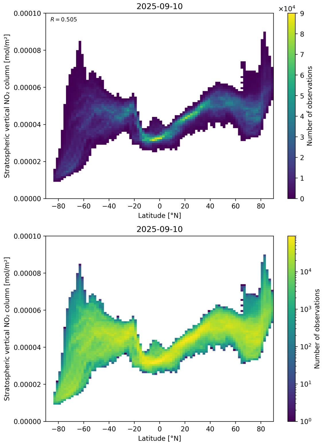
Figure 87: Scatter density plot of “Latitude” against “Stratospheric vertical \text{NO}_2 column” for 2025-09-10 to 2025-09-11.
