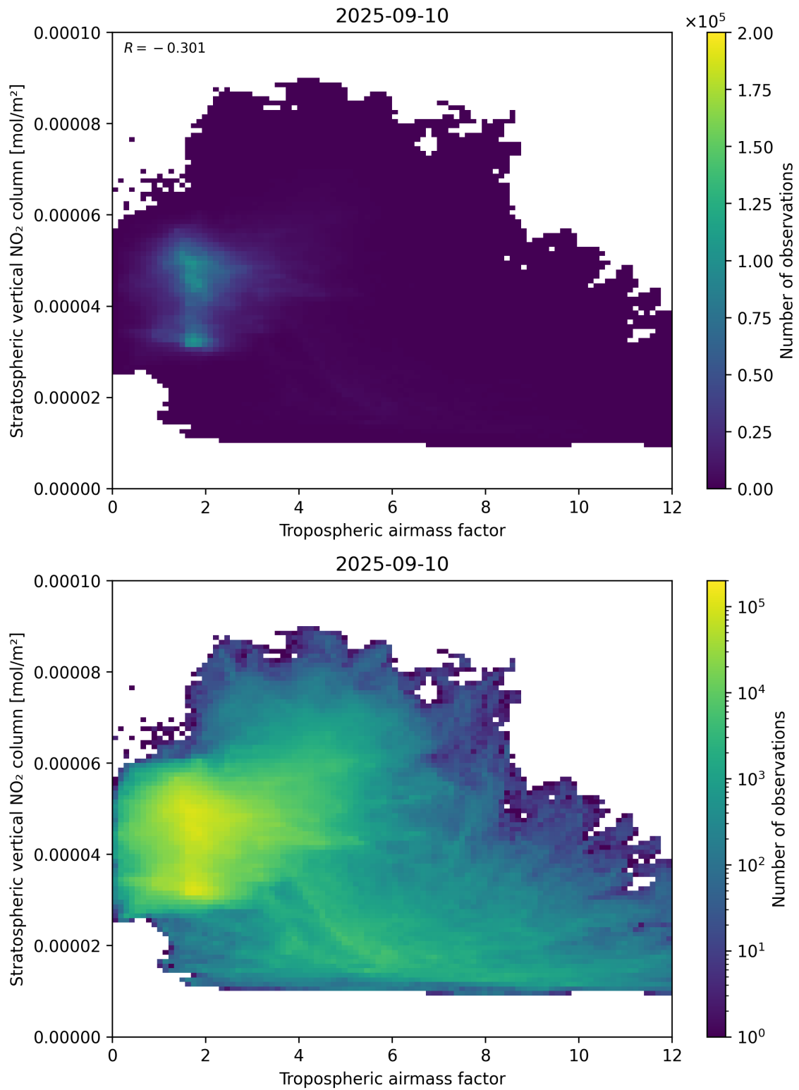
Figure 74: Scatter density plot of “Tropospheric airmass factor” against “Stratospheric vertical NO 2 column” for 2025-09-10 to 2025-09-11.
