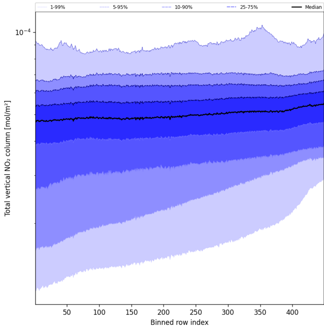
Figure 55: Along track statistics of “Total vertical NO 2 column” for 2025-09-10 to 2025-09-11
