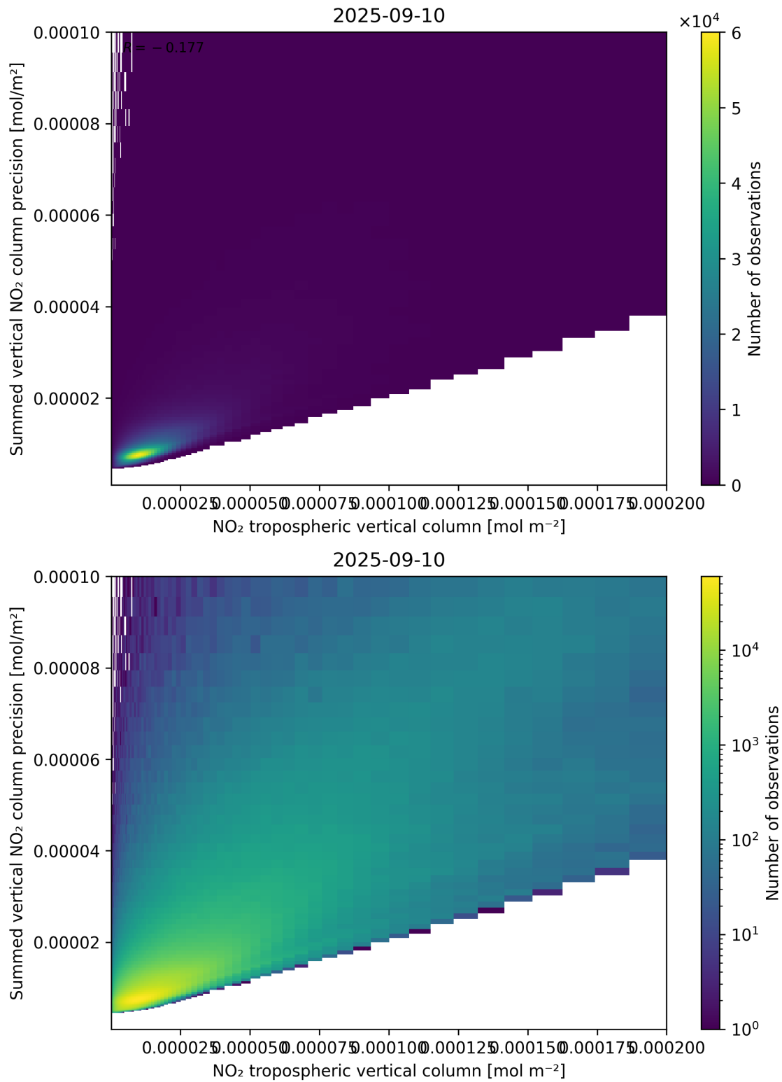
Figure 127: Scatter density plot of “NO 2 tropospheric vertical column” against “Summed vertical NO 2 column precision” for 2025-09-10 to 2025-09-11.
