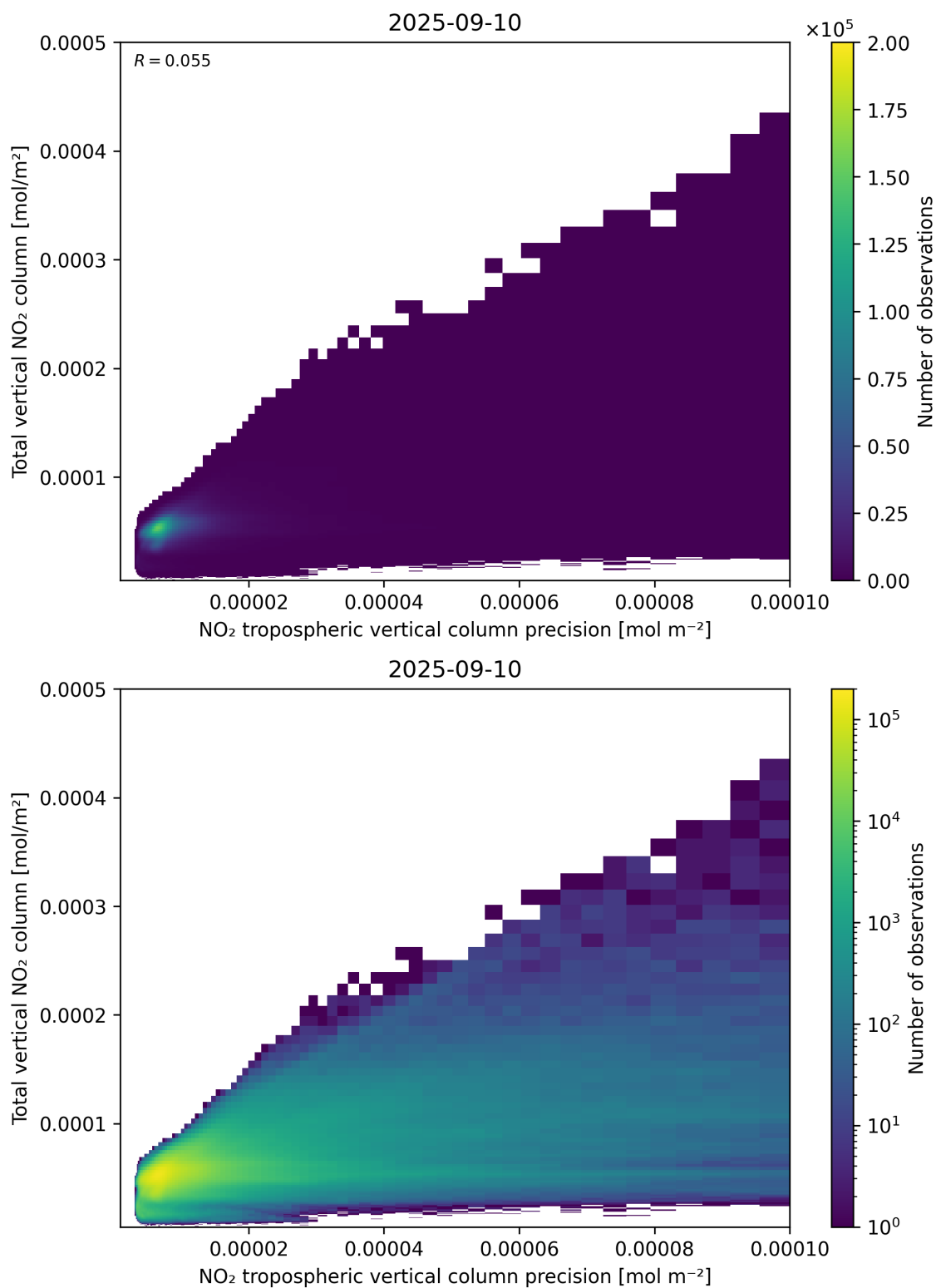
Figure 138: Scatter density plot of “NO 2 tropospheric vertical column precision” against “Total vertical NO 2 column” for 2025-09-10 to 2025-09-11.
