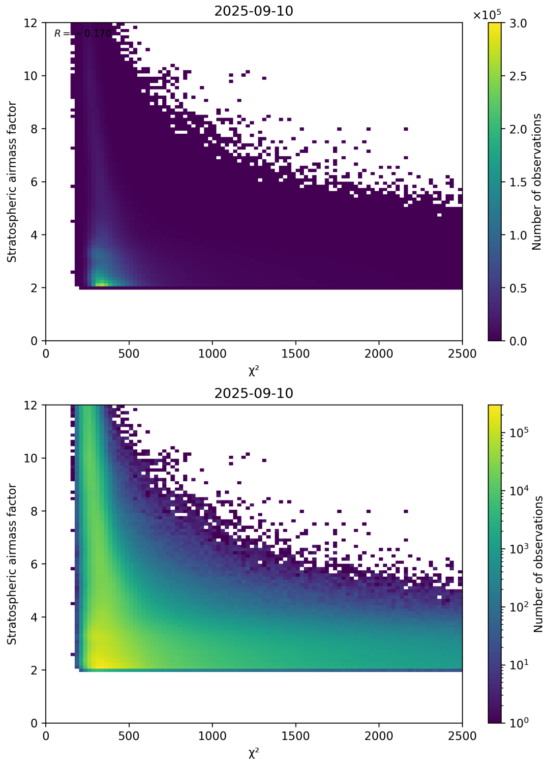
Figure 81: Scatter density plot of “ \chi^2 ” against “Stratospheric airmass factor” for 2025-09-10 to 2025-09-11.
