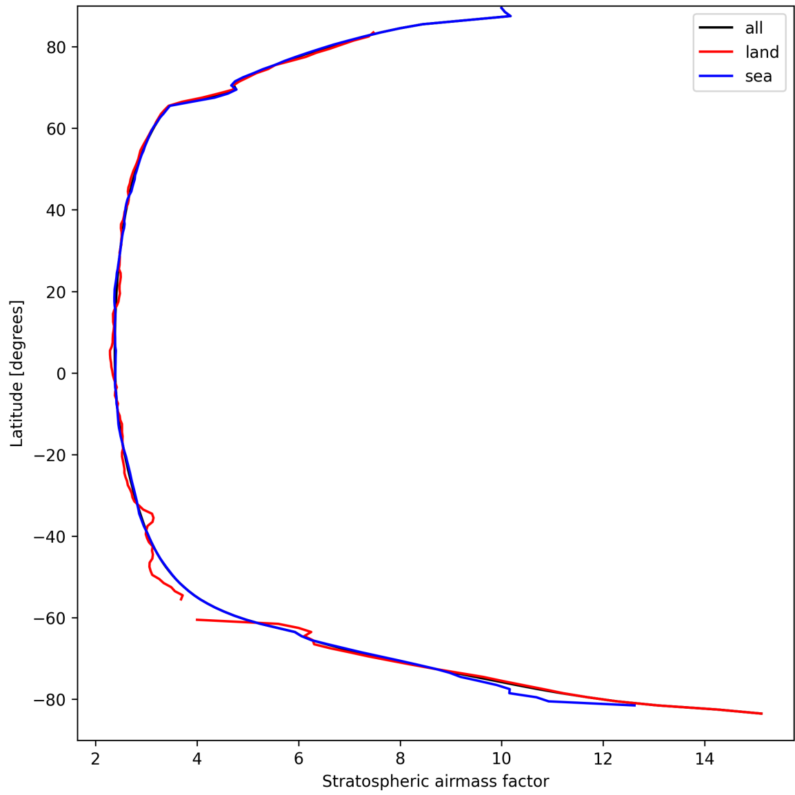
Figure 27: Zonal average of “Stratospheric airmass factor” for 2025-09-10 to 2025-09-11.
