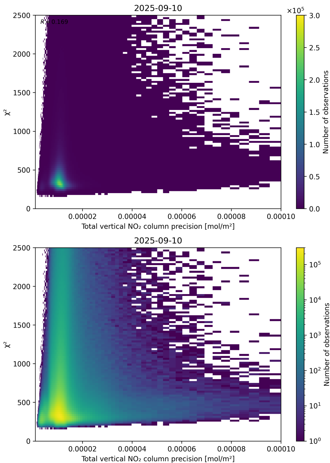
Figure 116: Scatter density plot of “Total vertical NO 2 column precision” against “ \chi^2 ” for 2025-09-10 to 2025-09-11.
