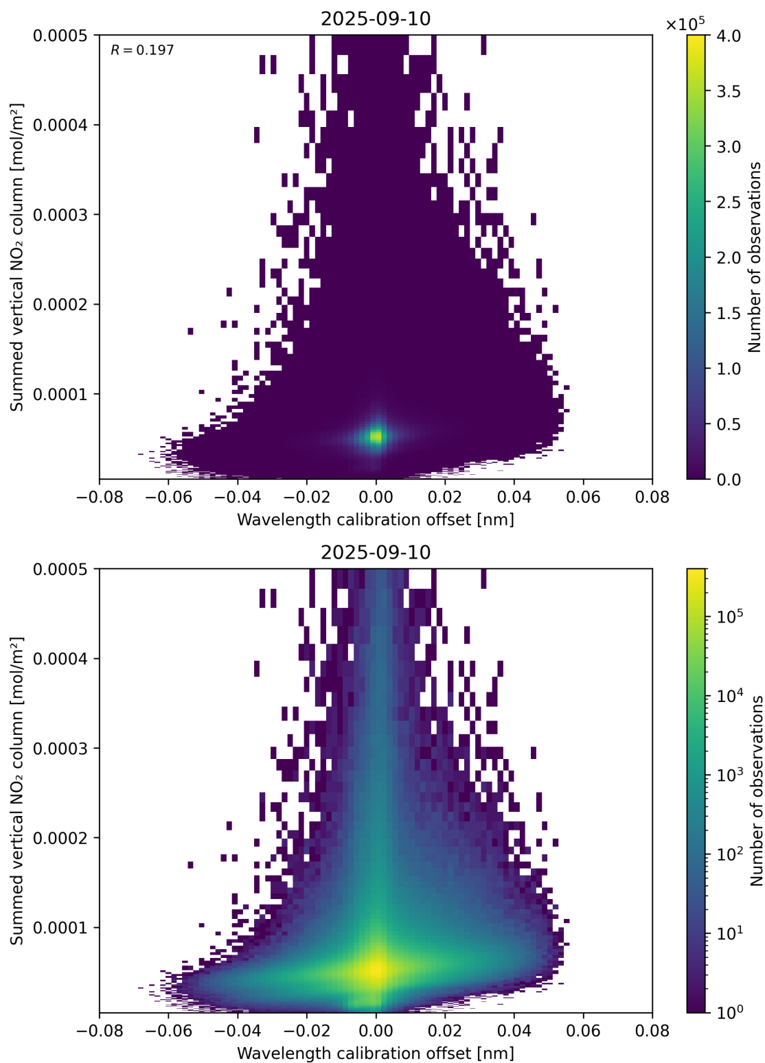
Figure 177: Scatter density plot of “Wavelength calibration offset” against “Summed vertical NO 2 column” for 2025-09-10 to 2025-09-11.
