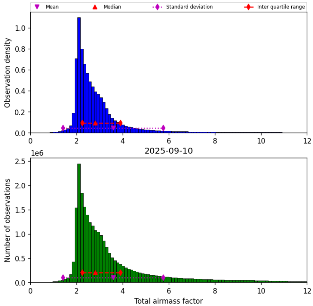
Figure 32: Histogram of “Total airmass factor” for 2025-09-10 to 2025-09-11
