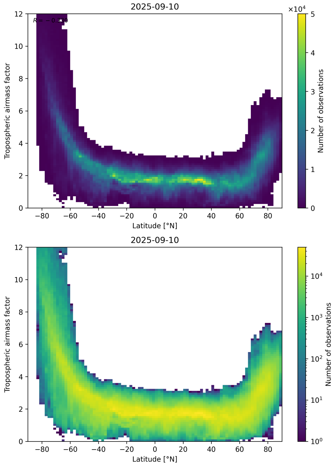
Figure 85: Scatter density plot of “Latitude” against “Tropospheric air mass factor” for 2025-09-10 to 2025-09-11.
