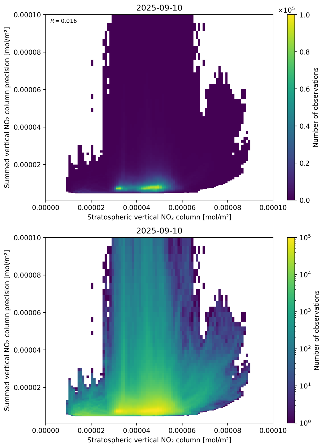
Figure 99: Scatter density plot of “Stratospheric vertical NO 2 column” against “Summed vertical NO 2 column precision” for 2025-09-10 to 2025-09-11.
