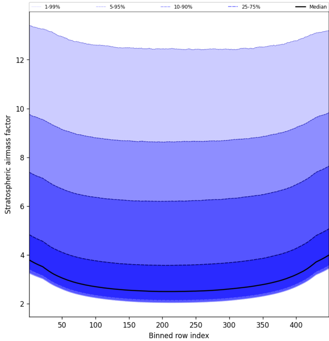
Figure 61: Along track statistics of “Stratospheric air mass factor” for 2025-09-10 to 2025-09-11
