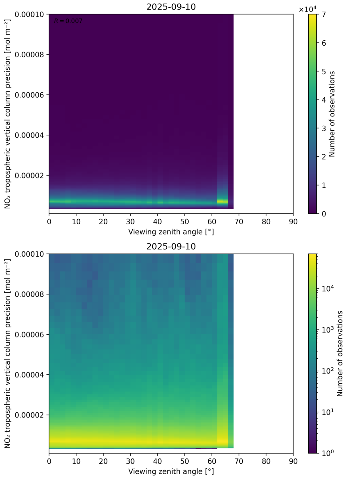
Figure 170: Scatter density plot of “Viewing zenith angle” against “NO 2 tropospheric vertical column precision” for 2025-09-10 to 2025-09-11.
