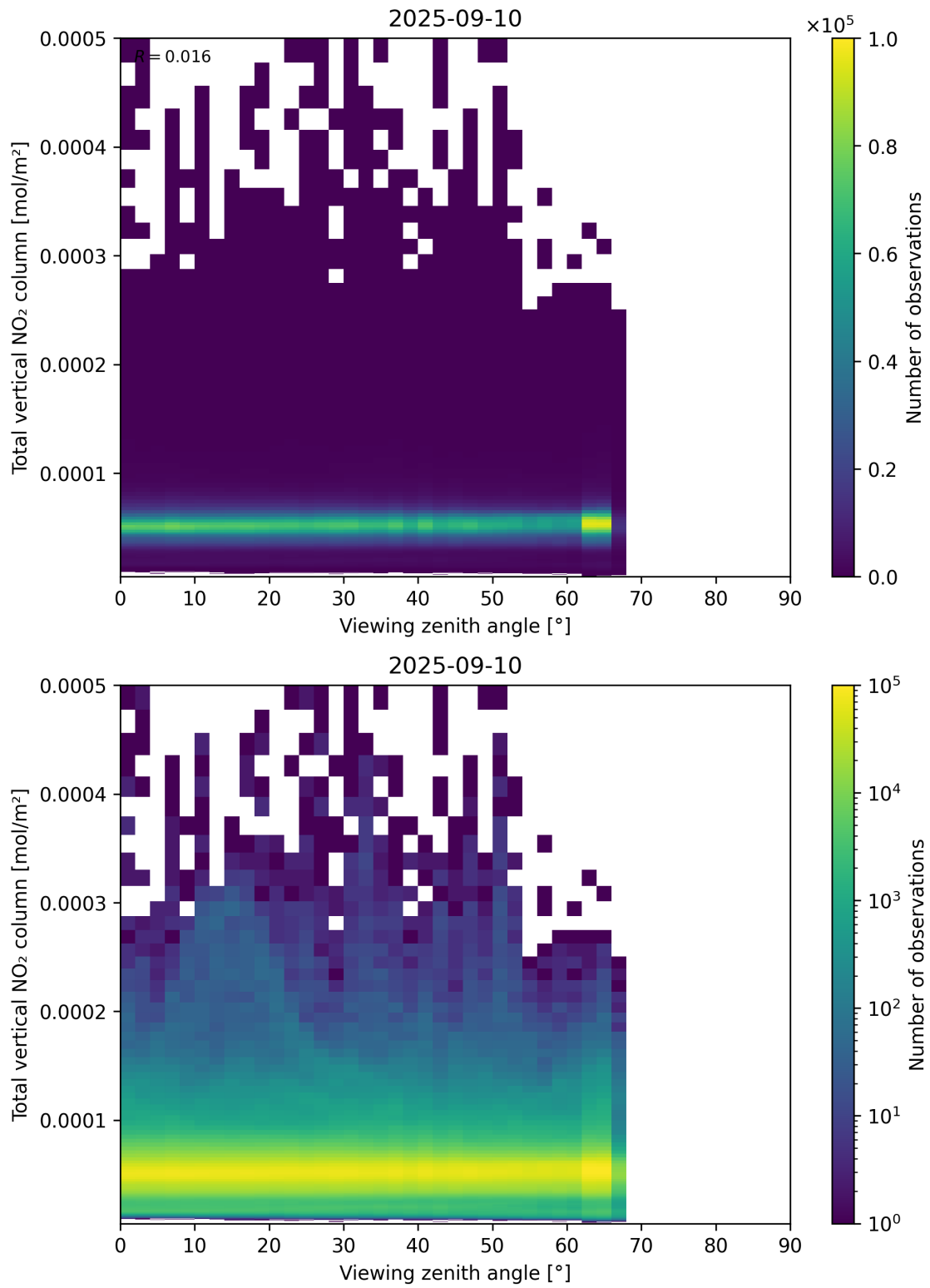
Figure 167: Scatter density plot of “Viewing zenith angle” against “Total vertical NO 2 column” for 2025-09-10 to 2025-09-11.
