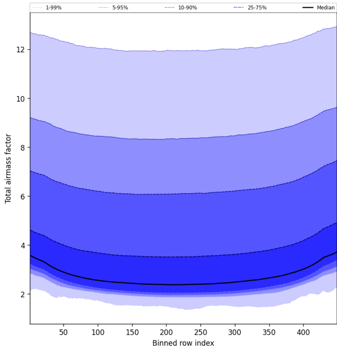
Figure 49: Along track statistics of “Total airmass factor” for 2025-09-10 to 2025-09-11
