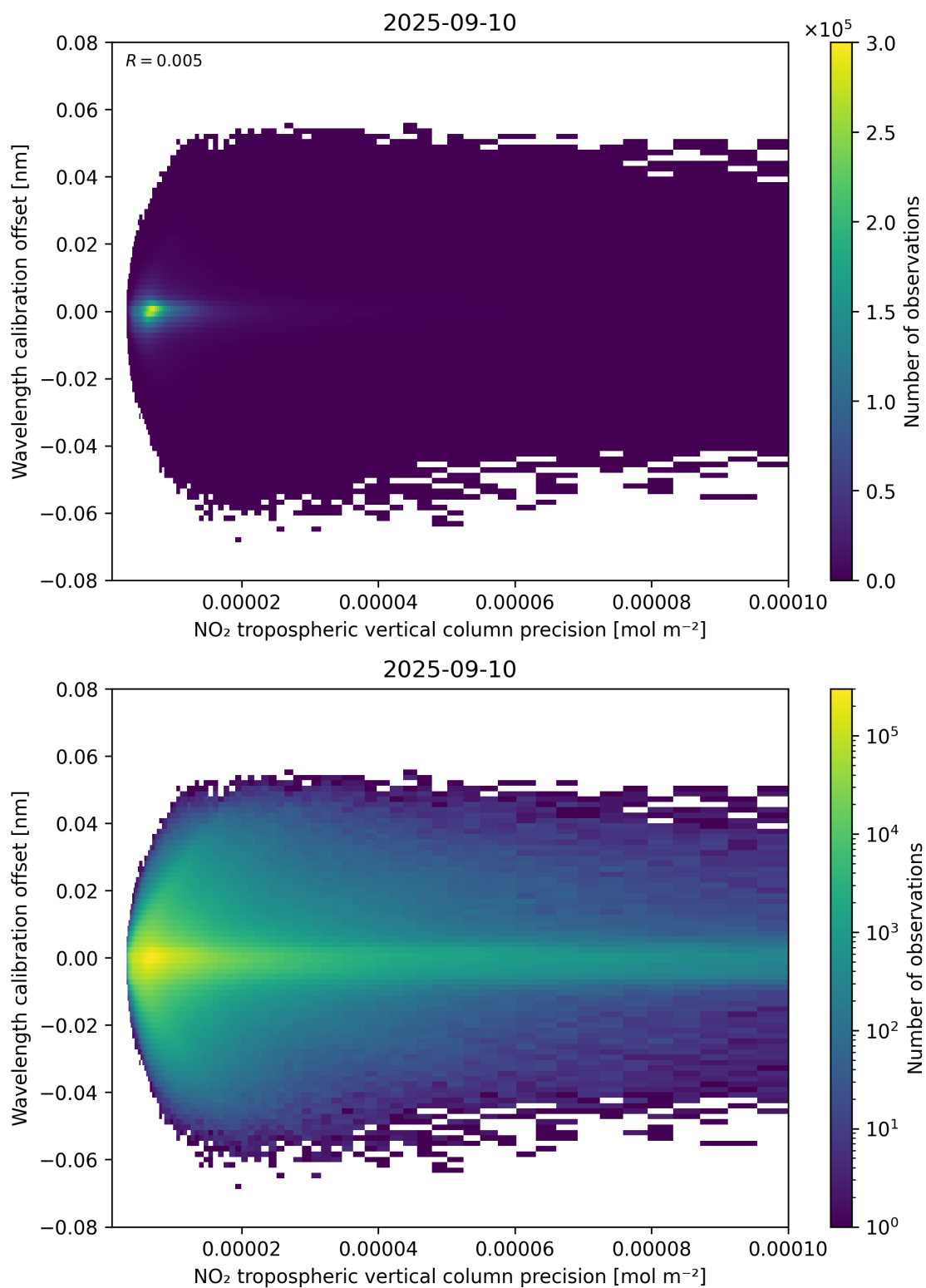
Figure 141: Scatter density plot of “NO 2 tropospheric vertical column precision” against “Wavelength calibration offset” for 2025-09-10 to 2025-09-11.
