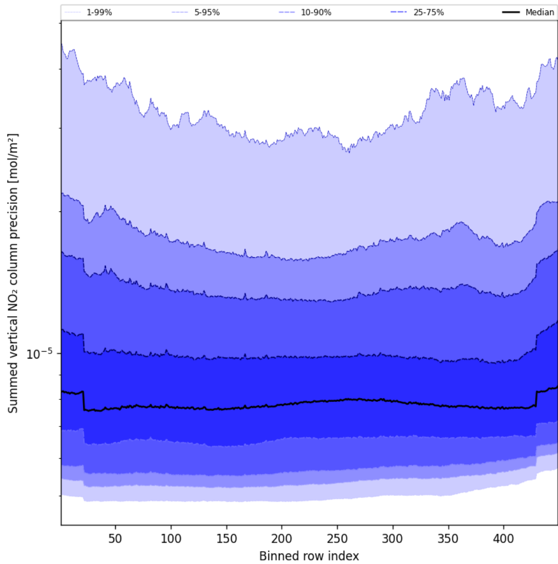
Figure 58: Along track statistics of “Summed vertical NO 2 column precision” for 2025-09-10 to 2025-09-11
