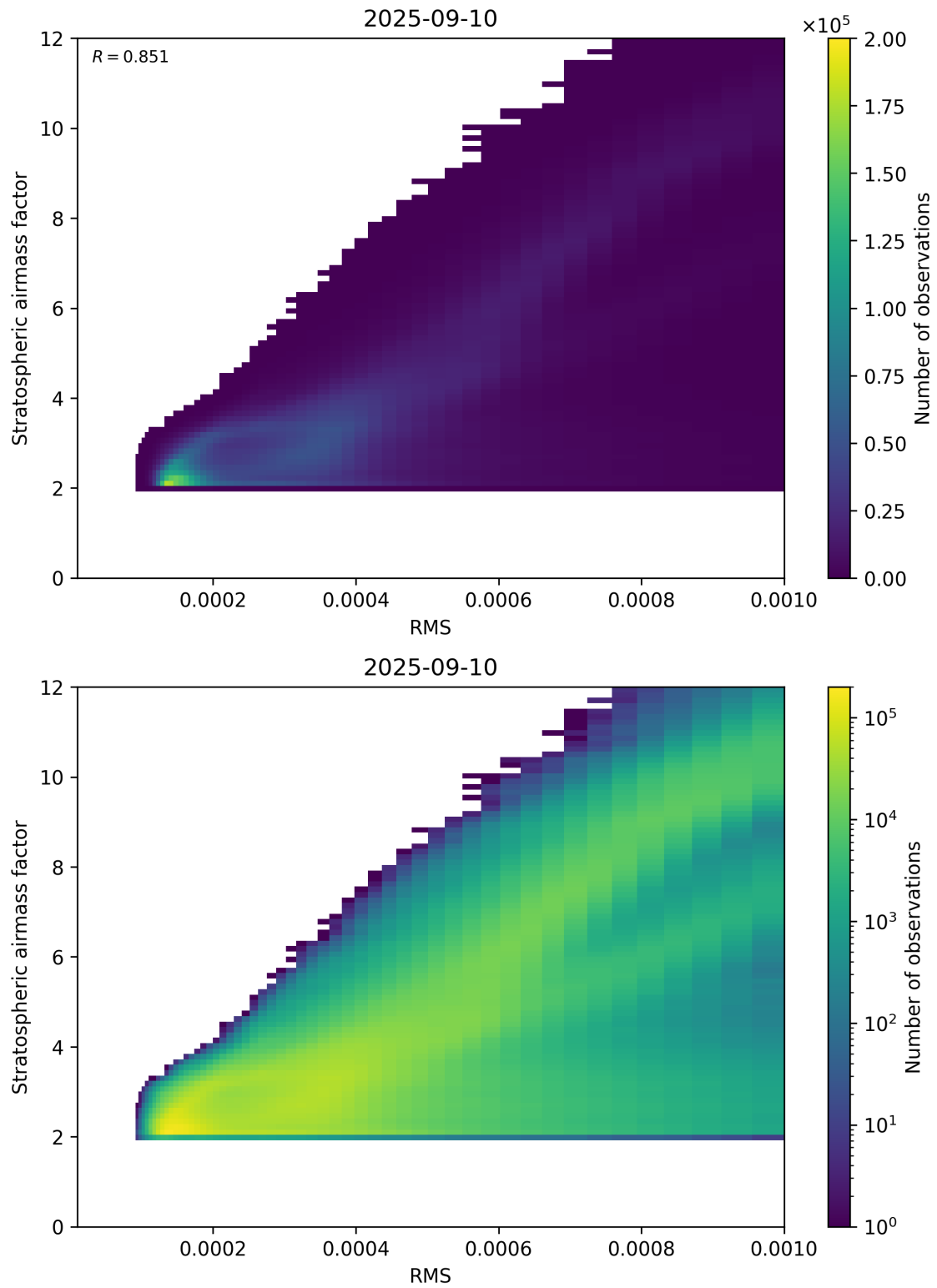
Figure 144: Scatter density plot of “RMS” against “Stratospheric airmass factor” for 2025-09-10 to 2025-09-11.
