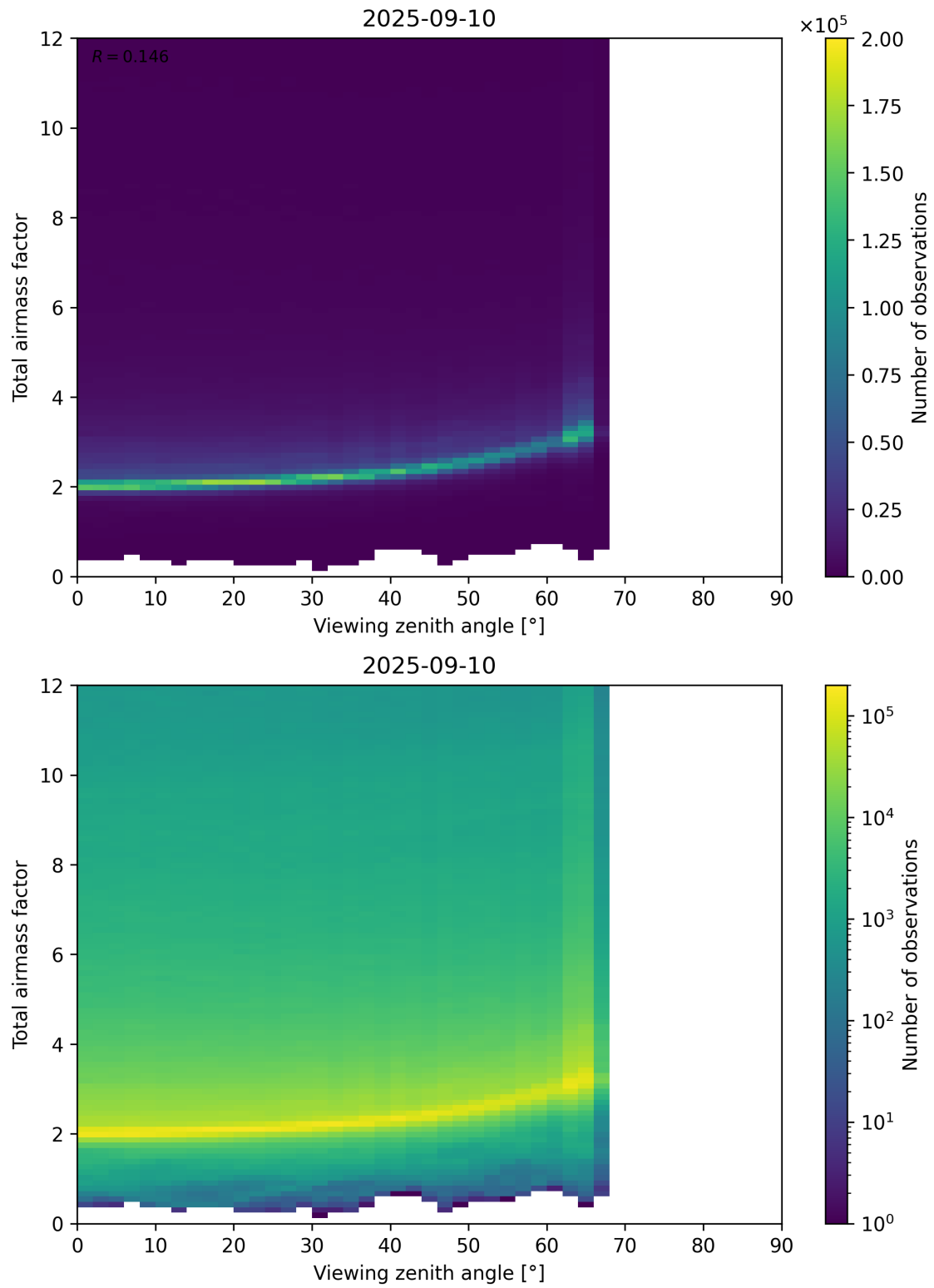
Figure 160: Scatter density plot of “Viewing zenith angle” against “Total airmass factor” for 2025-09-10 to 2025-09-11.
