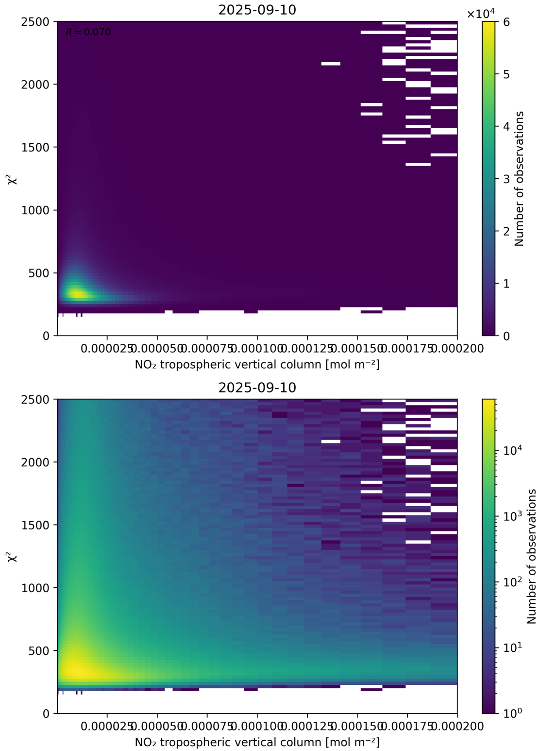
Figure 124: Scatter density plot of “NO 2 tropospheric vertical column” against “ \chi^2 ” for 2025-09-10 to 2025-09-11.
