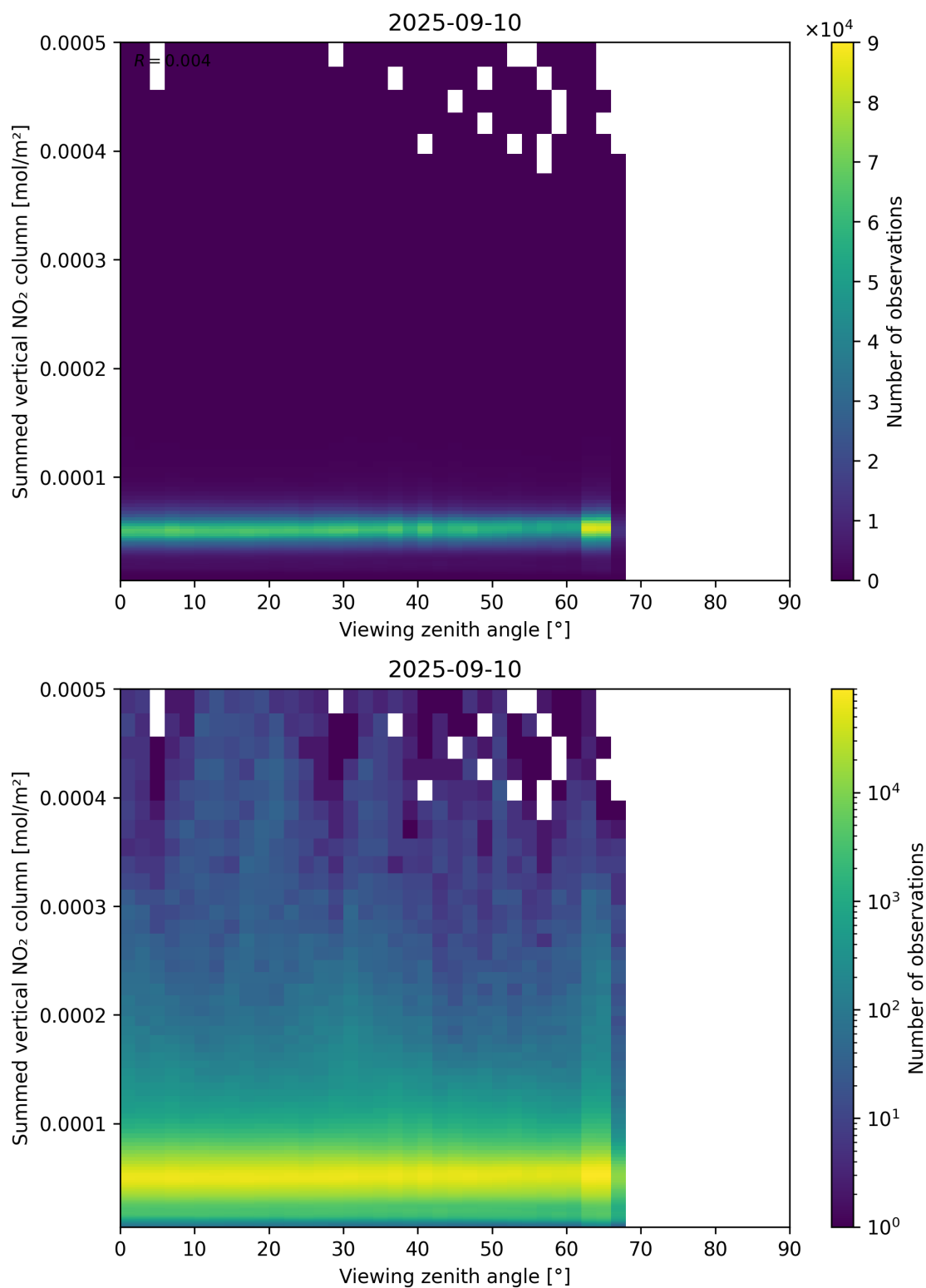
Figure 165: Scatter density plot of “Viewing zenith angle” against “Summed vertical NO 2 column” for 2025-09-10 to 2025-09-11.
