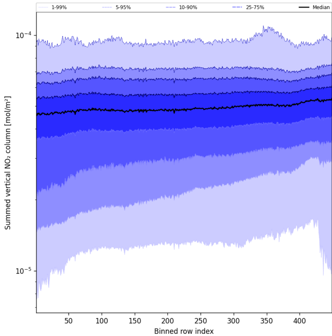
Figure 57: Along track statistics of “Summed vertical NO 2 column” for 2025-09-10 to 2025-09-11
