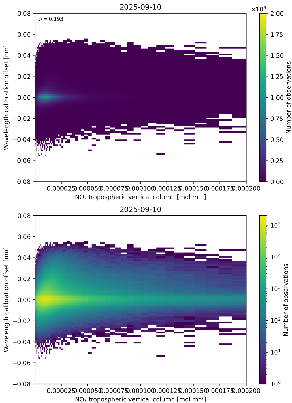
Figure 143: Scatter density plot of “NO 2 tropospheric vertical column” against “Wavelength calibration offset” for 2025-09-10 to 2025-09-11.
