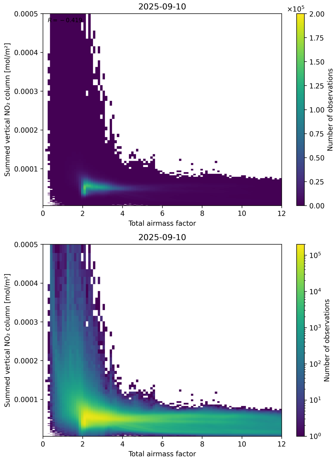
Figure 65: Scatter density plot of “Total airmass factor” against “Summed vertical NO 2 column” for 2025-09-10 to 2025-09-11.
