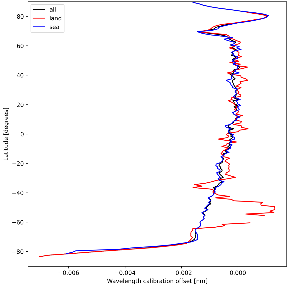
Figure 18: Zonal average of “Wavelength calibration offset” for 2025-09-10 to 2025-09-11.
