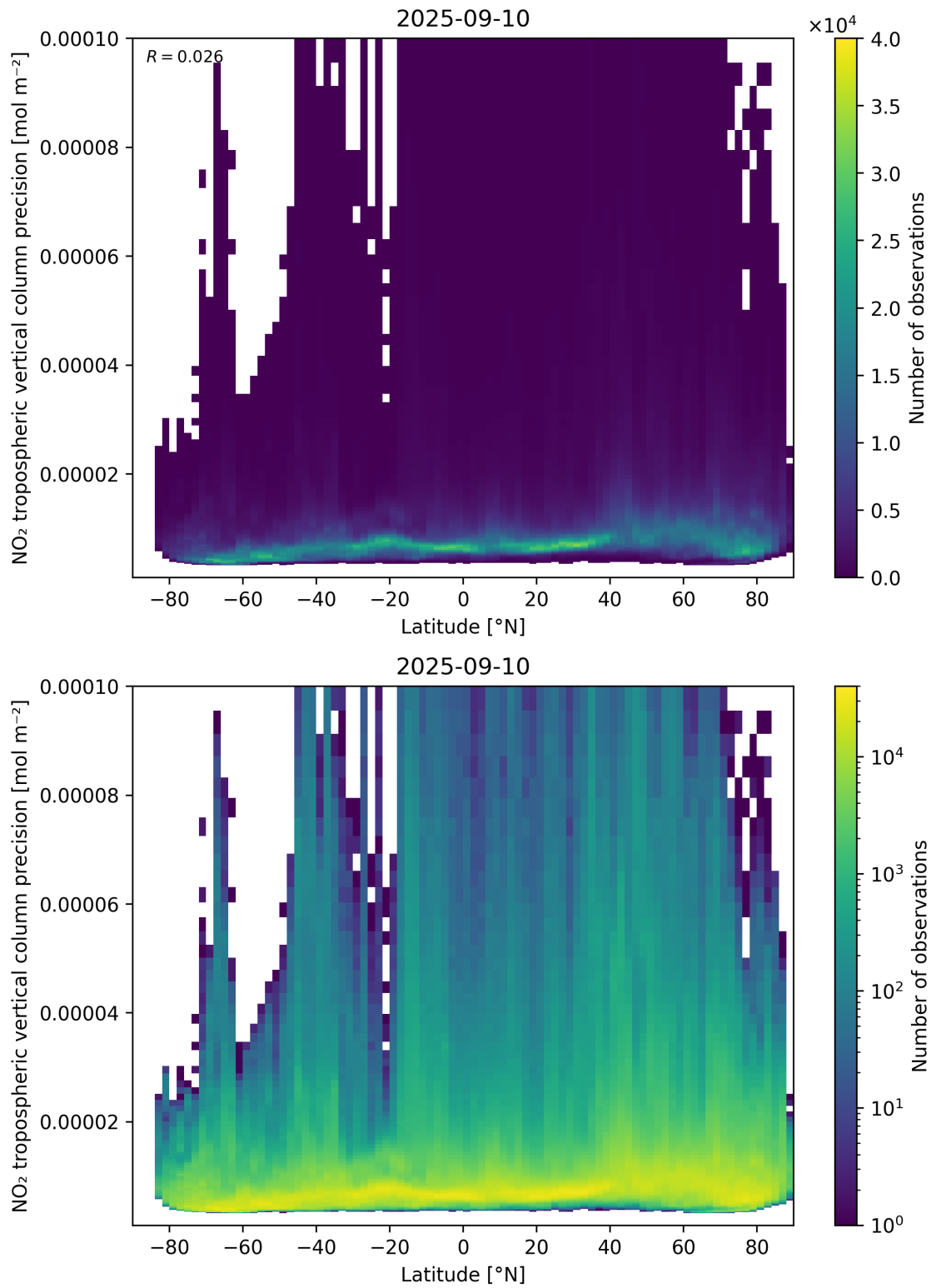
Figure 93: Scatter density plot of “Latitude” against “NO 2 tropospheric vertical column precision” for 2025-09-10 to 2025-09-11.
