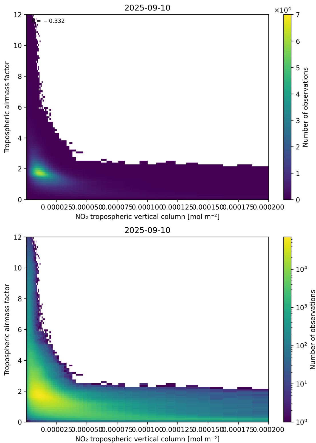
Figure 123: Scatter density plot of “NO 2 tropospheric vertical column” against “Tropospheric air mass factor” for 2025-09-10 to 2025-09-11.
