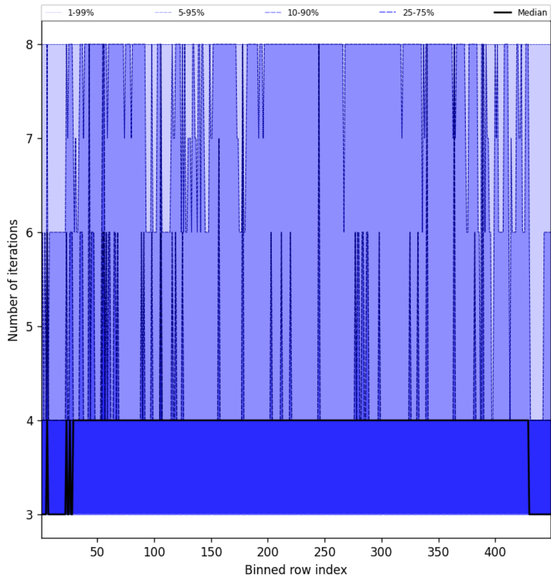
Figure 51: Along track statistics of “Number of iterations” for 2025-09-10 to 2025-09-11
