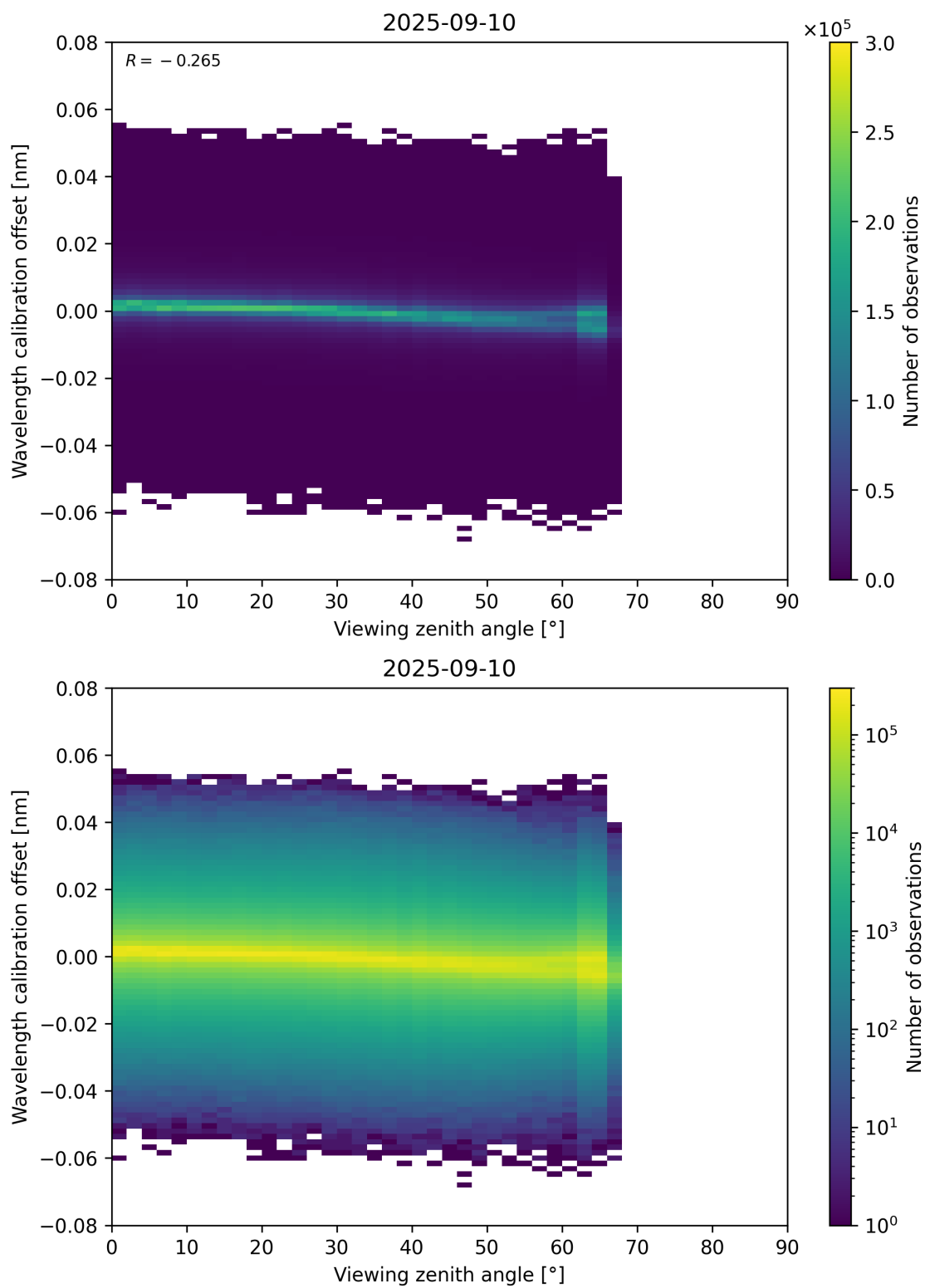
Figure 173: Scatter density plot of “Viewing zenith angle” against “Wavelength calibration offset” for 2025-09-10 to 2025-09-11.
