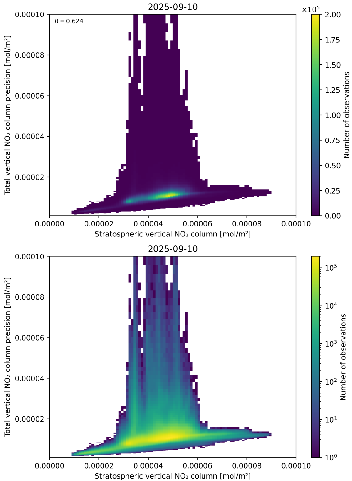
Figure 101: Scatter density plot of “Stratospheric vertical NO 2 column” against “Total vertical NO 2 column precision” for 2025-09-10 to 2025-09-11.
