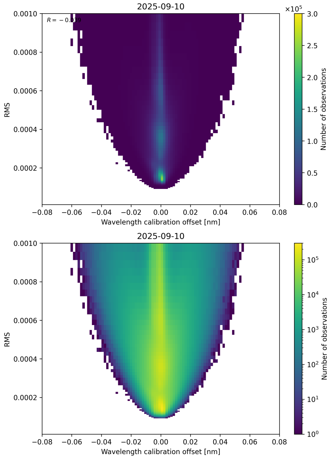
Figure 181: Scatter density plot of “Wavelength calibration offset” against “RMS” for 2025-09-10 to 2025-09-11.
