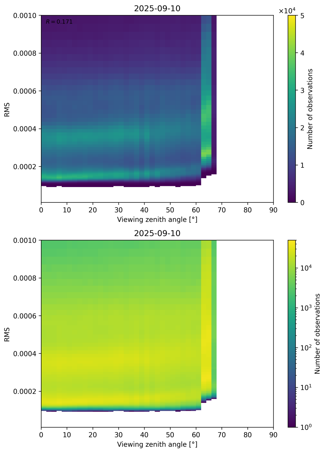
Figure 171: Scatter density plot of “Viewing zenith angle” against “RMS” for 2025-09-10 to 2025-09-11.
