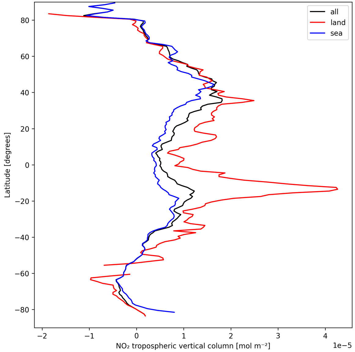
Figure 12: Zonal average of “NO 2 tropospheric vertical column” for 2025-09-10 to 2025-09-11.
