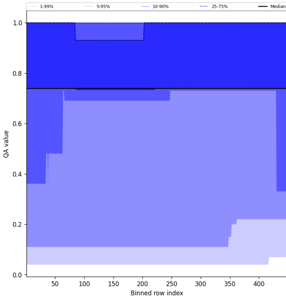
Figure 45: Along track statistics of “QA value” for 2025-09-10 to 2025-09-11
