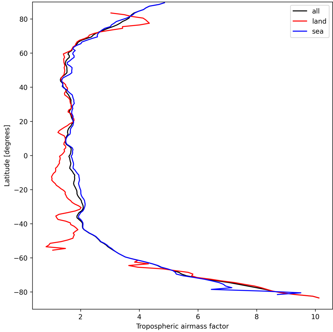
Figure 14: Zonal average of “Tropospheric airmass factor” for 2025-09-10 to 2025-09-11.
