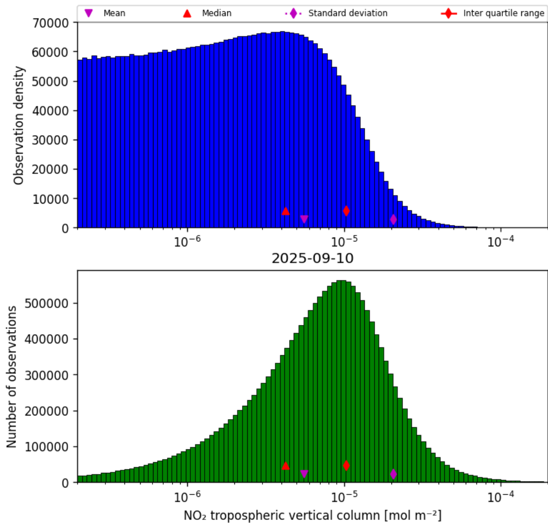
Figure 29: Histogram of “NO 2 tropospheric vertical column” for 2025-09-10 to 2025-09-11
