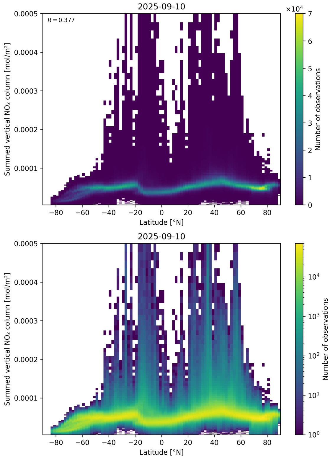
Figure 88: Scatter density plot of “Latitude” against “Summed vertical NO 2 column” for 2025-09-10 to 2025-09-11.
