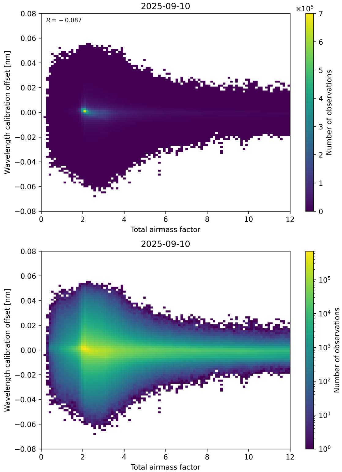
Figure 70: Scatter density plot of “Total airmass factor” against “Wavelength calibration offset” for 2025-09-10 to 2025-09-11.
