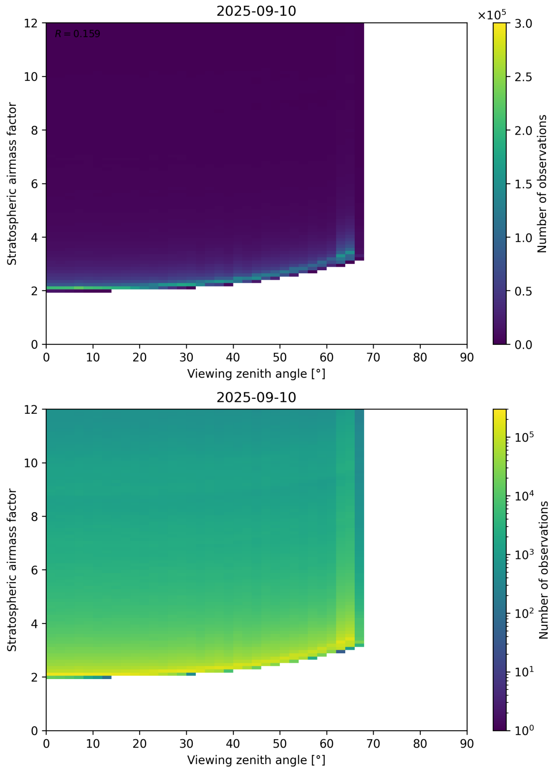
Figure 159: Scatter density plot of “Viewing zenith angle” against “Stratospheric airmass factor” for 2025-09-10 to 2025-09-11.
