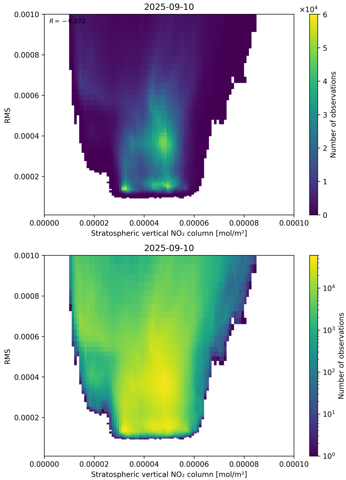
Figure 102: Scatter density plot of “Stratospheric vertical NO 2 column” against “RMS” for 2025-09-10 to 2025-09-11.
