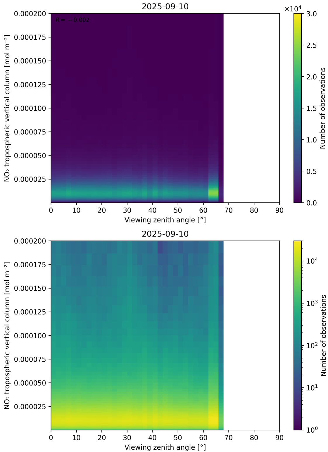
Figure 169: Scatter density plot of “Viewing zenith angle” against “NO 2 tropospheric vertical column” for 2025-09-10 to 2025-09-11.
