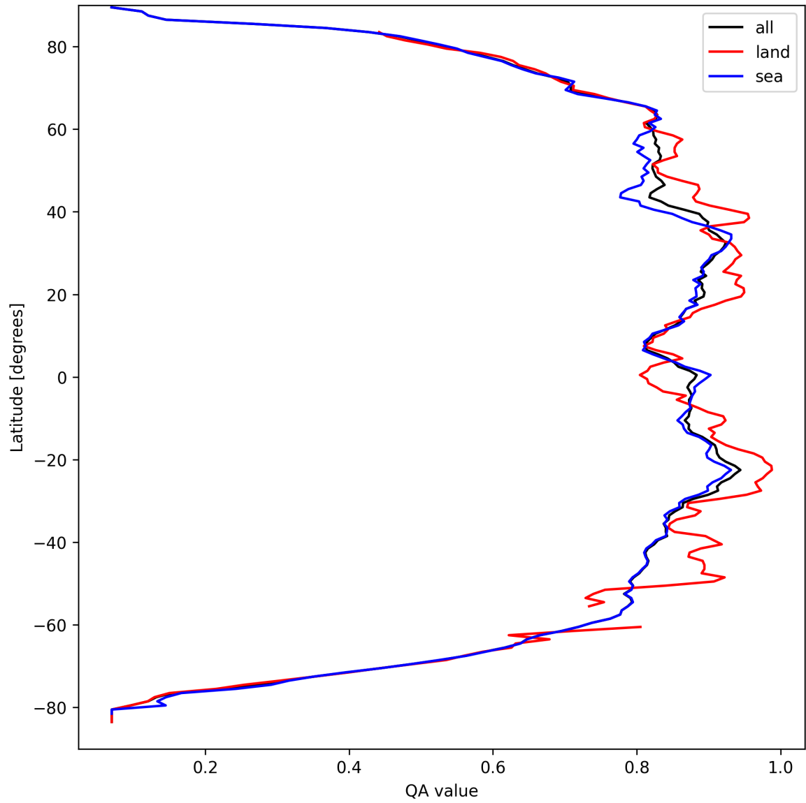
Figure 11: Zonal average of “QA value” for 2025-09-10 to 2025-09-11.
