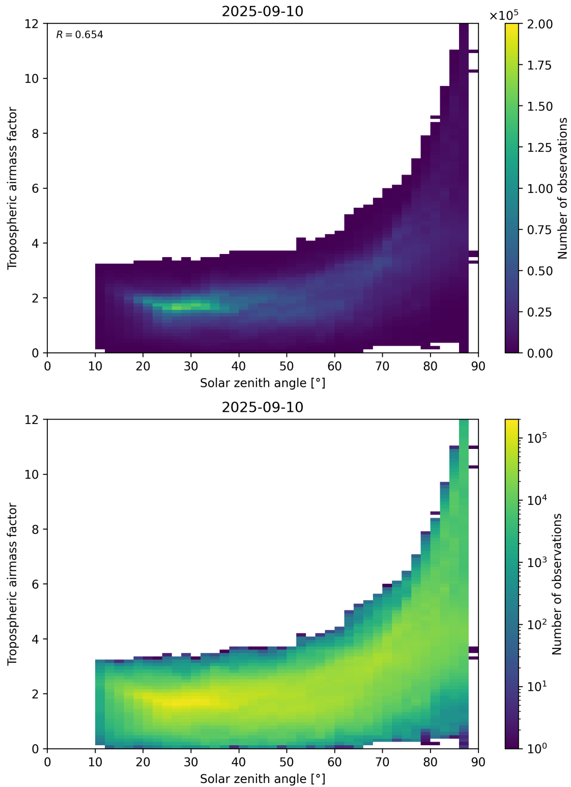
Figure 147: Scatter density plot of “Solar zenith angle” against “Tropospheric airmass factor” for 2025-09-10 to 2025-09-11.
