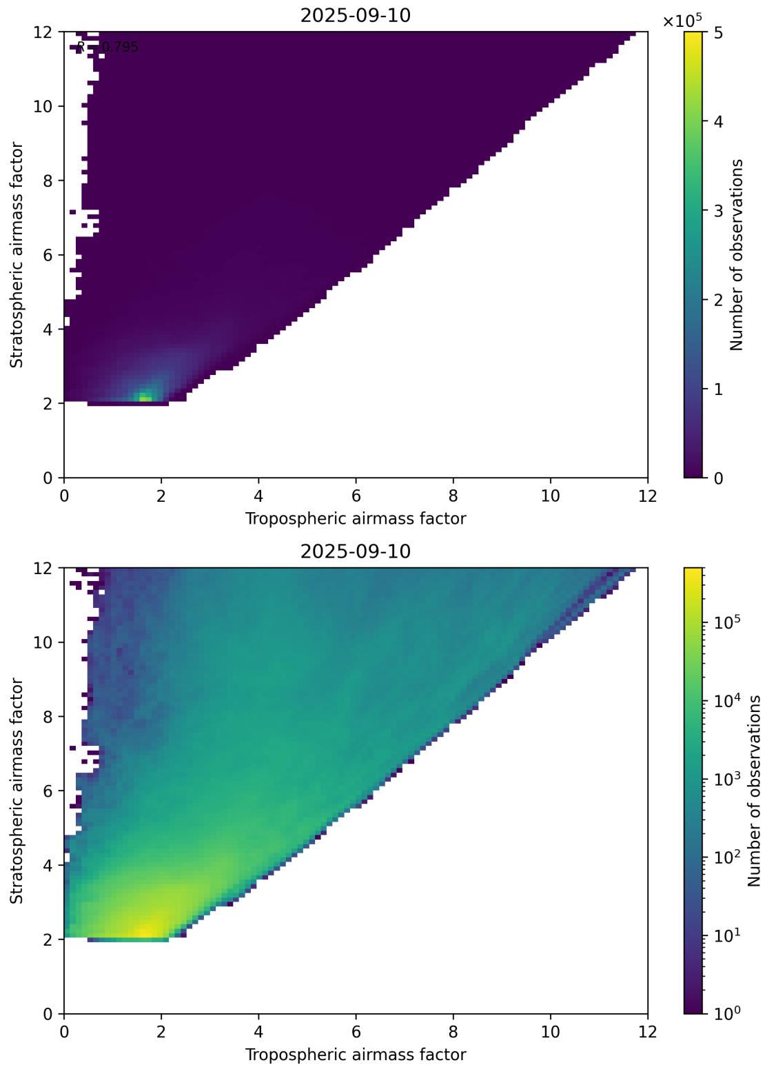
Figure 71: Scatter density plot of “Tropospheric airmass factor” against “Stratospheric airmass factor” for 2025-09-10 to 2025-09-11.
