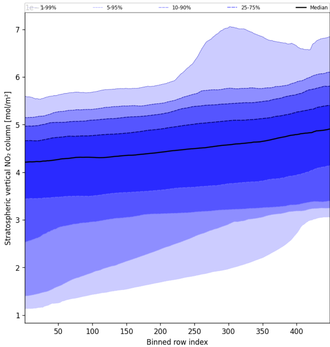
Figure 53: Along track statistics of “Stratospheric vertical NO 2 column” for 2025-09-10 to 2025-09-11
