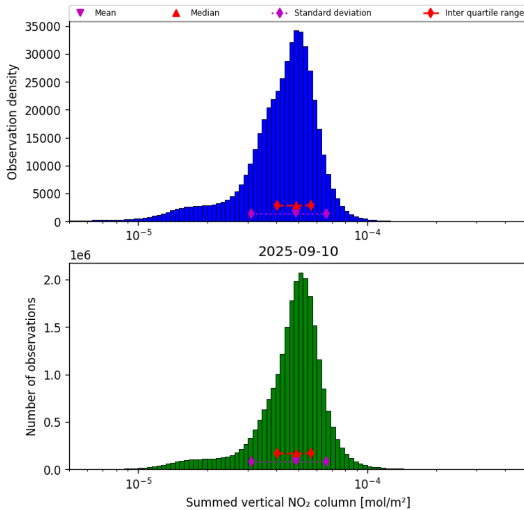
Figure 40: Histogram of “Summed vertical NO 2 column” for 2025-09-10 to 2025-09-11
