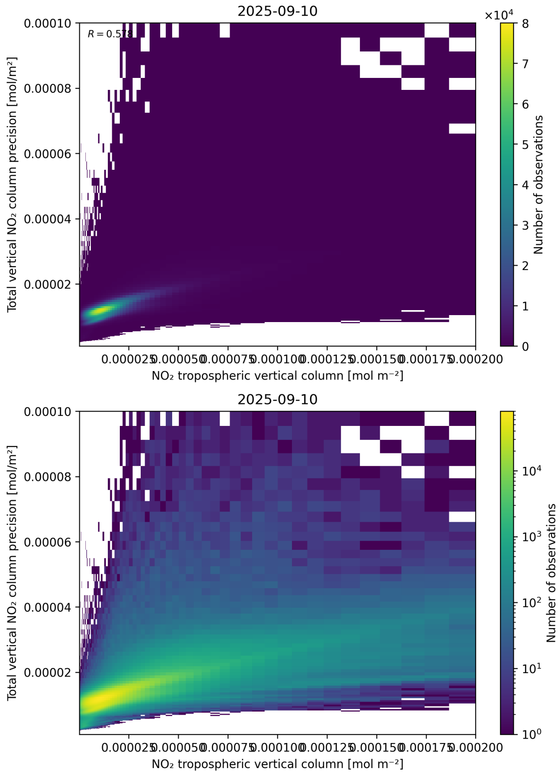
Figure 129: Scatter density plot of “NO 2 tropospheric vertical column” against “Total vertical NO 2 column precision” for 2025-09-10 to 2025-09-11.
