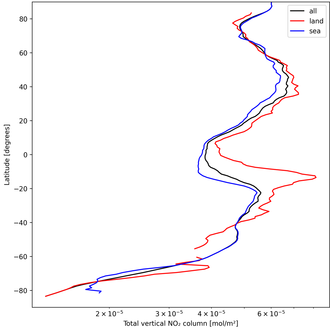
Figure 21: Zonal average of “Total vertical NO 2 column” for 2025-09-10 to 2025-09-11.
