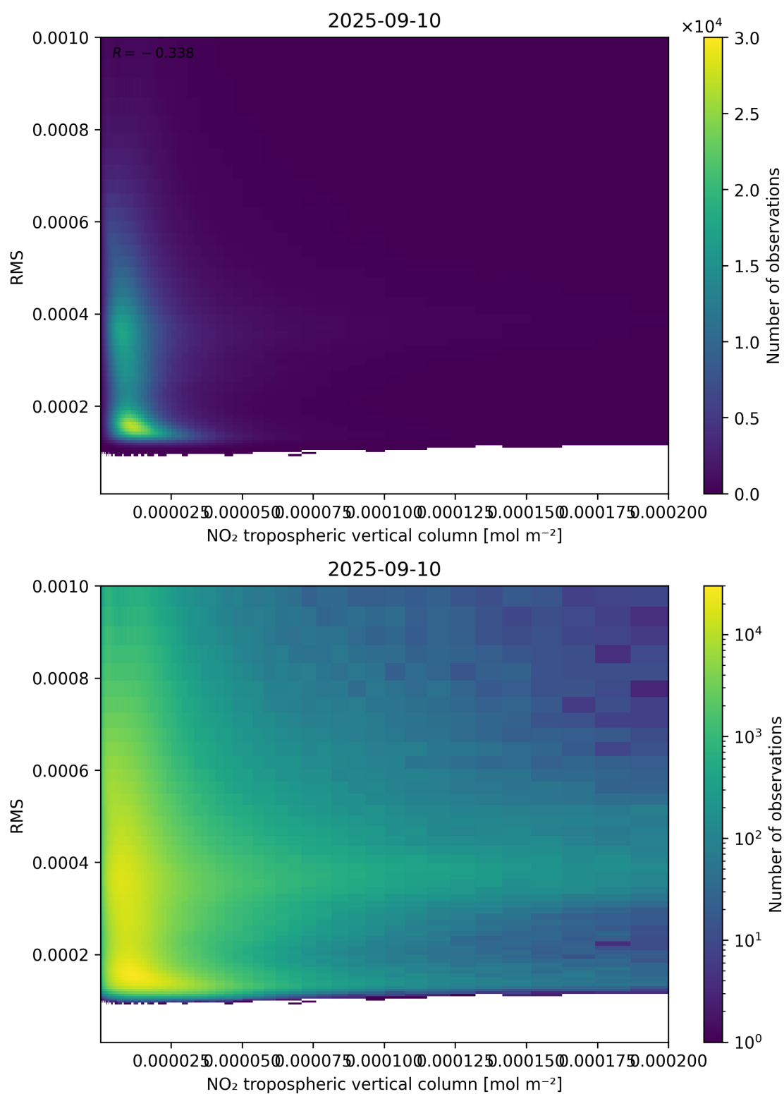
Figure 142: Scatter density plot of “NO 2 tropospheric vertical column” against “RMS” for 2025-09-10 to 2025-09-11.
