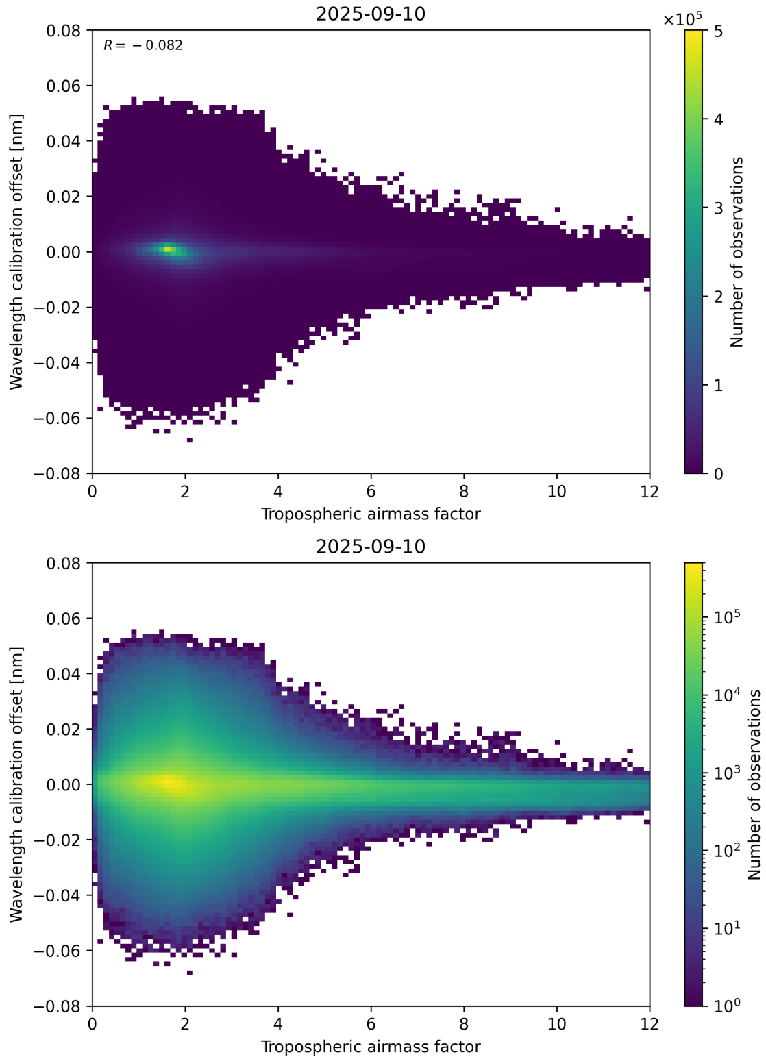
Figure 80: Scatter density plot of “Tropospheric airmass factor” against “Wavelength calibration offset” for 2025-09-10 to 2025-09-11.
