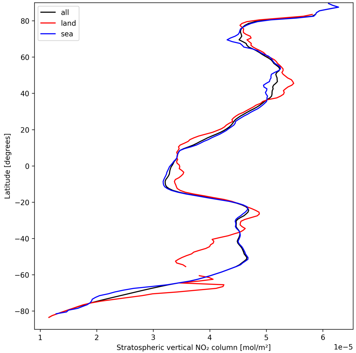
Figure 19: Zonal average of “Stratospheric vertical NO 2 column” for 2025-09-10 to 2025-09-11.
