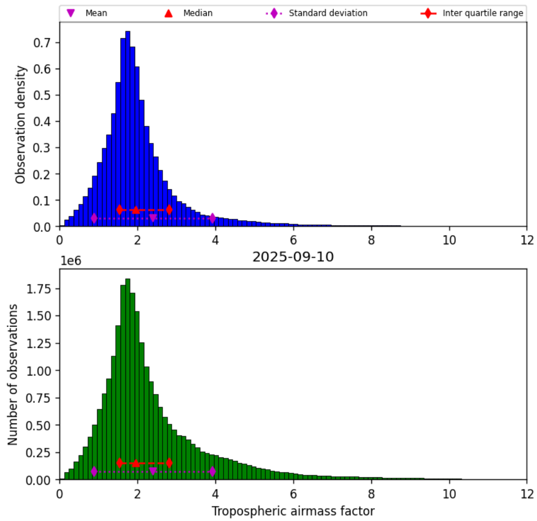
Figure 31: Histogram of “Tropospheric airmass factor” for 2025-09-10 to 2025-09-11
