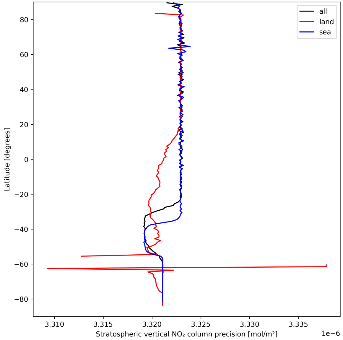
Figure 20: Zonal average of “Stratospheric vertical NO 2 column precision” for 2025-09-10 to 2025-09-11.
