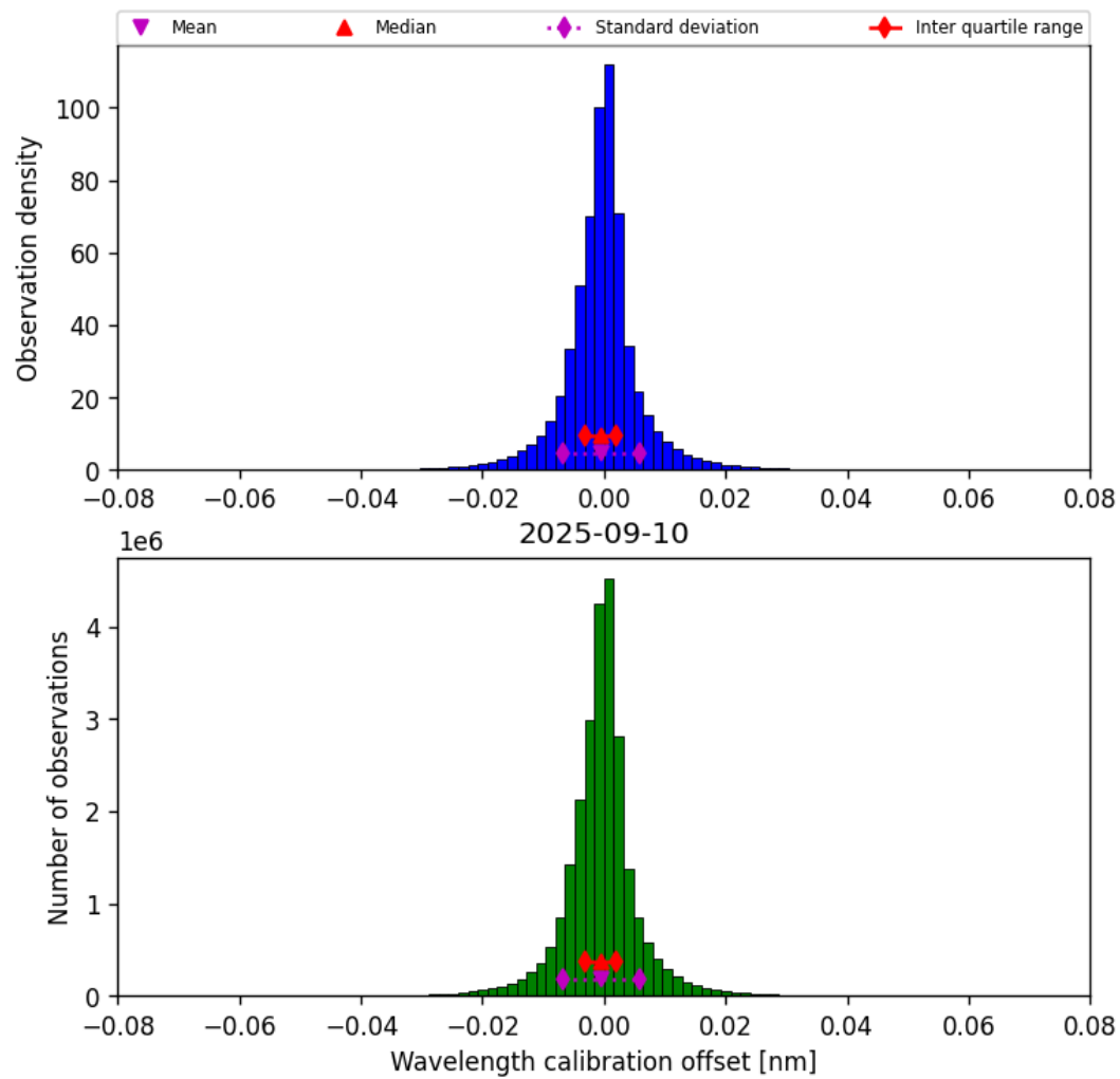
Figure 35: Histogram of “Wavelength calibration offset” for 2025-09-10 to 2025-09-11
