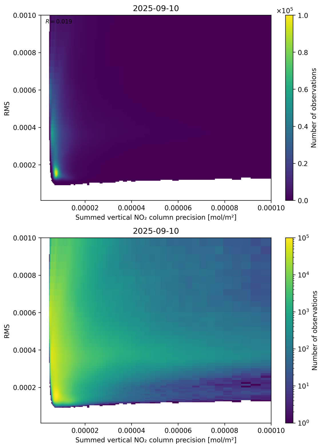
Figure 108: Scatter density plot of “Summed vertical NO 2 column precision” against “RMS” for 2025-09-10 to 2025-09-11.
