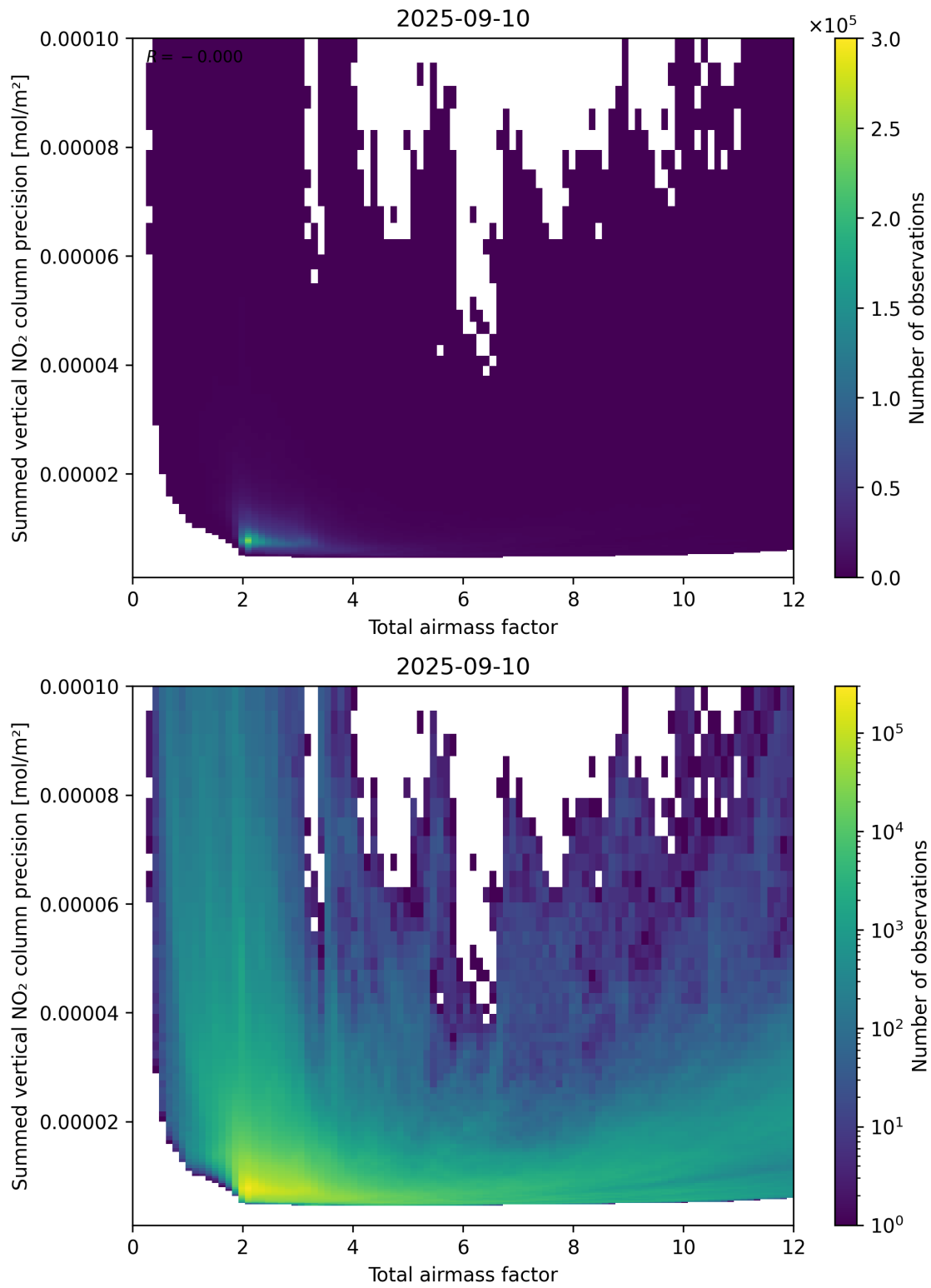
Figure 66: Scatter density plot of “Total airmass factor” against “Summed vertical NO 2 column precision” for 2025-09-10 to 2025-09-11.
