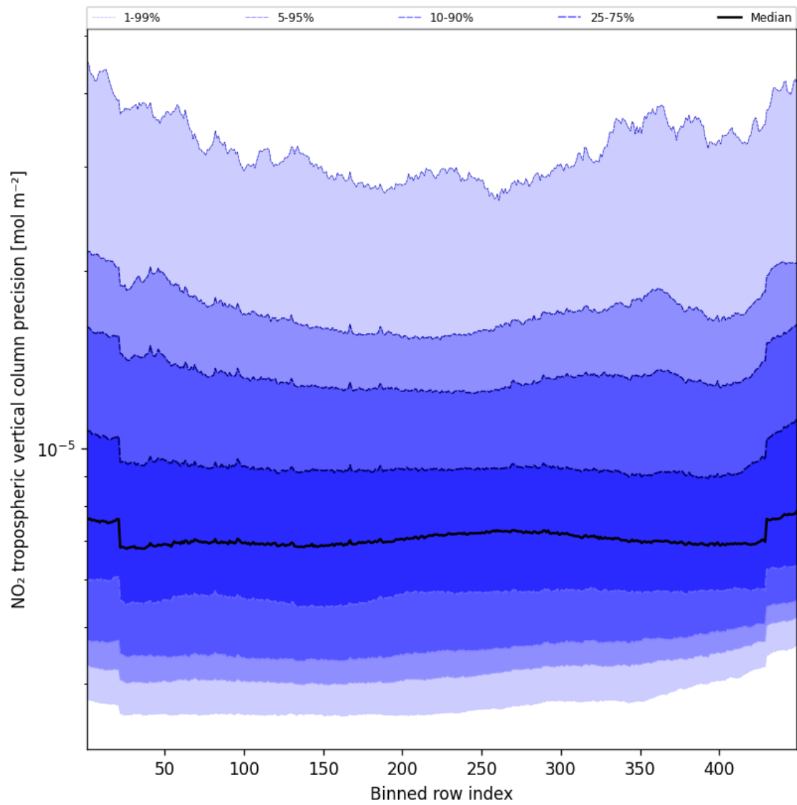
Figure 47: Along track statistics of “NO 2 tropospheric vertical column precision” for 2025-09-10 to 2025-09-11
