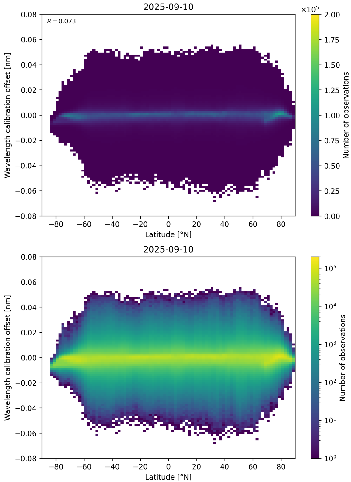
Figure 95: Scatter density plot of “Latitude” against “Wavelength calibration offset” for 2025-09-10 to 2025-09-11.
