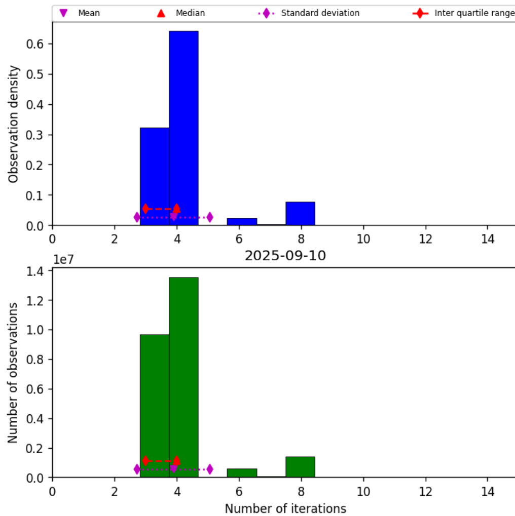
Figure 34: Histogram of “Number of iterations” for 2025-09-10 to 2025-09-11
