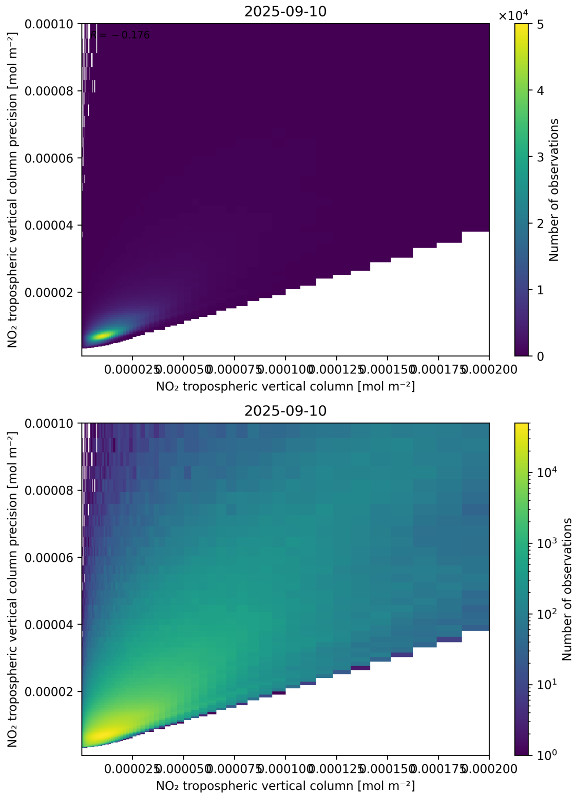
Figure 130: Scatter density plot of “NO 2 tropospheric vertical column” against “NO 2 tropospheric vertical column precision” for 2025-09-10 to 2025-09-11.
