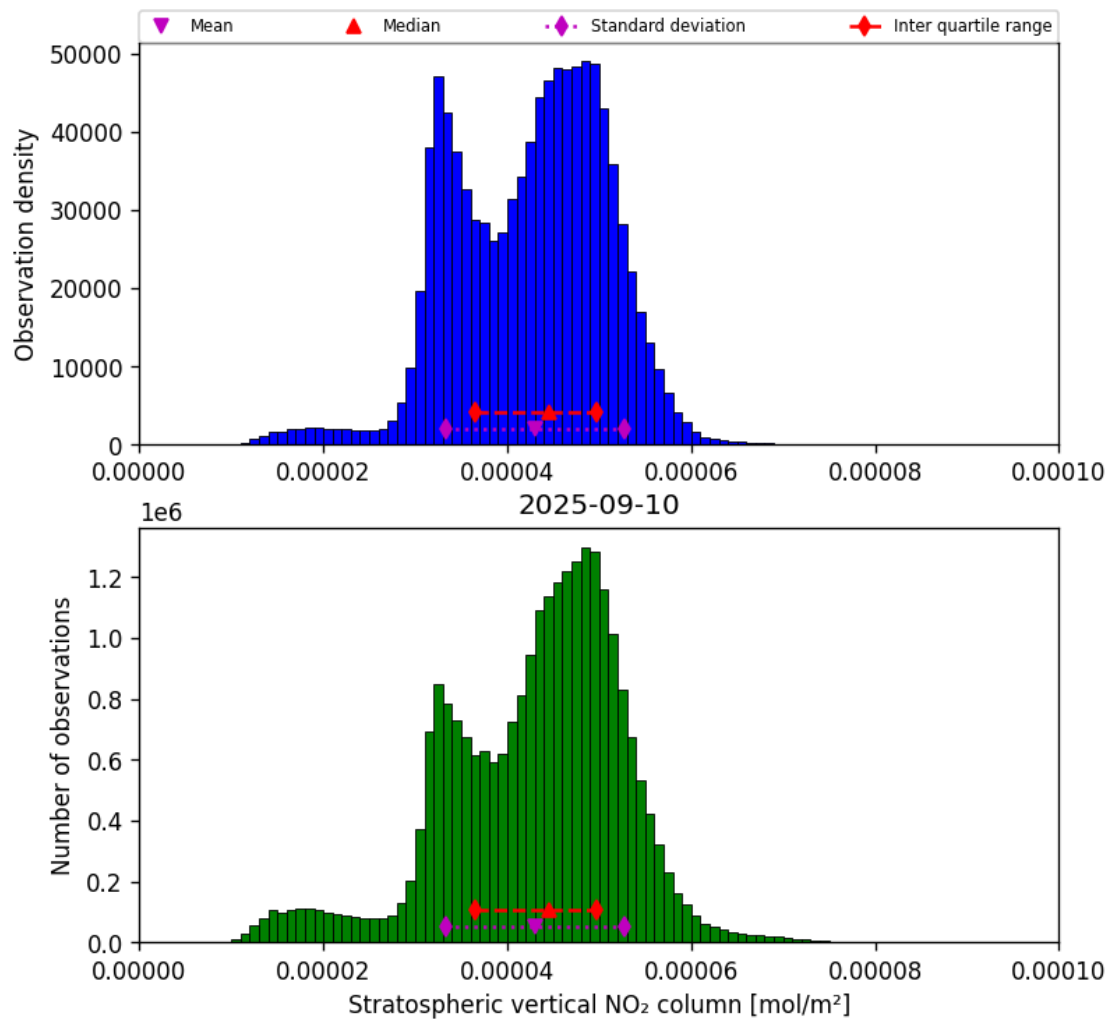
Figure 36: Histogram of “Stratospheric vertical NO 2 column” for 2025-09-10 to 2025-09-11
