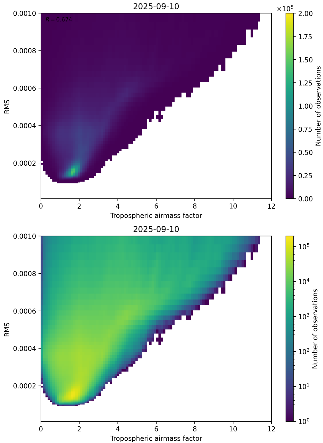
Figure 79: Scatter density plot of “Tropospheric airmass factor” against “RMS” for 2025-09-10 to 2025-09-11.
