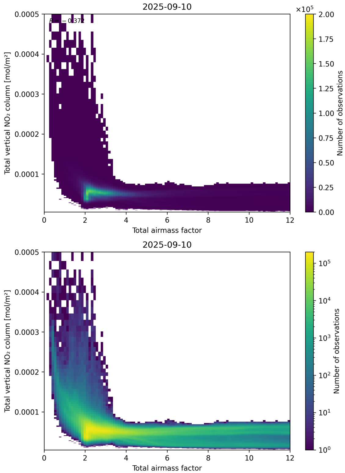
Figure 67: Scatter density plot of “Total airmass factor” against “Total vertical NO 2 column” for 2025-09-10 to 2025-09-11.
