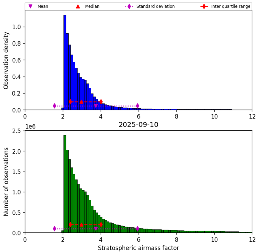
Figure 44: Histogram of “Stratospheric airmass factor” for 2025-09-10 to 2025-09-11
