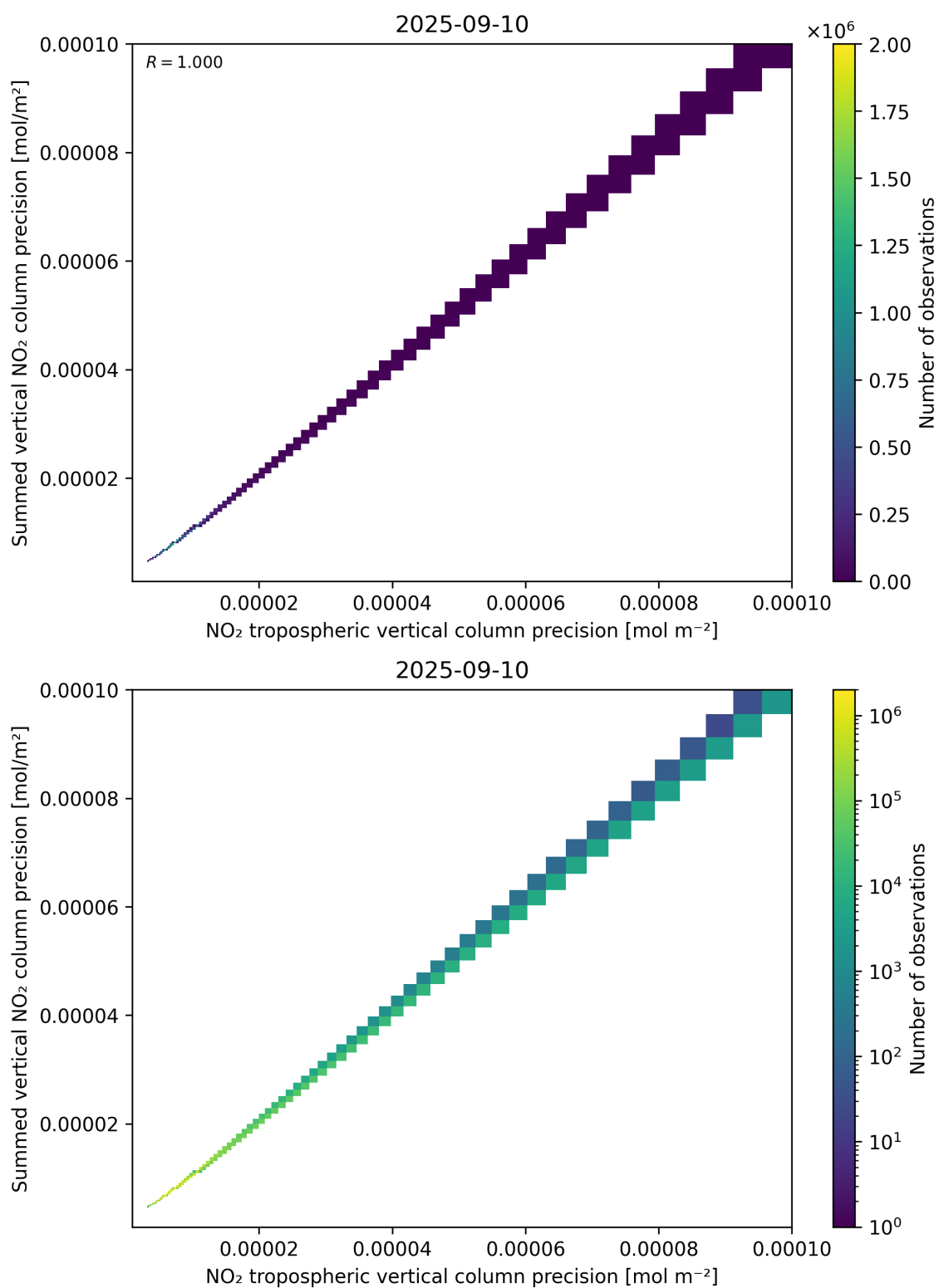
Figure 137: Scatter density plot of “NO 2 tropospheric vertical column precision” against “Summed vertical NO 2 column precision” for 2025-09-10 to 2025-09-11.
