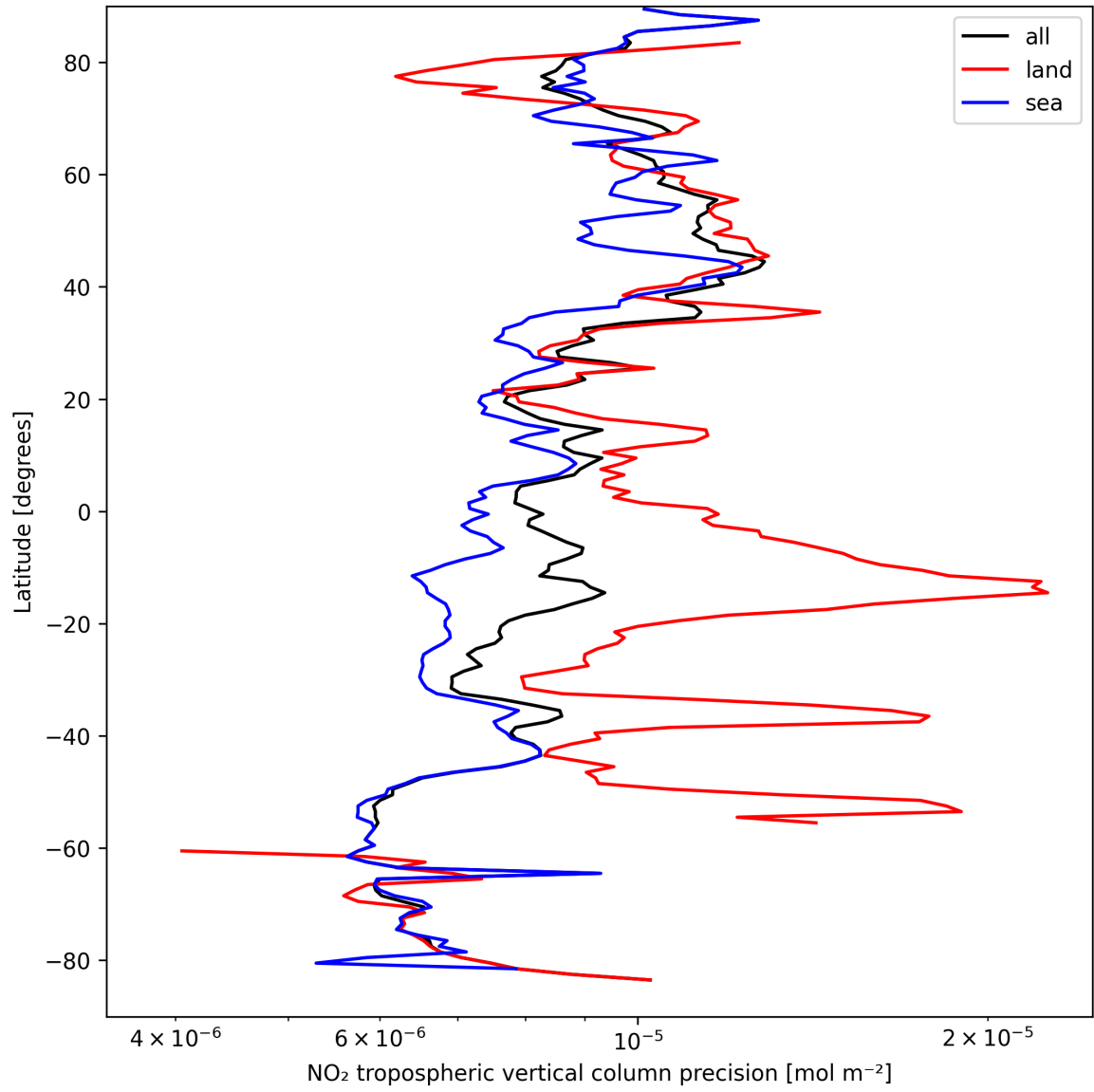
Figure 13: Zonal average of “NO 2 tropospheric vertical column precision” for 2025-09-10 to 2025-09-11.
