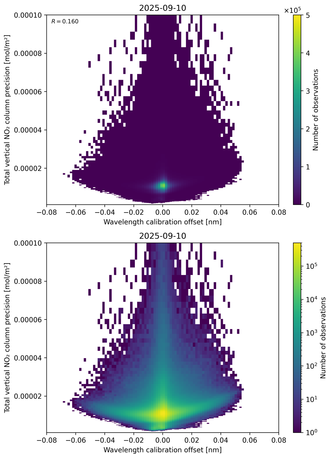
Figure 180: Scatter density plot of “Wavelength calibration offset” against “Total vertical NO 2 column precision” for 2025-09-10 to 2025-09-11.
