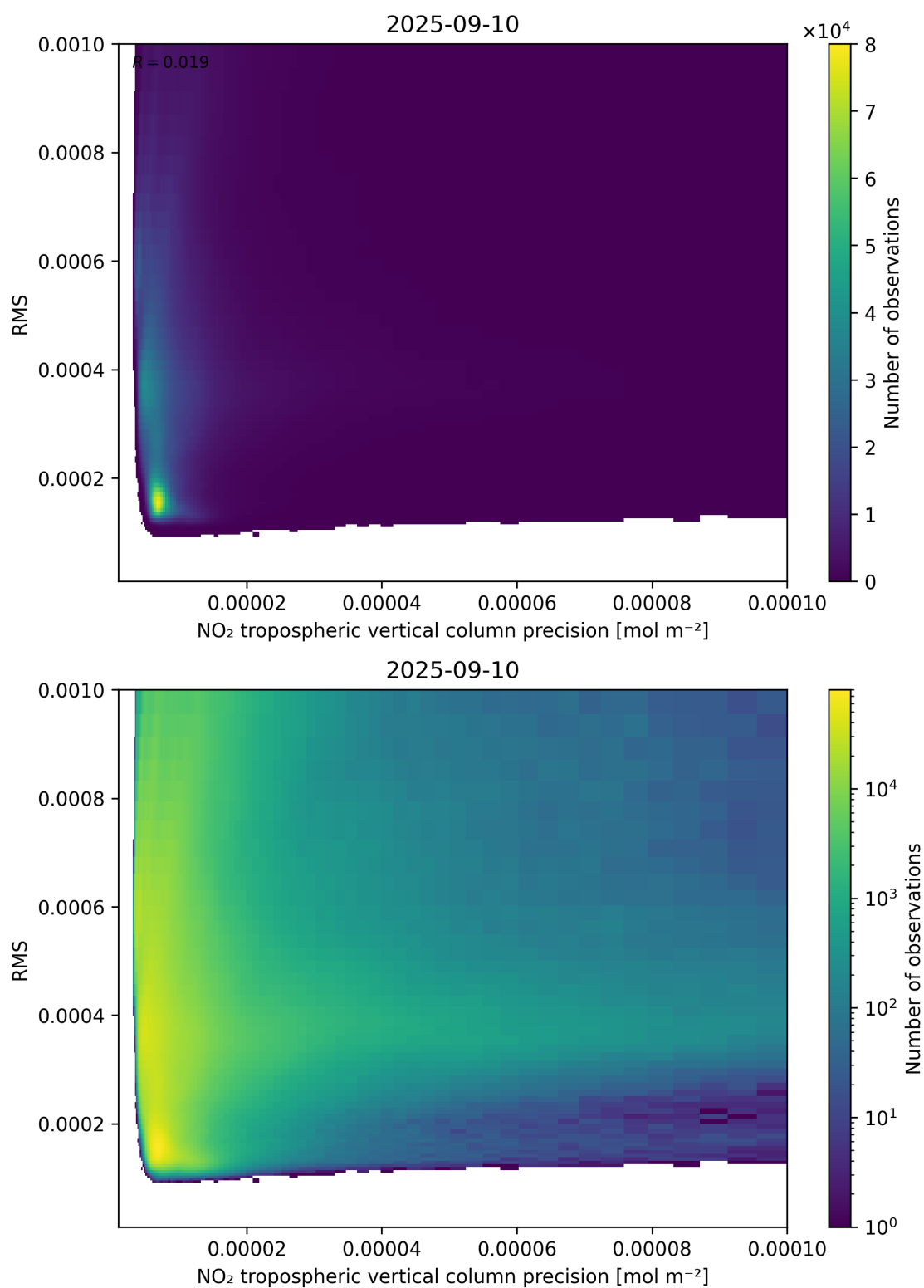
Figure 140: Scatter density plot of “NO 2 tropospheric vertical column precision” against “RMS” for 2025-09-10 to 2025-09-11.
