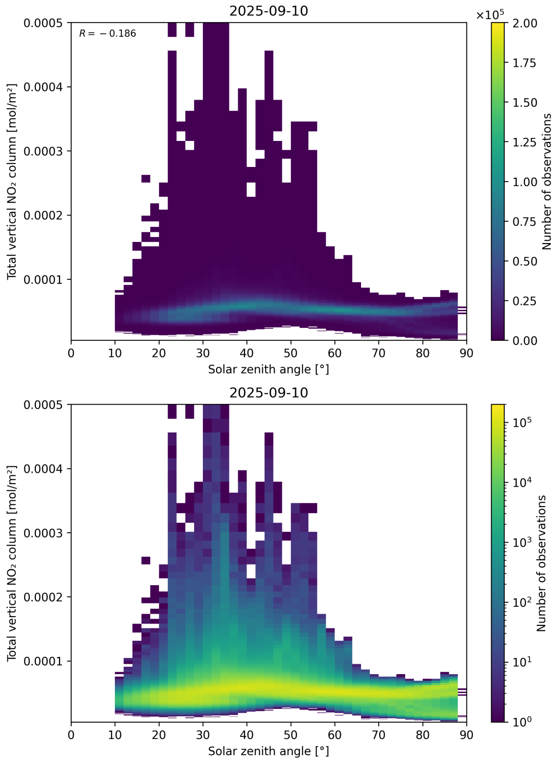
Figure 153: Scatter density plot of “Solar zenith angle” against “Total vertical NO 2 column” for 2025-09-10 to 2025-09-11.
