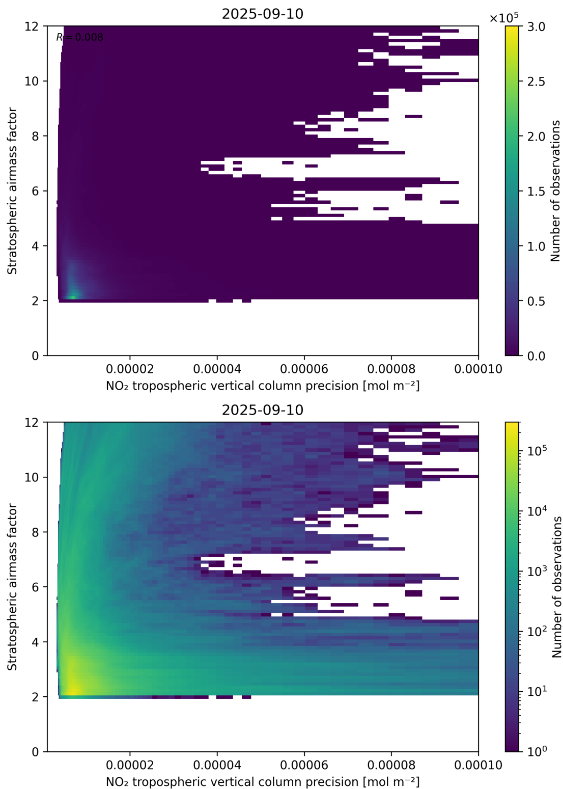
Figure 131: Scatter density plot of “NO 2 tropospheric vertical column precision” against “Stratospheric airmass factor” for 2025-09-10 to 2025-09-11.
