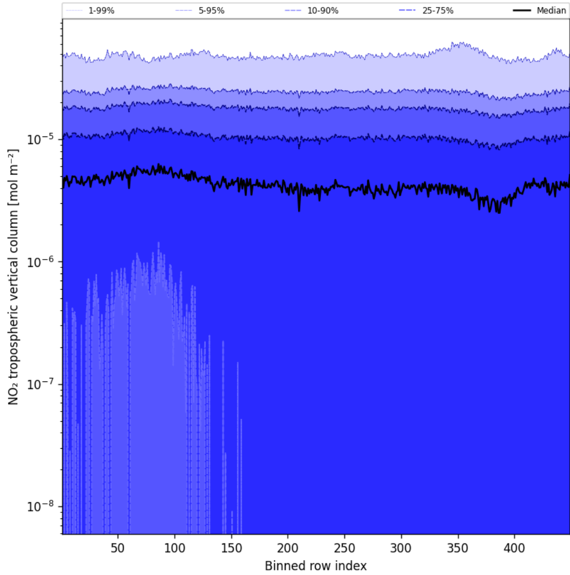
Figure 46: Along track statistics of “NO 2 tropospheric vertical column” for 2025-09-10 to 2025-09-11
