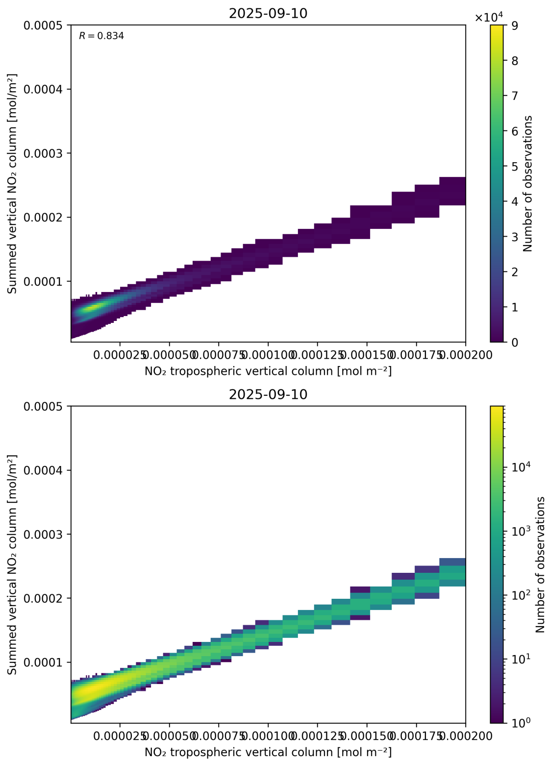
Figure 126: Scatter density plot of “NO 2 tropospheric vertical column” against “Summed vertical NO 2 column” for 2025-09-10 to 2025-09-11.
