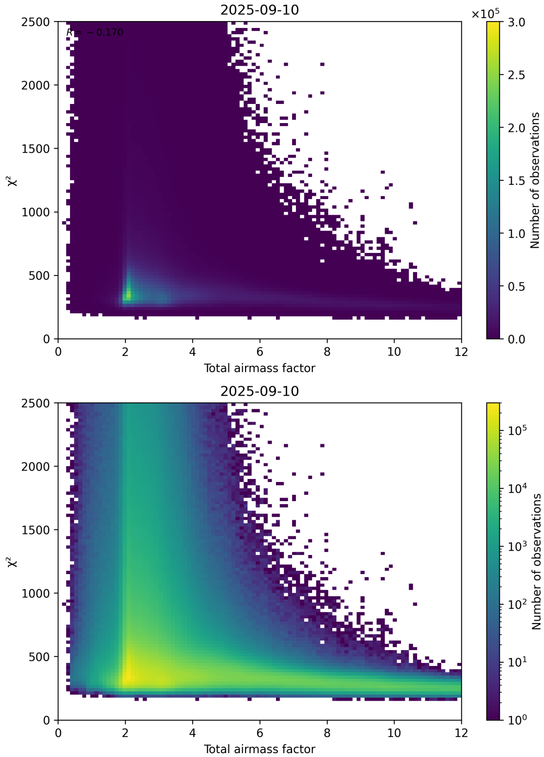
Figure 63: Scatter density plot of “Total airmass factor” against “ \chi^2 ” for 2025-09-10 to 2025-09-11.
