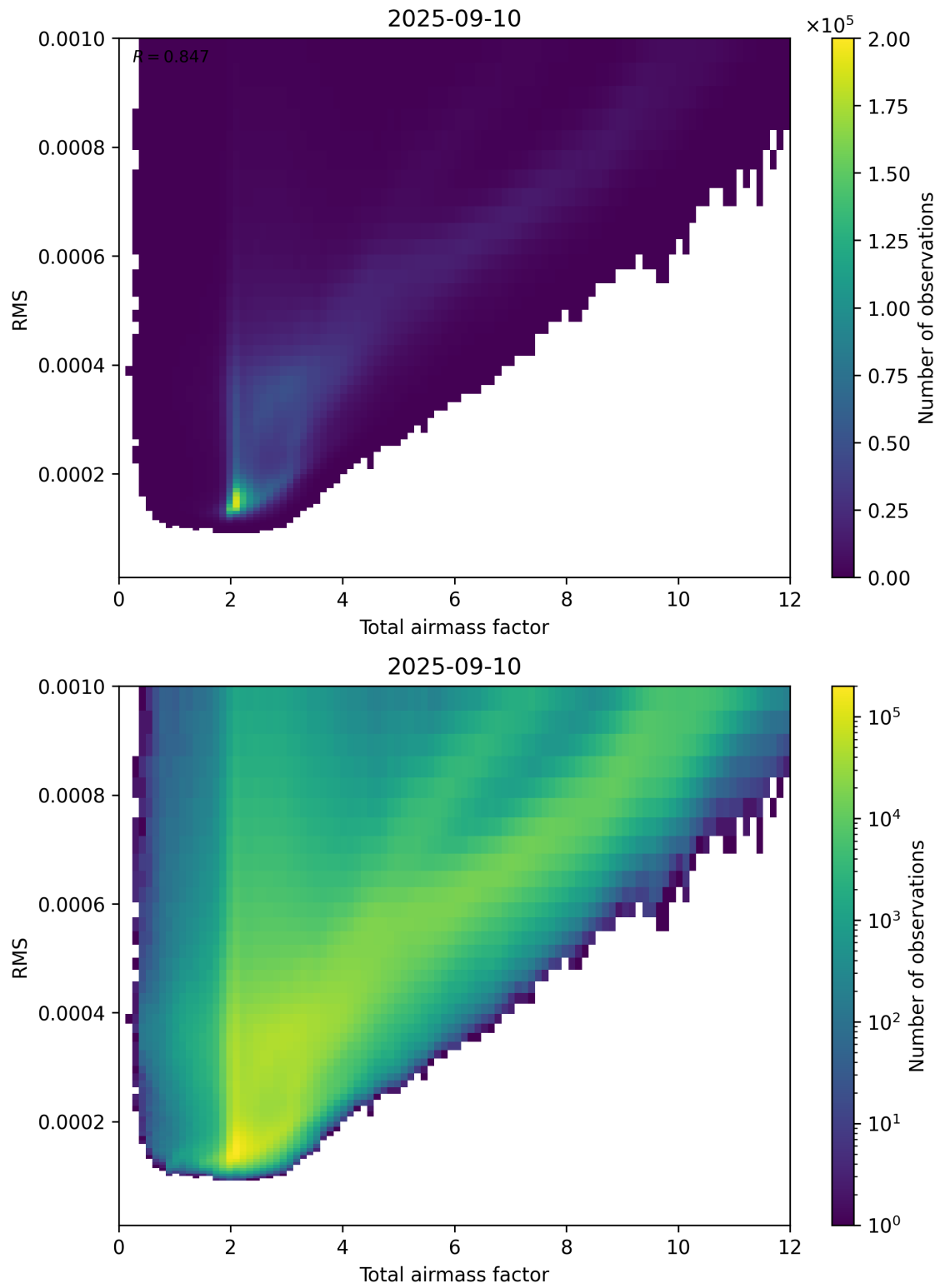
Figure 69: Scatter density plot of “Total airmass factor” against “RMS” for 2025-09-10 to 2025-09-11.
