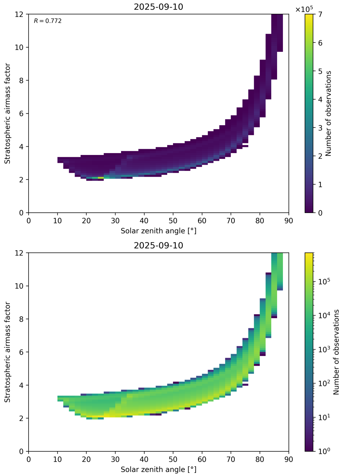
Figure 145: Scatter density plot of “Solar zenith angle” against “Stratospheric airmass factor” for 2025-09-10 to 2025-09-11.
