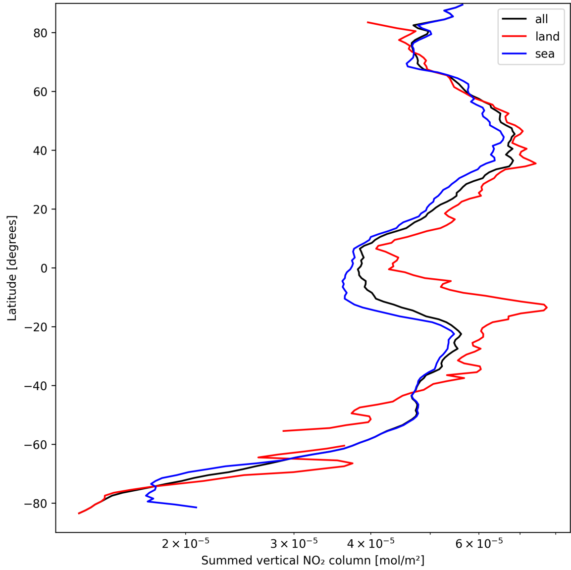
Figure 23: Zonal average of “Summed vertical NO 2 column” for 2025-09-10 to 2025-09-11.
