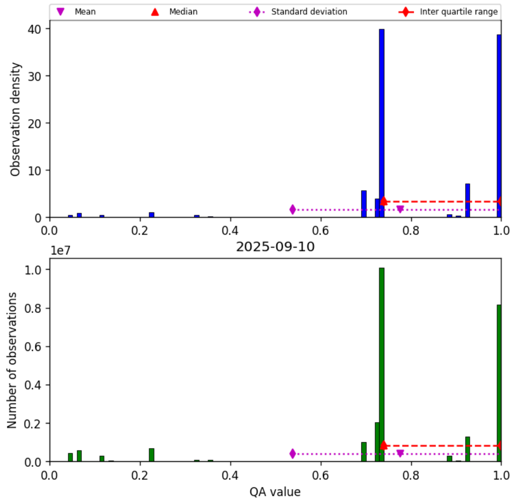
Figure 28: Histogram of “QA value” for 2025-09-10 to 2025-09-11
