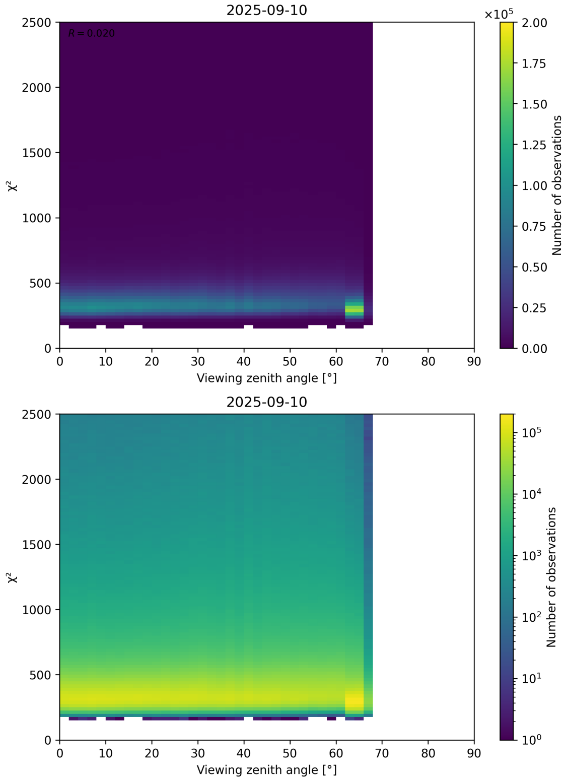
Figure 162: Scatter density plot of “Viewing zenith angle” against “ \chi^2 ” for 2025-09-10 to 2025-09-11.
