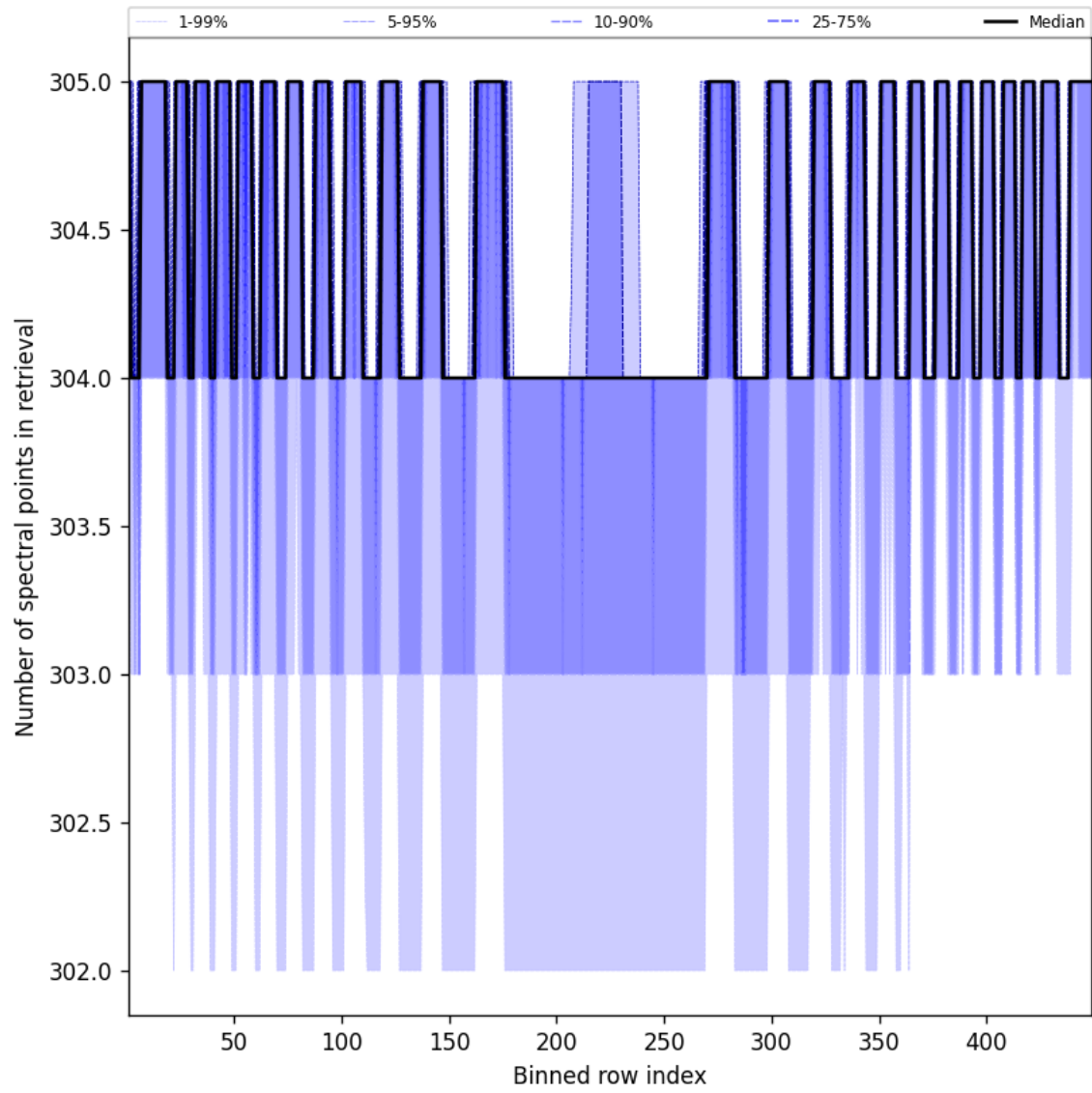
Figure 50: Along track statistics of “Number of spectral points in retrieval” for 2025-09-10 to 2025-09-11
