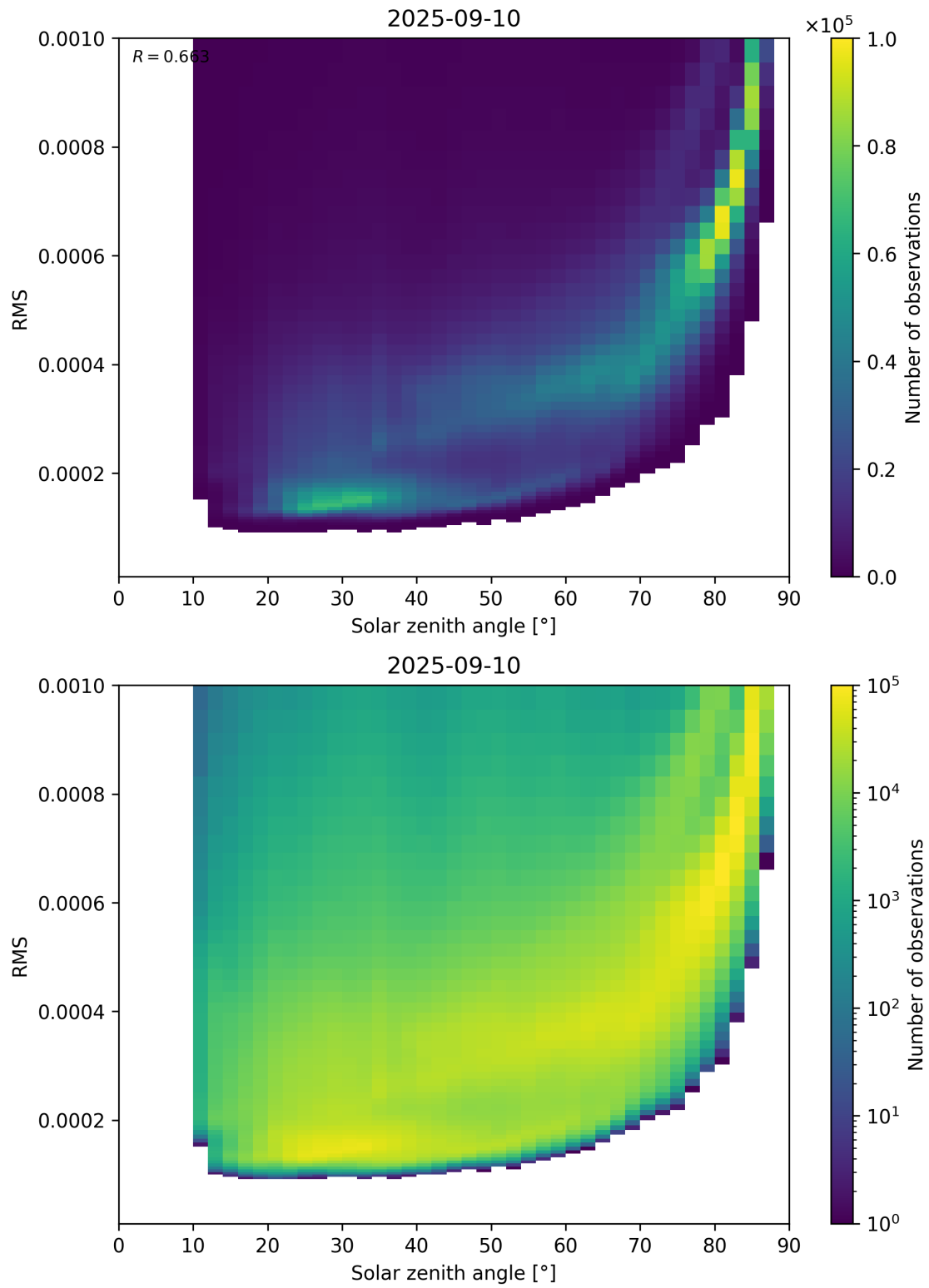
Figure 157: Scatter density plot of “Solar zenith angle” against “RMS” for 2025-09-10 to 2025-09-11.
