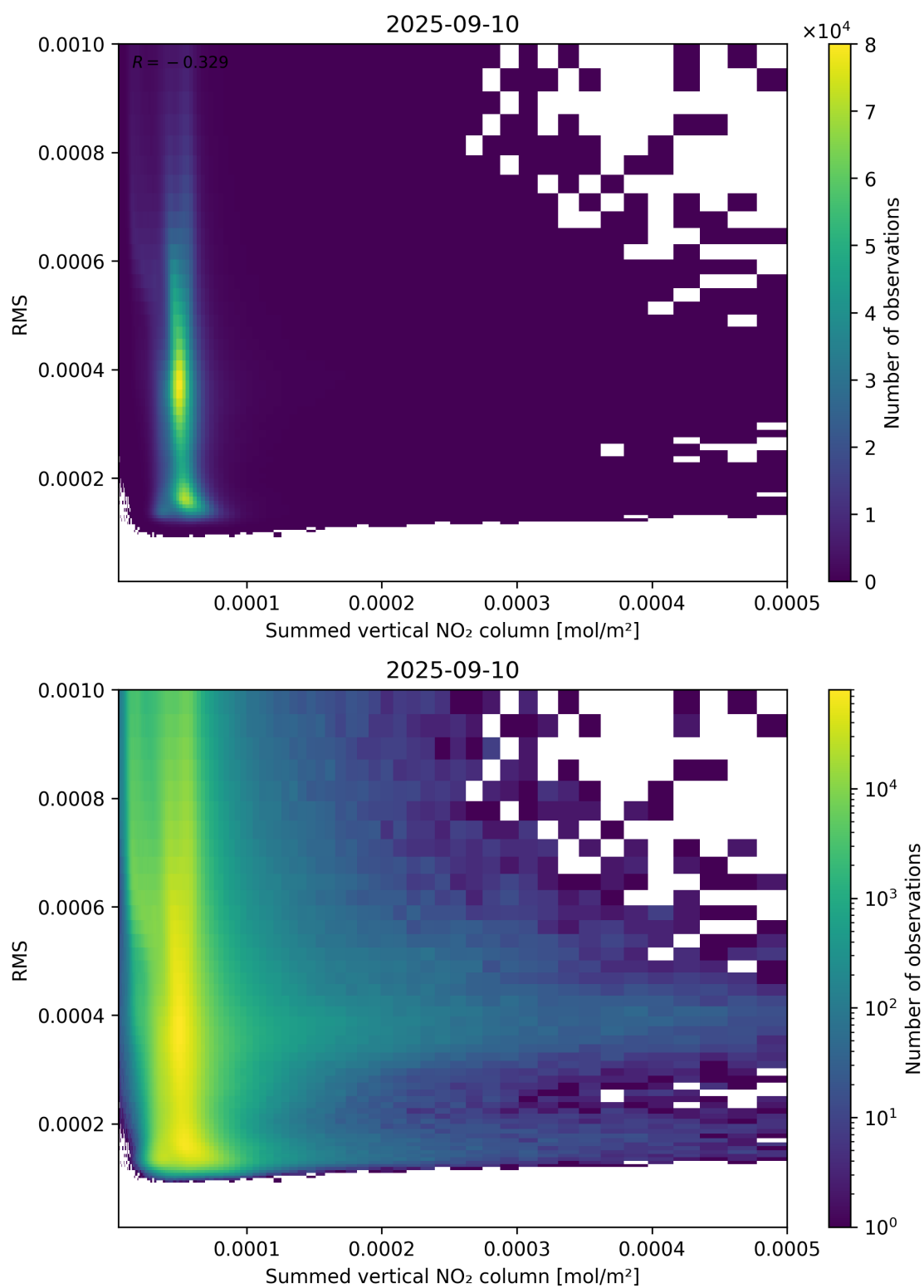
Figure 109: Scatter density plot of “Summed vertical NO 2 column” against “RMS” for 2025-09-10 to 2025-09-11.
