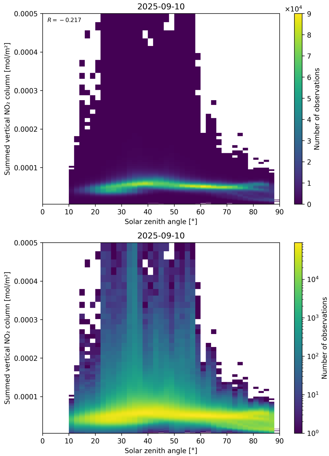
Figure 151: Scatter density plot of “Solar zenith angle” against “Summed vertical NO 2 column” for 2025-09-10 to 2025-09-11.
