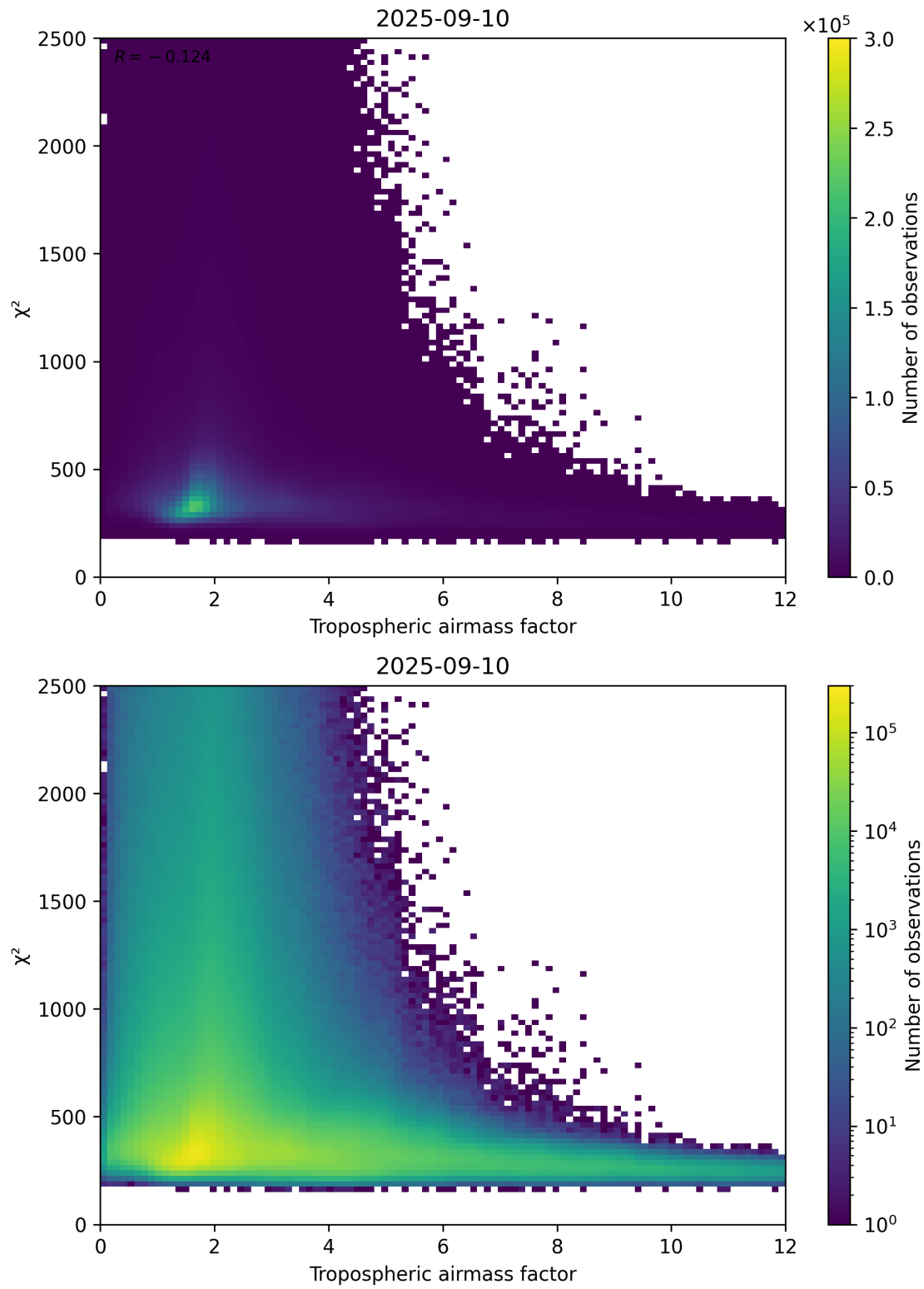
Figure 73: Scatter density plot of “Tropospheric airmass factor” against “ \chi^2 ” for 2025-09-10 to 2025-09-11.
