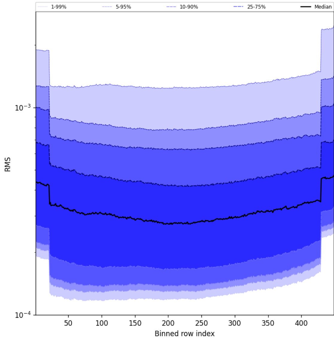
Figure 60: Along track statistics of “RMS” for 2025-09-10 to 2025-09-11
