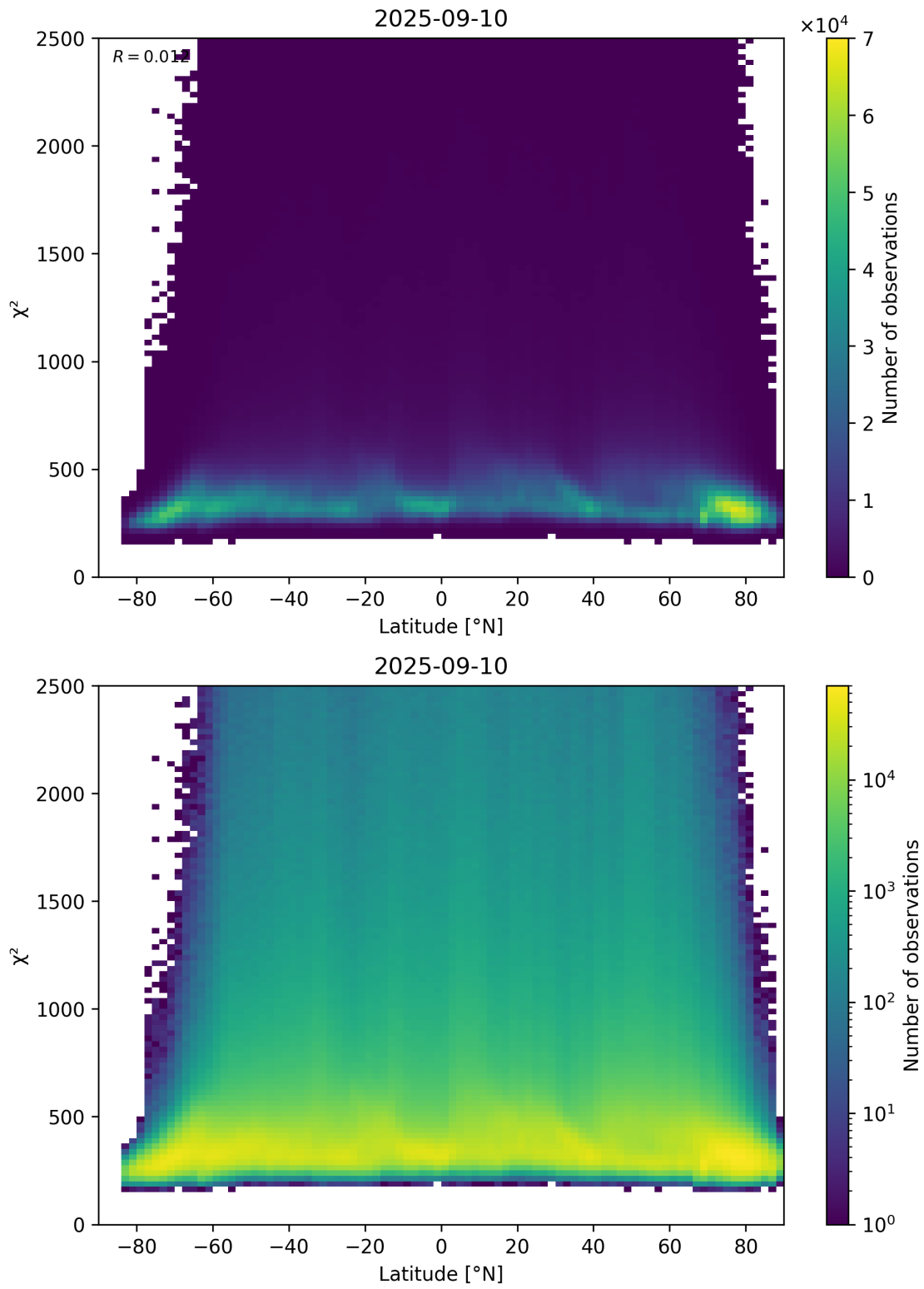
Figure 86: Scatter density plot of “Latitude” against “ \chi^2 ” for 2025-09-10 to 2025-09-11.
