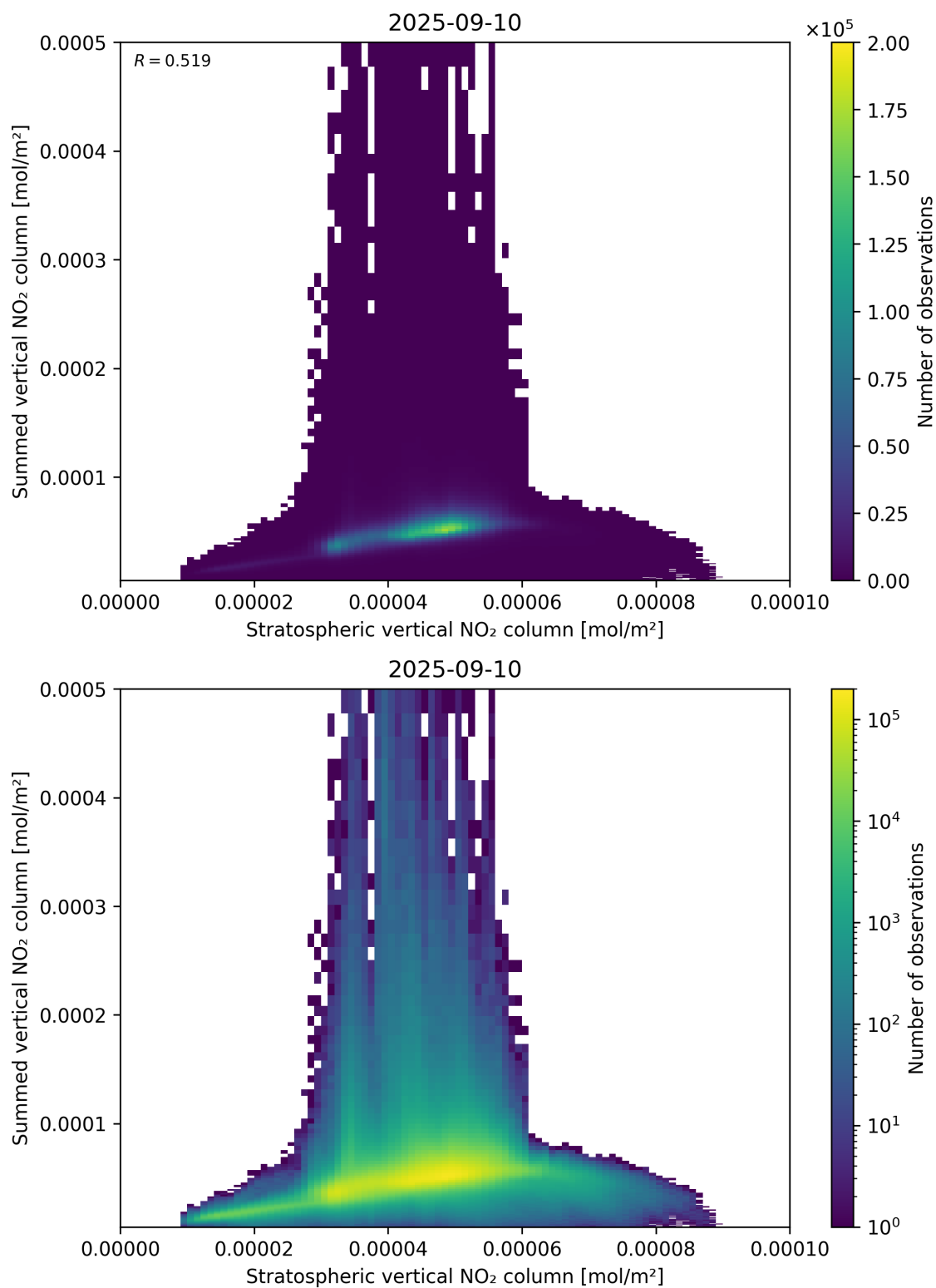
Figure 98: Scatter density plot of “Stratospheric vertical NO 2 column” against “Summed vertical NO 2 column” for 2025-09-10 to 2025-09-11.
