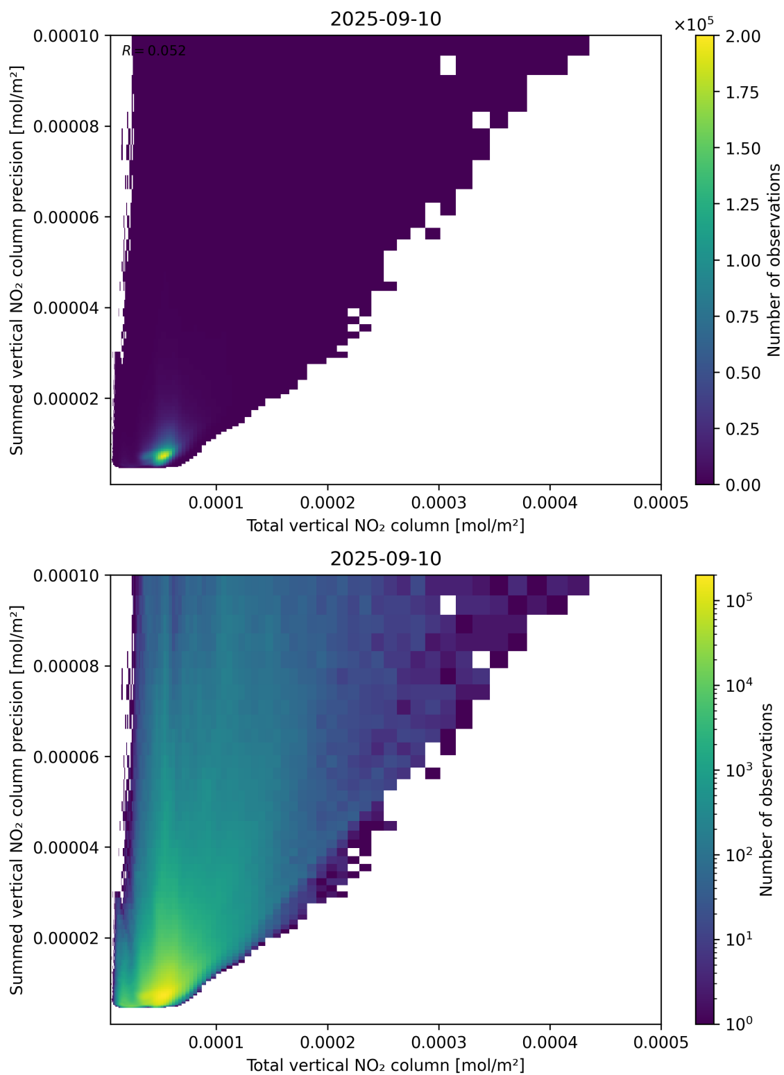
Figure 113: Scatter density plot of “Total vertical NO 2 column” against “Summed vertical NO 2 column precision” for 2025-09-10 to 2025-09-11.
