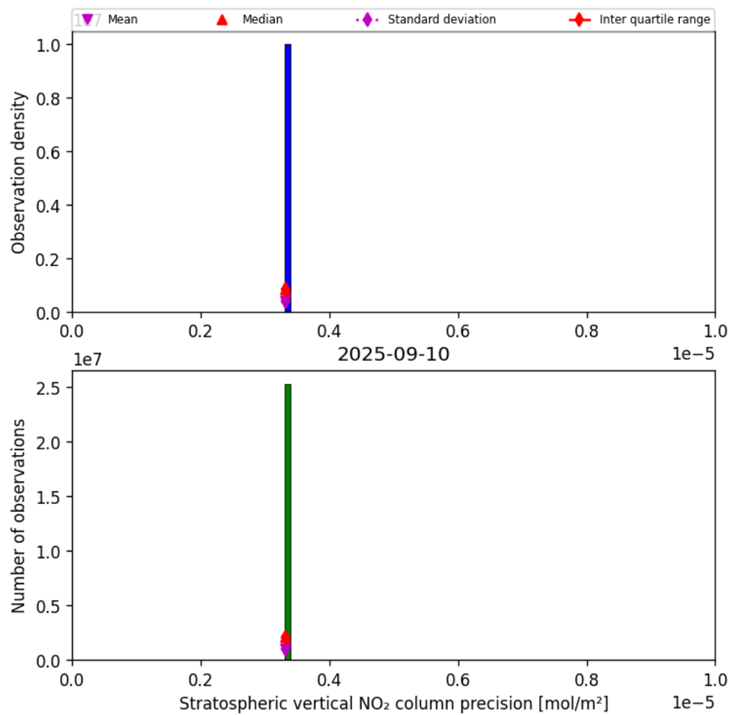
Figure 37: Histogram of “Stratospheric vertical NO 2 column precision” for 2025-09-10 to 2025-09-11
