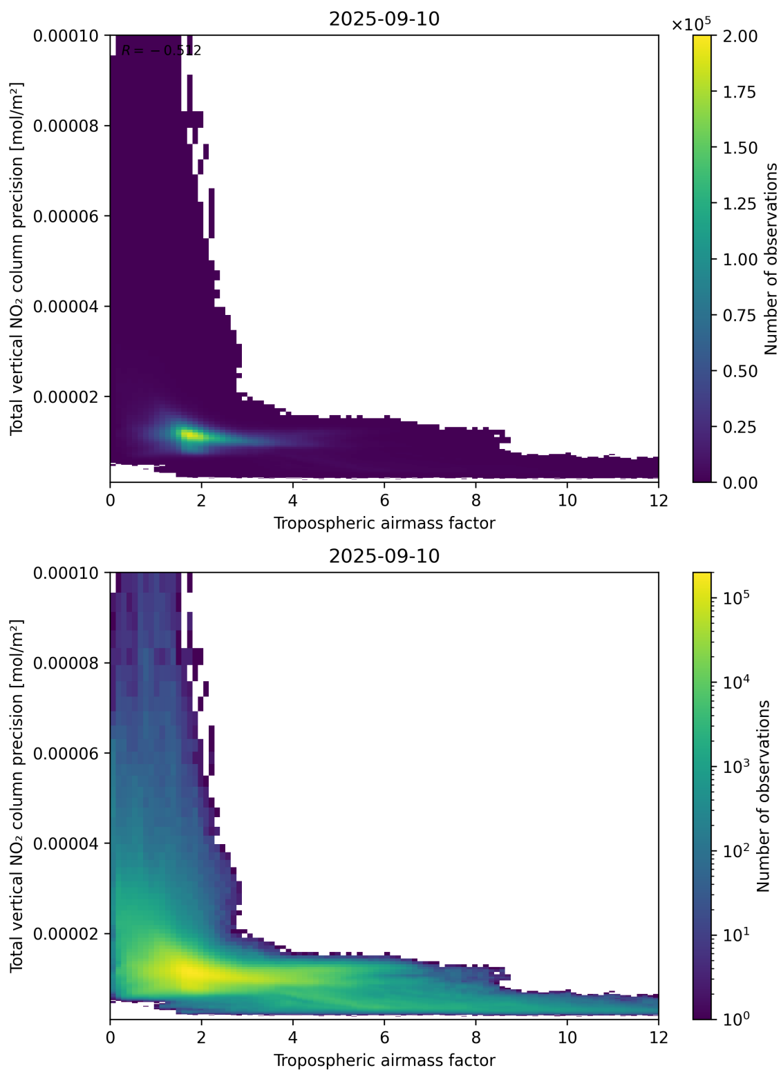
Figure 78: Scatter density plot of “Tropospheric airmass factor” against “Total vertical NO 2 column precision” for 2025-09-10 to 2025-09-11.
