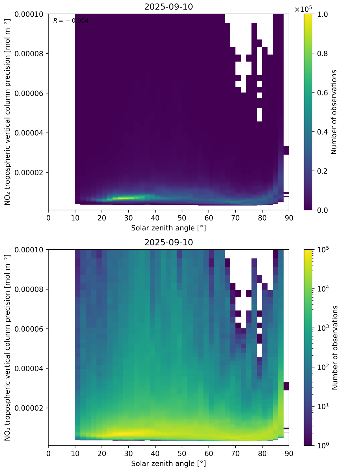
Figure 156: Scatter density plot of “Solar zenith angle” against “NO 2 tropospheric vertical column precision” for 2025-09-10 to 2025-09-11.
