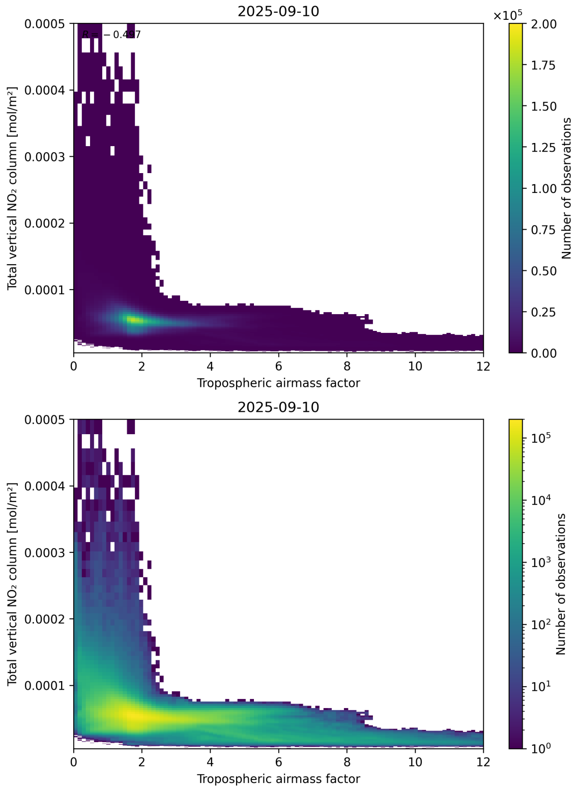
Figure 77: Scatter density plot of “Tropospheric airmass factor” against “Total vertical NO 2 column” for 2025-09-10 to 2025-09-11.
