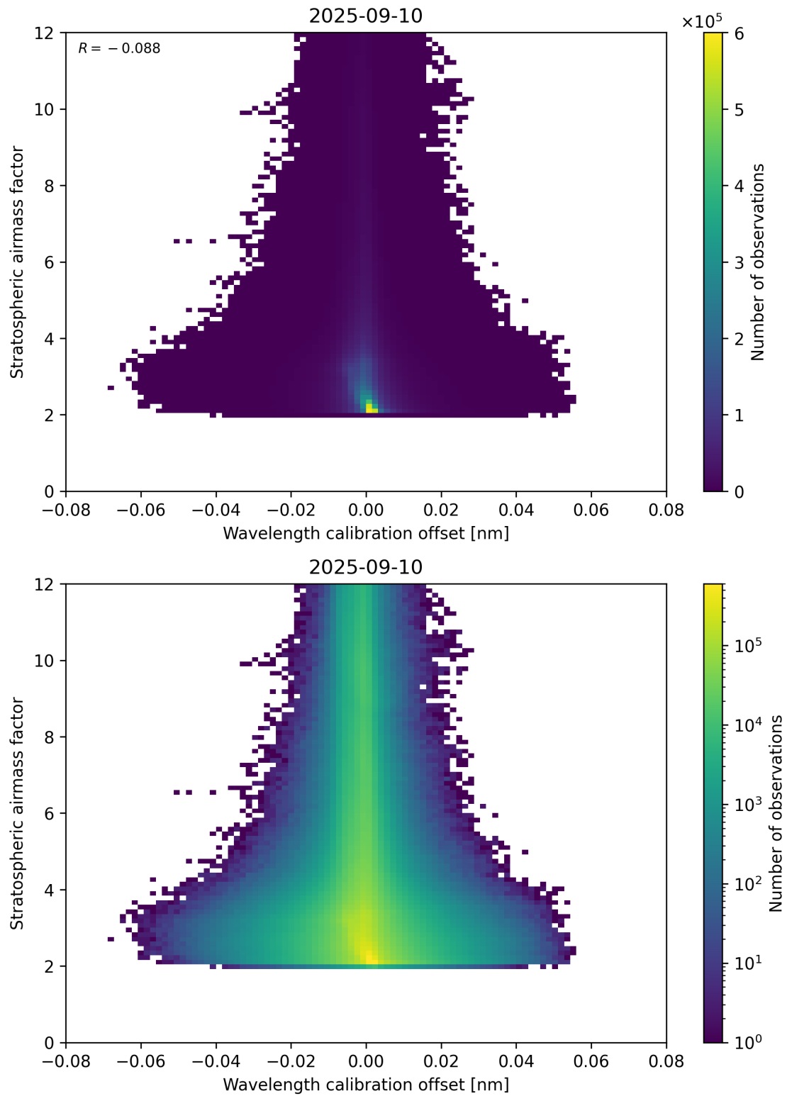
Figure 174: Scatter density plot of “Wavelength calibration offset” against “Stratospheric airmass factor” for 2025-09-10 to 2025-09-11.
