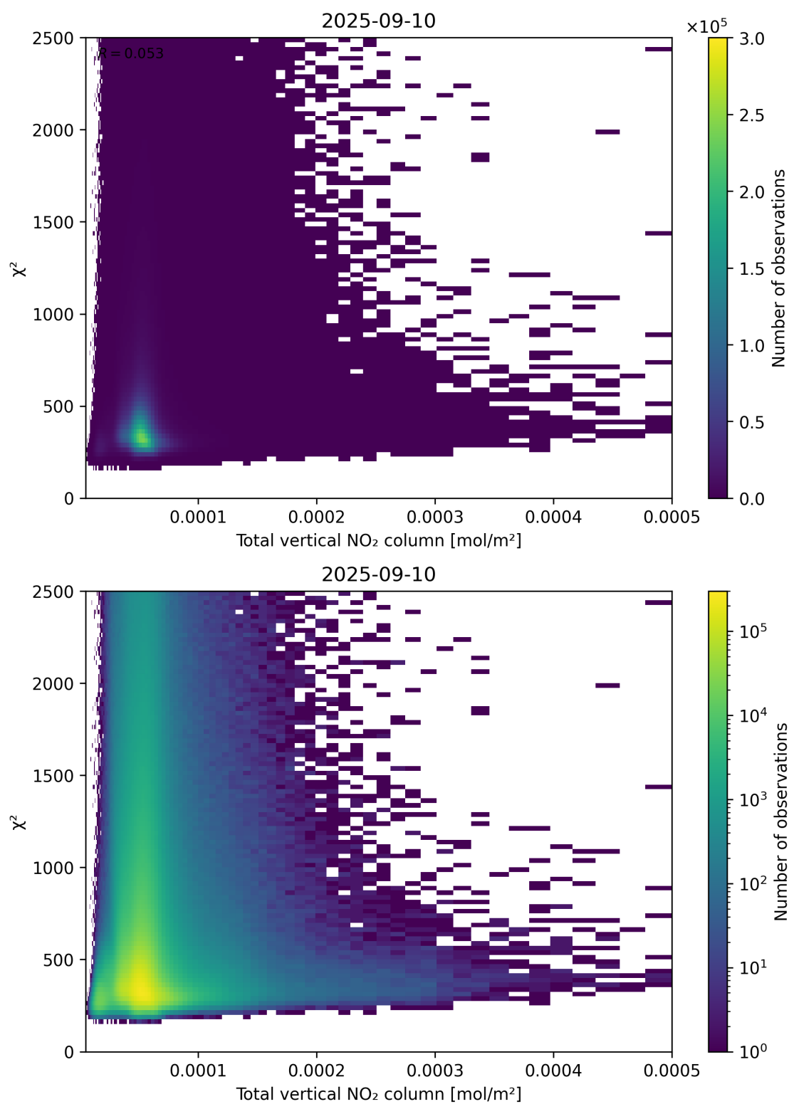
Figure 111: Scatter density plot of “Total vertical NO 2 column” against “ \chi^2 ” for 2025-09-10 to 2025-09-11.
