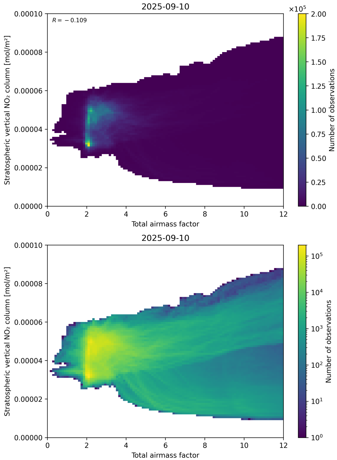
Figure 64: Scatter density plot of “Total airmass factor” against “Stratospheric vertical \text{NO}_2 column” for 2025-09-10 to 2025-09-11.
