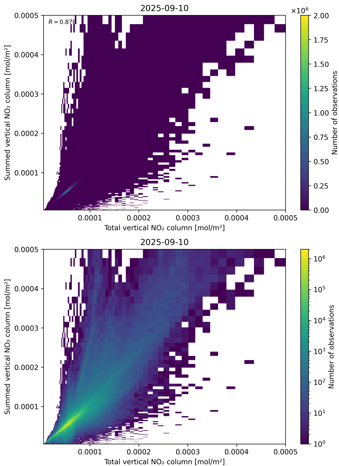
Figure 112: Scatter density plot of “Total vertical NO 2 column” against “Summed vertical NO 2 column” for 2025-09-10 to 2025-09-11.
