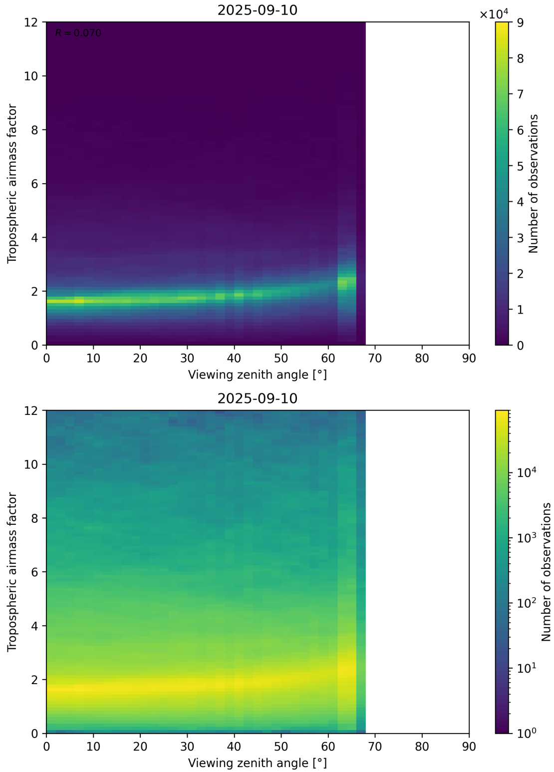
Figure 161: Scatter density plot of “Viewing zenith angle” against “Tropospheric airmass factor” for 2025-09-10 to 2025-09-11.
