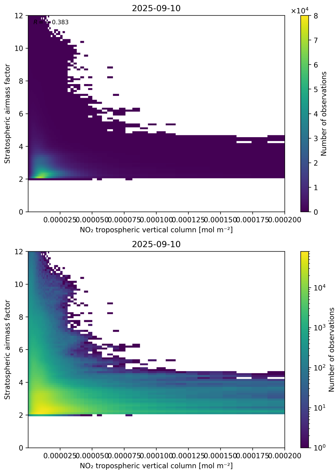
Figure 121: Scatter density plot of “NO 2 tropospheric vertical column” against “Stratospheric airmass factor” for 2025-09-10 to 2025-09-11.
