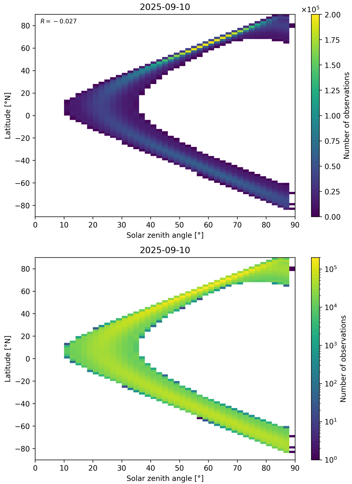
Figure 149: Scatter density plot of “Solar zenith angle” against “Latitude” for 2025-09-10 to 2025-09-11.
