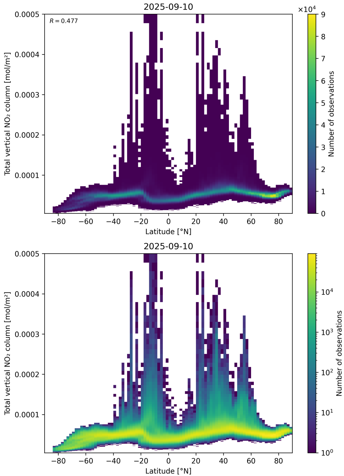
Figure 90: Scatter density plot of “Latitude” against “Total vertical NO 2 column” for 2025-09-10 to 2025-09-11.
