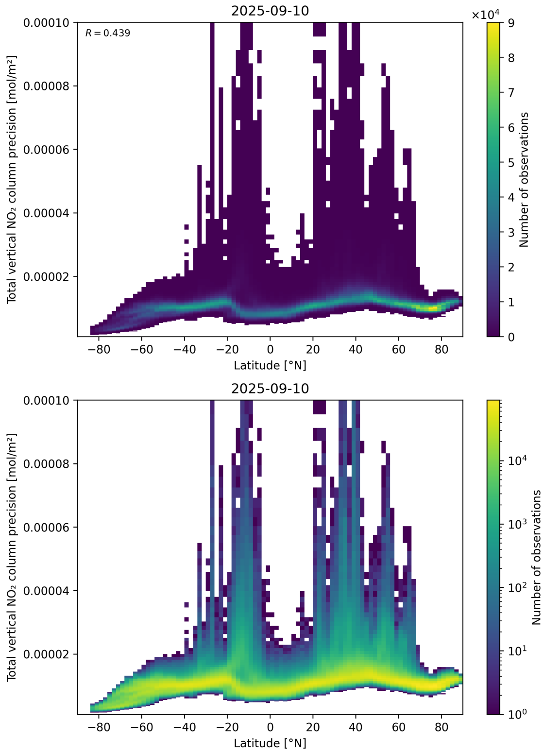
Figure 91: Scatter density plot of “Latitude” against “Total vertical NO 2 column precision” for 2025-09-10 to 2025-09-11.
