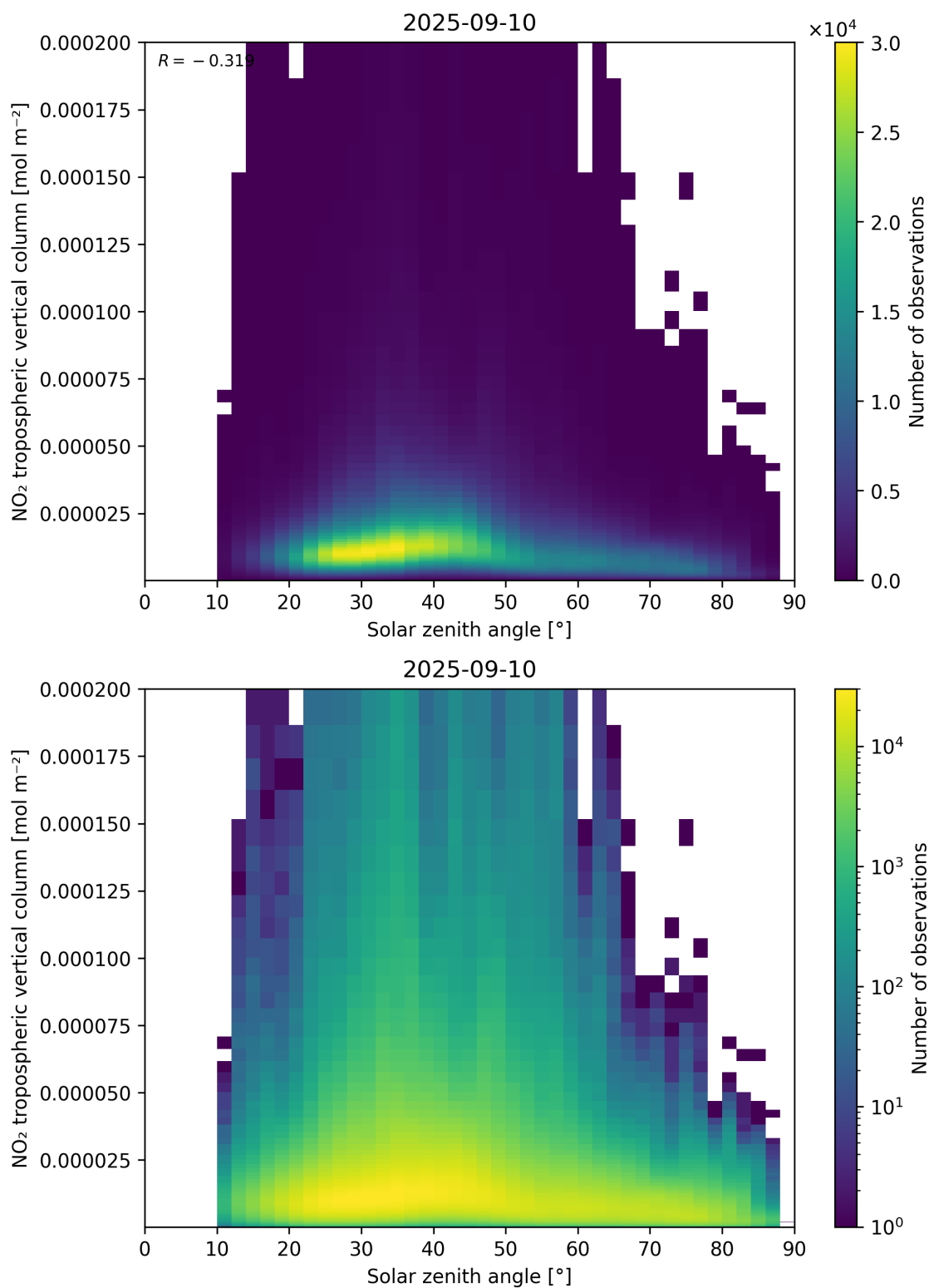
Figure 155: Scatter density plot of “Solar zenith angle” against “NO 2 tropospheric vertical column” for 2025-09-10 to 2025-09-11.
