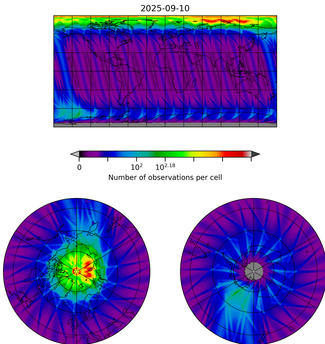
Figure 10: Map of the number of observations for 2025-09-10 to 2025-09-11
