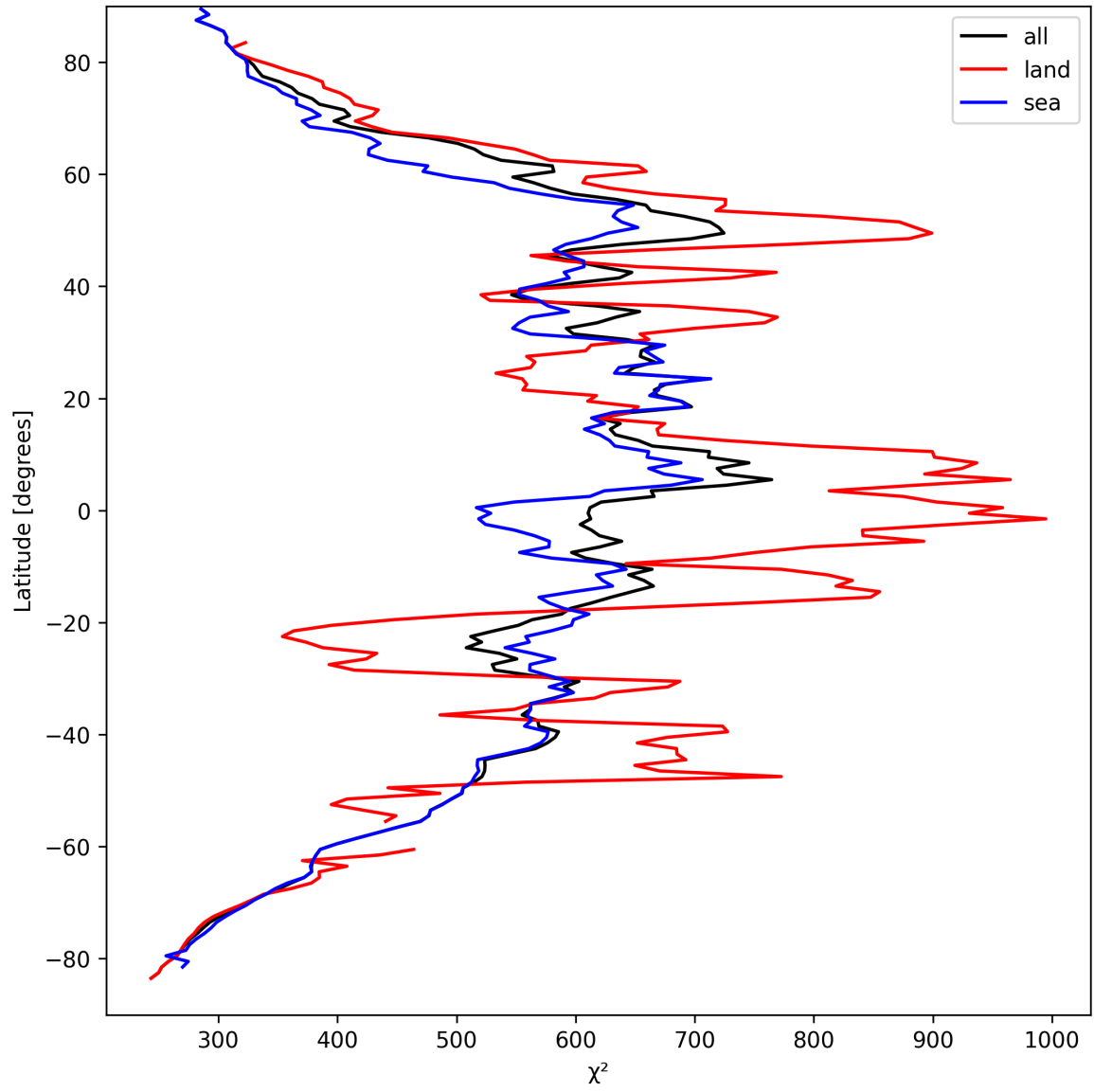
Figure 25: Zonal average of “ \chi^2 ” for 2025-09-10 to 2025-09-11.
