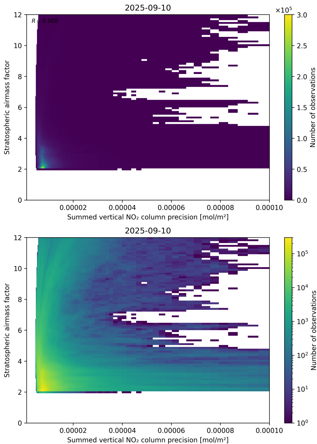
Figure 106: Scatter density plot of “Summed vertical NO 2 column precision” against “Stratospheric airmass factor” for 2025-09-10 to 2025-09-11.
