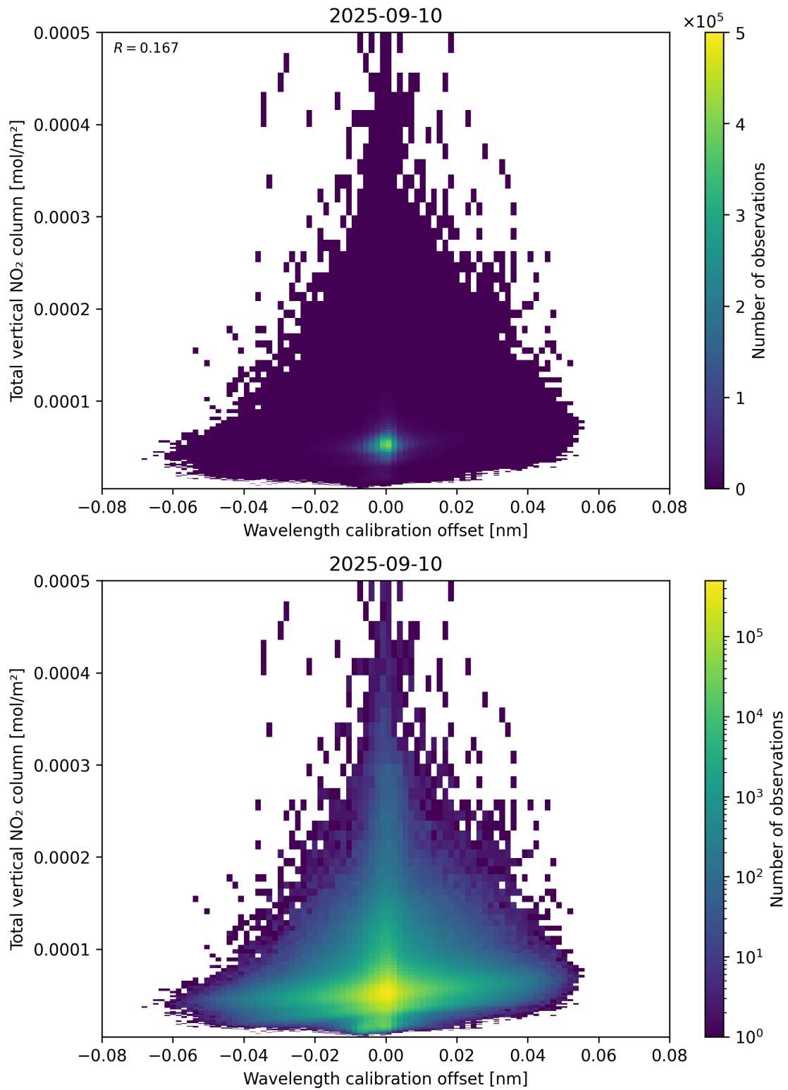
Figure 179: Scatter density plot of “Wavelength calibration offset” against “Total vertical NO 2 column” for 2025-09-10 to 2025-09-11.
