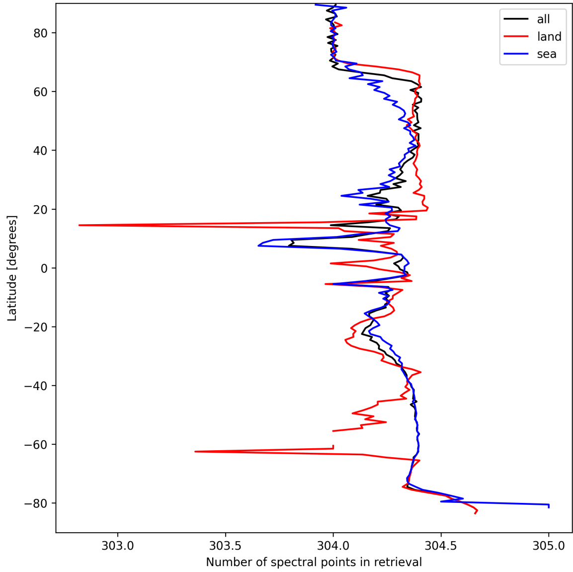
Figure 16: Zonal average of “Number of spectral points in retrieval” for 2025-09-10 to 2025-09-11.
