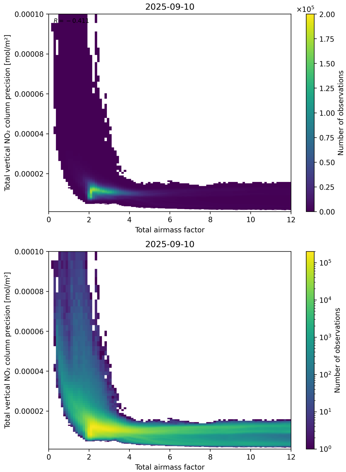
Figure 68: Scatter density plot of “Total airmass factor” against “Total vertical NO 2 column precision” for 2025-09-10 to 2025-09-11.
