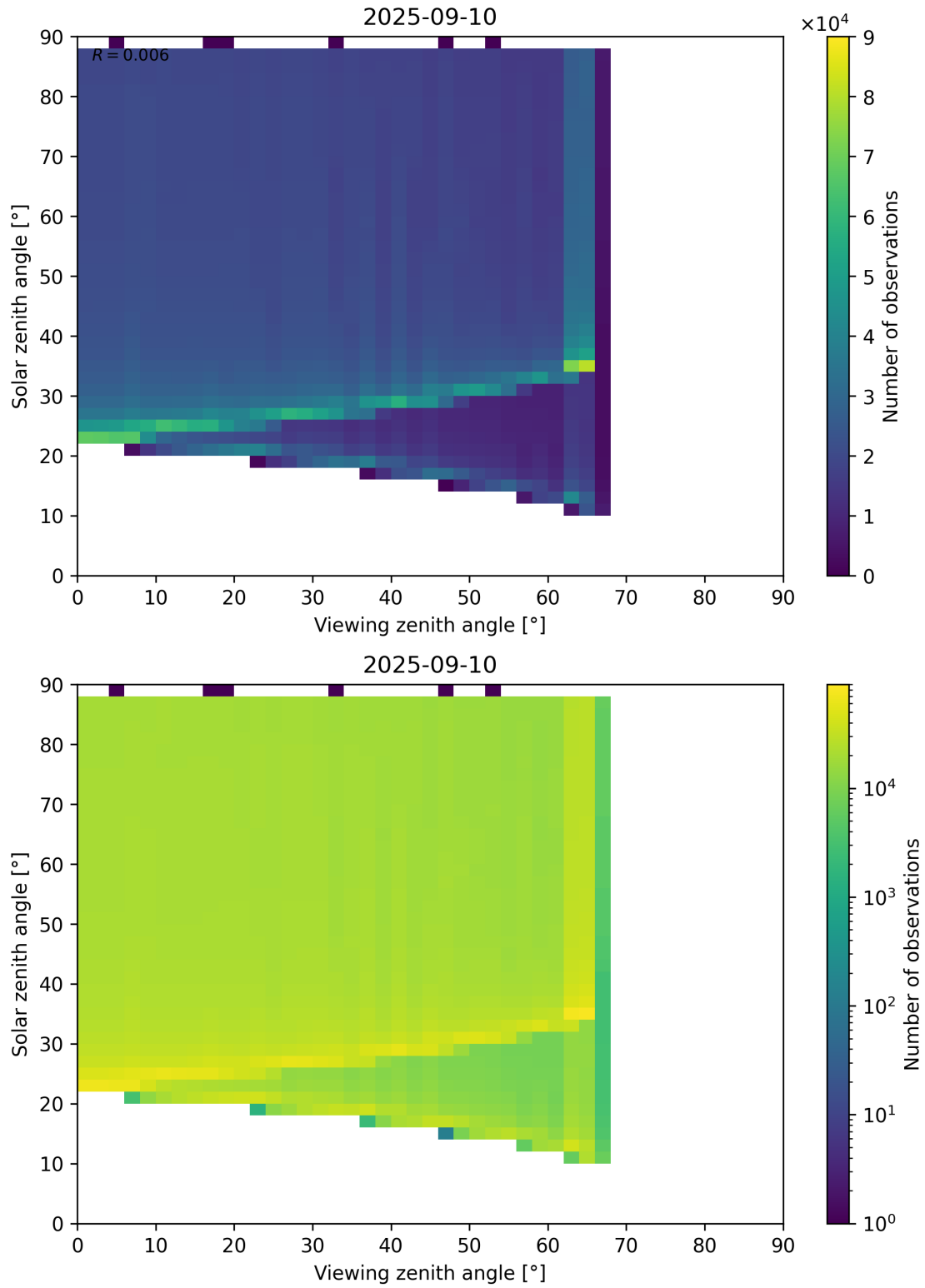
Figure 172: Scatter density plot of “Viewing zenith angle” against “Solar zenith angle” for 2025-09-10 to 2025-09-11.
