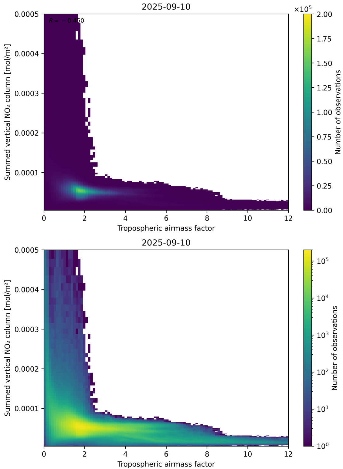
Figure 75: Scatter density plot of “Tropospheric air mass factor” against “Summed vertical NO 2 column” for 2025-09-10 to 2025-09-11.
