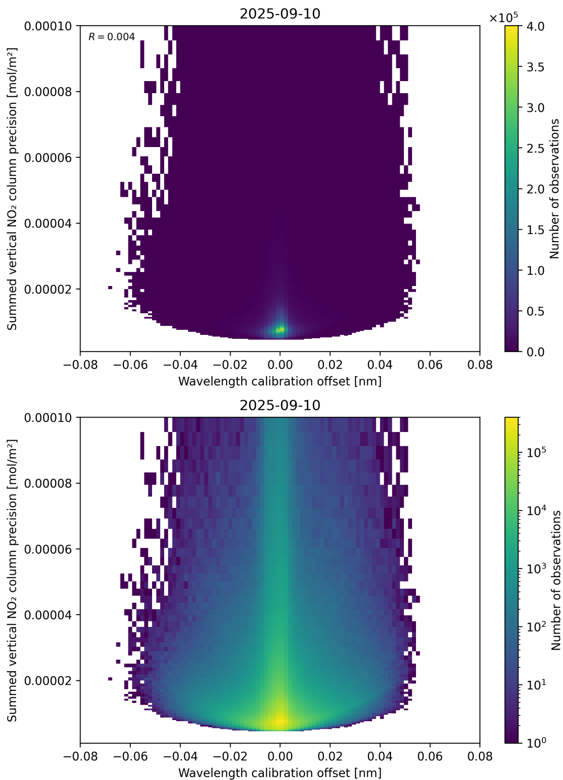
Figure 178: Scatter density plot of “Wavelength calibration offset” against “Summed vertical NO 2 column precision” for 2025-09-10 to 2025-09-11.
