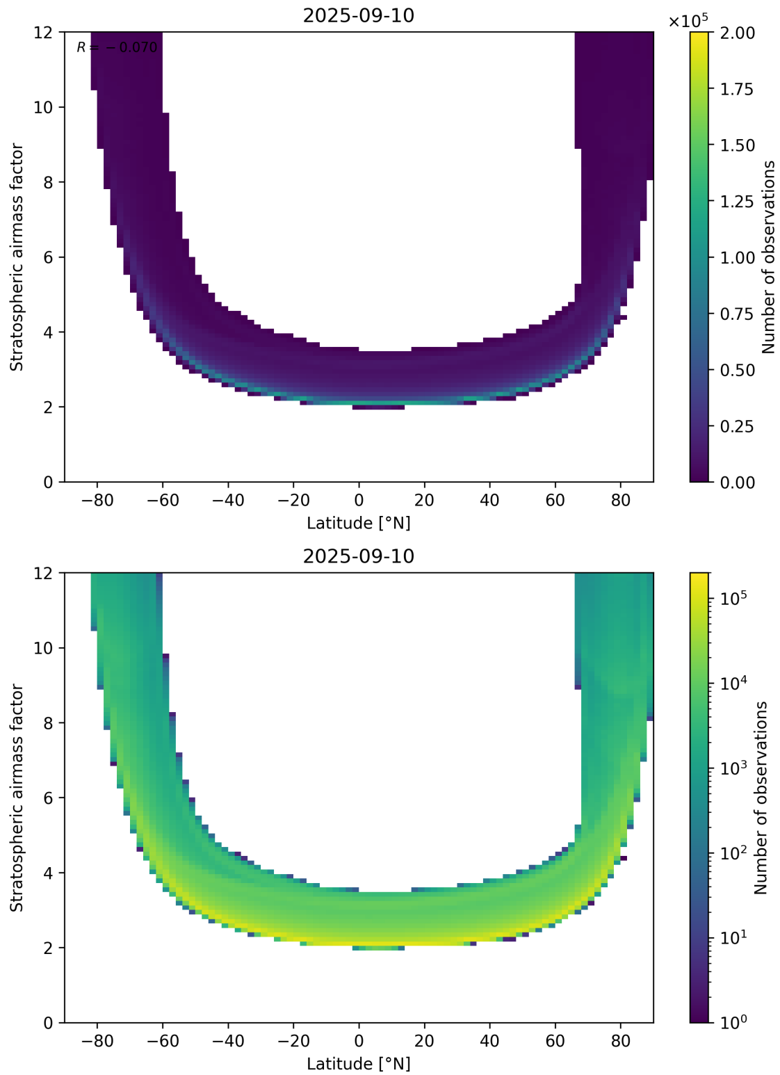
Figure 83: Scatter density plot of “Latitude” against “Stratospheric airmass factor” for 2025-09-10 to 2025-09-11.
