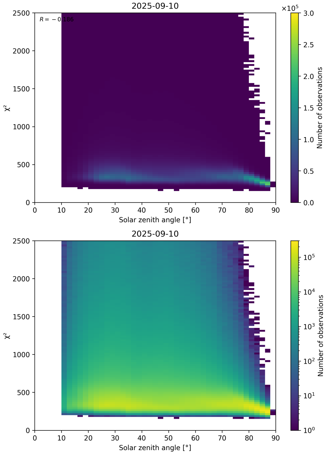
Figure 148: Scatter density plot of “Solar zenith angle” against “ \chi^2 ” for 2025-09-10 to 2025-09-11.
