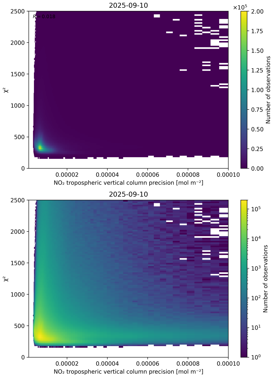
Figure 134: Scatter density plot of “NO 2 tropospheric vertical column precision” against “ \chi^2 ” for 2025-09-10 to 2025-09-11.
