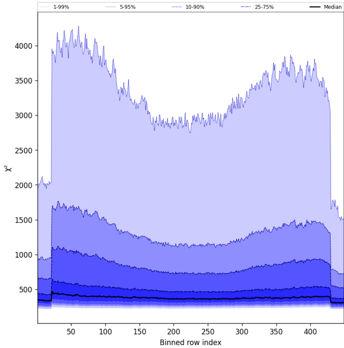
Figure 59: Along track statistics of “ \chi^2 ” for 2025-09-10 to 2025-09-11
