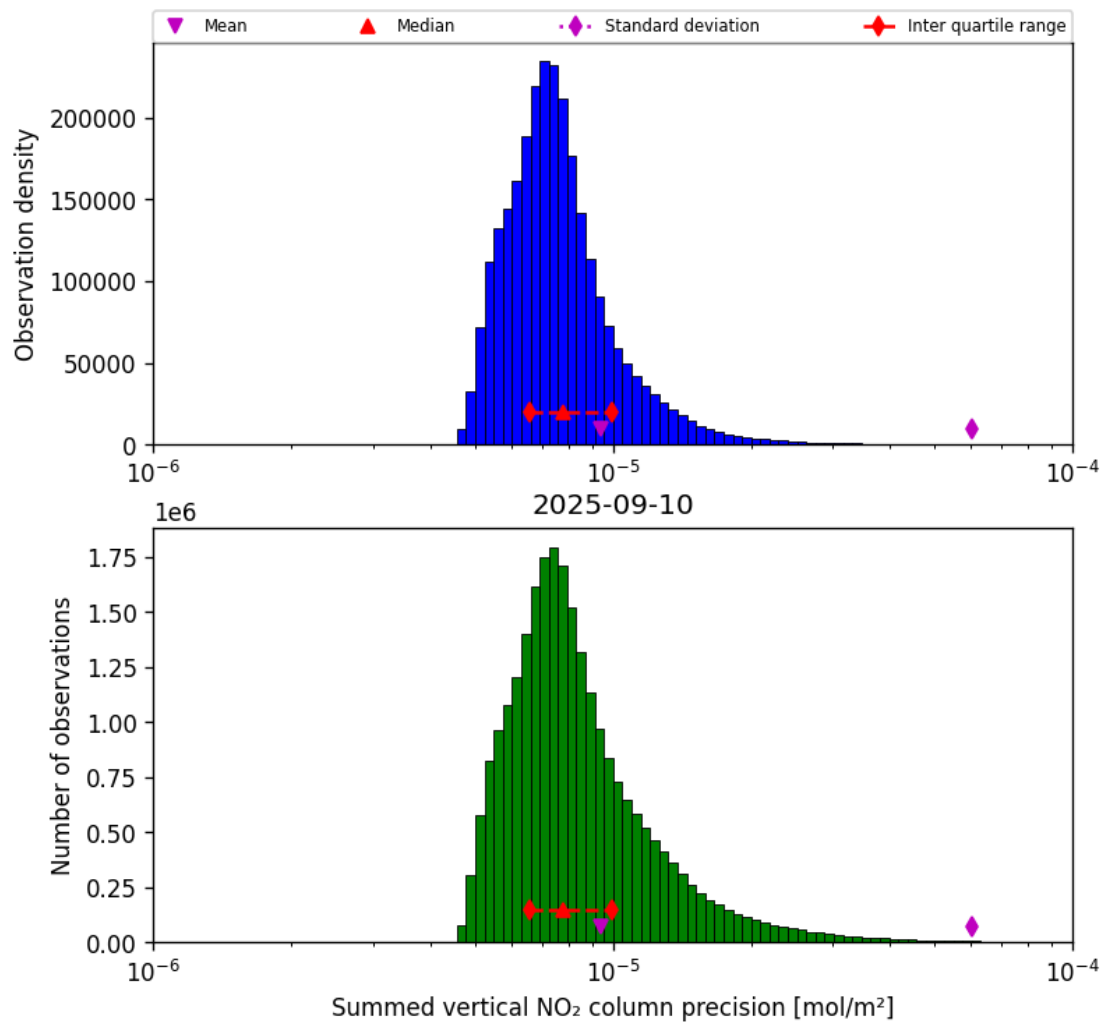
Figure 41: Histogram of “Summed vertical NO 2 column precision” for 2025-09-10 to 2025-09-11
