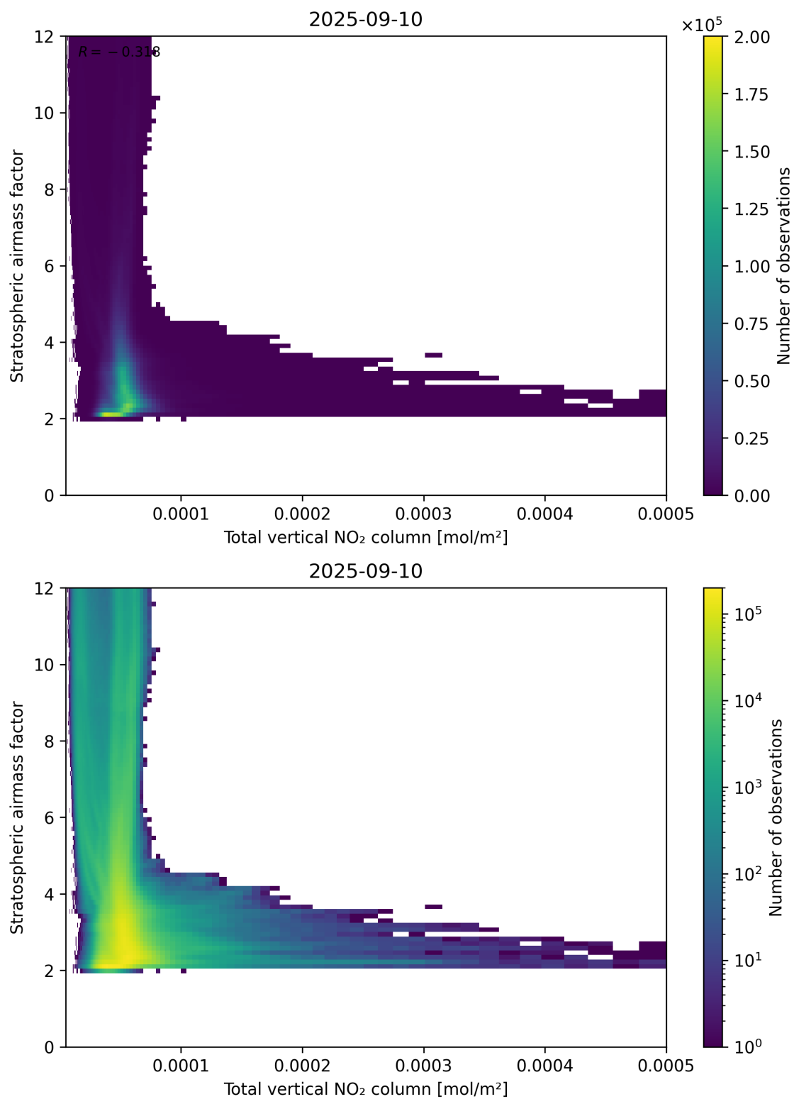
Figure 110: Scatter density plot of “Total vertical NO 2 column” against “Stratospheric airmass factor” for 2025-09-10 to 2025-09-11.
