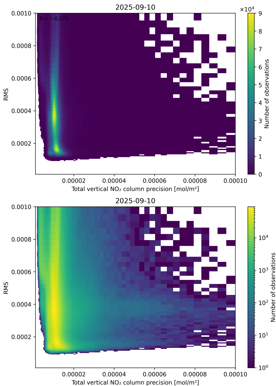
Figure 119: Scatter density plot of “Total vertical NO 2 column precision” against “RMS” for 2025-09-10 to 2025-09-11.
