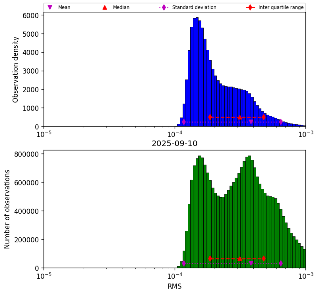
Figure 43: Histogram of “RMS” for 2025-09-10 to 2025-09-11
