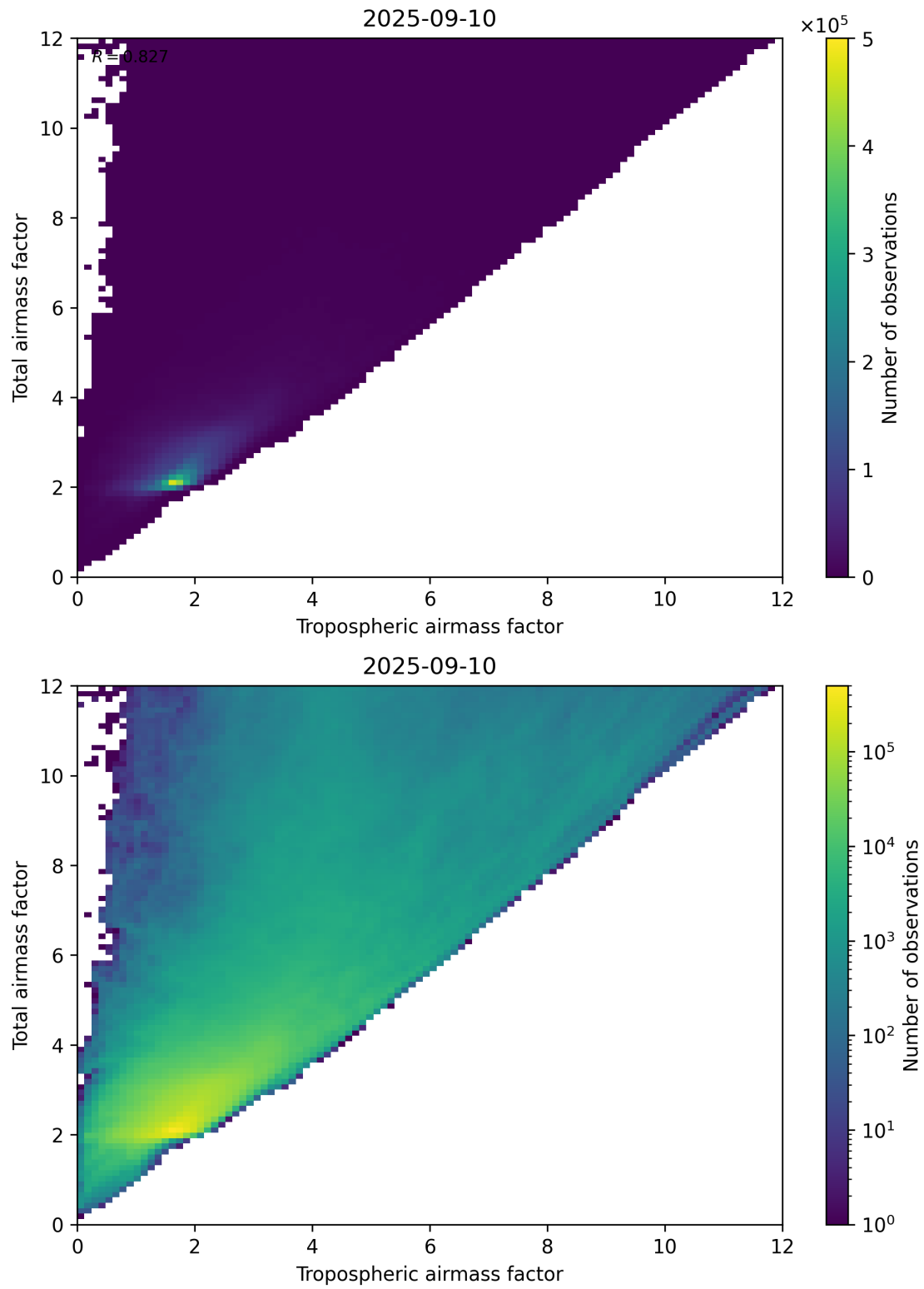
Figure 72: Scatter density plot of “Tropospheric airmass factor” against “Total airmass factor” for 2025-09-10 to 2025-09-11.
