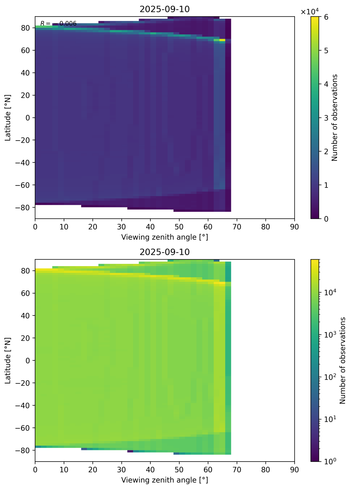
Figure 163: Scatter density plot of “Viewing zenith angle” against “Latitude” for 2025-09-10 to 2025-09-11.
