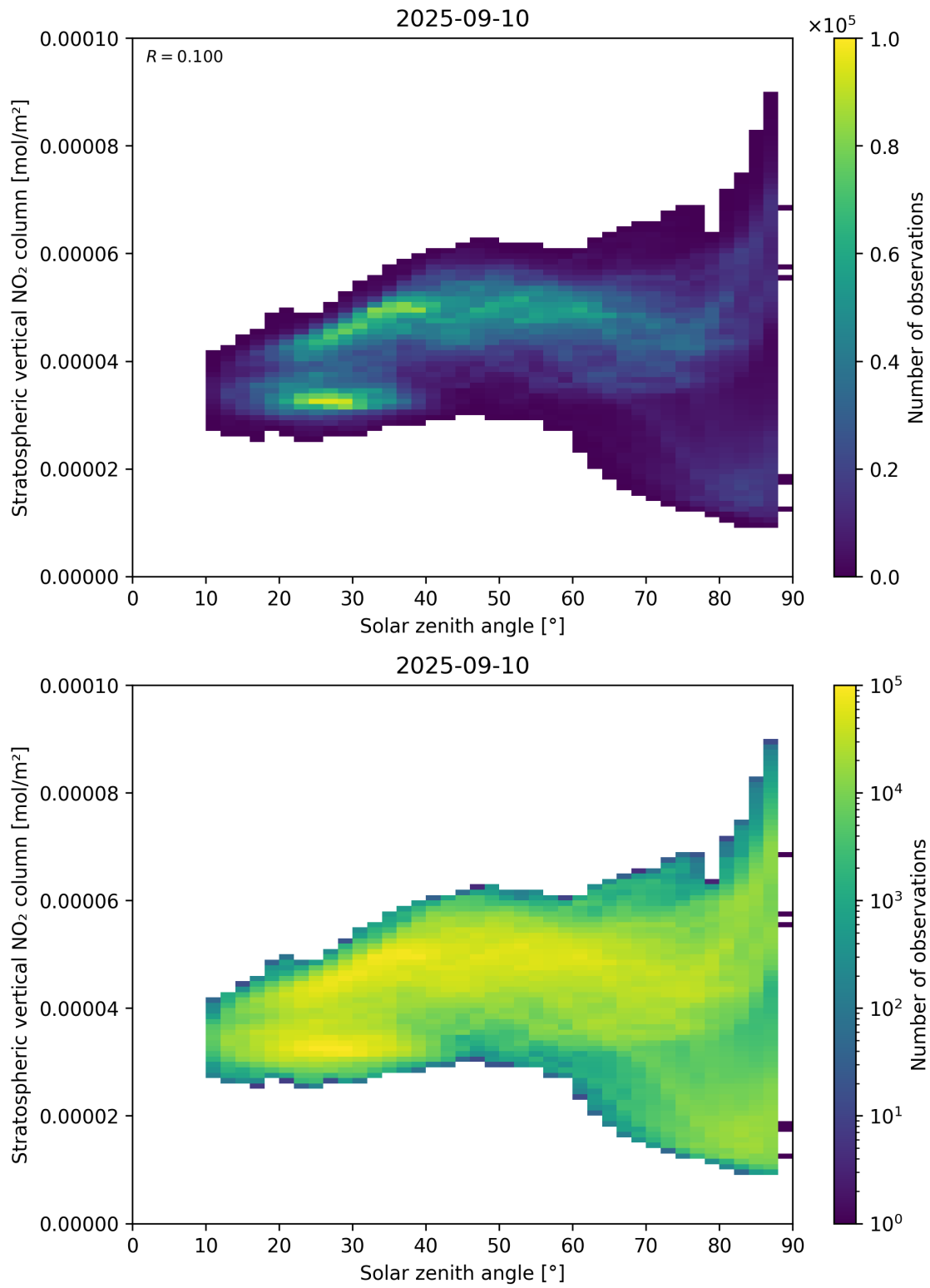
Figure 150: Scatter density plot of “Solar zenith angle” against “Stratospheric vertical NO 2 column” for 2025-09-10 to 2025-09-11.
