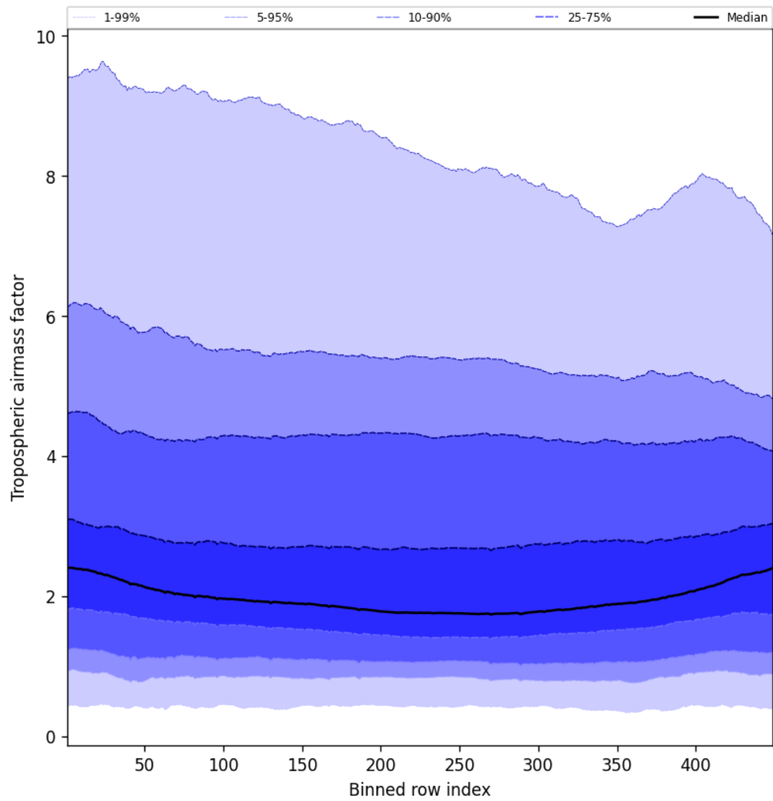
Figure 48: Along track statistics of “Tropospheric air mass factor” for 2025-09-10 to 2025-09-11
