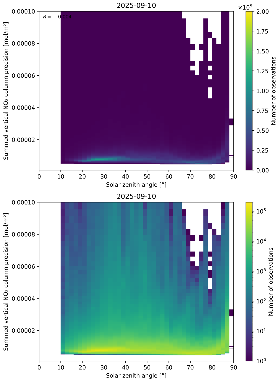
Figure 152: Scatter density plot of “Solar zenith angle” against “Summed vertical NO 2 column precision” for 2025-09-10 to 2025-09-11.
