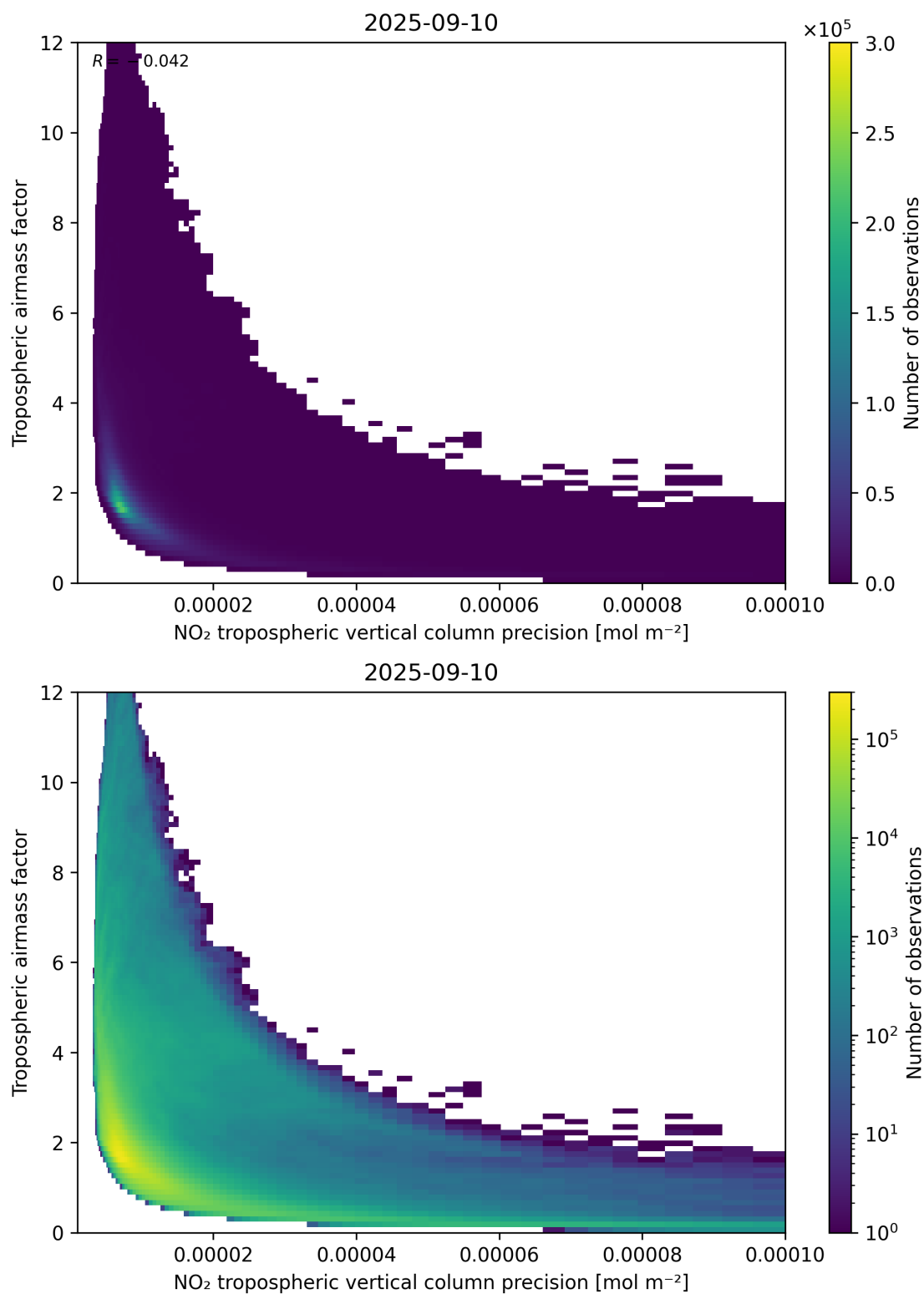
Figure 133: Scatter density plot of “NO 2 tropospheric vertical column precision” against “Tropospheric airmass factor” for 2025-09-10 to 2025-09-11.
