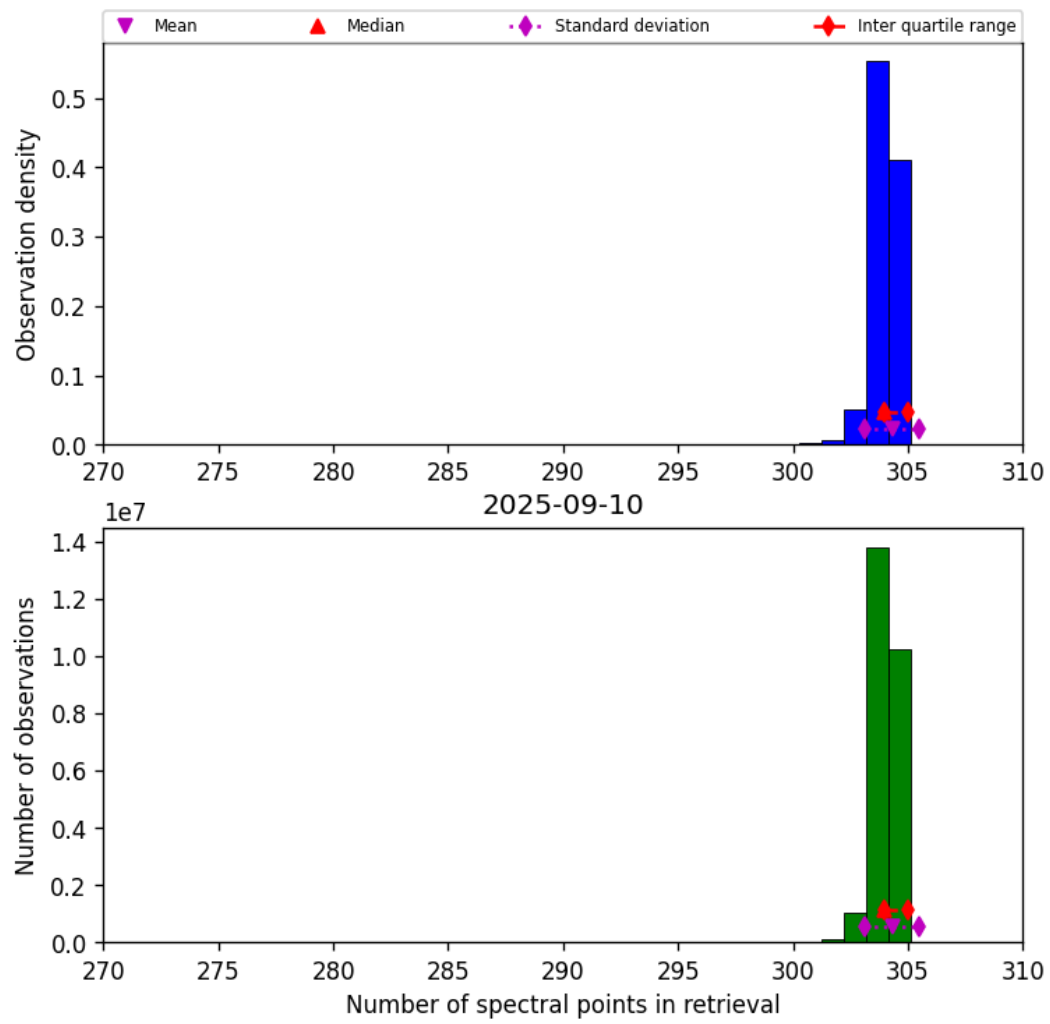
Figure 33: Histogram of “Number of spectral points in retrieval” for 2025-09-10 to 2025-09-11
