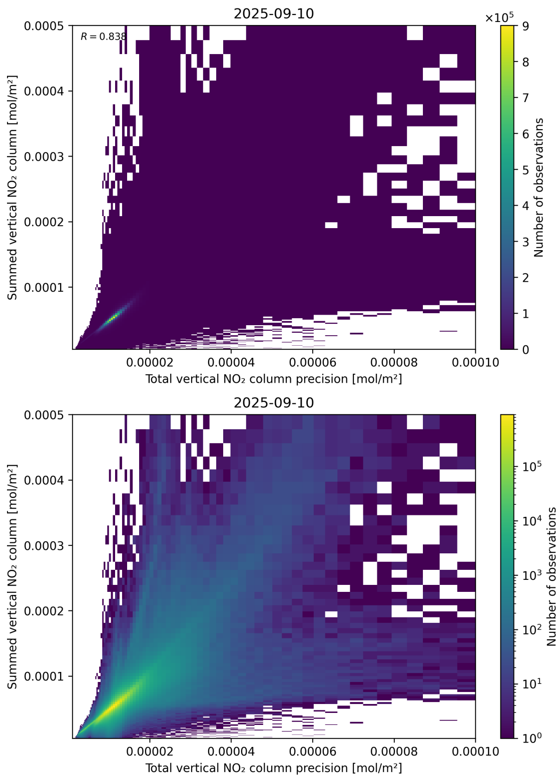
Figure 117: Scatter density plot of “Total vertical NO 2 column precision” against “Summed vertical NO 2 column” for 2025-09-10 to 2025-09-11.
