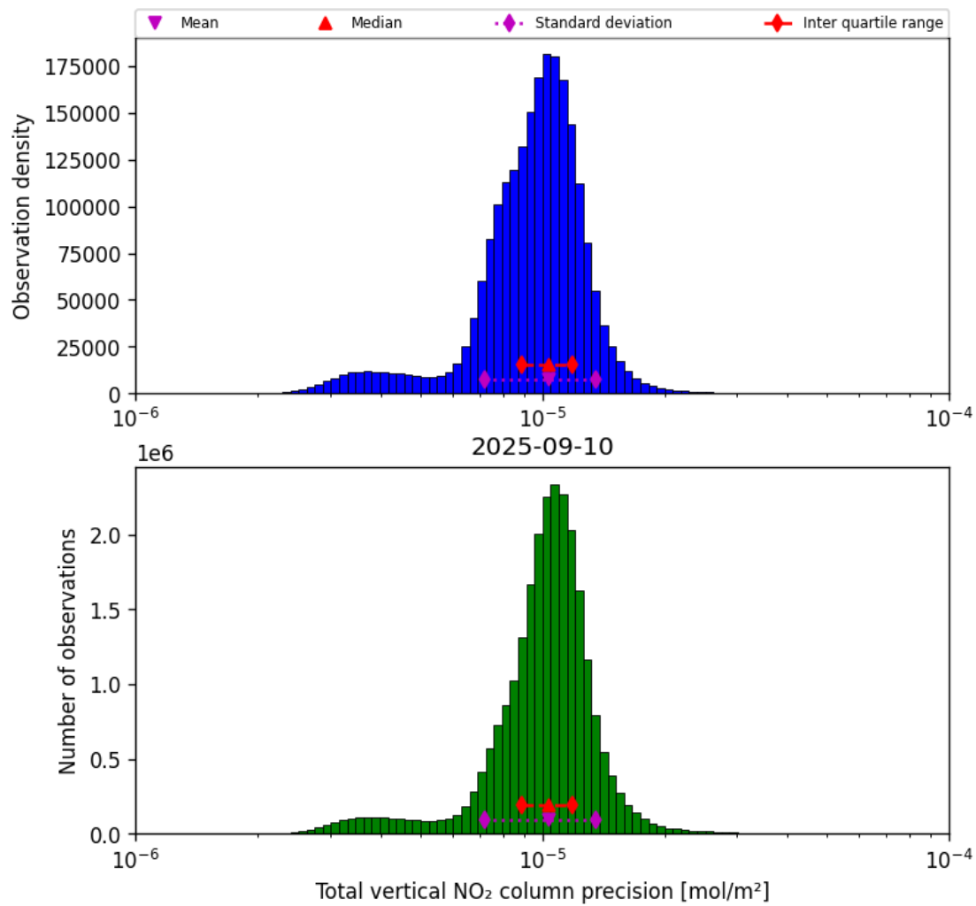
Figure 39: Histogram of “Total vertical NO 2 column precision” for 2025-09-10 to 2025-09-11
