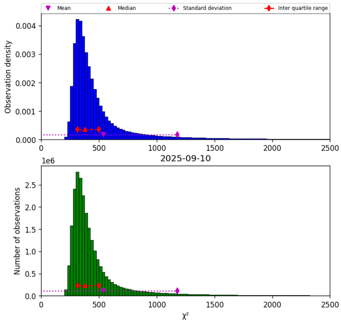
Figure 42: Histogram of “ \chi^2 ” for 2025-09-10 to 2025-09-11
