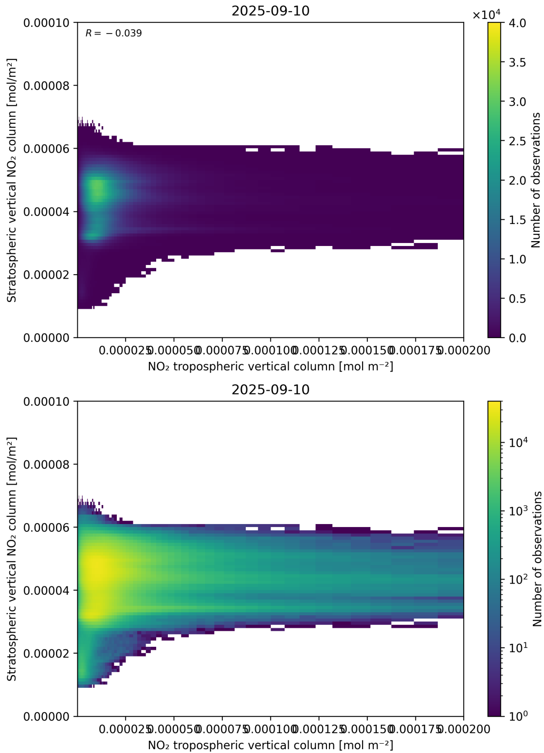
Figure 125: Scatter density plot of “NO 2 tropospheric vertical column” against “Stratospheric vertical NO 2 column” for 2025-09-10 to 2025-09-11.
