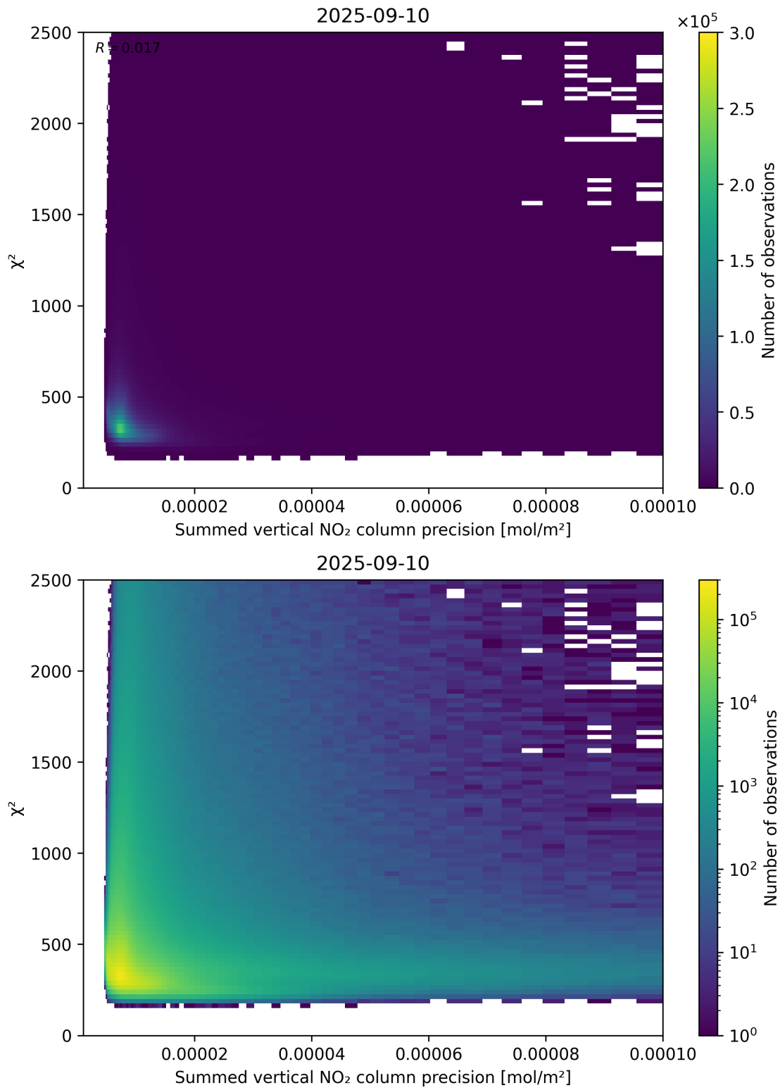
Figure 107: Scatter density plot of “Summed vertical NO 2 column precision” against “ \chi^2 ” for 2025-09-10 to 2025-09-11.
