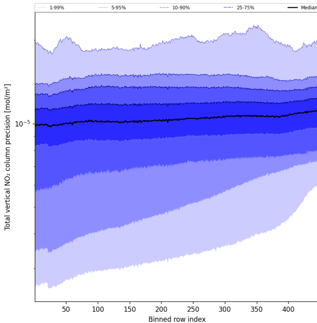
Figure 56: Along track statistics of “Total vertical NO 2 column precision” for 2025-09-10 to 2025-09-11
