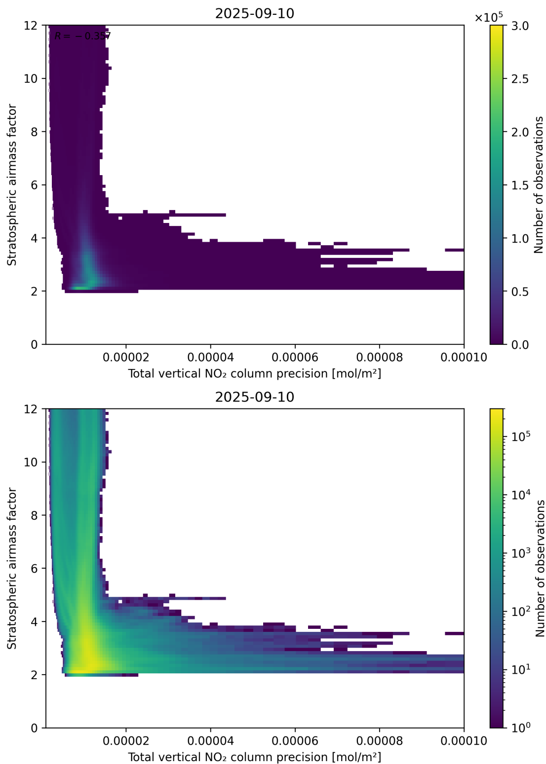
Figure 115: Scatter density plot of “Total vertical NO 2 column precision” against “Stratospheric air mass factor” for 2025-09-10 to 2025-09-11.
