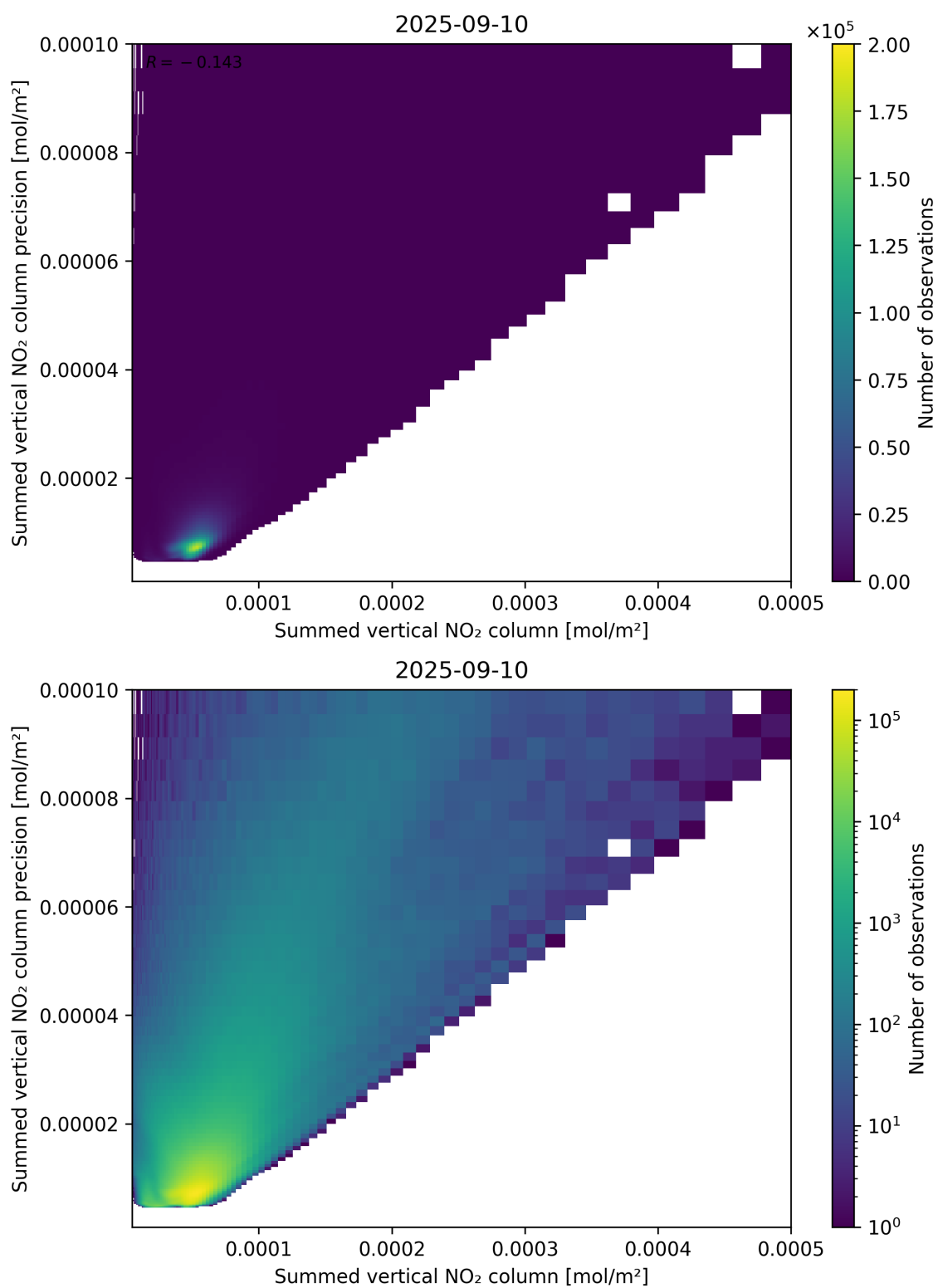
Figure 105: Scatter density plot of “Summed vertical NO 2 column” against “Summed vertical NO 2 column precision” for 2025-09-10 to 2025-09-11.
