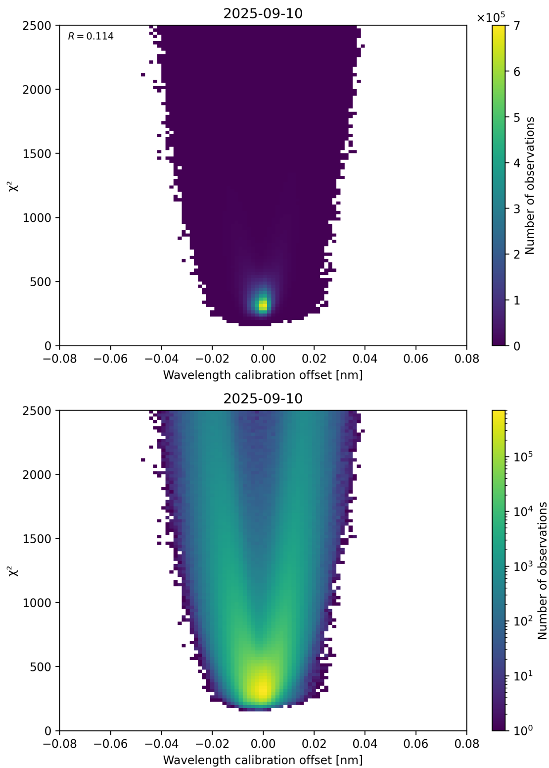
Figure 175: Scatter density plot of “Wavelength calibration offset” against “ \chi^2 ” for 2025-09-10 to 2025-09-11.
