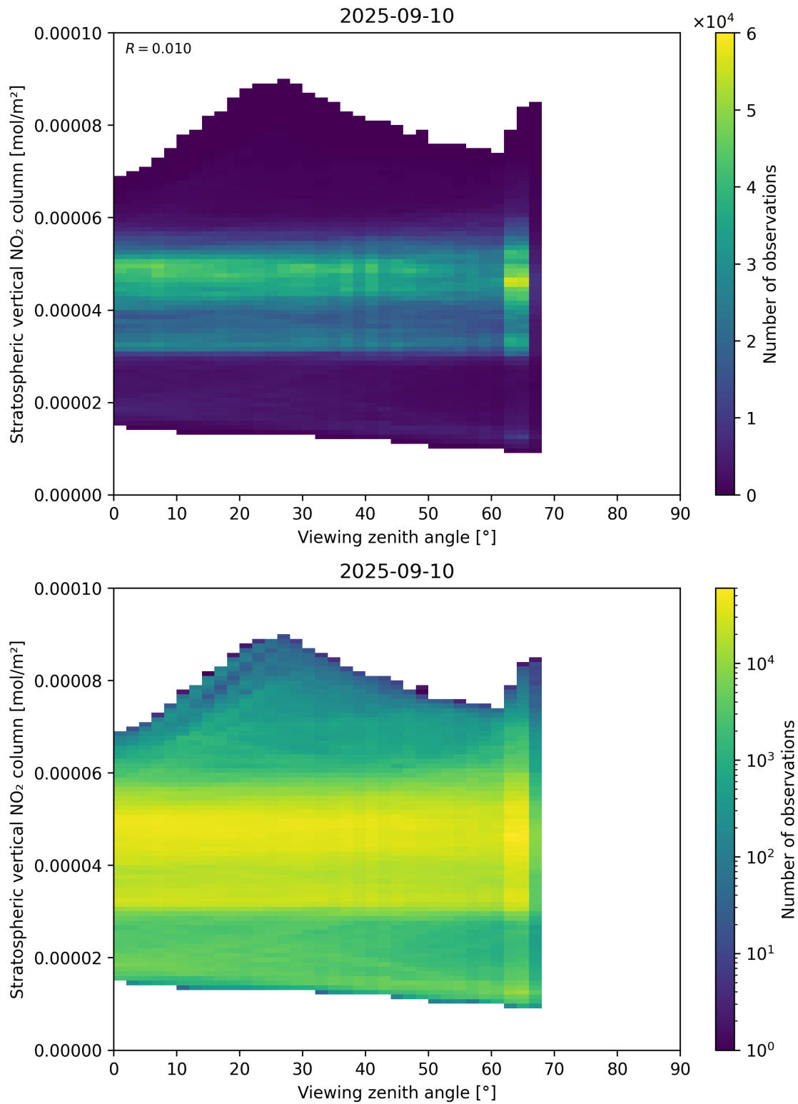
Figure 164: Scatter density plot of “Viewing zenith angle” against “Stratospheric vertical NO 2 column” for 2025-09-10 to 2025-09-11.
