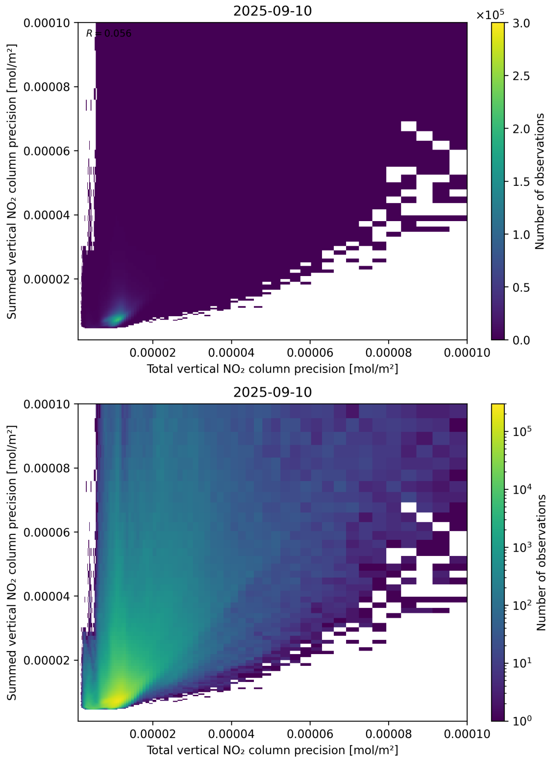
Figure 118: Scatter density plot of “Total vertical NO 2 column precision” against “Summed vertical NO 2 column precision” for 2025-09-10 to 2025-09-11.
