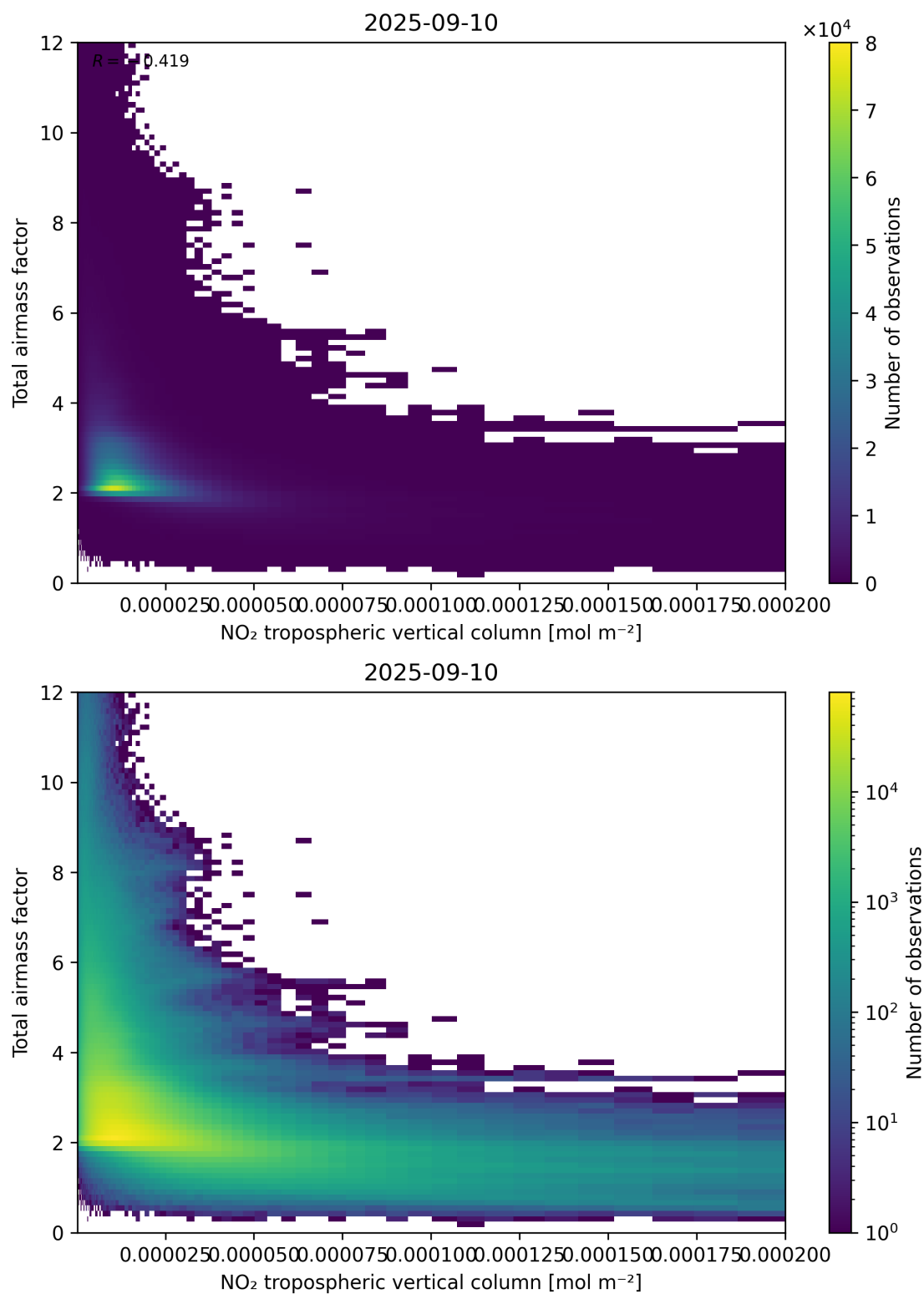
Figure 122: Scatter density plot of “NO 2 tropospheric vertical column” against “Total air mass factor” for 2025-09-10 to 2025-09-11.
