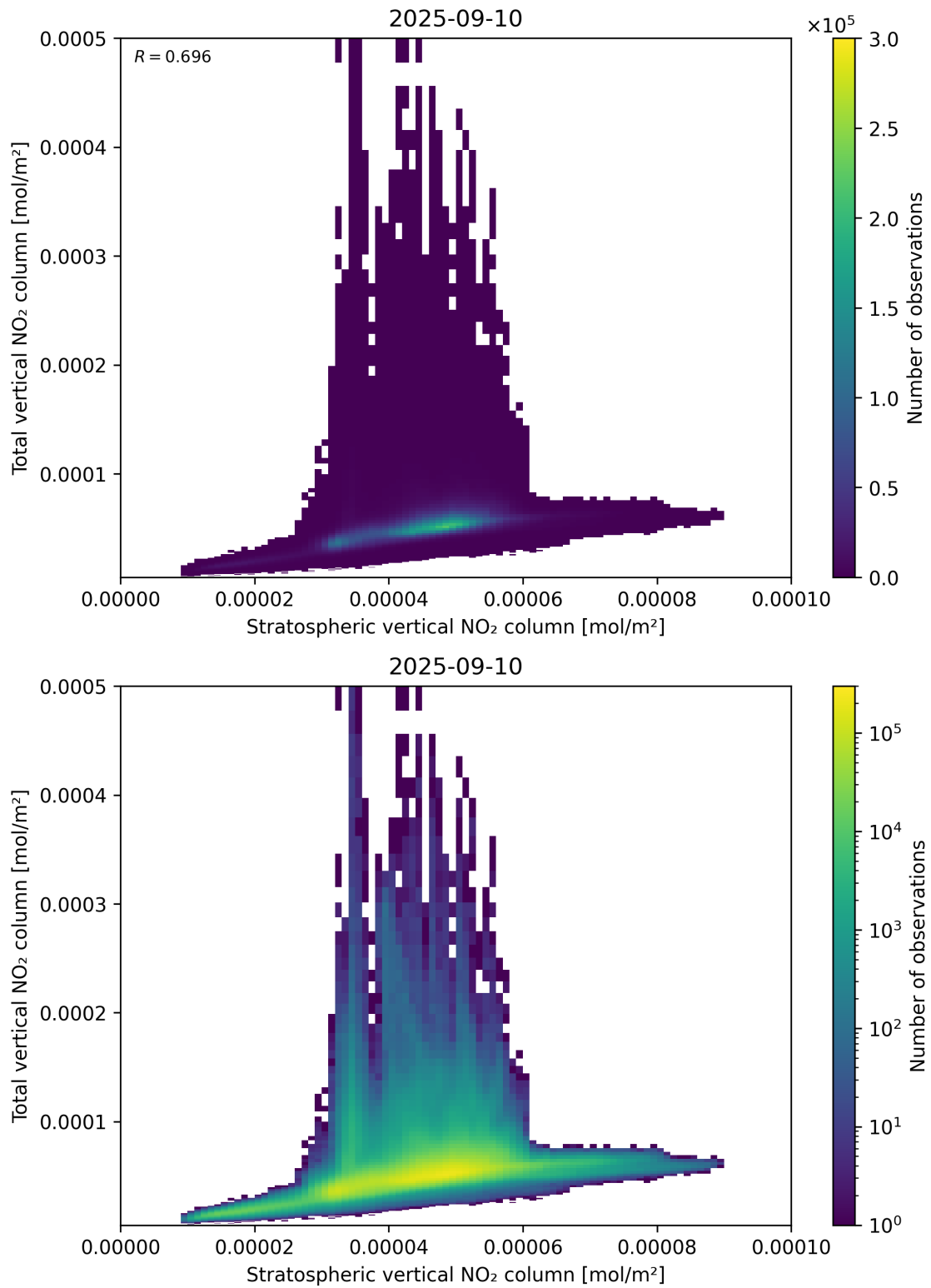
Figure 100: Scatter density plot of “Stratospheric vertical NO 2 column” against “Total vertical NO 2 column” for 2025-09-10 to 2025-09-11.
