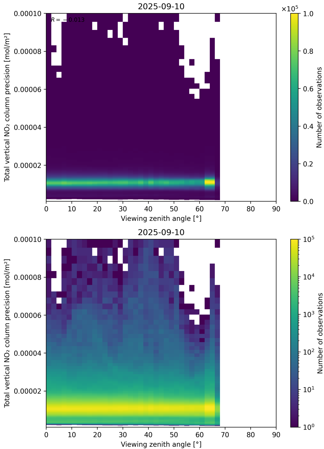
Figure 168: Scatter density plot of “Viewing zenith angle” against “Total vertical NO 2 column precision” for 2025-09-10 to 2025-09-11.
