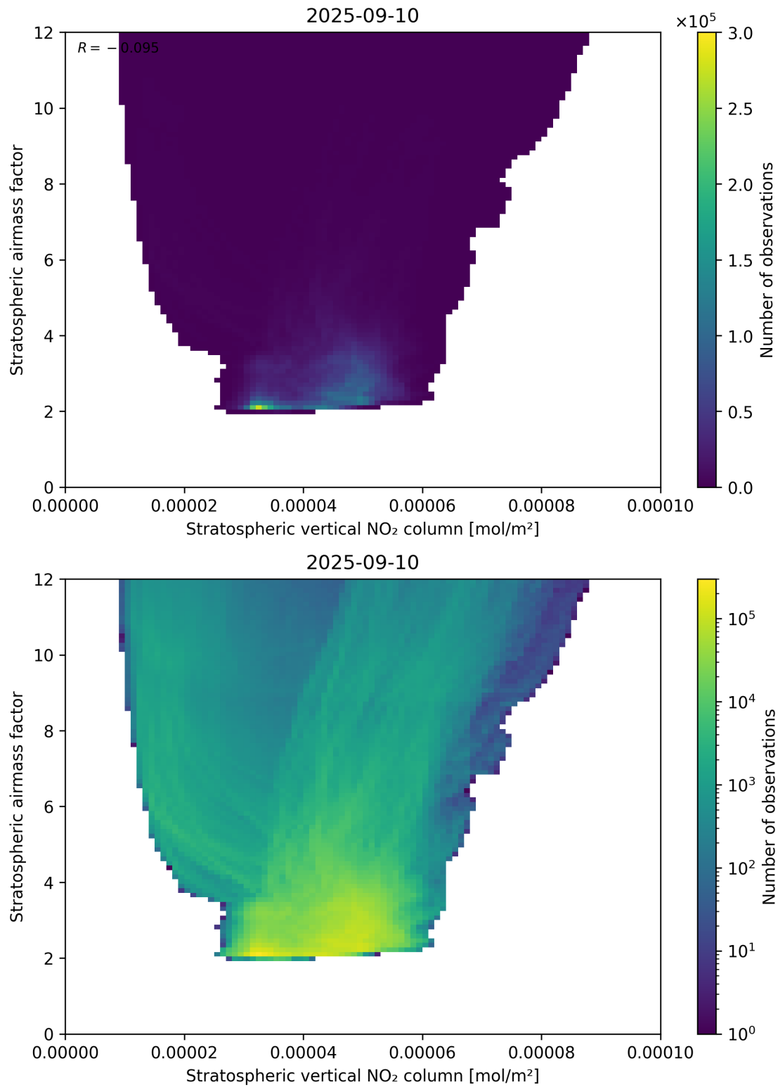
Figure 96: Scatter density plot of “Stratospheric vertical NO 2 column” against “Stratospheric airmass factor” for 2025-09-10 to 2025-09-11.
