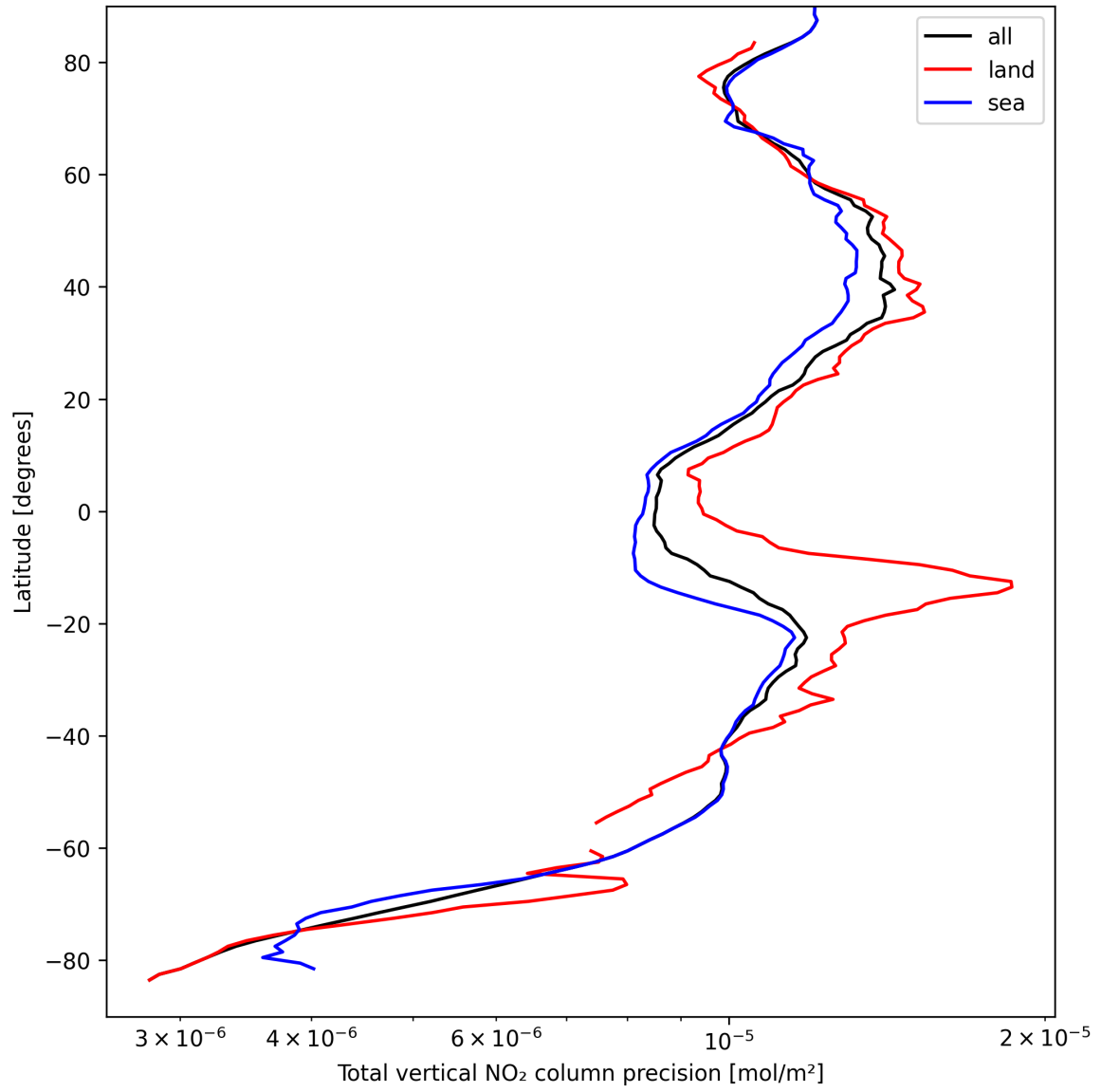
Figure 22: Zonal average of “Total vertical NO 2 column precision” for 2025-09-10 to 2025-09-11.
