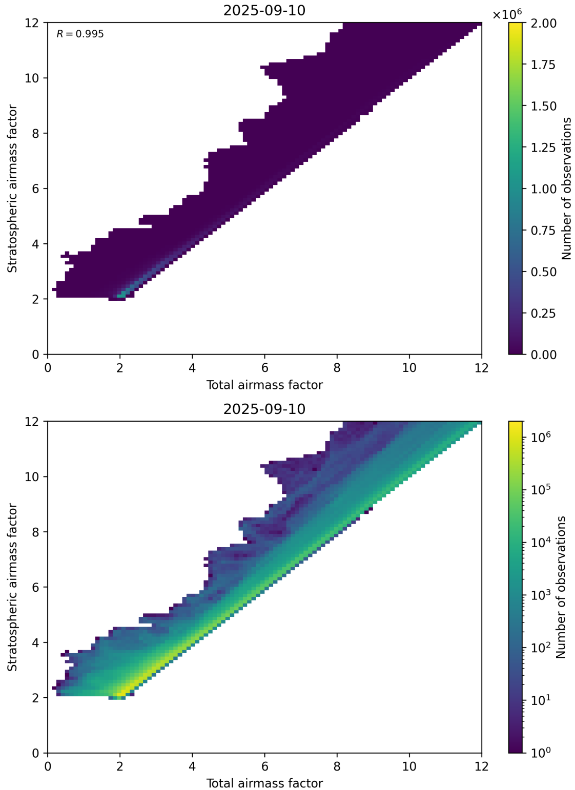
Figure 62: Scatter density plot of “Total airmass factor” against “Stratospheric airmass factor” for 2025-09-10 to 2025-09-11.
