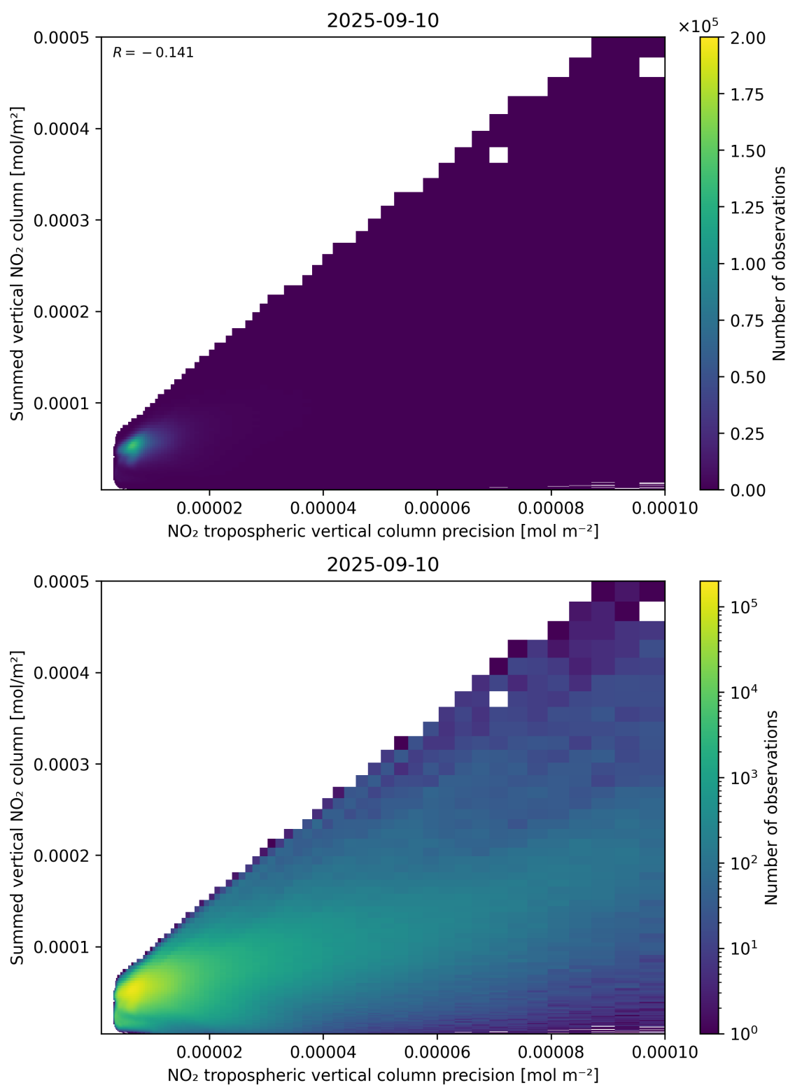
Figure 136: Scatter density plot of “NO 2 tropospheric vertical column precision” against “Summed vertical NO 2 column” for 2025-09-10 to 2025-09-11.
