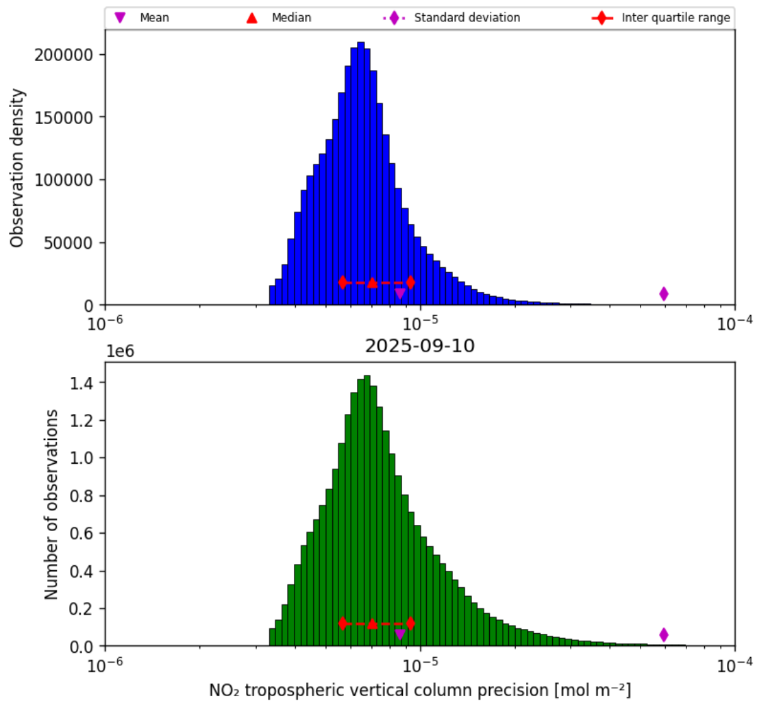
Figure 30: Histogram of “NO 2 tropospheric vertical column precision” for 2025-09-10 to 2025-09-11
