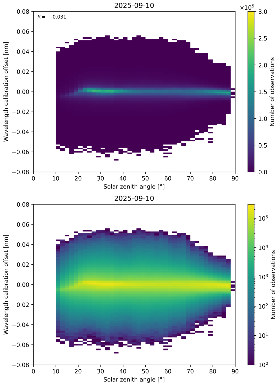
Figure 158: Scatter density plot of “Solar zenith angle” against “Wavelength calibration offset” for 2025-09-10 to 2025-09-11.
