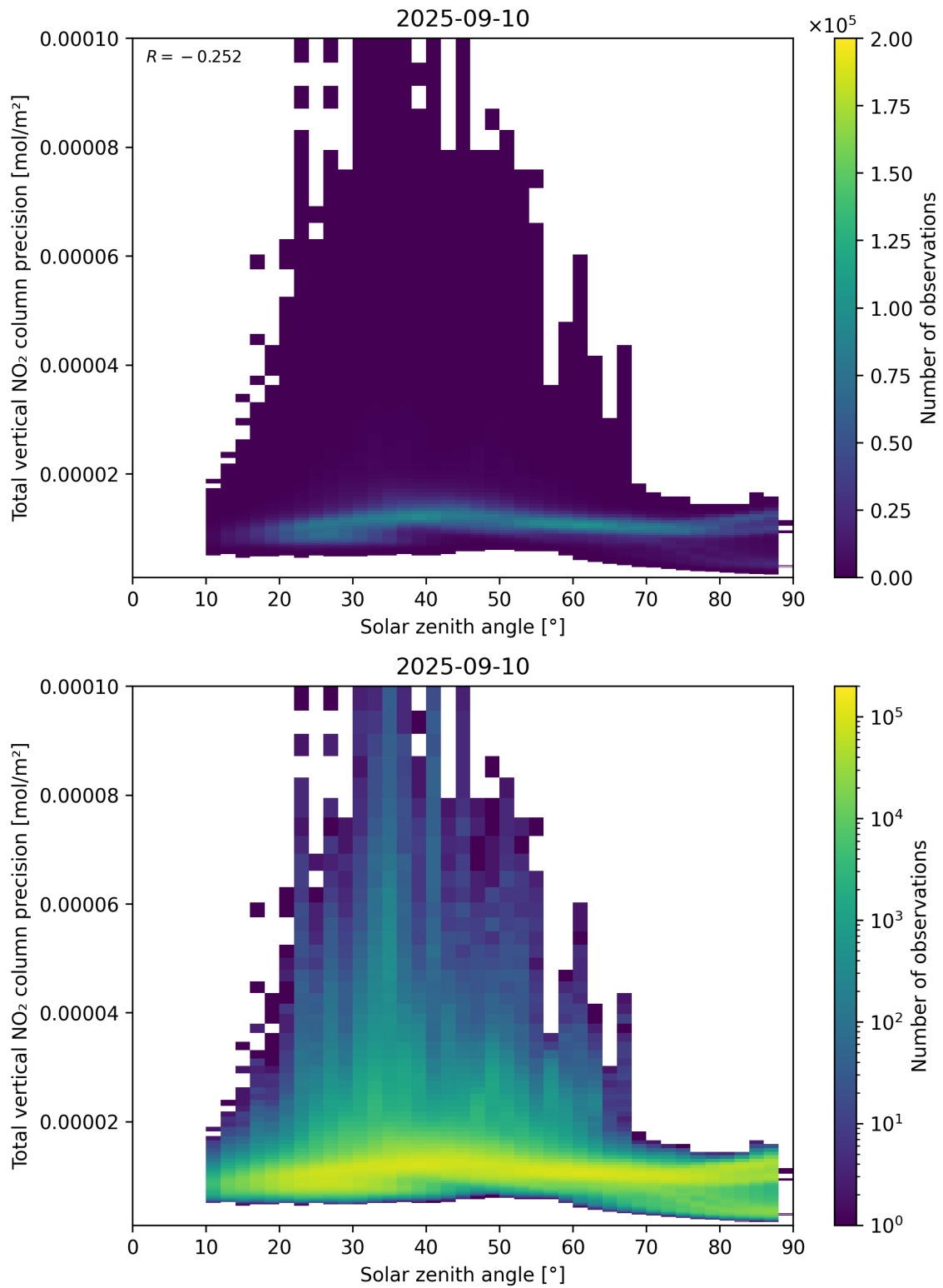
Figure 154: Scatter density plot of “Solar zenith angle” against “Total vertical NO 2 column precision” for 2025-09-10 to 2025-09-11.
