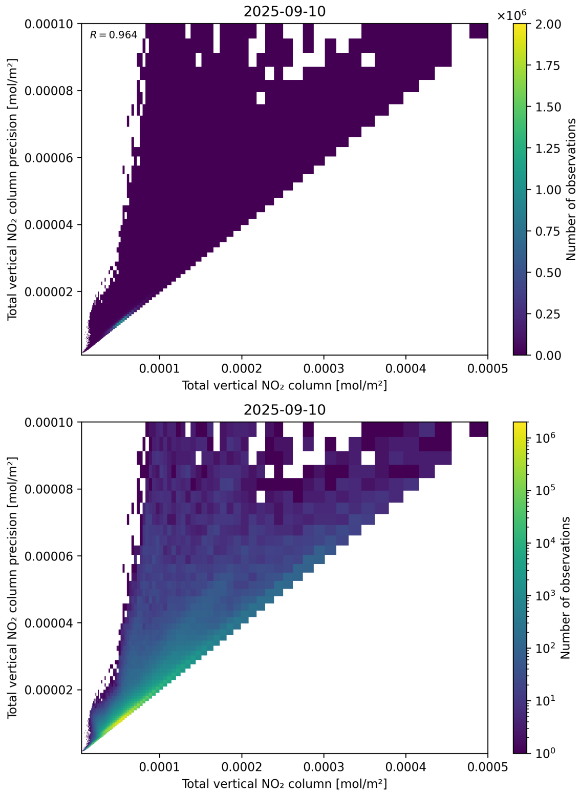
Figure 114: Scatter density plot of “Total vertical NO 2 column” against “Total vertical NO 2 column precision” for 2025-09-10 to 2025-09-11.
