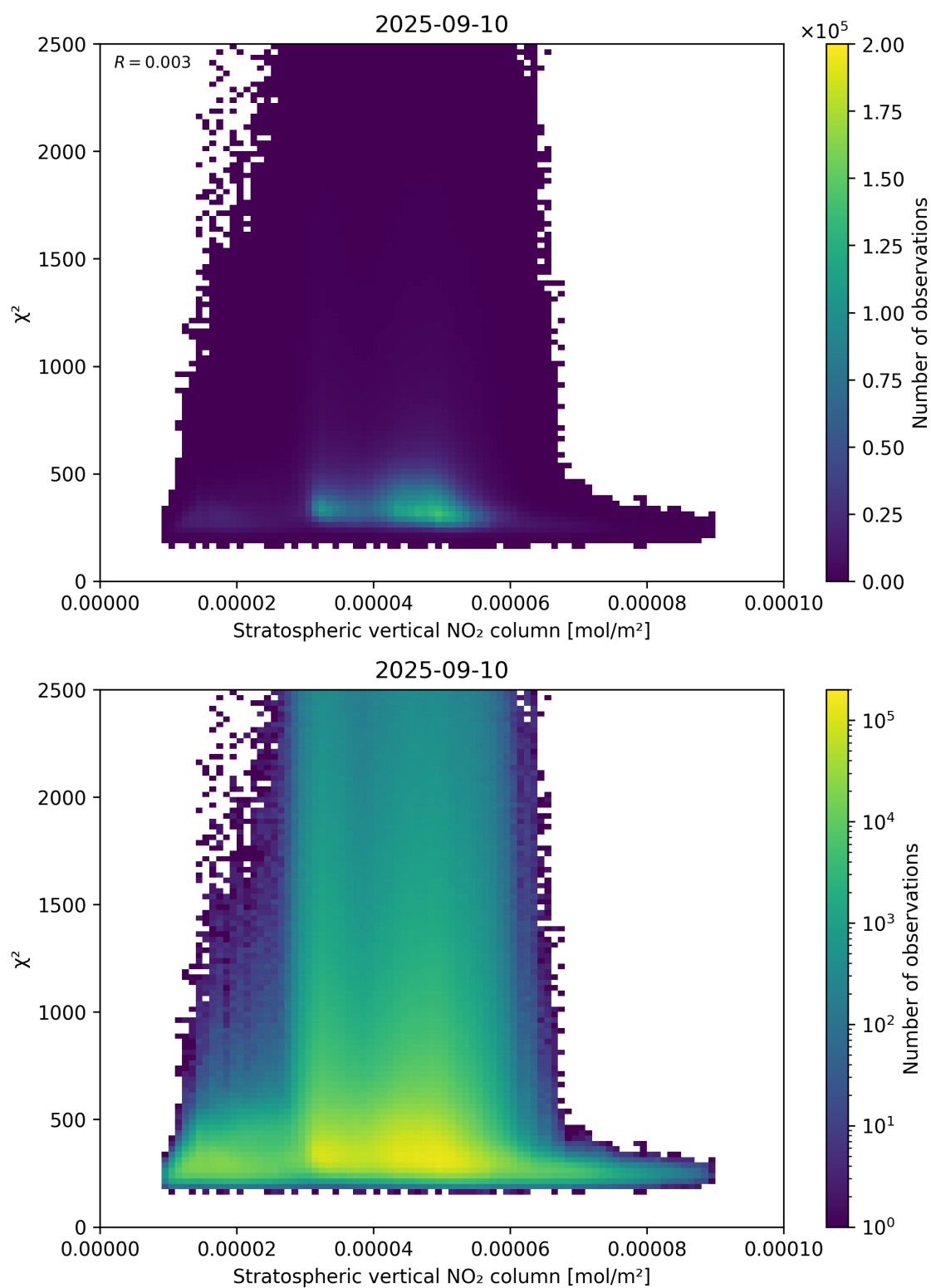
Figure 97: Scatter density plot of “Stratospheric vertical NO 2 column” against “ \chi^2 ” for 2025-09-10 to 2025-09-11.
