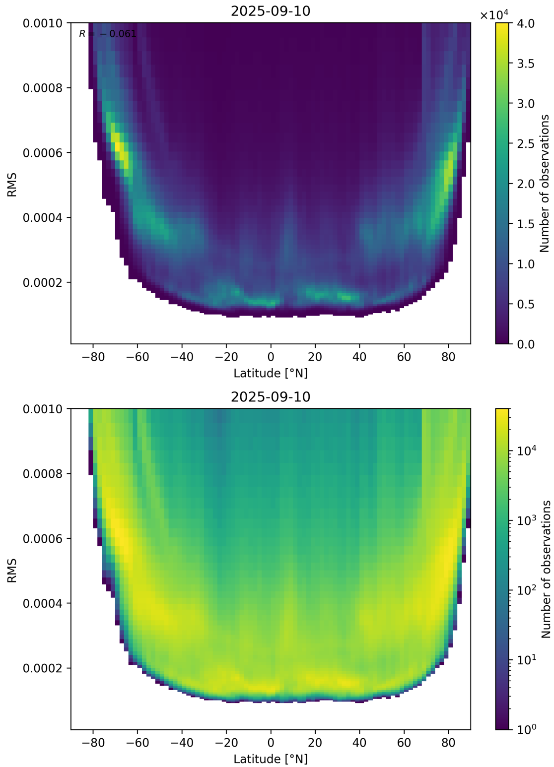
Figure 94: Scatter density plot of “Latitude” against “RMS” for 2025-09-10 to 2025-09-11.
