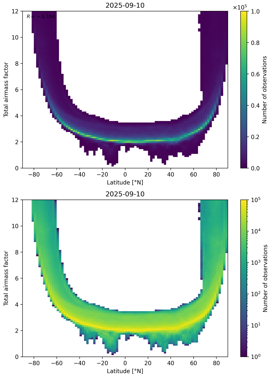
Figure 84: Scatter density plot of “Latitude” against “Total airmass factor” for 2025-09-10 to 2025-09-11.
