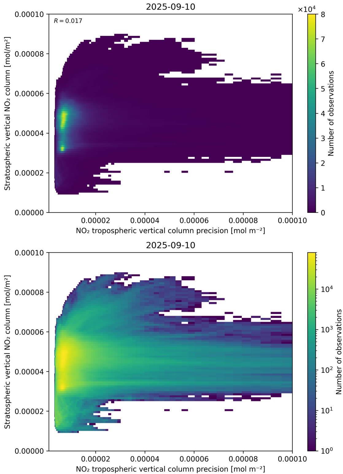
Figure 135: Scatter density plot of “NO 2 tropospheric vertical column precision” against “Stratospheric vertical NO 2 column” for 2025-09-10 to 2025-09-11.
