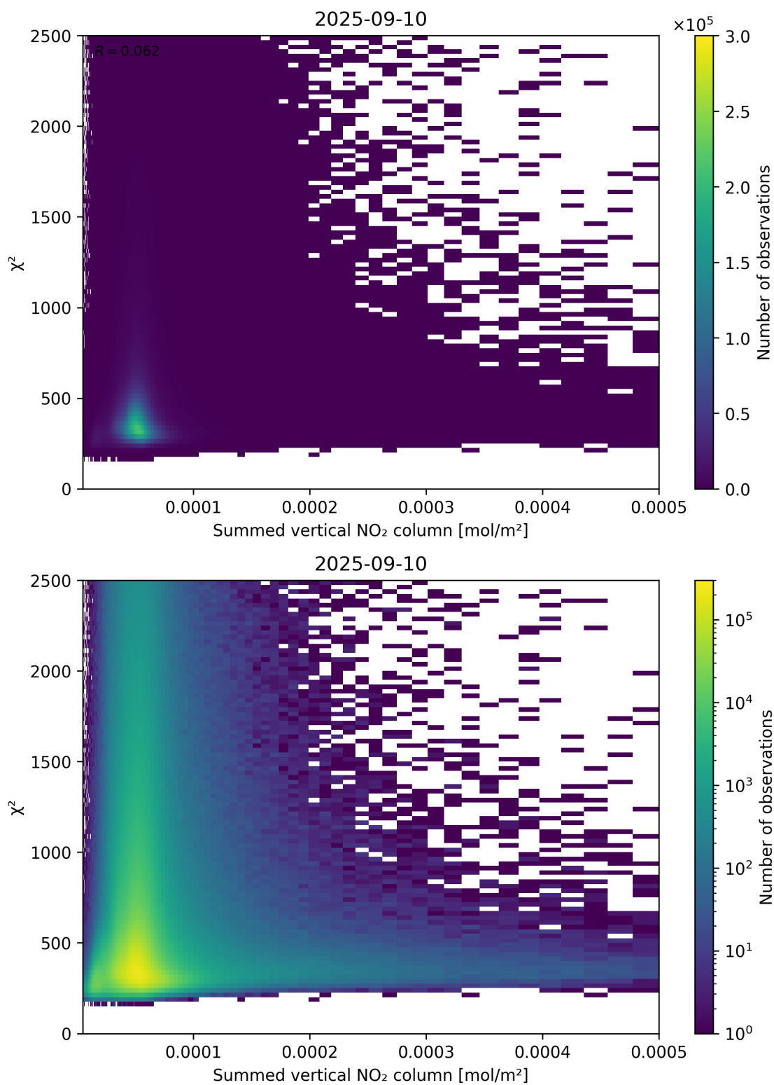
Figure 104: Scatter density plot of “Summed vertical NO 2 column” against “ \chi^2 ” for 2025-09-10 to 2025-09-11.
