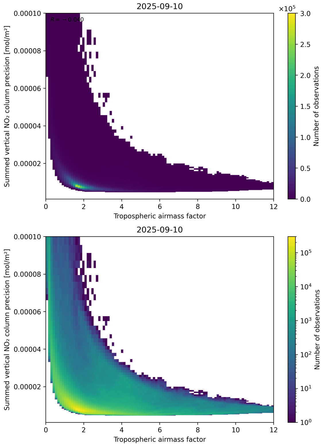
Figure 76: Scatter density plot of “Tropospheric air mass factor” against “Summed vertical NO 2 column precision” for 2025-09-10 to 2025-09-11.
