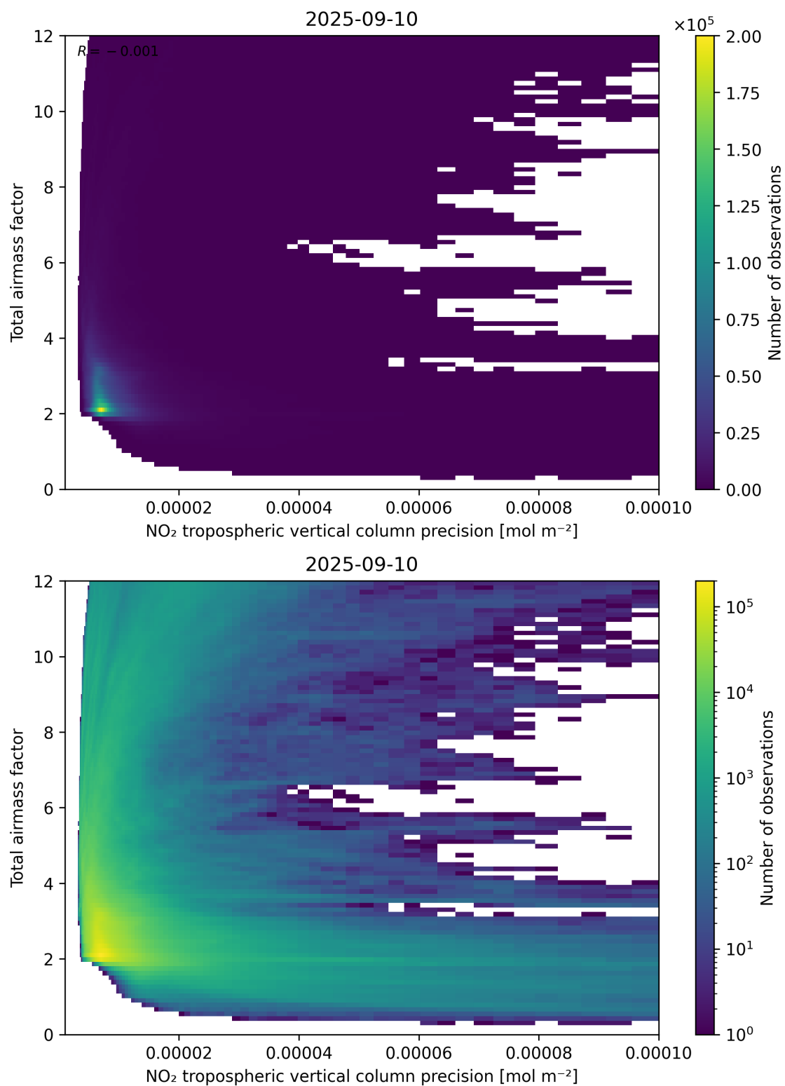
Figure 132: Scatter density plot of “NO 2 tropospheric vertical column precision” against “Total air mass factor” for 2025-09-10 to 2025-09-11.
