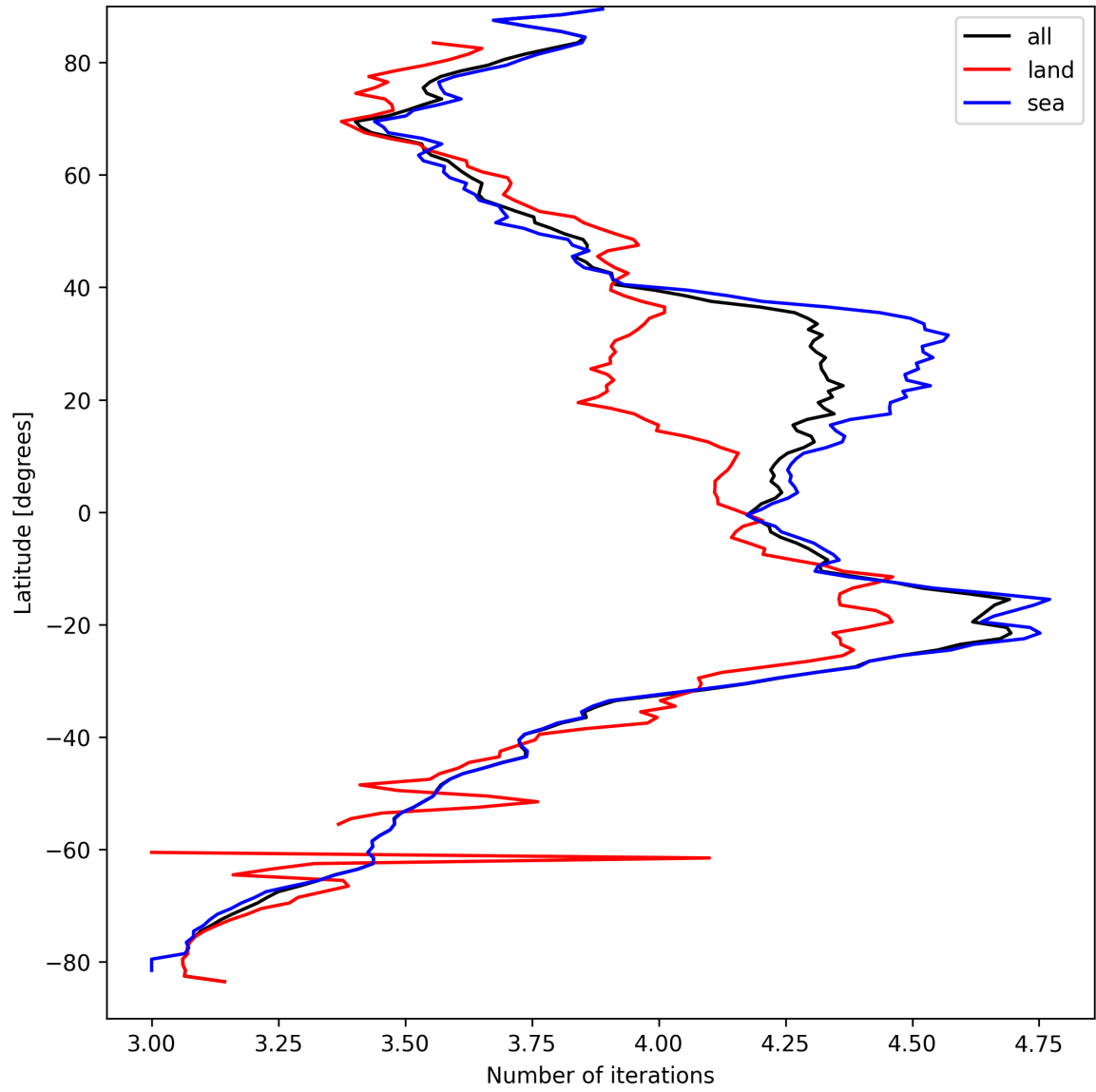
Figure 17: Zonal average of “Number of iterations” for 2025-09-10 to 2025-09-11.
