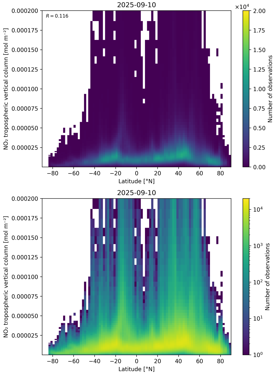
Figure 92: Scatter density plot of “Latitude” against “NO 2 tropospheric vertical column” for 2025-09-10 to 2025-09-11.
