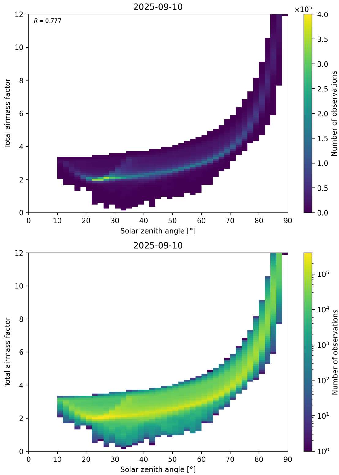
Figure 146: Scatter density plot of “Solar zenith angle” against “Total airmass factor” for 2025-09-10 to 2025-09-11.
