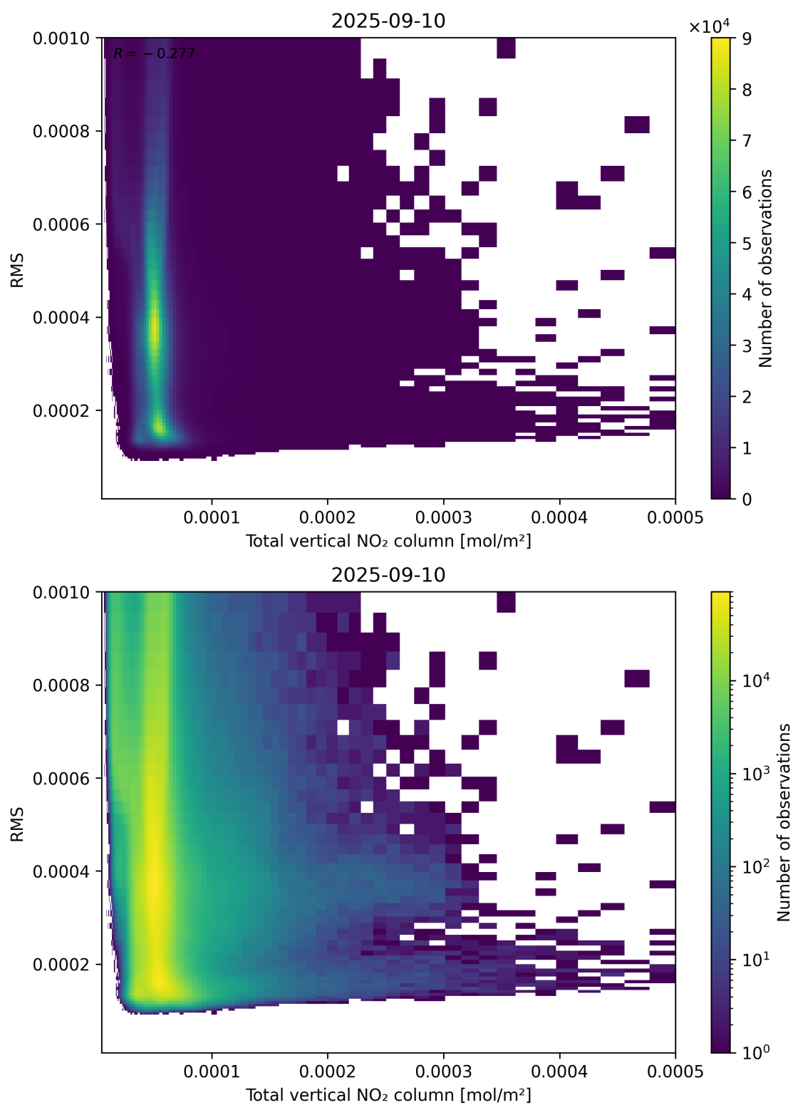
Figure 120: Scatter density plot of “Total vertical NO 2 column” against “RMS” for 2025-09-10 to 2025-09-11.
