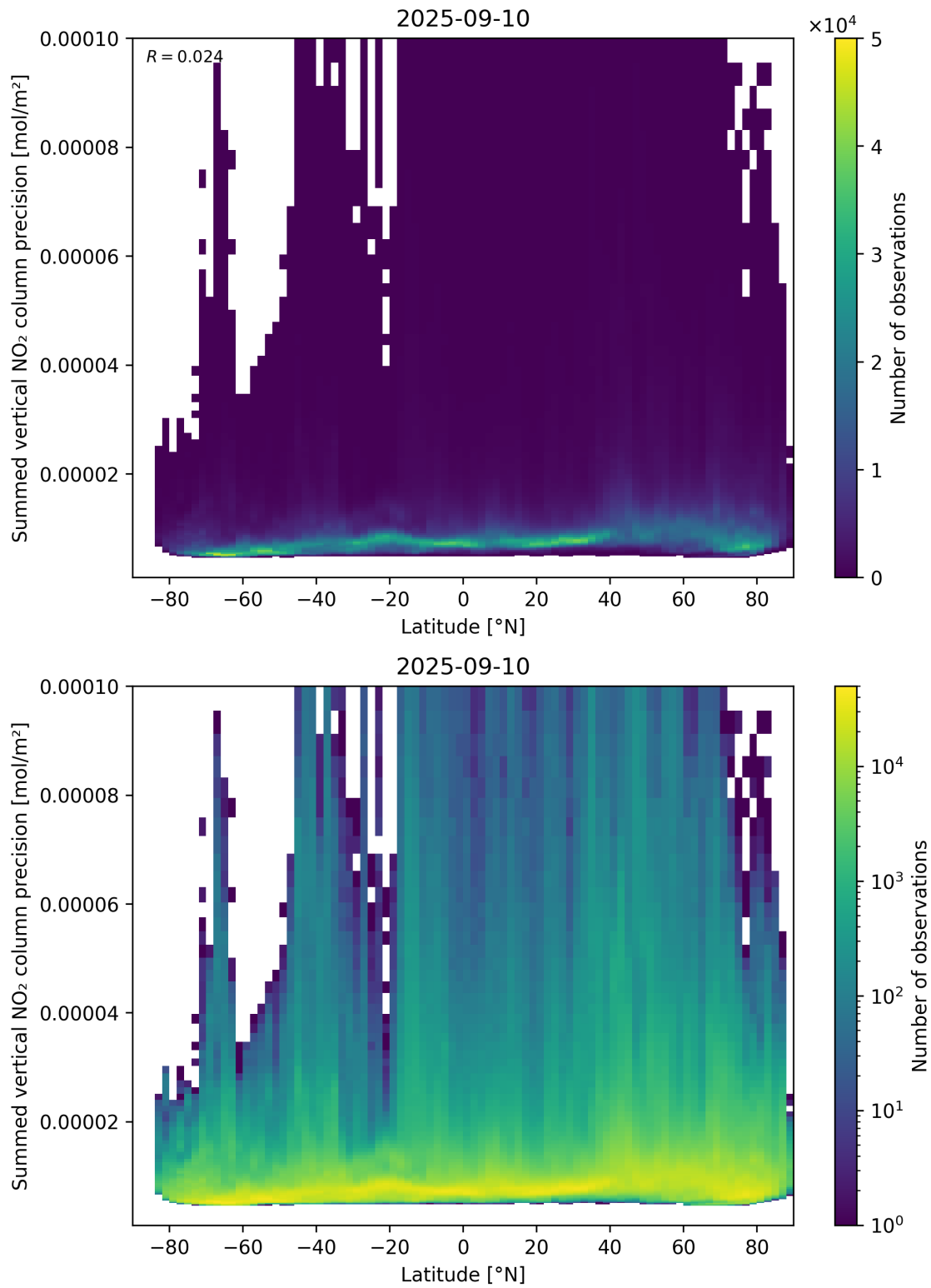
Figure 89: Scatter density plot of “Latitude” against “Summed vertical NO 2 column precision” for 2025-09-10 to 2025-09-11.
