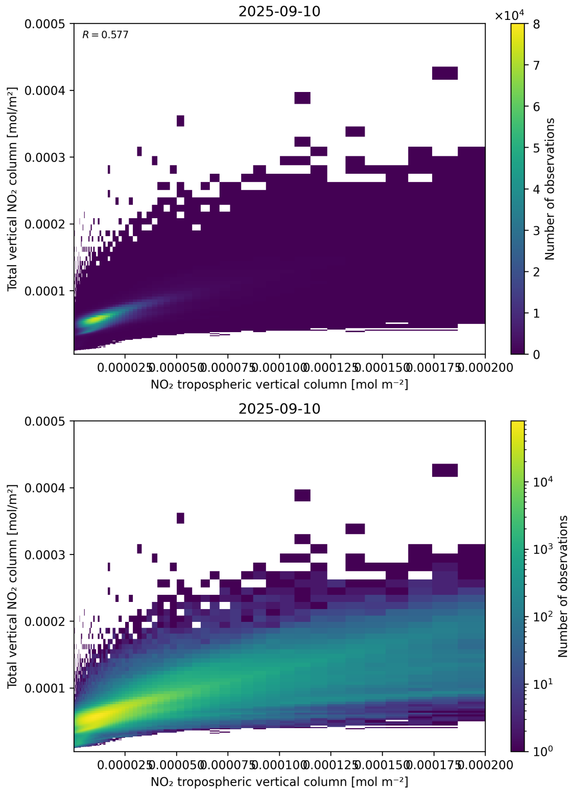
Figure 128: Scatter density plot of “NO 2 tropospheric vertical column” against “Total vertical NO 2 column” for 2025-09-10 to 2025-09-11.
