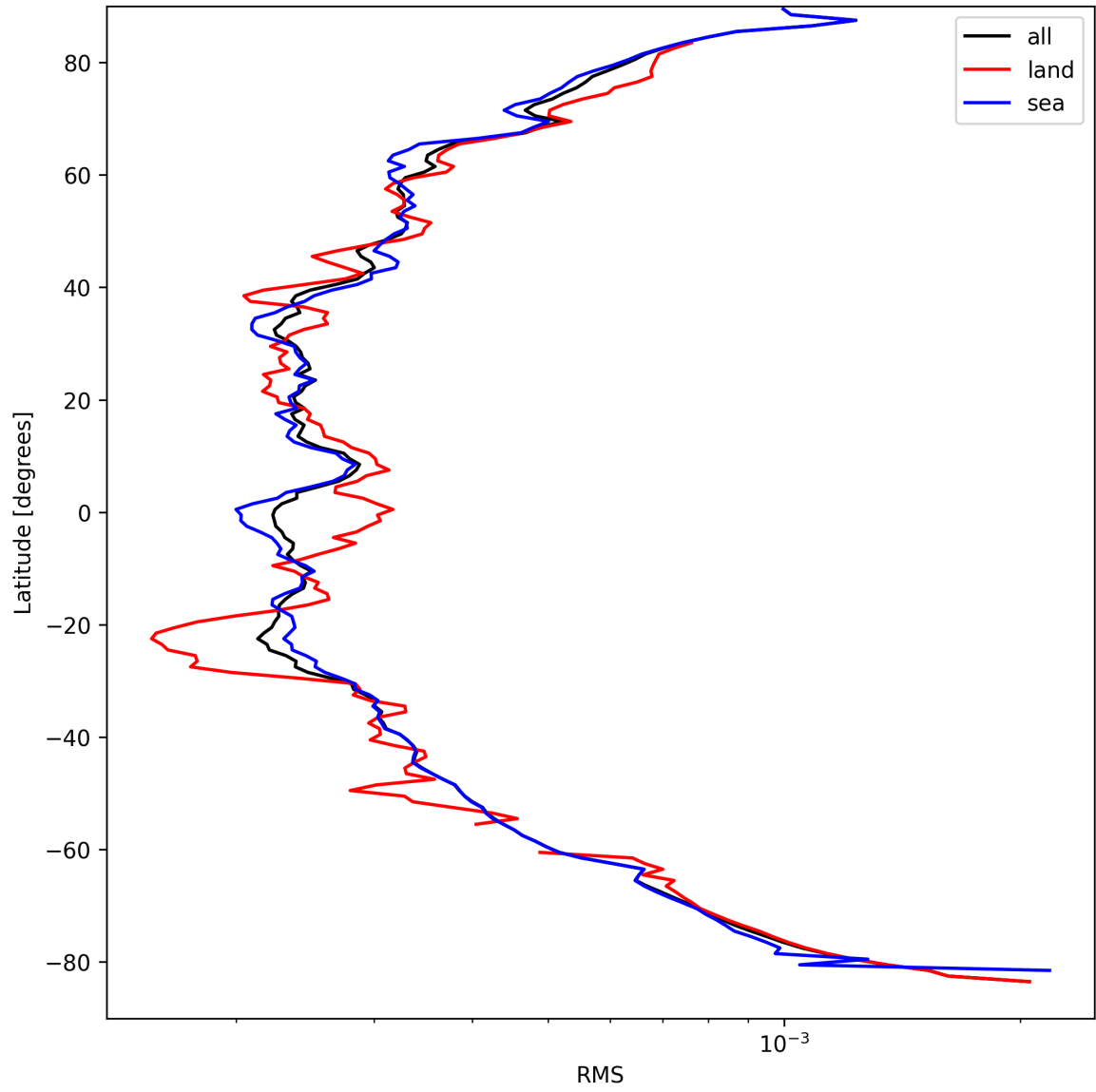
Figure 26: Zonal average of “RMS” for 2025-09-10 to 2025-09-11.
