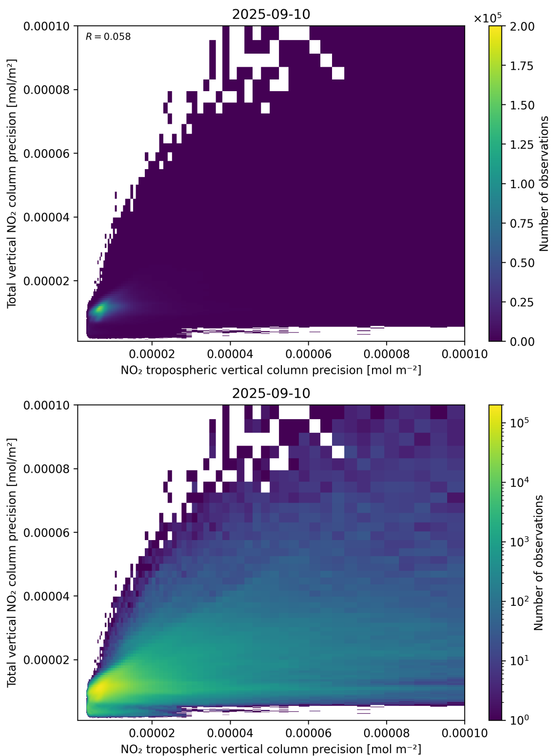
Figure 139: Scatter density plot of “NO 2 tropospheric vertical column precision” against “Total vertical NO 2 column precision” for 2025-09-10 to 2025-09-11.
