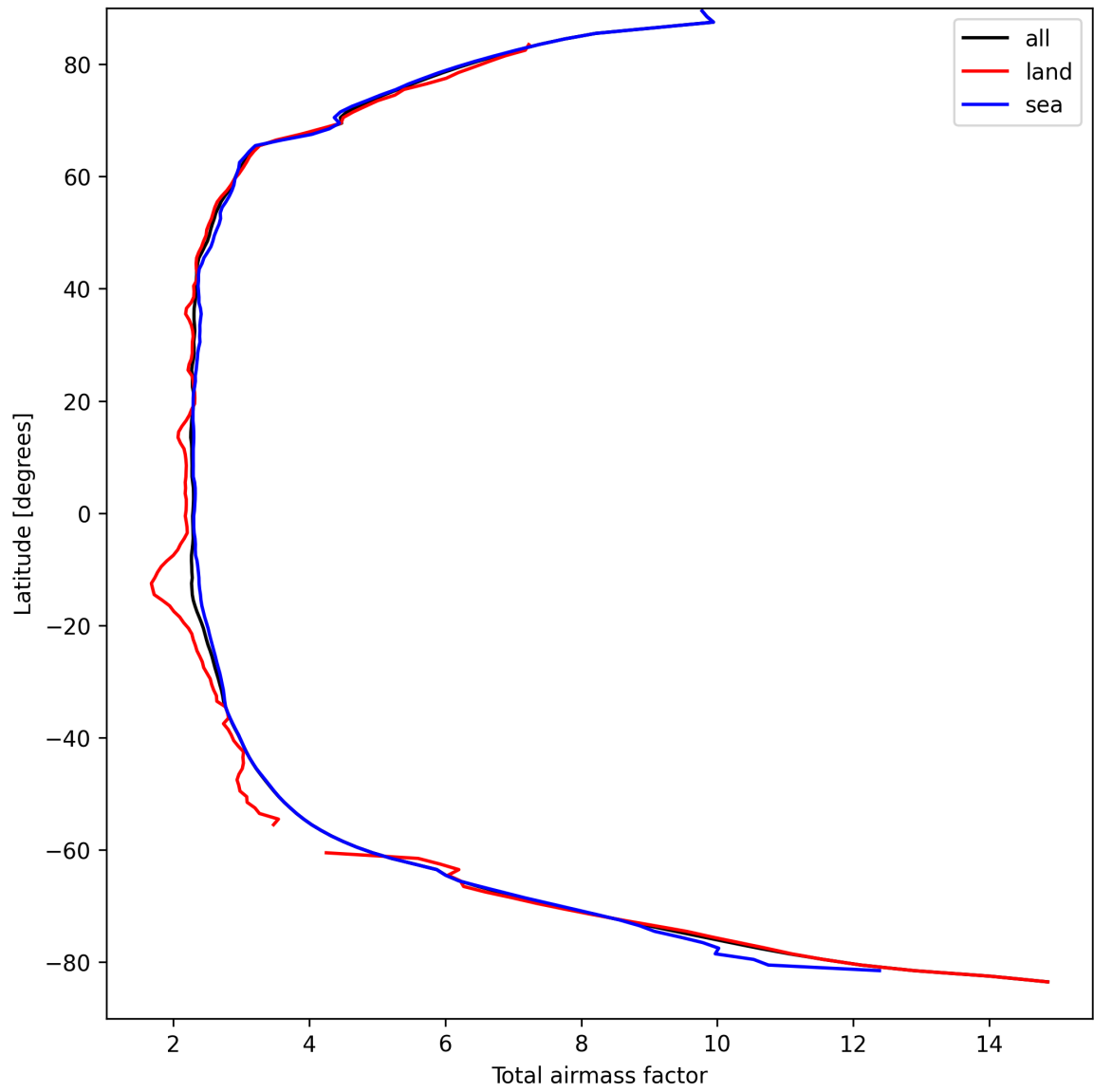
Figure 15: Zonal average of “Total airmass factor” for 2025-09-10 to 2025-09-11.
