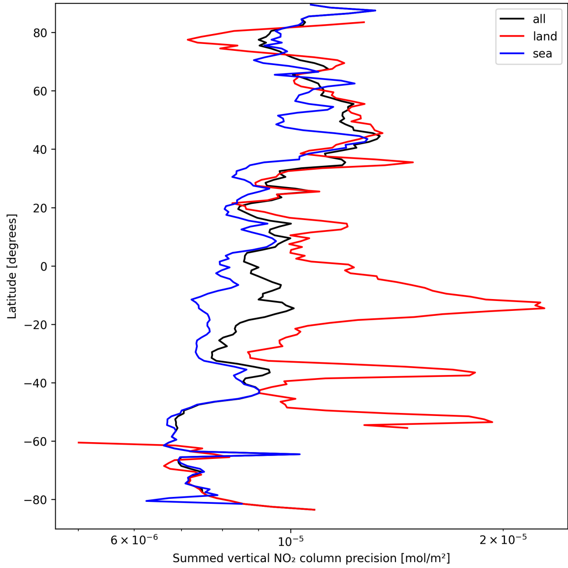
Figure 24: Zonal average of “Summed vertical NO 2 column precision” for 2025-09-10 to 2025-09-11.
