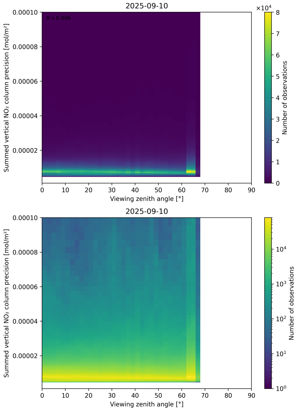
Figure 166: Scatter density plot of “Viewing zenith angle” against “Summed vertical NO 2 column precision” for 2025-09-10 to 2025-09-11.
