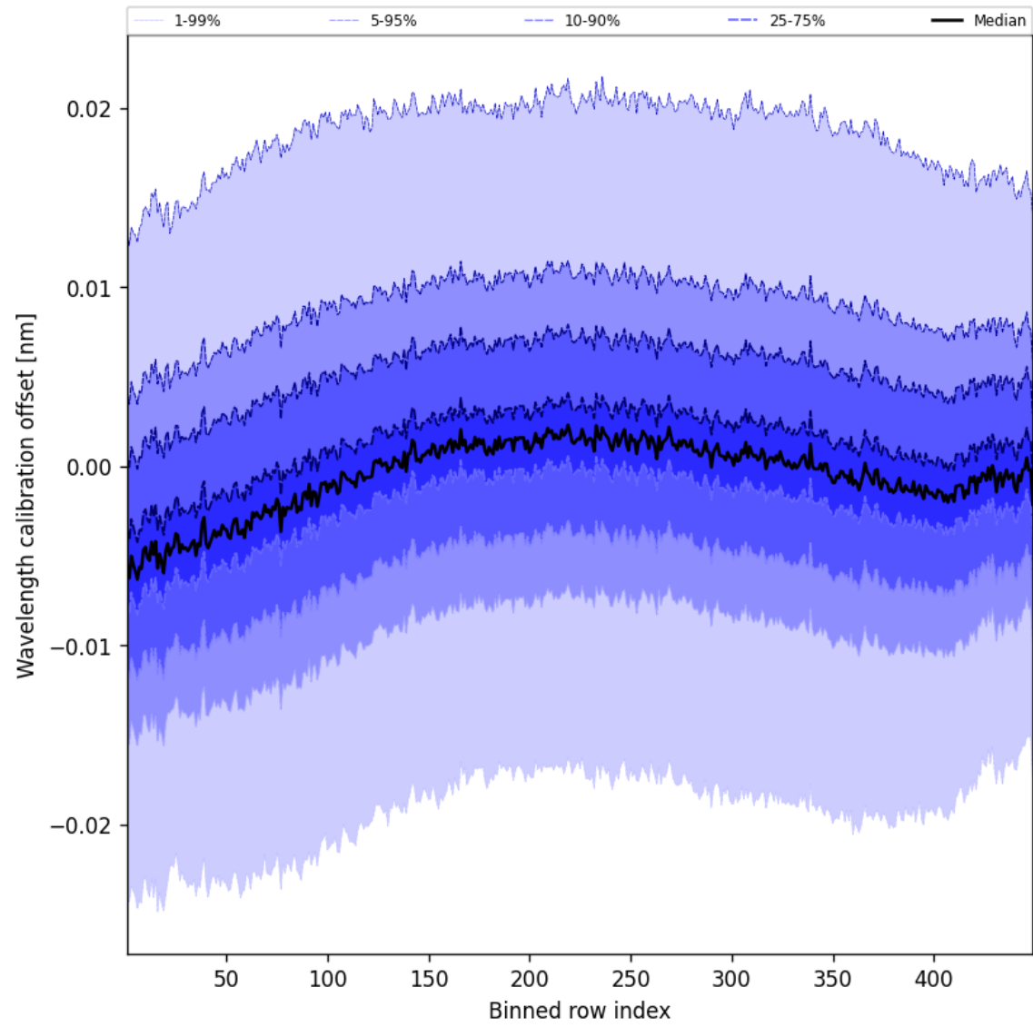
Figure 52: Along track statistics of “Wavelength calibration offset” for 2025-09-10 to 2025-09-11
