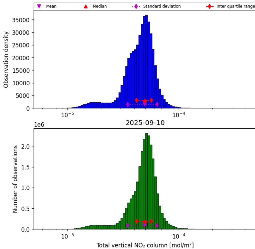
Figure 38: Histogram of “Total vertical NO 2 column” for 2025-09-10 to 2025-09-11
