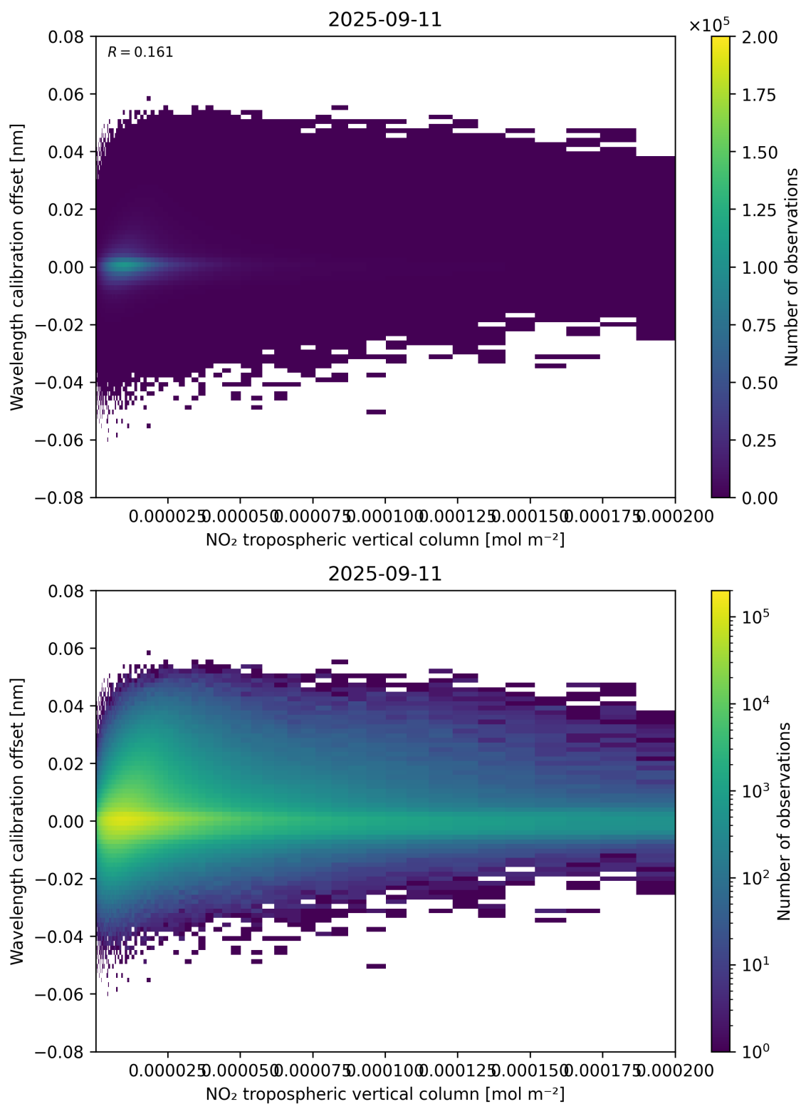
Figure 143: Scatter density plot of “NO 2 tropospheric vertical column” against “Wavelength calibration offset” for 2025-09-10 to 2025-09-12.
