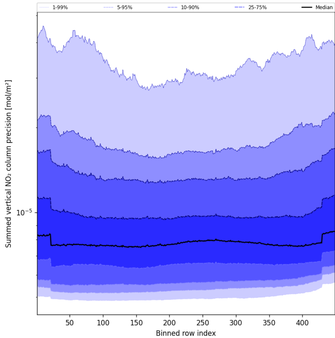
Figure 58: Along track statistics of “Summed vertical NO 2 column precision” for 2025-09-10 to 2025-09-12
