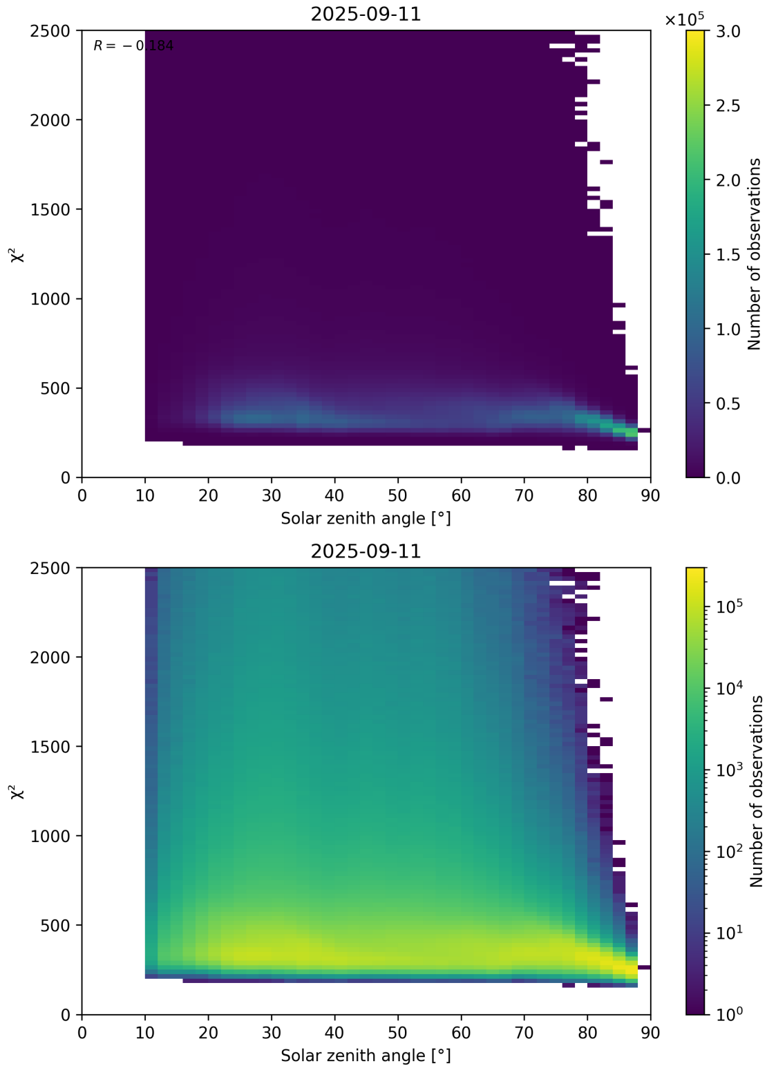
Figure 148: Scatter density plot of “Solar zenith angle” against “ \chi^2 ” for 2025-09-10 to 2025-09-12.
