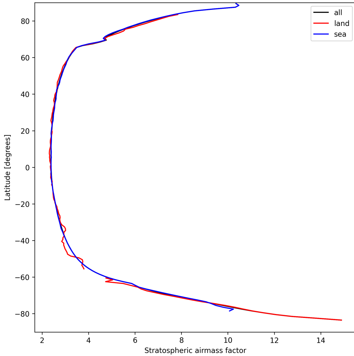
Figure 27: Zonal average of “Stratospheric airmass factor” for 2025-09-10 to 2025-09-12.
