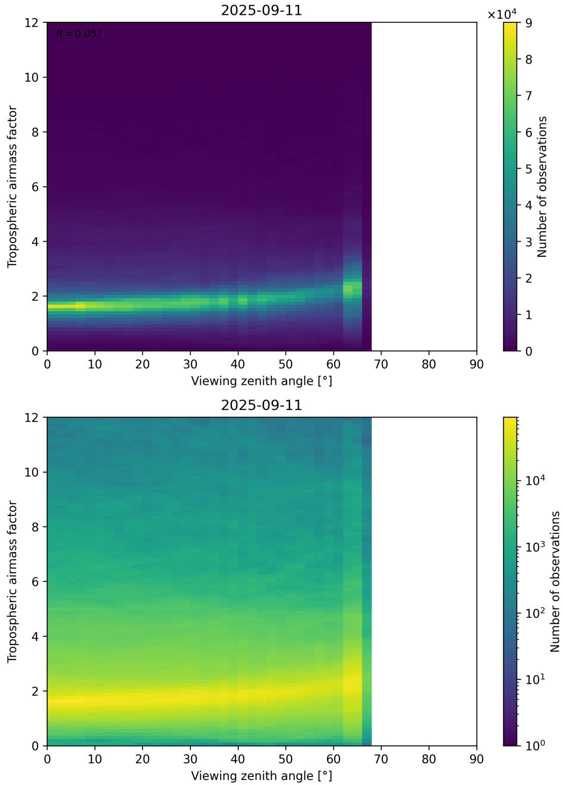
Figure 161: Scatter density plot of “Viewing zenith angle” against “Tropospheric airmass factor” for 2025-09-10 to 2025-09-12.
