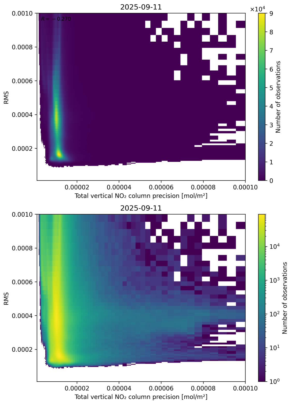
Figure 119: Scatter density plot of “Total vertical NO 2 column precision” against “RMS” for 2025-09-10 to 2025-09-12.
