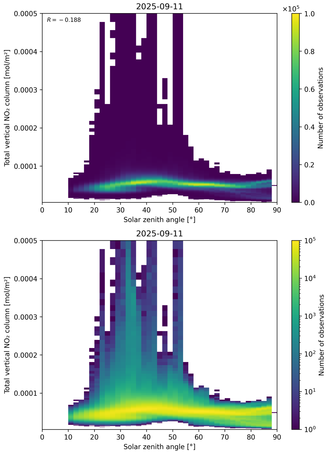
Figure 153: Scatter density plot of “Solar zenith angle” against “Total vertical NO 2 column” for 2025-09-10 to 2025-09-12.
