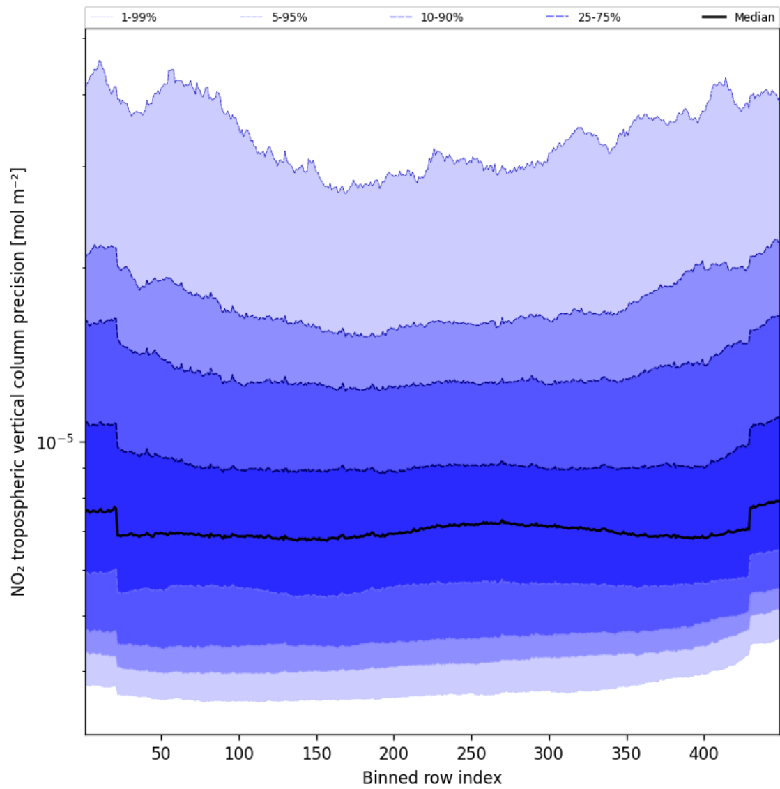
Figure 47: Along track statistics of “NO 2 tropospheric vertical column precision” for 2025-09-10 to 2025-09-12
