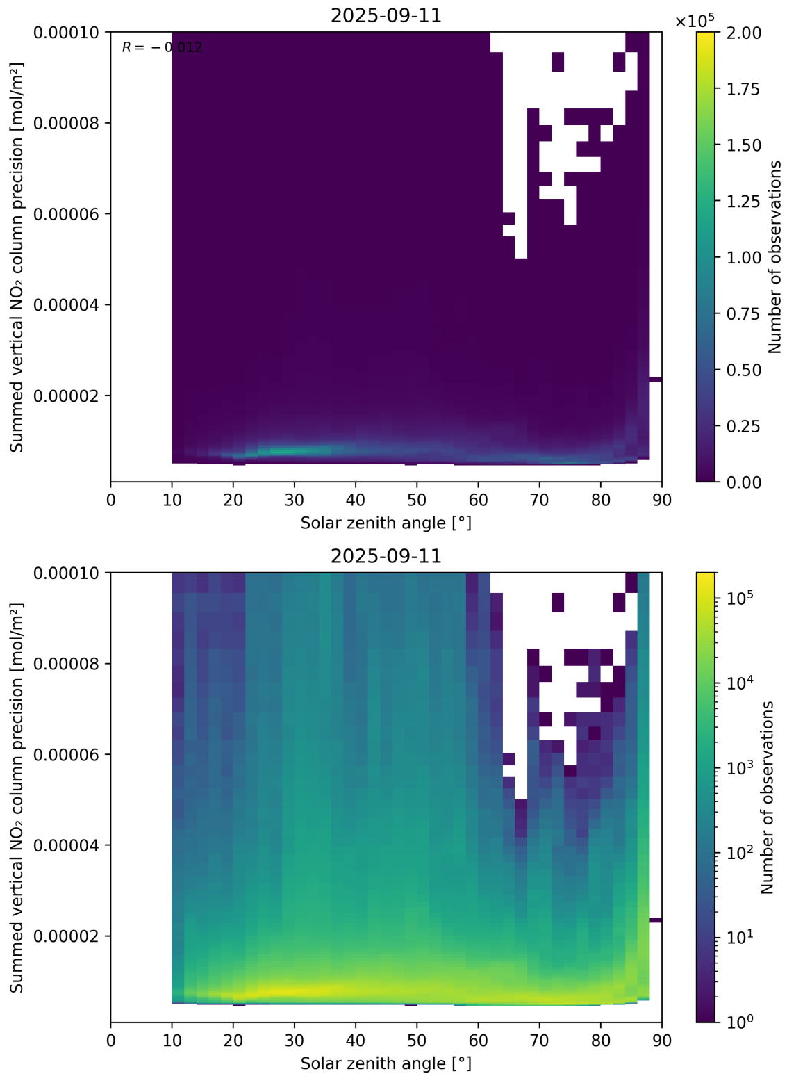
Figure 152: Scatter density plot of “Solar zenith angle” against “Summed vertical NO 2 column precision” for 2025-09-10 to 2025-09-12.
