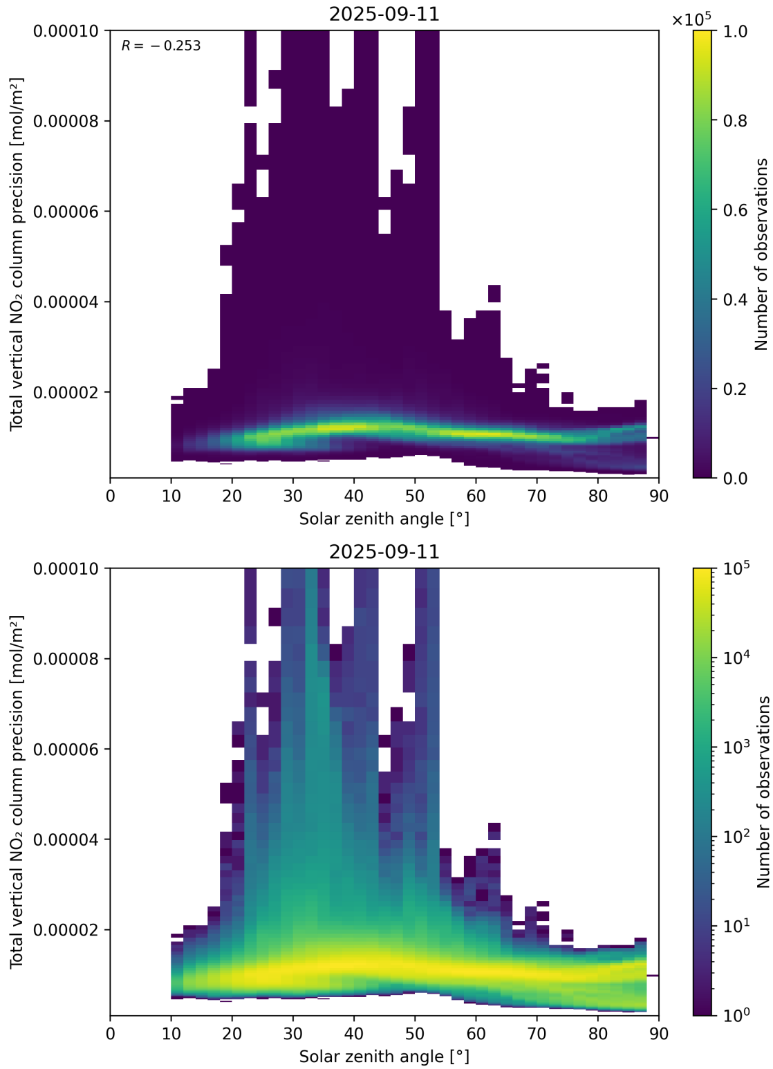
Figure 154: Scatter density plot of “Solar zenith angle” against “Total vertical NO 2 column precision” for 2025-09-10 to 2025-09-12.
