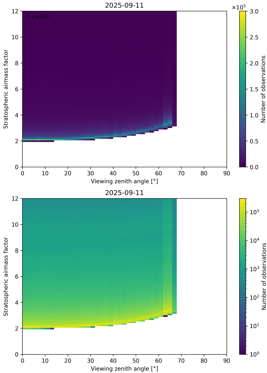
Figure 159: Scatter density plot of “Viewing zenith angle” against “Stratospheric airmass factor” for 2025-09-10 to 2025-09-12.
