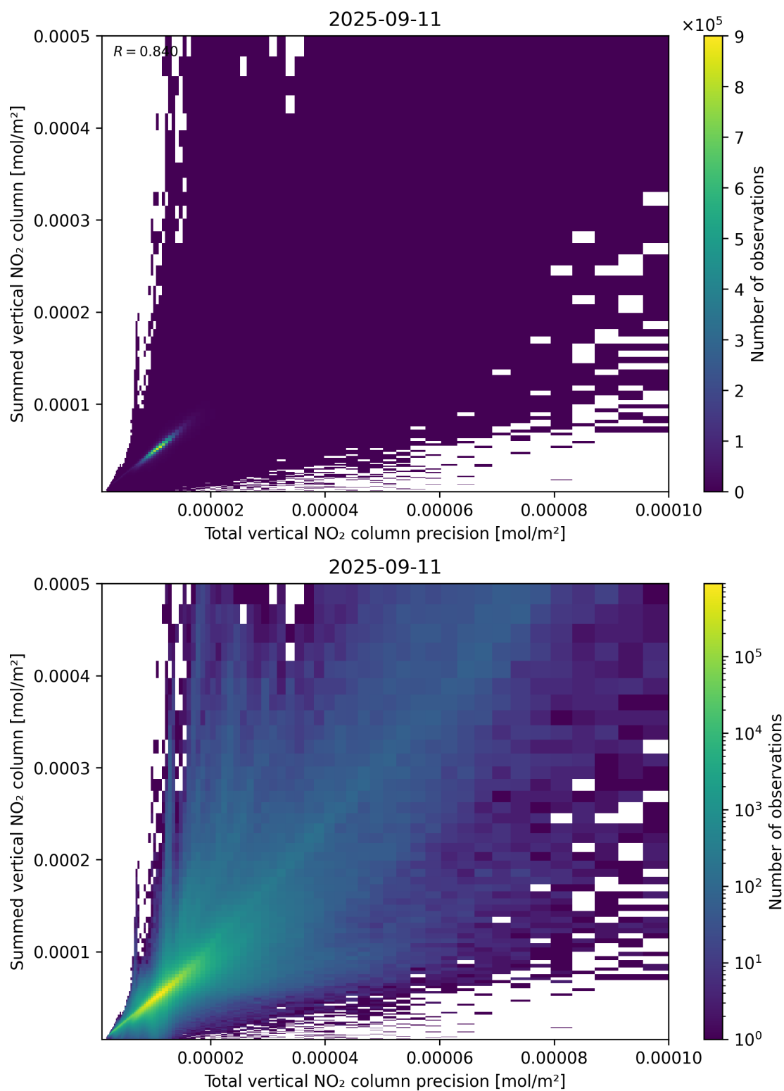
Figure 117: Scatter density plot of “Total vertical NO 2 column precision” against “Summed vertical NO 2 column” for 2025-09-10 to 2025-09-12.
