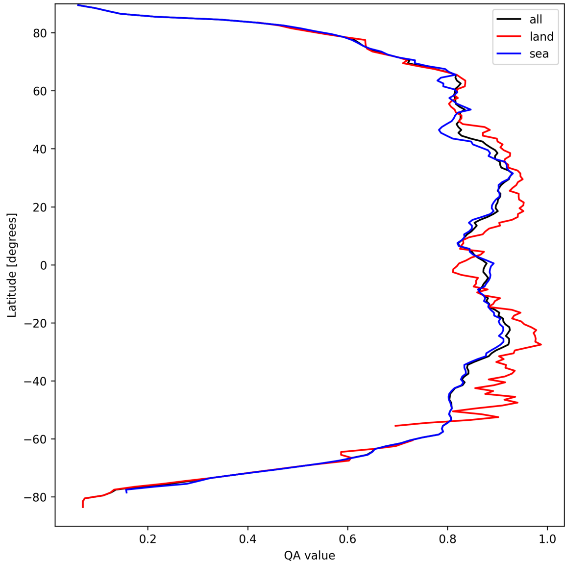
Figure 11: Zonal average of “QA value” for 2025-09-10 to 2025-09-12.
