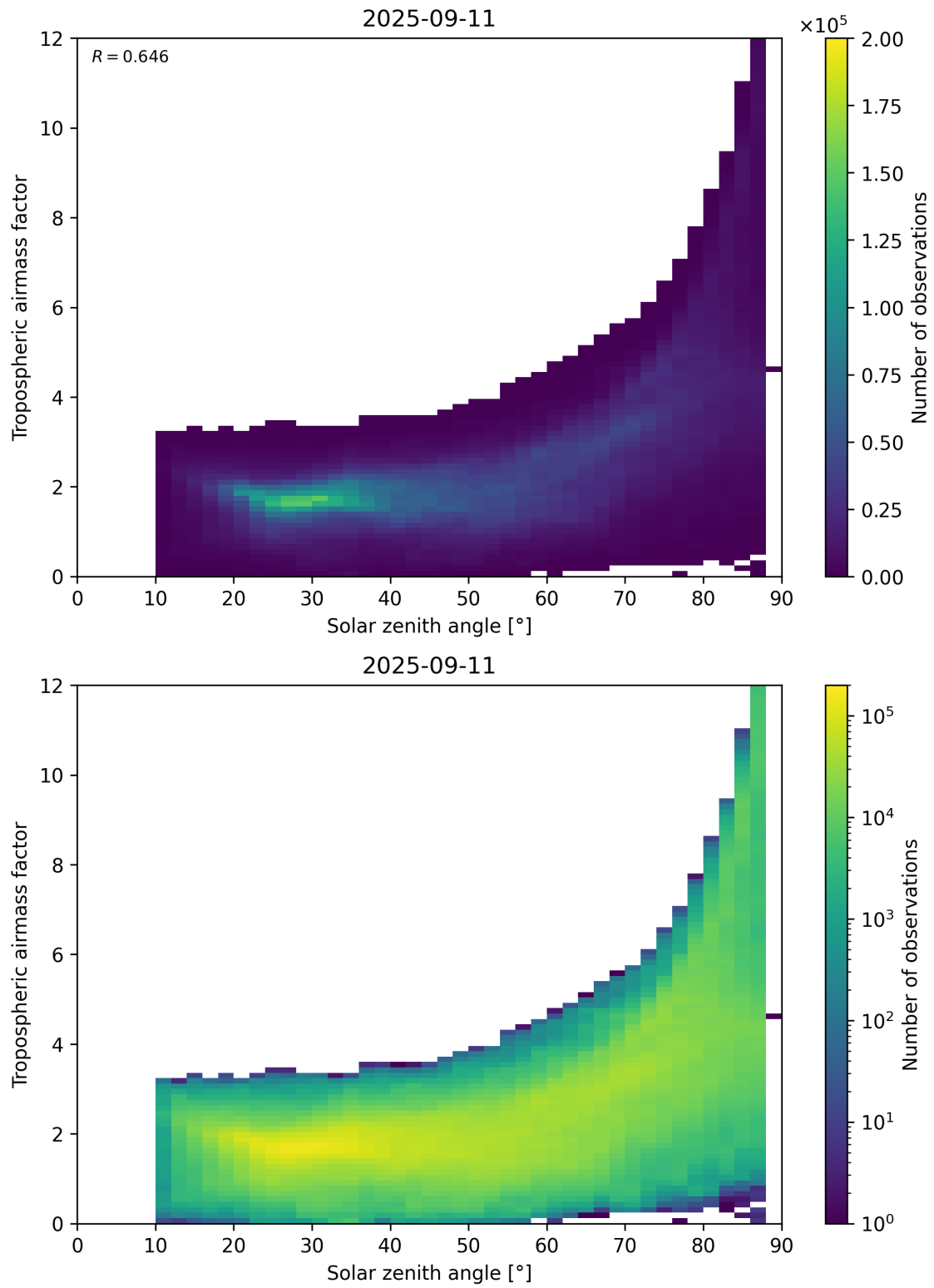
Figure 147: Scatter density plot of “Solar zenith angle” against “Tropospheric airmass factor” for 2025-09-10 to 2025-09-12.
