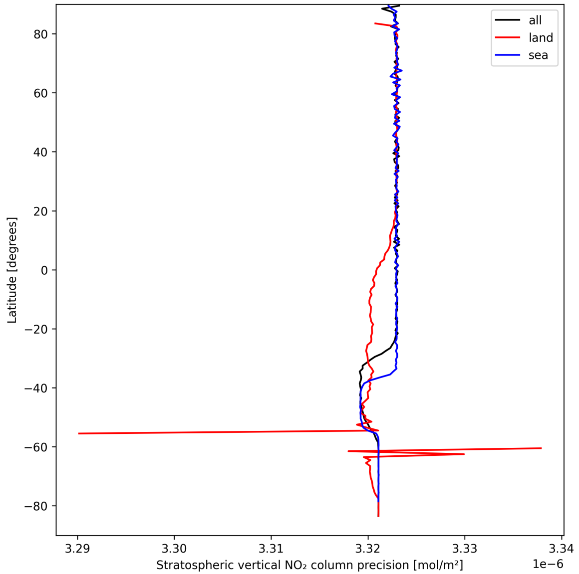
Figure 20: Zonal average of “Stratospheric vertical NO 2 column precision” for 2025-09-10 to 2025-09-12.
