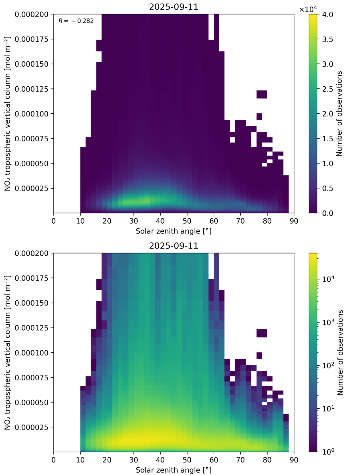
Figure 155: Scatter density plot of “Solar zenith angle” against “NO 2 tropospheric vertical column” for 2025-09-10 to 2025-09-12.
