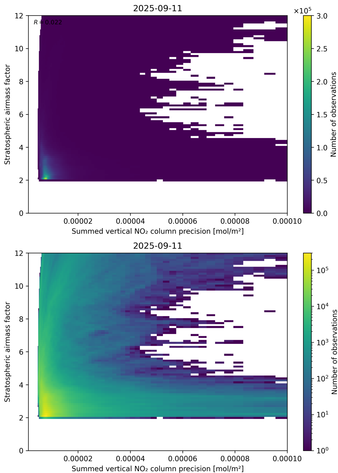
Figure 106: Scatter density plot of “Summed vertical NO 2 column precision” against “Stratospheric airmass factor” for 2025-09-10 to 2025-09-12.
