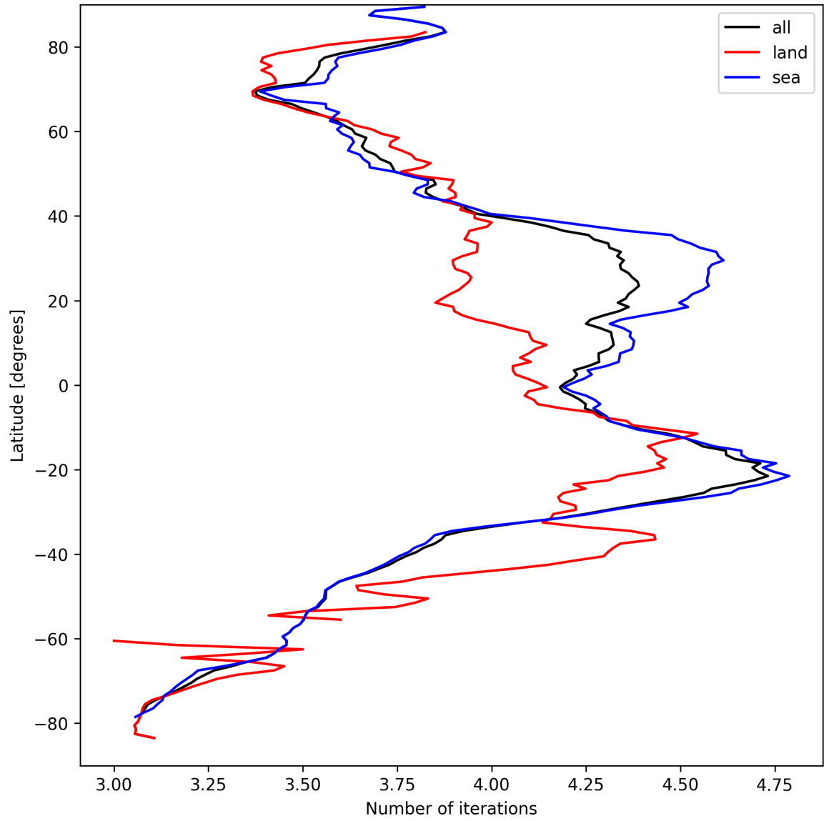
Figure 17: Zonal average of “Number of iterations” for 2025-09-10 to 2025-09-12.
