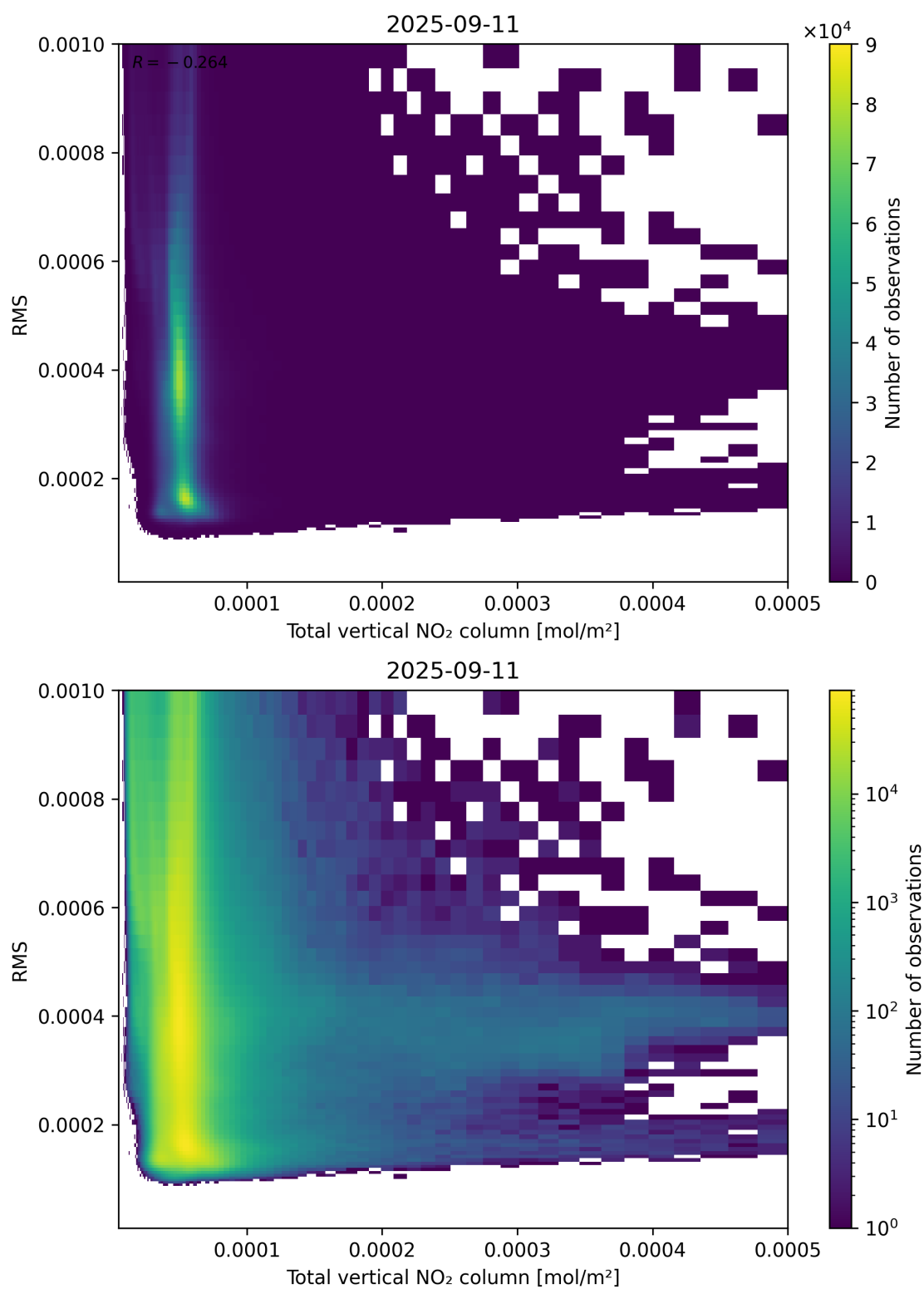
Figure 120: Scatter density plot of “Total vertical NO 2 column” against “RMS” for 2025-09-10 to 2025-09-12.
