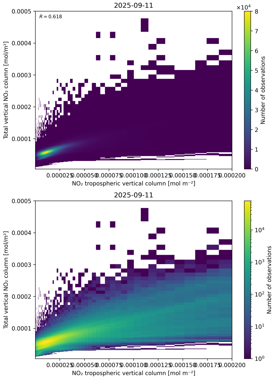
Figure 128: Scatter density plot of “NO 2 tropospheric vertical column” against “Total vertical NO 2 column” for 2025-09-10 to 2025-09-12.
