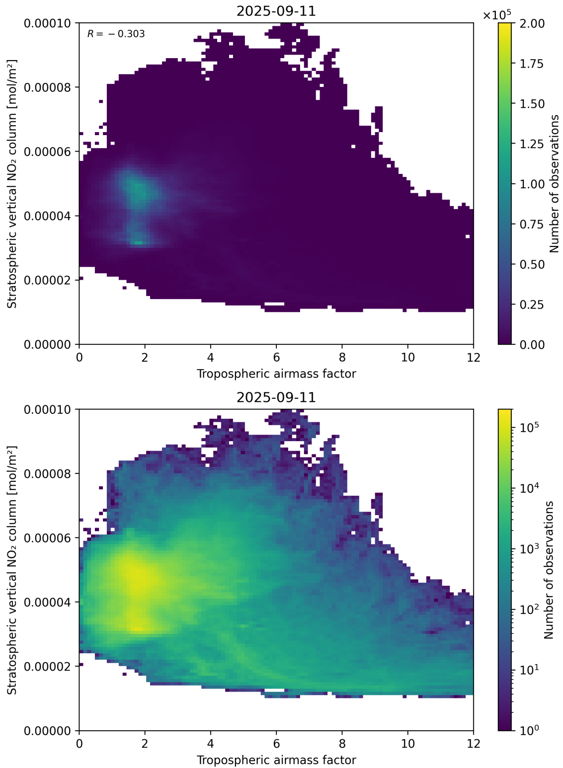
Figure 74: Scatter density plot of “Tropospheric airmass factor” against “Stratospheric vertical NO 2 column” for 2025-09-10 to 2025-09-12.
