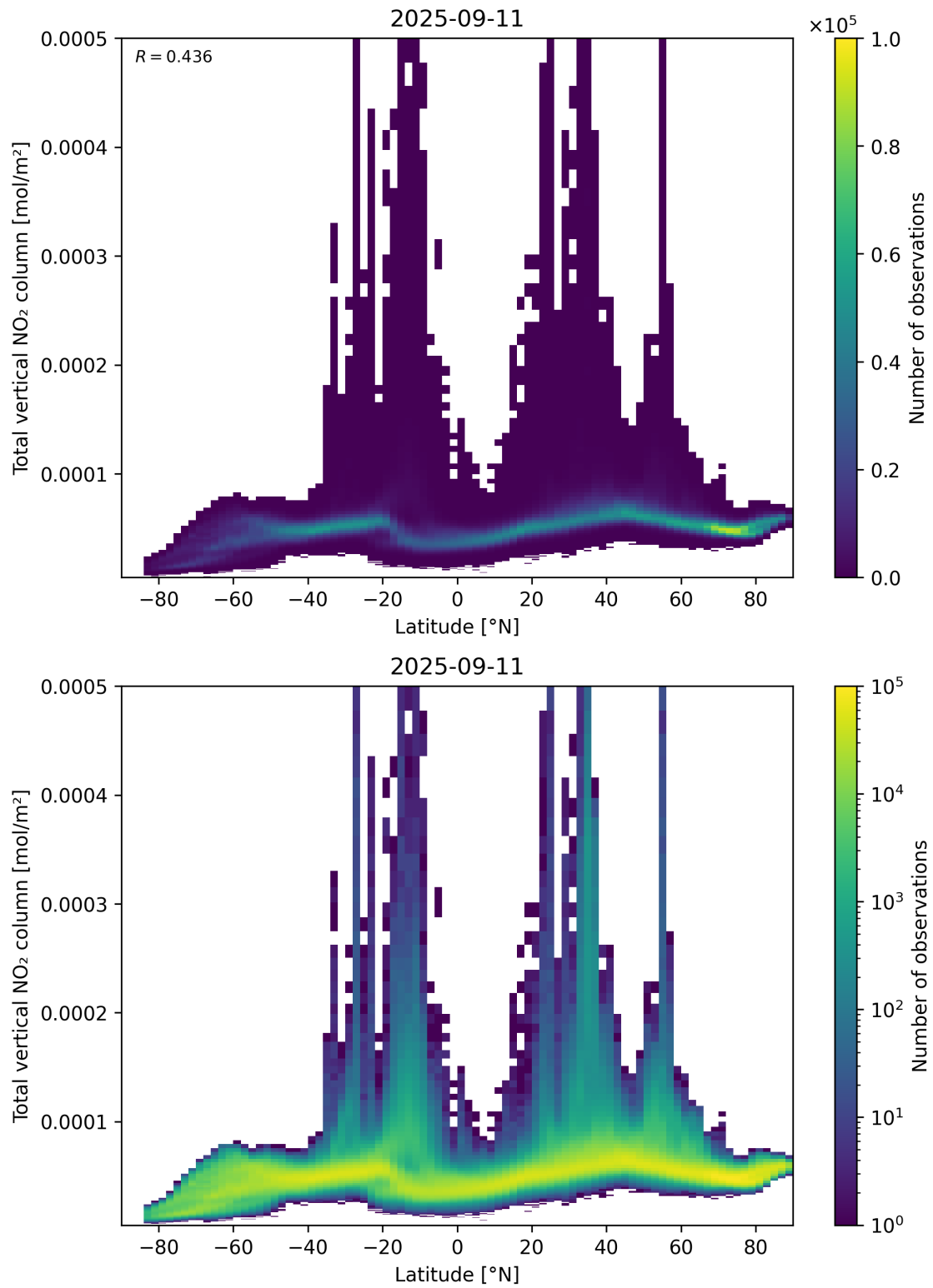
Figure 90: Scatter density plot of “Latitude” against “Total vertical NO 2 column” for 2025-09-10 to 2025-09-12.
