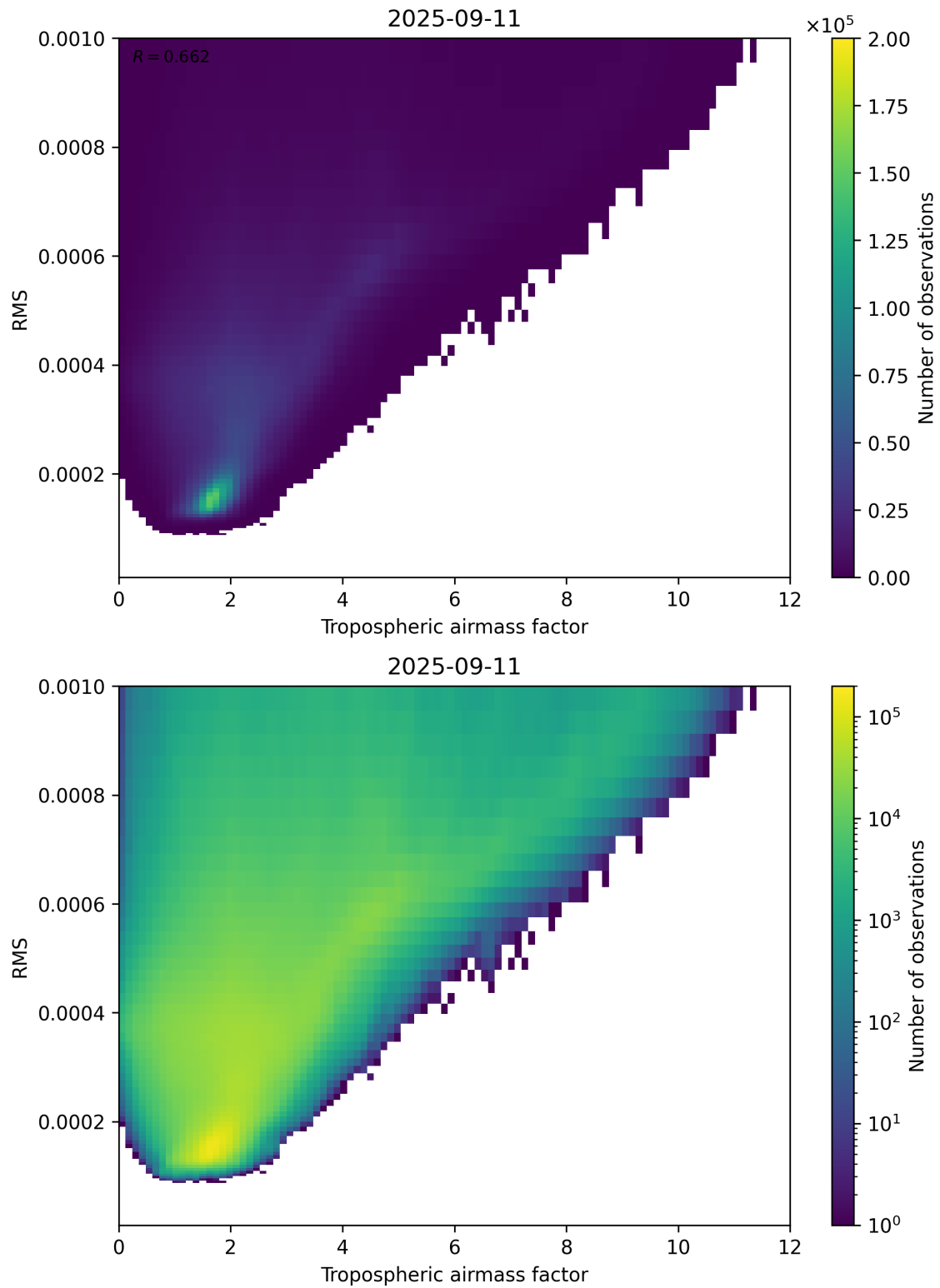
Figure 79: Scatter density plot of “Tropospheric airmass factor” against “RMS” for 2025-09-10 to 2025-09-12.
