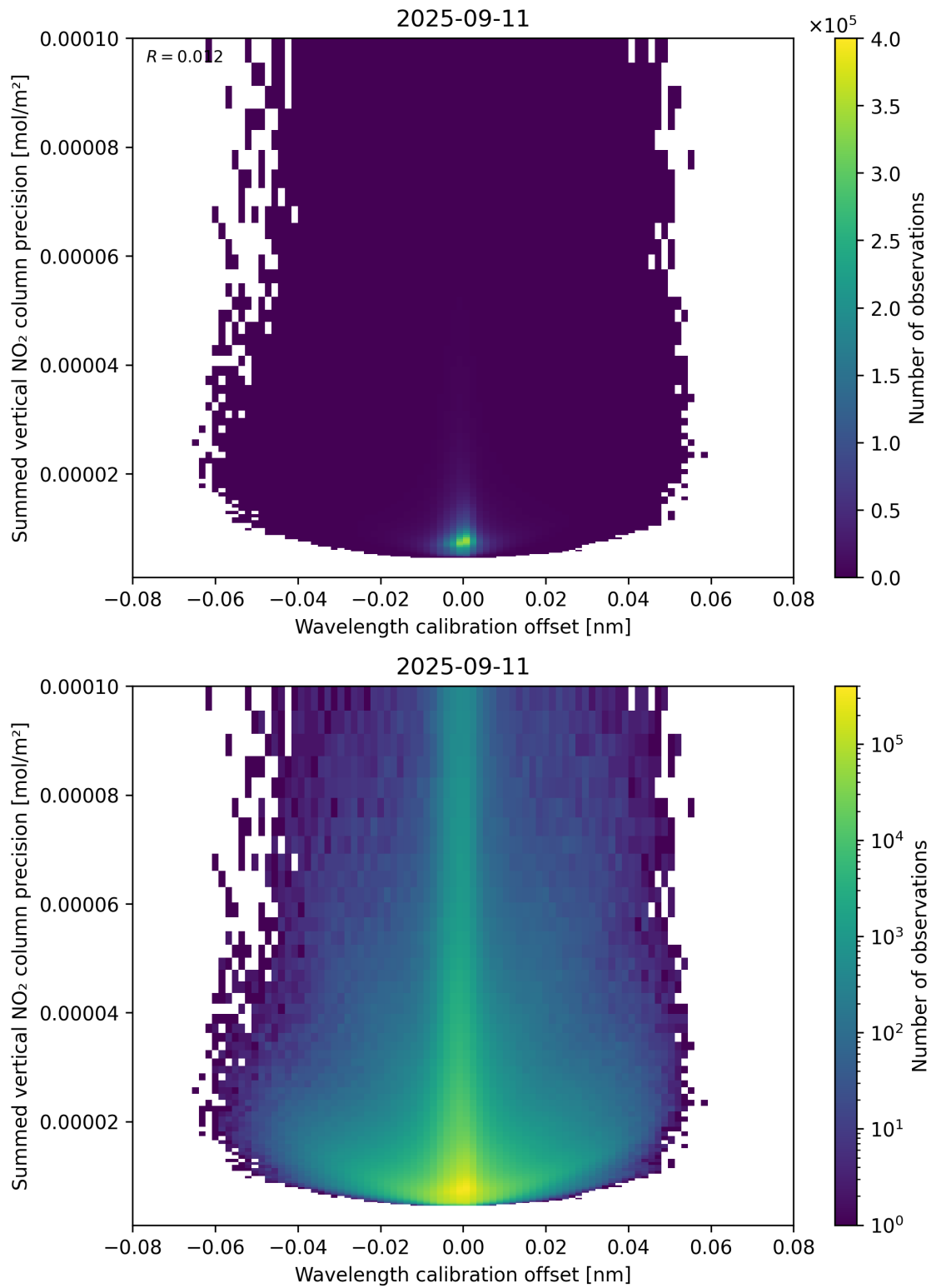
Figure 178: Scatter density plot of “Wavelength calibration offset” against “Summed vertical NO 2 column precision” for 2025-09-10 to 2025-09-12.
