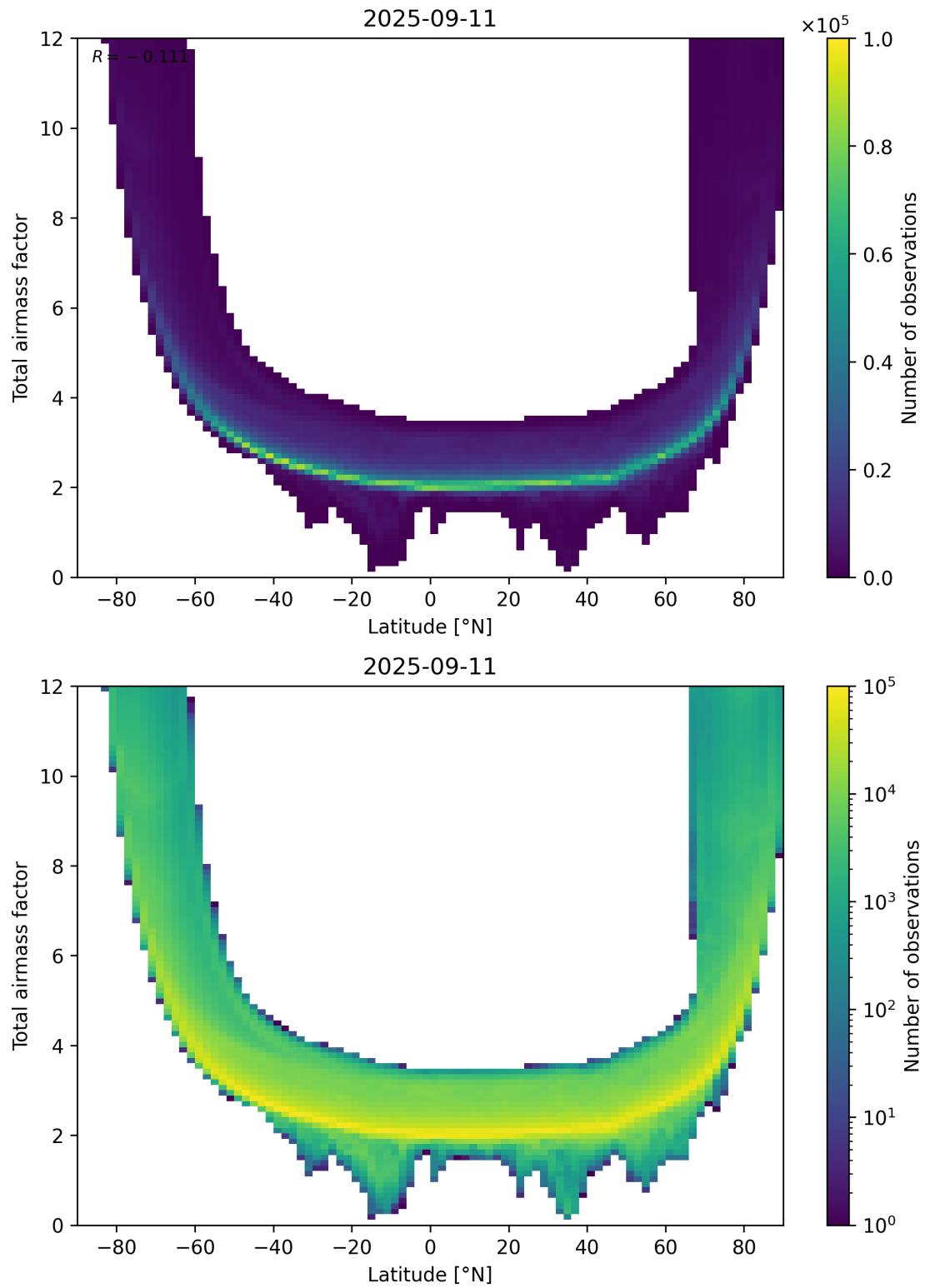
Figure 84: Scatter density plot of “Latitude” against “Total airmass factor” for 2025-09-10 to 2025-09-12.
