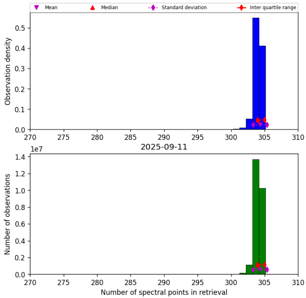
Figure 33: Histogram of “Number of spectral points in retrieval” for 2025-09-10 to 2025-09-12
