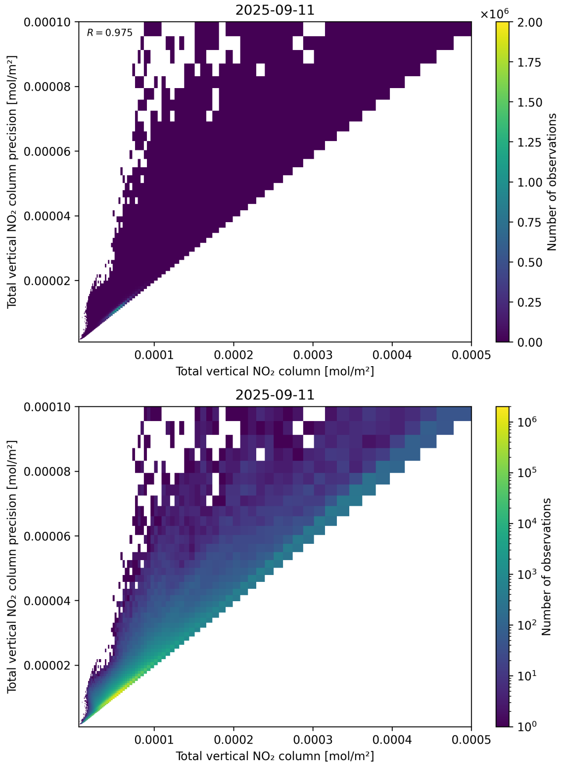
Figure 114: Scatter density plot of “Total vertical NO 2 column” against “Total vertical NO 2 column precision” for 2025-09-10 to 2025-09-12.
