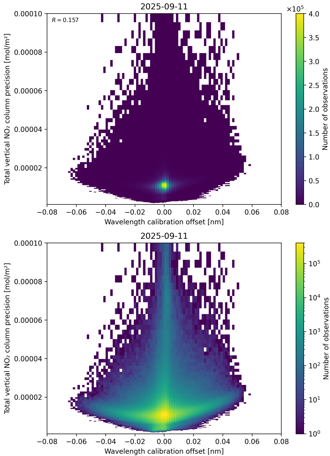
Figure 180: Scatter density plot of “Wavelength calibration offset” against “Total vertical NO 2 column precision” for 2025-09-10 to 2025-09-12.
