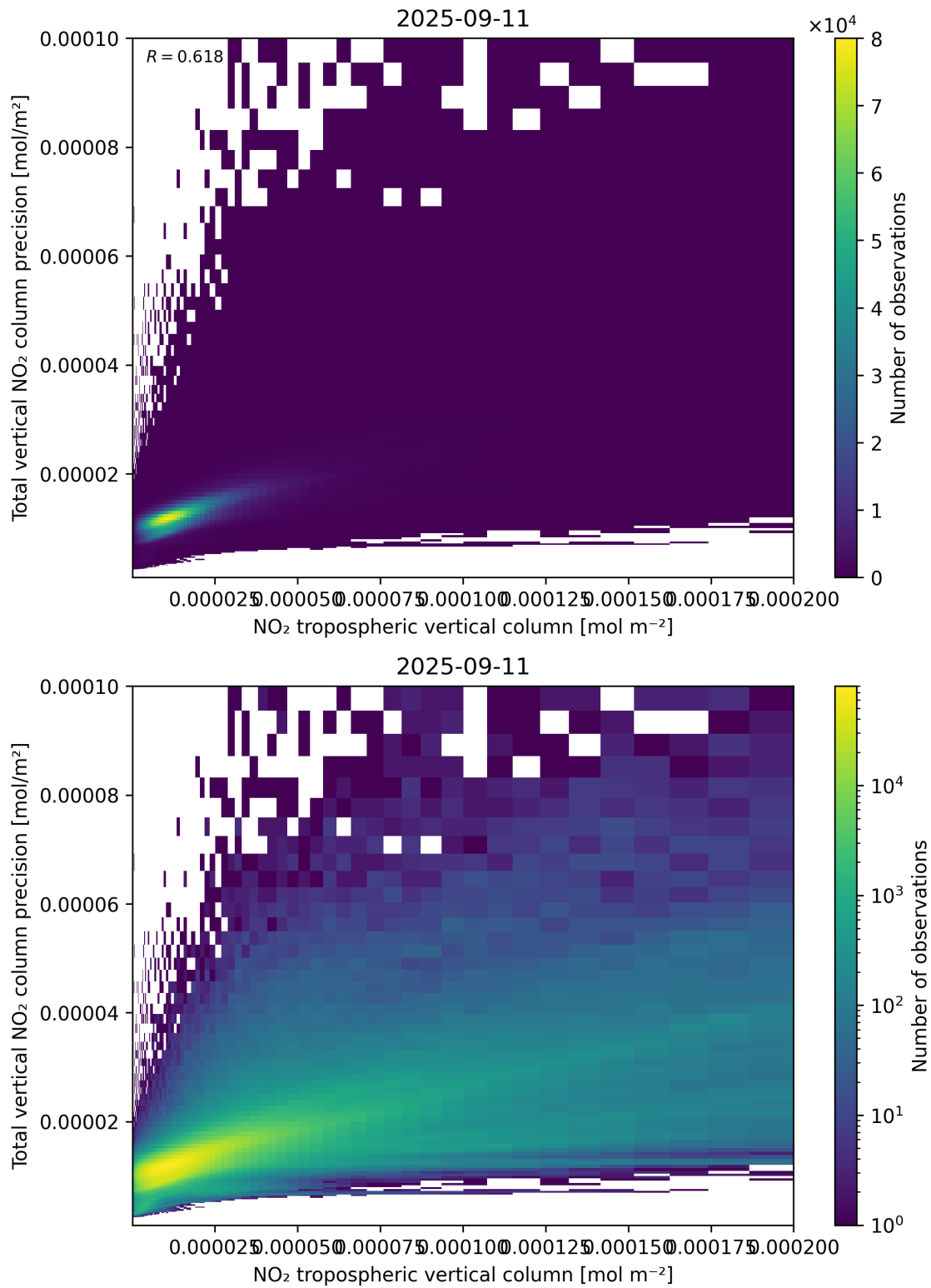
Figure 129: Scatter density plot of “NO 2 tropospheric vertical column” against “Total vertical NO 2 column precision” for 2025-09-10 to 2025-09-12.
