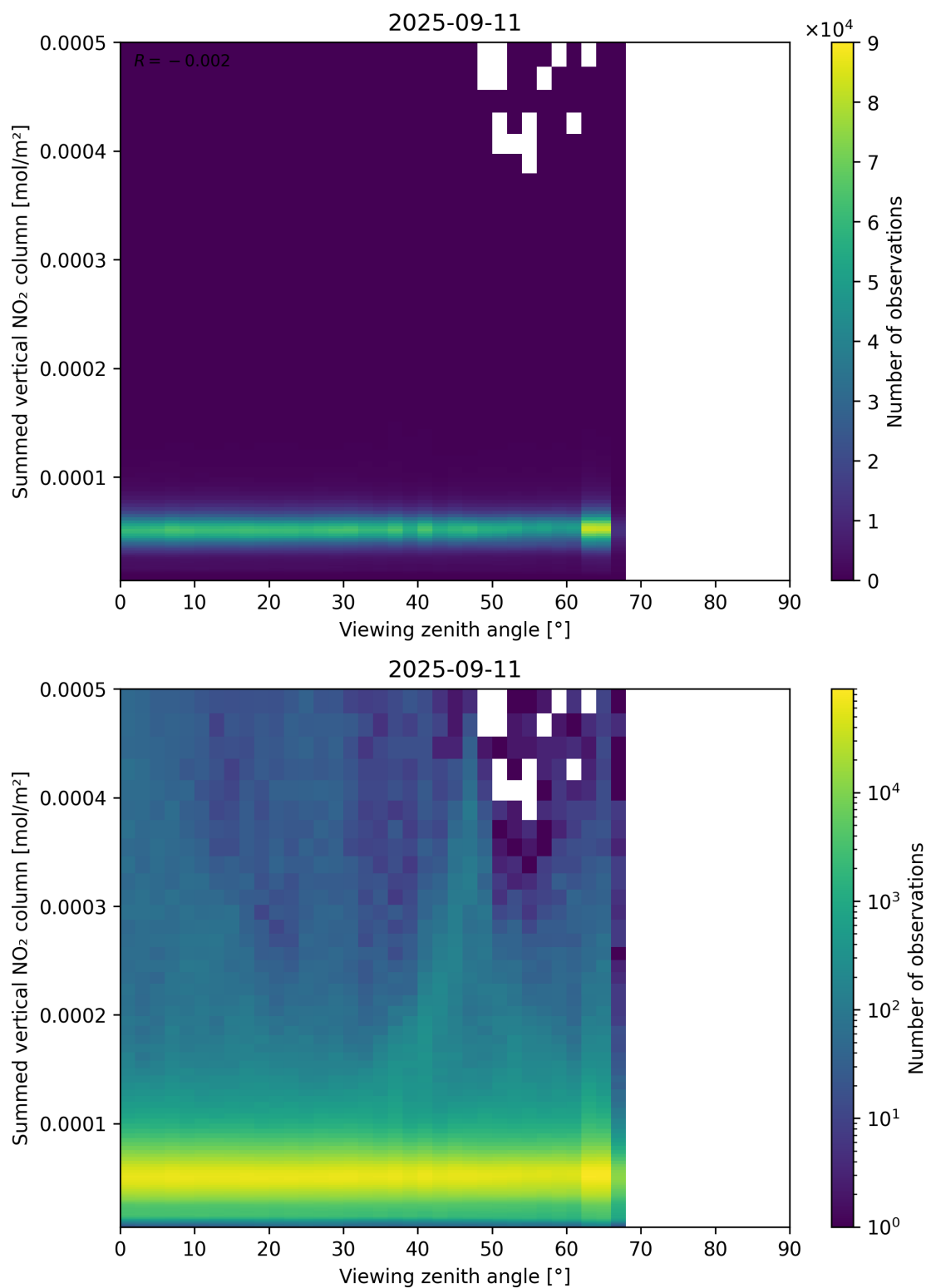
Figure 165: Scatter density plot of “Viewing zenith angle” against “Summed vertical NO 2 column” for 2025-09-10 to 2025-09-12.
