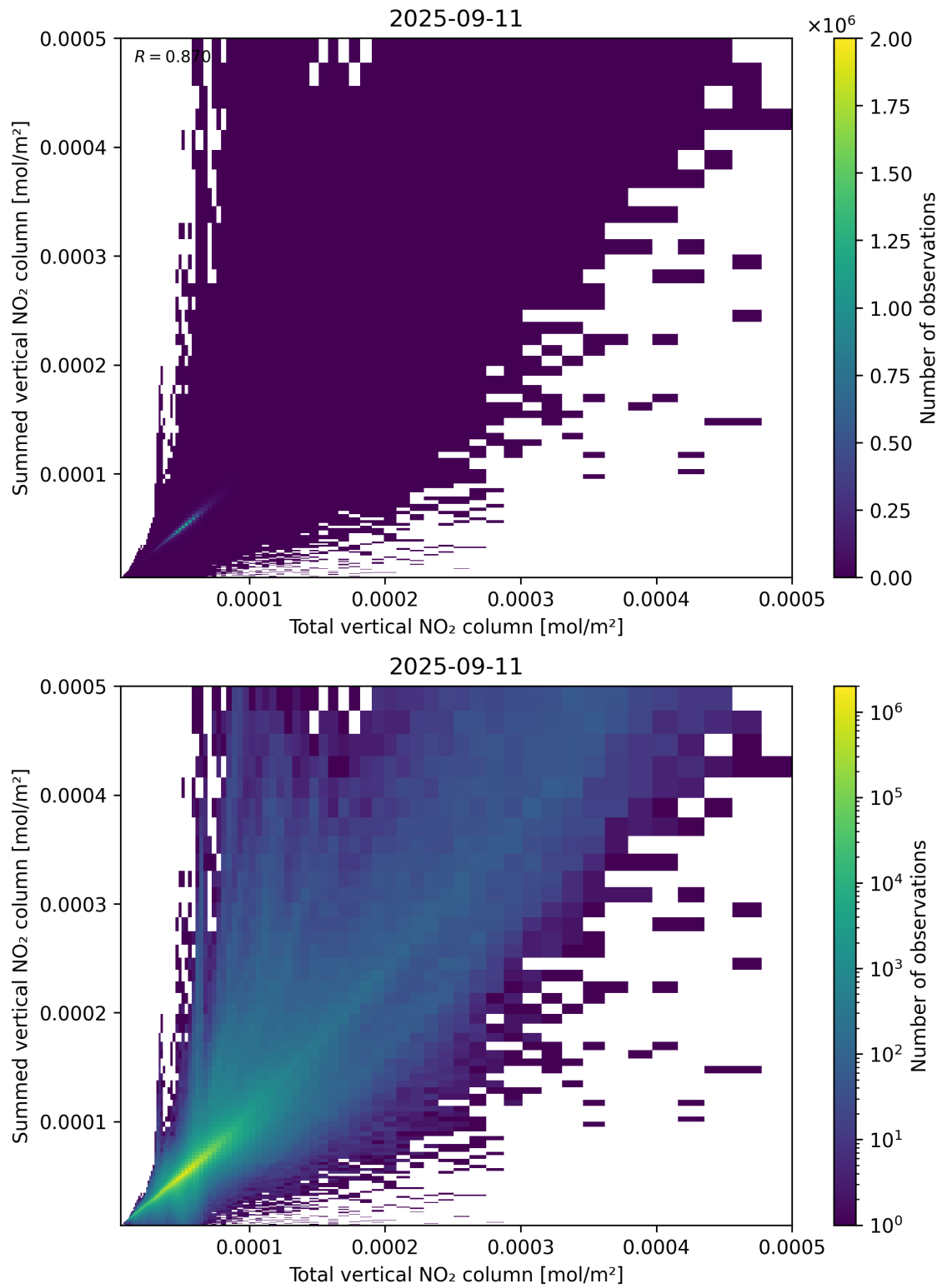
Figure 112: Scatter density plot of “Total vertical NO 2 column” against “Summed vertical NO 2 column” for 2025-09-10 to 2025-09-12.
