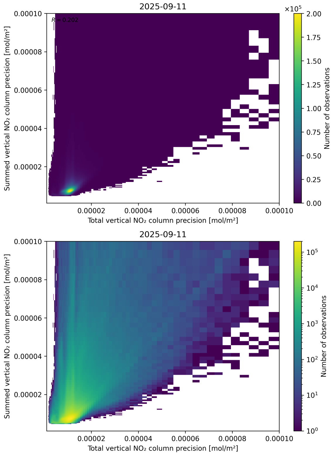
Figure 118: Scatter density plot of “Total vertical NO 2 column precision” against “Summed vertical NO 2 column precision” for 2025-09-10 to 2025-09-12.
