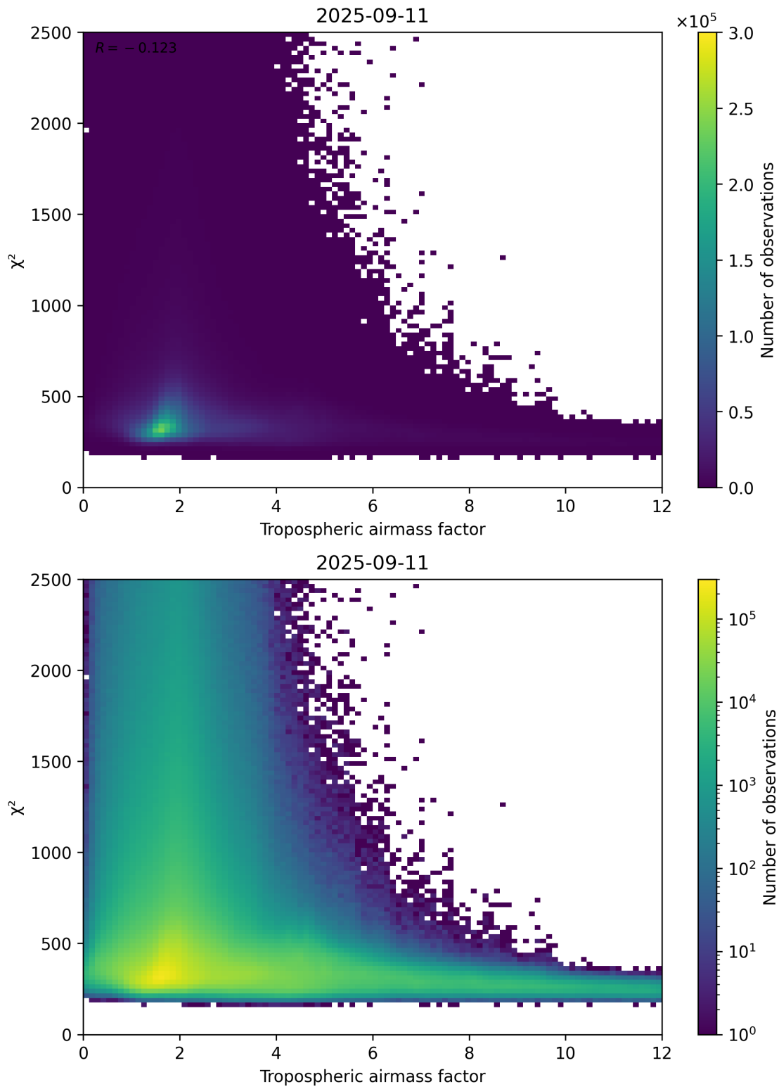
Figure 73: Scatter density plot of “Tropospheric airmass factor” against “ \chi^2 ” for 2025-09-10 to 2025-09-12.
