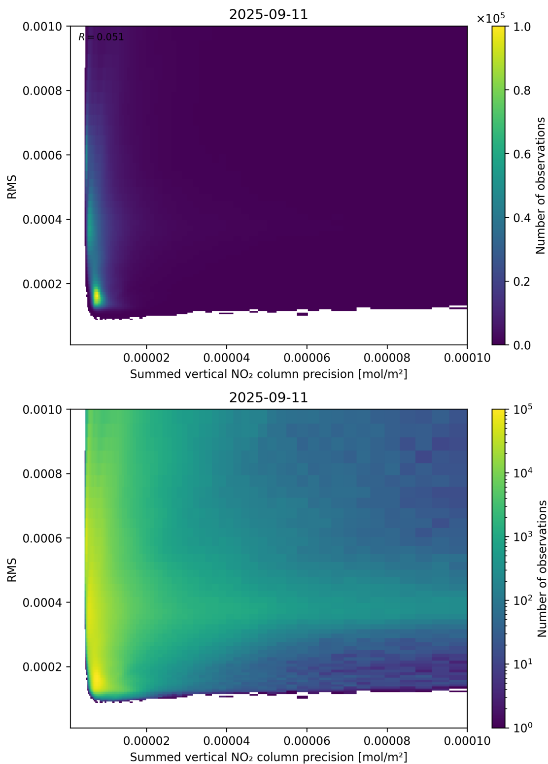
Figure 108: Scatter density plot of “Summed vertical NO 2 column precision” against “RMS” for 2025-09-10 to 2025-09-12.
