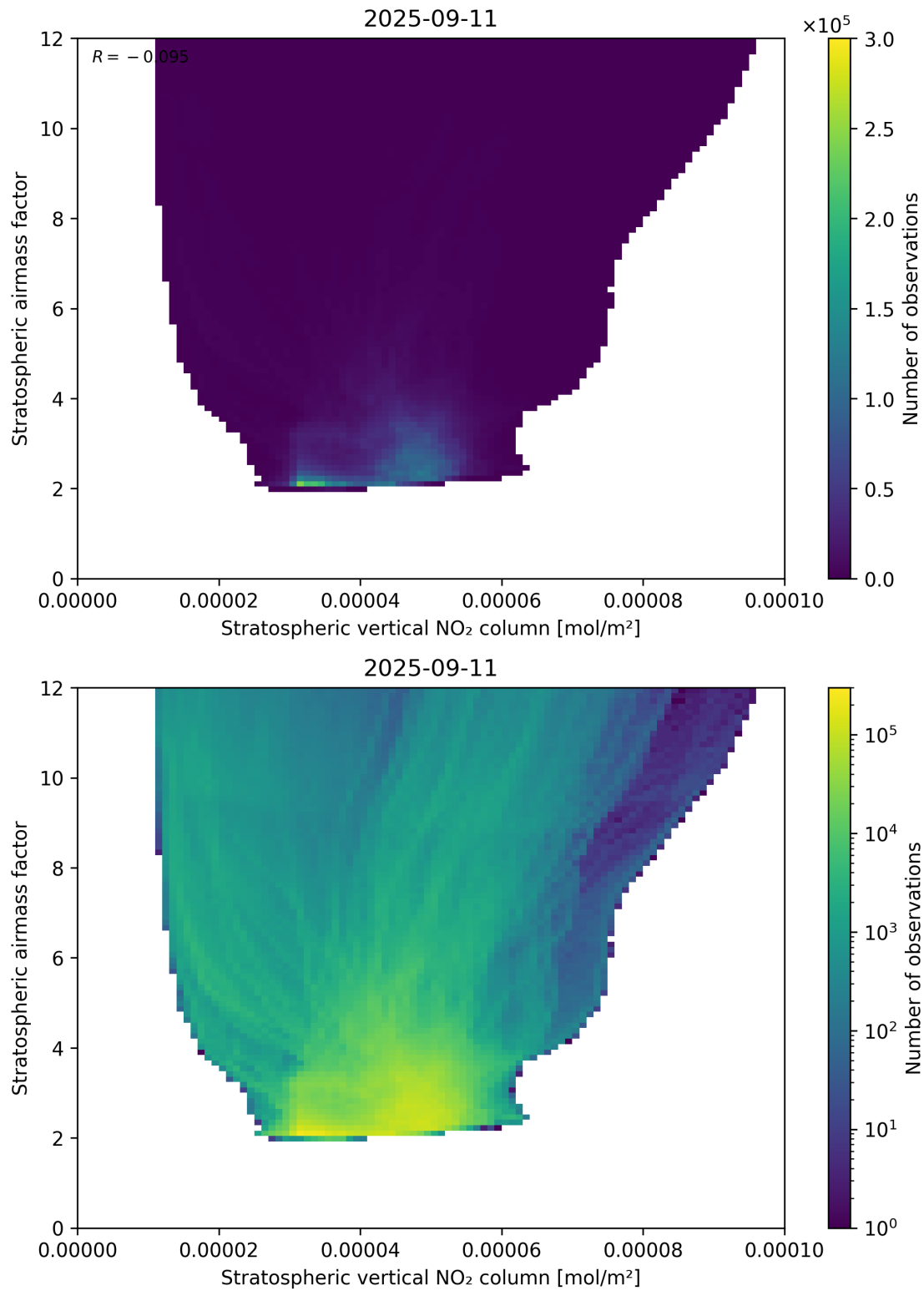
Figure 96: Scatter density plot of “Stratospheric vertical NO 2 column” against “Stratospheric airmass factor” for 2025-09-10 to 2025-09-12.
