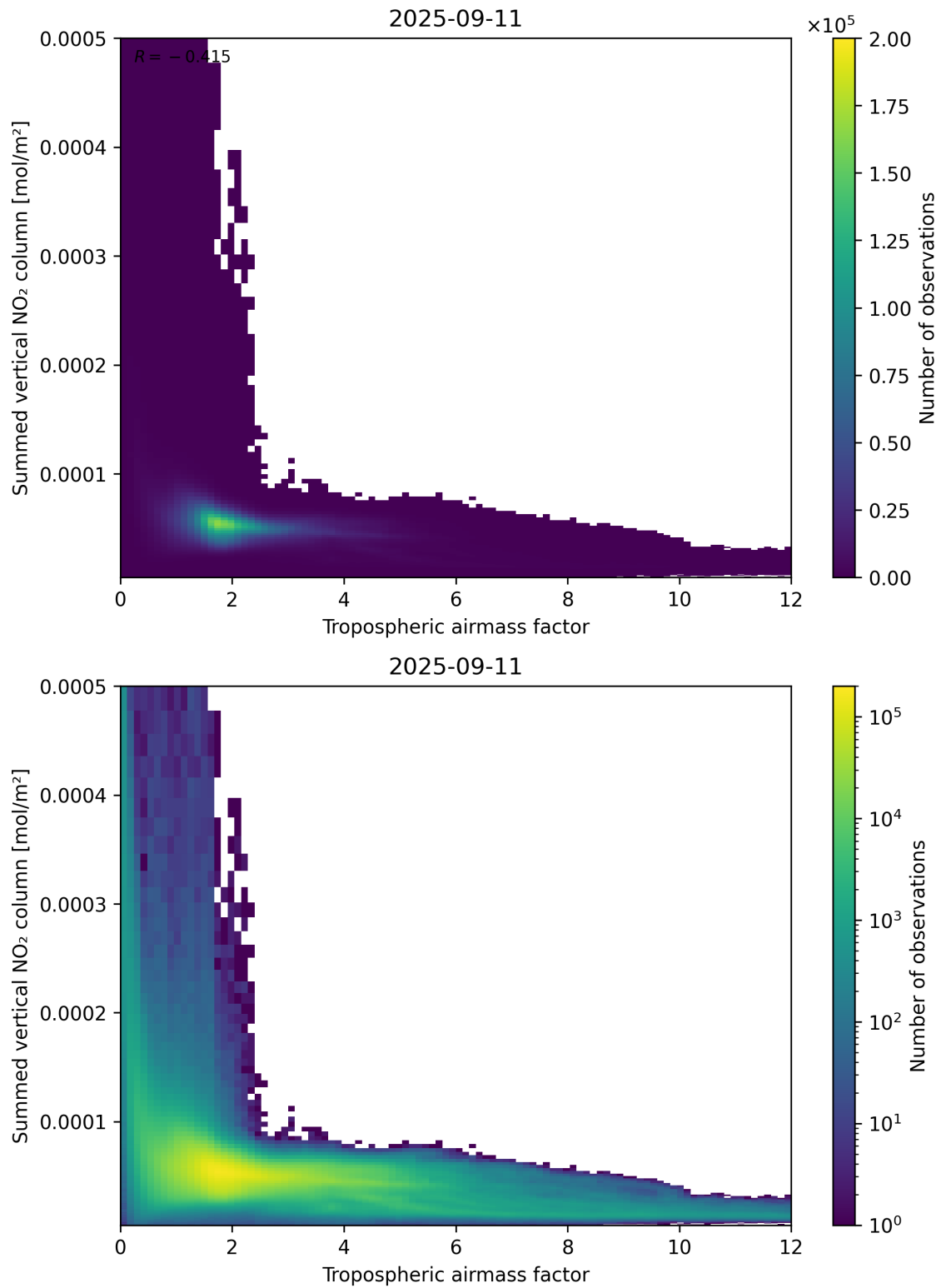
Figure 75: Scatter density plot of “Tropospheric airmass factor” against “Summed vertical NO 2 column” for 2025-09-10 to 2025-09-12.
