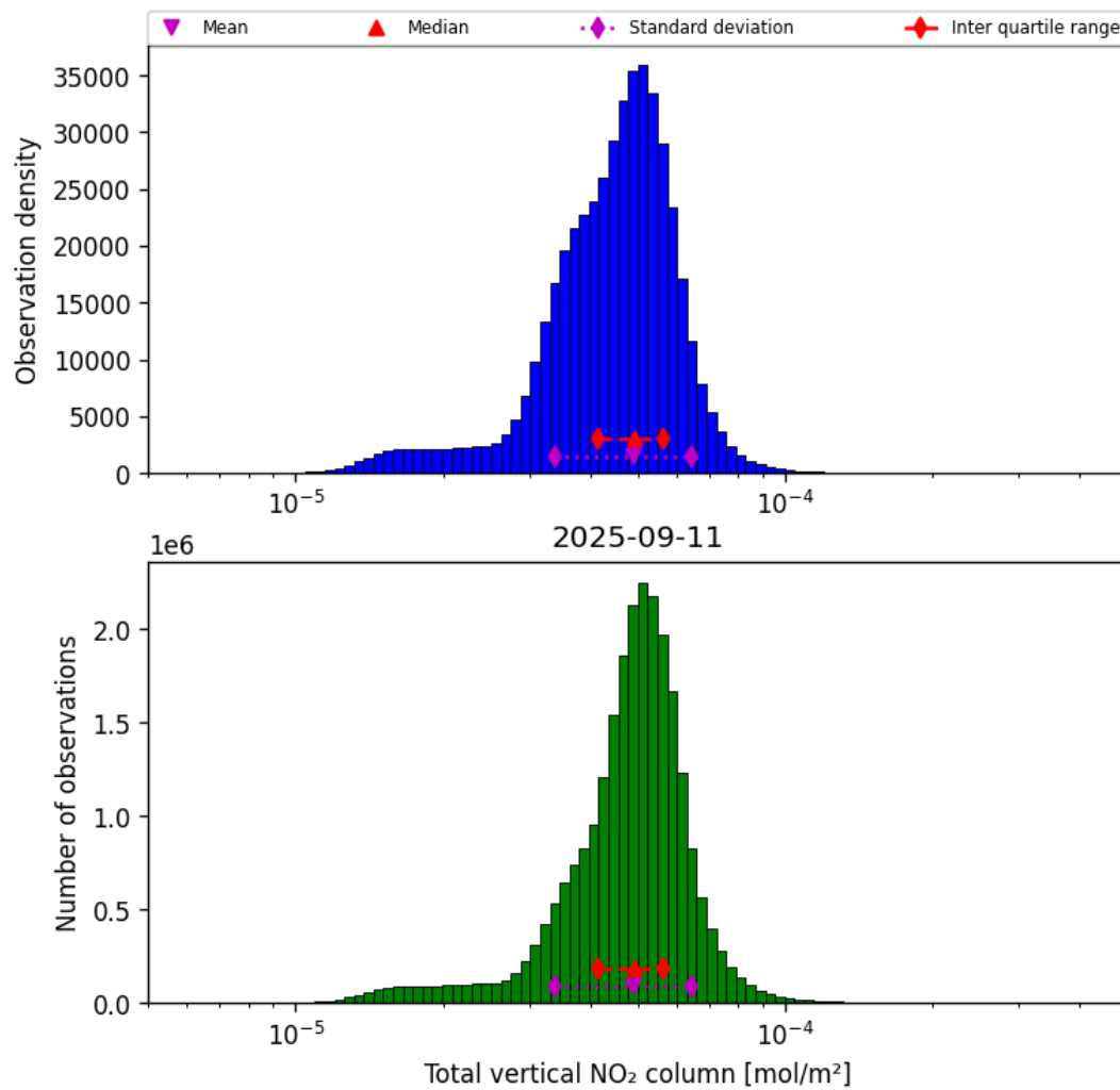
Figure 38: Histogram of “Total vertical NO 2 column” for 2025-09-10 to 2025-09-12
