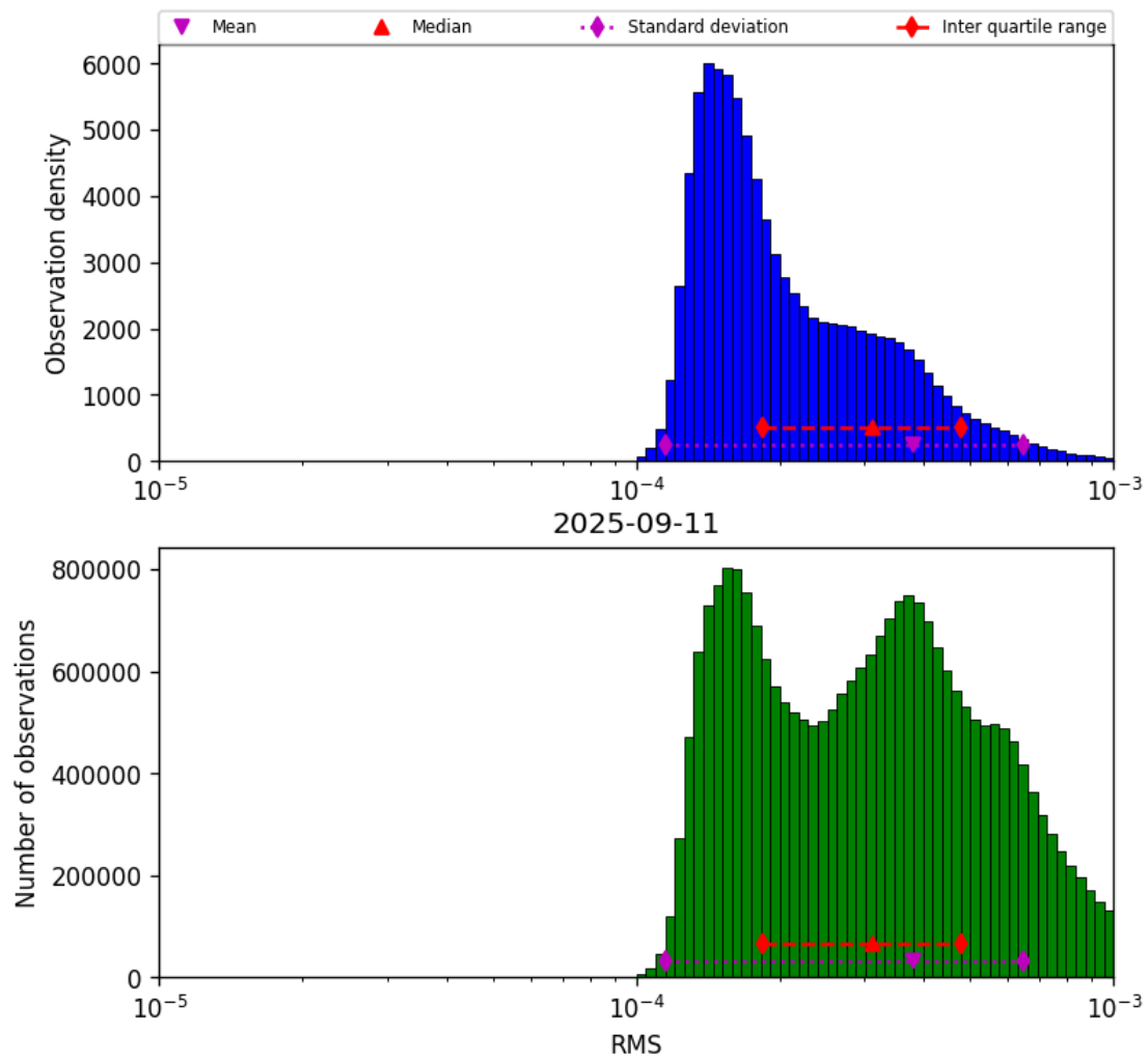
Figure 43: Histogram of “RMS” for 2025-09-10 to 2025-09-12
