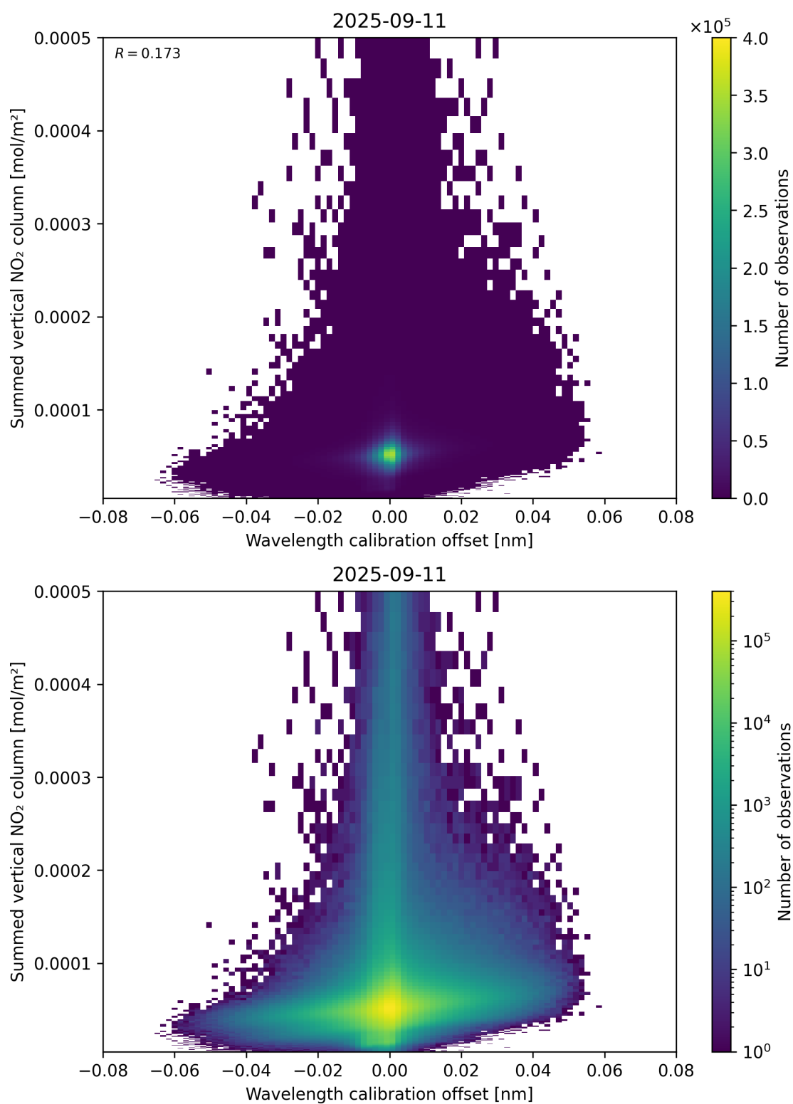
Figure 177: Scatter density plot of “Wavelength calibration offset” against “Summed vertical NO 2 column” for 2025-09-10 to 2025-09-12.
