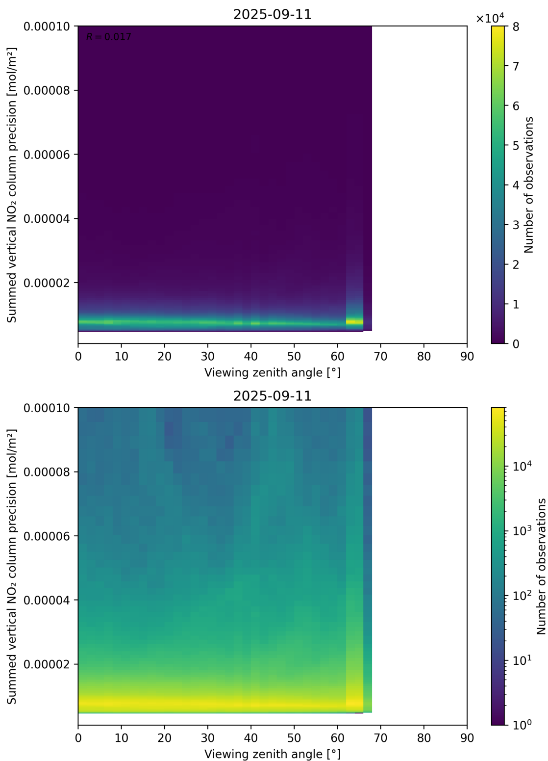
Figure 166: Scatter density plot of “Viewing zenith angle” against “Summed vertical NO 2 column precision” for 2025-09-10 to 2025-09-12.
