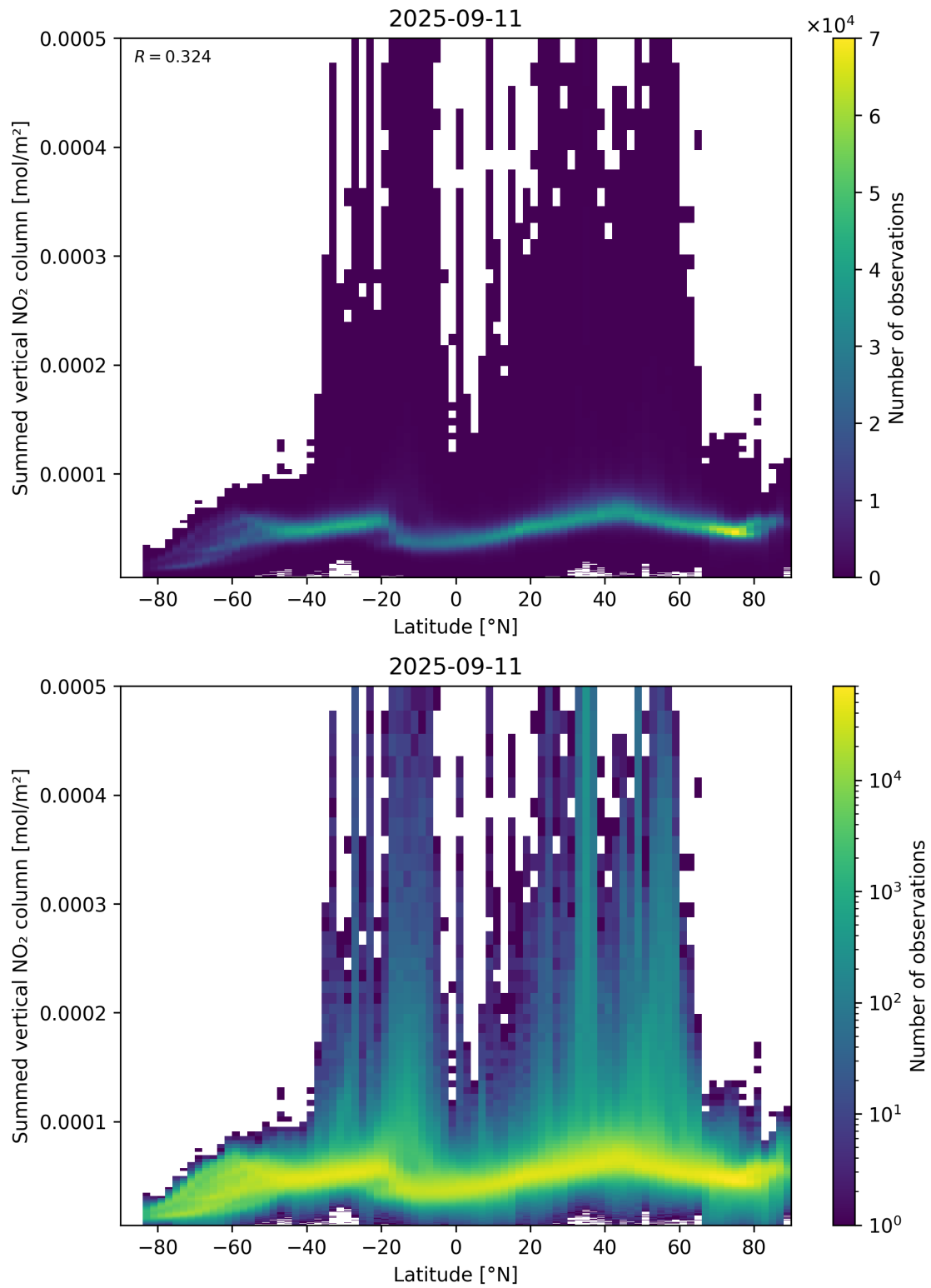
Figure 88: Scatter density plot of “Latitude” against “Summed vertical NO 2 column” for 2025-09-10 to 2025-09-12.
