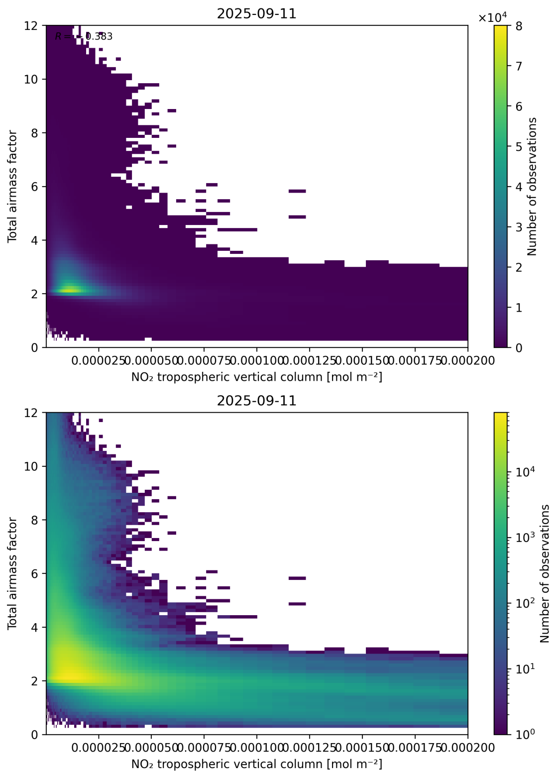
Figure 122: Scatter density plot of “NO 2 tropospheric vertical column” against “Total air mass factor” for 2025-09-10 to 2025-09-12.
