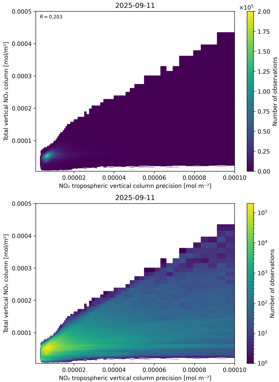
Figure 138: Scatter density plot of “NO 2 tropospheric vertical column precision” against “Total vertical NO 2 column” for 2025-09-10 to 2025-09-12.
