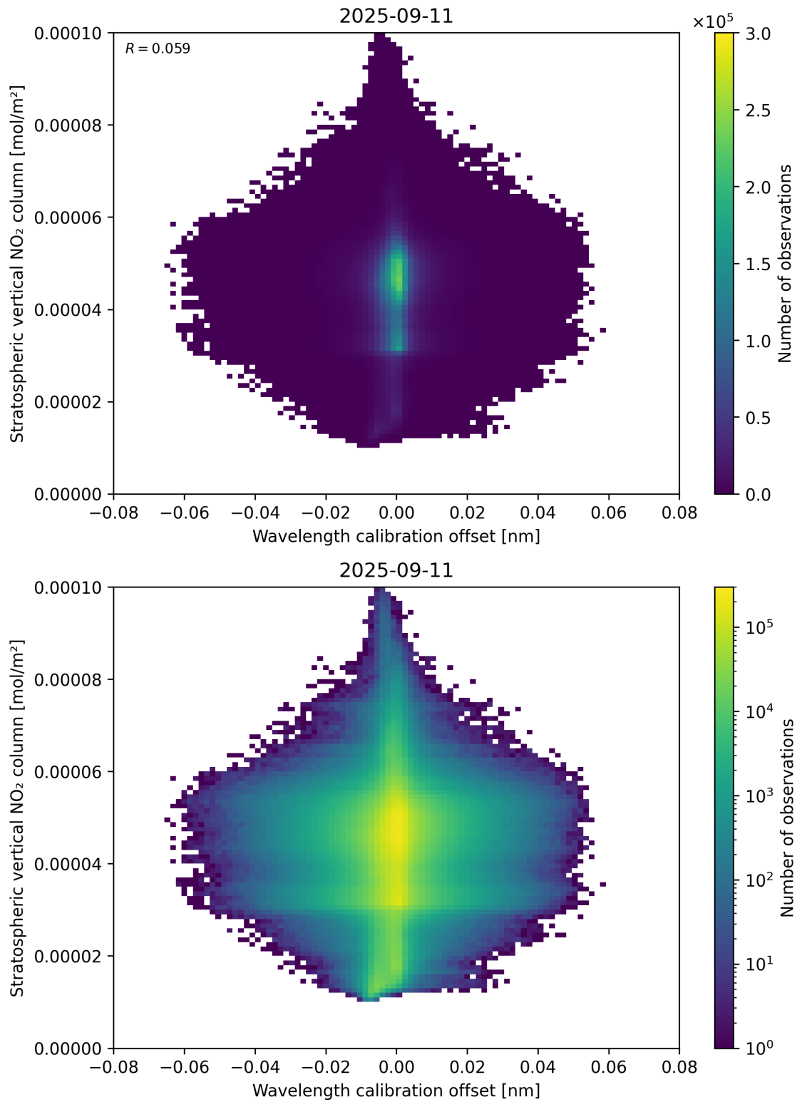
Figure 176: Scatter density plot of “Wavelength calibration offset” against “Stratospheric vertical NO 2 column” for 2025-09-10 to 2025-09-12.
