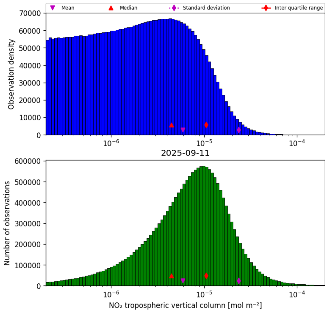
Figure 29: Histogram of “NO 2 tropospheric vertical column” for 2025-09-10 to 2025-09-12
