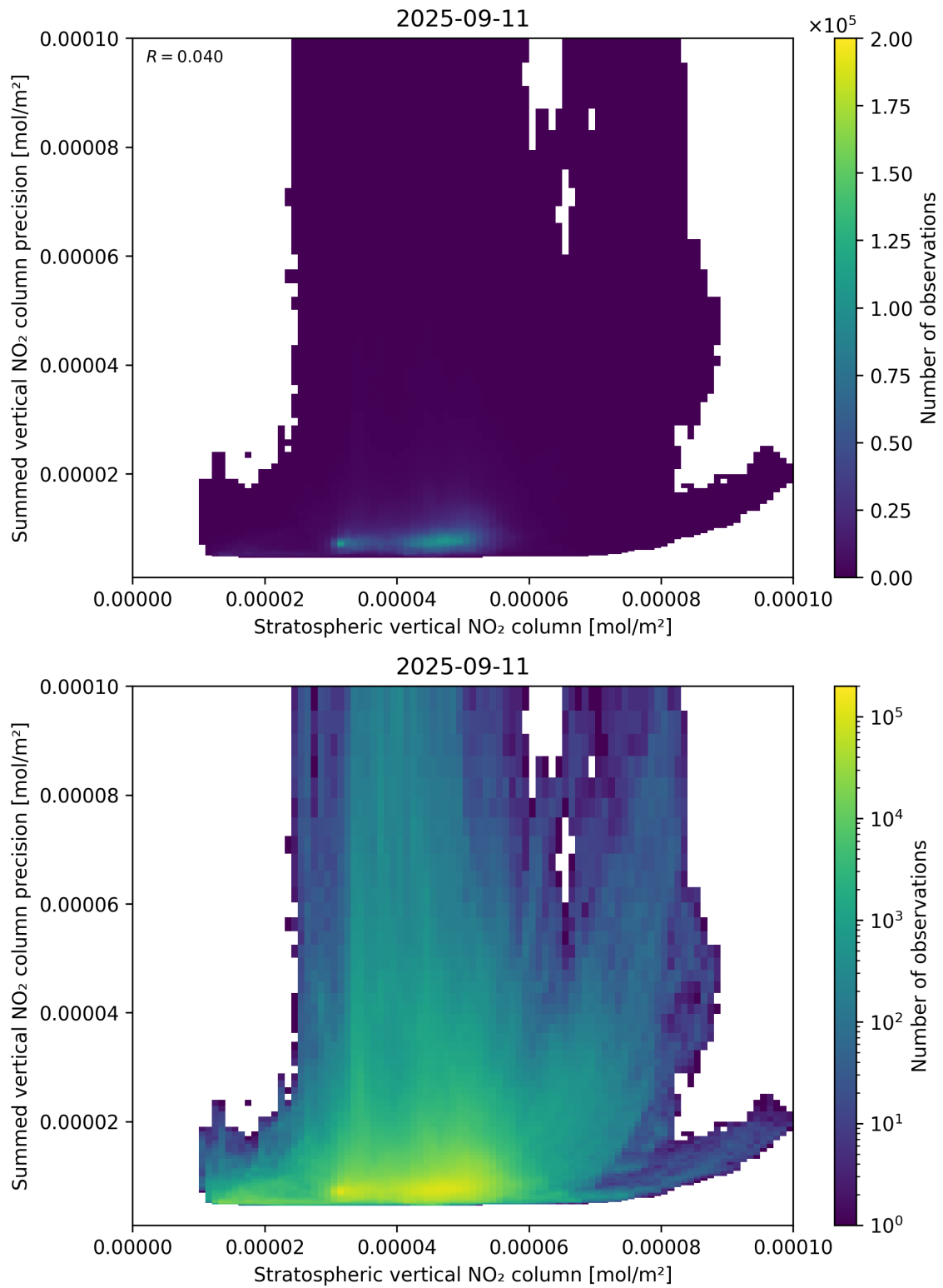
Figure 99: Scatter density plot of “Stratospheric vertical NO 2 column” against “Summed vertical NO 2 column precision” for 2025-09-10 to 2025-09-12.
