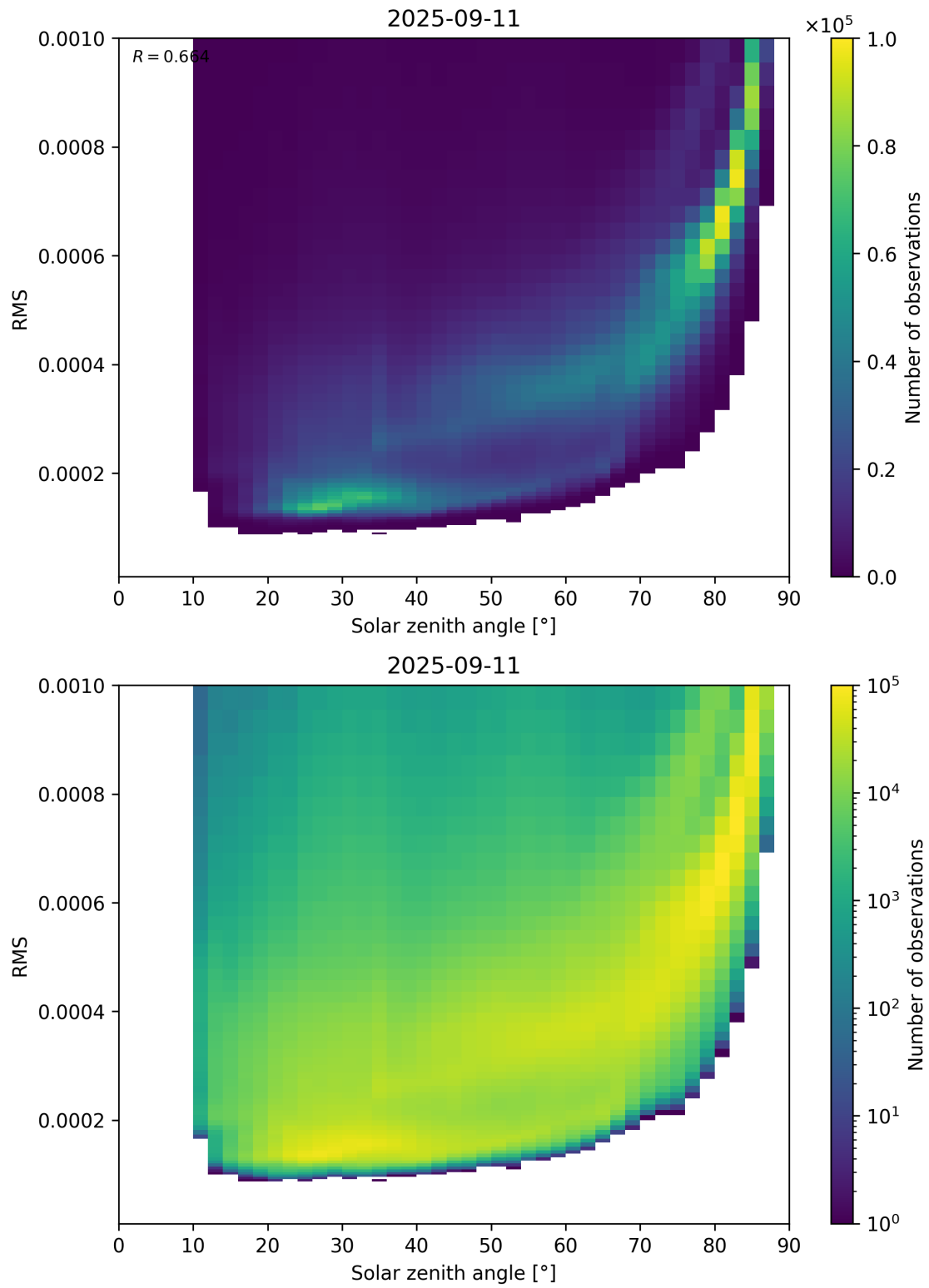
Figure 157: Scatter density plot of “Solar zenith angle” against “RMS” for 2025-09-10 to 2025-09-12.
