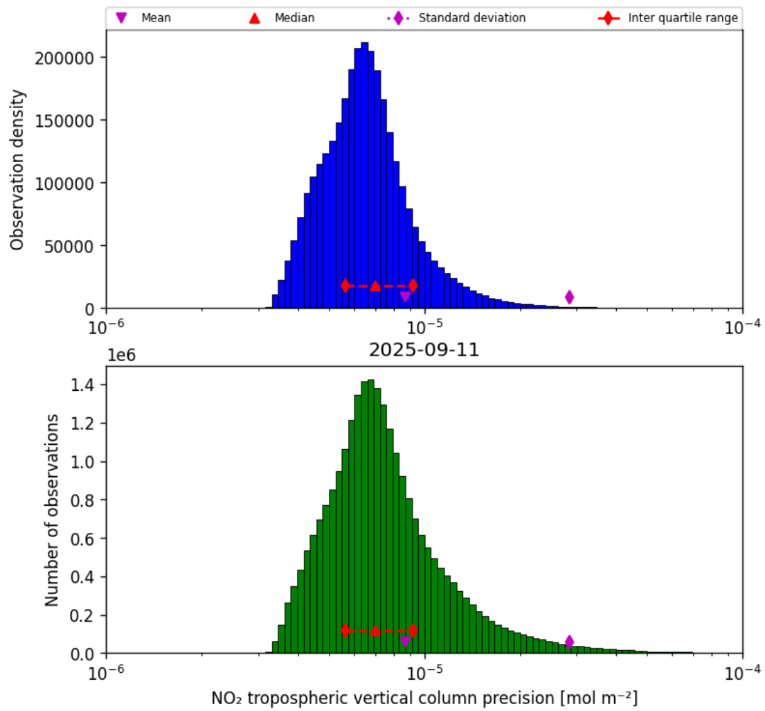
Figure 30: Histogram of “NO 2 tropospheric vertical column precision” for 2025-09-10 to 2025-09-12
