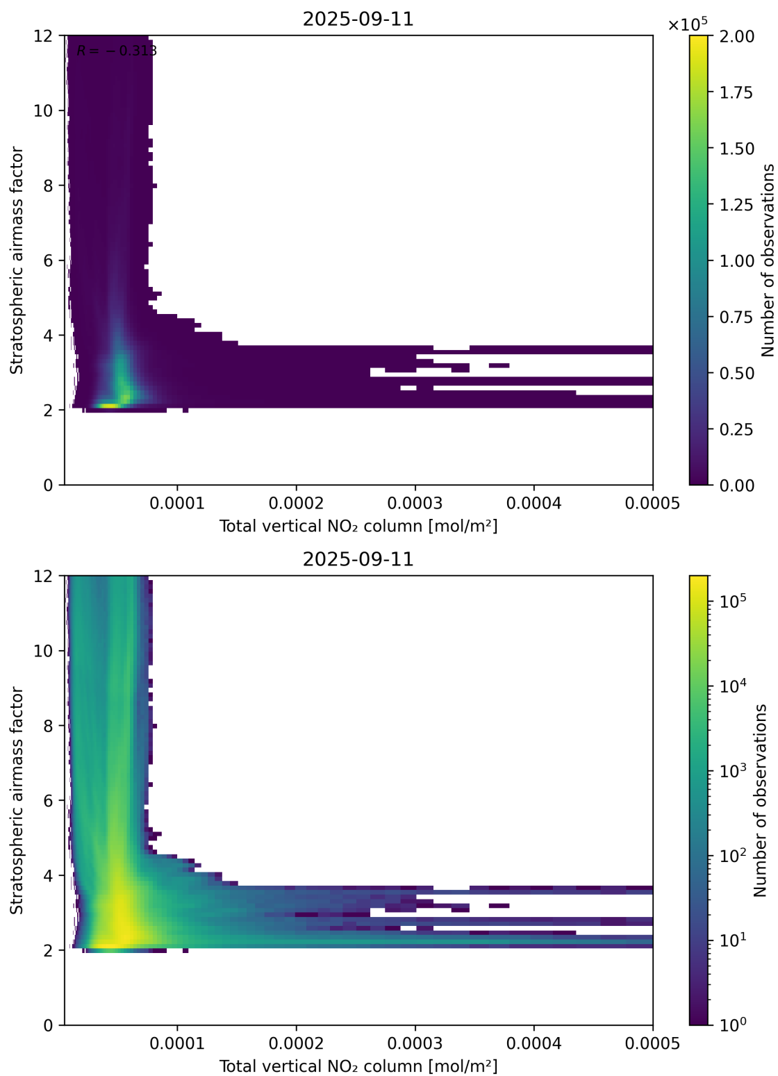
Figure 110: Scatter density plot of “Total vertical NO 2 column” against “Stratospheric airmass factor” for 2025-09-10 to 2025-09-12.
