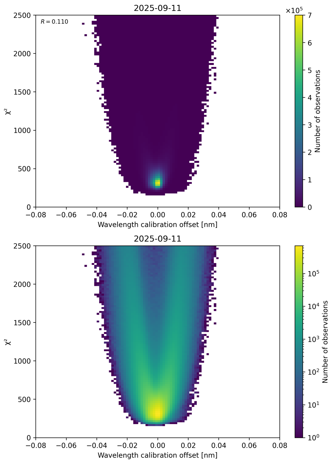
Figure 175: Scatter density plot of “Wavelength calibration offset” against “ \chi^2 ” for 2025-09-10 to 2025-09-12.
