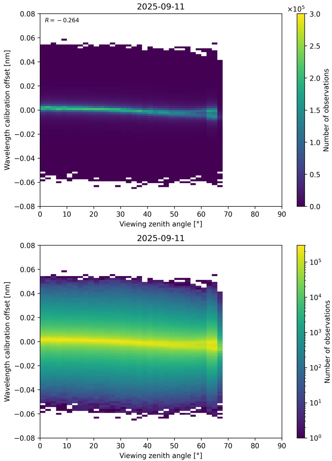
Figure 173: Scatter density plot of “Viewing zenith angle” against “Wavelength calibration offset” for 2025-09-10 to 2025-09-12.
