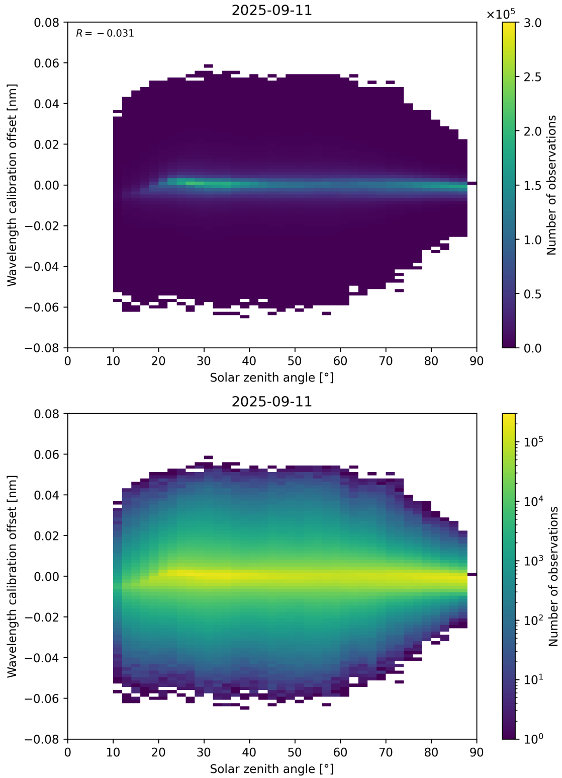
Figure 158: Scatter density plot of “Solar zenith angle” against “Wavelength calibration offset” for 2025-09-10 to 2025-09-12.
