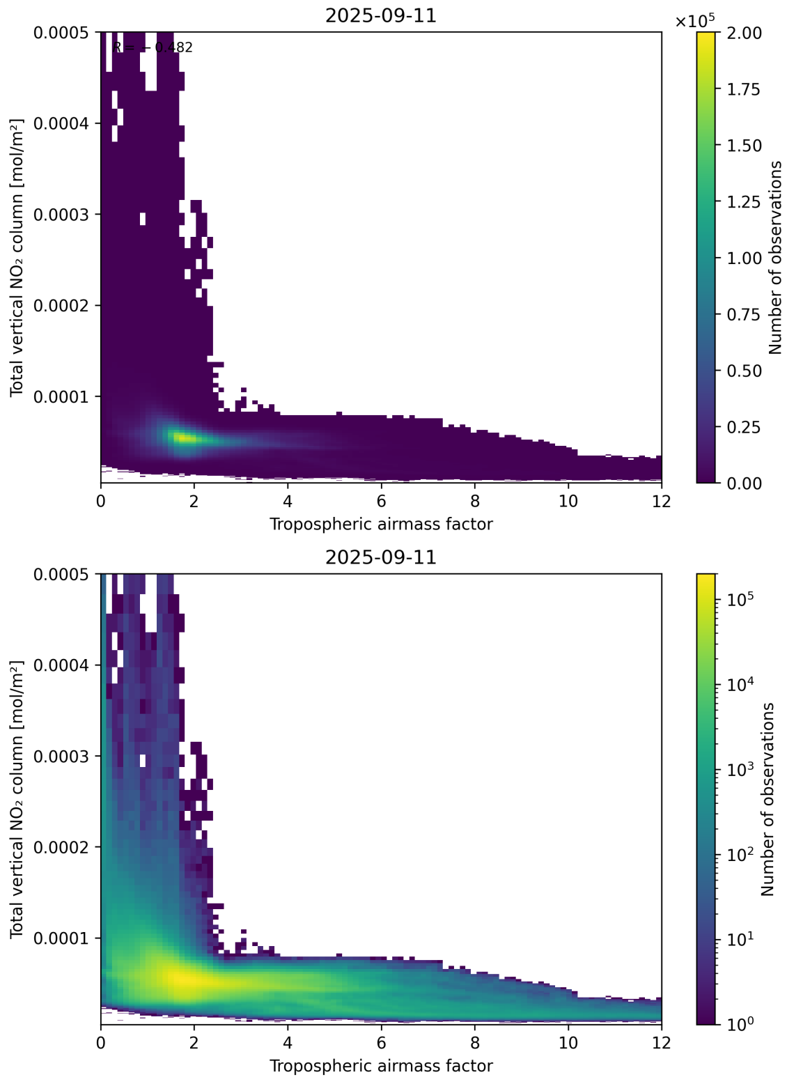
Figure 77: Scatter density plot of “Tropospheric airmass factor” against “Total vertical NO 2 column” for 2025-09-10 to 2025-09-12.
