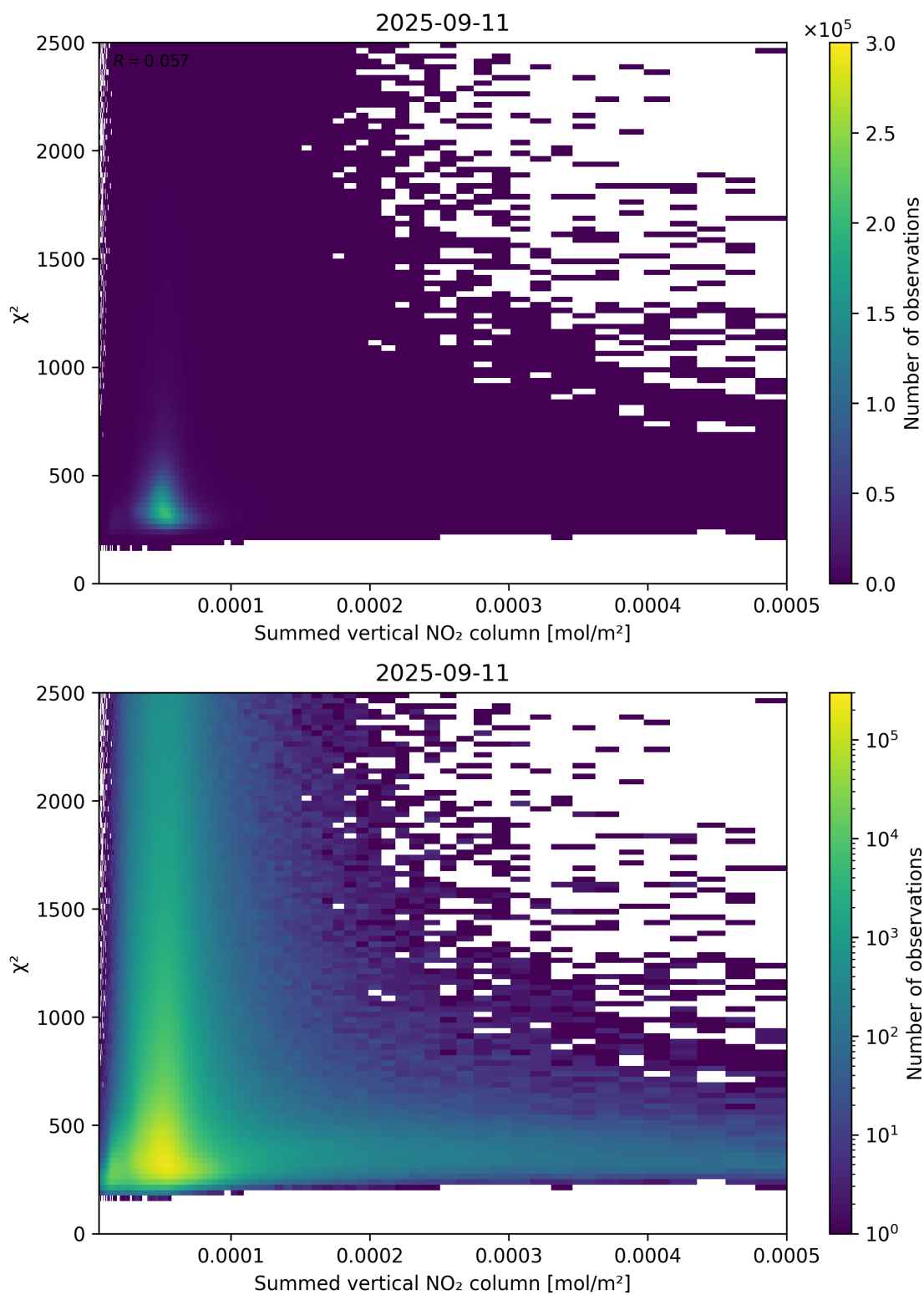
Figure 104: Scatter density plot of “Summed vertical NO 2 column” against “ \chi^2 ” for 2025-09-10 to 2025-09-12.
