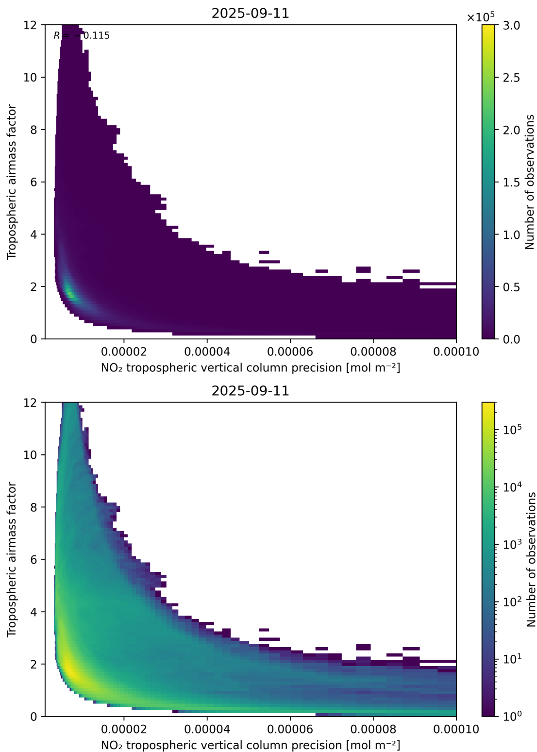
Figure 133: Scatter density plot of “NO 2 tropospheric vertical column precision” against “Tropospheric air mass factor” for 2025-09-10 to 2025-09-12.
