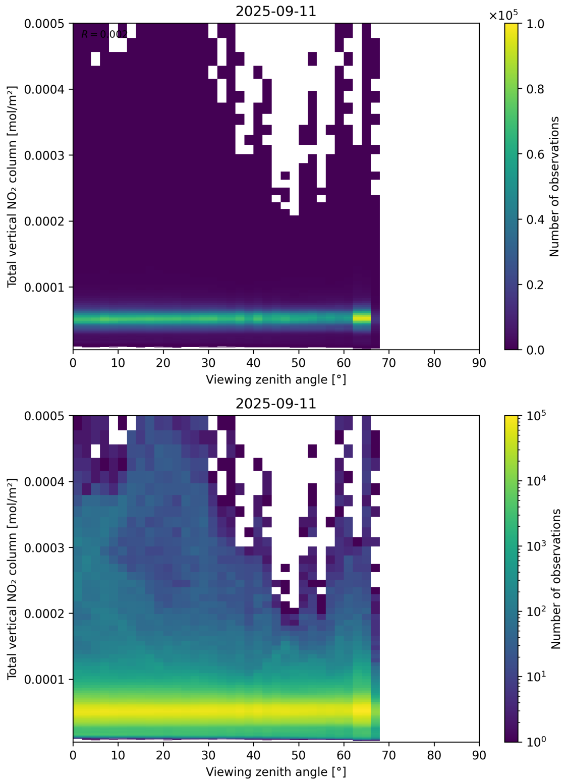
Figure 167: Scatter density plot of “Viewing zenith angle” against “Total vertical NO 2 column” for 2025-09-10 to 2025-09-12.
