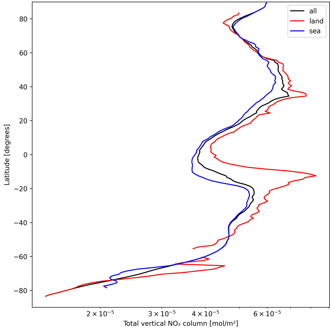
Figure 21: Zonal average of “Total vertical NO 2 column” for 2025-09-10 to 2025-09-12.
