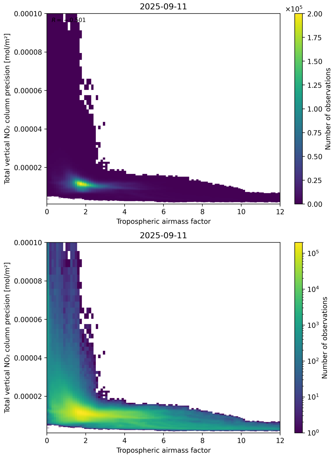
Figure 78: Scatter density plot of “Tropospheric air mass factor” against “Total vertical NO 2 column precision” for 2025-09-10 to 2025-09-12.
