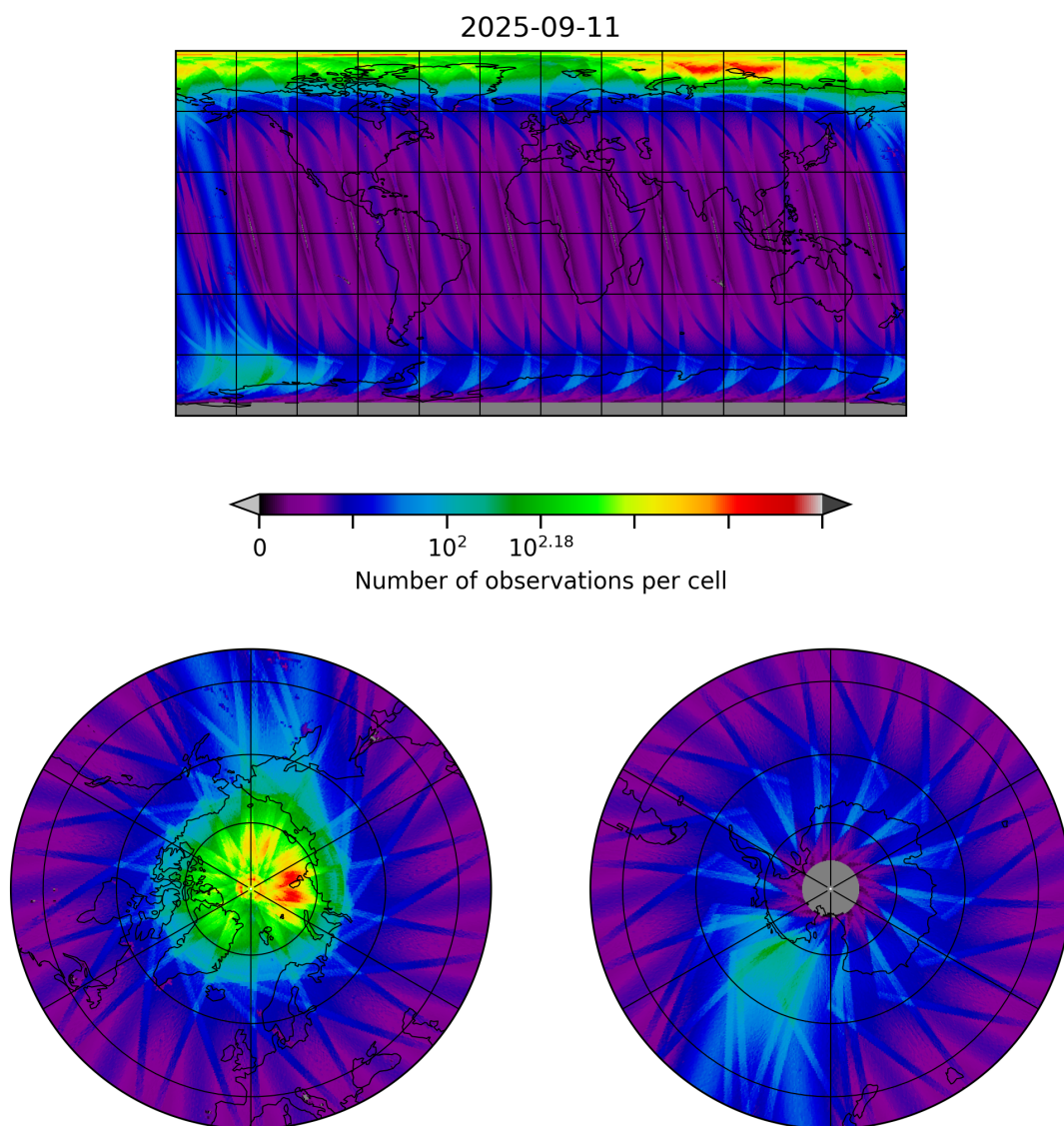
Figure 10: Map of the number of observations for 2025-09-10 to 2025-09-12
