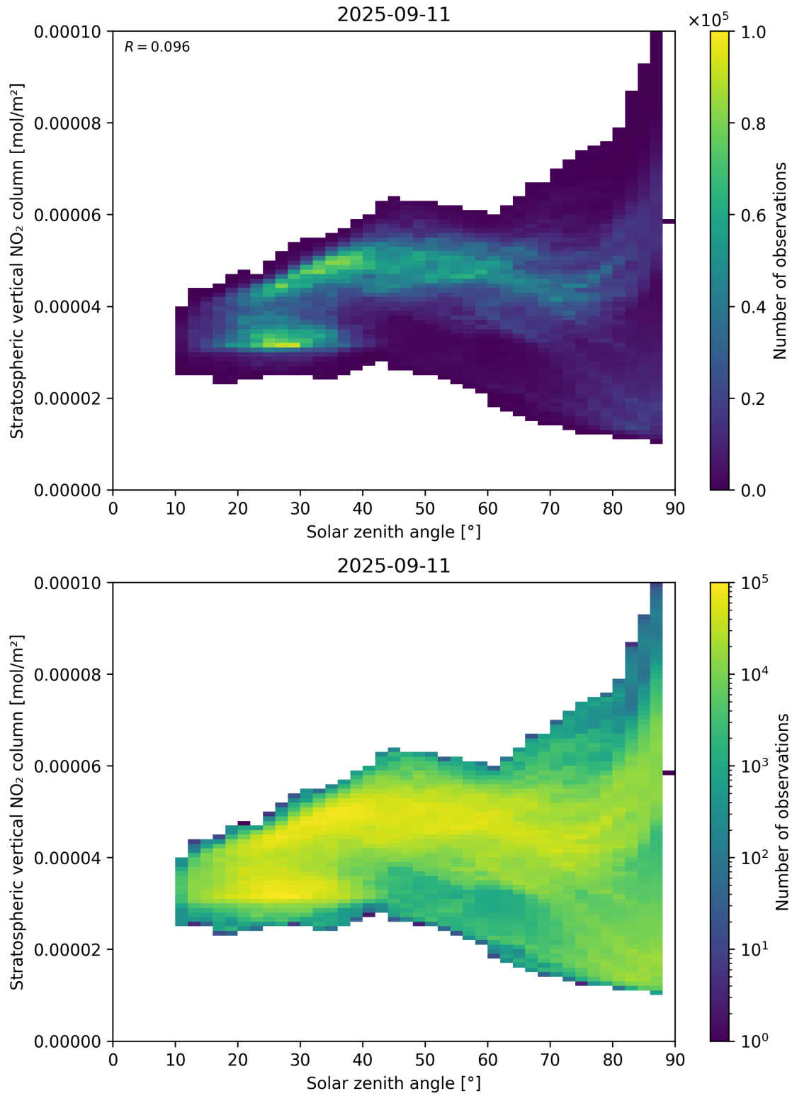
Figure 150: Scatter density plot of “Solar zenith angle” against “Stratospheric vertical NO 2 column” for 2025-09-10 to 2025-09-12.
