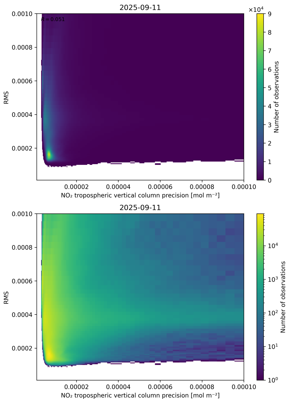
Figure 140: Scatter density plot of “NO 2 tropospheric vertical column precision” against “RMS” for 2025-09-10 to 2025-09-12.
