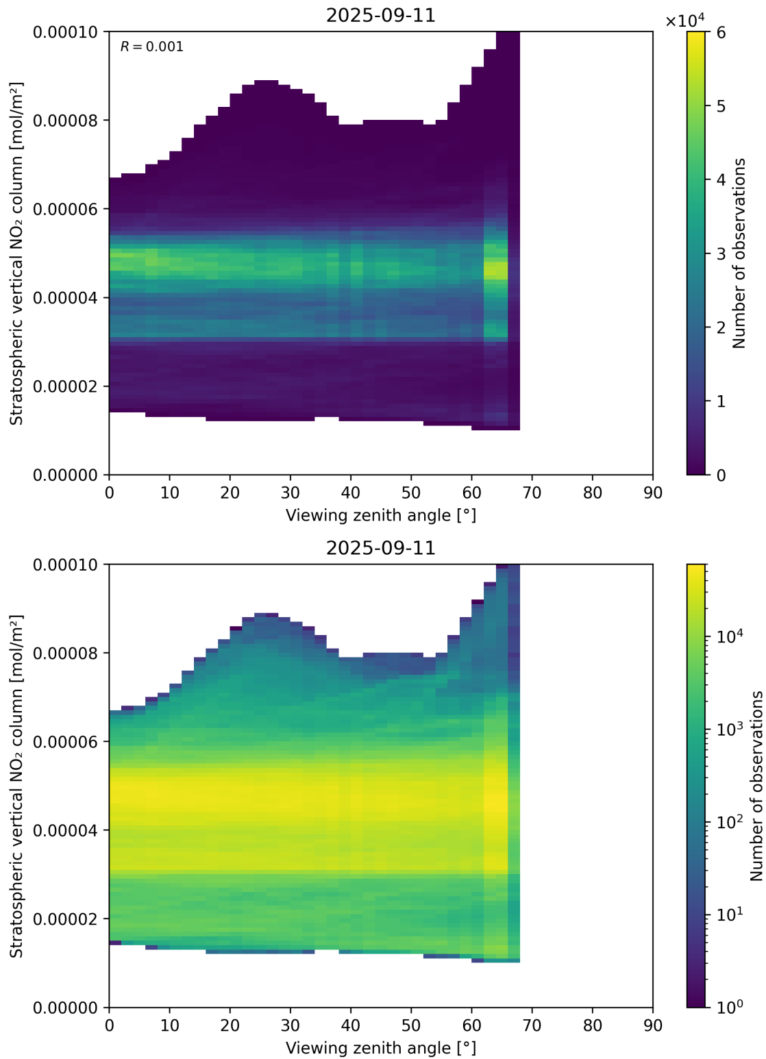
Figure 164: Scatter density plot of “Viewing zenith angle” against “Stratospheric vertical NO 2 column” for 2025-09-10 to 2025-09-12.
