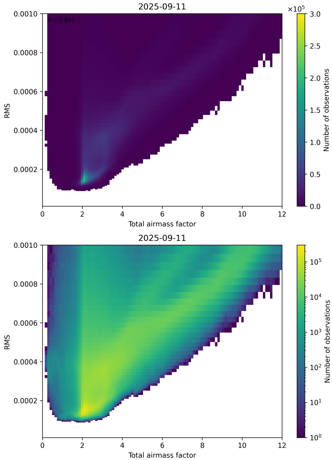
Figure 69: Scatter density plot of “Total airmass factor” against “RMS” for 2025-09-10 to 2025-09-12.
