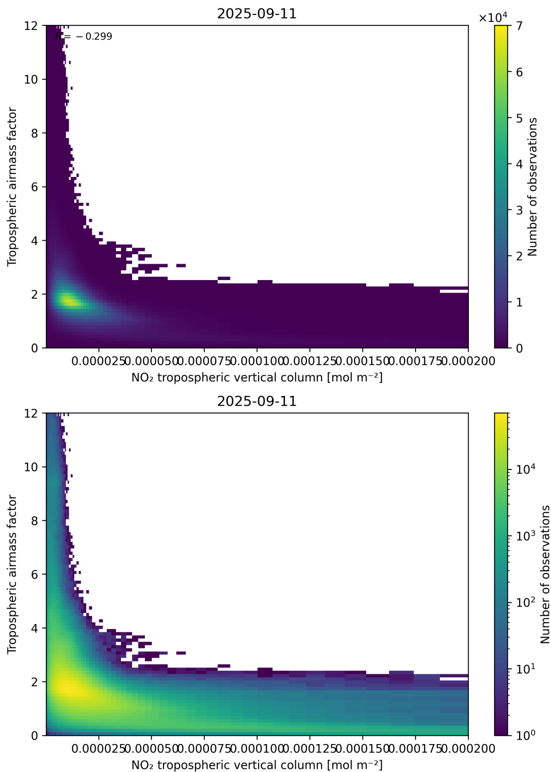
Figure 123: Scatter density plot of “NO 2 tropospheric vertical column” against “Tropospheric air mass factor” for 2025-09-10 to 2025-09-12.
