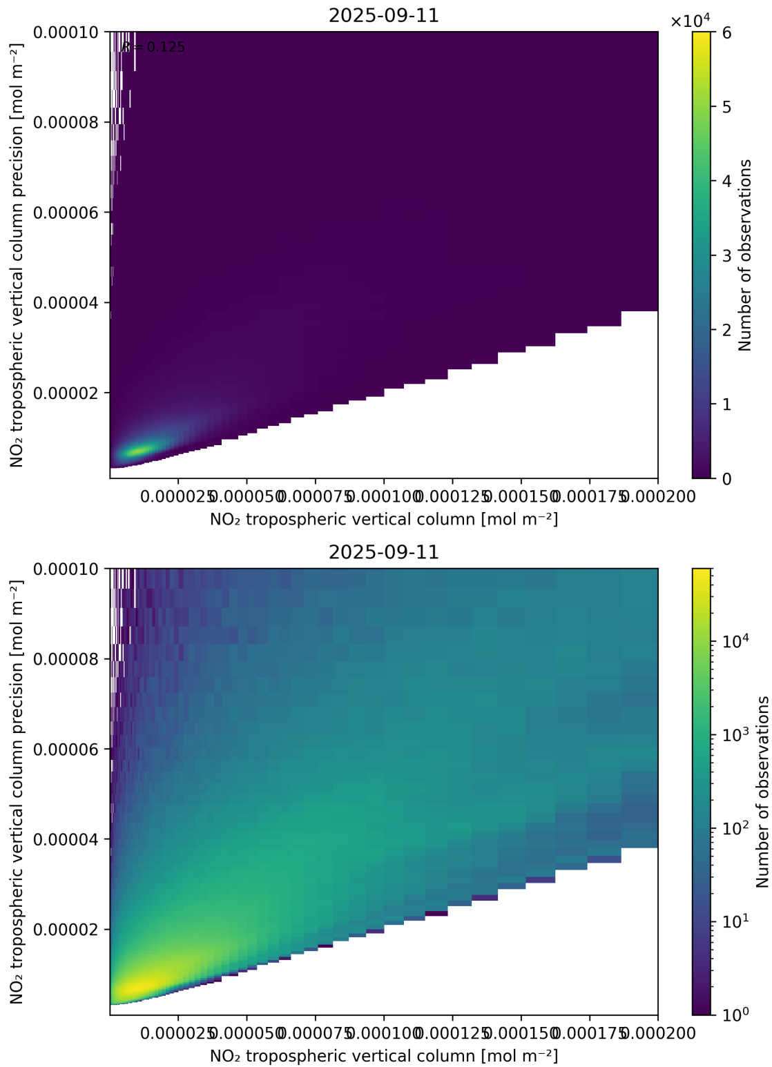
Figure 130: Scatter density plot of “NO 2 tropospheric vertical column” against “NO 2 tropospheric vertical column precision” for 2025-09-10 to 2025-09-12.
