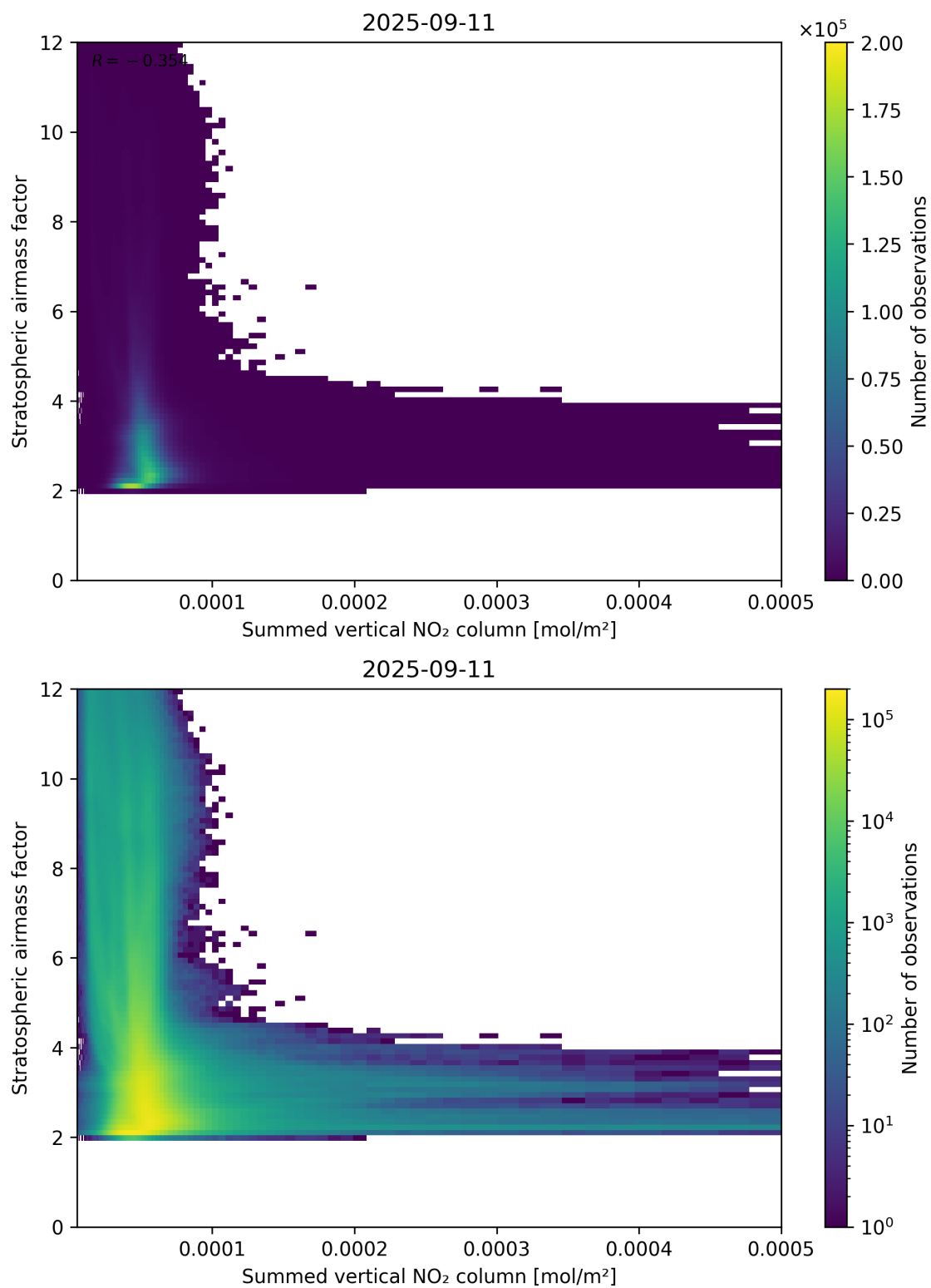
Figure 103: Scatter density plot of “Summed vertical NO 2 column” against “Stratospheric airmass factor” for 2025-09-10 to 2025-09-12.
