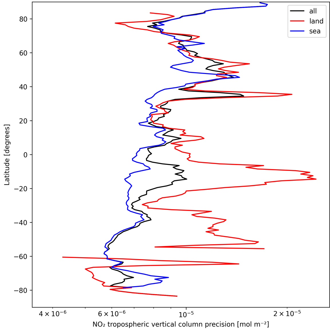
Figure 13: Zonal average of “NO 2 tropospheric vertical column precision” for 2025-09-10 to 2025-09-12.
