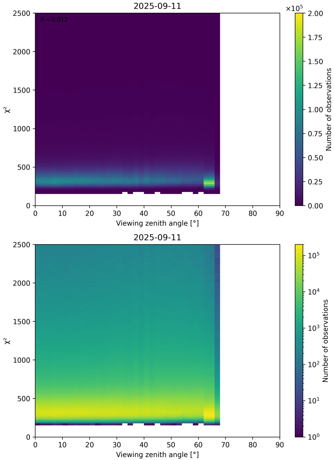
Figure 162: Scatter density plot of “Viewing zenith angle” against “ \chi^2 ” for 2025-09-10 to 2025-09-12.
