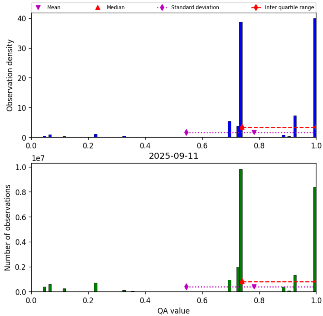
Figure 28: Histogram of “QA value” for 2025-09-10 to 2025-09-12
