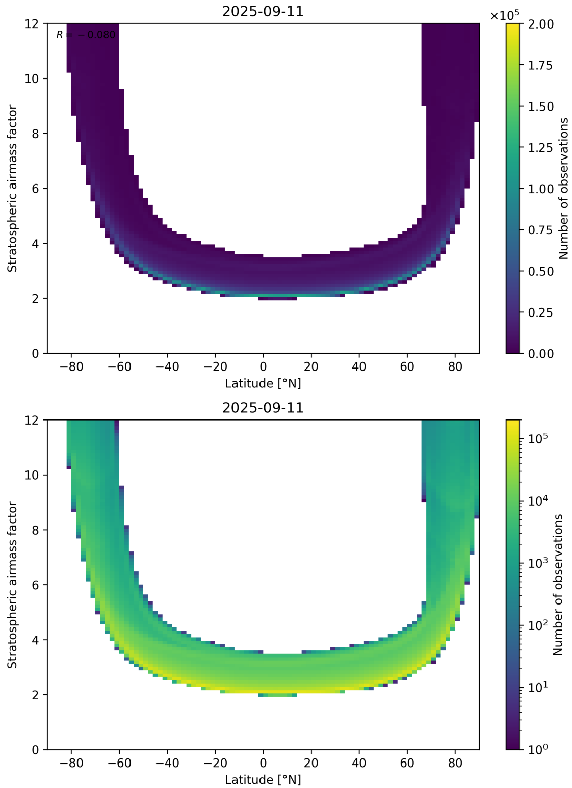
Figure 83: Scatter density plot of “Latitude” against “Stratospheric air mass factor” for 2025-09-10 to 2025-09-12.
