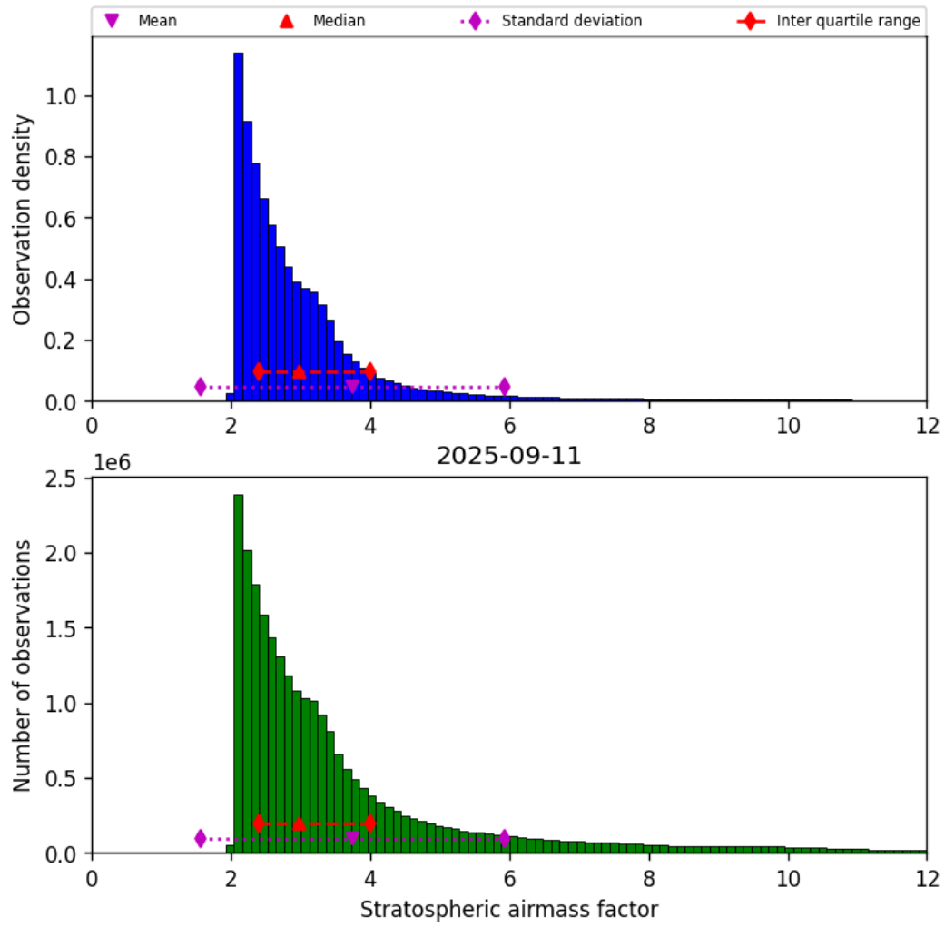
Figure 44: Histogram of “Stratospheric airmass factor” for 2025-09-10 to 2025-09-12
