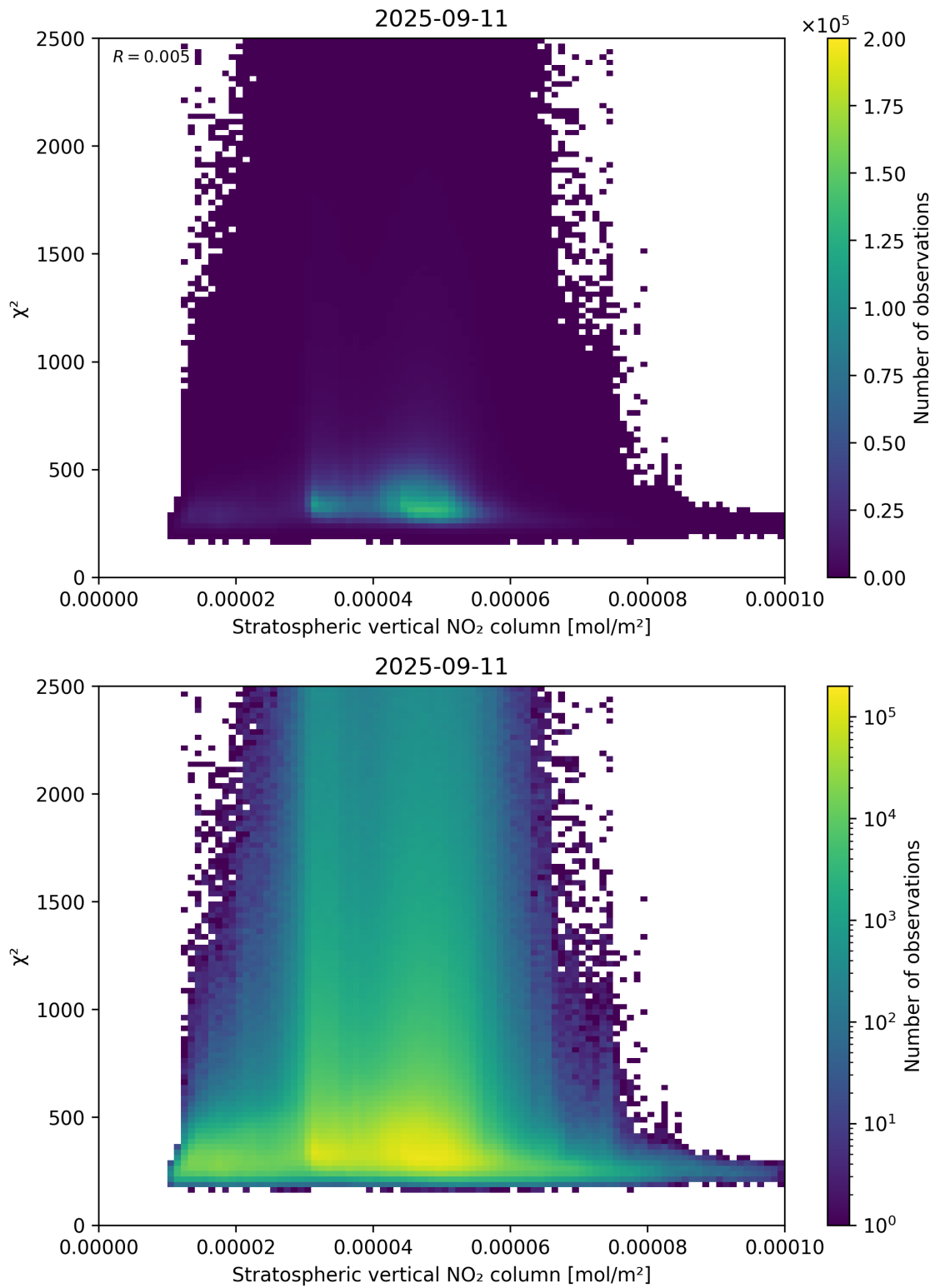
Figure 97: Scatter density plot of “Stratospheric vertical NO 2 column” against “ \chi^2 ” for 2025-09-10 to 2025-09-12.
