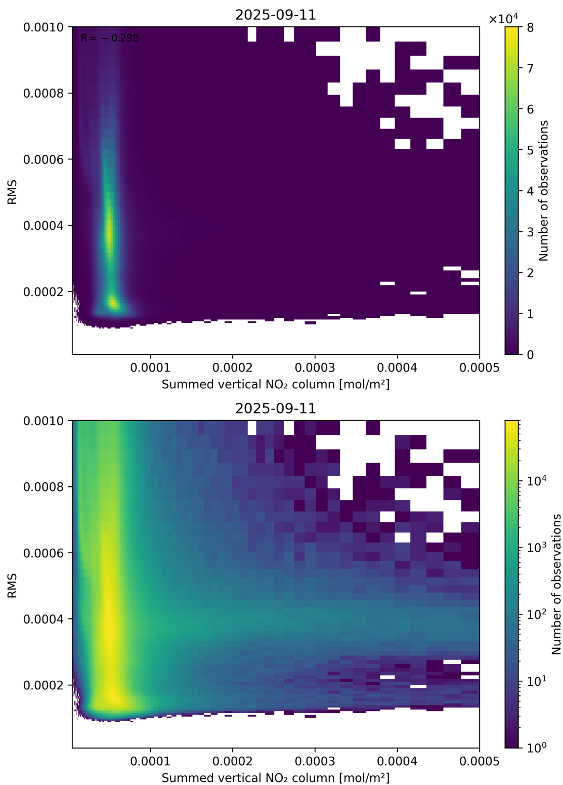
Figure 109: Scatter density plot of “Summed vertical NO 2 column” against “RMS” for 2025-09-10 to 2025-09-12.
