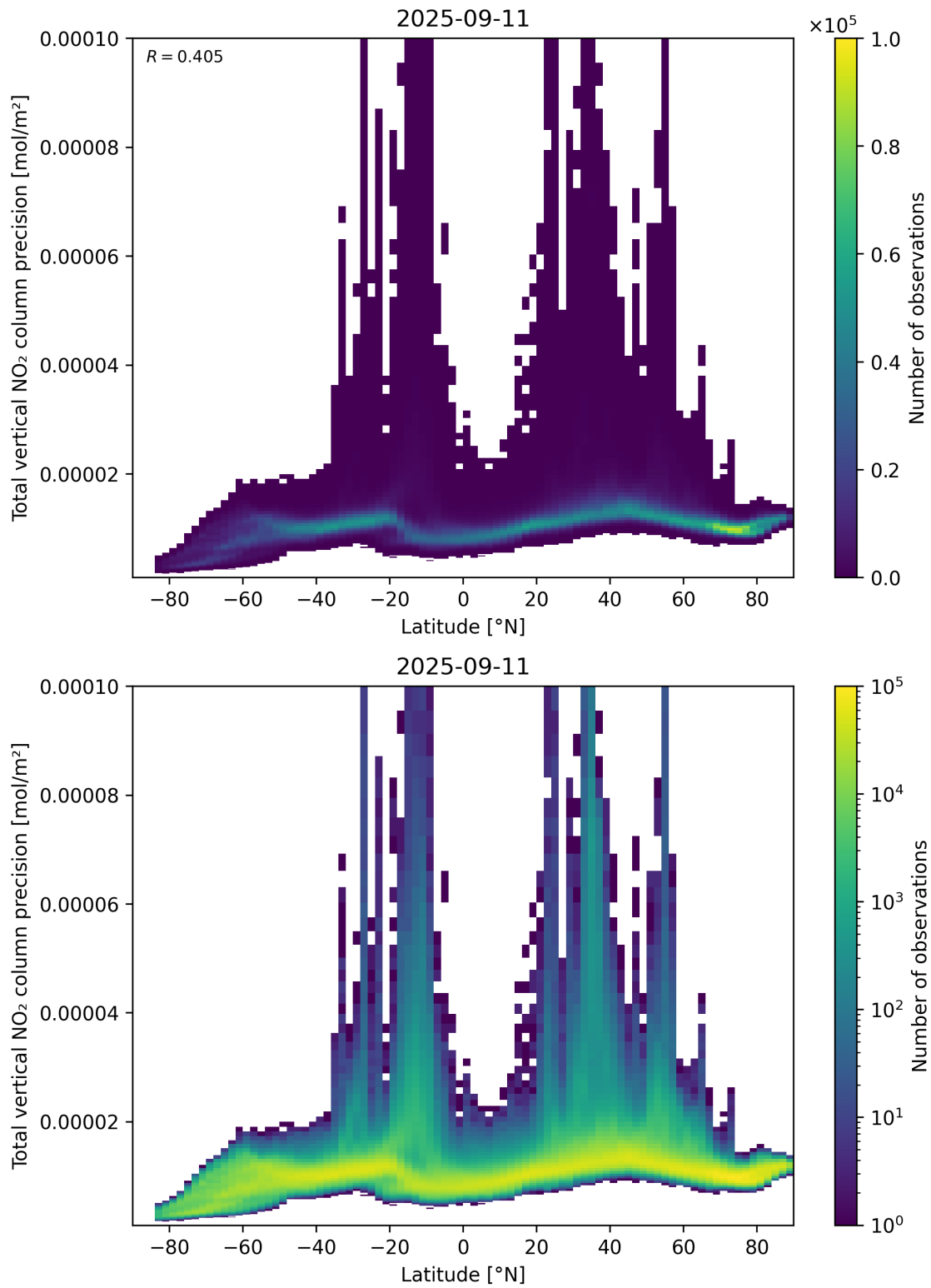
Figure 91: Scatter density plot of “Latitude” against “Total vertical NO 2 column precision” for 2025-09-10 to 2025-09-12.
