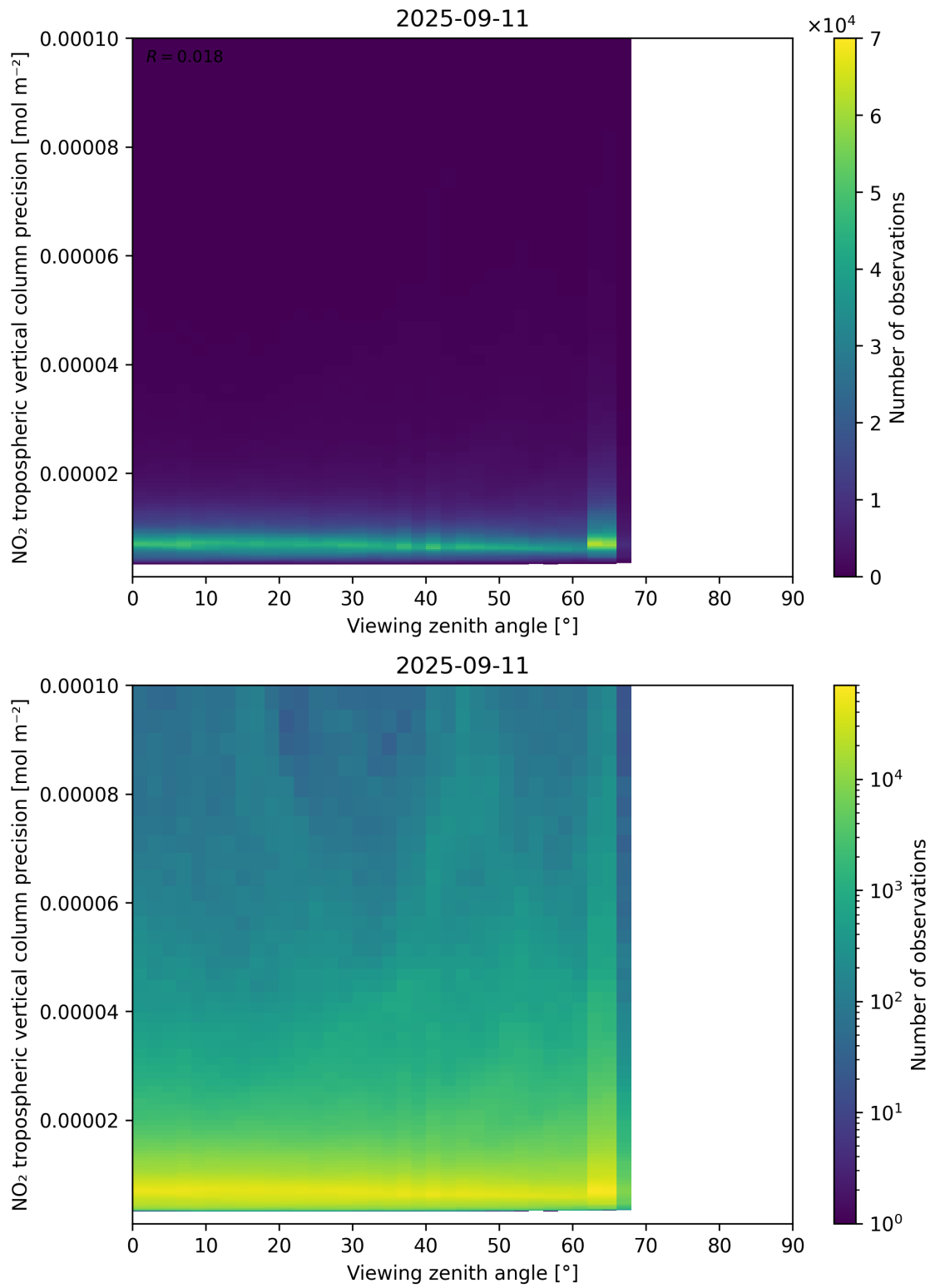
Figure 170: Scatter density plot of “Viewing zenith angle” against “NO 2 tropospheric vertical column precision” for 2025-09-10 to 2025-09-12.
