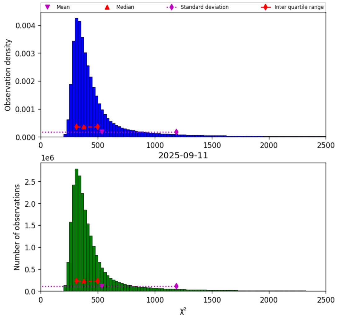
Figure 42: Histogram of " \chi^2 " for 2025-09-10 to 2025-09-12
