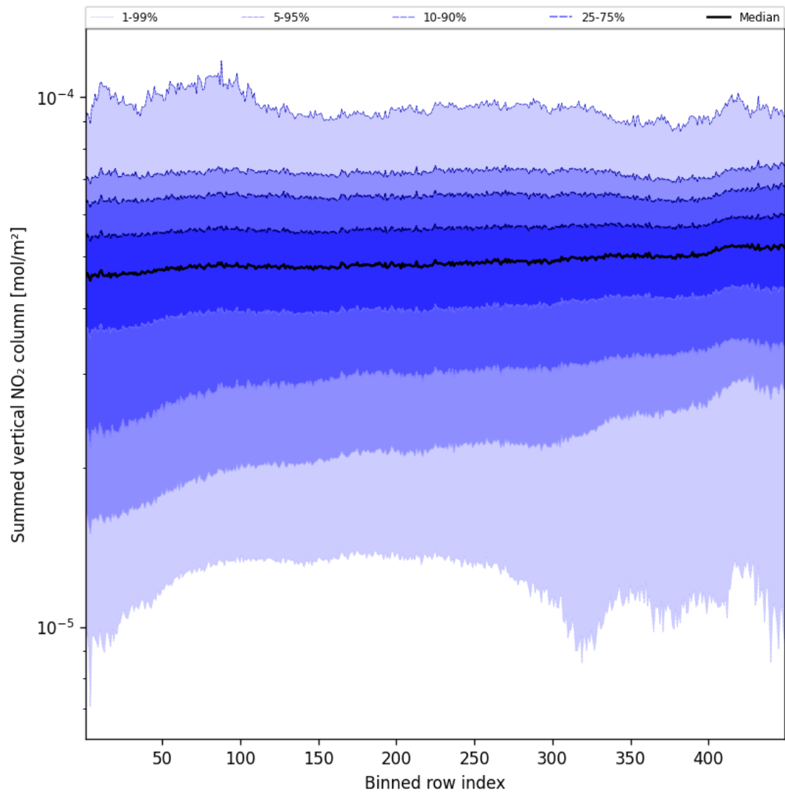
Figure 57: Along track statistics of “Summed vertical NO 2 column” for 2025-09-10 to 2025-09-12
