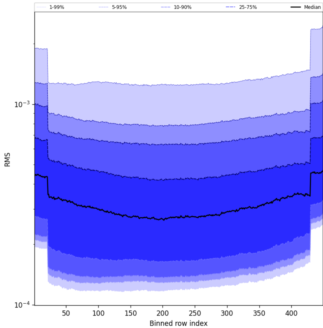
Figure 60: Along track statistics of “RMS” for 2025-09-10 to 2025-09-12
