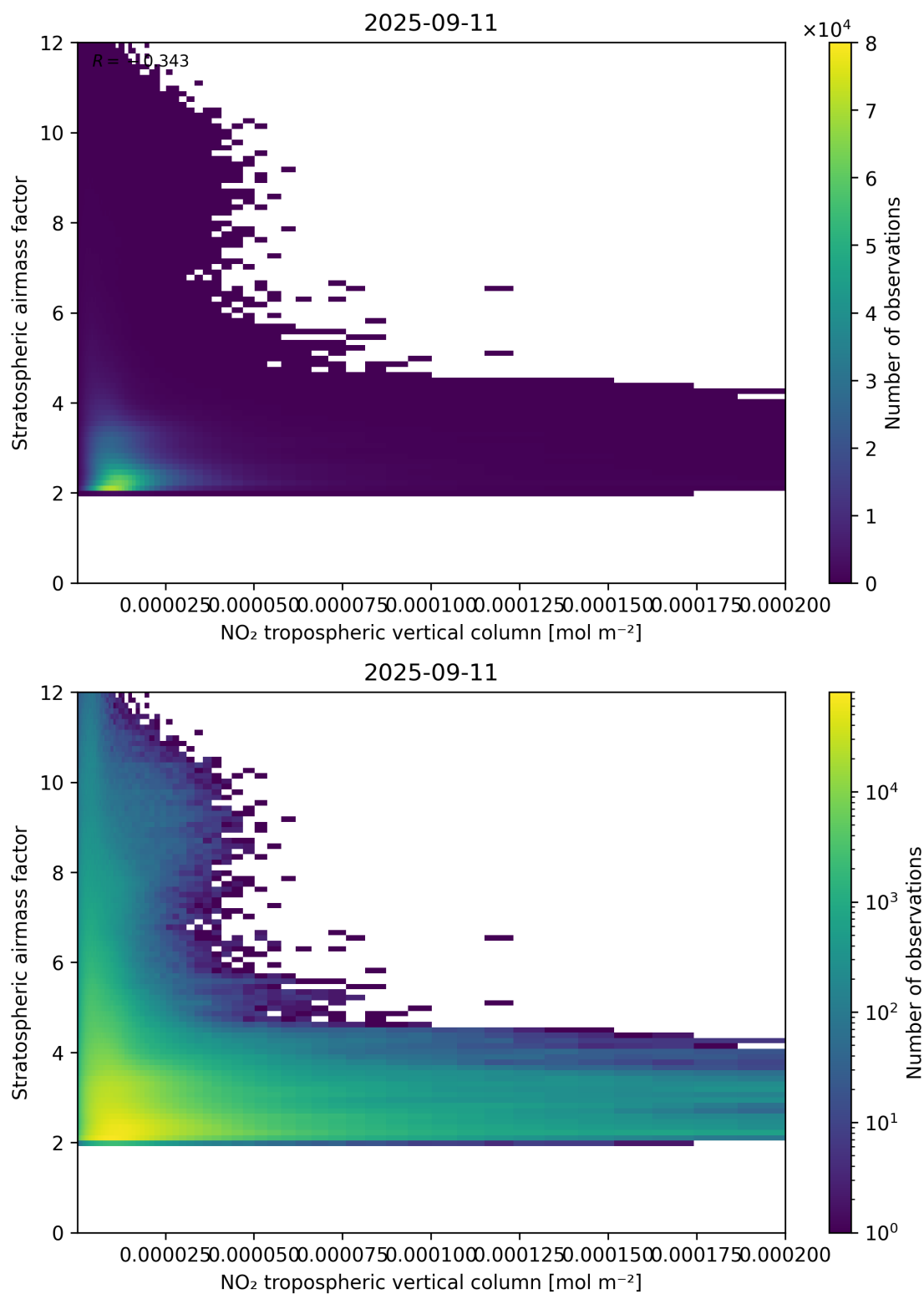
Figure 121: Scatter density plot of “NO 2 tropospheric vertical column” against “Stratospheric air mass factor” for 2025-09-10 to 2025-09-12.
