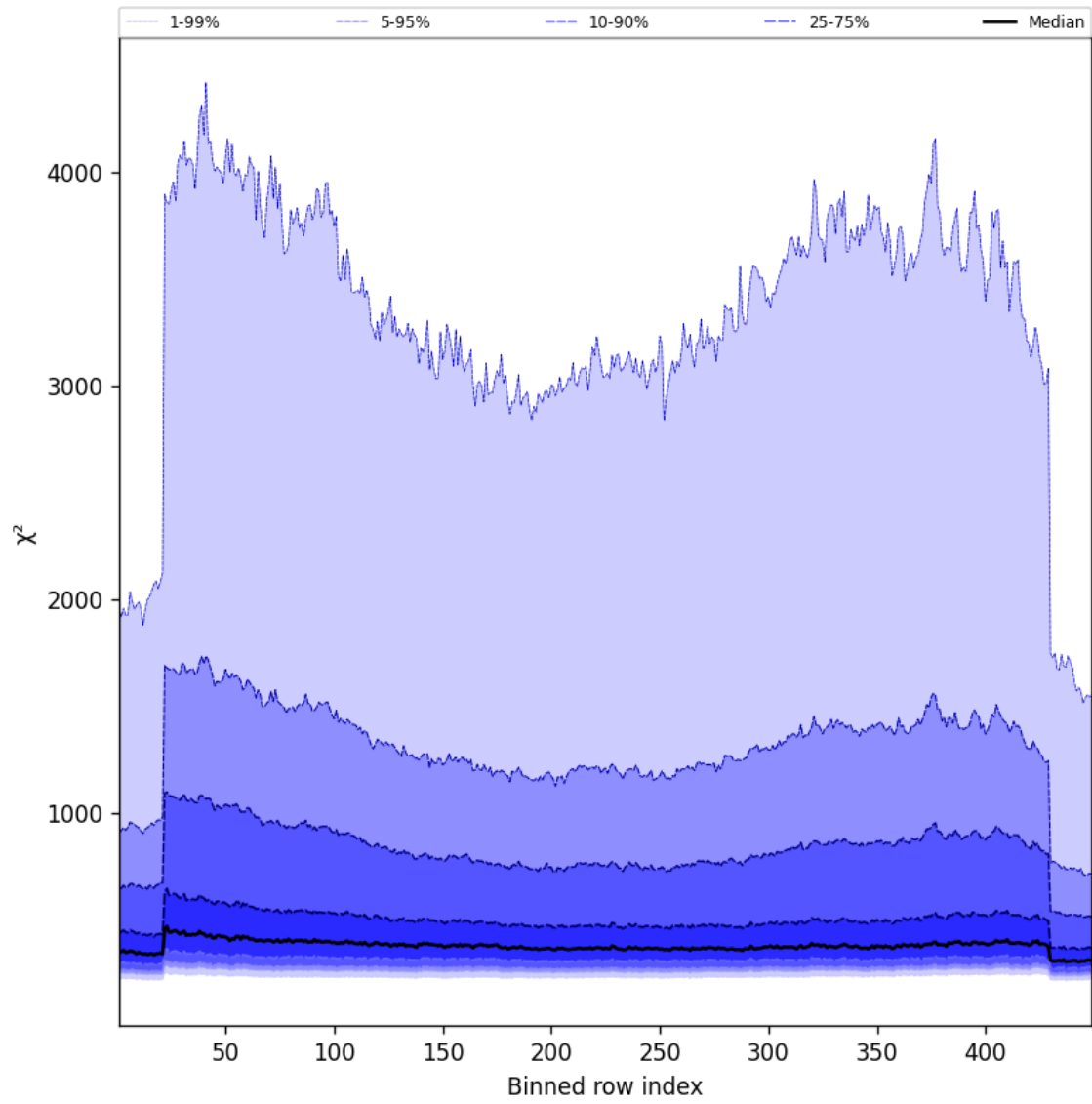
Figure 59: Along track statistics of “ \chi^2 ” for 2025-09-10 to 2025-09-12
