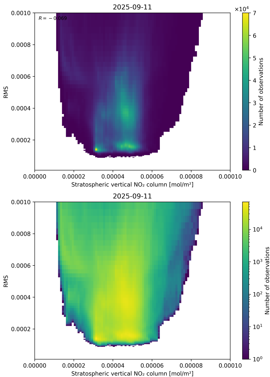
Figure 102: Scatter density plot of “Stratospheric vertical NO 2 column” against “RMS” for 2025-09-10 to 2025-09-12.
