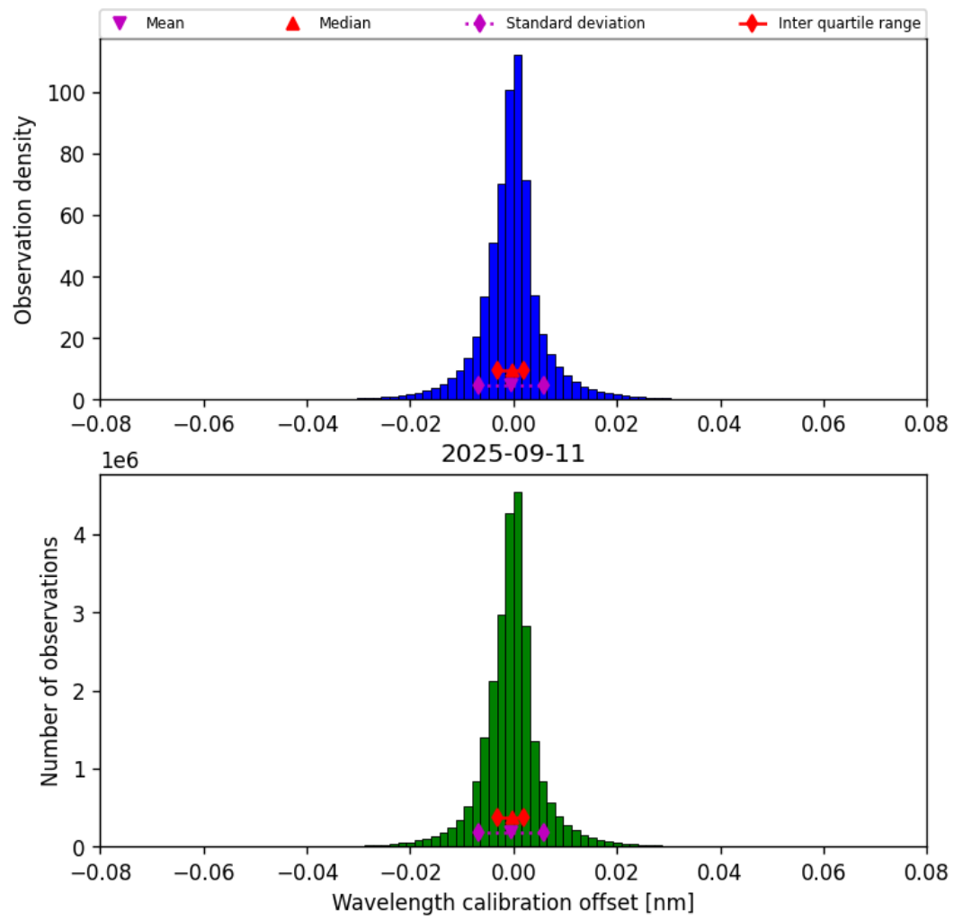
Figure 35: Histogram of “Wavelength calibration offset” for 2025-09-10 to 2025-09-12
