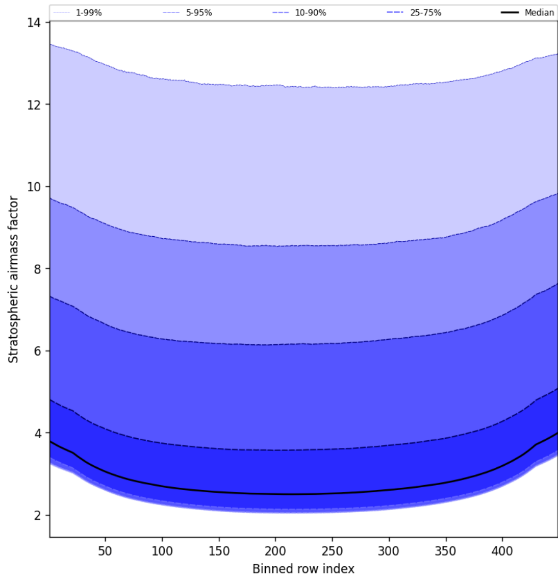
Figure 61: Along track statistics of “Stratospheric airmass factor” for 2025-09-10 to 2025-09-12
