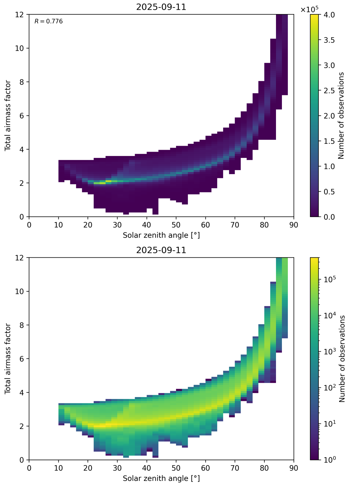
Figure 146: Scatter density plot of “Solar zenith angle” against “Total airmass factor” for 2025-09-10 to 2025-09-12.
