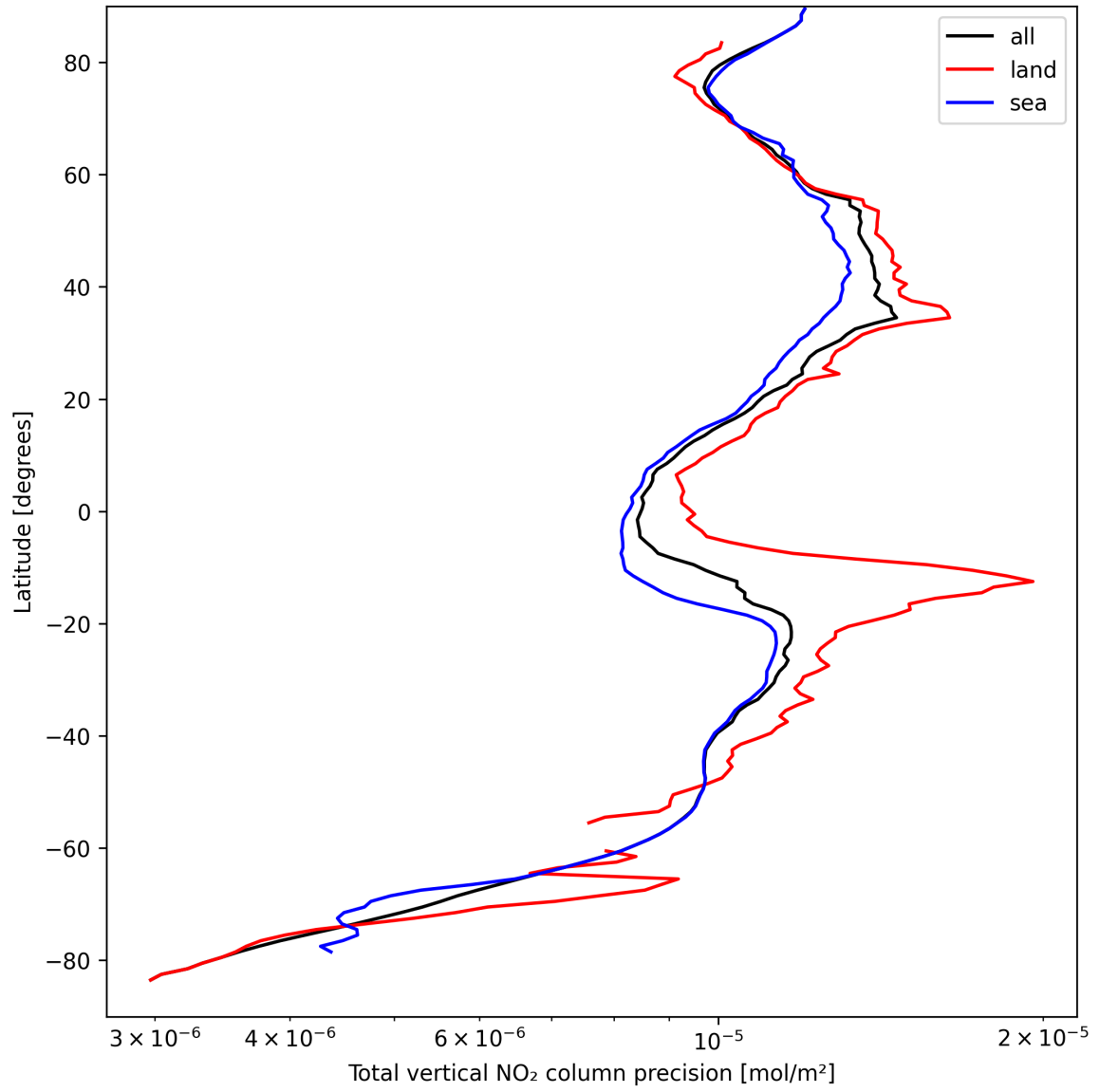
Figure 22: Zonal average of “Total vertical NO 2 column precision” for 2025-09-10 to 2025-09-12.
