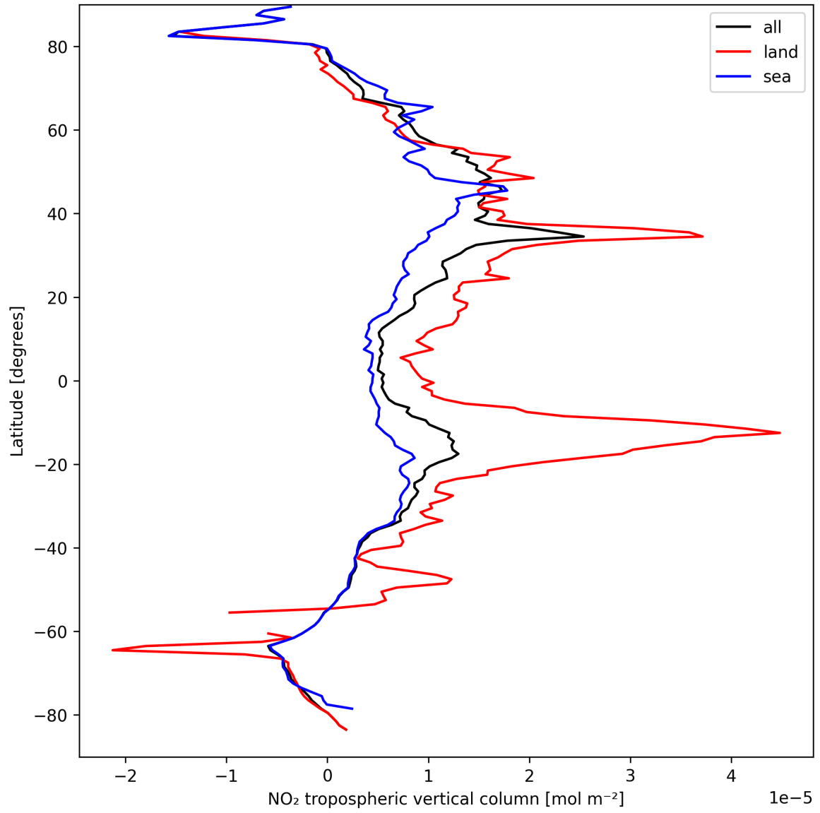
Figure 12: Zonal average of “NO 2 tropospheric vertical column” for 2025-09-10 to 2025-09-12.
