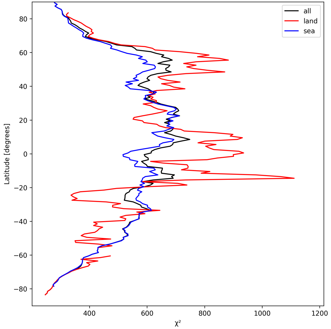
Figure 25: Zonal average of “ \chi^2 ” for 2025-09-10 to 2025-09-12.
