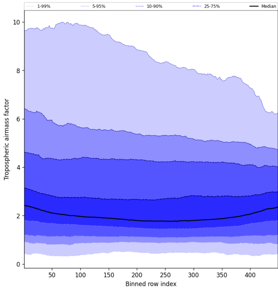
Figure 48: Along track statistics of “Tropospheric airmass factor” for 2025-09-10 to 2025-09-12
