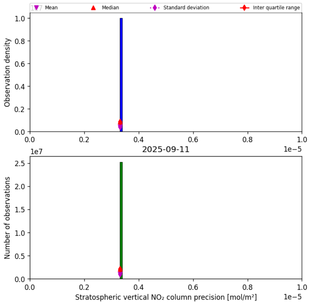
Figure 37: Histogram of “Stratospheric vertical NO 2 column precision” for 2025-09-10 to 2025-09-12
