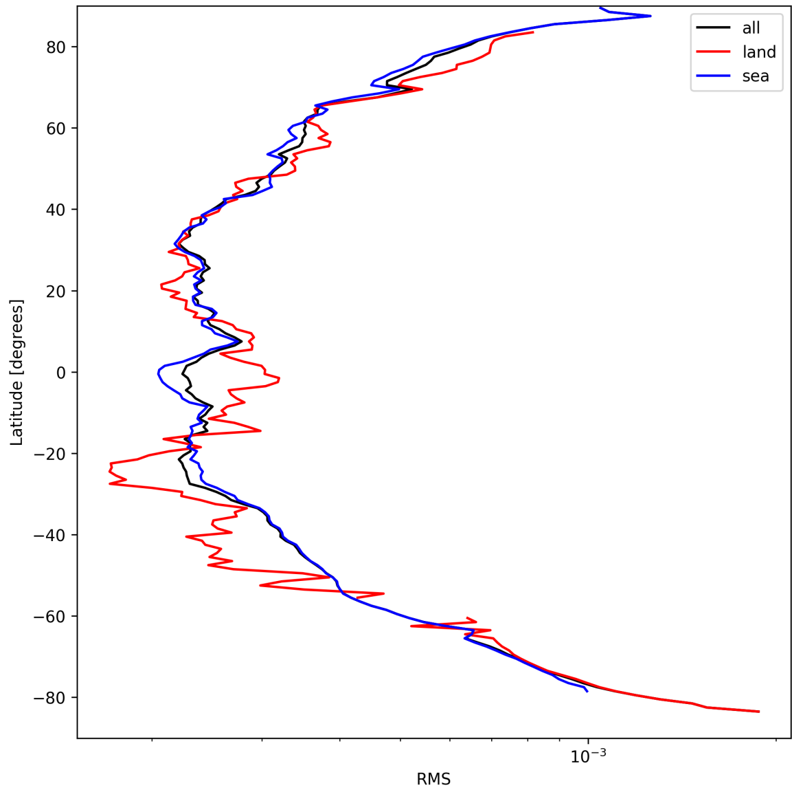
Figure 26: Zonal average of “RMS” for 2025-09-10 to 2025-09-12.
