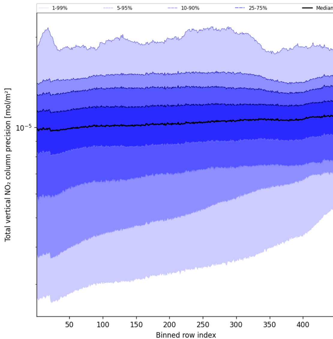
Figure 56: Along track statistics of “Total vertical NO 2 column precision” for 2025-09-10 to 2025-09-12
