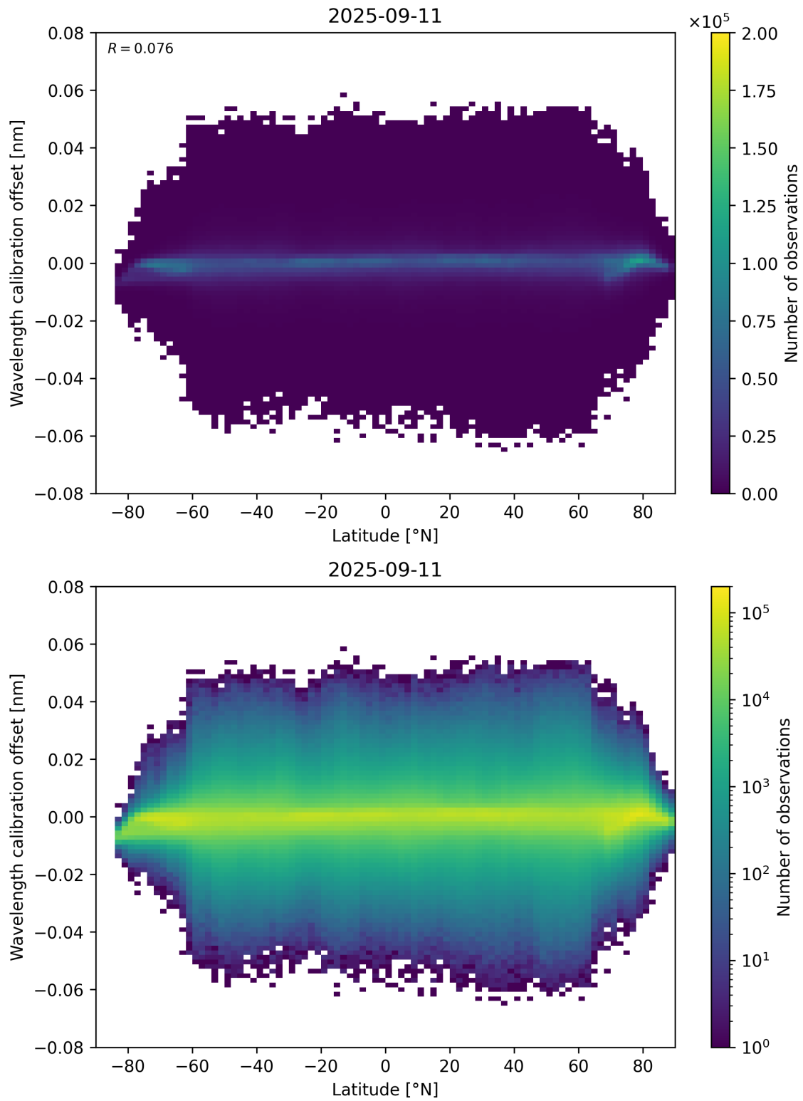
Figure 95: Scatter density plot of “Latitude” against “Wavelength calibration offset” for 2025-09-10 to 2025-09-12.
