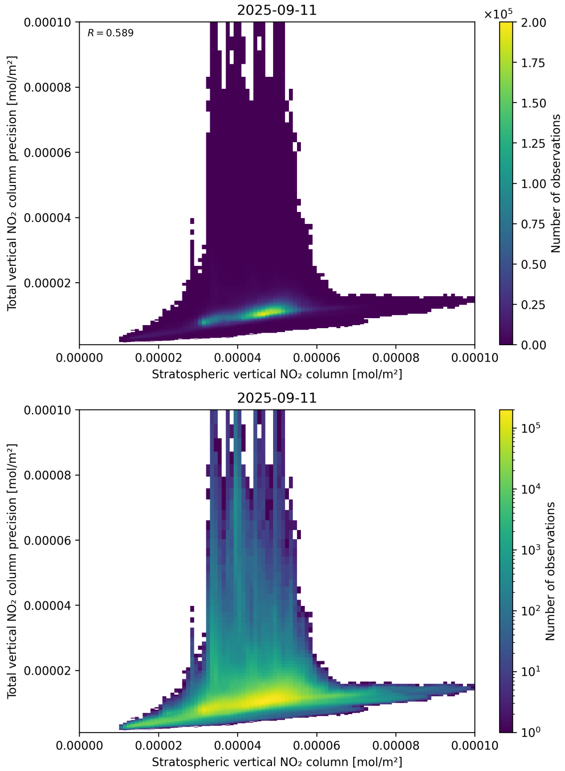
Figure 101: Scatter density plot of “Stratospheric vertical NO 2 column” against “Total vertical NO 2 column precision” for 2025-09-10 to 2025-09-12.
