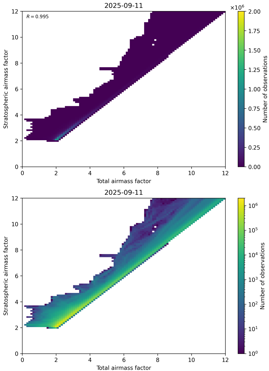
Figure 62: Scatter density plot of “Total airmass factor” against “Stratospheric airmass factor” for 2025-09-10 to 2025-09-12.
