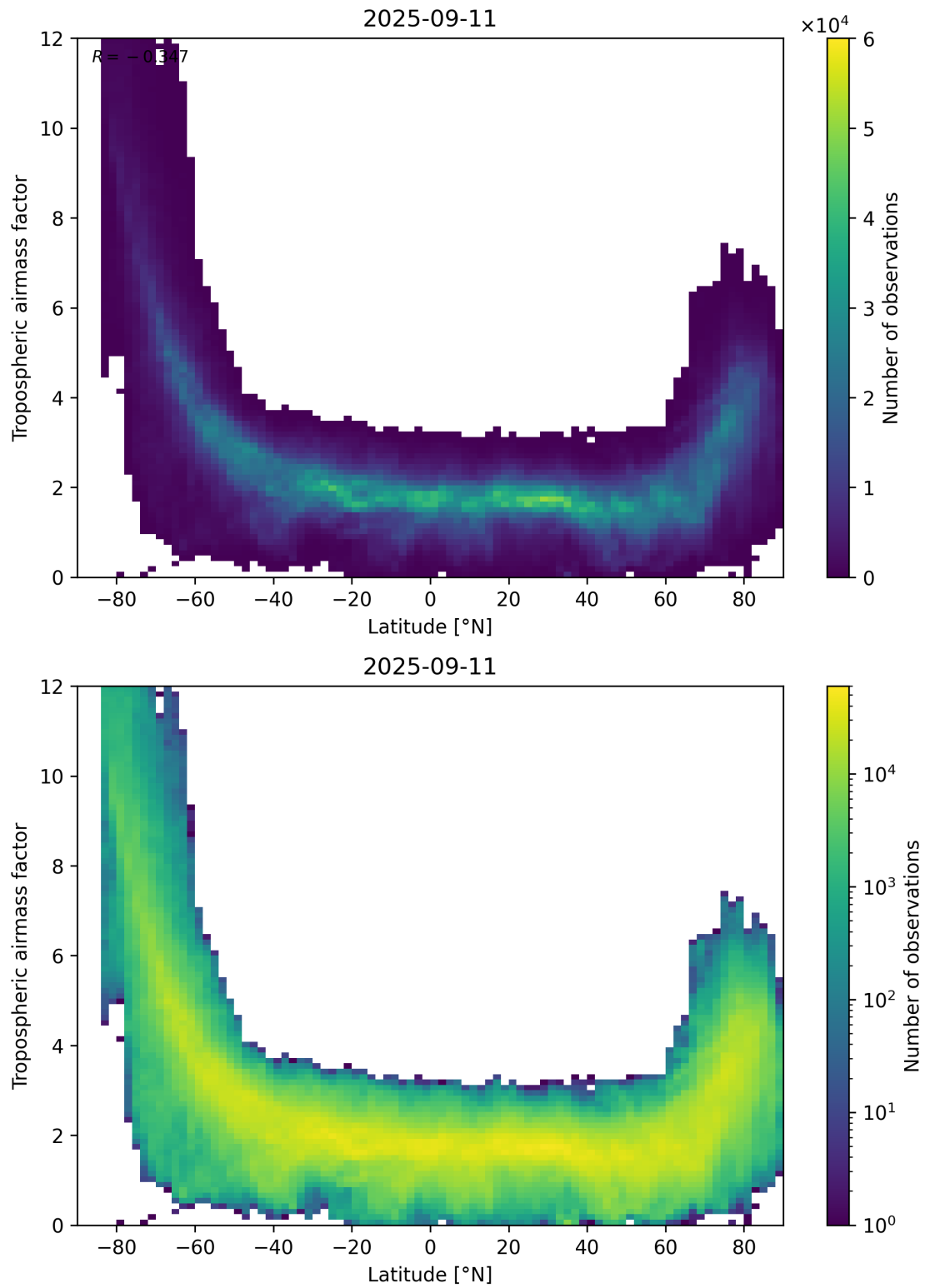
Figure 85: Scatter density plot of “Latitude” against “Tropospheric air mass factor” for 2025-09-10 to 2025-09-12.
