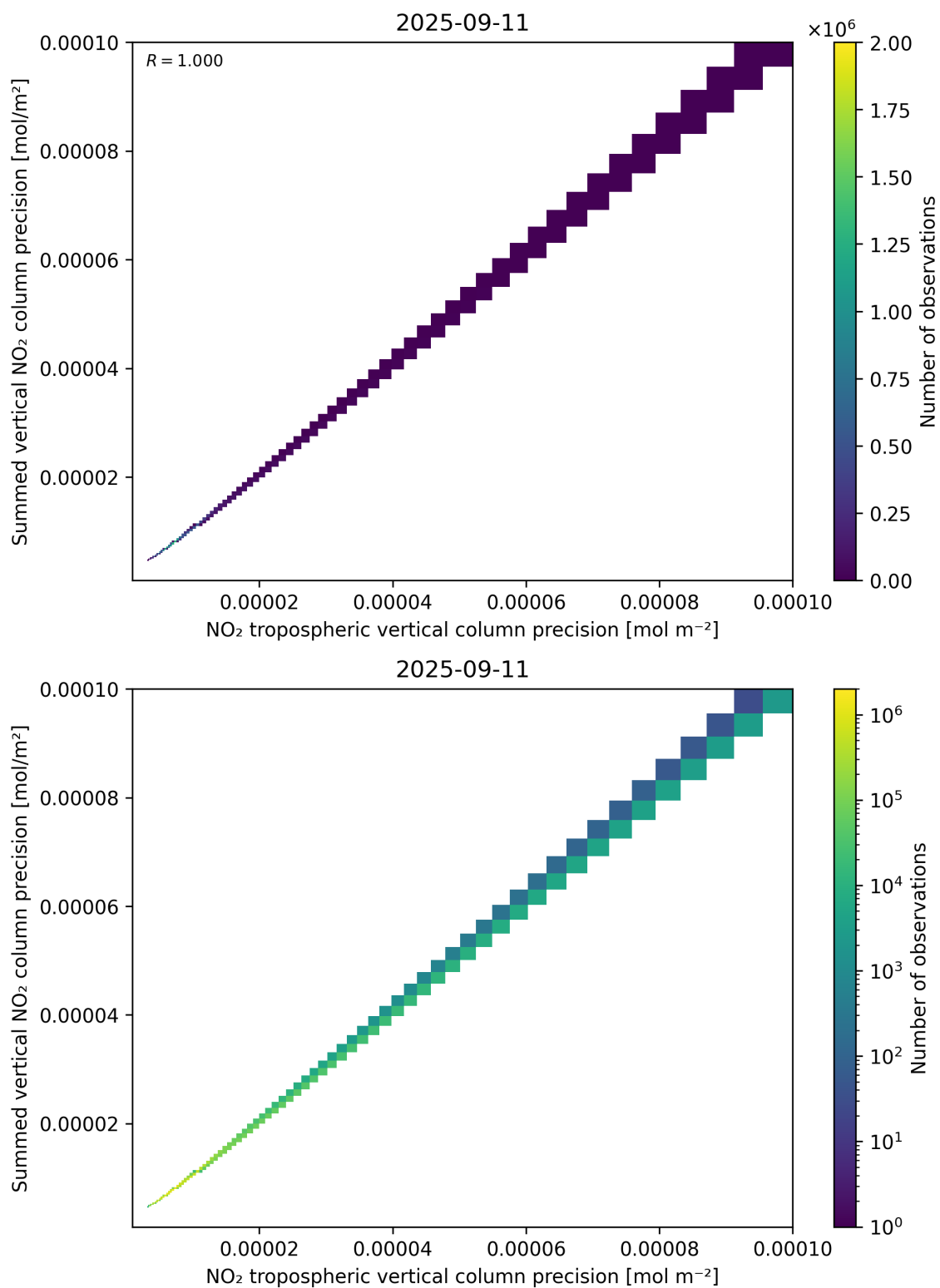
Figure 137: Scatter density plot of “NO 2 tropospheric vertical column precision” against “Summed vertical NO 2 column precision” for 2025-09-10 to 2025-09-12.
