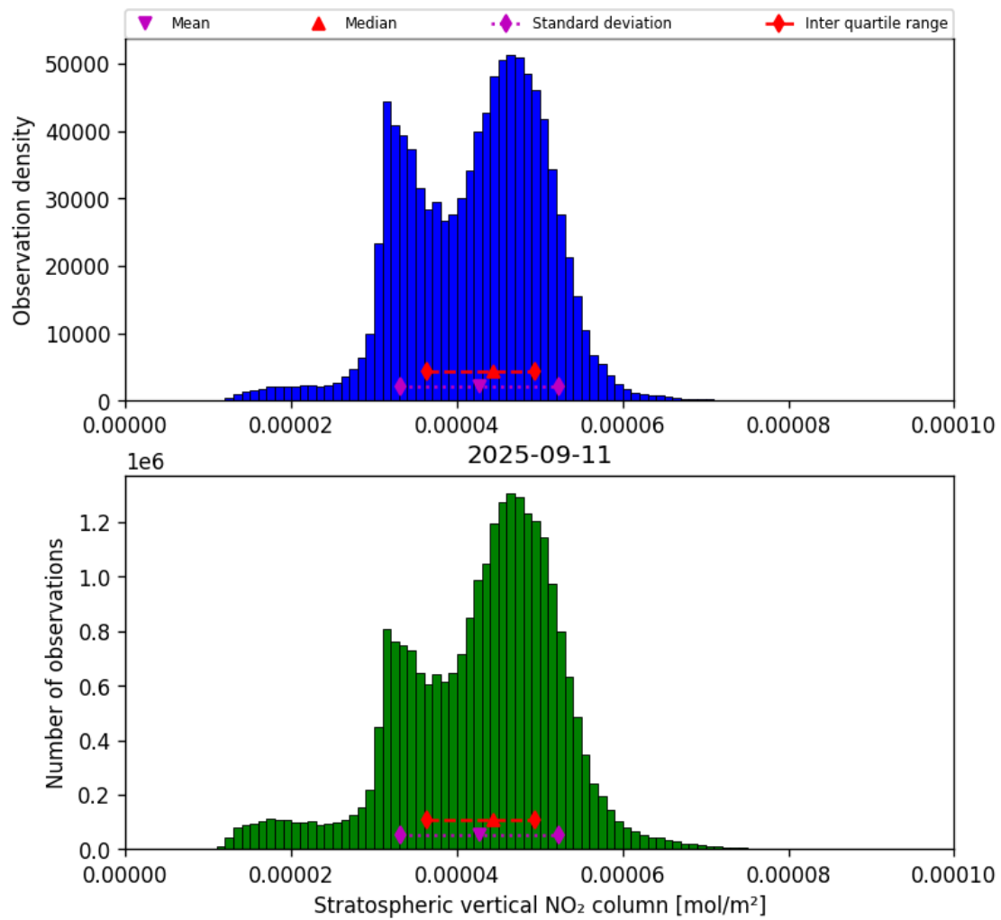
Figure 36: Histogram of “Stratospheric vertical NO 2 column” for 2025-09-10 to 2025-09-12
