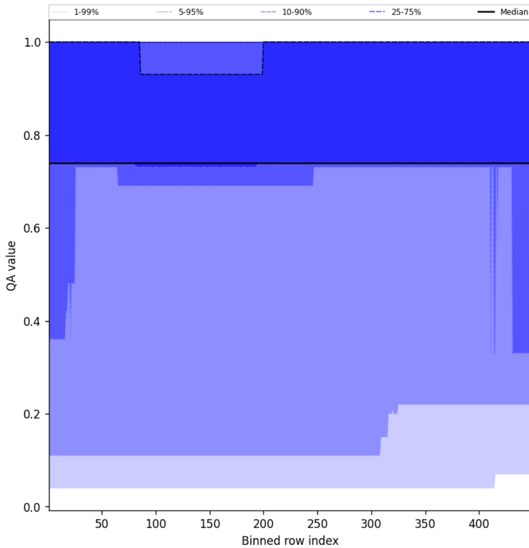
Figure 45: Along track statistics of “QA value” for 2025-09-10 to 2025-09-12
