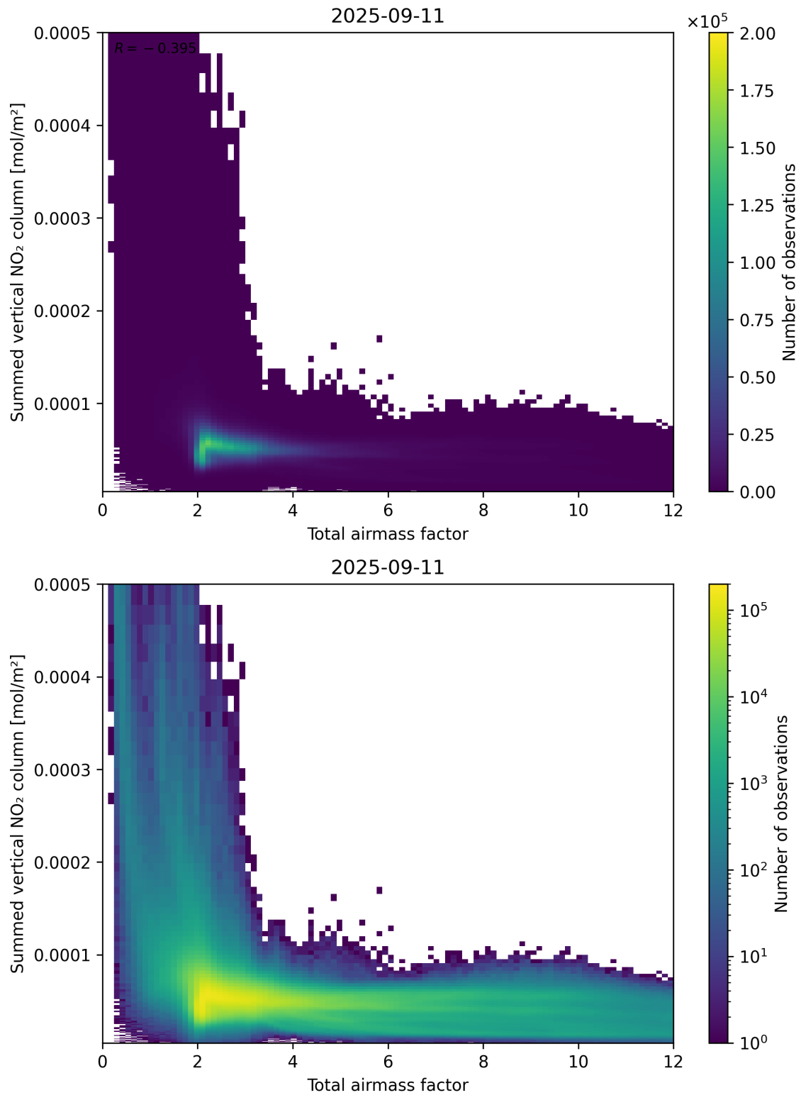
Figure 65: Scatter density plot of “Total airmass factor” against “Summed vertical NO 2 column” for 2025-09-10 to 2025-09-12.
