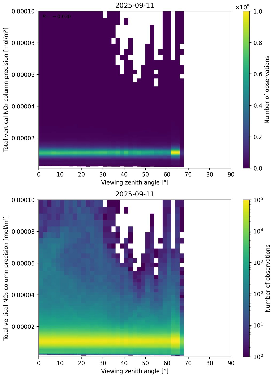
Figure 168: Scatter density plot of “Viewing zenith angle” against “Total vertical NO 2 column precision” for 2025-09-10 to 2025-09-12.
