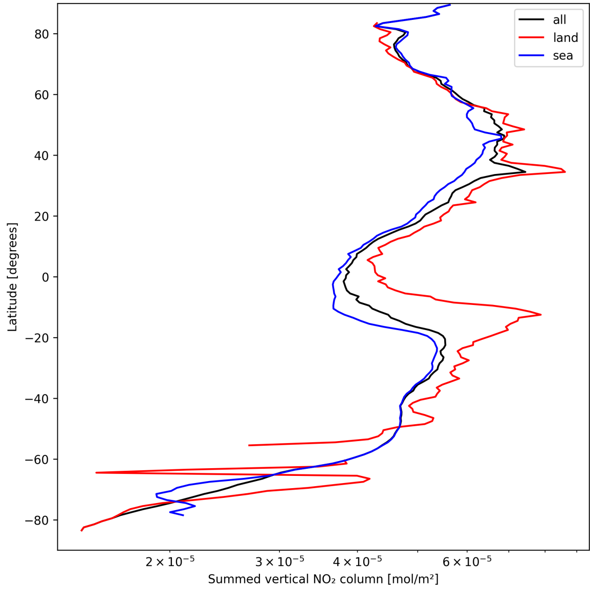
Figure 23: Zonal average of “Summed vertical NO 2 column” for 2025-09-10 to 2025-09-12.
