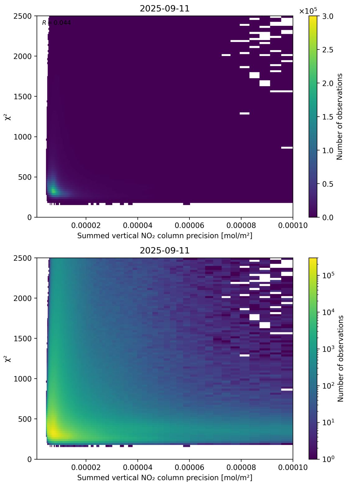
Figure 107: Scatter density plot of “Summed vertical NO 2 column precision” against “ \chi^2 ” for 2025-09-10 to 2025-09-12.
