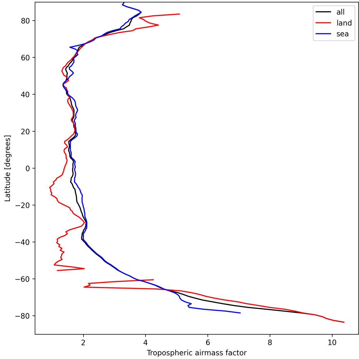
Figure 14: Zonal average of “Tropospheric air mass factor” for 2025-09-10 to 2025-09-12.
