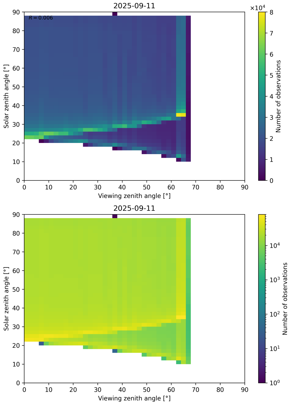
Figure 172: Scatter density plot of “Viewing zenith angle” against “Solar zenith angle” for 2025-09-10 to 2025-09-12.
