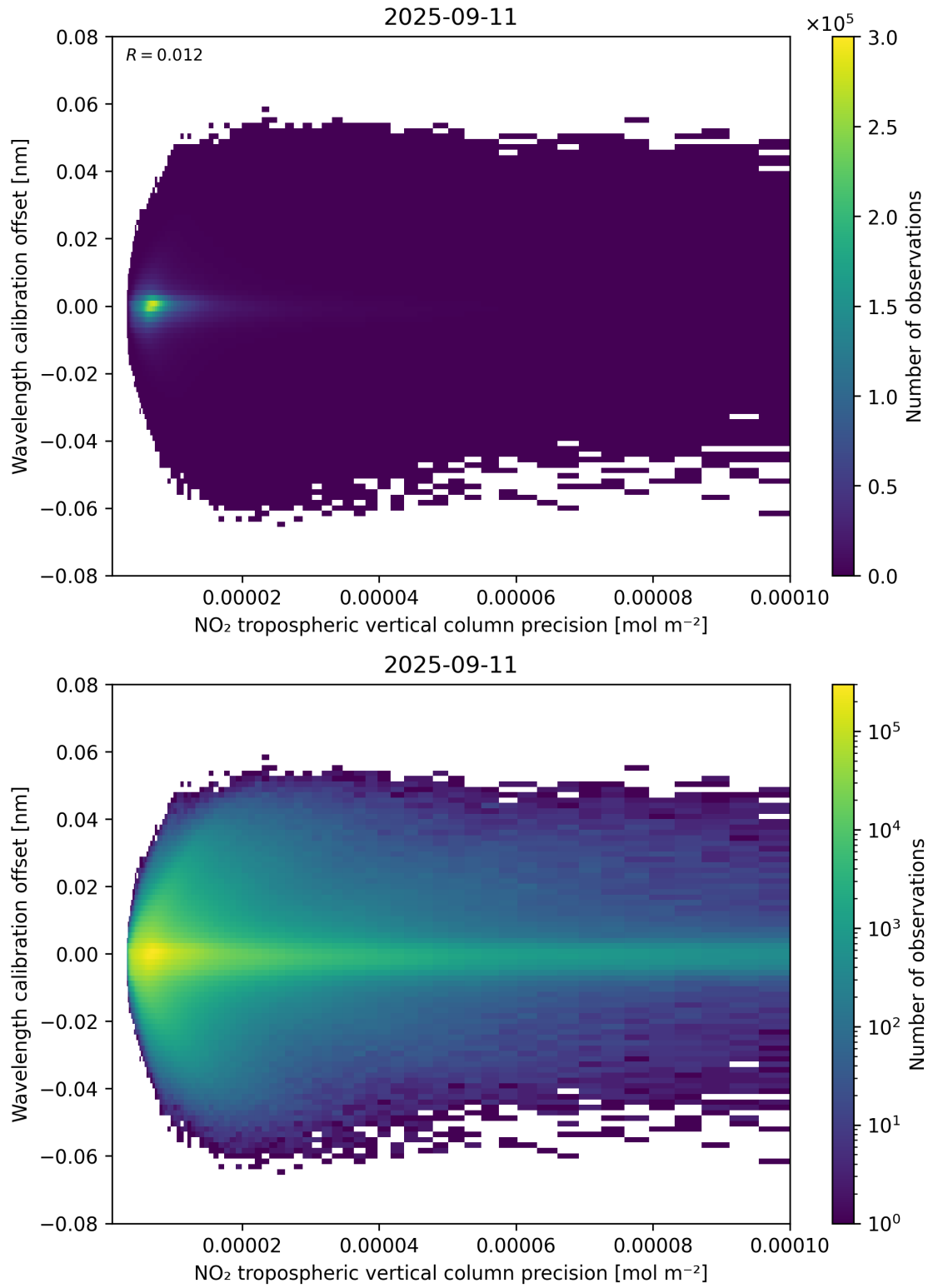
Figure 141: Scatter density plot of “NO 2 tropospheric vertical column precision” against “Wavelength calibration offset” for 2025-09-10 to 2025-09-12.
