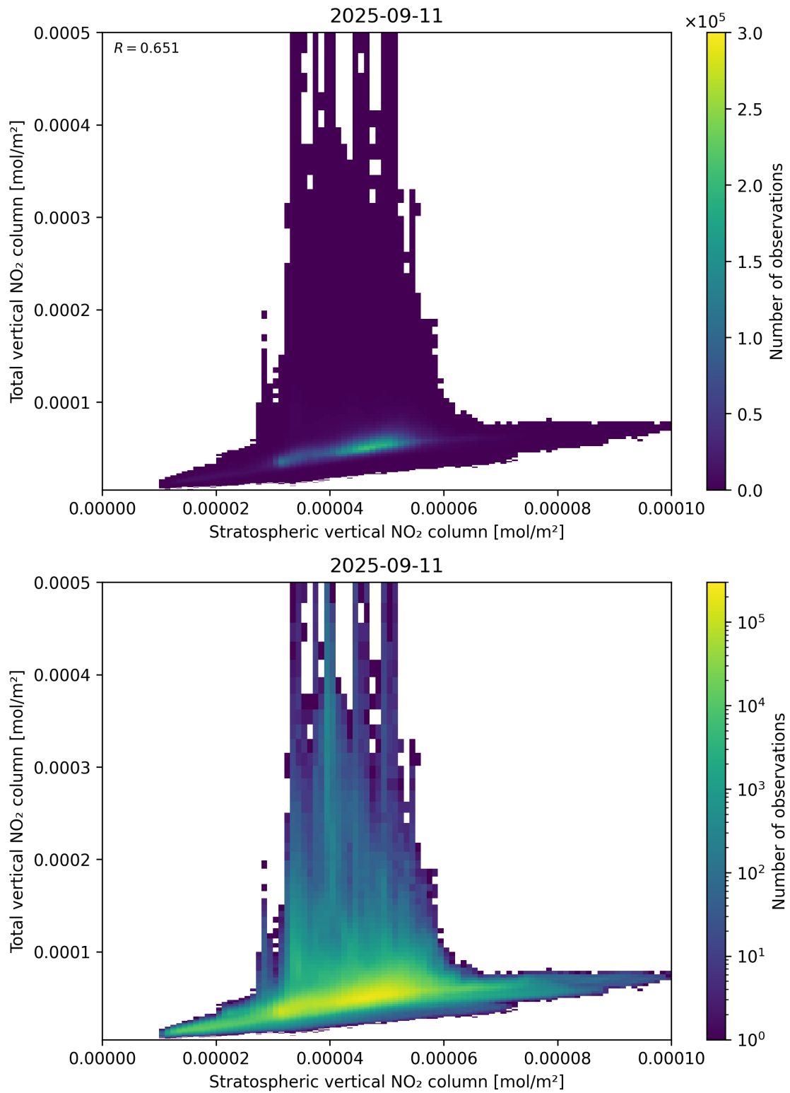
Figure 100: Scatter density plot of “Stratospheric vertical NO 2 column” against “Total vertical NO 2 column” for 2025-09-10 to 2025-09-12.
