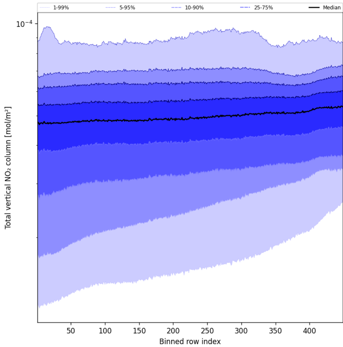
Figure 55: Along track statistics of “Total vertical NO 2 column” for 2025-09-10 to 2025-09-12
