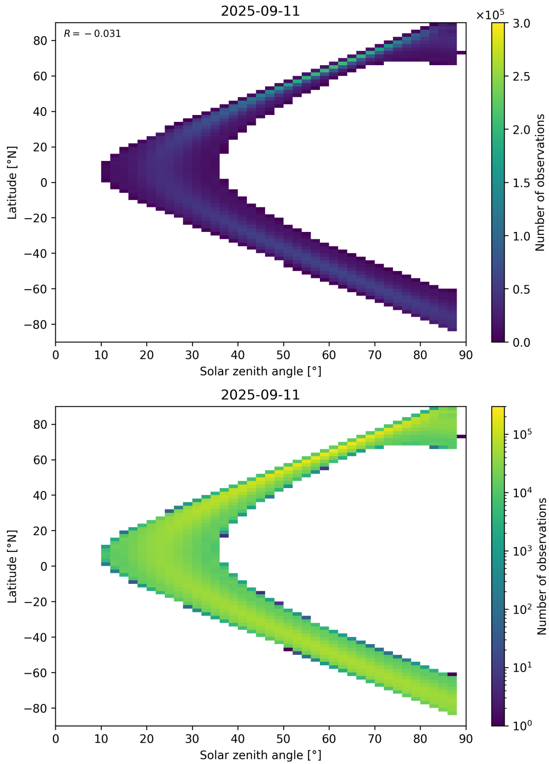
Figure 149: Scatter density plot of “Solar zenith angle” against “Latitude” for 2025-09-10 to 2025-09-12.
