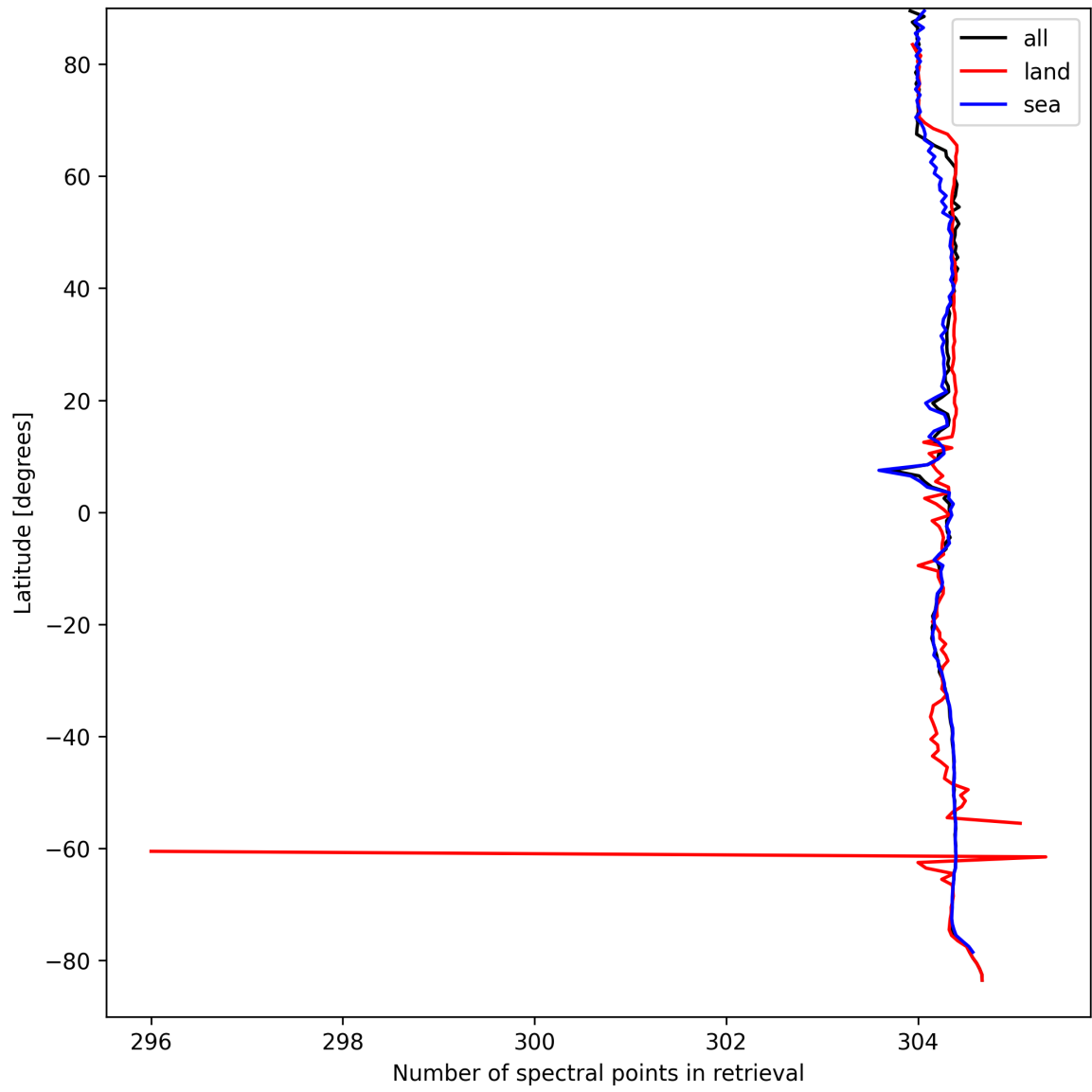
Figure 16: Zonal average of “Number of spectral points in retrieval” for 2025-09-10 to 2025-09-12.
