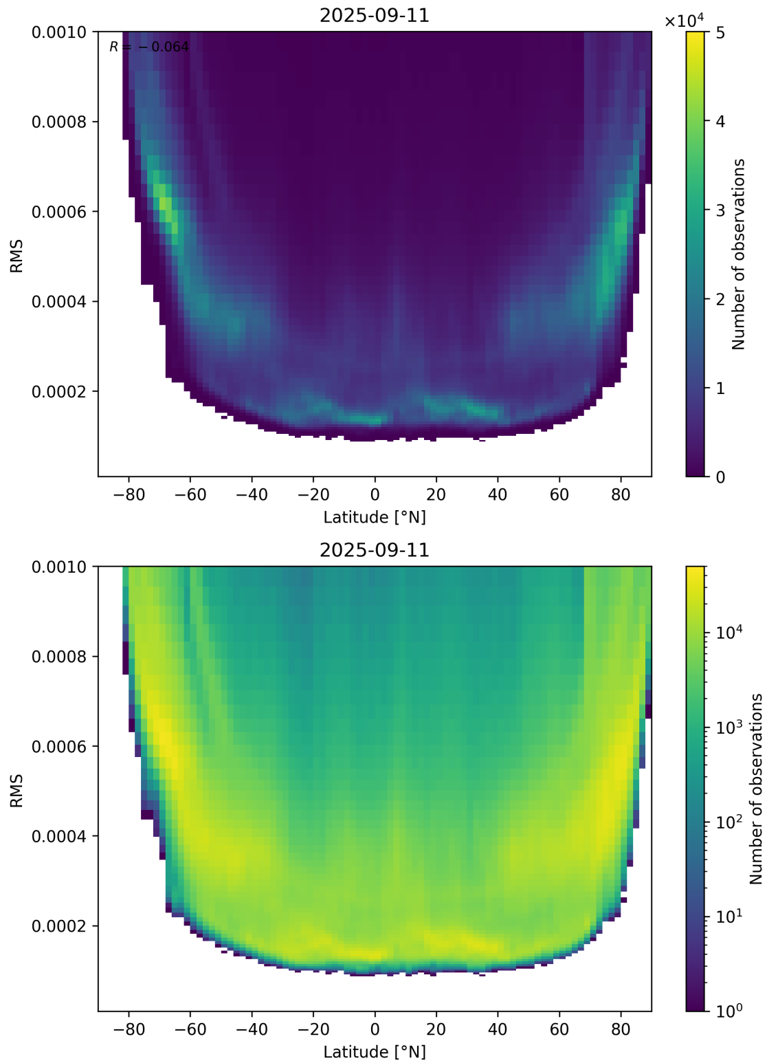
Figure 94: Scatter density plot of “Latitude” against “RMS” for 2025-09-10 to 2025-09-12.
