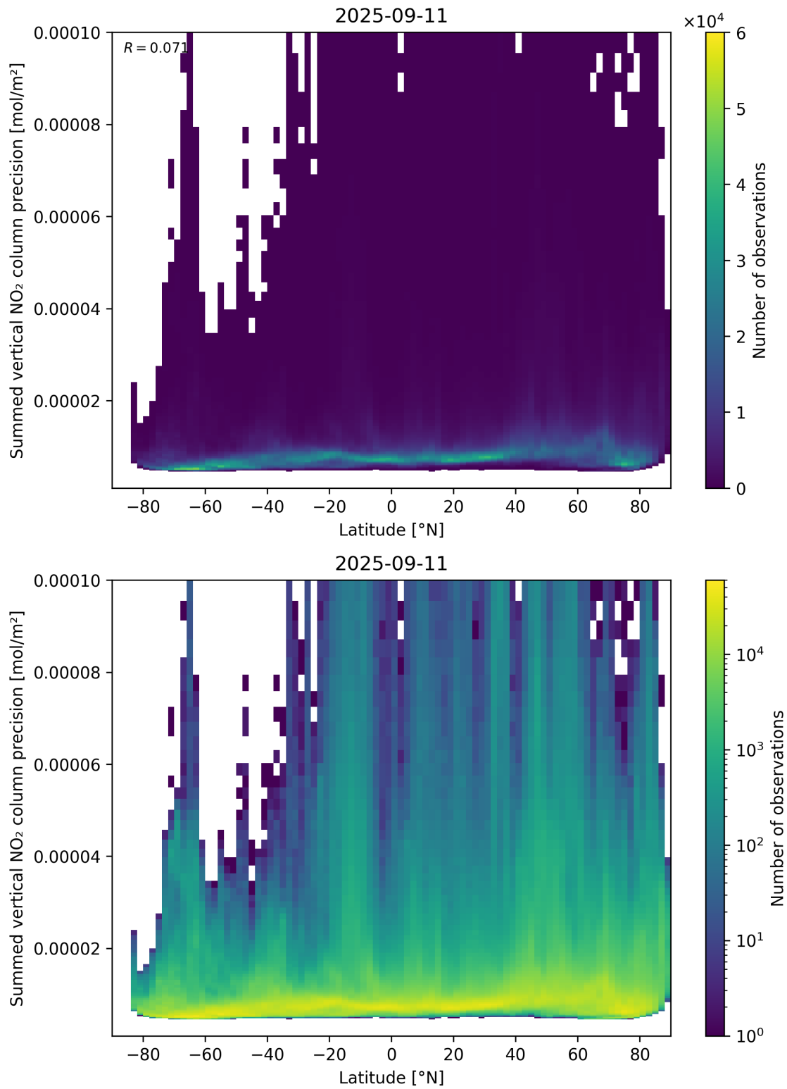
Figure 89: Scatter density plot of “Latitude” against “Summed vertical NO 2 column precision” for 2025-09-10 to 2025-09-12.
