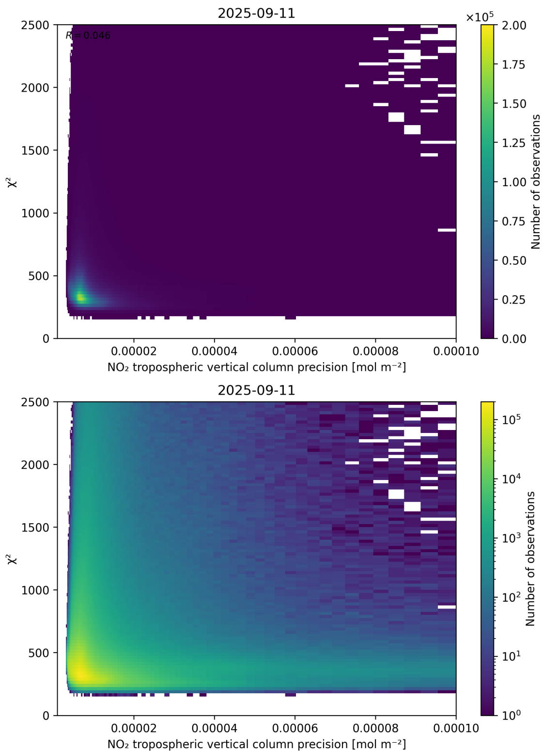
Figure 134: Scatter density plot of “NO 2 tropospheric vertical column precision” against “ \chi^2 ” for 2025-09-10 to 2025-09-12.
