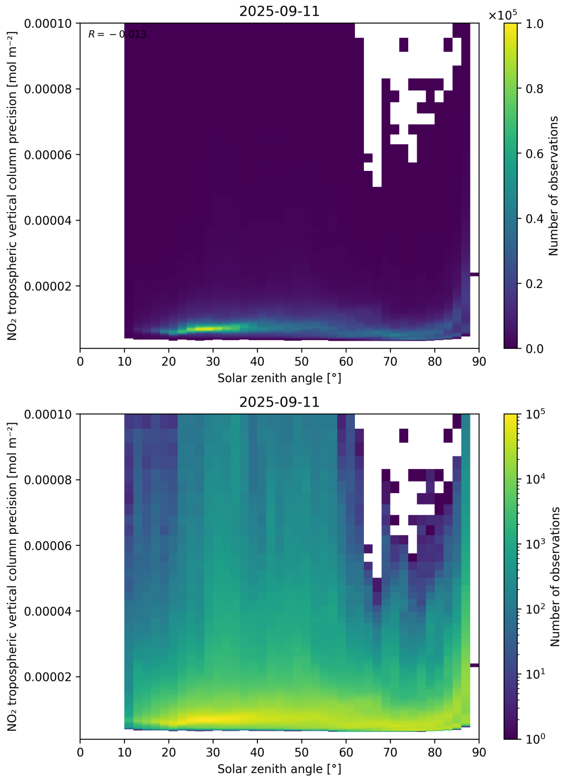
Figure 156: Scatter density plot of “Solar zenith angle” against “NO 2 tropospheric vertical column precision” for 2025-09-10 to 2025-09-12.
