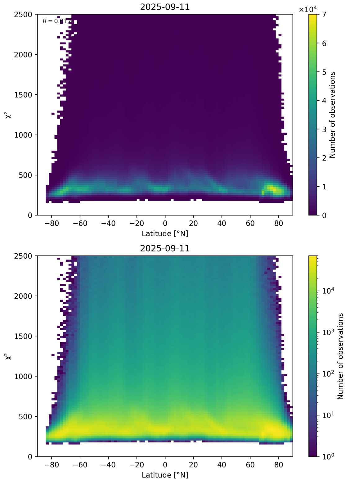
Figure 86: Scatter density plot of “Latitude” against “ \chi^2 ” for 2025-09-10 to 2025-09-12.
