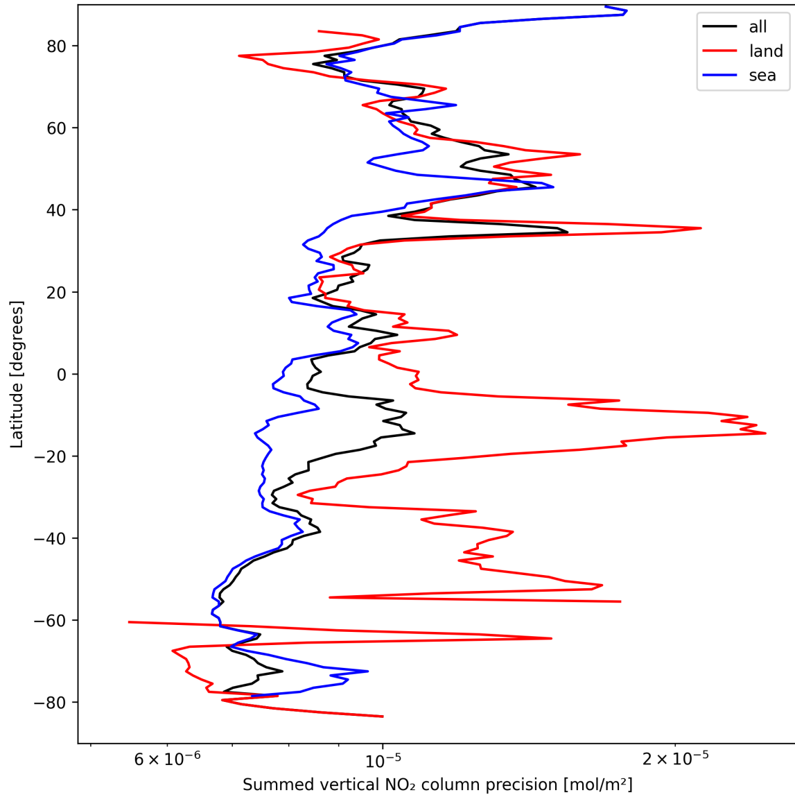
Figure 24: Zonal average of “Summed vertical NO 2 column precision” for 2025-09-10 to 2025-09-12.
