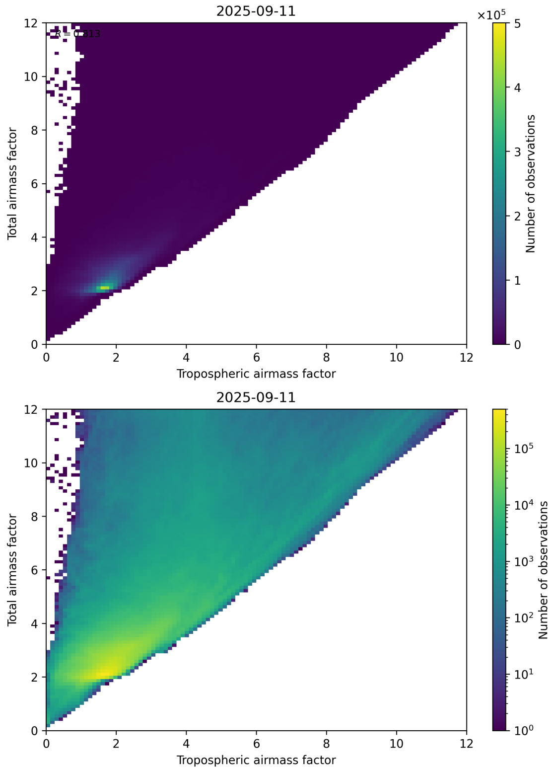
Figure 72: Scatter density plot of “Tropospheric airmass factor” against “Total airmass factor” for 2025-09-10 to 2025-09-12.
