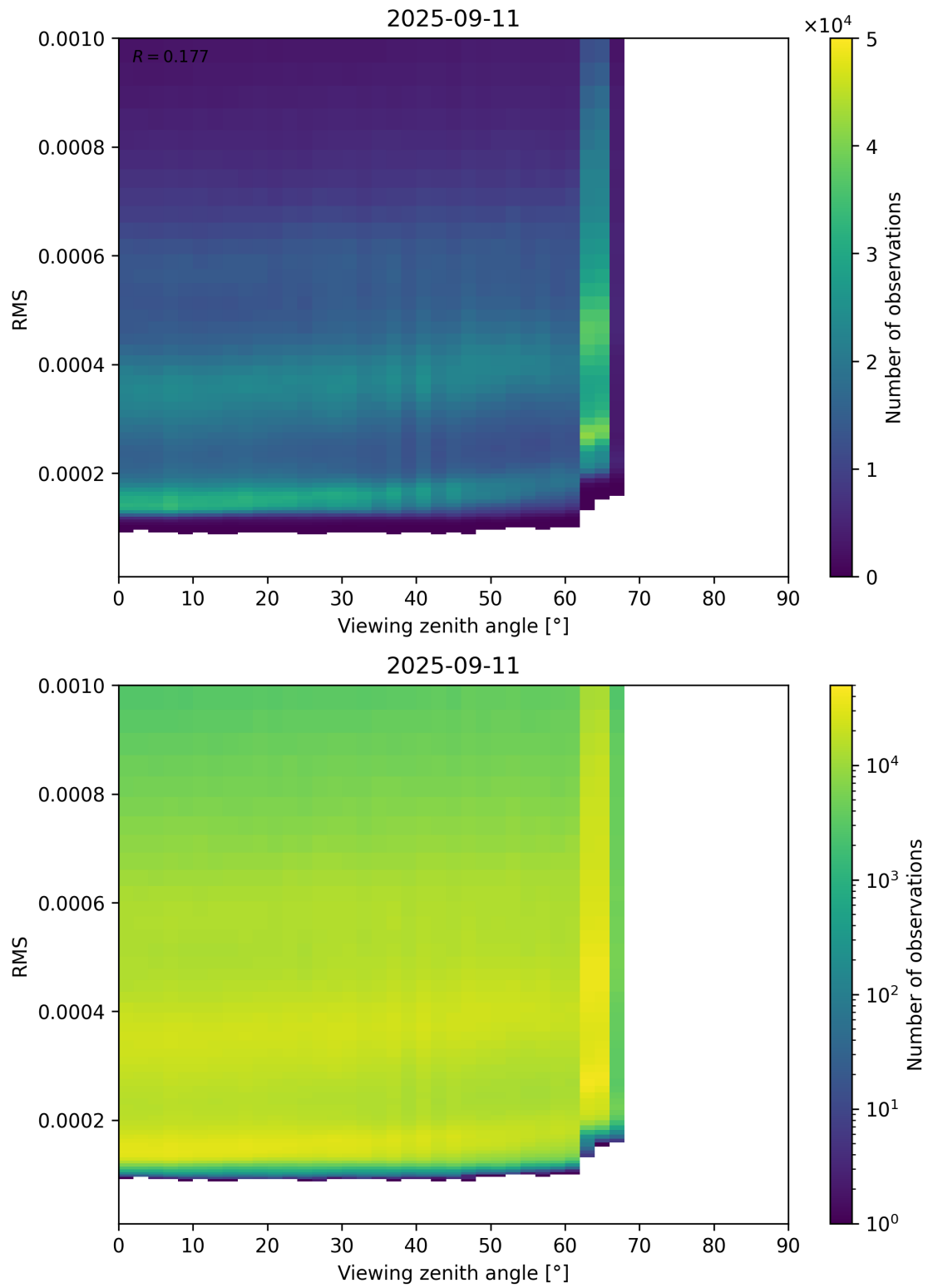
Figure 171: Scatter density plot of “Viewing zenith angle” against “RMS” for 2025-09-10 to 2025-09-12.
