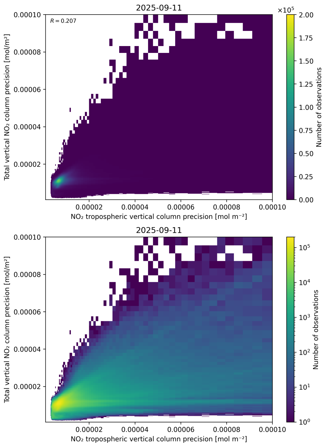
Figure 139: Scatter density plot of “NO 2 tropospheric vertical column precision” against “Total vertical NO 2 column precision” for 2025-09-10 to 2025-09-12.
