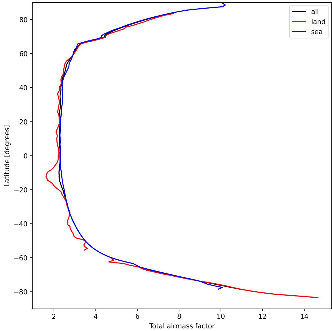
Figure 15: Zonal average of “Total airmass factor” for 2025-09-10 to 2025-09-12.
