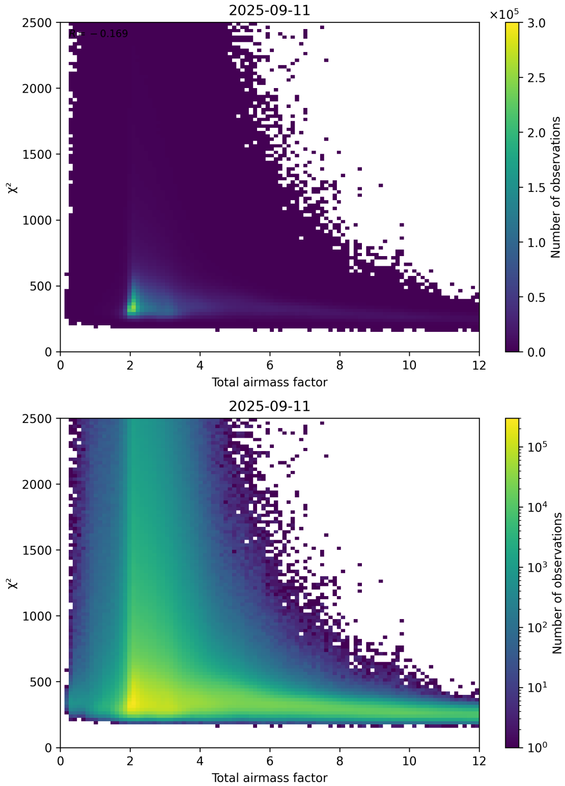
Figure 63: Scatter density plot of “Total airmass factor” against “ \chi^2 ” for 2025-09-10 to 2025-09-12.
