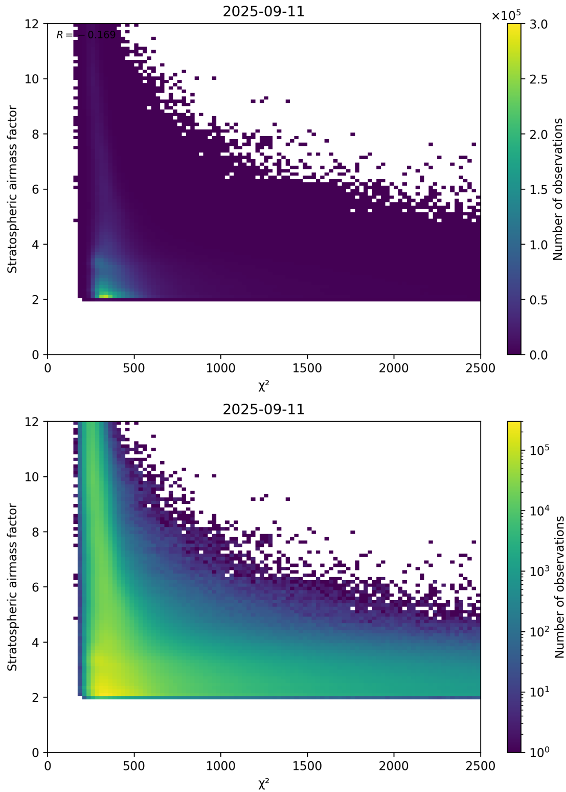
Figure 81: Scatter density plot of “ \chi^2 ” against “Stratospheric airmass factor” for 2025-09-10 to 2025-09-12.
