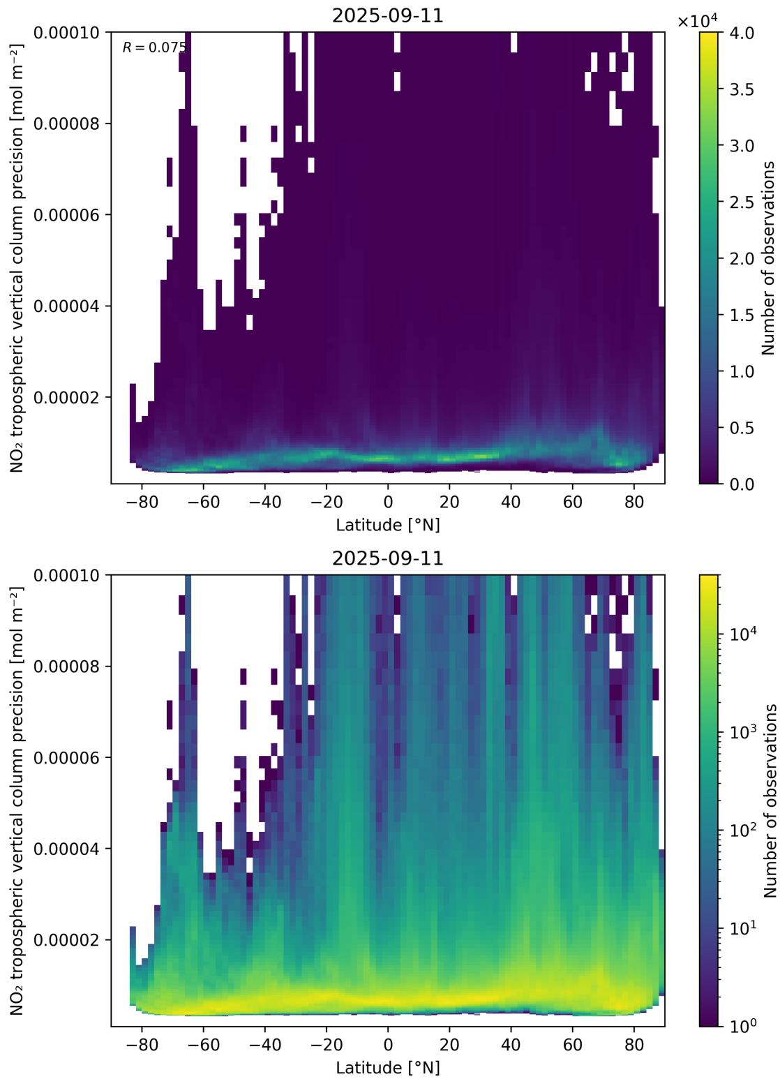
Figure 93: Scatter density plot of “Latitude” against “NO 2 tropospheric vertical column precision” for 2025-09-10 to 2025-09-12.
