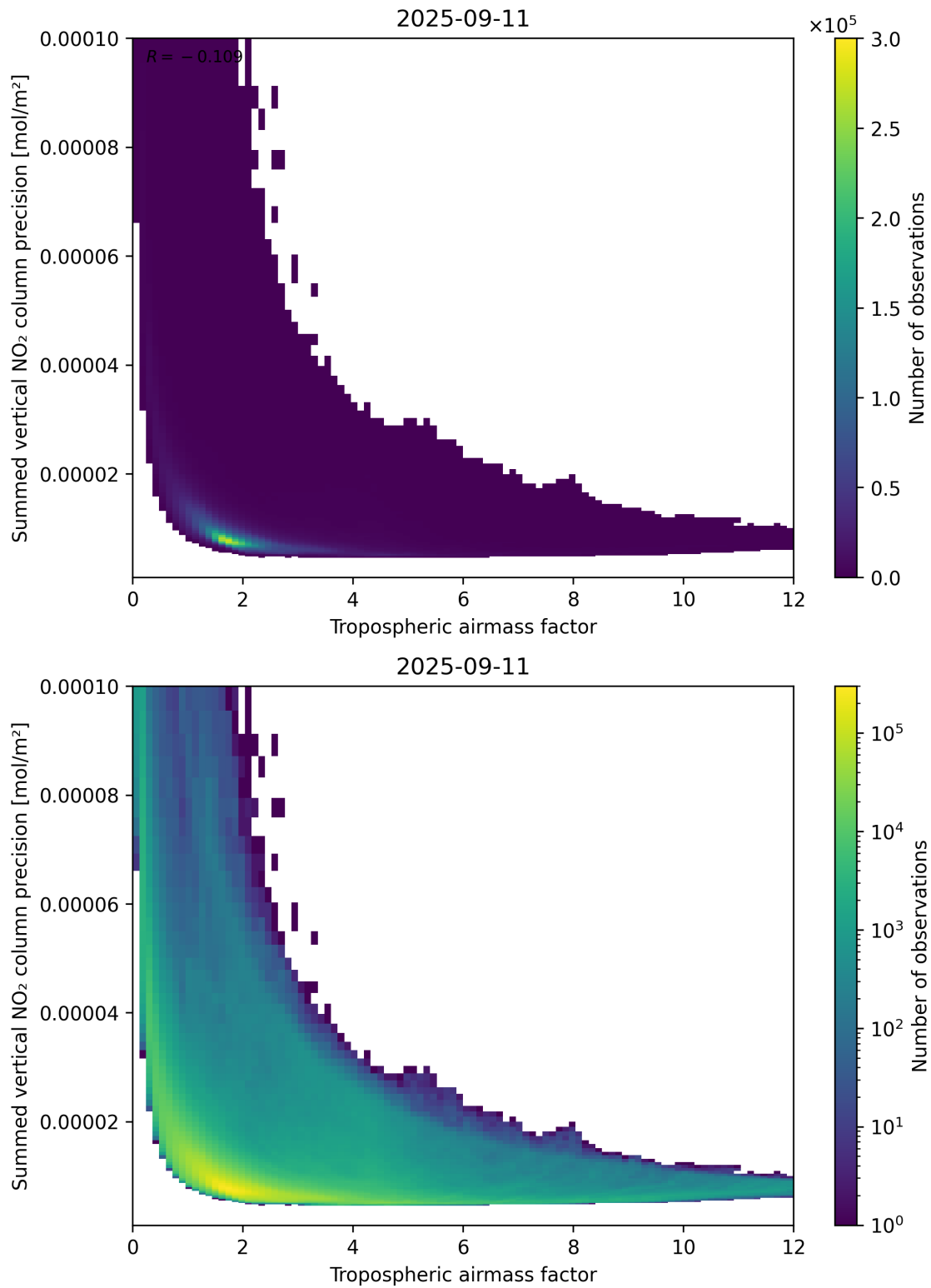
Figure 76: Scatter density plot of “Tropospheric airmass factor” against “Summed vertical NO 2 column precision” for 2025-09-10 to 2025-09-12.
