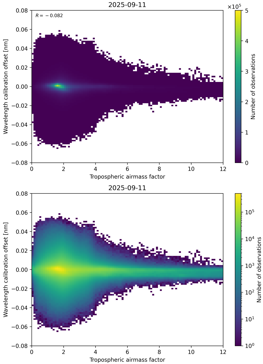
Figure 80: Scatter density plot of “Tropospheric airmass factor” against “Wavelength calibration offset” for 2025-09-10 to 2025-09-12.
