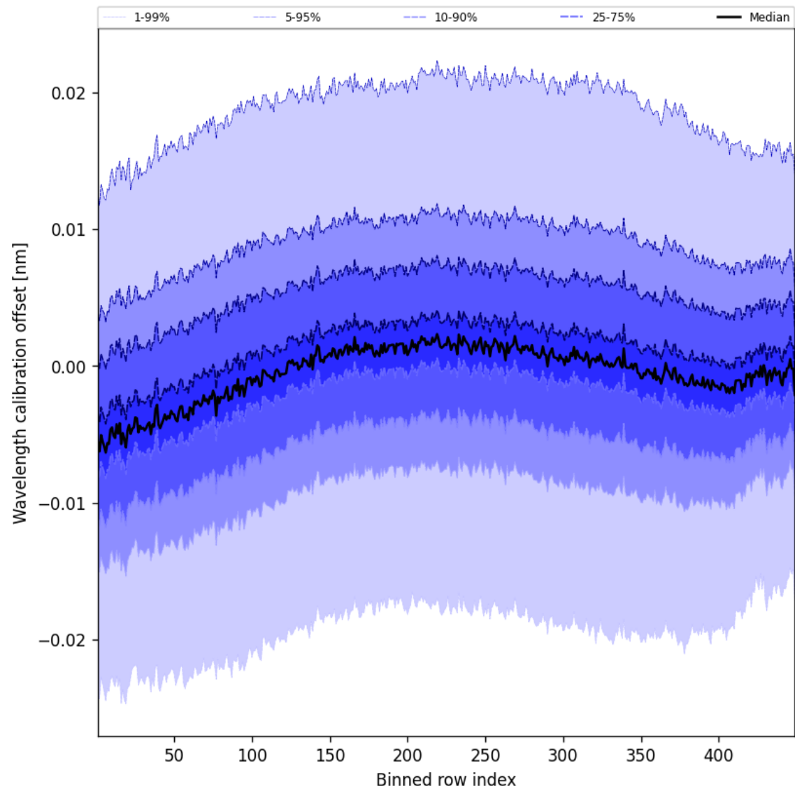
Figure 52: Along track statistics of “Wavelength calibration offset” for 2025-09-10 to 2025-09-12
