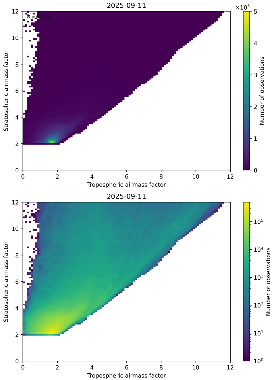
Figure 71: Scatter density plot of “Tropospheric airmass factor” against “Stratospheric airmass factor” for 2025-09-10 to 2025-09-12.
