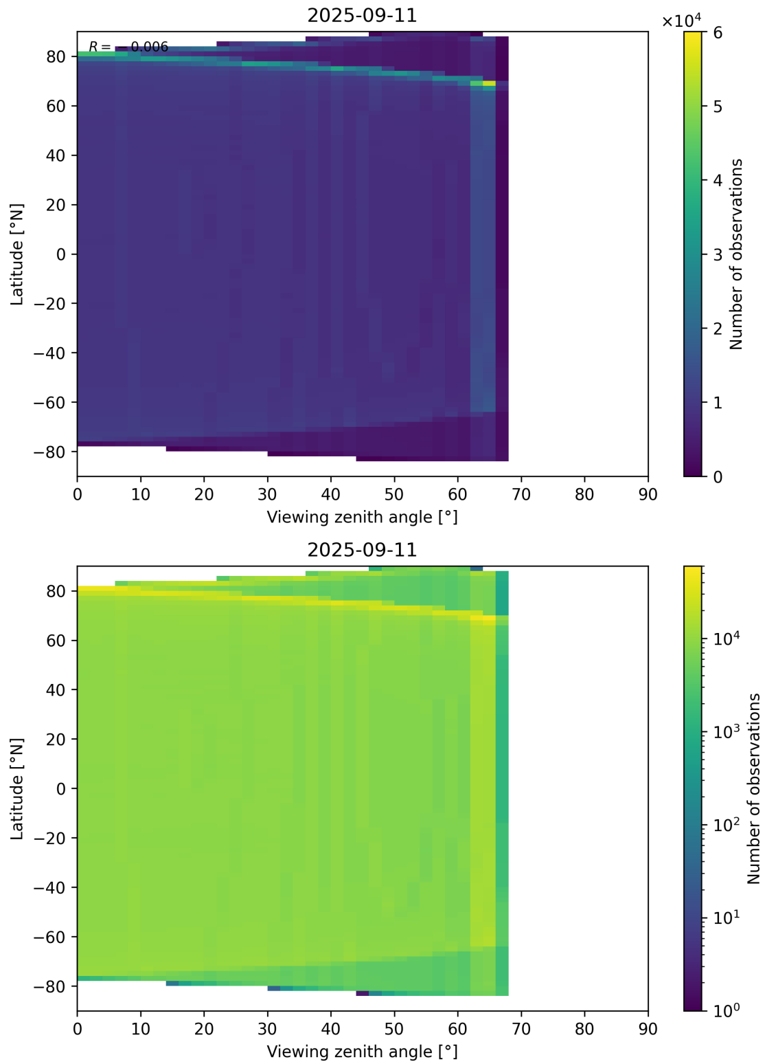
Figure 163: Scatter density plot of “Viewing zenith angle” against “Latitude” for 2025-09-10 to 2025-09-12.
