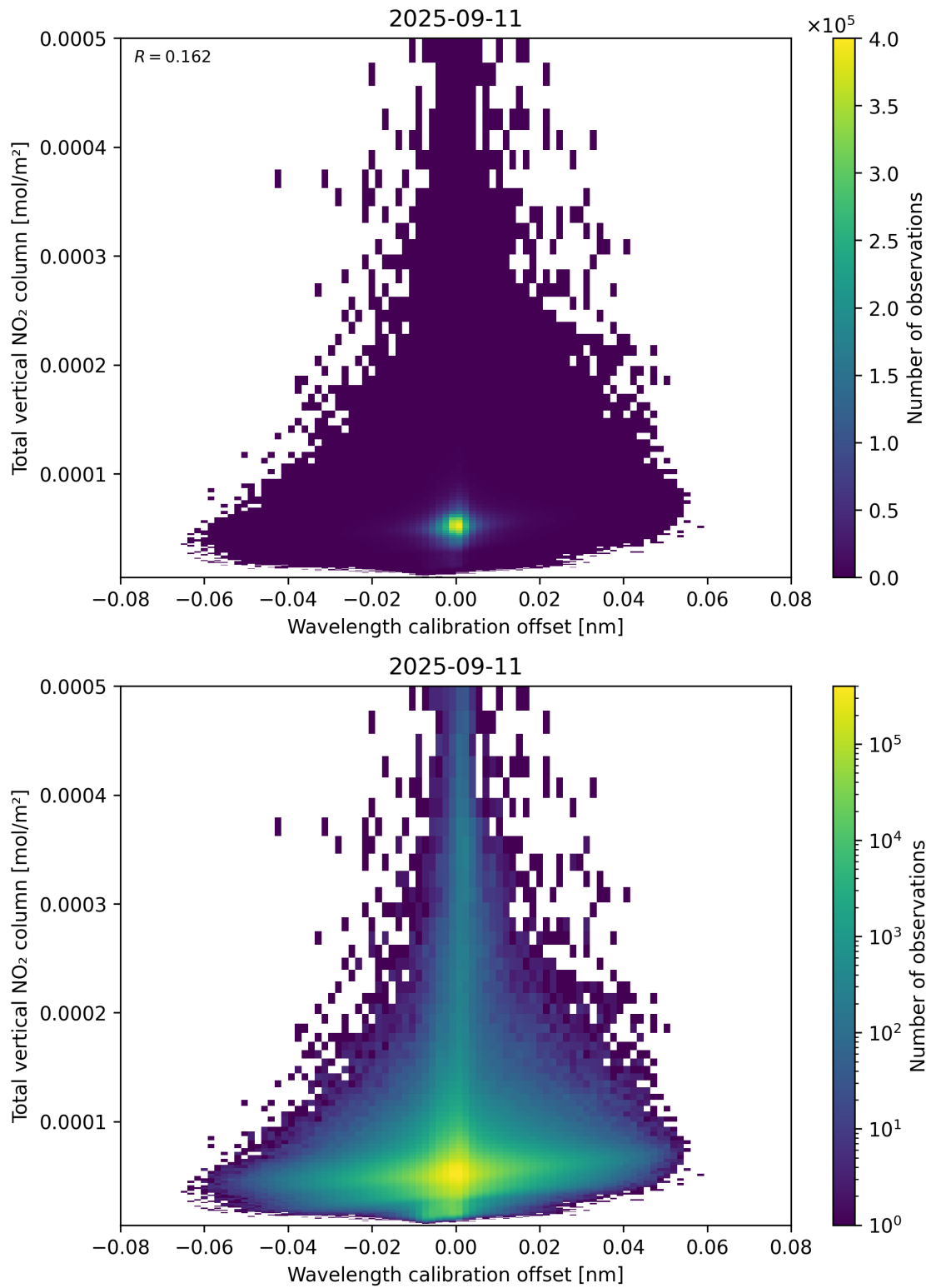
Figure 179: Scatter density plot of “Wavelength calibration offset” against “Total vertical NO 2 column” for 2025-09-10 to 2025-09-12.
