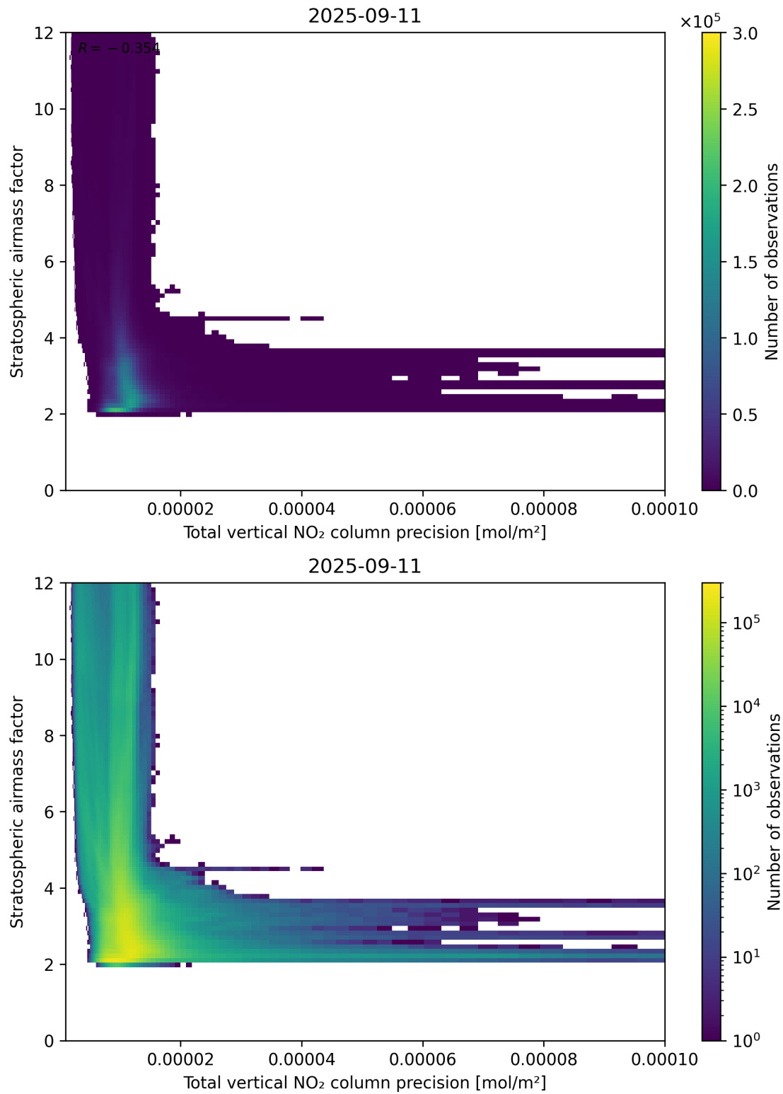
Figure 115: Scatter density plot of “Total vertical NO 2 column precision” against “Stratospheric air mass factor” for 2025-09-10 to 2025-09-12.
