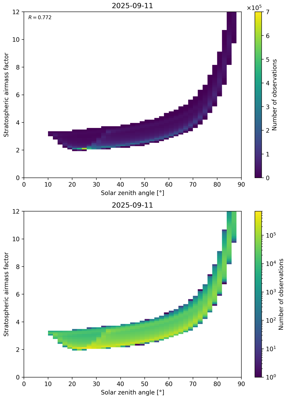
Figure 145: Scatter density plot of “Solar zenith angle” against “Stratospheric airmass factor” for 2025-09-10 to 2025-09-12.
