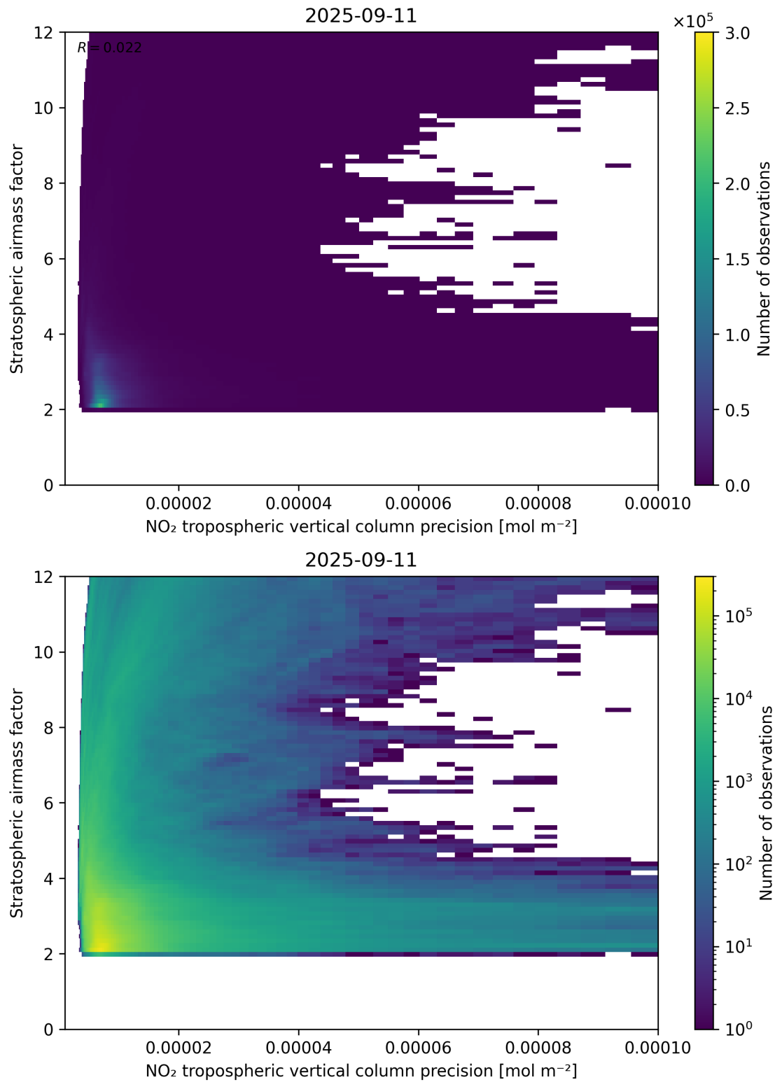
Figure 131: Scatter density plot of “NO 2 tropospheric vertical column precision” against “Stratospheric airmass factor” for 2025-09-10 to 2025-09-12.
