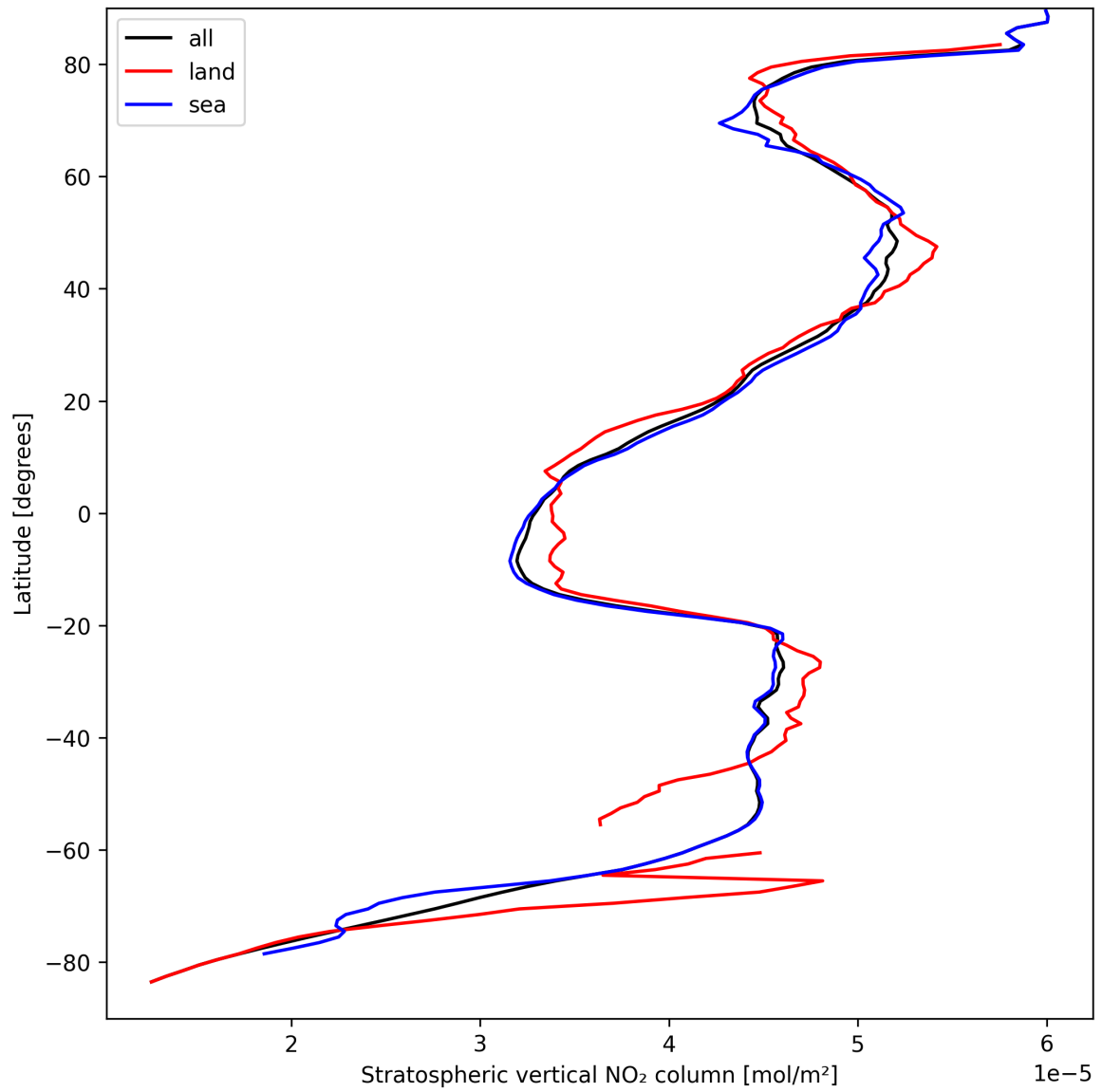
Figure 19: Zonal average of “Stratospheric vertical NO 2 column” for 2025-09-10 to 2025-09-12.
