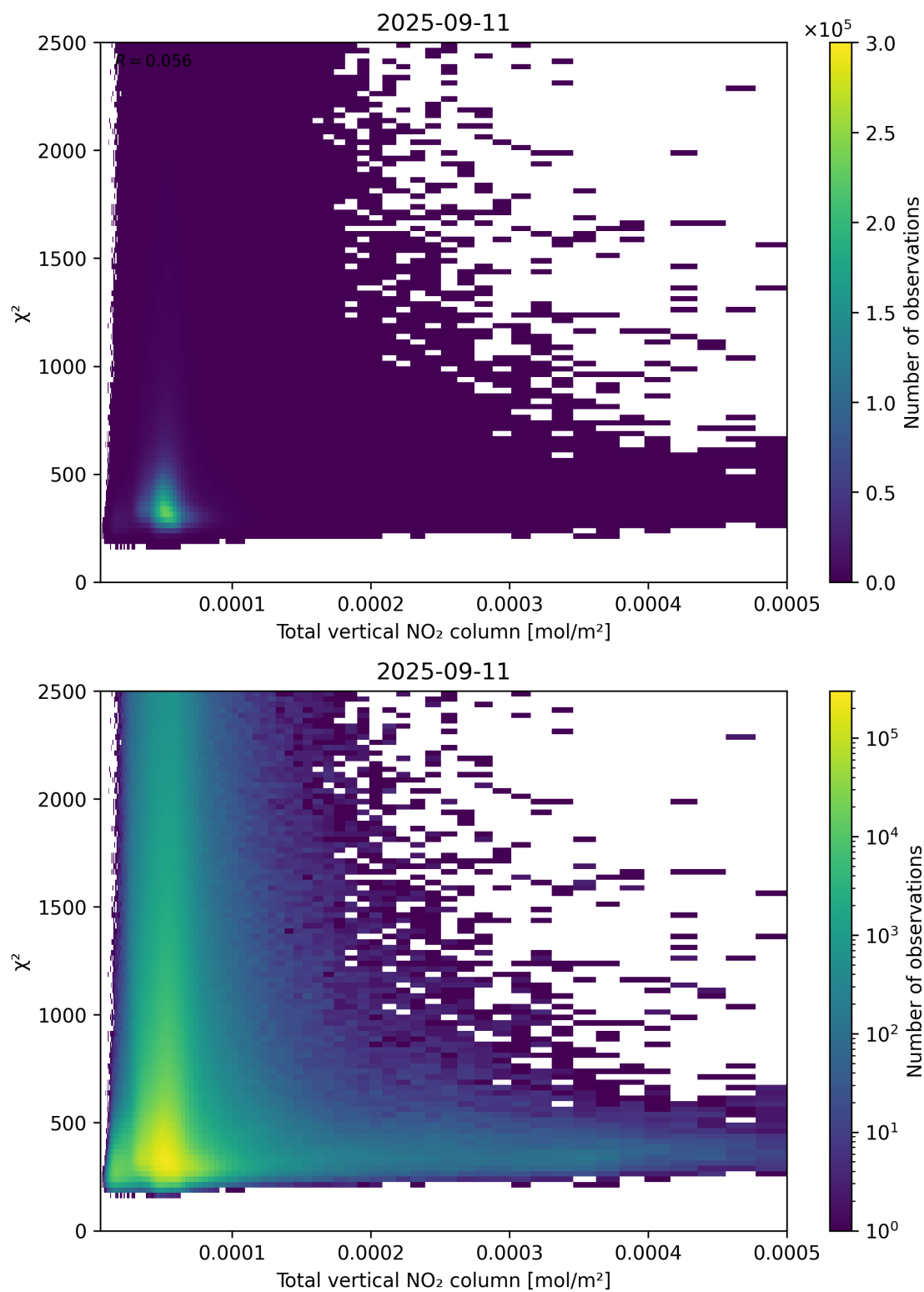
Figure 111: Scatter density plot of “Total vertical NO 2 column” against “ \chi^2 ” for 2025-09-10 to 2025-09-12.
