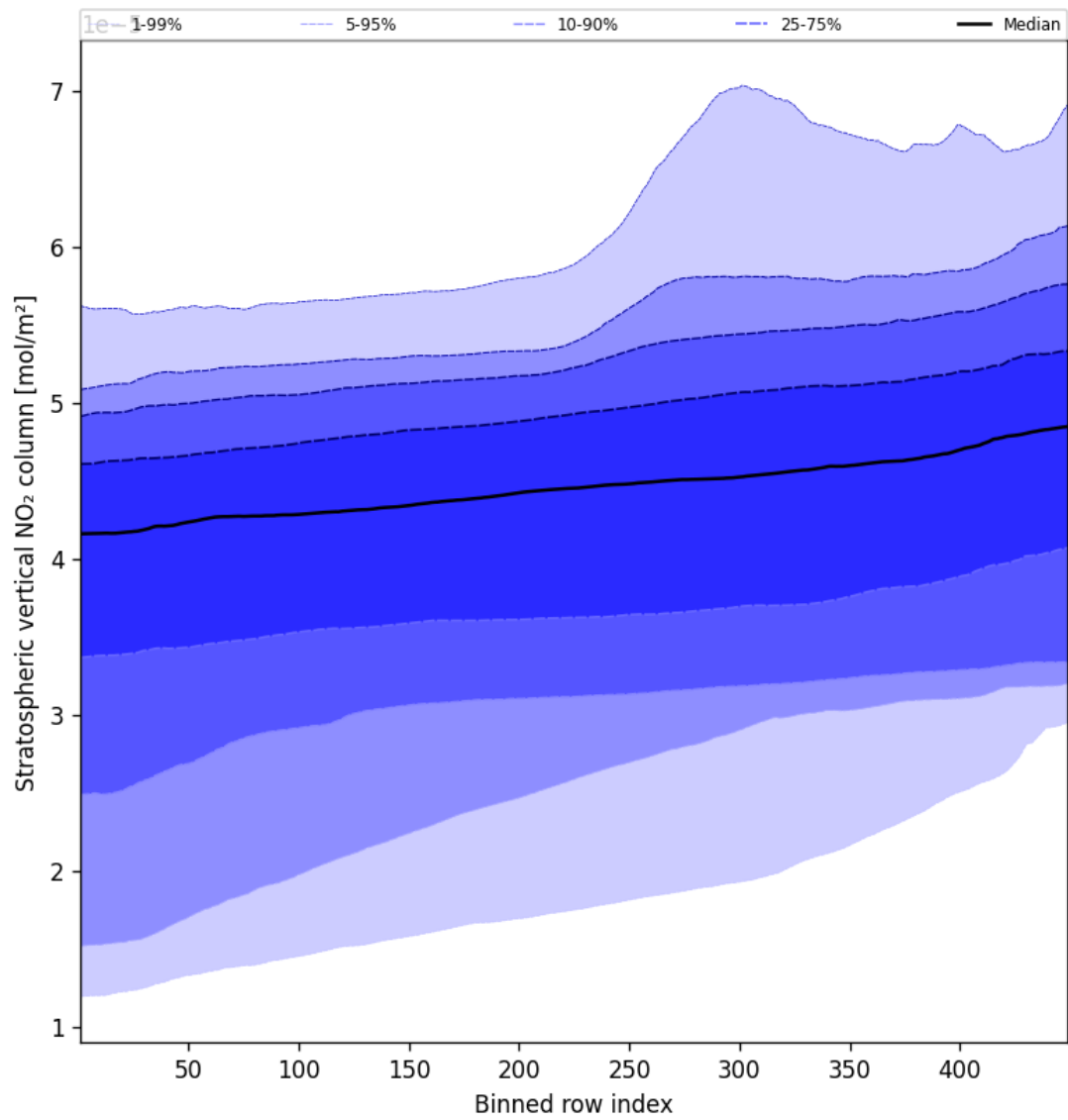
Figure 53: Along track statistics of “Stratospheric vertical NO 2 column” for 2025-09-10 to 2025-09-12
