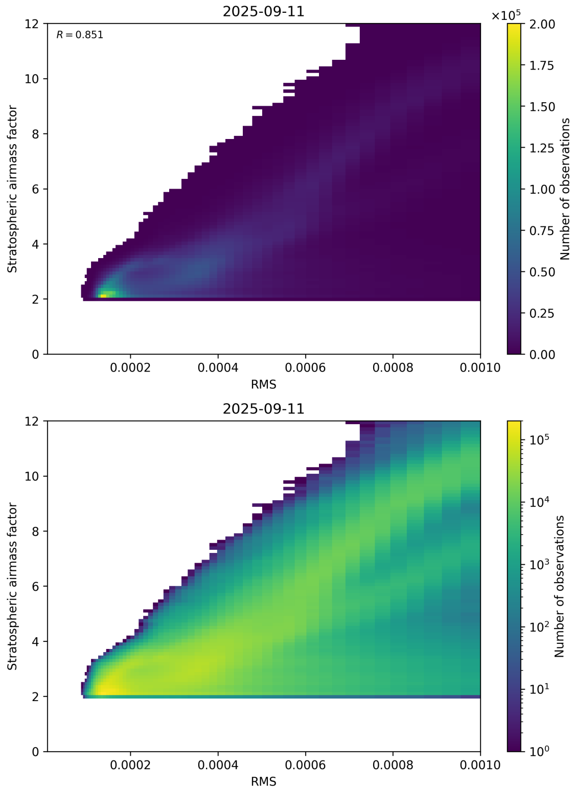
Figure 144: Scatter density plot of “RMS” against “Stratospheric airmass factor” for 2025-09-10 to 2025-09-12.
