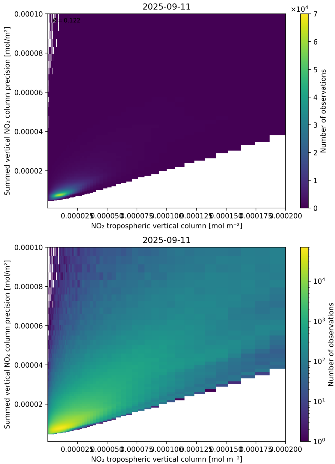
Figure 127: Scatter density plot of “NO 2 tropospheric vertical column” against “Summed vertical NO 2 column precision” for 2025-09-10 to 2025-09-12.
