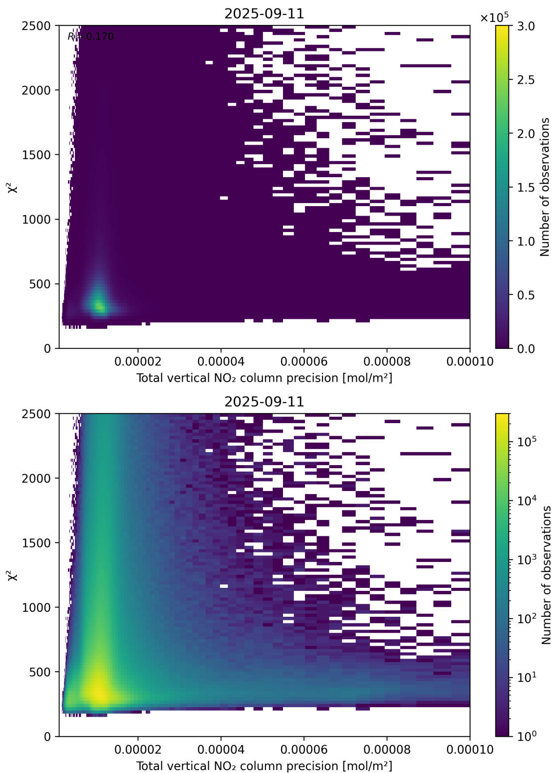
Figure 116: Scatter density plot of “Total vertical NO 2 column precision” against “ \chi^2 ” for 2025-09-10 to 2025-09-12.
