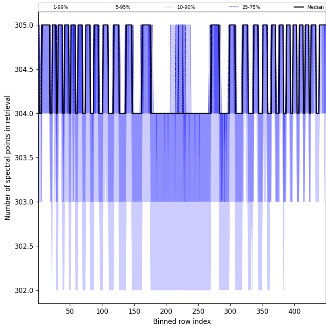
Figure 50: Along track statistics of “Number of spectral points in retrieval” for 2025-09-10 to 2025-09-12
