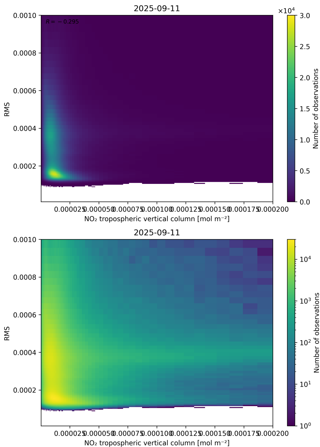
Figure 142: Scatter density plot of “NO 2 tropospheric vertical column” against “RMS” for 2025-09-10 to 2025-09-12.
