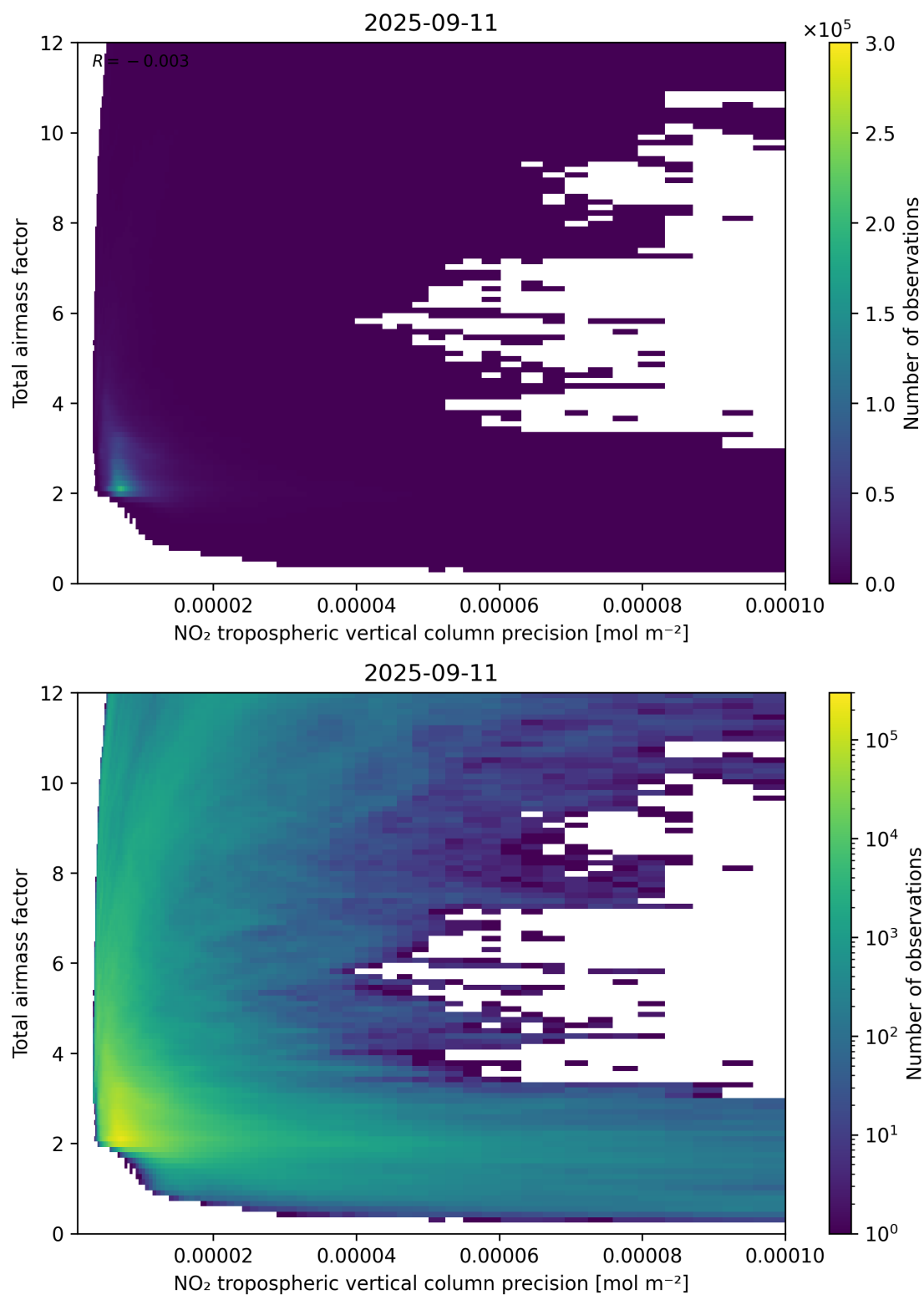
Figure 132: Scatter density plot of “NO 2 tropospheric vertical column precision” against “Total air mass factor” for 2025-09-10 to 2025-09-12.
