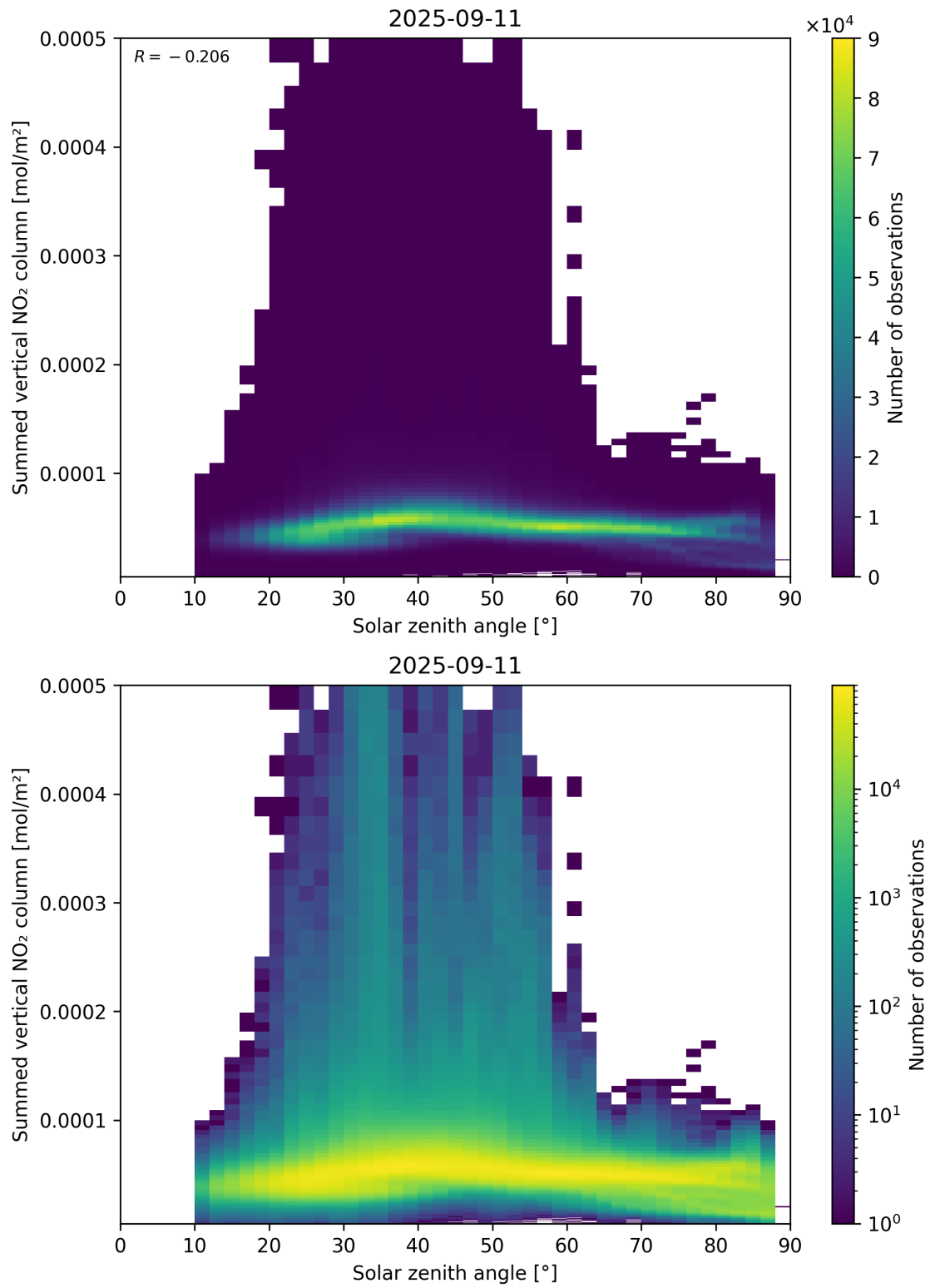
Figure 151: Scatter density plot of “Solar zenith angle” against “Summed vertical NO 2 column” for 2025-09-10 to 2025-09-12.
