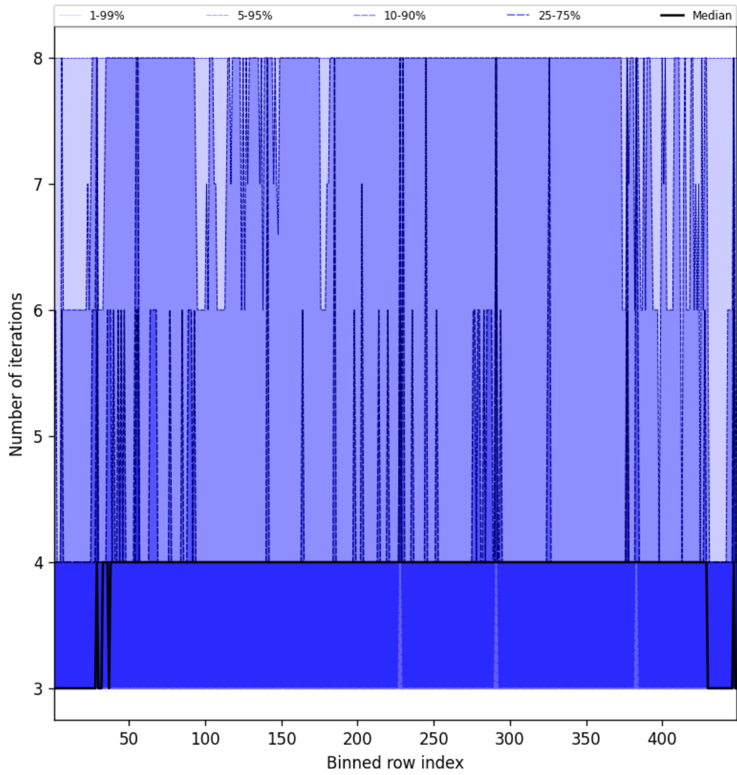
Figure 51: Along track statistics of “Number of iterations” for 2025-09-10 to 2025-09-12
