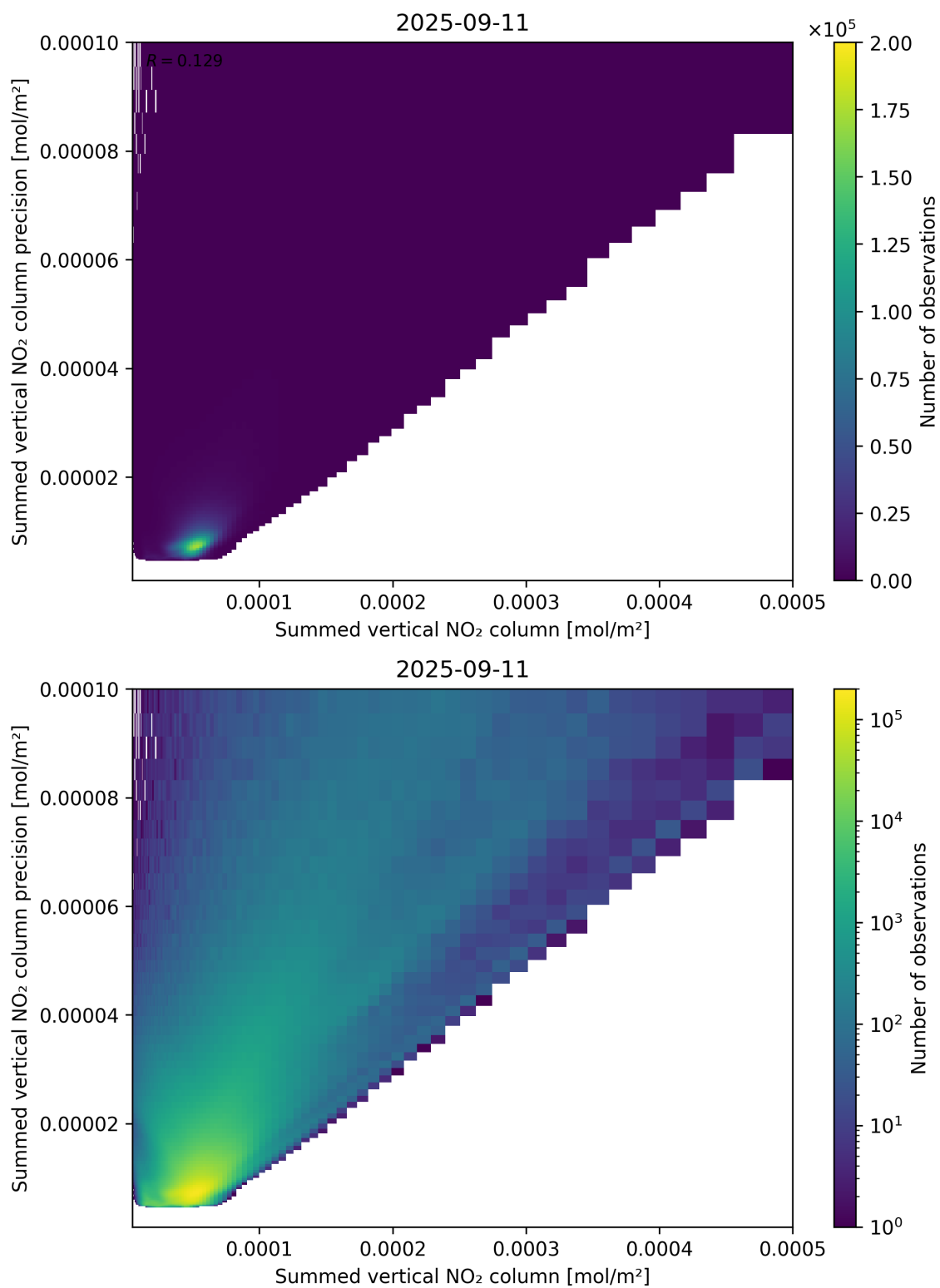
Figure 105: Scatter density plot of “Summed vertical NO 2 column” against “Summed vertical NO 2 column precision” for 2025-09-10 to 2025-09-12.
