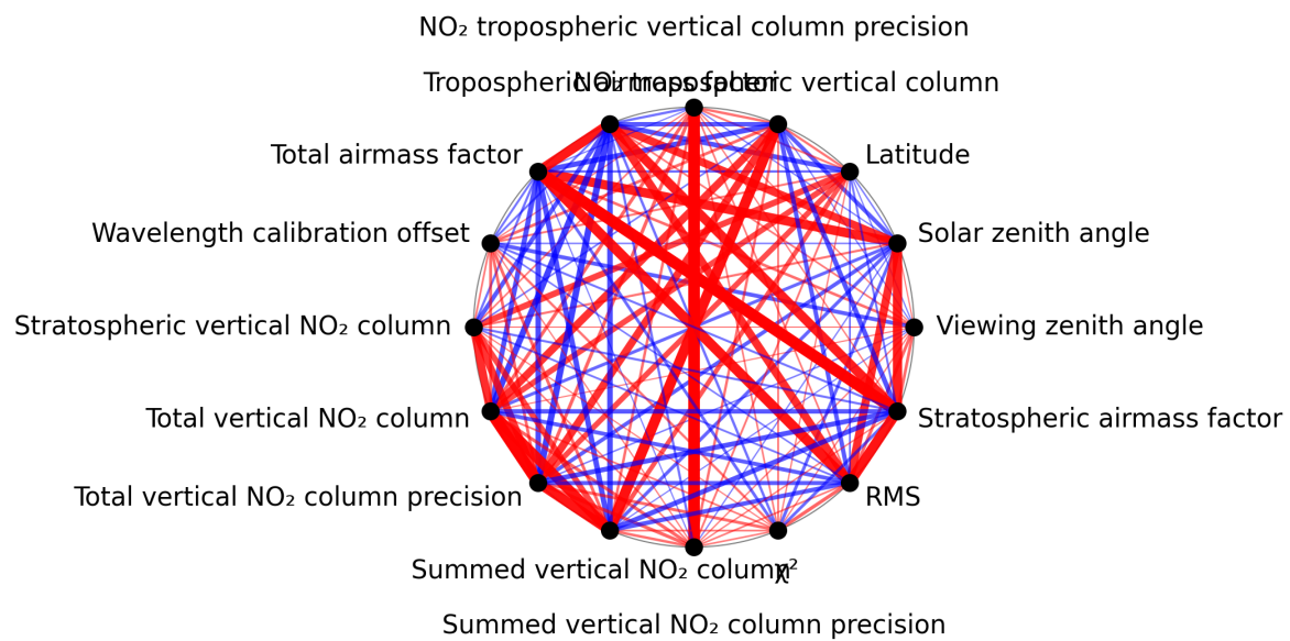
Figure 1: Map of correlation graph for 2025-09-10 to 2025-09-12.
