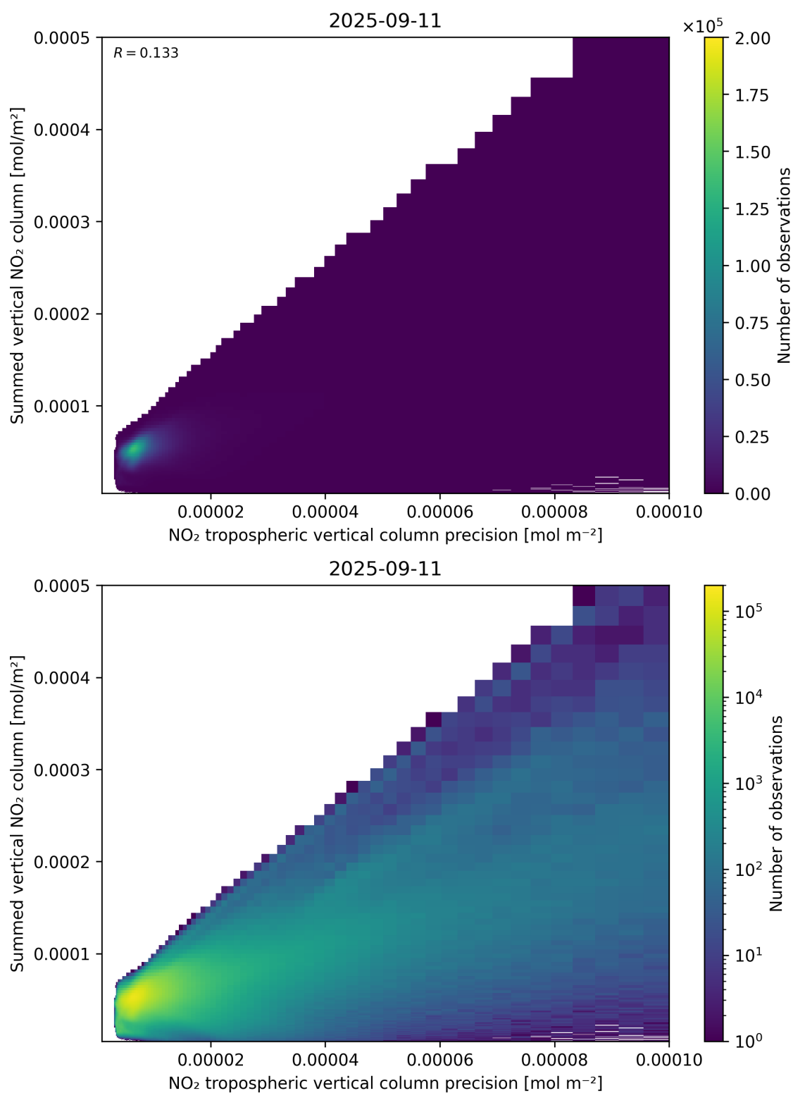
Figure 136: Scatter density plot of “NO 2 tropospheric vertical column precision” against “Summed vertical NO 2 column” for 2025-09-10 to 2025-09-12.
