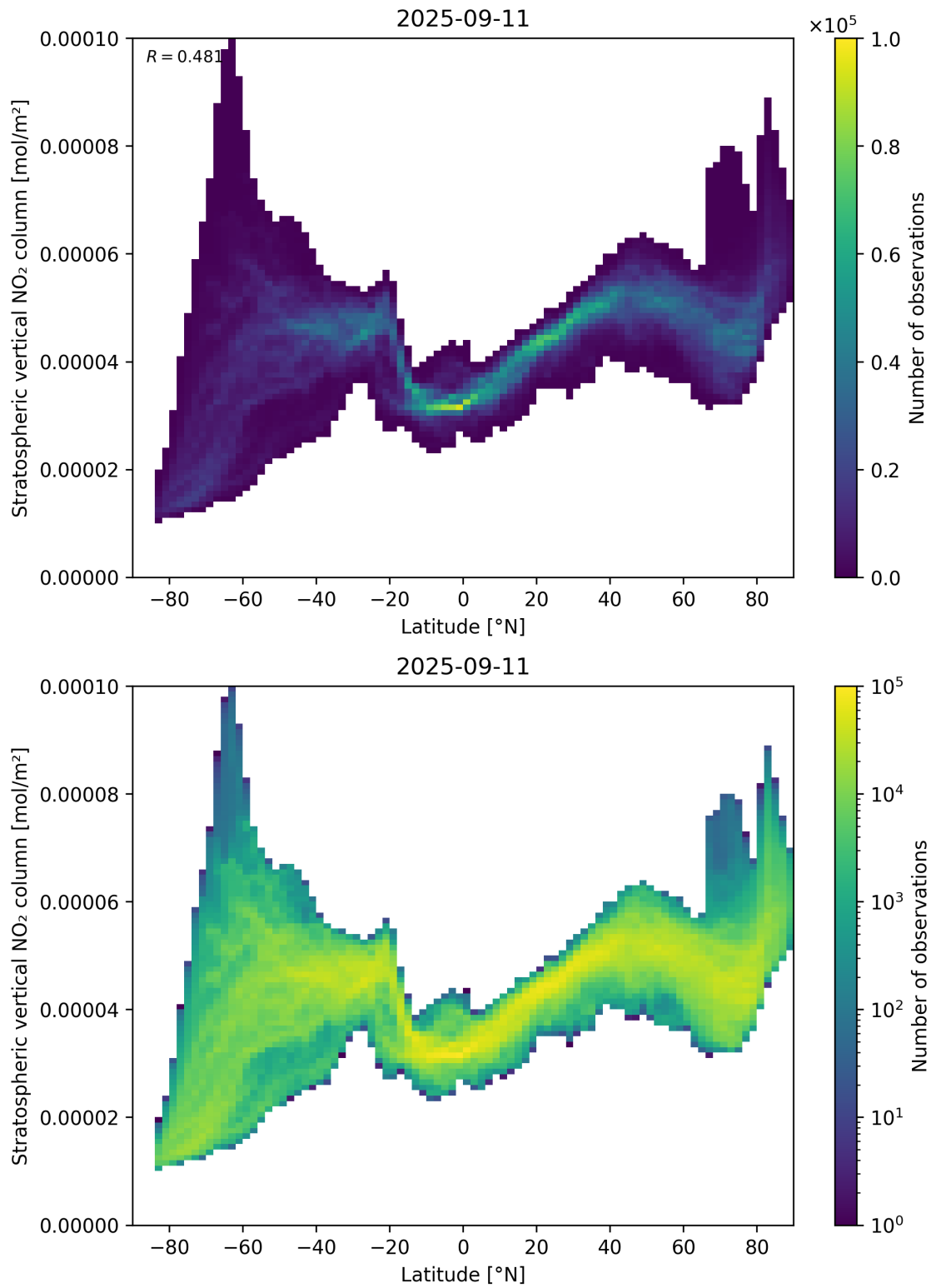
Figure 87: Scatter density plot of “Latitude” against “Stratospheric vertical NO 2 column” for 2025-09-10 to 2025-09-12.
