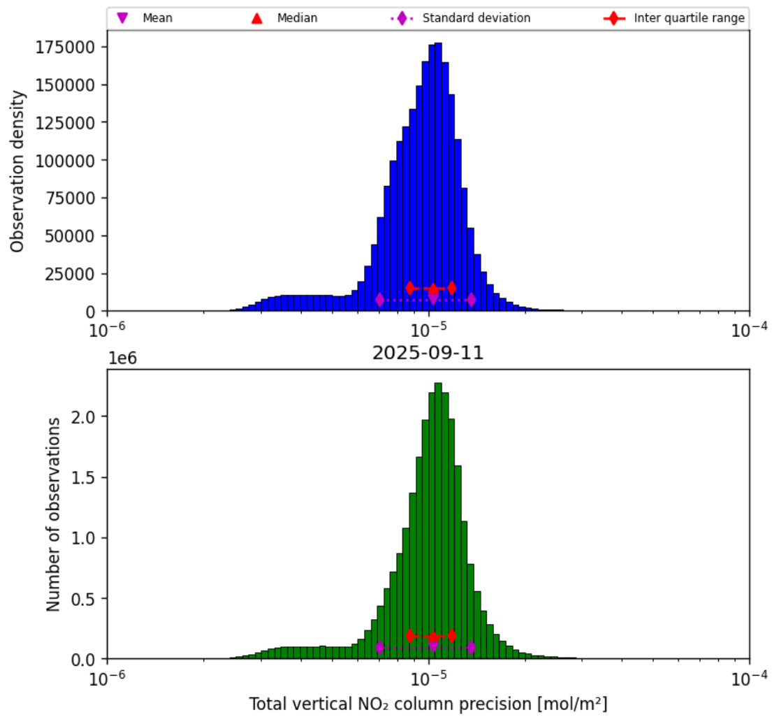
Figure 39: Histogram of “Total vertical NO 2 column precision” for 2025-09-10 to 2025-09-12
