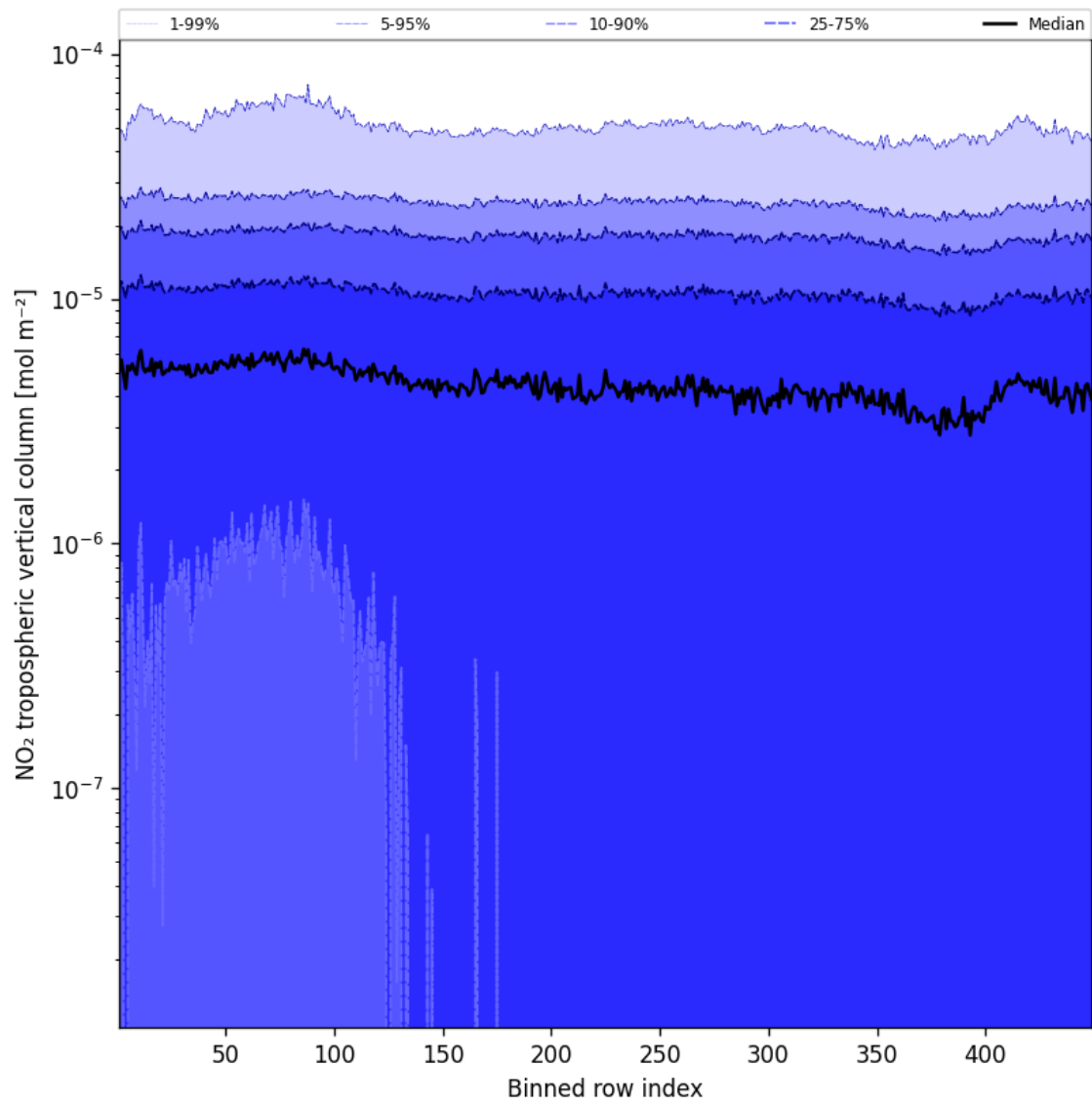
Figure 46: Along track statistics of “NO 2 tropospheric vertical column” for 2025-09-10 to 2025-09-12
