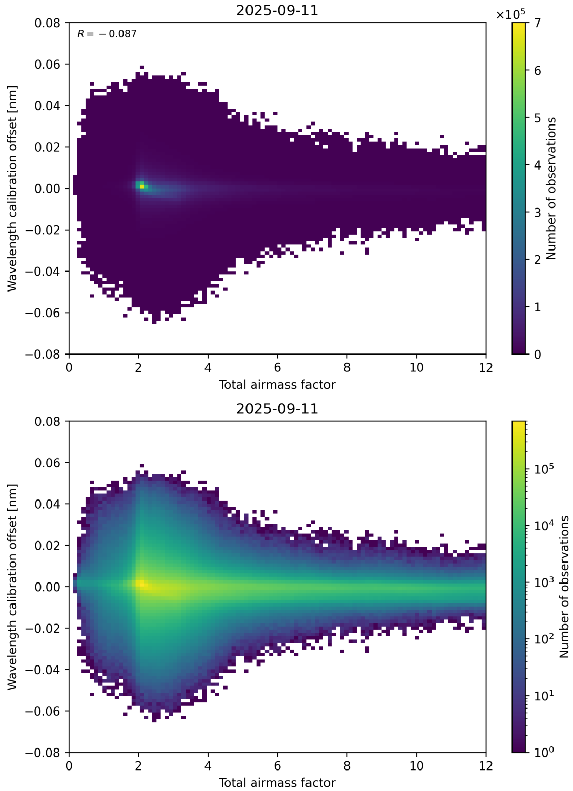
Figure 70: Scatter density plot of “Total airmass factor” against “Wavelength calibration offset” for 2025-09-10 to 2025-09-12.
