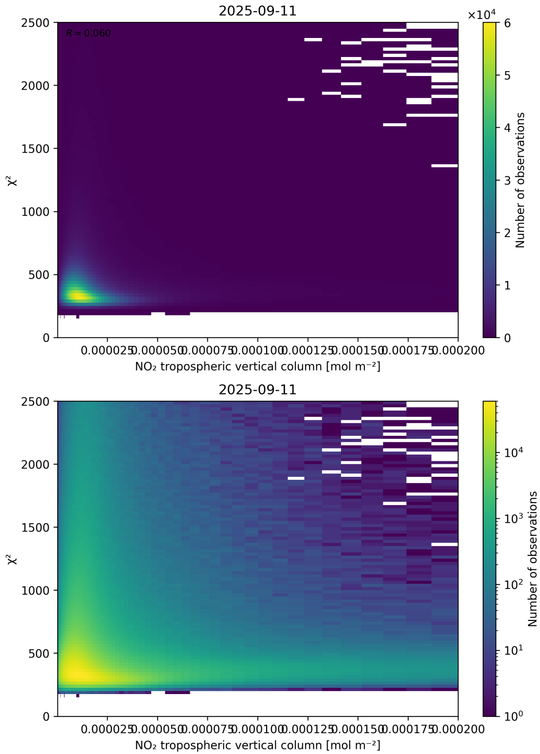
Figure 124: Scatter density plot of “NO 2 tropospheric vertical column” against “ \chi^2 ” for 2025-09-10 to 2025-09-12.
