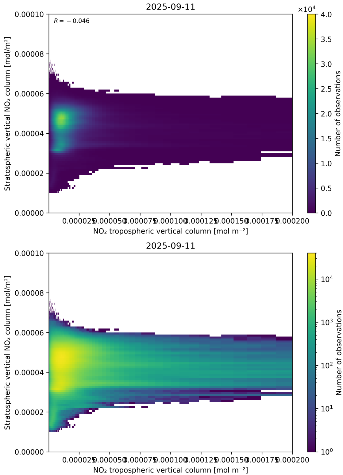
Figure 125: Scatter density plot of “NO 2 tropospheric vertical column” against “Stratospheric vertical NO 2 column” for 2025-09-10 to 2025-09-12.
