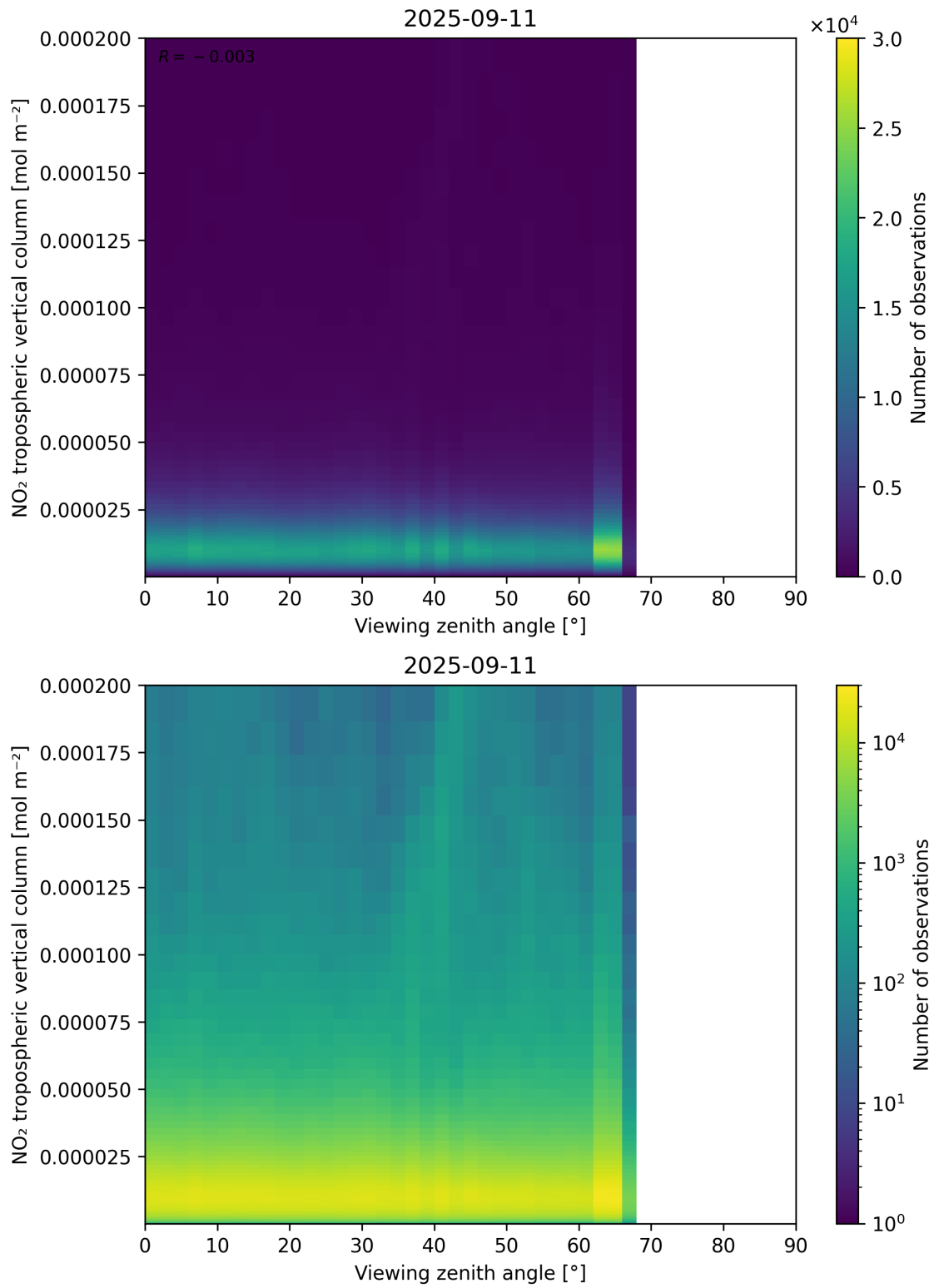
Figure 169: Scatter density plot of “Viewing zenith angle” against “NO 2 tropospheric vertical column” for 2025-09-10 to 2025-09-12.
