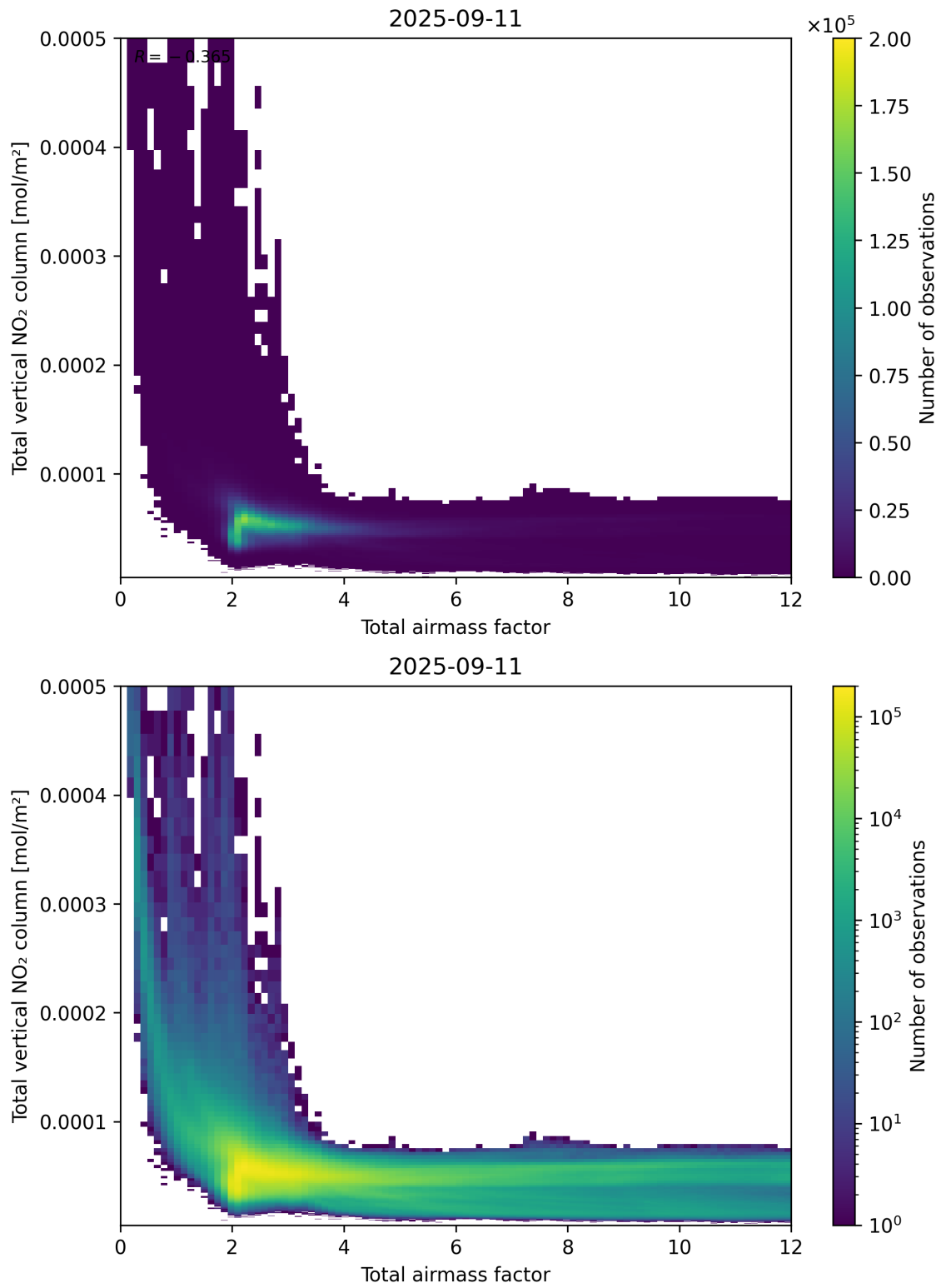
Figure 67: Scatter density plot of “Total airmass factor” against “Total vertical NO 2 column” for 2025-09-10 to 2025-09-12.
