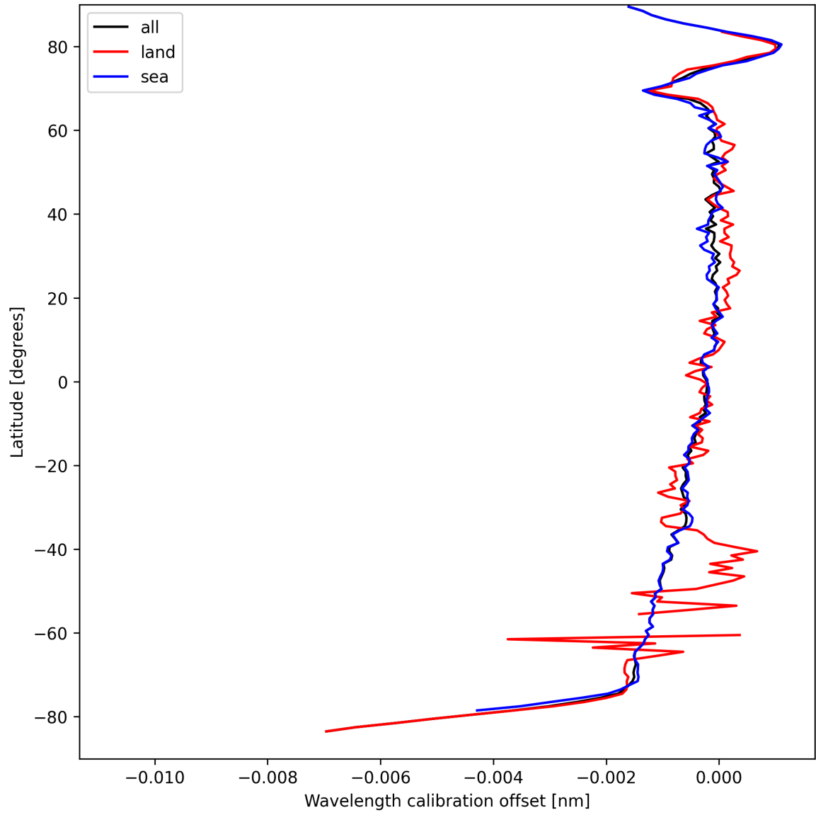
Figure 18: Zonal average of “Wavelength calibration offset” for 2025-09-10 to 2025-09-12.
