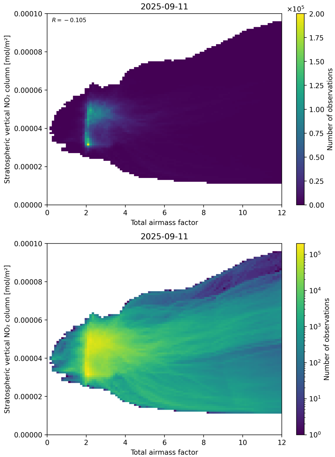
Figure 64: Scatter density plot of “Total airmass factor” against “Stratospheric vertical NO 2 column” for 2025-09-10 to 2025-09-12.
