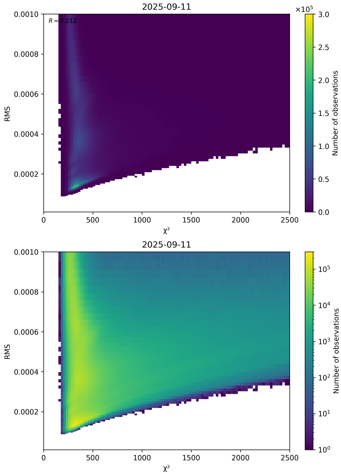
Figure 82: Scatter density plot of “ \chi^2 ” against “RMS” for 2025-09-10 to 2025-09-12.
