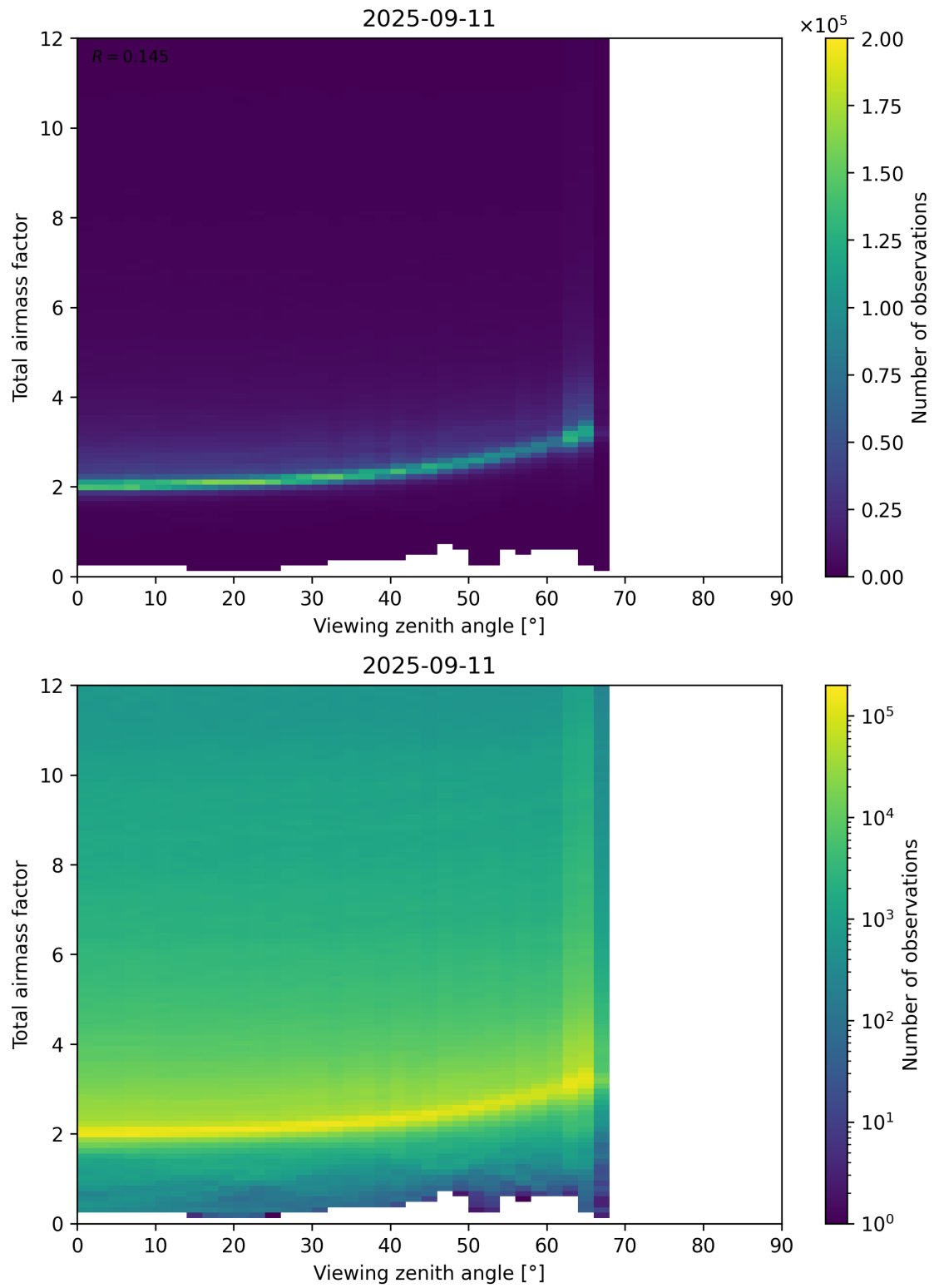
Figure 160: Scatter density plot of “Viewing zenith angle” against “Total airmass factor” for 2025-09-10 to 2025-09-12.
