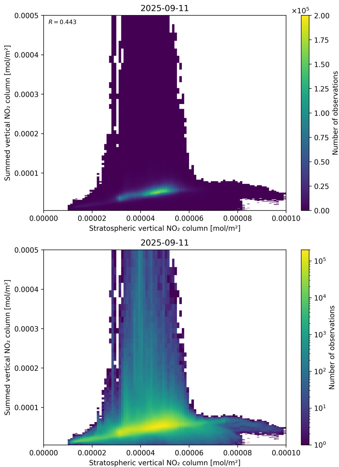
Figure 98: Scatter density plot of “Stratospheric vertical NO 2 column” against “Summed vertical NO 2 column” for 2025-09-10 to 2025-09-12.
