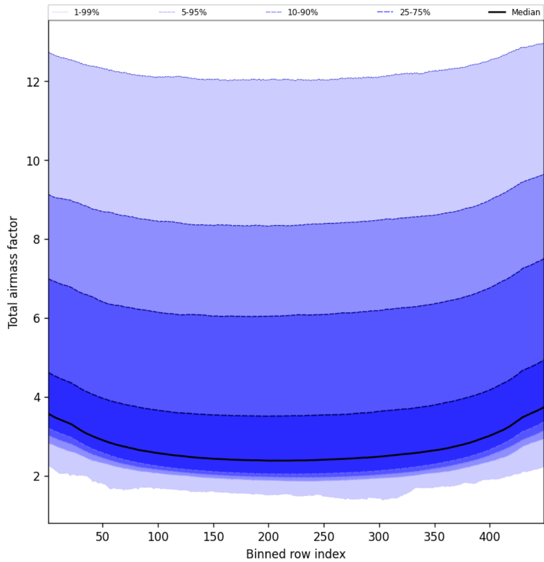
Figure 49: Along track statistics of “Total airmass factor” for 2025-09-10 to 2025-09-12
