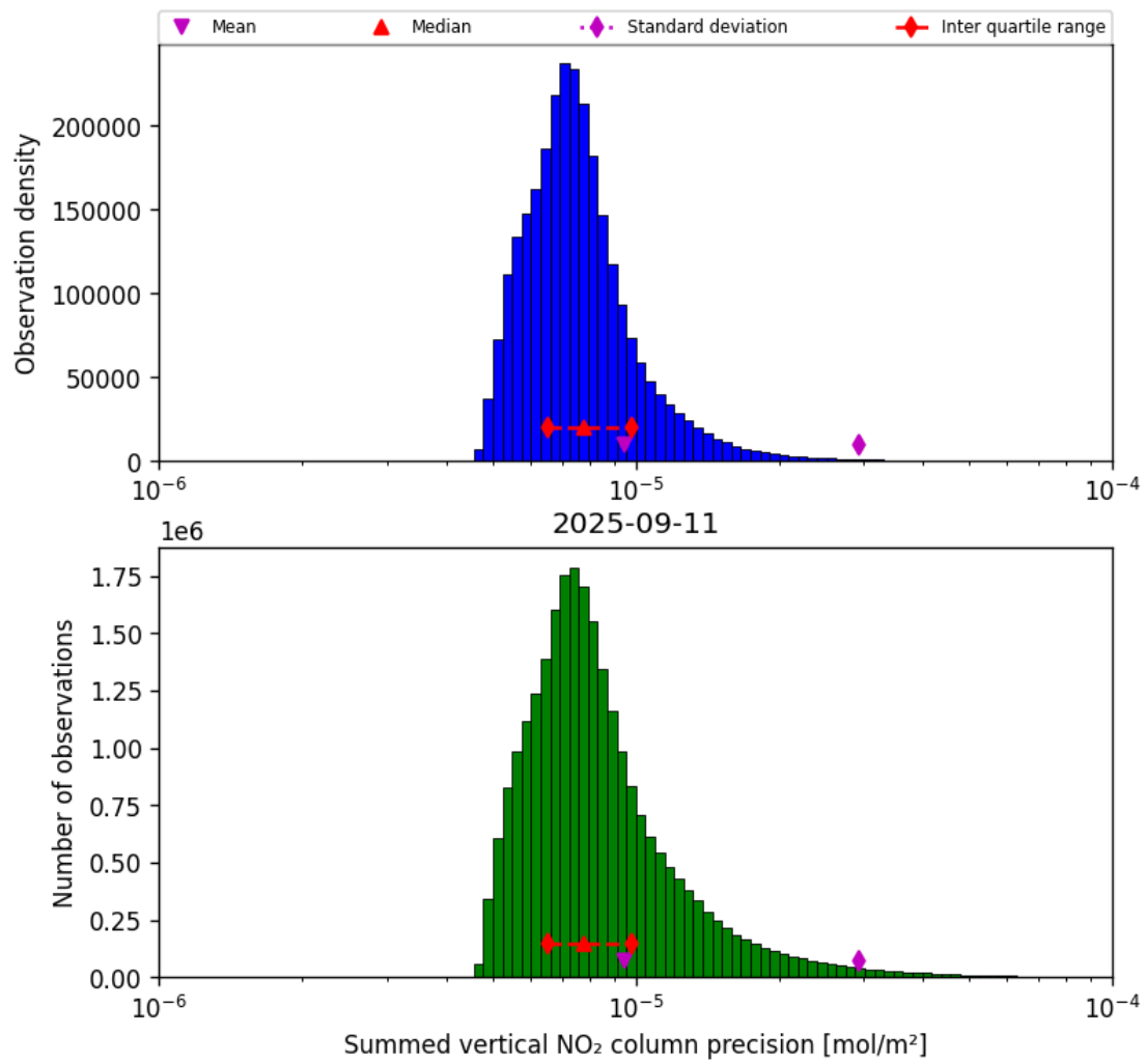
Figure 41: Histogram of “Summed vertical NO 2 column precision” for 2025-09-10 to 2025-09-12
