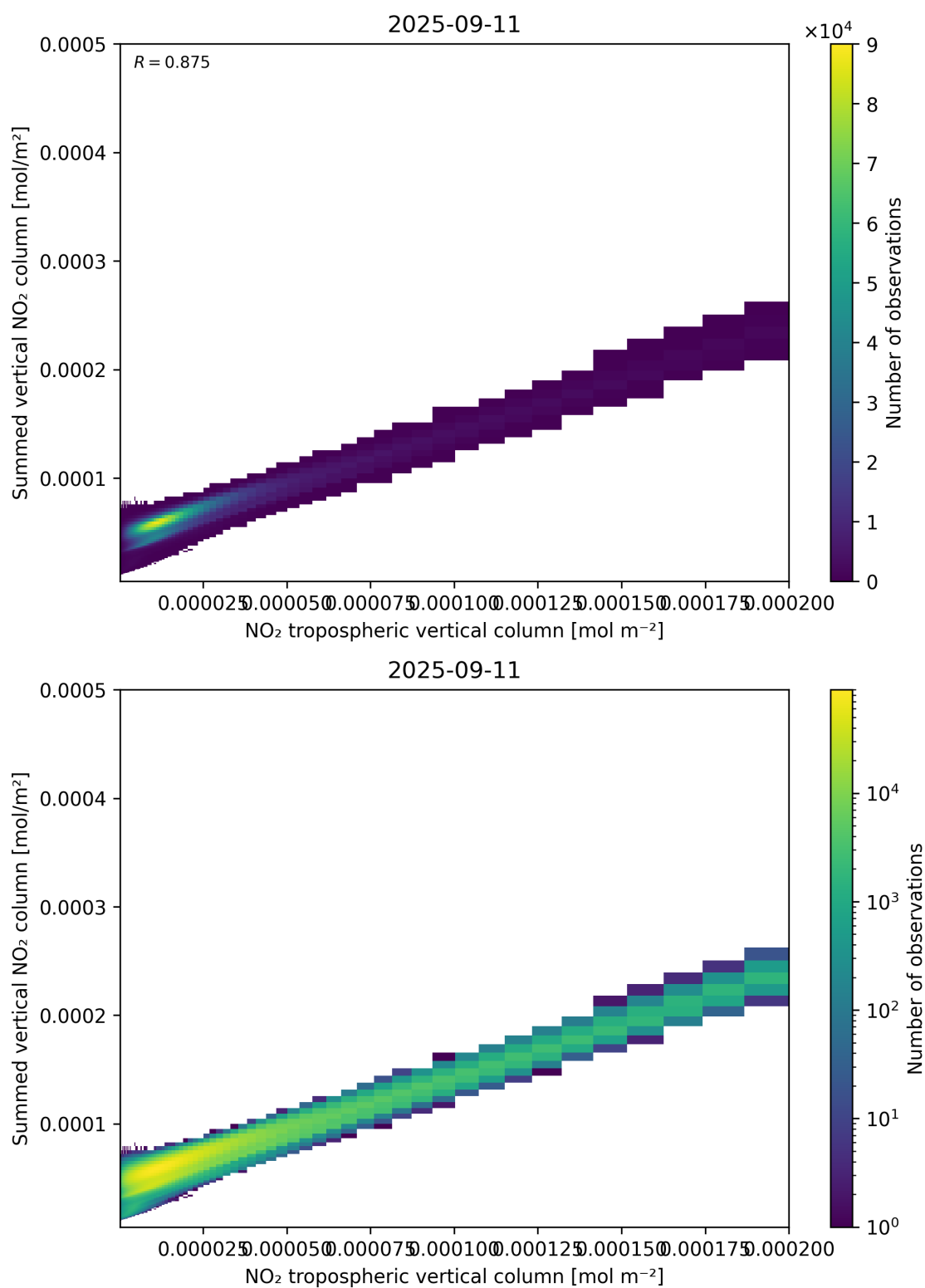
Figure 126: Scatter density plot of “NO 2 tropospheric vertical column” against “Summed vertical NO 2 column” for 2025-09-10 to 2025-09-12.
