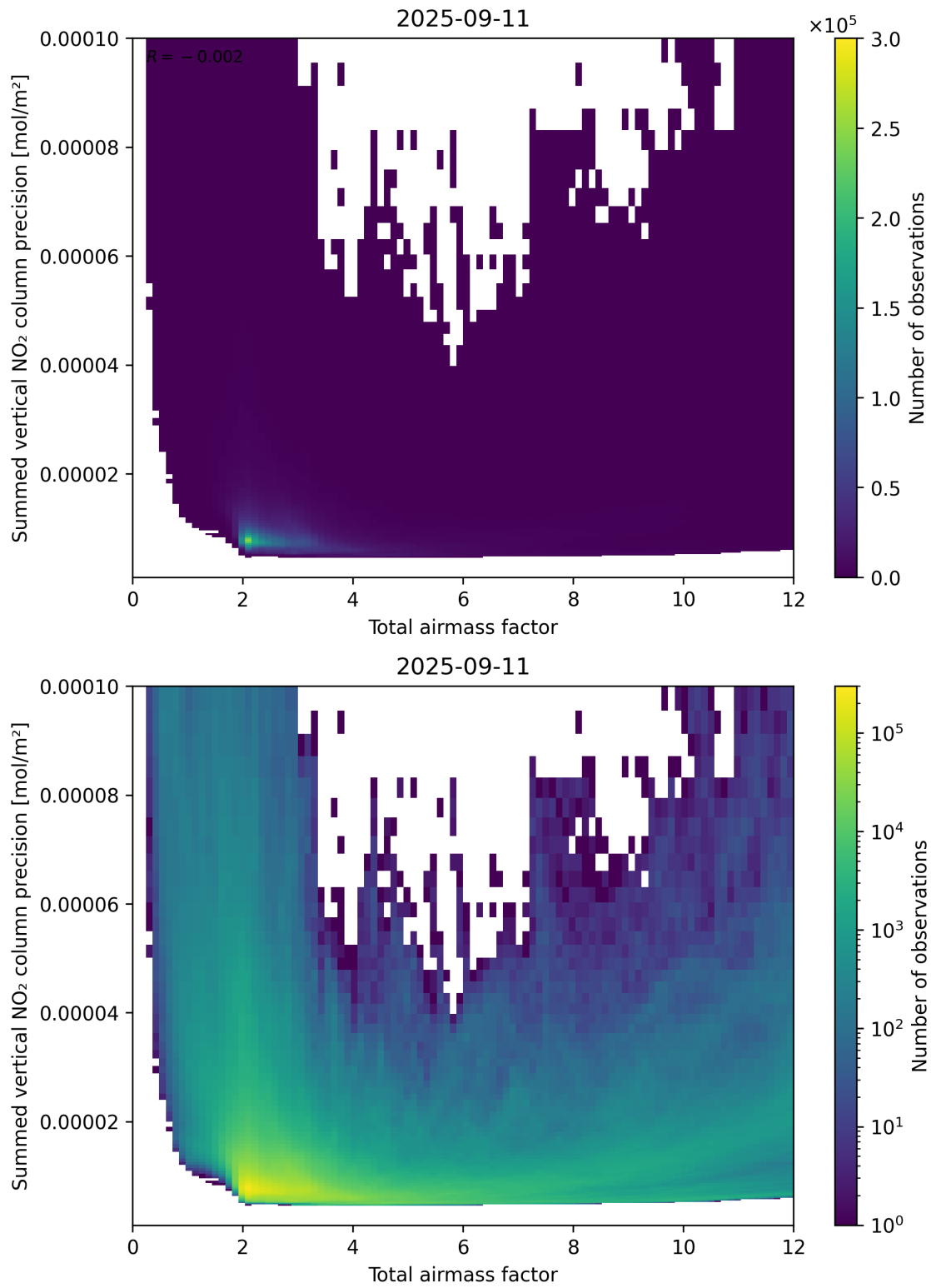
Figure 66: Scatter density plot of “Total airmass factor” against “Summed vertical NO 2 column precision” for 2025-09-10 to 2025-09-12.
