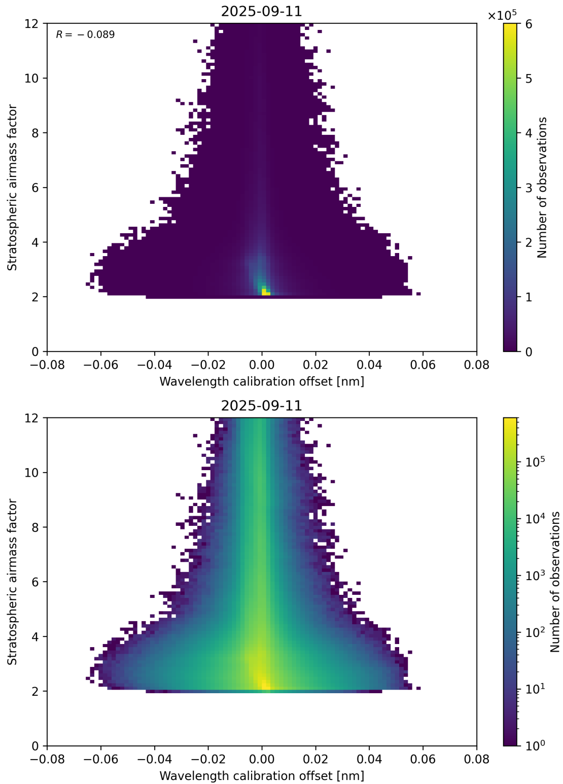
Figure 174: Scatter density plot of “Wavelength calibration offset” against “Stratospheric airmass factor” for 2025-09-10 to 2025-09-12.
