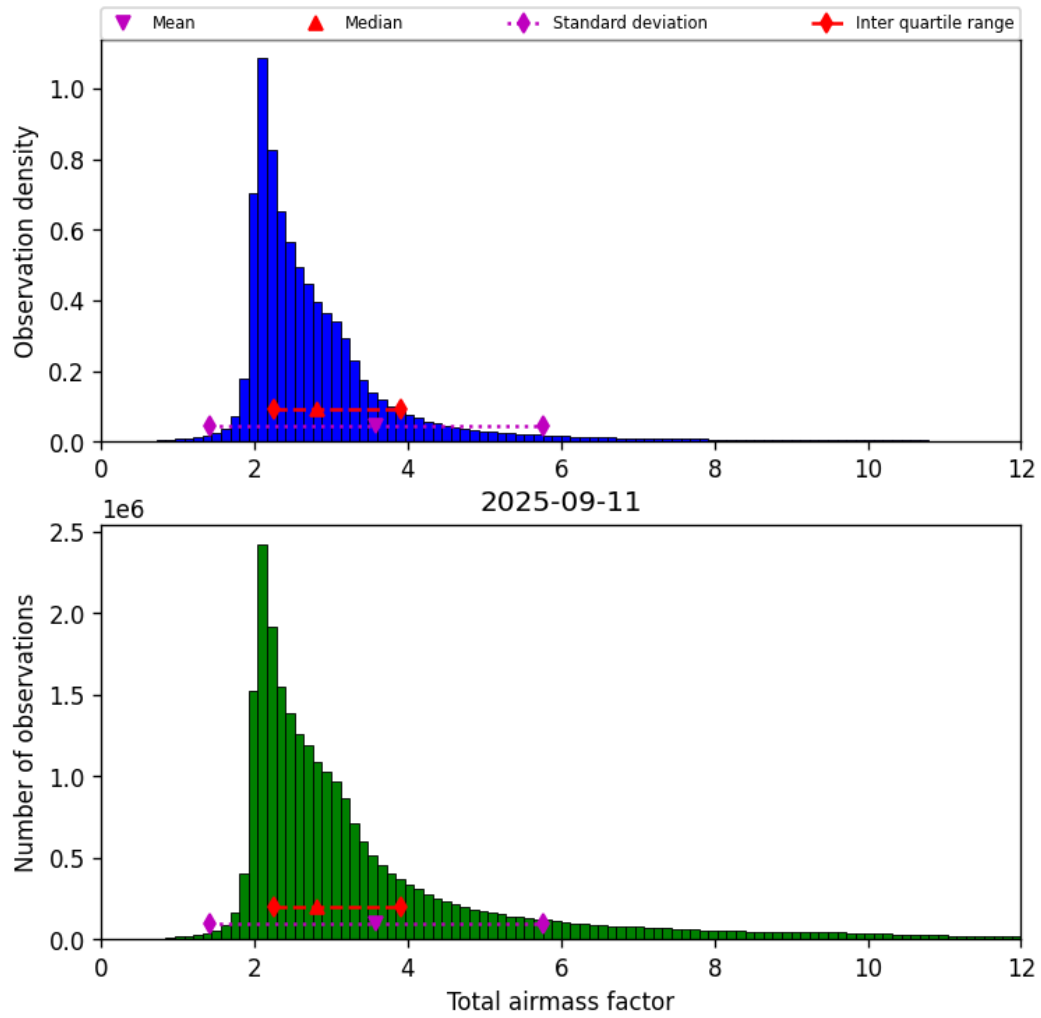
Figure 32: Histogram of “Total airmass factor” for 2025-09-10 to 2025-09-12
