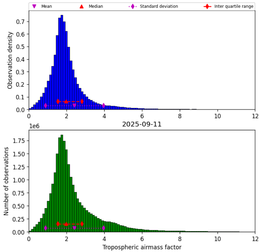
Figure 31: Histogram of “Tropospheric airmass factor” for 2025-09-10 to 2025-09-12
