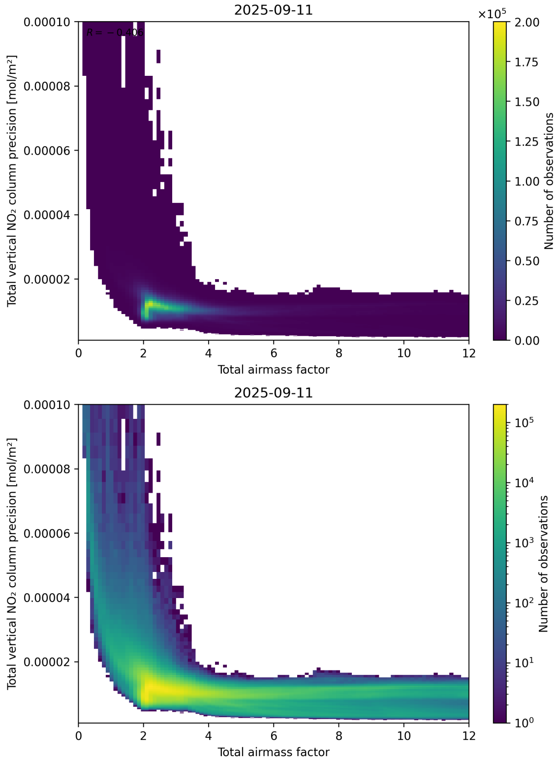
Figure 68: Scatter density plot of “Total airmass factor” against “Total vertical NO 2 column precision” for 2025-09-10 to 2025-09-12.
