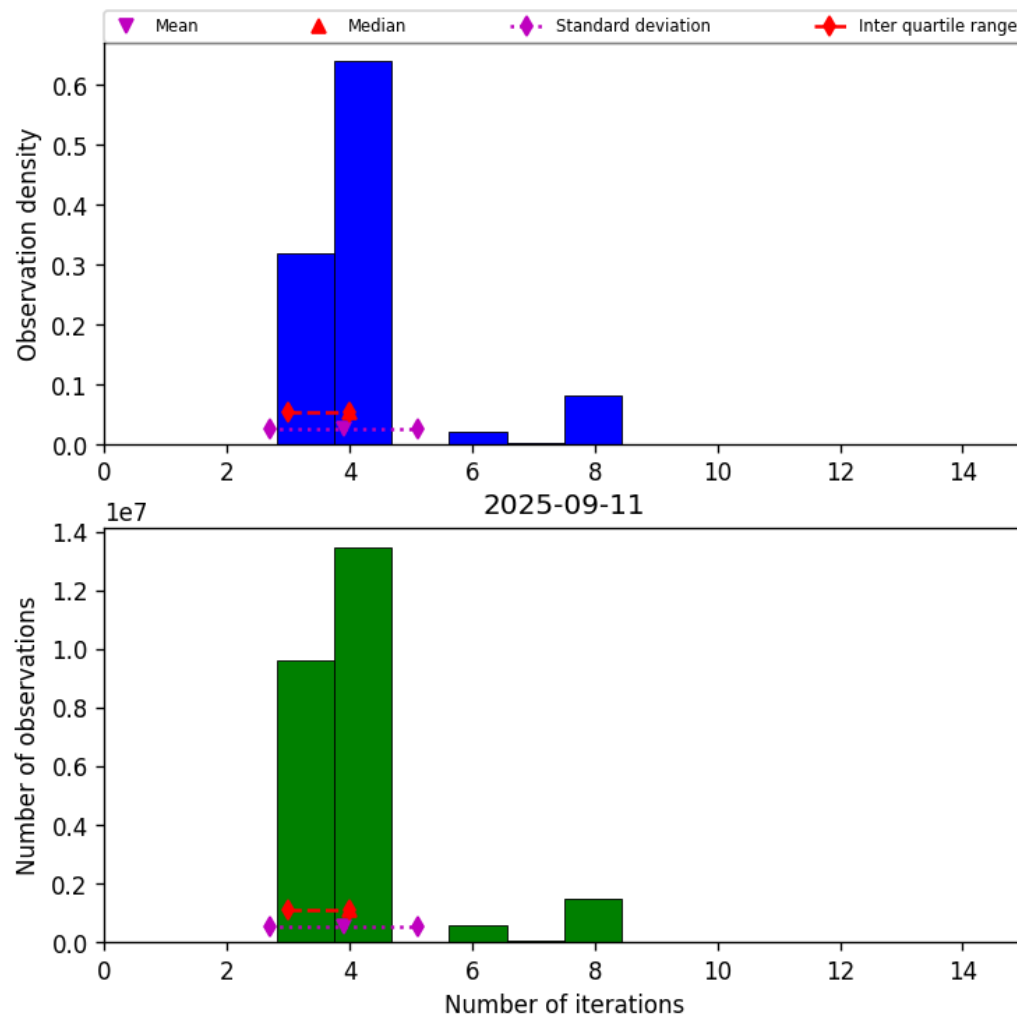
Figure 34: Histogram of “Number of iterations” for 2025-09-10 to 2025-09-12
