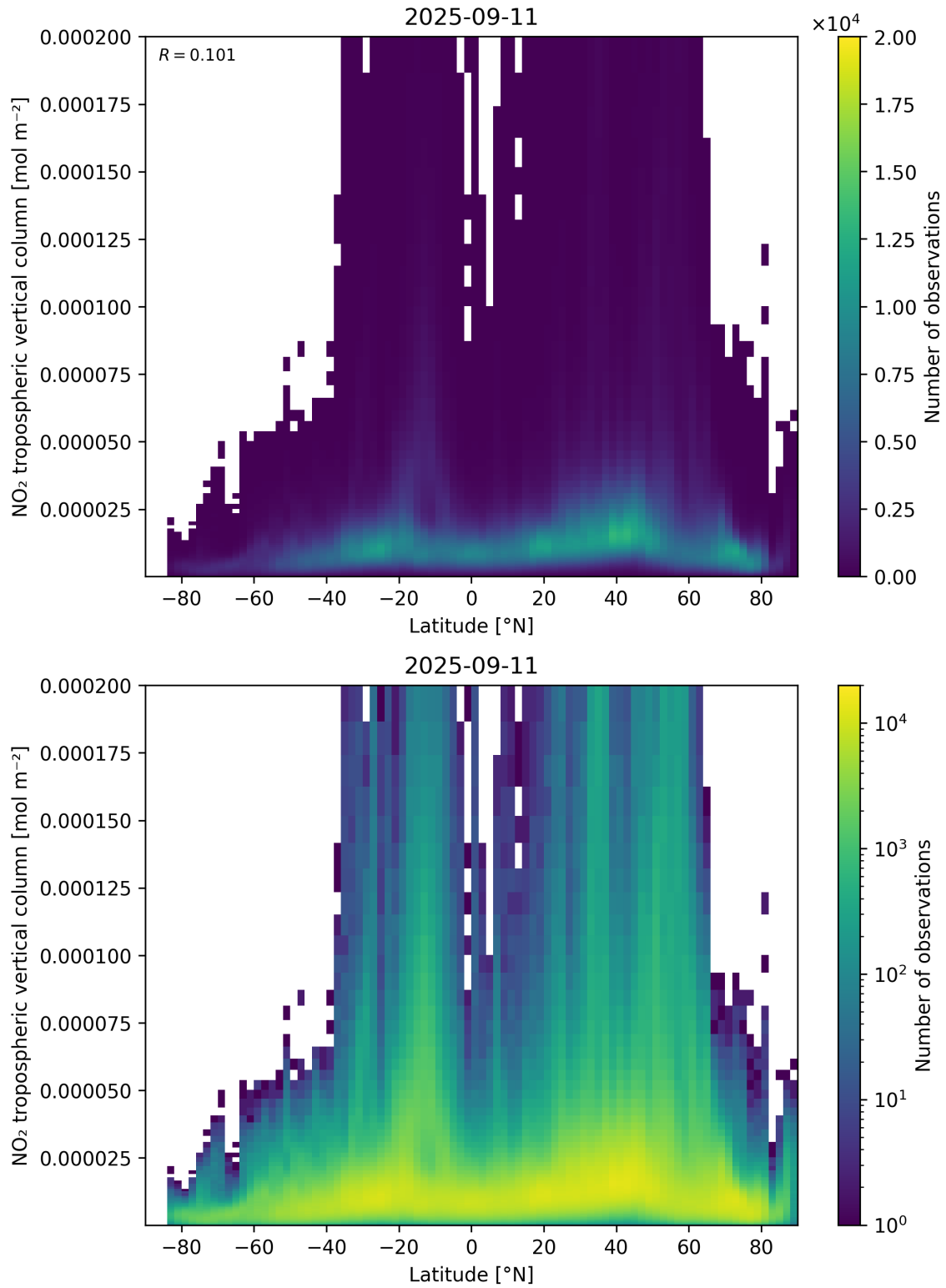
Figure 92: Scatter density plot of “Latitude” against “NO 2 tropospheric vertical column” for 2025-09-10 to 2025-09-12.
