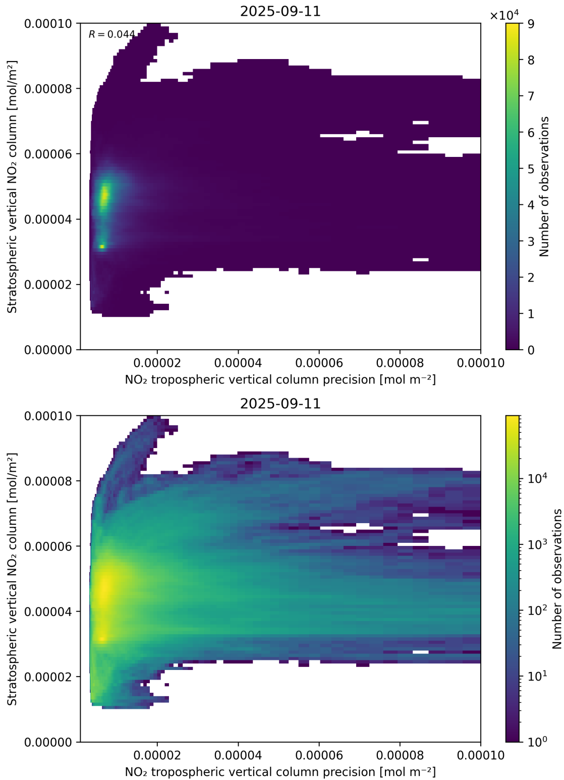
Figure 135: Scatter density plot of “NO 2 tropospheric vertical column precision” against “Stratospheric vertical NO 2 column” for 2025-09-10 to 2025-09-12.
