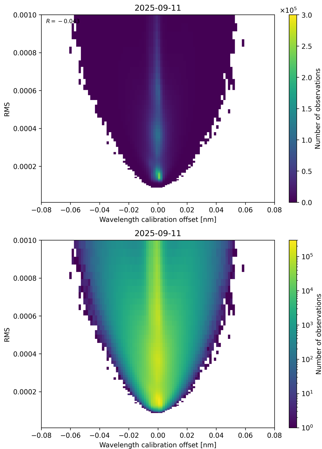
Figure 181: Scatter density plot of “Wavelength calibration offset” against “RMS” for 2025-09-10 to 2025-09-12.
