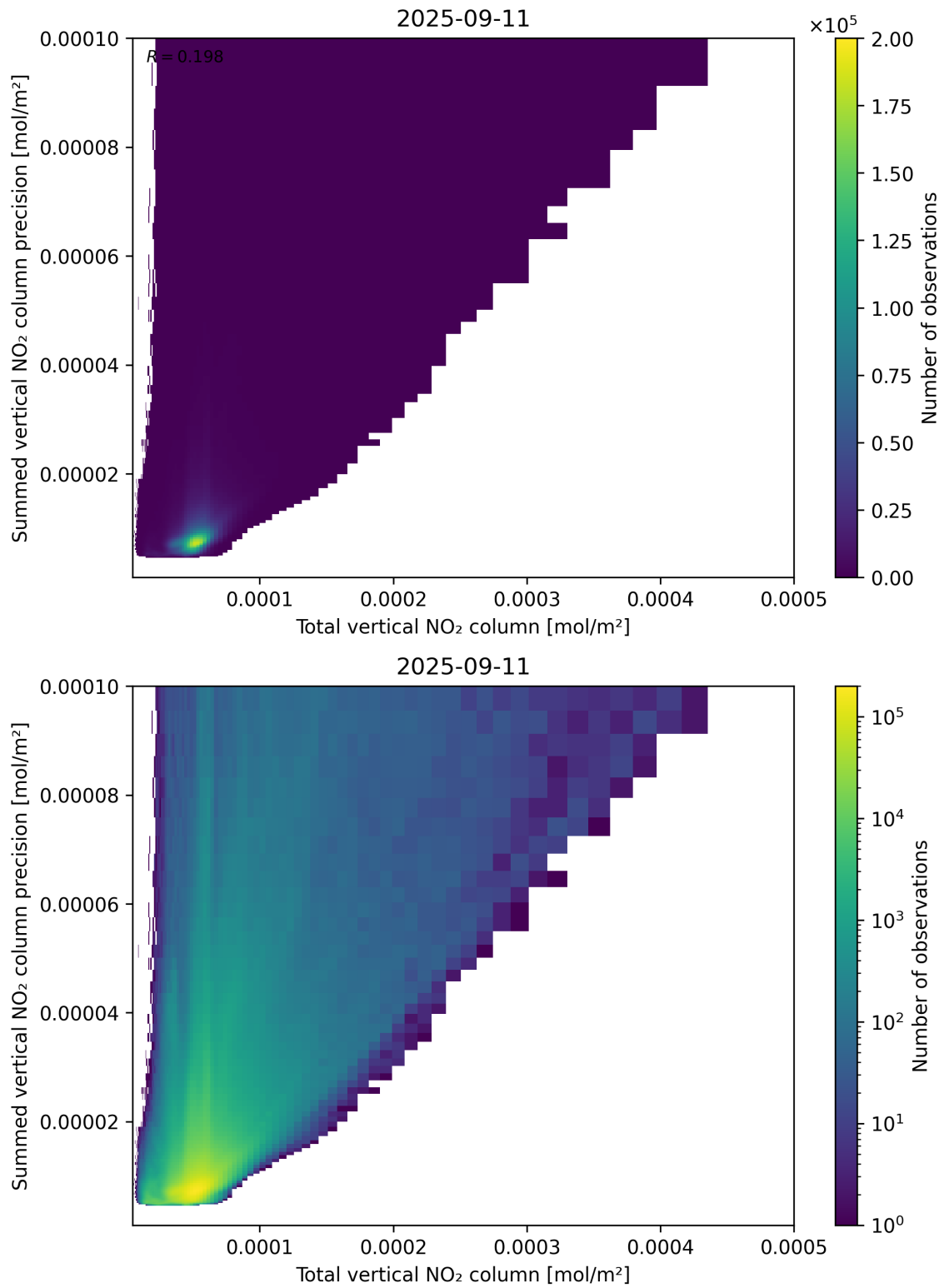
Figure 113: Scatter density plot of “Total vertical NO 2 column” against “Summed vertical NO 2 column precision” for 2025-09-10 to 2025-09-12.
