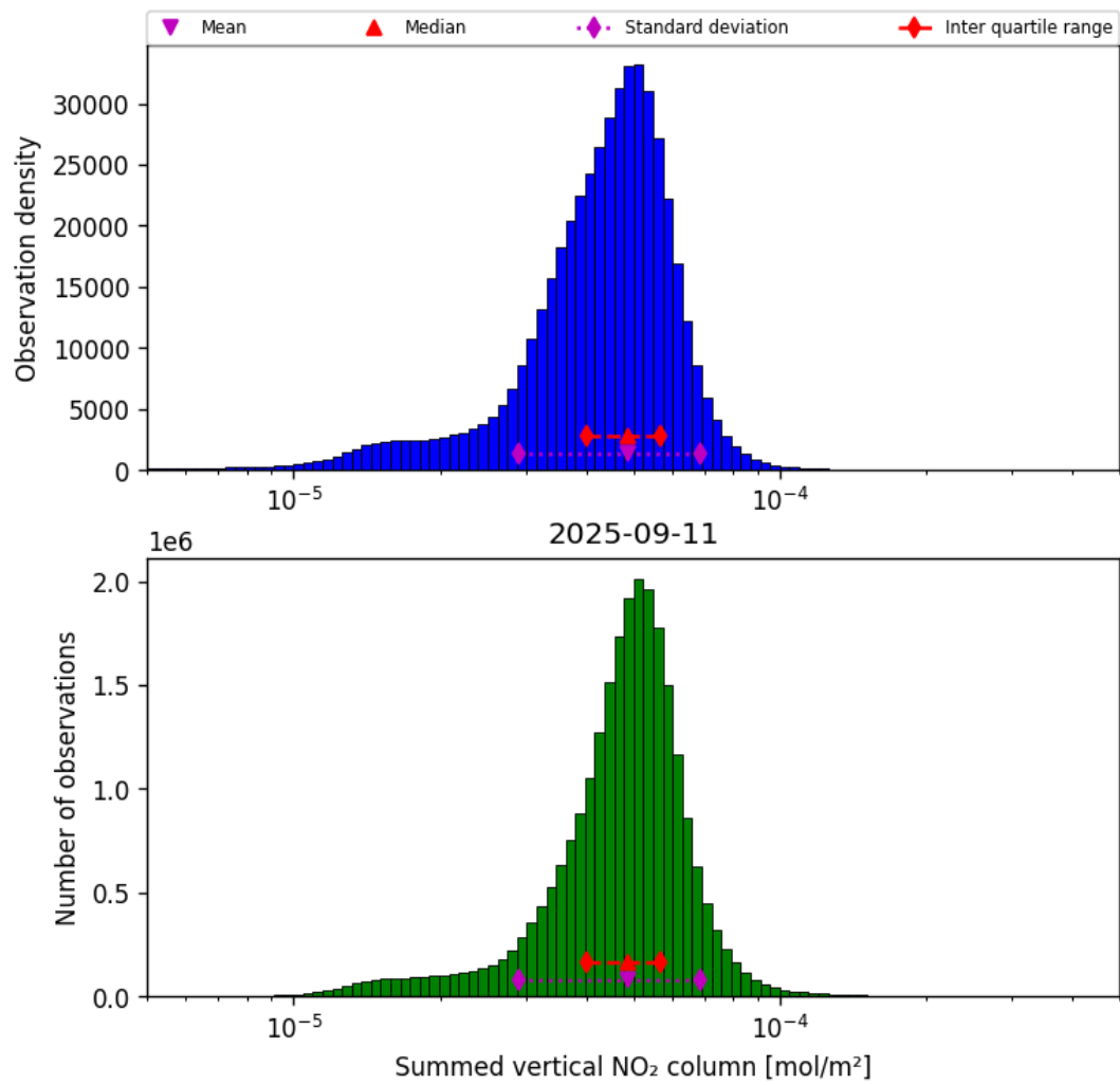
Figure 40: Histogram of “Summed vertical NO 2 column” for 2025-09-10 to 2025-09-12
