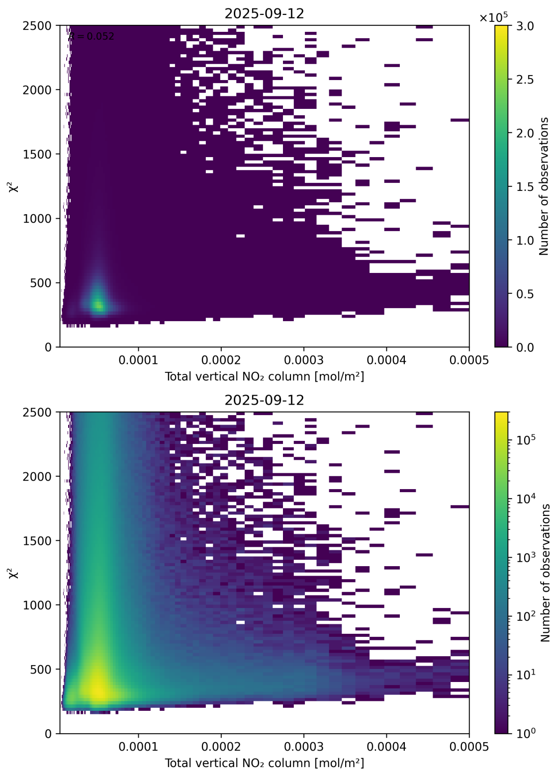
Figure 111: Scatter density plot of “Total vertical NO 2 column” against “ \chi^2 ” for 2025-09-11 to 2025-09-13.
