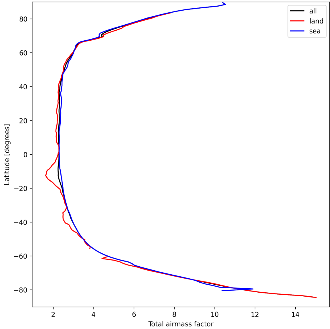
Figure 15: Zonal average of “Total airmass factor” for 2025-09-11 to 2025-09-13.
