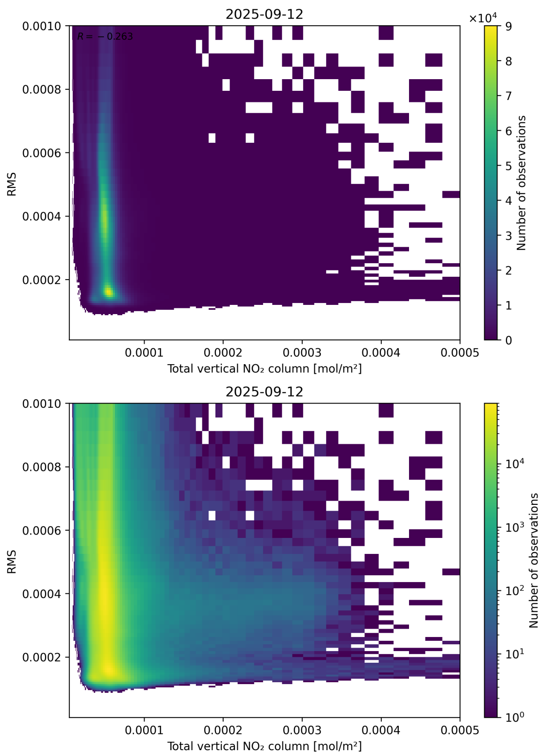
Figure 120: Scatter density plot of “Total vertical NO 2 column” against “RMS” for 2025-09-11 to 2025-09-13.
