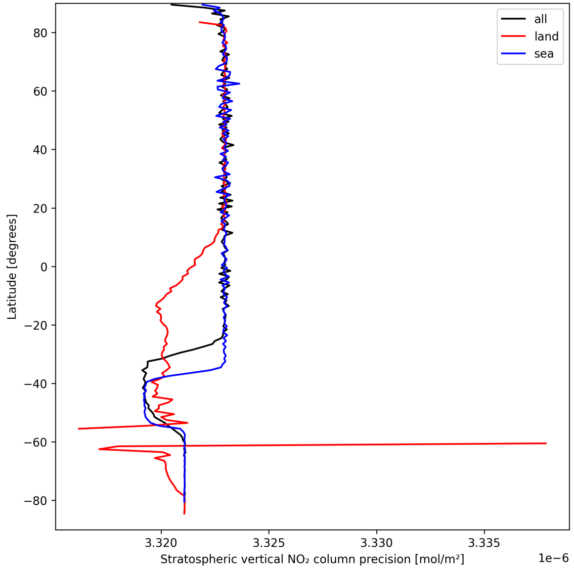
Figure 20: Zonal average of “Stratospheric vertical NO 2 column precision” for 2025-09-11 to 2025-09-13.
