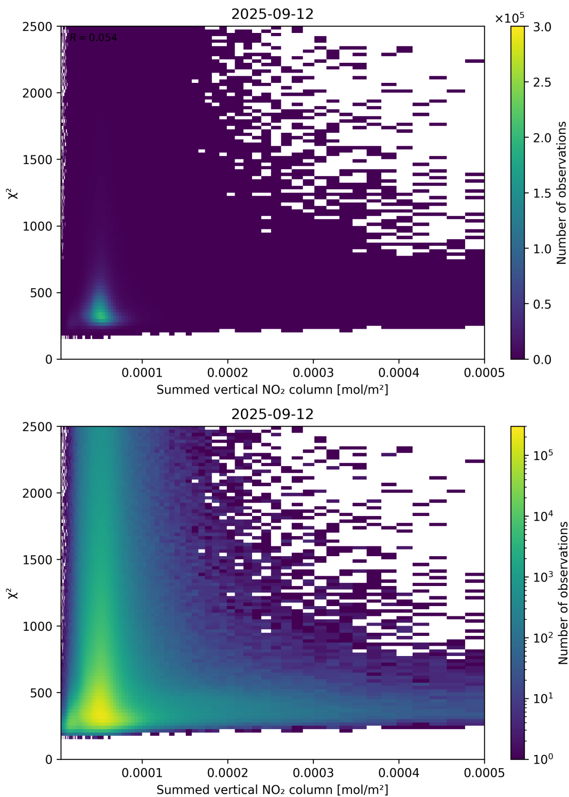
Figure 104: Scatter density plot of “Summed vertical NO 2 column” against “ \chi^2 ” for 2025-09-11 to 2025-09-13.
