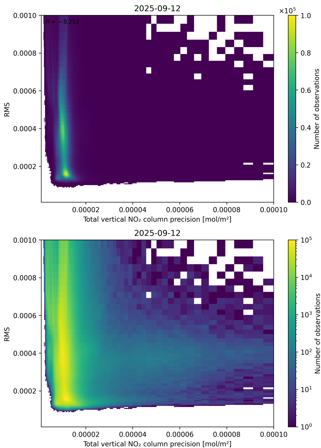
Figure 119: Scatter density plot of “Total vertical NO 2 column precision” against “RMS” for 2025-09-11 to 2025-09-13.
