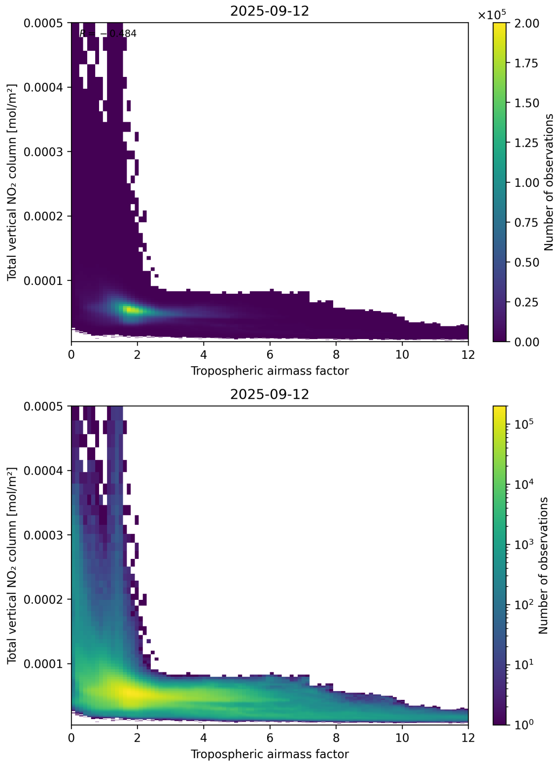
Figure 77: Scatter density plot of “Tropospheric airmass factor” against “Total vertical NO 2 column” for 2025-09-11 to 2025-09-13.
