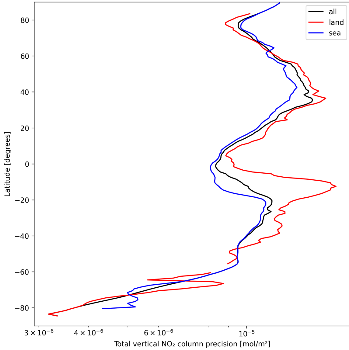
Figure 22: Zonal average of “Total vertical NO 2 column precision” for 2025-09-11 to 2025-09-13.
