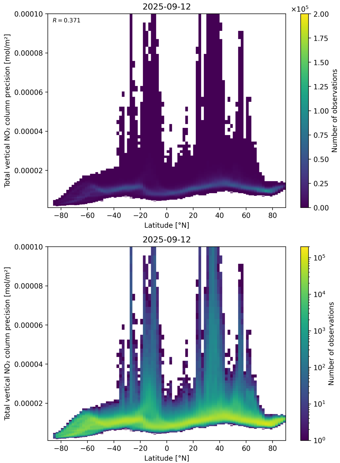
Figure 91: Scatter density plot of “Latitude” against “Total vertical NO 2 column precision” for 2025-09-11 to 2025-09-13.
