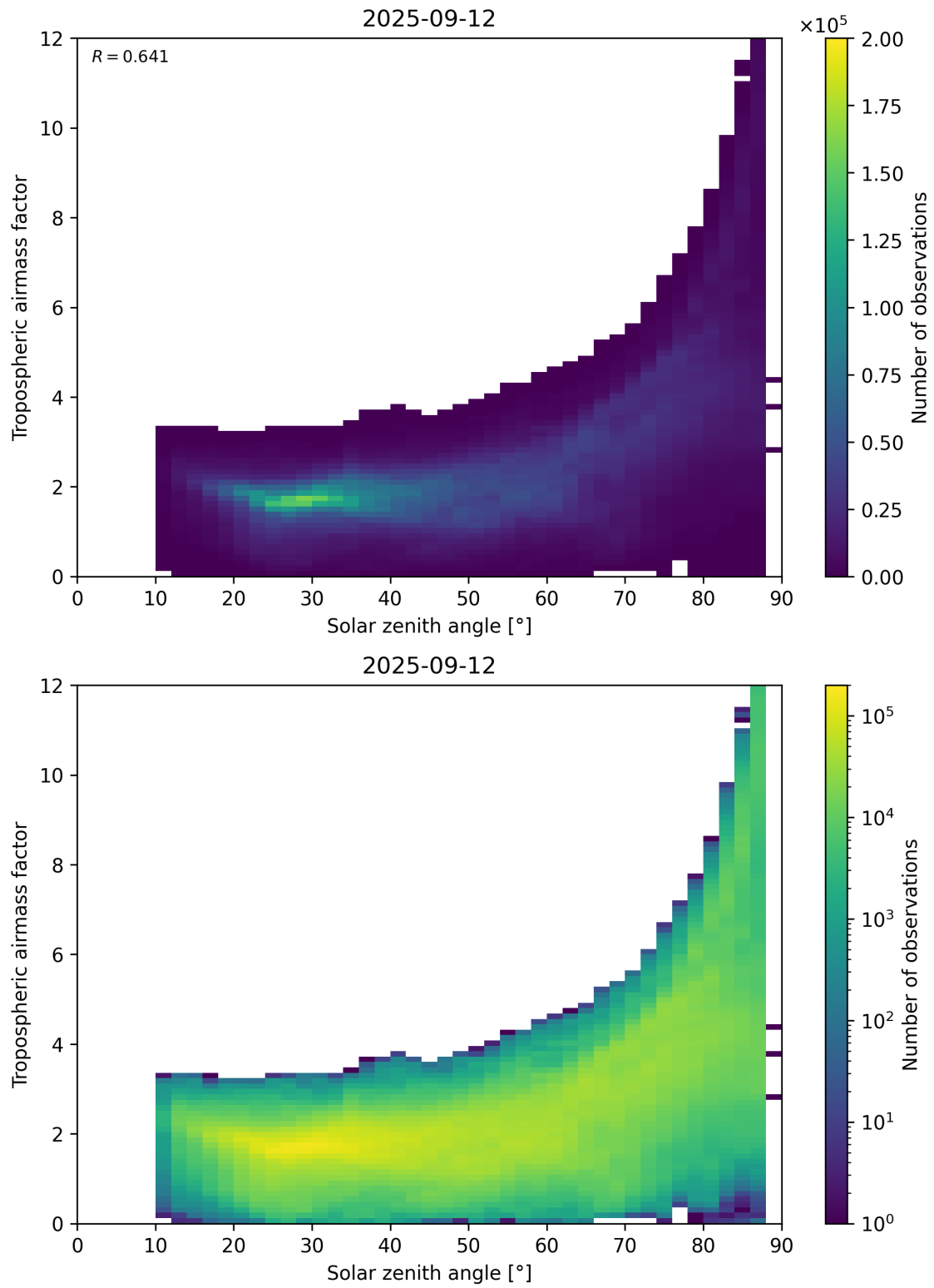
Figure 147: Scatter density plot of “Solar zenith angle” against “Tropospheric airmass factor” for 2025-09-11 to 2025-09-13.
