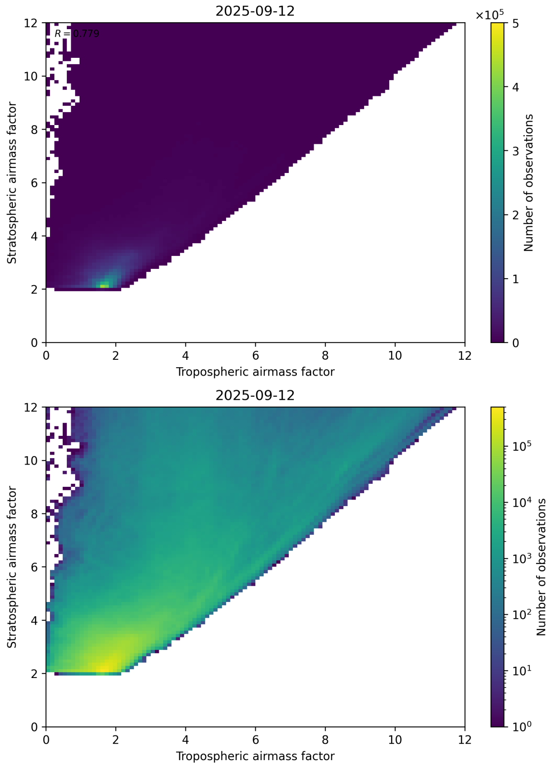
Figure 71: Scatter density plot of “Tropospheric airmass factor” against “Stratospheric airmass factor” for 2025-09-11 to 2025-09-13.
