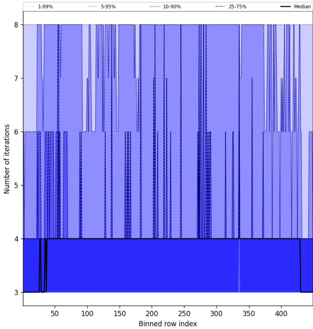
Figure 51: Along track statistics of “Number of iterations” for 2025-09-11 to 2025-09-13
