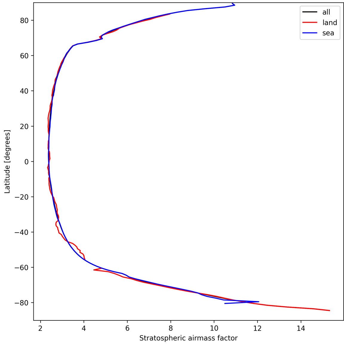
Figure 27: Zonal average of “Stratospheric airmass factor” for 2025-09-11 to 2025-09-13.
