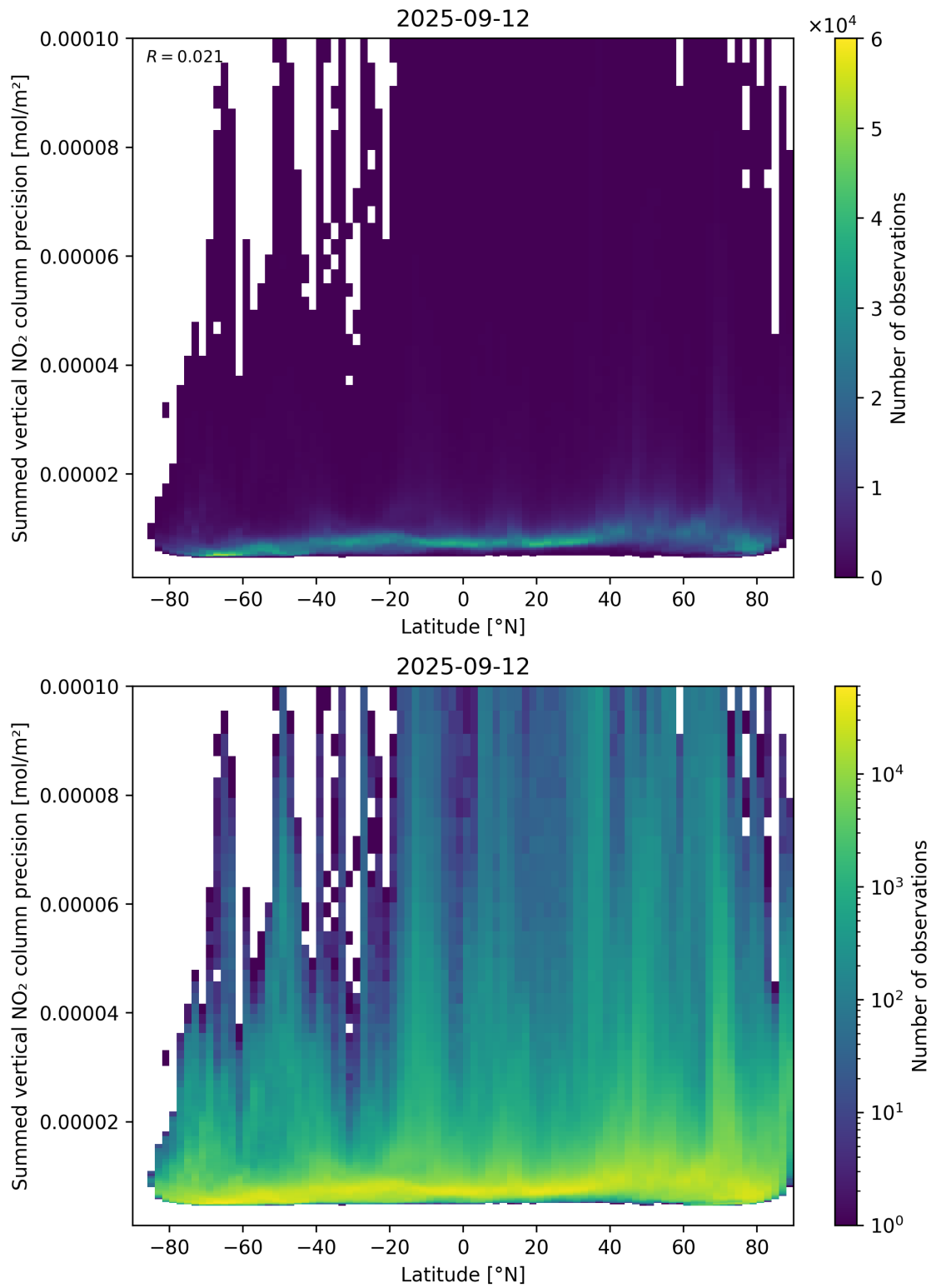
Figure 89: Scatter density plot of “Latitude” against “Summed vertical NO 2 column precision” for 2025-09-11 to 2025-09-13.
