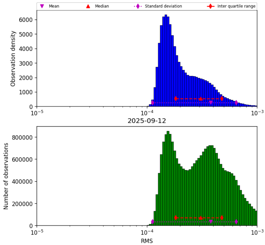
Figure 43: Histogram of “RMS” for 2025-09-11 to 2025-09-13
