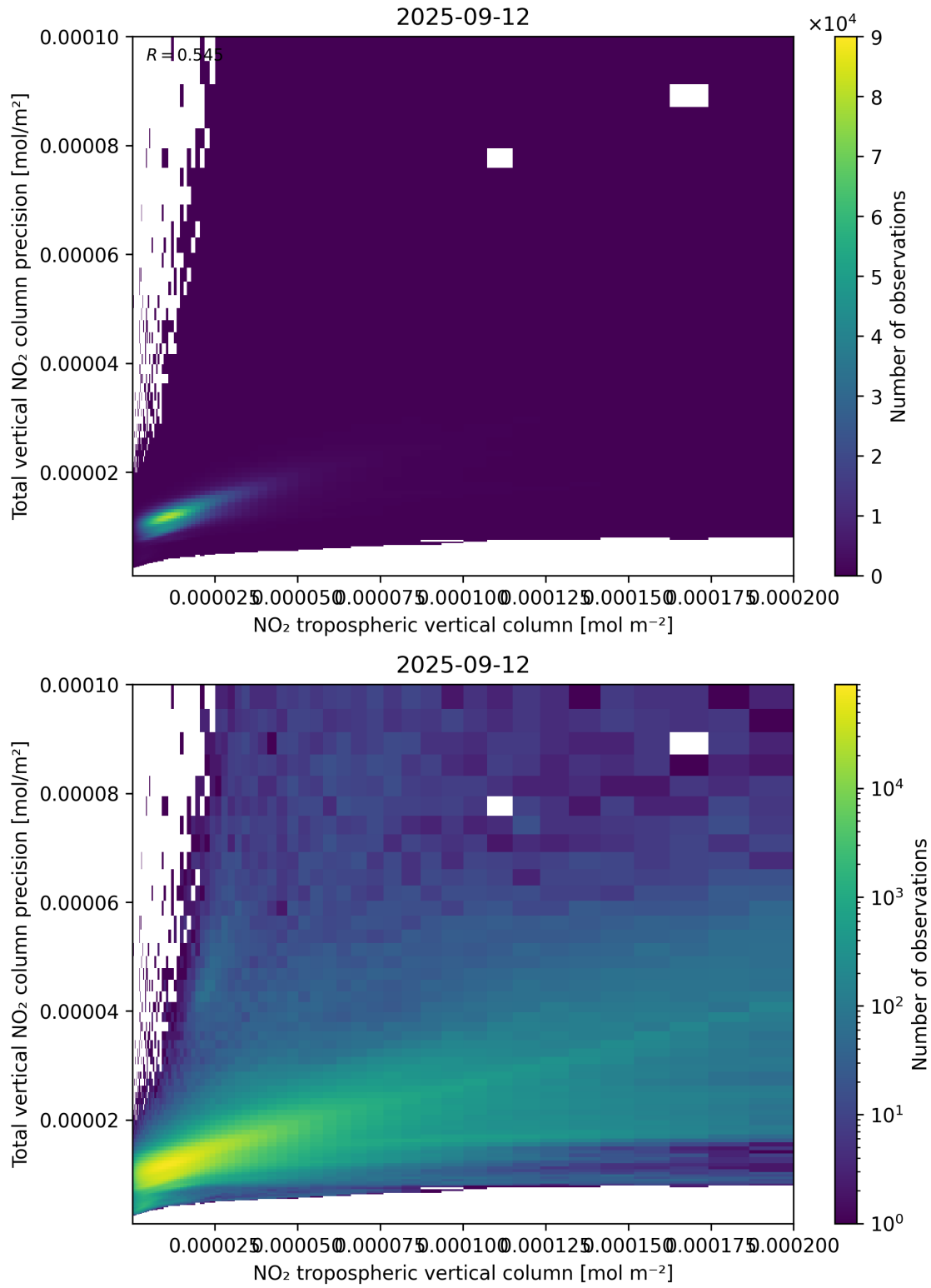
Figure 129: Scatter density plot of “NO 2 tropospheric vertical column” against “Total vertical NO 2 column precision” for 2025-09-11 to 2025-09-13.
