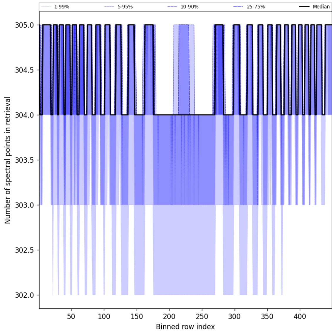
Figure 50: Along track statistics of “Number of spectral points in retrieval” for 2025-09-11 to 2025-09-13
