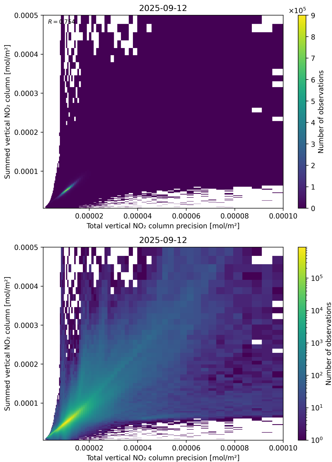
Figure 117: Scatter density plot of “Total vertical NO 2 column precision” against “Summed vertical NO 2 column” for 2025-09-11 to 2025-09-13.
