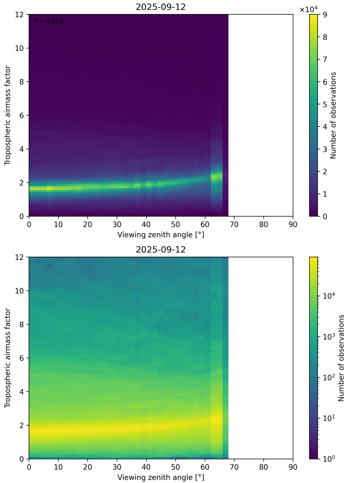
Figure 161: Scatter density plot of “Viewing zenith angle” against “Tropospheric airmass factor” for 2025-09-11 to 2025-09-13.
