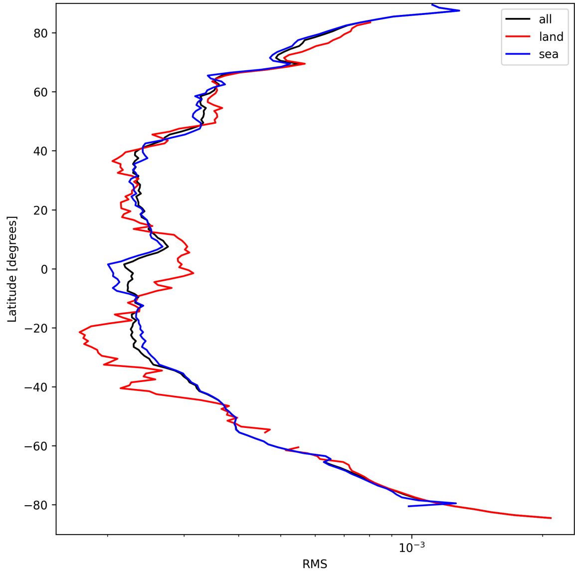
Figure 26: Zonal average of “RMS” for 2025-09-11 to 2025-09-13.
