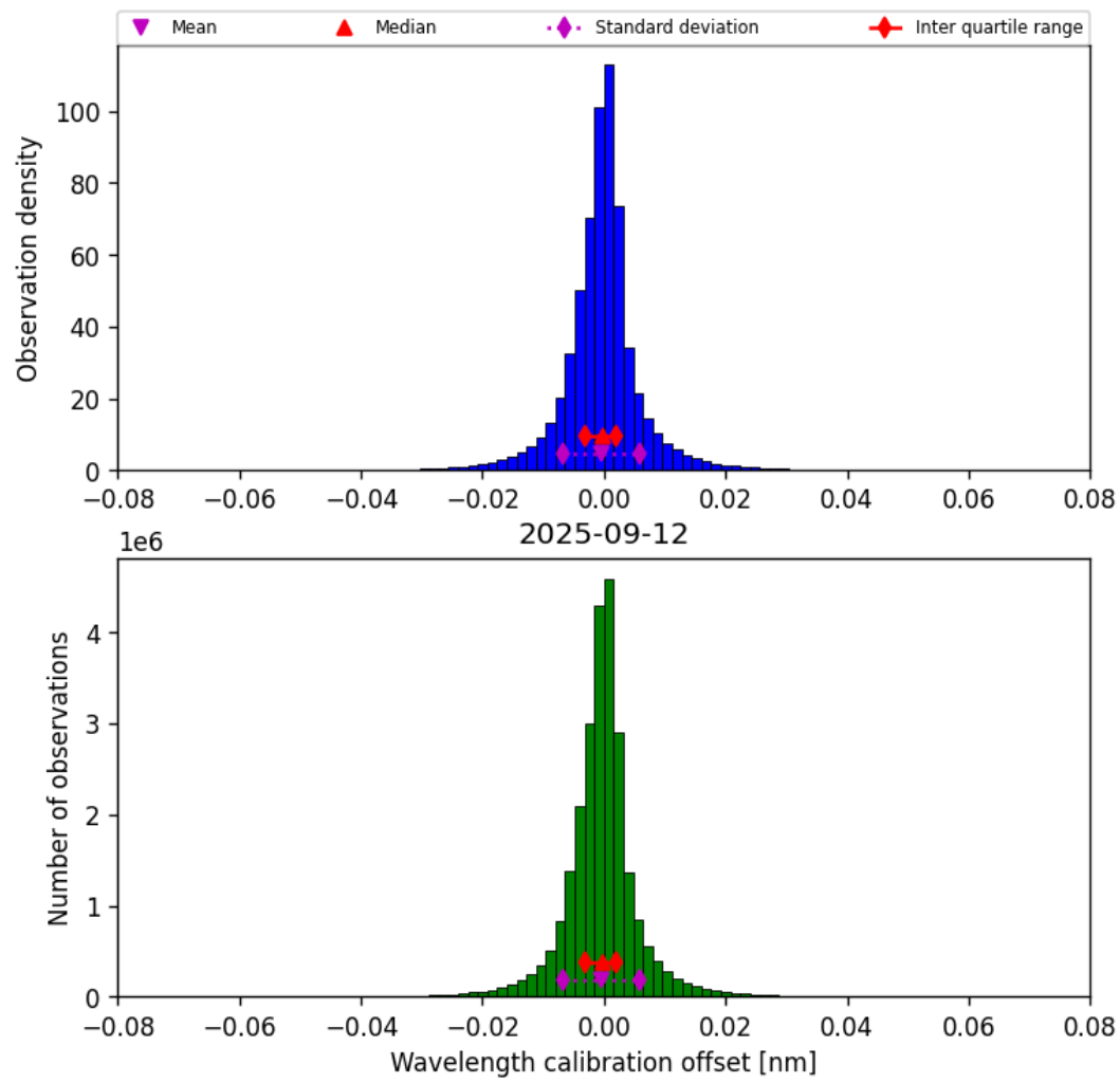
Figure 35: Histogram of “Wavelength calibration offset” for 2025-09-11 to 2025-09-13
