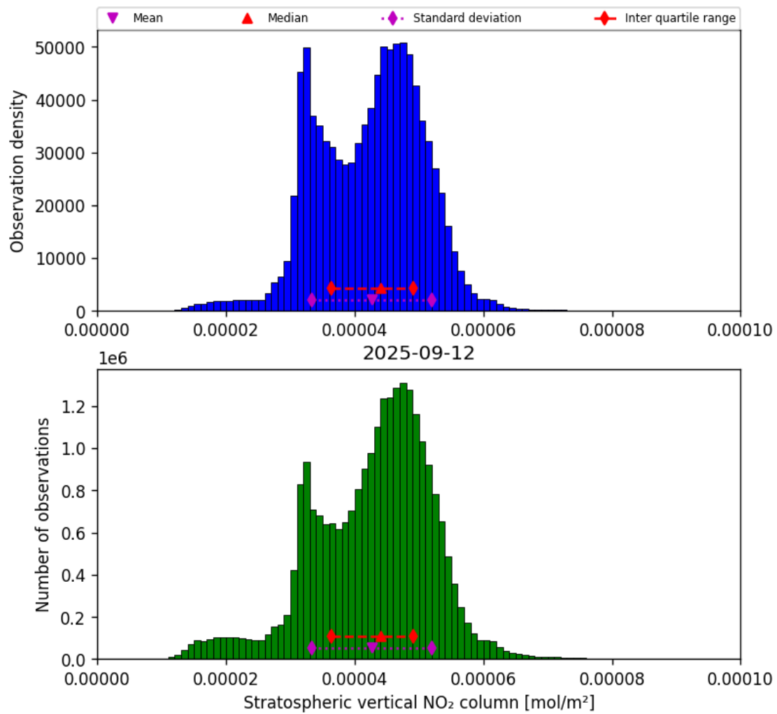
Figure 36: Histogram of “Stratospheric vertical NO 2 column” for 2025-09-11 to 2025-09-13
