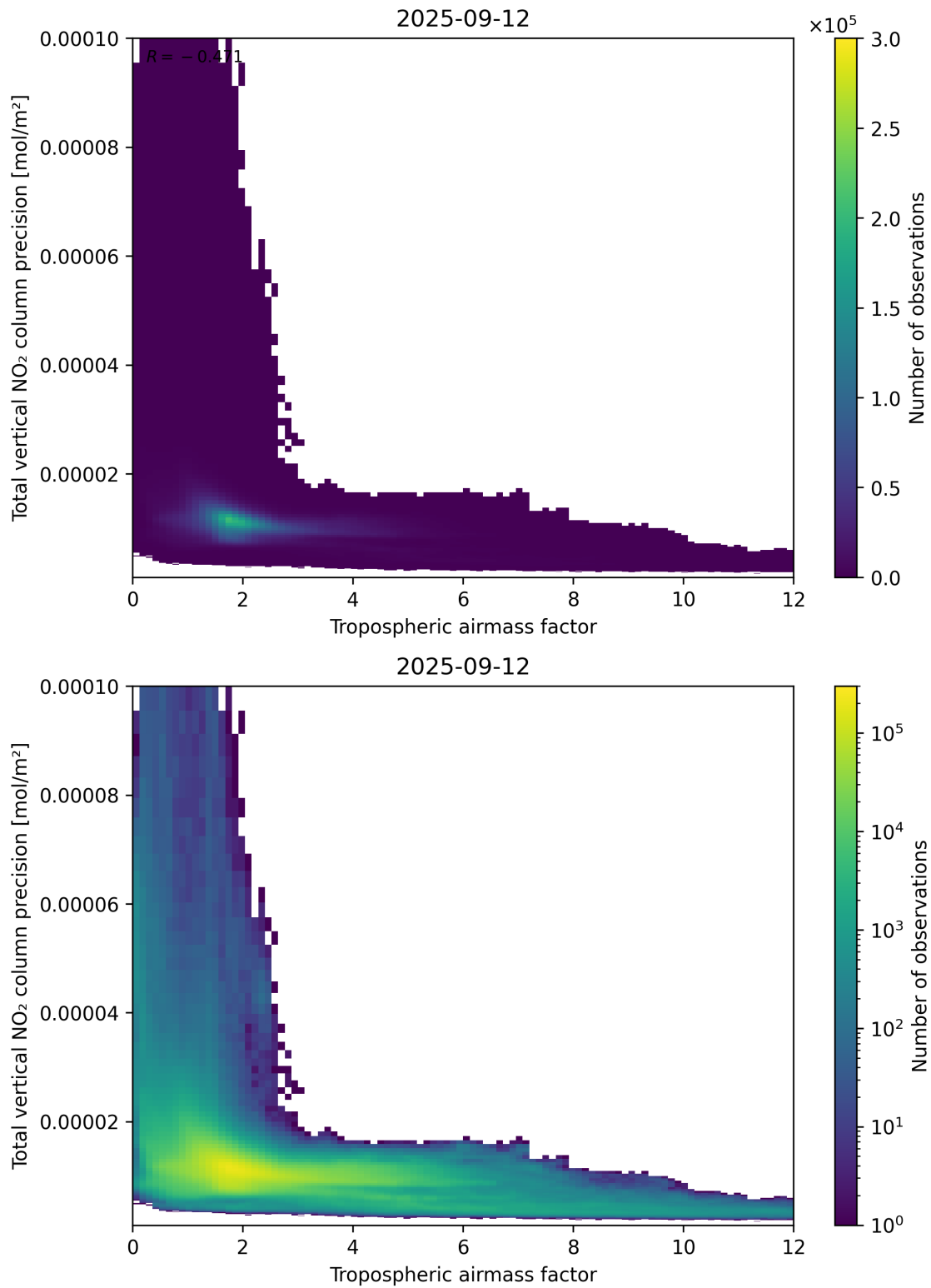
Figure 78: Scatter density plot of “Tropospheric air mass factor” against “Total vertical NO 2 column precision” for 2025-09-11 to 2025-09-13.
