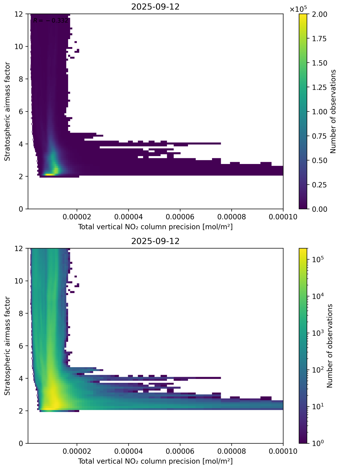
Figure 115: Scatter density plot of “Total vertical NO 2 column precision” against “Stratospheric air mass factor” for 2025-09-11 to 2025-09-13.
