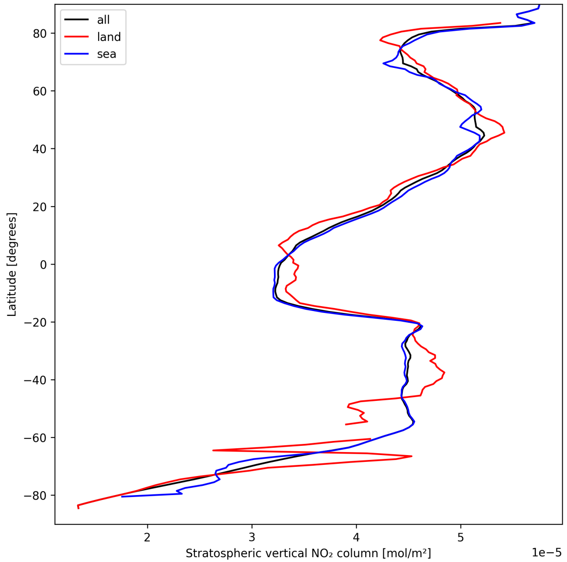
Figure 19: Zonal average of “Stratospheric vertical NO 2 column” for 2025-09-11 to 2025-09-13.
