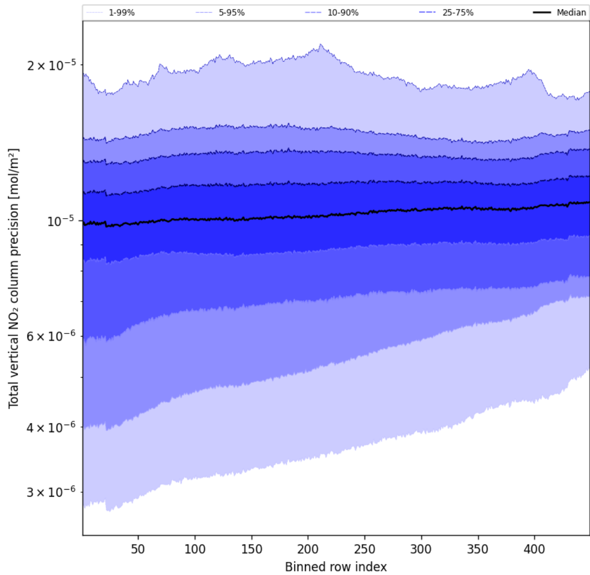
Figure 56: Along track statistics of “Total vertical NO 2 column precision” for 2025-09-11 to 2025-09-13
