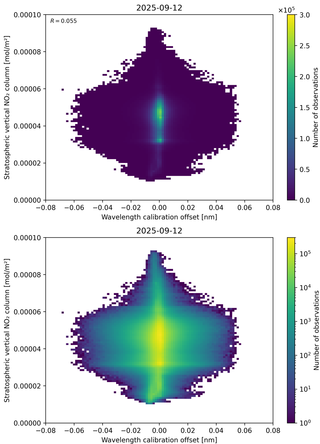
Figure 176: Scatter density plot of “Wavelength calibration offset” against “Stratospheric vertical NO 2 column” for 2025-09-11 to 2025-09-13.
