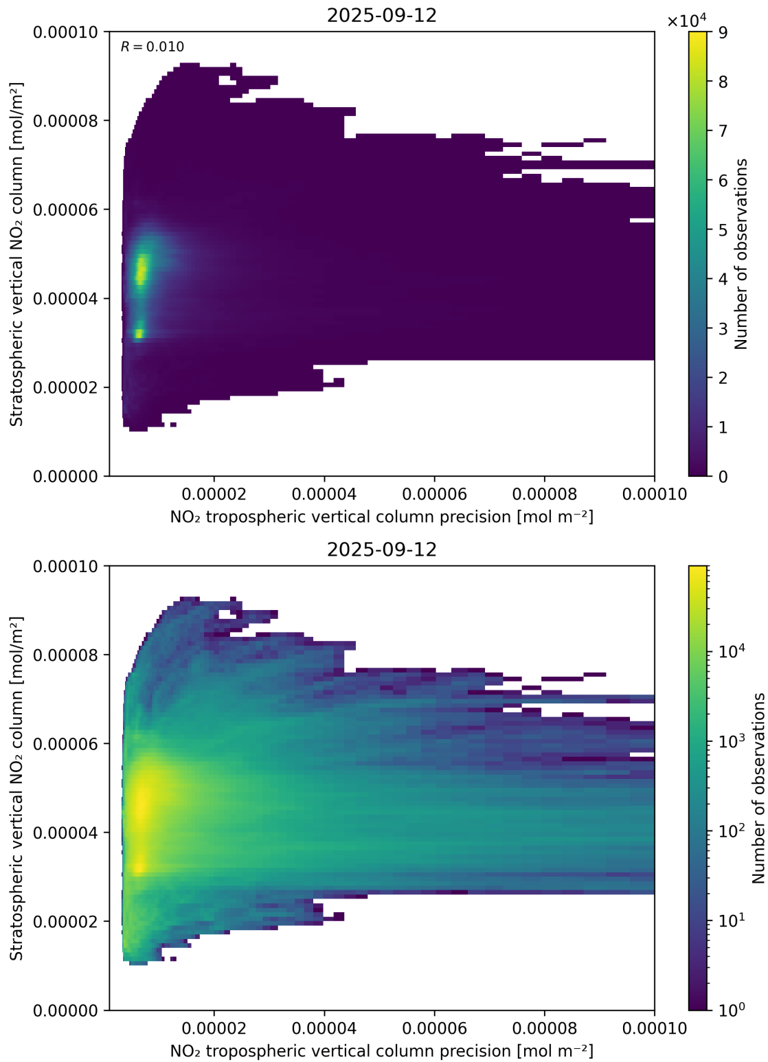
Figure 135: Scatter density plot of “NO 2 tropospheric vertical column precision” against “Stratospheric vertical NO 2 column” for 2025-09-11 to 2025-09-13.
