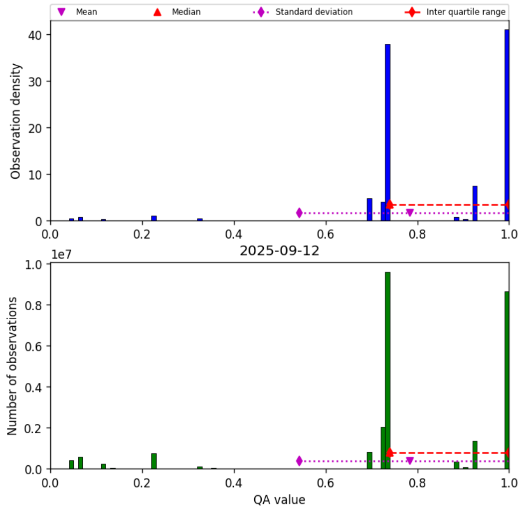
Figure 28: Histogram of “QA value” for 2025-09-11 to 2025-09-13
