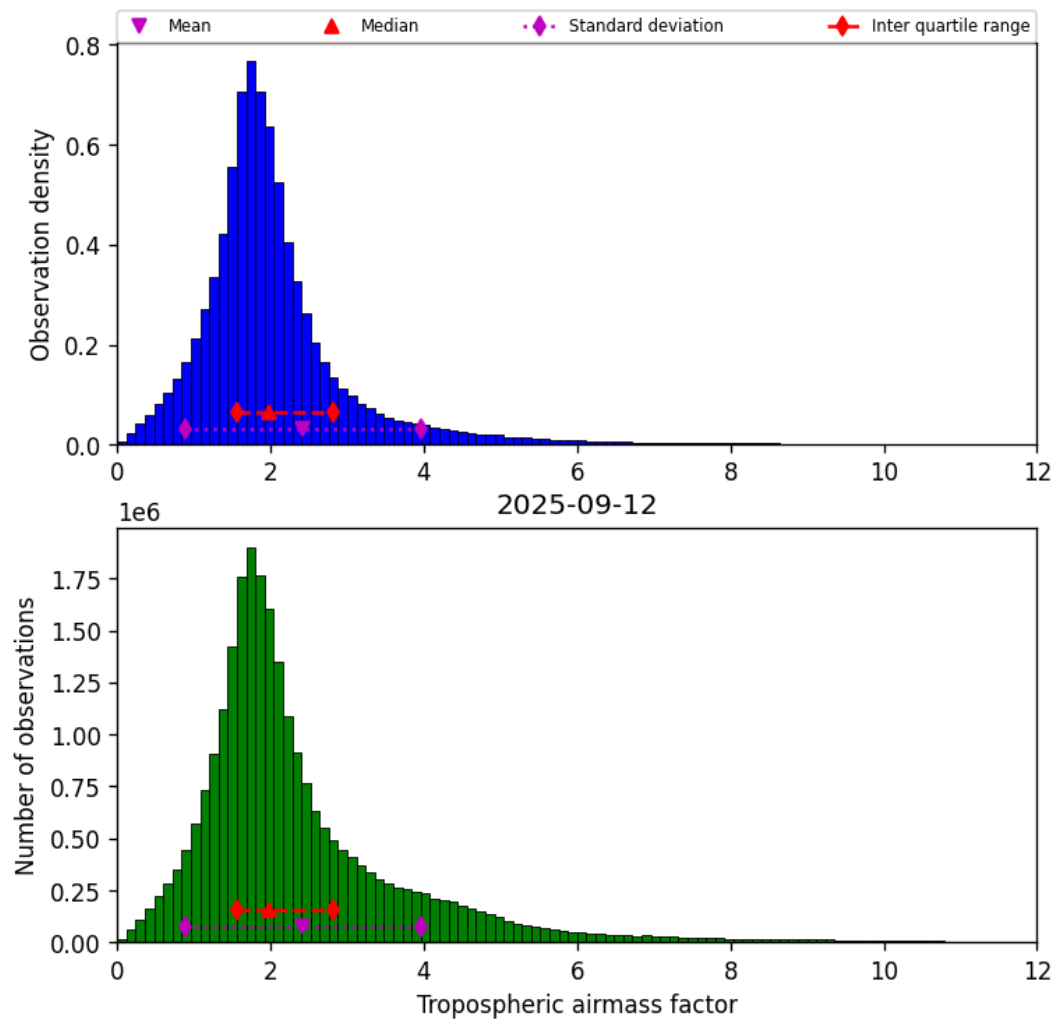
Figure 31: Histogram of “Tropospheric airmass factor” for 2025-09-11 to 2025-09-13
