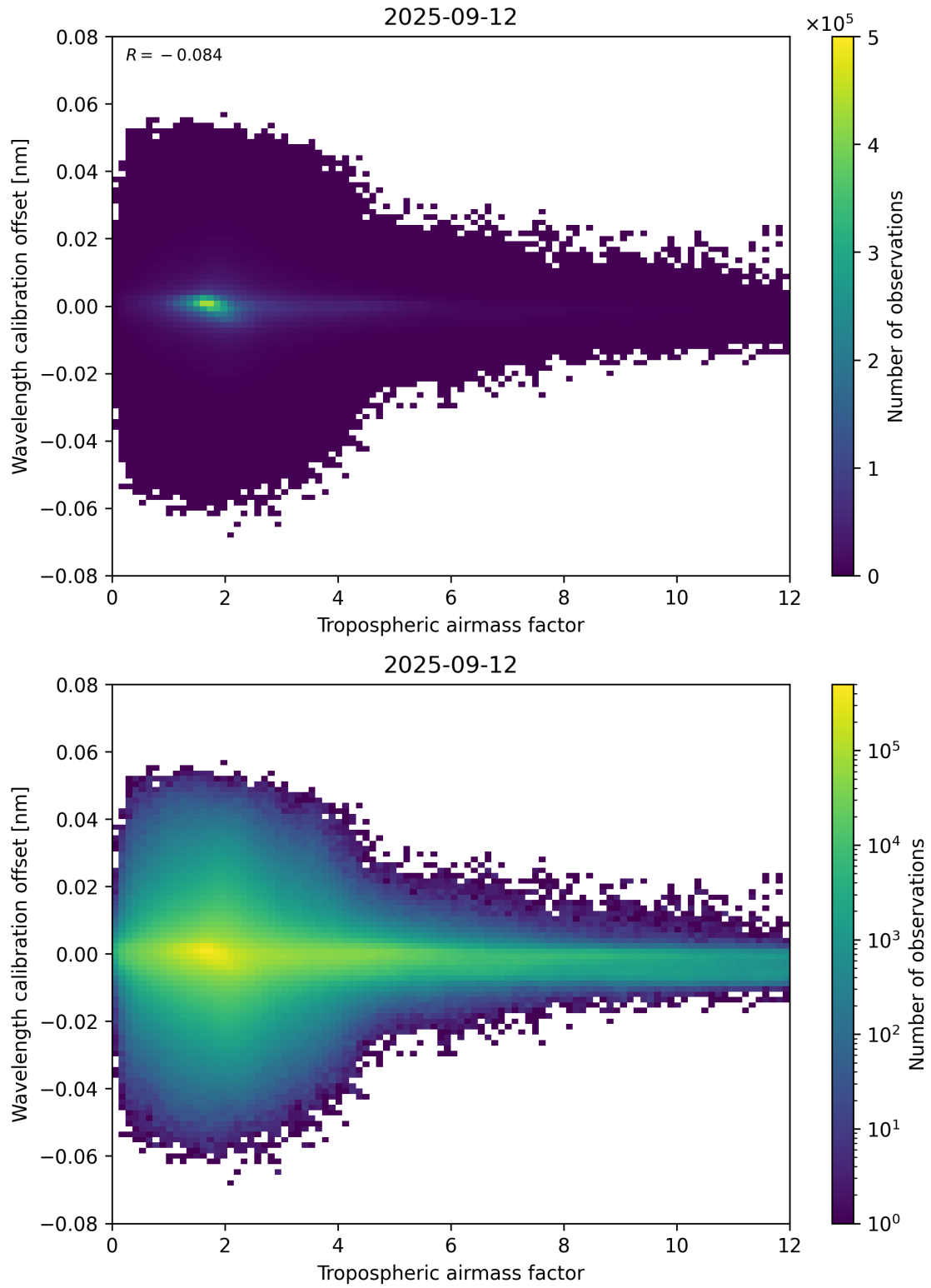
Figure 80: Scatter density plot of “Tropospheric airmass factor” against “Wavelength calibration offset” for 2025-09-11 to 2025-09-13.
