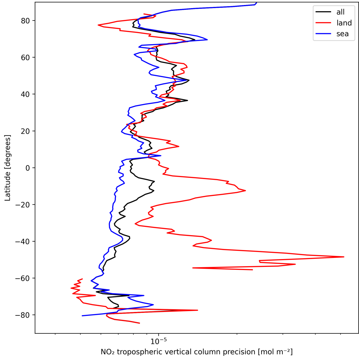
Figure 13: Zonal average of “NO 2 tropospheric vertical column precision” for 2025-09-11 to 2025-09-13.
