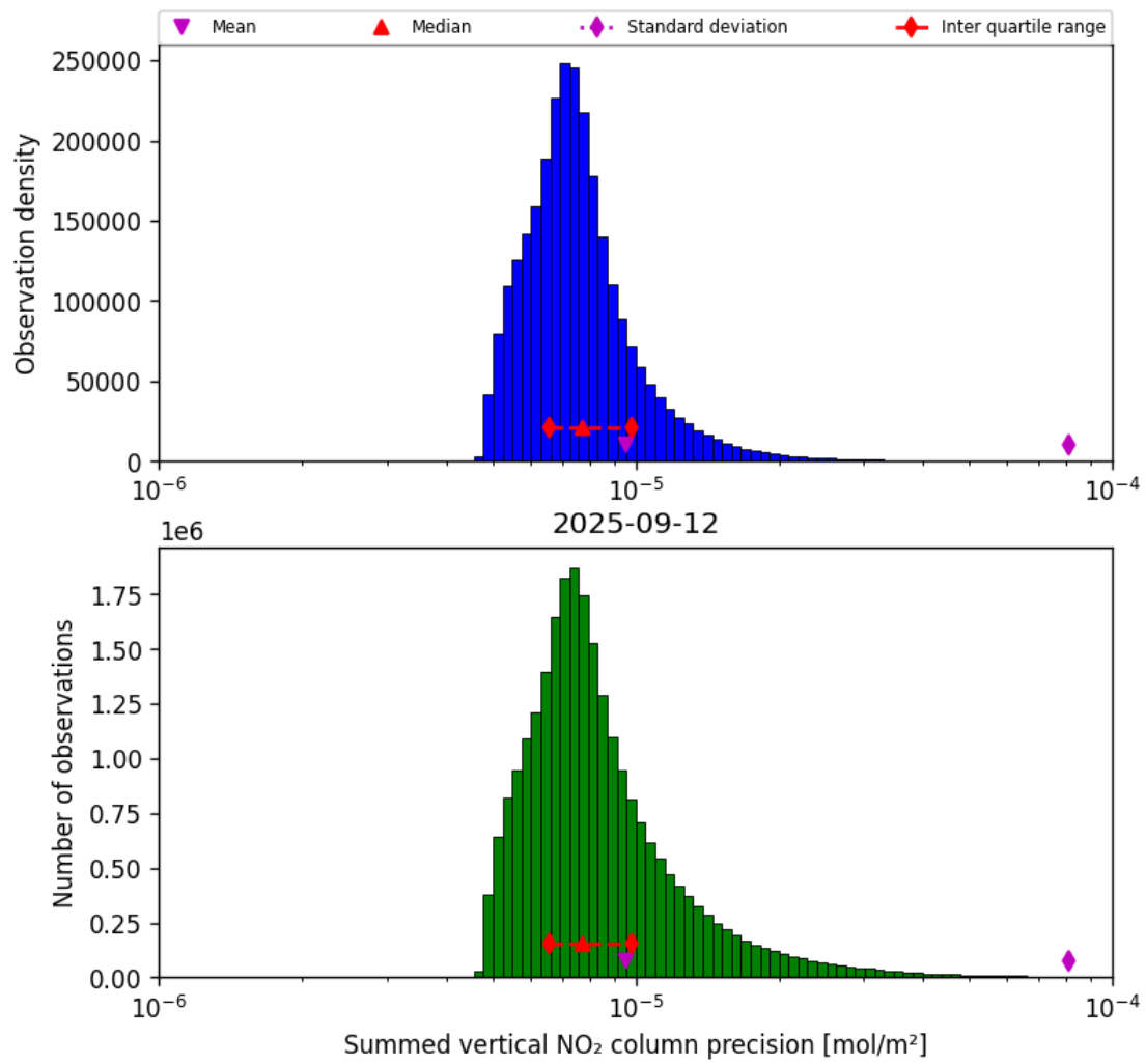
Figure 41: Histogram of "Summed vertical NO 2 column precision" for 2025-09-11 to 2025-09-13
