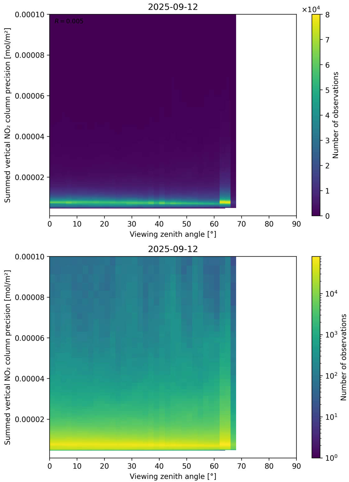
Figure 166: Scatter density plot of “Viewing zenith angle” against “Summed vertical NO 2 column precision” for 2025-09-11 to 2025-09-13.
