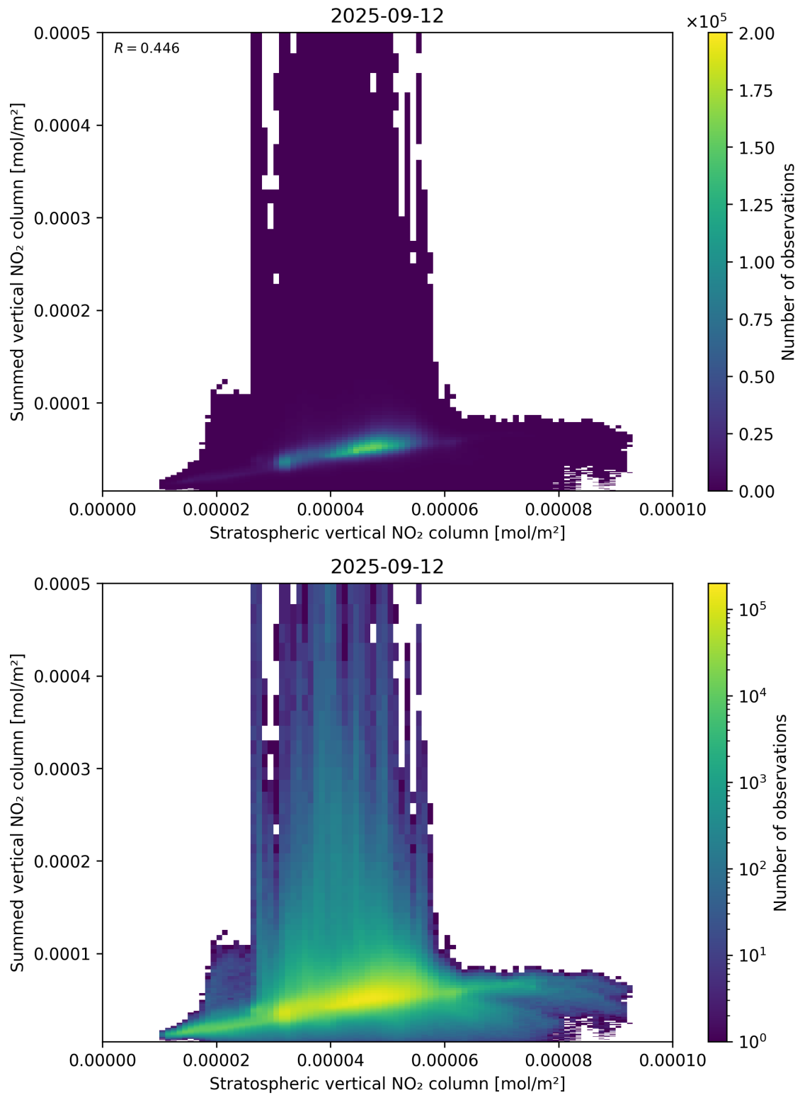
Figure 98: Scatter density plot of “Stratospheric vertical NO 2 column” against “Summed vertical NO 2 column” for 2025-09-11 to 2025-09-13.
