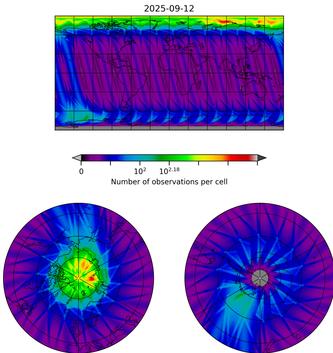
Figure 10: Map of the number of observations for 2025-09-11 to 2025-09-13
