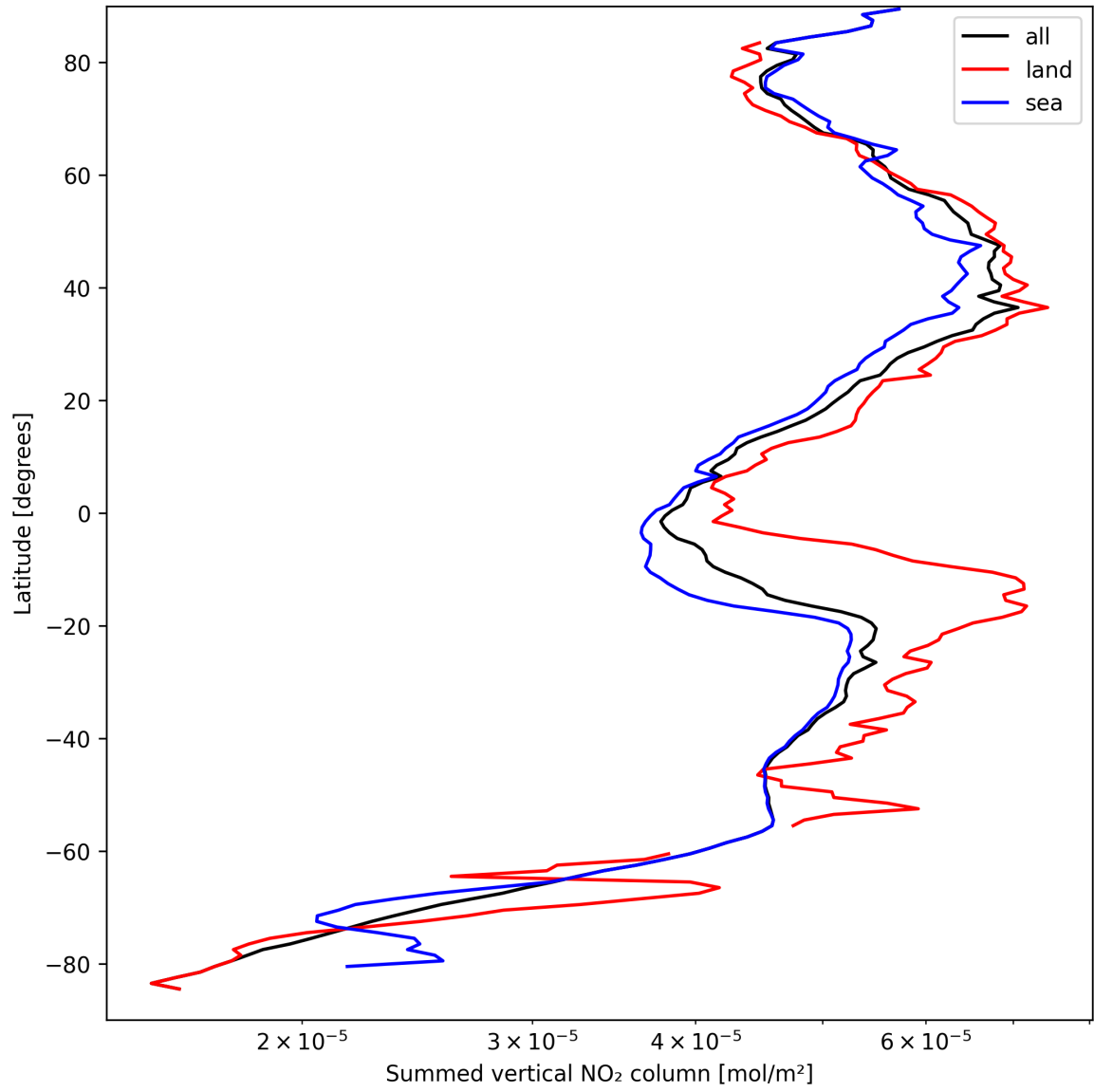
Figure 23: Zonal average of “Summed vertical NO 2 column” for 2025-09-11 to 2025-09-13.
