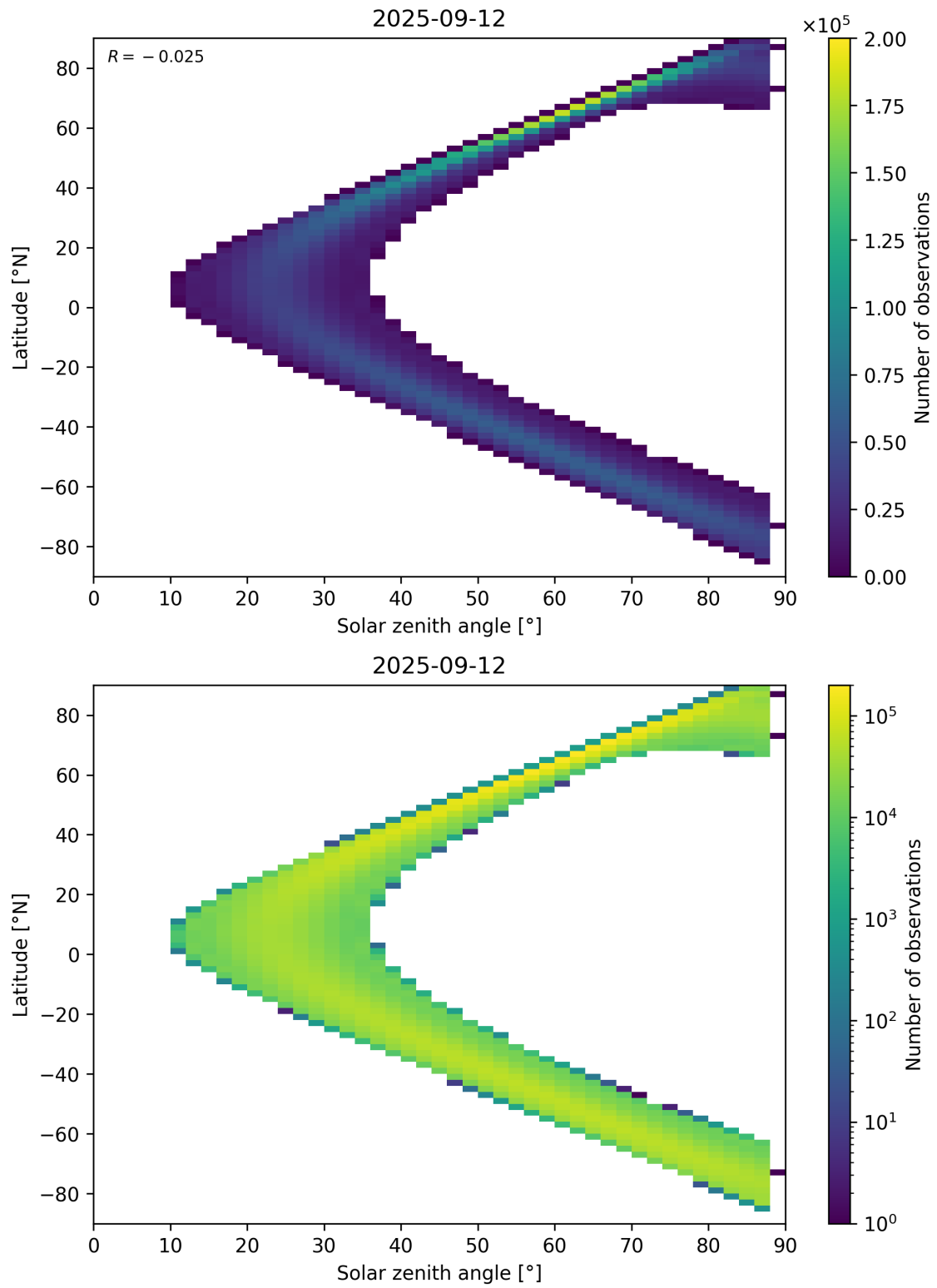
Figure 149: Scatter density plot of “Solar zenith angle” against “Latitude” for 2025-09-11 to 2025-09-13.
