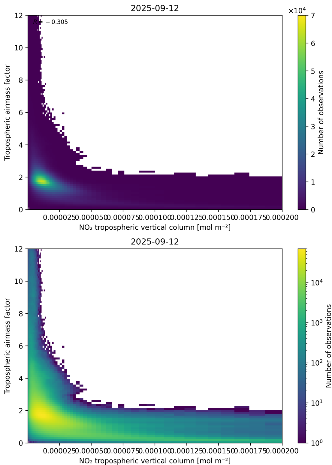
Figure 123: Scatter density plot of “NO 2 tropospheric vertical column” against “Tropospheric air mass factor” for 2025-09-11 to 2025-09-13.
