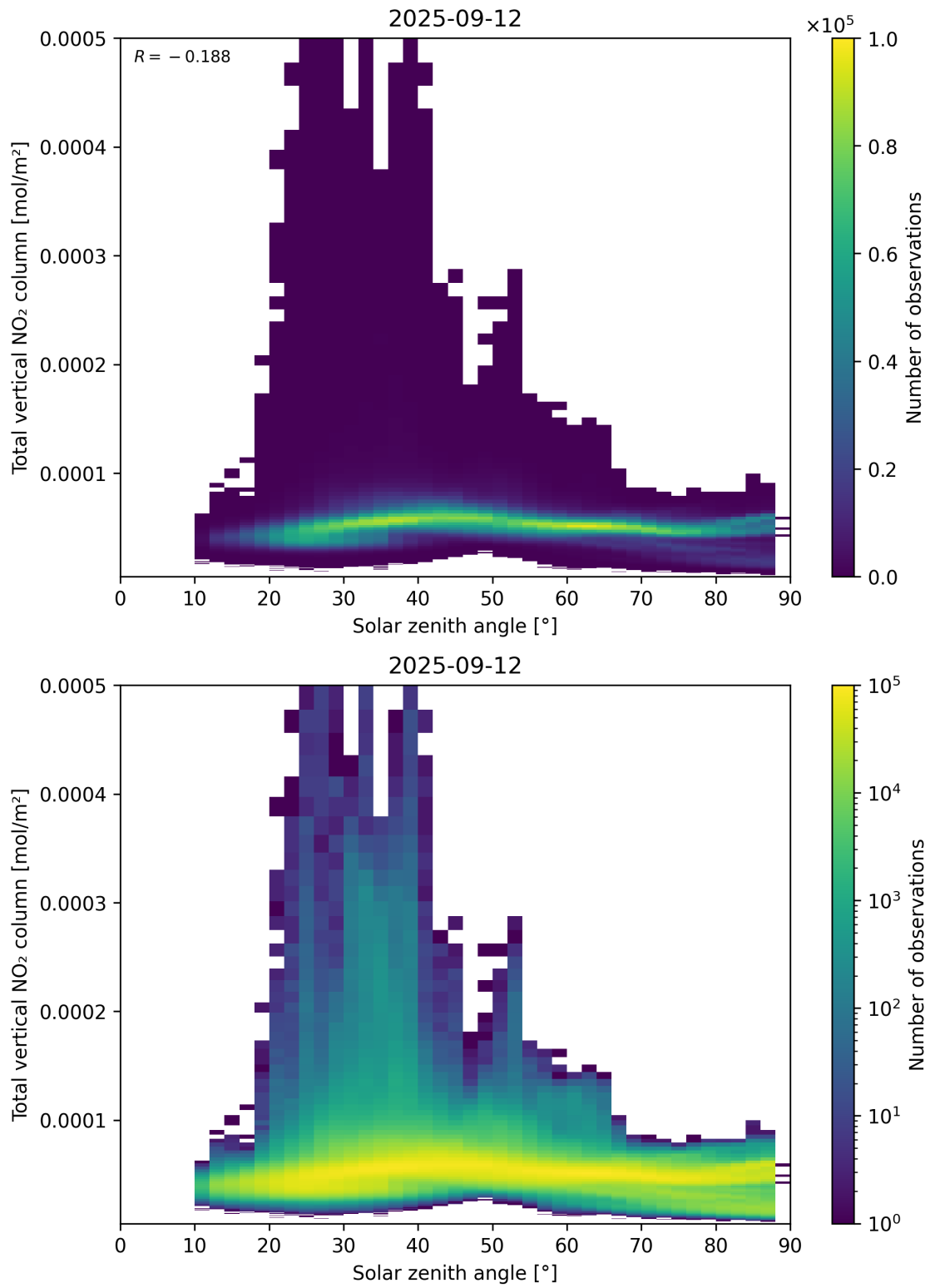
Figure 153: Scatter density plot of “Solar zenith angle” against “Total vertical NO 2 column” for 2025-09-11 to 2025-09-13.
