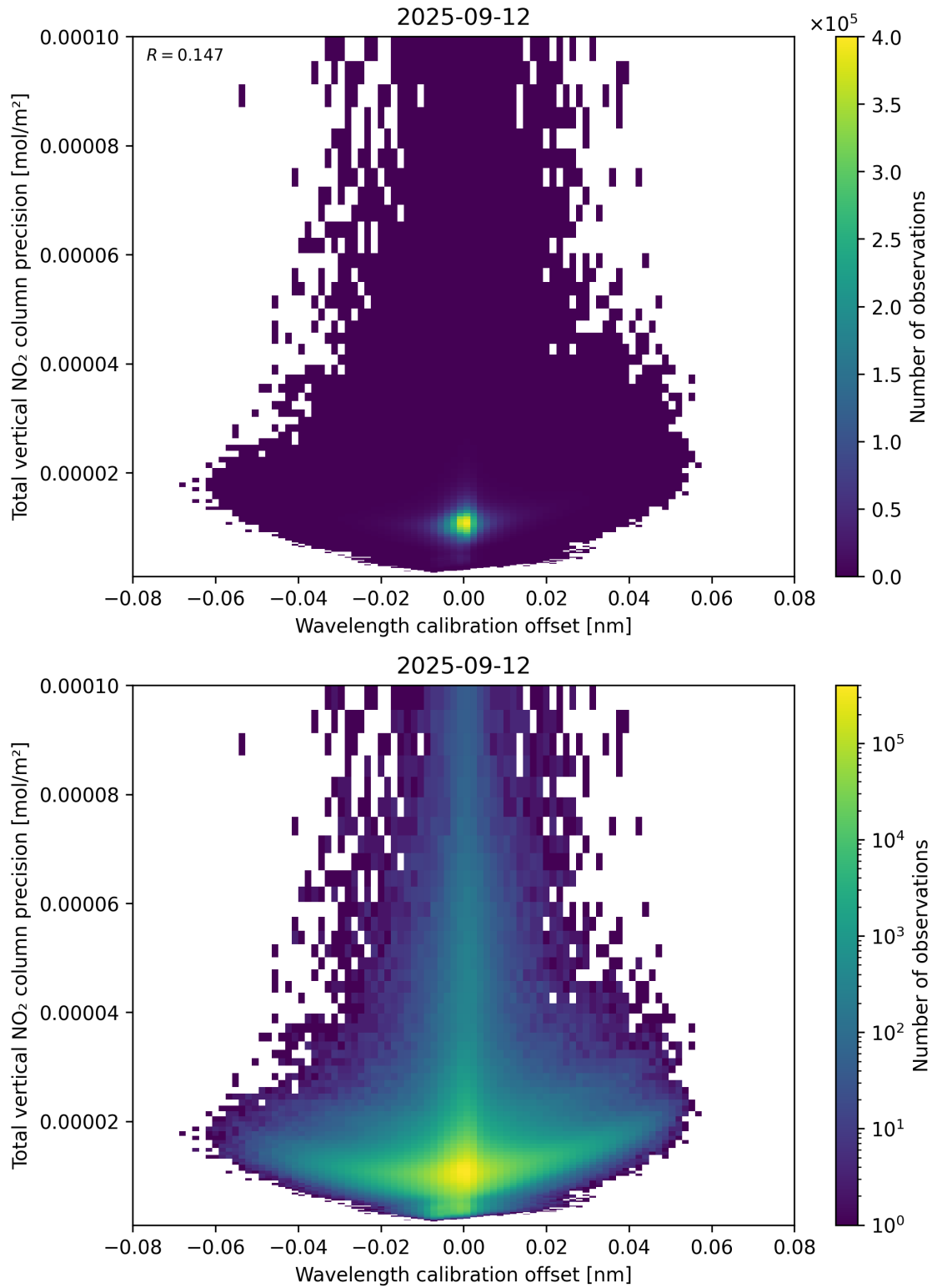
Figure 180: Scatter density plot of “Wavelength calibration offset” against “Total vertical NO 2 column precision” for 2025-09-11 to 2025-09-13.
