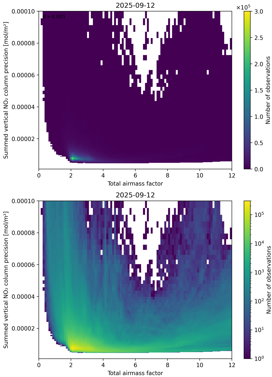
Figure 66: Scatter density plot of “Total airmass factor” against “Summed vertical NO 2 column precision” for 2025-09-11 to 2025-09-13.
