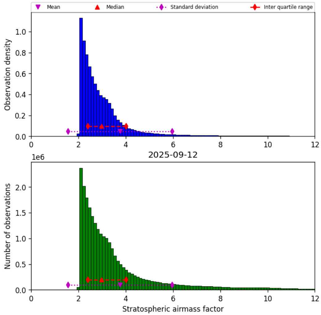
Figure 44: Histogram of “Stratospheric airmass factor” for 2025-09-11 to 2025-09-13
