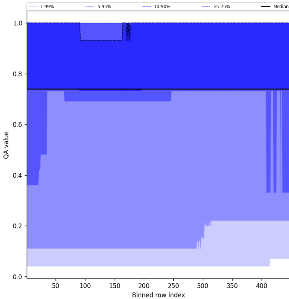
Figure 45: Along track statistics of "QA value" for 2025-09-11 to 2025-09-13
