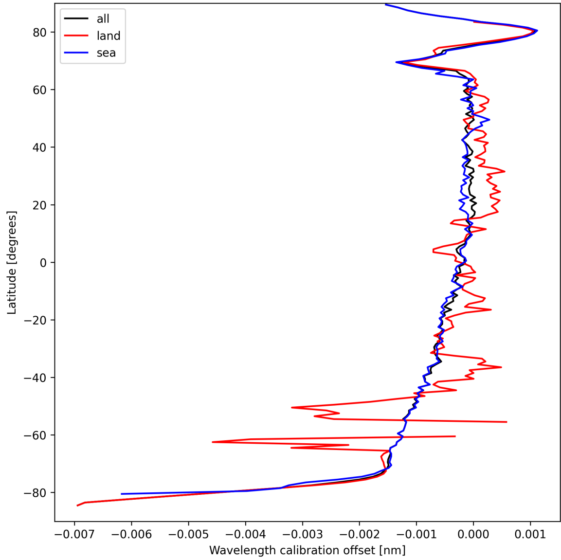
Figure 18: Zonal average of “Wavelength calibration offset” for 2025-09-11 to 2025-09-13.
