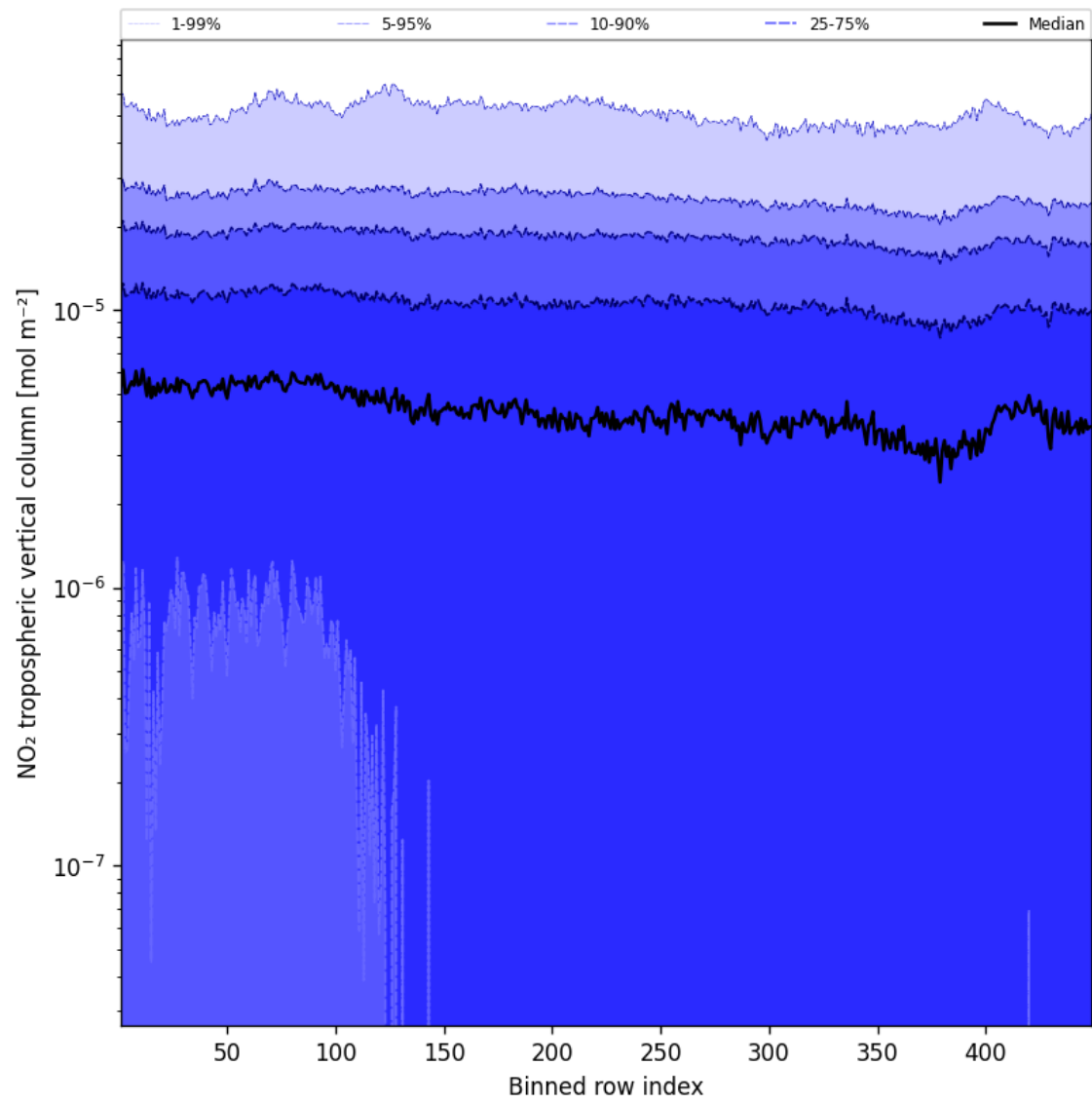
Figure 46: Along track statistics of “NO 2 tropospheric vertical column” for 2025-09-11 to 2025-09-13
