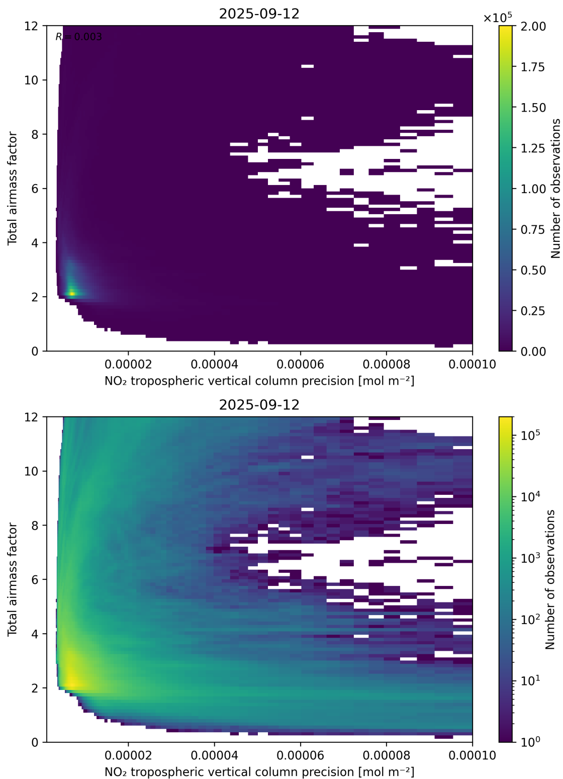
Figure 132: Scatter density plot of “NO 2 tropospheric vertical column precision” against “Total air mass factor” for 2025-09-11 to 2025-09-13.
