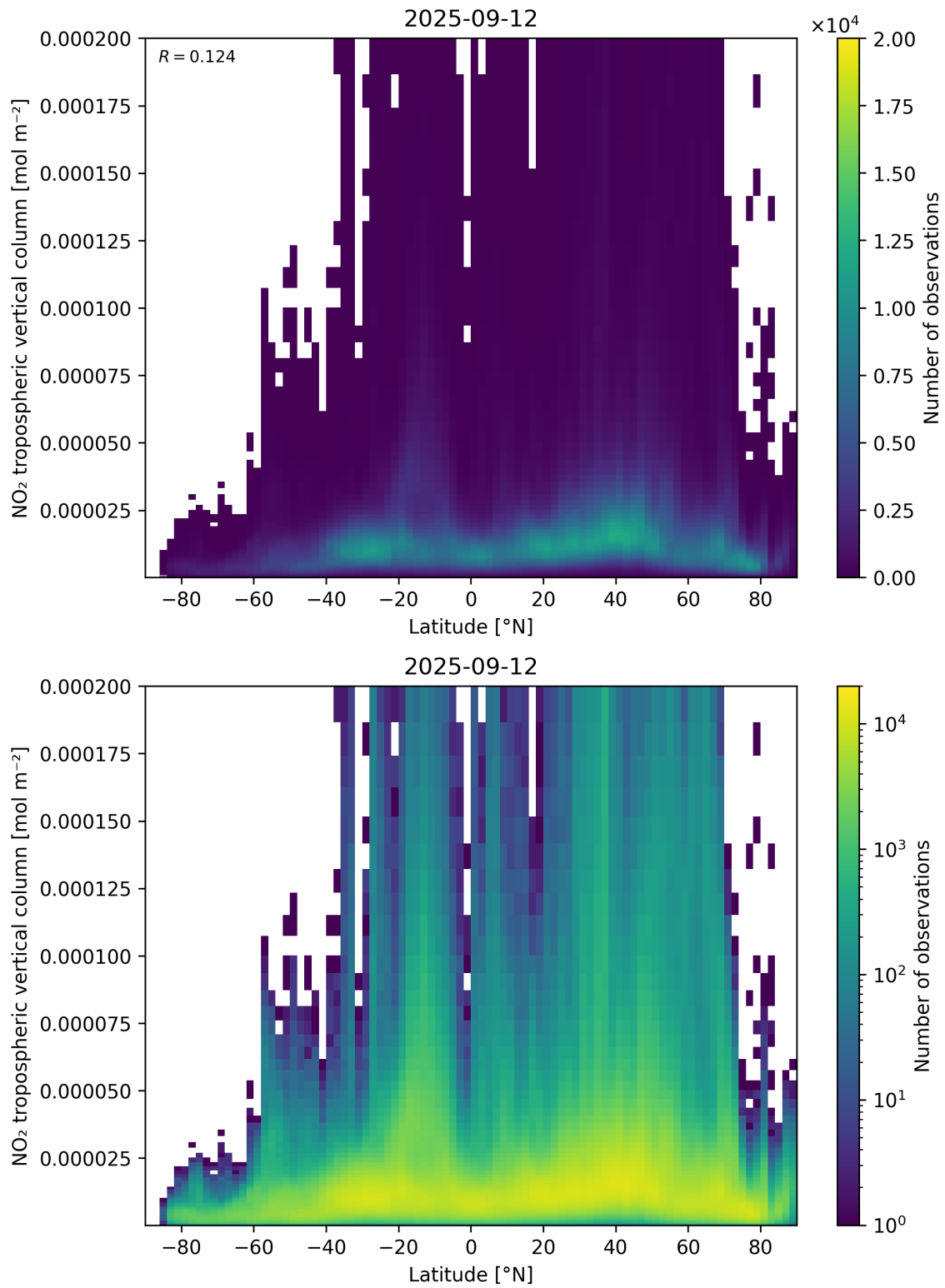
Figure 92: Scatter density plot of “Latitude” against “NO 2 tropospheric vertical column” for 2025-09-11 to 2025-09-13.
