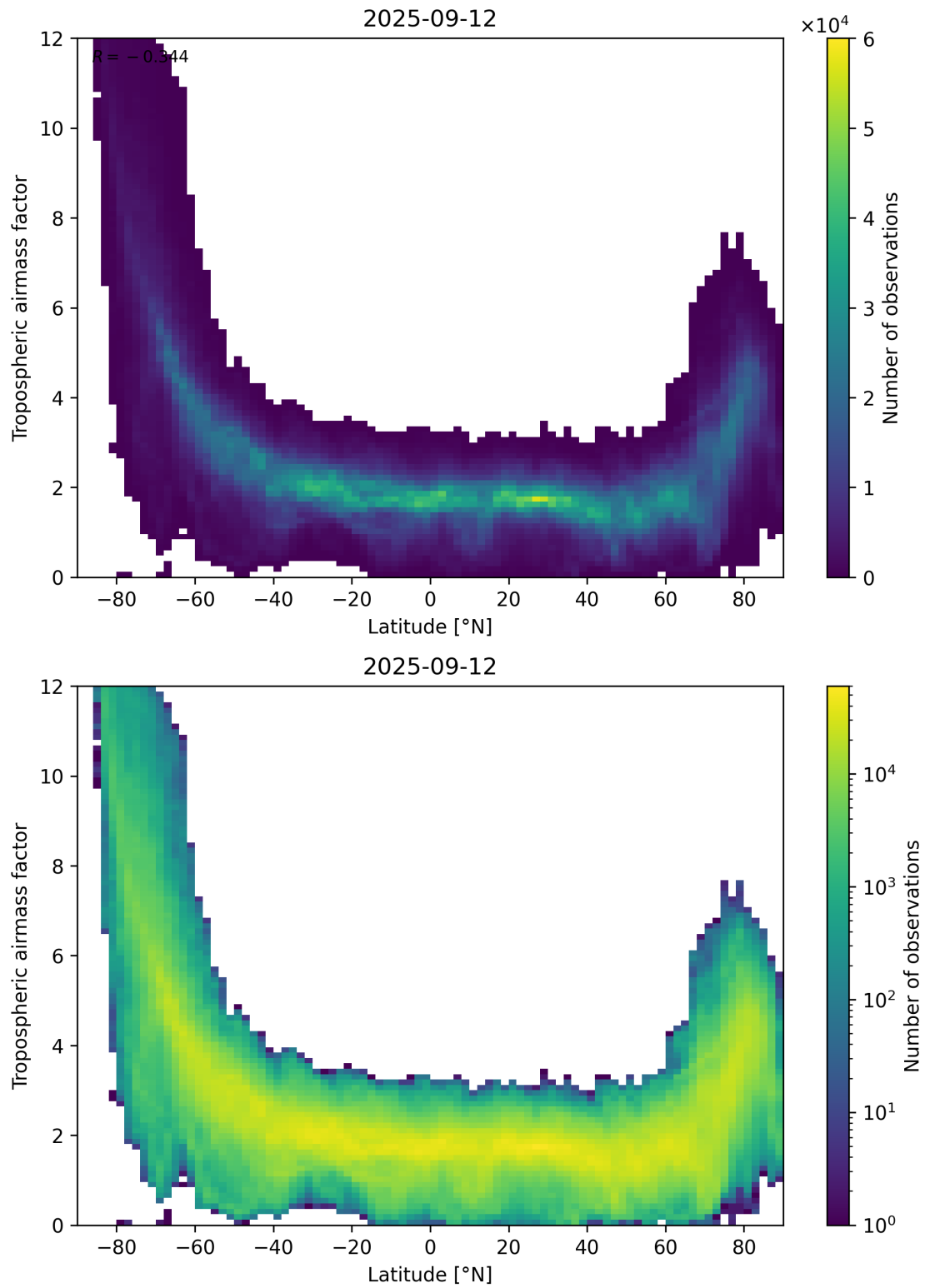
Figure 85: Scatter density plot of “Latitude” against “Tropospheric airmass factor” for 2025-09-11 to 2025-09-13.
