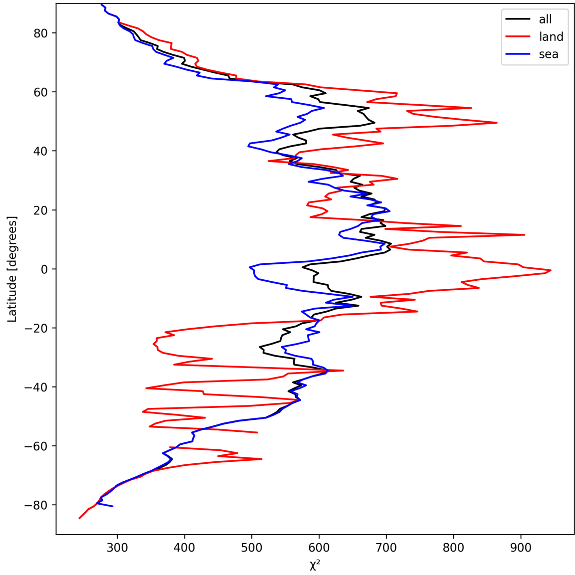
Figure 25: Zonal average of “ \chi^2 ” for 2025-09-11 to 2025-09-13.
