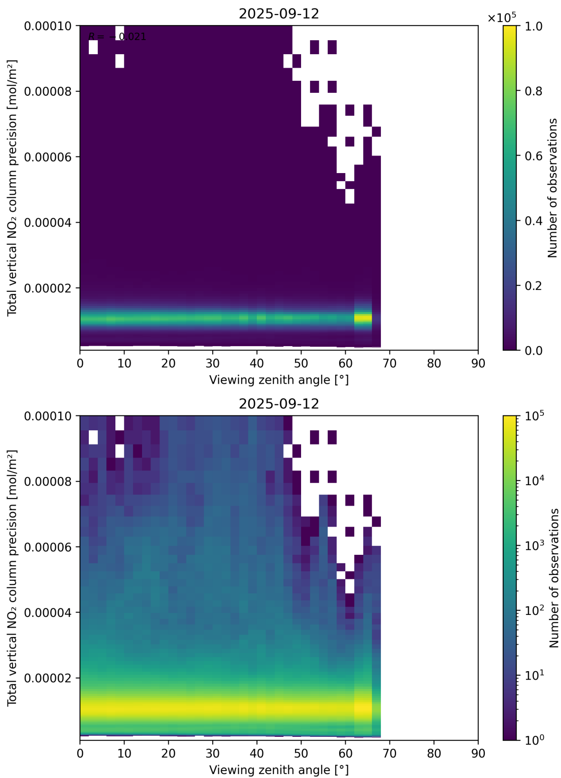
Figure 168: Scatter density plot of “Viewing zenith angle” against “Total vertical NO 2 column precision” for 2025-09-11 to 2025-09-13.
