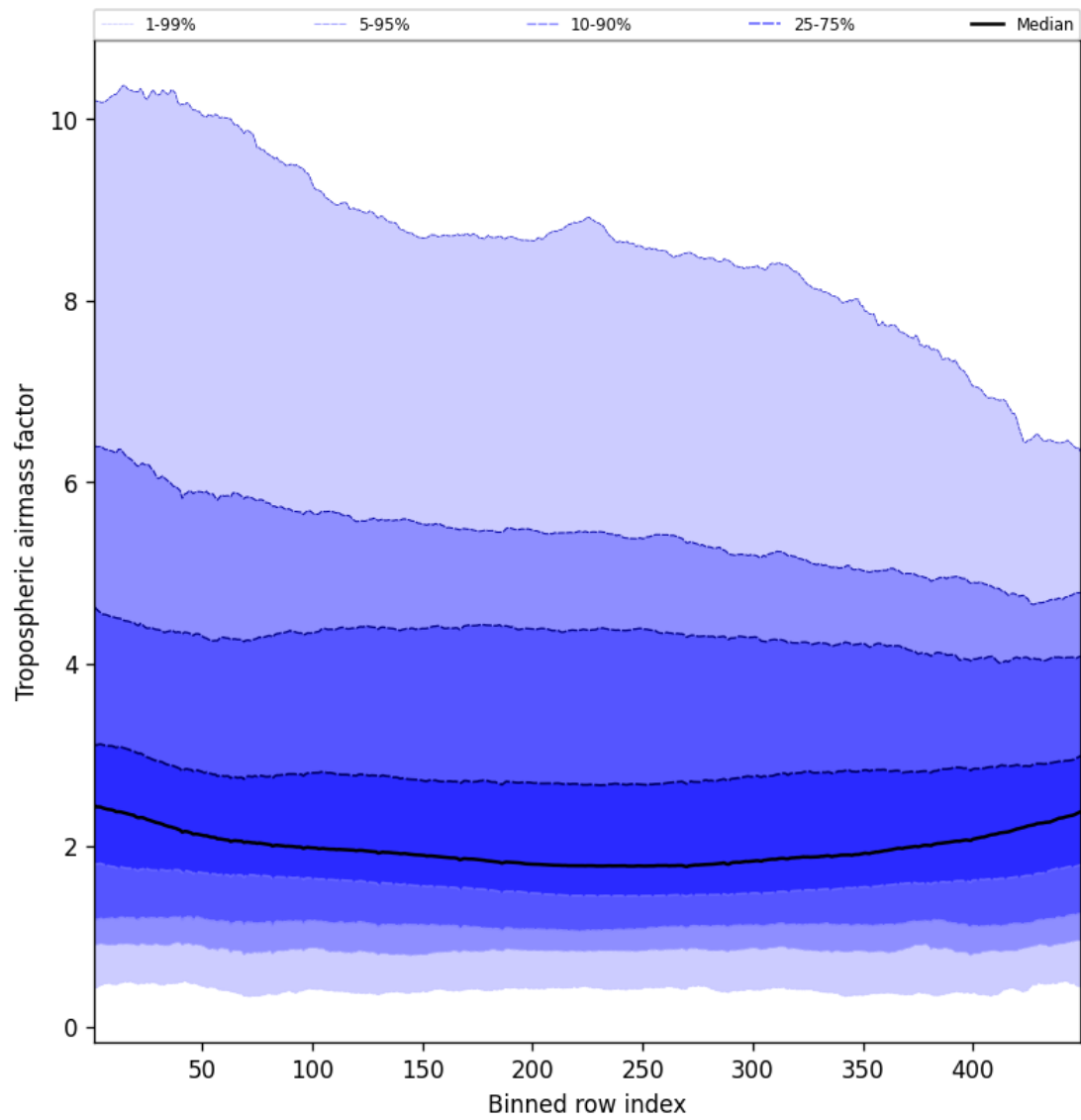
Figure 48: Along track statistics of “Tropospheric air mass factor” for 2025-09-11 to 2025-09-13
