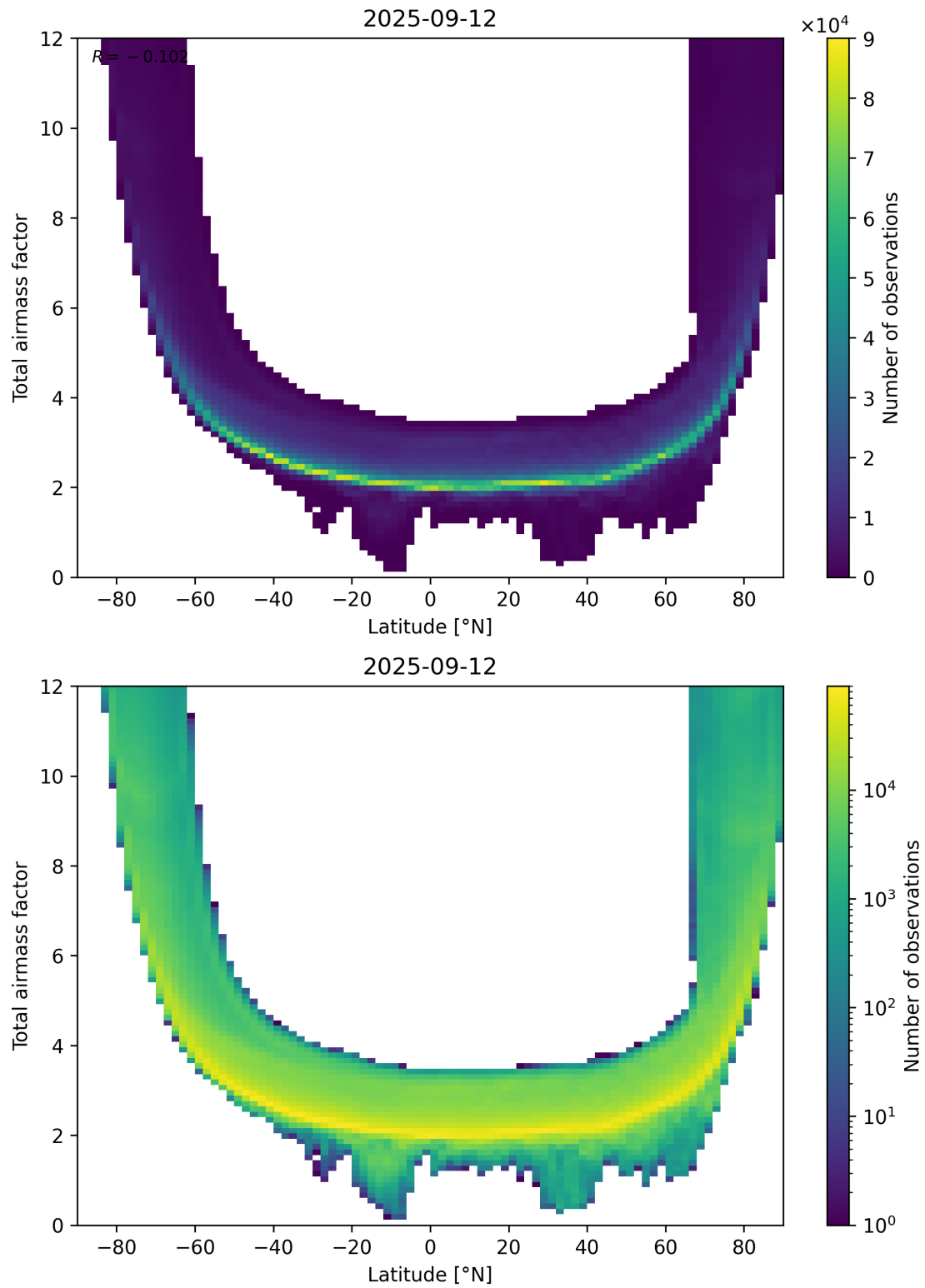
Figure 84: Scatter density plot of “Latitude” against “Total airmass factor” for 2025-09-11 to 2025-09-13.
