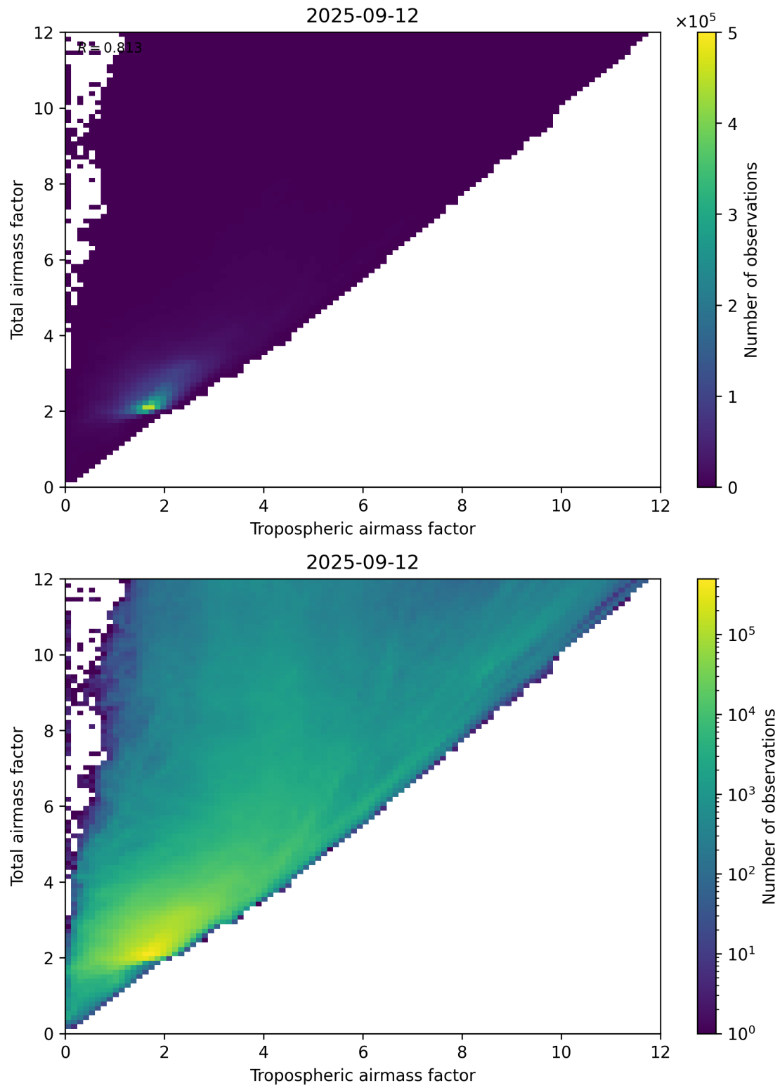
Figure 72: Scatter density plot of “Tropospheric airmass factor” against “Total airmass factor” for 2025-09-11 to 2025-09-13.
