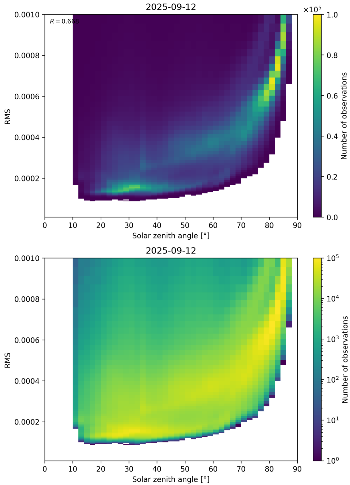
Figure 157: Scatter density plot of “Solar zenith angle” against “RMS” for 2025-09-11 to 2025-09-13.
