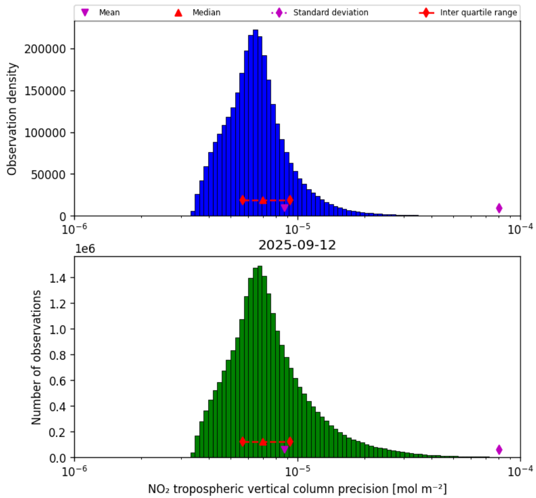
Figure 30: Histogram of “NO 2 tropospheric vertical column precision” for 2025-09-11 to 2025-09-13
