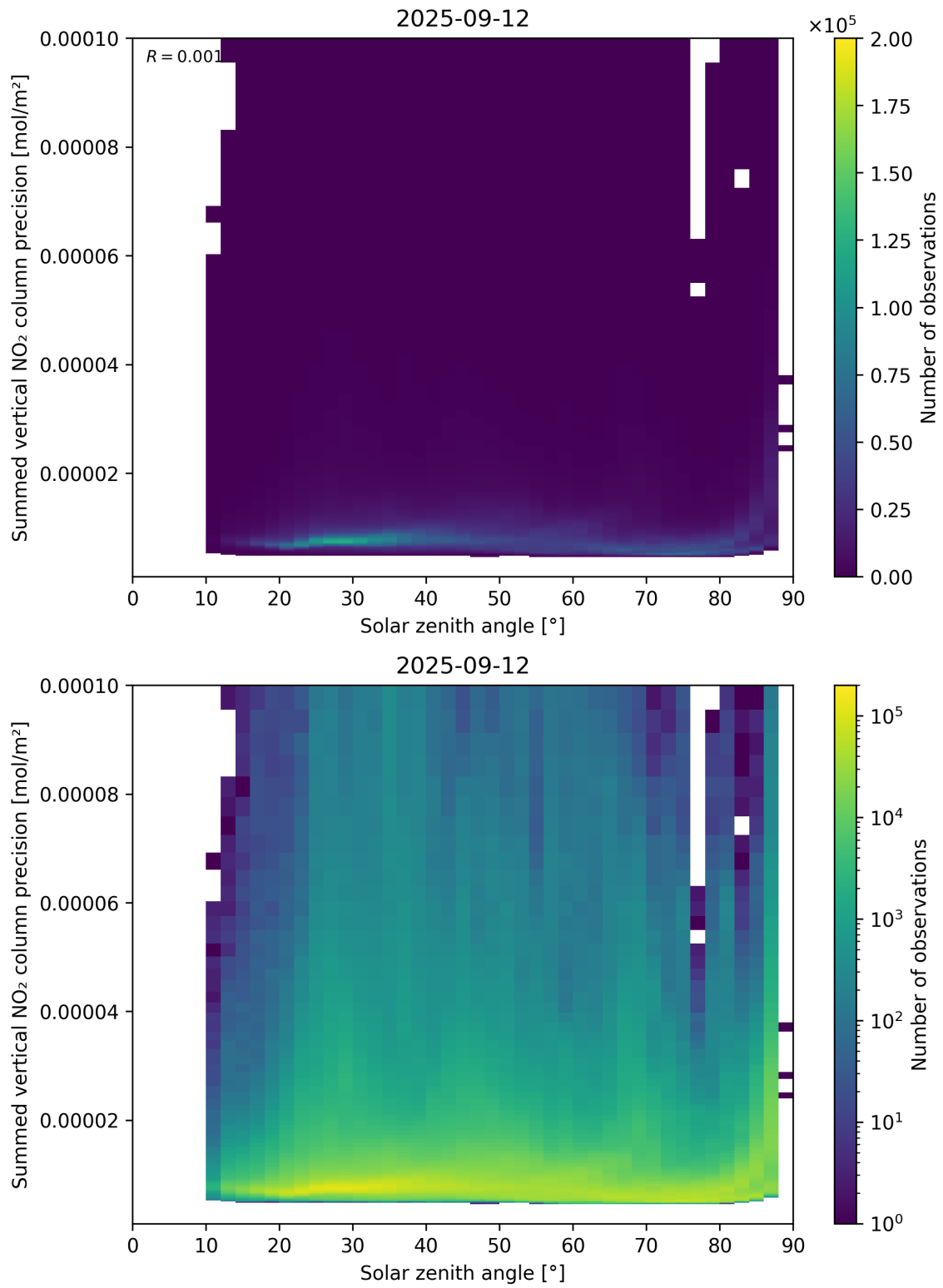
Figure 152: Scatter density plot of “Solar zenith angle” against “Summed vertical NO 2 column precision” for 2025-09-11 to 2025-09-13.
