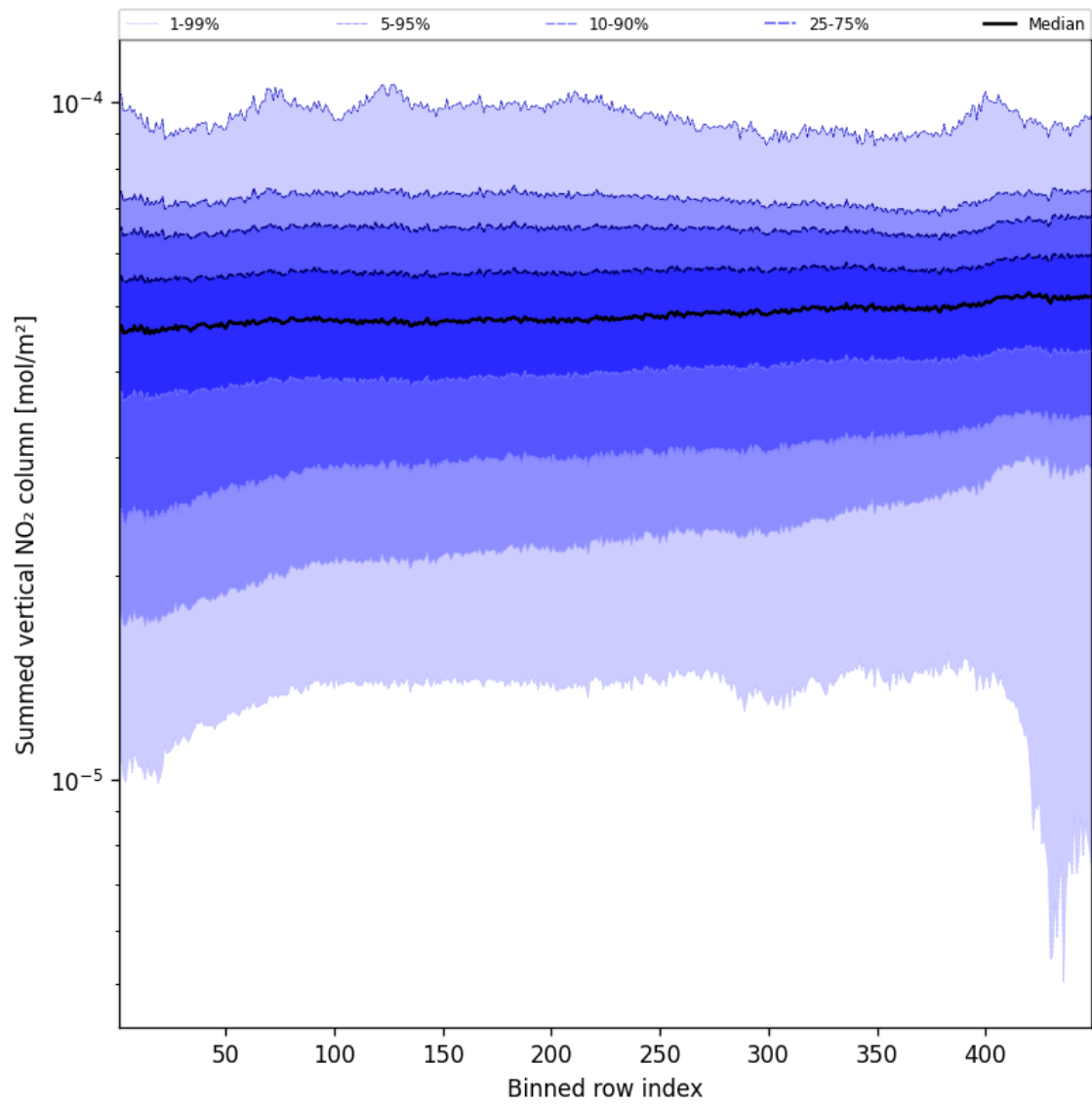
Figure 57: Along track statistics of “Summed vertical NO 2 column” for 2025-09-11 to 2025-09-13
