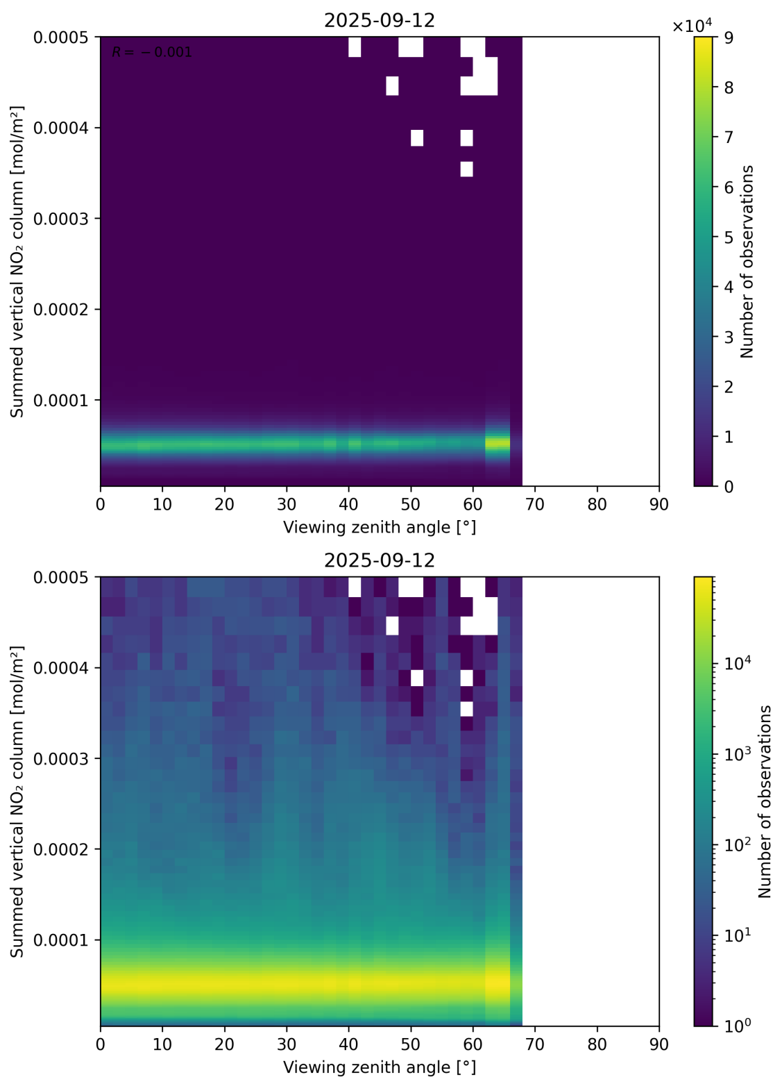
Figure 165: Scatter density plot of “Viewing zenith angle” against “Summed vertical NO 2 column” for 2025-09-11 to 2025-09-13.
