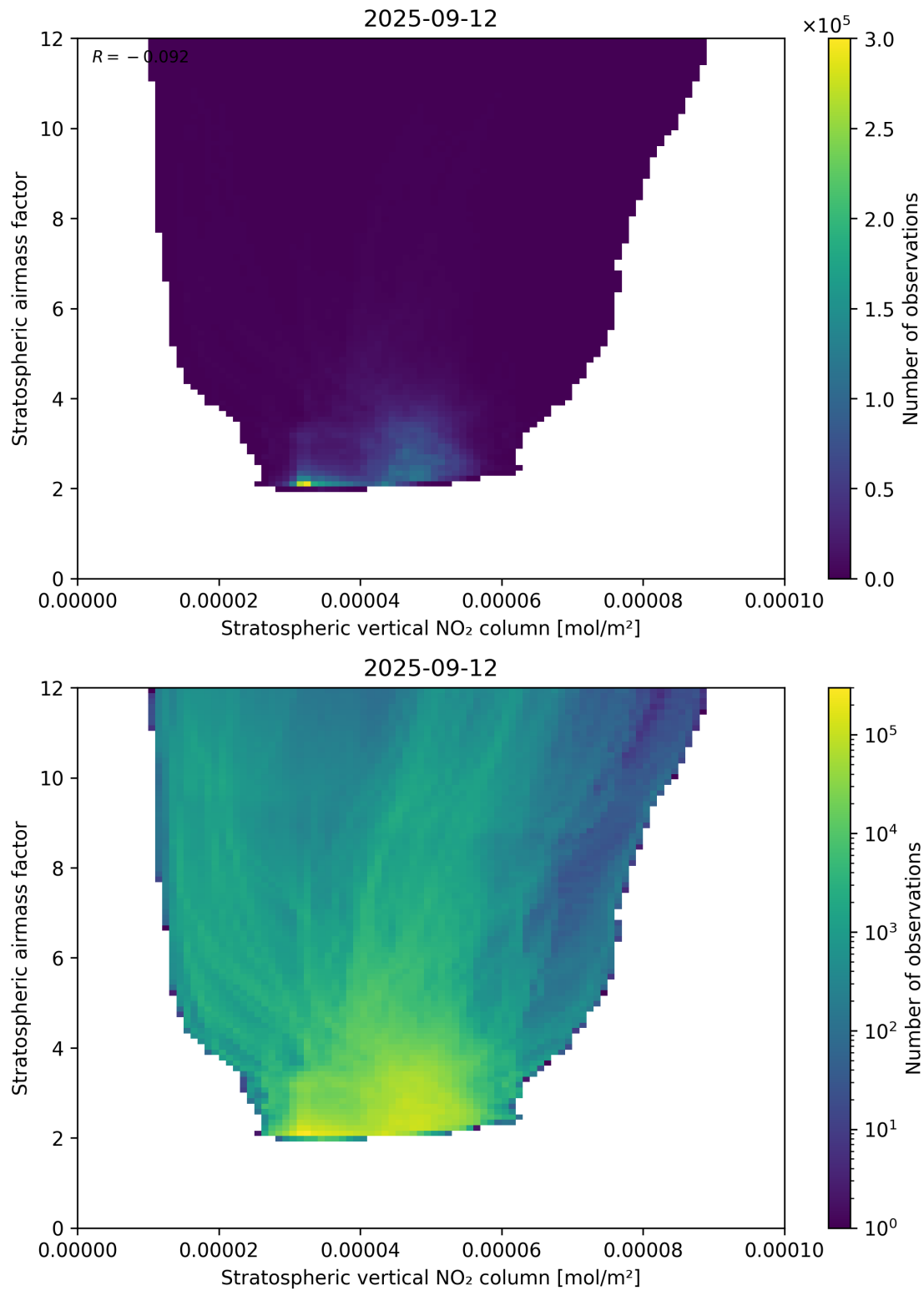
Figure 96: Scatter density plot of “Stratospheric vertical NO 2 column” against “Stratospheric airmass factor” for 2025-09-11 to 2025-09-13.
