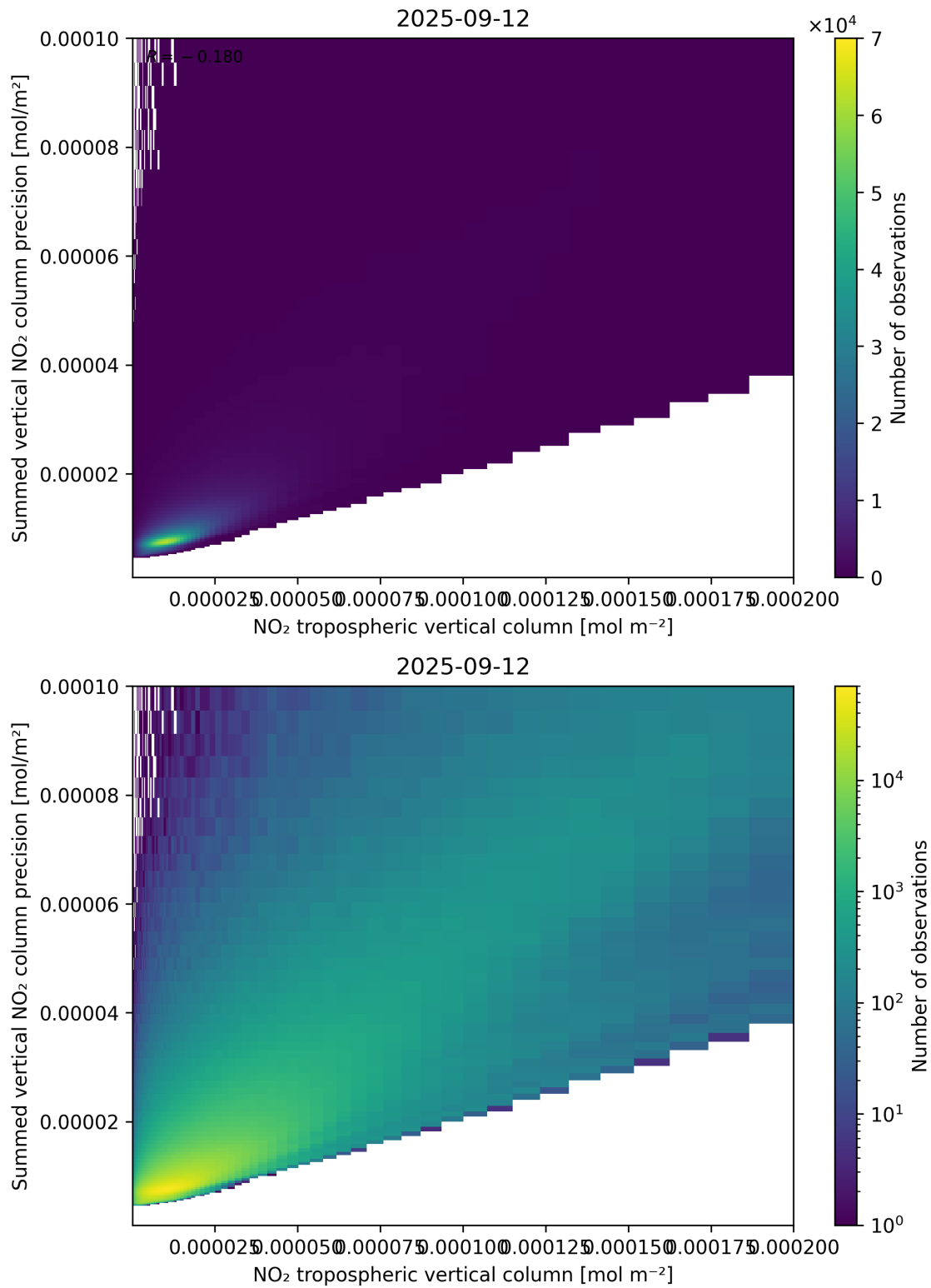
Figure 127: Scatter density plot of “NO 2 tropospheric vertical column” against “Summed vertical NO 2 column precision” for 2025-09-11 to 2025-09-13.
