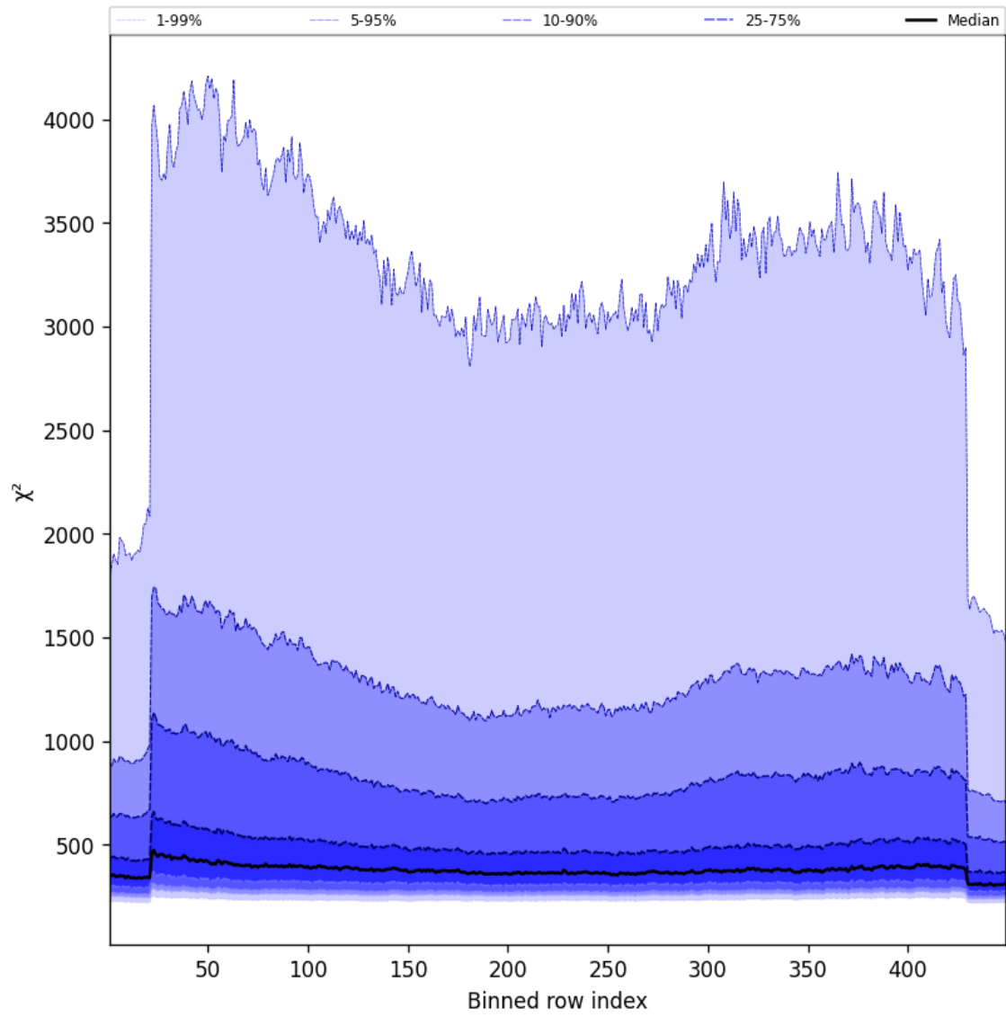
Figure 59: Along track statistics of “ \chi^2 ” for 2025-09-11 to 2025-09-13
