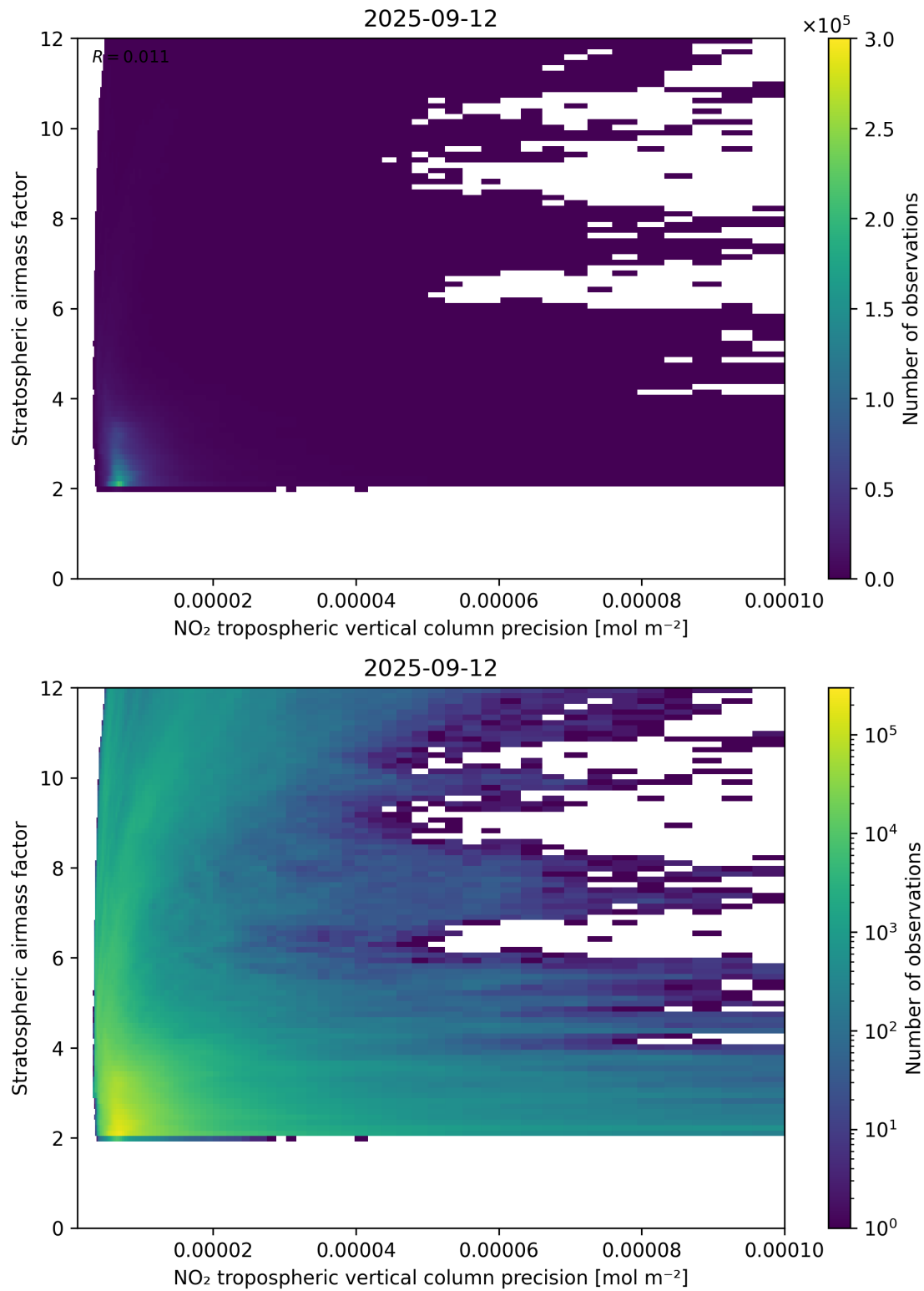
Figure 131: Scatter density plot of “NO 2 tropospheric vertical column precision” against “Stratospheric airmass factor” for 2025-09-11 to 2025-09-13.
