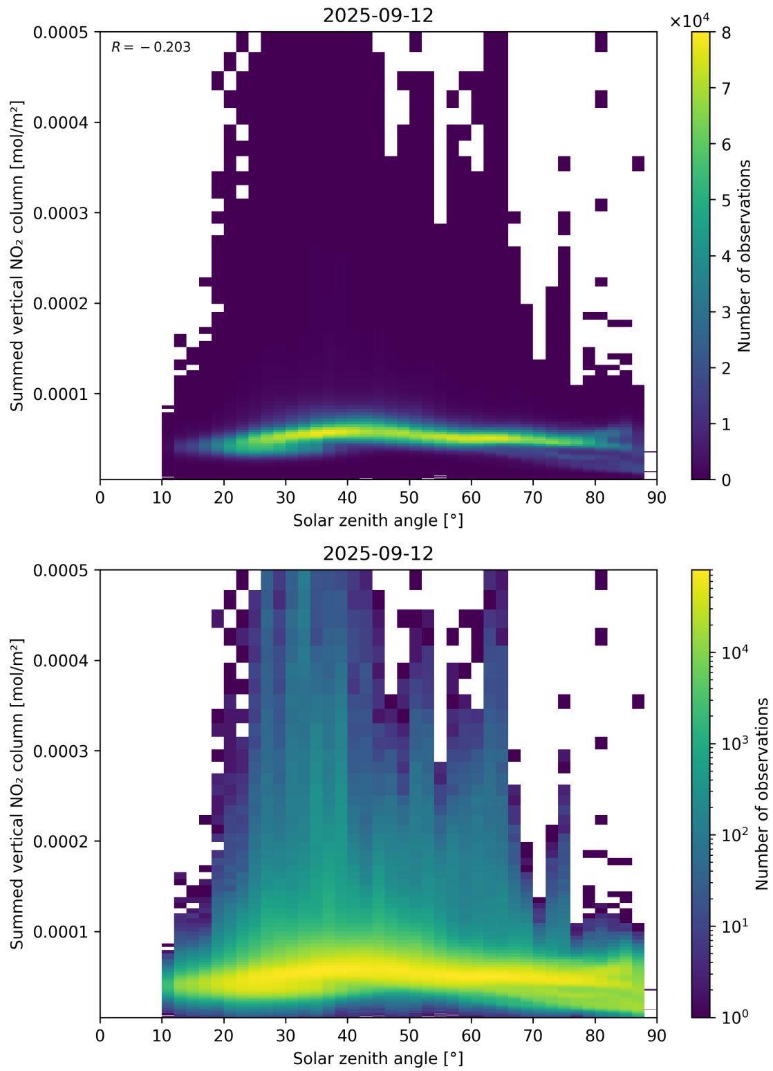
Figure 151: Scatter density plot of “Solar zenith angle” against “Summed vertical NO 2 column” for 2025-09-11 to 2025-09-13.
