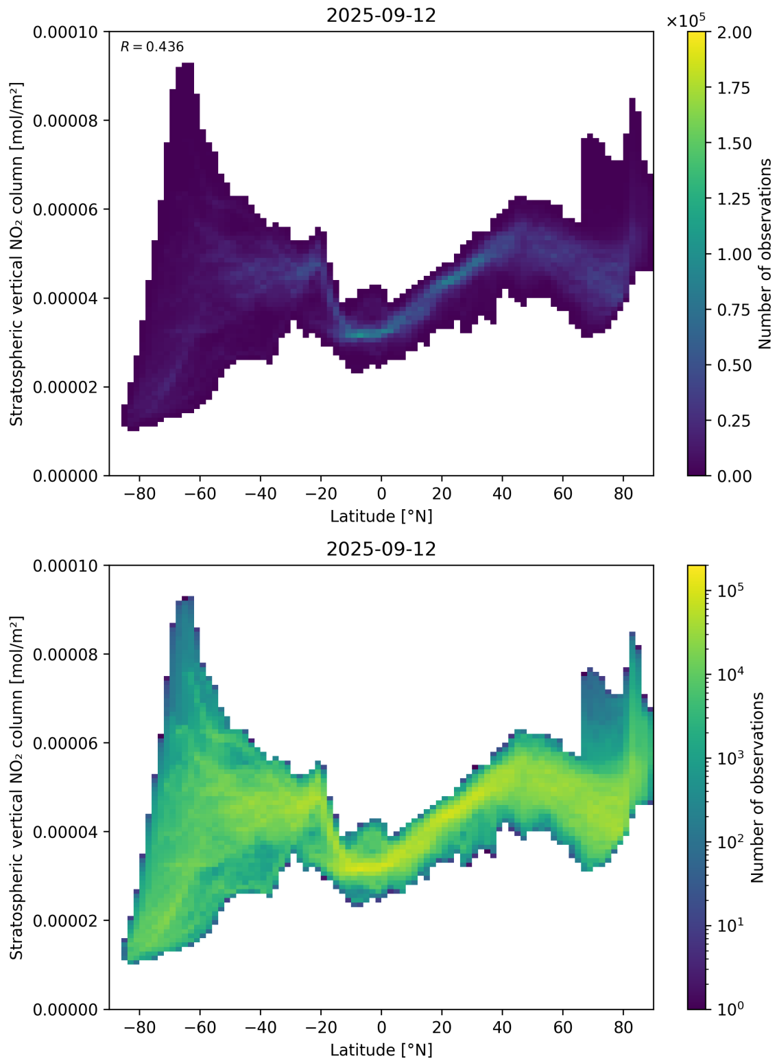
Figure 87: Scatter density plot of “Latitude” against “Stratospheric vertical NO 2 column” for 2025-09-11 to 2025-09-13.
