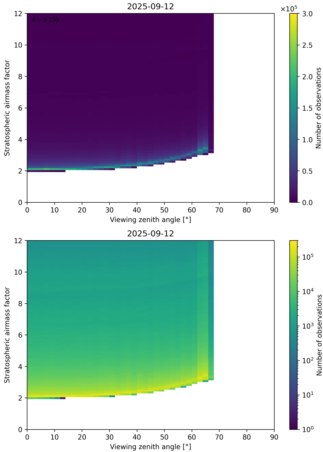
Figure 159: Scatter density plot of “Viewing zenith angle” against “Stratospheric airmass factor” for 2025-09-11 to 2025-09-13.
