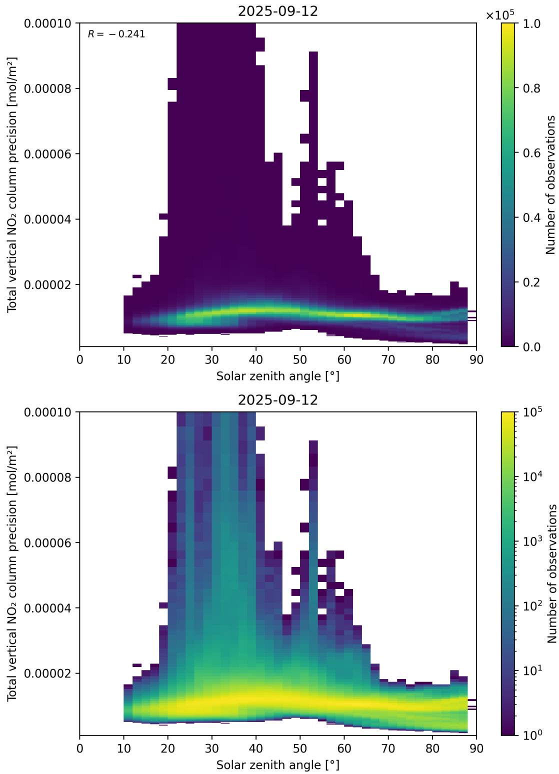
Figure 154: Scatter density plot of “Solar zenith angle” against “Total vertical NO 2 column precision” for 2025-09-11 to 2025-09-13.
