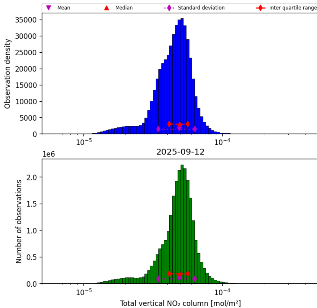
Figure 38: Histogram of “Total vertical NO 2 column” for 2025-09-11 to 2025-09-13
