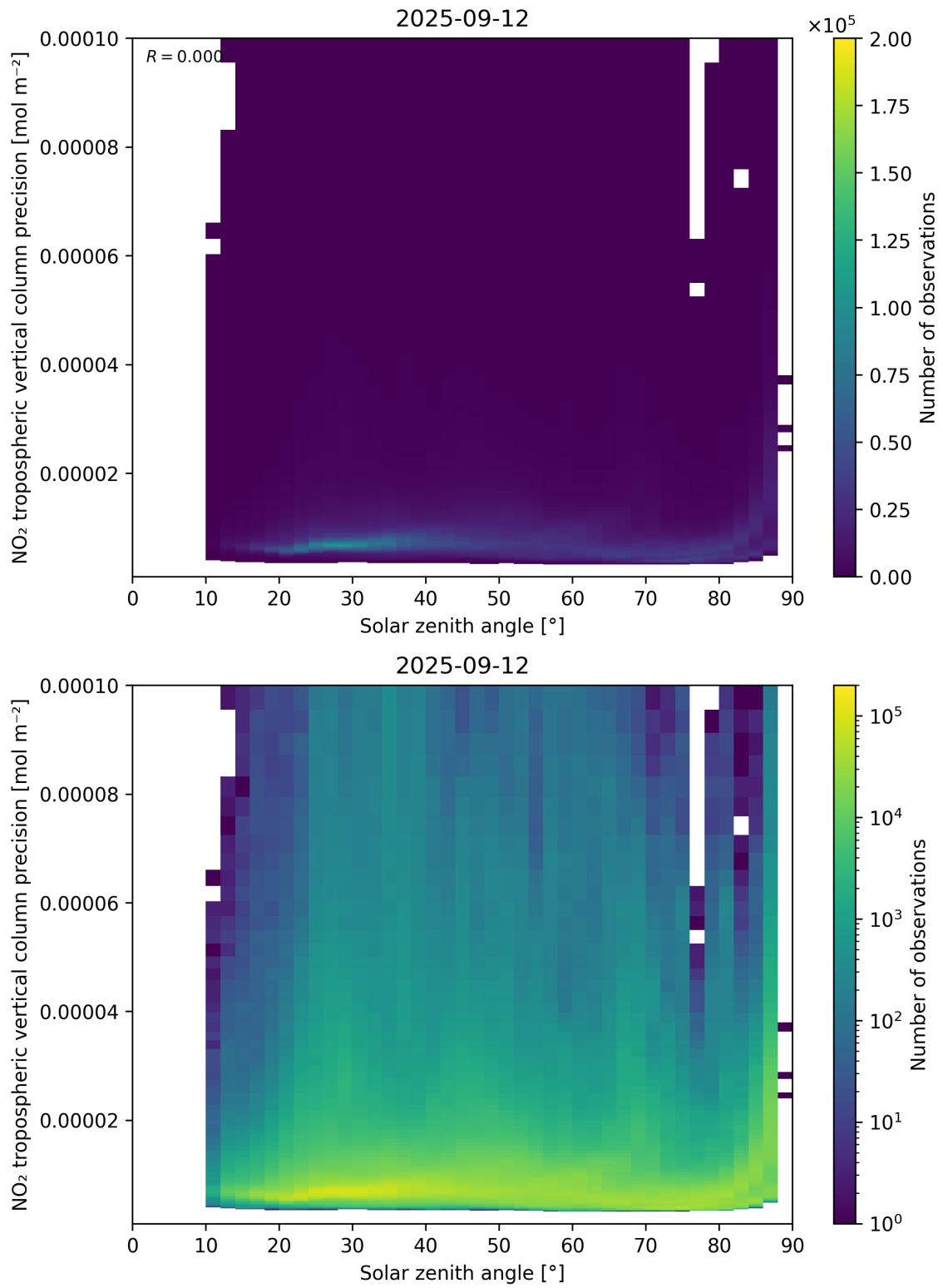
Figure 156: Scatter density plot of “Solar zenith angle” against “NO 2 tropospheric vertical column precision” for 2025-09-11 to 2025-09-13.
