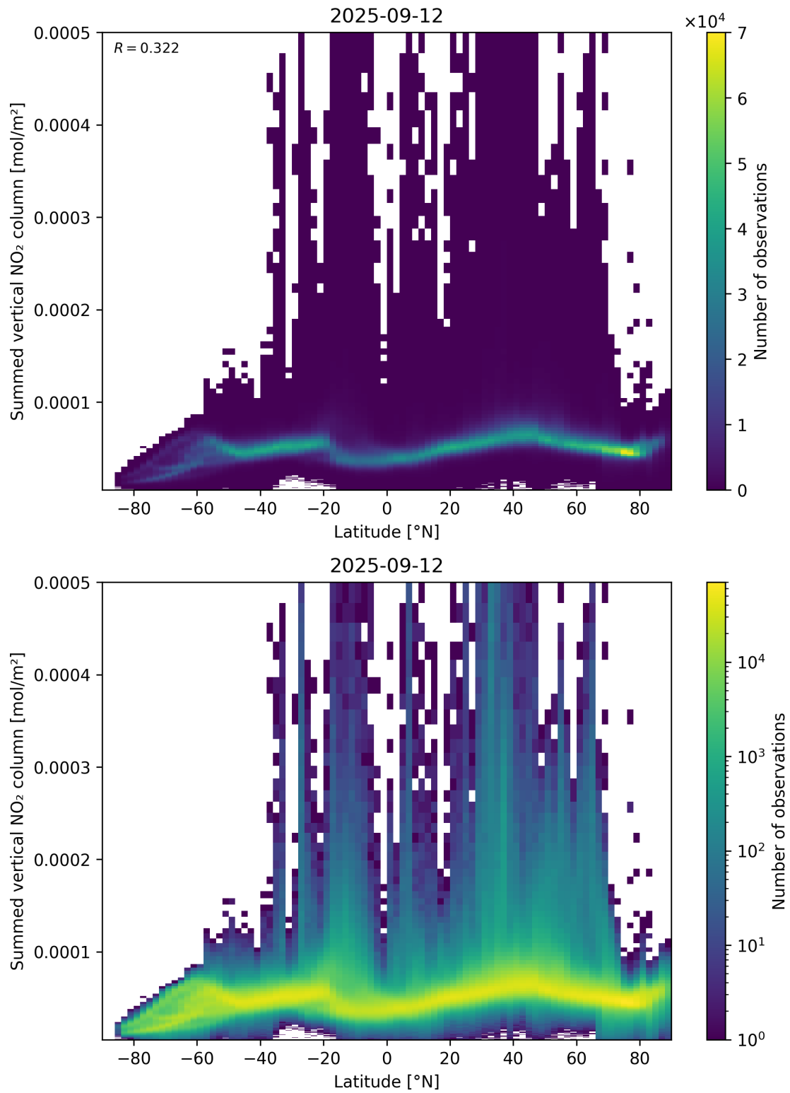
Figure 88: Scatter density plot of “Latitude” against “Summed vertical NO 2 column” for 2025-09-11 to 2025-09-13.
