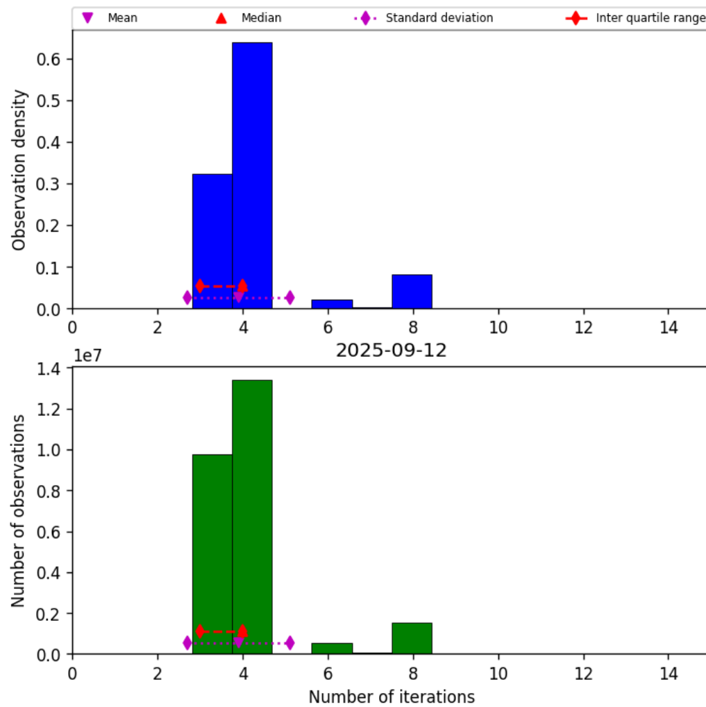
Figure 34: Histogram of “Number of iterations” for 2025-09-11 to 2025-09-13
