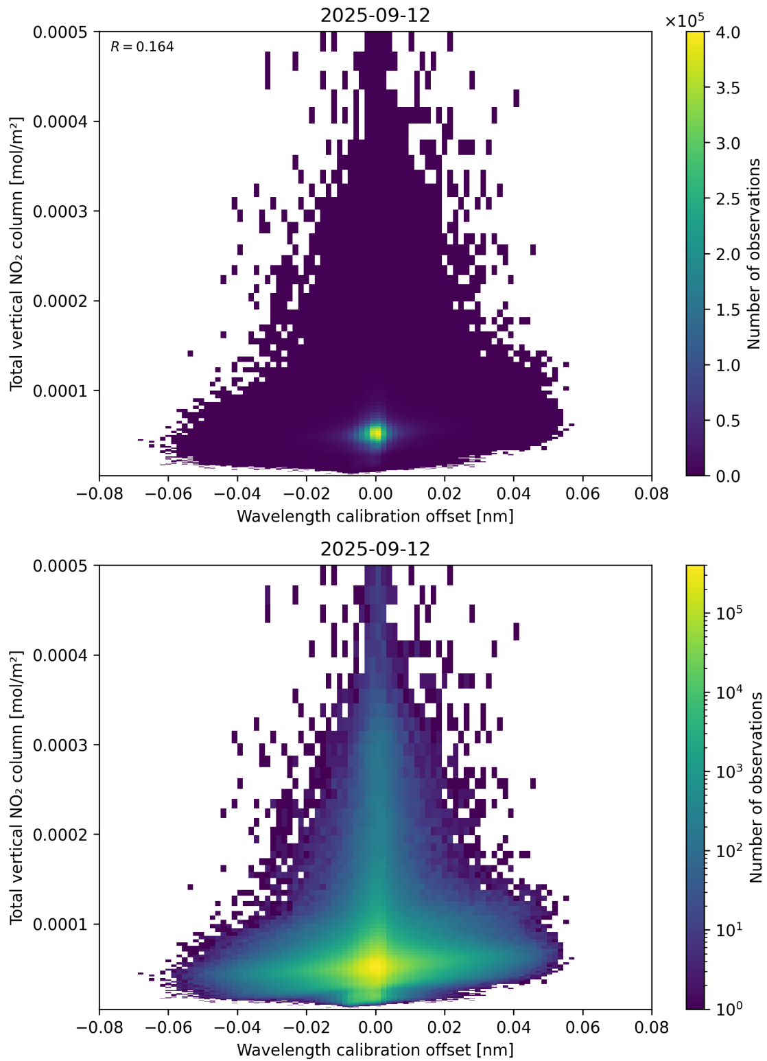
Figure 179: Scatter density plot of “Wavelength calibration offset” against “Total vertical NO 2 column” for 2025-09-11 to 2025-09-13.
