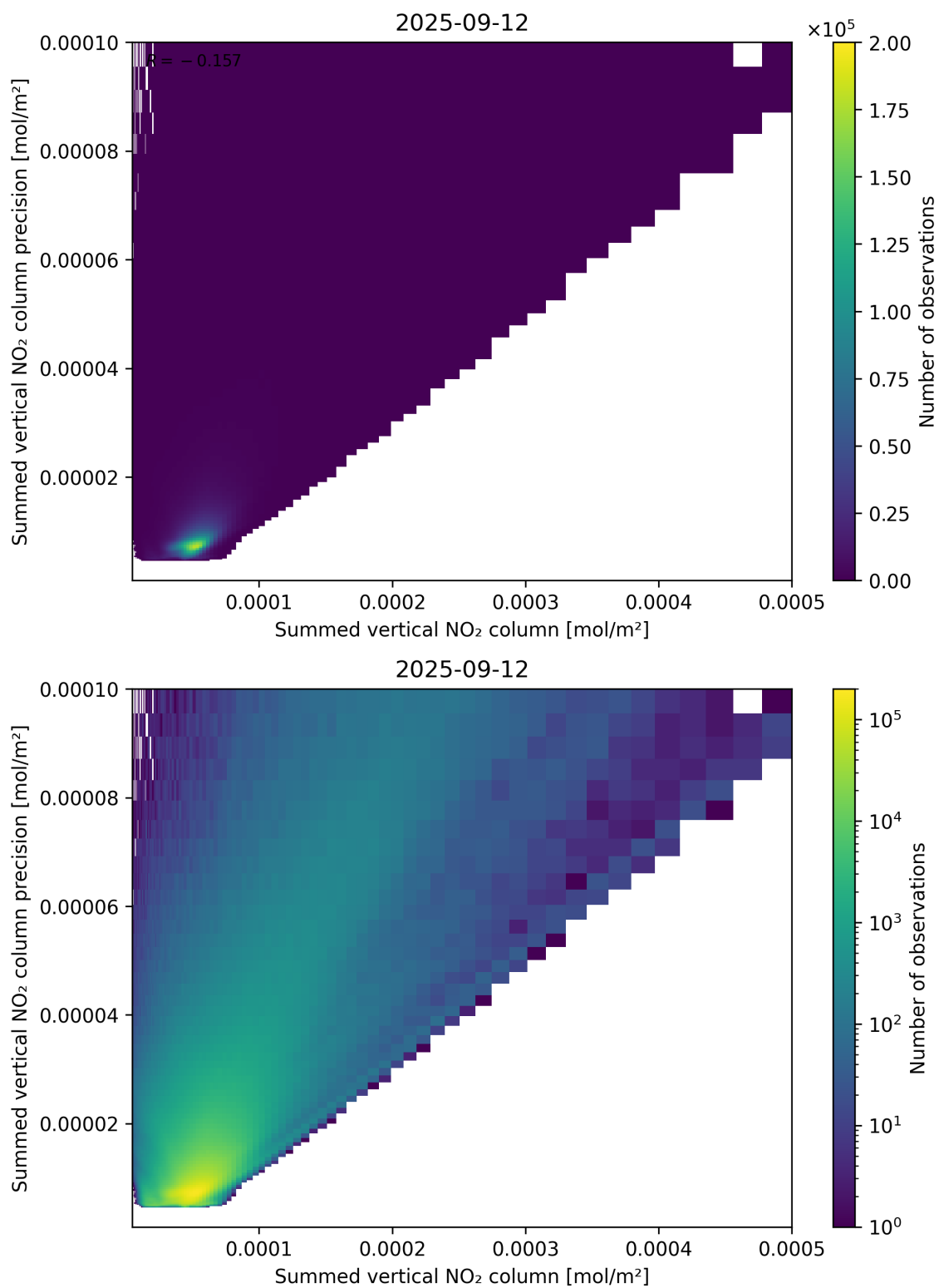
Figure 105: Scatter density plot of “Summed vertical NO 2 column” against “Summed vertical NO 2 column precision” for 2025-09-11 to 2025-09-13.
