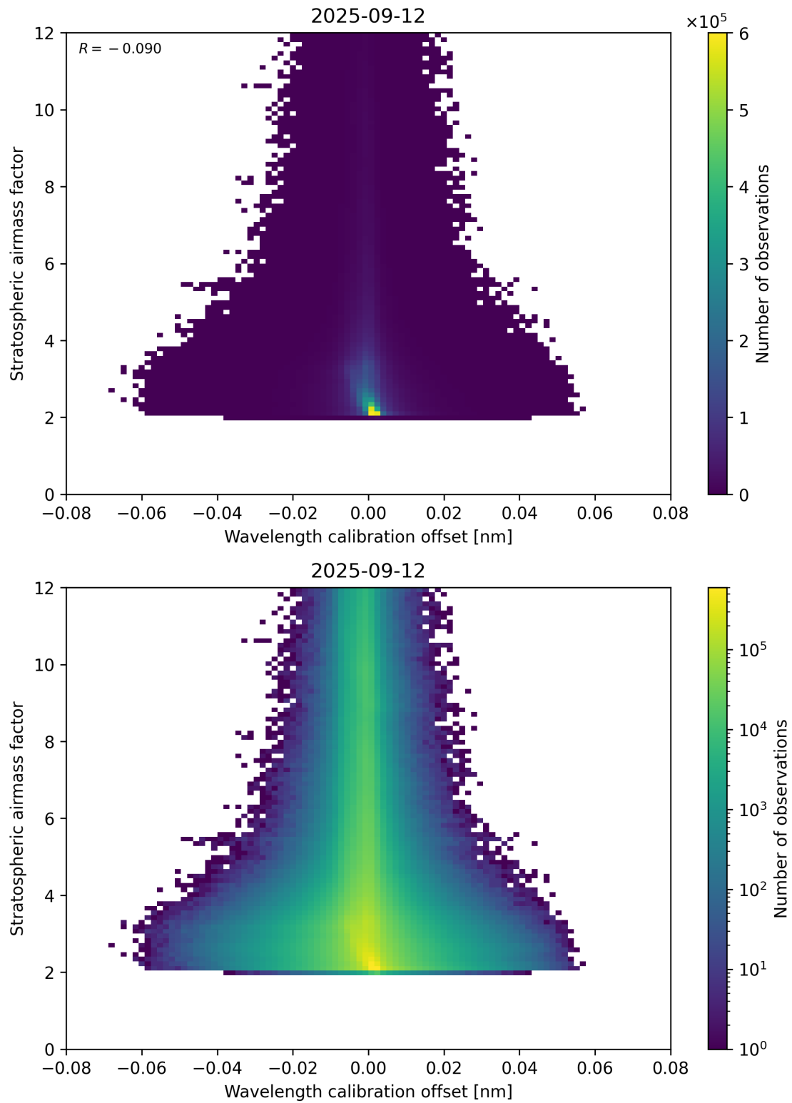
Figure 174: Scatter density plot of “Wavelength calibration offset” against “Stratospheric airmass factor” for 2025-09-11 to 2025-09-13.
