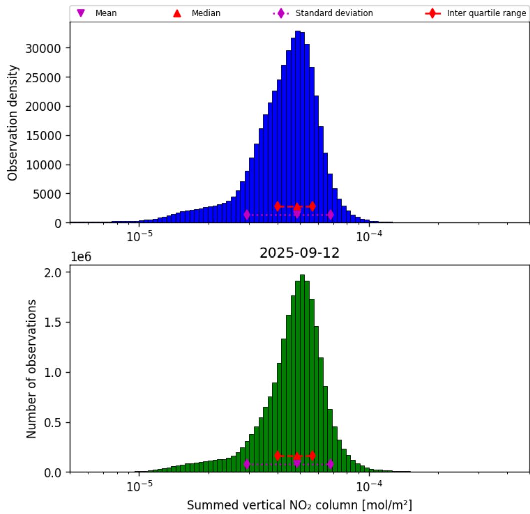
Figure 40: Histogram of “Summed vertical NO 2 column” for 2025-09-11 to 2025-09-13
