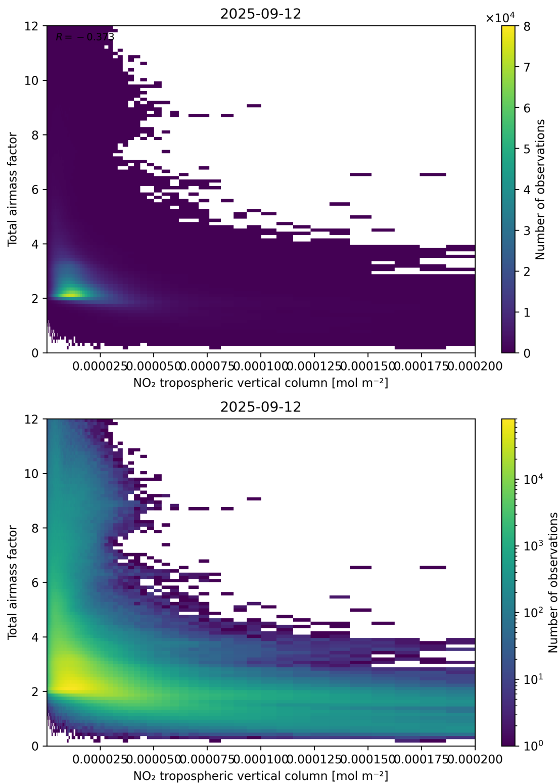
Figure 122: Scatter density plot of “NO 2 tropospheric vertical column” against “Total air mass factor” for 2025-09-11 to 2025-09-13.
