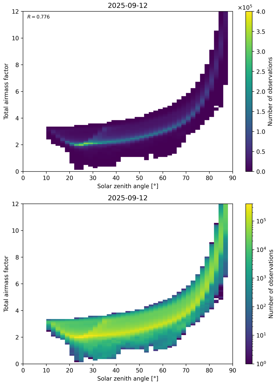
Figure 146: Scatter density plot of “Solar zenith angle” against “Total airmass factor” for 2025-09-11 to 2025-09-13.
