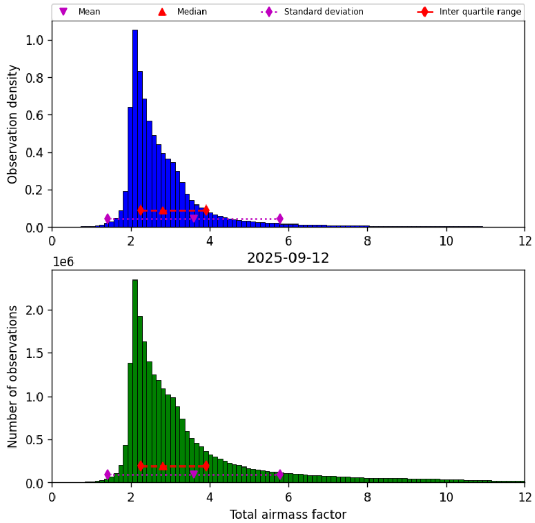
Figure 32: Histogram of “Total airmass factor” for 2025-09-11 to 2025-09-13
