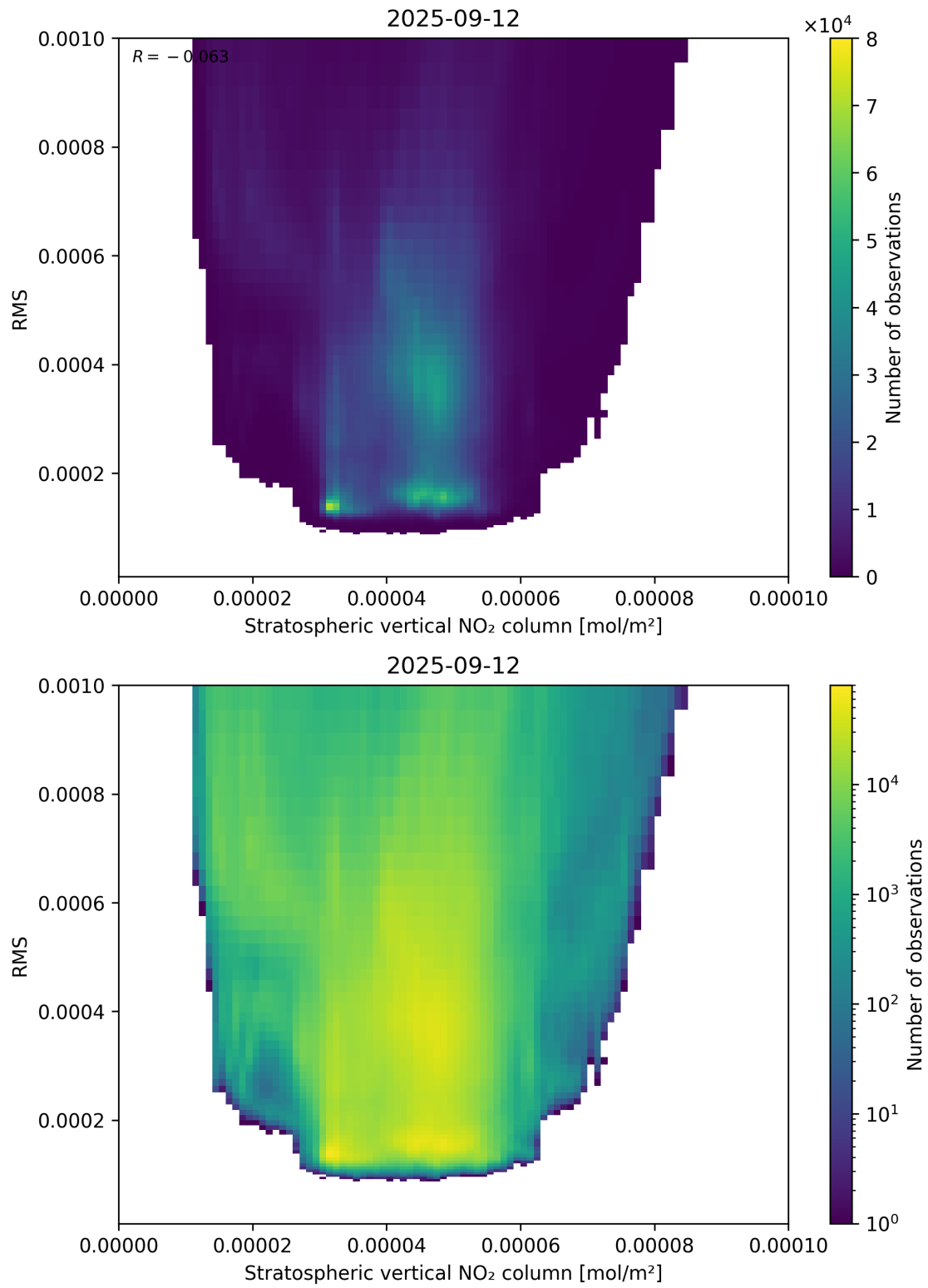
Figure 102: Scatter density plot of “Stratospheric vertical NO 2 column” against “RMS” for 2025-09-11 to 2025-09-13.
