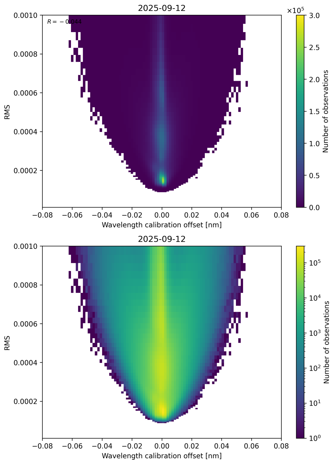
Figure 181: Scatter density plot of “Wavelength calibration offset” against “RMS” for 2025-09-11 to 2025-09-13.
