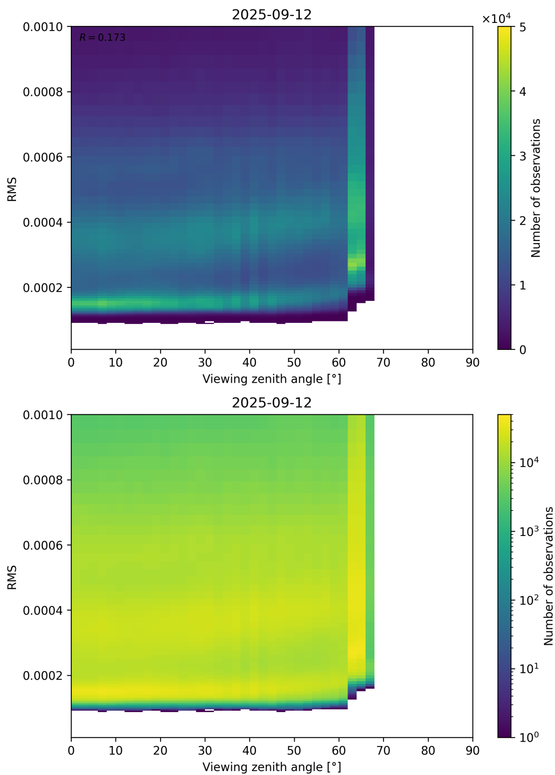
Figure 171: Scatter density plot of “Viewing zenith angle” against “RMS” for 2025-09-11 to 2025-09-13.
