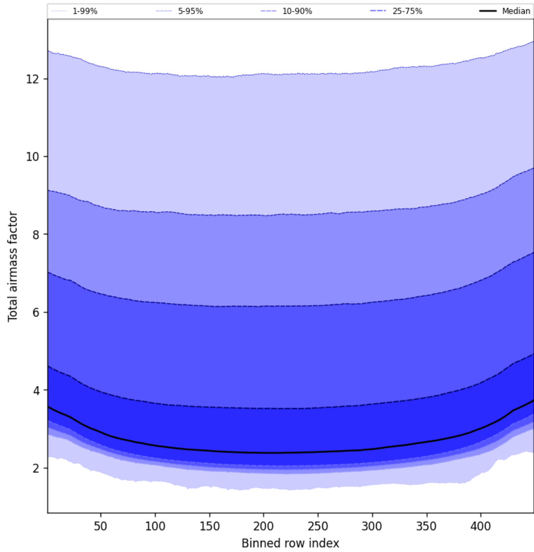
Figure 49: Along track statistics of “Total airmass factor” for 2025-09-11 to 2025-09-13
