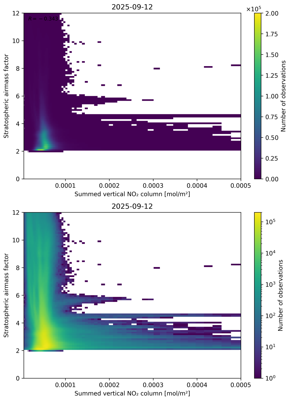
Figure 103: Scatter density plot of “Summed vertical NO 2 column” against “Stratospheric air mass factor” for 2025-09-11 to 2025-09-13.
