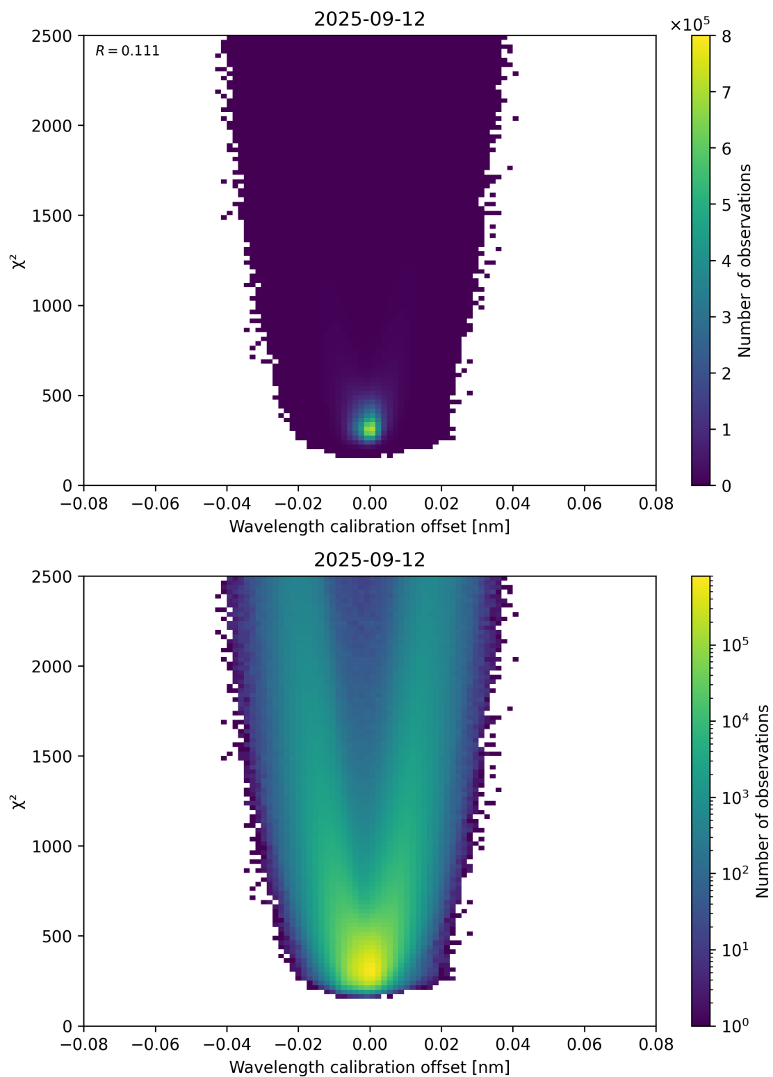
Figure 175: Scatter density plot of “Wavelength calibration offset” against “ \chi^2 ” for 2025-09-11 to 2025-09-13.
