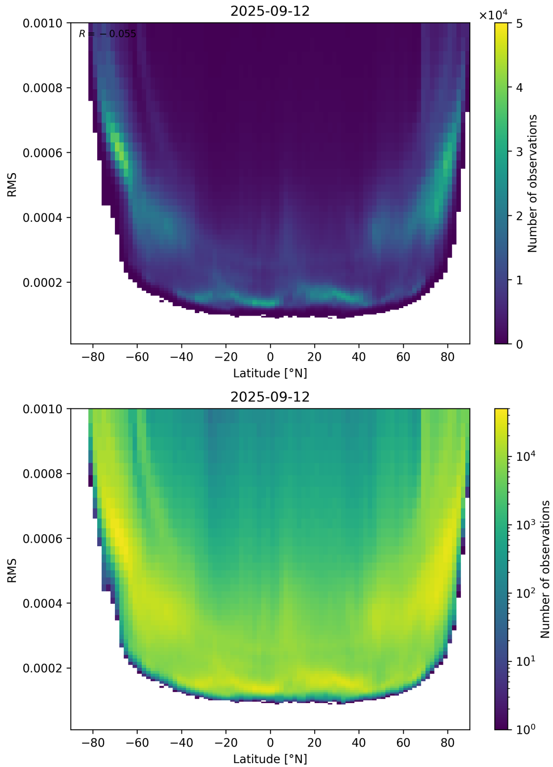
Figure 94: Scatter density plot of “Latitude” against “RMS” for 2025-09-11 to 2025-09-13.
