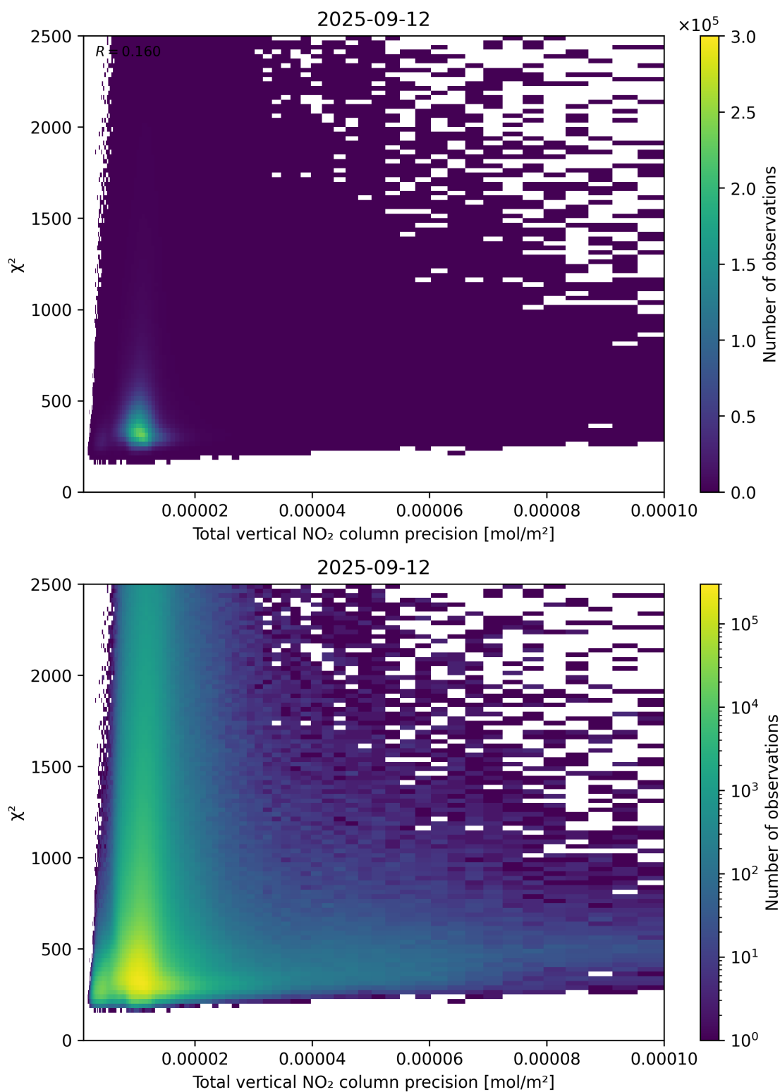
Figure 116: Scatter density plot of “Total vertical NO 2 column precision” against “ \chi^2 ” for 2025-09-11 to 2025-09-13.
