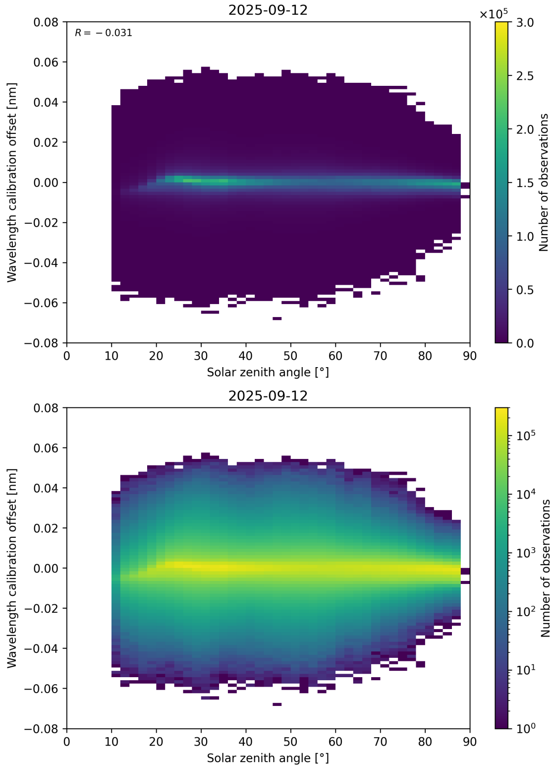
Figure 158: Scatter density plot of “Solar zenith angle” against “Wavelength calibration offset” for 2025-09-11 to 2025-09-13.
