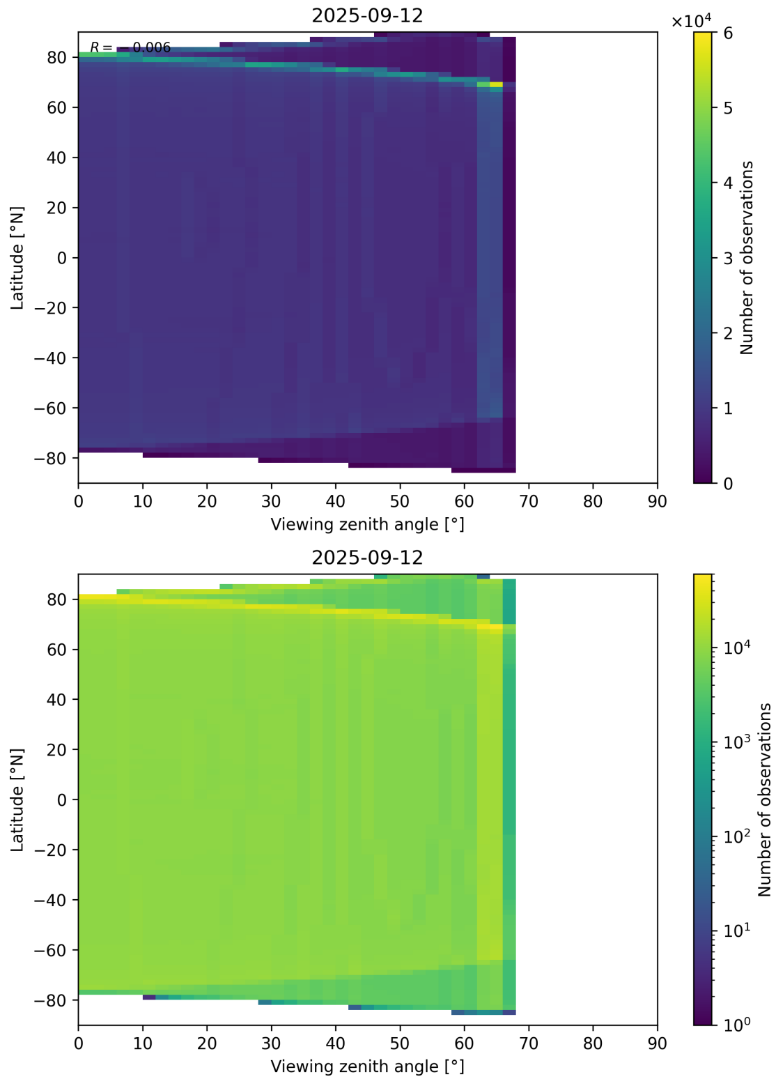
Figure 163: Scatter density plot of “Viewing zenith angle” against “Latitude” for 2025-09-11 to 2025-09-13.
