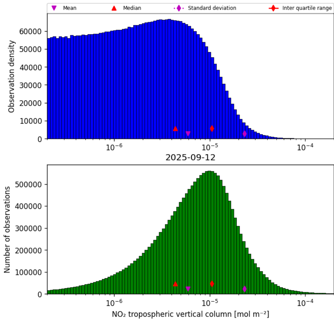
Figure 29: Histogram of “NO 2 tropospheric vertical column” for 2025-09-11 to 2025-09-13
