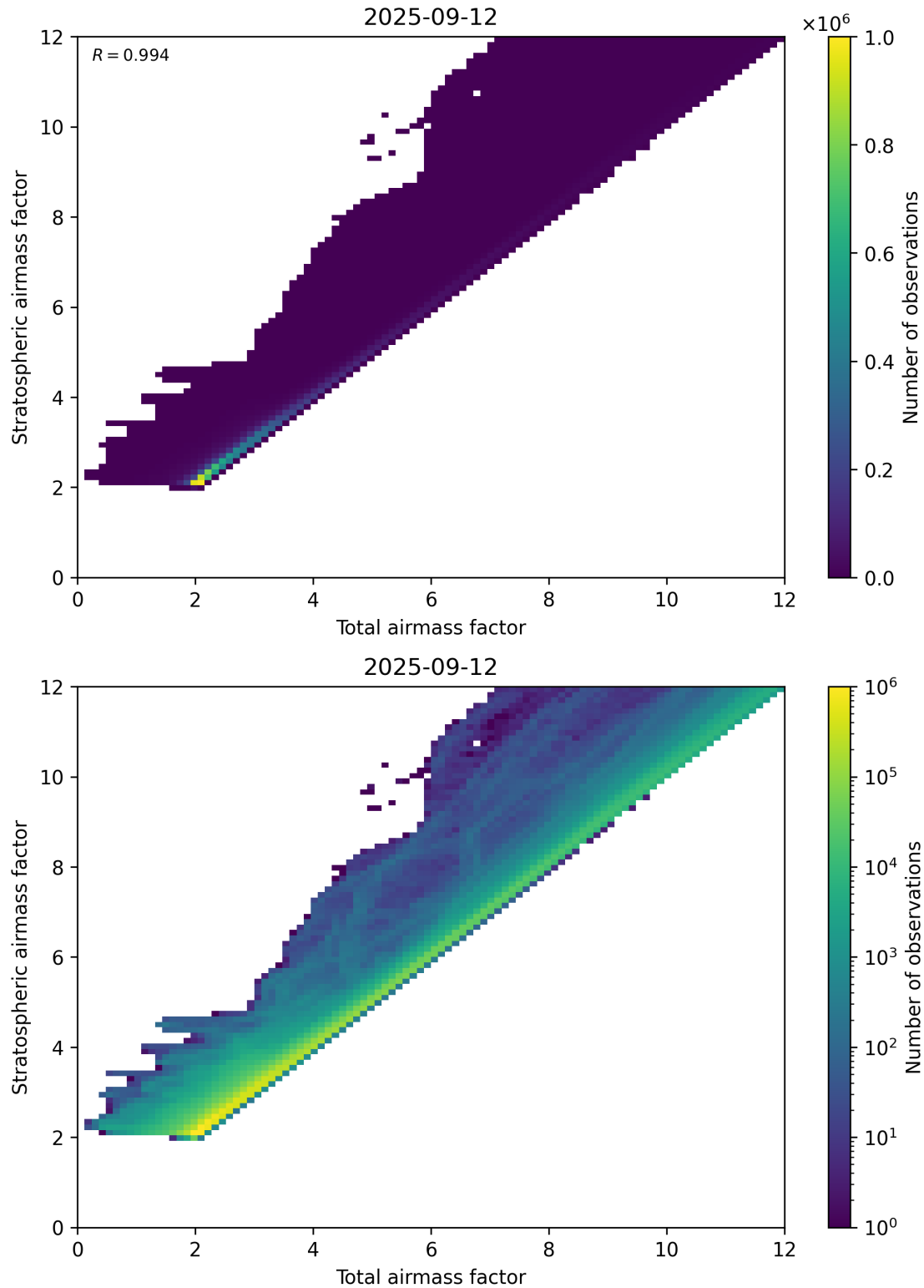
Figure 62: Scatter density plot of “Total airmass factor” against “Stratospheric airmass factor” for 2025-09-11 to 2025-09-13.
