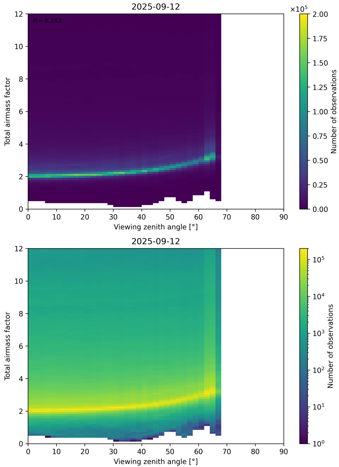
Figure 160: Scatter density plot of “Viewing zenith angle” against “Total airmass factor” for 2025-09-11 to 2025-09-13.
