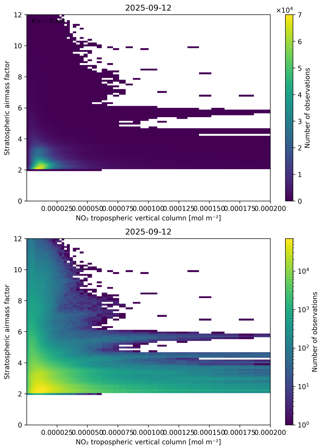
Figure 121: Scatter density plot of “NO 2 tropospheric vertical column” against “Stratospheric air mass factor” for 2025-09-11 to 2025-09-13.
