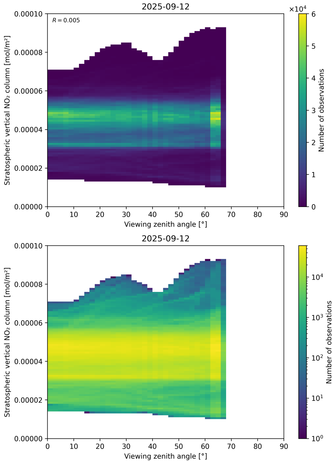
Figure 164: Scatter density plot of “Viewing zenith angle” against “Stratospheric vertical NO 2 column” for 2025-09-11 to 2025-09-13.
