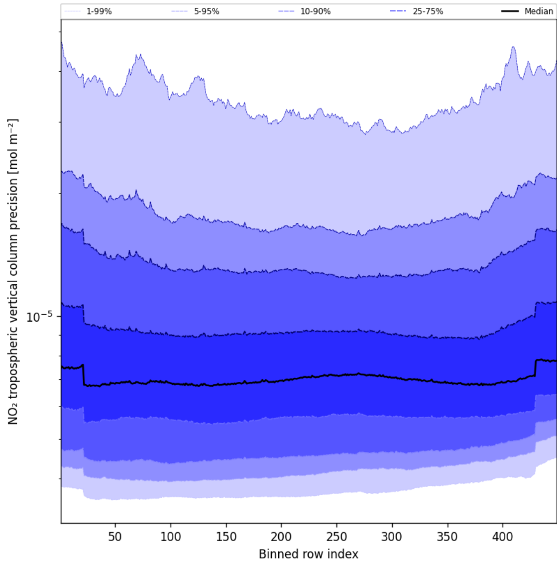
Figure 47: Along track statistics of “NO 2 tropospheric vertical column precision” for 2025-09-11 to 2025-09-13
