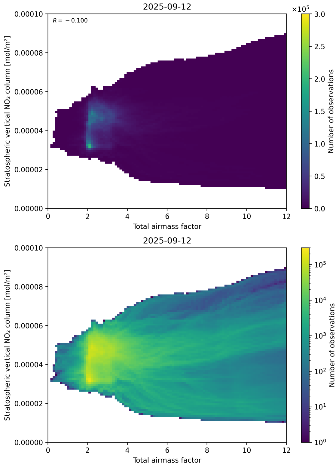
Figure 64: Scatter density plot of “Total airmass factor” against “Stratospheric vertical NO 2 column” for 2025-09-11 to 2025-09-13.
