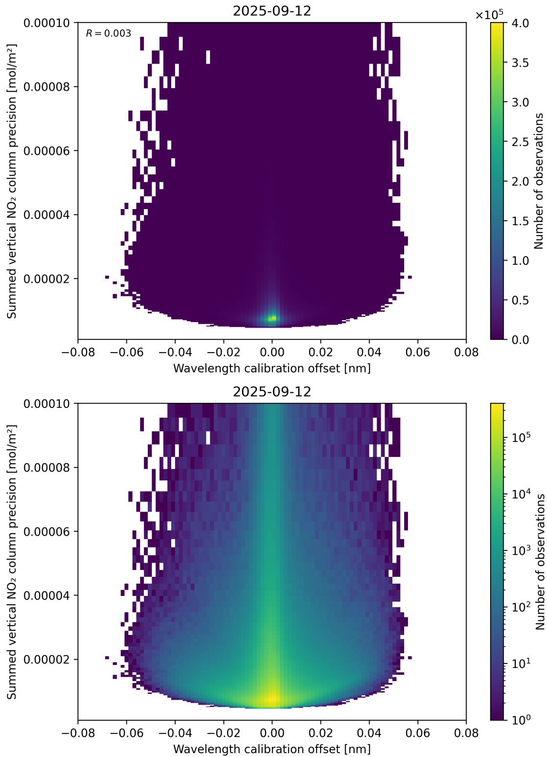
Figure 178: Scatter density plot of “Wavelength calibration offset” against “Summed vertical NO 2 column precision” for 2025-09-11 to 2025-09-13.
