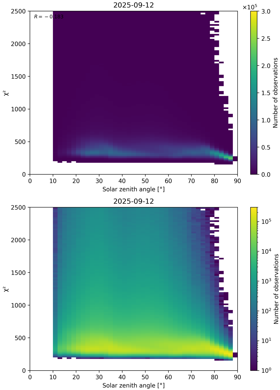
Figure 148: Scatter density plot of “Solar zenith angle” against “ \chi^2 ” for 2025-09-11 to 2025-09-13.
