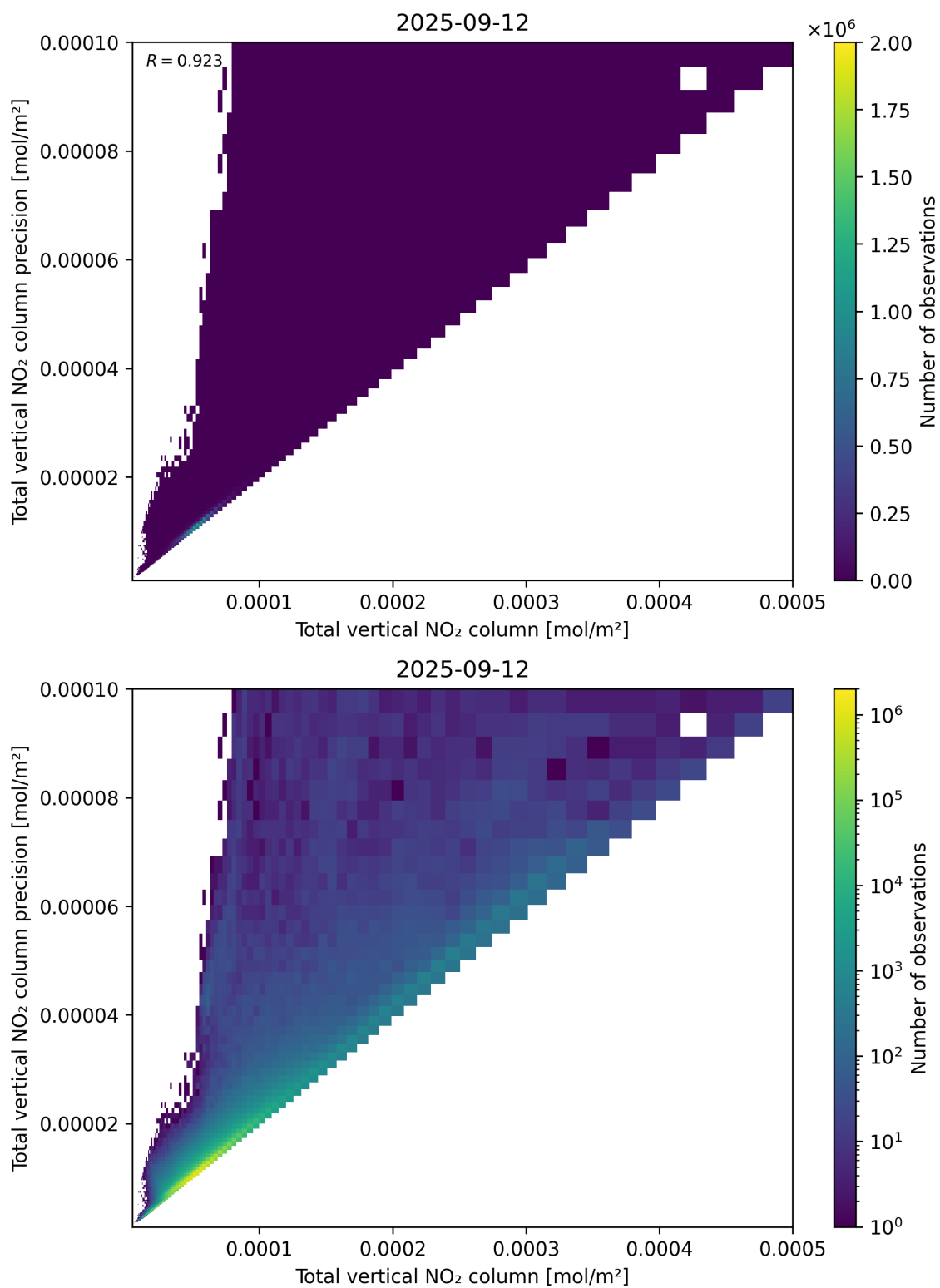
Figure 114: Scatter density plot of “Total vertical NO 2 column” against “Total vertical NO 2 column precision” for 2025-09-11 to 2025-09-13.
