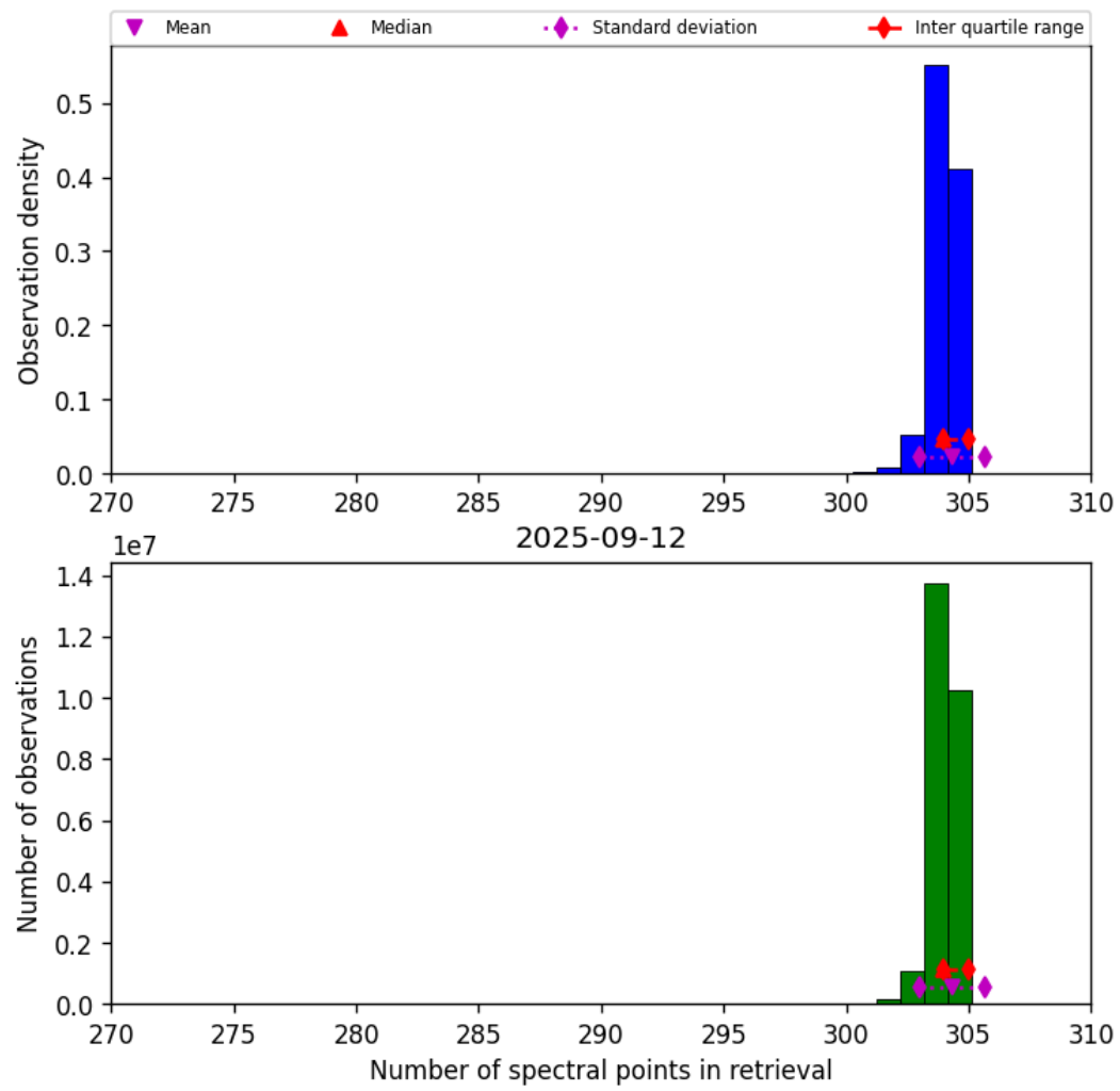
Figure 33: Histogram of “Number of spectral points in retrieval” for 2025-09-11 to 2025-09-13
