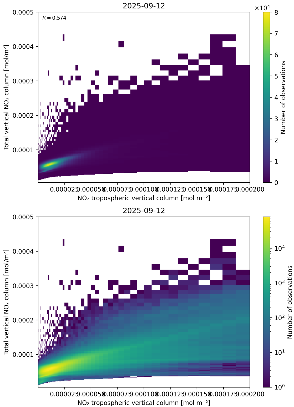
Figure 128: Scatter density plot of “NO 2 tropospheric vertical column” against “Total vertical NO 2 column” for 2025-09-11 to 2025-09-13.
