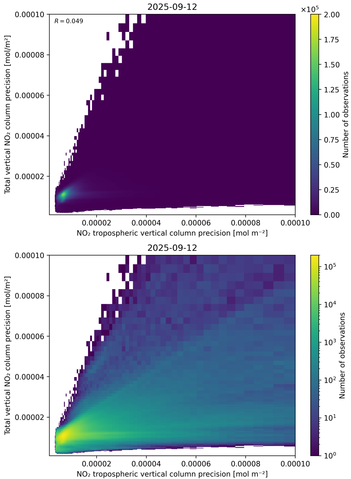
Figure 139: Scatter density plot of “NO 2 tropospheric vertical column precision” against “Total vertical NO 2 column precision” for 2025-09-11 to 2025-09-13.
