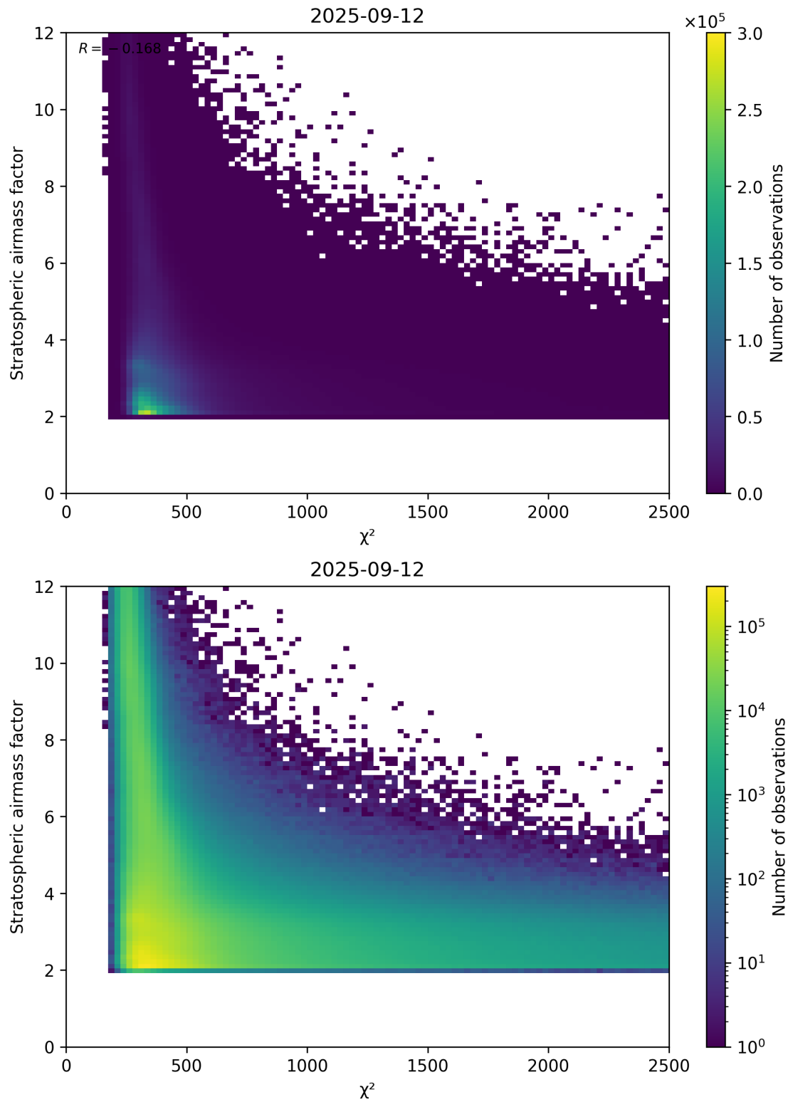
Figure 81: Scatter density plot of “ \chi^2 ” against “Stratospheric airmass factor” for 2025-09-11 to 2025-09-13.
