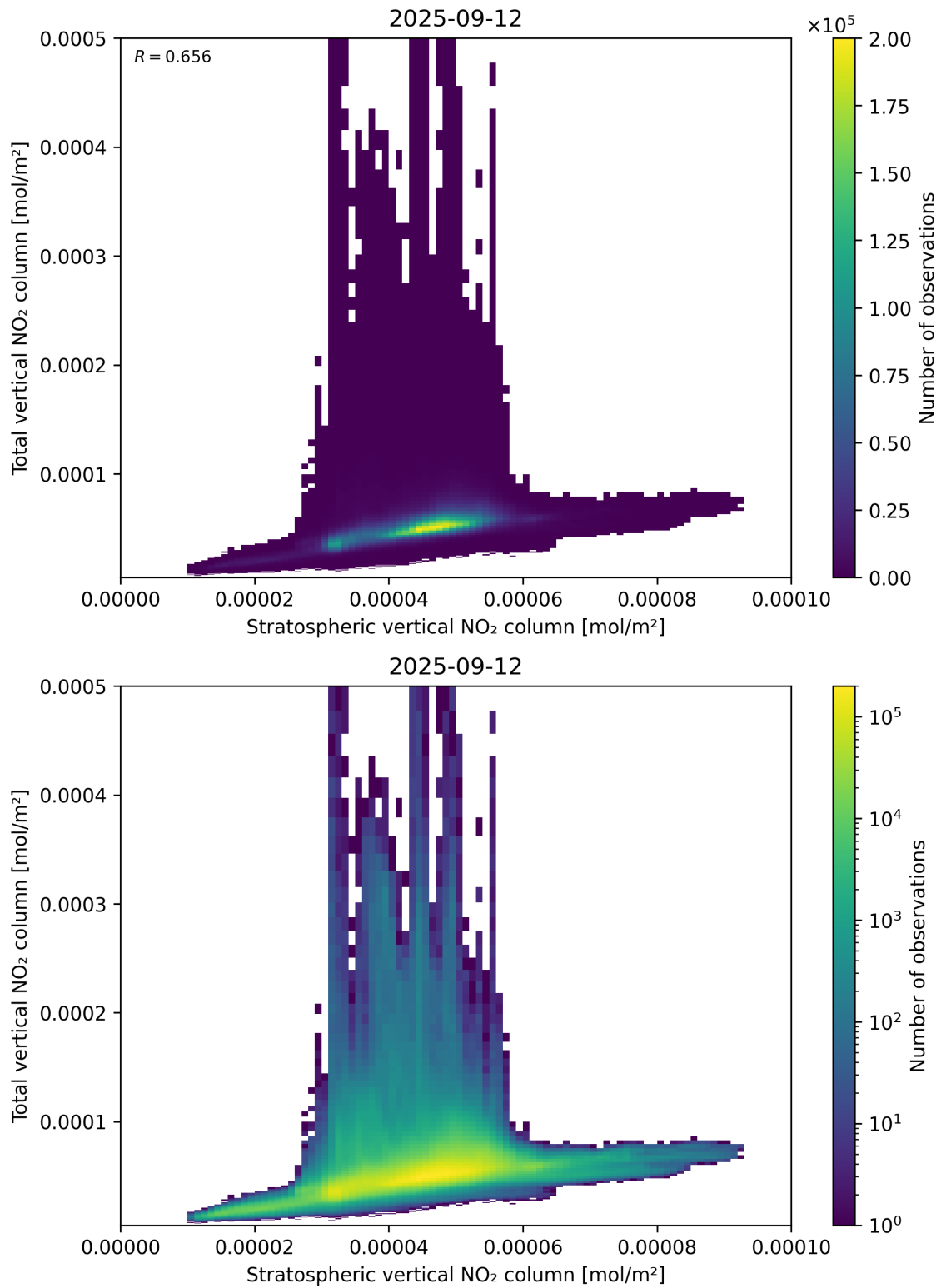
Figure 100: Scatter density plot of “Stratospheric vertical NO 2 column” against “Total vertical NO 2 column” for 2025-09-11 to 2025-09-13.
