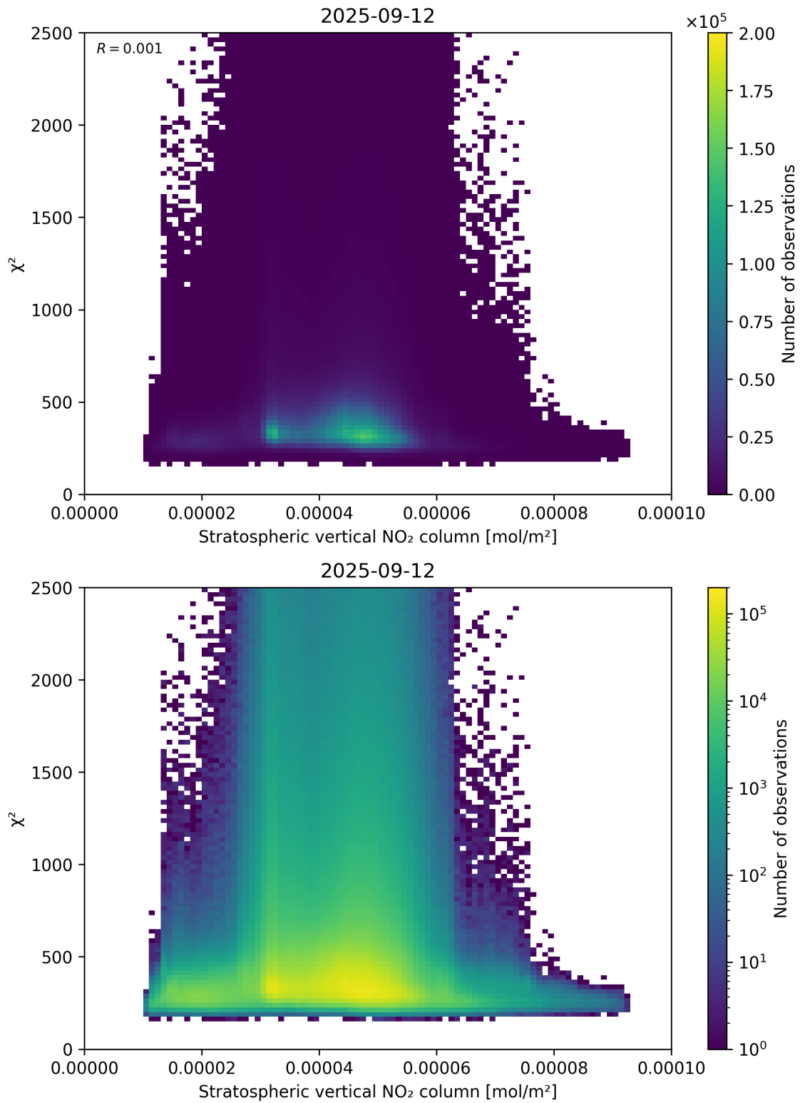
Figure 97: Scatter density plot of “Stratospheric vertical NO 2 column” against “ \chi^2 ” for 2025-09-11 to 2025-09-13.
