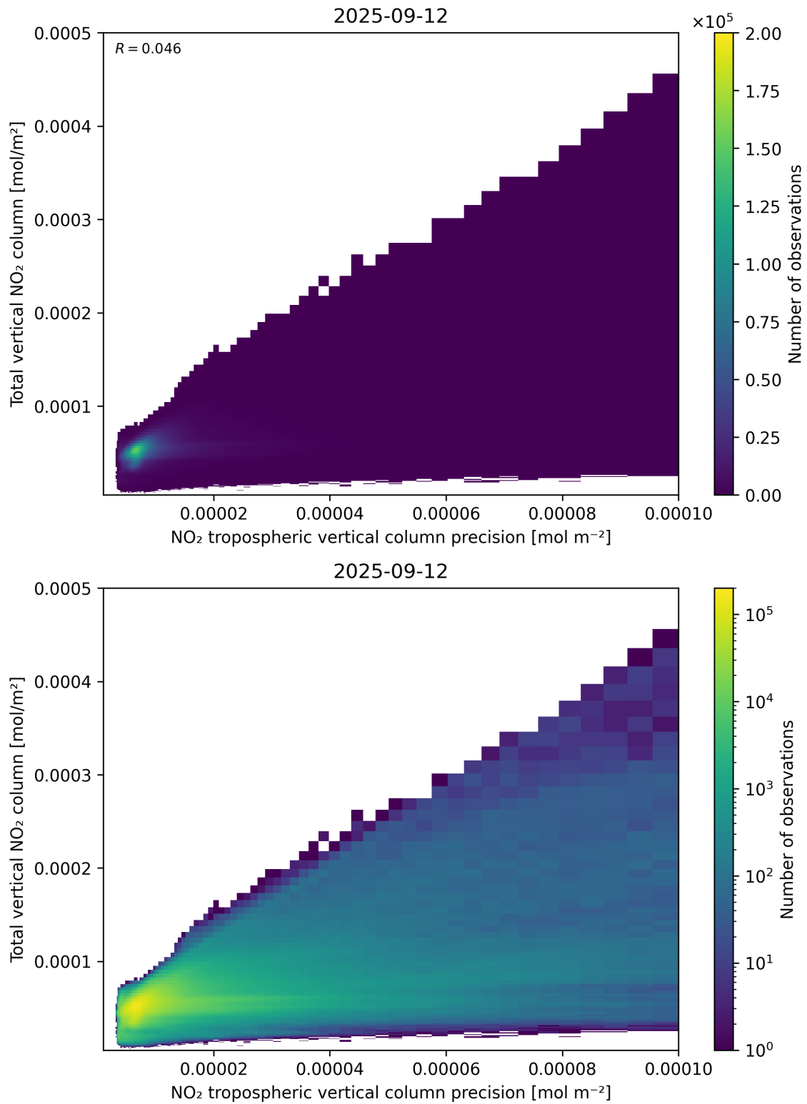
Figure 138: Scatter density plot of “NO 2 tropospheric vertical column precision” against “Total vertical NO 2 column” for 2025-09-11 to 2025-09-13.
