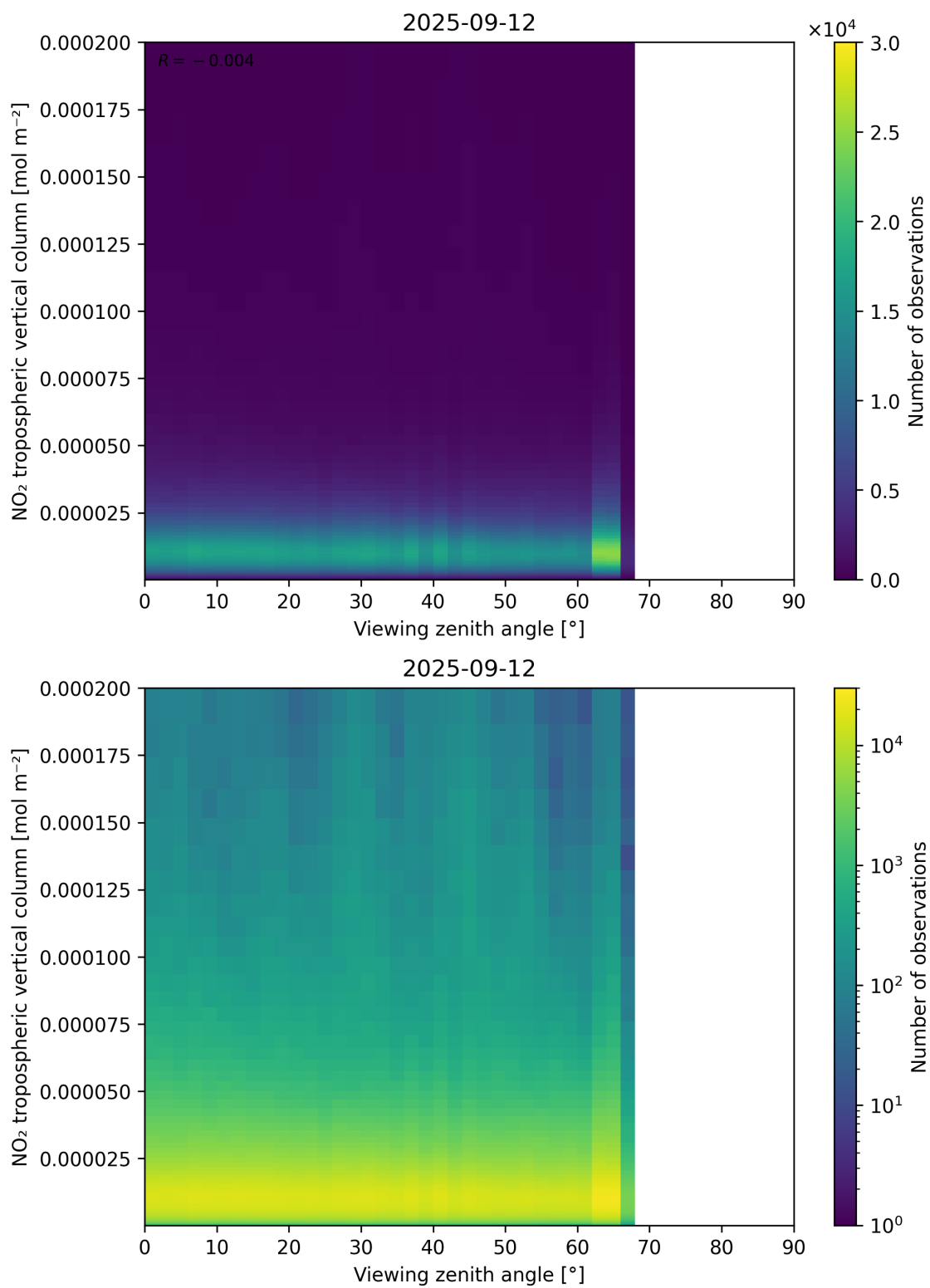
Figure 169: Scatter density plot of “Viewing zenith angle” against “NO 2 tropospheric vertical column” for 2025-09-11 to 2025-09-13.
