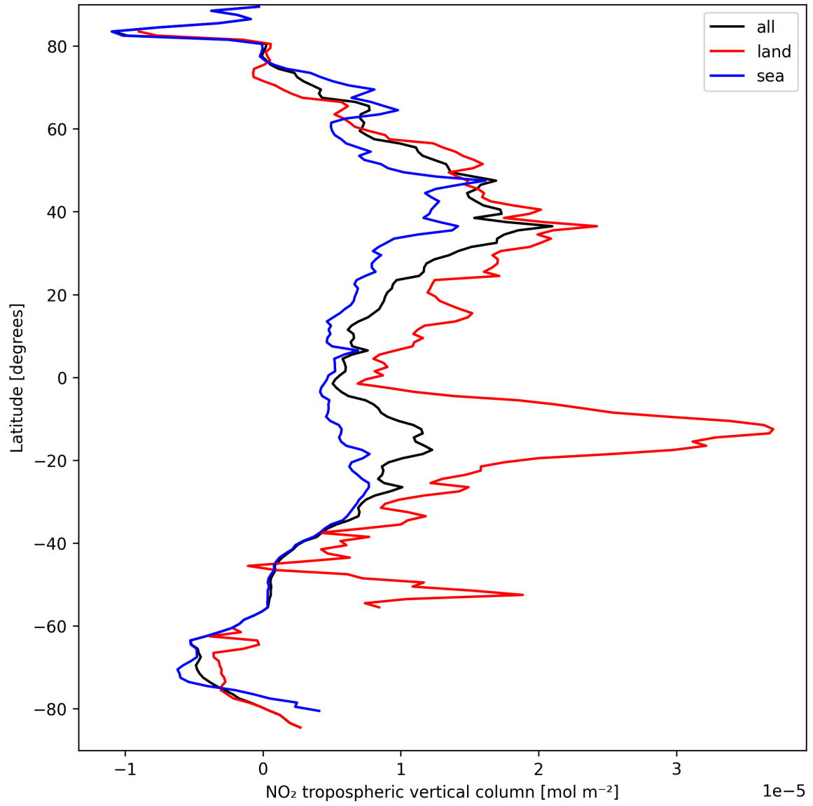
Figure 12: Zonal average of “NO 2 tropospheric vertical column” for 2025-09-11 to 2025-09-13.
