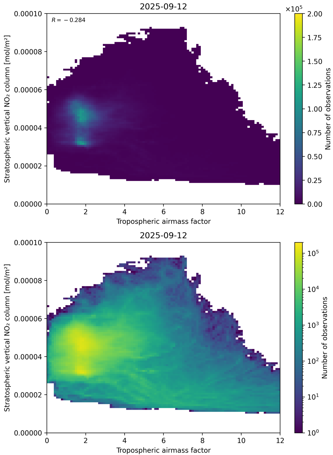
Figure 74: Scatter density plot of “Tropospheric air mass factor” against “Stratospheric vertical NO 2 column” for 2025-09-11 to 2025-09-13.
