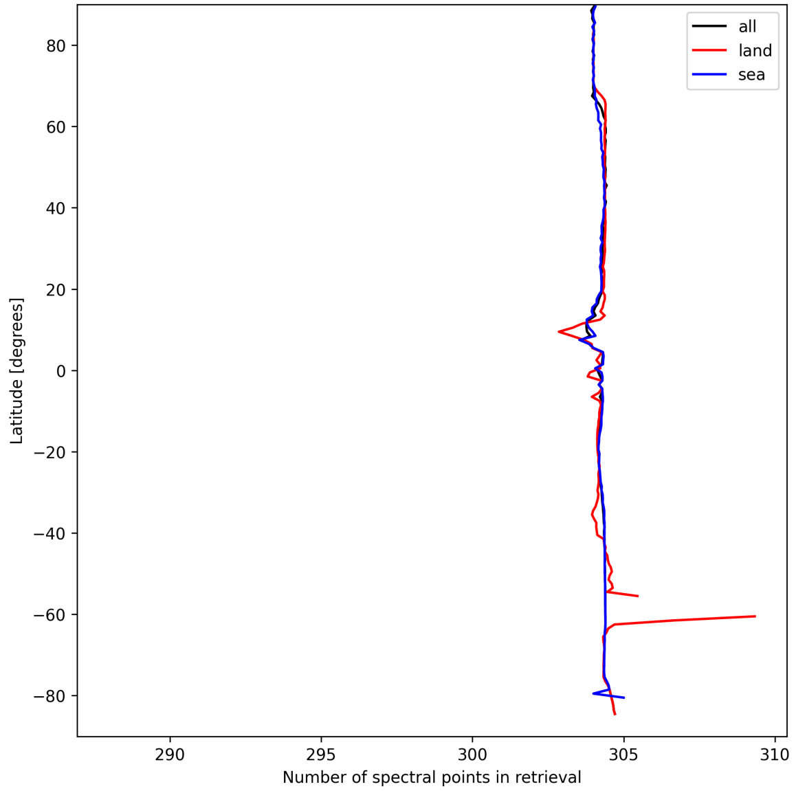
Figure 16: Zonal average of “Number of spectral points in retrieval” for 2025-09-11 to 2025-09-13.
