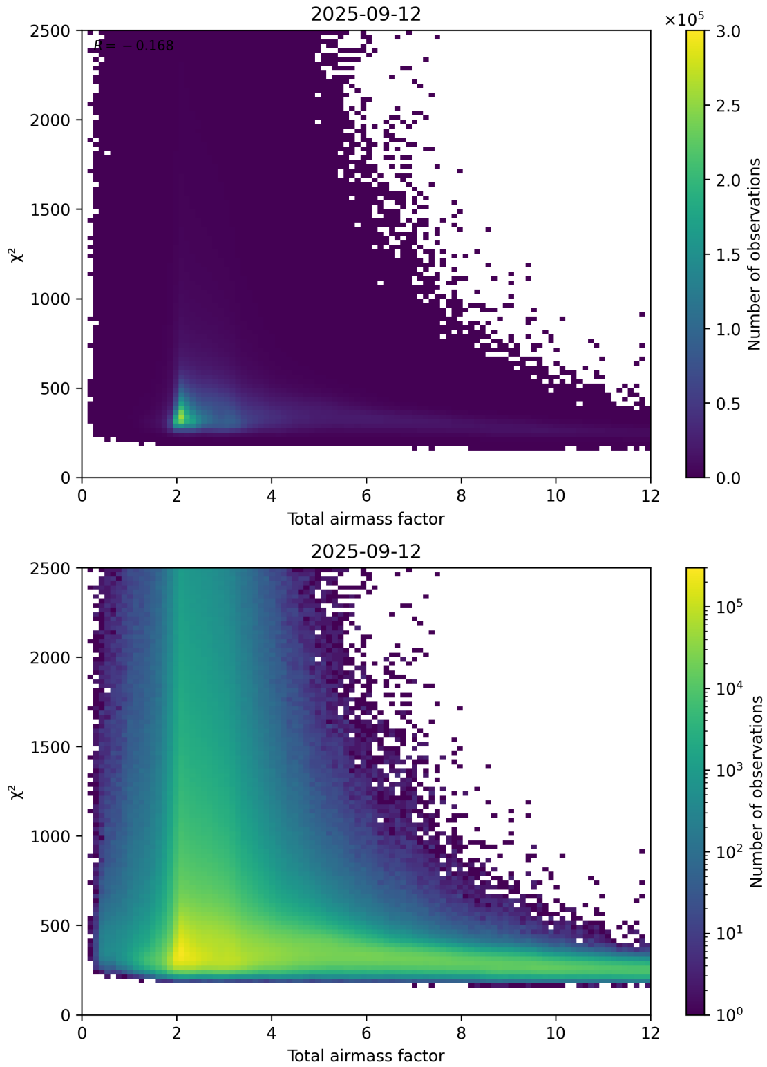
Figure 63: Scatter density plot of “Total airmass factor” against “ \chi^2 ” for 2025-09-11 to 2025-09-13.
