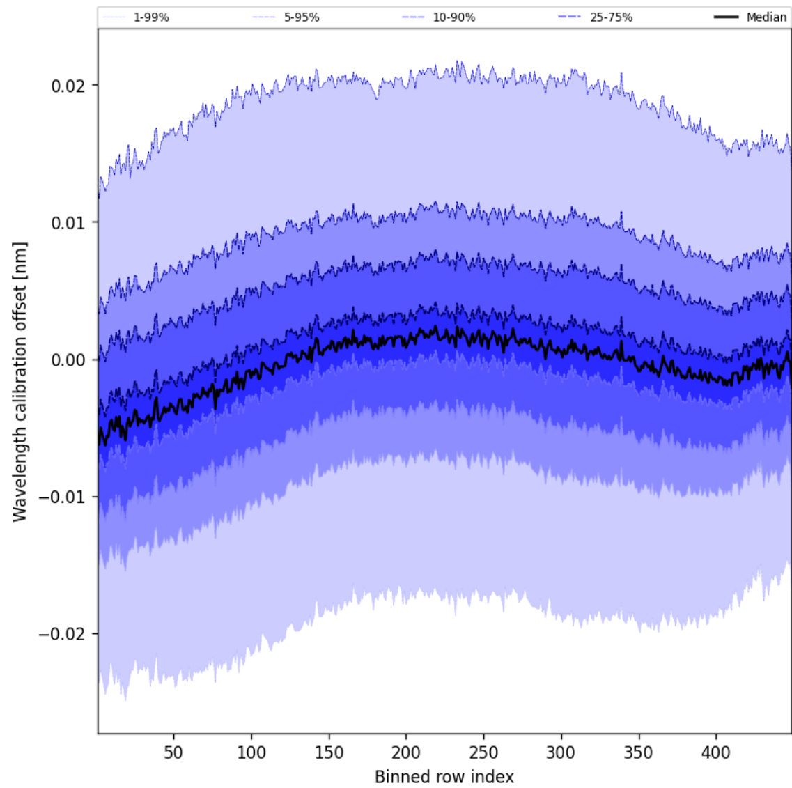
Figure 52: Along track statistics of “Wavelength calibration offset” for 2025-09-11 to 2025-09-13
