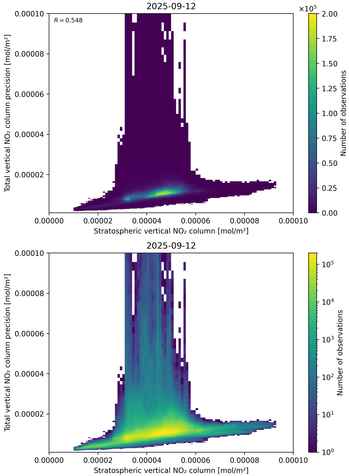
Figure 101: Scatter density plot of “Stratospheric vertical NO 2 column” against “Total vertical NO 2 column precision” for 2025-09-11 to 2025-09-13.
