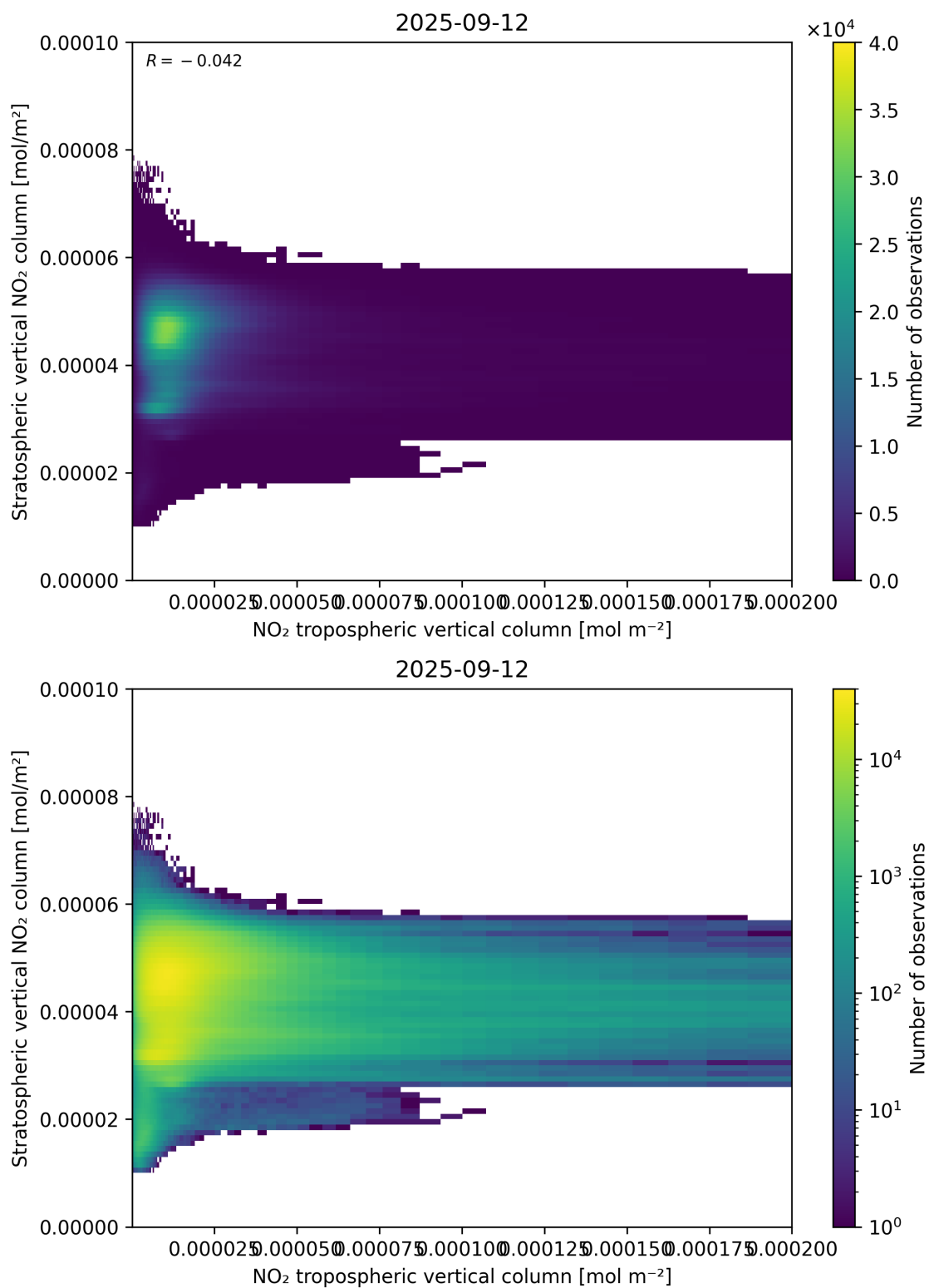
Figure 125: Scatter density plot of “NO 2 tropospheric vertical column” against “Stratospheric vertical NO 2 column” for 2025-09-11 to 2025-09-13.
