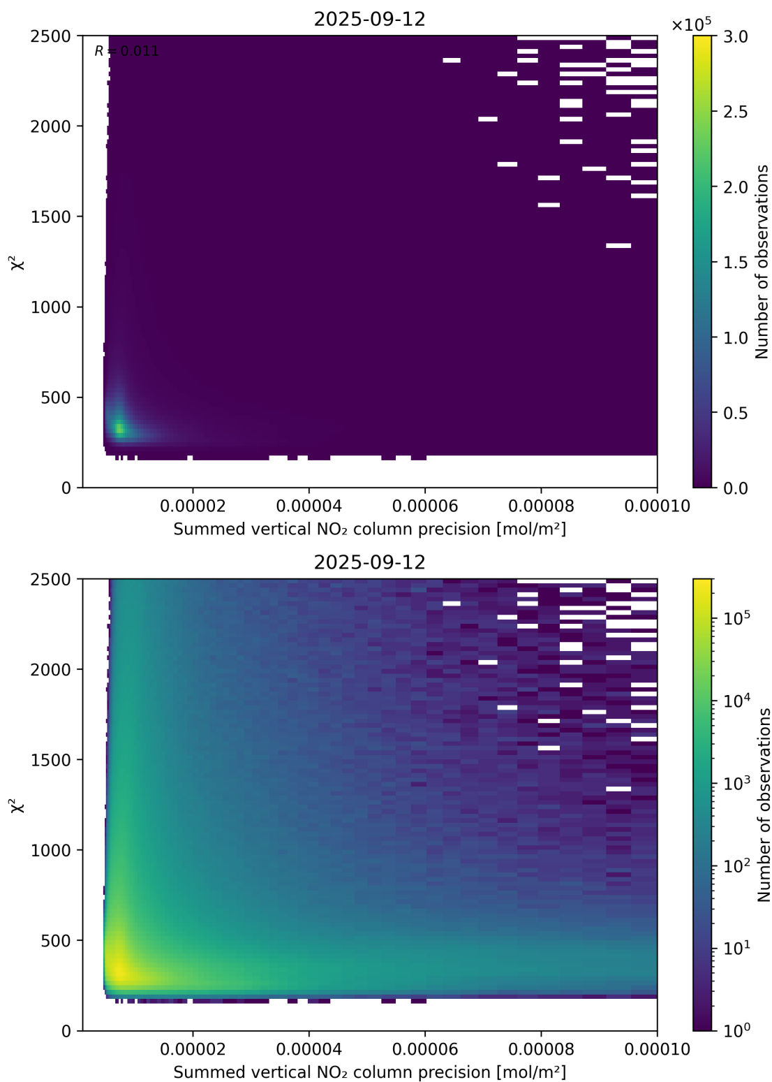
Figure 107: Scatter density plot of “Summed vertical NO 2 column precision” against “ \chi^2 ” for 2025-09-11 to 2025-09-13.
