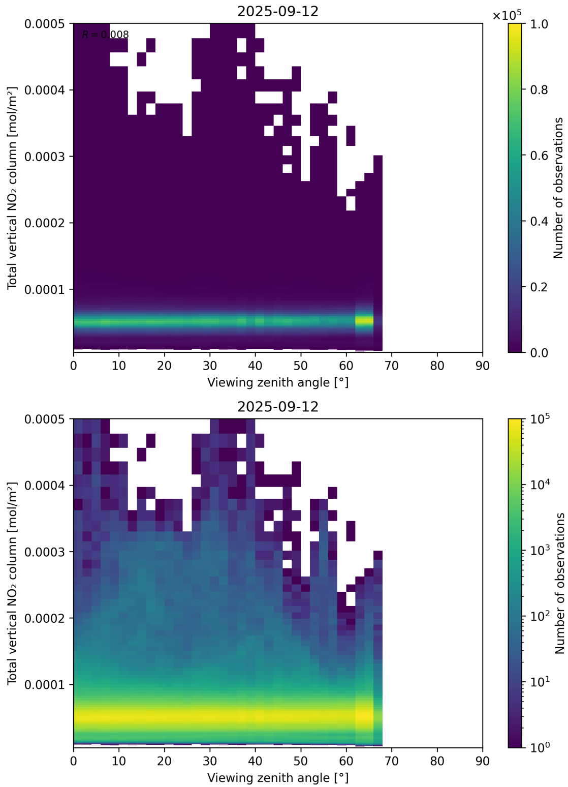
Figure 167: Scatter density plot of “Viewing zenith angle” against “Total vertical NO 2 column” for 2025-09-11 to 2025-09-13.
