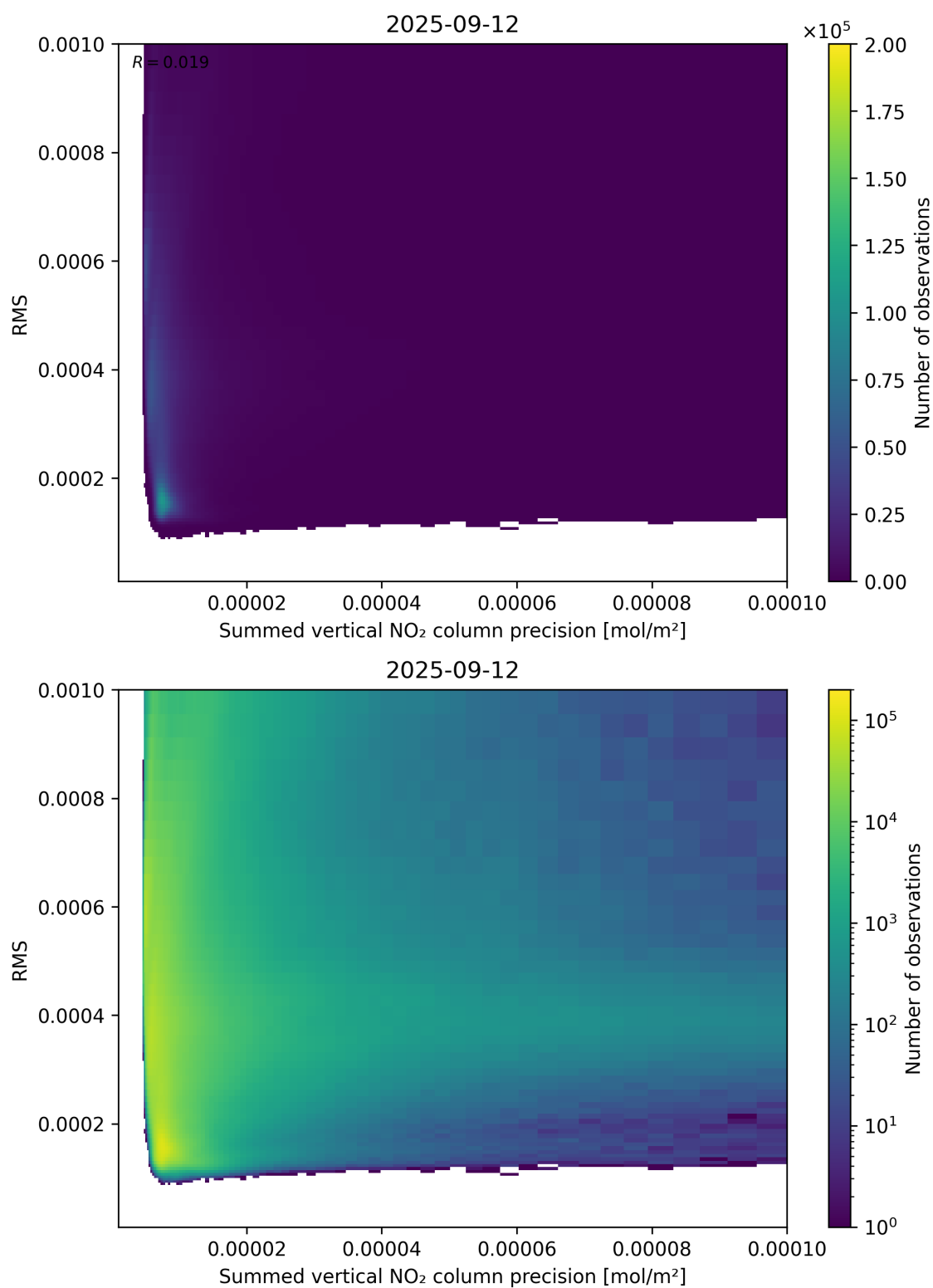
Figure 108: Scatter density plot of “Summed vertical NO 2 column precision” against “RMS” for 2025-09-11 to 2025-09-13.
