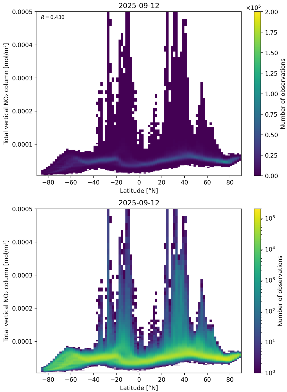
Figure 90: Scatter density plot of “Latitude” against “Total vertical NO 2 column” for 2025-09-11 to 2025-09-13.
