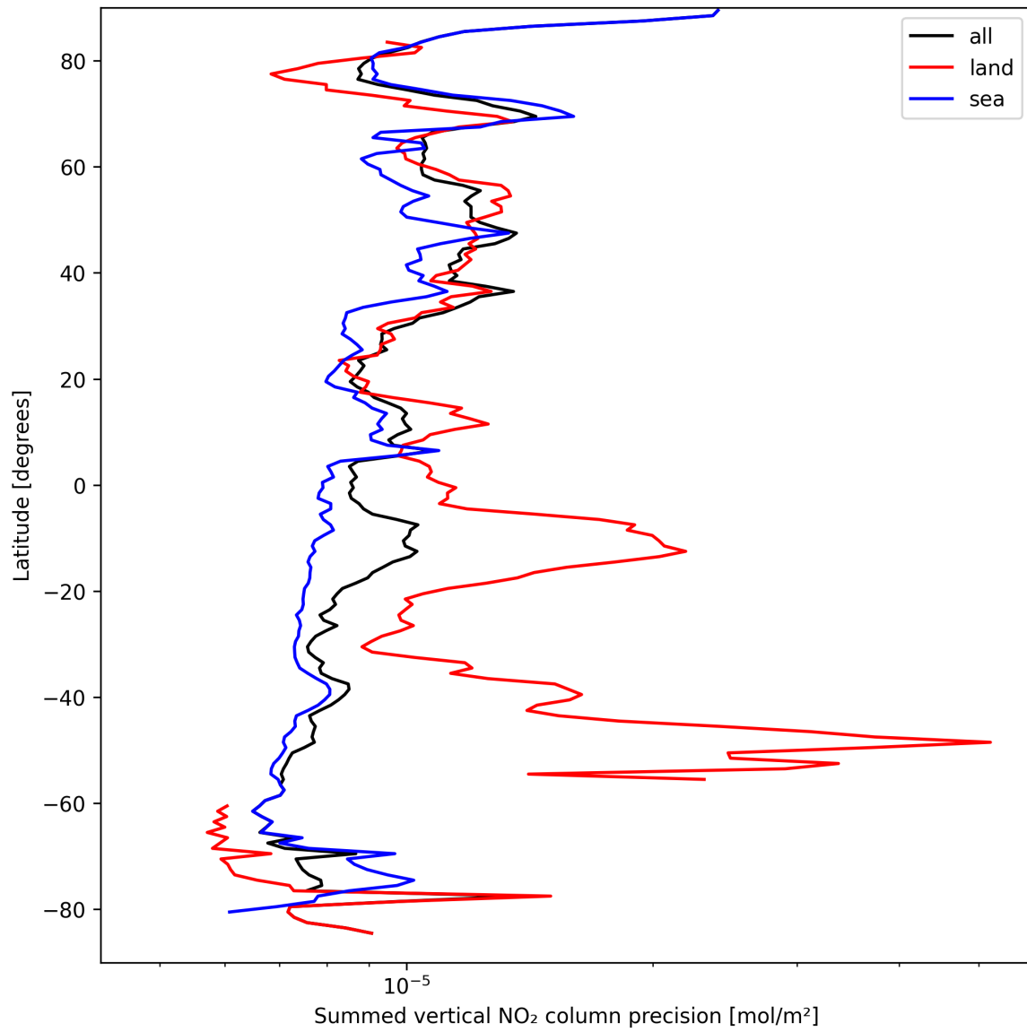
Figure 24: Zonal average of “Summed vertical NO 2 column precision” for 2025-09-11 to 2025-09-13.
