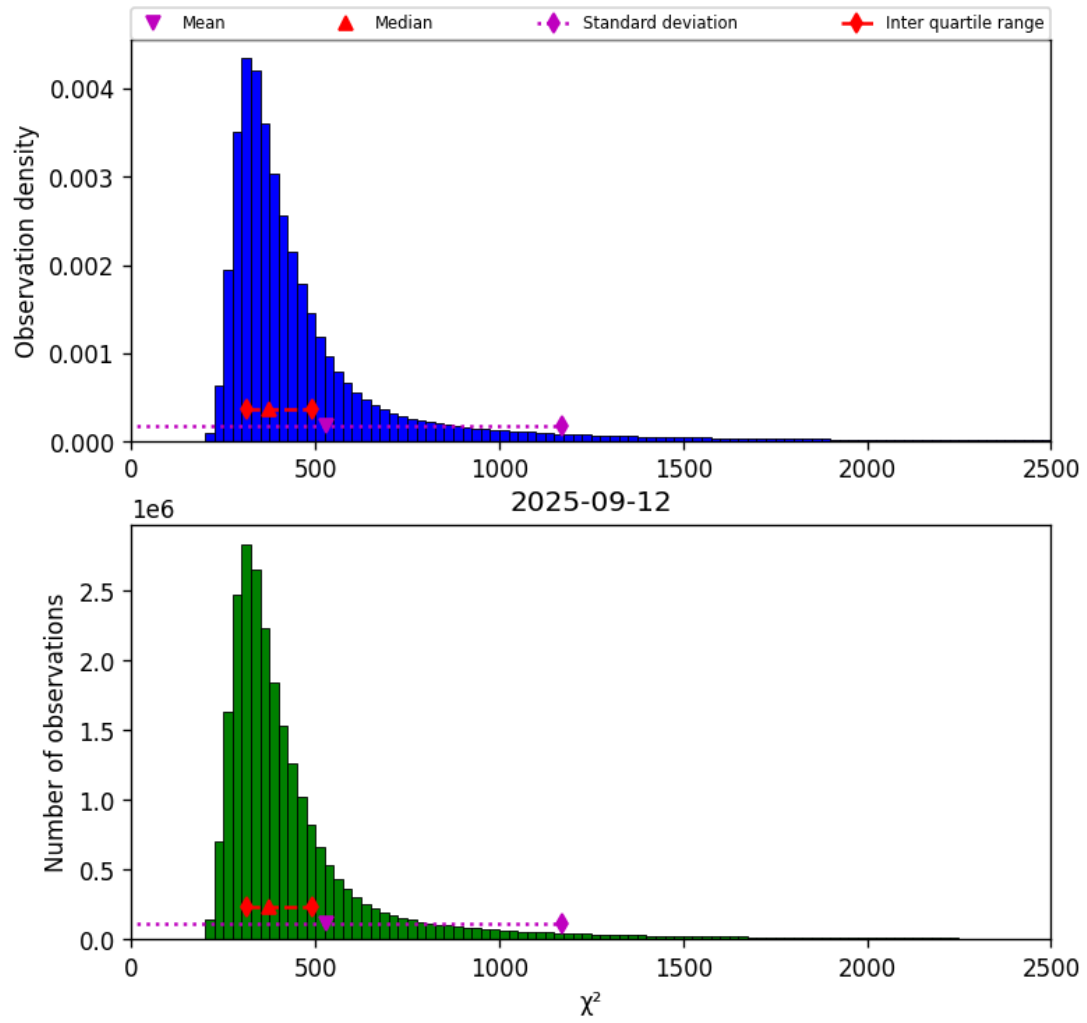
Figure 42: Histogram of “ \chi^2 ” for 2025-09-11 to 2025-09-13
