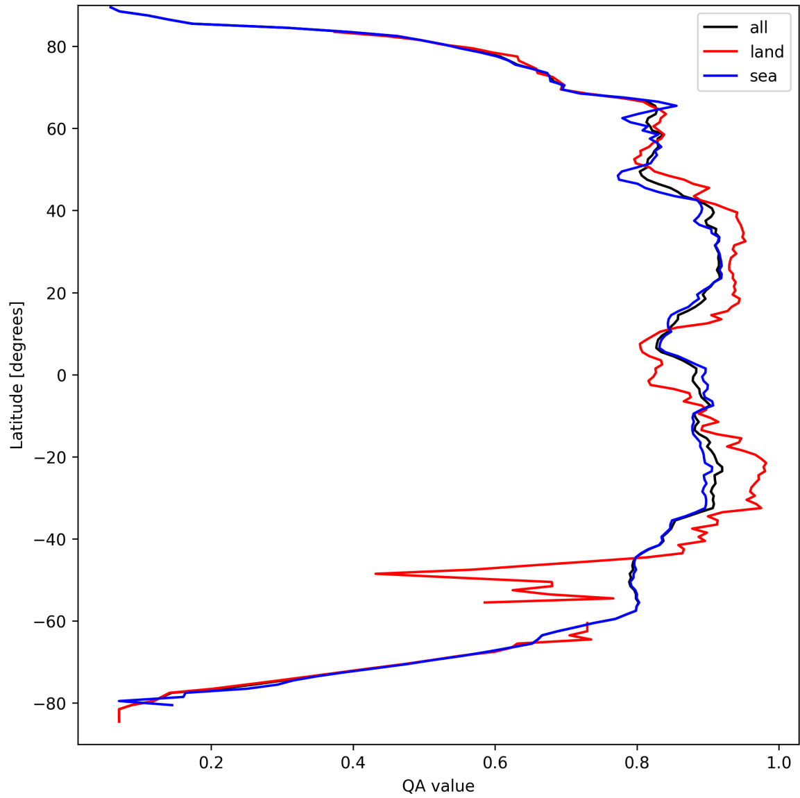
Figure 11: Zonal average of “QA value” for 2025-09-11 to 2025-09-13.
