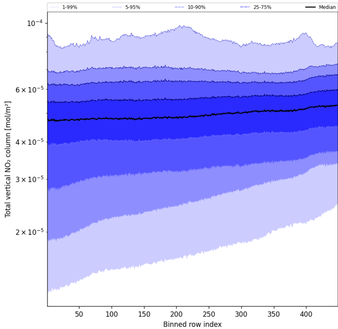
Figure 55: Along track statistics of “Total vertical NO 2 column” for 2025-09-11 to 2025-09-13
