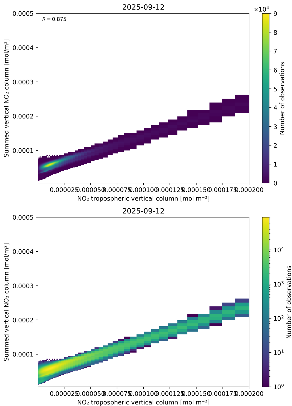
Figure 126: Scatter density plot of “NO 2 tropospheric vertical column” against “Summed vertical NO 2 column” for 2025-09-11 to 2025-09-13.
