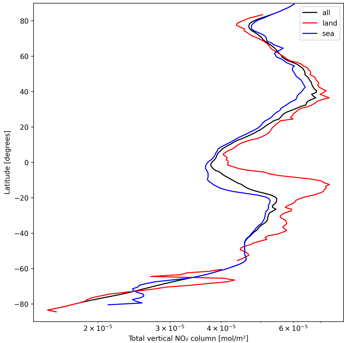
Figure 21: Zonal average of “Total vertical NO 2 column” for 2025-09-11 to 2025-09-13.
