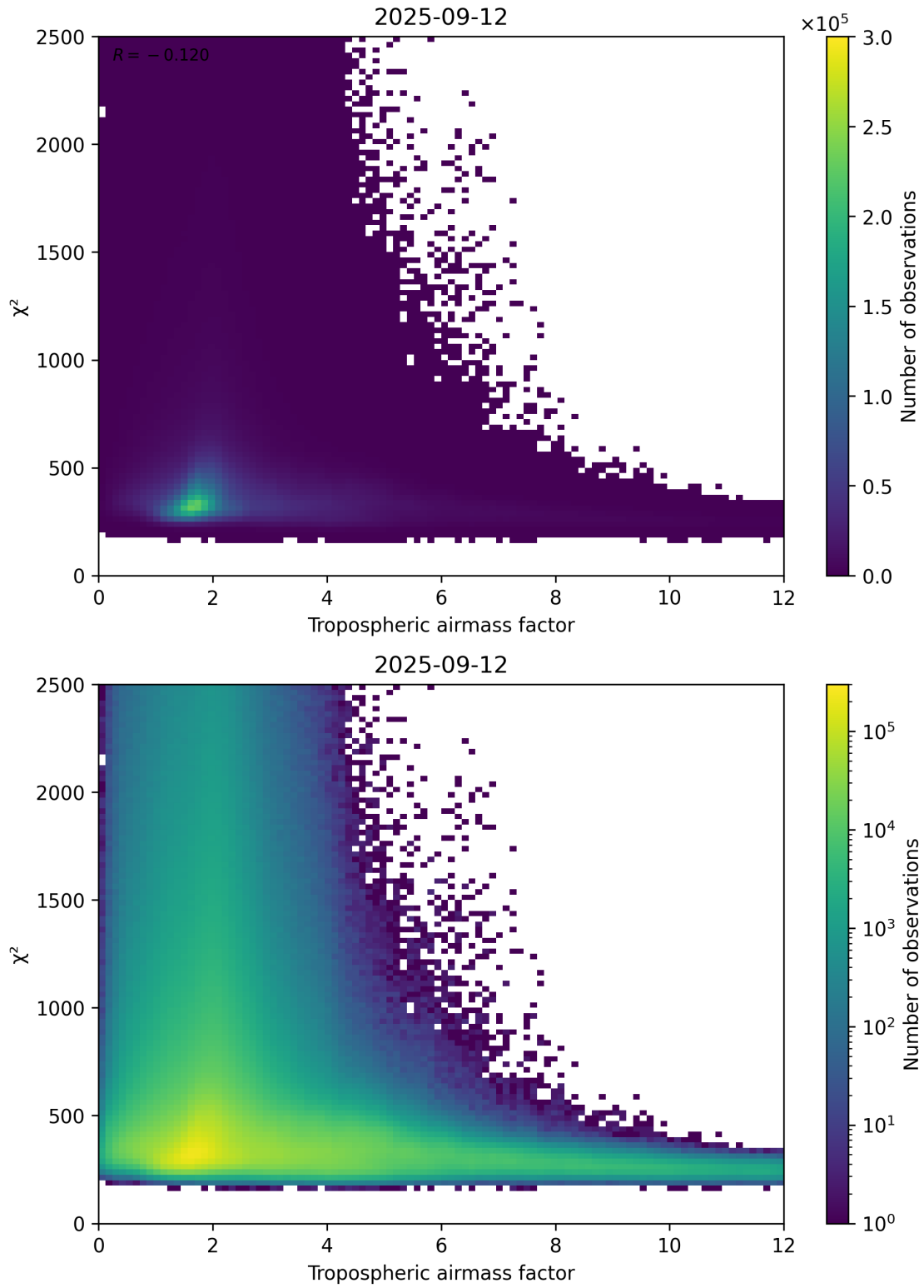
Figure 73: Scatter density plot of “Tropospheric airmass factor” against “ \chi^2 ” for 2025-09-11 to 2025-09-13.
