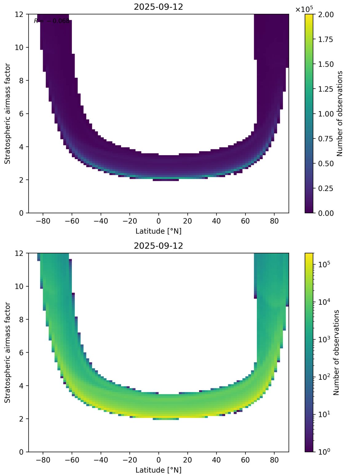
Figure 83: Scatter density plot of “Latitude” against “Stratospheric air mass factor” for 2025-09-11 to 2025-09-13.
