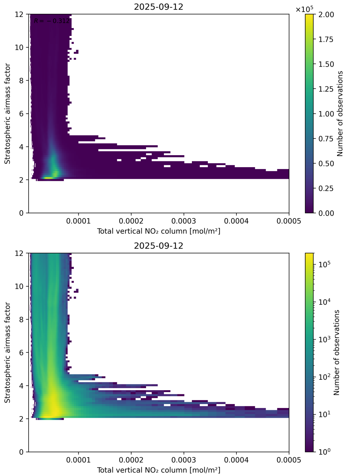
Figure 110: Scatter density plot of “Total vertical NO 2 column” against “Stratospheric airmass factor” for 2025-09-11 to 2025-09-13.
