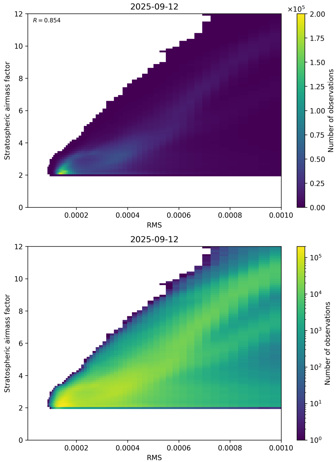
Figure 144: Scatter density plot of “RMS” against “Stratospheric airmass factor” for 2025-09-11 to 2025-09-13.
