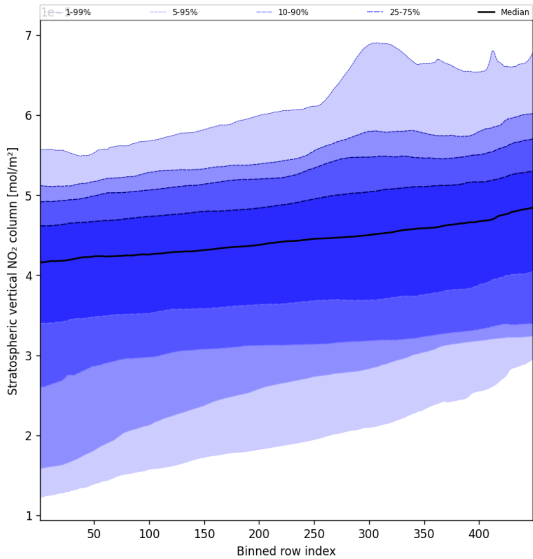
Figure 53: Along track statistics of “Stratospheric vertical NO 2 column” for 2025-09-11 to 2025-09-13
