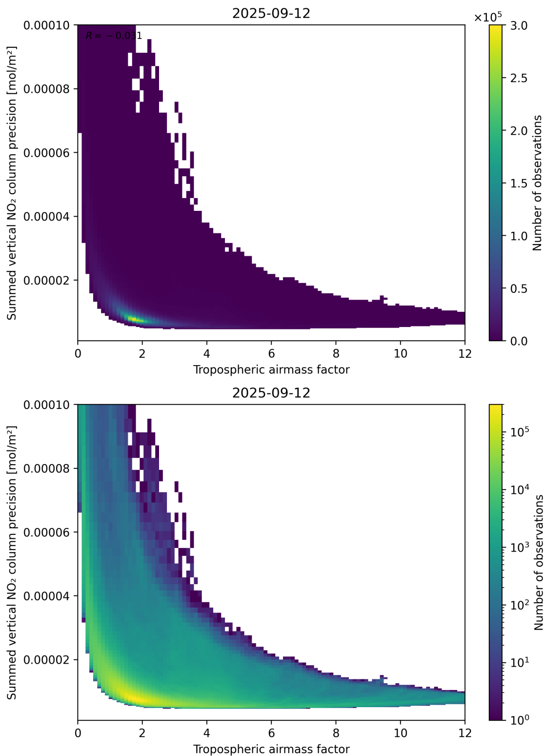
Figure 76: Scatter density plot of “Tropospheric air mass factor” against “Summed vertical NO 2 column precision” for 2025-09-11 to 2025-09-13.
