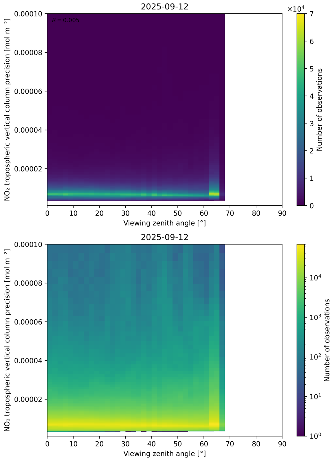
Figure 170: Scatter density plot of “Viewing zenith angle” against “NO 2 tropospheric vertical column precision” for 2025-09-11 to 2025-09-13.
