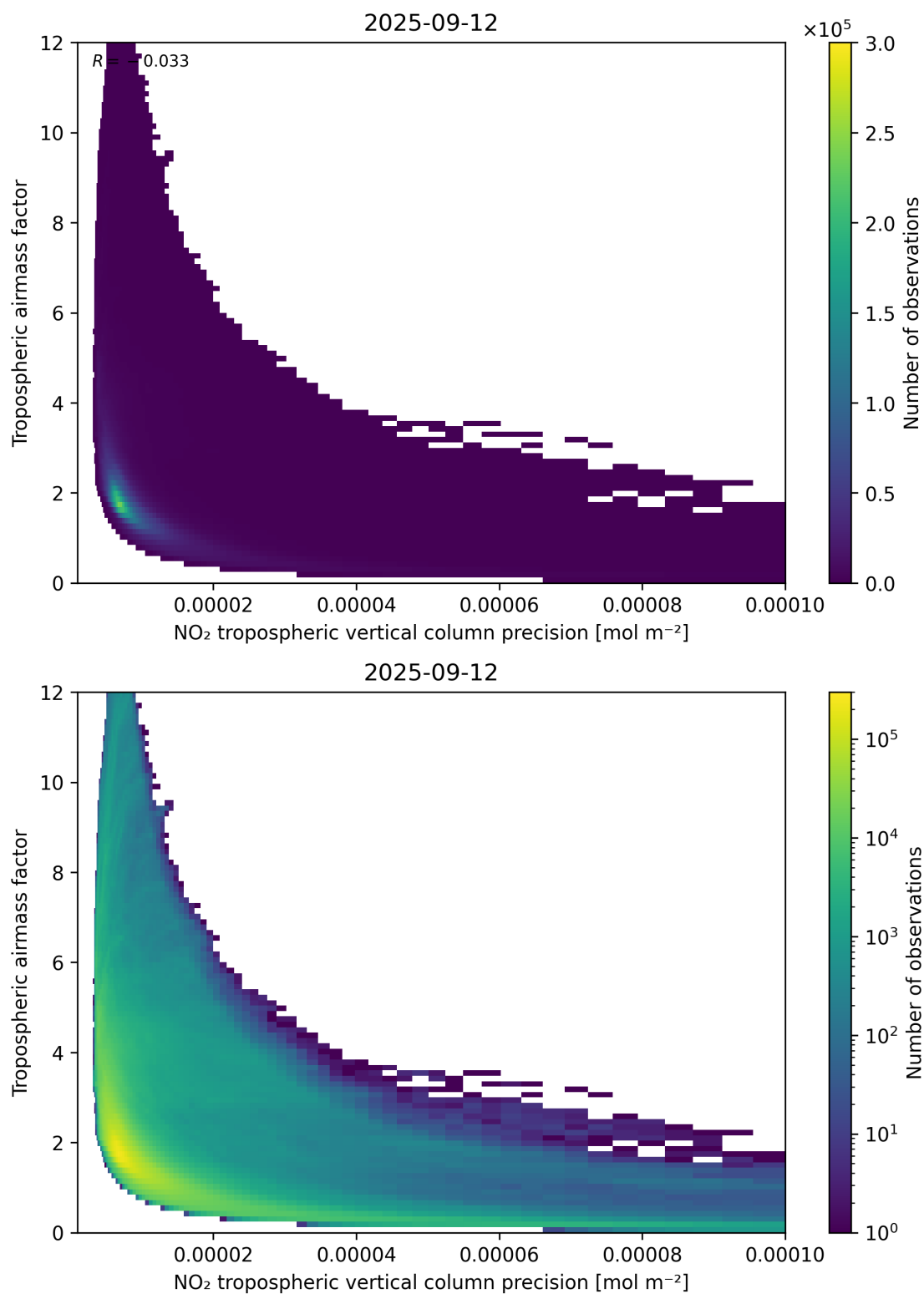
Figure 133: Scatter density plot of “NO 2 tropospheric vertical column precision” against “Tropospheric air mass factor” for 2025-09-11 to 2025-09-13.
