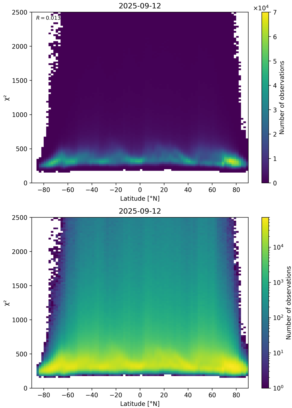
Figure 86: Scatter density plot of “Latitude” against “ \chi^2 ” for 2025-09-11 to 2025-09-13.
