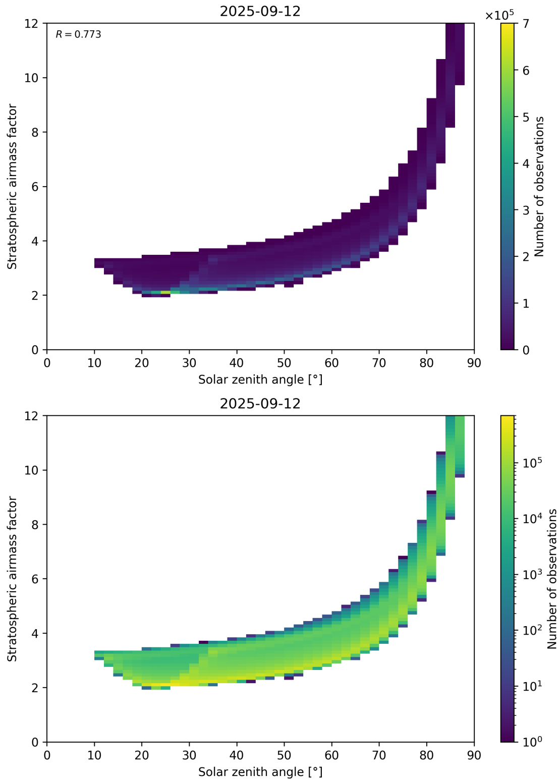
Figure 145: Scatter density plot of “Solar zenith angle” against “Stratospheric airmass factor” for 2025-09-11 to 2025-09-13.
