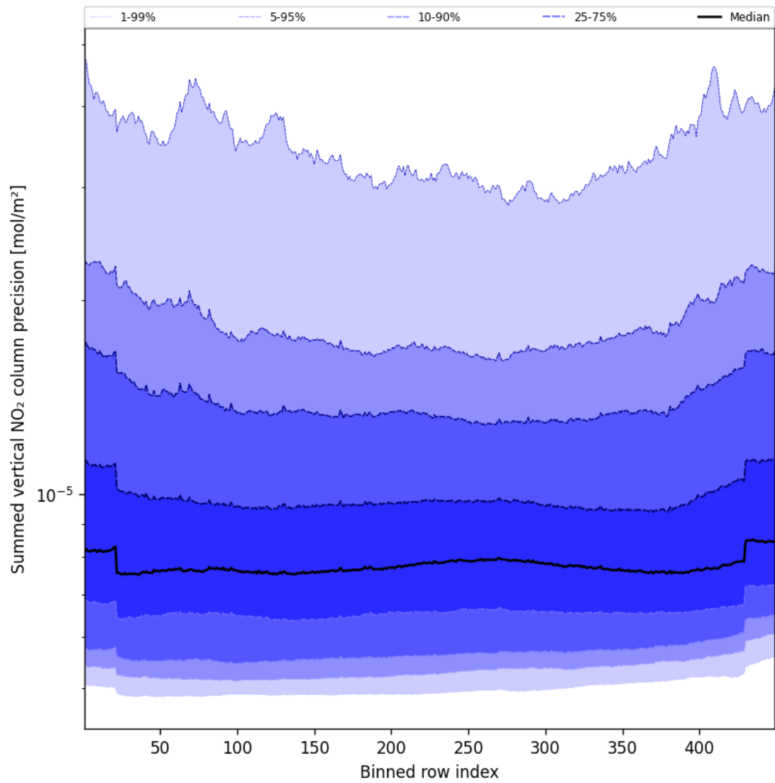
Figure 58: Along track statistics of “Summed vertical NO 2 column precision” for 2025-09-11 to 2025-09-13
