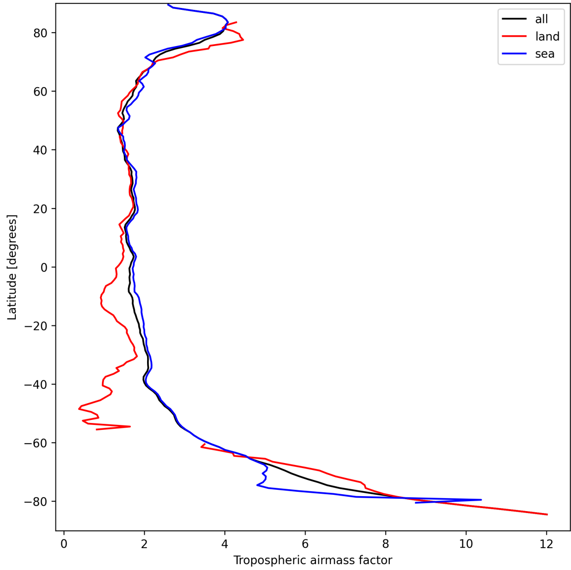
Figure 14: Zonal average of “Tropospheric airmass factor” for 2025-09-11 to 2025-09-13.
