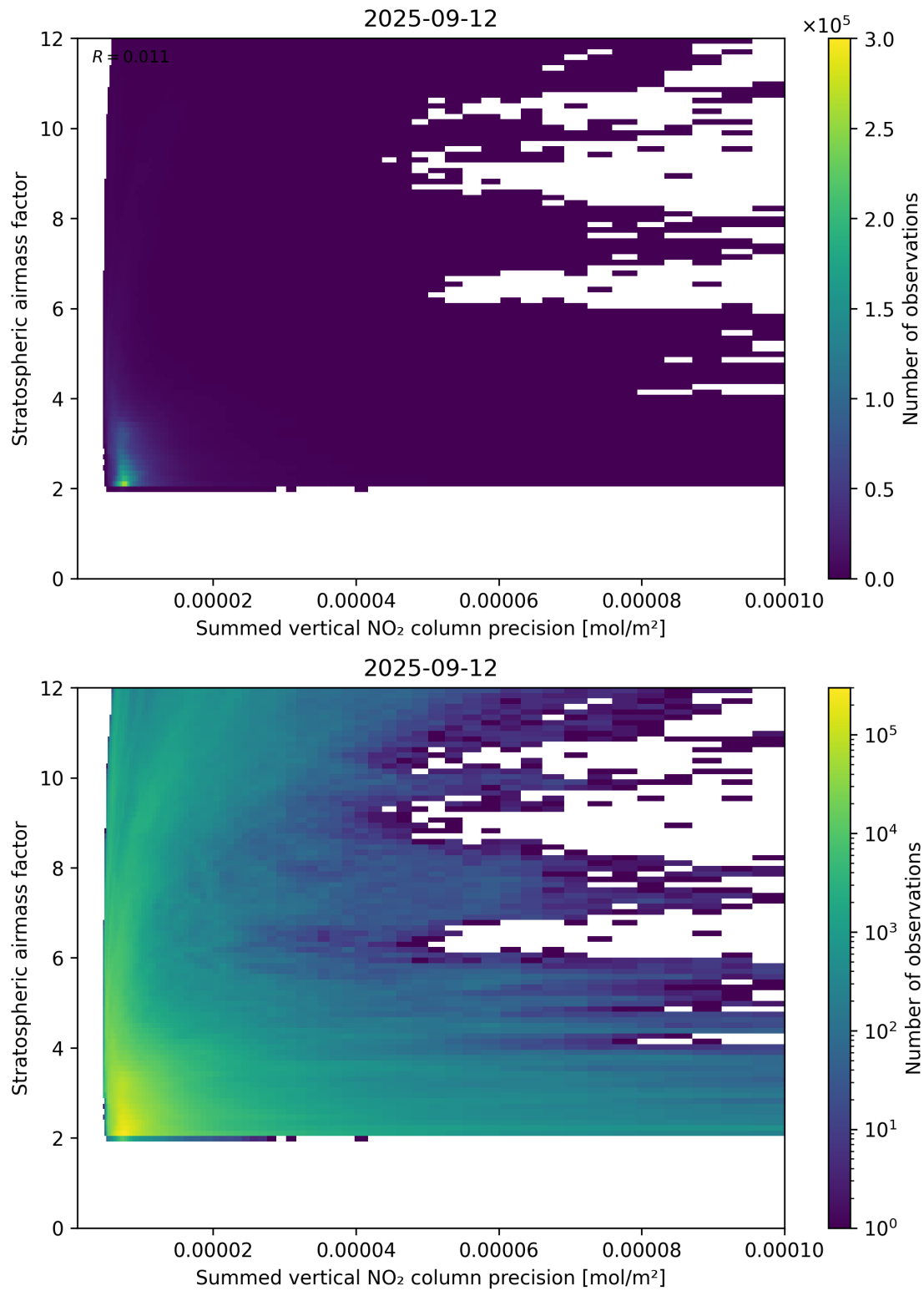
Figure 106: Scatter density plot of “Summed vertical NO 2 column precision” against “Stratospheric airmass factor” for 2025-09-11 to 2025-09-13.
