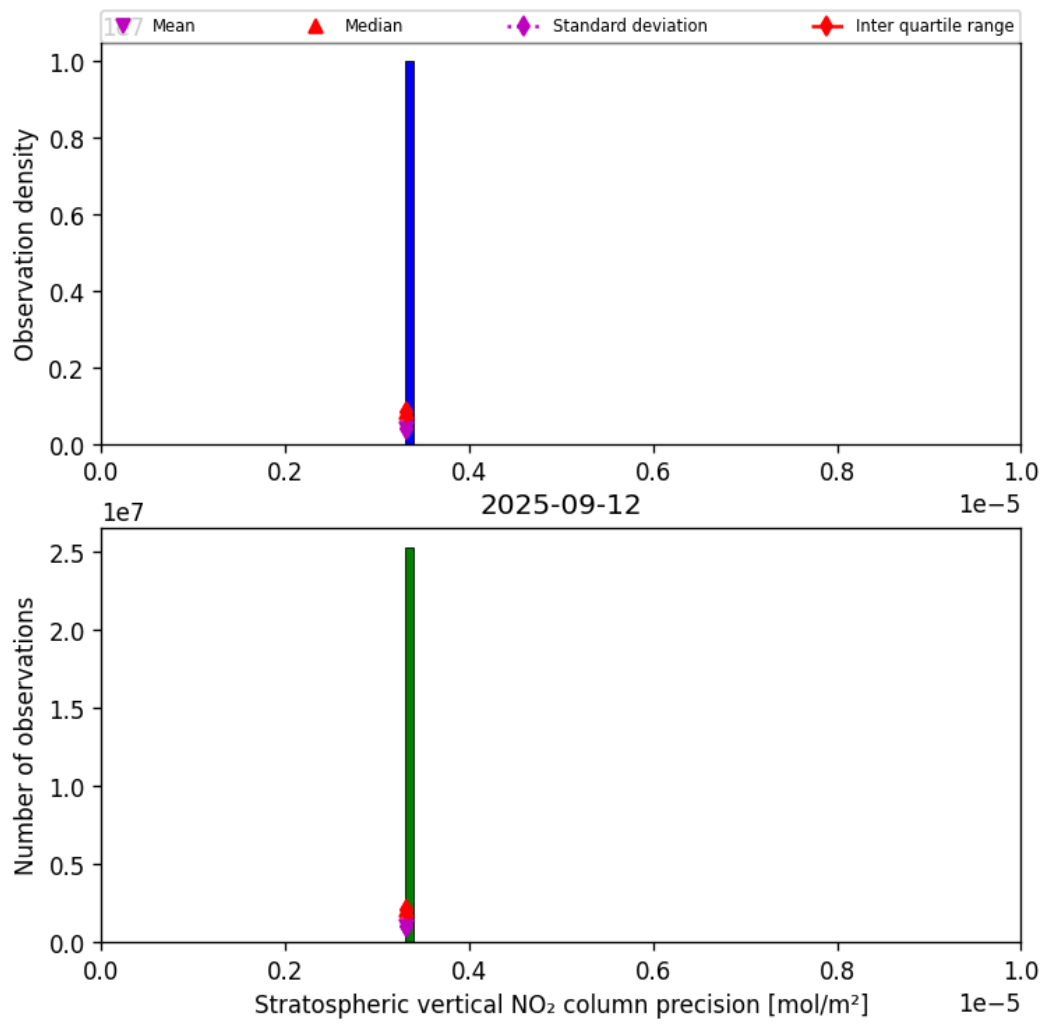
Figure 37: Histogram of “Stratospheric vertical NO 2 column precision” for 2025-09-11 to 2025-09-13
