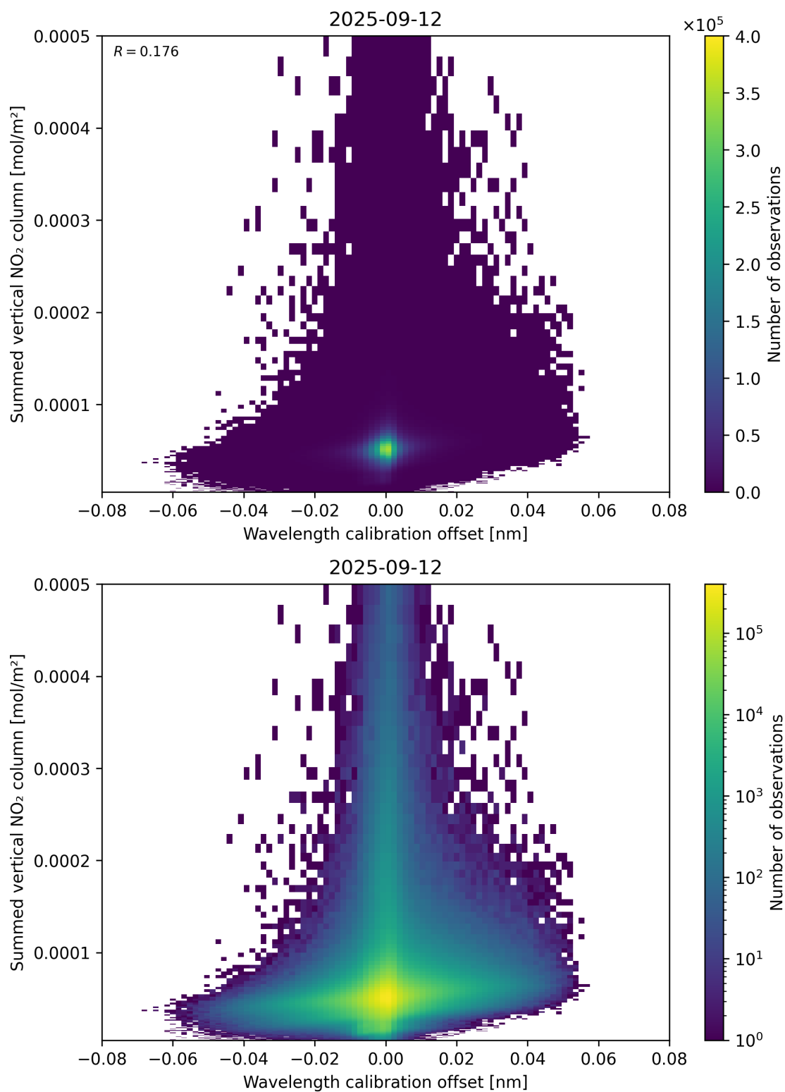
Figure 177: Scatter density plot of “Wavelength calibration offset” against “Summed vertical NO 2 column” for 2025-09-11 to 2025-09-13.
