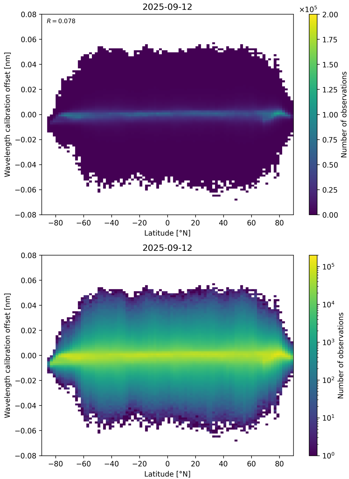
Figure 95: Scatter density plot of “Latitude” against “Wavelength calibration offset” for 2025-09-11 to 2025-09-13.
