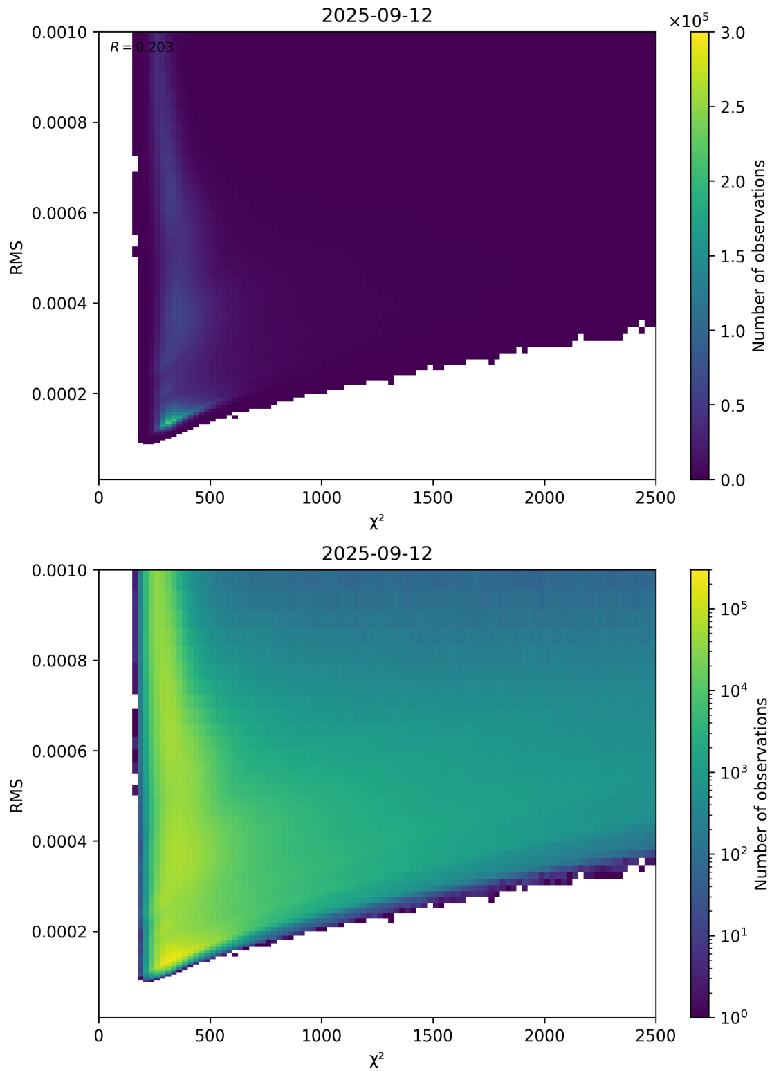
Figure 82: Scatter density plot of “ \chi^2 ” against “RMS” for 2025-09-11 to 2025-09-13.
