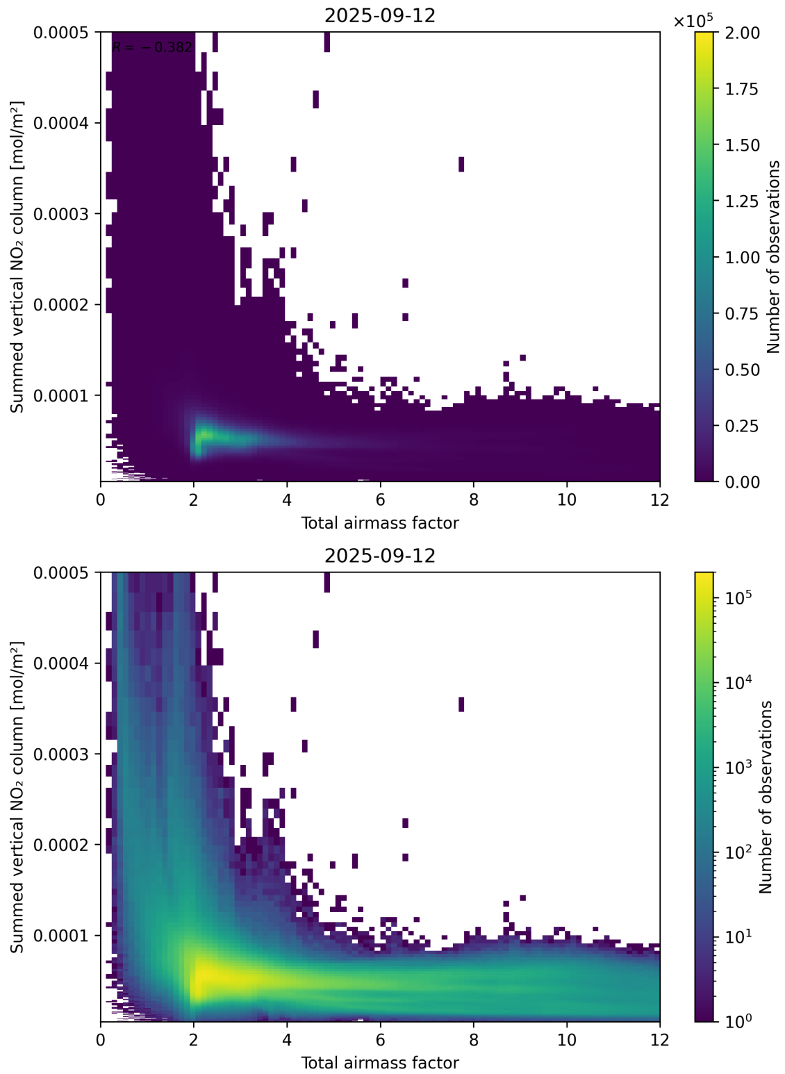
Figure 65: Scatter density plot of “Total airmass factor” against “Summed vertical NO 2 column” for 2025-09-11 to 2025-09-13.
