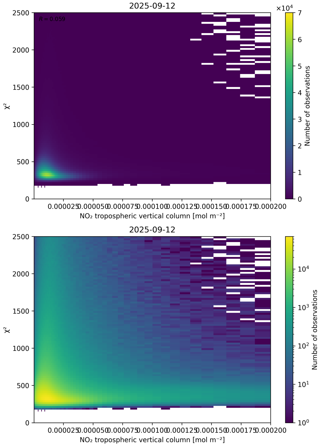
Figure 124: Scatter density plot of “NO 2 tropospheric vertical column” against “ \chi^2 ” for 2025-09-11 to 2025-09-13.
