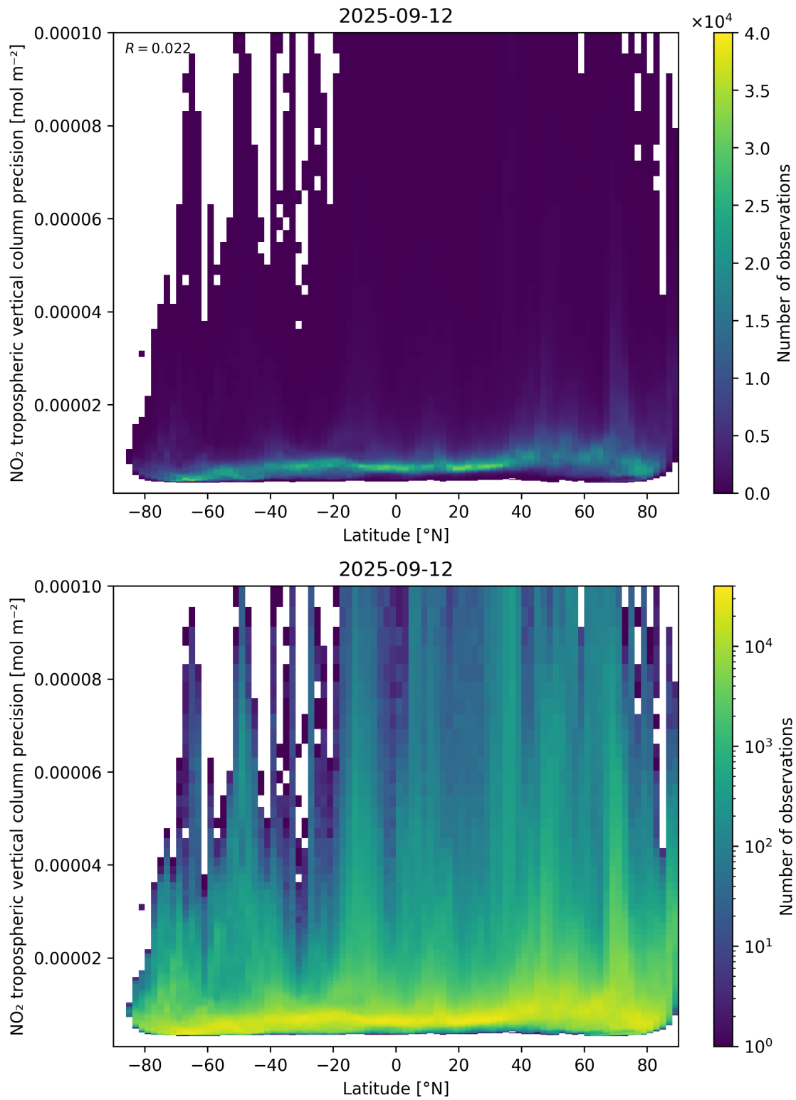
Figure 93: Scatter density plot of “Latitude” against “NO 2 tropospheric vertical column precision” for 2025-09-11 to 2025-09-13.
