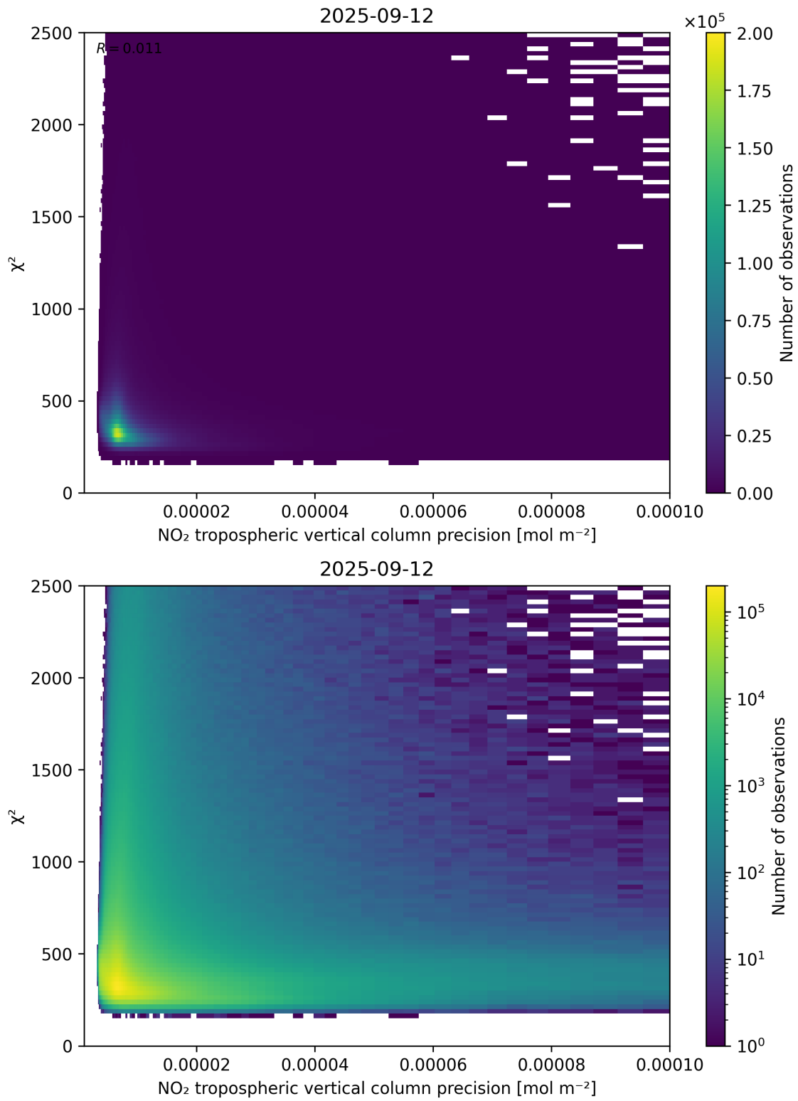
Figure 134: Scatter density plot of “NO 2 tropospheric vertical column precision” against “ \chi^2 ” for 2025-09-11 to 2025-09-13.
