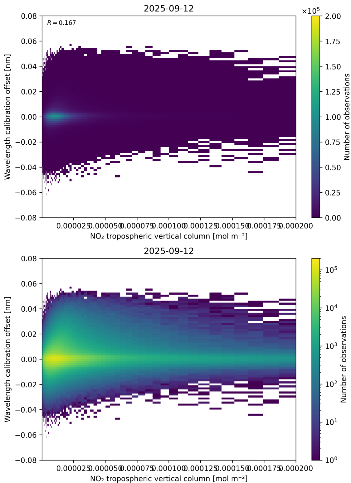
Figure 143: Scatter density plot of “NO 2 tropospheric vertical column” against “Wavelength calibration offset” for 2025-09-11 to 2025-09-13.
