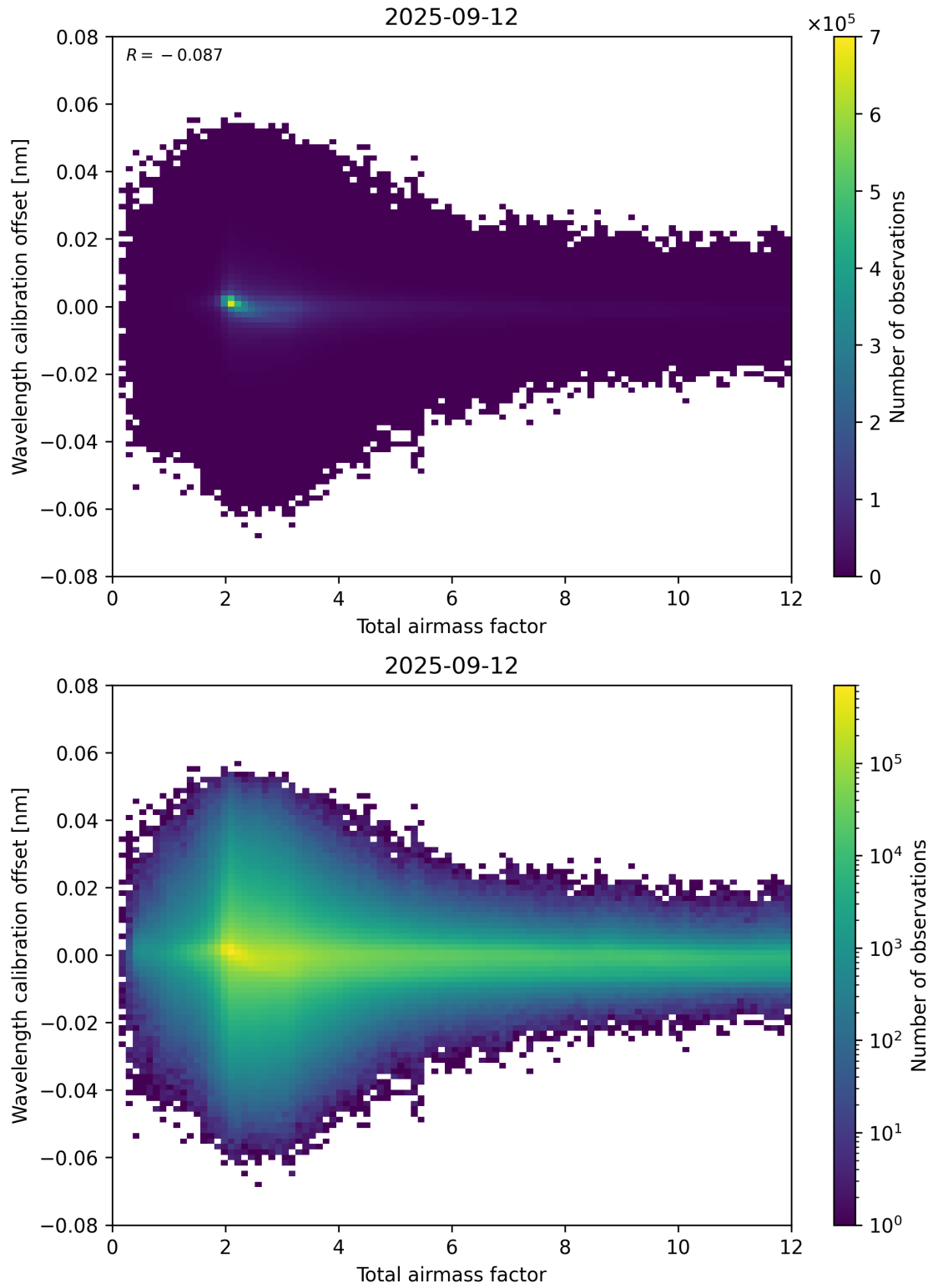
Figure 70: Scatter density plot of “Total airmass factor” against “Wavelength calibration offset” for 2025-09-11 to 2025-09-13.
