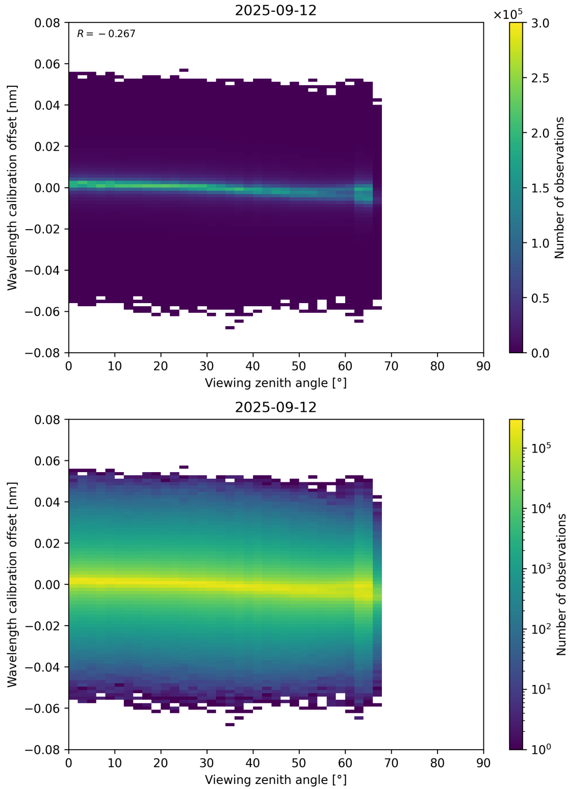
Figure 173: Scatter density plot of “Viewing zenith angle” against “Wavelength calibration offset” for 2025-09-11 to 2025-09-13.
