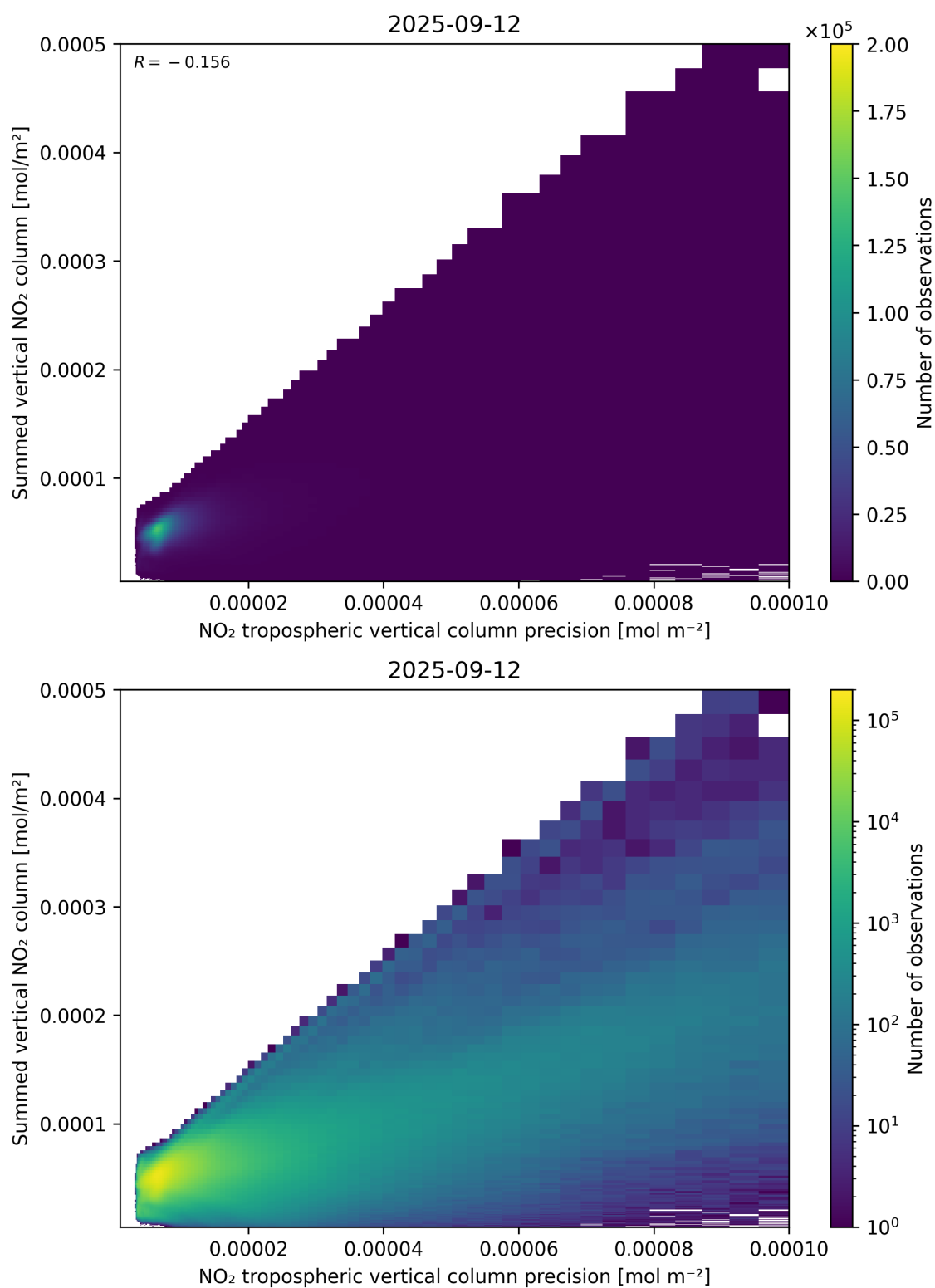
Figure 136: Scatter density plot of “NO 2 tropospheric vertical column precision” against “Summed vertical NO 2 column” for 2025-09-11 to 2025-09-13.
