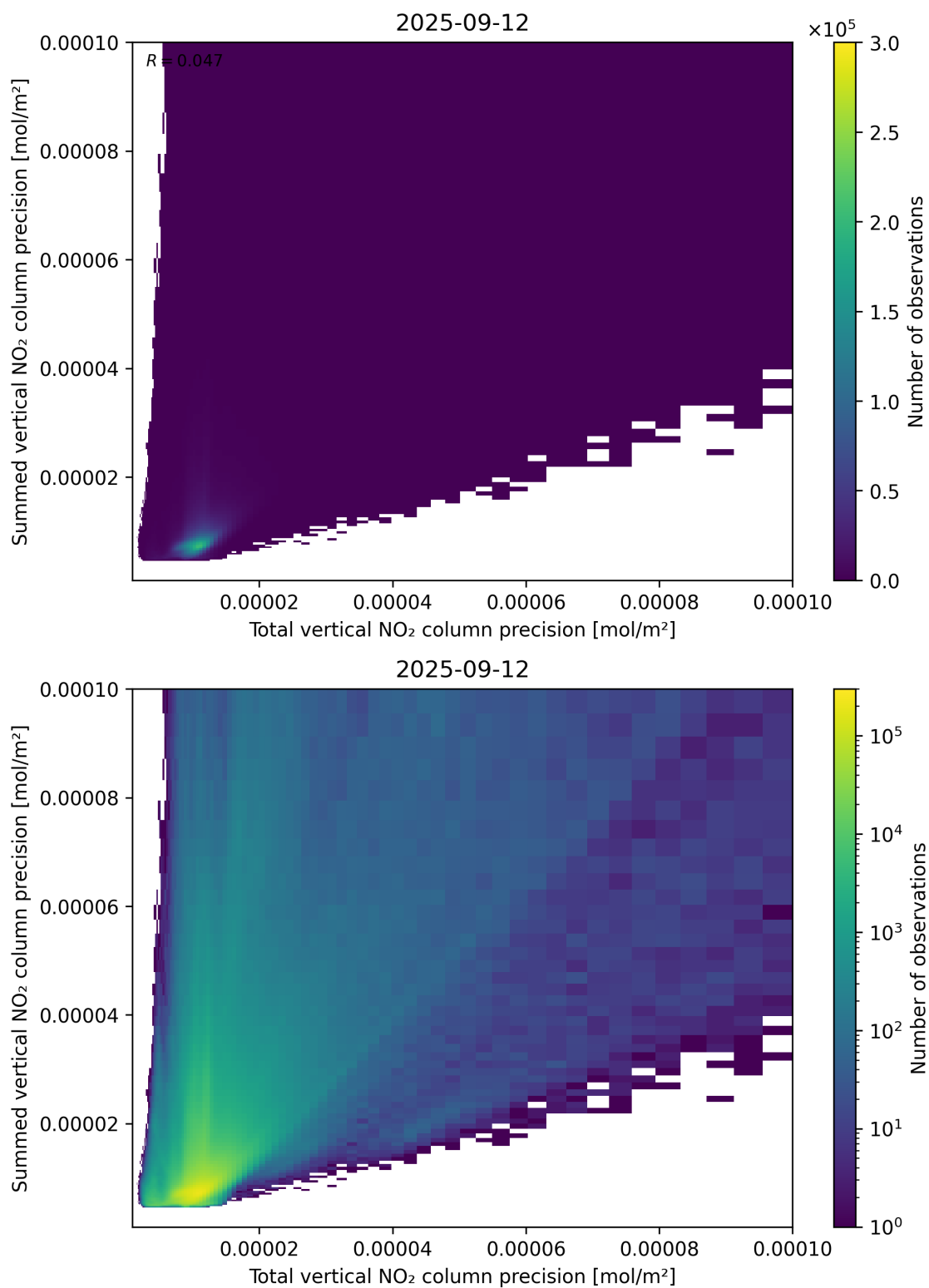
Figure 118: Scatter density plot of “Total vertical NO 2 column precision” against “Summed vertical NO 2 column precision” for 2025-09-11 to 2025-09-13.
