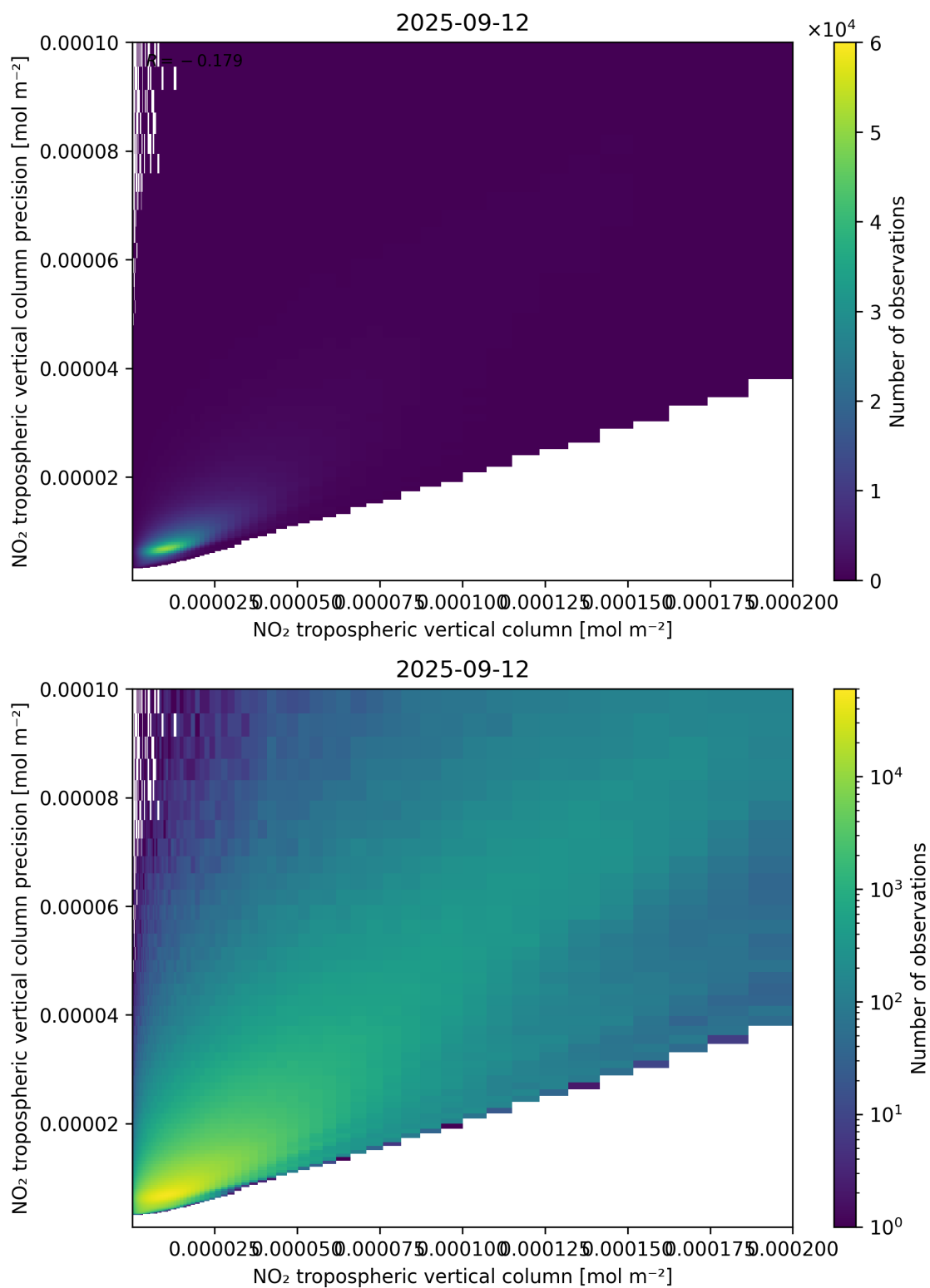
Figure 130: Scatter density plot of “NO 2 tropospheric vertical column” against “NO 2 tropospheric vertical column precision” for 2025-09-11 to 2025-09-13.
