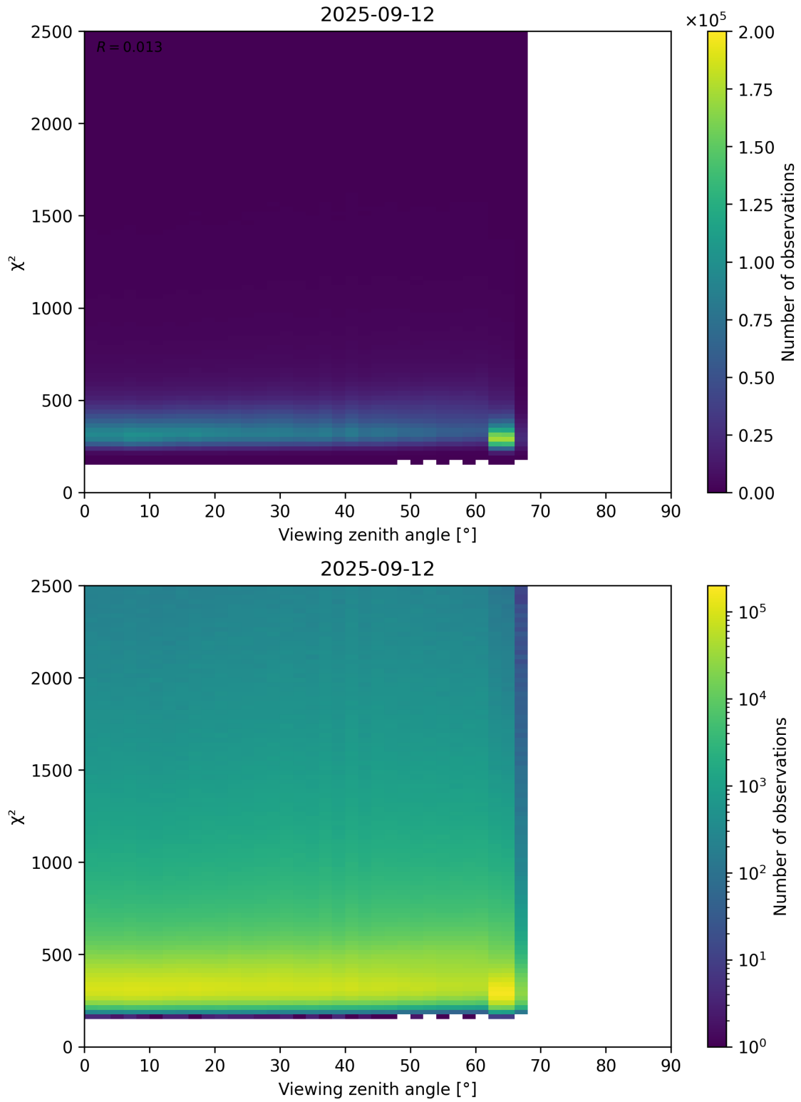
Figure 162: Scatter density plot of “Viewing zenith angle” against “ \chi^2 ” for 2025-09-11 to 2025-09-13.
