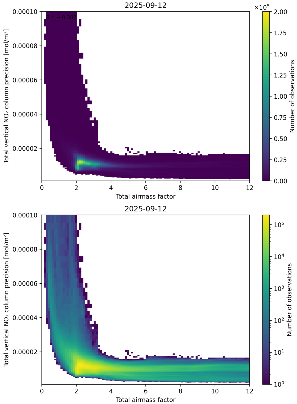
Figure 68: Scatter density plot of “Total airmass factor” against “Total vertical NO 2 column precision” for 2025-09-11 to 2025-09-13.
