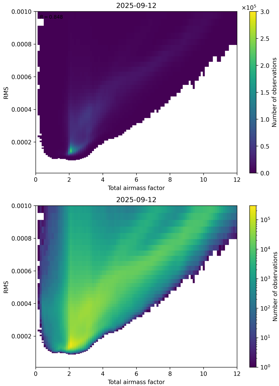
Figure 69: Scatter density plot of “Total airmass factor” against “RMS” for 2025-09-11 to 2025-09-13.
