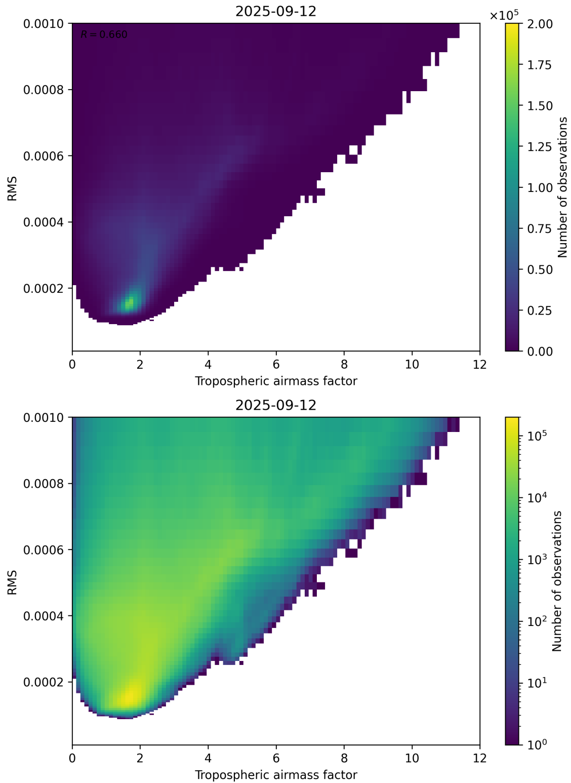
Figure 79: Scatter density plot of “Tropospheric airmass factor” against “RMS” for 2025-09-11 to 2025-09-13.
