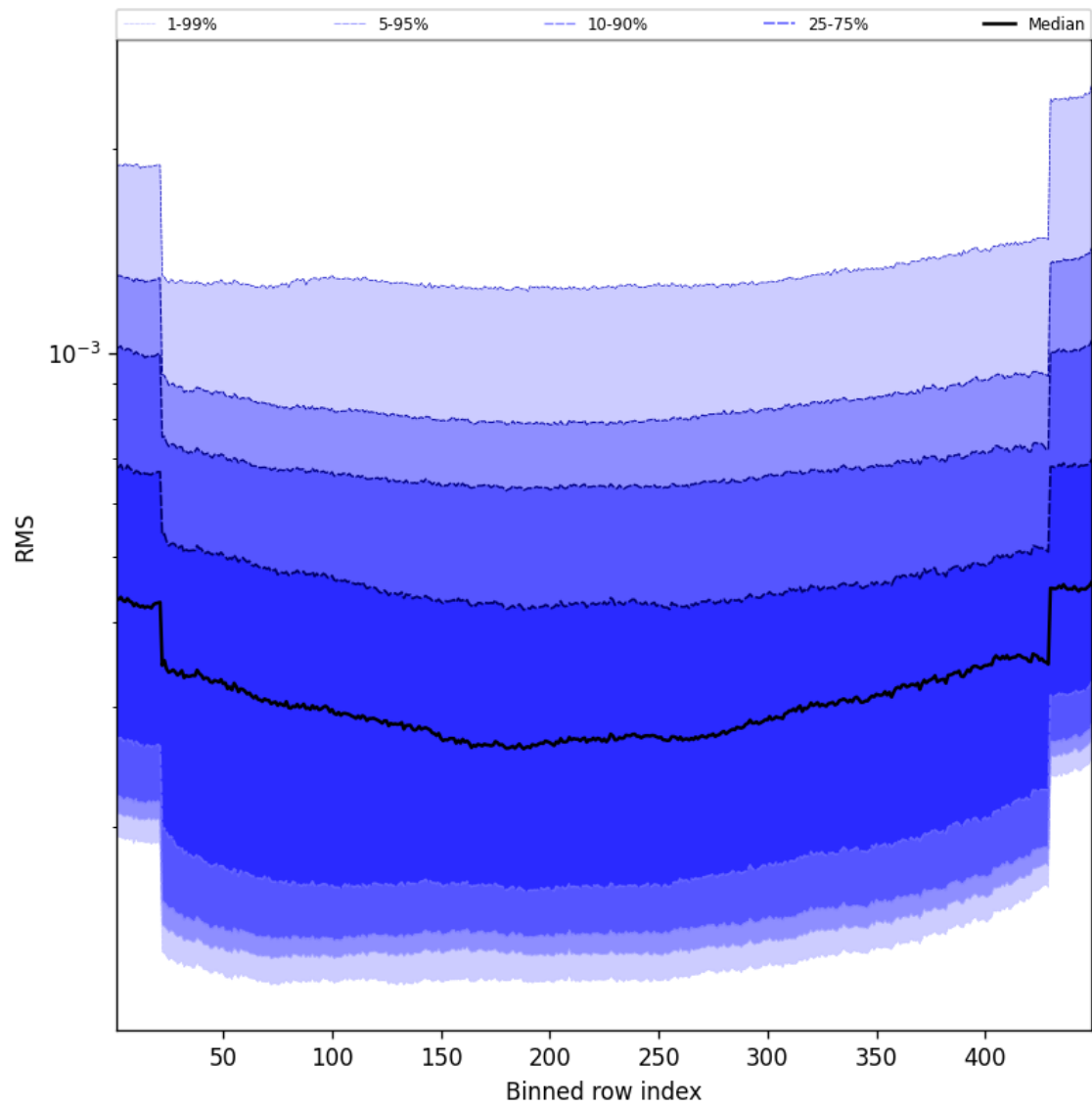
Figure 60: Along track statistics of “RMS” for 2025-09-11 to 2025-09-13
