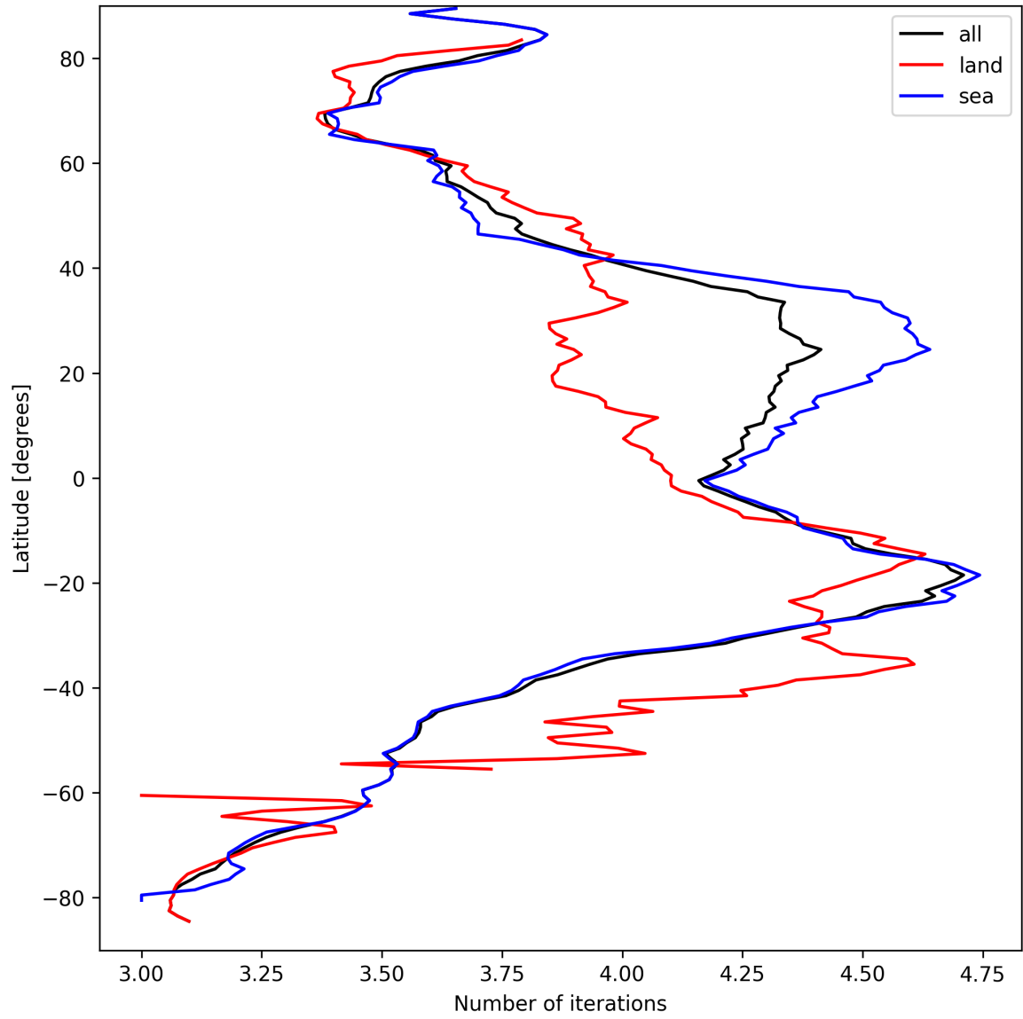
Figure 17: Zonal average of “Number of iterations” for 2025-09-11 to 2025-09-13.
