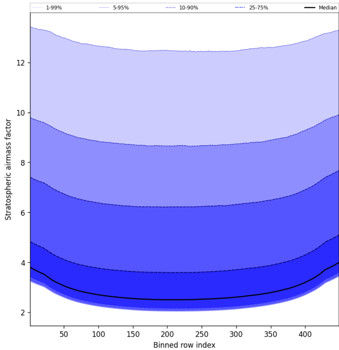
Figure 61: Along track statistics of “Stratospheric airmass factor” for 2025-09-11 to 2025-09-13
