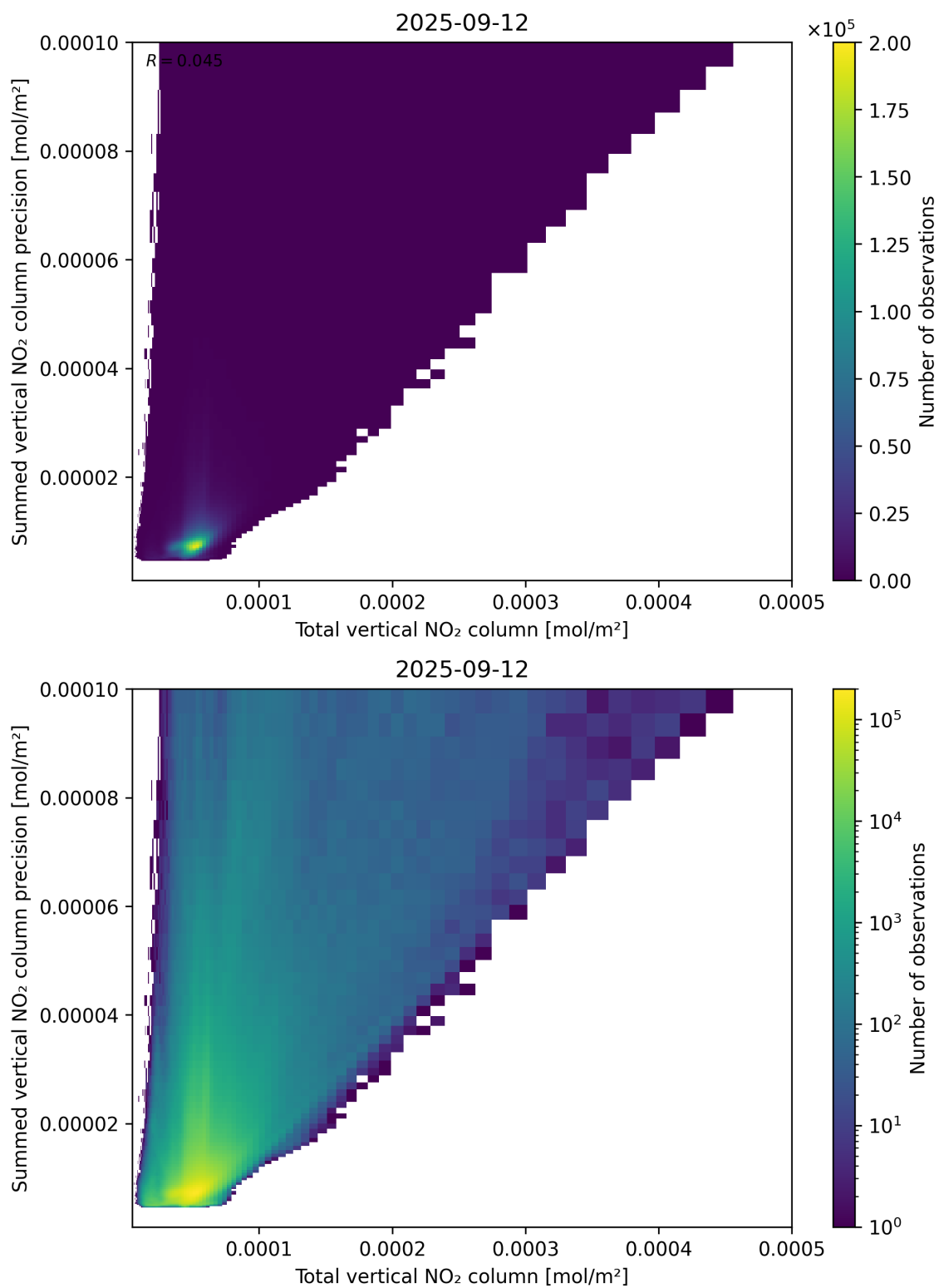
Figure 113: Scatter density plot of “Total vertical NO 2 column” against “Summed vertical NO 2 column precision” for 2025-09-11 to 2025-09-13.
