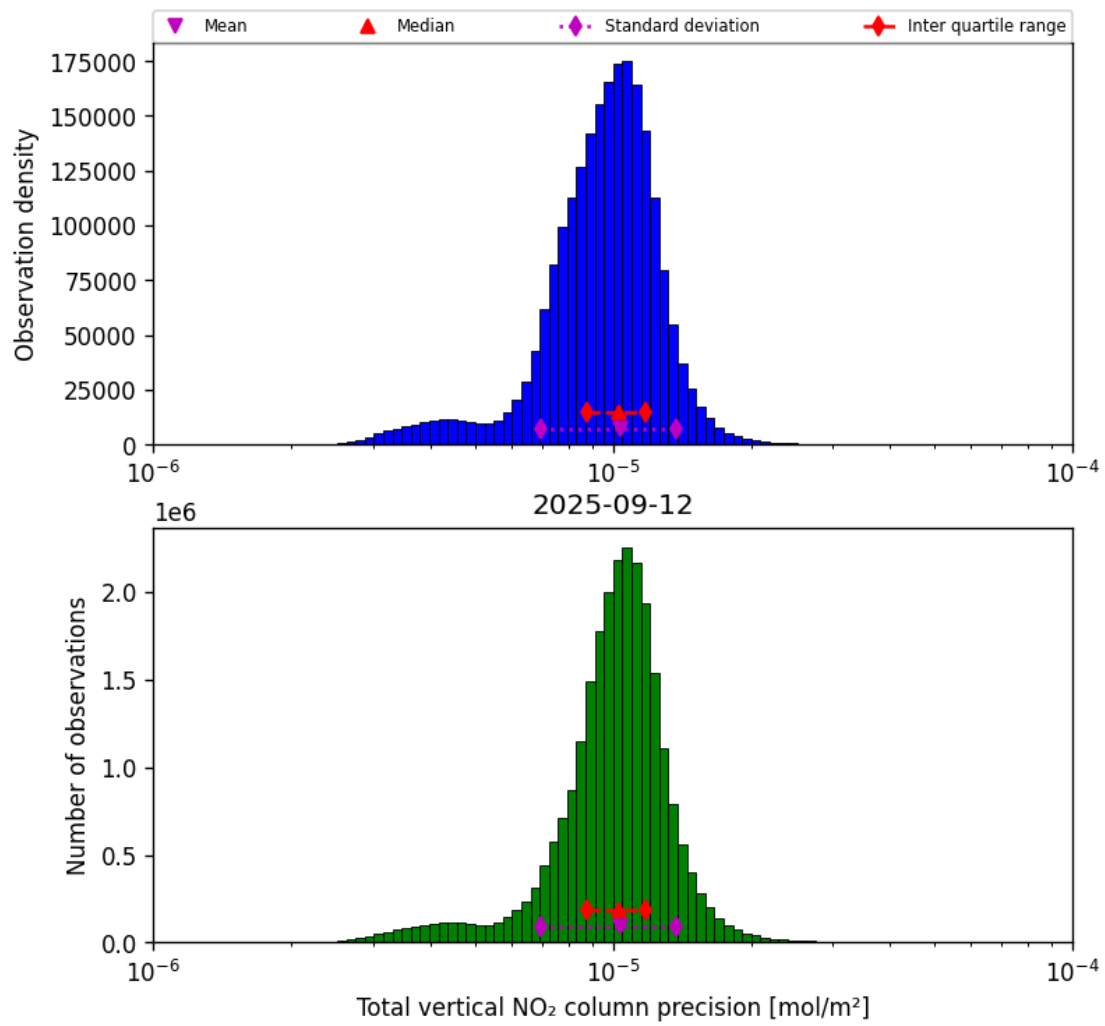
Figure 39: Histogram of “Total vertical NO 2 column precision” for 2025-09-11 to 2025-09-13
