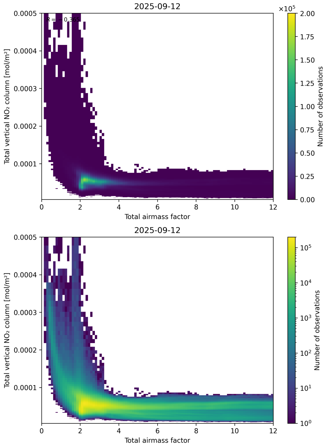
Figure 67: Scatter density plot of “Total airmass factor” against “Total vertical NO 2 column” for 2025-09-11 to 2025-09-13.
