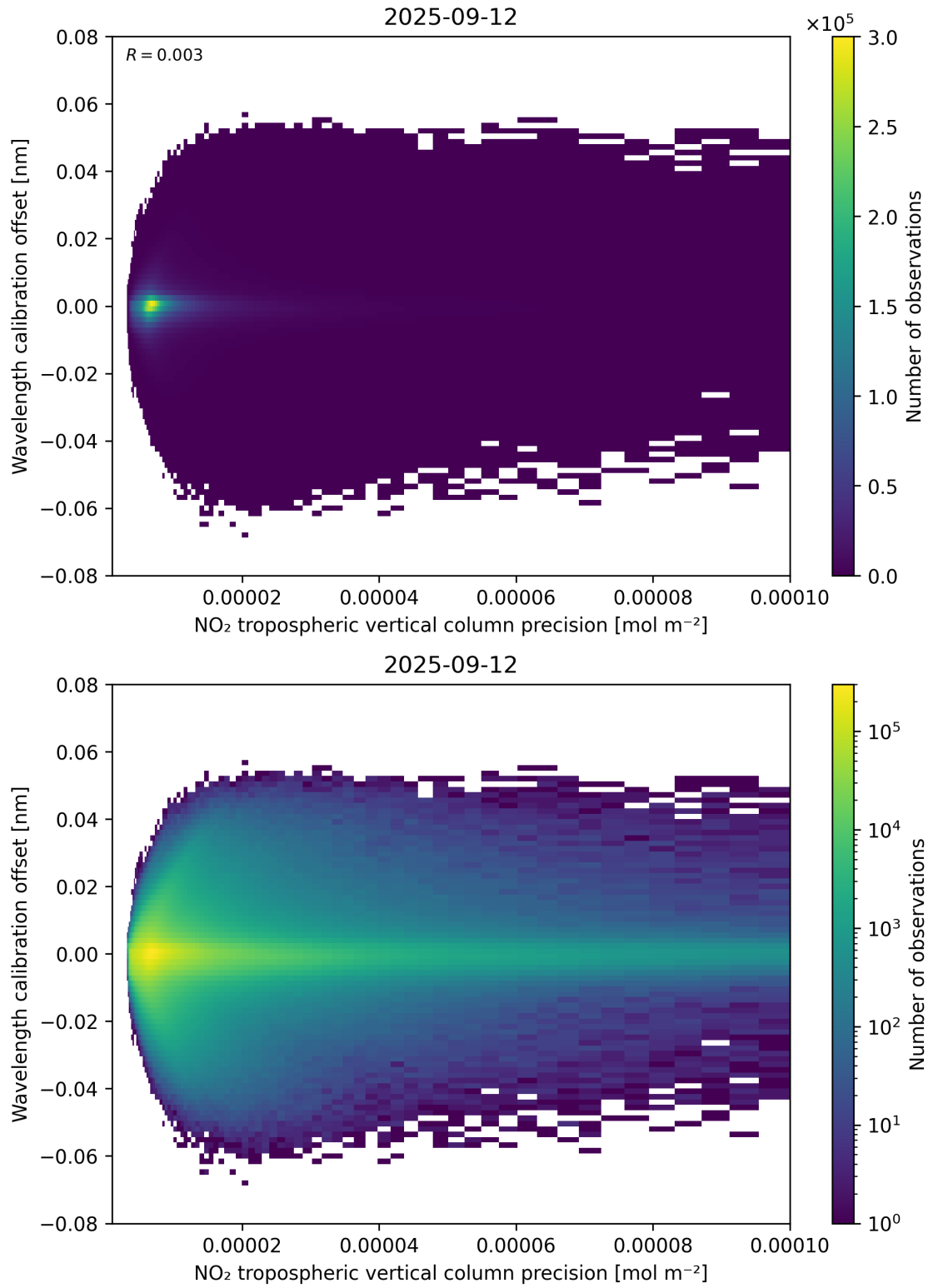
Figure 141: Scatter density plot of “NO 2 tropospheric vertical column precision” against “Wavelength calibration offset” for 2025-09-11 to 2025-09-13.
