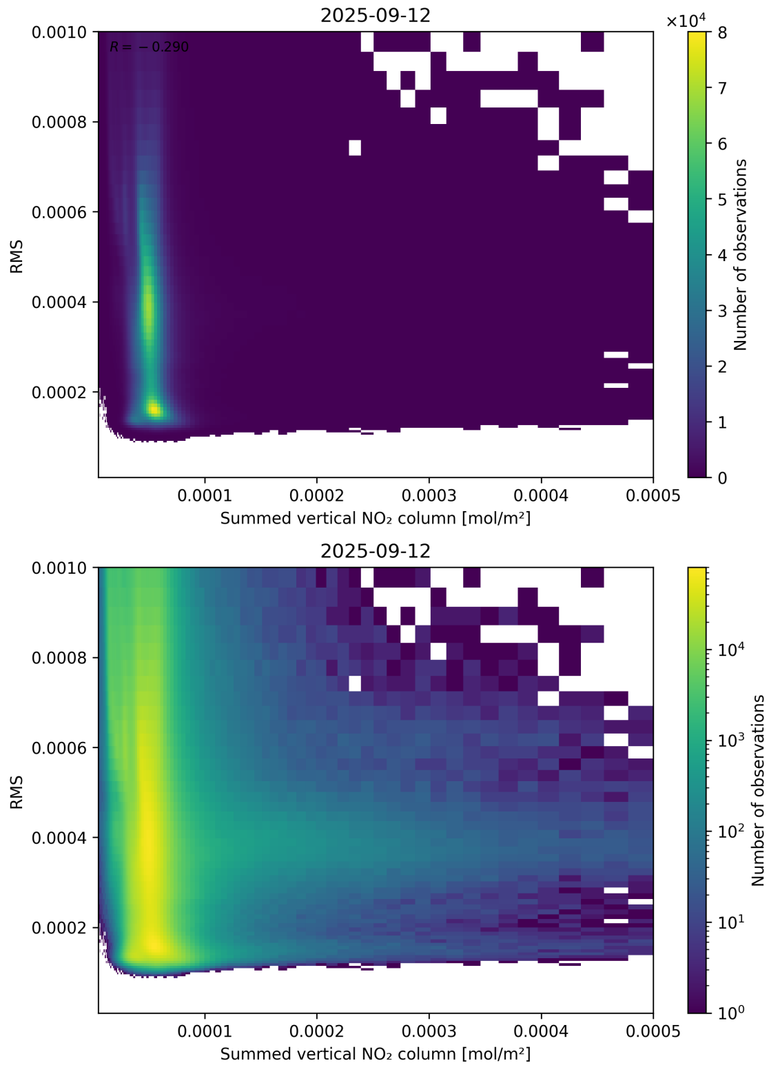
Figure 109: Scatter density plot of “Summed vertical NO 2 column” against “RMS” for 2025-09-11 to 2025-09-13.
