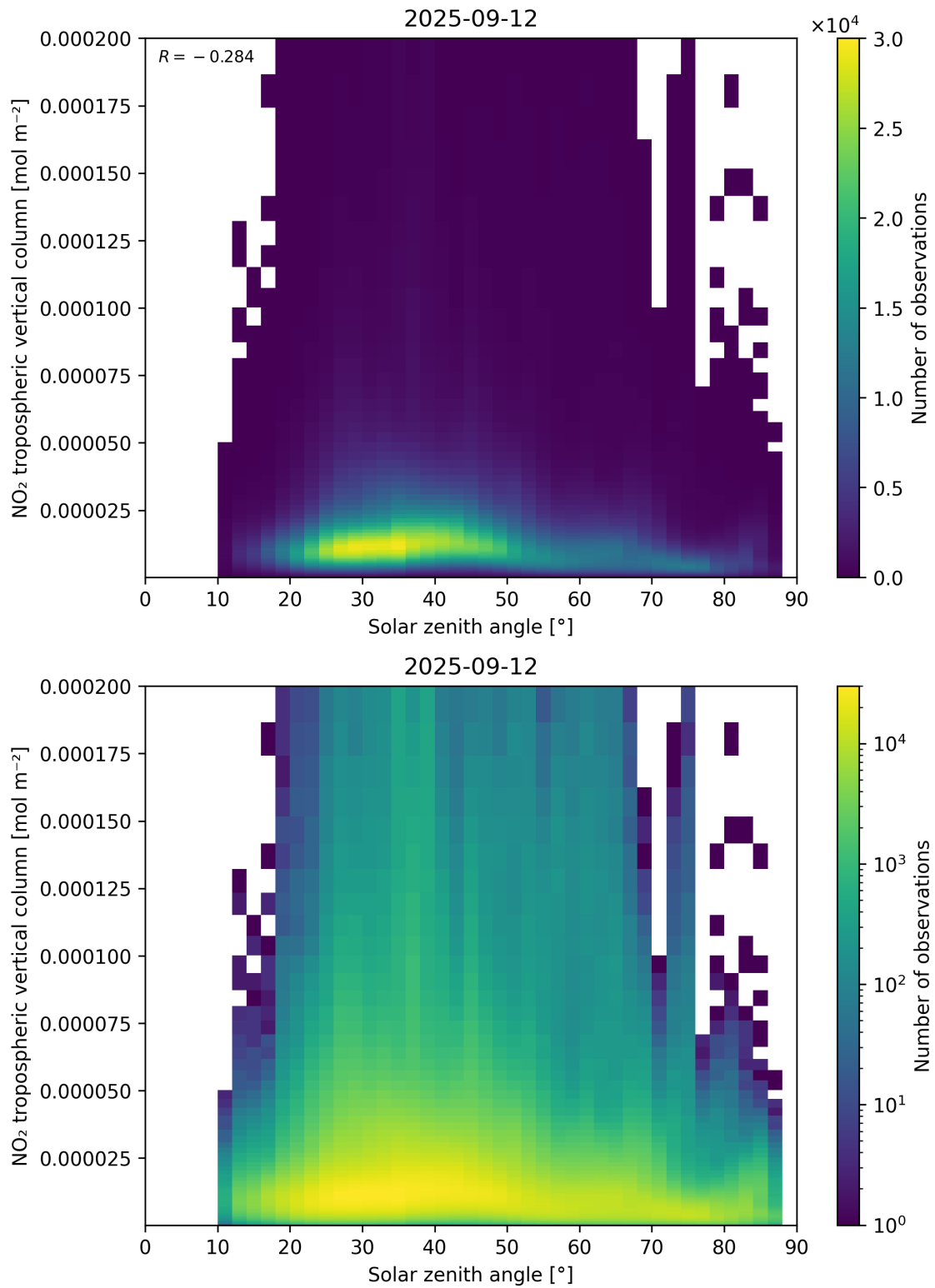
Figure 155: Scatter density plot of “Solar zenith angle” against “NO 2 tropospheric vertical column” for 2025-09-11 to 2025-09-13.
