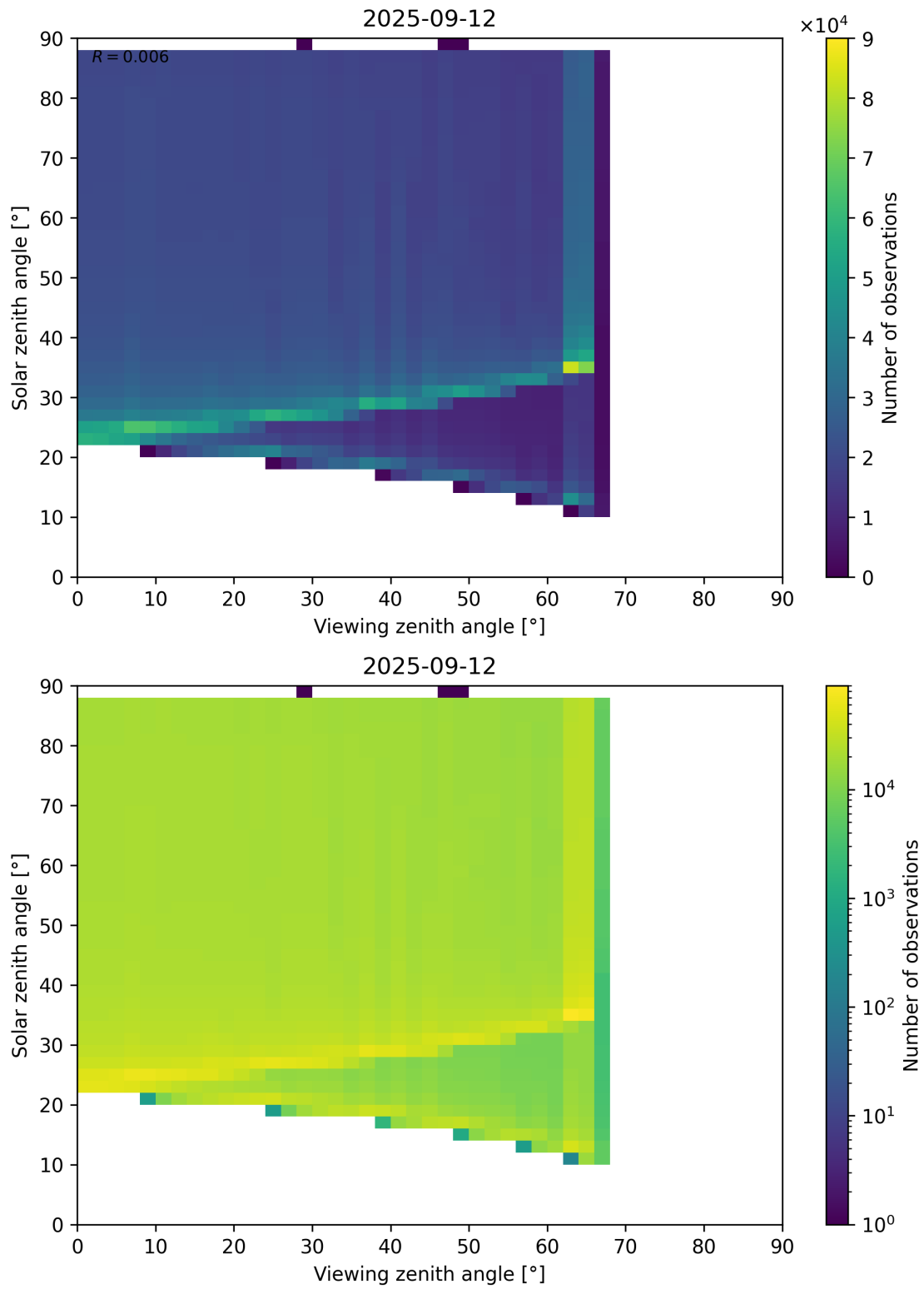
Figure 172: Scatter density plot of “Viewing zenith angle” against “Solar zenith angle” for 2025-09-11 to 2025-09-13.
