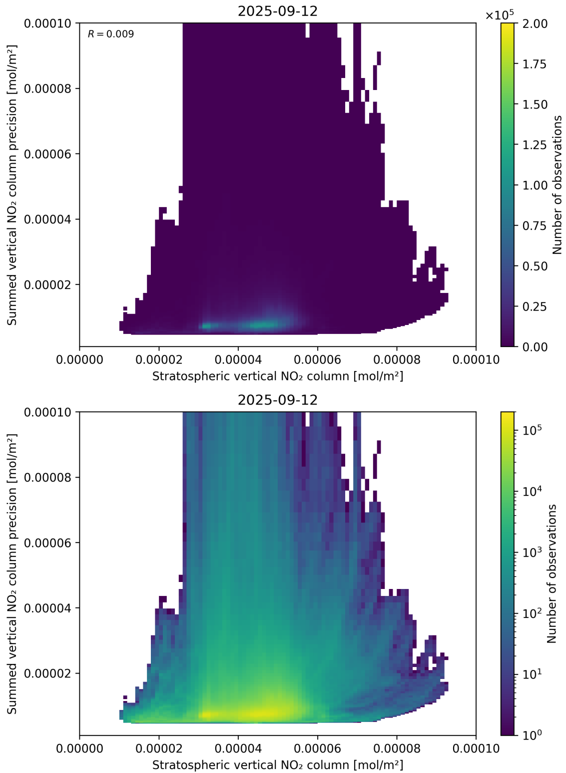
Figure 99: Scatter density plot of “Stratospheric vertical NO 2 column” against “Summed vertical NO 2 column precision” for 2025-09-11 to 2025-09-13.
