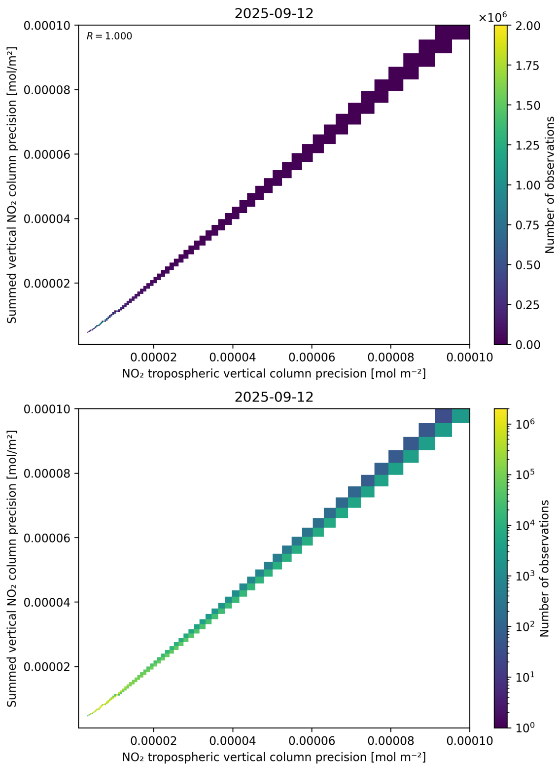
Figure 137: Scatter density plot of “NO 2 tropospheric vertical column precision” against “Summed vertical NO 2 column precision” for 2025-09-11 to 2025-09-13.
