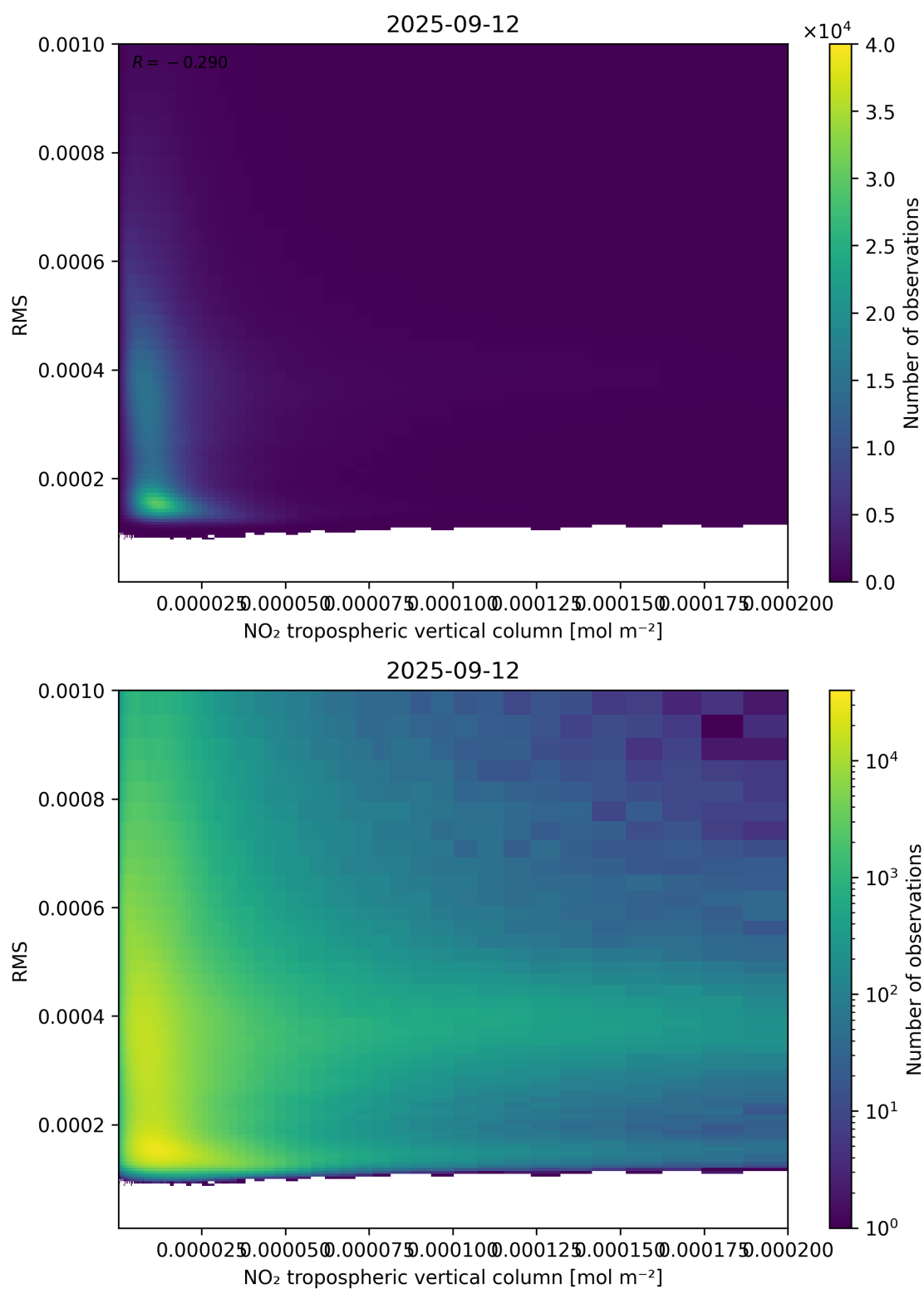
Figure 142: Scatter density plot of “NO 2 tropospheric vertical column” against “RMS” for 2025-09-11 to 2025-09-13.
