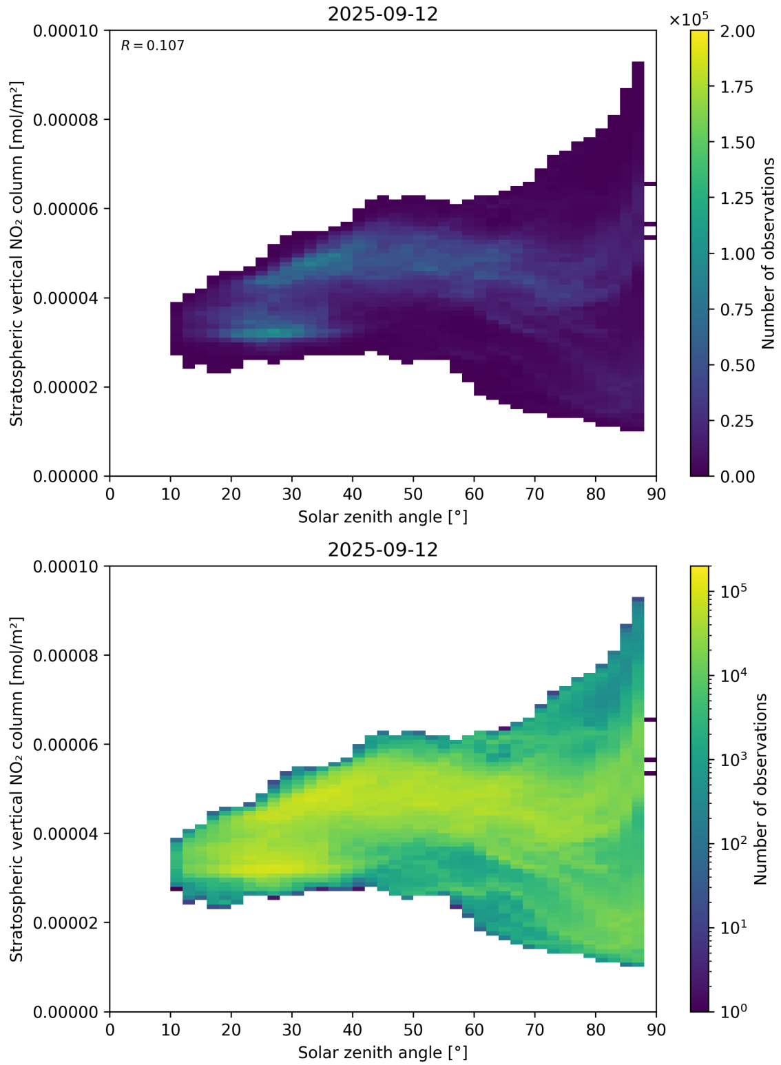
Figure 150: Scatter density plot of “Solar zenith angle” against “Stratospheric vertical NO 2 column” for 2025-09-11 to 2025-09-13.
