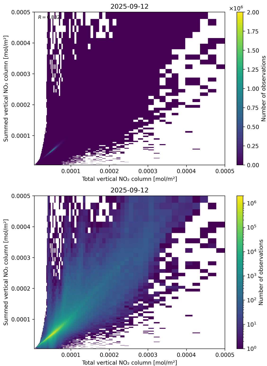
Figure 112: Scatter density plot of “Total vertical NO 2 column” against “Summed vertical NO 2 column” for 2025-09-11 to 2025-09-13.
