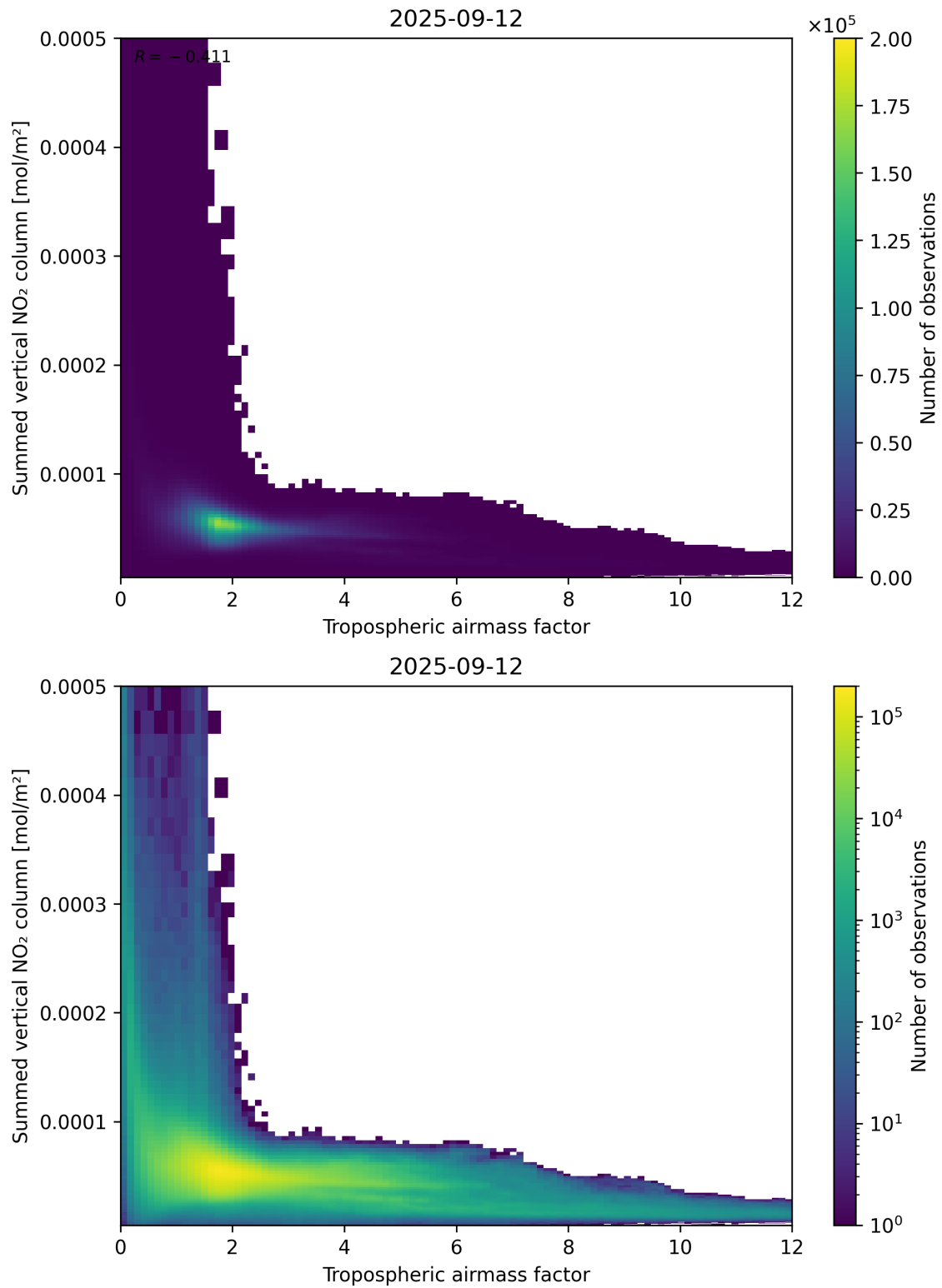
Figure 75: Scatter density plot of “Tropospheric air mass factor” against “Summed vertical NO 2 column” for 2025-09-11 to 2025-09-13.
