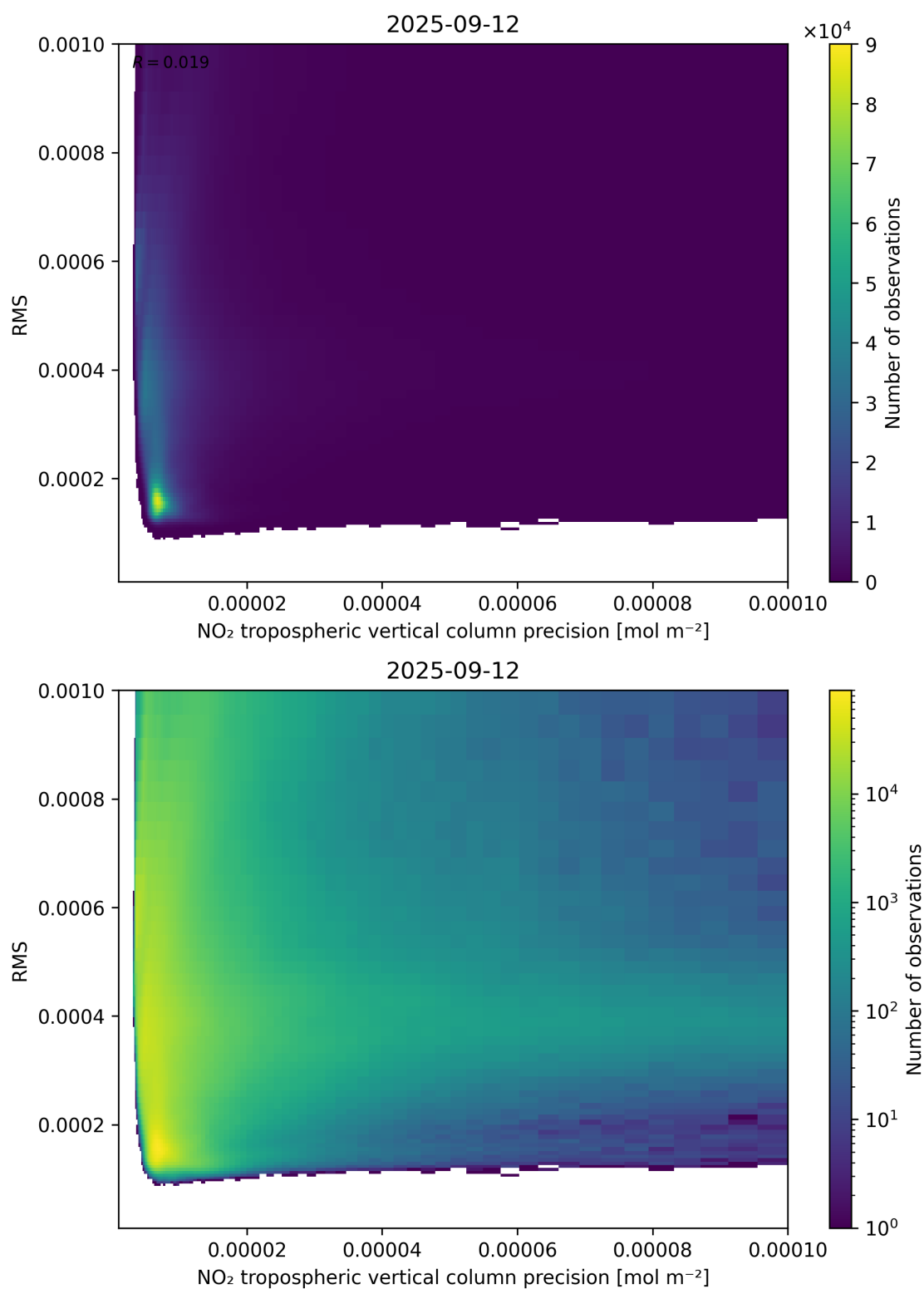
Figure 140: Scatter density plot of “NO 2 tropospheric vertical column precision” against “RMS” for 2025-09-11 to 2025-09-13.
