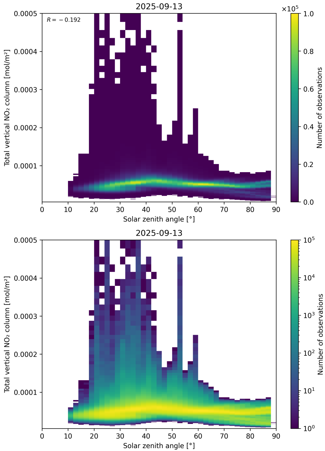
Figure 153: Scatter density plot of “Solar zenith angle” against “Total vertical NO 2 column” for 2025-09-12 to 2025-09-14.
