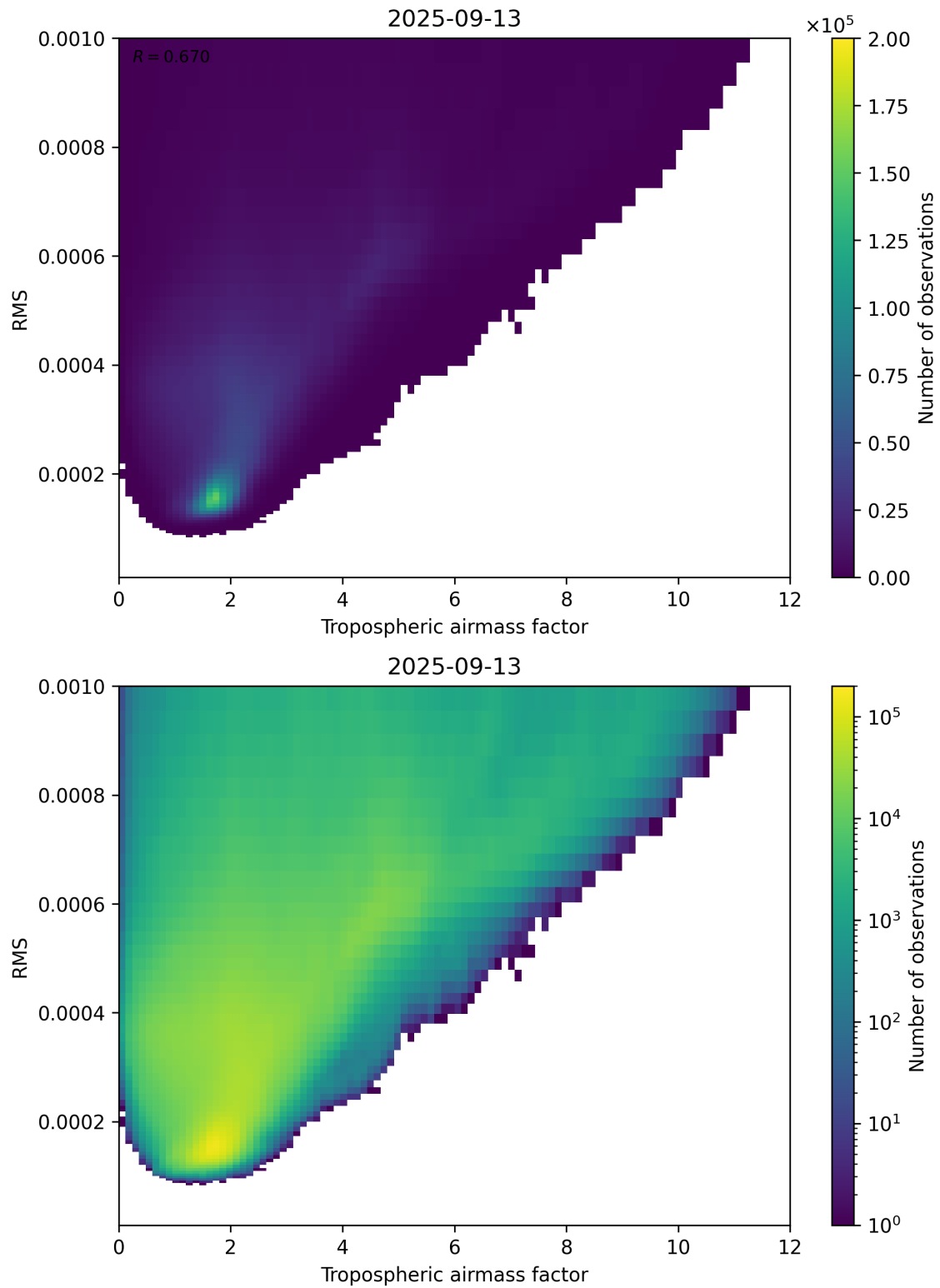
Figure 79: Scatter density plot of “Tropospheric airmass factor” against “RMS” for 2025-09-12 to 2025-09-14.
