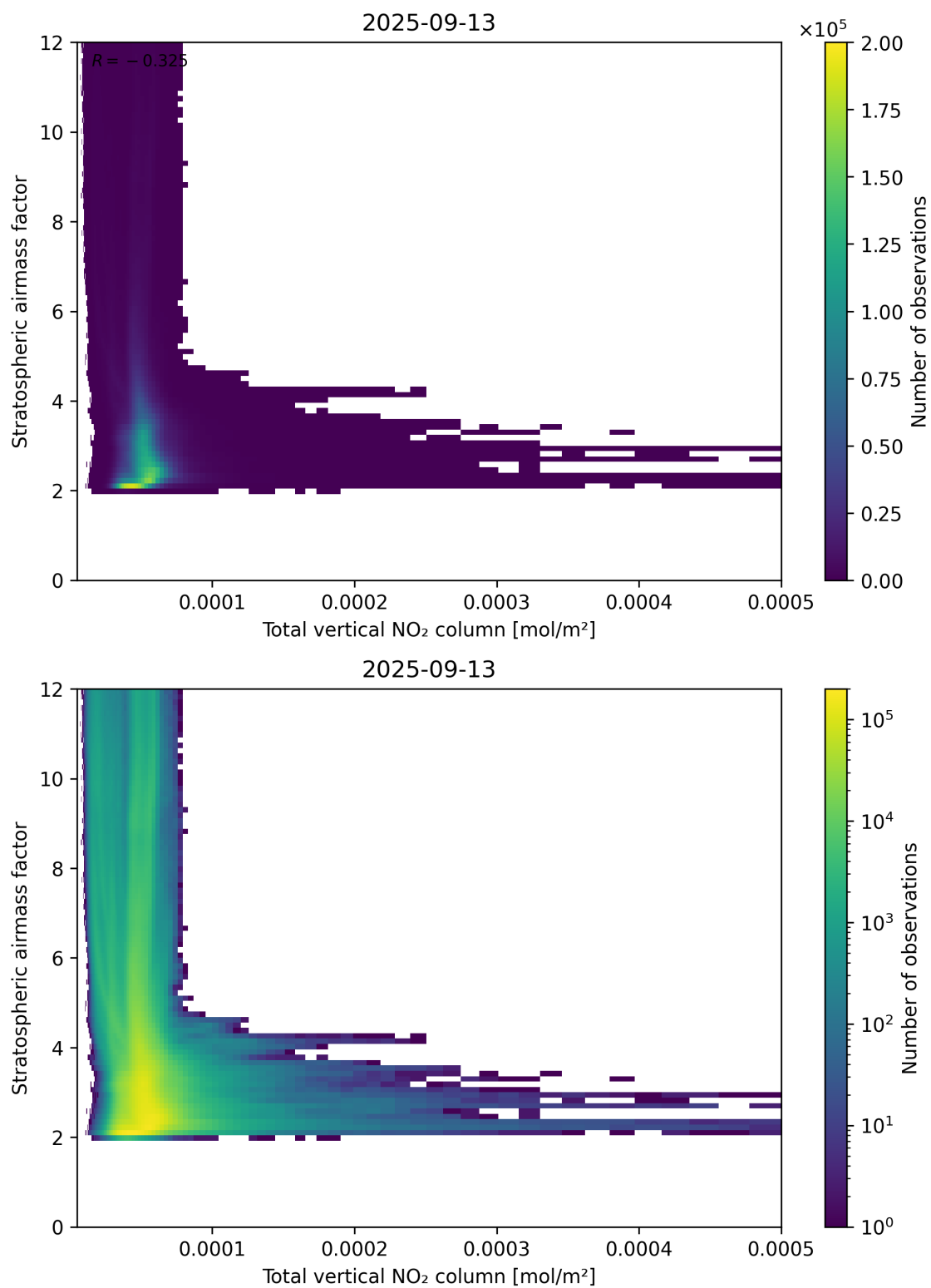
Figure 110: Scatter density plot of “Total vertical NO 2 column” against “Stratospheric airmass factor” for 2025-09-12 to 2025-09-14.
