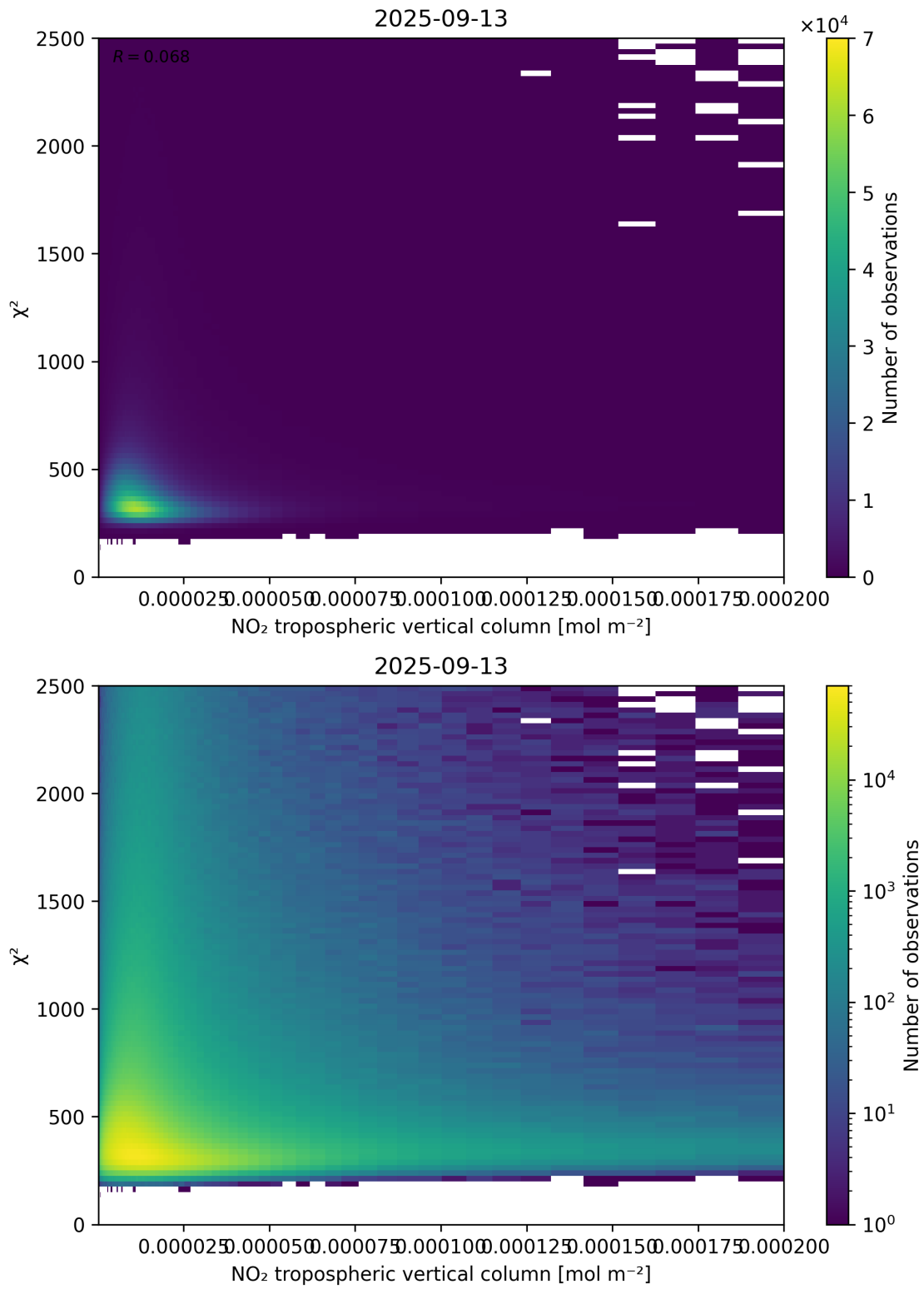
Figure 124: Scatter density plot of “NO 2 tropospheric vertical column” against “ \chi^2 ” for 2025-09-12 to 2025-09-14.
