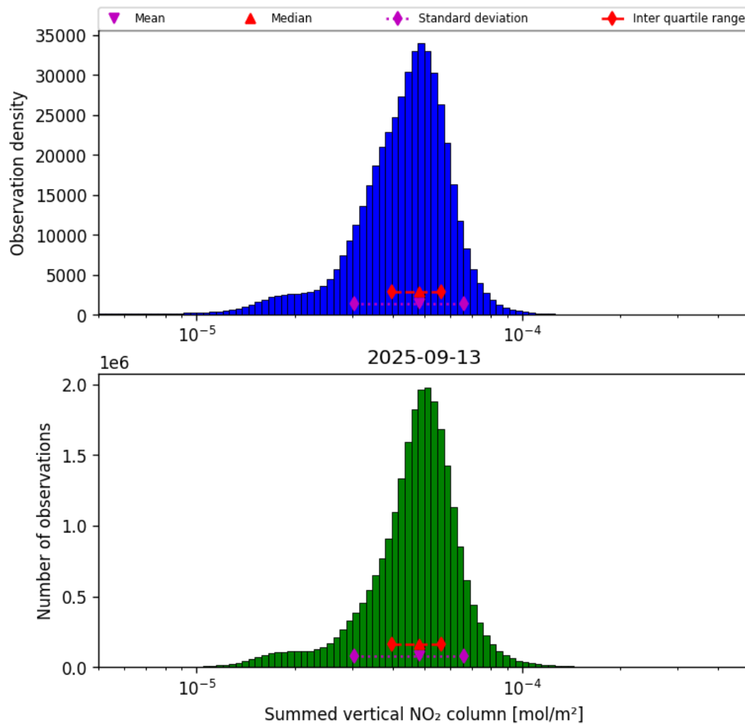
Figure 40: Histogram of “Summed vertical NO 2 column” for 2025-09-12 to 2025-09-14
