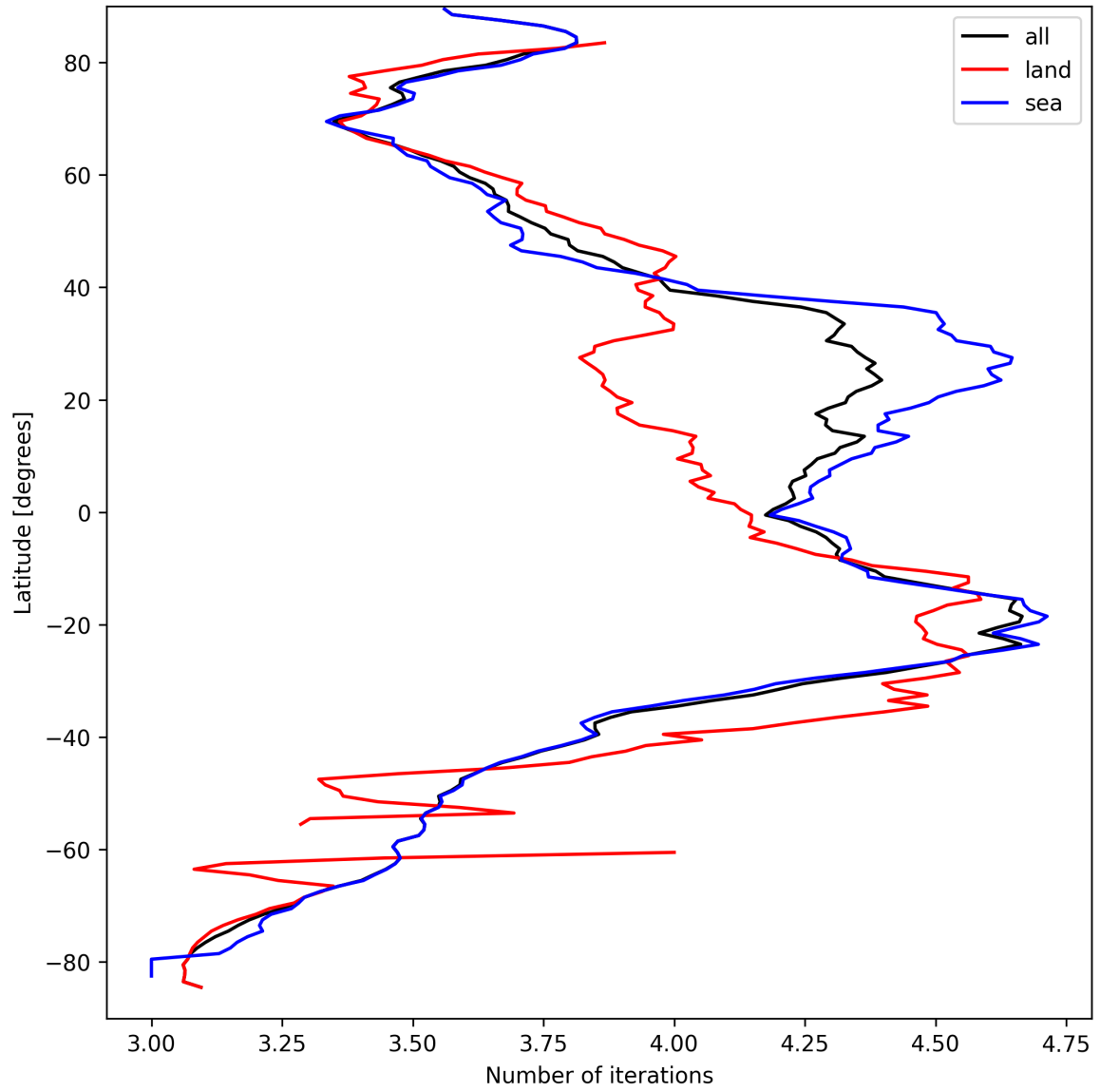
Figure 17: Zonal average of “Number of iterations” for 2025-09-12 to 2025-09-14.
