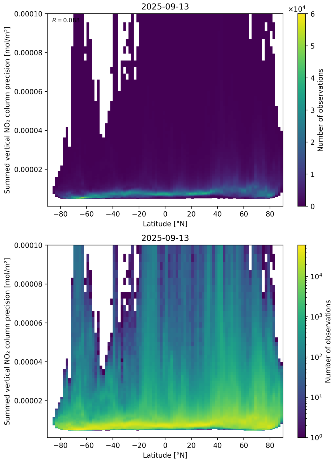
Figure 89: Scatter density plot of “Latitude” against “Summed vertical NO 2 column precision” for 2025-09-12 to 2025-09-14.
