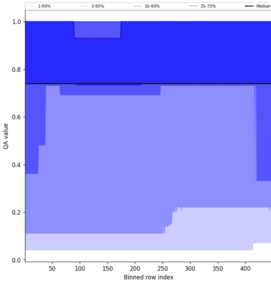
Figure 45: Along track statistics of “QA value” for 2025-09-12 to 2025-09-14
