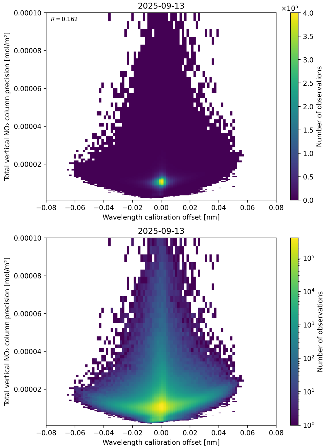
Figure 180: Scatter density plot of “Wavelength calibration offset” against “Total vertical NO 2 column precision” for 2025-09-12 to 2025-09-14.
