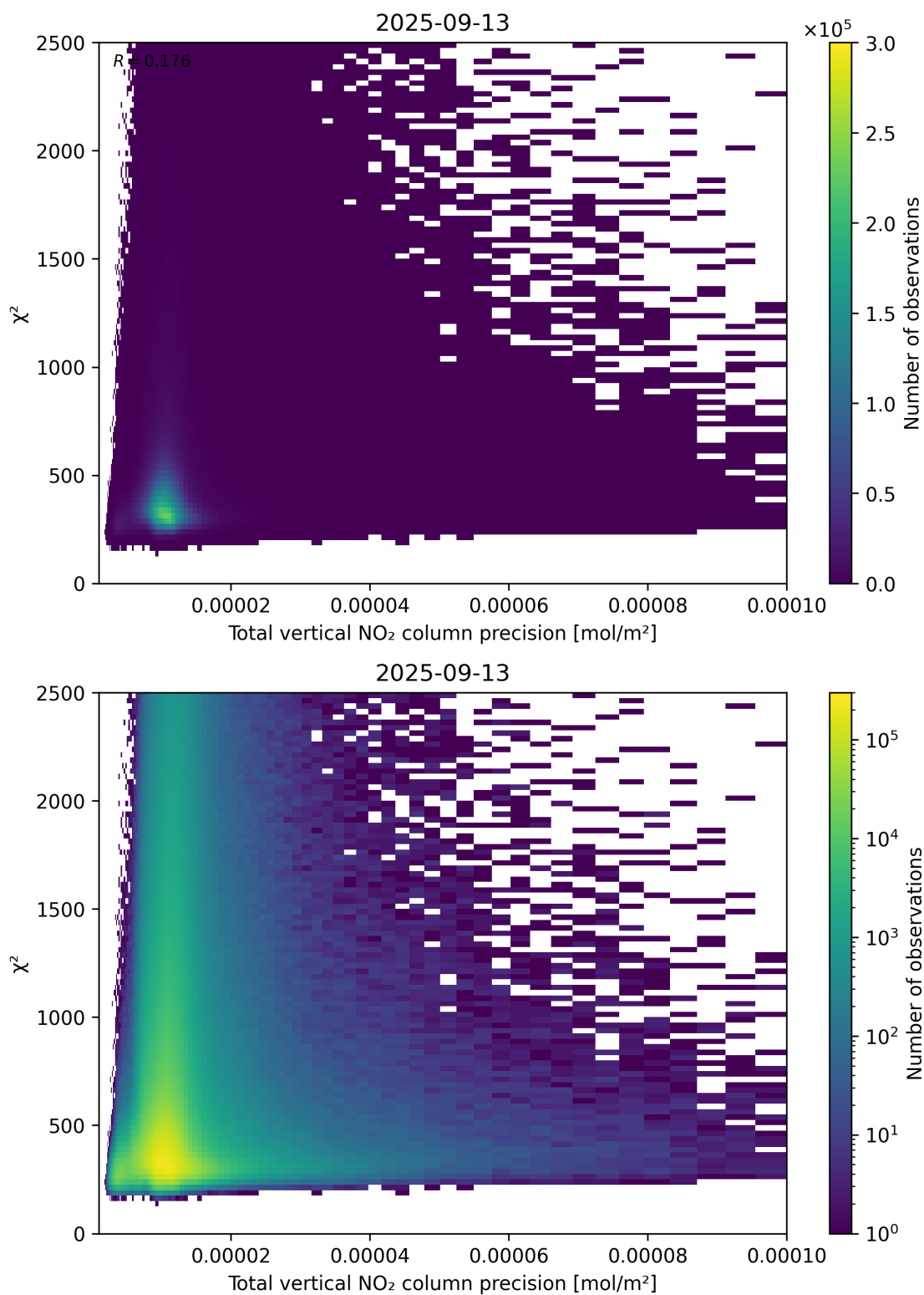
Figure 116: Scatter density plot of “Total vertical NO 2 column precision” against “ \chi^2 ” for 2025-09-12 to 2025-09-14.
