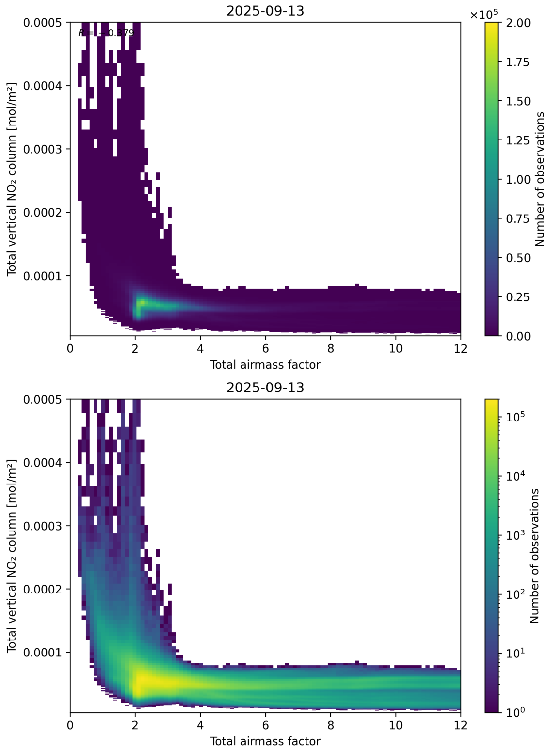
Figure 67: Scatter density plot of “Total airmass factor” against “Total vertical NO 2 column” for 2025-09-12 to 2025-09-14.
