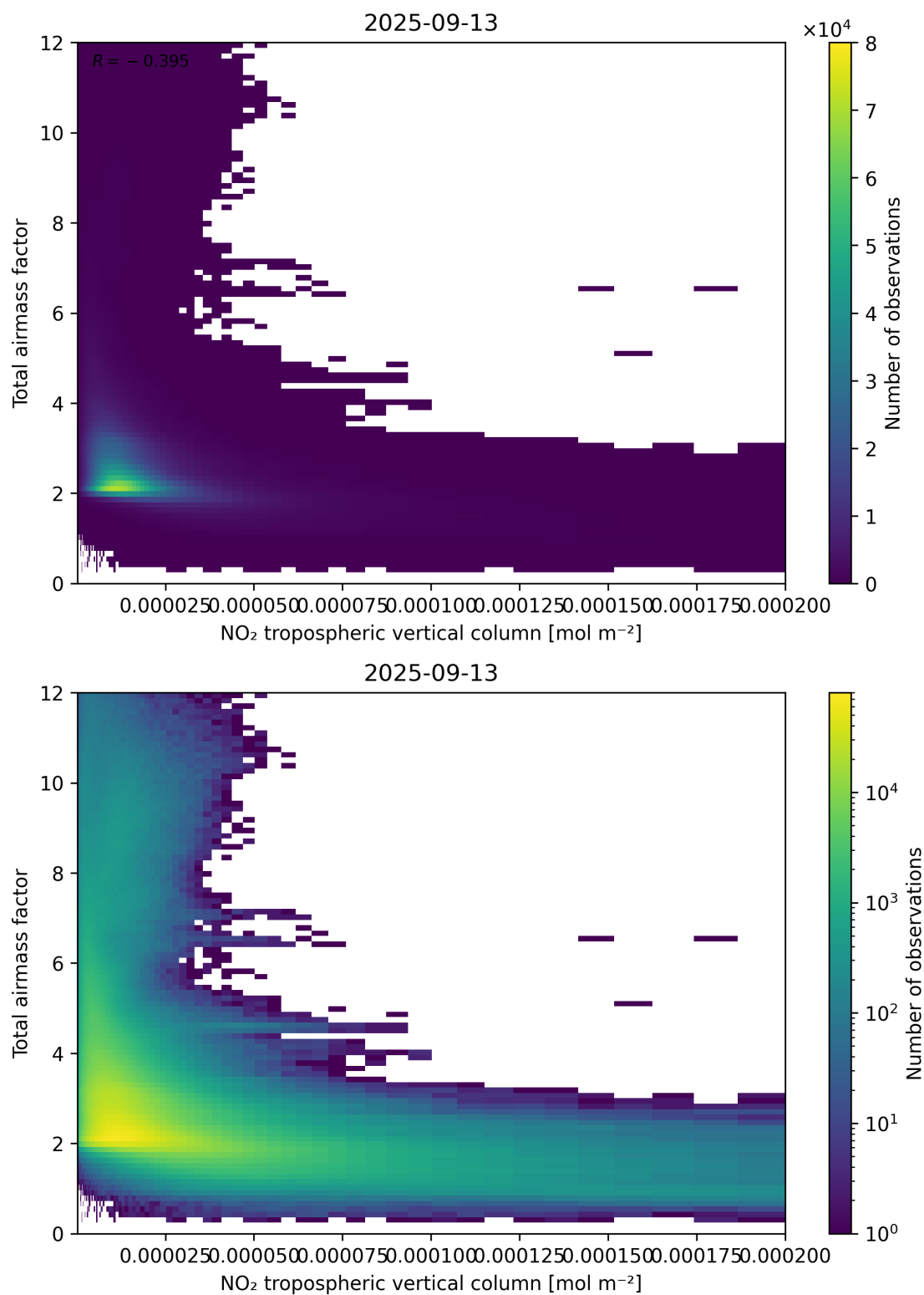
Figure 122: Scatter density plot of “NO 2 tropospheric vertical column” against “Total air mass factor” for 2025-09-12 to 2025-09-14.
