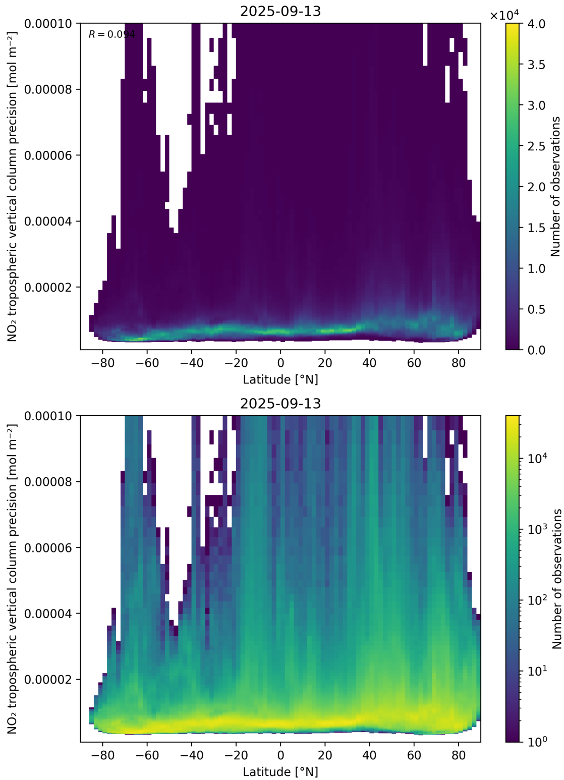
Figure 93: Scatter density plot of “Latitude” against “NO 2 tropospheric vertical column precision” for 2025-09-12 to 2025-09-14.
