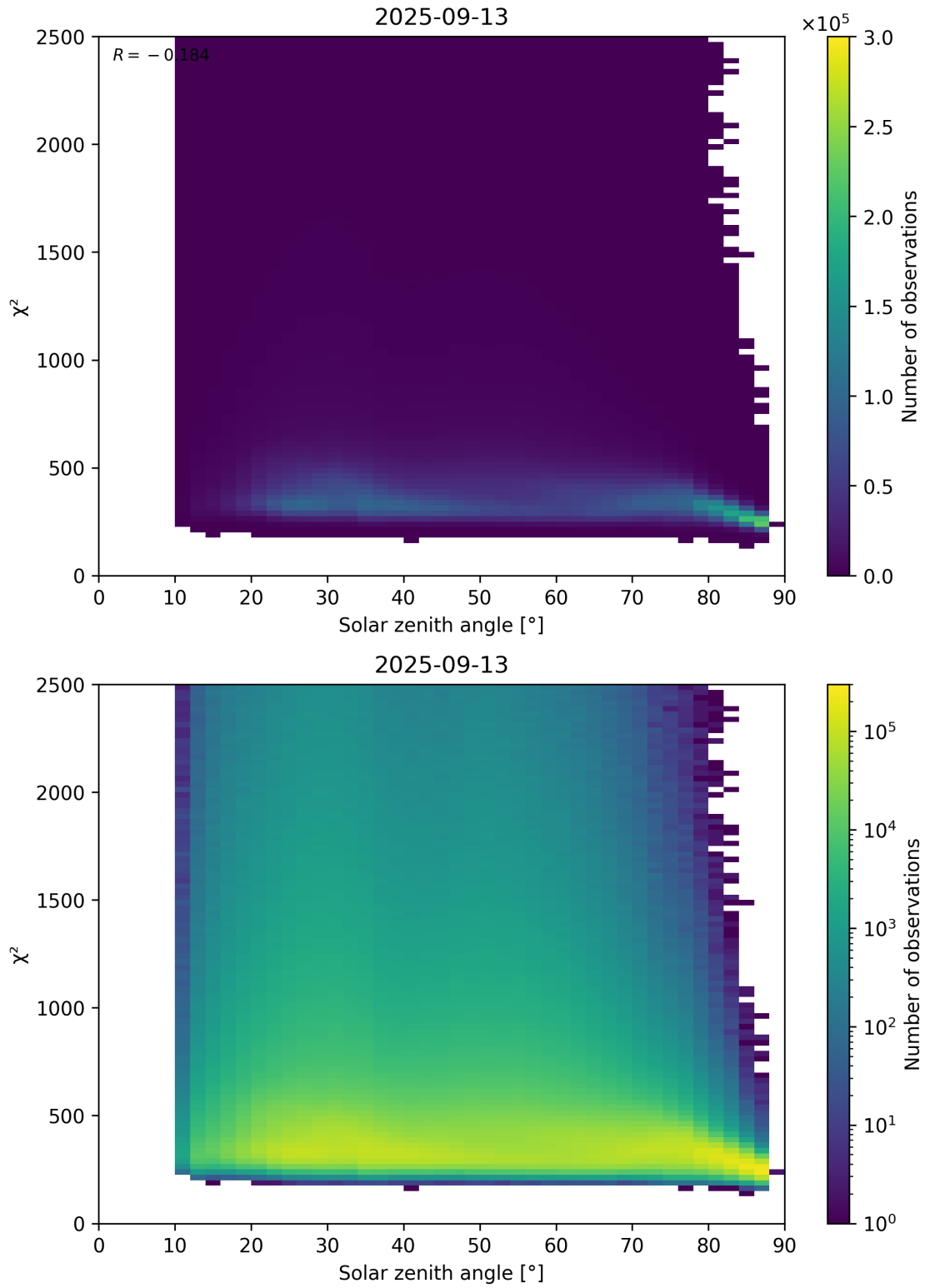
Figure 148: Scatter density plot of “Solar zenith angle” against “ \chi^2 ” for 2025-09-12 to 2025-09-14.
