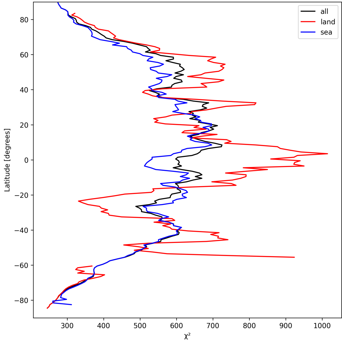
Figure 25: Zonal average of “ \chi^2 ” for 2025-09-12 to 2025-09-14.
