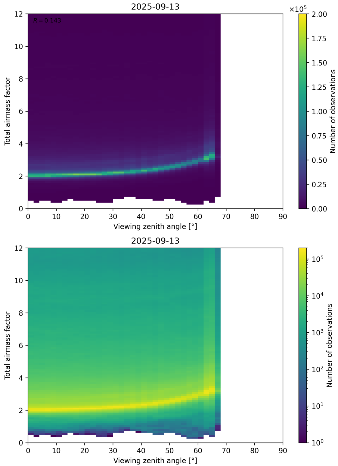
Figure 160: Scatter density plot of “Viewing zenith angle” against “Total airmass factor” for 2025-09-12 to 2025-09-14.
