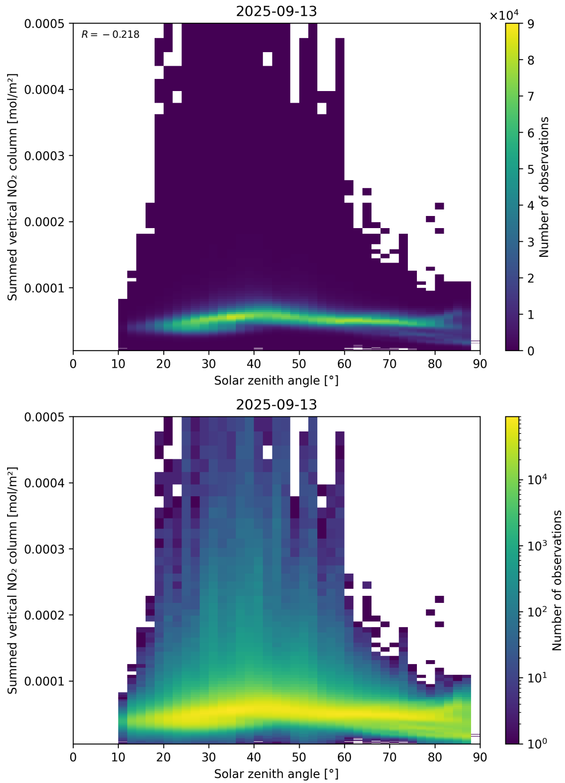
Figure 151: Scatter density plot of “Solar zenith angle” against “Summed vertical NO 2 column” for 2025-09-12 to 2025-09-14.
