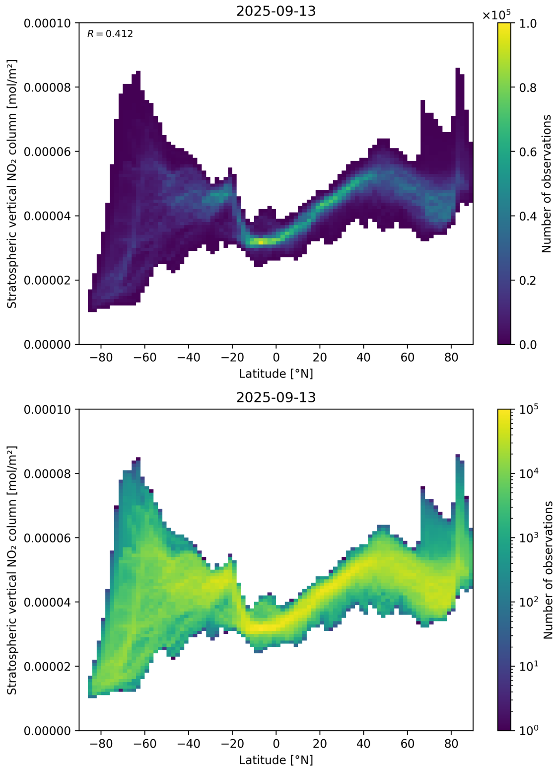
Figure 87: Scatter density plot of “Latitude” against “Stratospheric vertical NO 2 column” for 2025-09-12 to 2025-09-14.
