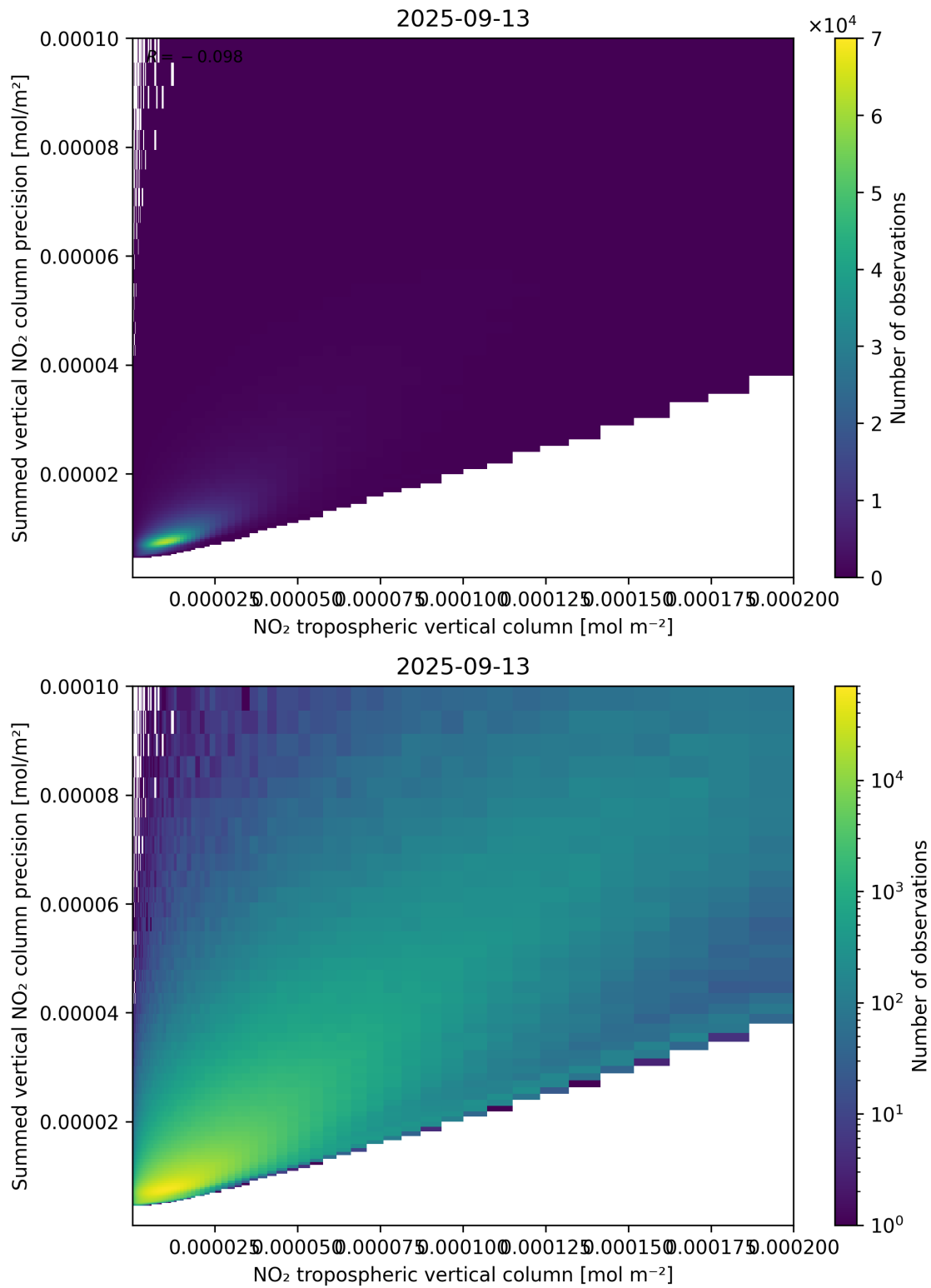
Figure 127: Scatter density plot of “NO 2 tropospheric vertical column” against “Summed vertical NO 2 column precision” for 2025-09-12 to 2025-09-14.
