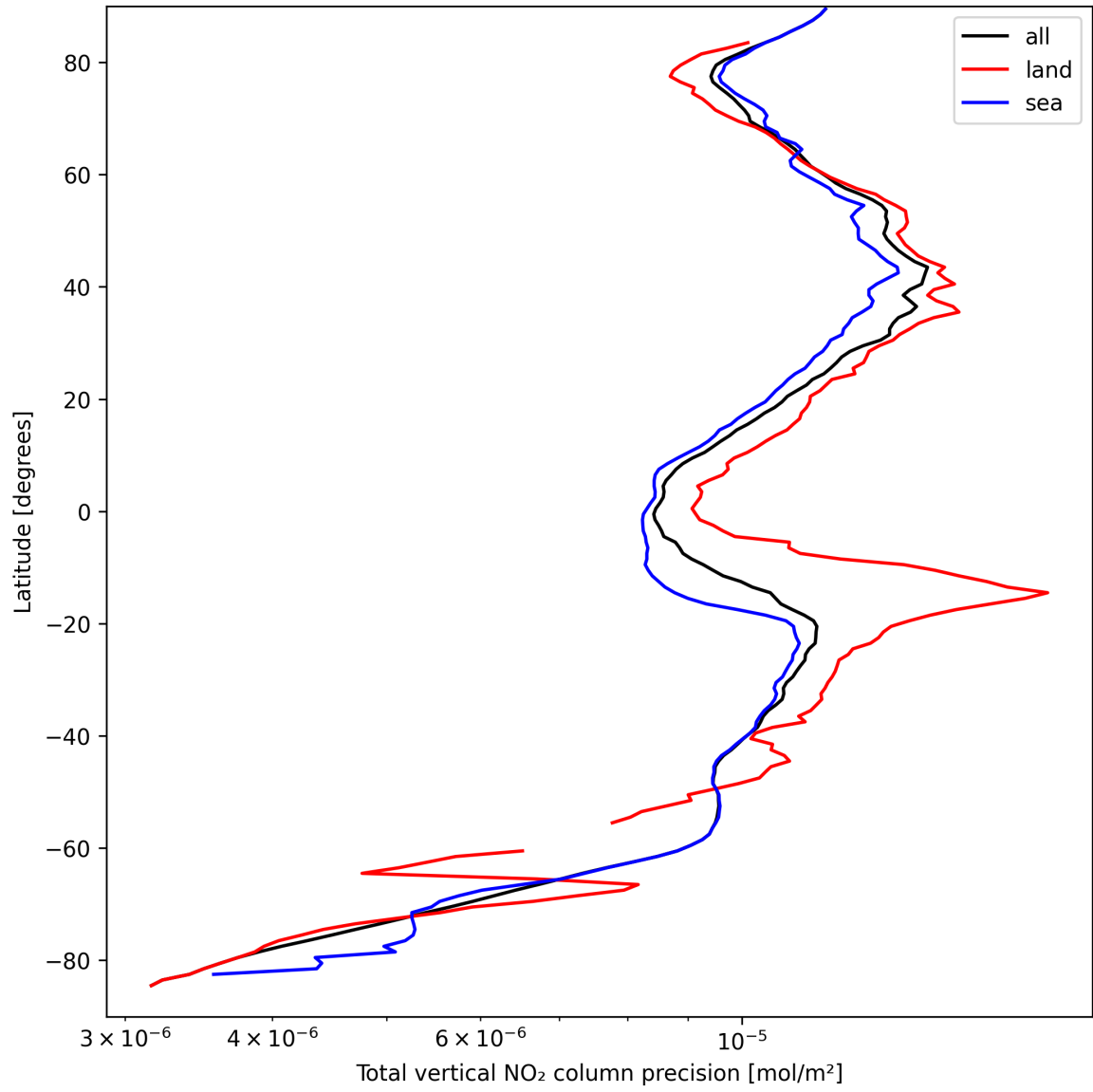
Figure 22: Zonal average of “Total vertical NO 2 column precision” for 2025-09-12 to 2025-09-14.
