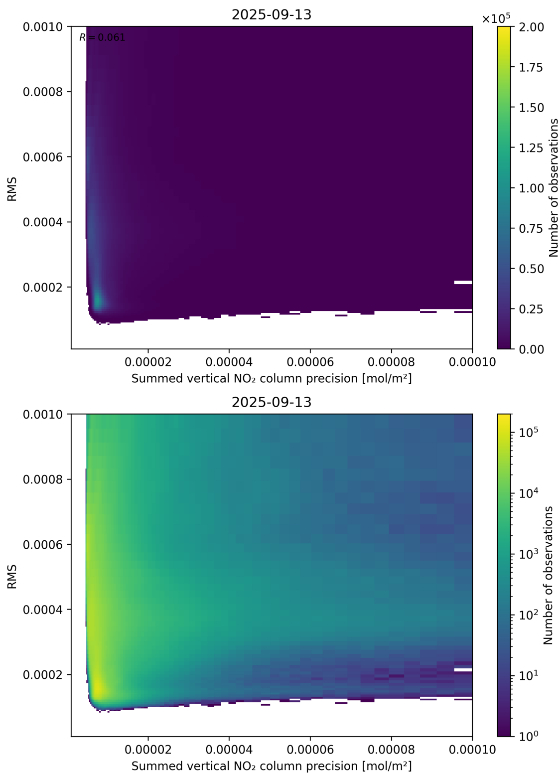
Figure 108: Scatter density plot of “Summed vertical NO 2 column precision” against “RMS” for 2025-09-12 to 2025-09-14.
