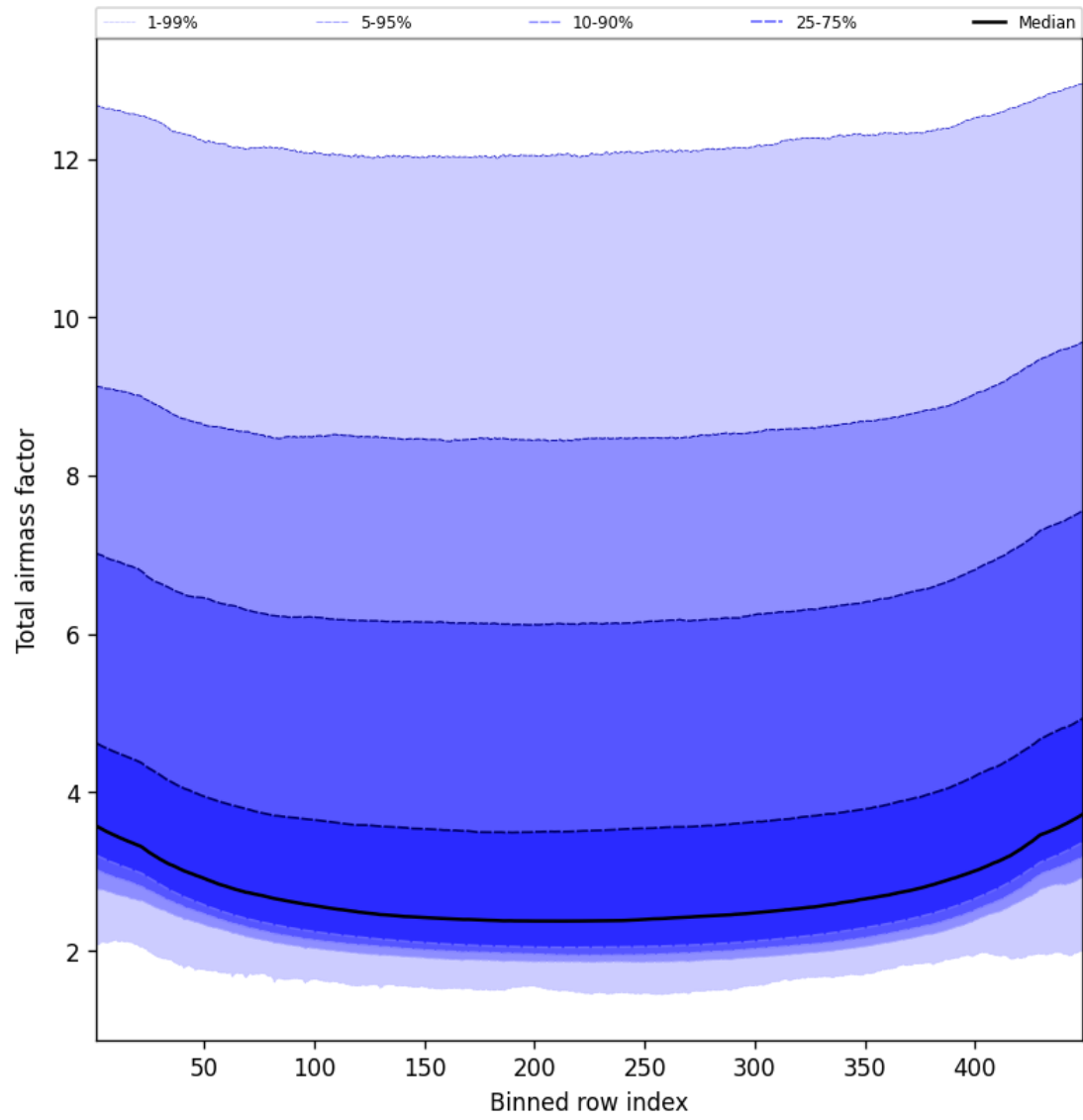
Figure 49: Along track statistics of “Total airmass factor” for 2025-09-12 to 2025-09-14
