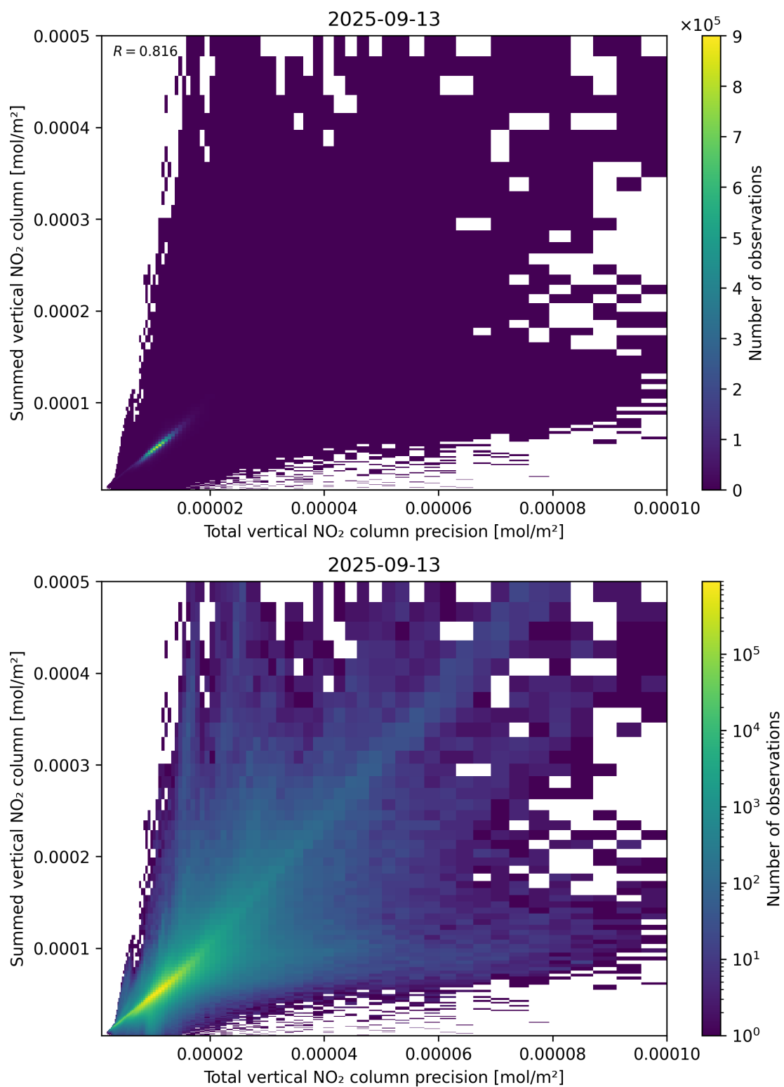
Figure 117: Scatter density plot of “Total vertical NO 2 column precision” against “Summed vertical NO 2 column” for 2025-09-12 to 2025-09-14.
