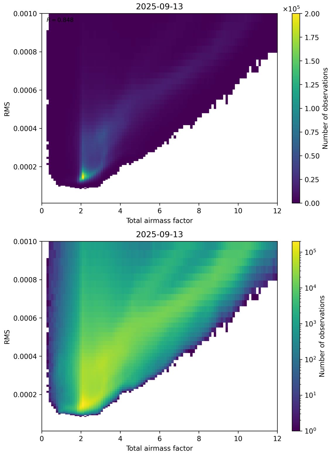
Figure 69: Scatter density plot of “Total airmass factor” against “RMS” for 2025-09-12 to 2025-09-14.
