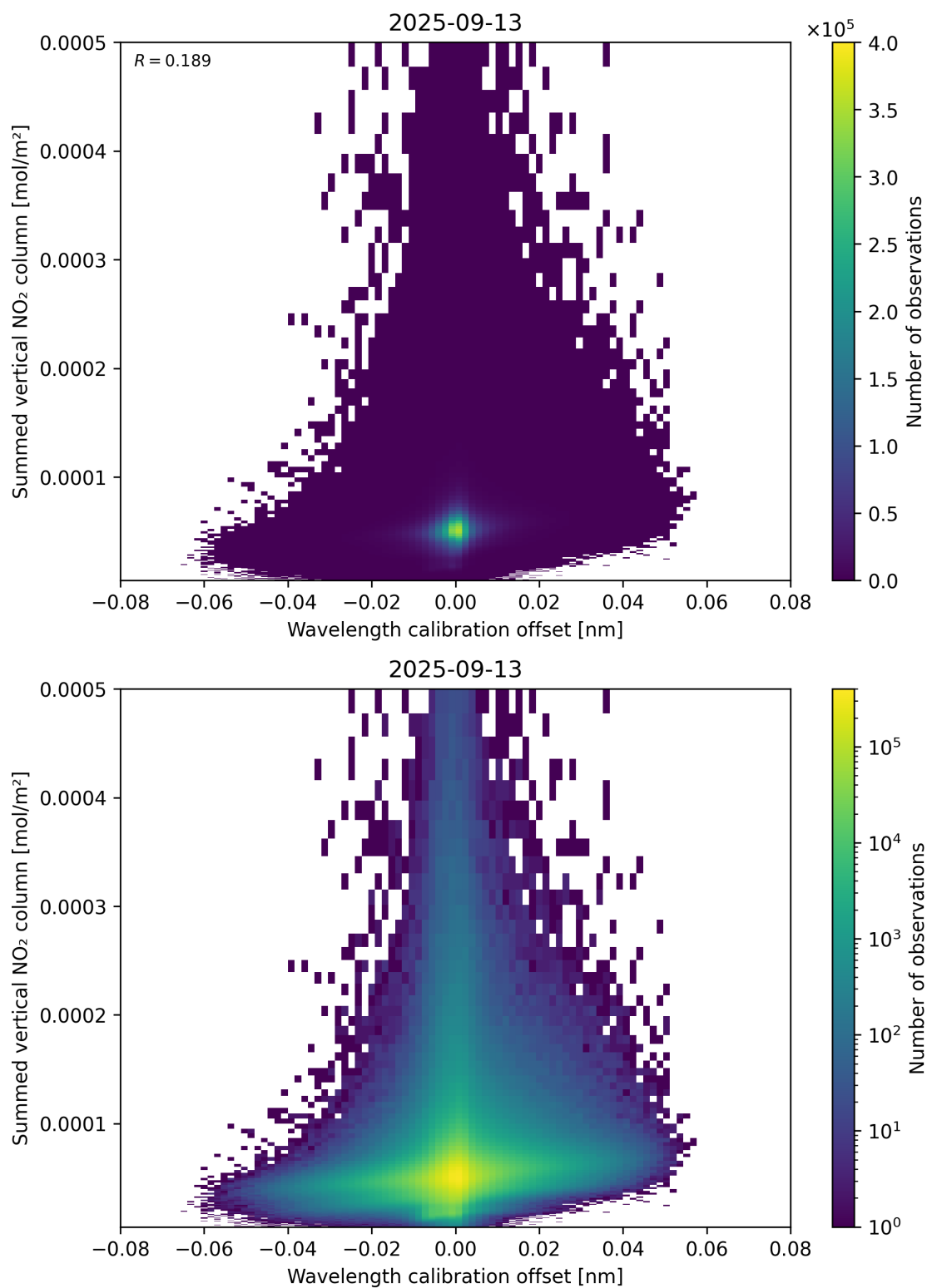
Figure 177: Scatter density plot of “Wavelength calibration offset” against “Summed vertical NO 2 column” for 2025-09-12 to 2025-09-14.
