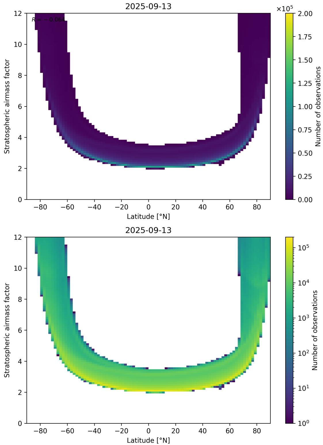
Figure 83: Scatter density plot of “Latitude” against “Stratospheric air mass factor” for 2025-09-12 to 2025-09-14.
