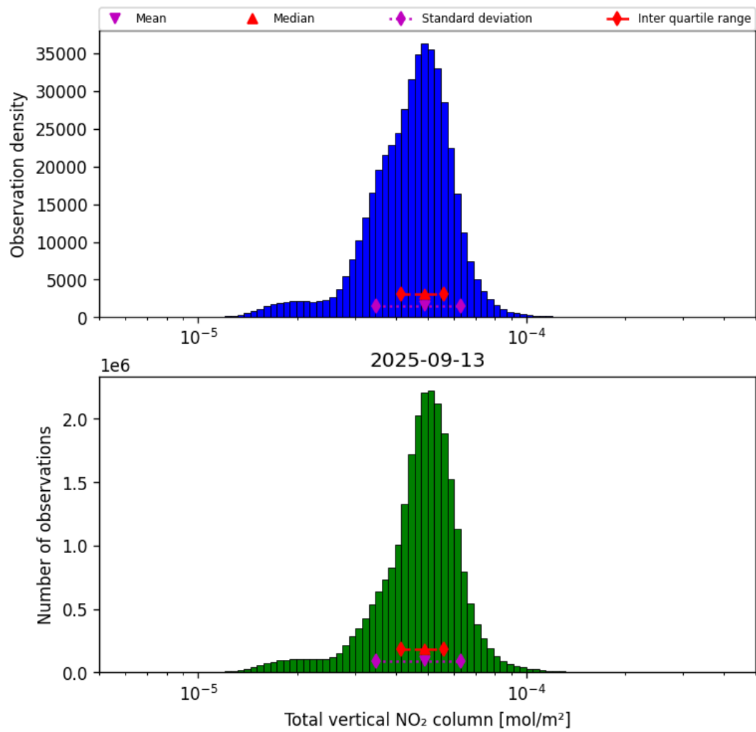
Figure 38: Histogram of “Total vertical NO 2 column” for 2025-09-12 to 2025-09-14
