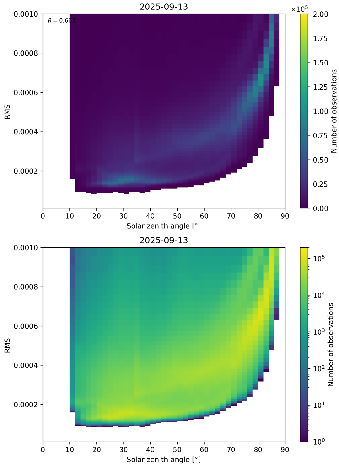
Figure 157: Scatter density plot of “Solar zenith angle” against “RMS” for 2025-09-12 to 2025-09-14.
