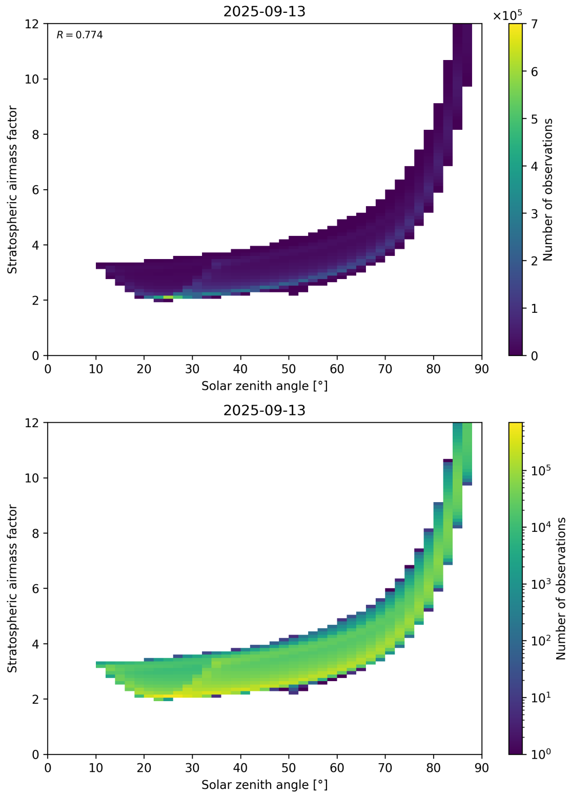
Figure 145: Scatter density plot of “Solar zenith angle” against “Stratospheric airmass factor” for 2025-09-12 to 2025-09-14.
