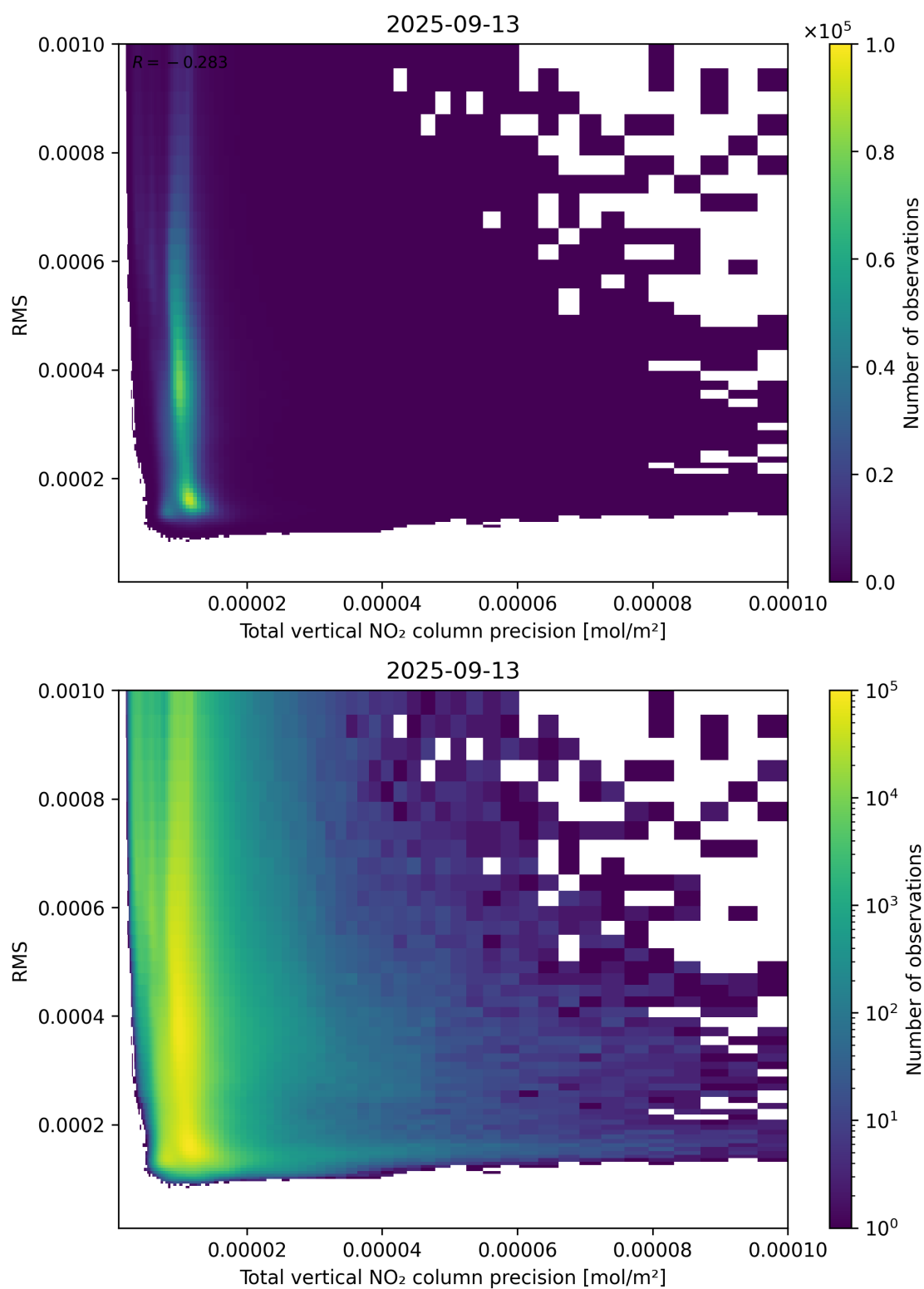
Figure 119: Scatter density plot of “Total vertical NO 2 column precision” against “RMS” for 2025-09-12 to 2025-09-14.
