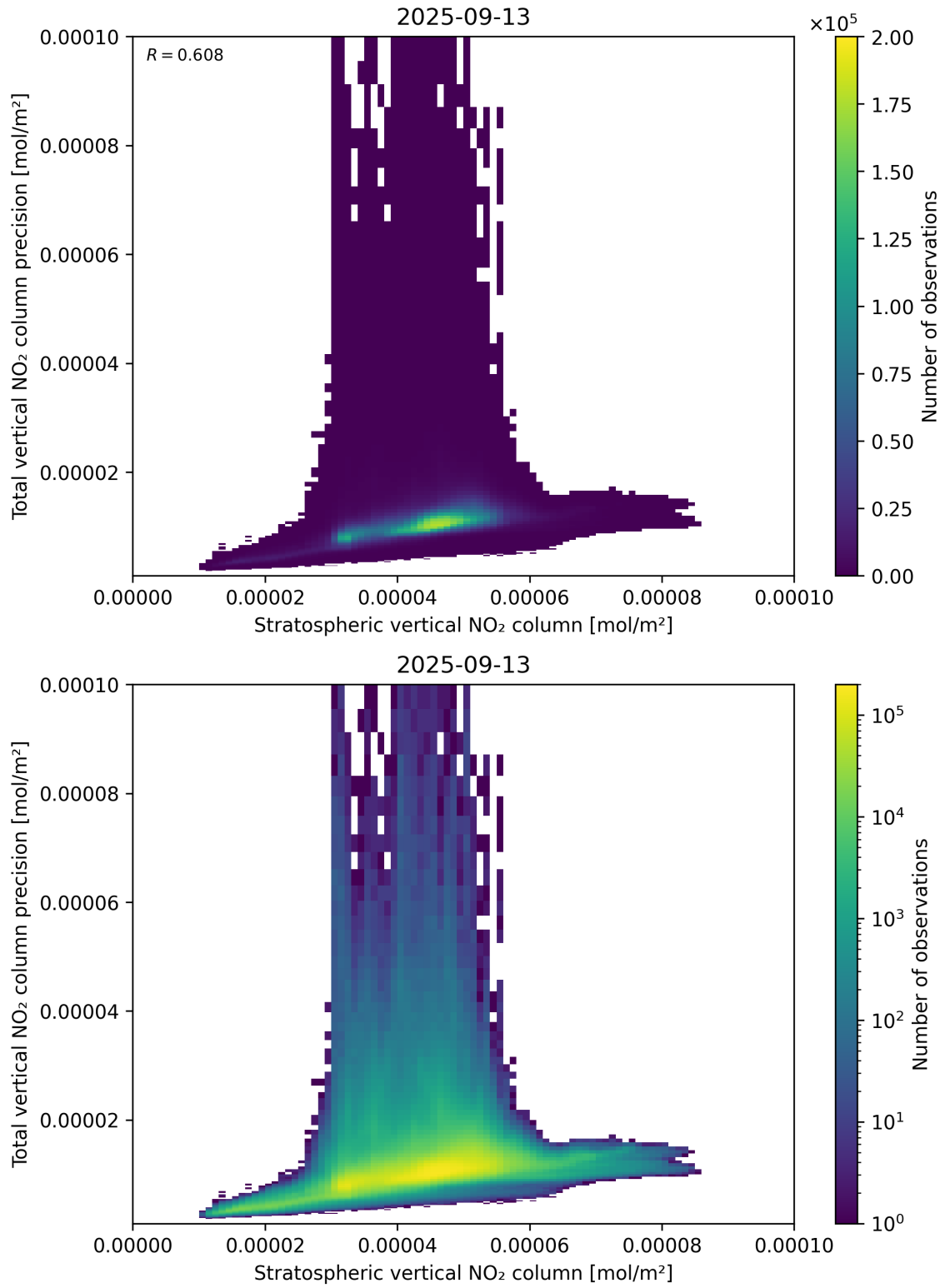
Figure 101: Scatter density plot of “Stratospheric vertical NO 2 column” against “Total vertical NO 2 column precision” for 2025-09-12 to 2025-09-14.
