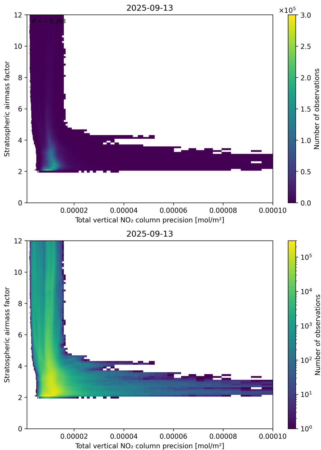
Figure 115: Scatter density plot of “Total vertical NO 2 column precision” against “Stratospheric air mass factor” for 2025-09-12 to 2025-09-14.
