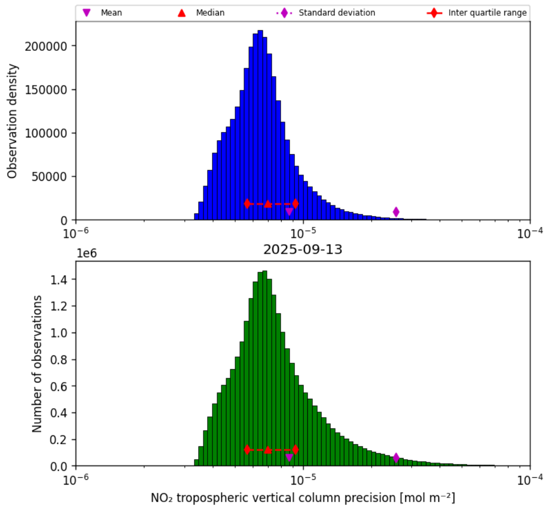
Figure 30: Histogram of “NO 2 tropospheric vertical column precision” for 2025-09-12 to 2025-09-14
