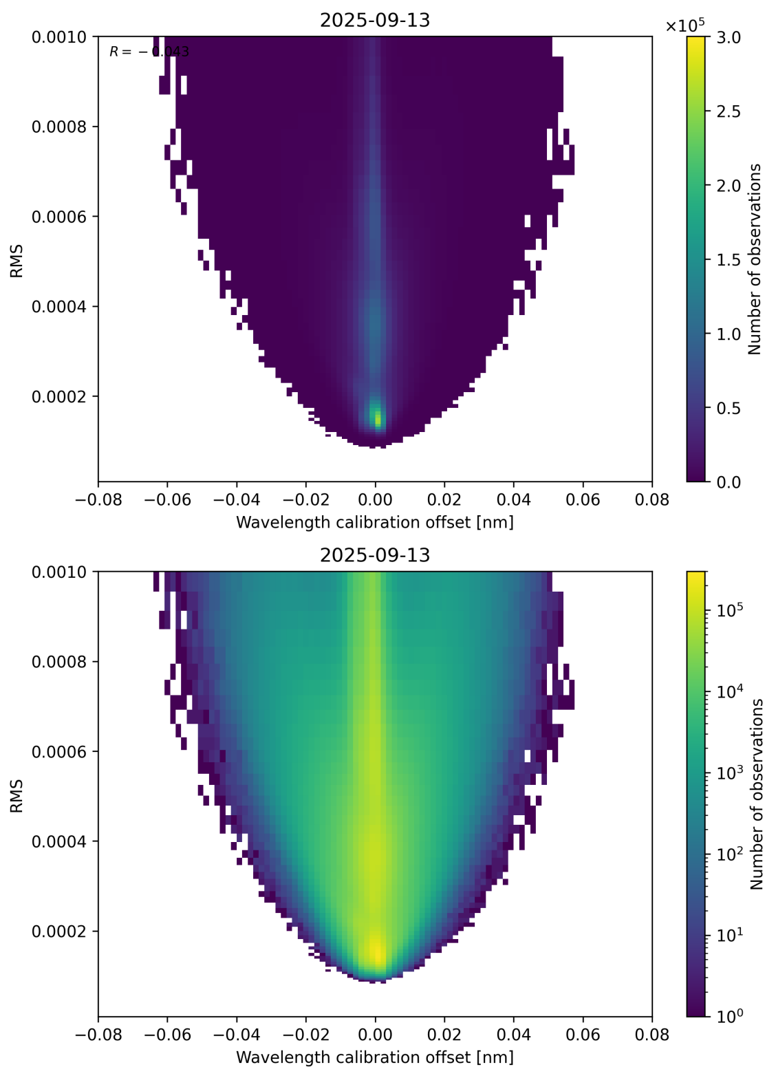
Figure 181: Scatter density plot of “Wavelength calibration offset” against “RMS” for 2025-09-12 to 2025-09-14.
