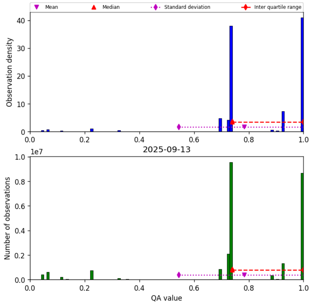
Figure 28: Histogram of “QA value” for 2025-09-12 to 2025-09-14
