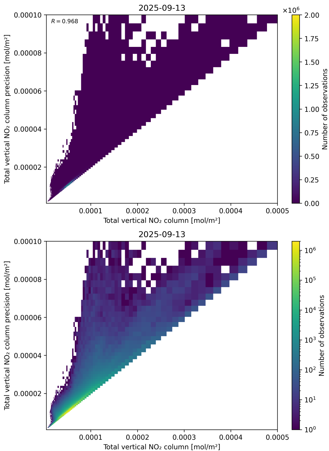
Figure 114: Scatter density plot of “Total vertical NO 2 column” against “Total vertical NO 2 column precision” for 2025-09-12 to 2025-09-14.
