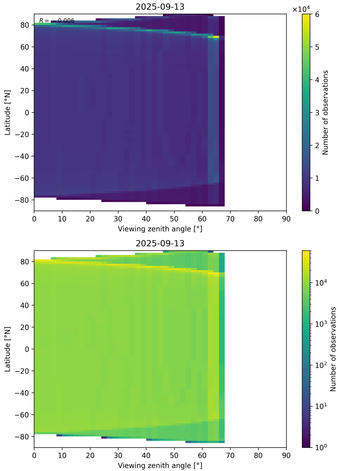
Figure 163: Scatter density plot of “Viewing zenith angle” against “Latitude” for 2025-09-12 to 2025-09-14.
