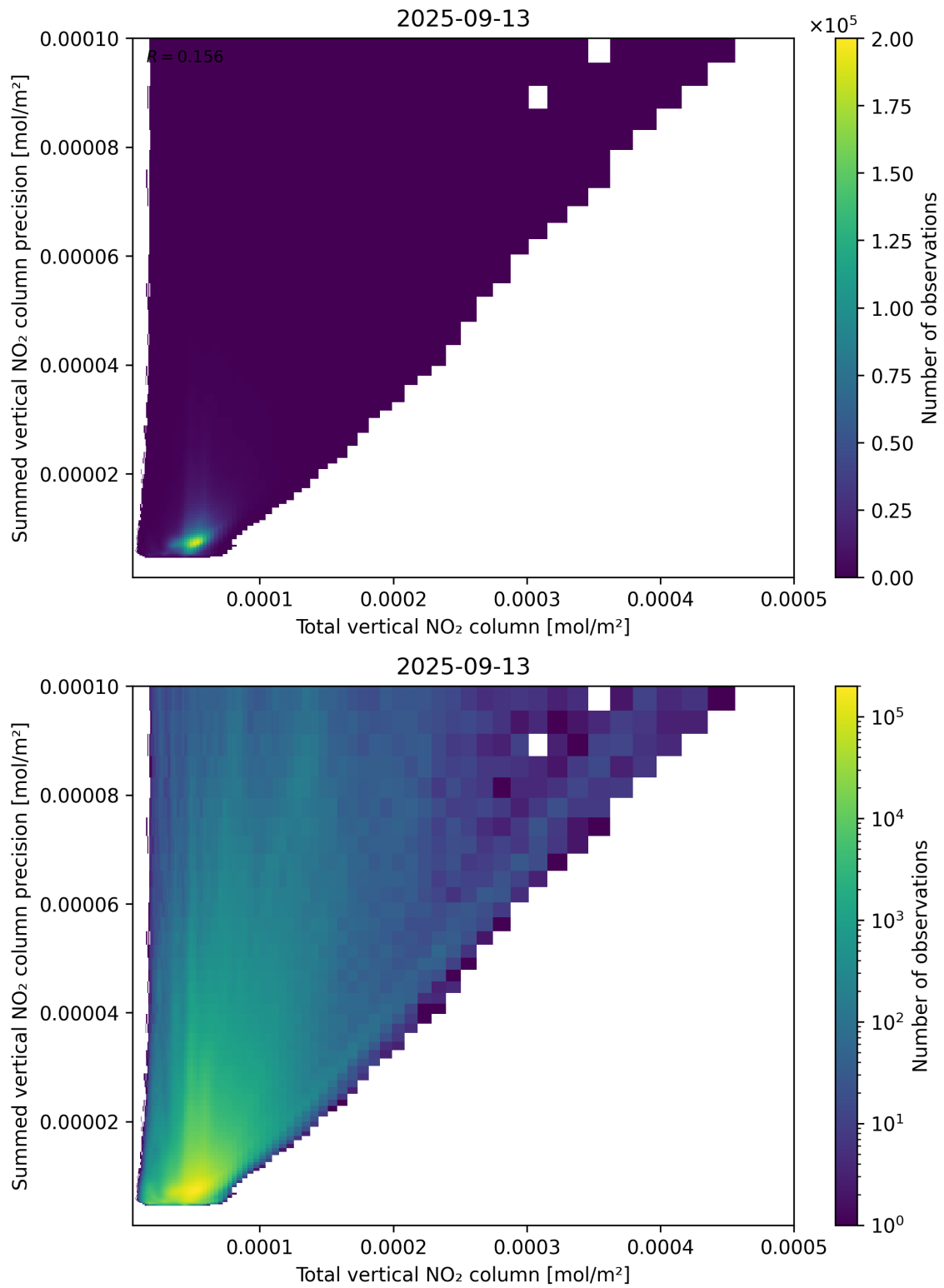
Figure 113: Scatter density plot of “Total vertical NO 2 column” against “Summed vertical NO 2 column precision” for 2025-09-12 to 2025-09-14.
