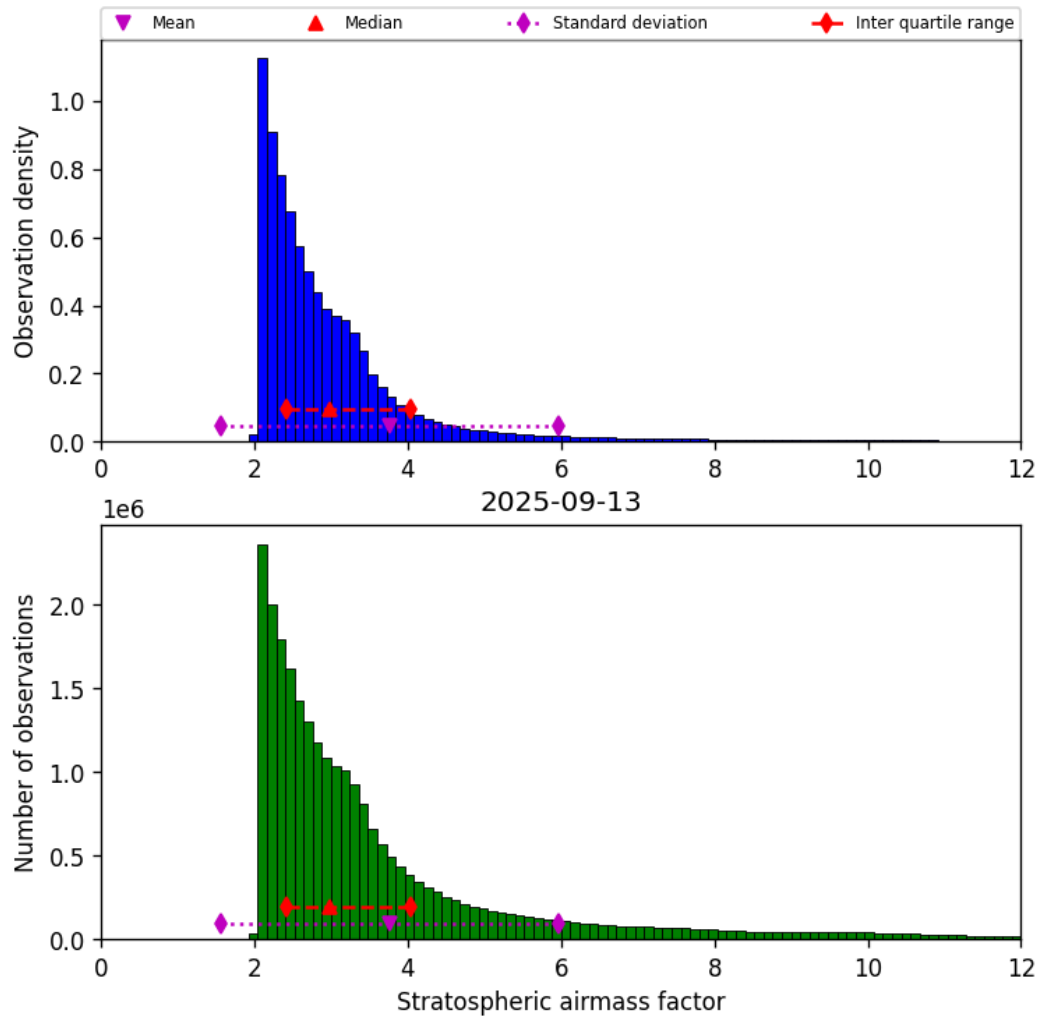
Figure 44: Histogram of “Stratospheric airmass factor” for 2025-09-12 to 2025-09-14
