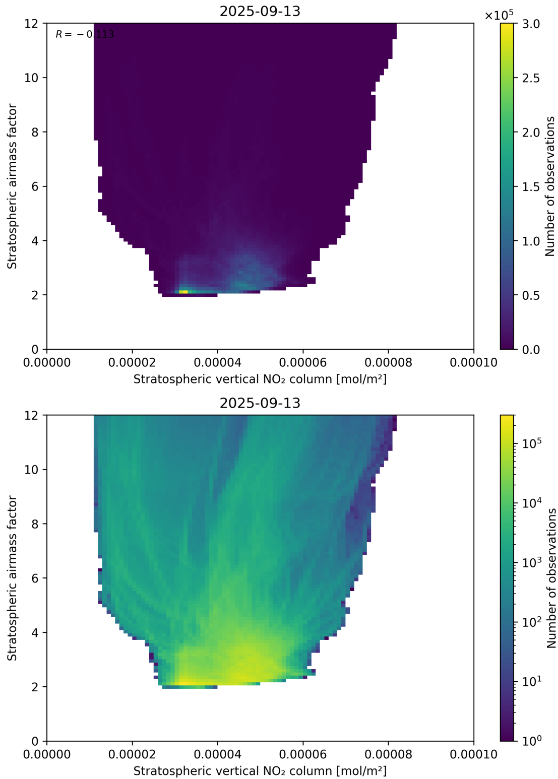
Figure 96: Scatter density plot of “Stratospheric vertical NO 2 column” against “Stratospheric airmass factor” for 2025-09-12 to 2025-09-14.
