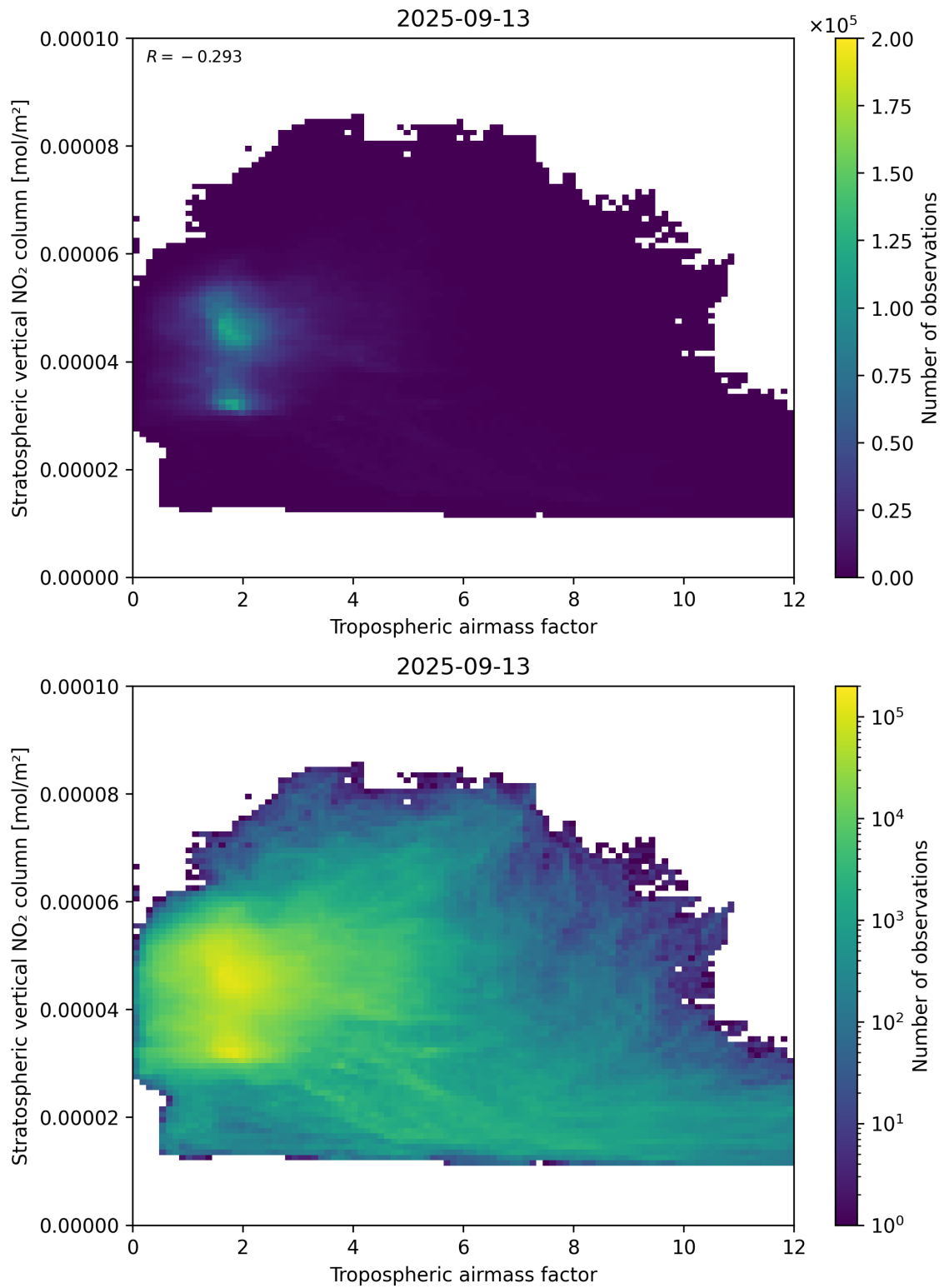
Figure 74: Scatter density plot of “Tropospheric airmass factor” against “Stratospheric vertical NO 2 column” for 2025-09-12 to 2025-09-14.
