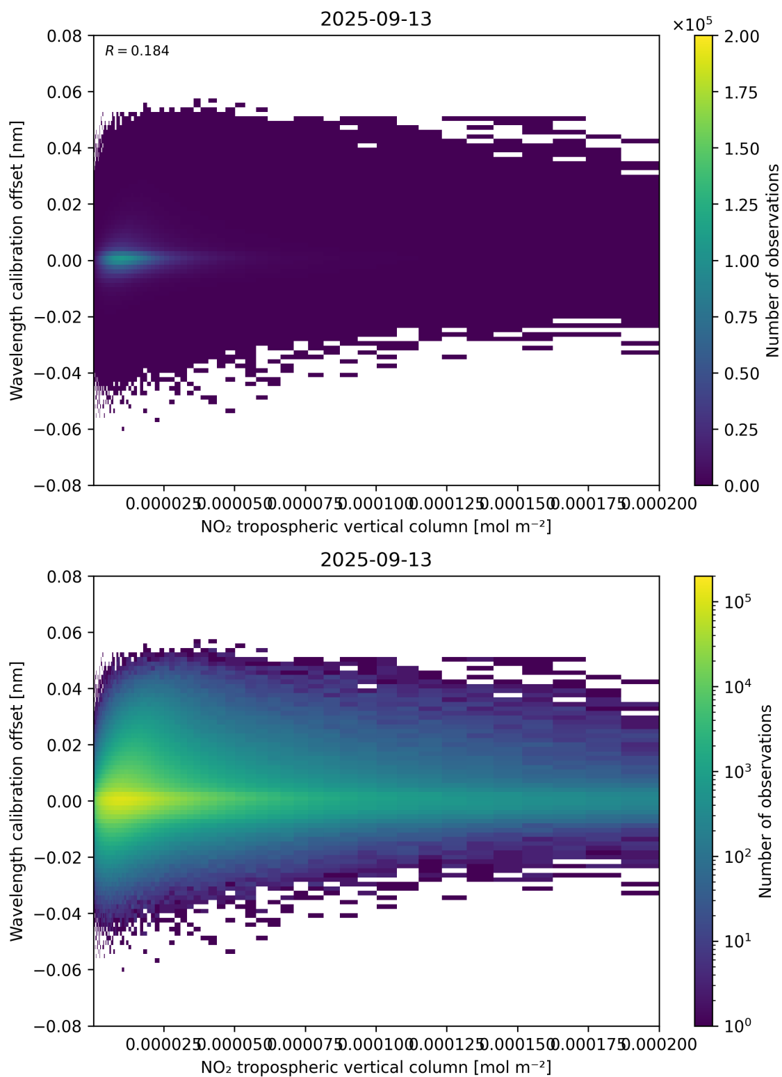
Figure 143: Scatter density plot of “NO 2 tropospheric vertical column” against “Wavelength calibration offset” for 2025-09-12 to 2025-09-14.
