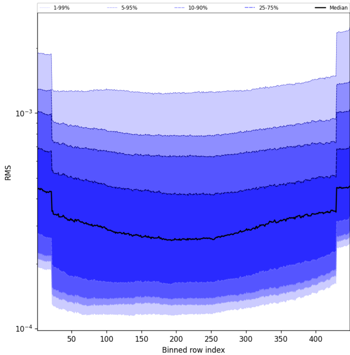
Figure 60: Along track statistics of “RMS” for 2025-09-12 to 2025-09-14
