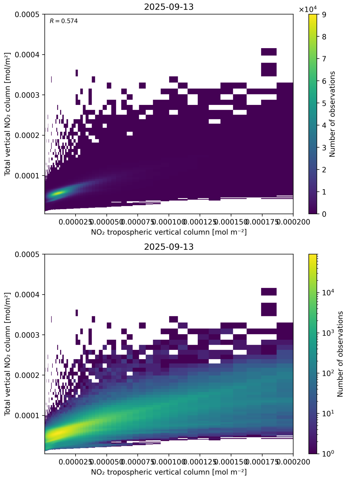
Figure 128: Scatter density plot of “NO 2 tropospheric vertical column” against “Total vertical NO 2 column” for 2025-09-12 to 2025-09-14.
