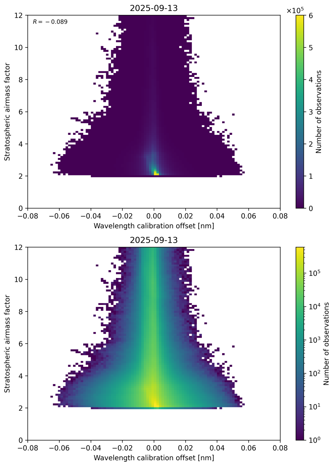
Figure 174: Scatter density plot of “Wavelength calibration offset” against “Stratospheric airmass factor” for 2025-09-12 to 2025-09-14.
