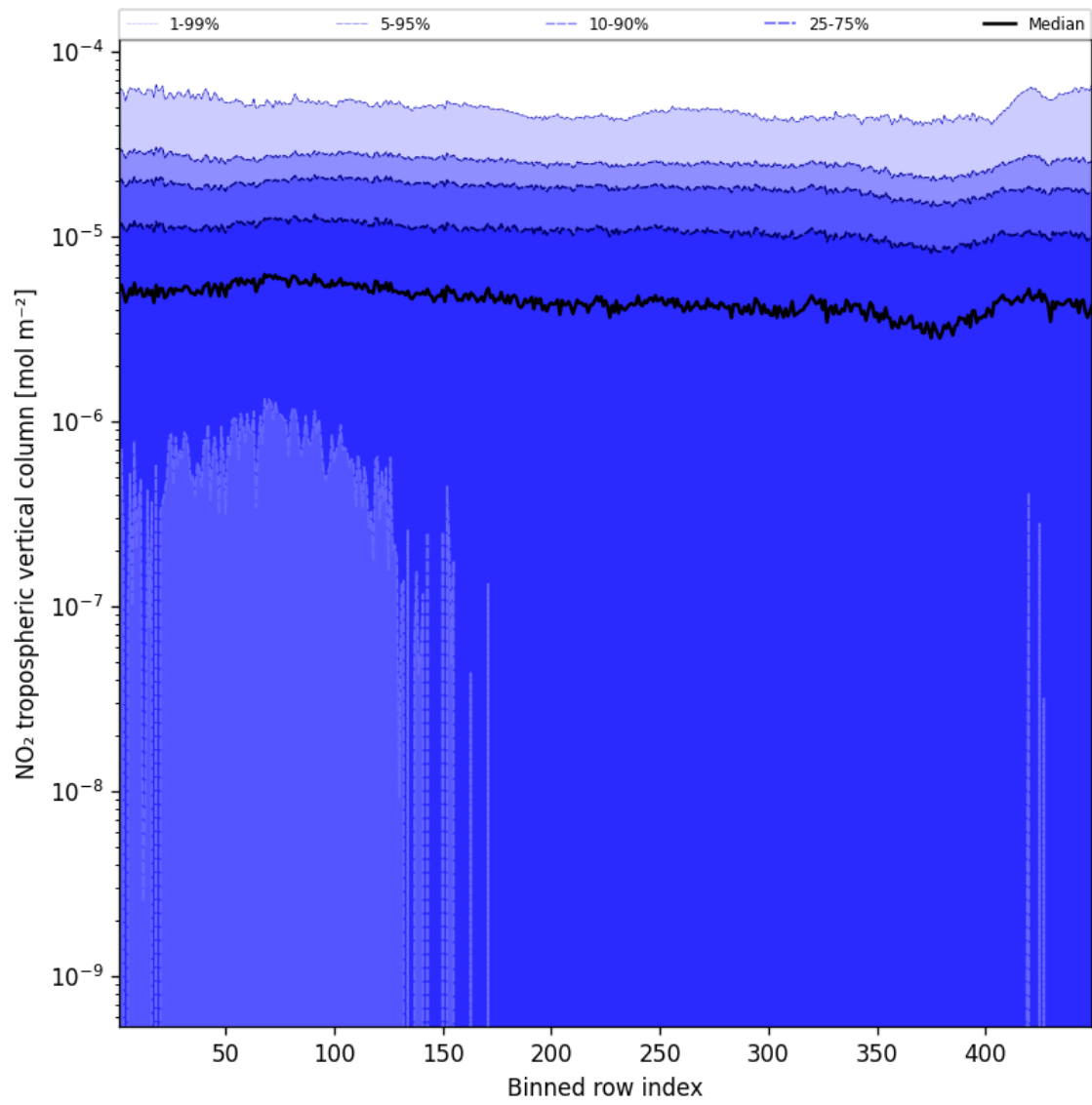
Figure 46: Along track statistics of “NO 2 tropospheric vertical column” for 2025-09-12 to 2025-09-14
