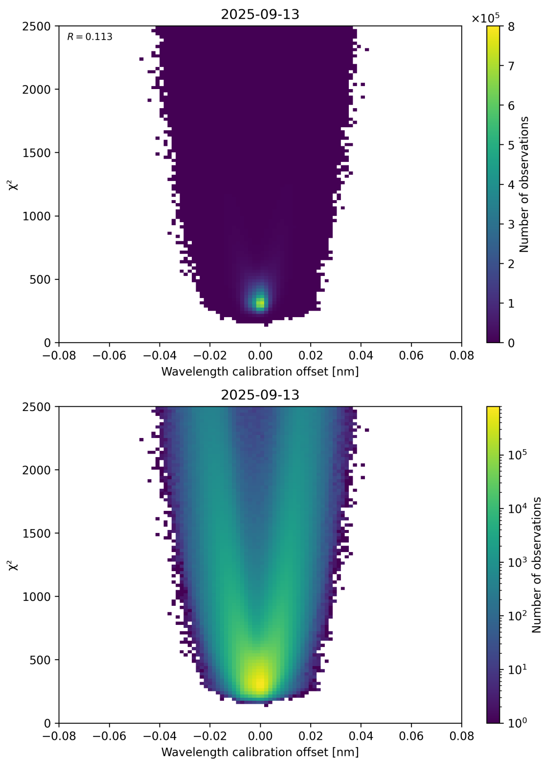
Figure 175: Scatter density plot of “Wavelength calibration offset” against “ \chi^2 ” for 2025-09-12 to 2025-09-14.
