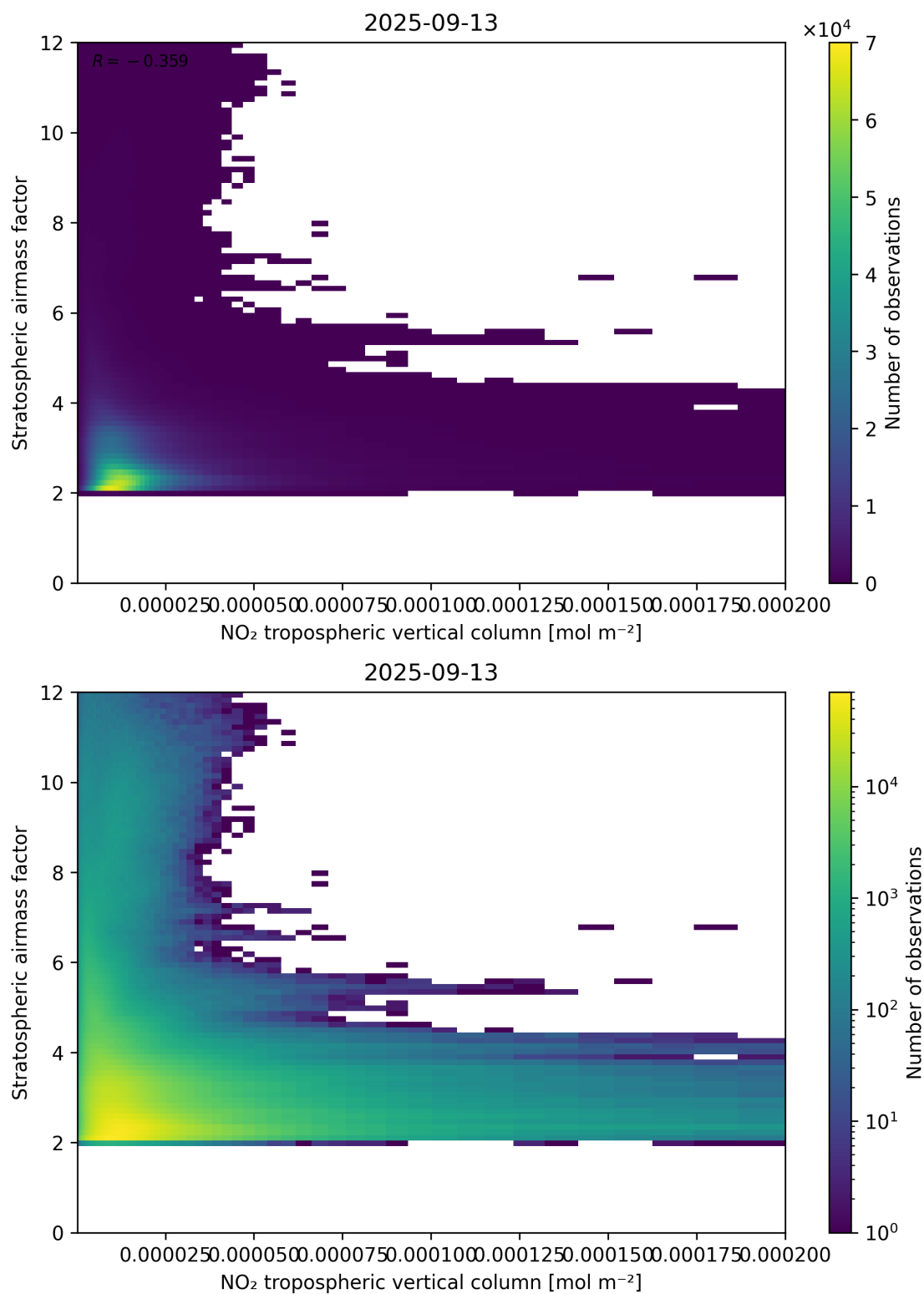
Figure 121: Scatter density plot of “NO 2 tropospheric vertical column” against “Stratospheric airmass factor” for 2025-09-12 to 2025-09-14.
