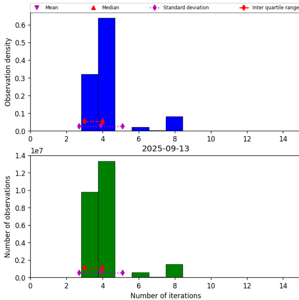
Figure 34: Histogram of “Number of iterations” for 2025-09-12 to 2025-09-14
