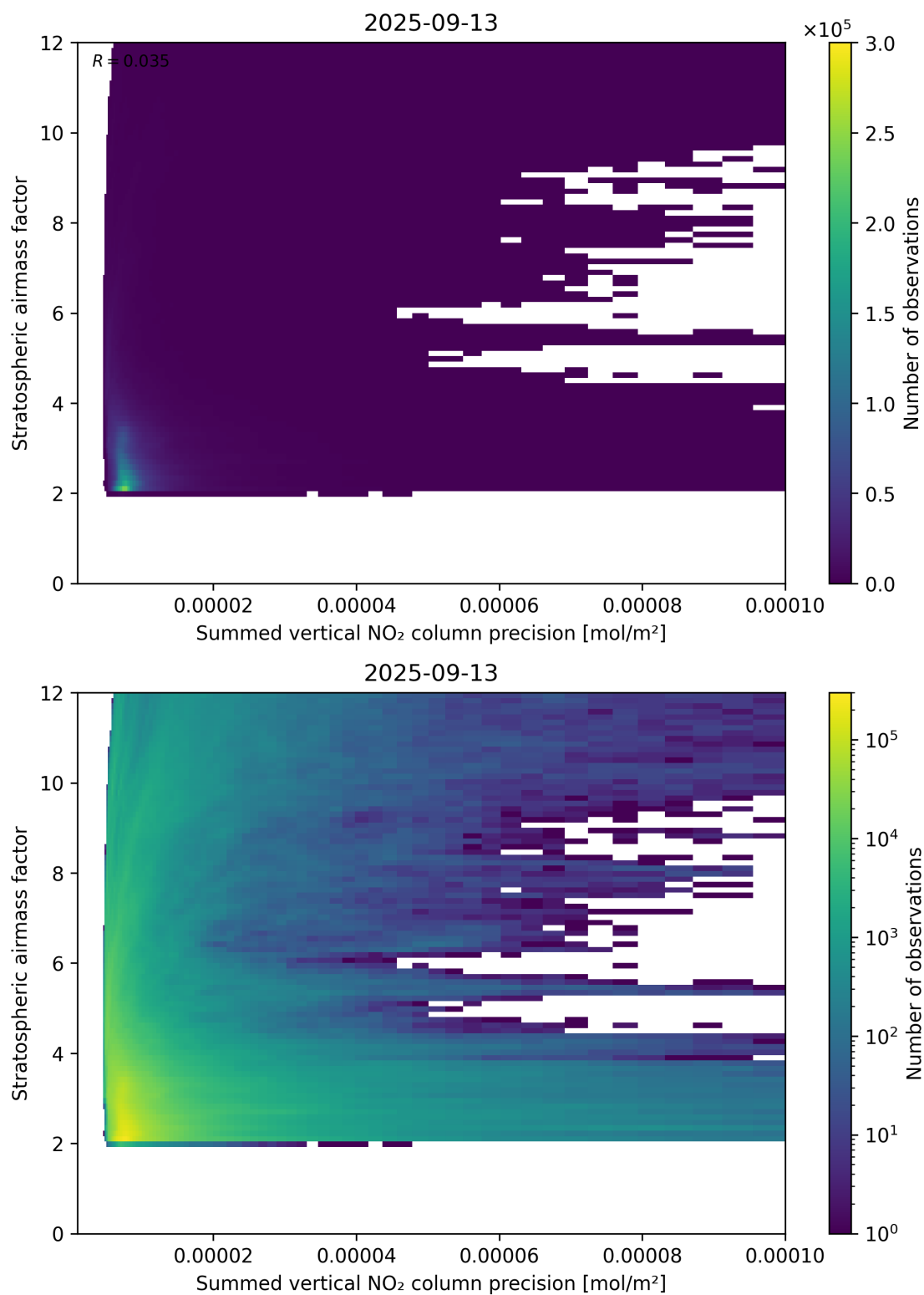
Figure 106: Scatter density plot of “Summed vertical NO 2 column precision” against “Stratospheric airmass factor” for 2025-09-12 to 2025-09-14.
