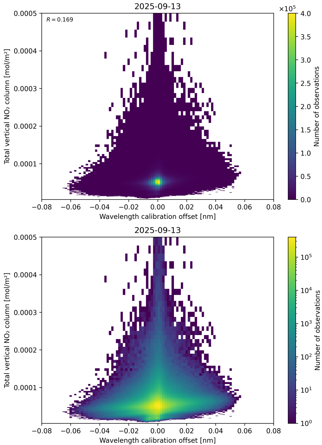
Figure 179: Scatter density plot of “Wavelength calibration offset” against “Total vertical NO 2 column” for 2025-09-12 to 2025-09-14.
