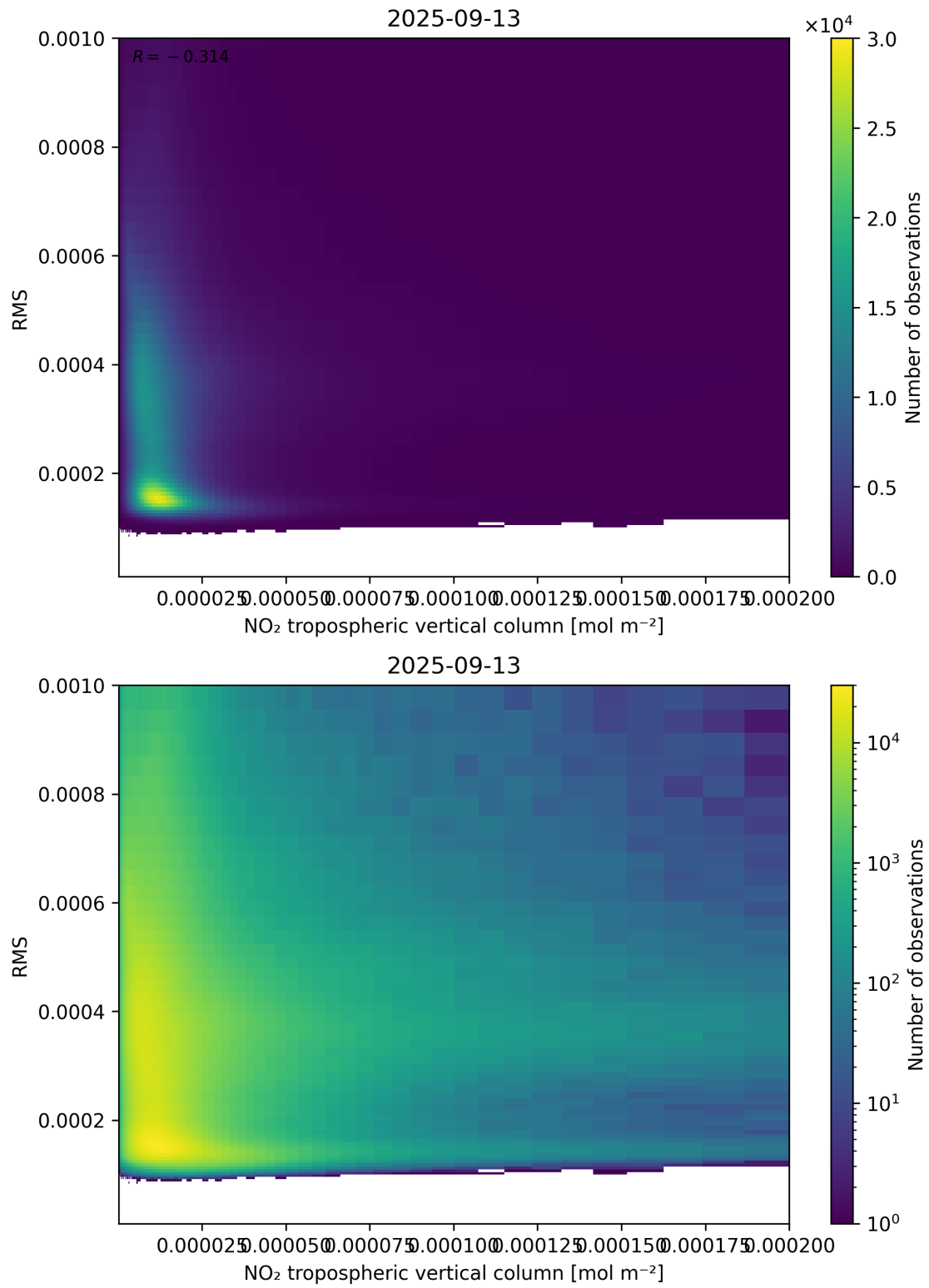
Figure 142: Scatter density plot of “NO 2 tropospheric vertical column” against “RMS” for 2025-09-12 to 2025-09-14.
