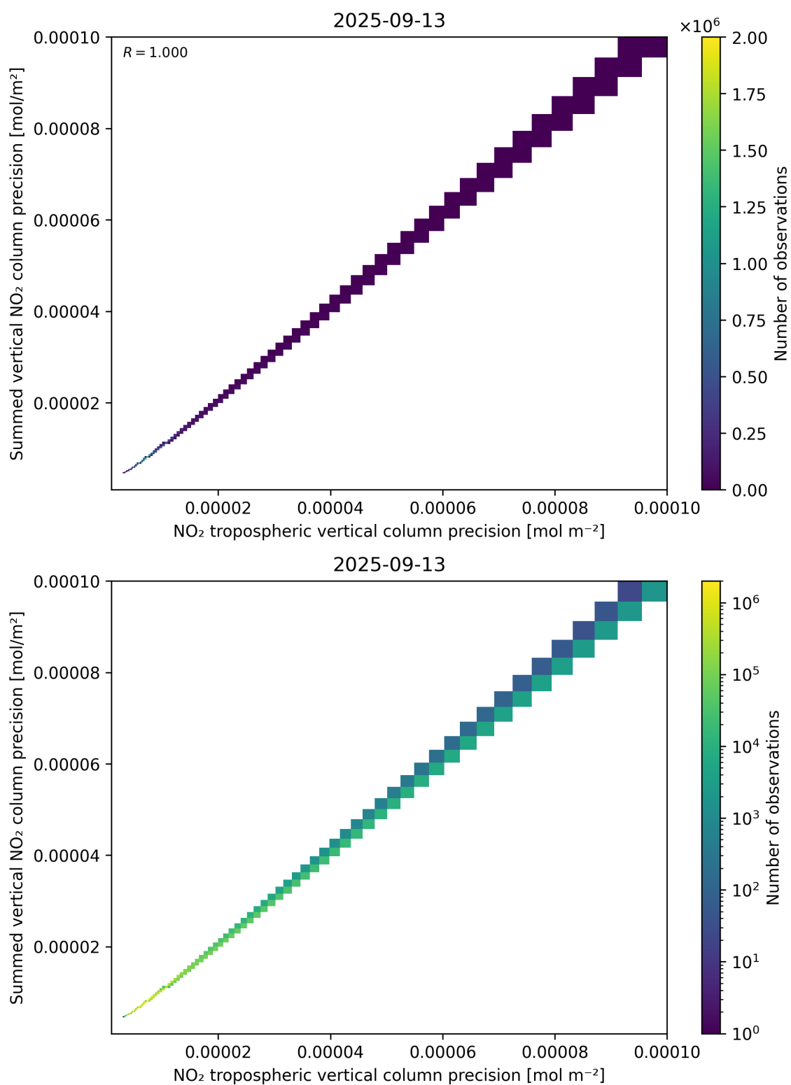
Figure 137: Scatter density plot of “NO 2 tropospheric vertical column precision” against “Summed vertical NO 2 column precision” for 2025-09-12 to 2025-09-14.
