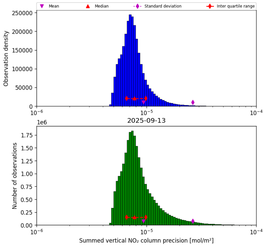
Figure 41: Histogram of “Summed vertical NO 2 column precision” for 2025-09-12 to 2025-09-14
