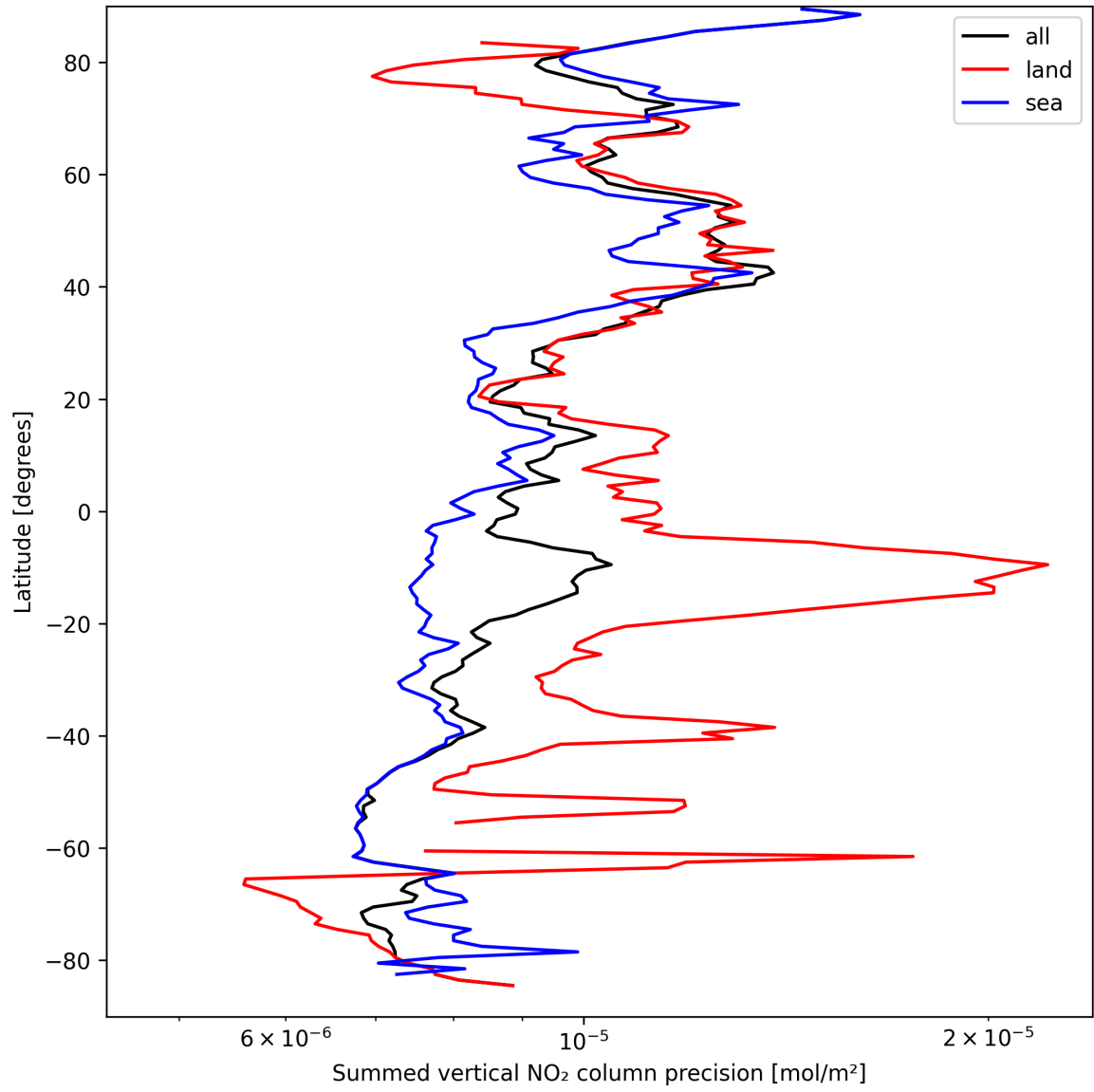
Figure 24: Zonal average of “Summed vertical NO 2 column precision” for 2025-09-12 to 2025-09-14.
