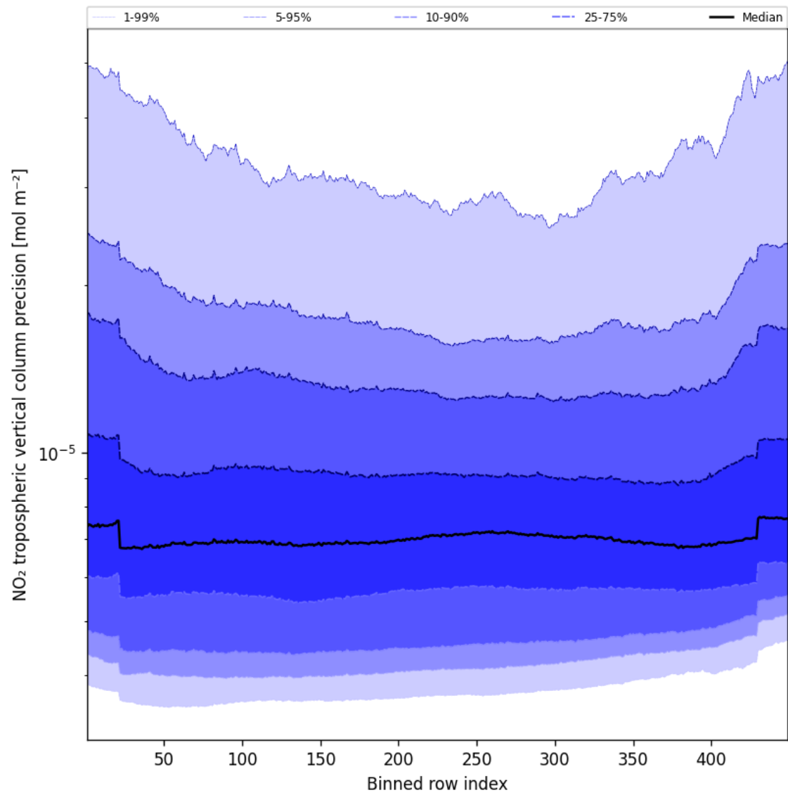
Figure 47: Along track statistics of “NO 2 tropospheric vertical column precision” for 2025-09-12 to 2025-09-14
