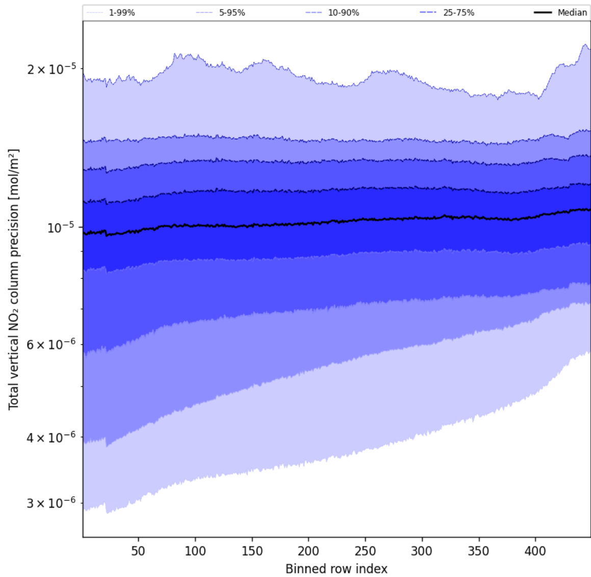
Figure 56: Along track statistics of “Total vertical NO 2 column precision” for 2025-09-12 to 2025-09-14
