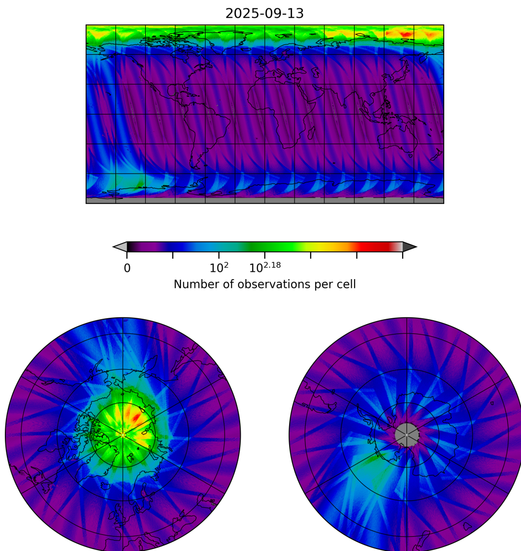
Figure 10: Map of the number of observations for 2025-09-12 to 2025-09-14
