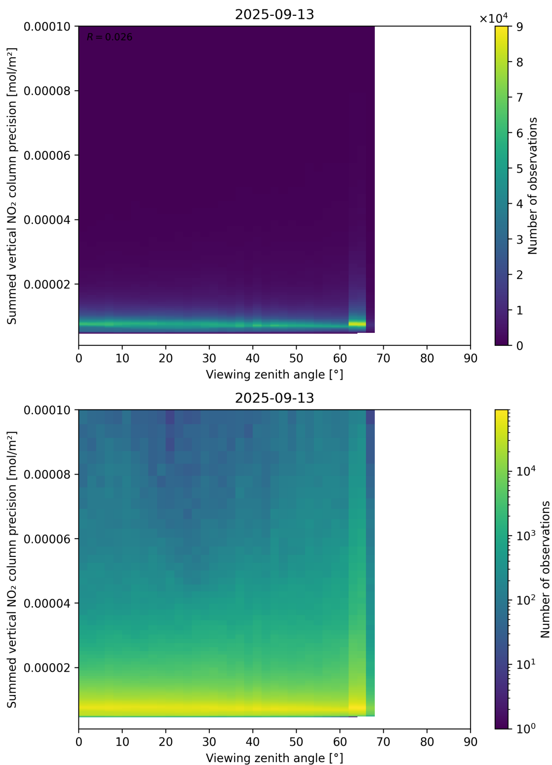
Figure 166: Scatter density plot of “Viewing zenith angle” against “Summed vertical NO 2 column precision” for 2025-09-12 to 2025-09-14.
