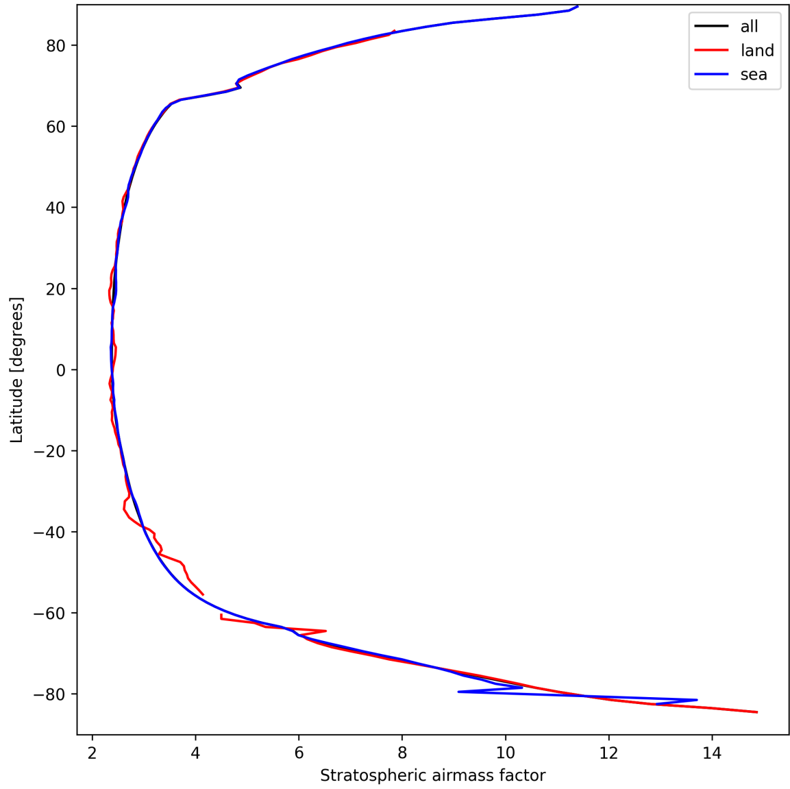
Figure 27: Zonal average of “Stratospheric air mass factor” for 2025-09-12 to 2025-09-14.
