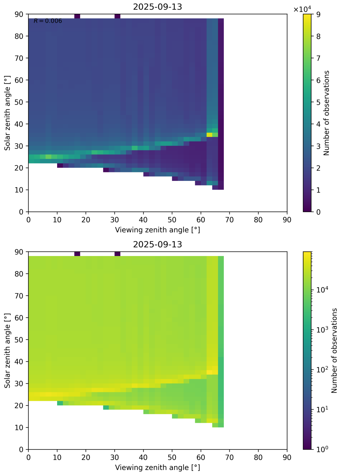
Figure 172: Scatter density plot of “Viewing zenith angle” against “Solar zenith angle” for 2025-09-12 to 2025-09-14.
