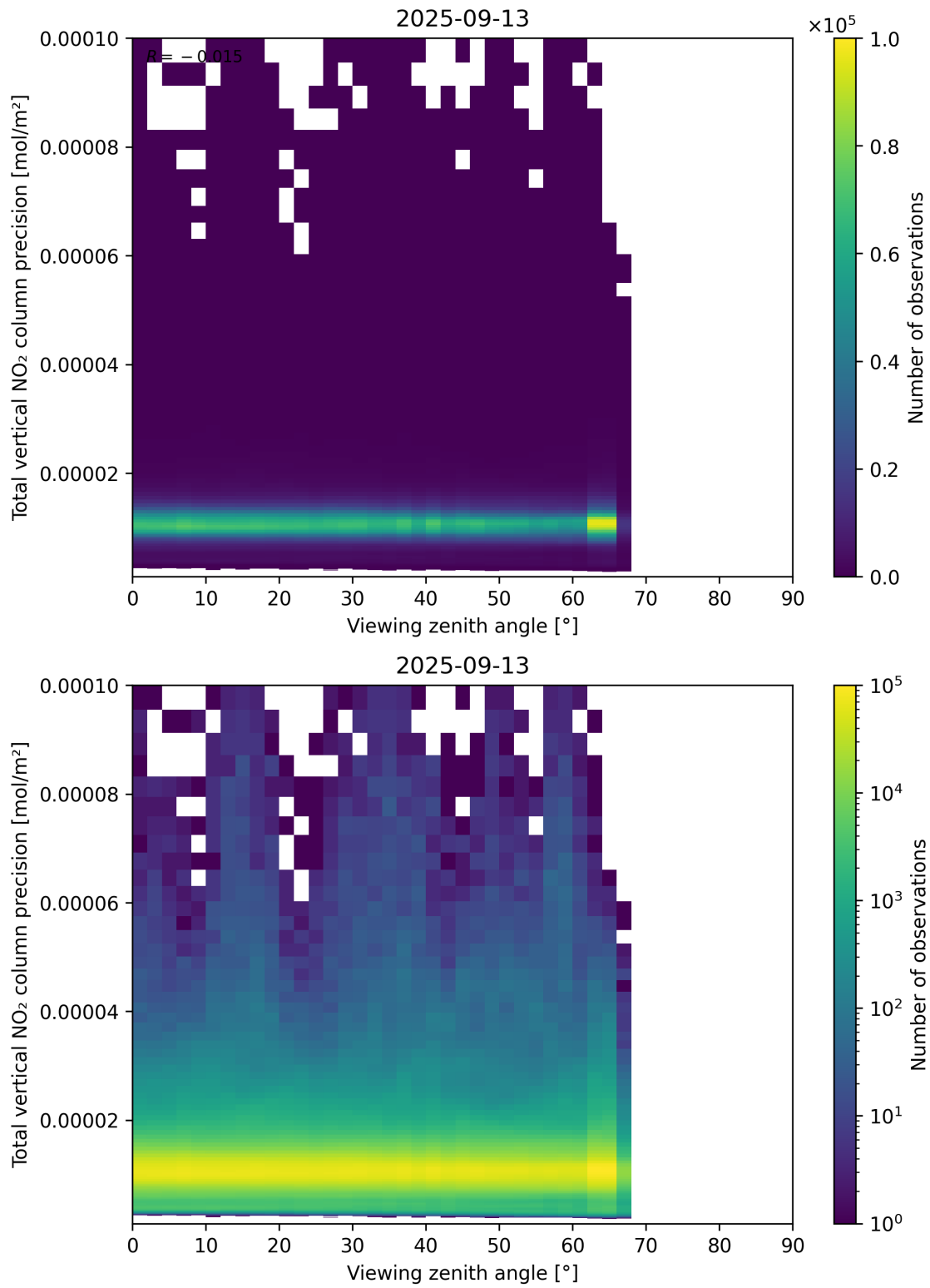
Figure 168: Scatter density plot of “Viewing zenith angle” against “Total vertical NO 2 column precision” for 2025-09-12 to 2025-09-14.
