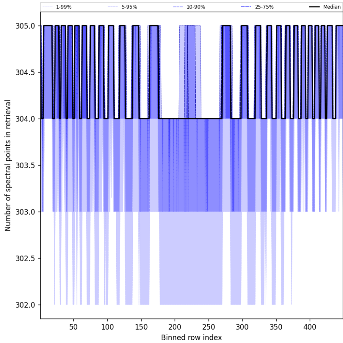
Figure 50: Along track statistics of “Number of spectral points in retrieval” for 2025-09-12 to 2025-09-14
