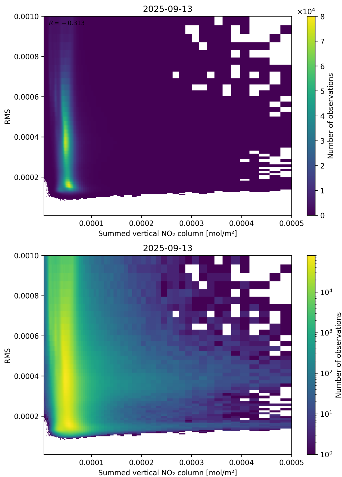
Figure 109: Scatter density plot of “Summed vertical NO 2 column” against “RMS” for 2025-09-12 to 2025-09-14.
