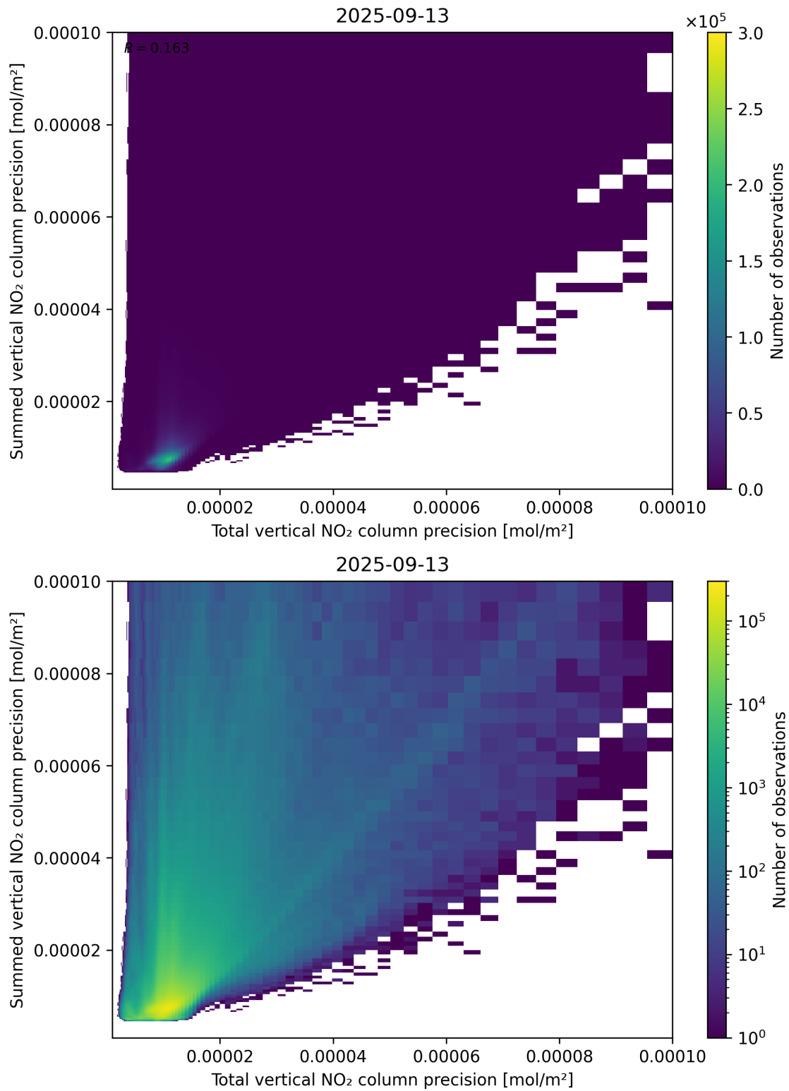
Figure 118: Scatter density plot of “Total vertical NO 2 column precision” against “Summed vertical NO 2 column precision” for 2025-09-12 to 2025-09-14.
