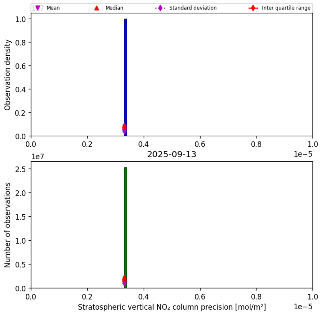
Figure 37: Histogram of “Stratospheric vertical NO 2 column precision” for 2025-09-12 to 2025-09-14
