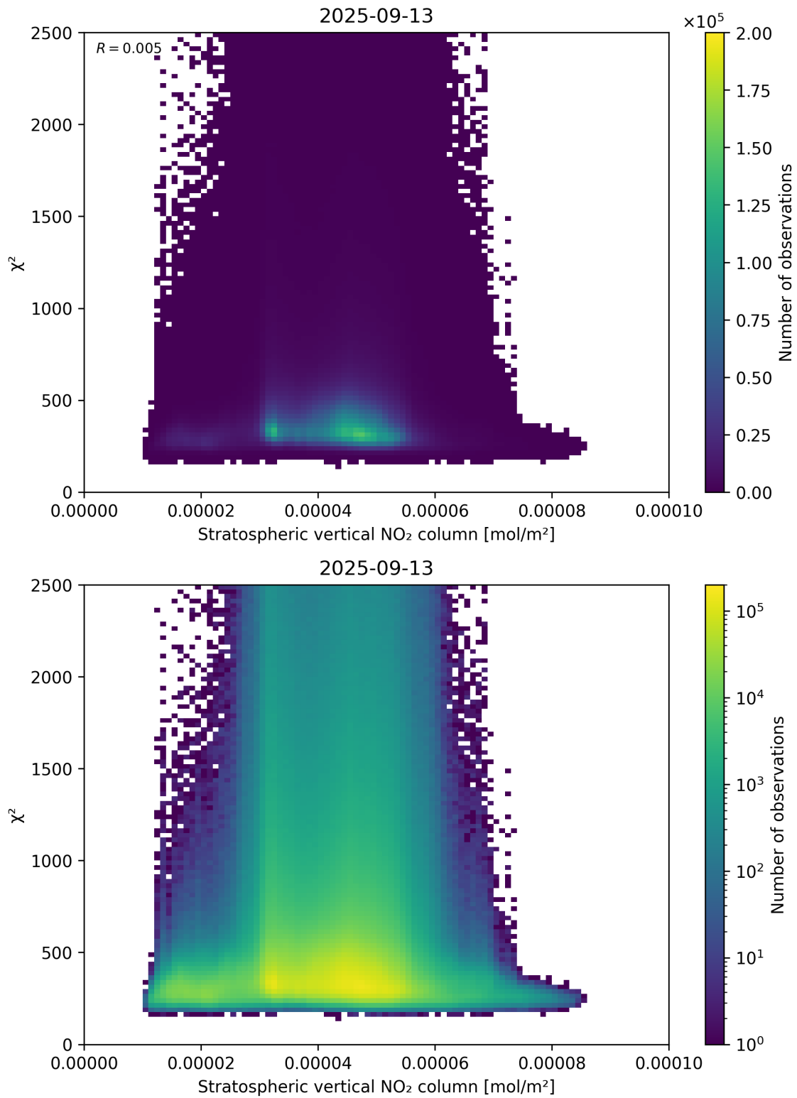
Figure 97: Scatter density plot of “Stratospheric vertical NO 2 column” against “ \chi^2 ” for 2025-09-12 to 2025-09-14.
