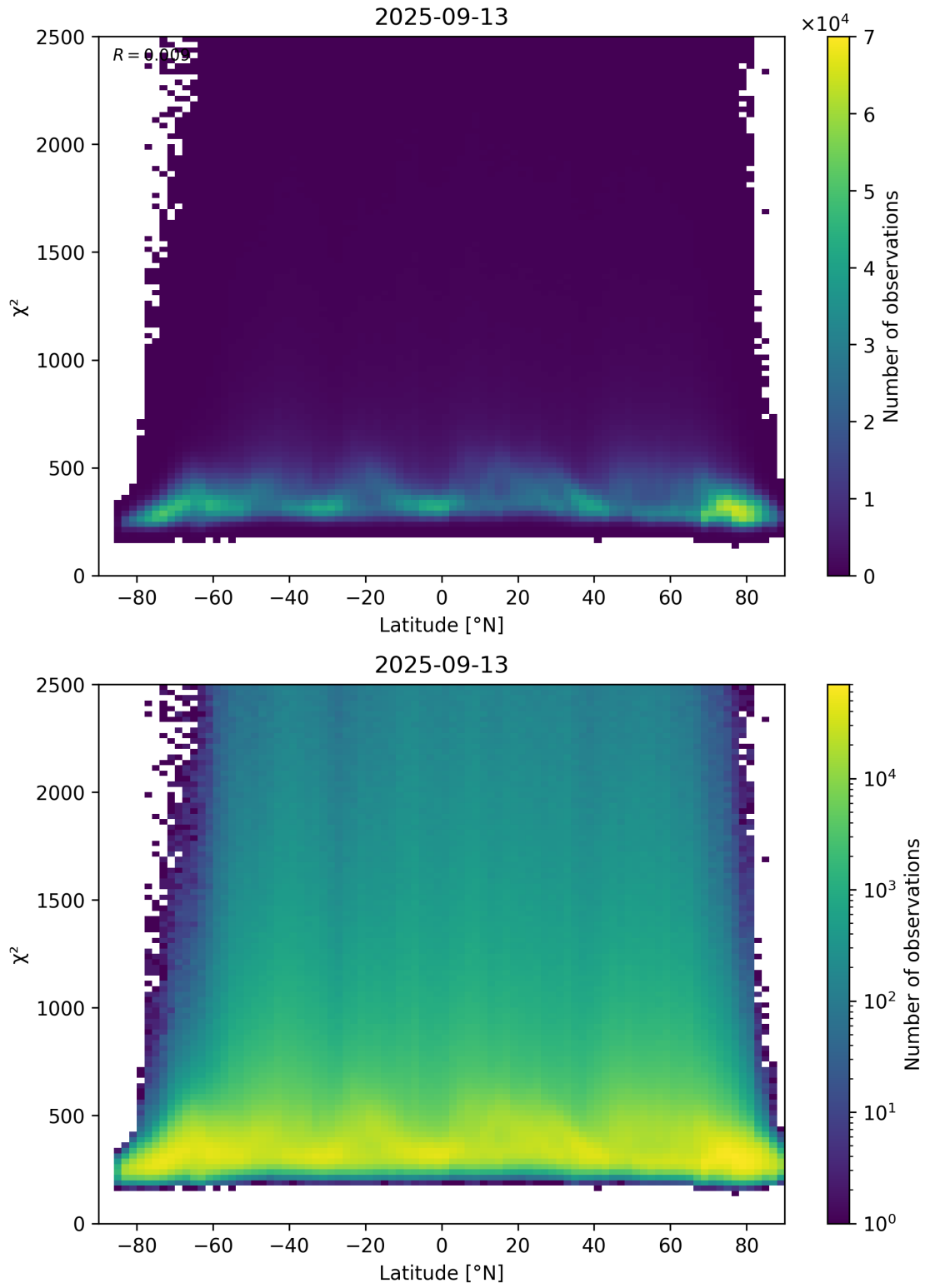
Figure 86: Scatter density plot of “Latitude” against “ \chi^2 ” for 2025-09-12 to 2025-09-14.
