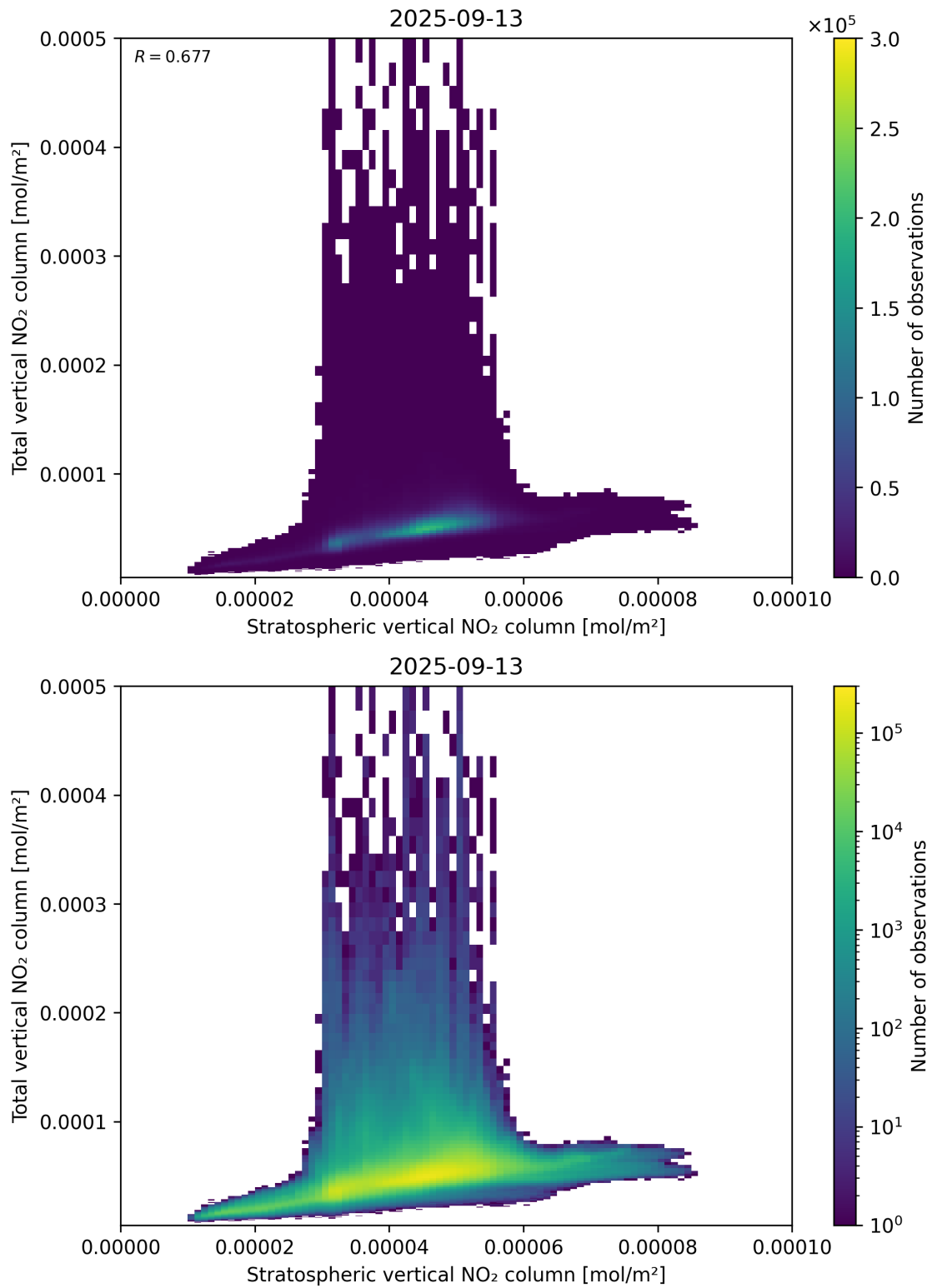
Figure 100: Scatter density plot of “Stratospheric vertical NO 2 column” against “Total vertical NO 2 column” for 2025-09-12 to 2025-09-14.
