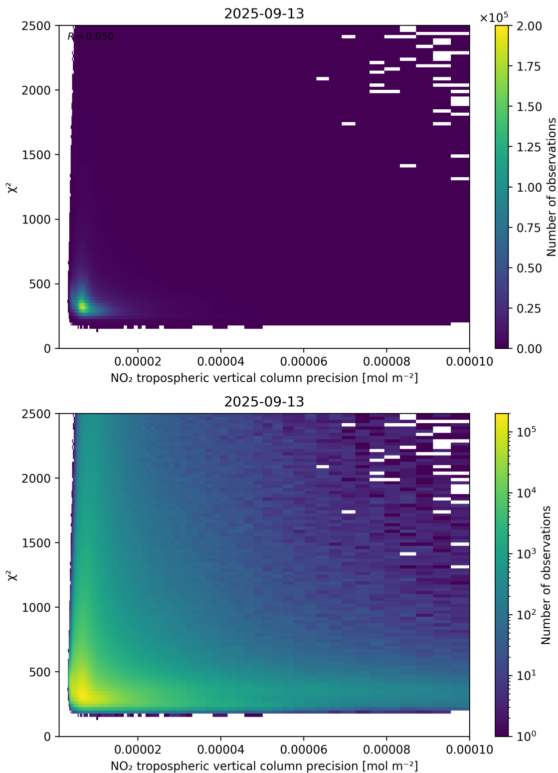
Figure 134: Scatter density plot of “NO 2 tropospheric vertical column precision” against “ \chi^2 ” for 2025-09-12 to 2025-09-14.
