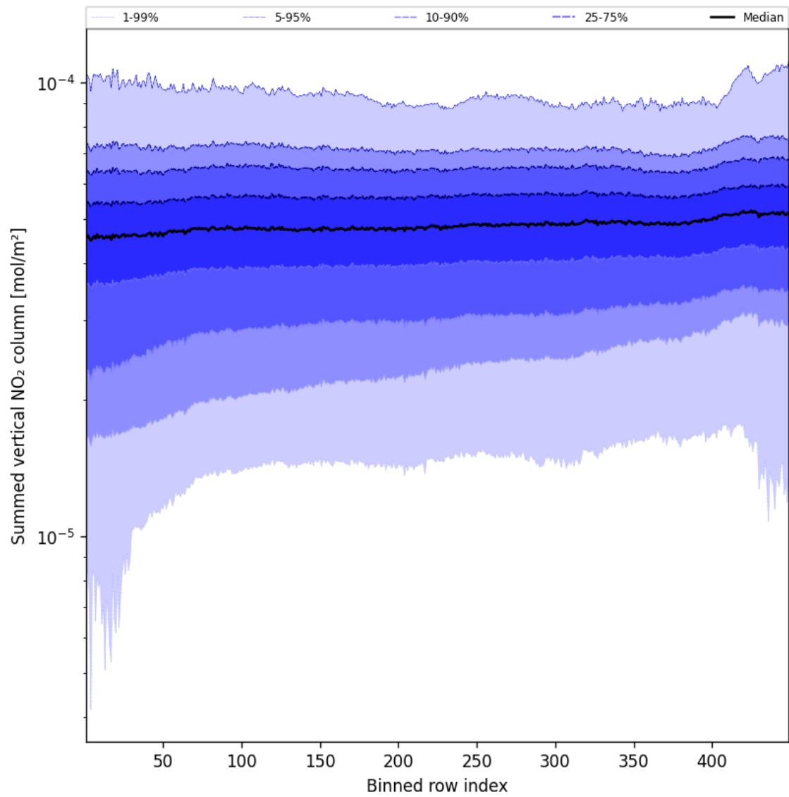
Figure 57: Along track statistics of “Summed vertical NO 2 column” for 2025-09-12 to 2025-09-14
