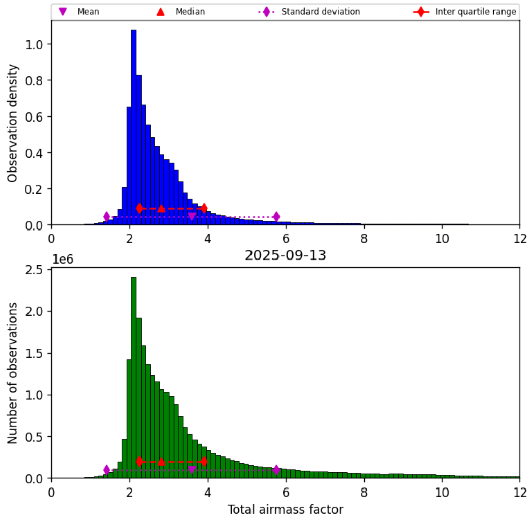
Figure 32: Histogram of “Total airmass factor” for 2025-09-12 to 2025-09-14
