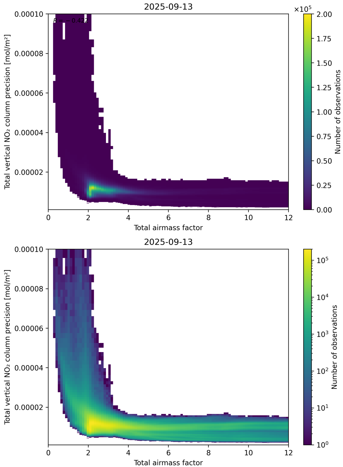
Figure 68: Scatter density plot of “Total airmass factor” against “Total vertical NO 2 column precision” for 2025-09-12 to 2025-09-14.
