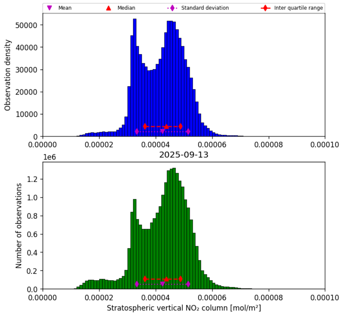
Figure 36: Histogram of “Stratospheric vertical NO 2 column” for 2025-09-12 to 2025-09-14
