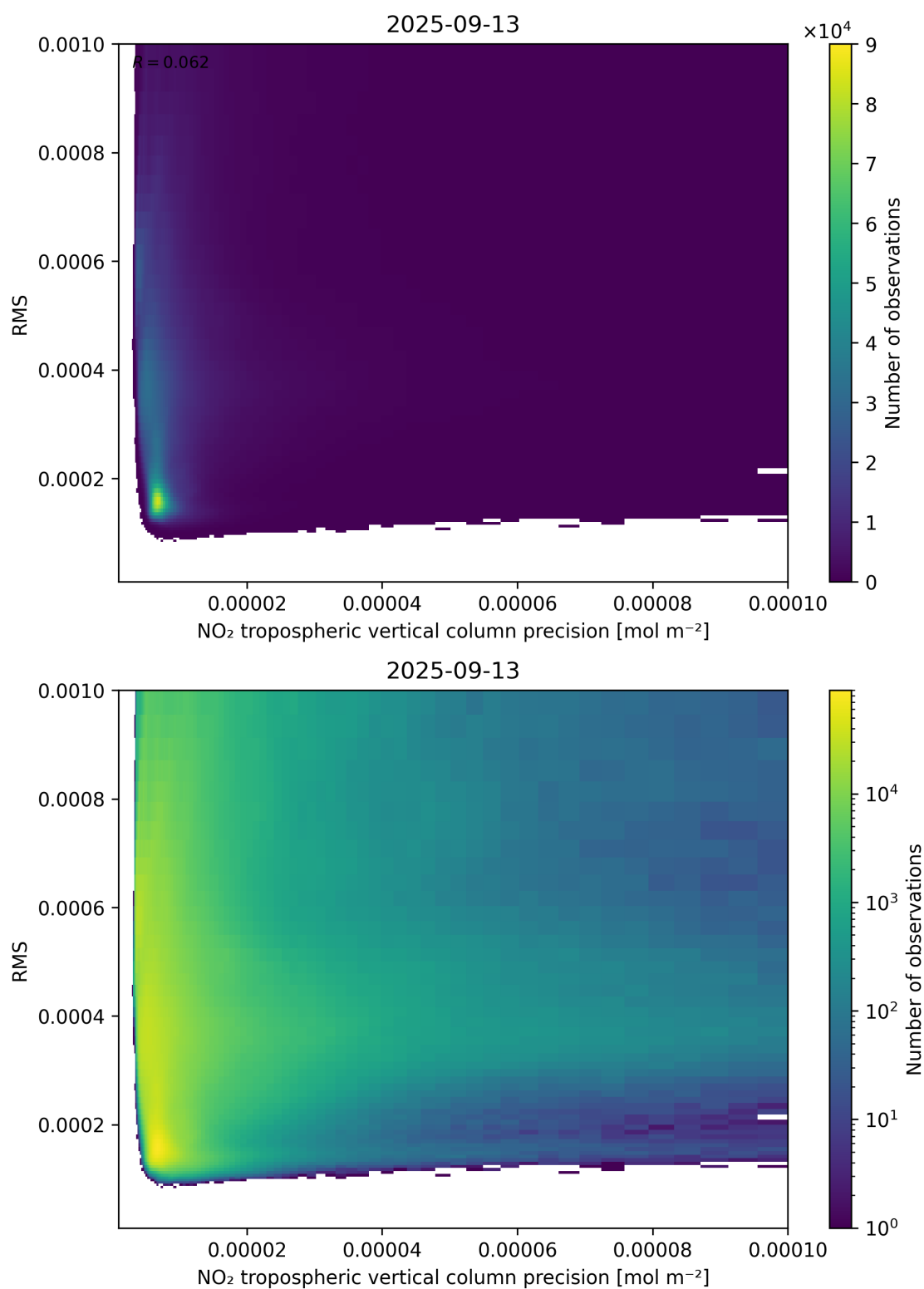
Figure 140: Scatter density plot of “NO 2 tropospheric vertical column precision” against “RMS” for 2025-09-12 to 2025-09-14.
