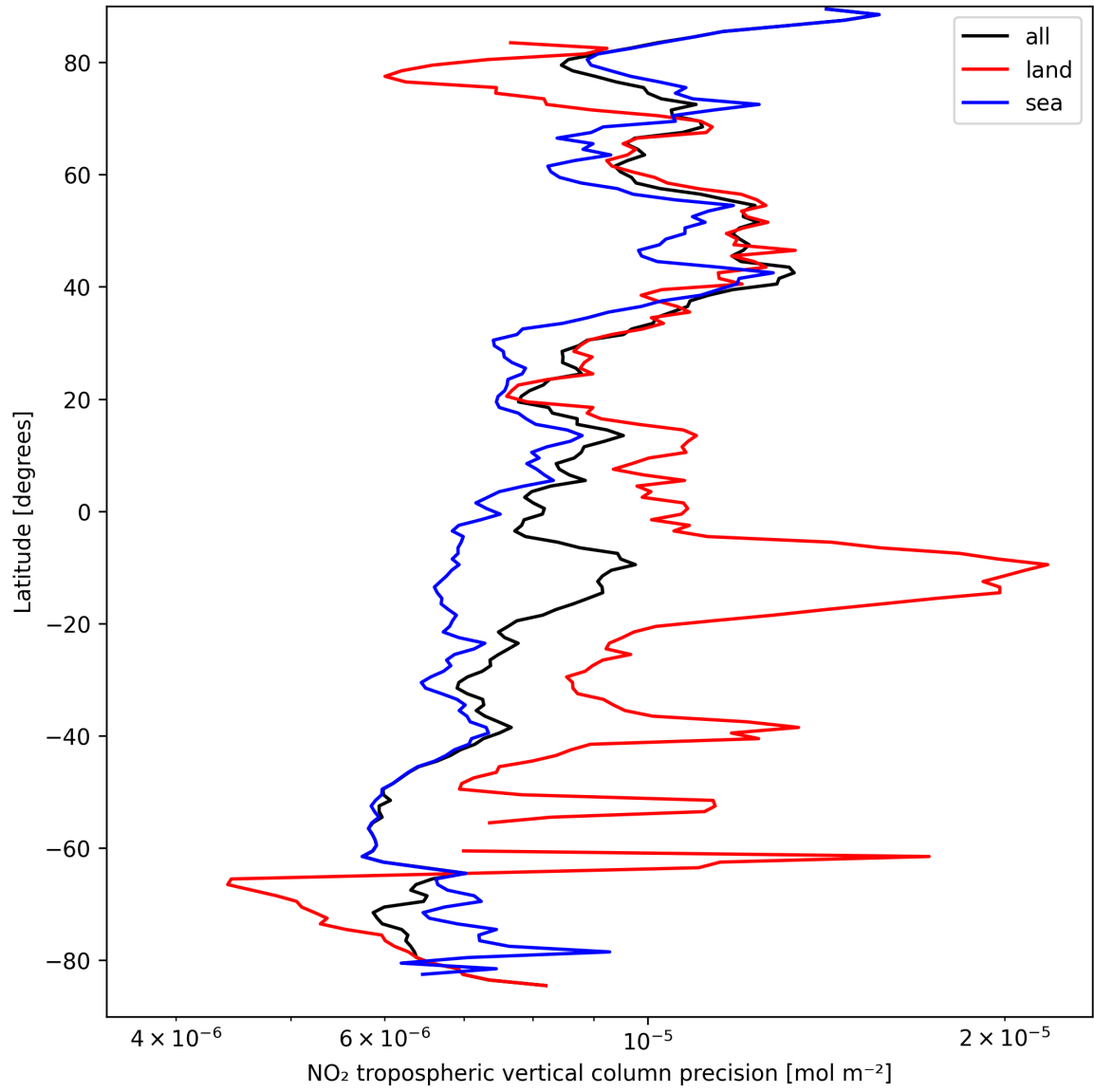
Figure 13: Zonal average of “NO 2 tropospheric vertical column precision” for 2025-09-12 to 2025-09-14.
