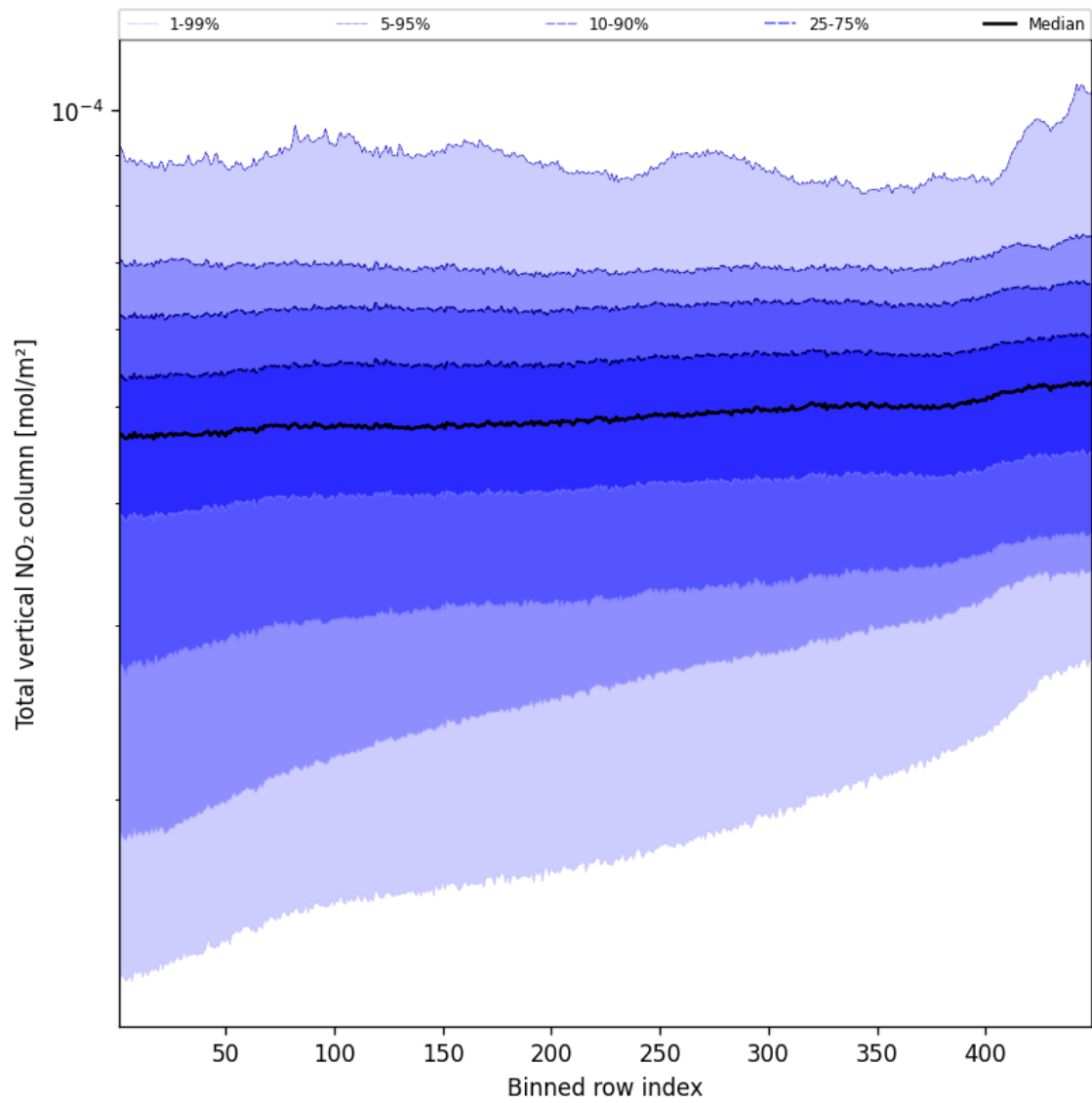
Figure 55: Along track statistics of “Total vertical NO 2 column” for 2025-09-12 to 2025-09-14
