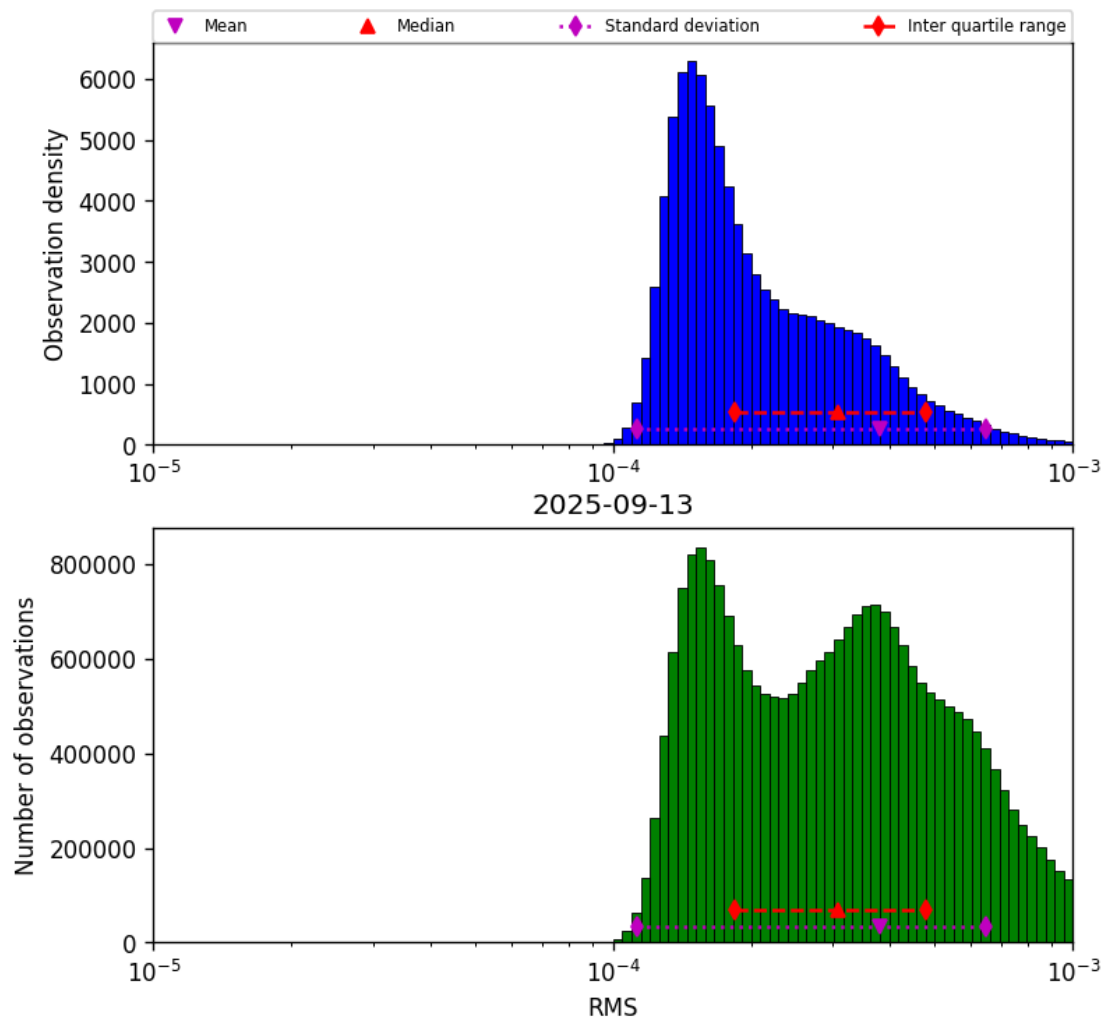
Figure 43: Histogram of “RMS” for 2025-09-12 to 2025-09-14
