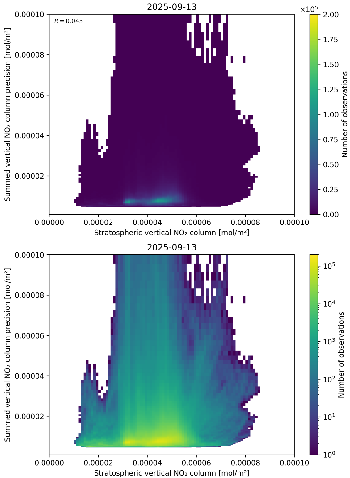
Figure 99: Scatter density plot of “Stratospheric vertical NO 2 column” against “Summed vertical NO 2 column precision” for 2025-09-12 to 2025-09-14.
