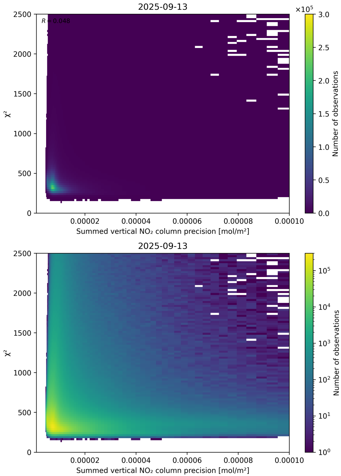
Figure 107: Scatter density plot of “Summed vertical NO 2 column precision” against “ \chi^2 ” for 2025-09-12 to 2025-09-14.
