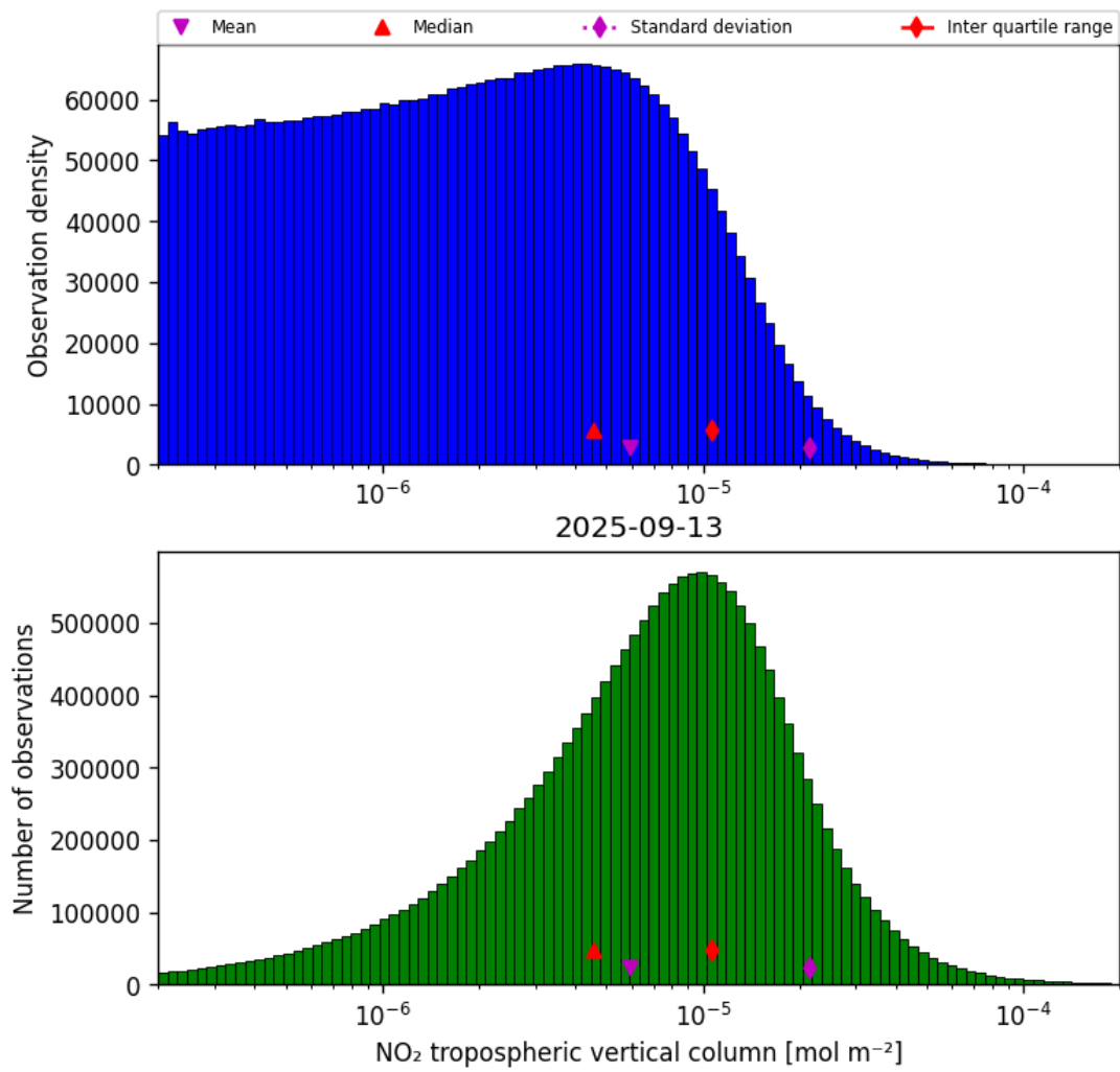
Figure 29: Histogram of “NO 2 tropospheric vertical column” for 2025-09-12 to 2025-09-14
