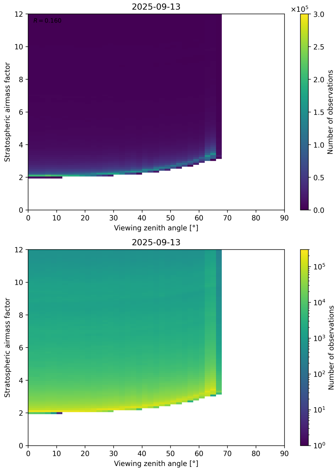
Figure 159: Scatter density plot of “Viewing zenith angle” against “Stratospheric airmass factor” for 2025-09-12 to 2025-09-14.
