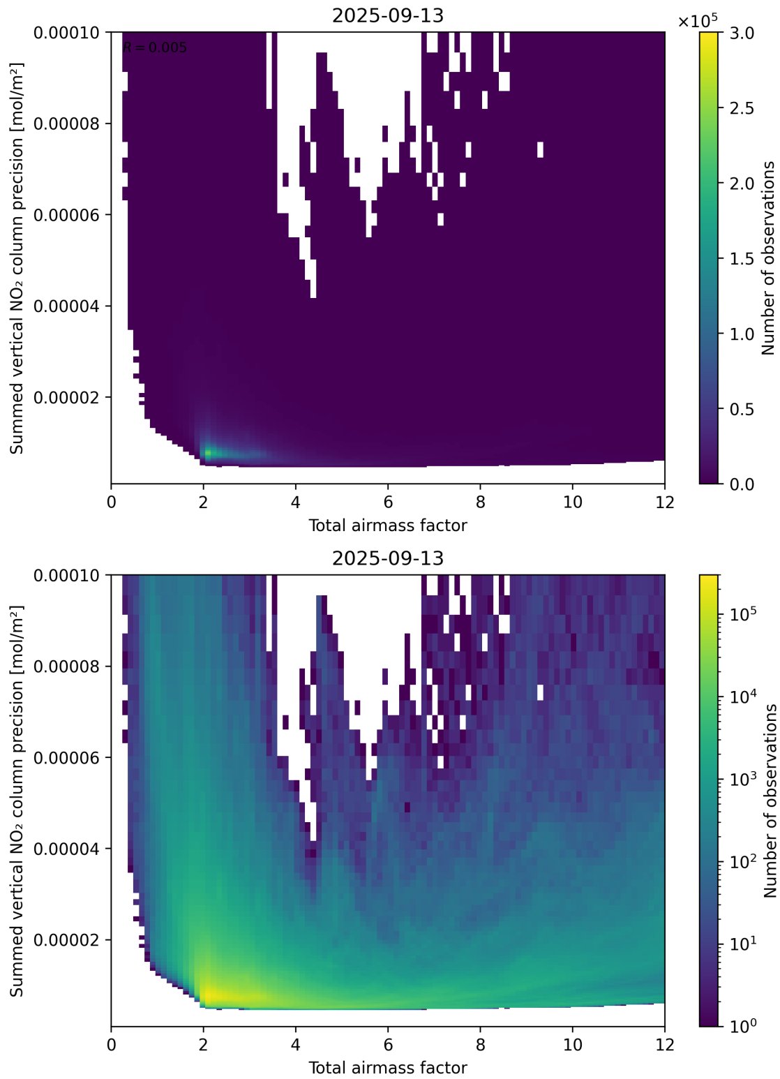
Figure 66: Scatter density plot of “Total airmass factor” against “Summed vertical NO 2 column precision” for 2025-09-12 to 2025-09-14.
