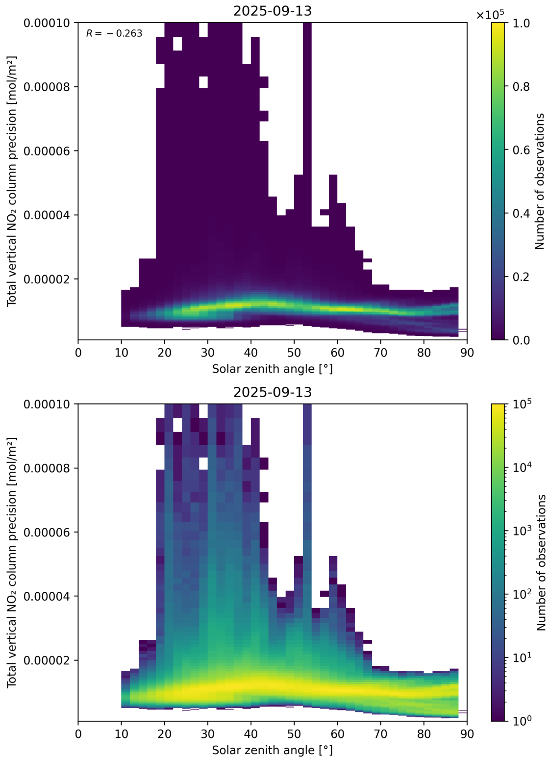
Figure 154: Scatter density plot of “Solar zenith angle” against “Total vertical NO 2 column precision” for 2025-09-12 to 2025-09-14.
