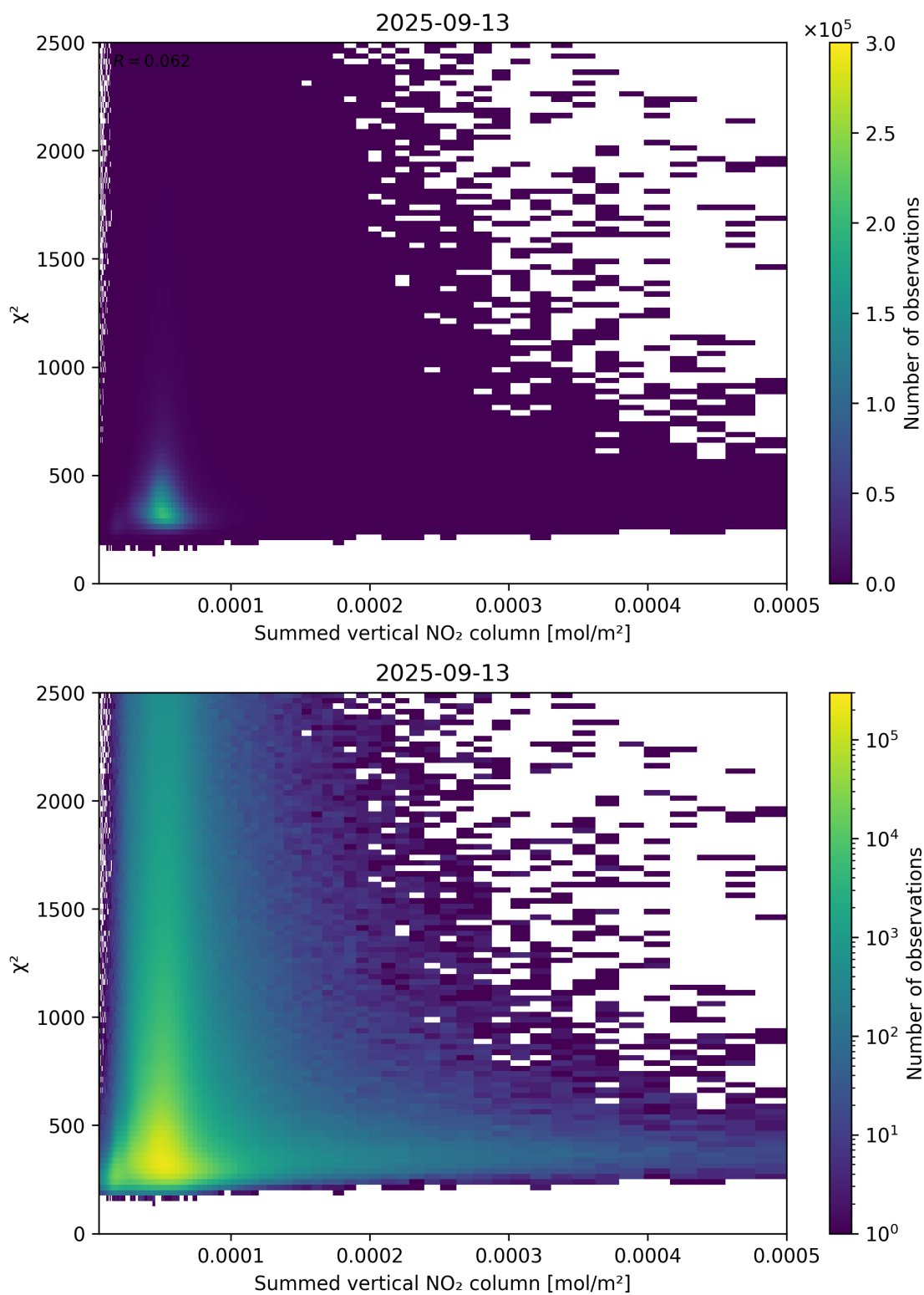
Figure 104: Scatter density plot of “Summed vertical NO 2 column” against “ \chi^2 ” for 2025-09-12 to 2025-09-14.
