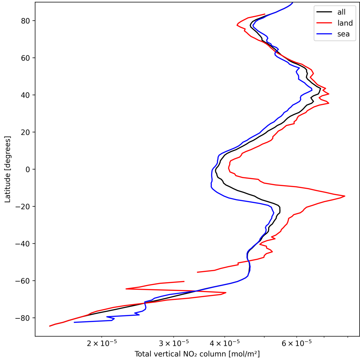
Figure 21: Zonal average of “Total vertical NO 2 column” for 2025-09-12 to 2025-09-14.
