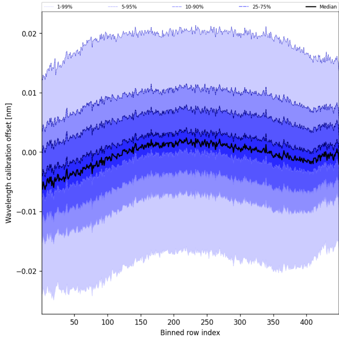
Figure 52: Along track statistics of “Wavelength calibration offset” for 2025-09-12 to 2025-09-14
