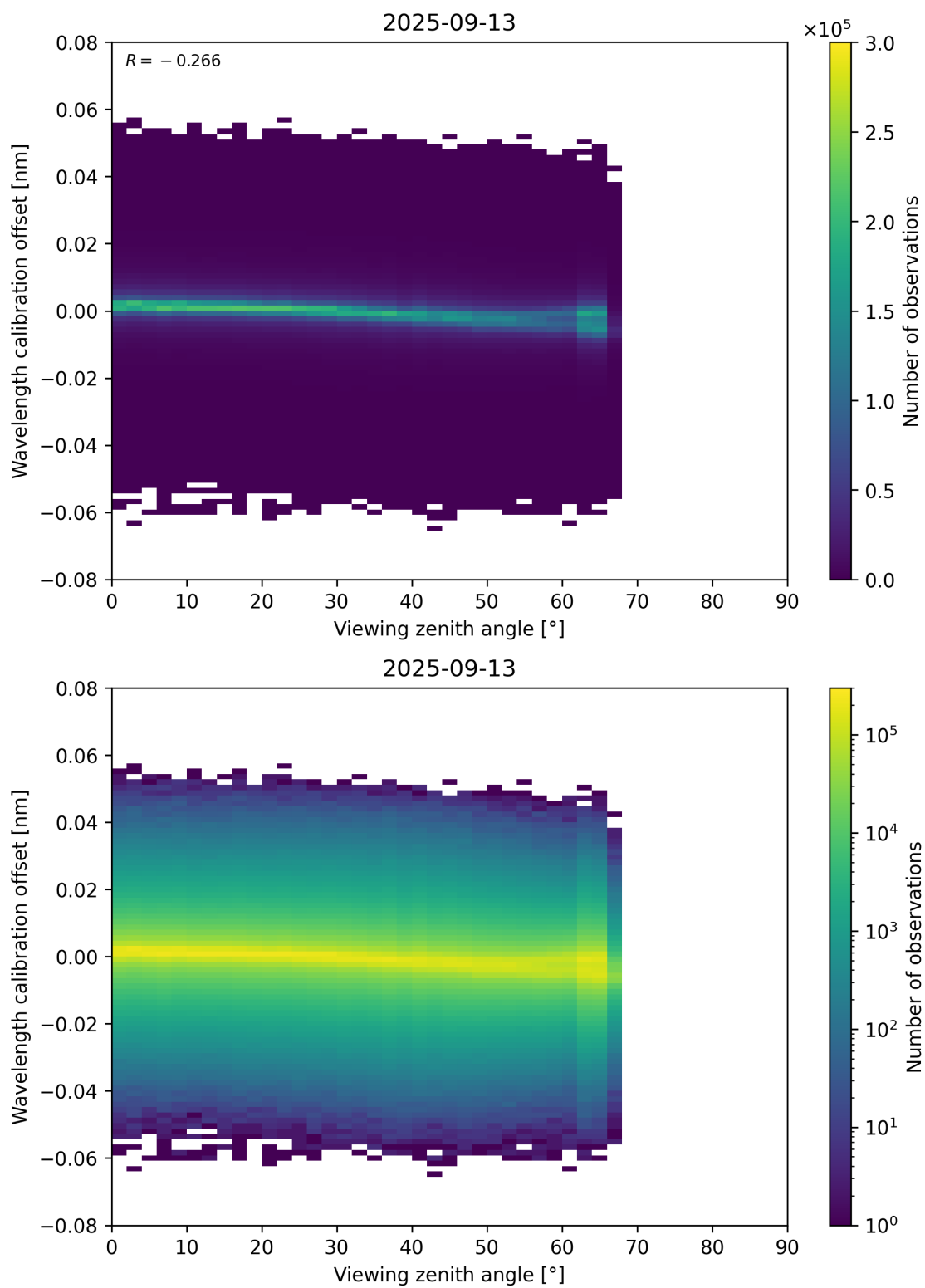
Figure 173: Scatter density plot of “Viewing zenith angle” against “Wavelength calibration offset” for 2025-09-12 to 2025-09-14.
