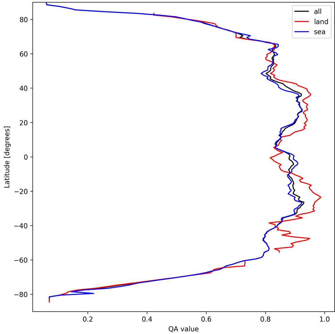
Figure 11: Zonal average of “QA value” for 2025-09-12 to 2025-09-14.
