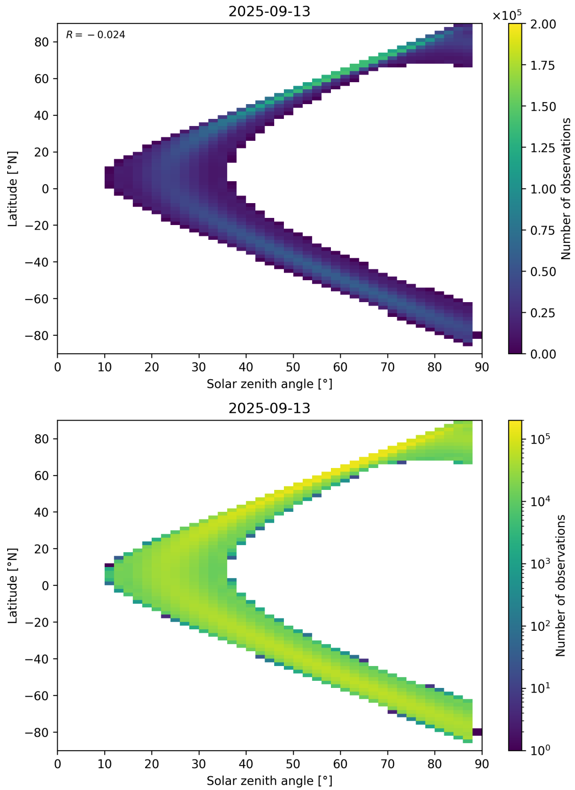
Figure 149: Scatter density plot of “Solar zenith angle” against “Latitude” for 2025-09-12 to 2025-09-14.
