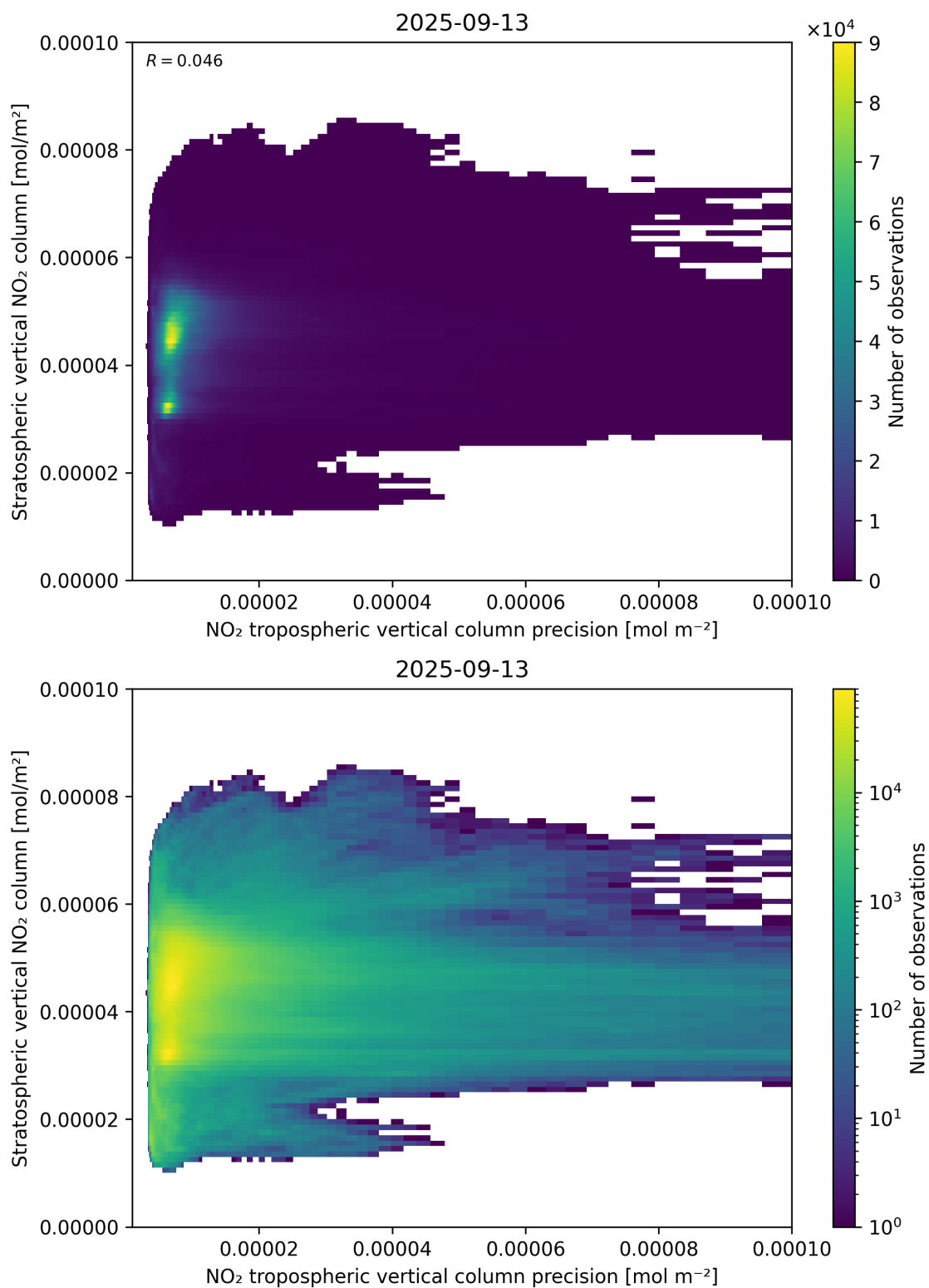
Figure 135: Scatter density plot of “NO 2 tropospheric vertical column precision” against “Stratospheric vertical NO 2 column” for 2025-09-12 to 2025-09-14.
