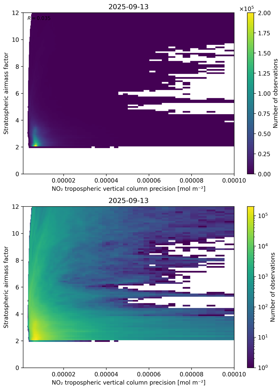
Figure 131: Scatter density plot of “NO 2 tropospheric vertical column precision” against “Stratospheric airmass factor” for 2025-09-12 to 2025-09-14.
