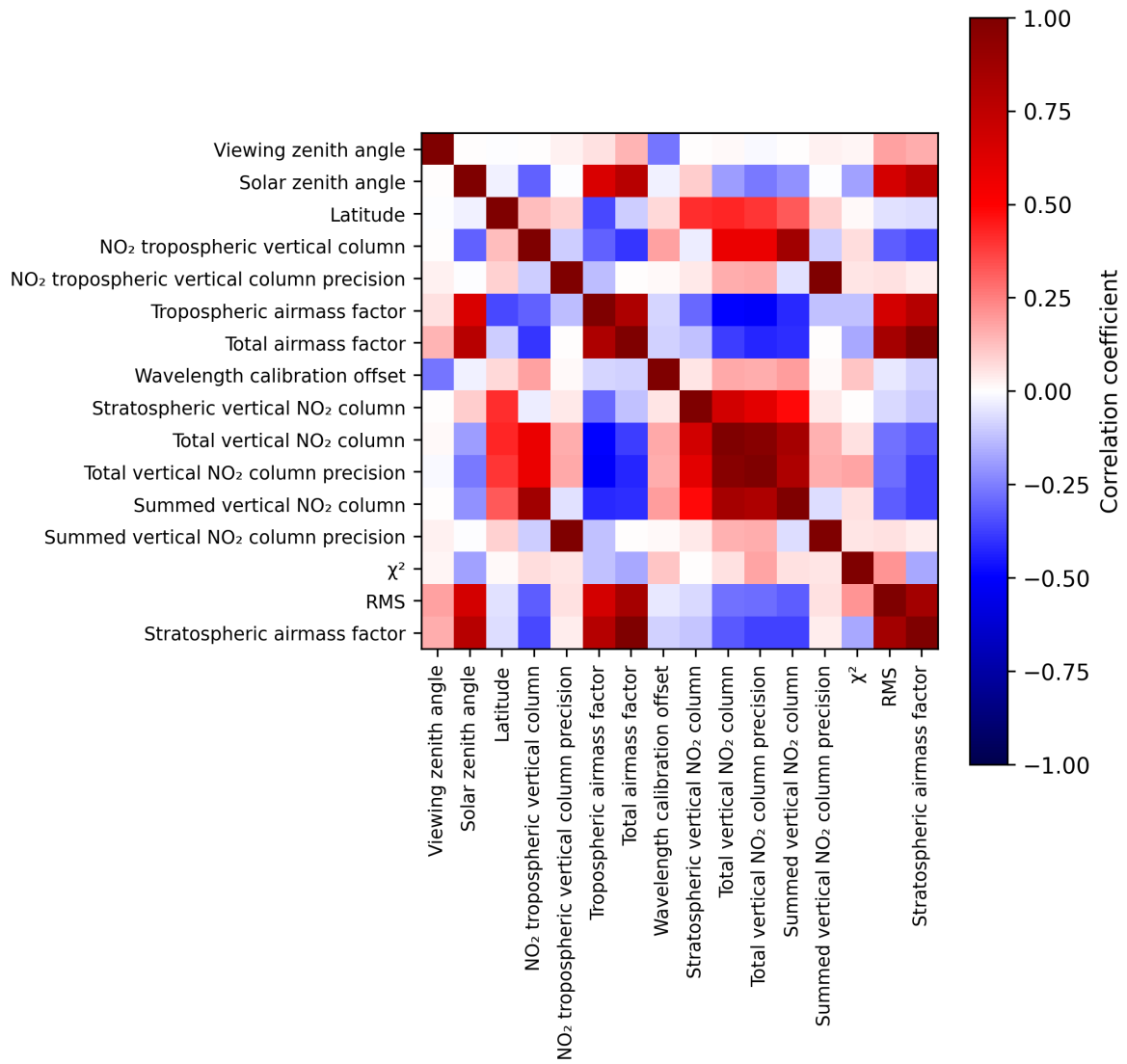
Figure 2: Map of correlation matrix for 2025-09-12 to 2025-09-14.
