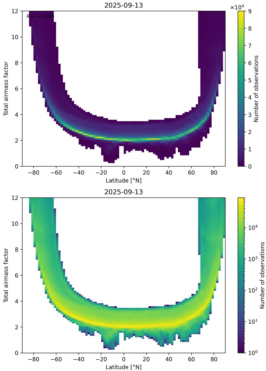
Figure 84: Scatter density plot of “Latitude” against “Total airmass factor” for 2025-09-12 to 2025-09-14.
