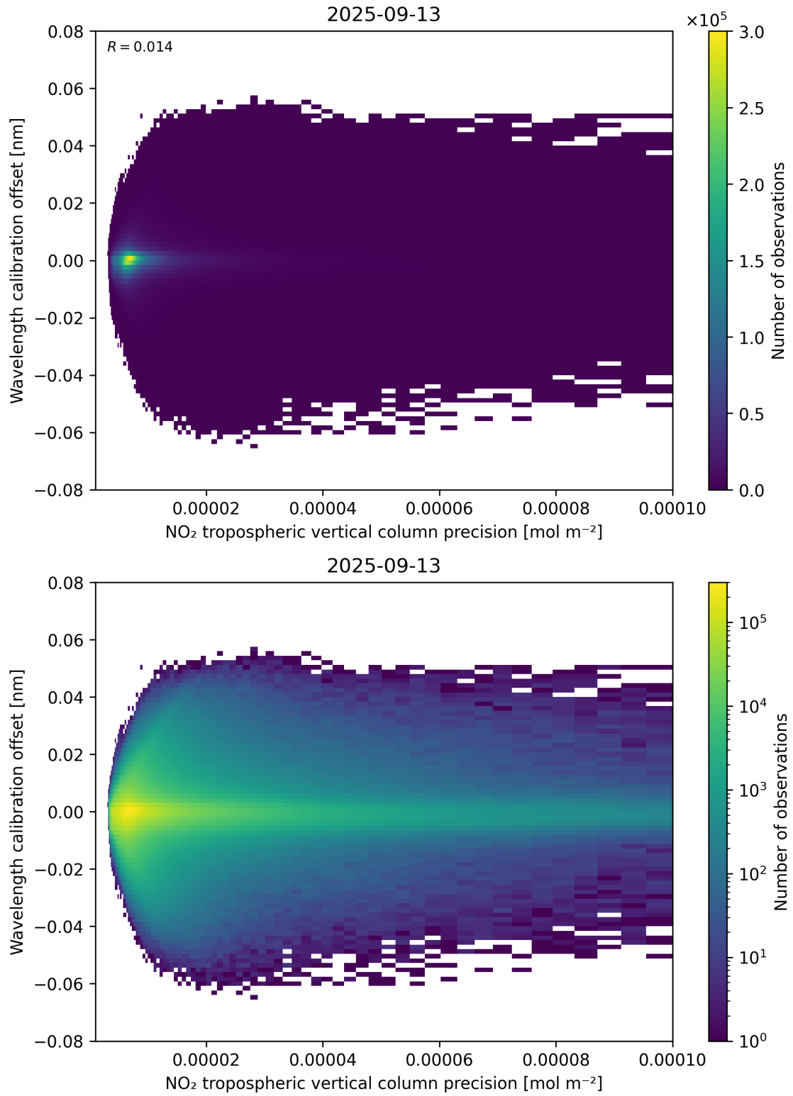
Figure 141: Scatter density plot of “NO 2 tropospheric vertical column precision” against “Wavelength calibration offset” for 2025-09-12 to 2025-09-14.
