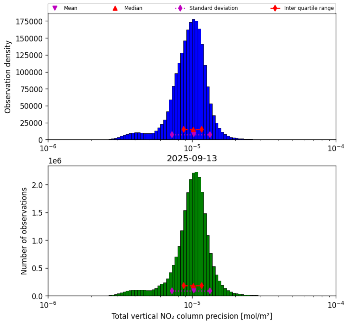
Figure 39: Histogram of “Total vertical NO 2 column precision” for 2025-09-12 to 2025-09-14
