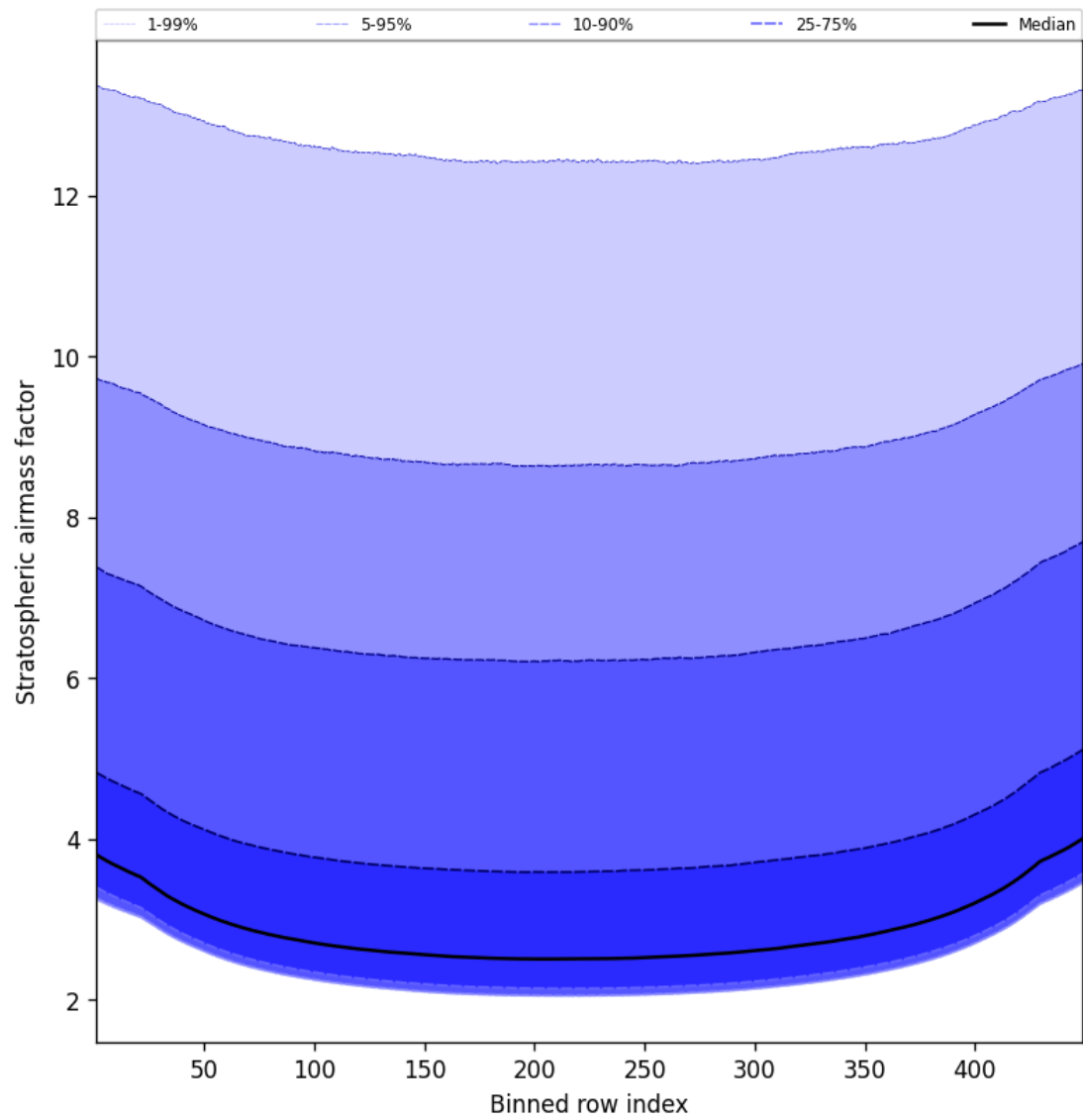
Figure 61: Along track statistics of “Stratospheric air mass factor” for 2025-09-12 to 2025-09-14
