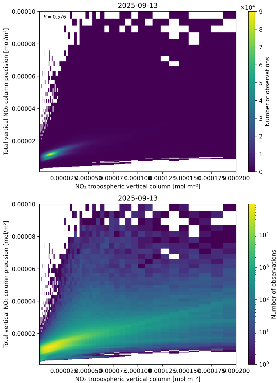
Figure 129: Scatter density plot of “NO 2 tropospheric vertical column” against “Total vertical NO 2 column precision” for 2025-09-12 to 2025-09-14.
