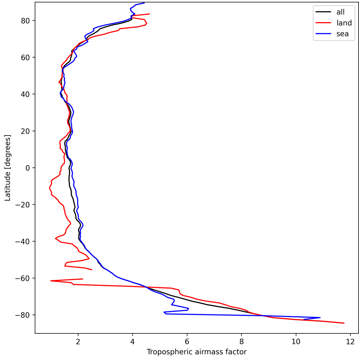
Figure 14: Zonal average of “Tropospheric airmass factor” for 2025-09-12 to 2025-09-14.
