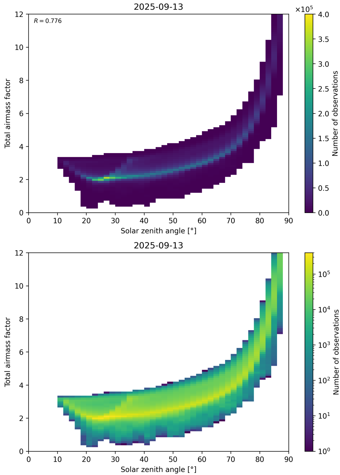
Figure 146: Scatter density plot of “Solar zenith angle” against “Total air mass factor” for 2025-09-12 to 2025-09-14.
