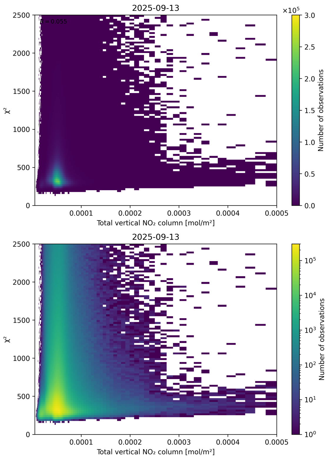
Figure 111: Scatter density plot of “Total vertical NO 2 column” against “ \chi^2 ” for 2025-09-12 to 2025-09-14.
