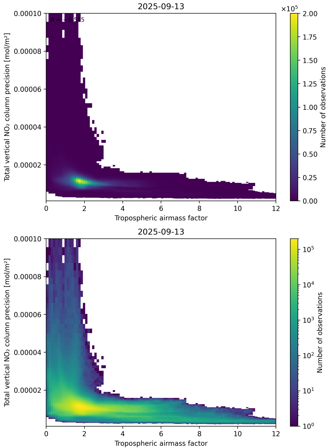
Figure 78: Scatter density plot of “Tropospheric airmass factor” against “Total vertical NO 2 column precision” for 2025-09-12 to 2025-09-14.
