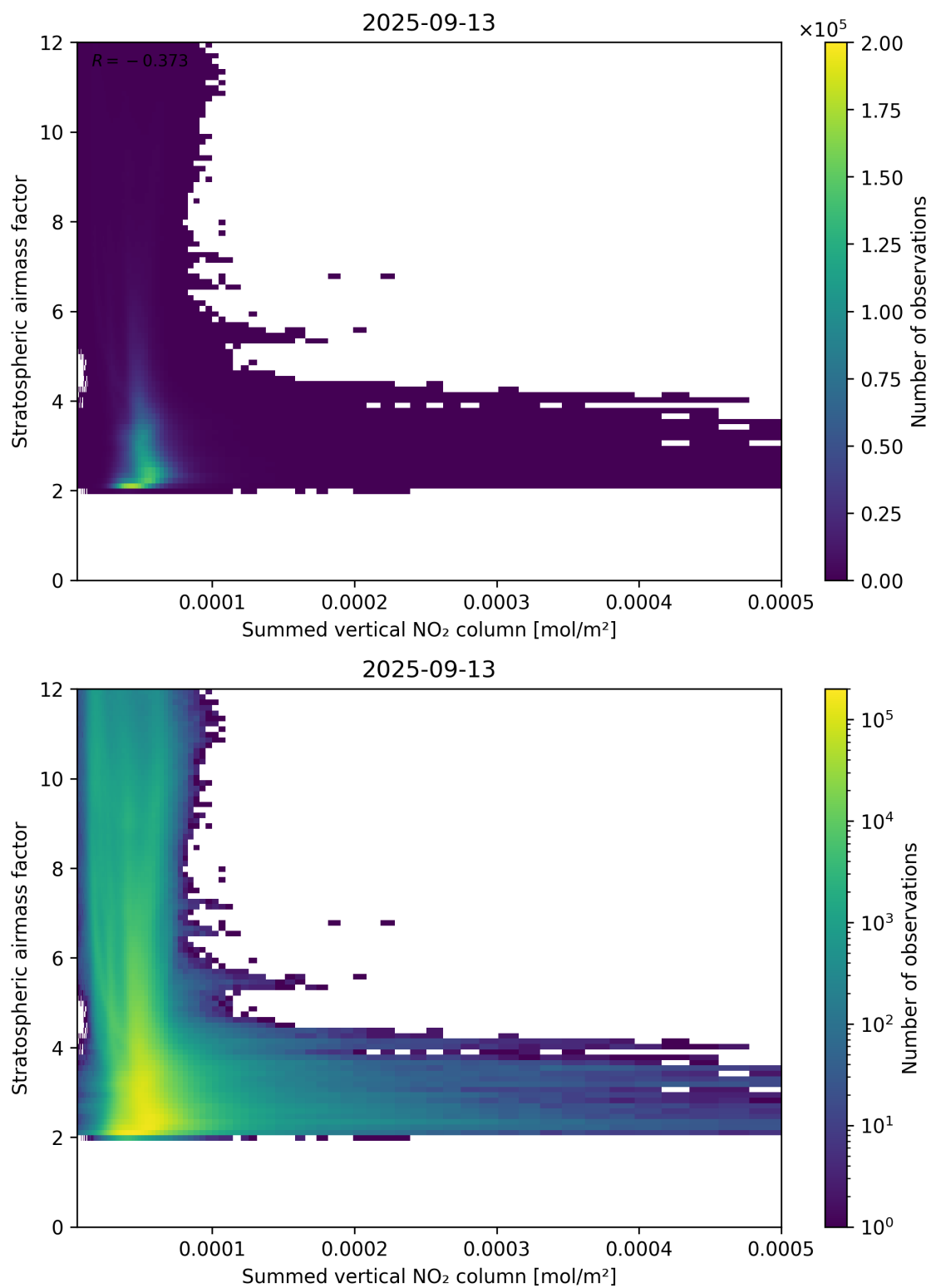
Figure 103: Scatter density plot of “Summed vertical NO 2 column” against “Stratospheric airmass factor” for 2025-09-12 to 2025-09-14.
