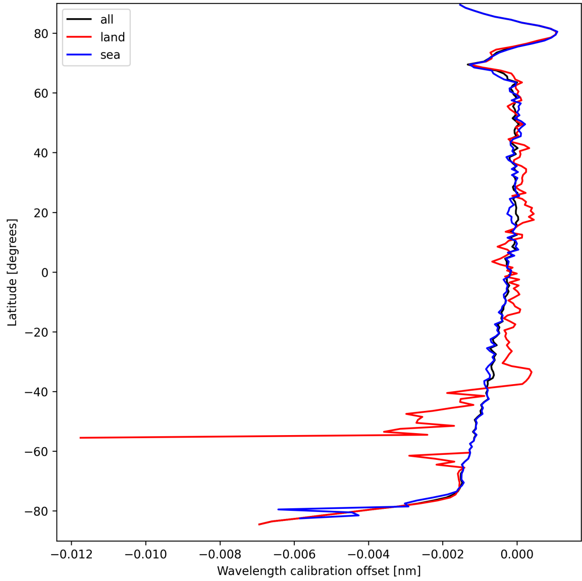
Figure 18: Zonal average of “Wavelength calibration offset” for 2025-09-12 to 2025-09-14.
