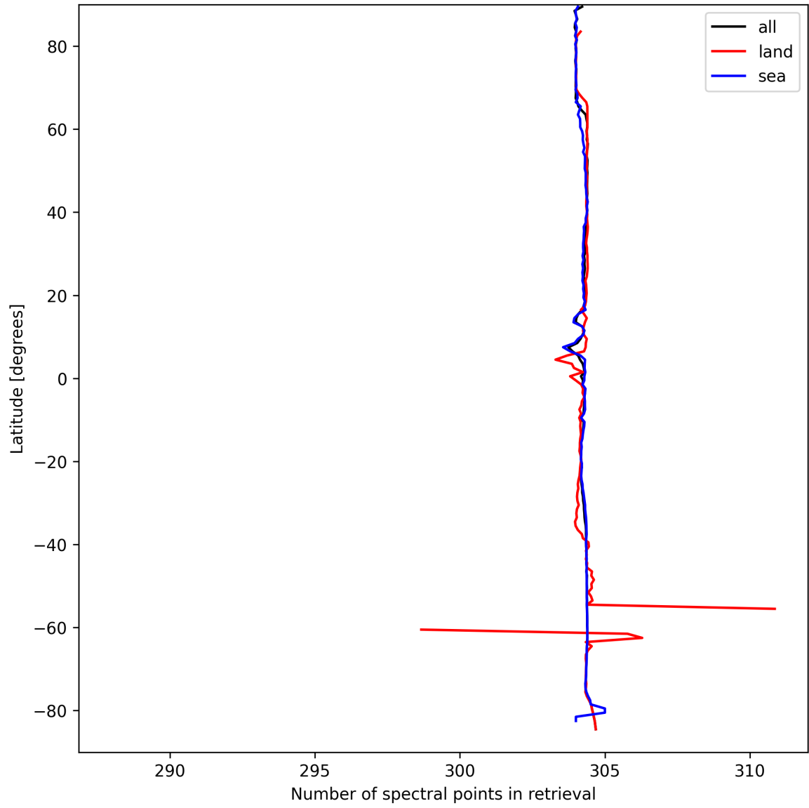
Figure 16: Zonal average of “Number of spectral points in retrieval” for 2025-09-12 to 2025-09-14.
