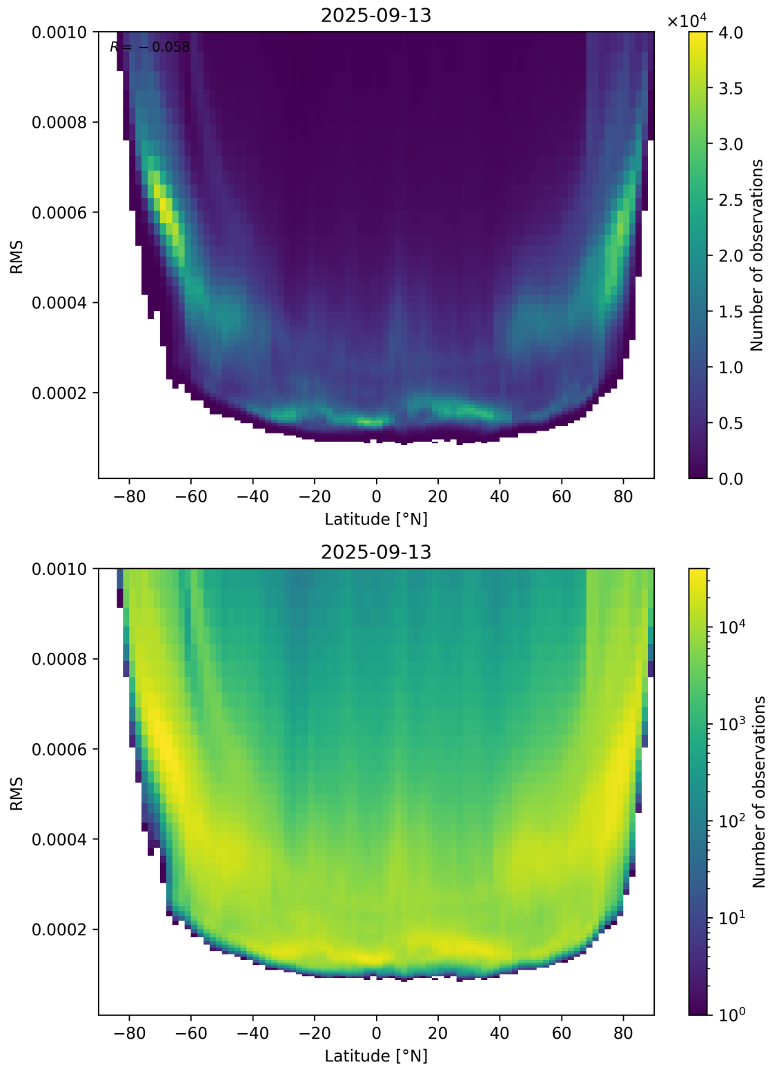
Figure 94: Scatter density plot of “Latitude” against “RMS” for 2025-09-12 to 2025-09-14.
