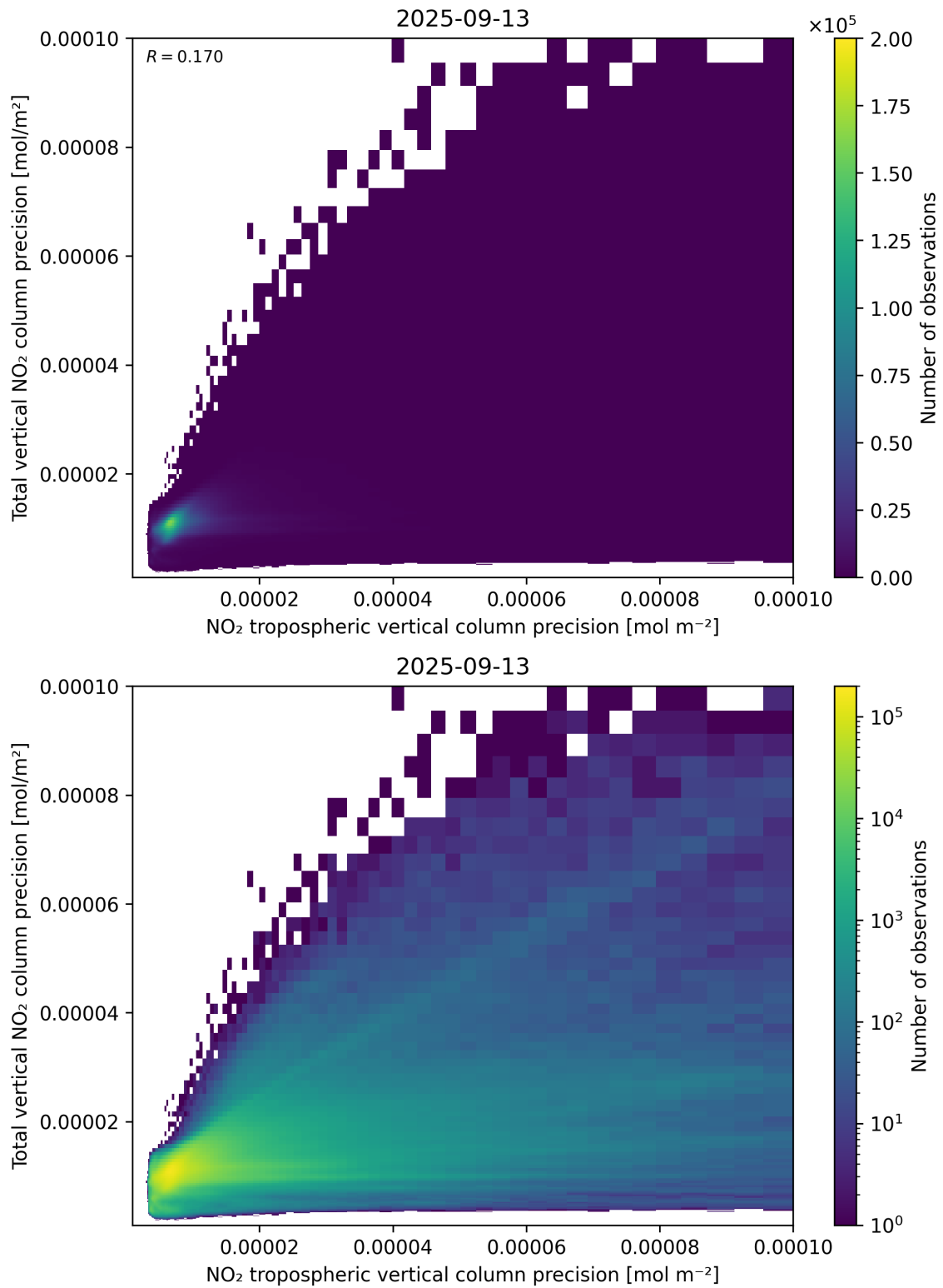
Figure 139: Scatter density plot of “NO 2 tropospheric vertical column precision” against “Total vertical NO 2 column precision” for 2025-09-12 to 2025-09-14.
