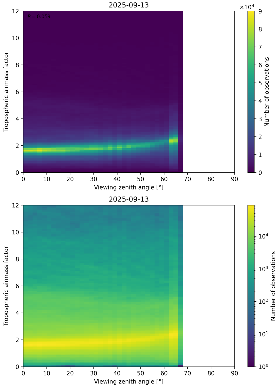
Figure 161: Scatter density plot of “Viewing zenith angle” against “Tropospheric airmass factor” for 2025-09-12 to 2025-09-14.
