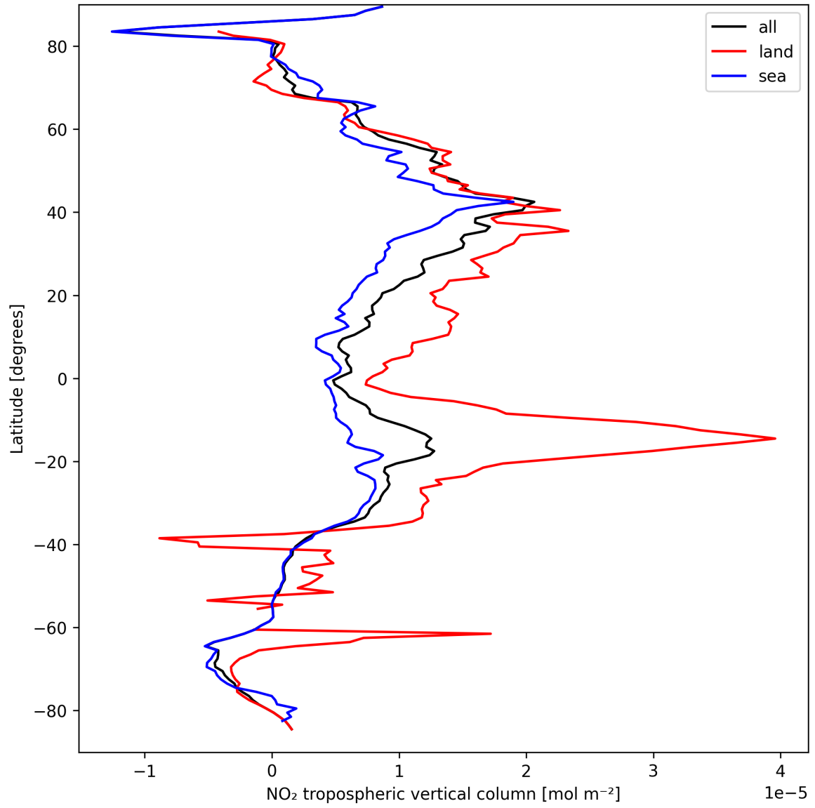
Figure 12: Zonal average of “NO 2 tropospheric vertical column” for 2025-09-12 to 2025-09-14.
