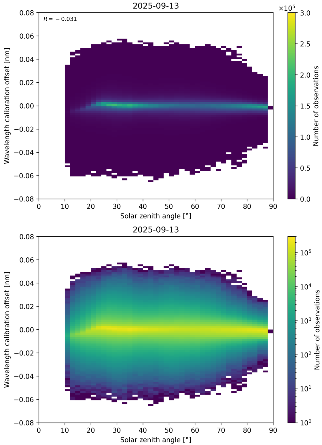
Figure 158: Scatter density plot of “Solar zenith angle” against “Wavelength calibration offset” for 2025-09-12 to 2025-09-14.
