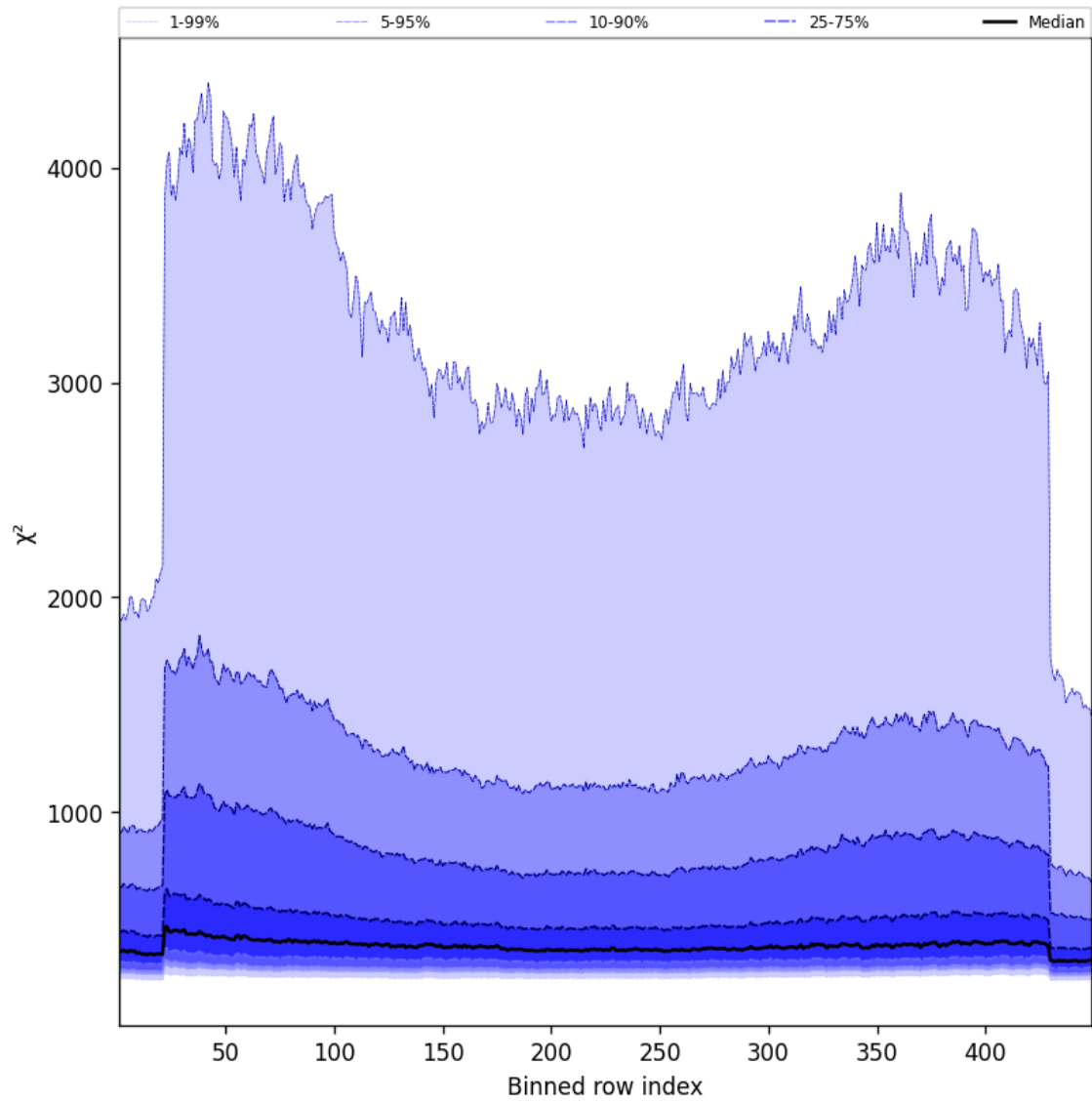
Figure 59: Along track statistics of “ \chi^2 ” for 2025-09-12 to 2025-09-14
