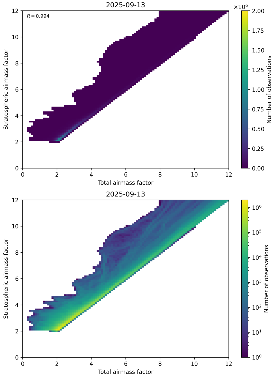
Figure 62: Scatter density plot of “Total airmass factor” against “Stratospheric airmass factor” for 2025-09-12 to 2025-09-14.
