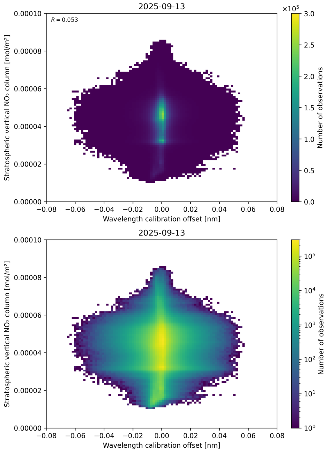
Figure 176: Scatter density plot of “Wavelength calibration offset” against “Stratospheric vertical NO 2 column” for 2025-09-12 to 2025-09-14.
