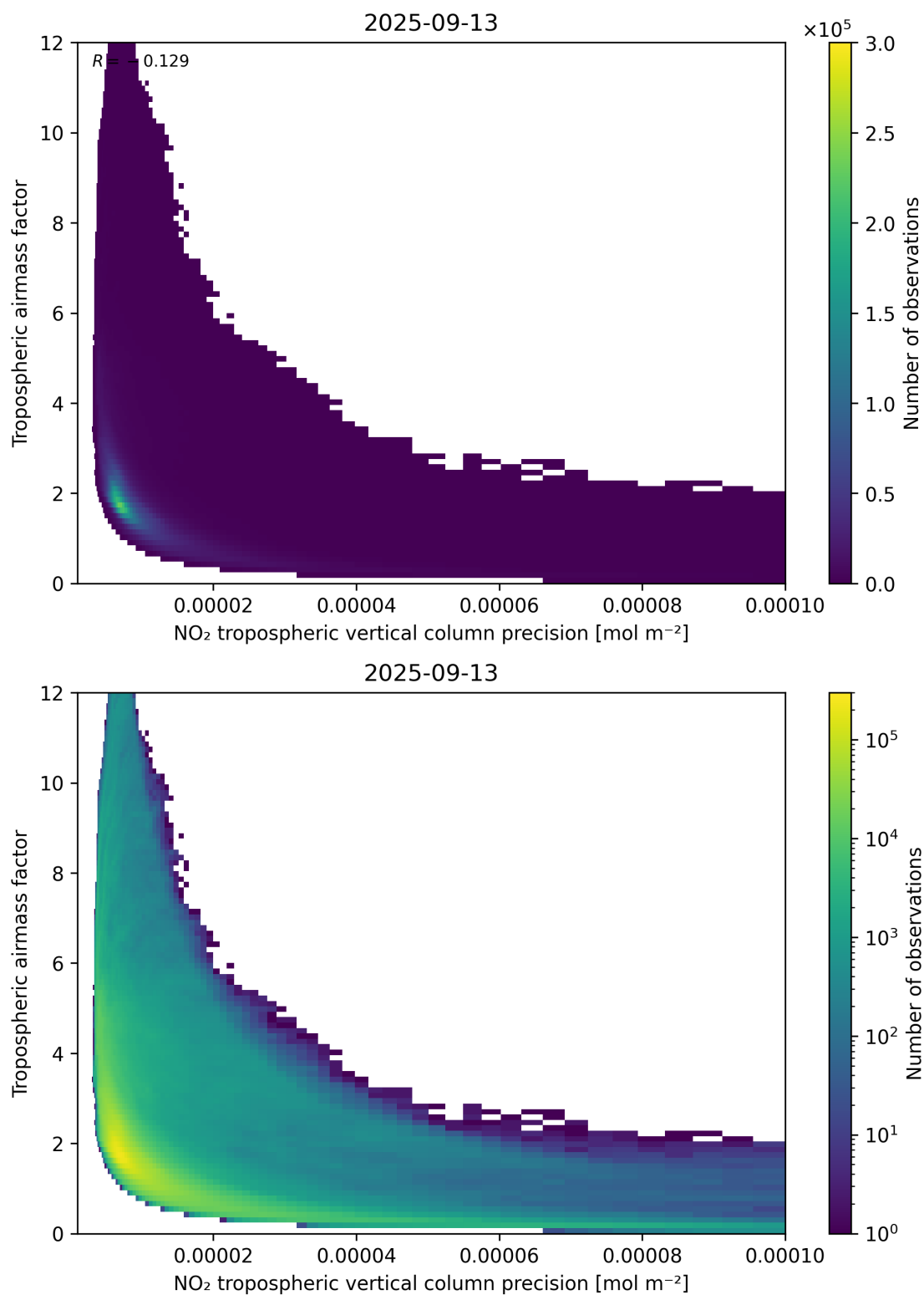
Figure 133: Scatter density plot of “NO 2 tropospheric vertical column precision” against “Tropospheric airmass factor” for 2025-09-12 to 2025-09-14.
