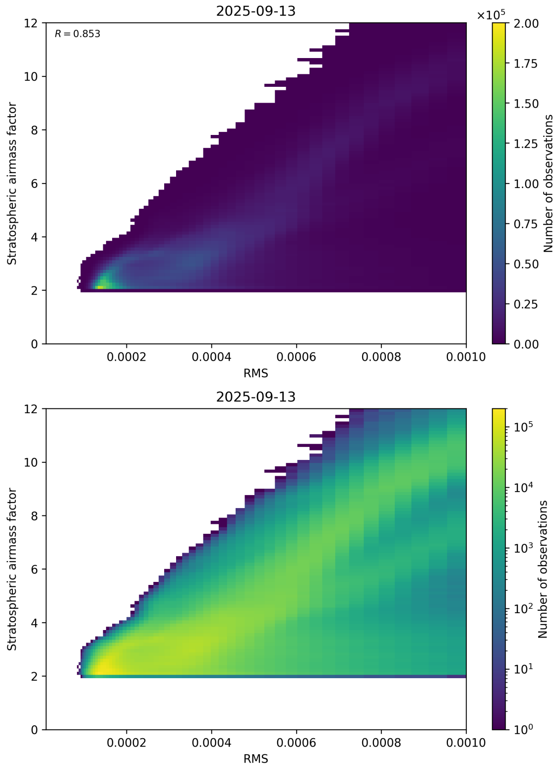
Figure 144: Scatter density plot of “RMS” against “Stratospheric airmass factor” for 2025-09-12 to 2025-09-14.
