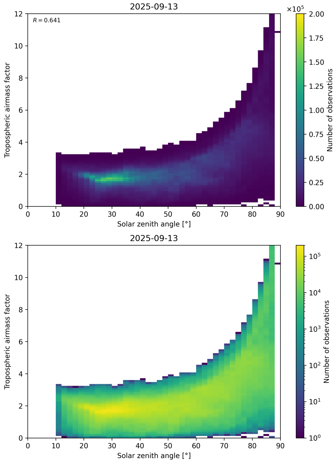
Figure 147: Scatter density plot of “Solar zenith angle” against “Tropospheric airmass factor” for 2025-09-12 to 2025-09-14.
