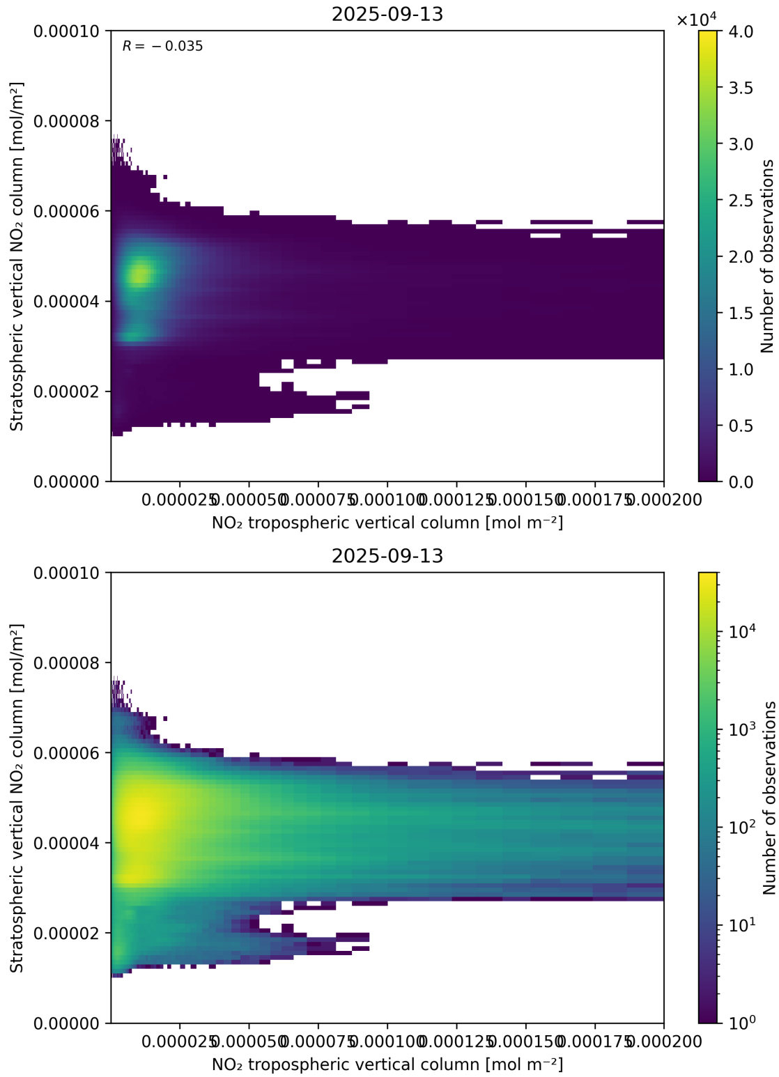
Figure 125: Scatter density plot of “NO 2 tropospheric vertical column” against “Stratospheric vertical NO 2 column” for 2025-09-12 to 2025-09-14.
