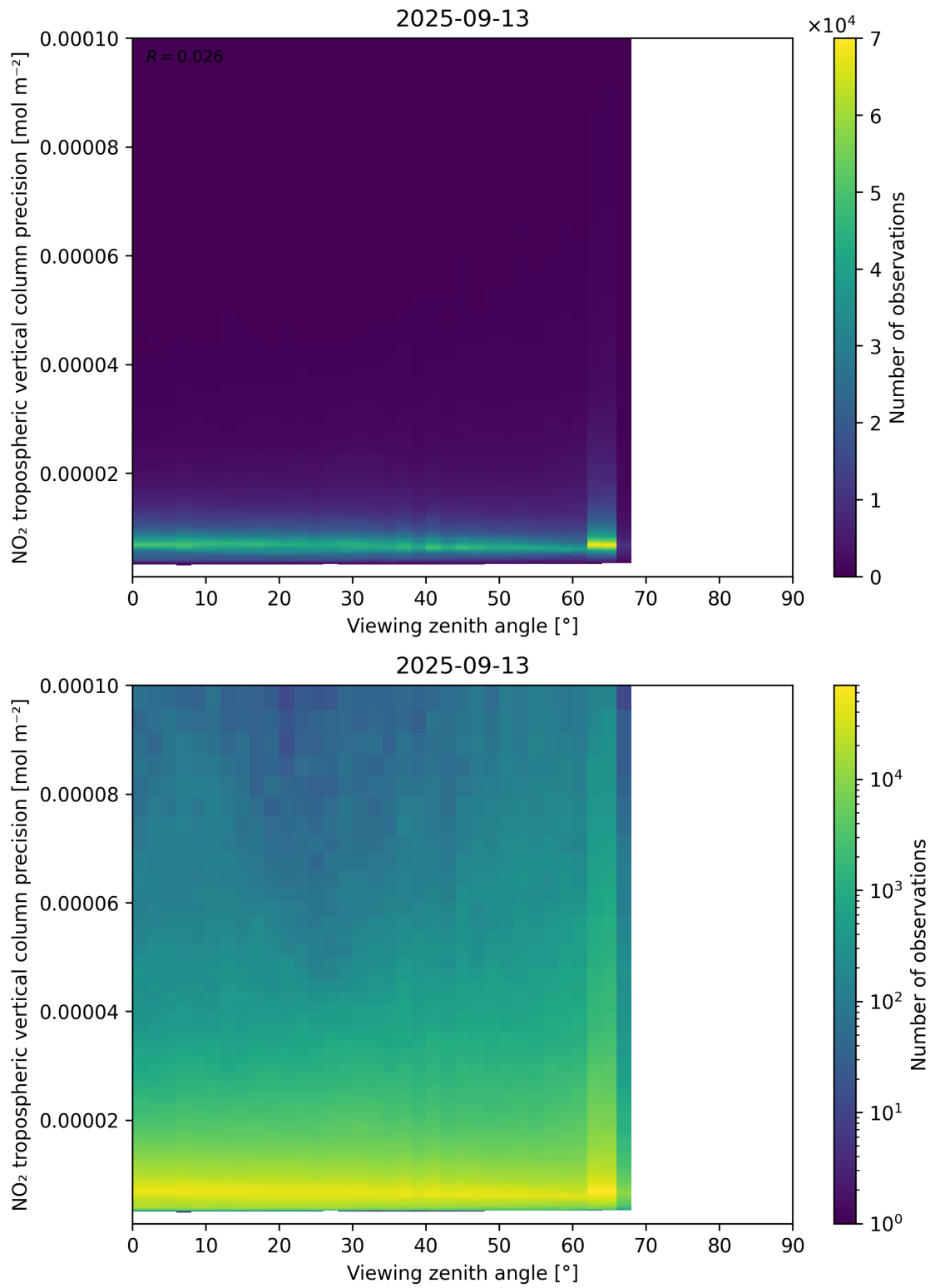
Figure 170: Scatter density plot of “Viewing zenith angle” against “NO 2 tropospheric vertical column precision” for 2025-09-12 to 2025-09-14.
