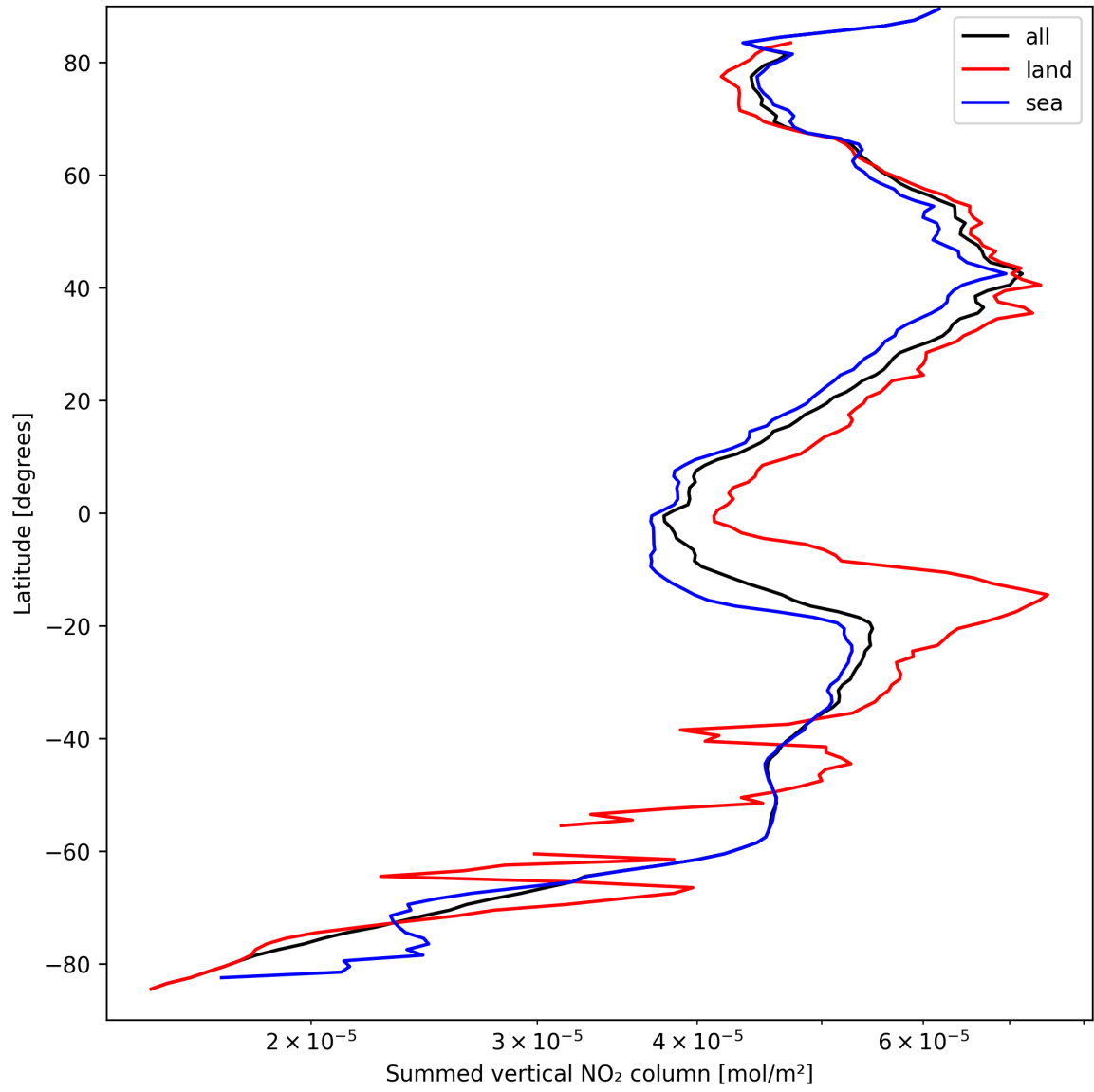
Figure 23: Zonal average of “Summed vertical NO 2 column” for 2025-09-12 to 2025-09-14.
