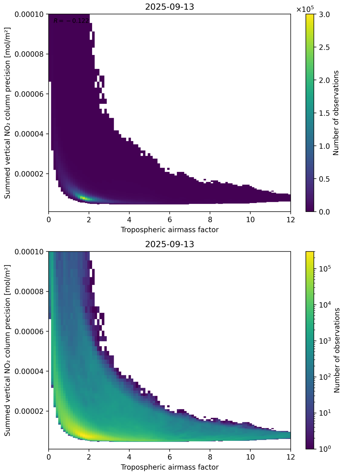
Figure 76: Scatter density plot of “Tropospheric air mass factor” against “Summed vertical NO 2 column precision” for 2025-09-12 to 2025-09-14.
