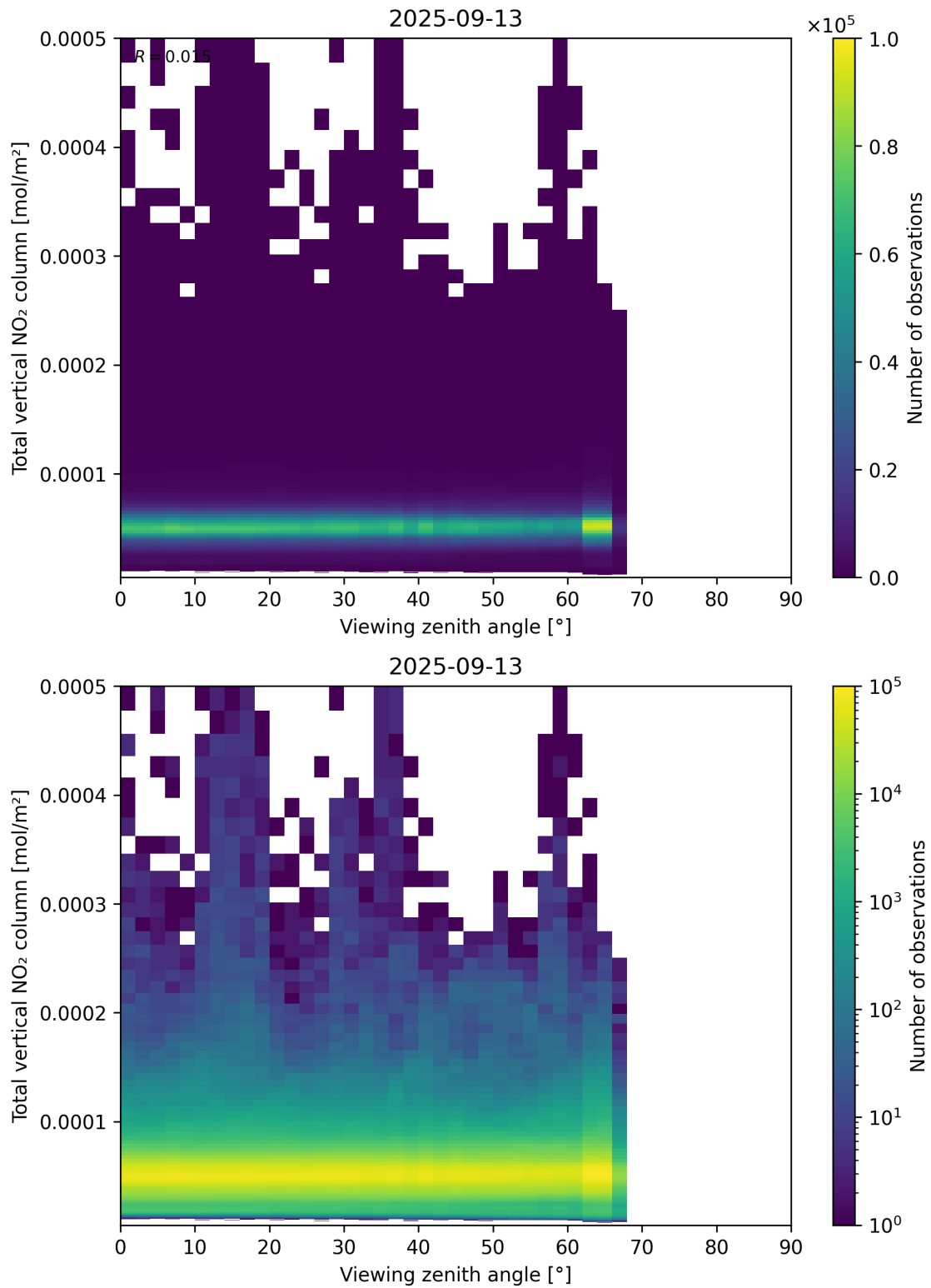
Figure 167: Scatter density plot of “Viewing zenith angle” against “Total vertical NO 2 column” for 2025-09-12 to 2025-09-14.
