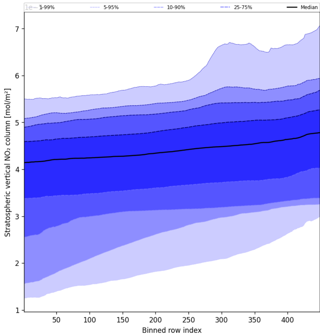
Figure 53: Along track statistics of “Stratospheric vertical NO 2 column” for 2025-09-12 to 2025-09-14
