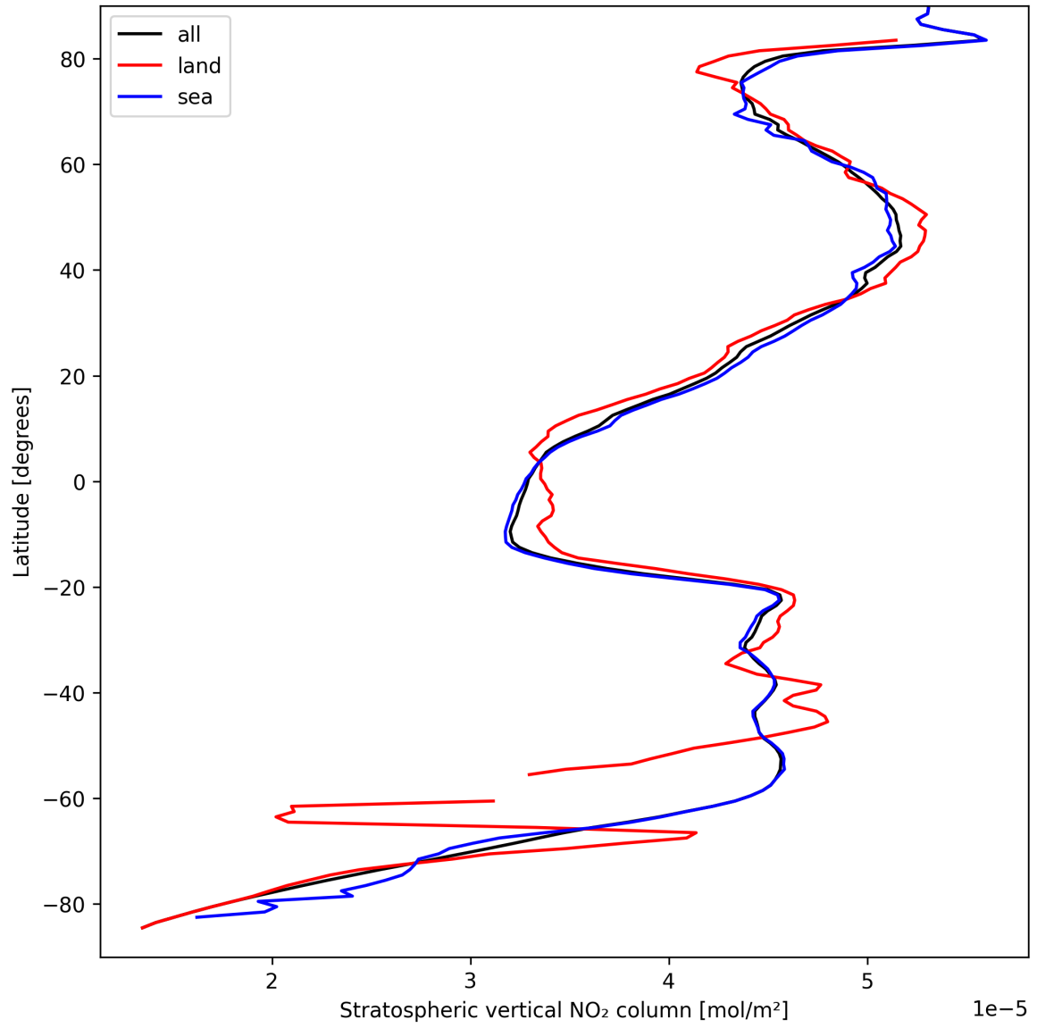
Figure 19: Zonal average of “Stratospheric vertical NO 2 column” for 2025-09-12 to 2025-09-14.
