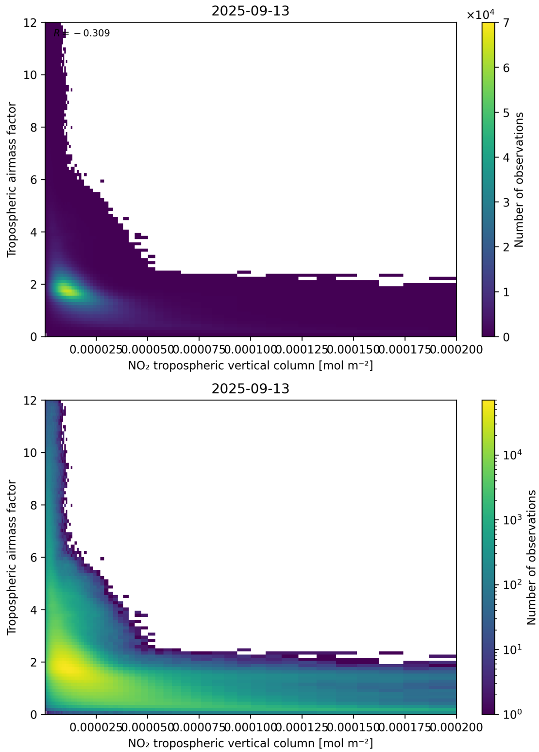
Figure 123: Scatter density plot of “NO 2 tropospheric vertical column” against “Tropospheric air mass factor” for 2025-09-12 to 2025-09-14.
