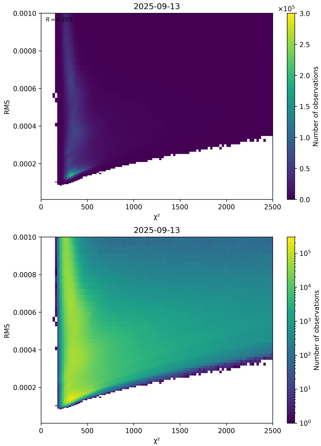
Figure 82: Scatter density plot of “ \chi^2 ” against “RMS” for 2025-09-12 to 2025-09-14.
