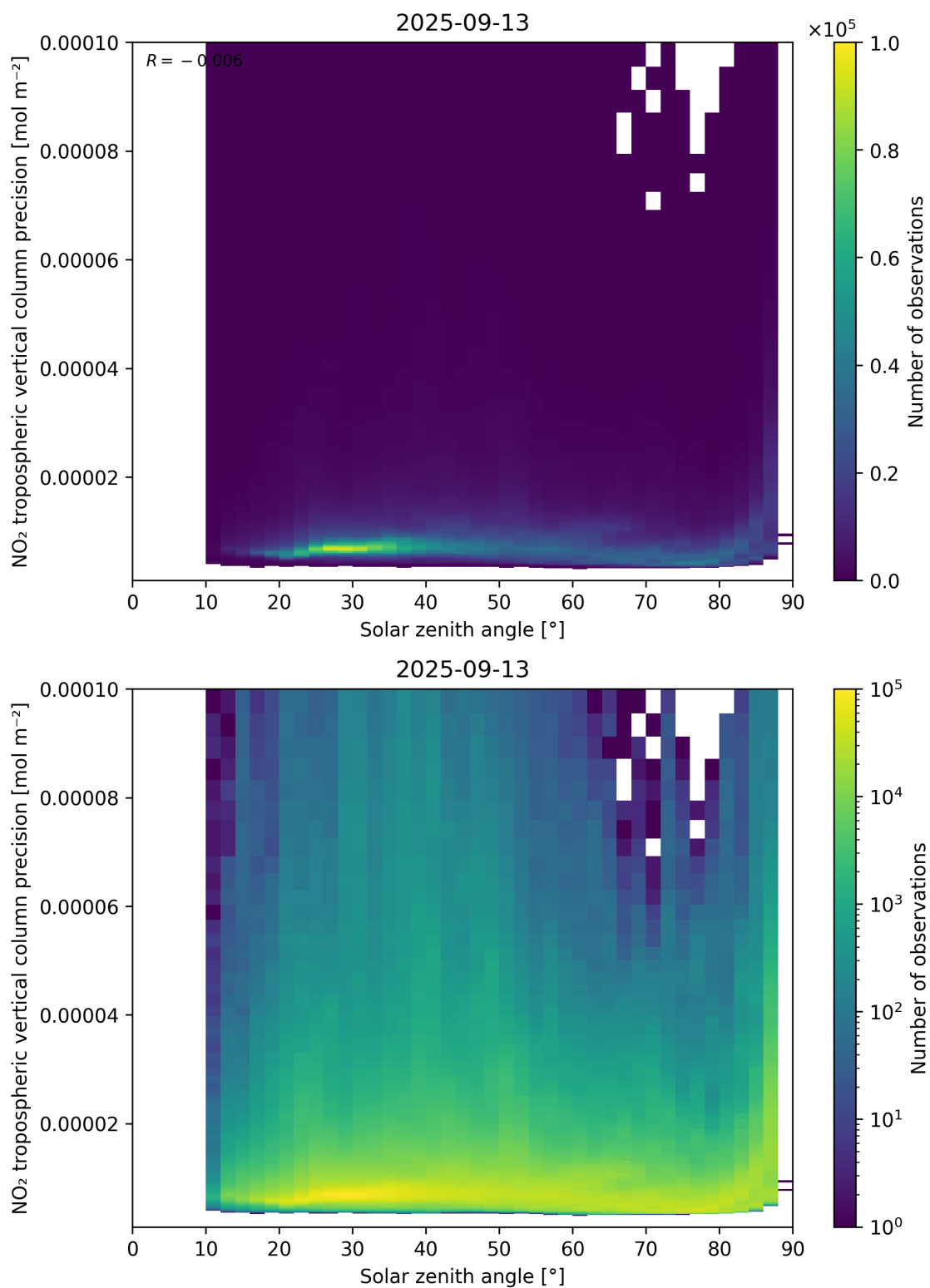
Figure 156: Scatter density plot of “Solar zenith angle” against “NO 2 tropospheric vertical column precision” for 2025-09-12 to 2025-09-14.
