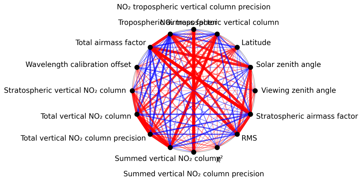
Figure 1: Map of correlation graph for 2025-09-12 to 2025-09-14.
