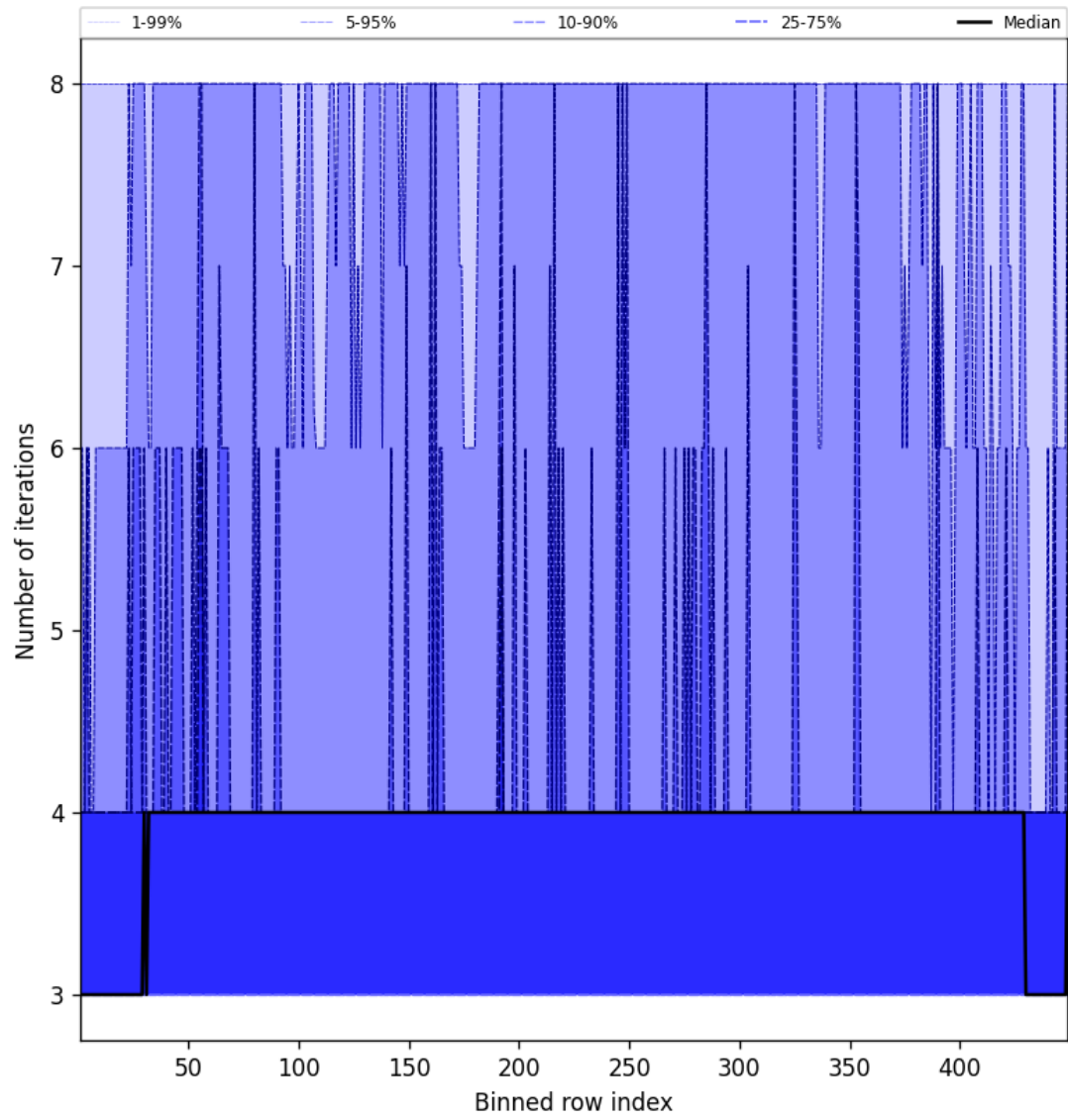
Figure 51: Along track statistics of “Number of iterations” for 2025-09-12 to 2025-09-14
