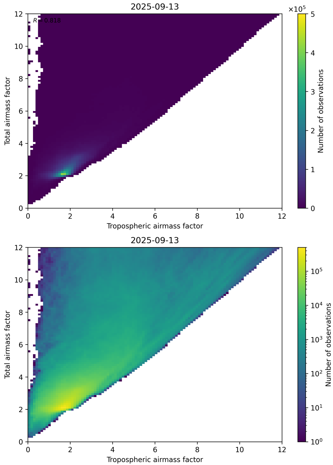
Figure 72: Scatter density plot of “Tropospheric airmass factor” against “Total airmass factor” for 2025-09-12 to 2025-09-14.
