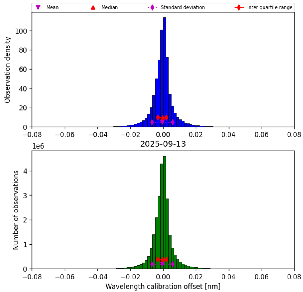
Figure 35: Histogram of “Wavelength calibration offset” for 2025-09-12 to 2025-09-14
