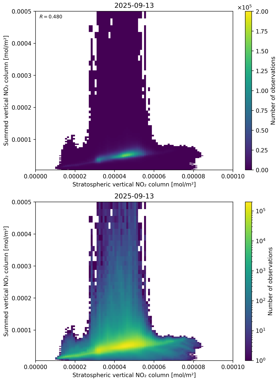
Figure 98: Scatter density plot of “Stratospheric vertical NO 2 column” against “Summed vertical NO 2 column” for 2025-09-12 to 2025-09-14.
