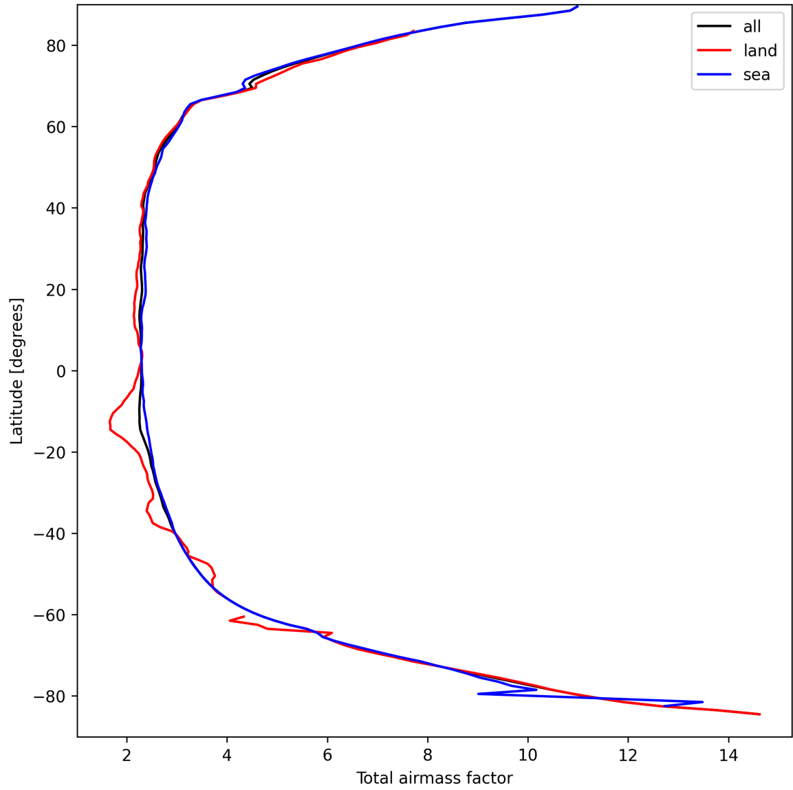
Figure 15: Zonal average of “Total airmass factor” for 2025-09-12 to 2025-09-14.
