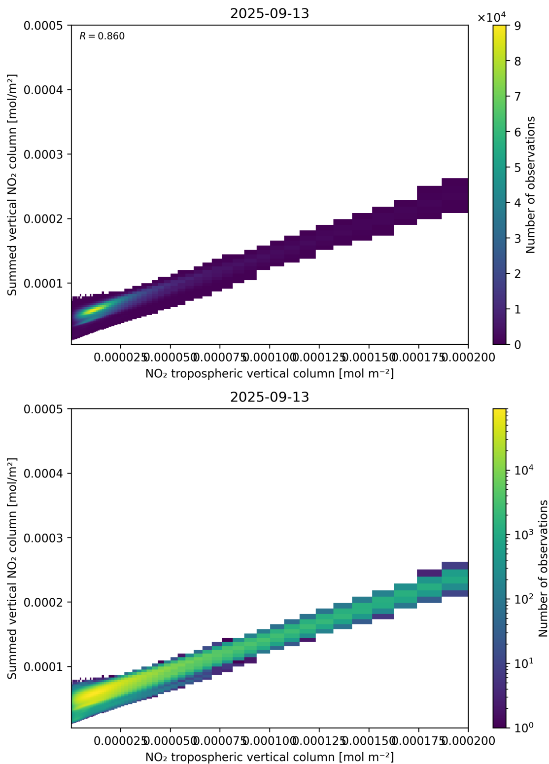
Figure 126: Scatter density plot of “NO 2 tropospheric vertical column” against “Summed vertical NO 2 column” for 2025-09-12 to 2025-09-14.
