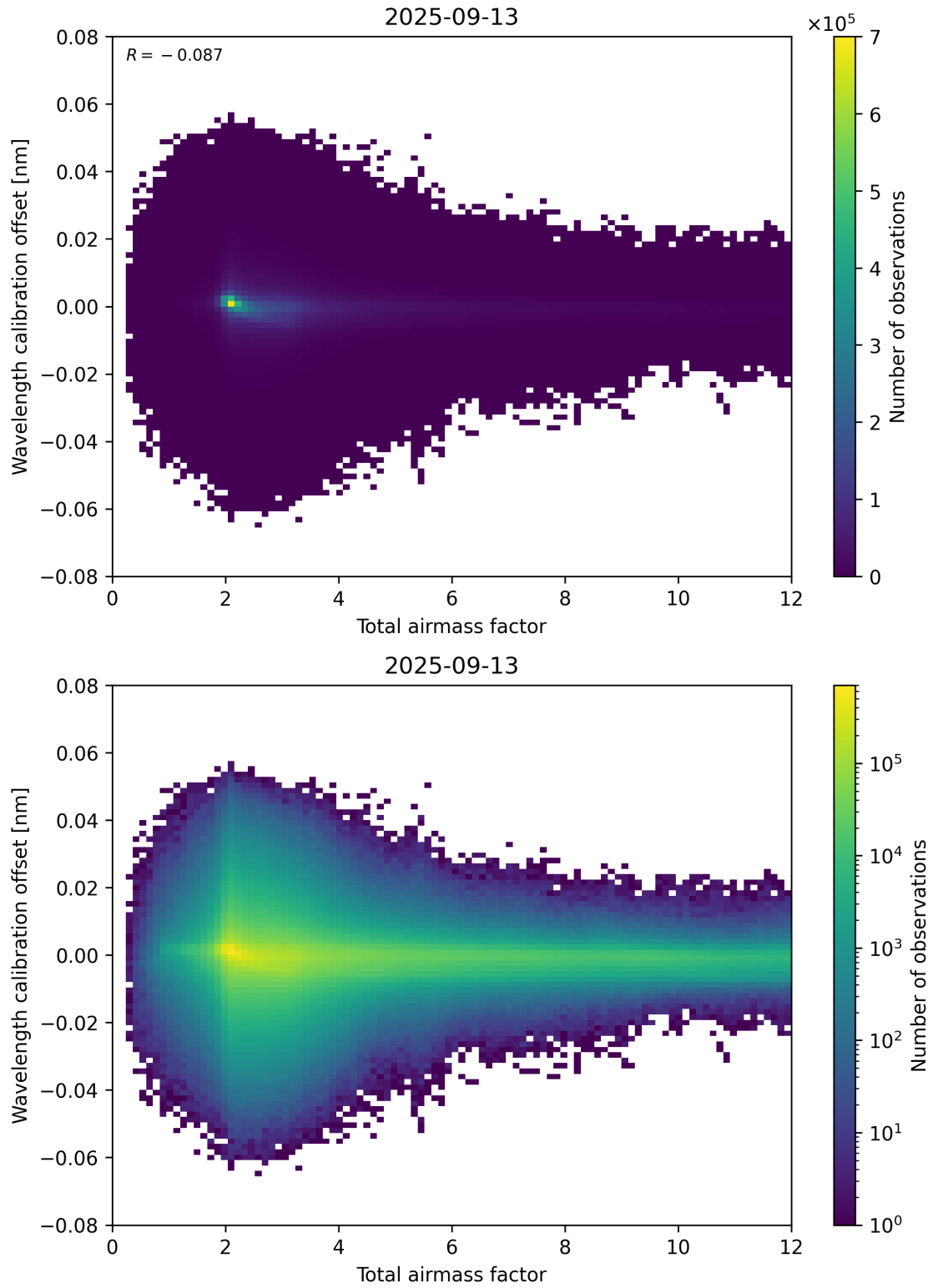
Figure 70: Scatter density plot of “Total airmass factor” against “Wavelength calibration offset” for 2025-09-12 to 2025-09-14.
