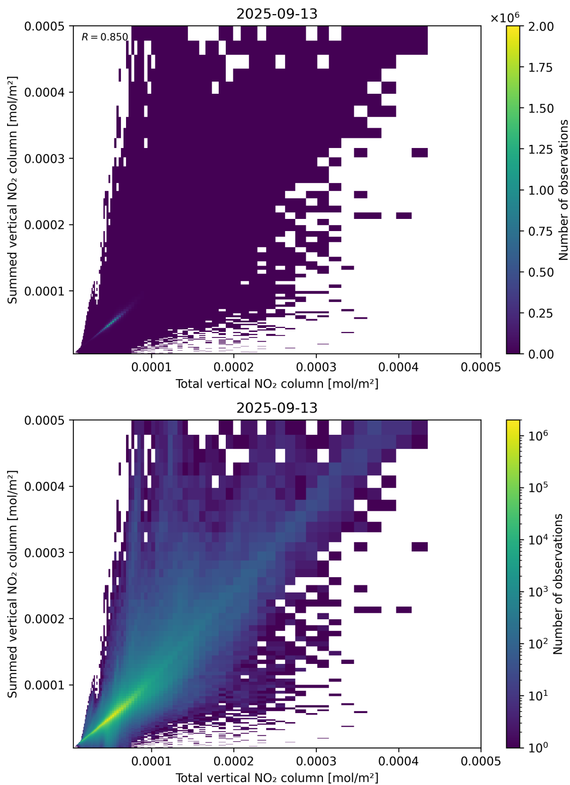
Figure 112: Scatter density plot of “Total vertical NO 2 column” against “Summed vertical NO 2 column” for 2025-09-12 to 2025-09-14.
