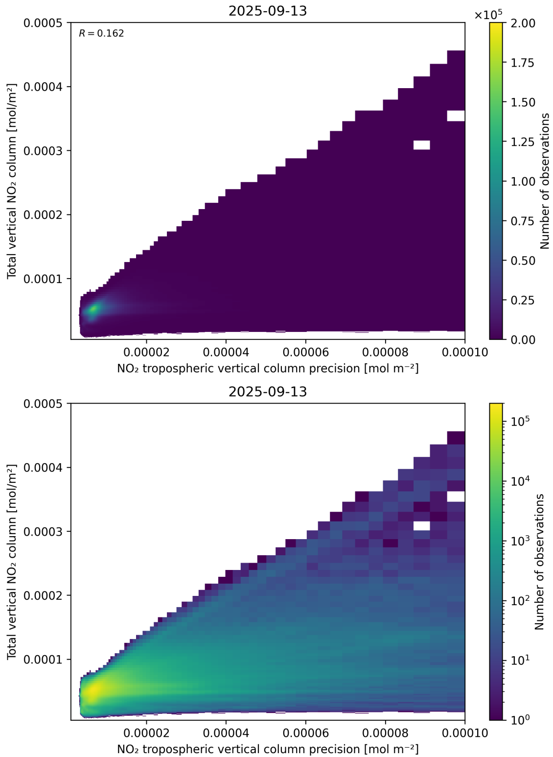
Figure 138: Scatter density plot of “NO 2 tropospheric vertical column precision” against “Total vertical NO 2 column” for 2025-09-12 to 2025-09-14.
