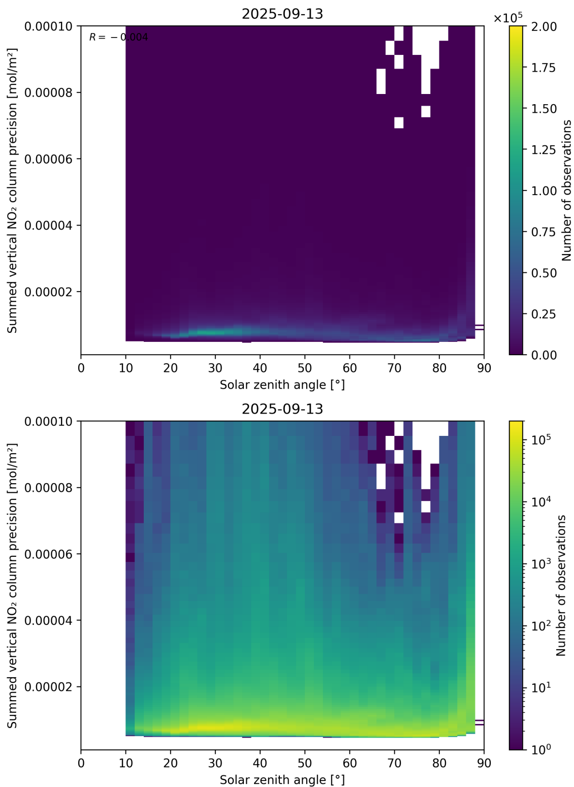
Figure 152: Scatter density plot of “Solar zenith angle” against “Summed vertical NO 2 column precision” for 2025-09-12 to 2025-09-14.
