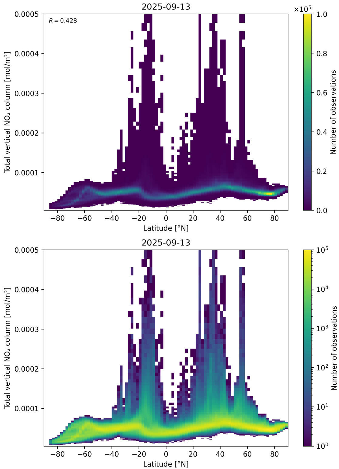
Figure 90: Scatter density plot of “Latitude” against “Total vertical NO 2 column” for 2025-09-12 to 2025-09-14.
