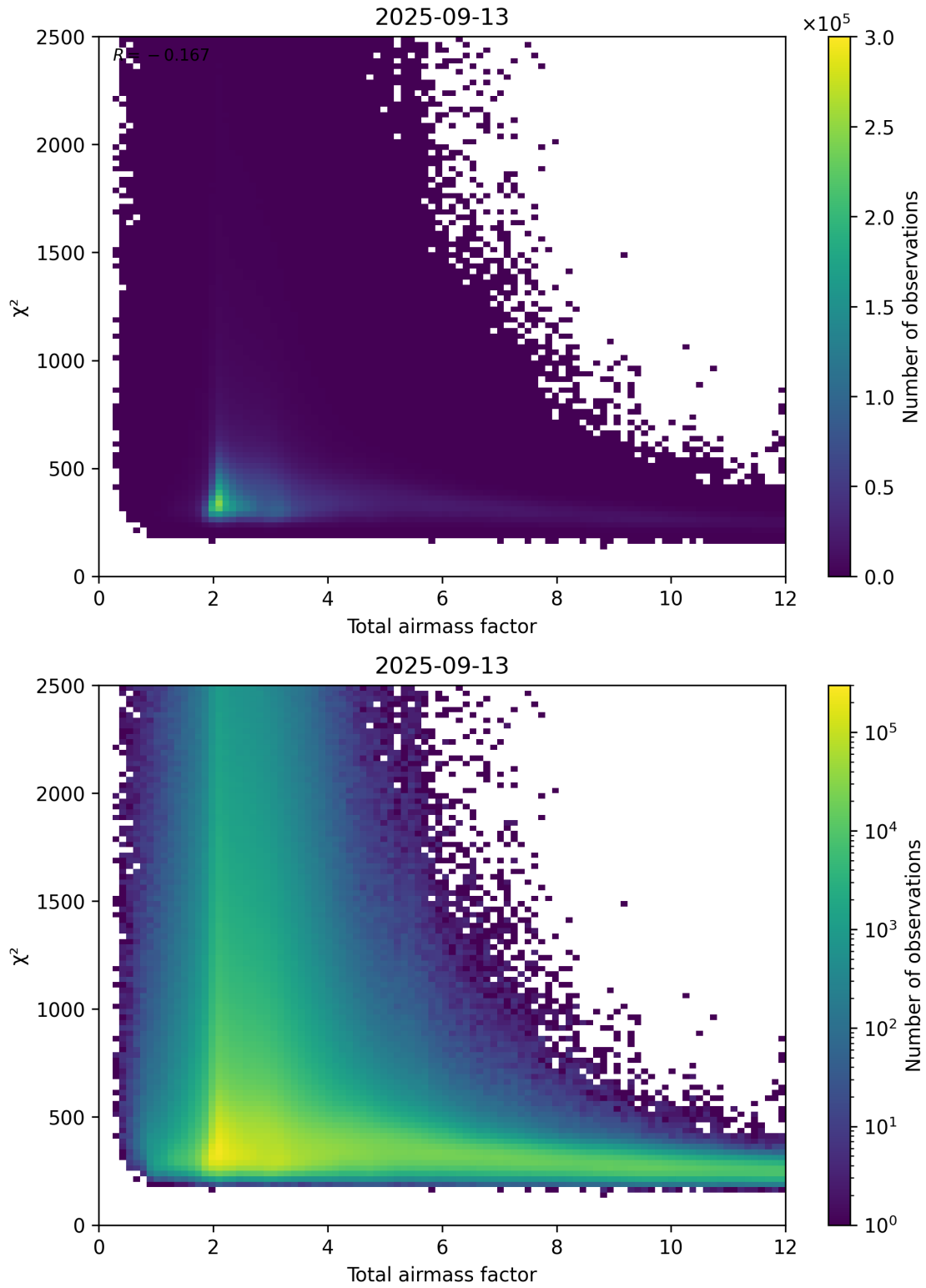
Figure 63: Scatter density plot of “Total airmass factor” against “ \chi^2 ” for 2025-09-12 to 2025-09-14.
