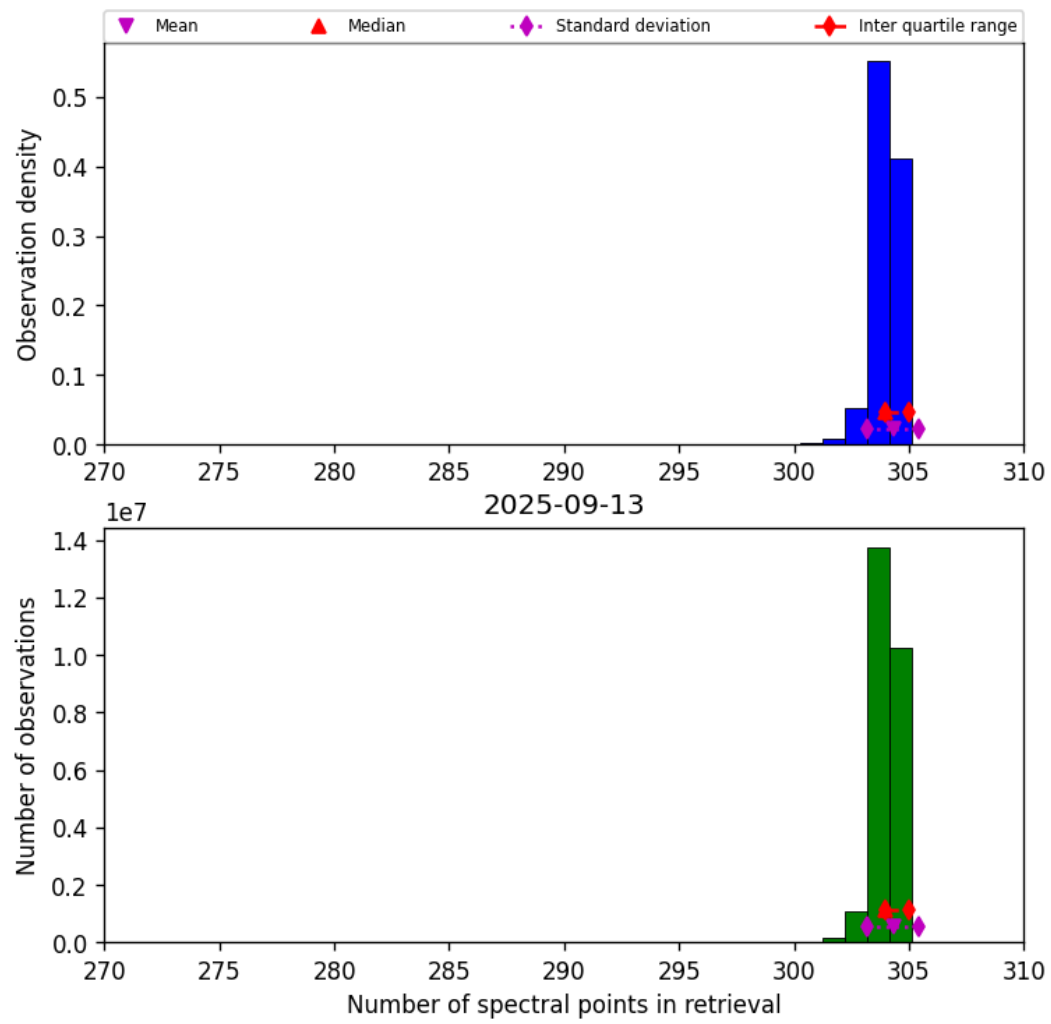
Figure 33: Histogram of “Number of spectral points in retrieval” for 2025-09-12 to 2025-09-14
