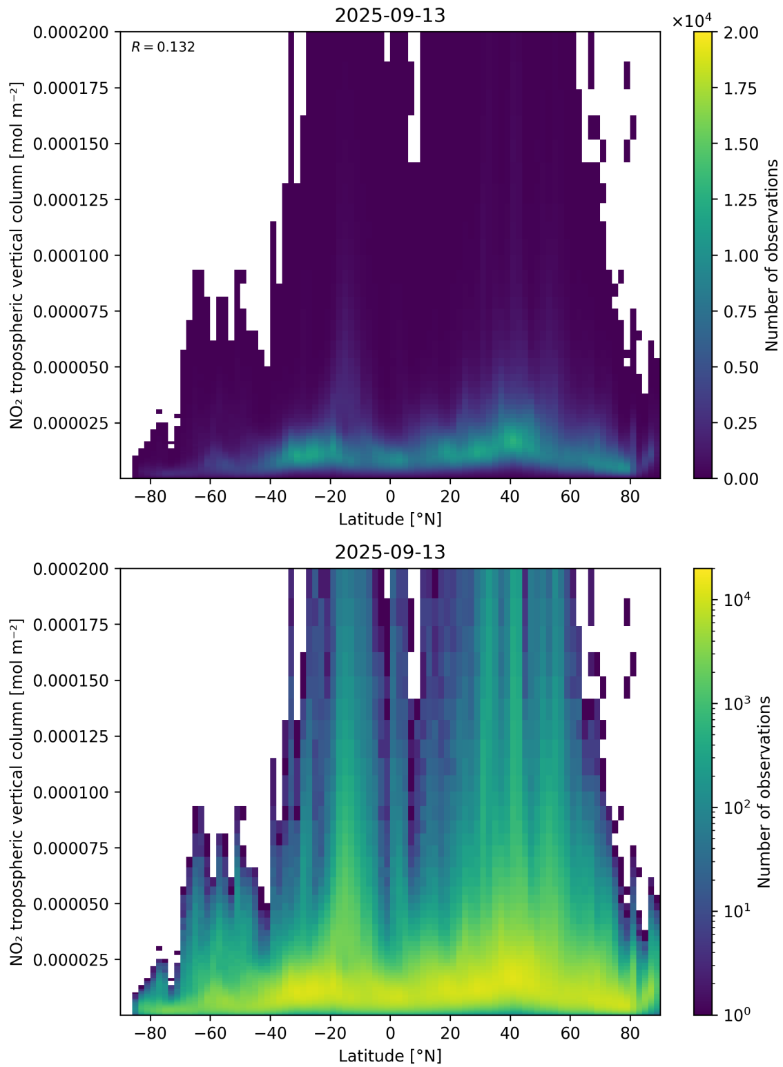
Figure 92: Scatter density plot of “Latitude” against “NO 2 tropospheric vertical column” for 2025-09-12 to 2025-09-14.
