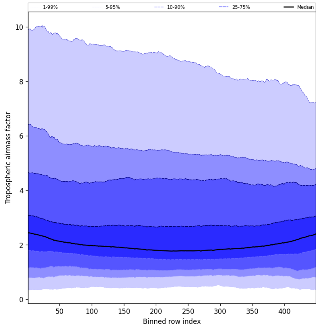
Figure 48: Along track statistics of “Tropospheric air mass factor” for 2025-09-12 to 2025-09-14
