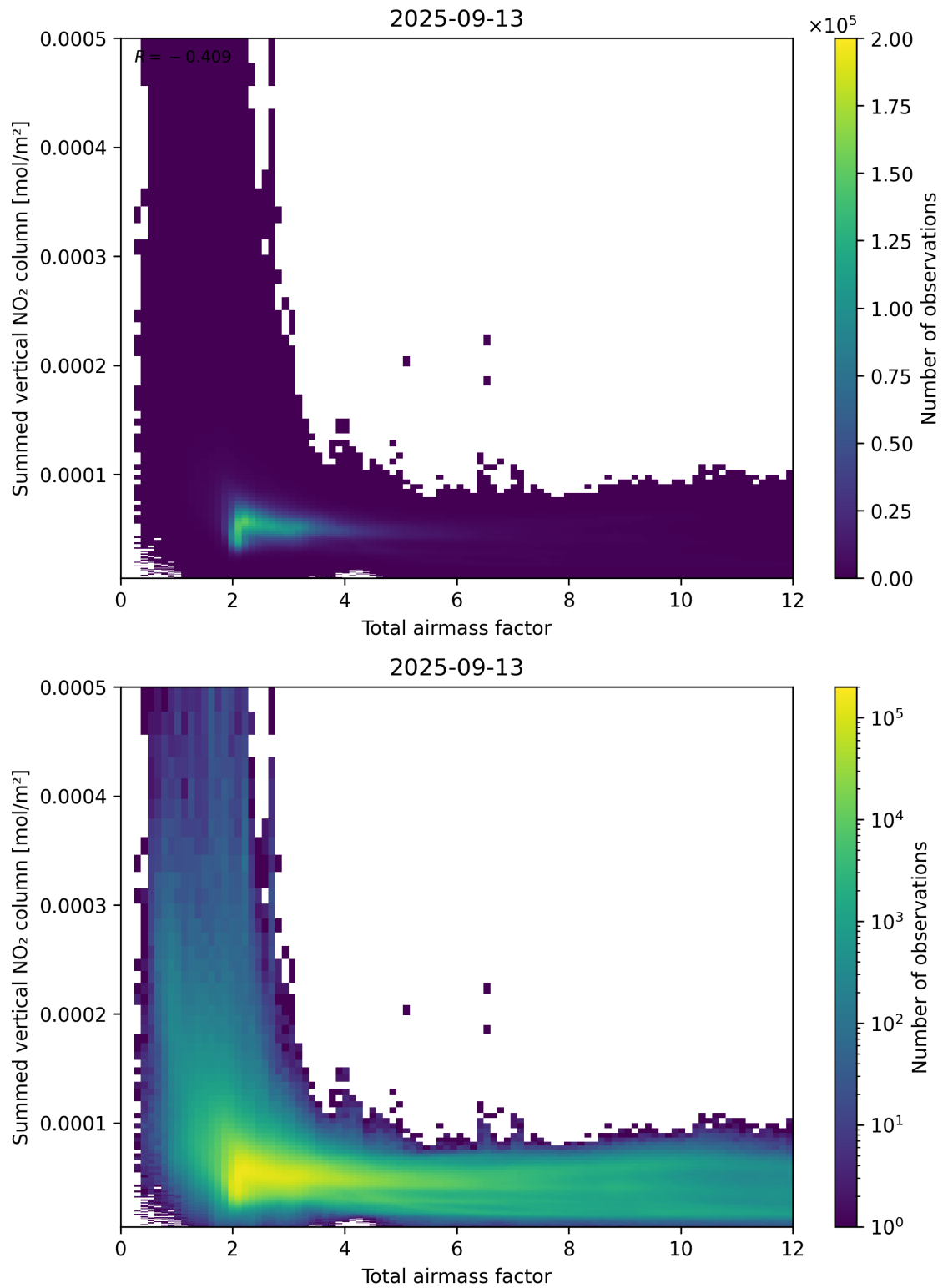
Figure 65: Scatter density plot of “Total airmass factor” against “Summed vertical NO 2 column” for 2025-09-12 to 2025-09-14.
