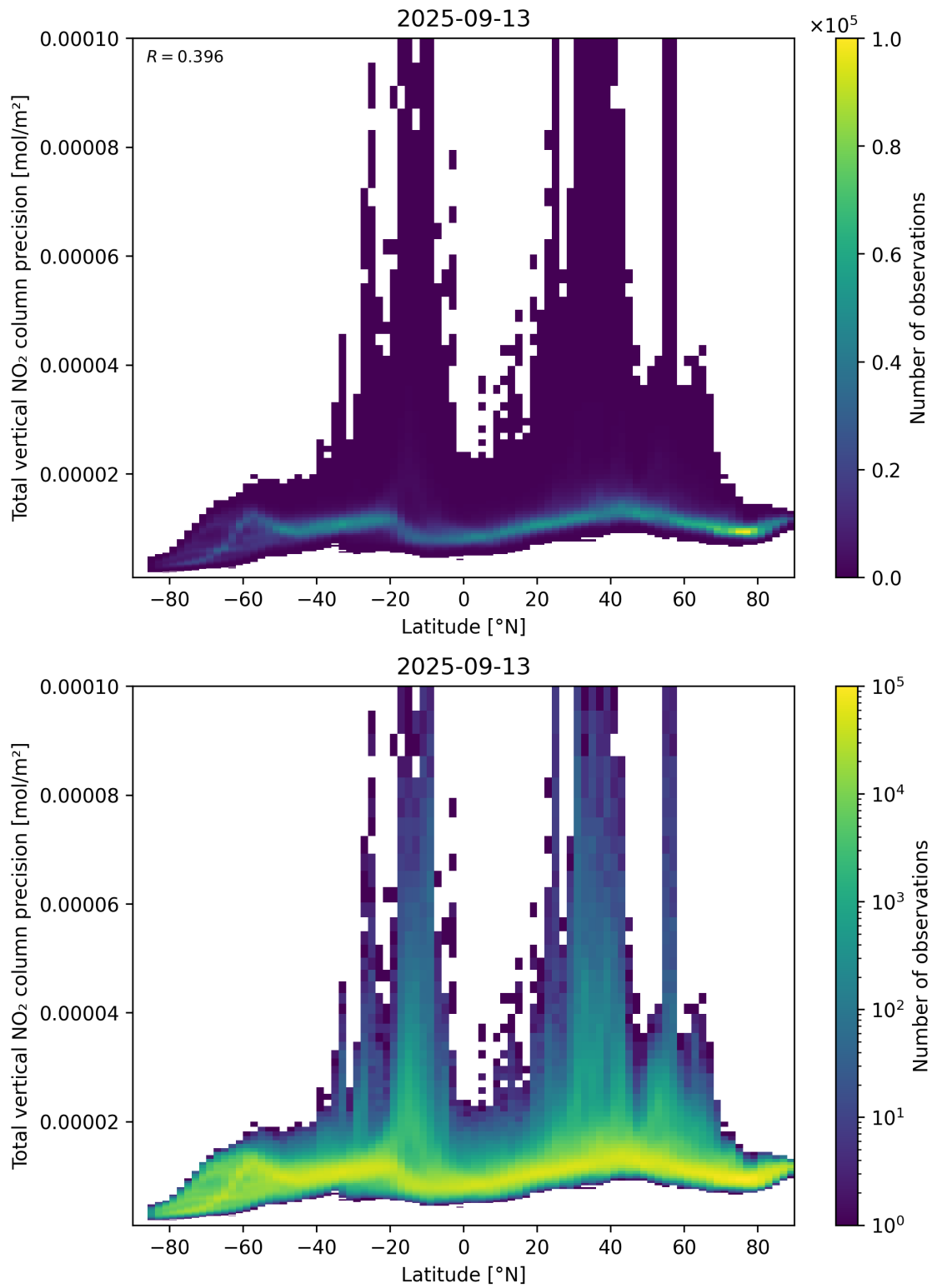
Figure 91: Scatter density plot of “Latitude” against “Total vertical NO 2 column precision” for 2025-09-12 to 2025-09-14.
