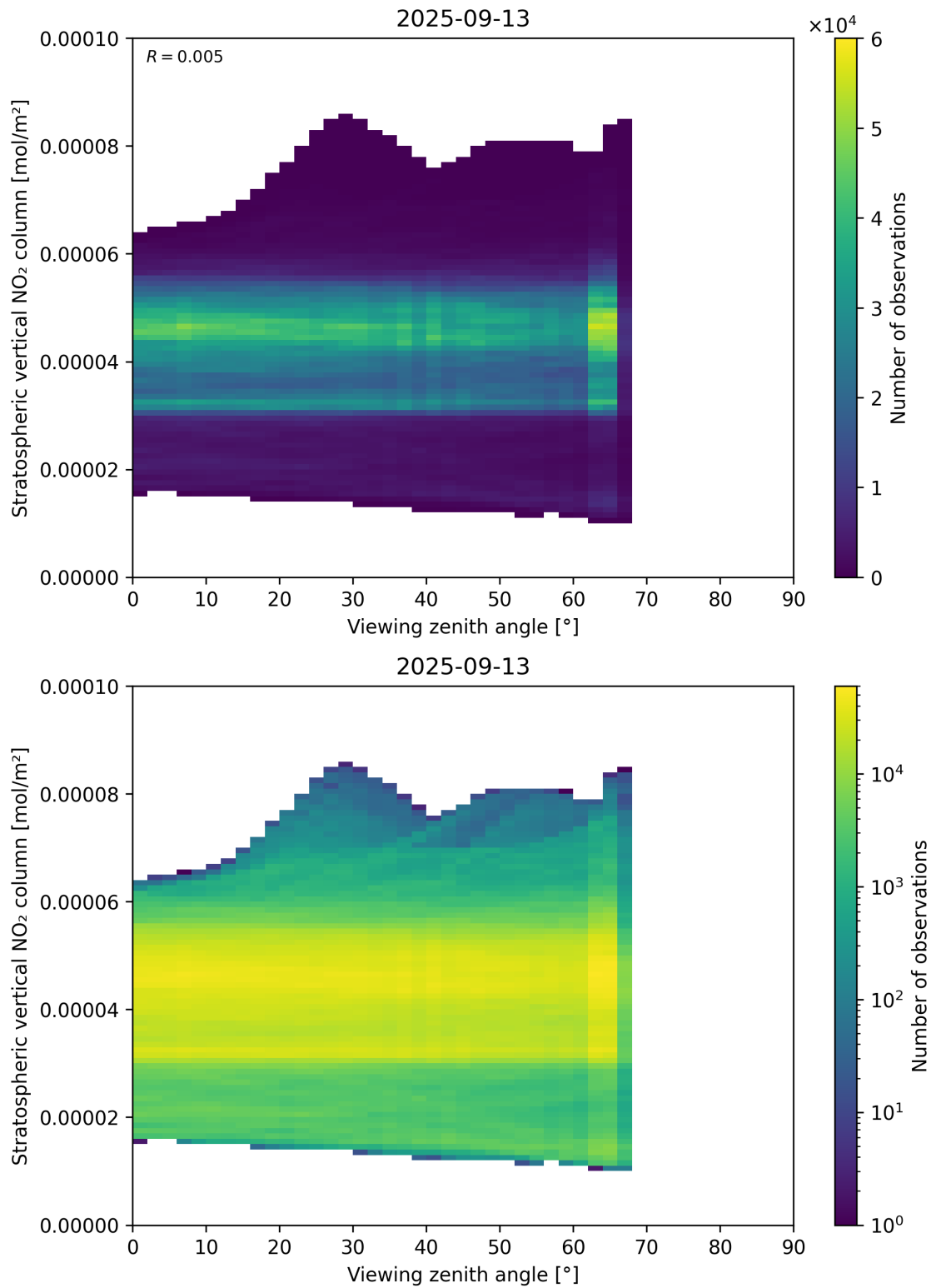
Figure 164: Scatter density plot of “Viewing zenith angle” against “Stratospheric vertical NO 2 column” for 2025-09-12 to 2025-09-14.
