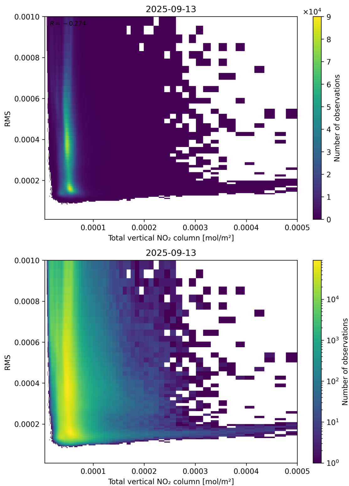
Figure 120: Scatter density plot of “Total vertical NO 2 column” against “RMS” for 2025-09-12 to 2025-09-14.
