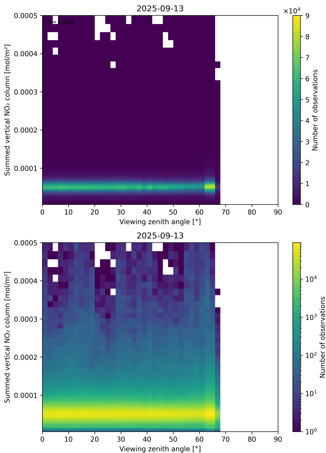
Figure 165: Scatter density plot of “Viewing zenith angle” against “Summed vertical NO 2 column” for 2025-09-12 to 2025-09-14.
