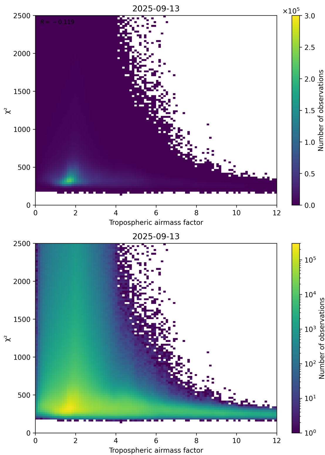
Figure 73: Scatter density plot of “Tropospheric airmass factor” against “ \chi^2 ” for 2025-09-12 to 2025-09-14.
