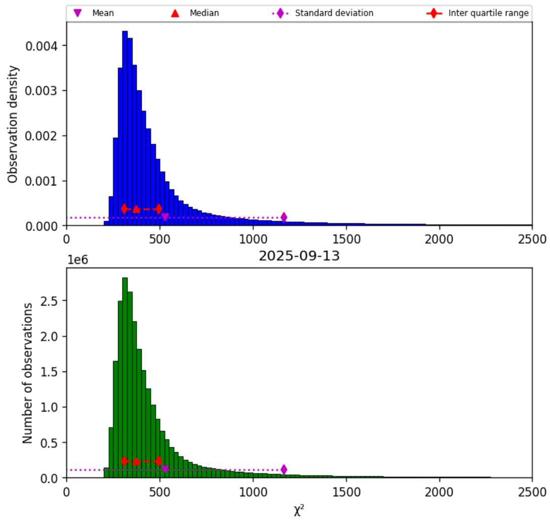
Figure 42: Histogram of “ \chi^2 ” for 2025-09-12 to 2025-09-14
