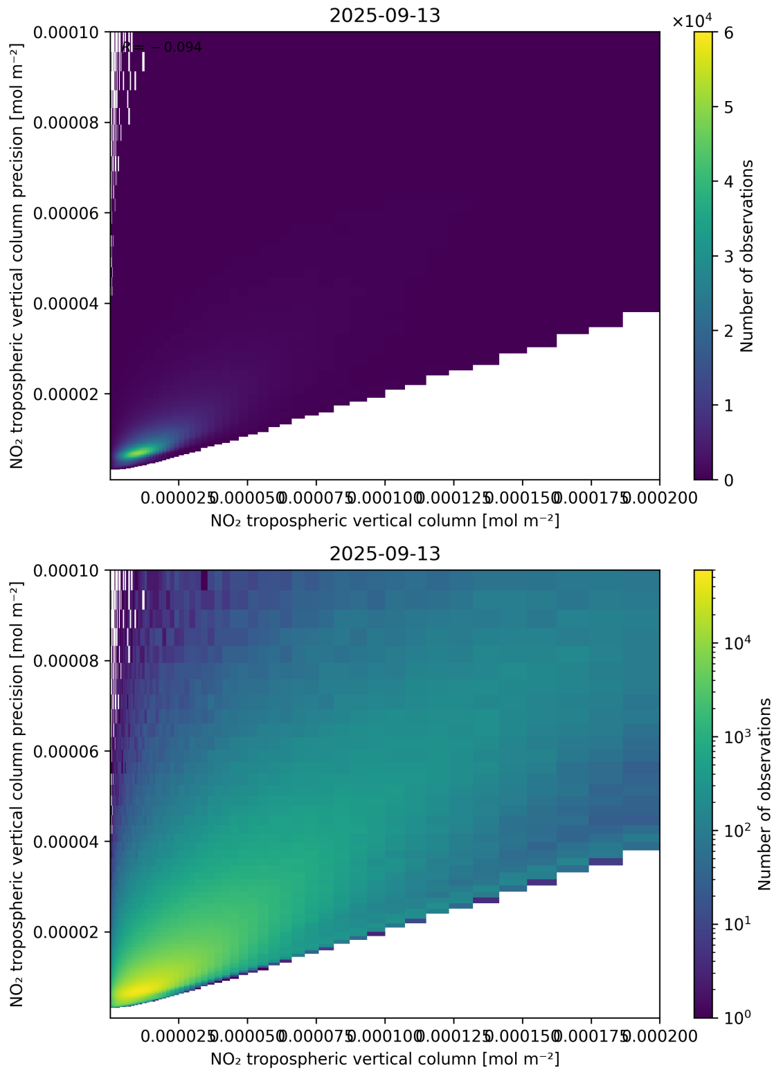
Figure 130: Scatter density plot of “NO 2 tropospheric vertical column” against “NO 2 tropospheric vertical column precision” for 2025-09-12 to 2025-09-14.
