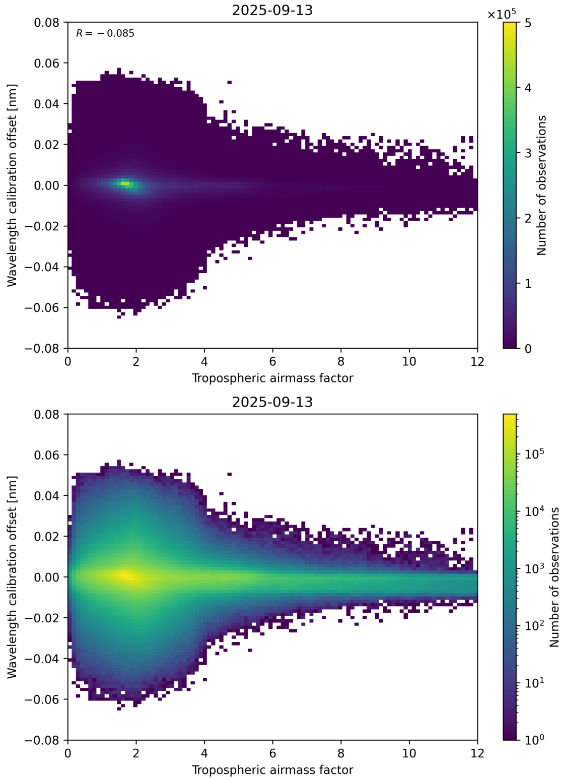
Figure 80: Scatter density plot of “Tropospheric airmass factor” against “Wavelength calibration offset” for 2025-09-12 to 2025-09-14.
