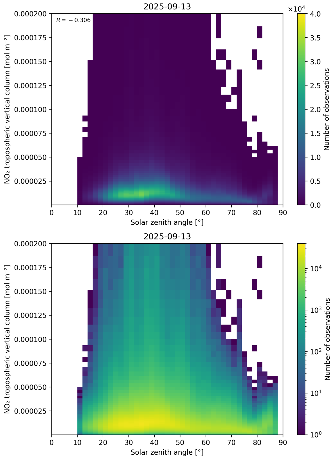
Figure 155: Scatter density plot of “Solar zenith angle” against “NO 2 tropospheric vertical column” for 2025-09-12 to 2025-09-14.
