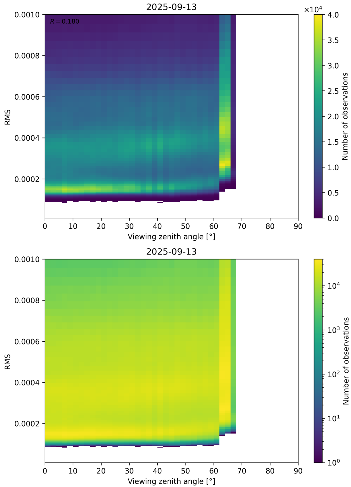
Figure 171: Scatter density plot of “Viewing zenith angle” against “RMS” for 2025-09-12 to 2025-09-14.
