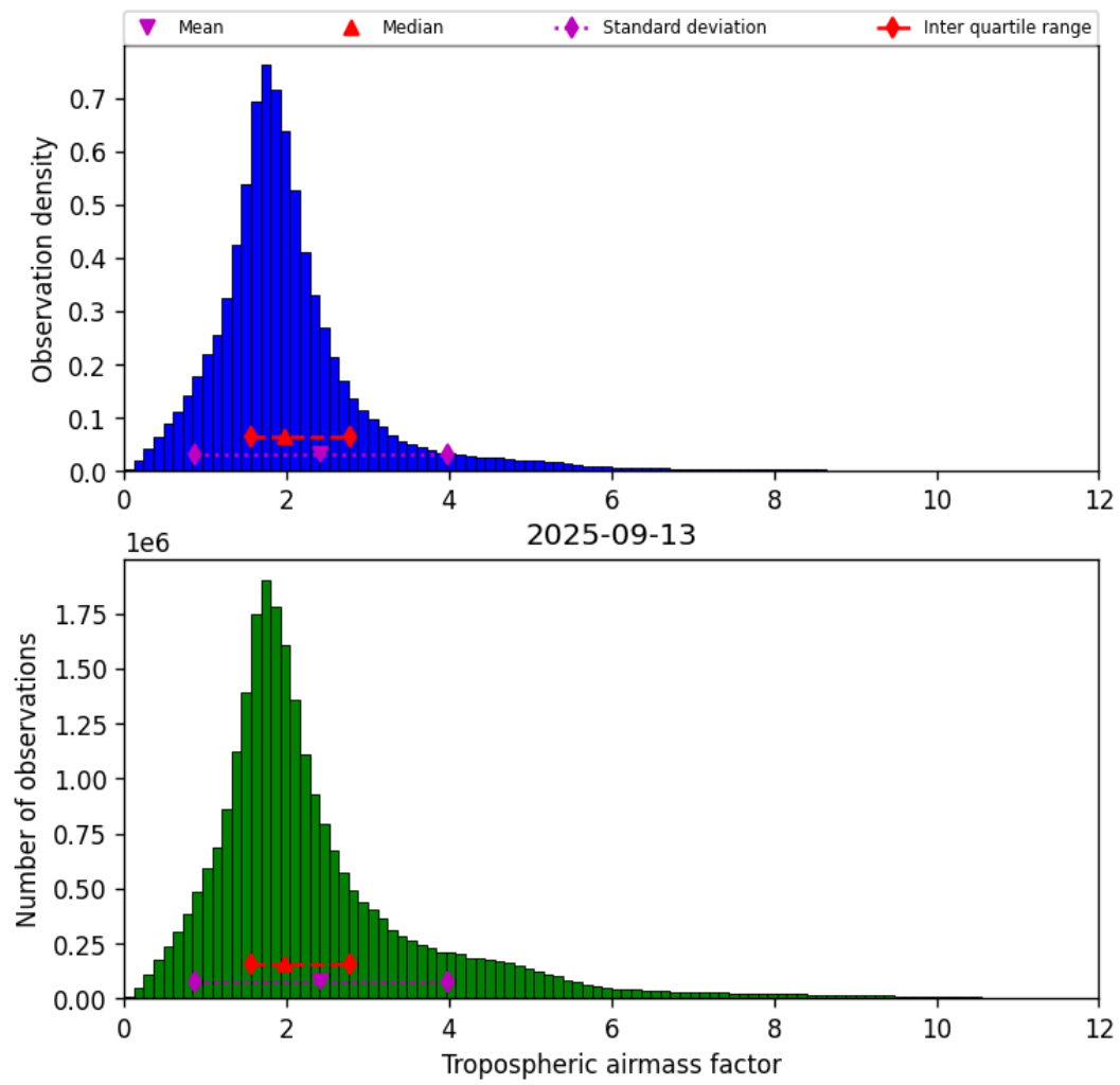
Figure 31: Histogram of “Tropospheric airmass factor” for 2025-09-12 to 2025-09-14
