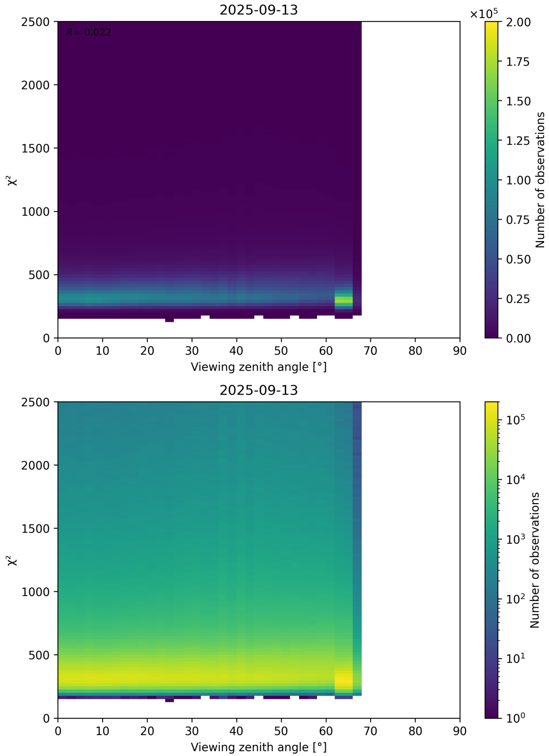
Figure 162: Scatter density plot of “Viewing zenith angle” against “ \chi^2 ” for 2025-09-12 to 2025-09-14.
