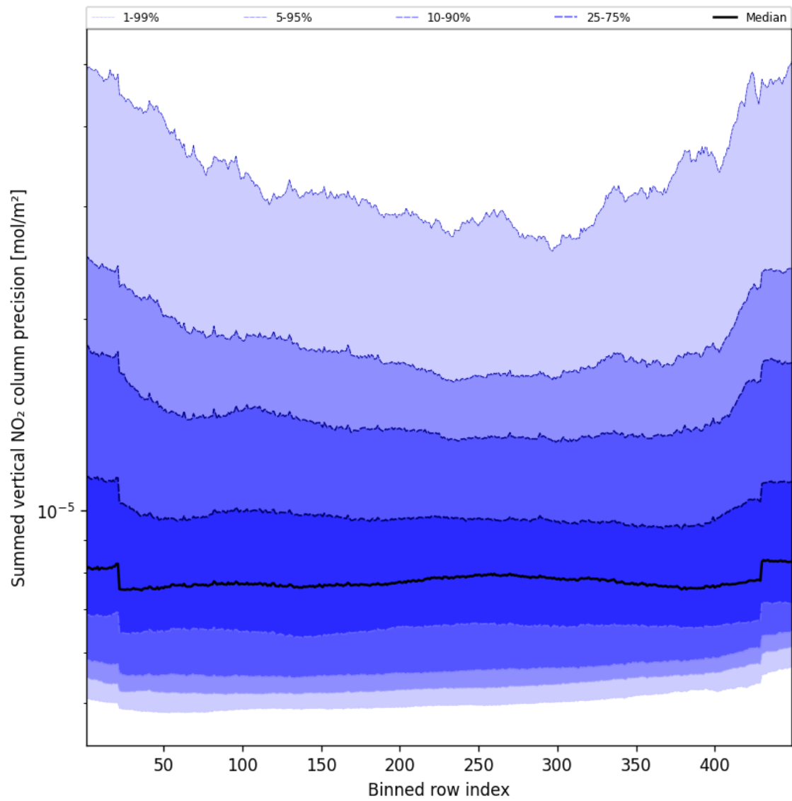
Figure 58: Along track statistics of “Summed vertical NO 2 column precision” for 2025-09-12 to 2025-09-14
