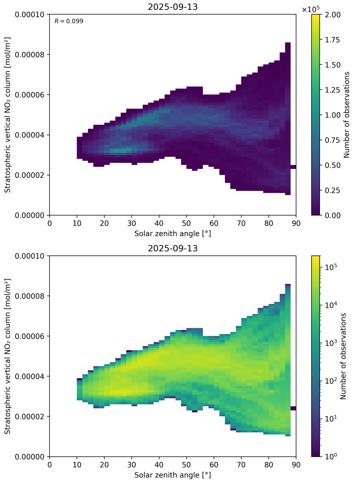
Figure 150: Scatter density plot of “Solar zenith angle” against “Stratospheric vertical \text{NO}_2 column” for 2025-09-12 to 2025-09-14.
