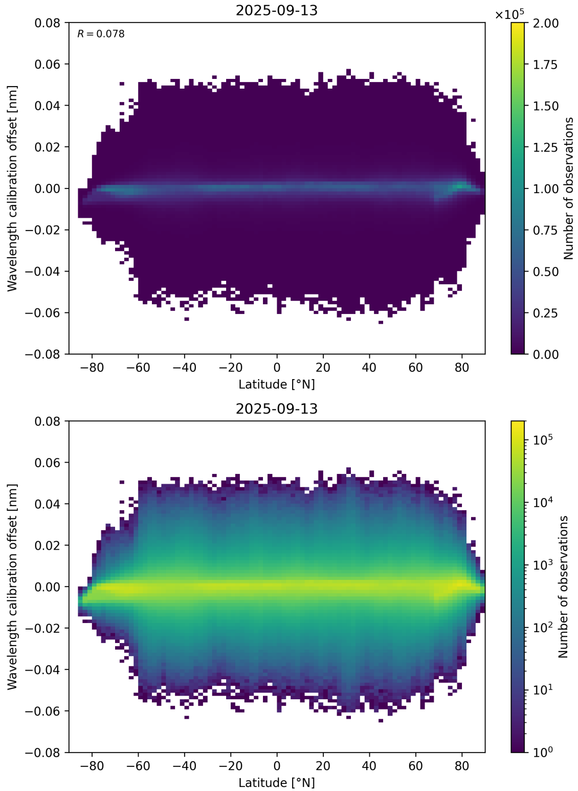
Figure 95: Scatter density plot of “Latitude” against “Wavelength calibration offset” for 2025-09-12 to 2025-09-14.
