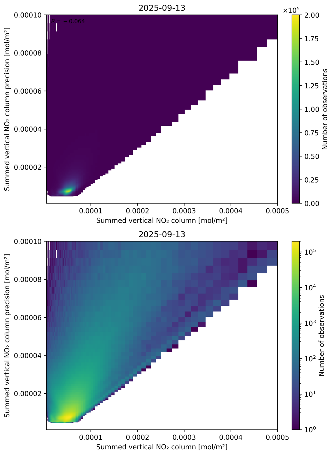
Figure 105: Scatter density plot of “Summed vertical NO 2 column” against “Summed vertical NO 2 column precision” for 2025-09-12 to 2025-09-14.
