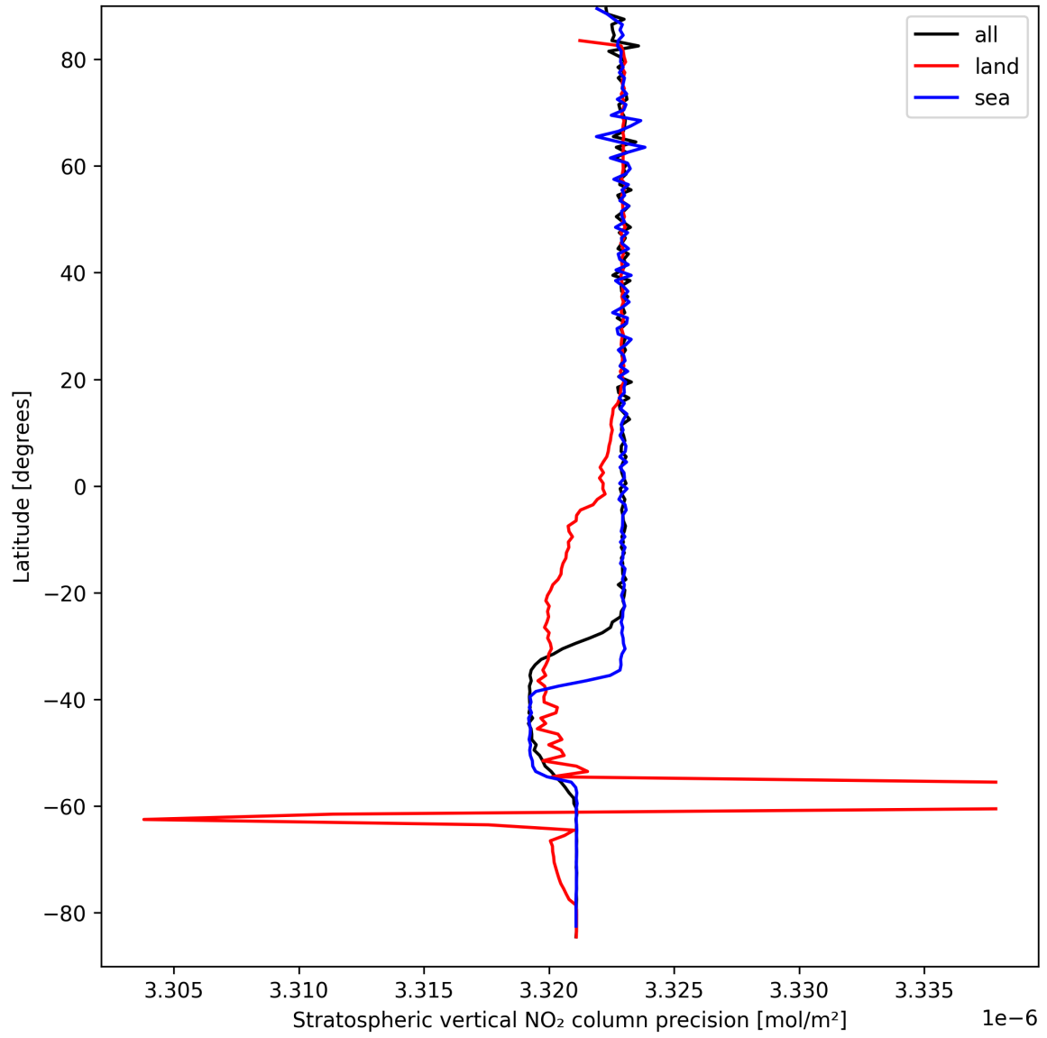
Figure 20: Zonal average of “Stratospheric vertical NO 2 column precision” for 2025-09-12 to 2025-09-14.
