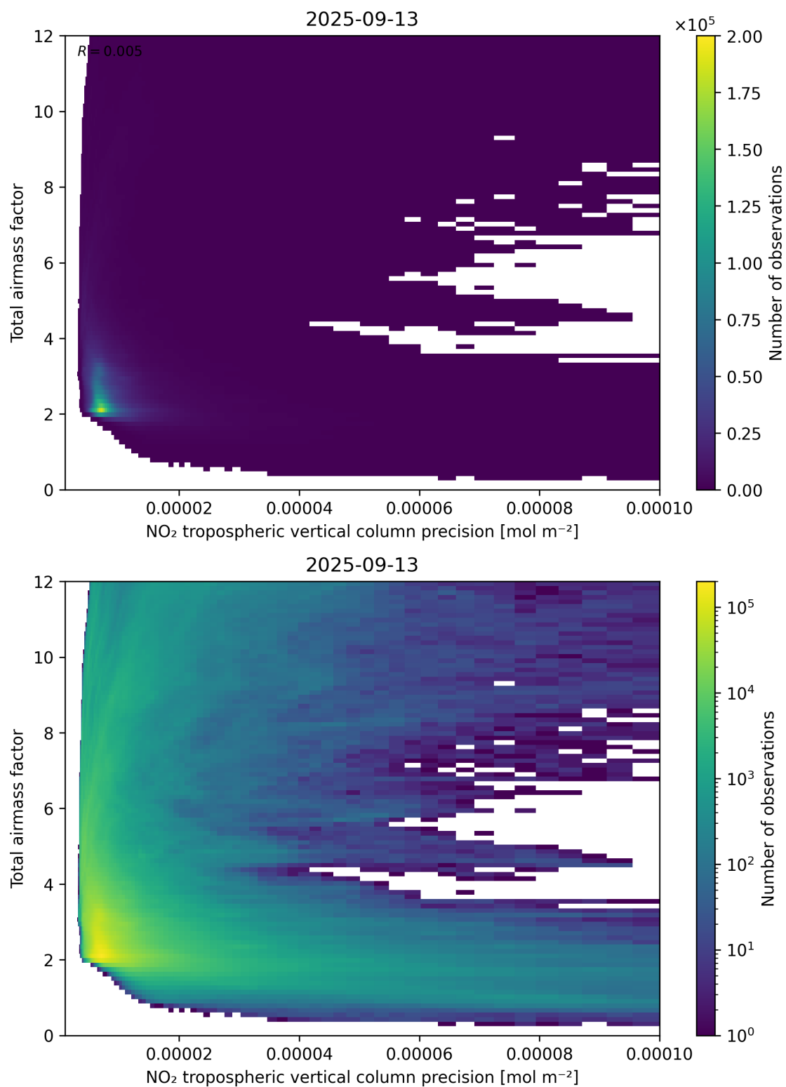
Figure 132: Scatter density plot of “NO 2 tropospheric vertical column precision” against “Total air mass factor” for 2025-09-12 to 2025-09-14.
