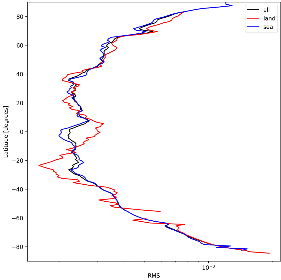
Figure 26: Zonal average of “RMS” for 2025-09-12 to 2025-09-14.
