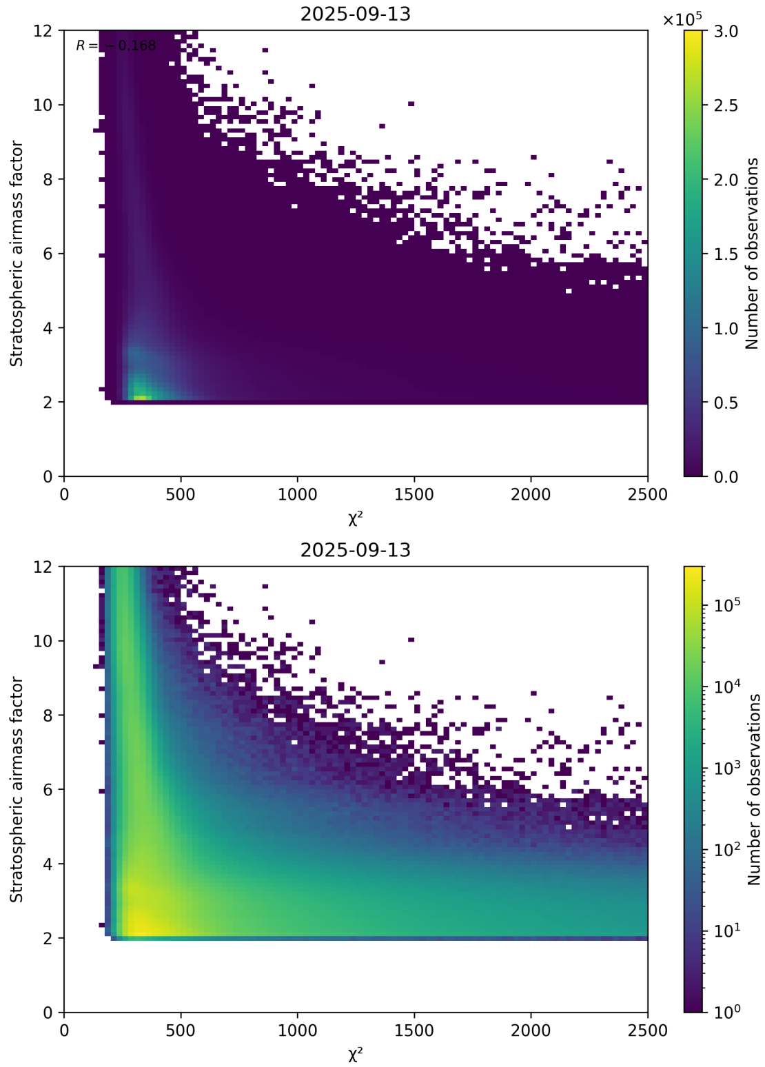
Figure 81: Scatter density plot of “ \chi^2 ” against “Stratospheric airmass factor” for 2025-09-12 to 2025-09-14.
