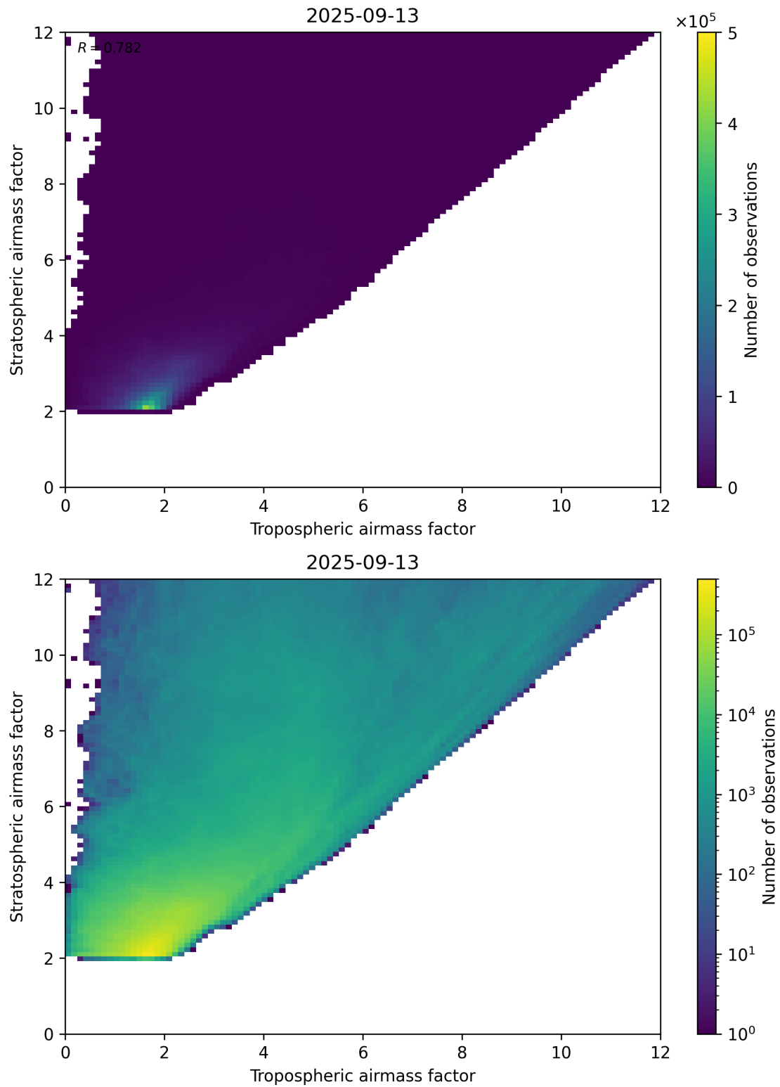
Figure 71: Scatter density plot of “Tropospheric airmass factor” against “Stratospheric airmass factor” for 2025-09-12 to 2025-09-14.
