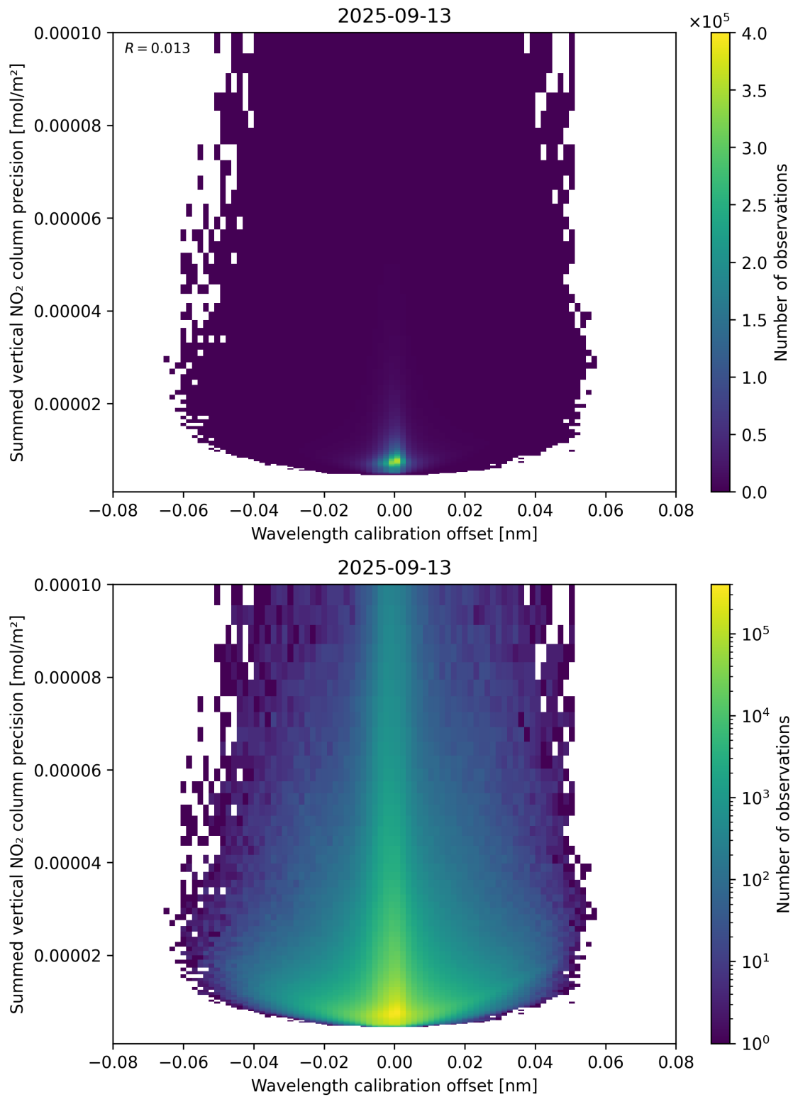
Figure 178: Scatter density plot of “Wavelength calibration offset” against “Summed vertical NO 2 column precision” for 2025-09-12 to 2025-09-14.
