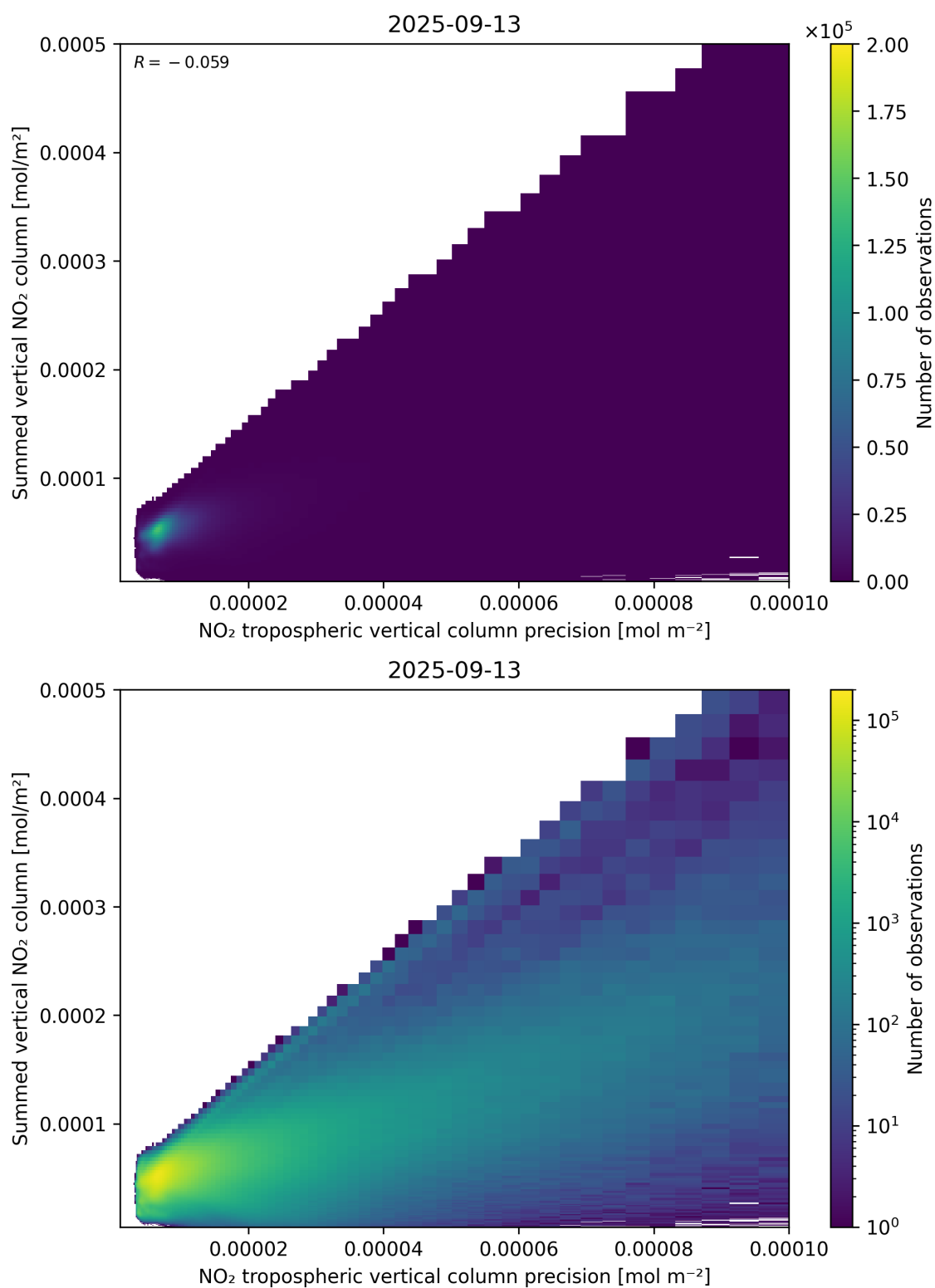
Figure 136: Scatter density plot of “NO 2 tropospheric vertical column precision” against “Summed vertical NO 2 column” for 2025-09-12 to 2025-09-14.
