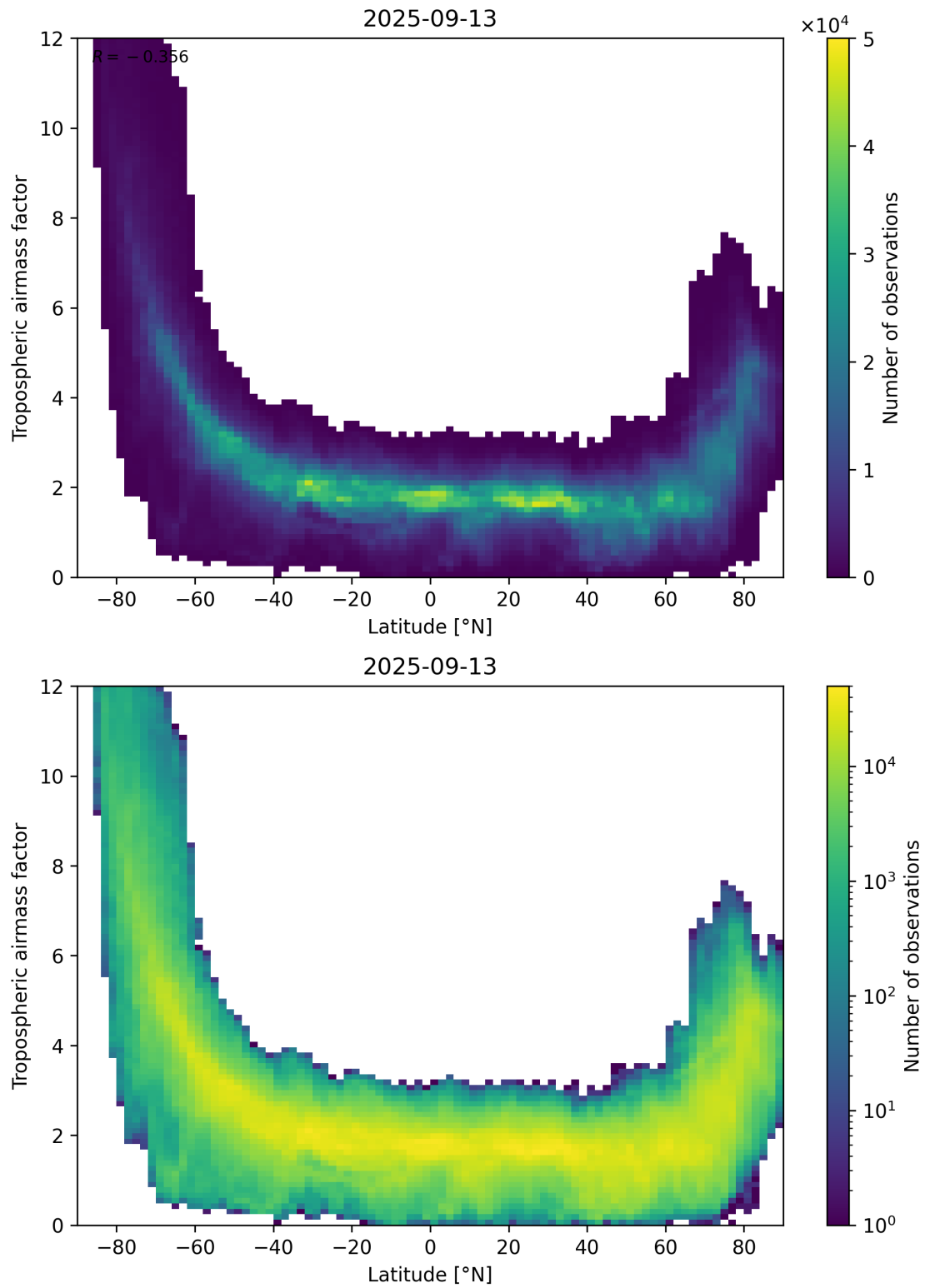
Figure 85: Scatter density plot of “Latitude” against “Tropospheric airmass factor” for 2025-09-12 to 2025-09-14.
