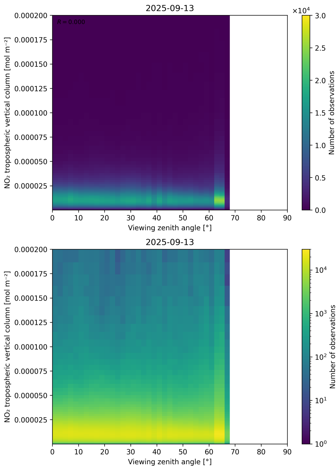
Figure 169: Scatter density plot of “Viewing zenith angle” against “NO 2 tropospheric vertical column” for 2025-09-12 to 2025-09-14.
