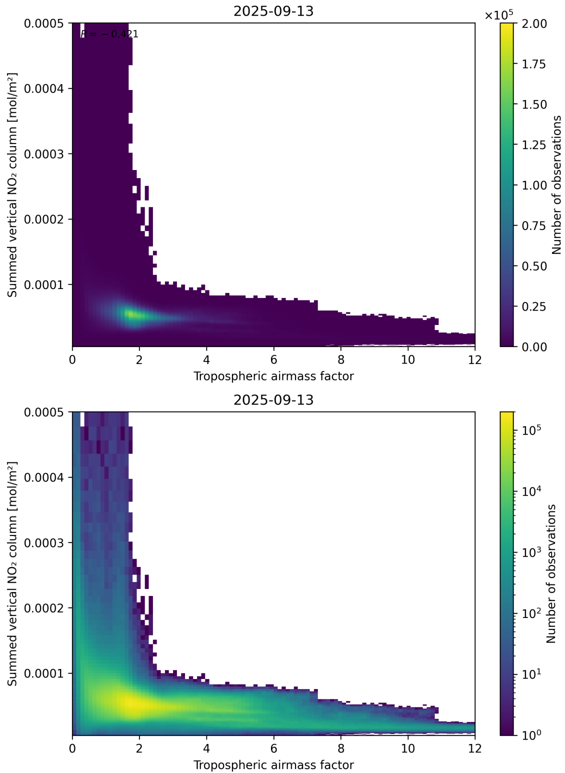
Figure 75: Scatter density plot of “Tropospheric air mass factor” against “Summed vertical NO 2 column” for 2025-09-12 to 2025-09-14.
