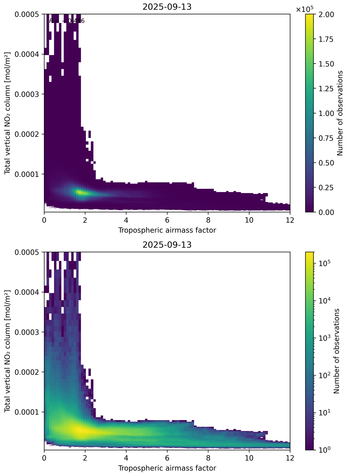
Figure 77: Scatter density plot of “Tropospheric airmass factor” against “Total vertical NO 2 column” for 2025-09-12 to 2025-09-14.
