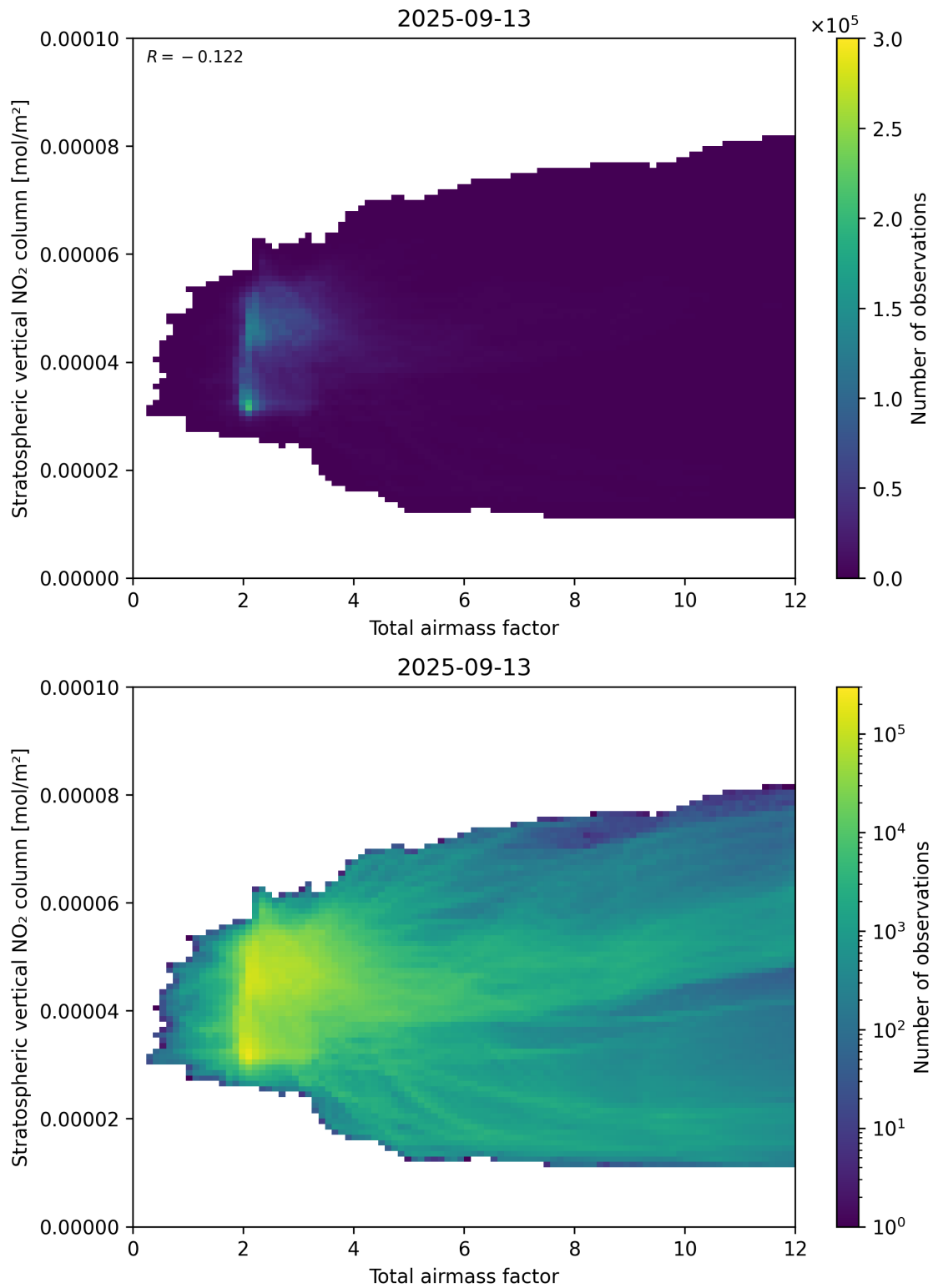
Figure 64: Scatter density plot of “Total airmass factor” against “Stratospheric vertical NO 2 column” for 2025-09-12 to 2025-09-14.
