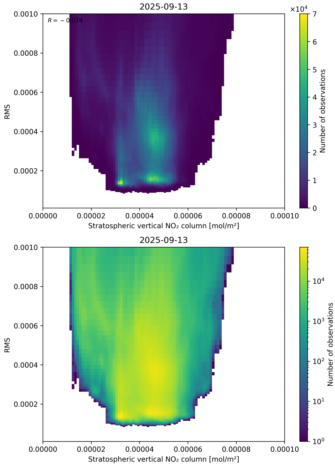
Figure 102: Scatter density plot of “Stratospheric vertical NO 2 column” against “RMS” for 2025-09-12 to 2025-09-14.
