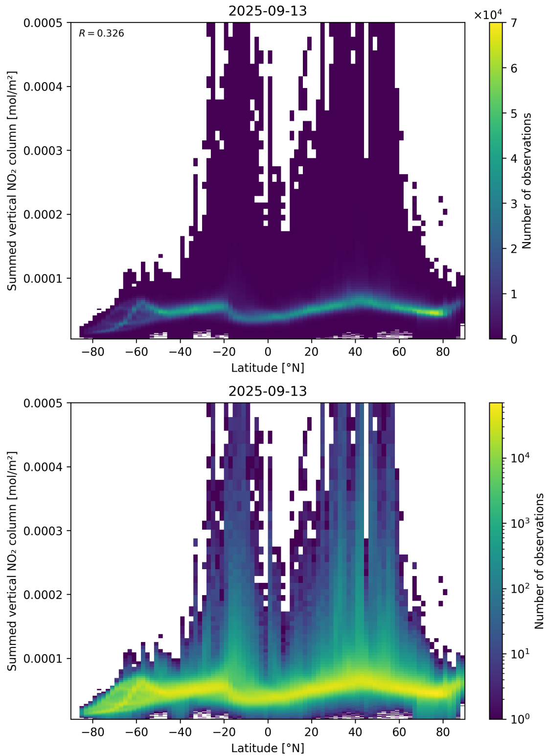
Figure 88: Scatter density plot of “Latitude” against “Summed vertical NO 2 column” for 2025-09-12 to 2025-09-14.
