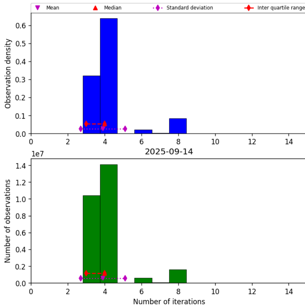
Figure 34: Histogram of “Number of iterations” for 2025-09-13 to 2025-09-15
