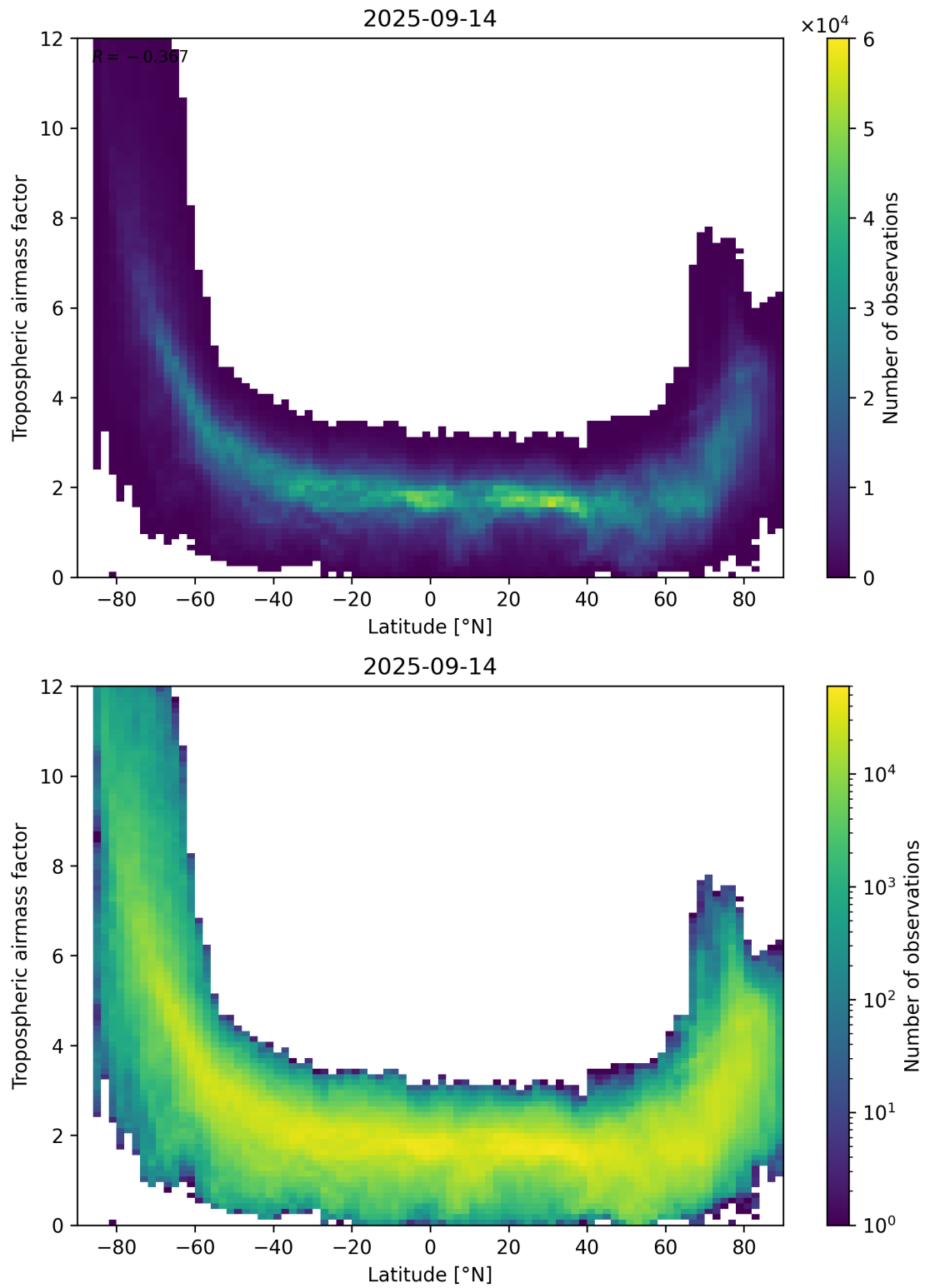
Figure 85: Scatter density plot of “Latitude” against “Tropospheric airmass factor” for 2025-09-13 to 2025-09-15.
