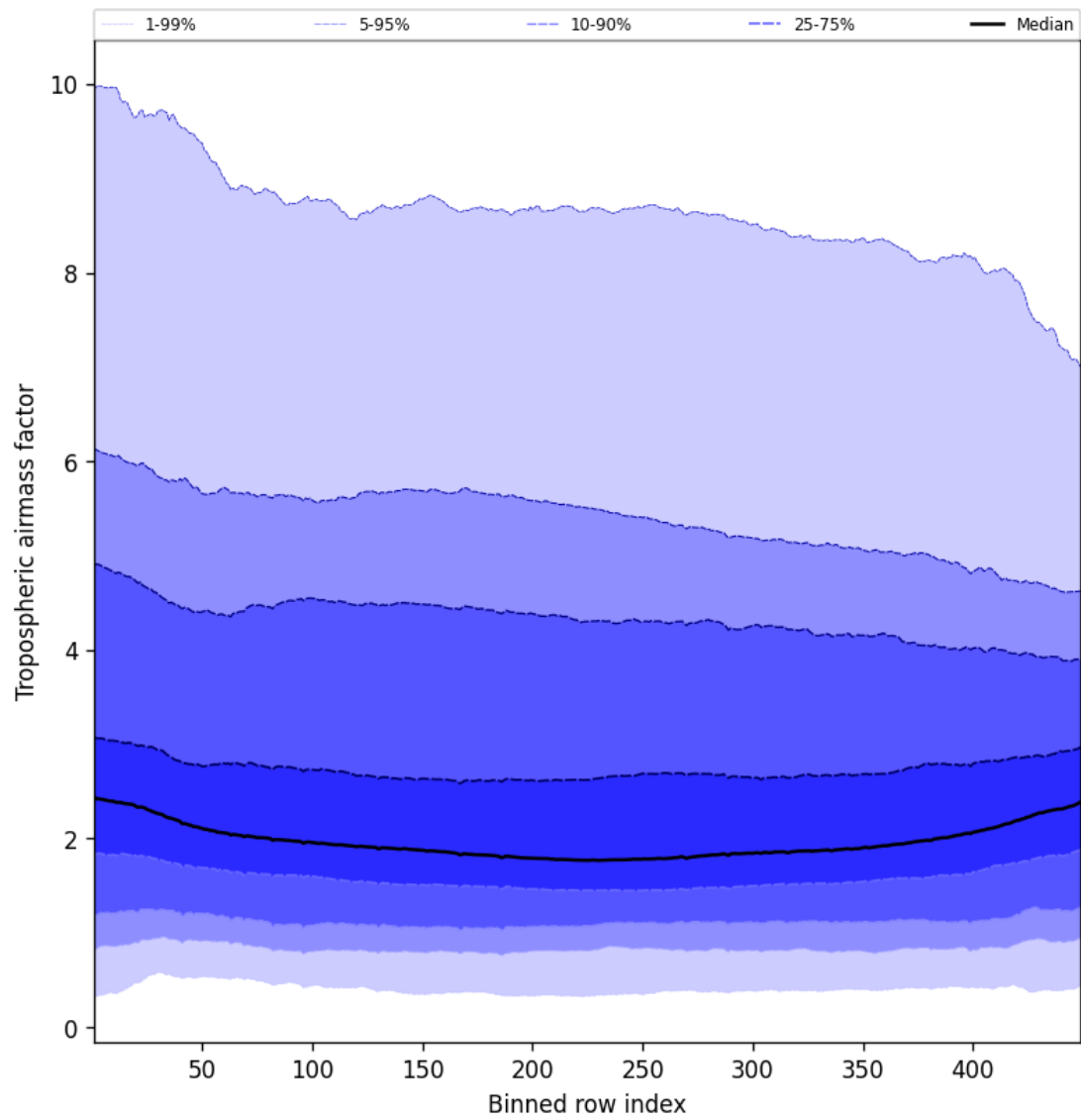
Figure 48: Along track statistics of “Tropospheric air mass factor” for 2025-09-13 to 2025-09-15
