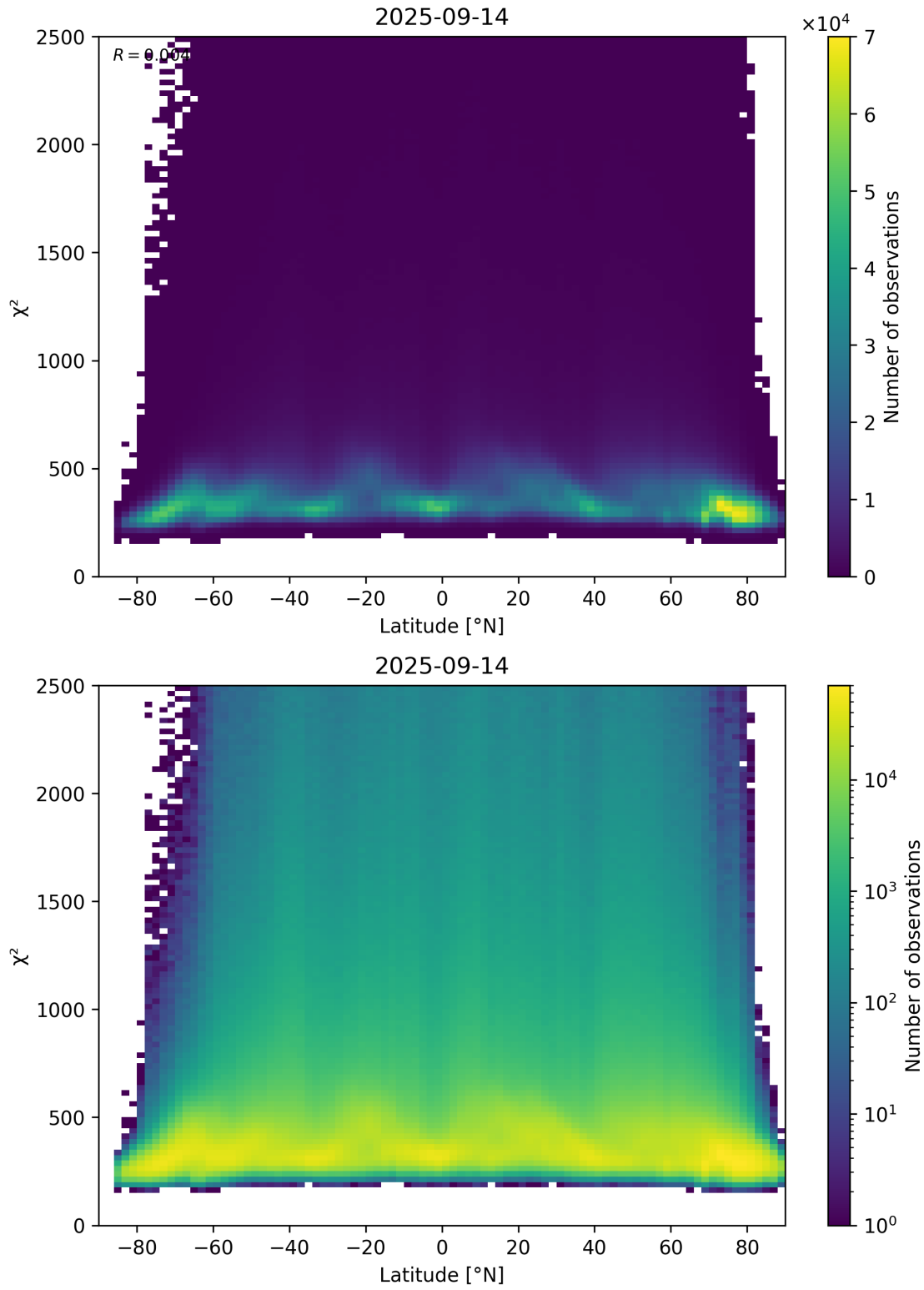
Figure 86: Scatter density plot of “Latitude” against “ \chi^2 ” for 2025-09-13 to 2025-09-15.
