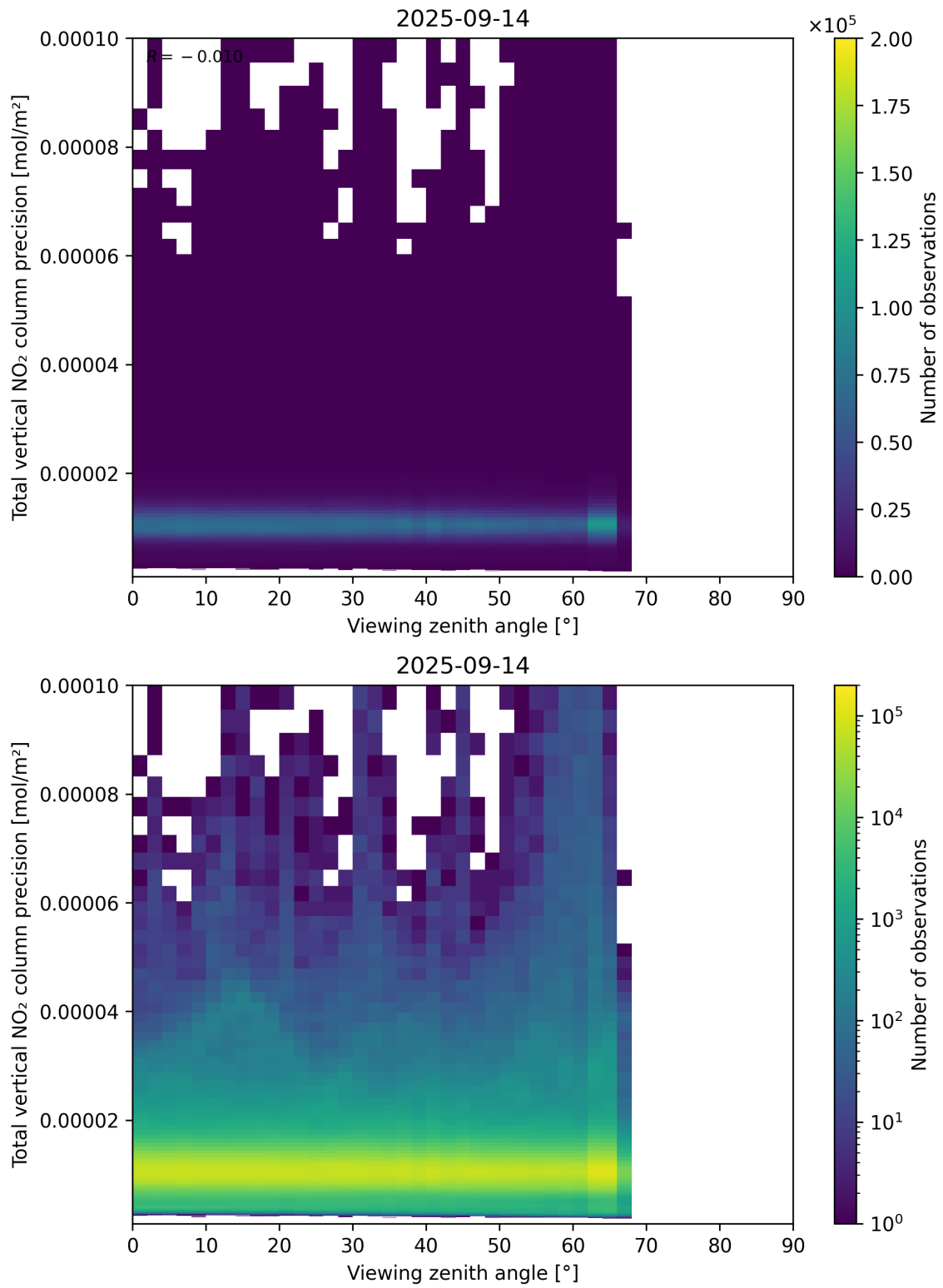
Figure 168: Scatter density plot of “Viewing zenith angle” against “Total vertical NO 2 column precision” for 2025-09-13 to 2025-09-15.
