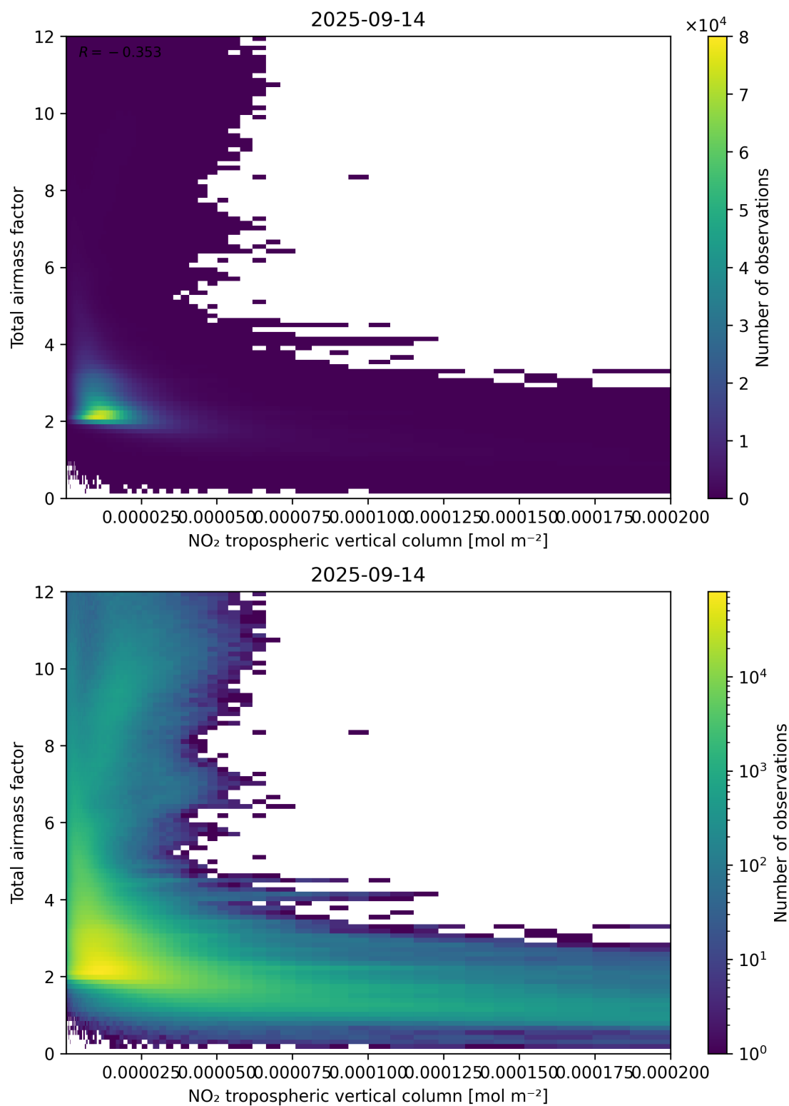
Figure 122: Scatter density plot of “NO 2 tropospheric vertical column” against “Total air mass factor” for 2025-09-13 to 2025-09-15.
