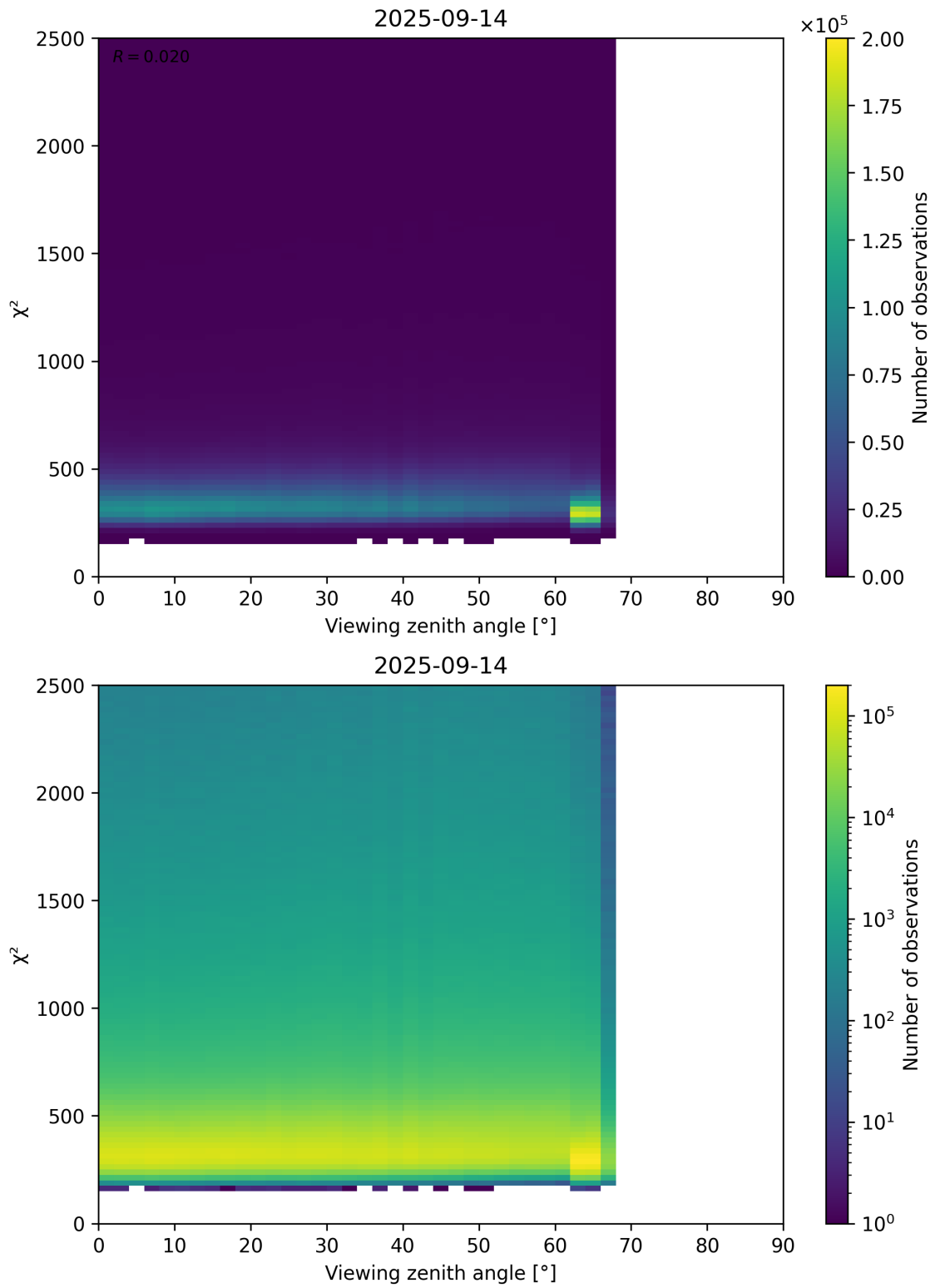
Figure 162: Scatter density plot of “Viewing zenith angle” against “ \chi^2 ” for 2025-09-13 to 2025-09-15.
