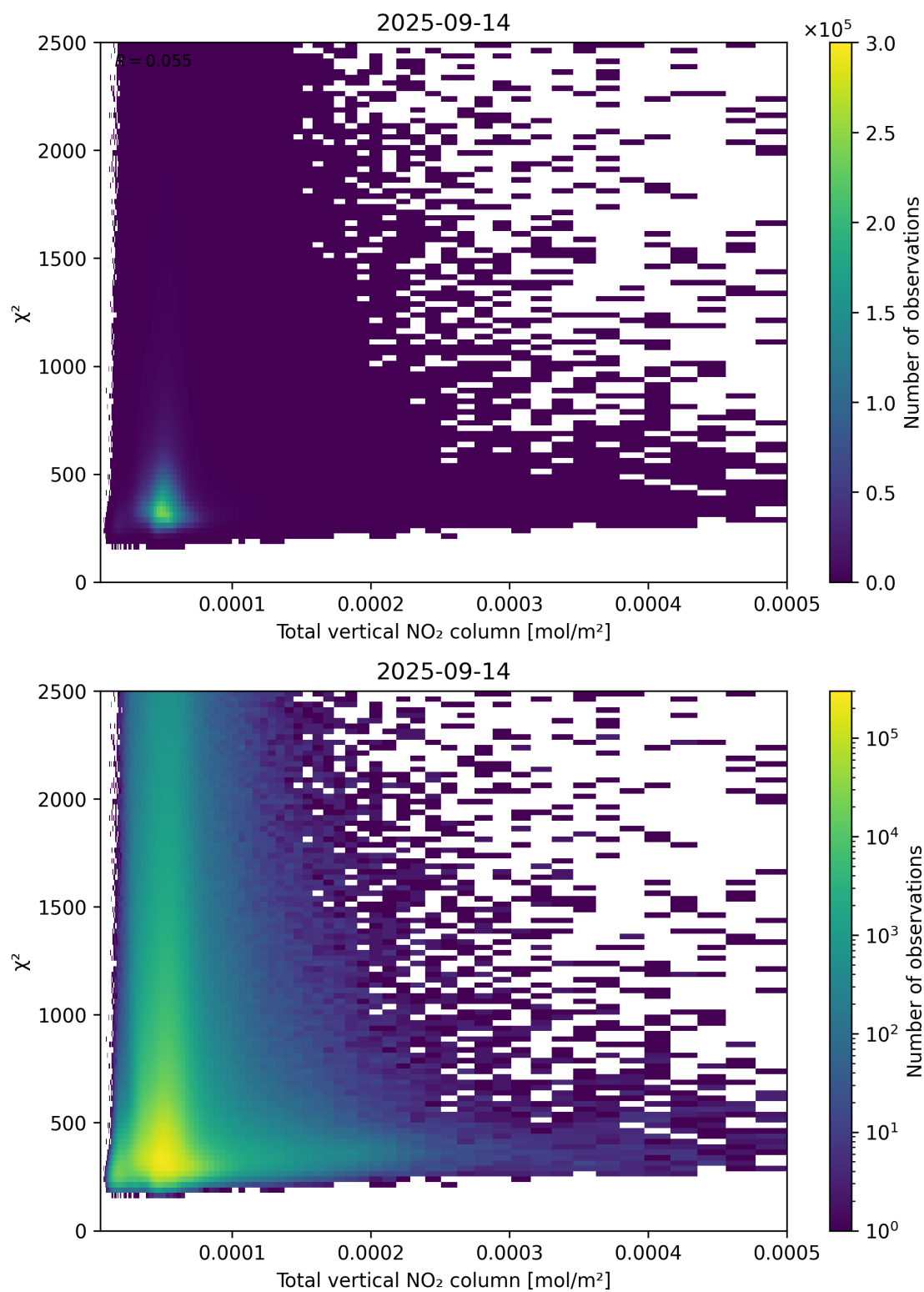
Figure 111: Scatter density plot of “Total vertical NO 2 column” against “ \chi^2 ” for 2025-09-13 to 2025-09-15.
