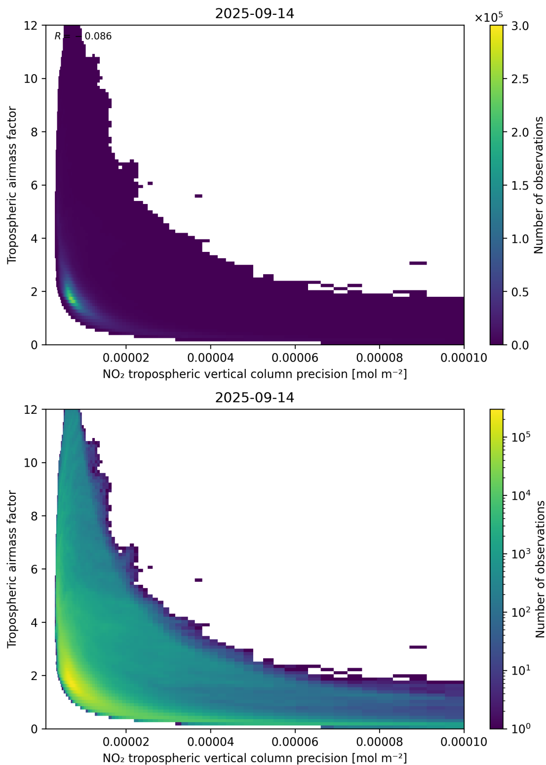
Figure 133: Scatter density plot of “NO 2 tropospheric vertical column precision” against “Tropospheric air mass factor” for 2025-09-13 to 2025-09-15.
