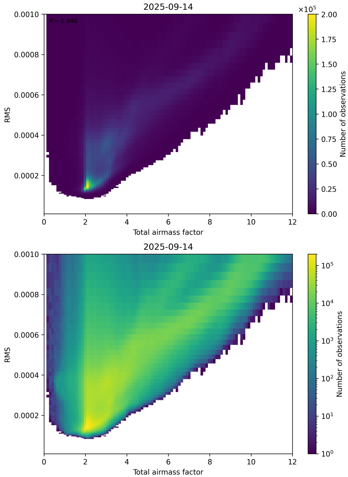
Figure 69: Scatter density plot of “Total airmass factor” against “RMS” for 2025-09-13 to 2025-09-15.
