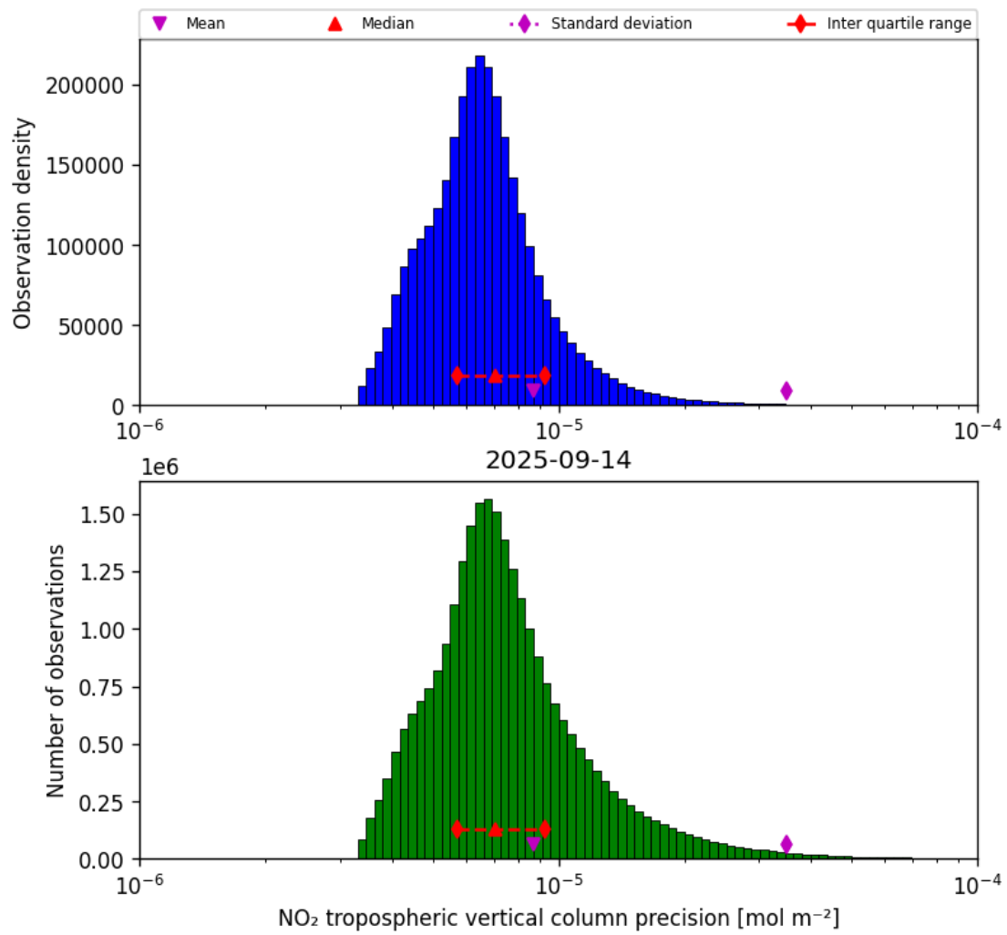
Figure 30: Histogram of “NO 2 tropospheric vertical column precision” for 2025-09-13 to 2025-09-15
