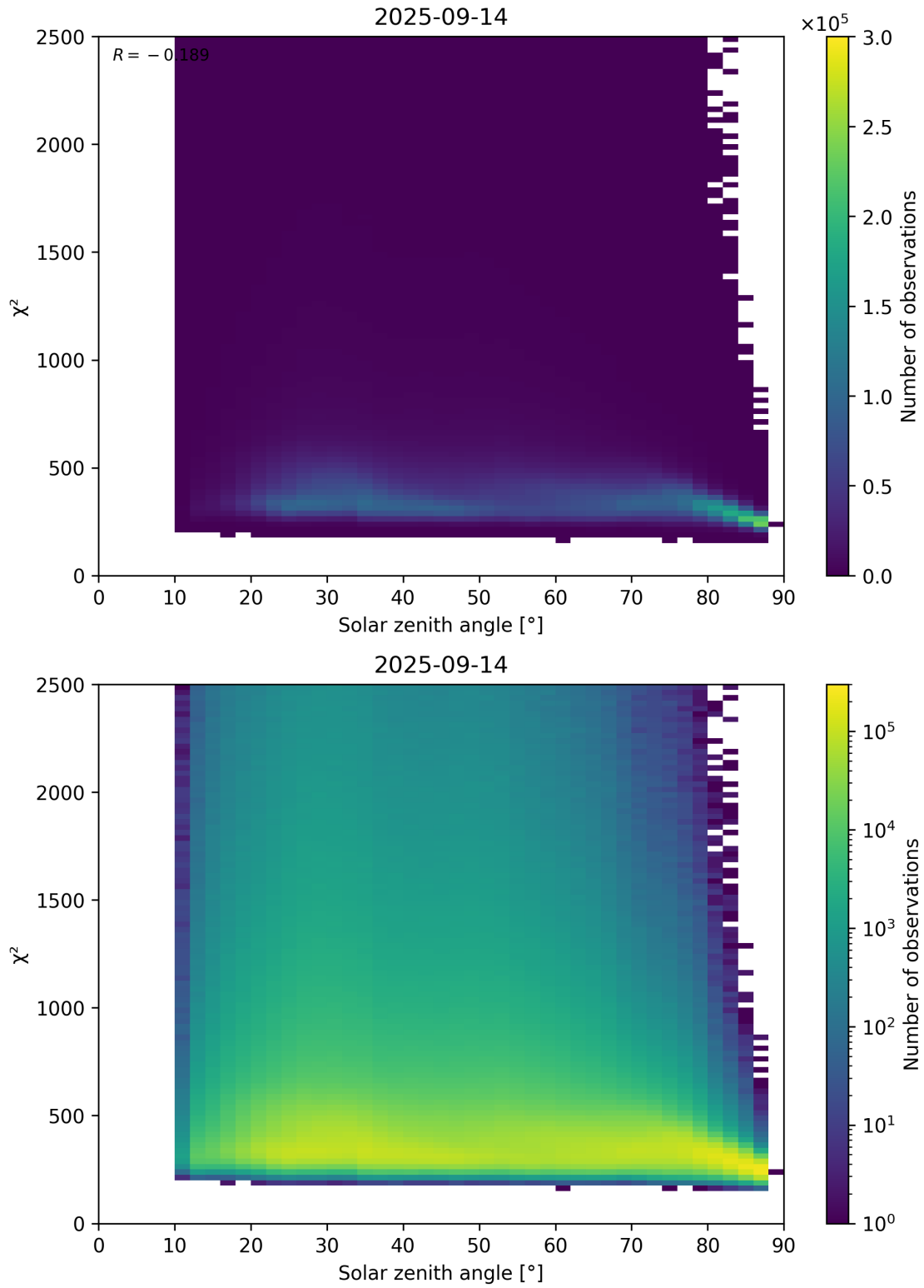
Figure 148: Scatter density plot of “Solar zenith angle” against “ \chi^2 ” for 2025-09-13 to 2025-09-15.
