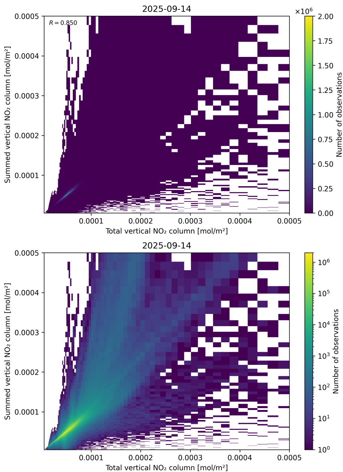
Figure 112: Scatter density plot of “Total vertical NO 2 column” against “Summed vertical NO 2 column” for 2025-09-13 to 2025-09-15.
