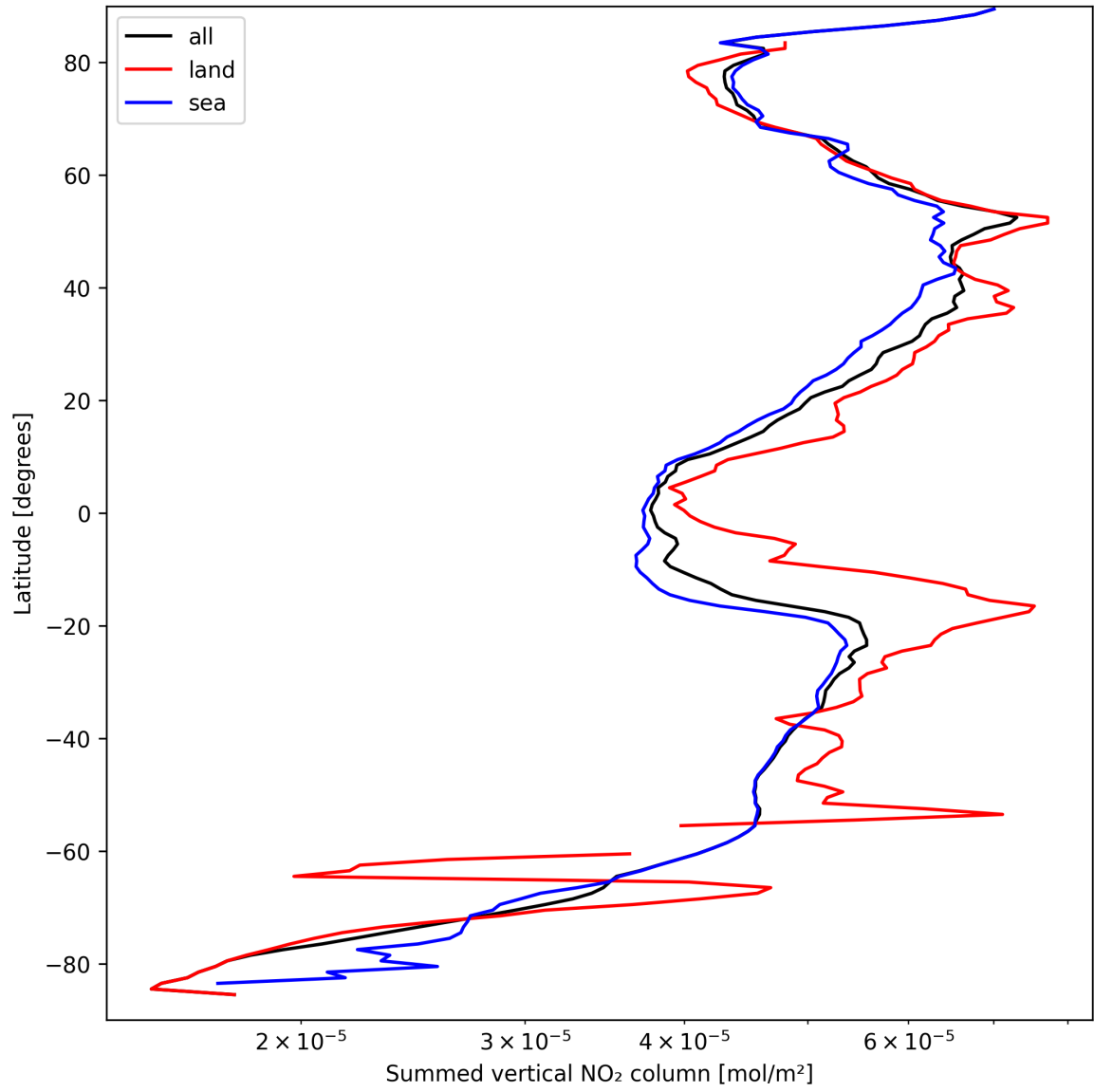
Figure 23: Zonal average of “Summed vertical NO 2 column” for 2025-09-13 to 2025-09-15.
