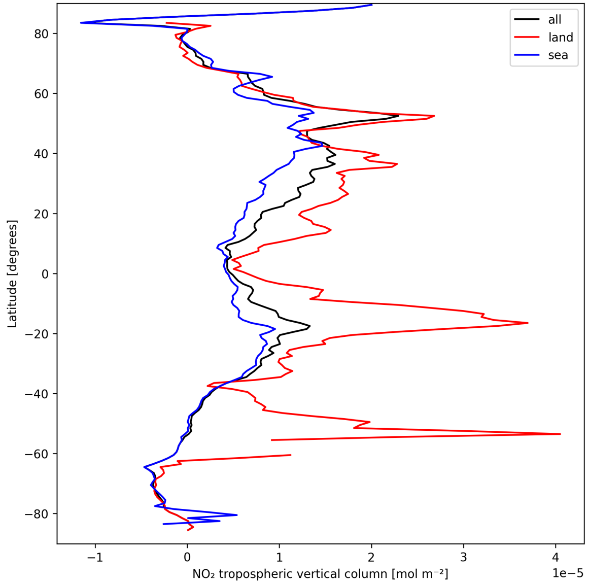
Figure 12: Zonal average of “NO 2 tropospheric vertical column” for 2025-09-13 to 2025-09-15.
