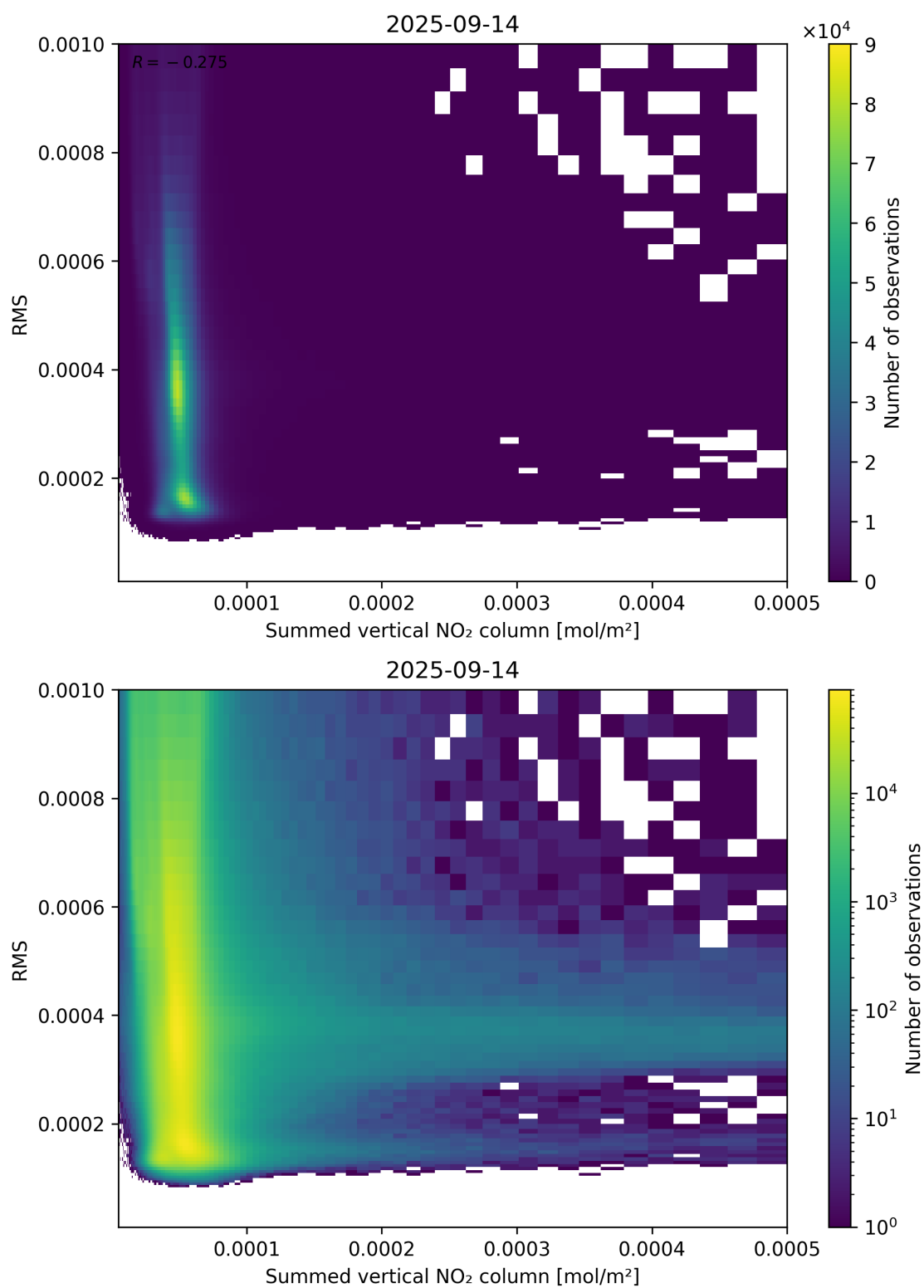
Figure 109: Scatter density plot of “Summed vertical NO 2 column” against “RMS” for 2025-09-13 to 2025-09-15.
