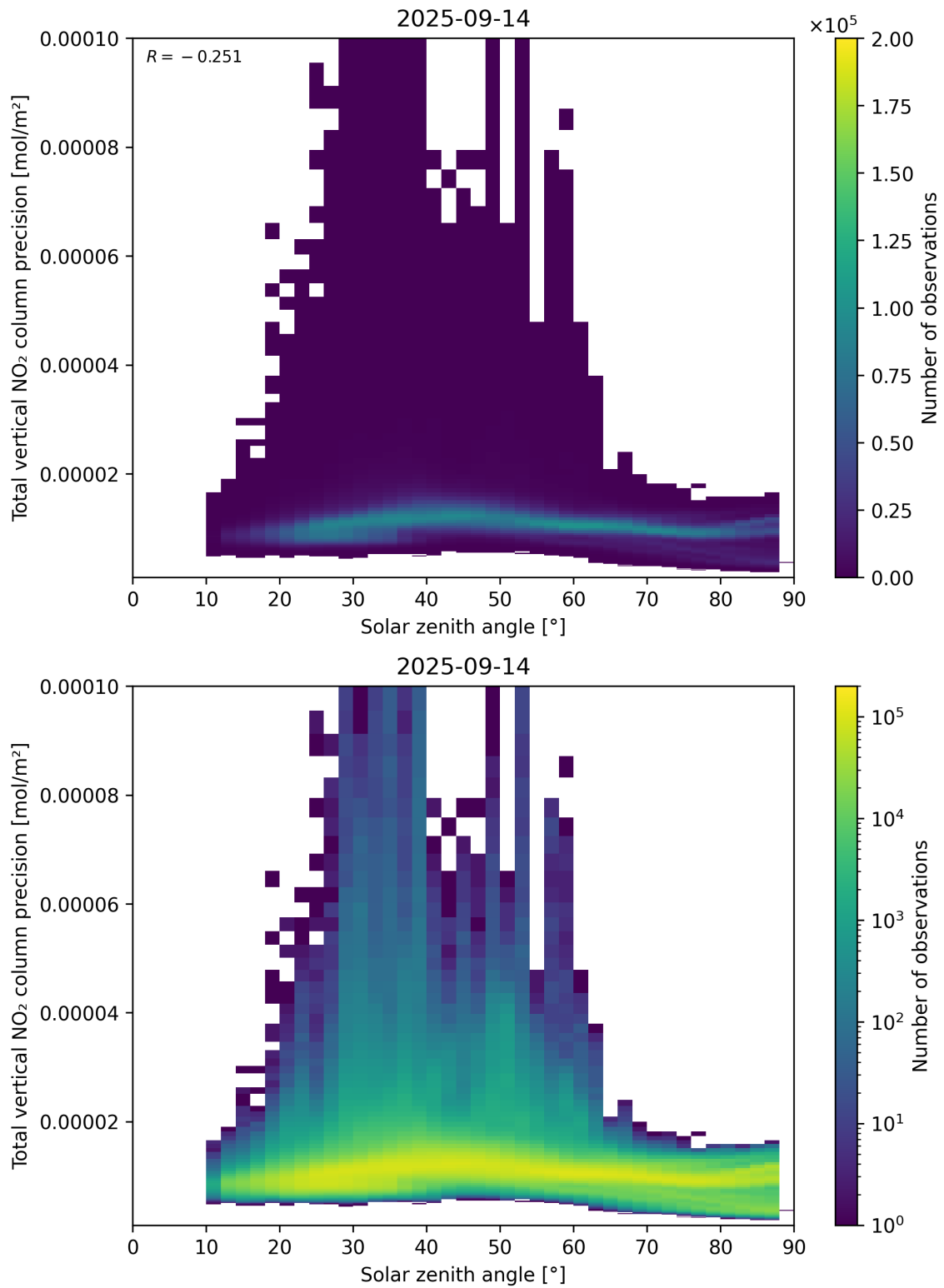
Figure 154: Scatter density plot of “Solar zenith angle” against “Total vertical NO 2 column precision” for 2025-09-13 to 2025-09-15.
