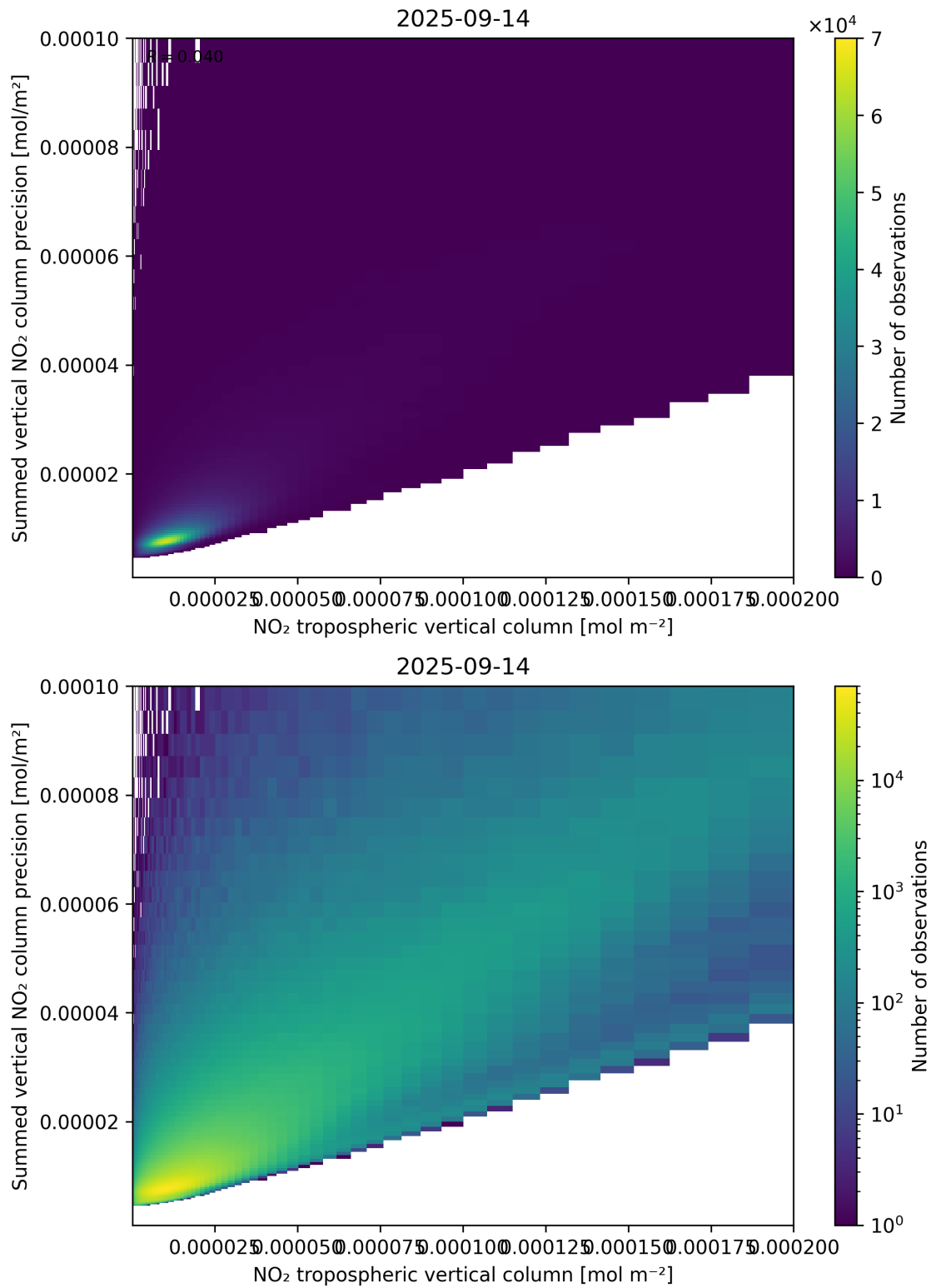
Figure 127: Scatter density plot of “NO 2 tropospheric vertical column” against “Summed vertical NO 2 column precision” for 2025-09-13 to 2025-09-15.
