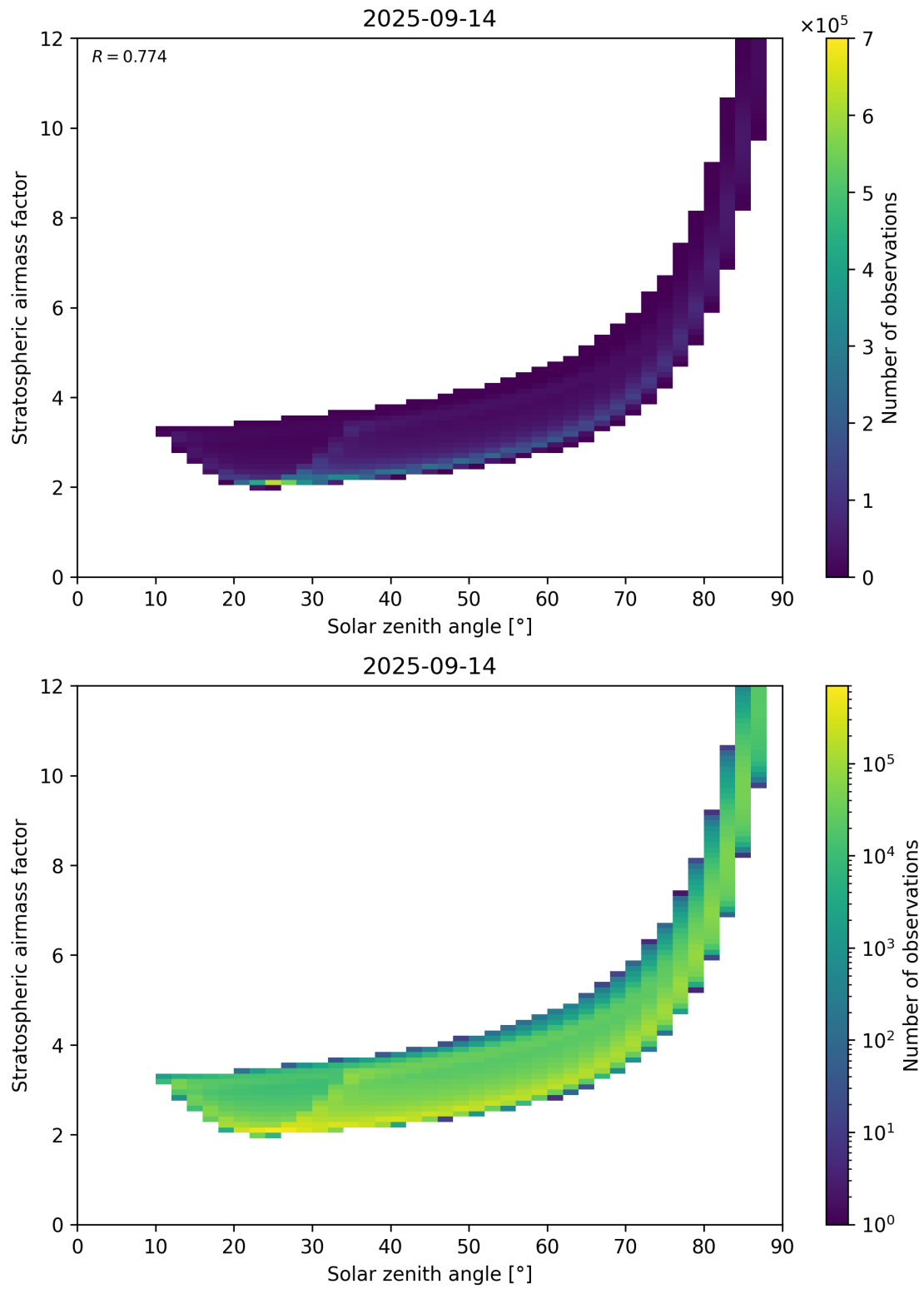
Figure 145: Scatter density plot of “Solar zenith angle” against “Stratospheric airmass factor” for 2025-09-13 to 2025-09-15.
