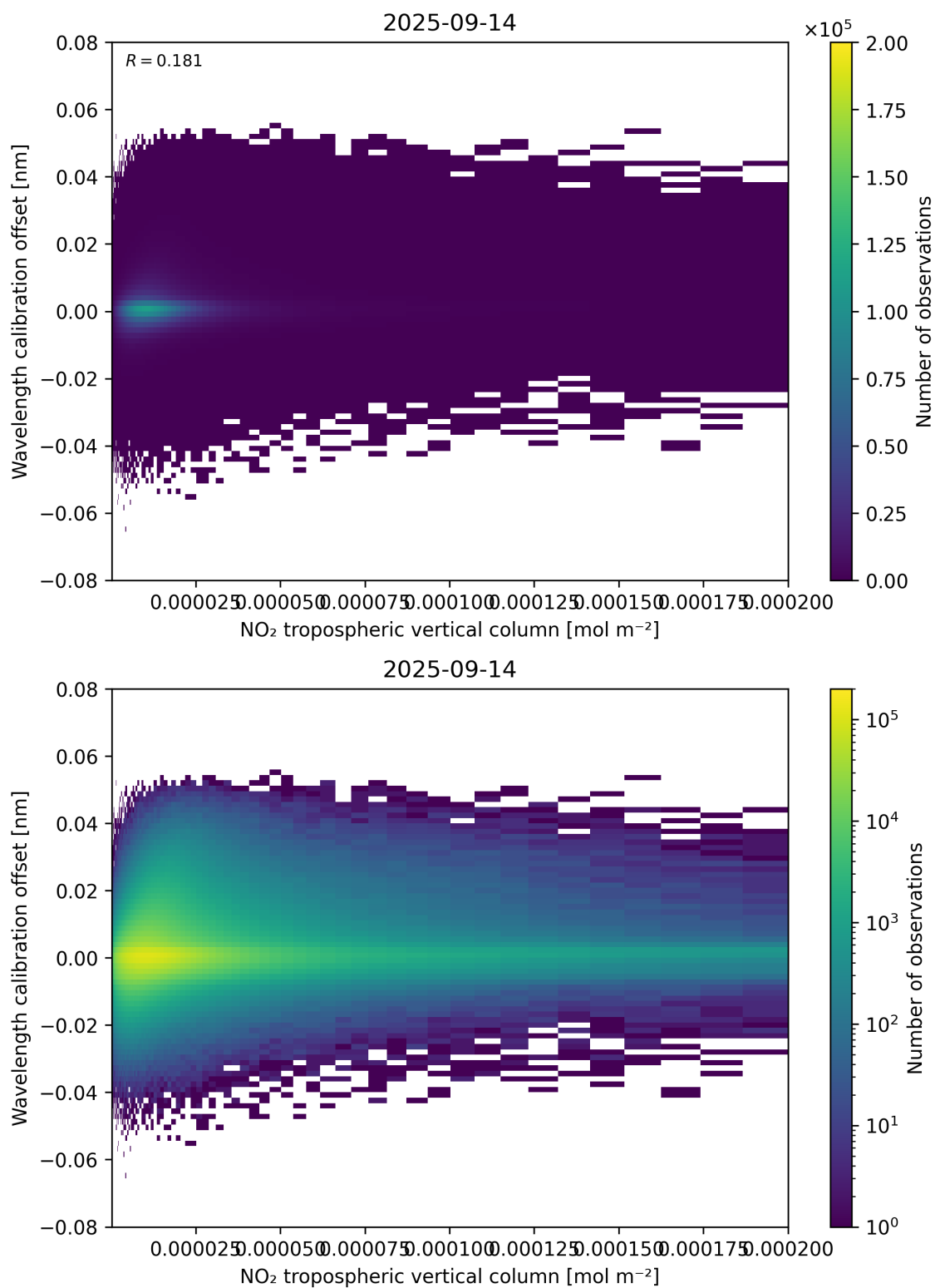
Figure 143: Scatter density plot of “NO 2 tropospheric vertical column” against “Wavelength calibration offset” for 2025-09-13 to 2025-09-15.
