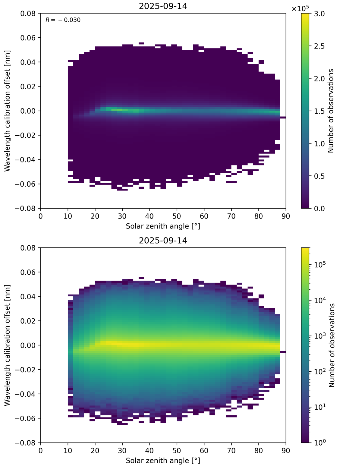
Figure 158: Scatter density plot of “Solar zenith angle” against “Wavelength calibration offset” for 2025-09-13 to 2025-09-15.
