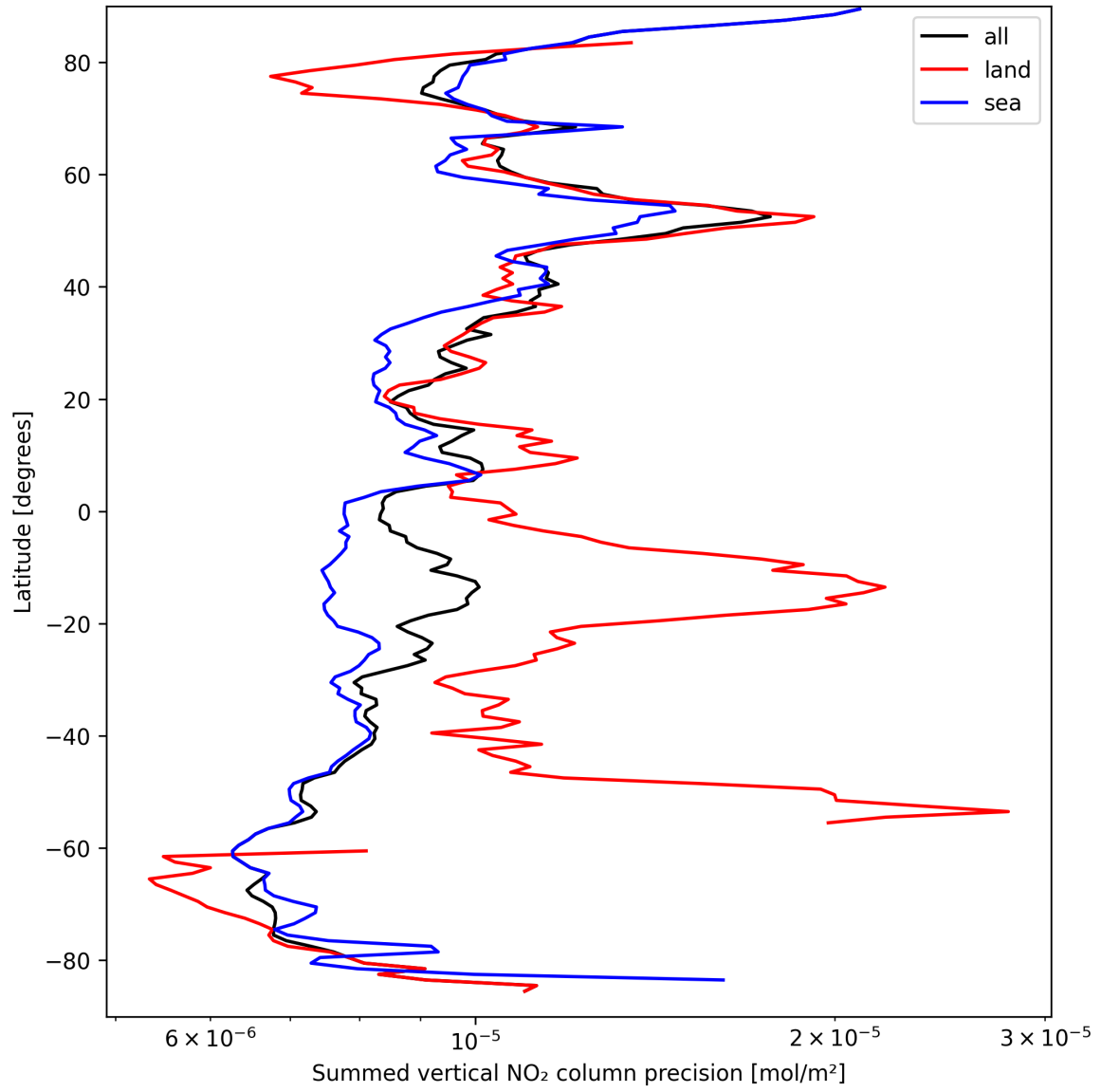
Figure 24: Zonal average of “Summed vertical NO 2 column precision” for 2025-09-13 to 2025-09-15.
