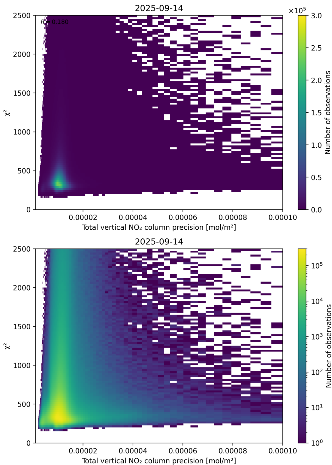
Figure 116: Scatter density plot of “Total vertical NO 2 column precision” against “ \chi^2 ” for 2025-09-13 to 2025-09-15.
