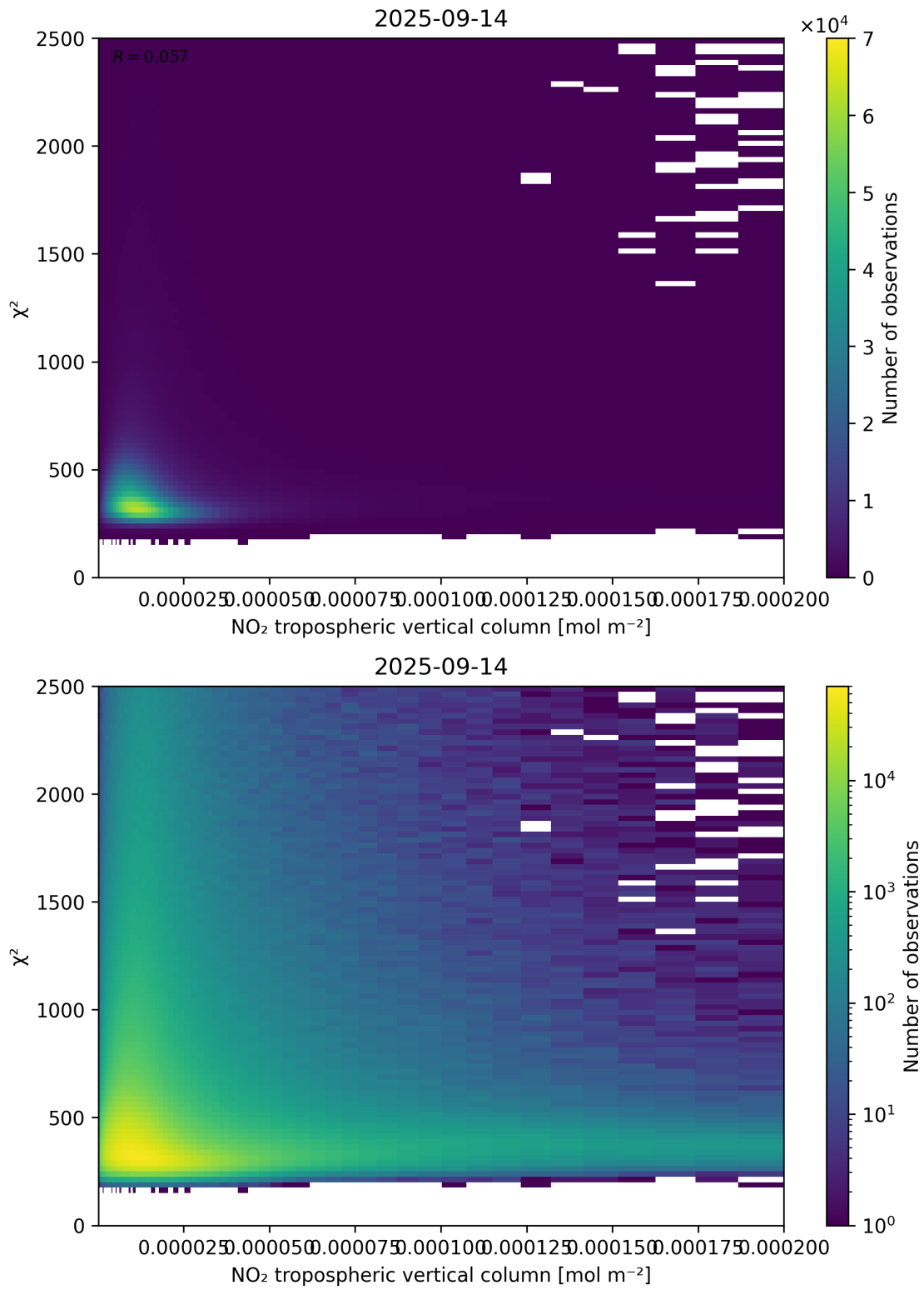
Figure 124: Scatter density plot of “NO 2 tropospheric vertical column” against “ \chi^2 ” for 2025-09-13 to 2025-09-15.
