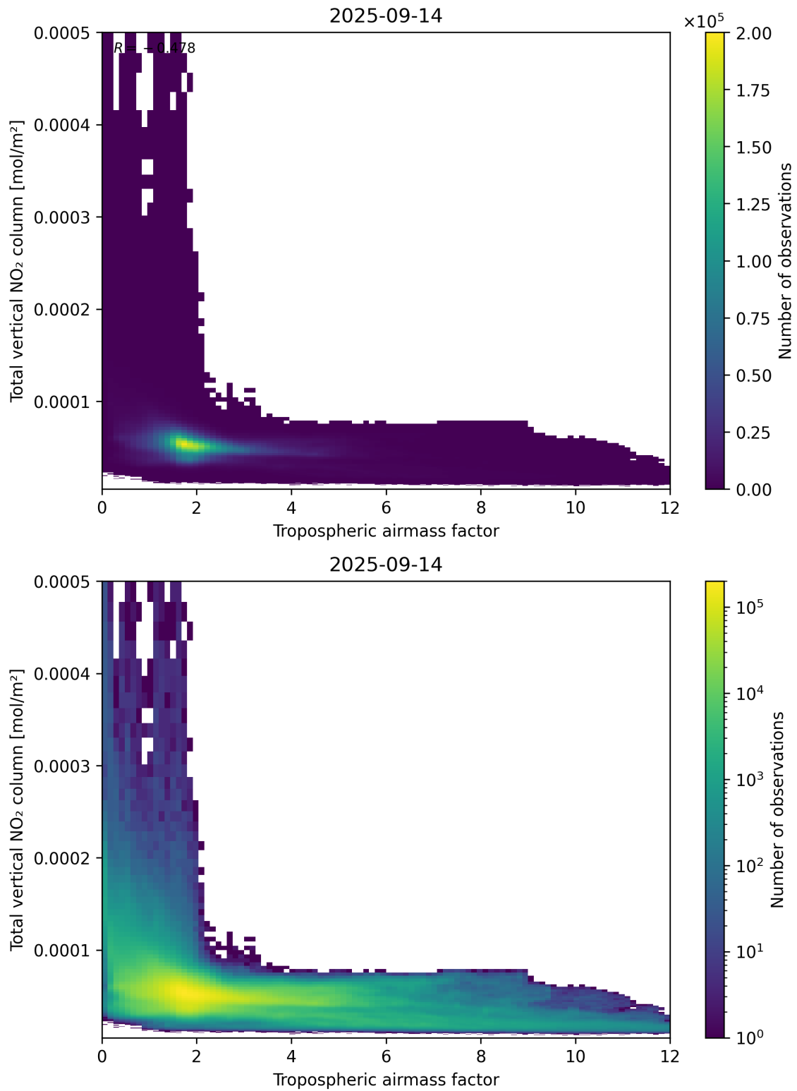
Figure 77: Scatter density plot of “Tropospheric airmass factor” against “Total vertical NO 2 column” for 2025-09-13 to 2025-09-15.
