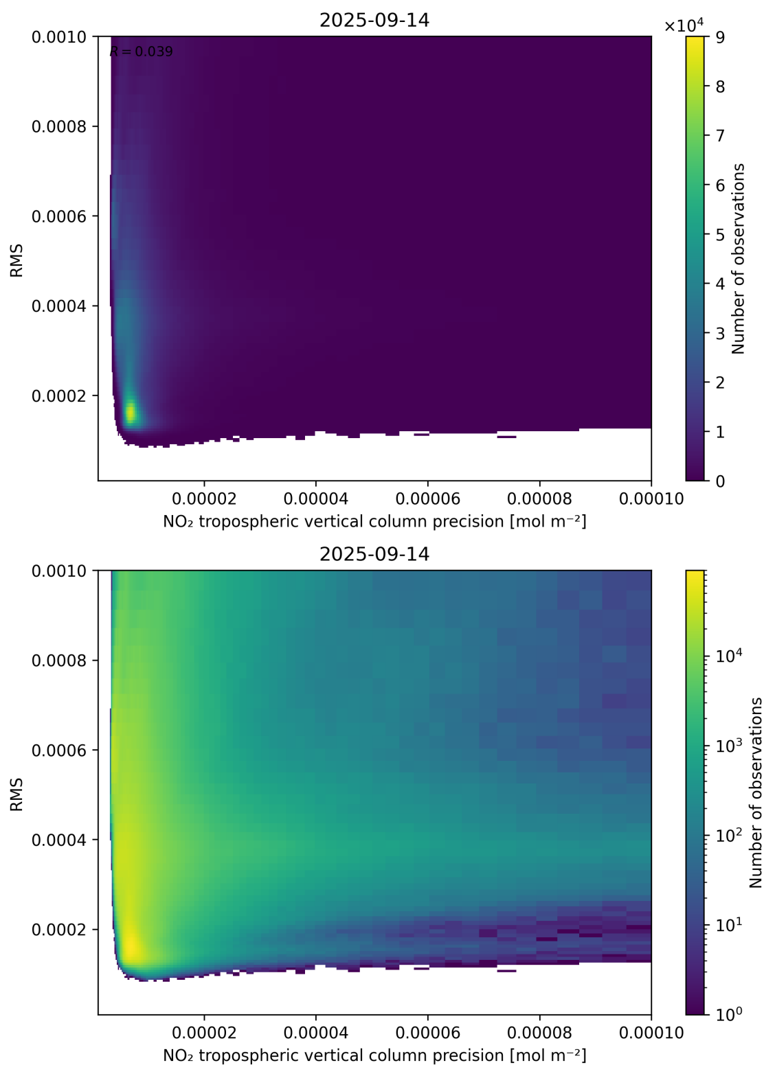
Figure 140: Scatter density plot of “NO 2 tropospheric vertical column precision” against “RMS” for 2025-09-13 to 2025-09-15.
