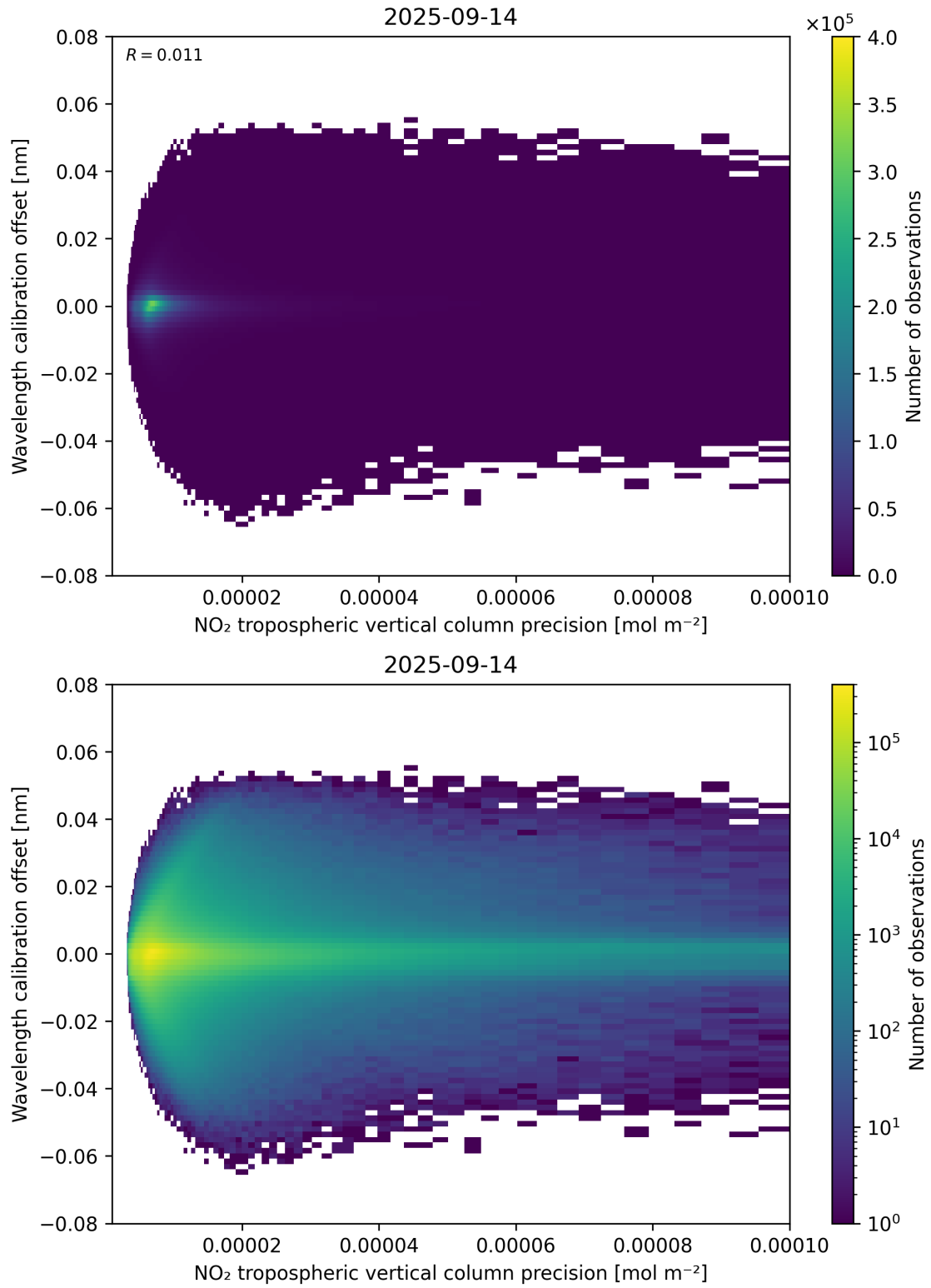
Figure 141: Scatter density plot of “NO 2 tropospheric vertical column precision” against “Wavelength calibration offset” for 2025-09-13 to 2025-09-15.
