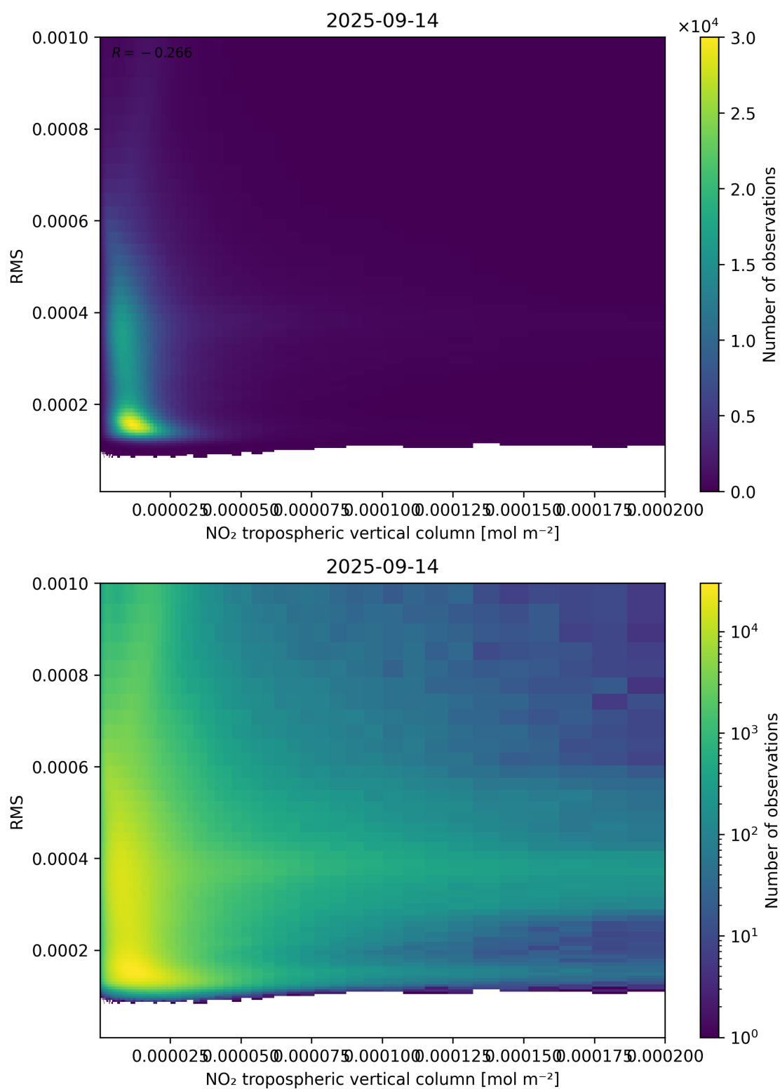
Figure 142: Scatter density plot of “NO 2 tropospheric vertical column” against “RMS” for 2025-09-13 to 2025-09-15.
