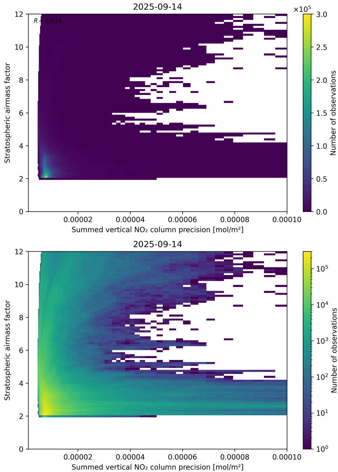
Figure 106: Scatter density plot of “Summed vertical NO 2 column precision” against “Stratospheric airmass factor” for 2025-09-13 to 2025-09-15.
