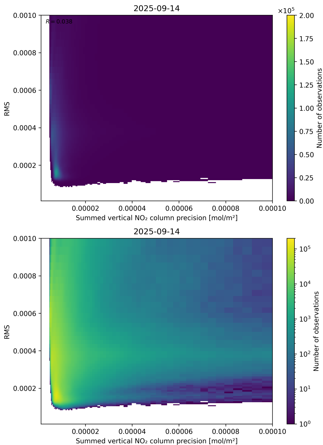
Figure 108: Scatter density plot of “Summed vertical NO 2 column precision” against “RMS” for 2025-09-13 to 2025-09-15.
