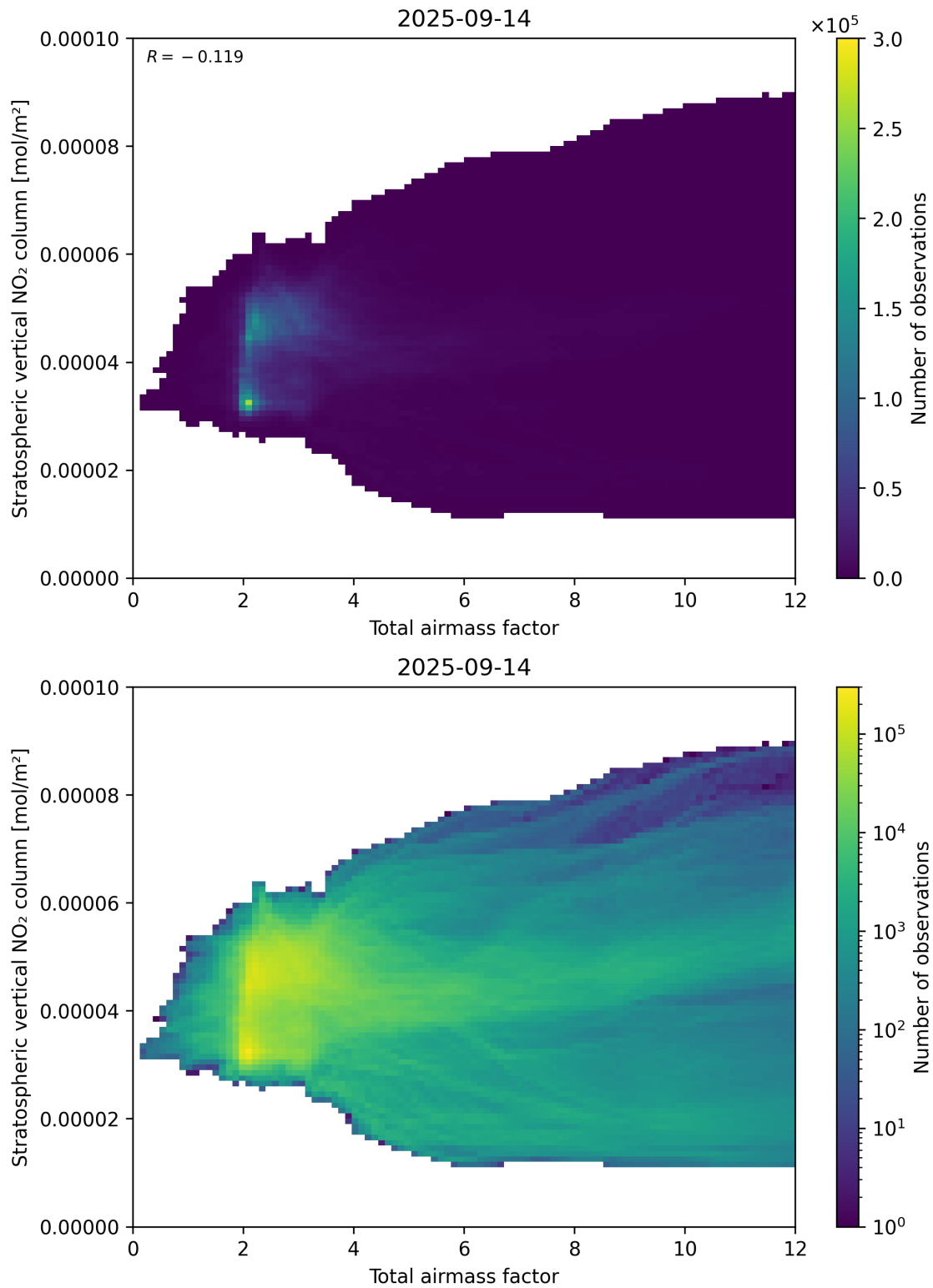
Figure 64: Scatter density plot of “Total airmass factor” against “Stratospheric vertical NO 2 column” for 2025-09-13 to 2025-09-15.
