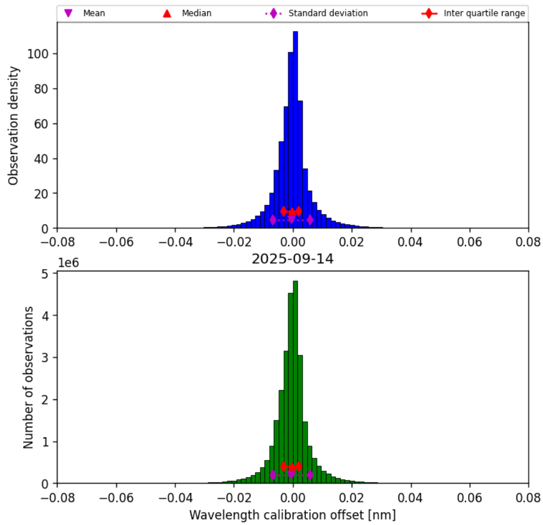
Figure 35: Histogram of “Wavelength calibration offset” for 2025-09-13 to 2025-09-15
