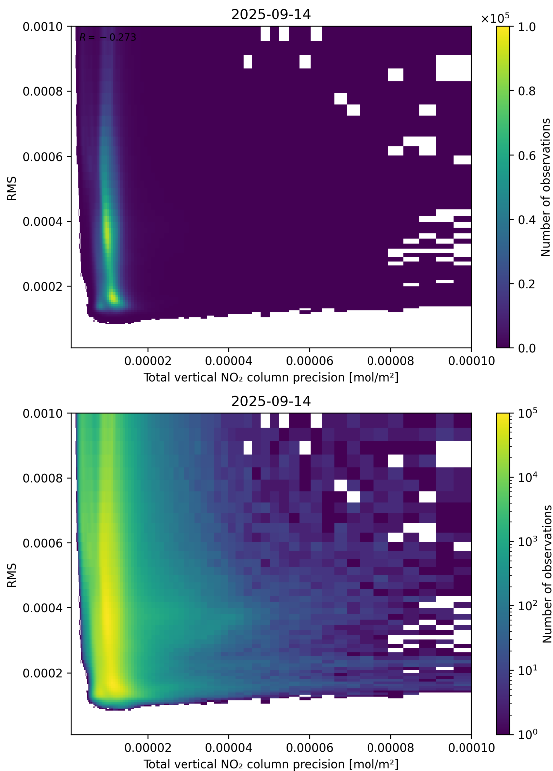
Figure 119: Scatter density plot of “Total vertical NO 2 column precision” against “RMS” for 2025-09-13 to 2025-09-15.
