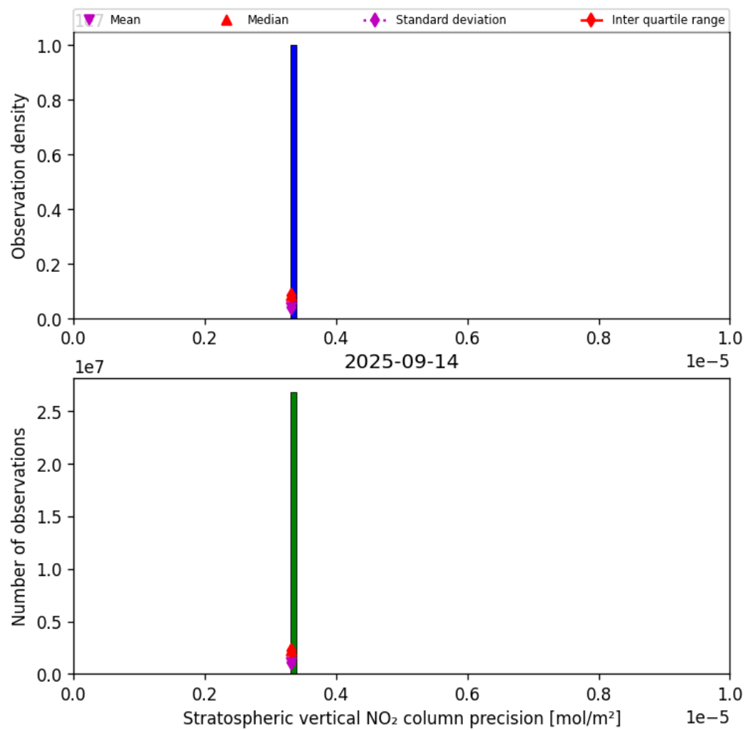
Figure 37: Histogram of “Stratospheric vertical NO 2 column precision” for 2025-09-13 to 2025-09-15
