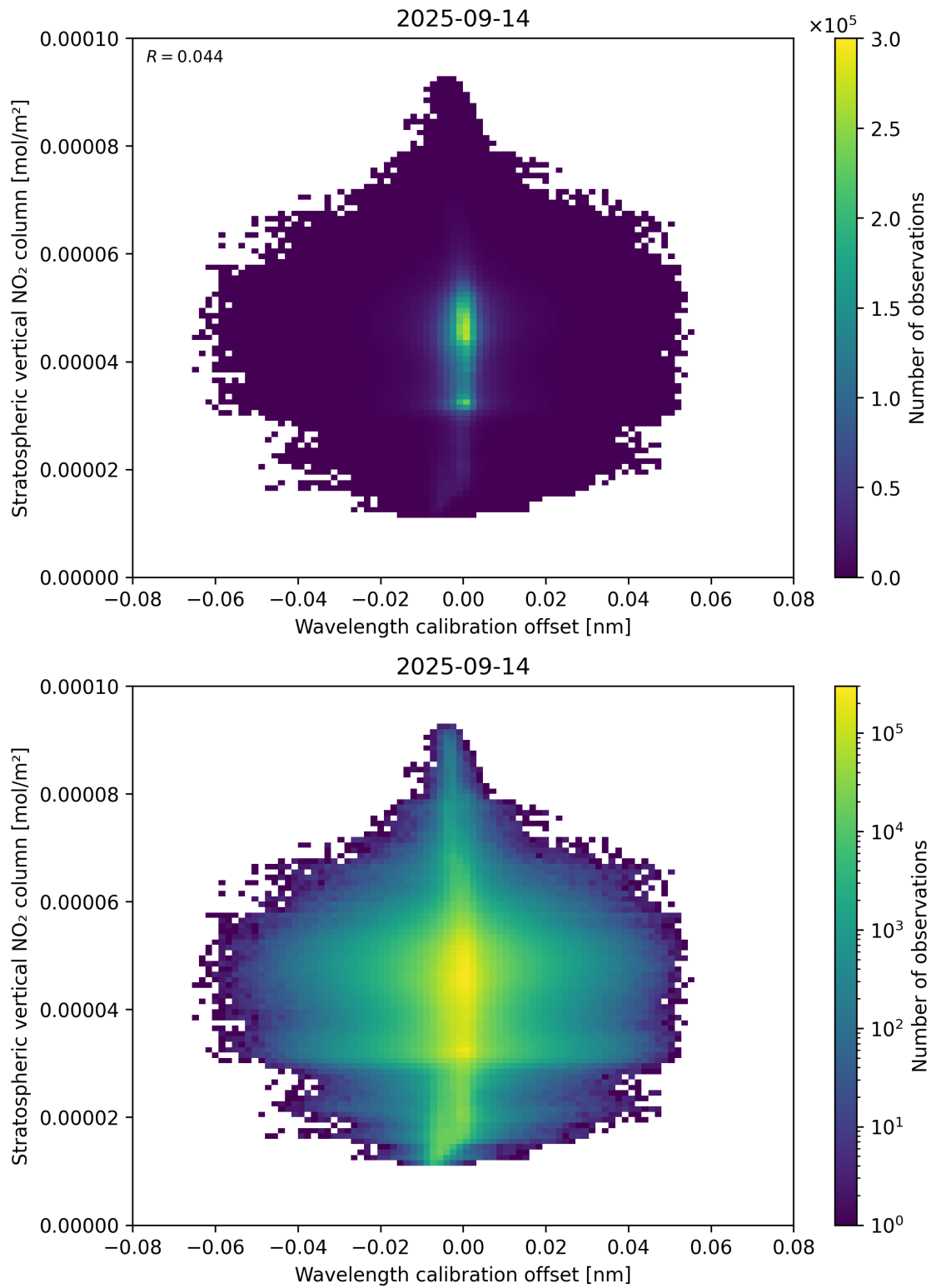
Figure 176: Scatter density plot of “Wavelength calibration offset” against “Stratospheric vertical NO 2 column” for 2025-09-13 to 2025-09-15.
