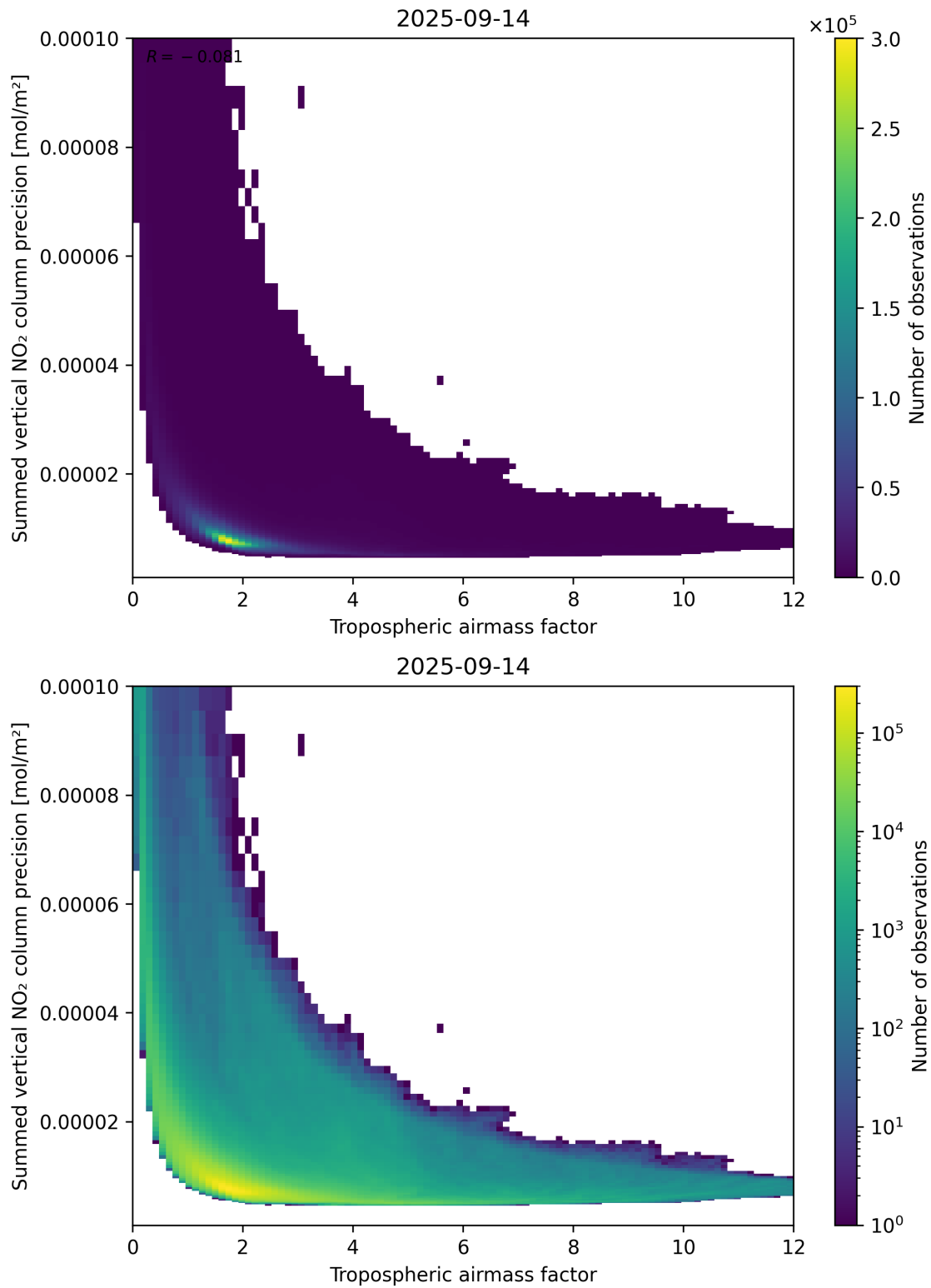
Figure 76: Scatter density plot of “Tropospheric air mass factor” against “Summed vertical NO 2 column precision” for 2025-09-13 to 2025-09-15.
