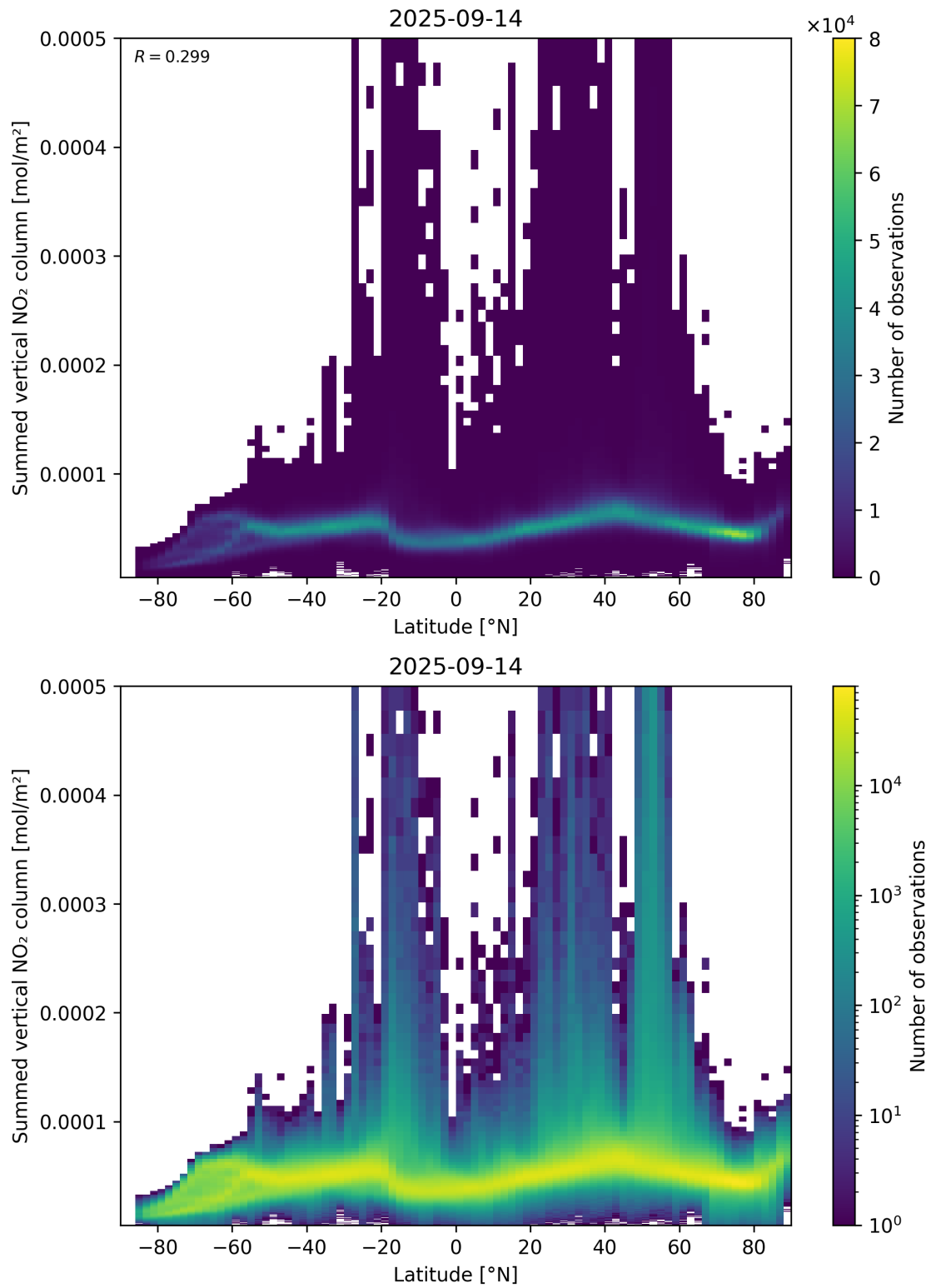
Figure 88: Scatter density plot of “Latitude” against “Summed vertical NO 2 column” for 2025-09-13 to 2025-09-15.
