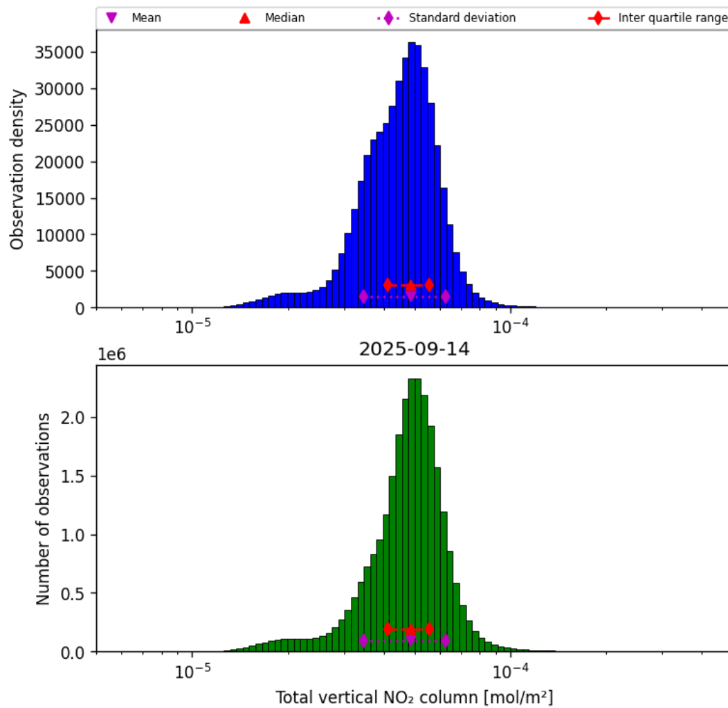
Figure 38: Histogram of “Total vertical NO 2 column” for 2025-09-13 to 2025-09-15
