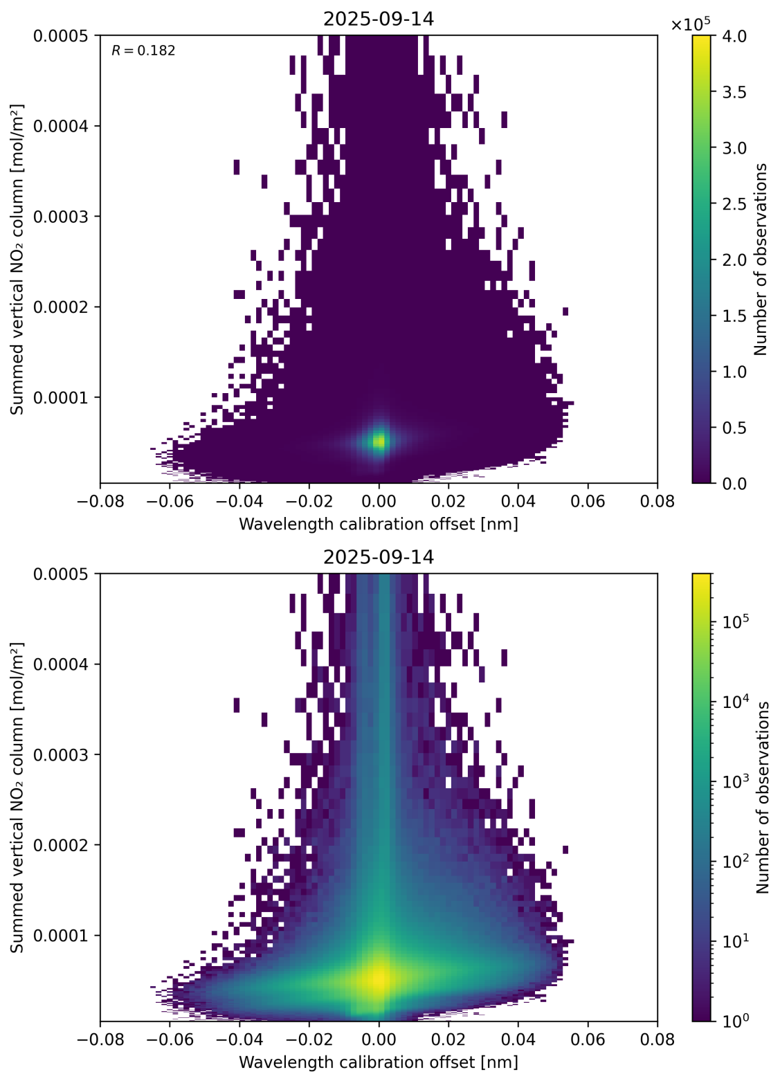
Figure 177: Scatter density plot of “Wavelength calibration offset” against “Summed vertical NO 2 column” for 2025-09-13 to 2025-09-15.
