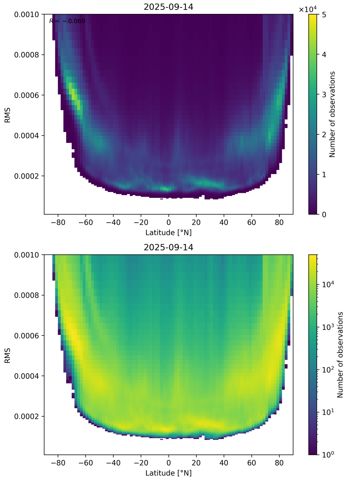
Figure 94: Scatter density plot of “Latitude” against “RMS” for 2025-09-13 to 2025-09-15.
