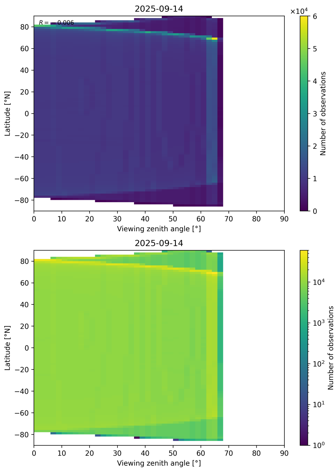
Figure 163: Scatter density plot of “Viewing zenith angle” against “Latitude” for 2025-09-13 to 2025-09-15.
