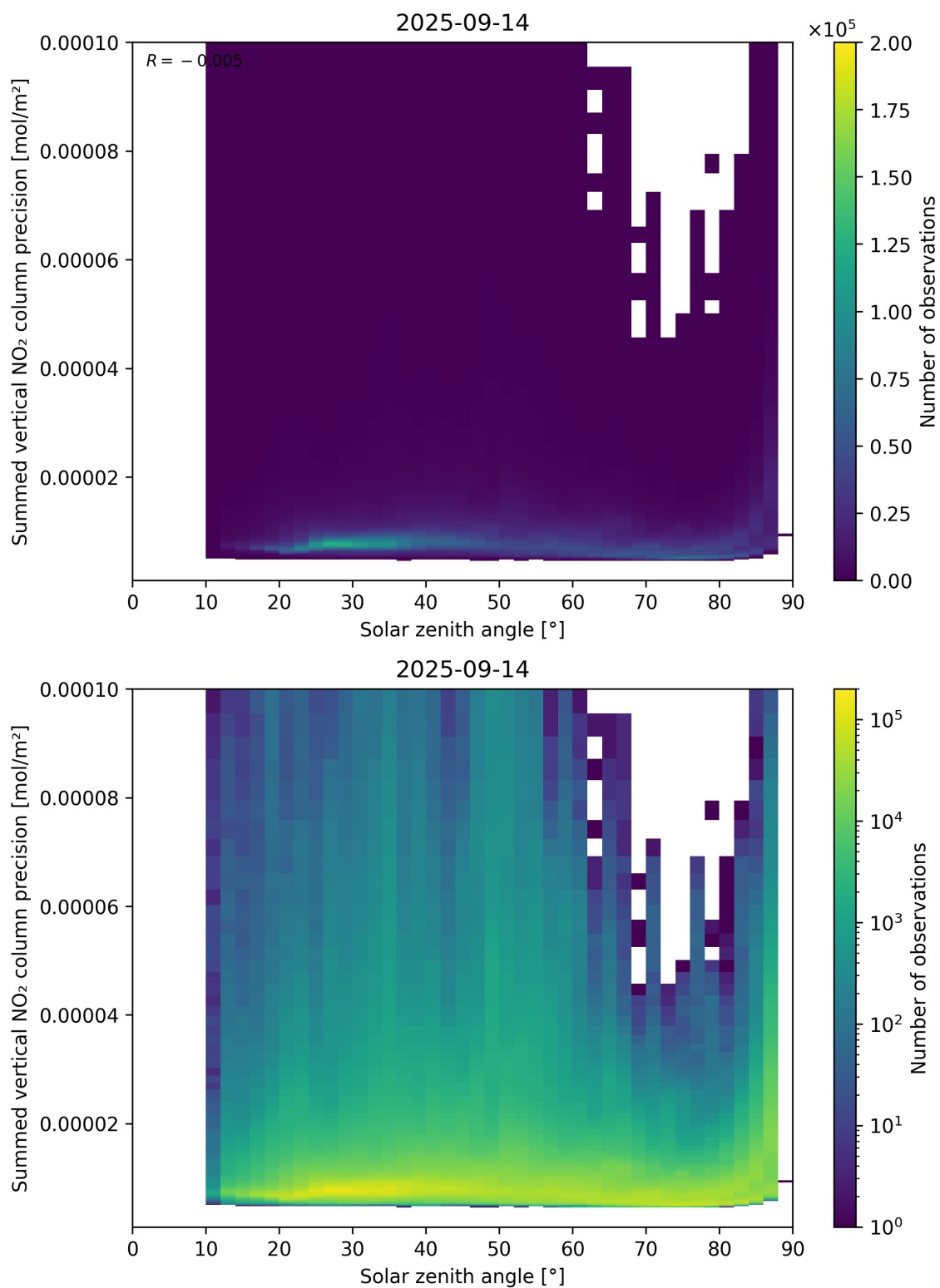
Figure 152: Scatter density plot of “Solar zenith angle” against “Summed vertical NO 2 column precision” for 2025-09-13 to 2025-09-15.
