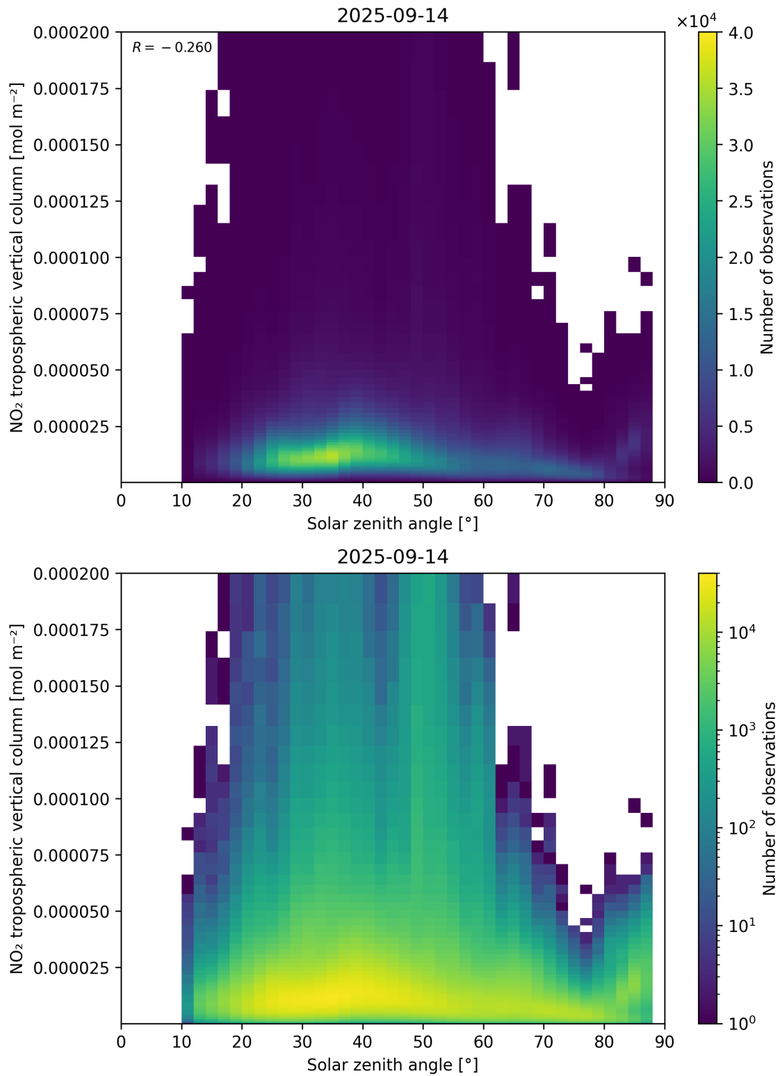
Figure 155: Scatter density plot of “Solar zenith angle” against “NO 2 tropospheric vertical column” for 2025-09-13 to 2025-09-15.
