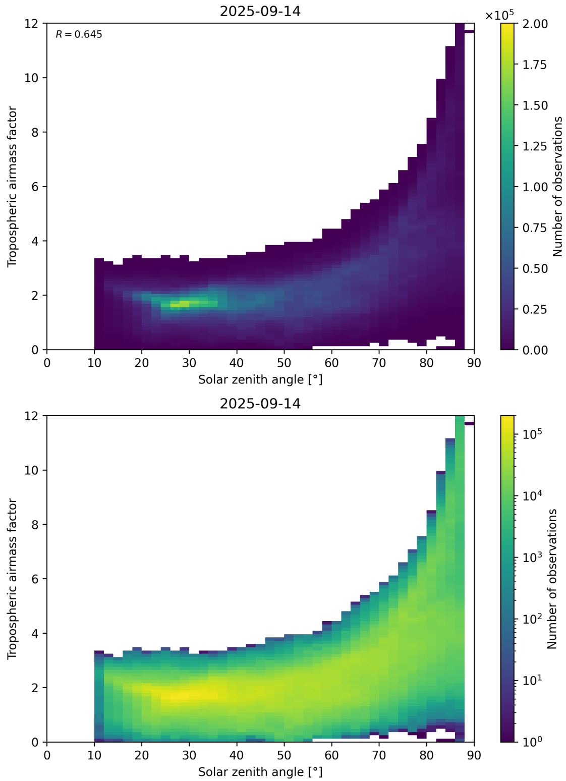
Figure 147: Scatter density plot of “Solar zenith angle” against “Tropospheric airmass factor” for 2025-09-13 to 2025-09-15.
