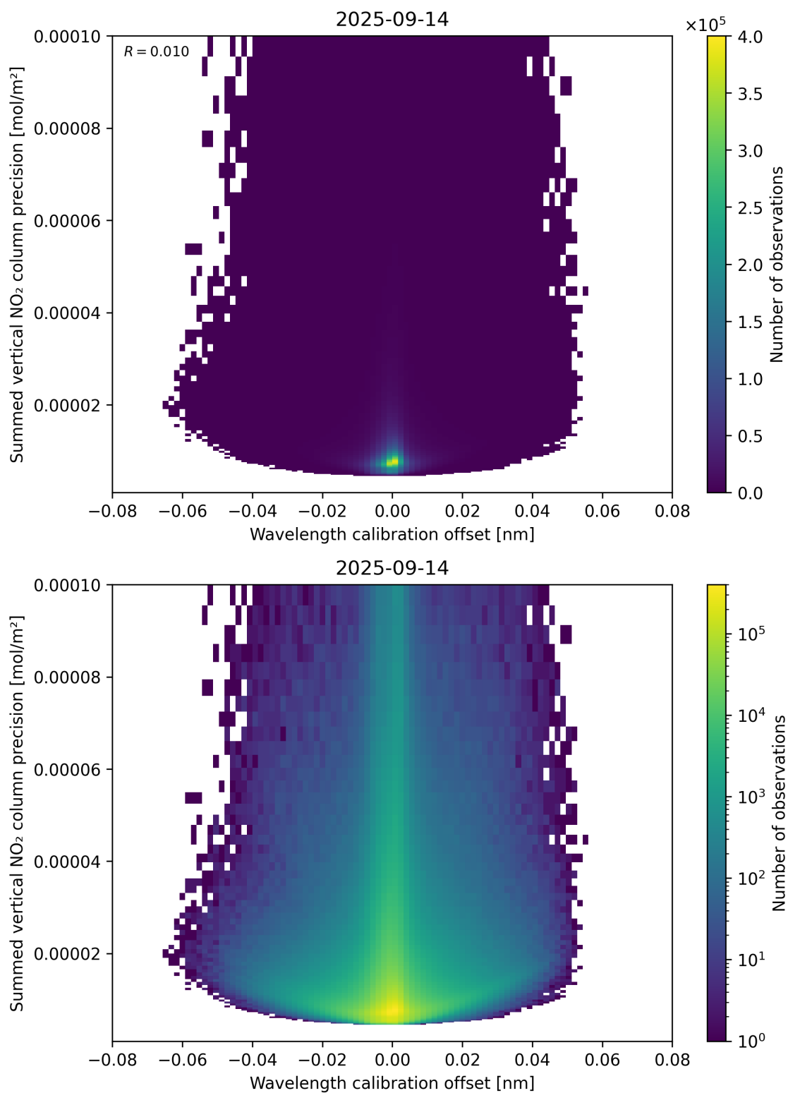
Figure 178: Scatter density plot of “Wavelength calibration offset” against “Summed vertical NO 2 column precision” for 2025-09-13 to 2025-09-15.
