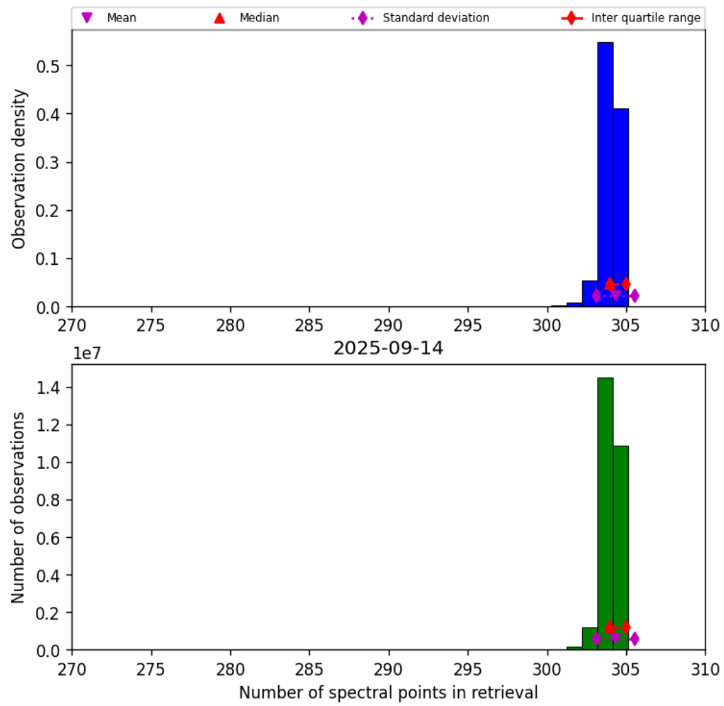
Figure 33: Histogram of “Number of spectral points in retrieval” for 2025-09-13 to 2025-09-15
