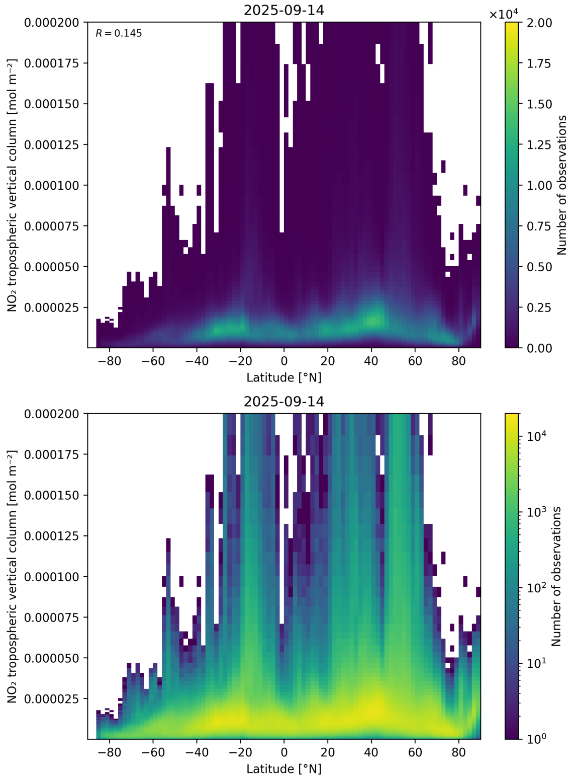
Figure 92: Scatter density plot of “Latitude” against “NO 2 tropospheric vertical column” for 2025-09-13 to 2025-09-15.
