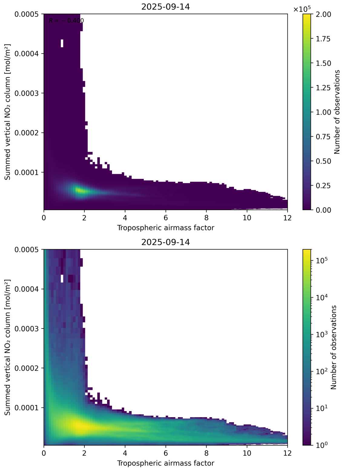
Figure 75: Scatter density plot of “Tropospheric air mass factor” against “Summed vertical NO 2 column” for 2025-09-13 to 2025-09-15.
