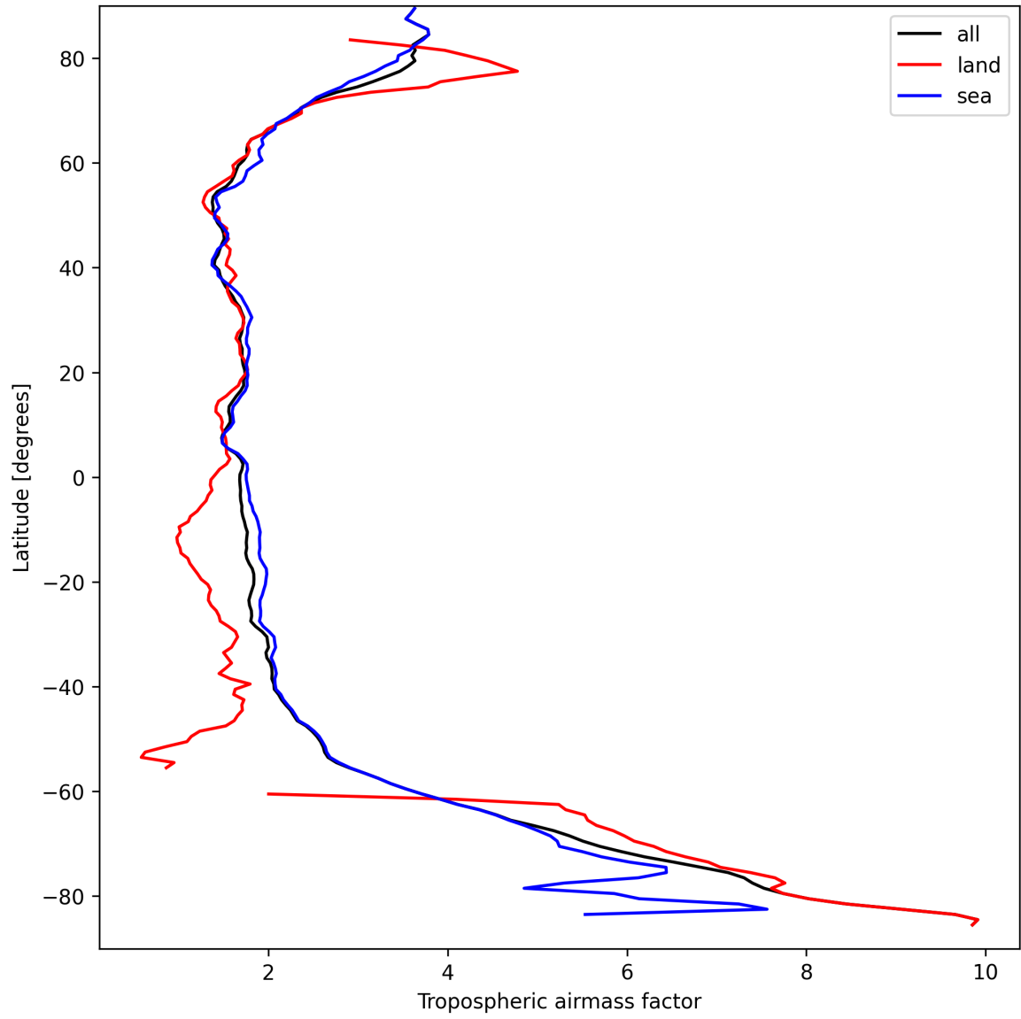
Figure 14: Zonal average of “Tropospheric airmass factor” for 2025-09-13 to 2025-09-15.
