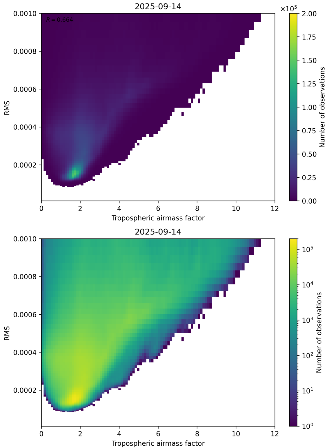
Figure 79: Scatter density plot of “Tropospheric airmass factor” against “RMS” for 2025-09-13 to 2025-09-15.
