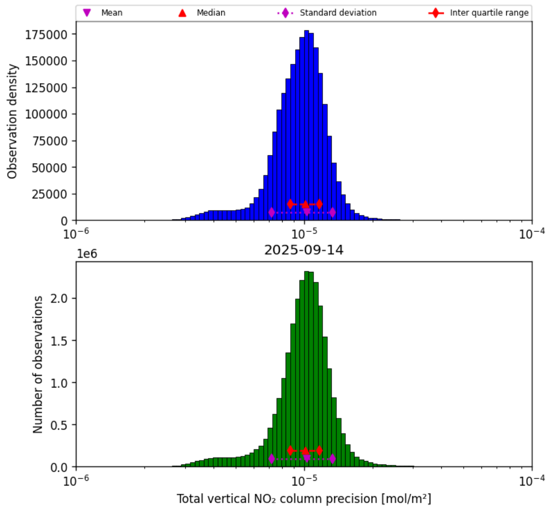
Figure 39: Histogram of “Total vertical NO 2 column precision” for 2025-09-13 to 2025-09-15
