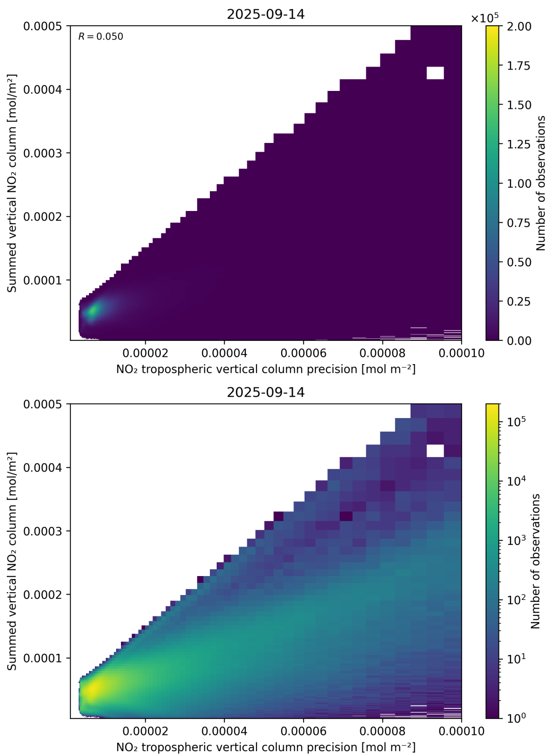
Figure 136: Scatter density plot of “NO 2 tropospheric vertical column precision” against “Summed vertical NO 2 column” for 2025-09-13 to 2025-09-15.
