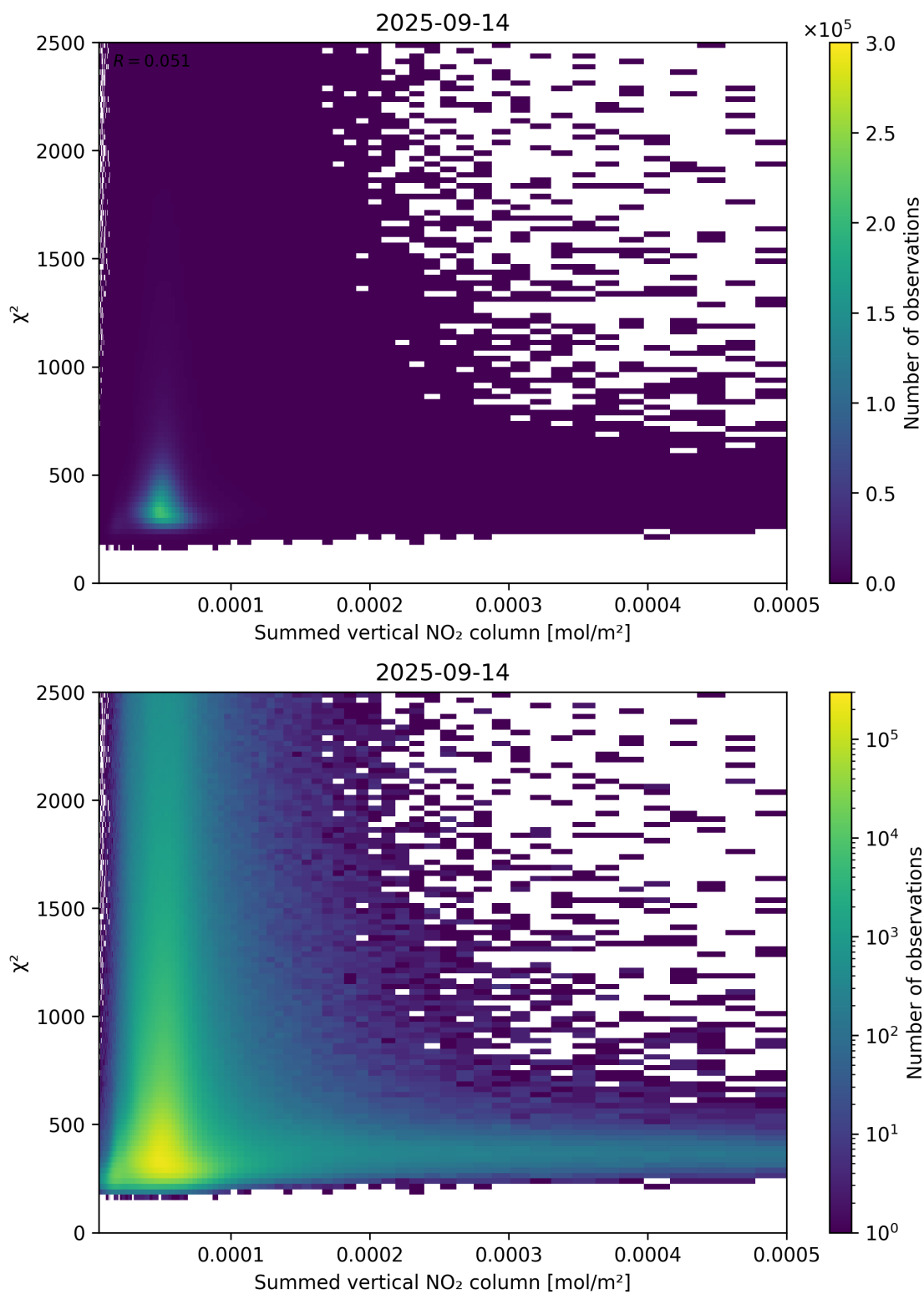
Figure 104: Scatter density plot of “Summed vertical NO 2 column” against “ \chi^2 ” for 2025-09-13 to 2025-09-15.
