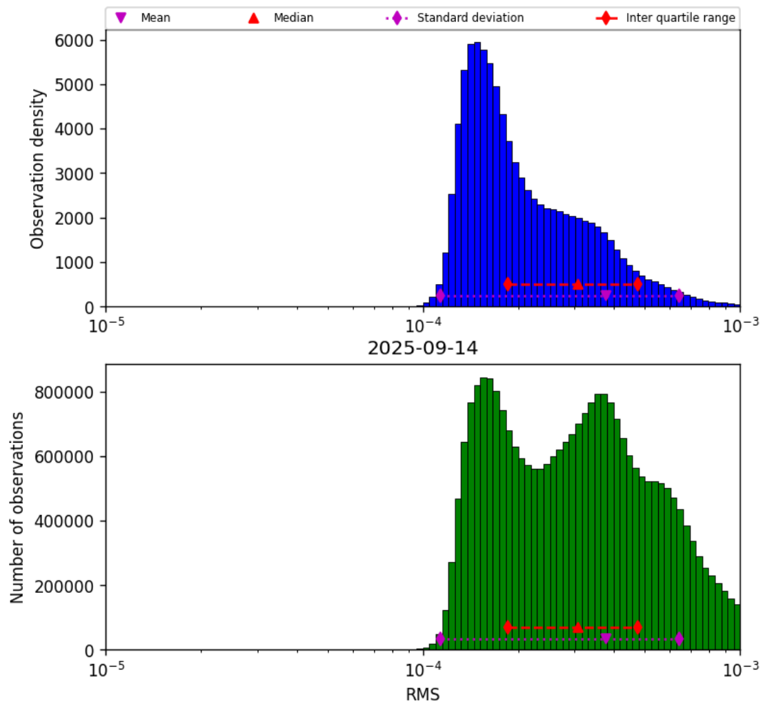
Figure 43: Histogram of “RMS” for 2025-09-13 to 2025-09-15
