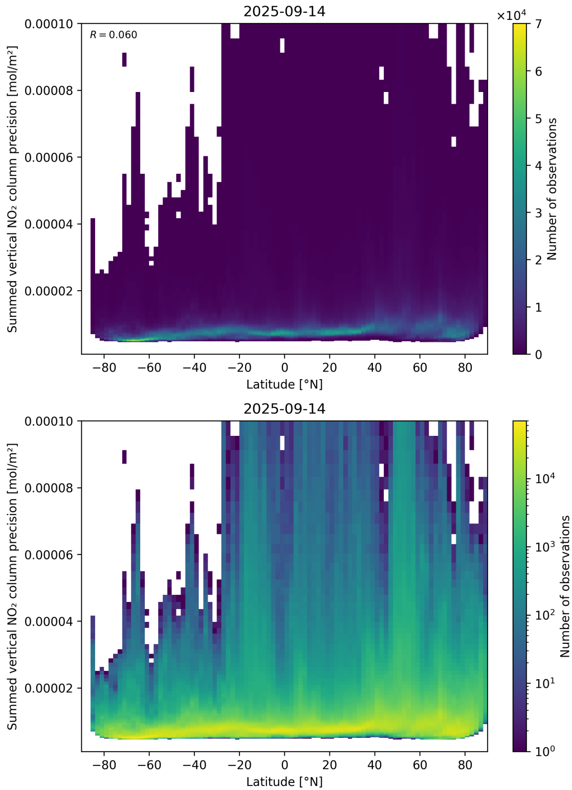
Figure 89: Scatter density plot of “Latitude” against “Summed vertical NO 2 column precision” for 2025-09-13 to 2025-09-15.
