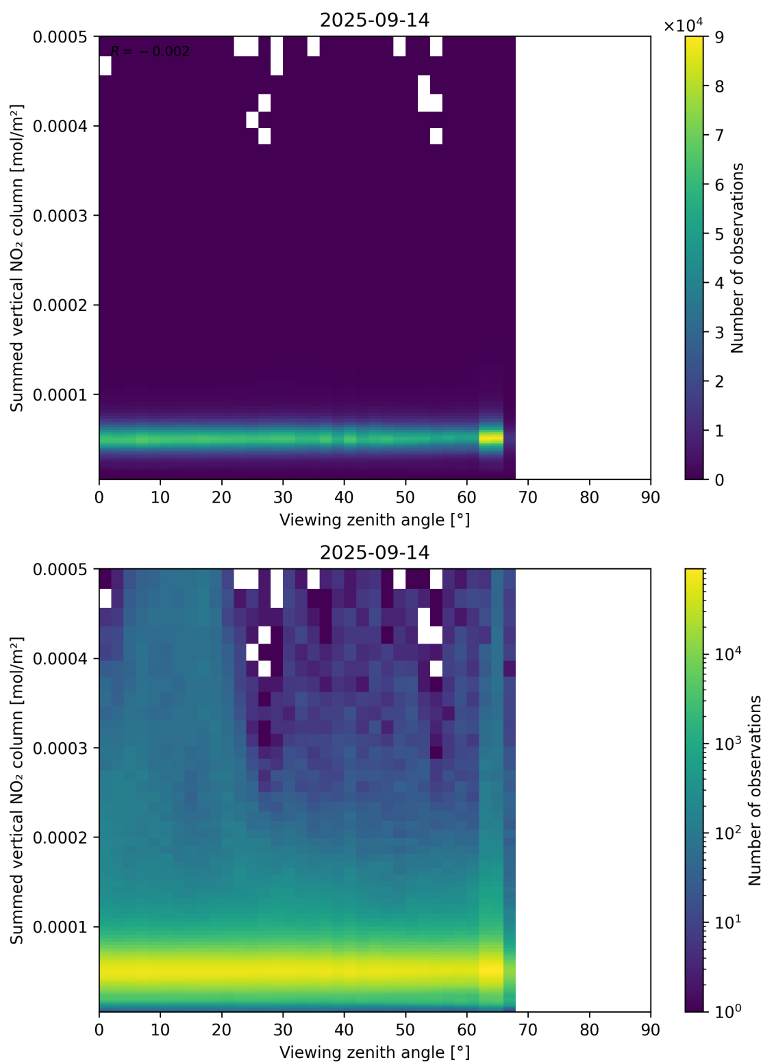
Figure 165: Scatter density plot of “Viewing zenith angle” against “Summed vertical NO 2 column” for 2025-09-13 to 2025-09-15.
