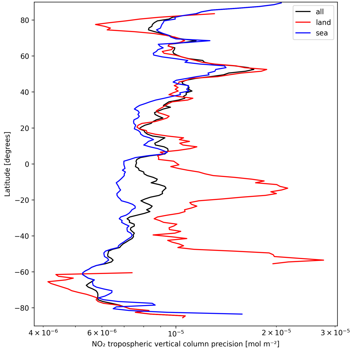
Figure 13: Zonal average of “NO 2 tropospheric vertical column precision” for 2025-09-13 to 2025-09-15.
