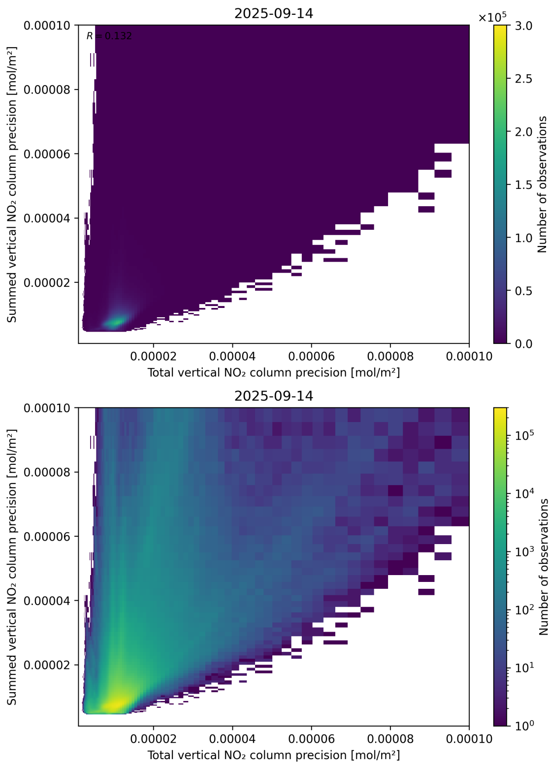
Figure 118: Scatter density plot of “Total vertical NO 2 column precision” against “Summed vertical NO 2 column precision” for 2025-09-13 to 2025-09-15.
