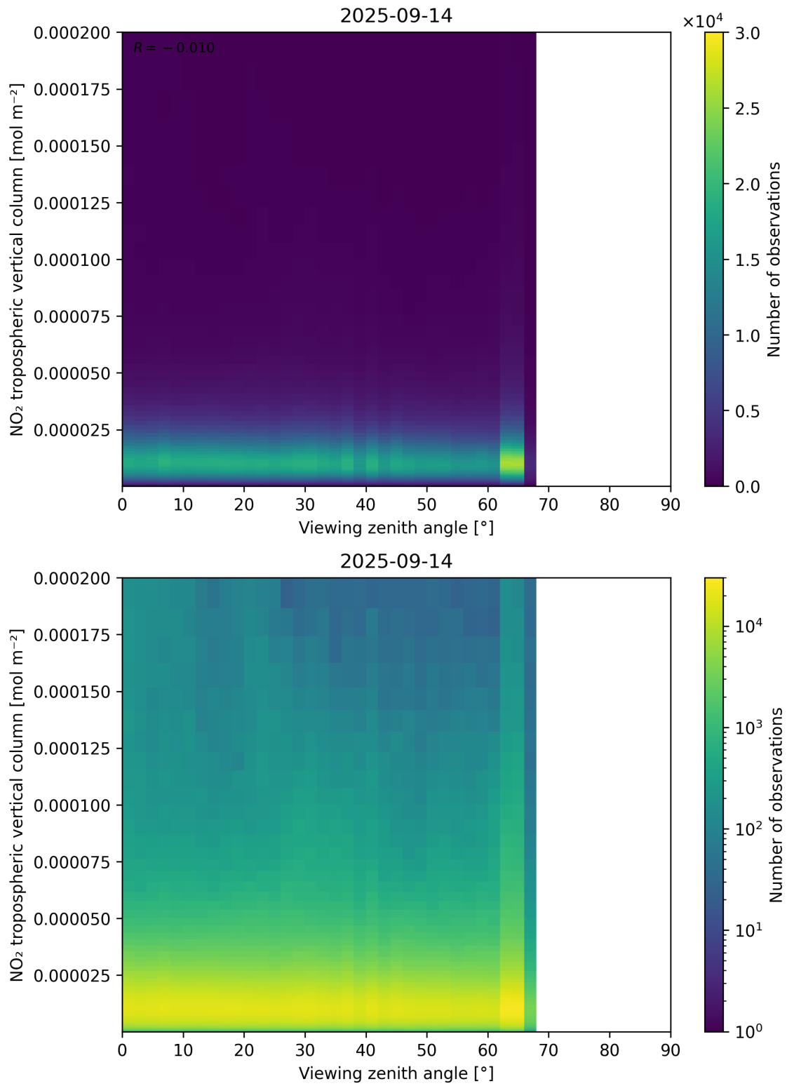
Figure 169: Scatter density plot of “Viewing zenith angle” against “NO 2 tropospheric vertical column” for 2025-09-13 to 2025-09-15.
