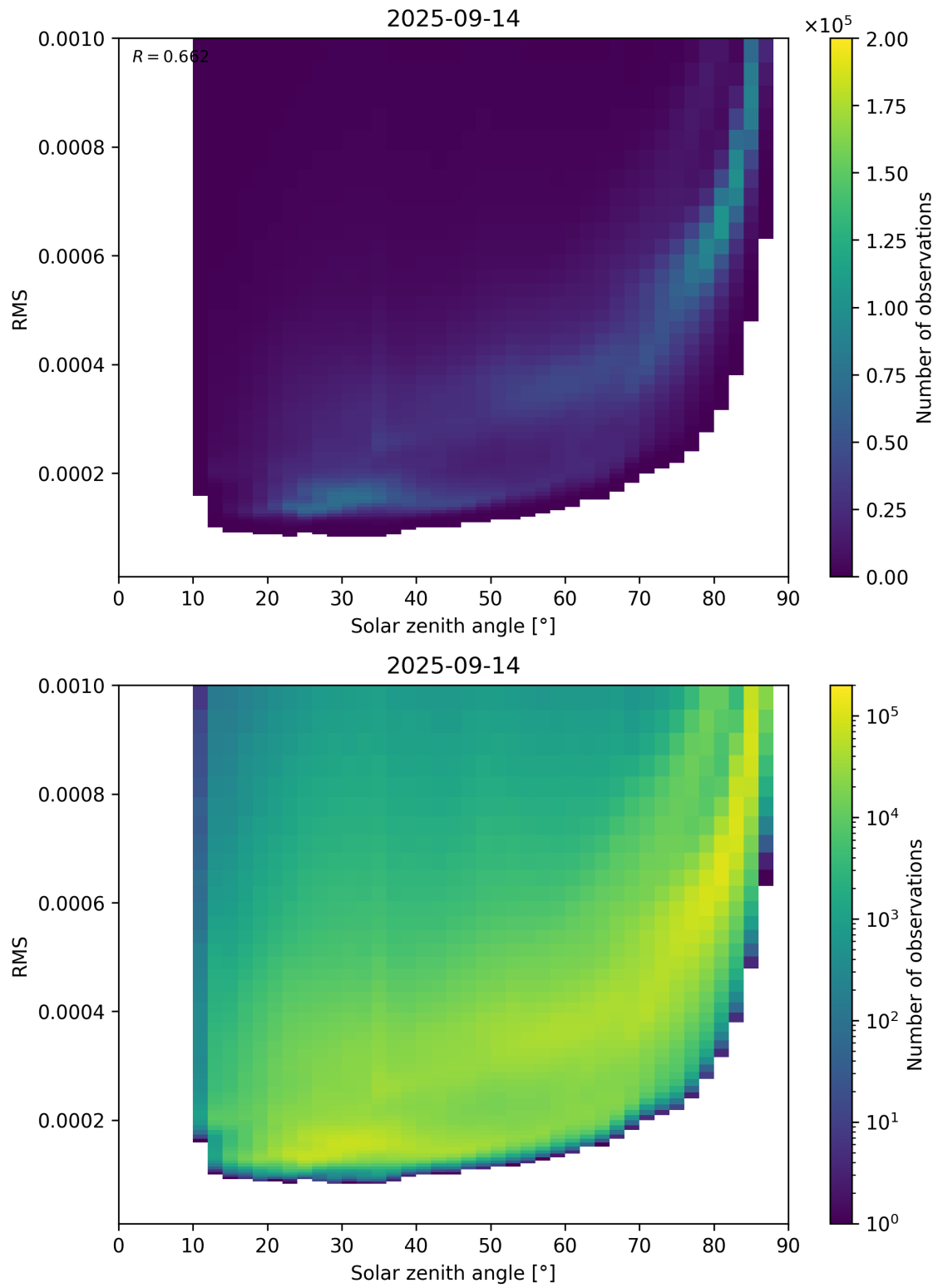
Figure 157: Scatter density plot of “Solar zenith angle” against “RMS” for 2025-09-13 to 2025-09-15.
