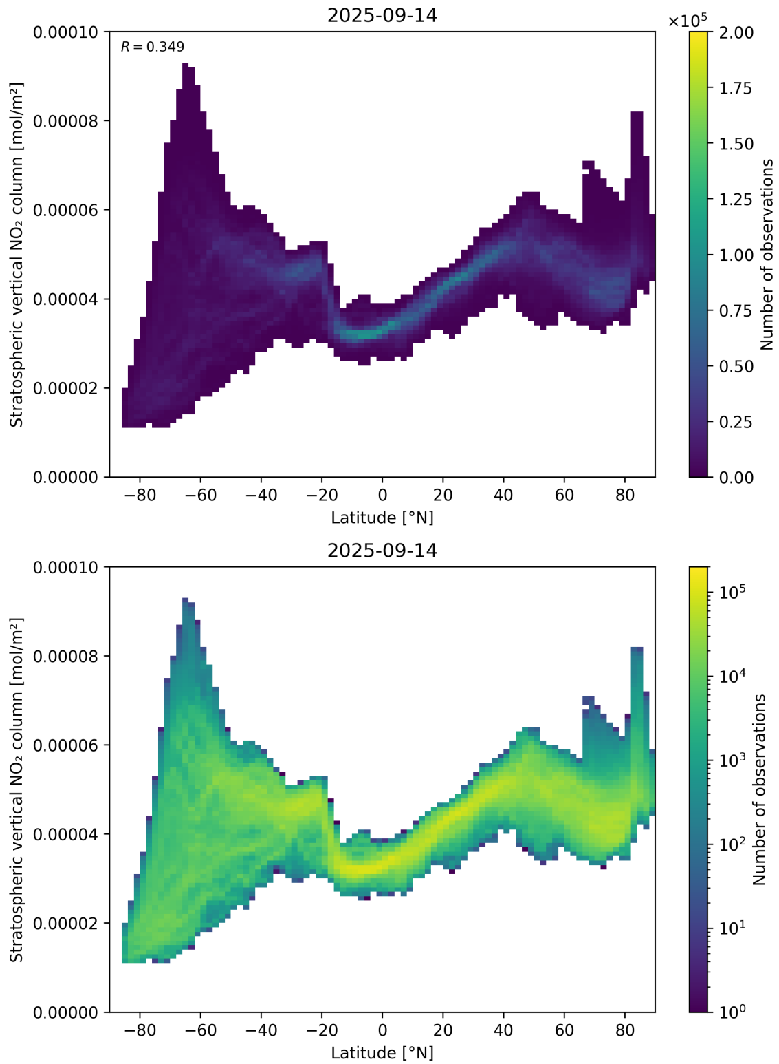
Figure 87: Scatter density plot of “Latitude” against “Stratospheric vertical NO 2 column” for 2025-09-13 to 2025-09-15.
