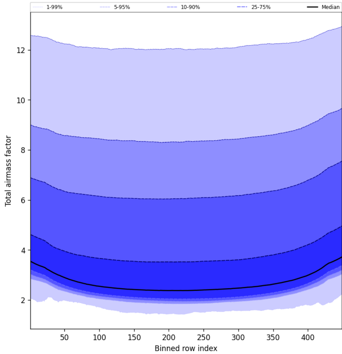
Figure 49: Along track statistics of “Total airmass factor” for 2025-09-13 to 2025-09-15
