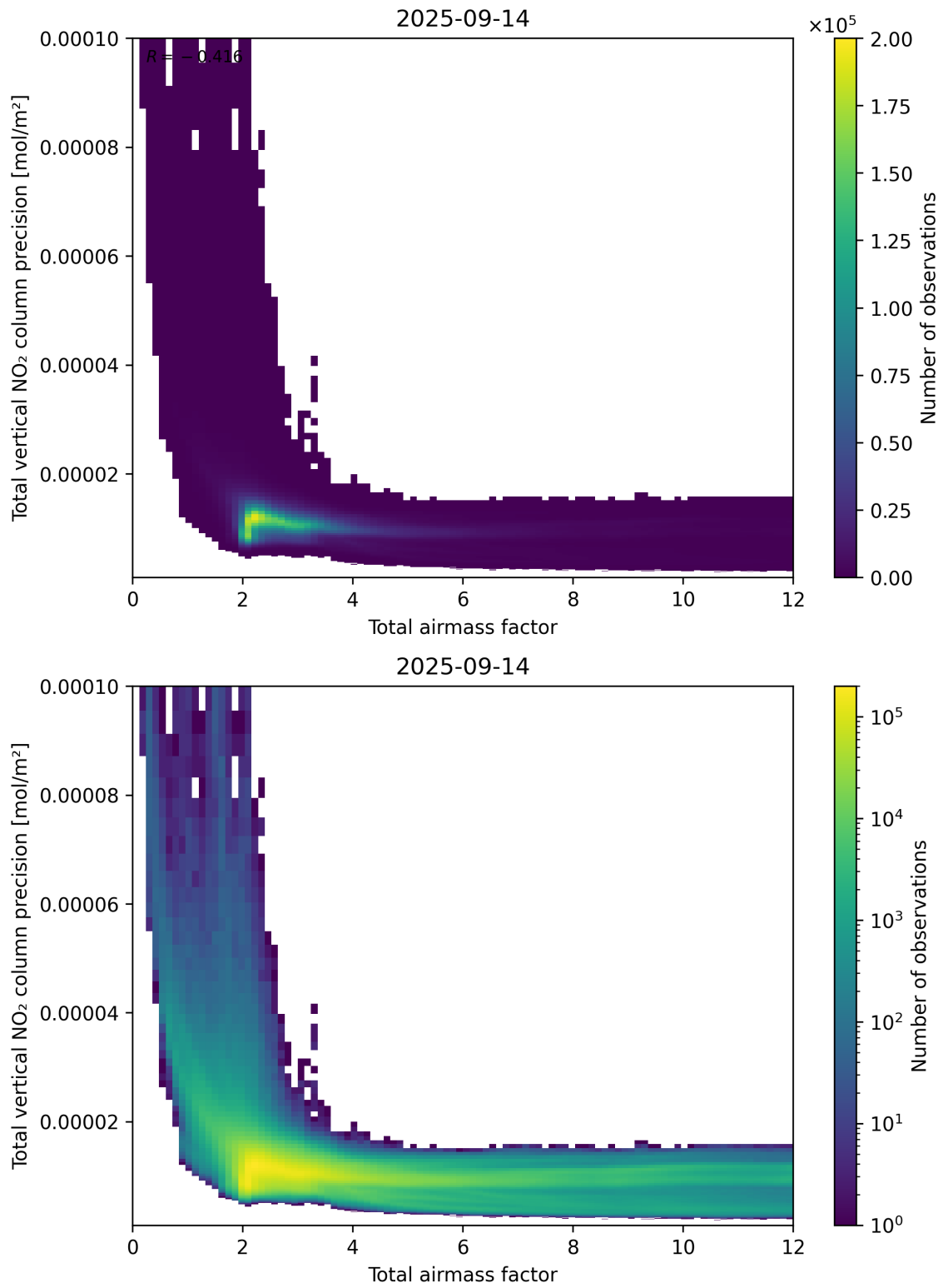
Figure 68: Scatter density plot of “Total airmass factor” against “Total vertical NO 2 column precision” for 2025-09-13 to 2025-09-15.
