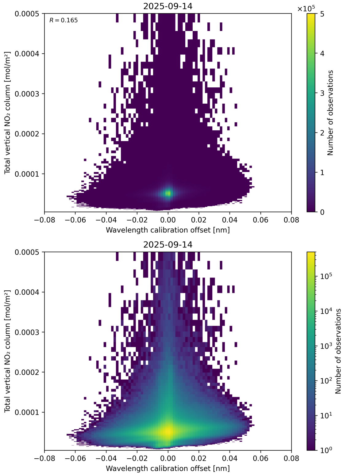
Figure 179: Scatter density plot of “Wavelength calibration offset” against “Total vertical NO 2 column” for 2025-09-13 to 2025-09-15.
