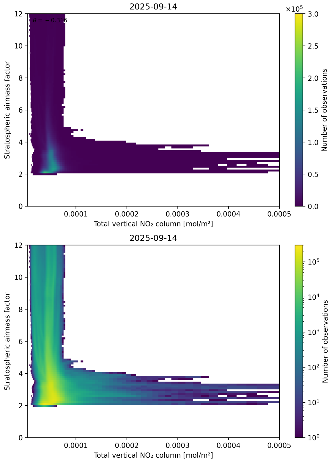
Figure 110: Scatter density plot of “Total vertical NO 2 column” against “Stratospheric airmass factor” for 2025-09-13 to 2025-09-15.
