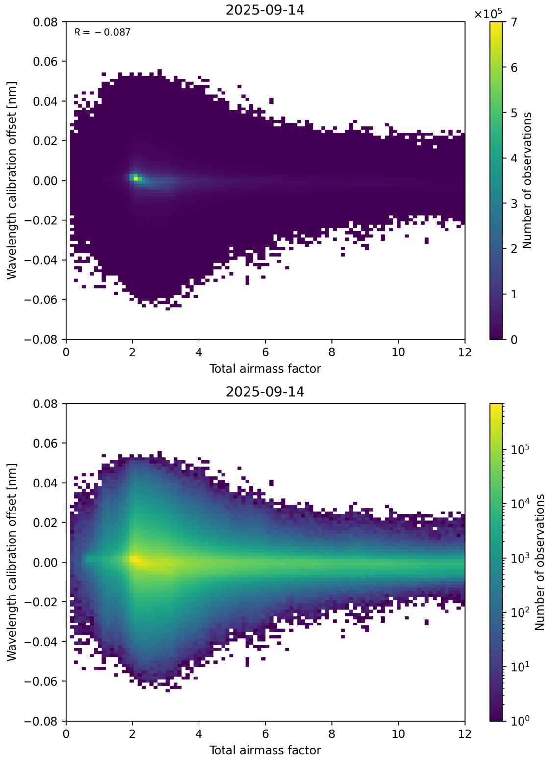
Figure 70: Scatter density plot of “Total airmass factor” against “Wavelength calibration offset” for 2025-09-13 to 2025-09-15.
