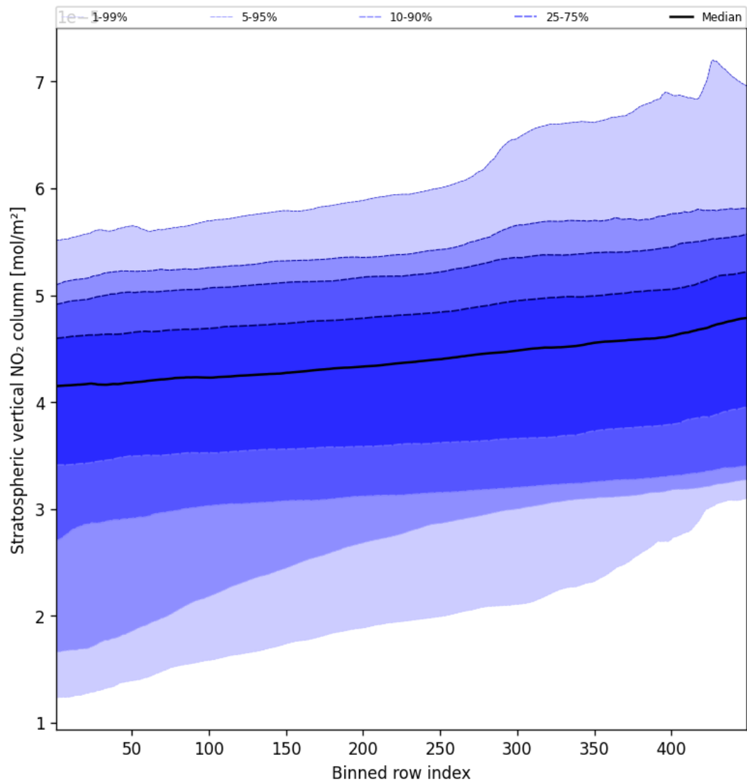
Figure 53: Along track statistics of “Stratospheric vertical NO 2 column” for 2025-09-13 to 2025-09-15
