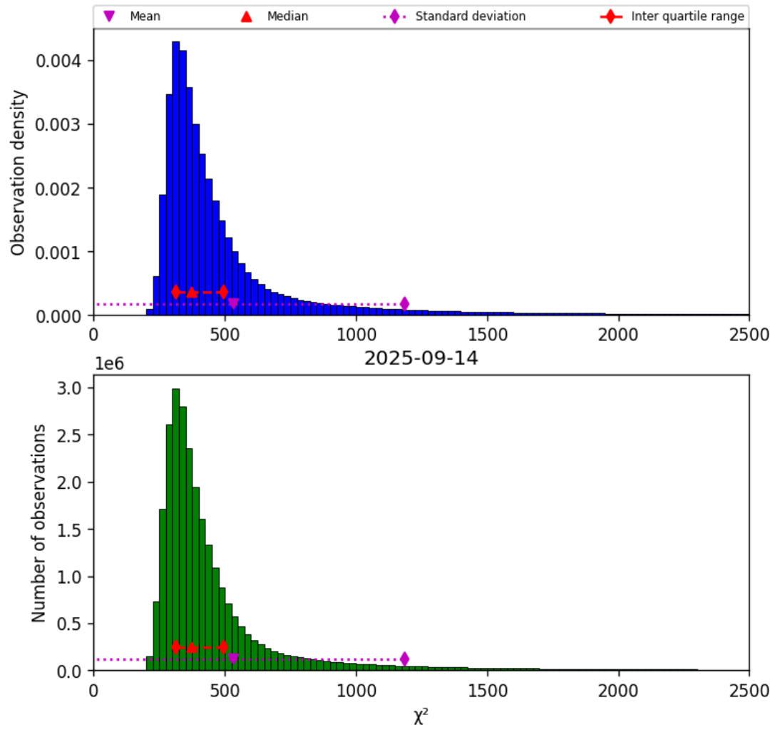
Figure 42: Histogram of “ \chi^2 ” for 2025-09-13 to 2025-09-15
