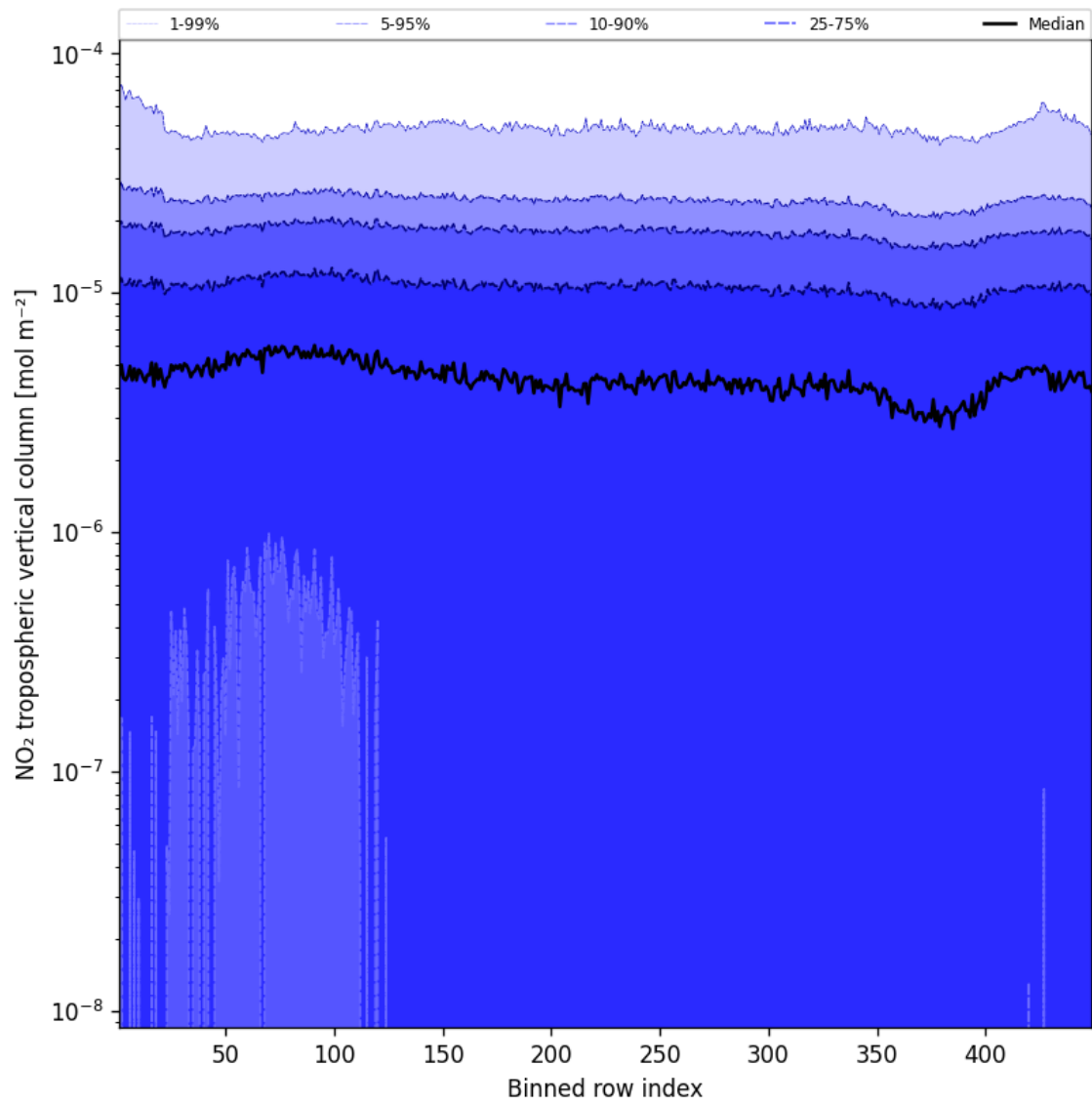
Figure 46: Along track statistics of “NO 2 tropospheric vertical column” for 2025-09-13 to 2025-09-15
