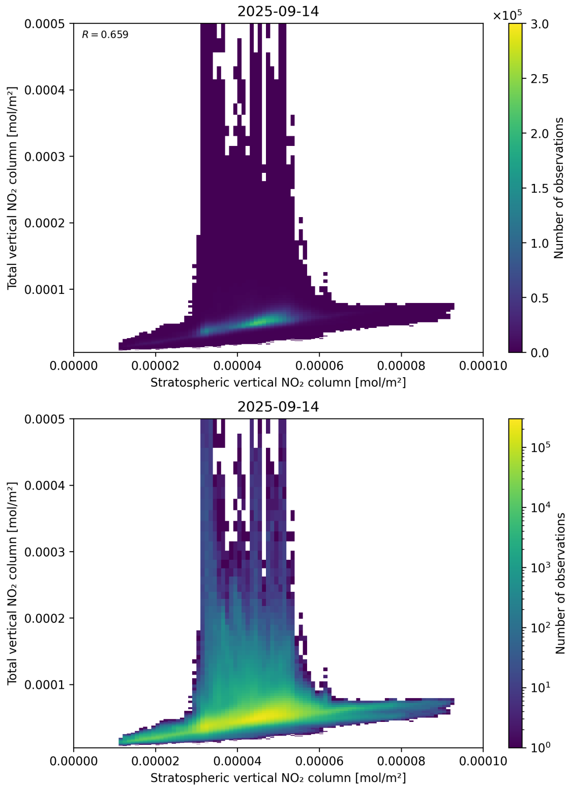
Figure 100: Scatter density plot of “Stratospheric vertical NO 2 column” against “Total vertical NO 2 column” for 2025-09-13 to 2025-09-15.
