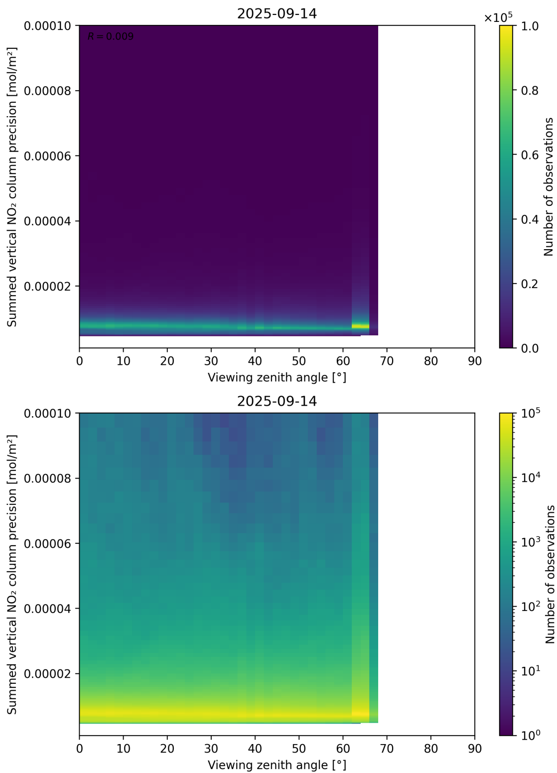
Figure 166: Scatter density plot of “Viewing zenith angle” against “Summed vertical NO 2 column precision” for 2025-09-13 to 2025-09-15.
