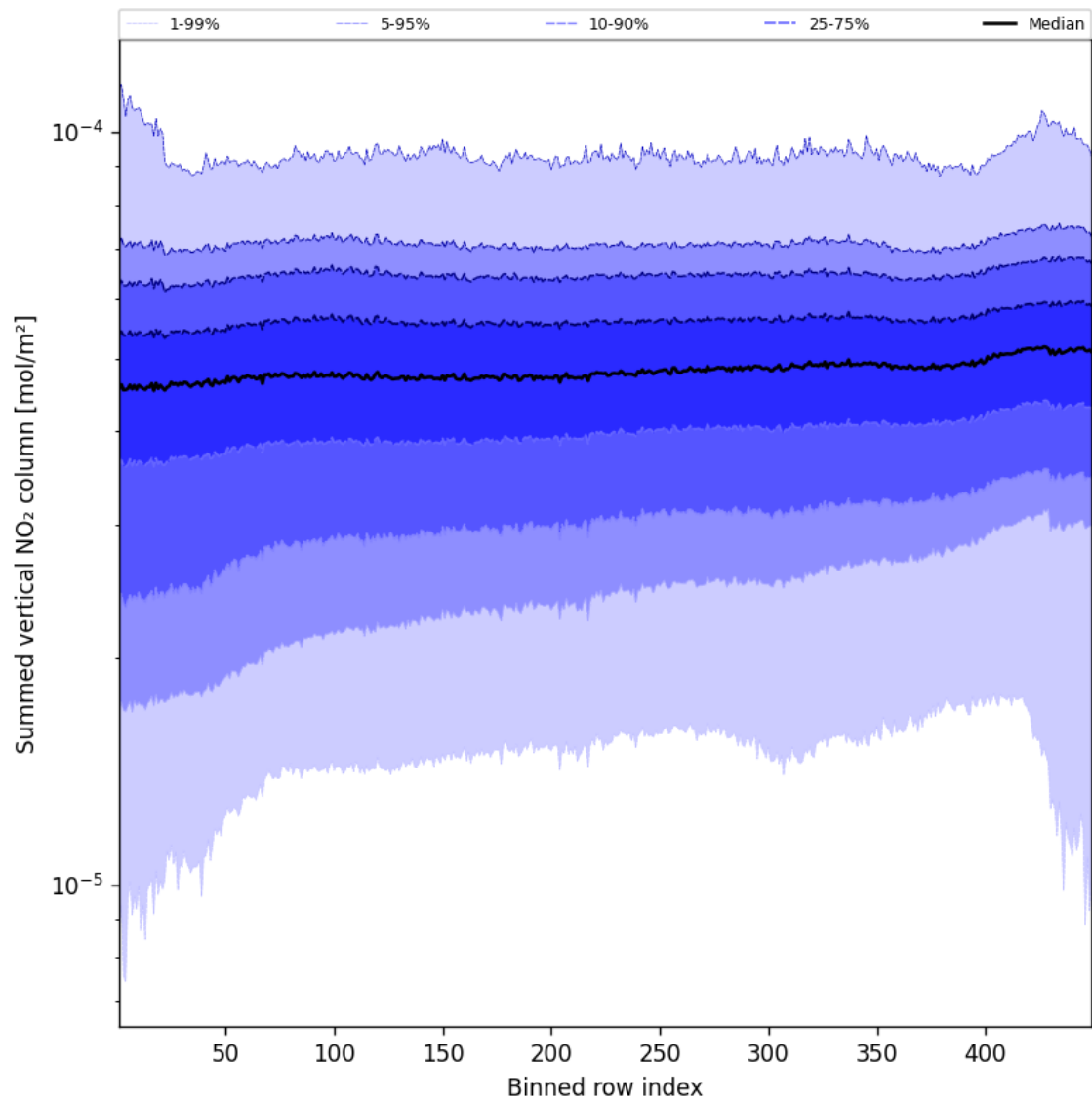
Figure 57: Along track statistics of “Summed vertical NO 2 column” for 2025-09-13 to 2025-09-15
