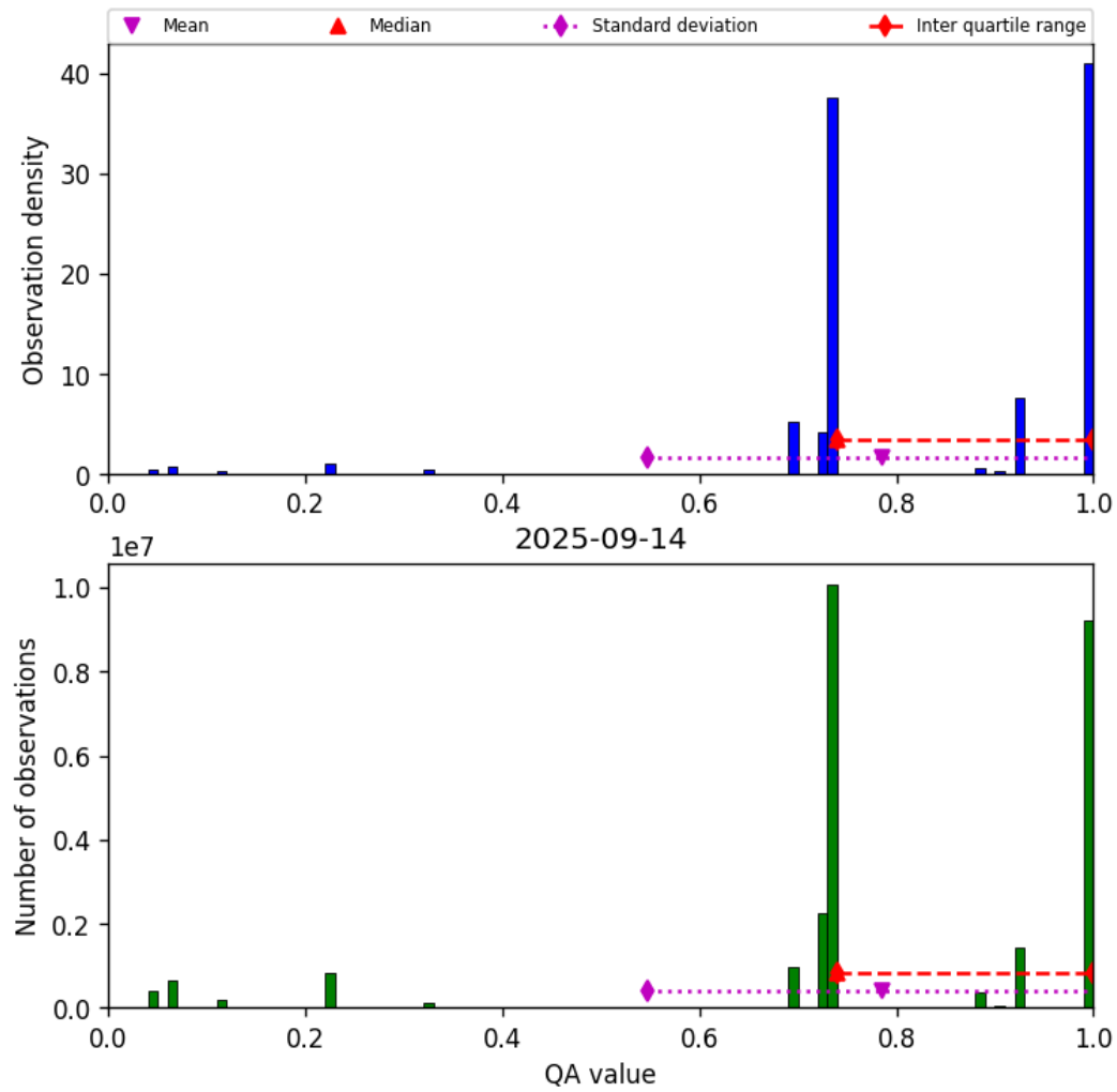
Figure 28: Histogram of “QA value” for 2025-09-13 to 2025-09-15
