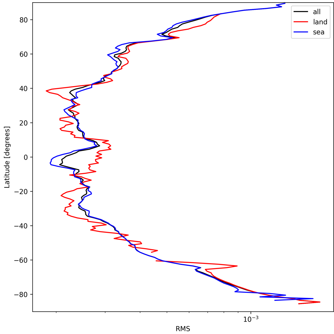
Figure 26: Zonal average of “RMS” for 2025-09-13 to 2025-09-15.
