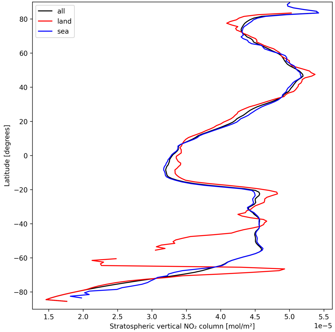
Figure 19: Zonal average of “Stratospheric vertical NO 2 column” for 2025-09-13 to 2025-09-15.
