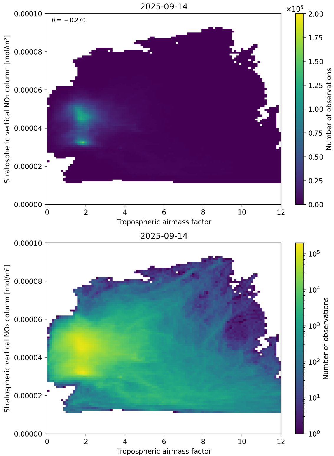
Figure 74: Scatter density plot of “Tropospheric airmass factor” against “Stratospheric vertical NO 2 column” for 2025-09-13 to 2025-09-15.
