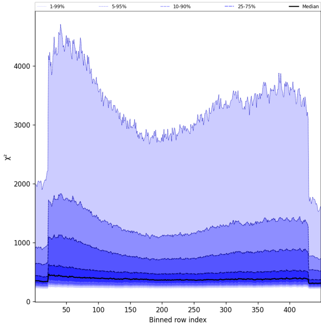
Figure 59: Along track statistics of “ \chi^2 ” for 2025-09-13 to 2025-09-15
