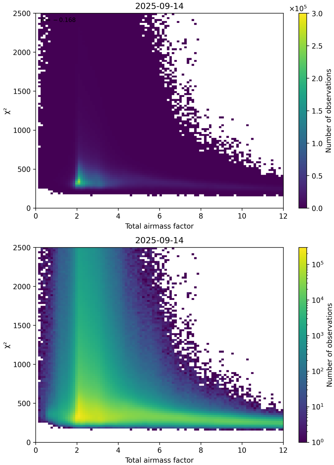
Figure 63: Scatter density plot of “Total airmass factor” against “ \chi^2 ” for 2025-09-13 to 2025-09-15.
