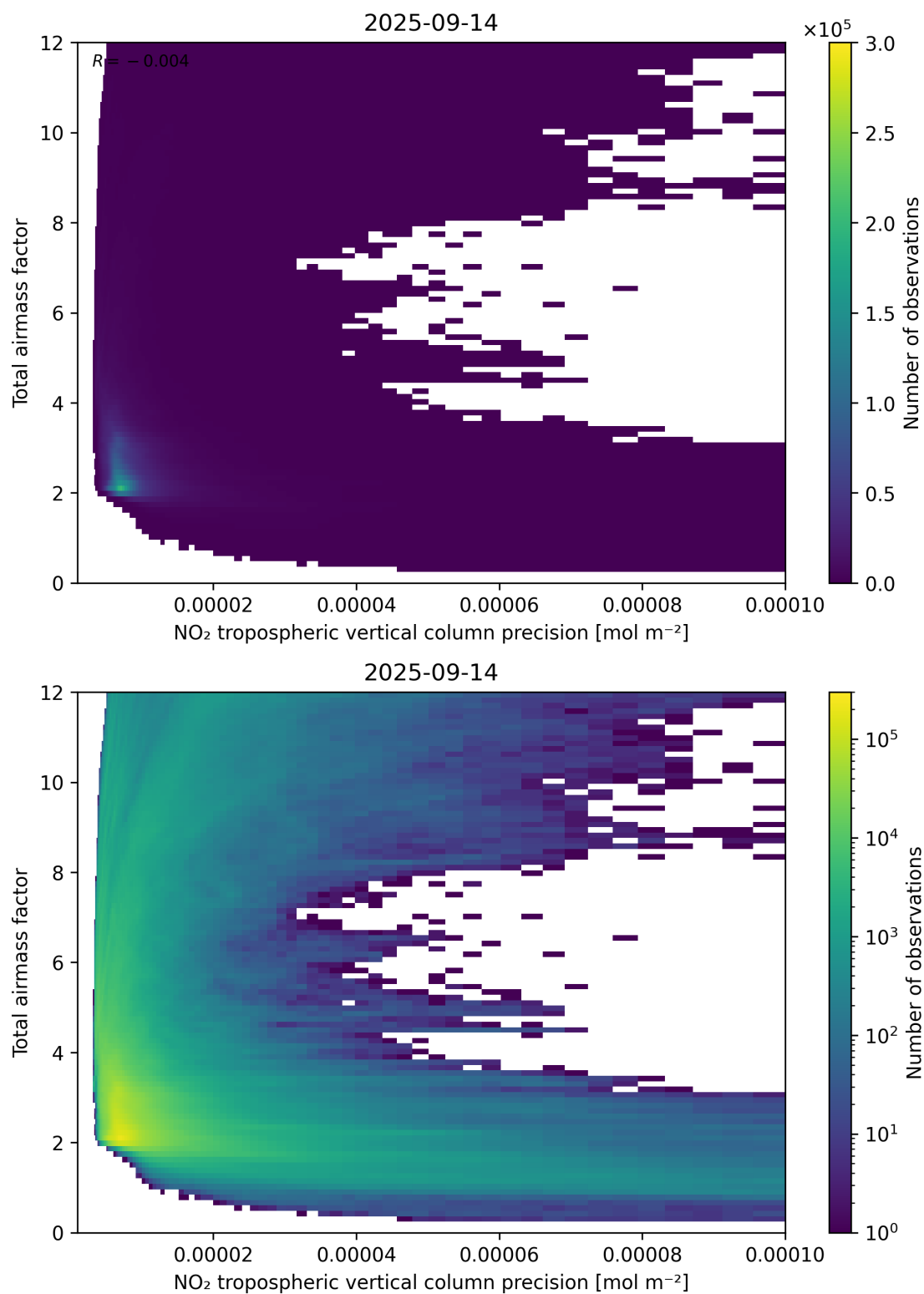
Figure 132: Scatter density plot of “NO 2 tropospheric vertical column precision” against “Total airmass factor” for 2025-09-13 to 2025-09-15.
