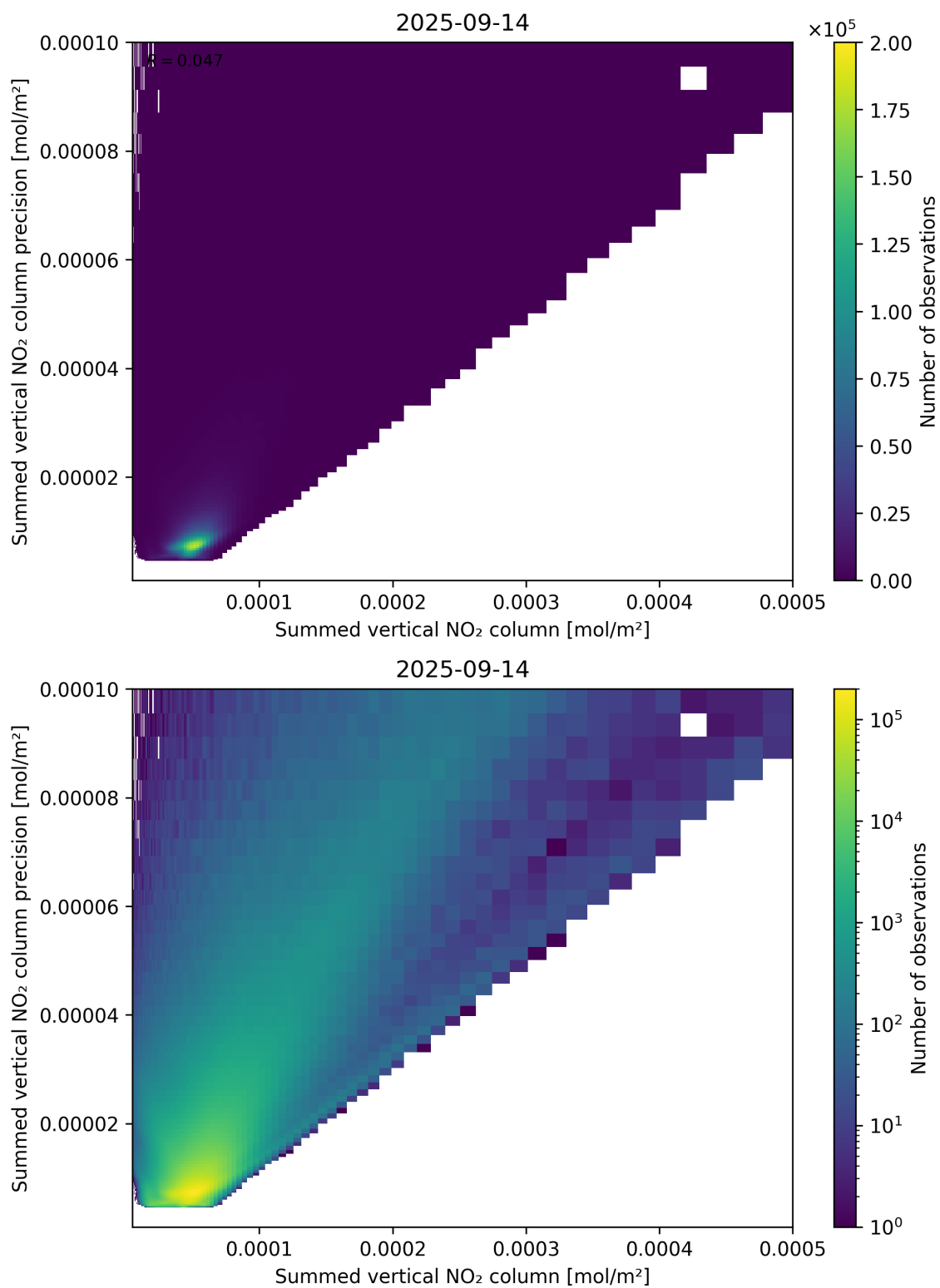
Figure 105: Scatter density plot of “Summed vertical NO 2 column” against “Summed vertical NO 2 column precision” for 2025-09-13 to 2025-09-15.
