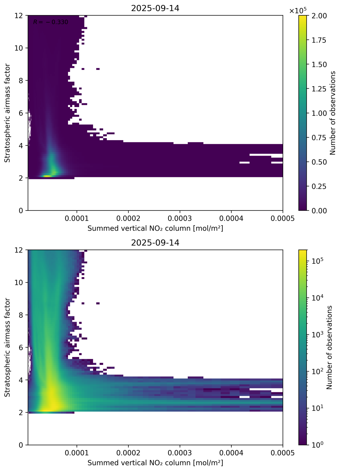
Figure 103: Scatter density plot of “Summed vertical NO 2 column” against “Stratospheric air mass factor” for 2025-09-13 to 2025-09-15.
