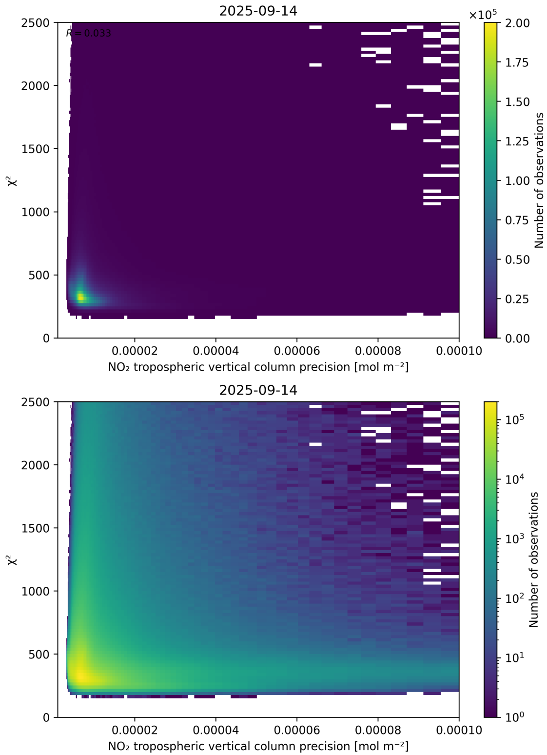
Figure 134: Scatter density plot of “NO 2 tropospheric vertical column precision” against “ \chi^2 ” for 2025-09-13 to 2025-09-15.
