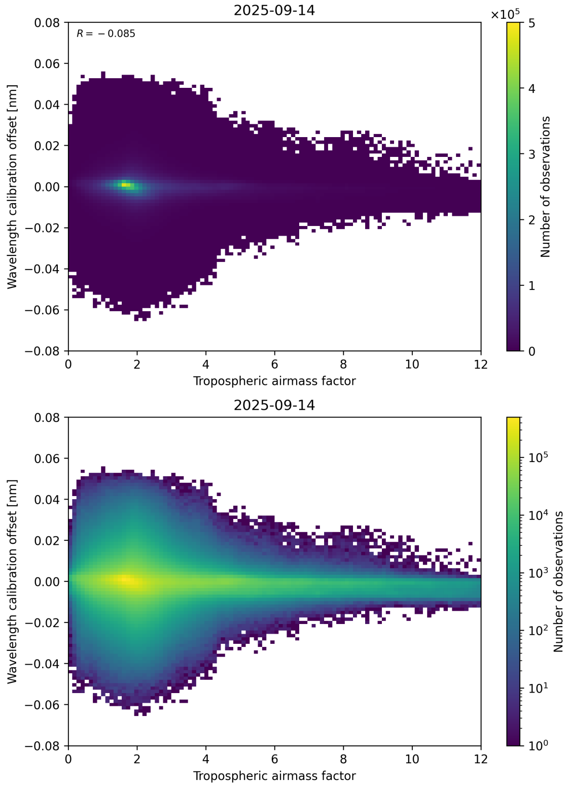
Figure 80: Scatter density plot of “Tropospheric airmass factor” against “Wavelength calibration offset” for 2025-09-13 to 2025-09-15.
