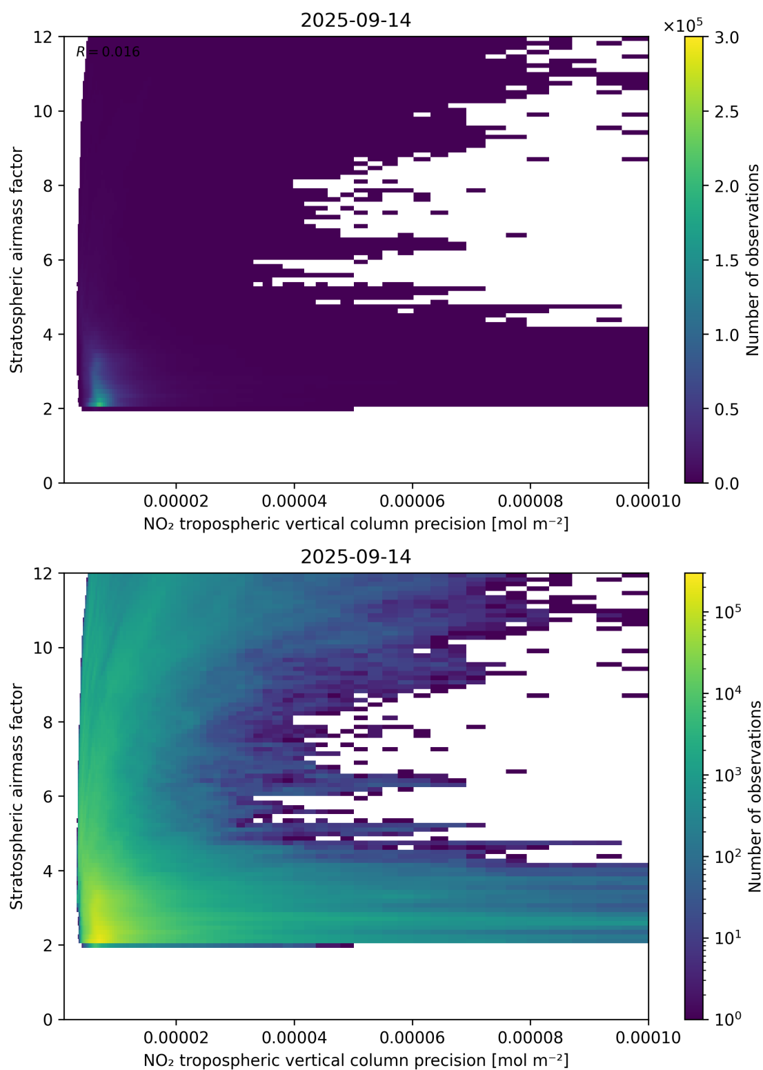
Figure 131: Scatter density plot of “NO 2 tropospheric vertical column precision” against “Stratospheric airmass factor” for 2025-09-13 to 2025-09-15.
