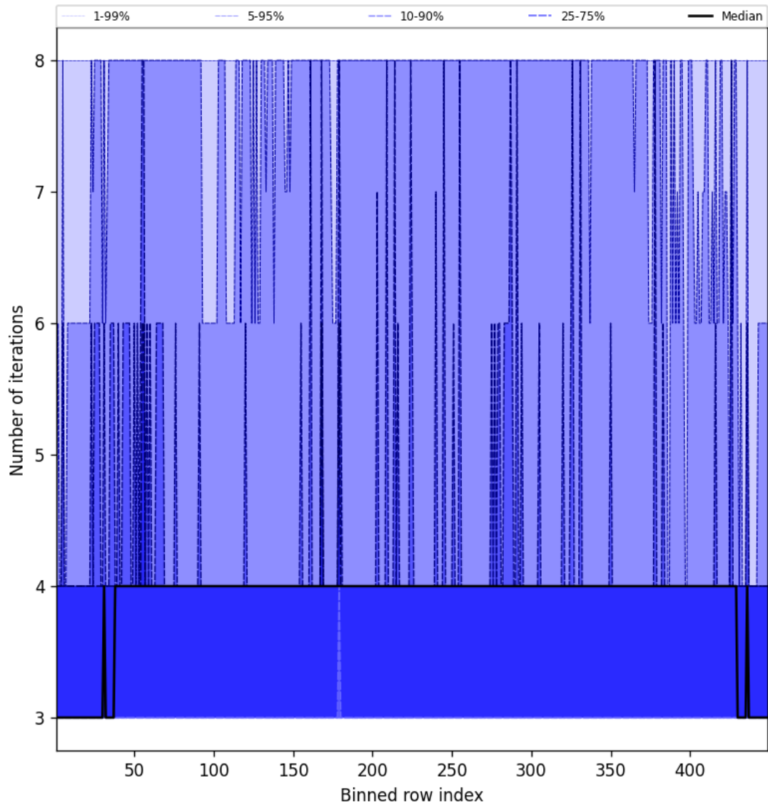
Figure 51: Along track statistics of “Number of iterations” for 2025-09-13 to 2025-09-15
