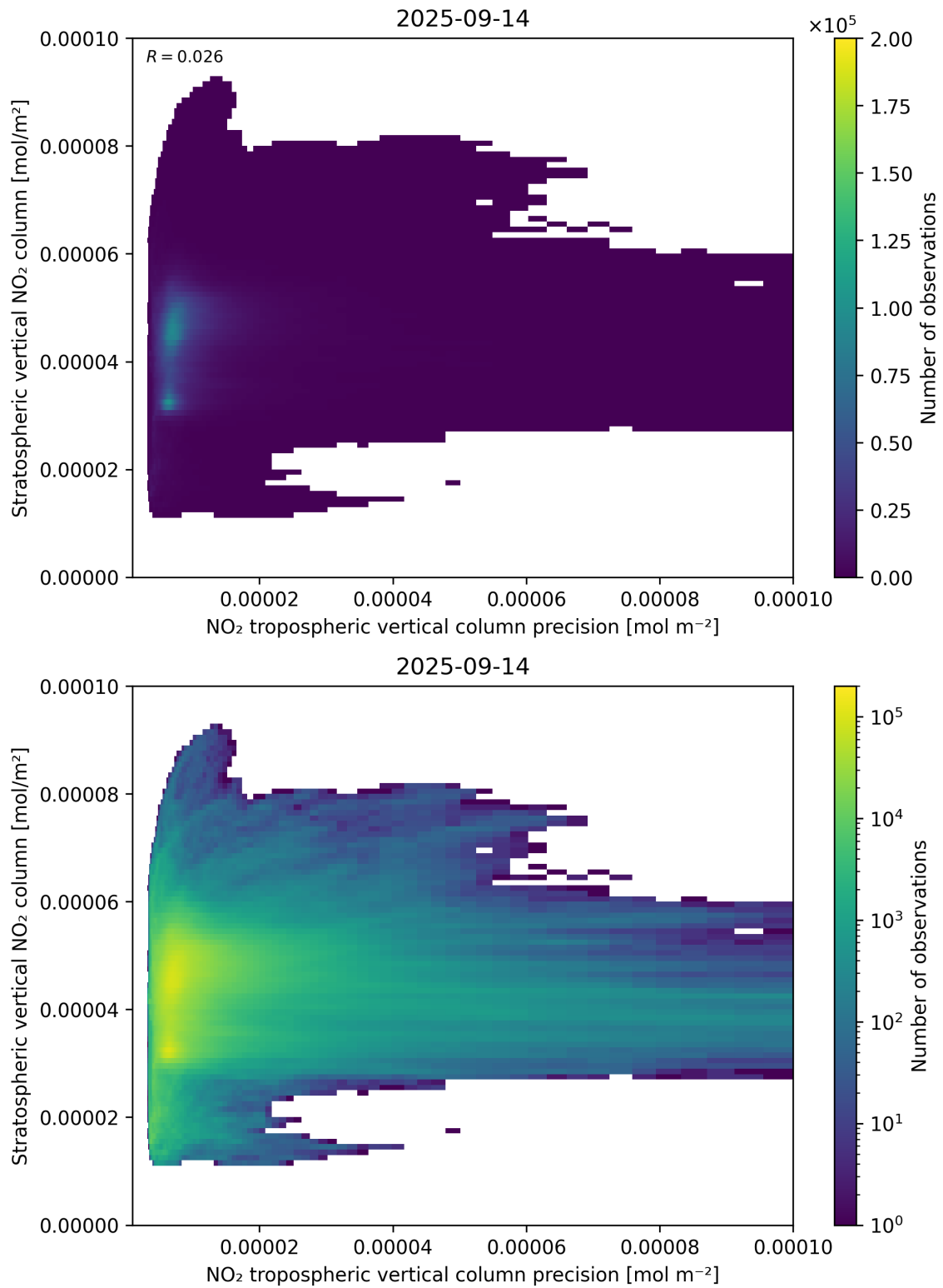
Figure 135: Scatter density plot of “NO 2 tropospheric vertical column precision” against “Stratospheric vertical NO 2 column” for 2025-09-13 to 2025-09-15.
