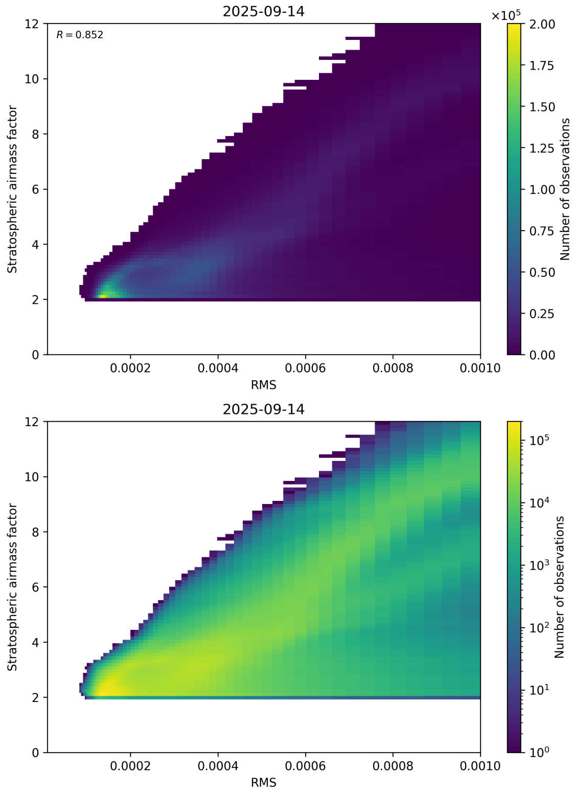
Figure 144: Scatter density plot of “RMS” against “Stratospheric airmass factor” for 2025-09-13 to 2025-09-15.
