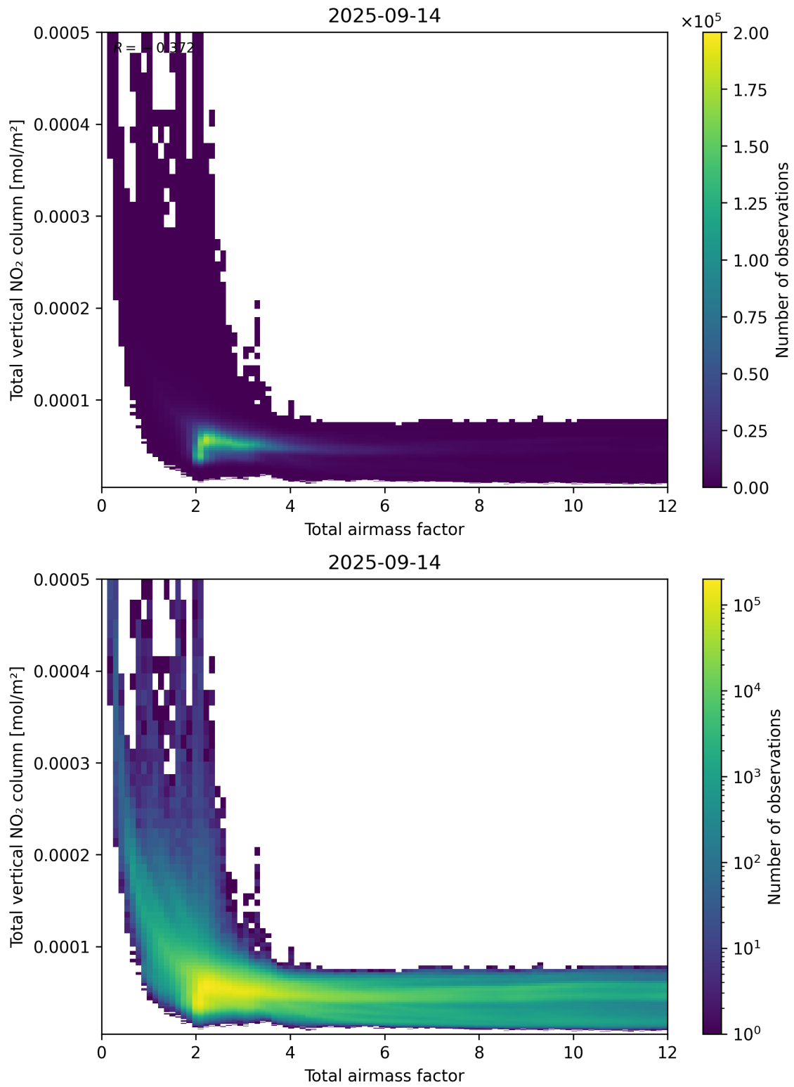
Figure 67: Scatter density plot of “Total airmass factor” against “Total vertical NO 2 column” for 2025-09-13 to 2025-09-15.
