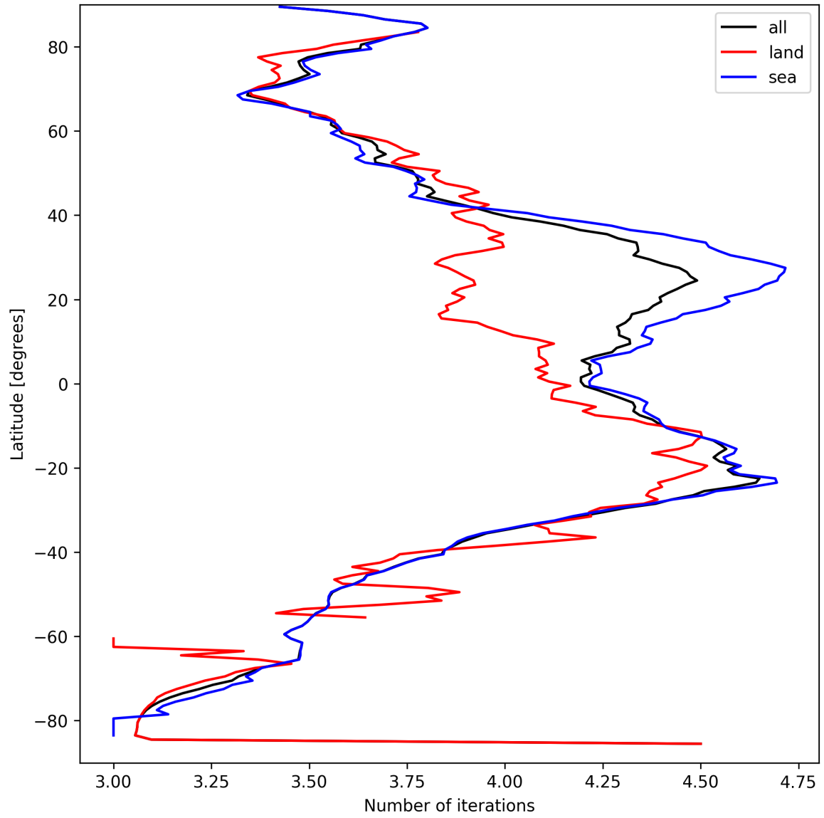
Figure 17: Zonal average of “Number of iterations” for 2025-09-13 to 2025-09-15.
