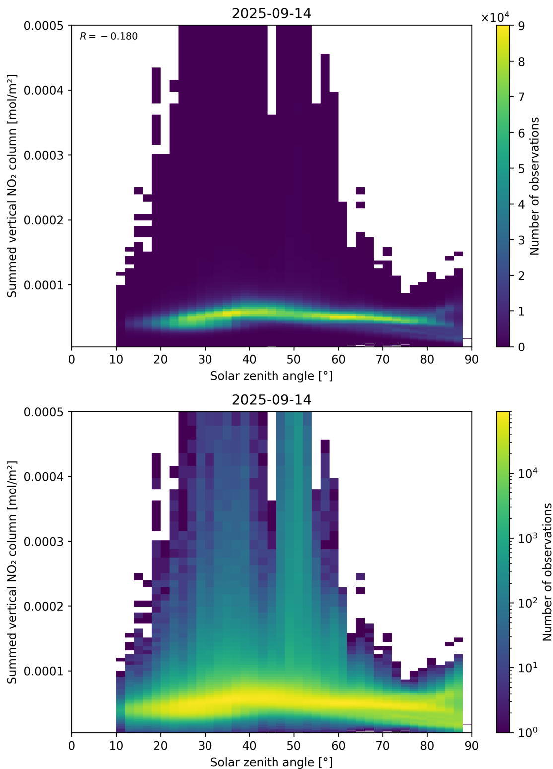
Figure 151: Scatter density plot of “Solar zenith angle” against “Summed vertical NO 2 column” for 2025-09-13 to 2025-09-15.
