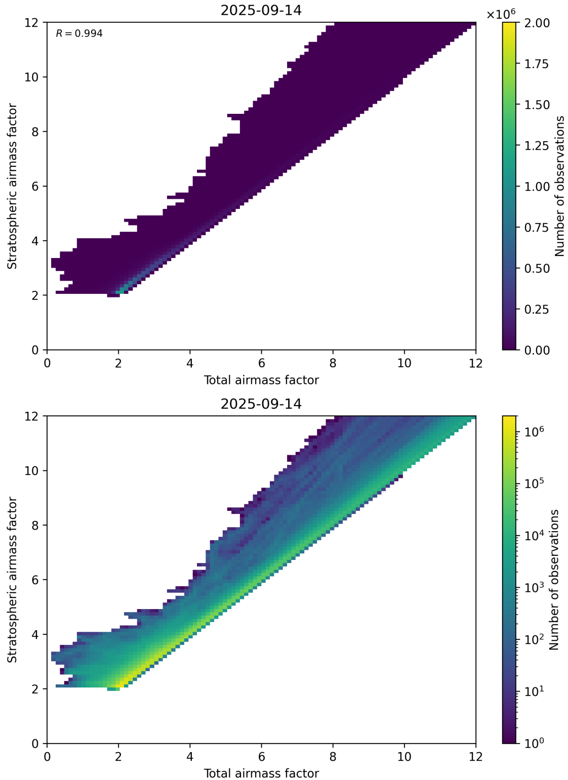
Figure 62: Scatter density plot of “Total airmass factor” against “Stratospheric airmass factor” for 2025-09-13 to 2025-09-15.
