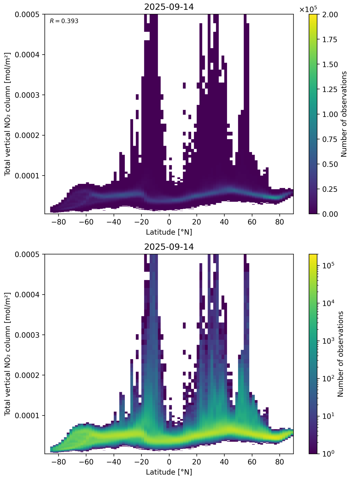
Figure 90: Scatter density plot of “Latitude” against “Total vertical NO 2 column” for 2025-09-13 to 2025-09-15.
