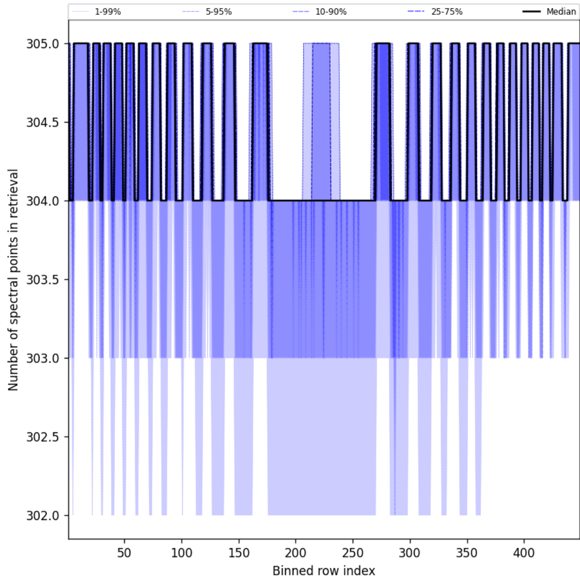
Figure 50: Along track statistics of “Number of spectral points in retrieval” for 2025-09-13 to 2025-09-15
