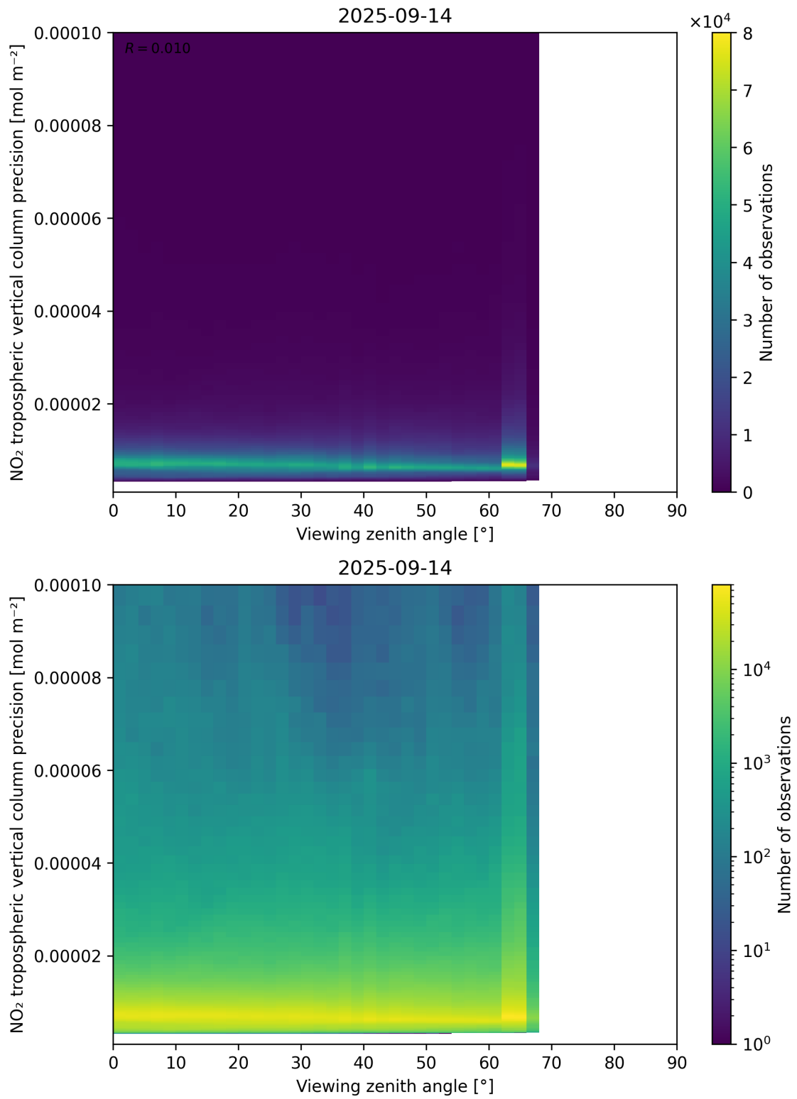
Figure 170: Scatter density plot of “Viewing zenith angle” against “NO 2 tropospheric vertical column precision” for 2025-09-13 to 2025-09-15.
