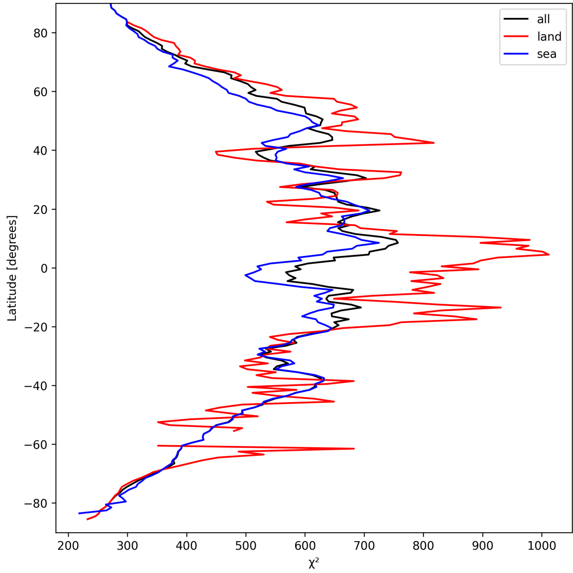
Figure 25: Zonal average of “ \chi^2 ” for 2025-09-13 to 2025-09-15.
