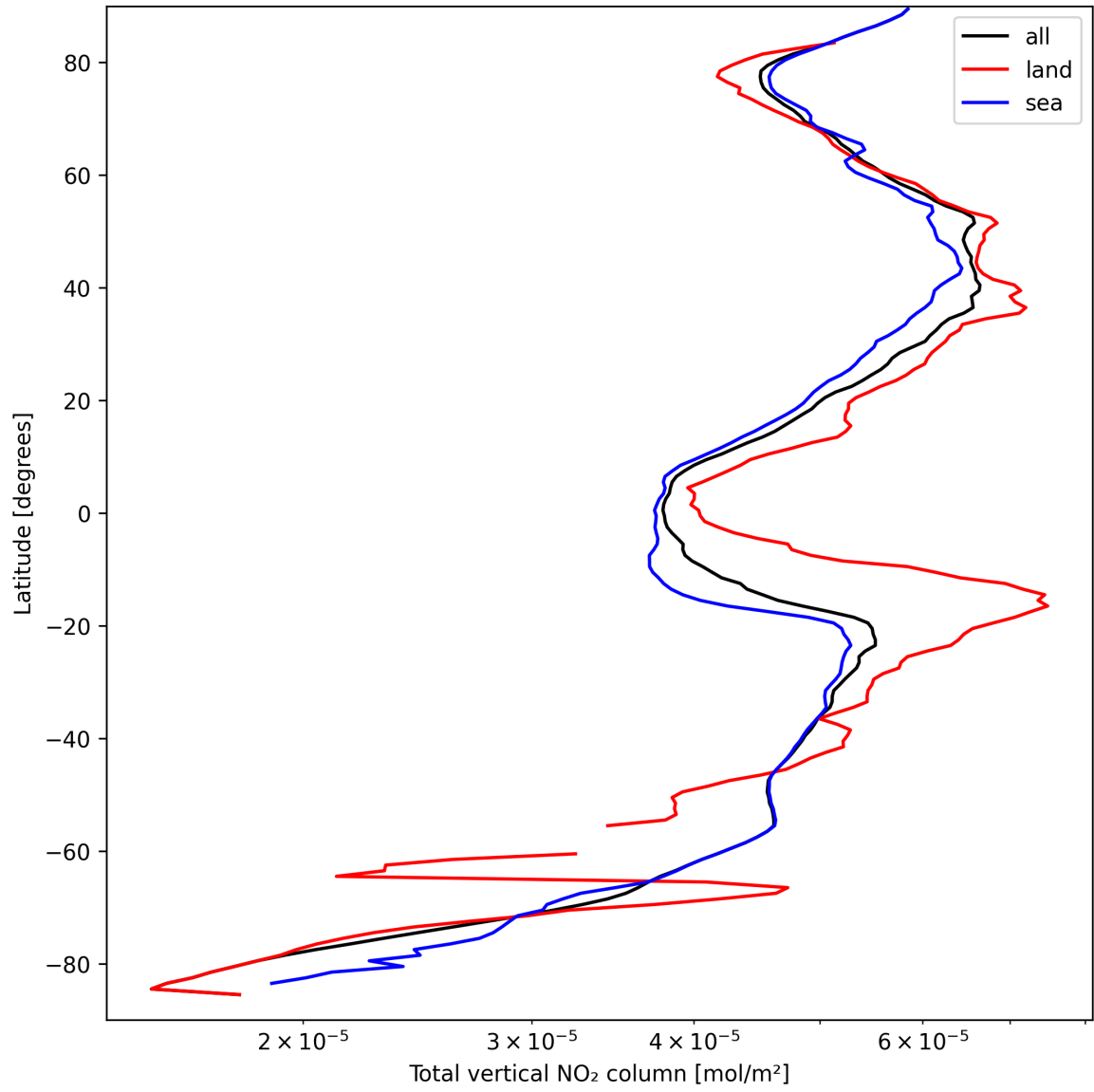
Figure 21: Zonal average of “Total vertical NO 2 column” for 2025-09-13 to 2025-09-15.
