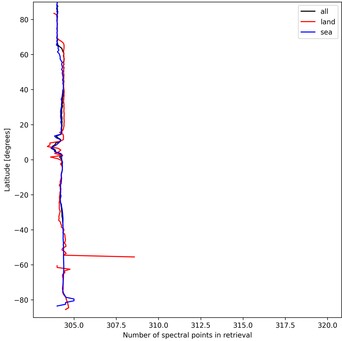
Figure 16: Zonal average of “Number of spectral points in retrieval” for 2025-09-13 to 2025-09-15.
