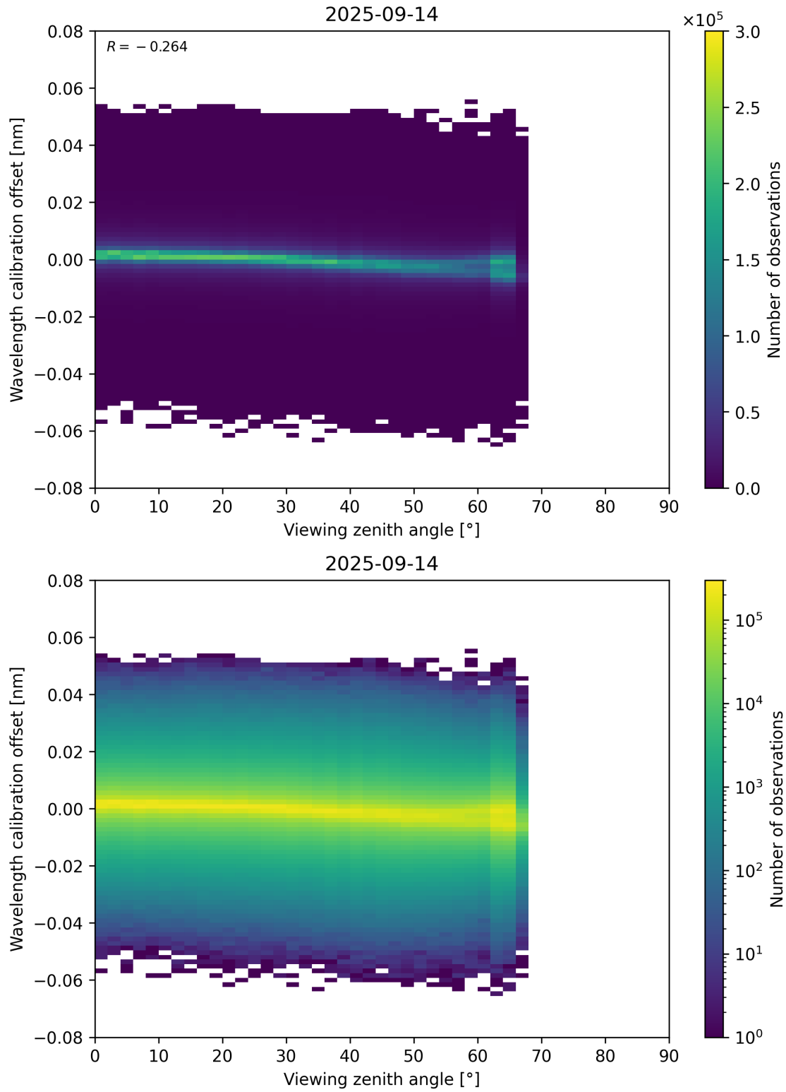
Figure 173: Scatter density plot of “Viewing zenith angle” against “Wavelength calibration offset” for 2025-09-13 to 2025-09-15.
