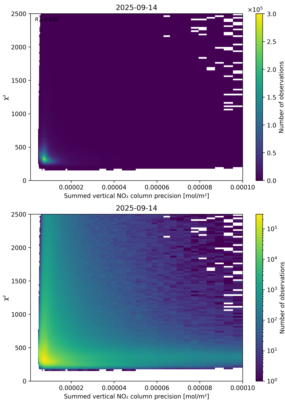
Figure 107: Scatter density plot of “Summed vertical NO 2 column precision” against “ \chi^2 ” for 2025-09-13 to 2025-09-15.
