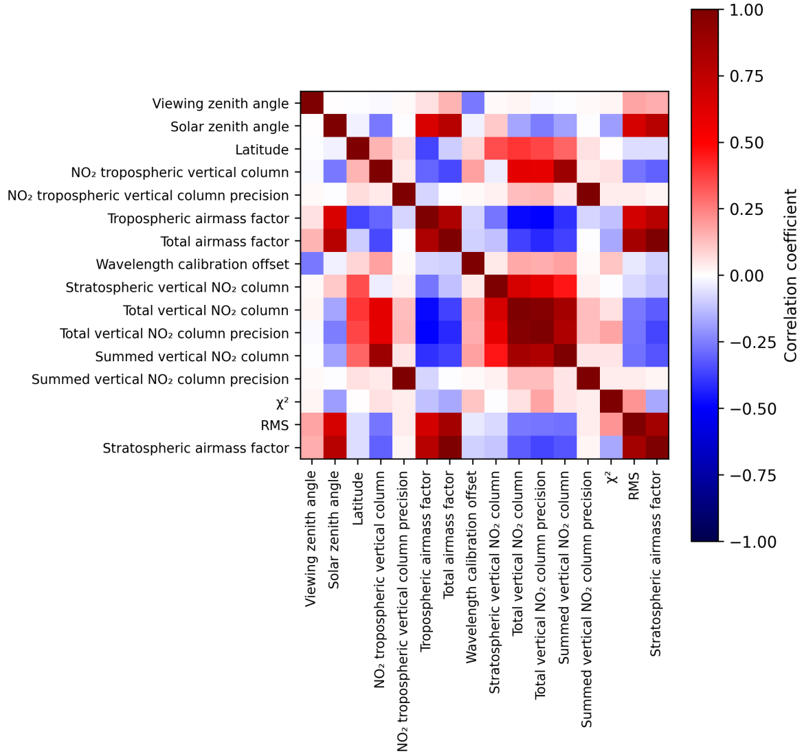
Figure 2: Map of correlation matrix for 2025-09-13 to 2025-09-15.
