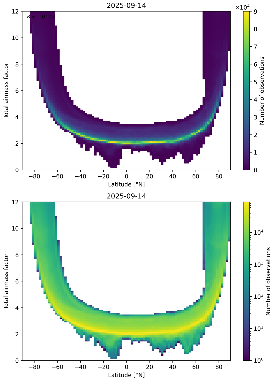
Figure 84: Scatter density plot of “Latitude” against “Total airmass factor” for 2025-09-13 to 2025-09-15.
