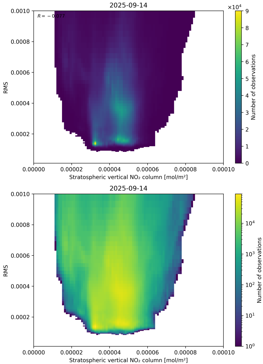
Figure 102: Scatter density plot of “Stratospheric vertical NO 2 column” against “RMS” for 2025-09-13 to 2025-09-15.
