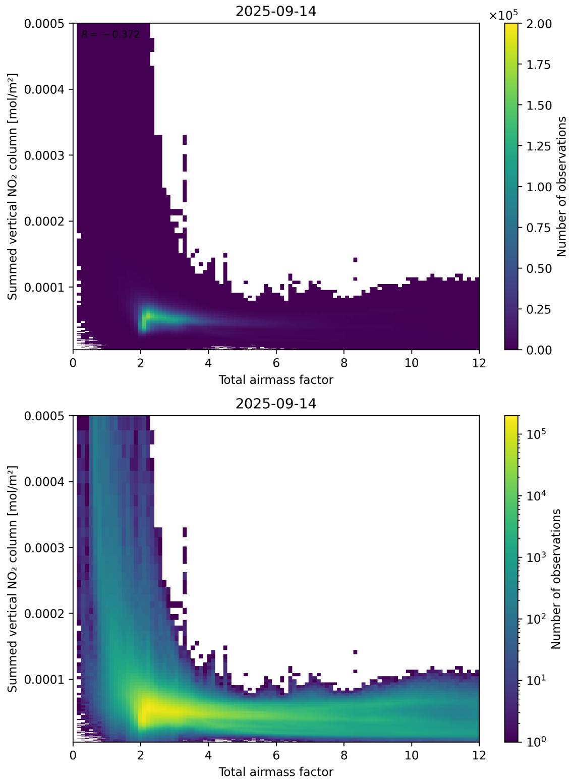
Figure 65: Scatter density plot of “Total airmass factor” against “Summed vertical NO 2 column” for 2025-09-13 to 2025-09-15.
