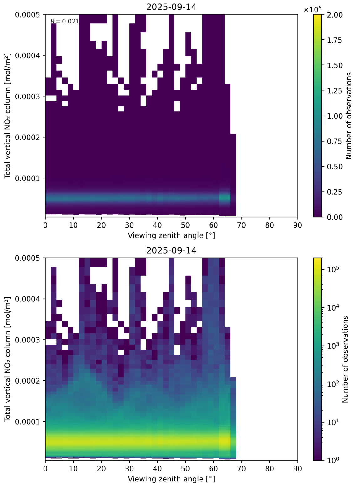
Figure 167: Scatter density plot of “Viewing zenith angle” against “Total vertical NO 2 column” for 2025-09-13 to 2025-09-15.
