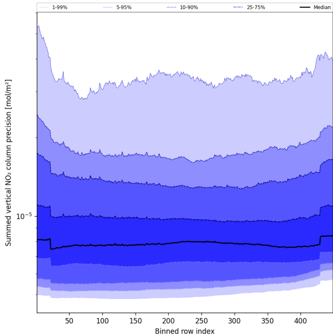
Figure 58: Along track statistics of “Summed vertical NO 2 column precision” for 2025-09-13 to 2025-09-15
