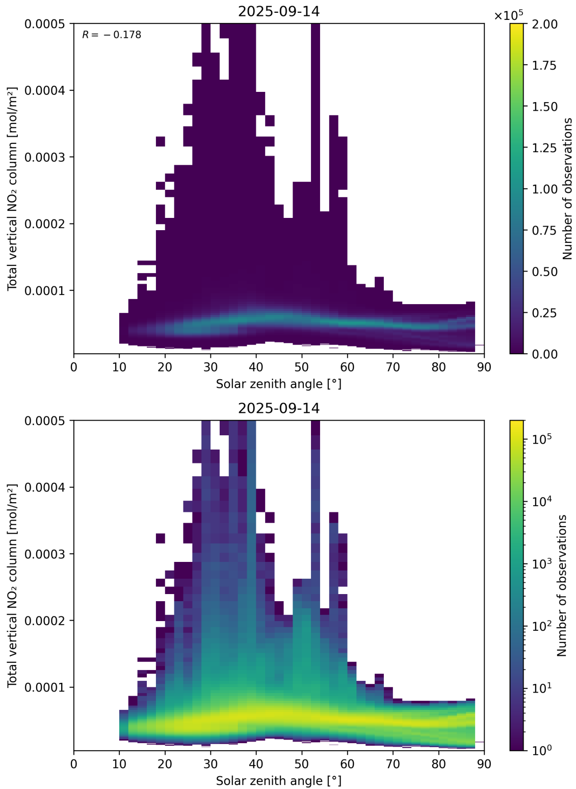
Figure 153: Scatter density plot of “Solar zenith angle” against “Total vertical NO 2 column” for 2025-09-13 to 2025-09-15.
