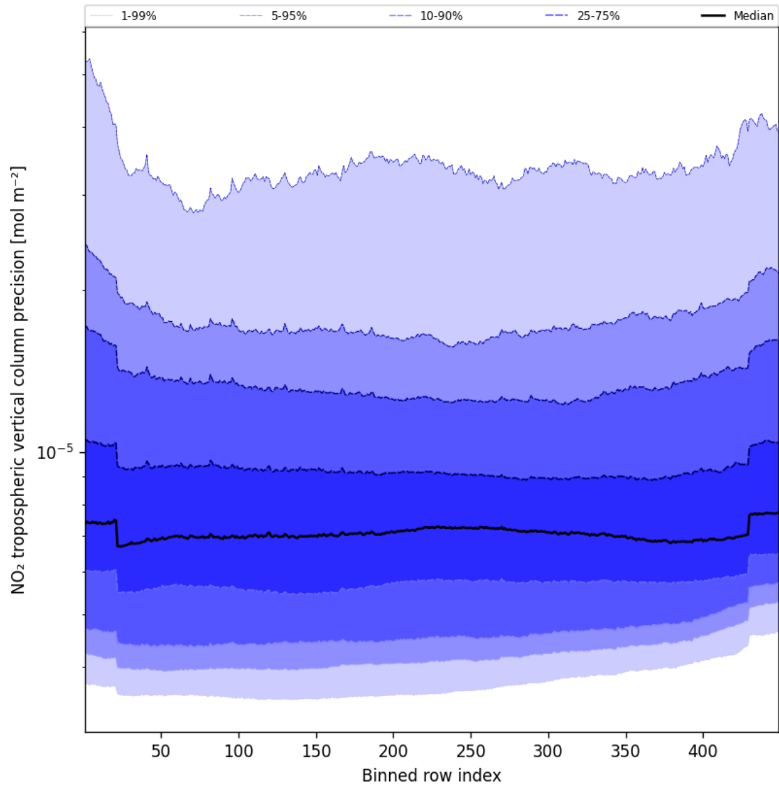
Figure 47: Along track statistics of “NO 2 tropospheric vertical column precision” for 2025-09-13 to 2025-09-15
