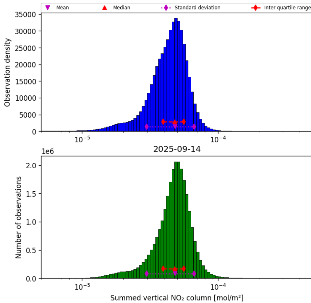
Figure 40: Histogram of “Summed vertical NO 2 column” for 2025-09-13 to 2025-09-15
