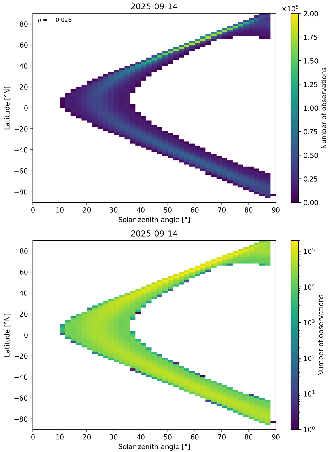
Figure 149: Scatter density plot of “Solar zenith angle” against “Latitude” for 2025-09-13 to 2025-09-15.
