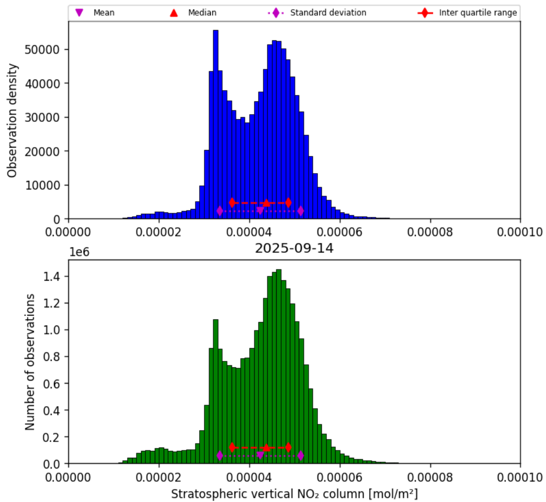
Figure 36: Histogram of “Stratospheric vertical NO 2 column” for 2025-09-13 to 2025-09-15
