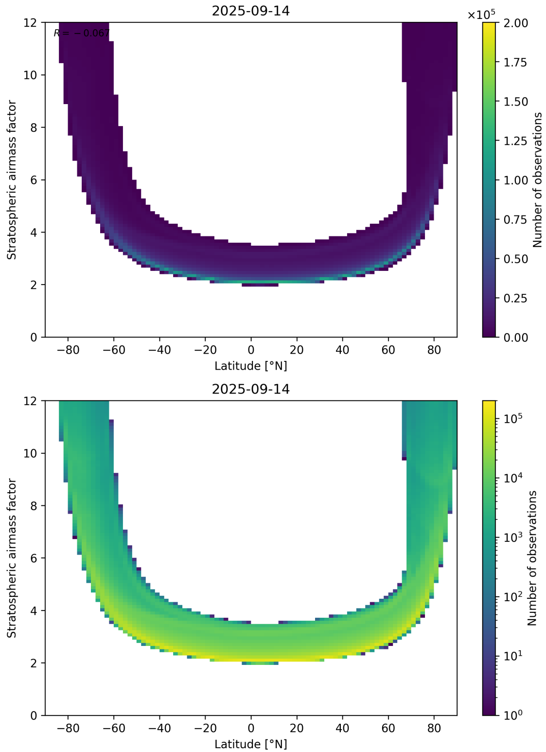
Figure 83: Scatter density plot of “Latitude” against “Stratospheric airmass factor” for 2025-09-13 to 2025-09-15.
