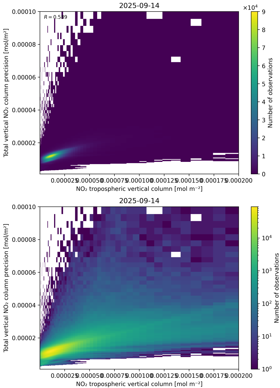
Figure 129: Scatter density plot of “NO 2 tropospheric vertical column” against “Total vertical NO 2 column precision” for 2025-09-13 to 2025-09-15.
