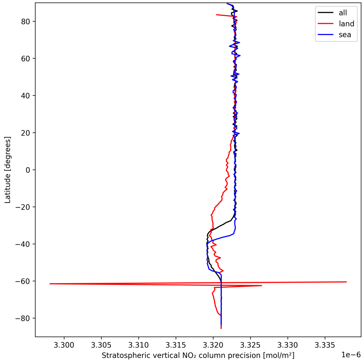
Figure 20: Zonal average of “Stratospheric vertical NO 2 column precision” for 2025-09-13 to 2025-09-15.
