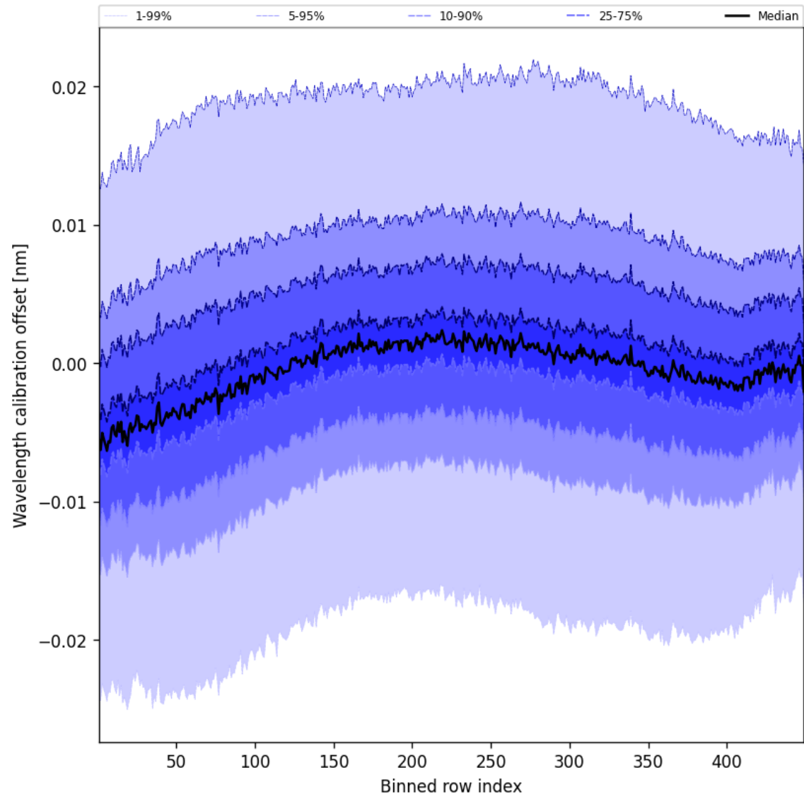
Figure 52: Along track statistics of “Wavelength calibration offset” for 2025-09-13 to 2025-09-15
