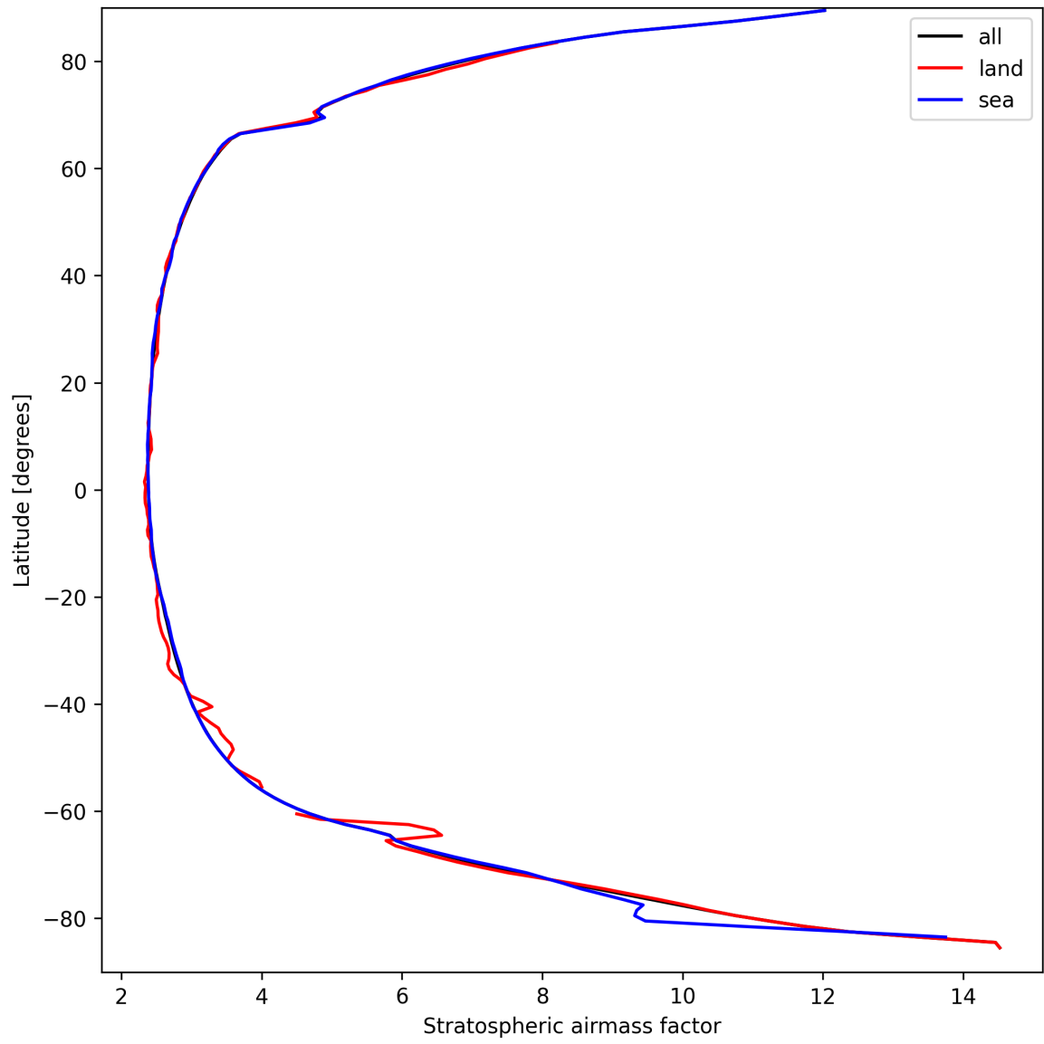
Figure 27: Zonal average of “Stratospheric airmass factor” for 2025-09-13 to 2025-09-15.
