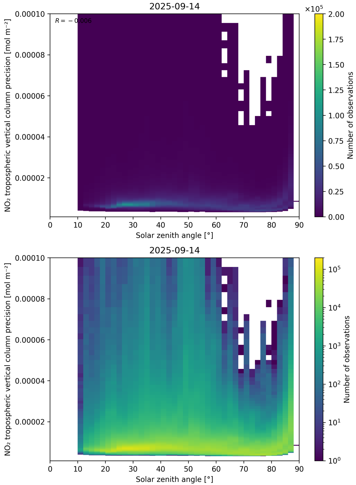
Figure 156: Scatter density plot of “Solar zenith angle” against “NO 2 tropospheric vertical column precision” for 2025-09-13 to 2025-09-15.
