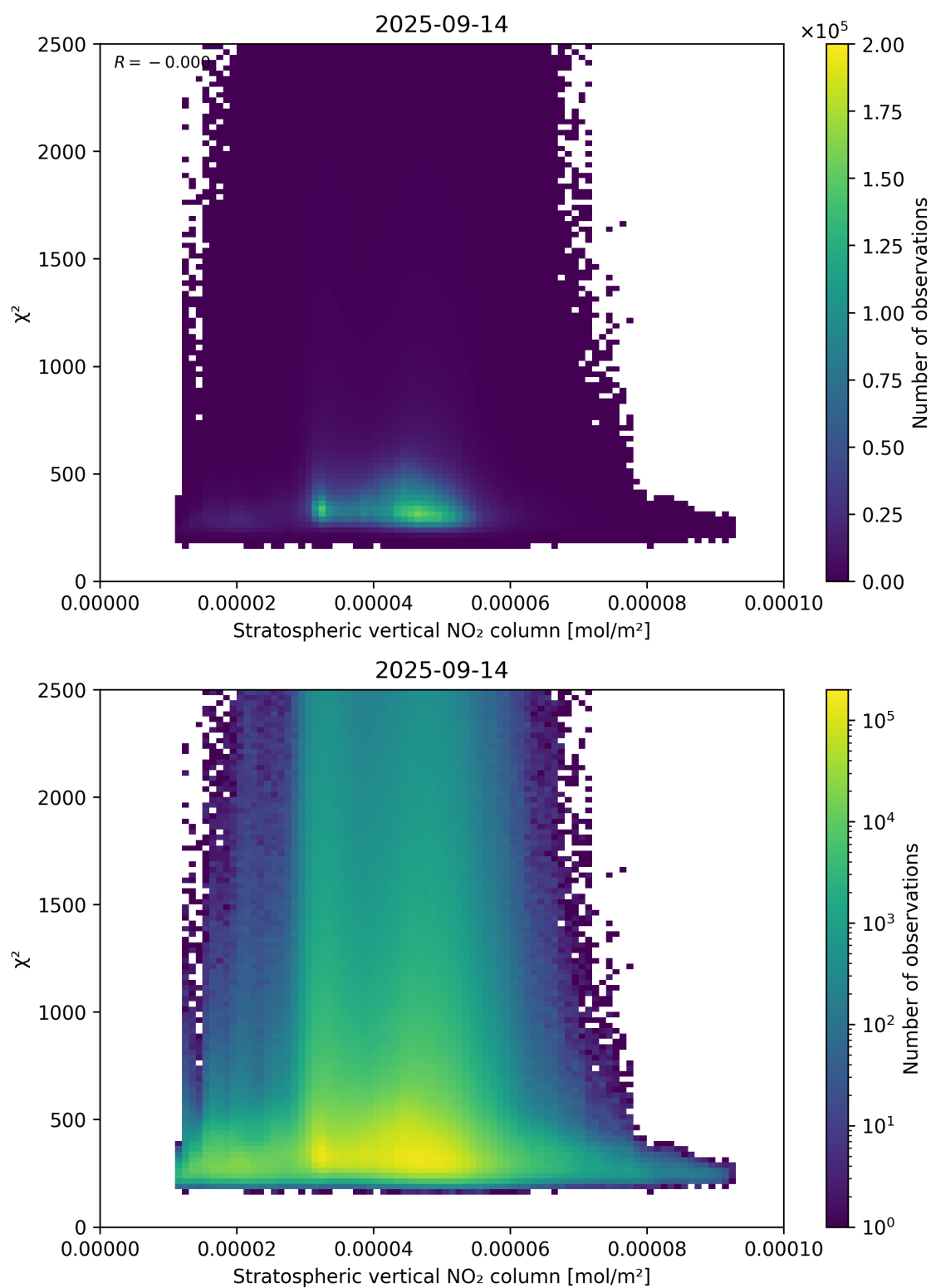
Figure 97: Scatter density plot of “Stratospheric vertical NO 2 column” against “ \chi^2 ” for 2025-09-13 to 2025-09-15.
