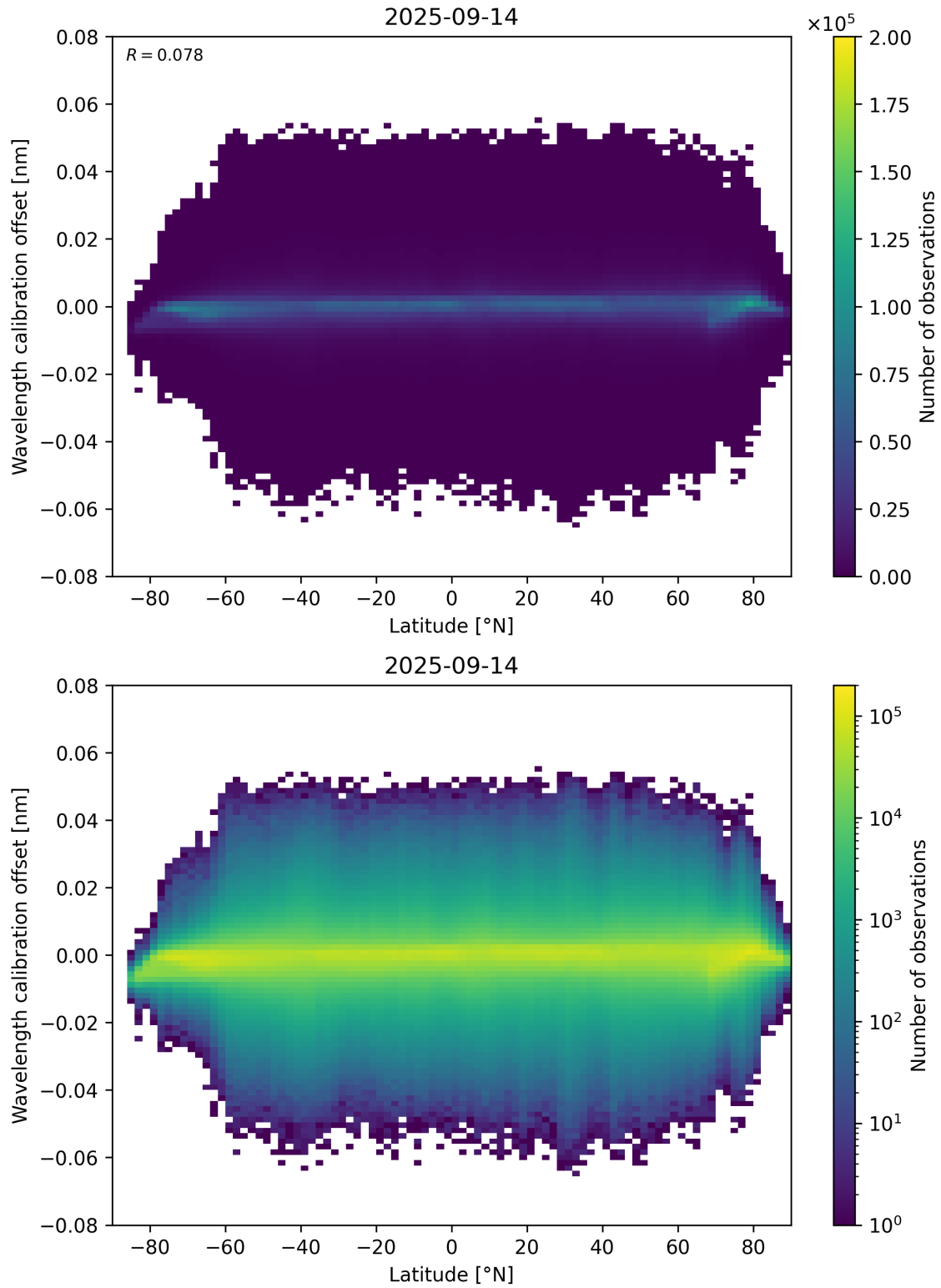
Figure 95: Scatter density plot of “Latitude” against “Wavelength calibration offset” for 2025-09-13 to 2025-09-15.
