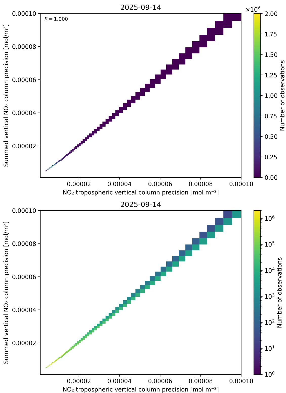
Figure 137: Scatter density plot of “NO 2 tropospheric vertical column precision” against “Summed vertical NO 2 column precision” for 2025-09-13 to 2025-09-15.
