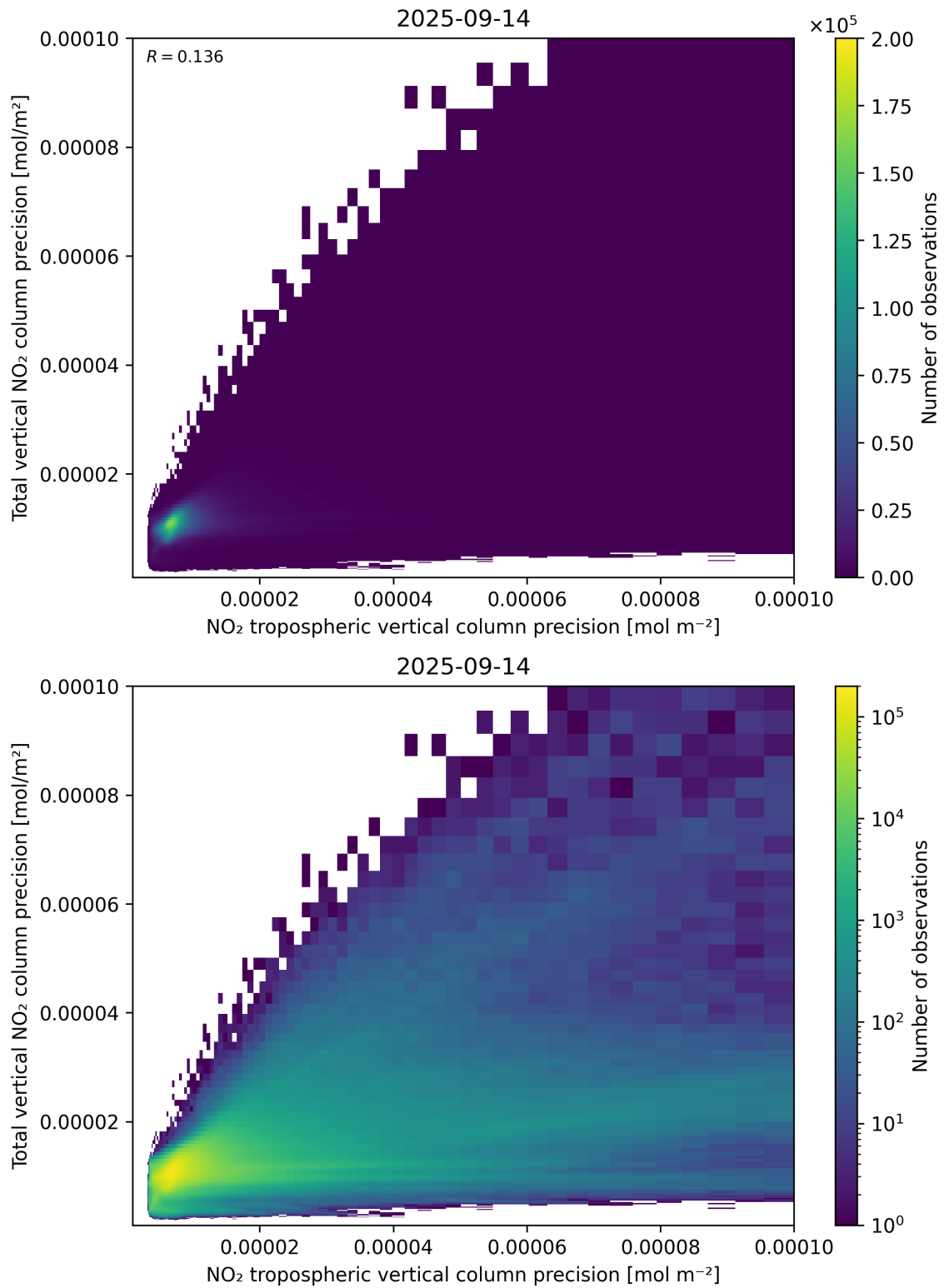
Figure 139: Scatter density plot of “NO 2 tropospheric vertical column precision” against “Total vertical NO 2 column precision” for 2025-09-13 to 2025-09-15.
