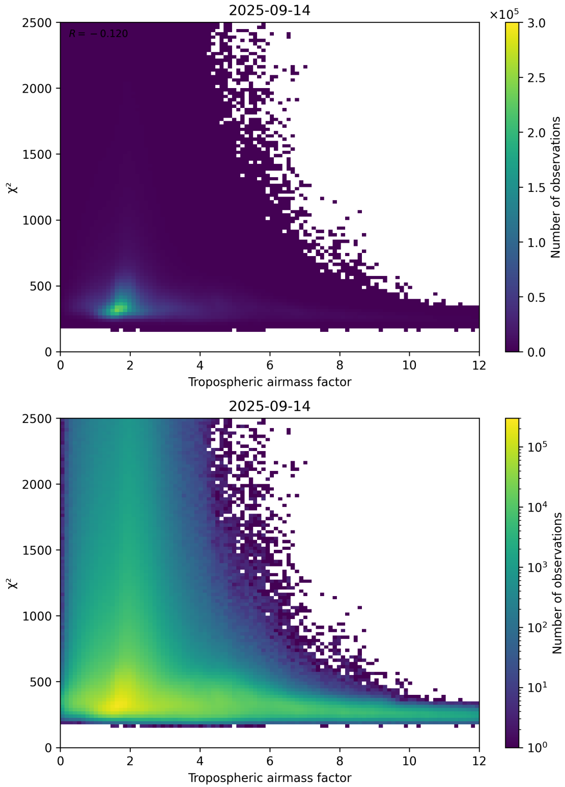
Figure 73: Scatter density plot of “Tropospheric airmass factor” against “ \chi^2 ” for 2025-09-13 to 2025-09-15.
