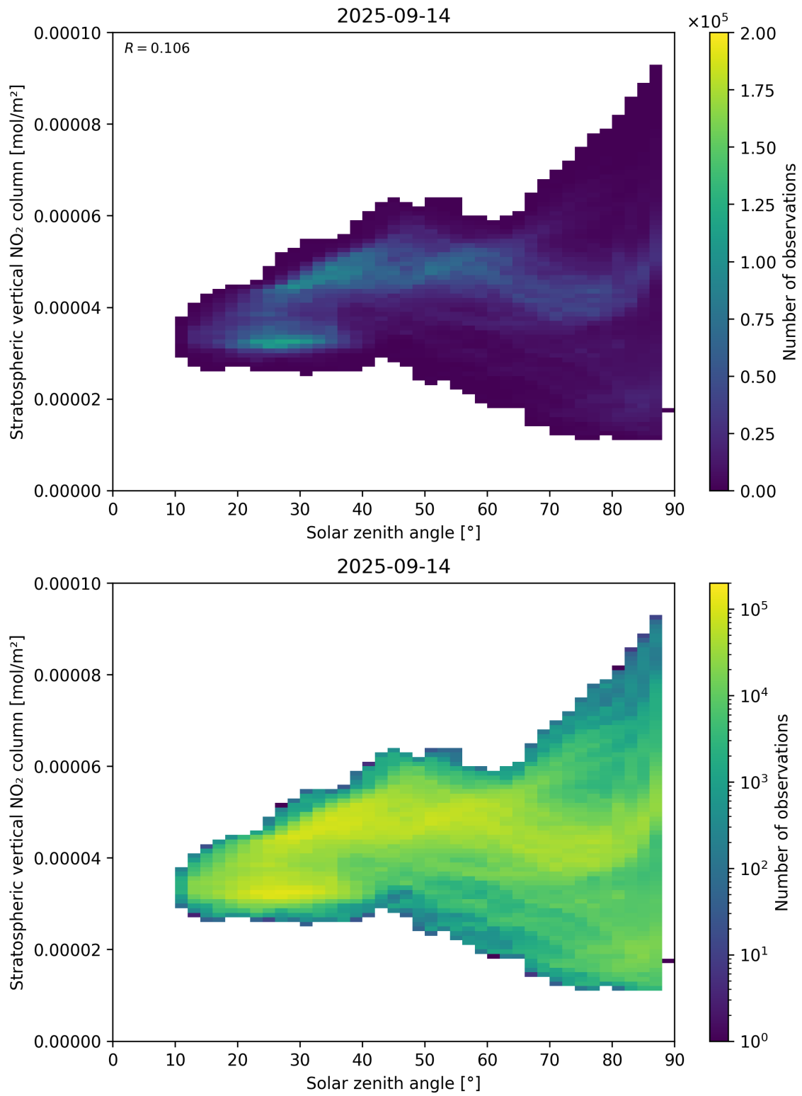
Figure 150: Scatter density plot of “Solar zenith angle” against “Stratospheric vertical NO 2 column” for 2025-09-13 to 2025-09-15.
