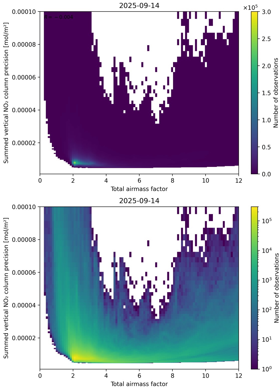
Figure 66: Scatter density plot of “Total airmass factor” against “Summed vertical NO 2 column precision” for 2025-09-13 to 2025-09-15.
