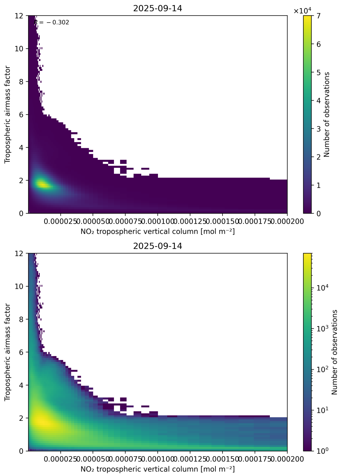
Figure 123: Scatter density plot of “NO 2 tropospheric vertical column” against “Tropospheric air mass factor” for 2025-09-13 to 2025-09-15.
