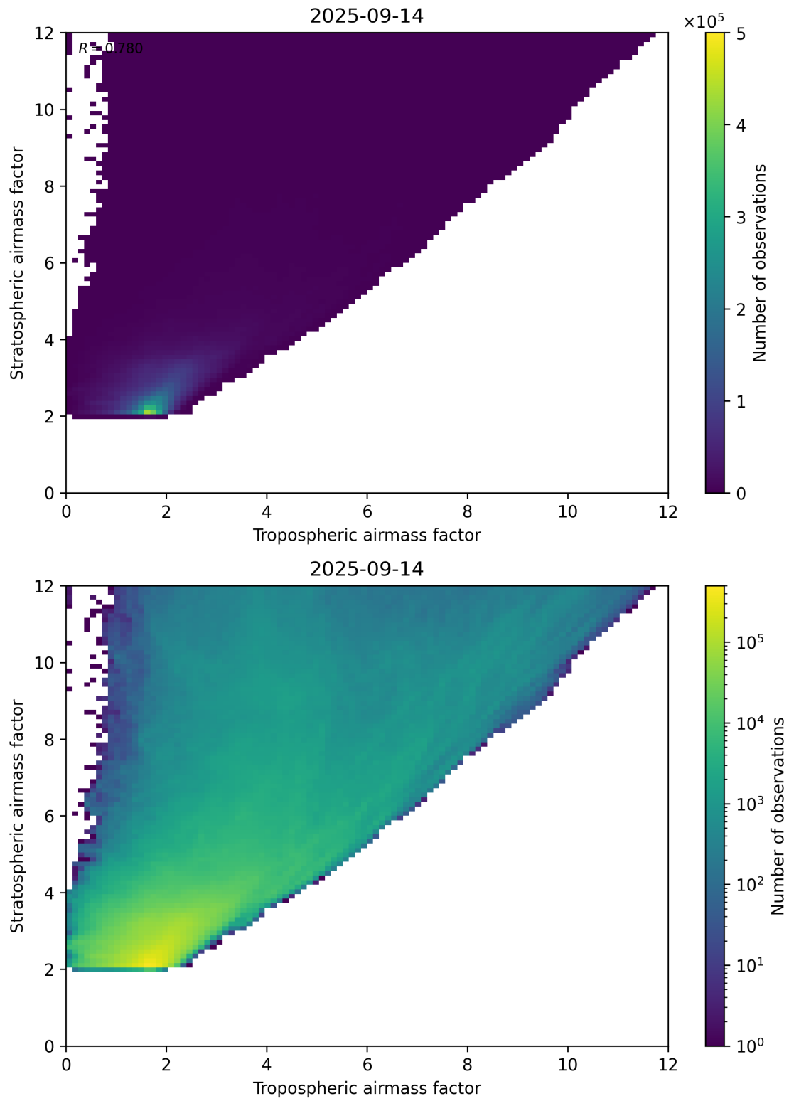
Figure 71: Scatter density plot of “Tropospheric airmass factor” against “Stratospheric airmass factor” for 2025-09-13 to 2025-09-15.
