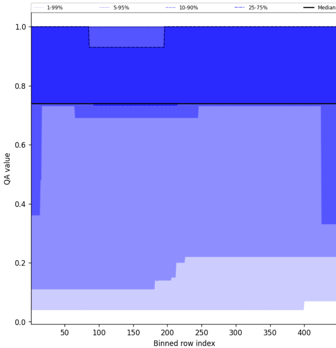
Figure 45: Along track statistics of “QA value” for 2025-09-13 to 2025-09-15
