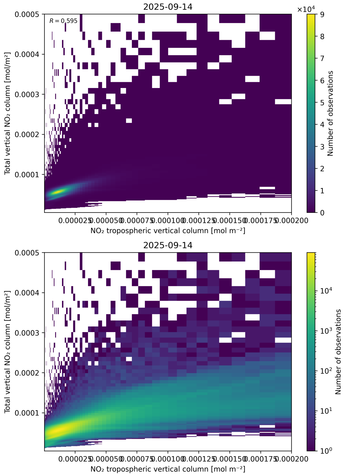
Figure 128: Scatter density plot of “NO 2 tropospheric vertical column” against “Total vertical NO 2 column” for 2025-09-13 to 2025-09-15.
