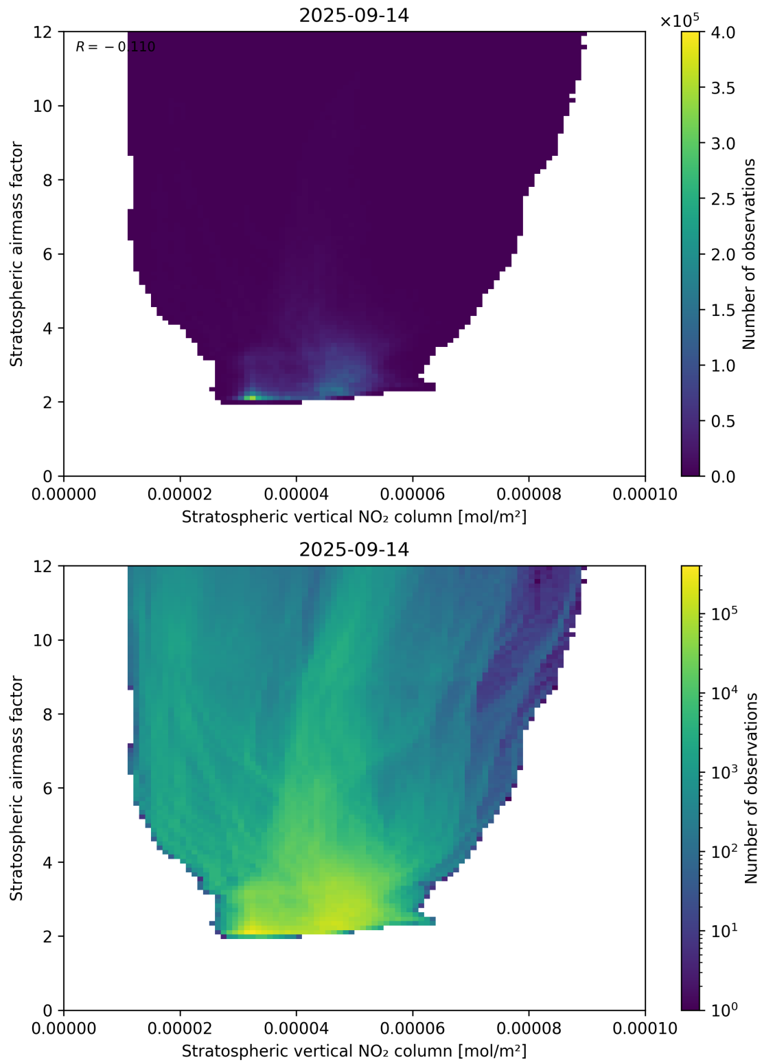
Figure 96: Scatter density plot of “Stratospheric vertical NO 2 column” against “Stratospheric airmass factor” for 2025-09-13 to 2025-09-15.
