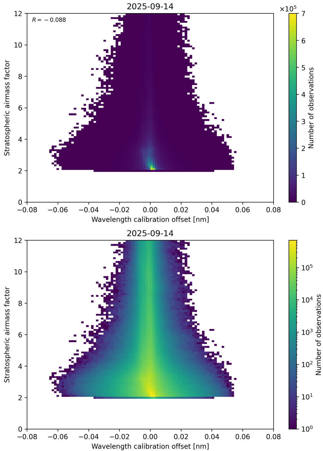
Figure 174: Scatter density plot of “Wavelength calibration offset” against “Stratospheric airmass factor” for 2025-09-13 to 2025-09-15.
