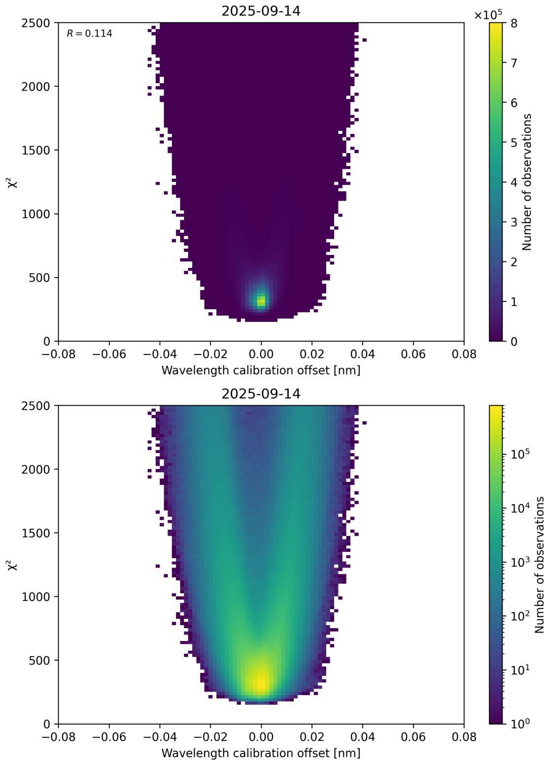
Figure 175: Scatter density plot of “Wavelength calibration offset” against “ \chi^2 ” for 2025-09-13 to 2025-09-15.
