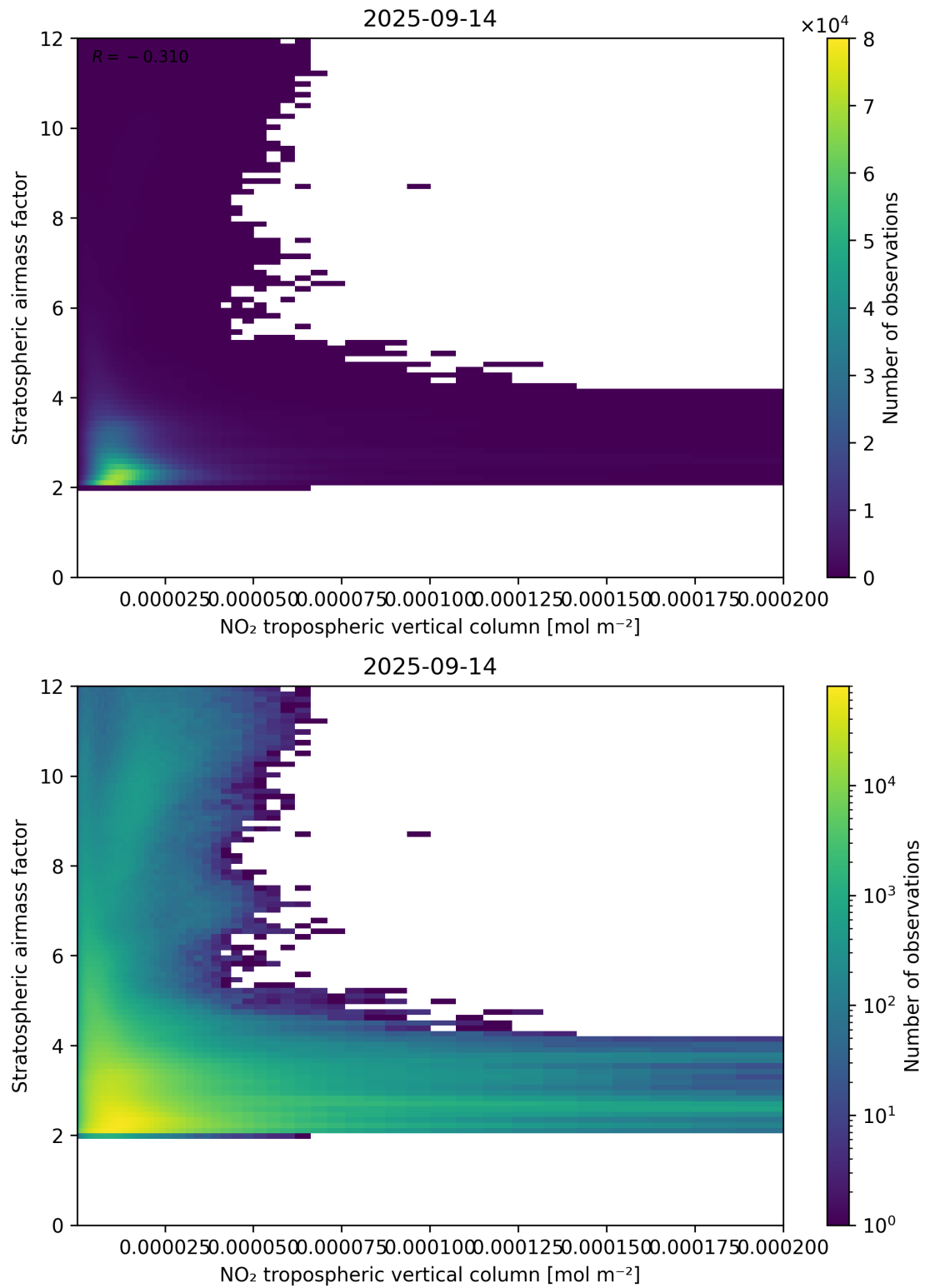
Figure 121: Scatter density plot of “NO 2 tropospheric vertical column” against “Stratospheric air mass factor” for 2025-09-13 to 2025-09-15.
