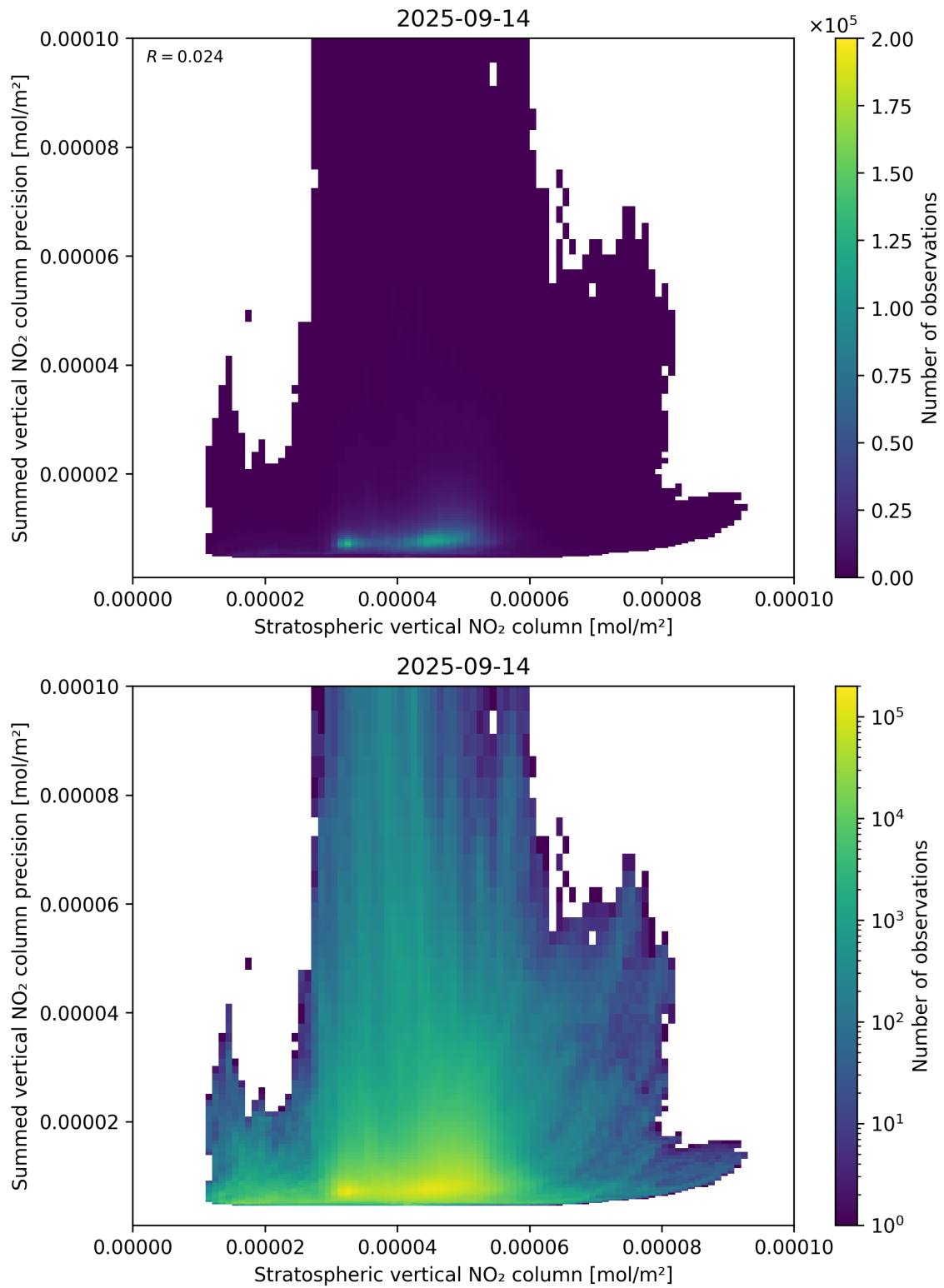
Figure 99: Scatter density plot of “Stratospheric vertical NO 2 column” against “Summed vertical NO 2 column precision” for 2025-09-13 to 2025-09-15.
