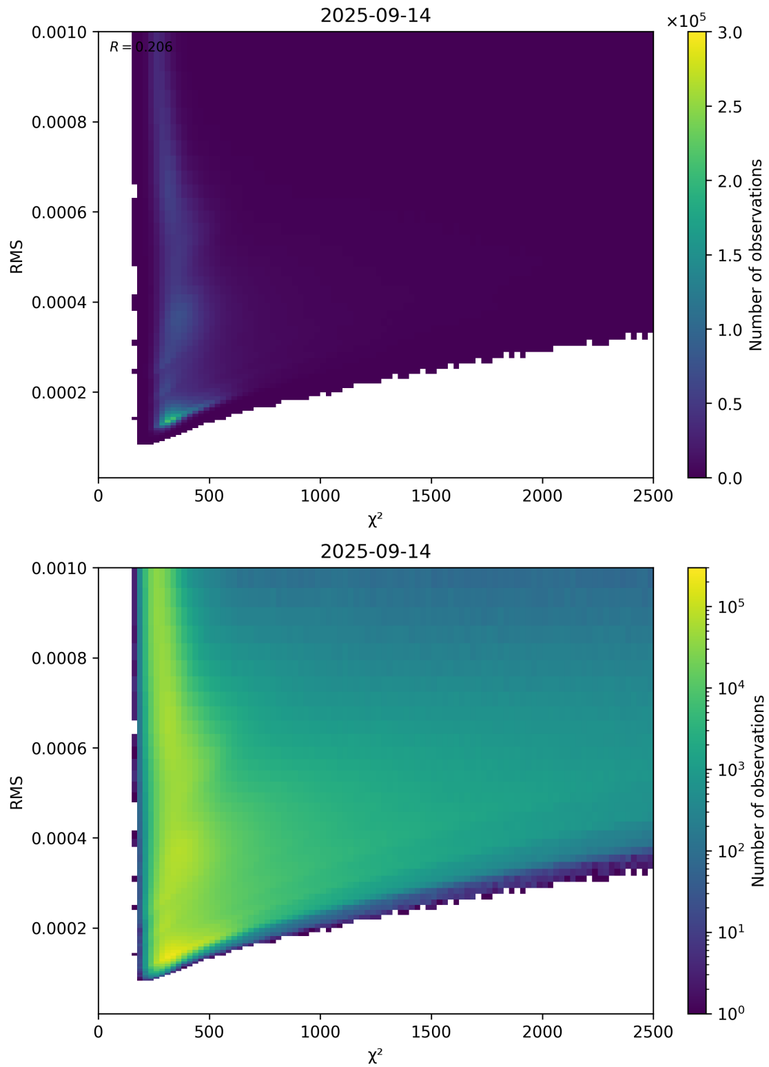
Figure 82: Scatter density plot of “ \chi^2 ” against “RMS” for 2025-09-13 to 2025-09-15.
