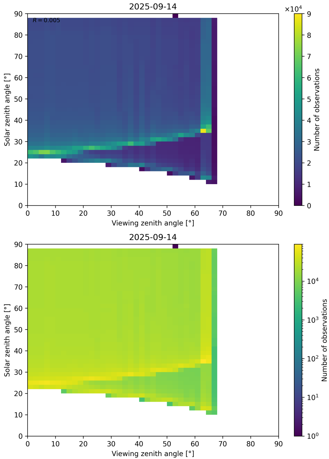
Figure 172: Scatter density plot of “Viewing zenith angle” against “Solar zenith angle” for 2025-09-13 to 2025-09-15.
