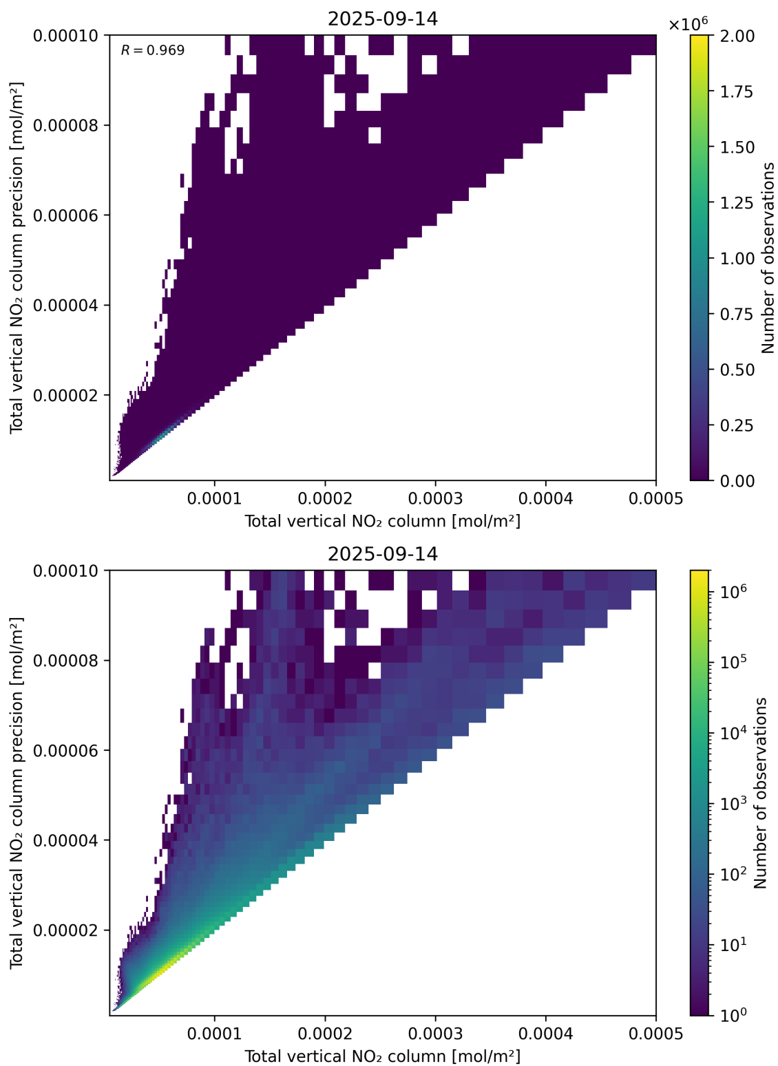
Figure 114: Scatter density plot of “Total vertical NO 2 column” against “Total vertical NO 2 column precision” for 2025-09-13 to 2025-09-15.
