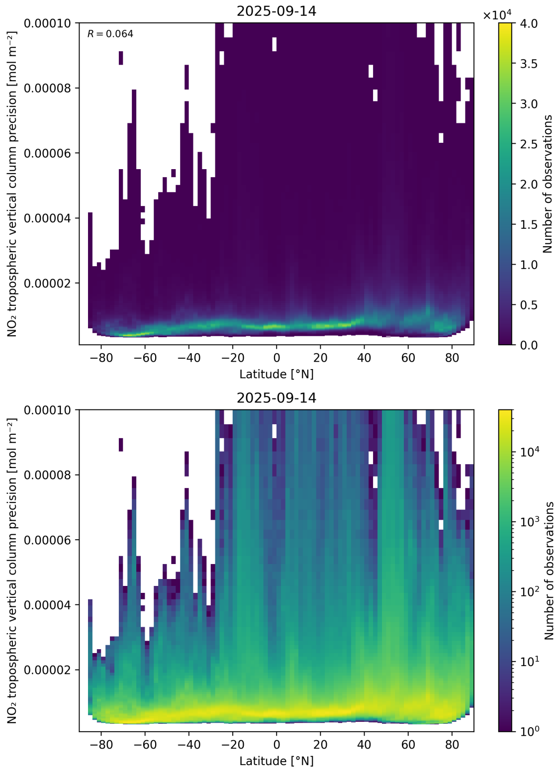
Figure 93: Scatter density plot of “Latitude” against “NO 2 tropospheric vertical column precision” for 2025-09-13 to 2025-09-15.
