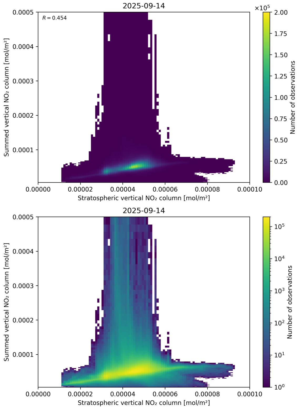
Figure 98: Scatter density plot of “Stratospheric vertical NO 2 column” against “Summed vertical NO 2 column” for 2025-09-13 to 2025-09-15.
