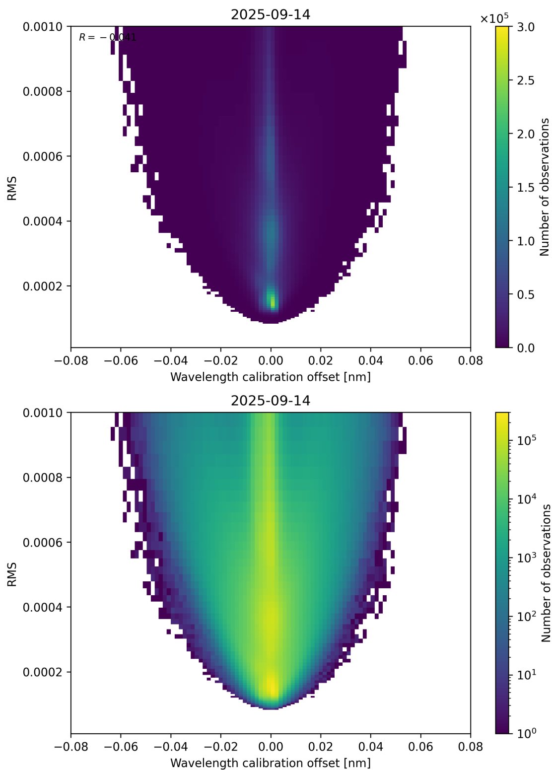
Figure 181: Scatter density plot of “Wavelength calibration offset” against “RMS” for 2025-09-13 to 2025-09-15.
