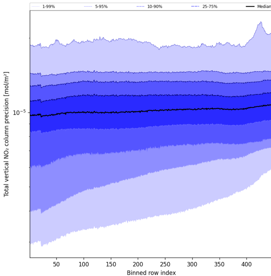
Figure 56: Along track statistics of “Total vertical NO 2 column precision” for 2025-09-13 to 2025-09-15
