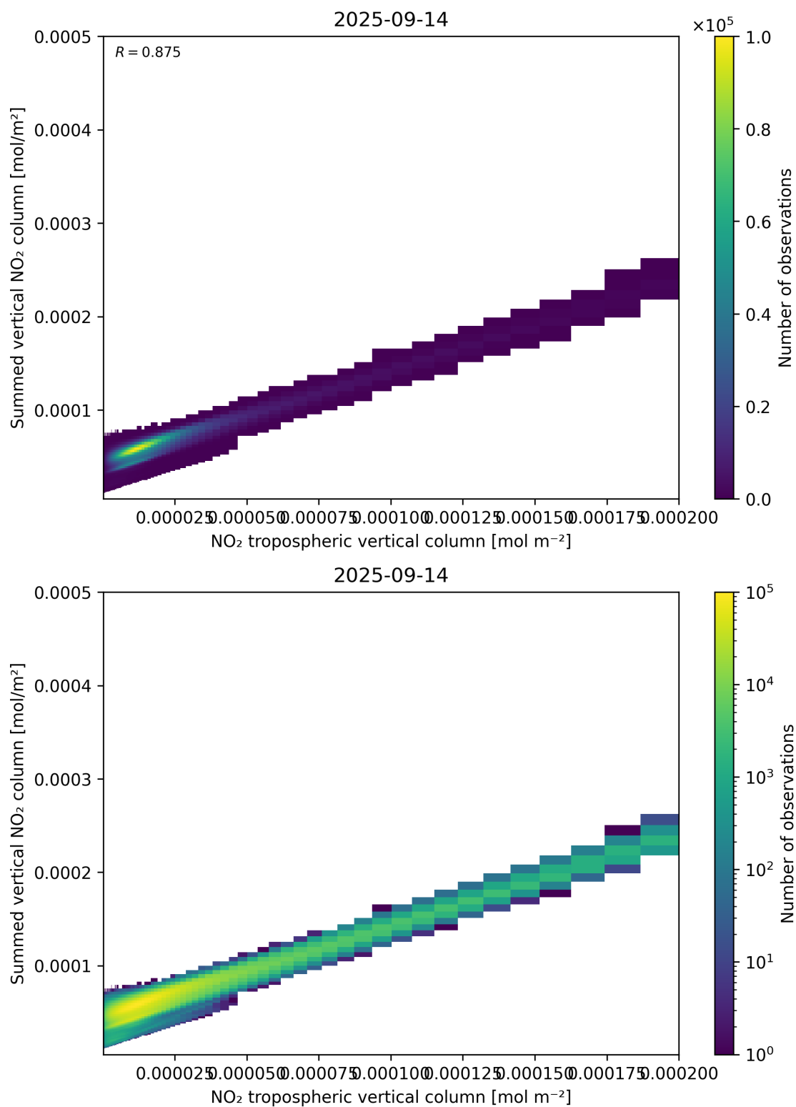
Figure 126: Scatter density plot of “NO 2 tropospheric vertical column” against “Summed vertical NO 2 column” for 2025-09-13 to 2025-09-15.
