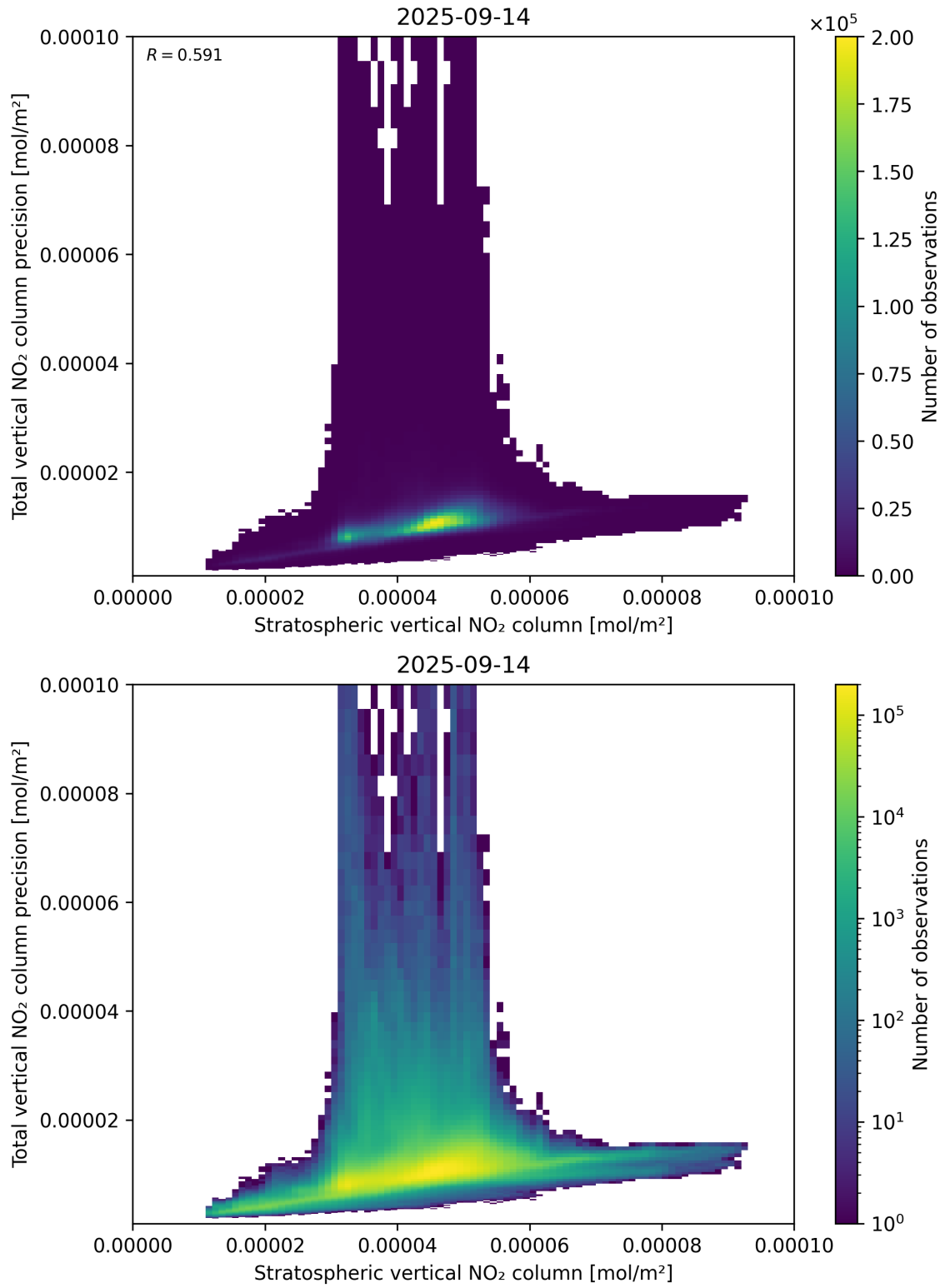
Figure 101: Scatter density plot of “Stratospheric vertical NO 2 column” against “Total vertical NO 2 column precision” for 2025-09-13 to 2025-09-15.
