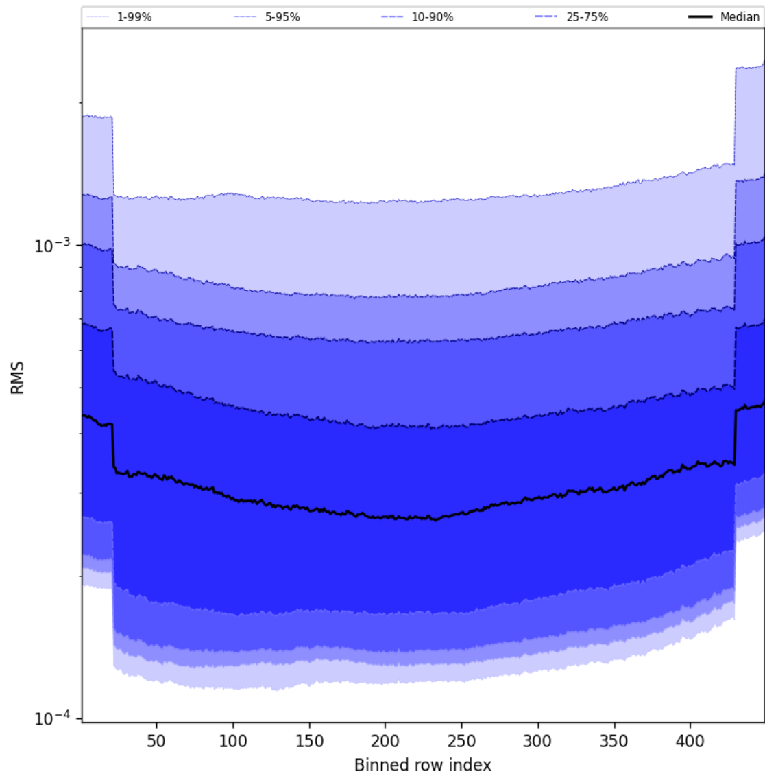
Figure 60: Along track statistics of “RMS” for 2025-09-13 to 2025-09-15
