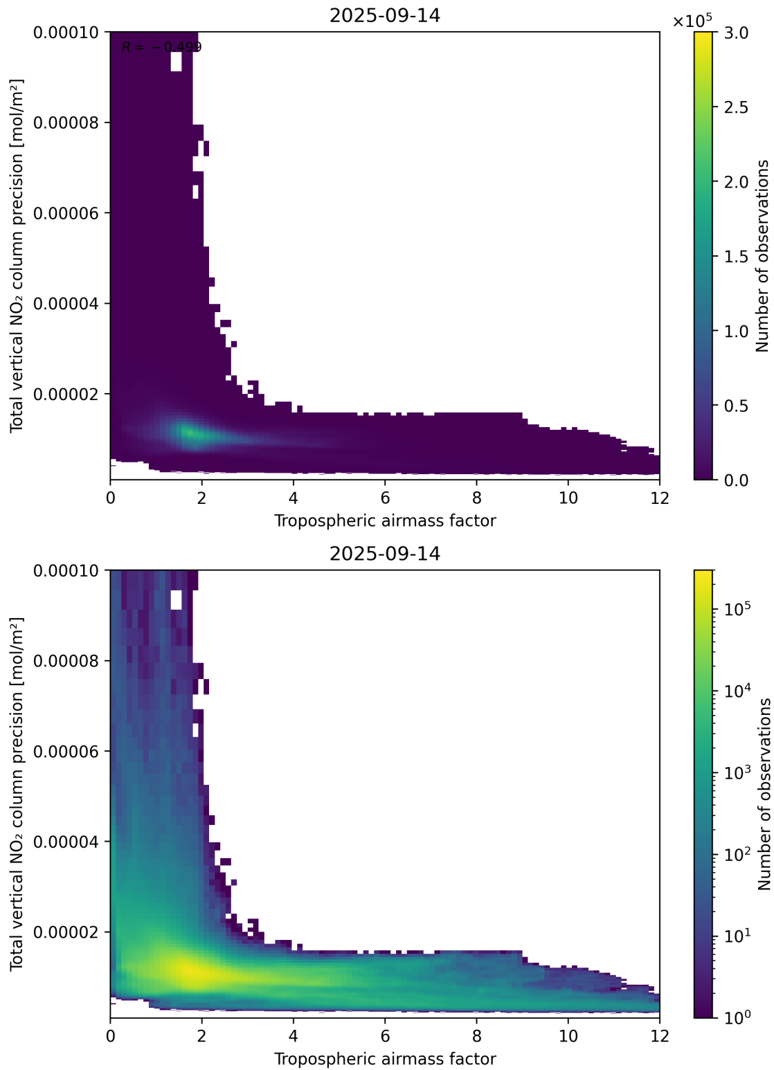
Figure 78: Scatter density plot of “Tropospheric air mass factor” against “Total vertical NO 2 column precision” for 2025-09-13 to 2025-09-15.
