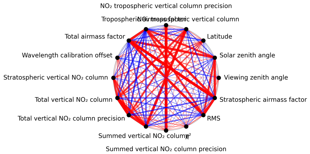
Figure 1: Map of correlation graph for 2025-09-13 to 2025-09-15.
