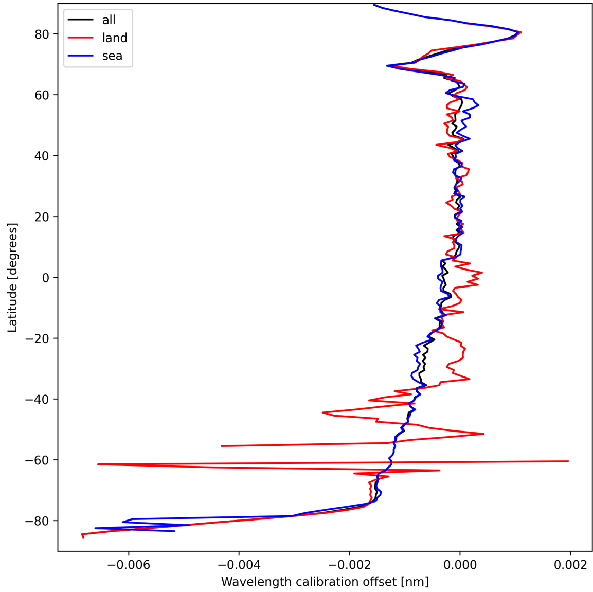
Figure 18: Zonal average of “Wavelength calibration offset” for 2025-09-13 to 2025-09-15.
