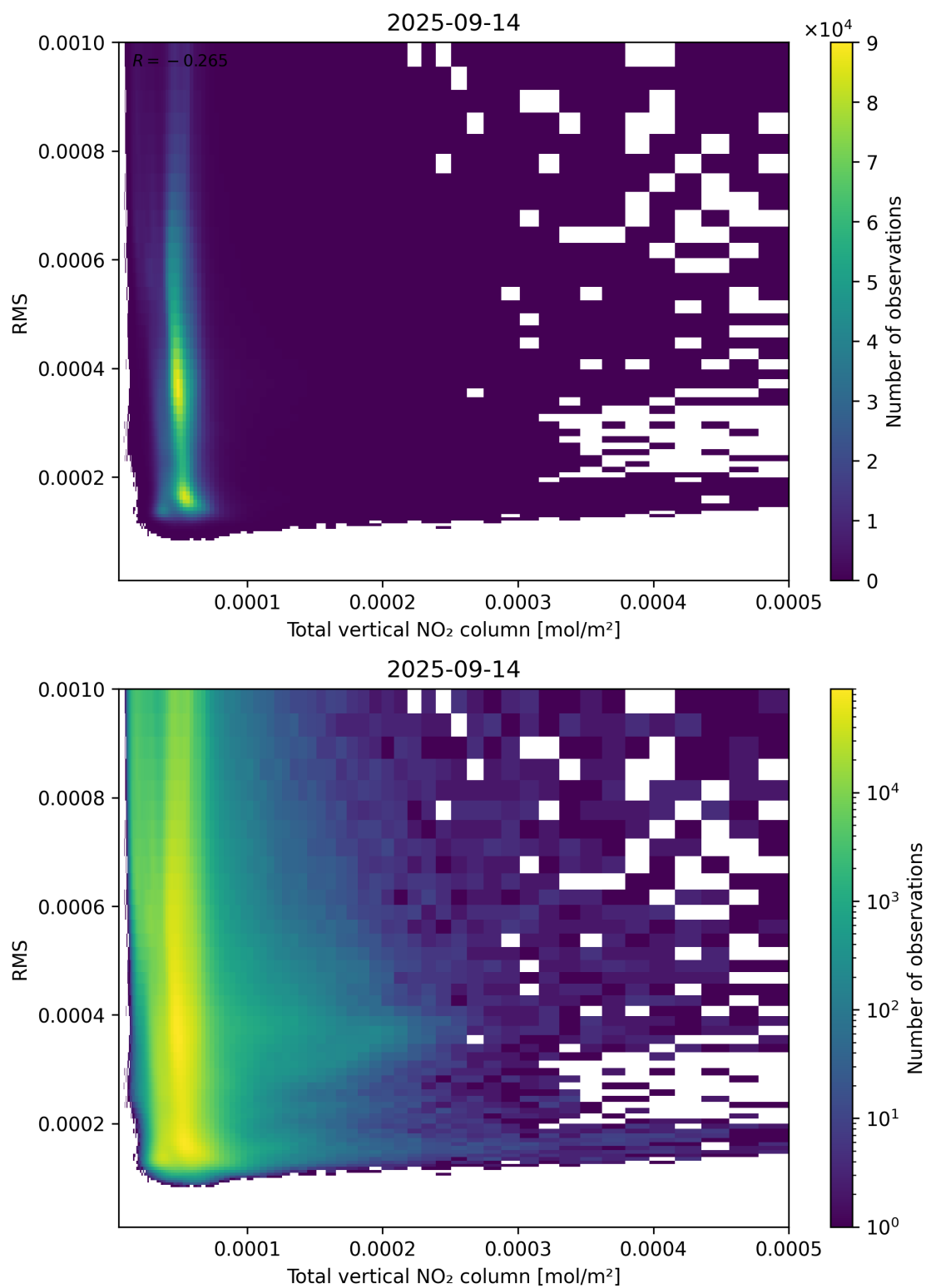
Figure 120: Scatter density plot of “Total vertical NO 2 column” against “RMS” for 2025-09-13 to 2025-09-15.
