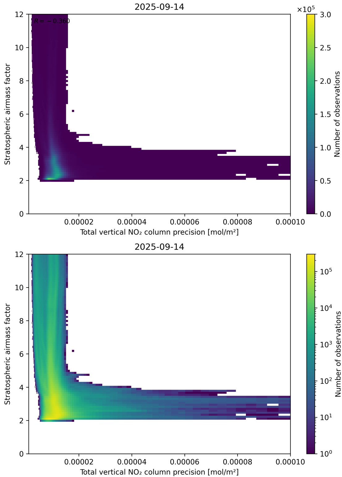
Figure 115: Scatter density plot of “Total vertical NO 2 column precision” against “Stratospheric air mass factor” for 2025-09-13 to 2025-09-15.
