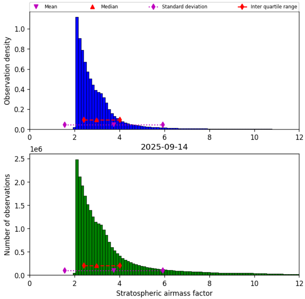
Figure 44: Histogram of “Stratospheric airmass factor” for 2025-09-13 to 2025-09-15
