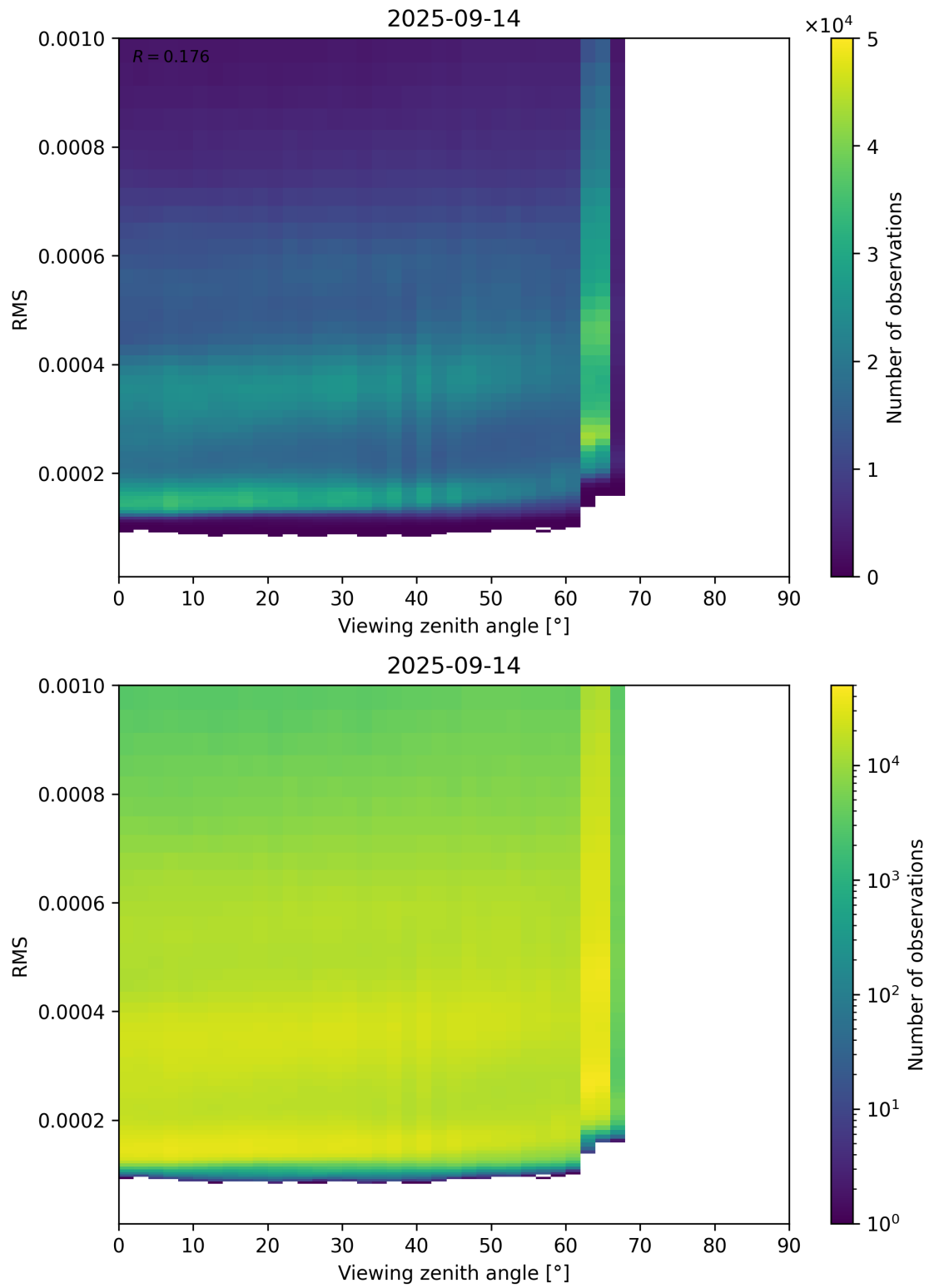
Figure 171: Scatter density plot of “Viewing zenith angle” against “RMS” for 2025-09-13 to 2025-09-15.
