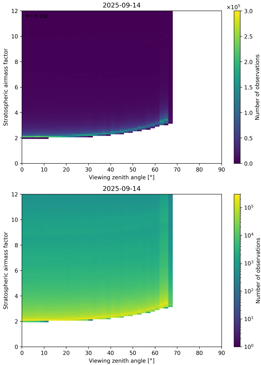
Figure 159: Scatter density plot of “Viewing zenith angle” against “Stratospheric airmass factor” for 2025-09-13 to 2025-09-15.
