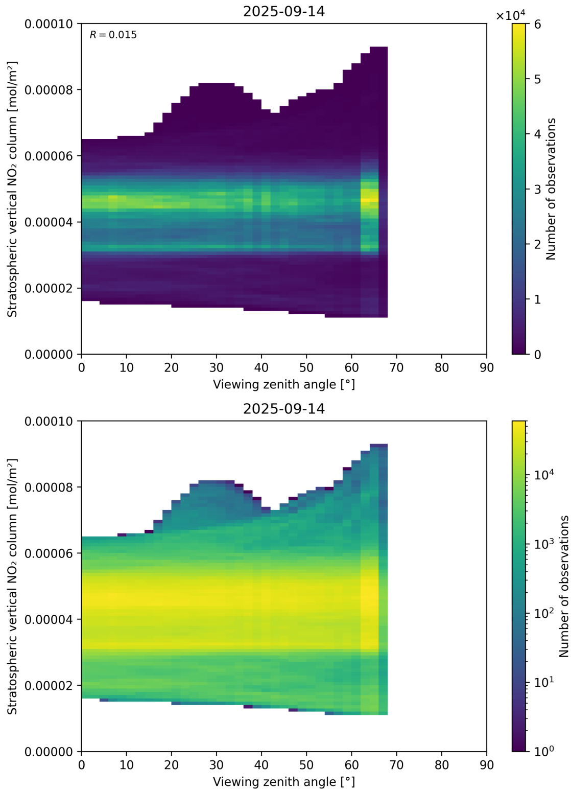
Figure 164: Scatter density plot of “Viewing zenith angle” against “Stratospheric vertical NO 2 column” for 2025-09-13 to 2025-09-15.
