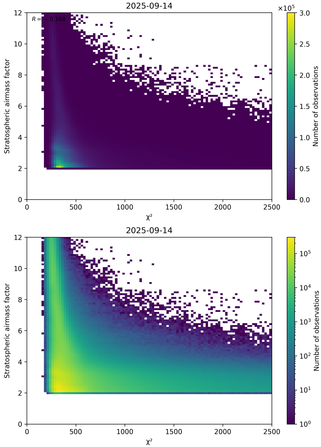
Figure 81: Scatter density plot of “ \chi^2 ” against “Stratospheric airmass factor” for 2025-09-13 to 2025-09-15.
