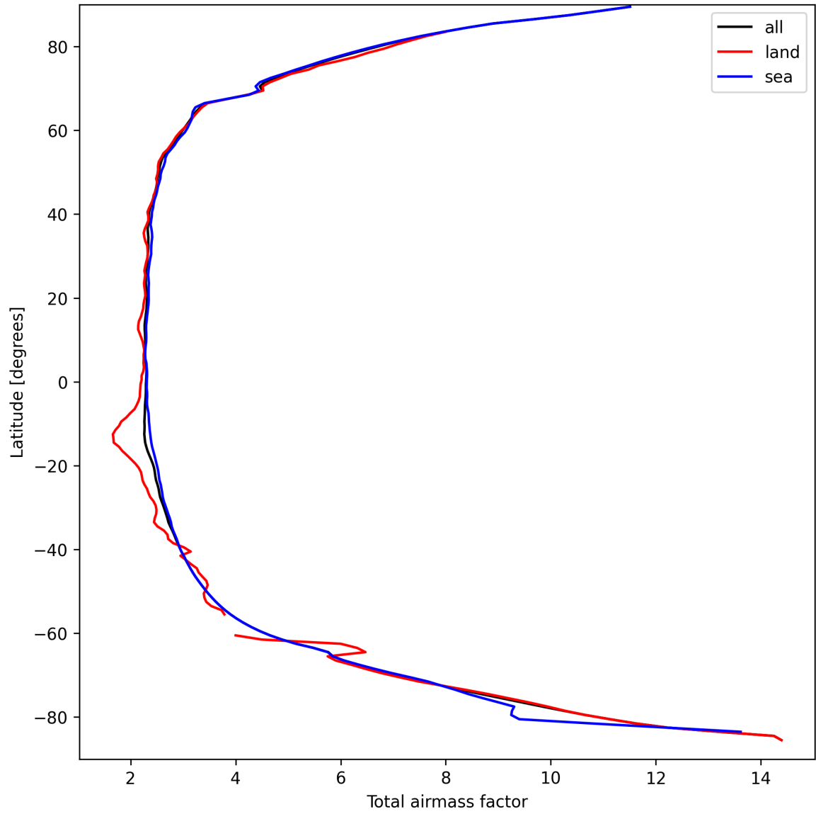
Figure 15: Zonal average of “Total airmass factor” for 2025-09-13 to 2025-09-15.
