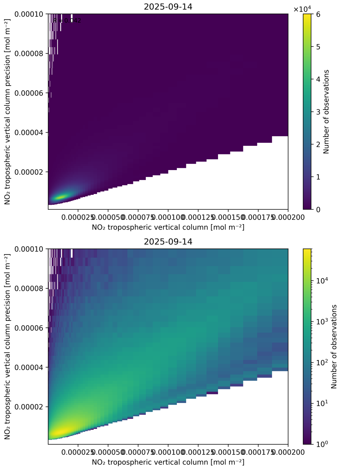
Figure 130: Scatter density plot of “NO 2 tropospheric vertical column” against “NO 2 tropospheric vertical column precision” for 2025-09-13 to 2025-09-15.
