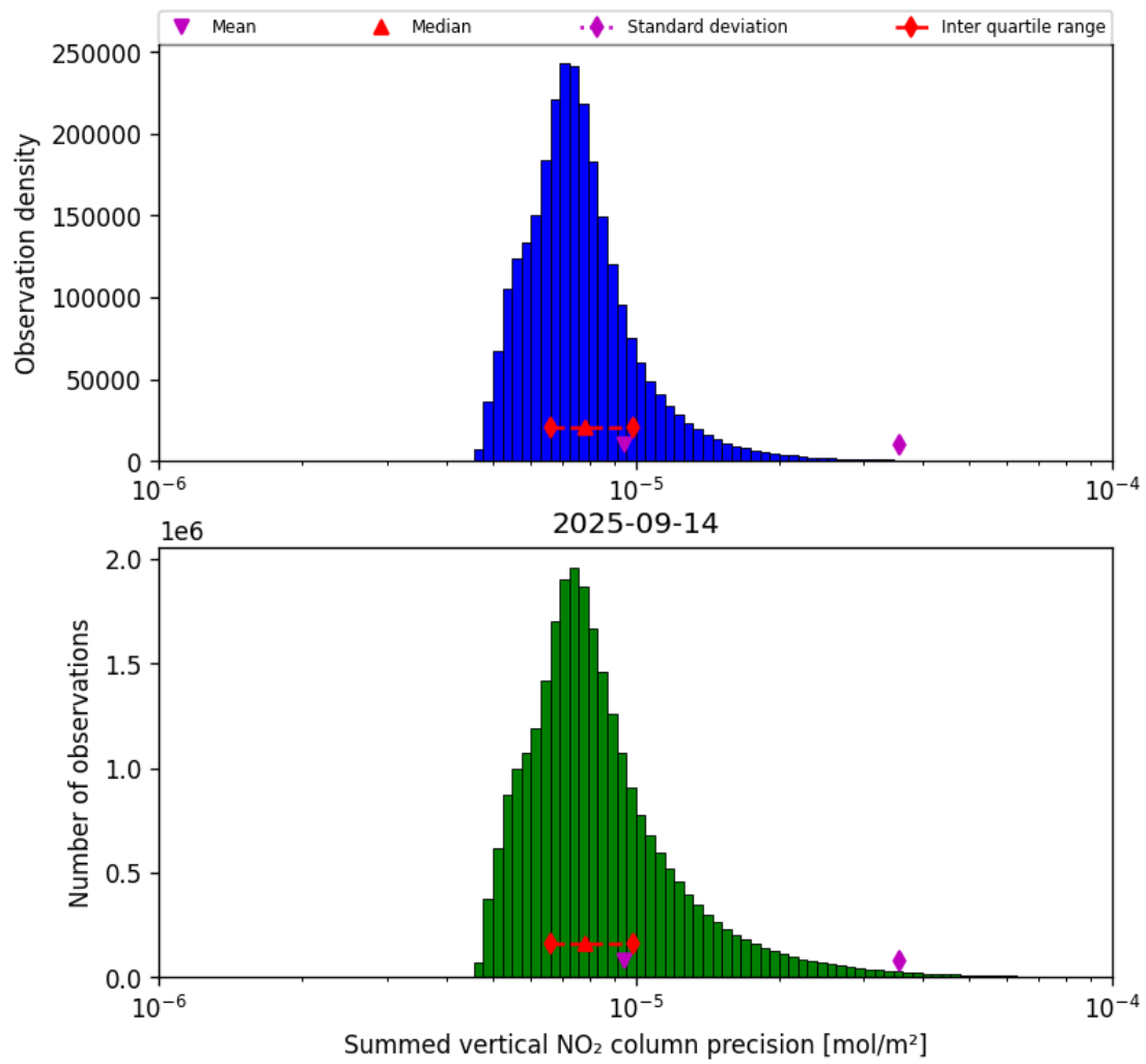
Figure 41: Histogram of "Summed vertical NO 2 column precision" for 2025-09-13 to 2025-09-15
