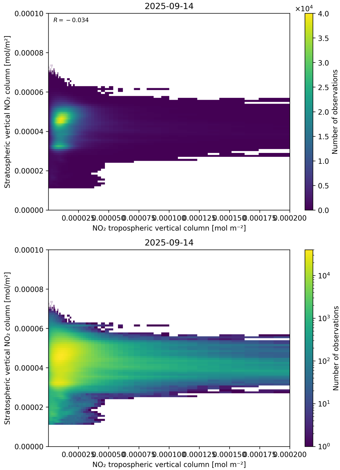
Figure 125: Scatter density plot of “NO 2 tropospheric vertical column” against “Stratospheric vertical NO 2 column” for 2025-09-13 to 2025-09-15.
