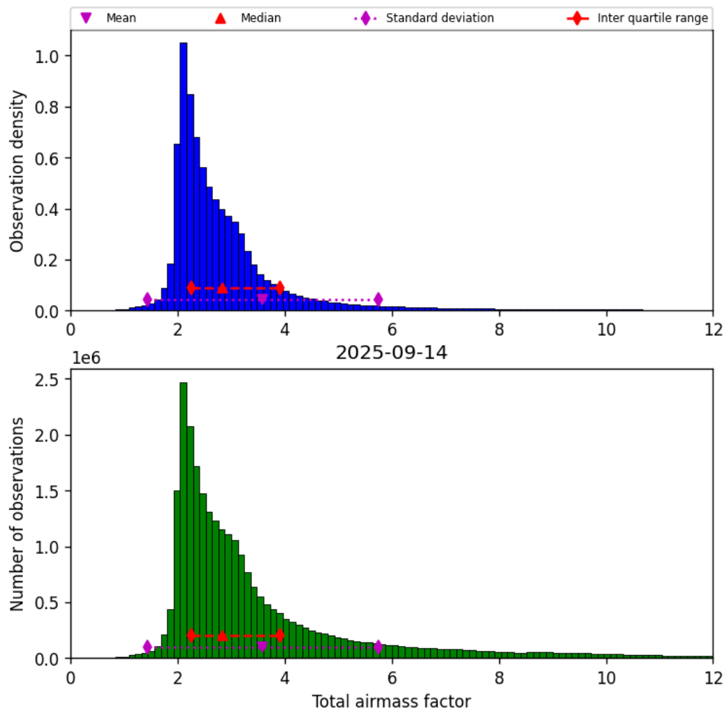
Figure 32: Histogram of “Total airmass factor” for 2025-09-13 to 2025-09-15
