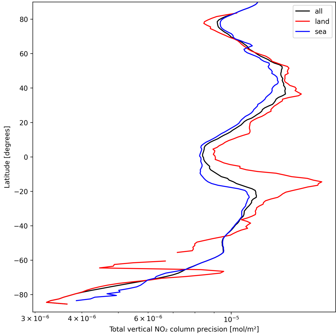
Figure 22: Zonal average of “Total vertical NO 2 column precision” for 2025-09-13 to 2025-09-15.
