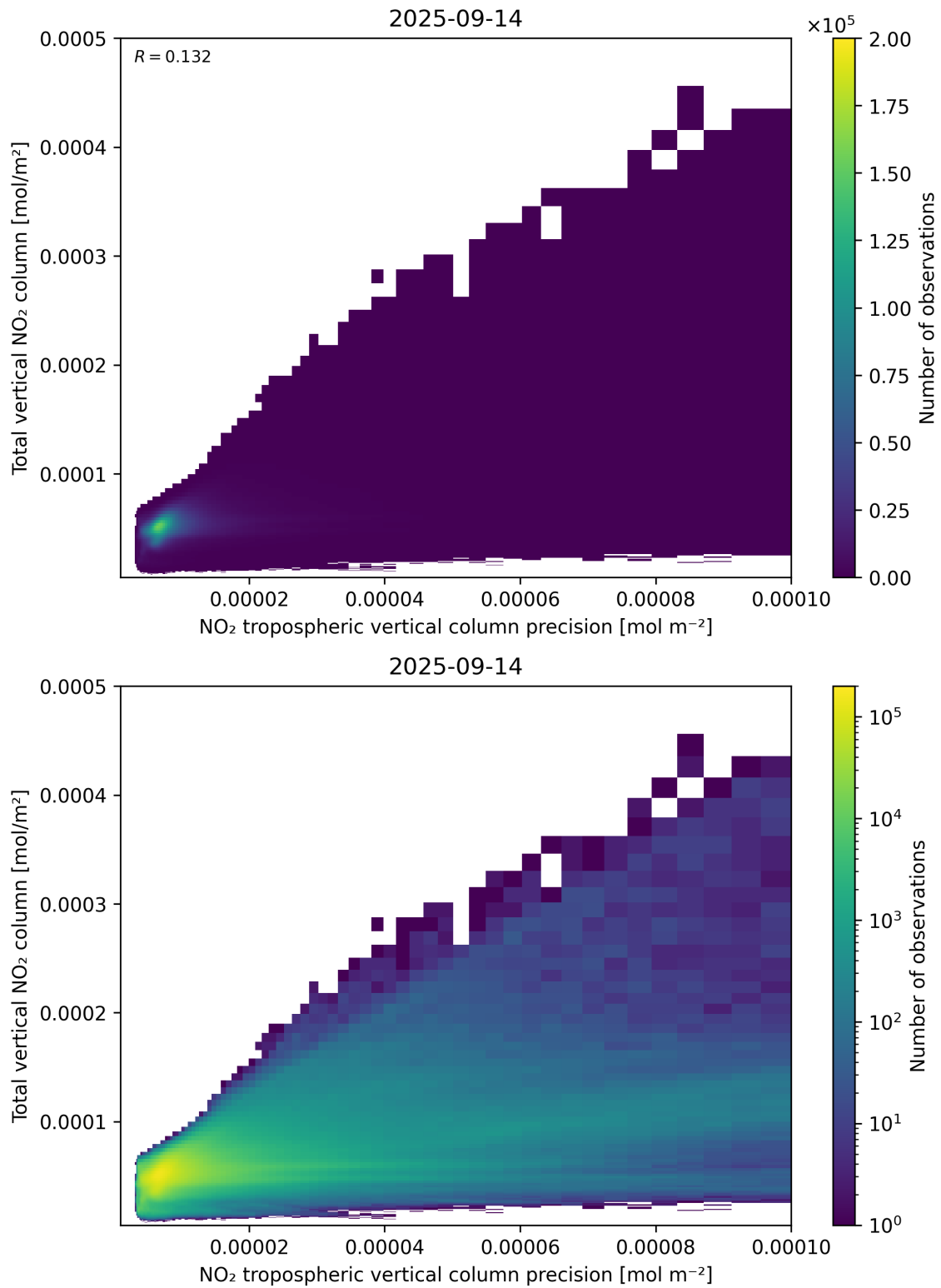
Figure 138: Scatter density plot of “NO 2 tropospheric vertical column precision” against “Total vertical NO 2 column” for 2025-09-13 to 2025-09-15.
