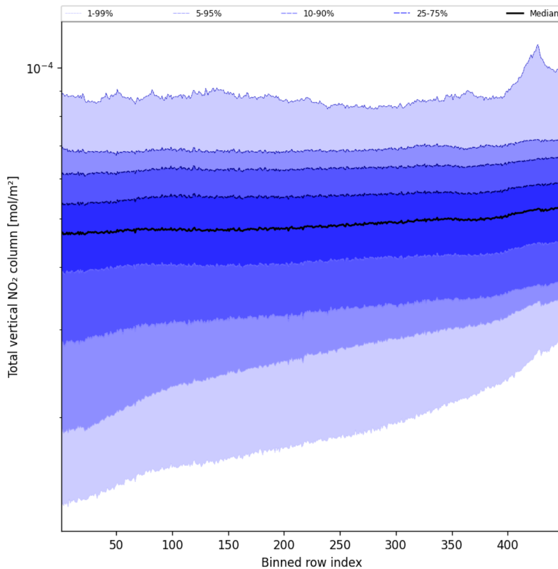
Figure 55: Along track statistics of “Total vertical NO 2 column” for 2025-09-13 to 2025-09-15
