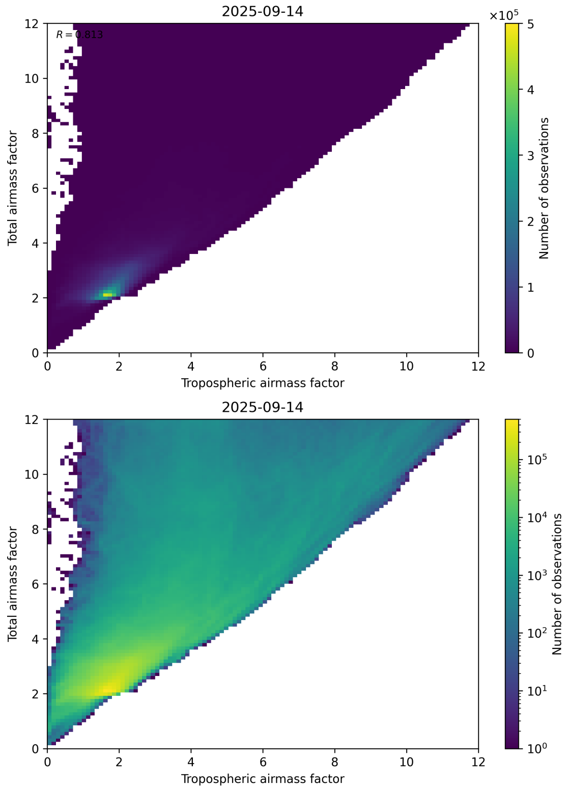
Figure 72: Scatter density plot of “Tropospheric airmass factor” against “Total airmass factor” for 2025-09-13 to 2025-09-15.
