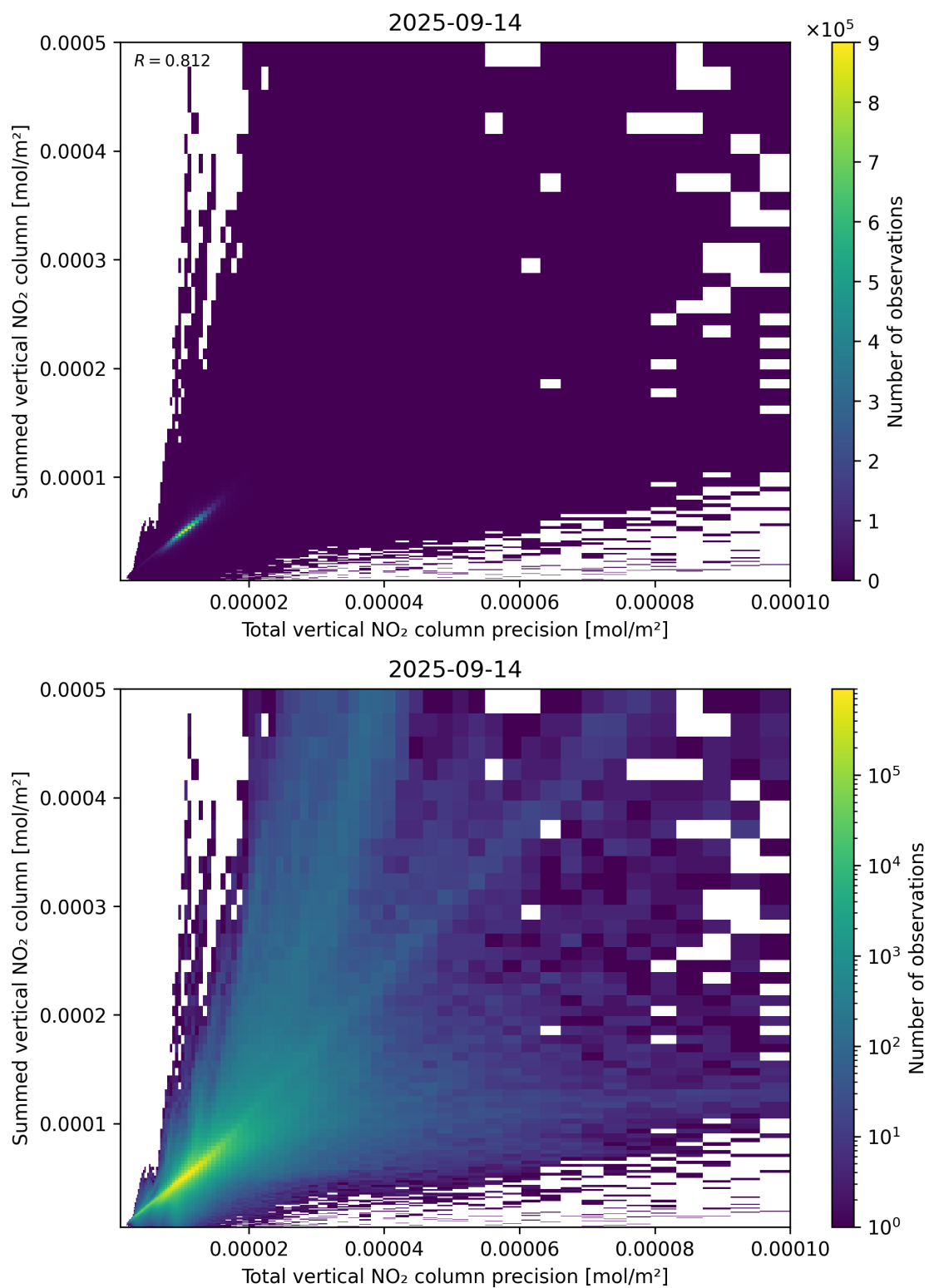
Figure 117: Scatter density plot of “Total vertical NO 2 column precision” against “Summed vertical NO 2 column” for 2025-09-13 to 2025-09-15.
