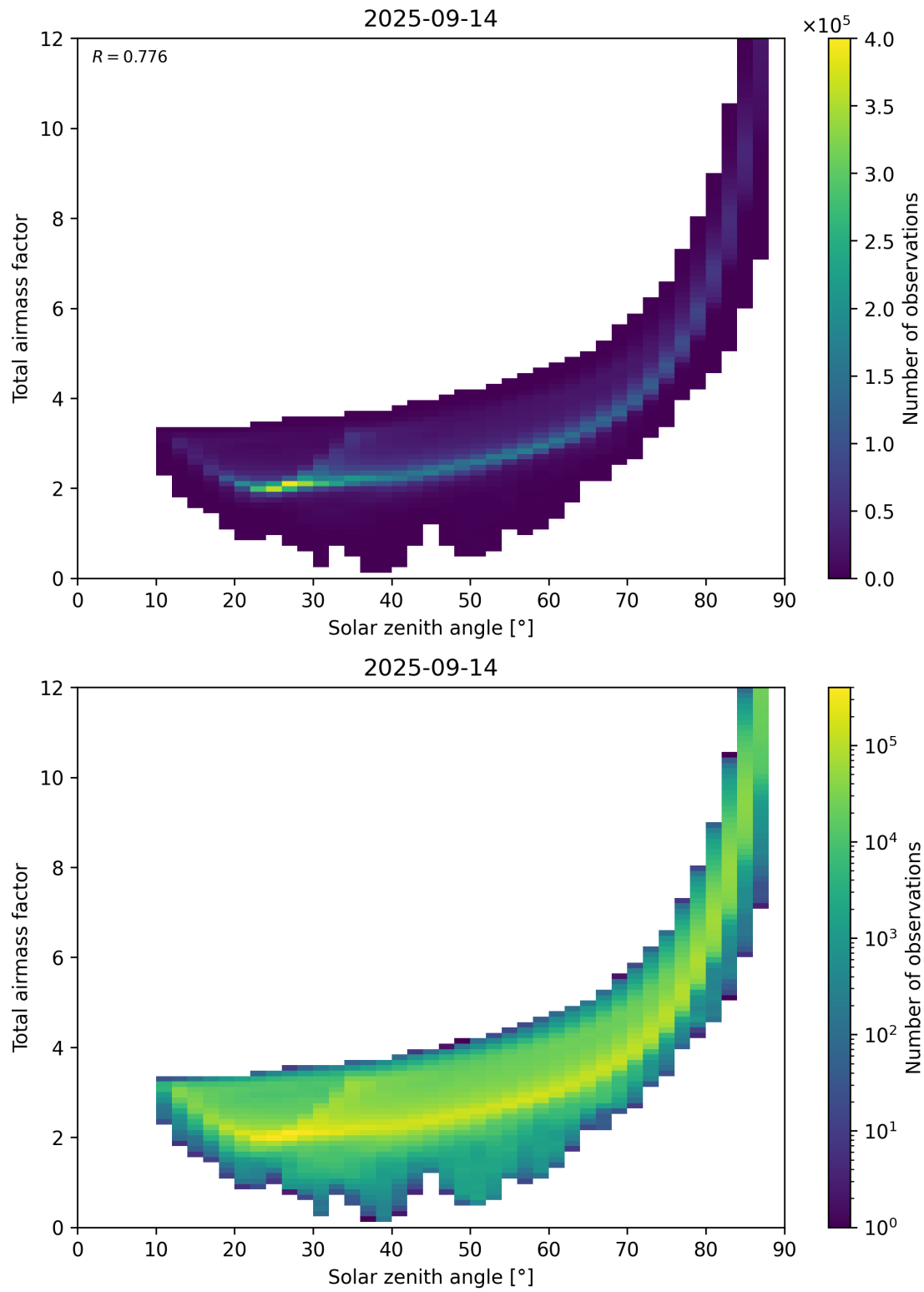
Figure 146: Scatter density plot of “Solar zenith angle” against “Total air mass factor” for 2025-09-13 to 2025-09-15.
