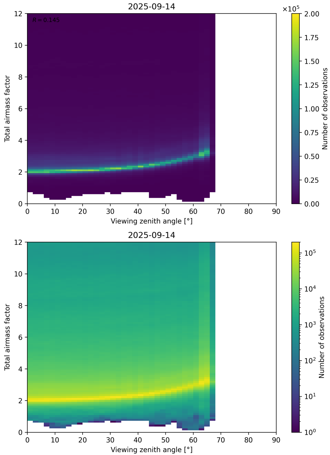
Figure 160: Scatter density plot of “Viewing zenith angle” against “Total airmass factor” for 2025-09-13 to 2025-09-15.
