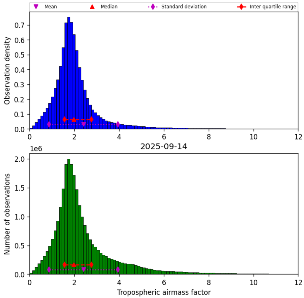
Figure 31: Histogram of “Tropospheric airmass factor” for 2025-09-13 to 2025-09-15
