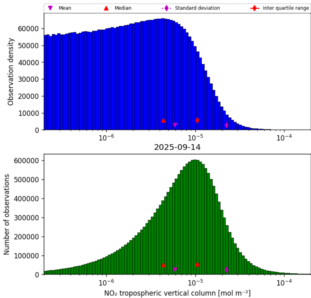
Figure 29: Histogram of “NO 2 tropospheric vertical column” for 2025-09-13 to 2025-09-15
