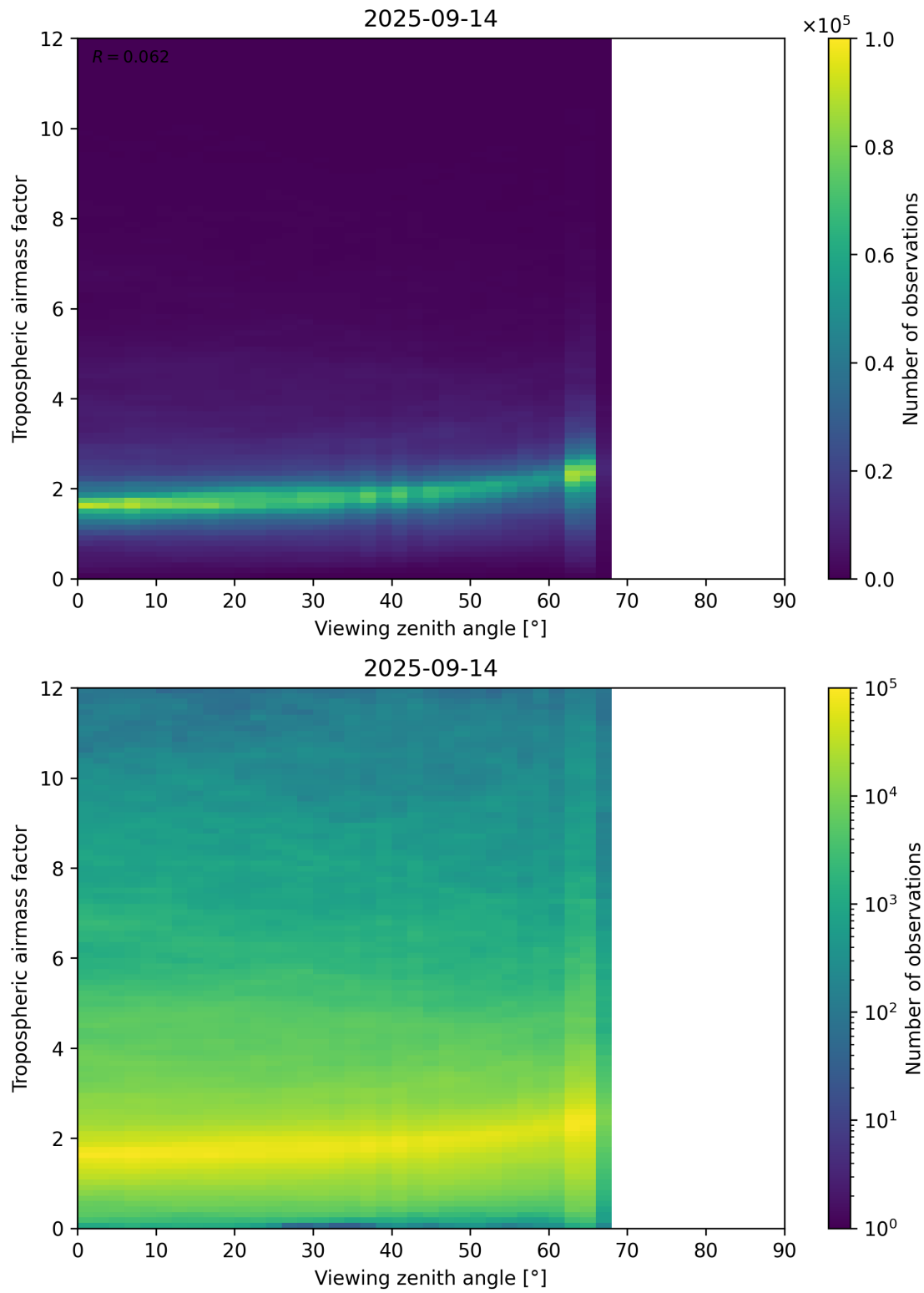
Figure 161: Scatter density plot of “Viewing zenith angle” against “Tropospheric airmass factor” for 2025-09-13 to 2025-09-15.
