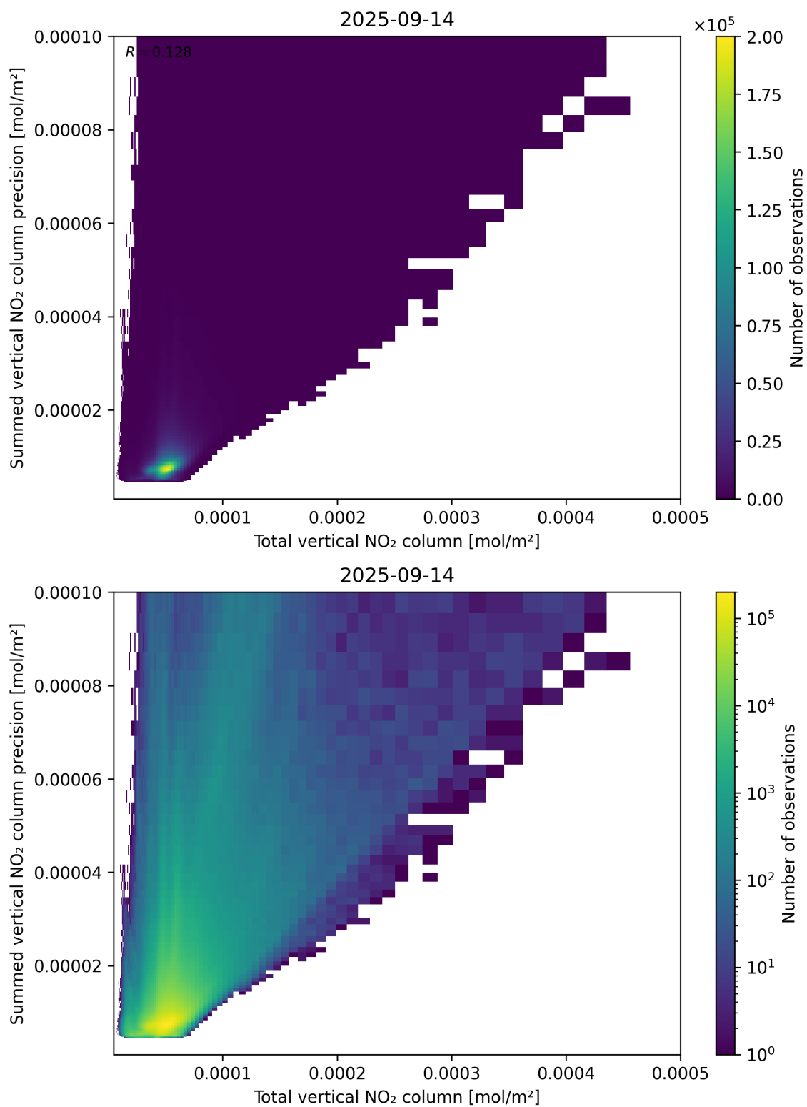
Figure 113: Scatter density plot of “Total vertical NO 2 column” against “Summed vertical NO 2 column precision” for 2025-09-13 to 2025-09-15.
