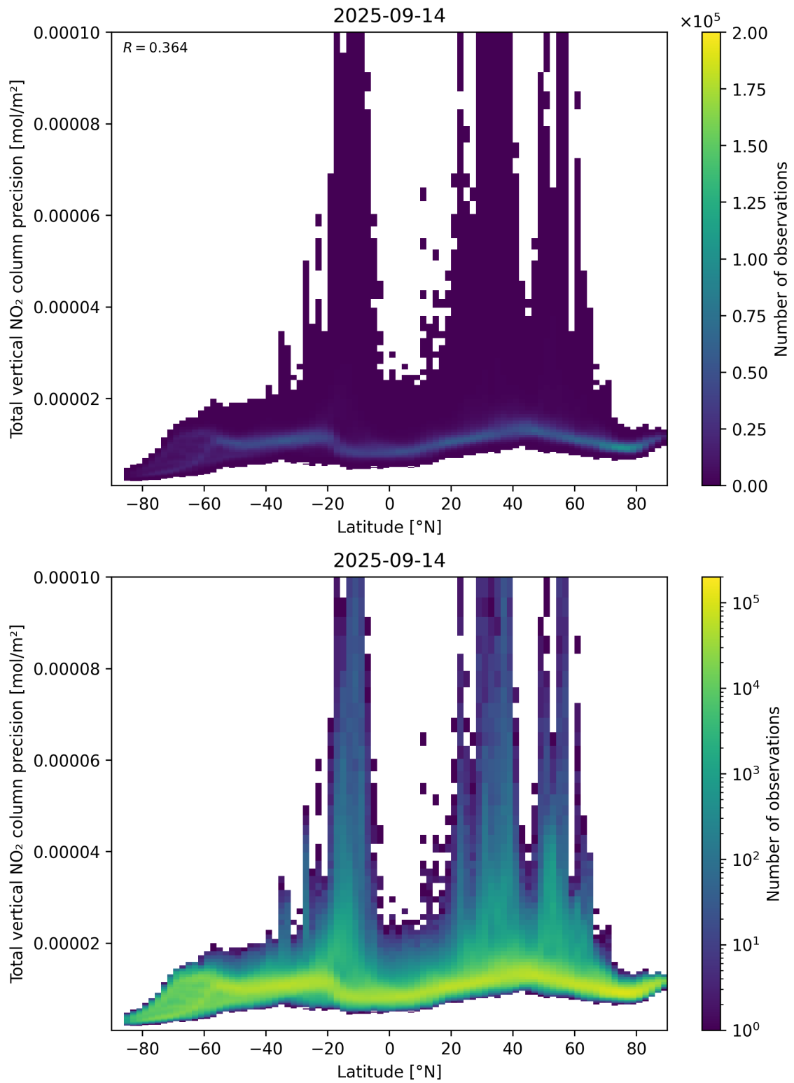
Figure 91: Scatter density plot of “Latitude” against “Total vertical NO 2 column precision” for 2025-09-13 to 2025-09-15.
