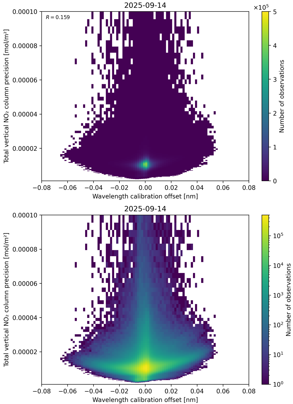
Figure 180: Scatter density plot of “Wavelength calibration offset” against “Total vertical NO 2 column precision” for 2025-09-13 to 2025-09-15.
