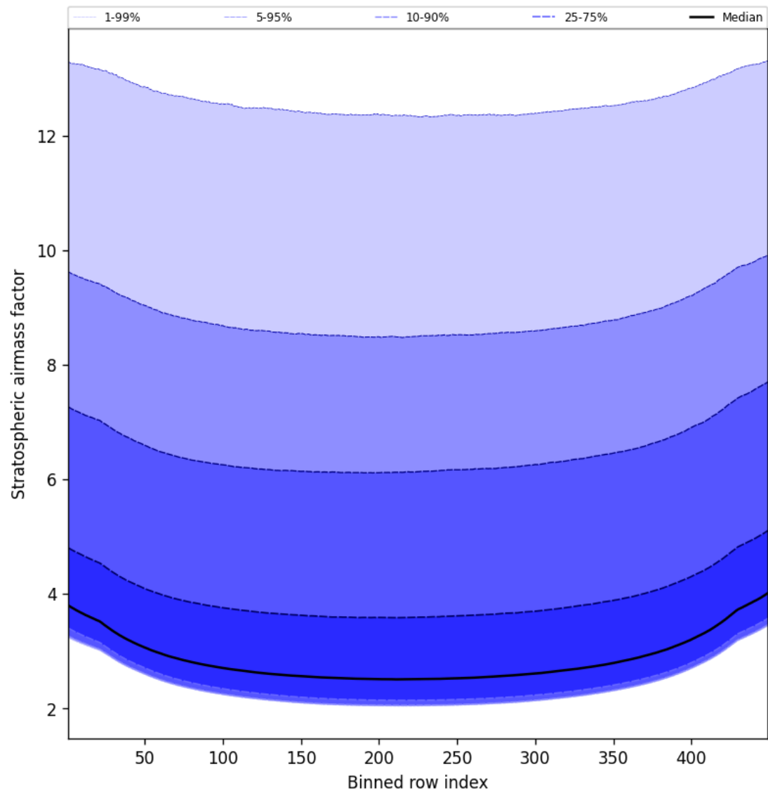
Figure 61: Along track statistics of “Stratospheric airmass factor” for 2025-09-13 to 2025-09-15
