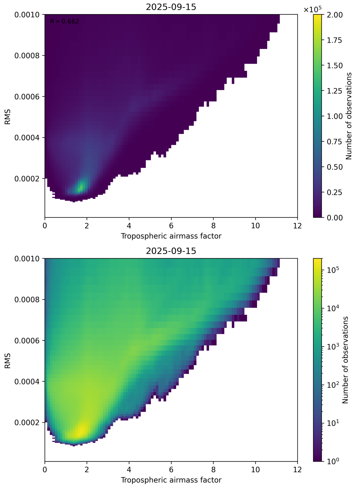
Figure 79: Scatter density plot of “Tropospheric airmass factor” against “RMS” for 2025-09-15 to 2025-09-16.
