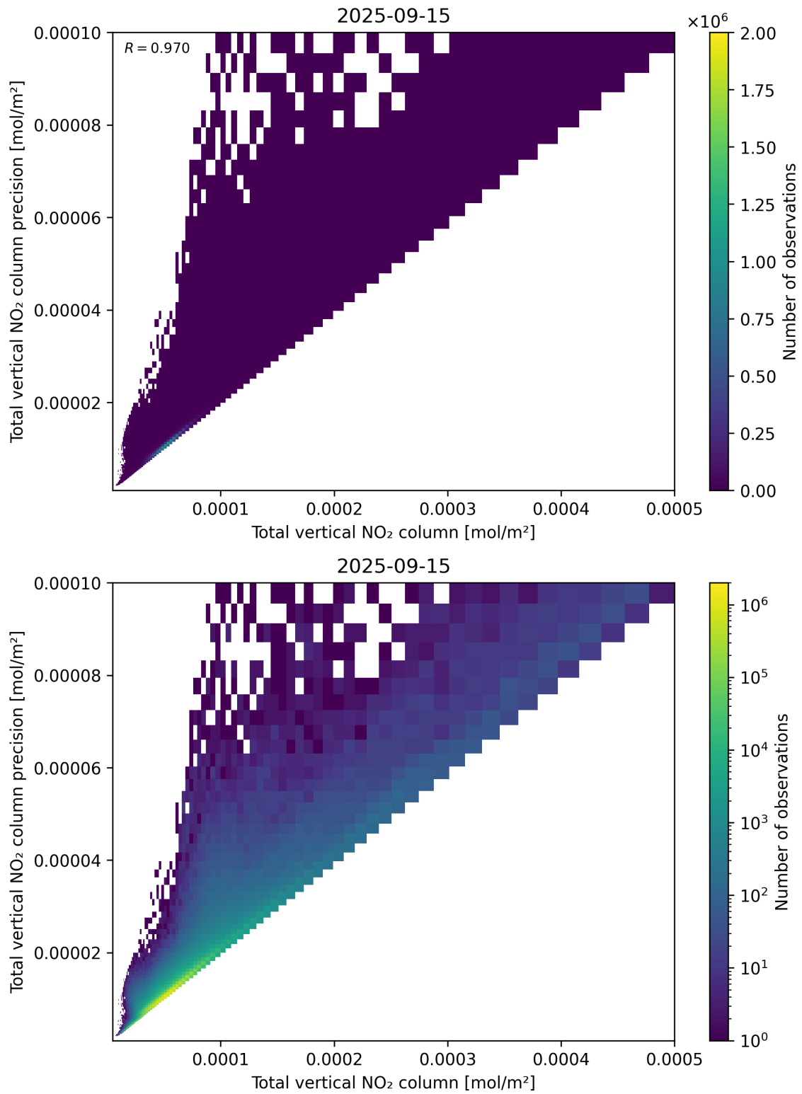
Figure 114: Scatter density plot of “Total vertical NO 2 column” against “Total vertical NO 2 column precision” for 2025-09-15 to 2025-09-16.
