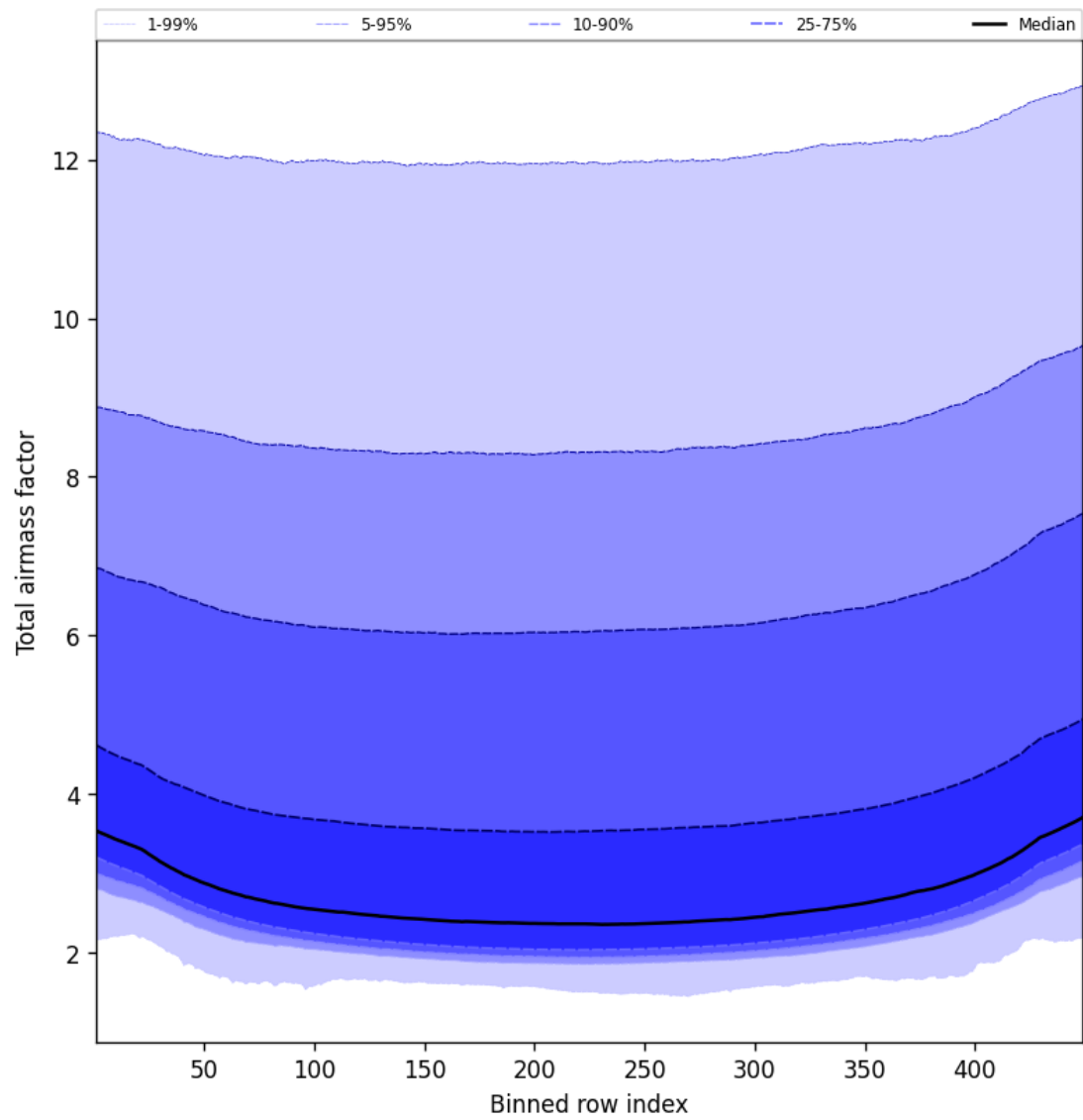
Figure 49: Along track statistics of “Total airmass factor” for 2025-09-15 to 2025-09-16
