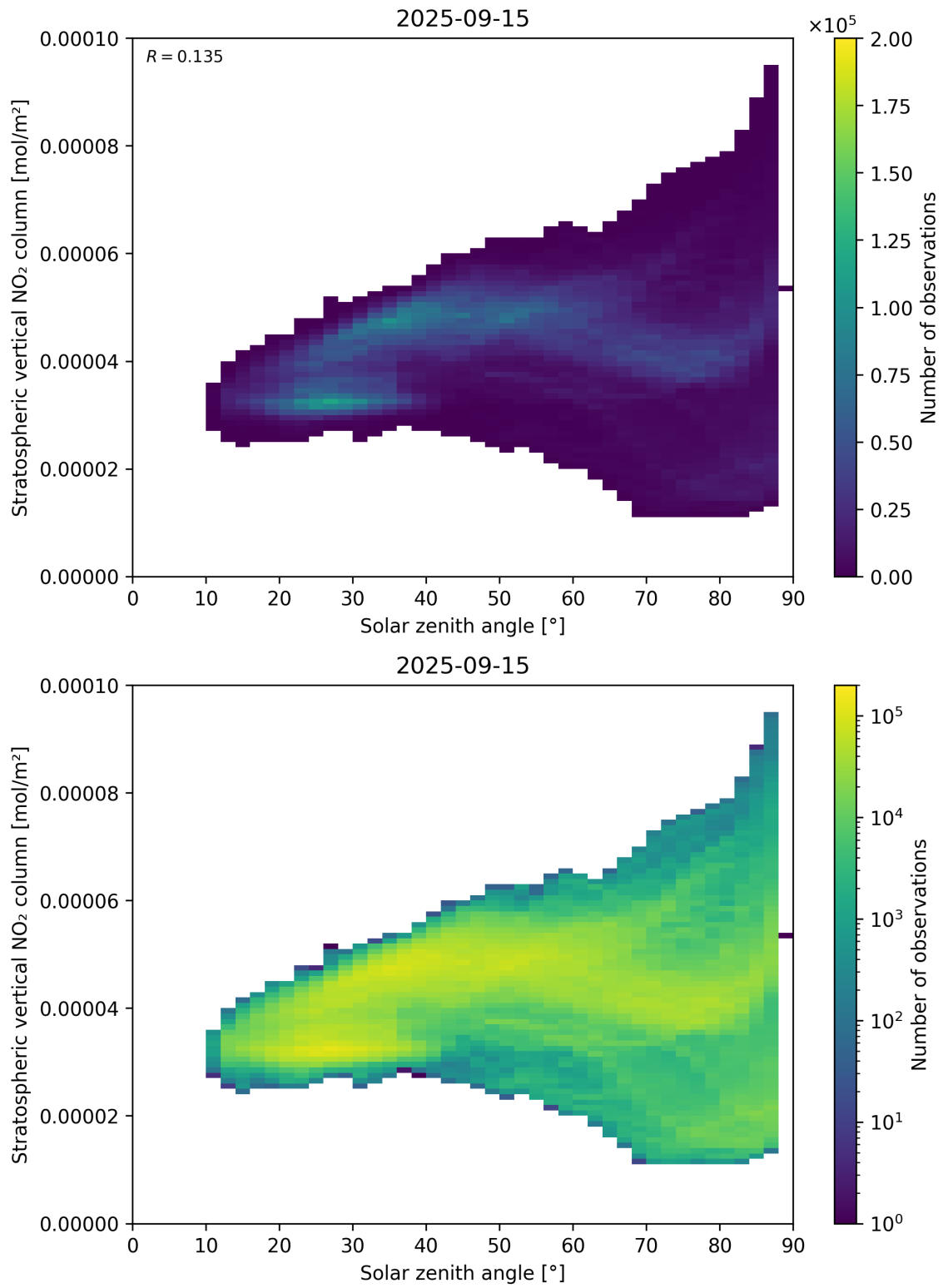
Figure 150: Scatter density plot of “Solar zenith angle” against “Stratospheric vertical NO 2 column” for 2025-09-15 to 2025-09-16.
