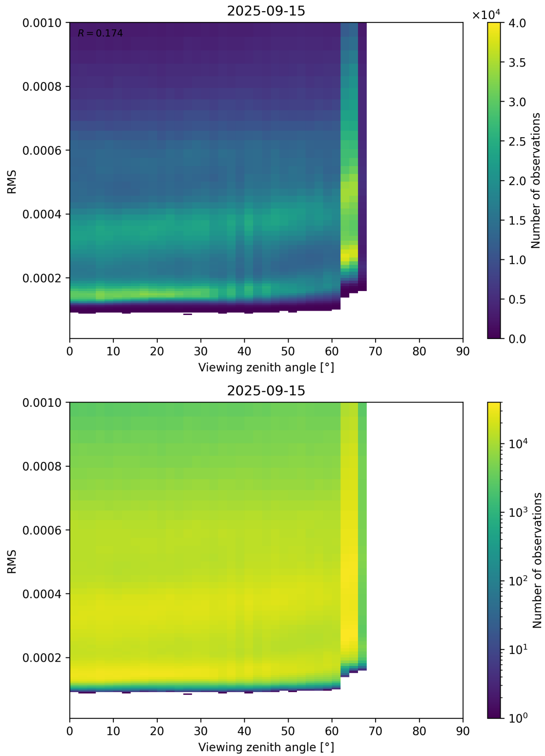
Figure 171: Scatter density plot of “Viewing zenith angle” against “RMS” for 2025-09-15 to 2025-09-16.
