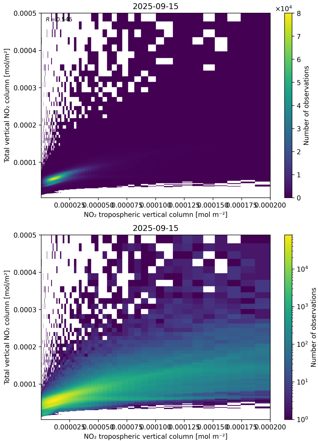
Figure 128: Scatter density plot of “NO 2 tropospheric vertical column” against “Total vertical NO 2 column” for 2025-09-15 to 2025-09-16.
