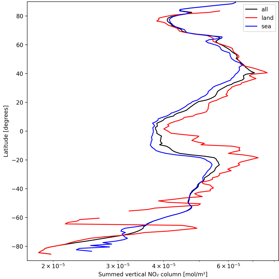
Figure 23: Zonal average of “Summed vertical NO 2 column” for 2025-09-15 to 2025-09-16.
