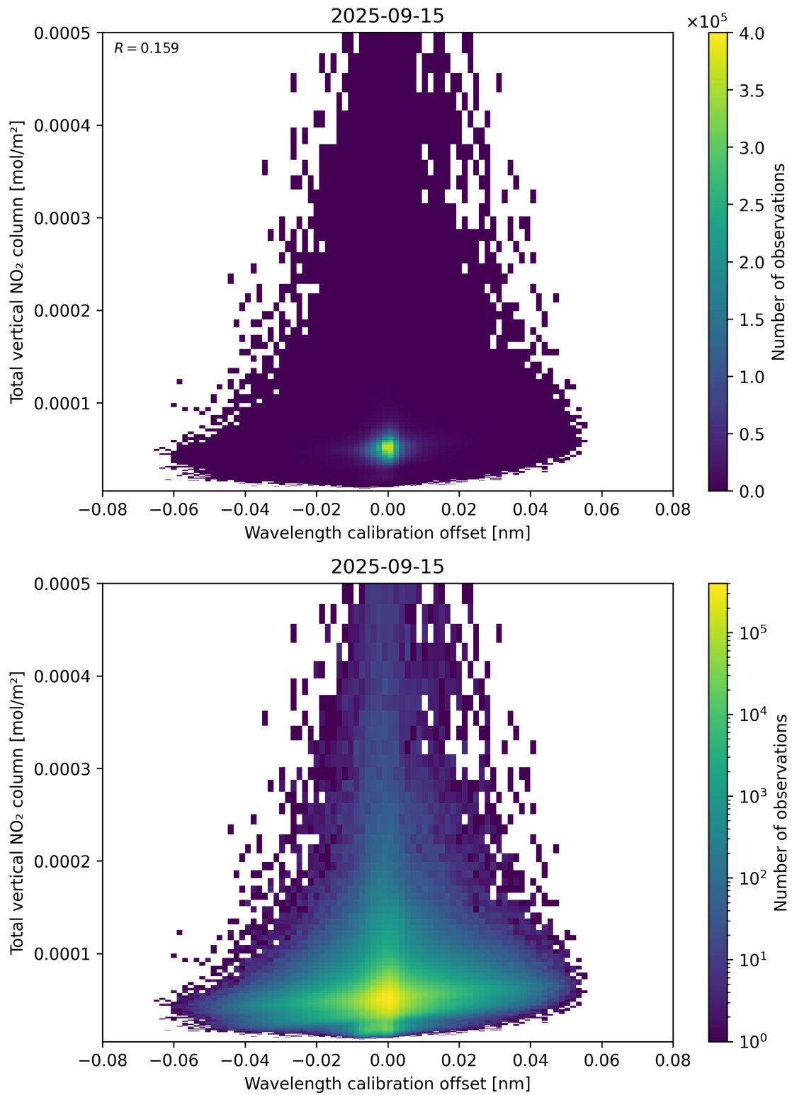
Figure 179: Scatter density plot of “Wavelength calibration offset” against “Total vertical NO 2 column” for 2025-09-15 to 2025-09-16.
