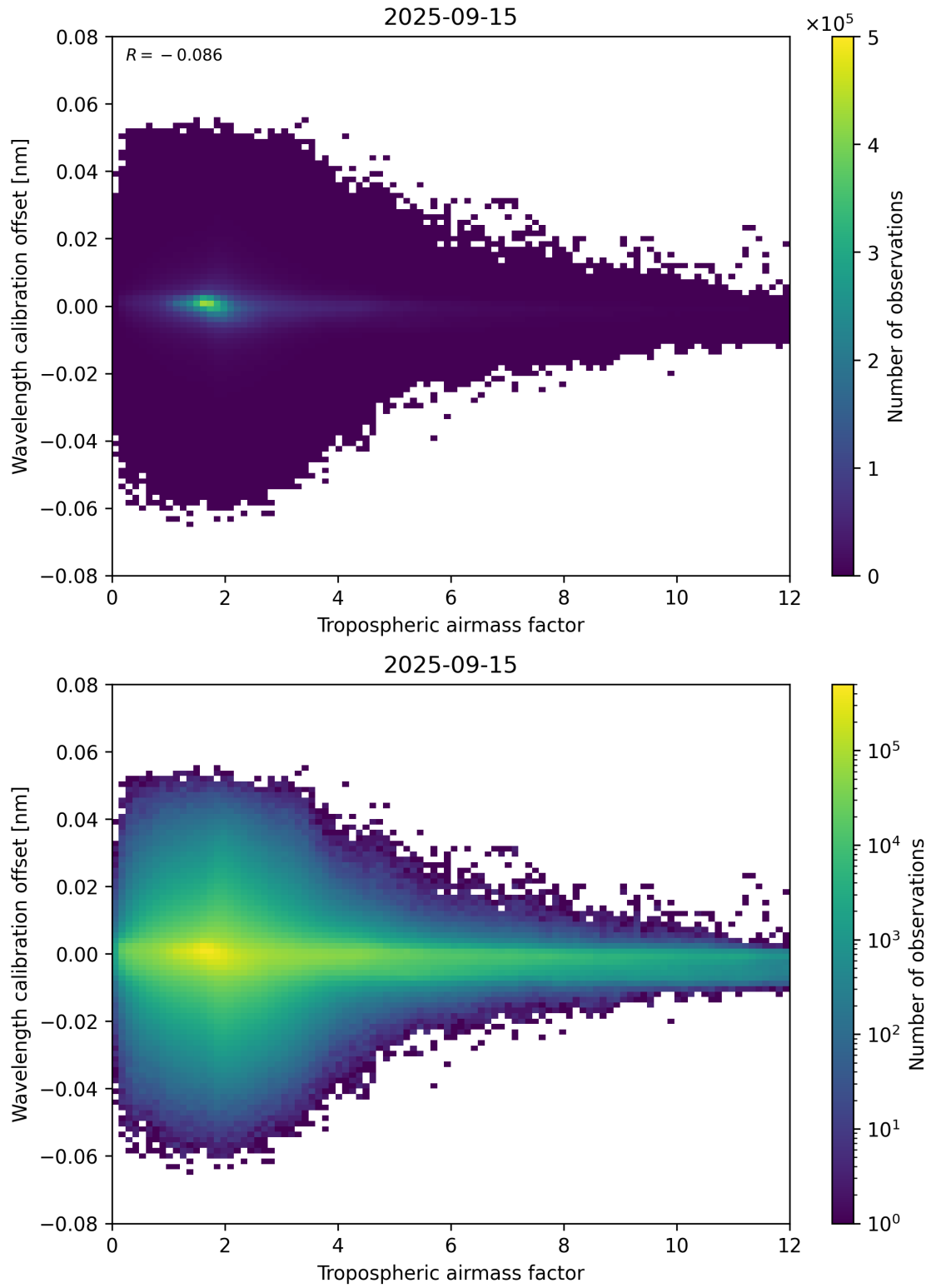
Figure 80: Scatter density plot of “Tropospheric airmass factor” against “Wavelength calibration offset” for 2025-09-15 to 2025-09-16.
