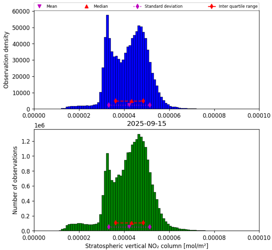
Figure 36: Histogram of “Stratospheric vertical NO 2 column” for 2025-09-15 to 2025-09-16
