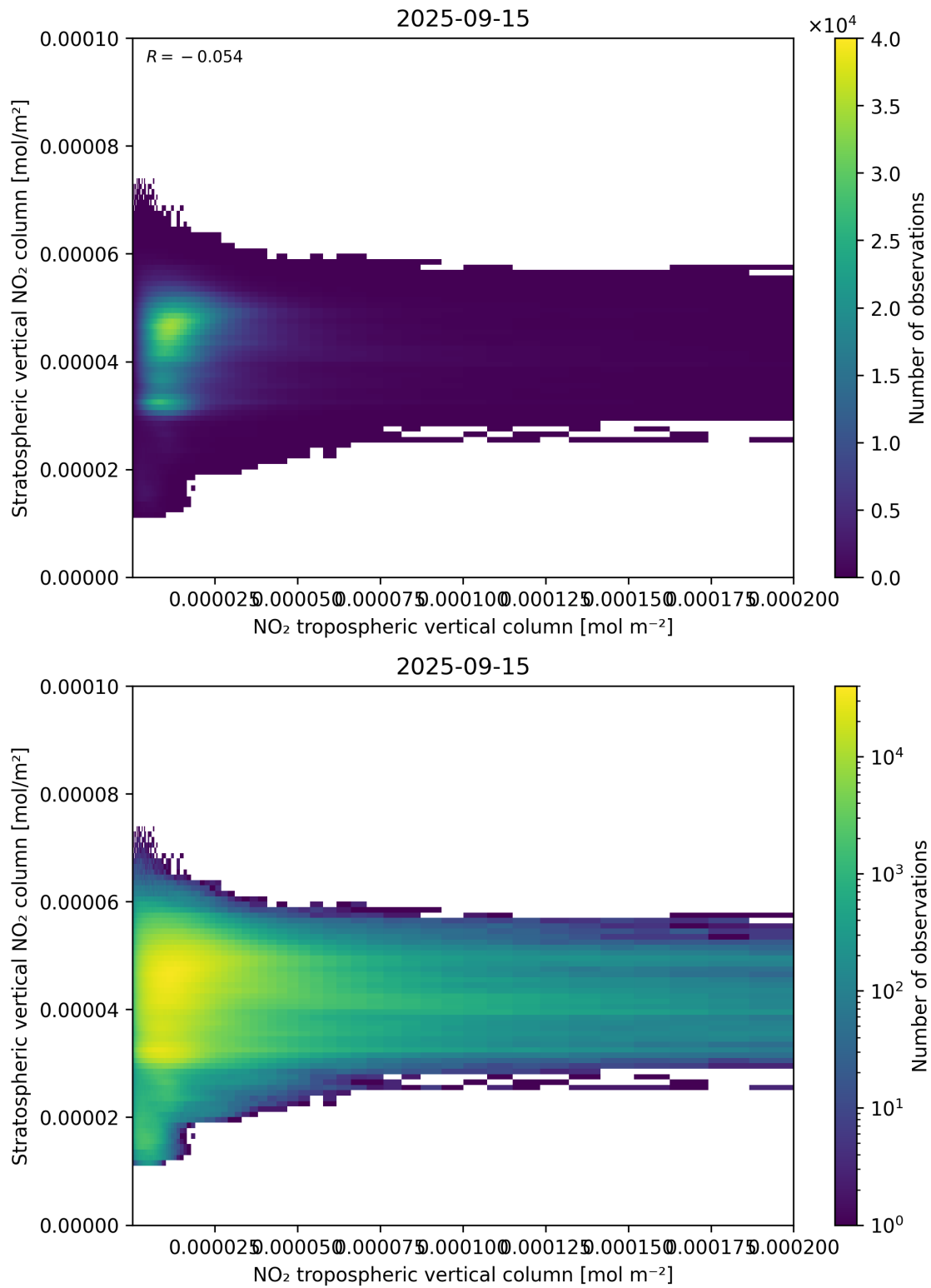
Figure 125: Scatter density plot of “NO 2 tropospheric vertical column” against “Stratospheric vertical NO 2 column” for 2025-09-15 to 2025-09-16.
