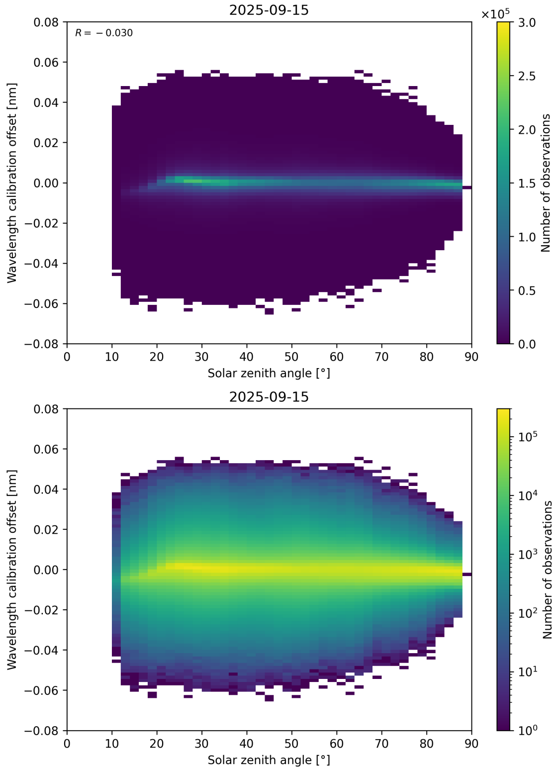
Figure 158: Scatter density plot of “Solar zenith angle” against “Wavelength calibration offset” for 2025-09-15 to 2025-09-16.
