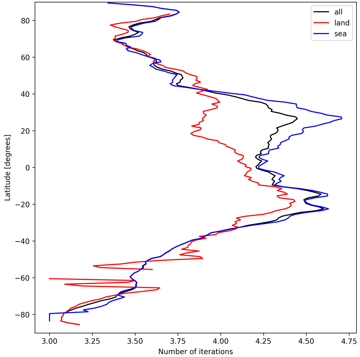
Figure 17: Zonal average of “Number of iterations” for 2025-09-15 to 2025-09-16.
