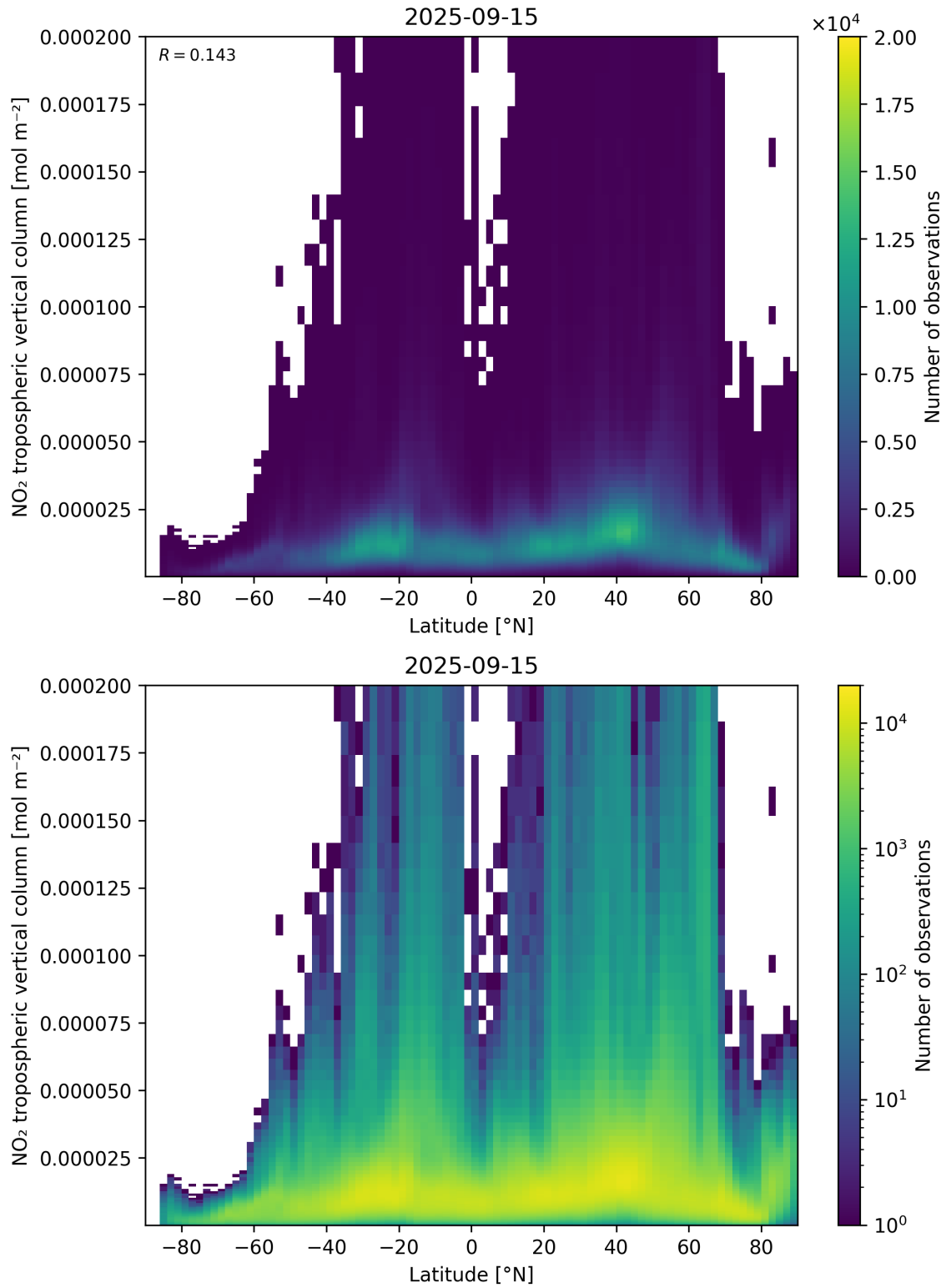
Figure 92: Scatter density plot of “Latitude” against “NO 2 tropospheric vertical column” for 2025-09-15 to 2025-09-16.
