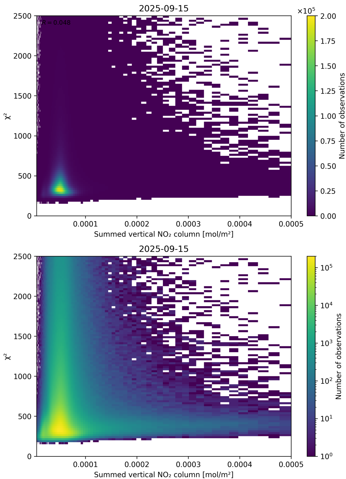
Figure 104: Scatter density plot of “Summed vertical NO 2 column” against “ \chi^2 ” for 2025-09-15 to 2025-09-16.
