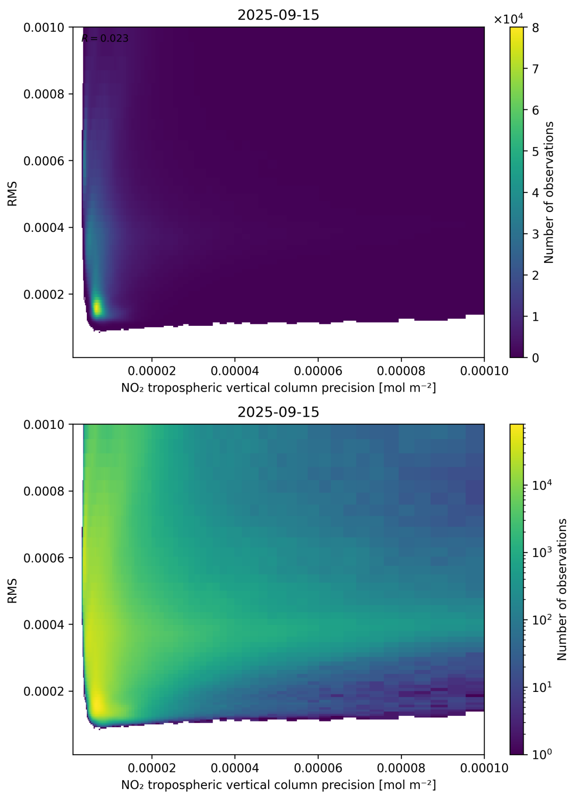
Figure 140: Scatter density plot of “NO 2 tropospheric vertical column precision” against “RMS” for 2025-09-15 to 2025-09-16.
