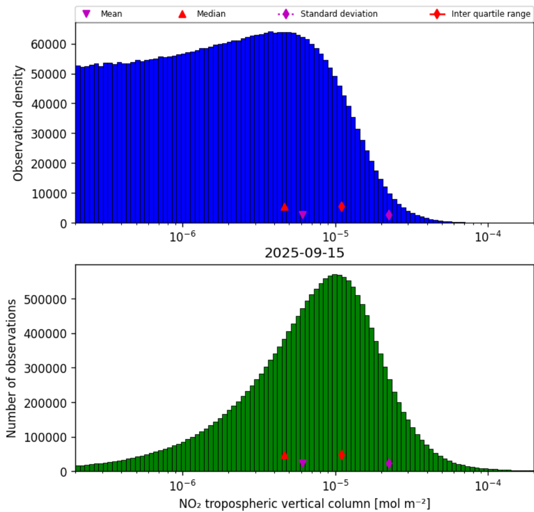
Figure 29: Histogram of “NO 2 tropospheric vertical column” for 2025-09-15 to 2025-09-16
