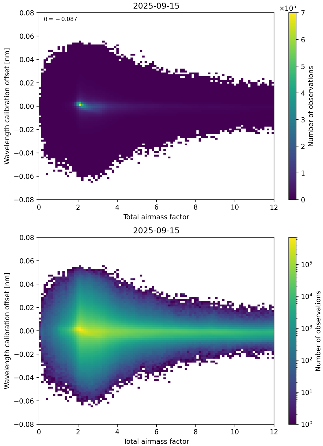
Figure 70: Scatter density plot of “Total airmass factor” against “Wavelength calibration offset” for 2025-09-15 to 2025-09-16.
