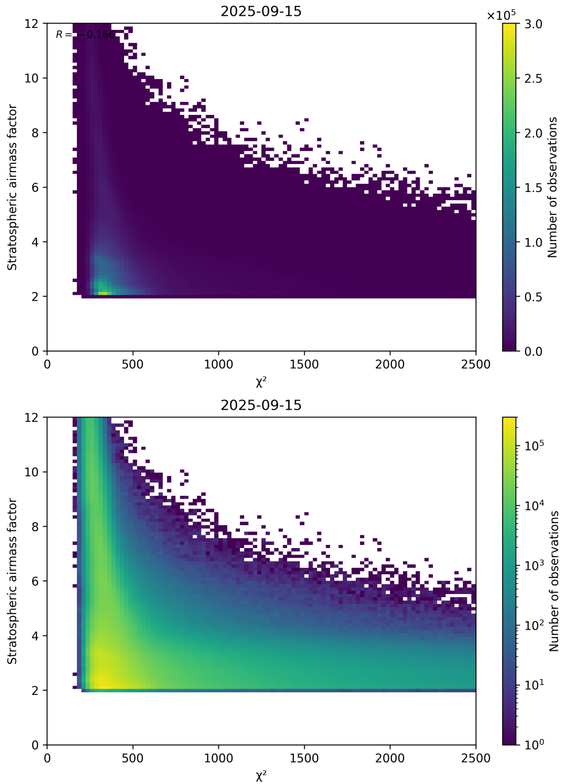
Figure 81: Scatter density plot of “ \chi^2 ” against “Stratospheric airmass factor” for 2025-09-15 to 2025-09-16.
