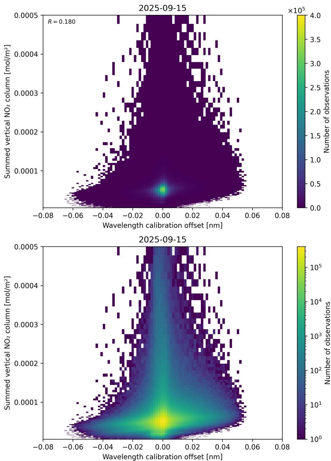
Figure 177: Scatter density plot of “Wavelength calibration offset” against “Summed vertical NO 2 column” for 2025-09-15 to 2025-09-16.
