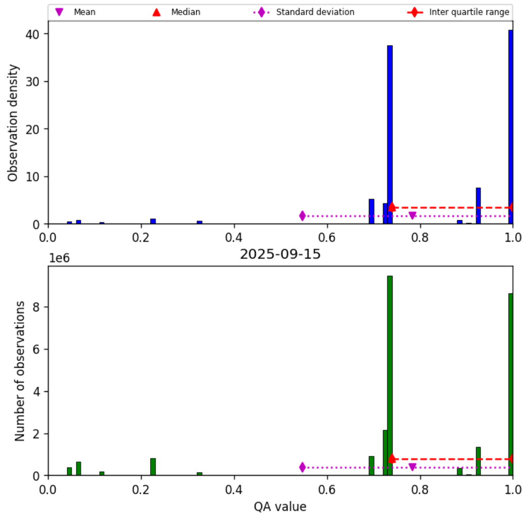
Figure 28: Histogram of “QA value” for 2025-09-15 to 2025-09-16
