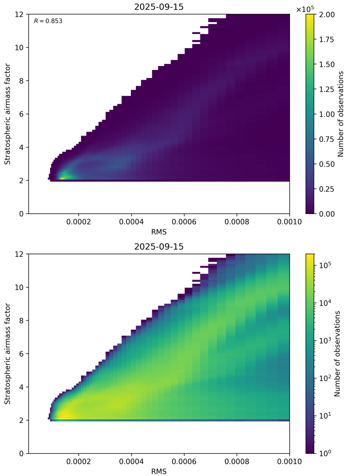
Figure 144: Scatter density plot of “RMS” against “Stratospheric airmass factor” for 2025-09-15 to 2025-09-16.
