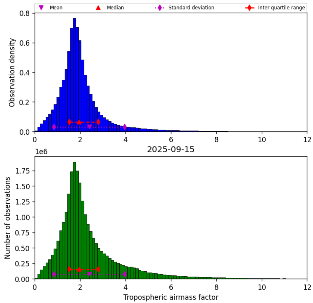
Figure 31: Histogram of “Tropospheric airmass factor” for 2025-09-15 to 2025-09-16
