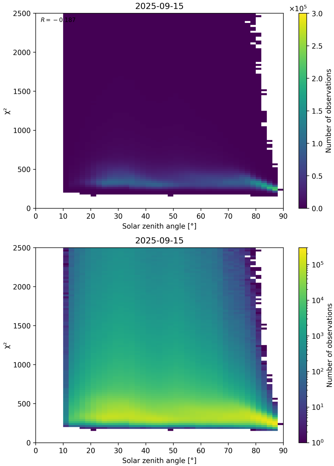
Figure 148: Scatter density plot of “Solar zenith angle” against “ \chi^2 ” for 2025-09-15 to 2025-09-16.
