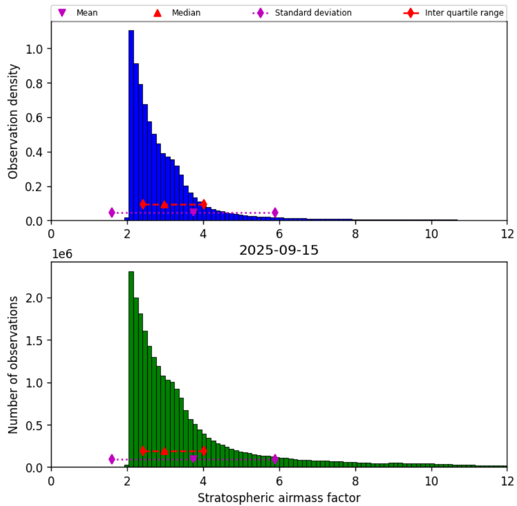
Figure 44: Histogram of “Stratospheric airmass factor” for 2025-09-15 to 2025-09-16
