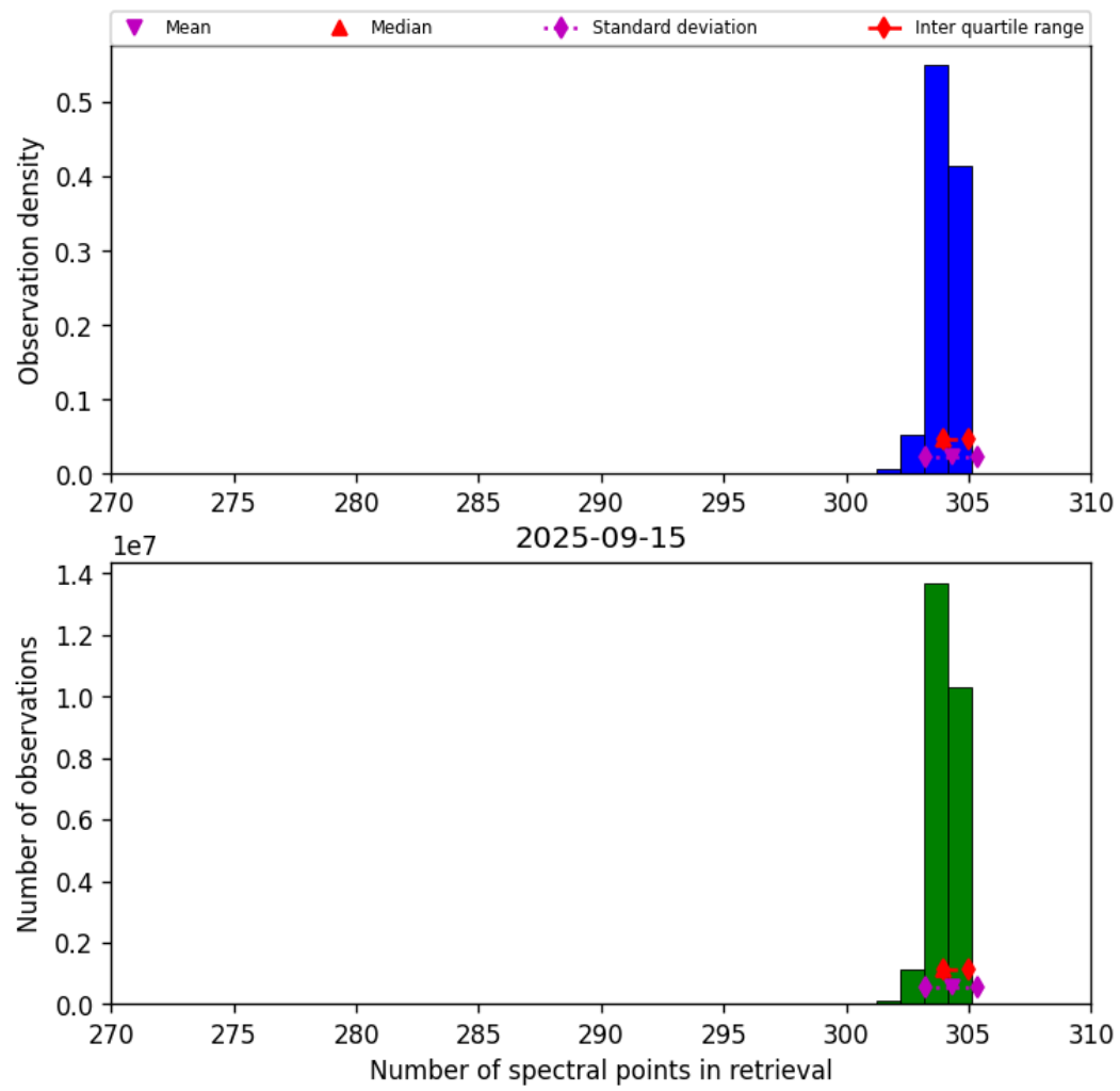
Figure 33: Histogram of “Number of spectral points in retrieval” for 2025-09-15 to 2025-09-16
