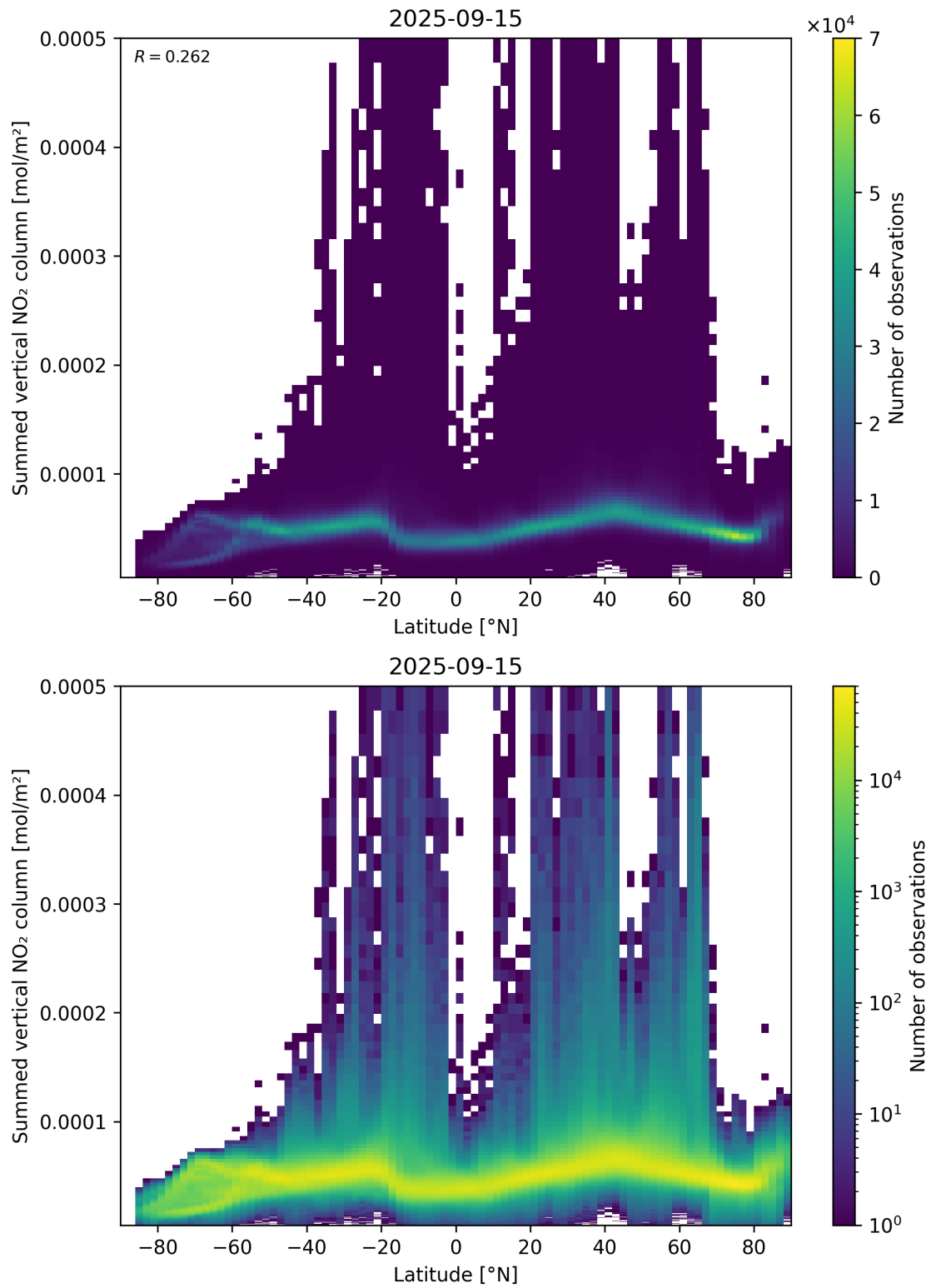
Figure 88: Scatter density plot of “Latitude” against “Summed vertical NO 2 column” for 2025-09-15 to 2025-09-16.
