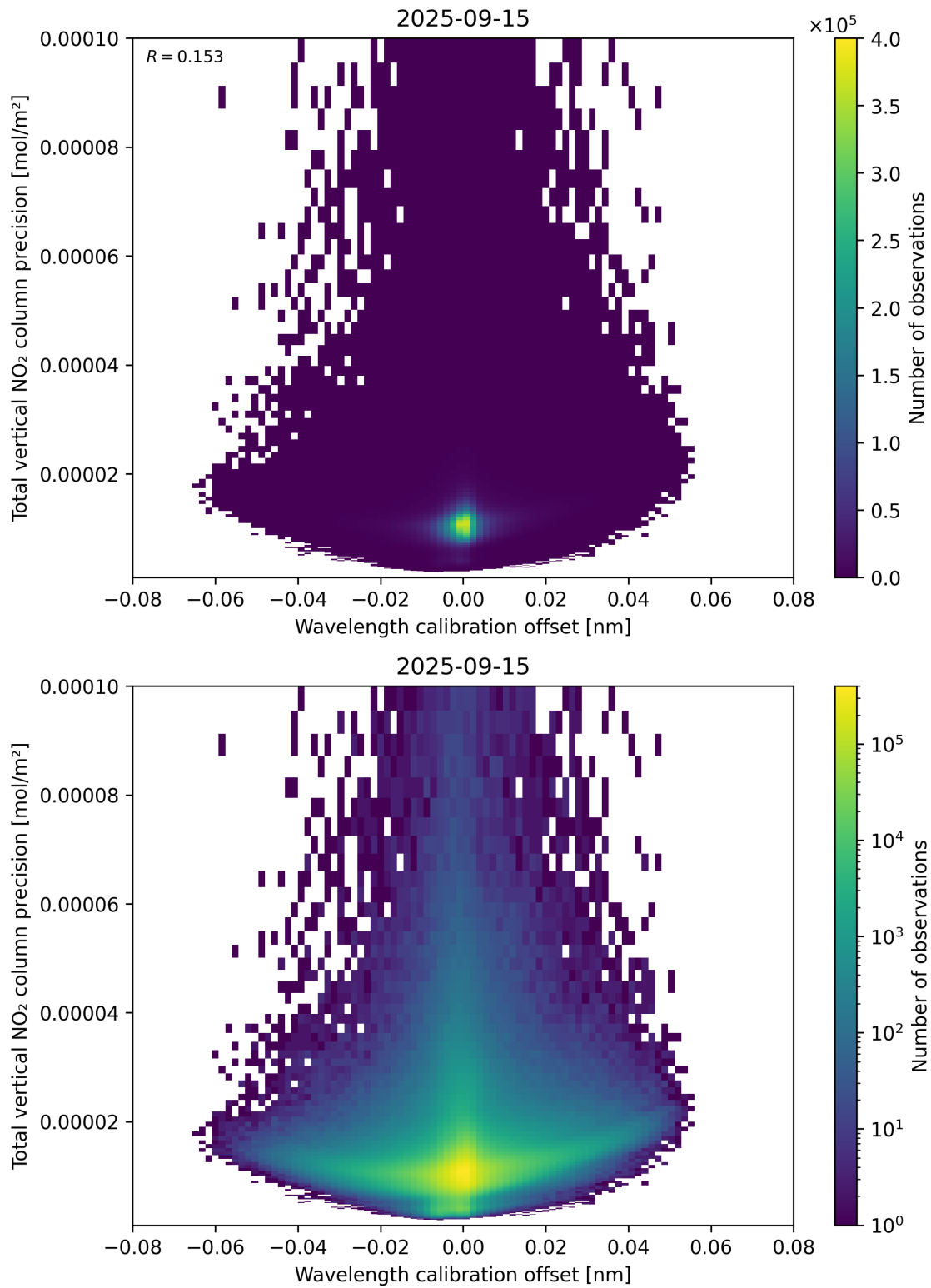
Figure 180: Scatter density plot of “Wavelength calibration offset” against “Total vertical NO 2 column precision” for 2025-09-15 to 2025-09-16.
