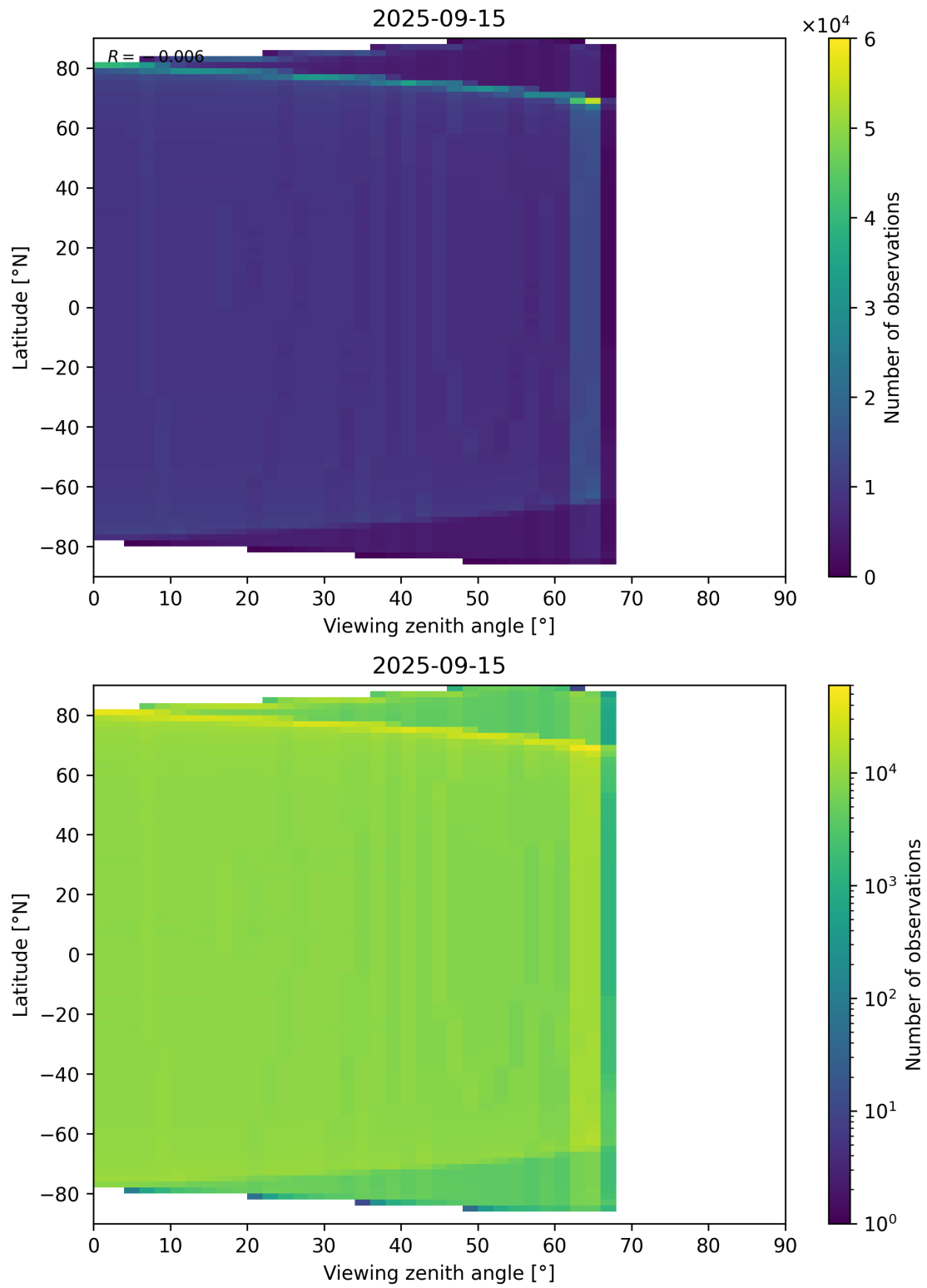
Figure 163: Scatter density plot of “Viewing zenith angle” against “Latitude” for 2025-09-15 to 2025-09-16.
