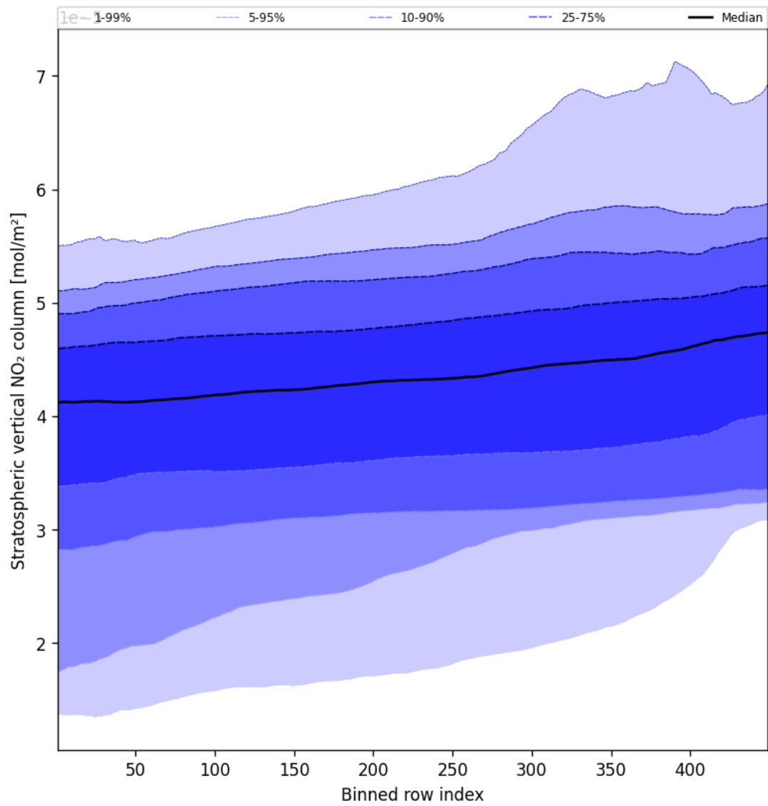
Figure 53: Along track statistics of “Stratospheric vertical NO 2 column” for 2025-09-15 to 2025-09-16
