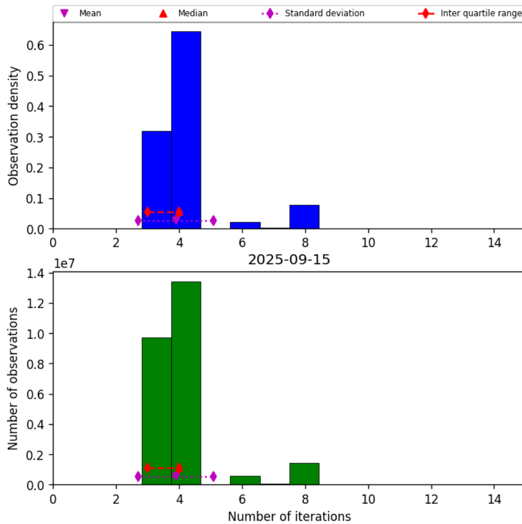
Figure 34: Histogram of “Number of iterations” for 2025-09-15 to 2025-09-16
