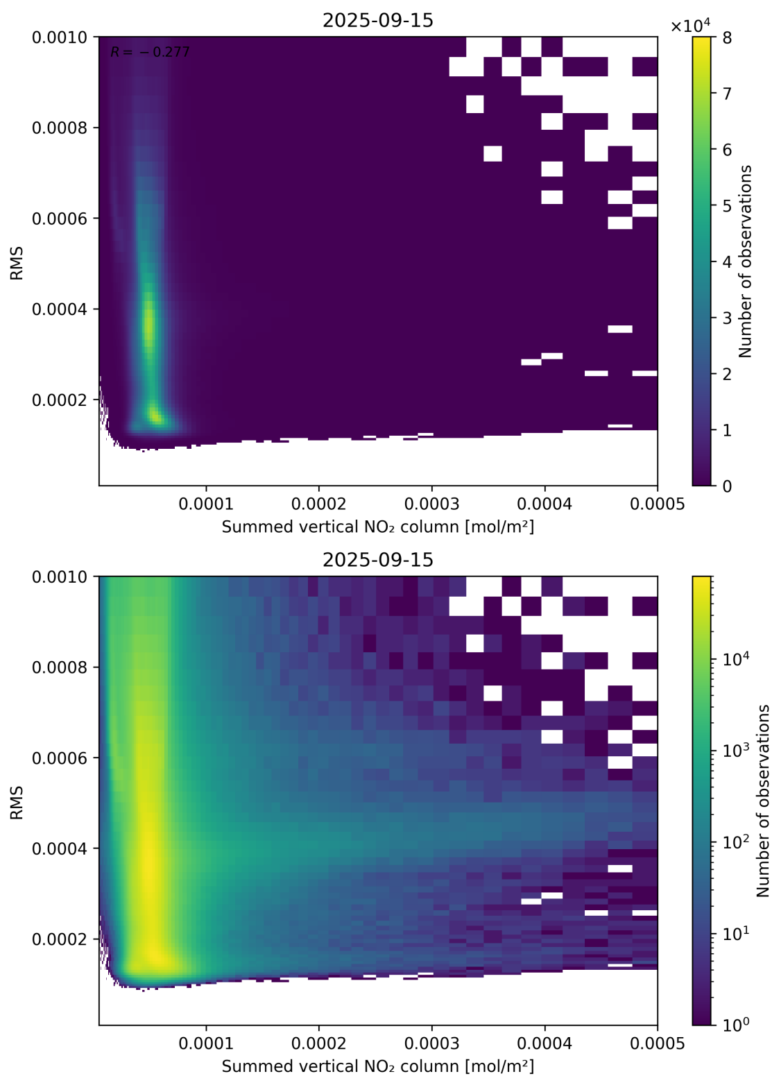
Figure 109: Scatter density plot of “Summed vertical NO 2 column” against “RMS” for 2025-09-15 to 2025-09-16.
