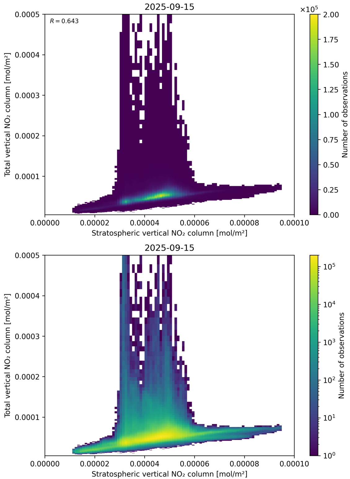
Figure 100: Scatter density plot of “Stratospheric vertical NO 2 column” against “Total vertical NO 2 column” for 2025-09-15 to 2025-09-16.
