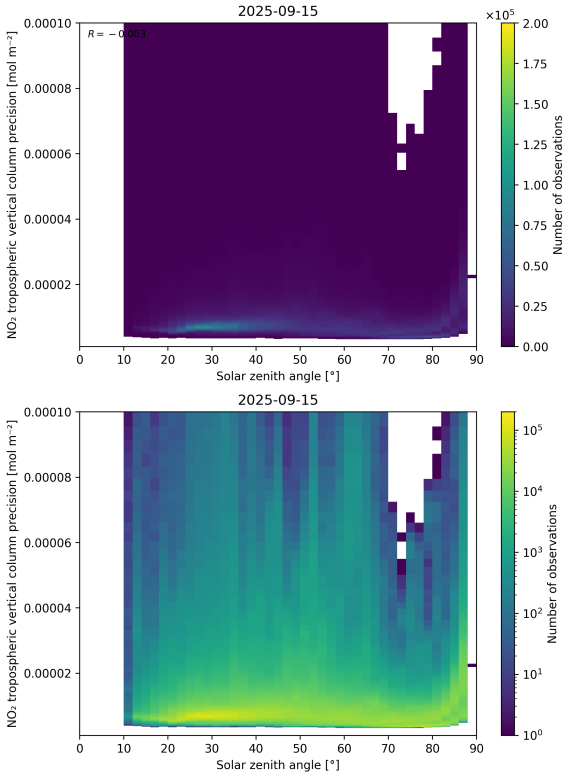
Figure 156: Scatter density plot of “Solar zenith angle” against “NO 2 tropospheric vertical column precision” for 2025-09-15 to 2025-09-16.
