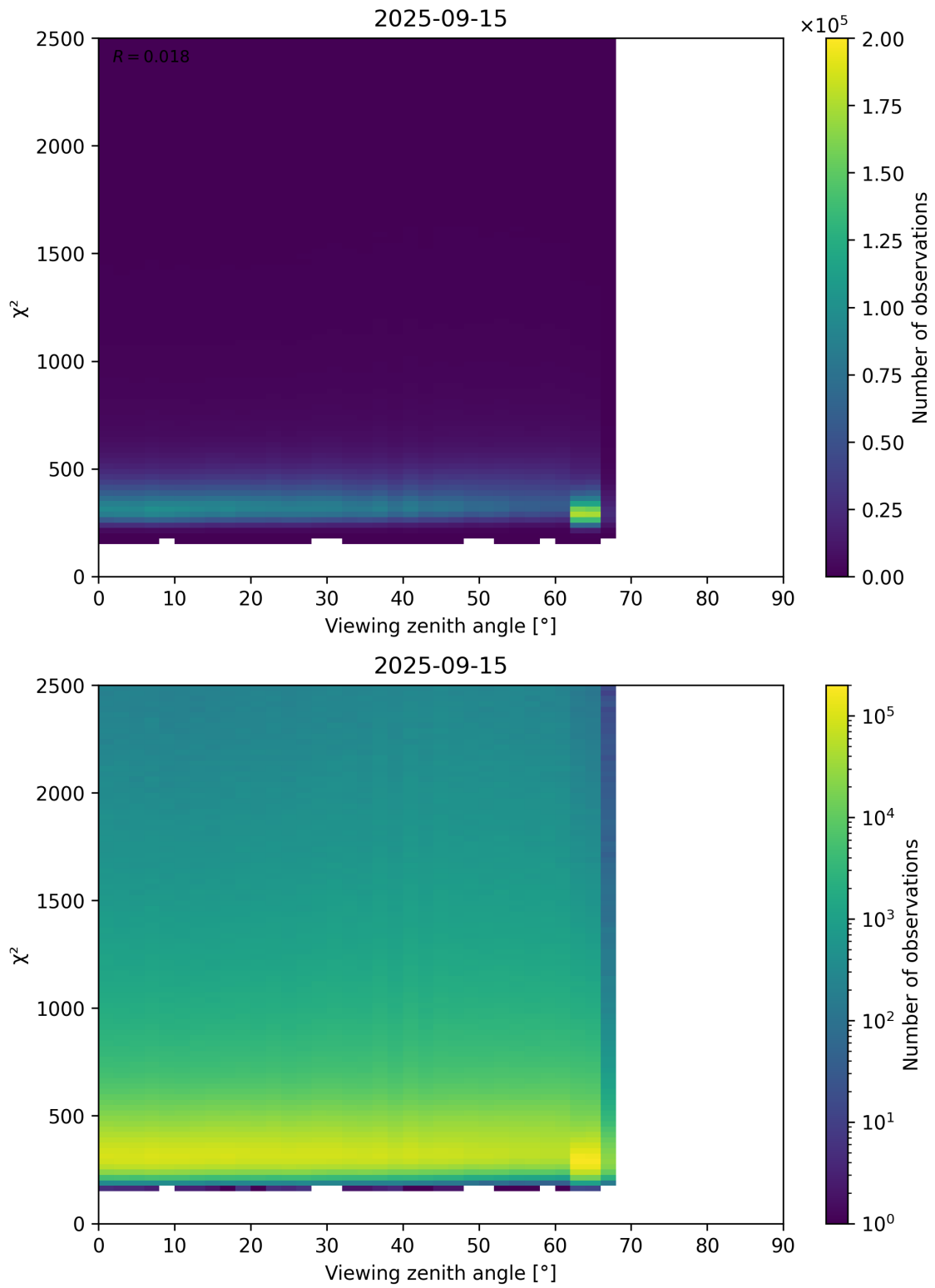
Figure 162: Scatter density plot of “Viewing zenith angle” against “ \chi^2 ” for 2025-09-15 to 2025-09-16.
