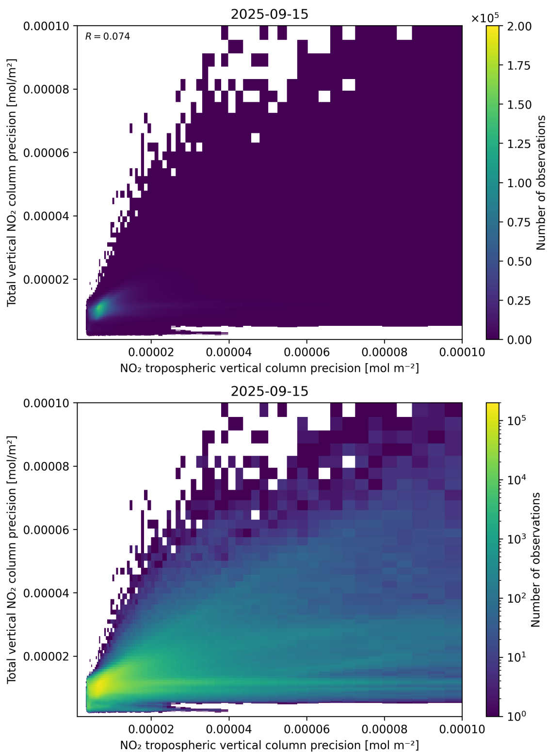
Figure 139: Scatter density plot of “NO 2 tropospheric vertical column precision” against “Total vertical NO 2 column precision” for 2025-09-15 to 2025-09-16.
