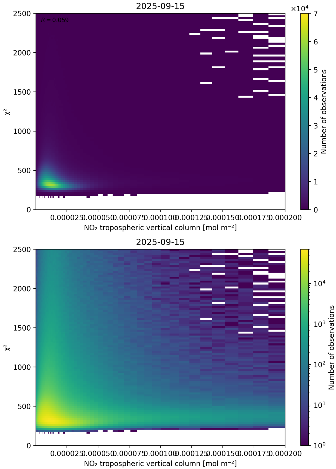
Figure 124: Scatter density plot of “NO 2 tropospheric vertical column” against “ \chi^2 ” for 2025-09-15 to 2025-09-16.
