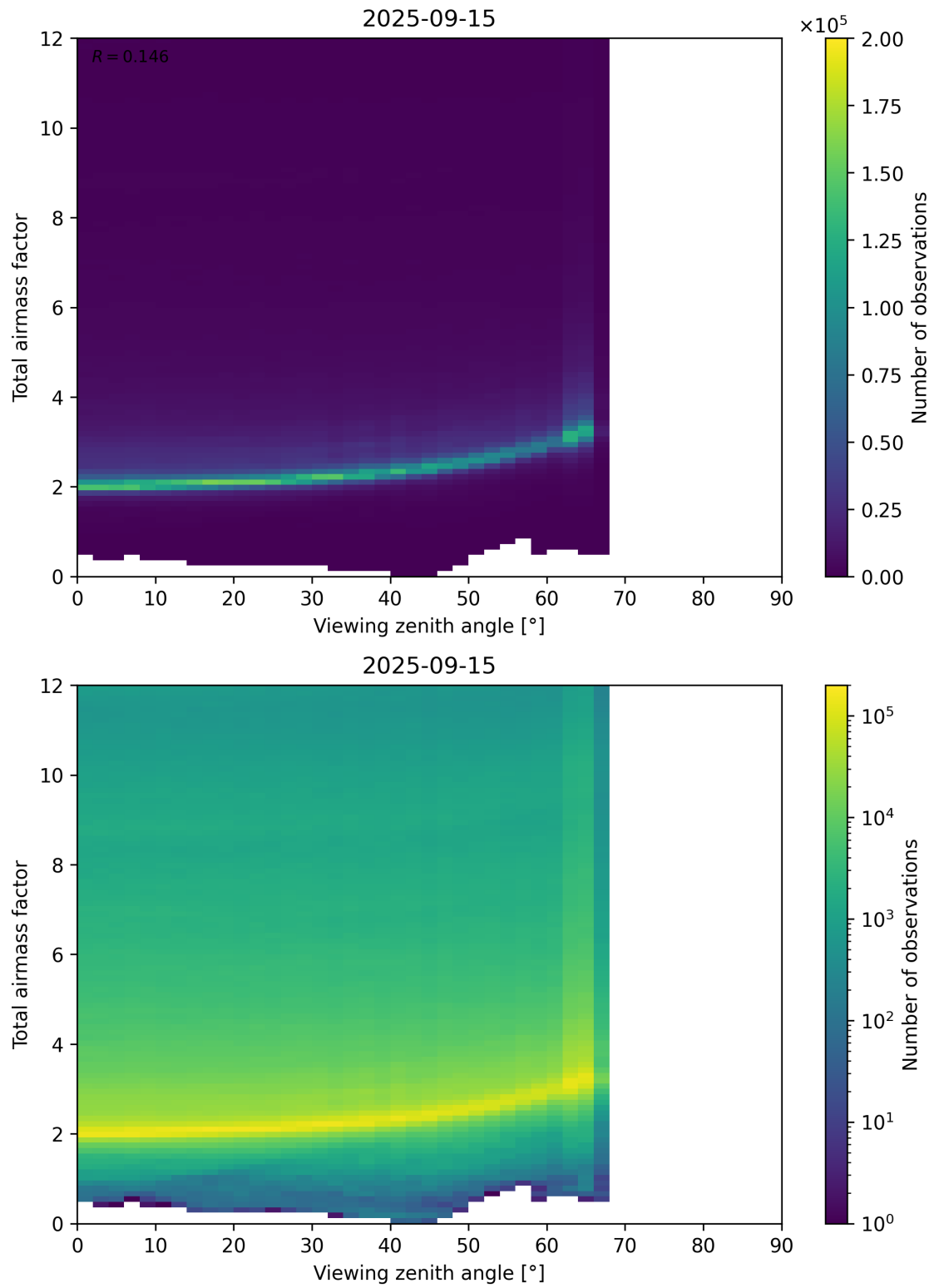
Figure 160: Scatter density plot of “Viewing zenith angle” against “Total airmass factor” for 2025-09-15 to 2025-09-16.
