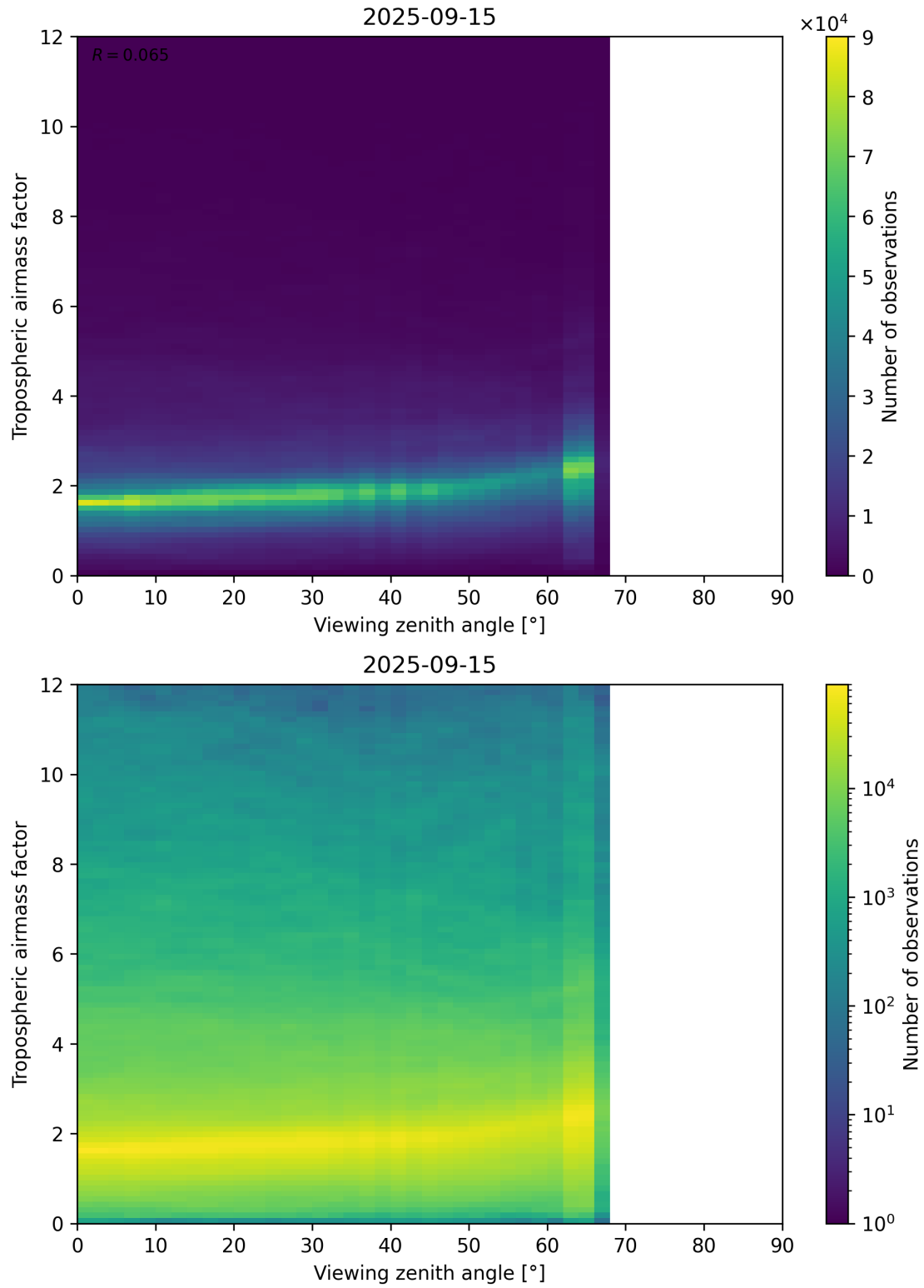
Figure 161: Scatter density plot of “Viewing zenith angle” against “Tropospheric airmass factor” for 2025-09-15 to 2025-09-16.
