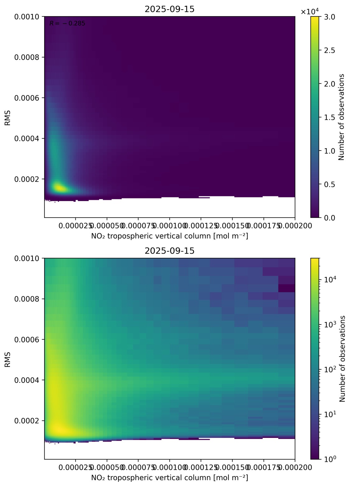
Figure 142: Scatter density plot of “NO 2 tropospheric vertical column” against “RMS” for 2025-09-15 to 2025-09-16.
