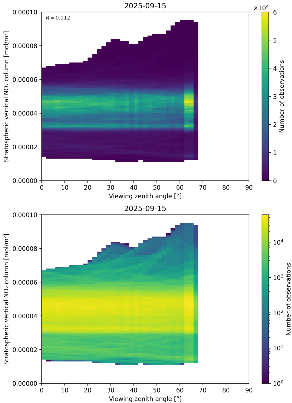
Figure 164: Scatter density plot of “Viewing zenith angle” against “Stratospheric vertical NO 2 column” for 2025-09-15 to 2025-09-16.
