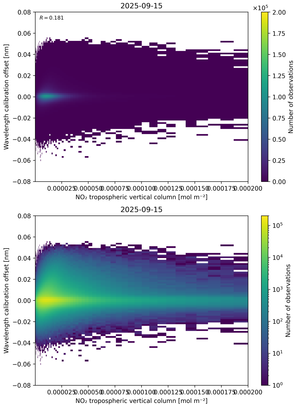
Figure 143: Scatter density plot of “NO 2 tropospheric vertical column” against “Wavelength calibration offset” for 2025-09-15 to 2025-09-16.
