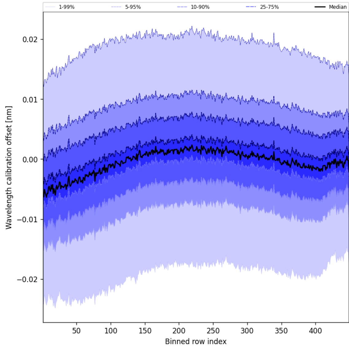
Figure 52: Along track statistics of “Wavelength calibration offset” for 2025-09-15 to 2025-09-16
