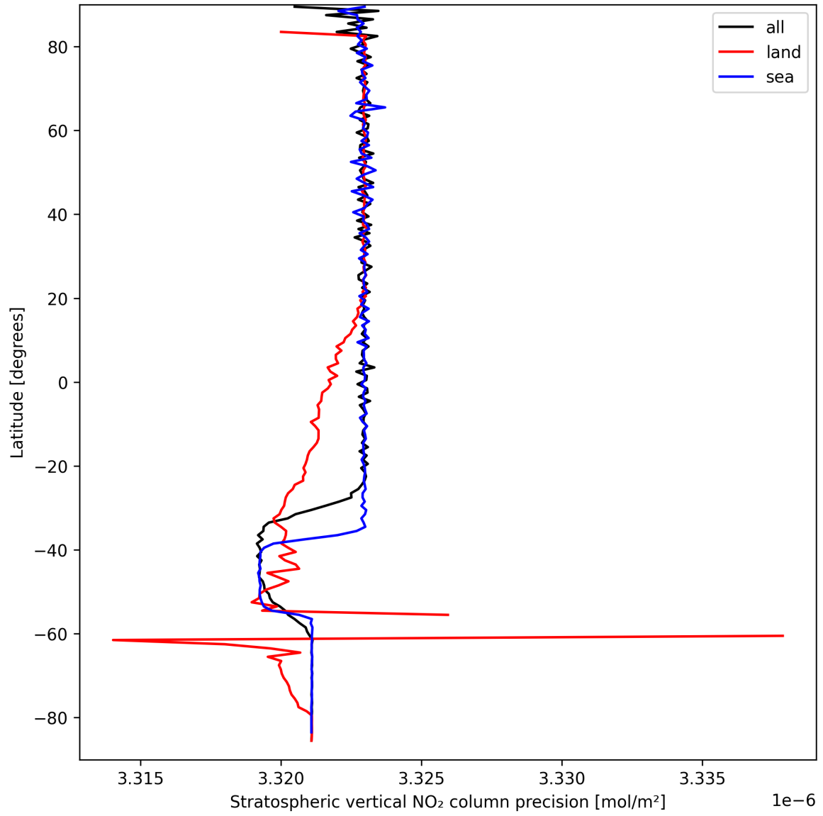
Figure 20: Zonal average of “Stratospheric vertical NO 2 column precision” for 2025-09-15 to 2025-09-16.
