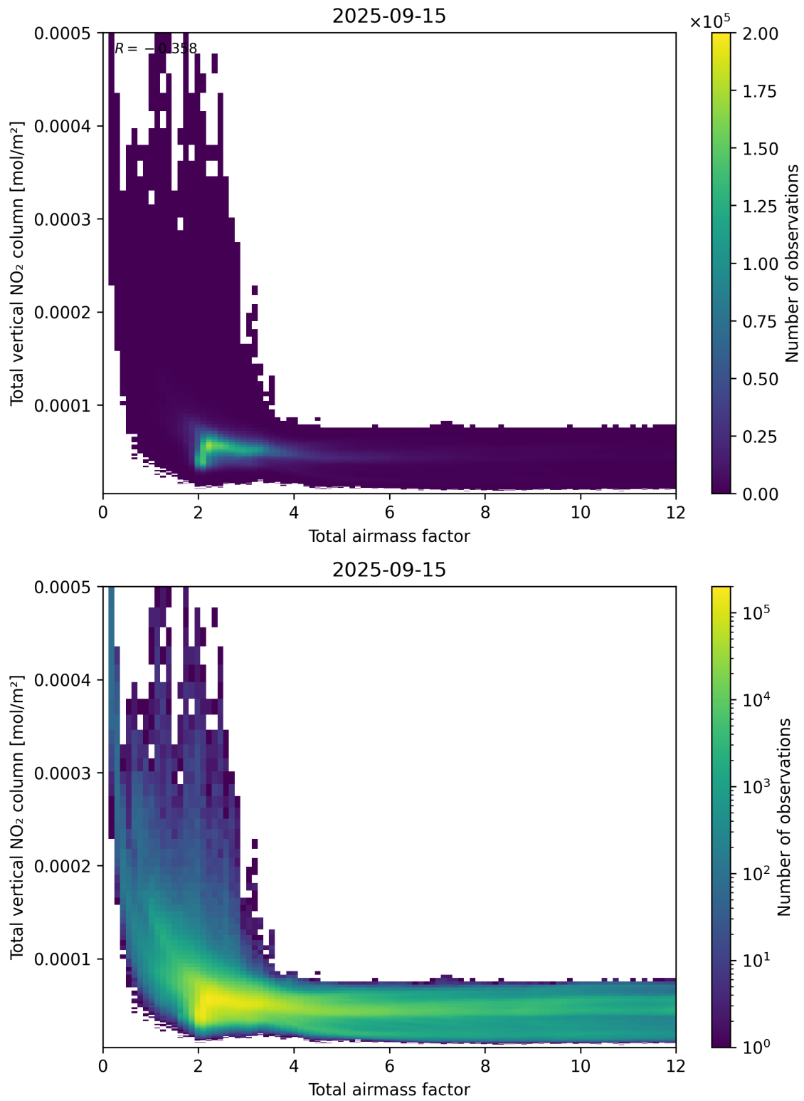
Figure 67: Scatter density plot of “Total airmass factor” against “Total vertical NO 2 column” for 2025-09-15 to 2025-09-16.
