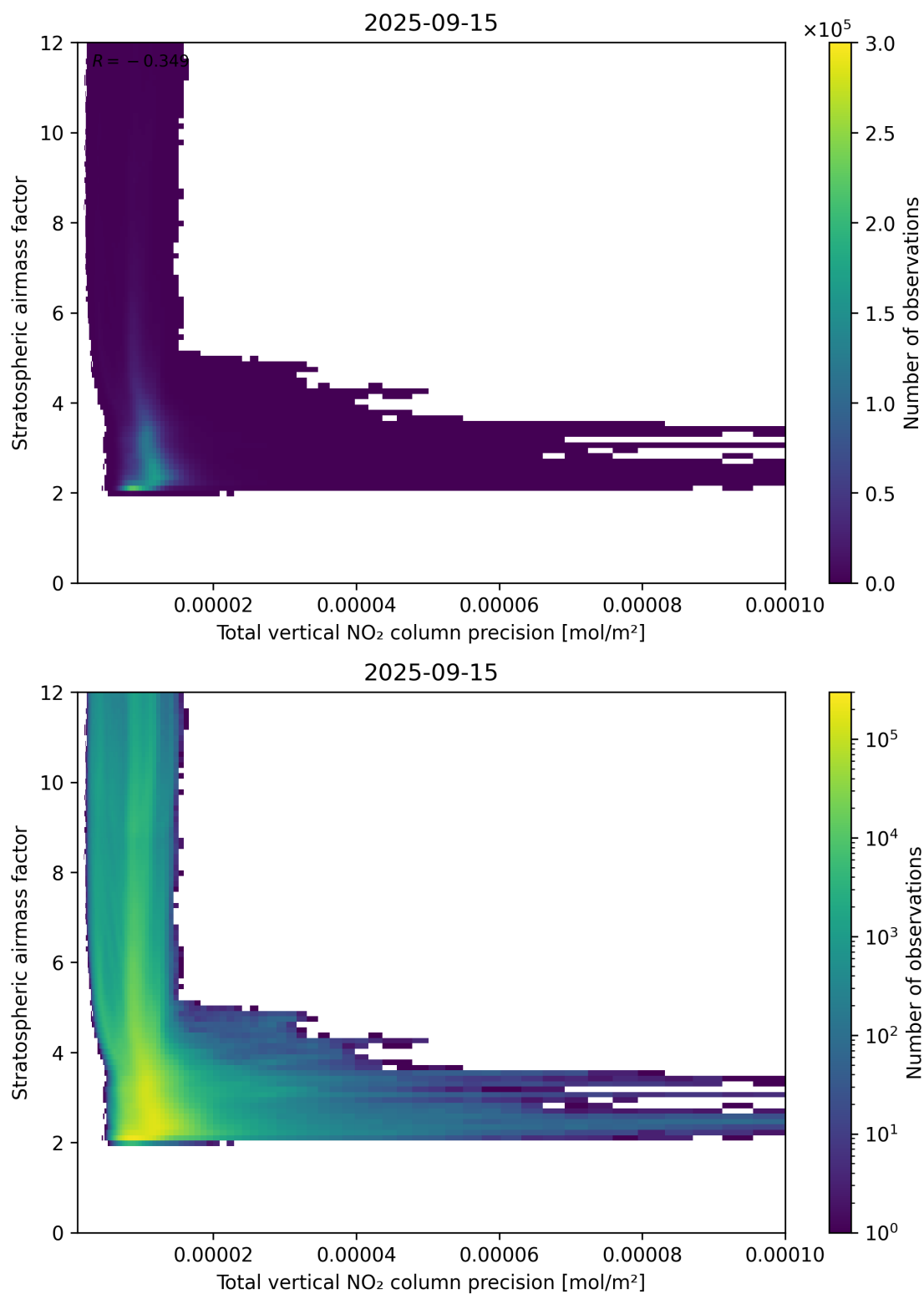
Figure 115: Scatter density plot of “Total vertical NO 2 column precision” against “Stratospheric airmass factor” for 2025-09-15 to 2025-09-16.
