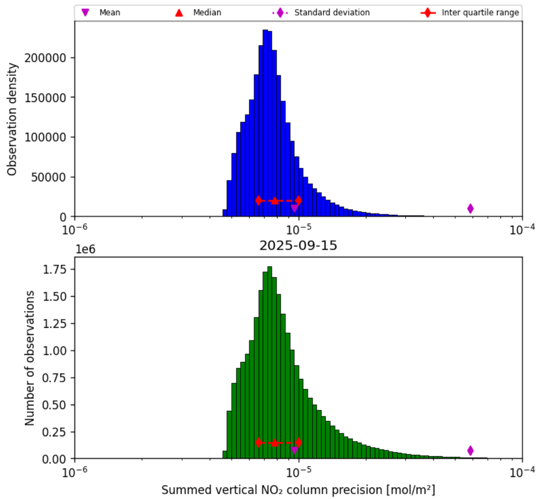
Figure 41: Histogram of “Summed vertical NO 2 column precision” for 2025-09-15 to 2025-09-16
