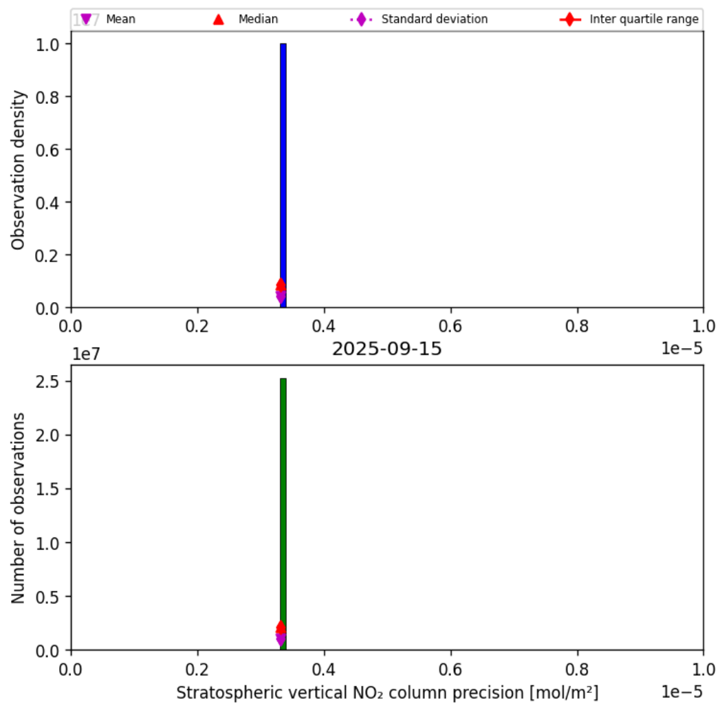
Figure 37: Histogram of “Stratospheric vertical NO 2 column precision” for 2025-09-15 to 2025-09-16
