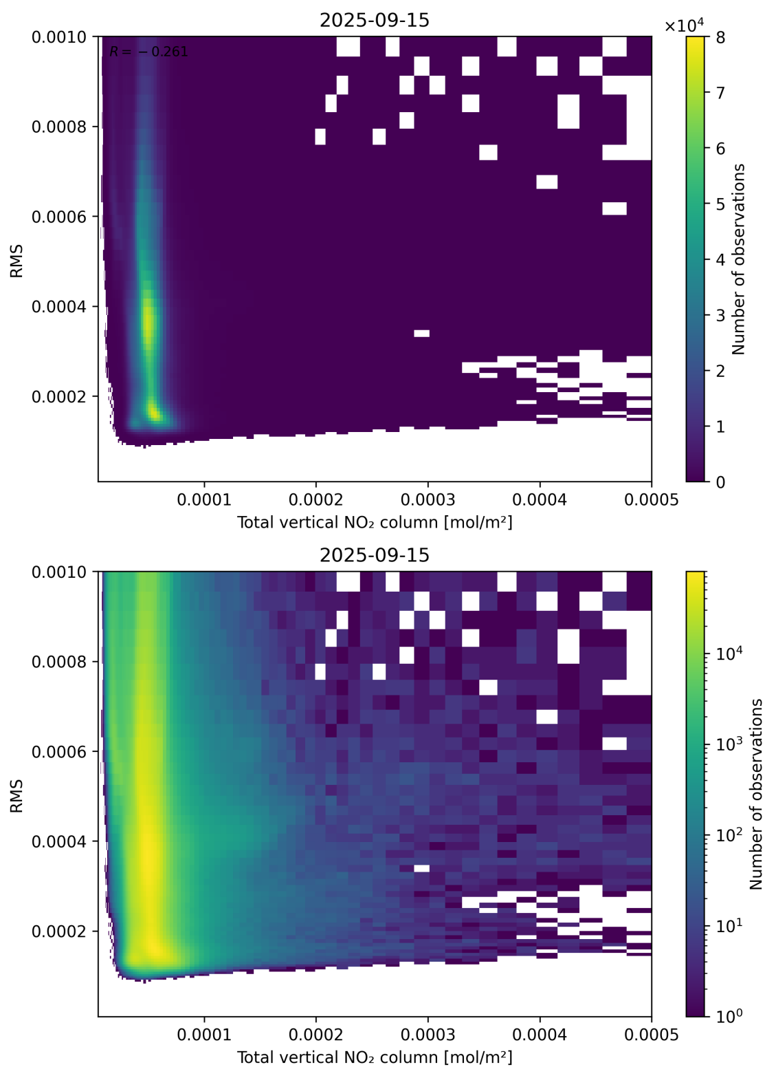
Figure 120: Scatter density plot of “Total vertical NO 2 column” against “RMS” for 2025-09-15 to 2025-09-16.
