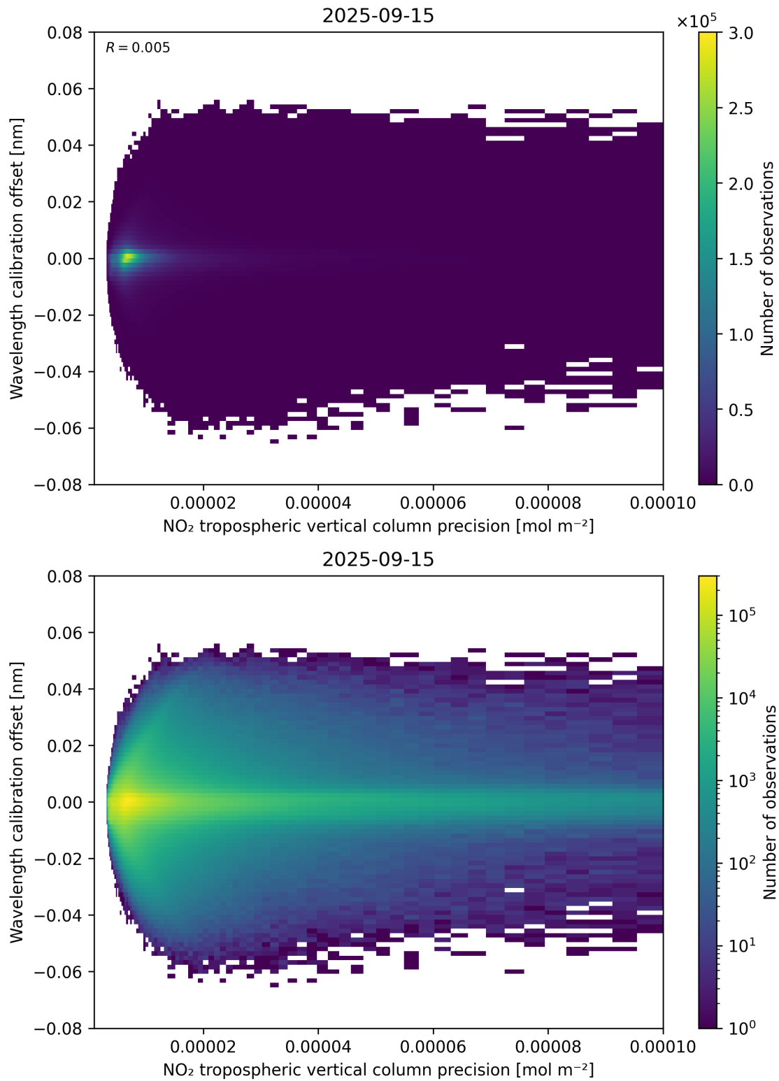
Figure 141: Scatter density plot of “NO 2 tropospheric vertical column precision” against “Wavelength calibration offset” for 2025-09-15 to 2025-09-16.
