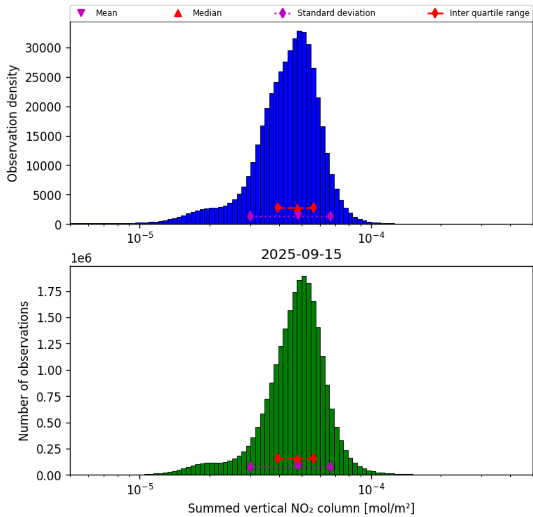
Figure 40: Histogram of “Summed vertical NO 2 column” for 2025-09-15 to 2025-09-16
