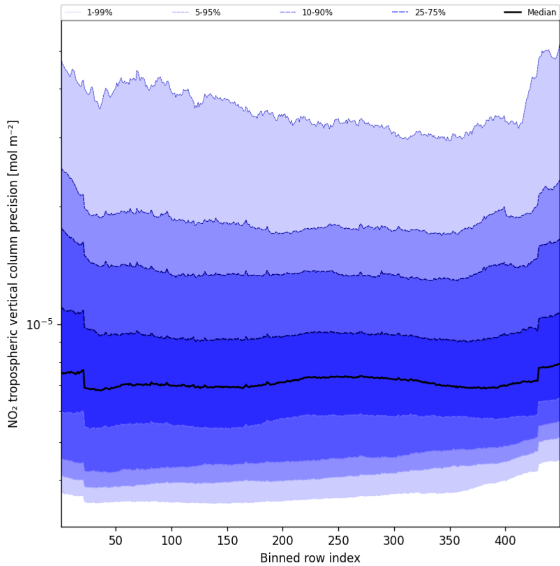
Figure 47: Along track statistics of “NO 2 tropospheric vertical column precision” for 2025-09-15 to 2025-09-16
