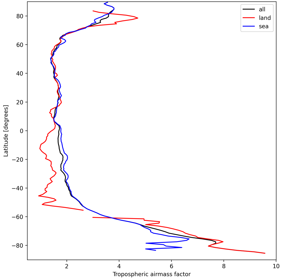
Figure 14: Zonal average of “Tropospheric airmass factor” for 2025-09-15 to 2025-09-16.
