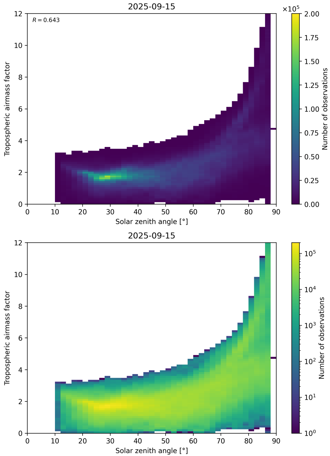
Figure 147: Scatter density plot of “Solar zenith angle” against “Tropospheric airmass factor” for 2025-09-15 to 2025-09-16.
