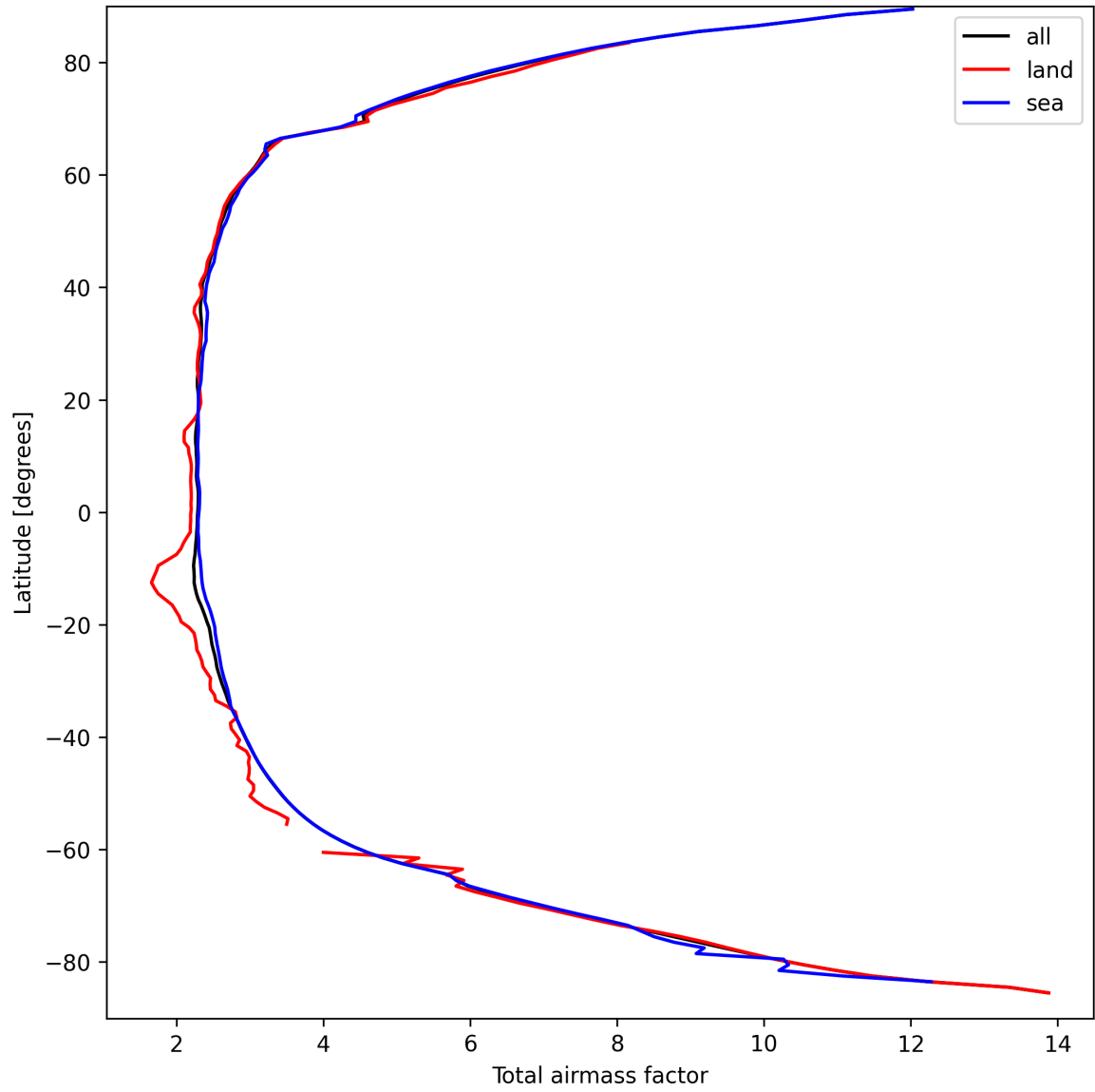
Figure 15: Zonal average of “Total airmass factor” for 2025-09-15 to 2025-09-16.
