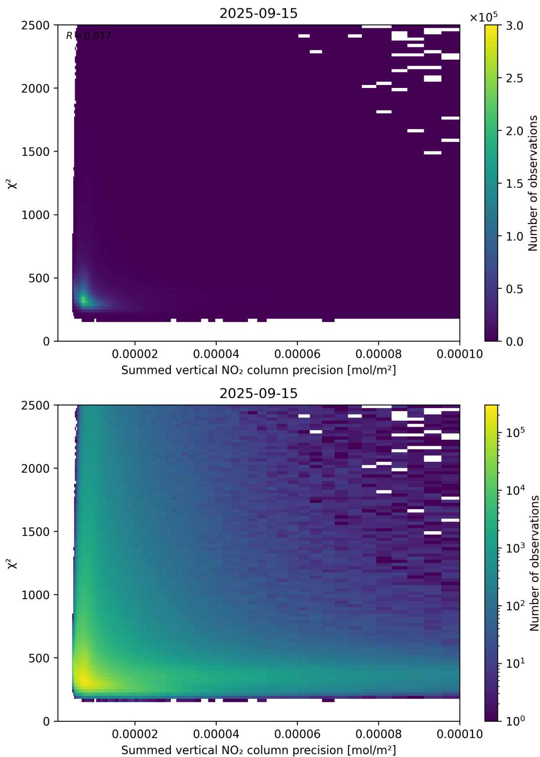
Figure 107: Scatter density plot of “Summed vertical NO 2 column precision” against “ \chi^2 ” for 2025-09-15 to 2025-09-16.
