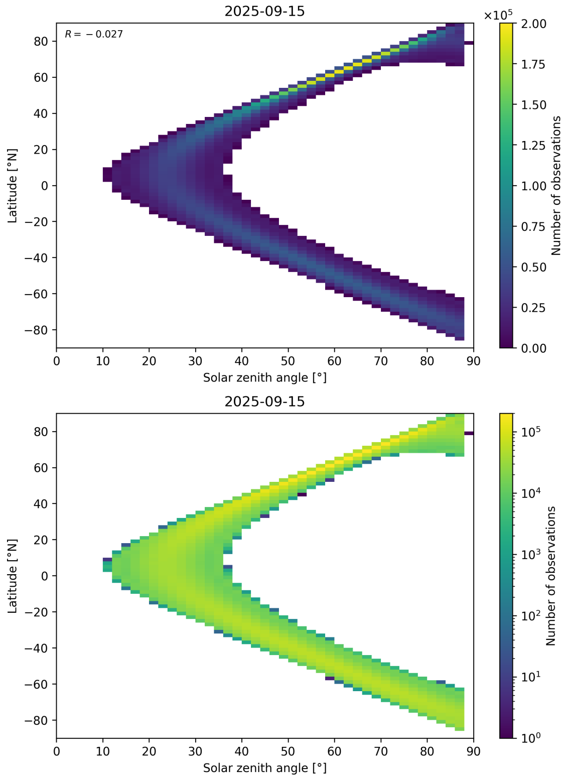
Figure 149: Scatter density plot of “Solar zenith angle” against “Latitude” for 2025-09-15 to 2025-09-16.
