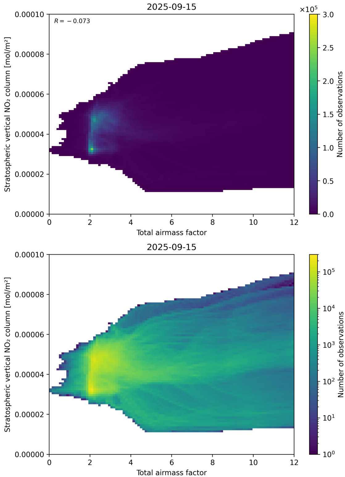
Figure 64: Scatter density plot of “Total airmass factor” against “Stratospheric vertical NO 2 column” for 2025-09-15 to 2025-09-16.
