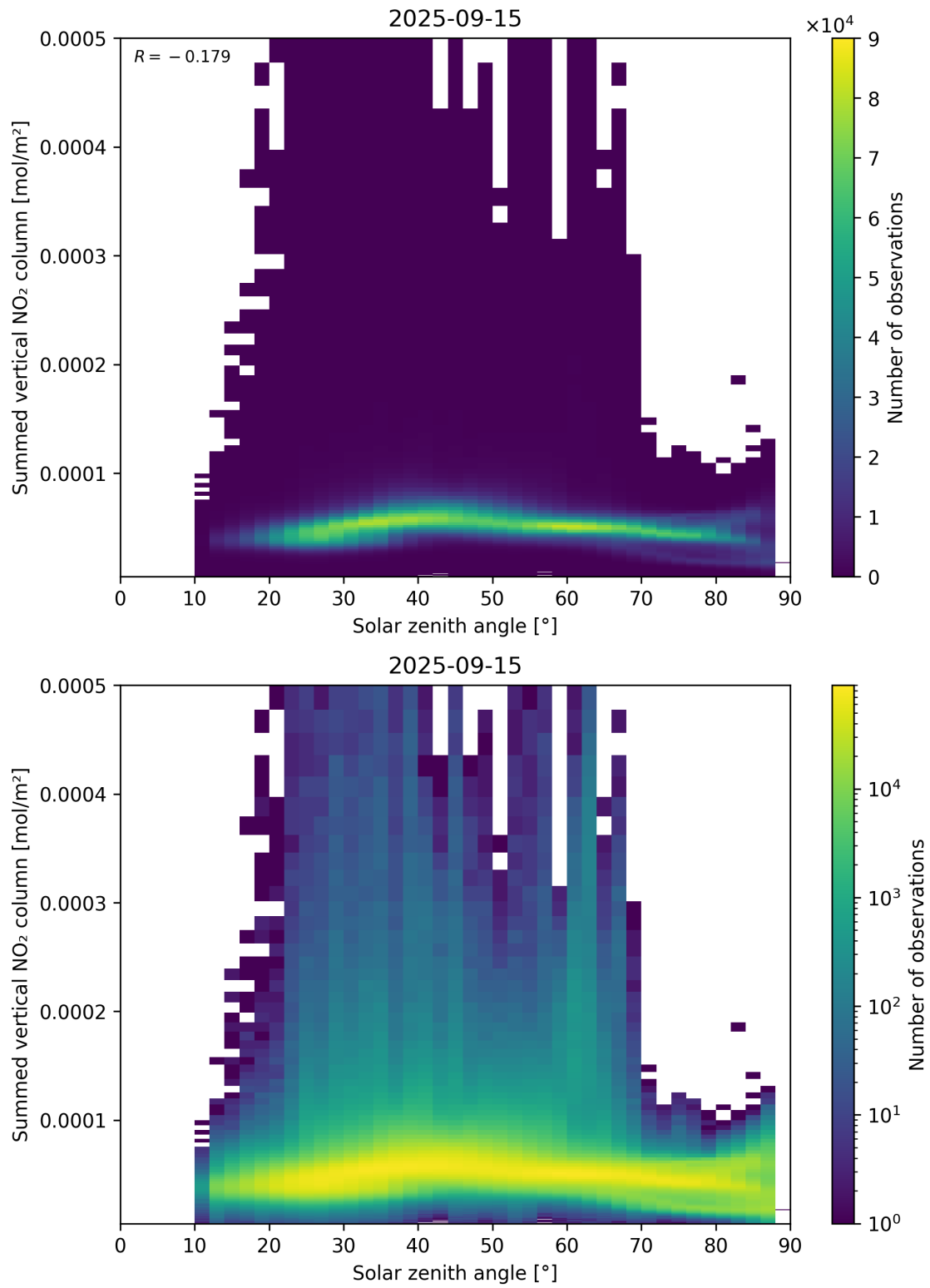
Figure 151: Scatter density plot of “Solar zenith angle” against “Summed vertical NO 2 column” for 2025-09-15 to 2025-09-16.
