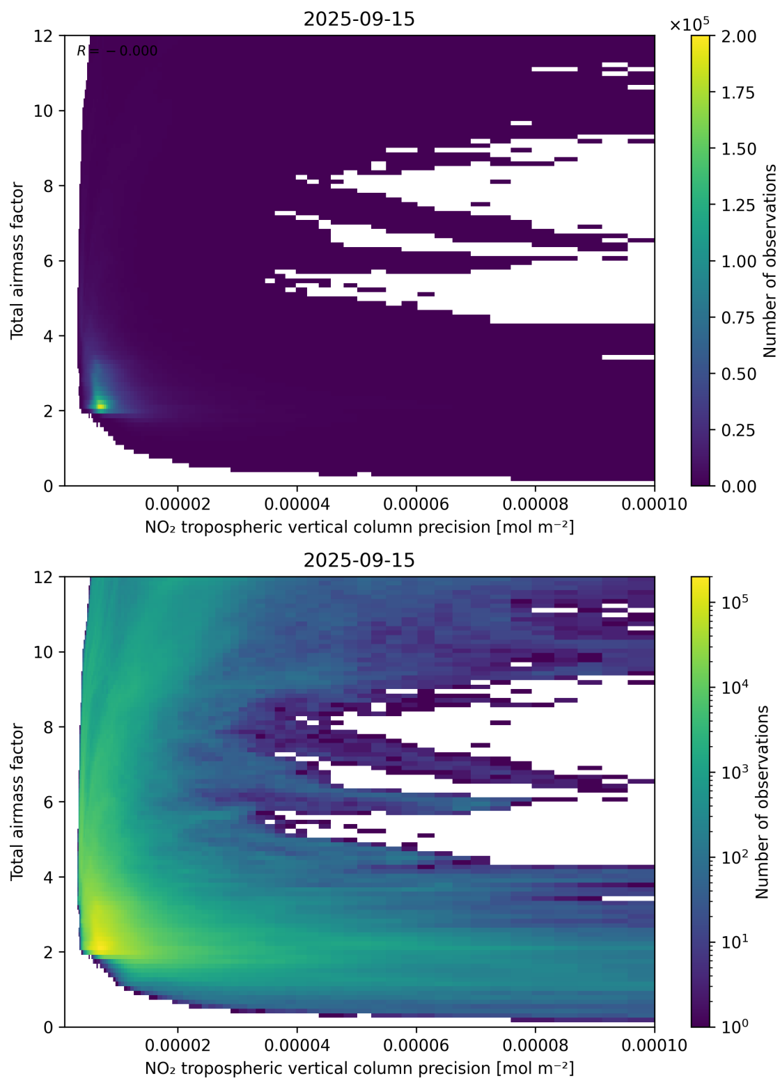
Figure 132: Scatter density plot of “NO 2 tropospheric vertical column precision” against “Total air mass factor” for 2025-09-15 to 2025-09-16.
