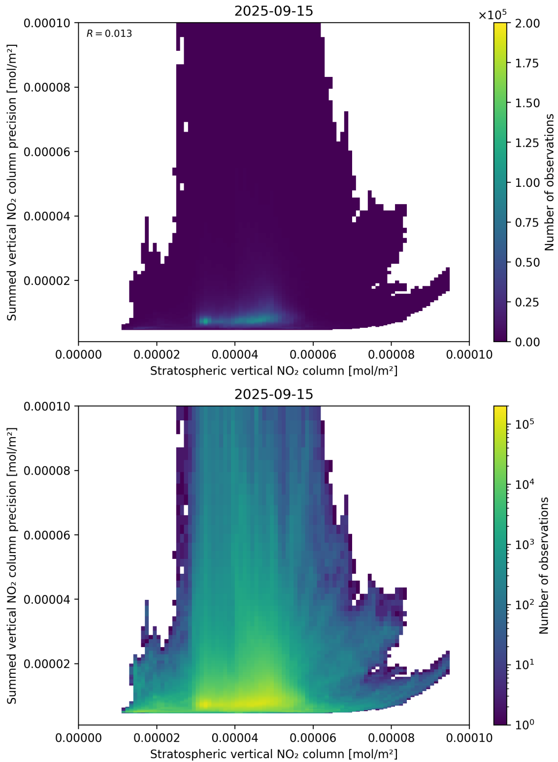
Figure 99: Scatter density plot of “Stratospheric vertical NO 2 column” against “Summed vertical NO 2 column precision” for 2025-09-15 to 2025-09-16.
