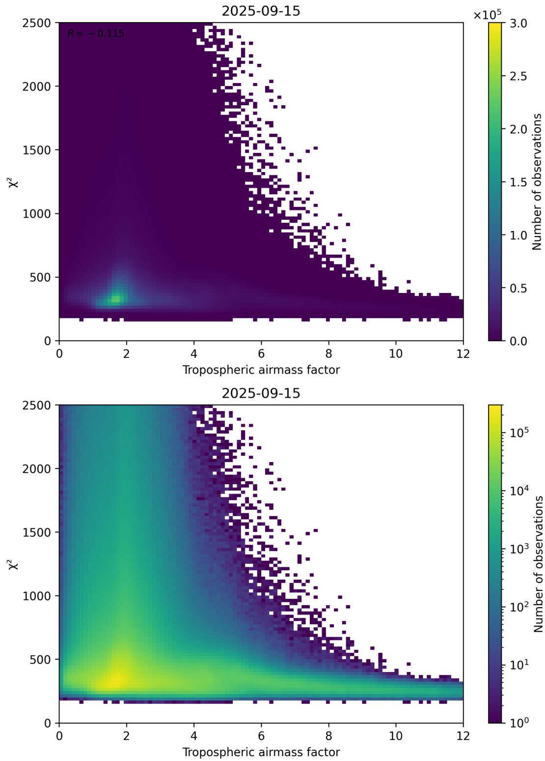
Figure 73: Scatter density plot of “Tropospheric airmass factor” against “ \chi^2 ” for 2025-09-15 to 2025-09-16.
