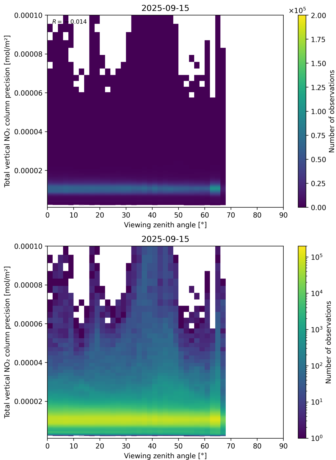
Figure 168: Scatter density plot of “Viewing zenith angle” against “Total vertical NO 2 column precision” for 2025-09-15 to 2025-09-16.
