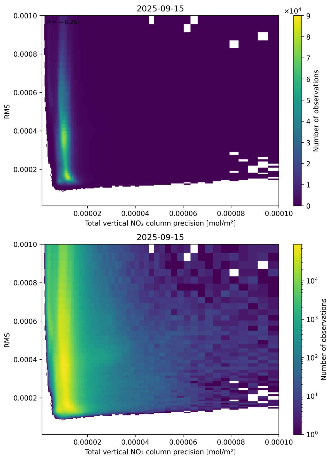
Figure 119: Scatter density plot of “Total vertical NO 2 column precision” against “RMS” for 2025-09-15 to 2025-09-16.
