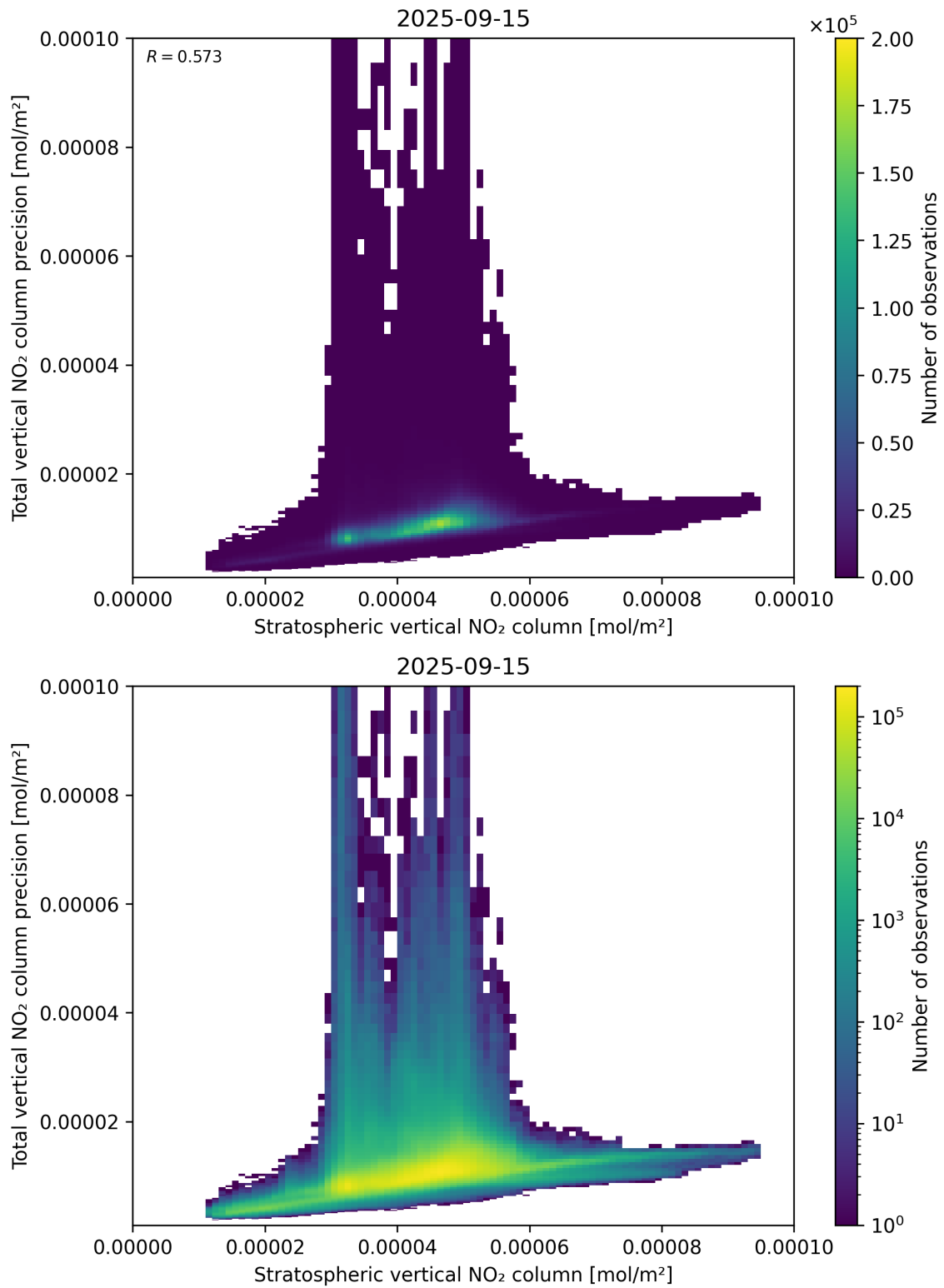
Figure 101: Scatter density plot of “Stratospheric vertical NO 2 column” against “Total vertical NO 2 column precision” for 2025-09-15 to 2025-09-16.
