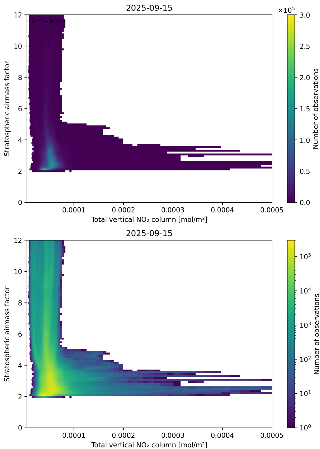
Figure 110: Scatter density plot of “Total vertical NO 2 column” against “Stratospheric airmass factor” for 2025-09-15 to 2025-09-16.
