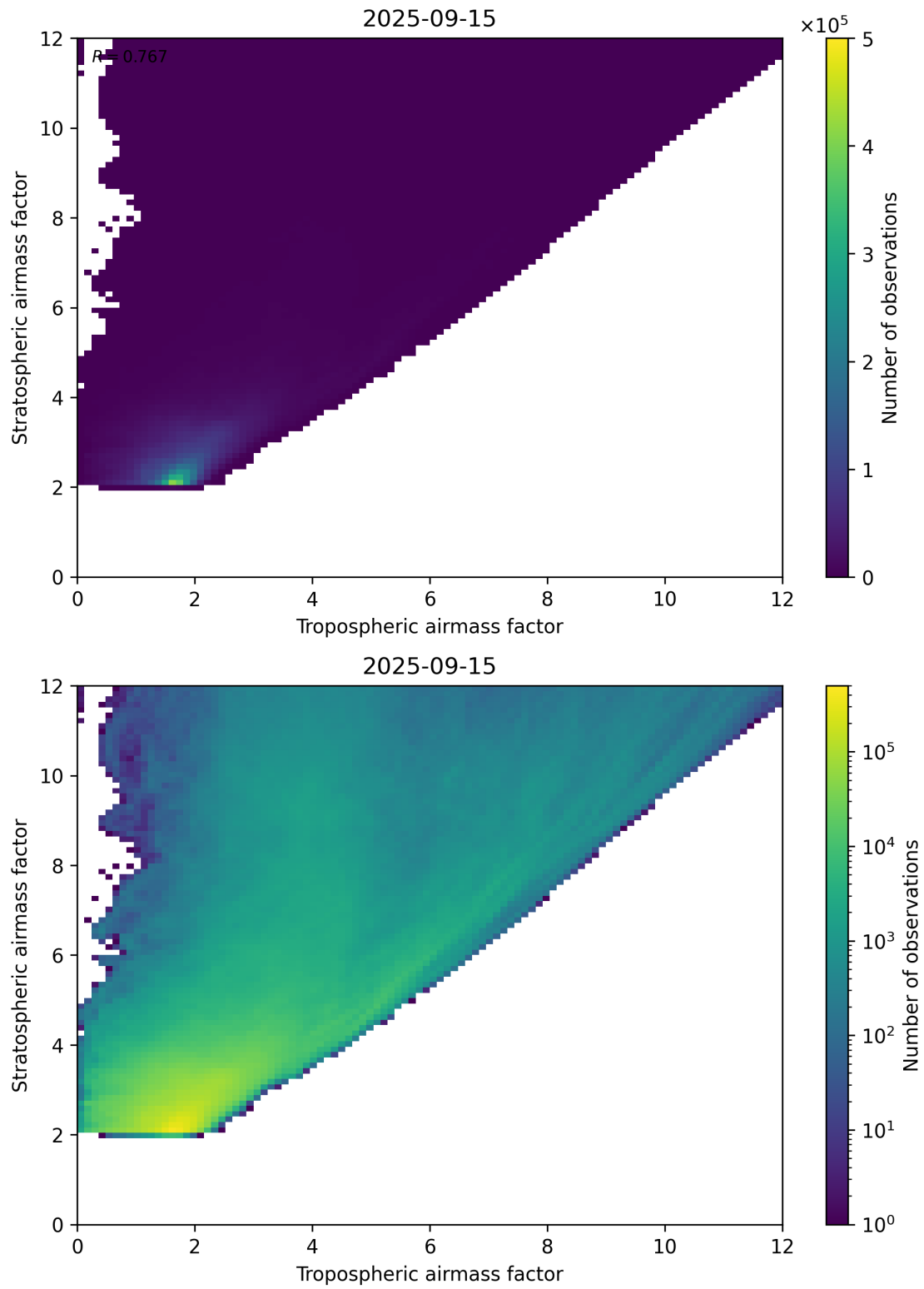
Figure 71: Scatter density plot of “Tropospheric airmass factor” against “Stratospheric airmass factor” for 2025-09-15 to 2025-09-16.
