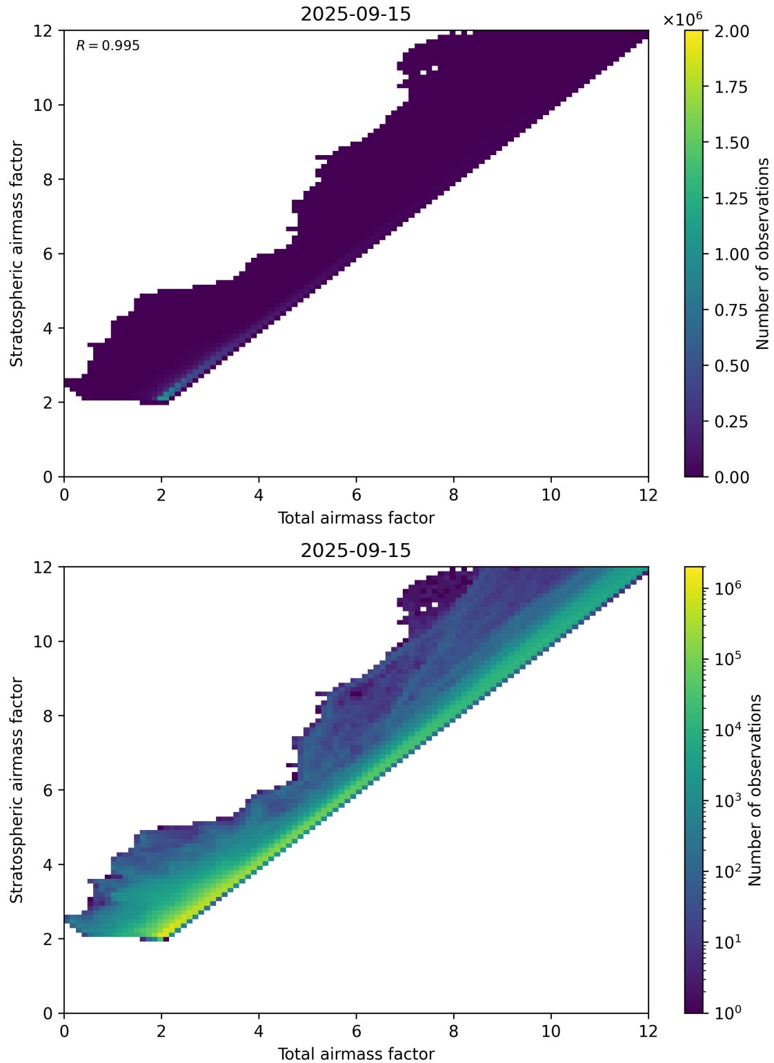
Figure 62: Scatter density plot of “Total airmass factor” against “Stratospheric airmass factor” for 2025-09-15 to 2025-09-16.
