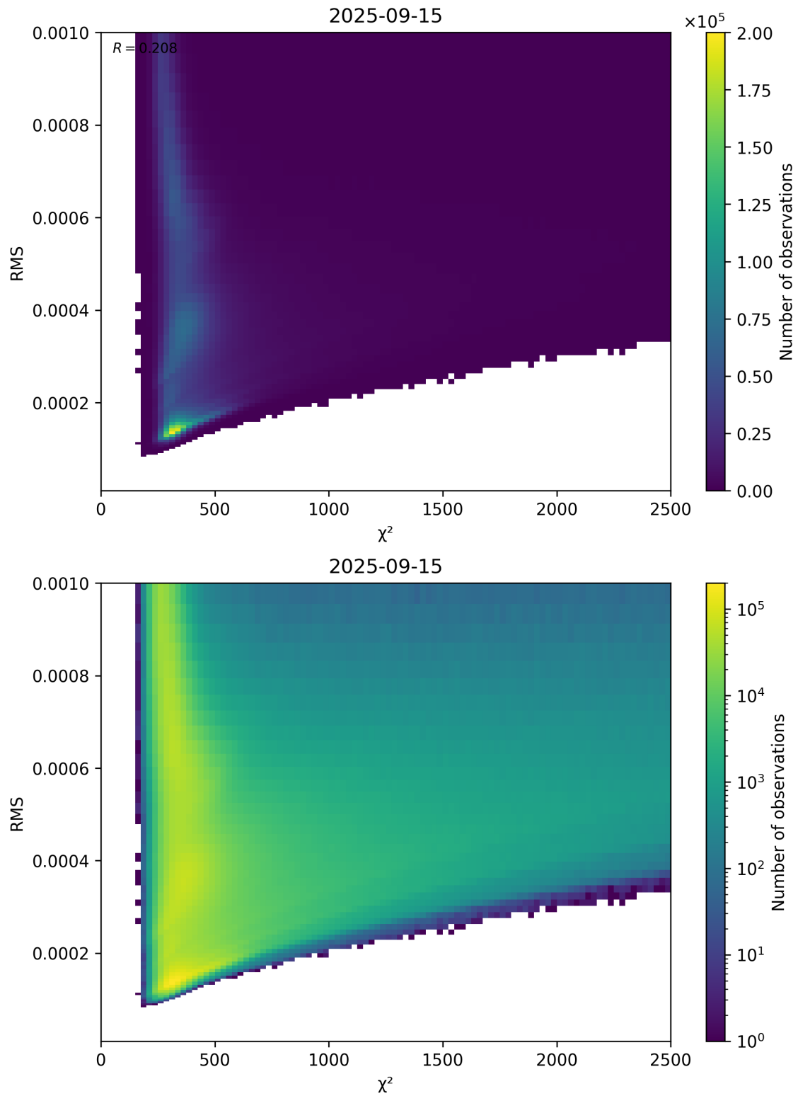
Figure 82: Scatter density plot of “ \chi^2 ” against “RMS” for 2025-09-15 to 2025-09-16.
