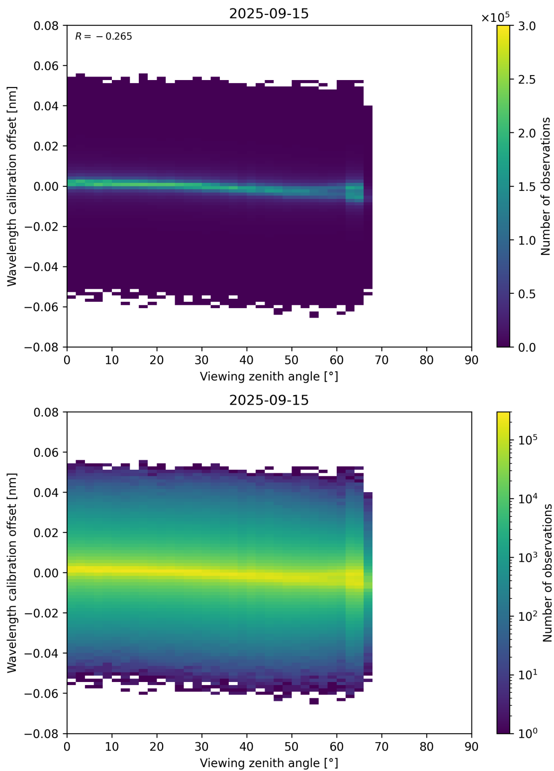
Figure 173: Scatter density plot of “Viewing zenith angle” against “Wavelength calibration offset” for 2025-09-15 to 2025-09-16.
