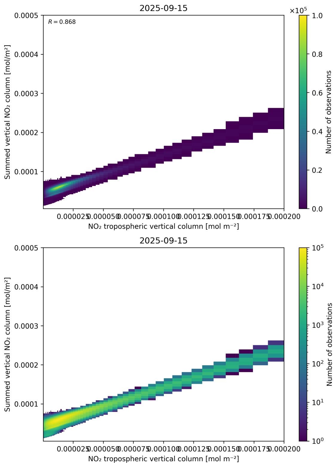
Figure 126: Scatter density plot of “NO 2 tropospheric vertical column” against “Summed vertical NO 2 column” for 2025-09-15 to 2025-09-16.
