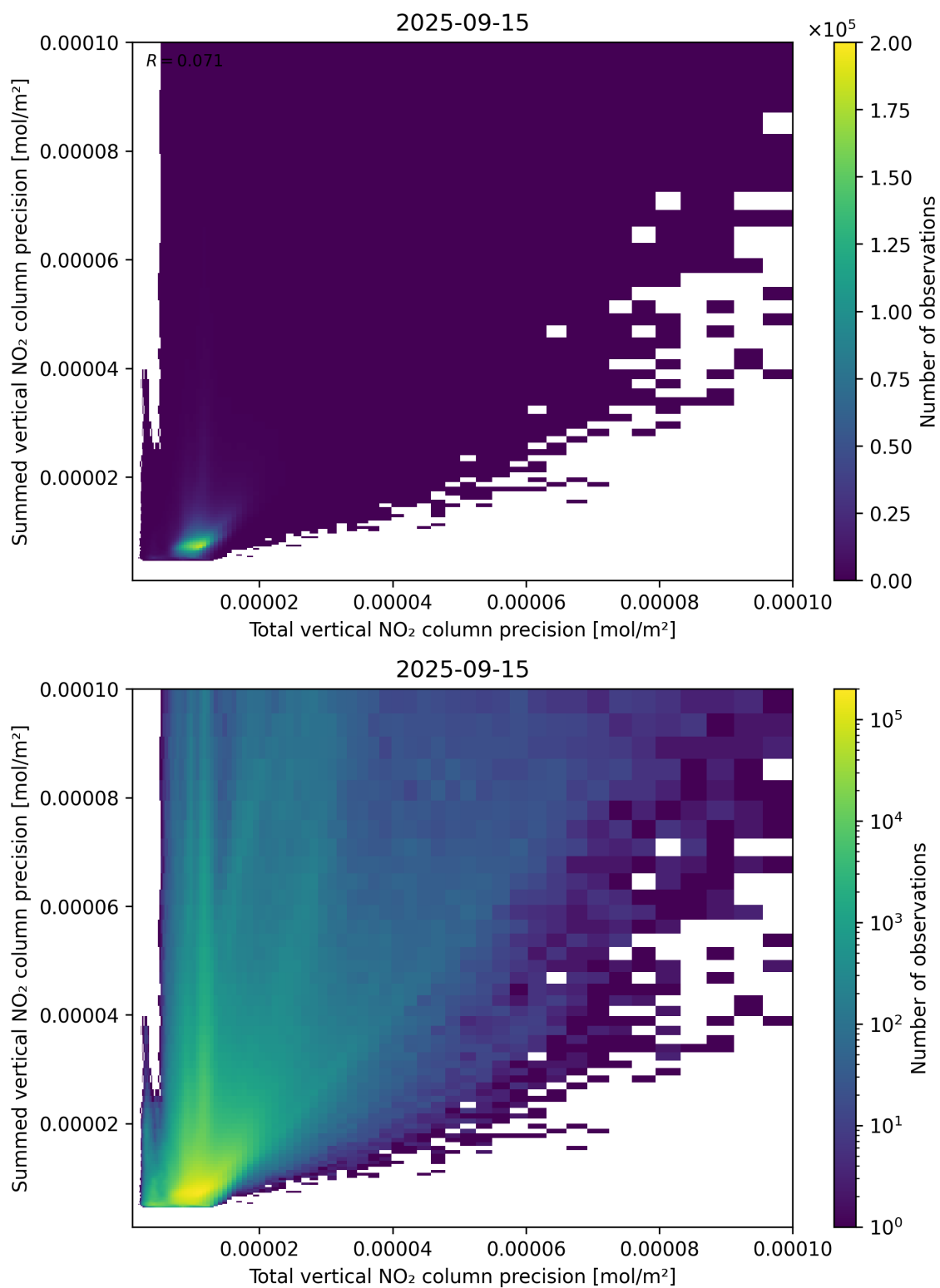
Figure 118: Scatter density plot of “Total vertical NO 2 column precision” against “Summed vertical NO 2 column precision” for 2025-09-15 to 2025-09-16.
