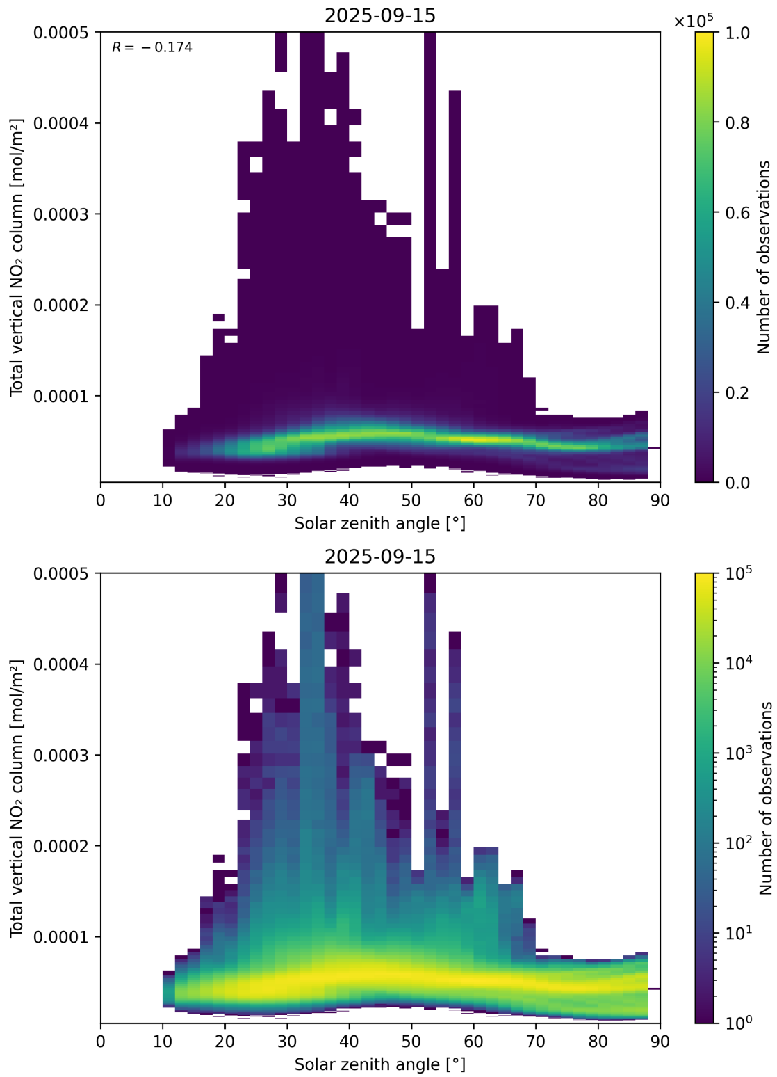
Figure 153: Scatter density plot of “Solar zenith angle” against “Total vertical NO 2 column” for 2025-09-15 to 2025-09-16.
