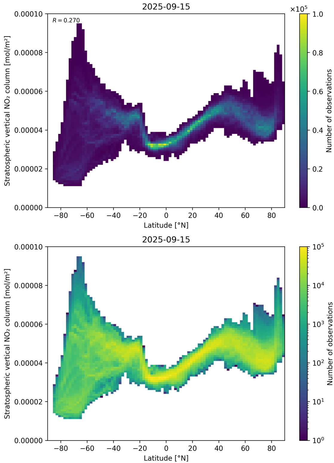
Figure 87: Scatter density plot of “Latitude” against “Stratospheric vertical NO 2 column” for 2025-09-15 to 2025-09-16.
