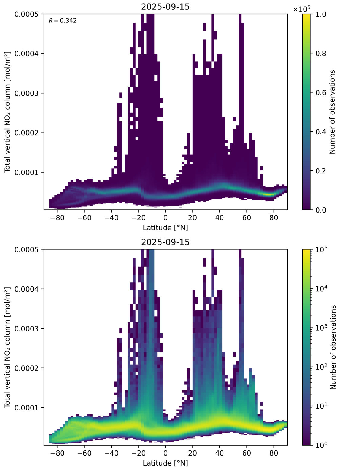
Figure 90: Scatter density plot of “Latitude” against “Total vertical NO 2 column” for 2025-09-15 to 2025-09-16.
