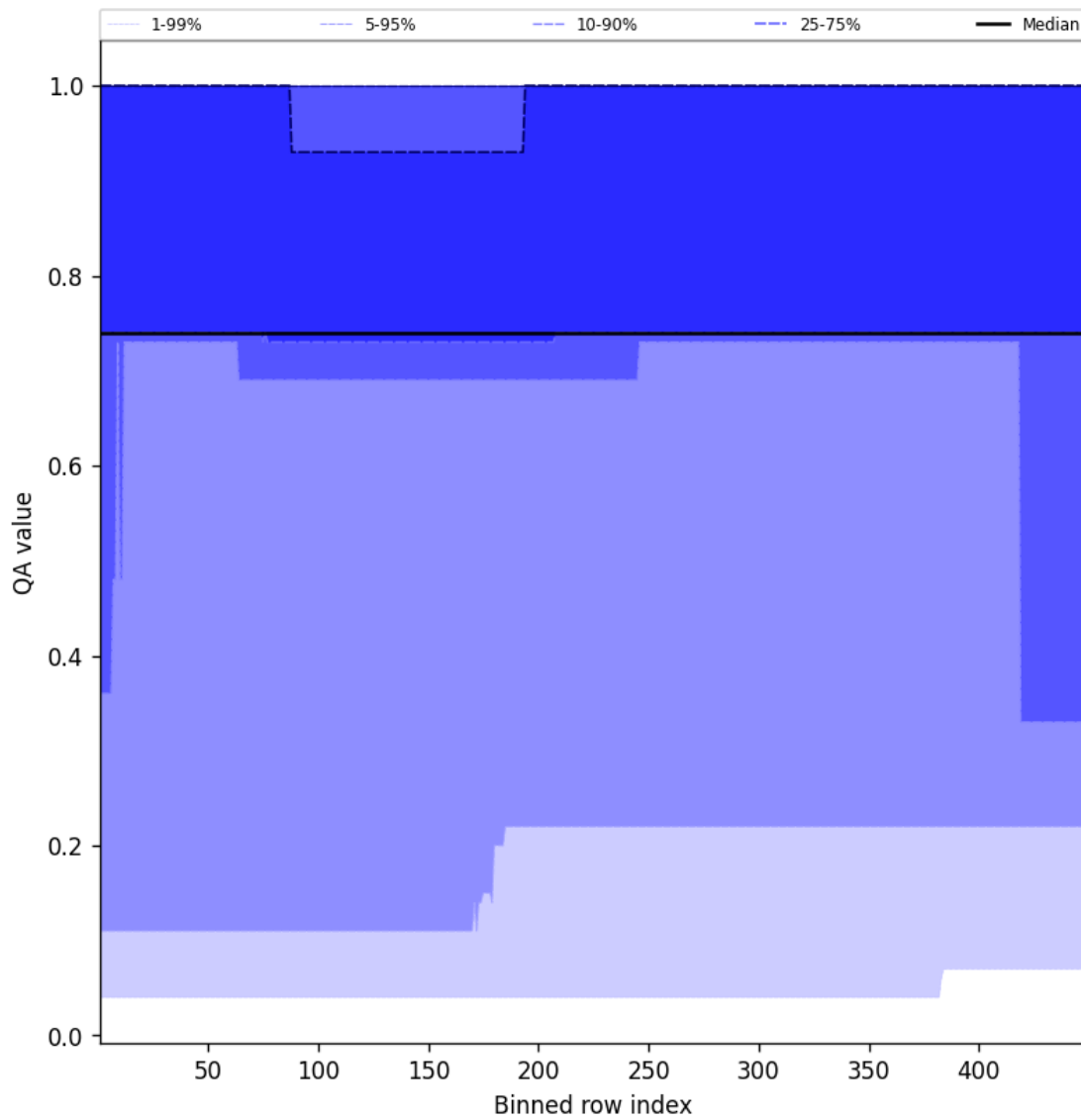
Figure 45: Along track statistics of “QA value” for 2025-09-15 to 2025-09-16
