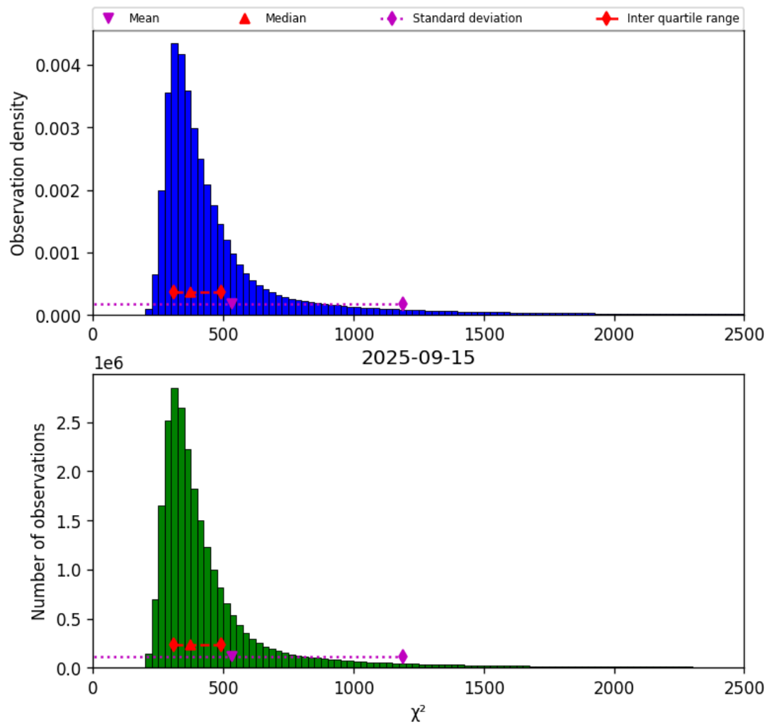
Figure 42: Histogram of “ \chi^2 ” for 2025-09-15 to 2025-09-16
