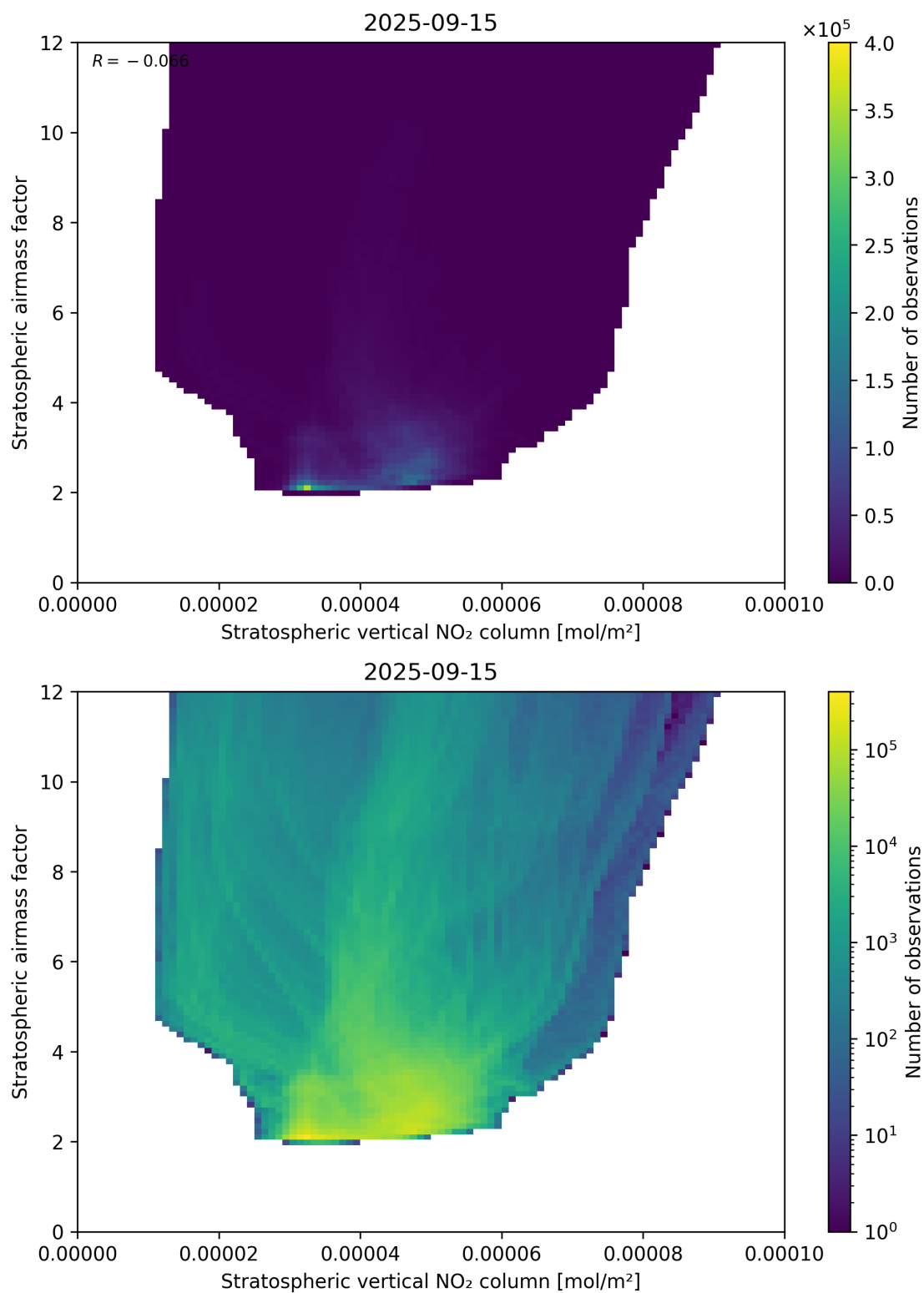
Figure 96: Scatter density plot of “Stratospheric vertical NO 2 column” against “Stratospheric airmass factor” for 2025-09-15 to 2025-09-16.
