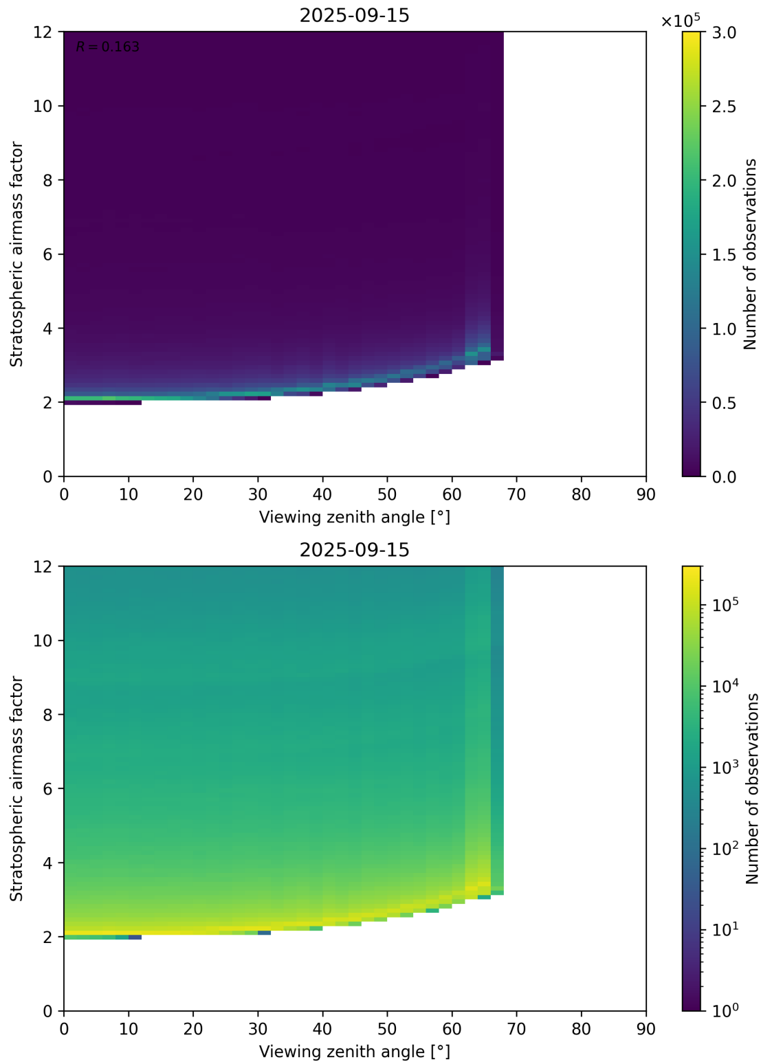
Figure 159: Scatter density plot of “Viewing zenith angle” against “Stratospheric airmass factor” for 2025-09-15 to 2025-09-16.
