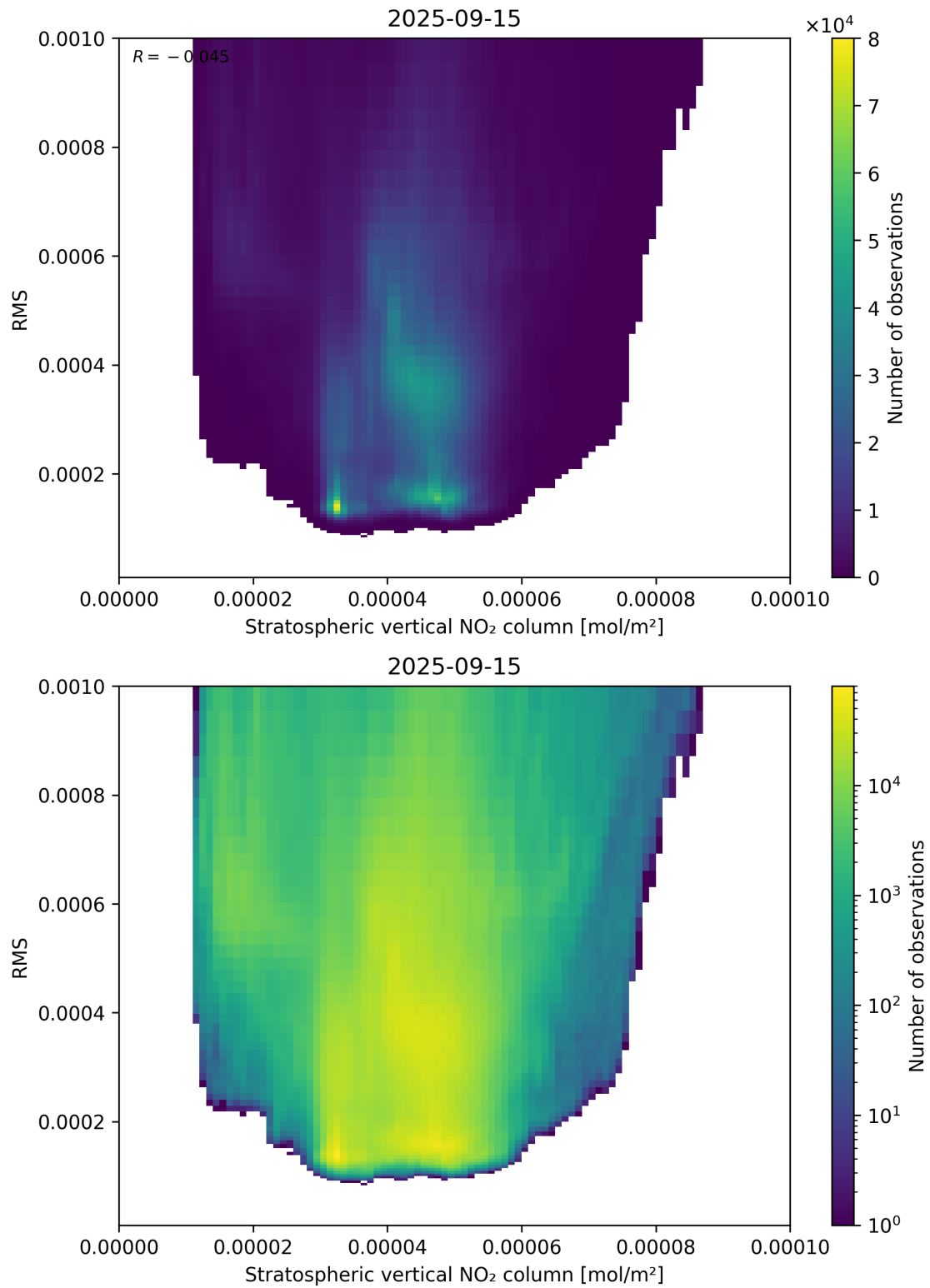
Figure 102: Scatter density plot of “Stratospheric vertical NO 2 column” against “RMS” for 2025-09-15 to 2025-09-16.
