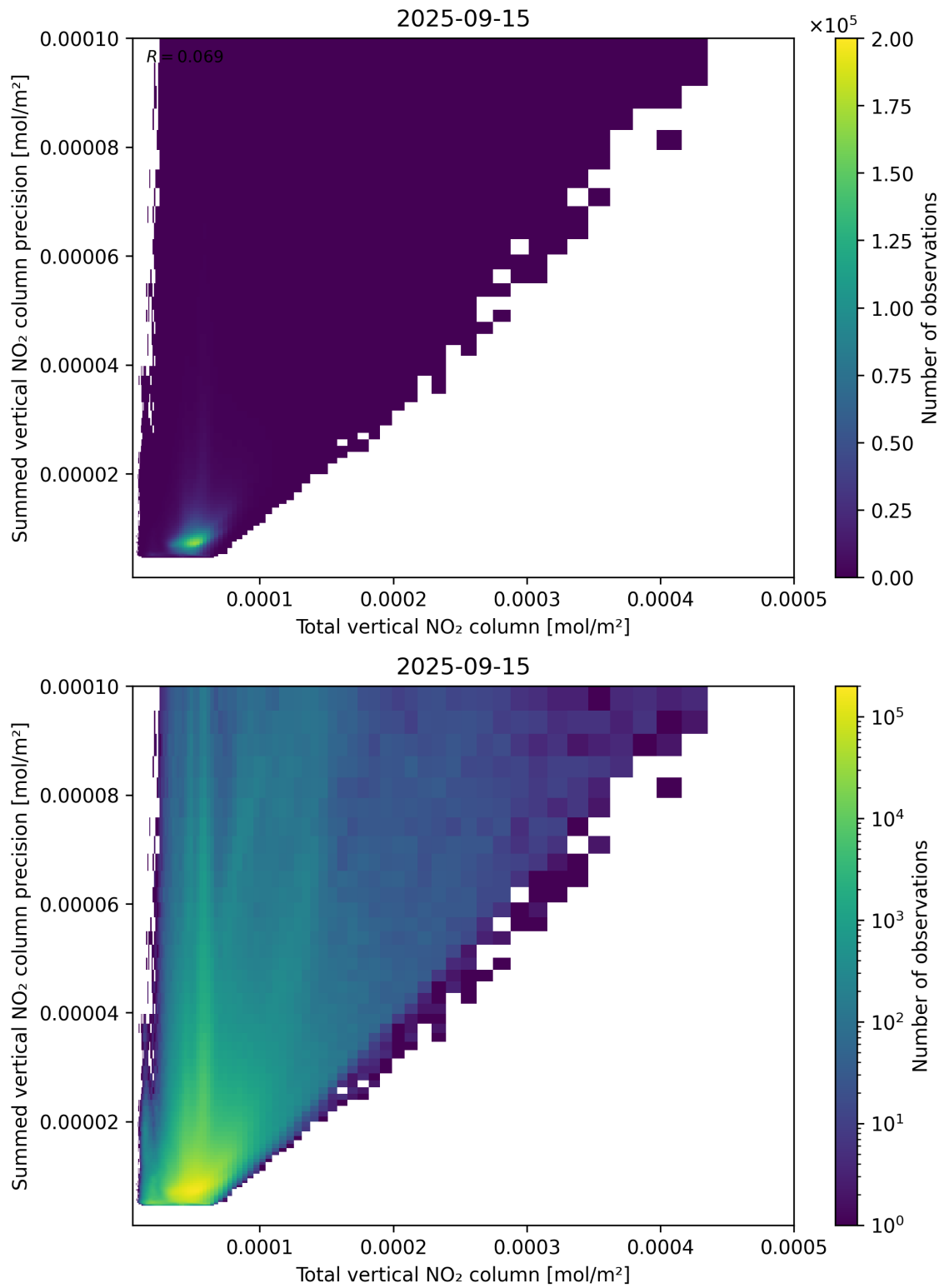
Figure 113: Scatter density plot of “Total vertical NO 2 column” against “Summed vertical NO 2 column precision” for 2025-09-15 to 2025-09-16.
