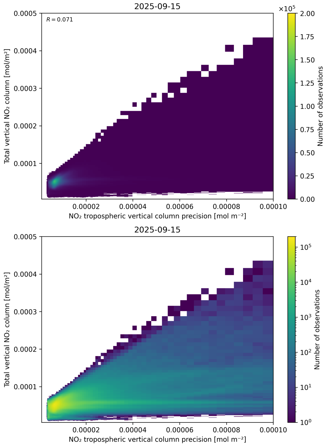
Figure 138: Scatter density plot of “NO 2 tropospheric vertical column precision” against “Total vertical NO 2 column” for 2025-09-15 to 2025-09-16.
