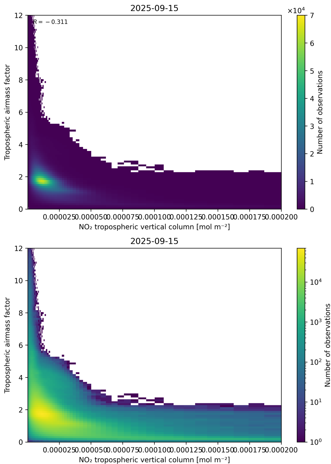
Figure 123: Scatter density plot of “NO 2 tropospheric vertical column” against “Tropospheric air mass factor” for 2025-09-15 to 2025-09-16.
