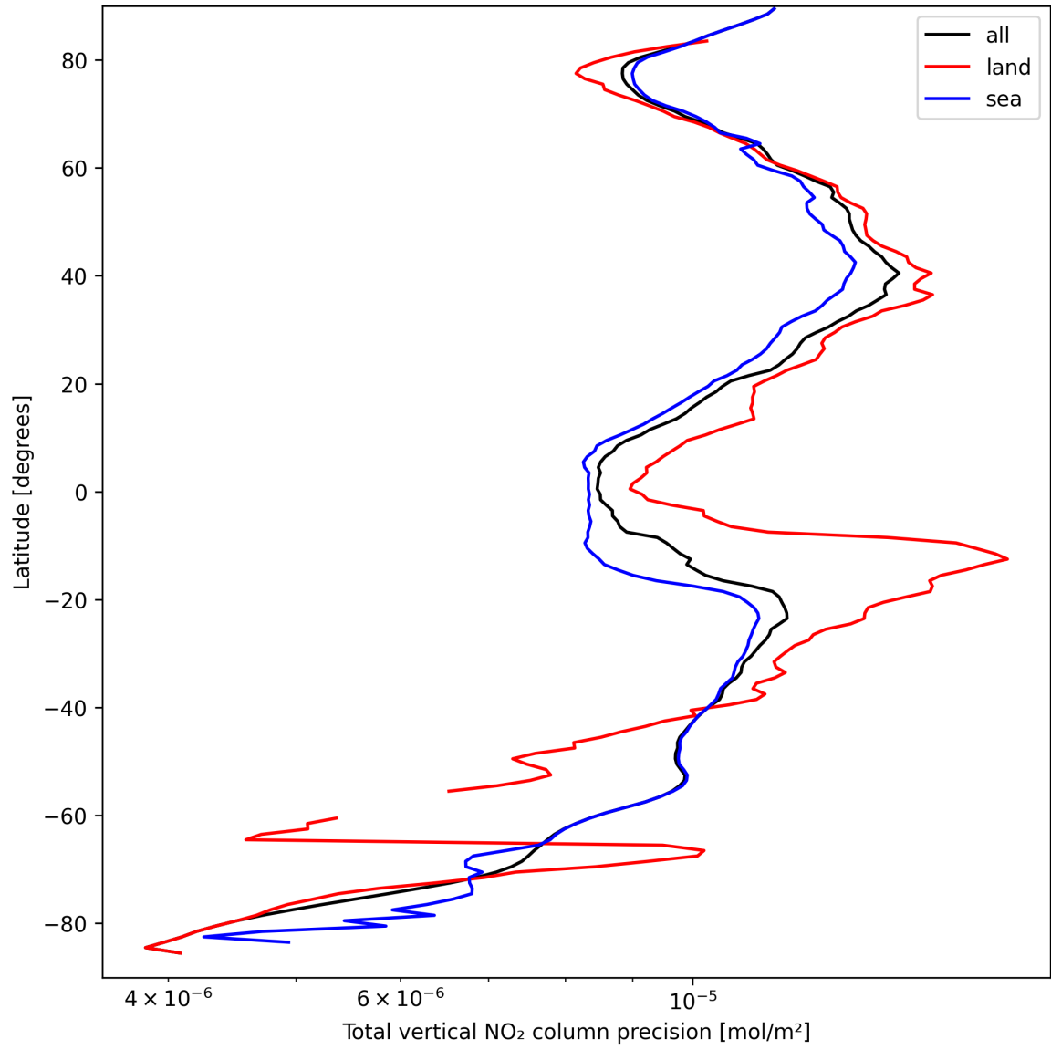
Figure 22: Zonal average of “Total vertical NO 2 column precision” for 2025-09-15 to 2025-09-16.
