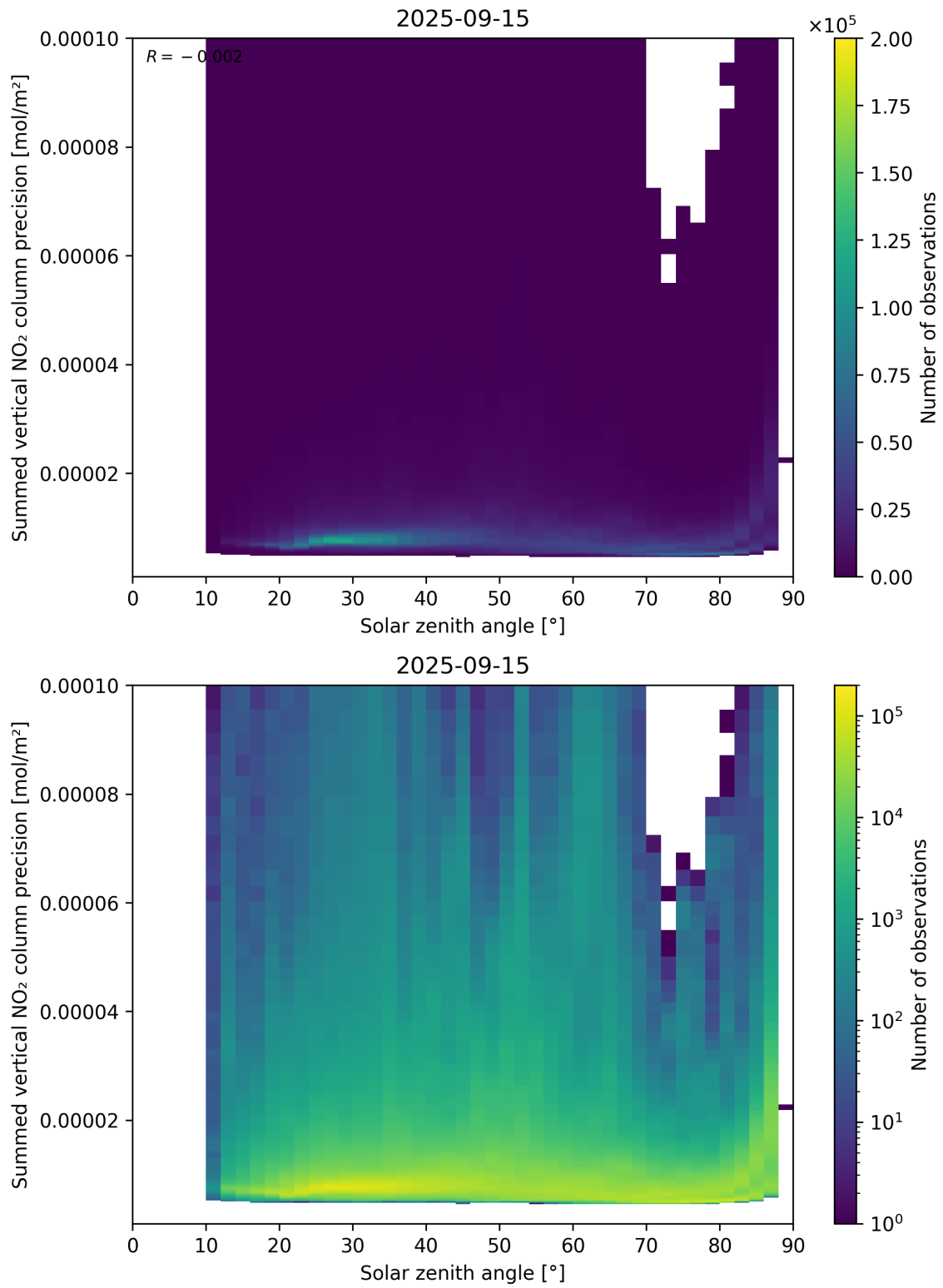
Figure 152: Scatter density plot of “Solar zenith angle” against “Summed vertical NO 2 column precision” for 2025-09-15 to 2025-09-16.
