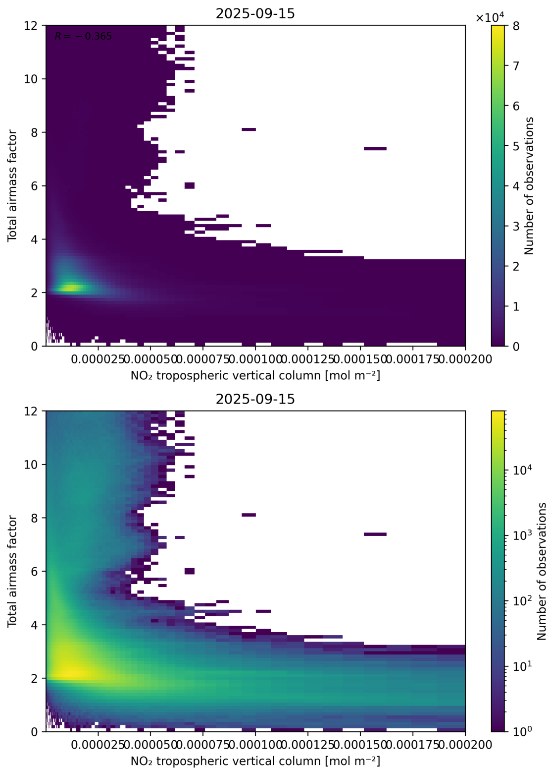
Figure 122: Scatter density plot of “NO 2 tropospheric vertical column” against “Total air mass factor” for 2025-09-15 to 2025-09-16.
