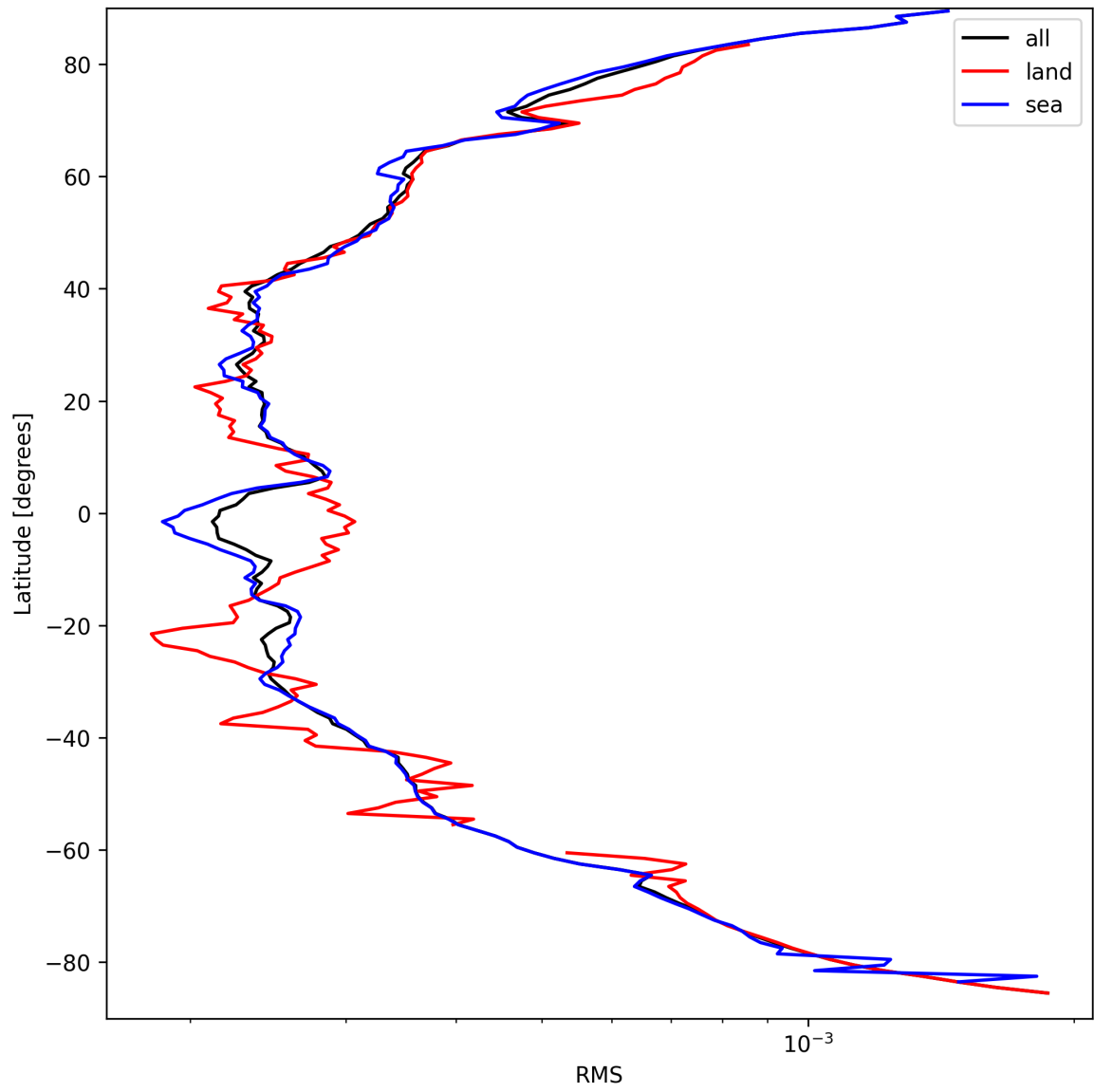
Figure 26: Zonal average of “RMS” for 2025-09-15 to 2025-09-16.
