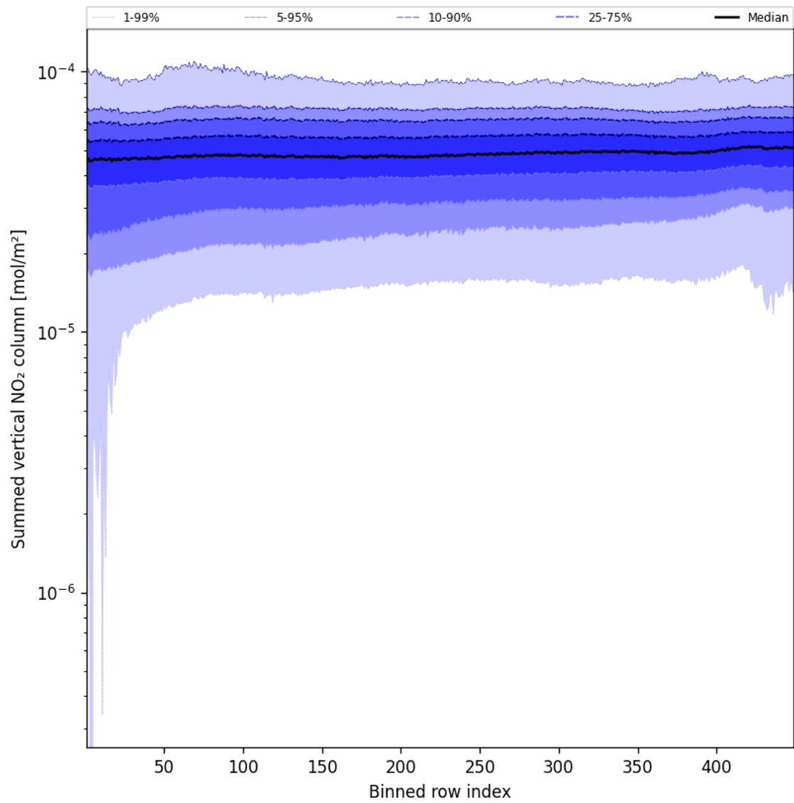
Figure 57: Along track statistics of “Summed vertical NO 2 column” for 2025-09-15 to 2025-09-16
