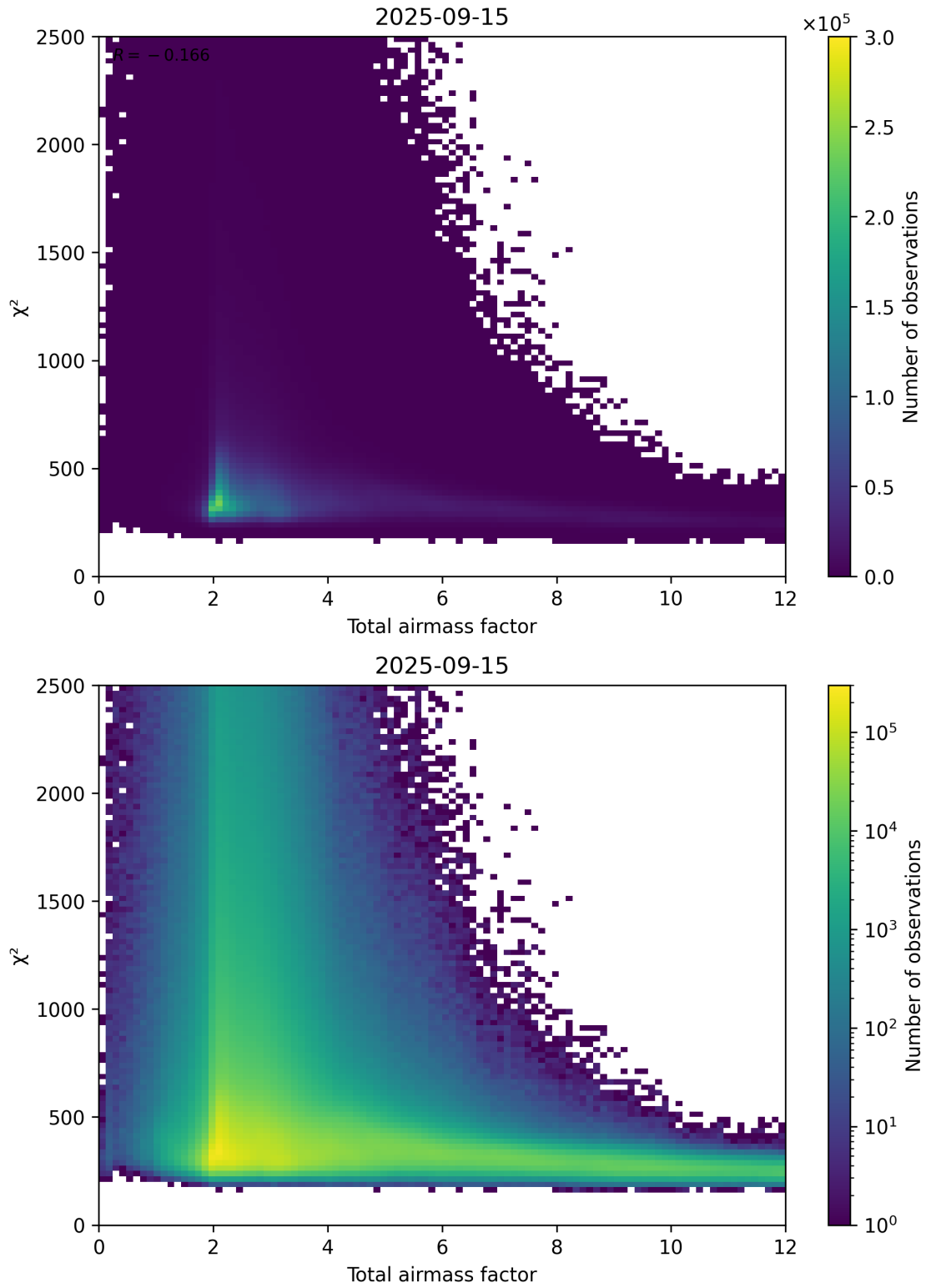
Figure 63: Scatter density plot of “Total airmass factor” against “ \chi^2 ” for 2025-09-15 to 2025-09-16.
