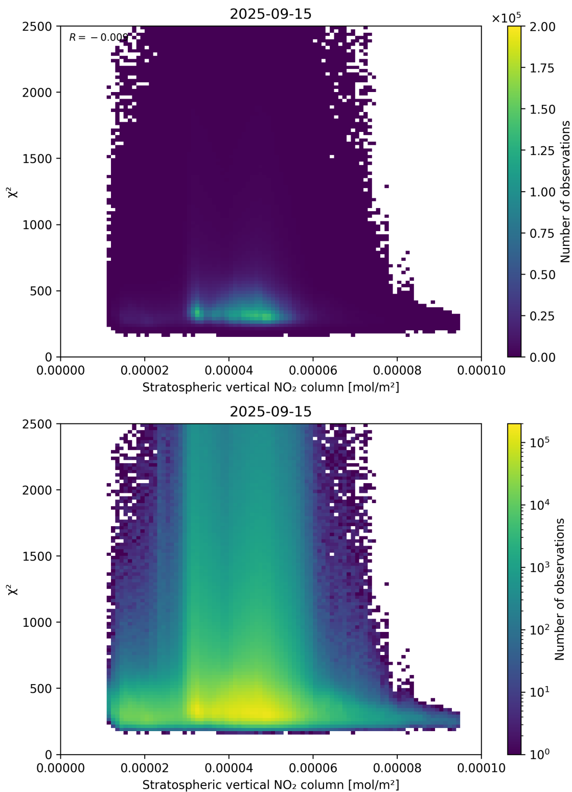
Figure 97: Scatter density plot of “Stratospheric vertical NO 2 column” against “ \chi^2 ” for 2025-09-15 to 2025-09-16.
