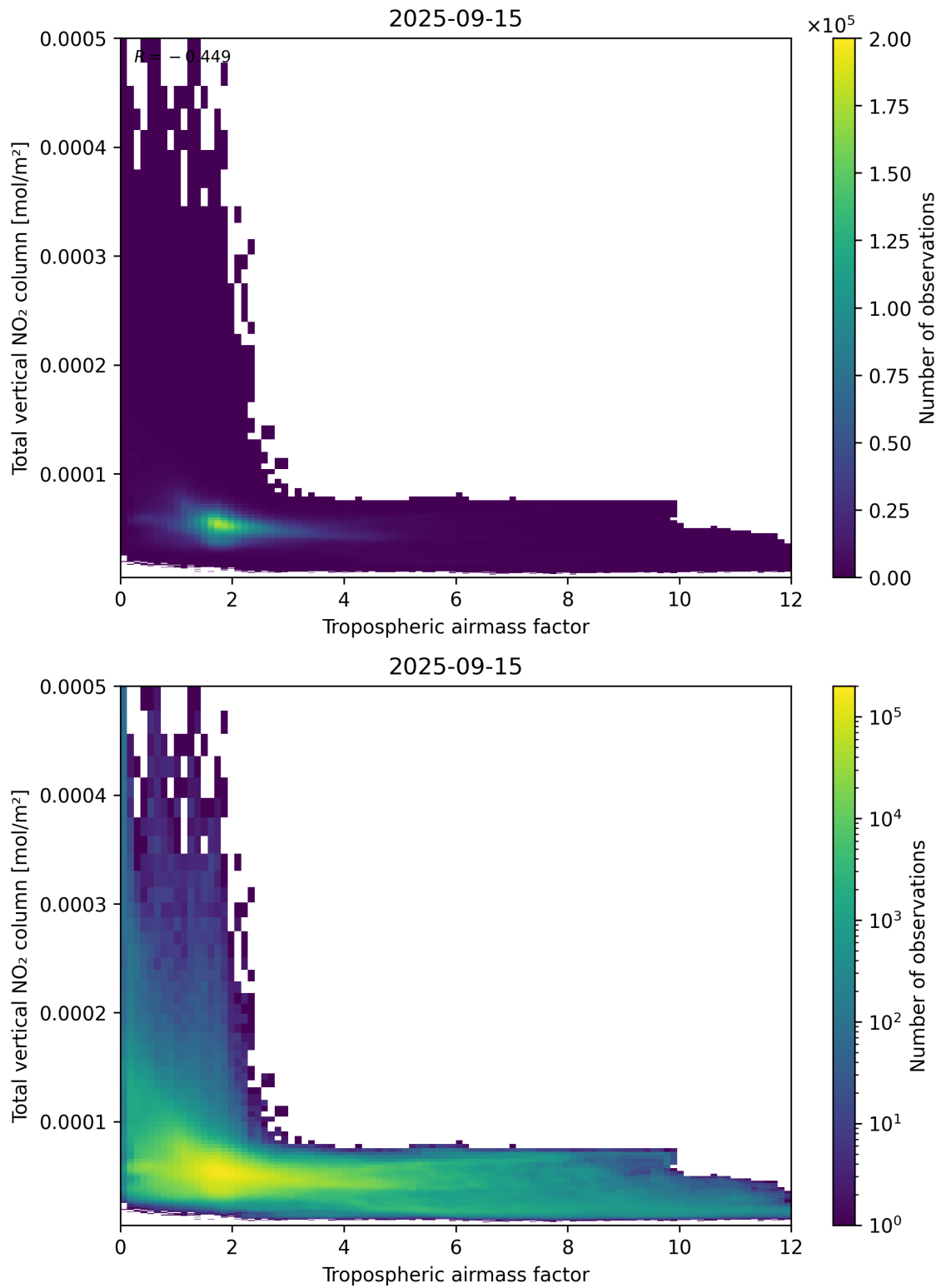
Figure 77: Scatter density plot of “Tropospheric airmass factor” against “Total vertical NO 2 column” for 2025-09-15 to 2025-09-16.
