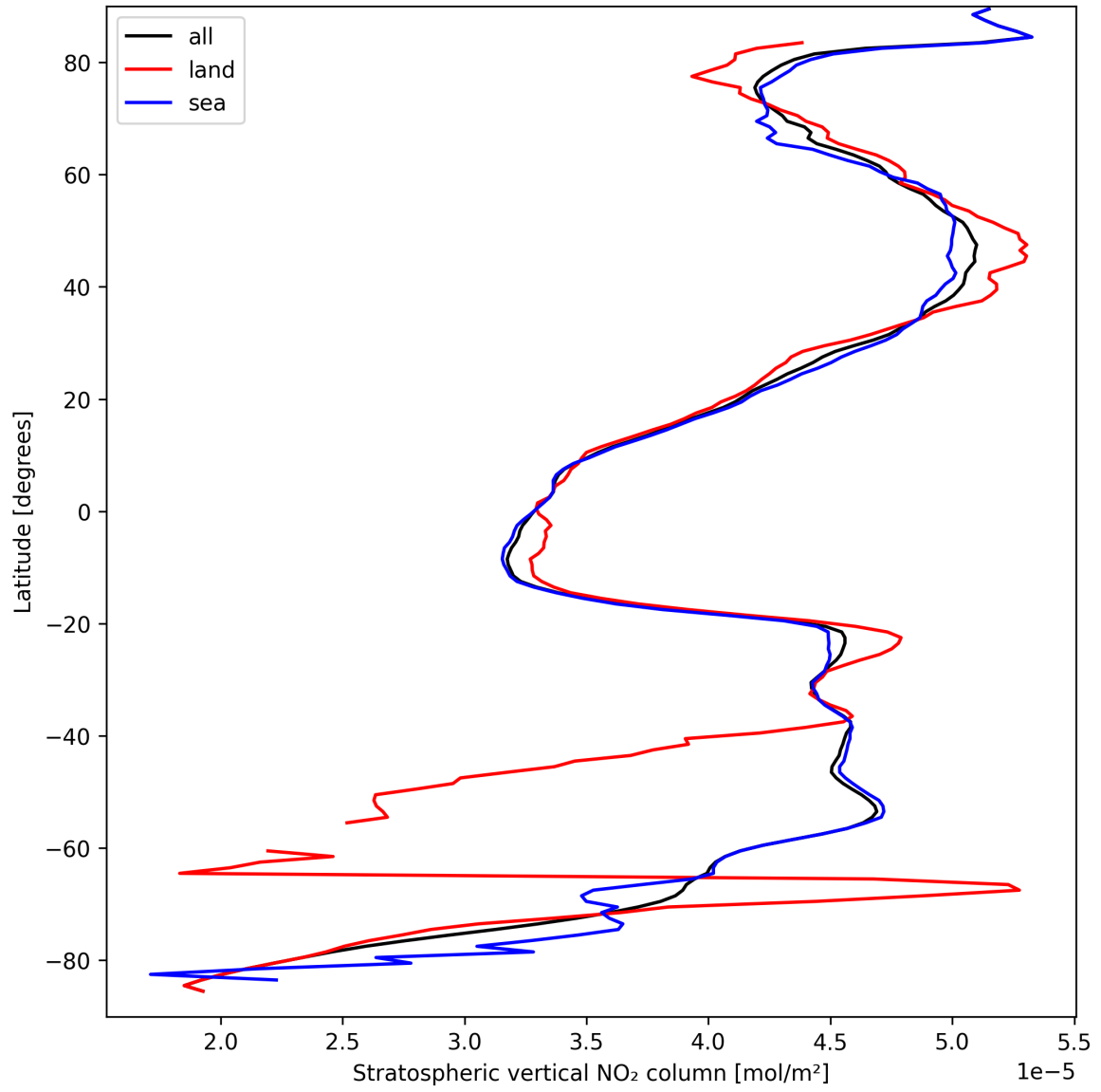
Figure 19: Zonal average of “Stratospheric vertical NO 2 column” for 2025-09-15 to 2025-09-16.
