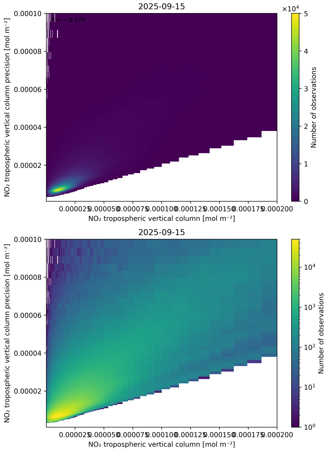
Figure 130: Scatter density plot of “NO 2 tropospheric vertical column” against “NO 2 tropospheric vertical column precision” for 2025-09-15 to 2025-09-16.
