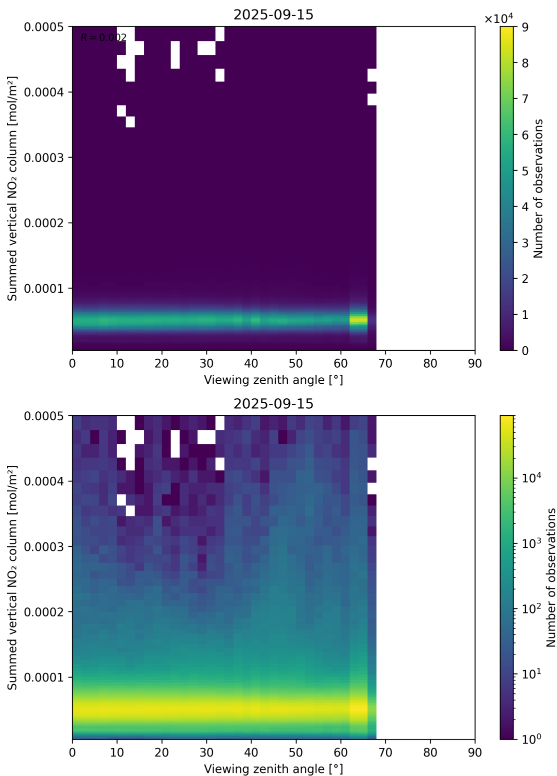
Figure 165: Scatter density plot of “Viewing zenith angle” against “Summed vertical NO 2 column” for 2025-09-15 to 2025-09-16.
