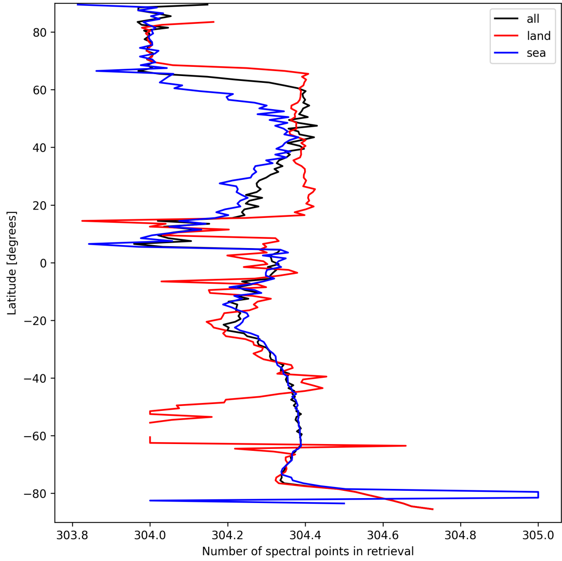
Figure 16: Zonal average of “Number of spectral points in retrieval” for 2025-09-15 to 2025-09-16.
