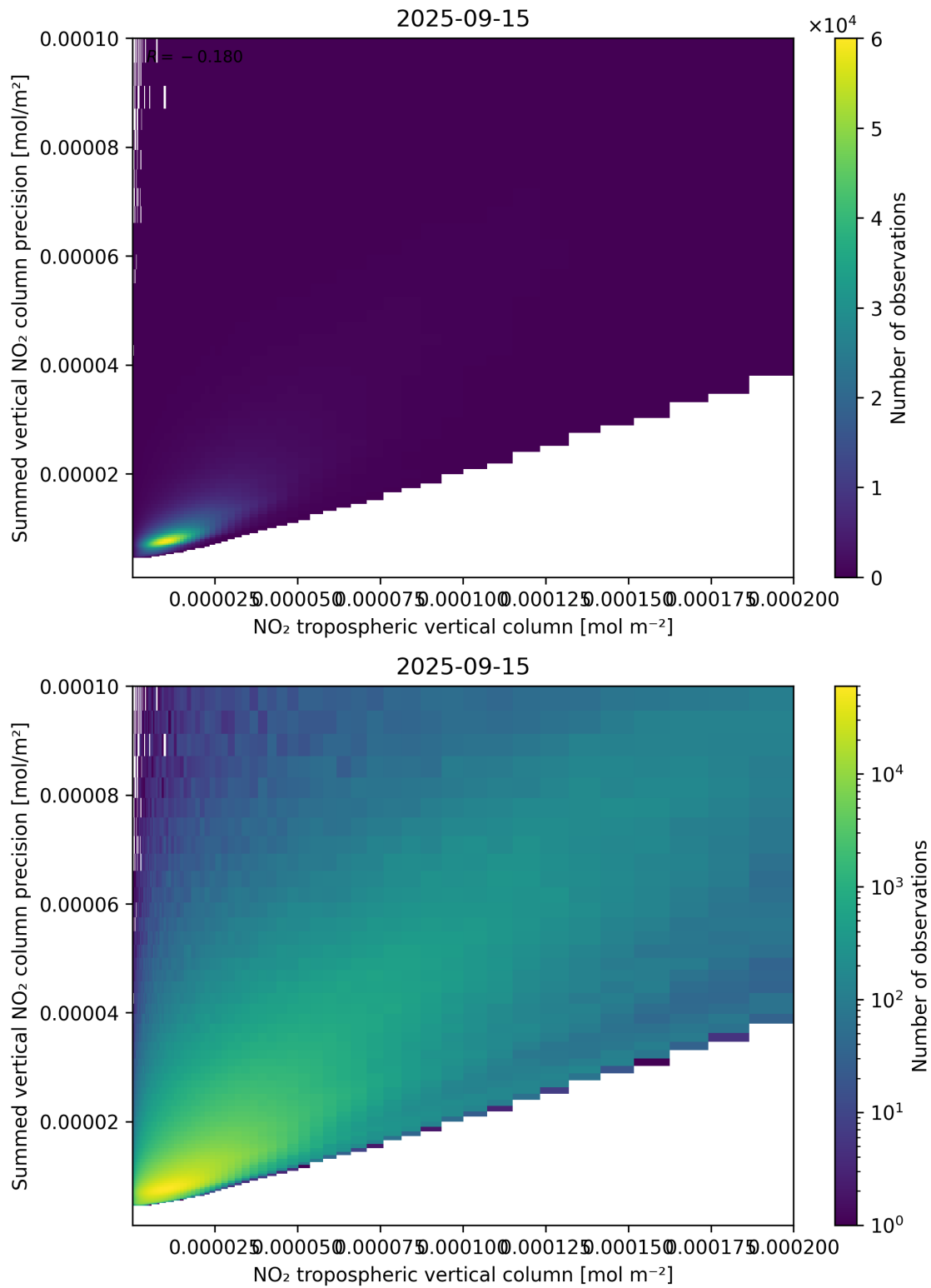
Figure 127: Scatter density plot of “NO 2 tropospheric vertical column” against “Summed vertical NO 2 column precision” for 2025-09-15 to 2025-09-16.
