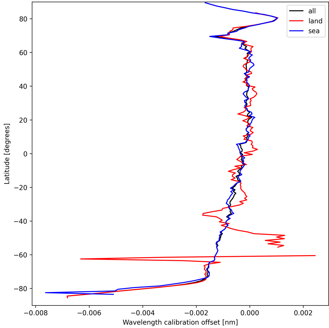
Figure 18: Zonal average of “Wavelength calibration offset” for 2025-09-15 to 2025-09-16.
