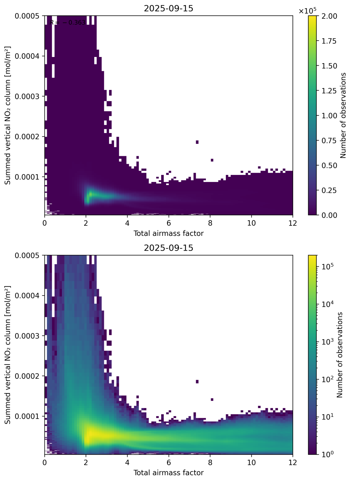
Figure 65: Scatter density plot of “Total airmass factor” against “Summed vertical NO 2 column” for 2025-09-15 to 2025-09-16.
