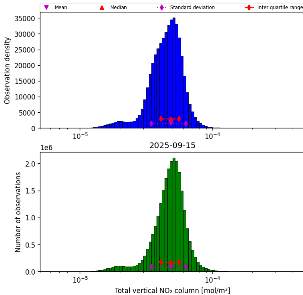
Figure 38: Histogram of “Total vertical NO 2 column” for 2025-09-15 to 2025-09-16
