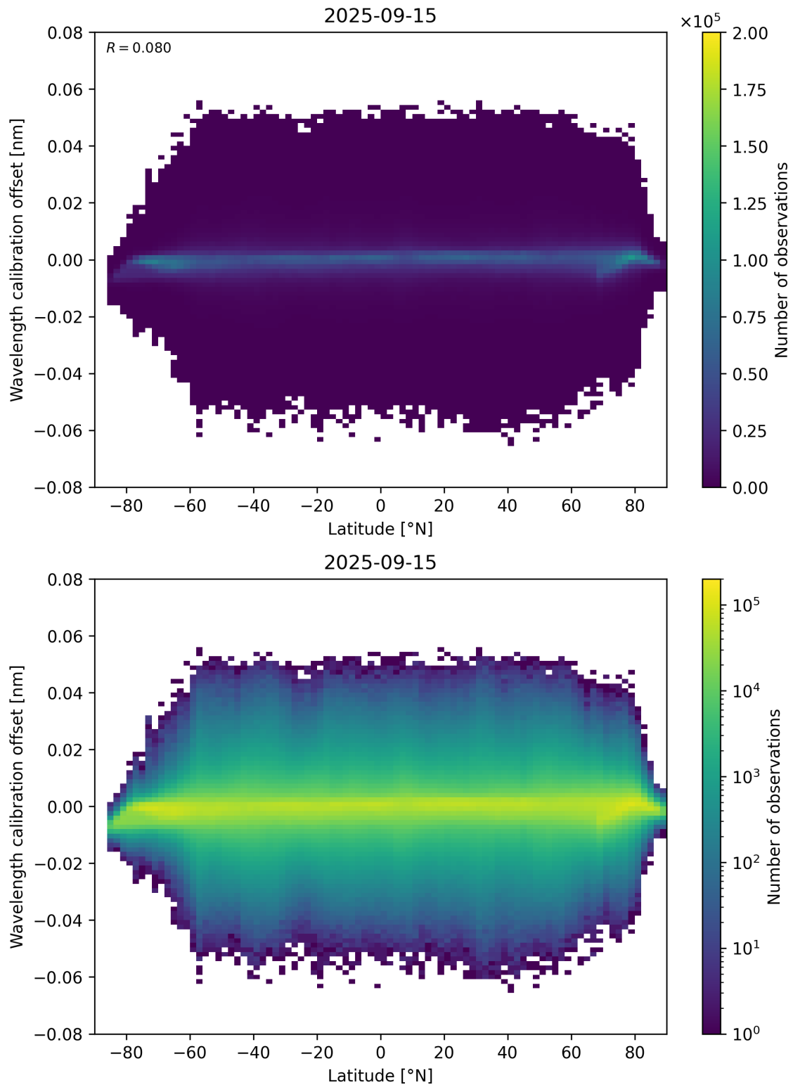
Figure 95: Scatter density plot of “Latitude” against “Wavelength calibration offset” for 2025-09-15 to 2025-09-16.
