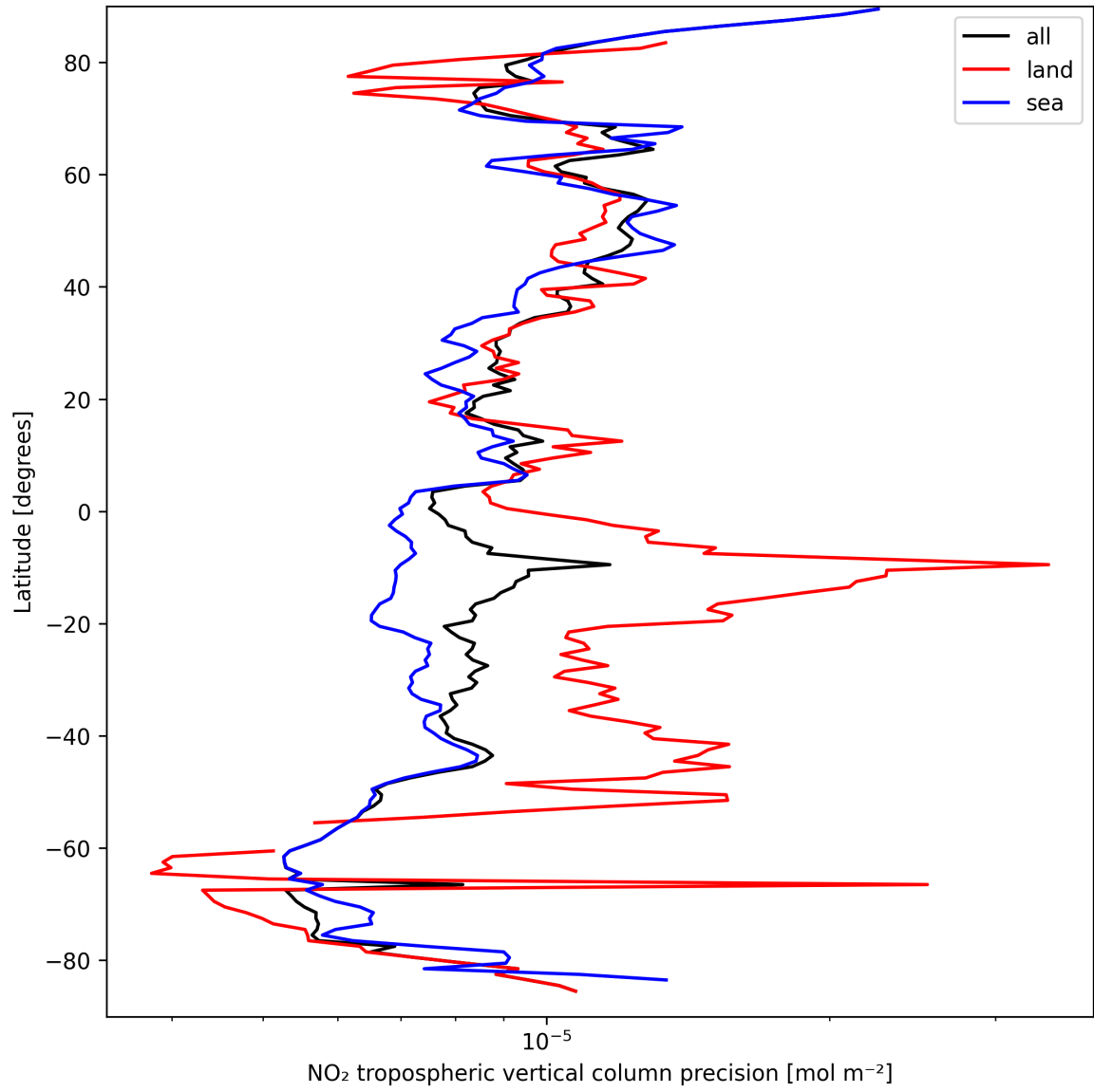
Figure 13: Zonal average of “NO 2 tropospheric vertical column precision” for 2025-09-15 to 2025-09-16.
