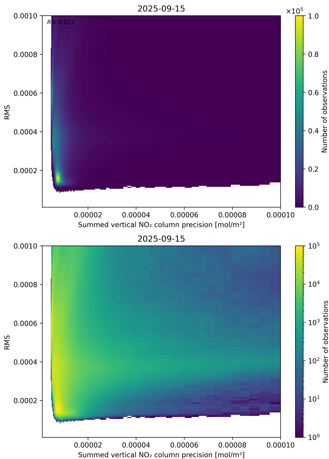
Figure 108: Scatter density plot of “Summed vertical NO 2 column precision” against “RMS” for 2025-09-15 to 2025-09-16.
