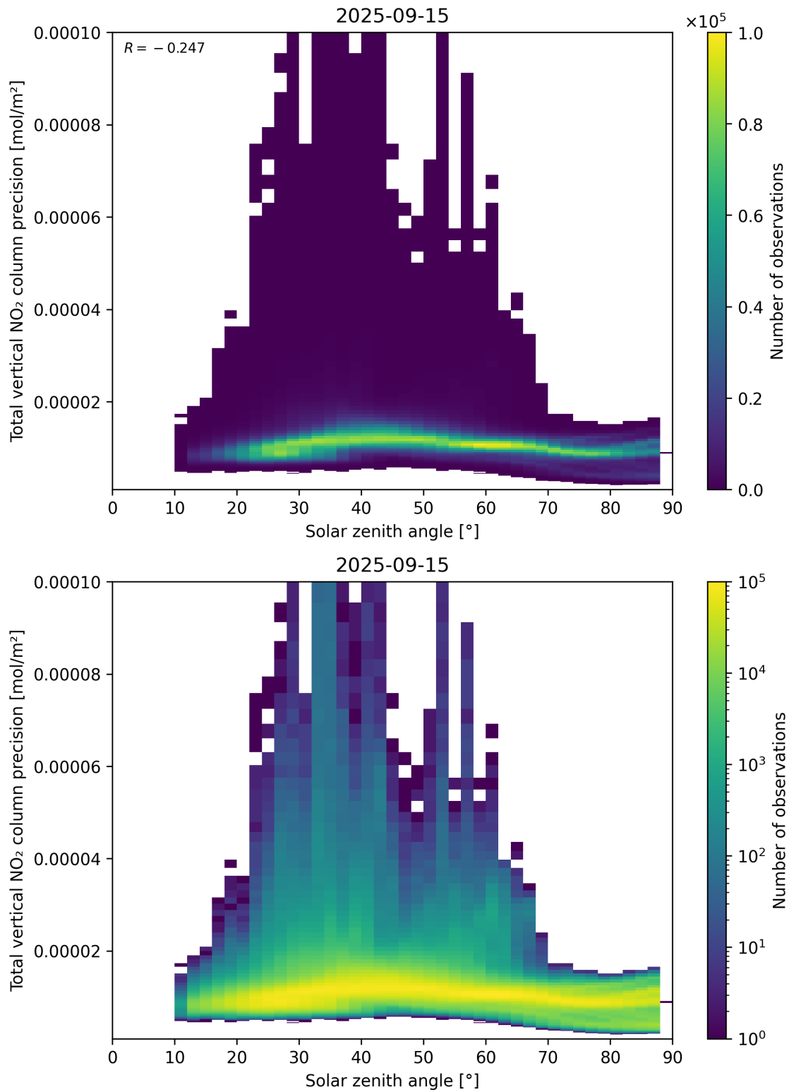
Figure 154: Scatter density plot of “Solar zenith angle” against “Total vertical NO 2 column precision” for 2025-09-15 to 2025-09-16.
