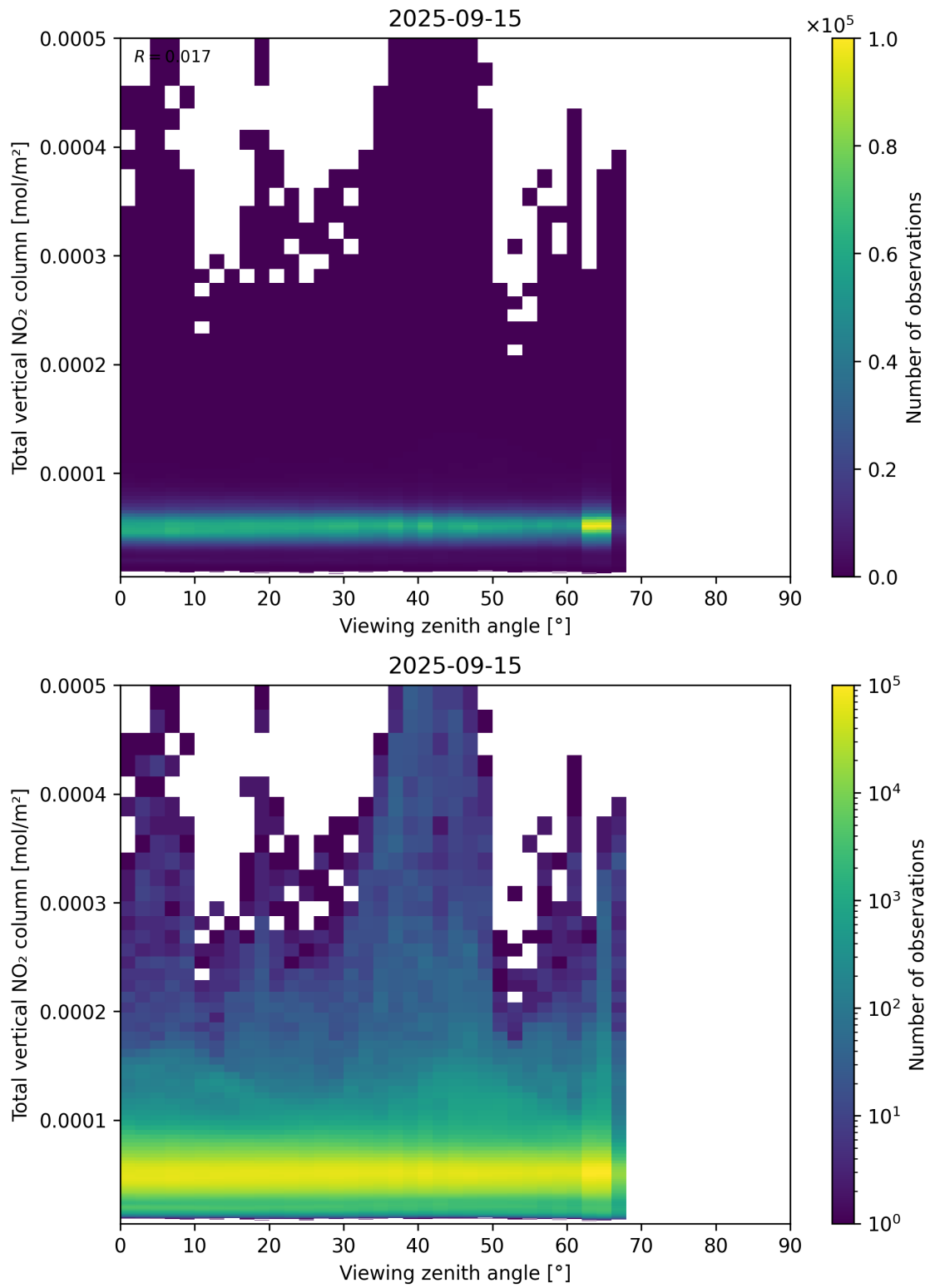
Figure 167: Scatter density plot of “Viewing zenith angle” against “Total vertical NO 2 column” for 2025-09-15 to 2025-09-16.
