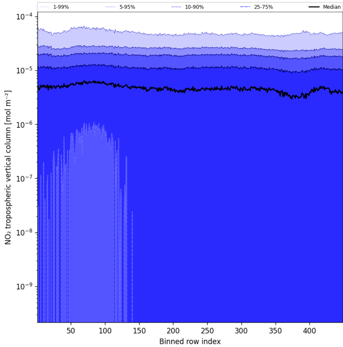
Figure 46: Along track statistics of “ \text{NO}_2 tropospheric vertical column” for 2025-09-15 to 2025-09-16
