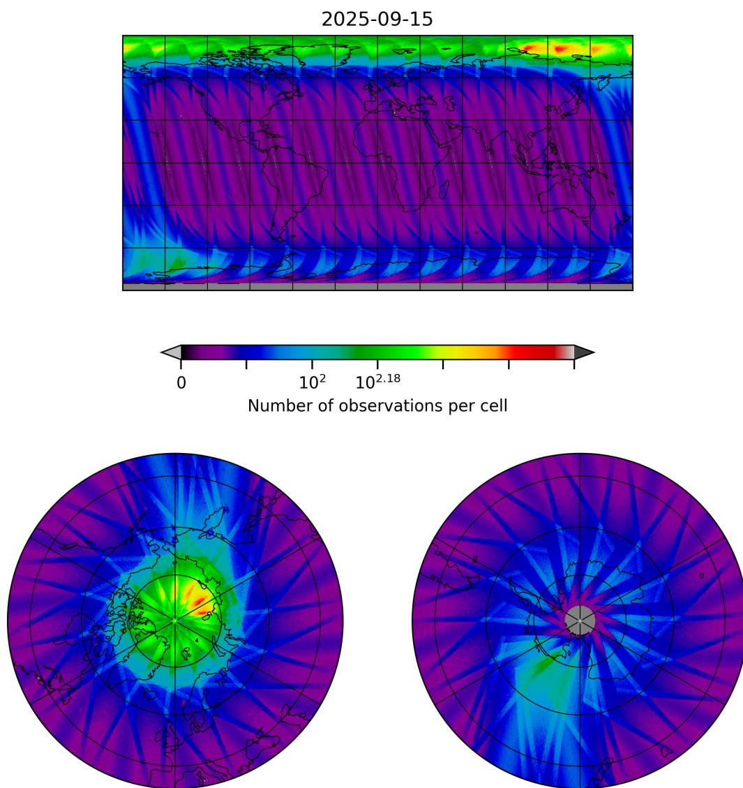
Figure 10: Map of the number of observations for 2025-09-15 to 2025-09-16
