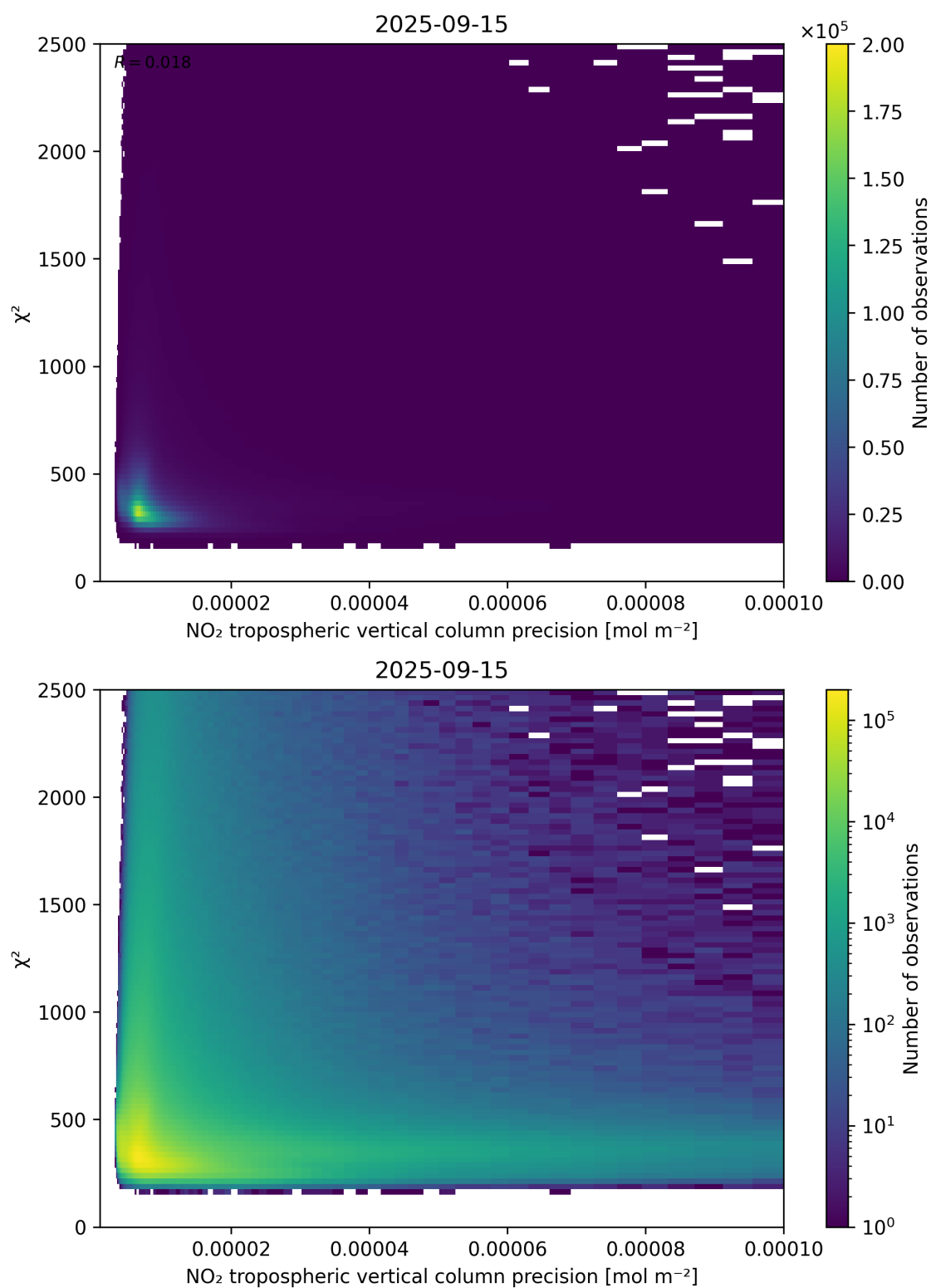
Figure 134: Scatter density plot of “NO 2 tropospheric vertical column precision” against “ \chi^2 ” for 2025-09-15 to 2025-09-16.
