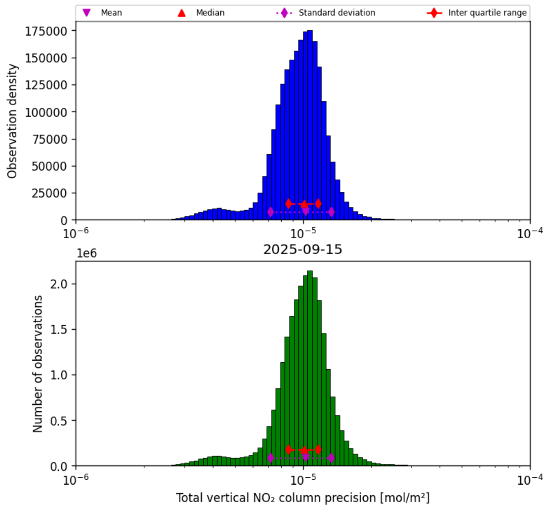
Figure 39: Histogram of “Total vertical NO 2 column precision” for 2025-09-15 to 2025-09-16
