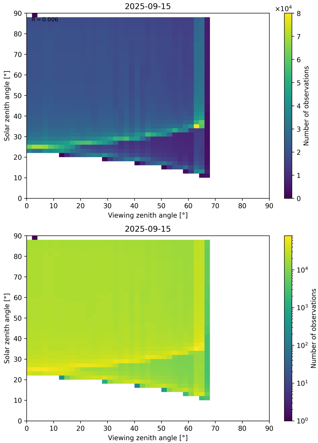
Figure 172: Scatter density plot of “Viewing zenith angle” against “Solar zenith angle” for 2025-09-15 to 2025-09-16.
