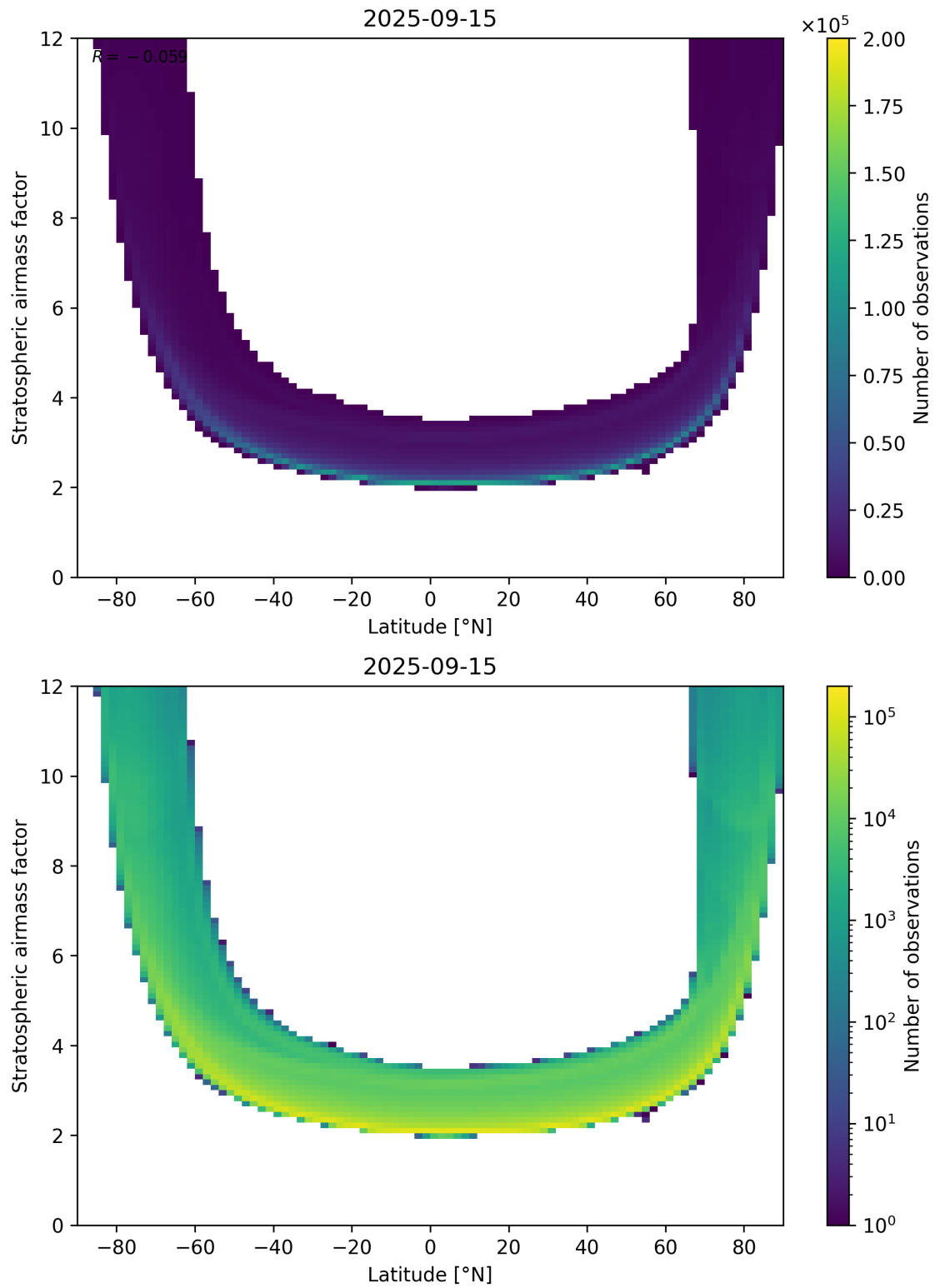
Figure 83: Scatter density plot of “Latitude” against “Stratospheric air mass factor” for 2025-09-15 to 2025-09-16.
