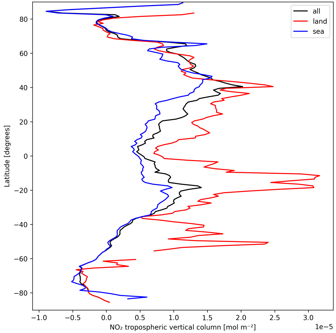
Figure 12: Zonal average of “NO 2 tropospheric vertical column” for 2025-09-15 to 2025-09-16.
