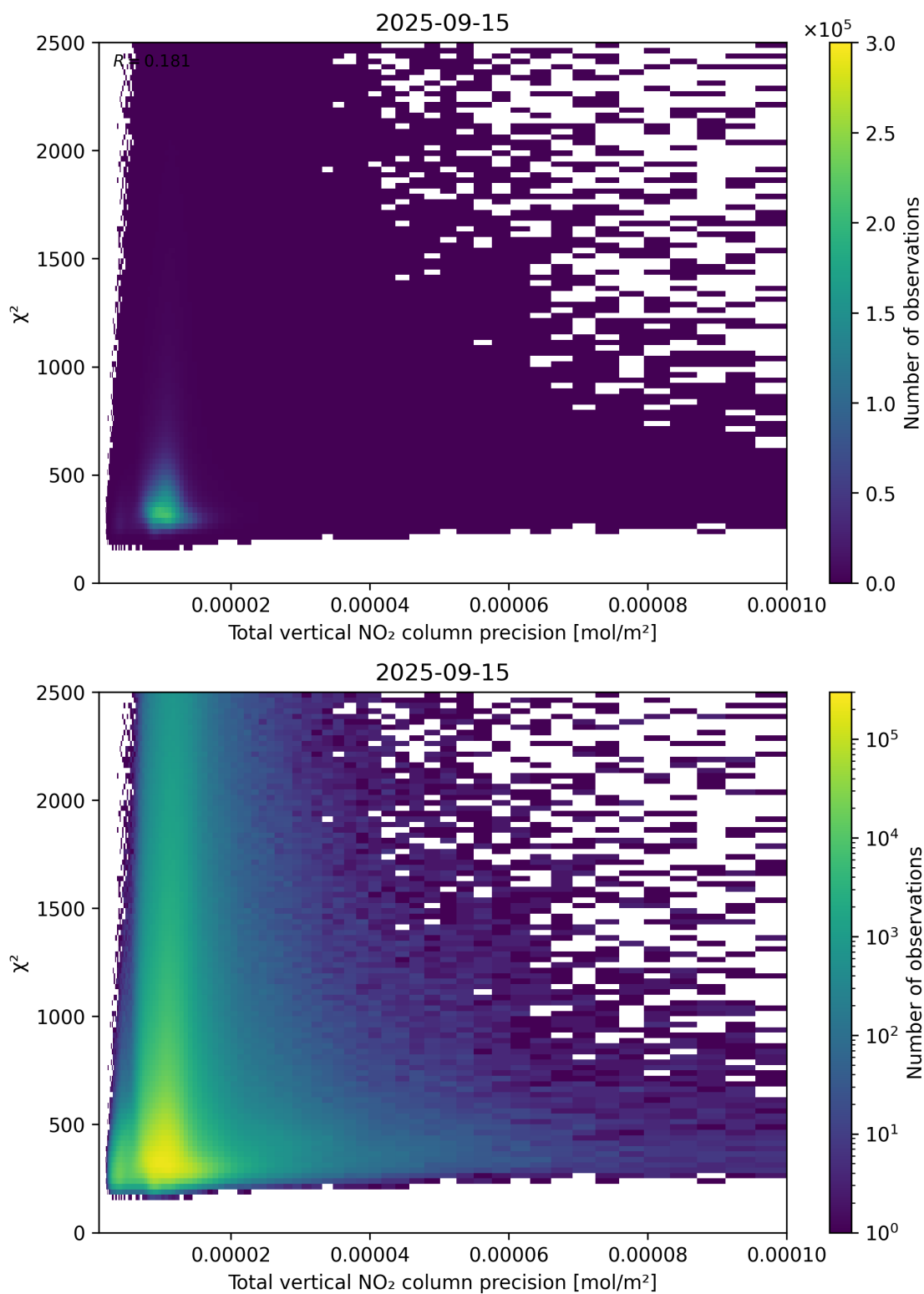
Figure 116: Scatter density plot of “Total vertical NO 2 column precision” against “ \chi^2 ” for 2025-09-15 to 2025-09-16.
