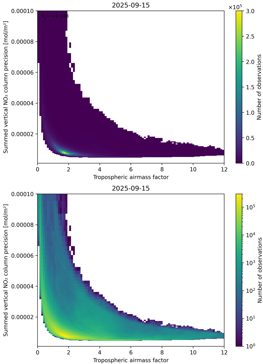
Figure 76: Scatter density plot of “Tropospheric air mass factor” against “Summed vertical NO 2 column precision” for 2025-09-15 to 2025-09-16.
