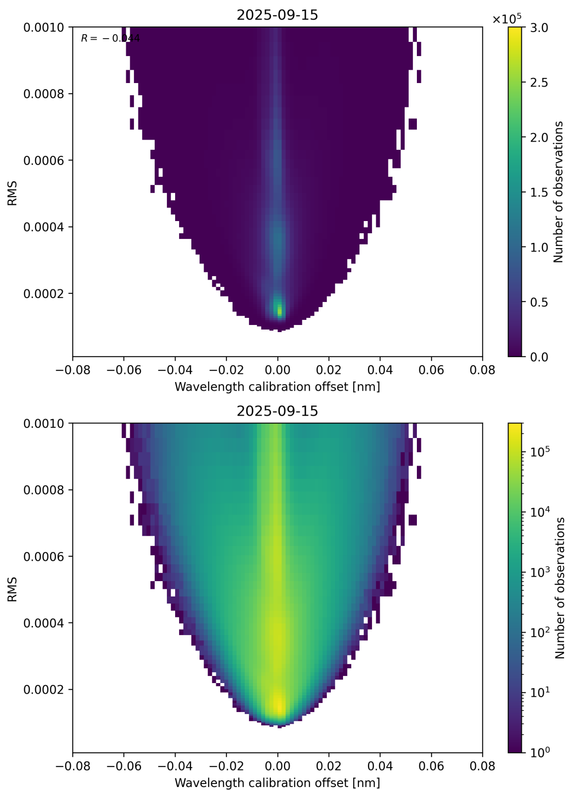
Figure 181: Scatter density plot of “Wavelength calibration offset” against “RMS” for 2025-09-15 to 2025-09-16.
