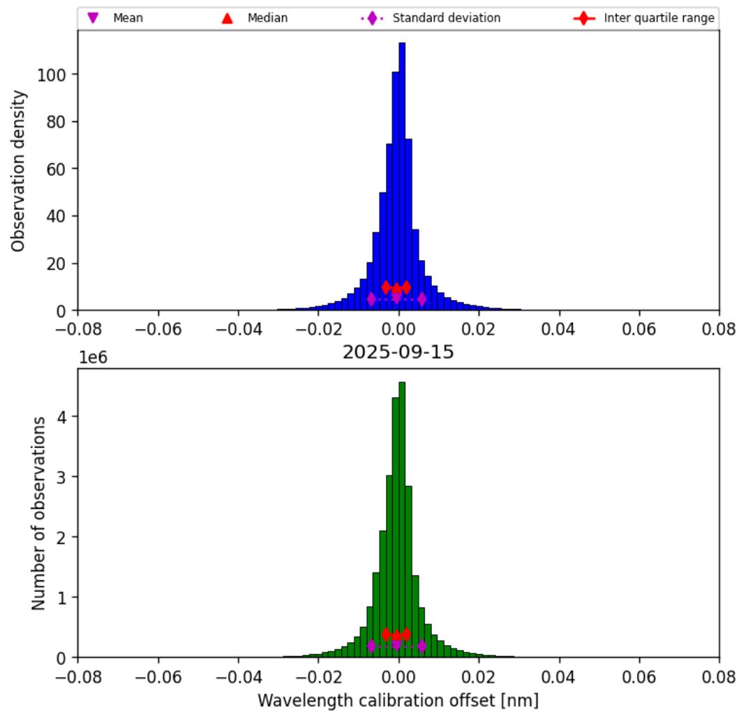
Figure 35: Histogram of “Wavelength calibration offset” for 2025-09-15 to 2025-09-16
