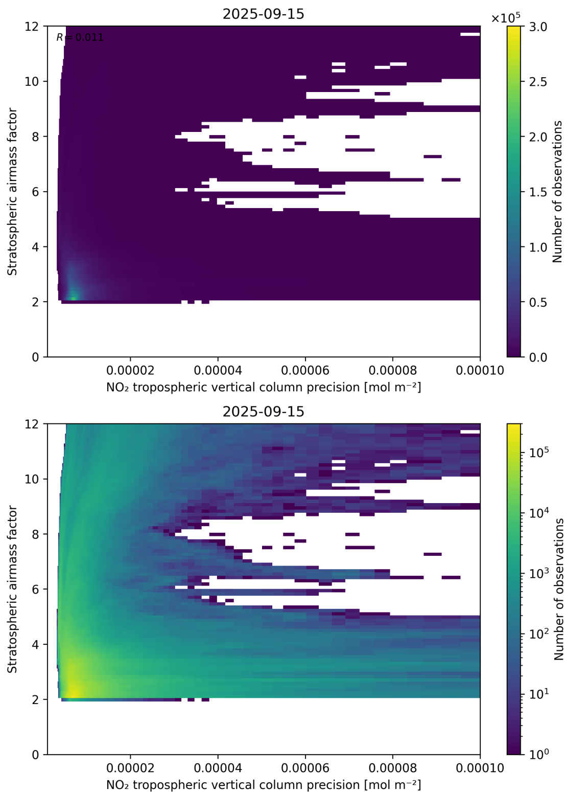
Figure 131: Scatter density plot of “NO 2 tropospheric vertical column precision” against “Stratospheric airmass factor” for 2025-09-15 to 2025-09-16.
