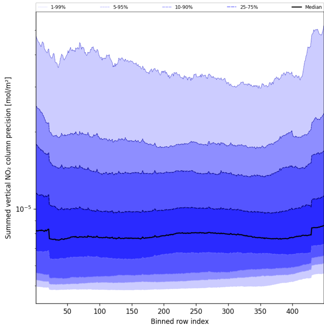
Figure 58: Along track statistics of “Summed vertical NO 2 column precision” for 2025-09-15 to 2025-09-16
