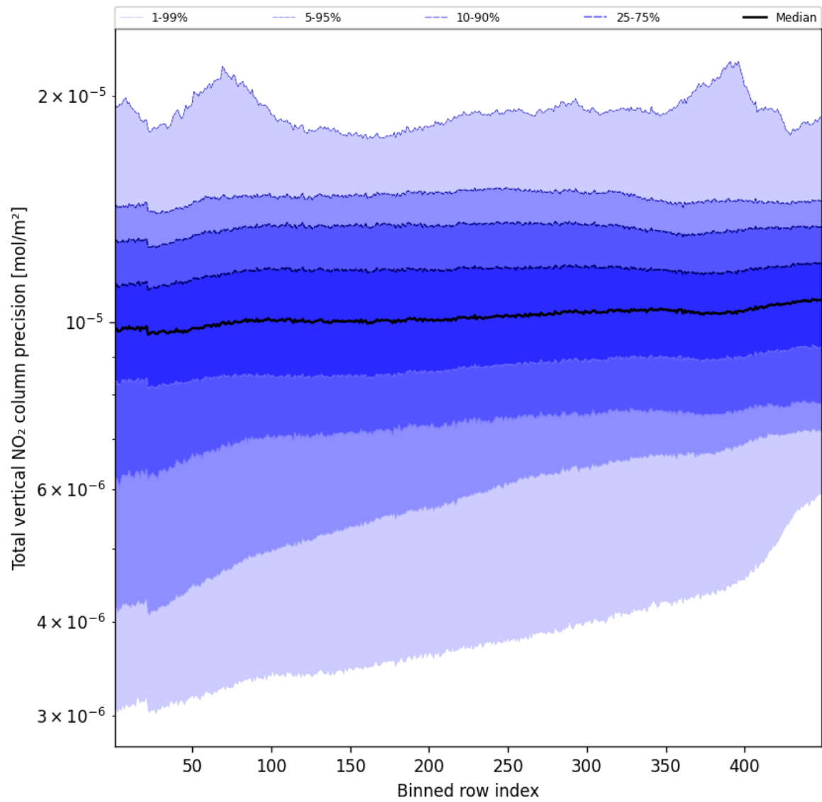
Figure 56: Along track statistics of “Total vertical NO 2 column precision” for 2025-09-15 to 2025-09-16
