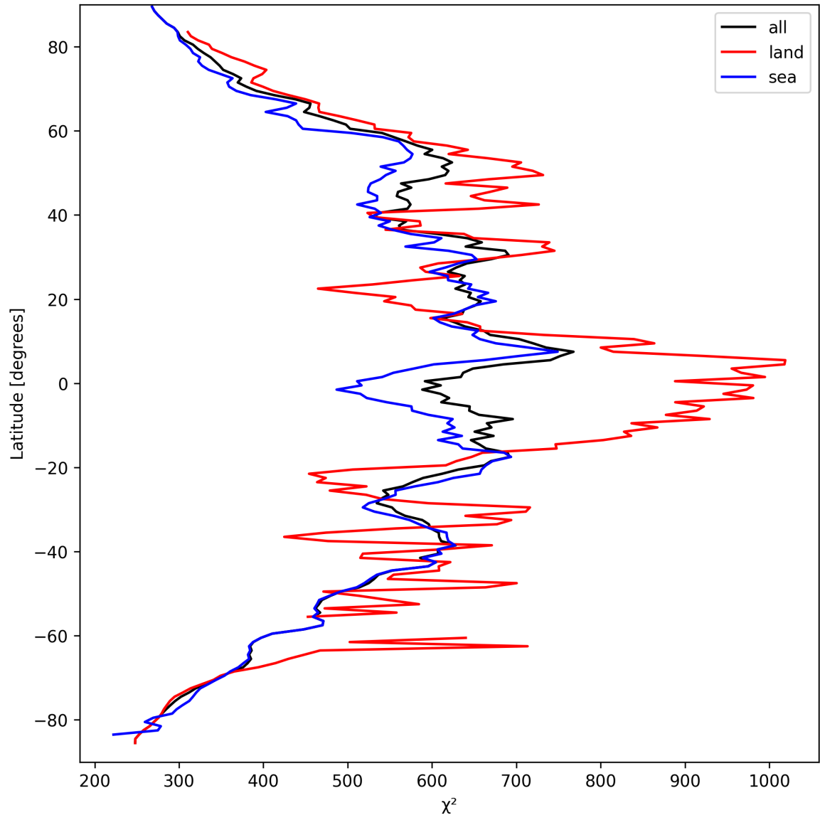
Figure 25: Zonal average of “ \chi^2 ” for 2025-09-15 to 2025-09-16.
