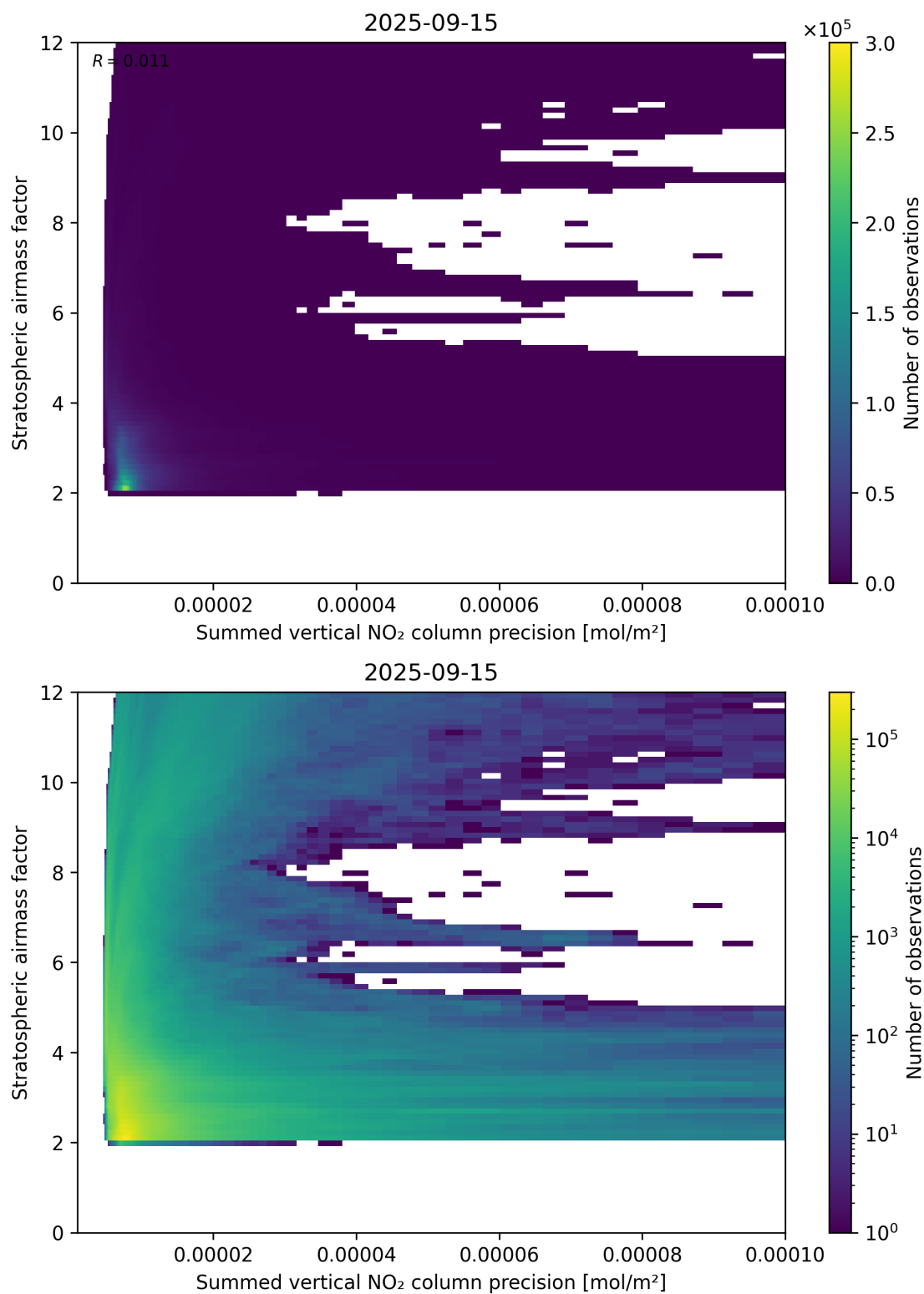
Figure 106: Scatter density plot of “Summed vertical NO 2 column precision” against “Stratospheric airmass factor” for 2025-09-15 to 2025-09-16.
