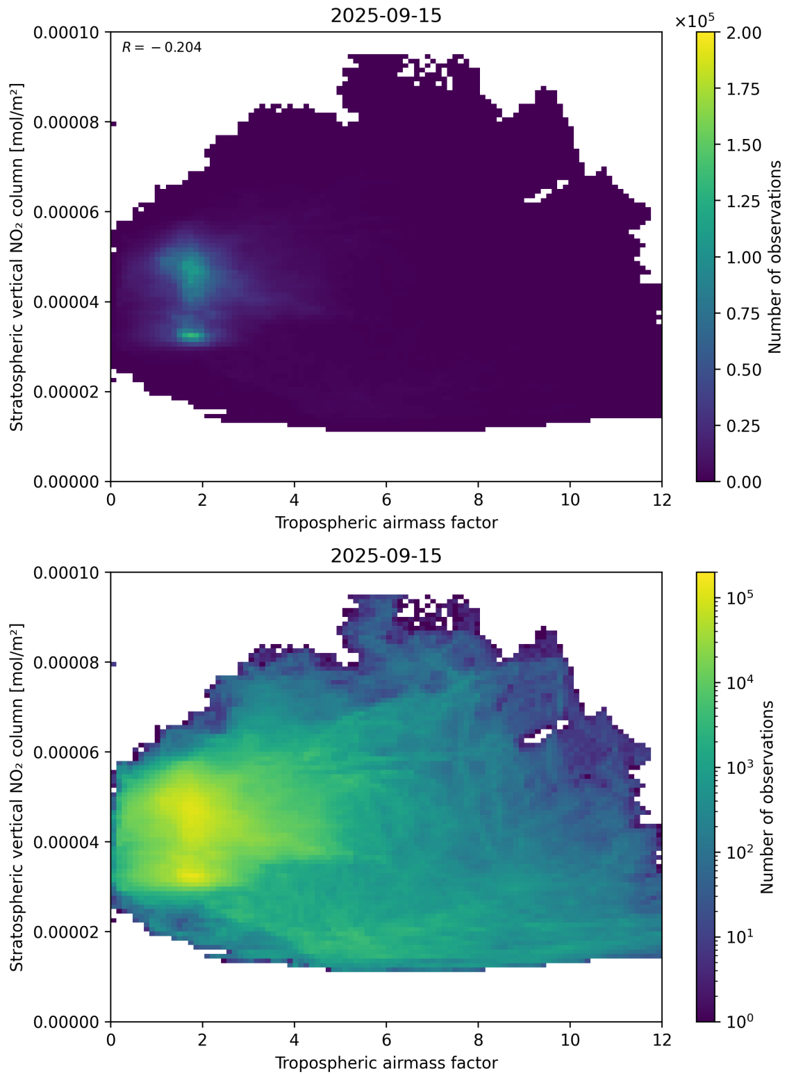
Figure 74: Scatter density plot of “Tropospheric air mass factor” against “Stratospheric vertical NO 2 column” for 2025-09-15 to 2025-09-16.
