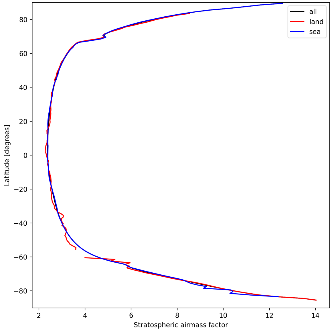
Figure 27: Zonal average of “Stratospheric airmass factor” for 2025-09-15 to 2025-09-16.
