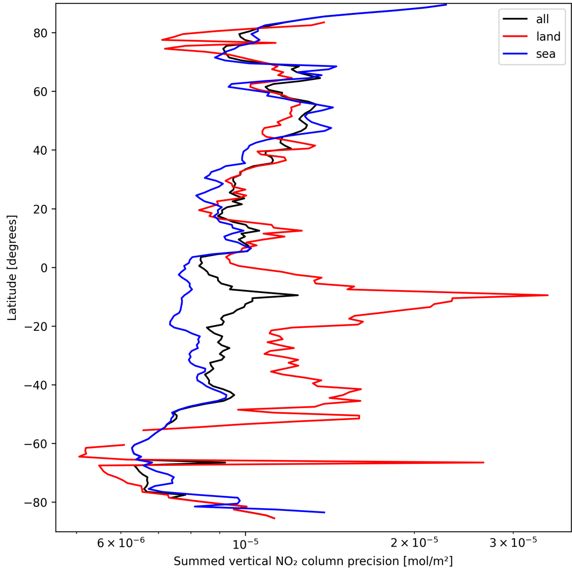
Figure 24: Zonal average of “Summed vertical NO 2 column precision” for 2025-09-15 to 2025-09-16.
