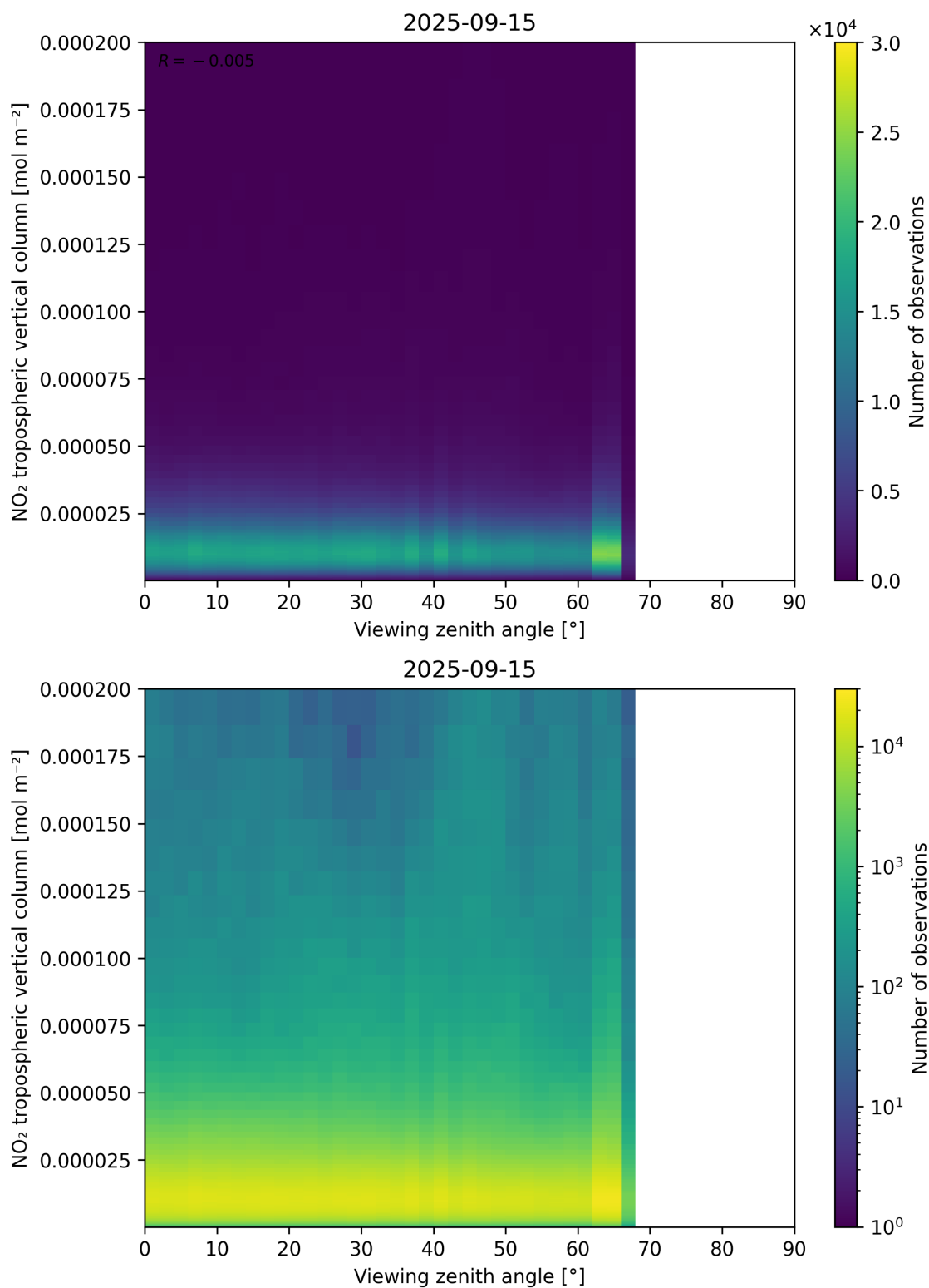
Figure 169: Scatter density plot of “Viewing zenith angle” against “NO 2 tropospheric vertical column” for 2025-09-15 to 2025-09-16.
