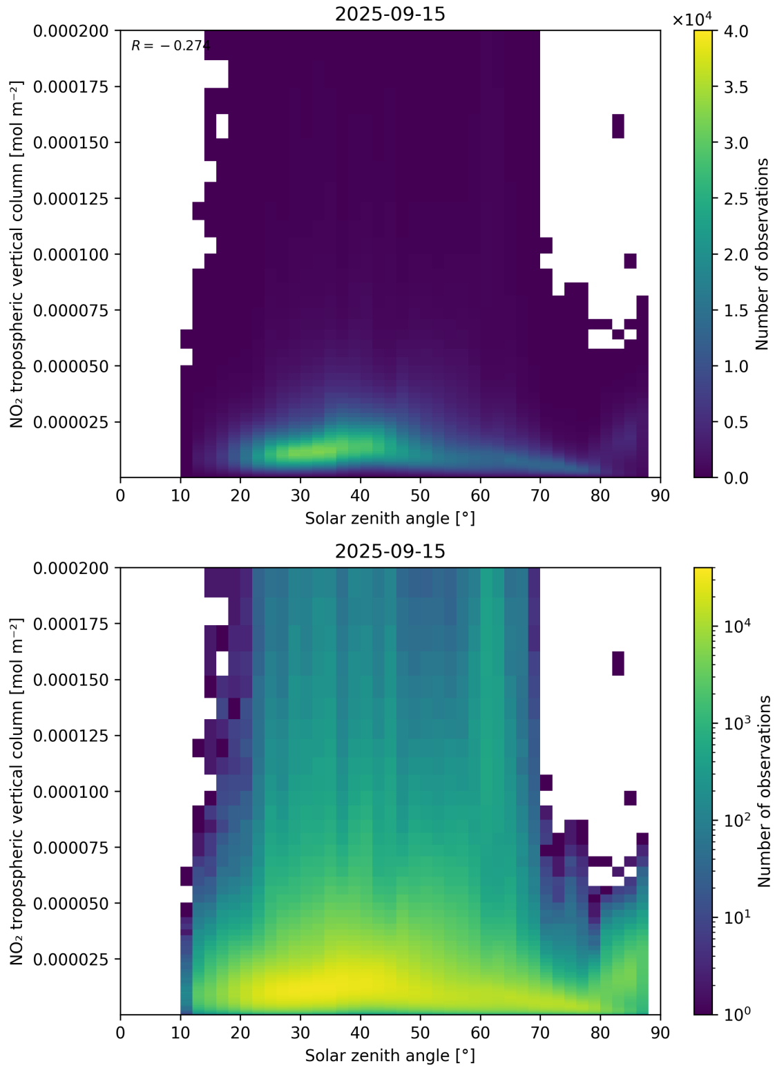
Figure 155: Scatter density plot of “Solar zenith angle” against “NO 2 tropospheric vertical column” for 2025-09-15 to 2025-09-16.
