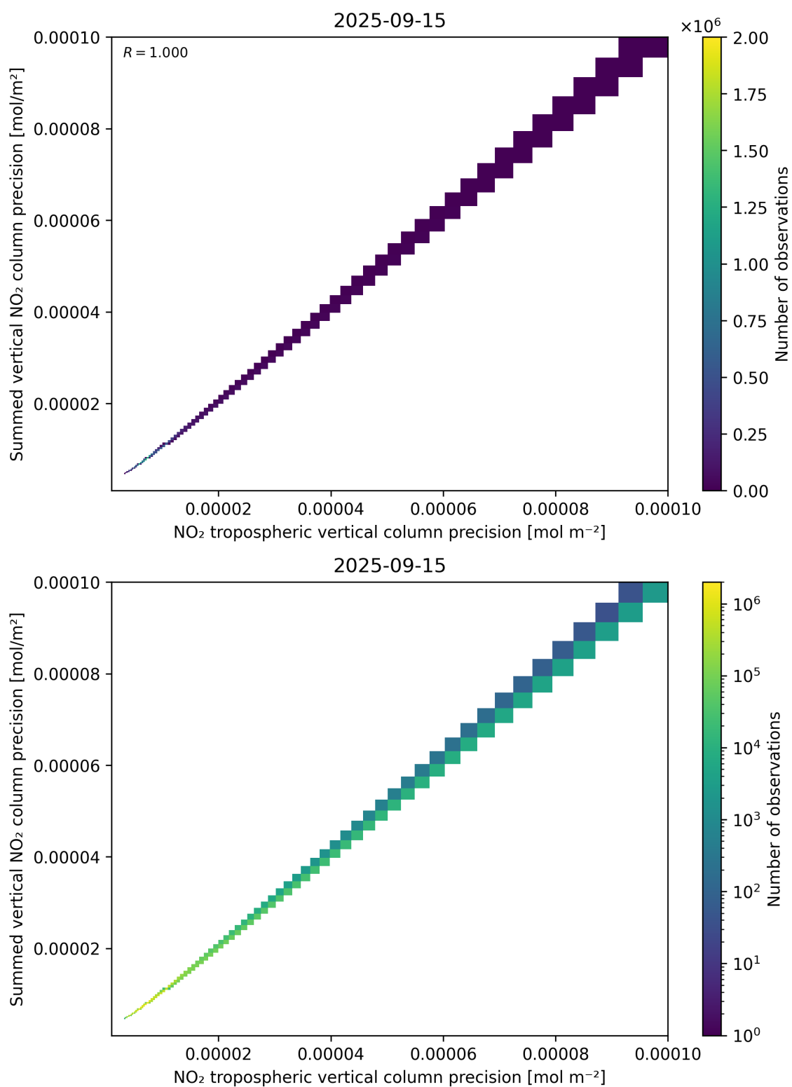
Figure 137: Scatter density plot of “NO 2 tropospheric vertical column precision” against “Summed vertical NO 2 column precision” for 2025-09-15 to 2025-09-16.
