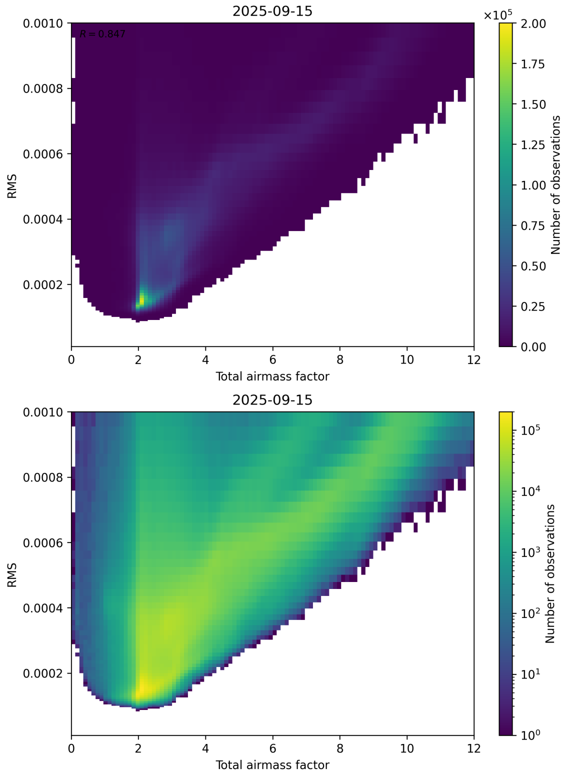
Figure 69: Scatter density plot of “Total airmass factor” against “RMS” for 2025-09-15 to 2025-09-16.
