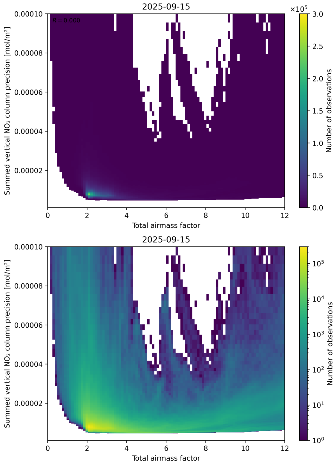
Figure 66: Scatter density plot of “Total airmass factor” against “Summed vertical NO 2 column precision” for 2025-09-15 to 2025-09-16.
