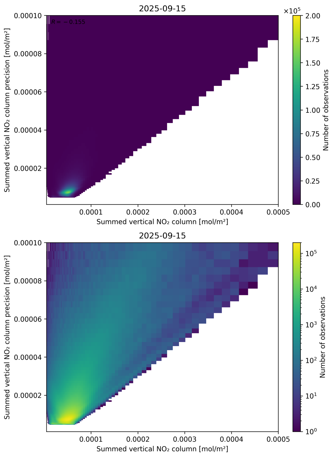
Figure 105: Scatter density plot of “Summed vertical NO 2 column” against “Summed vertical NO 2 column precision” for 2025-09-15 to 2025-09-16.
