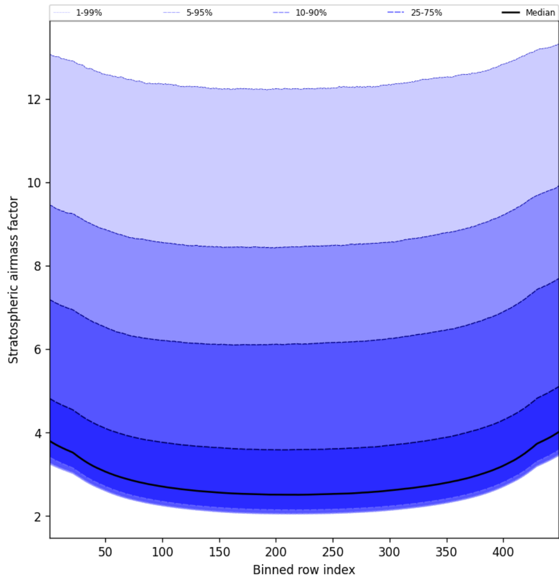
Figure 61: Along track statistics of “Stratospheric airmass factor” for 2025-09-15 to 2025-09-16
