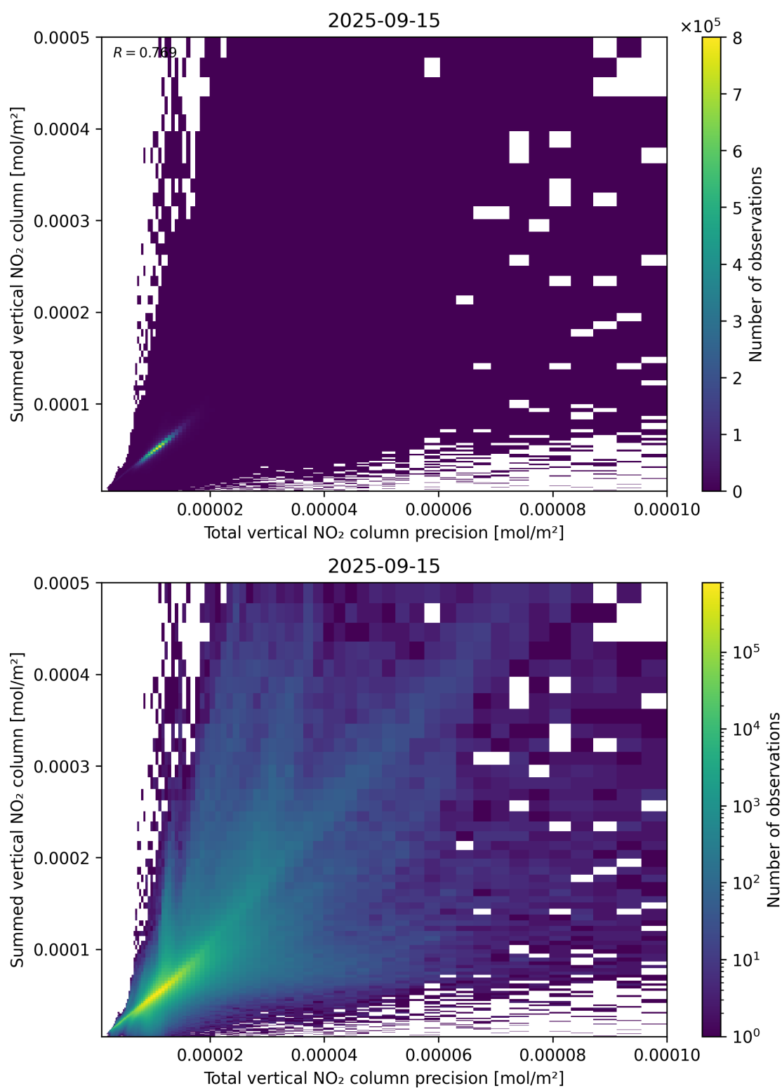
Figure 117: Scatter density plot of “Total vertical NO 2 column precision” against “Summed vertical NO 2 column” for 2025-09-15 to 2025-09-16.
