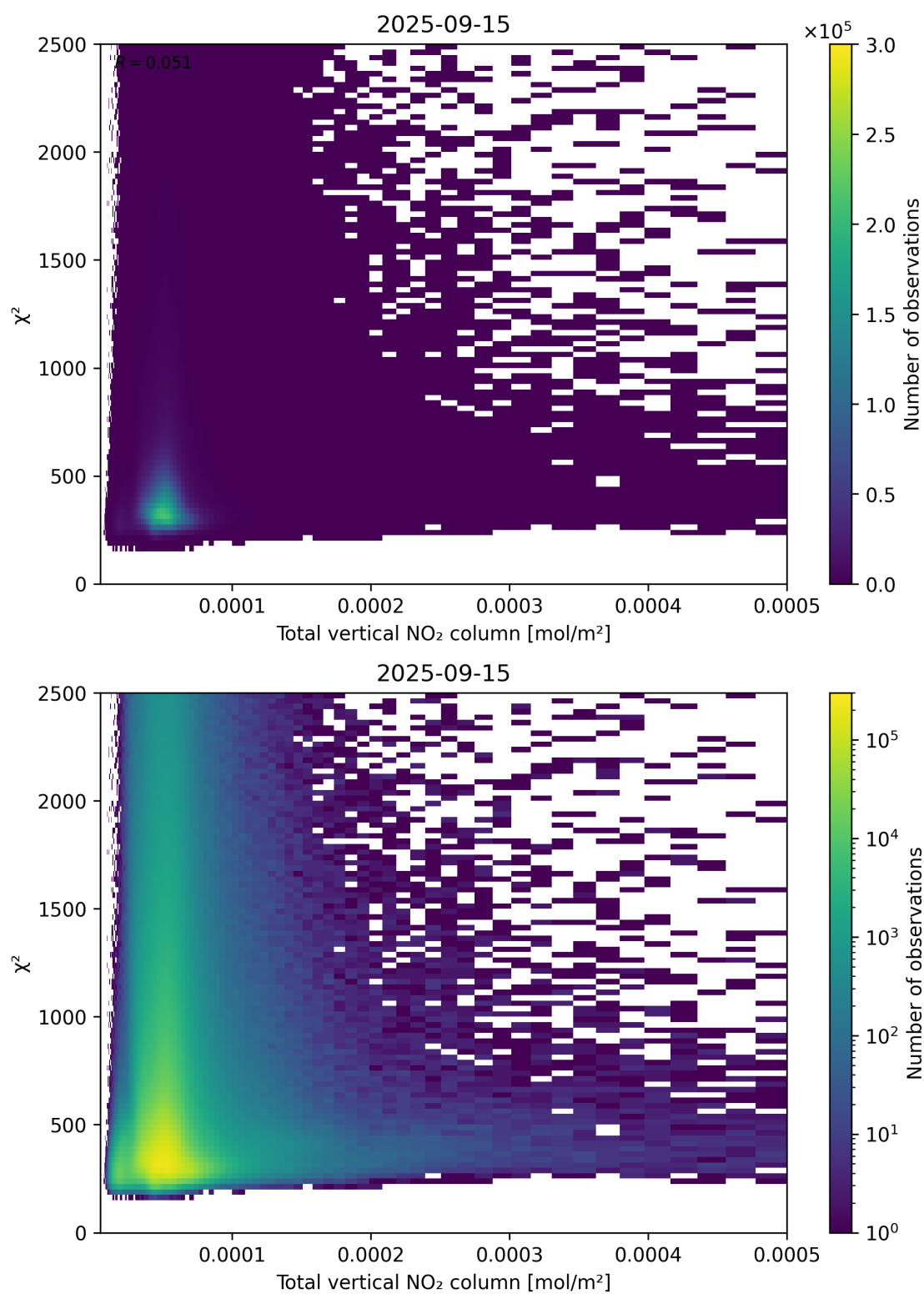
Figure 111: Scatter density plot of “Total vertical NO 2 column” against “ \chi^2 ” for 2025-09-15 to 2025-09-16.
