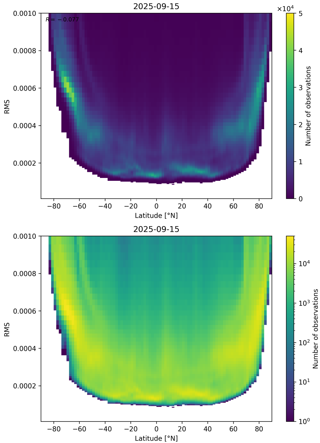
Figure 94: Scatter density plot of “Latitude” against “RMS” for 2025-09-15 to 2025-09-16.
