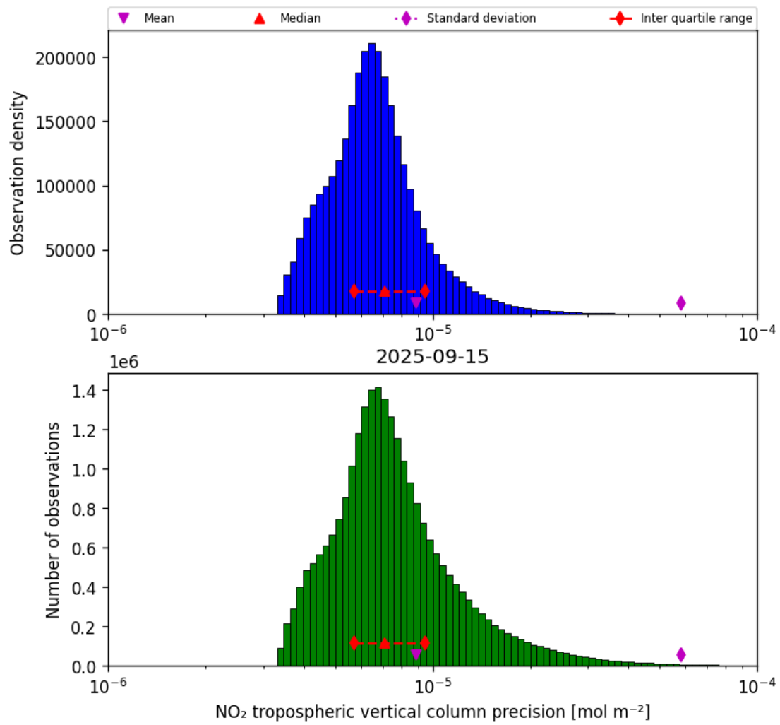
Figure 30: Histogram of “NO 2 tropospheric vertical column precision” for 2025-09-15 to 2025-09-16
