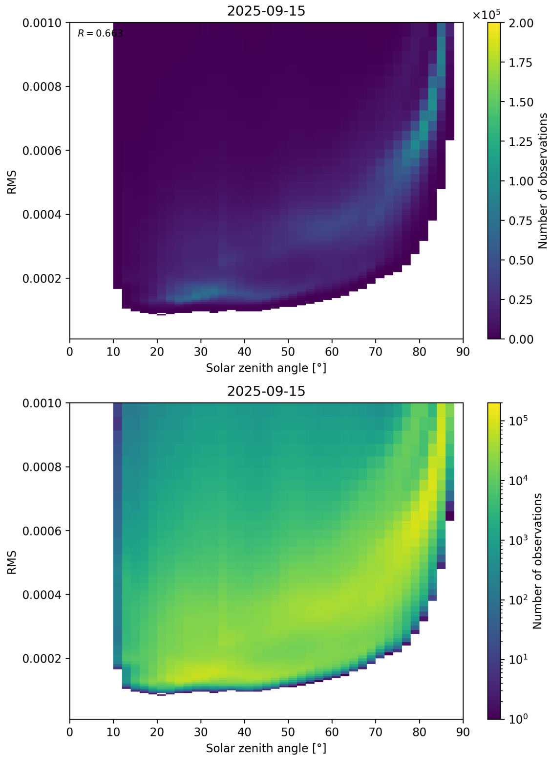
Figure 157: Scatter density plot of “Solar zenith angle” against “RMS” for 2025-09-15 to 2025-09-16.
