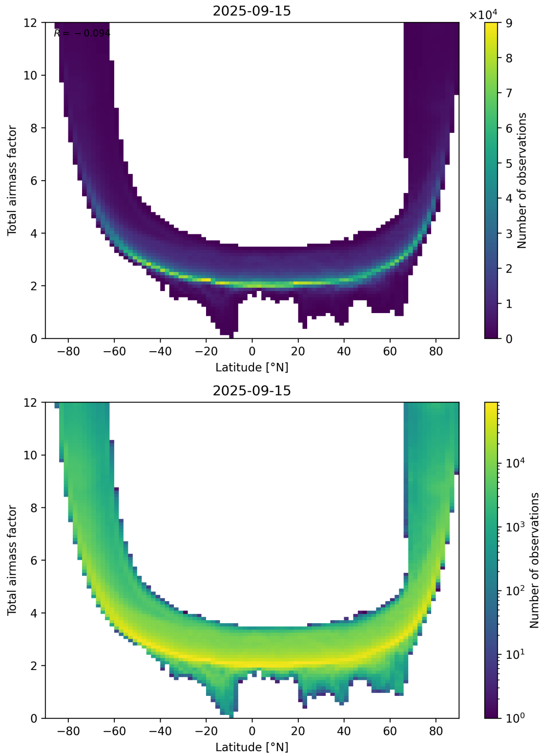
Figure 84: Scatter density plot of “Latitude” against “Total airmass factor” for 2025-09-15 to 2025-09-16.
