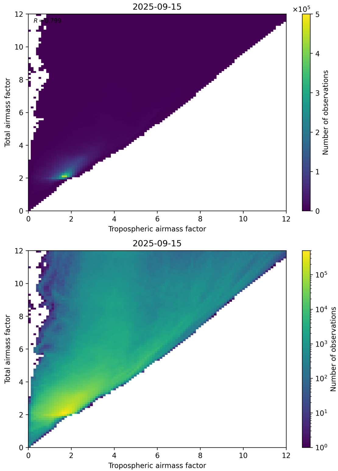
Figure 72: Scatter density plot of “Tropospheric airmass factor” against “Total airmass factor” for 2025-09-15 to 2025-09-16.
