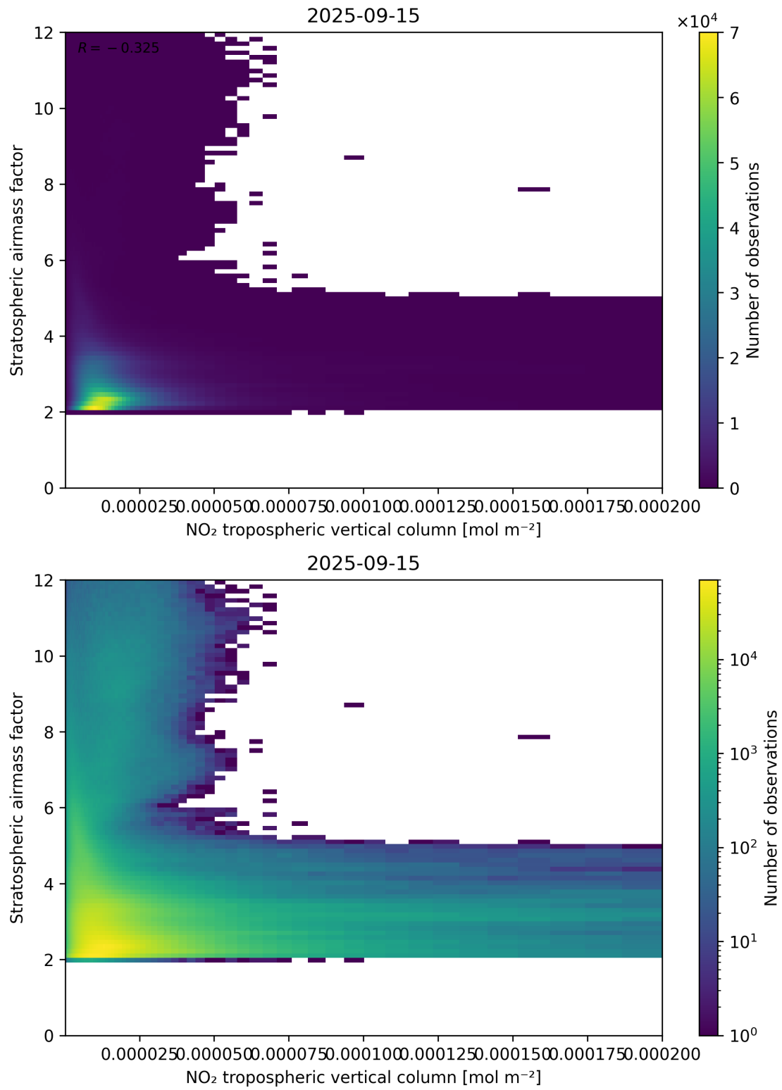
Figure 121: Scatter density plot of “NO 2 tropospheric vertical column” against “Stratospheric air mass factor” for 2025-09-15 to 2025-09-16.
