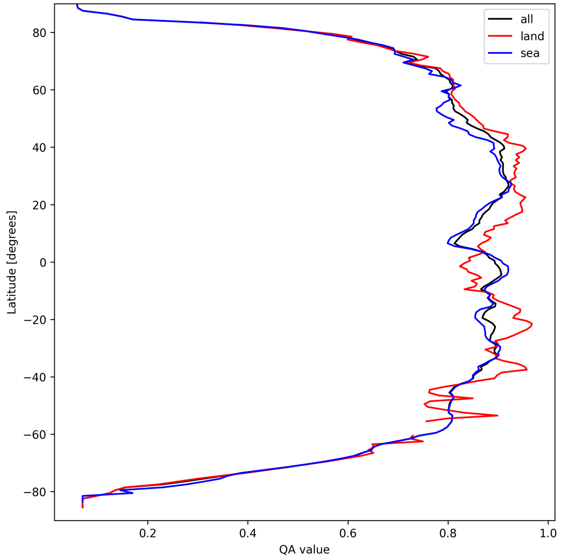
Figure 11: Zonal average of “QA value” for 2025-09-15 to 2025-09-16.
