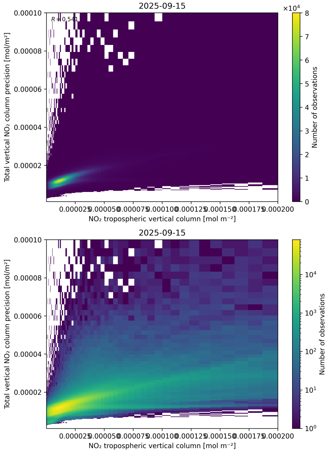
Figure 129: Scatter density plot of “NO 2 tropospheric vertical column” against “Total vertical NO 2 column precision” for 2025-09-15 to 2025-09-16.
