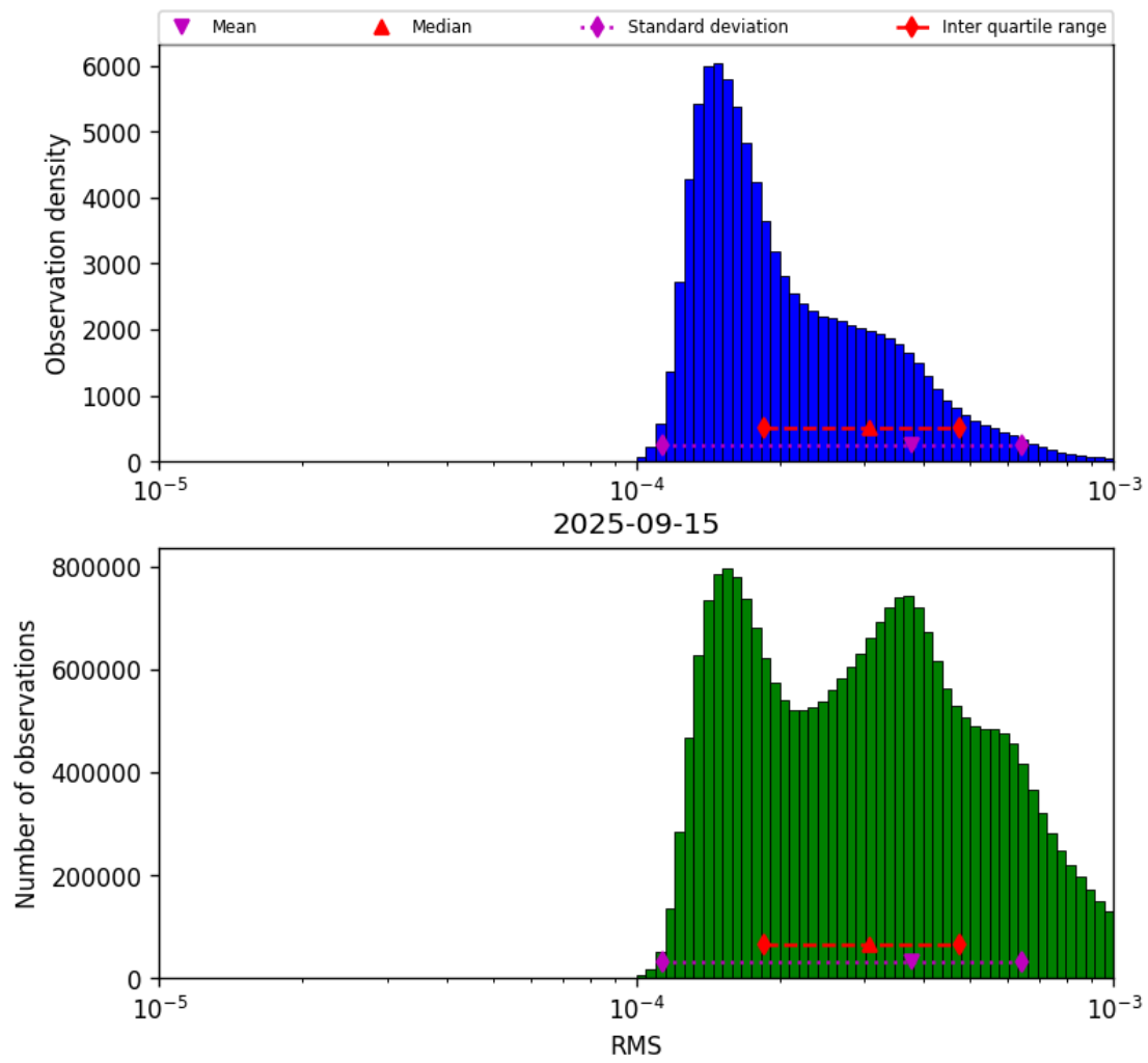
Figure 43: Histogram of “RMS” for 2025-09-15 to 2025-09-16
