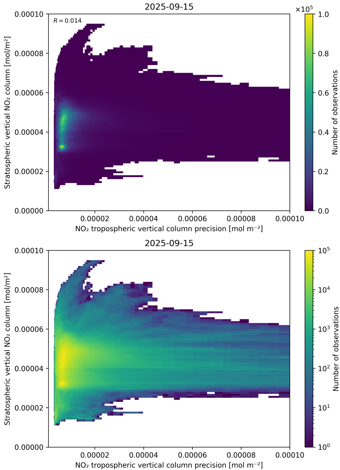
Figure 135: Scatter density plot of “NO 2 tropospheric vertical column precision” against “Stratospheric vertical NO 2 column” for 2025-09-15 to 2025-09-16.
