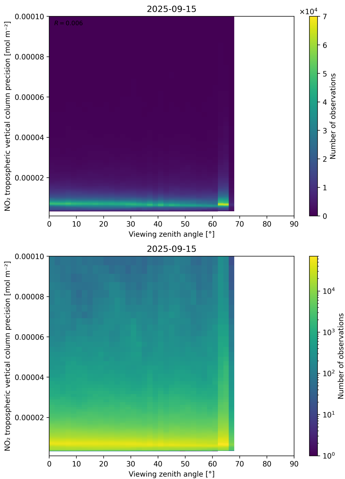
Figure 170: Scatter density plot of “Viewing zenith angle” against “NO 2 tropospheric vertical column precision” for 2025-09-15 to 2025-09-16.
