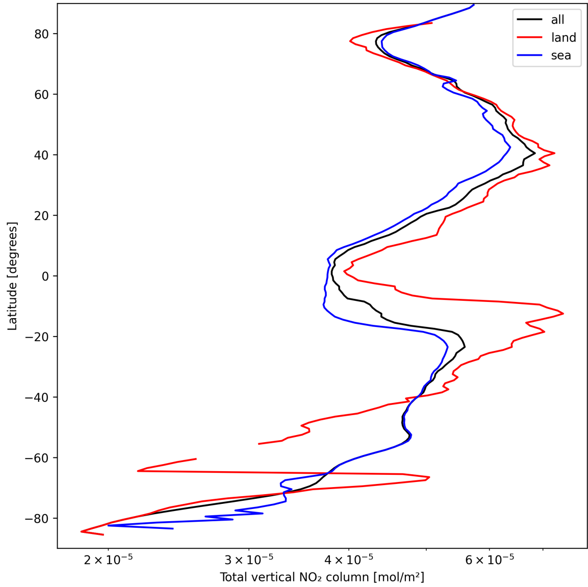
Figure 21: Zonal average of “Total vertical NO 2 column” for 2025-09-15 to 2025-09-16.
