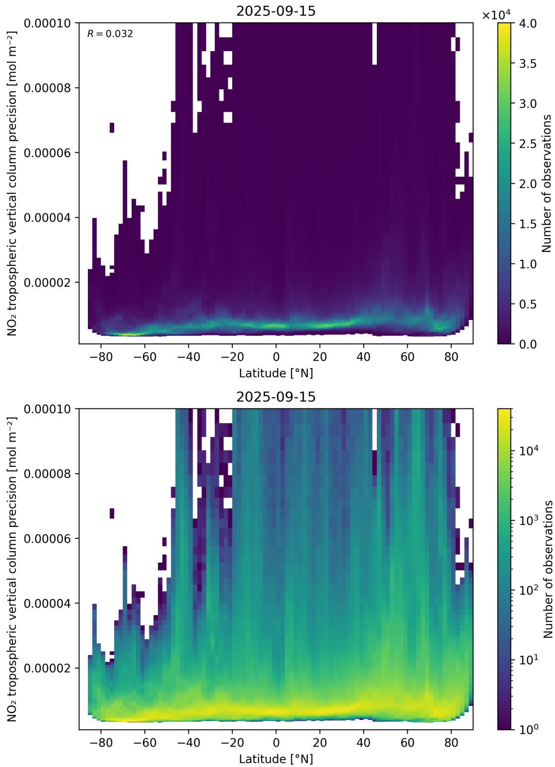
Figure 93: Scatter density plot of “Latitude” against “NO 2 tropospheric vertical column precision” for 2025-09-15 to 2025-09-16.
