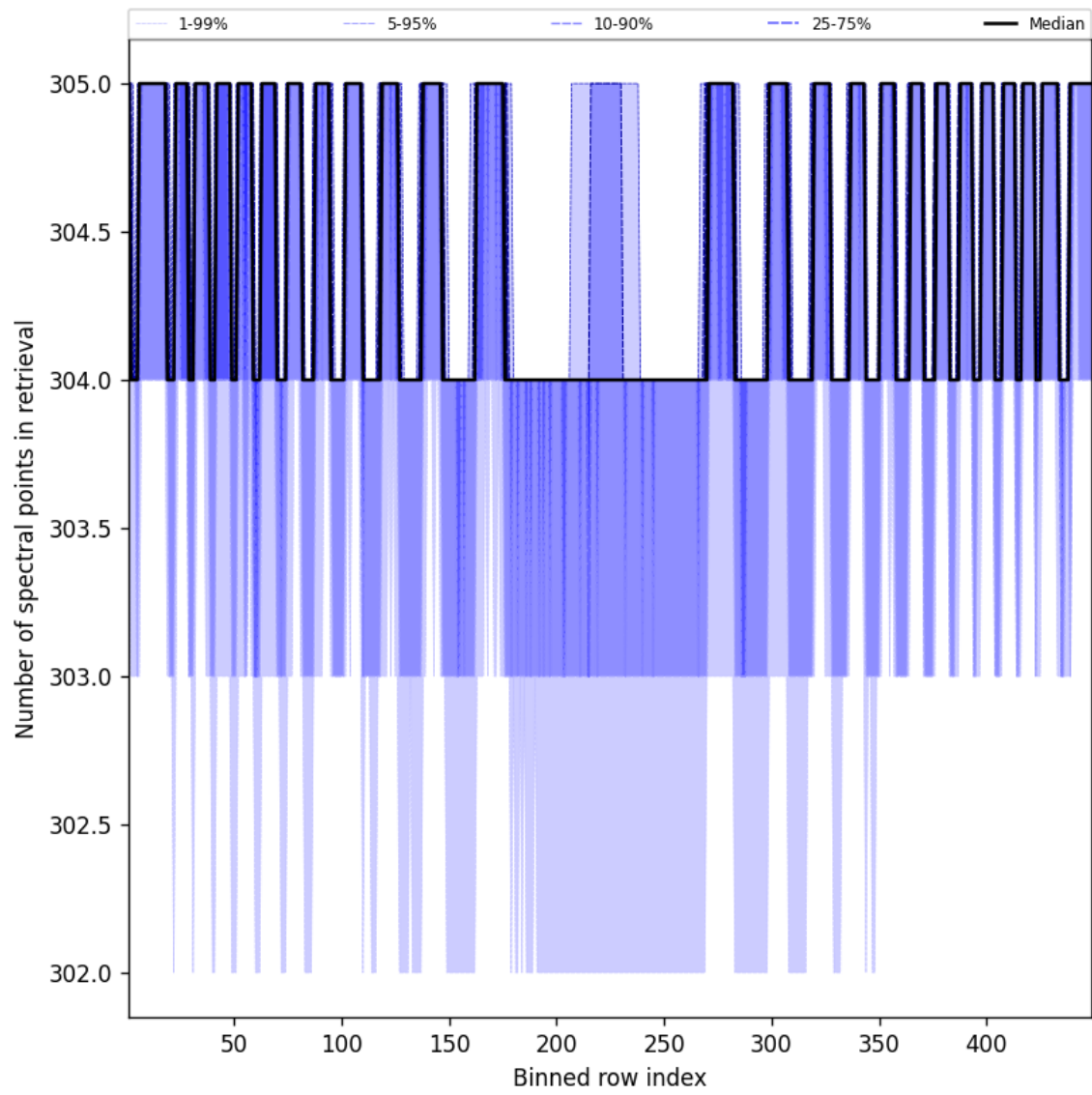
Figure 50: Along track statistics of “Number of spectral points in retrieval” for 2025-09-15 to 2025-09-16
