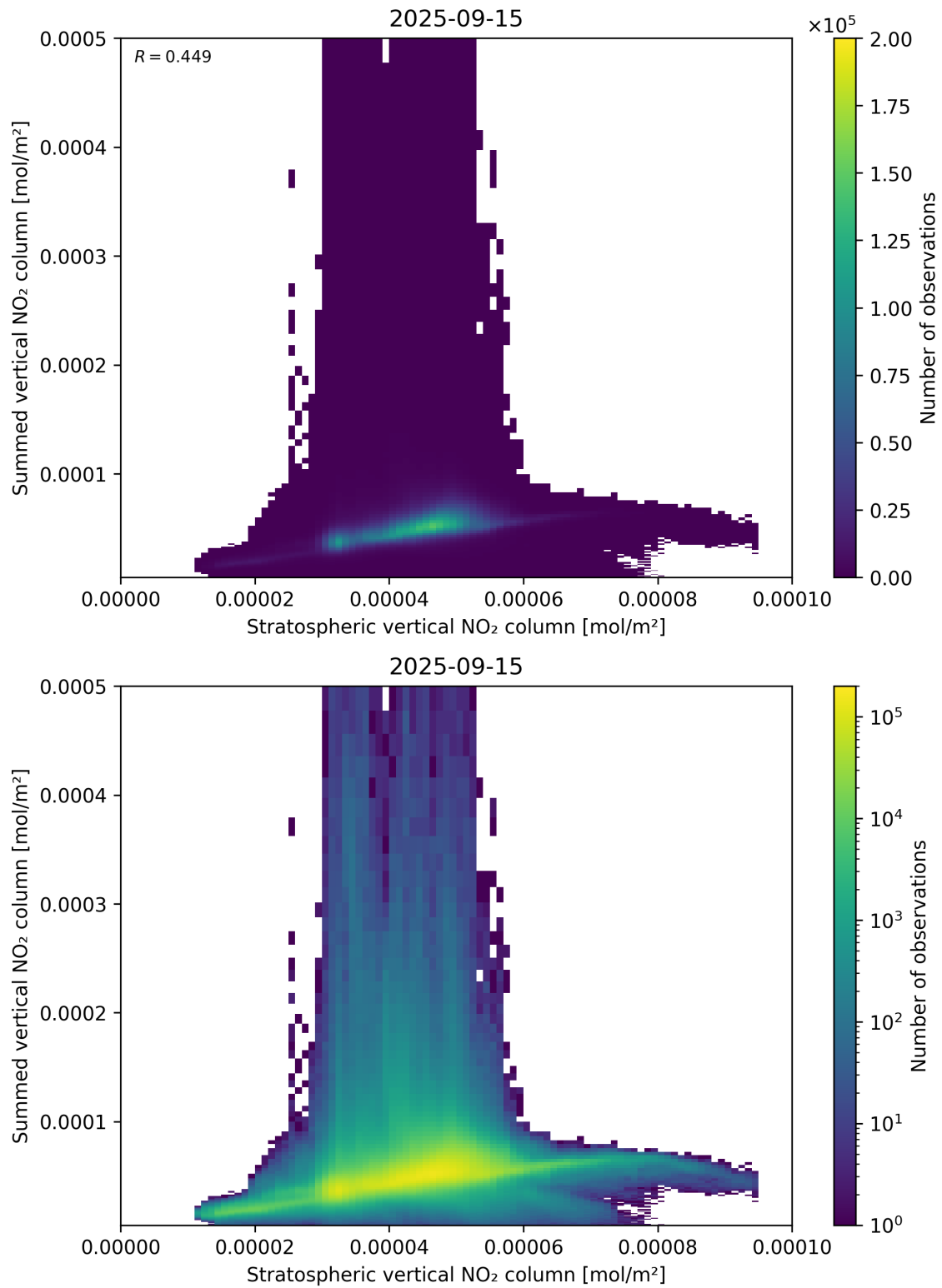
Figure 98: Scatter density plot of “Stratospheric vertical NO 2 column” against “Summed vertical NO 2 column” for 2025-09-15 to 2025-09-16.
