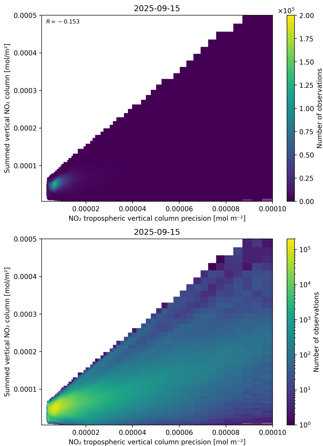
Figure 136: Scatter density plot of “NO 2 tropospheric vertical column precision” against “Summed vertical NO 2 column” for 2025-09-15 to 2025-09-16.
