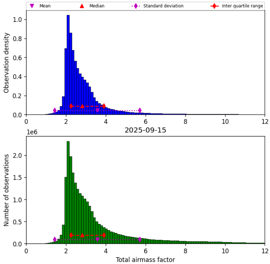
Figure 32: Histogram of “Total airmass factor” for 2025-09-15 to 2025-09-16
