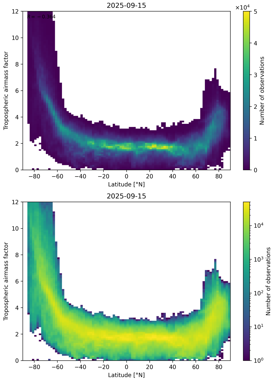
Figure 85: Scatter density plot of “Latitude” against “Tropospheric air mass factor” for 2025-09-15 to 2025-09-16.
