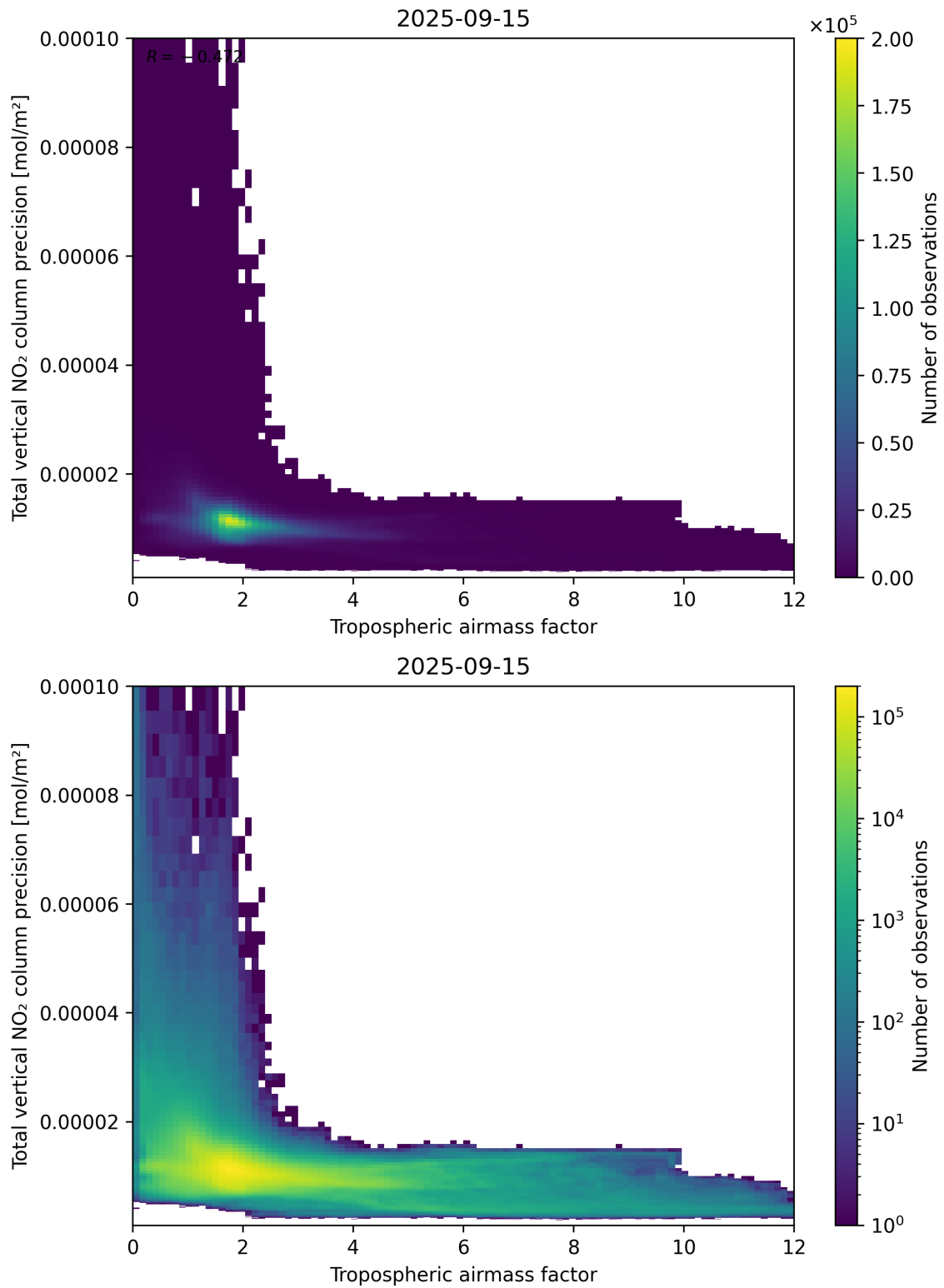
Figure 78: Scatter density plot of “Tropospheric air mass factor” against “Total vertical NO 2 column precision” for 2025-09-15 to 2025-09-16.
