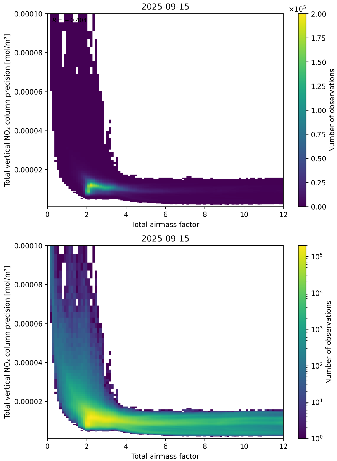
Figure 68: Scatter density plot of “Total airmass factor” against “Total vertical NO 2 column precision” for 2025-09-15 to 2025-09-16.
