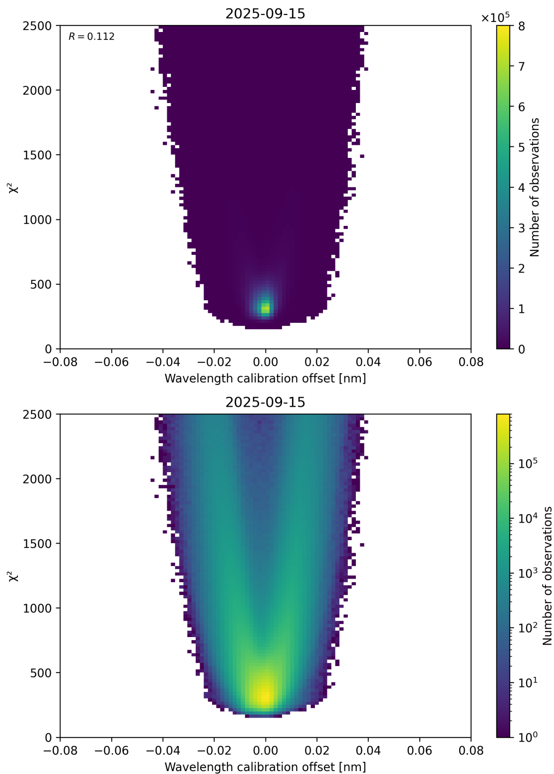
Figure 175: Scatter density plot of “Wavelength calibration offset” against “ \chi^2 ” for 2025-09-15 to 2025-09-16.
