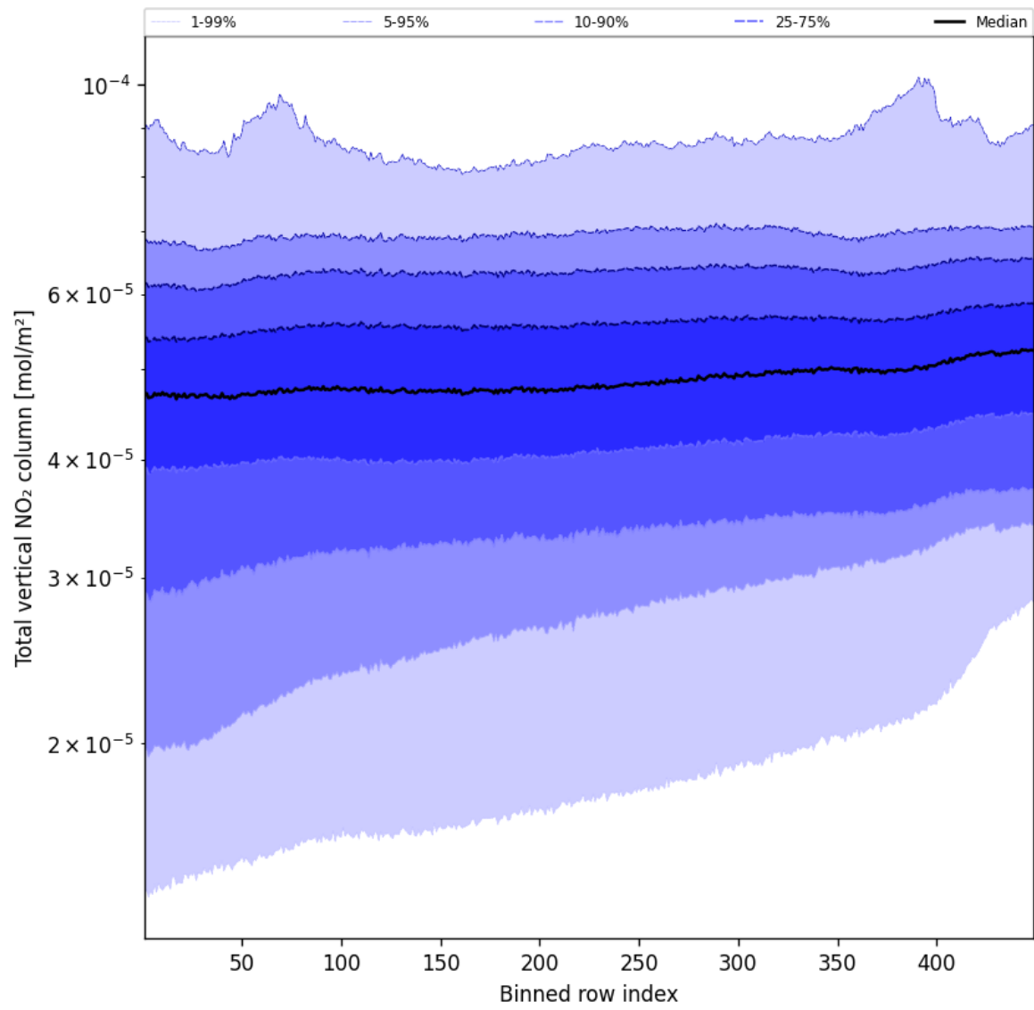
Figure 55: Along track statistics of “Total vertical NO 2 column” for 2025-09-15 to 2025-09-16
