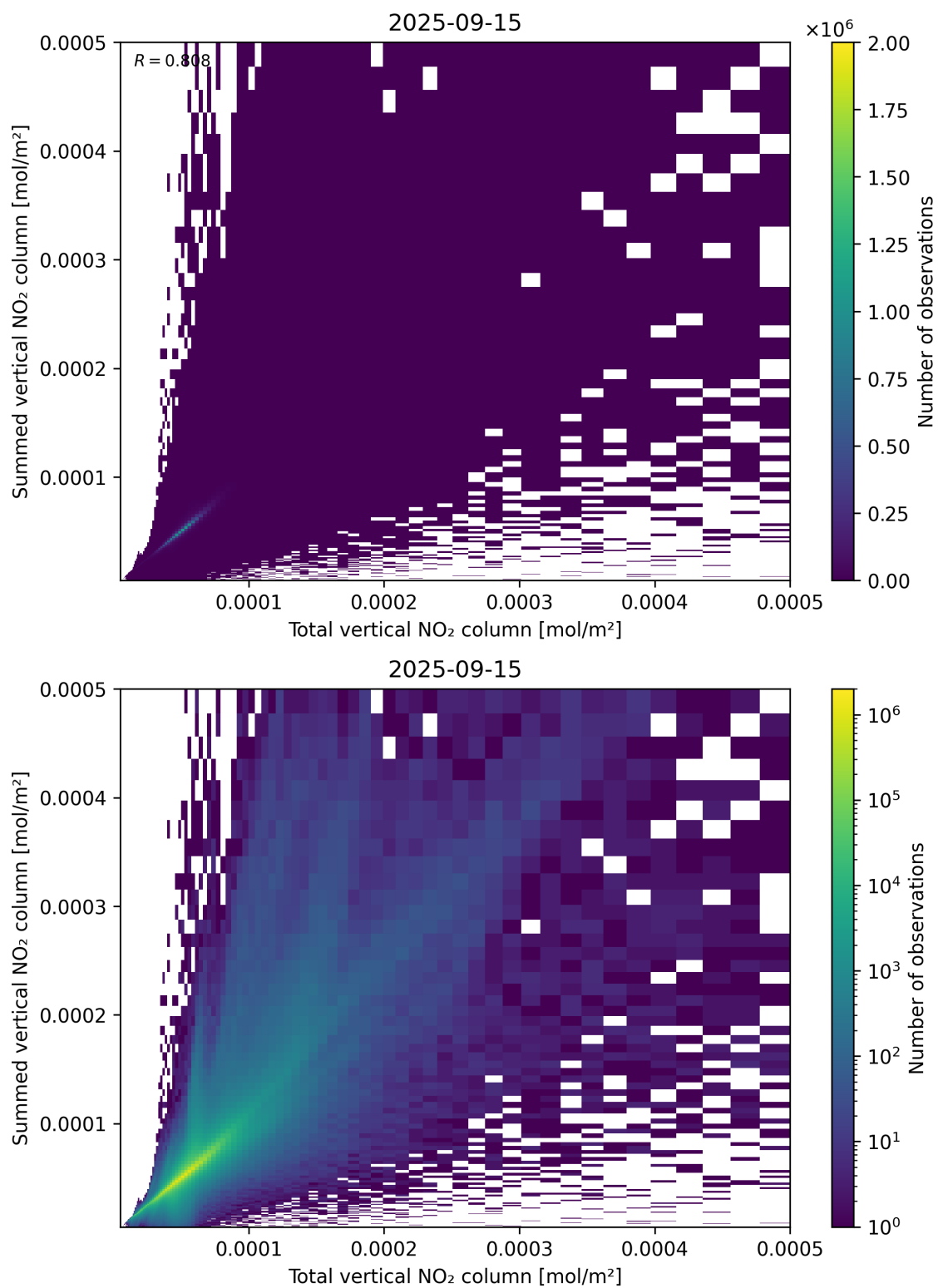
Figure 112: Scatter density plot of “Total vertical NO 2 column” against “Summed vertical NO 2 column” for 2025-09-15 to 2025-09-16.
