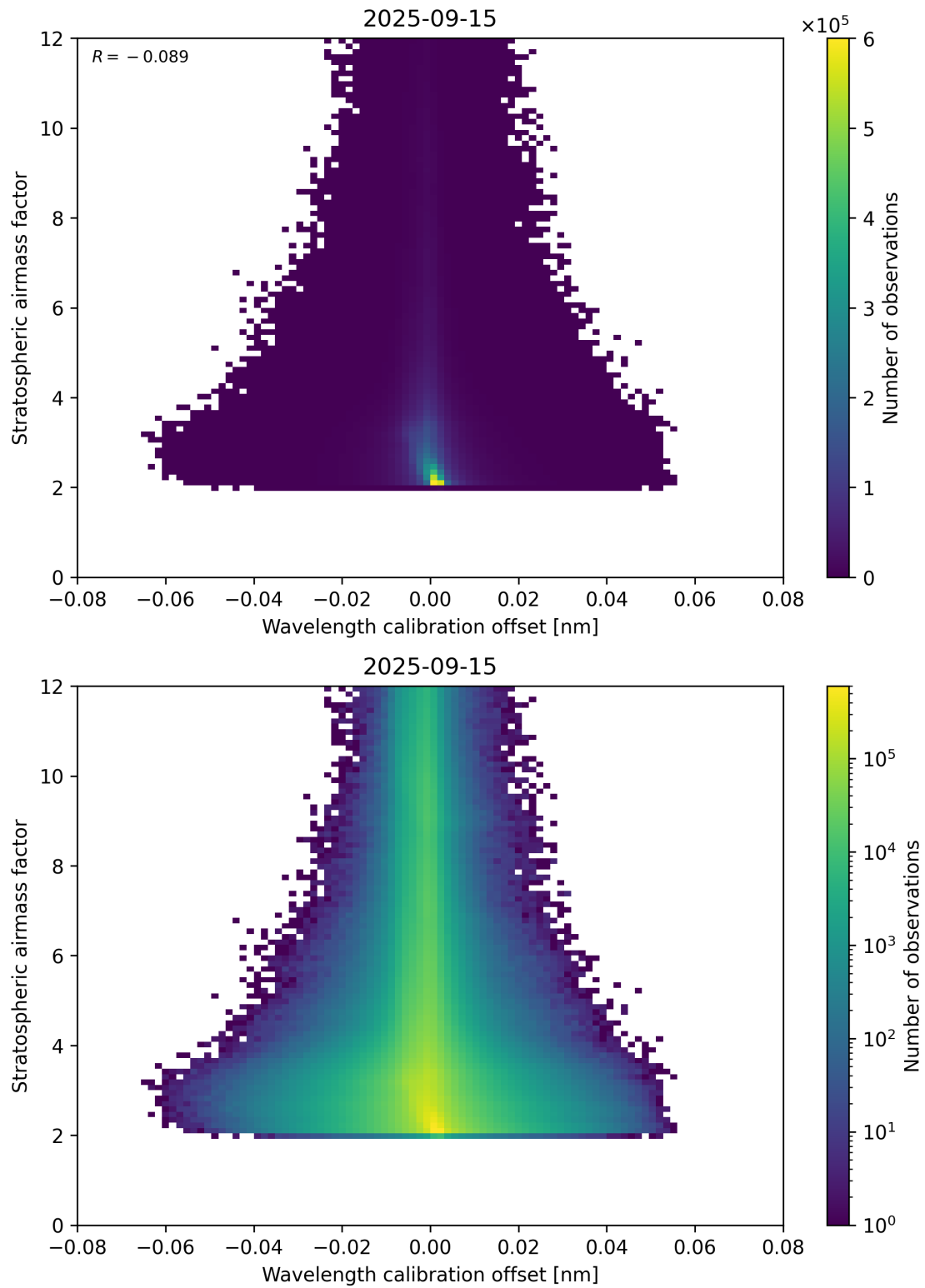
Figure 174: Scatter density plot of “Wavelength calibration offset” against “Stratospheric airmass factor” for 2025-09-15 to 2025-09-16.
