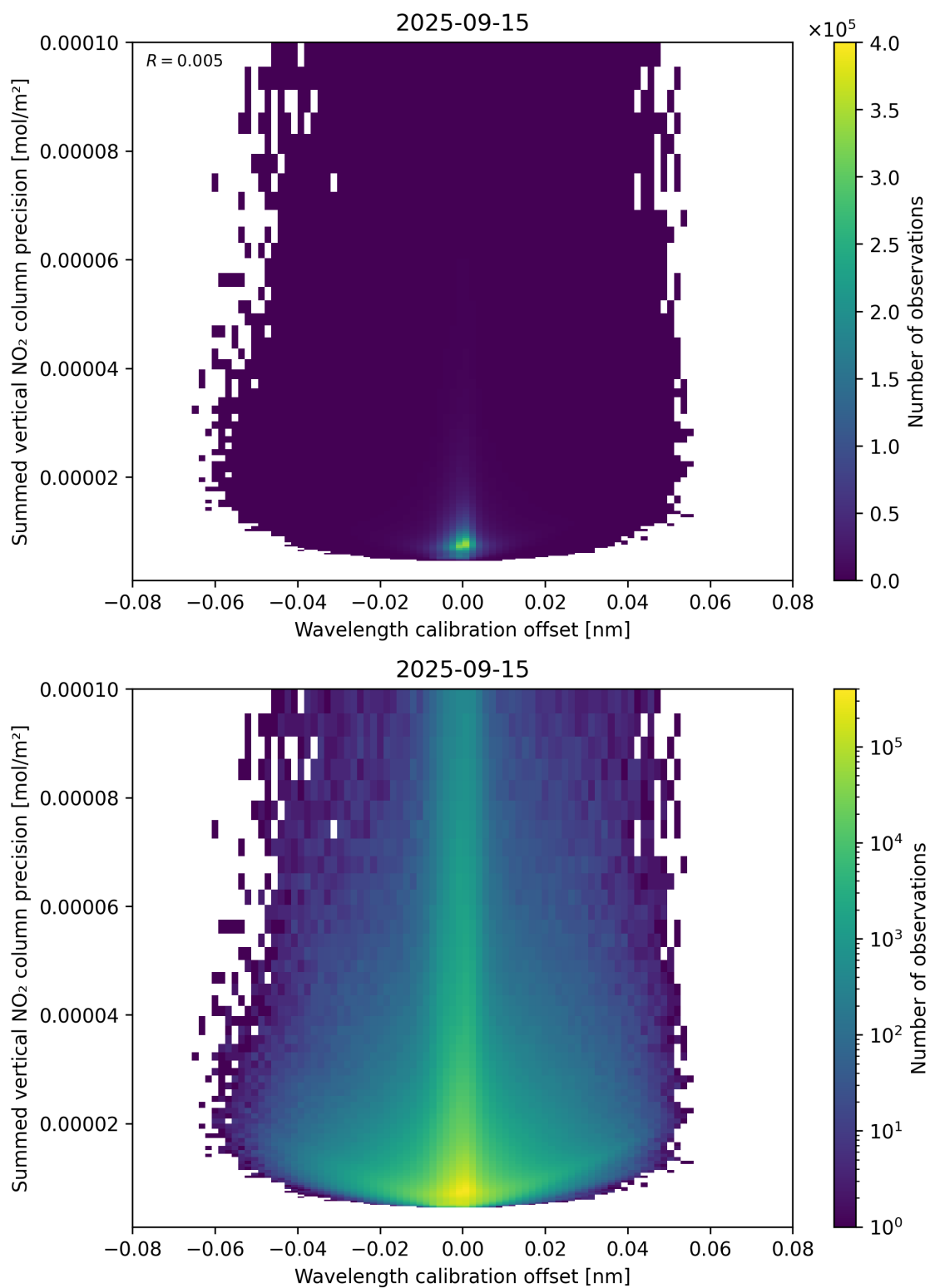
Figure 178: Scatter density plot of “Wavelength calibration offset” against “Summed vertical NO 2 column precision” for 2025-09-15 to 2025-09-16.
