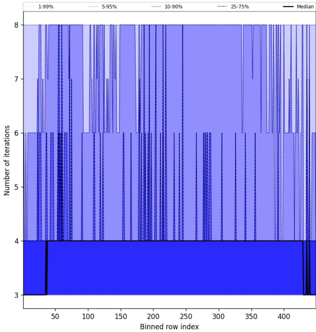
Figure 51: Along track statistics of “Number of iterations” for 2025-09-15 to 2025-09-16
