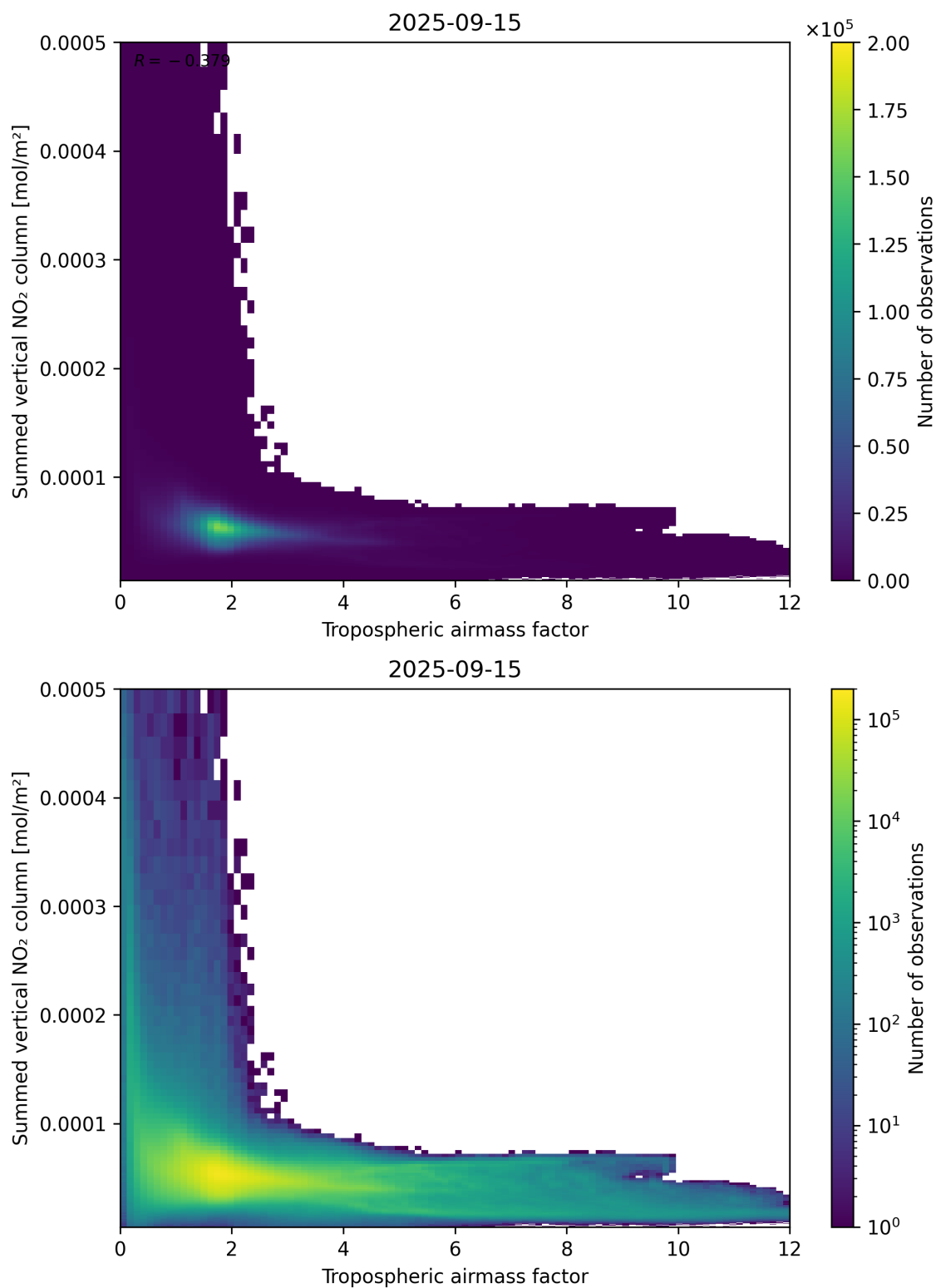
Figure 75: Scatter density plot of “Tropospheric air mass factor” against “Summed vertical NO 2 column” for 2025-09-15 to 2025-09-16.
