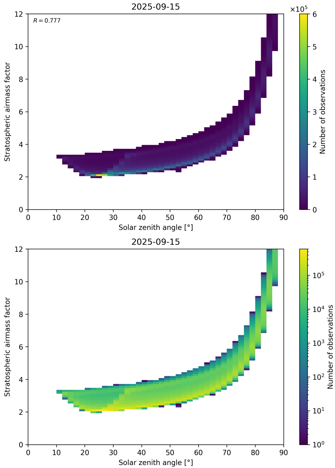
Figure 145: Scatter density plot of “Solar zenith angle” against “Stratospheric airmass factor” for 2025-09-15 to 2025-09-16.
