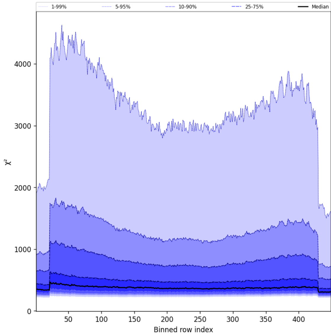
Figure 59: Along track statistics of “ \chi^2 ” for 2025-09-15 to 2025-09-16
