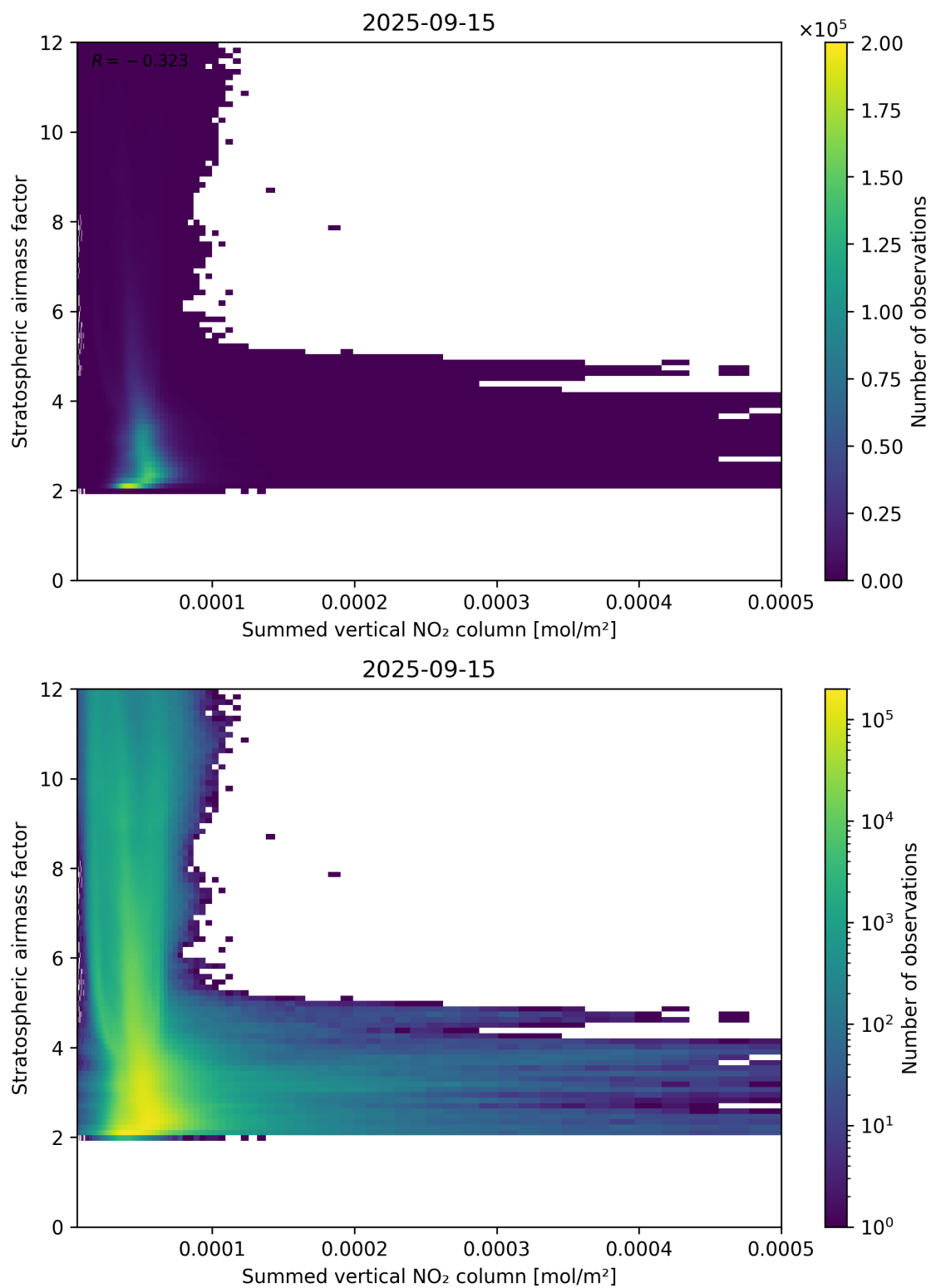
Figure 103: Scatter density plot of “Summed vertical NO 2 column” against “Stratospheric airmass factor” for 2025-09-15 to 2025-09-16.
