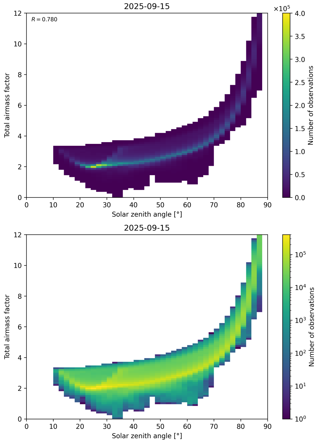
Figure 146: Scatter density plot of “Solar zenith angle” against “Total air mass factor” for 2025-09-15 to 2025-09-16.
