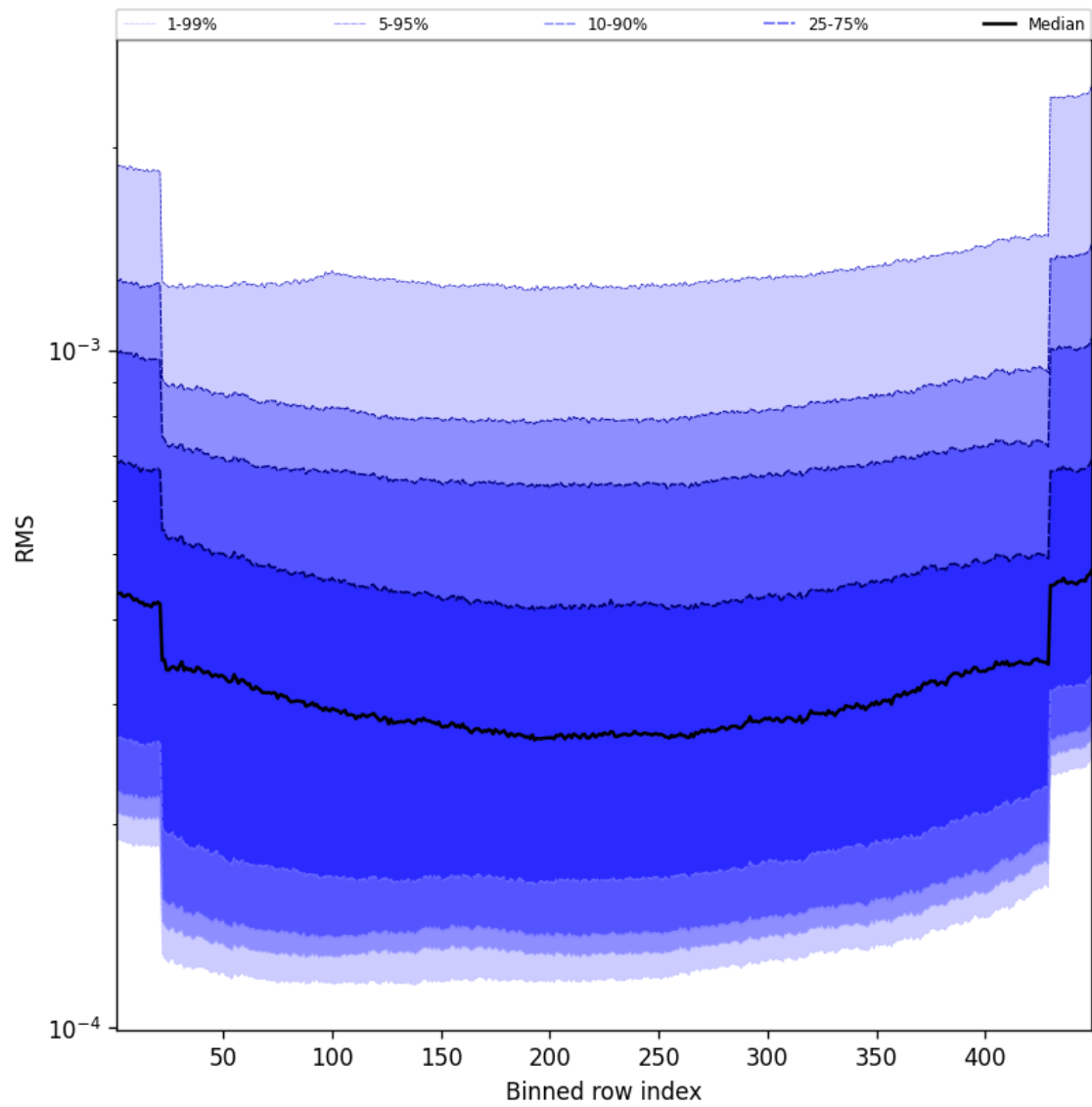
Figure 60: Along track statistics of “RMS” for 2025-09-15 to 2025-09-16
