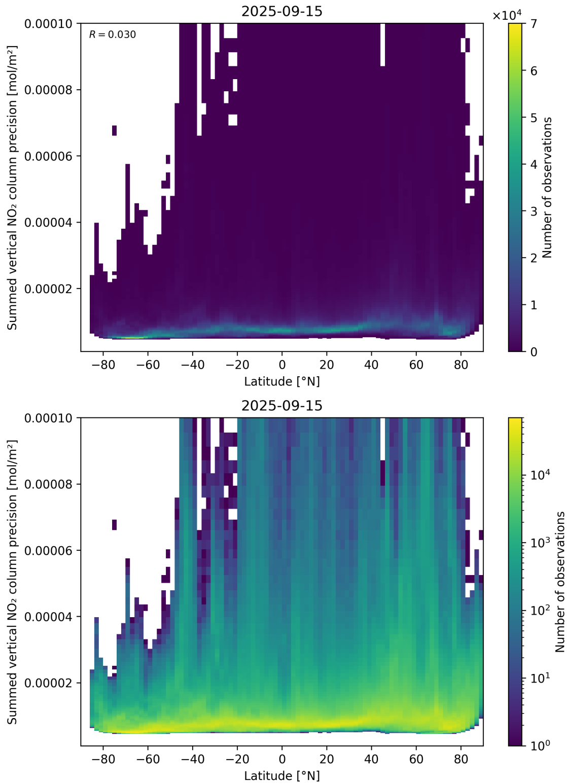
Figure 89: Scatter density plot of “Latitude” against “Summed vertical NO 2 column precision” for 2025-09-15 to 2025-09-16.
