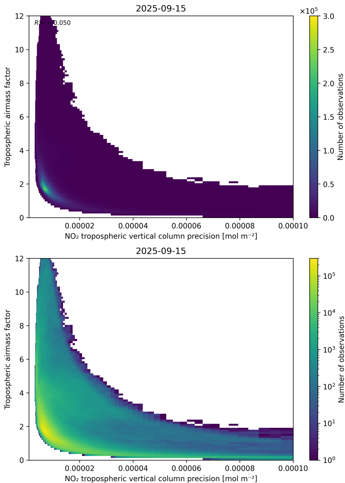
Figure 133: Scatter density plot of “NO 2 tropospheric vertical column precision” against “Tropospheric airmass factor” for 2025-09-15 to 2025-09-16.
