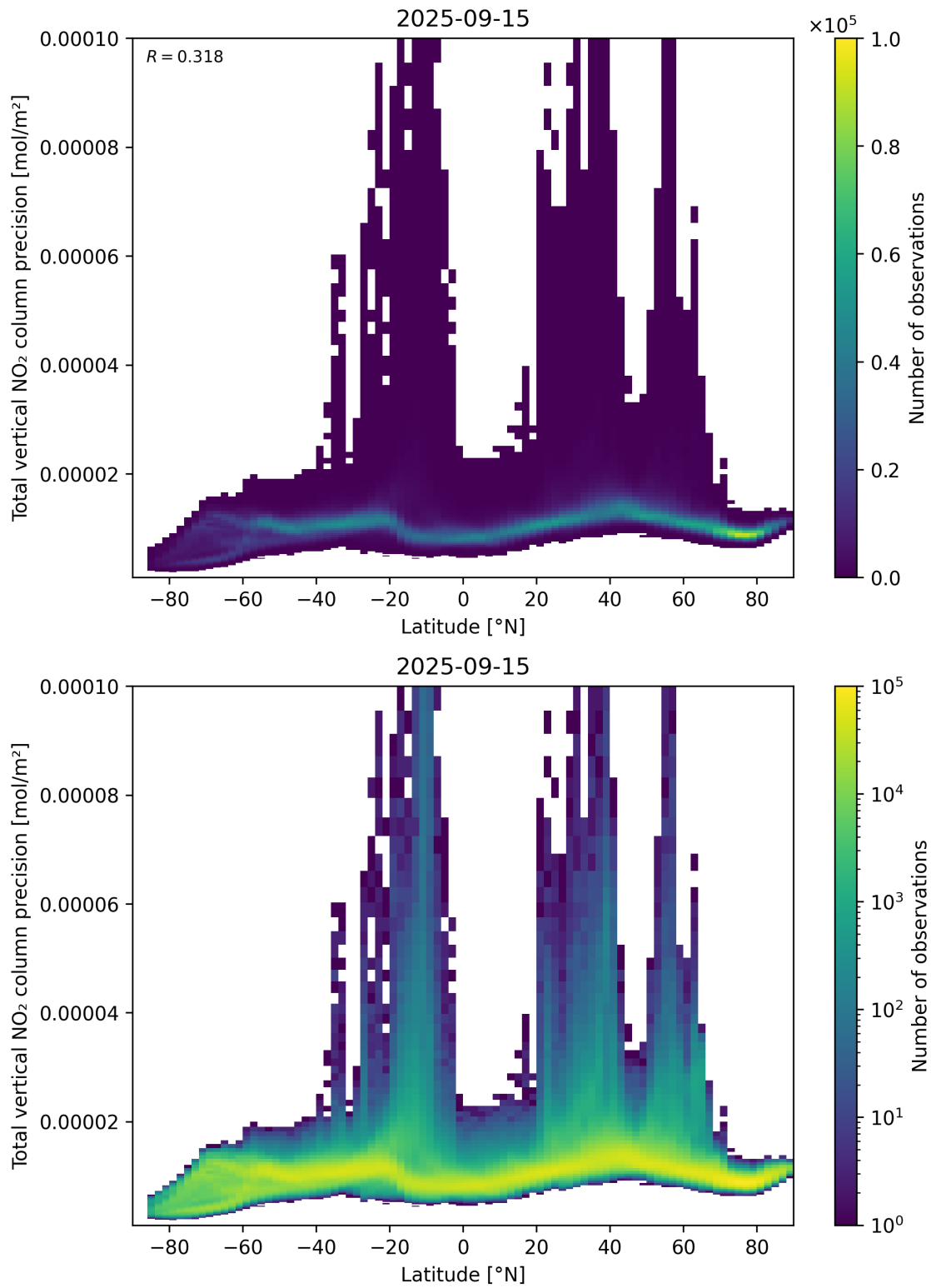
Figure 91: Scatter density plot of “Latitude” against “Total vertical NO 2 column precision” for 2025-09-15 to 2025-09-16.
