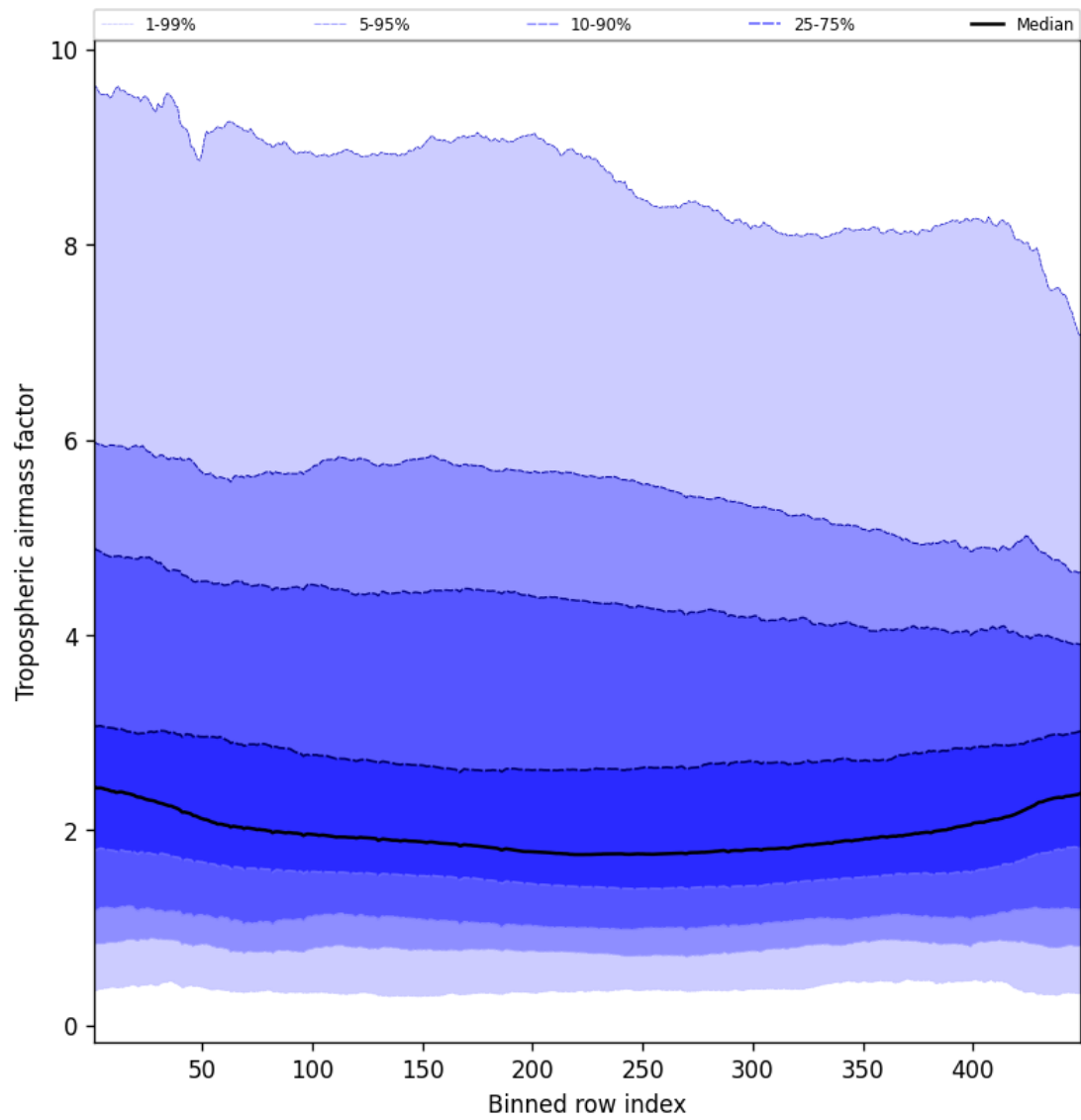
Figure 48: Along track statistics of “Tropospheric airmass factor” for 2025-09-15 to 2025-09-16
