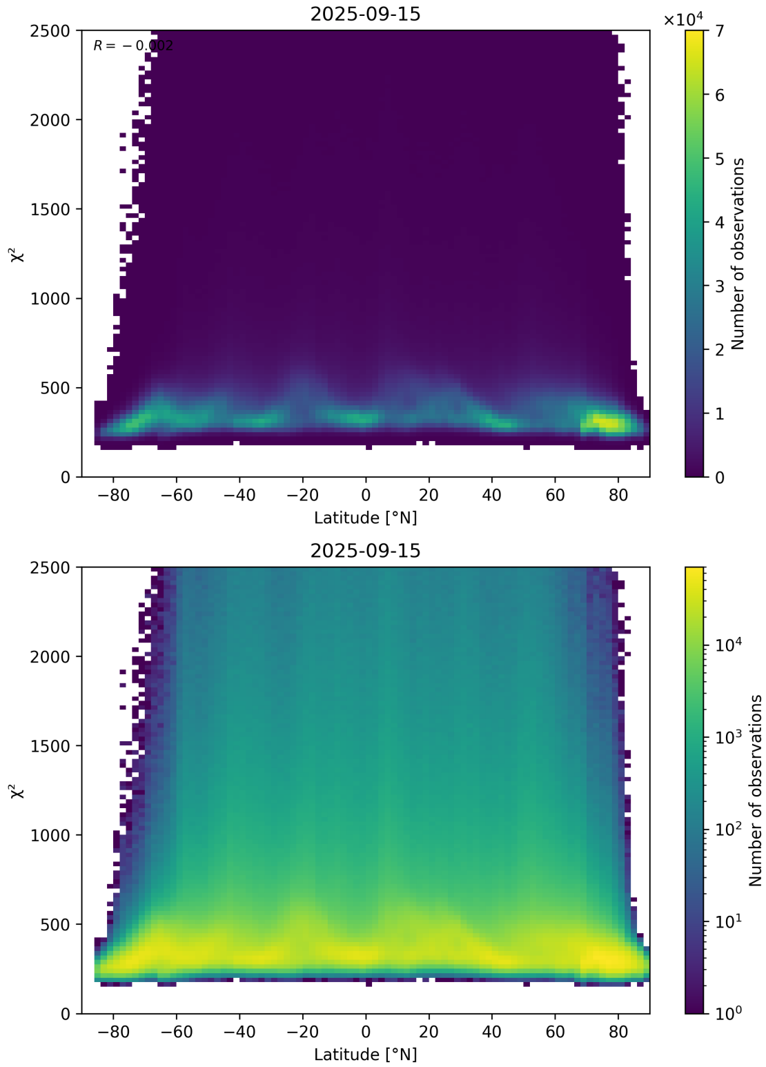
Figure 86: Scatter density plot of “Latitude” against “ \chi^2 ” for 2025-09-15 to 2025-09-16.
