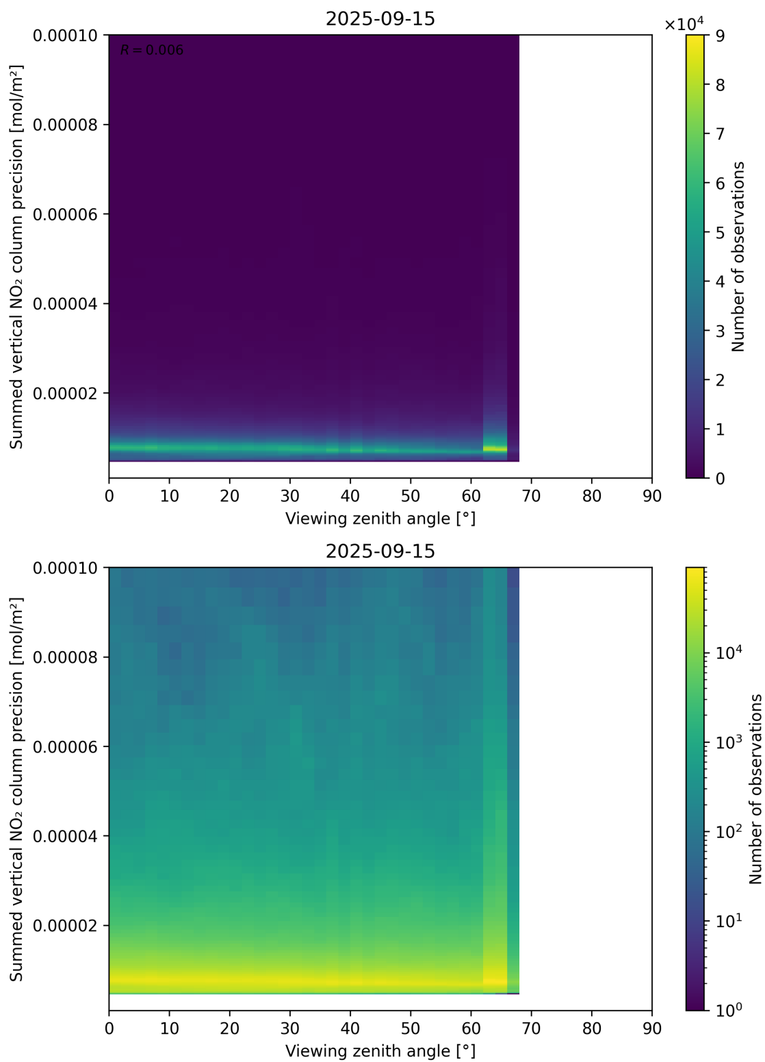
Figure 166: Scatter density plot of “Viewing zenith angle” against “Summed vertical NO 2 column precision” for 2025-09-15 to 2025-09-16.
