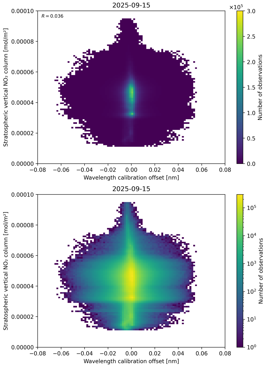
Figure 176: Scatter density plot of “Wavelength calibration offset” against “Stratospheric vertical NO 2 column” for 2025-09-15 to 2025-09-16.
