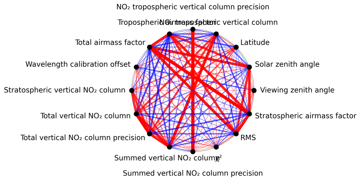
Figure 1: Map of correlation graph for 2025-09-15 to 2025-09-16.
