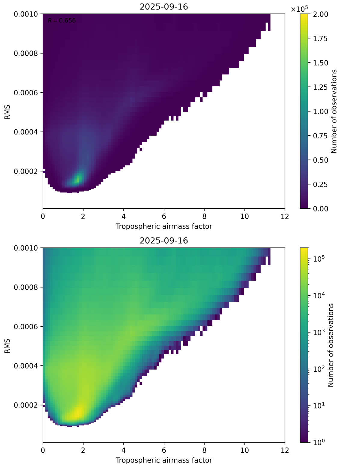
Figure 79: Scatter density plot of “Tropospheric airmass factor” against “RMS” for 2025-09-15 to 2025-09-17.
