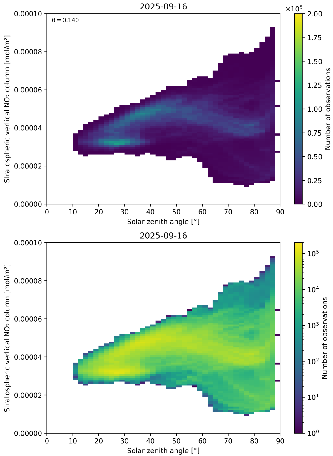
Figure 150: Scatter density plot of “Solar zenith angle” against “Stratospheric vertical NO 2 column” for 2025-09-15 to 2025-09-17.
