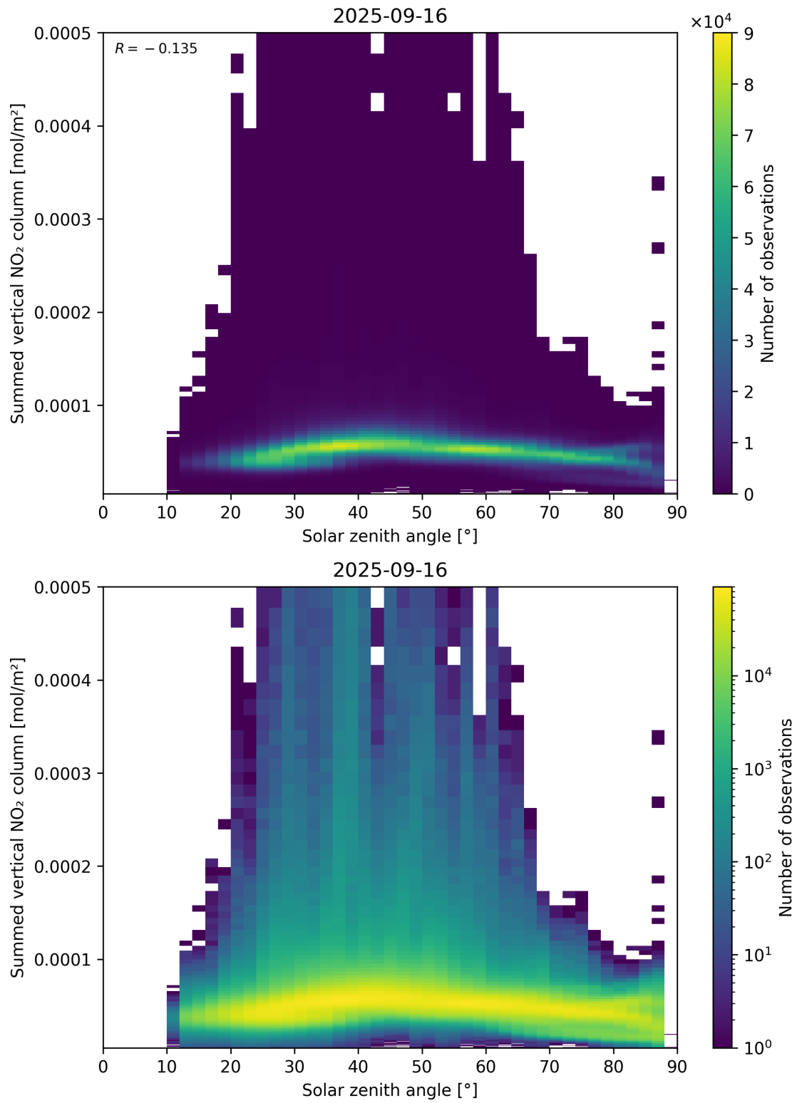
Figure 151: Scatter density plot of “Solar zenith angle” against “Summed vertical NO 2 column” for 2025-09-15 to 2025-09-17.
