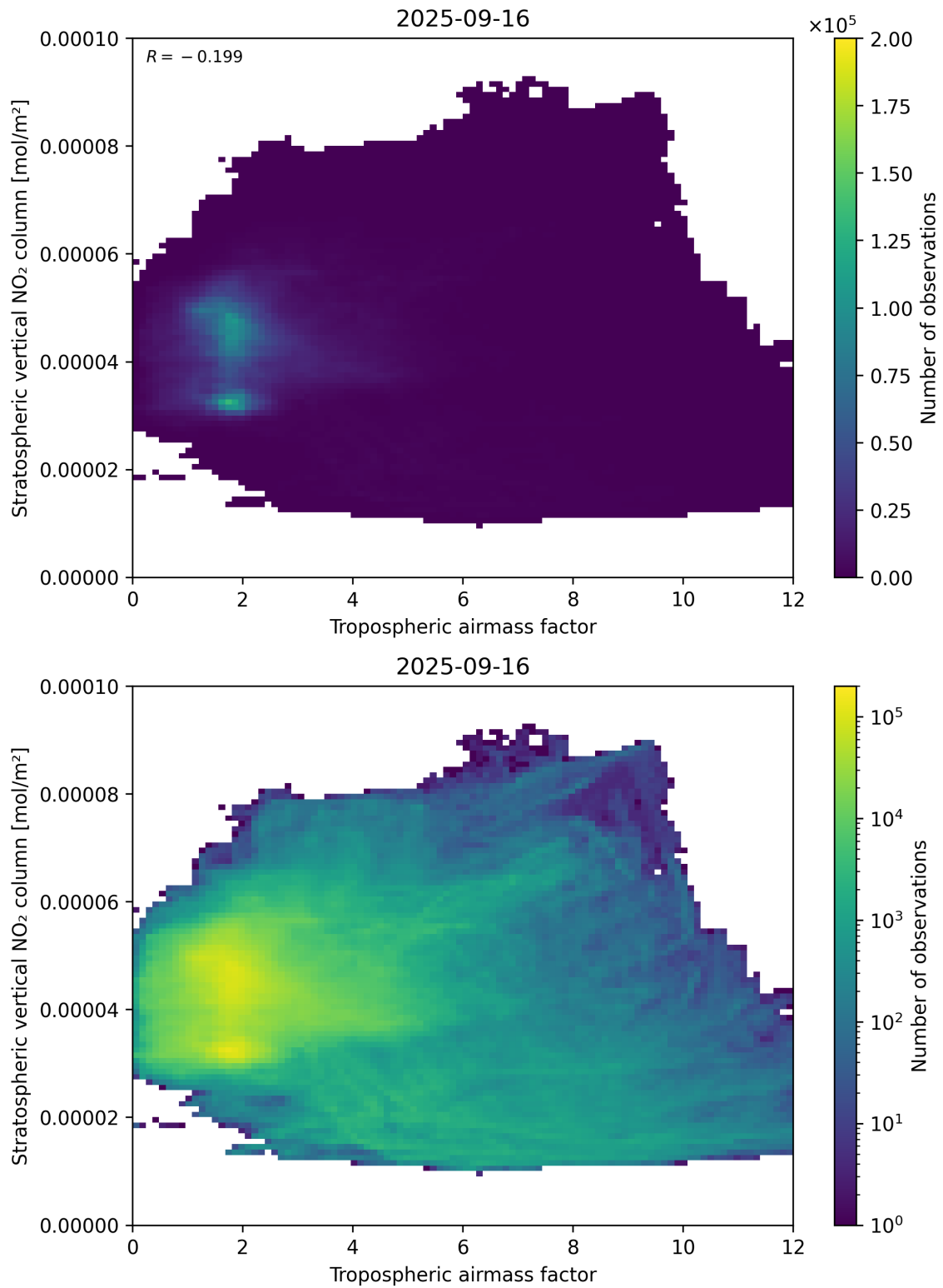
Figure 74: Scatter density plot of “Tropospheric air mass factor” against “Stratospheric vertical NO 2 column” for 2025-09-15 to 2025-09-17.
