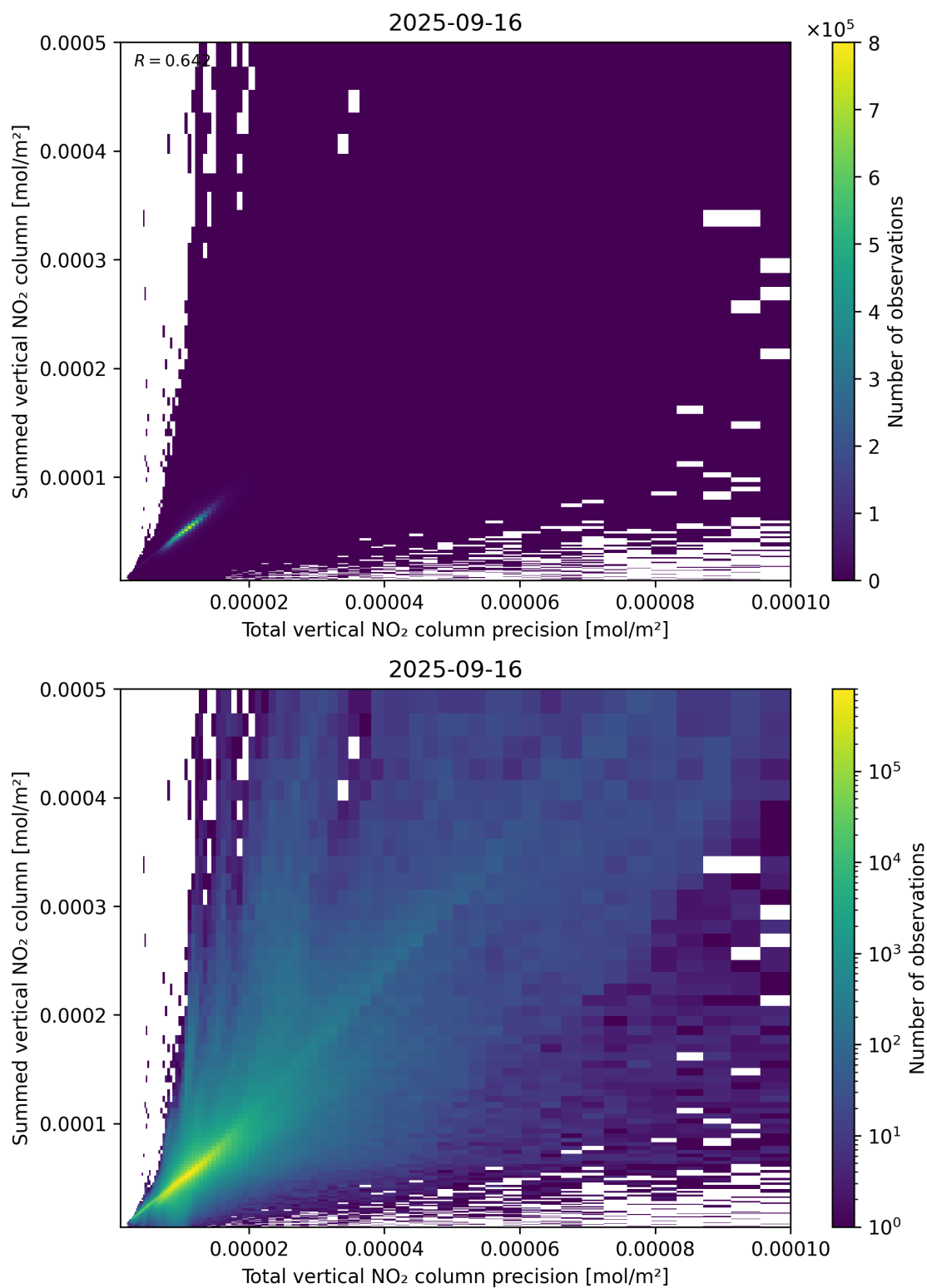
Figure 117: Scatter density plot of “Total vertical NO 2 column precision” against “Summed vertical NO 2 column” for 2025-09-15 to 2025-09-17.
