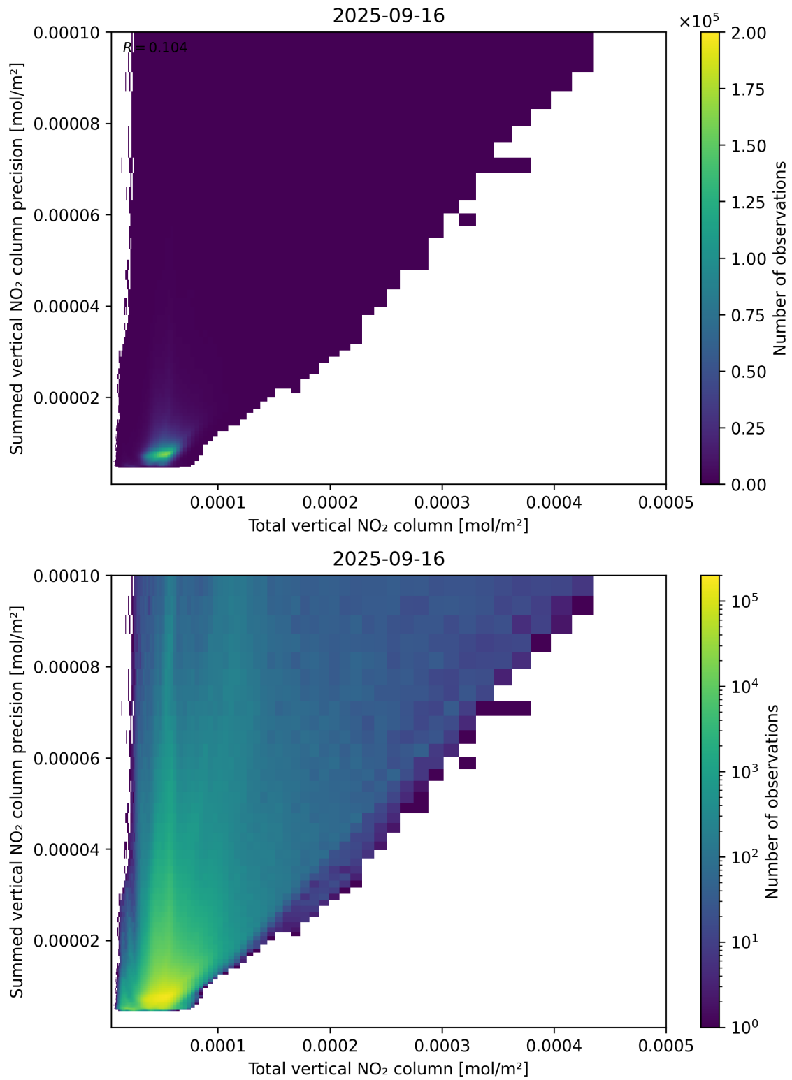
Figure 113: Scatter density plot of “Total vertical NO 2 column” against “Summed vertical NO 2 column precision” for 2025-09-15 to 2025-09-17.
