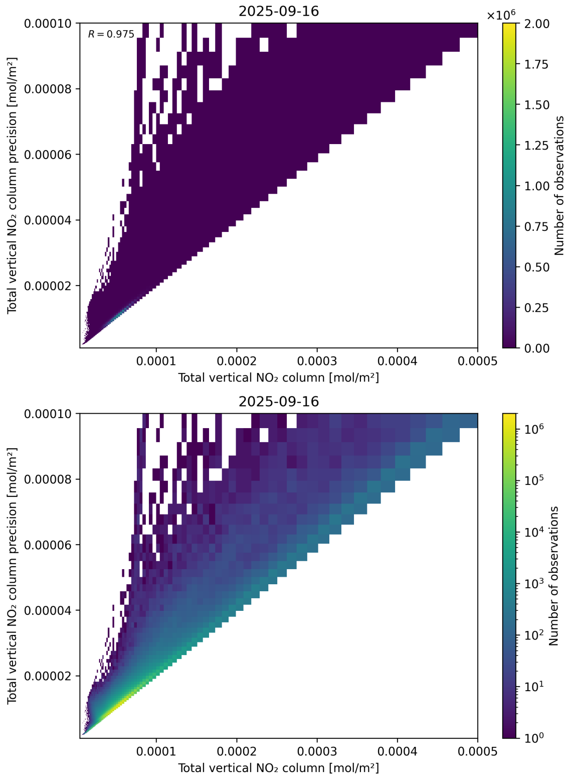
Figure 114: Scatter density plot of “Total vertical NO 2 column” against “Total vertical NO 2 column precision” for 2025-09-15 to 2025-09-17.
