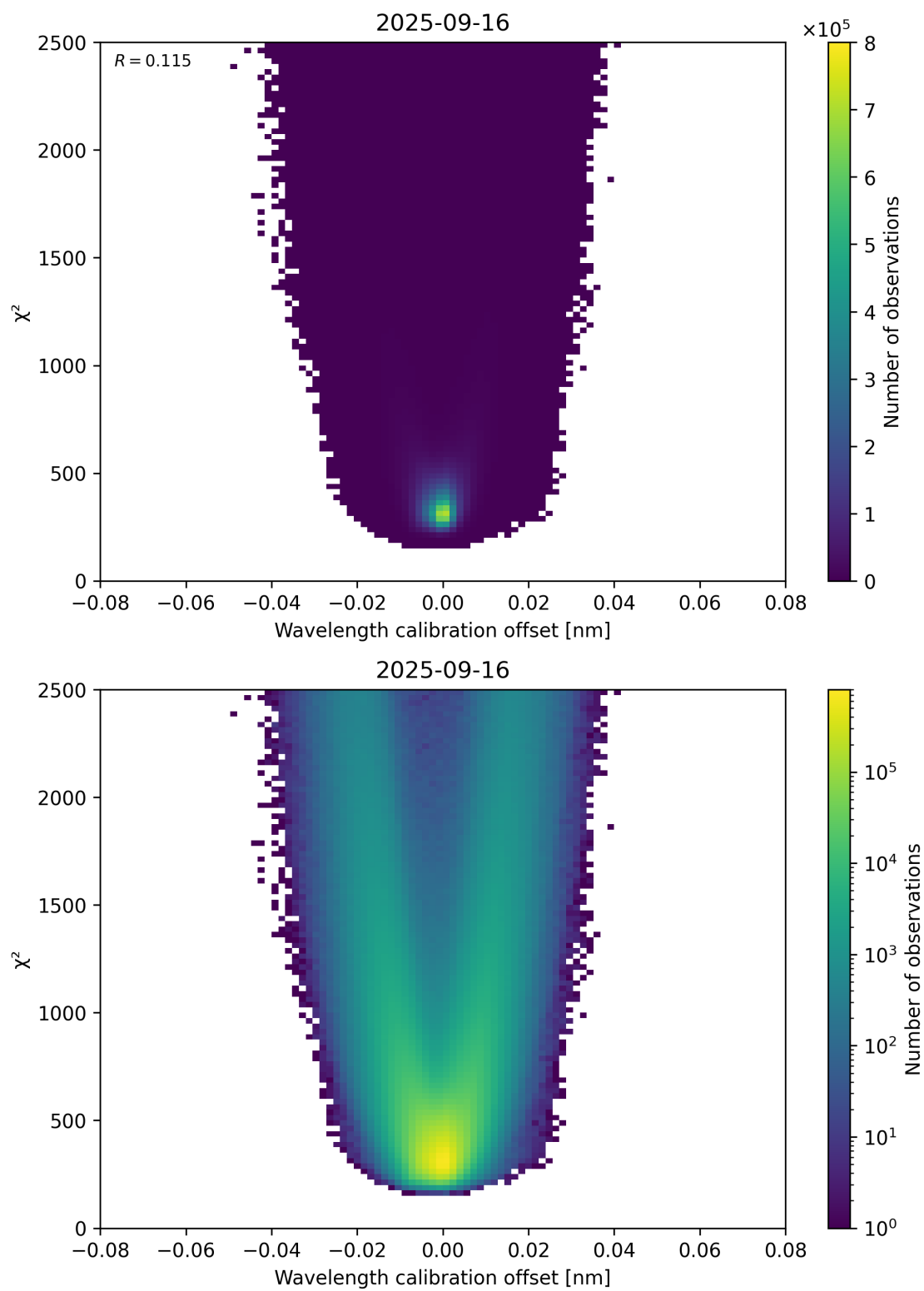
Figure 175: Scatter density plot of “Wavelength calibration offset” against “ \chi^2 ” for 2025-09-15 to 2025-09-17.
