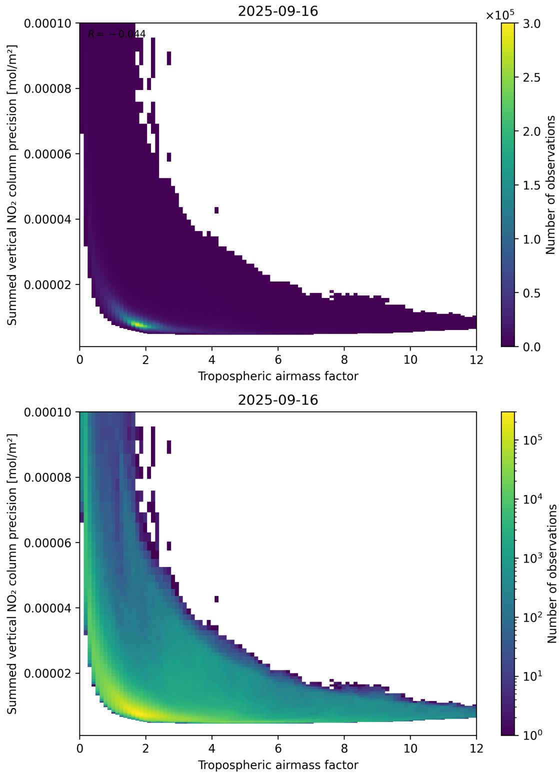
Figure 76: Scatter density plot of “Tropospheric air mass factor” against “Summed vertical NO 2 column precision” for 2025-09-15 to 2025-09-17.
