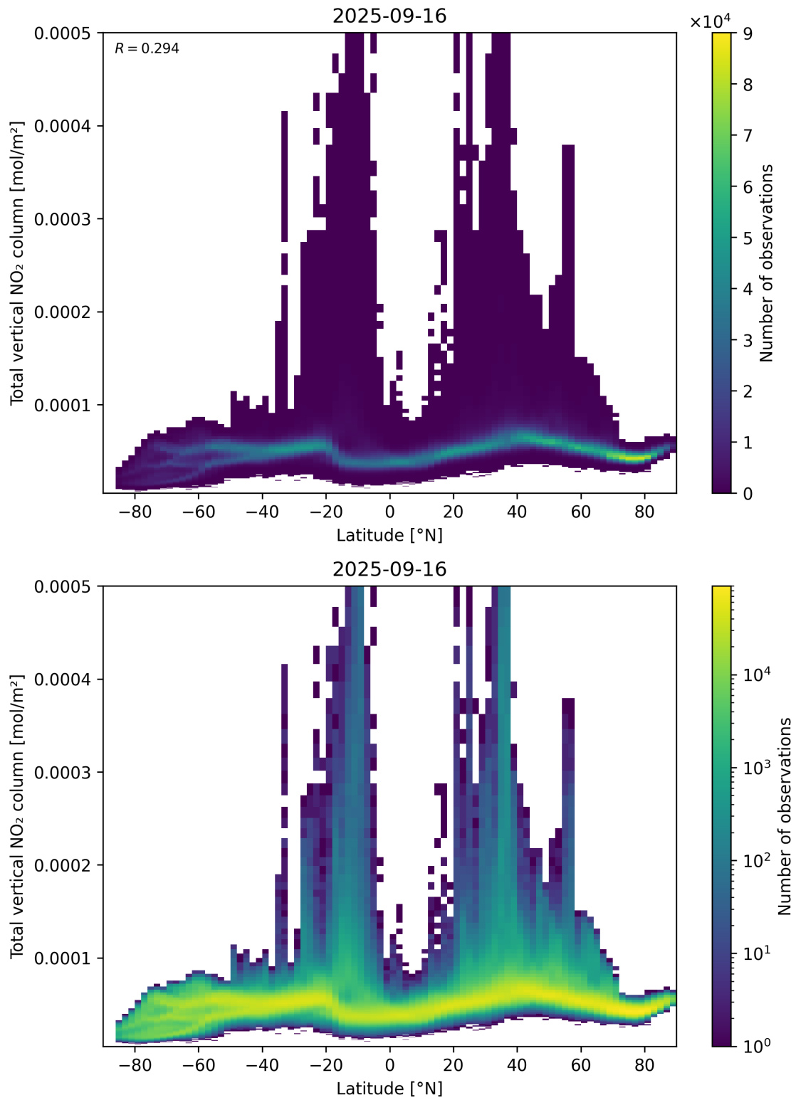
Figure 90: Scatter density plot of “Latitude” against “Total vertical NO 2 column” for 2025-09-15 to 2025-09-17.
