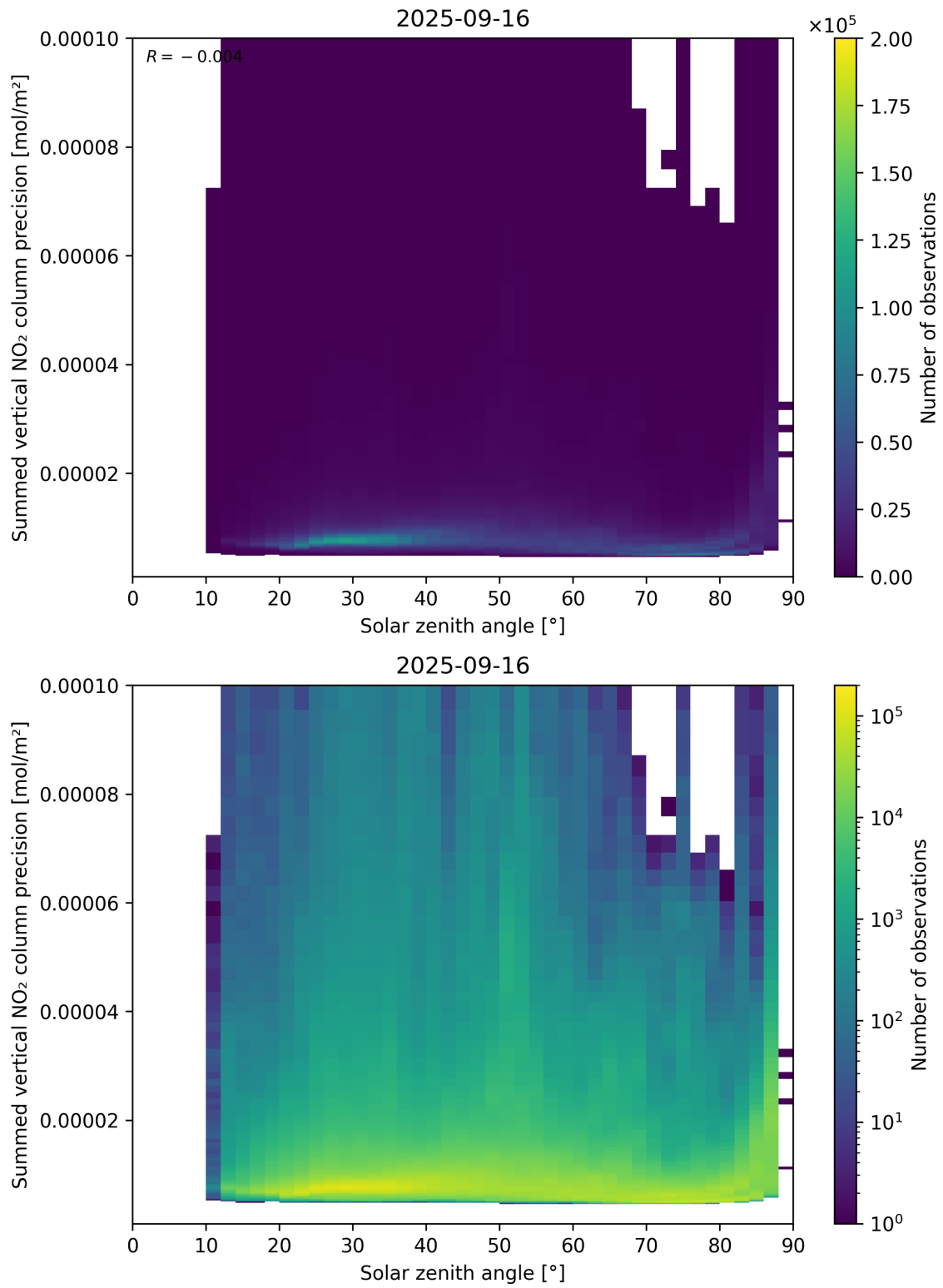
Figure 152: Scatter density plot of “Solar zenith angle” against “Summed vertical NO 2 column precision” for 2025-09-15 to 2025-09-17.
