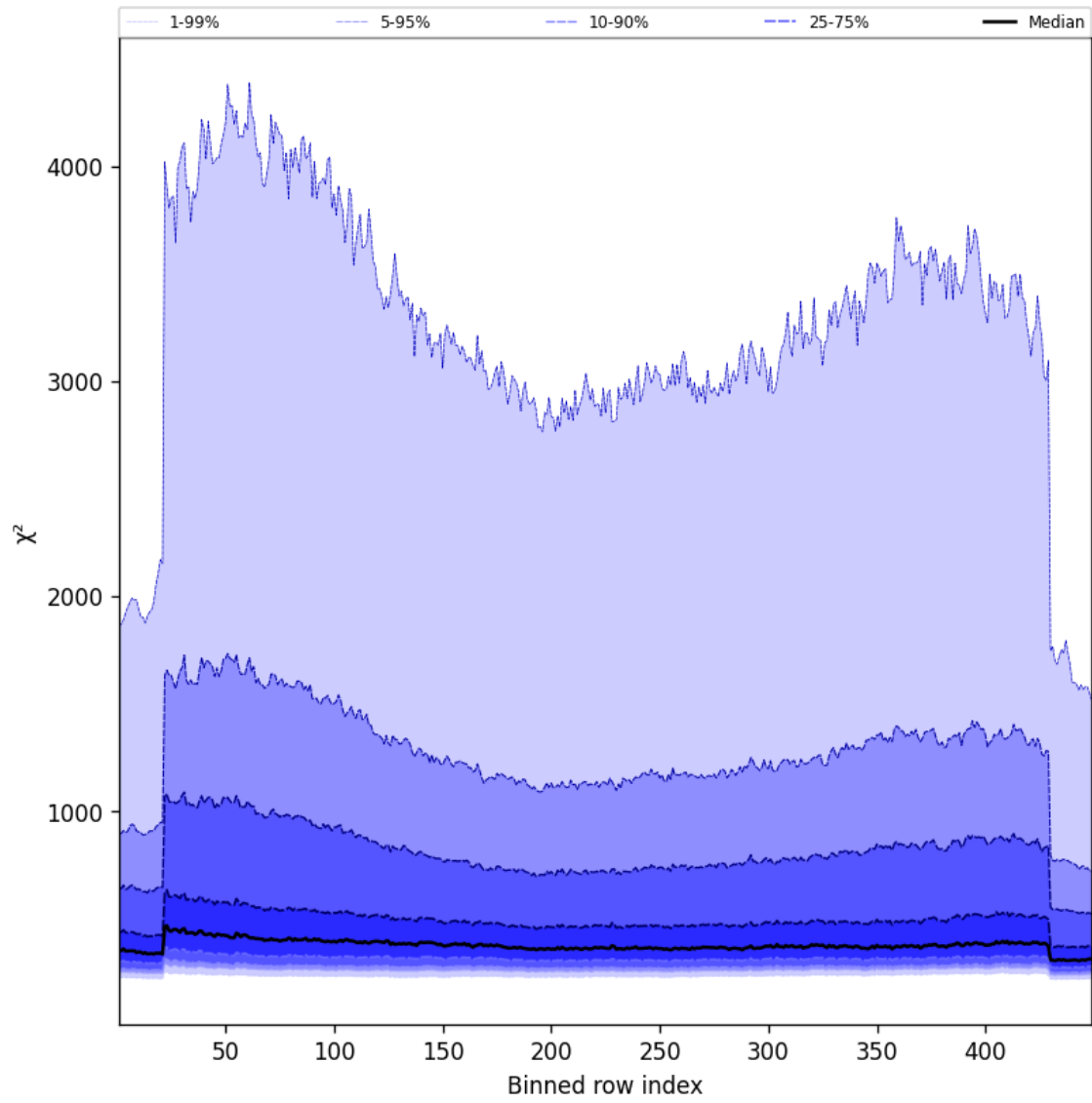
Figure 59: Along track statistics of “ \chi^2 ” for 2025-09-15 to 2025-09-17
