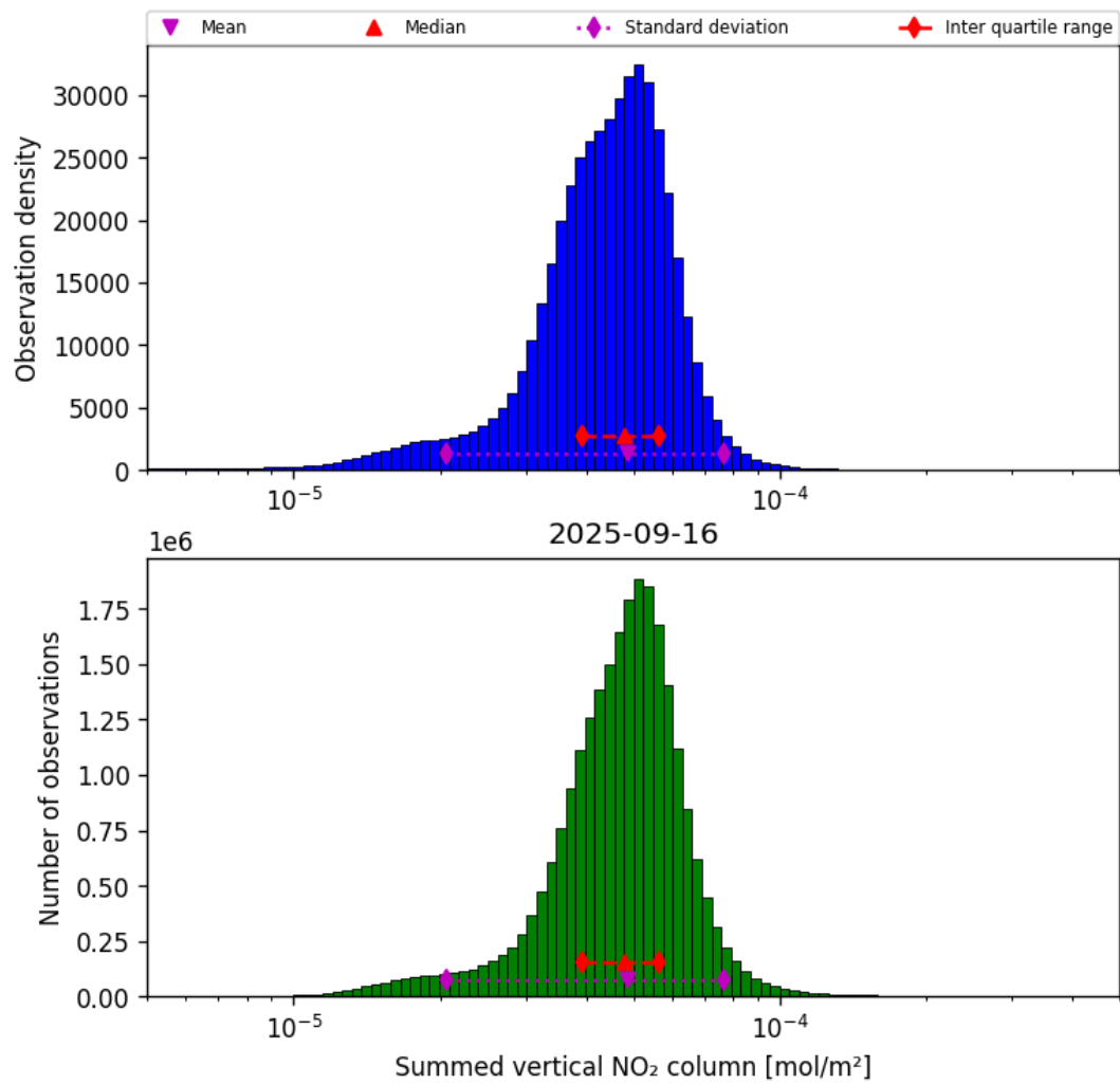
Figure 40: Histogram of “Summed vertical NO 2 column” for 2025-09-15 to 2025-09-17
