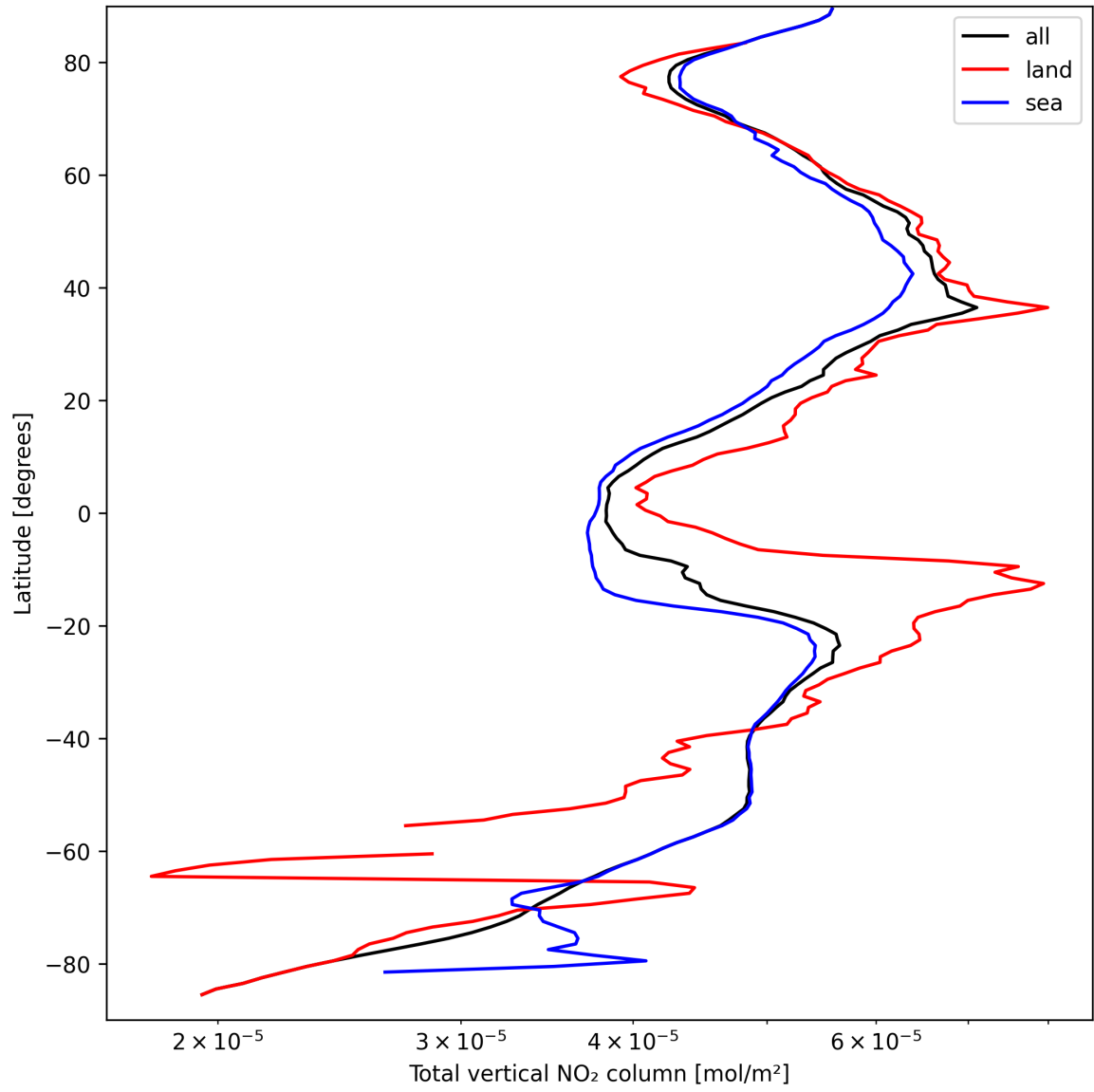
Figure 21: Zonal average of “Total vertical NO 2 column” for 2025-09-15 to 2025-09-17.
