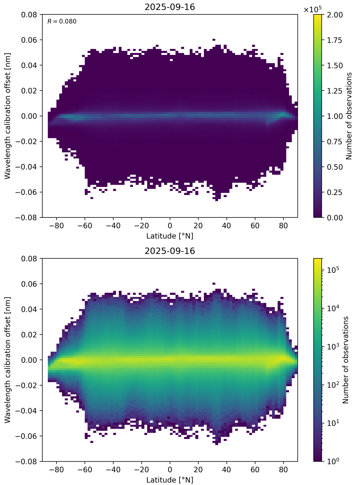
Figure 95: Scatter density plot of “Latitude” against “Wavelength calibration offset” for 2025-09-15 to 2025-09-17.
