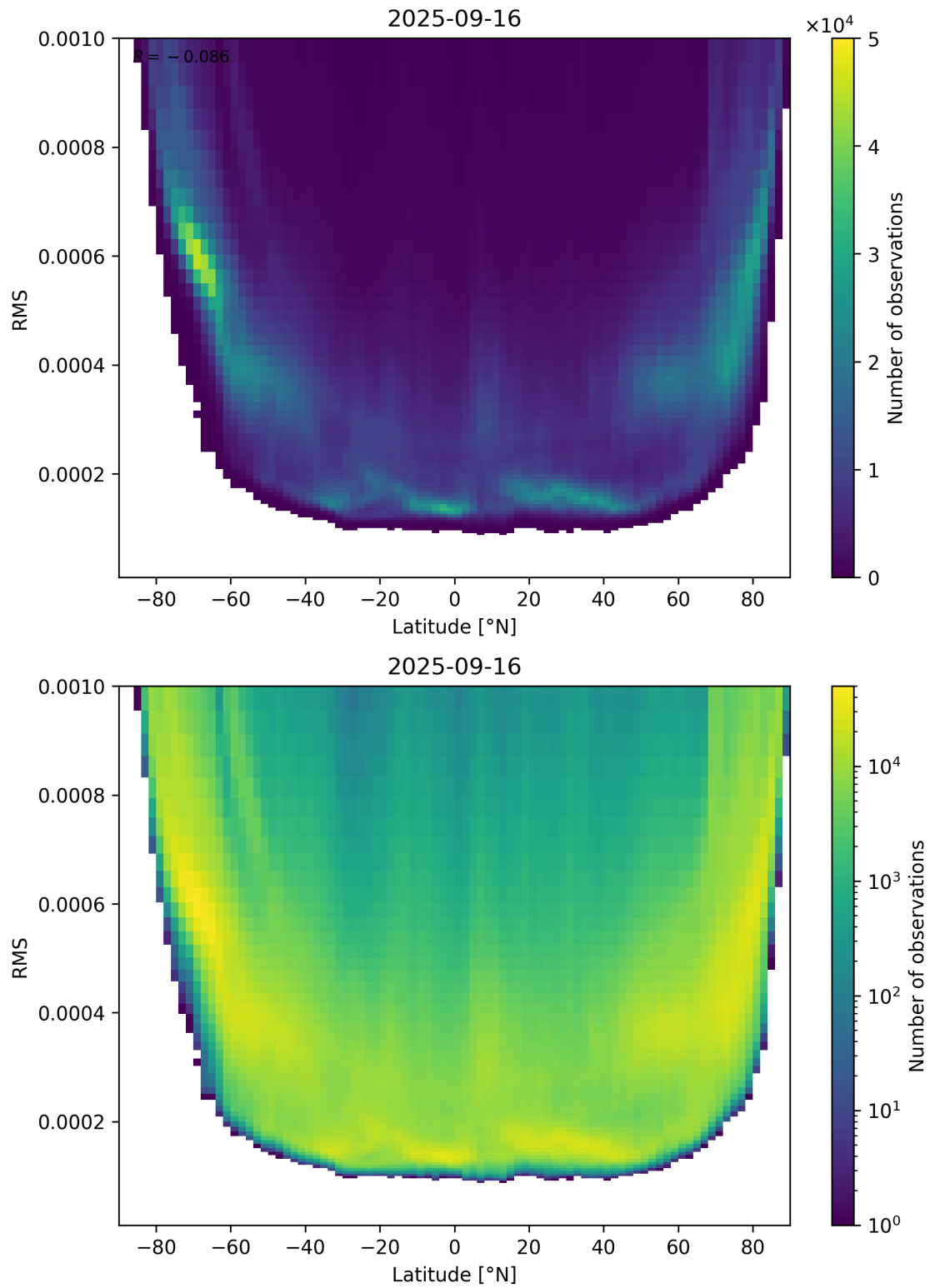
Figure 94: Scatter density plot of “Latitude” against “RMS” for 2025-09-15 to 2025-09-17.
