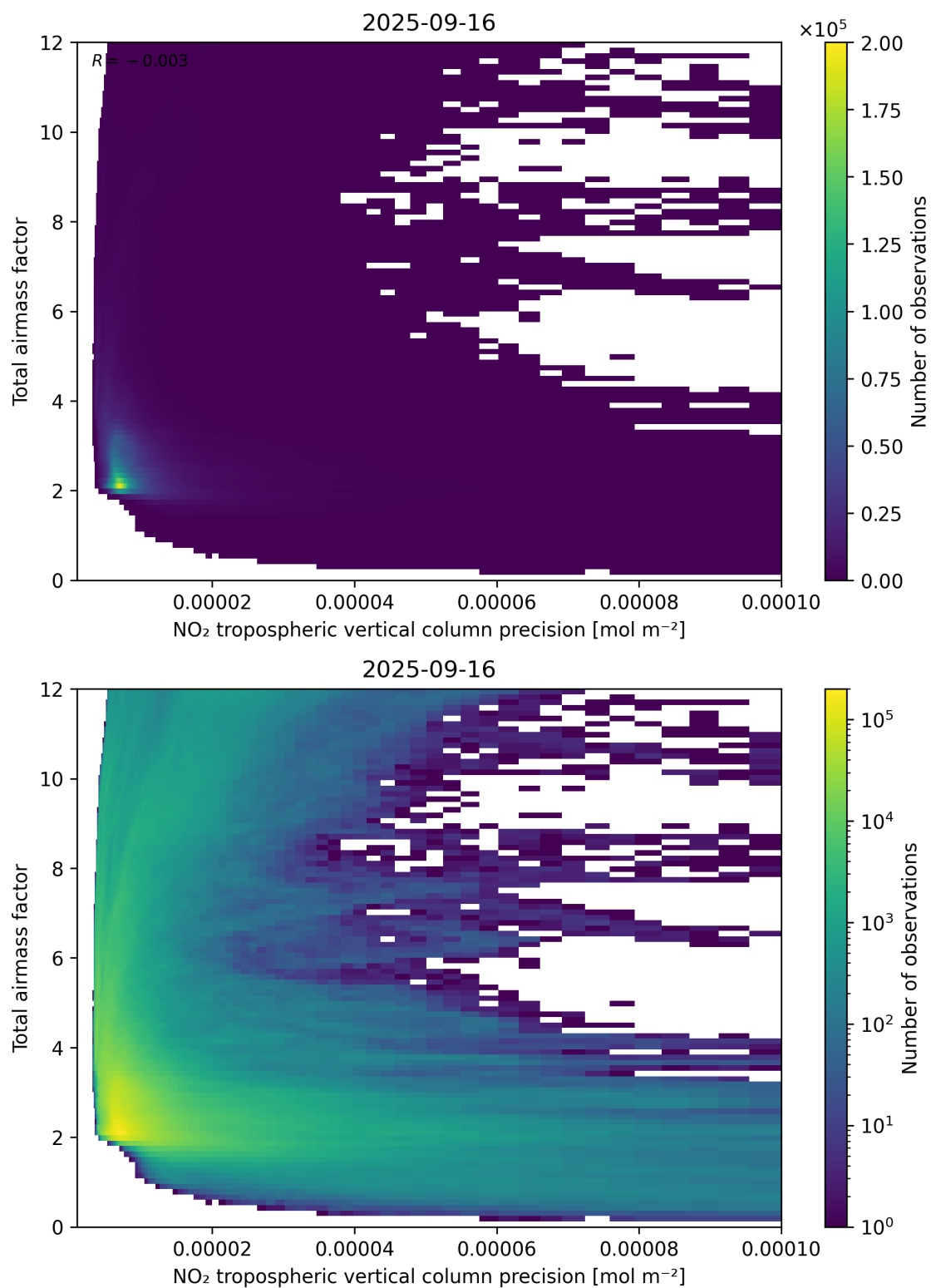
Figure 132: Scatter density plot of “NO 2 tropospheric vertical column precision” against “Total air mass factor” for 2025-09-15 to 2025-09-17.
