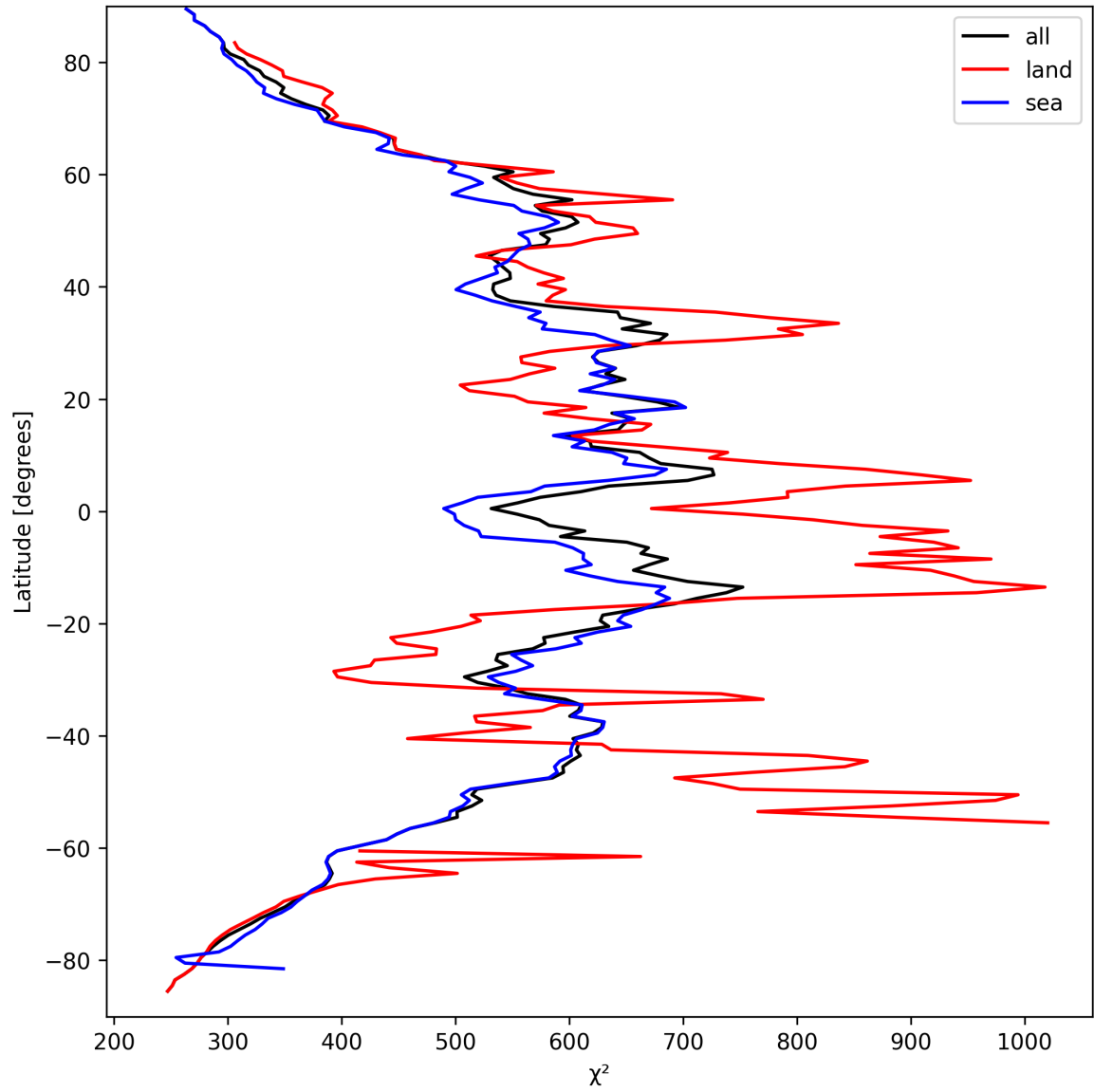
Figure 25: Zonal average of “ \chi^2 ” for 2025-09-15 to 2025-09-17.
