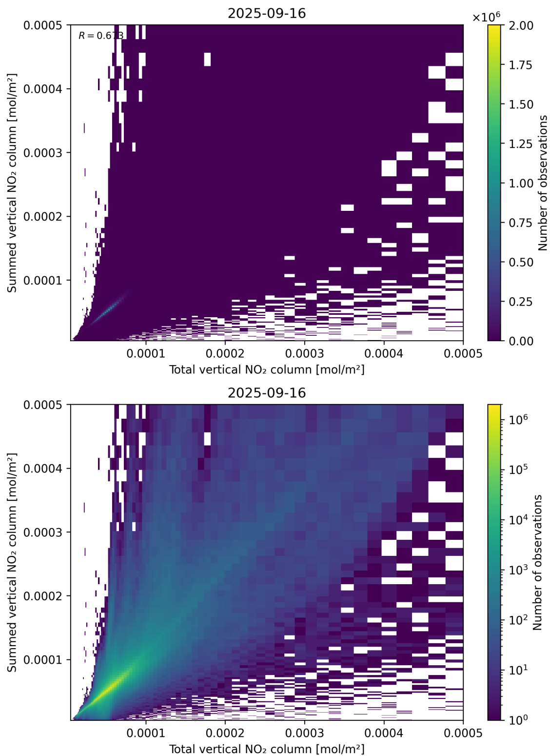
Figure 112: Scatter density plot of “Total vertical NO 2 column” against “Summed vertical NO 2 column” for 2025-09-15 to 2025-09-17.
