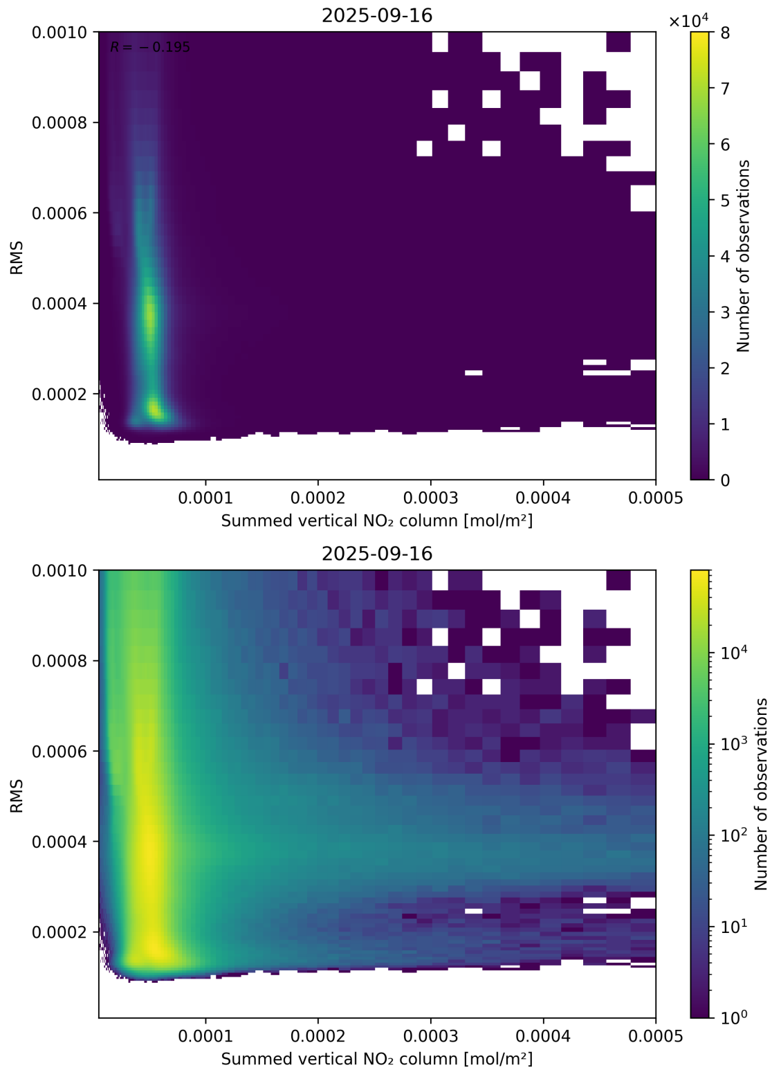
Figure 109: Scatter density plot of “Summed vertical NO 2 column” against “RMS” for 2025-09-15 to 2025-09-17.
