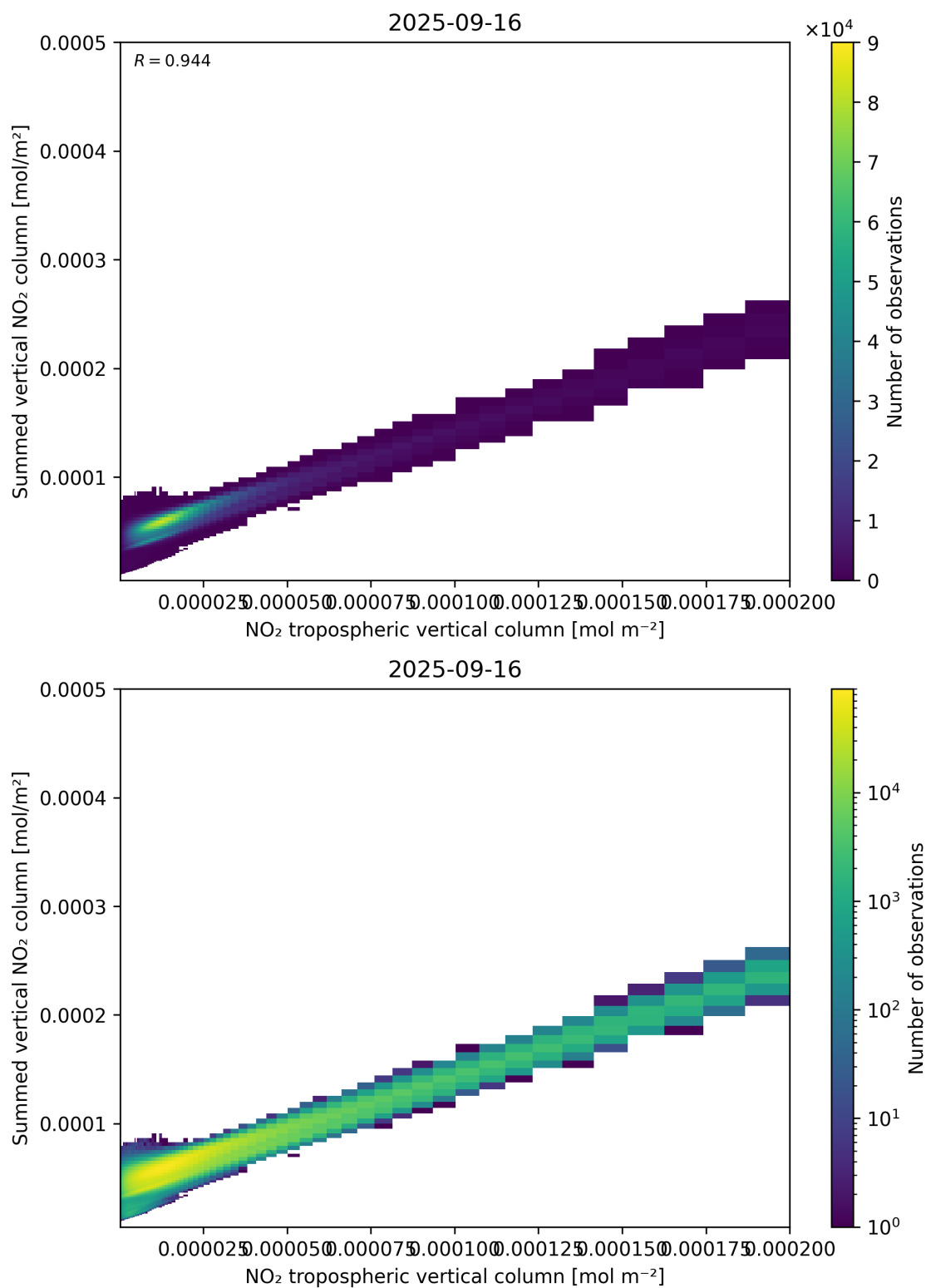
Figure 126: Scatter density plot of “NO 2 tropospheric vertical column” against “Summed vertical NO 2 column” for 2025-09-15 to 2025-09-17.
