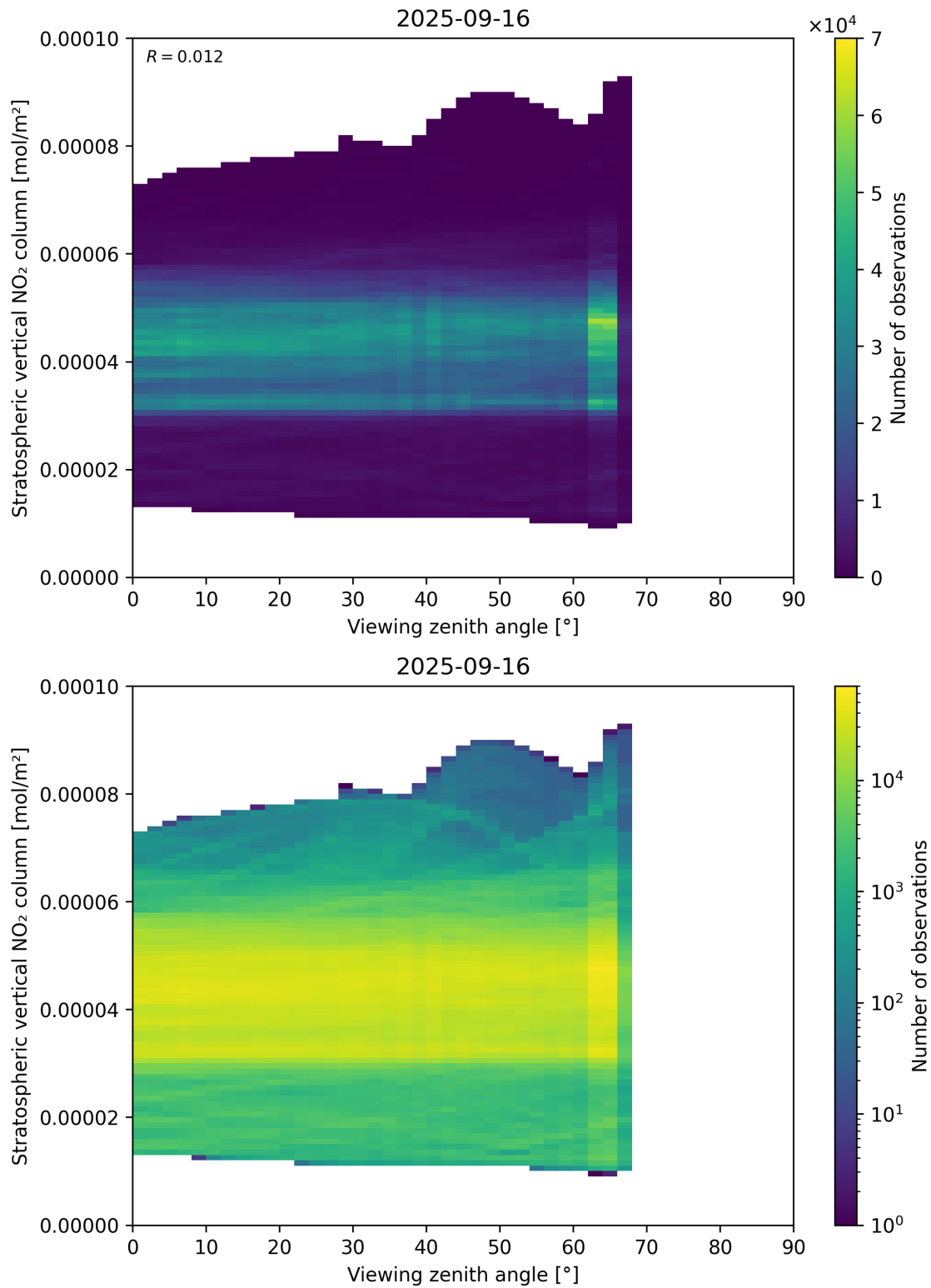
Figure 164: Scatter density plot of “Viewing zenith angle” against “Stratospheric vertical NO 2 column” for 2025-09-15 to 2025-09-17.
