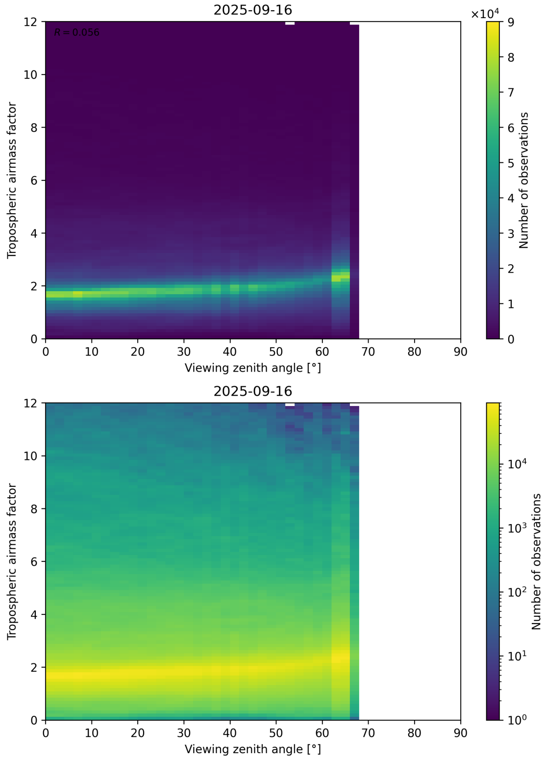
Figure 161: Scatter density plot of “Viewing zenith angle” against “Tropospheric airmass factor” for 2025-09-15 to 2025-09-17.
