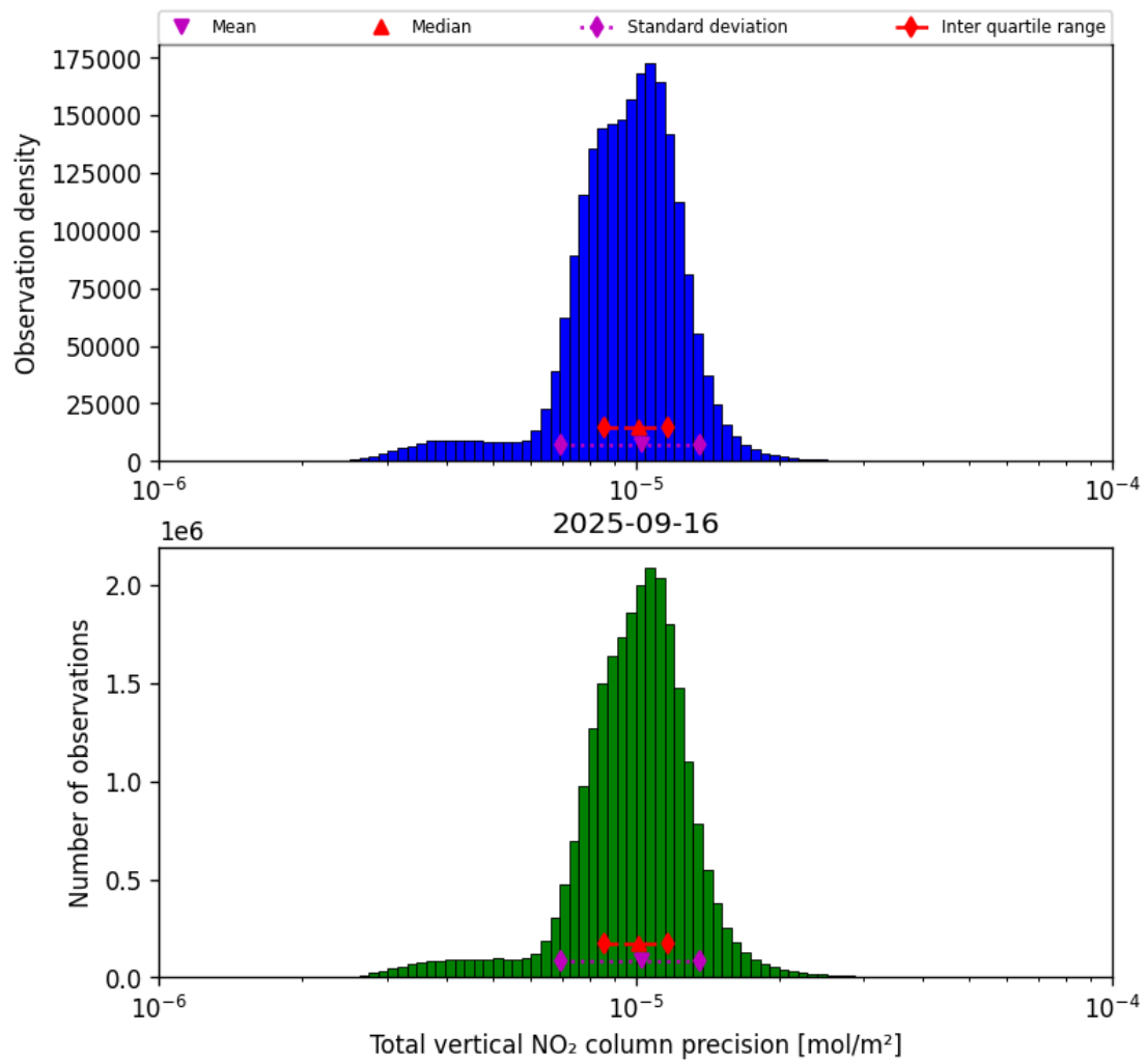
Figure 39: Histogram of “Total vertical NO 2 column precision” for 2025-09-15 to 2025-09-17
