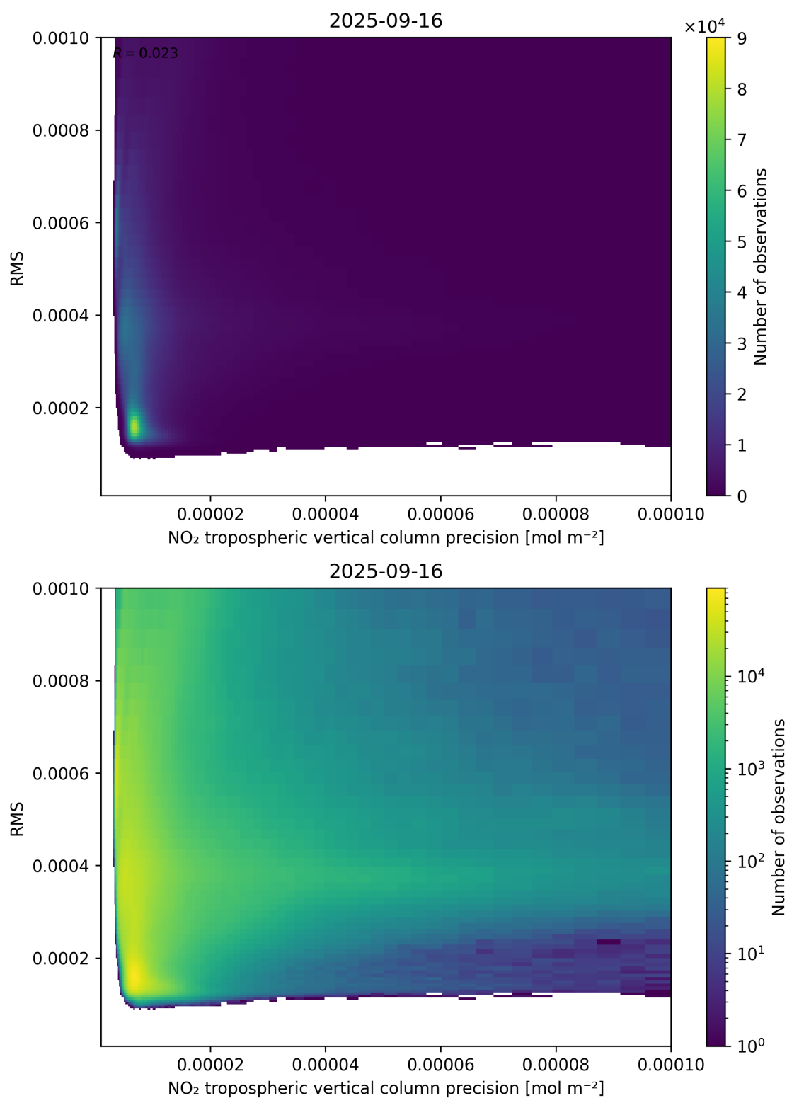
Figure 140: Scatter density plot of “NO 2 tropospheric vertical column precision” against “RMS” for 2025-09-15 to 2025-09-17.
