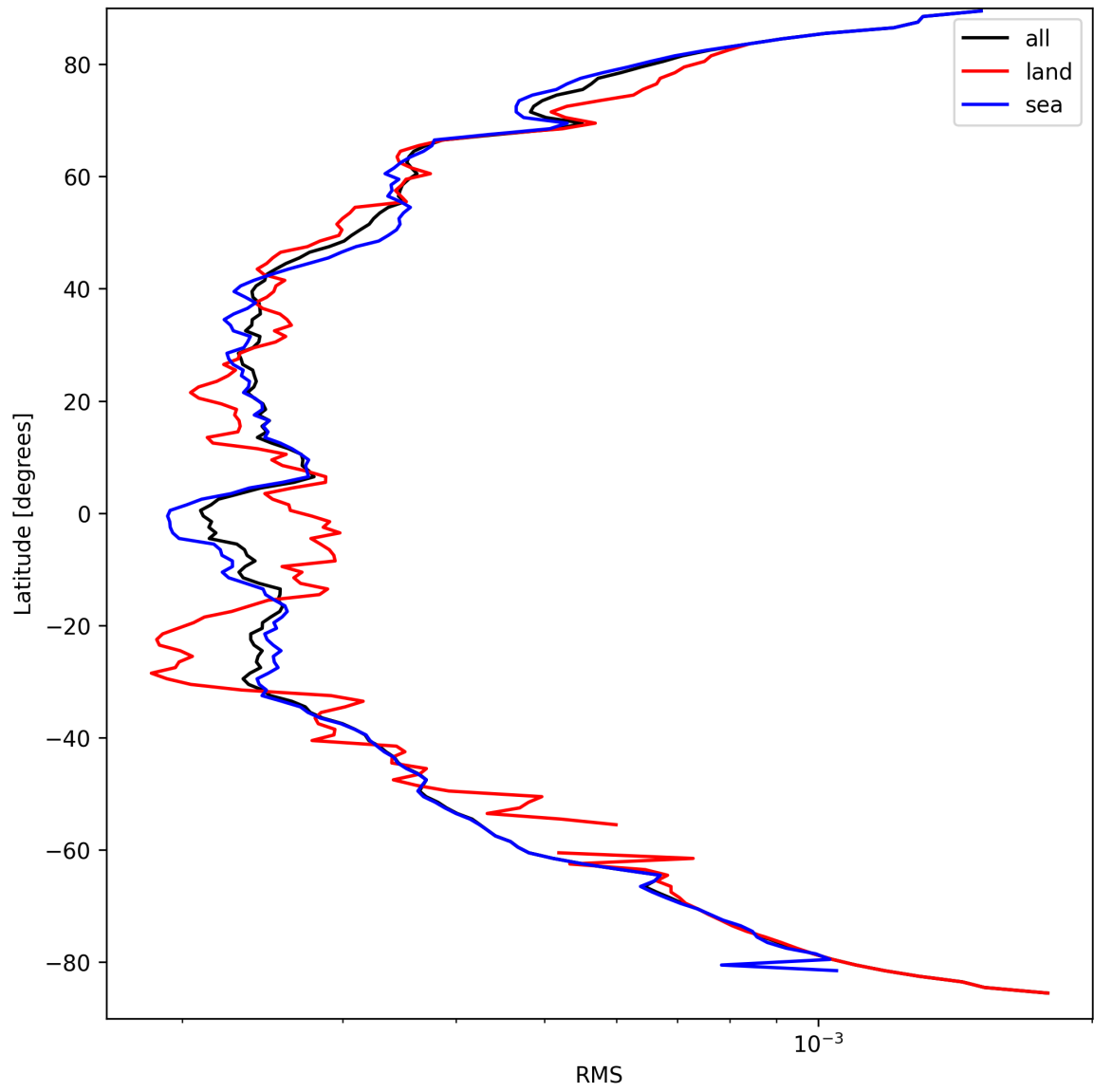
Figure 26: Zonal average of “RMS” for 2025-09-15 to 2025-09-17.
