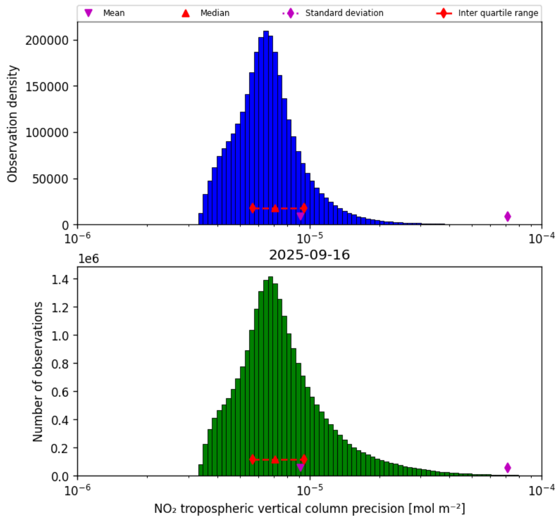
Figure 30: Histogram of “NO 2 tropospheric vertical column precision” for 2025-09-15 to 2025-09-17
