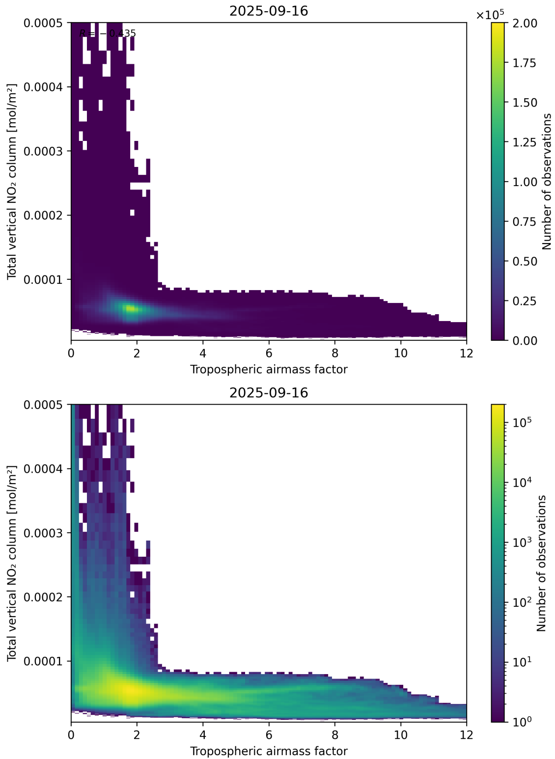
Figure 77: Scatter density plot of “Tropospheric airmass factor” against “Total vertical NO 2 column” for 2025-09-15 to 2025-09-17.
