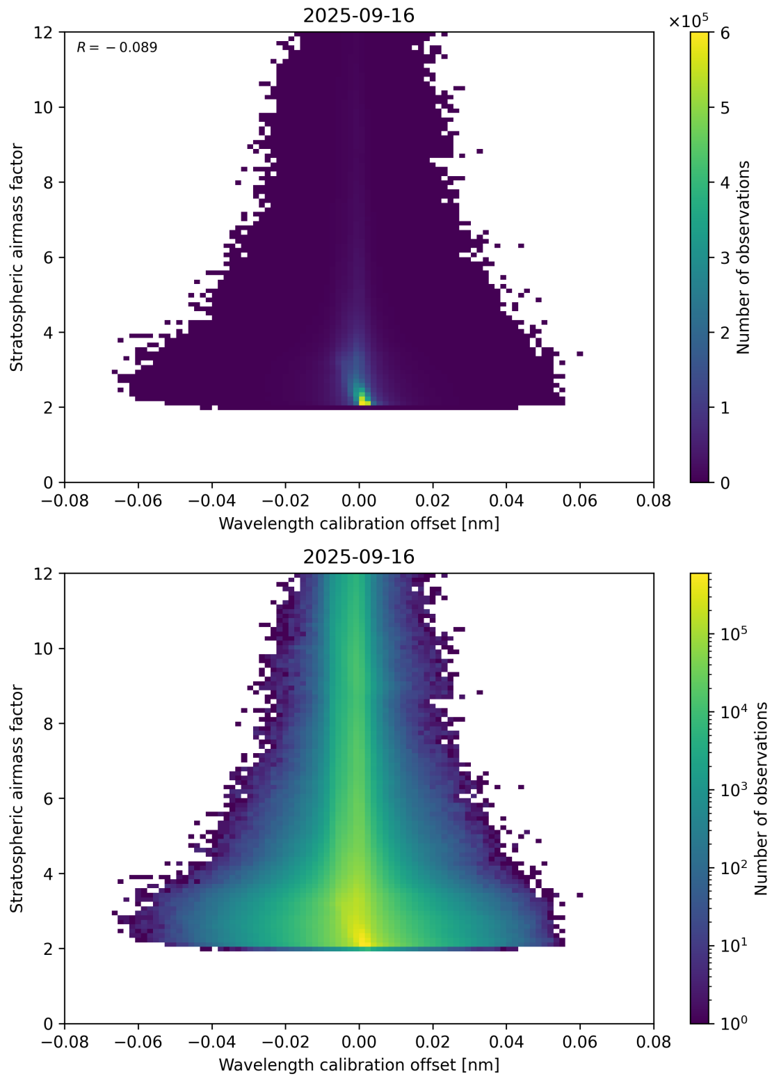
Figure 174: Scatter density plot of “Wavelength calibration offset” against “Stratospheric airmass factor” for 2025-09-15 to 2025-09-17.
