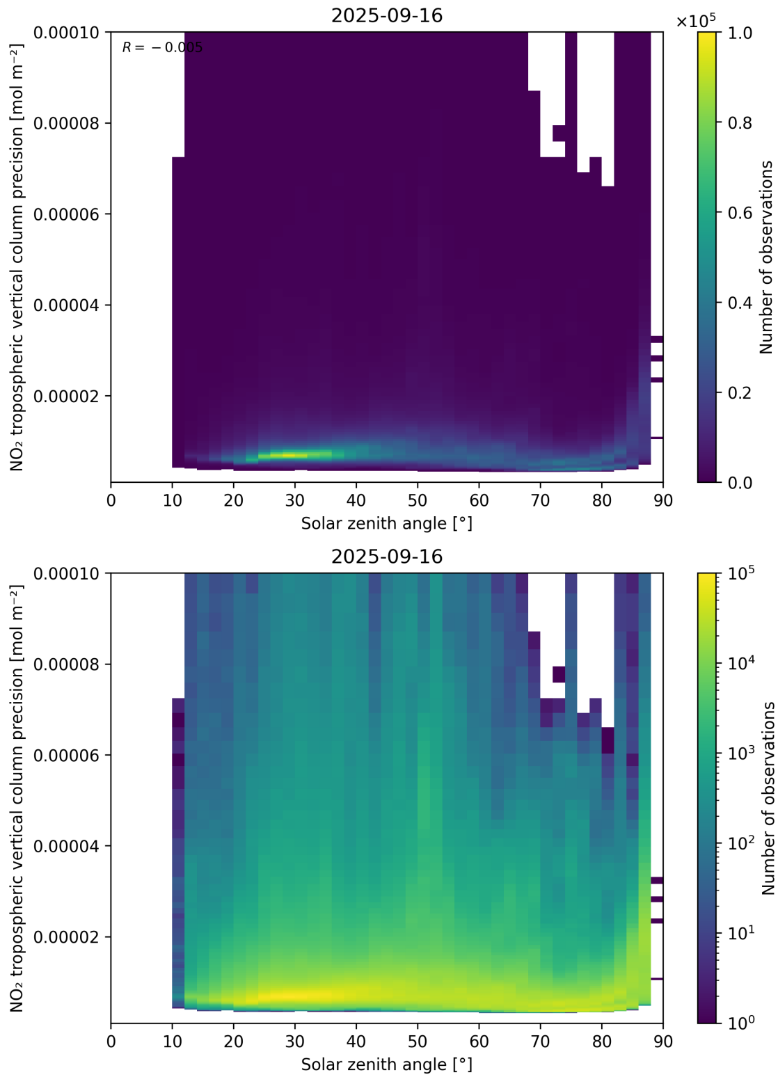
Figure 156: Scatter density plot of “Solar zenith angle” against “NO 2 tropospheric vertical column precision” for 2025-09-15 to 2025-09-17.
