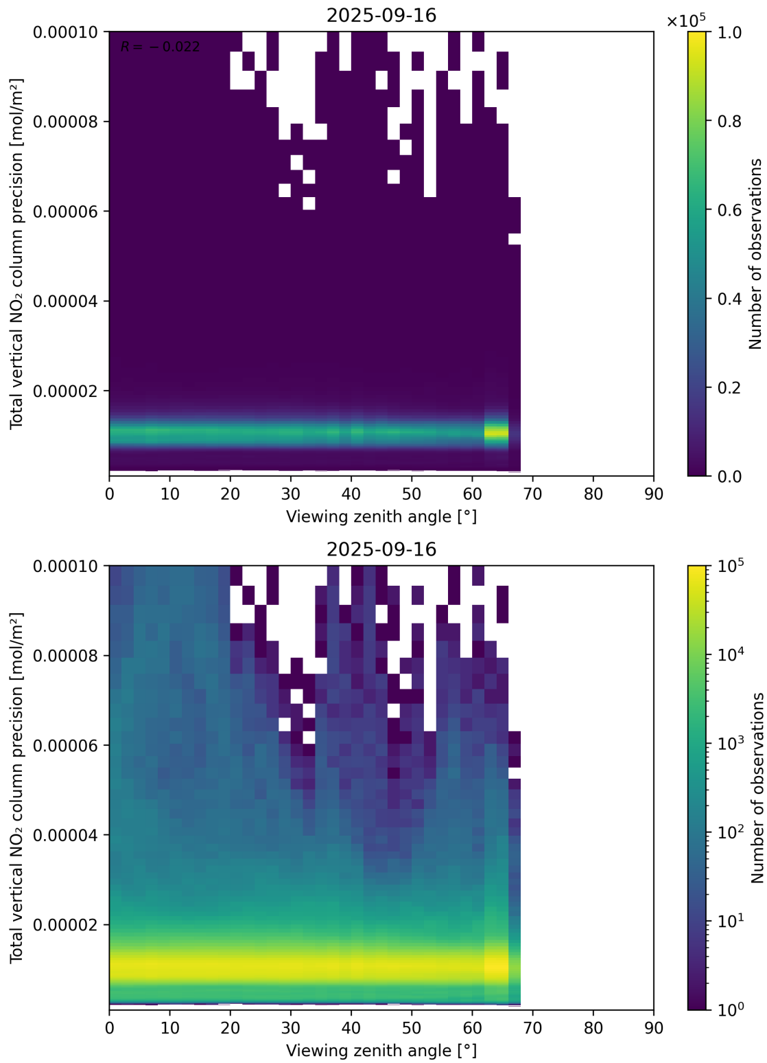
Figure 168: Scatter density plot of “Viewing zenith angle” against “Total vertical NO 2 column precision” for 2025-09-15 to 2025-09-17.
