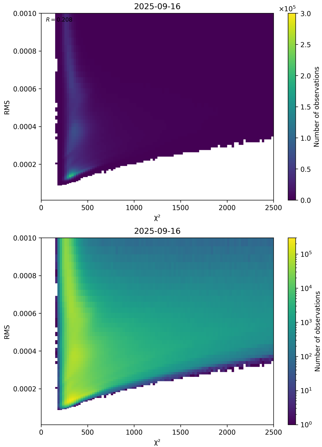
Figure 82: Scatter density plot of “ \chi^2 ” against “RMS” for 2025-09-15 to 2025-09-17.
