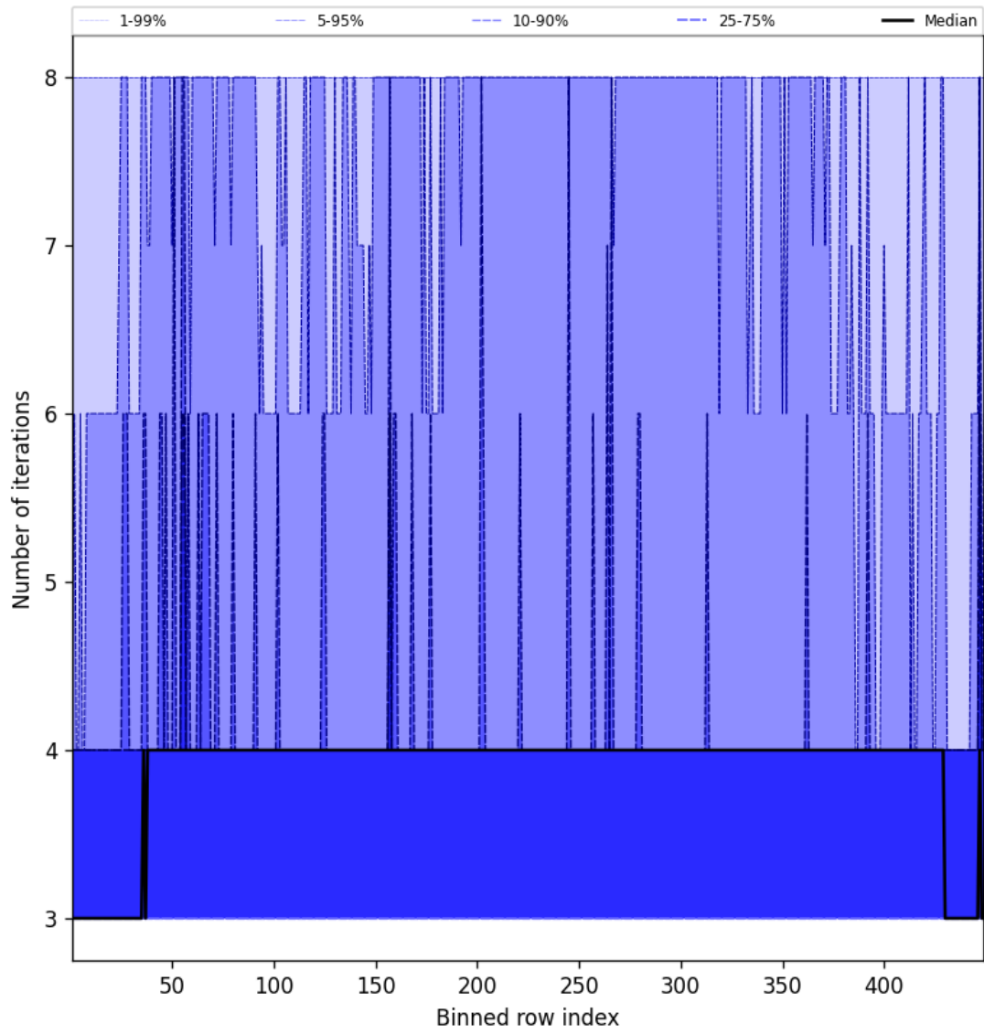
Figure 51: Along track statistics of “Number of iterations” for 2025-09-15 to 2025-09-17
