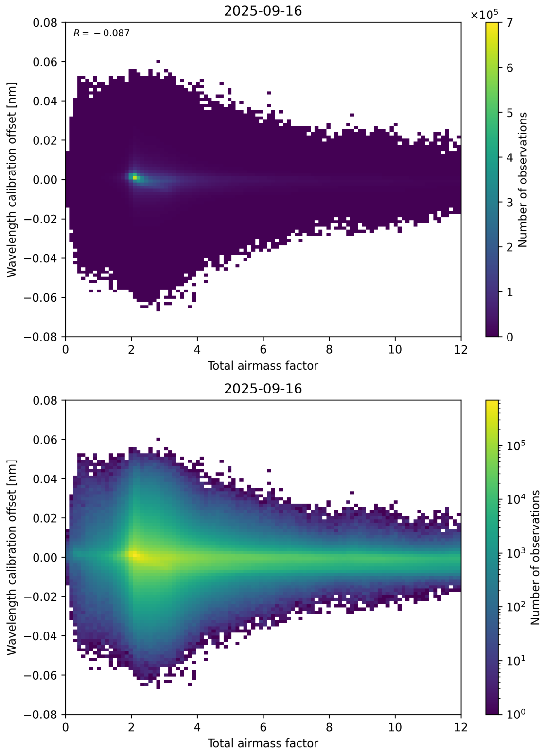
Figure 70: Scatter density plot of “Total airmass factor” against “Wavelength calibration offset” for 2025-09-15 to 2025-09-17.
