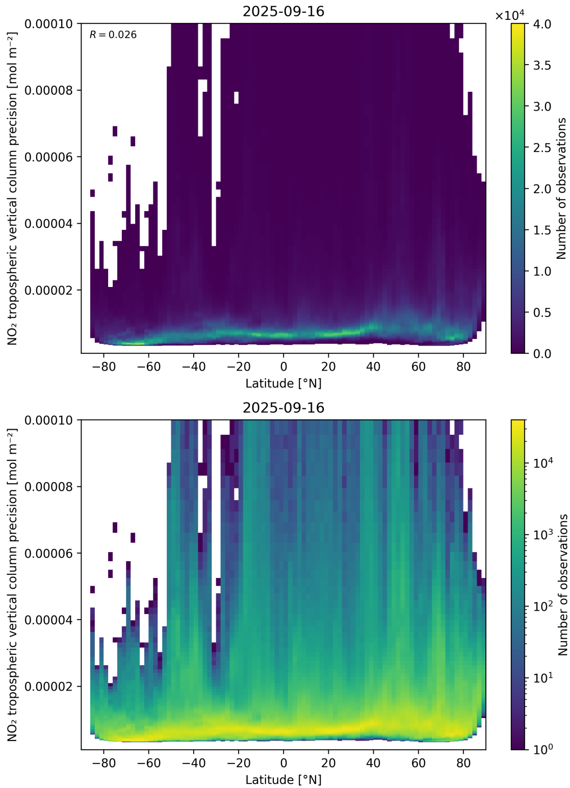
Figure 93: Scatter density plot of “Latitude” against “NO 2 tropospheric vertical column precision” for 2025-09-15 to 2025-09-17.
