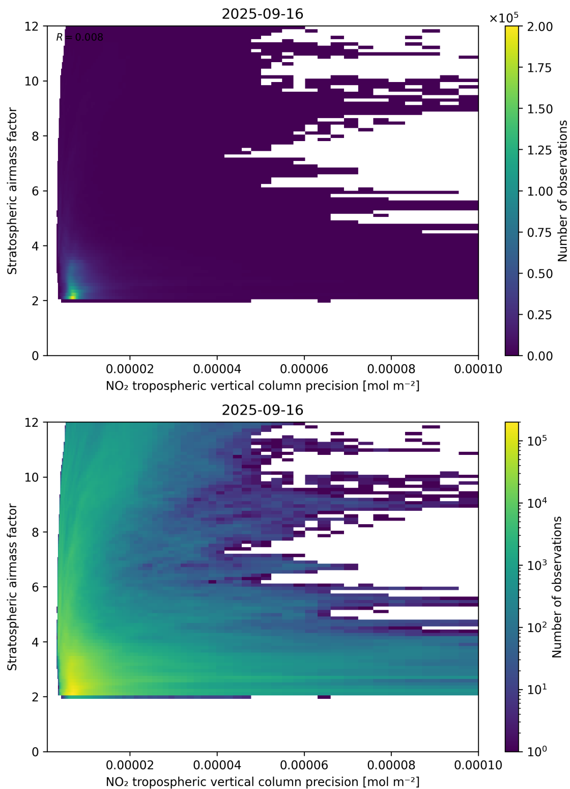
Figure 131: Scatter density plot of “NO 2 tropospheric vertical column precision” against “Stratospheric airmass factor” for 2025-09-15 to 2025-09-17.
