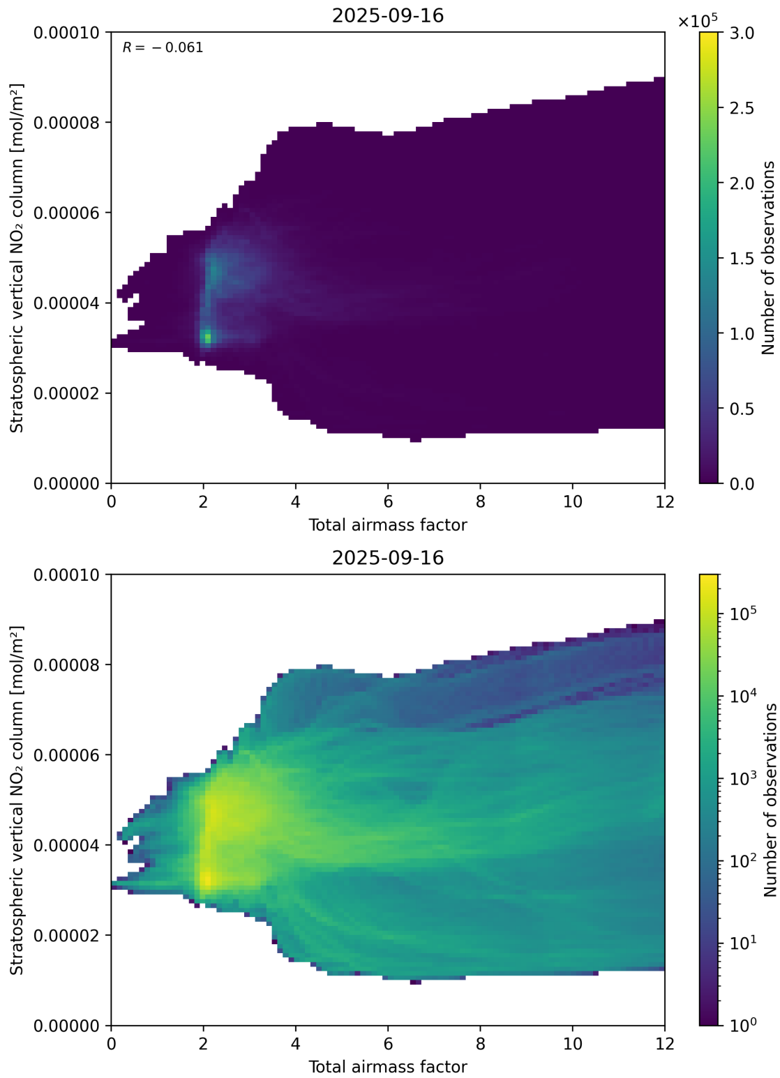
Figure 64: Scatter density plot of “Total airmass factor” against “Stratospheric vertical NO 2 column” for 2025-09-15 to 2025-09-17.
