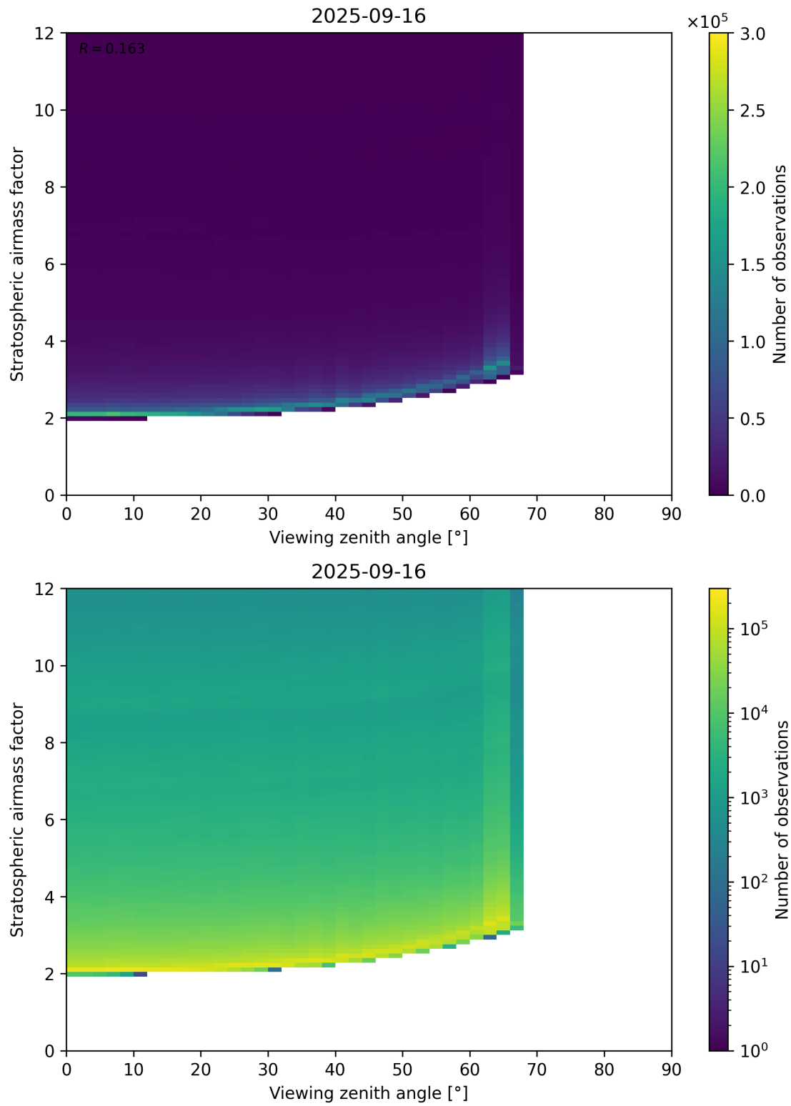
Figure 159: Scatter density plot of “Viewing zenith angle” against “Stratospheric airmass factor” for 2025-09-15 to 2025-09-17.
