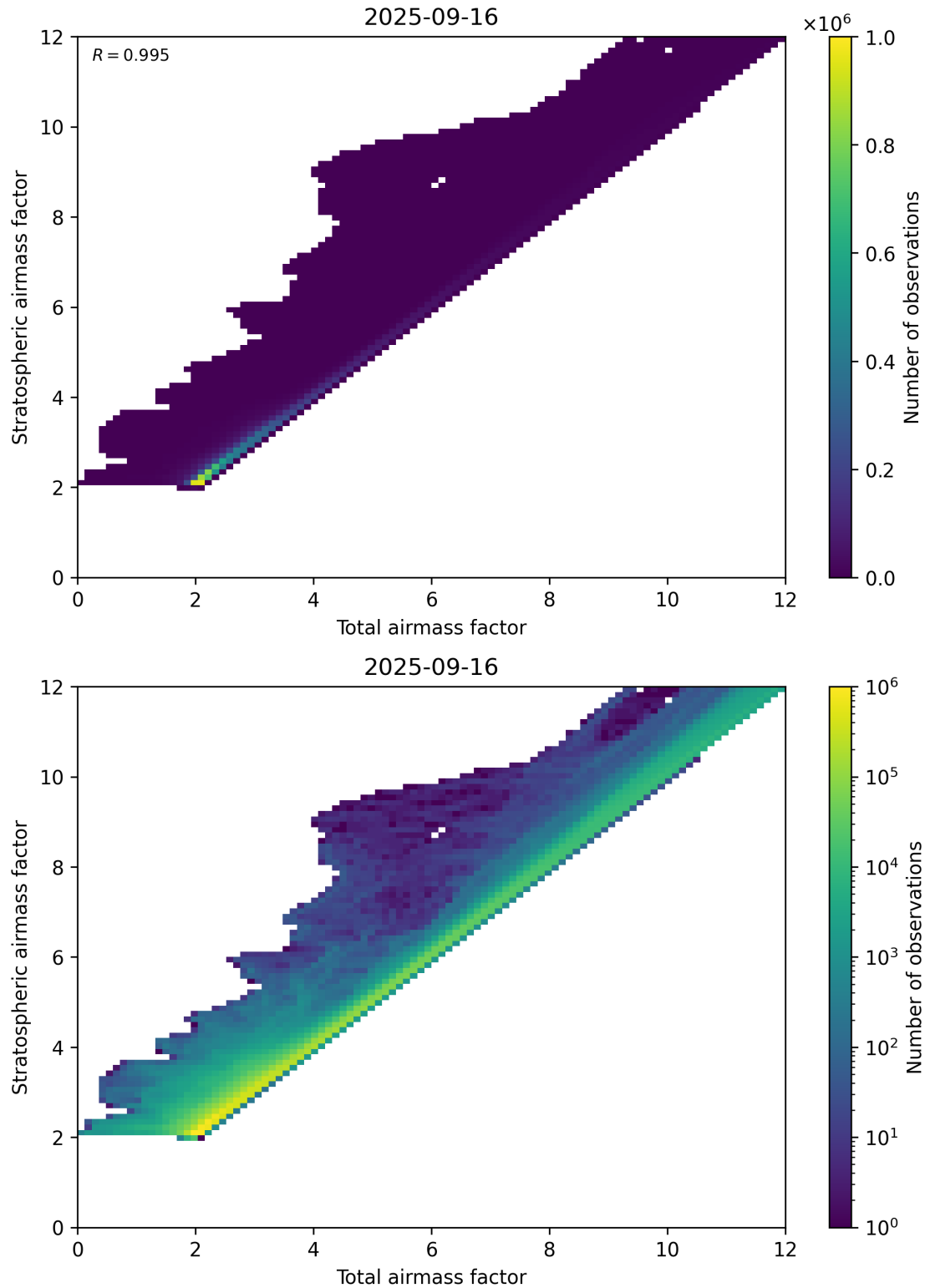
Figure 62: Scatter density plot of “Total airmass factor” against “Stratospheric airmass factor” for 2025-09-15 to 2025-09-17.
