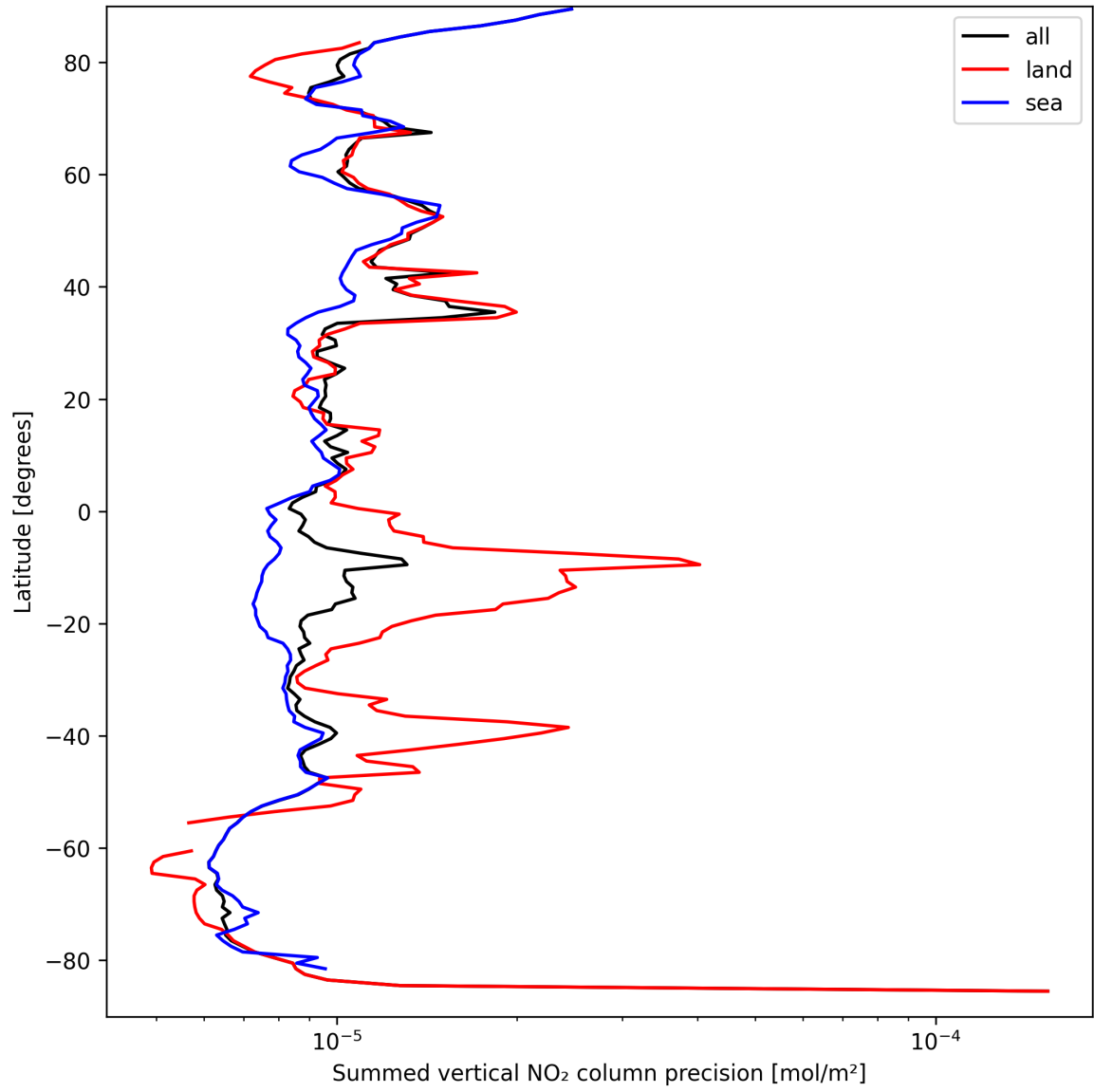
Figure 24: Zonal average of “Summed vertical NO 2 column precision” for 2025-09-15 to 2025-09-17.
