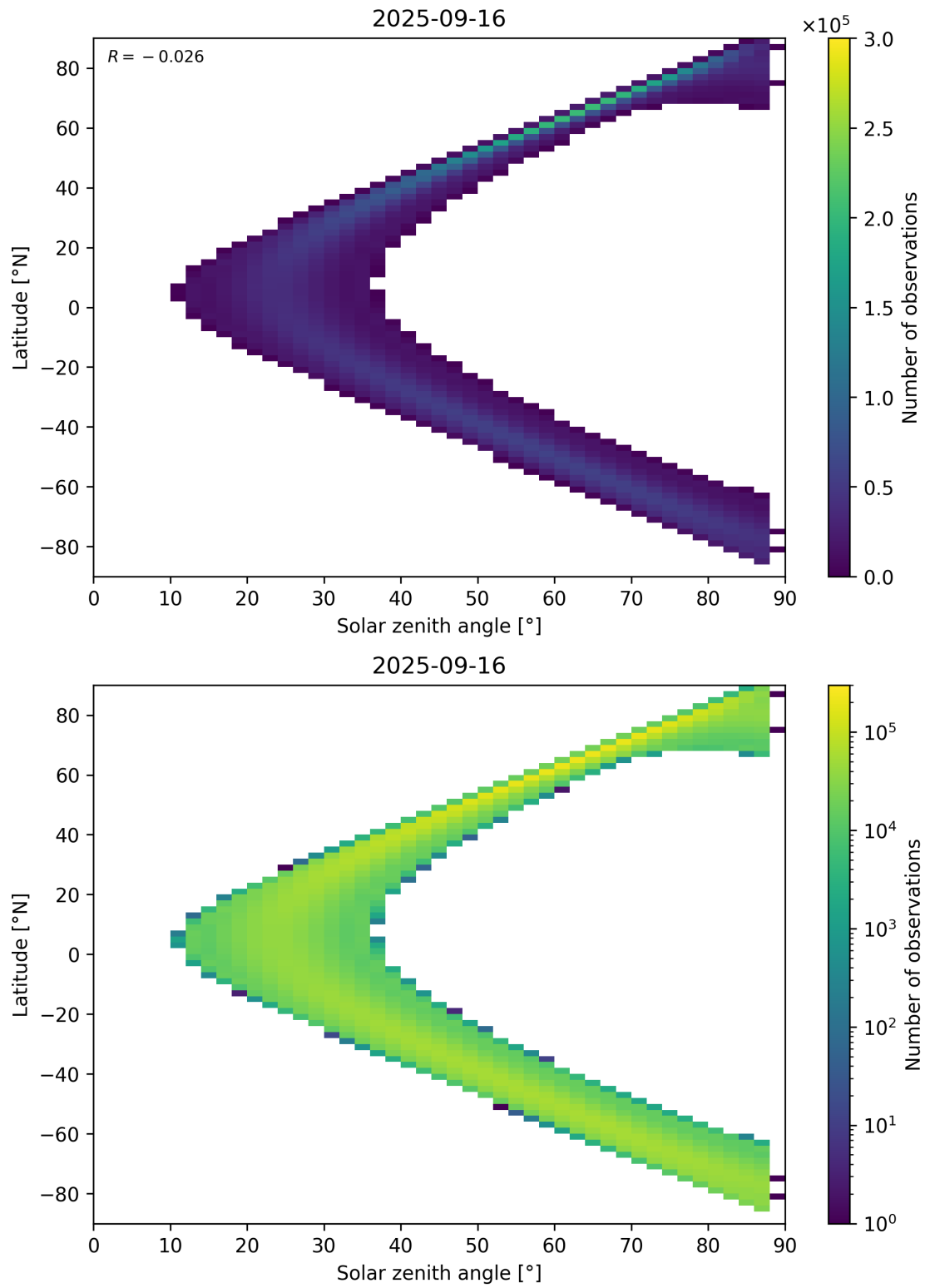
Figure 149: Scatter density plot of “Solar zenith angle” against “Latitude” for 2025-09-15 to 2025-09-17.
