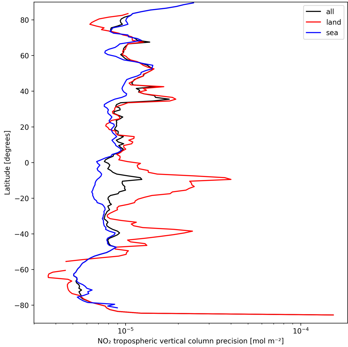
Figure 13: Zonal average of “NO 2 tropospheric vertical column precision” for 2025-09-15 to 2025-09-17.
