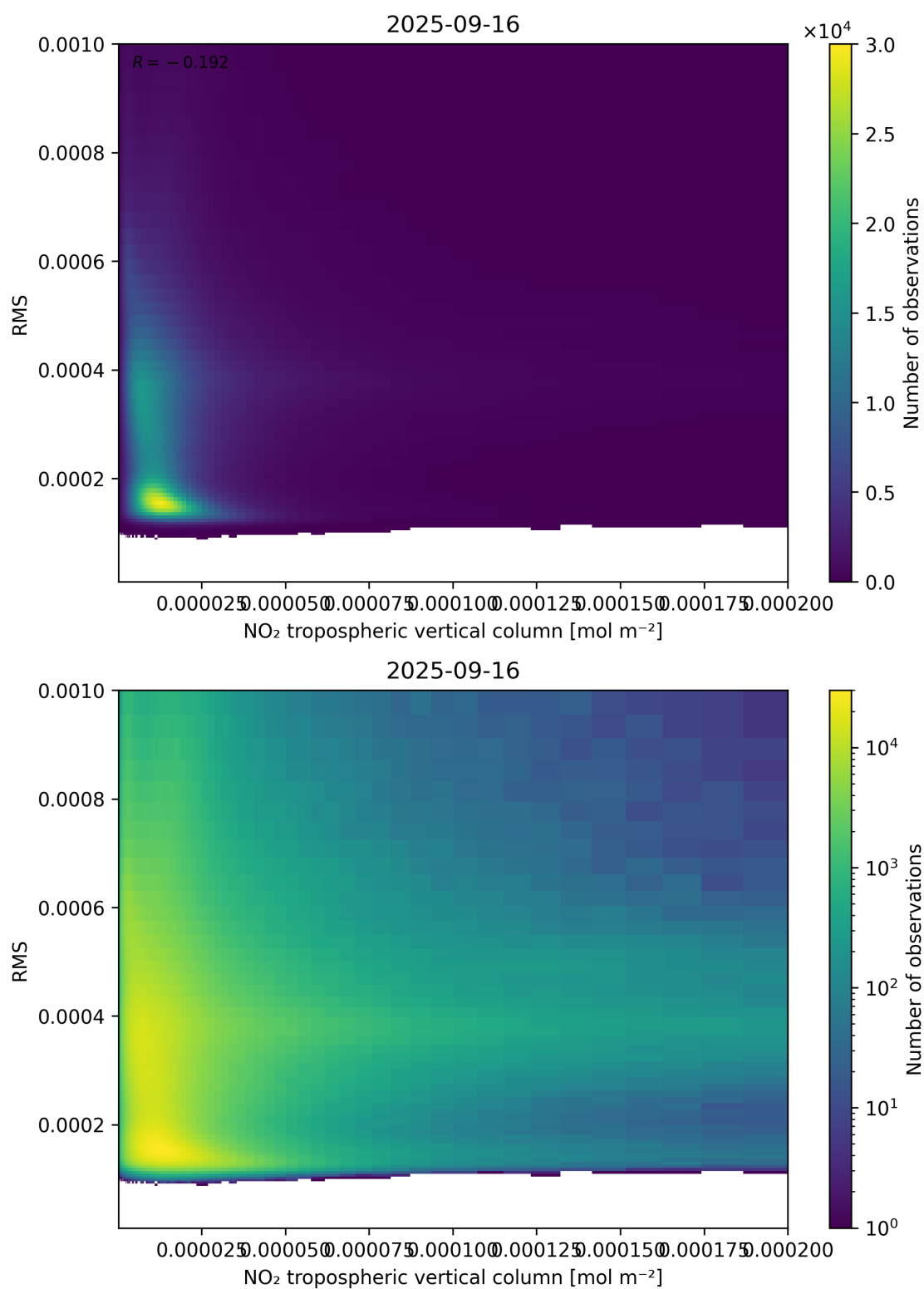
Figure 142: Scatter density plot of “NO 2 tropospheric vertical column” against “RMS” for 2025-09-15 to 2025-09-17.
