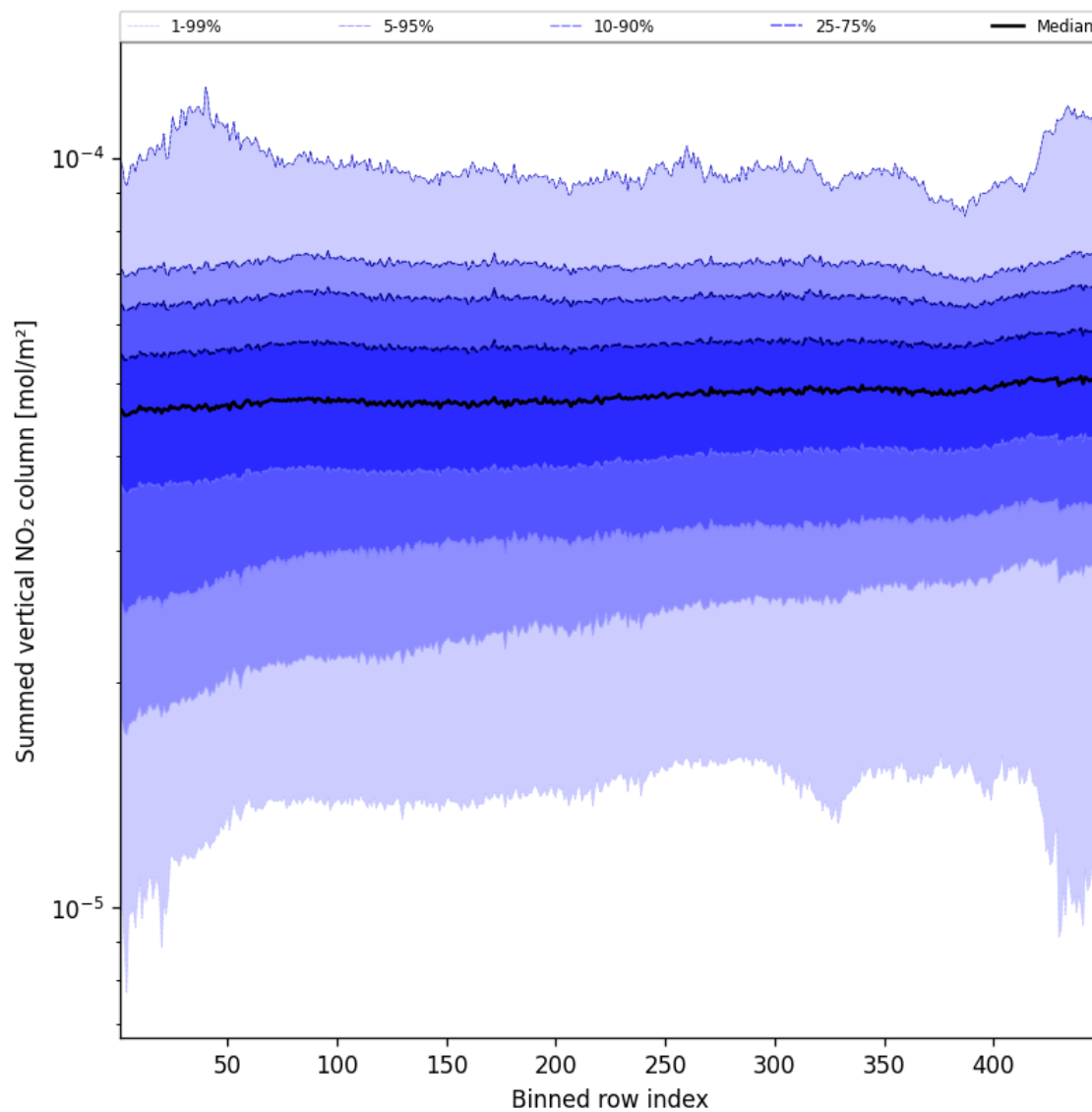
Figure 57: Along track statistics of “Summed vertical NO 2 column” for 2025-09-15 to 2025-09-17
