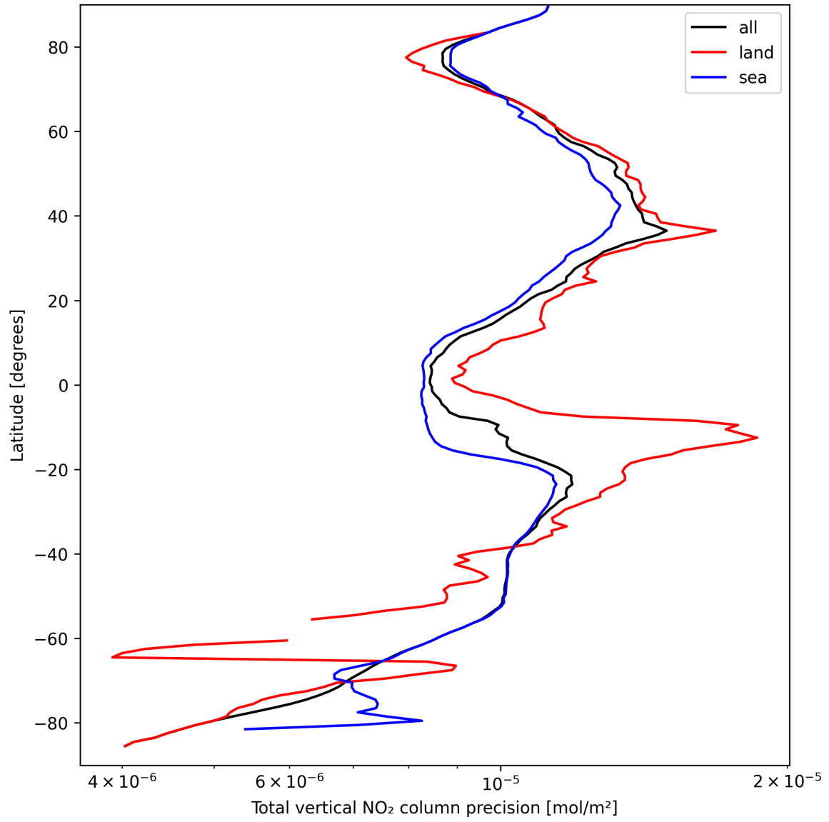
Figure 22: Zonal average of “Total vertical NO 2 column precision” for 2025-09-15 to 2025-09-17.
