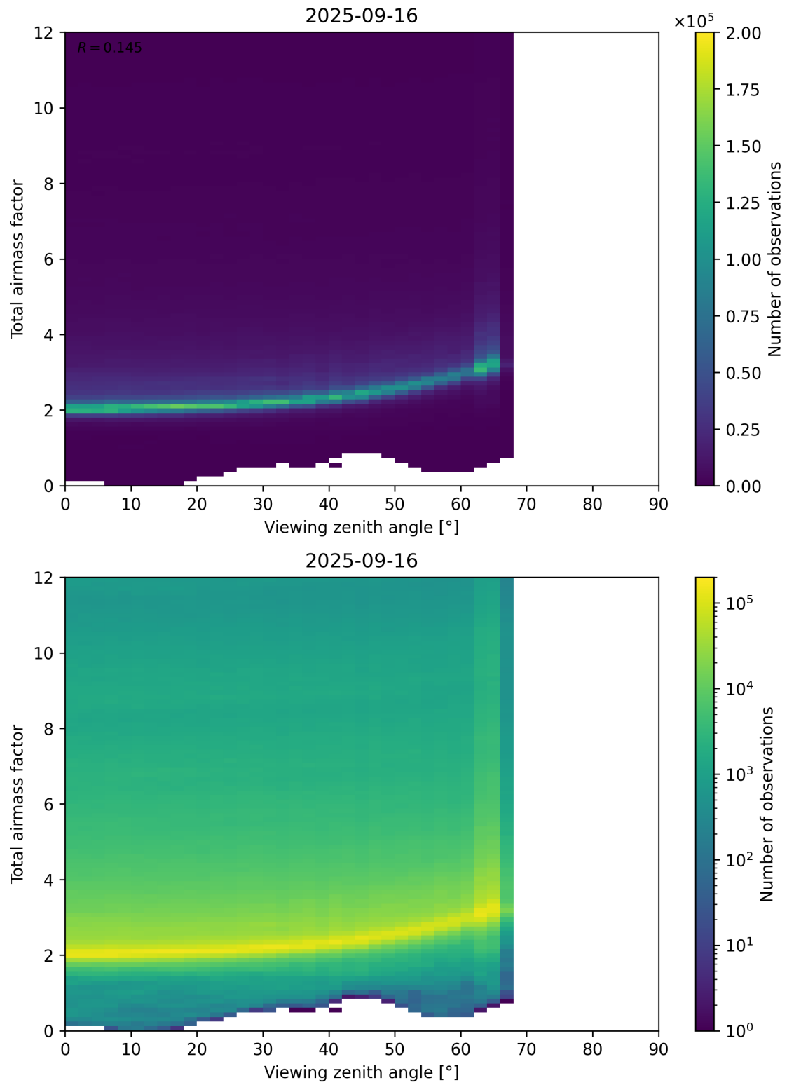
Figure 160: Scatter density plot of “Viewing zenith angle” against “Total airmass factor” for 2025-09-15 to 2025-09-17.
