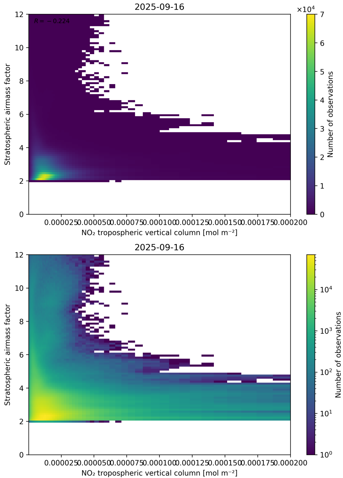
Figure 121: Scatter density plot of “NO 2 tropospheric vertical column” against “Stratospheric air mass factor” for 2025-09-15 to 2025-09-17.
