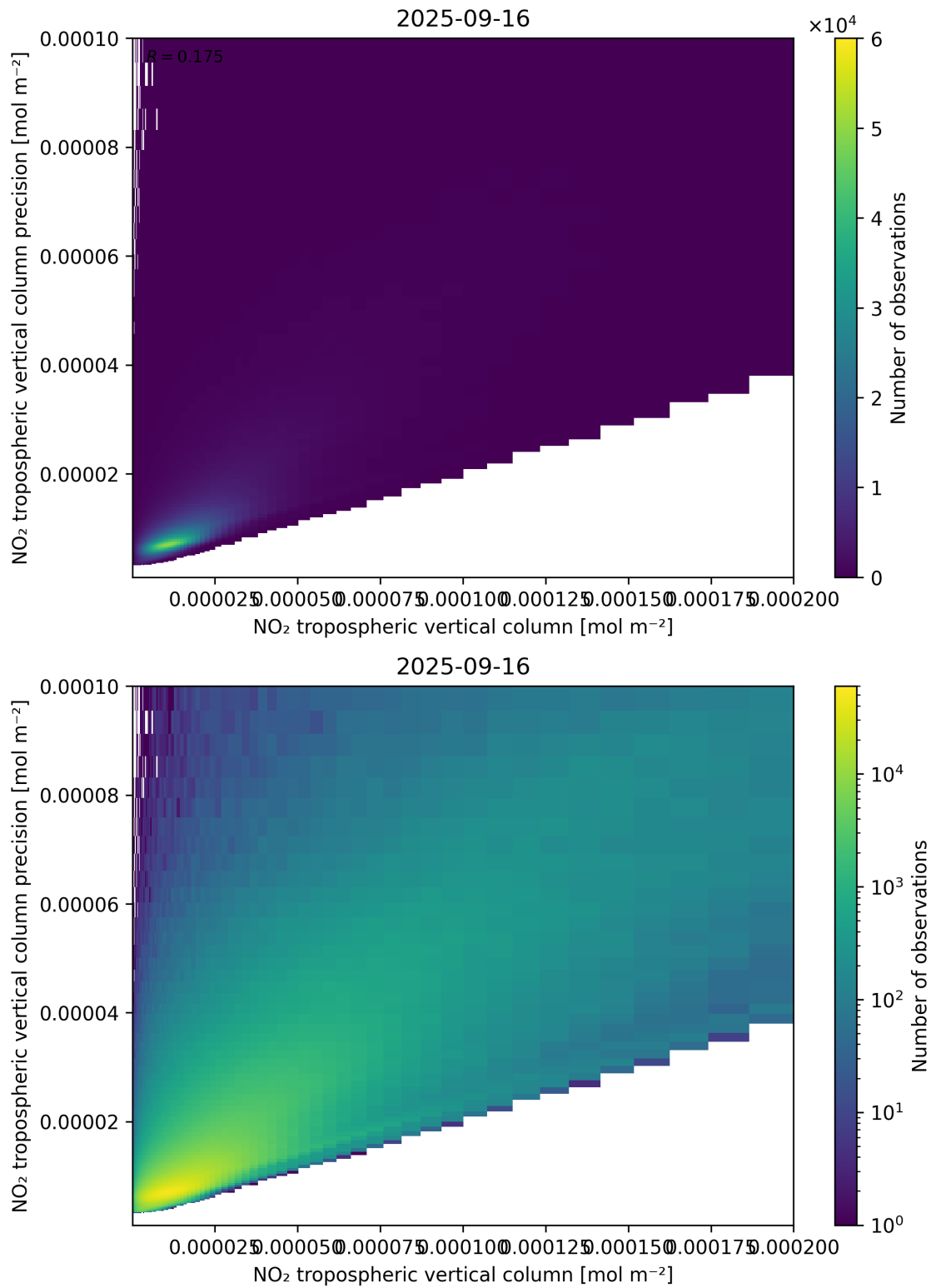
Figure 130: Scatter density plot of “NO 2 tropospheric vertical column” against “NO 2 tropospheric vertical column precision” for 2025-09-15 to 2025-09-17.
