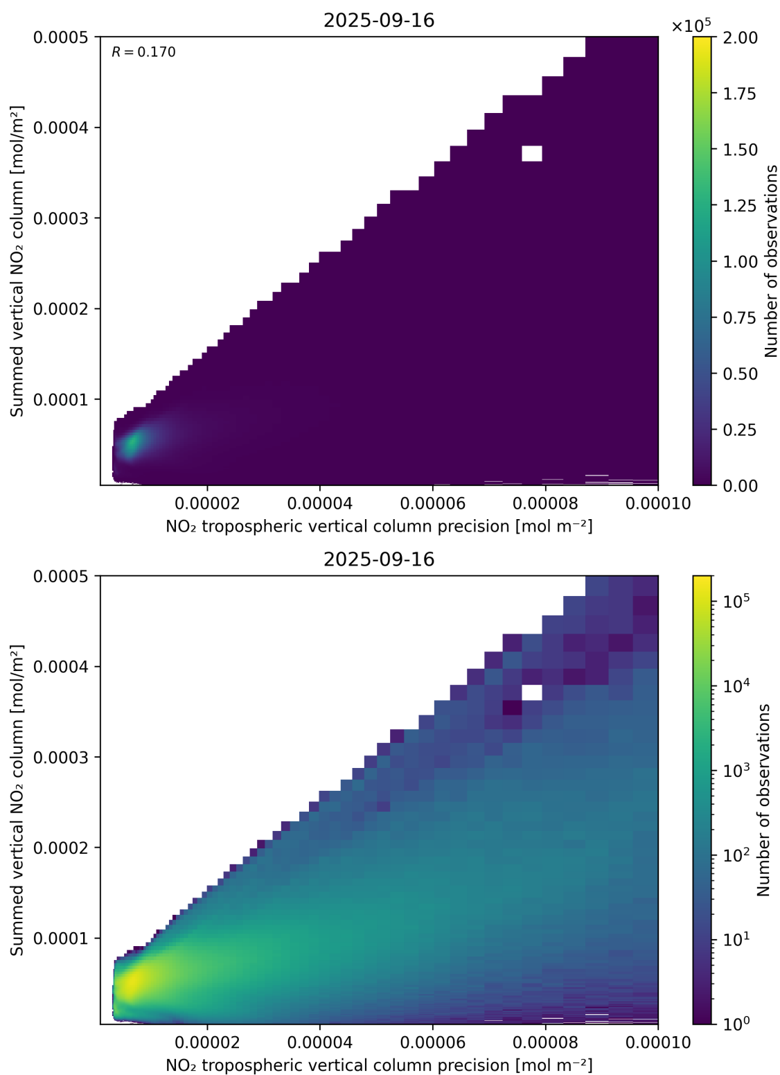
Figure 136: Scatter density plot of “NO 2 tropospheric vertical column precision” against “Summed vertical NO 2 column” for 2025-09-15 to 2025-09-17.
