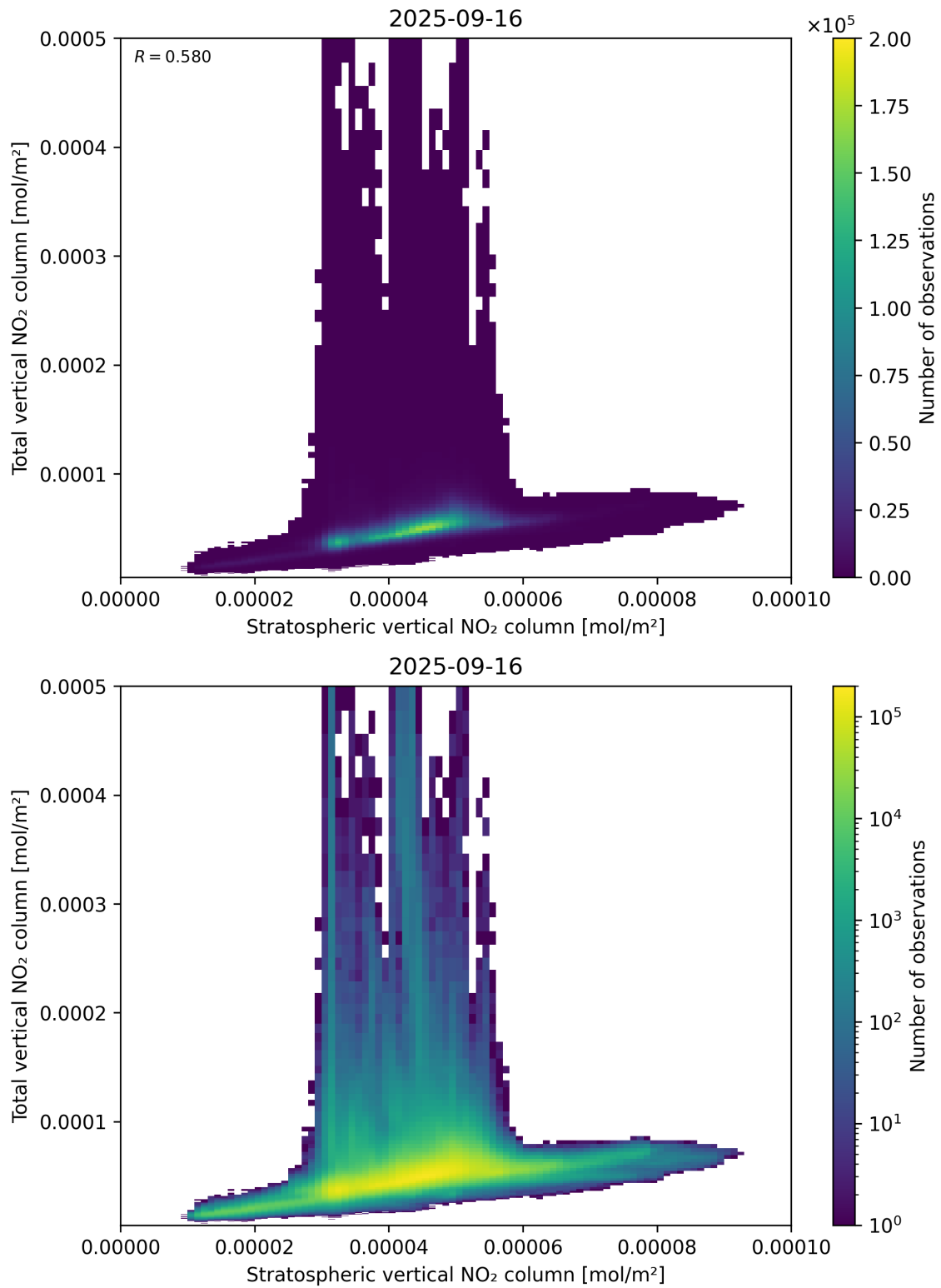
Figure 100: Scatter density plot of “Stratospheric vertical NO 2 column” against “Total vertical NO 2 column” for 2025-09-15 to 2025-09-17.
