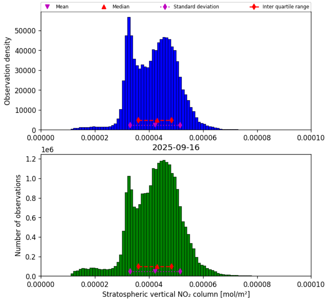
Figure 36: Histogram of “Stratospheric vertical NO 2 column” for 2025-09-15 to 2025-09-17
