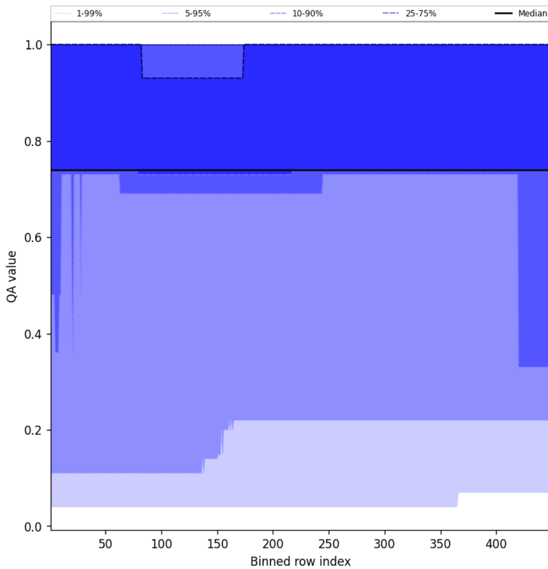
Figure 45: Along track statistics of “QA value” for 2025-09-15 to 2025-09-17
