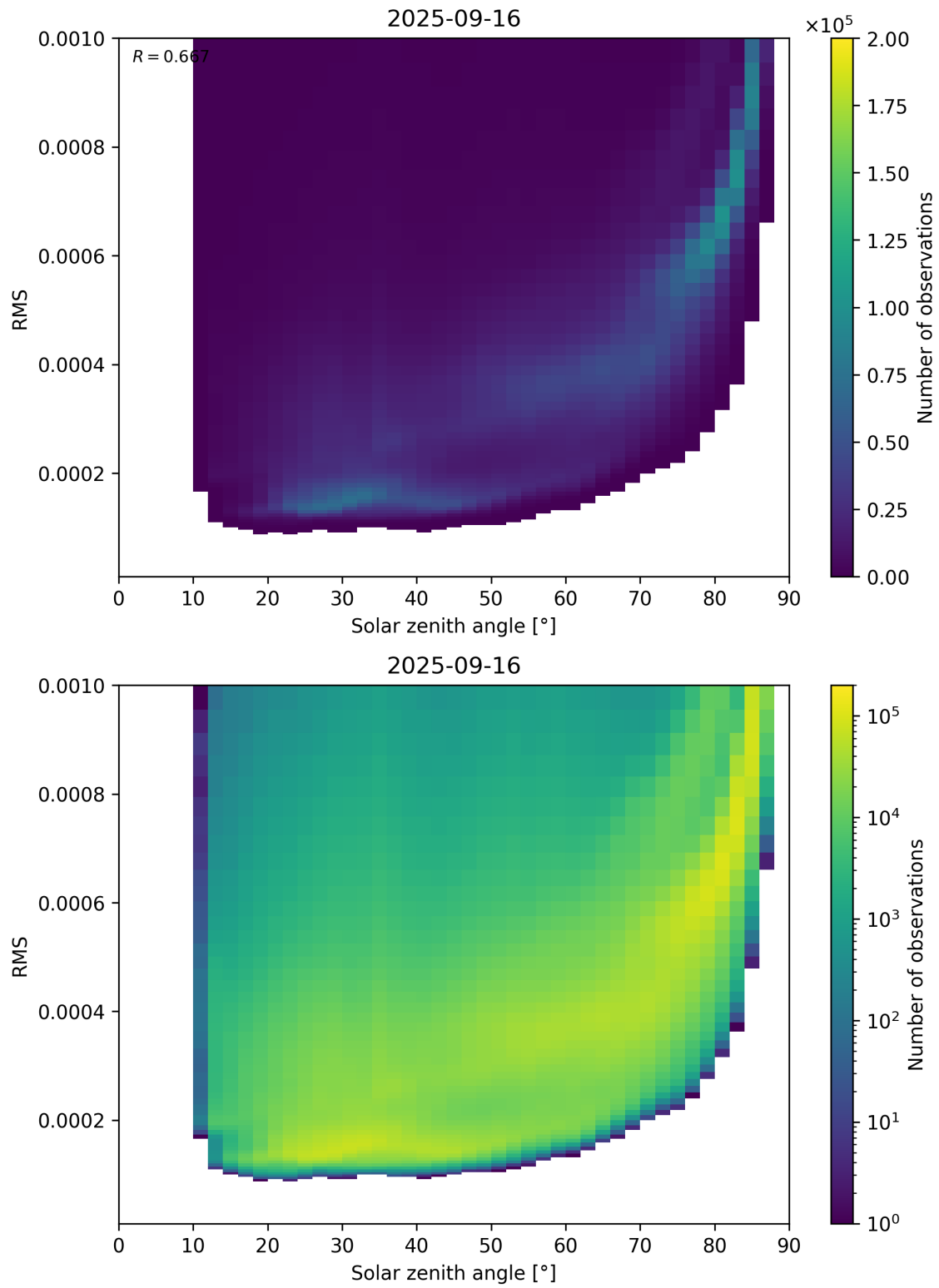
Figure 157: Scatter density plot of “Solar zenith angle” against “RMS” for 2025-09-15 to 2025-09-17.
