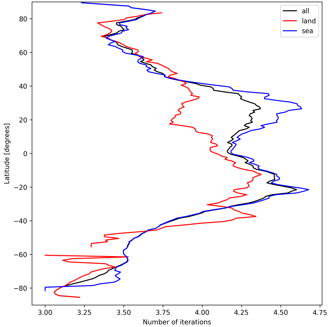
Figure 17: Zonal average of “Number of iterations” for 2025-09-15 to 2025-09-17.
