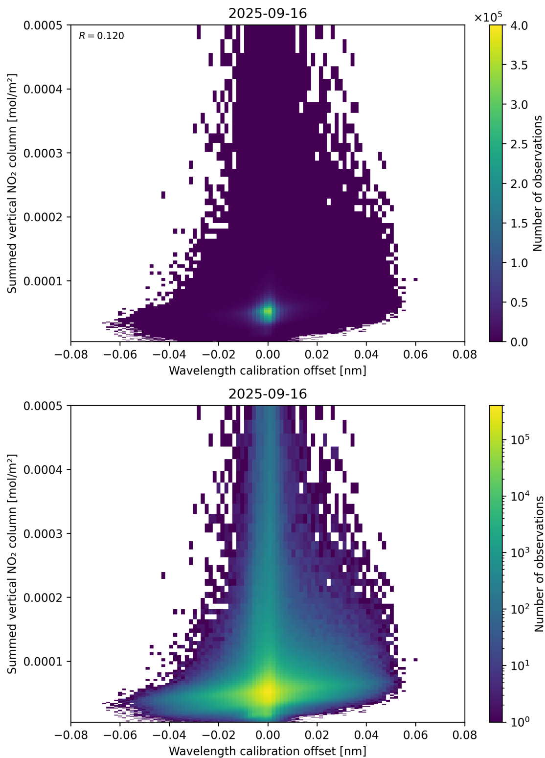
Figure 177: Scatter density plot of “Wavelength calibration offset” against “Summed vertical NO 2 column” for 2025-09-15 to 2025-09-17.
