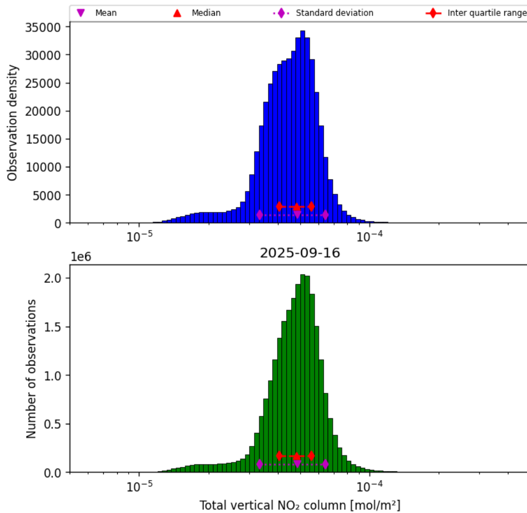
Figure 38: Histogram of “Total vertical NO 2 column” for 2025-09-15 to 2025-09-17
