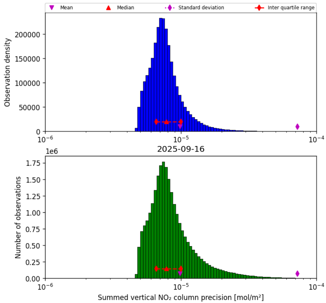
Figure 41: Histogram of "Summed vertical NO 2 column precision" for 2025-09-15 to 2025-09-17
