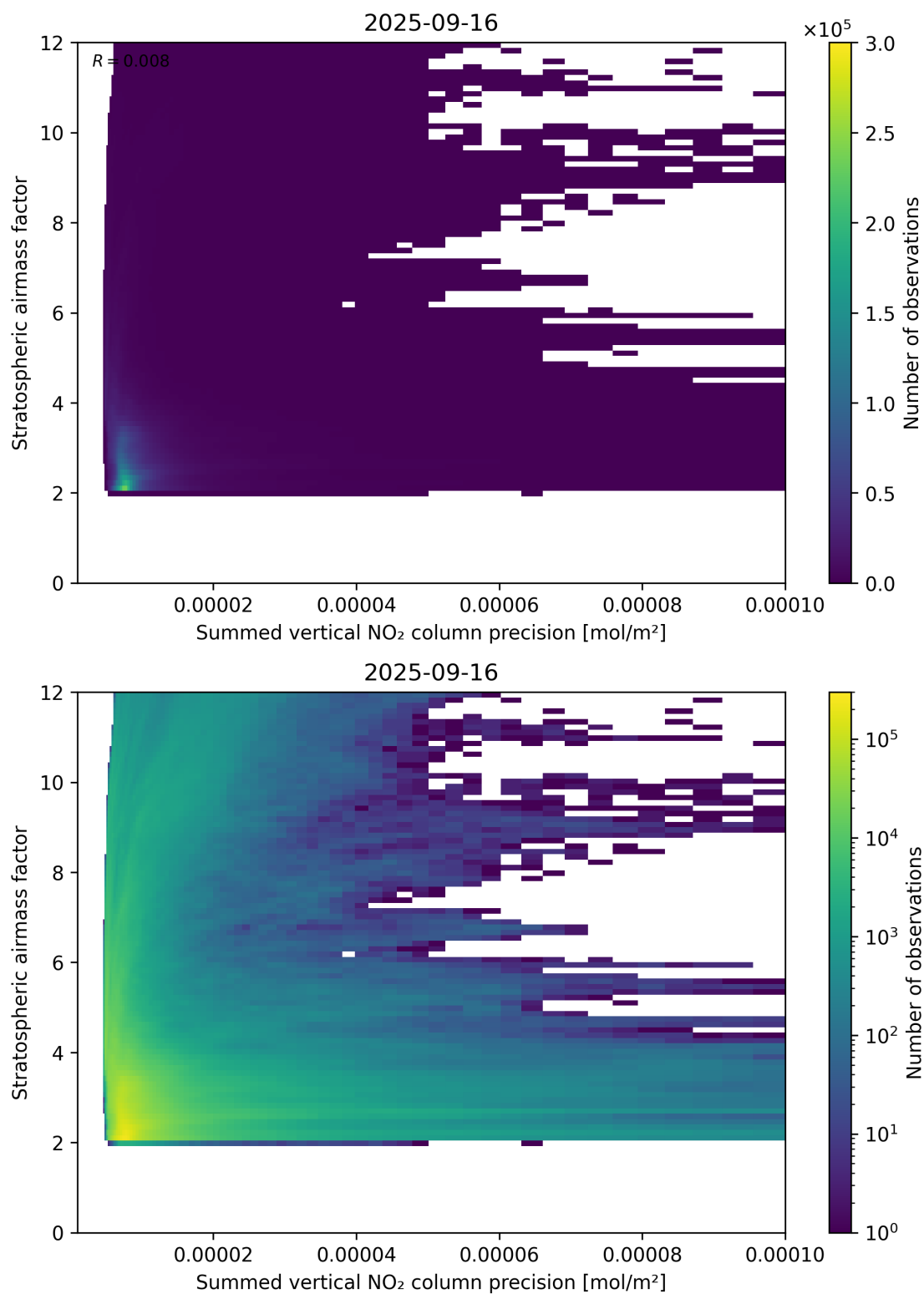
Figure 106: Scatter density plot of “Summed vertical NO 2 column precision” against “Stratospheric airmass factor” for 2025-09-15 to 2025-09-17.
