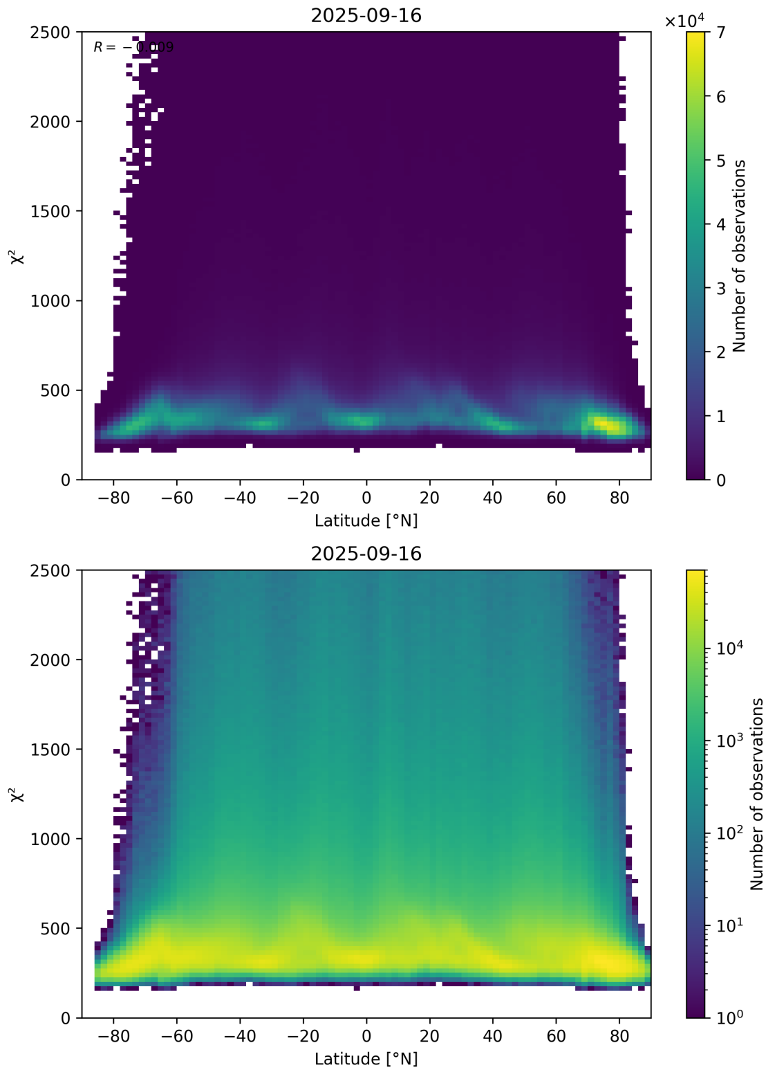
Figure 86: Scatter density plot of “Latitude” against “ \chi^2 ” for 2025-09-15 to 2025-09-17.
