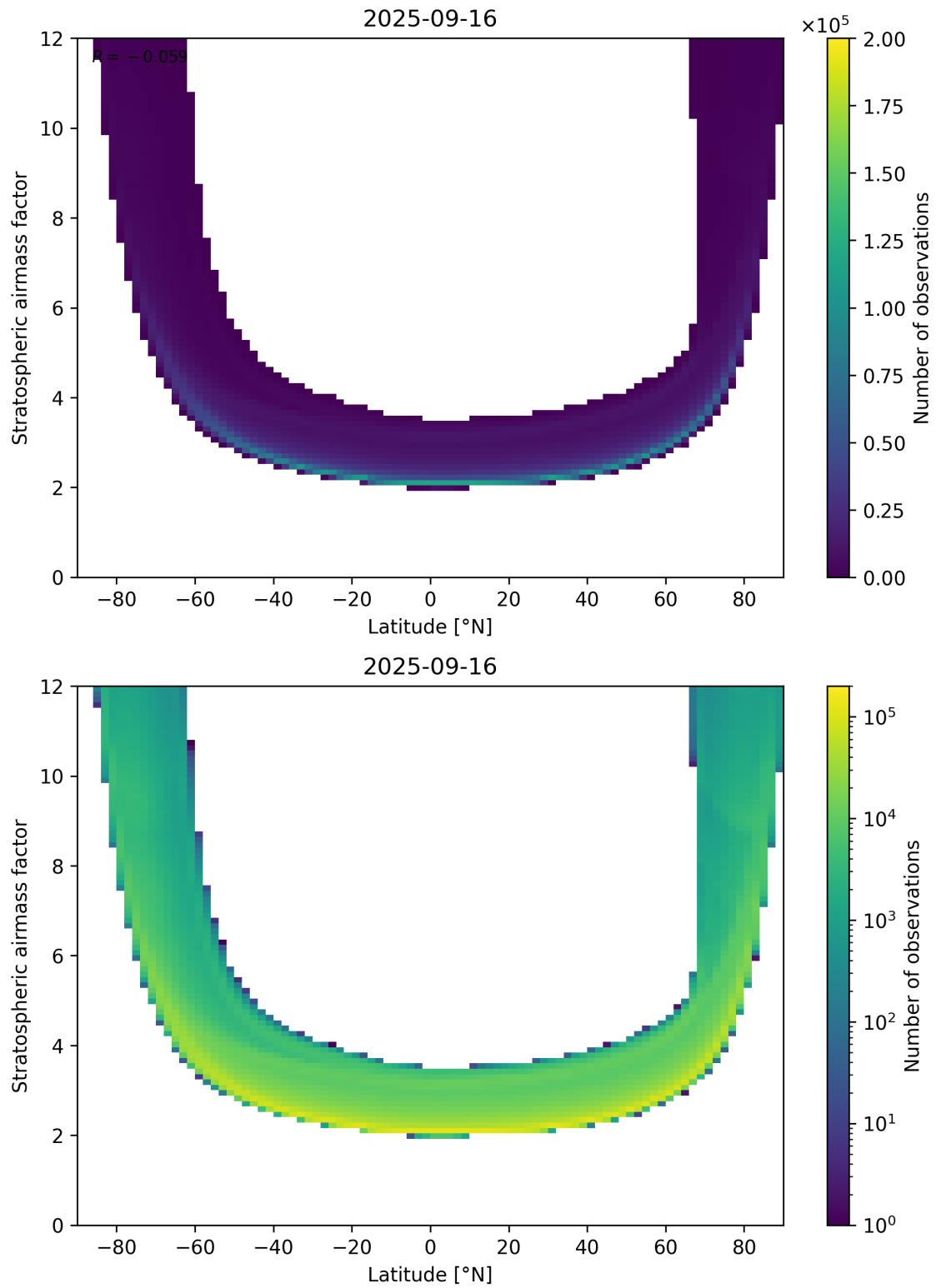
Figure 83: Scatter density plot of “Latitude” against “Stratospheric airmass factor” for 2025-09-15 to 2025-09-17.
