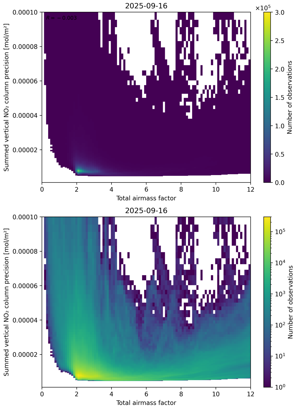
Figure 66: Scatter density plot of “Total airmass factor” against “Summed vertical NO 2 column precision” for 2025-09-15 to 2025-09-17.
