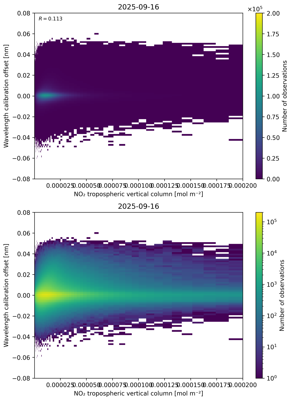
Figure 143: Scatter density plot of “NO 2 tropospheric vertical column” against “Wavelength calibration offset” for 2025-09-15 to 2025-09-17.
