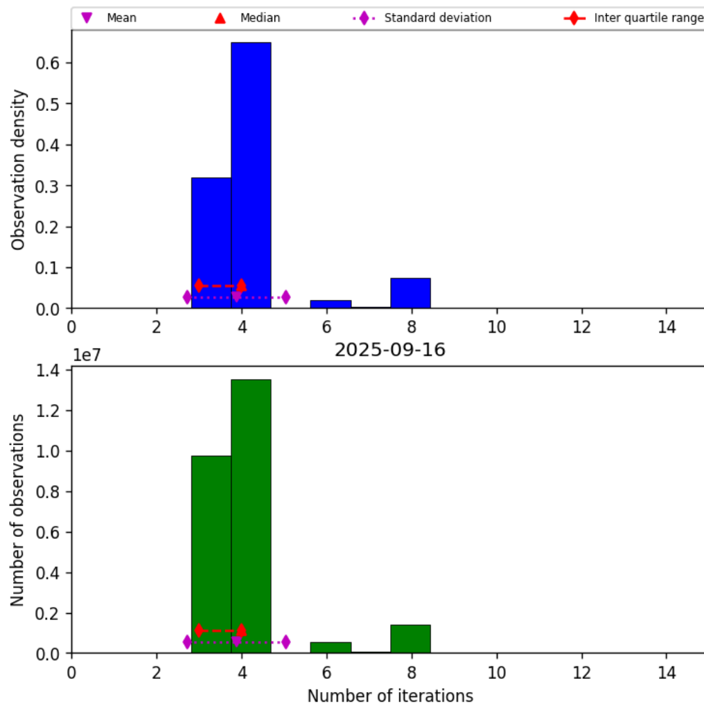
Figure 34: Histogram of “Number of iterations” for 2025-09-15 to 2025-09-17
