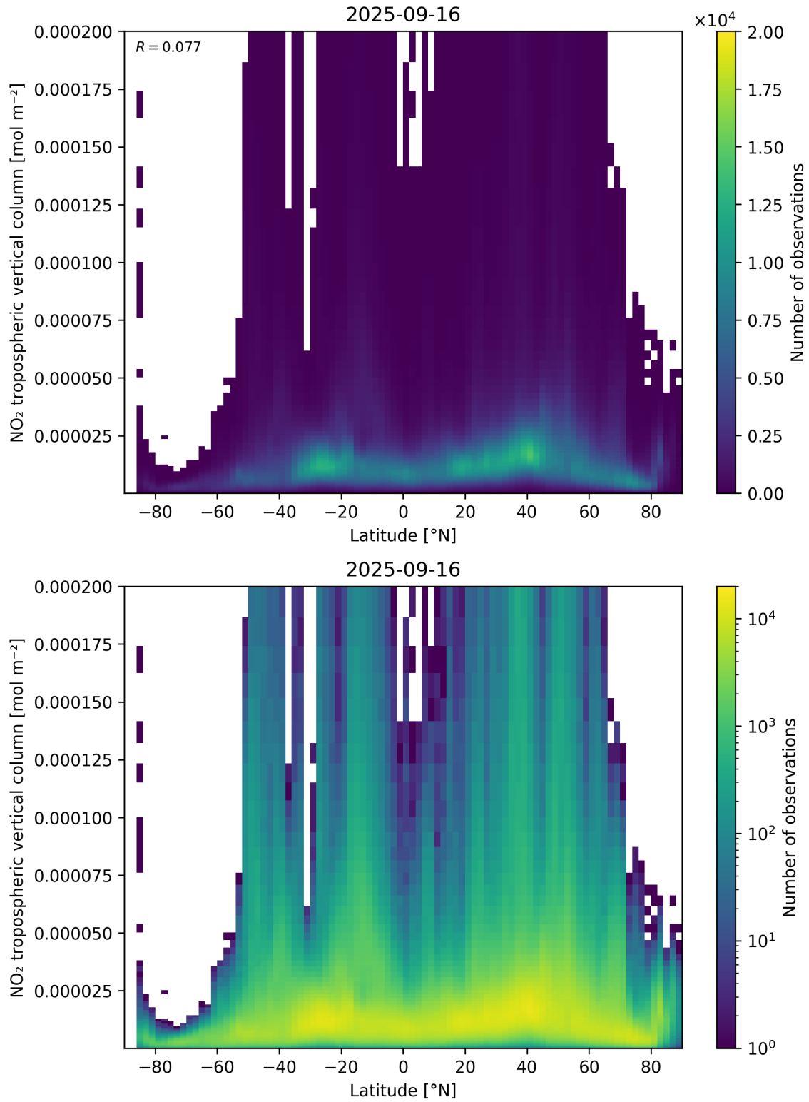
Figure 92: Scatter density plot of “Latitude” against “NO 2 tropospheric vertical column” for 2025-09-15 to 2025-09-17.
