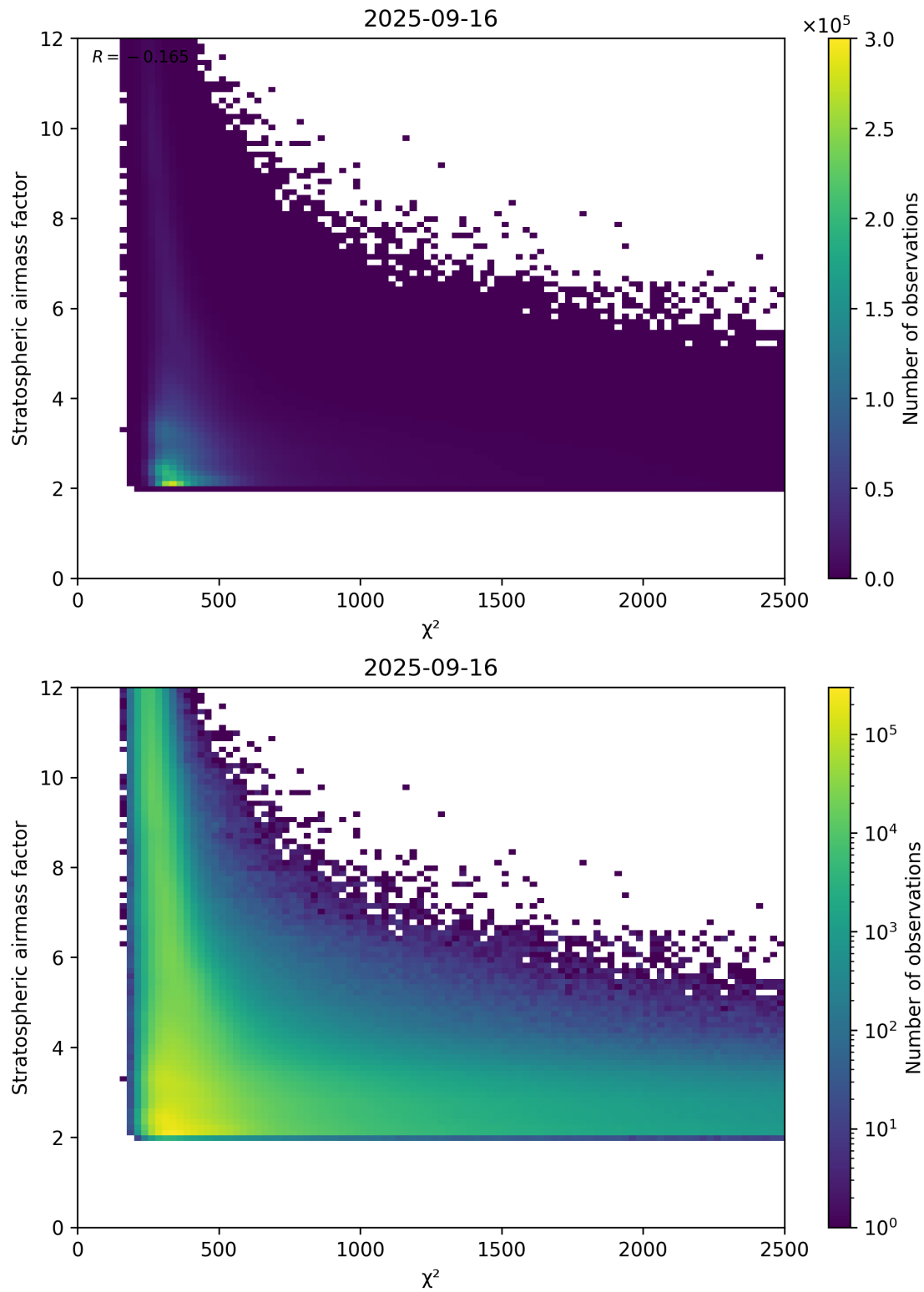
Figure 81: Scatter density plot of “ \chi^2 ” against “Stratospheric airmass factor” for 2025-09-15 to 2025-09-17.
