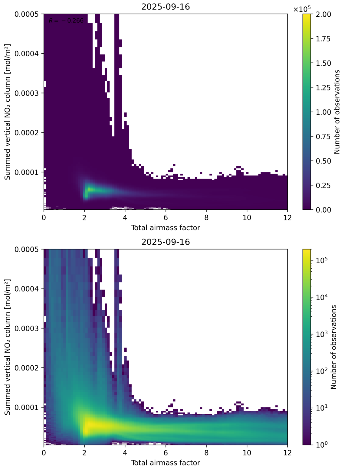
Figure 65: Scatter density plot of “Total airmass factor” against “Summed vertical NO 2 column” for 2025-09-15 to 2025-09-17.
