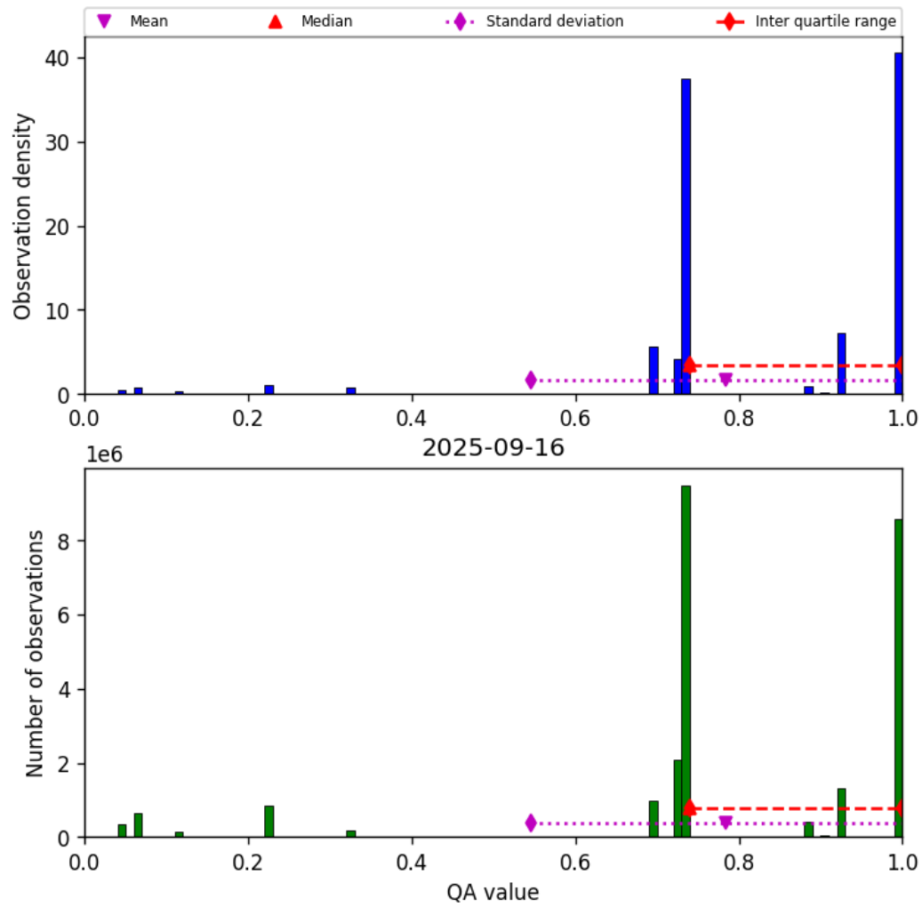
Figure 28: Histogram of “QA value” for 2025-09-15 to 2025-09-17
