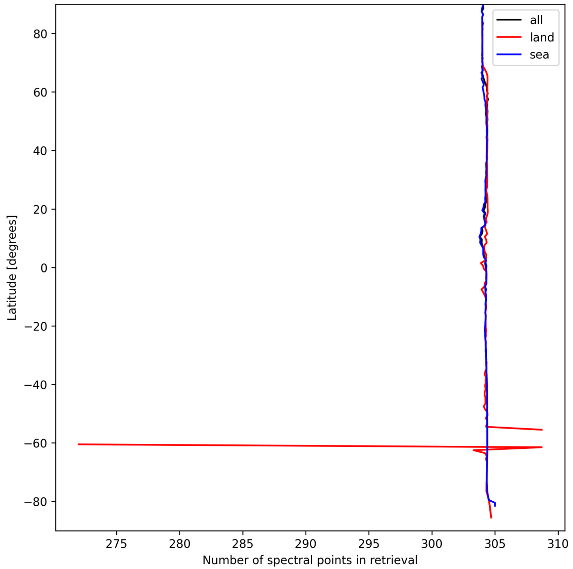
Figure 16: Zonal average of “Number of spectral points in retrieval” for 2025-09-15 to 2025-09-17.
