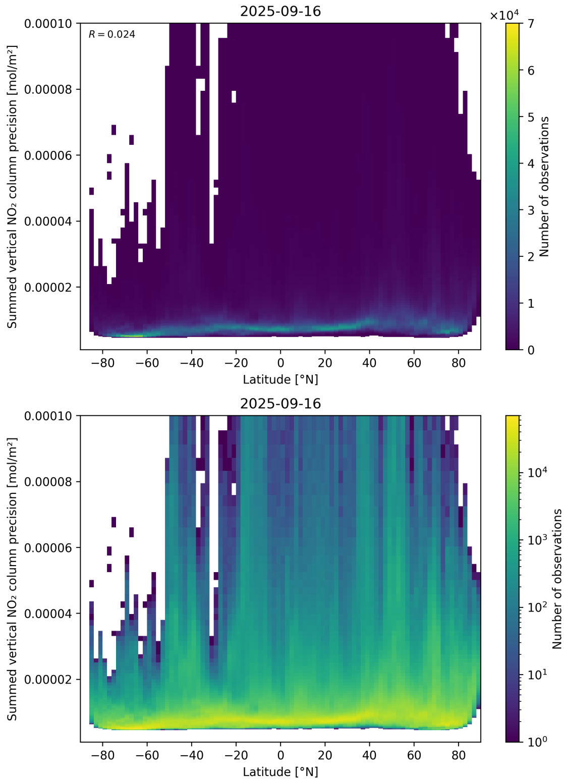
Figure 89: Scatter density plot of “Latitude” against “Summed vertical NO 2 column precision” for 2025-09-15 to 2025-09-17.
