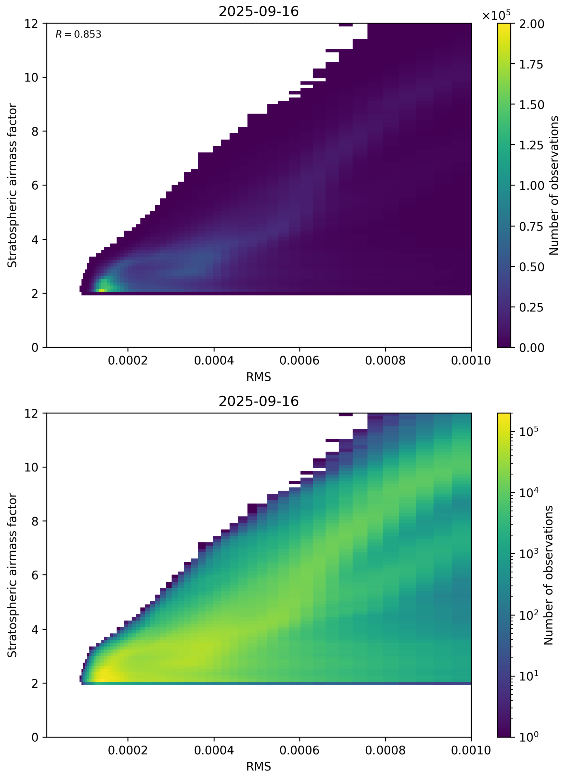
Figure 144: Scatter density plot of “RMS” against “Stratospheric airmass factor” for 2025-09-15 to 2025-09-17.
