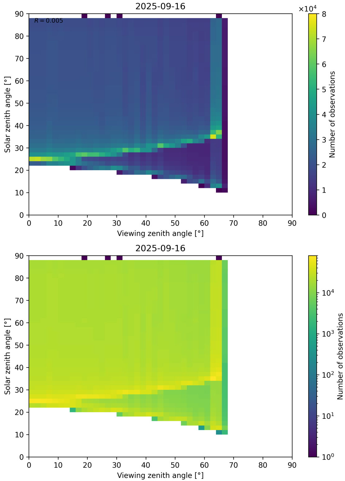
Figure 172: Scatter density plot of “Viewing zenith angle” against “Solar zenith angle” for 2025-09-15 to 2025-09-17.
