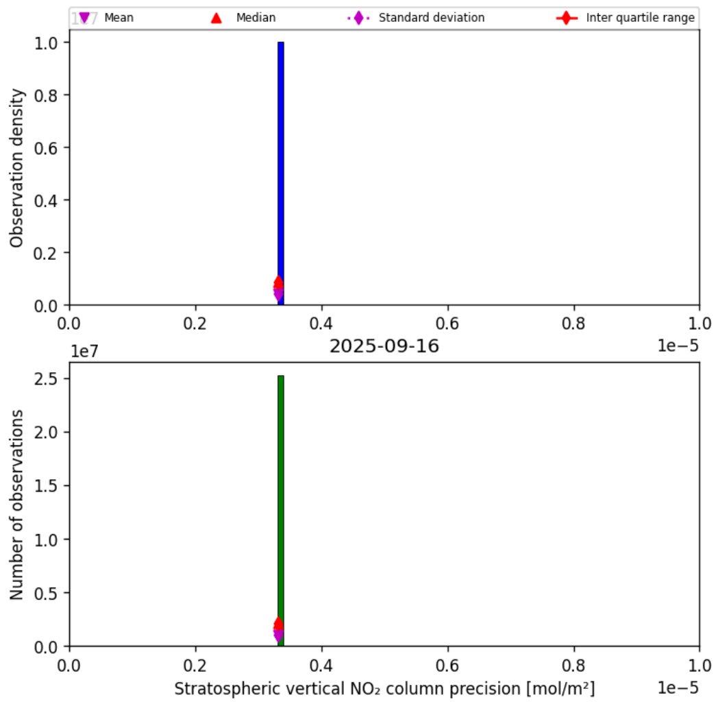
Figure 37: Histogram of “Stratospheric vertical NO 2 column precision” for 2025-09-15 to 2025-09-17
