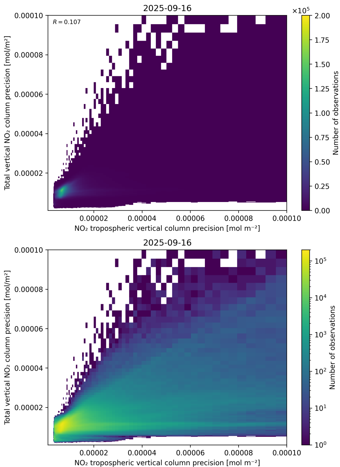
Figure 139: Scatter density plot of “NO 2 tropospheric vertical column precision” against “Total vertical NO 2 column precision” for 2025-09-15 to 2025-09-17.
