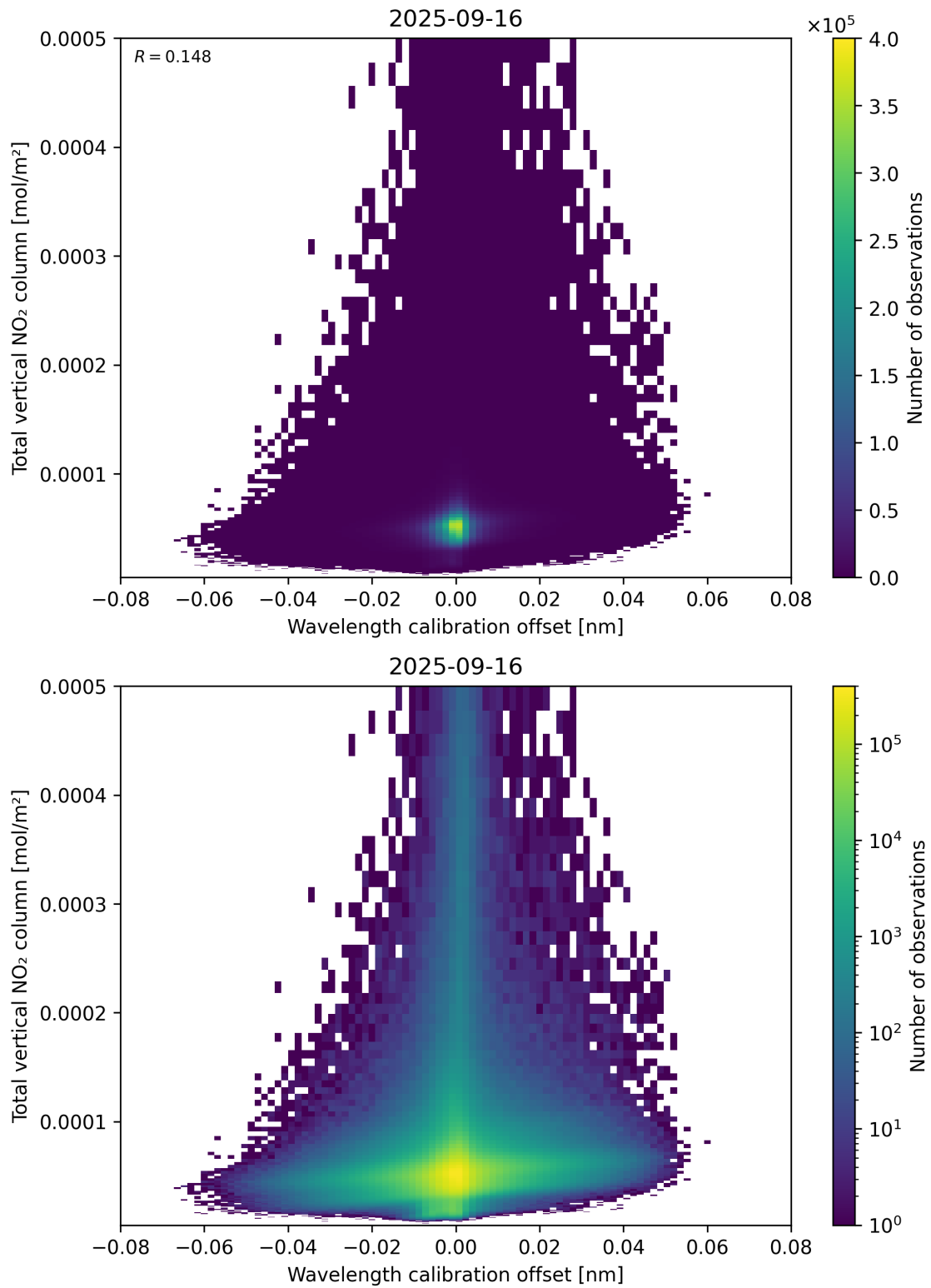
Figure 179: Scatter density plot of “Wavelength calibration offset” against “Total vertical NO 2 column” for 2025-09-15 to 2025-09-17.
