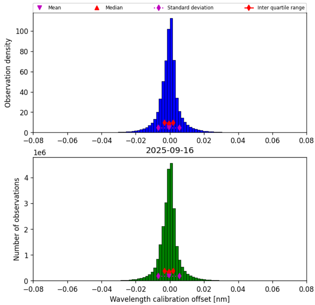
Figure 35: Histogram of “Wavelength calibration offset” for 2025-09-15 to 2025-09-17
