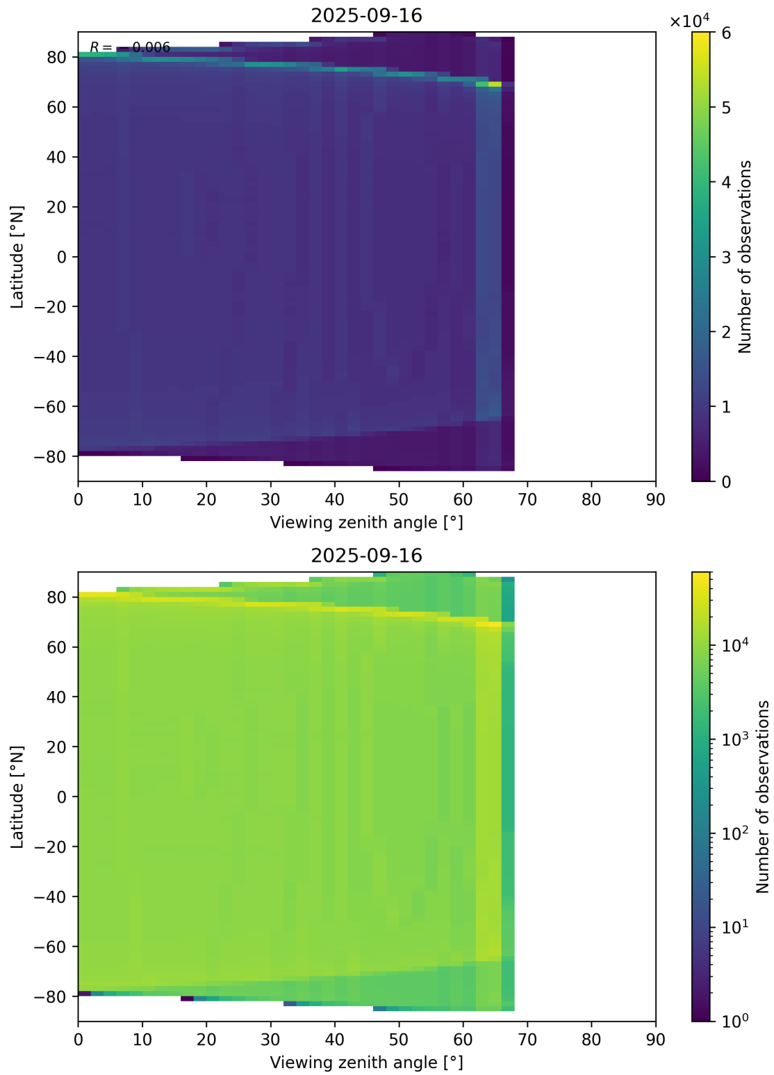
Figure 163: Scatter density plot of “Viewing zenith angle” against “Latitude” for 2025-09-15 to 2025-09-17.
