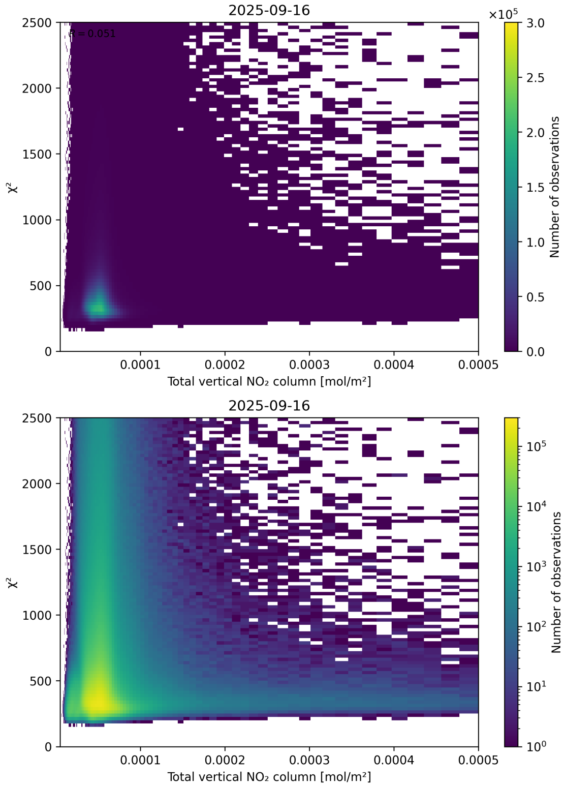
Figure 111: Scatter density plot of “Total vertical NO 2 column” against “ \chi^2 ” for 2025-09-15 to 2025-09-17.
