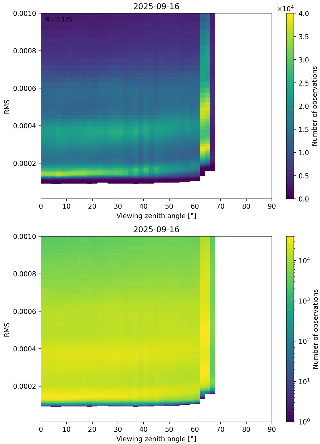
Figure 171: Scatter density plot of “Viewing zenith angle” against “RMS” for 2025-09-15 to 2025-09-17.
