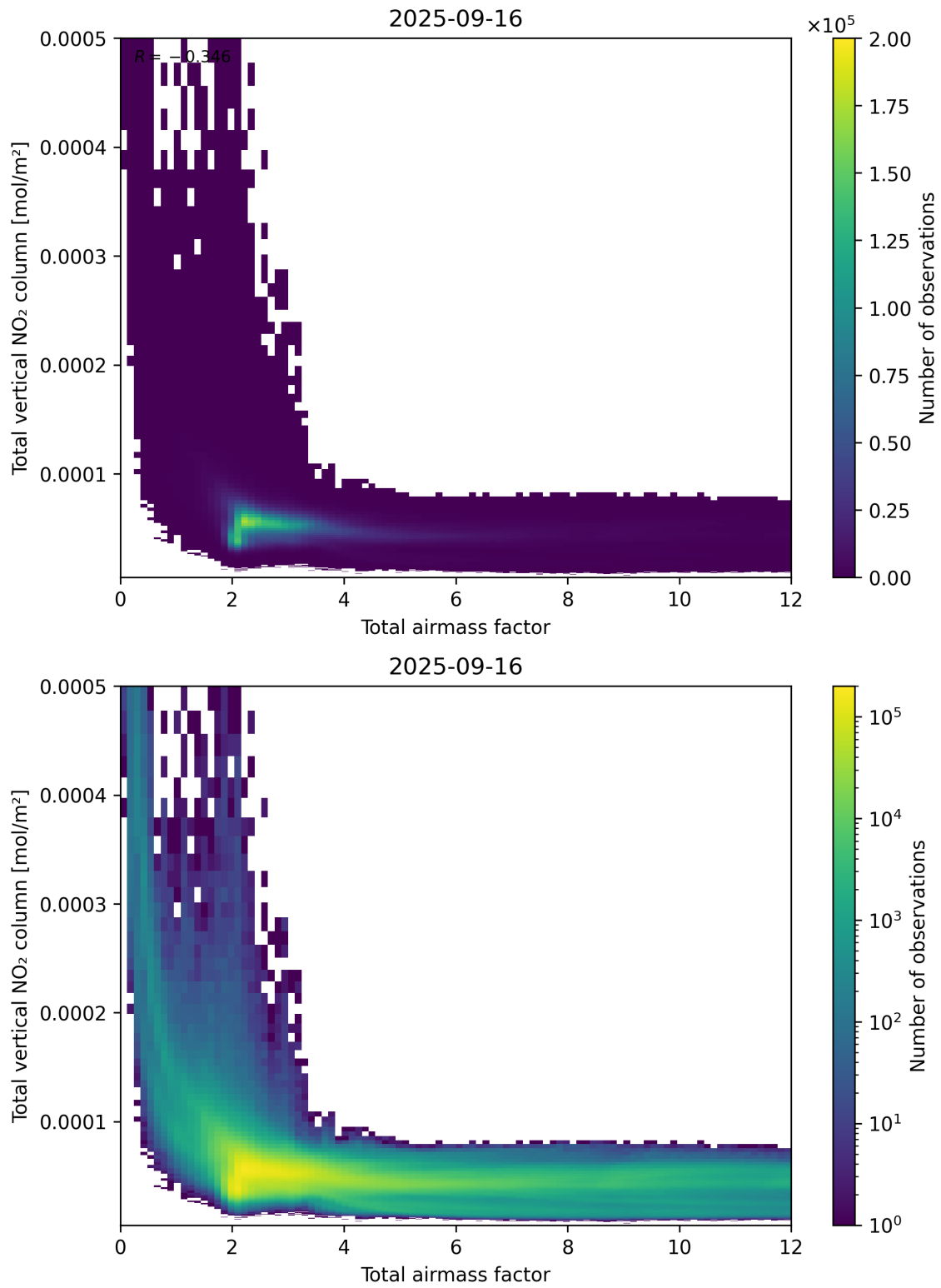
Figure 67: Scatter density plot of “Total airmass factor” against “Total vertical NO 2 column” for 2025-09-15 to 2025-09-17.
