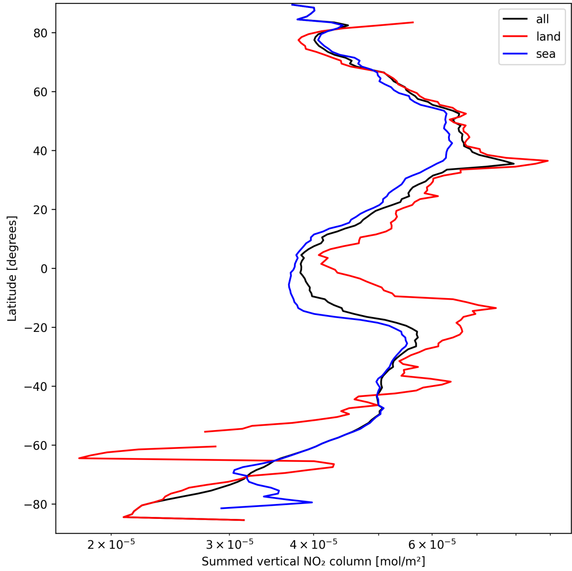
Figure 23: Zonal average of “Summed vertical NO 2 column” for 2025-09-15 to 2025-09-17.
