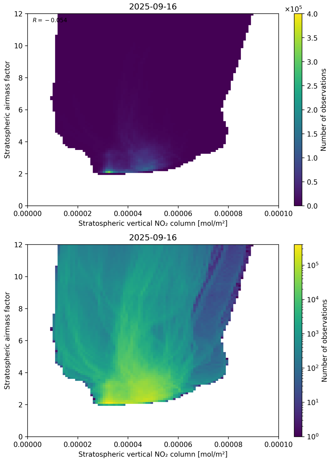
Figure 96: Scatter density plot of “Stratospheric vertical NO 2 column” against “Stratospheric airmass factor” for 2025-09-15 to 2025-09-17.
