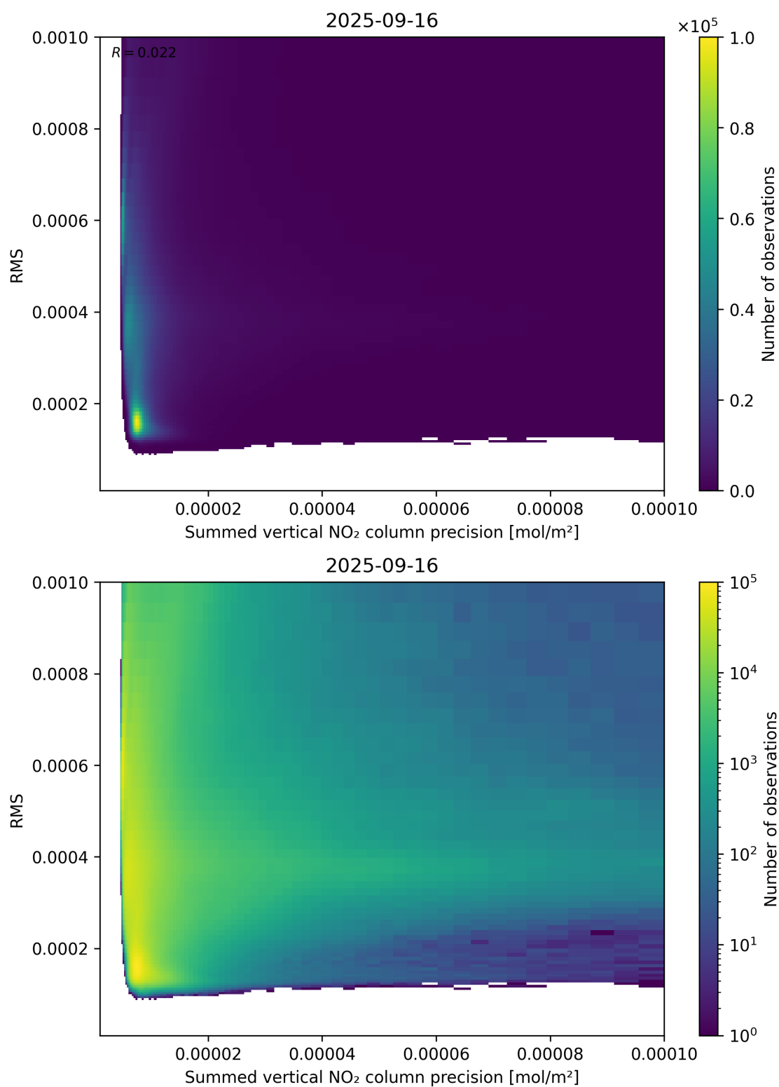
Figure 108: Scatter density plot of “Summed vertical NO 2 column precision” against “RMS” for 2025-09-15 to 2025-09-17.
