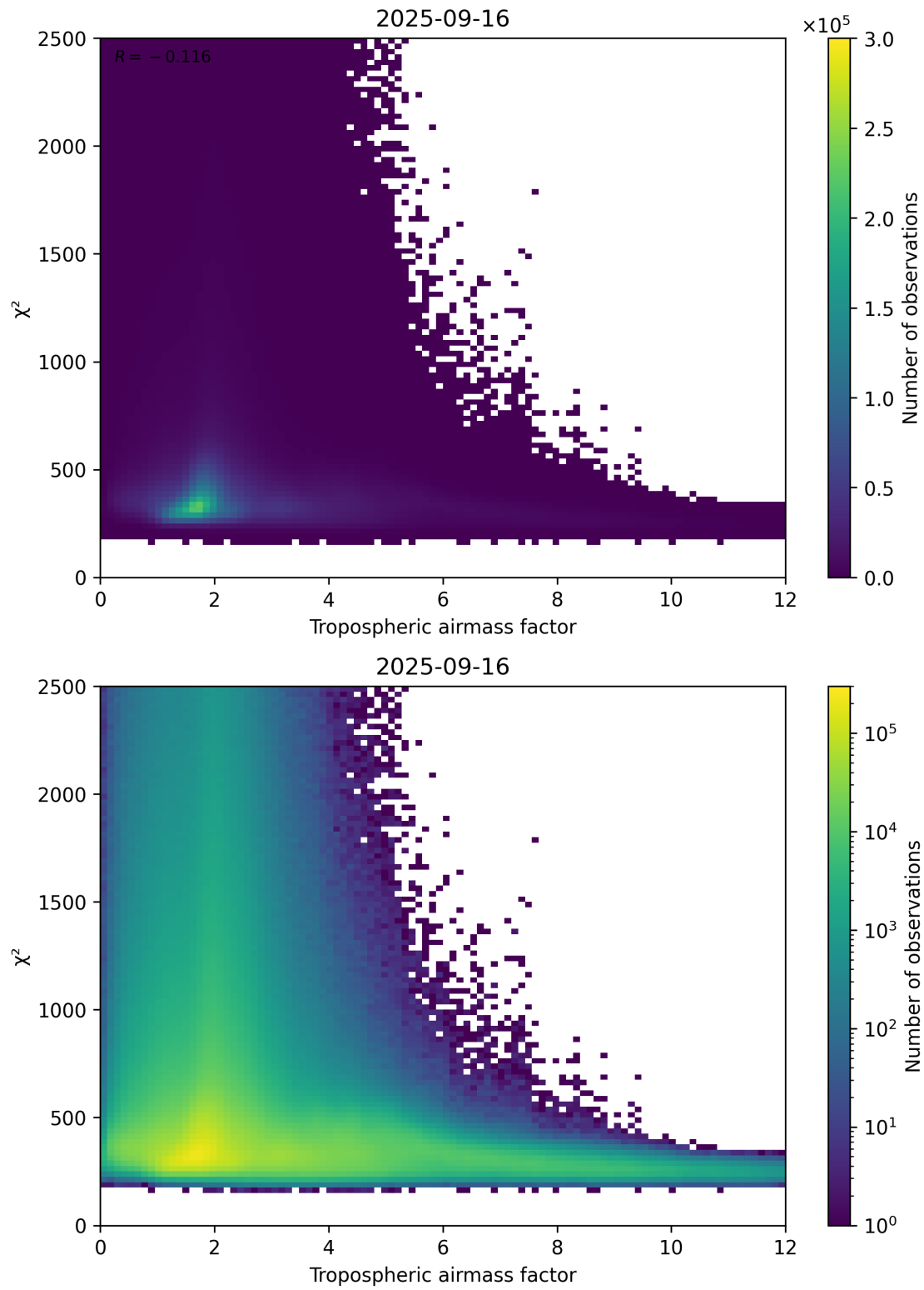
Figure 73: Scatter density plot of “Tropospheric airmass factor” against “ \chi^2 ” for 2025-09-15 to 2025-09-17.
