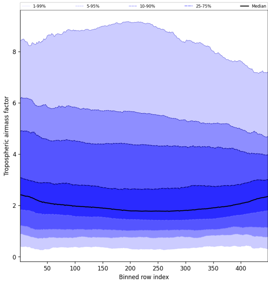
Figure 48: Along track statistics of “Tropospheric airmass factor” for 2025-09-15 to 2025-09-17
