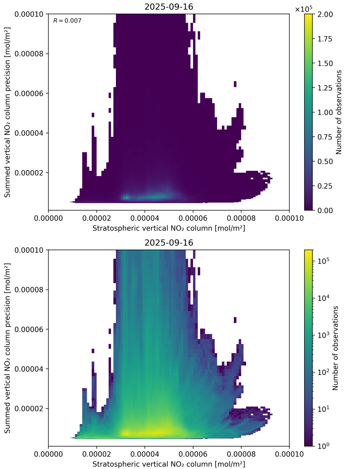
Figure 99: Scatter density plot of “Stratospheric vertical NO 2 column” against “Summed vertical NO 2 column precision” for 2025-09-15 to 2025-09-17.
