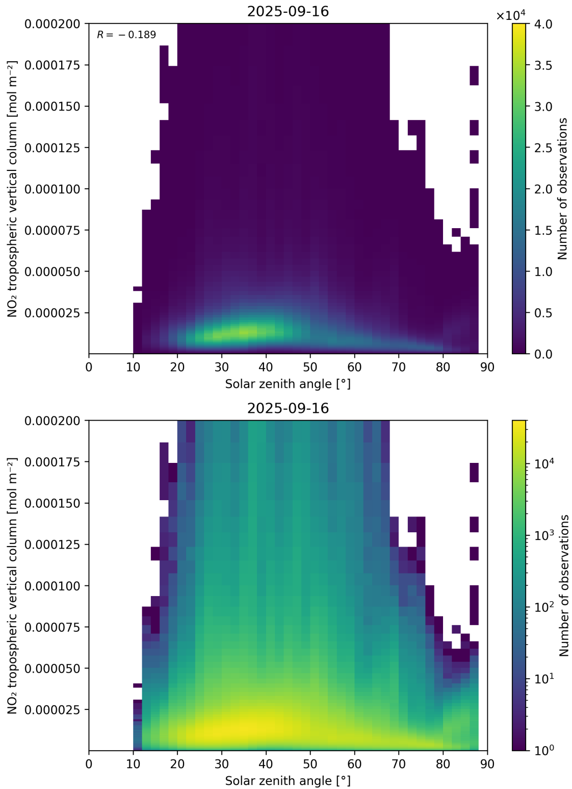
Figure 155: Scatter density plot of “Solar zenith angle” against “NO 2 tropospheric vertical column” for 2025-09-15 to 2025-09-17.
