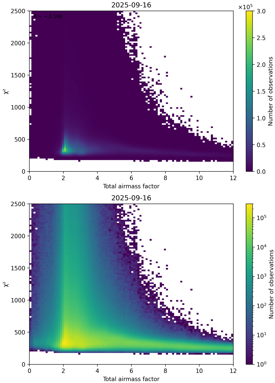
Figure 63: Scatter density plot of “Total airmass factor” against “ \chi^2 ” for 2025-09-15 to 2025-09-17.
