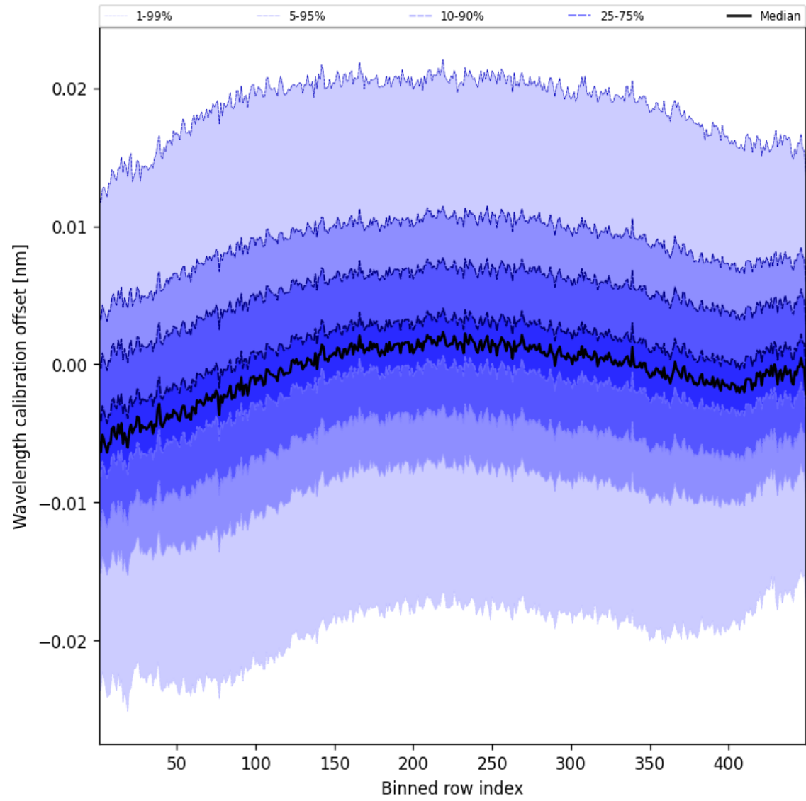
Figure 52: Along track statistics of “Wavelength calibration offset” for 2025-09-15 to 2025-09-17
