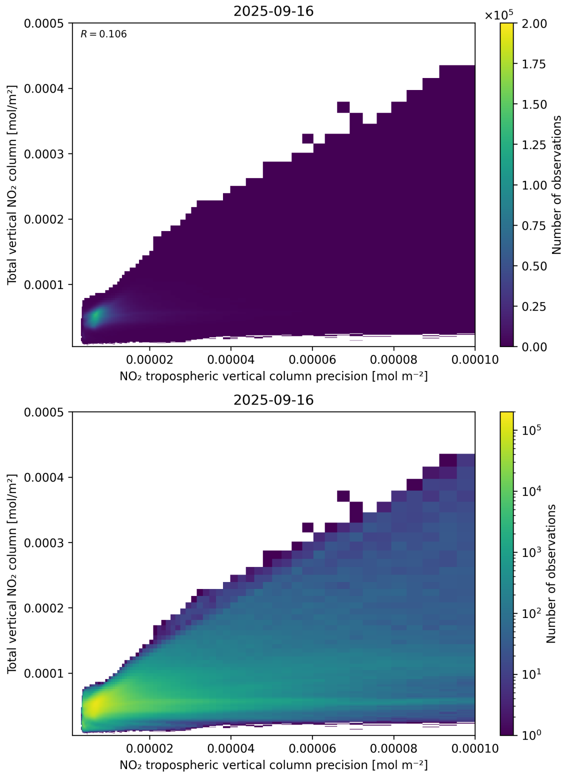
Figure 138: Scatter density plot of “NO 2 tropospheric vertical column precision” against “Total vertical NO 2 column” for 2025-09-15 to 2025-09-17.
