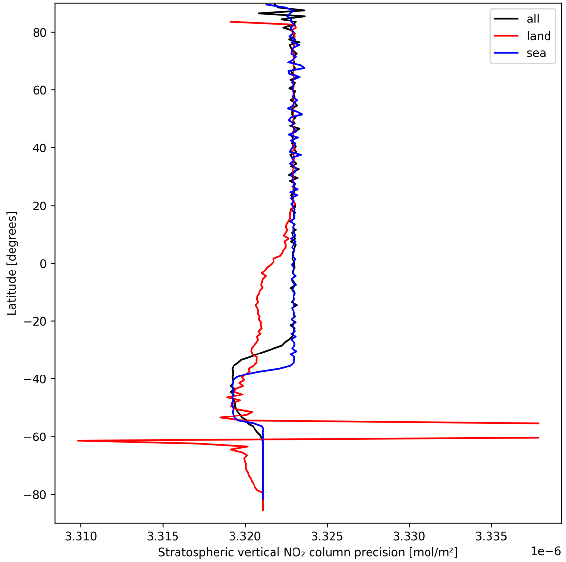
Figure 20: Zonal average of "Stratospheric vertical NO 2 column precision" for 2025-09-15 to 2025-09-17.
