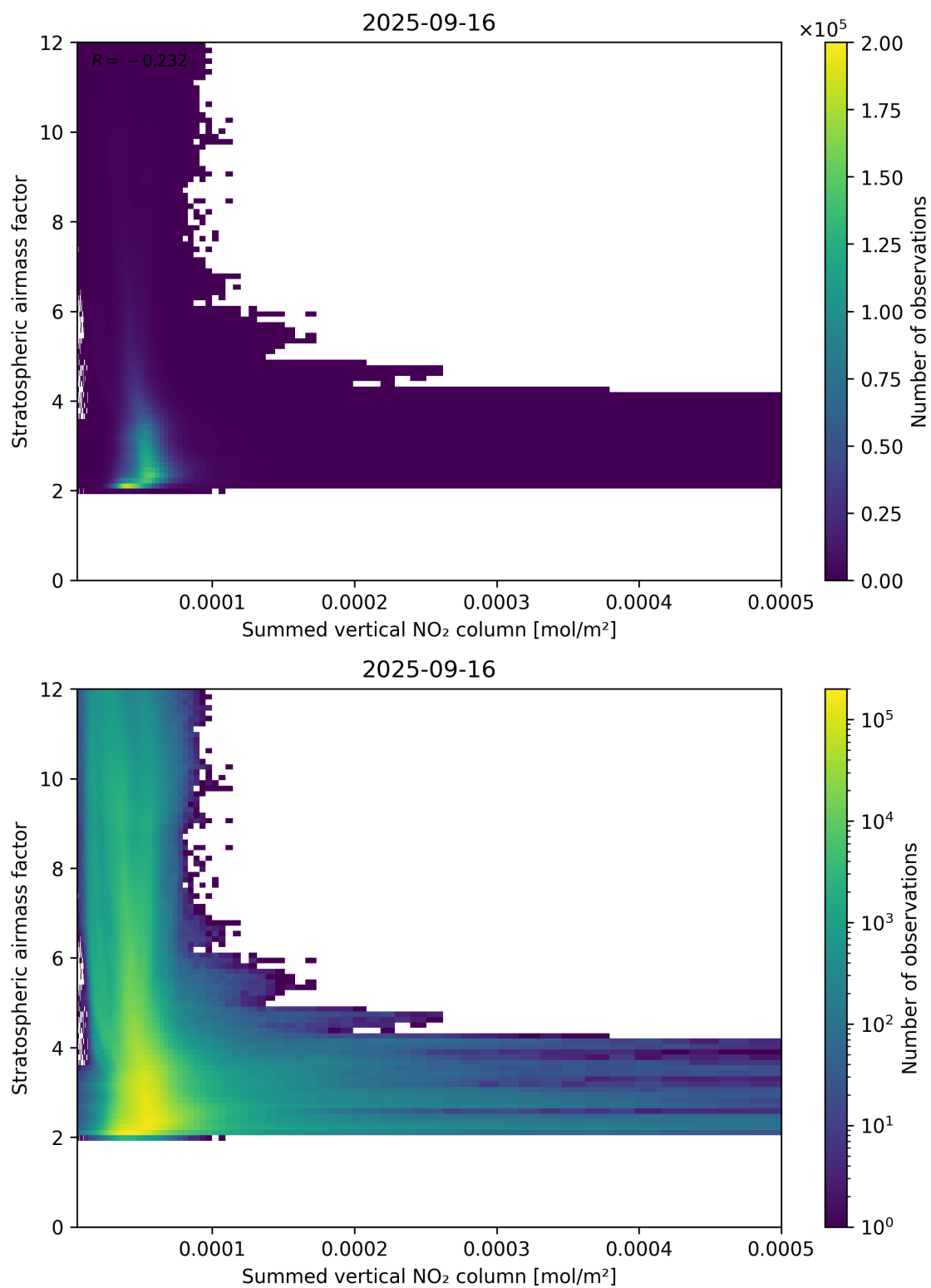
Figure 103: Scatter density plot of “Summed vertical NO 2 column” against “Stratospheric airmass factor” for 2025-09-15 to 2025-09-17.
