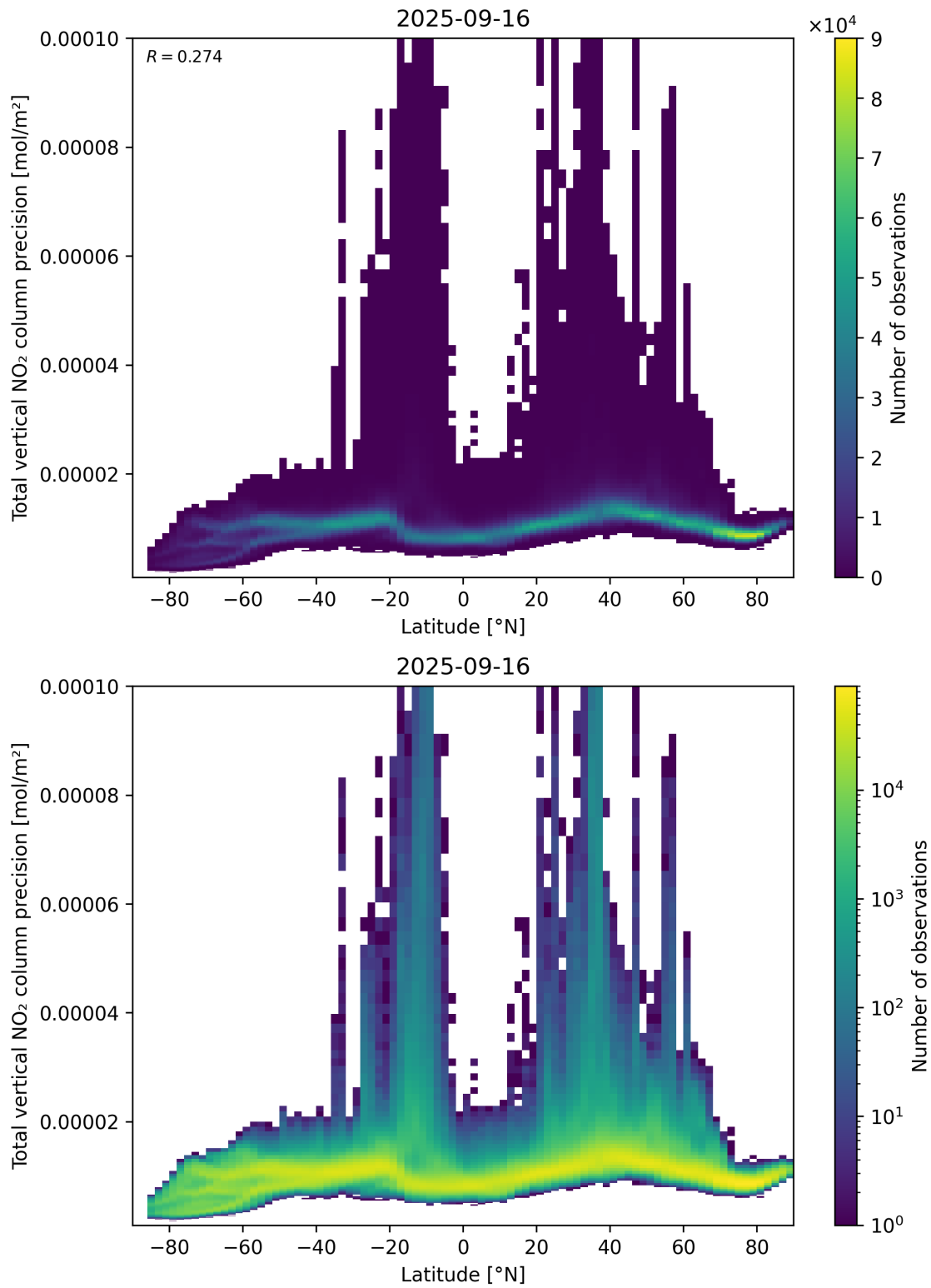
Figure 91: Scatter density plot of “Latitude” against “Total vertical NO 2 column precision” for 2025-09-15 to 2025-09-17.
