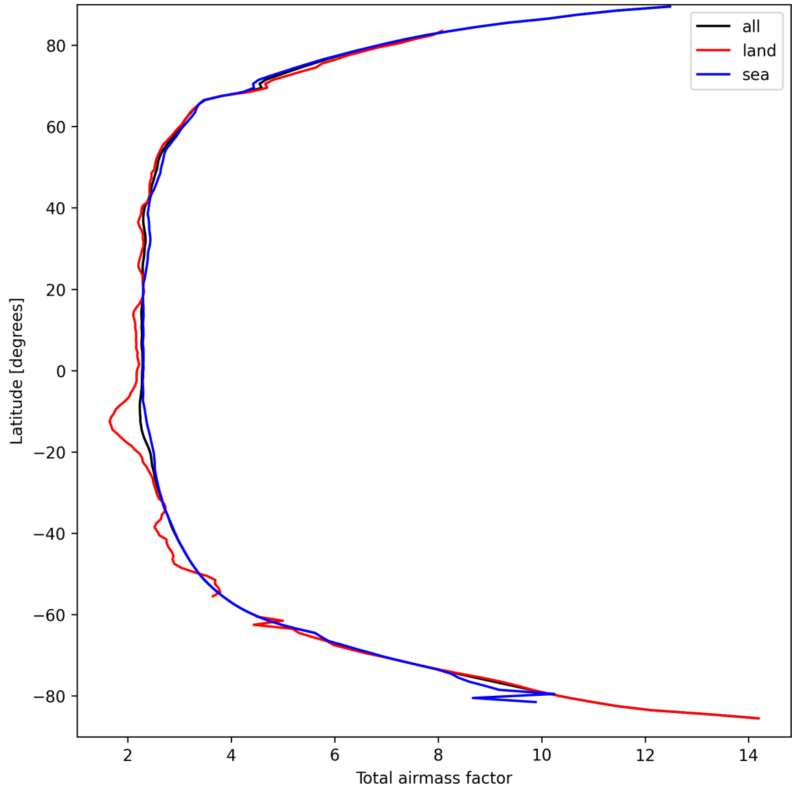
Figure 15: Zonal average of “Total airmass factor” for 2025-09-15 to 2025-09-17.
