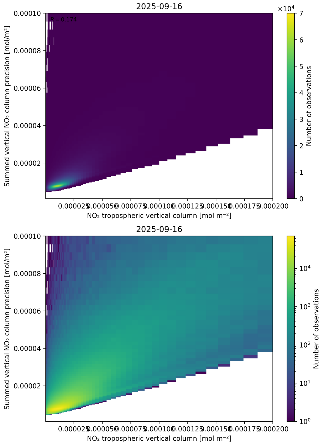
Figure 127: Scatter density plot of “NO 2 tropospheric vertical column” against “Summed vertical NO 2 column precision” for 2025-09-15 to 2025-09-17.
