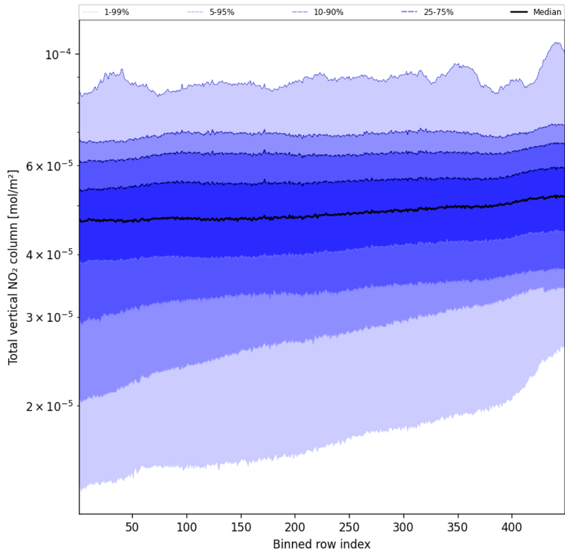
Figure 55: Along track statistics of “Total vertical NO 2 column” for 2025-09-15 to 2025-09-17
