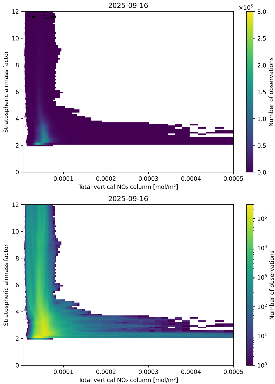
Figure 110: Scatter density plot of “Total vertical NO 2 column” against “Stratospheric airmass factor” for 2025-09-15 to 2025-09-17.
