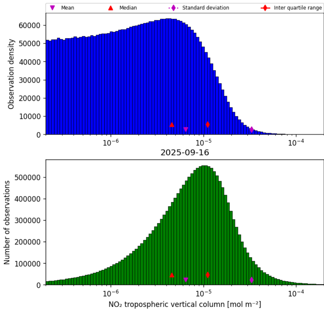
Figure 29: Histogram of “NO 2 tropospheric vertical column” for 2025-09-15 to 2025-09-17
