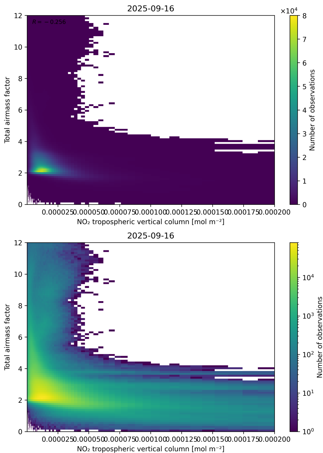
Figure 122: Scatter density plot of “NO 2 tropospheric vertical column” against “Total airmass factor” for 2025-09-15 to 2025-09-17.
