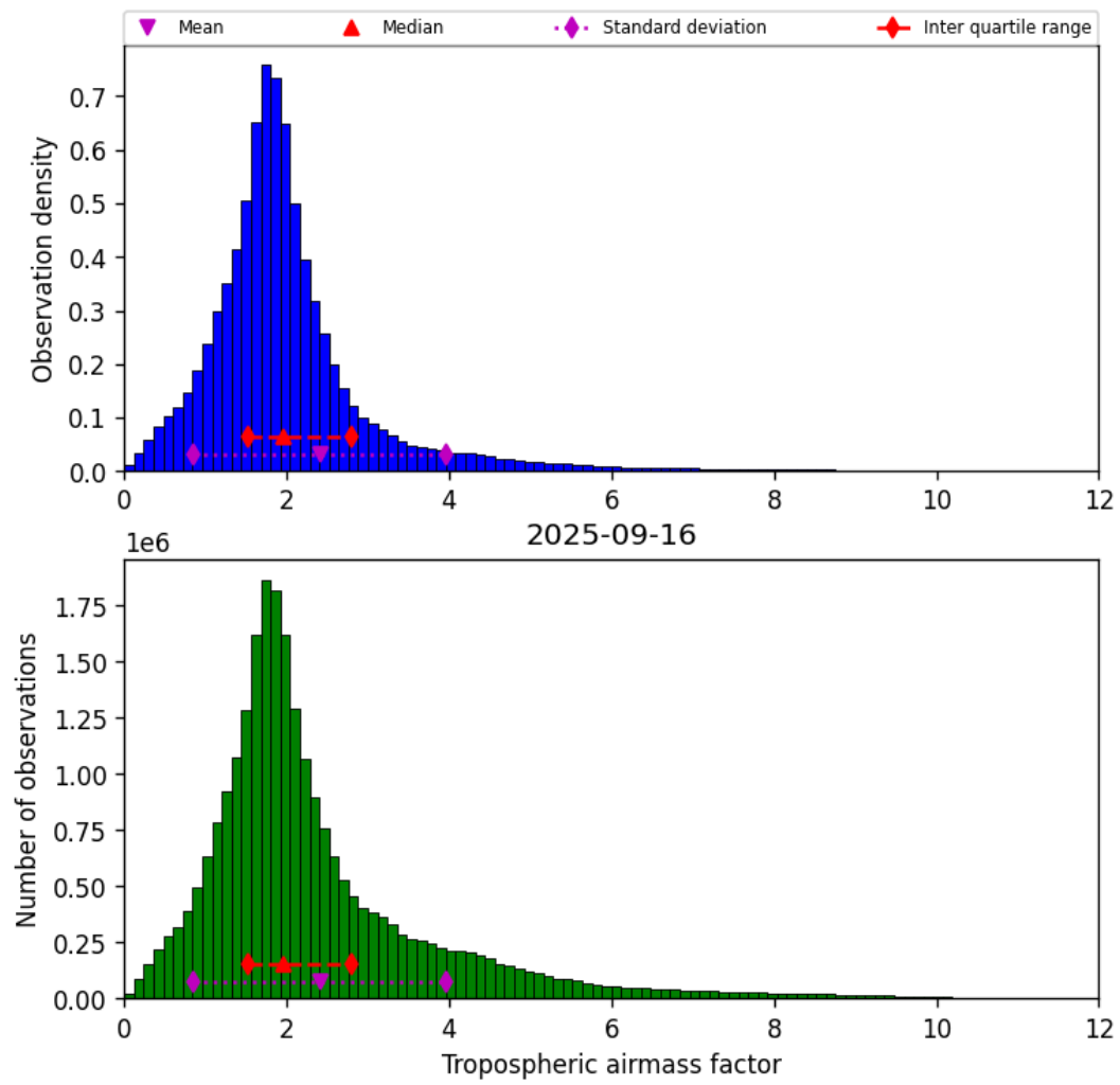
Figure 31: Histogram of “Tropospheric airmass factor” for 2025-09-15 to 2025-09-17
