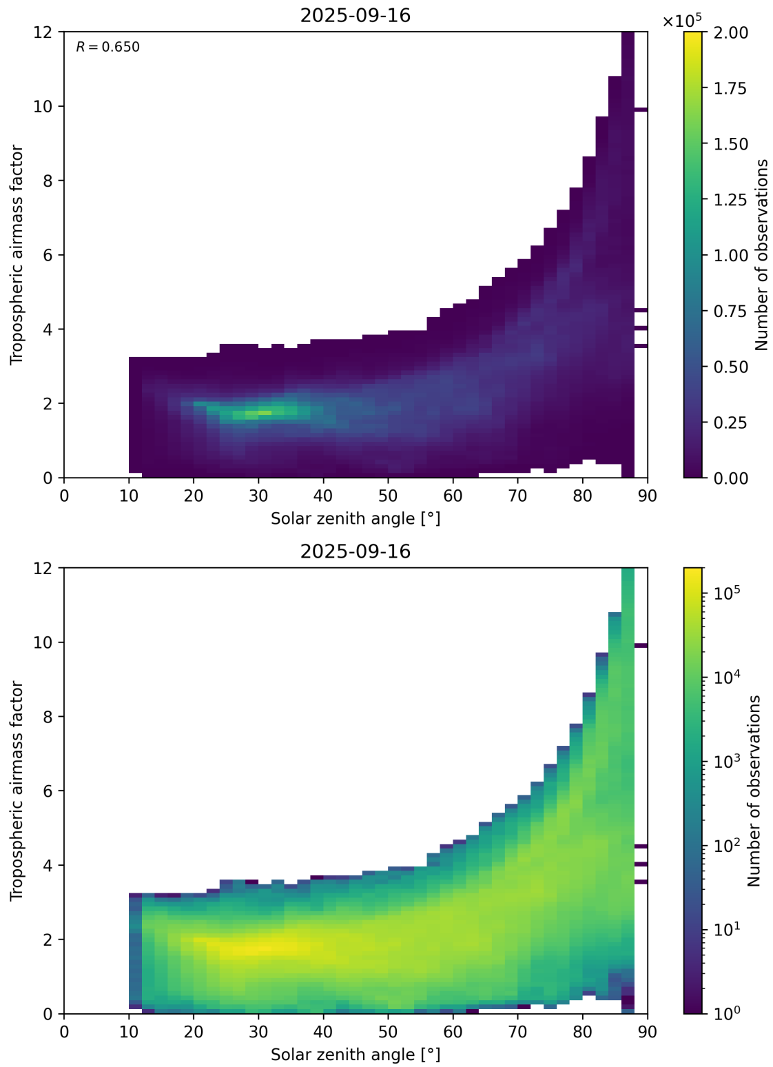
Figure 147: Scatter density plot of “Solar zenith angle” against “Tropospheric airmass factor” for 2025-09-15 to 2025-09-17.
