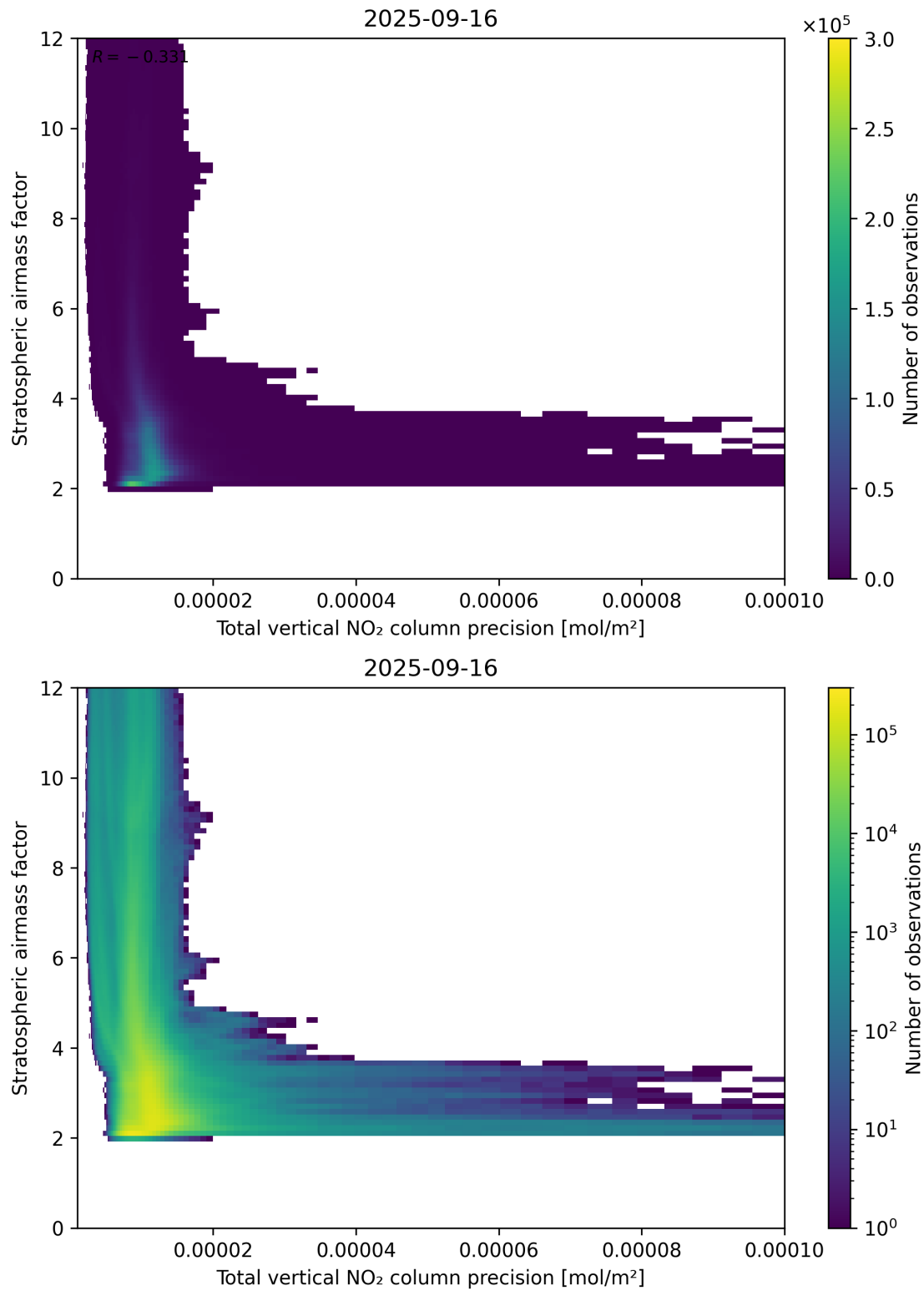
Figure 115: Scatter density plot of “Total vertical NO 2 column precision” against “Stratospheric air mass factor” for 2025-09-15 to 2025-09-17.
