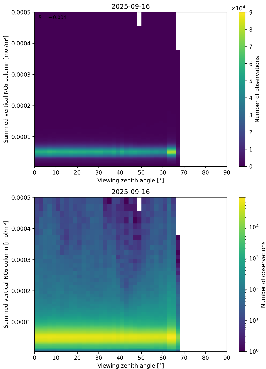
Figure 165: Scatter density plot of “Viewing zenith angle” against “Summed vertical NO 2 column” for 2025-09-15 to 2025-09-17.
