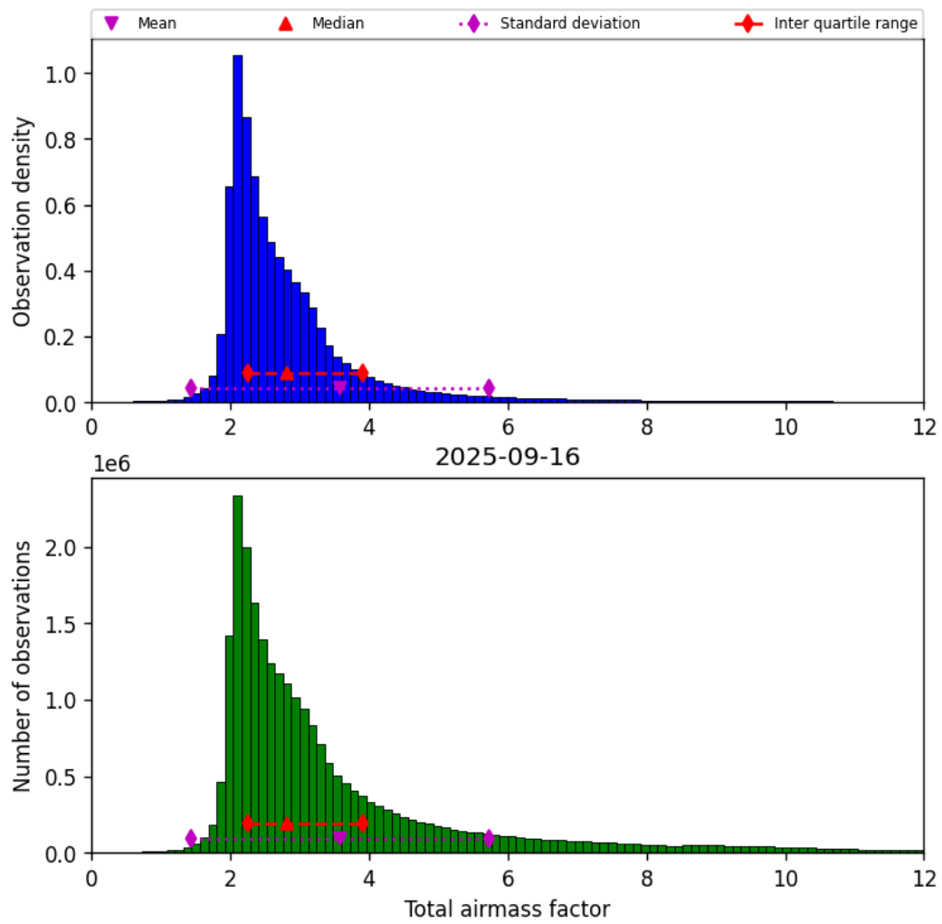
Figure 32: Histogram of “Total airmass factor” for 2025-09-15 to 2025-09-17
