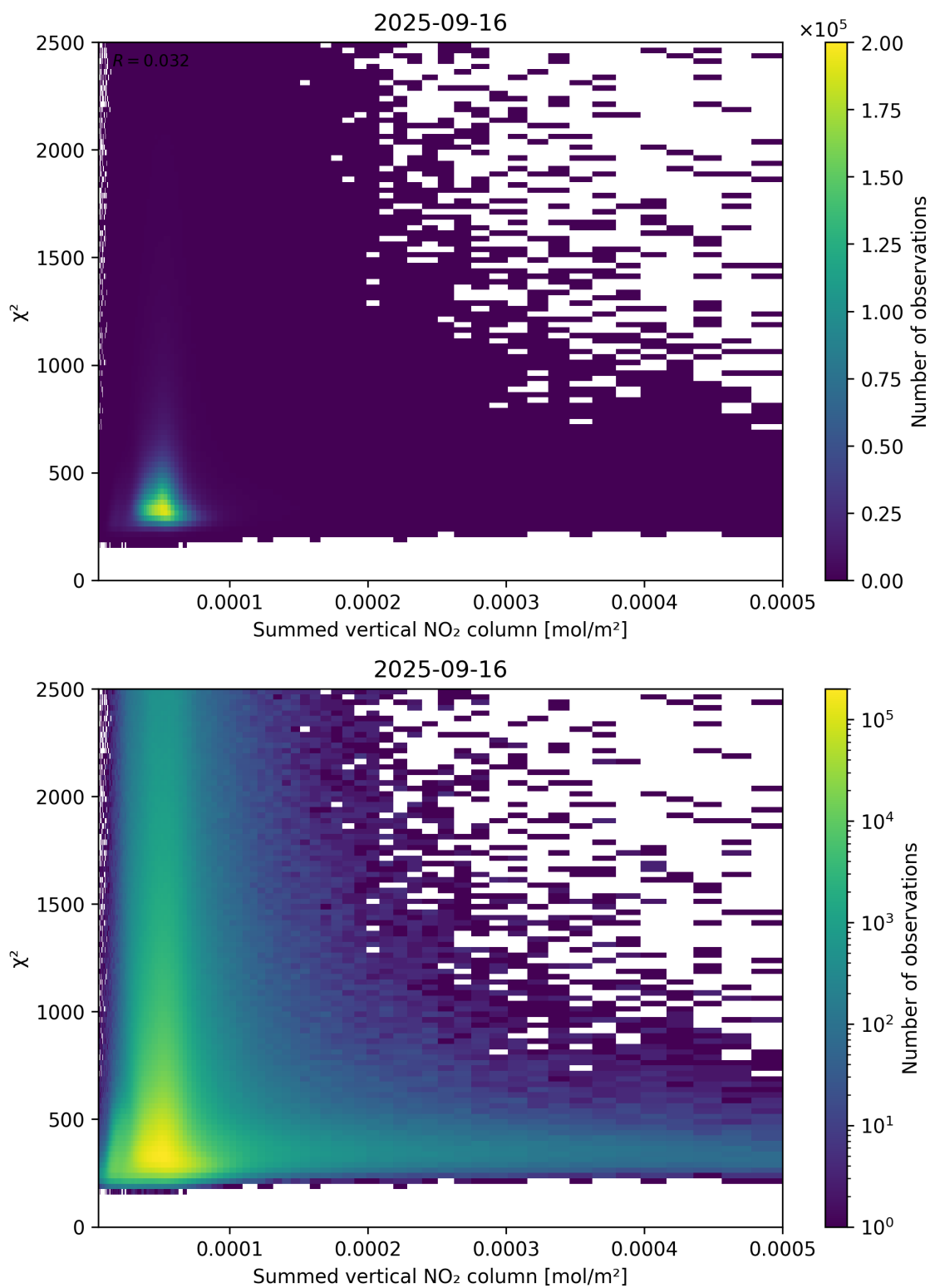
Figure 104: Scatter density plot of “Summed vertical NO 2 column” against “ \chi^2 ” for 2025-09-15 to 2025-09-17.
