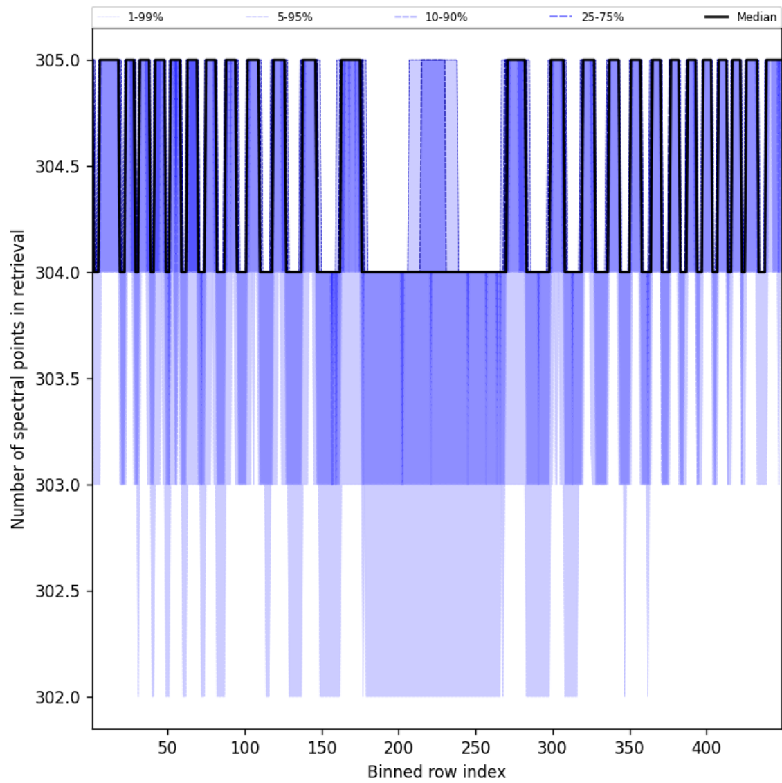
Figure 50: Along track statistics of “Number of spectral points in retrieval” for 2025-09-15 to 2025-09-17
