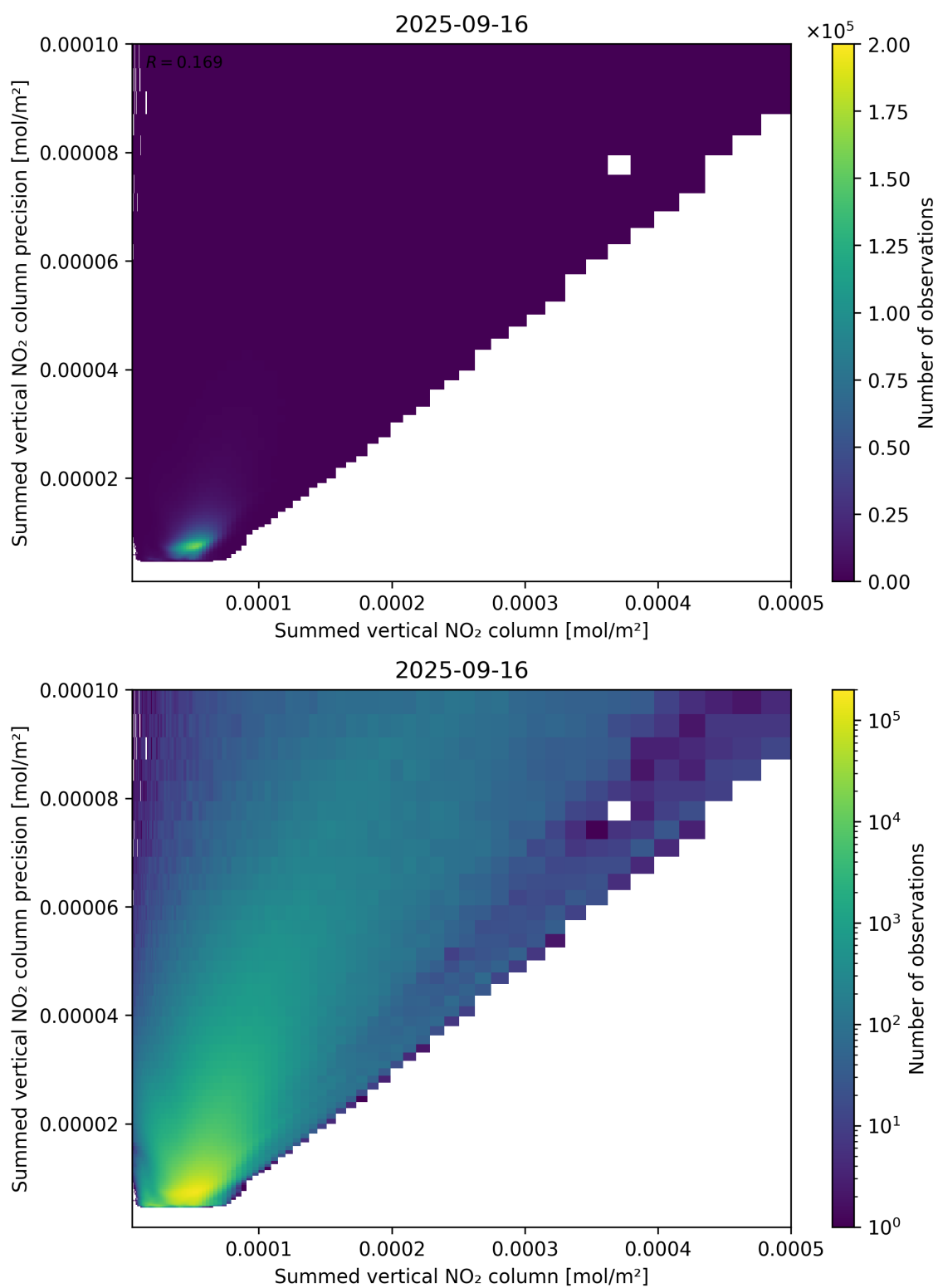
Figure 105: Scatter density plot of “Summed vertical NO 2 column” against “Summed vertical NO 2 column precision” for 2025-09-15 to 2025-09-17.
