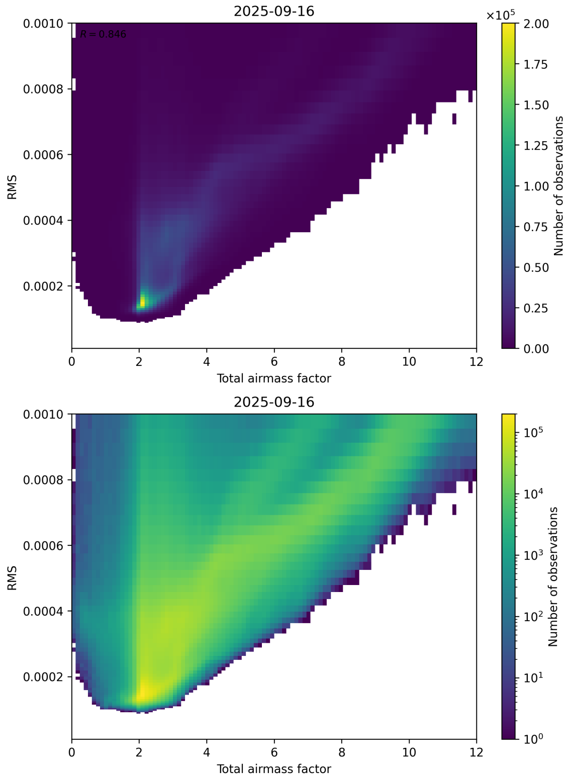
Figure 69: Scatter density plot of “Total airmass factor” against “RMS” for 2025-09-15 to 2025-09-17.
