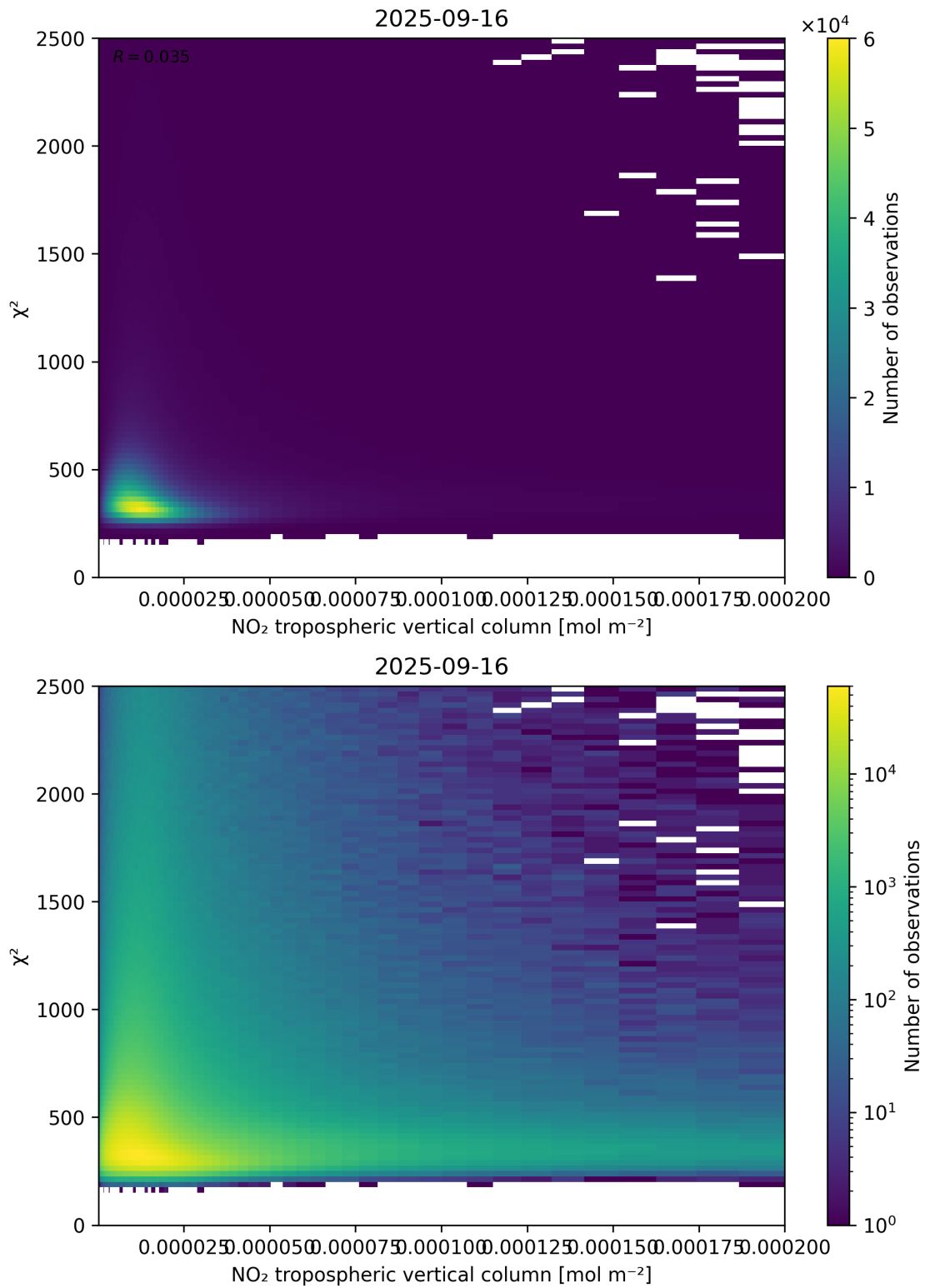
Figure 124: Scatter density plot of “NO 2 tropospheric vertical column” against “ \chi^2 ” for 2025-09-15 to 2025-09-17.
