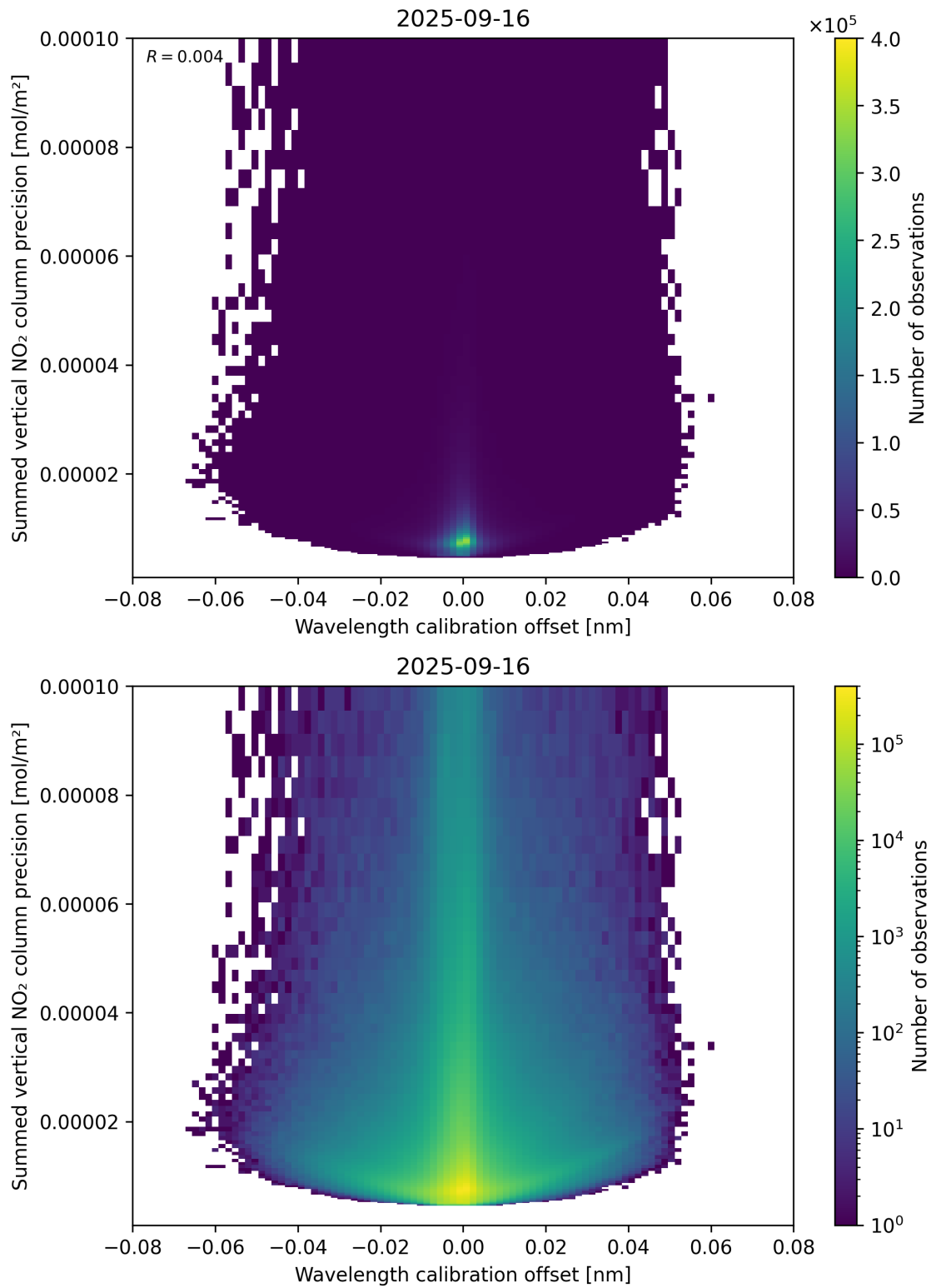
Figure 178: Scatter density plot of “Wavelength calibration offset” against “Summed vertical NO 2 column precision” for 2025-09-15 to 2025-09-17.
