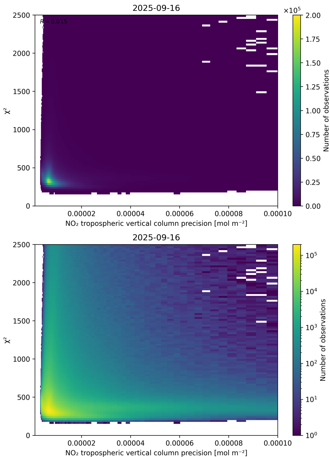
Figure 134: Scatter density plot of “NO 2 tropospheric vertical column precision” against “ \chi^2 ” for 2025-09-15 to 2025-09-17.
