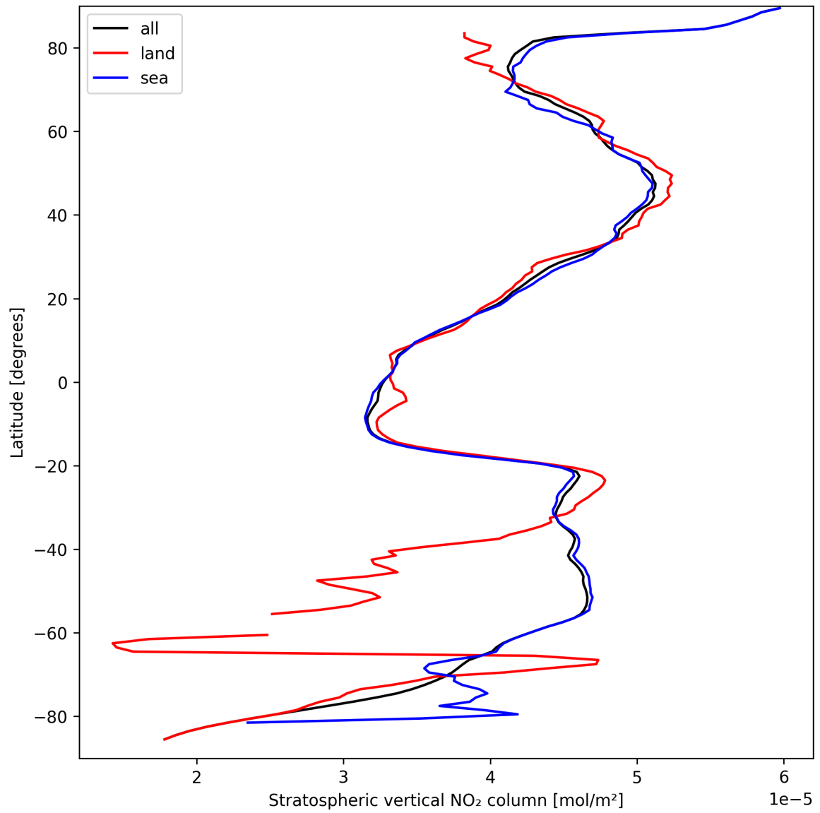
Figure 19: Zonal average of “Stratospheric vertical NO 2 column” for 2025-09-15 to 2025-09-17.
