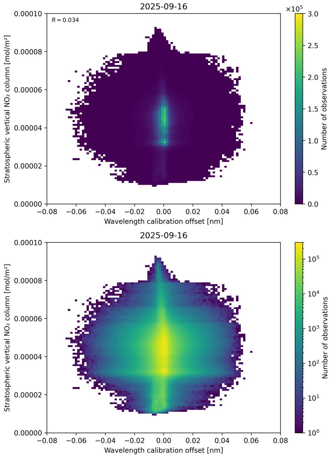
Figure 176: Scatter density plot of “Wavelength calibration offset” against “Stratospheric vertical NO 2 column” for 2025-09-15 to 2025-09-17.
