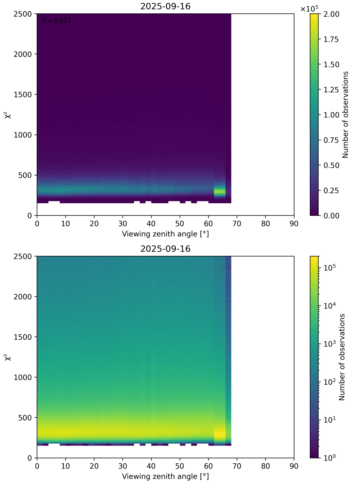
Figure 162: Scatter density plot of “Viewing zenith angle” against “ \chi^2 ” for 2025-09-15 to 2025-09-17.
