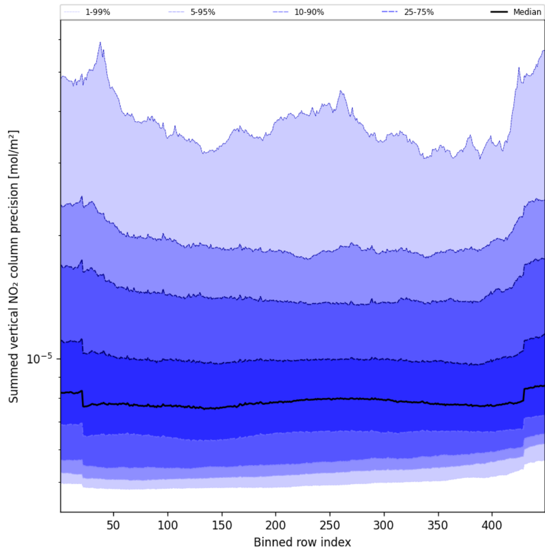
Figure 58: Along track statistics of “Summed vertical NO 2 column precision” for 2025-09-15 to 2025-09-17
