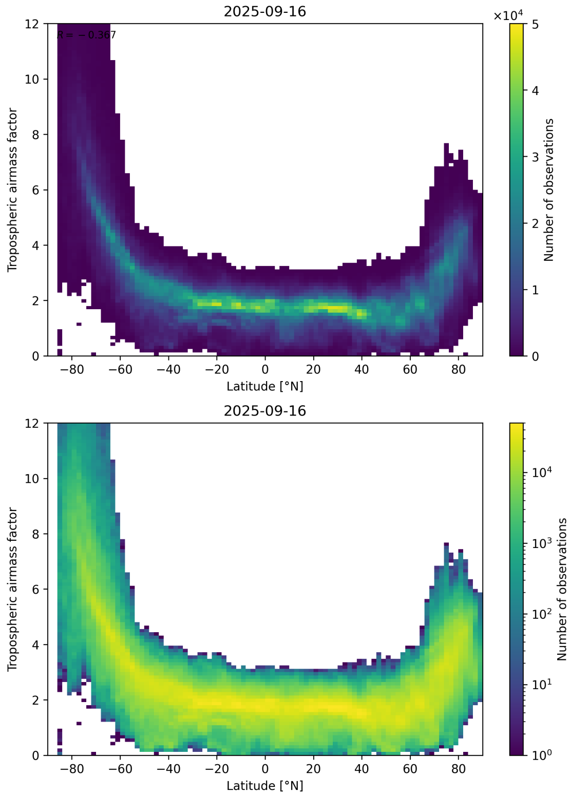
Figure 85: Scatter density plot of “Latitude” against “Tropospheric airmass factor” for 2025-09-15 to 2025-09-17.
