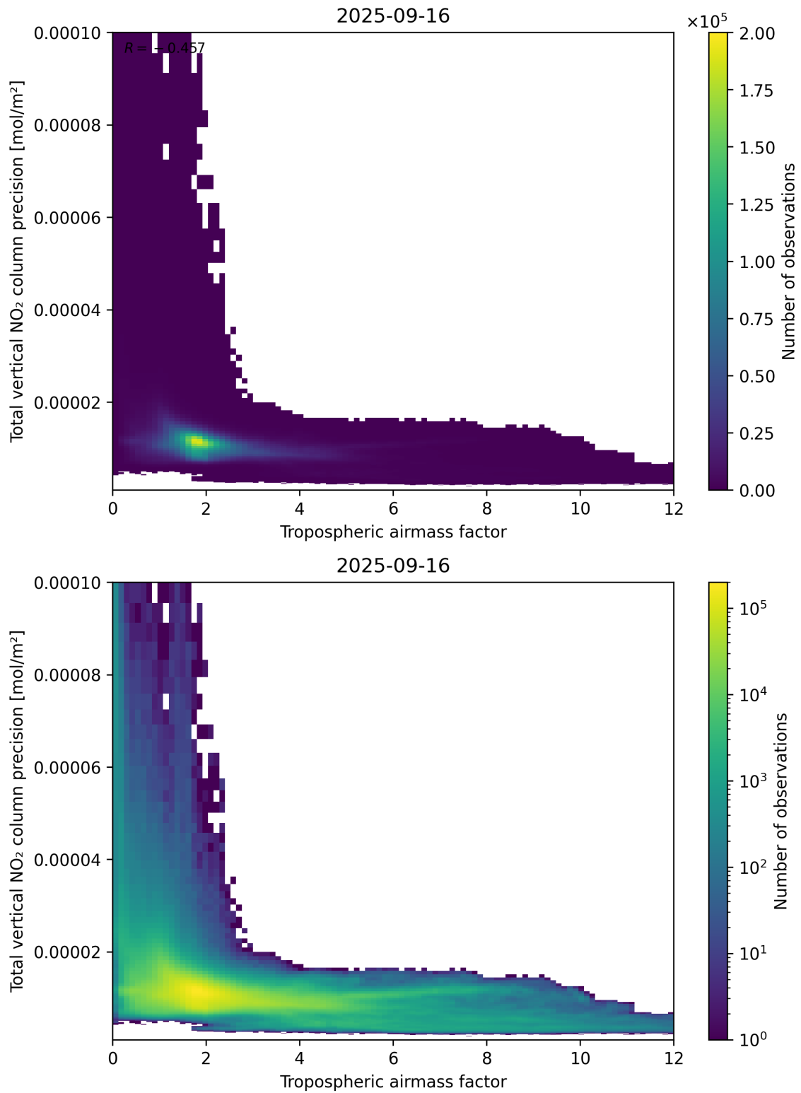
Figure 78: Scatter density plot of “Tropospheric air mass factor” against “Total vertical NO 2 column precision” for 2025-09-15 to 2025-09-17.
