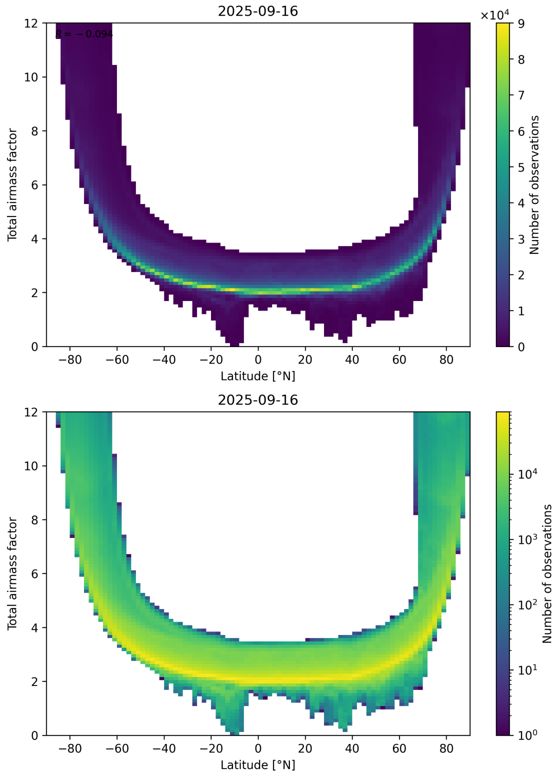
Figure 84: Scatter density plot of “Latitude” against “Total airmass factor” for 2025-09-15 to 2025-09-17.
