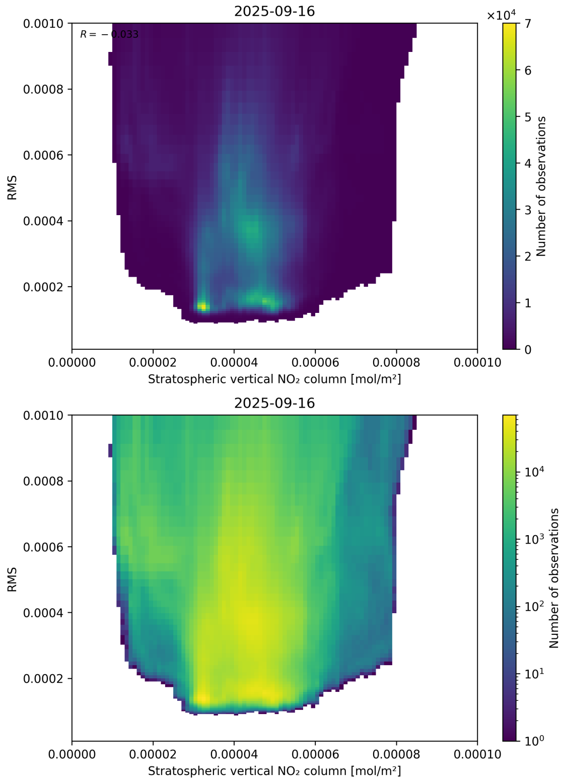
Figure 102: Scatter density plot of “Stratospheric vertical NO 2 column” against “RMS” for 2025-09-15 to 2025-09-17.
