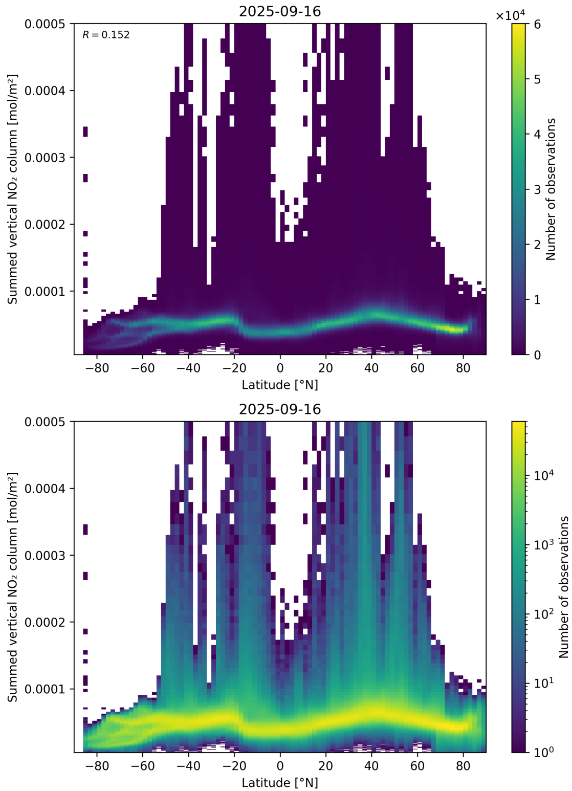
Figure 88: Scatter density plot of “Latitude” against “Summed vertical NO 2 column” for 2025-09-15 to 2025-09-17.
