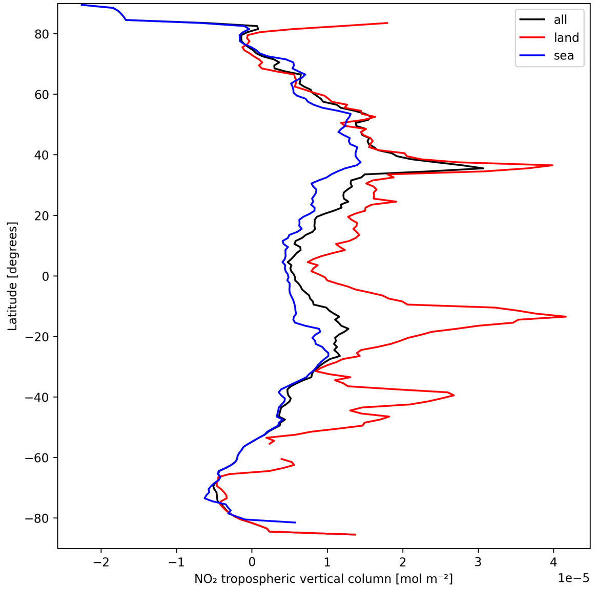
Figure 12: Zonal average of “NO 2 tropospheric vertical column” for 2025-09-15 to 2025-09-17.
