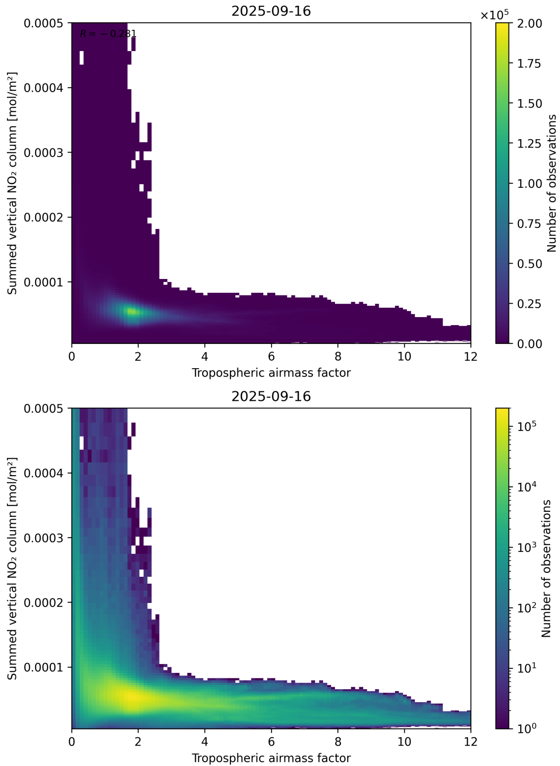
Figure 75: Scatter density plot of “Tropospheric airmass factor” against “Summed vertical NO 2 column” for 2025-09-15 to 2025-09-17.
