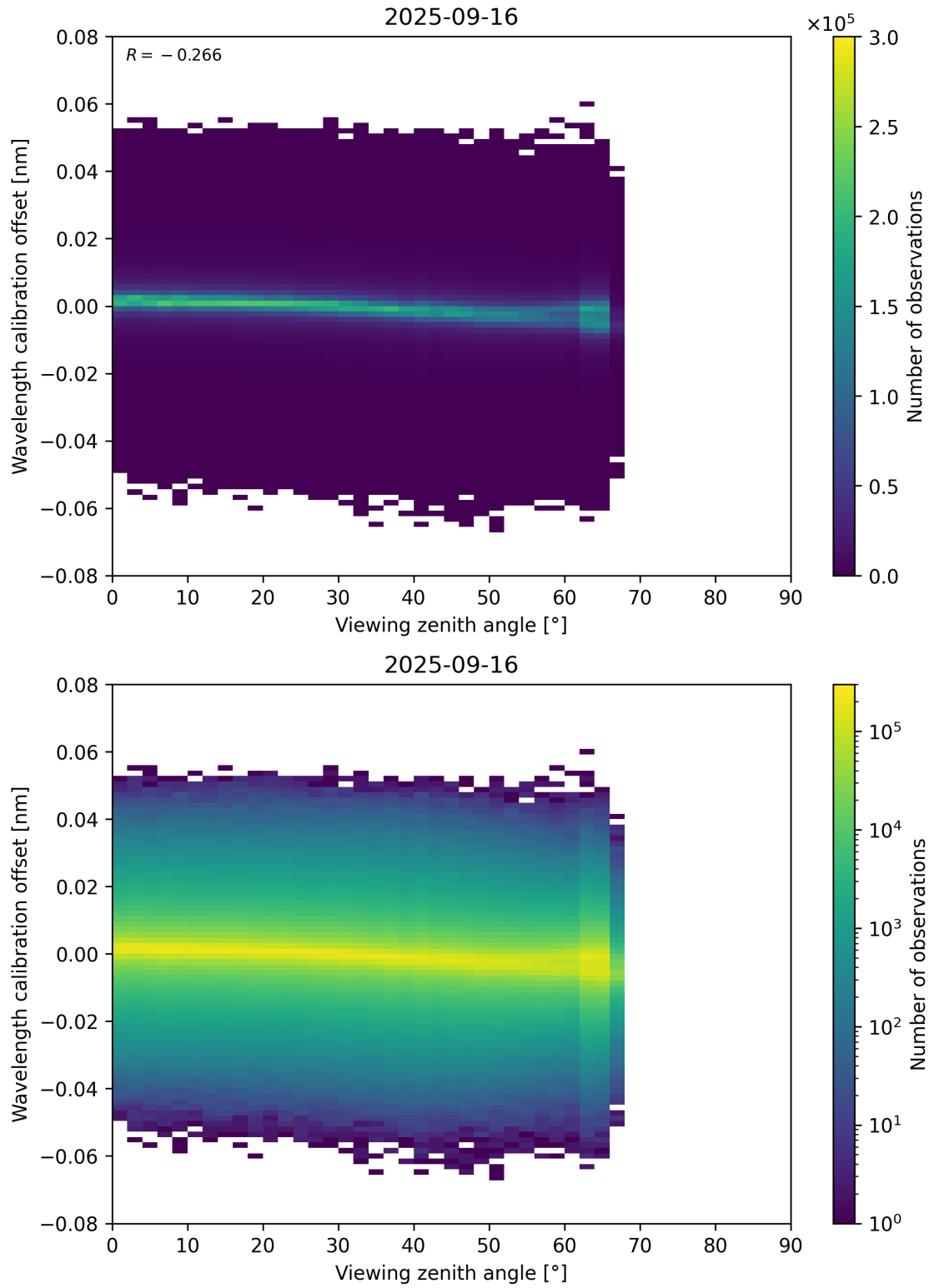
Figure 173: Scatter density plot of “Viewing zenith angle” against “Wavelength calibration offset” for 2025-09-15 to 2025-09-17.
