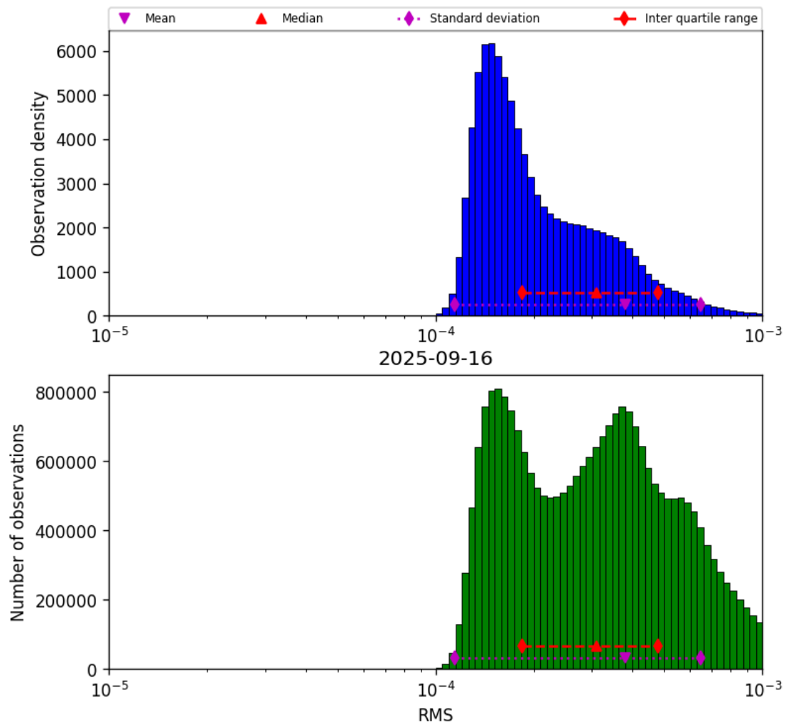
Figure 43: Histogram of “RMS” for 2025-09-15 to 2025-09-17
