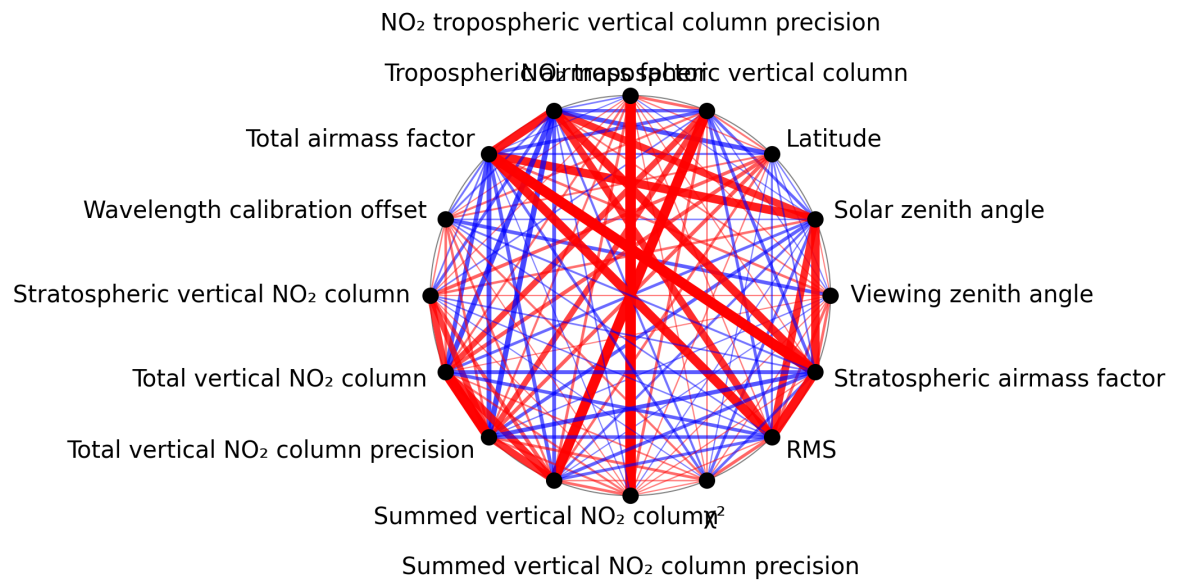
Figure 1: Map of correlation graph for 2025-09-15 to 2025-09-17.
