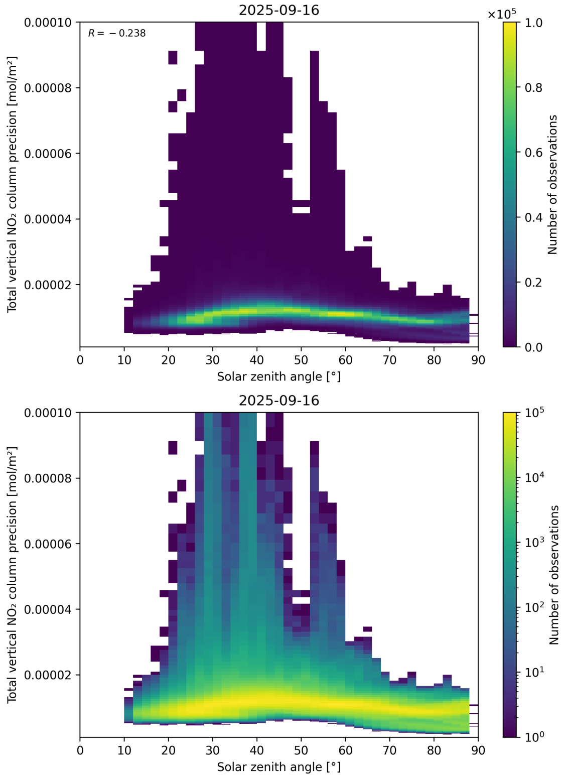
Figure 154: Scatter density plot of “Solar zenith angle” against “Total vertical NO 2 column precision” for 2025-09-15 to 2025-09-17.
