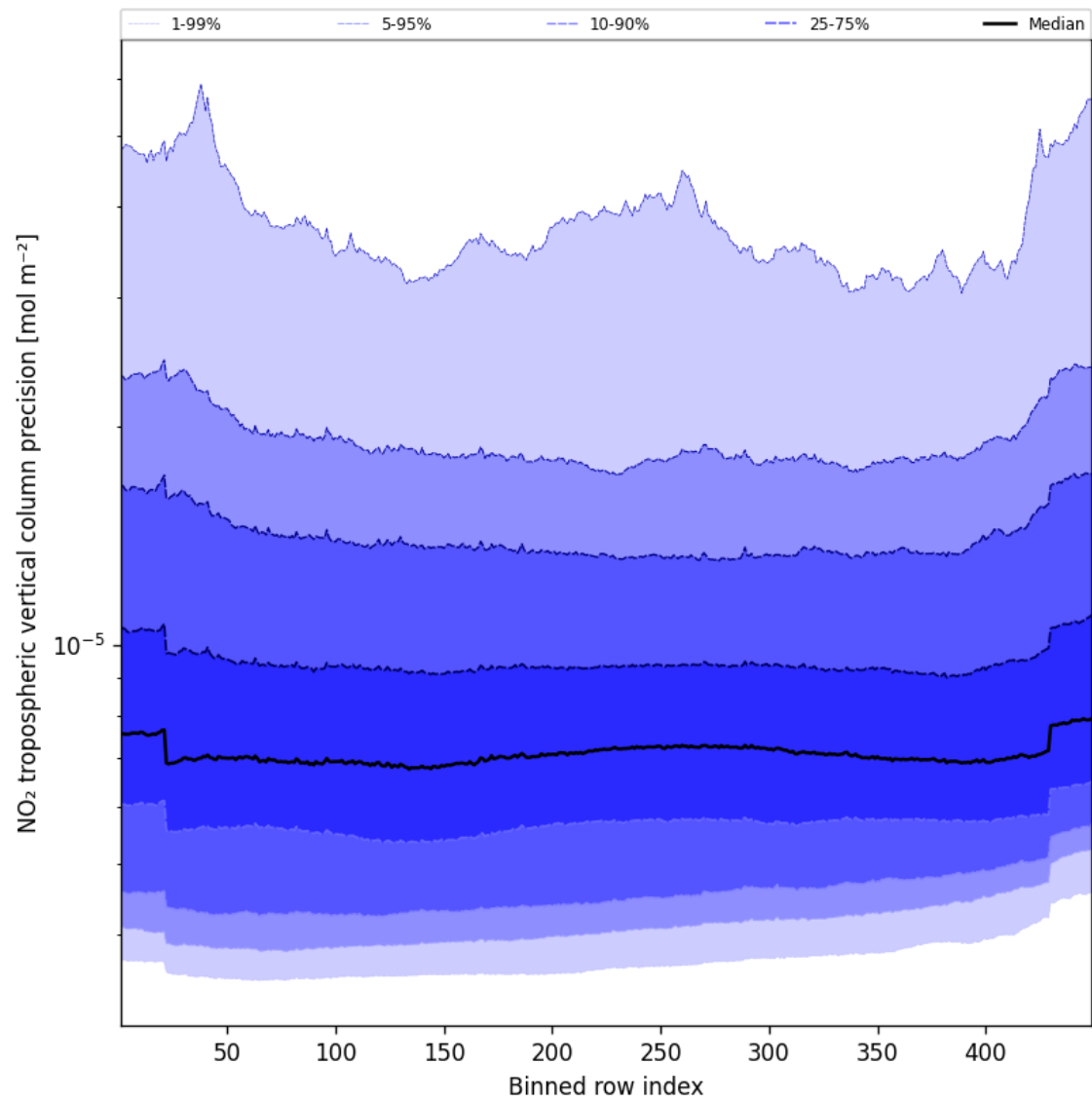
Figure 47: Along track statistics of “NO 2 tropospheric vertical column precision” for 2025-09-15 to 2025-09-17
