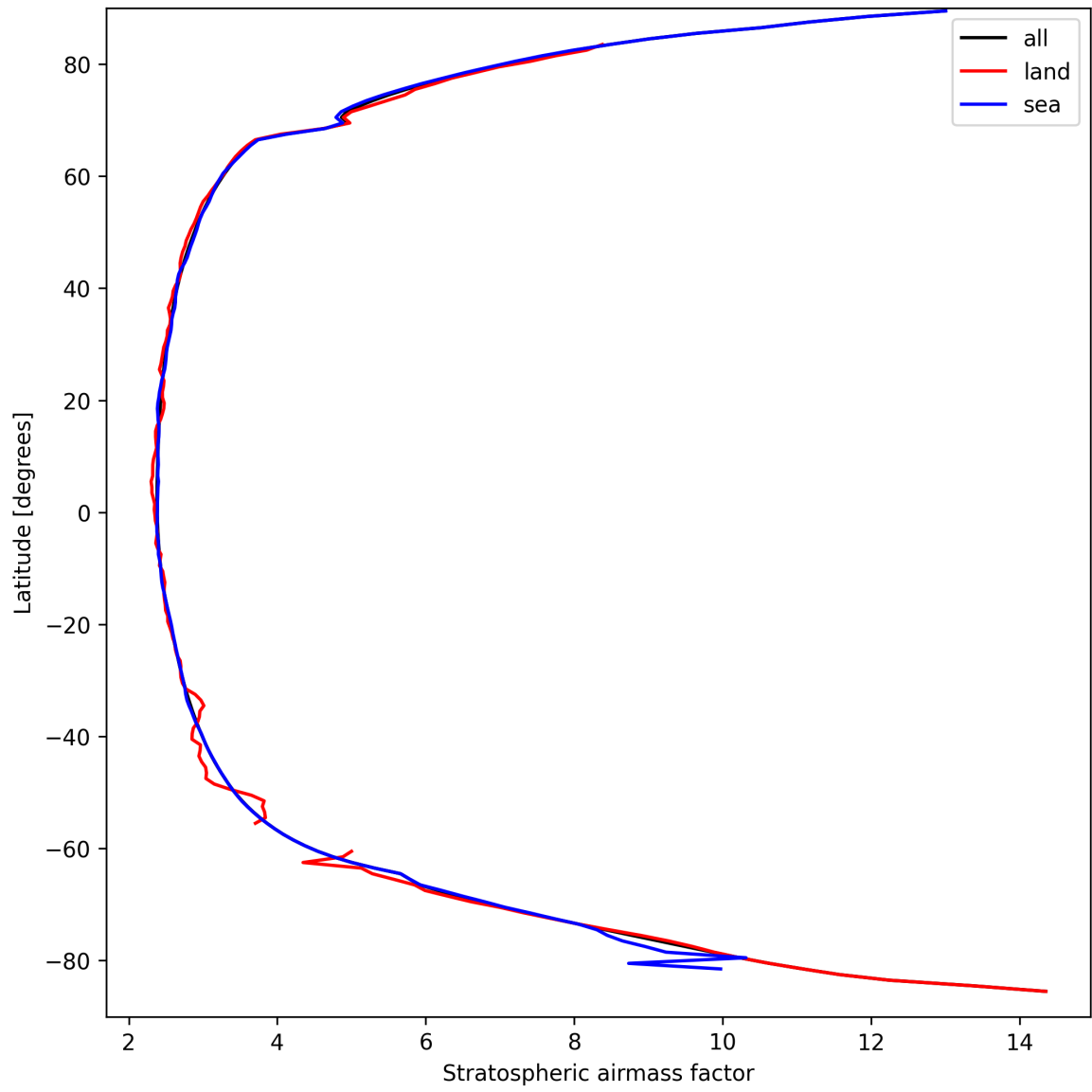
Figure 27: Zonal average of “Stratospheric airmass factor” for 2025-09-15 to 2025-09-17.
