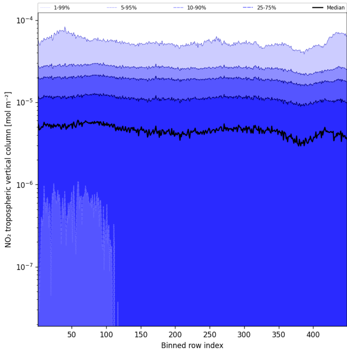
Figure 46: Along track statistics of “NO 2 tropospheric vertical column” for 2025-09-15 to 2025-09-17
