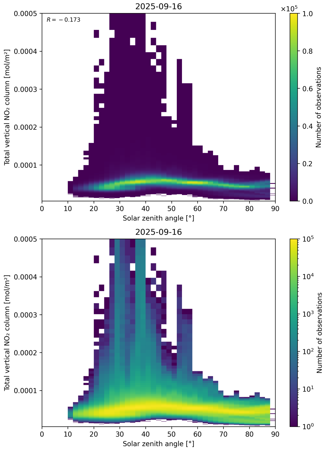
Figure 153: Scatter density plot of “Solar zenith angle” against “Total vertical NO 2 column” for 2025-09-15 to 2025-09-17.
