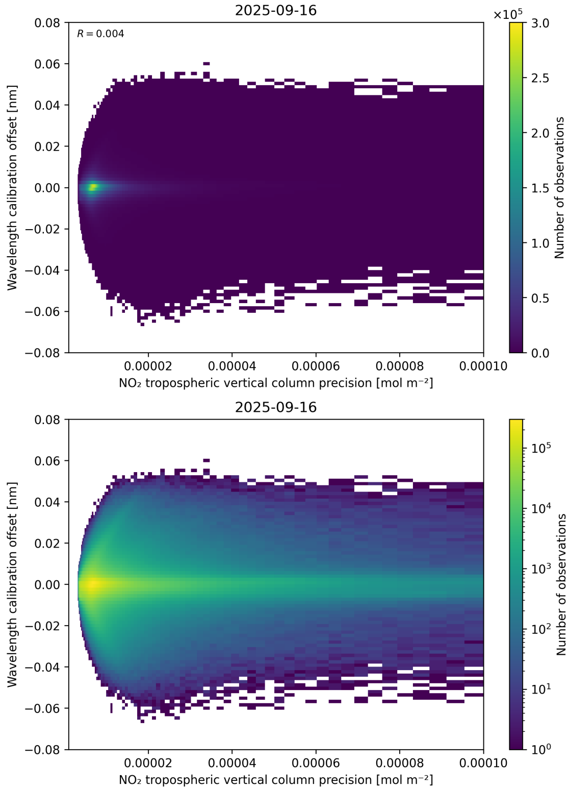
Figure 141: Scatter density plot of “NO 2 tropospheric vertical column precision” against “Wavelength calibration offset” for 2025-09-15 to 2025-09-17.
