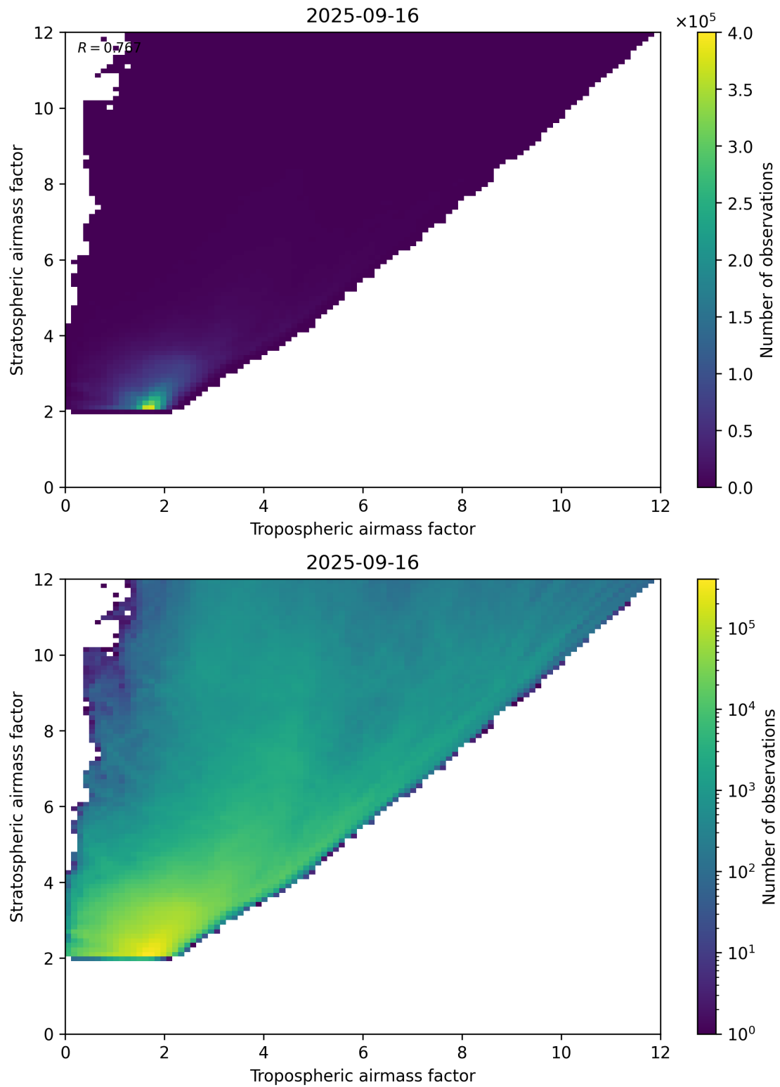
Figure 71: Scatter density plot of “Tropospheric airmass factor” against “Stratospheric airmass factor” for 2025-09-15 to 2025-09-17.
