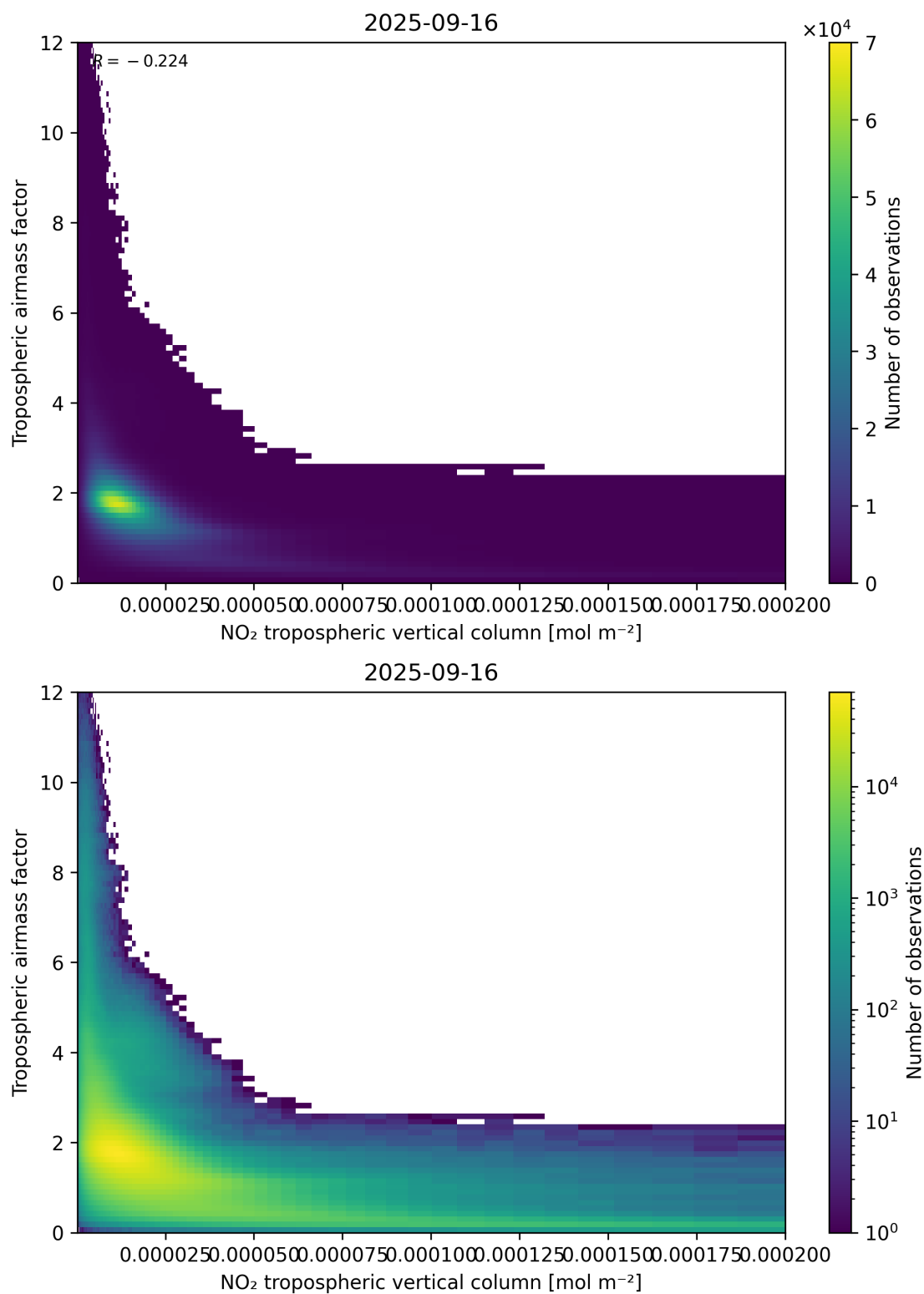
Figure 123: Scatter density plot of “NO 2 tropospheric vertical column” against “Tropospheric air mass factor” for 2025-09-15 to 2025-09-17.
