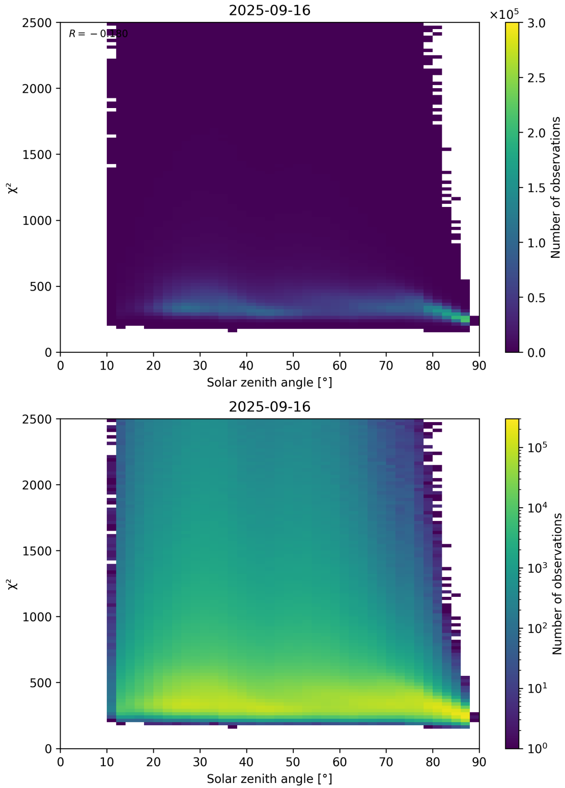
Figure 148: Scatter density plot of “Solar zenith angle” against “ \chi^2 ” for 2025-09-15 to 2025-09-17.
