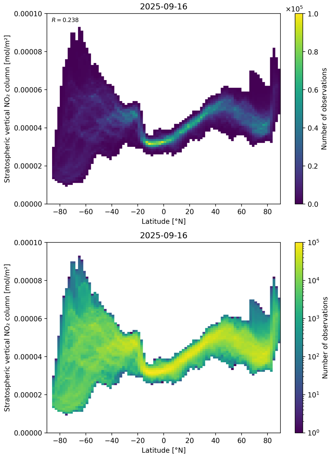
Figure 87: Scatter density plot of “Latitude” against “Stratospheric vertical NO 2 column” for 2025-09-15 to 2025-09-17.
