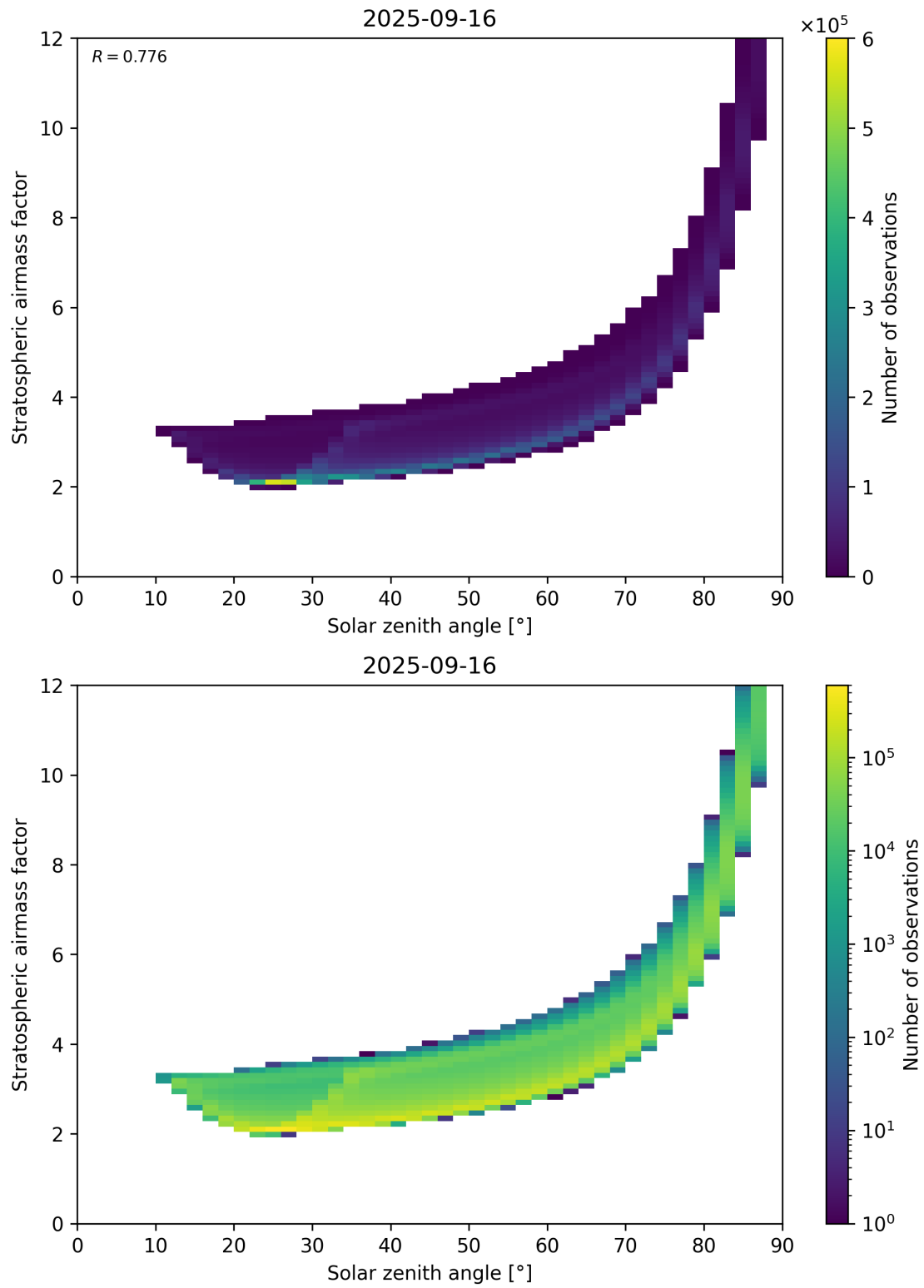
Figure 145: Scatter density plot of “Solar zenith angle” against “Stratospheric airmass factor” for 2025-09-15 to 2025-09-17.
