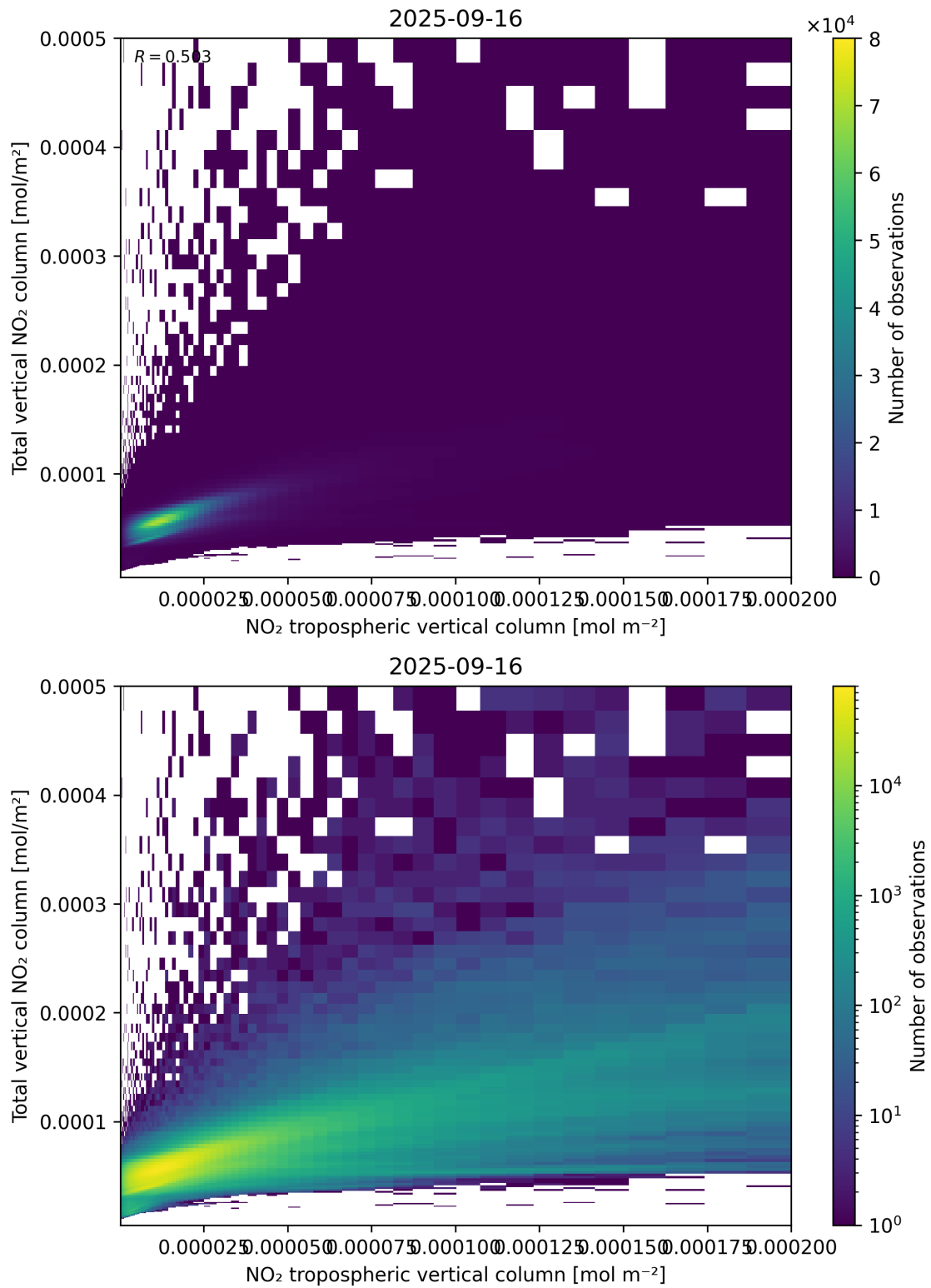
Figure 128: Scatter density plot of “NO 2 tropospheric vertical column” against “Total vertical NO 2 column” for 2025-09-15 to 2025-09-17.
