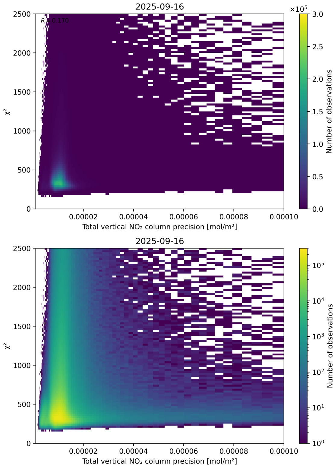
Figure 116: Scatter density plot of “Total vertical NO 2 column precision” against “ \chi^2 ” for 2025-09-15 to 2025-09-17.
