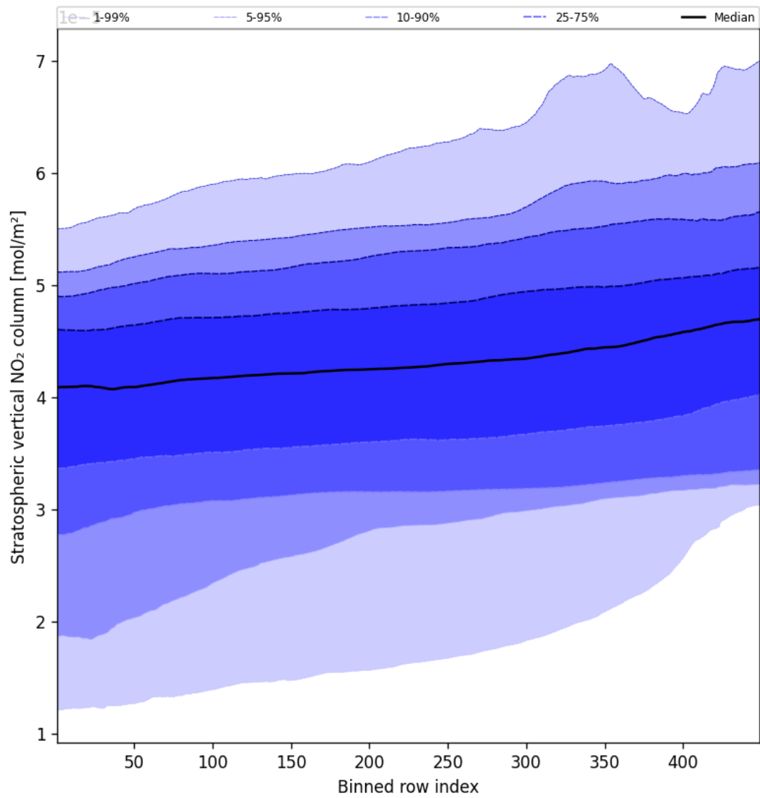
Figure 53: Along track statistics of “Stratospheric vertical NO 2 column” for 2025-09-15 to 2025-09-17
