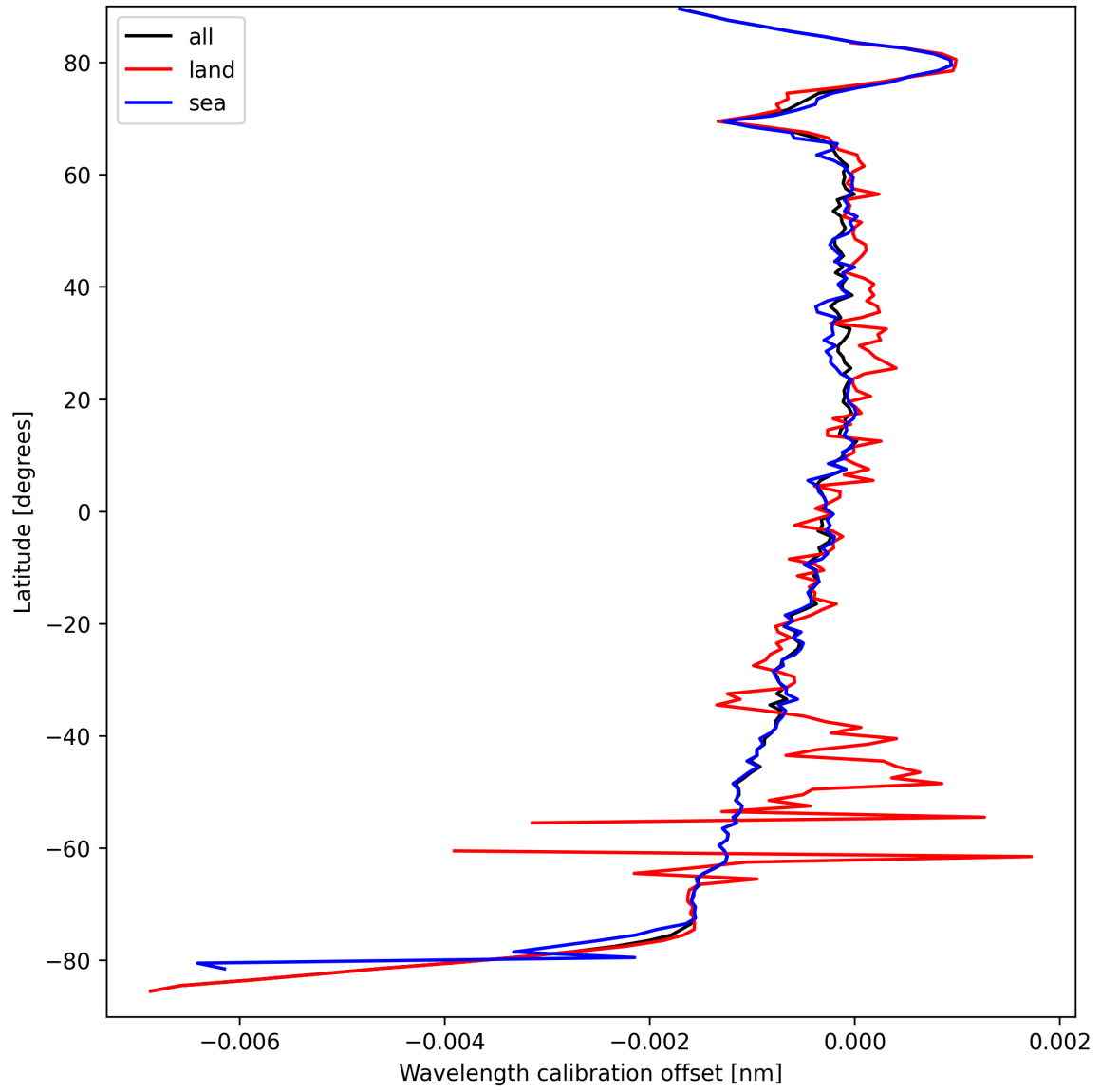
Figure 18: Zonal average of “Wavelength calibration offset” for 2025-09-15 to 2025-09-17.
