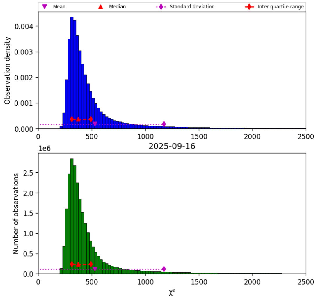
Figure 42: Histogram of " \chi^2 " for 2025-09-15 to 2025-09-17
