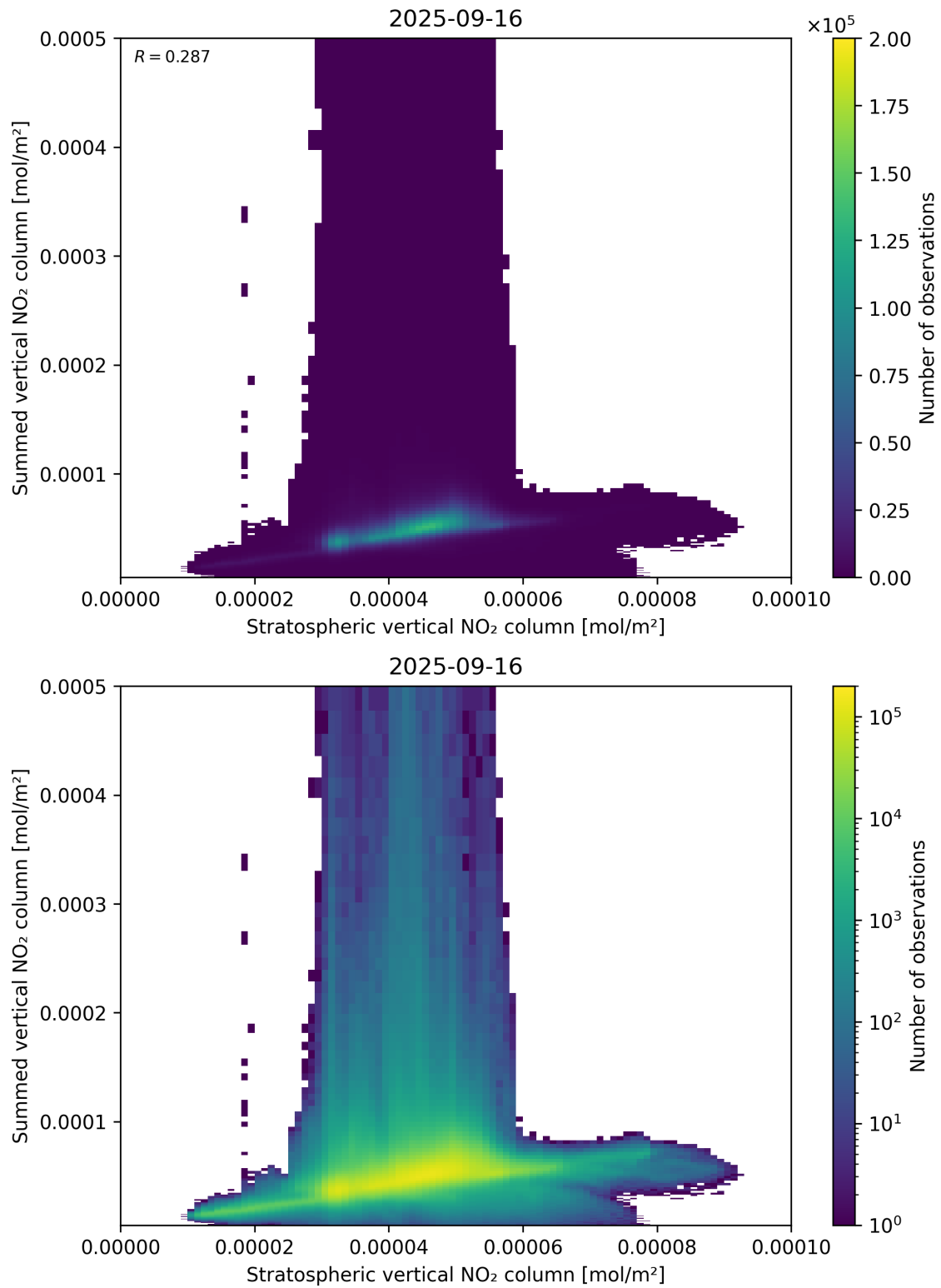
Figure 98: Scatter density plot of “Stratospheric vertical NO 2 column” against “Summed vertical NO 2 column” for 2025-09-15 to 2025-09-17.
