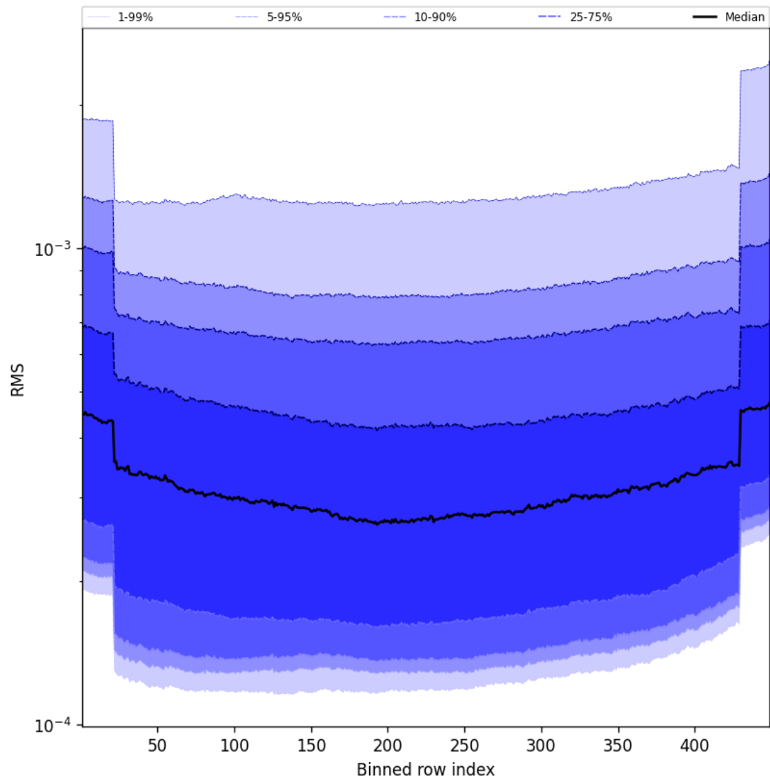
Figure 60: Along track statistics of “RMS” for 2025-09-15 to 2025-09-17
