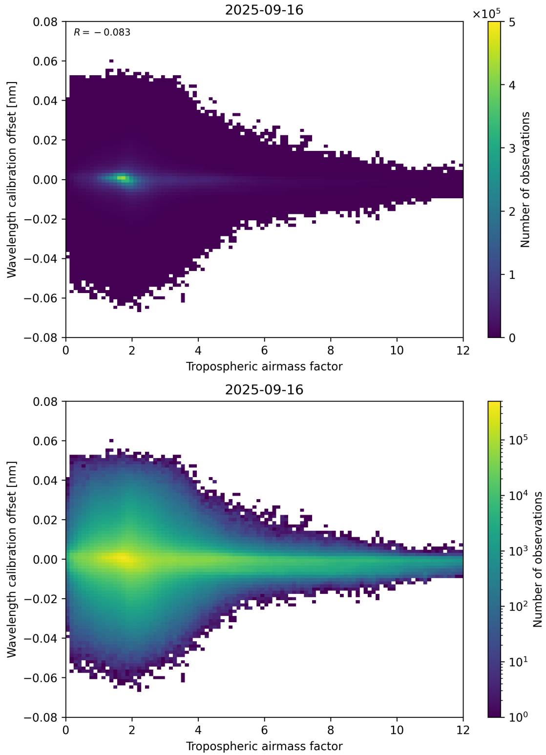
Figure 80: Scatter density plot of “Tropospheric airmass factor” against “Wavelength calibration offset” for 2025-09-15 to 2025-09-17.
