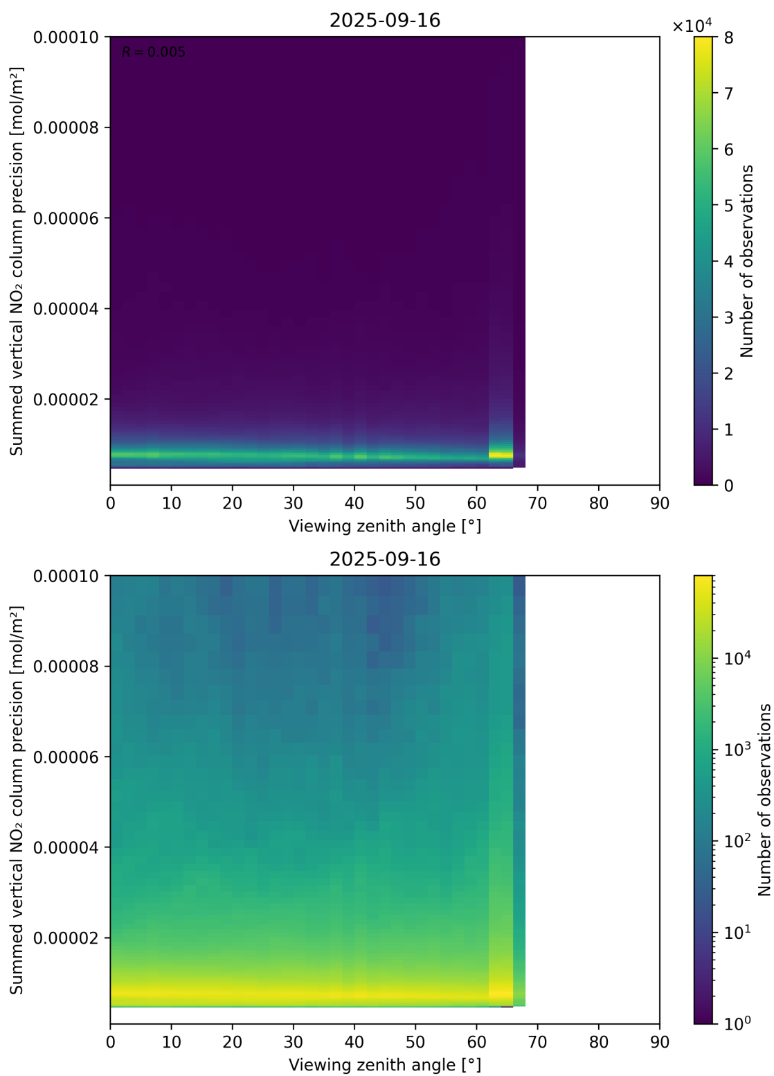
Figure 166: Scatter density plot of “Viewing zenith angle” against “Summed vertical NO 2 column precision” for 2025-09-15 to 2025-09-17.
