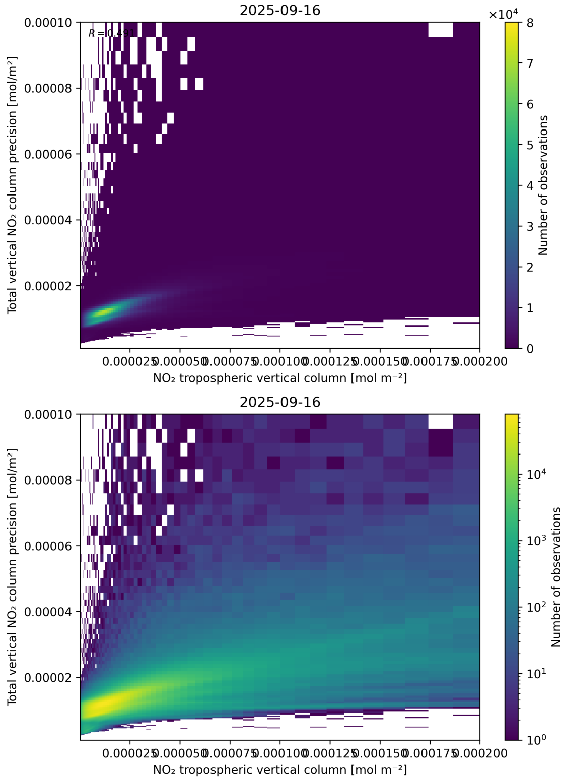
Figure 129: Scatter density plot of “NO 2 tropospheric vertical column” against “Total vertical NO 2 column precision” for 2025-09-15 to 2025-09-17.
