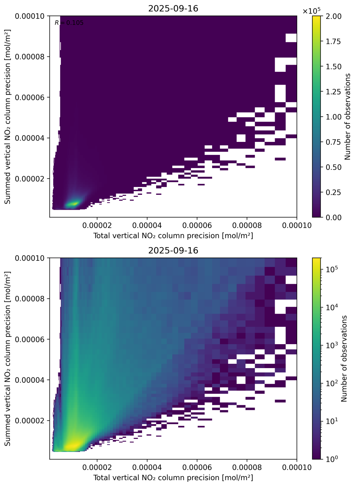
Figure 118: Scatter density plot of “Total vertical NO 2 column precision” against “Summed vertical NO 2 column precision” for 2025-09-15 to 2025-09-17.
