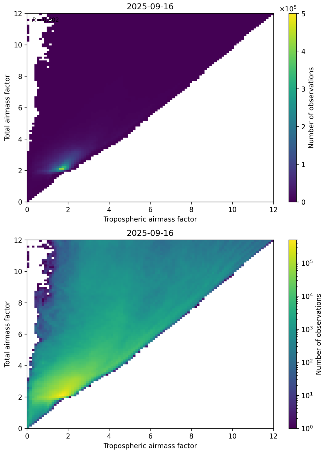
Figure 72: Scatter density plot of “Tropospheric airmass factor” against “Total airmass factor” for 2025-09-15 to 2025-09-17.
