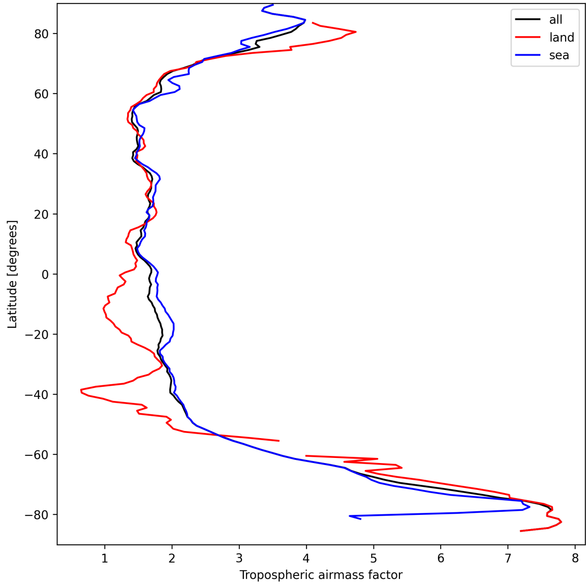
Figure 14: Zonal average of “Tropospheric air mass factor” for 2025-09-15 to 2025-09-17.
