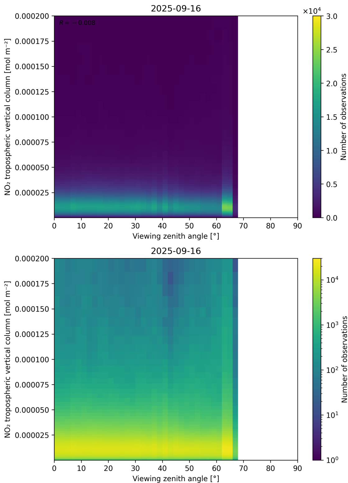
Figure 169: Scatter density plot of “Viewing zenith angle” against “NO 2 tropospheric vertical column” for 2025-09-15 to 2025-09-17.
