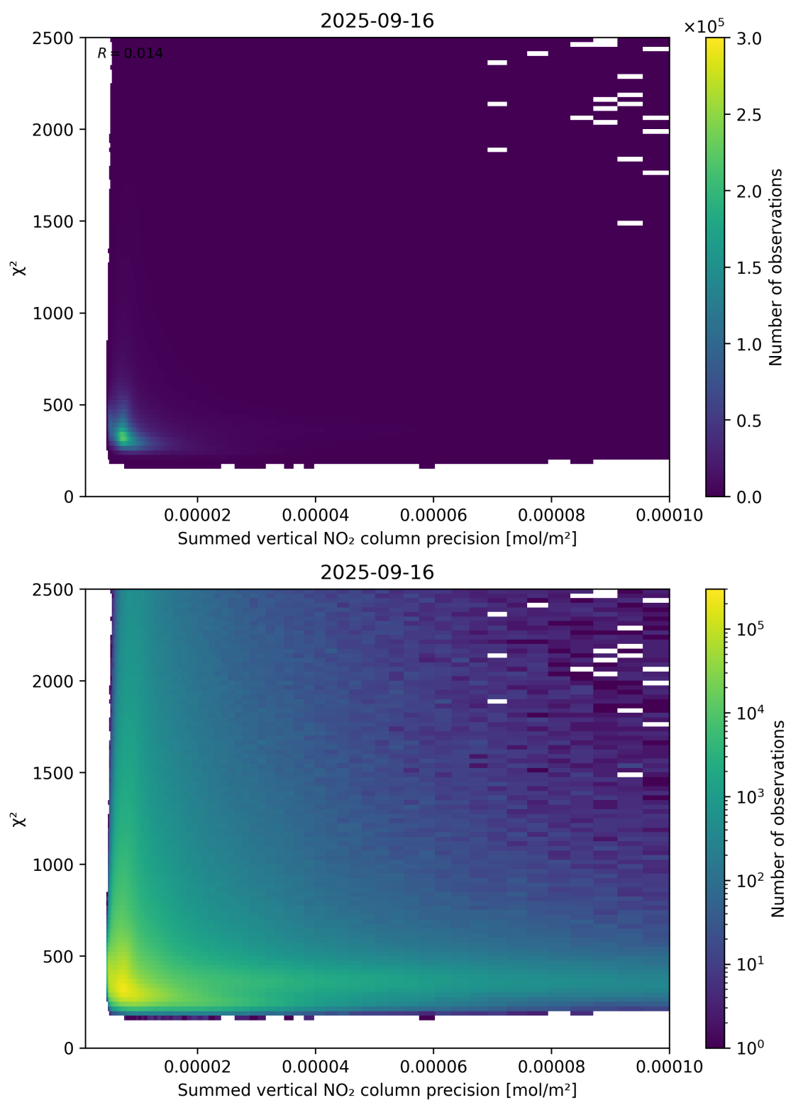
Figure 107: Scatter density plot of “Summed vertical NO 2 column precision” against “ \chi^2 ” for 2025-09-15 to 2025-09-17.
