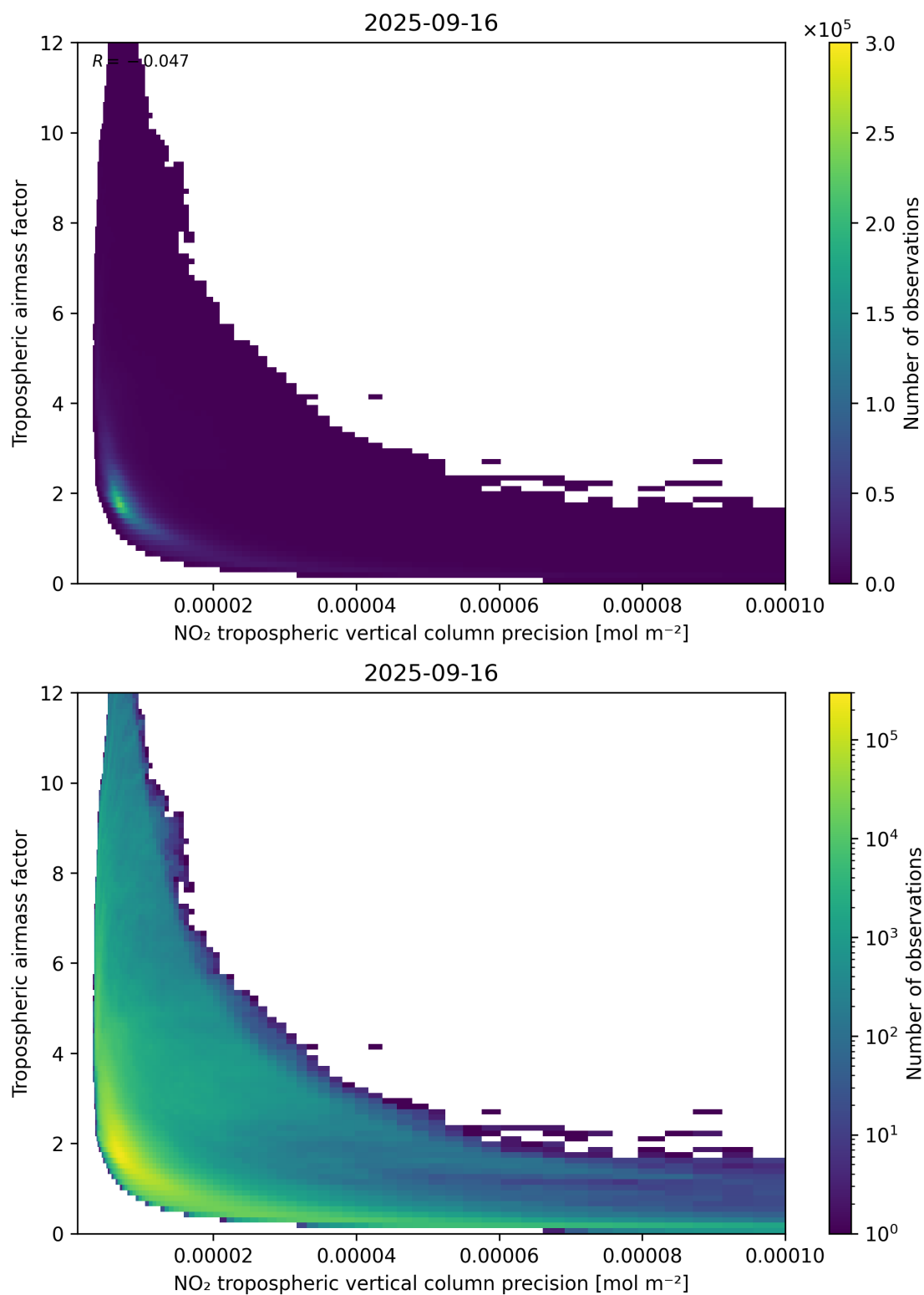
Figure 133: Scatter density plot of “NO 2 tropospheric vertical column precision” against “Tropospheric air mass factor” for 2025-09-15 to 2025-09-17.
