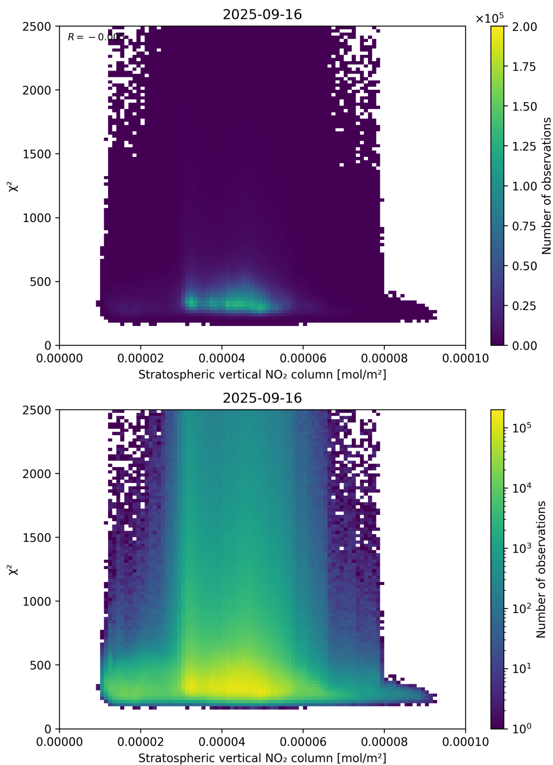
Figure 97: Scatter density plot of “Stratospheric vertical NO 2 column” against “ \chi^2 ” for 2025-09-15 to 2025-09-17.
