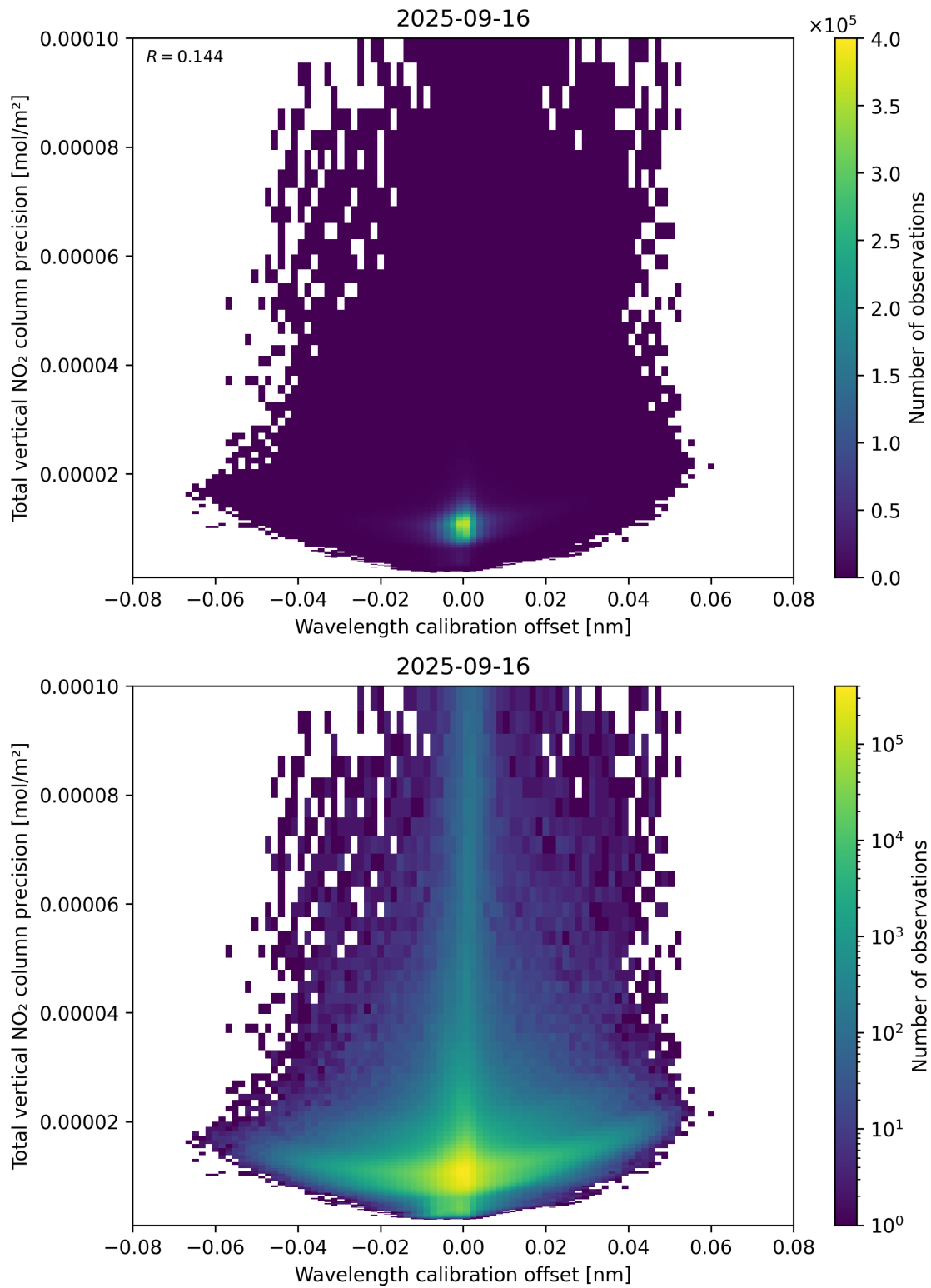
Figure 180: Scatter density plot of “Wavelength calibration offset” against “Total vertical NO 2 column precision” for 2025-09-15 to 2025-09-17.
