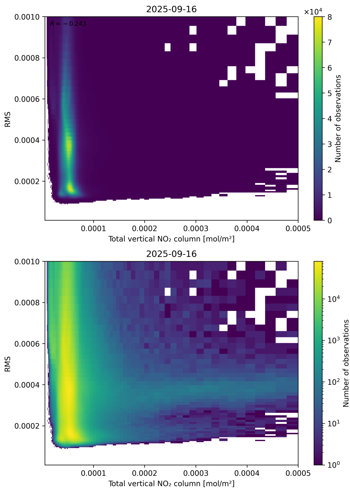
Figure 120: Scatter density plot of “Total vertical NO 2 column” against “RMS” for 2025-09-15 to 2025-09-17.
