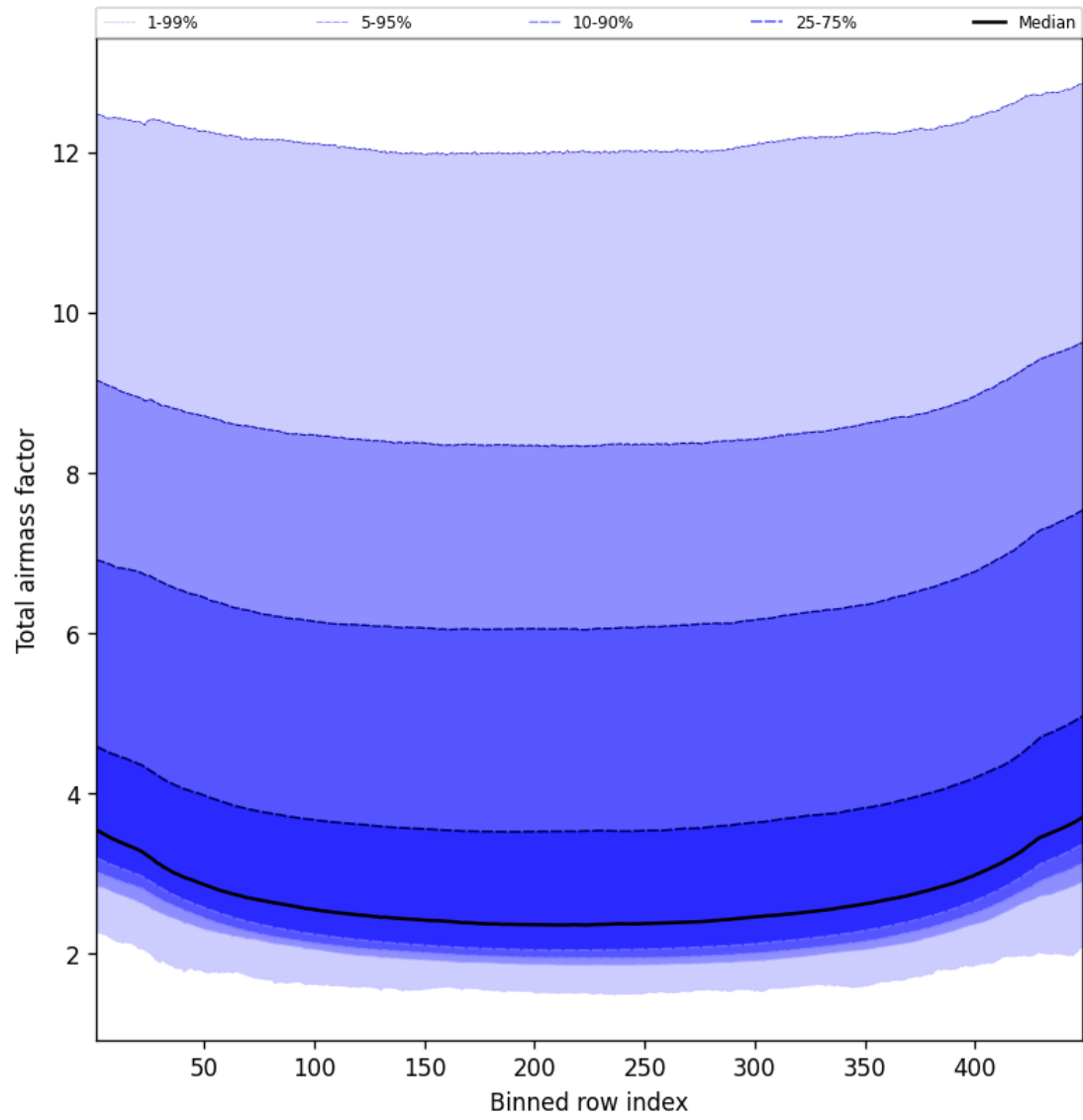
Figure 49: Along track statistics of “Total airmass factor” for 2025-09-15 to 2025-09-17
