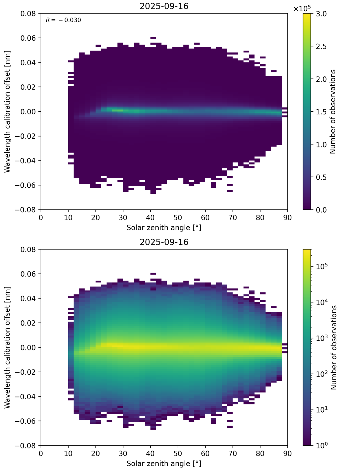
Figure 158: Scatter density plot of “Solar zenith angle” against “Wavelength calibration offset” for 2025-09-15 to 2025-09-17.
