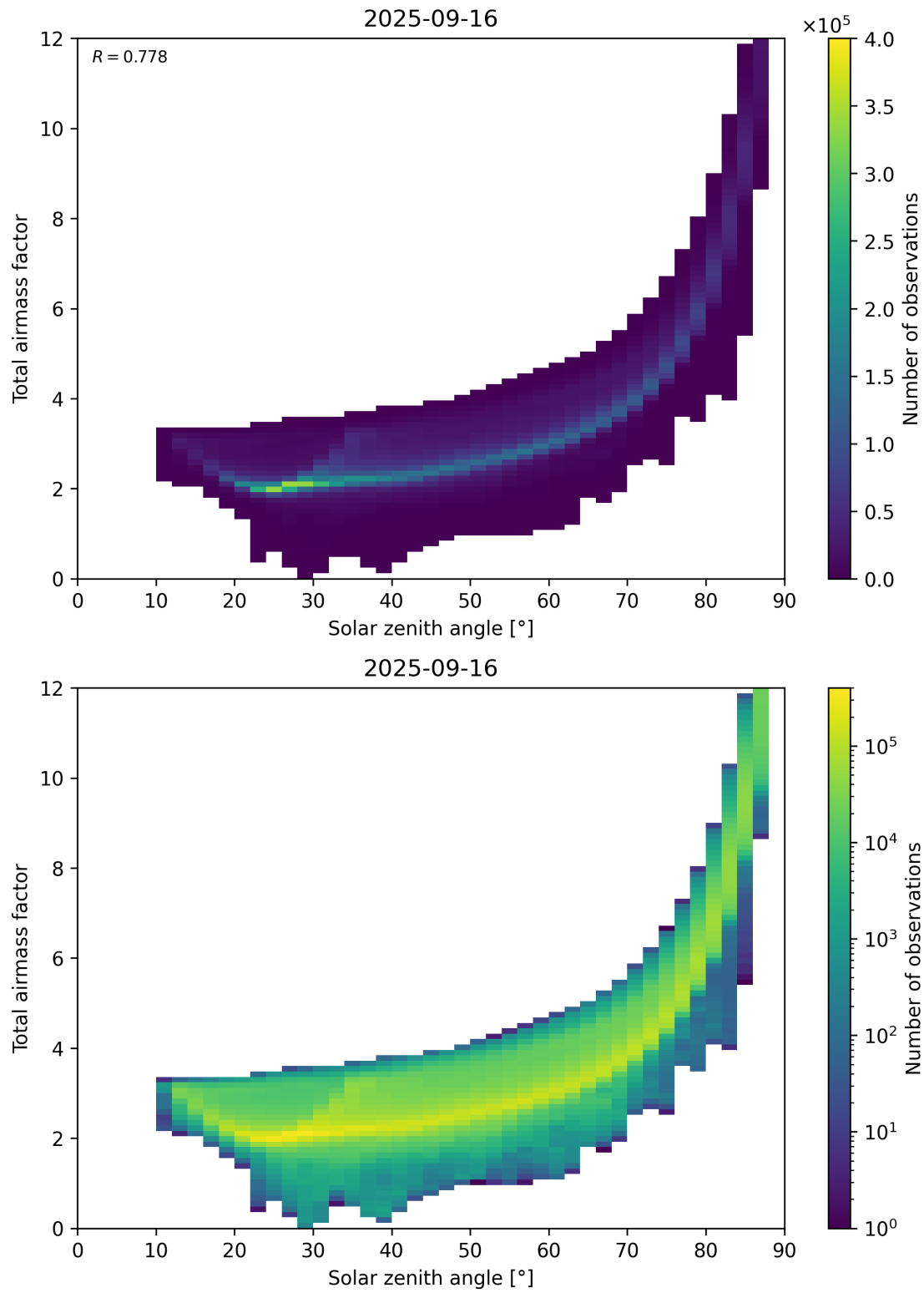
Figure 146: Scatter density plot of “Solar zenith angle” against “Total air mass factor” for 2025-09-15 to 2025-09-17.
