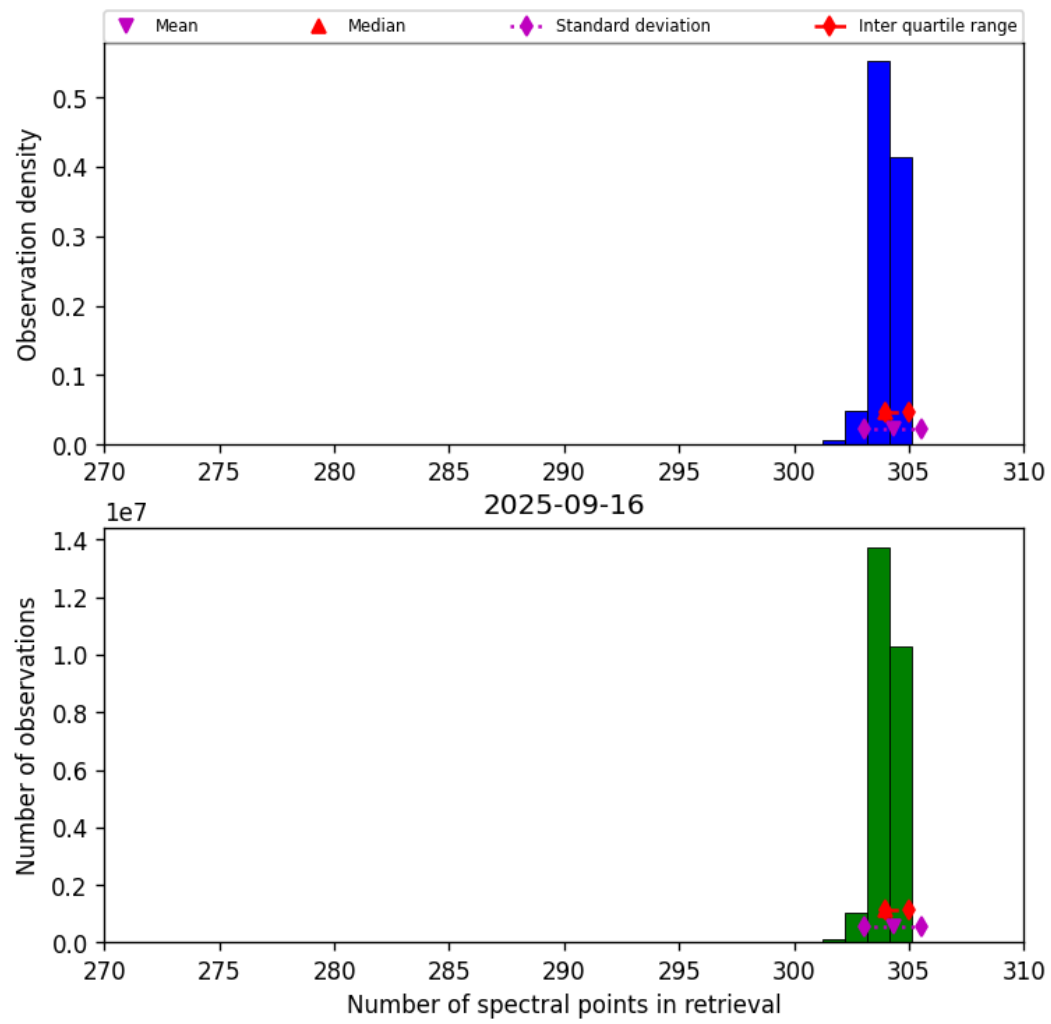
Figure 33: Histogram of “Number of spectral points in retrieval” for 2025-09-15 to 2025-09-17
