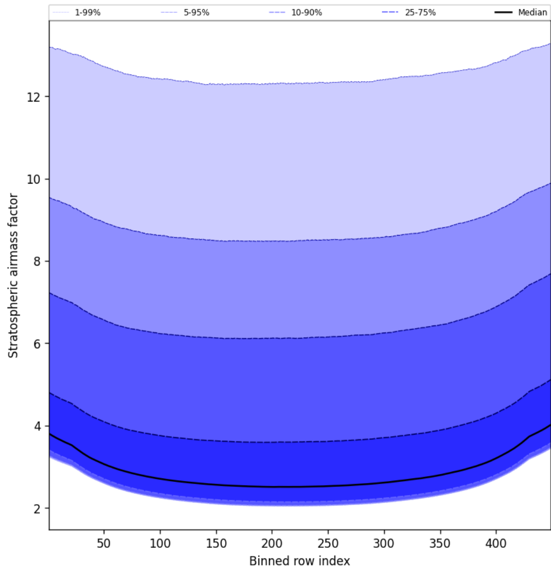
Figure 61: Along track statistics of “Stratospheric airmass factor” for 2025-09-15 to 2025-09-17
