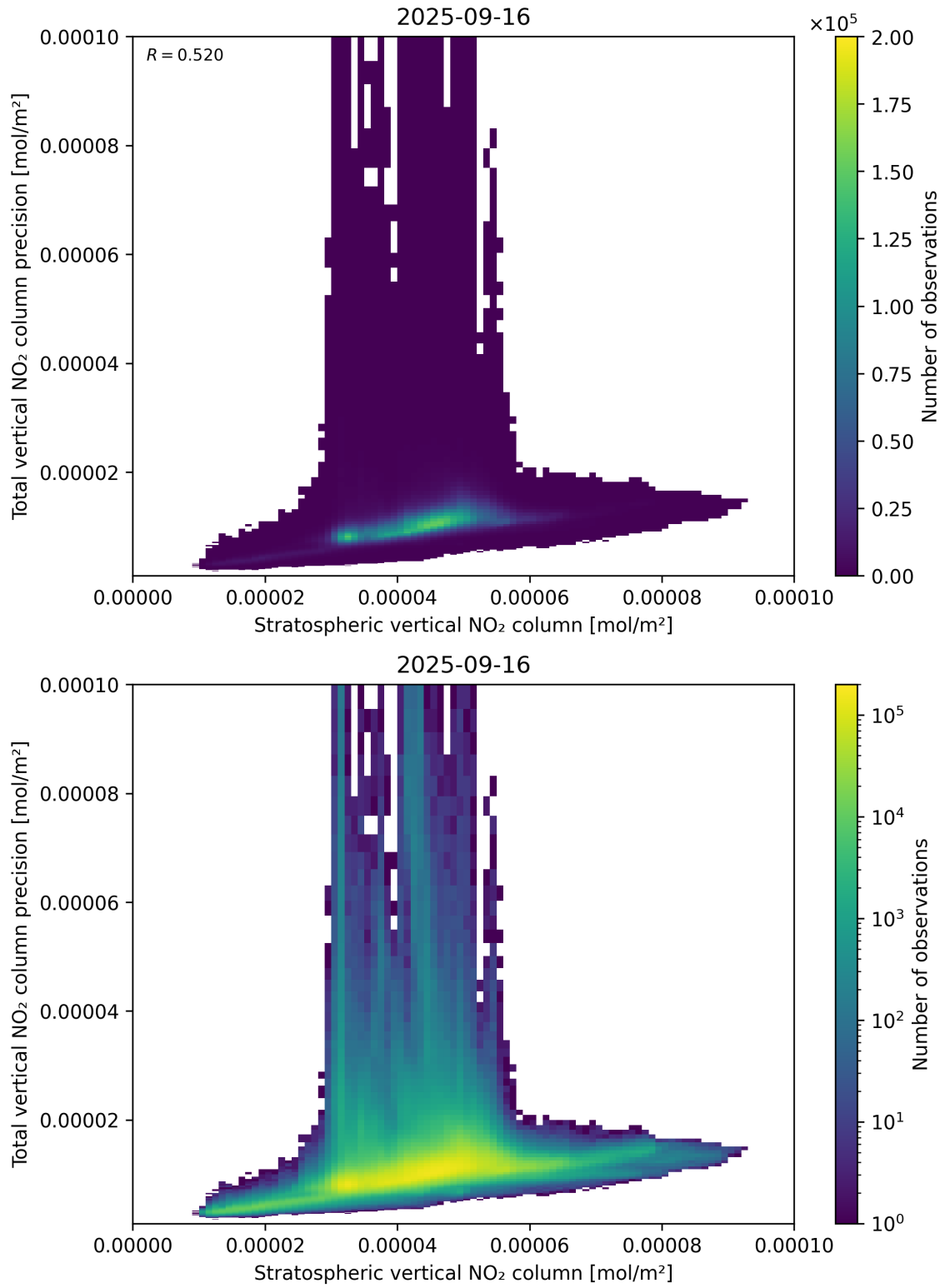
Figure 101: Scatter density plot of “Stratospheric vertical NO 2 column” against “Total vertical NO 2 column precision” for 2025-09-15 to 2025-09-17.
