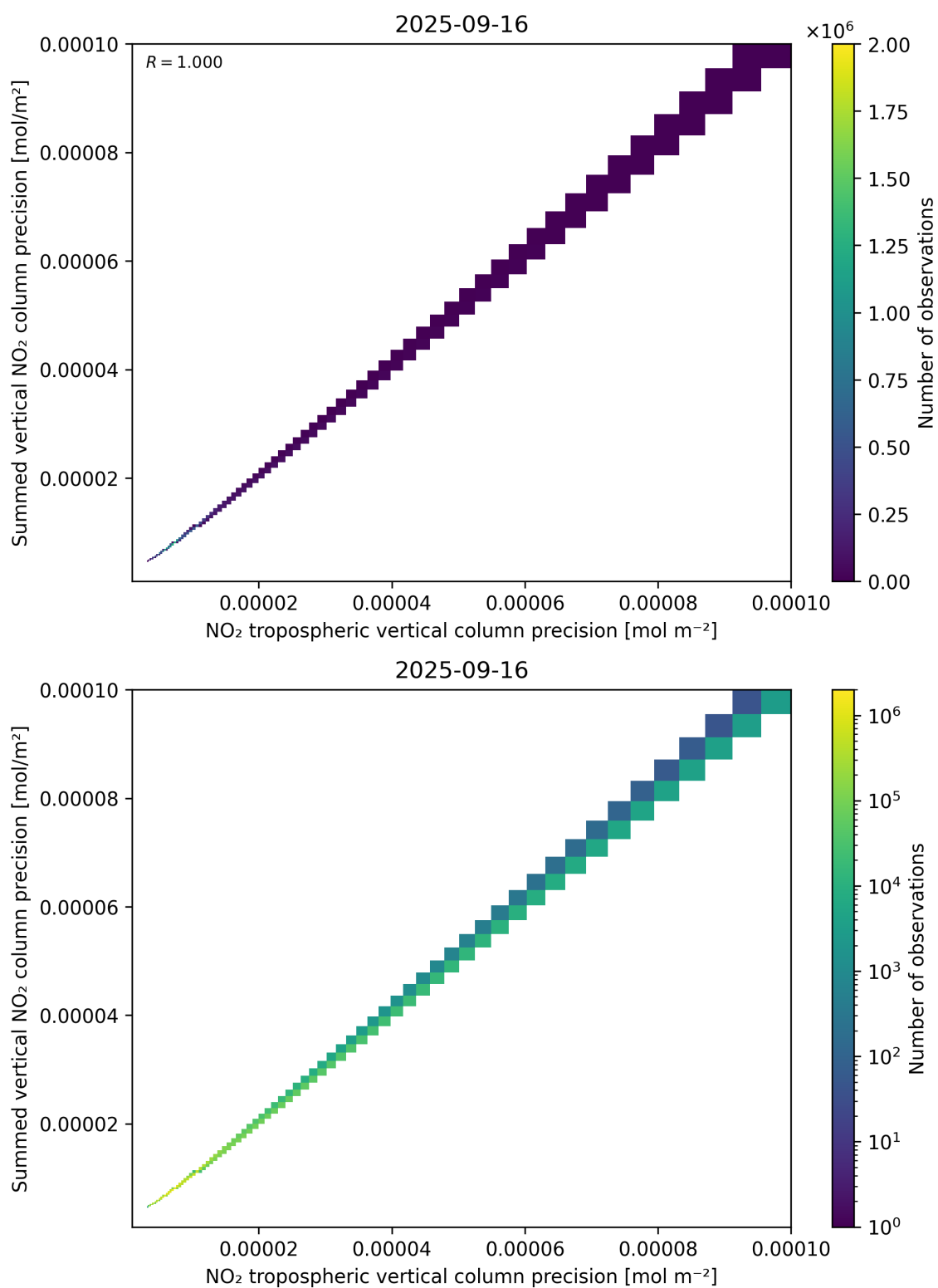
Figure 137: Scatter density plot of “NO 2 tropospheric vertical column precision” against “Summed vertical NO 2 column precision” for 2025-09-15 to 2025-09-17.
