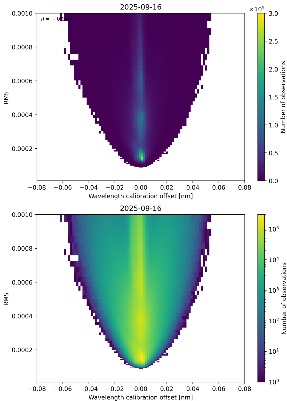
Figure 181: Scatter density plot of “Wavelength calibration offset” against “RMS” for 2025-09-15 to 2025-09-17.
