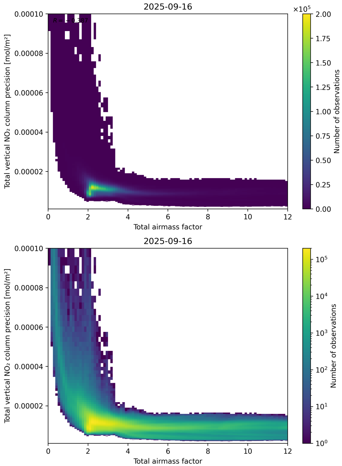
Figure 68: Scatter density plot of “Total airmass factor” against “Total vertical NO 2 column precision” for 2025-09-15 to 2025-09-17.
