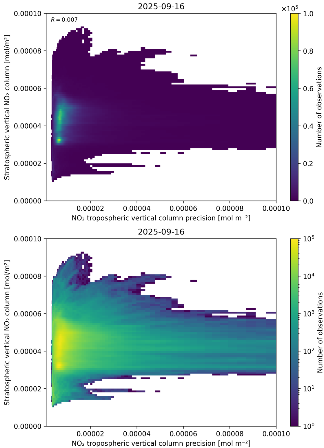
Figure 135: Scatter density plot of “NO 2 tropospheric vertical column precision” against “Stratospheric vertical NO 2 column” for 2025-09-15 to 2025-09-17.
