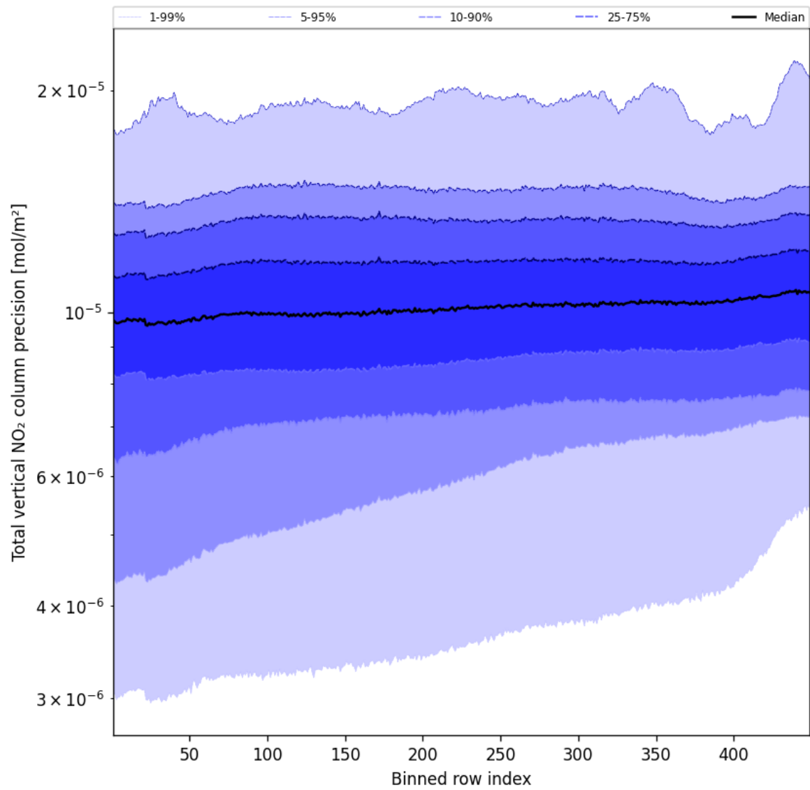
Figure 56: Along track statistics of “Total vertical NO 2 column precision” for 2025-09-15 to 2025-09-17
