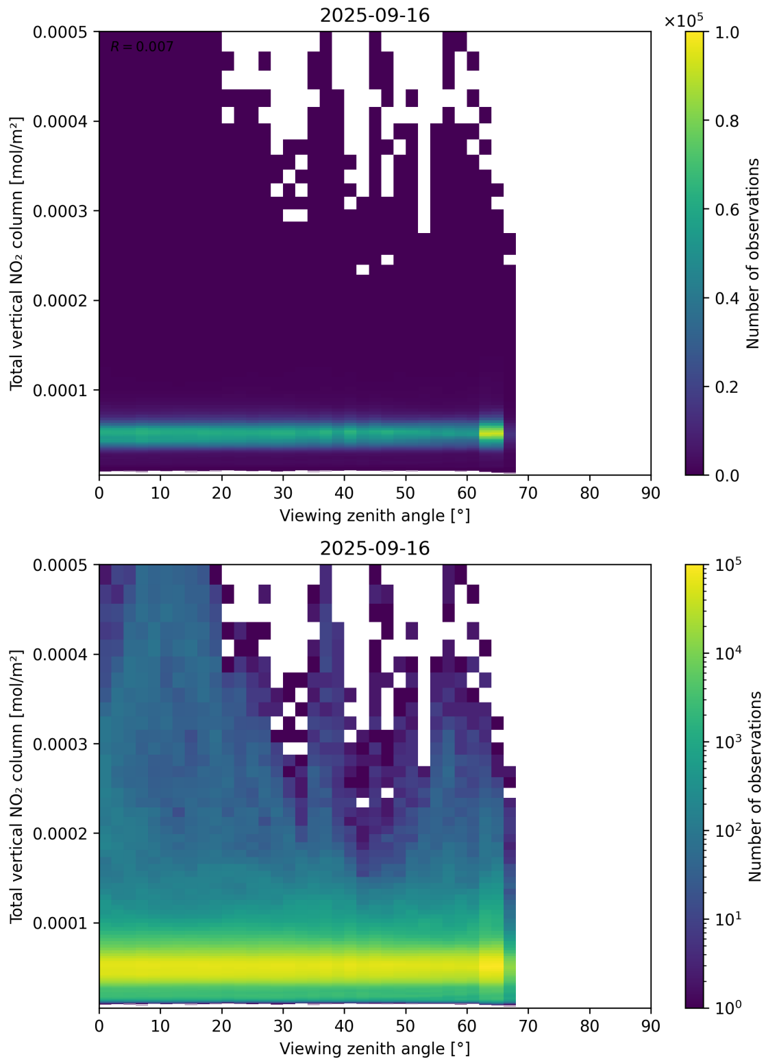
Figure 167: Scatter density plot of “Viewing zenith angle” against “Total vertical NO 2 column” for 2025-09-15 to 2025-09-17.
