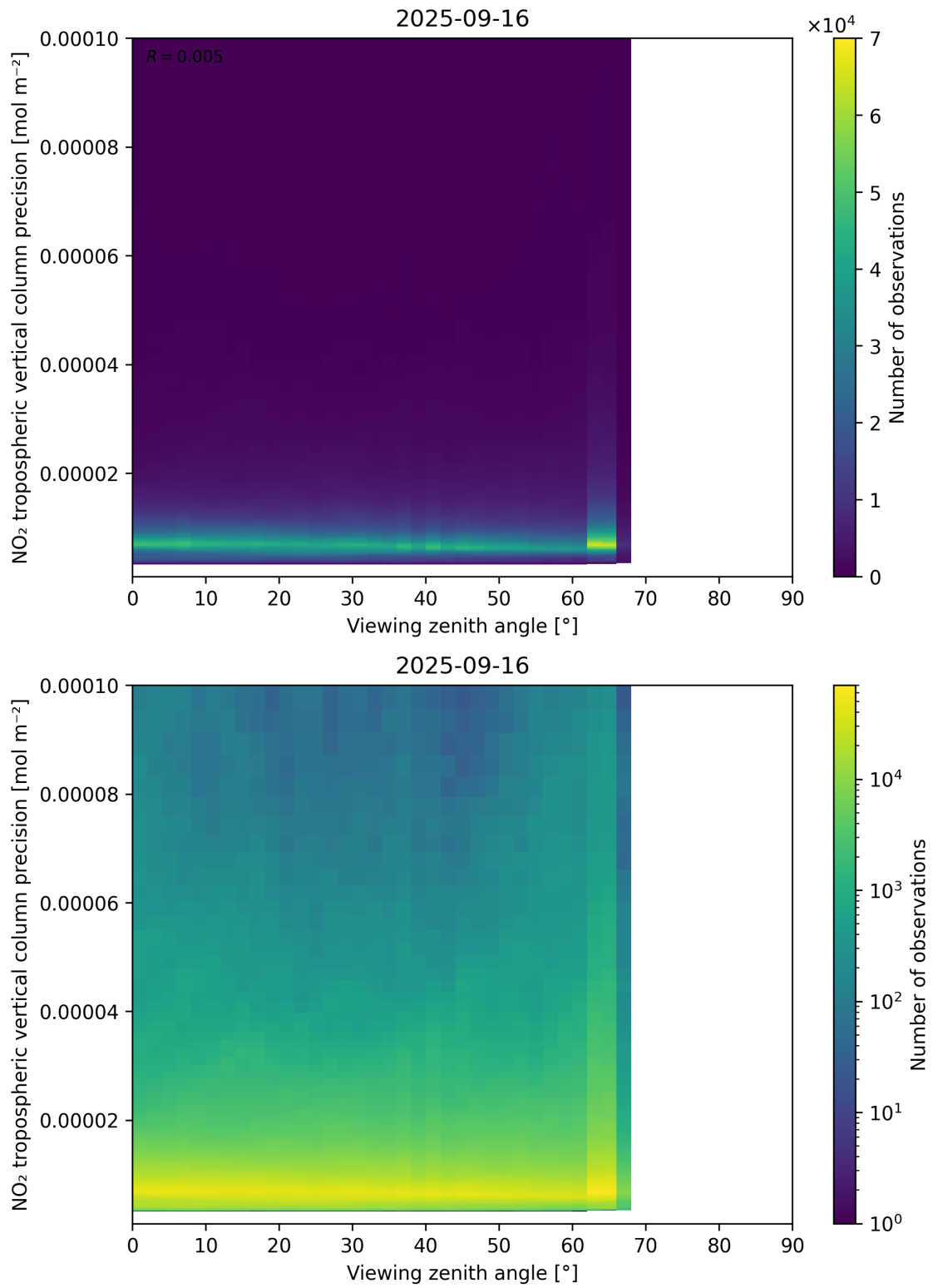
Figure 170: Scatter density plot of “Viewing zenith angle” against “NO 2 tropospheric vertical column precision” for 2025-09-15 to 2025-09-17.
