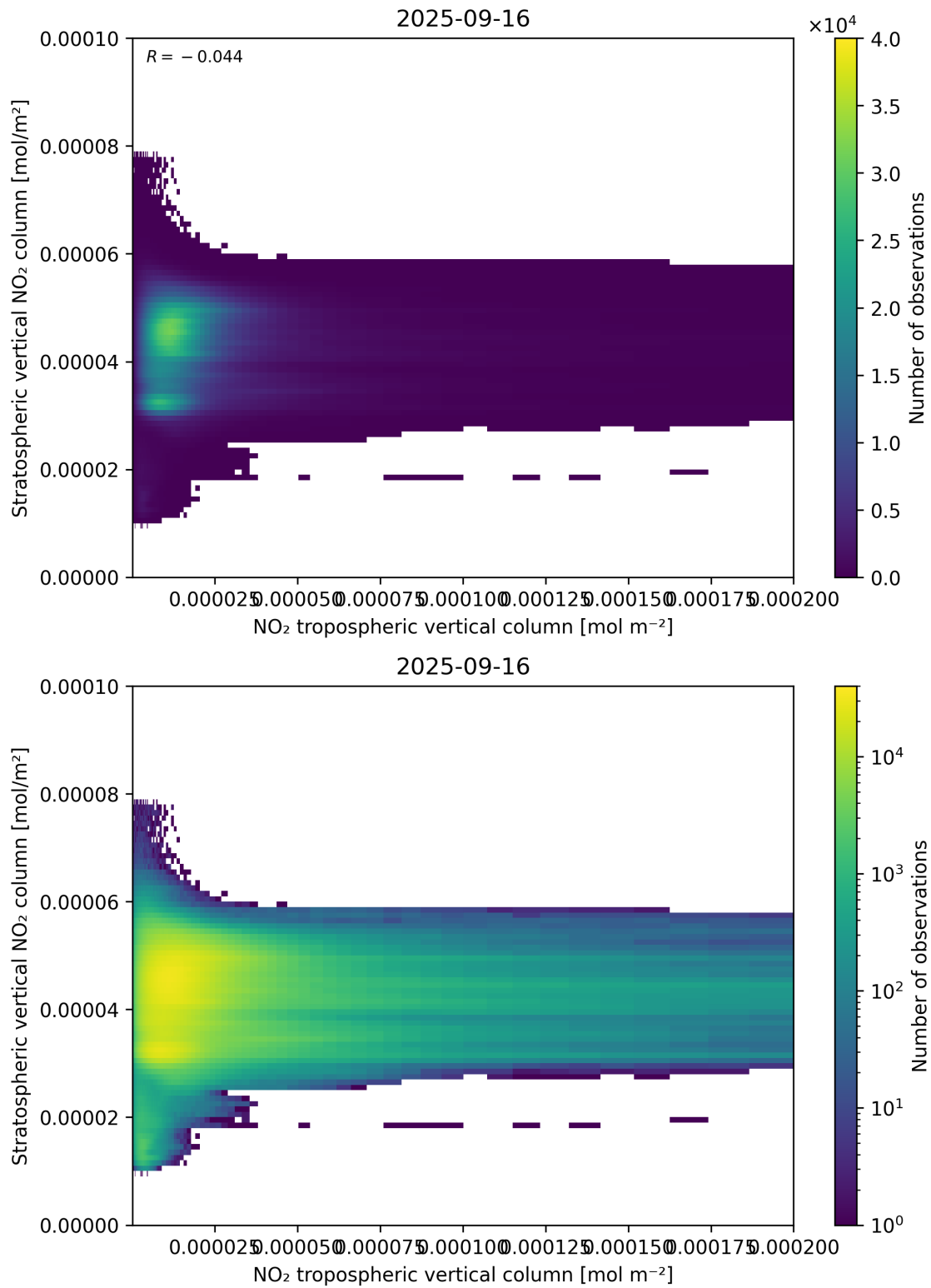
Figure 125: Scatter density plot of “NO 2 tropospheric vertical column” against “Stratospheric vertical NO 2 column” for 2025-09-15 to 2025-09-17.
