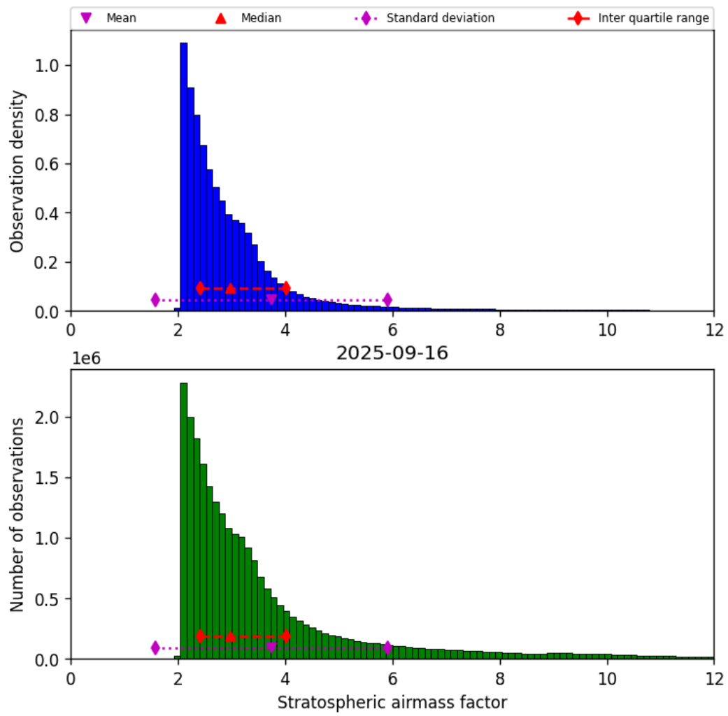
Figure 44: Histogram of “Stratospheric airmass factor” for 2025-09-15 to 2025-09-17
