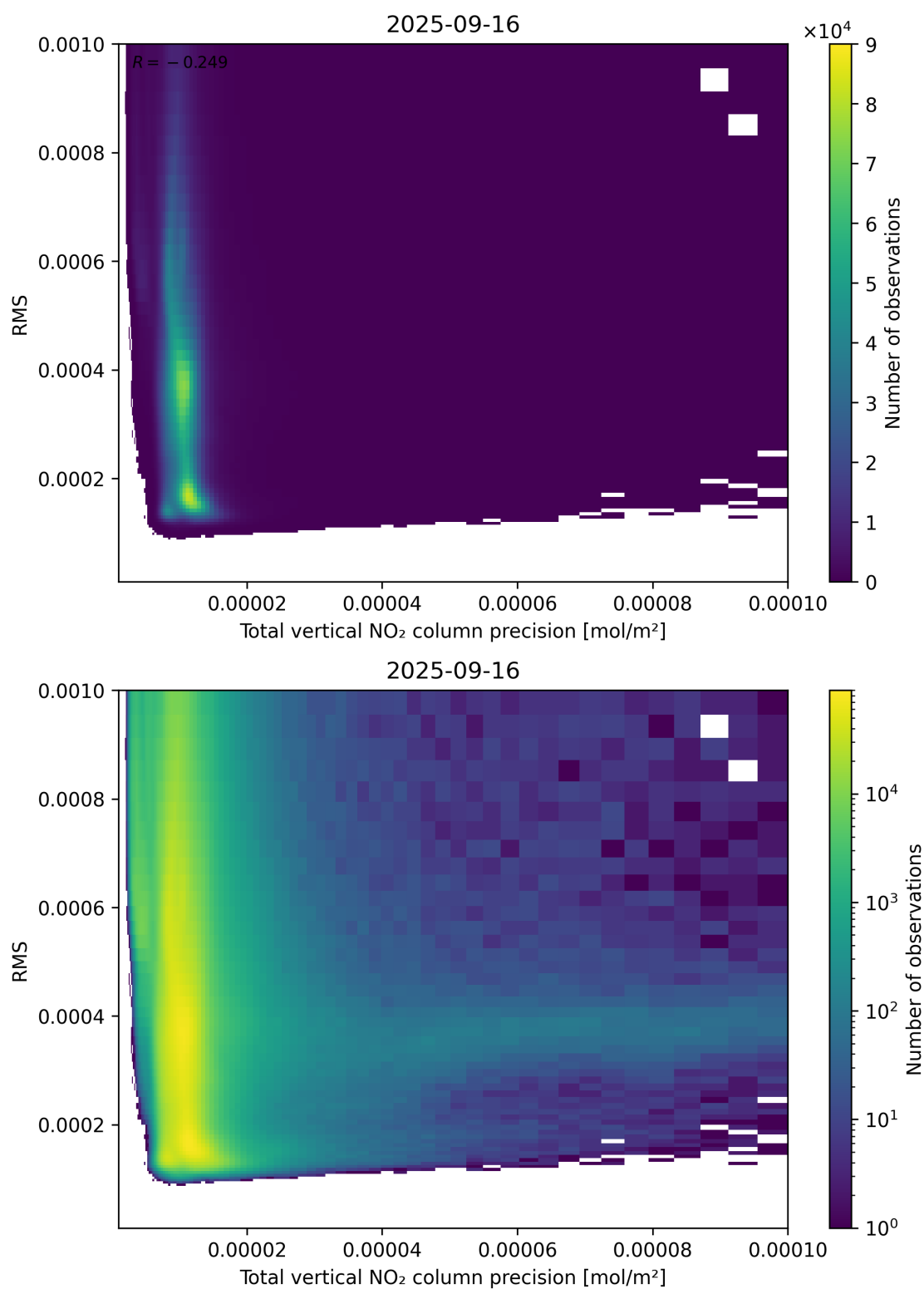
Figure 119: Scatter density plot of “Total vertical NO 2 column precision” against “RMS” for 2025-09-15 to 2025-09-17.
