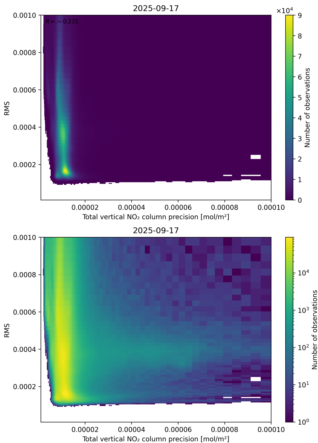
Figure 119: Scatter density plot of “Total vertical NO 2 column precision” against “RMS” for 2025-09-16 to 2025-09-18.
