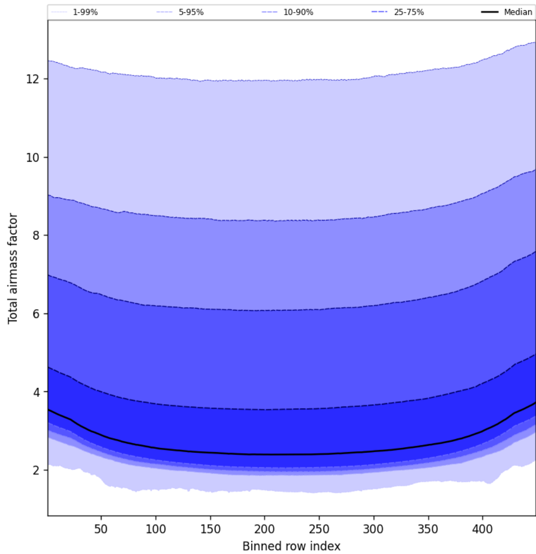
Figure 49: Along track statistics of “Total airmass factor” for 2025-09-16 to 2025-09-18
