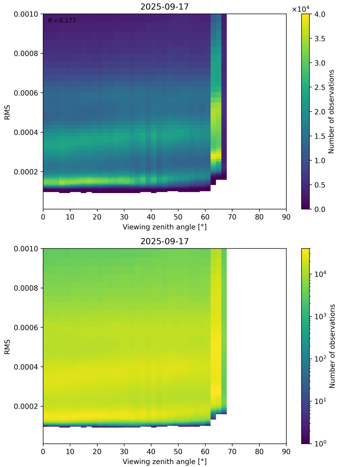
Figure 171: Scatter density plot of “Viewing zenith angle” against “RMS” for 2025-09-16 to 2025-09-18.
