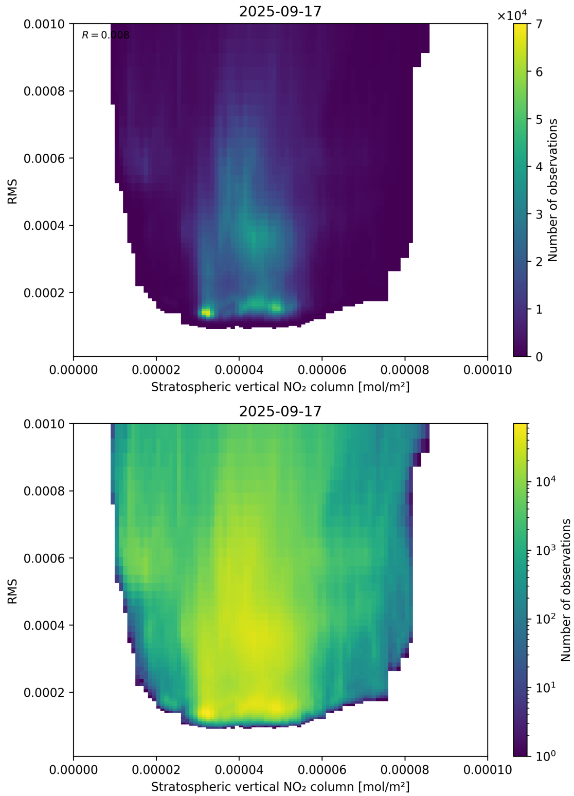
Figure 102: Scatter density plot of “Stratospheric vertical NO 2 column” against “RMS” for 2025-09-16 to 2025-09-18.
