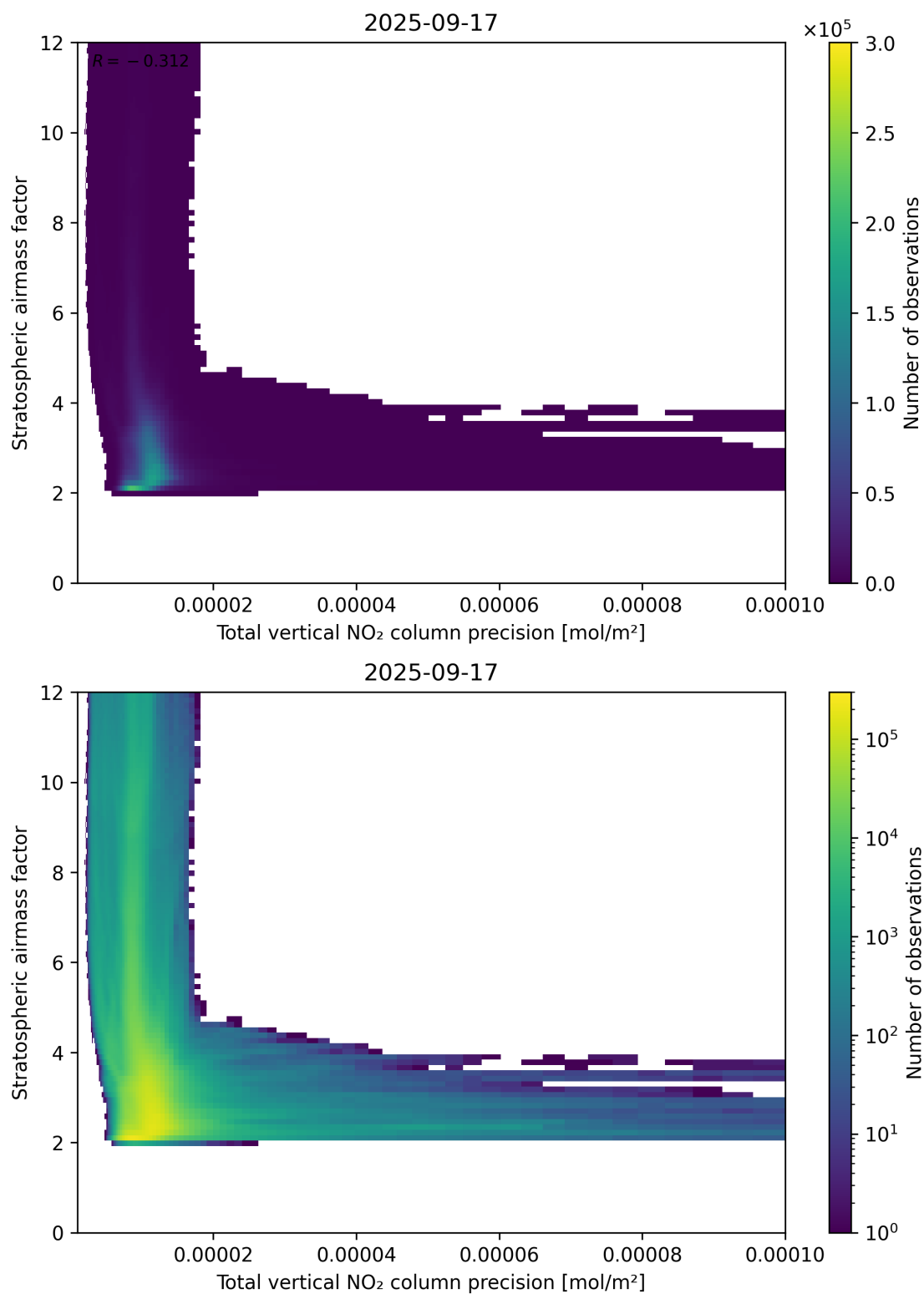
Figure 115: Scatter density plot of “Total vertical NO 2 column precision” against “Stratospheric air mass factor” for 2025-09-16 to 2025-09-18.
