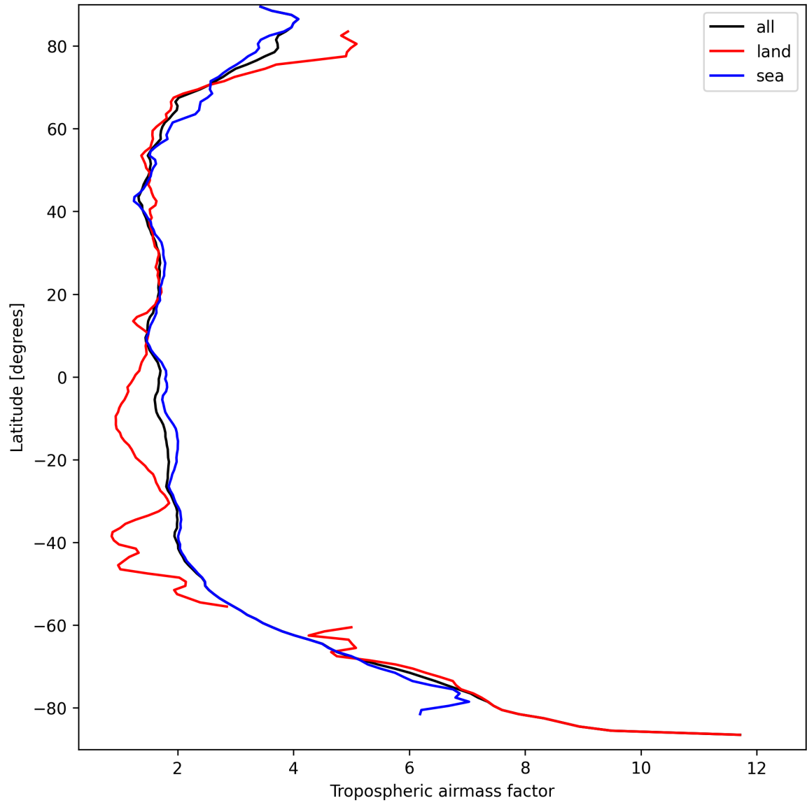
Figure 14: Zonal average of “Tropospheric air mass factor” for 2025-09-16 to 2025-09-18.
