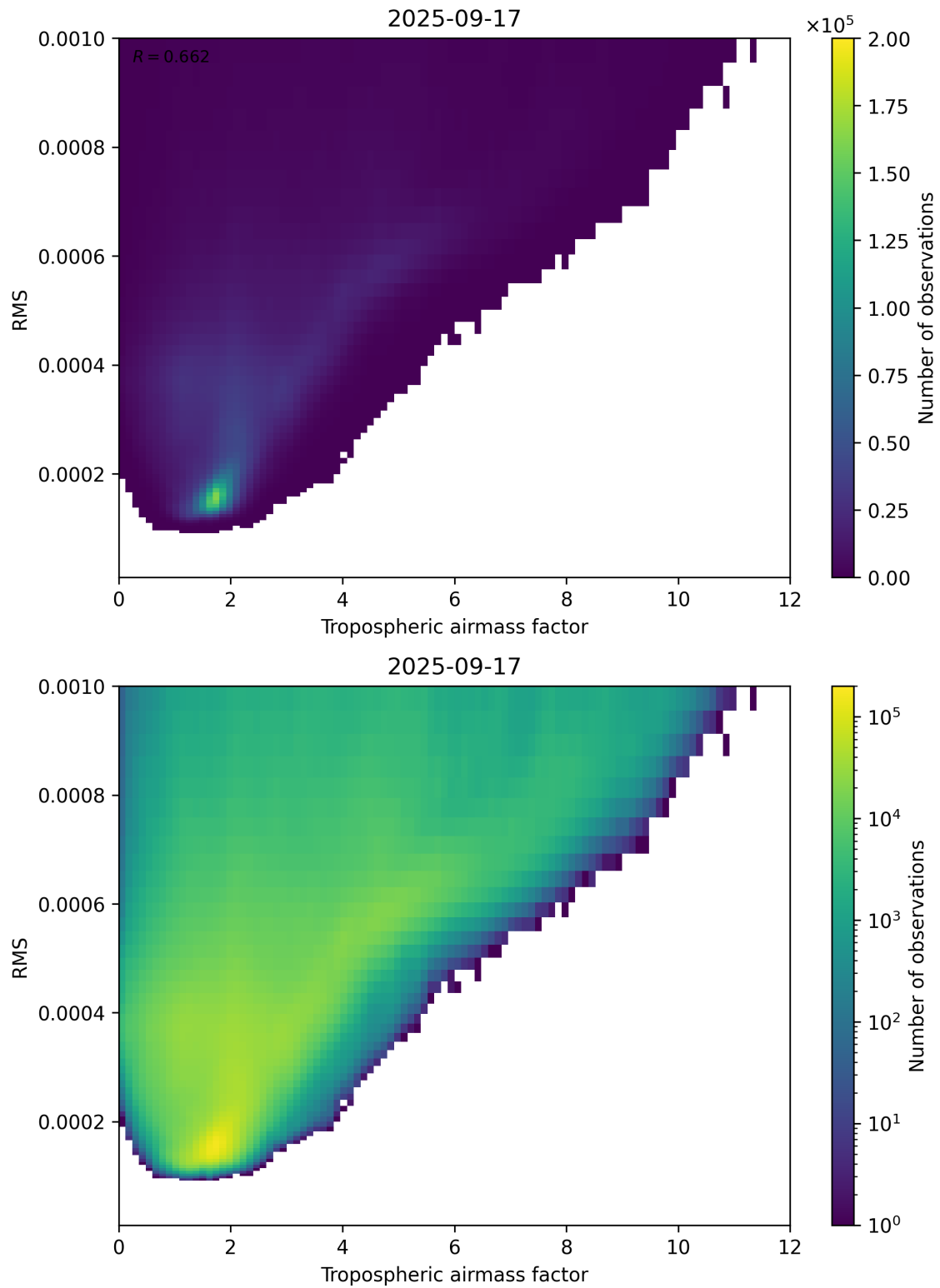
Figure 79: Scatter density plot of “Tropospheric airmass factor” against “RMS” for 2025-09-16 to 2025-09-18.
