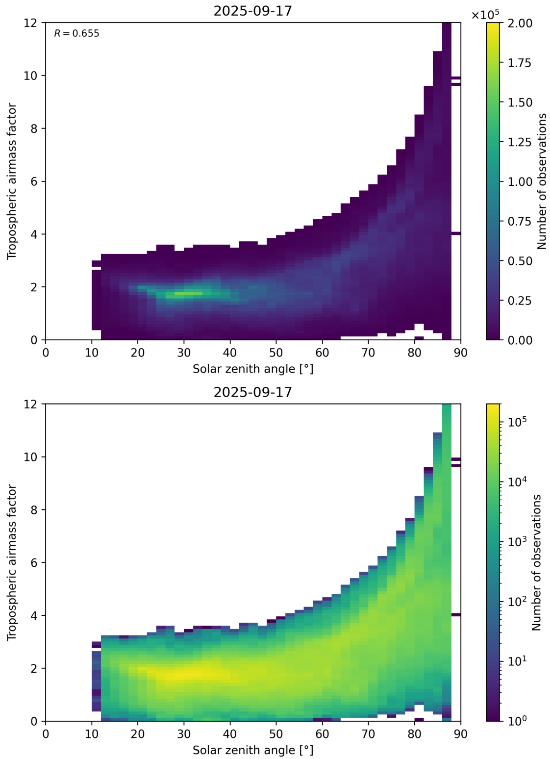
Figure 147: Scatter density plot of “Solar zenith angle” against “Tropospheric airmass factor” for 2025-09-16 to 2025-09-18.
