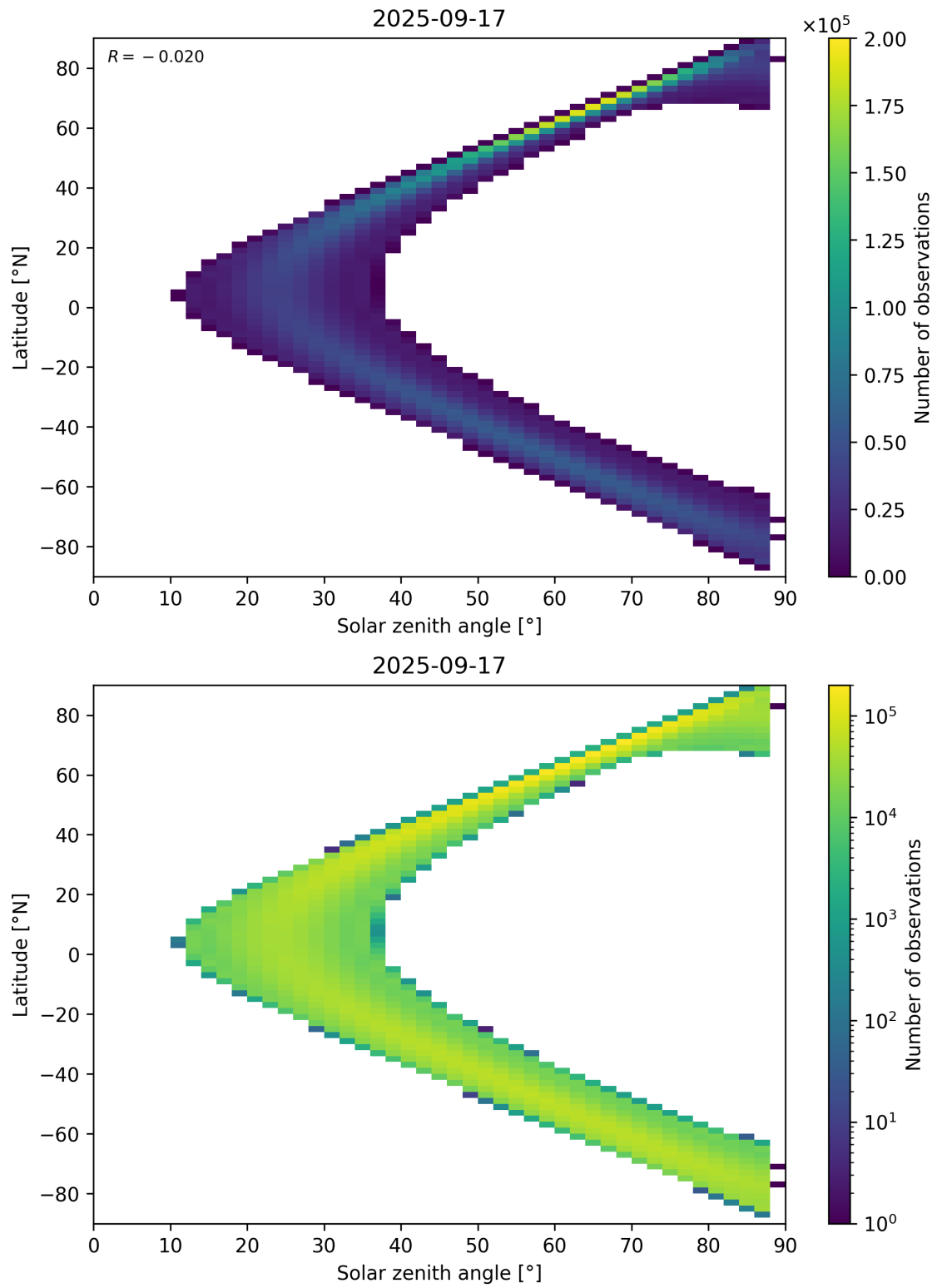
Figure 149: Scatter density plot of “Solar zenith angle” against “Latitude” for 2025-09-16 to 2025-09-18.
