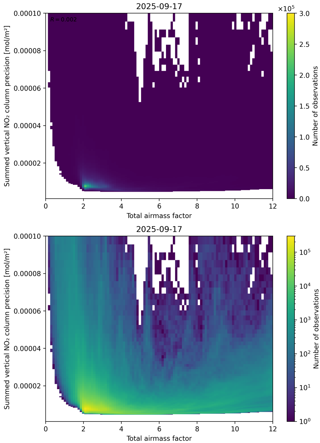
Figure 66: Scatter density plot of “Total airmass factor” against “Summed vertical NO 2 column precision” for 2025-09-16 to 2025-09-18.
