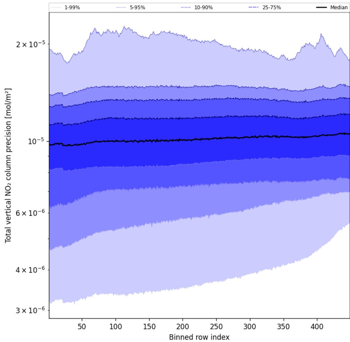
Figure 56: Along track statistics of “Total vertical NO 2 column precision” for 2025-09-16 to 2025-09-18
