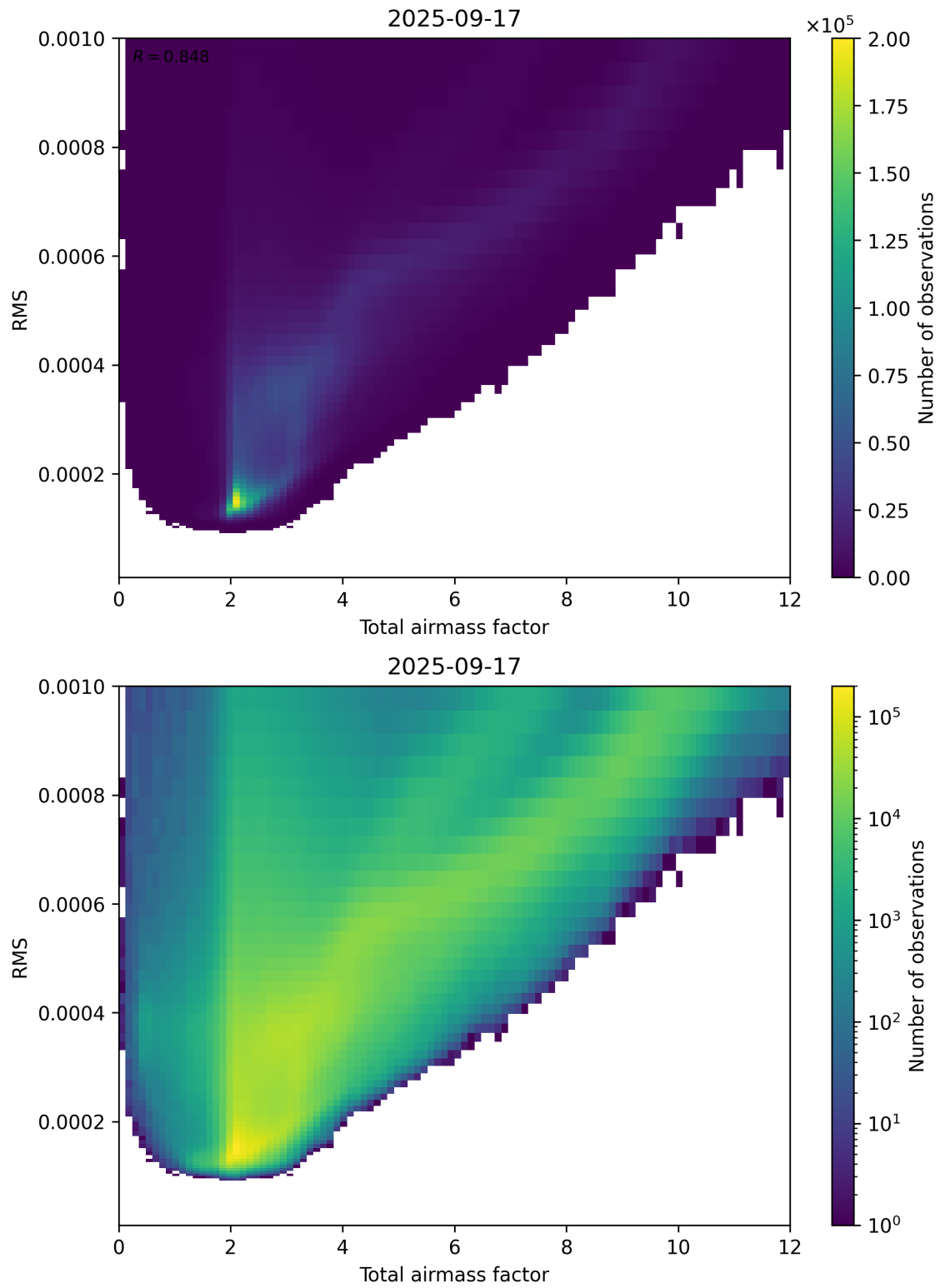
Figure 69: Scatter density plot of “Total airmass factor” against “RMS” for 2025-09-16 to 2025-09-18.
