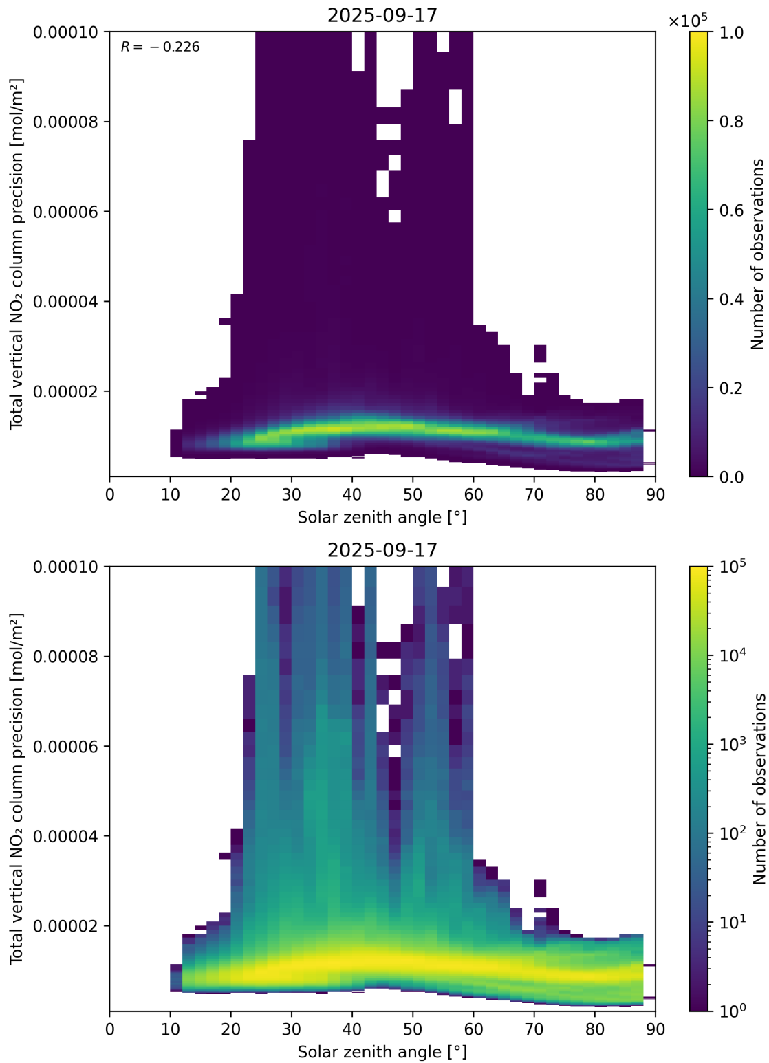
Figure 154: Scatter density plot of “Solar zenith angle” against “Total vertical NO 2 column precision” for 2025-09-16 to 2025-09-18.
