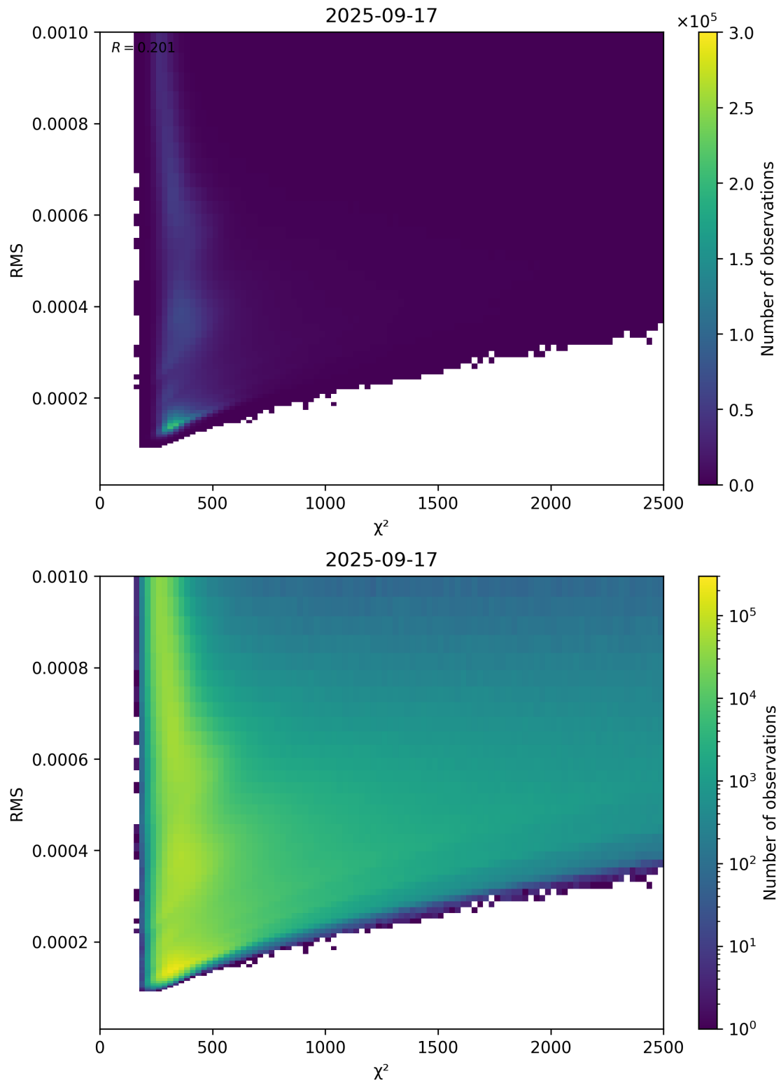
Figure 82: Scatter density plot of “ \chi^2 ” against “RMS” for 2025-09-16 to 2025-09-18.
