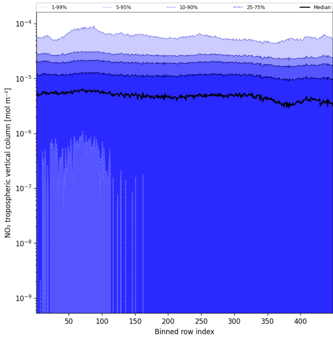
Figure 46: Along track statistics of “NO 2 tropospheric vertical column” for 2025-09-16 to 2025-09-18
