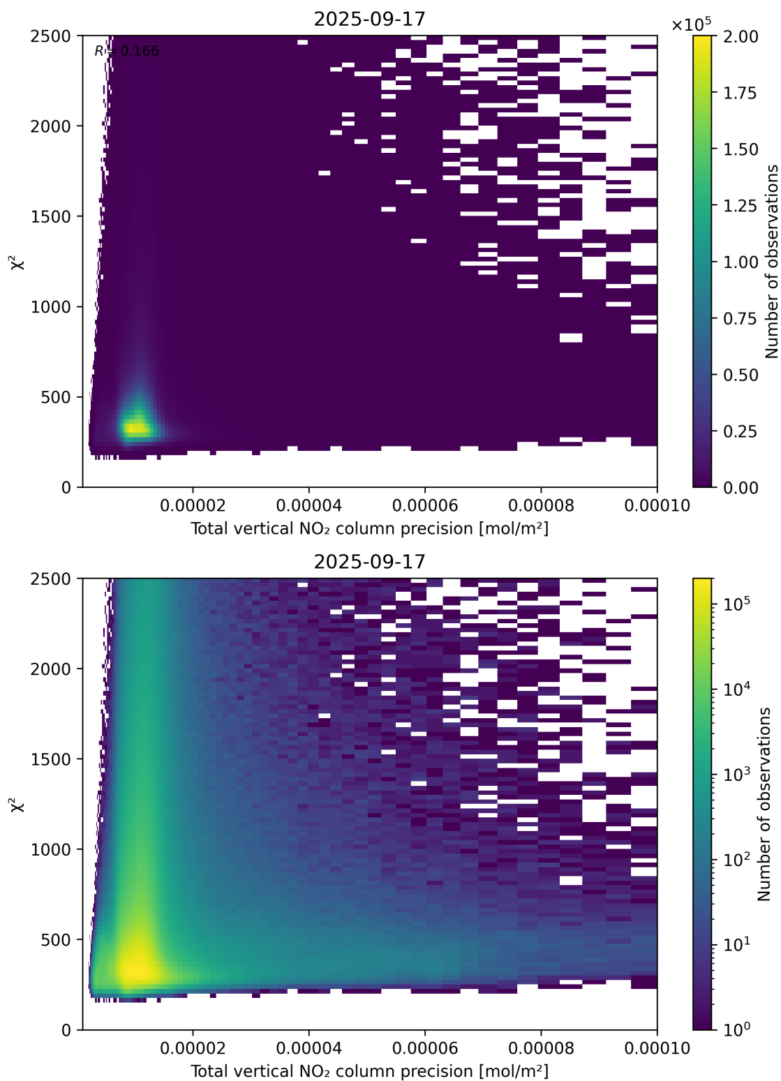
Figure 116: Scatter density plot of “Total vertical NO 2 column precision” against “ \chi^2 ” for 2025-09-16 to 2025-09-18.
