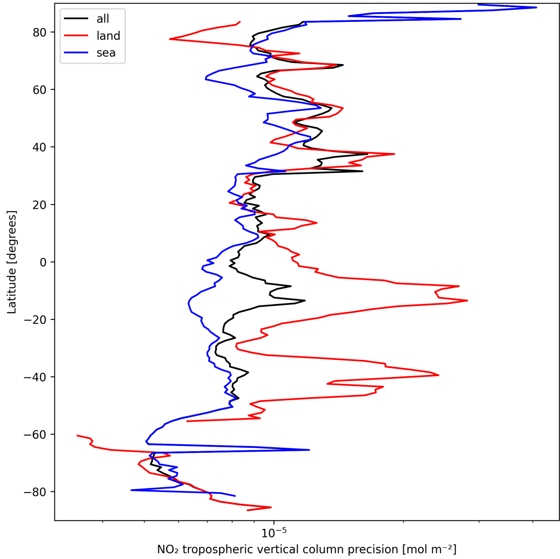
Figure 13: Zonal average of “NO 2 tropospheric vertical column precision” for 2025-09-16 to 2025-09-18.
