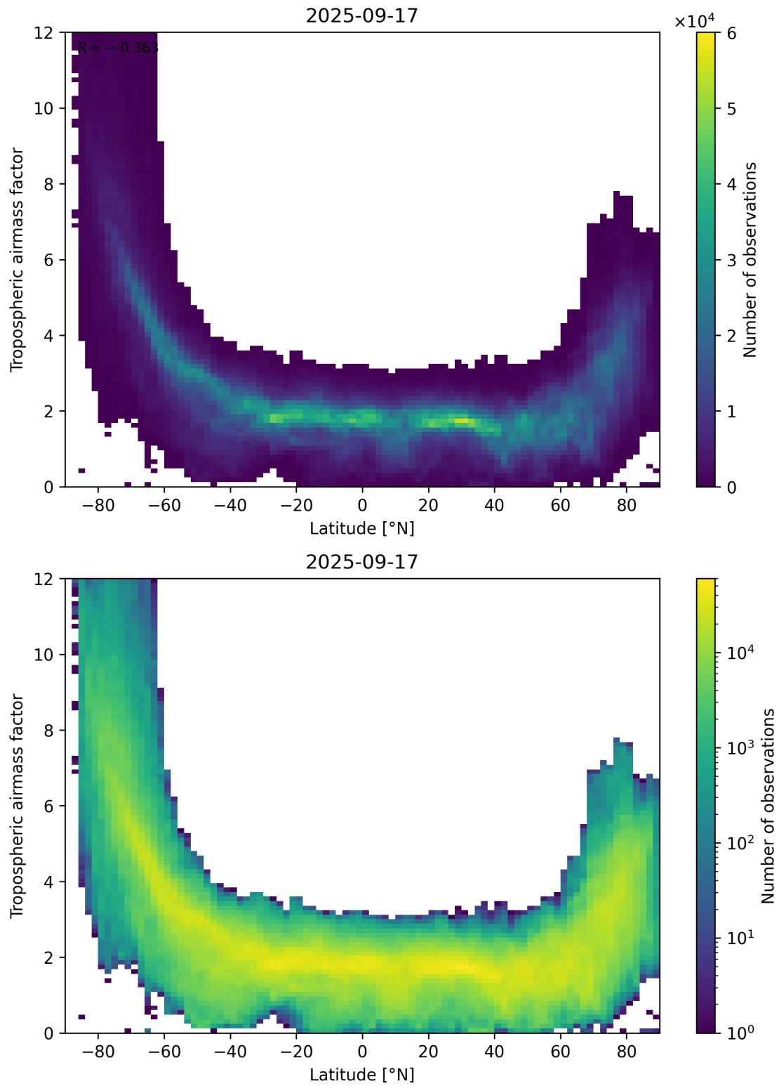
Figure 85: Scatter density plot of “Latitude” against “Tropospheric air mass factor” for 2025-09-16 to 2025-09-18.
