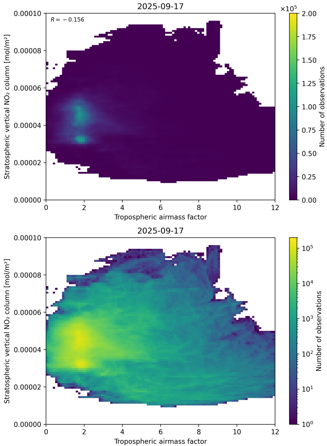
Figure 74: Scatter density plot of “Tropospheric air mass factor” against “Stratospheric vertical NO 2 column” for 2025-09-16 to 2025-09-18.
