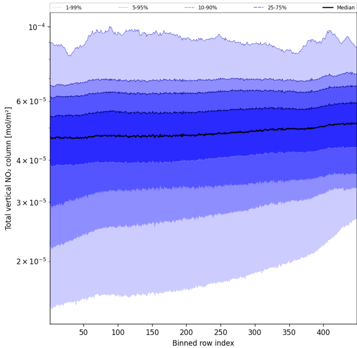
Figure 55: Along track statistics of “Total vertical NO 2 column” for 2025-09-16 to 2025-09-18
