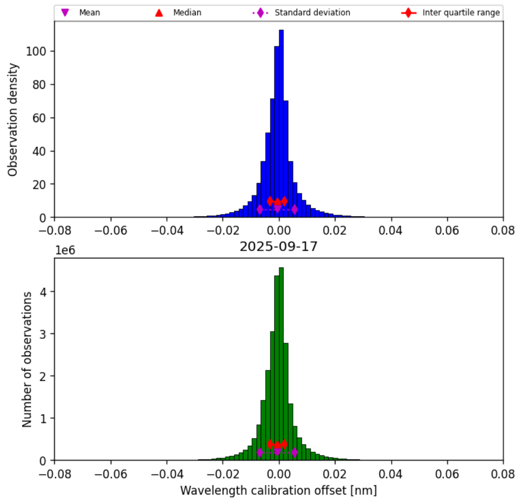
Figure 35: Histogram of “Wavelength calibration offset” for 2025-09-16 to 2025-09-18
