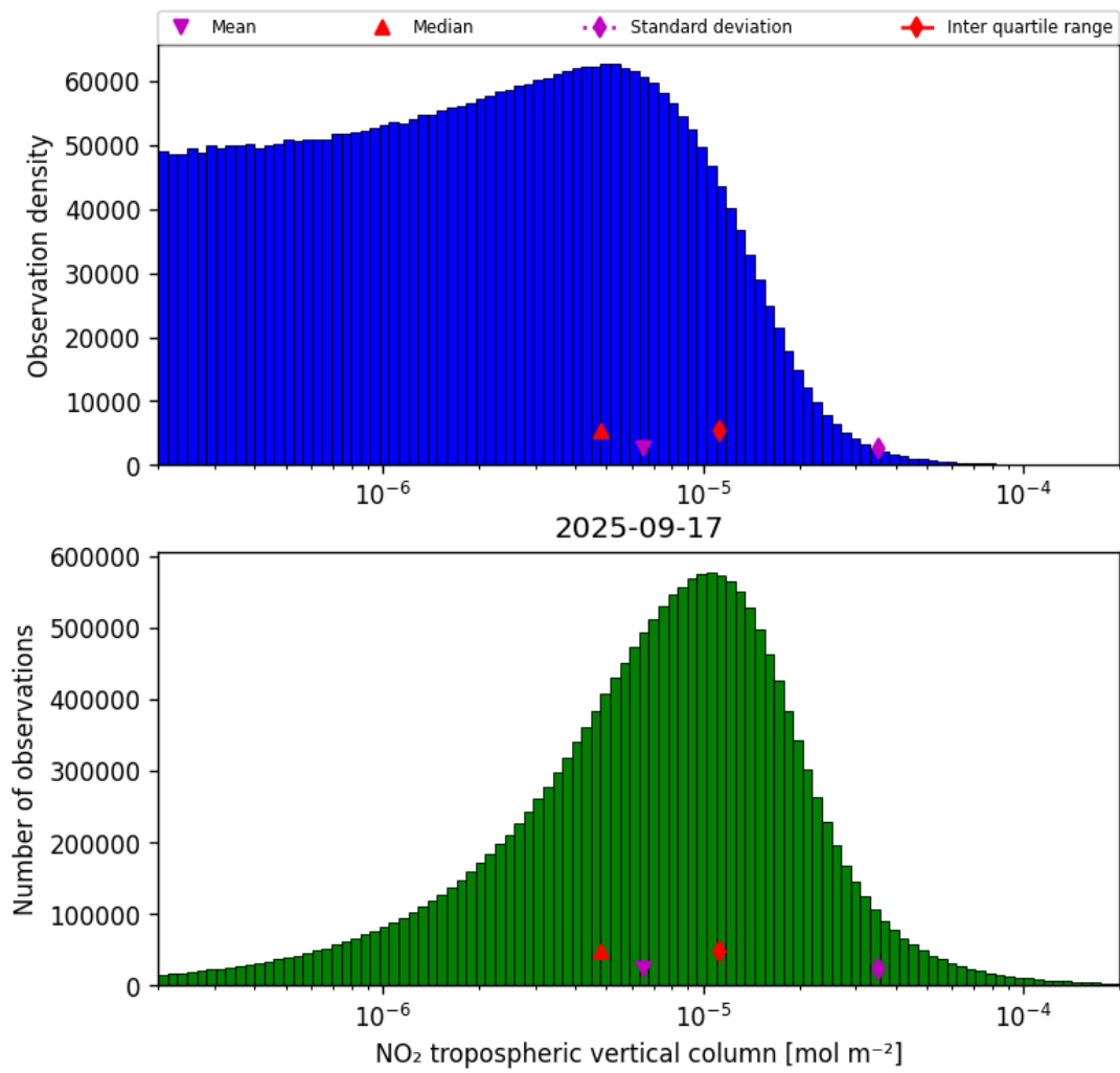
Figure 29: Histogram of “NO 2 tropospheric vertical column” for 2025-09-16 to 2025-09-18
