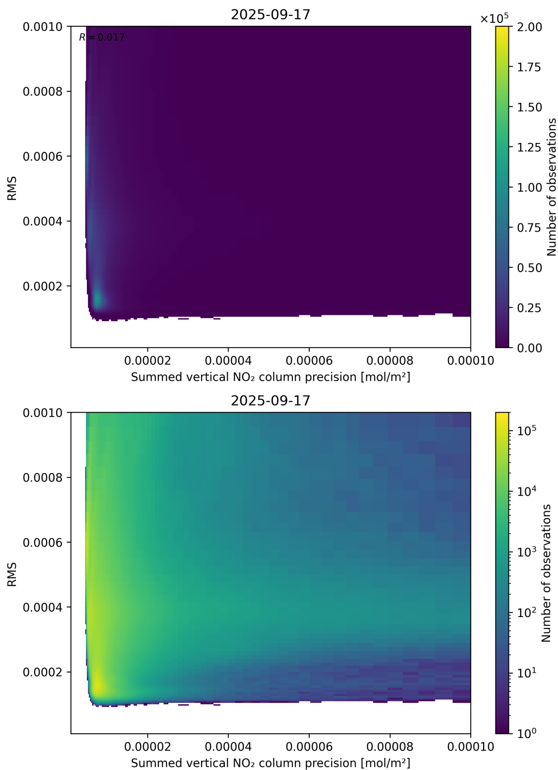
Figure 108: Scatter density plot of “Summed vertical NO 2 column precision” against “RMS” for 2025-09-16 to 2025-09-18.
