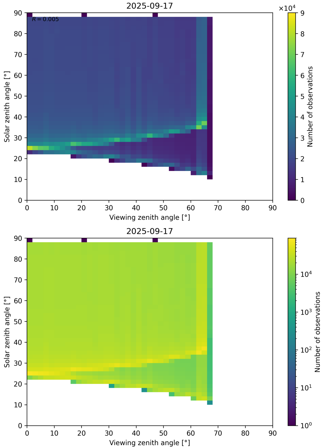
Figure 172: Scatter density plot of “Viewing zenith angle” against “Solar zenith angle” for 2025-09-16 to 2025-09-18.
