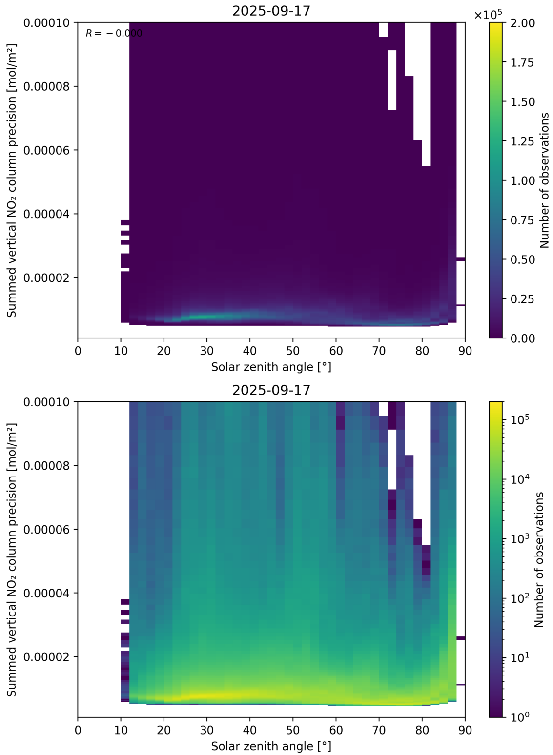
Figure 152: Scatter density plot of “Solar zenith angle” against “Summed vertical NO 2 column precision” for 2025-09-16 to 2025-09-18.
