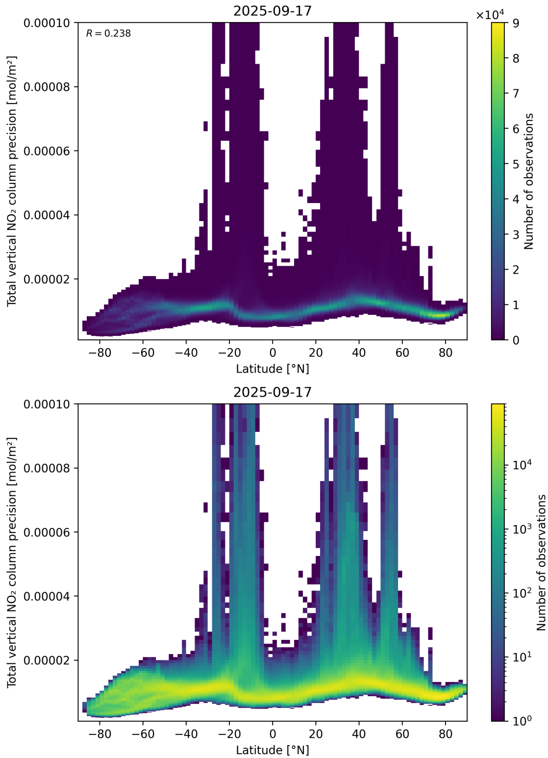
Figure 91: Scatter density plot of “Latitude” against “Total vertical NO 2 column precision” for 2025-09-16 to 2025-09-18.
