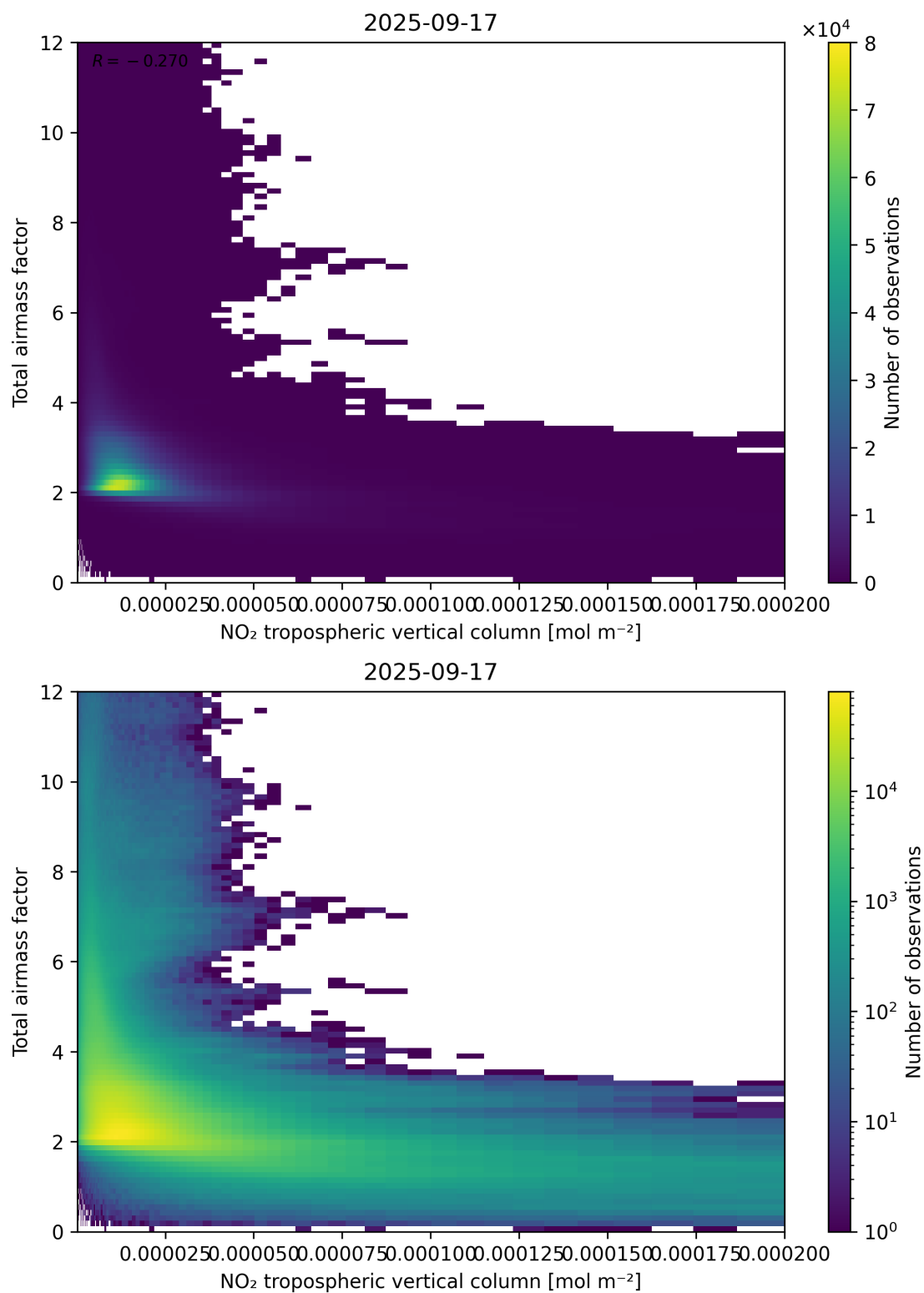
Figure 122: Scatter density plot of “NO 2 tropospheric vertical column” against “Total air mass factor” for 2025-09-16 to 2025-09-18.
