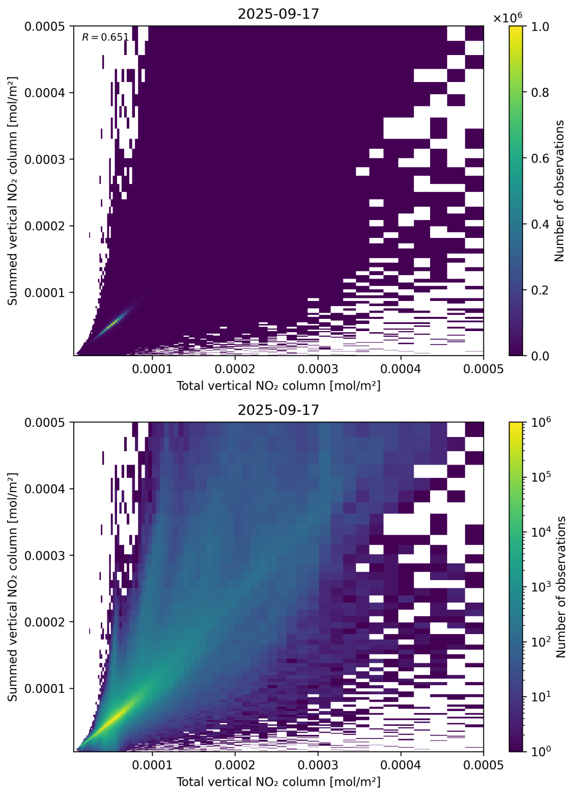
Figure 112: Scatter density plot of “Total vertical NO 2 column” against “Summed vertical NO 2 column” for 2025-09-16 to 2025-09-18.
