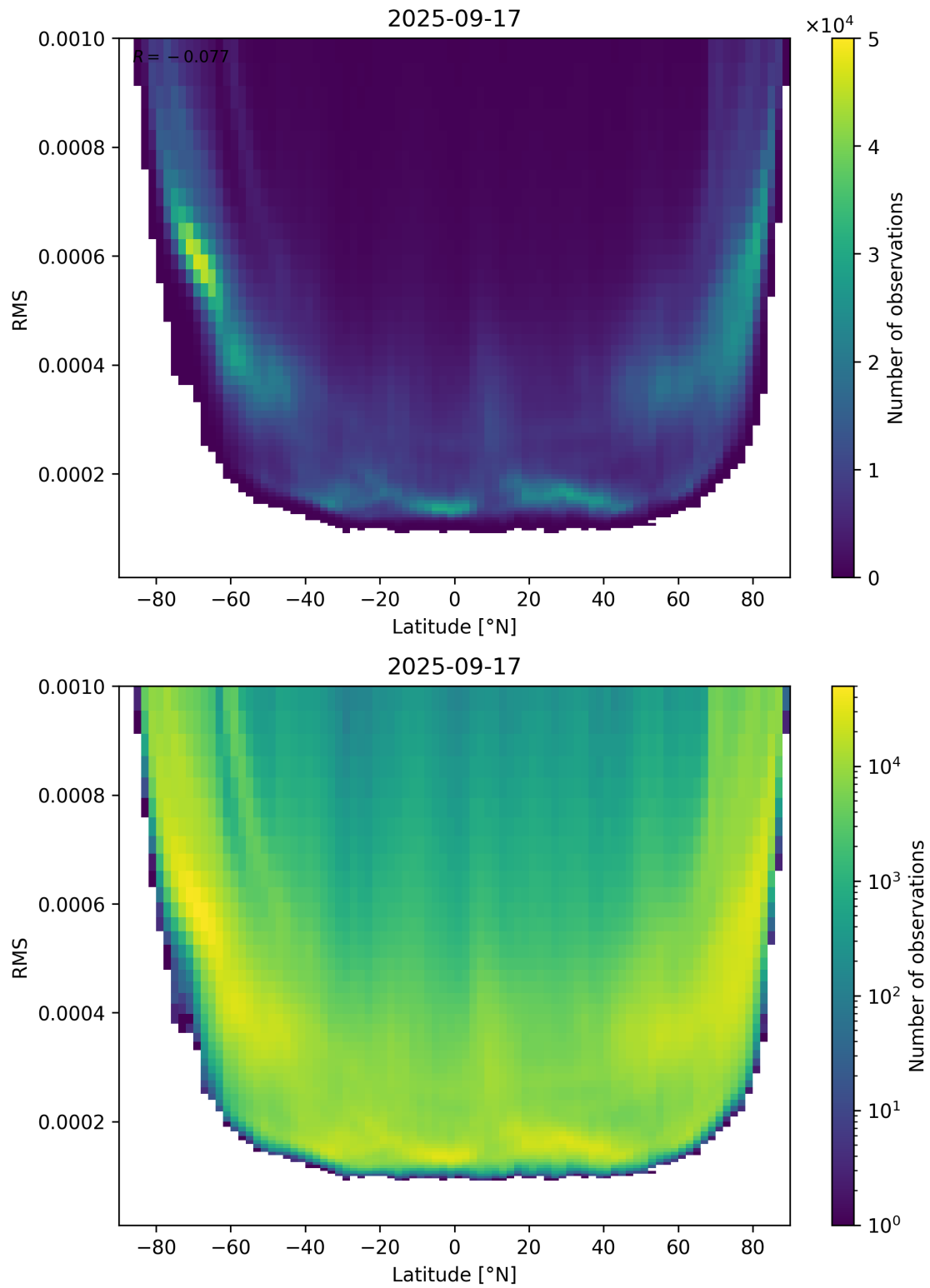
Figure 94: Scatter density plot of “Latitude” against “RMS” for 2025-09-16 to 2025-09-18.
