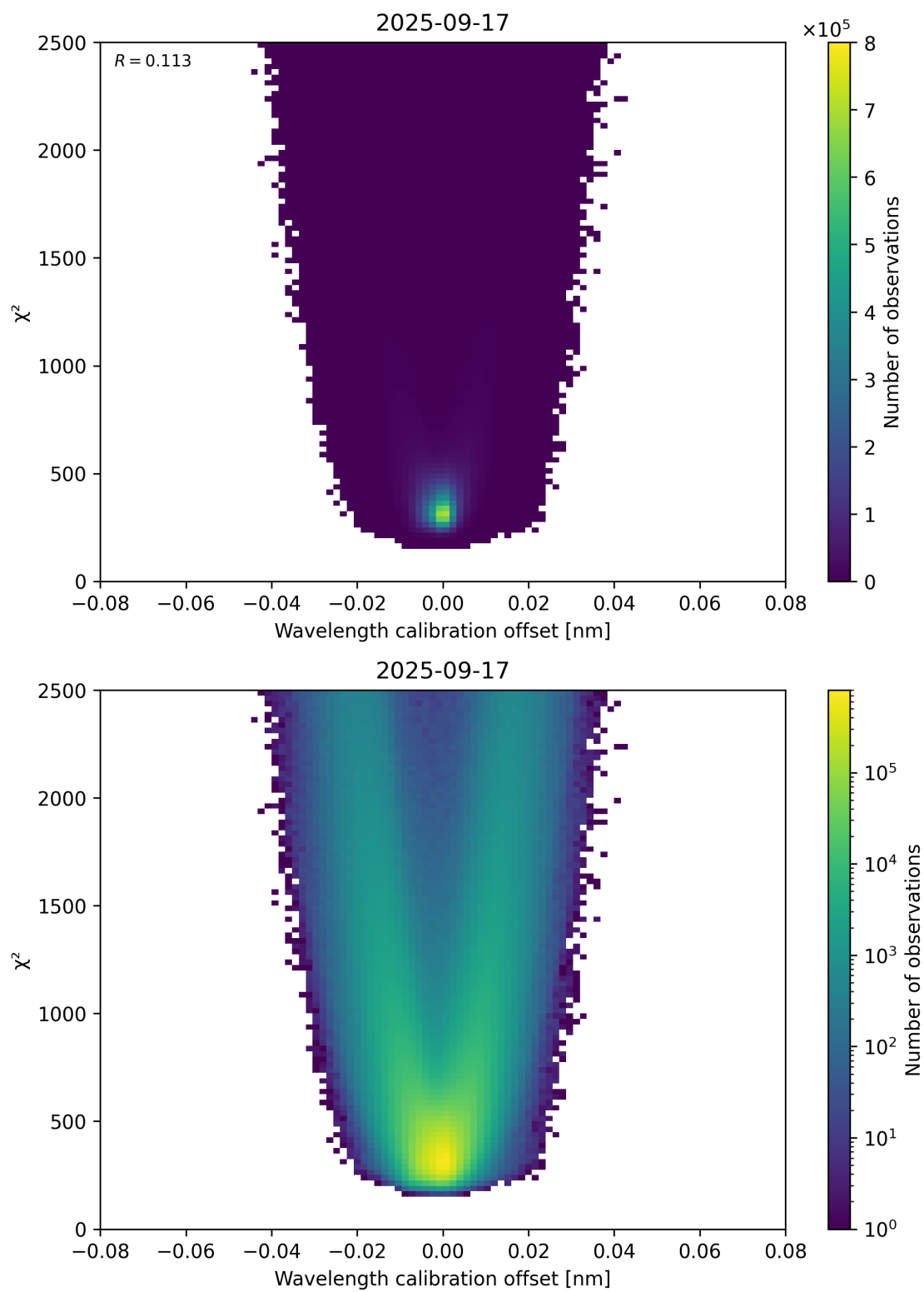
Figure 175: Scatter density plot of “Wavelength calibration offset” against “ \chi^2 ” for 2025-09-16 to 2025-09-18.
