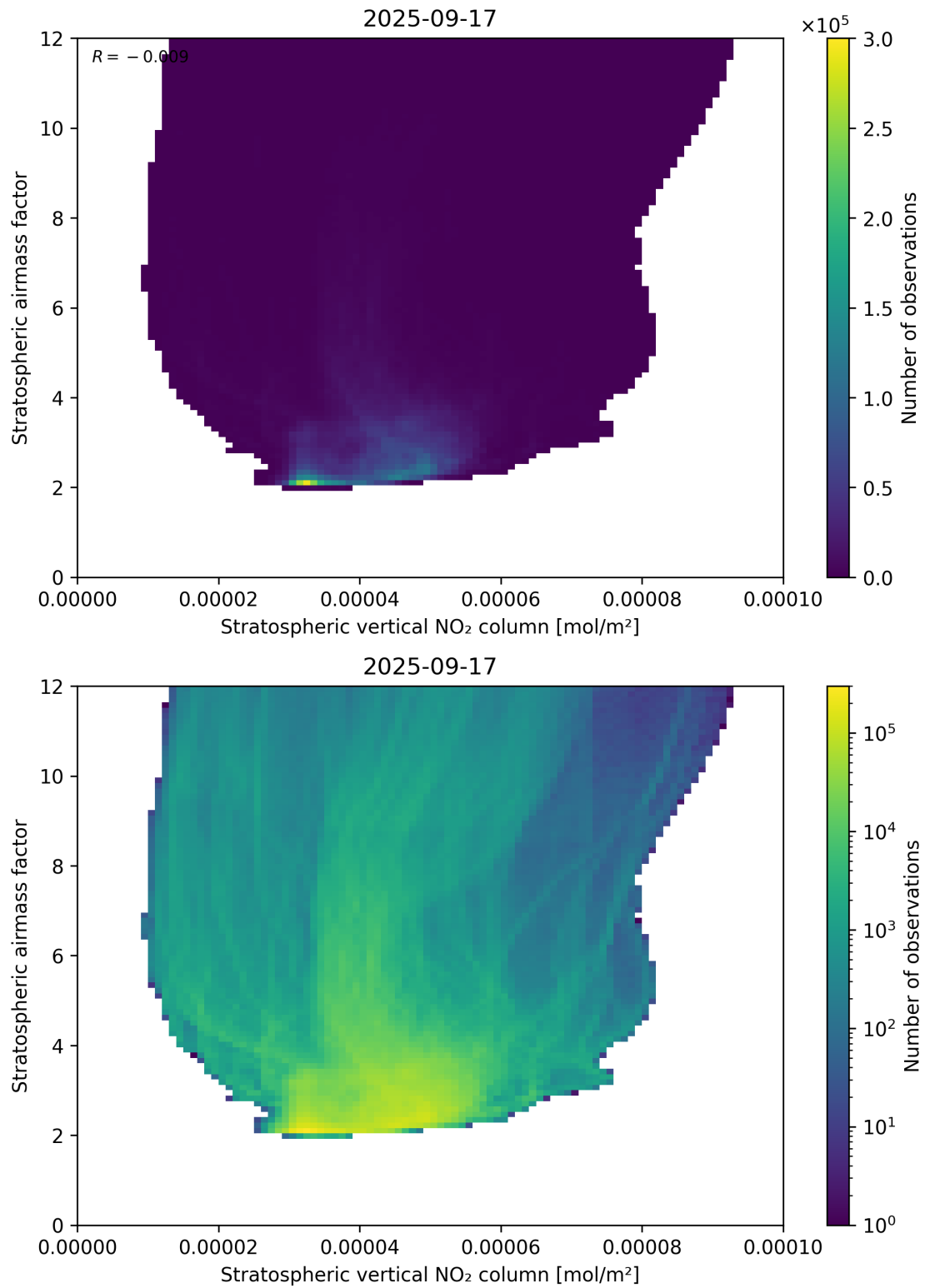
Figure 96: Scatter density plot of “Stratospheric vertical NO 2 column” against “Stratospheric airmass factor” for 2025-09-16 to 2025-09-18.
