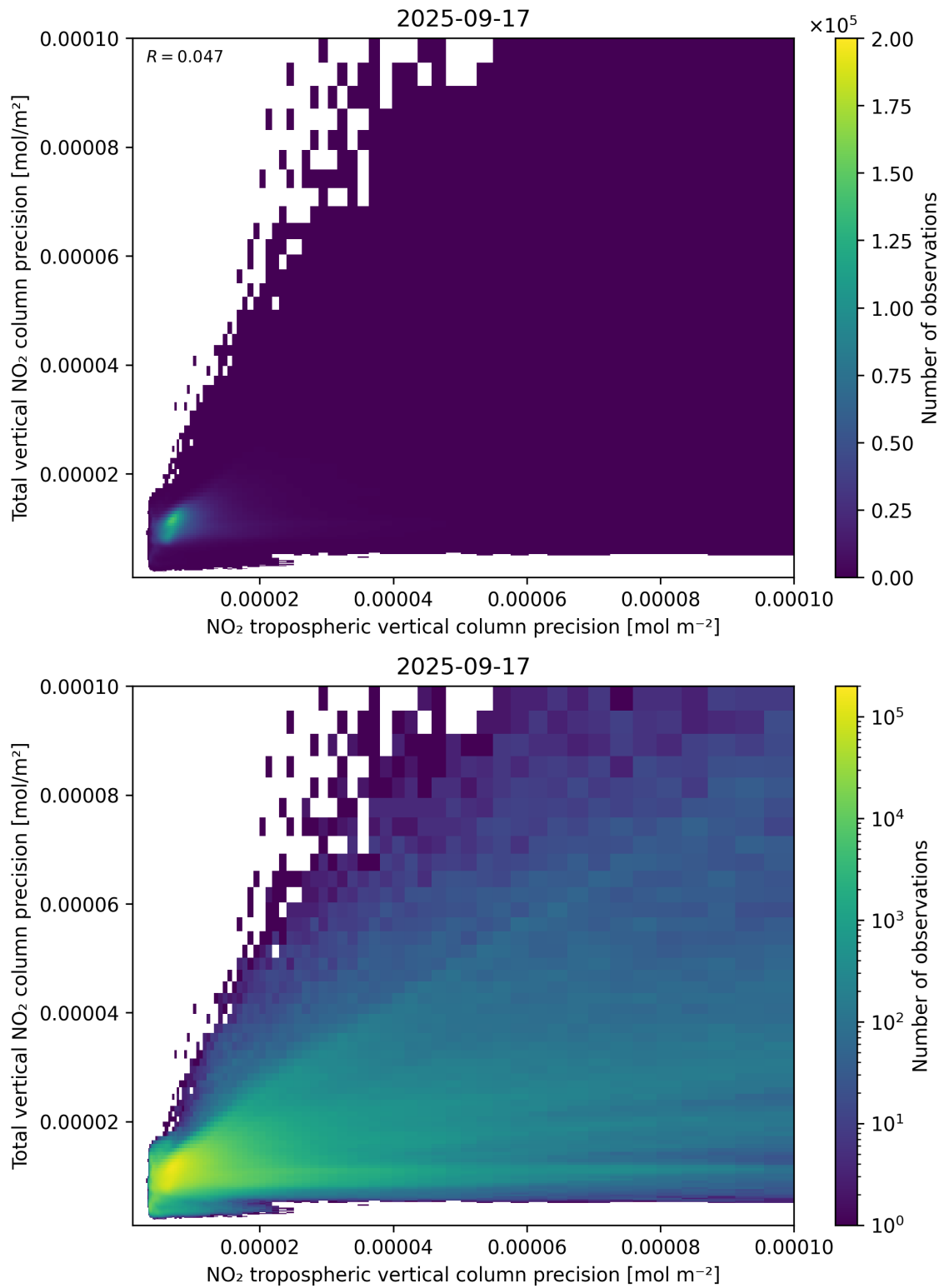
Figure 139: Scatter density plot of “NO 2 tropospheric vertical column precision” against “Total vertical NO 2 column precision” for 2025-09-16 to 2025-09-18.
