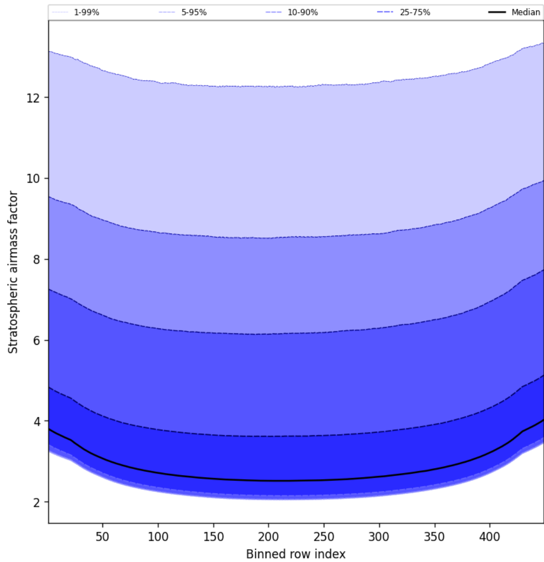
Figure 61: Along track statistics of “Stratospheric airmass factor” for 2025-09-16 to 2025-09-18
