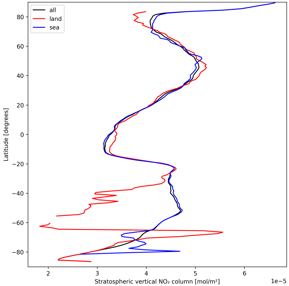
Figure 19: Zonal average of “Stratospheric vertical NO 2 column” for 2025-09-16 to 2025-09-18.
