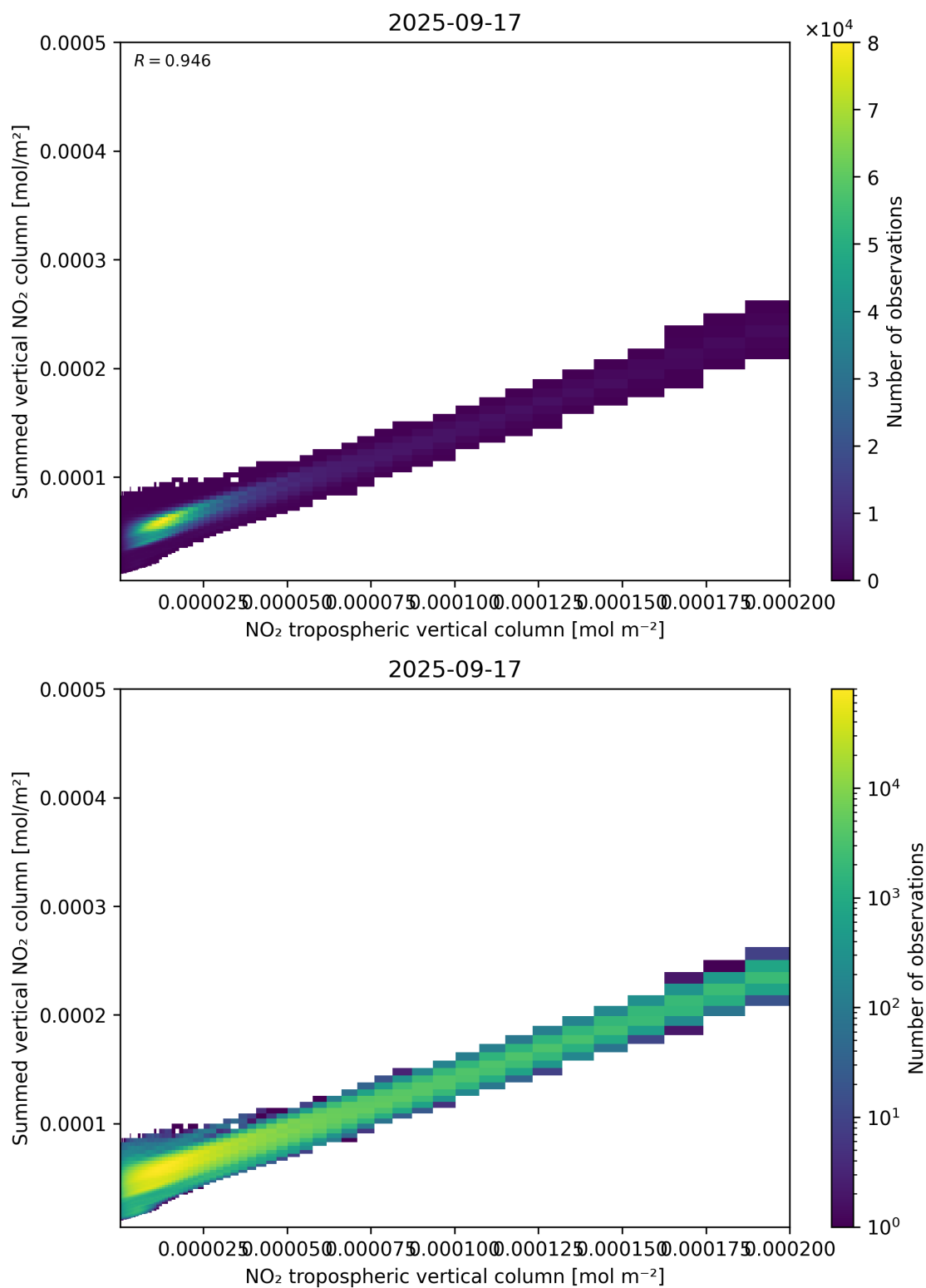
Figure 126: Scatter density plot of “NO 2 tropospheric vertical column” against “Summed vertical NO 2 column” for 2025-09-16 to 2025-09-18.
