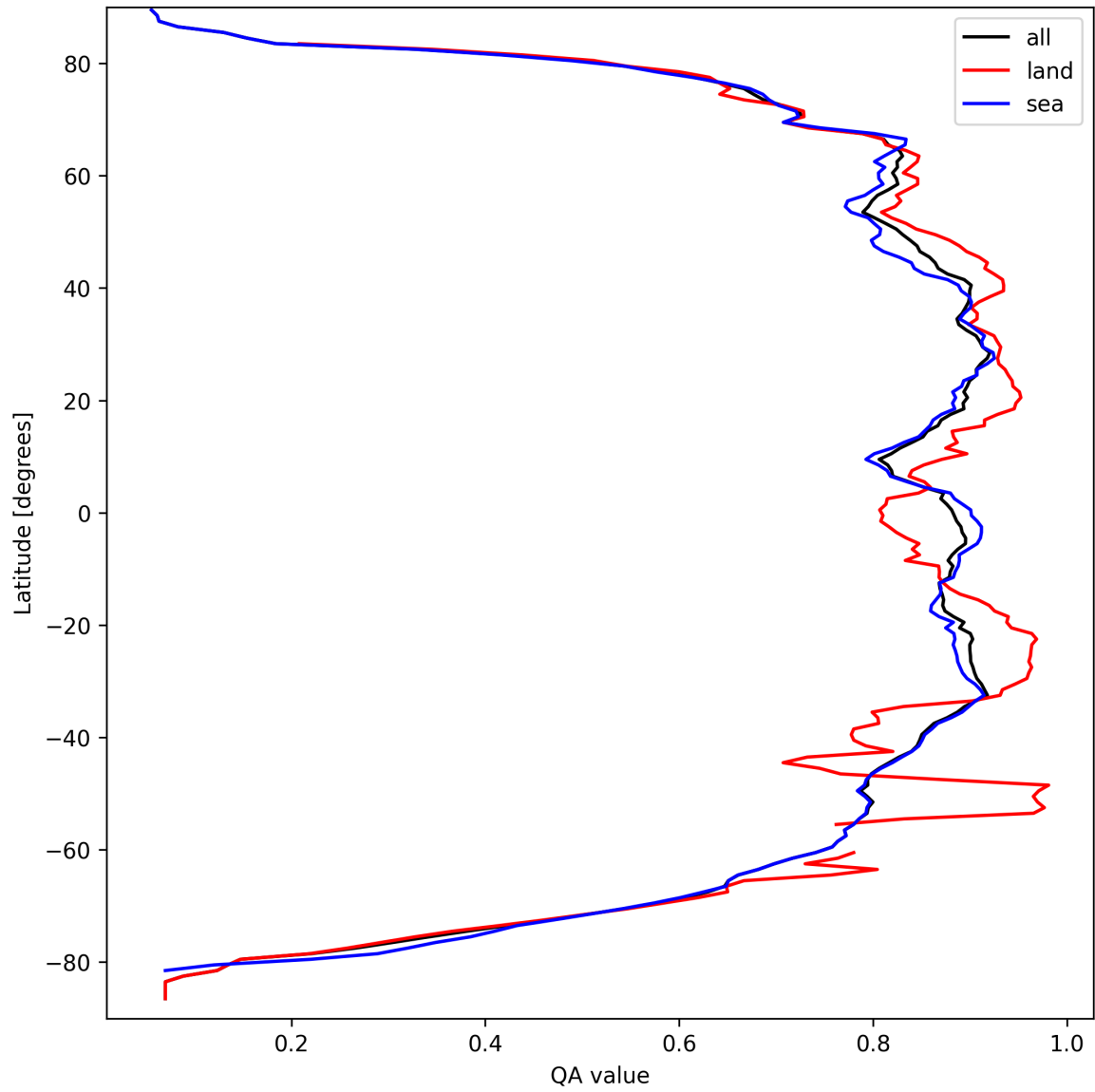
Figure 11: Zonal average of “QA value” for 2025-09-16 to 2025-09-18.
