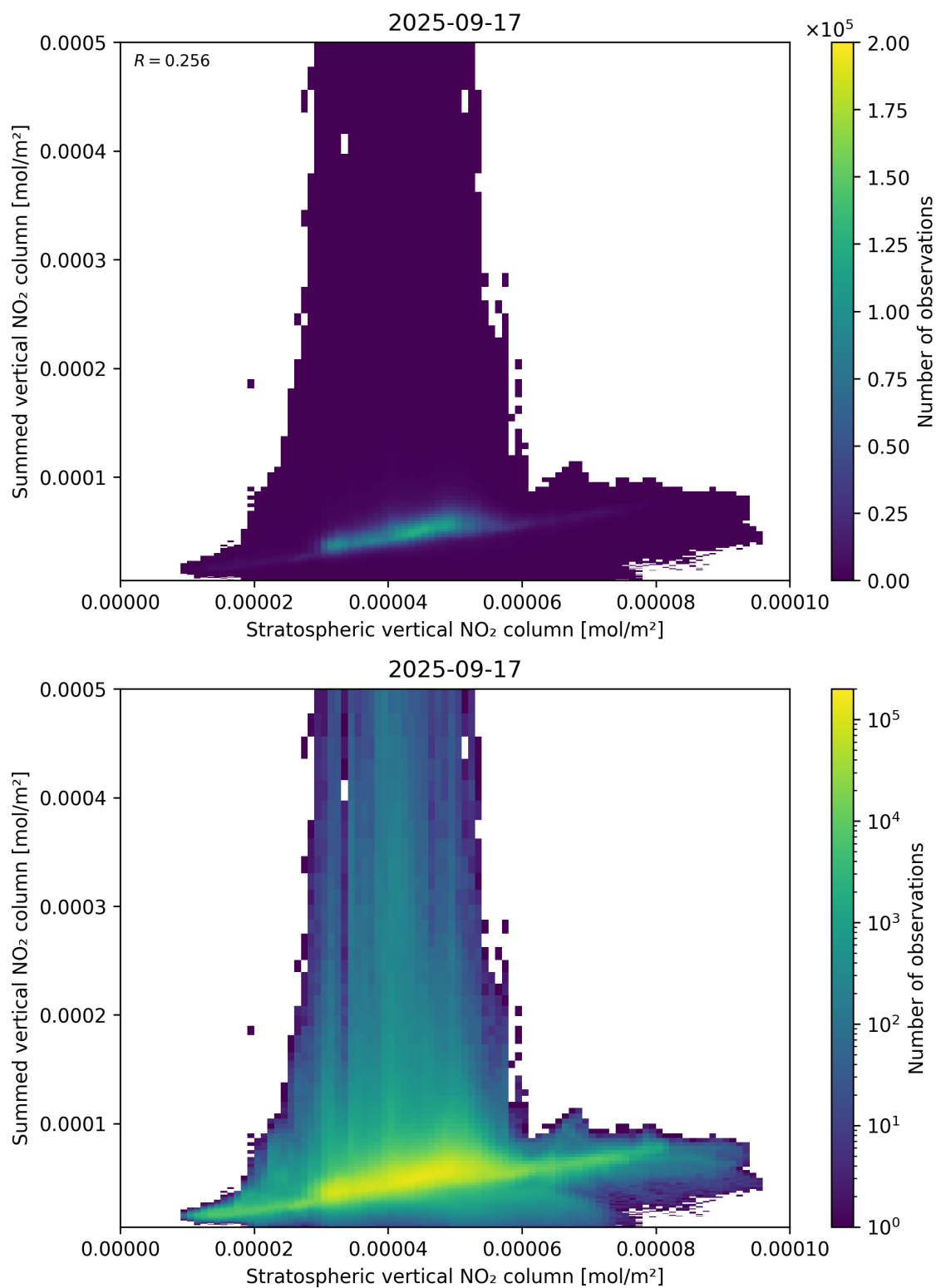
Figure 98: Scatter density plot of “Stratospheric vertical NO 2 column” against “Summed vertical NO 2 column” for 2025-09-16 to 2025-09-18.
