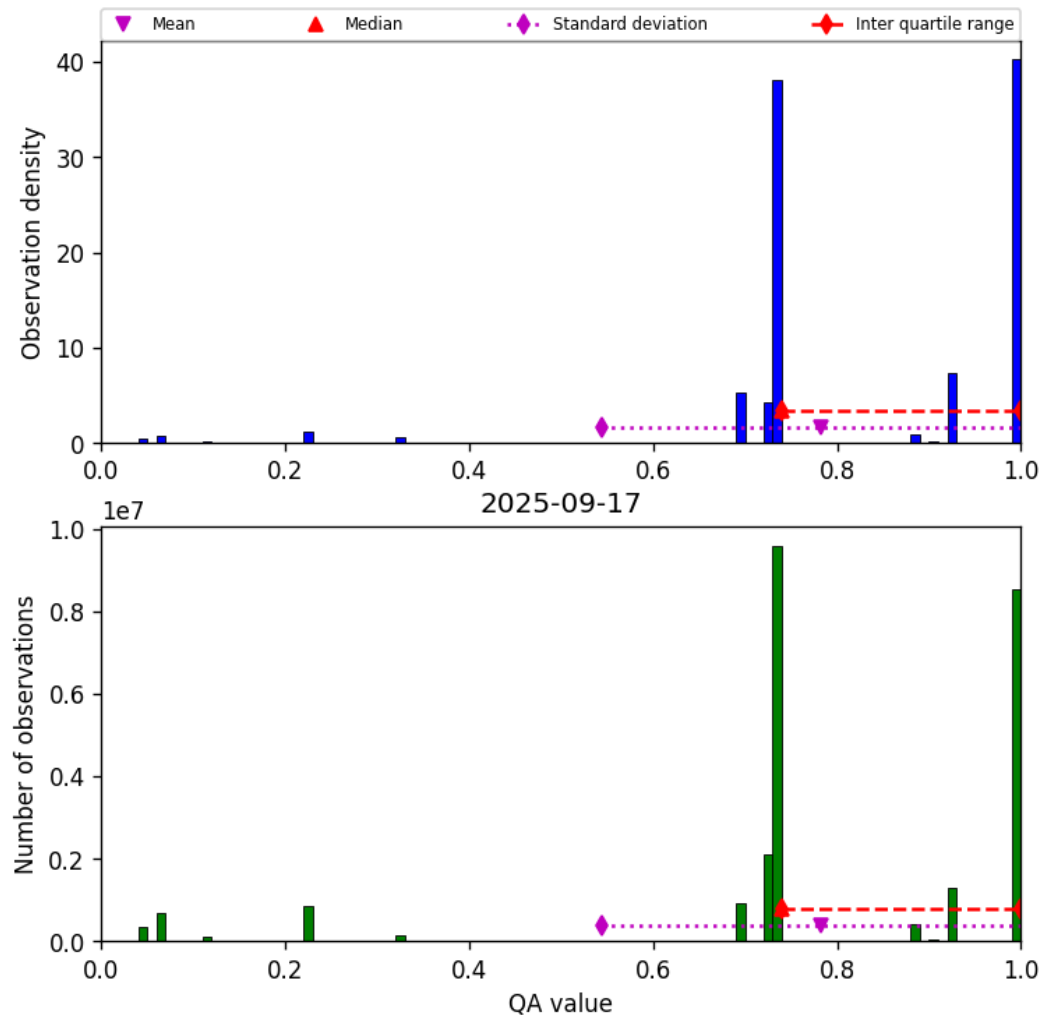
Figure 28: Histogram of “QA value” for 2025-09-16 to 2025-09-18
