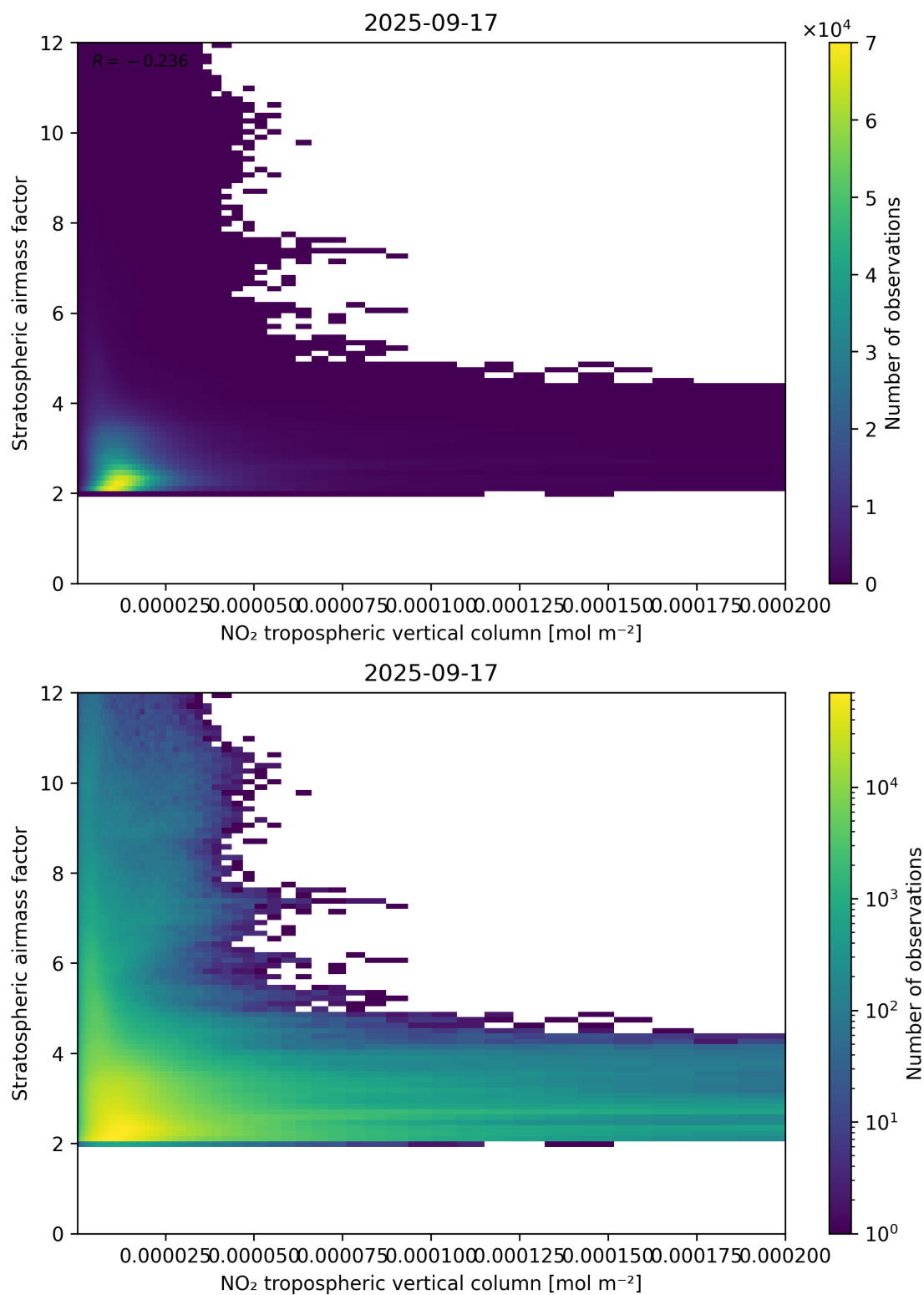
Figure 121: Scatter density plot of “NO 2 tropospheric vertical column” against “Stratospheric airmass factor” for 2025-09-16 to 2025-09-18.
