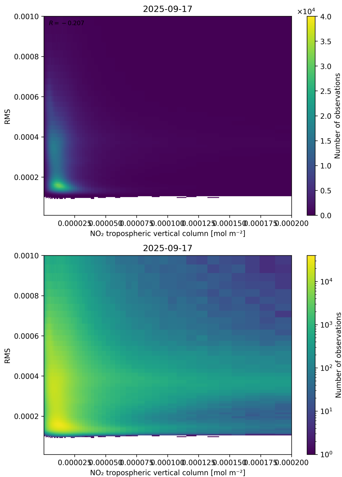
Figure 142: Scatter density plot of “NO 2 tropospheric vertical column” against “RMS” for 2025-09-16 to 2025-09-18.
