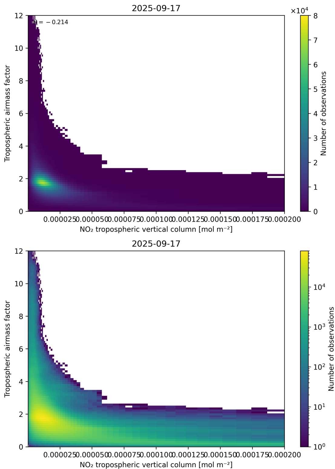
Figure 123: Scatter density plot of “NO 2 tropospheric vertical column” against “Tropospheric air mass factor” for 2025-09-16 to 2025-09-18.
