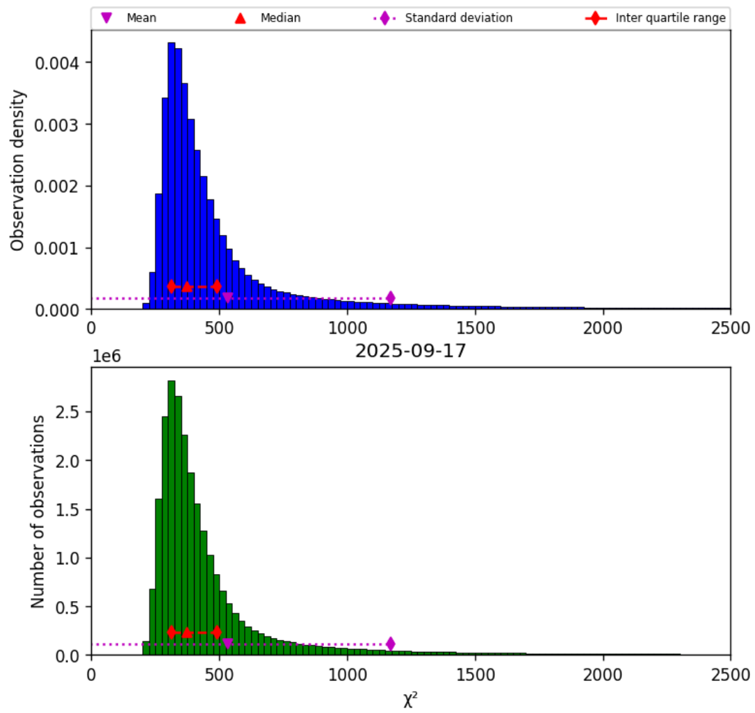
Figure 42: Histogram of “ \chi^2 ” for 2025-09-16 to 2025-09-18
