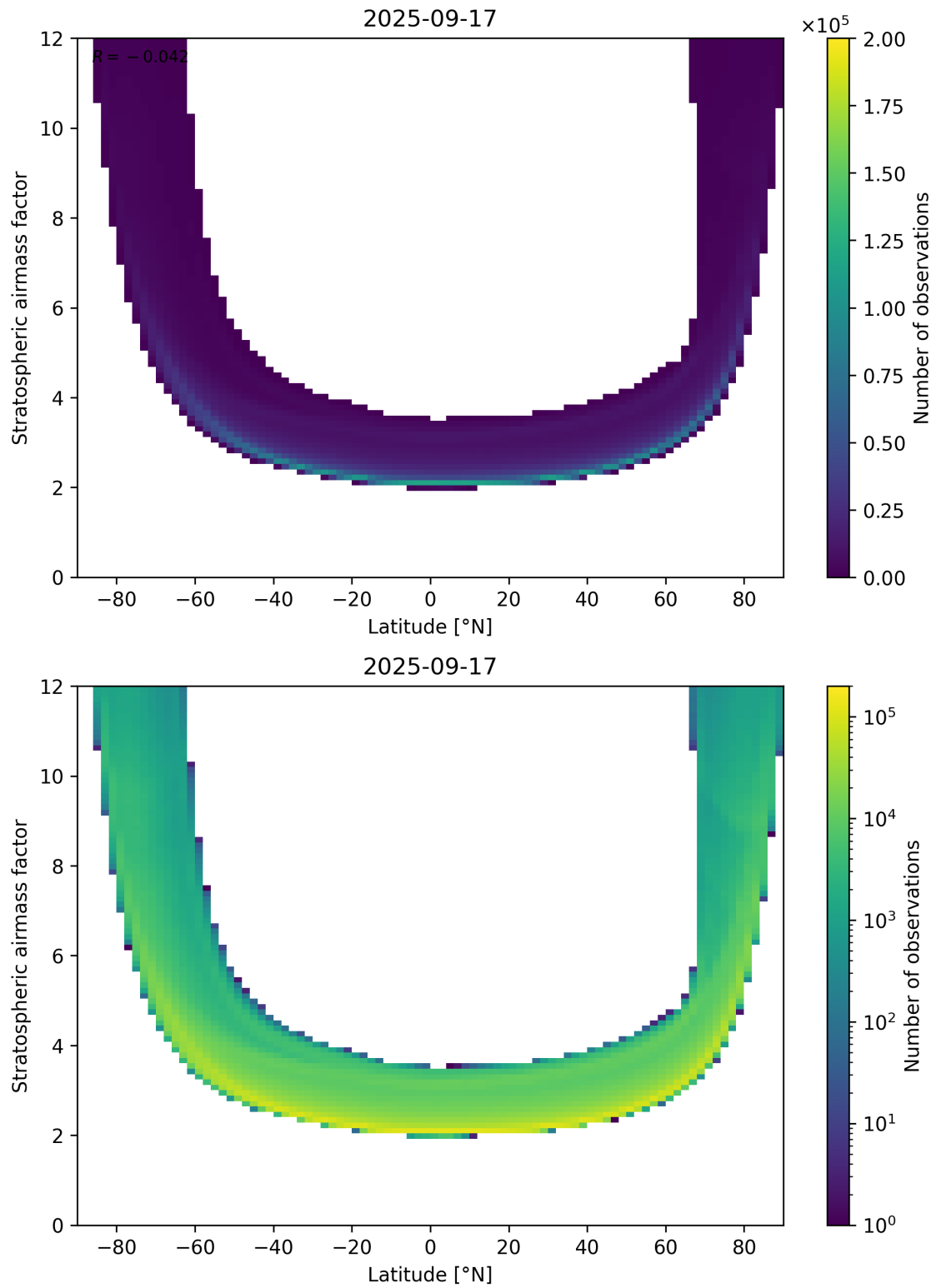
Figure 83: Scatter density plot of “Latitude” against “Stratospheric airmass factor” for 2025-09-16 to 2025-09-18.
