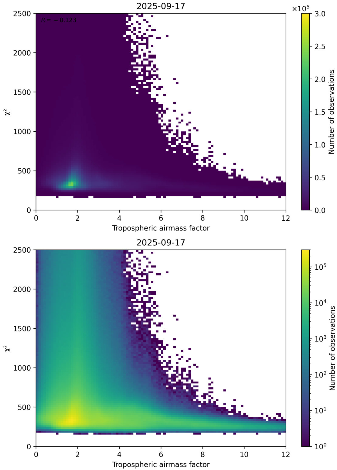
Figure 73: Scatter density plot of “Tropospheric airmass factor” against “ \chi^2 ” for 2025-09-16 to 2025-09-18.
