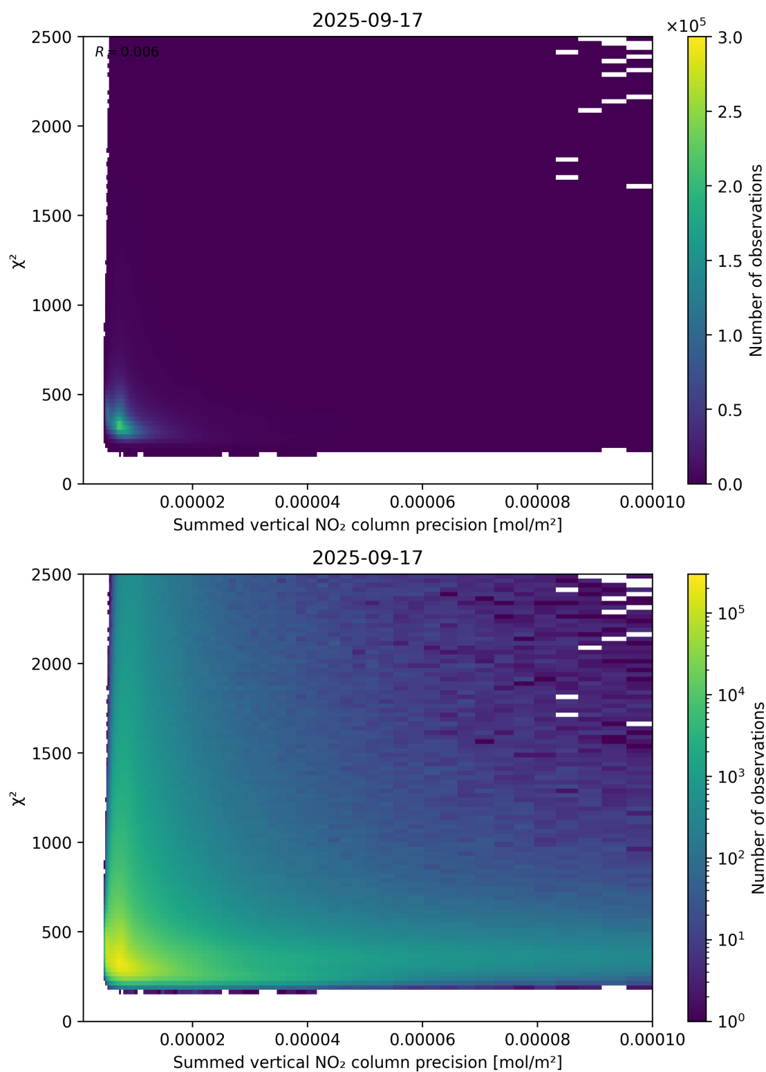
Figure 107: Scatter density plot of “Summed vertical NO 2 column precision” against “ \chi^2 ” for 2025-09-16 to 2025-09-18.
