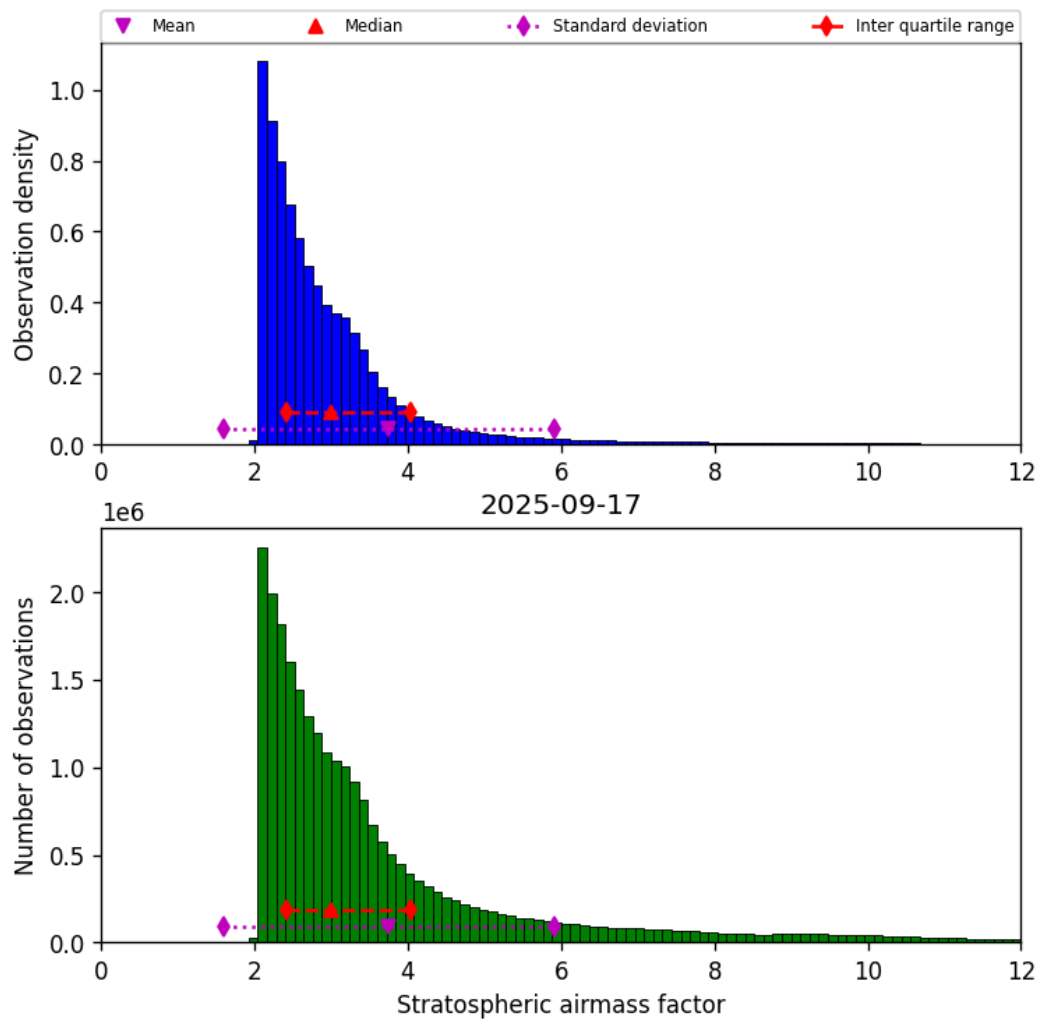
Figure 44: Histogram of “Stratospheric airmass factor” for 2025-09-16 to 2025-09-18
