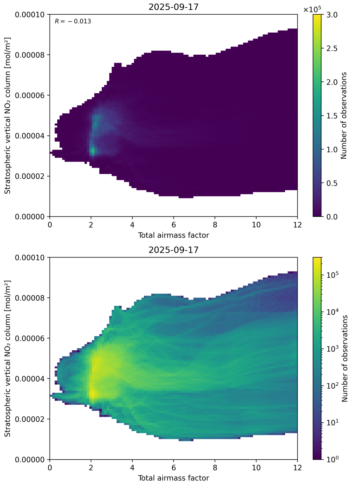
Figure 64: Scatter density plot of “Total airmass factor” against “Stratospheric vertical NO 2 column” for 2025-09-16 to 2025-09-18.
