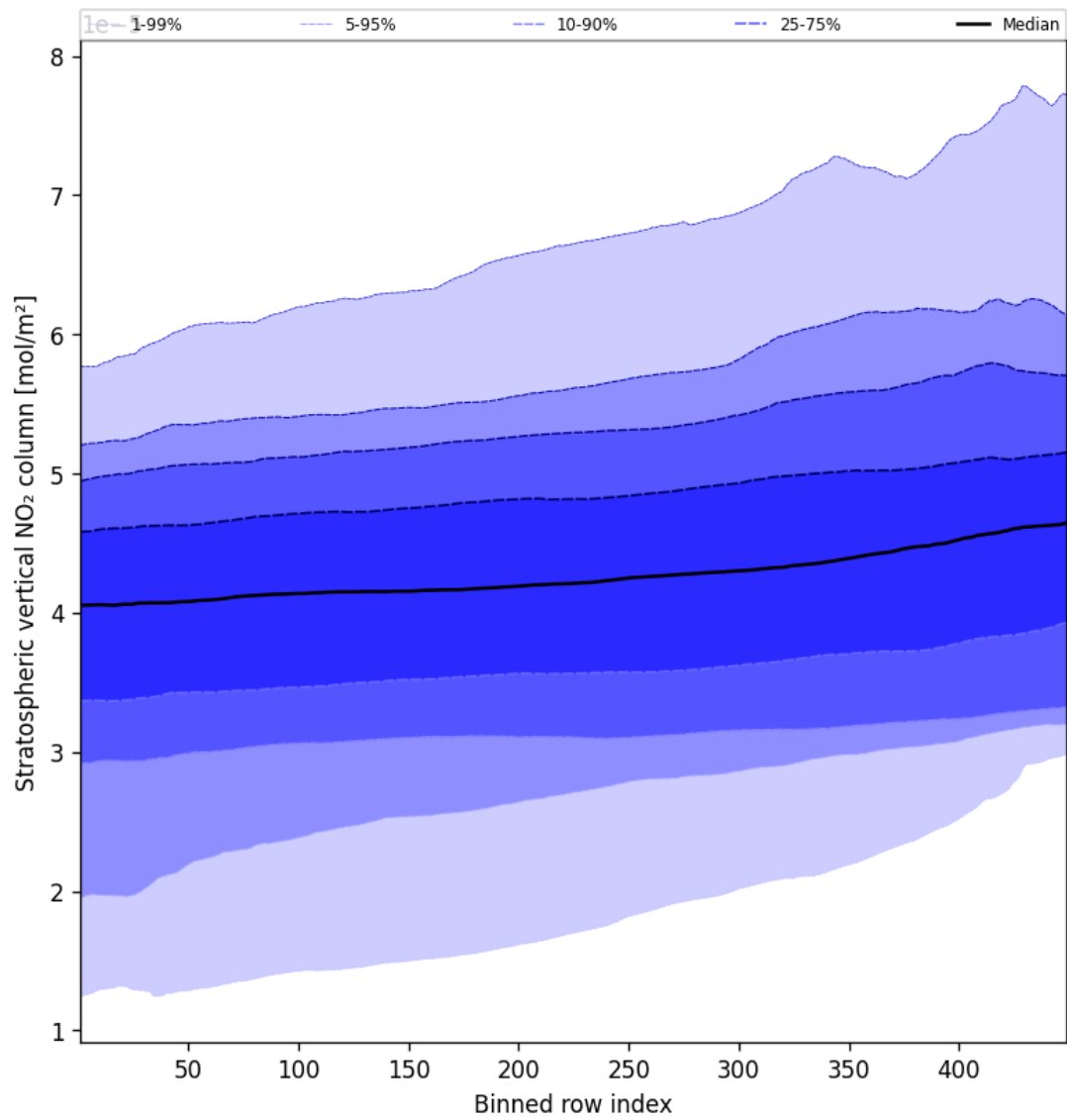
Figure 53: Along track statistics of “Stratospheric vertical NO 2 column” for 2025-09-16 to 2025-09-18
