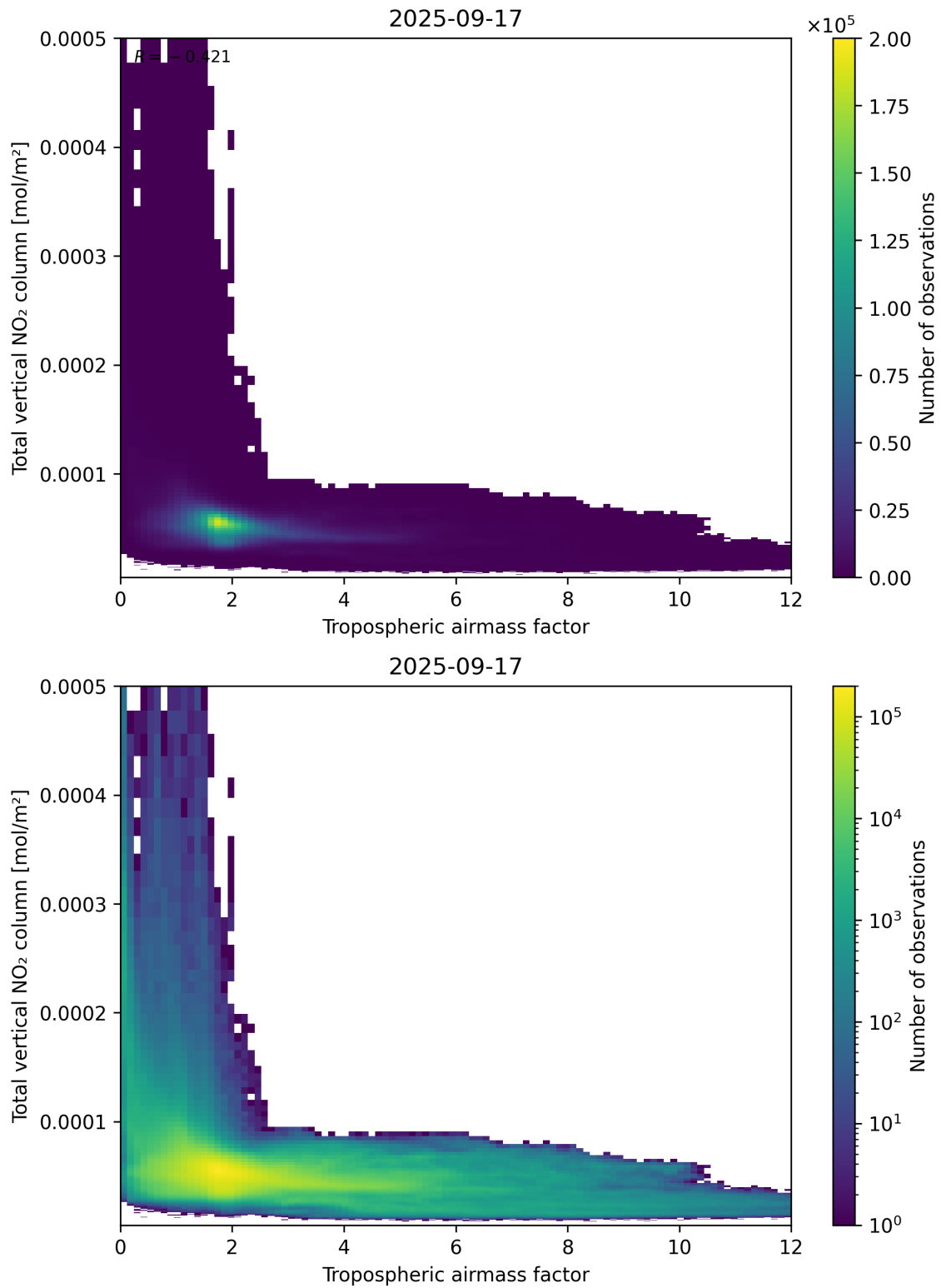
Figure 77: Scatter density plot of “Tropospheric airmass factor” against “Total vertical NO 2 column” for 2025-09-16 to 2025-09-18.
