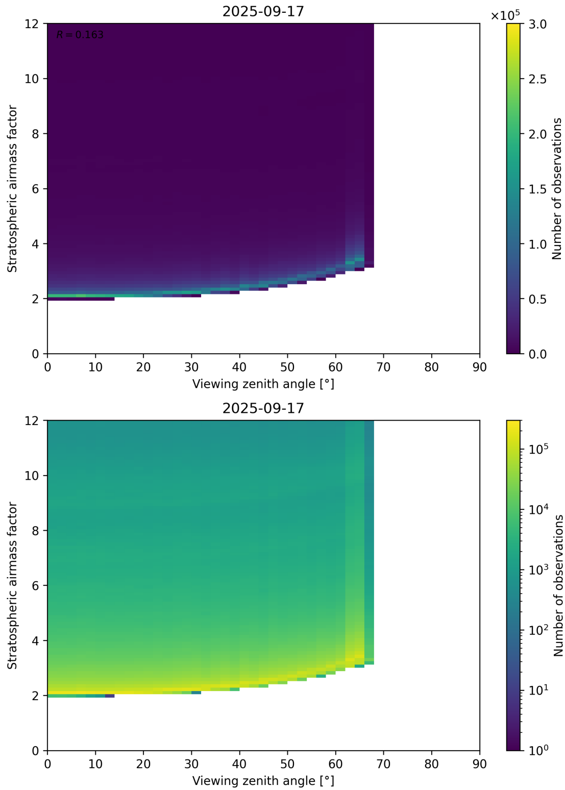
Figure 159: Scatter density plot of “Viewing zenith angle” against “Stratospheric airmass factor” for 2025-09-16 to 2025-09-18.
