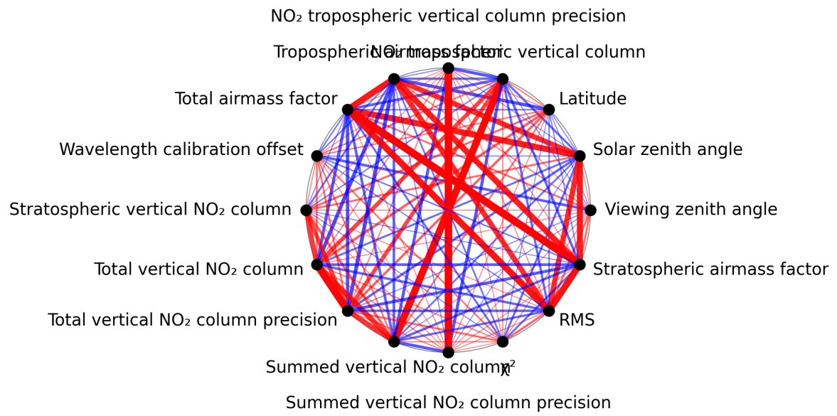
Figure 1: Map of correlation graph for 2025-09-16 to 2025-09-18.
