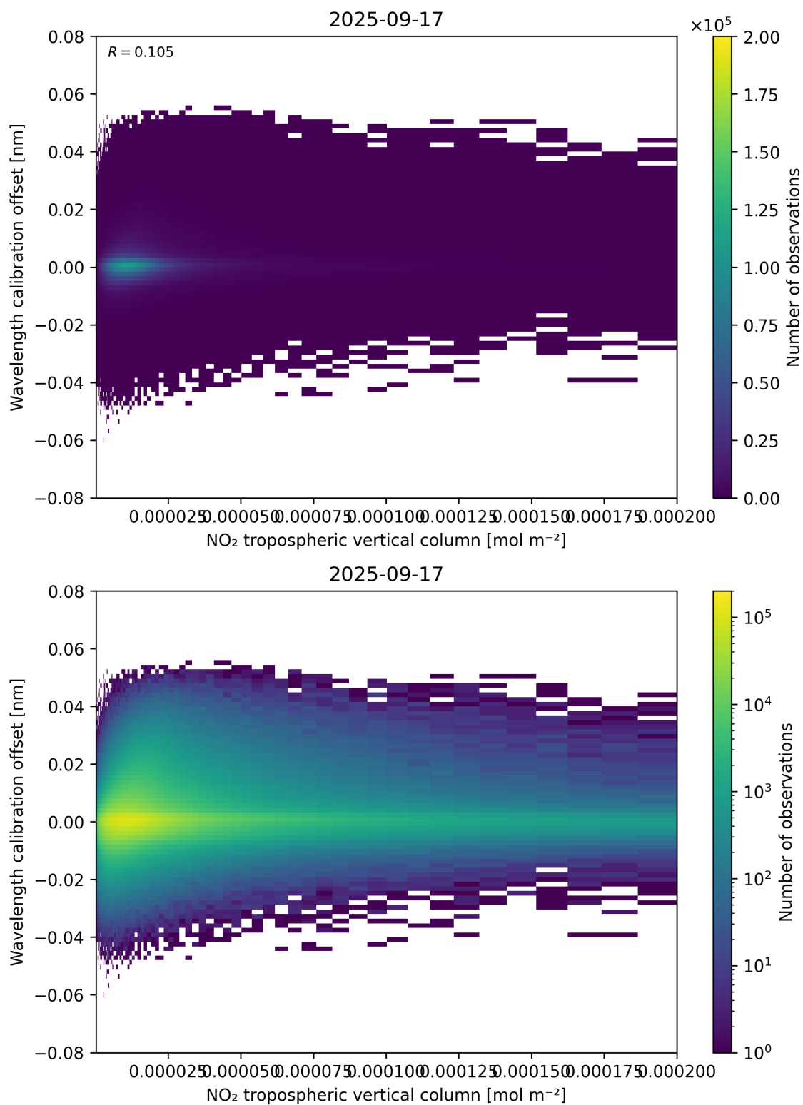
Figure 143: Scatter density plot of “NO 2 tropospheric vertical column” against “Wavelength calibration offset” for 2025-09-16 to 2025-09-18.
