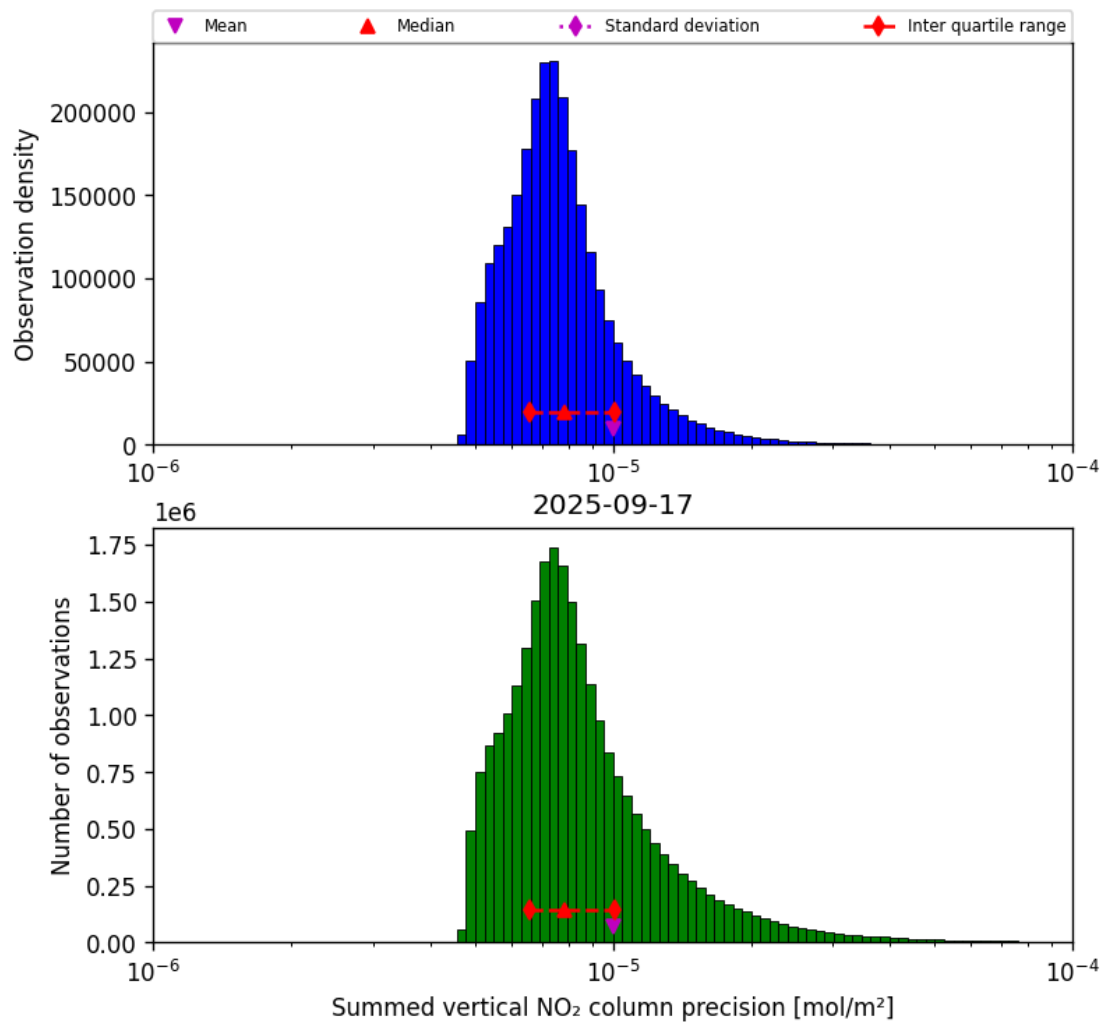
Figure 41: Histogram of "Summed vertical NO 2 column precision" for 2025-09-16 to 2025-09-18
