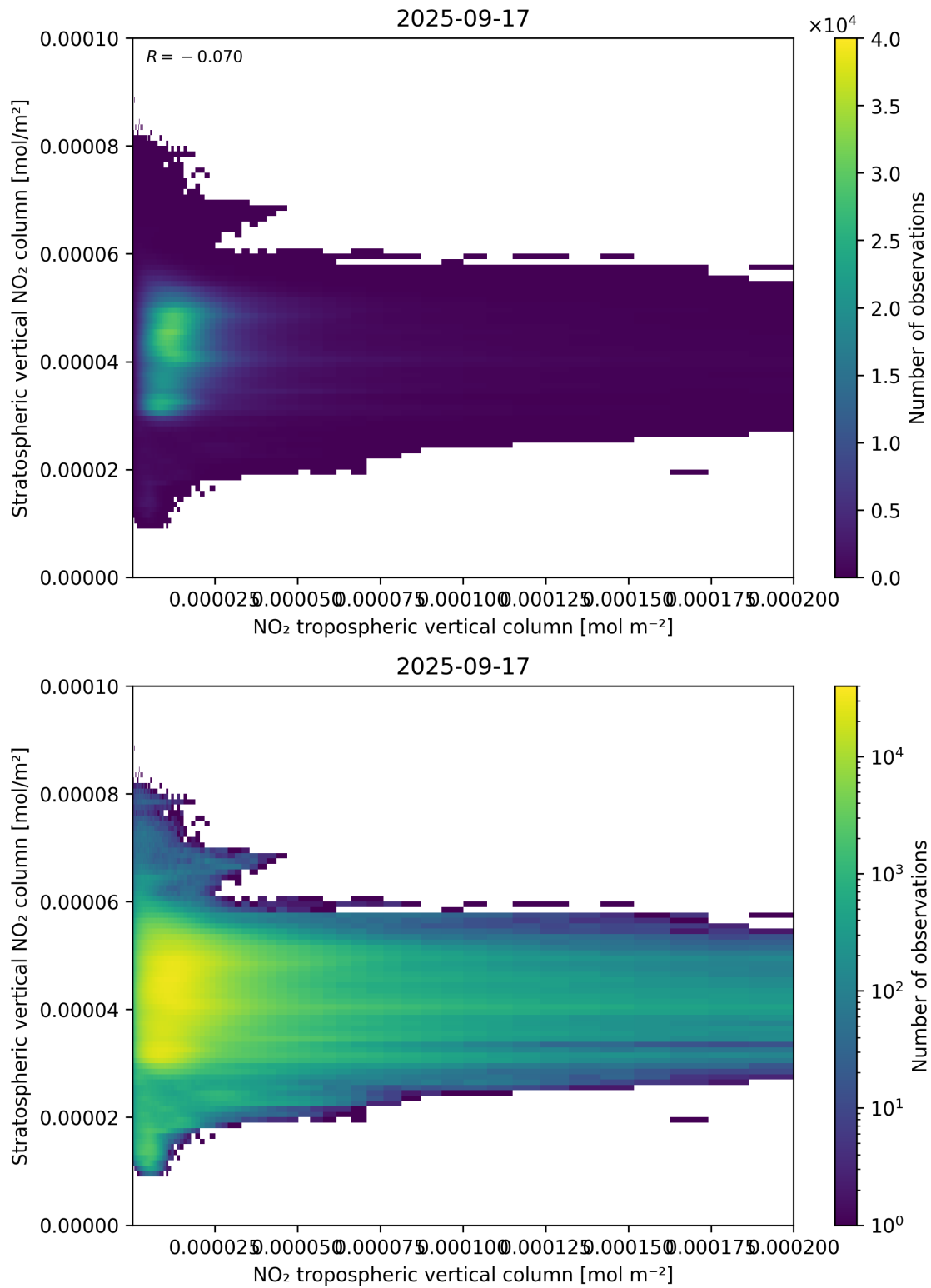
Figure 125: Scatter density plot of “NO 2 tropospheric vertical column” against “Stratospheric vertical NO 2 column” for 2025-09-16 to 2025-09-18.
