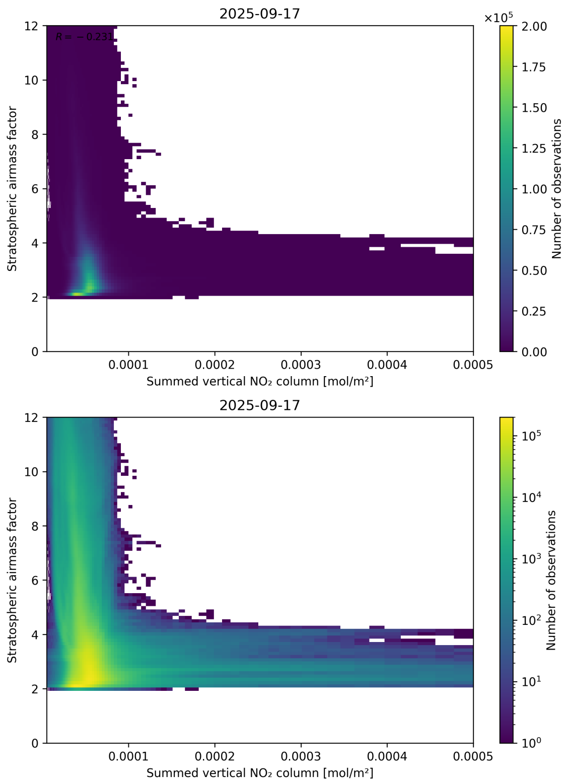
Figure 103: Scatter density plot of “Summed vertical NO 2 column” against “Stratospheric airmass factor” for 2025-09-16 to 2025-09-18.
