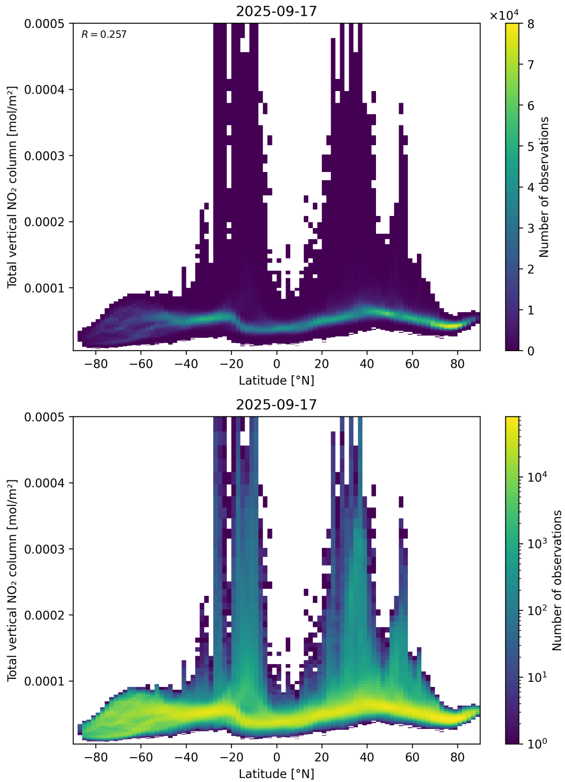
Figure 90: Scatter density plot of “Latitude” against “Total vertical NO 2 column” for 2025-09-16 to 2025-09-18.
