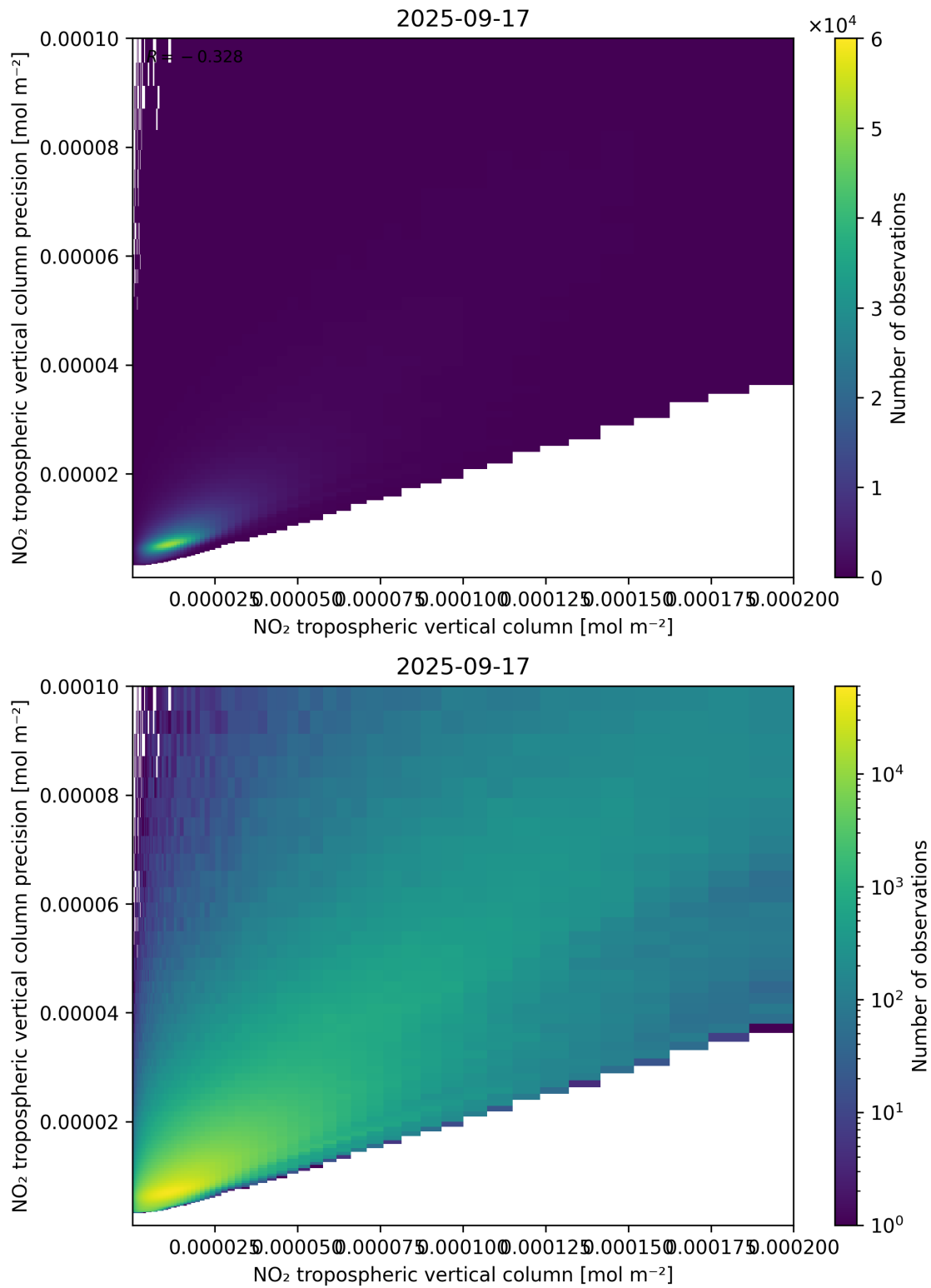
Figure 130: Scatter density plot of “NO 2 tropospheric vertical column” against “NO 2 tropospheric vertical column precision” for 2025-09-16 to 2025-09-18.
