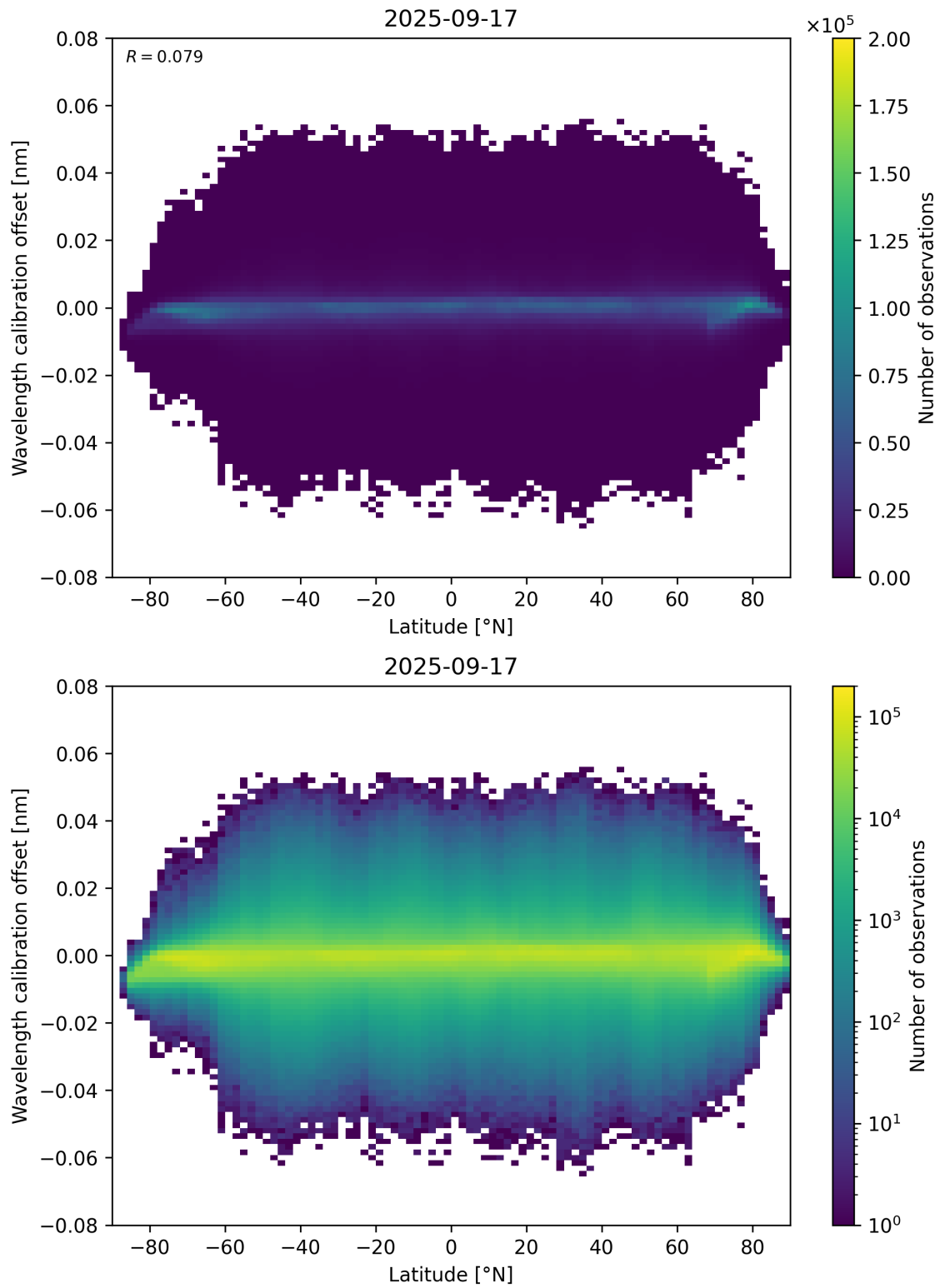
Figure 95: Scatter density plot of “Latitude” against “Wavelength calibration offset” for 2025-09-16 to 2025-09-18.
