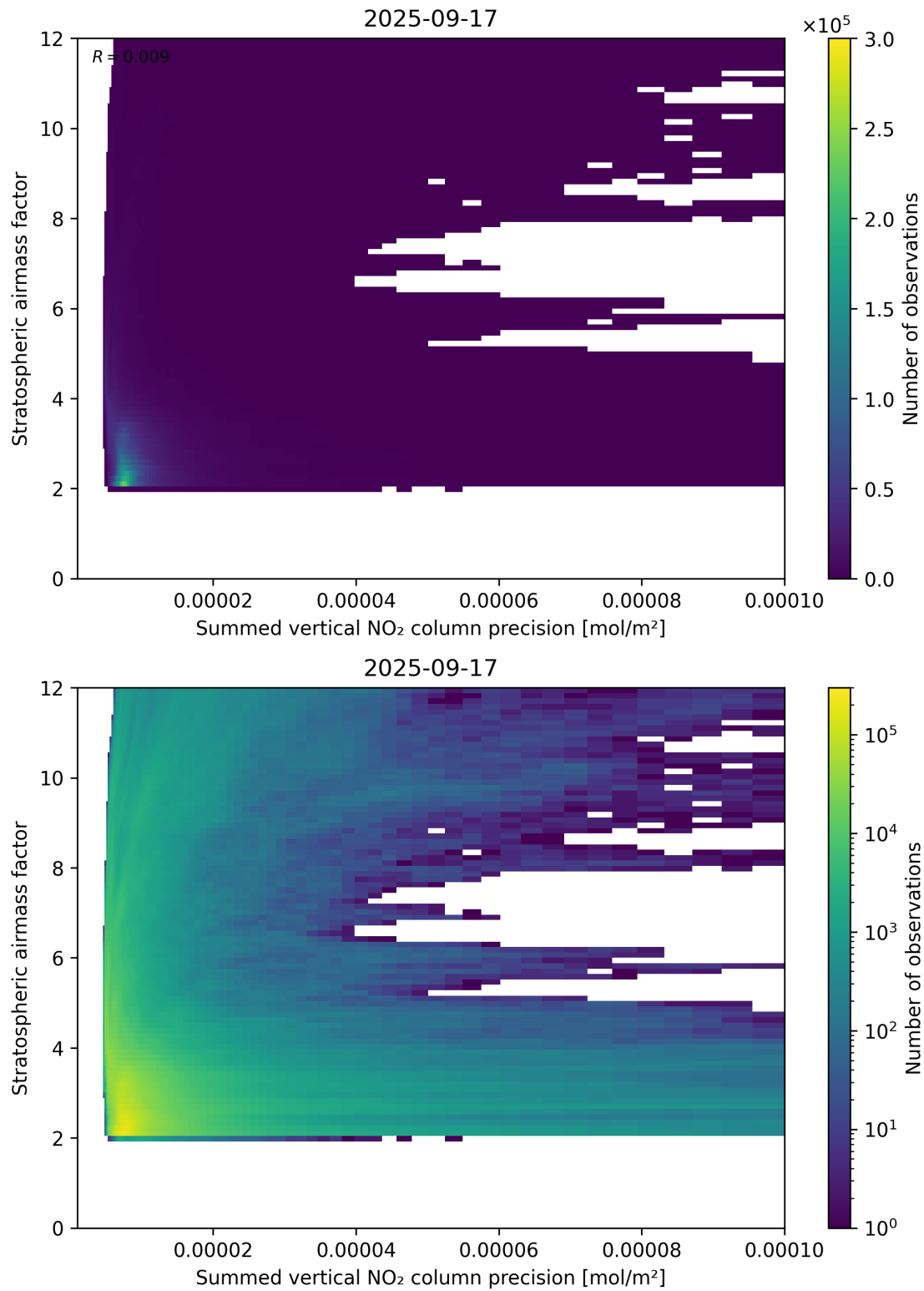
Figure 106: Scatter density plot of “Summed vertical NO 2 column precision” against “Stratospheric airmass factor” for 2025-09-16 to 2025-09-18.
