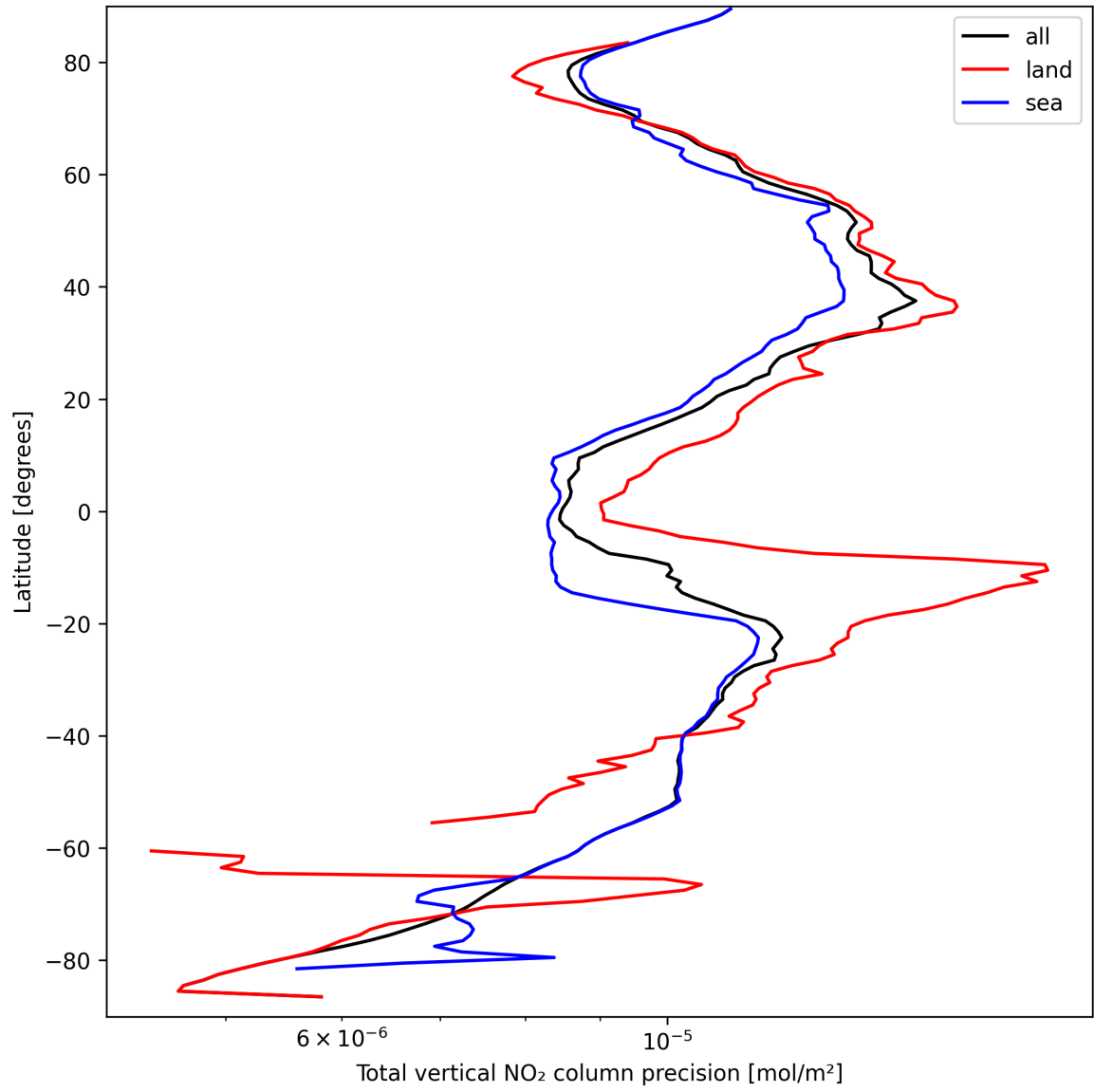
Figure 22: Zonal average of “Total vertical NO 2 column precision” for 2025-09-16 to 2025-09-18.
