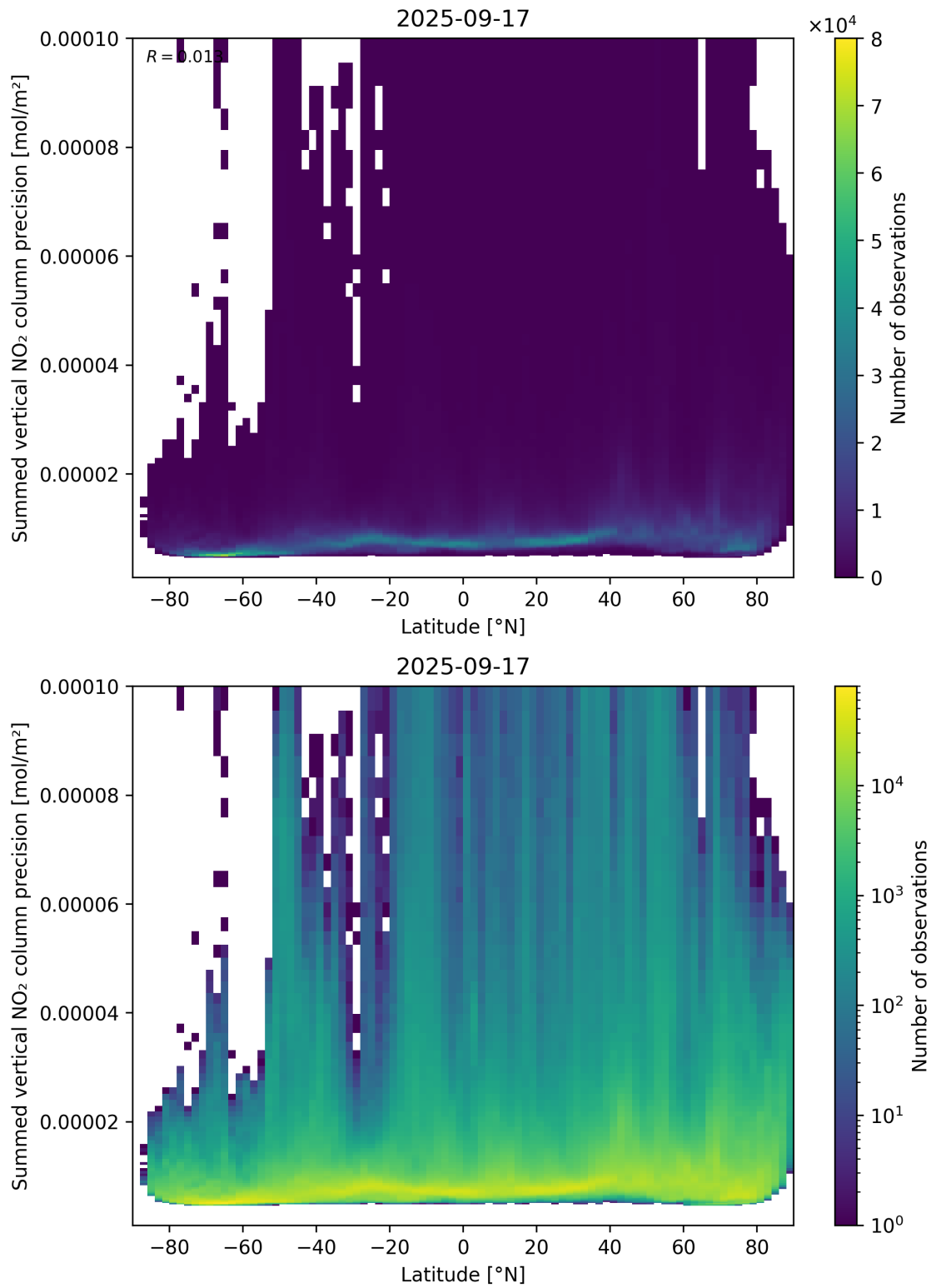
Figure 89: Scatter density plot of “Latitude” against “Summed vertical NO 2 column precision” for 2025-09-16 to 2025-09-18.
