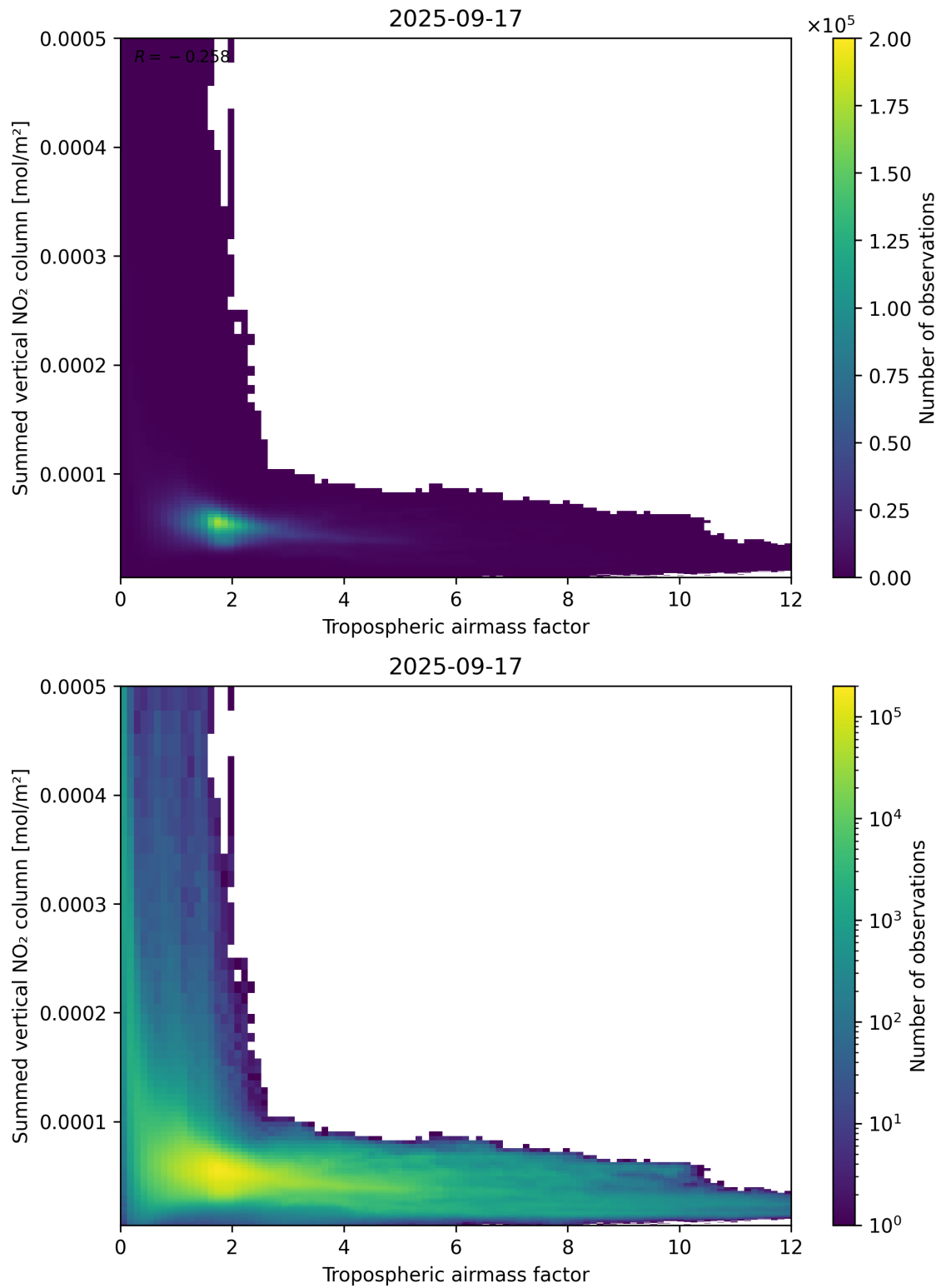
Figure 75: Scatter density plot of “Tropospheric air mass factor” against “Summed vertical NO 2 column” for 2025-09-16 to 2025-09-18.
