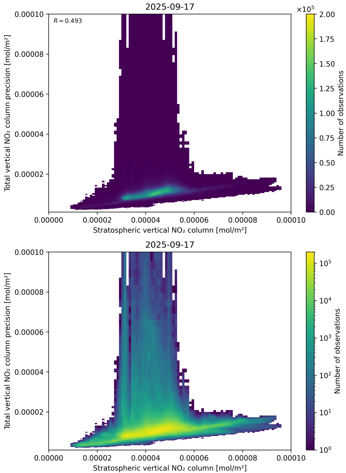
Figure 101: Scatter density plot of “Stratospheric vertical NO 2 column” against “Total vertical NO 2 column precision” for 2025-09-16 to 2025-09-18.
