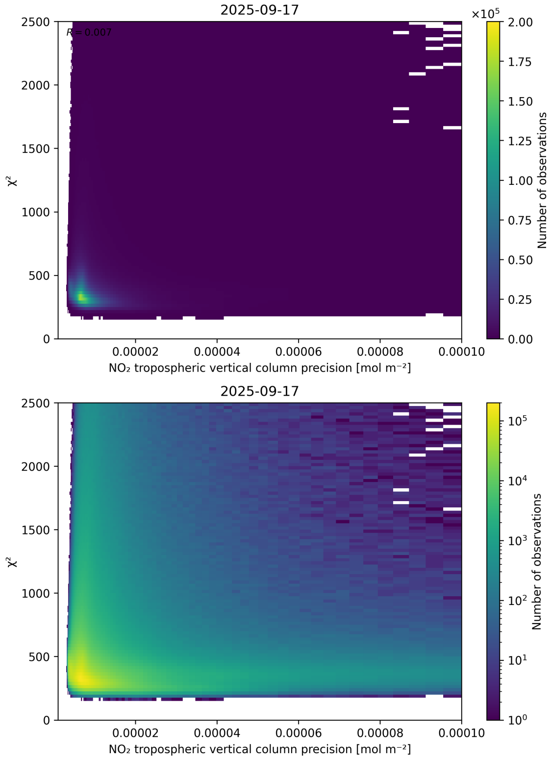
Figure 134: Scatter density plot of “NO 2 tropospheric vertical column precision” against “ \chi^2 ” for 2025-09-16 to 2025-09-18.
