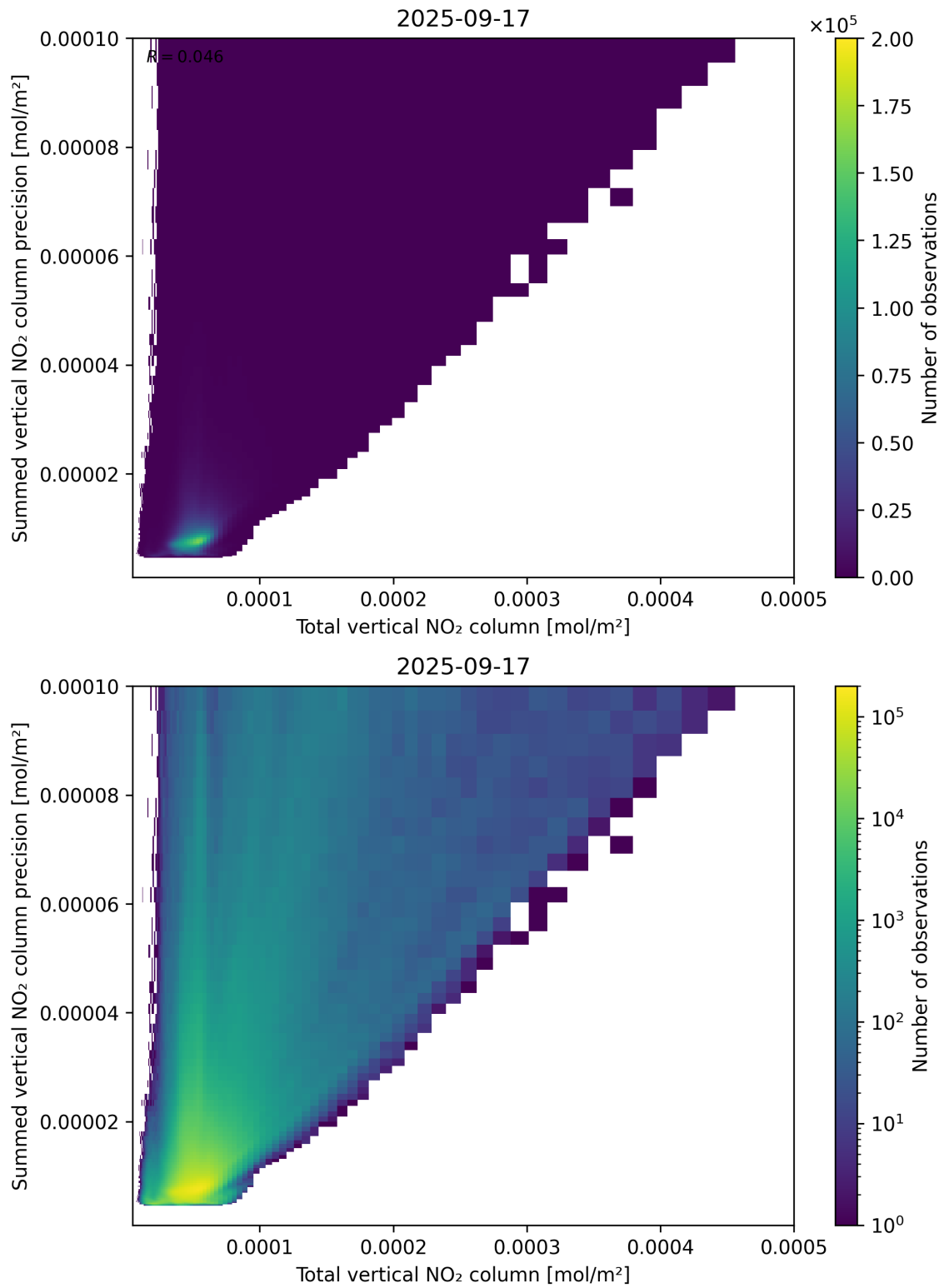
Figure 113: Scatter density plot of “Total vertical NO 2 column” against “Summed vertical NO 2 column precision” for 2025-09-16 to 2025-09-18.
