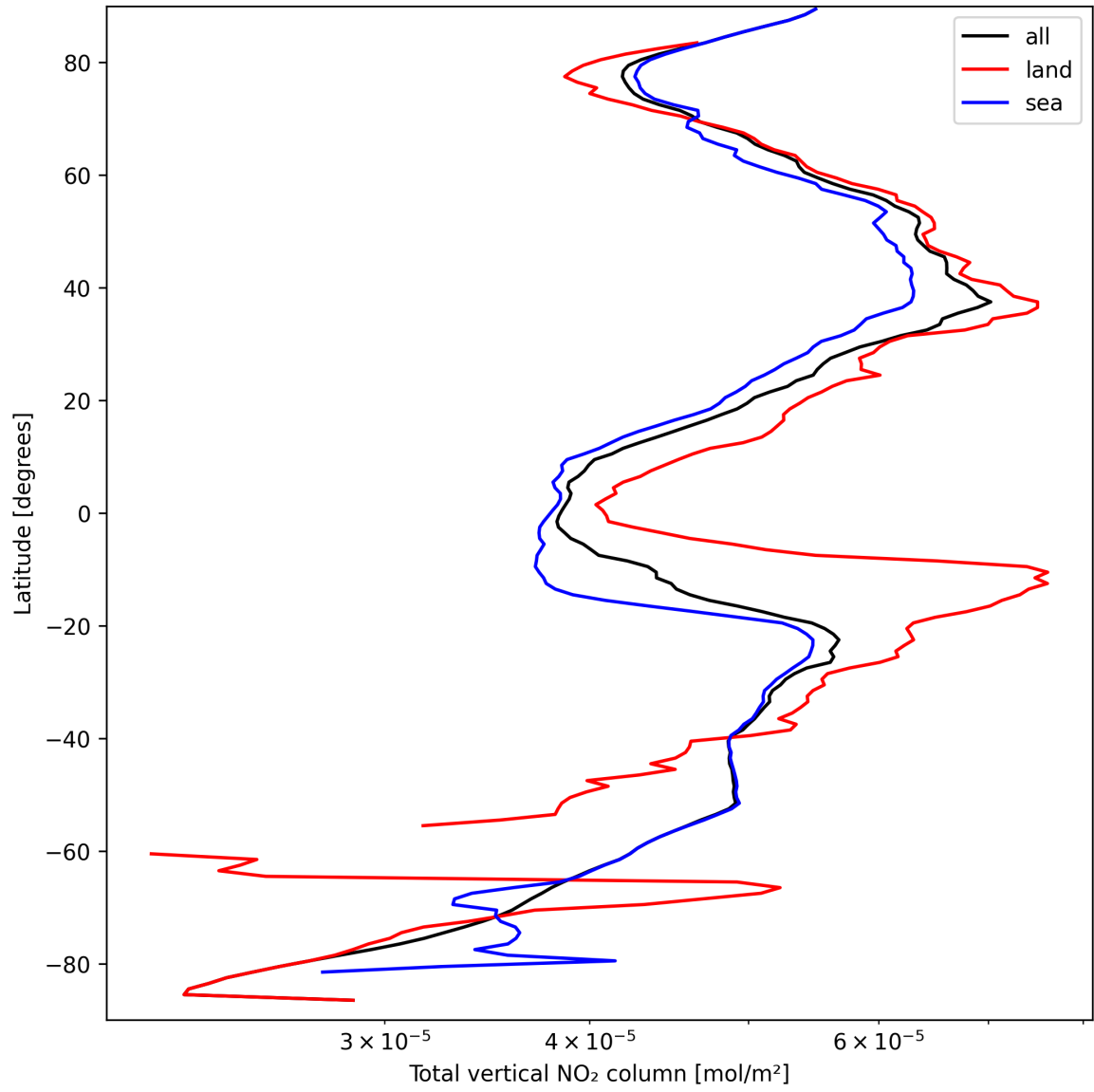
Figure 21: Zonal average of “Total vertical NO 2 column” for 2025-09-16 to 2025-09-18.
