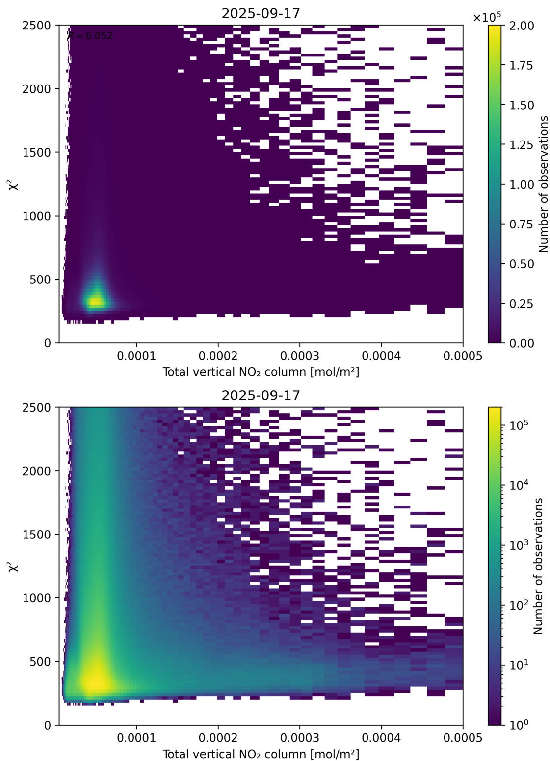
Figure 111: Scatter density plot of “Total vertical NO 2 column” against “ \chi^2 ” for 2025-09-16 to 2025-09-18.
