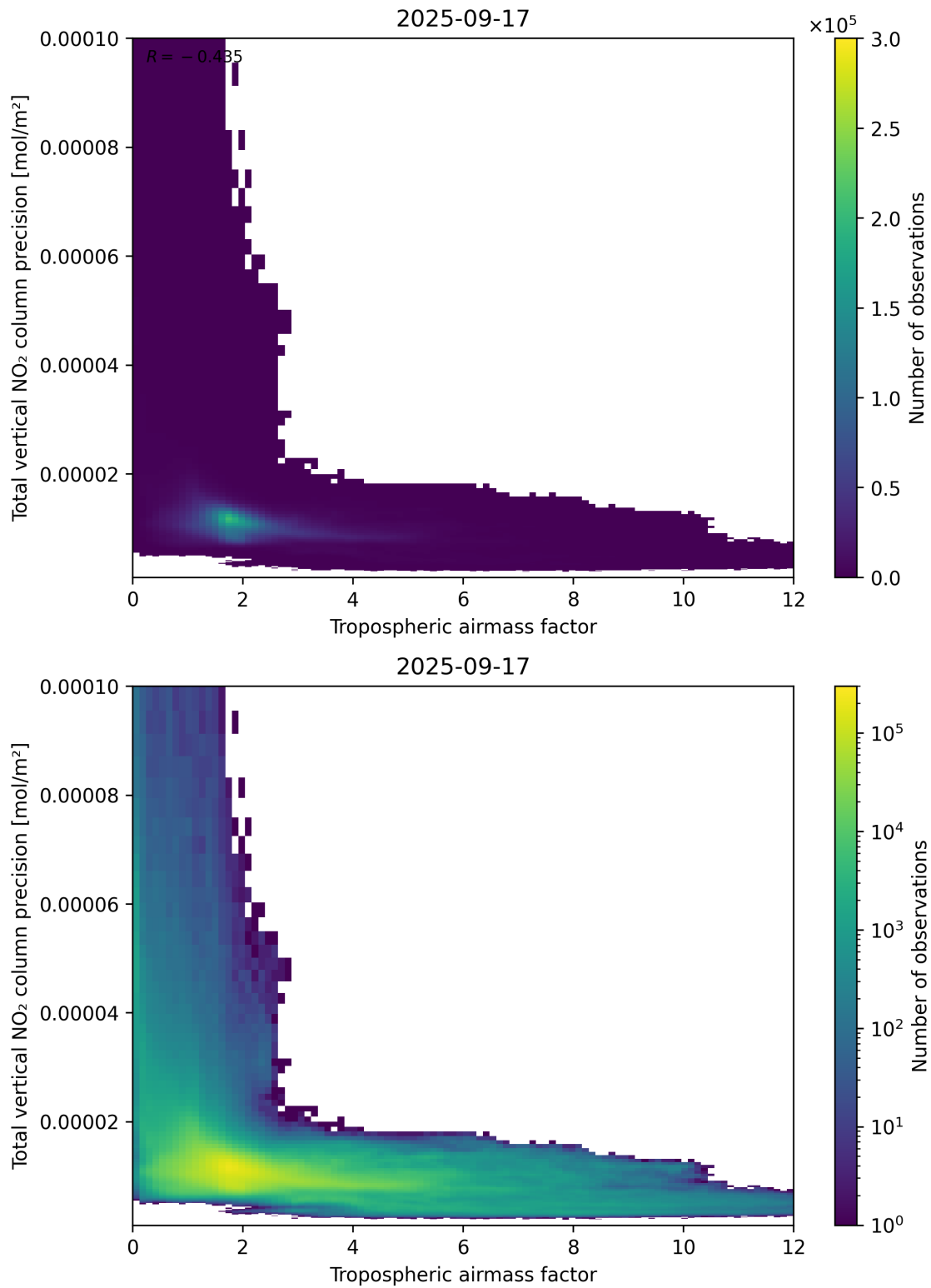
Figure 78: Scatter density plot of “Tropospheric air mass factor” against “Total vertical NO 2 column precision” for 2025-09-16 to 2025-09-18.
