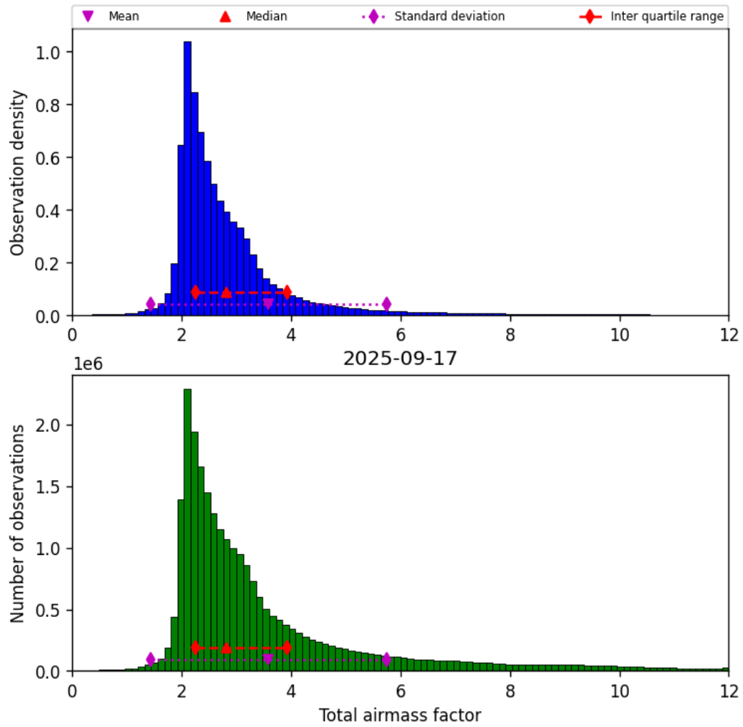
Figure 32: Histogram of “Total airmass factor” for 2025-09-16 to 2025-09-18
