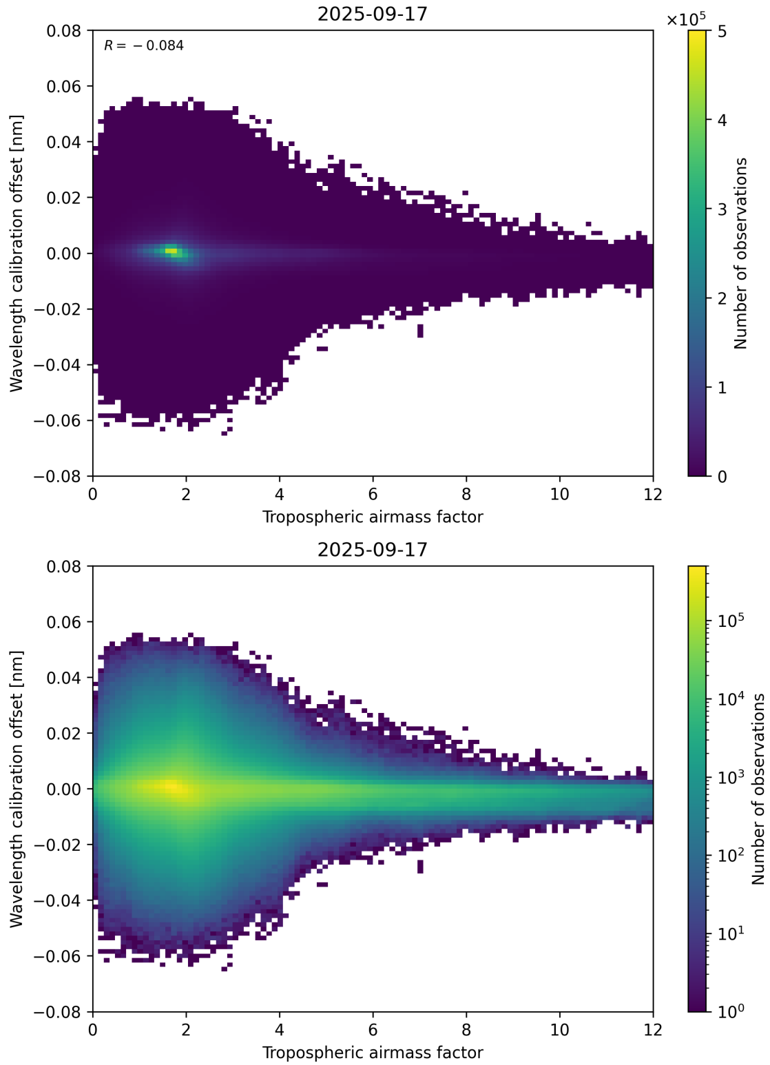
Figure 80: Scatter density plot of “Tropospheric airmass factor” against “Wavelength calibration offset” for 2025-09-16 to 2025-09-18.
