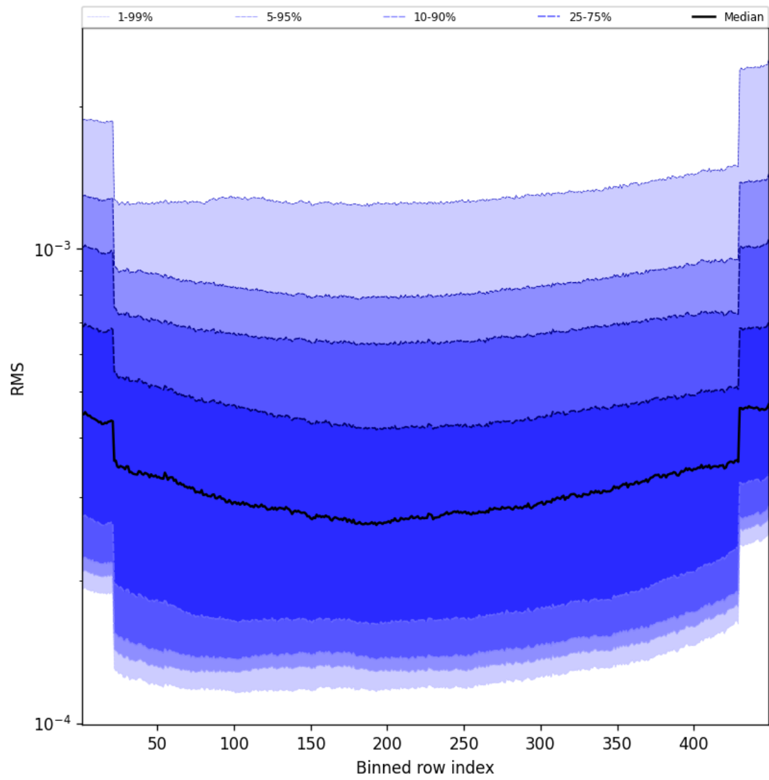
Figure 60: Along track statistics of “RMS” for 2025-09-16 to 2025-09-18
