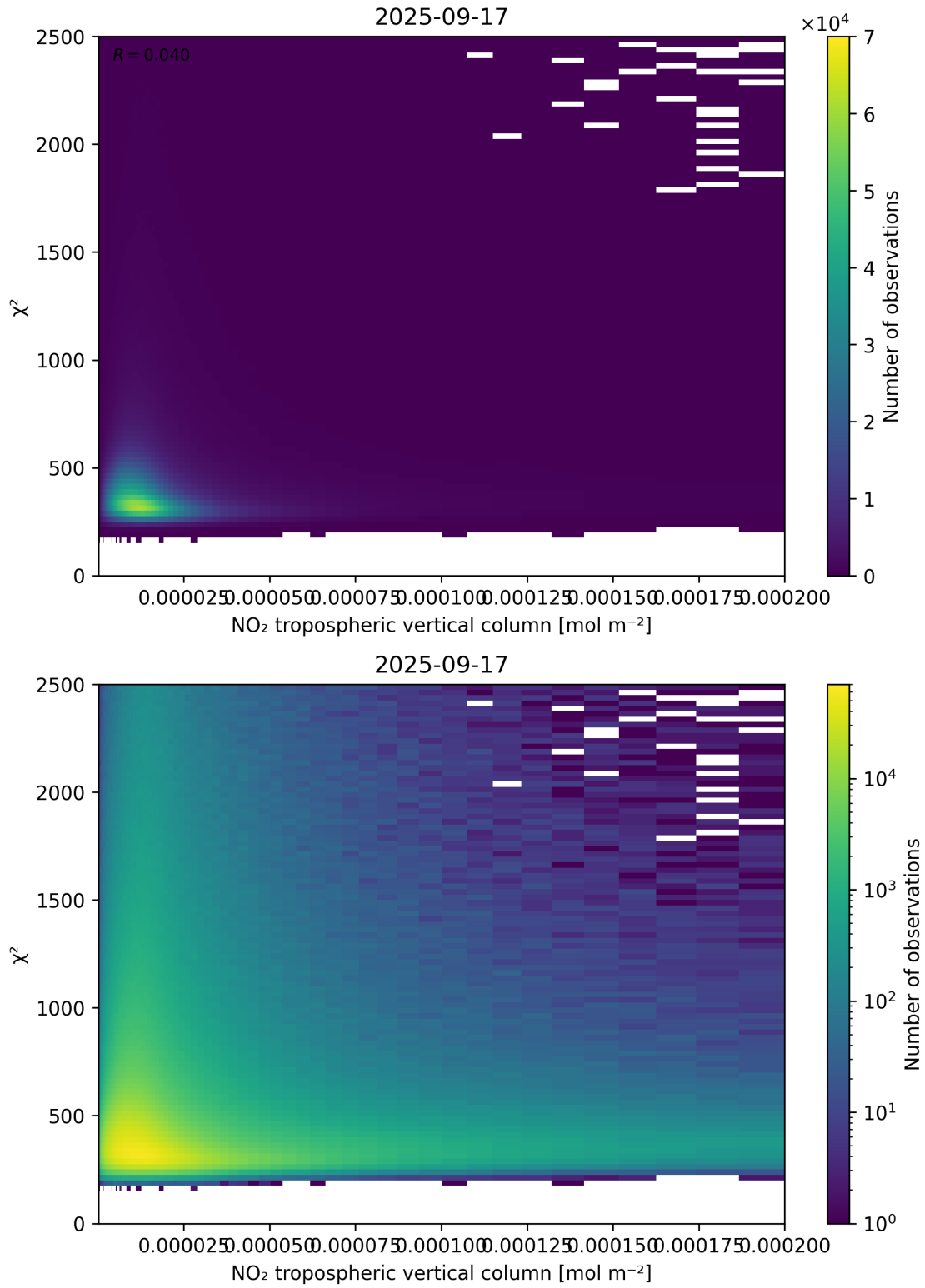
Figure 124: Scatter density plot of “NO 2 tropospheric vertical column” against “ \chi^2 ” for 2025-09-16 to 2025-09-18.
