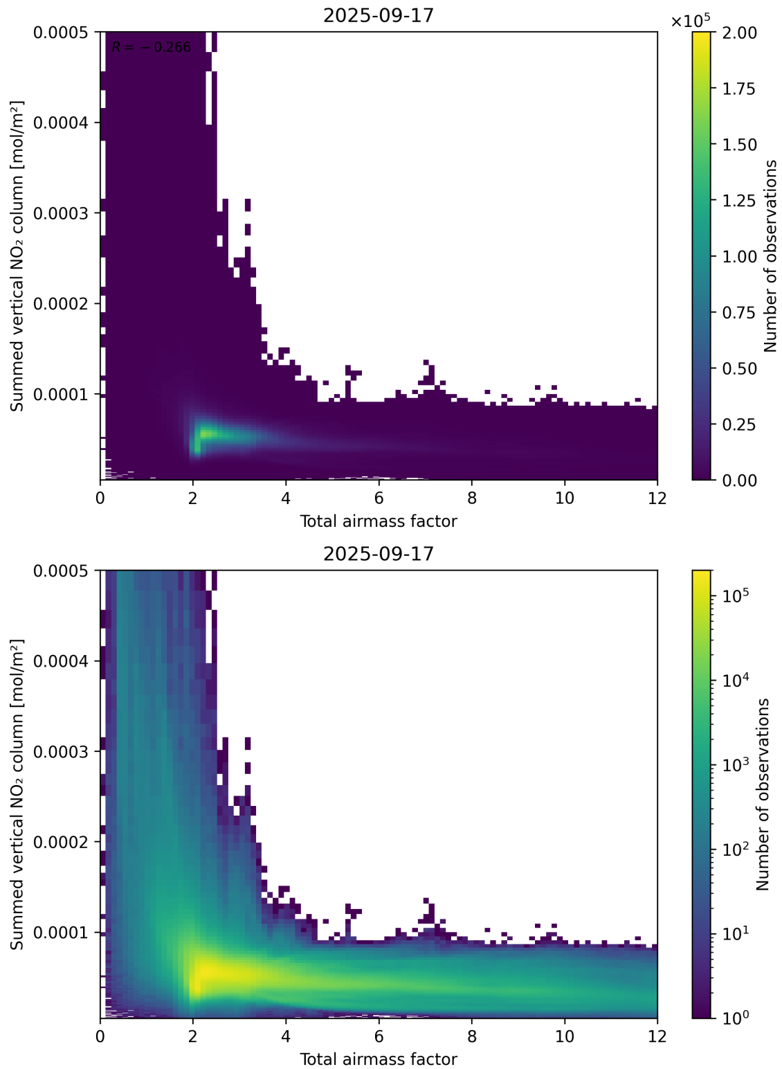
Figure 65: Scatter density plot of “Total airmass factor” against “Summed vertical NO 2 column” for 2025-09-16 to 2025-09-18.
