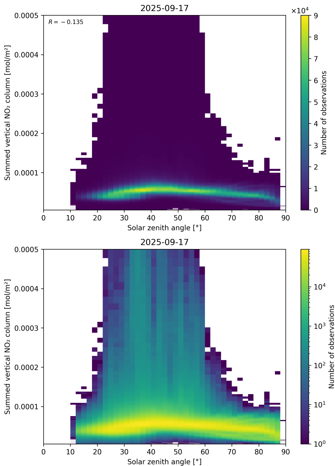
Figure 151: Scatter density plot of “Solar zenith angle” against “Summed vertical NO 2 column” for 2025-09-16 to 2025-09-18.
