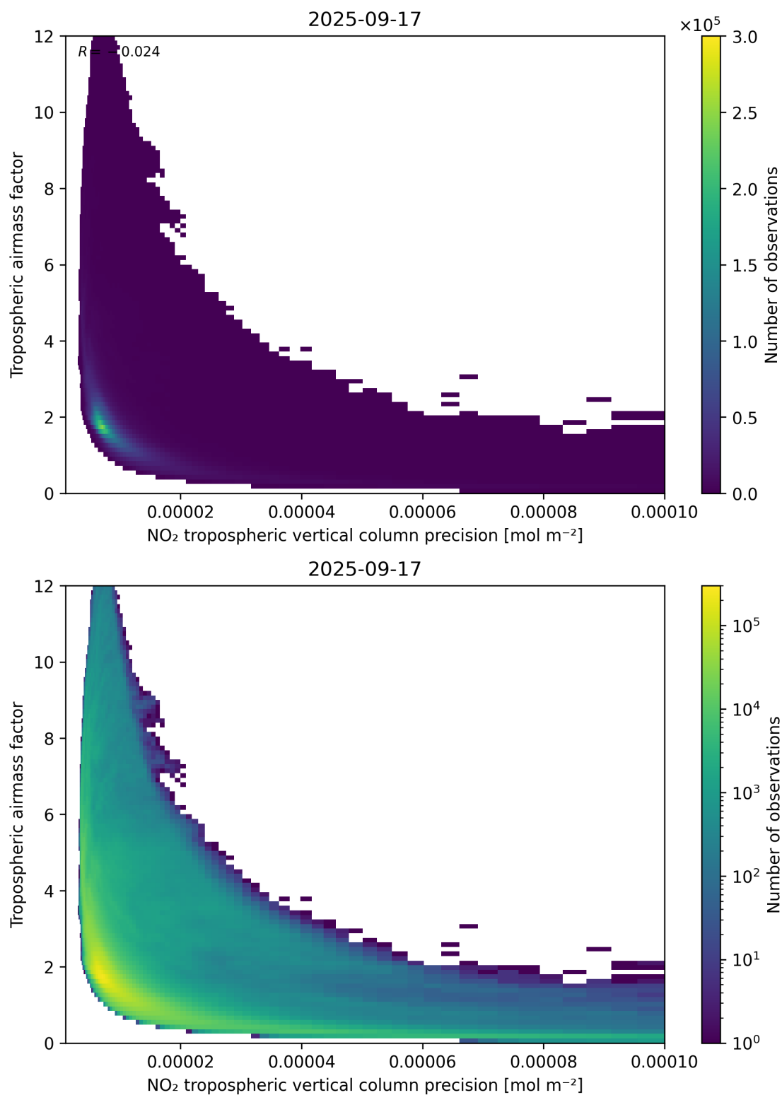
Figure 133: Scatter density plot of “NO 2 tropospheric vertical column precision” against “Tropospheric air mass factor” for 2025-09-16 to 2025-09-18.
