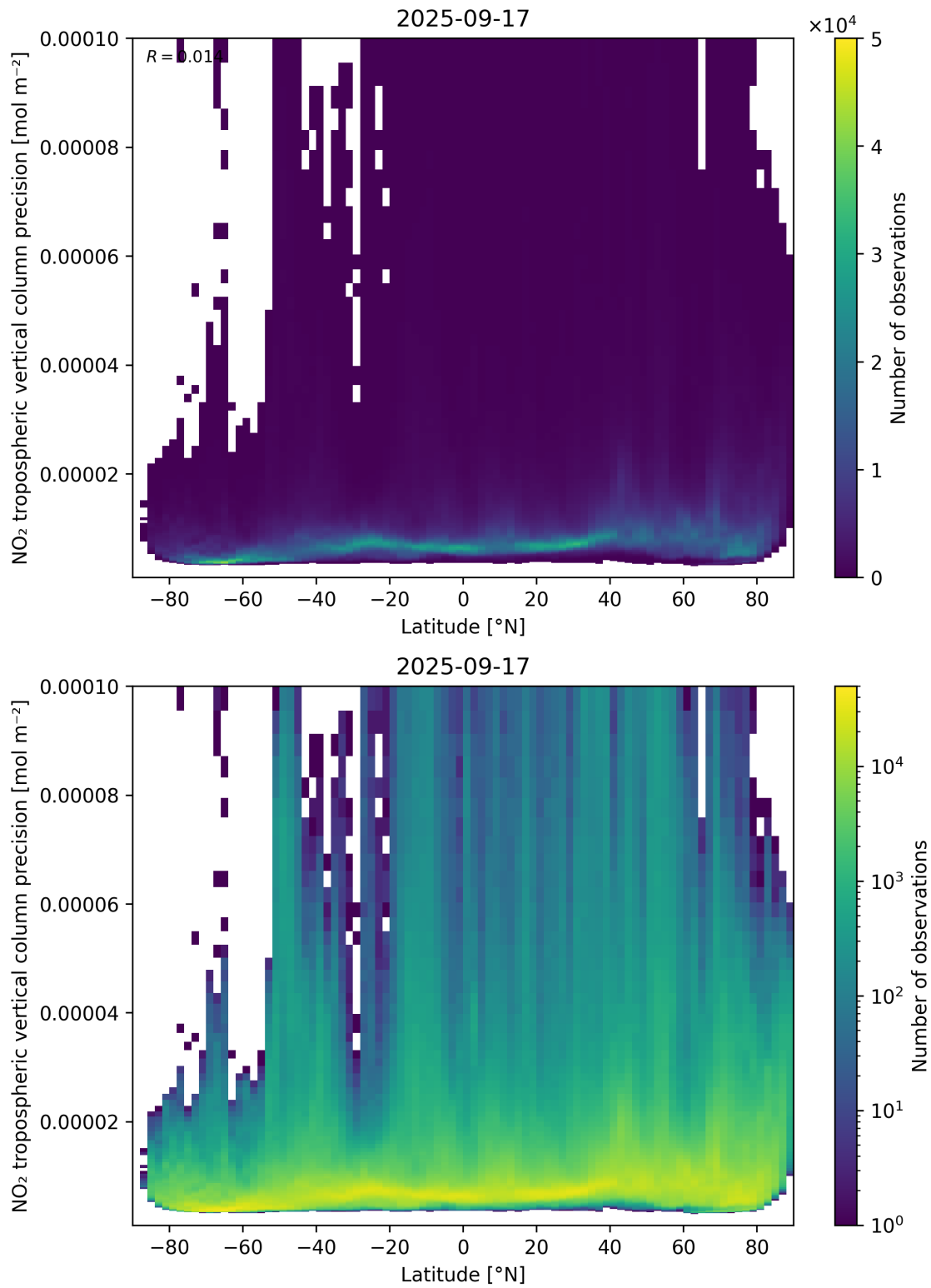
Figure 93: Scatter density plot of “Latitude” against “NO 2 tropospheric vertical column precision” for 2025-09-16 to 2025-09-18.
