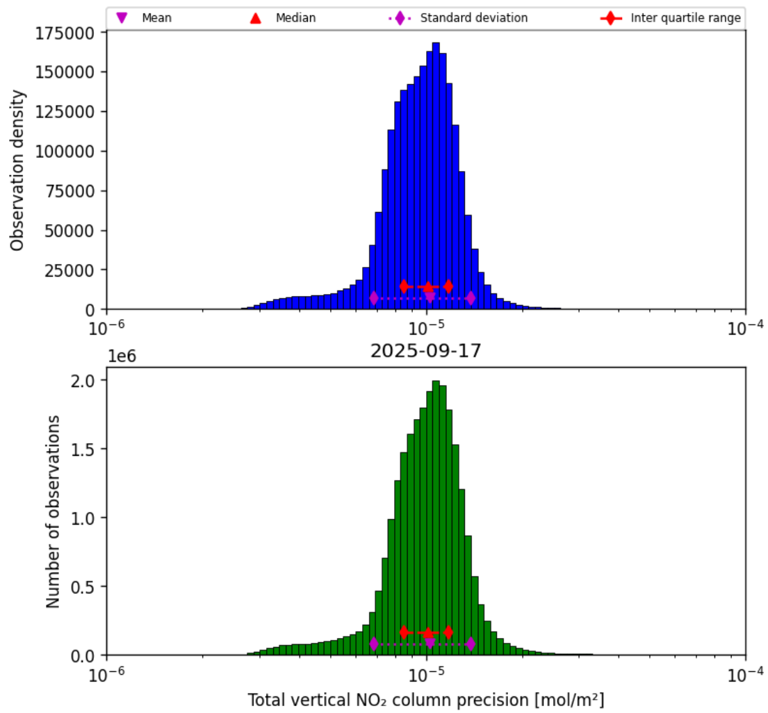
Figure 39: Histogram of “Total vertical NO 2 column precision” for 2025-09-16 to 2025-09-18
