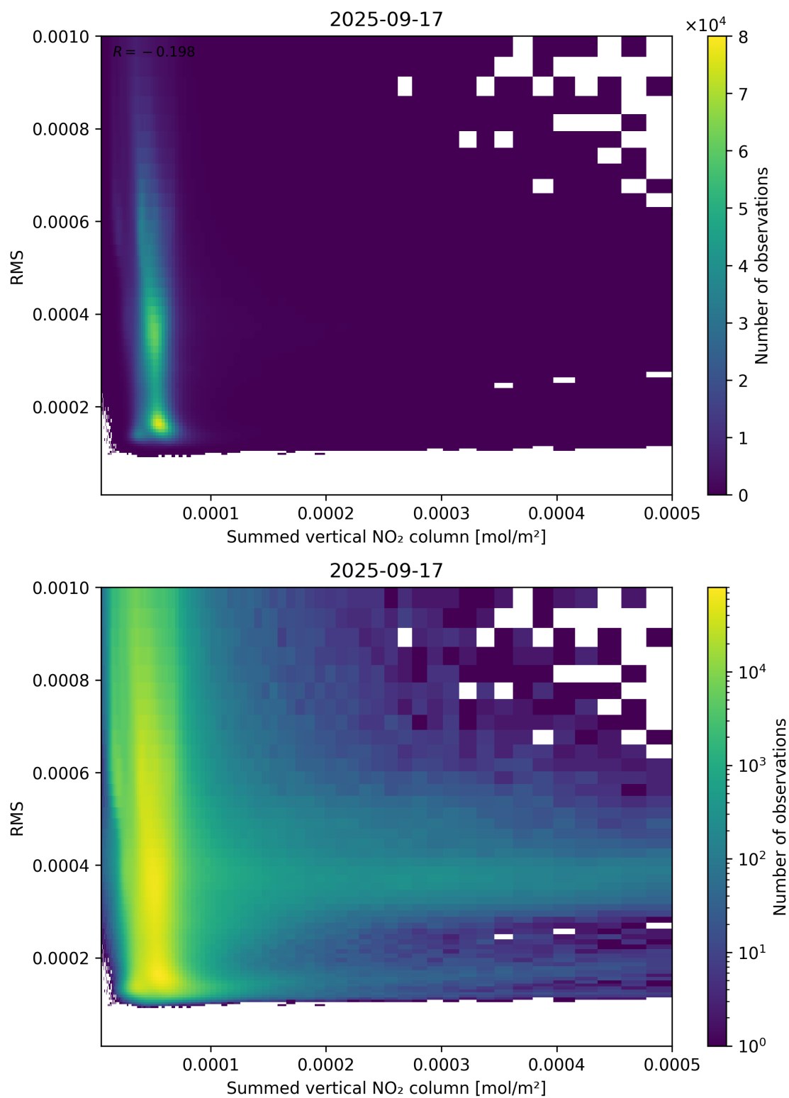
Figure 109: Scatter density plot of “Summed vertical NO 2 column” against “RMS” for 2025-09-16 to 2025-09-18.
