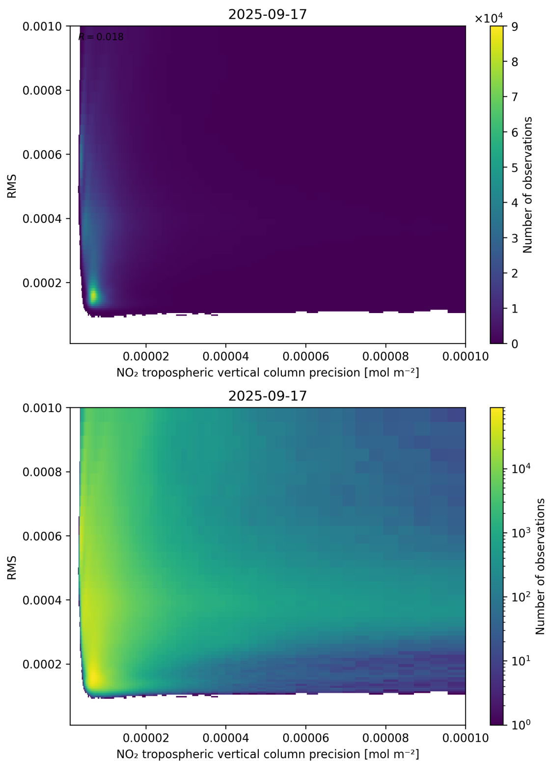
Figure 140: Scatter density plot of “NO 2 tropospheric vertical column precision” against “RMS” for 2025-09-16 to 2025-09-18.
