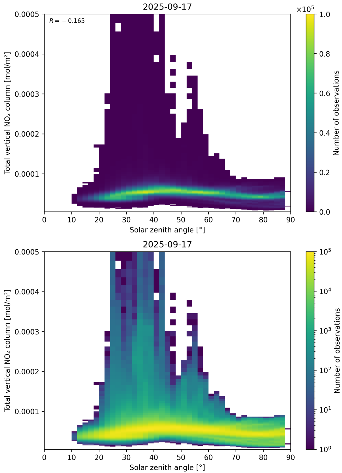
Figure 153: Scatter density plot of “Solar zenith angle” against “Total vertical NO 2 column” for 2025-09-16 to 2025-09-18.
