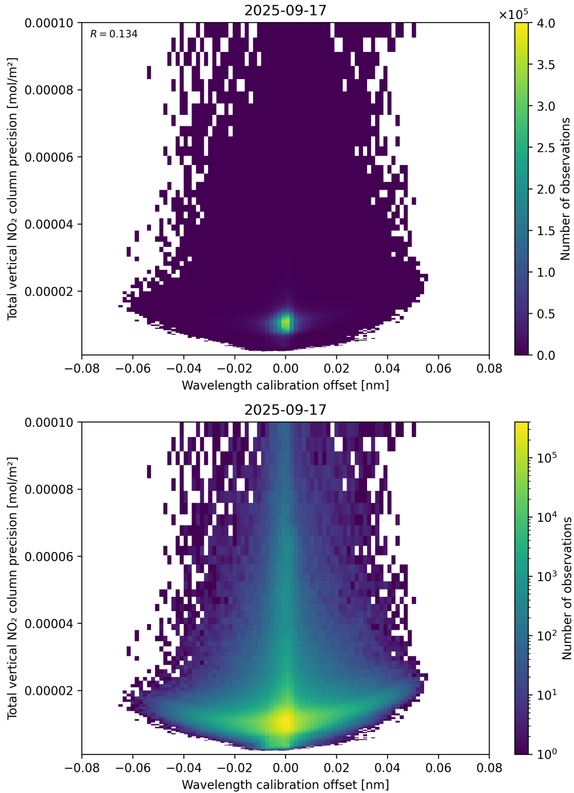
Figure 180: Scatter density plot of “Wavelength calibration offset” against “Total vertical NO 2 column precision” for 2025-09-16 to 2025-09-18.
