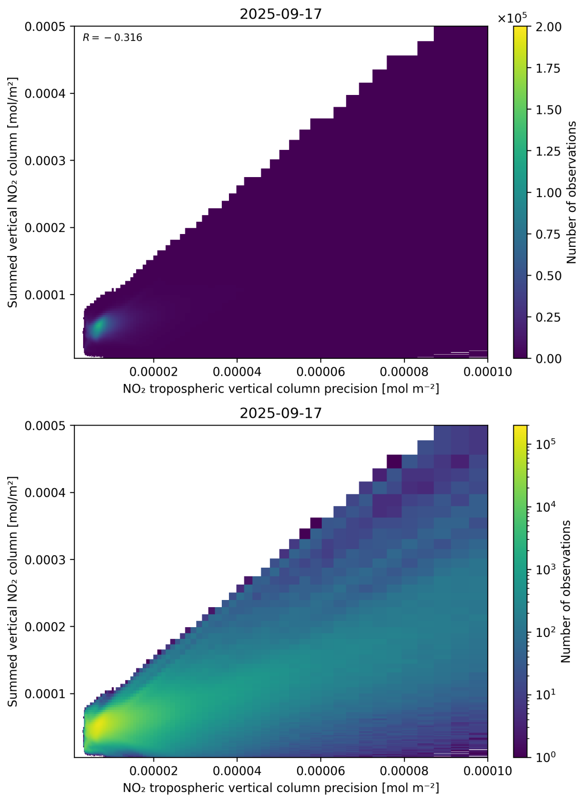
Figure 136: Scatter density plot of “NO 2 tropospheric vertical column precision” against “Summed vertical NO 2 column” for 2025-09-16 to 2025-09-18.
