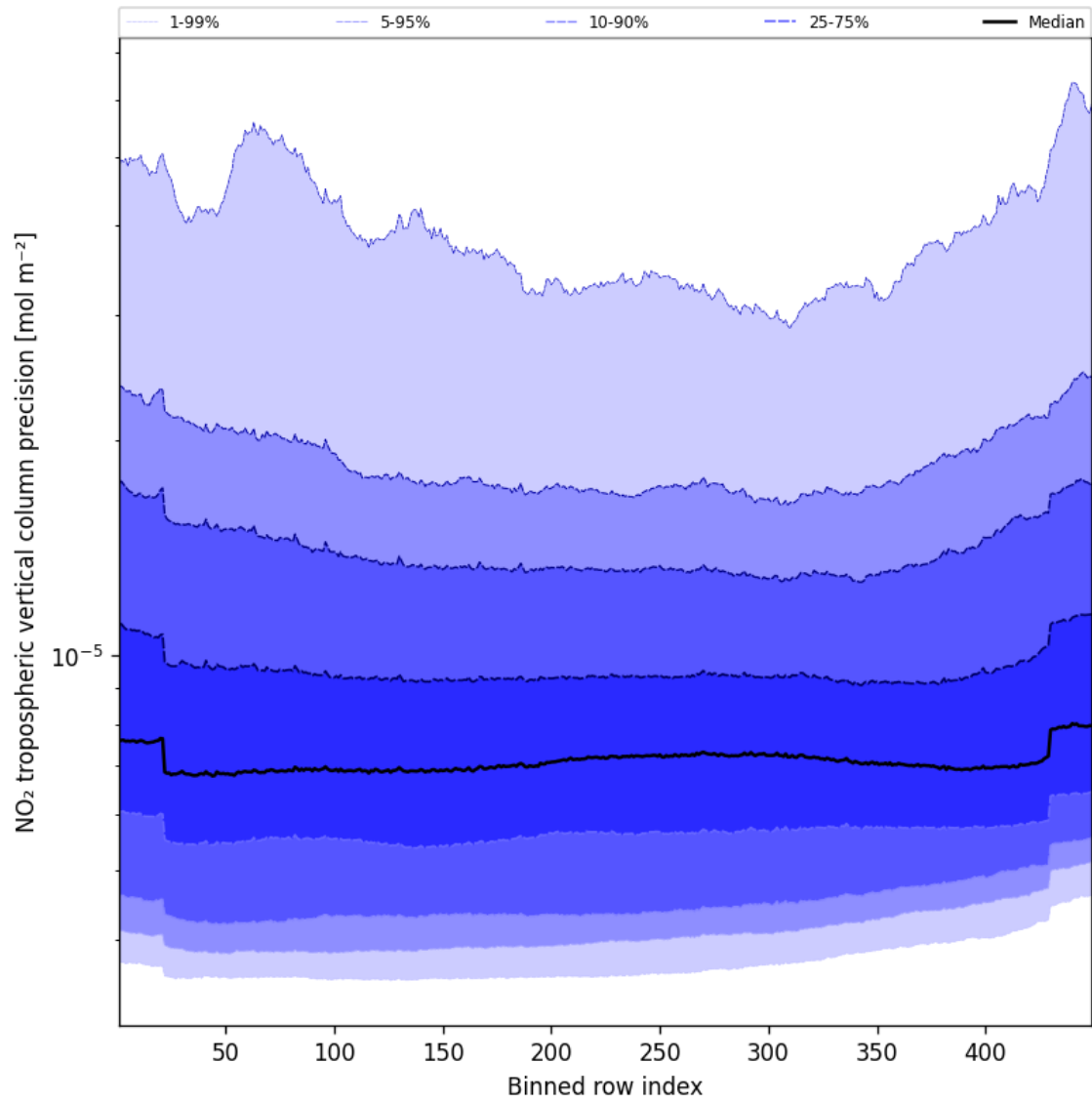
Figure 47: Along track statistics of “NO 2 tropospheric vertical column precision” for 2025-09-16 to 2025-09-18
