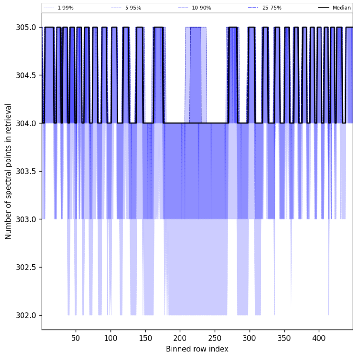
Figure 50: Along track statistics of “Number of spectral points in retrieval” for 2025-09-16 to 2025-09-18
