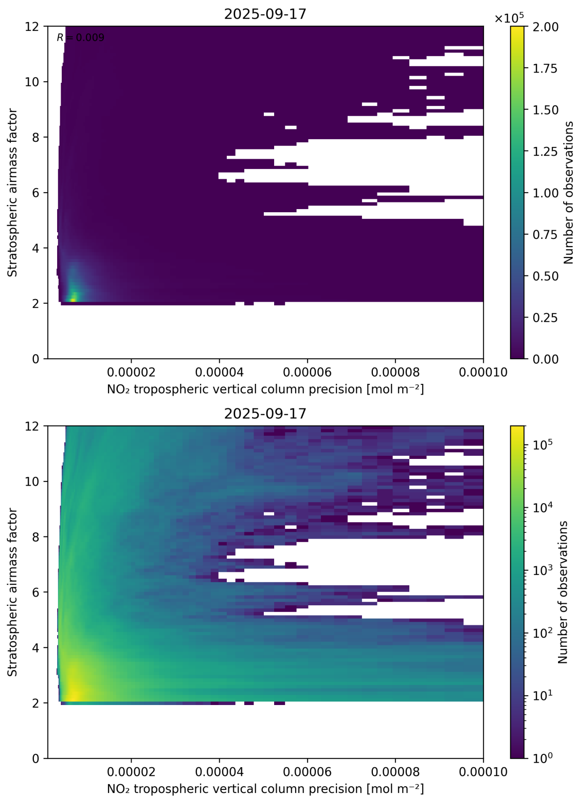
Figure 131: Scatter density plot of “NO 2 tropospheric vertical column precision” against “Stratospheric airmass factor” for 2025-09-16 to 2025-09-18.
