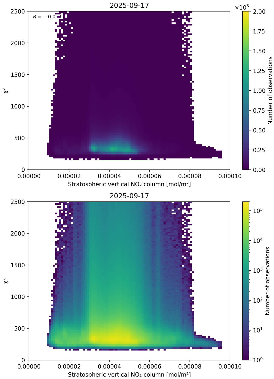
Figure 97: Scatter density plot of “Stratospheric vertical NO 2 column” against “ \chi^2 ” for 2025-09-16 to 2025-09-18.
