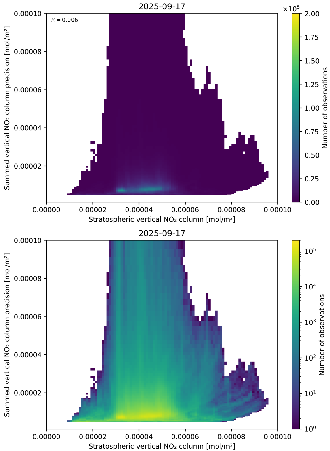
Figure 99: Scatter density plot of “Stratospheric vertical NO 2 column” against “Summed vertical NO 2 column precision” for 2025-09-16 to 2025-09-18.
