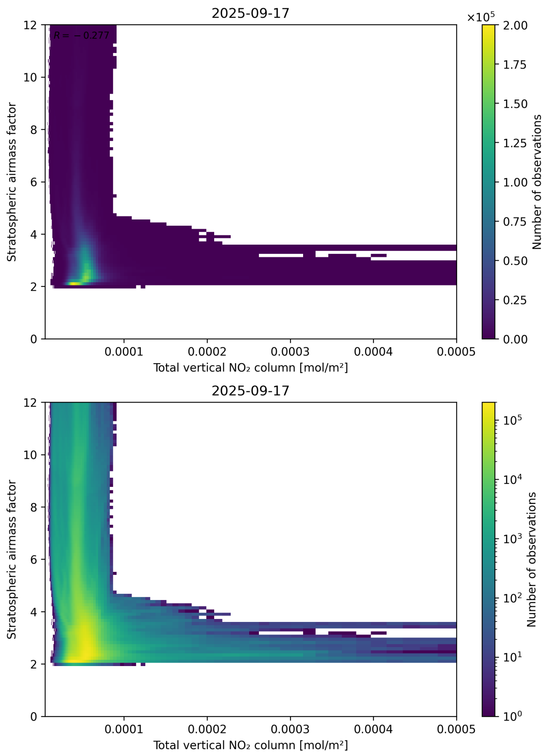
Figure 110: Scatter density plot of “Total vertical NO 2 column” against “Stratospheric airmass factor” for 2025-09-16 to 2025-09-18.
