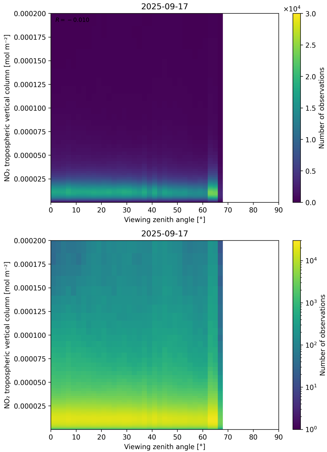
Figure 169: Scatter density plot of “Viewing zenith angle” against “NO 2 tropospheric vertical column” for 2025-09-16 to 2025-09-18.
