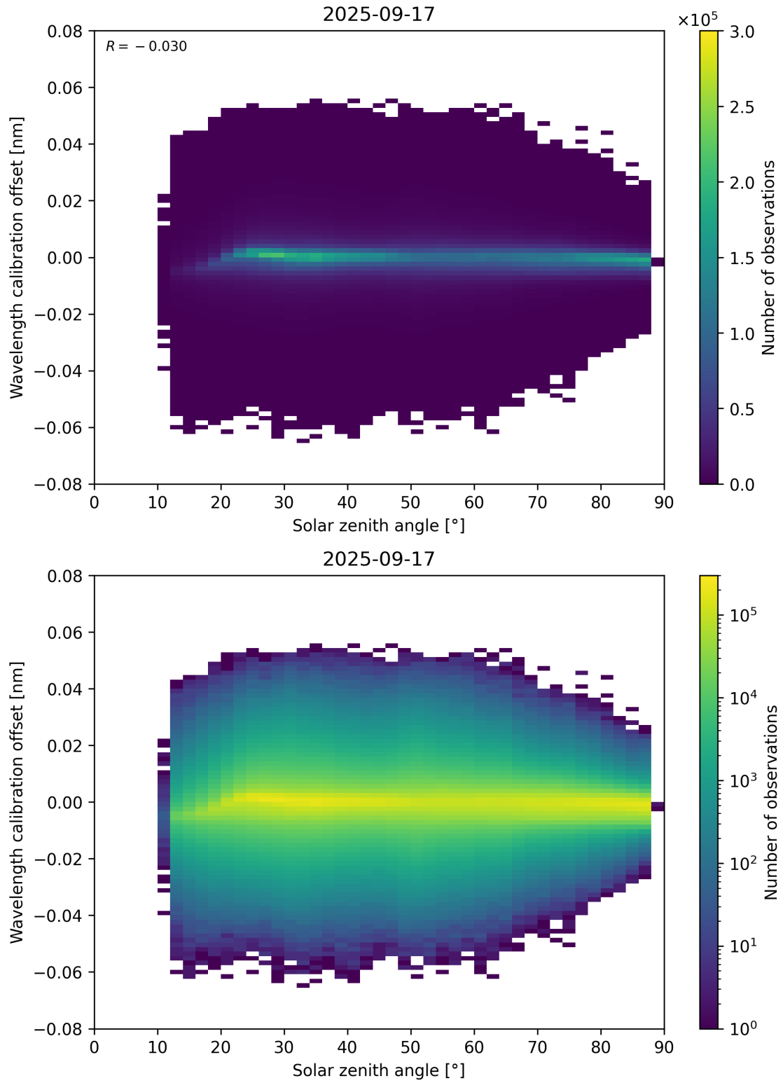
Figure 158: Scatter density plot of “Solar zenith angle” against “Wavelength calibration offset” for 2025-09-16 to 2025-09-18.
