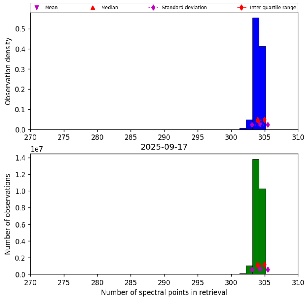
Figure 33: Histogram of “Number of spectral points in retrieval” for 2025-09-16 to 2025-09-18
