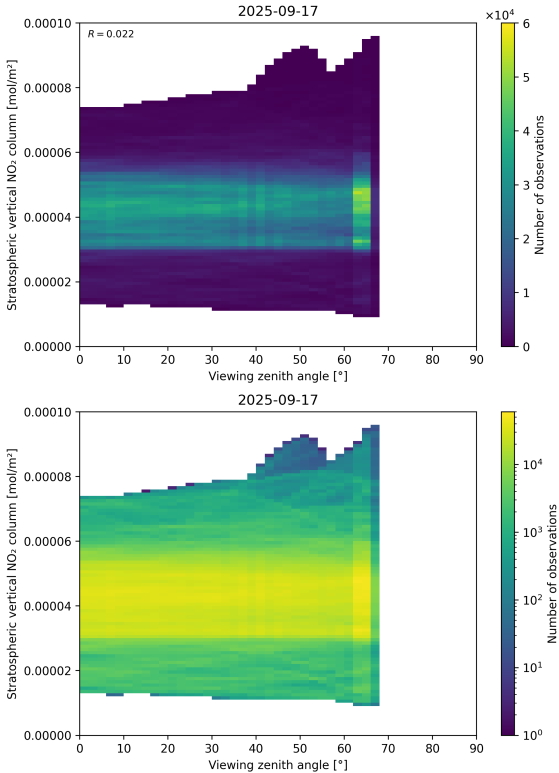
Figure 164: Scatter density plot of “Viewing zenith angle” against “Stratospheric vertical NO 2 column” for 2025-09-16 to 2025-09-18.
