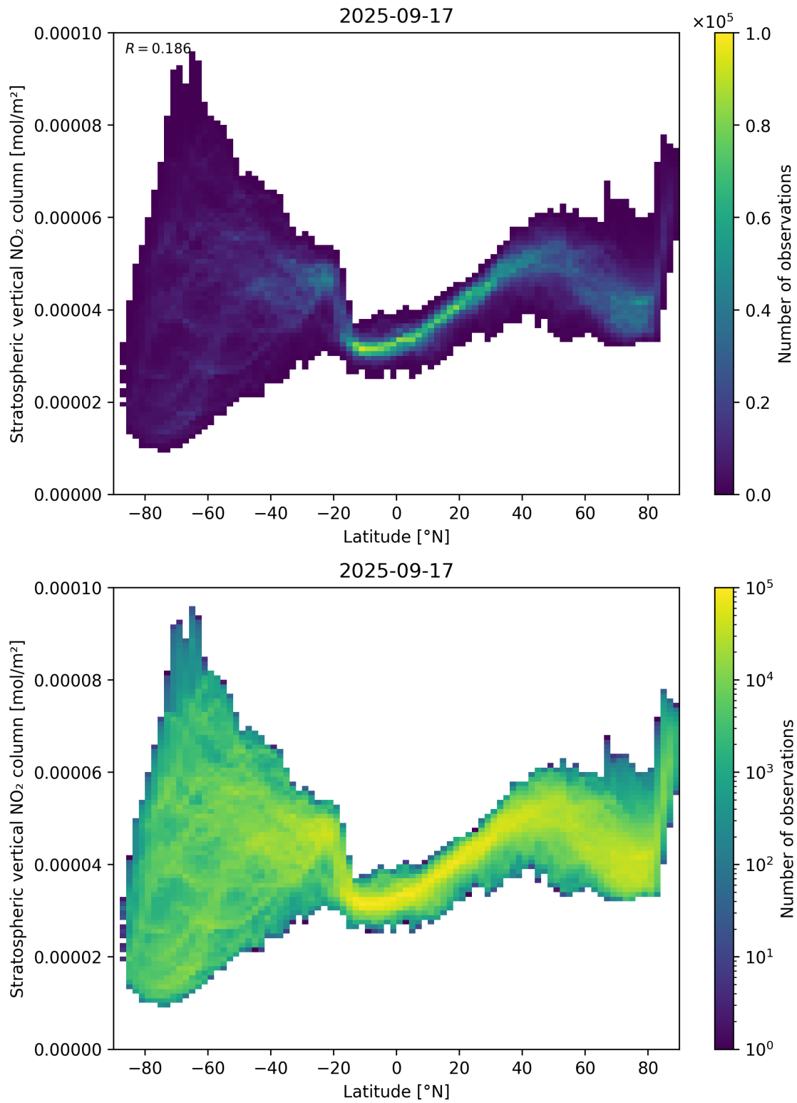
Figure 87: Scatter density plot of “Latitude” against “Stratospheric vertical NO 2 column” for 2025-09-16 to 2025-09-18.
