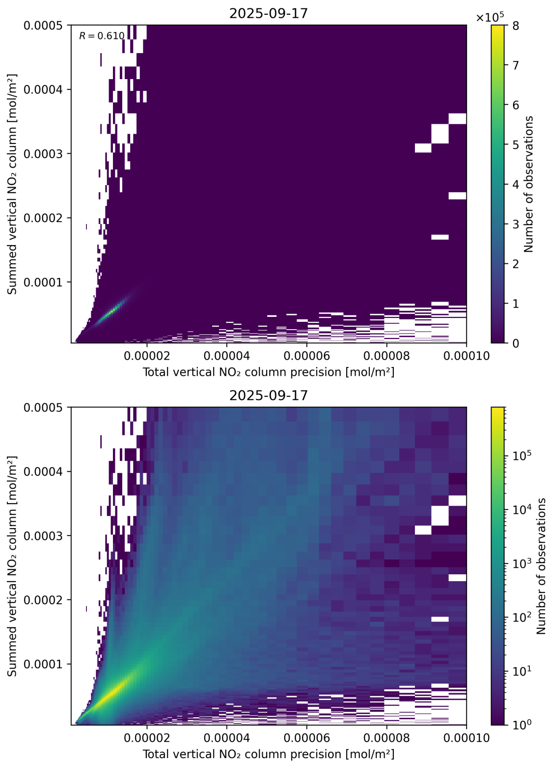
Figure 117: Scatter density plot of “Total vertical NO 2 column precision” against “Summed vertical NO 2 column” for 2025-09-16 to 2025-09-18.
