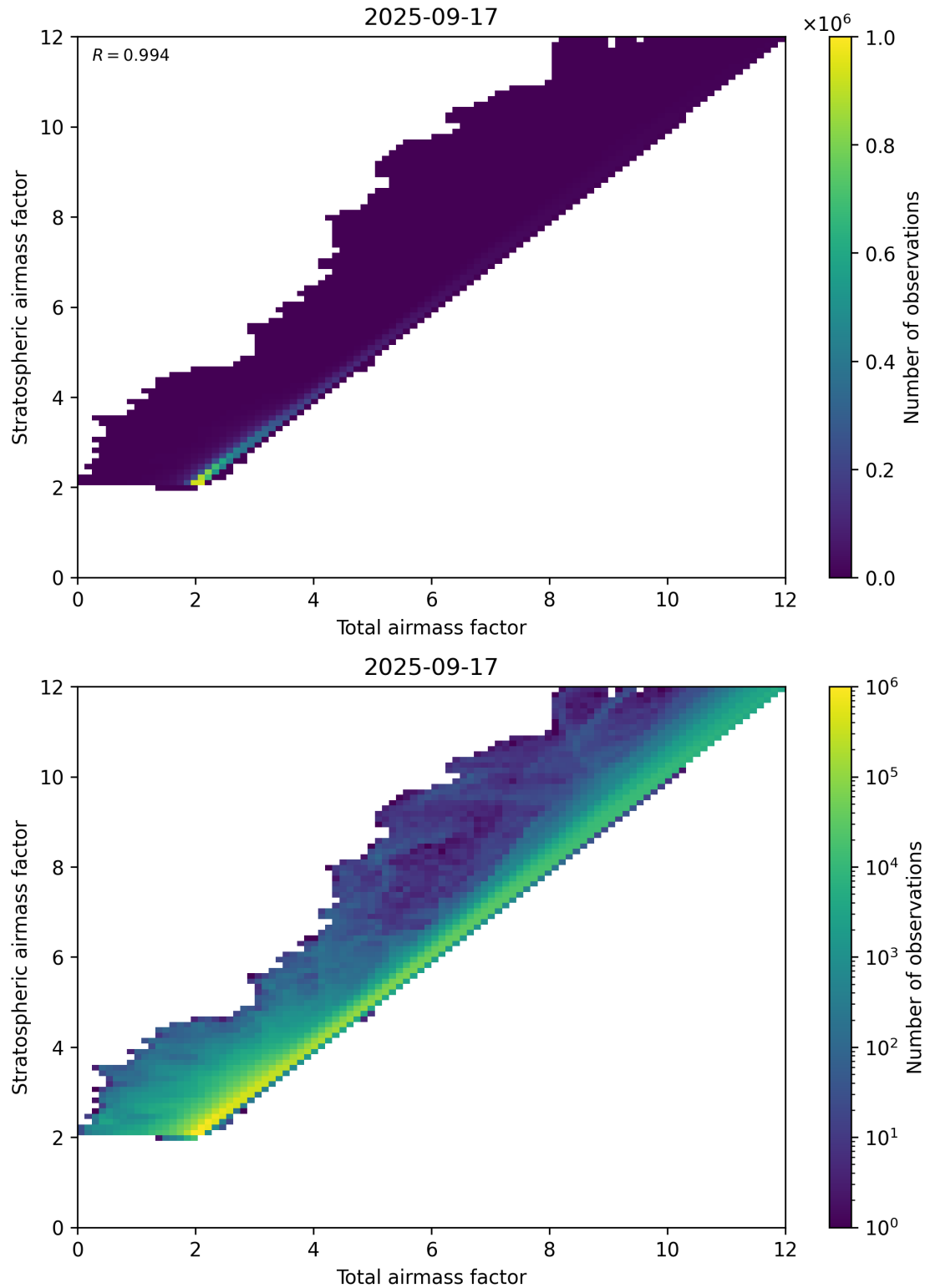
Figure 62: Scatter density plot of “Total airmass factor” against “Stratospheric airmass factor” for 2025-09-16 to 2025-09-18.
