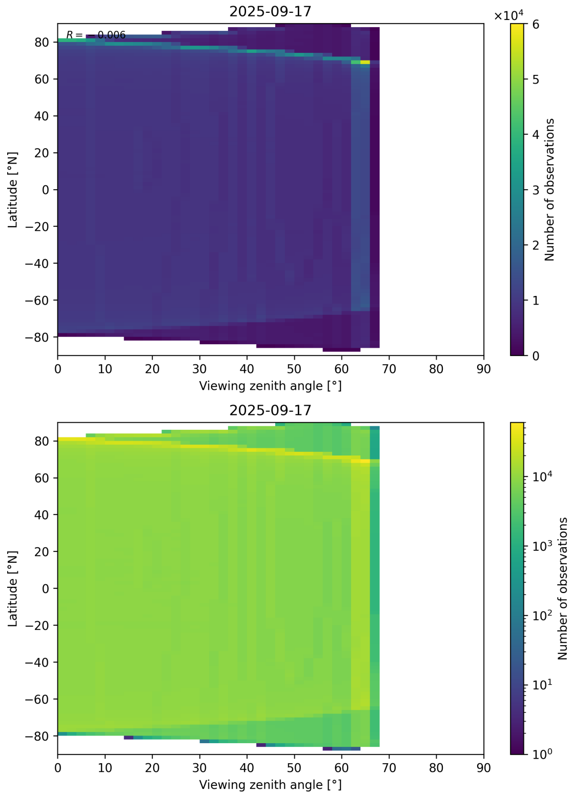
Figure 163: Scatter density plot of “Viewing zenith angle” against “Latitude” for 2025-09-16 to 2025-09-18.
