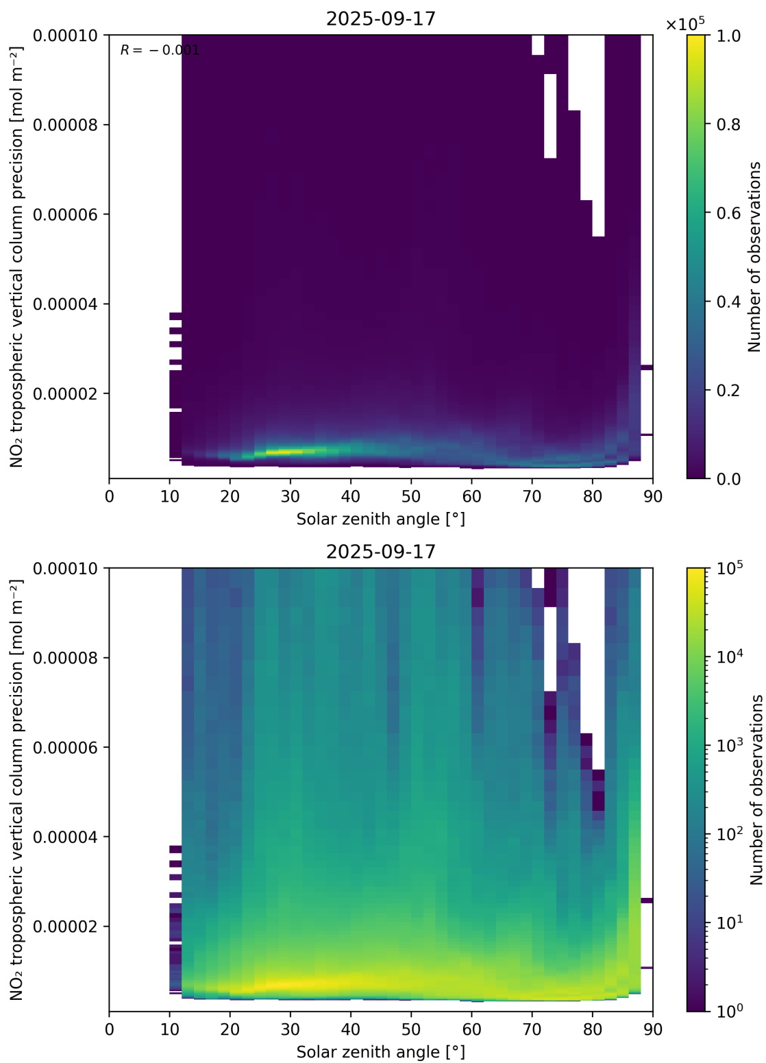
Figure 156: Scatter density plot of “Solar zenith angle” against “NO 2 tropospheric vertical column precision” for 2025-09-16 to 2025-09-18.
