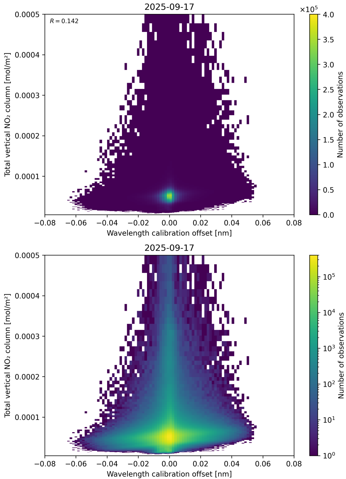
Figure 179: Scatter density plot of “Wavelength calibration offset” against “Total vertical NO 2 column” for 2025-09-16 to 2025-09-18.
