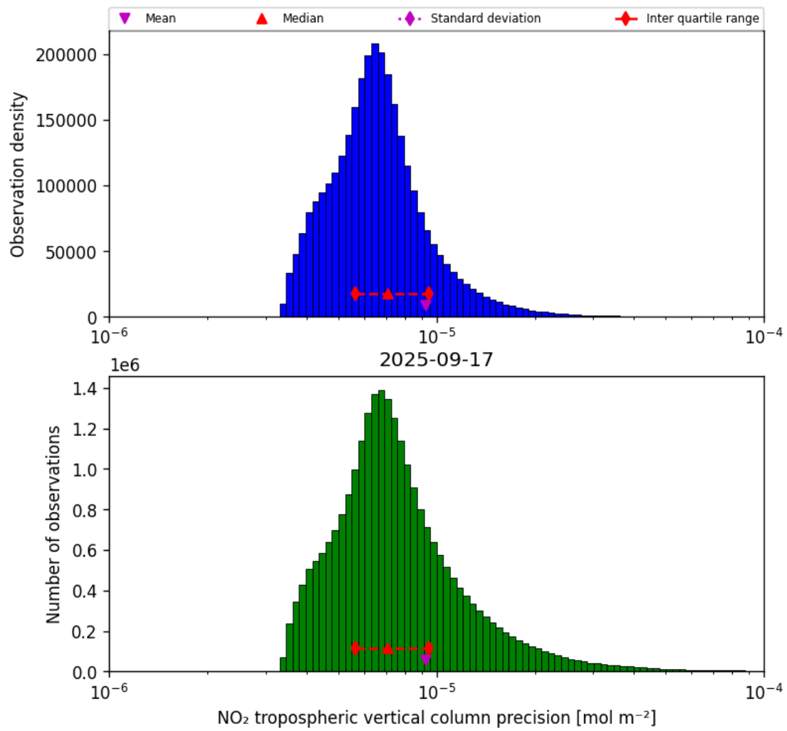
Figure 30: Histogram of “NO 2 tropospheric vertical column precision” for 2025-09-16 to 2025-09-18
