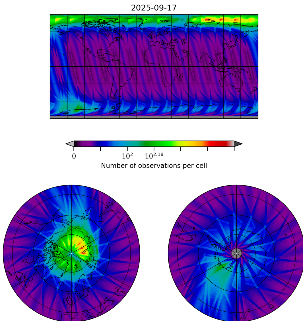
Figure 10: Map of the number of observations for 2025-09-16 to 2025-09-18
