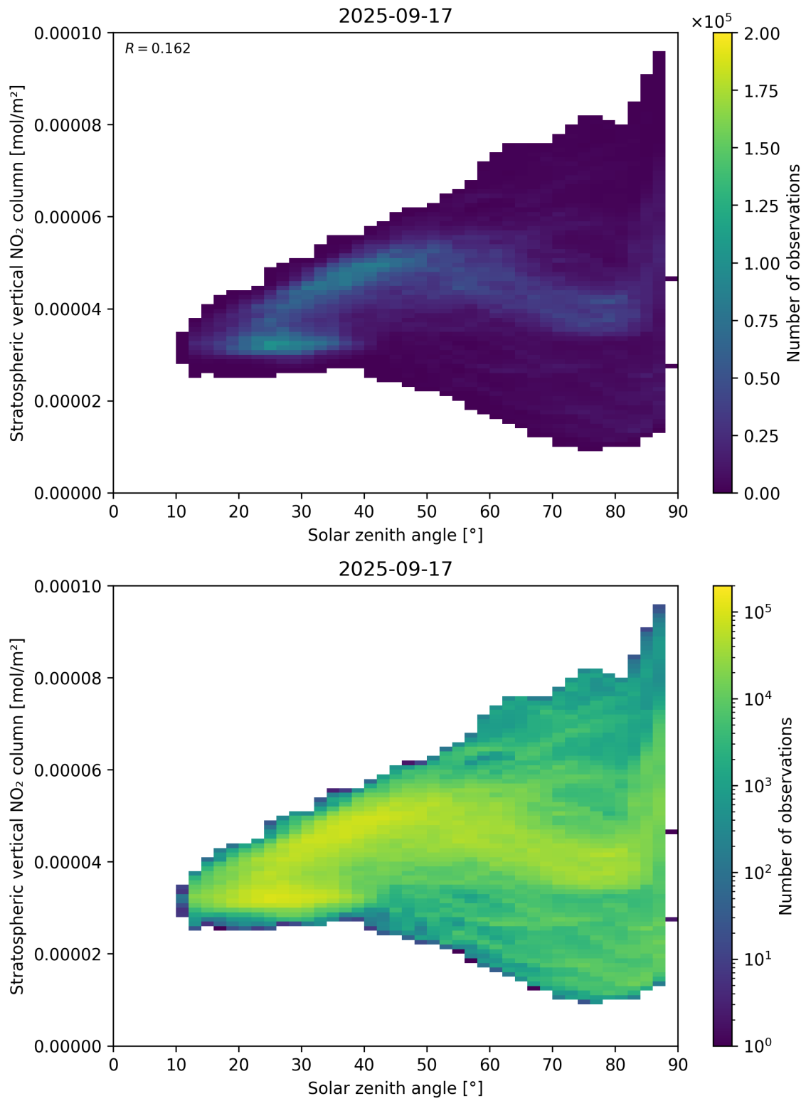
Figure 150: Scatter density plot of “Solar zenith angle” against “Stratospheric vertical NO 2 column” for 2025-09-16 to 2025-09-18.
