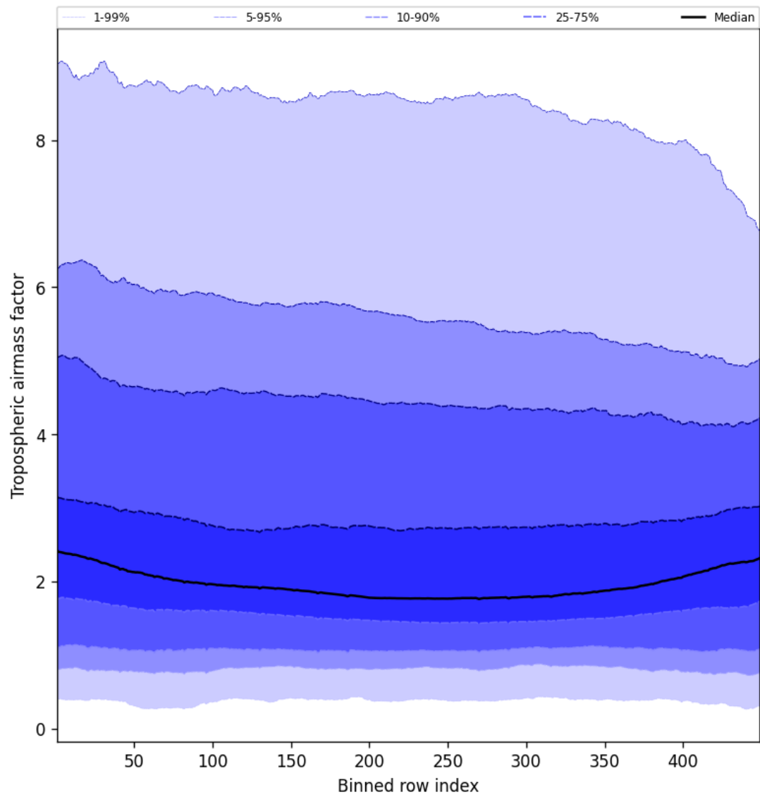
Figure 48: Along track statistics of “Tropospheric air mass factor” for 2025-09-16 to 2025-09-18
