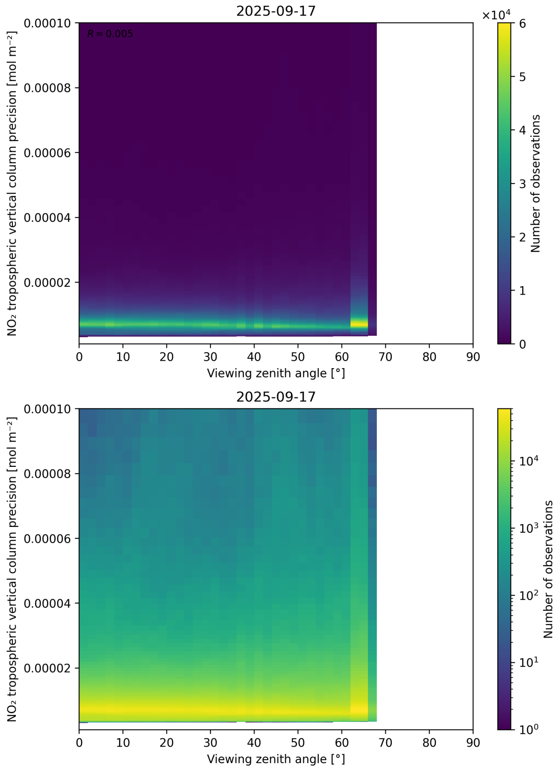
Figure 170: Scatter density plot of “Viewing zenith angle” against “NO 2 tropospheric vertical column precision” for 2025-09-16 to 2025-09-18.
