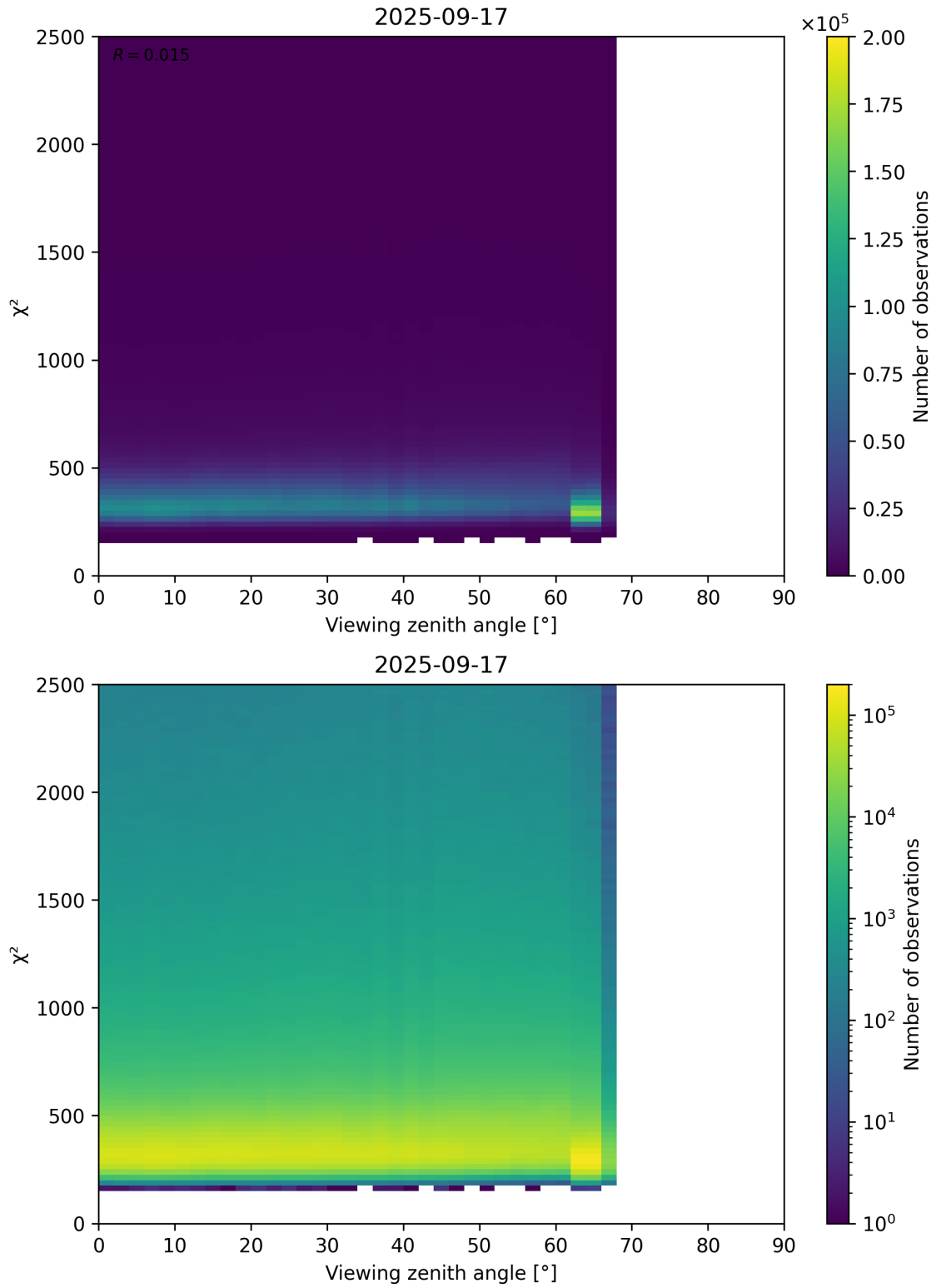
Figure 162: Scatter density plot of “Viewing zenith angle” against “ \chi^2 ” for 2025-09-16 to 2025-09-18.
