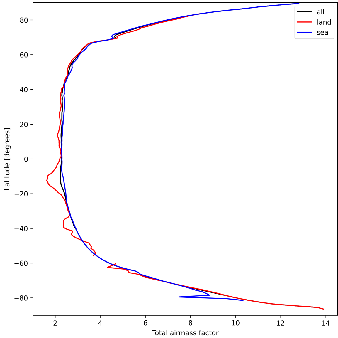
Figure 15: Zonal average of “Total airmass factor” for 2025-09-16 to 2025-09-18.
