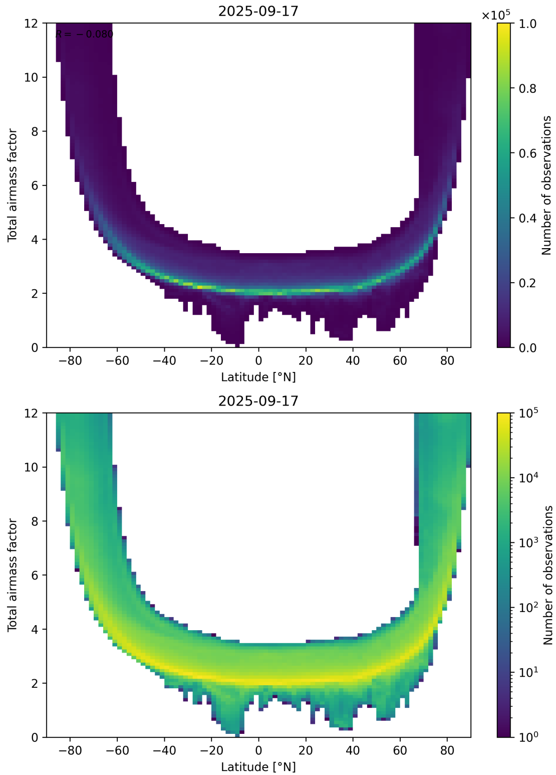
Figure 84: Scatter density plot of “Latitude” against “Total airmass factor” for 2025-09-16 to 2025-09-18.
