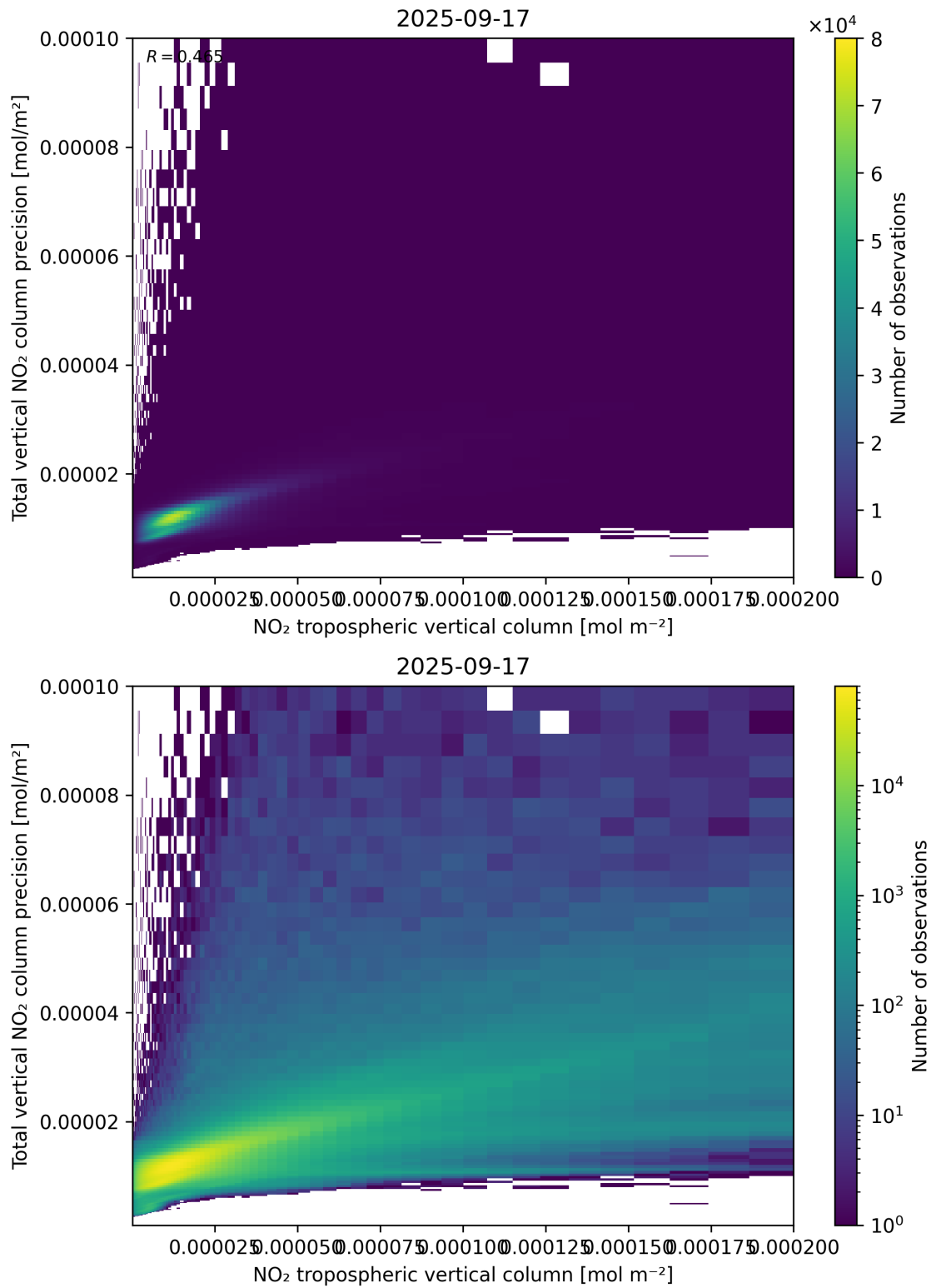
Figure 129: Scatter density plot of “NO 2 tropospheric vertical column” against “Total vertical NO 2 column precision” for 2025-09-16 to 2025-09-18.
