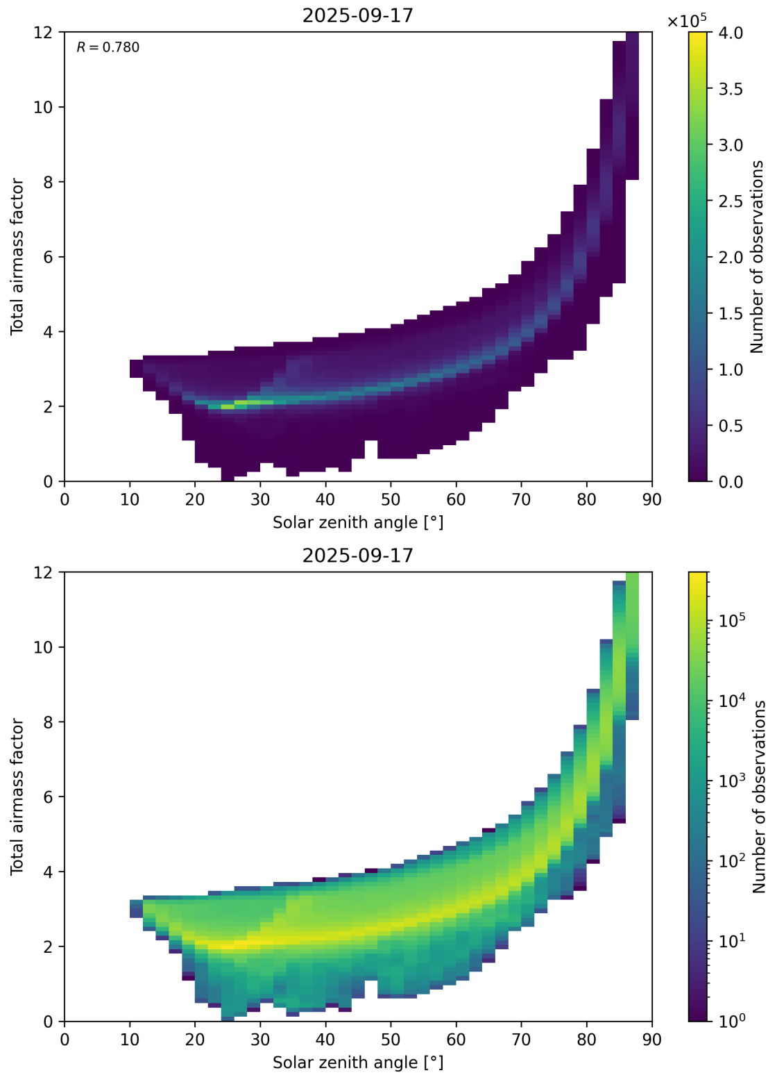
Figure 146: Scatter density plot of “Solar zenith angle” against “Total airmass factor” for 2025-09-16 to 2025-09-18.
