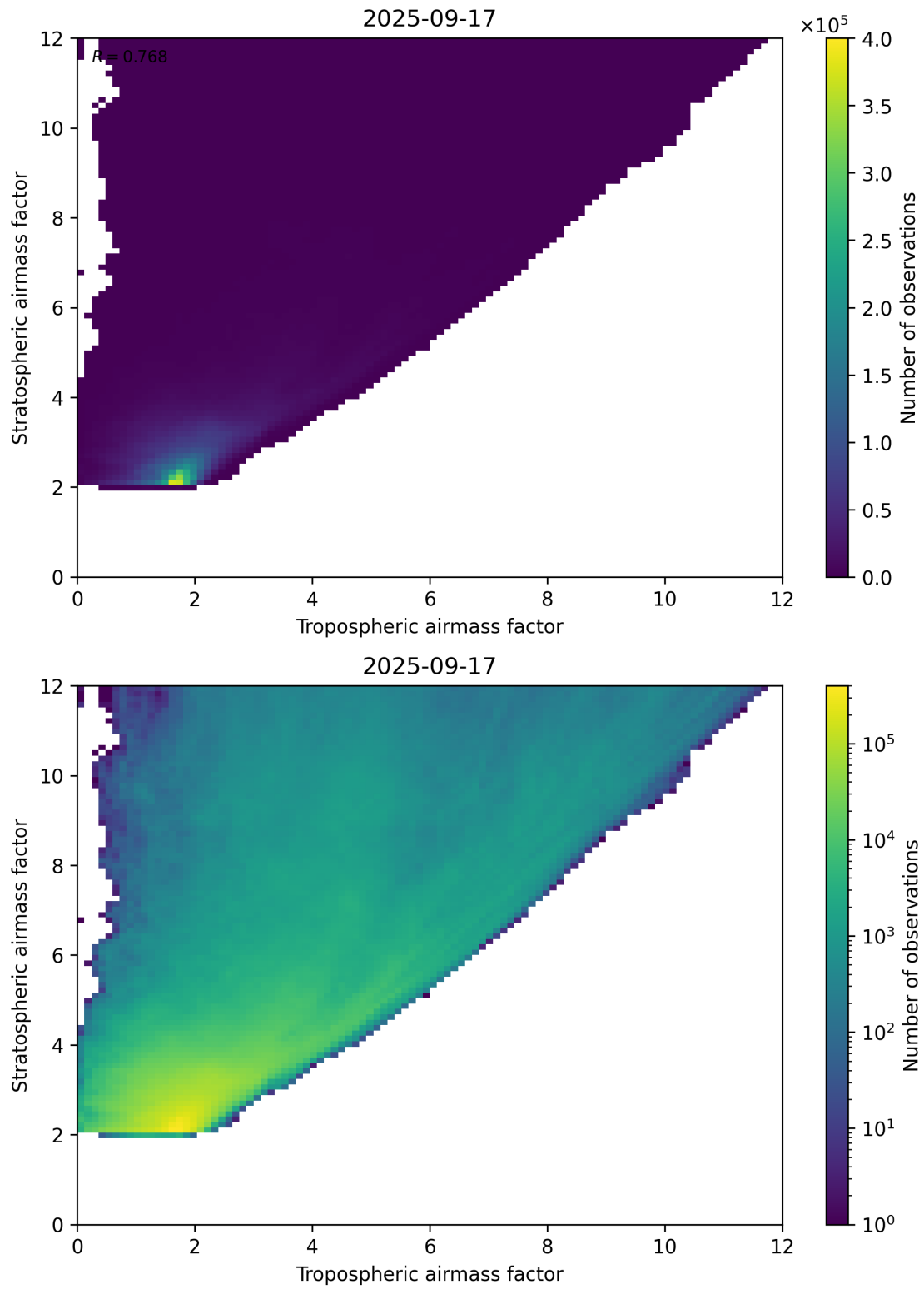
Figure 71: Scatter density plot of “Tropospheric airmass factor” against “Stratospheric airmass factor” for 2025-09-16 to 2025-09-18.
