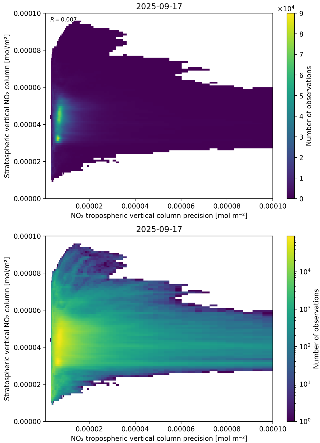
Figure 135: Scatter density plot of “NO 2 tropospheric vertical column precision” against “Stratospheric vertical NO 2 column” for 2025-09-16 to 2025-09-18.
