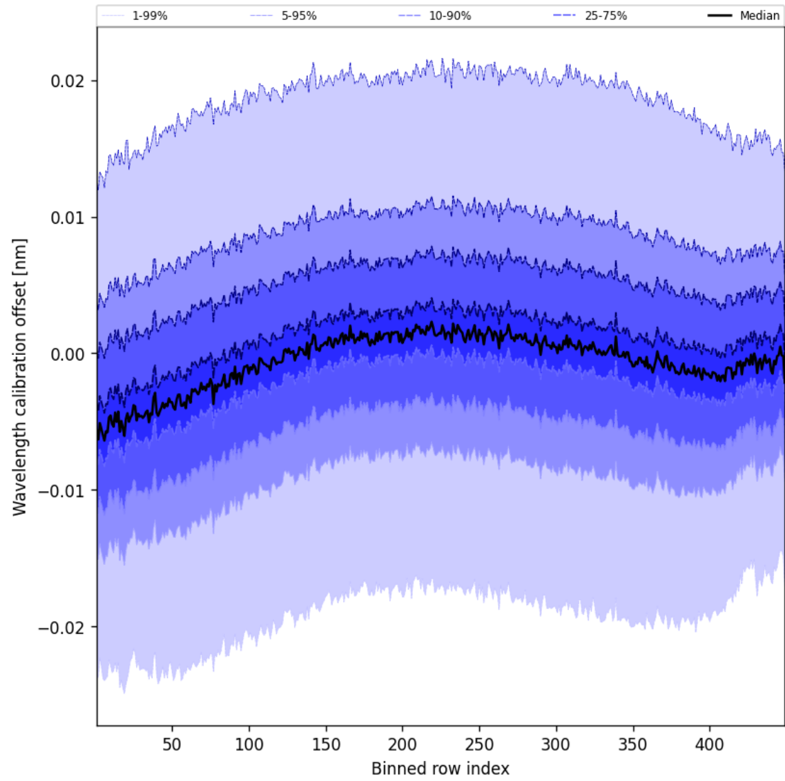
Figure 52: Along track statistics of “Wavelength calibration offset” for 2025-09-16 to 2025-09-18
