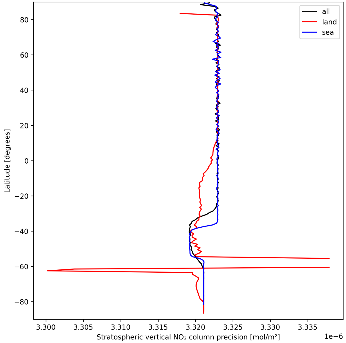
Figure 20: Zonal average of “Stratospheric vertical NO 2 column precision” for 2025-09-16 to 2025-09-18.
