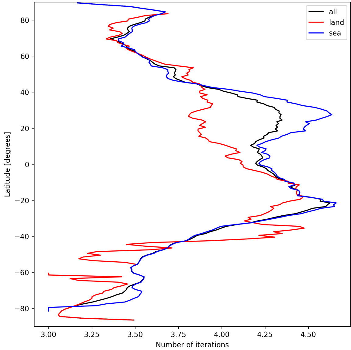
Figure 17: Zonal average of “Number of iterations” for 2025-09-16 to 2025-09-18.
