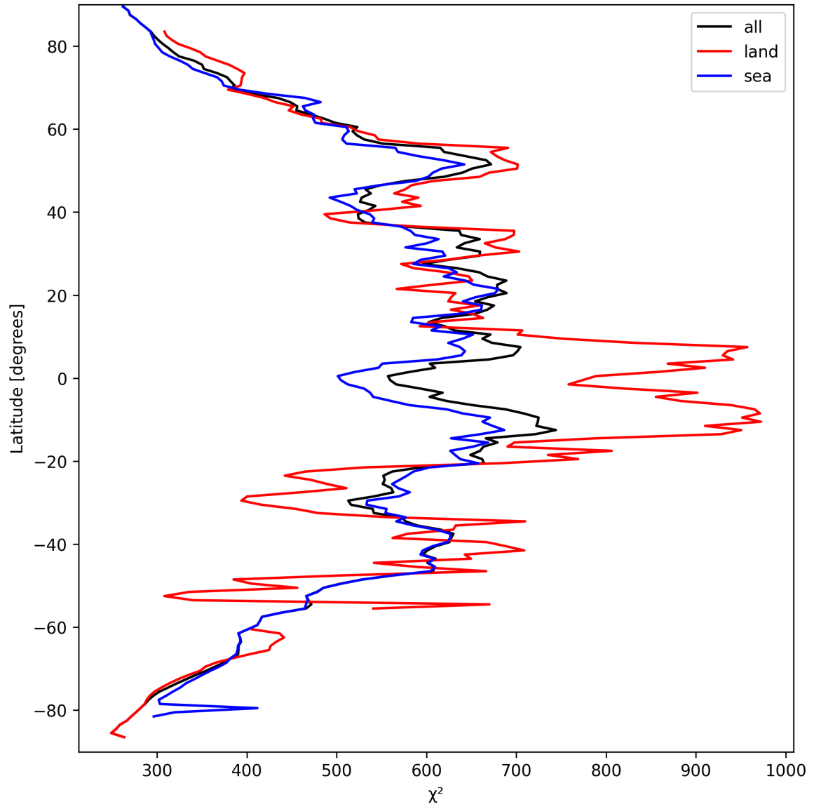
Figure 25: Zonal average of “ \chi^2 ” for 2025-09-16 to 2025-09-18.
