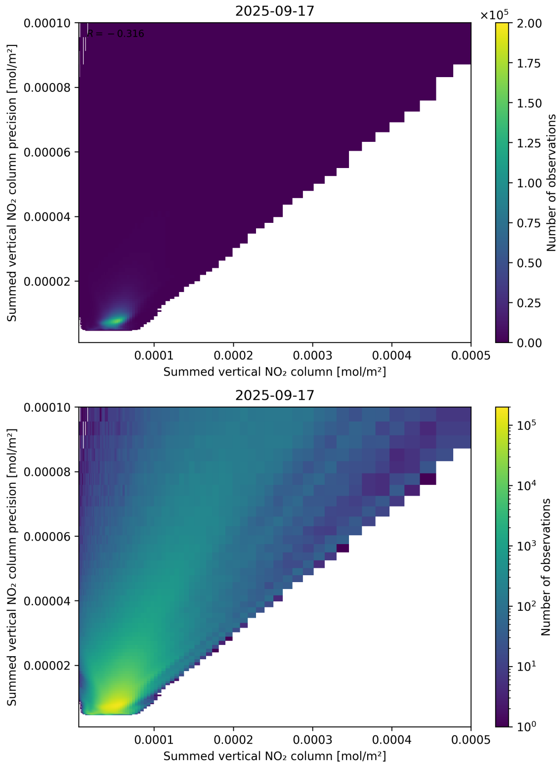
Figure 105: Scatter density plot of “Summed vertical NO 2 column” against “Summed vertical NO 2 column precision” for 2025-09-16 to 2025-09-18.
