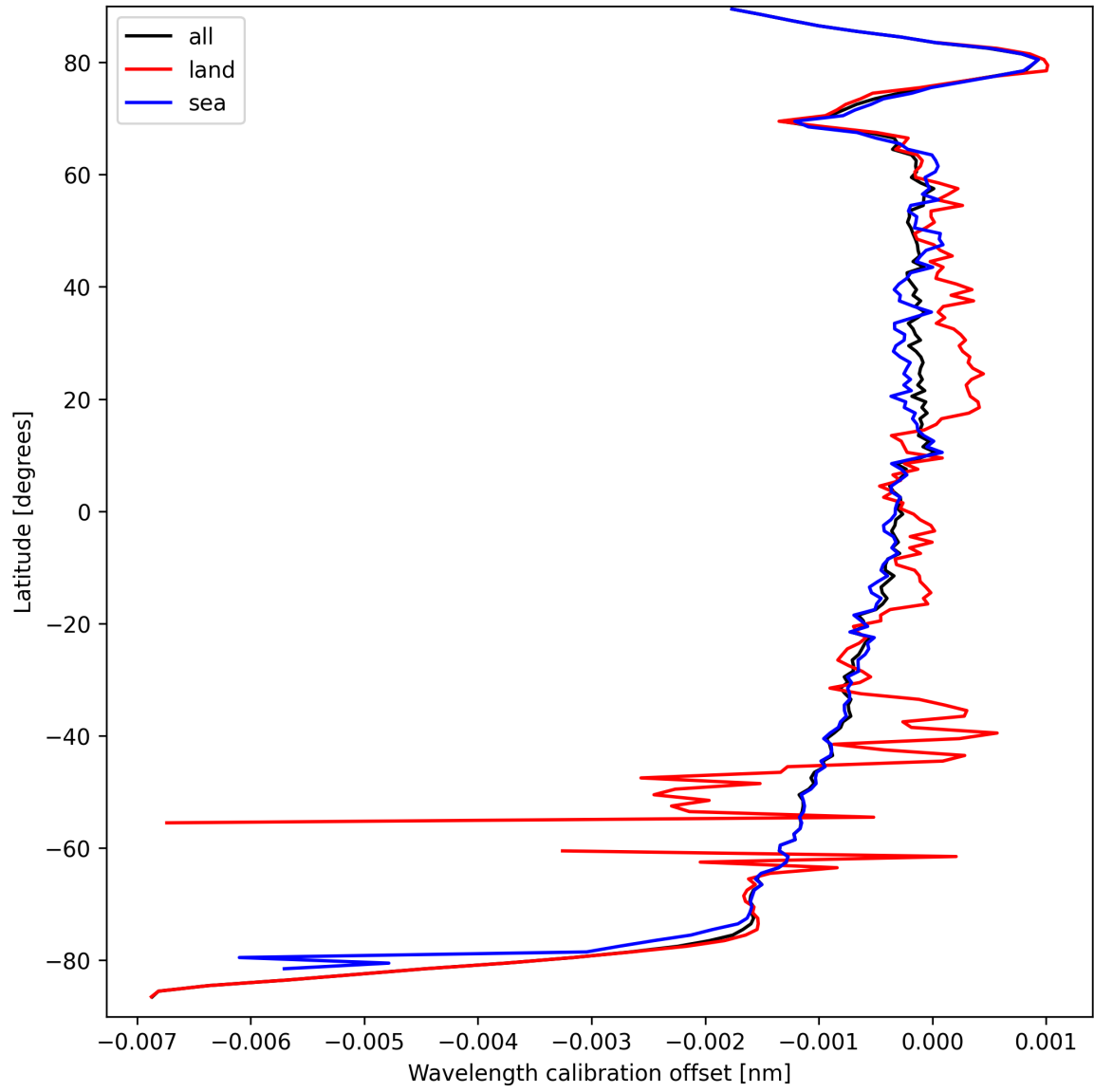
Figure 18: Zonal average of “Wavelength calibration offset” for 2025-09-16 to 2025-09-18.
