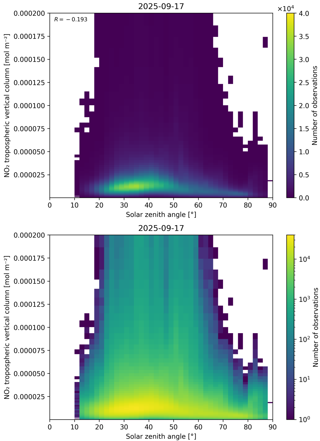
Figure 155: Scatter density plot of “Solar zenith angle” against “NO 2 tropospheric vertical column” for 2025-09-16 to 2025-09-18.
