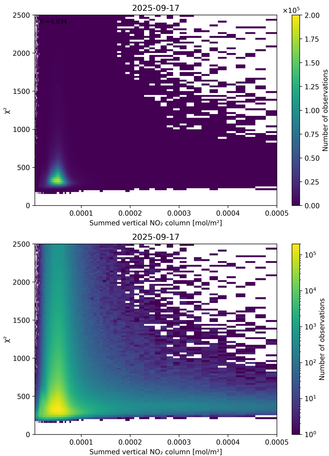
Figure 104: Scatter density plot of “Summed vertical NO 2 column” against “ \chi^2 ” for 2025-09-16 to 2025-09-18.
