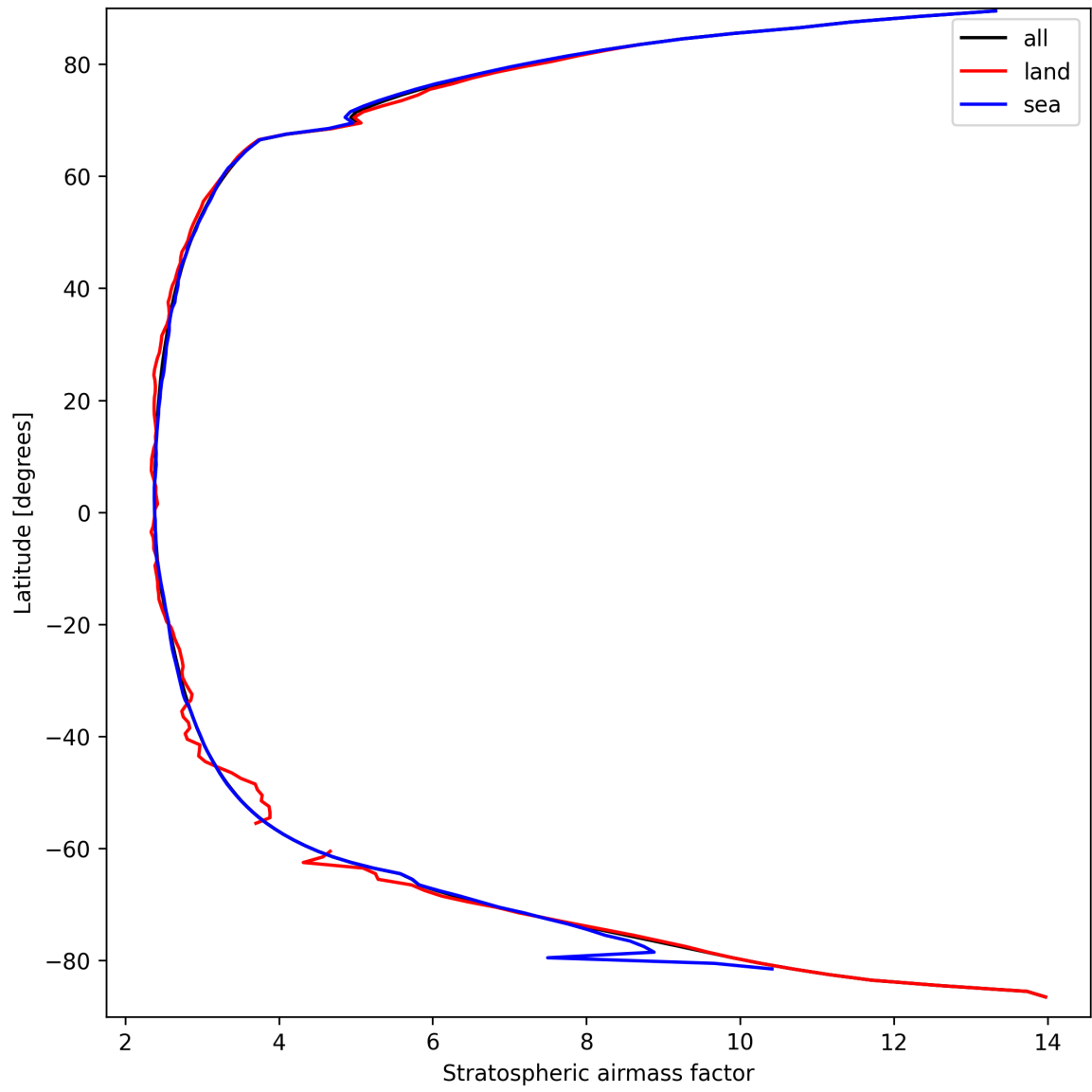
Figure 27: Zonal average of “Stratospheric airmass factor” for 2025-09-16 to 2025-09-18.
