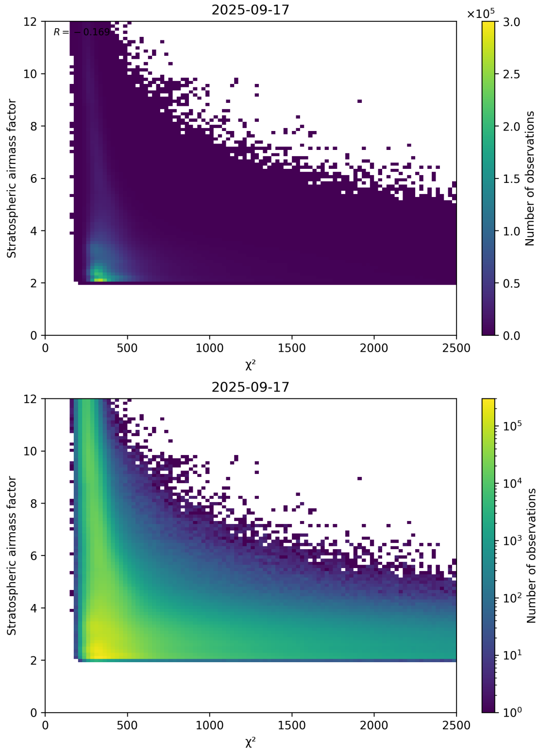
Figure 81: Scatter density plot of “ \chi^2 ” against “Stratospheric airmass factor” for 2025-09-16 to 2025-09-18.
