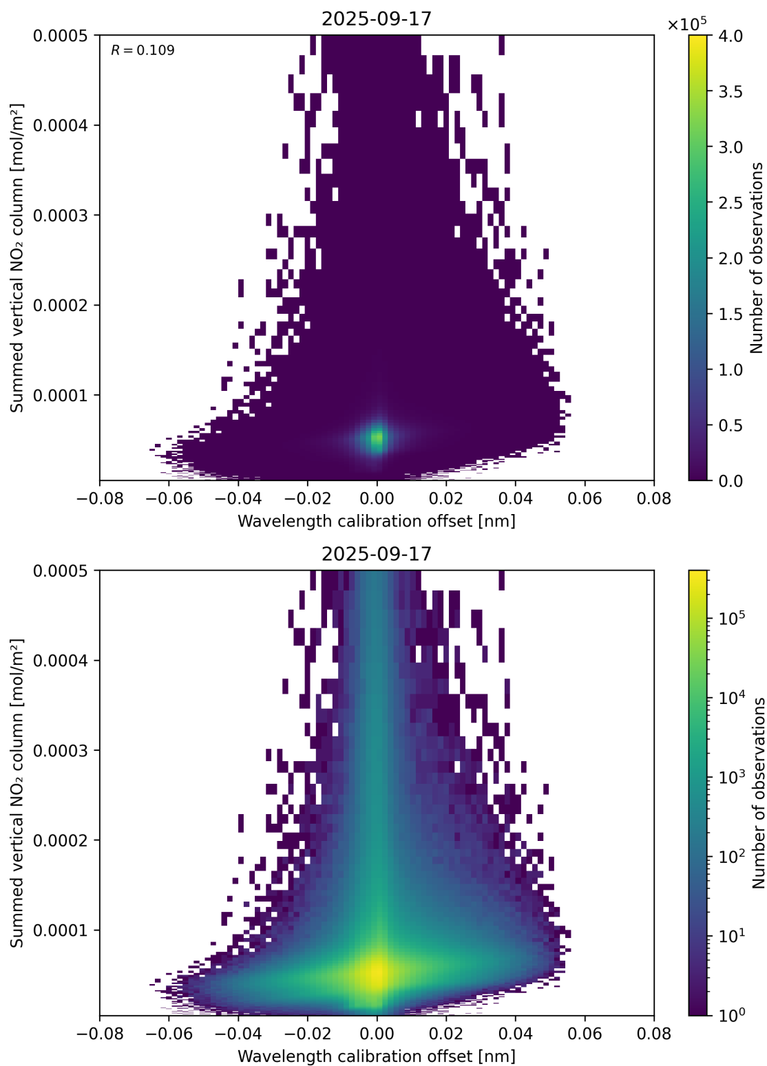
Figure 177: Scatter density plot of “Wavelength calibration offset” against “Summed vertical NO 2 column” for 2025-09-16 to 2025-09-18.
