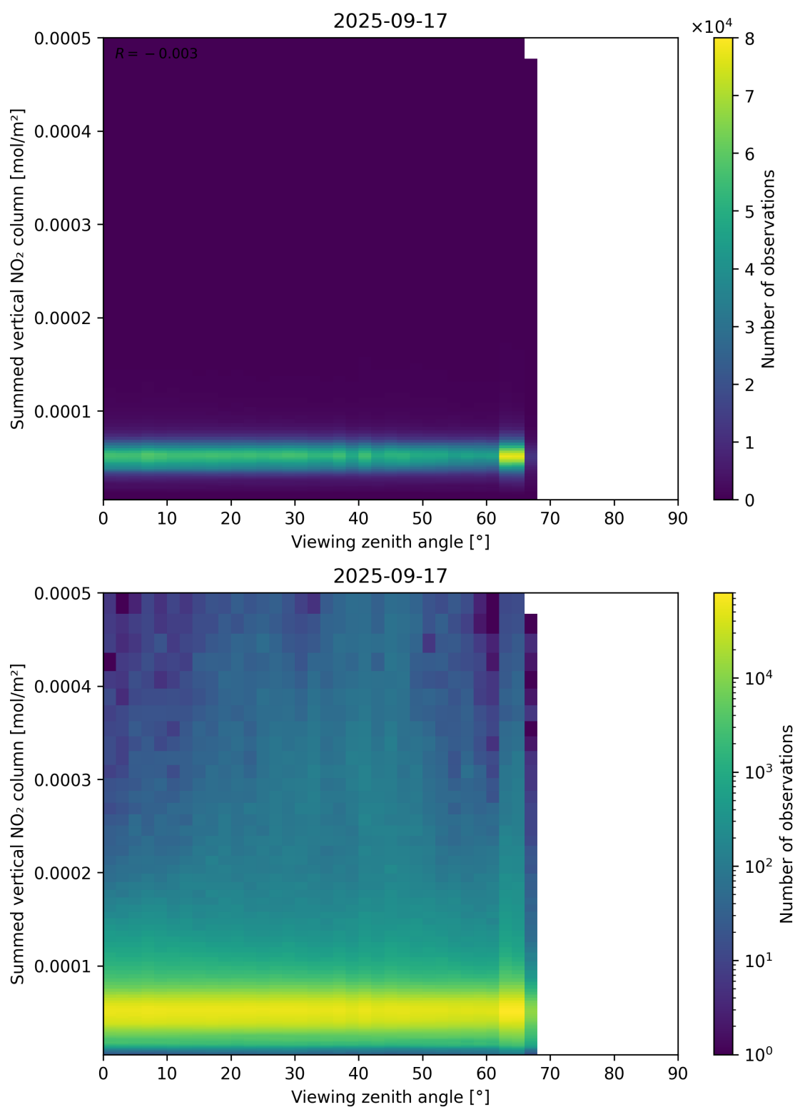
Figure 165: Scatter density plot of “Viewing zenith angle” against “Summed vertical NO 2 column” for 2025-09-16 to 2025-09-18.
