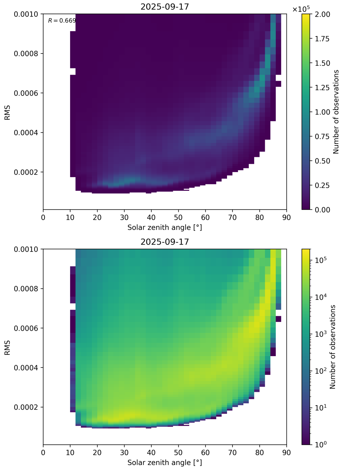
Figure 157: Scatter density plot of “Solar zenith angle” against “RMS” for 2025-09-16 to 2025-09-18.
