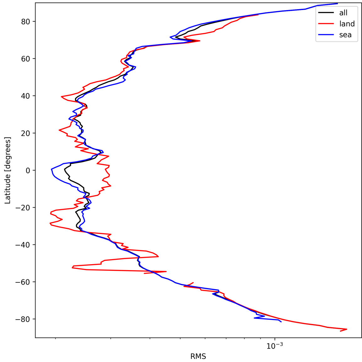
Figure 26: Zonal average of “RMS” for 2025-09-16 to 2025-09-18.
