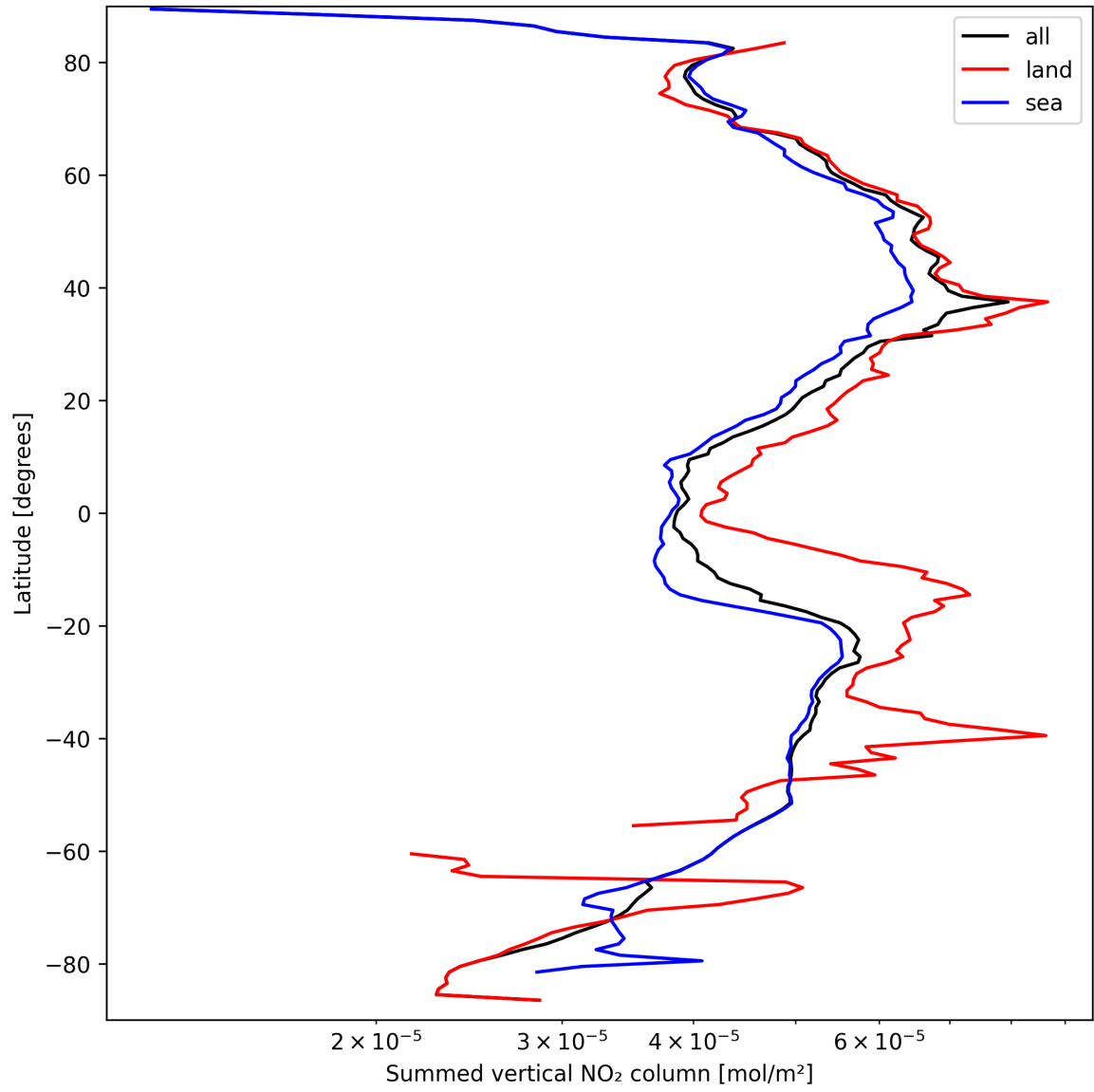
Figure 23: Zonal average of “Summed vertical NO 2 column” for 2025-09-16 to 2025-09-18.
