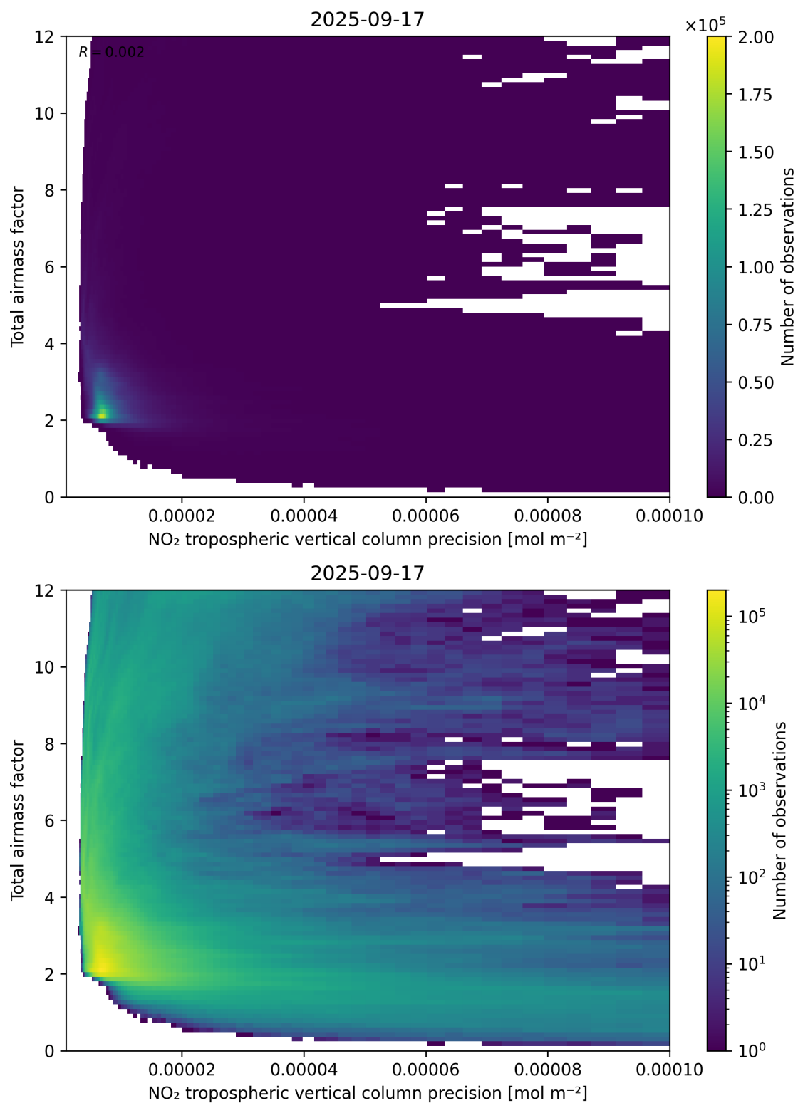
Figure 132: Scatter density plot of “NO 2 tropospheric vertical column precision” against “Total air mass factor” for 2025-09-16 to 2025-09-18.
