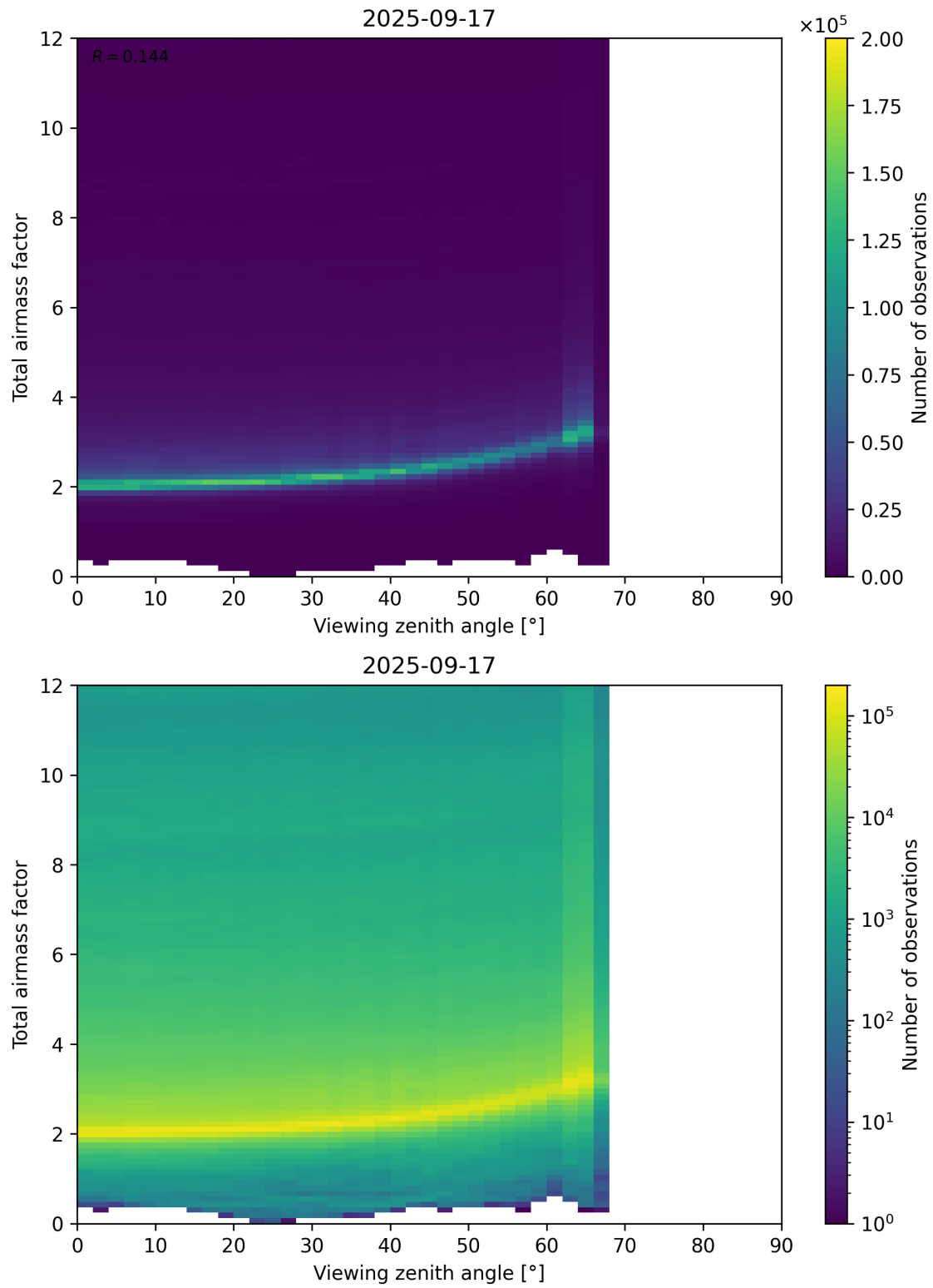
Figure 160: Scatter density plot of “Viewing zenith angle” against “Total airmass factor” for 2025-09-16 to 2025-09-18.
