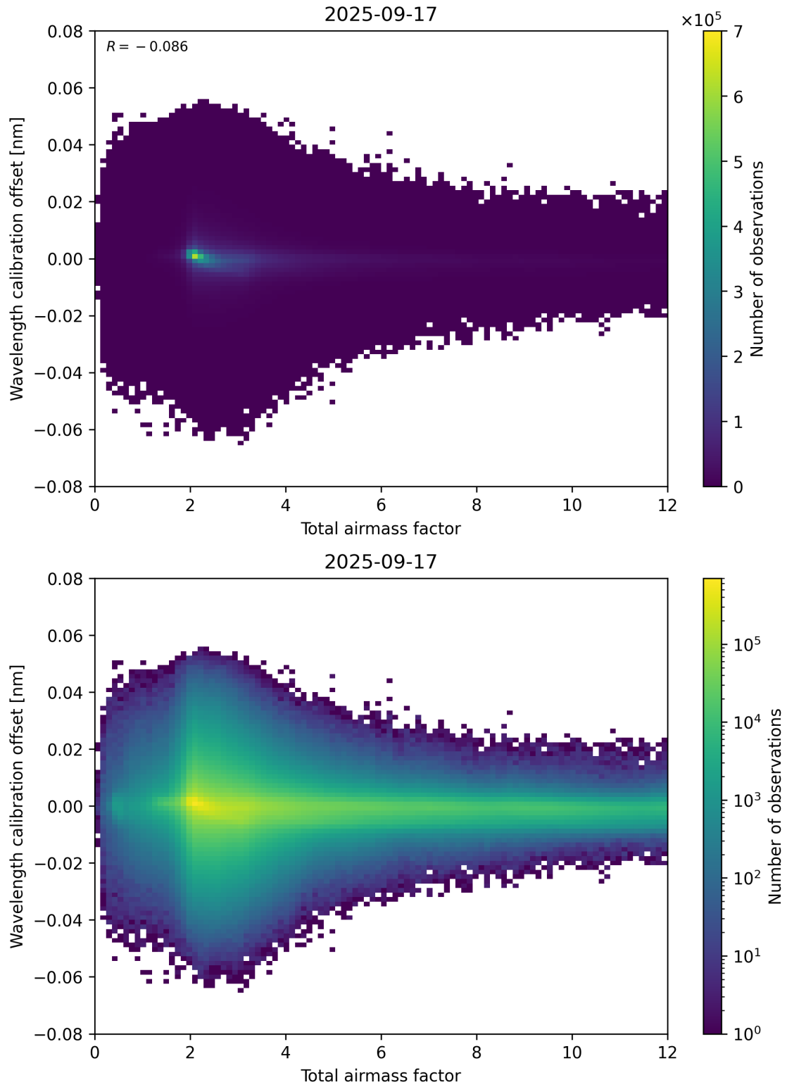
Figure 70: Scatter density plot of “Total airmass factor” against “Wavelength calibration offset” for 2025-09-16 to 2025-09-18.
