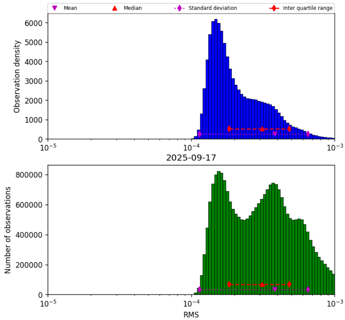
Figure 43: Histogram of “RMS” for 2025-09-16 to 2025-09-18
