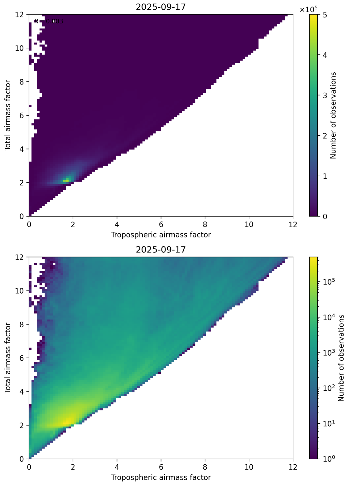
Figure 72: Scatter density plot of “Tropospheric airmass factor” against “Total airmass factor” for 2025-09-16 to 2025-09-18.
