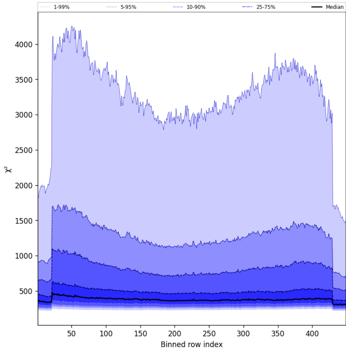
Figure 59: Along track statistics of “ \chi^2 ” for 2025-09-16 to 2025-09-18
