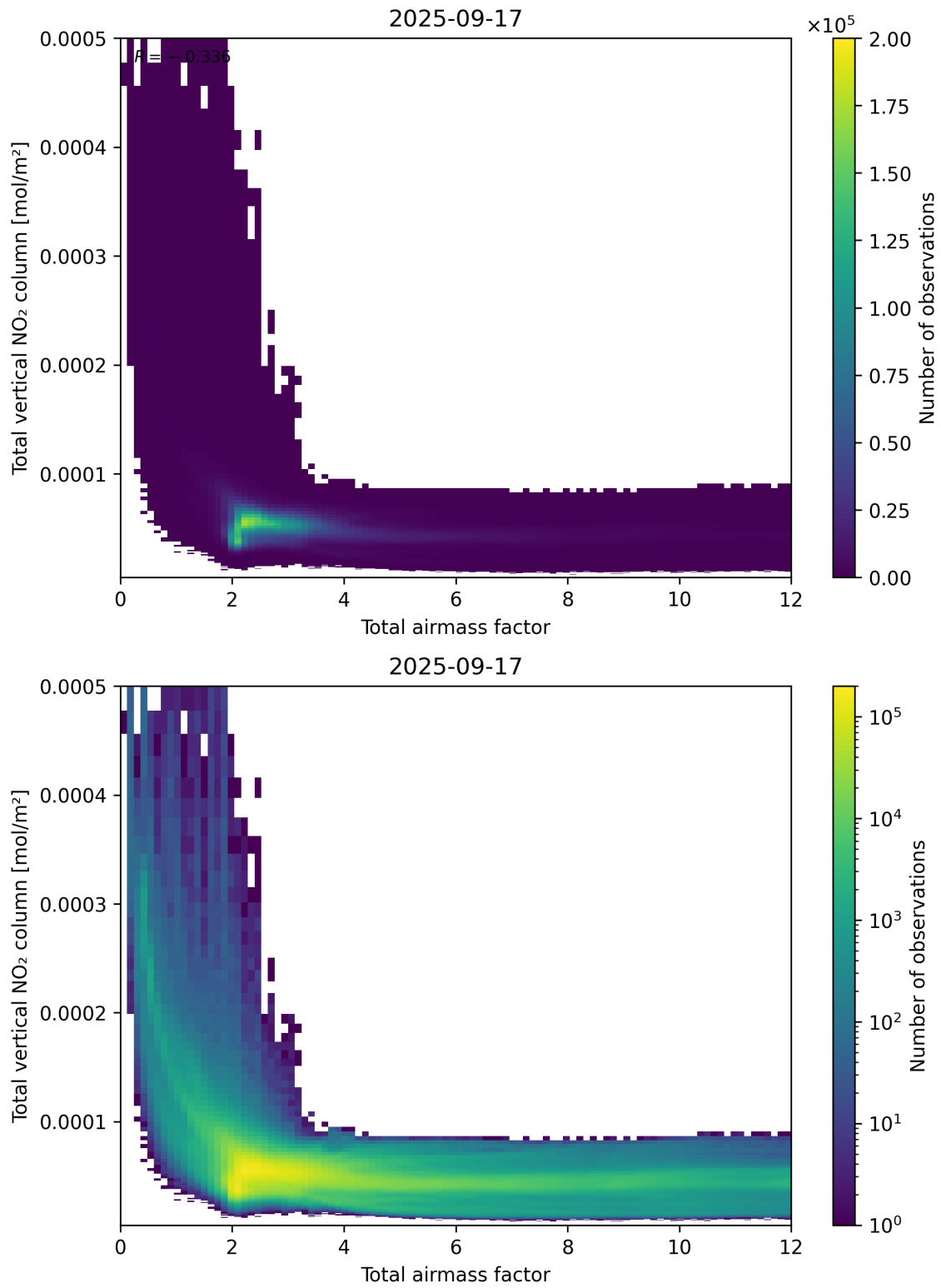
Figure 67: Scatter density plot of “Total airmass factor” against “Total vertical NO 2 column” for 2025-09-16 to 2025-09-18.
