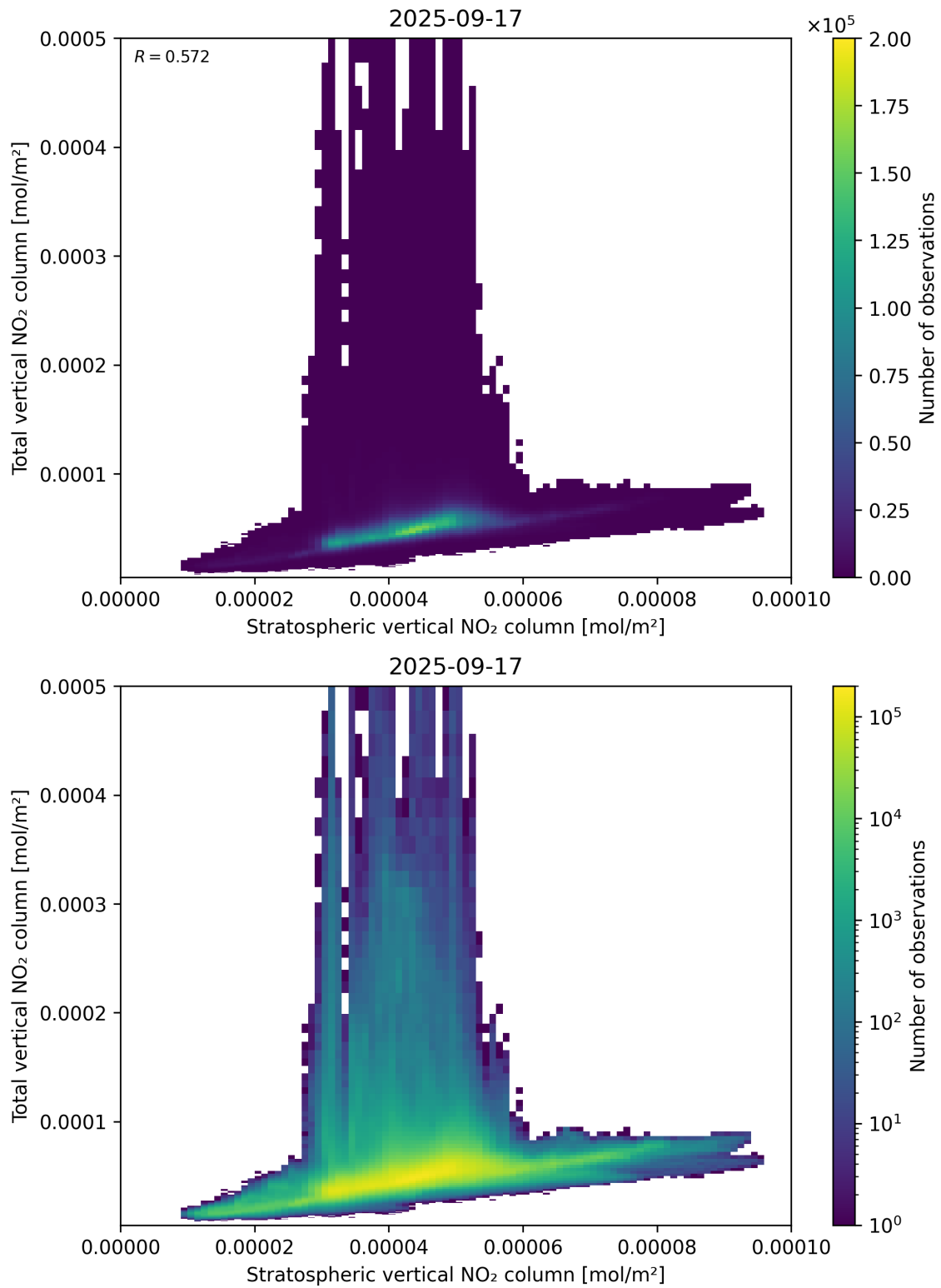
Figure 100: Scatter density plot of “Stratospheric vertical NO 2 column” against “Total vertical NO 2 column” for 2025-09-16 to 2025-09-18.
