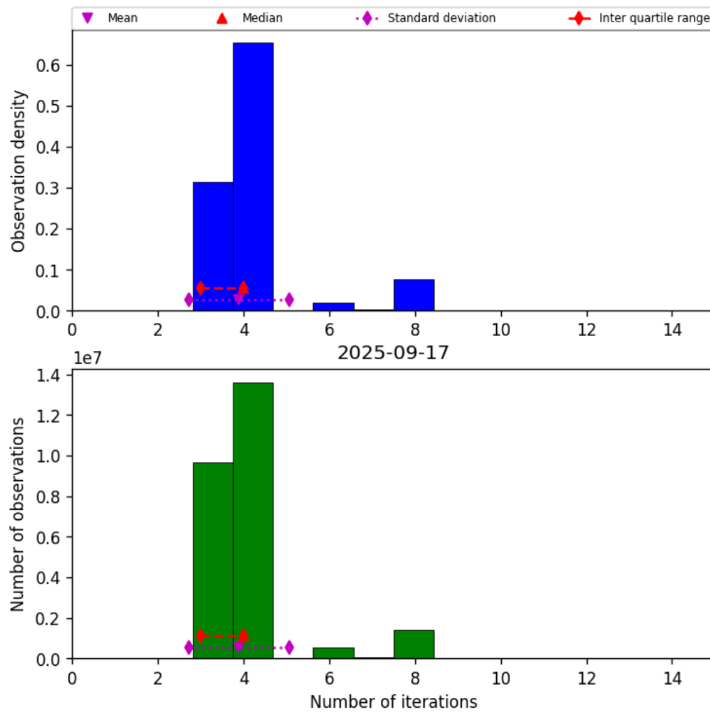
Figure 34: Histogram of “Number of iterations” for 2025-09-16 to 2025-09-18
