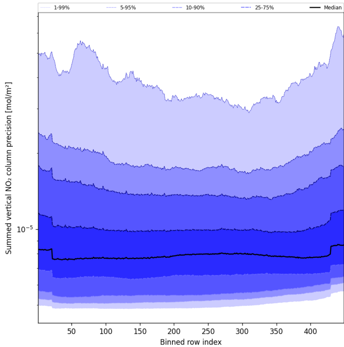
Figure 58: Along track statistics of “Summed vertical NO 2 column precision” for 2025-09-16 to 2025-09-18
