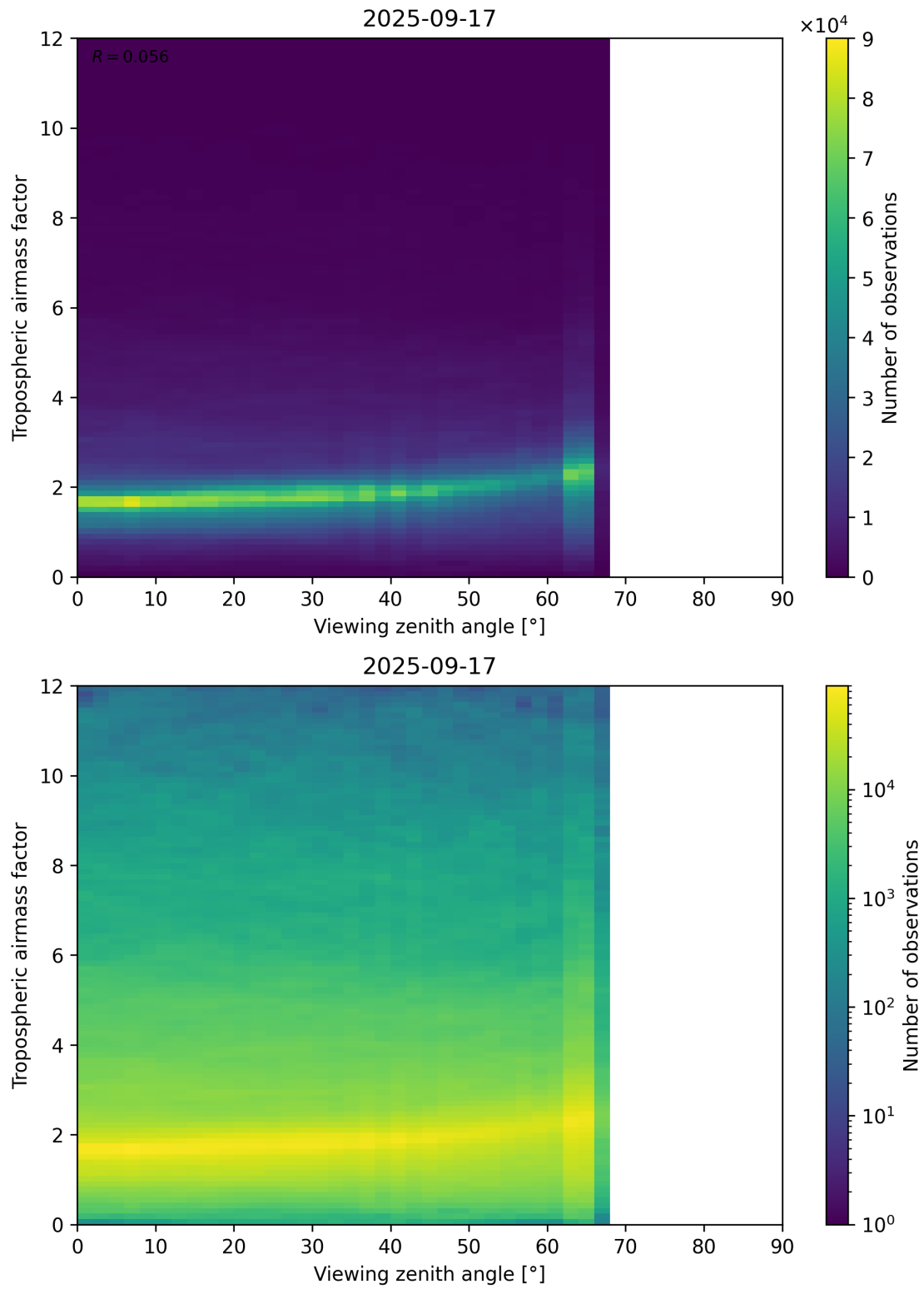
Figure 161: Scatter density plot of “Viewing zenith angle” against “Tropospheric airmass factor” for 2025-09-16 to 2025-09-18.
