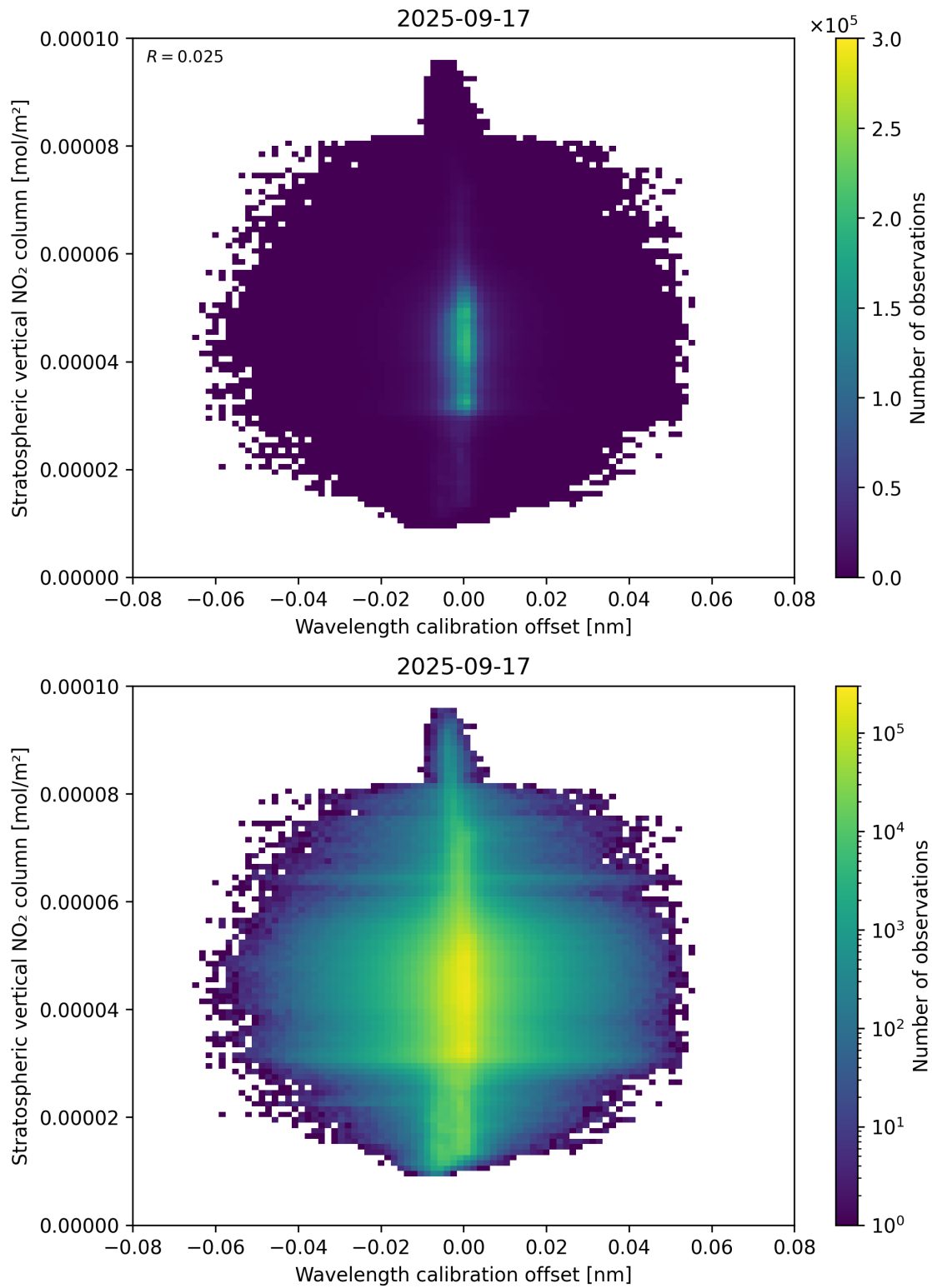
Figure 176: Scatter density plot of “Wavelength calibration offset” against “Stratospheric vertical NO 2 column” for 2025-09-16 to 2025-09-18.
