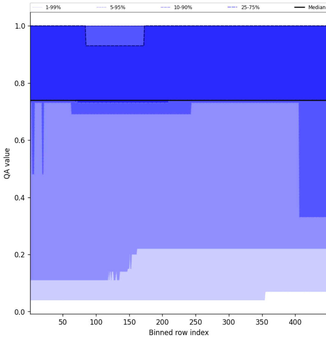
Figure 45: Along track statistics of “QA value” for 2025-09-16 to 2025-09-18
