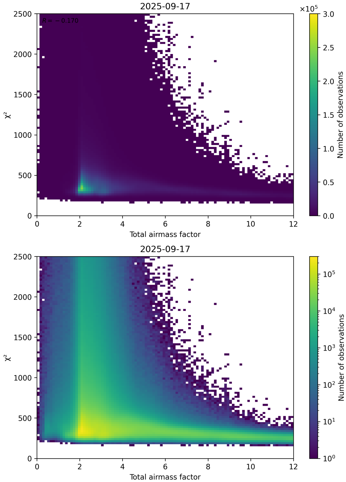
Figure 63: Scatter density plot of “Total airmass factor” against “ \chi^2 ” for 2025-09-16 to 2025-09-18.
