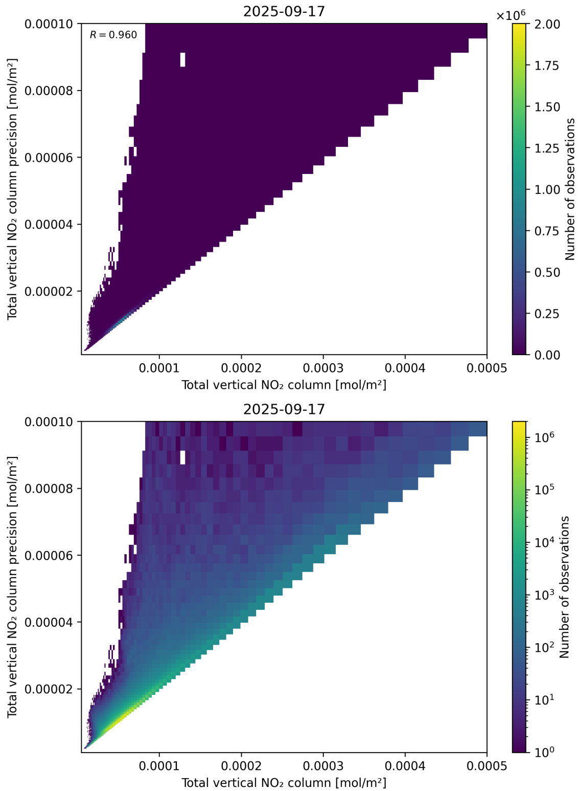
Figure 114: Scatter density plot of “Total vertical NO 2 column” against “Total vertical NO 2 column precision” for 2025-09-16 to 2025-09-18.
