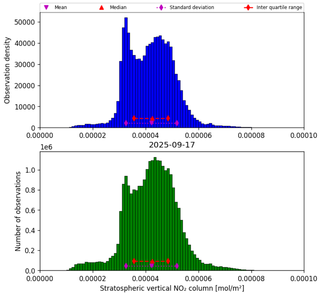
Figure 36: Histogram of “Stratospheric vertical NO 2 column” for 2025-09-16 to 2025-09-18
