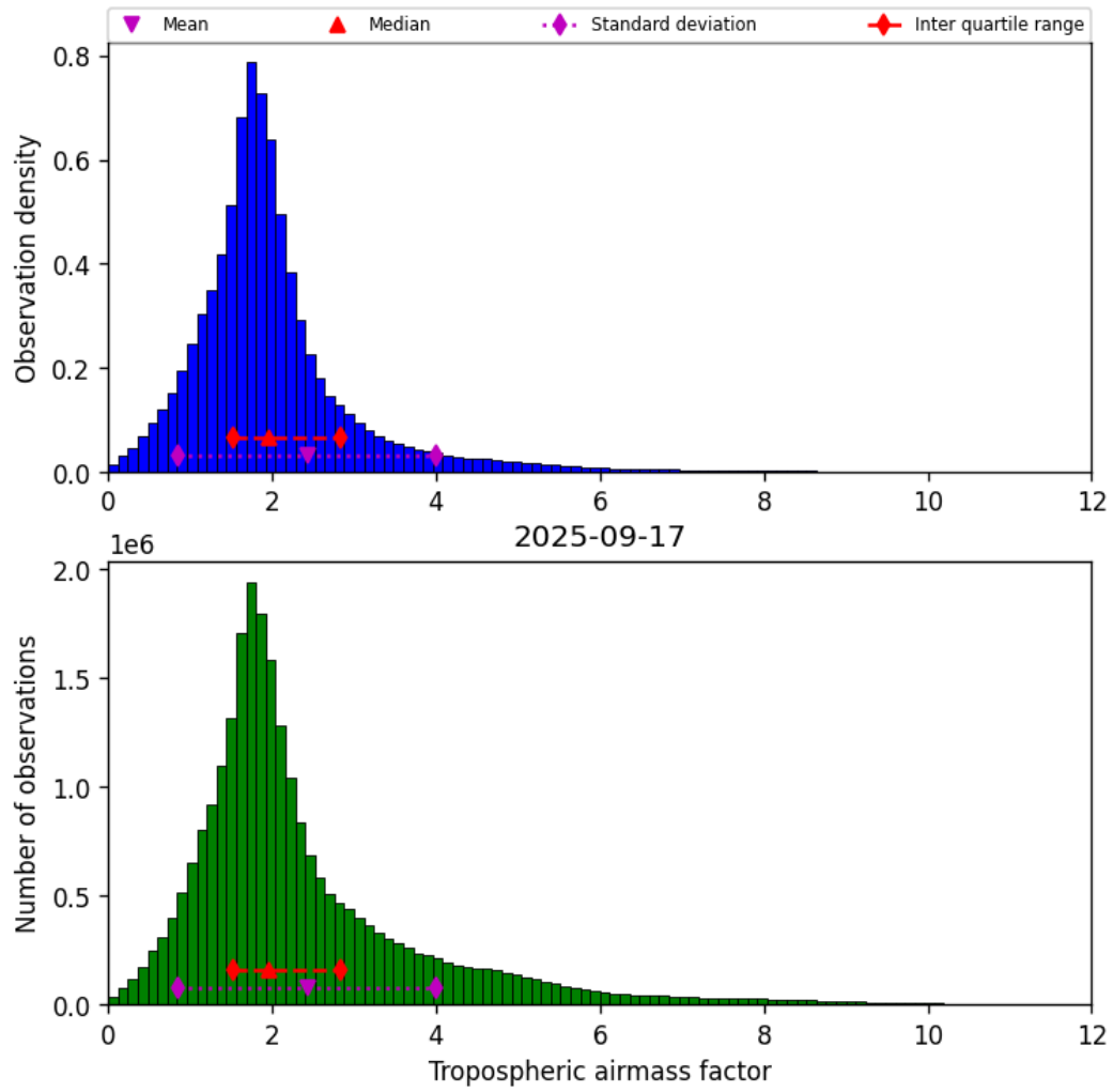
Figure 31: Histogram of “Tropospheric airmass factor” for 2025-09-16 to 2025-09-18
