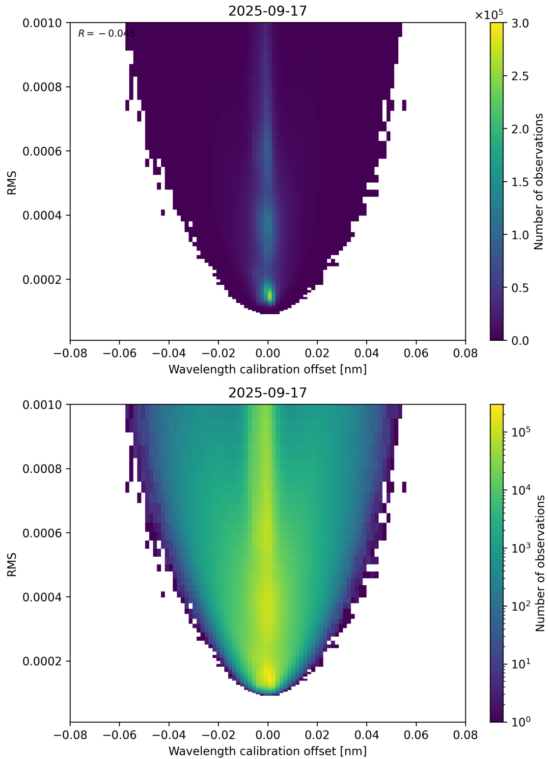
Figure 181: Scatter density plot of “Wavelength calibration offset” against “RMS” for 2025-09-16 to 2025-09-18.
