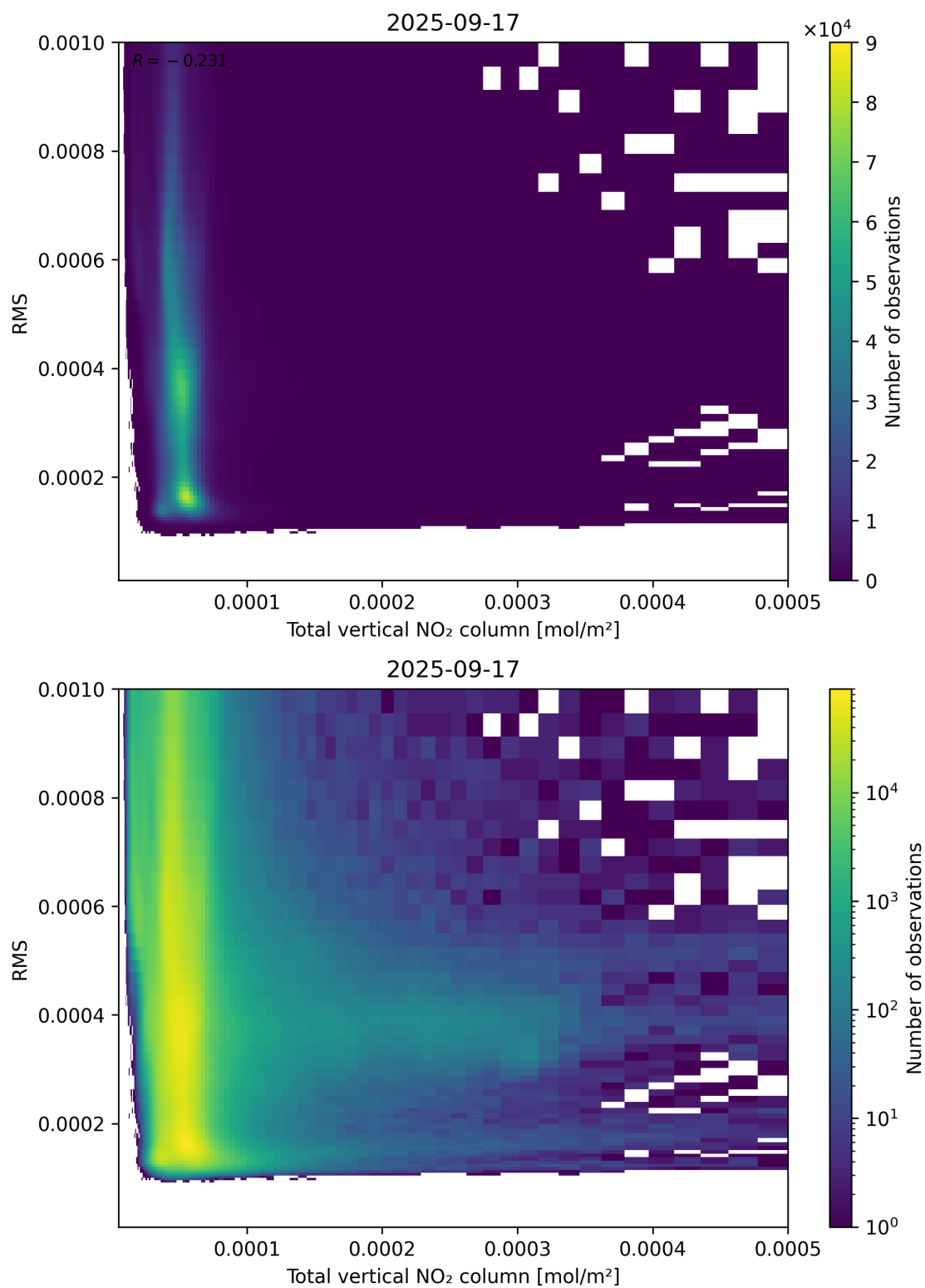
Figure 120: Scatter density plot of “Total vertical NO 2 column” against “RMS” for 2025-09-16 to 2025-09-18.
