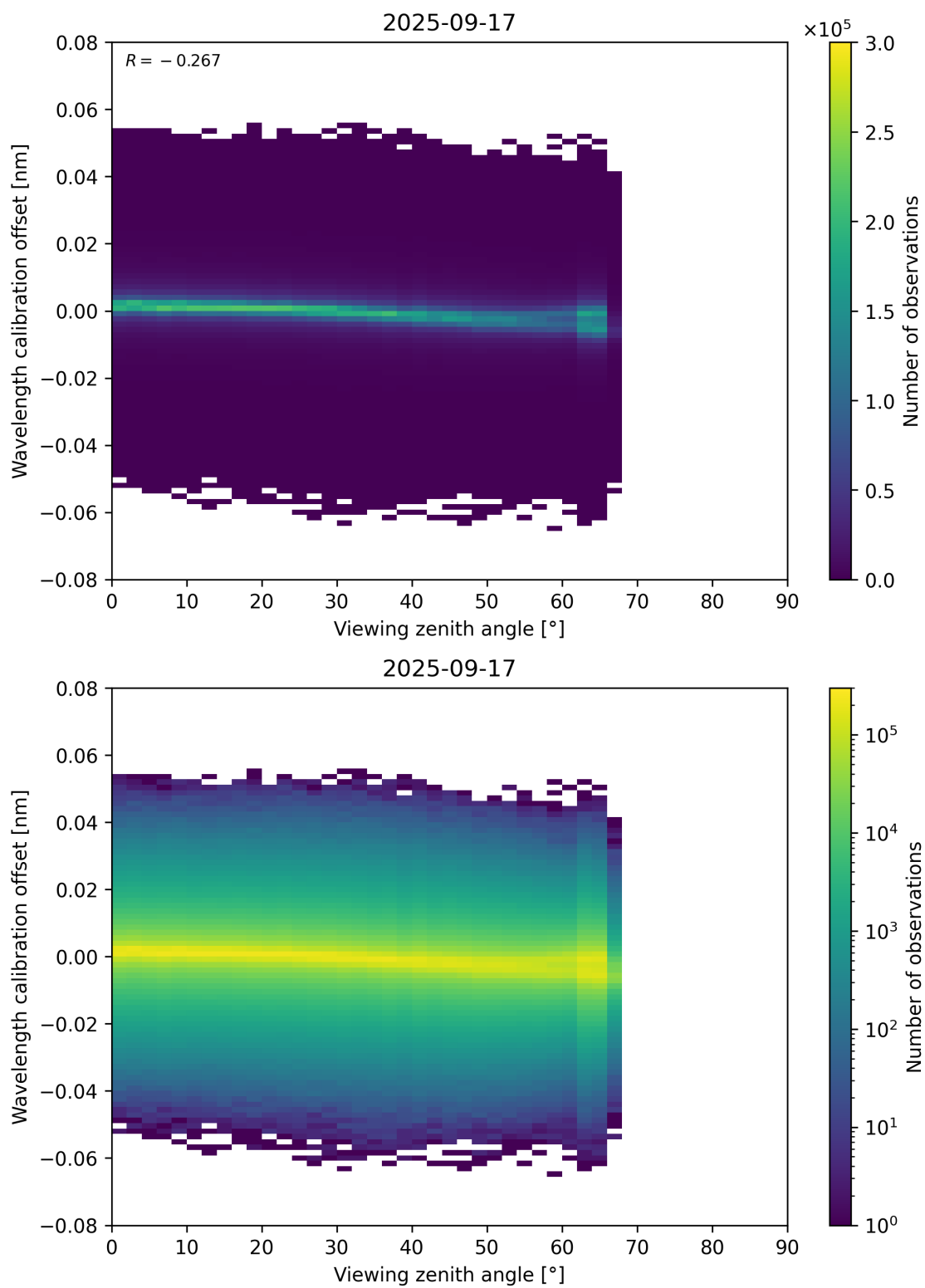
Figure 173: Scatter density plot of “Viewing zenith angle” against “Wavelength calibration offset” for 2025-09-16 to 2025-09-18.
