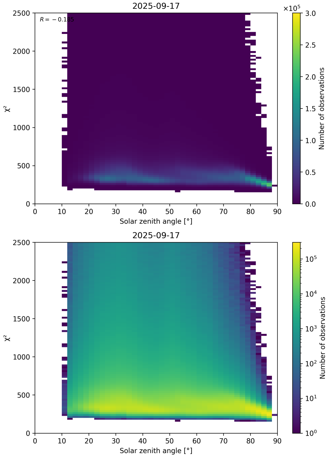
Figure 148: Scatter density plot of “Solar zenith angle” against “ \chi^2 ” for 2025-09-16 to 2025-09-18.
