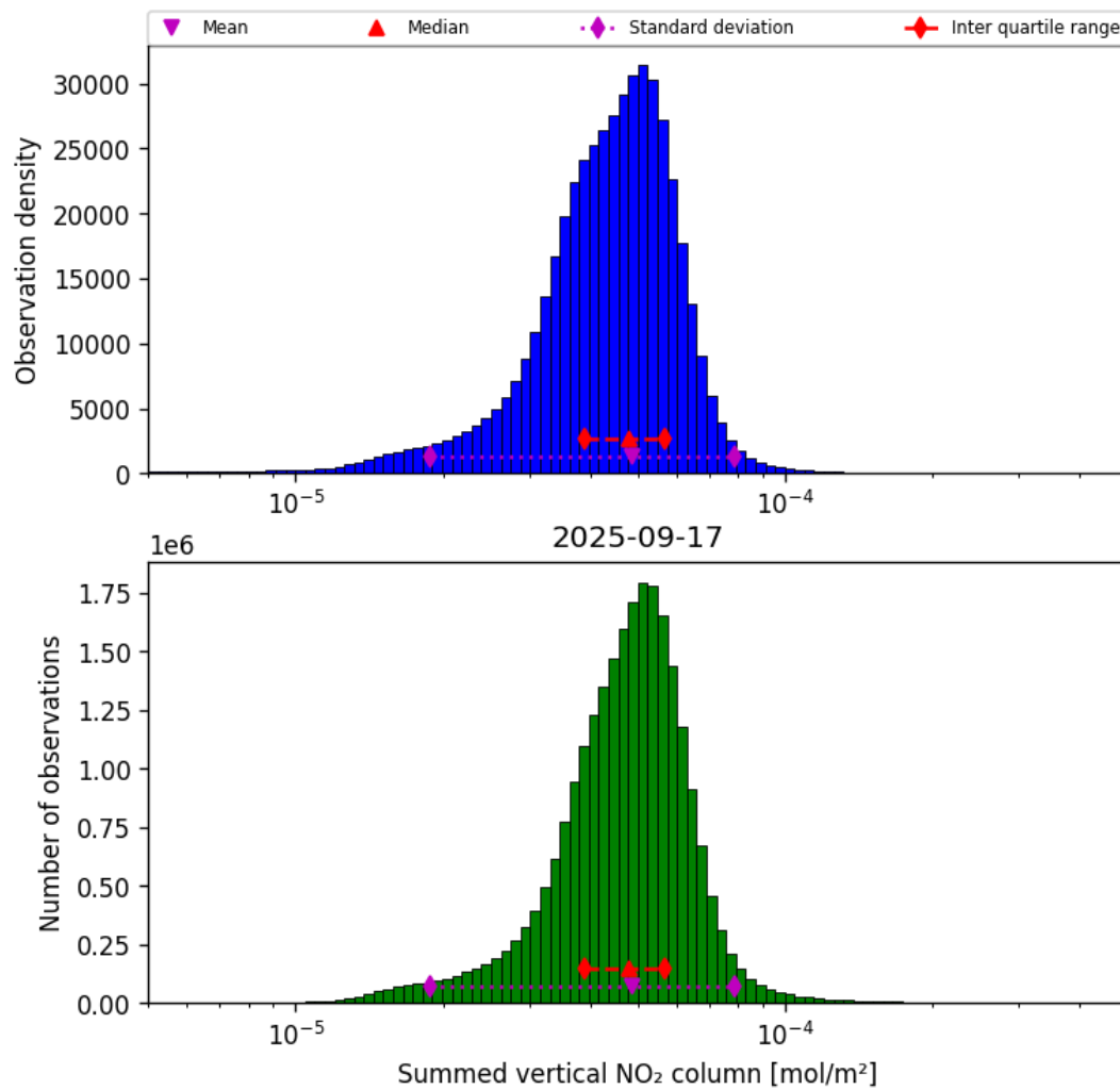
Figure 40: Histogram of “Summed vertical NO 2 column” for 2025-09-16 to 2025-09-18
