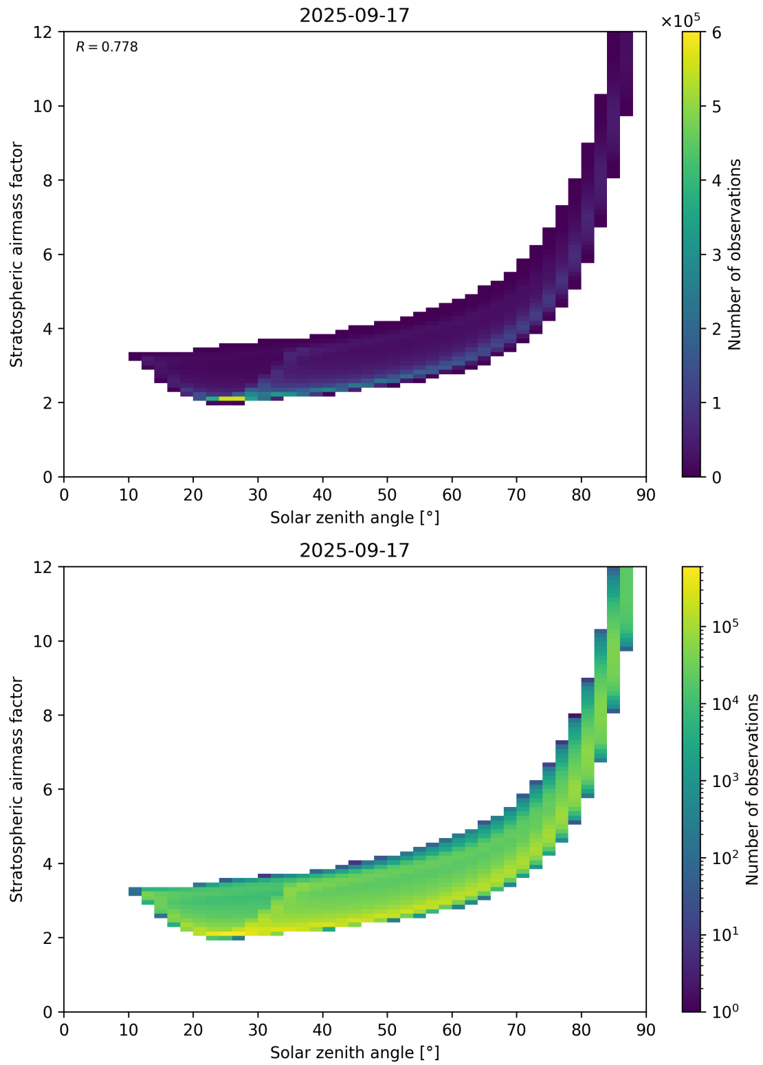
Figure 145: Scatter density plot of “Solar zenith angle” against “Stratospheric airmass factor” for 2025-09-16 to 2025-09-18.
