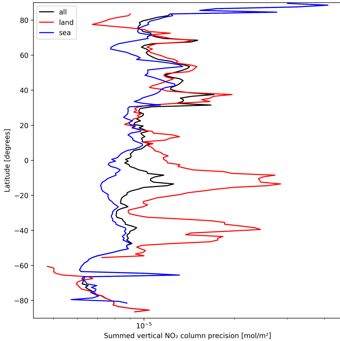
Figure 24: Zonal average of “Summed vertical NO 2 column precision” for 2025-09-16 to 2025-09-18.
