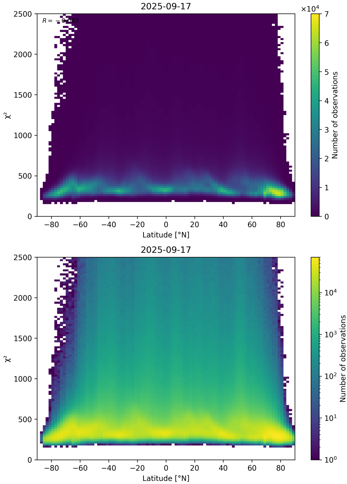
Figure 86: Scatter density plot of “Latitude” against “ \chi^2 ” for 2025-09-16 to 2025-09-18.
