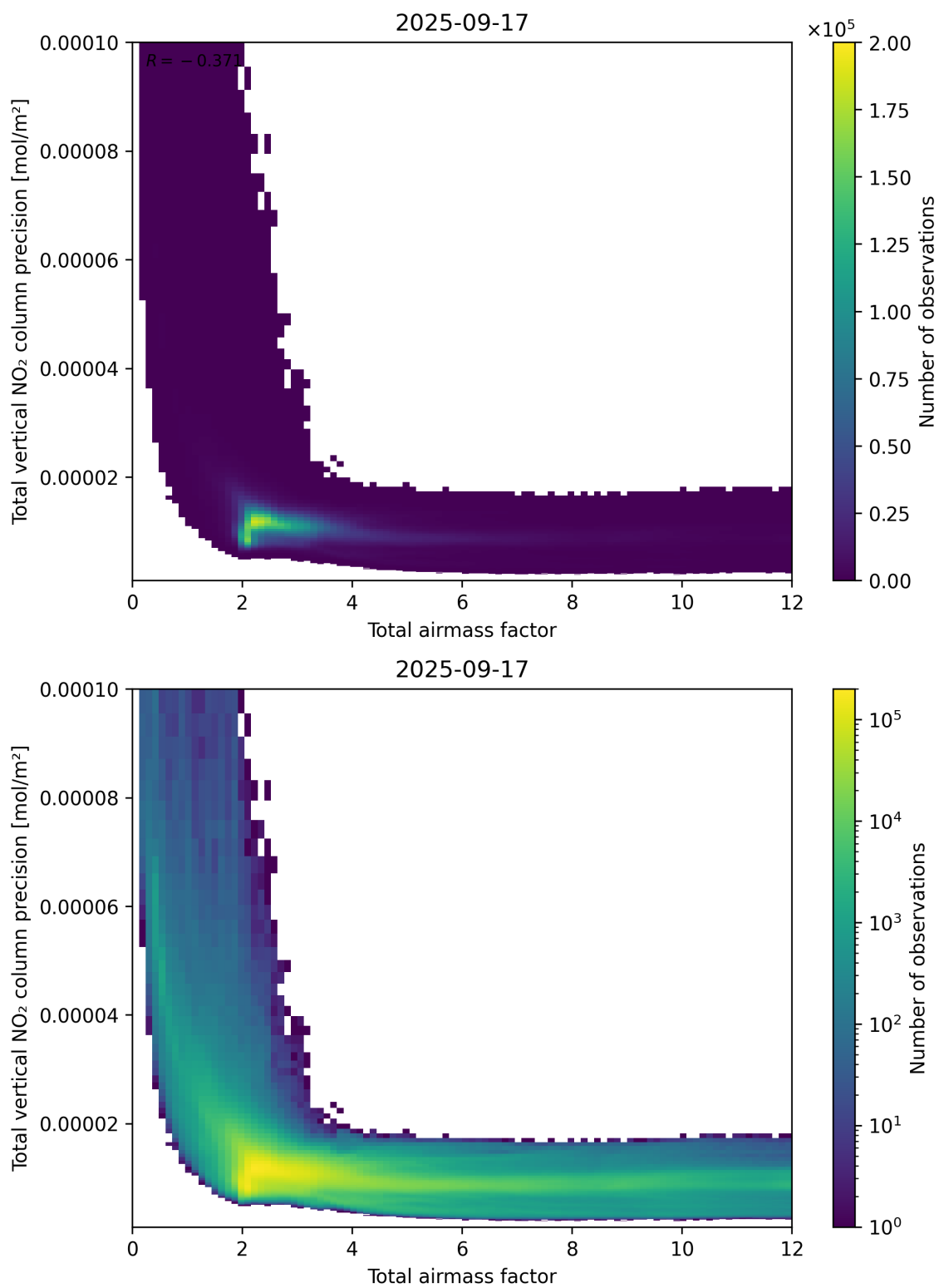
Figure 68: Scatter density plot of “Total airmass factor” against “Total vertical NO 2 column precision” for 2025-09-16 to 2025-09-18.
