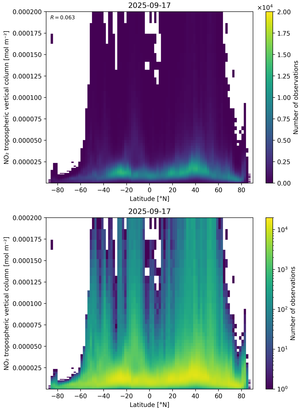
Figure 92: Scatter density plot of “Latitude” against “NO 2 tropospheric vertical column” for 2025-09-16 to 2025-09-18.
