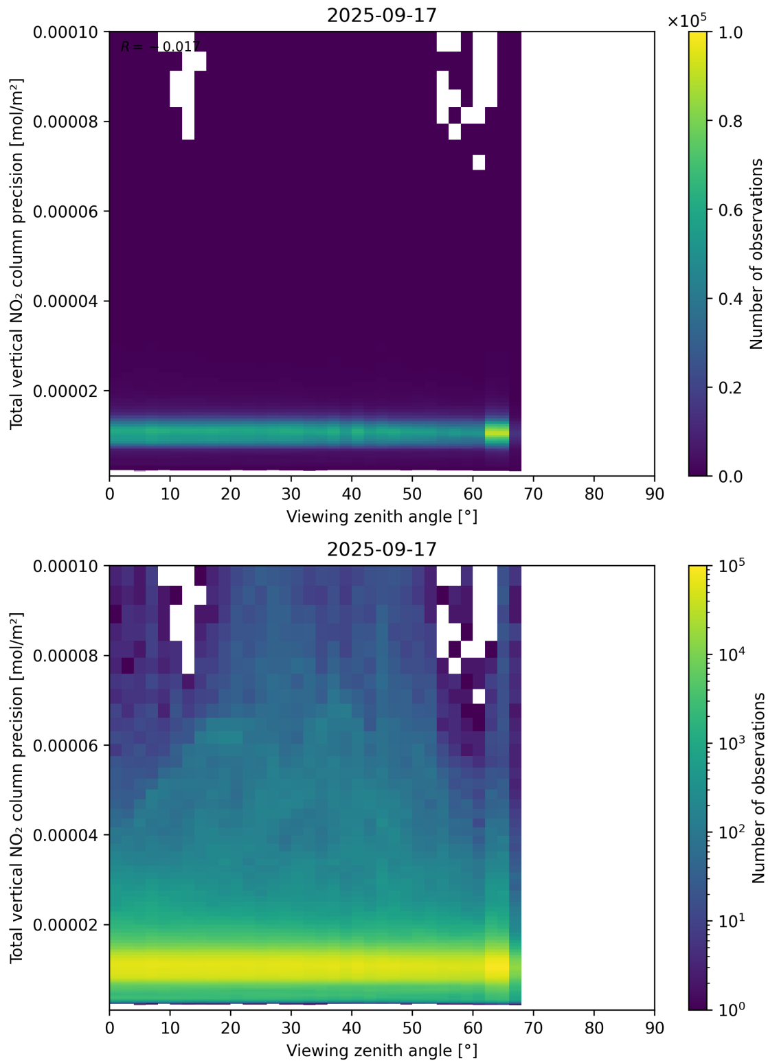
Figure 168: Scatter density plot of “Viewing zenith angle” against “Total vertical NO 2 column precision” for 2025-09-16 to 2025-09-18.
