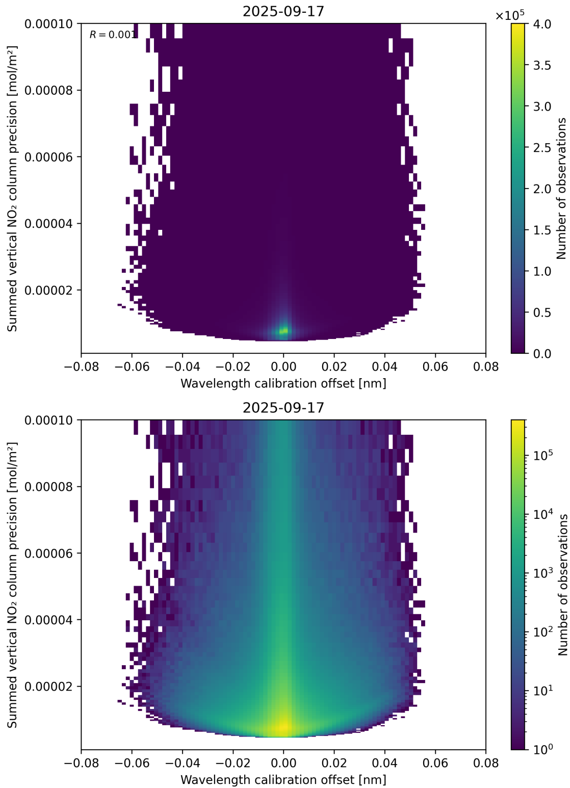
Figure 178: Scatter density plot of “Wavelength calibration offset” against “Summed vertical NO 2 column precision” for 2025-09-16 to 2025-09-18.
