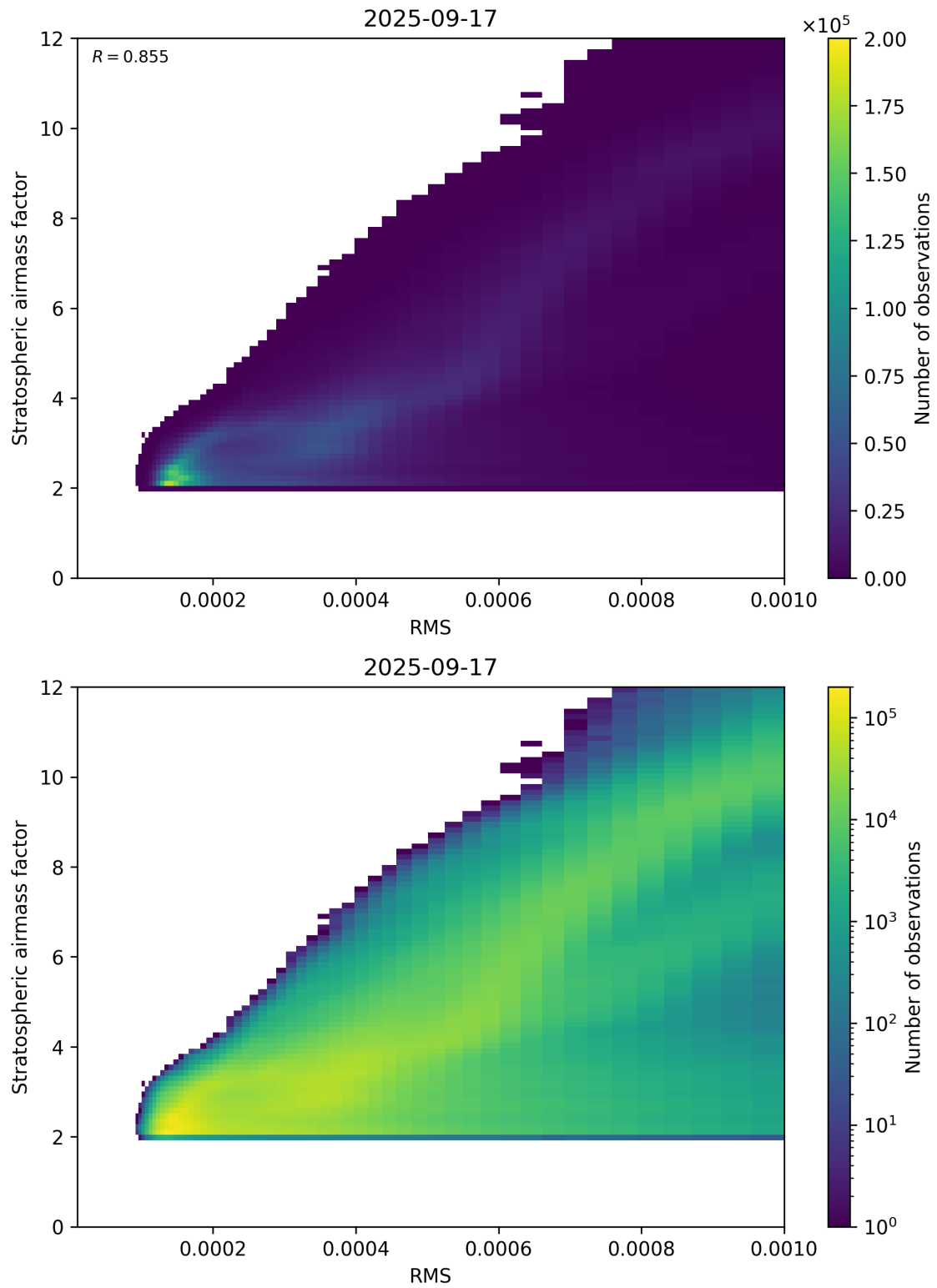
Figure 144: Scatter density plot of “RMS” against “Stratospheric airmass factor” for 2025-09-16 to 2025-09-18.
