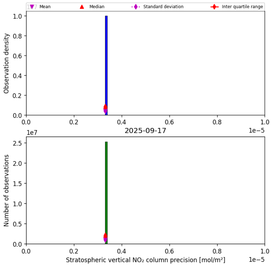
Figure 37: Histogram of “Stratospheric vertical NO 2 column precision” for 2025-09-16 to 2025-09-18
