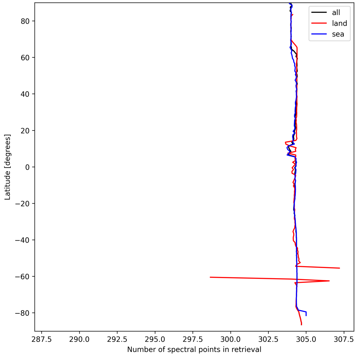
Figure 16: Zonal average of “Number of spectral points in retrieval” for 2025-09-16 to 2025-09-18.
