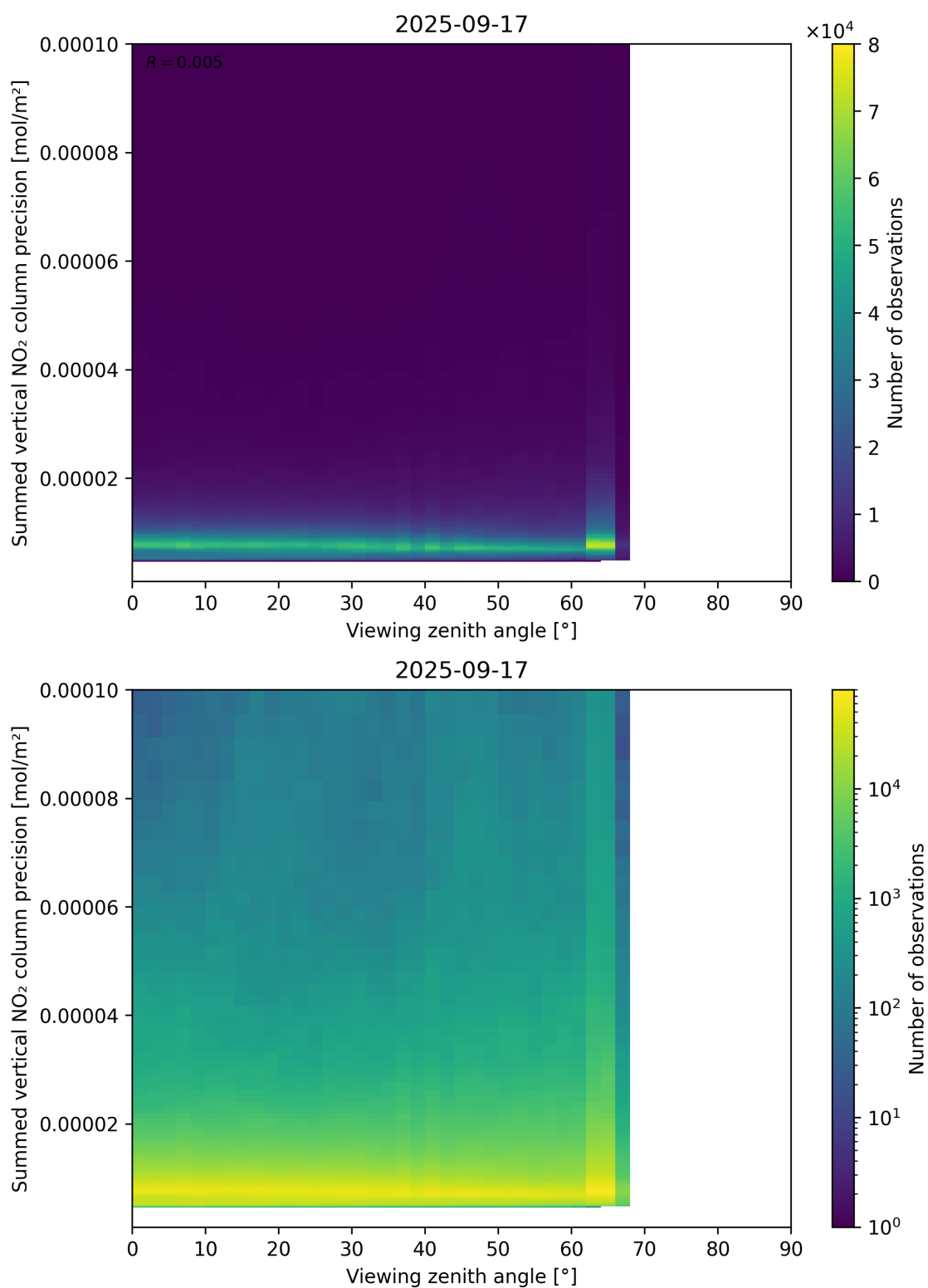
Figure 166: Scatter density plot of “Viewing zenith angle” against “Summed vertical NO 2 column precision” for 2025-09-16 to 2025-09-18.
