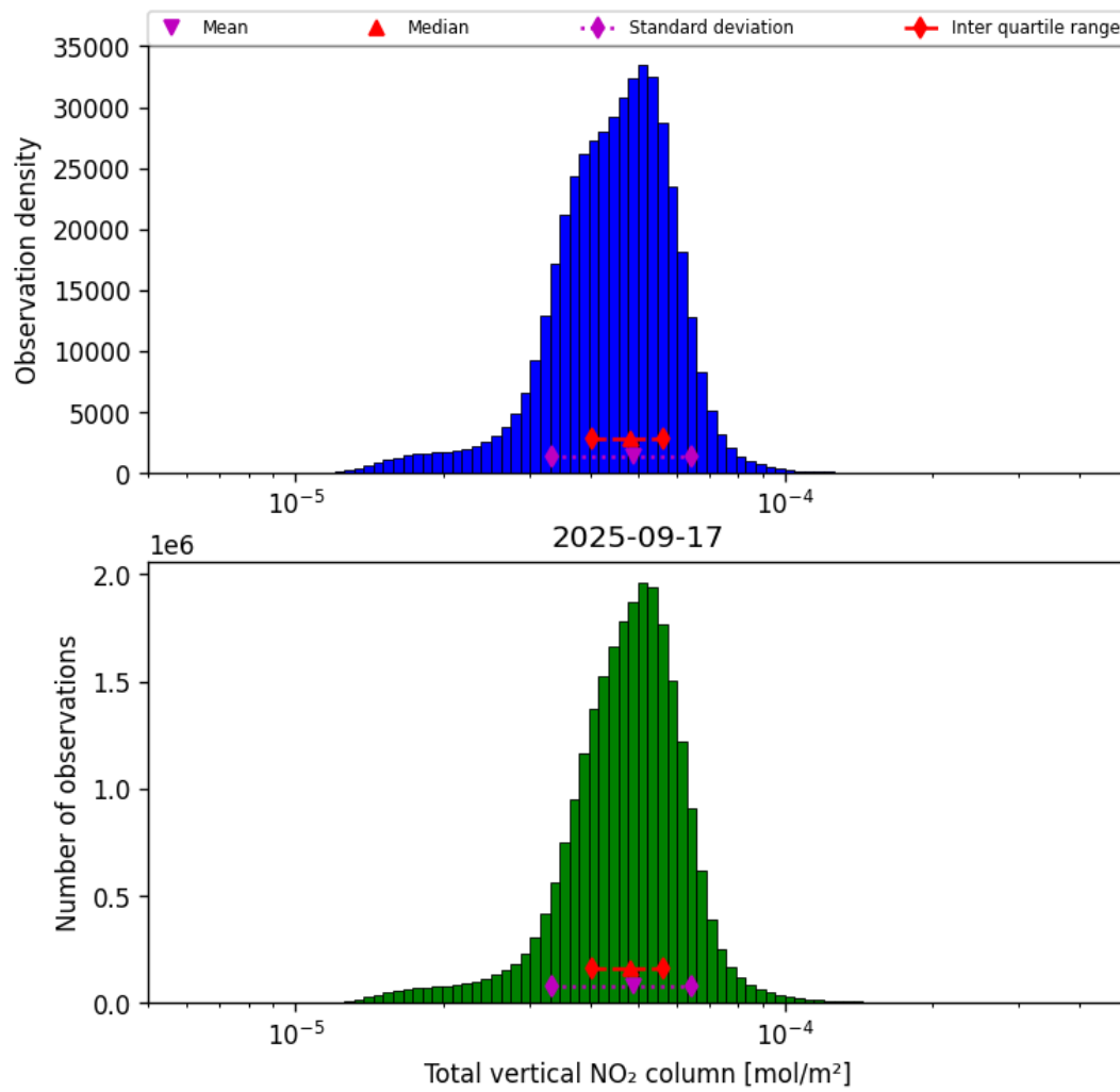
Figure 38: Histogram of "Total vertical NO 2 column" for 2025-09-16 to 2025-09-18
