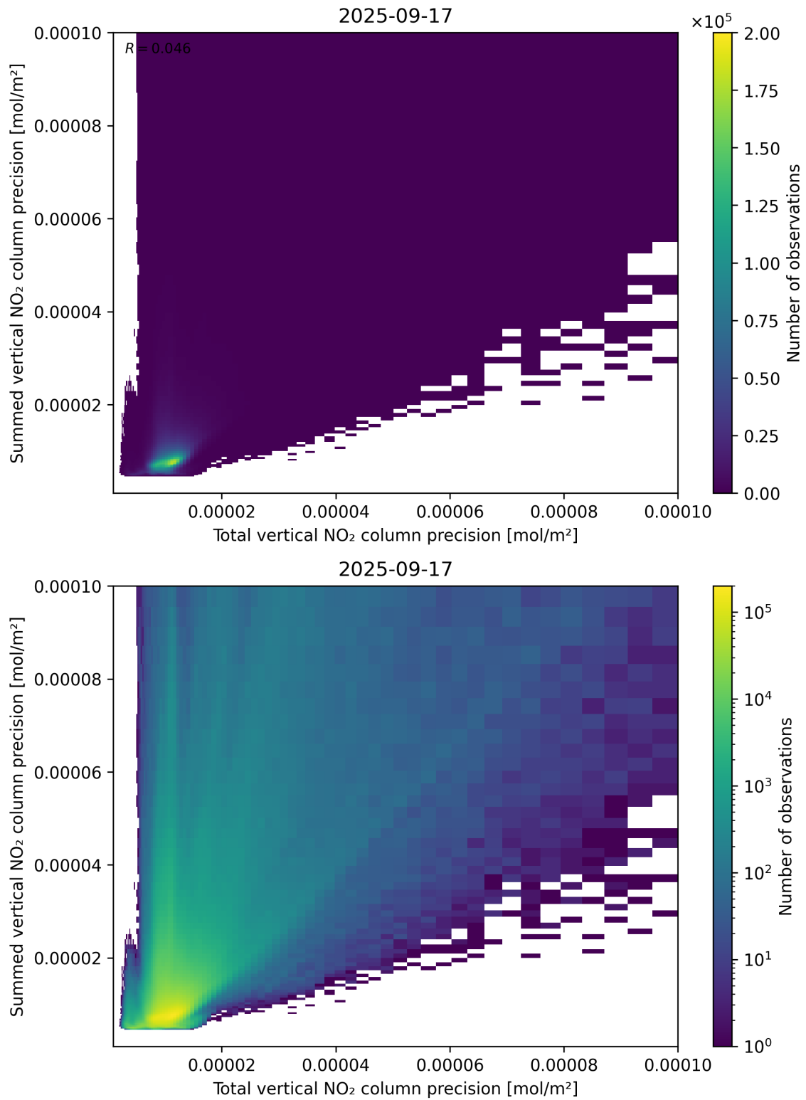
Figure 118: Scatter density plot of “Total vertical NO 2 column precision” against “Summed vertical NO 2 column precision” for 2025-09-16 to 2025-09-18.
