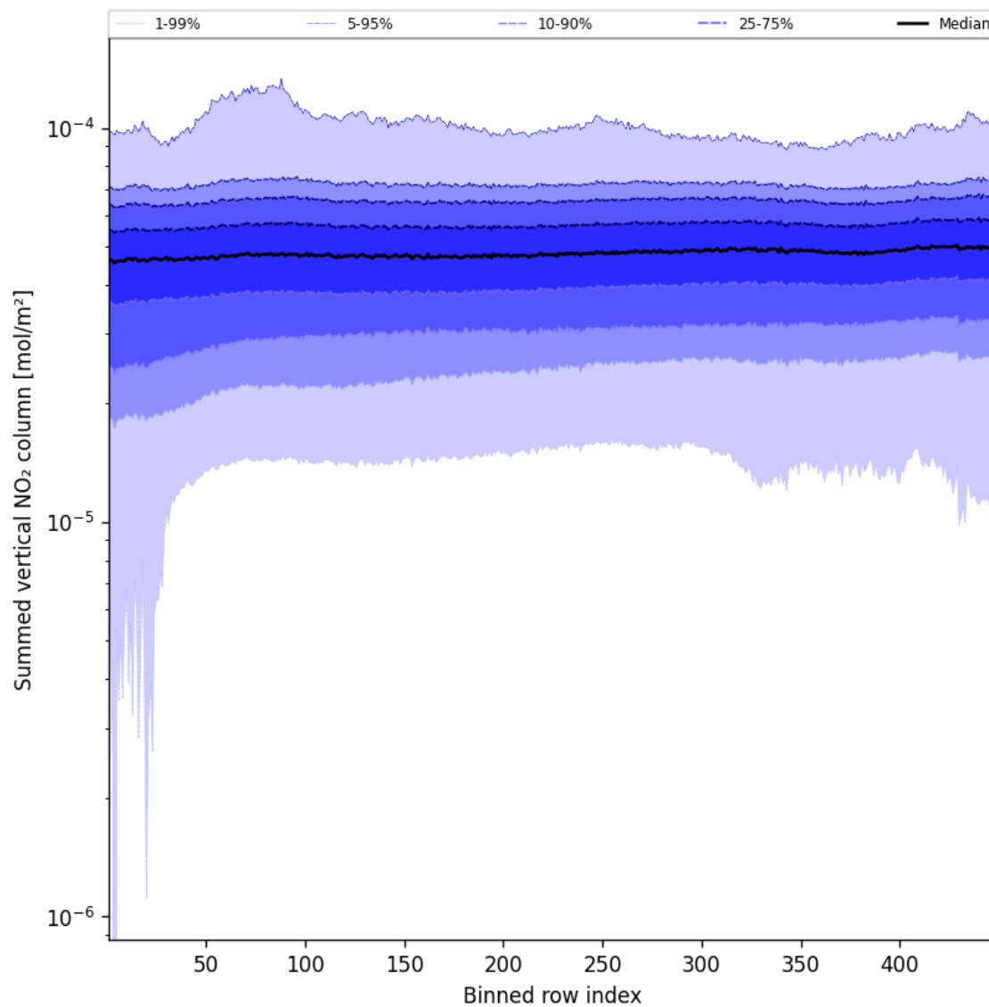
Figure 57: Along track statistics of “Summed vertical NO 2 column” for 2025-09-16 to 2025-09-18
