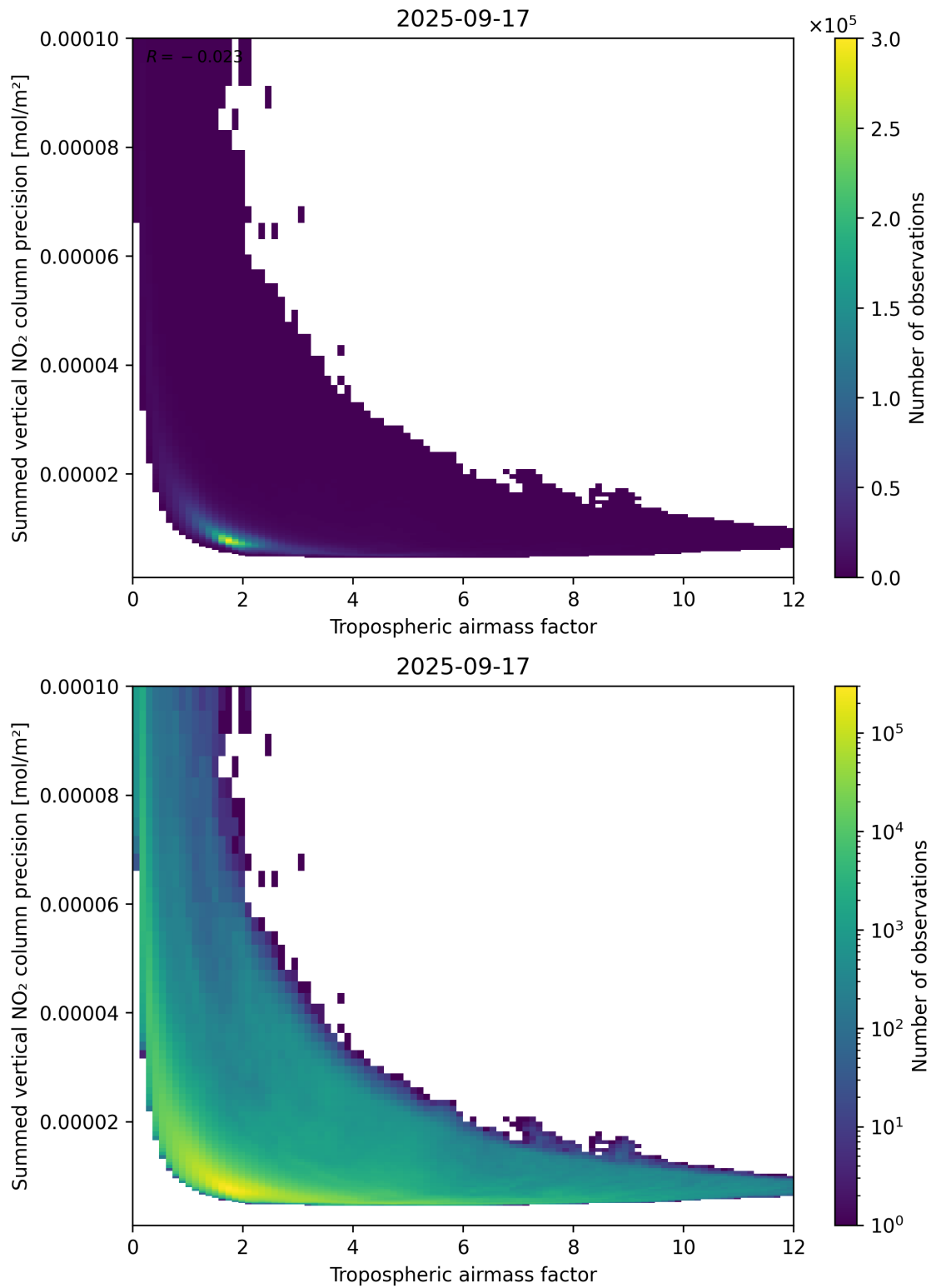
Figure 76: Scatter density plot of “Tropospheric air mass factor” against “Summed vertical NO 2 column precision” for 2025-09-16 to 2025-09-18.
