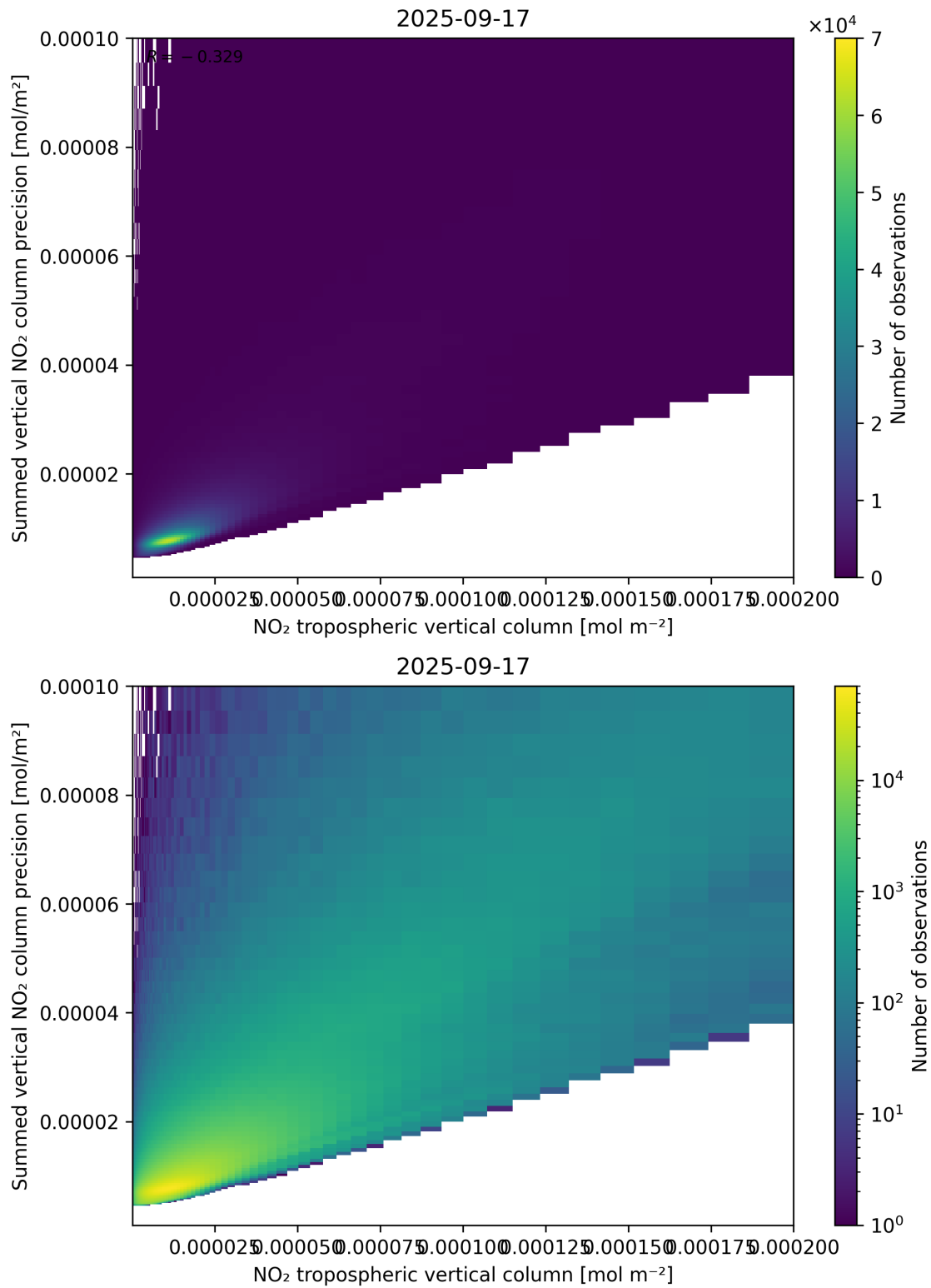
Figure 127: Scatter density plot of “NO 2 tropospheric vertical column” against “Summed vertical NO 2 column precision” for 2025-09-16 to 2025-09-18.
