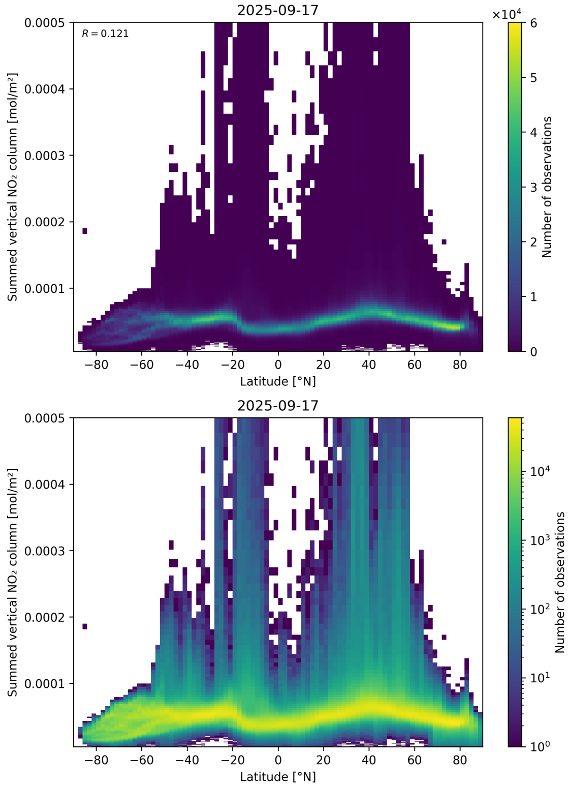
Figure 88: Scatter density plot of “Latitude” against “Summed vertical NO 2 column” for 2025-09-16 to 2025-09-18.
