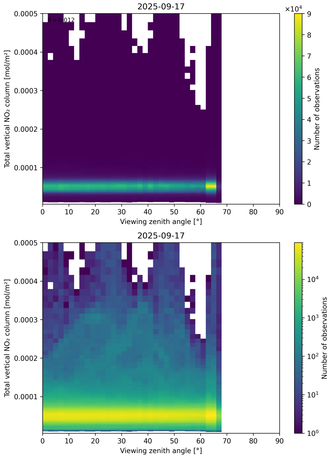
Figure 167: Scatter density plot of “Viewing zenith angle” against “Total vertical NO 2 column” for 2025-09-16 to 2025-09-18.
