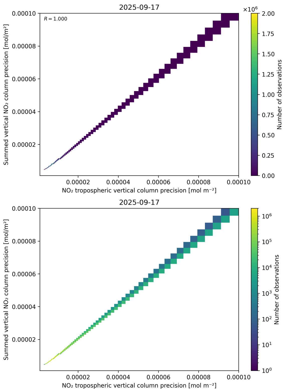
Figure 137: Scatter density plot of “NO 2 tropospheric vertical column precision” against “Summed vertical NO 2 column precision” for 2025-09-16 to 2025-09-18.
