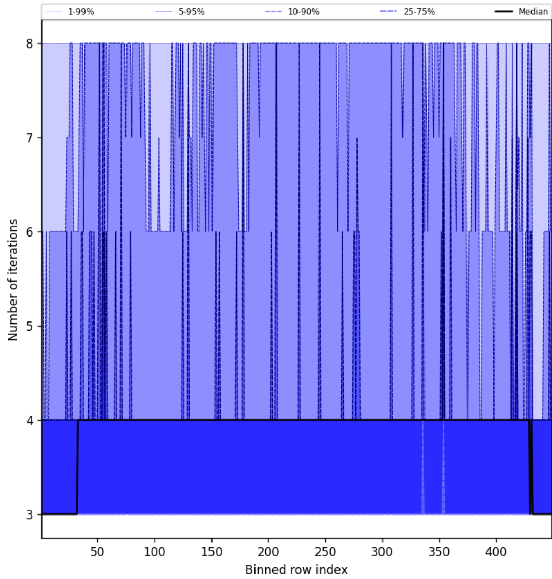
Figure 51: Along track statistics of “Number of iterations” for 2025-09-16 to 2025-09-18
