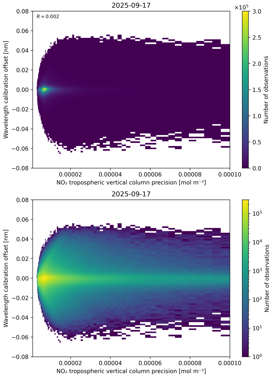
Figure 141: Scatter density plot of “NO 2 tropospheric vertical column precision” against “Wavelength calibration offset” for 2025-09-16 to 2025-09-18.
