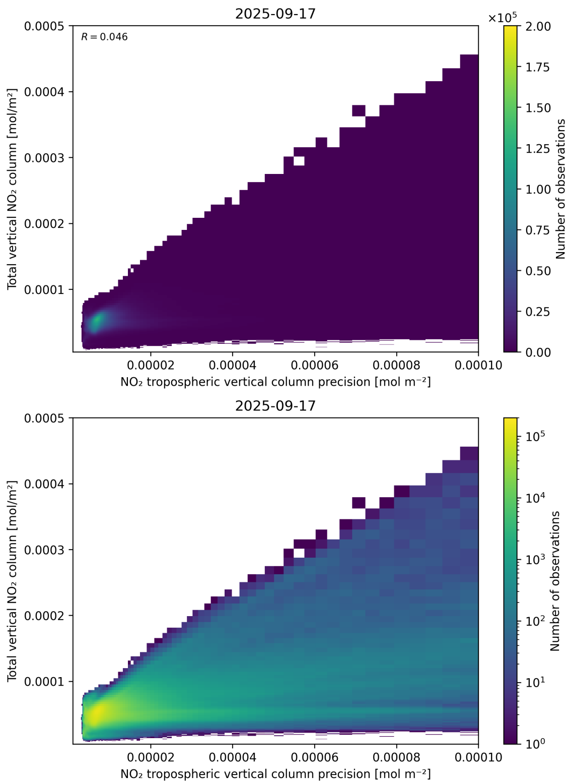
Figure 138: Scatter density plot of “NO 2 tropospheric vertical column precision” against “Total vertical NO 2 column” for 2025-09-16 to 2025-09-18.
