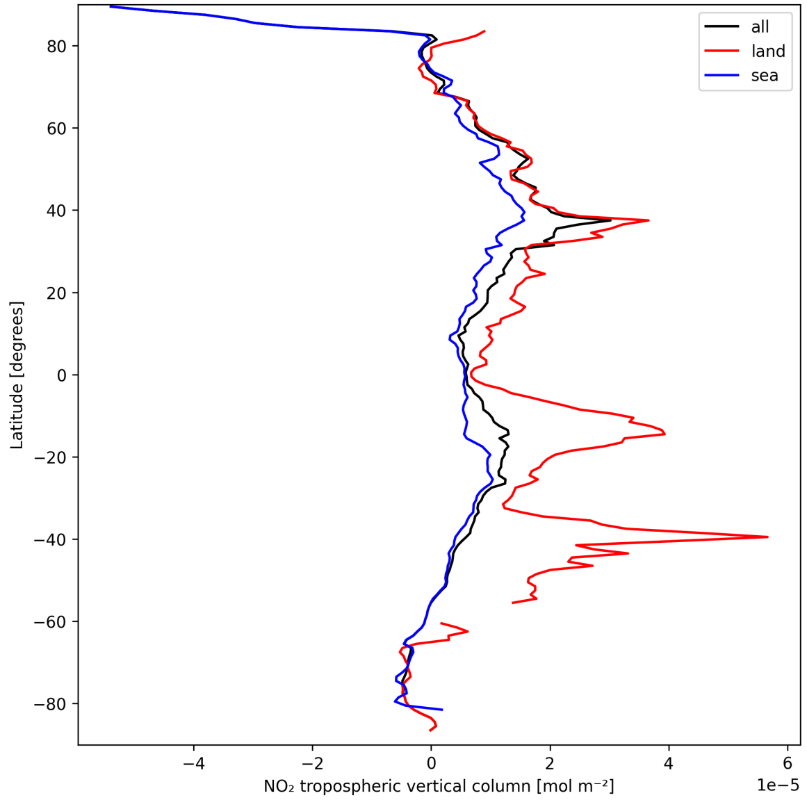
Figure 12: Zonal average of “NO 2 tropospheric vertical column” for 2025-09-16 to 2025-09-18.
