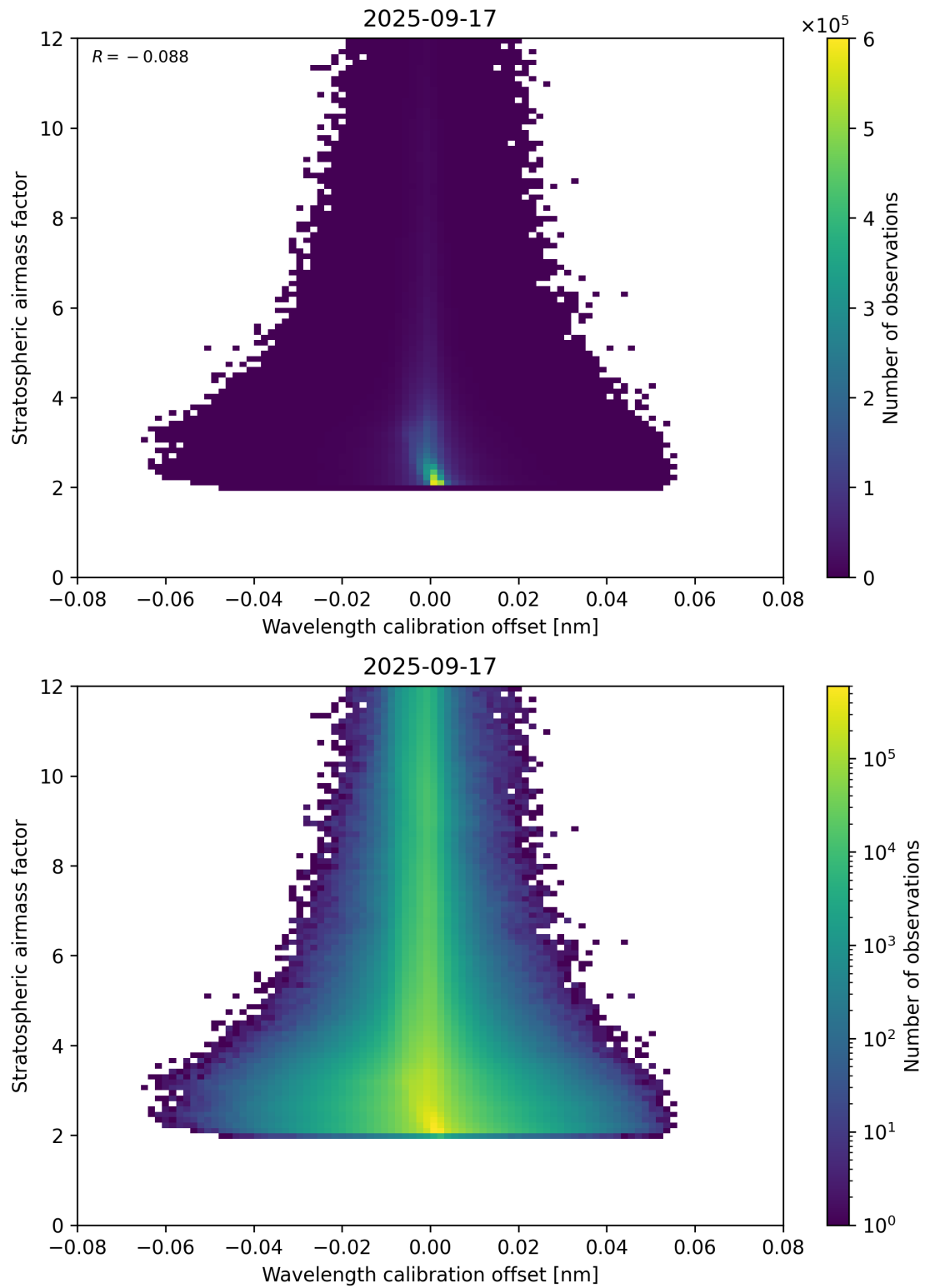
Figure 174: Scatter density plot of “Wavelength calibration offset” against “Stratospheric airmass factor” for 2025-09-16 to 2025-09-18.
