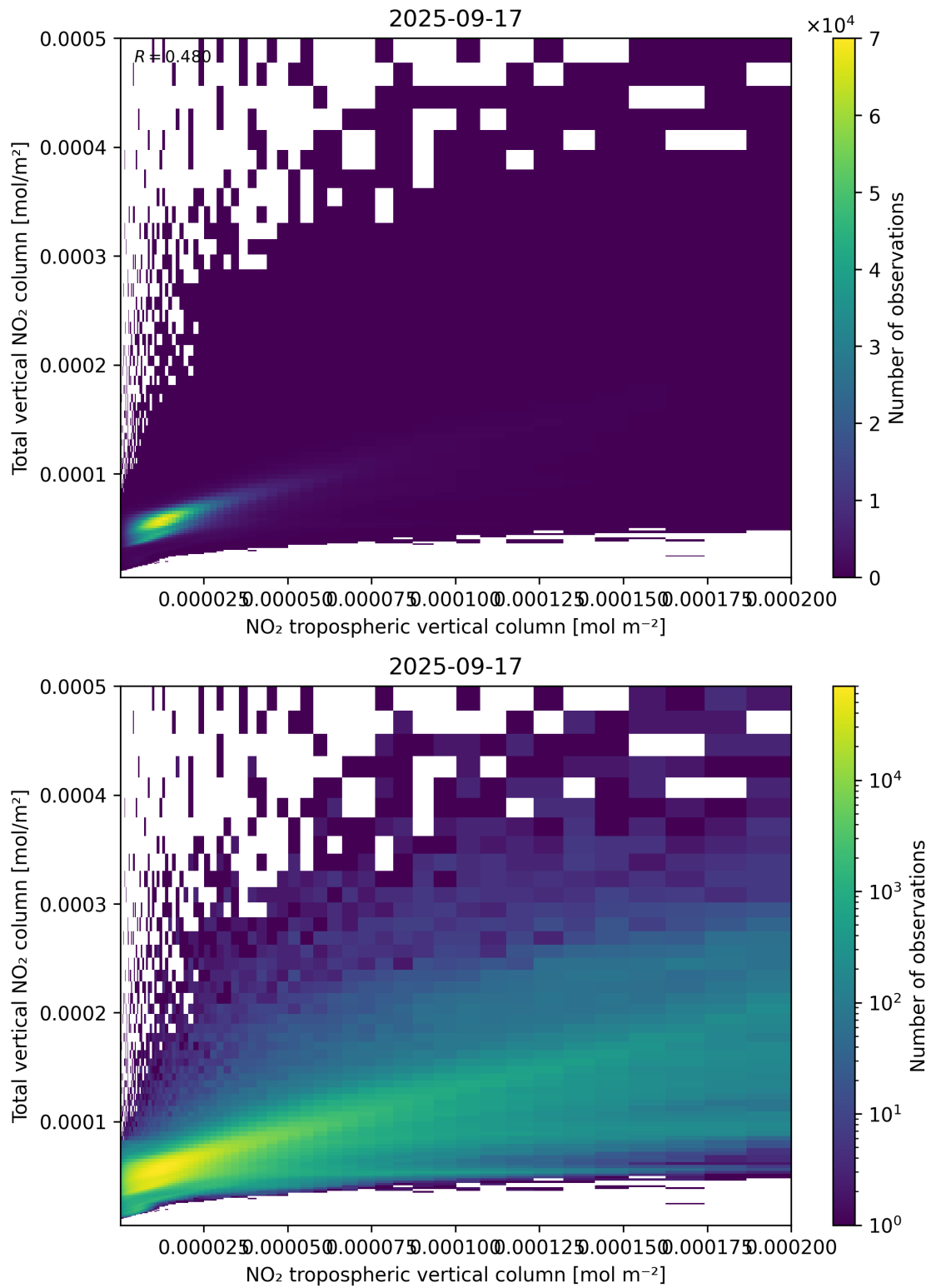
Figure 128: Scatter density plot of “NO 2 tropospheric vertical column” against “Total vertical NO 2 column” for 2025-09-16 to 2025-09-18.
