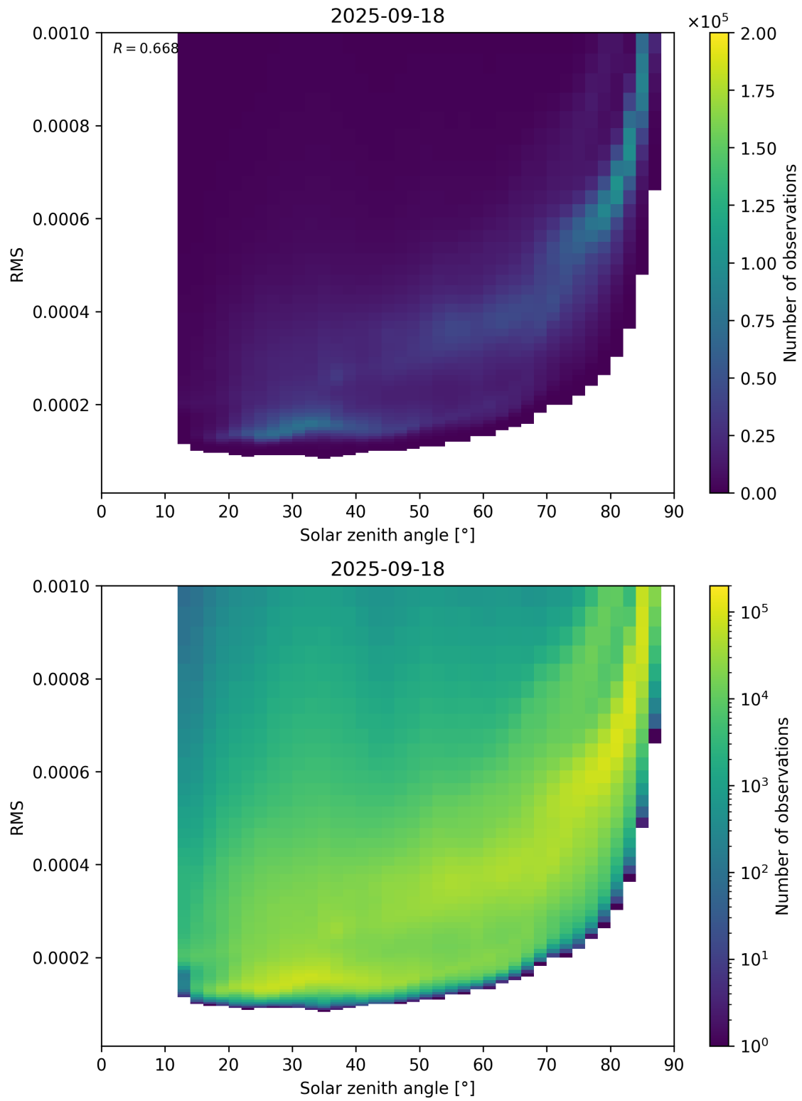
Figure 157: Scatter density plot of “Solar zenith angle” against “RMS” for 2025-09-17 to 2025-09-19.
