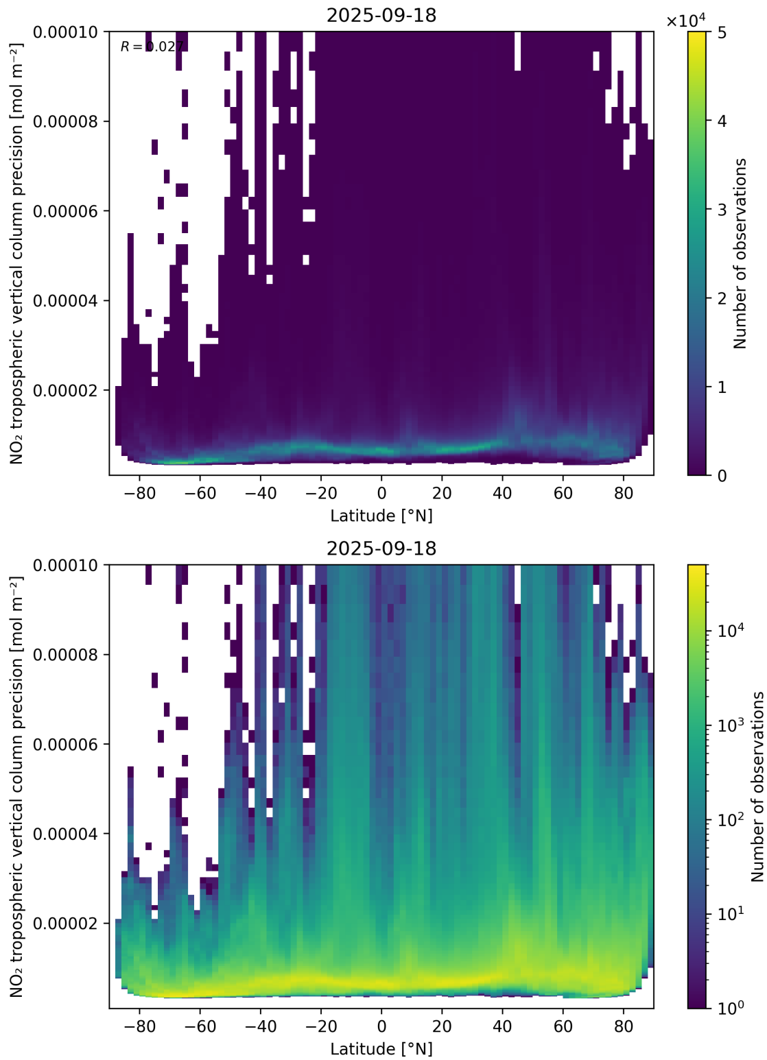
Figure 93: Scatter density plot of “Latitude” against “NO 2 tropospheric vertical column precision” for 2025-09-17 to 2025-09-19.
