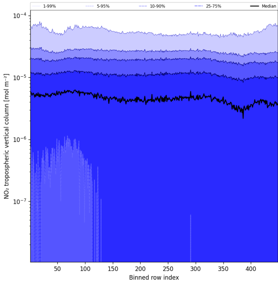
Figure 46: Along track statistics of “NO 2 tropospheric vertical column” for 2025-09-17 to 2025-09-19
