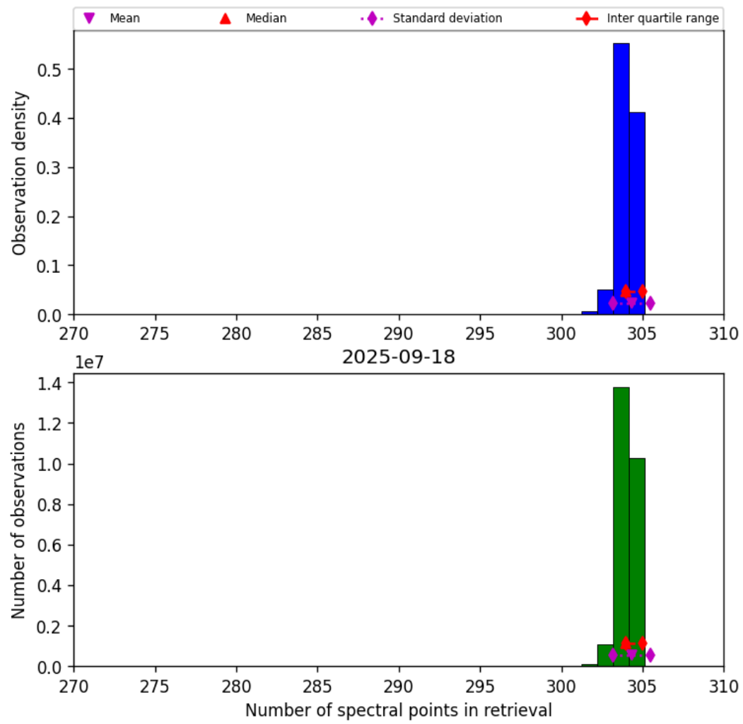
Figure 33: Histogram of “Number of spectral points in retrieval” for 2025-09-17 to 2025-09-19
