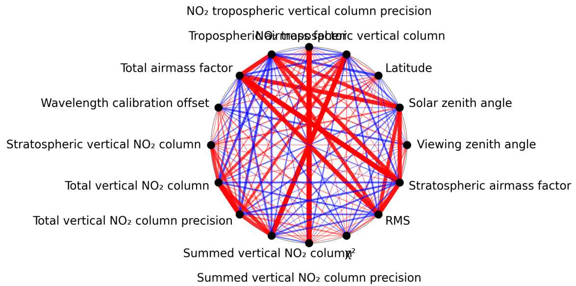
Figure 1: Map of correlation graph for 2025-09-17 to 2025-09-19.
