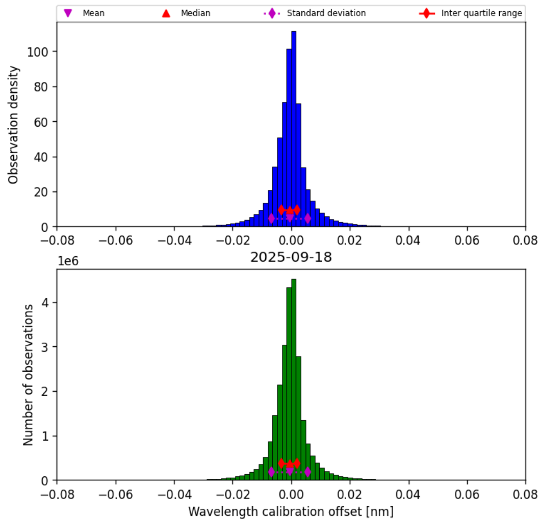
Figure 35: Histogram of “Wavelength calibration offset” for 2025-09-17 to 2025-09-19
