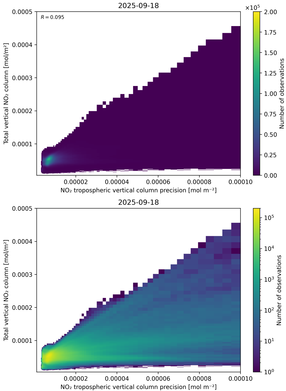
Figure 138: Scatter density plot of “NO 2 tropospheric vertical column precision” against “Total vertical NO 2 column” for 2025-09-17 to 2025-09-19.
