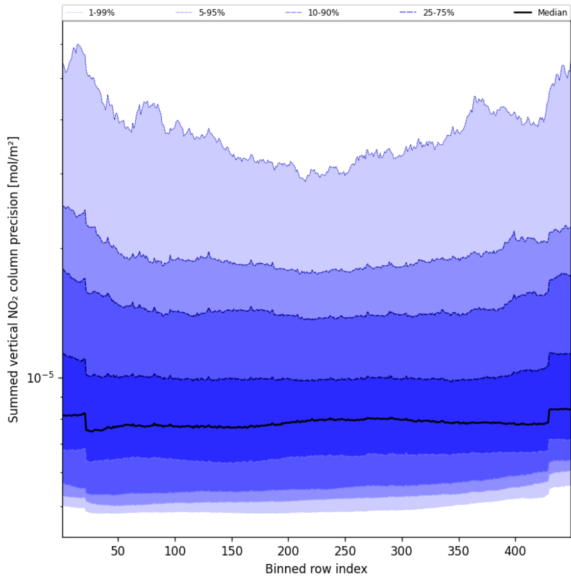
Figure 58: Along track statistics of “Summed vertical NO 2 column precision” for 2025-09-17 to 2025-09-19
