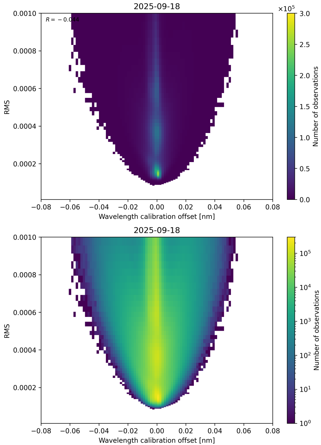
Figure 181: Scatter density plot of “Wavelength calibration offset” against “RMS” for 2025-09-17 to 2025-09-19.
