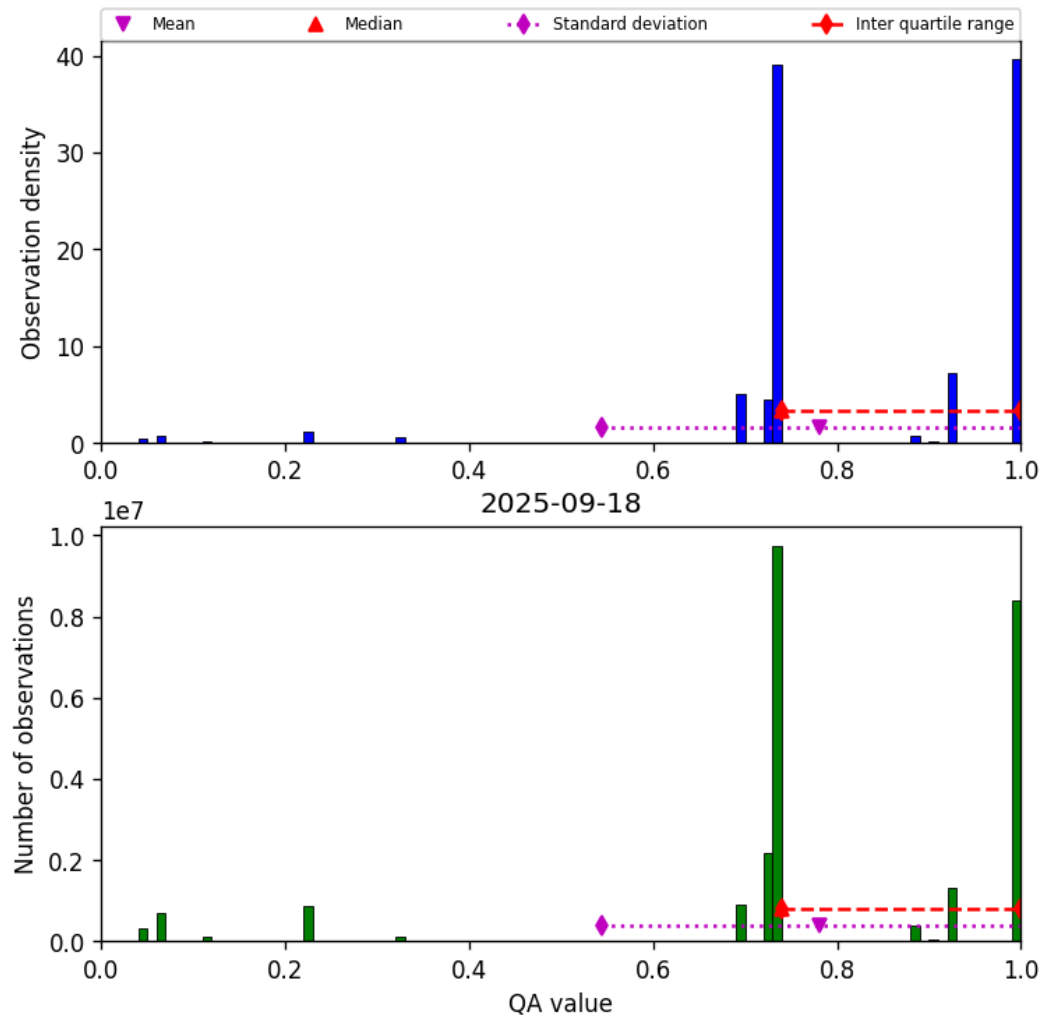
Figure 28: Histogram of “QA value” for 2025-09-17 to 2025-09-19
