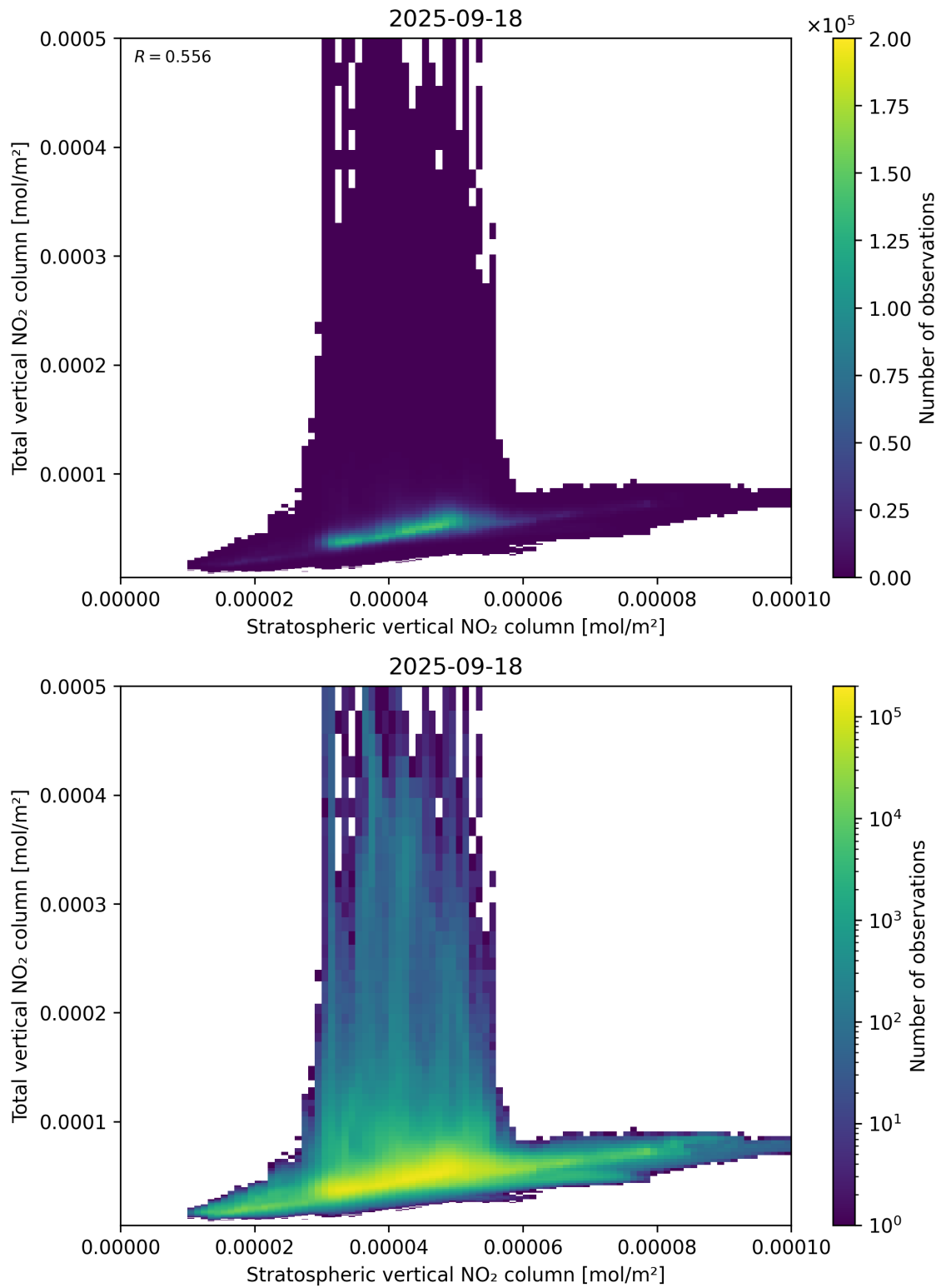
Figure 100: Scatter density plot of “Stratospheric vertical NO 2 column” against “Total vertical NO 2 column” for 2025-09-17 to 2025-09-19.
