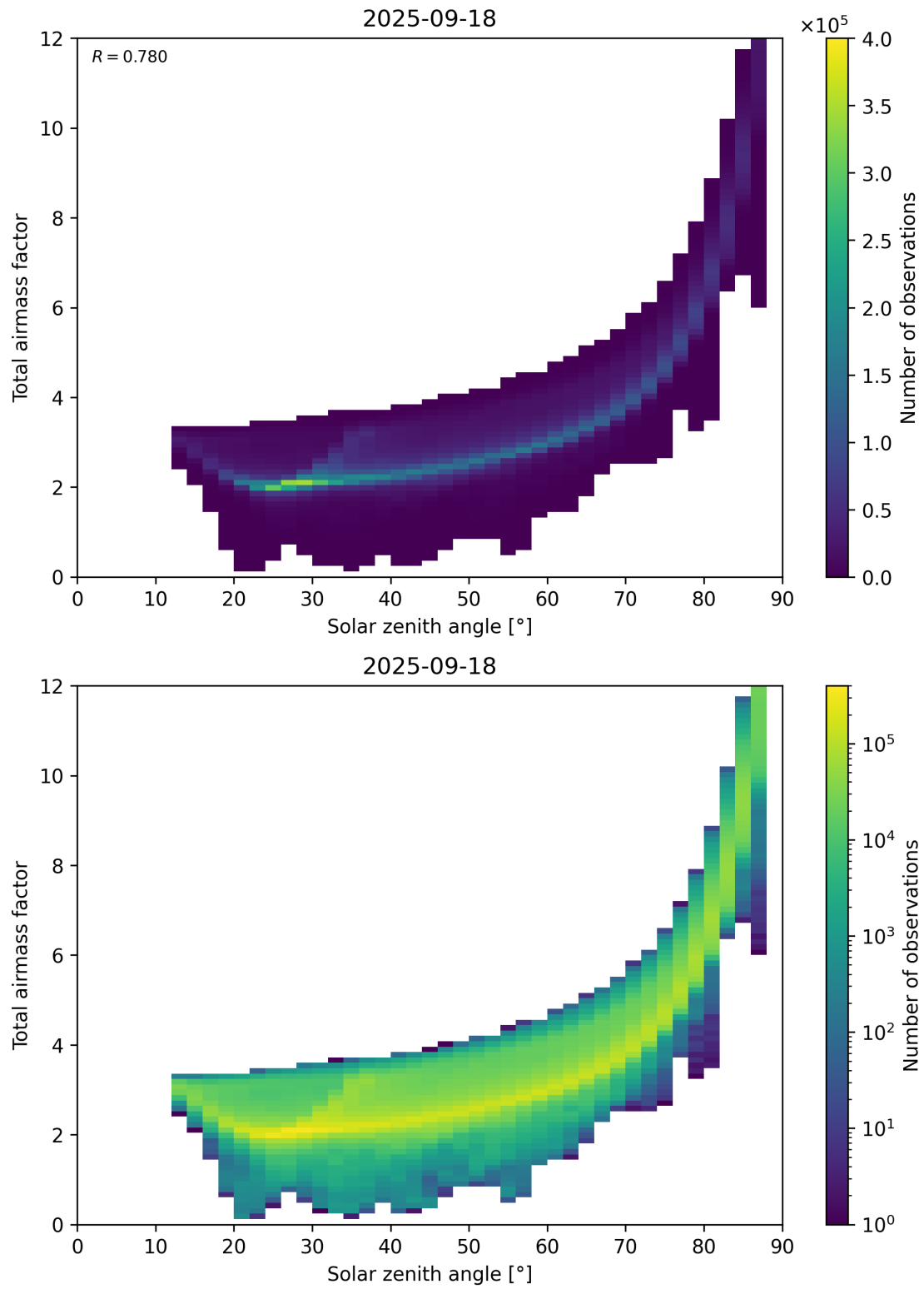
Figure 146: Scatter density plot of “Solar zenith angle” against “Total air mass factor” for 2025-09-17 to 2025-09-19.
