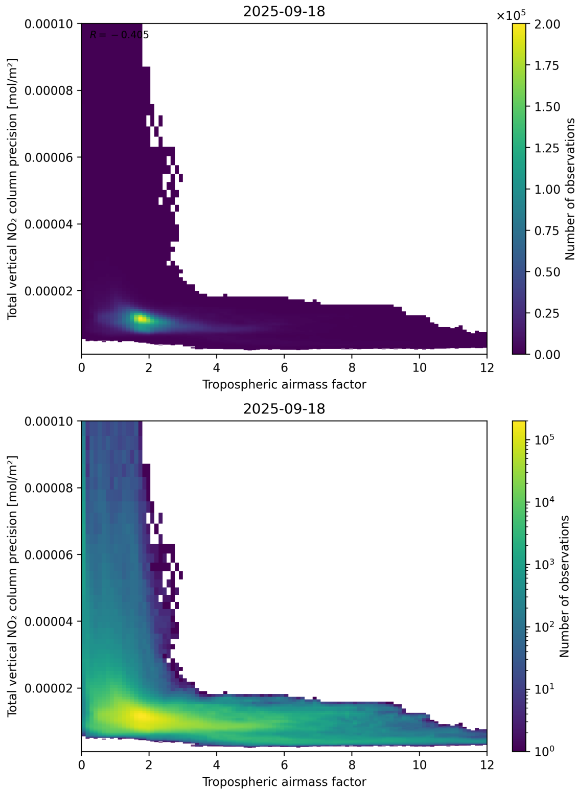
Figure 78: Scatter density plot of “Tropospheric air mass factor” against “Total vertical NO 2 column precision” for 2025-09-17 to 2025-09-19.
