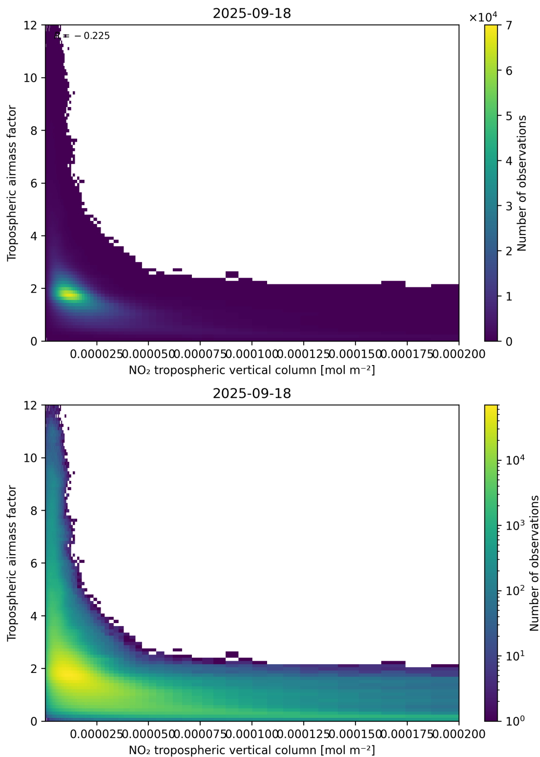
Figure 123: Scatter density plot of “NO 2 tropospheric vertical column” against “Tropospheric air mass factor” for 2025-09-17 to 2025-09-19.
