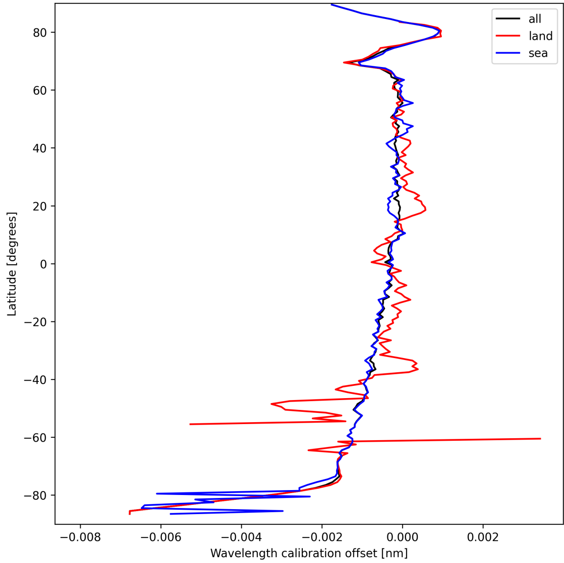
Figure 18: Zonal average of “Wavelength calibration offset” for 2025-09-17 to 2025-09-19.
