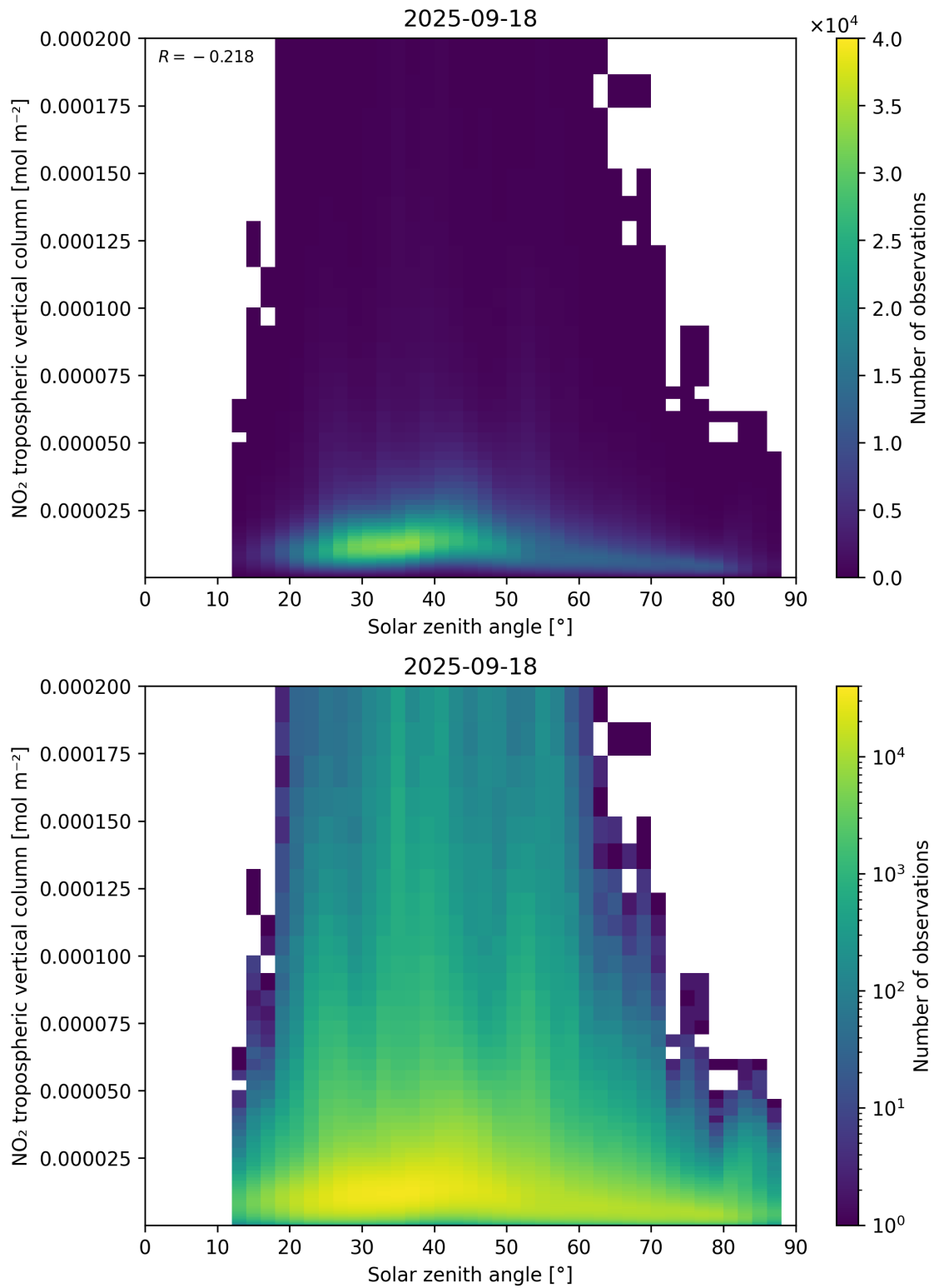
Figure 155: Scatter density plot of “Solar zenith angle” against “NO 2 tropospheric vertical column” for 2025-09-17 to 2025-09-19.
