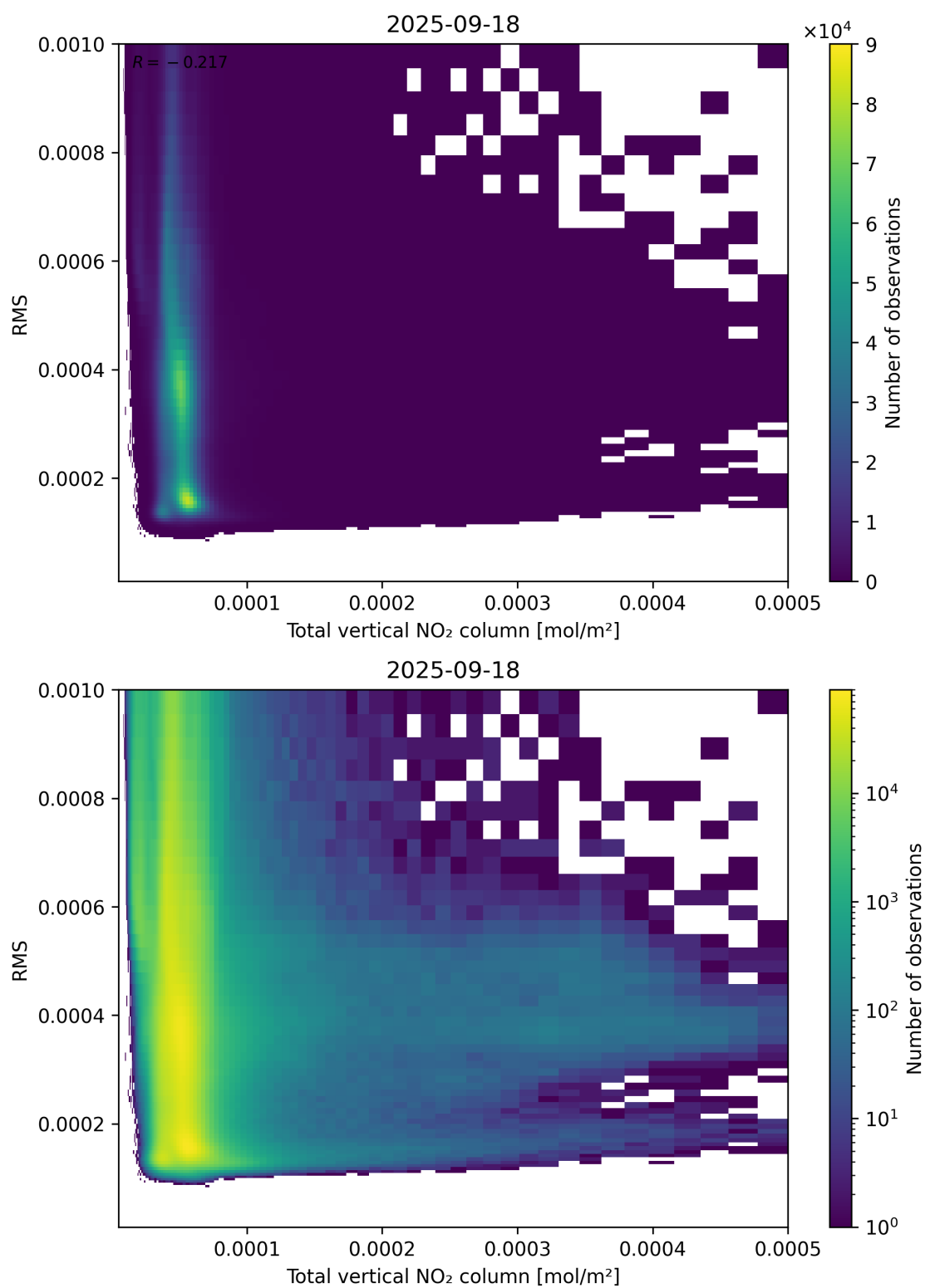
Figure 120: Scatter density plot of “Total vertical NO 2 column” against “RMS” for 2025-09-17 to 2025-09-19.
