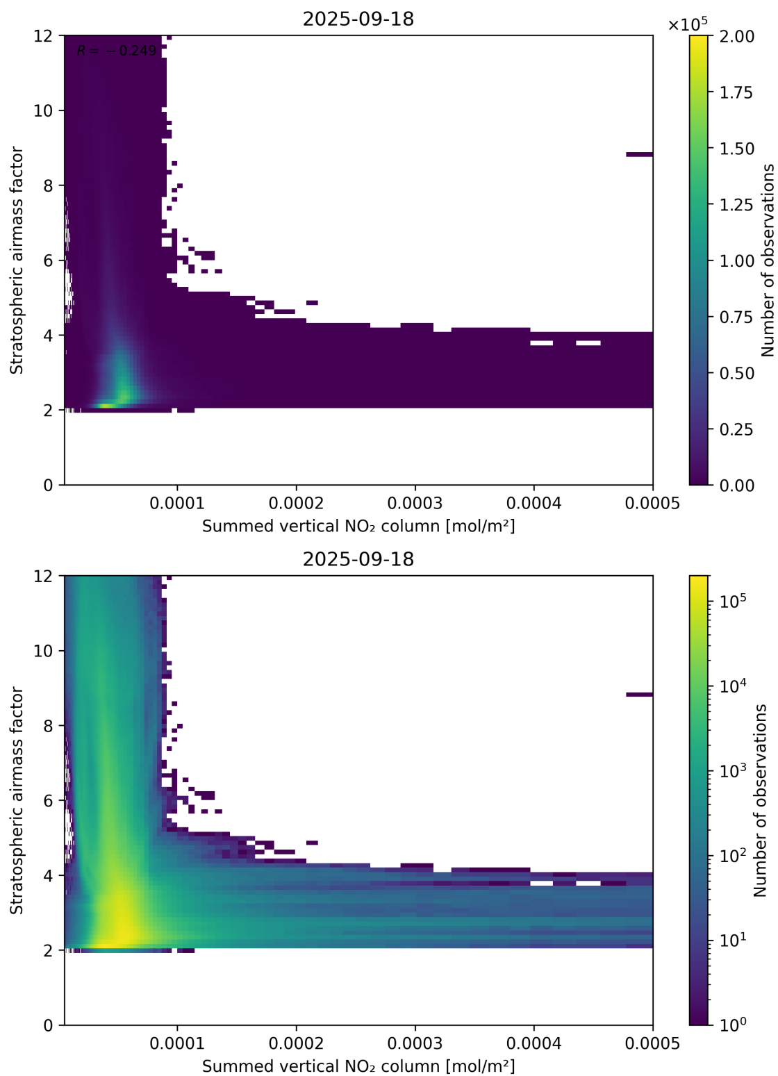
Figure 103: Scatter density plot of “Summed vertical NO 2 column” against “Stratospheric airmass factor” for 2025-09-17 to 2025-09-19.
