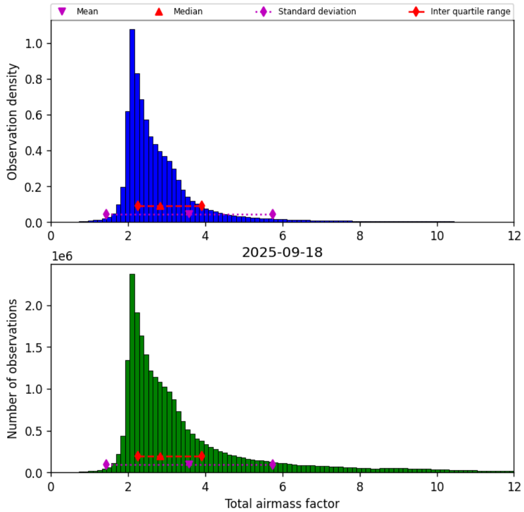
Figure 32: Histogram of “Total airmass factor” for 2025-09-17 to 2025-09-19
