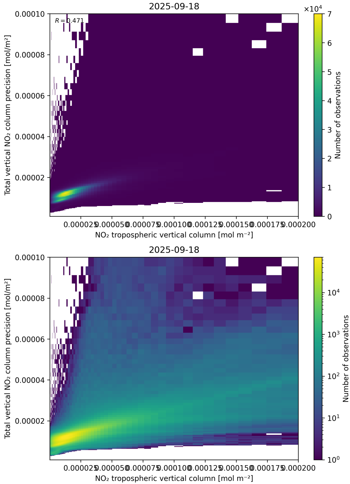
Figure 129: Scatter density plot of “NO 2 tropospheric vertical column” against “Total vertical NO 2 column precision” for 2025-09-17 to 2025-09-19.
