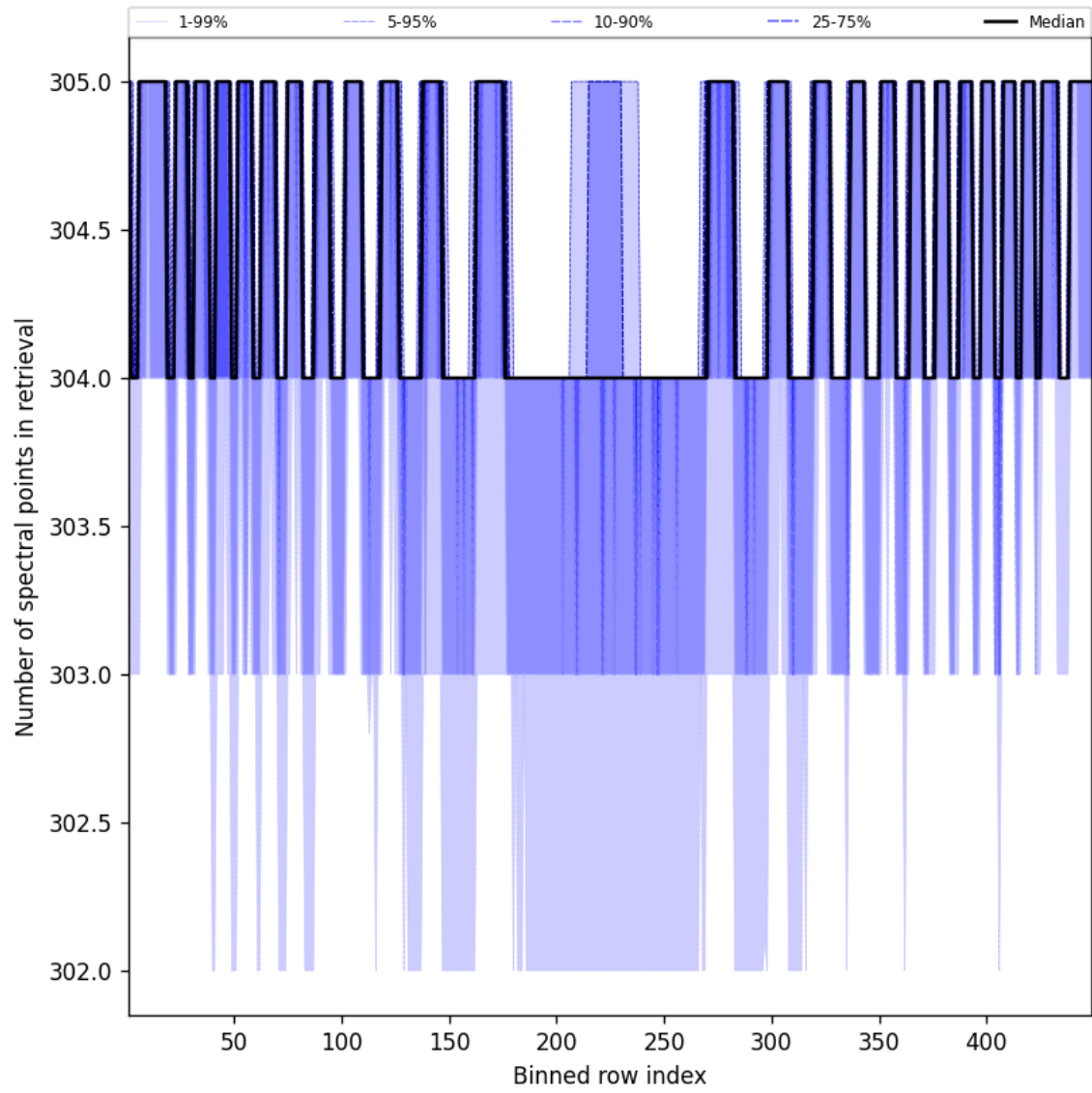
Figure 50: Along track statistics of “Number of spectral points in retrieval” for 2025-09-17 to 2025-09-19
