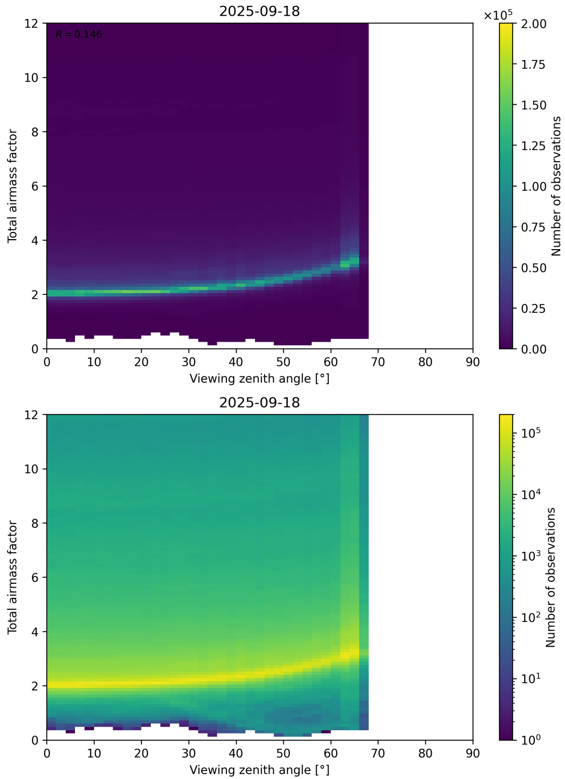
Figure 160: Scatter density plot of “Viewing zenith angle” against “Total airmass factor” for 2025-09-17 to 2025-09-19.
