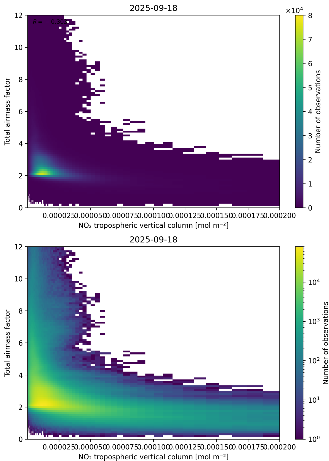
Figure 122: Scatter density plot of “NO 2 tropospheric vertical column” against “Total air mass factor” for 2025-09-17 to 2025-09-19.
