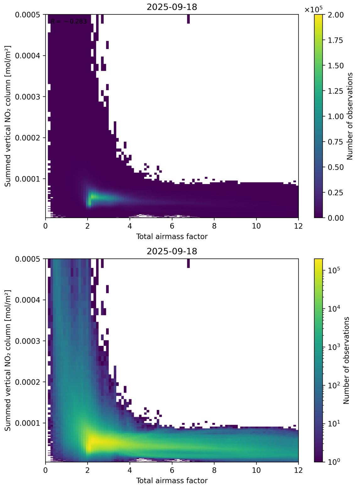
Figure 65: Scatter density plot of “Total airmass factor” against “Summed vertical NO 2 column” for 2025-09-17 to 2025-09-19.
