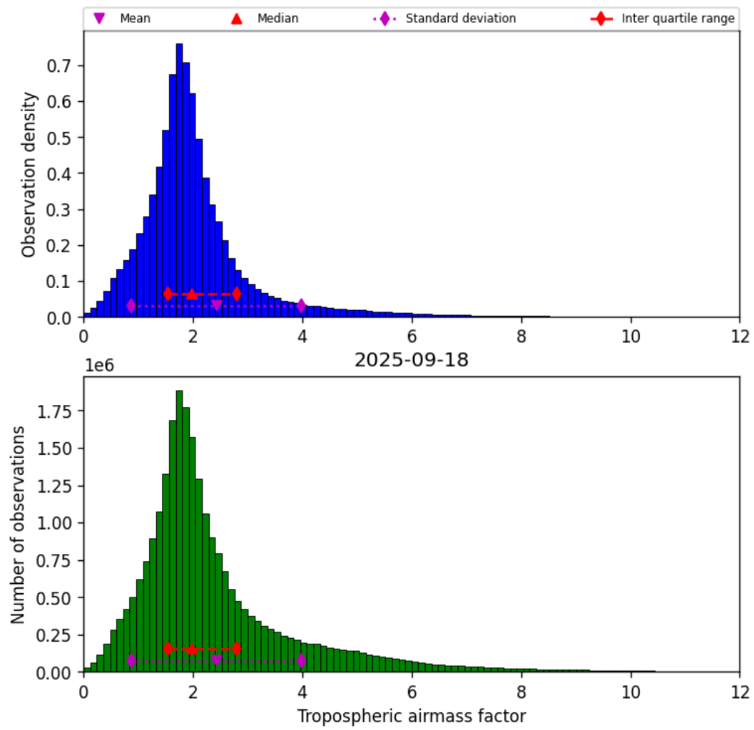
Figure 31: Histogram of “Tropospheric airmass factor” for 2025-09-17 to 2025-09-19
