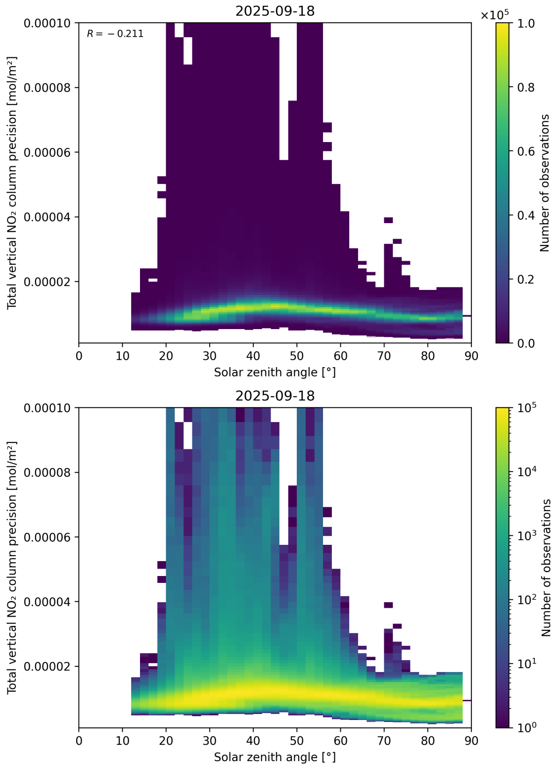
Figure 154: Scatter density plot of “Solar zenith angle” against “Total vertical NO 2 column precision” for 2025-09-17 to 2025-09-19.
