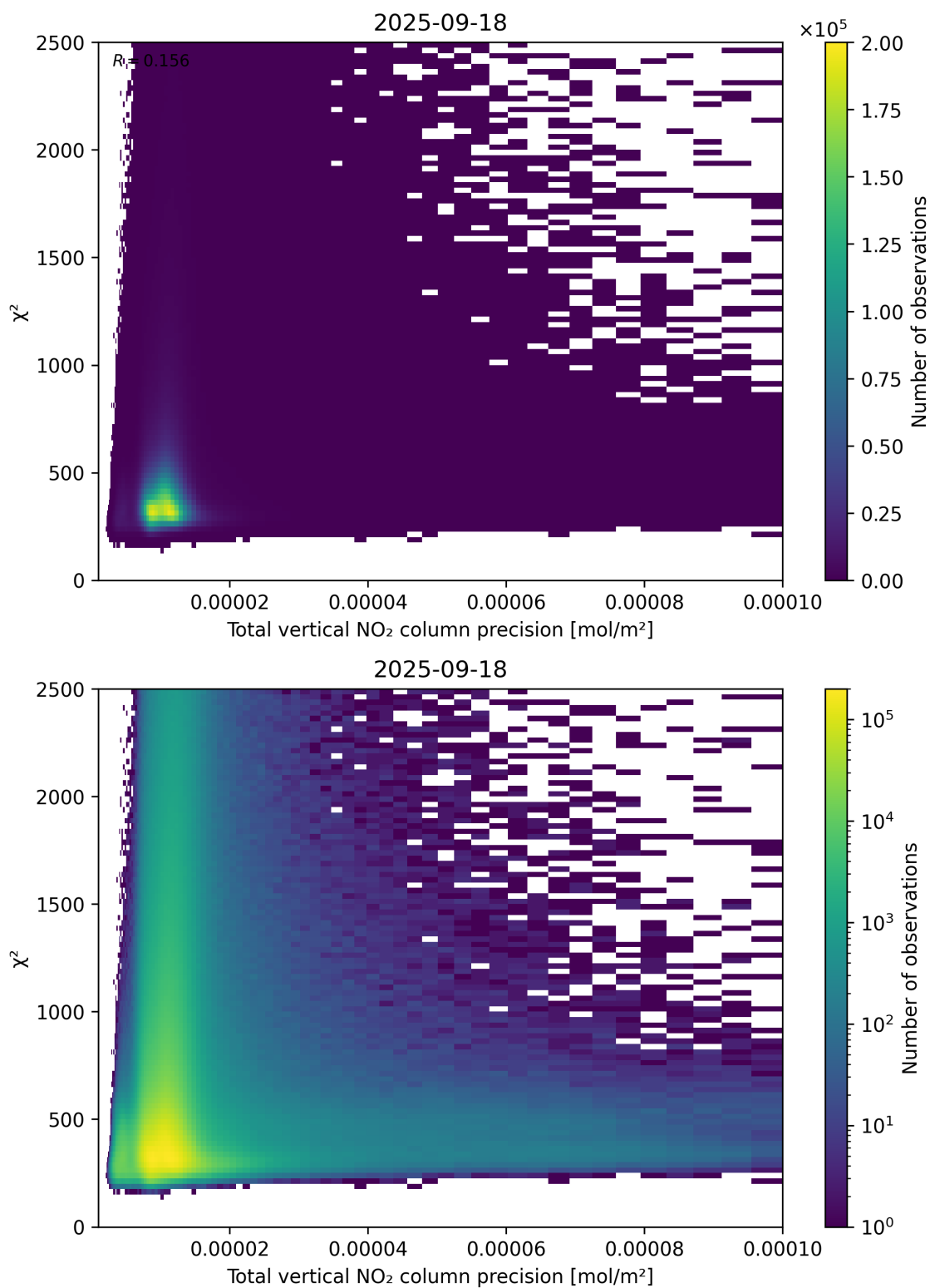
Figure 116: Scatter density plot of “Total vertical NO 2 column precision” against “ \chi^2 ” for 2025-09-17 to 2025-09-19.
