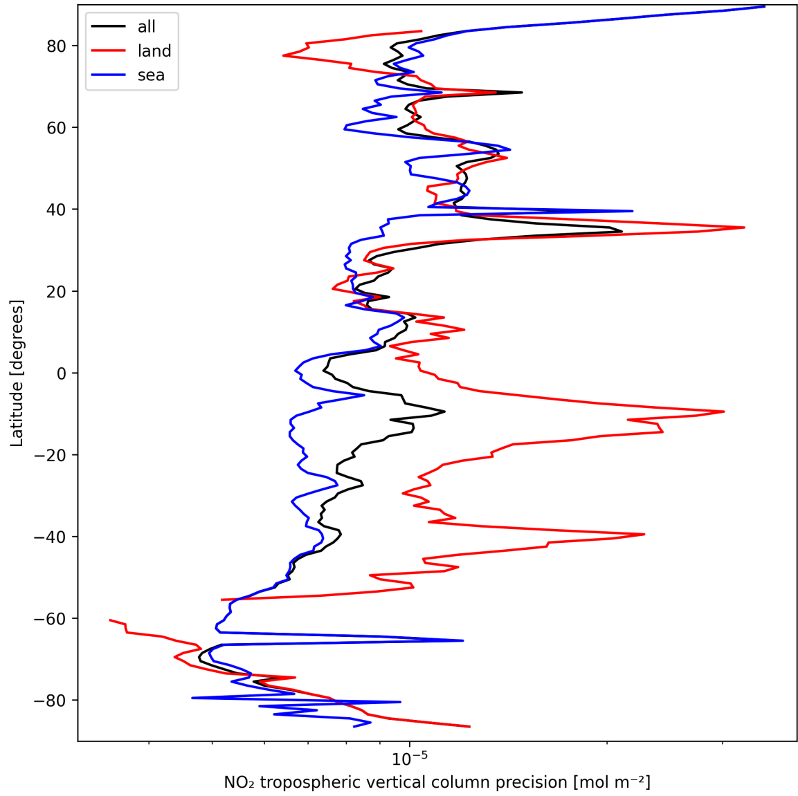
Figure 13: Zonal average of “NO 2 tropospheric vertical column precision” for 2025-09-17 to 2025-09-19.
