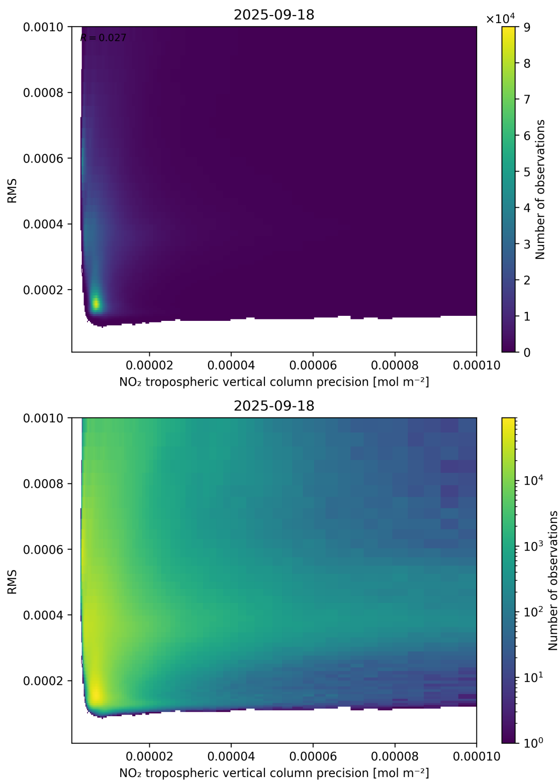
Figure 140: Scatter density plot of “NO 2 tropospheric vertical column precision” against “RMS” for 2025-09-17 to 2025-09-19.
