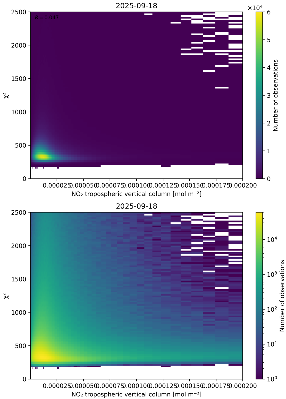
Figure 124: Scatter density plot of “NO 2 tropospheric vertical column” against “ \chi^2 ” for 2025-09-17 to 2025-09-19.
