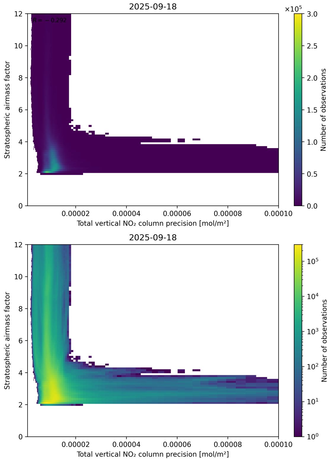
Figure 115: Scatter density plot of “Total vertical NO 2 column precision” against “Stratospheric airmass factor” for 2025-09-17 to 2025-09-19.
