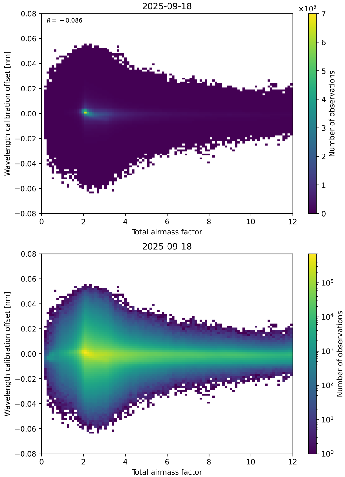
Figure 70: Scatter density plot of “Total airmass factor” against “Wavelength calibration offset” for 2025-09-17 to 2025-09-19.
