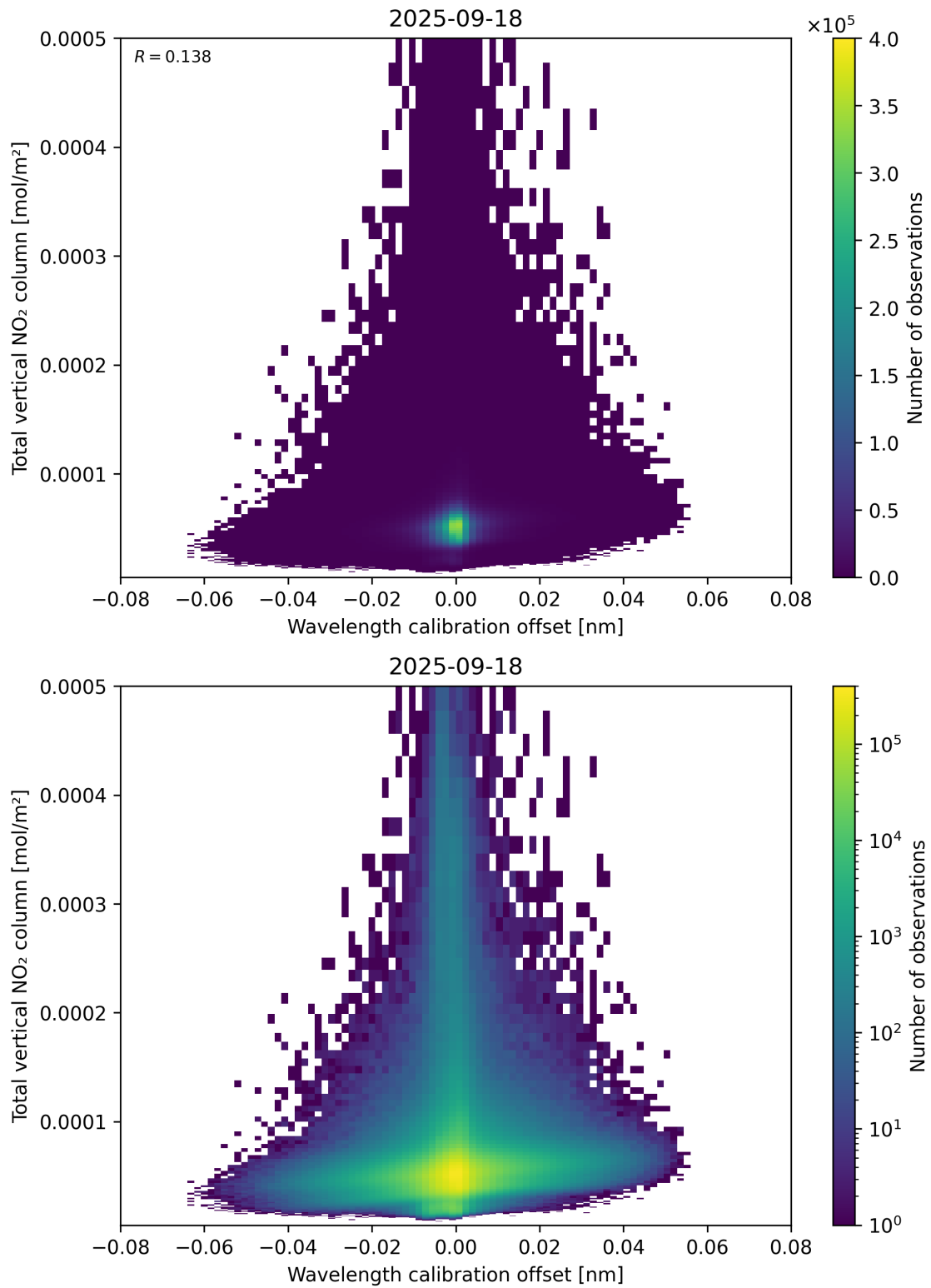
Figure 179: Scatter density plot of “Wavelength calibration offset” against “Total vertical NO 2 column” for 2025-09-17 to 2025-09-19.
