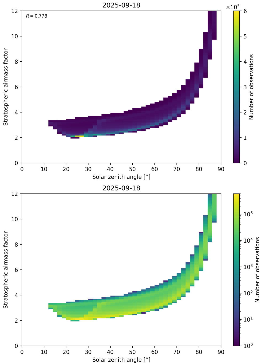
Figure 145: Scatter density plot of “Solar zenith angle” against “Stratospheric airmass factor” for 2025-09-17 to 2025-09-19.
