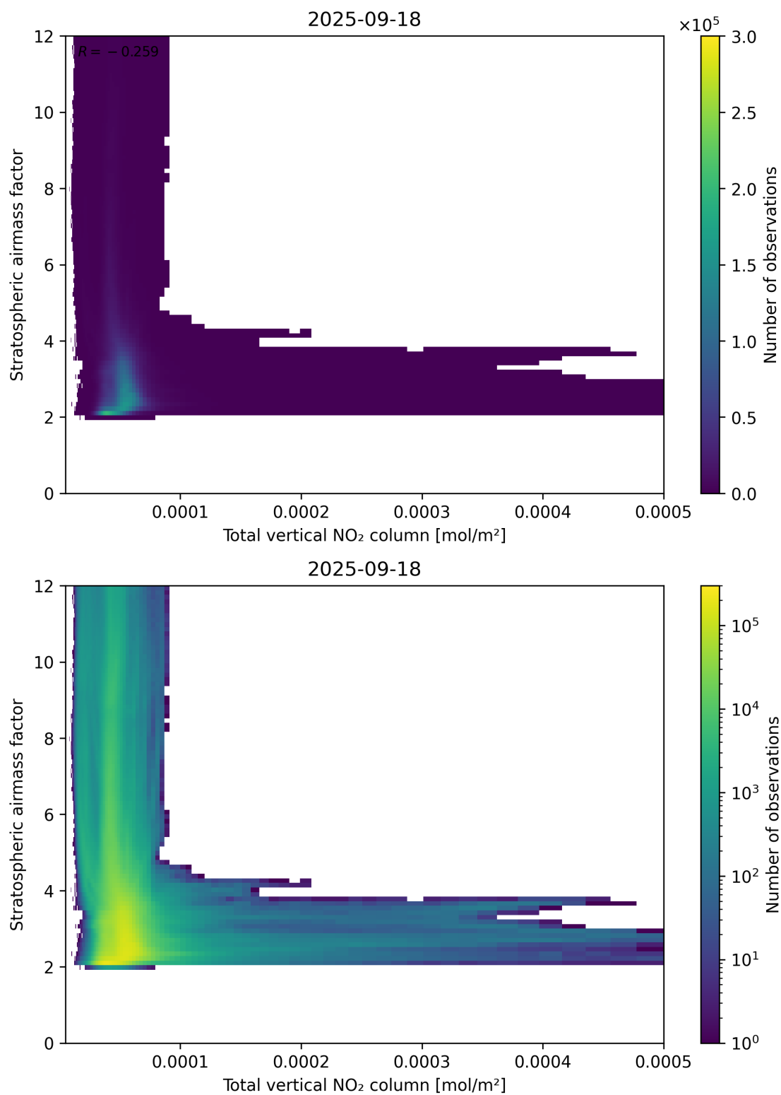
Figure 110: Scatter density plot of “Total vertical NO 2 column” against “Stratospheric airmass factor” for 2025-09-17 to 2025-09-19.
