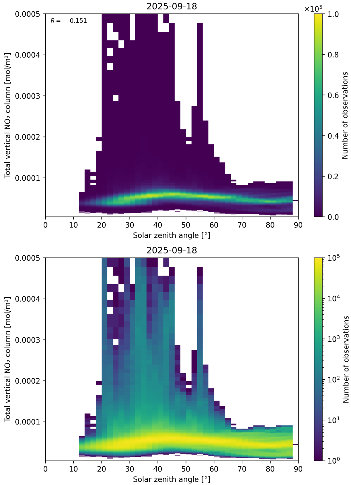
Figure 153: Scatter density plot of “Solar zenith angle” against “Total vertical NO 2 column” for 2025-09-17 to 2025-09-19.
