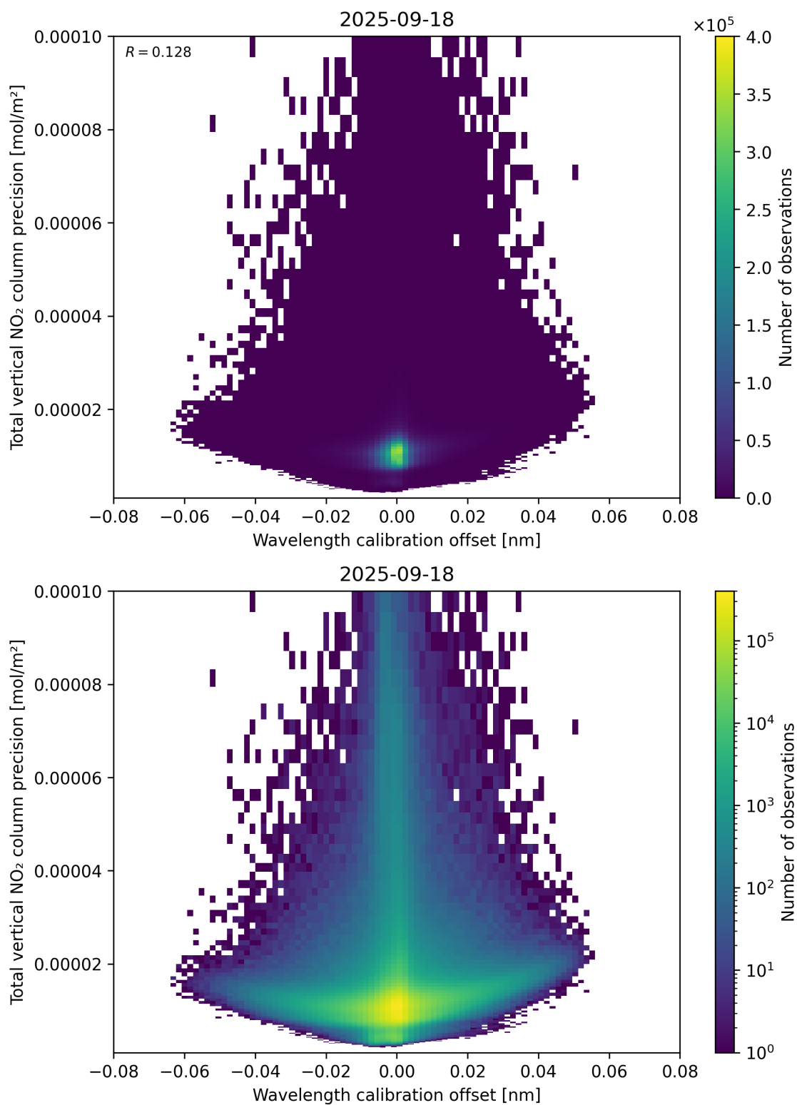
Figure 180: Scatter density plot of “Wavelength calibration offset” against “Total vertical NO 2 column precision” for 2025-09-17 to 2025-09-19.
