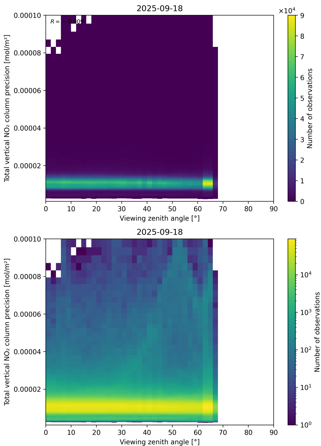
Figure 168: Scatter density plot of “Viewing zenith angle” against “Total vertical NO 2 column precision” for 2025-09-17 to 2025-09-19.
