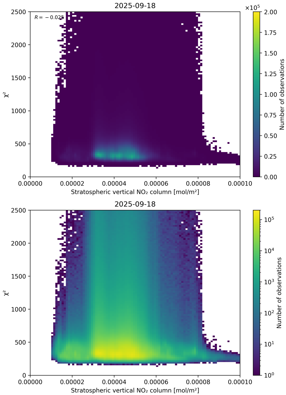
Figure 97: Scatter density plot of “Stratospheric vertical NO 2 column” against “ \chi^2 ” for 2025-09-17 to 2025-09-19.
