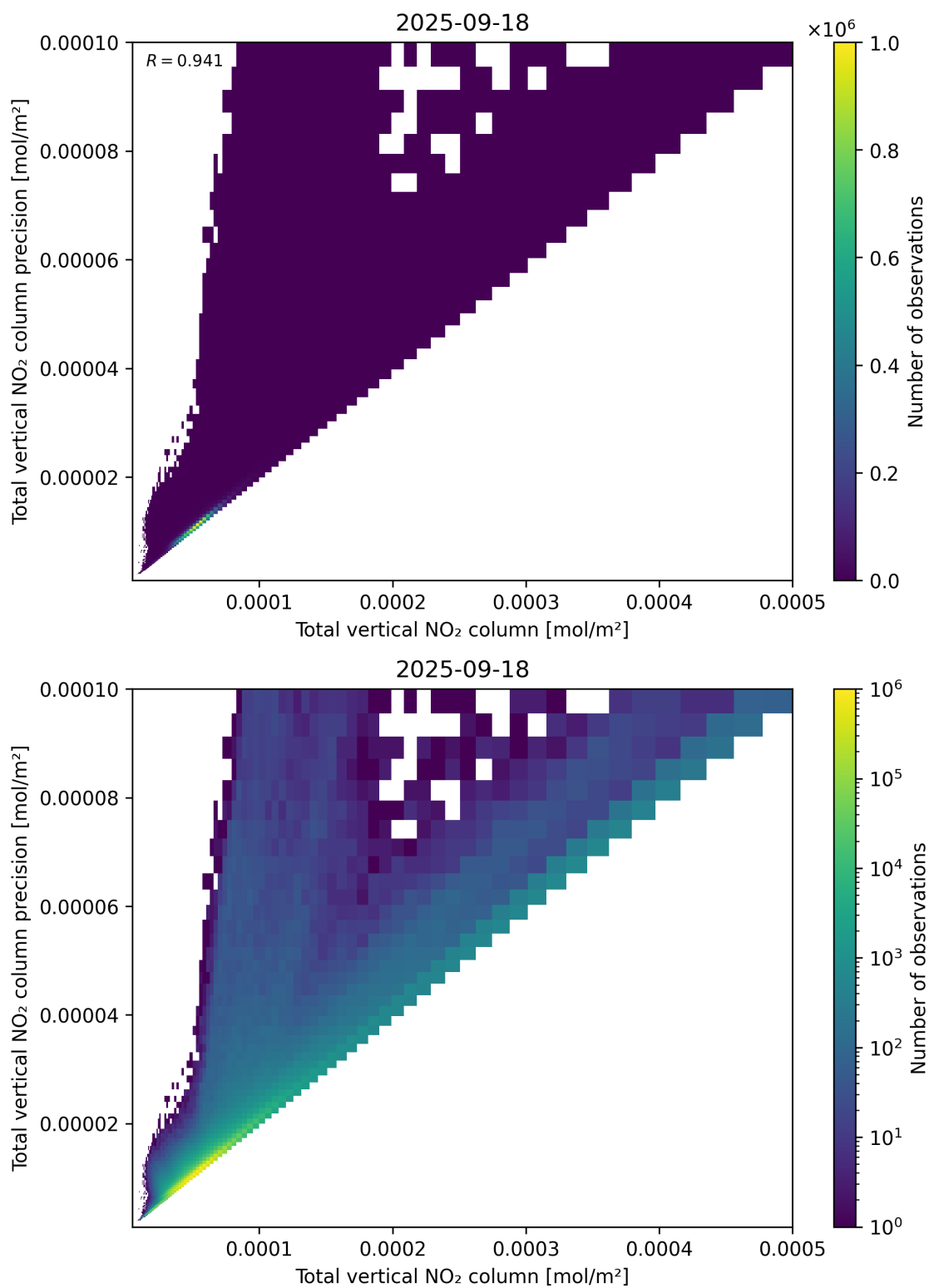
Figure 114: Scatter density plot of “Total vertical NO 2 column” against “Total vertical NO 2 column precision” for 2025-09-17 to 2025-09-19.
