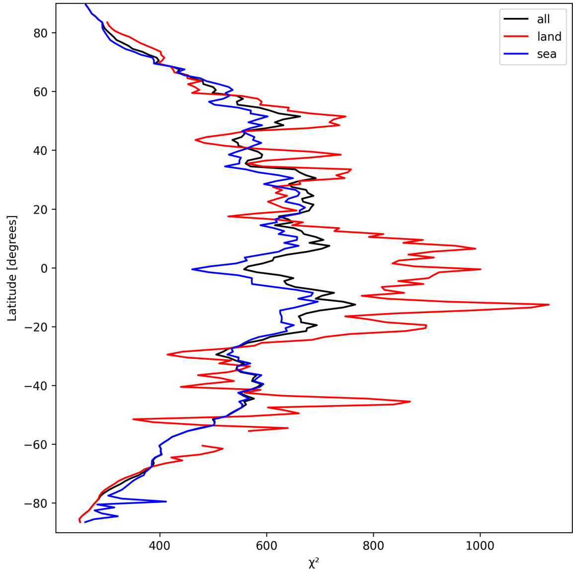
Figure 25: Zonal average of “ \chi^2 ” for 2025-09-17 to 2025-09-19.
