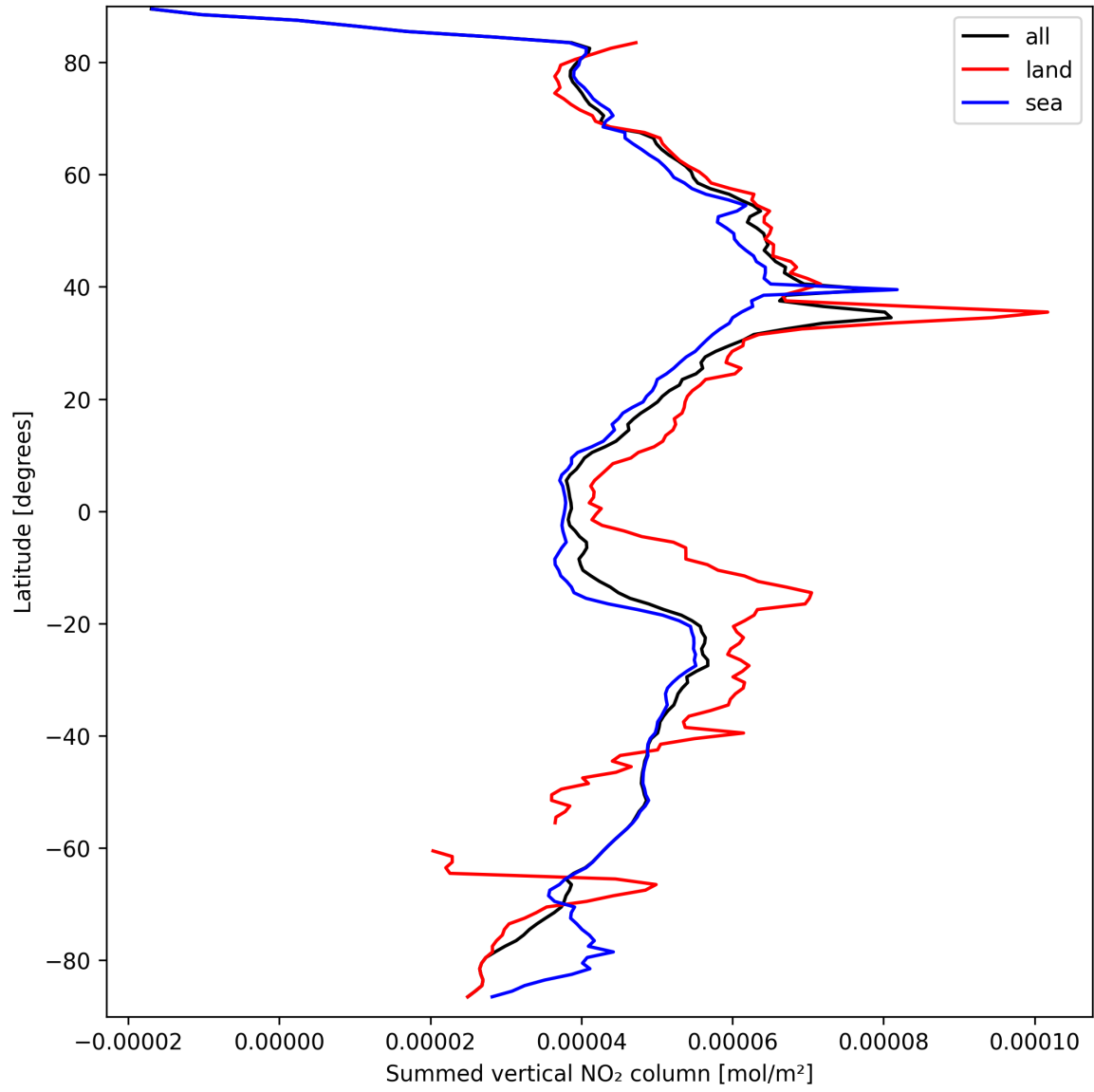
Figure 23: Zonal average of “Summed vertical NO 2 column” for 2025-09-17 to 2025-09-19.
