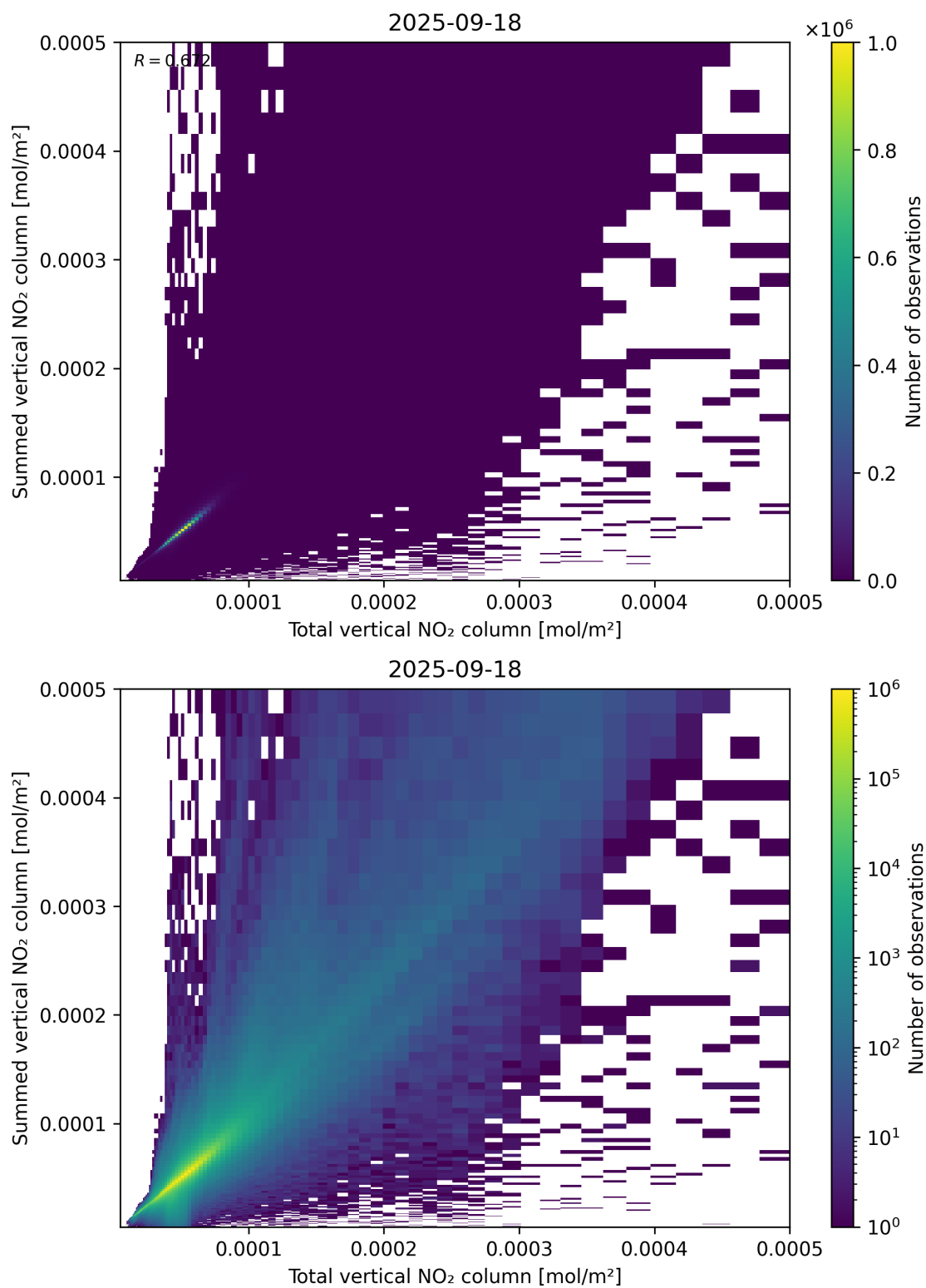
Figure 112: Scatter density plot of “Total vertical NO 2 column” against “Summed vertical NO 2 column” for 2025-09-17 to 2025-09-19.
