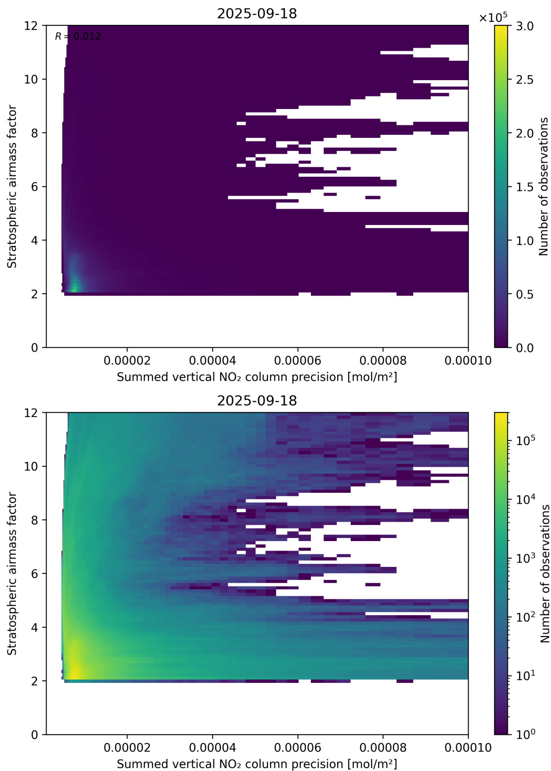
Figure 106: Scatter density plot of “Summed vertical NO 2 column precision” against “Stratospheric airmass factor” for 2025-09-17 to 2025-09-19.
