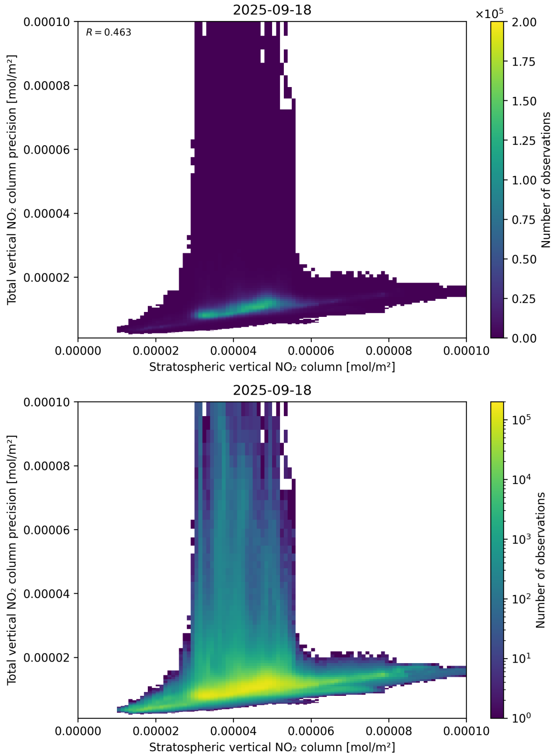
Figure 101: Scatter density plot of “Stratospheric vertical NO 2 column” against “Total vertical NO 2 column precision” for 2025-09-17 to 2025-09-19.
