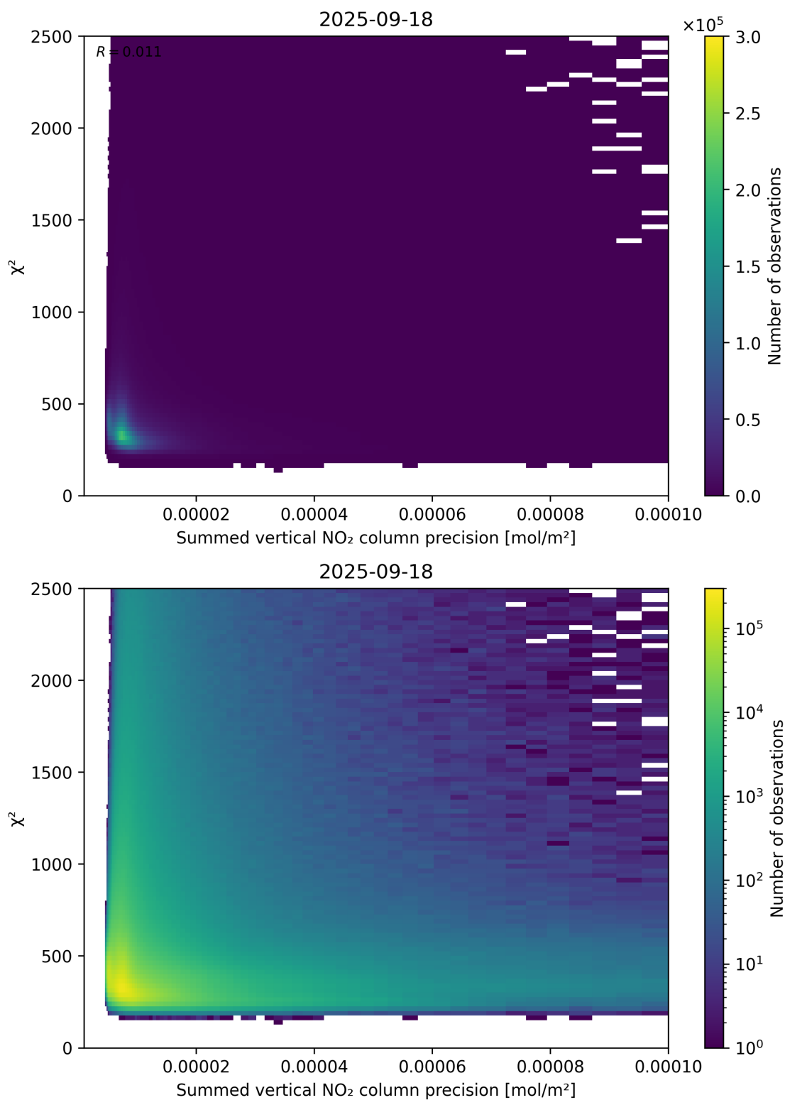
Figure 107: Scatter density plot of “Summed vertical NO 2 column precision” against “ \chi^2 ” for 2025-09-17 to 2025-09-19.
