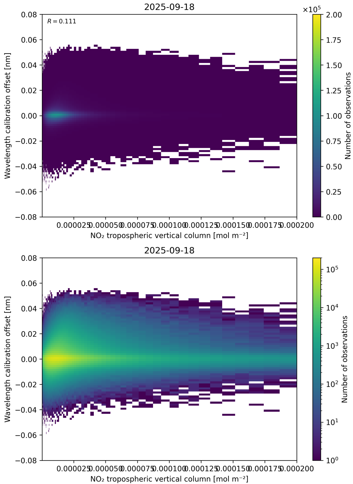
Figure 143: Scatter density plot of “NO 2 tropospheric vertical column” against “Wavelength calibration offset” for 2025-09-17 to 2025-09-19.
