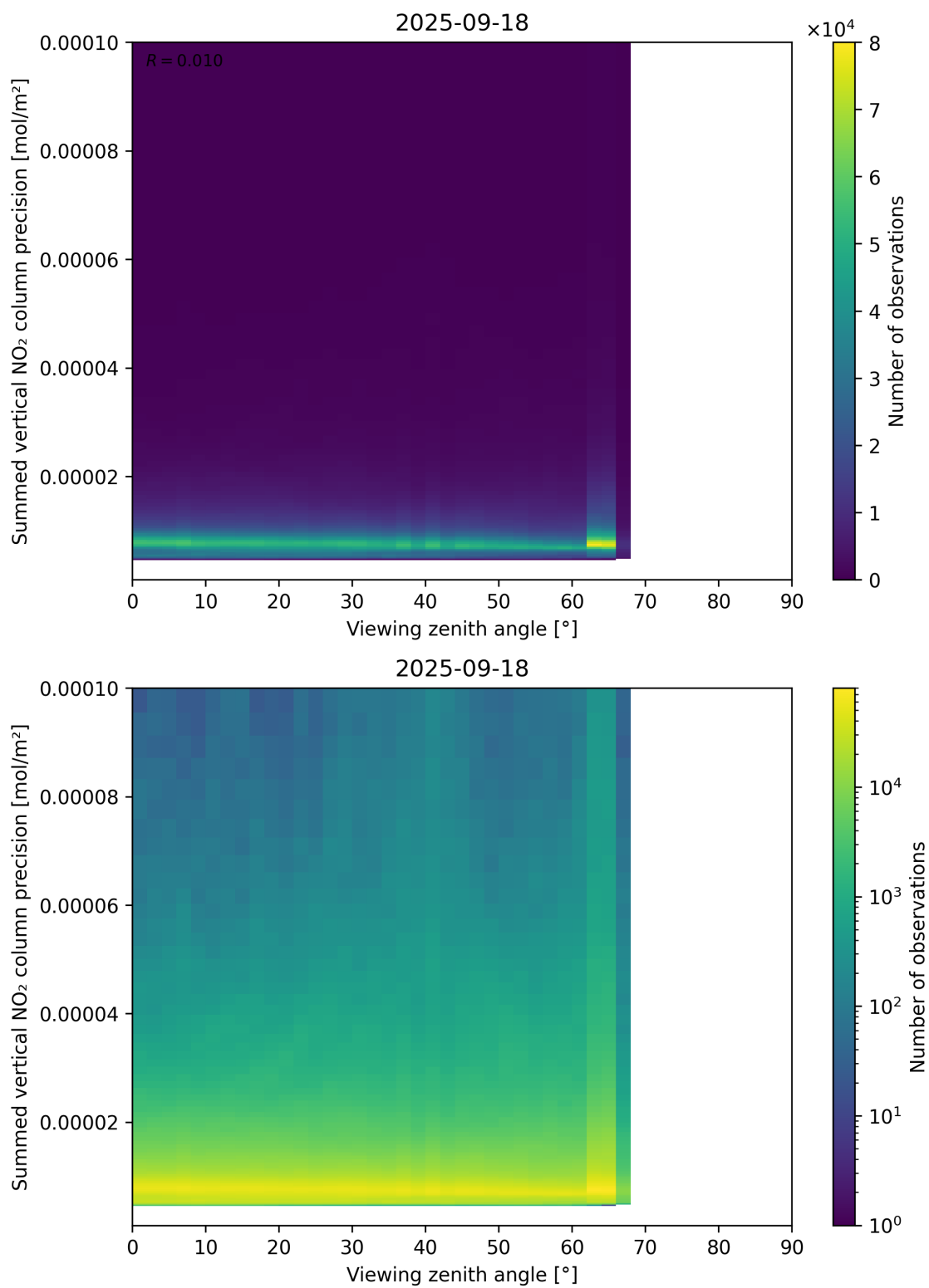
Figure 166: Scatter density plot of “Viewing zenith angle” against “Summed vertical NO 2 column precision” for 2025-09-17 to 2025-09-19.
