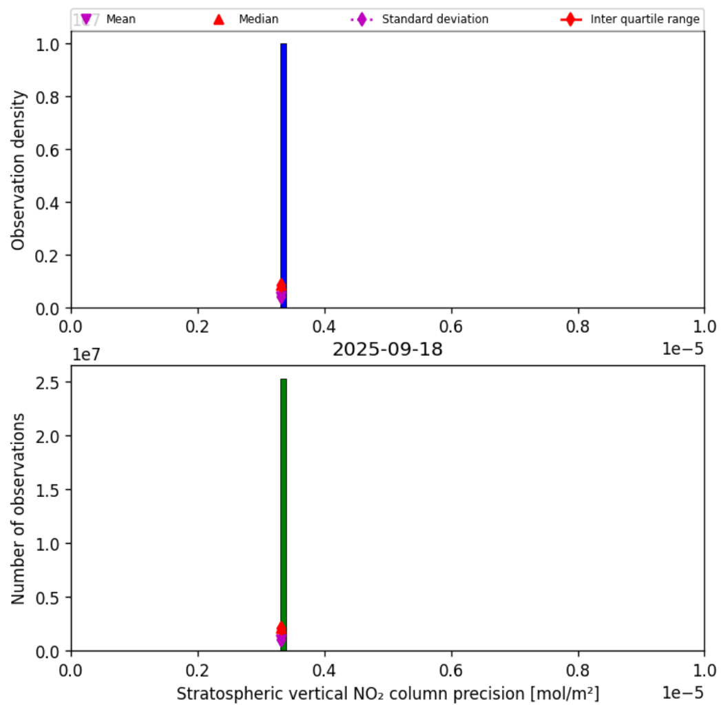
Figure 37: Histogram of “Stratospheric vertical NO 2 column precision” for 2025-09-17 to 2025-09-19
