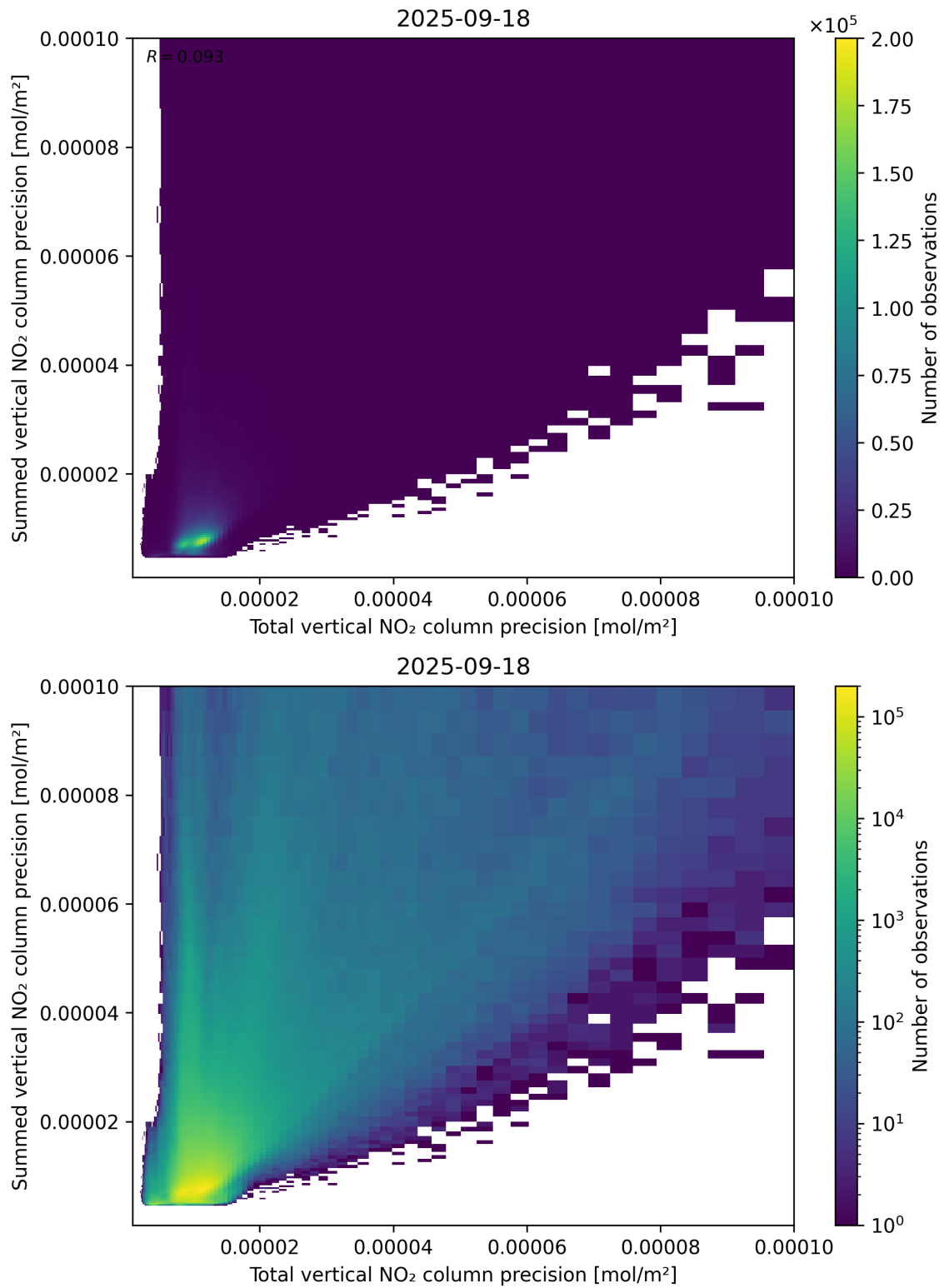
Figure 118: Scatter density plot of “Total vertical NO 2 column precision” against “Summed vertical NO 2 column precision” for 2025-09-17 to 2025-09-19.
