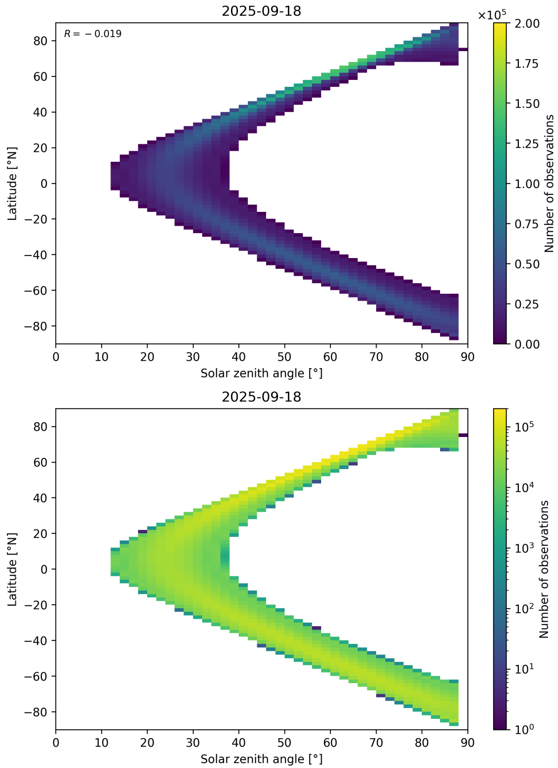
Figure 149: Scatter density plot of “Solar zenith angle” against “Latitude” for 2025-09-17 to 2025-09-19.
