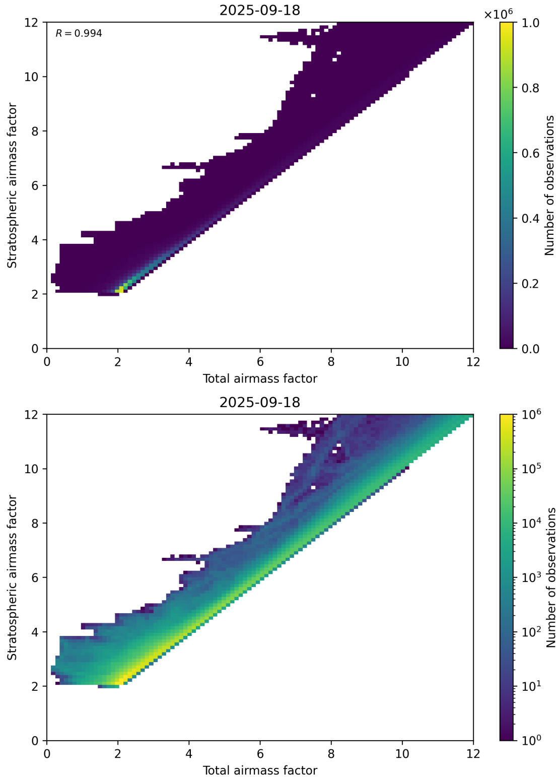
Figure 62: Scatter density plot of “Total airmass factor” against “Stratospheric airmass factor” for 2025-09-17 to 2025-09-19.
