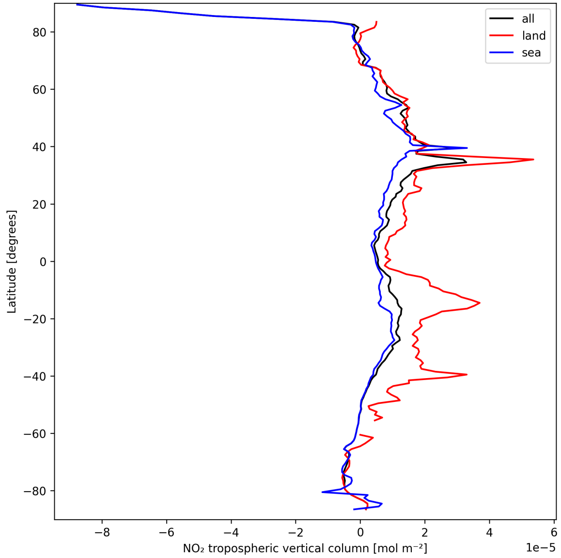
Figure 12: Zonal average of “NO 2 tropospheric vertical column” for 2025-09-17 to 2025-09-19.
