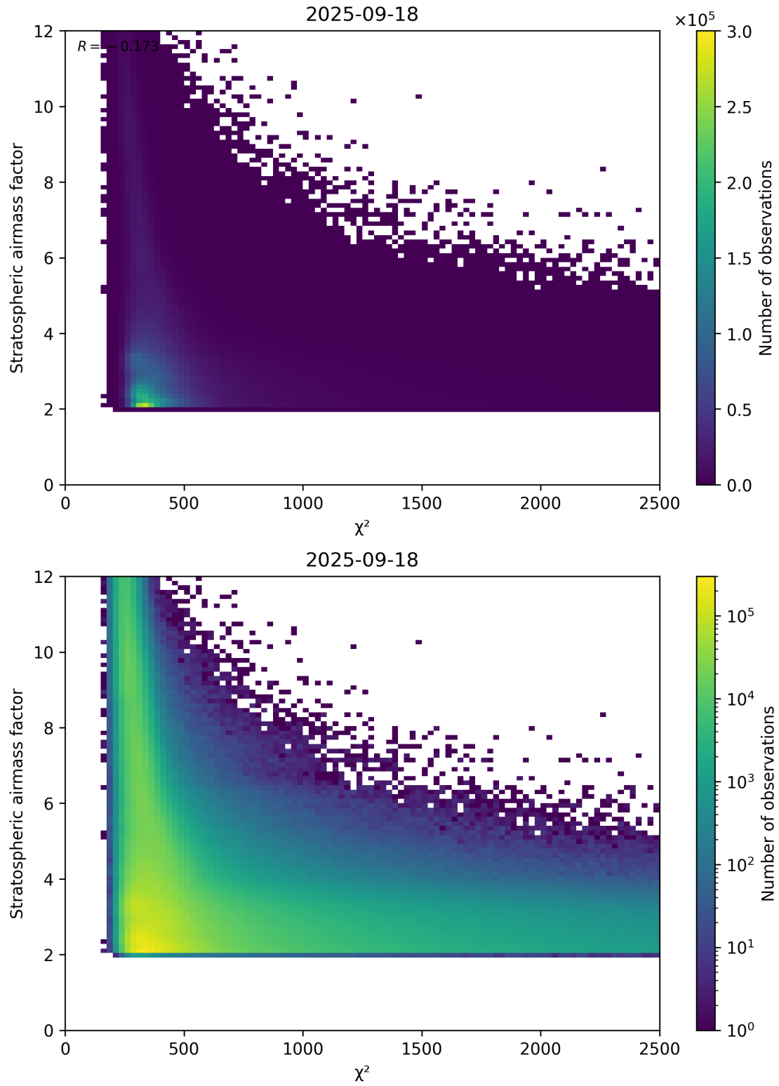
Figure 81: Scatter density plot of “ \chi^2 ” against “Stratospheric airmass factor” for 2025-09-17 to 2025-09-19.
