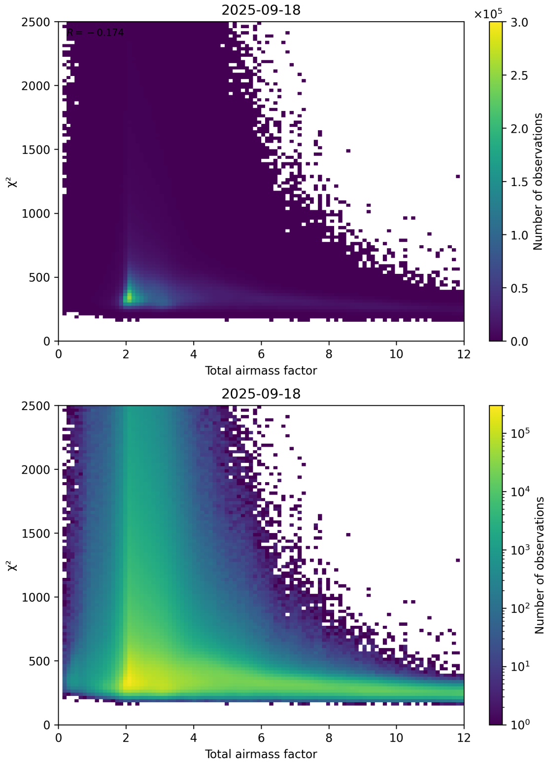
Figure 63: Scatter density plot of “Total airmass factor” against “ \chi^2 ” for 2025-09-17 to 2025-09-19.
