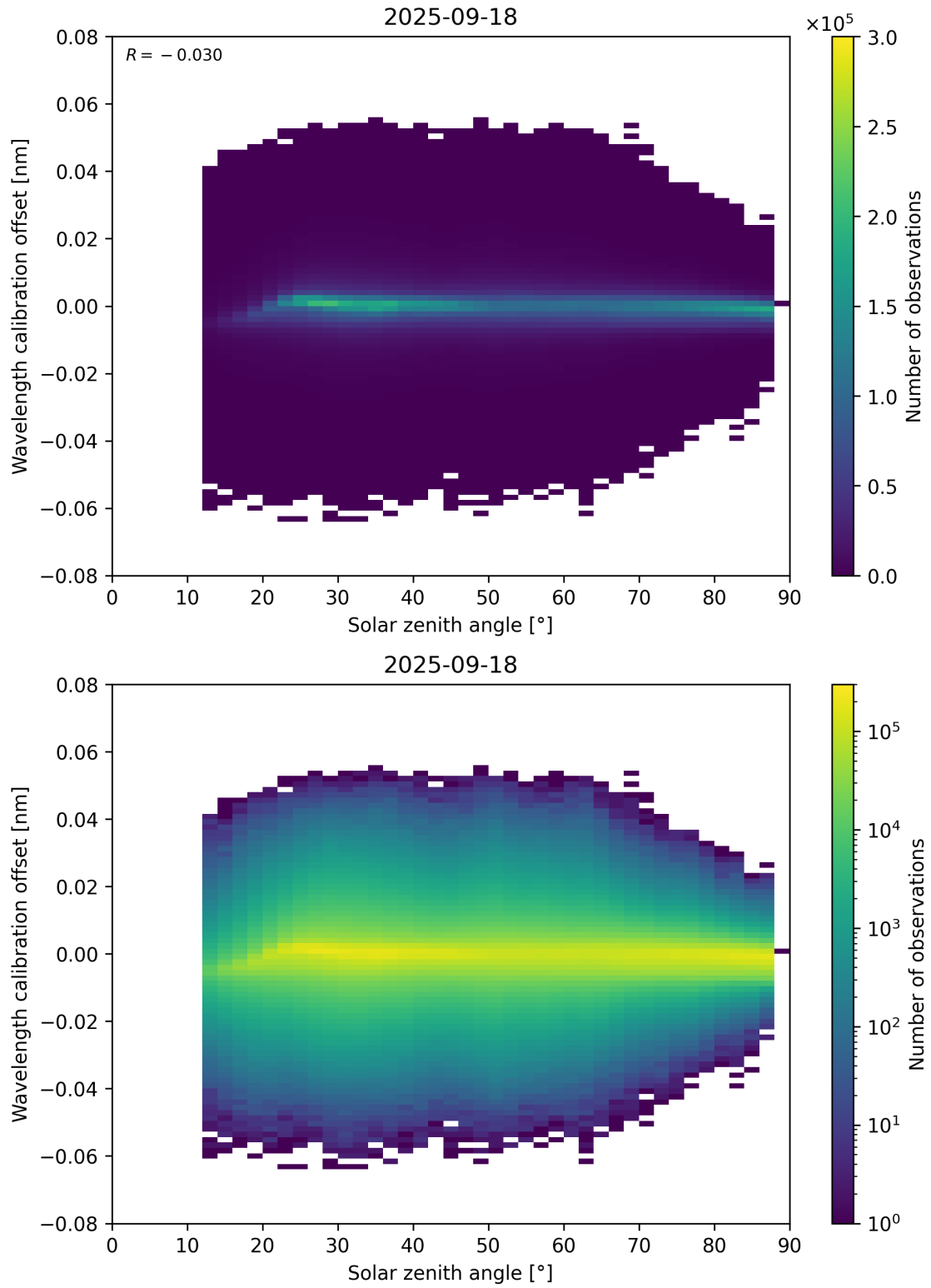
Figure 158: Scatter density plot of “Solar zenith angle” against “Wavelength calibration offset” for 2025-09-17 to 2025-09-19.
