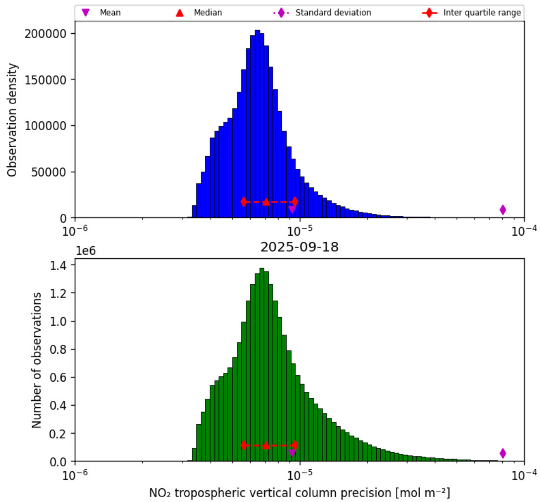
Figure 30: Histogram of “NO 2 tropospheric vertical column precision” for 2025-09-17 to 2025-09-19
