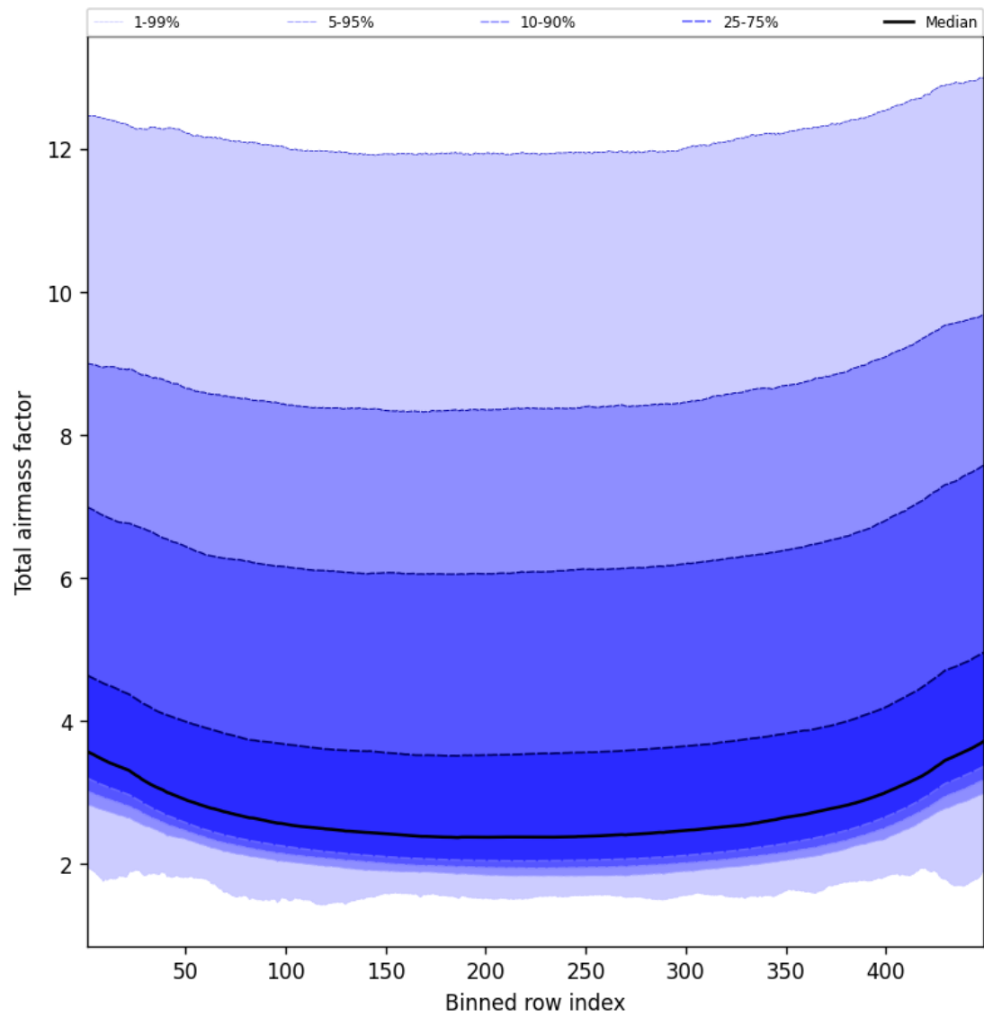
Figure 49: Along track statistics of “Total airmass factor” for 2025-09-17 to 2025-09-19
