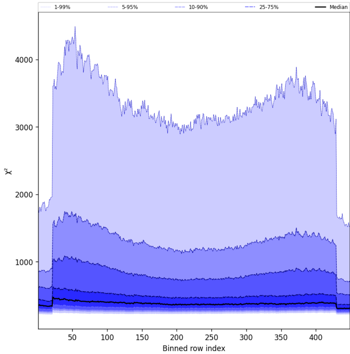
Figure 59: Along track statistics of “ \chi^2 ” for 2025-09-17 to 2025-09-19
