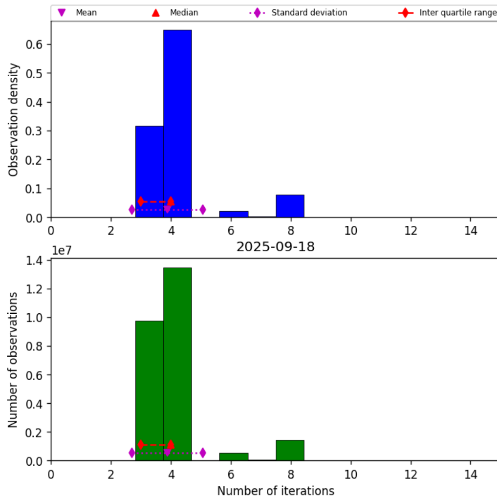
Figure 34: Histogram of “Number of iterations” for 2025-09-17 to 2025-09-19
