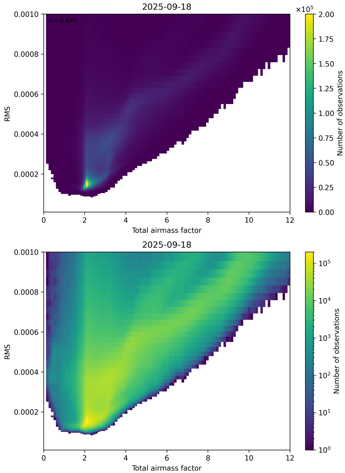
Figure 69: Scatter density plot of “Total airmass factor” against “RMS” for 2025-09-17 to 2025-09-19.
