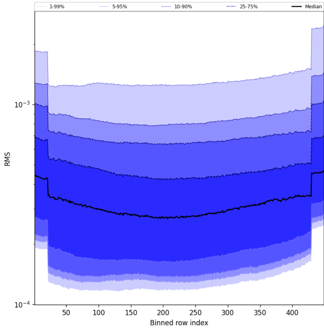
Figure 60: Along track statistics of “RMS” for 2025-09-17 to 2025-09-19
