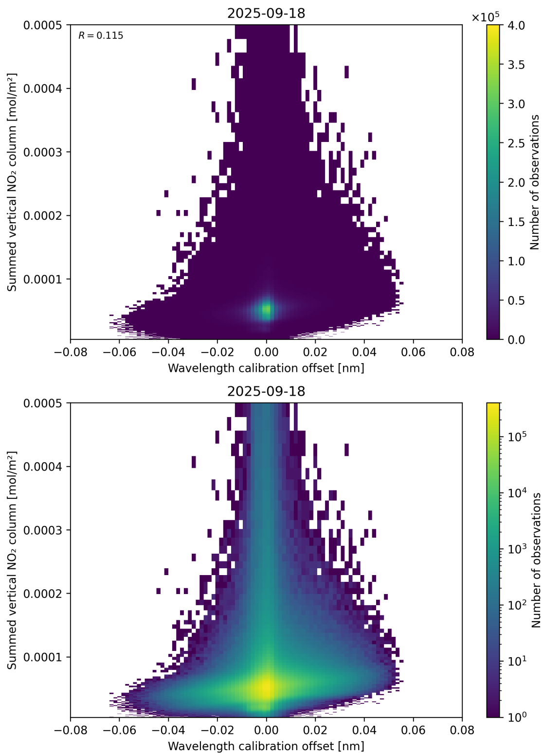
Figure 177: Scatter density plot of “Wavelength calibration offset” against “Summed vertical NO 2 column” for 2025-09-17 to 2025-09-19.
