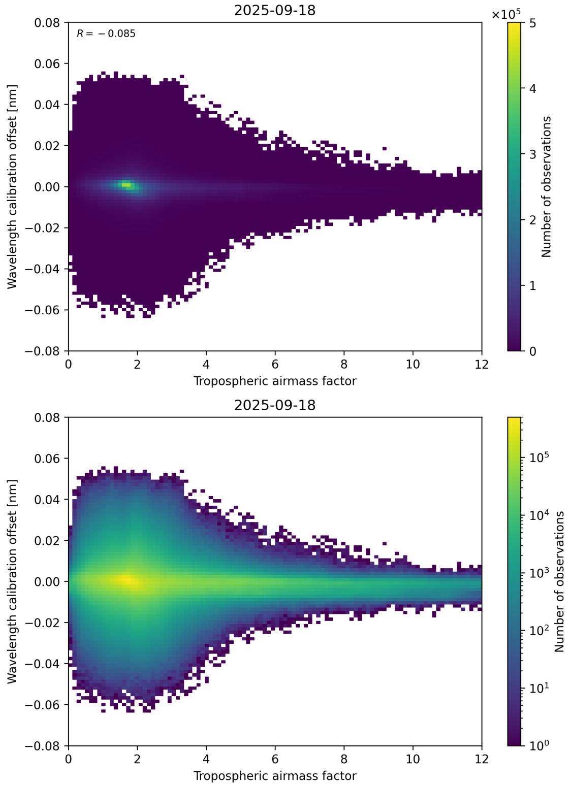
Figure 80: Scatter density plot of “Tropospheric airmass factor” against “Wavelength calibration offset” for 2025-09-17 to 2025-09-19.
