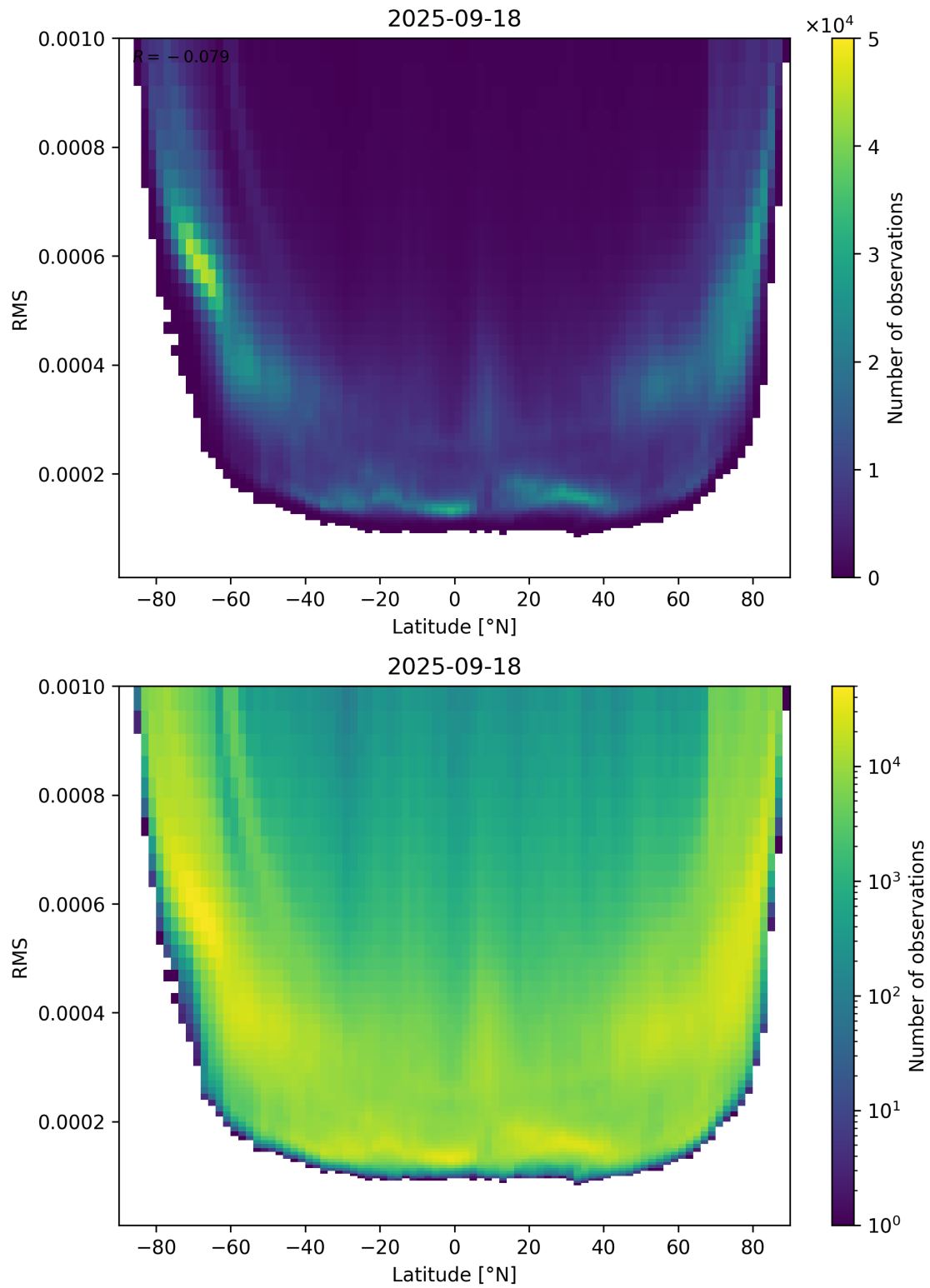
Figure 94: Scatter density plot of “Latitude” against “RMS” for 2025-09-17 to 2025-09-19.
