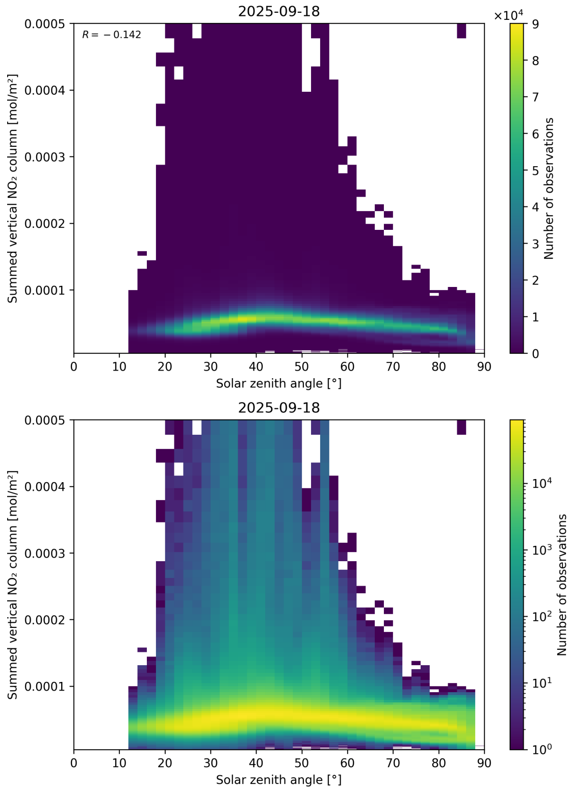
Figure 151: Scatter density plot of “Solar zenith angle” against “Summed vertical NO 2 column” for 2025-09-17 to 2025-09-19.
