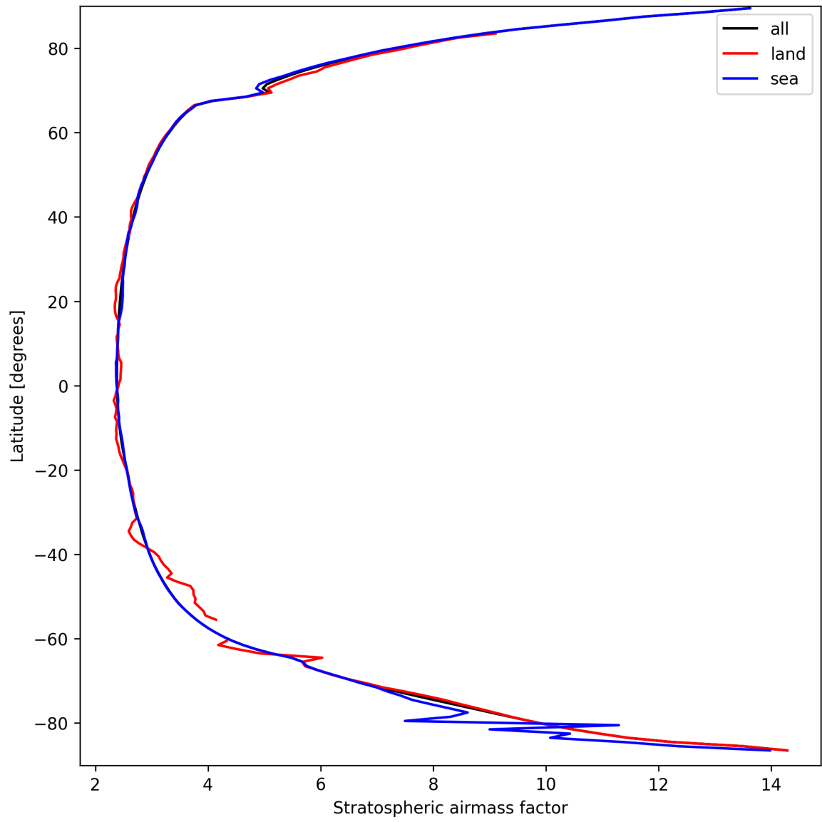
Figure 27: Zonal average of “Stratospheric air mass factor” for 2025-09-17 to 2025-09-19.
