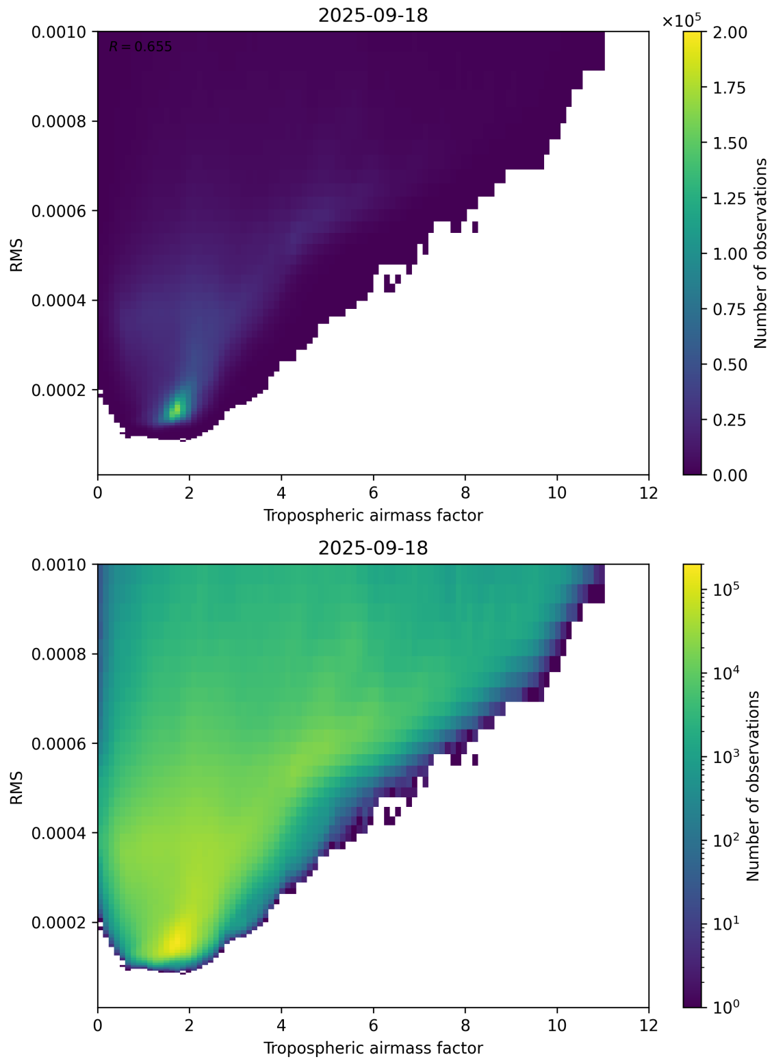
Figure 79: Scatter density plot of “Tropospheric airmass factor” against “RMS” for 2025-09-17 to 2025-09-19.
