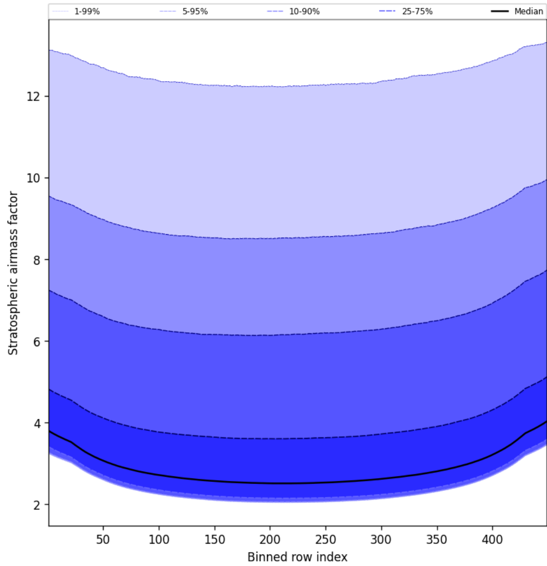
Figure 61: Along track statistics of “Stratospheric airmass factor” for 2025-09-17 to 2025-09-19
