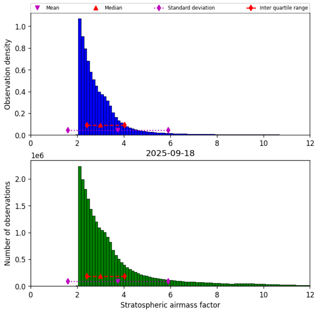
Figure 44: Histogram of “Stratospheric airmass factor” for 2025-09-17 to 2025-09-19
