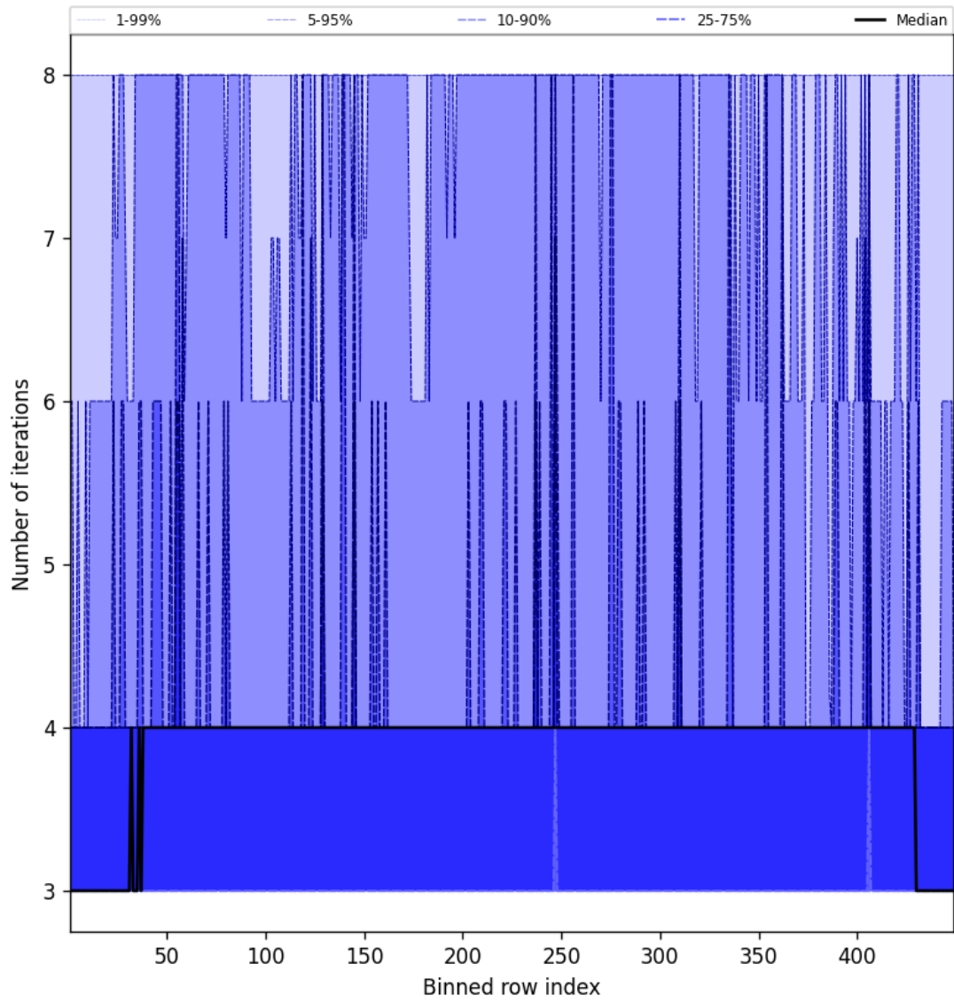
Figure 51: Along track statistics of “Number of iterations” for 2025-09-17 to 2025-09-19
