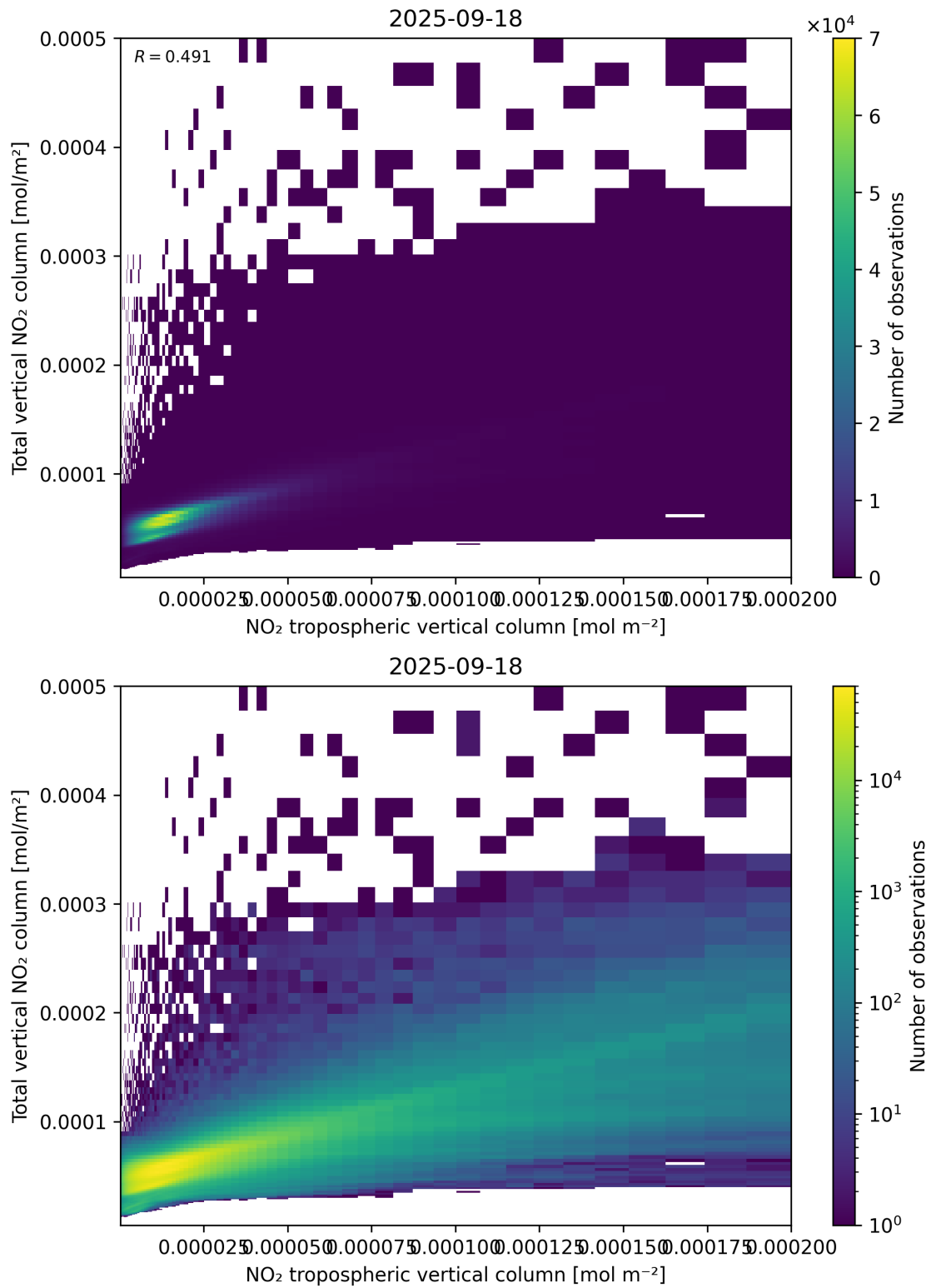
Figure 128: Scatter density plot of “NO 2 tropospheric vertical column” against “Total vertical NO 2 column” for 2025-09-17 to 2025-09-19.
