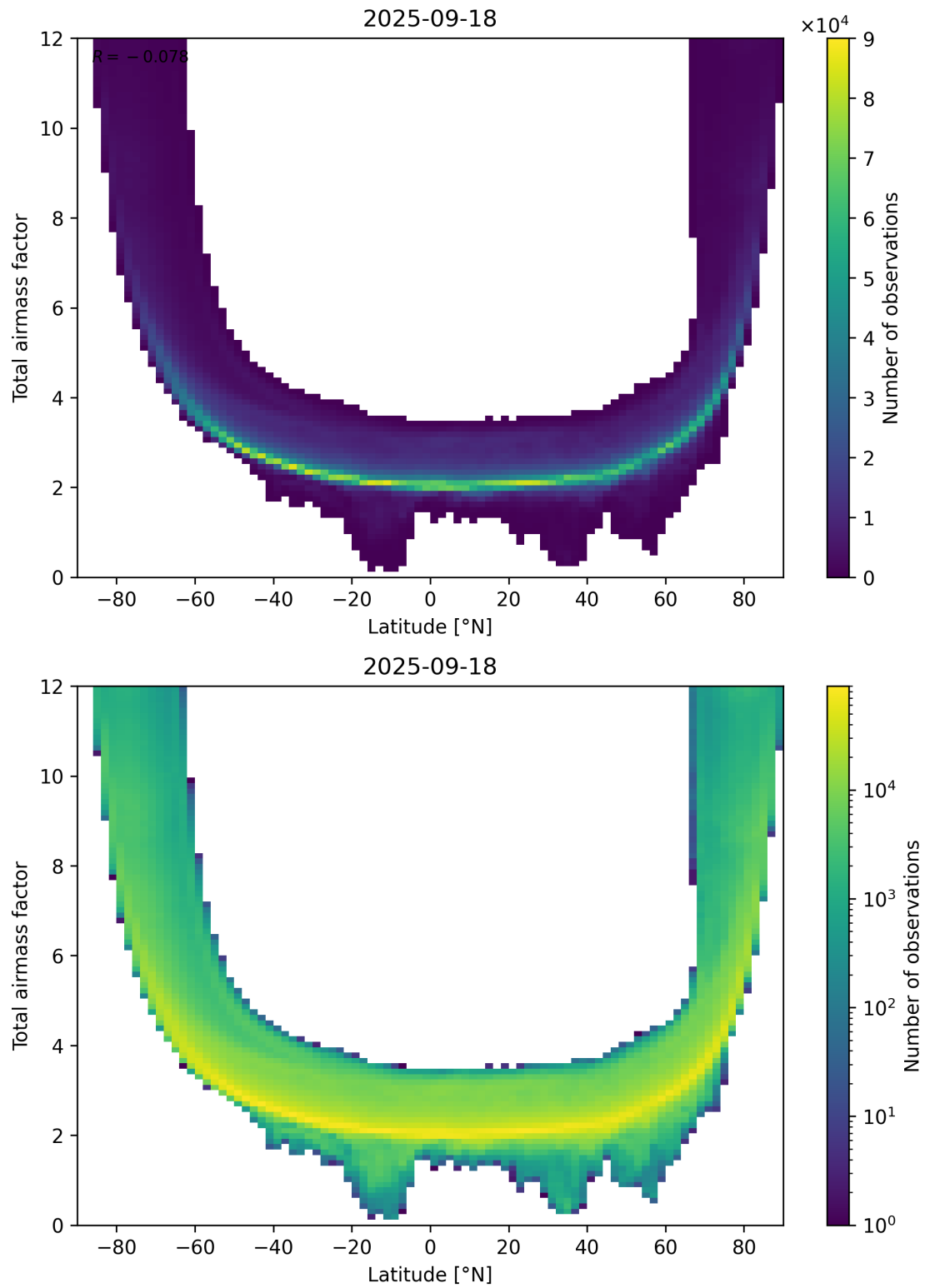
Figure 84: Scatter density plot of “Latitude” against “Total airmass factor” for 2025-09-17 to 2025-09-19.
