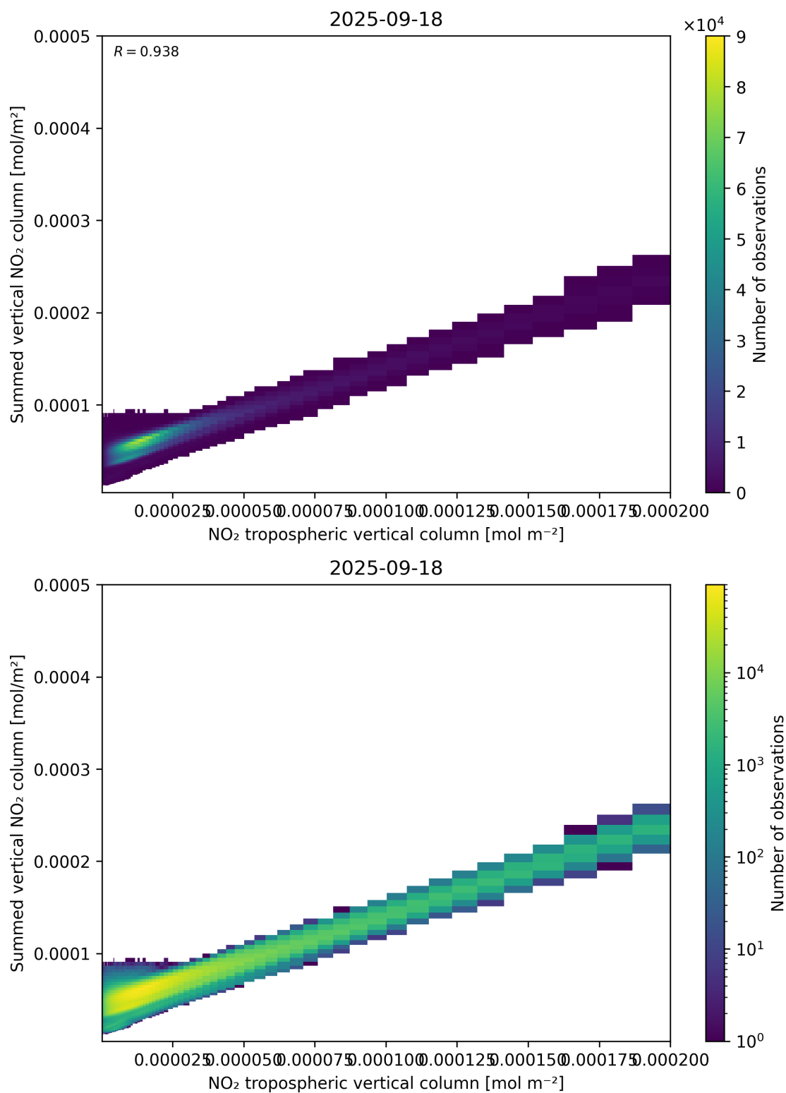
Figure 126: Scatter density plot of “NO 2 tropospheric vertical column” against “Summed vertical NO 2 column” for 2025-09-17 to 2025-09-19.
