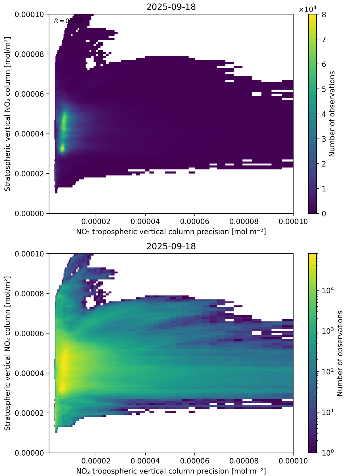
Figure 135: Scatter density plot of “NO 2 tropospheric vertical column precision” against “Stratospheric vertical NO 2 column” for 2025-09-17 to 2025-09-19.
