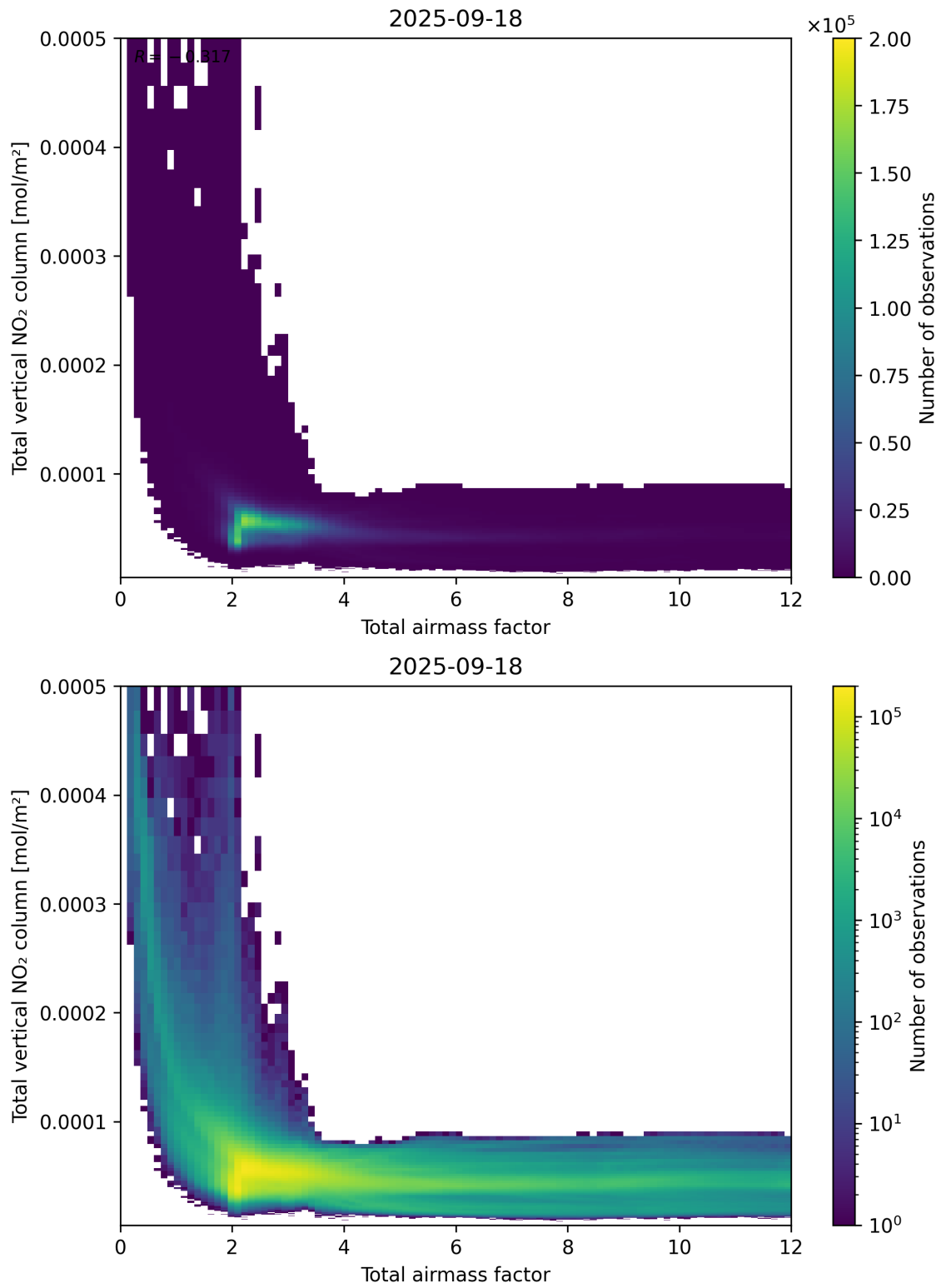
Figure 67: Scatter density plot of “Total airmass factor” against “Total vertical NO 2 column” for 2025-09-17 to 2025-09-19.
