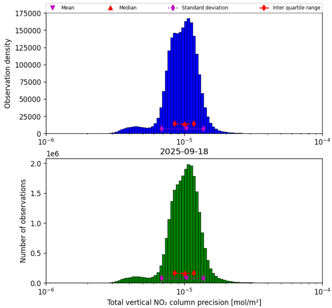
Figure 39: Histogram of “Total vertical NO 2 column precision” for 2025-09-17 to 2025-09-19
