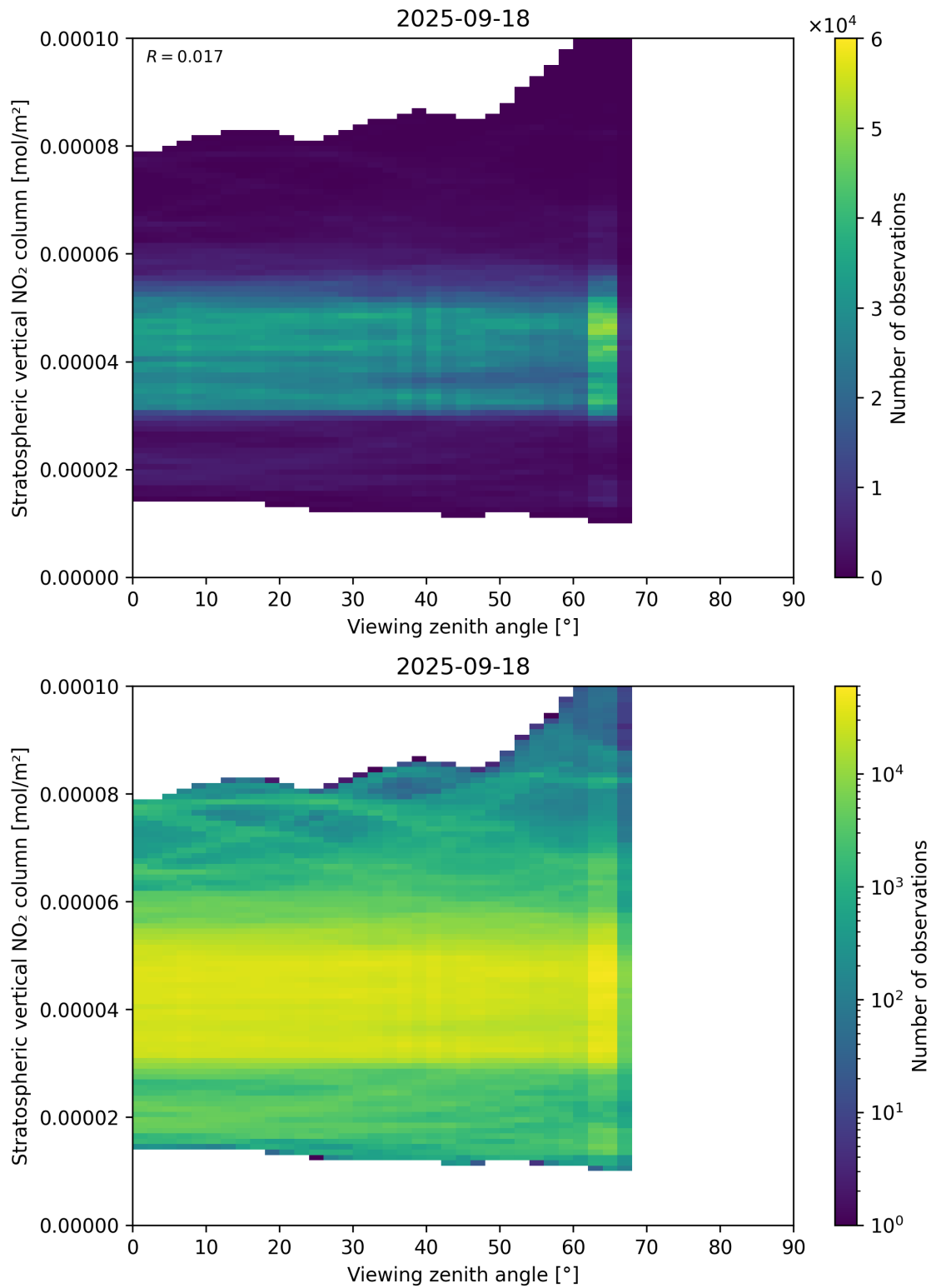
Figure 164: Scatter density plot of “Viewing zenith angle” against “Stratospheric vertical NO 2 column” for 2025-09-17 to 2025-09-19.
