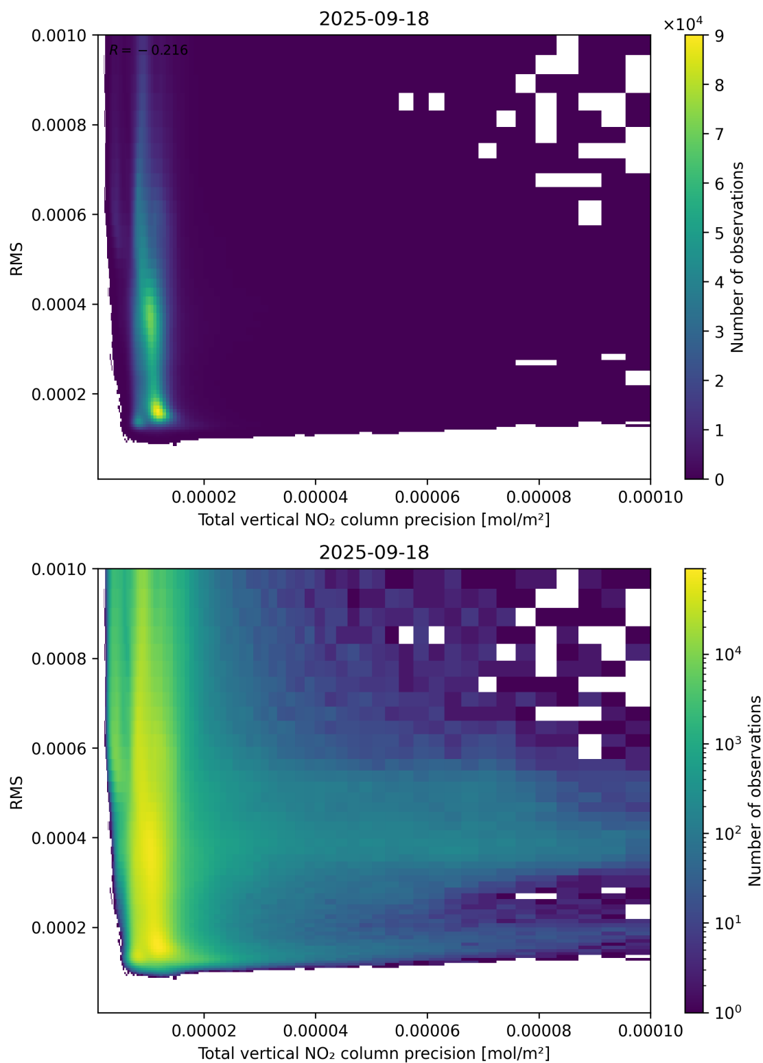
Figure 119: Scatter density plot of “Total vertical NO 2 column precision” against “RMS” for 2025-09-17 to 2025-09-19.
