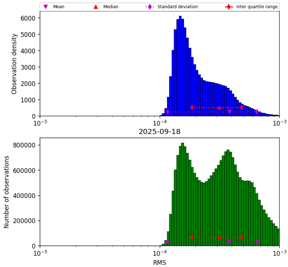
Figure 43: Histogram of “RMS” for 2025-09-17 to 2025-09-19
