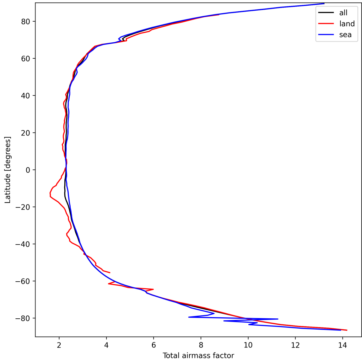
Figure 15: Zonal average of “Total airmass factor” for 2025-09-17 to 2025-09-19.
