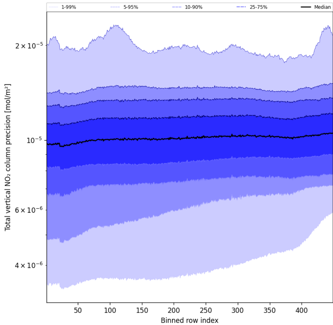
Figure 56: Along track statistics of "Total vertical NO 2 column precision" for 2025-09-17 to 2025-09-19
