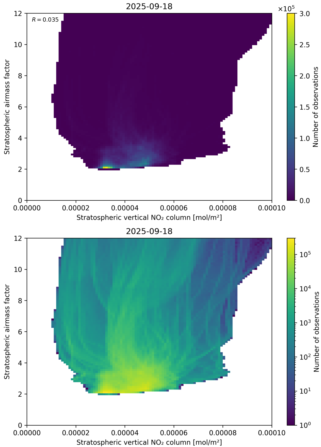
Figure 96: Scatter density plot of “Stratospheric vertical NO 2 column” against “Stratospheric airmass factor” for 2025-09-17 to 2025-09-19.
