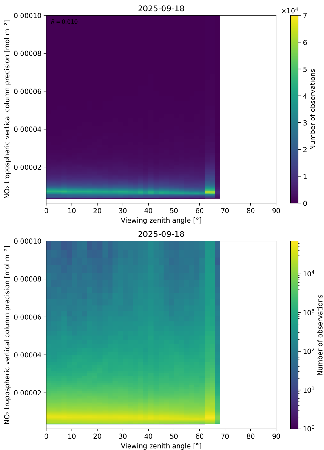
Figure 170: Scatter density plot of “Viewing zenith angle” against “NO 2 tropospheric vertical column precision” for 2025-09-17 to 2025-09-19.
