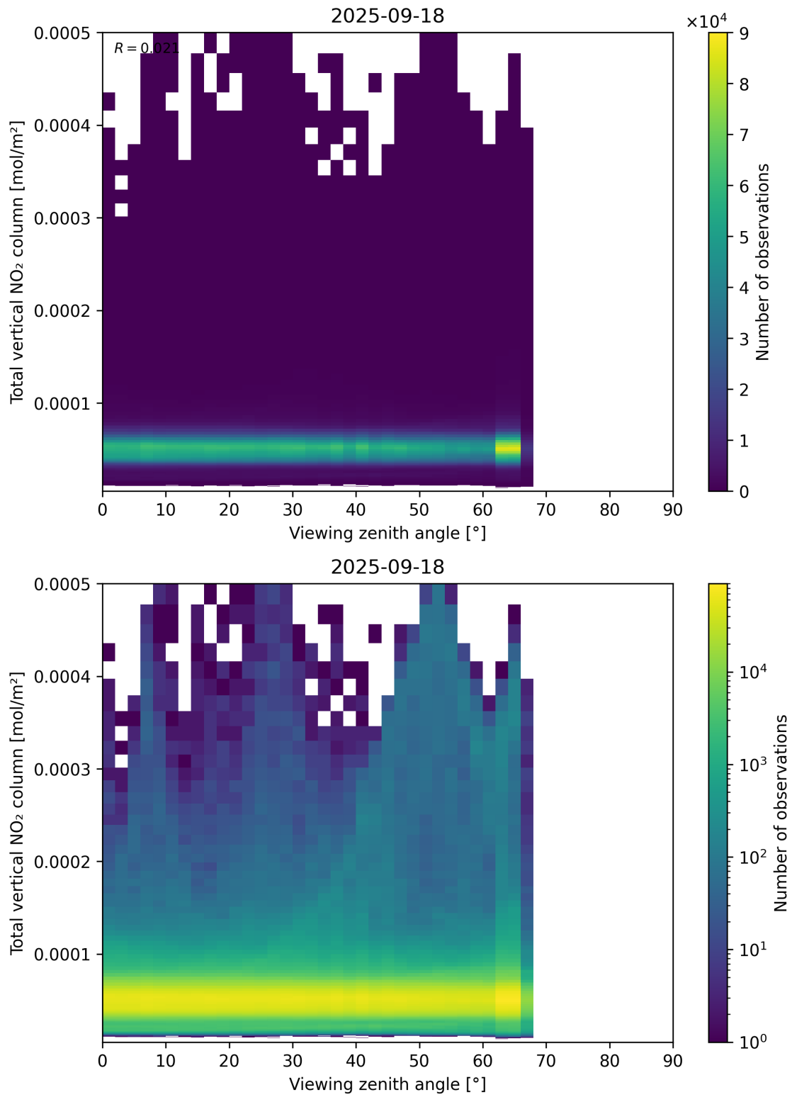
Figure 167: Scatter density plot of “Viewing zenith angle” against “Total vertical NO 2 column” for 2025-09-17 to 2025-09-19.
