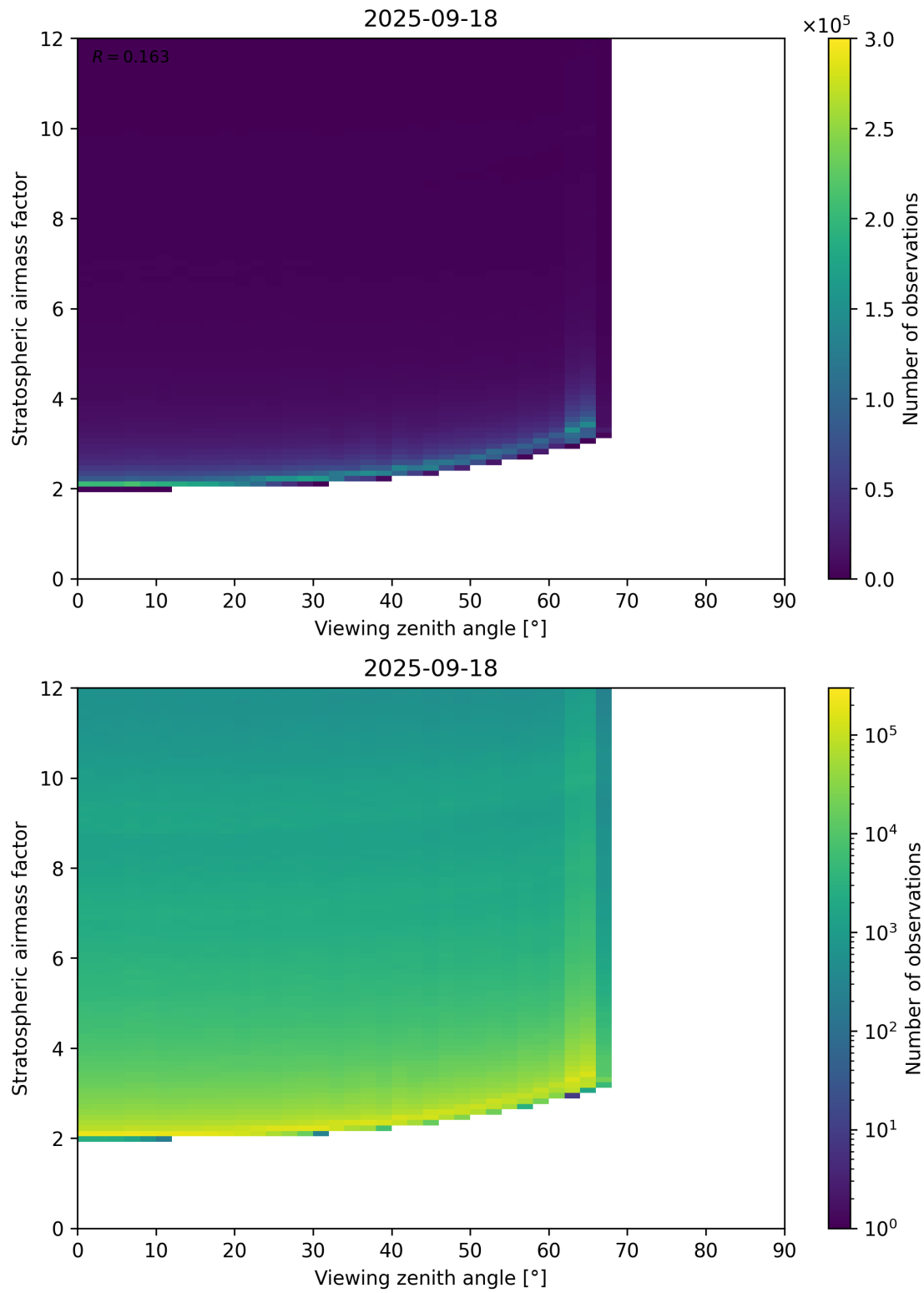
Figure 159: Scatter density plot of “Viewing zenith angle” against “Stratospheric airmass factor” for 2025-09-17 to 2025-09-19.
