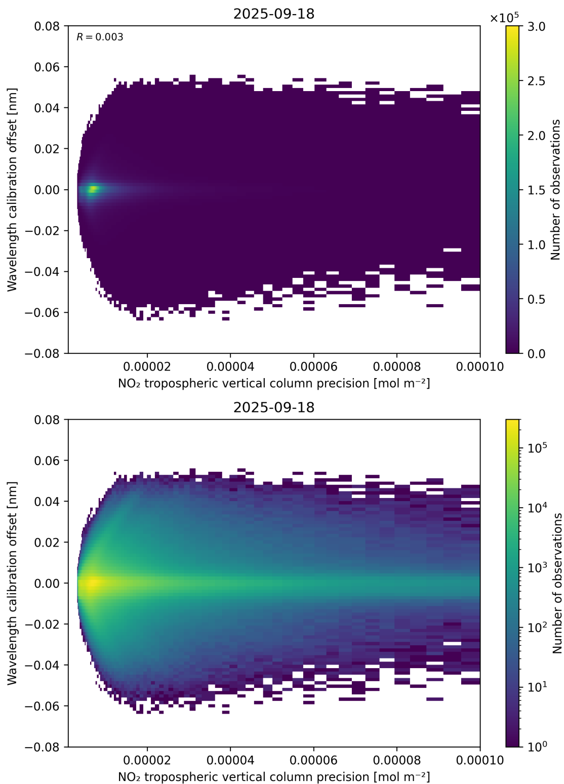
Figure 141: Scatter density plot of “NO 2 tropospheric vertical column precision” against “Wavelength calibration offset” for 2025-09-17 to 2025-09-19.
