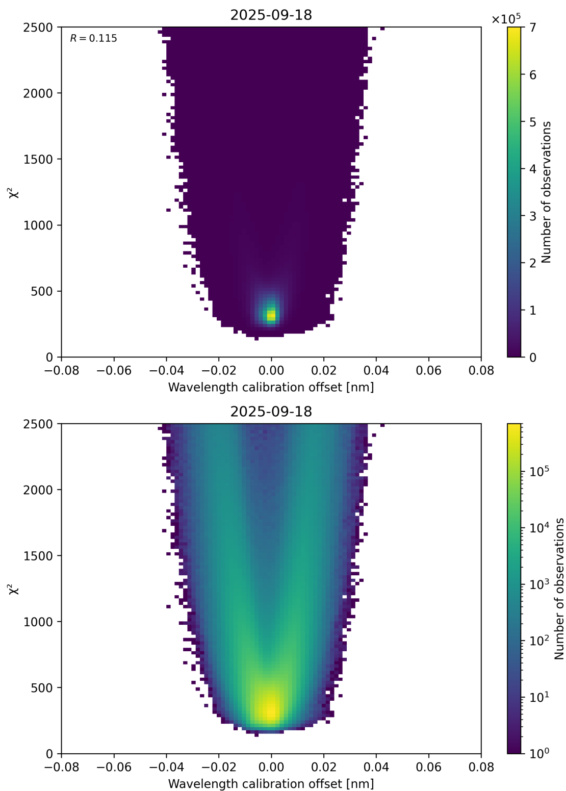
Figure 175: Scatter density plot of “Wavelength calibration offset” against “ \chi^2 ” for 2025-09-17 to 2025-09-19.
