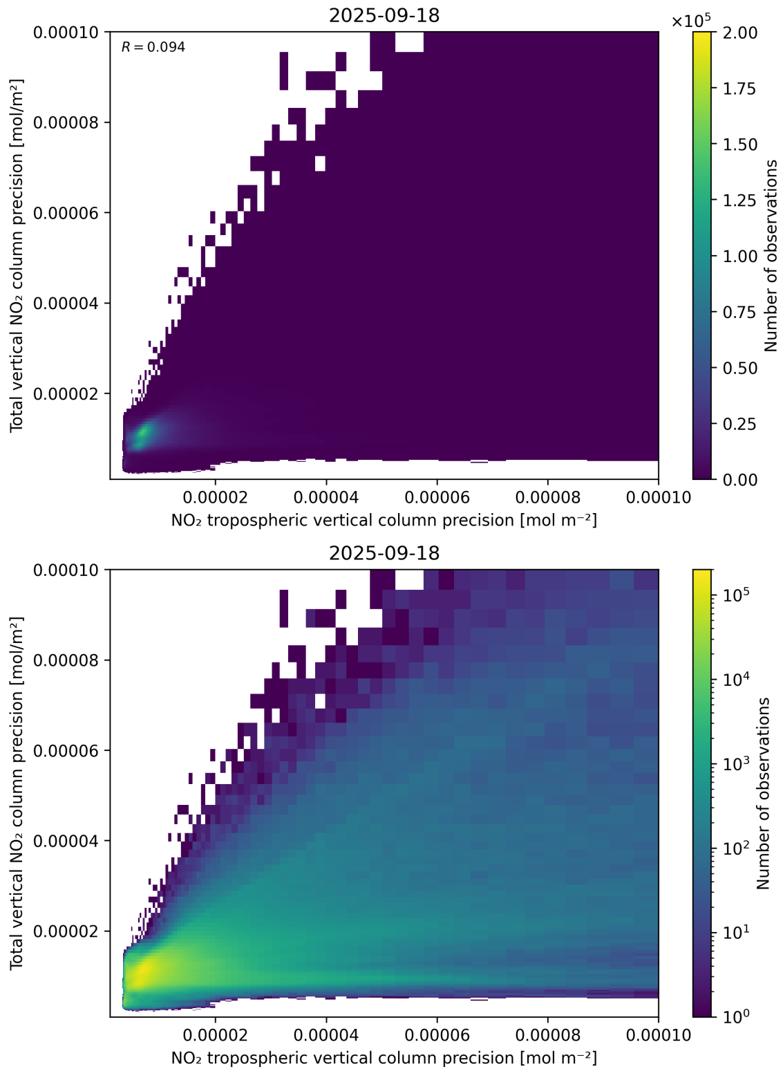
Figure 139: Scatter density plot of “NO 2 tropospheric vertical column precision” against “Total vertical NO 2 column precision” for 2025-09-17 to 2025-09-19.
