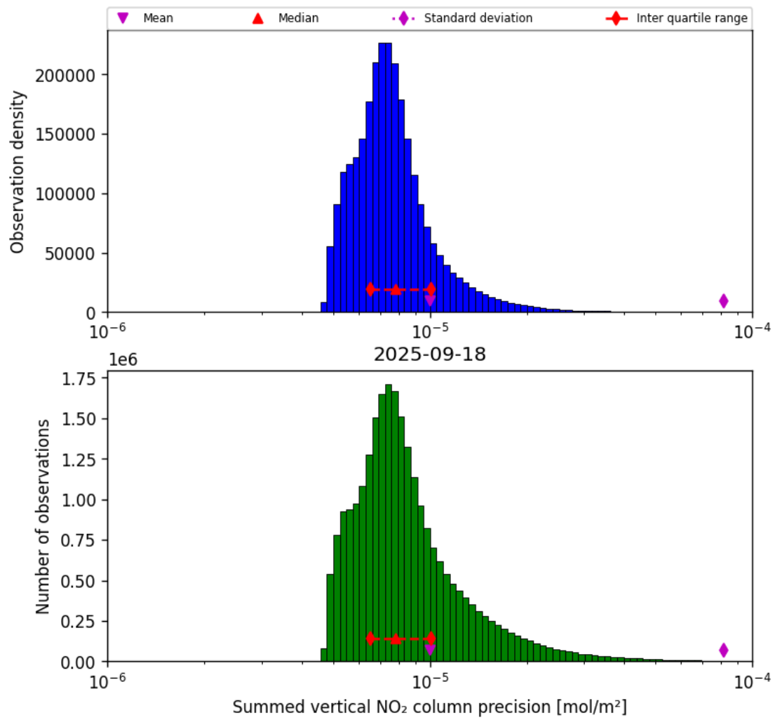
Figure 41: Histogram of "Summed vertical NO 2 column precision" for 2025-09-17 to 2025-09-19
