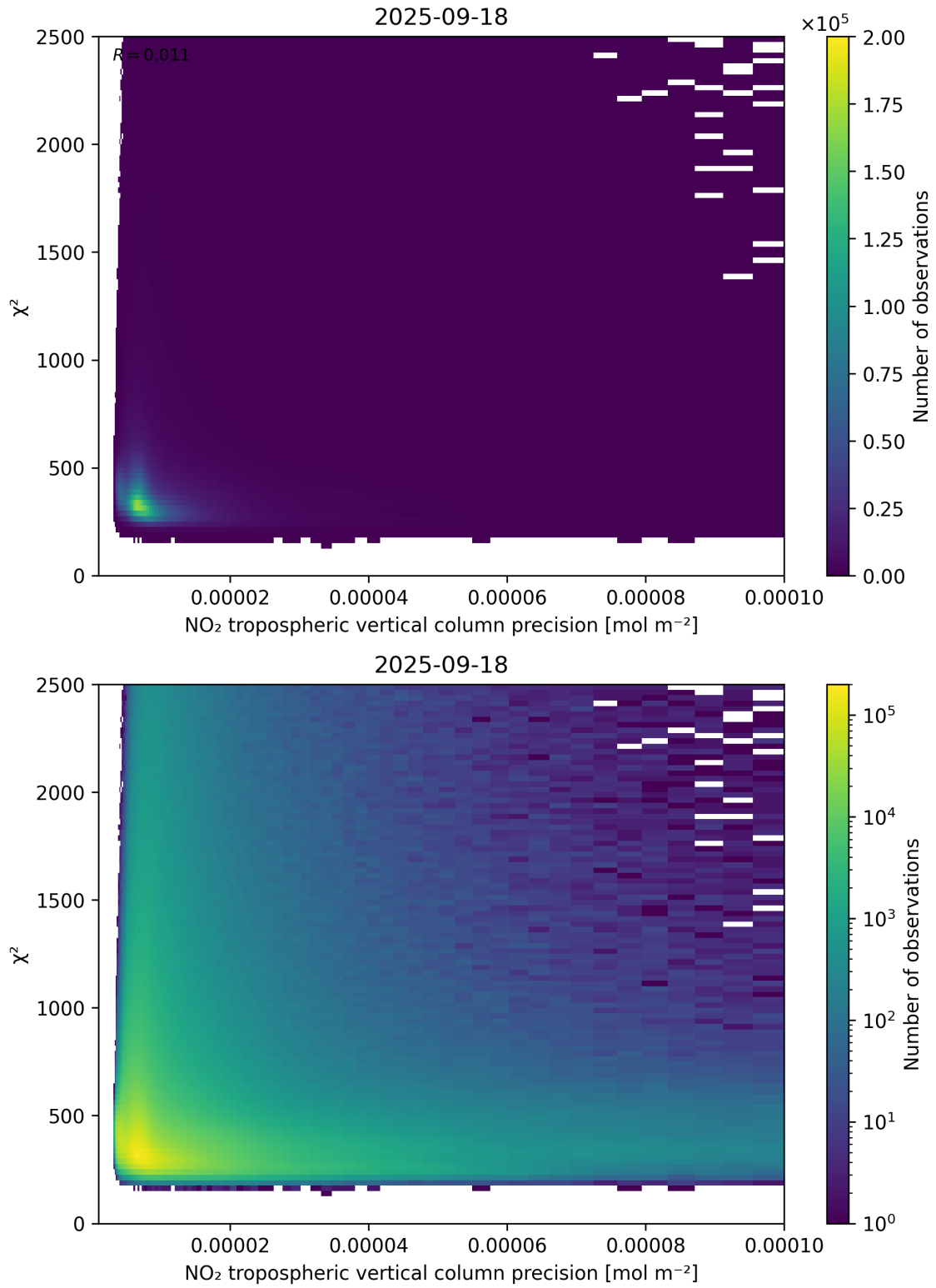
Figure 134: Scatter density plot of “NO 2 tropospheric vertical column precision” against “ \chi^2 ” for 2025-09-17 to 2025-09-19.
