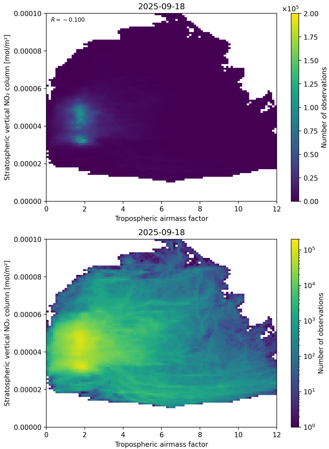
Figure 74: Scatter density plot of “Tropospheric air mass factor” against “Stratospheric vertical NO 2 column” for 2025-09-17 to 2025-09-19.
