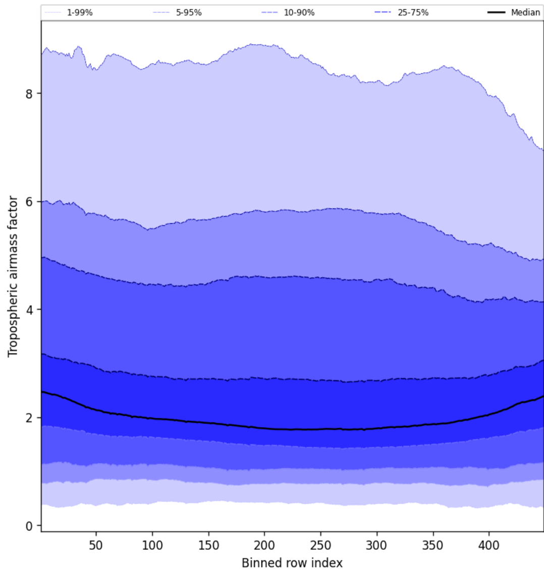
Figure 48: Along track statistics of “Tropospheric air mass factor” for 2025-09-17 to 2025-09-19
