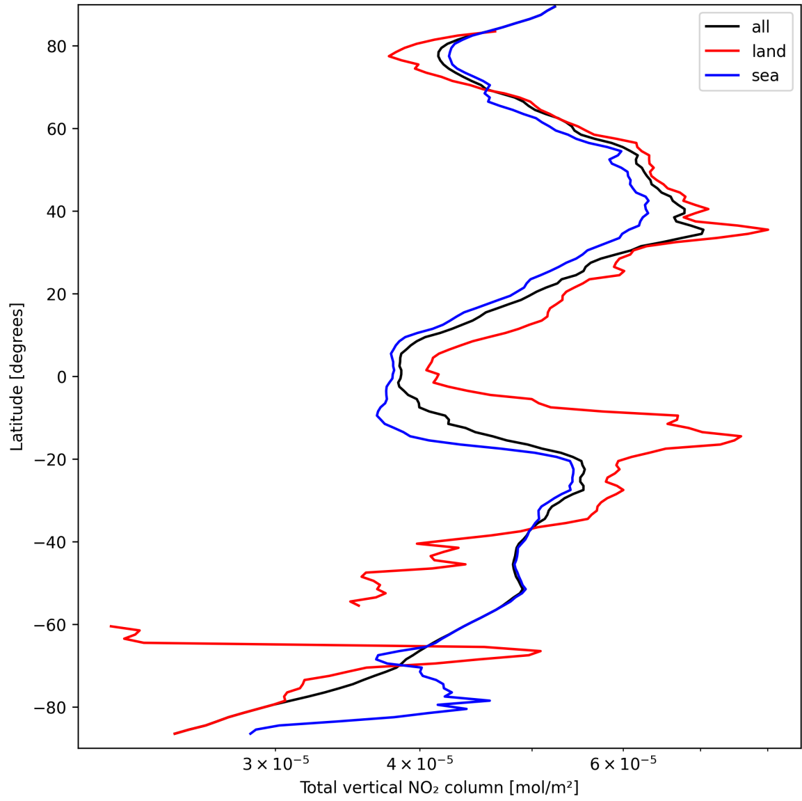
Figure 21: Zonal average of “Total vertical NO 2 column” for 2025-09-17 to 2025-09-19.
