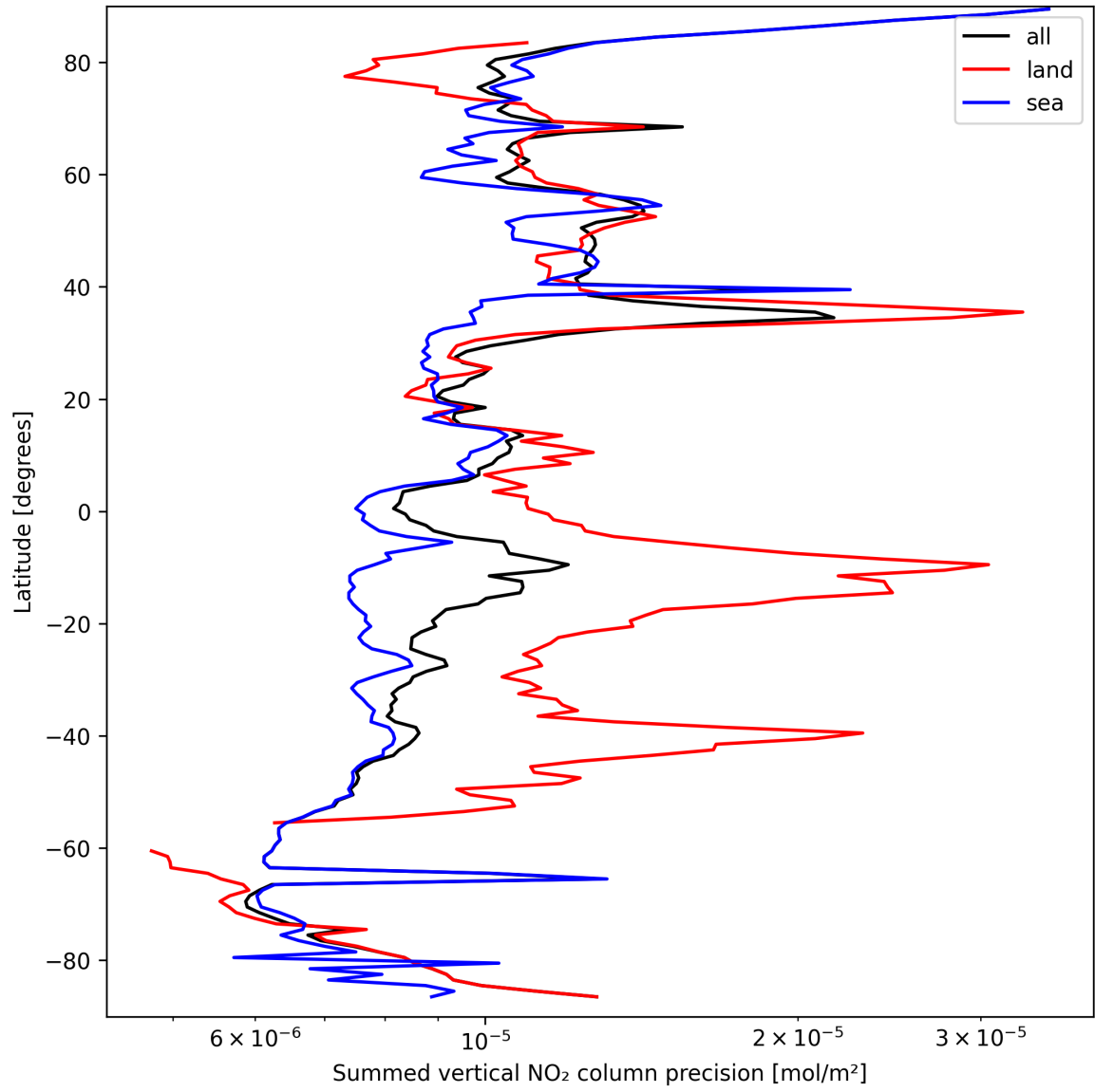
Figure 24: Zonal average of “Summed vertical NO 2 column precision” for 2025-09-17 to 2025-09-19.
