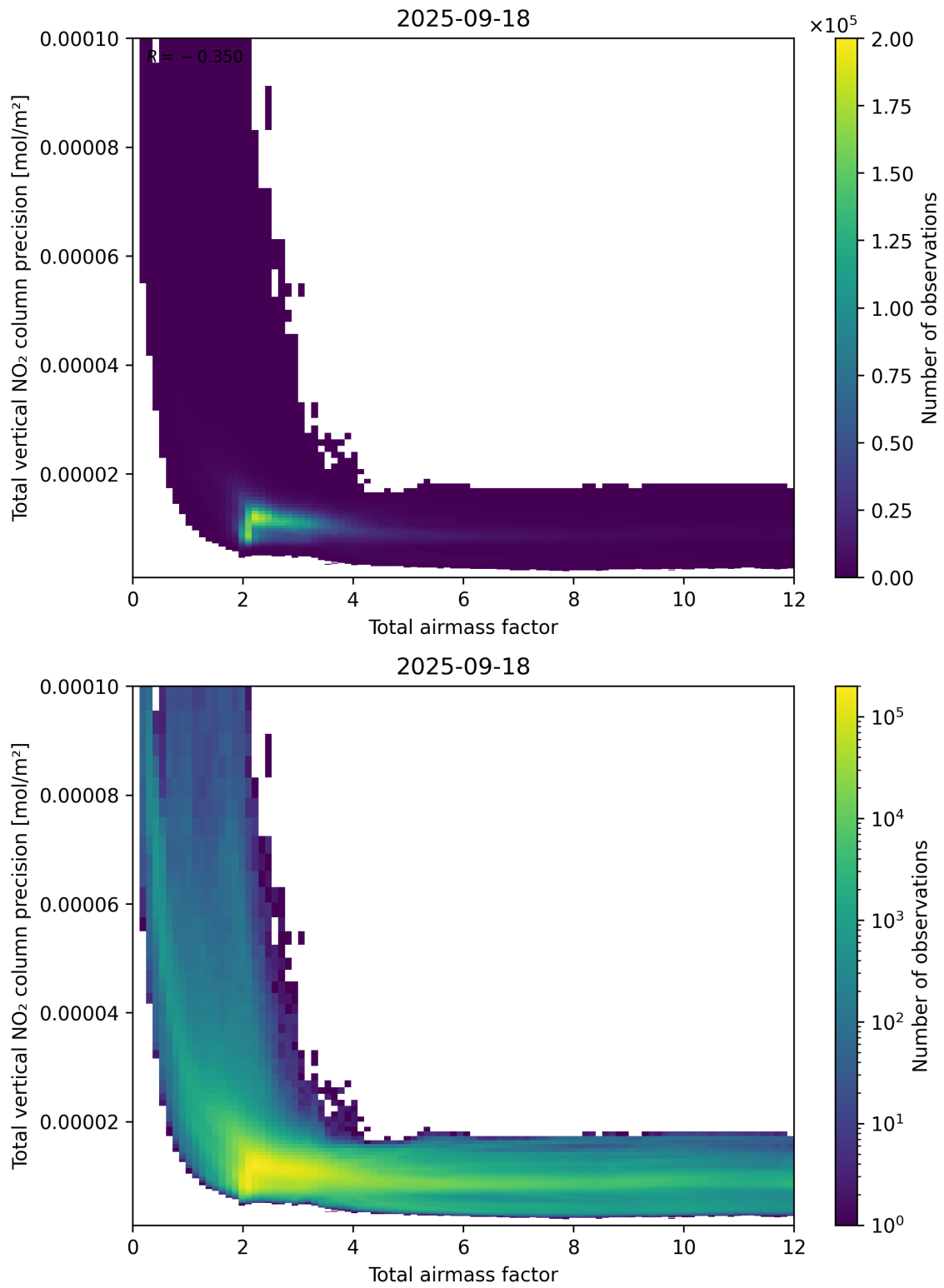
Figure 68: Scatter density plot of “Total airmass factor” against “Total vertical NO 2 column precision” for 2025-09-17 to 2025-09-19.
