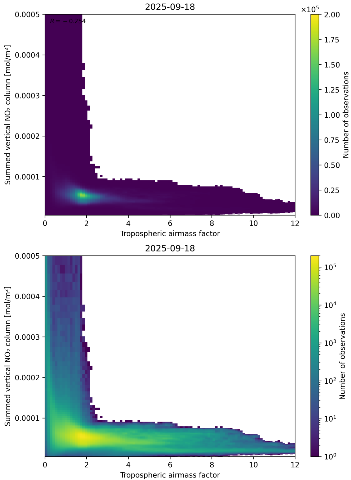
Figure 75: Scatter density plot of “Tropospheric airmass factor” against “Summed vertical NO 2 column” for 2025-09-17 to 2025-09-19.
