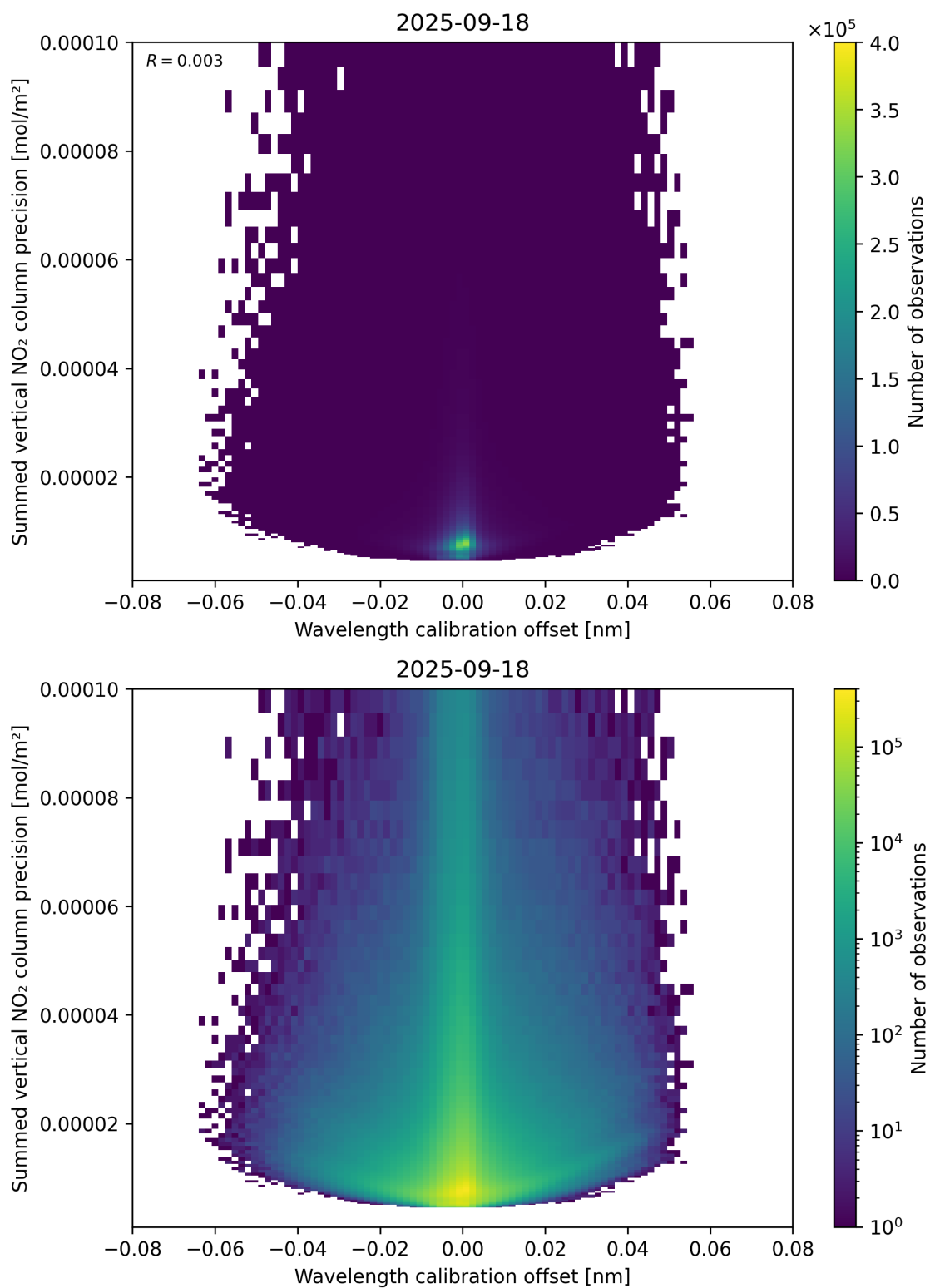
Figure 178: Scatter density plot of “Wavelength calibration offset” against “Summed vertical NO 2 column precision” for 2025-09-17 to 2025-09-19.
