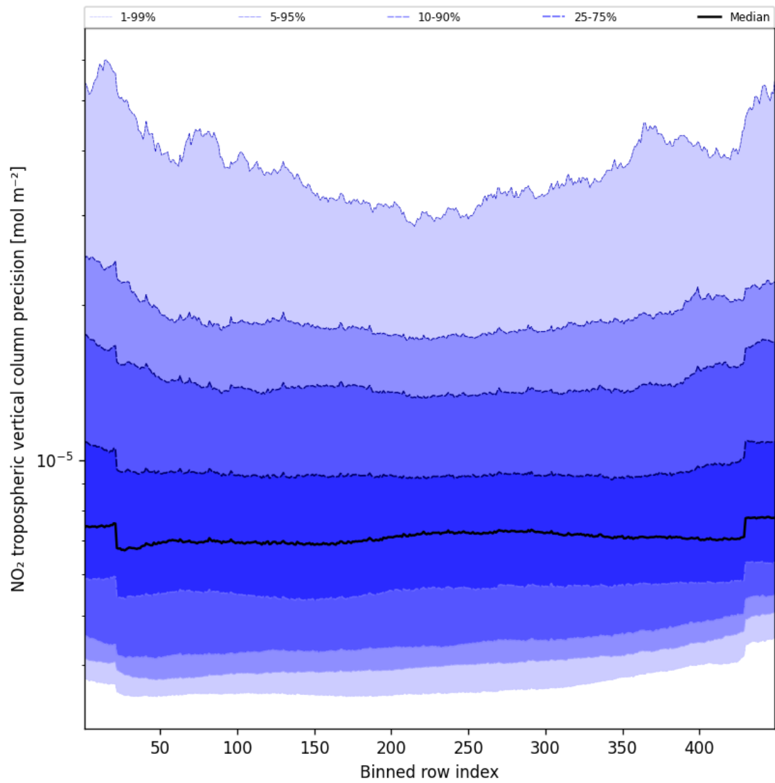
Figure 47: Along track statistics of “NO 2 tropospheric vertical column precision” for 2025-09-17 to 2025-09-19
