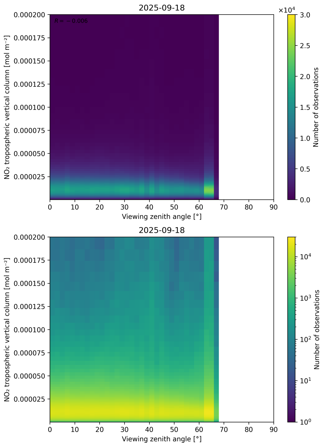
Figure 169: Scatter density plot of “Viewing zenith angle” against “NO 2 tropospheric vertical column” for 2025-09-17 to 2025-09-19.
