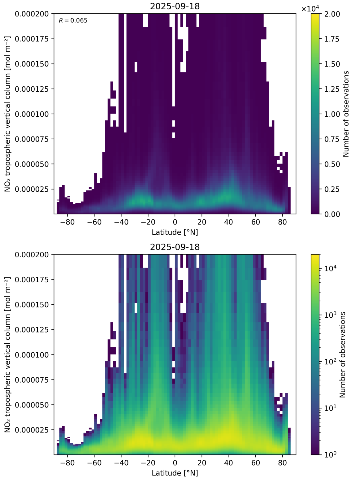
Figure 92: Scatter density plot of “Latitude” against “NO 2 tropospheric vertical column” for 2025-09-17 to 2025-09-19.
