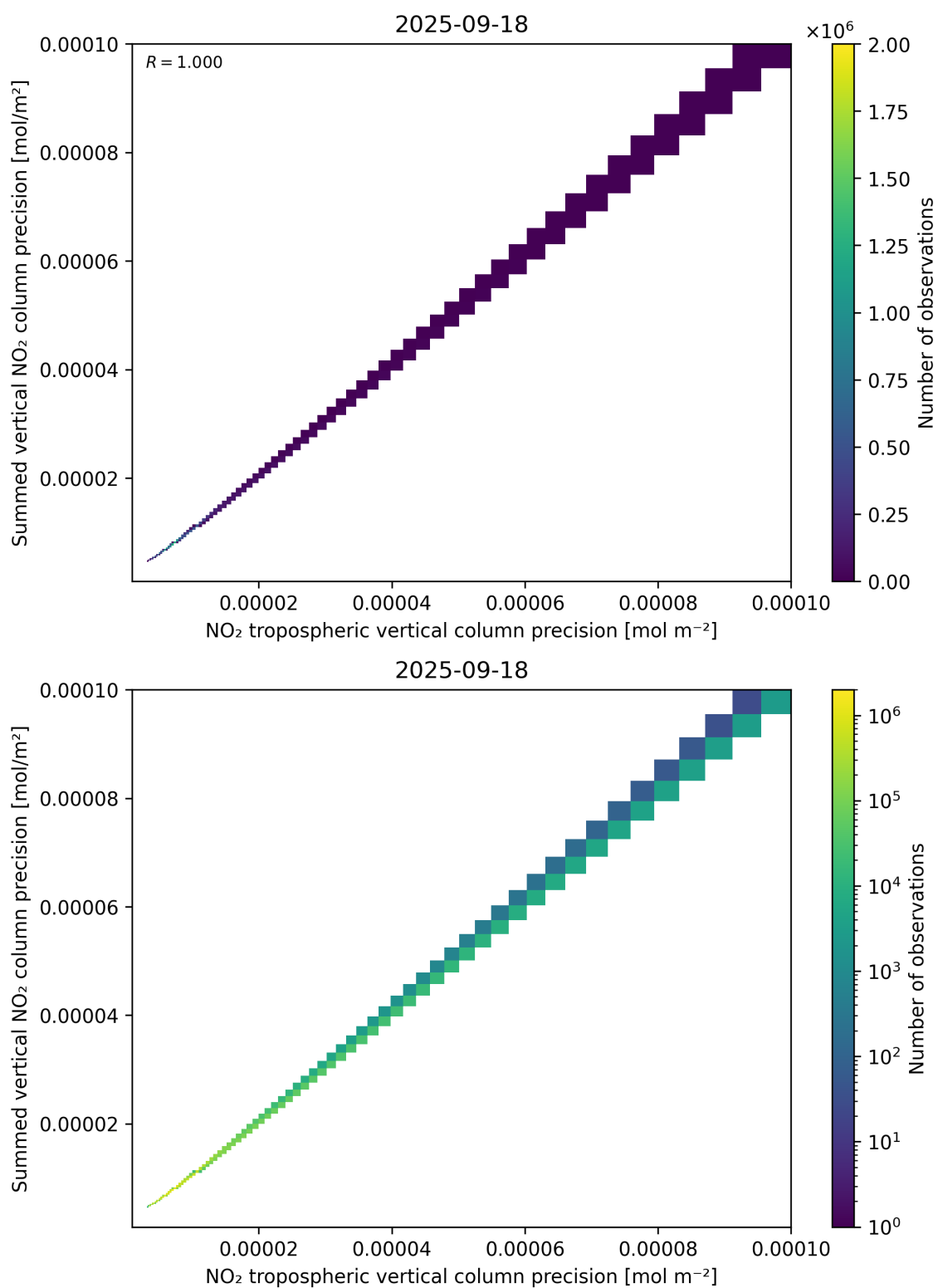
Figure 137: Scatter density plot of “NO 2 tropospheric vertical column precision” against “Summed vertical NO 2 column precision” for 2025-09-17 to 2025-09-19.
