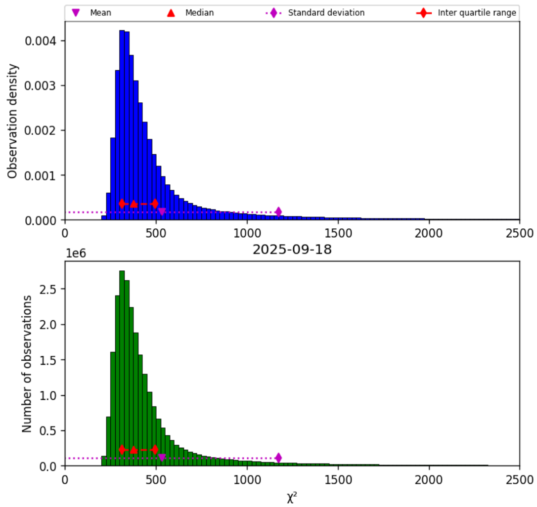
Figure 42: Histogram of “ \chi^2 ” for 2025-09-17 to 2025-09-19
