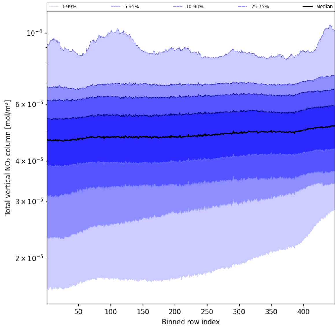
Figure 55: Along track statistics of “Total vertical NO 2 column” for 2025-09-17 to 2025-09-19
