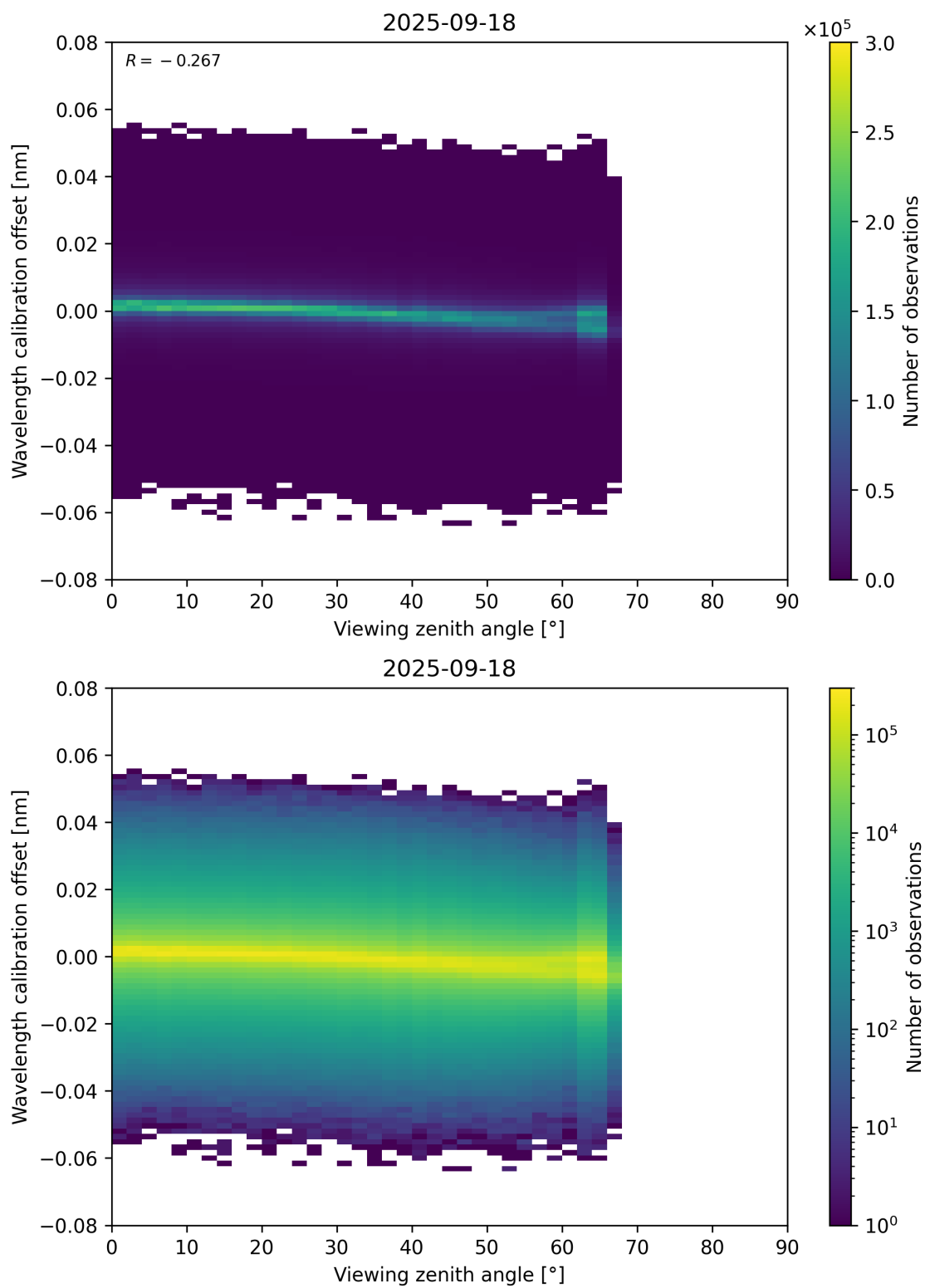
Figure 173: Scatter density plot of “Viewing zenith angle” against “Wavelength calibration offset” for 2025-09-17 to 2025-09-19.
