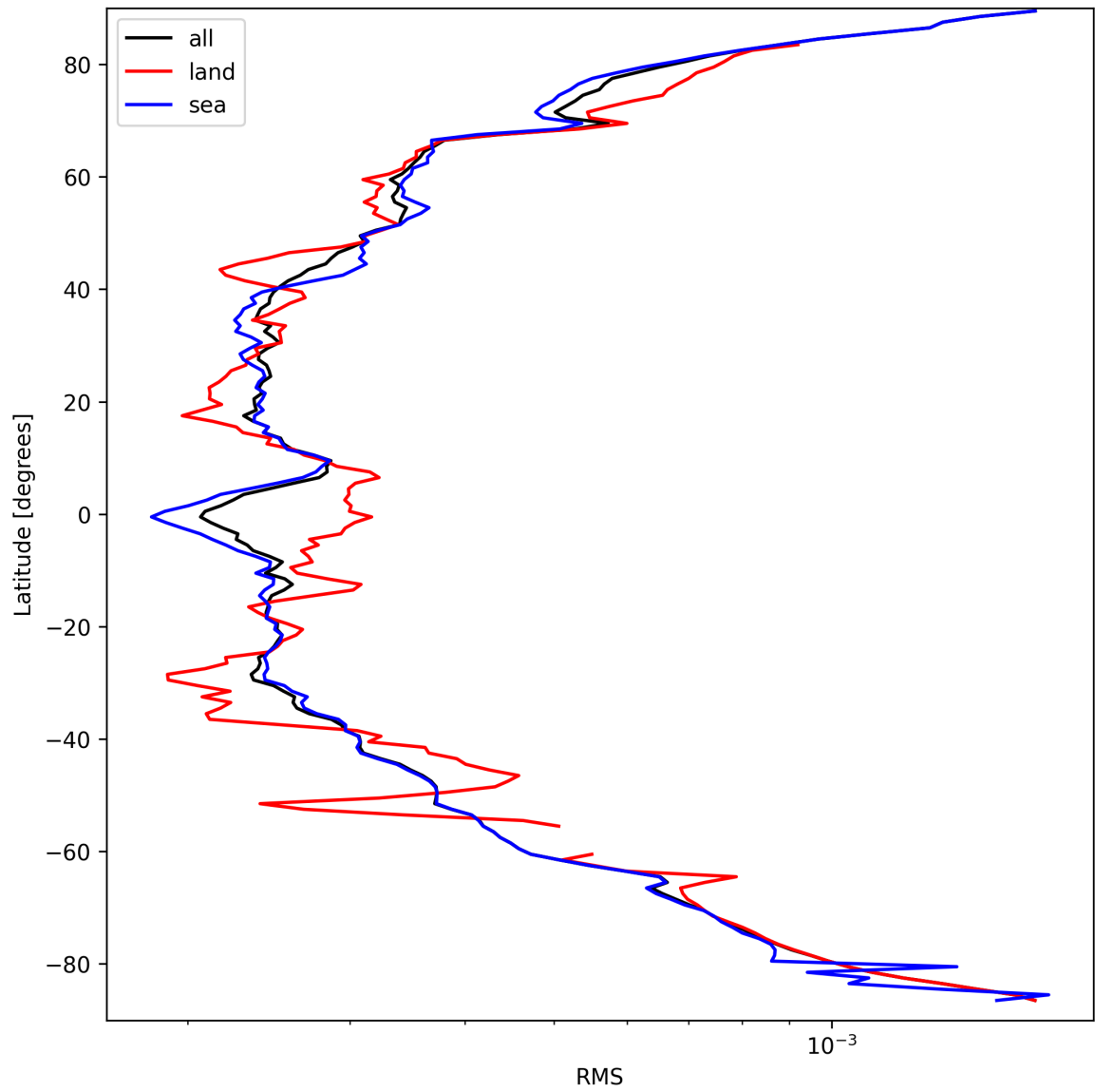
Figure 26: Zonal average of “RMS” for 2025-09-17 to 2025-09-19.
