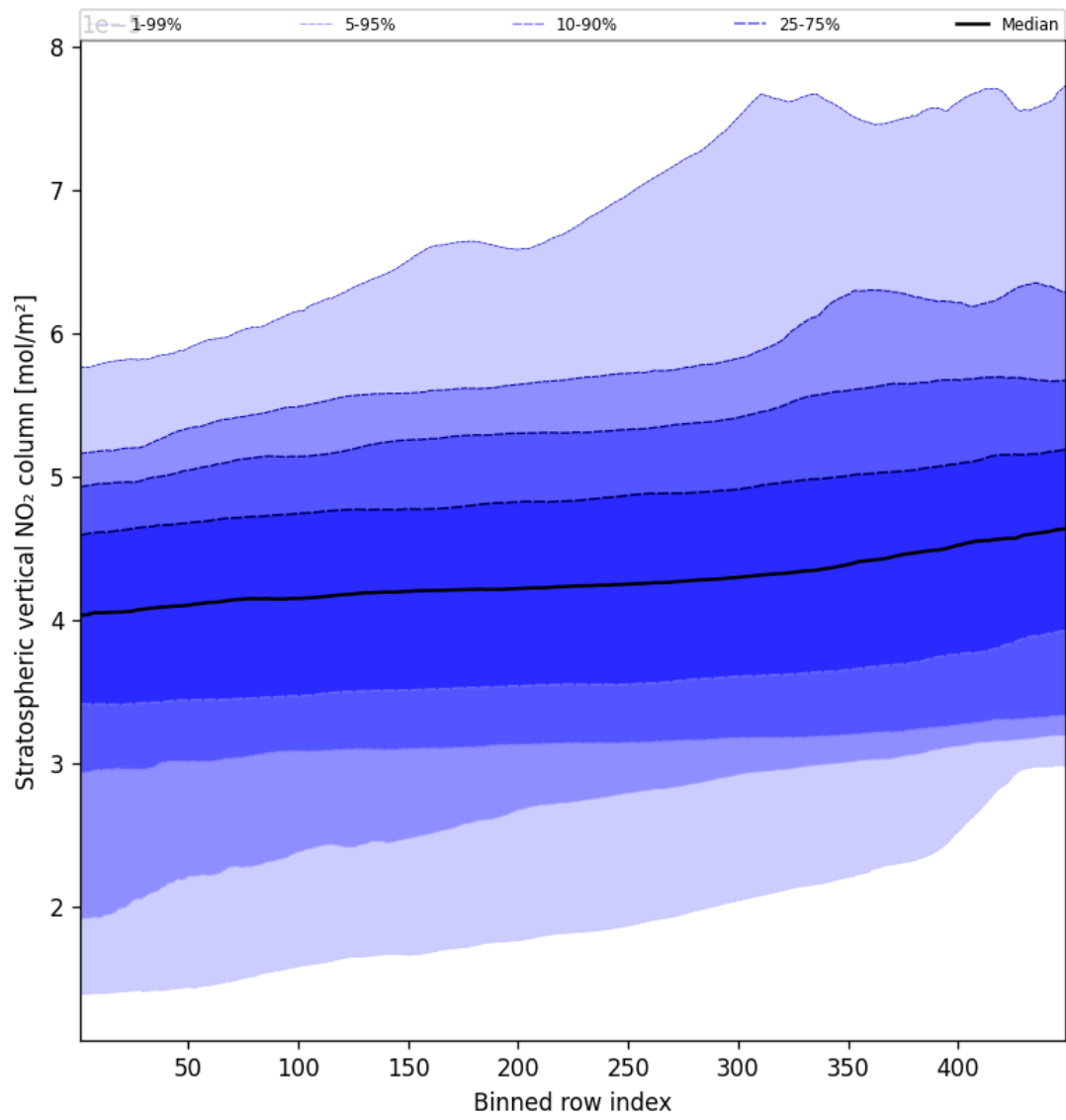
Figure 53: Along track statistics of “Stratospheric vertical NO 2 column” for 2025-09-17 to 2025-09-19
