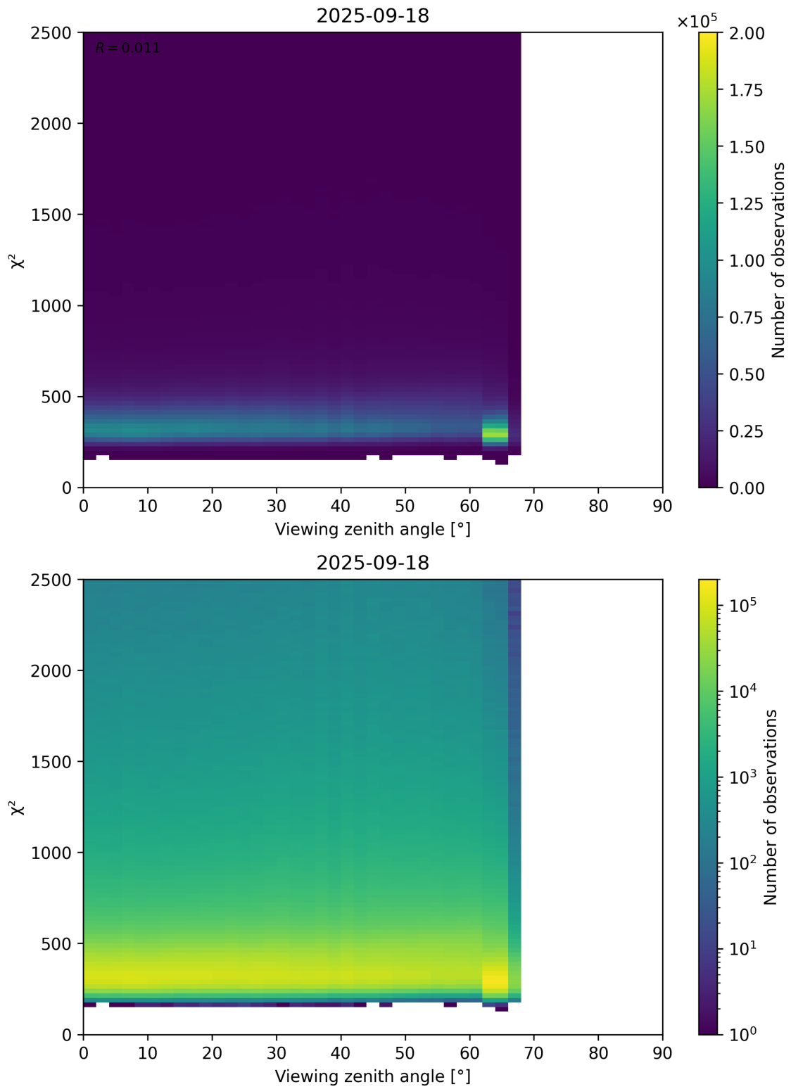
Figure 162: Scatter density plot of “Viewing zenith angle” against “ \chi^2 ” for 2025-09-17 to 2025-09-19.
