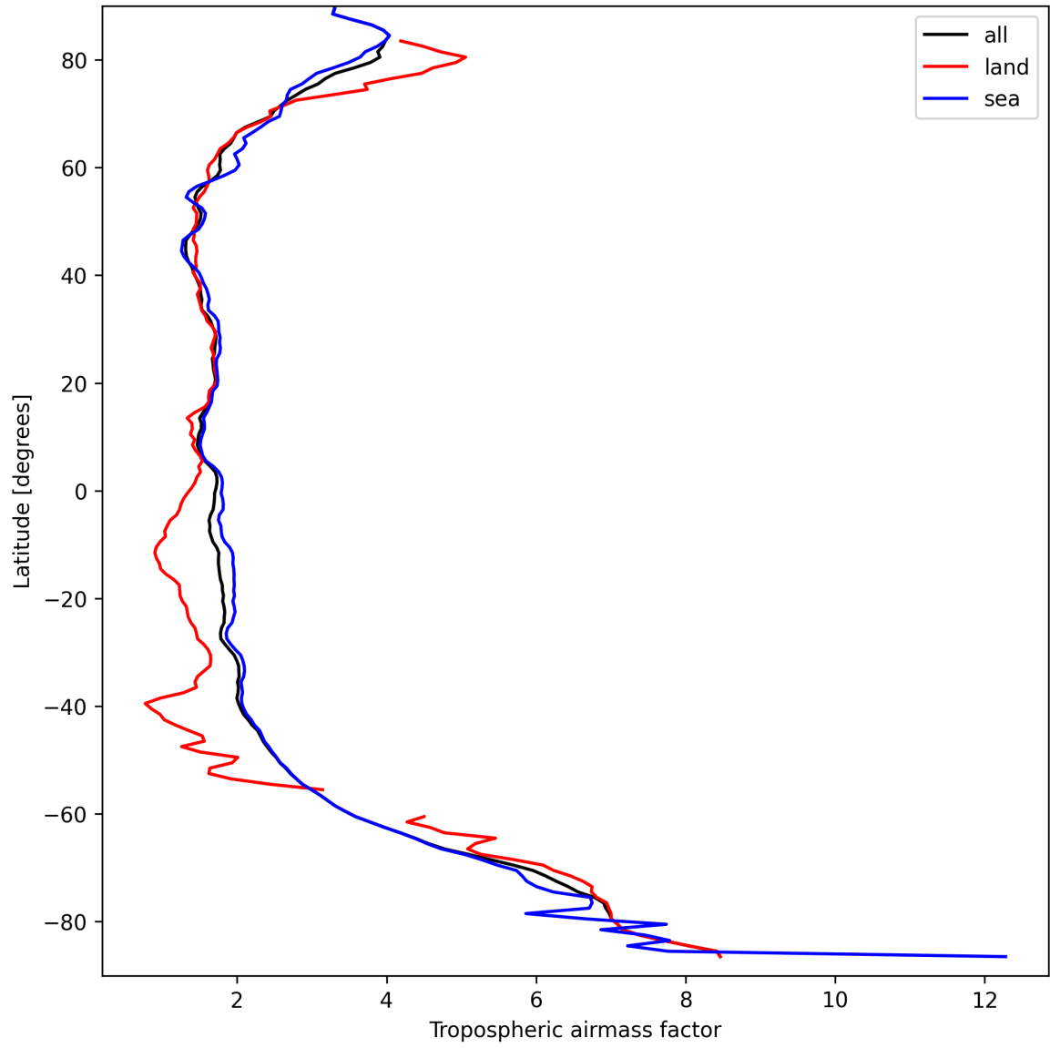
Figure 14: Zonal average of “Tropospheric airmass factor” for 2025-09-17 to 2025-09-19.
