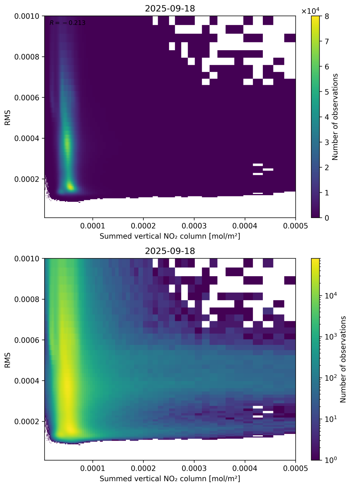
Figure 109: Scatter density plot of “Summed vertical NO 2 column” against “RMS” for 2025-09-17 to 2025-09-19.
