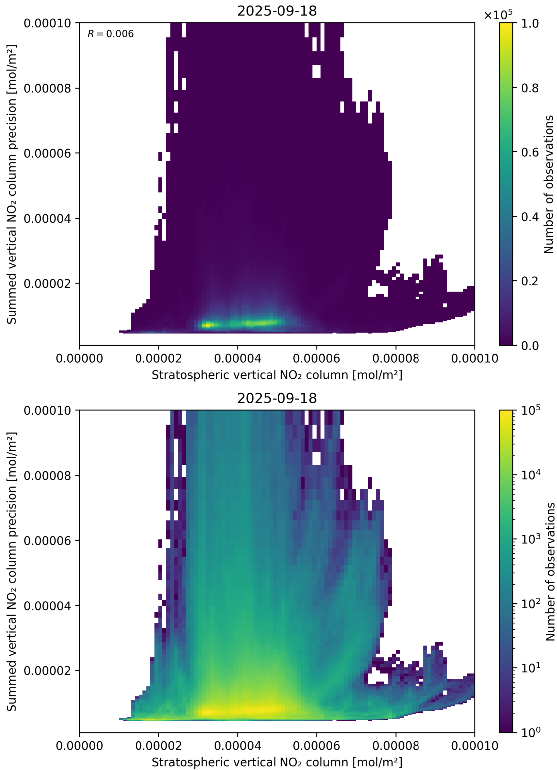
Figure 99: Scatter density plot of “Stratospheric vertical NO 2 column” against “Summed vertical NO 2 column precision” for 2025-09-17 to 2025-09-19.
