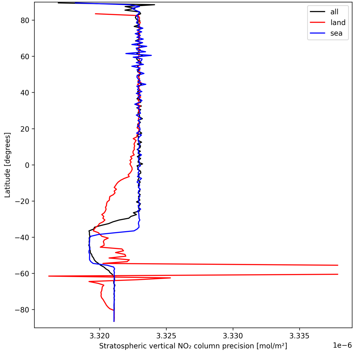
Figure 20: Zonal average of “Stratospheric vertical NO 2 column precision” for 2025-09-17 to 2025-09-19.
