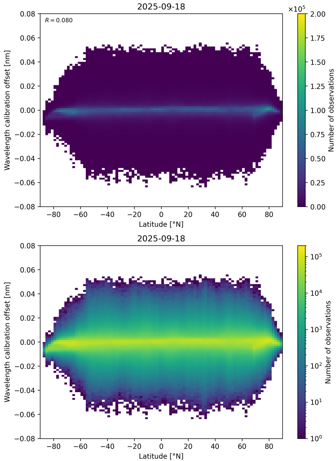
Figure 95: Scatter density plot of “Latitude” against “Wavelength calibration offset” for 2025-09-17 to 2025-09-19.
