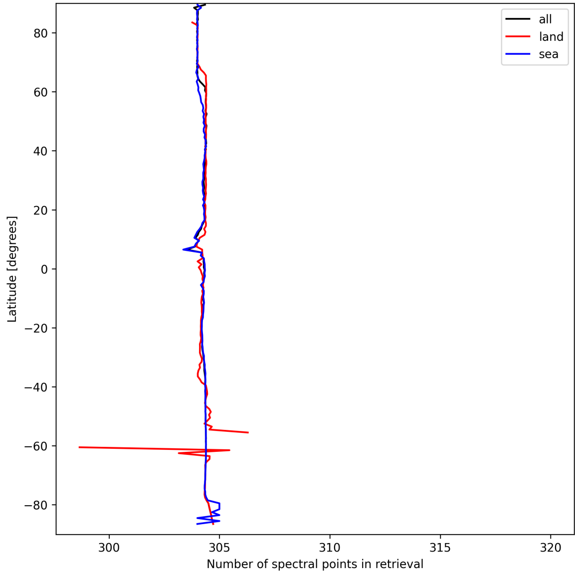
Figure 16: Zonal average of “Number of spectral points in retrieval” for 2025-09-17 to 2025-09-19.
