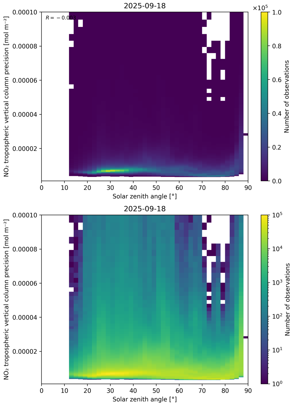
Figure 156: Scatter density plot of “Solar zenith angle” against “NO 2 tropospheric vertical column precision” for 2025-09-17 to 2025-09-19.
