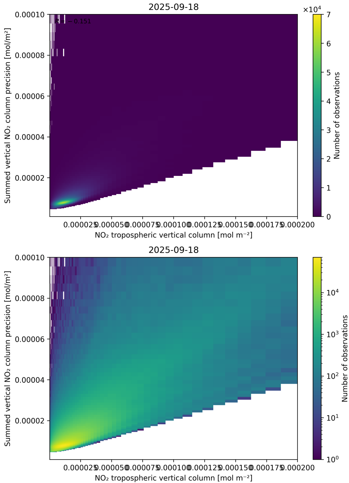
Figure 127: Scatter density plot of “NO 2 tropospheric vertical column” against “Summed vertical NO 2 column precision” for 2025-09-17 to 2025-09-19.
