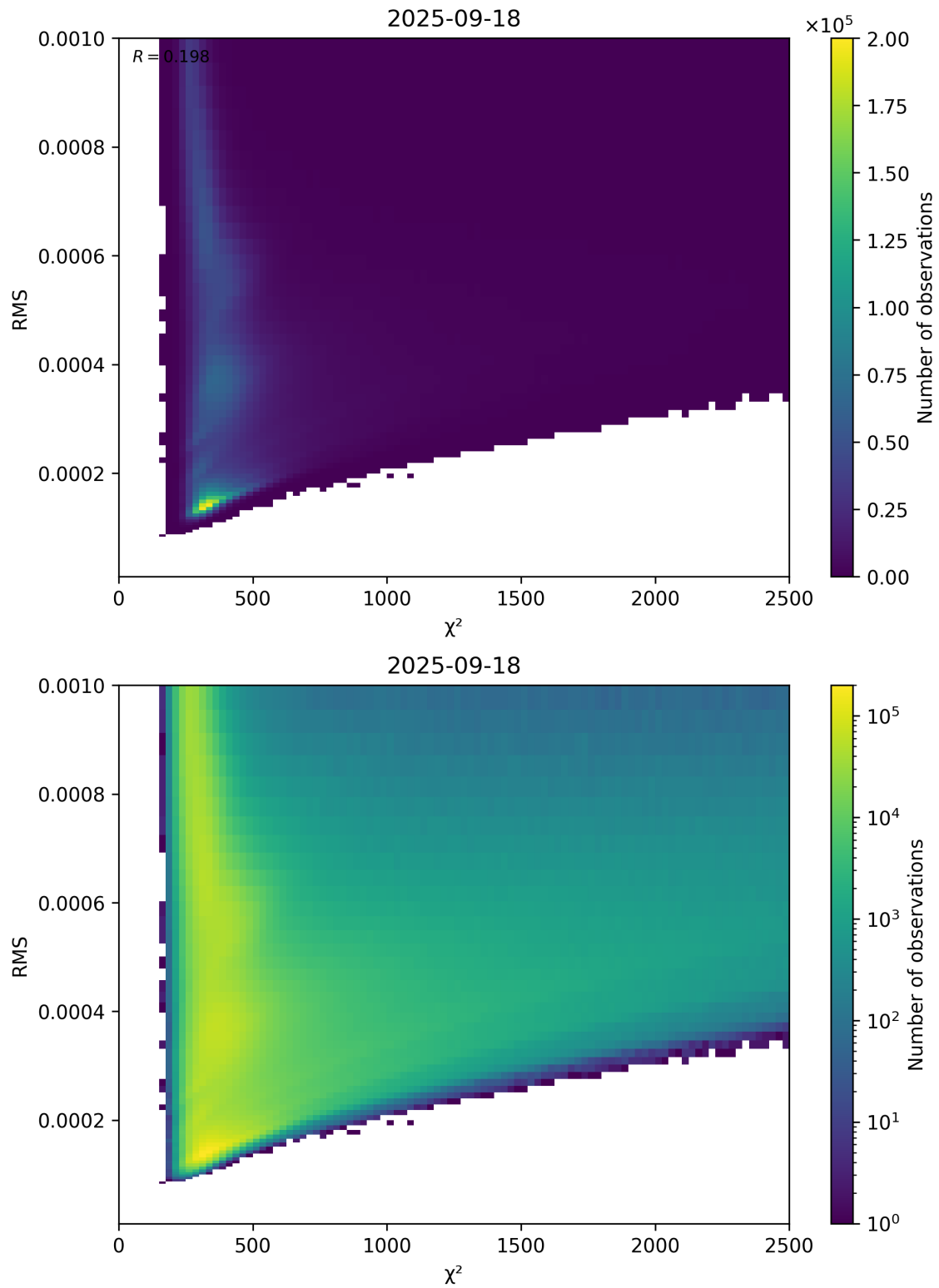
Figure 82: Scatter density plot of “ \chi^2 ” against “RMS” for 2025-09-17 to 2025-09-19.
