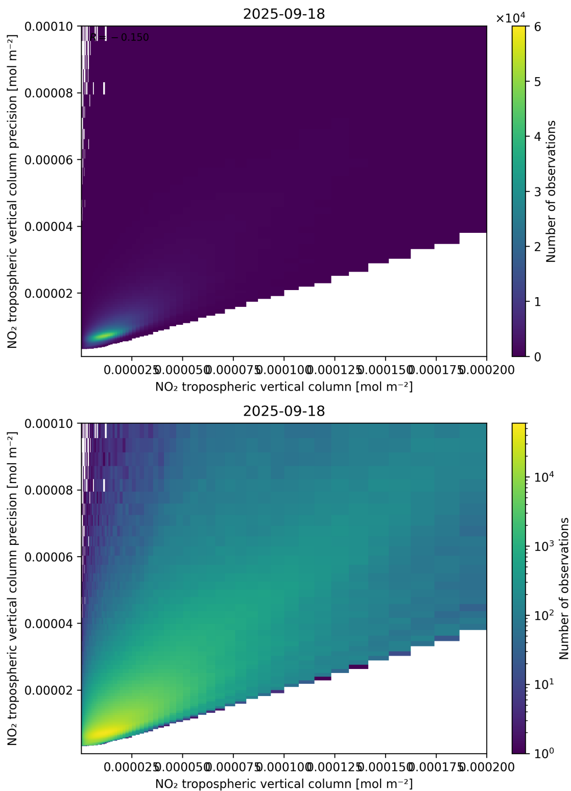
Figure 130: Scatter density plot of “NO 2 tropospheric vertical column” against “NO 2 tropospheric vertical column precision” for 2025-09-17 to 2025-09-19.
