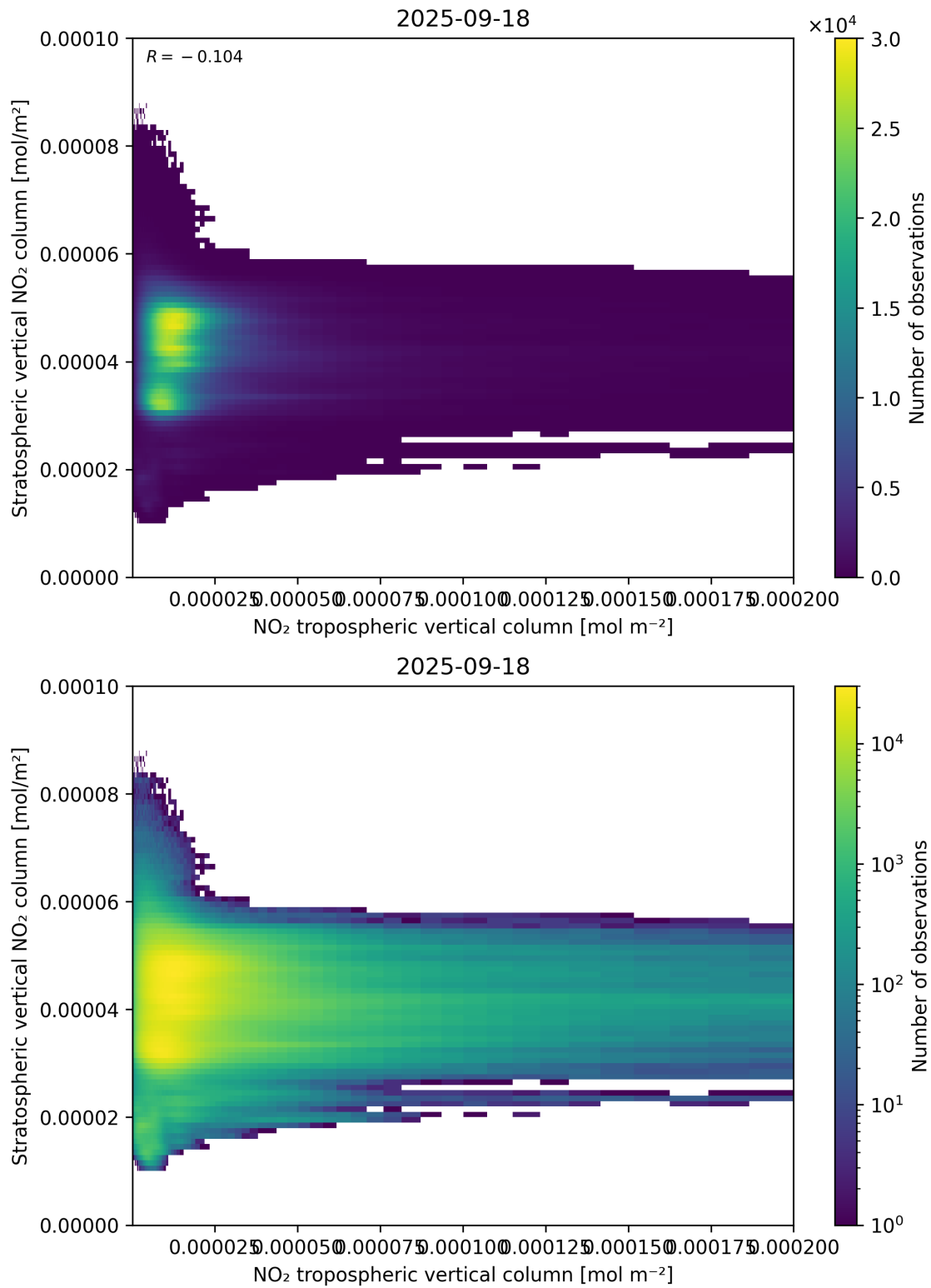
Figure 125: Scatter density plot of “NO 2 tropospheric vertical column” against “Stratospheric vertical NO 2 column” for 2025-09-17 to 2025-09-19.
