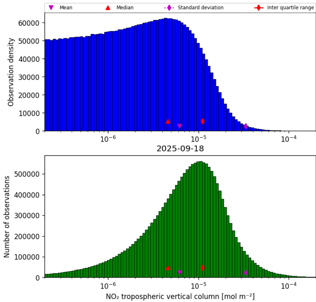
Figure 29: Histogram of “NO 2 tropospheric vertical column” for 2025-09-17 to 2025-09-19
