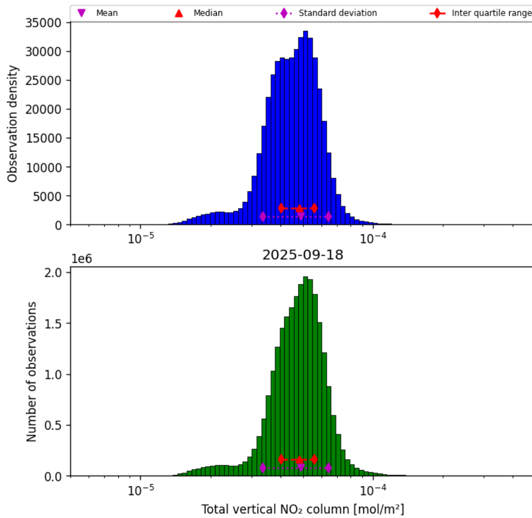
Figure 38: Histogram of “Total vertical NO 2 column” for 2025-09-17 to 2025-09-19
