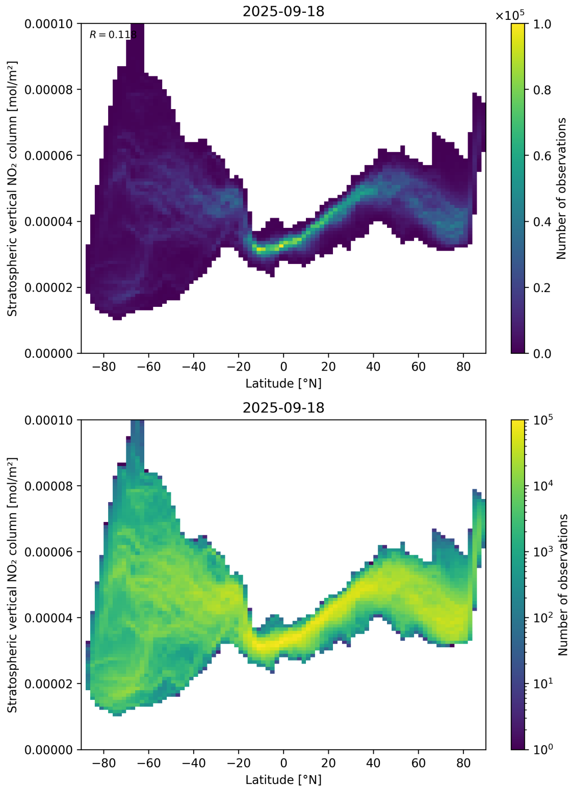
Figure 87: Scatter density plot of “Latitude” against “Stratospheric vertical NO 2 column” for 2025-09-17 to 2025-09-19.
