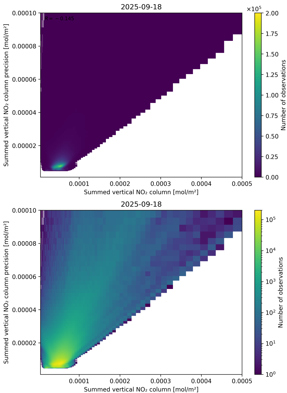
Figure 105: Scatter density plot of “Summed vertical NO 2 column” against “Summed vertical NO 2 column precision” for 2025-09-17 to 2025-09-19.
