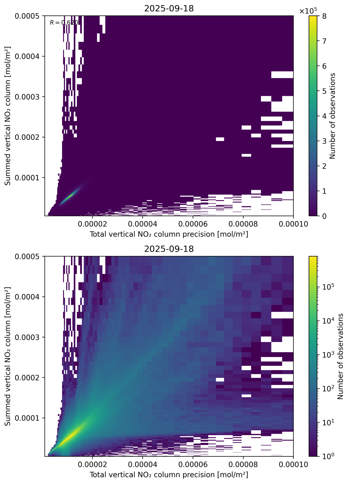
Figure 117: Scatter density plot of “Total vertical NO 2 column precision” against “Summed vertical NO 2 column” for 2025-09-17 to 2025-09-19.
