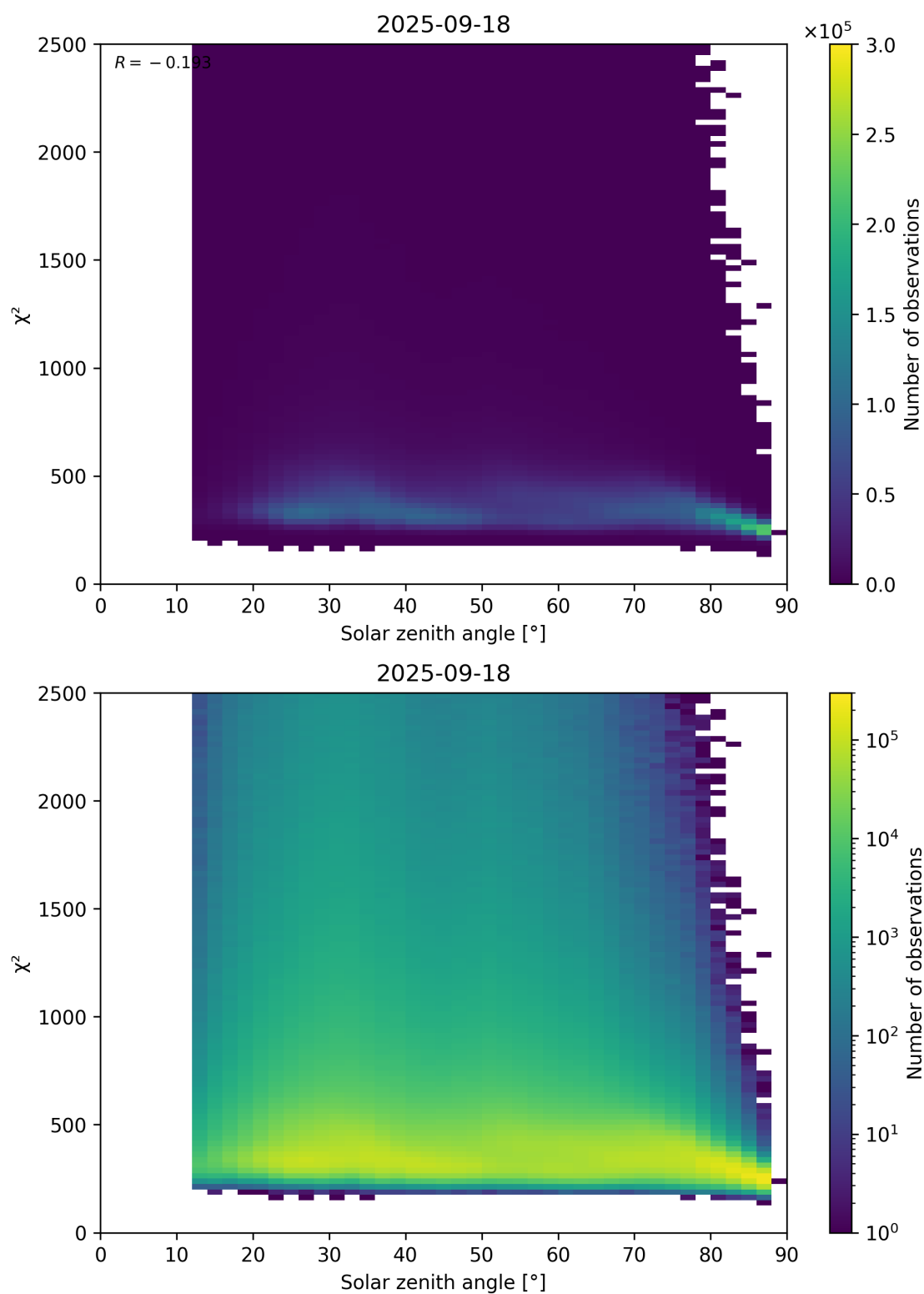
Figure 148: Scatter density plot of “Solar zenith angle” against “ \chi^2 ” for 2025-09-17 to 2025-09-19.
