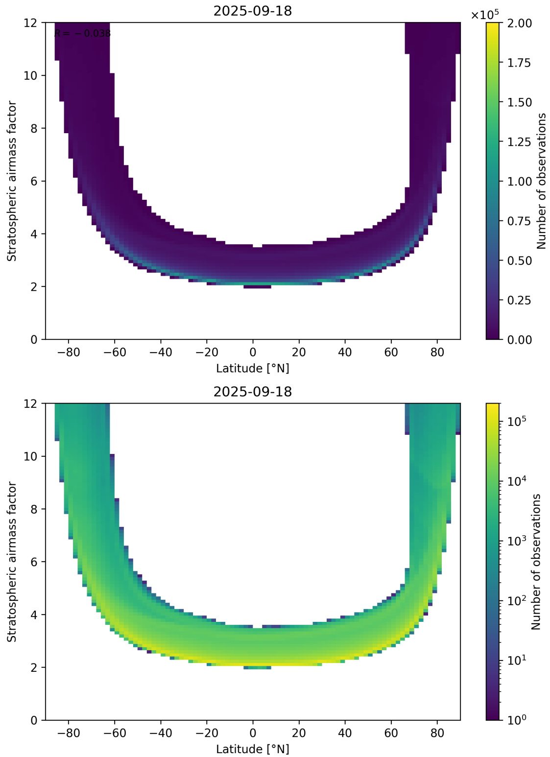
Figure 83: Scatter density plot of “Latitude” against “Stratospheric air mass factor” for 2025-09-17 to 2025-09-19.
