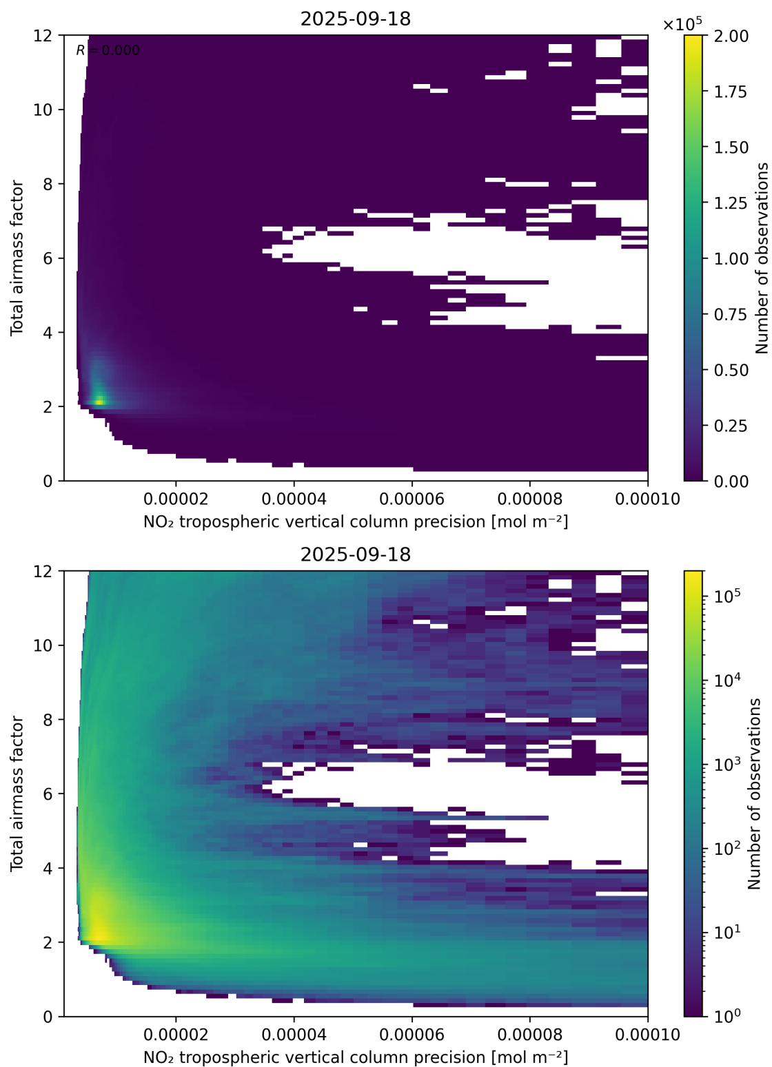
Figure 132: Scatter density plot of “NO 2 tropospheric vertical column precision” against “Total air mass factor” for 2025-09-17 to 2025-09-19.
