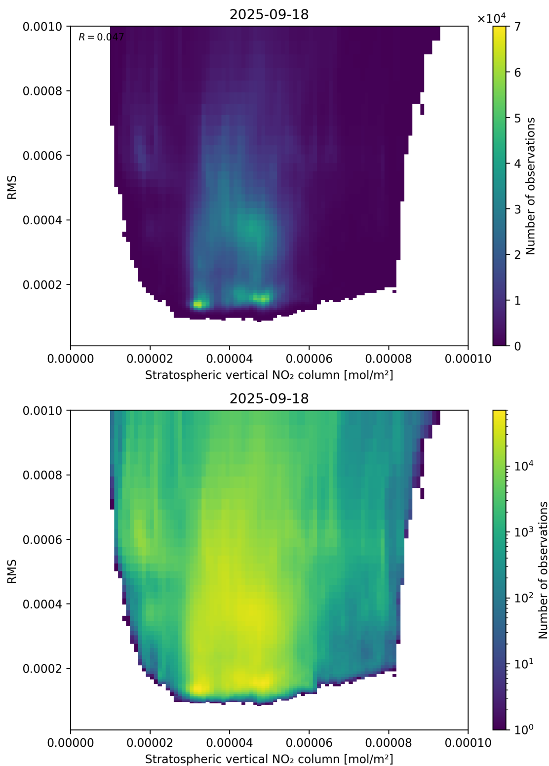
Figure 102: Scatter density plot of “Stratospheric vertical NO 2 column” against “RMS” for 2025-09-17 to 2025-09-19.
