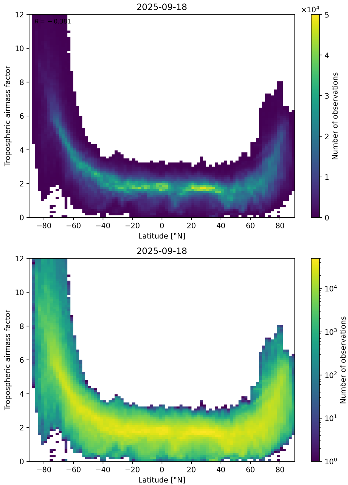
Figure 85: Scatter density plot of “Latitude” against “Tropospheric airmass factor” for 2025-09-17 to 2025-09-19.
