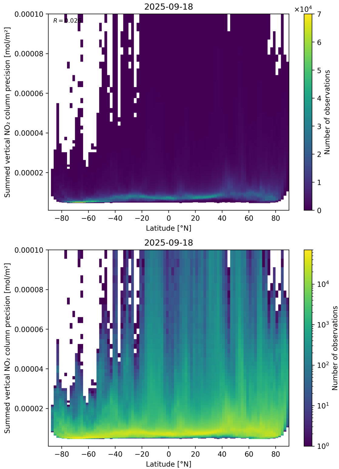
Figure 89: Scatter density plot of “Latitude” against “Summed vertical NO 2 column precision” for 2025-09-17 to 2025-09-19.
