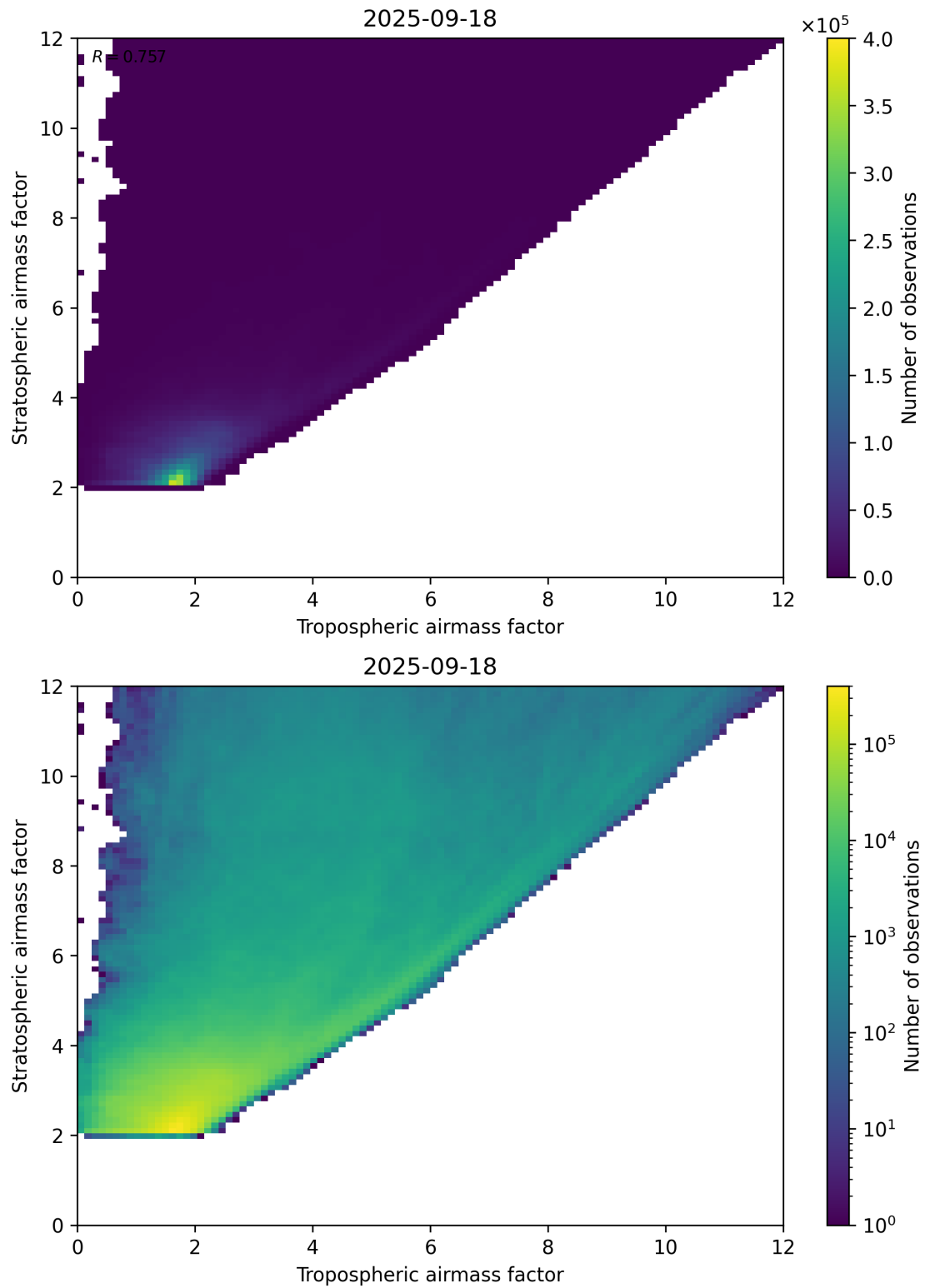
Figure 71: Scatter density plot of “Tropospheric airmass factor” against “Stratospheric airmass factor” for 2025-09-17 to 2025-09-19.
