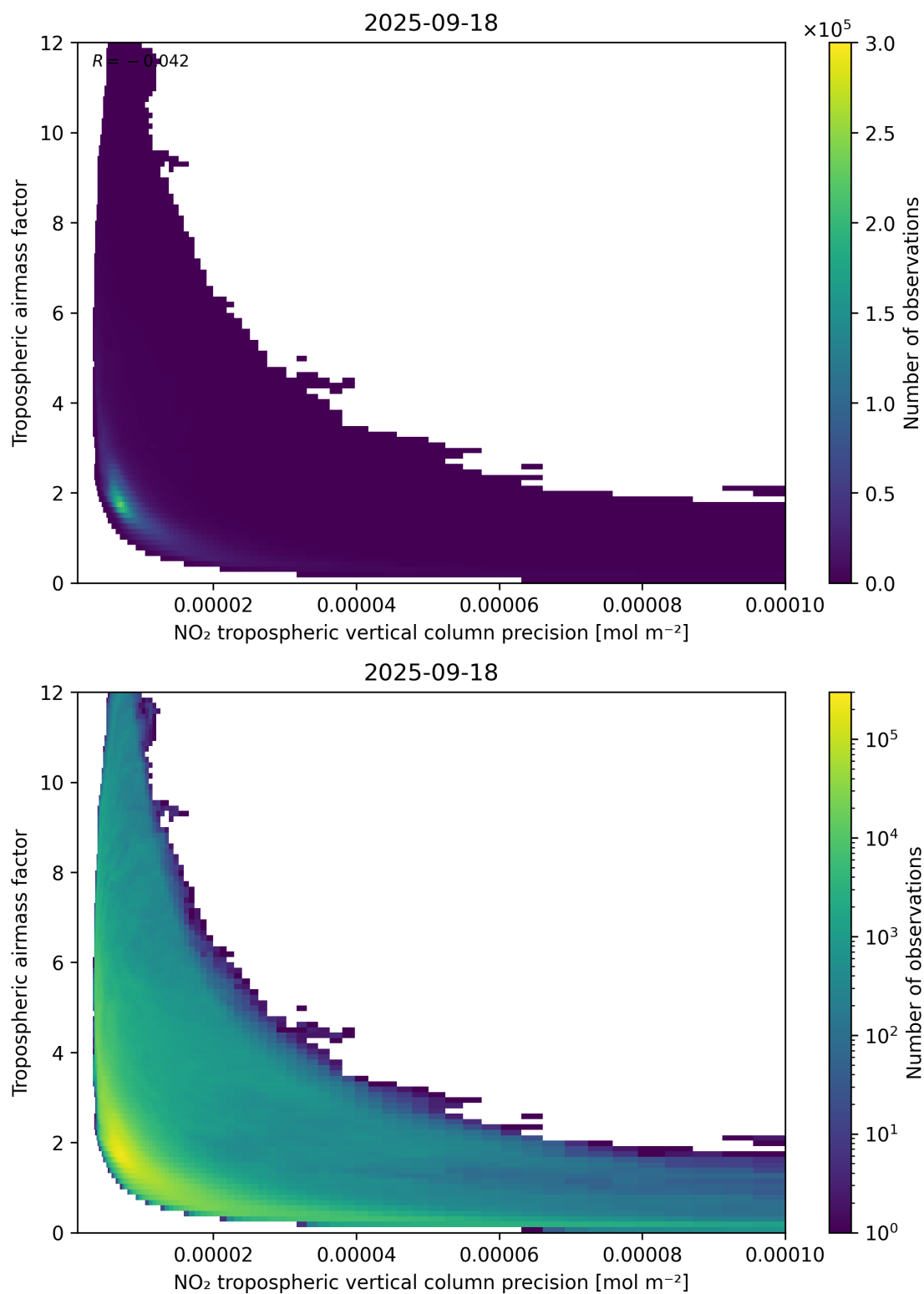
Figure 133: Scatter density plot of “NO 2 tropospheric vertical column precision” against “Tropospheric air mass factor” for 2025-09-17 to 2025-09-19.
