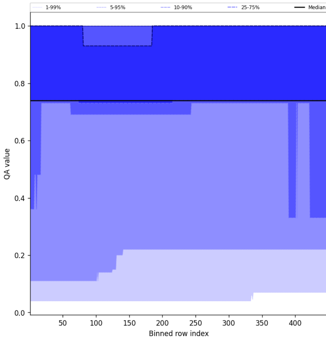
Figure 45: Along track statistics of "QA value" for 2025-09-17 to 2025-09-19
