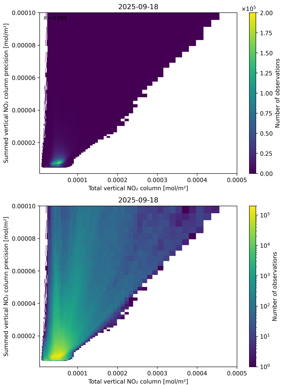
Figure 113: Scatter density plot of “Total vertical NO 2 column” against “Summed vertical NO 2 column precision” for 2025-09-17 to 2025-09-19.
