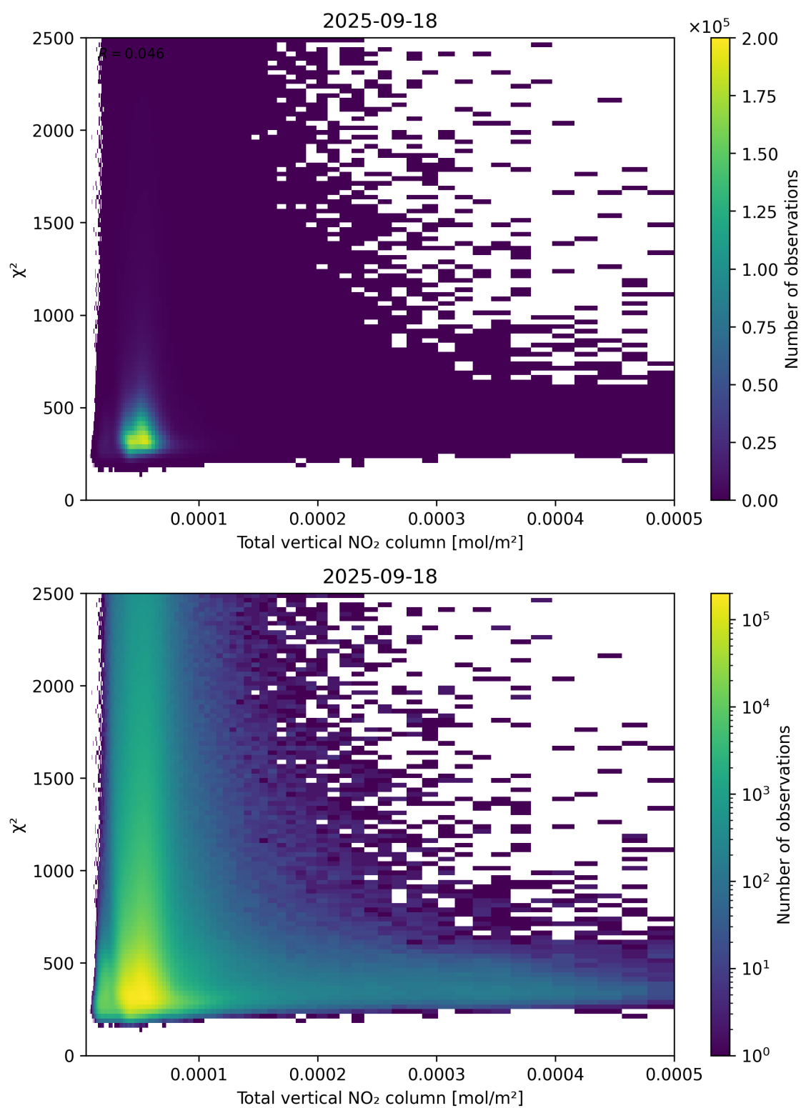
Figure 111: Scatter density plot of “Total vertical NO 2 column” against “ \chi^2 ” for 2025-09-17 to 2025-09-19.
