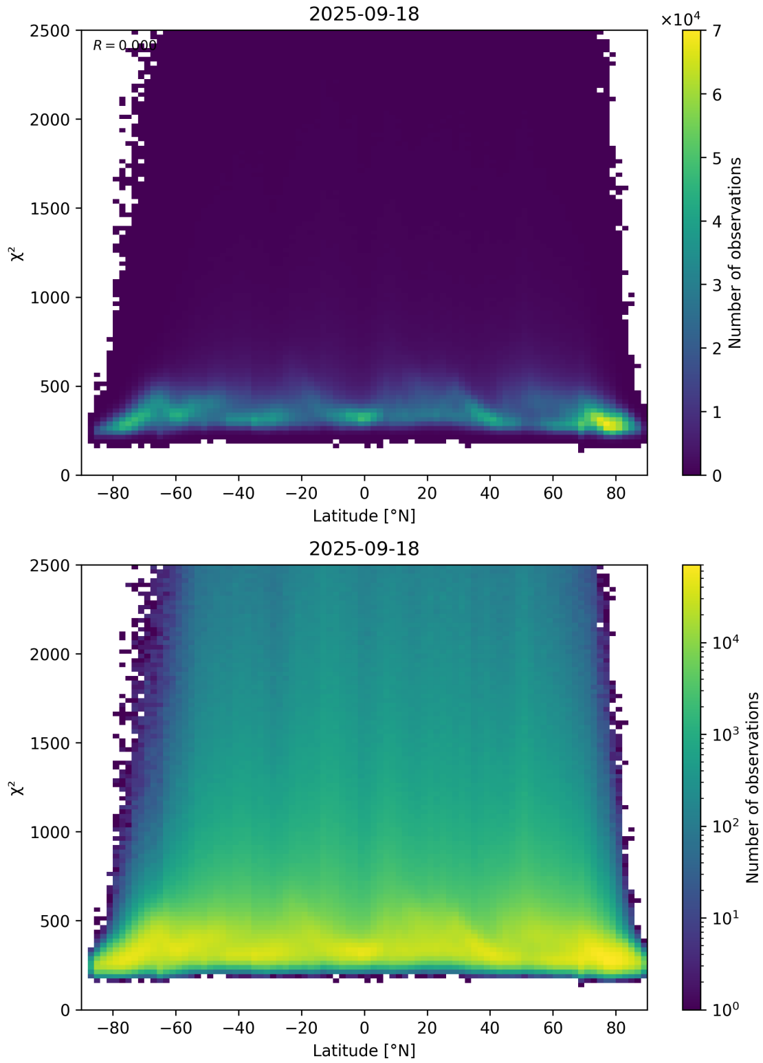
Figure 86: Scatter density plot of “Latitude” against “ \chi^2 ” for 2025-09-17 to 2025-09-19.
