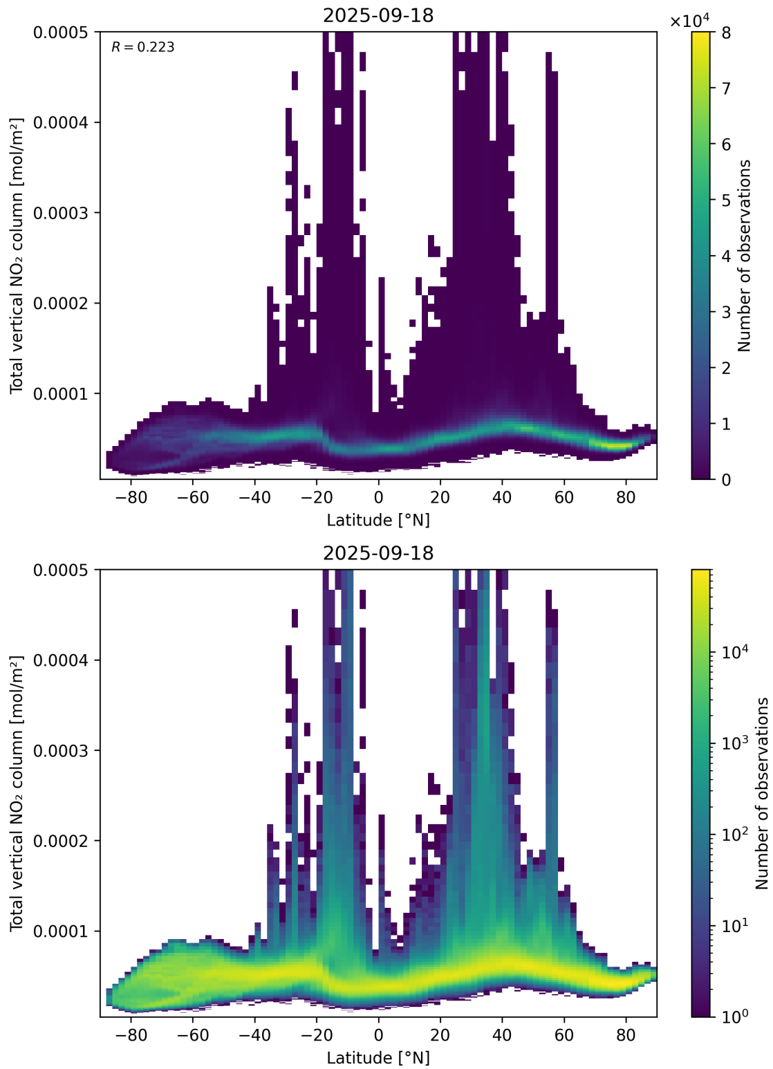
Figure 90: Scatter density plot of “Latitude” against “Total vertical NO 2 column” for 2025-09-17 to 2025-09-19.
