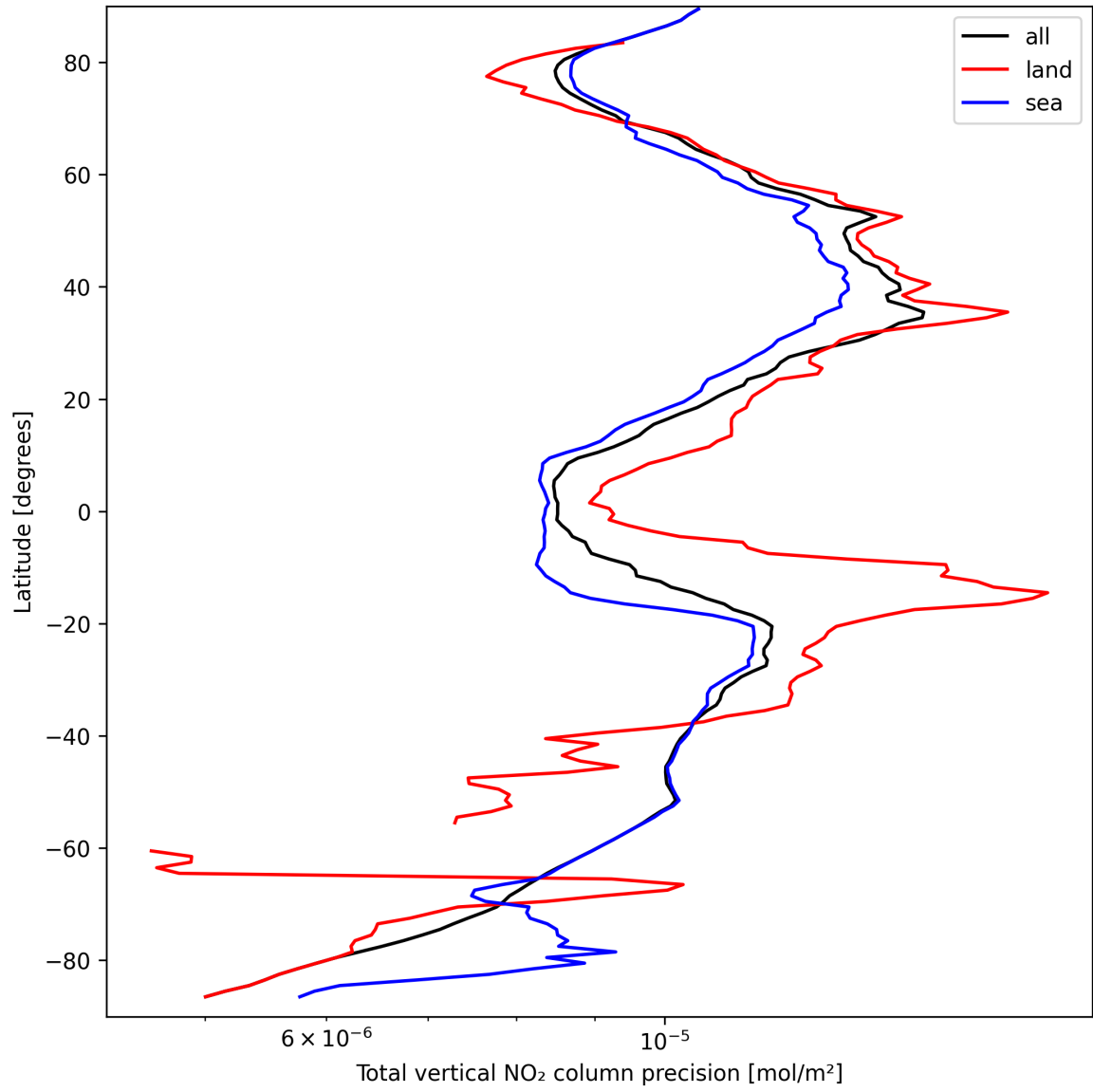
Figure 22: Zonal average of “Total vertical NO 2 column precision” for 2025-09-17 to 2025-09-19.
