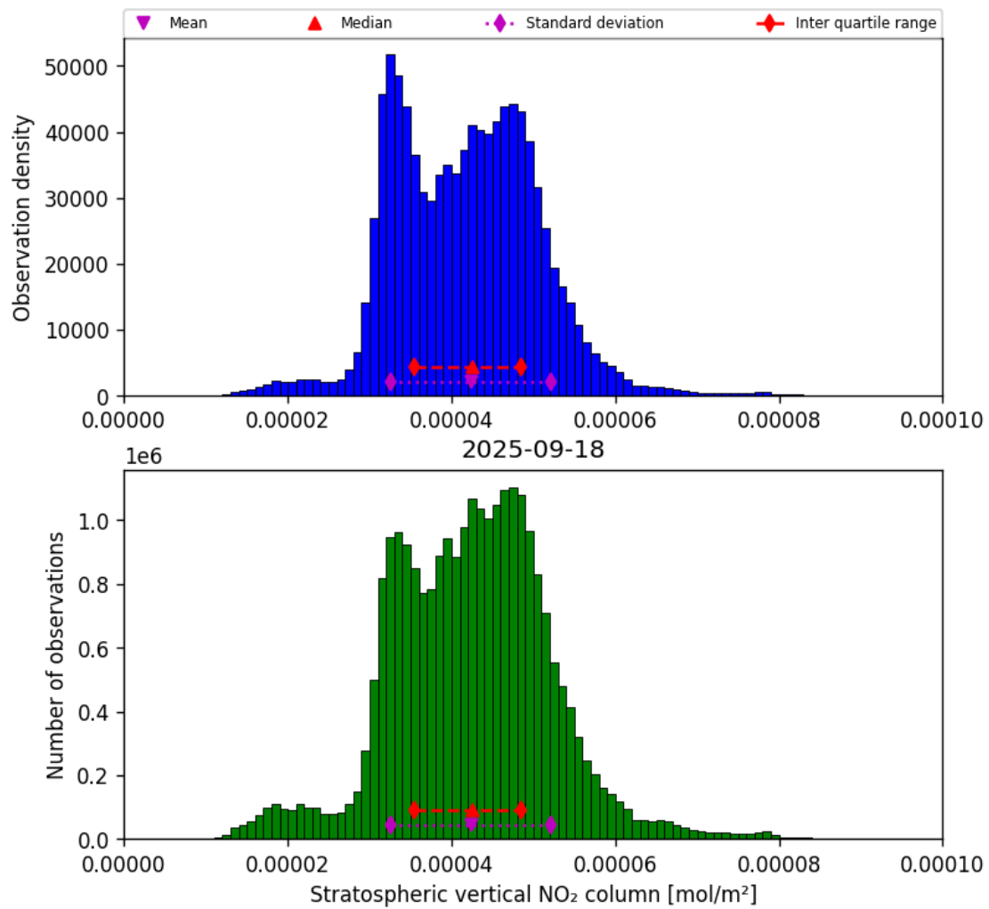
Figure 36: Histogram of “Stratospheric vertical NO 2 column” for 2025-09-17 to 2025-09-19
