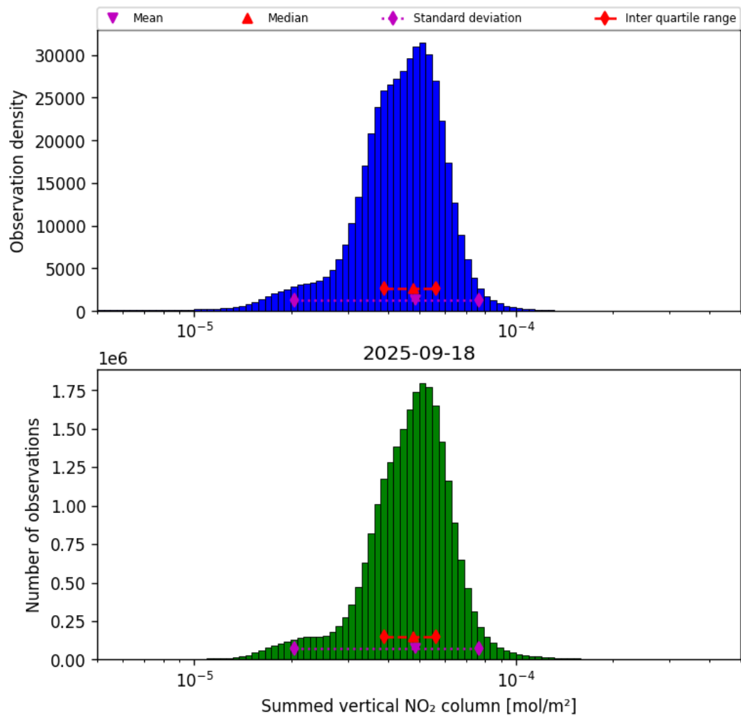
Figure 40: Histogram of “Summed vertical NO 2 column” for 2025-09-17 to 2025-09-19
