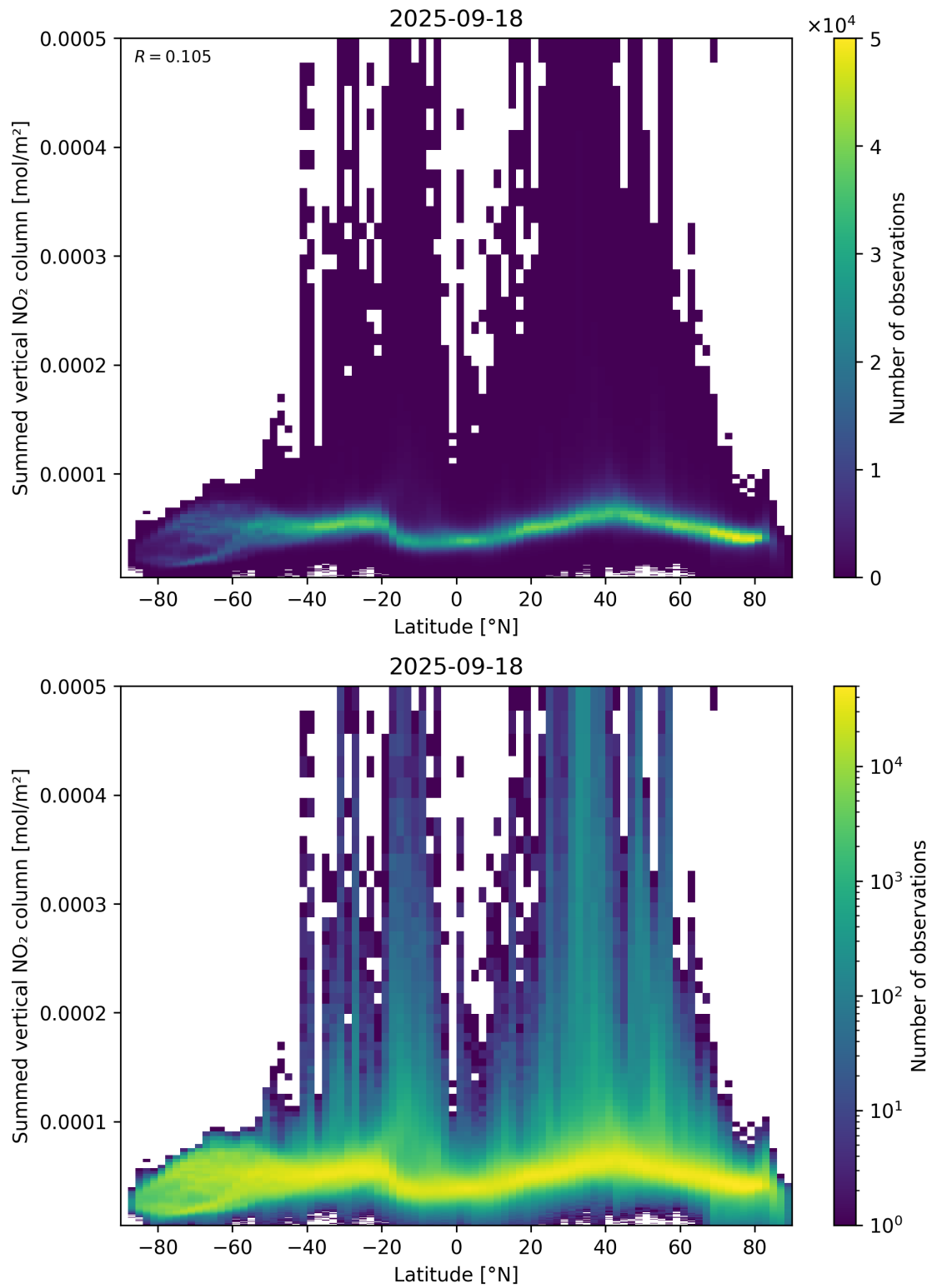
Figure 88: Scatter density plot of “Latitude” against “Summed vertical NO 2 column” for 2025-09-17 to 2025-09-19.
