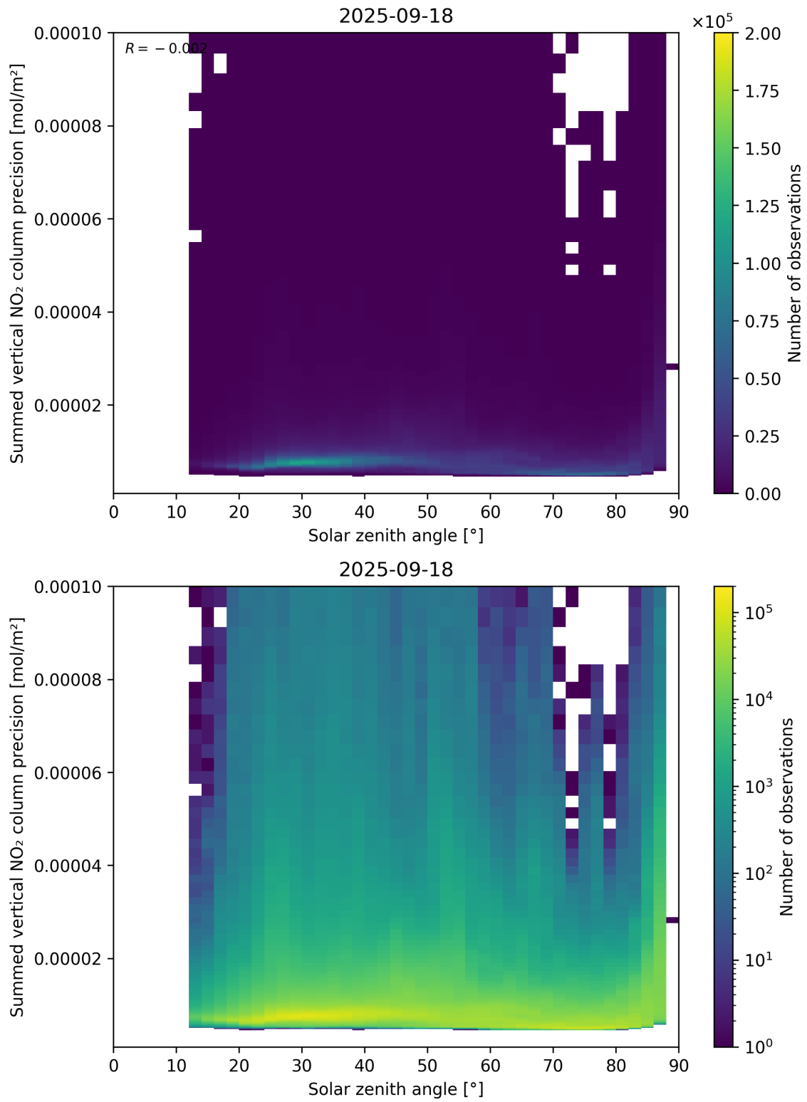
Figure 152: Scatter density plot of “Solar zenith angle” against “Summed vertical NO 2 column precision” for 2025-09-17 to 2025-09-19.
