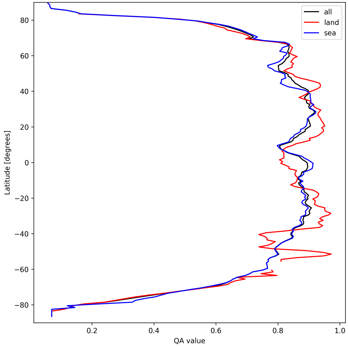
Figure 11: Zonal average of “QA value” for 2025-09-17 to 2025-09-19.
