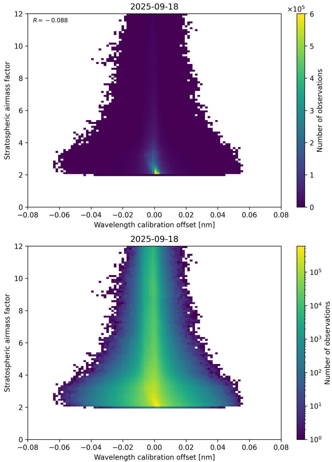
Figure 174: Scatter density plot of “Wavelength calibration offset” against “Stratospheric airmass factor” for 2025-09-17 to 2025-09-19.
