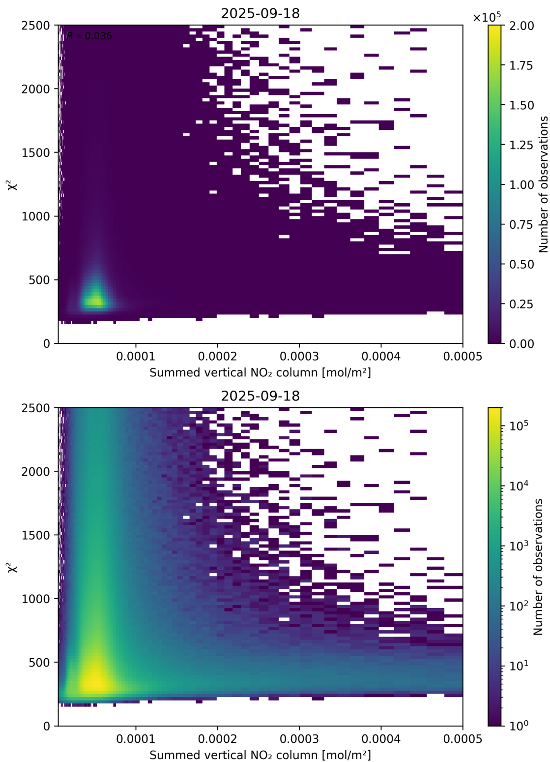
Figure 104: Scatter density plot of “Summed vertical NO 2 column” against “ \chi^2 ” for 2025-09-17 to 2025-09-19.
