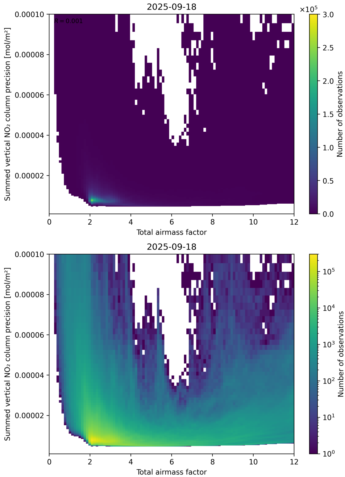
Figure 66: Scatter density plot of “Total airmass factor” against “Summed vertical NO 2 column precision” for 2025-09-17 to 2025-09-19.
