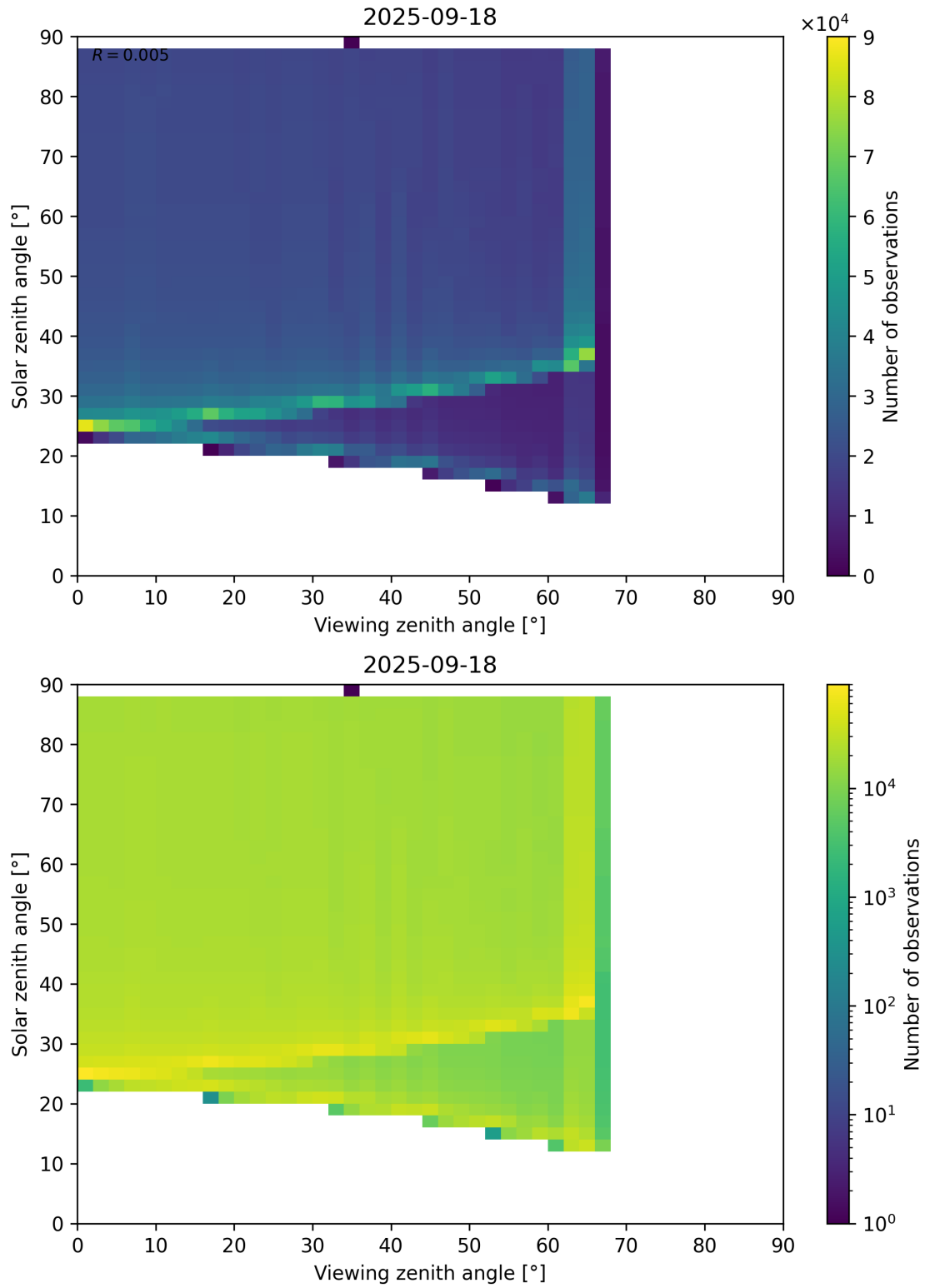
Figure 172: Scatter density plot of “Viewing zenith angle” against “Solar zenith angle” for 2025-09-17 to 2025-09-19.
