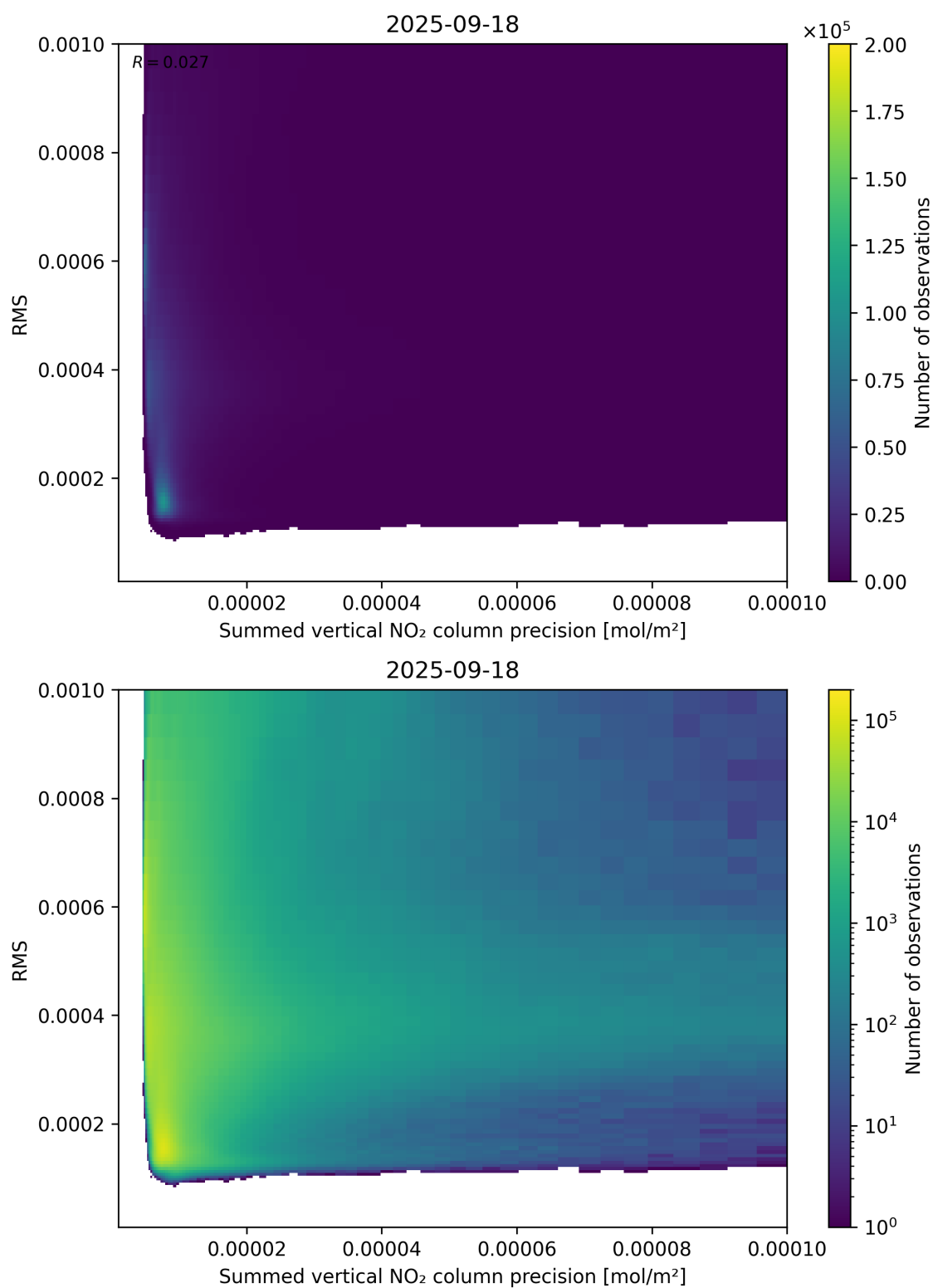
Figure 108: Scatter density plot of “Summed vertical NO 2 column precision” against “RMS” for 2025-09-17 to 2025-09-19.
