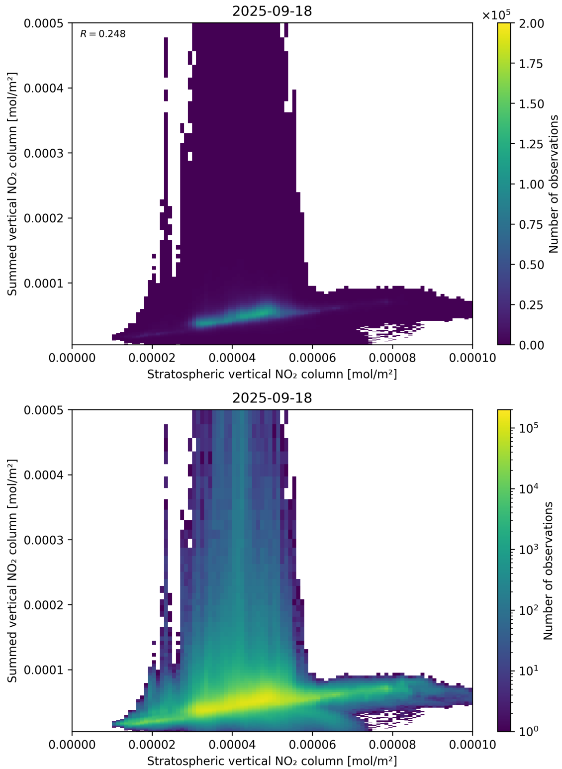
Figure 98: Scatter density plot of “Stratospheric vertical NO 2 column” against “Summed vertical NO 2 column” for 2025-09-17 to 2025-09-19.
