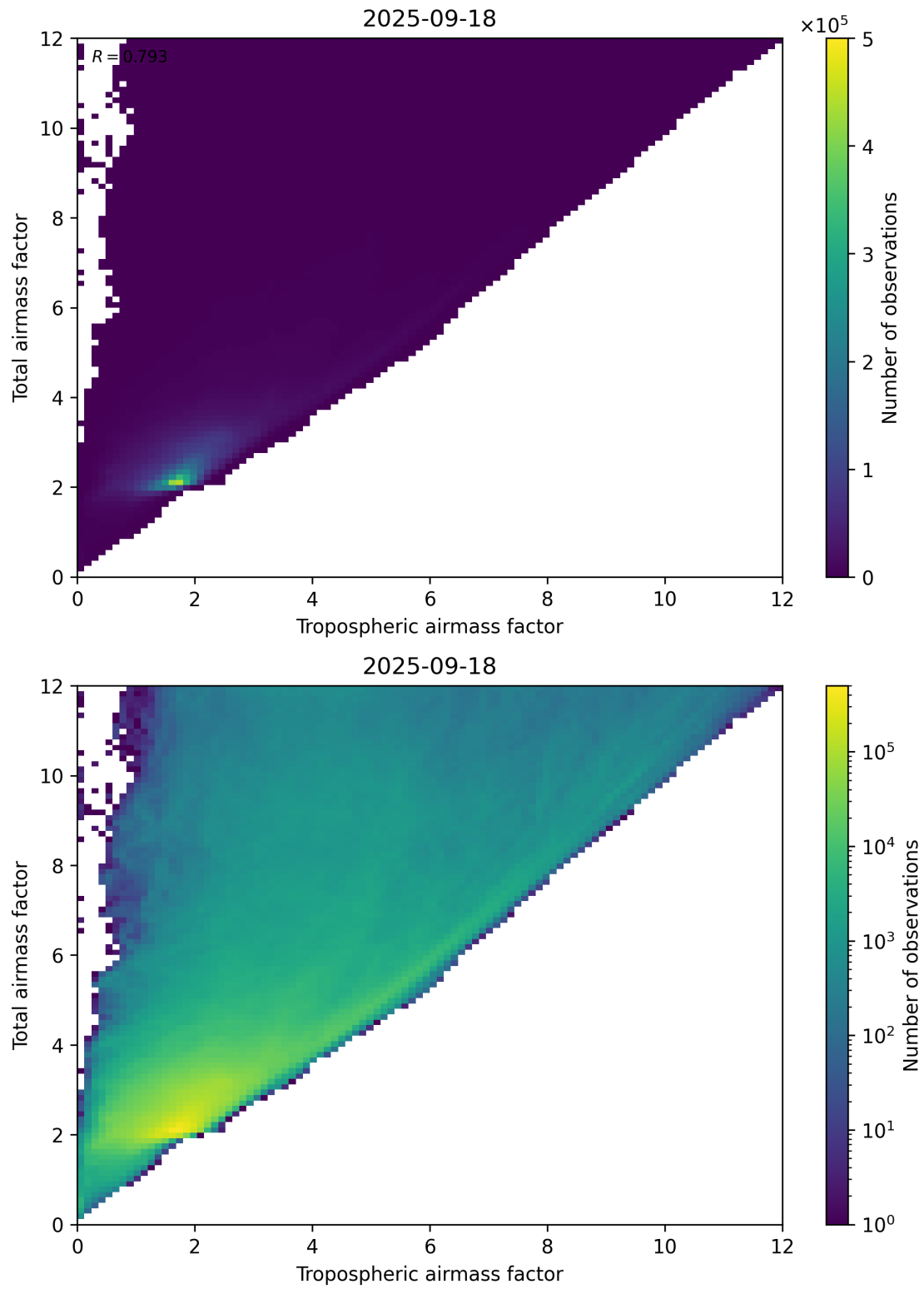
Figure 72: Scatter density plot of “Tropospheric airmass factor” against “Total airmass factor” for 2025-09-17 to 2025-09-19.
