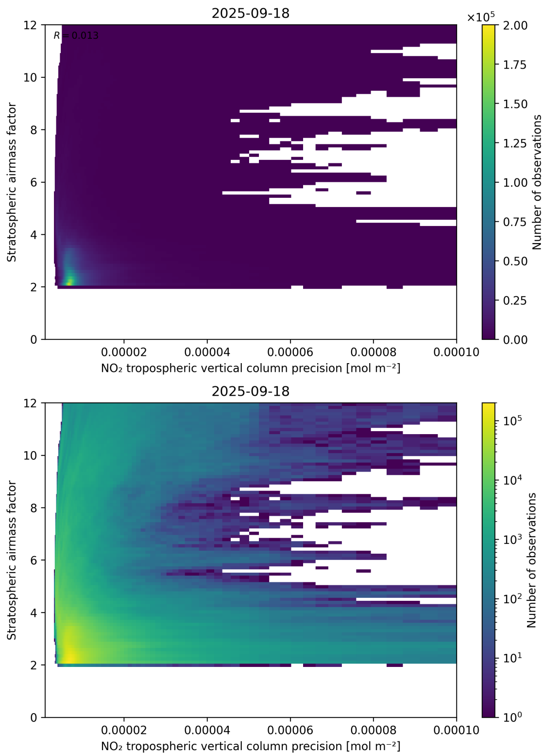
Figure 131: Scatter density plot of “NO 2 tropospheric vertical column precision” against “Stratospheric airmass factor” for 2025-09-17 to 2025-09-19.
