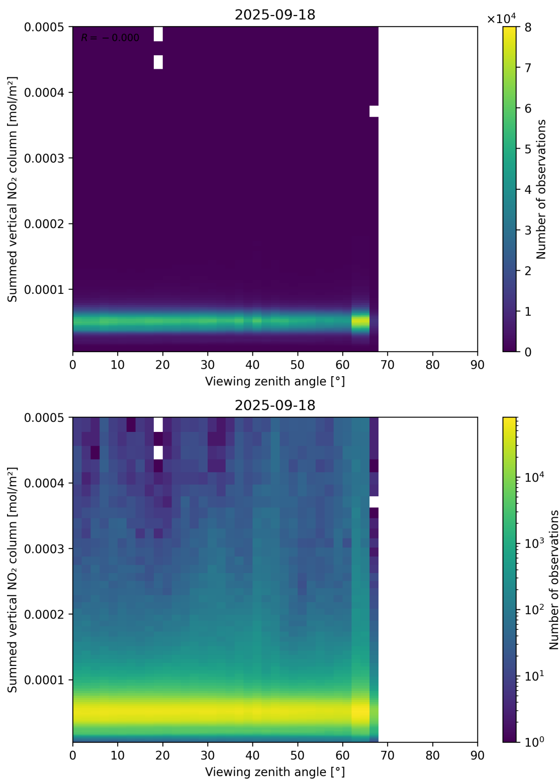
Figure 165: Scatter density plot of “Viewing zenith angle” against “Summed vertical NO 2 column” for 2025-09-17 to 2025-09-19.
