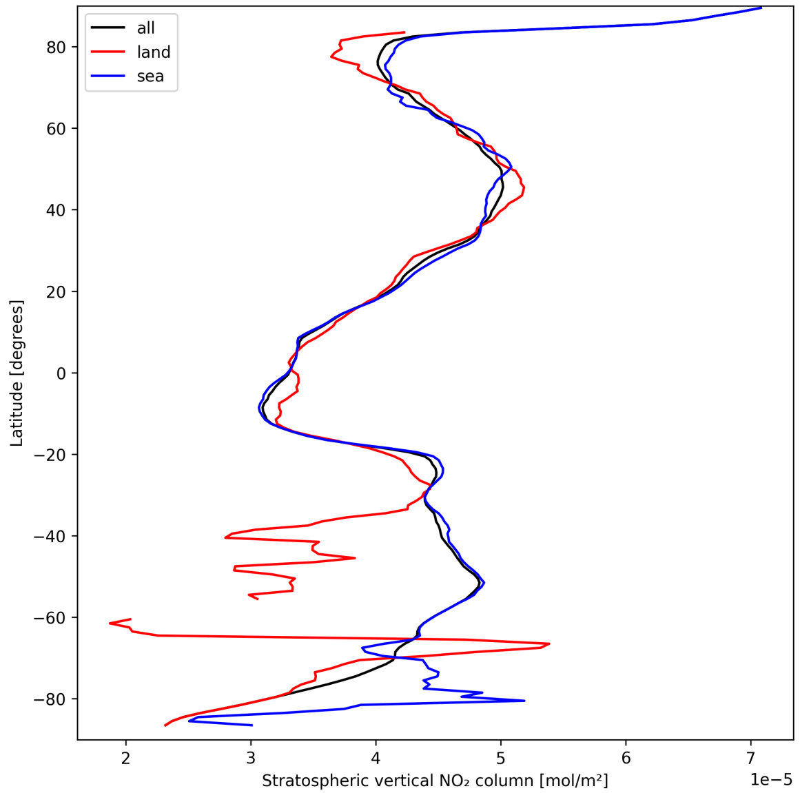
Figure 19: Zonal average of “Stratospheric vertical NO 2 column” for 2025-09-17 to 2025-09-19.
