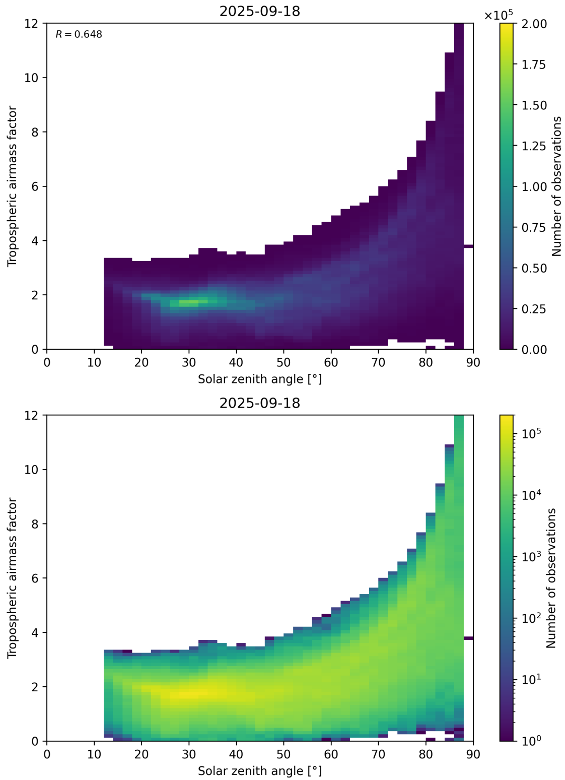
Figure 147: Scatter density plot of “Solar zenith angle” against “Tropospheric airmass factor” for 2025-09-17 to 2025-09-19.
