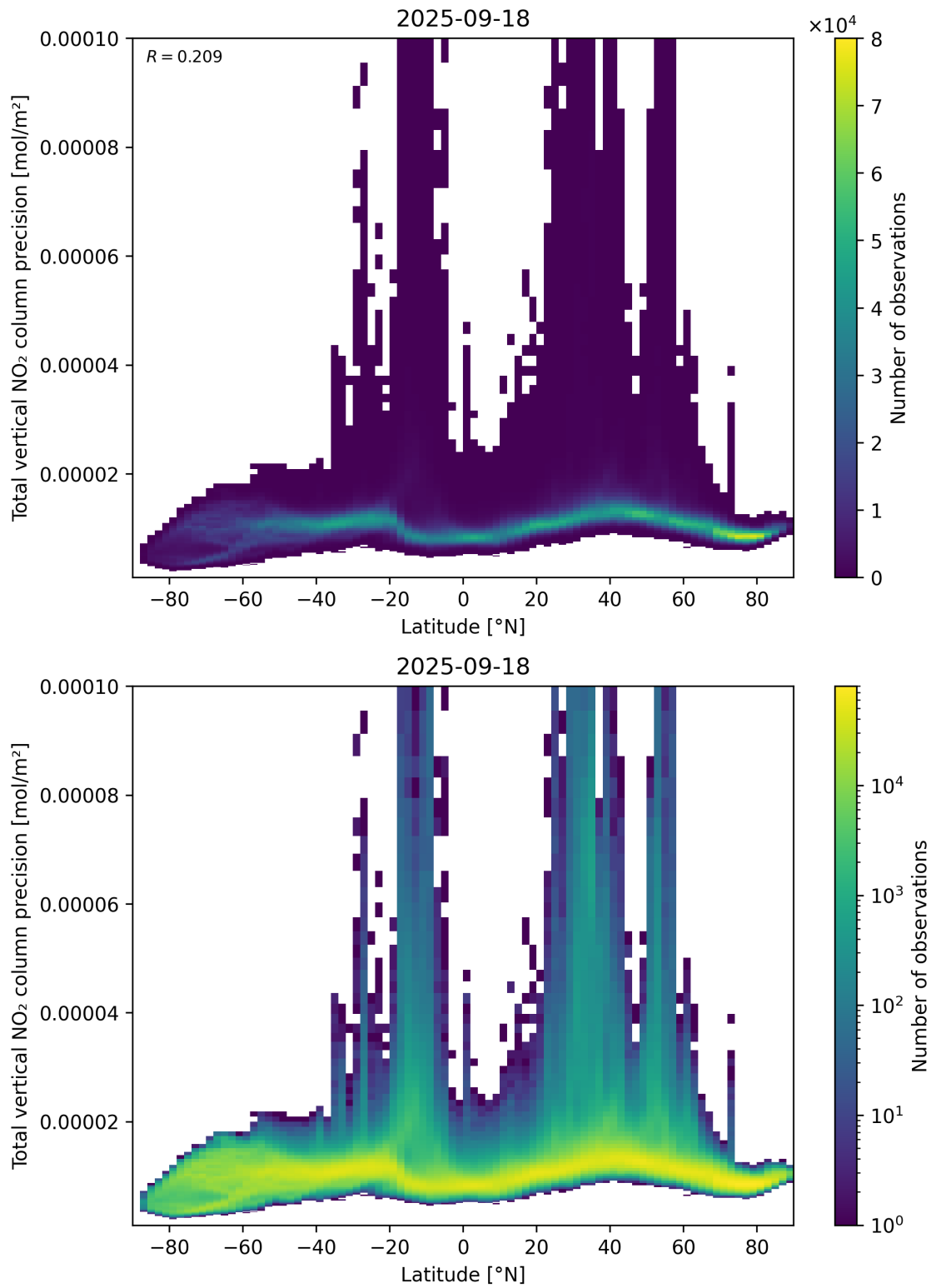
Figure 91: Scatter density plot of “Latitude” against “Total vertical NO 2 column precision” for 2025-09-17 to 2025-09-19.
