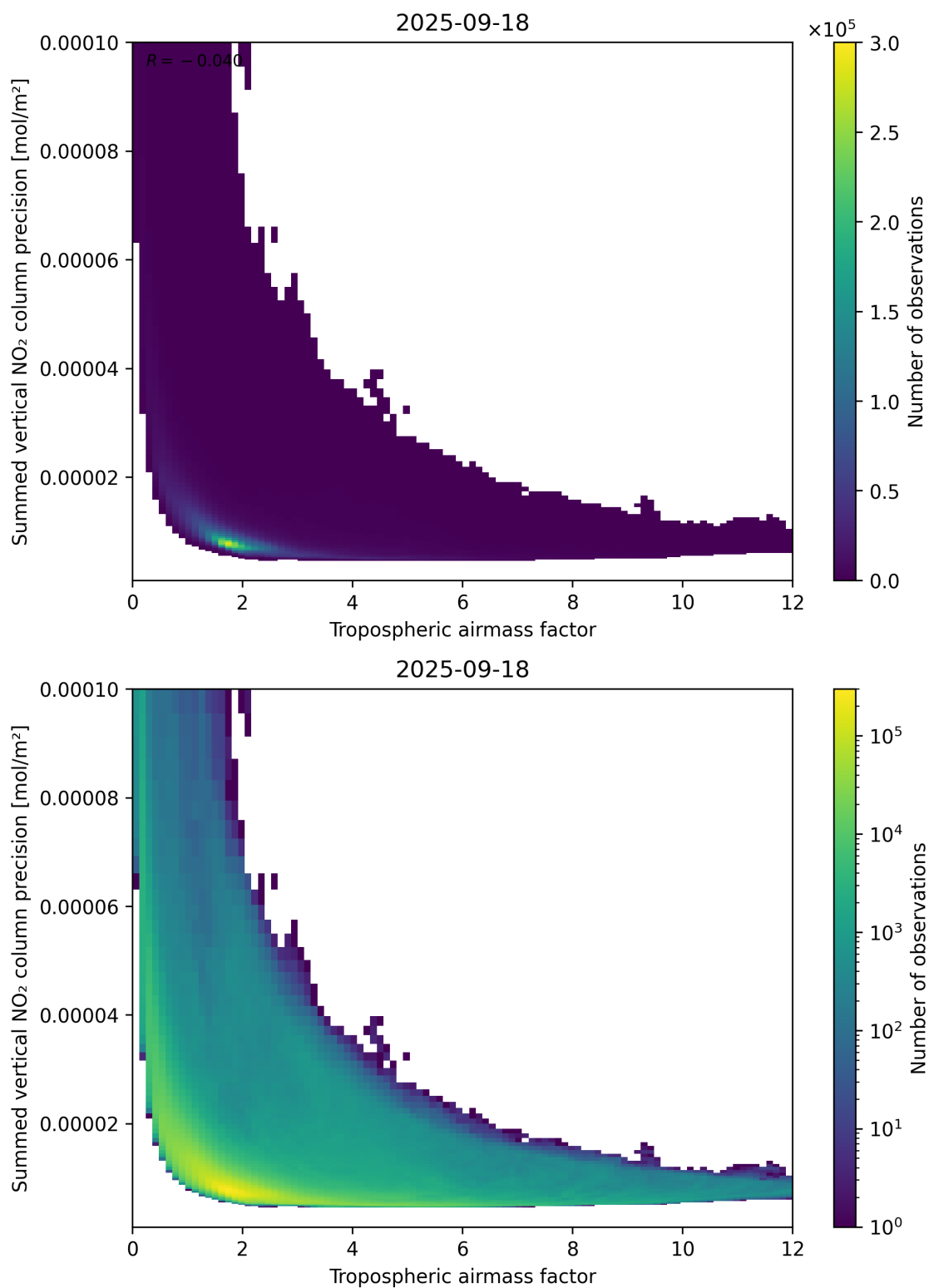
Figure 76: Scatter density plot of “Tropospheric air mass factor” against “Summed vertical NO 2 column precision” for 2025-09-17 to 2025-09-19.
