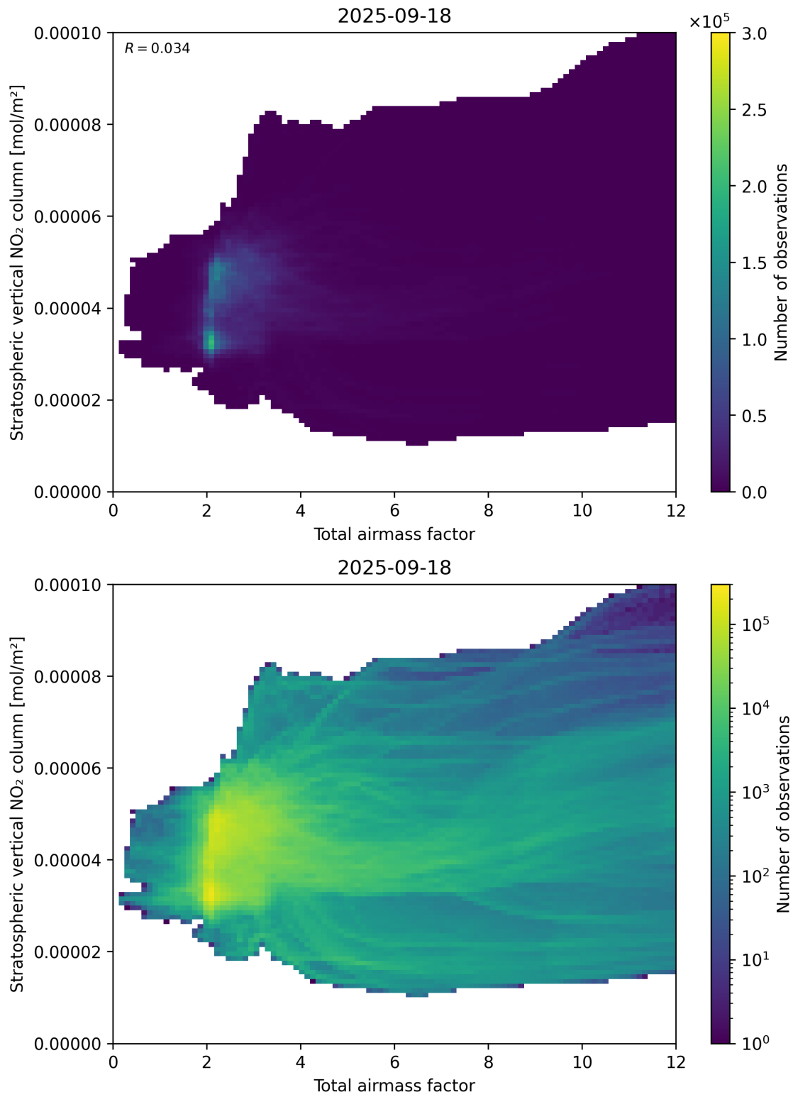
Figure 64: Scatter density plot of “Total airmass factor” against “Stratospheric vertical \text{NO}_2 column” for 2025-09-17 to 2025-09-19.
