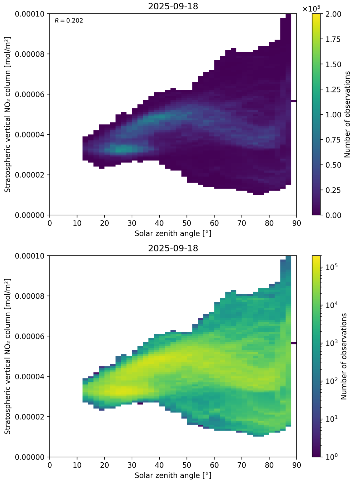
Figure 150: Scatter density plot of “Solar zenith angle” against “Stratospheric vertical NO 2 column” for 2025-09-17 to 2025-09-19.
