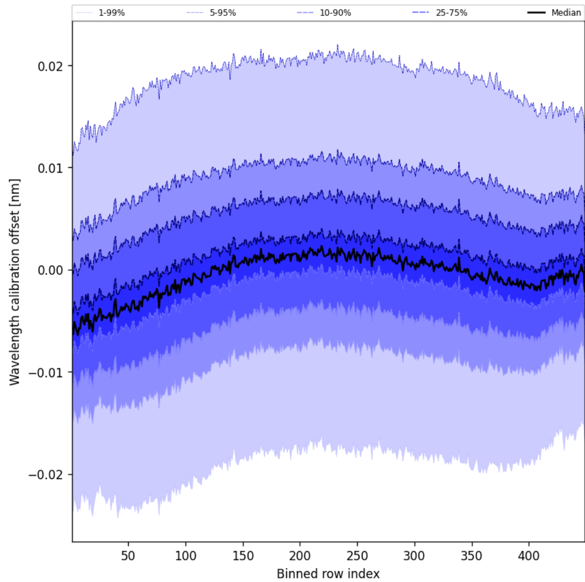
Figure 52: Along track statistics of “Wavelength calibration offset” for 2025-09-17 to 2025-09-19
