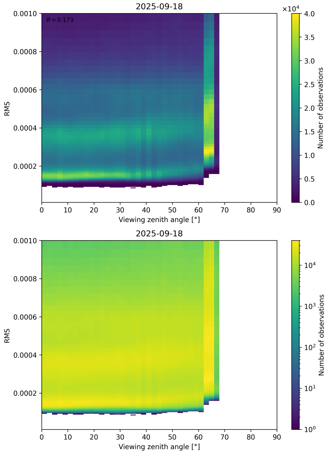
Figure 171: Scatter density plot of “Viewing zenith angle” against “RMS” for 2025-09-17 to 2025-09-19.
