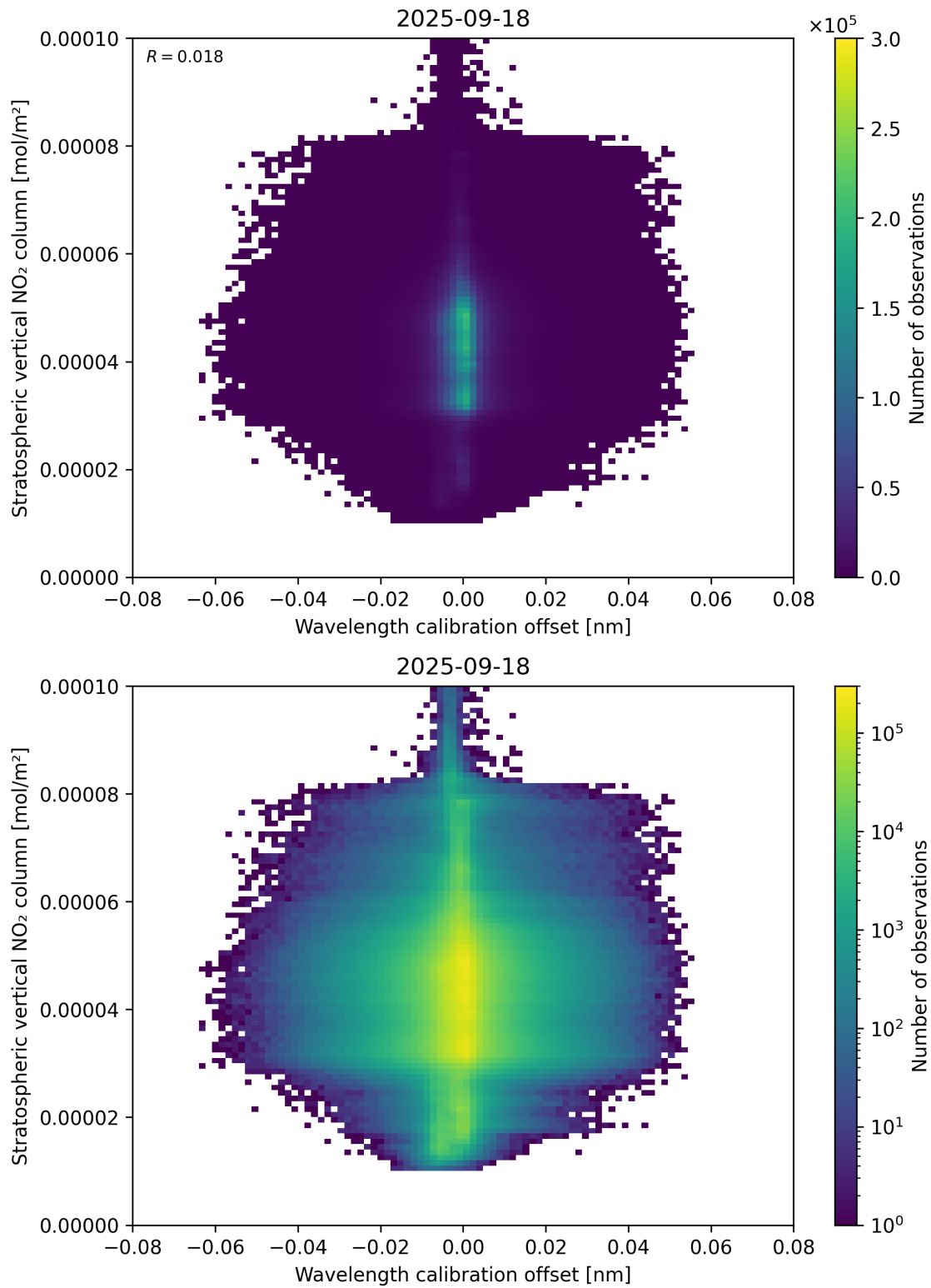
Figure 176: Scatter density plot of “Wavelength calibration offset” against “Stratospheric vertical NO 2 column” for 2025-09-17 to 2025-09-19.
