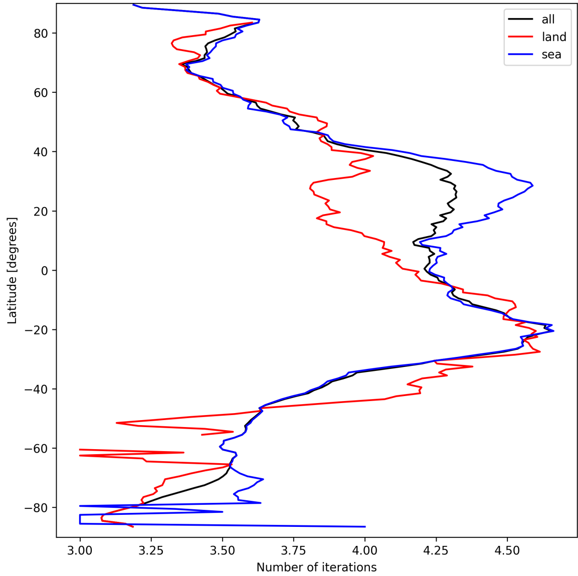
Figure 17: Zonal average of “Number of iterations” for 2025-09-17 to 2025-09-19.
