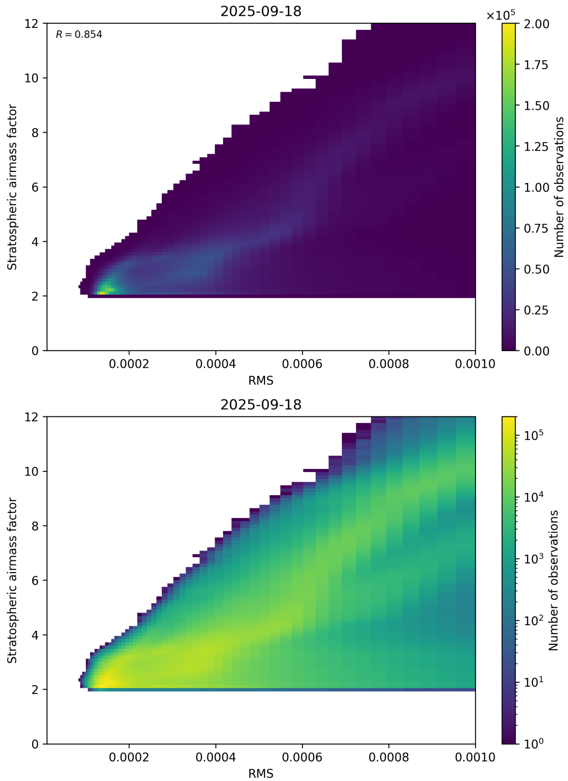
Figure 144: Scatter density plot of “RMS” against “Stratospheric airmass factor” for 2025-09-17 to 2025-09-19.
