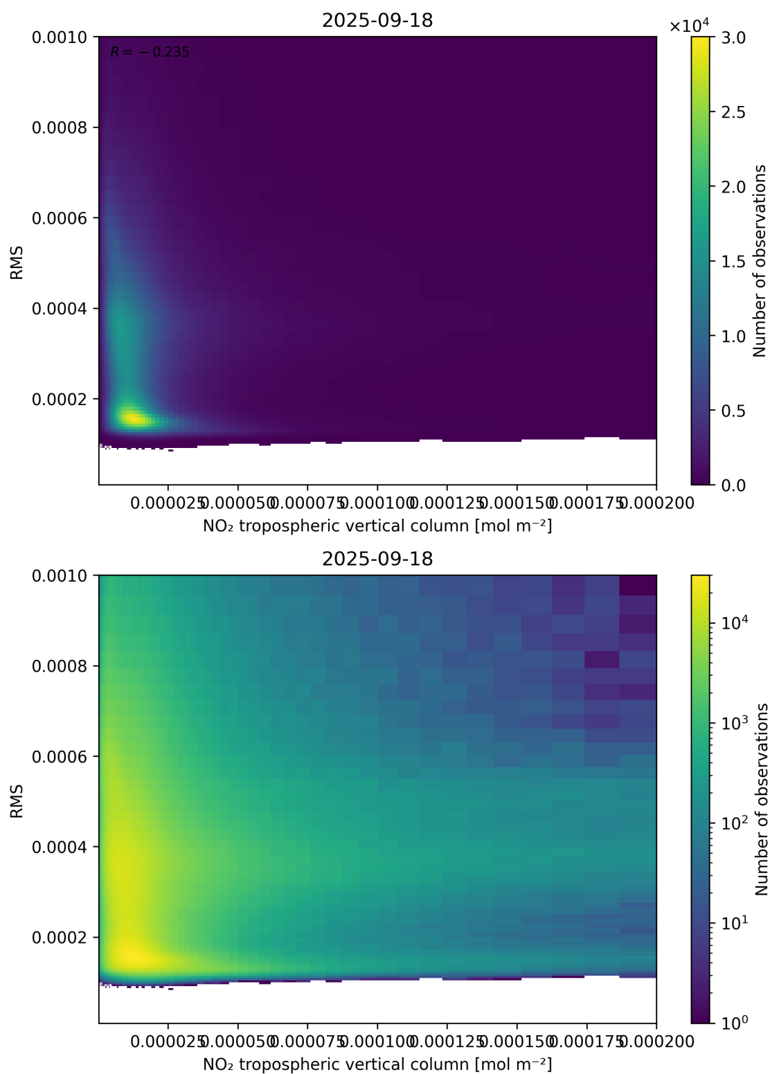
Figure 142: Scatter density plot of “NO 2 tropospheric vertical column” against “RMS” for 2025-09-17 to 2025-09-19.
