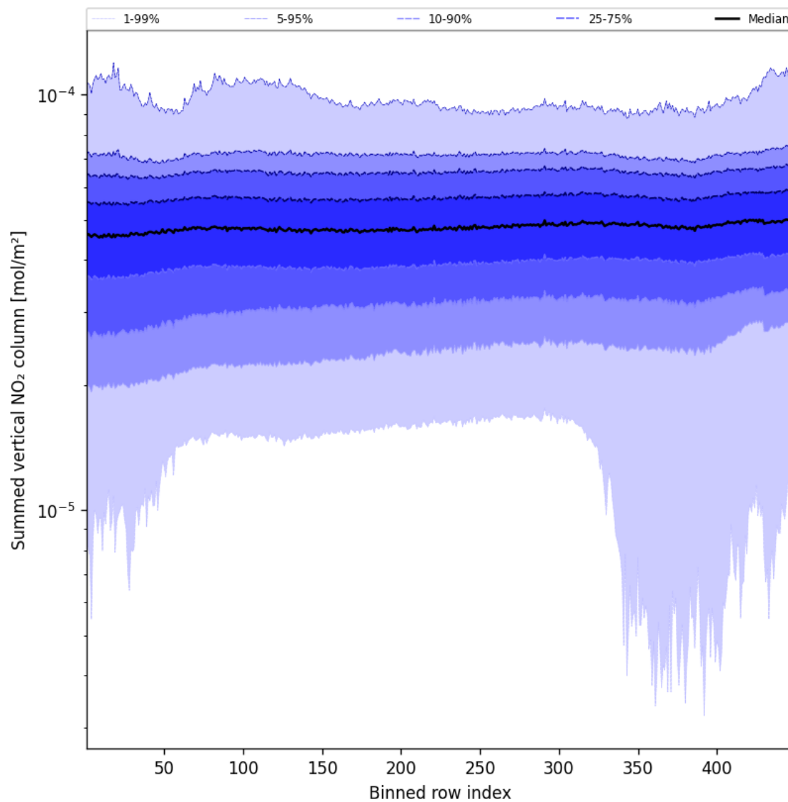
Figure 57: Along track statistics of “Summed vertical NO 2 column” for 2025-09-17 to 2025-09-19
