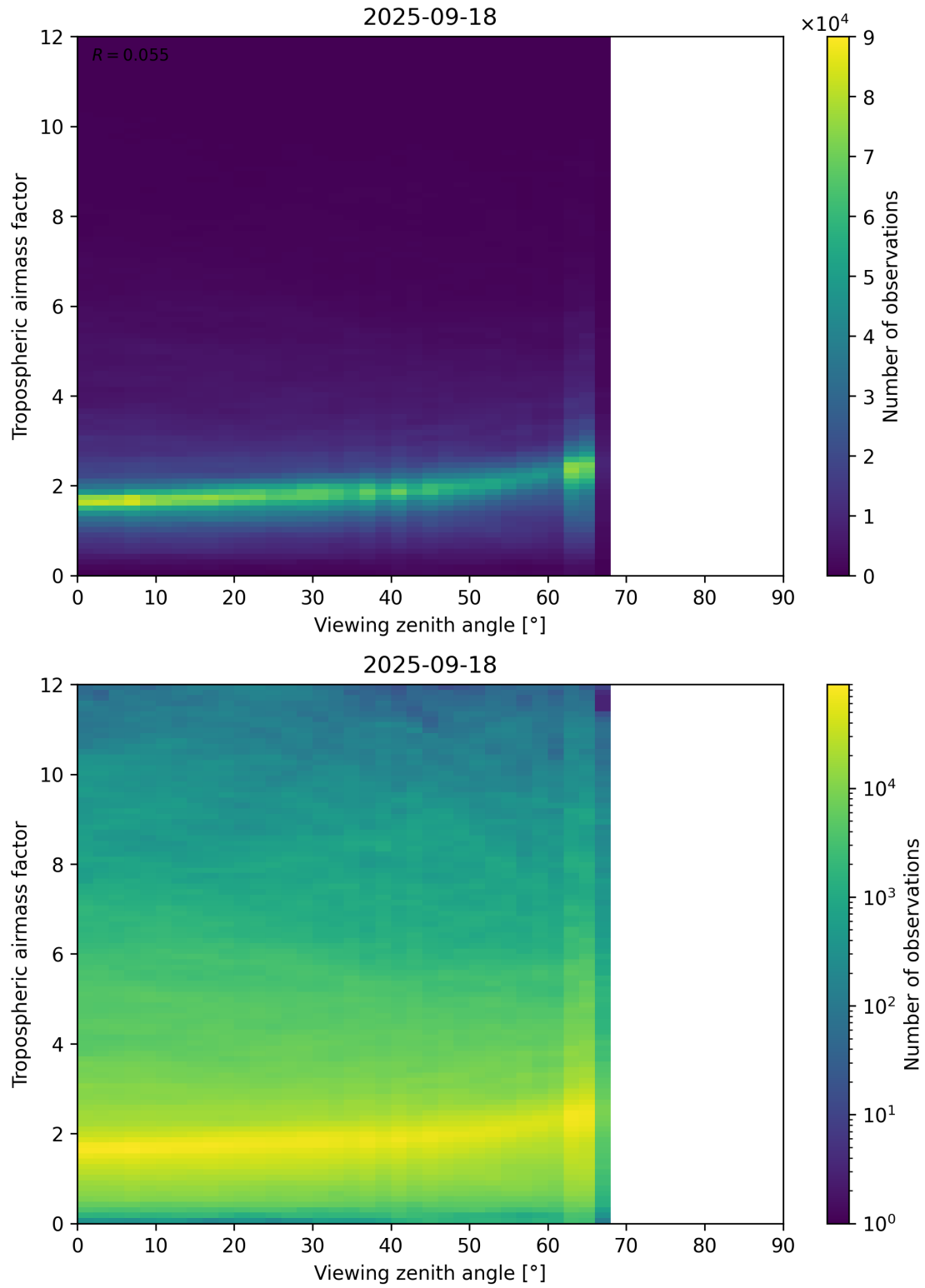
Figure 161: Scatter density plot of “Viewing zenith angle” against “Tropospheric airmass factor” for 2025-09-17 to 2025-09-19.
