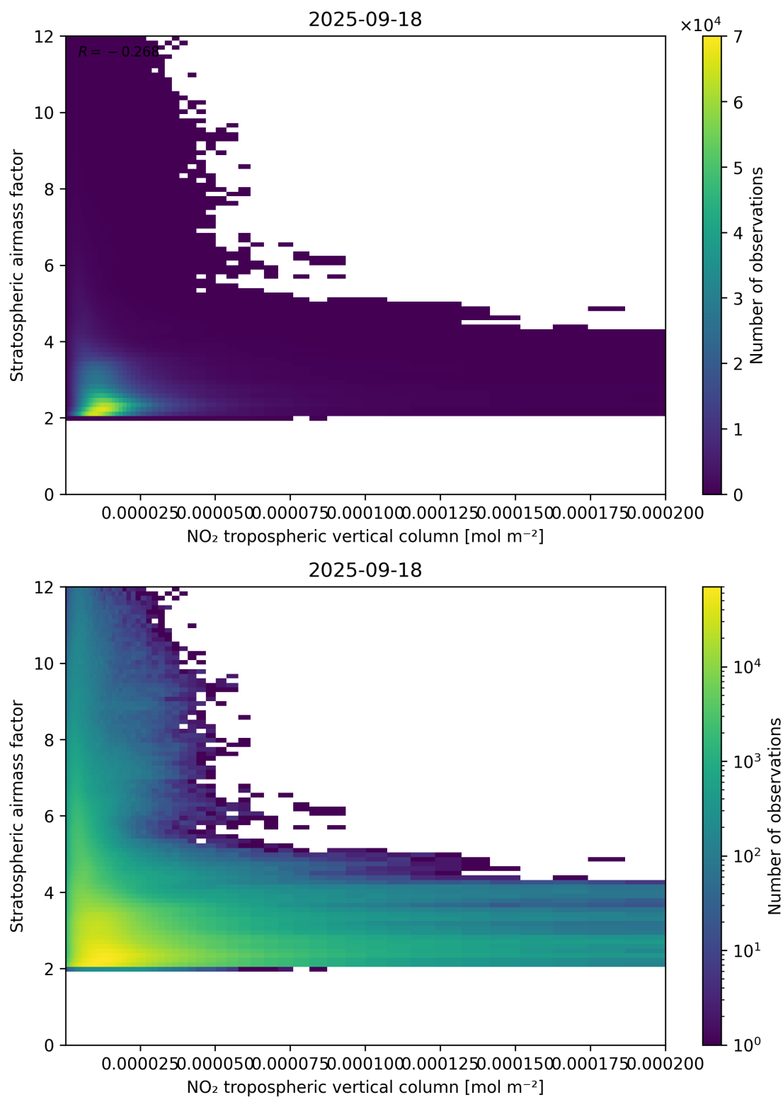
Figure 121: Scatter density plot of “NO 2 tropospheric vertical column” against “Stratospheric airmass factor” for 2025-09-17 to 2025-09-19.
