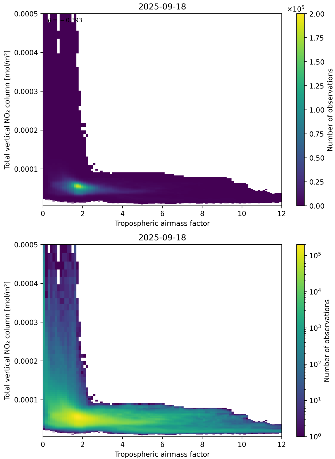
Figure 77: Scatter density plot of “Tropospheric airmass factor” against “Total vertical NO 2 column” for 2025-09-17 to 2025-09-19.
