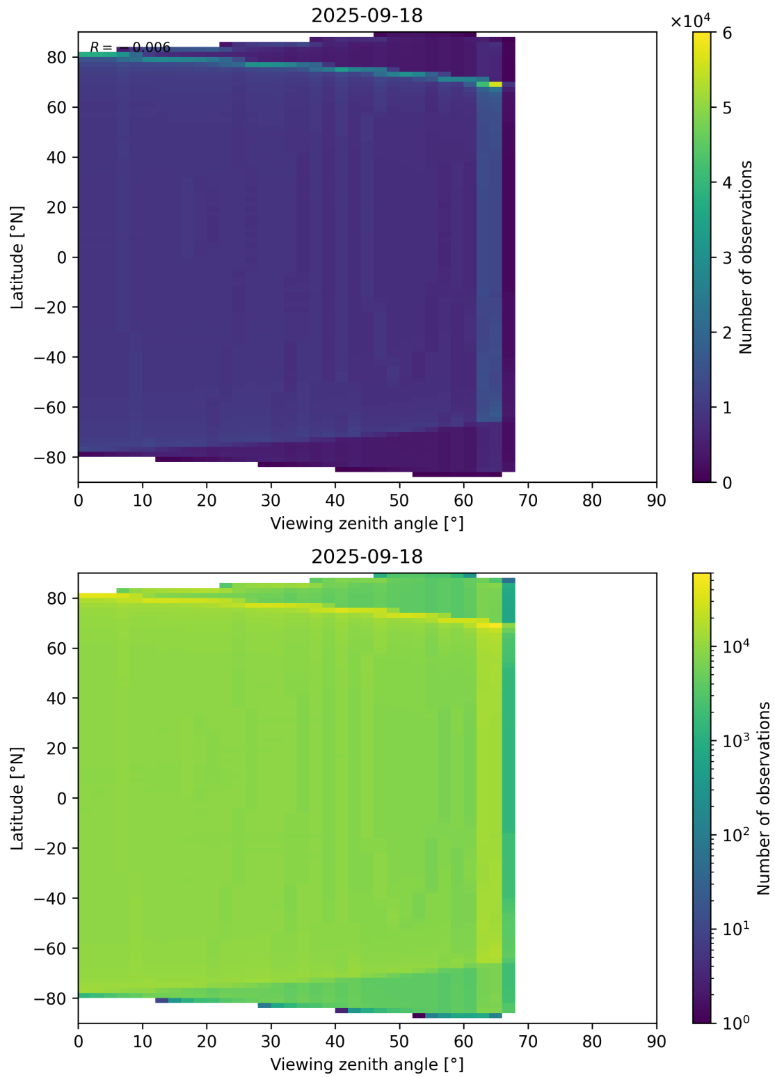
Figure 163: Scatter density plot of “Viewing zenith angle” against “Latitude” for 2025-09-17 to 2025-09-19.
