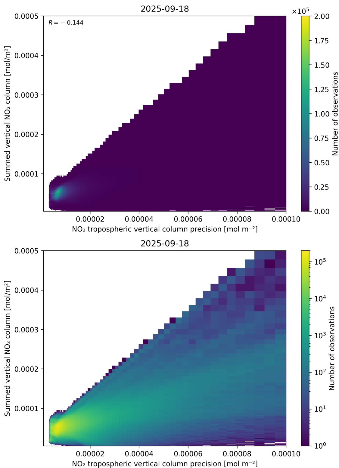
Figure 136: Scatter density plot of “NO 2 tropospheric vertical column precision” against “Summed vertical NO 2 column” for 2025-09-17 to 2025-09-19.
