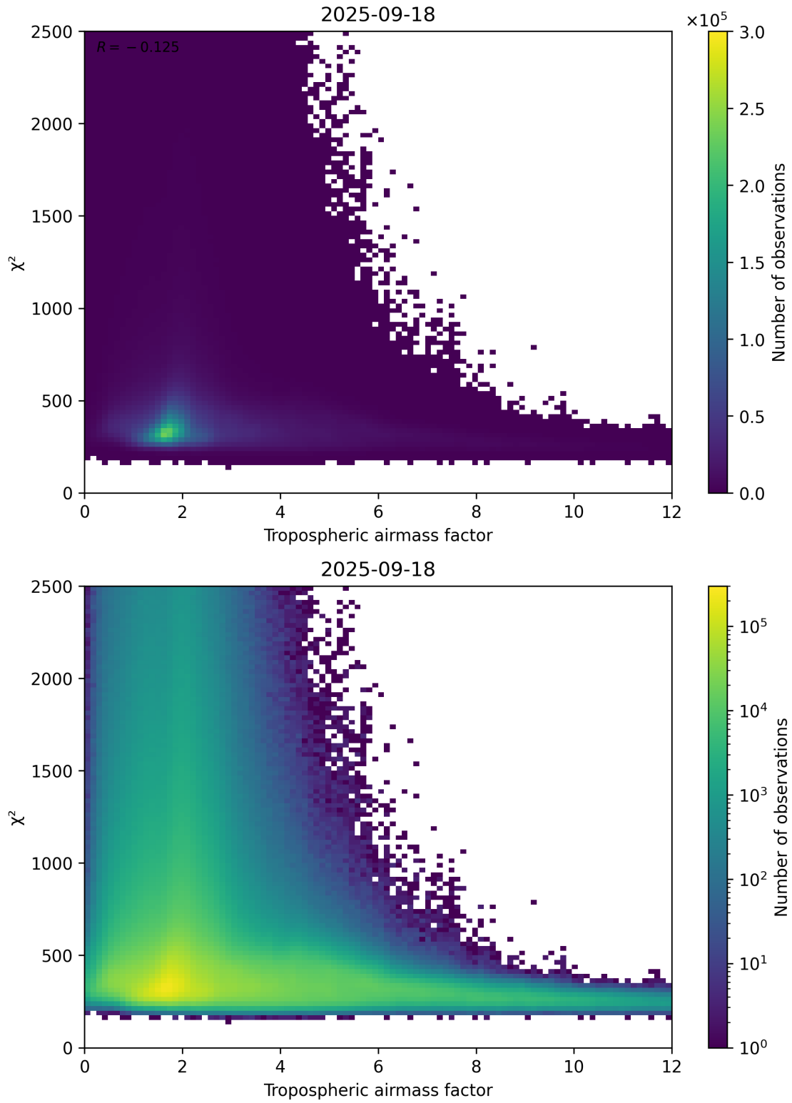
Figure 73: Scatter density plot of “Tropospheric airmass factor” against “ \chi^2 ” for 2025-09-17 to 2025-09-19.
