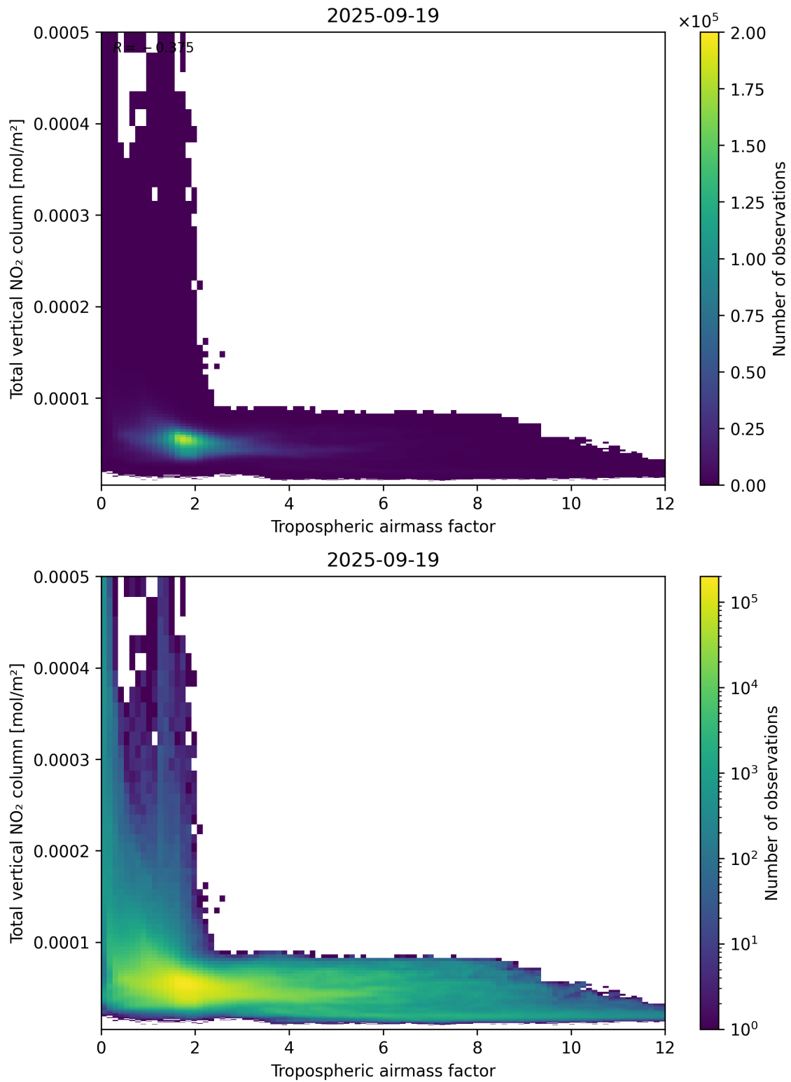
Figure 77: Scatter density plot of “Tropospheric airmass factor” against “Total vertical NO 2 column” for 2025-09-18 to 2025-09-20.
