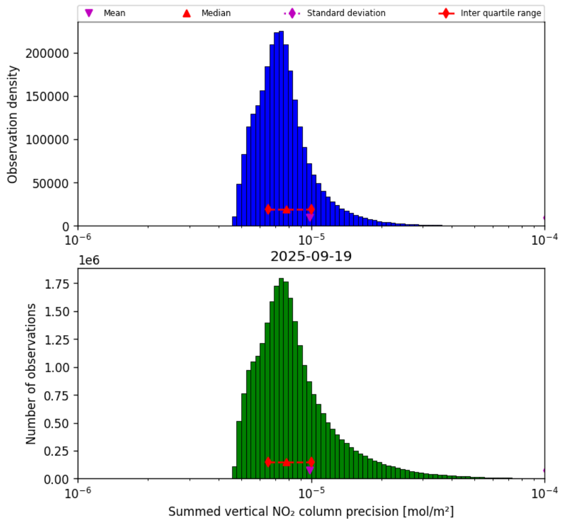
Figure 41: Histogram of “Summed vertical NO 2 column precision” for 2025-09-18 to 2025-09-20
