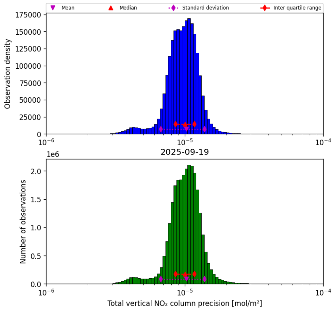
Figure 39: Histogram of “Total vertical NO 2 column precision” for 2025-09-18 to 2025-09-20
