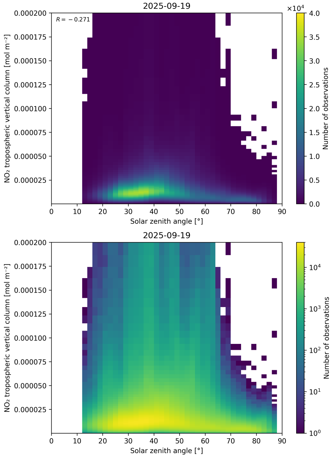
Figure 155: Scatter density plot of “Solar zenith angle” against “NO 2 tropospheric vertical column” for 2025-09-18 to 2025-09-20.
