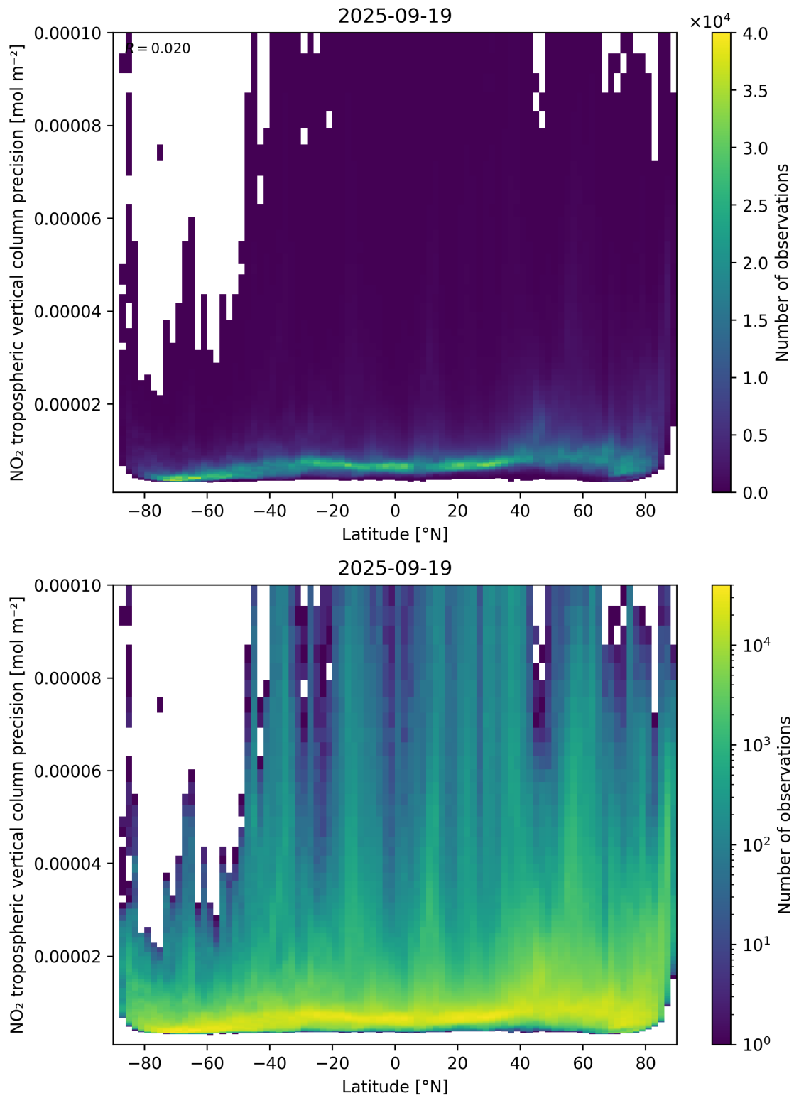
Figure 93: Scatter density plot of “Latitude” against “NO 2 tropospheric vertical column precision” for 2025-09-18 to 2025-09-20.
