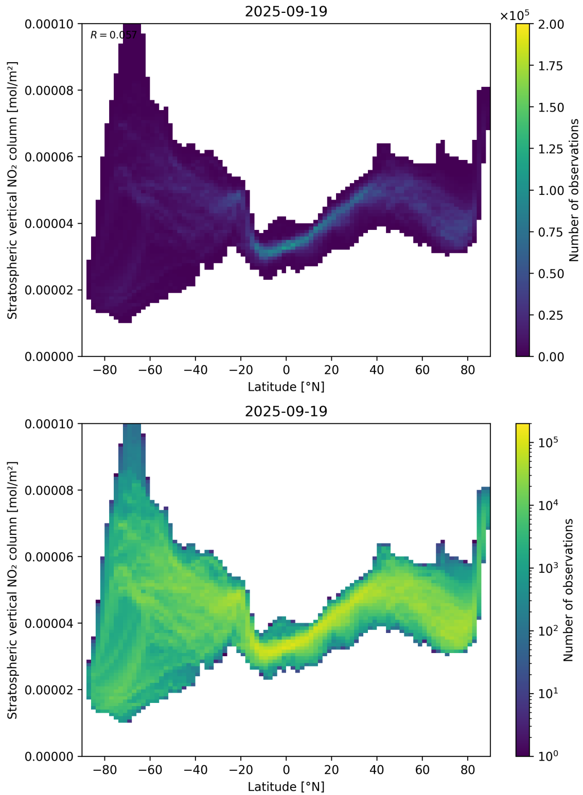
Figure 87: Scatter density plot of “Latitude” against “Stratospheric vertical NO 2 column” for 2025-09-18 to 2025-09-20.
