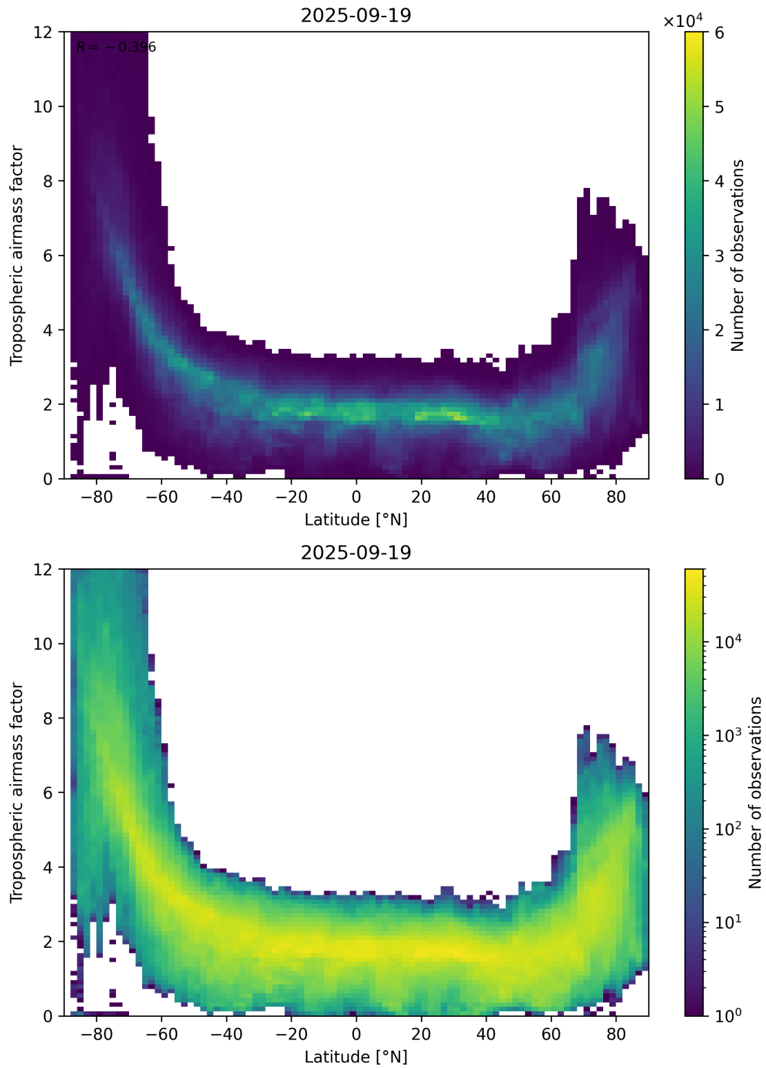
Figure 85: Scatter density plot of “Latitude” against “Tropospheric air mass factor” for 2025-09-18 to 2025-09-20.
