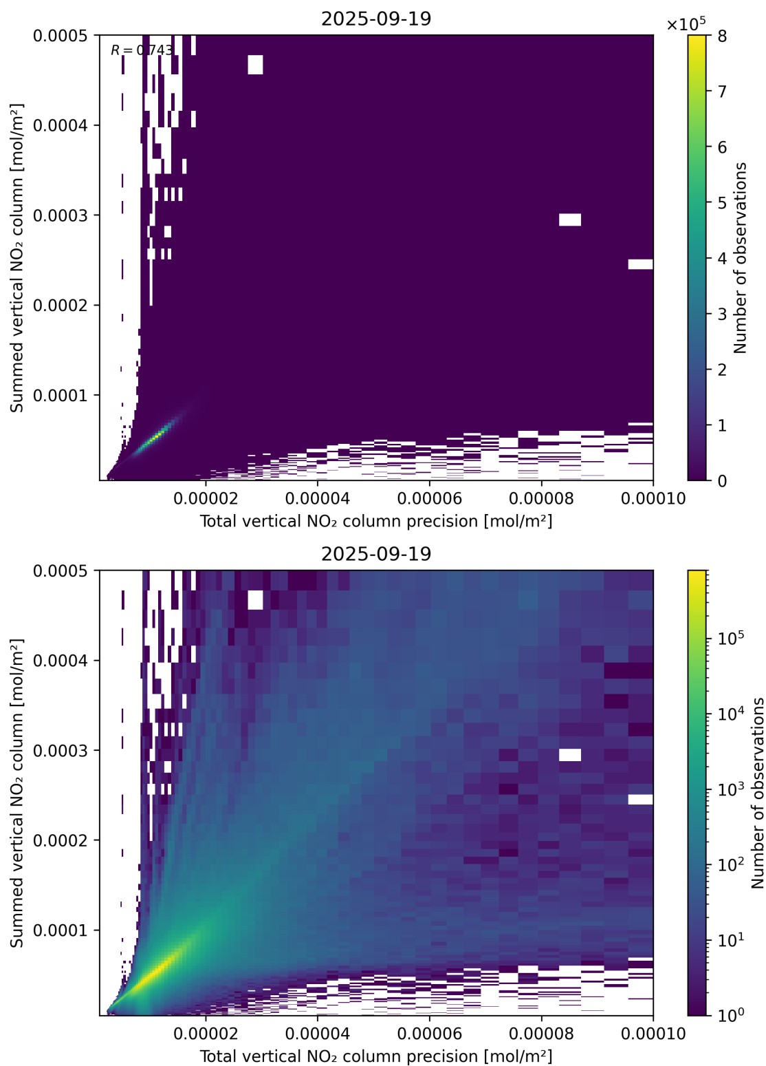
Figure 117: Scatter density plot of “Total vertical NO 2 column precision” against “Summed vertical NO 2 column” for 2025-09-18 to 2025-09-20.
