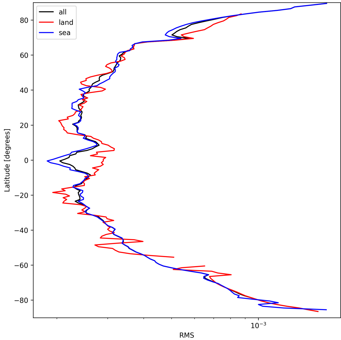
Figure 26: Zonal average of “RMS” for 2025-09-18 to 2025-09-20.
