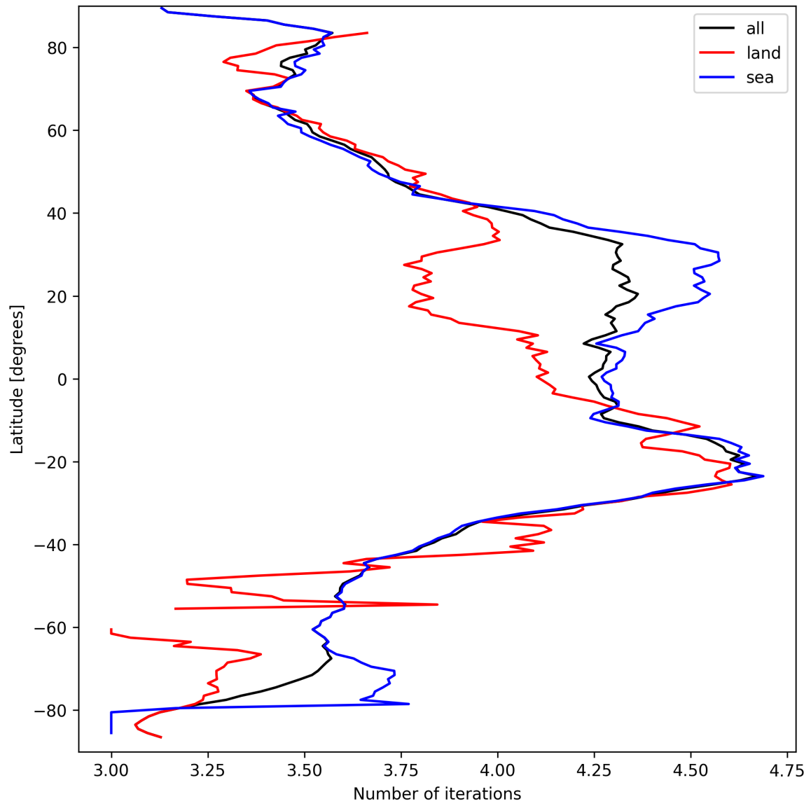
Figure 17: Zonal average of “Number of iterations” for 2025-09-18 to 2025-09-20.
