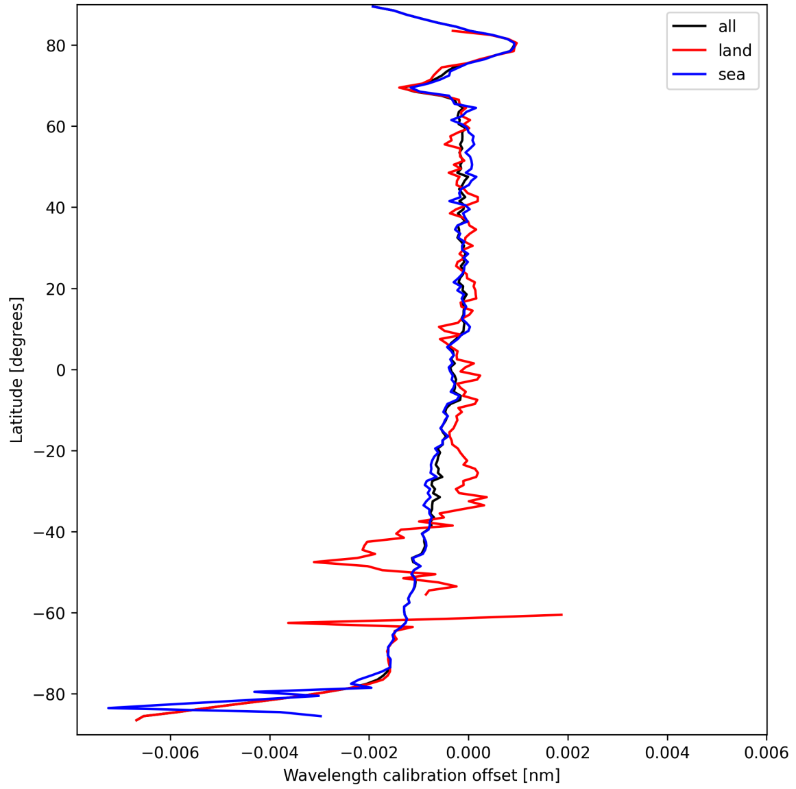
Figure 18: Zonal average of “Wavelength calibration offset” for 2025-09-18 to 2025-09-20.
