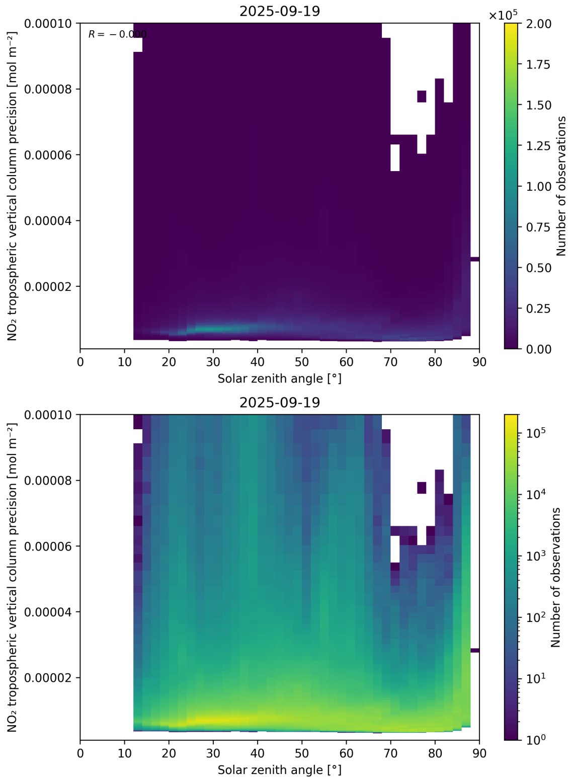
Figure 156: Scatter density plot of “Solar zenith angle” against “NO 2 tropospheric vertical column precision” for 2025-09-18 to 2025-09-20.
