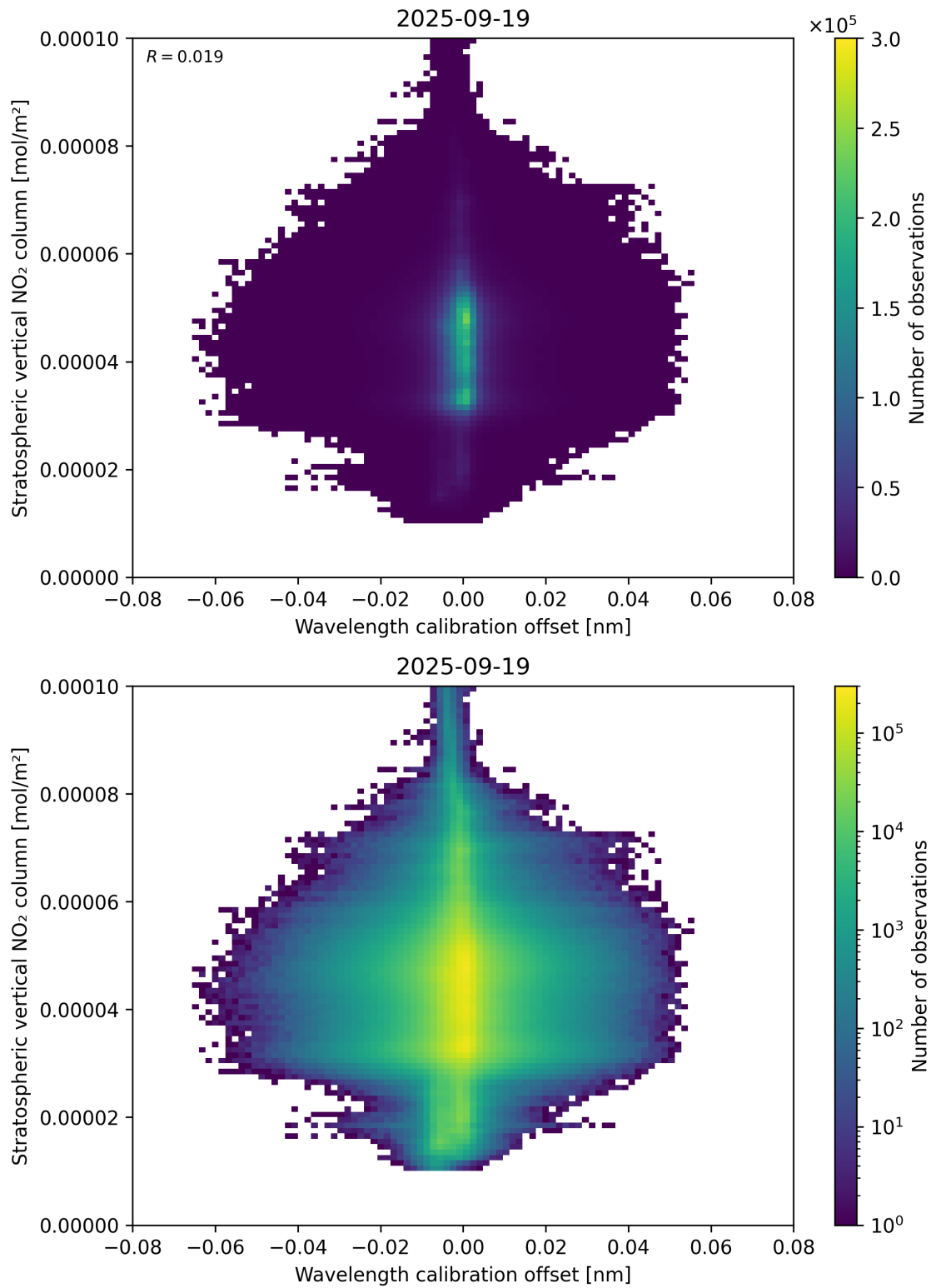
Figure 176: Scatter density plot of “Wavelength calibration offset” against “Stratospheric vertical NO 2 column” for 2025-09-18 to 2025-09-20.
