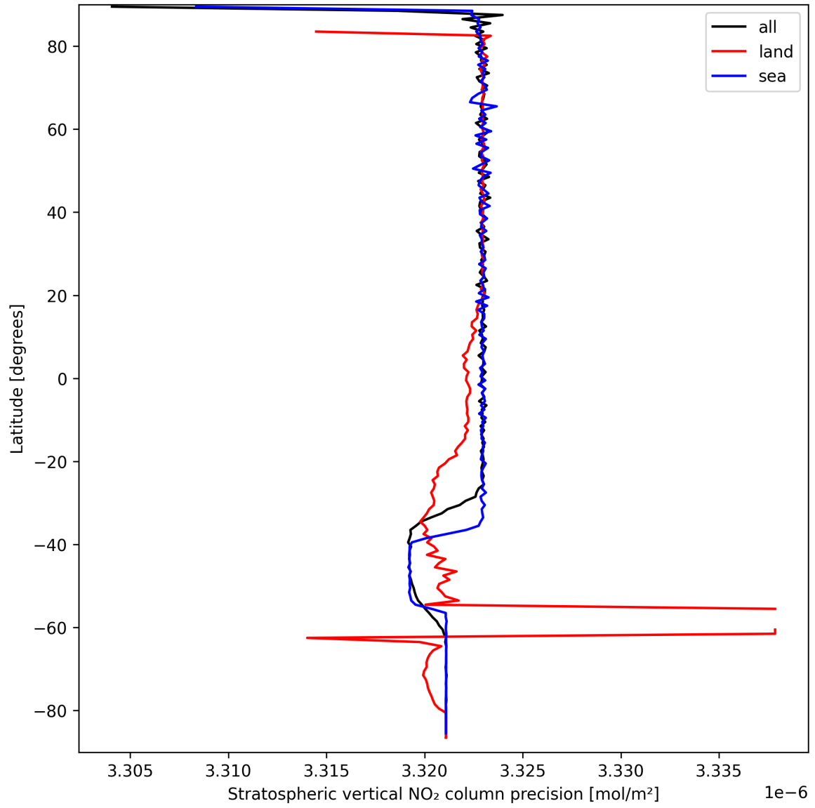
Figure 20: Zonal average of “Stratospheric vertical NO 2 column precision” for 2025-09-18 to 2025-09-20.
