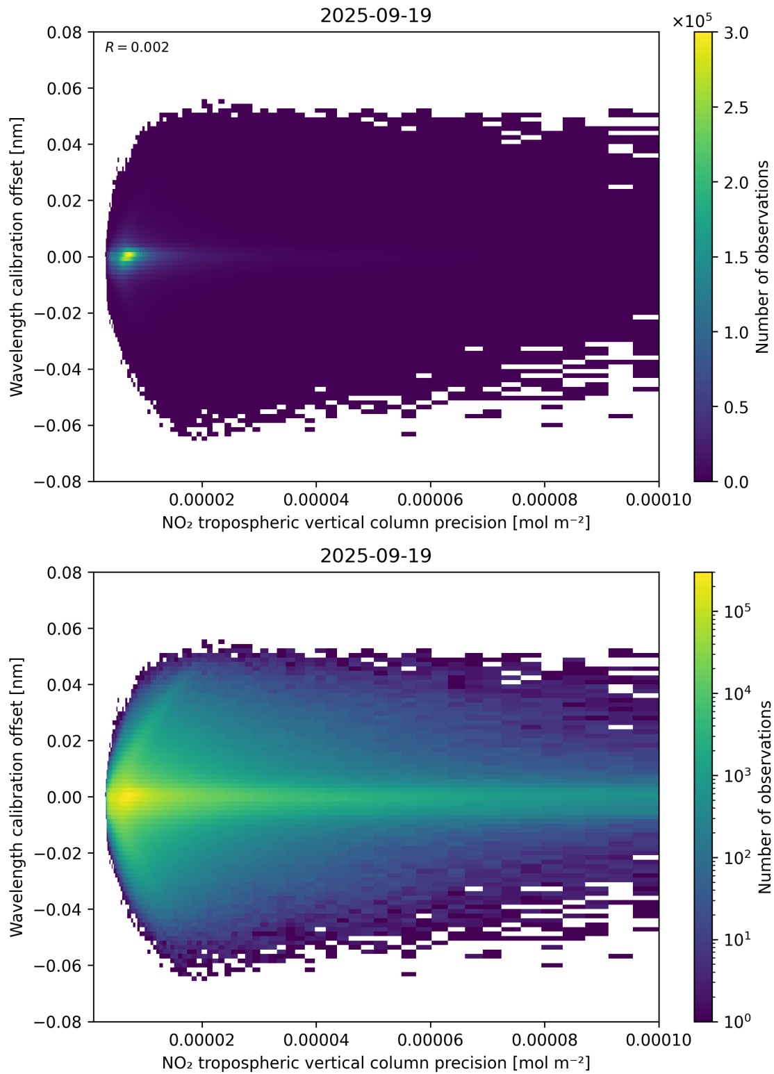
Figure 141: Scatter density plot of “NO 2 tropospheric vertical column precision” against “Wavelength calibration offset” for 2025-09-18 to 2025-09-20.
