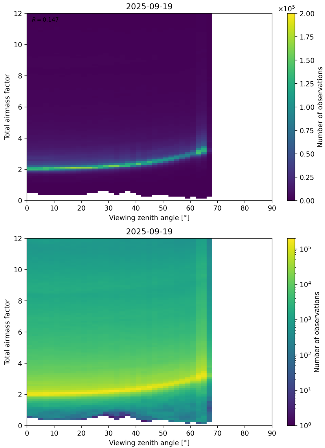
Figure 160: Scatter density plot of “Viewing zenith angle” against “Total airmass factor” for 2025-09-18 to 2025-09-20.
