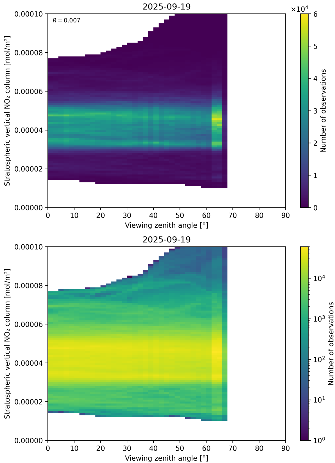
Figure 164: Scatter density plot of “Viewing zenith angle” against “Stratospheric vertical NO 2 column” for 2025-09-18 to 2025-09-20.
