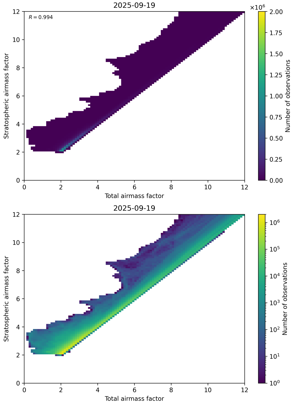
Figure 62: Scatter density plot of “Total airmass factor” against “Stratospheric airmass factor” for 2025-09-18 to 2025-09-20.
