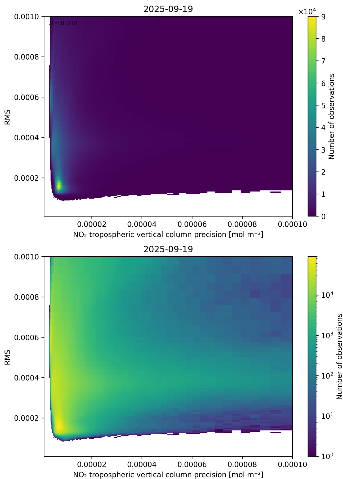
Figure 140: Scatter density plot of “NO 2 tropospheric vertical column precision” against “RMS” for 2025-09-18 to 2025-09-20.
