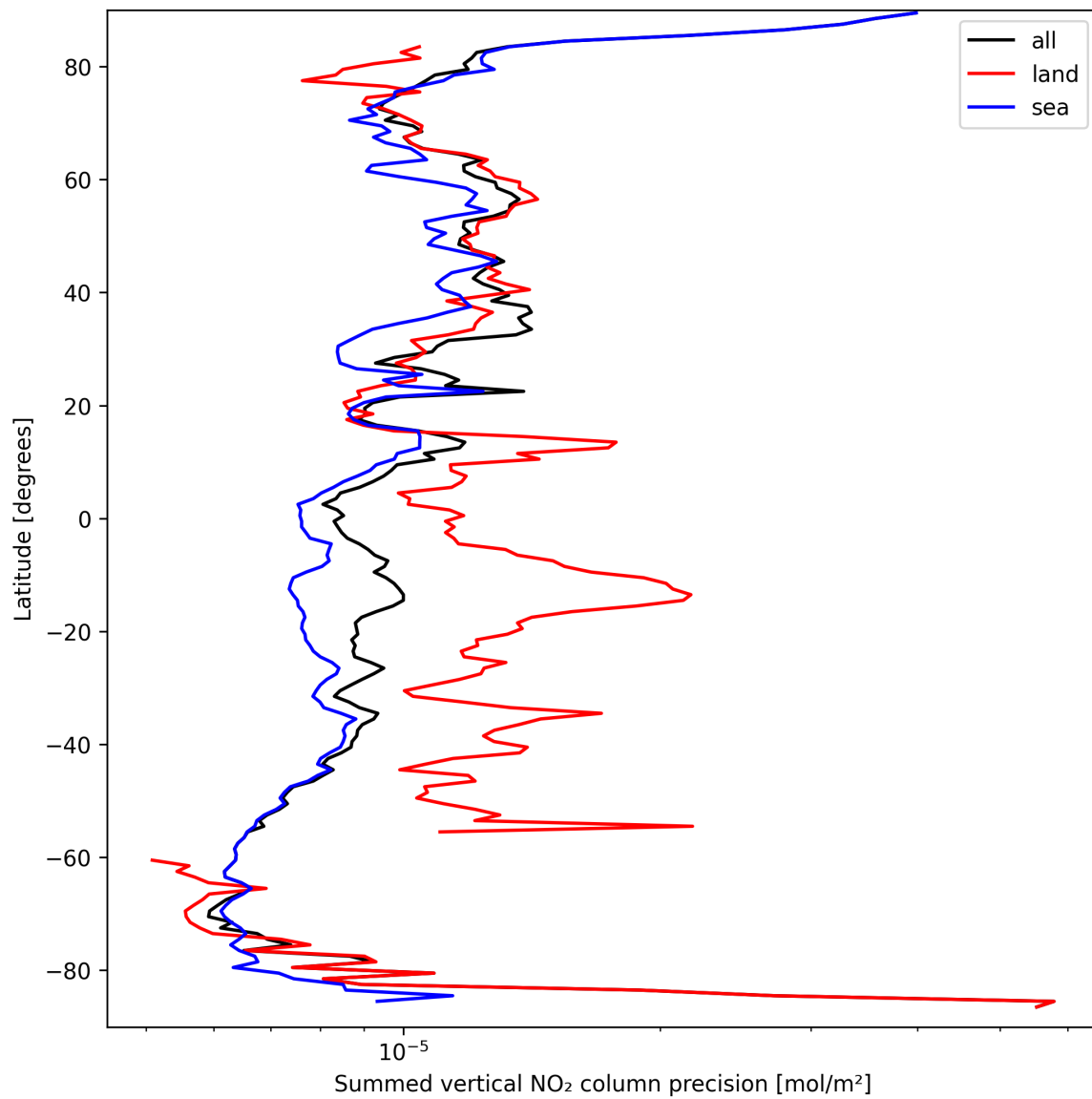
Figure 24: Zonal average of “Summed vertical NO 2 column precision” for 2025-09-18 to 2025-09-20.
