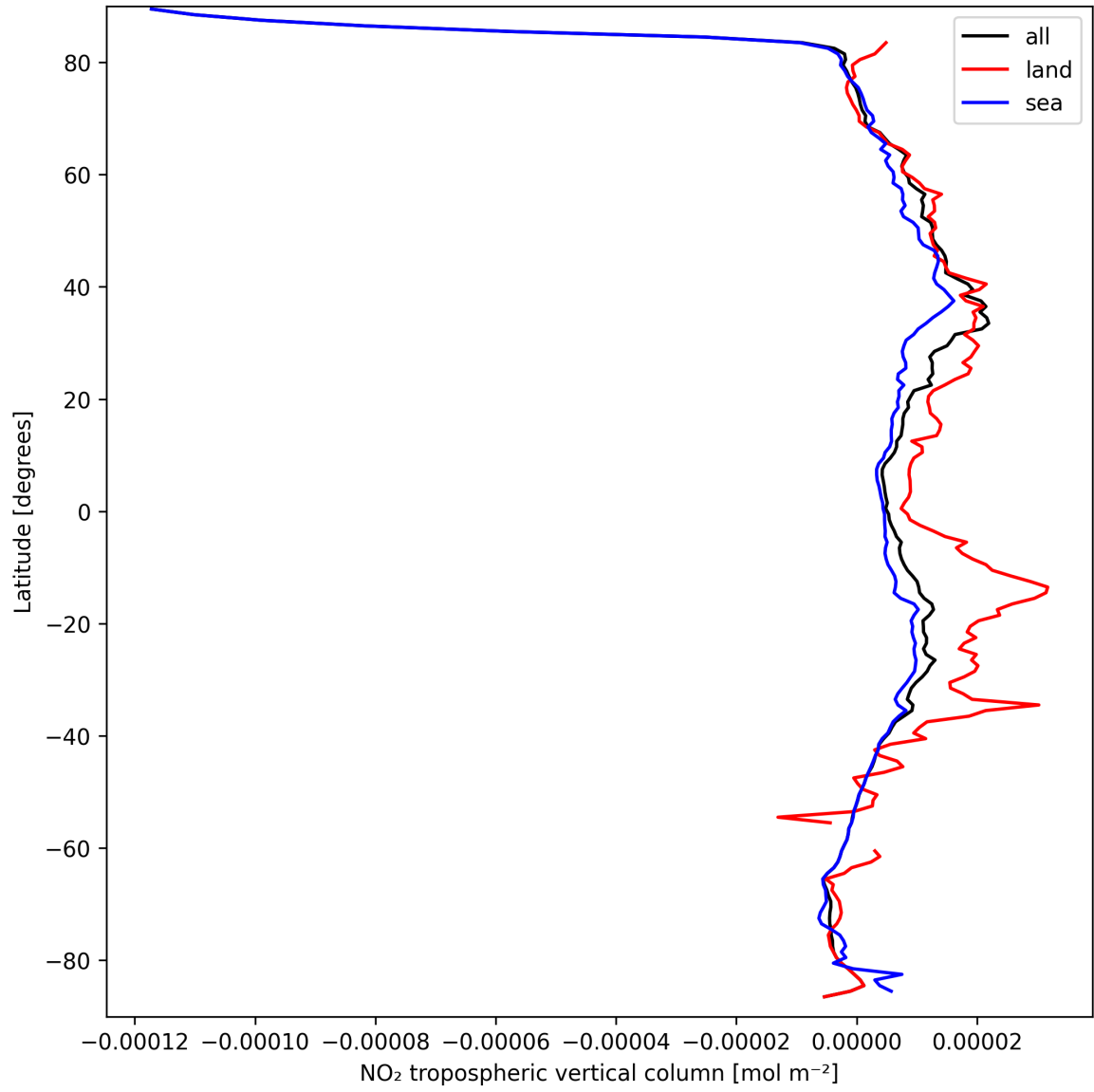
Figure 12: Zonal average of “NO 2 tropospheric vertical column” for 2025-09-18 to 2025-09-20.
