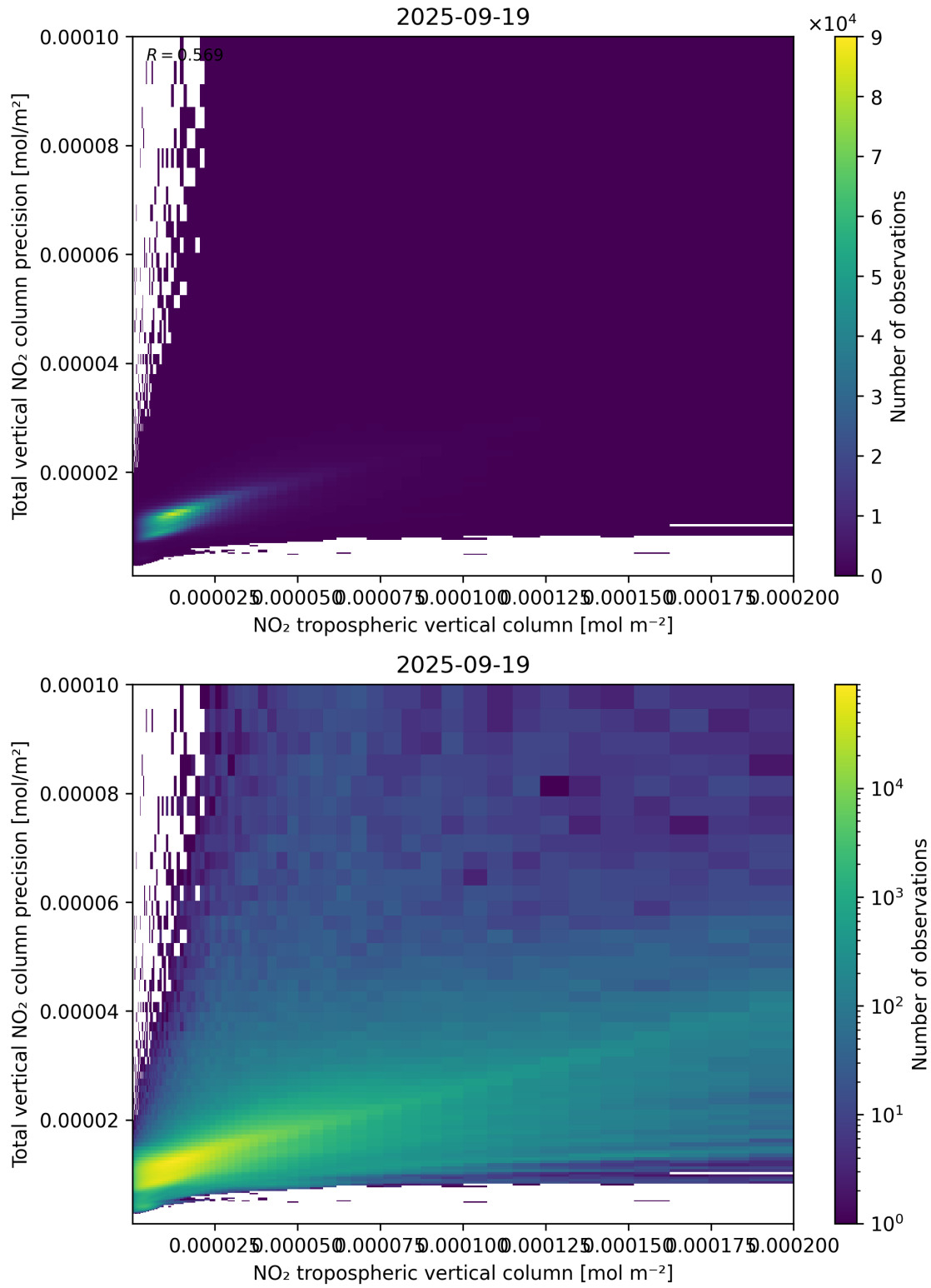
Figure 129: Scatter density plot of “NO 2 tropospheric vertical column” against “Total vertical NO 2 column precision” for 2025-09-18 to 2025-09-20.
