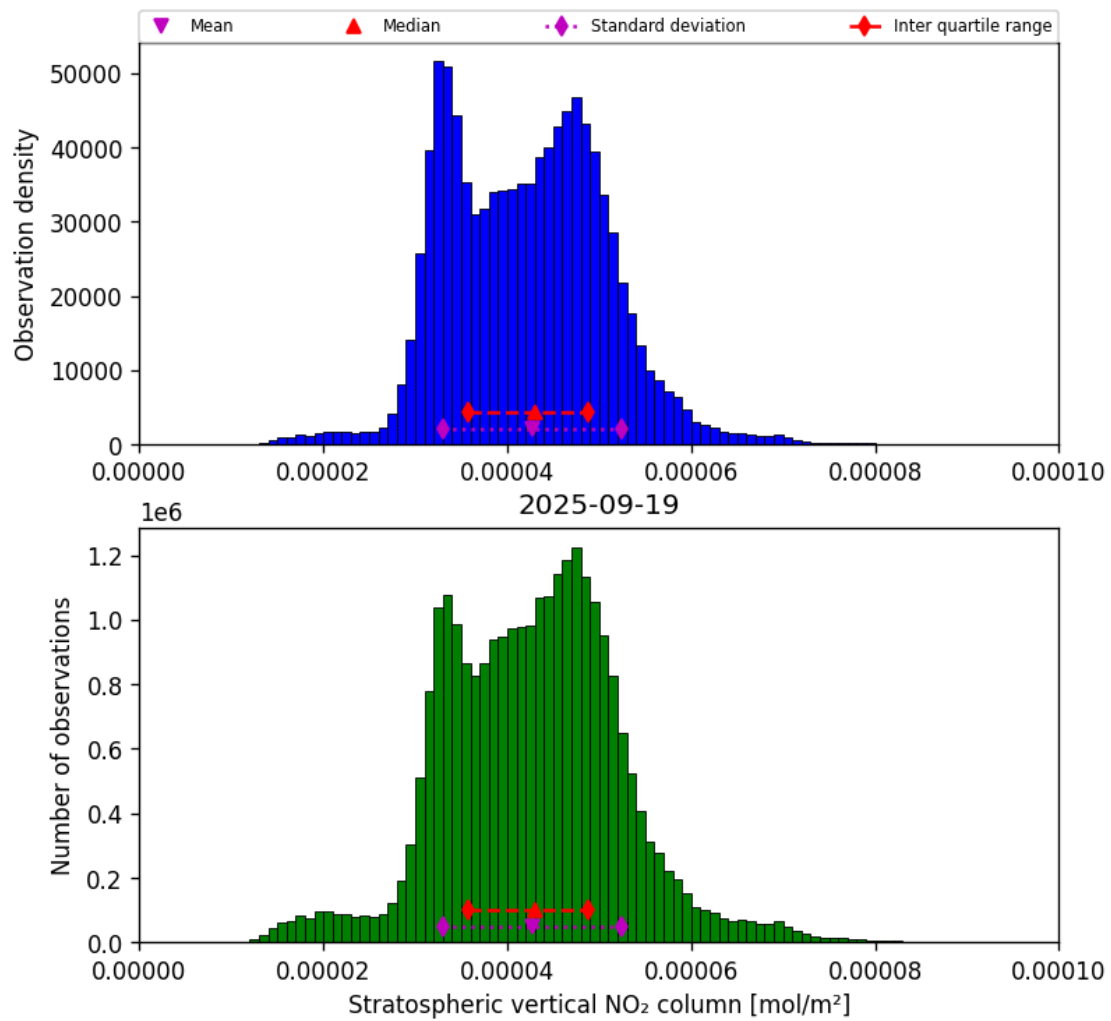
Figure 36: Histogram of “Stratospheric vertical NO 2 column” for 2025-09-18 to 2025-09-20
