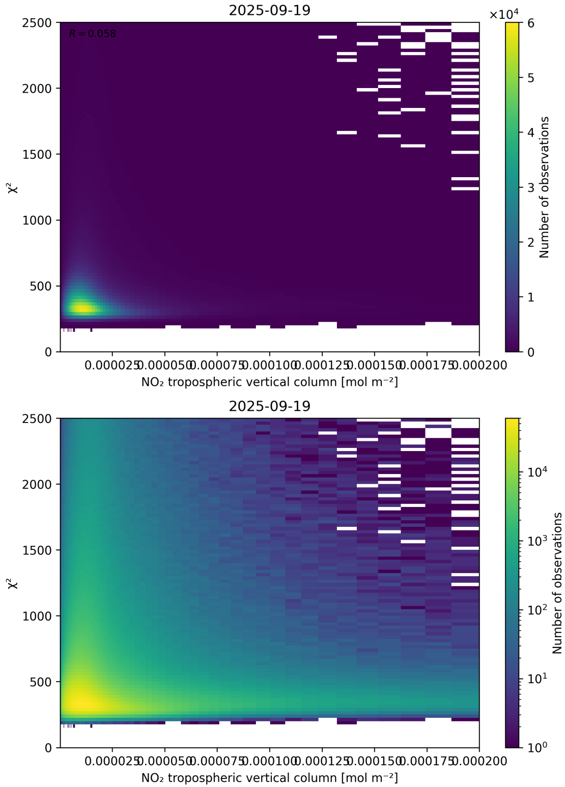
Figure 124: Scatter density plot of “NO 2 tropospheric vertical column” against “ \chi^2 ” for 2025-09-18 to 2025-09-20.
