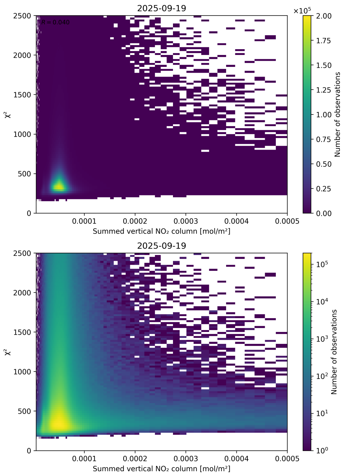
Figure 104: Scatter density plot of “Summed vertical NO 2 column” against “ \chi^2 ” for 2025-09-18 to 2025-09-20.
