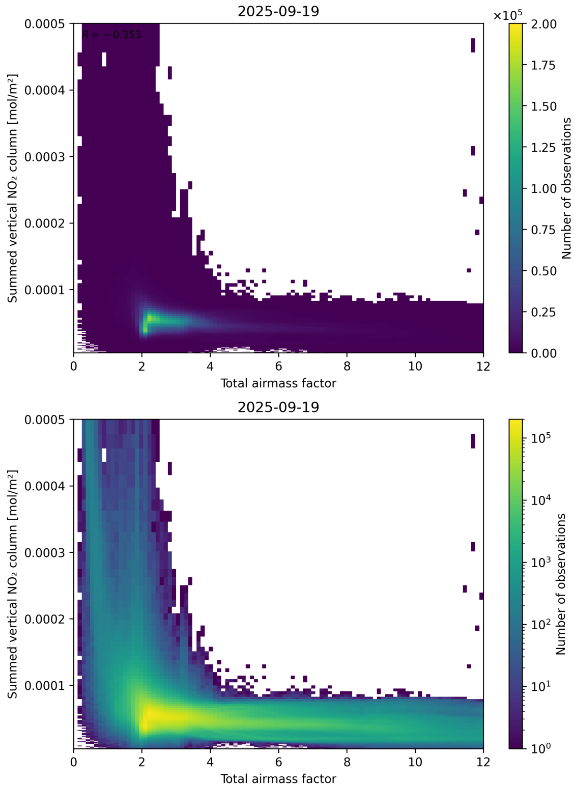
Figure 65: Scatter density plot of “Total airmass factor” against “Summed vertical NO 2 column” for 2025-09-18 to 2025-09-20.
