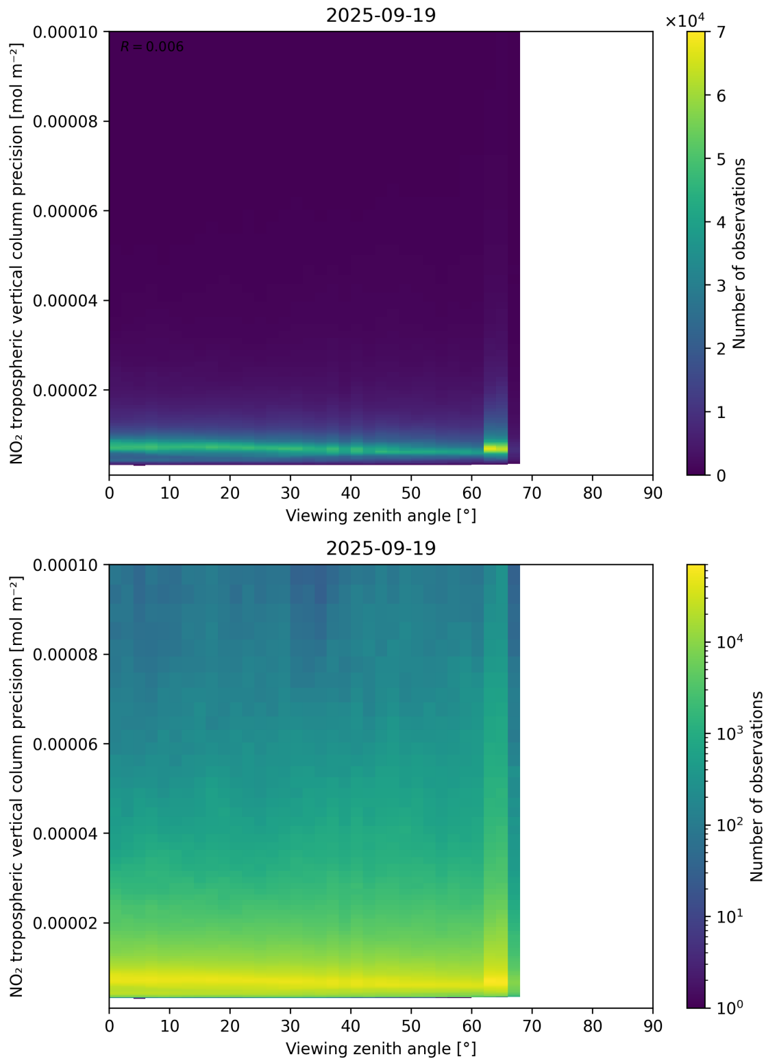
Figure 170: Scatter density plot of “Viewing zenith angle” against “NO 2 tropospheric vertical column precision” for 2025-09-18 to 2025-09-20.
