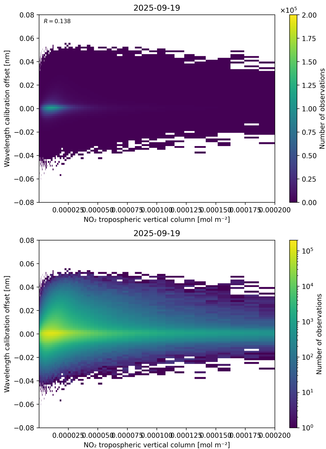
Figure 143: Scatter density plot of “NO 2 tropospheric vertical column” against “Wavelength calibration offset” for 2025-09-18 to 2025-09-20.
