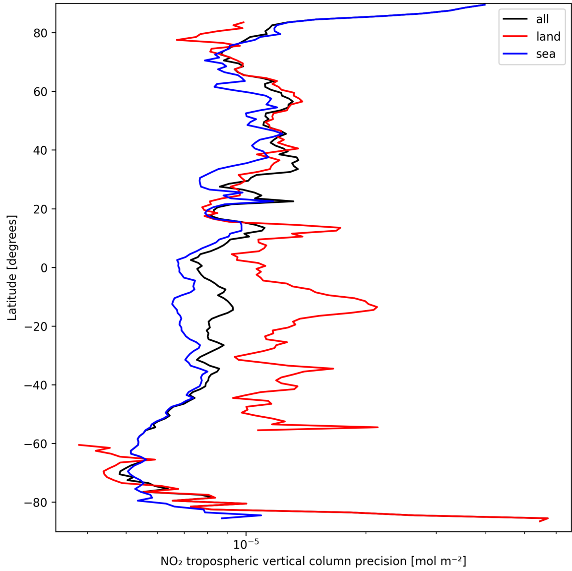
Figure 13: Zonal average of “NO 2 tropospheric vertical column precision” for 2025-09-18 to 2025-09-20.
