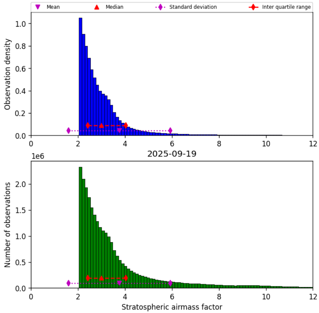
Figure 44: Histogram of “Stratospheric airmass factor” for 2025-09-18 to 2025-09-20
