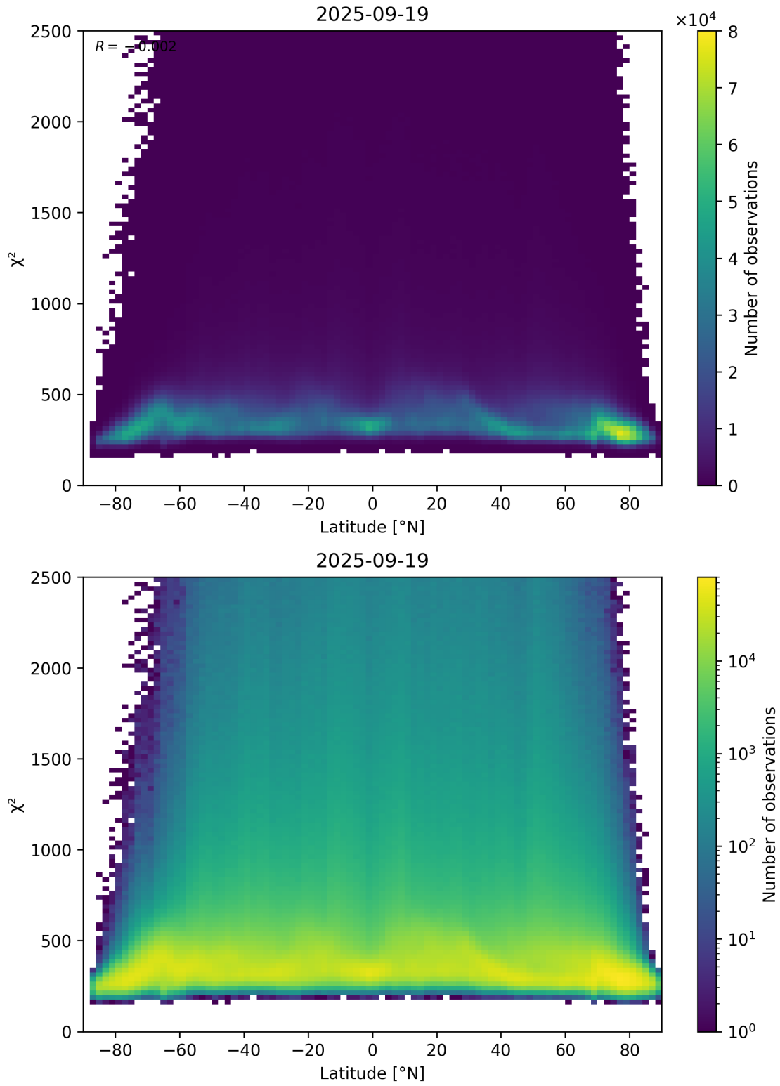
Figure 86: Scatter density plot of “Latitude” against “ \chi^2 ” for 2025-09-18 to 2025-09-20.
