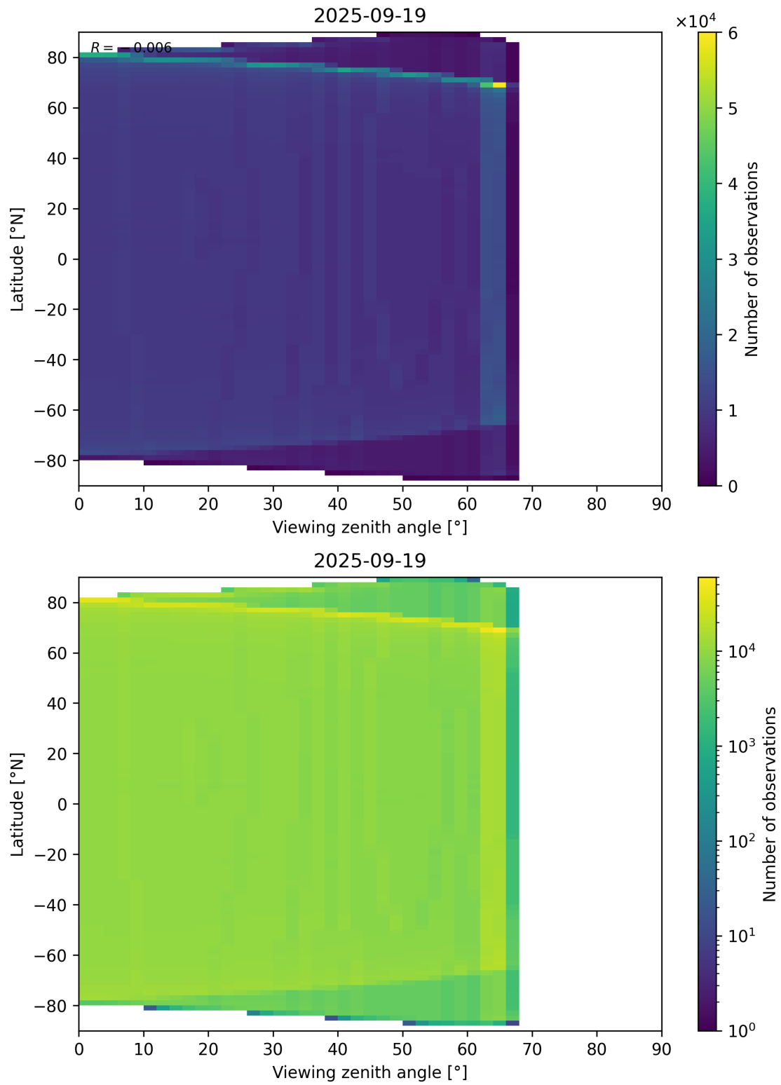
Figure 163: Scatter density plot of “Viewing zenith angle” against “Latitude” for 2025-09-18 to 2025-09-20.
