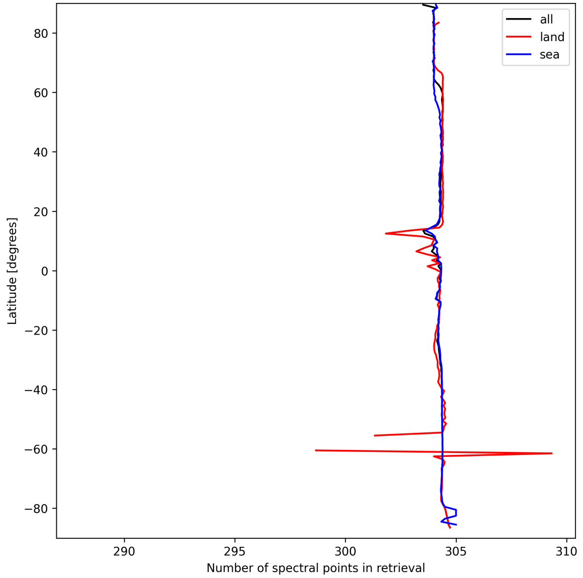
Figure 16: Zonal average of “Number of spectral points in retrieval” for 2025-09-18 to 2025-09-20.
