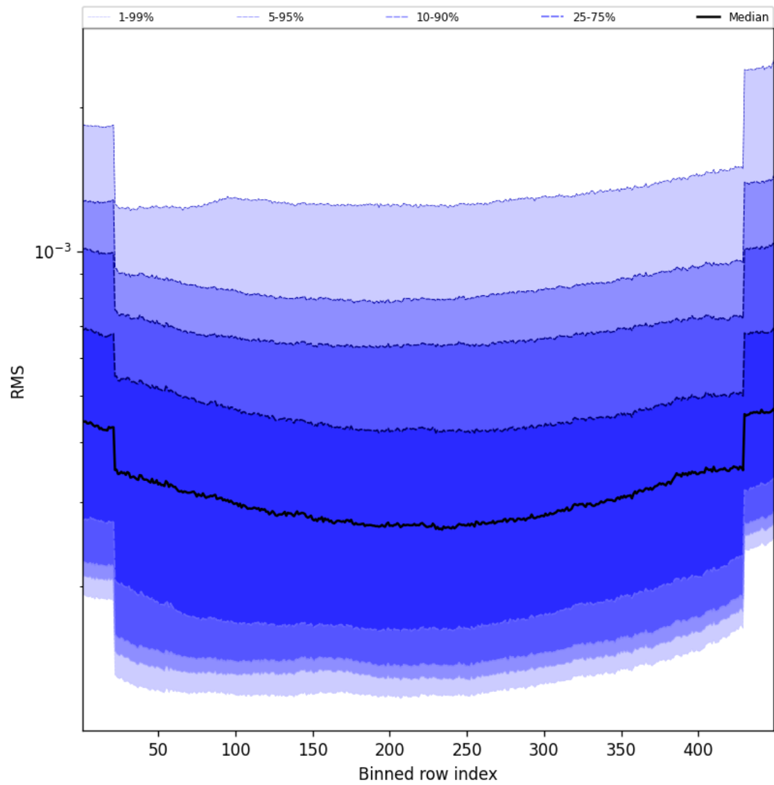
Figure 60: Along track statistics of “RMS” for 2025-09-18 to 2025-09-20
