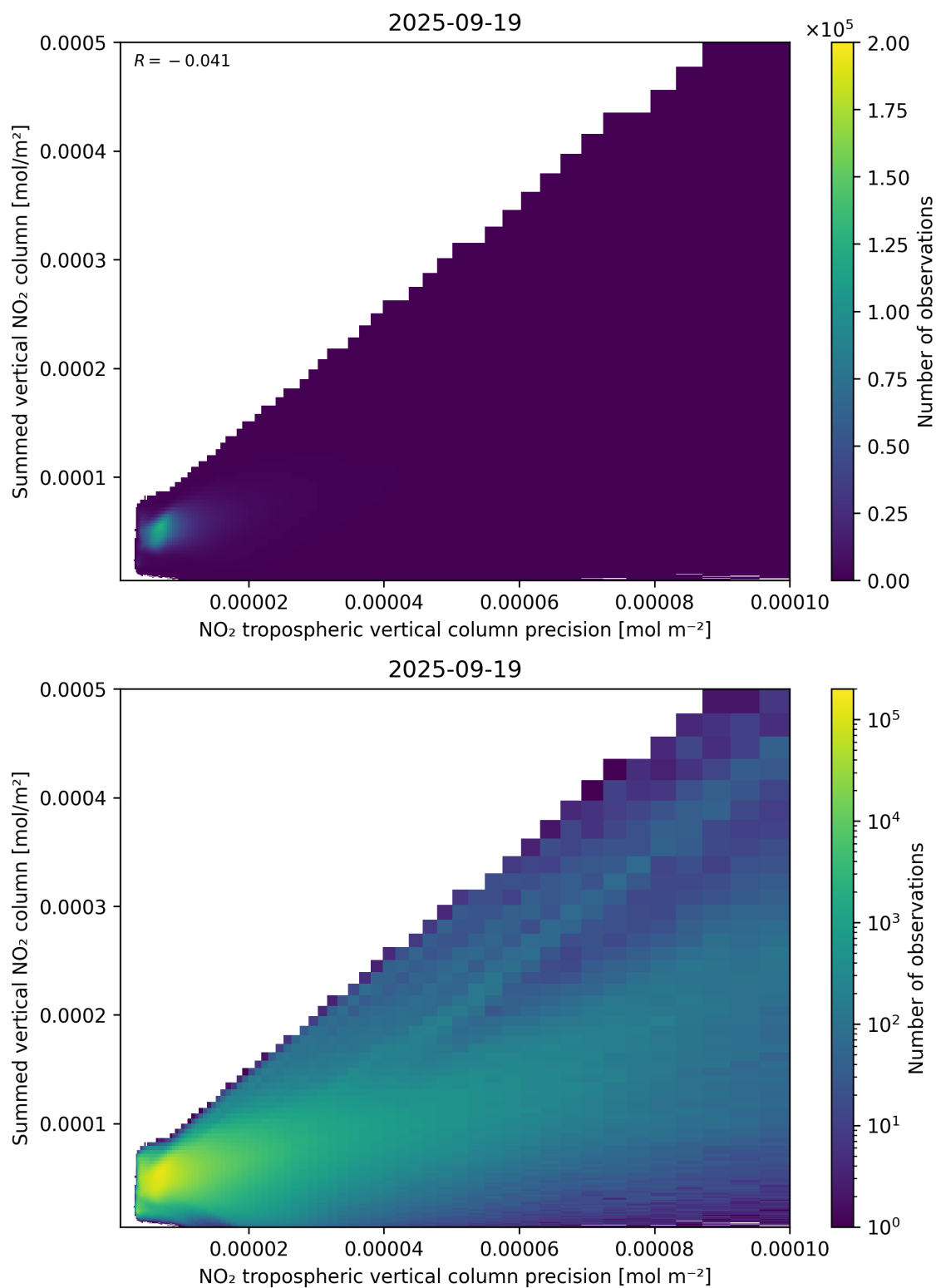
Figure 136: Scatter density plot of “NO 2 tropospheric vertical column precision” against “Summed vertical NO 2 column” for 2025-09-18 to 2025-09-20.
