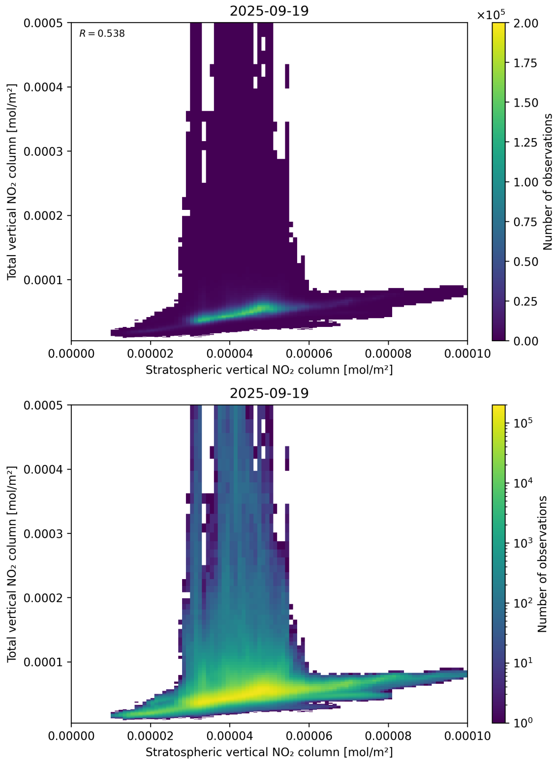
Figure 100: Scatter density plot of “Stratospheric vertical NO 2 column” against “Total vertical NO 2 column” for 2025-09-18 to 2025-09-20.
