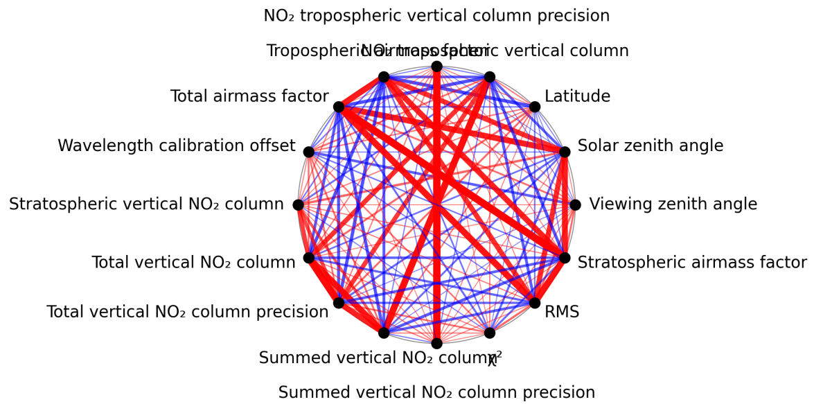
Figure 1: Map of correlation graph for 2025-09-18 to 2025-09-20.
