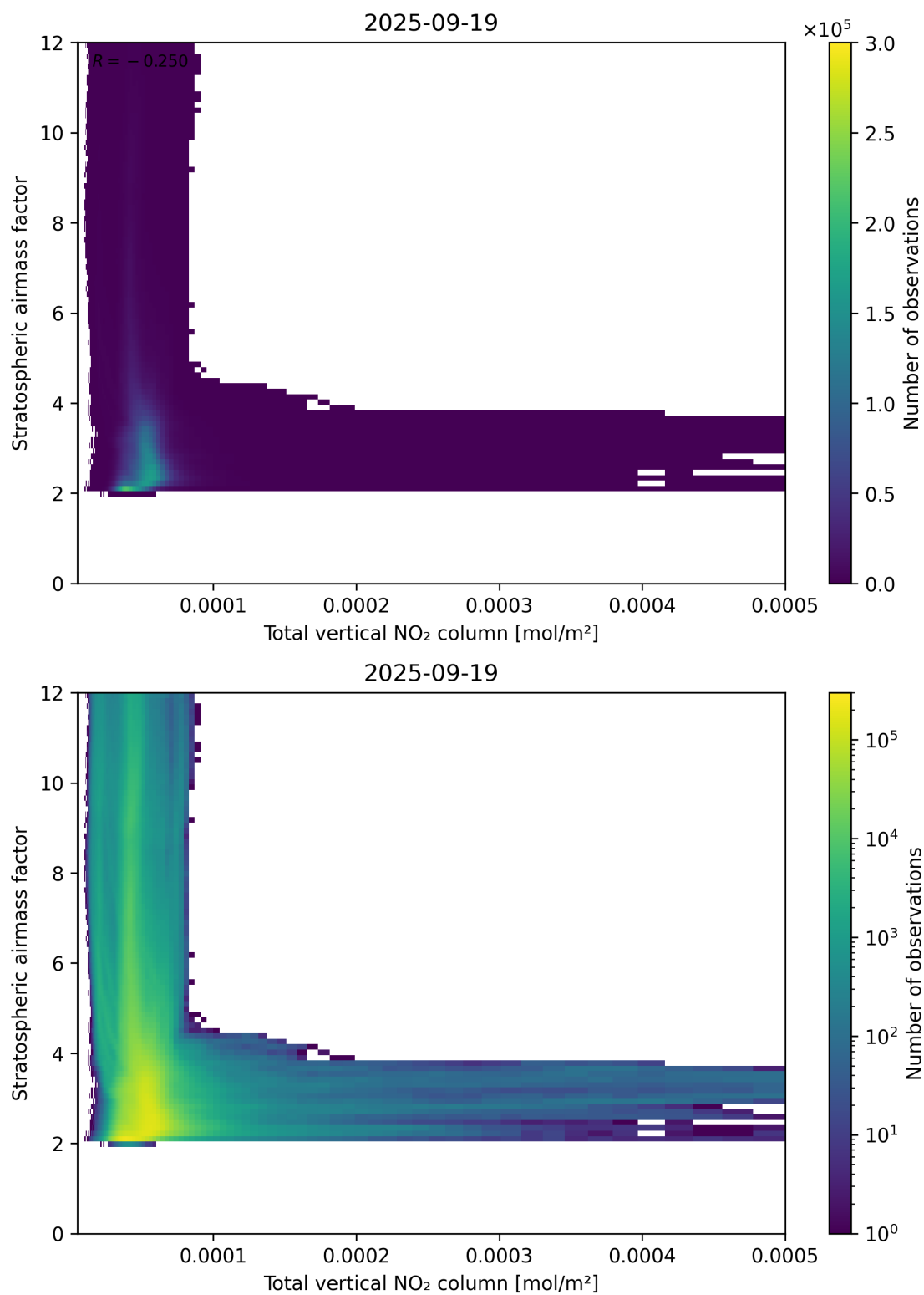
Figure 110: Scatter density plot of “Total vertical NO 2 column” against “Stratospheric airmass factor” for 2025-09-18 to 2025-09-20.
