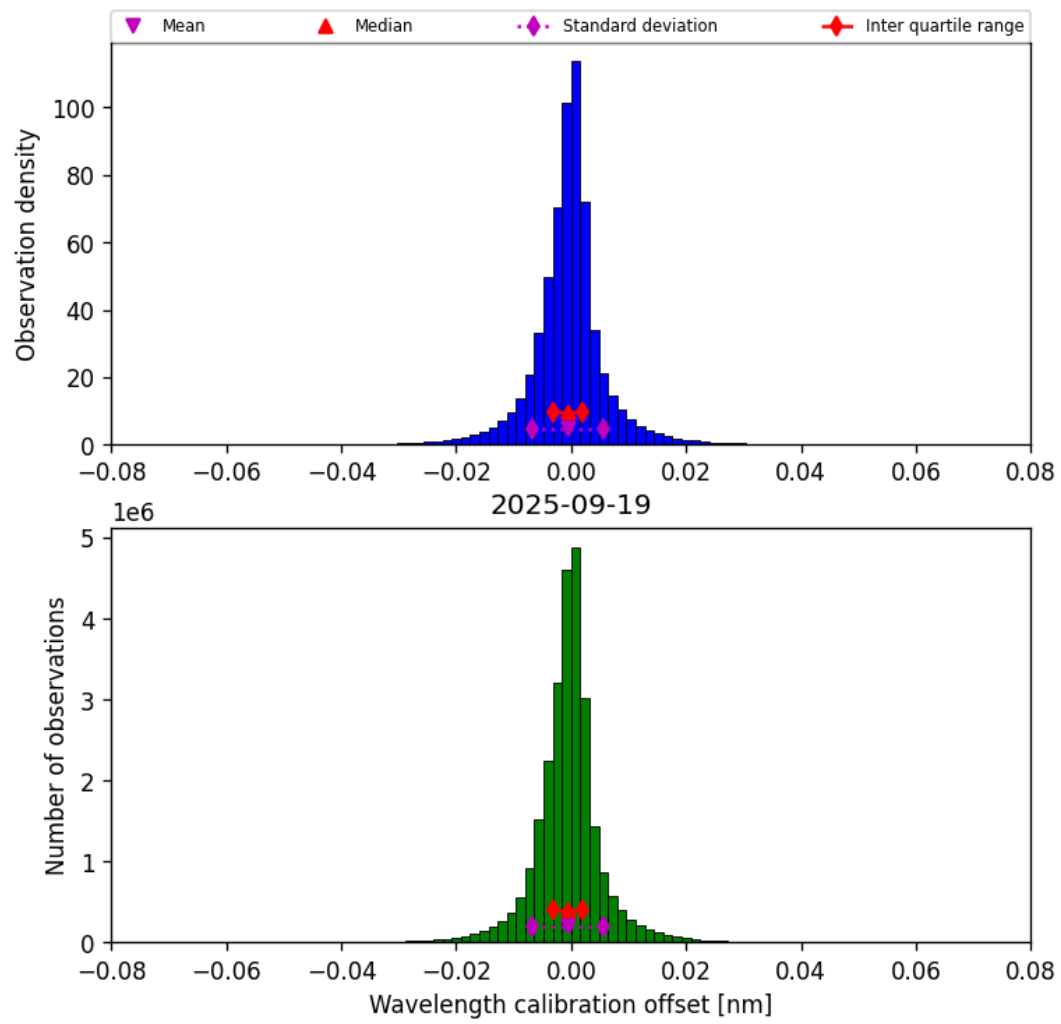
Figure 35: Histogram of “Wavelength calibration offset” for 2025-09-18 to 2025-09-20
