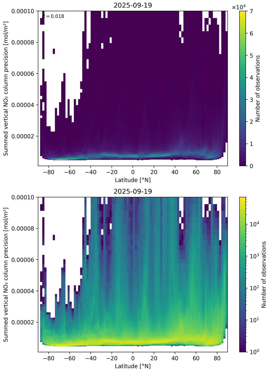
Figure 89: Scatter density plot of “Latitude” against “Summed vertical NO 2 column precision” for 2025-09-18 to 2025-09-20.
