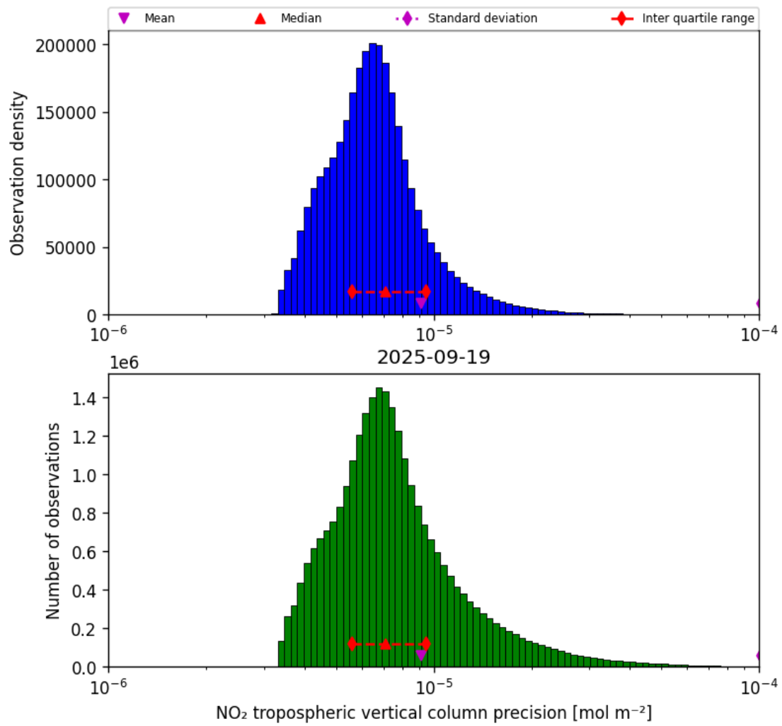
Figure 30: Histogram of “NO 2 tropospheric vertical column precision” for 2025-09-18 to 2025-09-20
