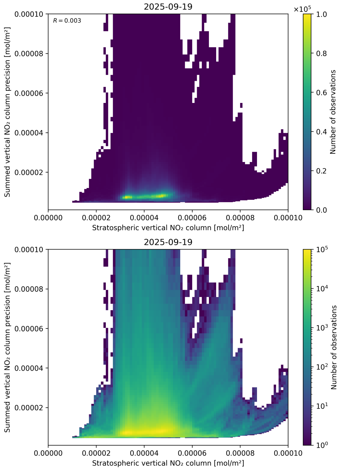
Figure 99: Scatter density plot of “Stratospheric vertical NO 2 column” against “Summed vertical NO 2 column precision” for 2025-09-18 to 2025-09-20.
