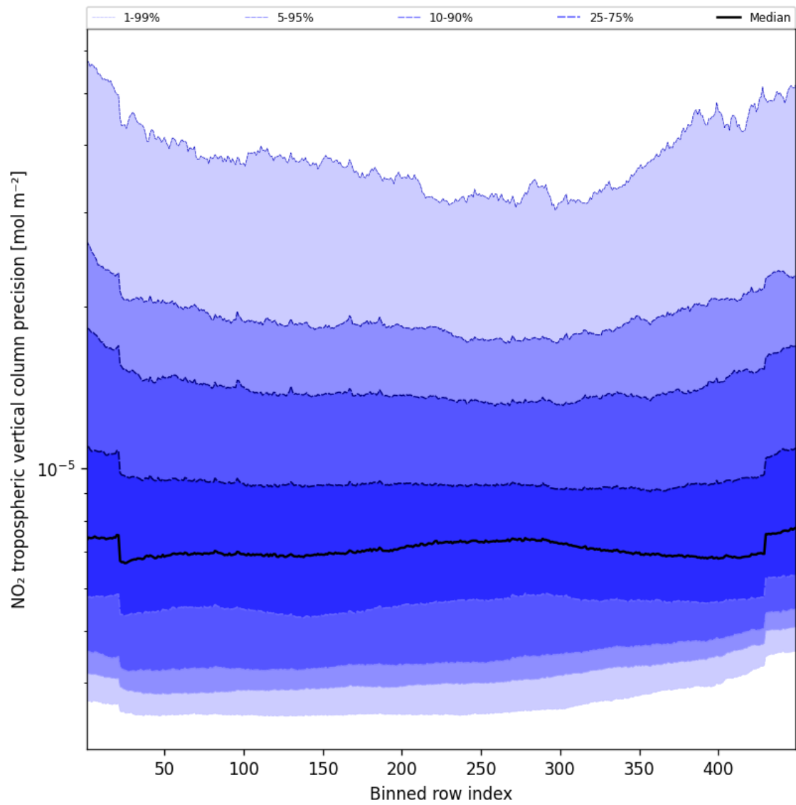
Figure 47: Along track statistics of “NO 2 tropospheric vertical column precision” for 2025-09-18 to 2025-09-20
