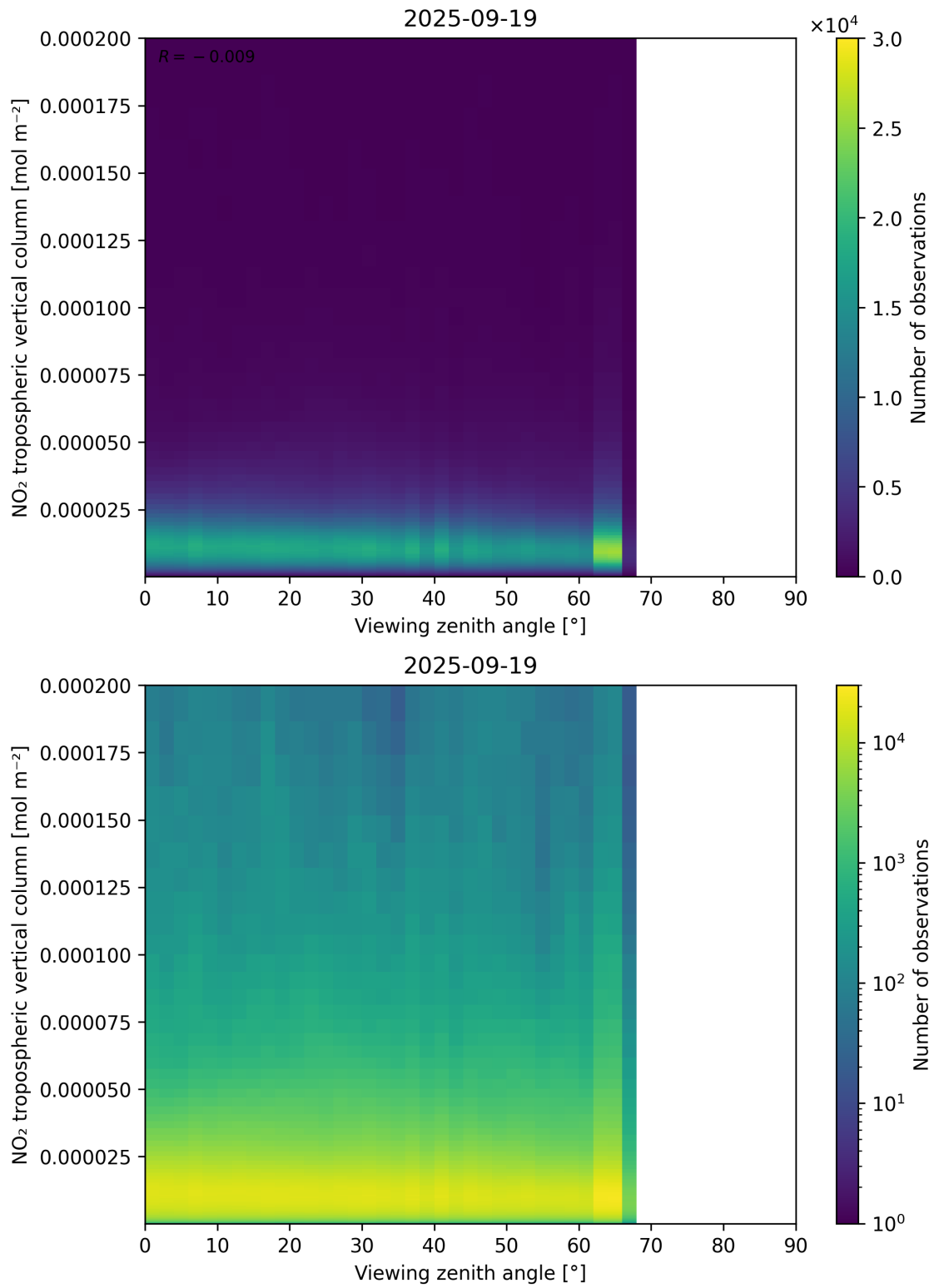
Figure 169: Scatter density plot of “Viewing zenith angle” against “NO 2 tropospheric vertical column” for 2025-09-18 to 2025-09-20.
