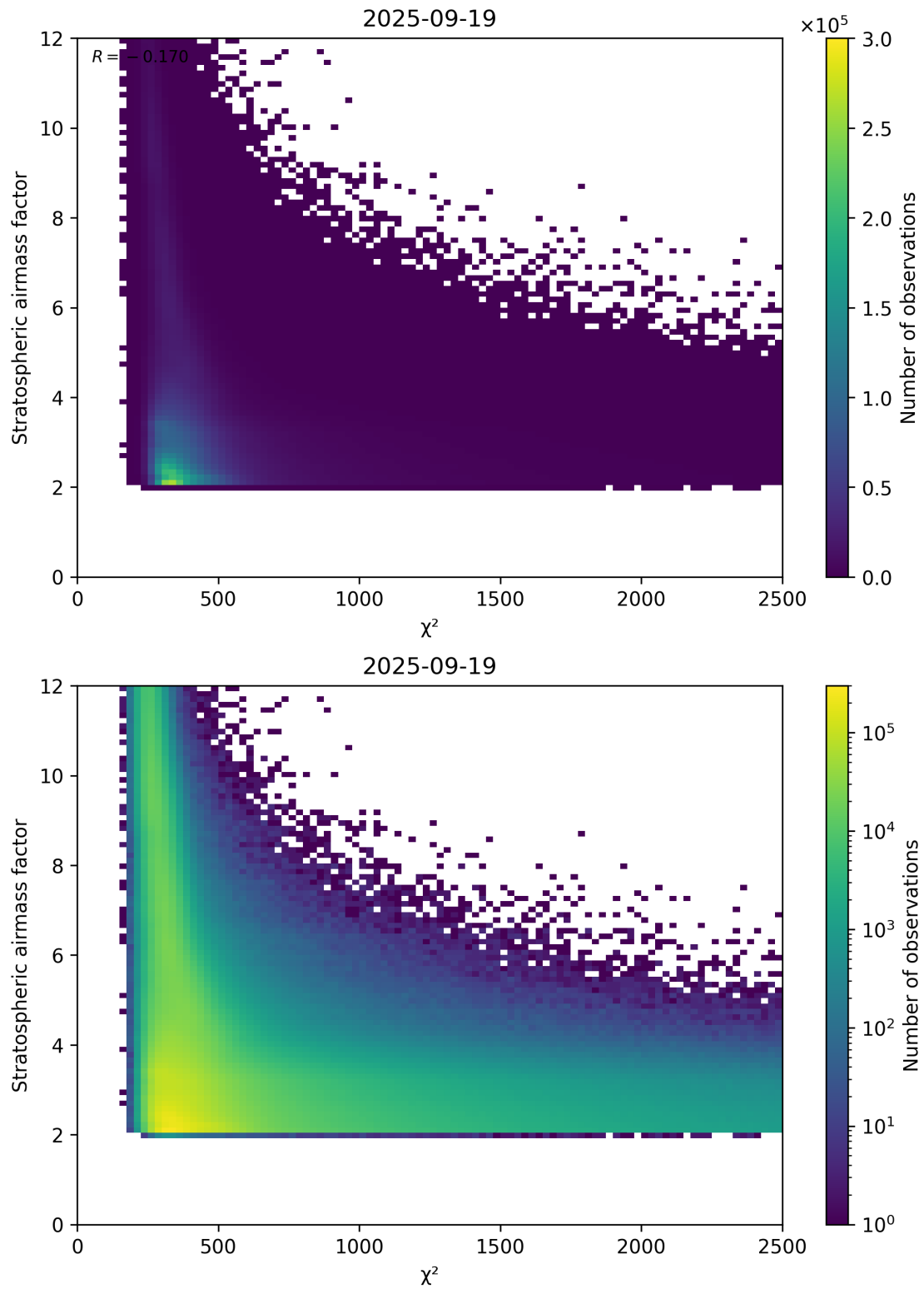
Figure 81: Scatter density plot of “ \chi^2 ” against “Stratospheric airmass factor” for 2025-09-18 to 2025-09-20.
