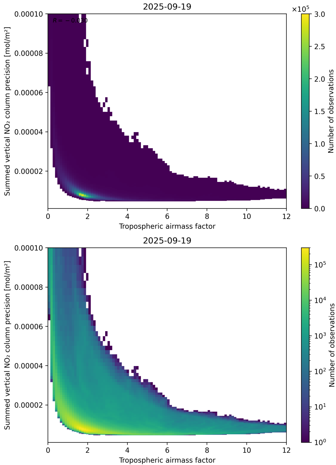
Figure 76: Scatter density plot of “Tropospheric air mass factor” against “Summed vertical NO 2 column precision” for 2025-09-18 to 2025-09-20.
