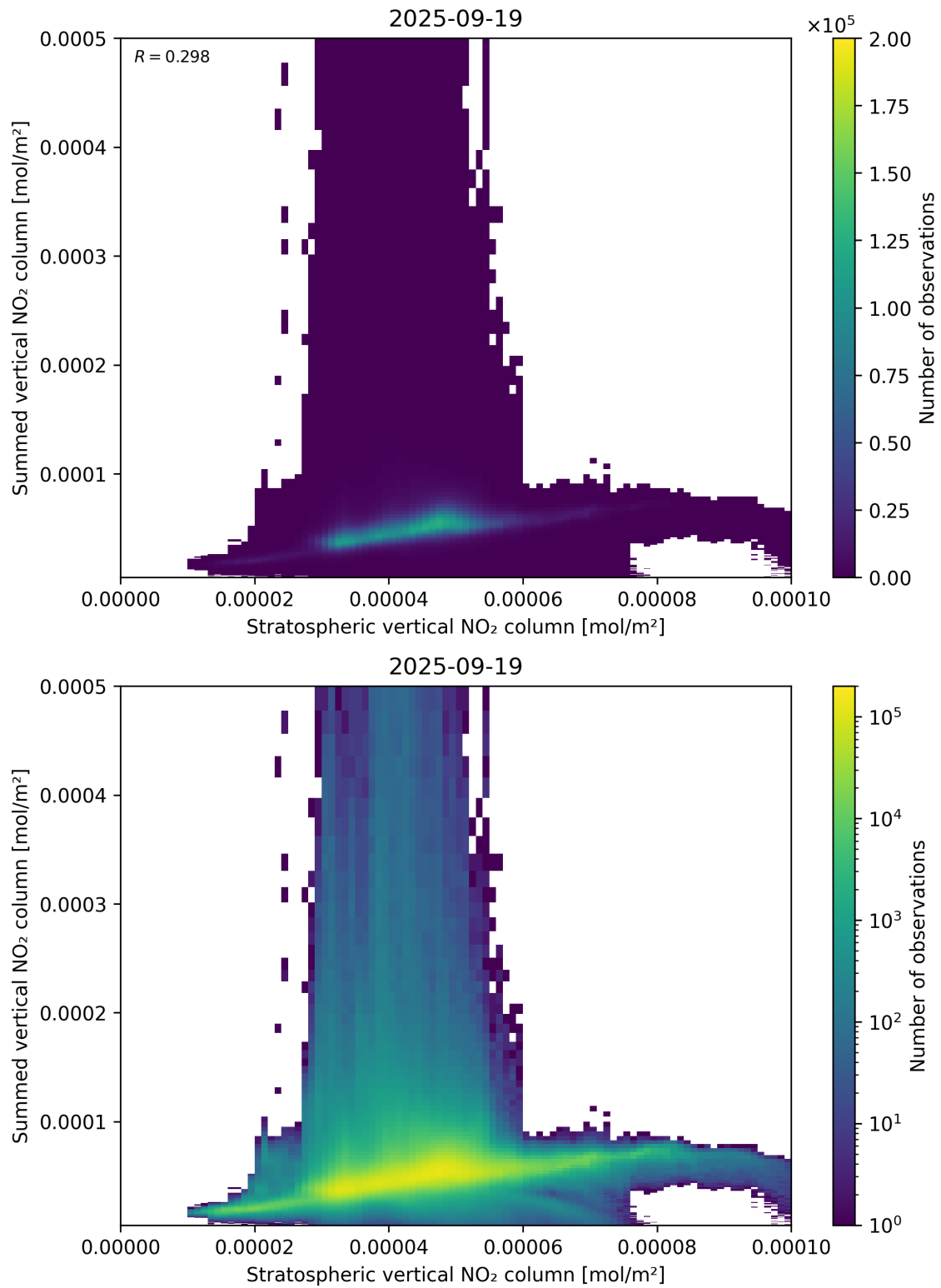
Figure 98: Scatter density plot of “Stratospheric vertical NO 2 column” against “Summed vertical NO 2 column” for 2025-09-18 to 2025-09-20.
