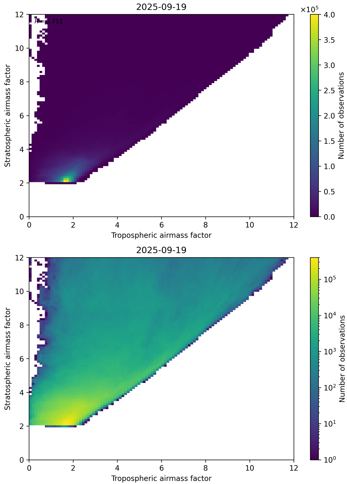
Figure 71: Scatter density plot of “Tropospheric airmass factor” against “Stratospheric airmass factor” for 2025-09-18 to 2025-09-20.
