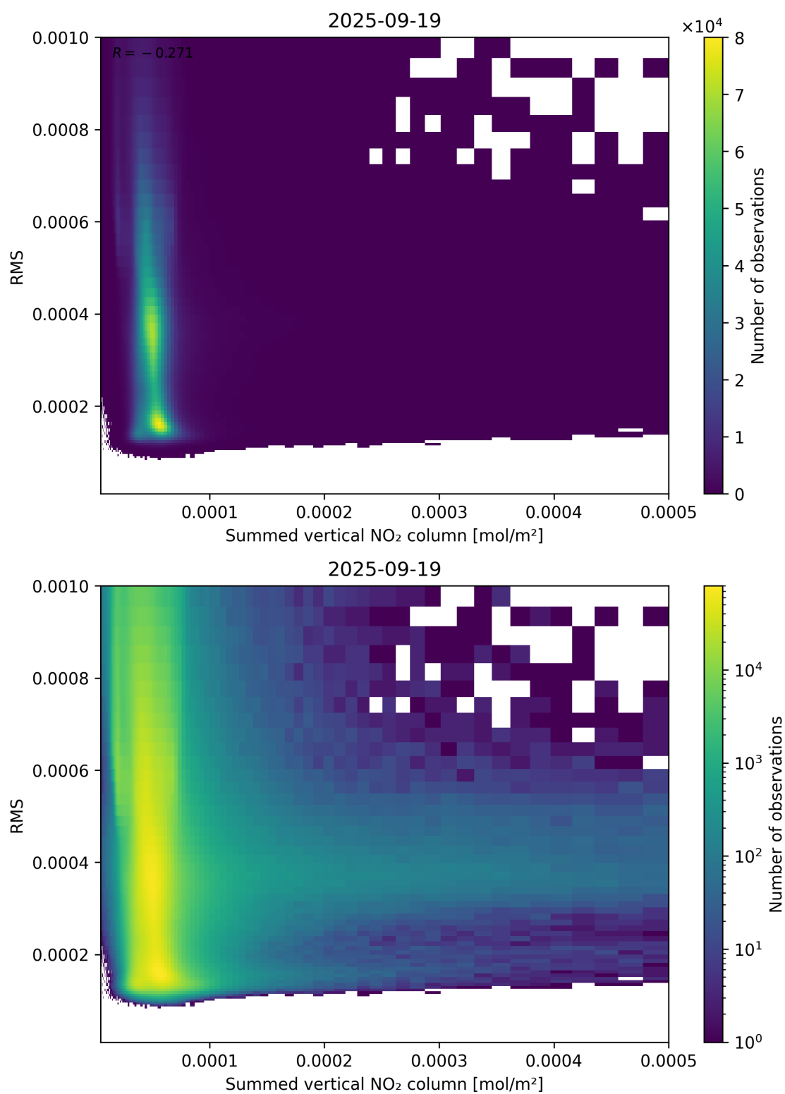
Figure 109: Scatter density plot of “Summed vertical NO 2 column” against “RMS” for 2025-09-18 to 2025-09-20.
