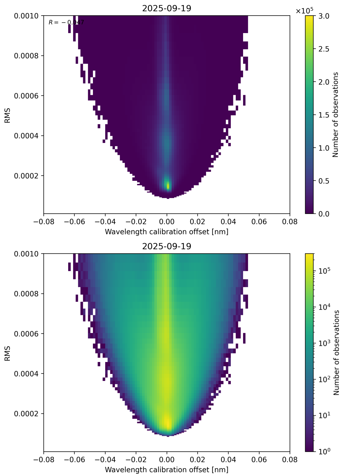
Figure 181: Scatter density plot of “Wavelength calibration offset” against “RMS” for 2025-09-18 to 2025-09-20.
