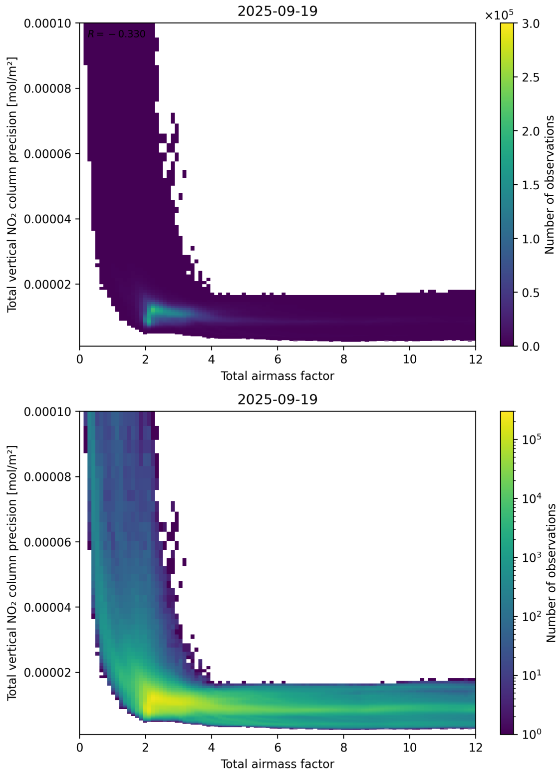
Figure 68: Scatter density plot of “Total airmass factor” against “Total vertical NO 2 column precision” for 2025-09-18 to 2025-09-20.
