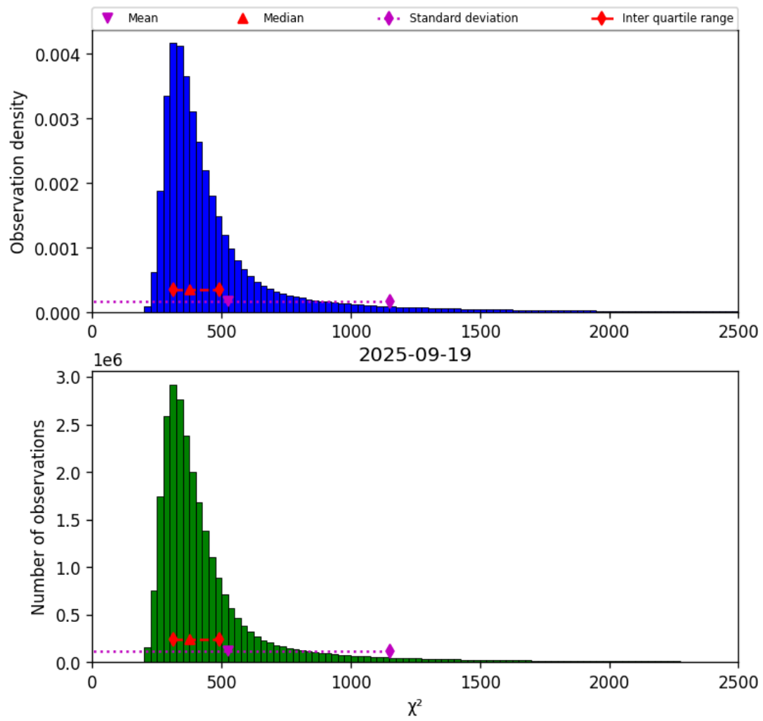
Figure 42: Histogram of “ \chi^2 ” for 2025-09-18 to 2025-09-20
