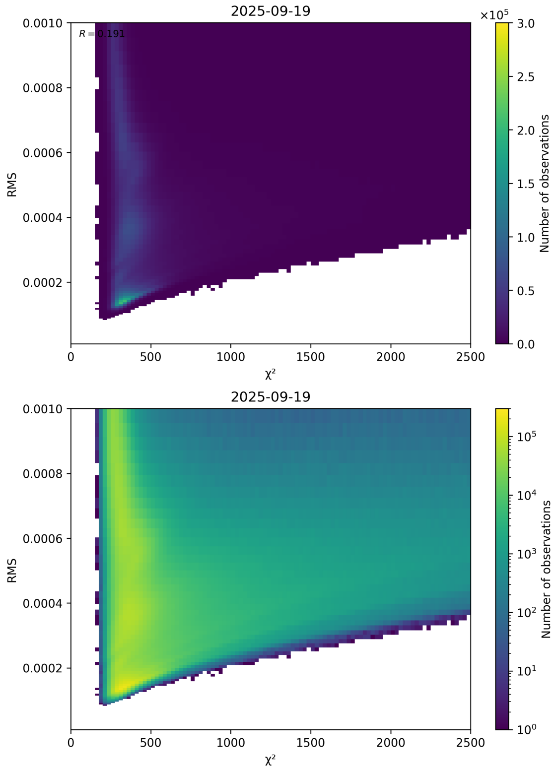
Figure 82: Scatter density plot of “ \chi^2 ” against “RMS” for 2025-09-18 to 2025-09-20.
