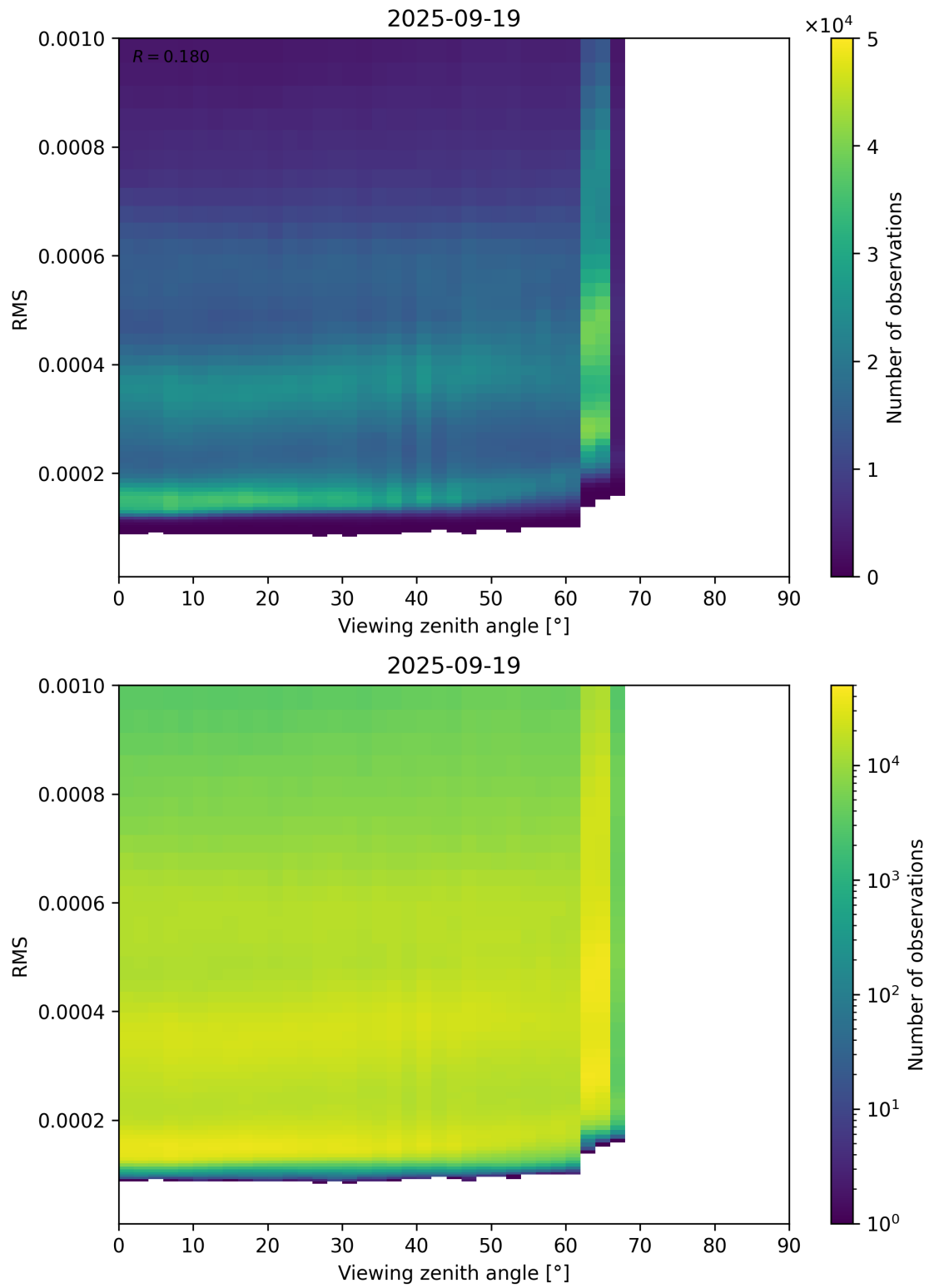
Figure 171: Scatter density plot of “Viewing zenith angle” against “RMS” for 2025-09-18 to 2025-09-20.
