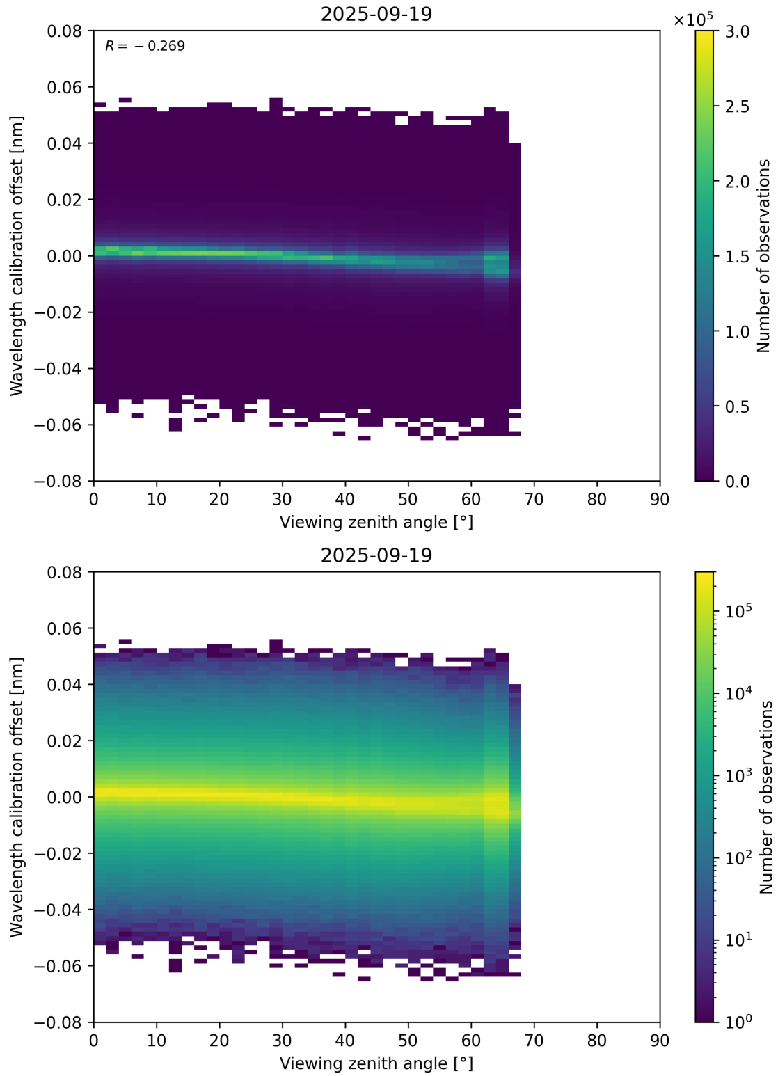
Figure 173: Scatter density plot of “Viewing zenith angle” against “Wavelength calibration offset” for 2025-09-18 to 2025-09-20.
