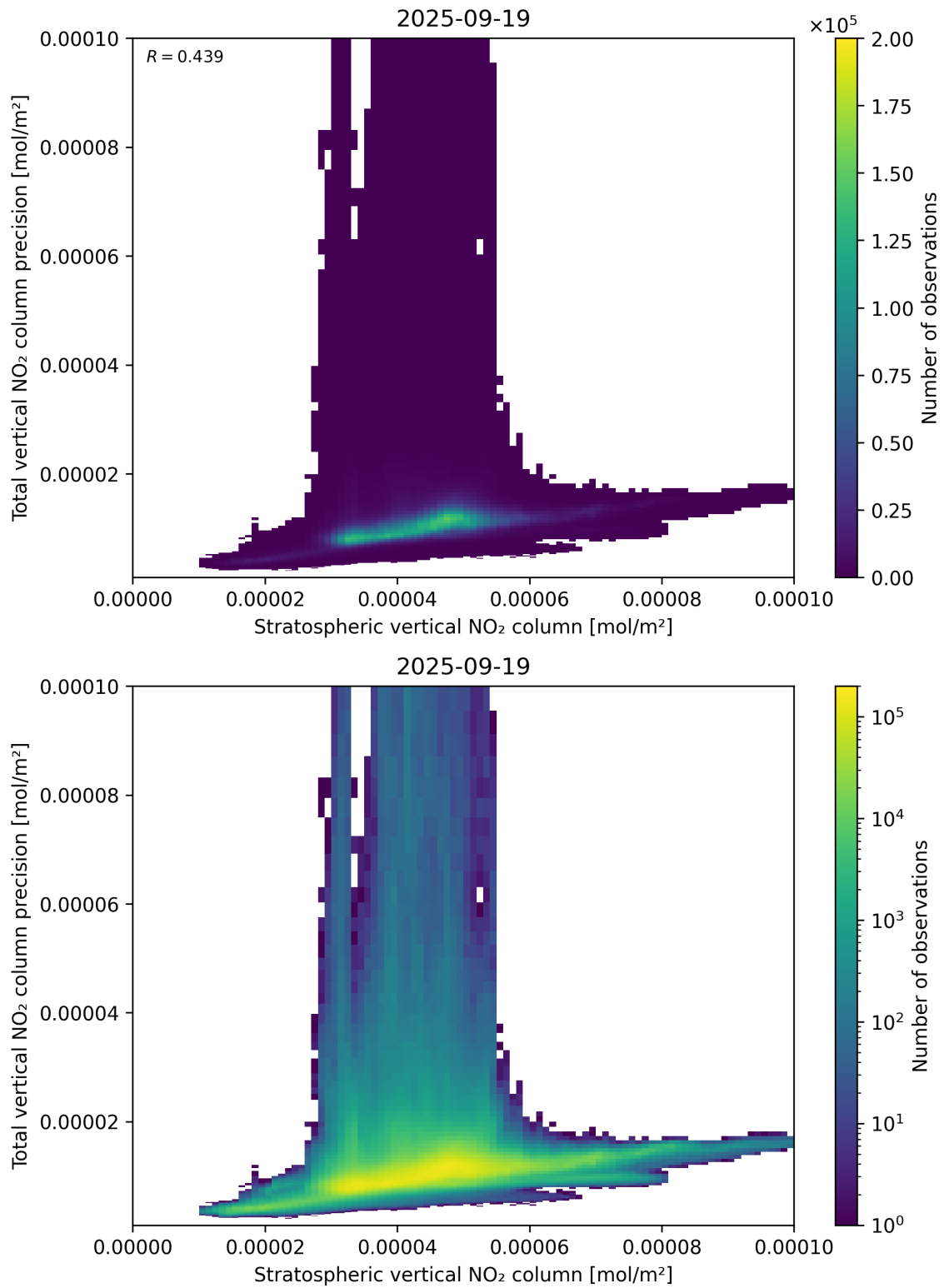
Figure 101: Scatter density plot of “Stratospheric vertical NO 2 column” against “Total vertical NO 2 column precision” for 2025-09-18 to 2025-09-20.
