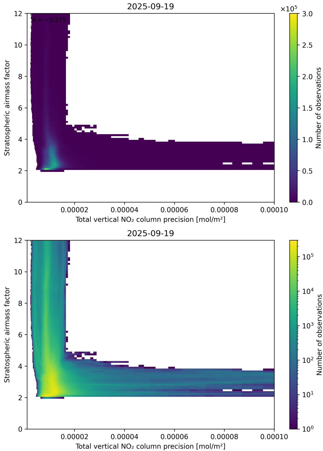
Figure 115: Scatter density plot of “Total vertical NO 2 column precision” against “Stratospheric air mass factor” for 2025-09-18 to 2025-09-20.
