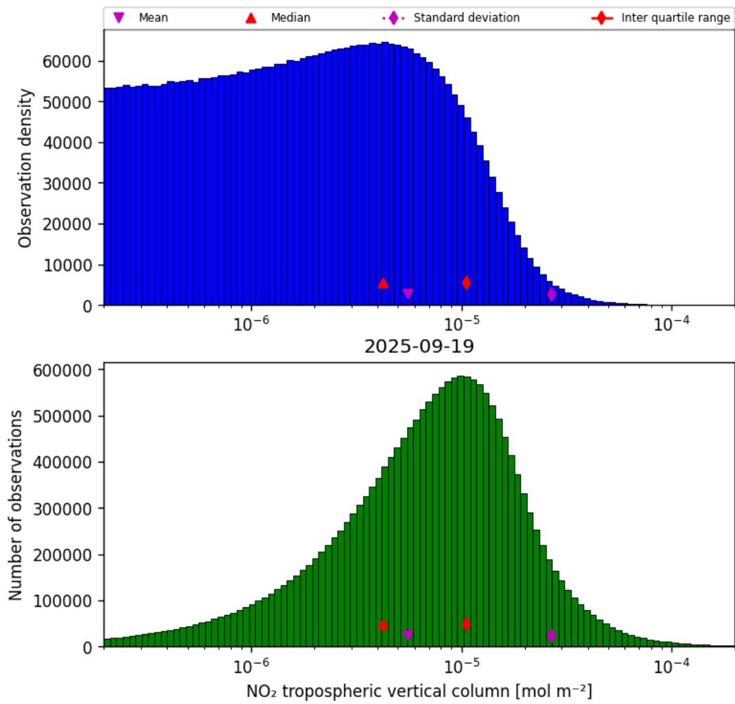
Figure 29: Histogram of “NO 2 tropospheric vertical column” for 2025-09-18 to 2025-09-20
