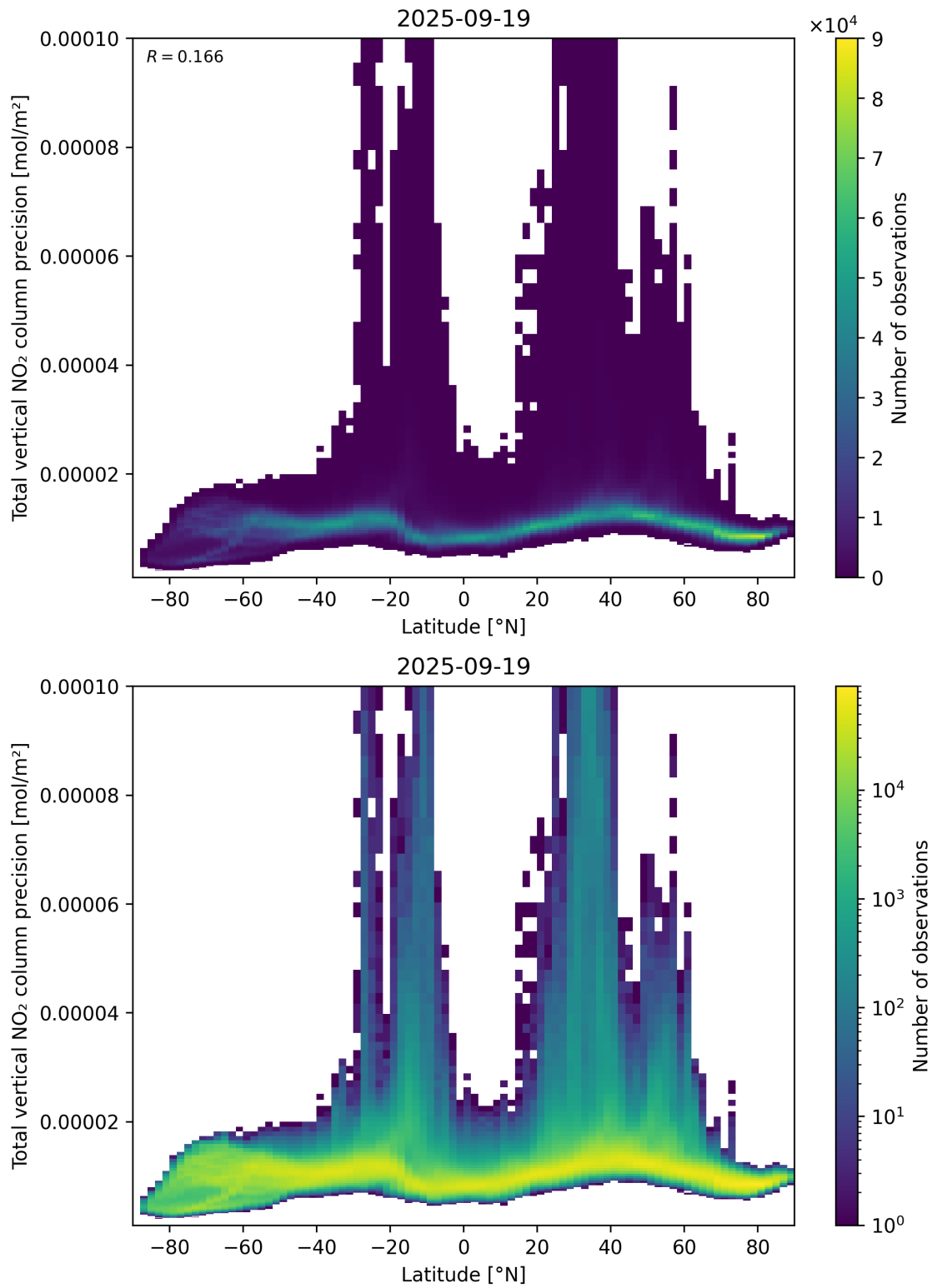
Figure 91: Scatter density plot of “Latitude” against “Total vertical NO 2 column precision” for 2025-09-18 to 2025-09-20.
