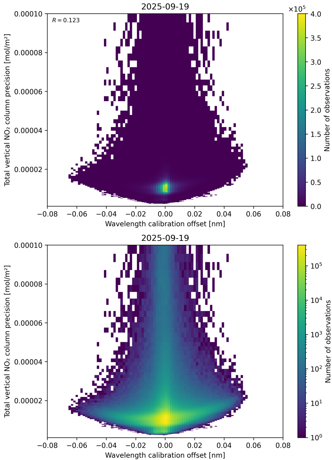
Figure 180: Scatter density plot of “Wavelength calibration offset” against “Total vertical NO 2 column precision” for 2025-09-18 to 2025-09-20.
