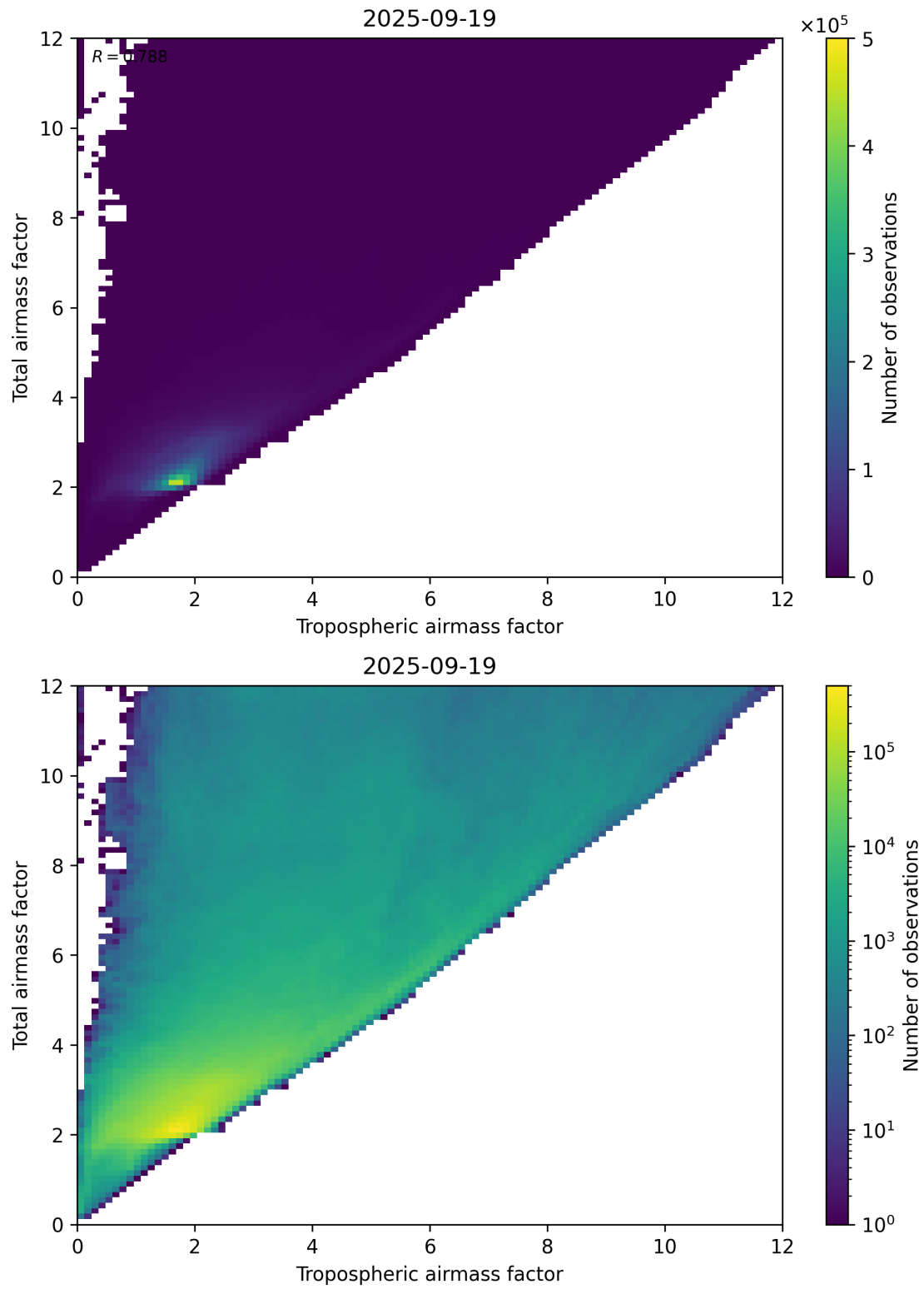
Figure 72: Scatter density plot of “Tropospheric airmass factor” against “Total airmass factor” for 2025-09-18 to 2025-09-20.
