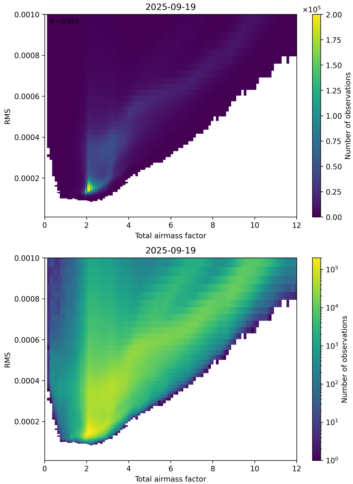
Figure 69: Scatter density plot of “Total airmass factor” against “RMS” for 2025-09-18 to 2025-09-20.
