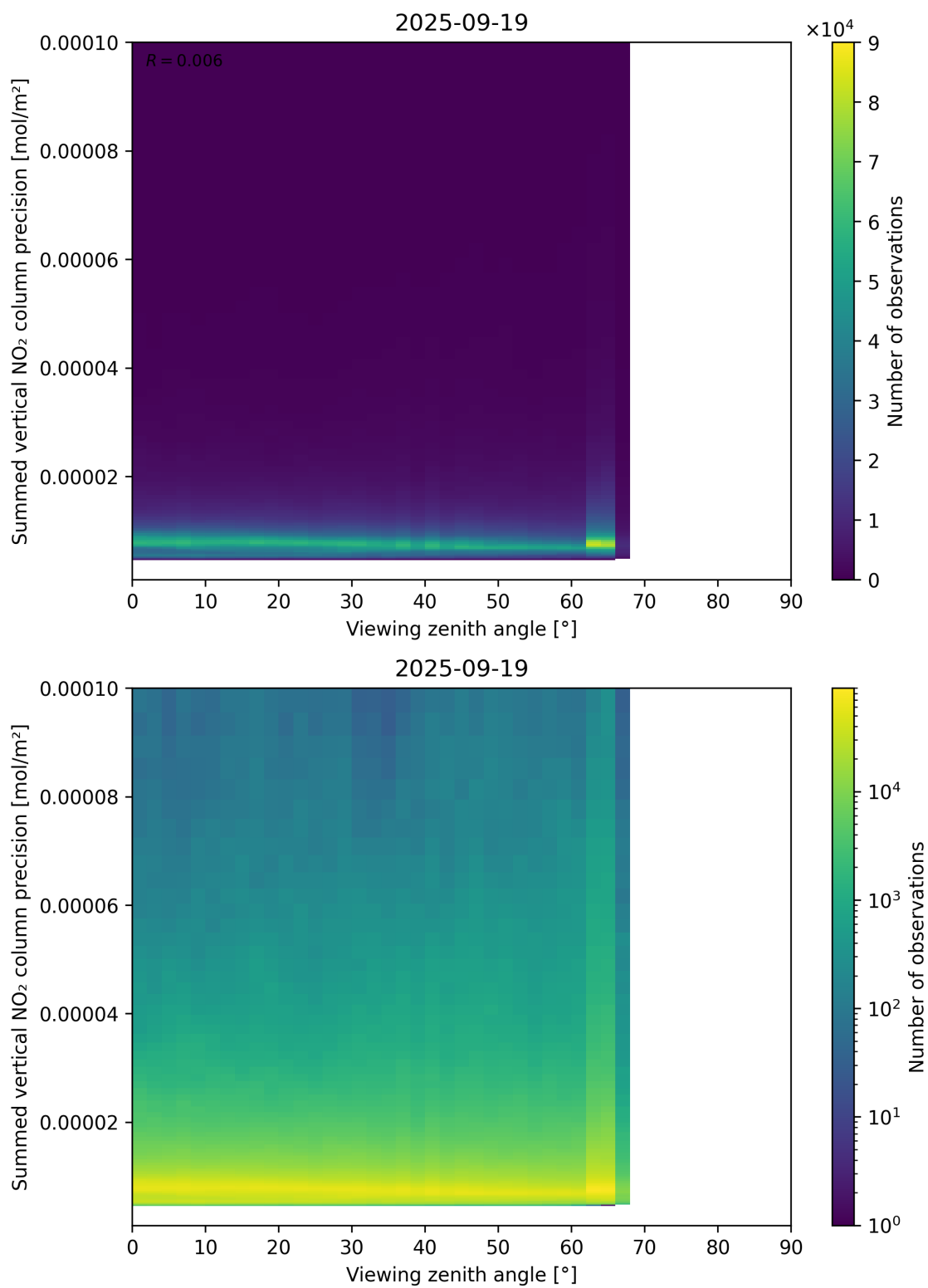
Figure 166: Scatter density plot of “Viewing zenith angle” against “Summed vertical NO 2 column precision” for 2025-09-18 to 2025-09-20.
