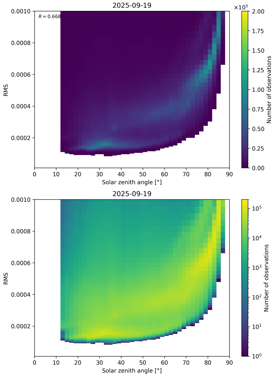
Figure 157: Scatter density plot of “Solar zenith angle” against “RMS” for 2025-09-18 to 2025-09-20.
