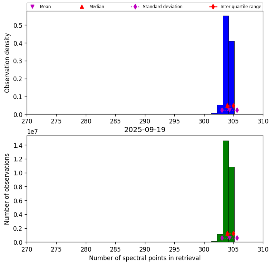
Figure 33: Histogram of “Number of spectral points in retrieval” for 2025-09-18 to 2025-09-20
