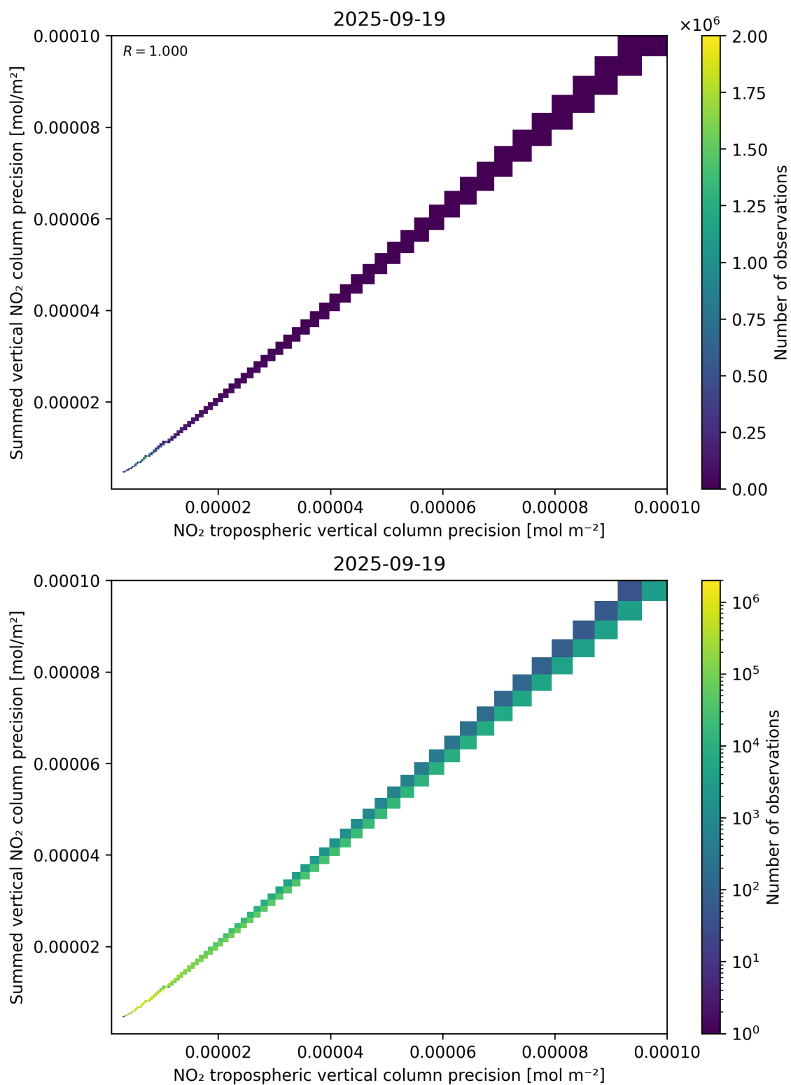
Figure 137: Scatter density plot of “NO 2 tropospheric vertical column precision” against “Summed vertical NO 2 column precision” for 2025-09-18 to 2025-09-20.
