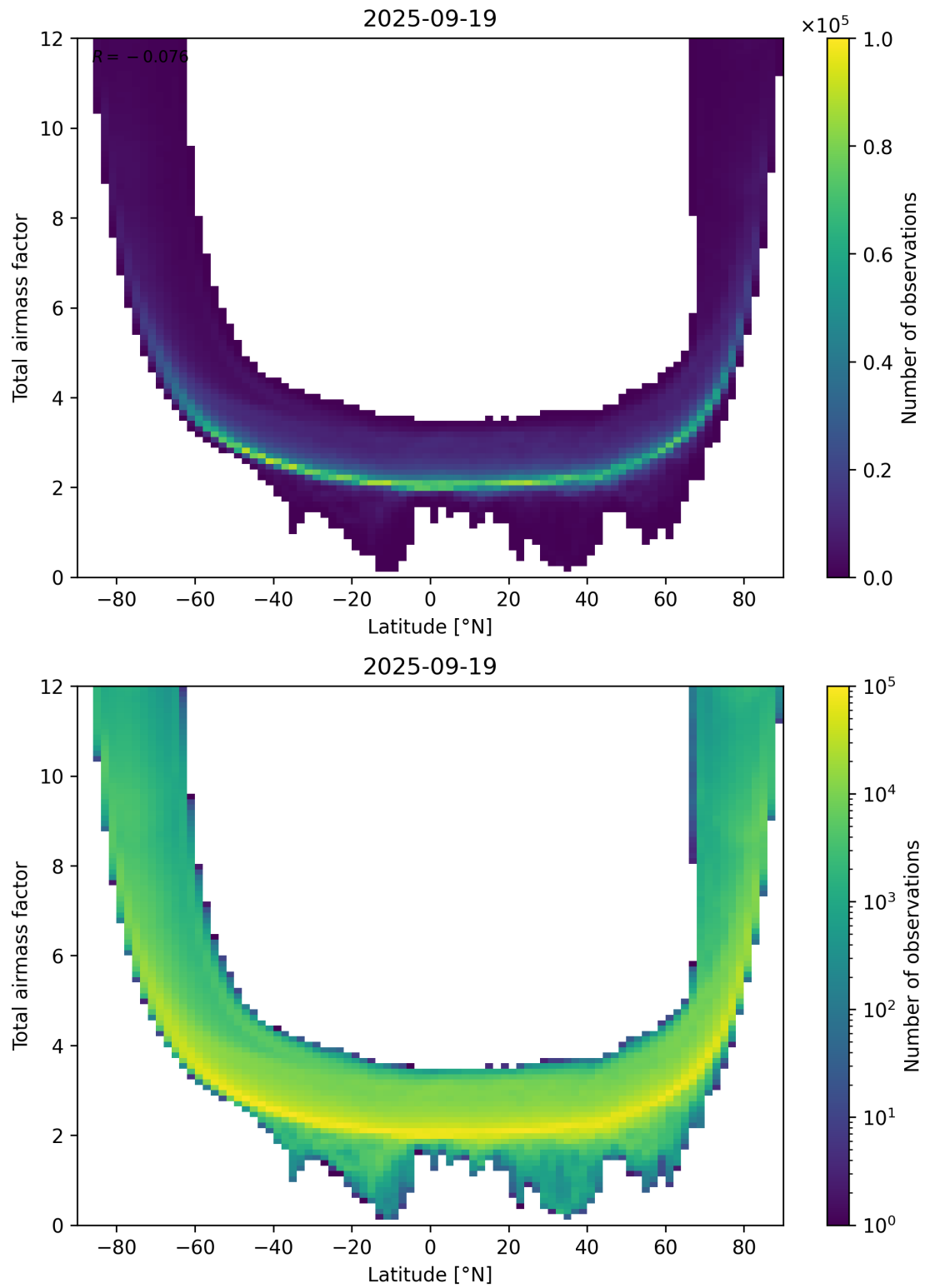
Figure 84: Scatter density plot of “Latitude” against “Total airmass factor” for 2025-09-18 to 2025-09-20.
