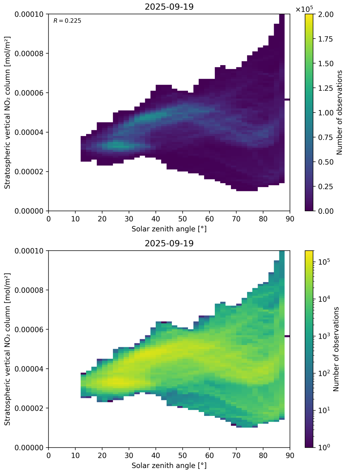
Figure 150: Scatter density plot of “Solar zenith angle” against “Stratospheric vertical NO 2 column” for 2025-09-18 to 2025-09-20.
