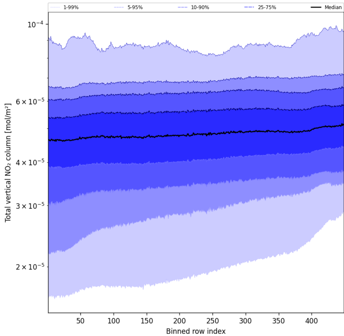
Figure 55: Along track statistics of “Total vertical NO 2 column” for 2025-09-18 to 2025-09-20
