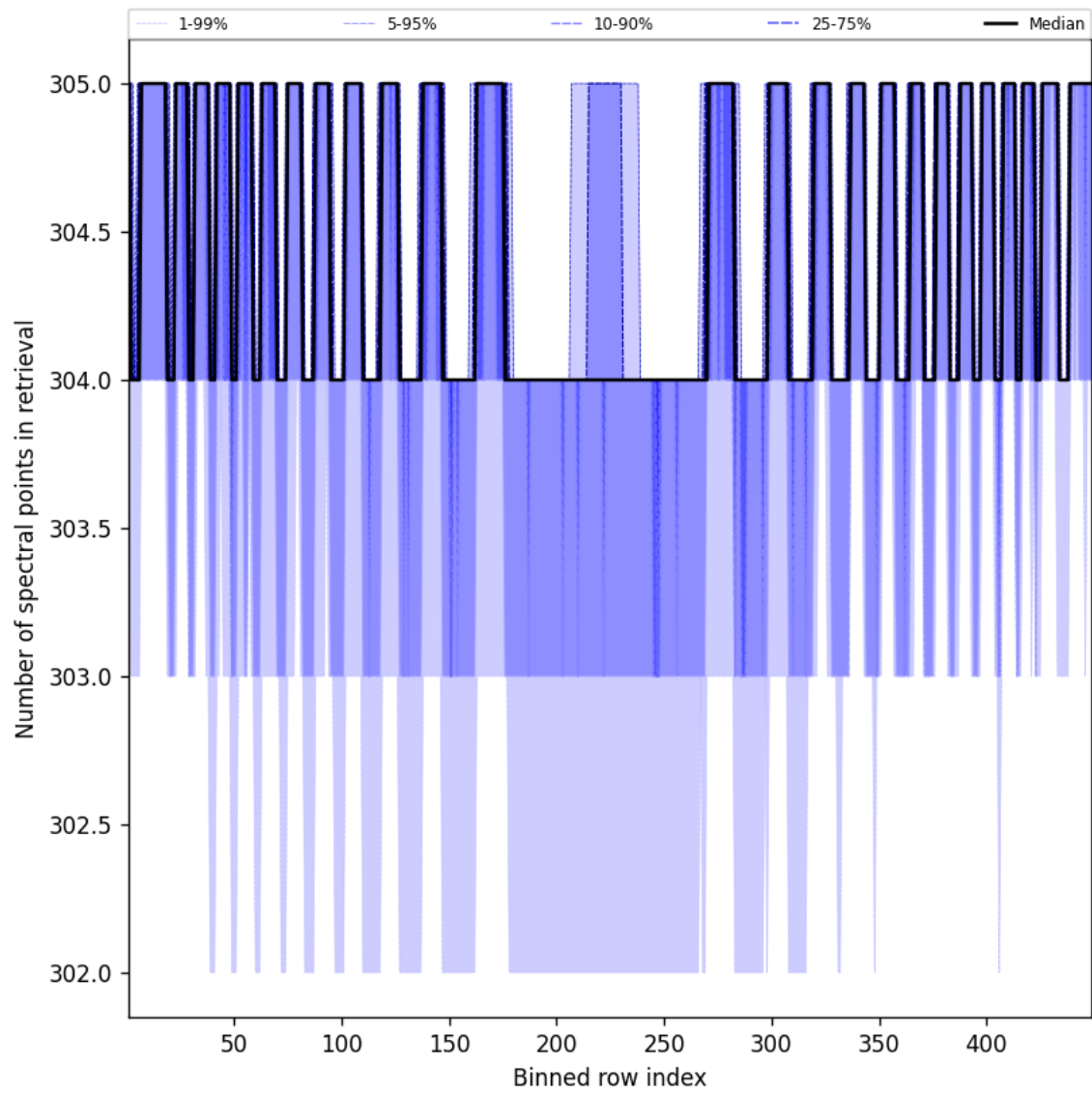
Figure 50: Along track statistics of “Number of spectral points in retrieval” for 2025-09-18 to 2025-09-20
