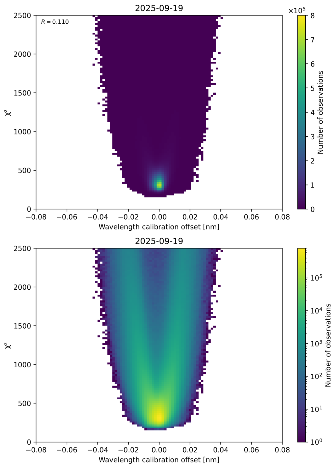
Figure 175: Scatter density plot of “Wavelength calibration offset” against “ \chi^2 ” for 2025-09-18 to 2025-09-20.
