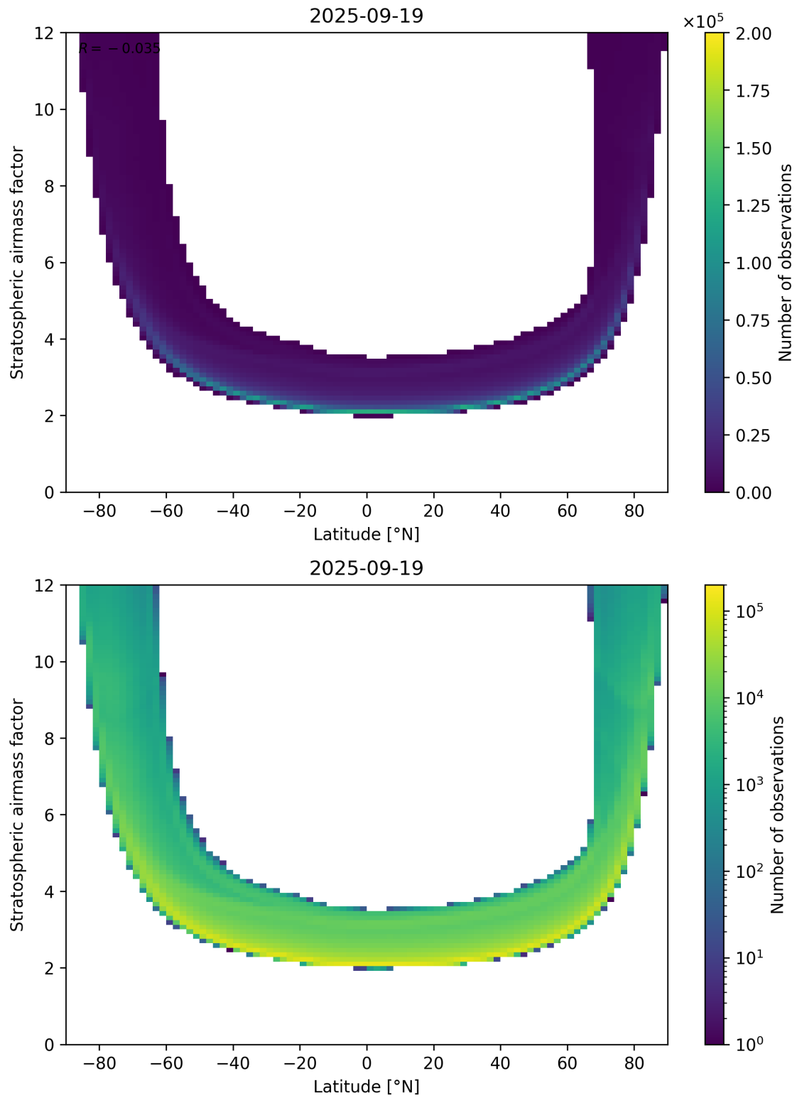
Figure 83: Scatter density plot of “Latitude” against “Stratospheric airmass factor” for 2025-09-18 to 2025-09-20.
