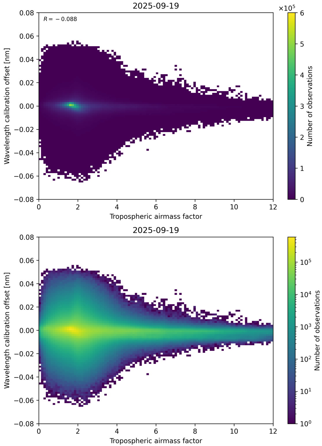
Figure 80: Scatter density plot of “Tropospheric airmass factor” against “Wavelength calibration offset” for 2025-09-18 to 2025-09-20.
