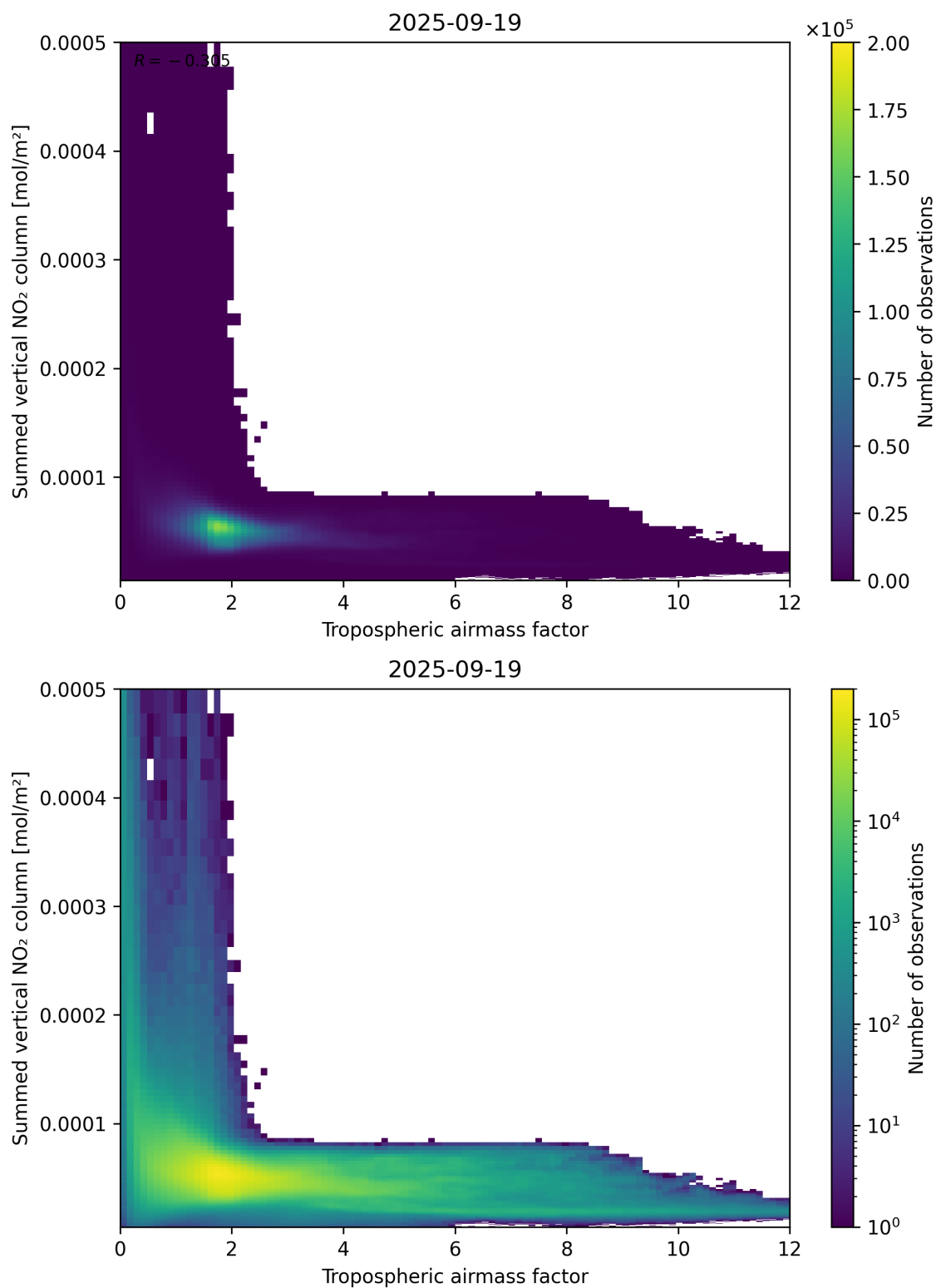
Figure 75: Scatter density plot of “Tropospheric airmass factor” against “Summed vertical NO 2 column” for 2025-09-18 to 2025-09-20.
