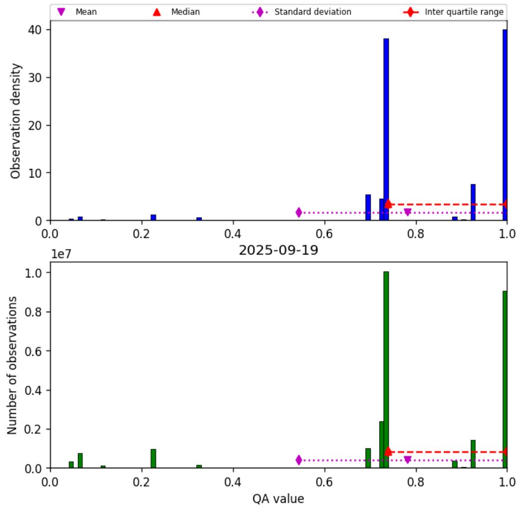
Figure 28: Histogram of “QA value” for 2025-09-18 to 2025-09-20
