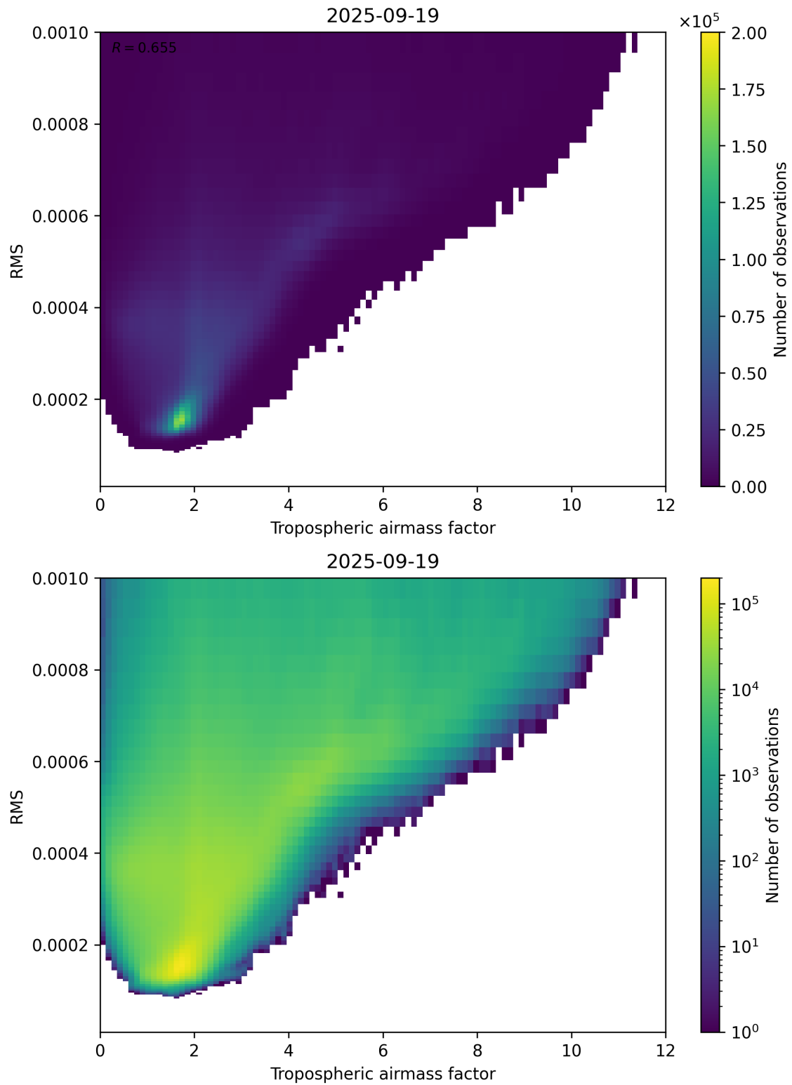
Figure 79: Scatter density plot of “Tropospheric airmass factor” against “RMS” for 2025-09-18 to 2025-09-20.
