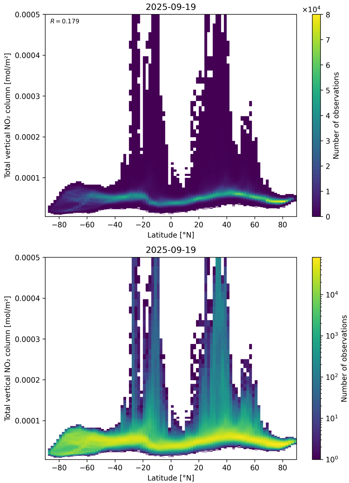
Figure 90: Scatter density plot of “Latitude” against “Total vertical NO 2 column” for 2025-09-18 to 2025-09-20.
