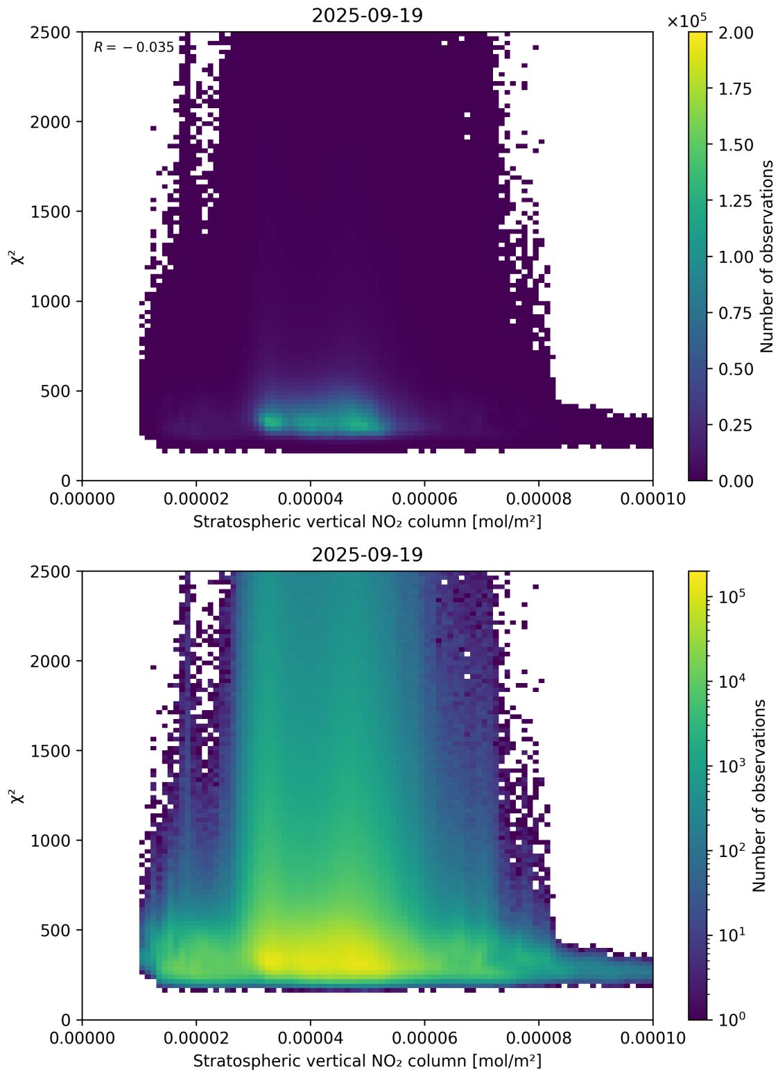
Figure 97: Scatter density plot of “Stratospheric vertical NO 2 column” against “ \chi^2 ” for 2025-09-18 to 2025-09-20.
