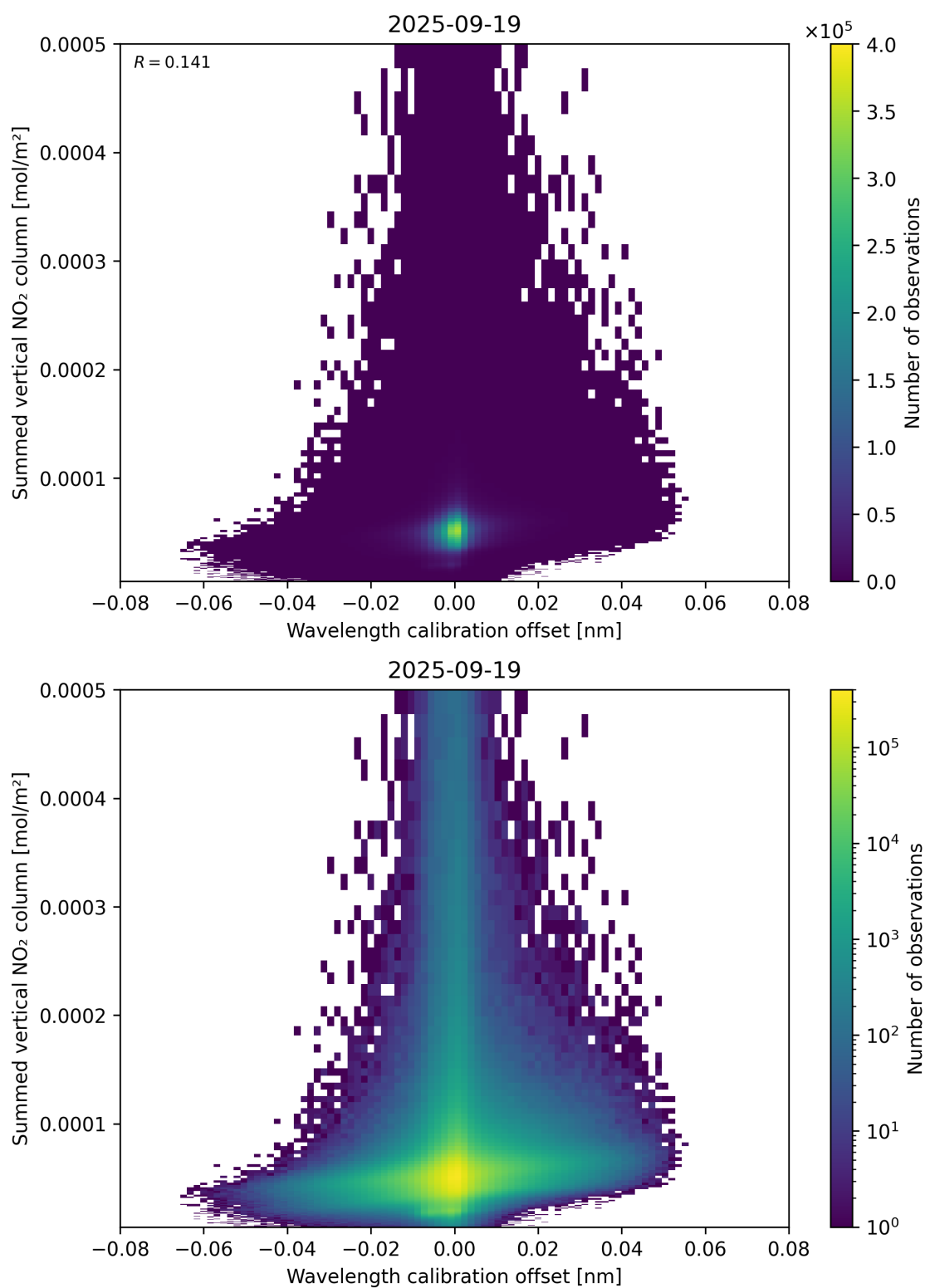
Figure 177: Scatter density plot of “Wavelength calibration offset” against “Summed vertical NO 2 column” for 2025-09-18 to 2025-09-20.
