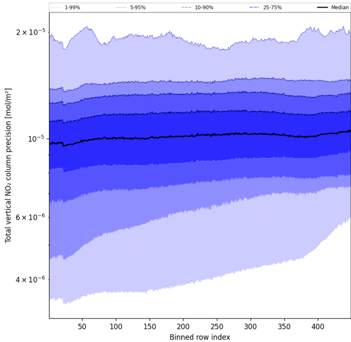
Figure 56: Along track statistics of “Total vertical NO 2 column precision” for 2025-09-18 to 2025-09-20
