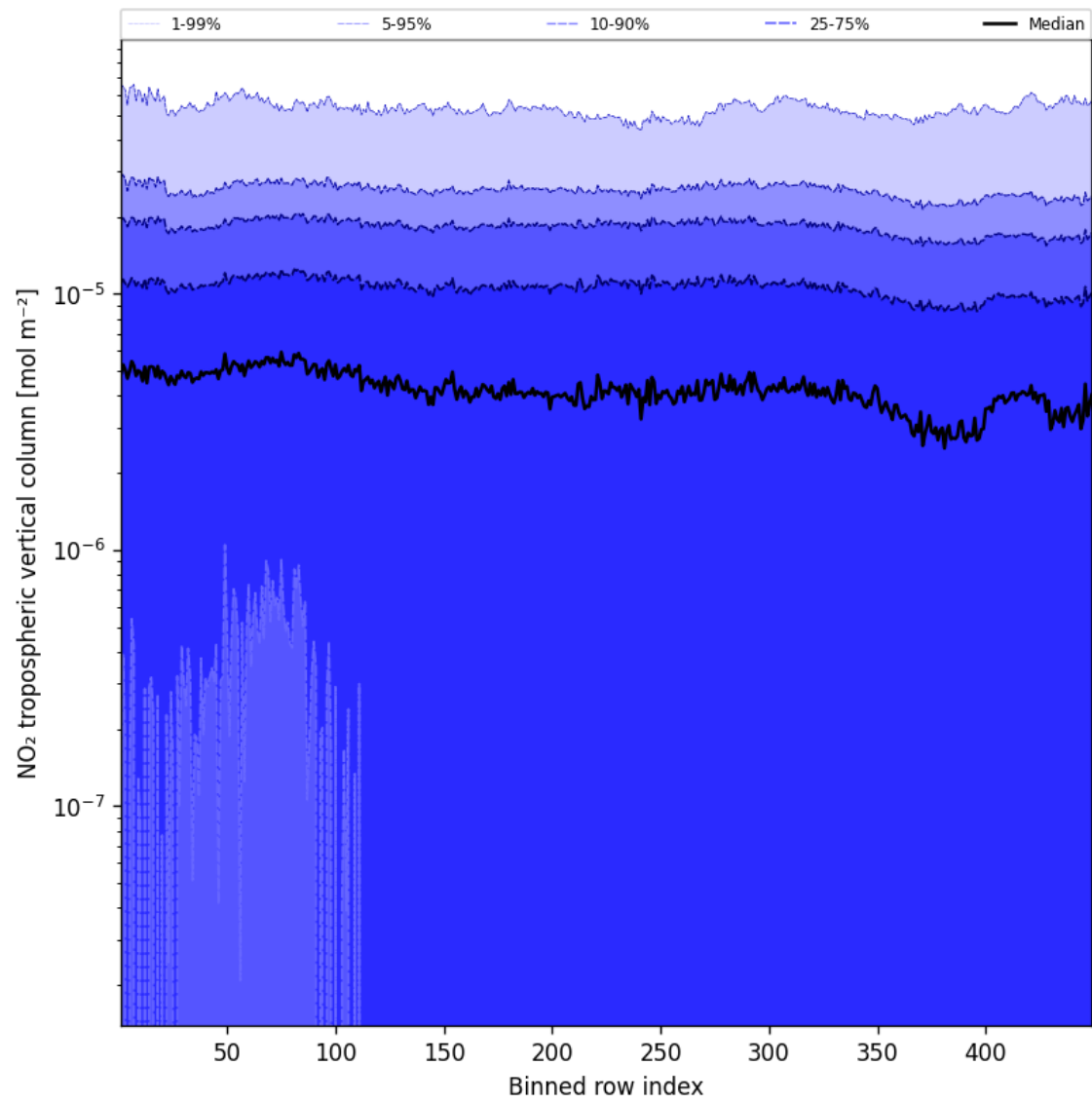
Figure 46: Along track statistics of “NO 2 tropospheric vertical column” for 2025-09-18 to 2025-09-20
