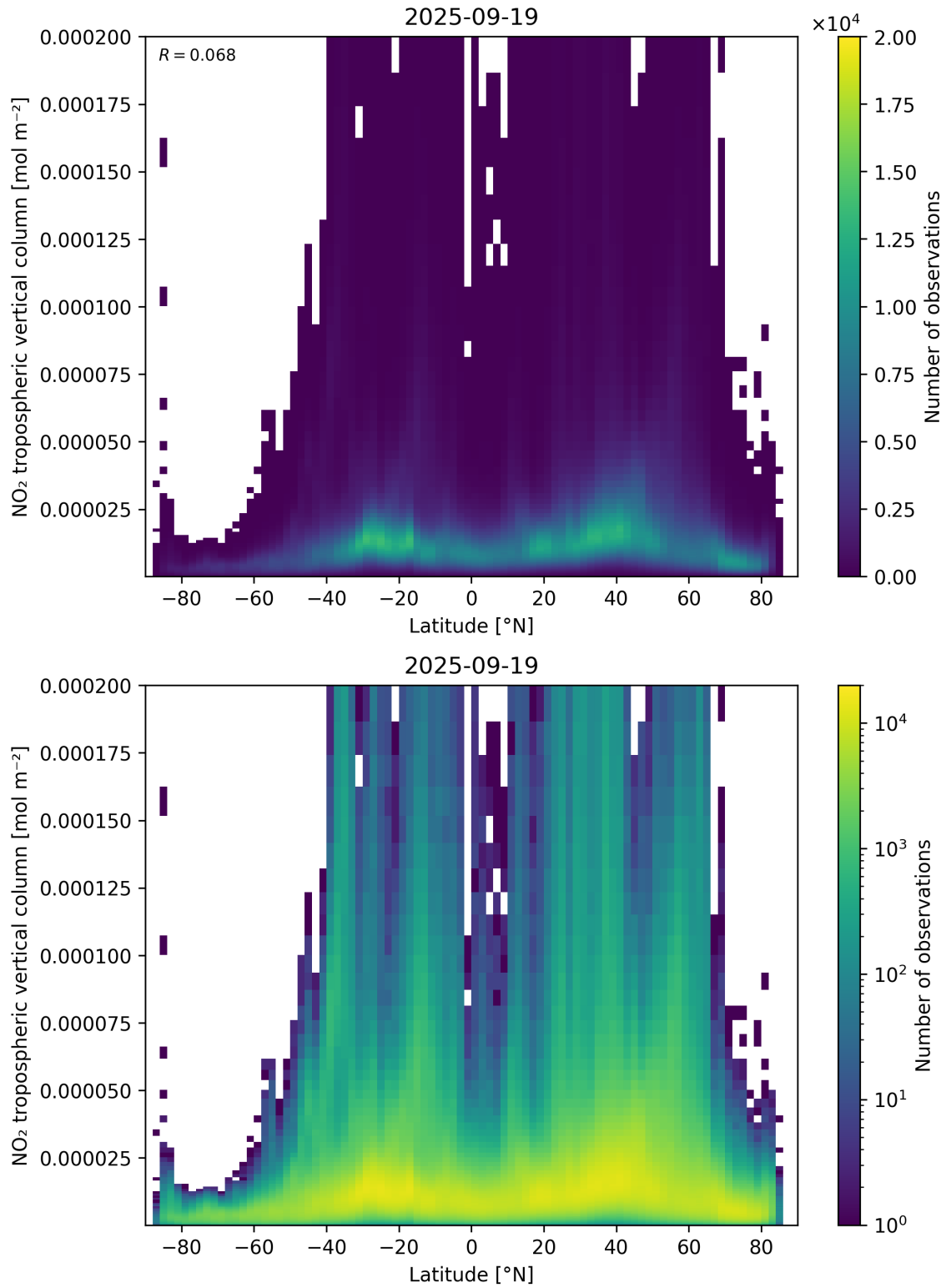
Figure 92: Scatter density plot of “Latitude” against “NO 2 tropospheric vertical column” for 2025-09-18 to 2025-09-20.
