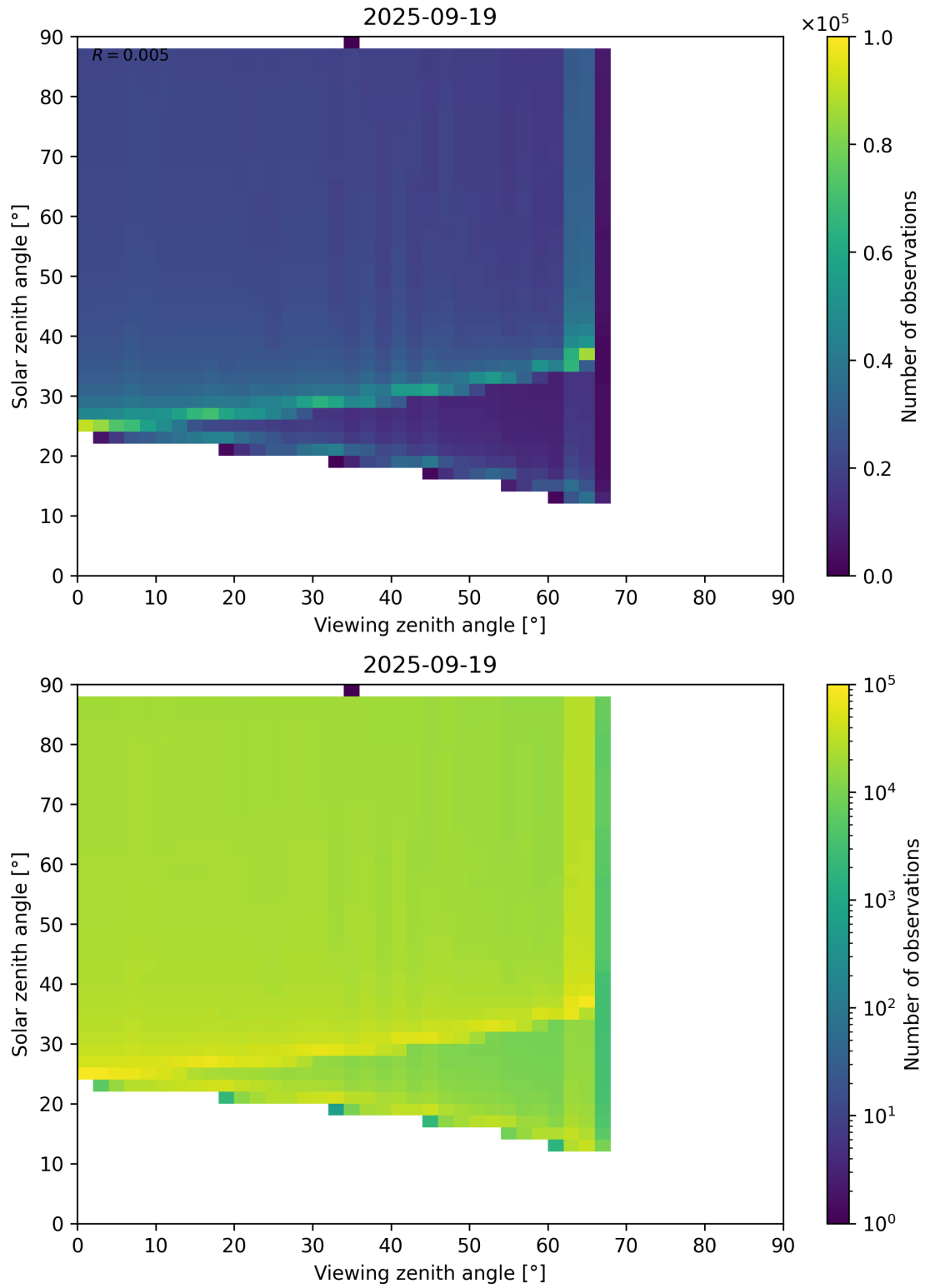
Figure 172: Scatter density plot of “Viewing zenith angle” against “Solar zenith angle” for 2025-09-18 to 2025-09-20.
