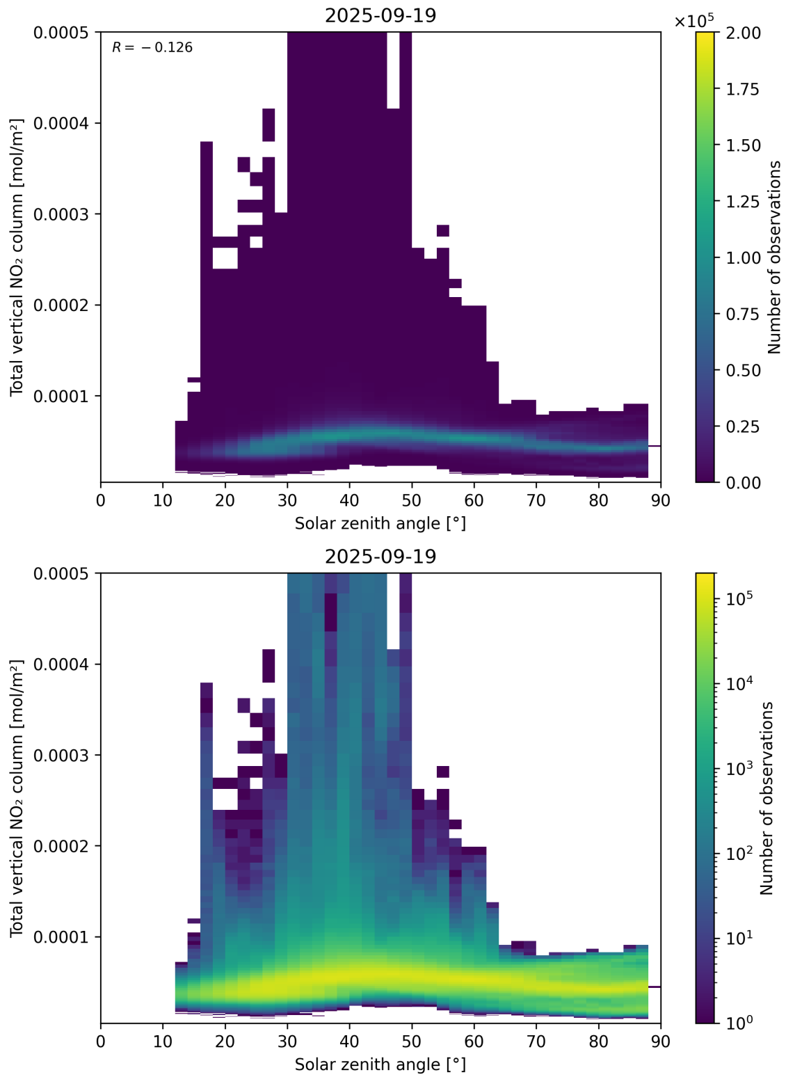
Figure 153: Scatter density plot of “Solar zenith angle” against “Total vertical NO 2 column” for 2025-09-18 to 2025-09-20.
