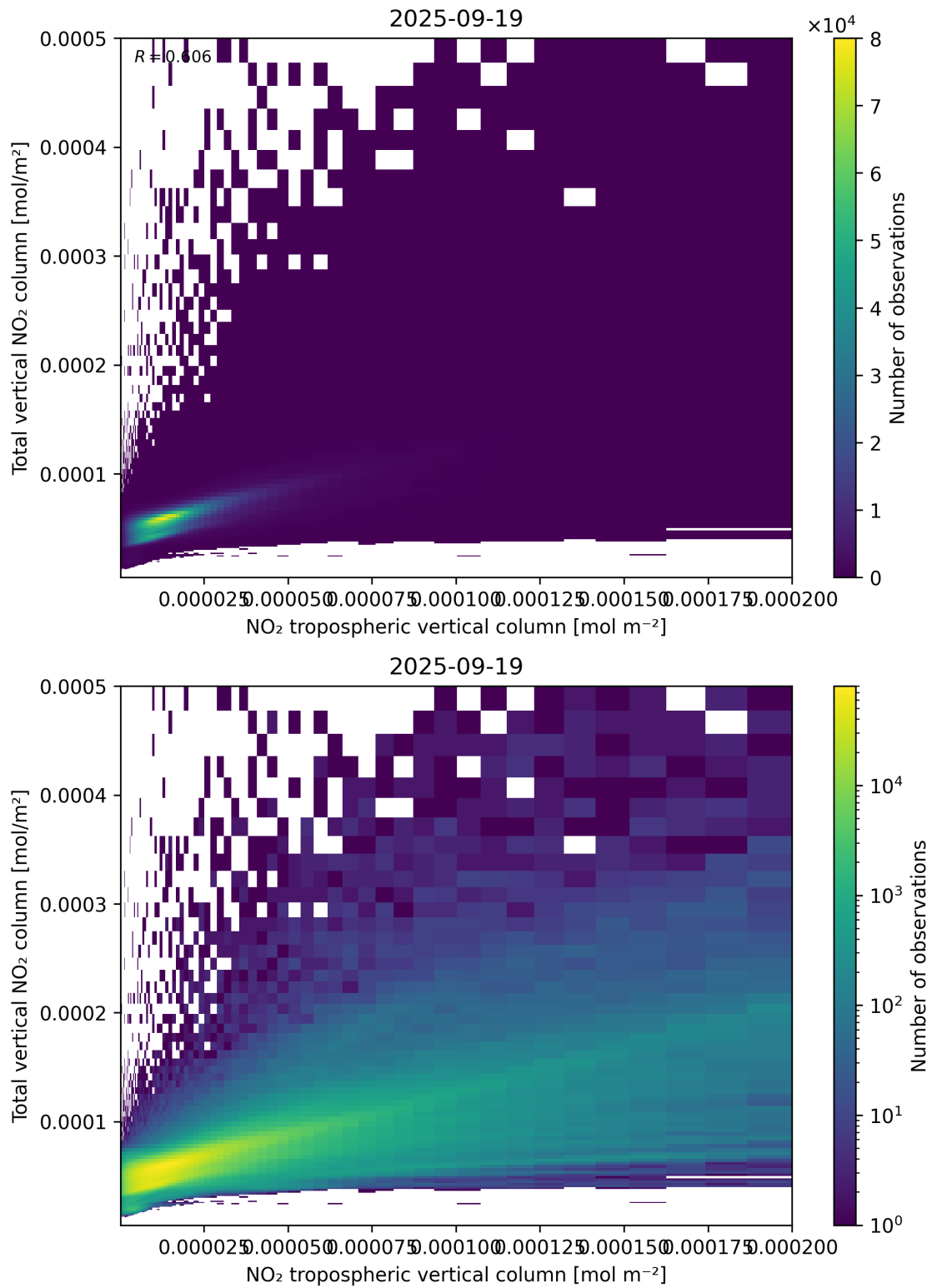
Figure 128: Scatter density plot of “NO 2 tropospheric vertical column” against “Total vertical NO 2 column” for 2025-09-18 to 2025-09-20.
