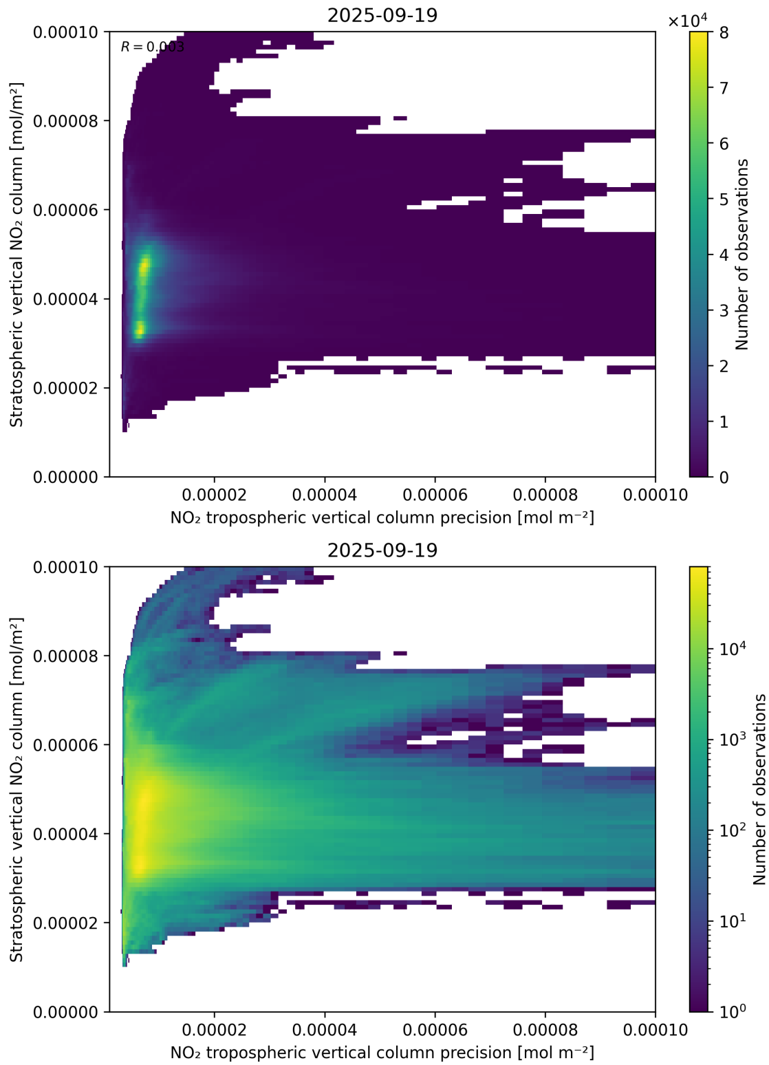
Figure 135: Scatter density plot of “NO 2 tropospheric vertical column precision” against “Stratospheric vertical NO 2 column” for 2025-09-18 to 2025-09-20.
