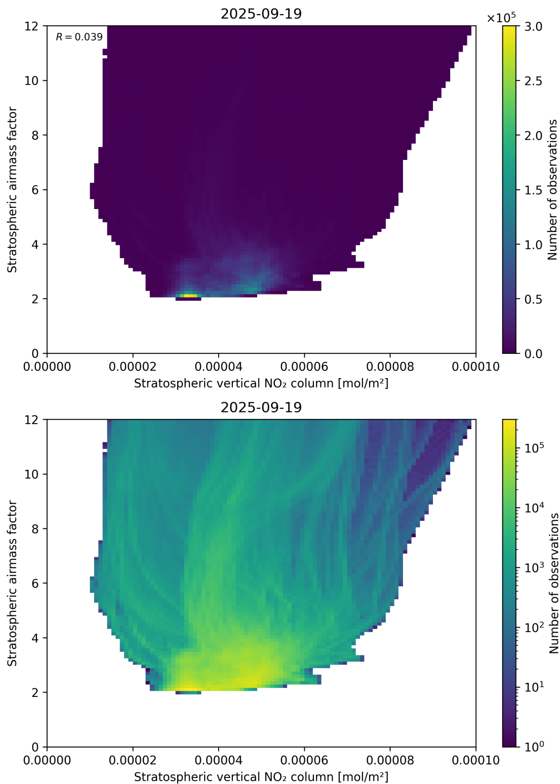
Figure 96: Scatter density plot of “Stratospheric vertical NO 2 column” against “Stratospheric airmass factor” for 2025-09-18 to 2025-09-20.
