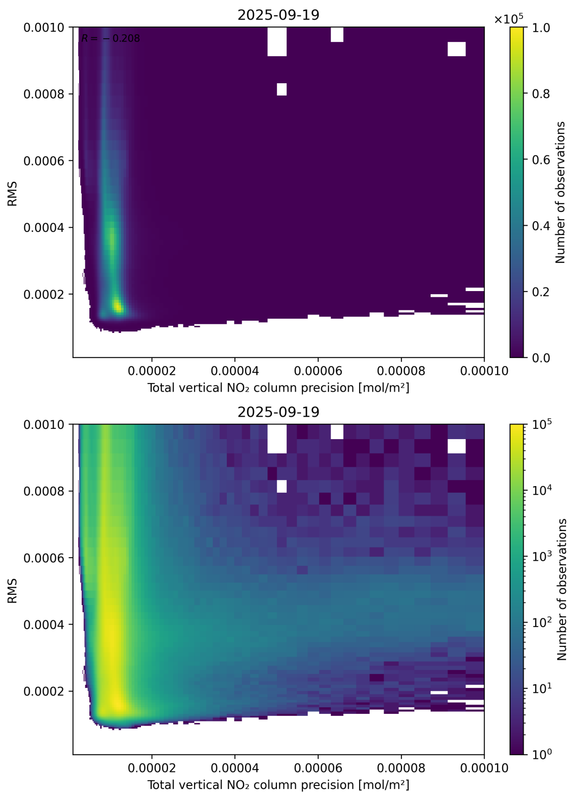
Figure 119: Scatter density plot of “Total vertical NO 2 column precision” against “RMS” for 2025-09-18 to 2025-09-20.
