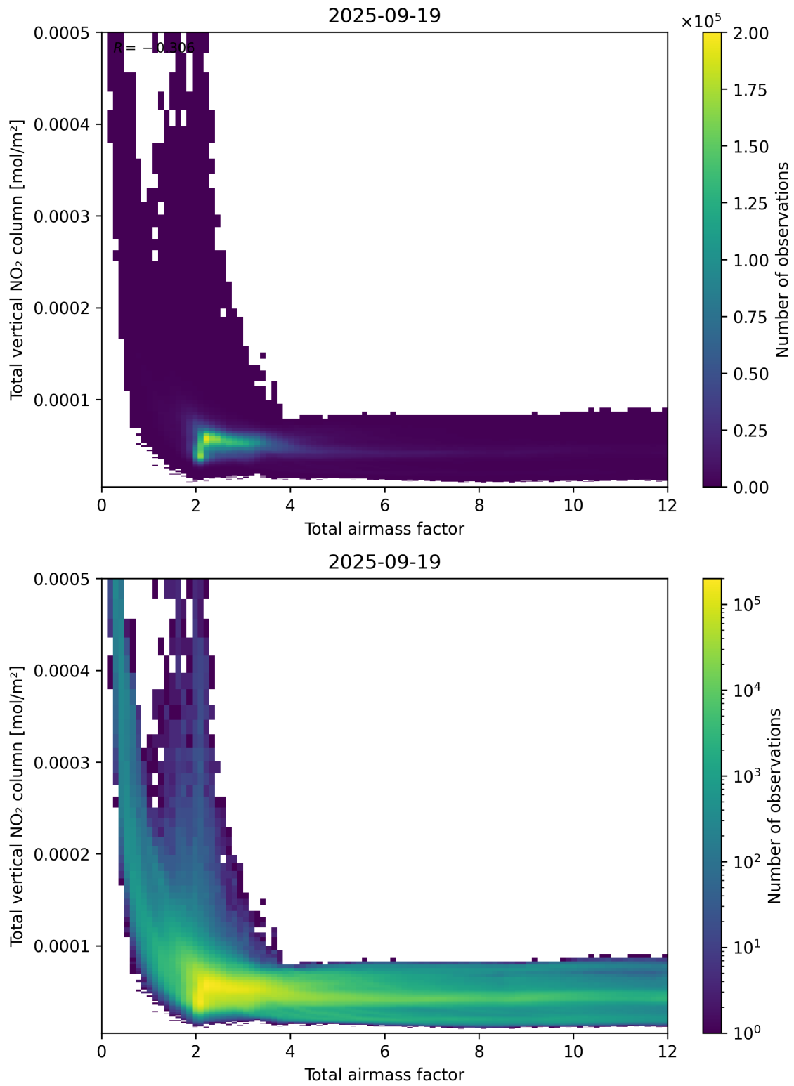
Figure 67: Scatter density plot of “Total airmass factor” against “Total vertical NO 2 column” for 2025-09-18 to 2025-09-20.
