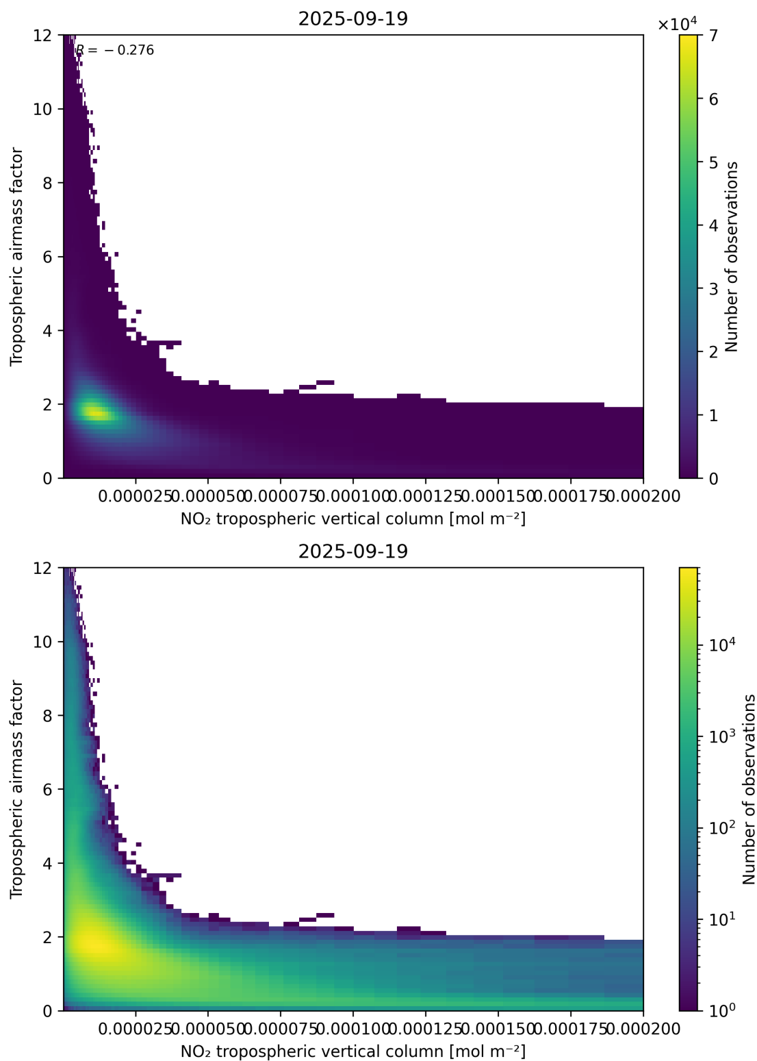
Figure 123: Scatter density plot of “NO 2 tropospheric vertical column” against “Tropospheric air mass factor” for 2025-09-18 to 2025-09-20.
