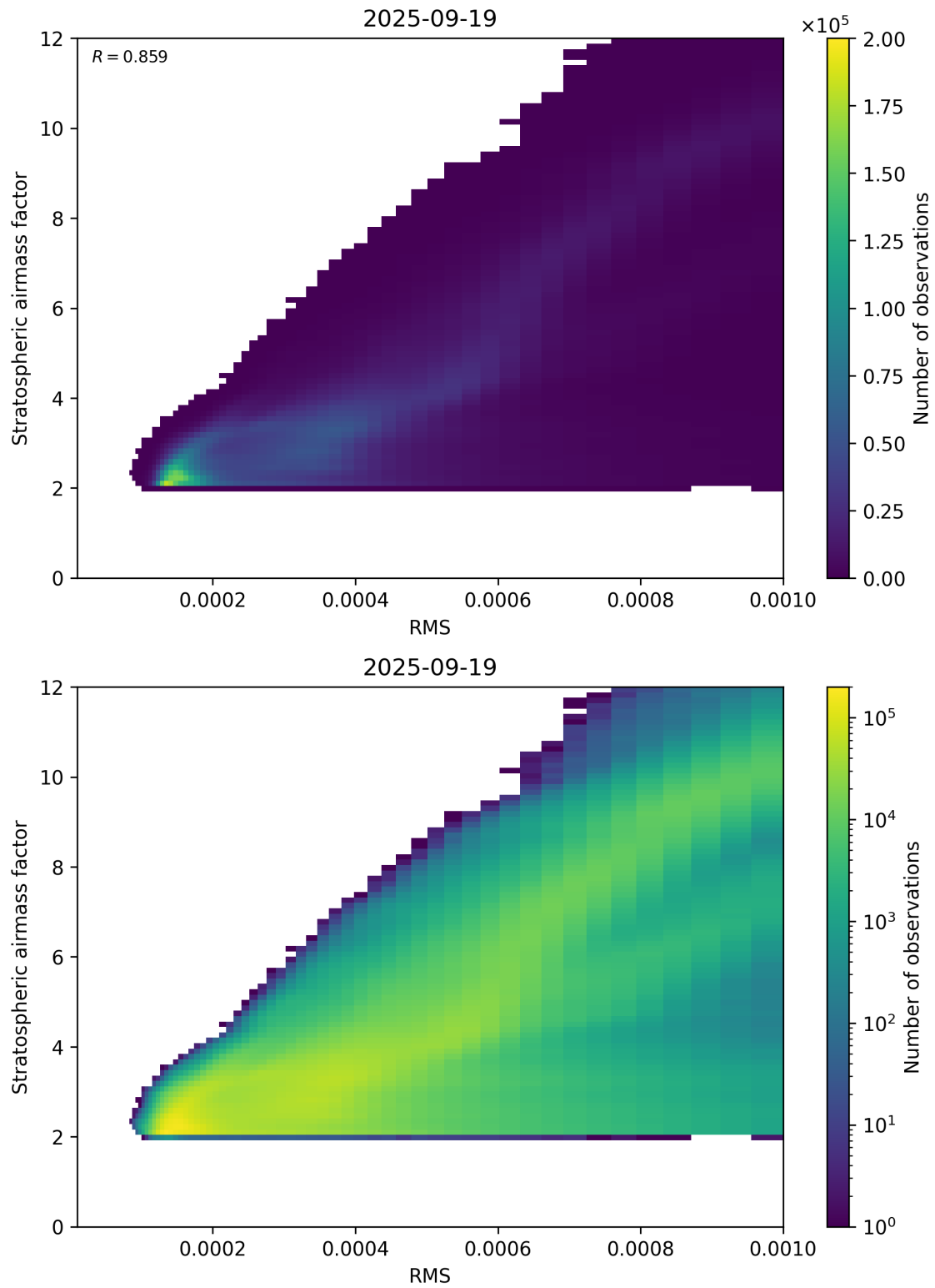
Figure 144: Scatter density plot of “RMS” against “Stratospheric airmass factor” for 2025-09-18 to 2025-09-20.
