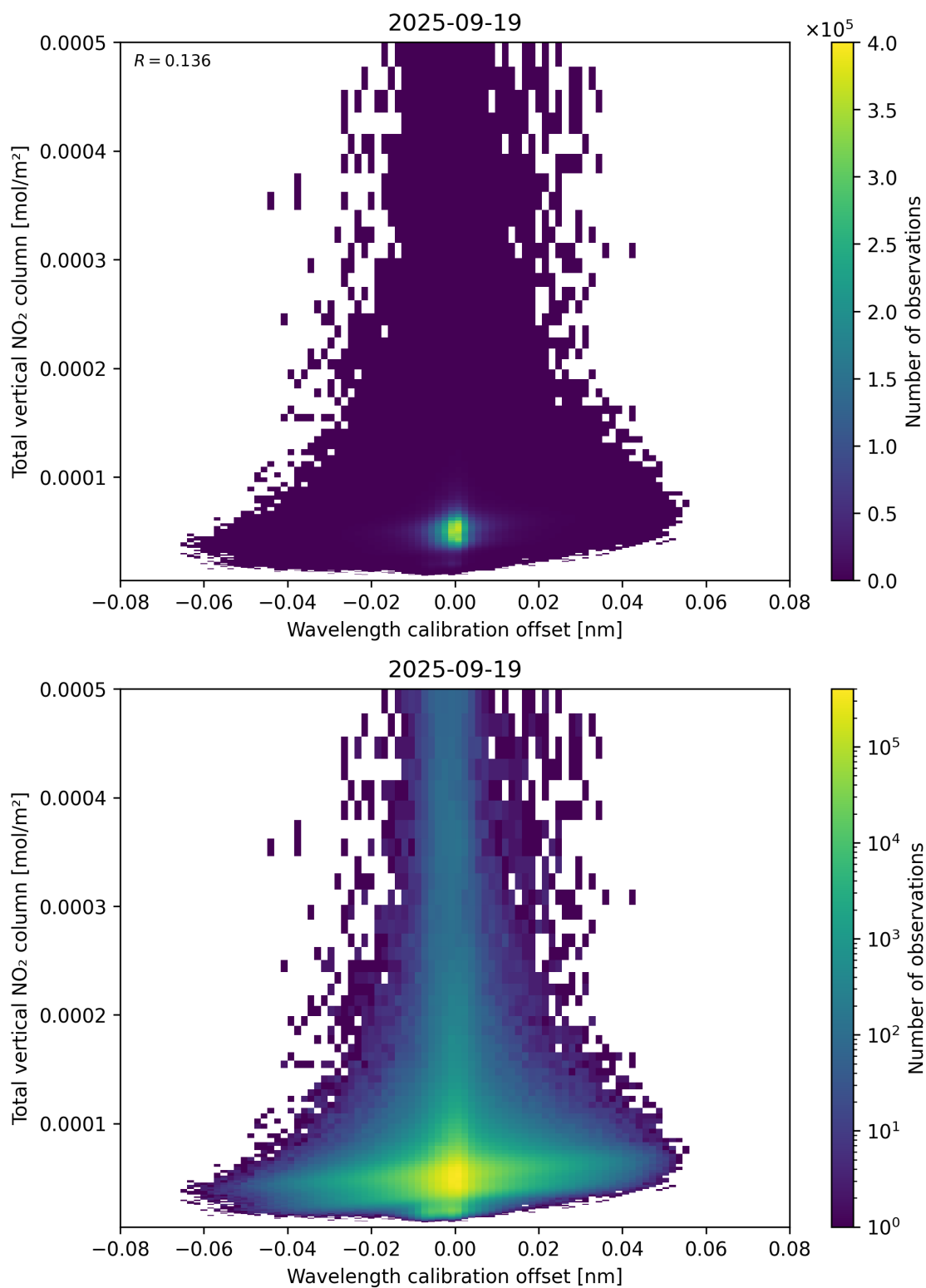
Figure 179: Scatter density plot of “Wavelength calibration offset” against “Total vertical NO 2 column” for 2025-09-18 to 2025-09-20.
