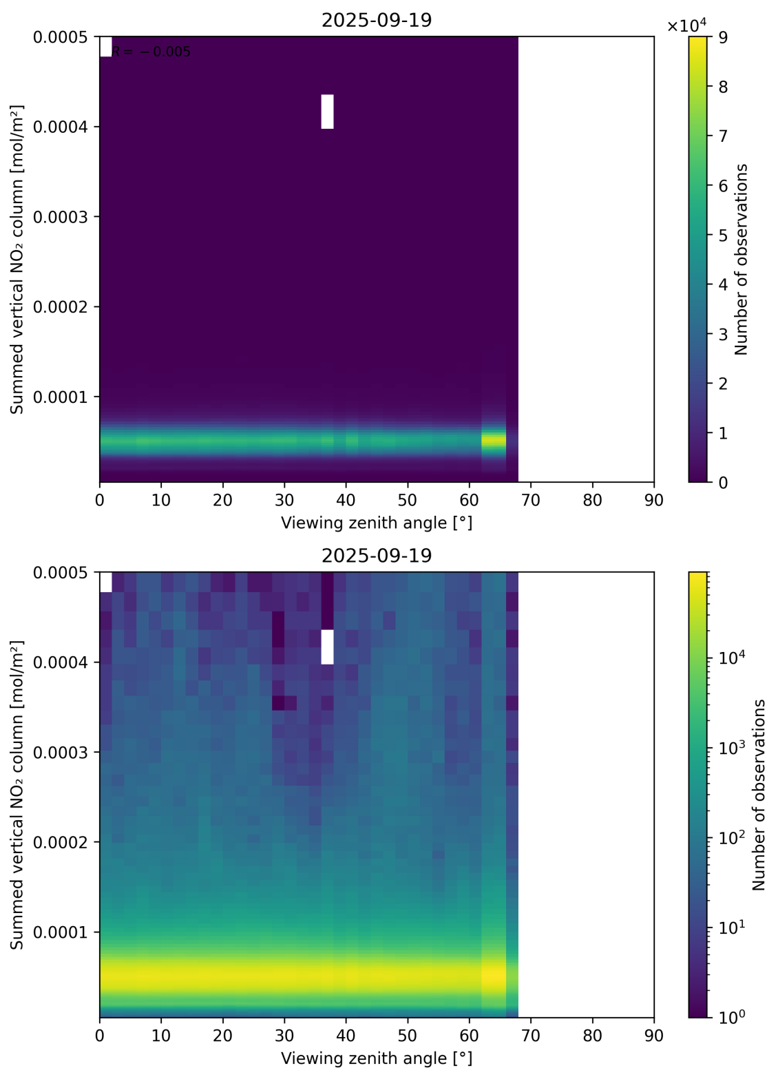
Figure 165: Scatter density plot of “Viewing zenith angle” against “Summed vertical NO 2 column” for 2025-09-18 to 2025-09-20.
