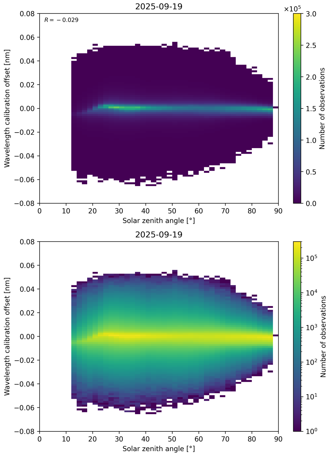
Figure 158: Scatter density plot of “Solar zenith angle” against “Wavelength calibration offset” for 2025-09-18 to 2025-09-20.
