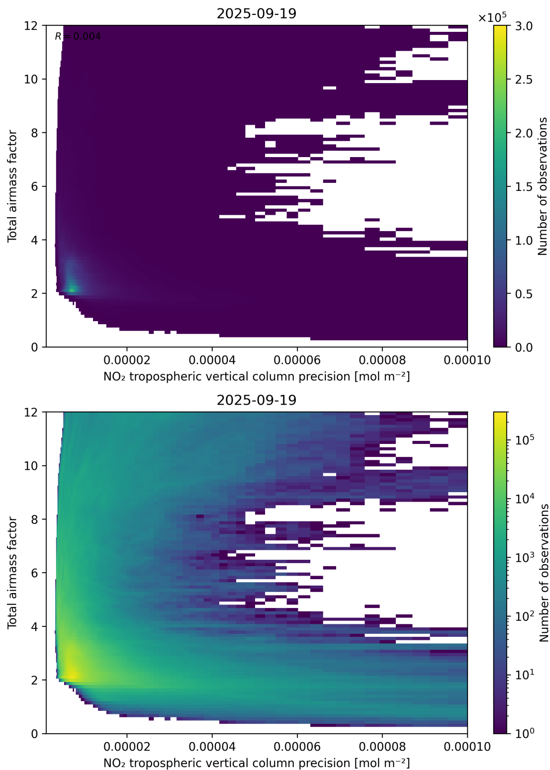
Figure 132: Scatter density plot of “NO 2 tropospheric vertical column precision” against “Total air mass factor” for 2025-09-18 to 2025-09-20.
