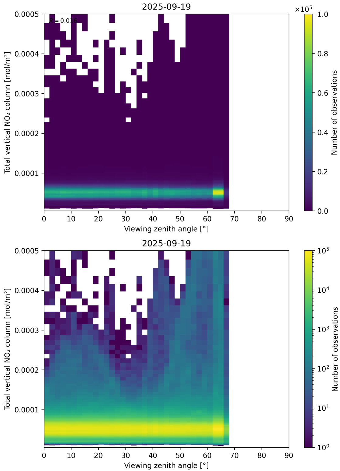
Figure 167: Scatter density plot of “Viewing zenith angle” against “Total vertical NO 2 column” for 2025-09-18 to 2025-09-20.
