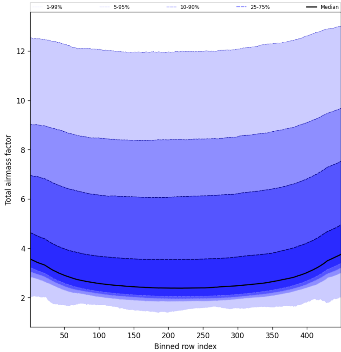
Figure 49: Along track statistics of “Total airmass factor” for 2025-09-18 to 2025-09-20
