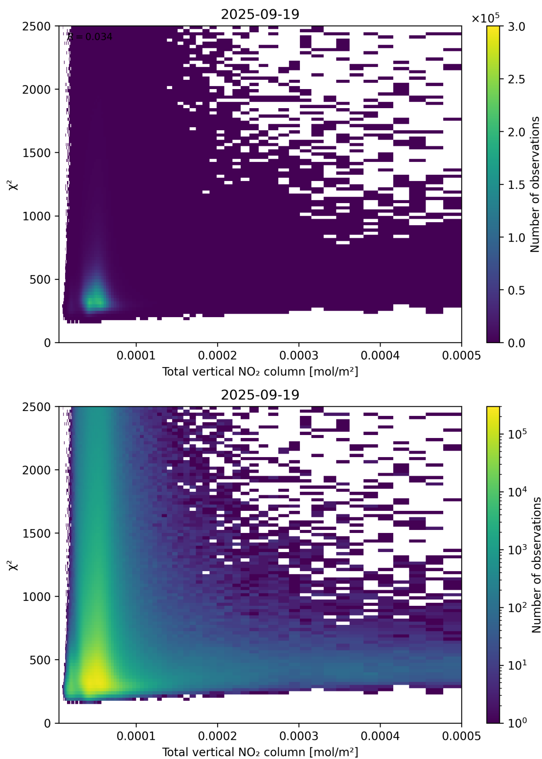
Figure 111: Scatter density plot of “Total vertical NO 2 column” against “ \chi^2 ” for 2025-09-18 to 2025-09-20.
