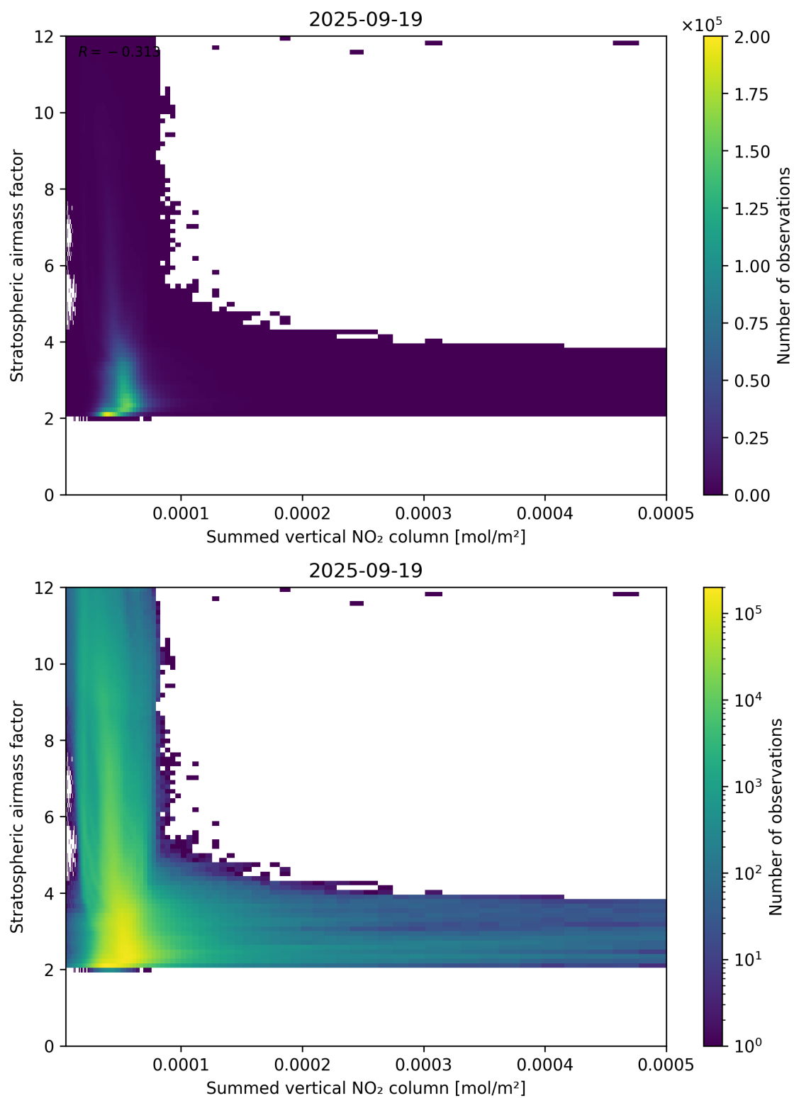
Figure 103: Scatter density plot of “Summed vertical NO 2 column” against “Stratospheric airmass factor” for 2025-09-18 to 2025-09-20.
