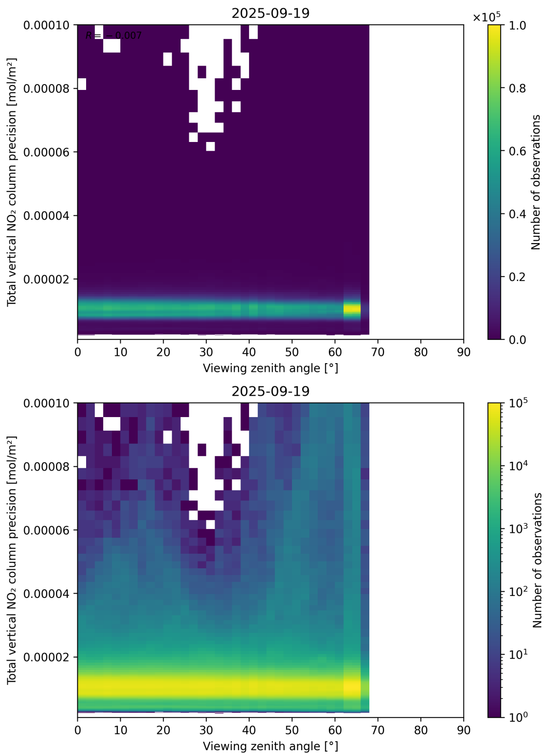
Figure 168: Scatter density plot of “Viewing zenith angle” against “Total vertical NO 2 column precision” for 2025-09-18 to 2025-09-20.
