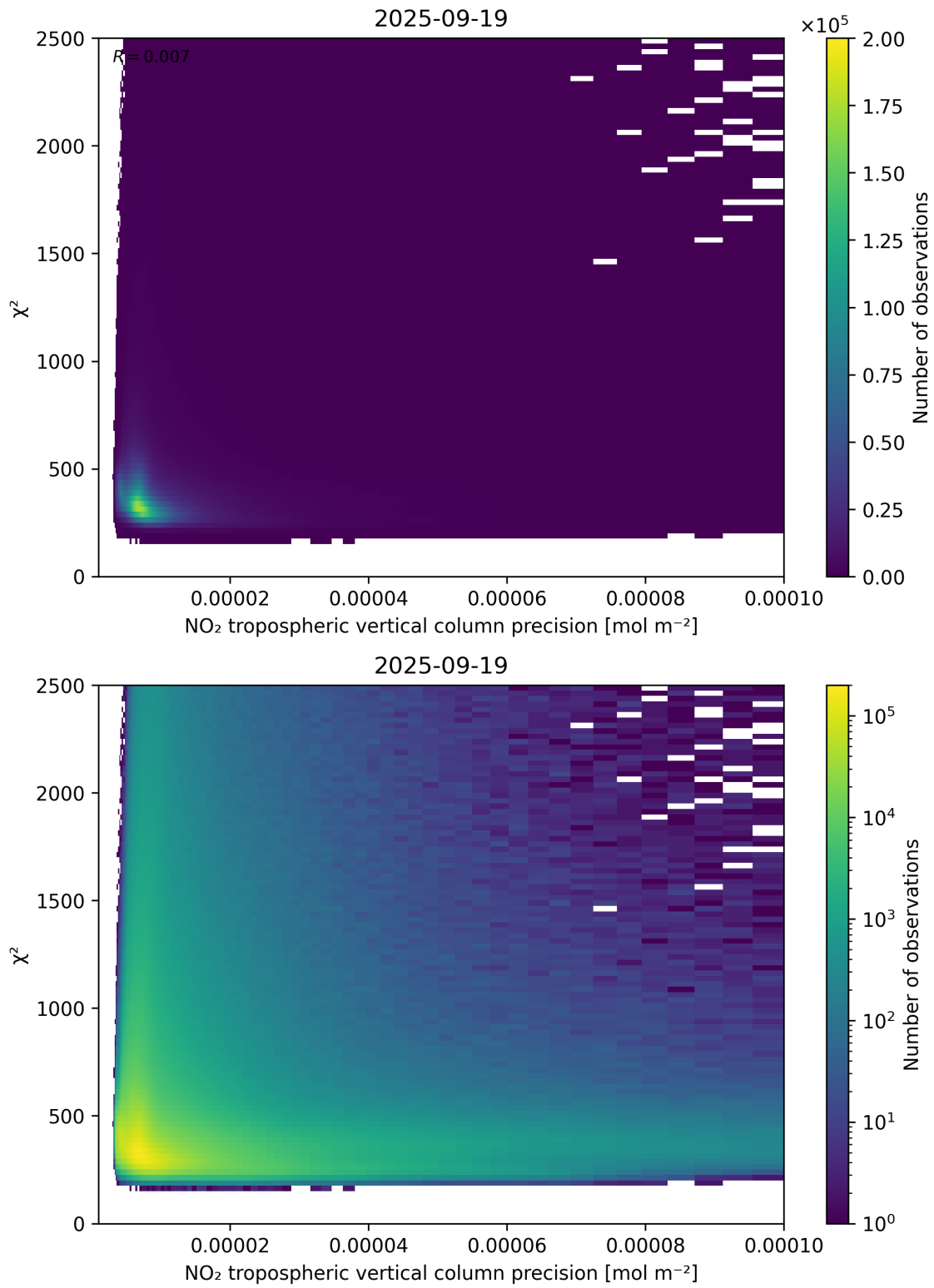
Figure 134: Scatter density plot of “NO 2 tropospheric vertical column precision” against “ \chi^2 ” for 2025-09-18 to 2025-09-20.
