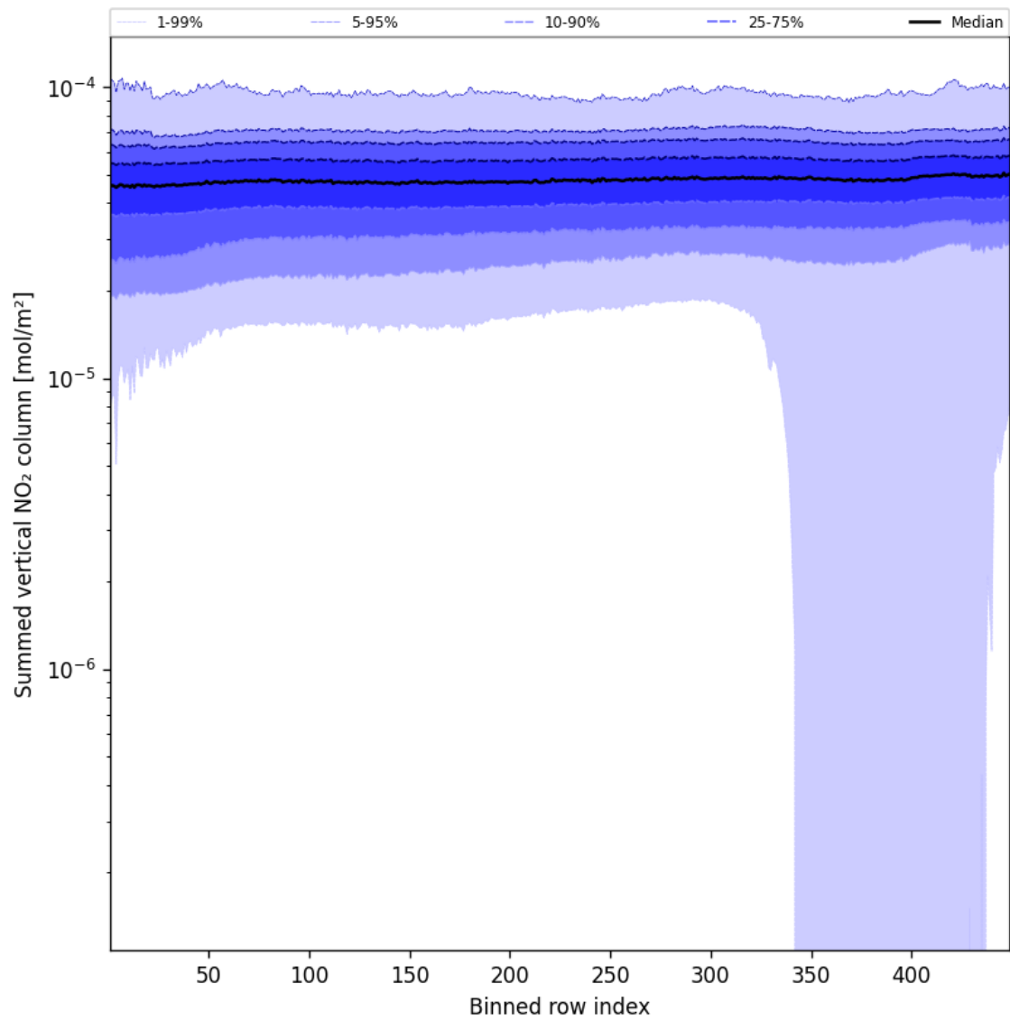
Figure 57: Along track statistics of “Summed vertical NO 2 column” for 2025-09-18 to 2025-09-20
