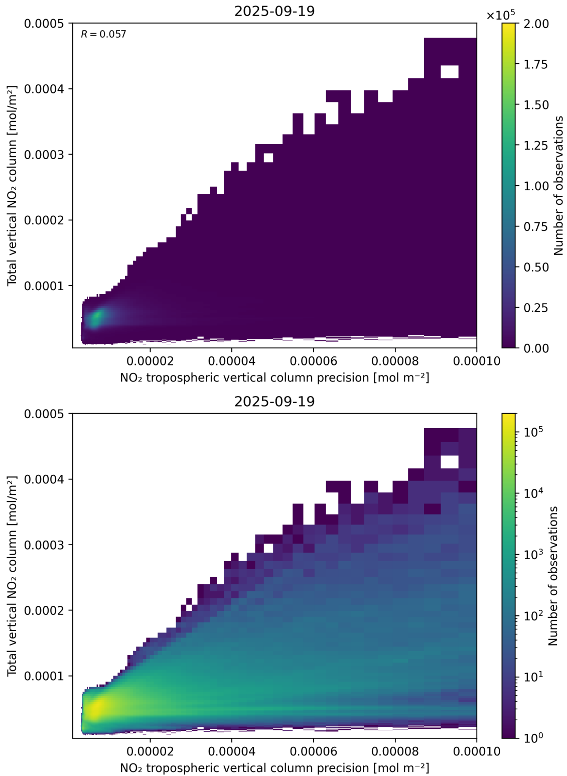
Figure 138: Scatter density plot of “NO 2 tropospheric vertical column precision” against “Total vertical NO 2 column” for 2025-09-18 to 2025-09-20.
