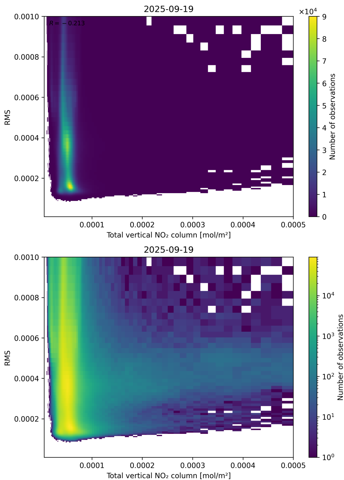
Figure 120: Scatter density plot of “Total vertical NO 2 column” against “RMS” for 2025-09-18 to 2025-09-20.
