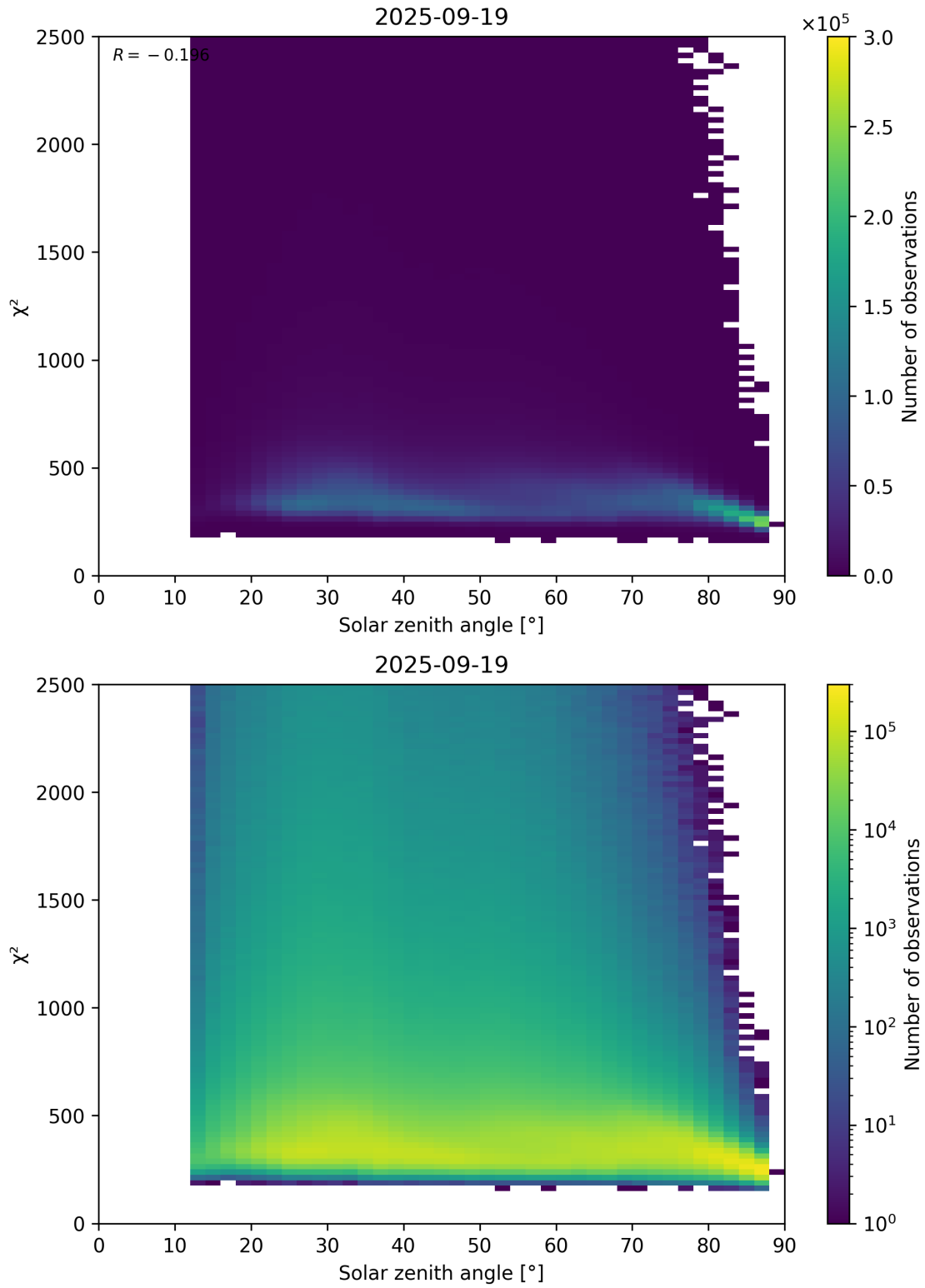
Figure 148: Scatter density plot of “Solar zenith angle” against “ \chi^2 ” for 2025-09-18 to 2025-09-20.
