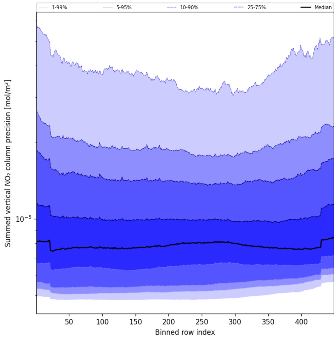
Figure 58: Along track statistics of “Summed vertical NO 2 column precision” for 2025-09-18 to 2025-09-20
