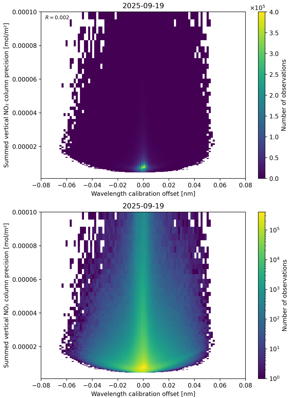
Figure 178: Scatter density plot of “Wavelength calibration offset” against “Summed vertical NO 2 column precision” for 2025-09-18 to 2025-09-20.
