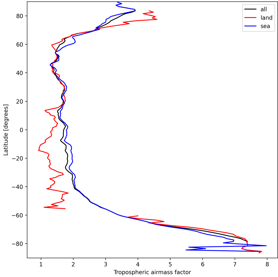
Figure 14: Zonal average of “Tropospheric airmass factor” for 2025-09-18 to 2025-09-20.
