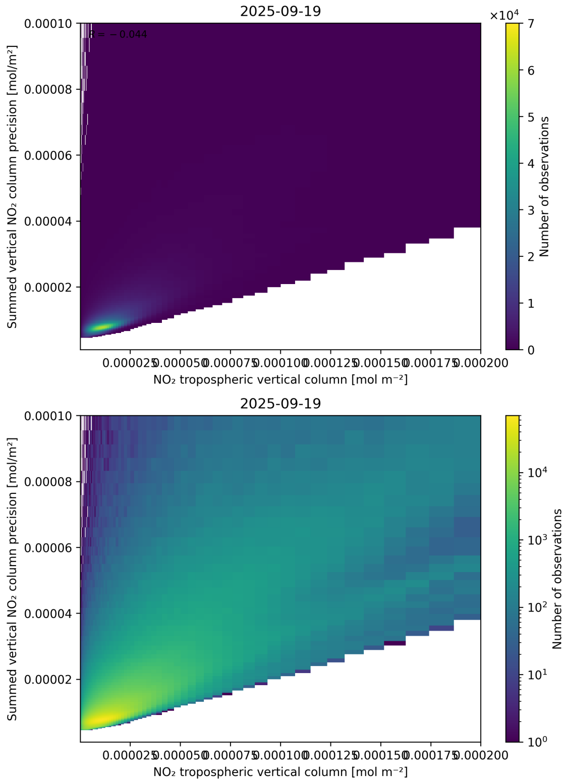
Figure 127: Scatter density plot of “NO 2 tropospheric vertical column” against “Summed vertical NO 2 column precision” for 2025-09-18 to 2025-09-20.
