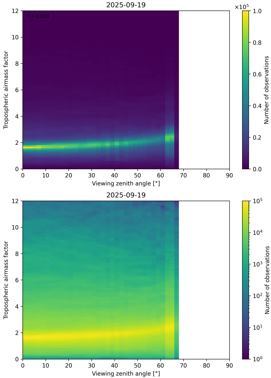
Figure 161: Scatter density plot of “Viewing zenith angle” against “Tropospheric airmass factor” for 2025-09-18 to 2025-09-20.
