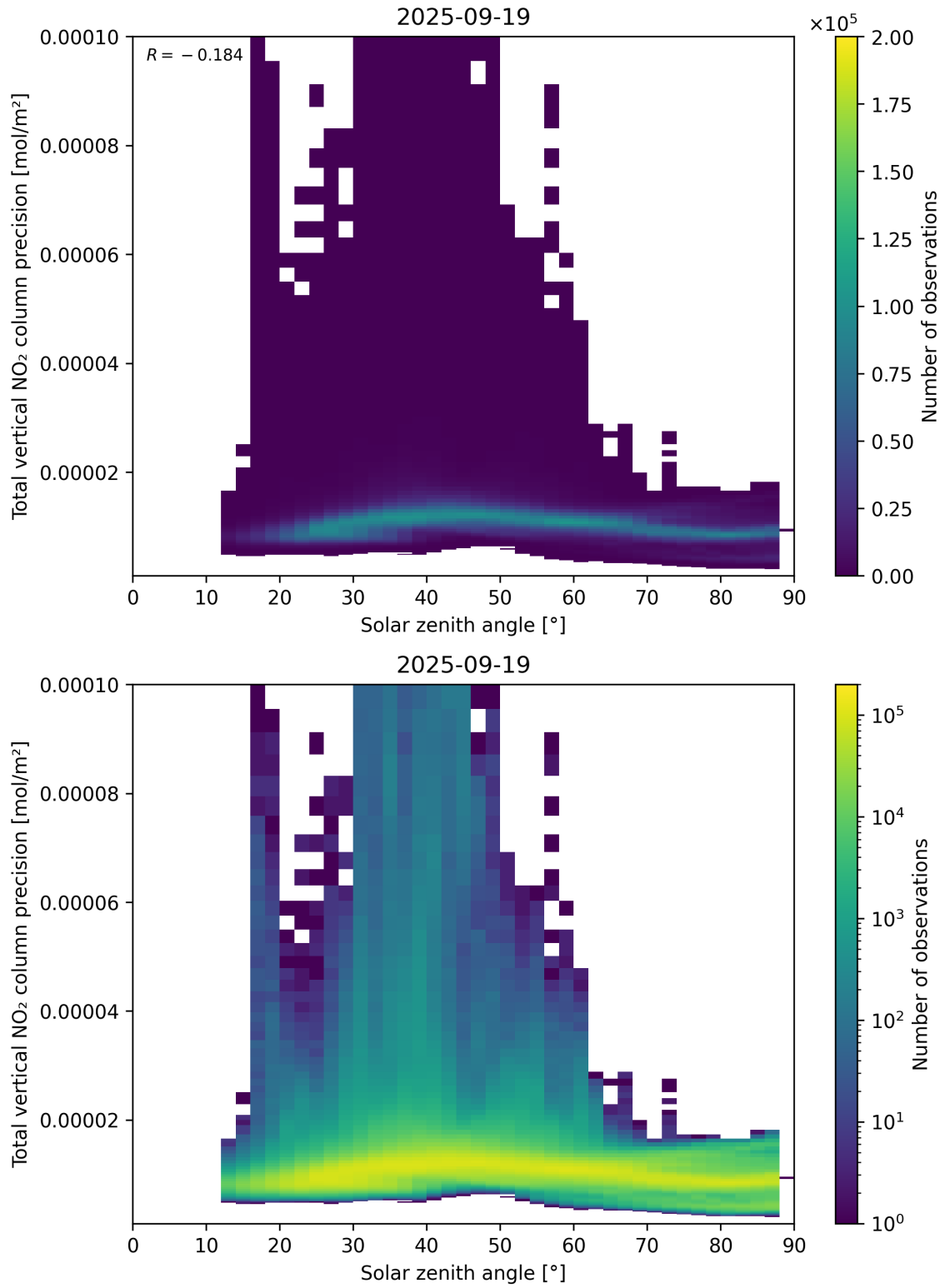
Figure 154: Scatter density plot of “Solar zenith angle” against “Total vertical NO 2 column precision” for 2025-09-18 to 2025-09-20.
