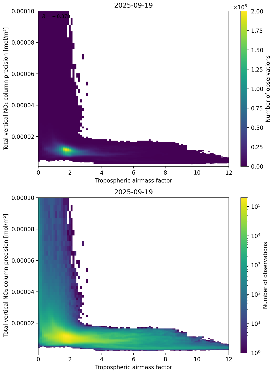
Figure 78: Scatter density plot of “Tropospheric air mass factor” against “Total vertical NO 2 column precision” for 2025-09-18 to 2025-09-20.
