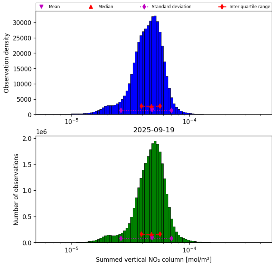
Figure 40: Histogram of “Summed vertical NO 2 column” for 2025-09-18 to 2025-09-20
