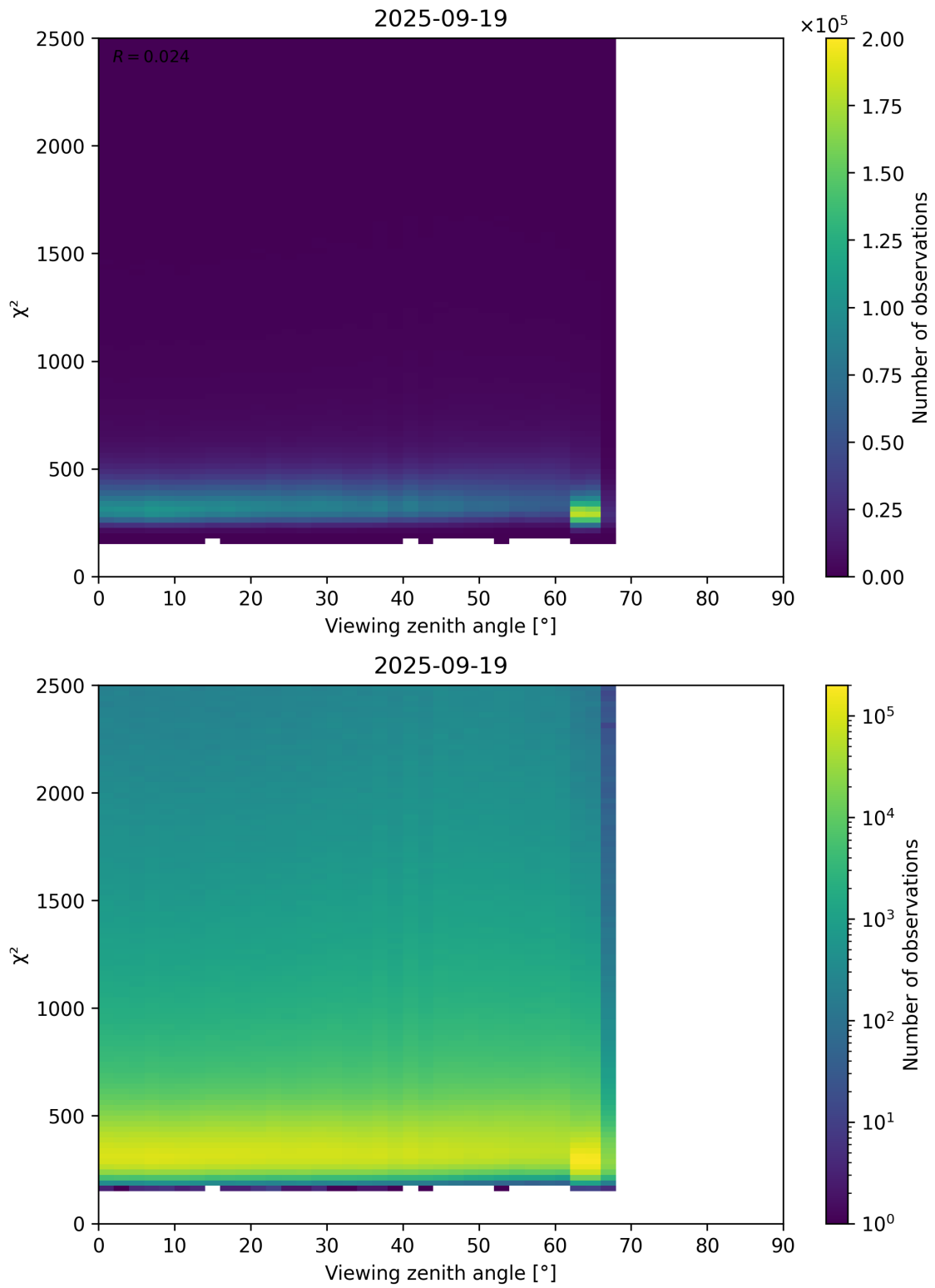
Figure 162: Scatter density plot of “Viewing zenith angle” against “ \chi^2 ” for 2025-09-18 to 2025-09-20.
