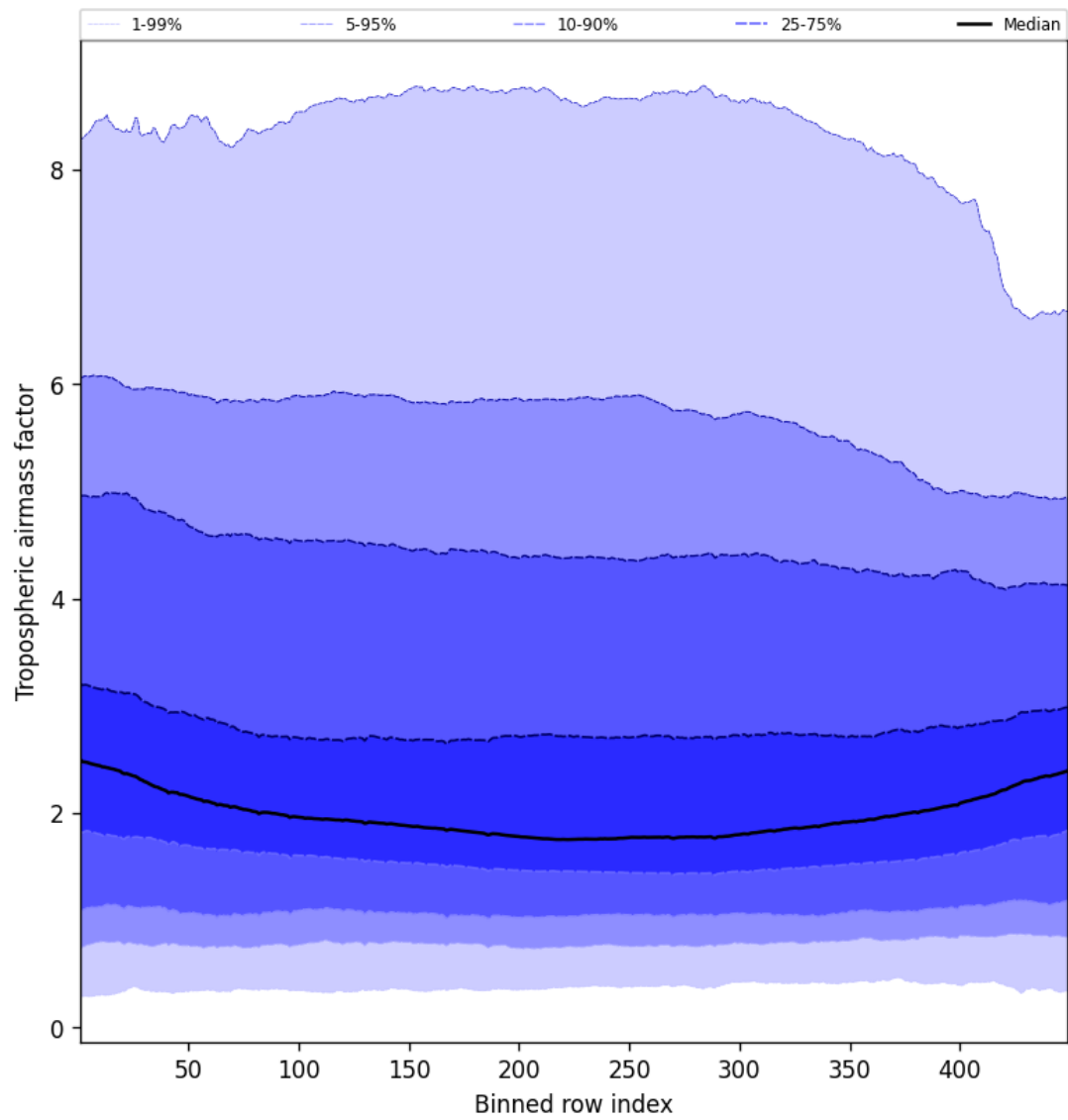
Figure 48: Along track statistics of “Tropospheric air mass factor” for 2025-09-18 to 2025-09-20
