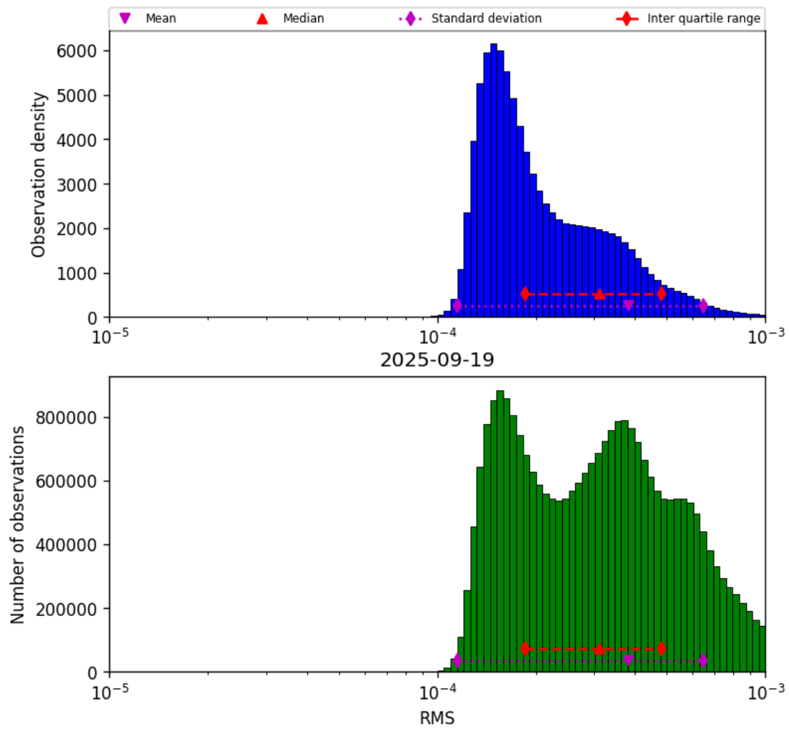
Figure 43: Histogram of “RMS” for 2025-09-18 to 2025-09-20
