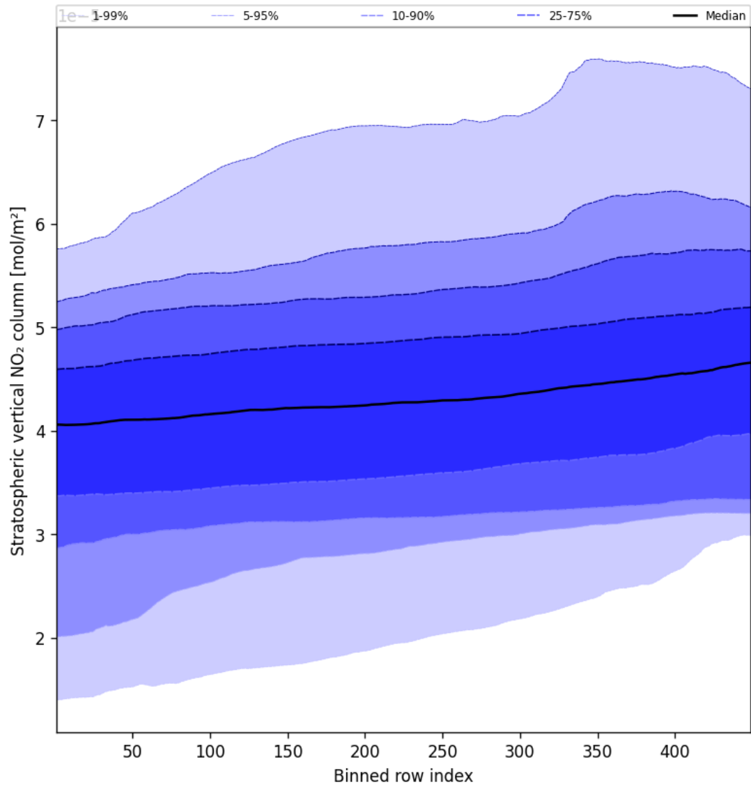
Figure 53: Along track statistics of “Stratospheric vertical NO 2 column” for 2025-09-18 to 2025-09-20
