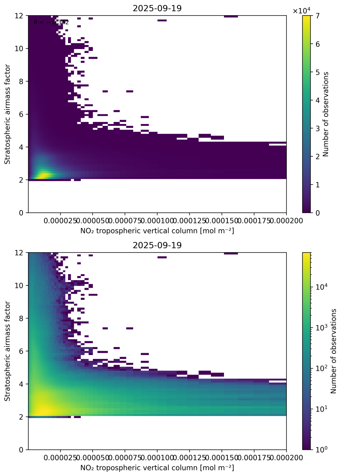
Figure 121: Scatter density plot of “NO 2 tropospheric vertical column” against “Stratospheric air mass factor” for 2025-09-18 to 2025-09-20.
