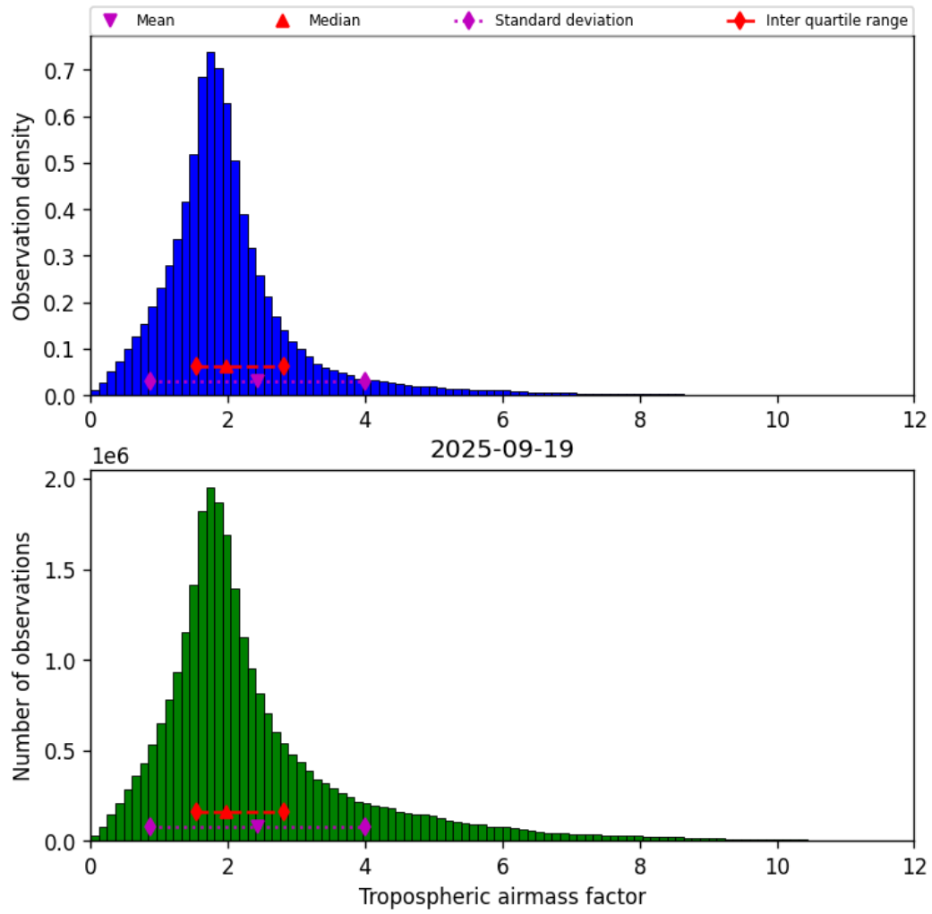
Figure 31: Histogram of “Tropospheric air mass factor” for 2025-09-18 to 2025-09-20
