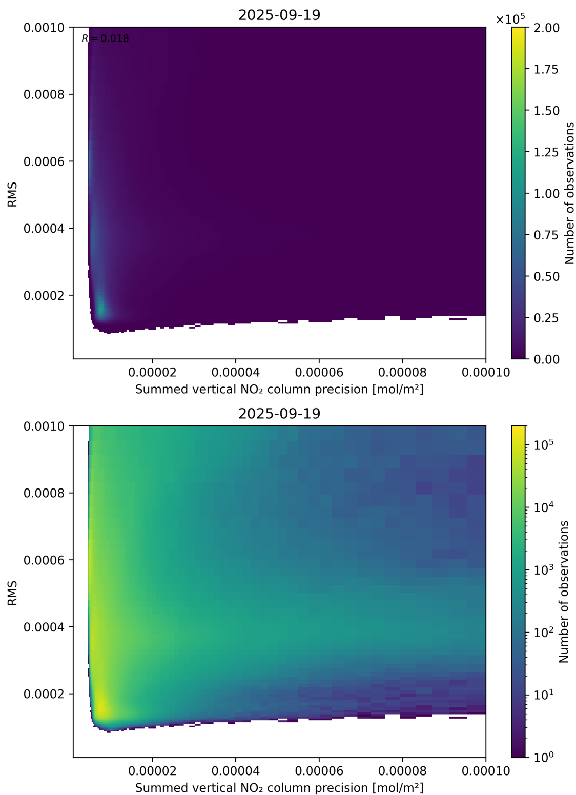
Figure 108: Scatter density plot of “Summed vertical NO 2 column precision” against “RMS” for 2025-09-18 to 2025-09-20.
