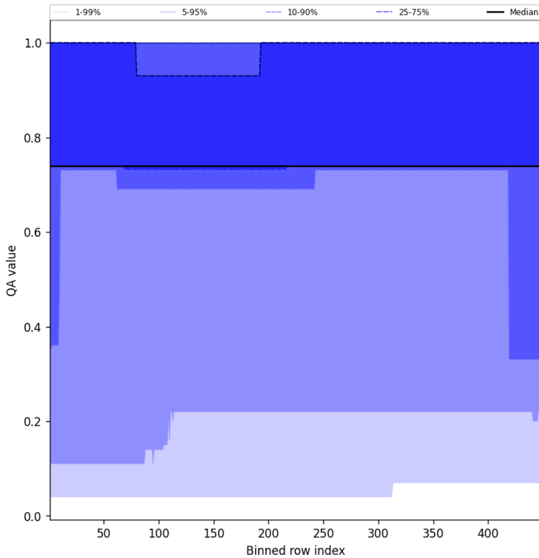
Figure 45: Along track statistics of “QA value” for 2025-09-18 to 2025-09-20
