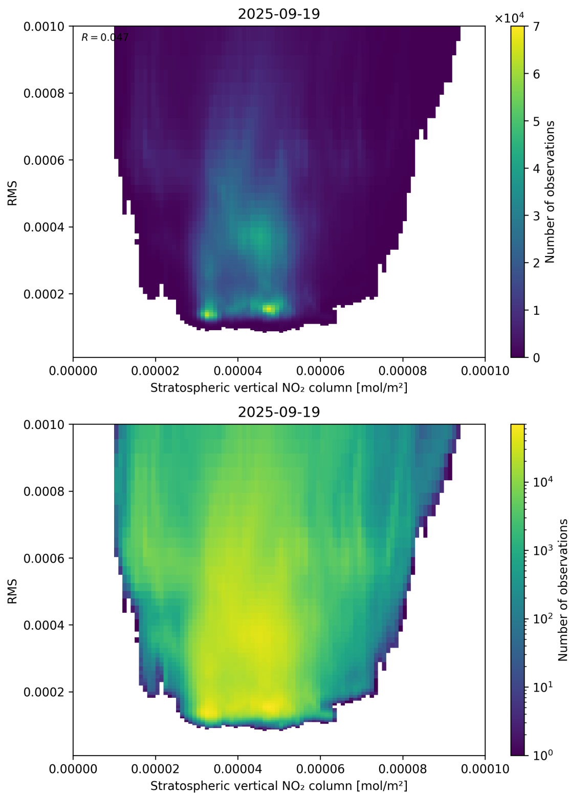
Figure 102: Scatter density plot of “Stratospheric vertical NO 2 column” against “RMS” for 2025-09-18 to 2025-09-20.
