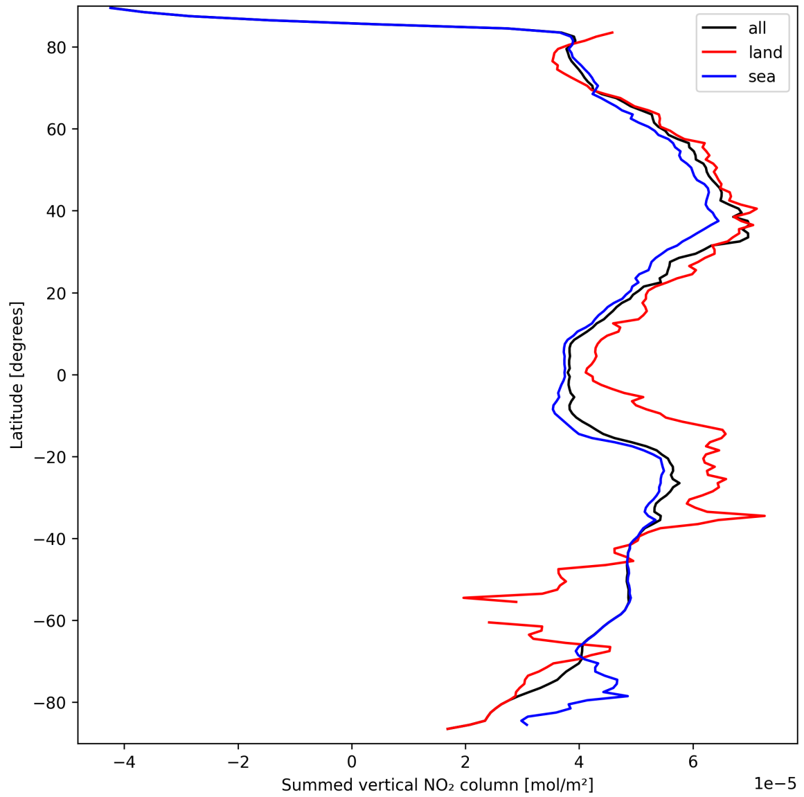
Figure 23: Zonal average of “Summed vertical NO 2 column” for 2025-09-18 to 2025-09-20.
