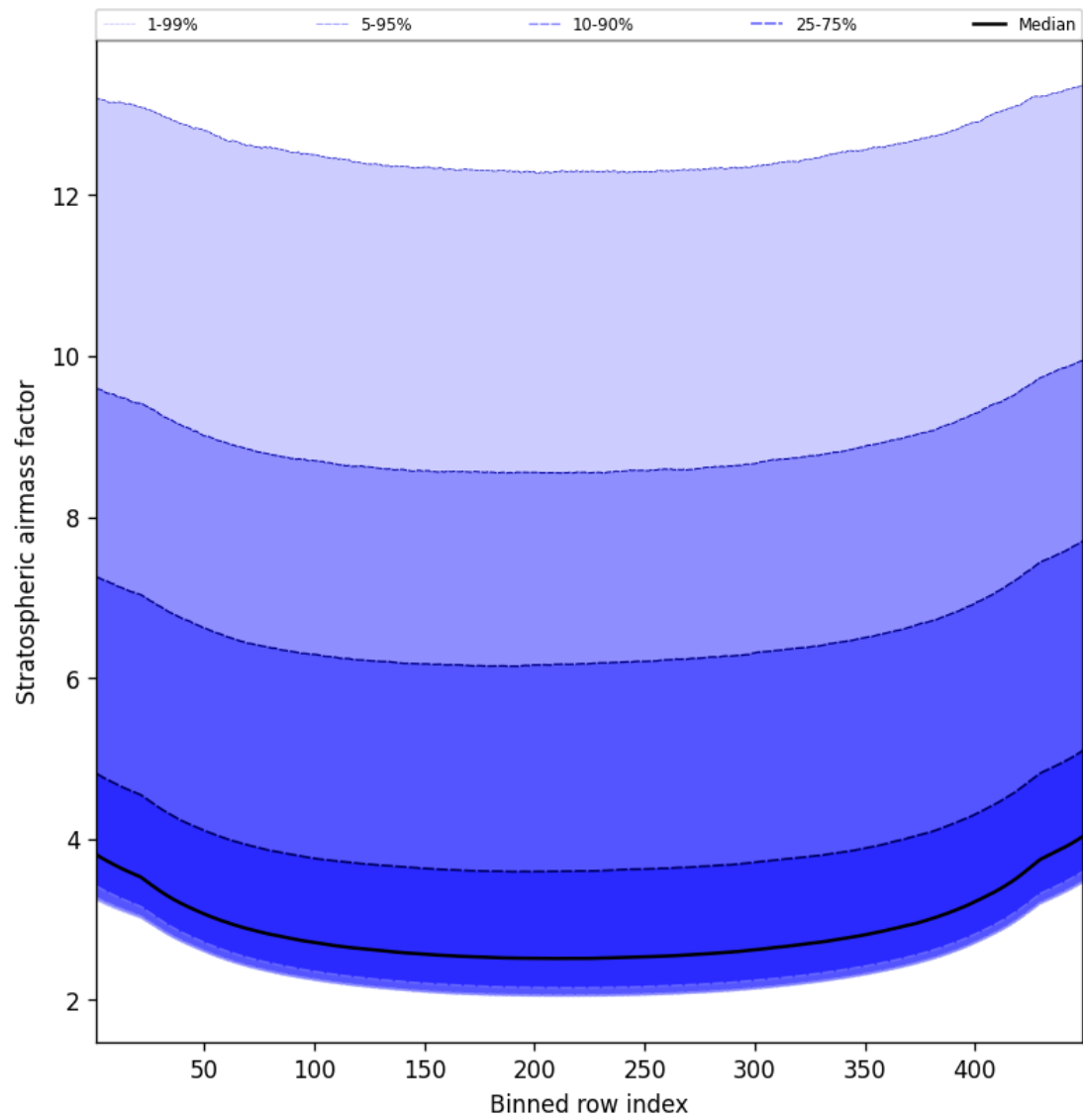
Figure 61: Along track statistics of “Stratospheric airmass factor” for 2025-09-18 to 2025-09-20
