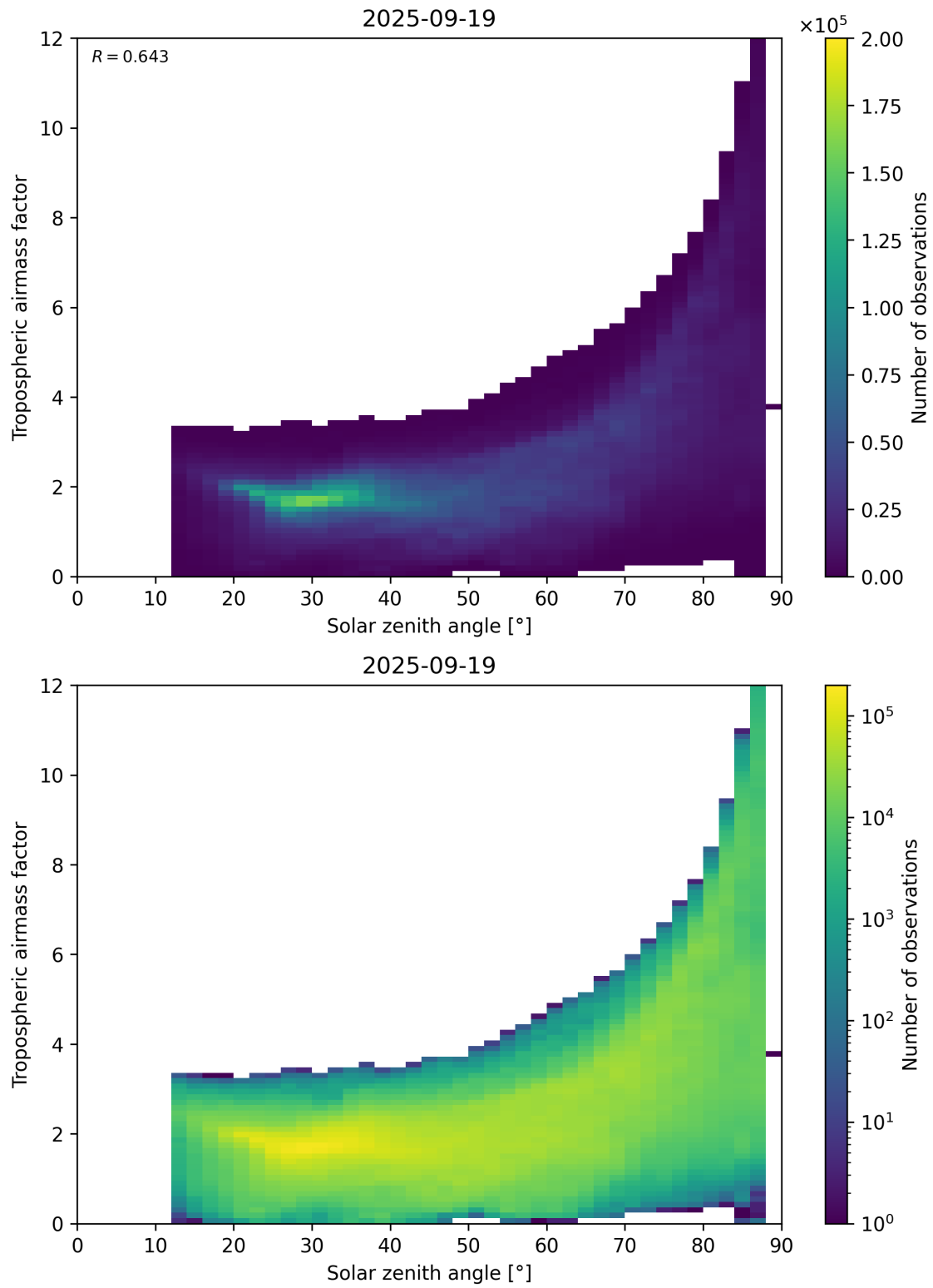
Figure 147: Scatter density plot of “Solar zenith angle” against “Tropospheric airmass factor” for 2025-09-18 to 2025-09-20.
