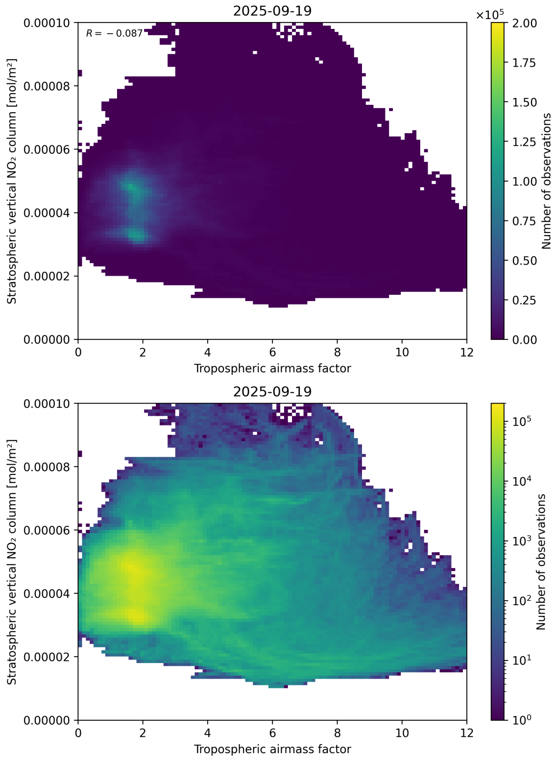
Figure 74: Scatter density plot of “Tropospheric airmass factor” against “Stratospheric vertical NO 2 column” for 2025-09-18 to 2025-09-20.
