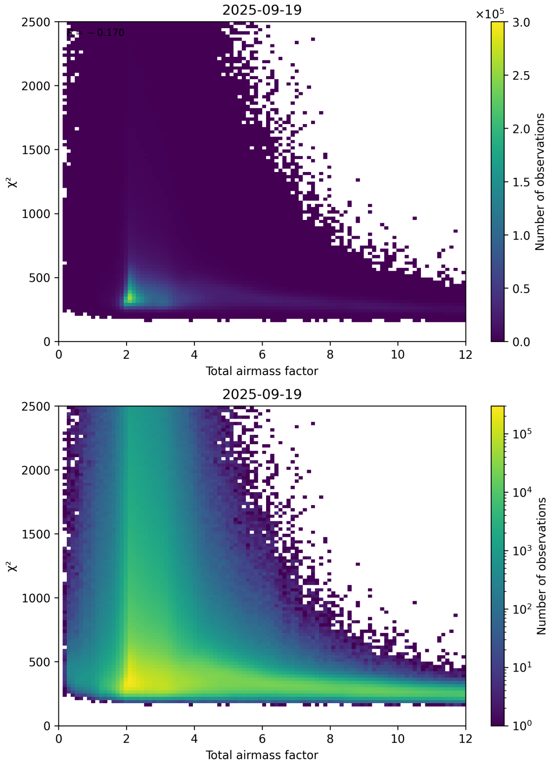
Figure 63: Scatter density plot of “Total airmass factor” against “ \chi^2 ” for 2025-09-18 to 2025-09-20.
