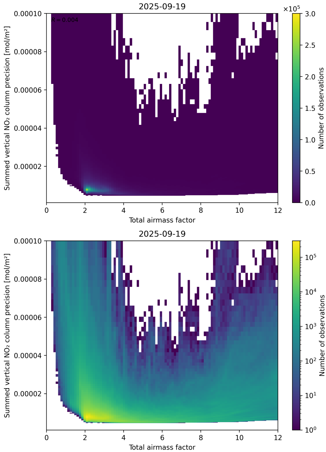
Figure 66: Scatter density plot of “Total airmass factor” against “Summed vertical NO 2 column precision” for 2025-09-18 to 2025-09-20.
