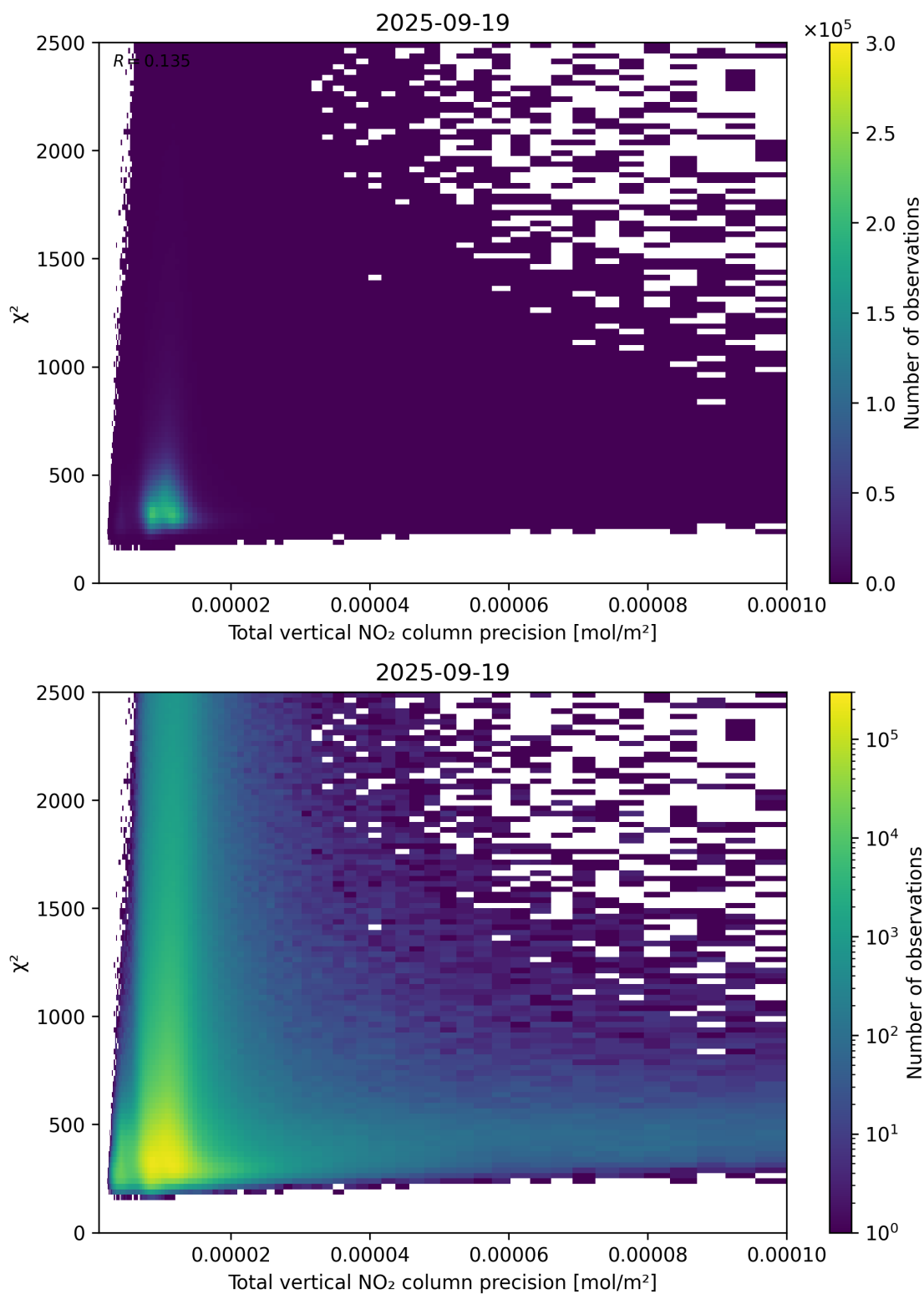
Figure 116: Scatter density plot of “Total vertical NO 2 column precision” against “ \chi^2 ” for 2025-09-18 to 2025-09-20.
