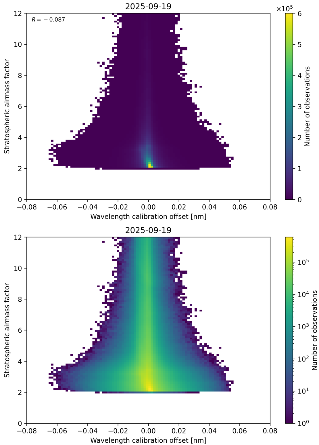
Figure 174: Scatter density plot of “Wavelength calibration offset” against “Stratospheric air mass factor” for 2025-09-18 to 2025-09-20.
