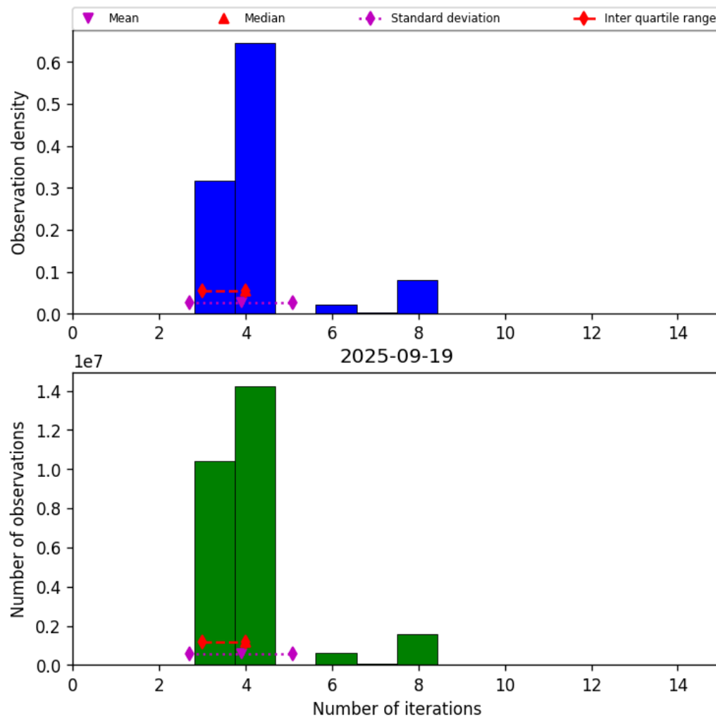
Figure 34: Histogram of “Number of iterations” for 2025-09-18 to 2025-09-20
