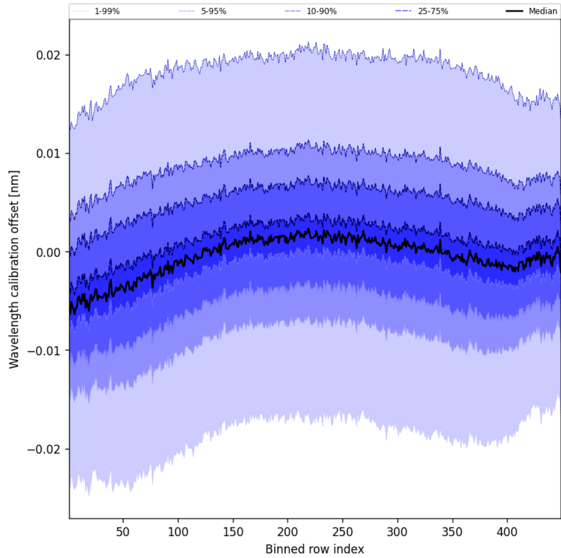
Figure 52: Along track statistics of “Wavelength calibration offset” for 2025-09-18 to 2025-09-20
