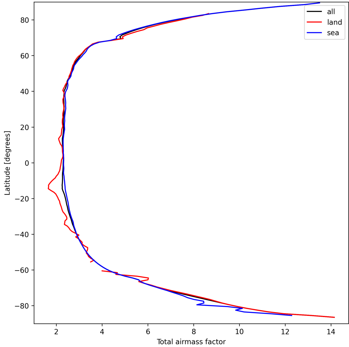
Figure 15: Zonal average of “Total airmass factor” for 2025-09-18 to 2025-09-20.
