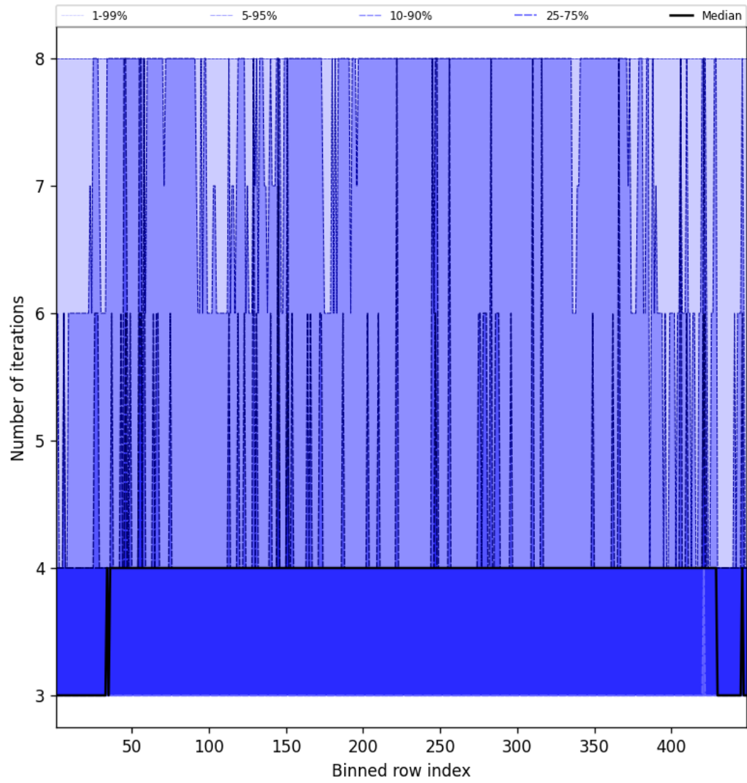
Figure 51: Along track statistics of “Number of iterations” for 2025-09-18 to 2025-09-20
