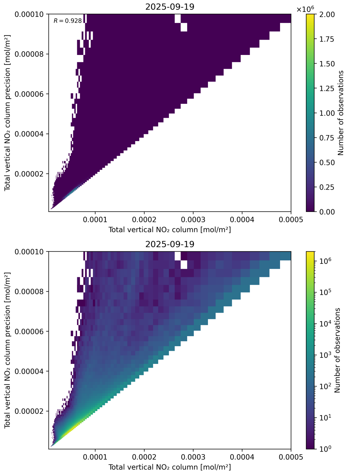
Figure 114: Scatter density plot of “Total vertical NO 2 column” against “Total vertical NO 2 column precision” for 2025-09-18 to 2025-09-20.
