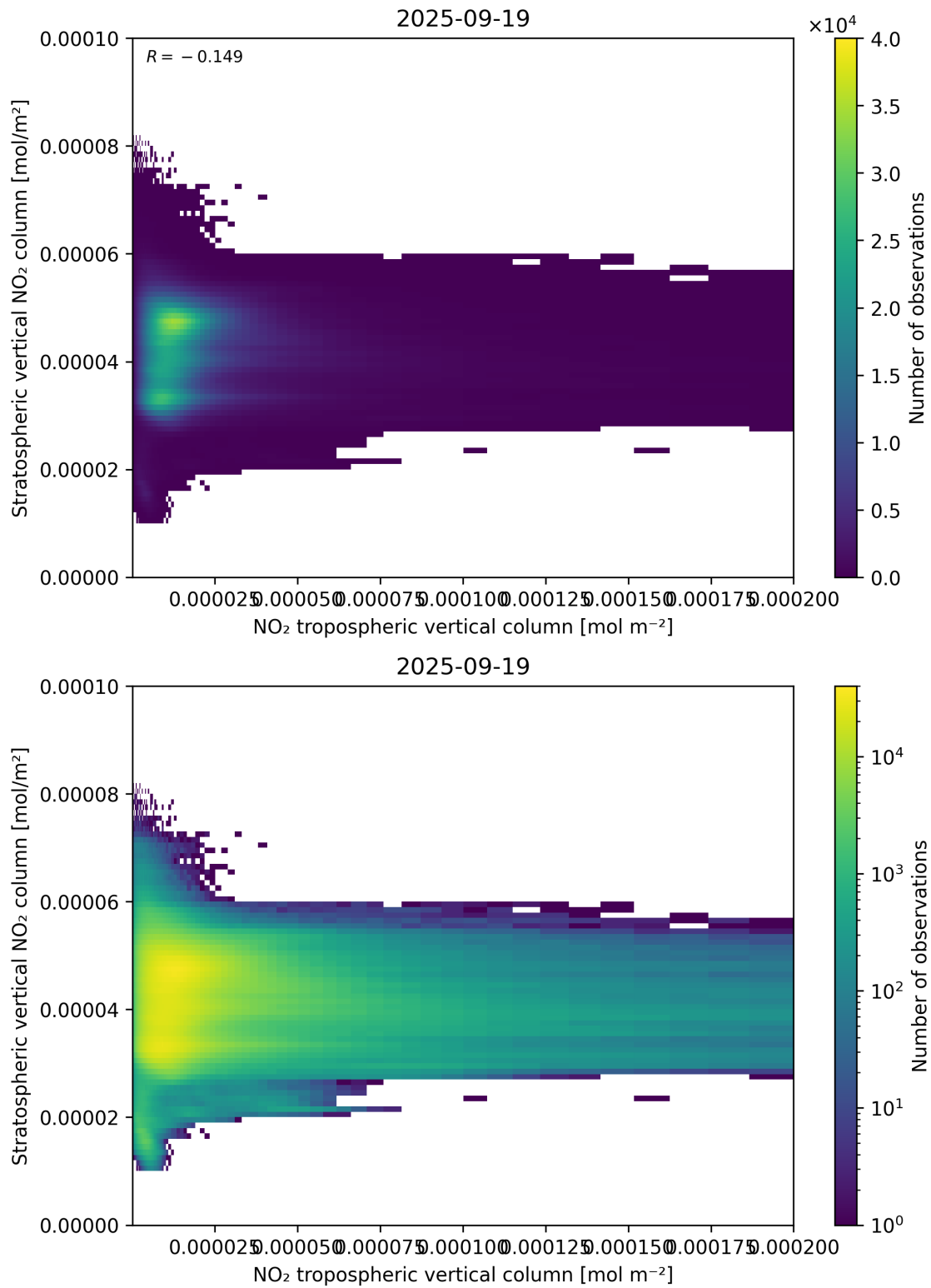
Figure 125: Scatter density plot of “NO 2 tropospheric vertical column” against “Stratospheric vertical NO 2 column” for 2025-09-18 to 2025-09-20.
