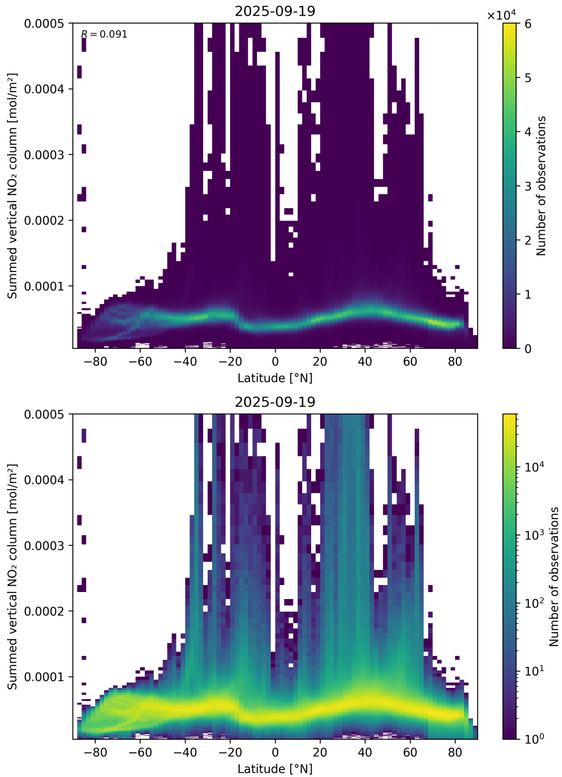
Figure 88: Scatter density plot of “Latitude” against “Summed vertical NO 2 column” for 2025-09-18 to 2025-09-20.
