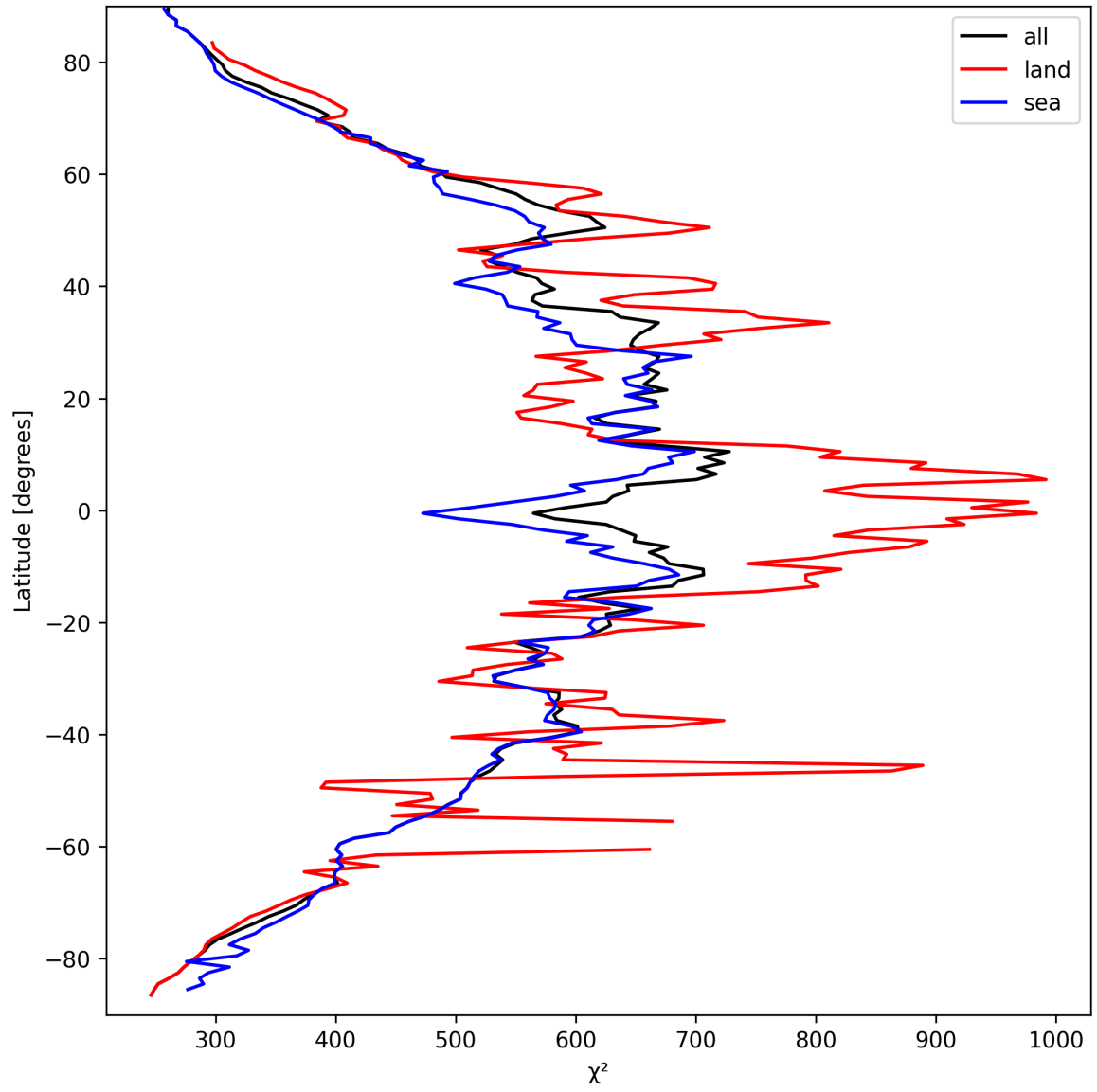
Figure 25: Zonal average of “ \chi^2 ” for 2025-09-18 to 2025-09-20.
