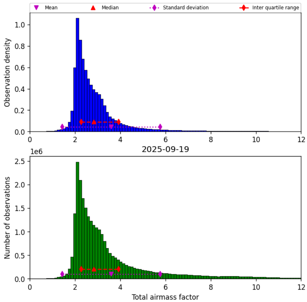
Figure 32: Histogram of “Total airmass factor” for 2025-09-18 to 2025-09-20
