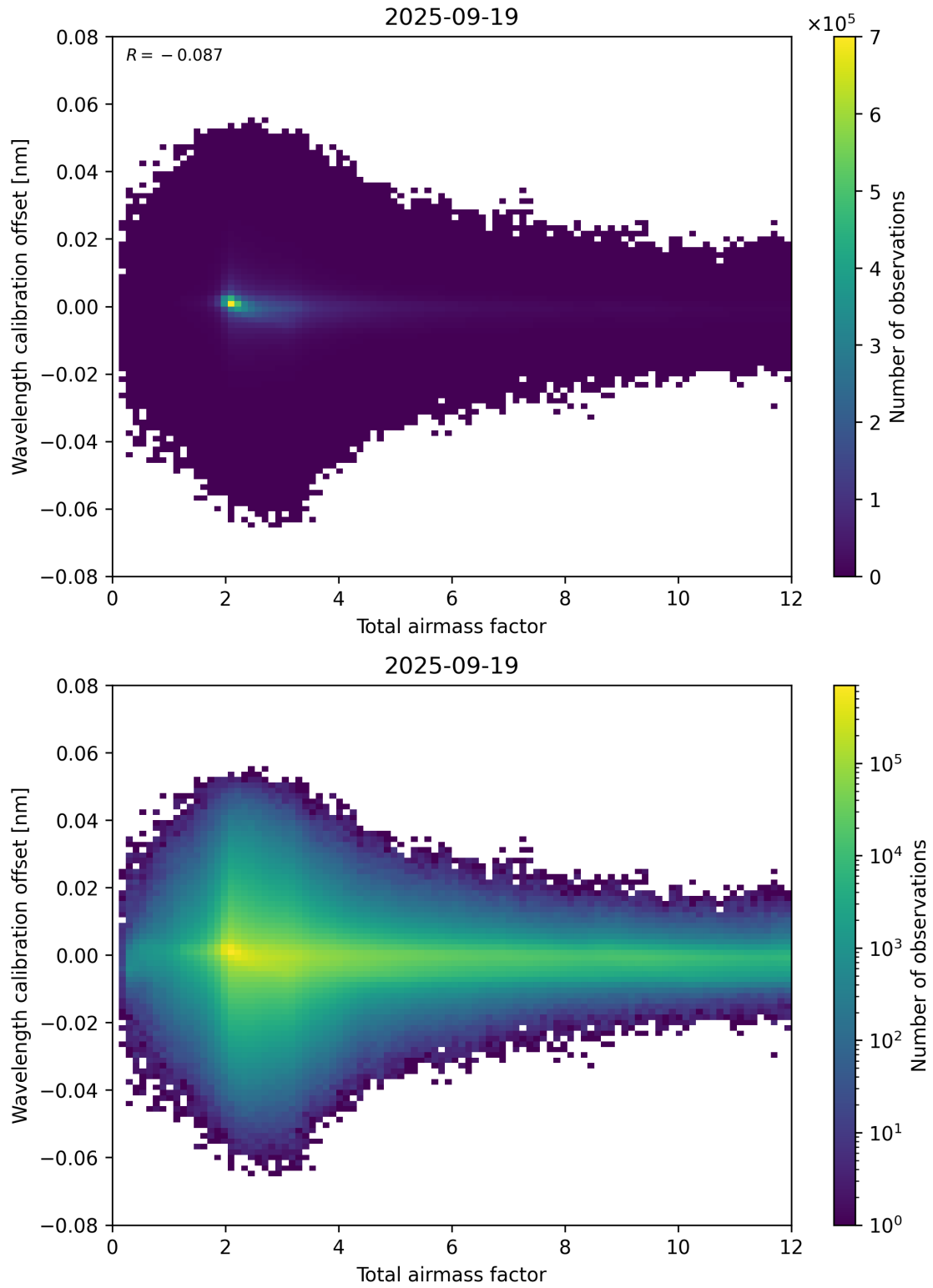
Figure 70: Scatter density plot of “Total airmass factor” against “Wavelength calibration offset” for 2025-09-18 to 2025-09-20.
