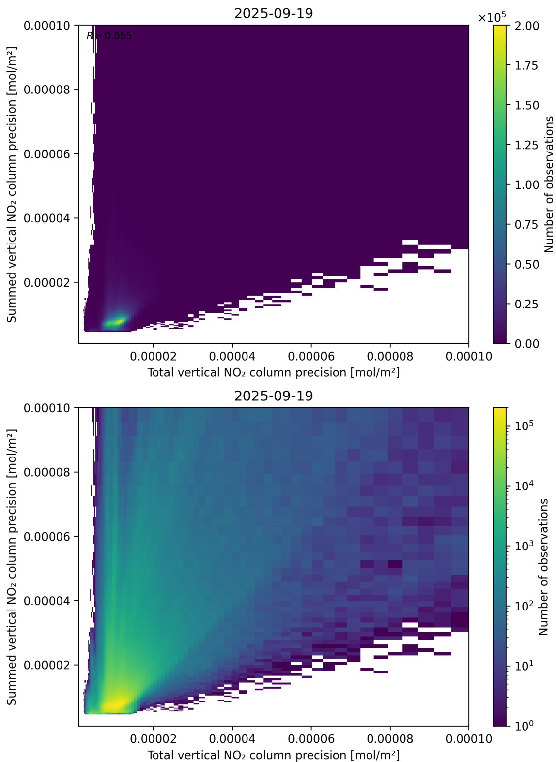
Figure 118: Scatter density plot of “Total vertical NO 2 column precision” against “Summed vertical NO 2 column precision” for 2025-09-18 to 2025-09-20.
