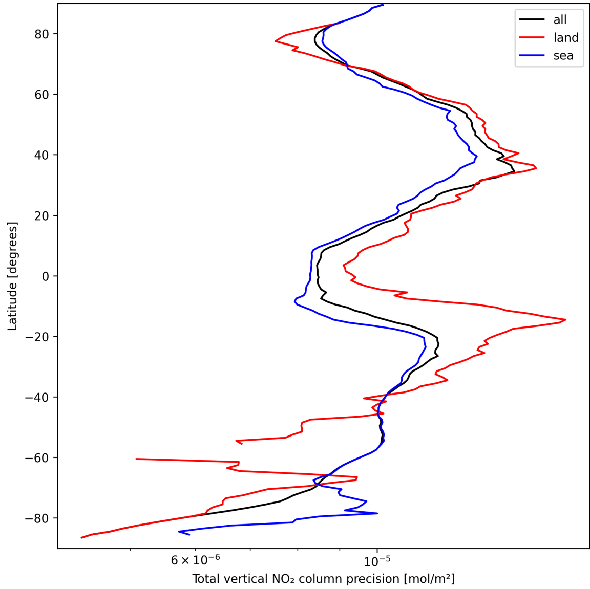
Figure 22: Zonal average of “Total vertical NO 2 column precision” for 2025-09-18 to 2025-09-20.
