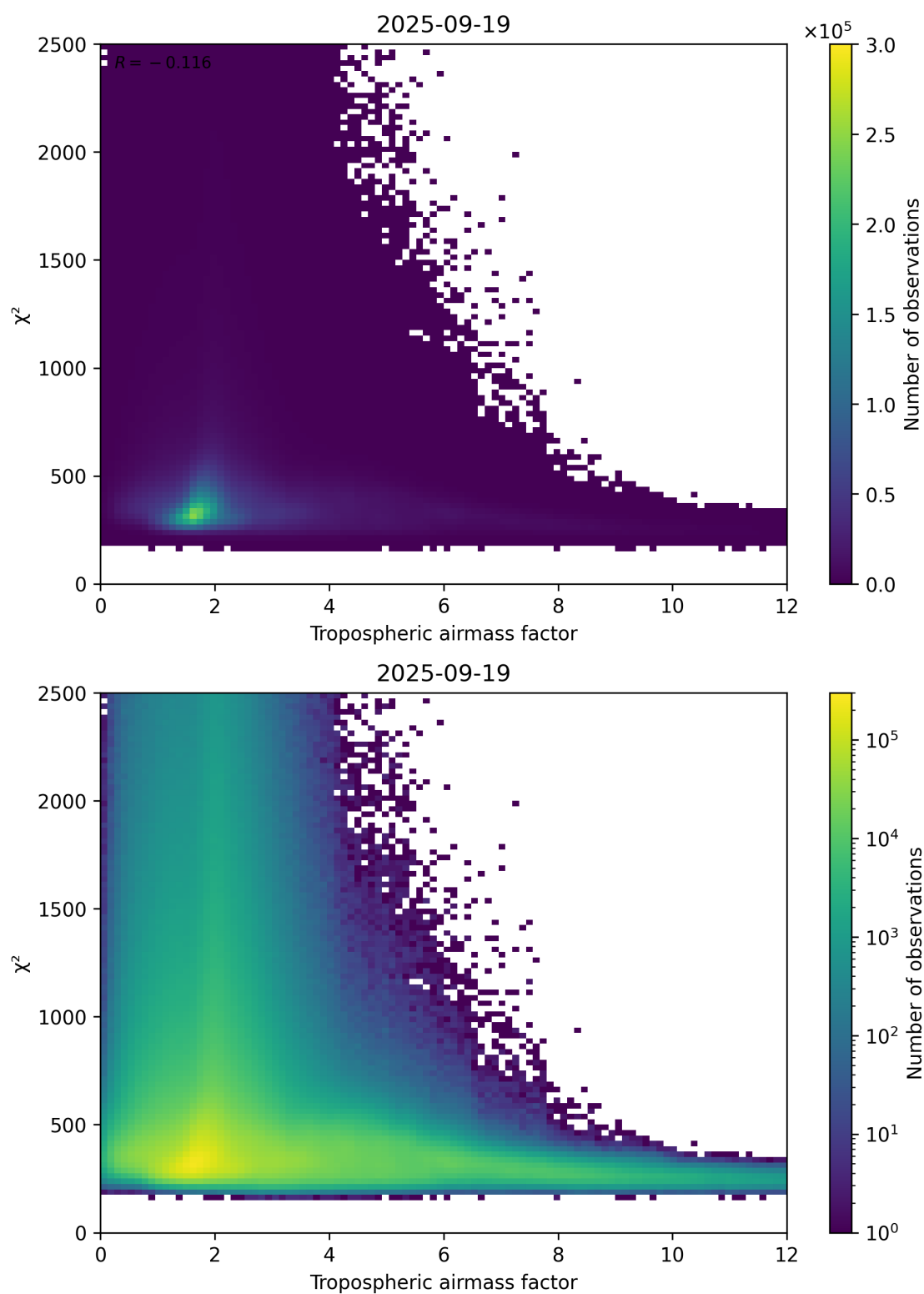
Figure 73: Scatter density plot of “Tropospheric airmass factor” against “ \chi^2 ” for 2025-09-18 to 2025-09-20.
