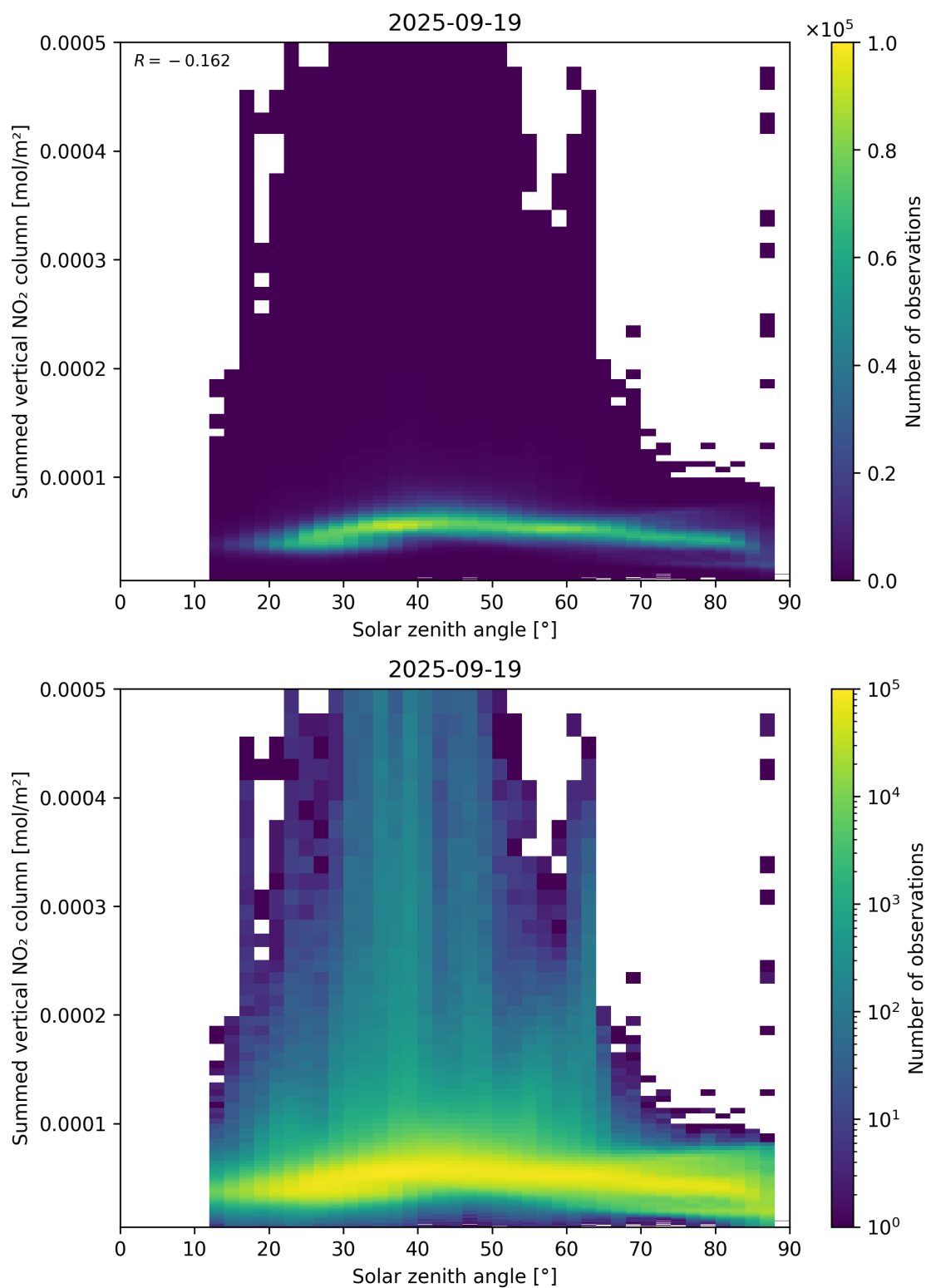
Figure 151: Scatter density plot of “Solar zenith angle” against “Summed vertical NO 2 column” for 2025-09-18 to 2025-09-20.
