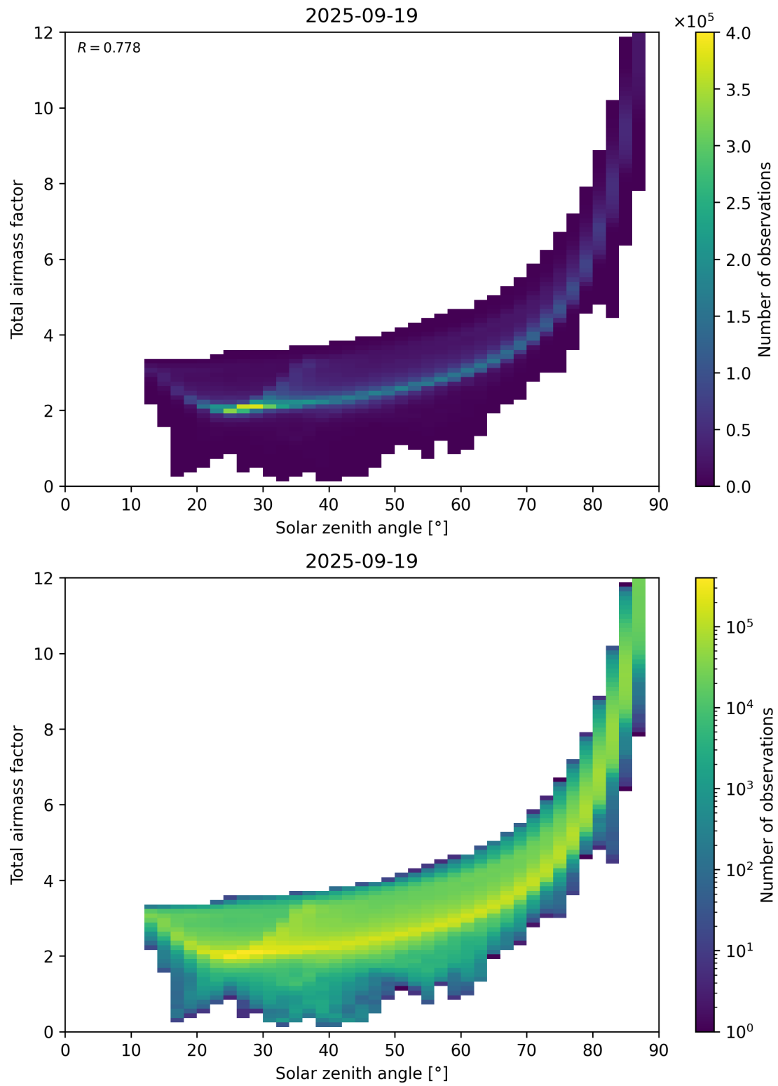
Figure 146: Scatter density plot of “Solar zenith angle” against “Total air mass factor” for 2025-09-18 to 2025-09-20.
