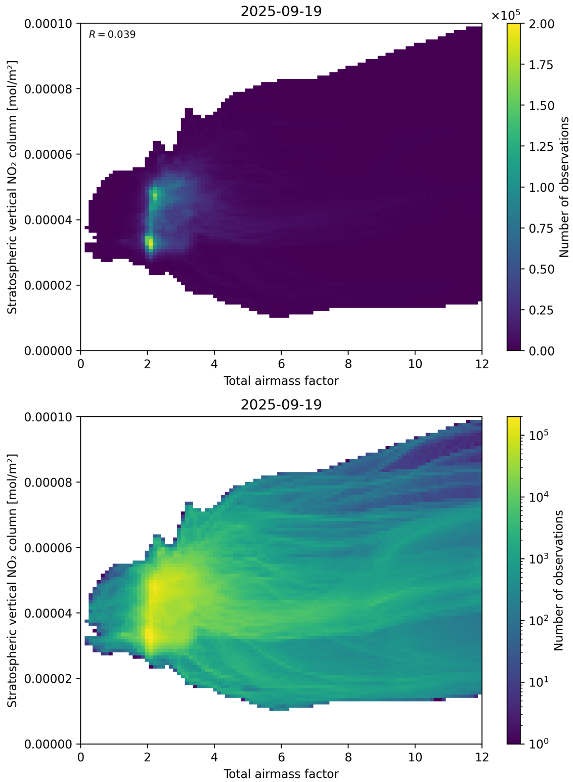
Figure 64: Scatter density plot of “Total airmass factor” against “Stratospheric vertical \text{NO}_2 column” for 2025-09-18 to 2025-09-20.
