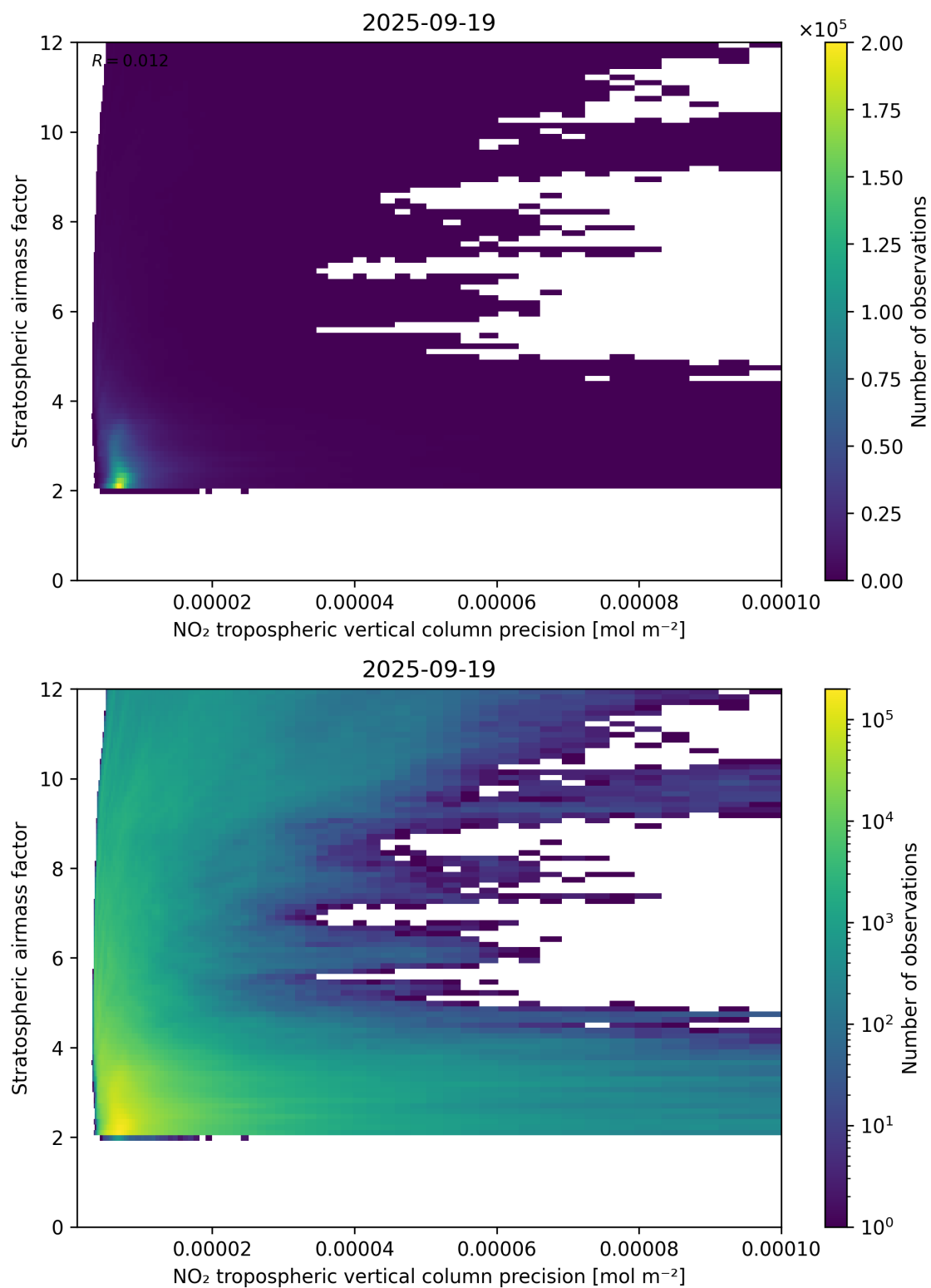
Figure 131: Scatter density plot of “NO 2 tropospheric vertical column precision” against “Stratospheric airmass factor” for 2025-09-18 to 2025-09-20.
