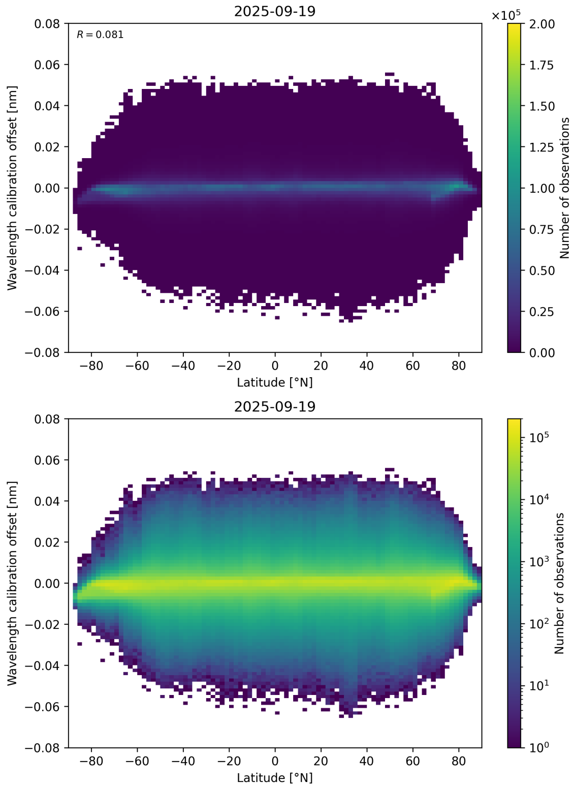
Figure 95: Scatter density plot of “Latitude” against “Wavelength calibration offset” for 2025-09-18 to 2025-09-20.
