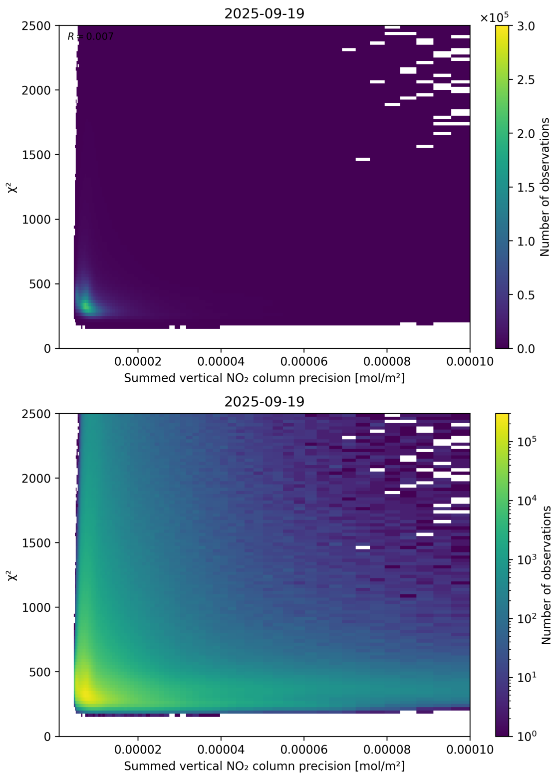
Figure 107: Scatter density plot of “Summed vertical NO 2 column precision” against “ \chi^2 ” for 2025-09-18 to 2025-09-20.
