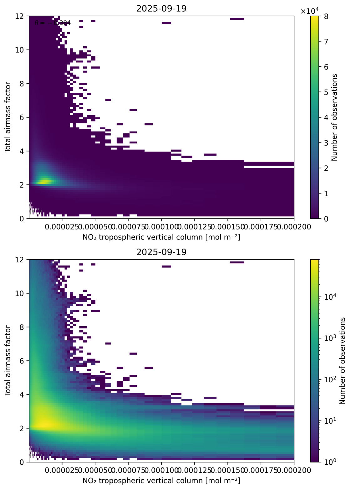
Figure 122: Scatter density plot of “NO 2 tropospheric vertical column” against “Total air mass factor” for 2025-09-18 to 2025-09-20.
