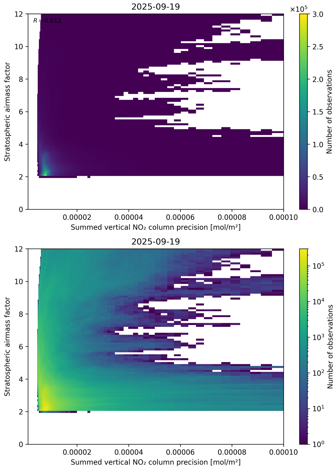
Figure 106: Scatter density plot of “Summed vertical NO 2 column precision” against “Stratospheric airmass factor” for 2025-09-18 to 2025-09-20.
