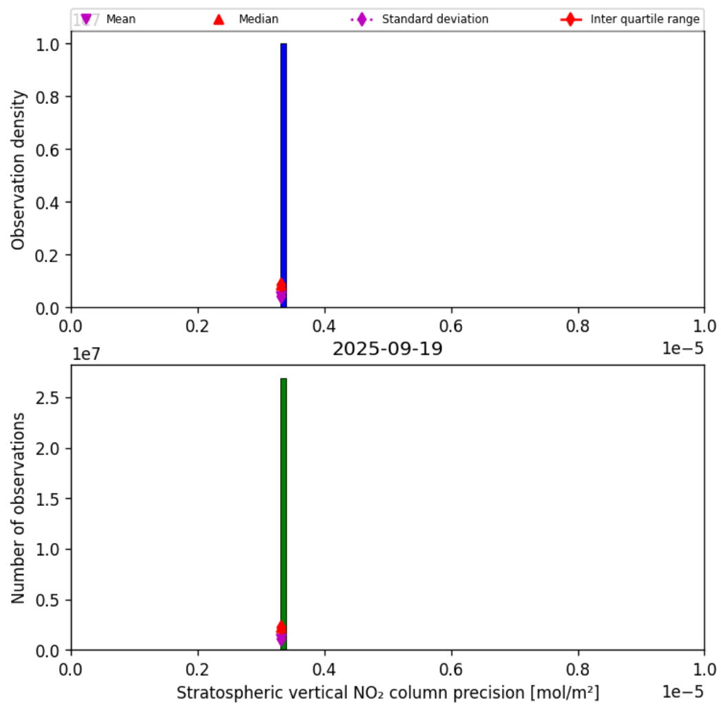
Figure 37: Histogram of “Stratospheric vertical NO 2 column precision” for 2025-09-18 to 2025-09-20
