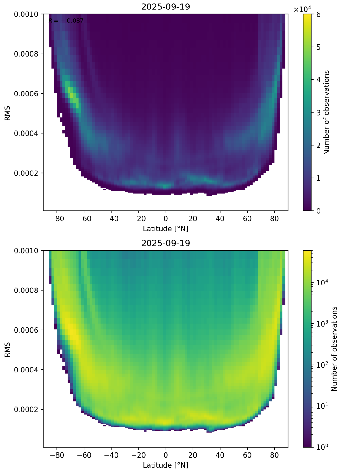
Figure 94: Scatter density plot of “Latitude” against “RMS” for 2025-09-18 to 2025-09-20.
