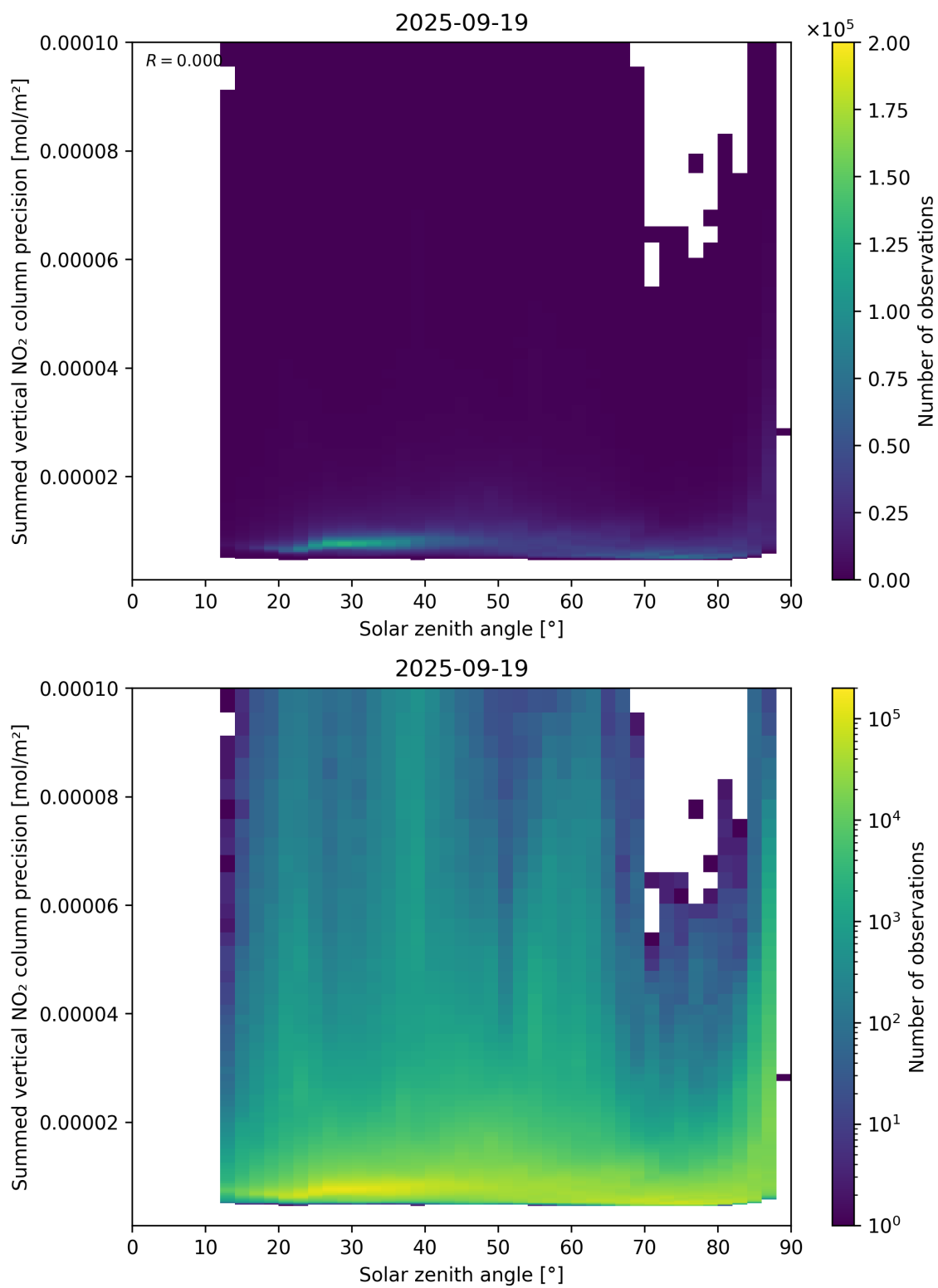
Figure 152: Scatter density plot of “Solar zenith angle” against “Summed vertical NO 2 column precision” for 2025-09-18 to 2025-09-20.
