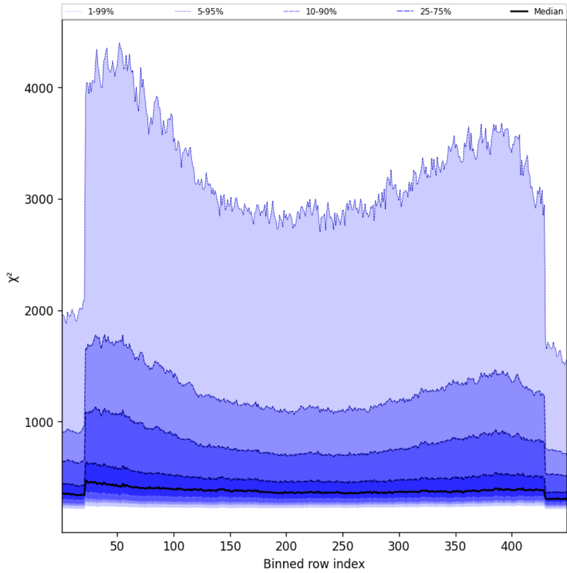
Figure 59: Along track statistics of “ \chi^2 ” for 2025-09-18 to 2025-09-20
