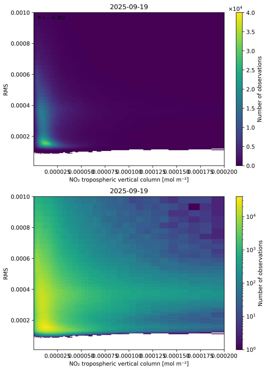
Figure 142: Scatter density plot of “NO 2 tropospheric vertical column” against “RMS” for 2025-09-18 to 2025-09-20.
