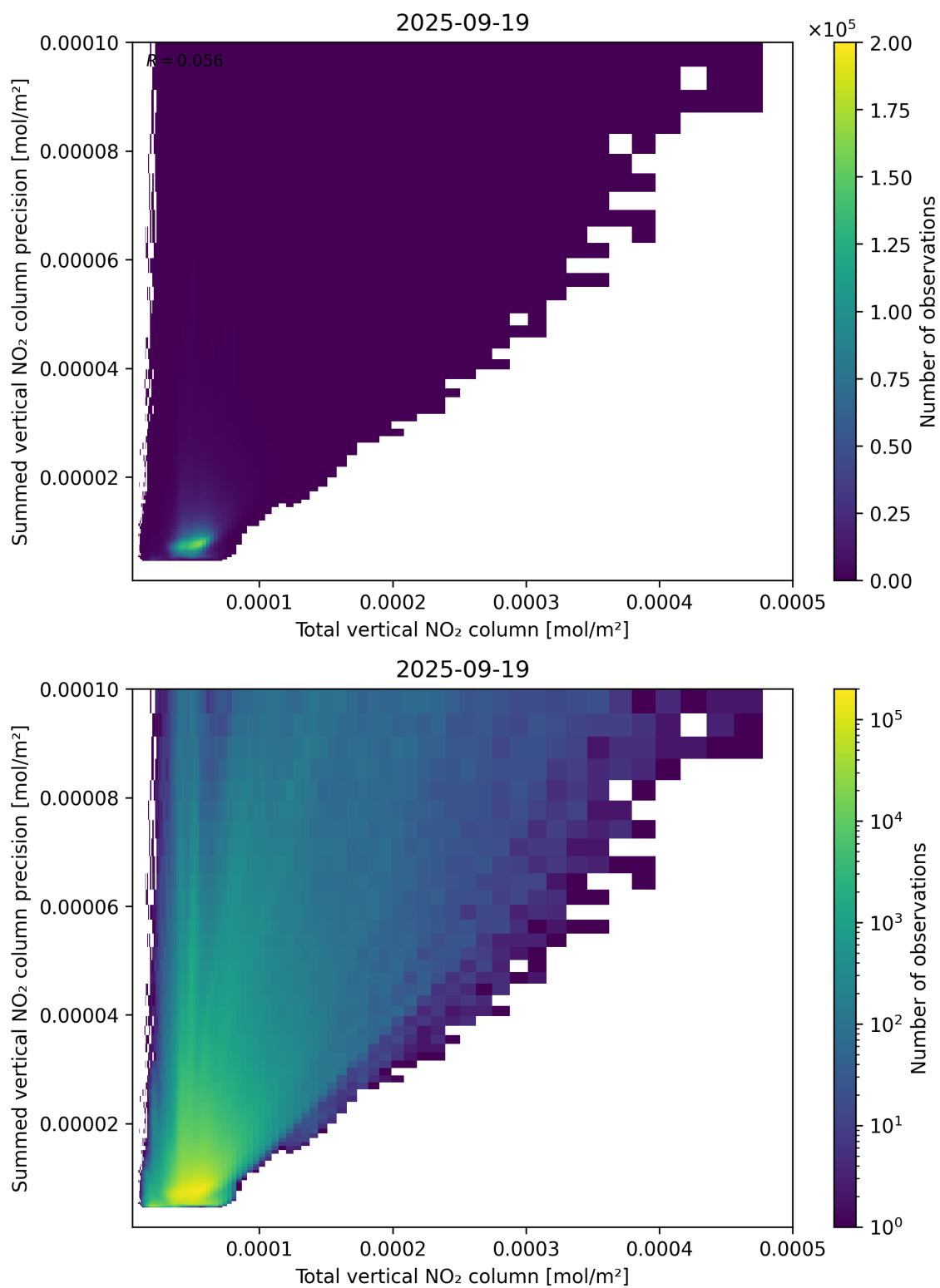
Figure 113: Scatter density plot of “Total vertical NO 2 column” against “Summed vertical NO 2 column precision” for 2025-09-18 to 2025-09-20.
