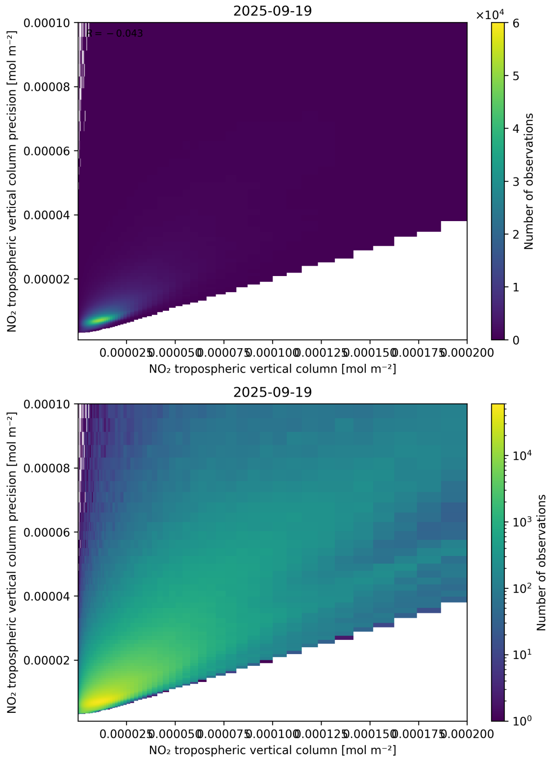
Figure 130: Scatter density plot of “NO 2 tropospheric vertical column” against “NO 2 tropospheric vertical column precision” for 2025-09-18 to 2025-09-20.
