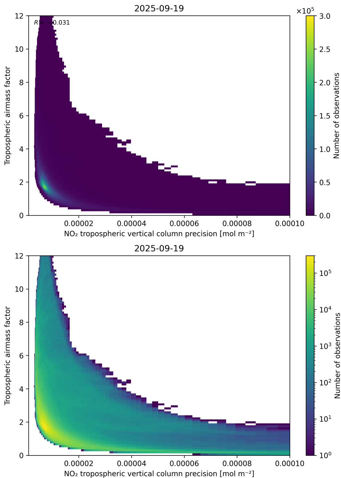
Figure 133: Scatter density plot of “NO 2 tropospheric vertical column precision” against “Tropospheric airmass factor” for 2025-09-18 to 2025-09-20.
