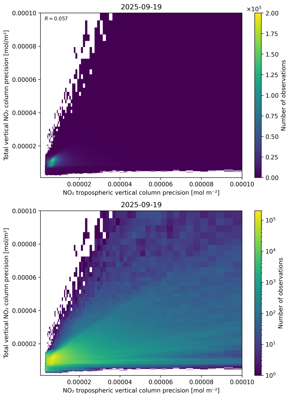
Figure 139: Scatter density plot of “NO 2 tropospheric vertical column precision” against “Total vertical NO 2 column precision” for 2025-09-18 to 2025-09-20.
