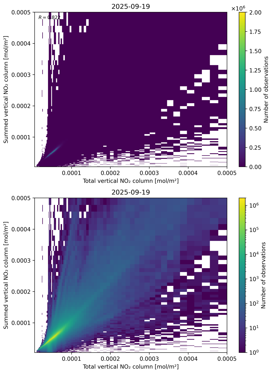
Figure 112: Scatter density plot of “Total vertical NO 2 column” against “Summed vertical NO 2 column” for 2025-09-18 to 2025-09-20.
