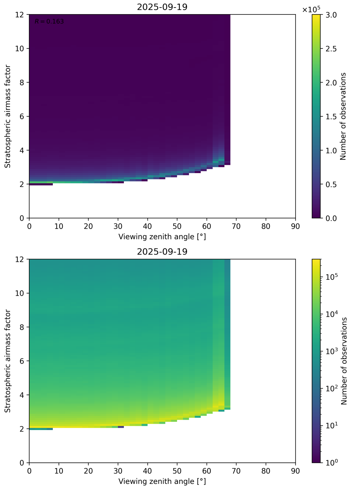
Figure 159: Scatter density plot of “Viewing zenith angle” against “Stratospheric airmass factor” for 2025-09-18 to 2025-09-20.
