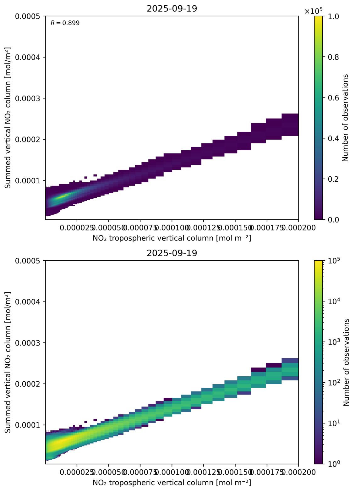
Figure 126: Scatter density plot of “NO 2 tropospheric vertical column” against “Summed vertical NO 2 column” for 2025-09-18 to 2025-09-20.
