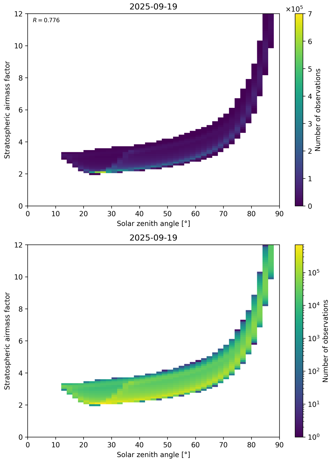
Figure 145: Scatter density plot of “Solar zenith angle” against “Stratospheric airmass factor” for 2025-09-18 to 2025-09-20.
