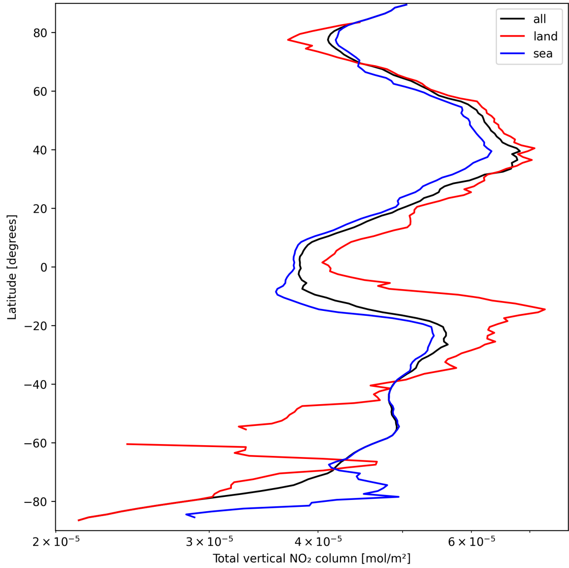
Figure 21: Zonal average of “Total vertical NO 2 column” for 2025-09-18 to 2025-09-20.
