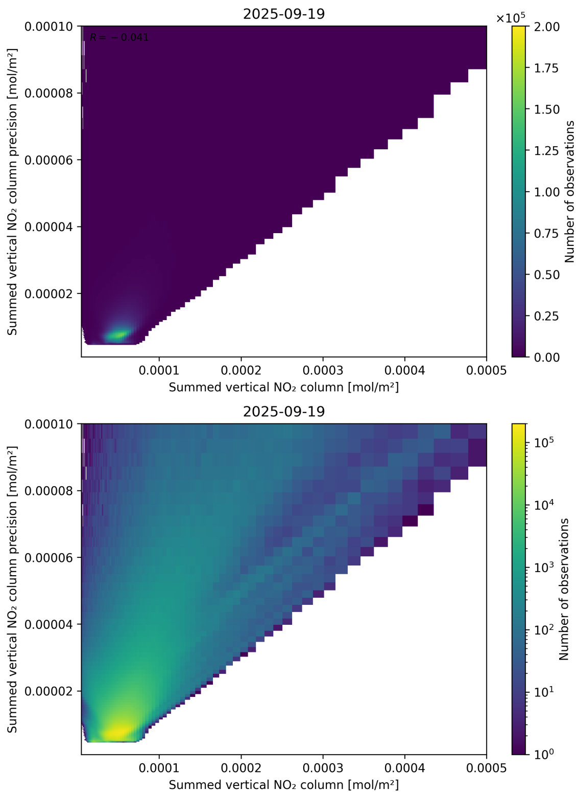
Figure 105: Scatter density plot of “Summed vertical NO 2 column” against “Summed vertical NO 2 column precision” for 2025-09-18 to 2025-09-20.
