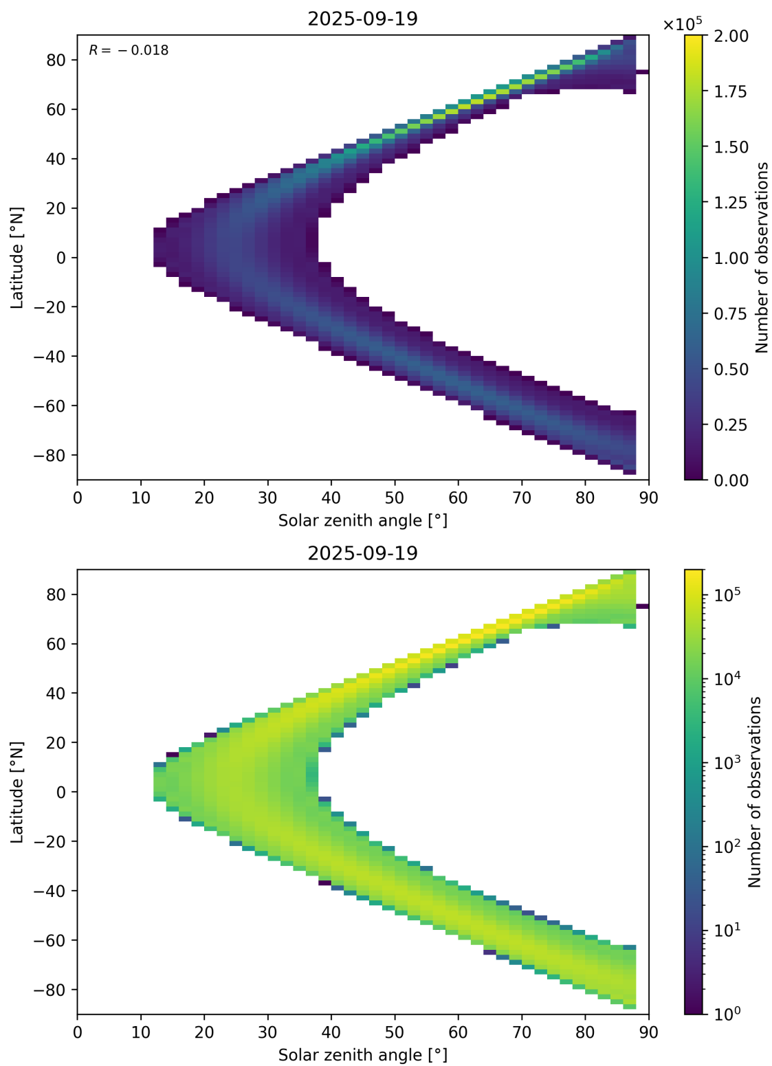
Figure 149: Scatter density plot of “Solar zenith angle” against “Latitude” for 2025-09-18 to 2025-09-20.
