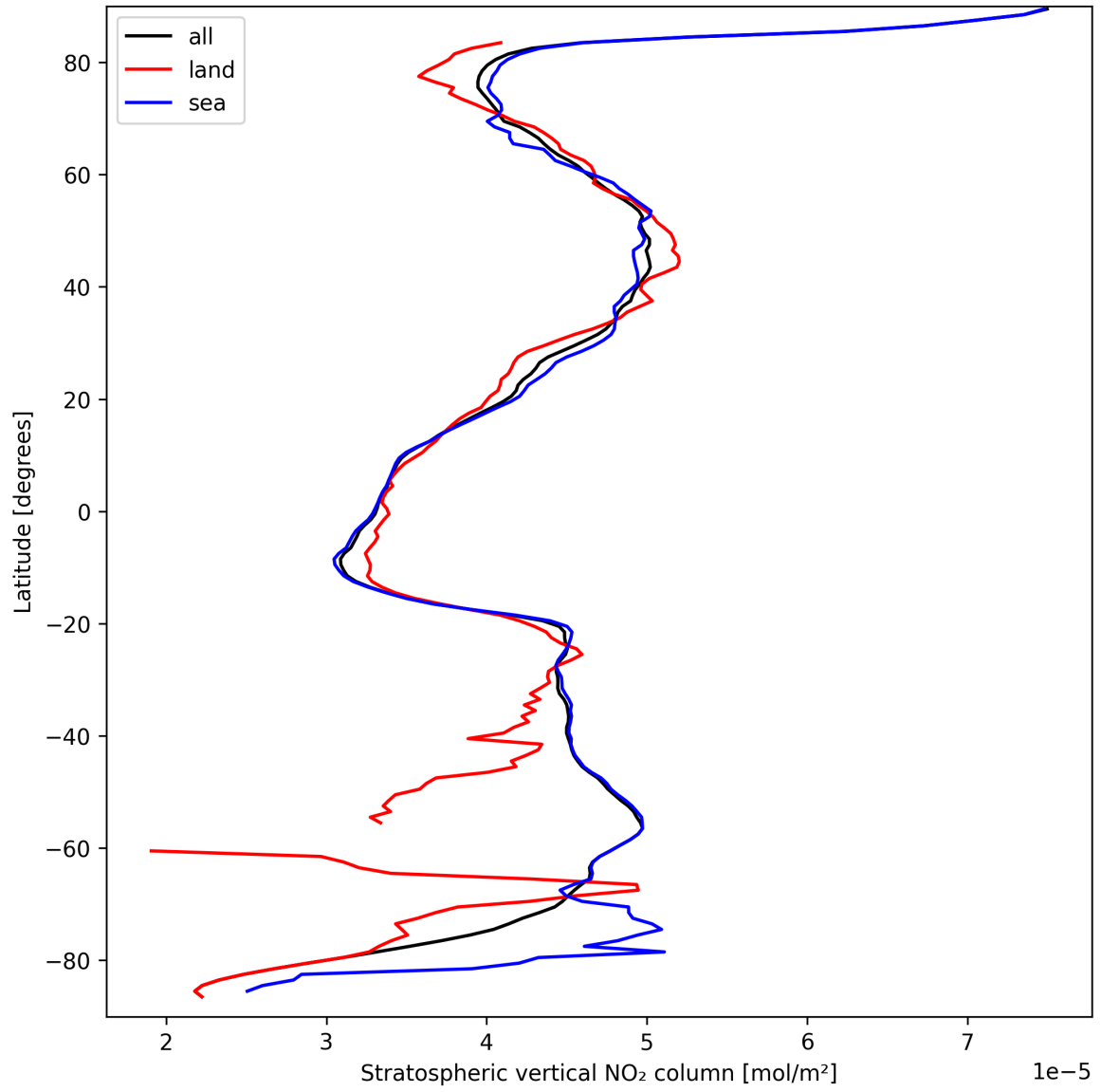
Figure 19: Zonal average of “Stratospheric vertical NO 2 column” for 2025-09-18 to 2025-09-20.
