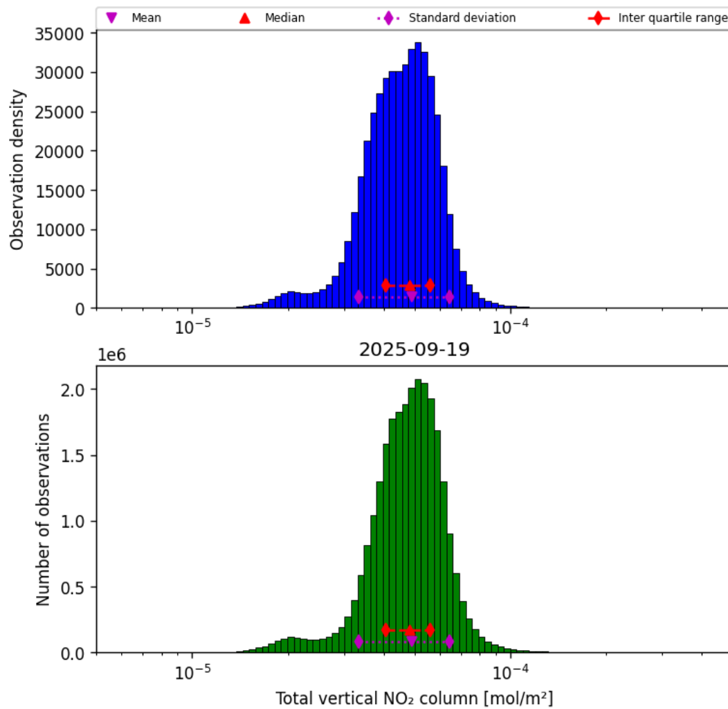
Figure 38: Histogram of “Total vertical NO 2 column” for 2025-09-18 to 2025-09-20
