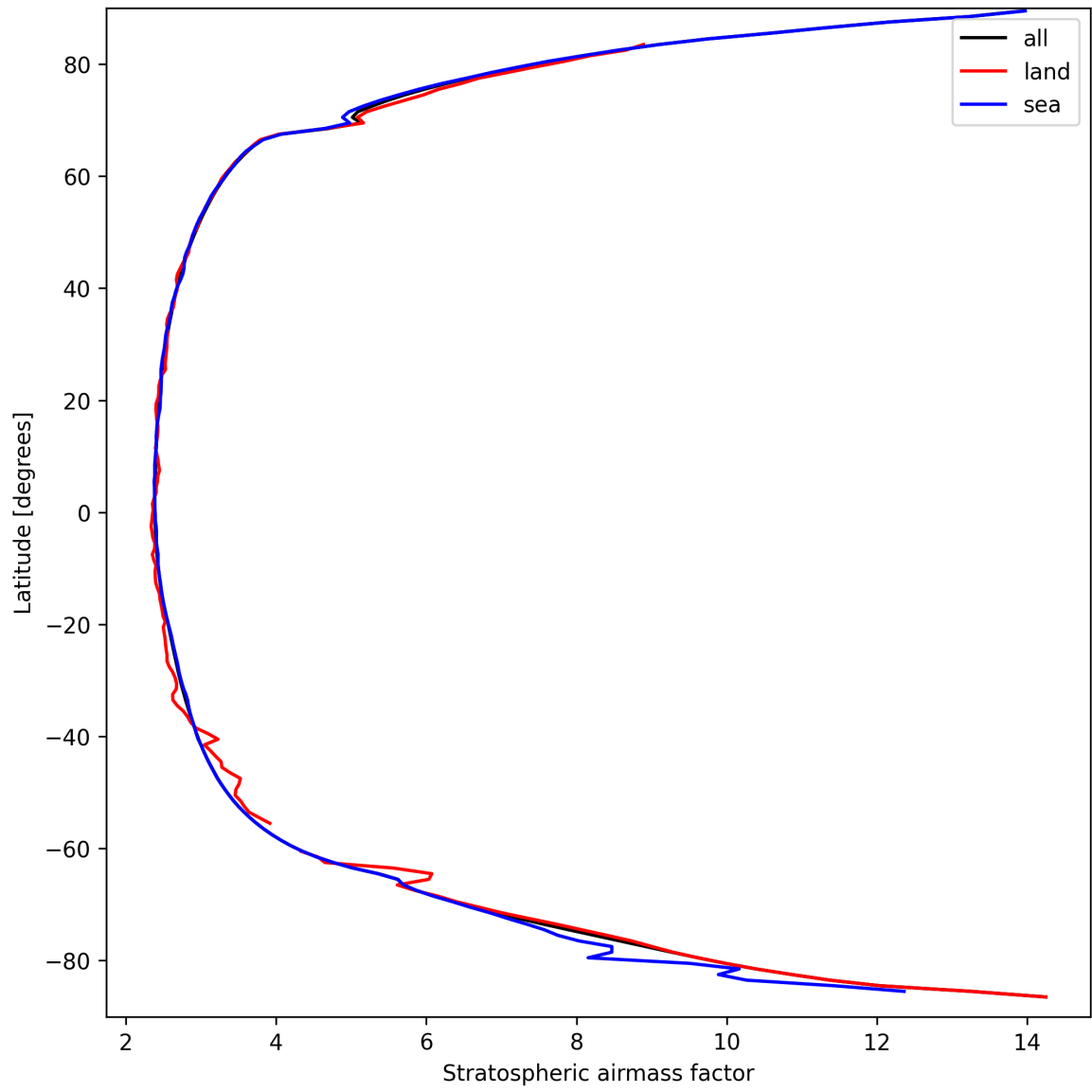
Figure 27: Zonal average of “Stratospheric airmass factor” for 2025-09-18 to 2025-09-20.
