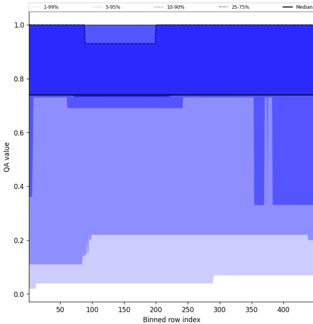
Figure 45: Along track statistics of "QA value" for 2025-09-20 to 2025-09-21
