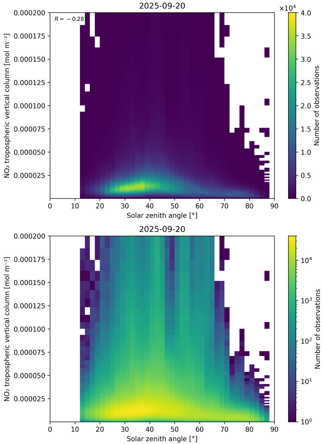
Figure 155: Scatter density plot of “Solar zenith angle” against “NO 2 tropospheric vertical column” for 2025-09-20 to 2025-09-21.
