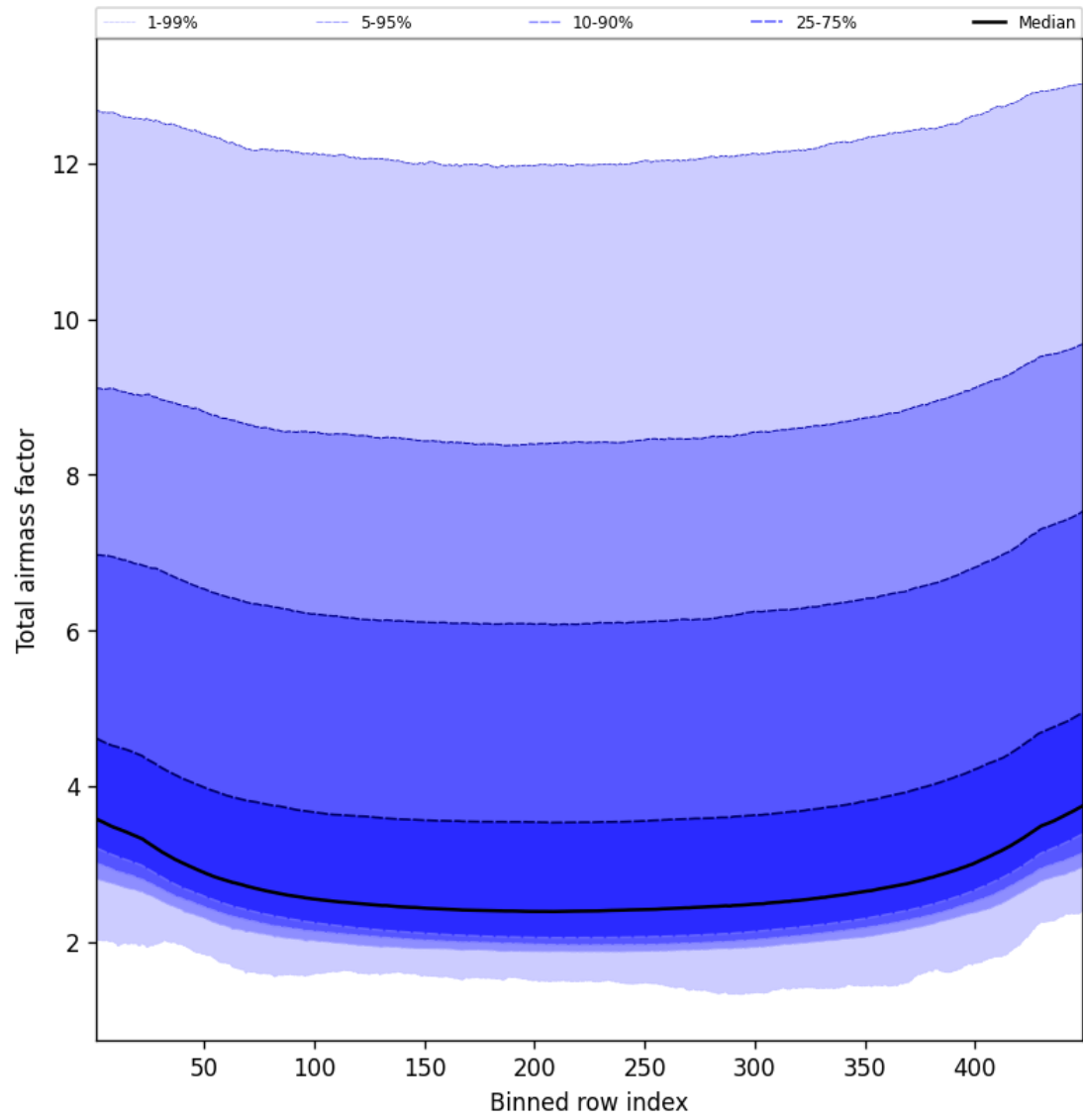
Figure 49: Along track statistics of “Total airmass factor” for 2025-09-20 to 2025-09-21
