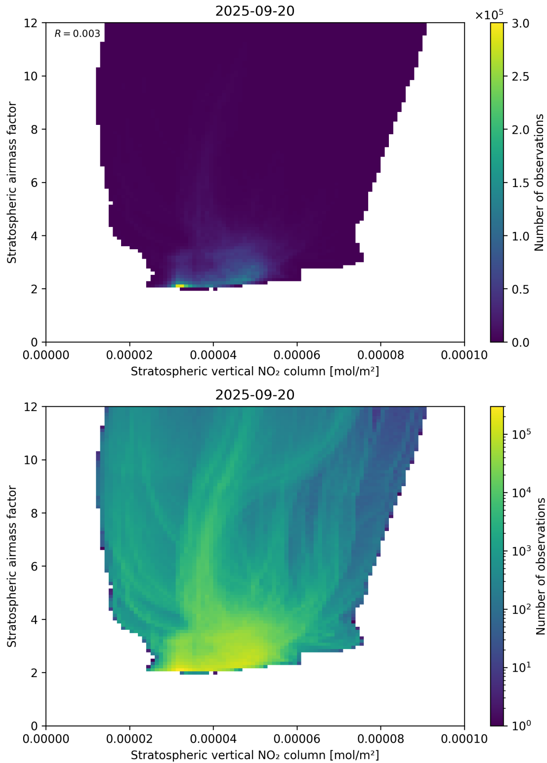
Figure 96: Scatter density plot of “Stratospheric vertical NO 2 column” against “Stratospheric airmass factor” for 2025-09-20 to 2025-09-21.
