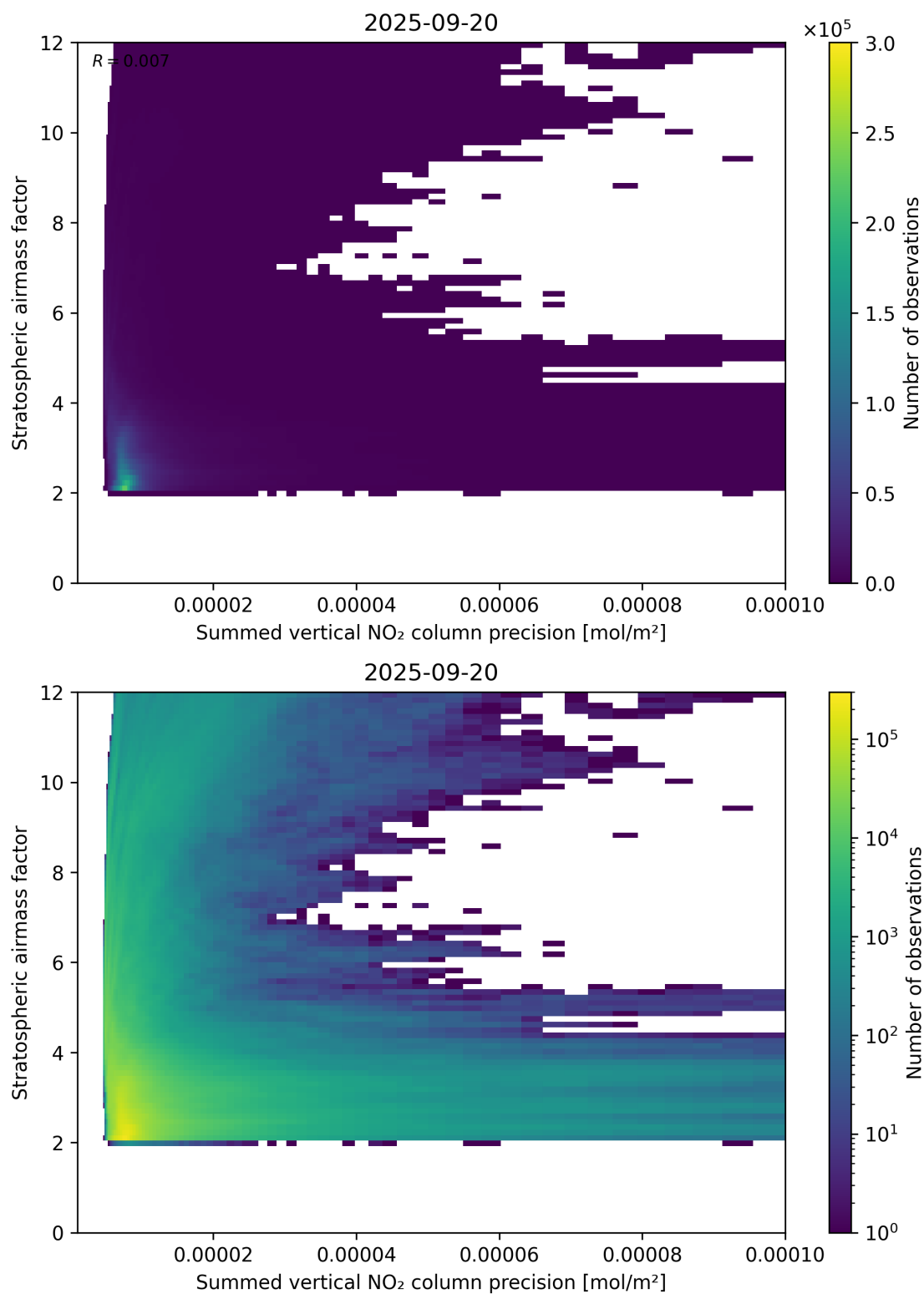
Figure 106: Scatter density plot of “Summed vertical NO 2 column precision” against “Stratospheric airmass factor” for 2025-09-20 to 2025-09-21.
