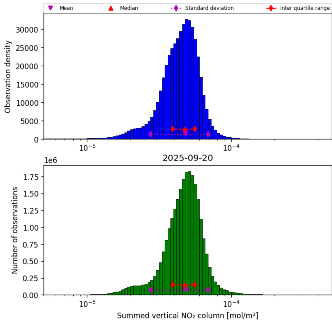
Figure 40: Histogram of “Summed vertical NO 2 column” for 2025-09-20 to 2025-09-21
