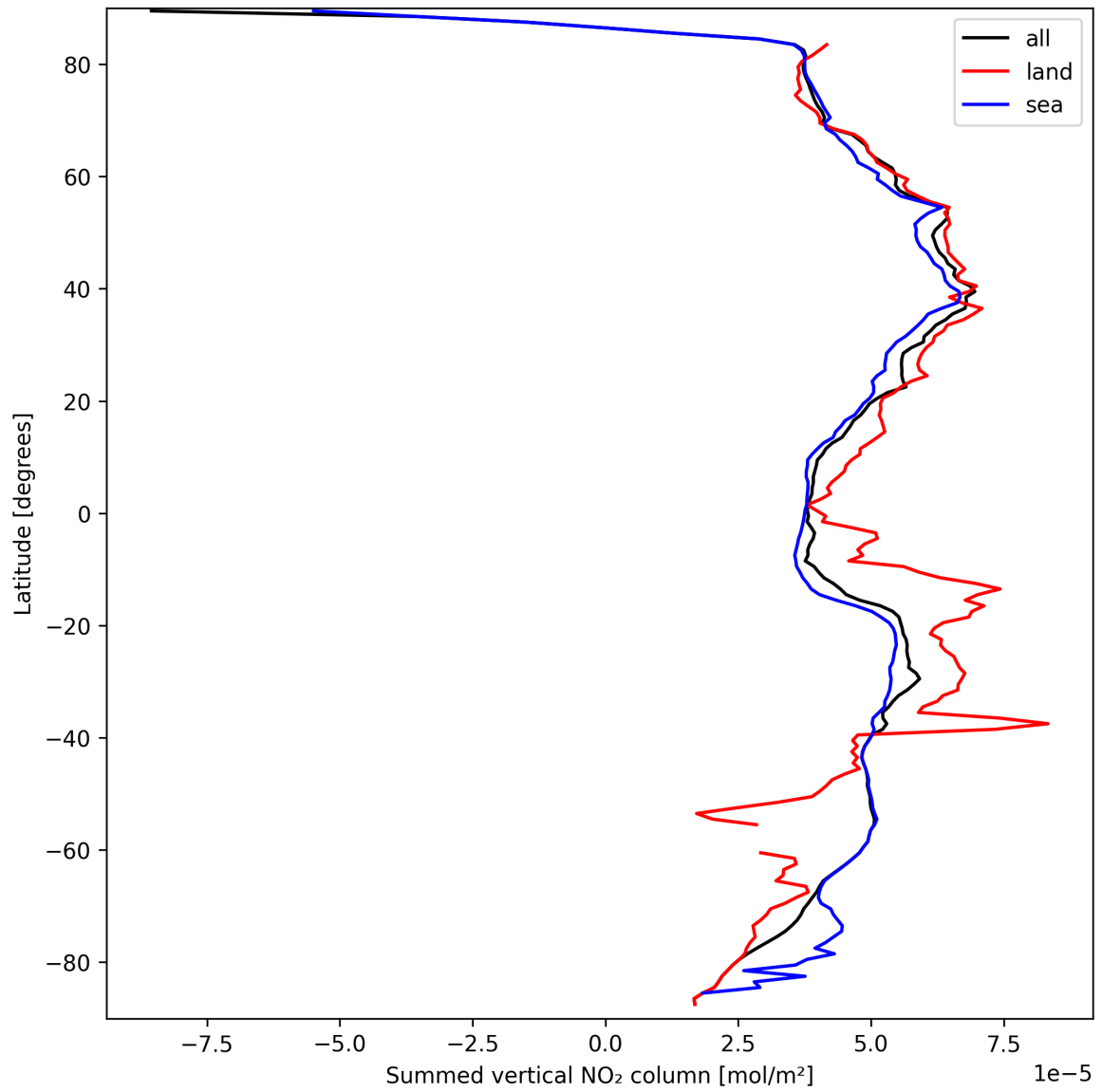
Figure 23: Zonal average of “Summed vertical NO 2 column” for 2025-09-20 to 2025-09-21.
