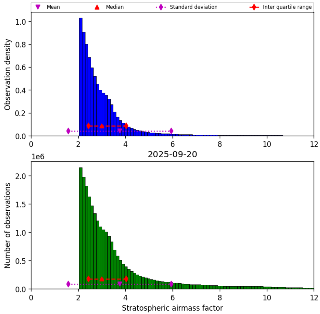
Figure 44: Histogram of “Stratospheric airmass factor” for 2025-09-20 to 2025-09-21
