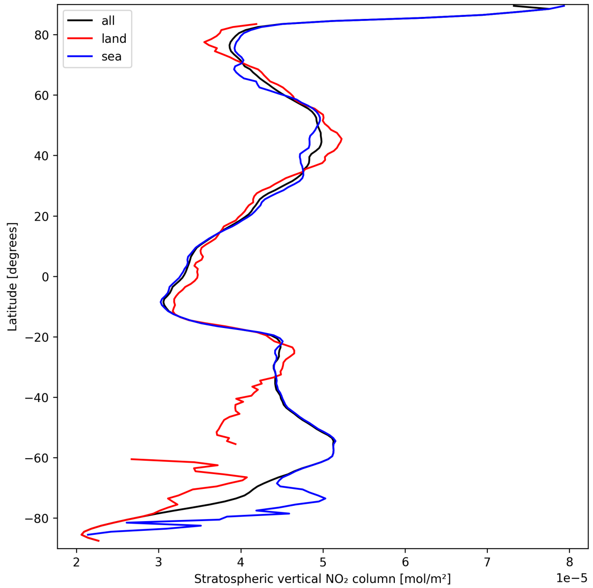
Figure 19: Zonal average of “Stratospheric vertical NO 2 column” for 2025-09-20 to 2025-09-21.
