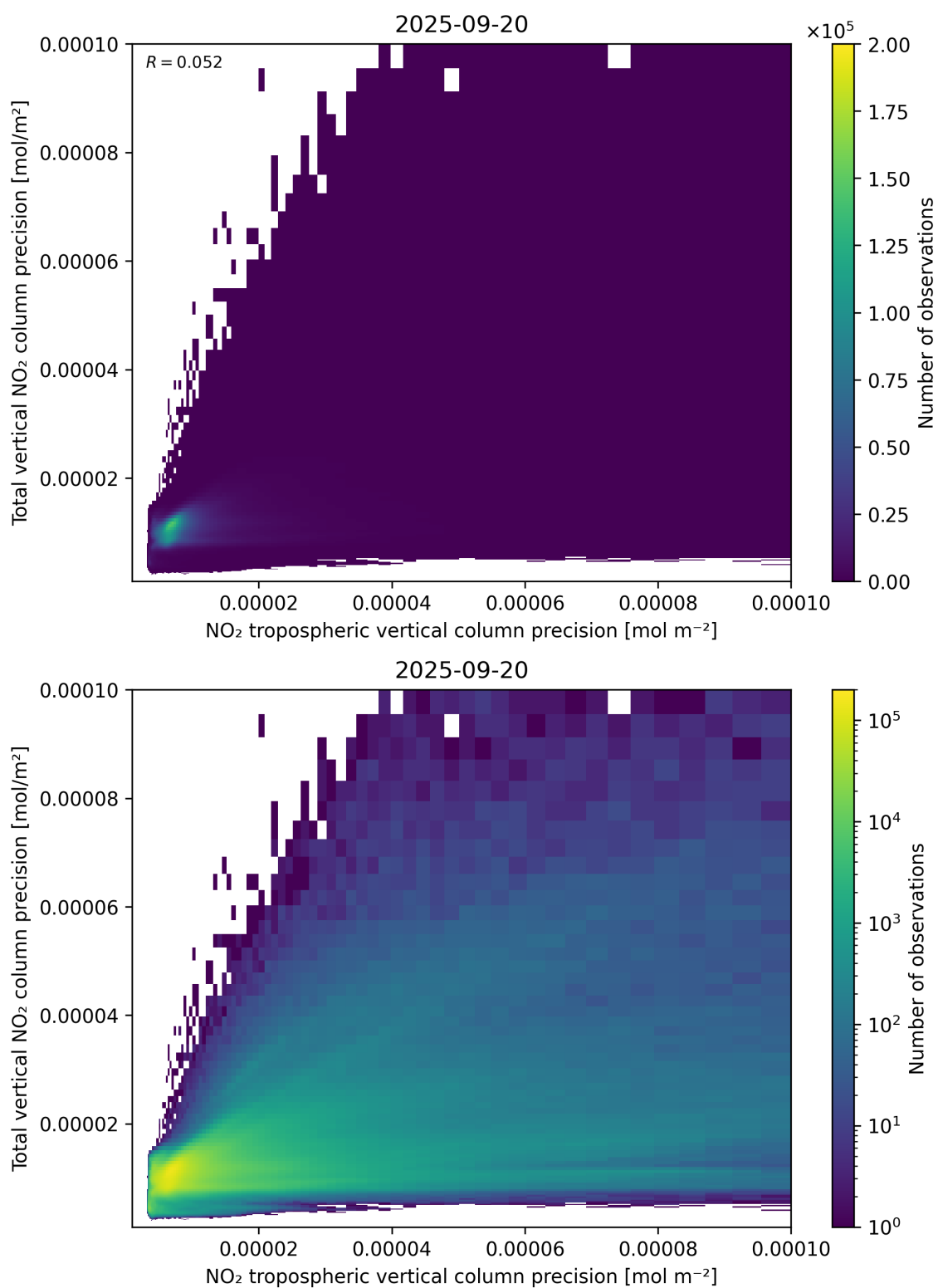
Figure 139: Scatter density plot of “NO 2 tropospheric vertical column precision” against “Total vertical NO 2 column precision” for 2025-09-20 to 2025-09-21.
