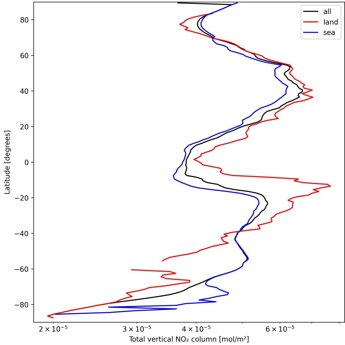
Figure 21: Zonal average of “Total vertical NO 2 column” for 2025-09-20 to 2025-09-21.
