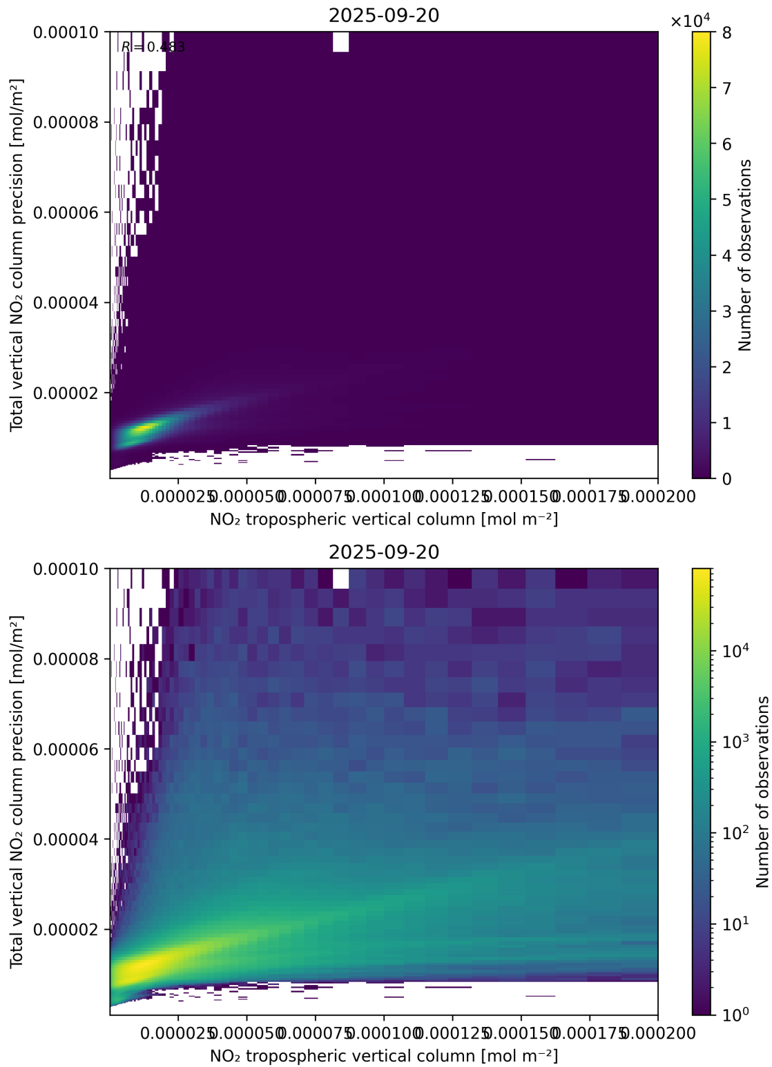
Figure 129: Scatter density plot of “NO 2 tropospheric vertical column” against “Total vertical NO 2 column precision” for 2025-09-20 to 2025-09-21.
