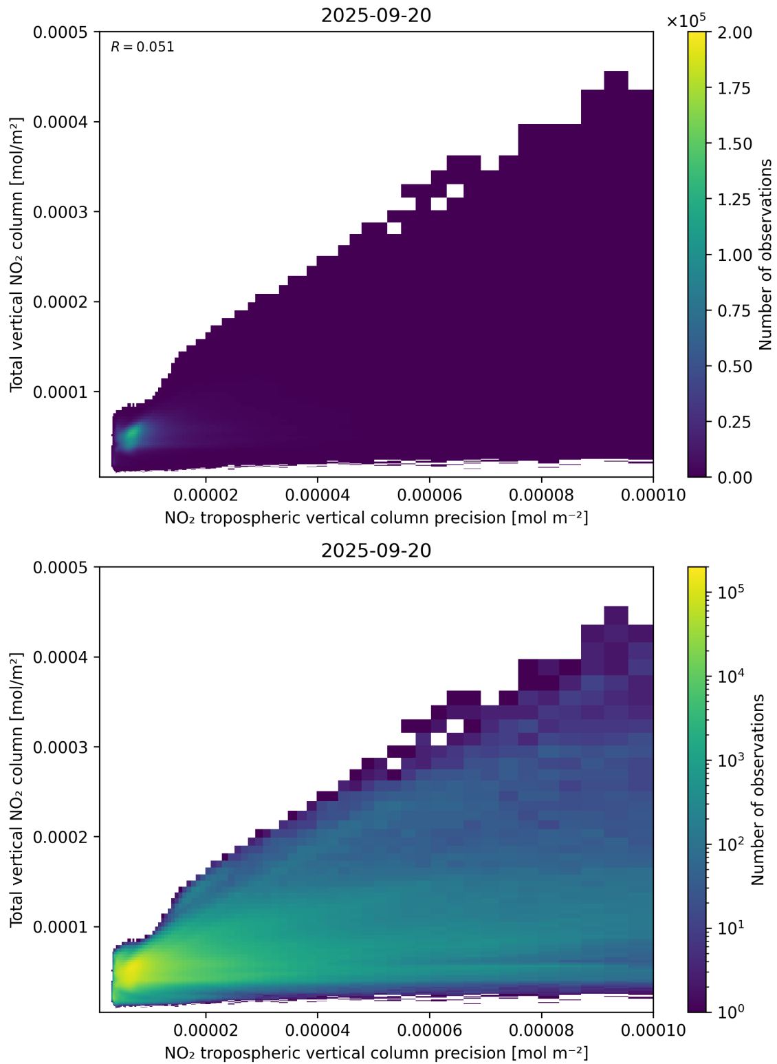
Figure 138: Scatter density plot of “NO 2 tropospheric vertical column precision” against “Total vertical NO 2 column” for 2025-09-20 to 2025-09-21.
