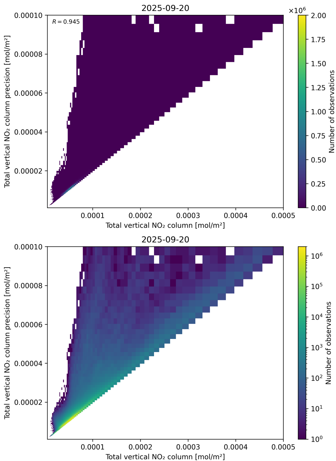
Figure 114: Scatter density plot of “Total vertical NO 2 column” against “Total vertical NO 2 column precision” for 2025-09-20 to 2025-09-21.
