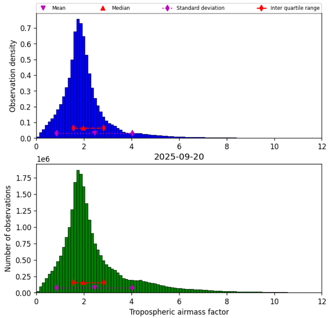
Figure 31: Histogram of “Tropospheric airmass factor” for 2025-09-20 to 2025-09-21
