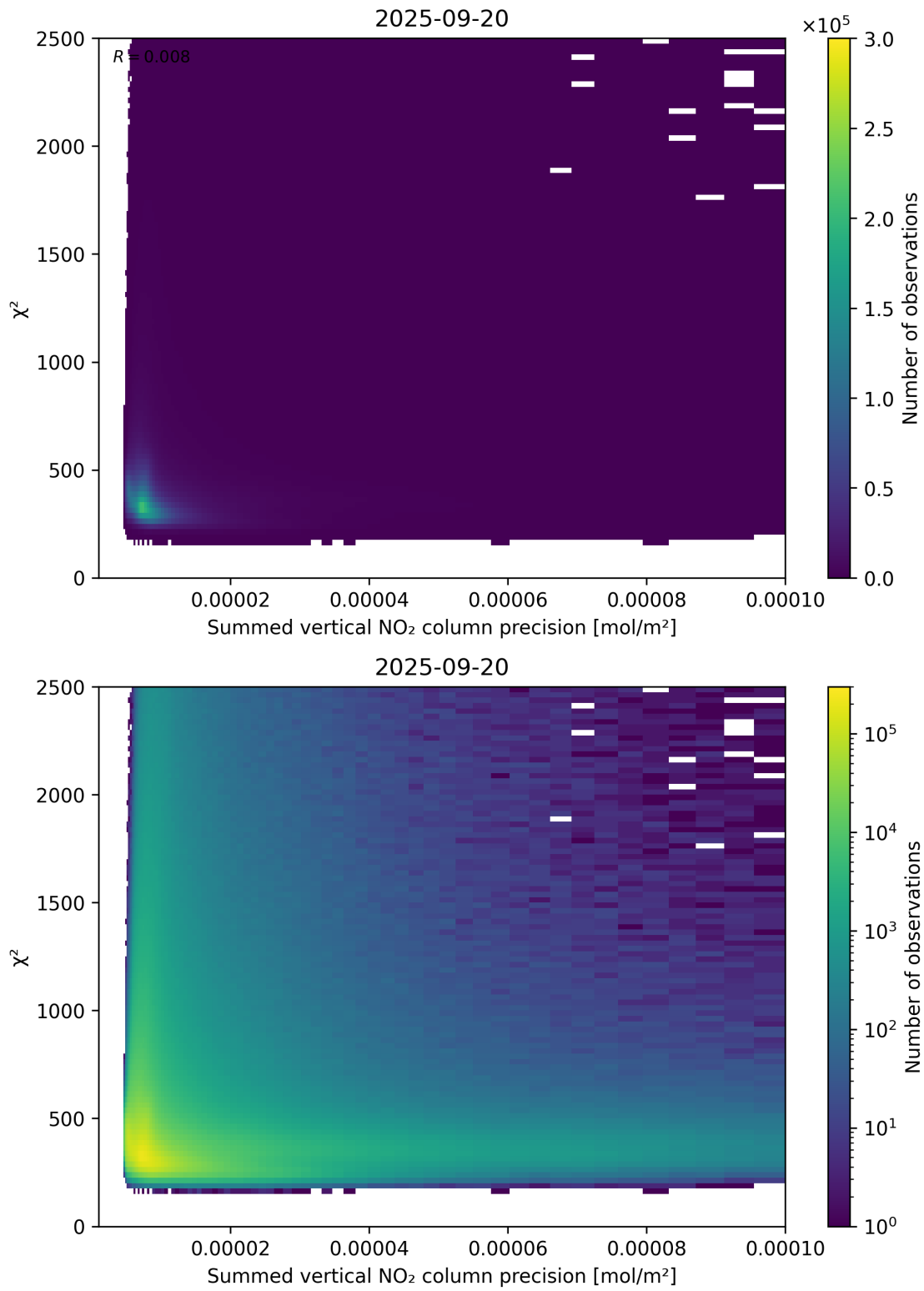
Figure 107: Scatter density plot of “Summed vertical NO 2 column precision” against “ \chi^2 ” for 2025-09-20 to 2025-09-21.
