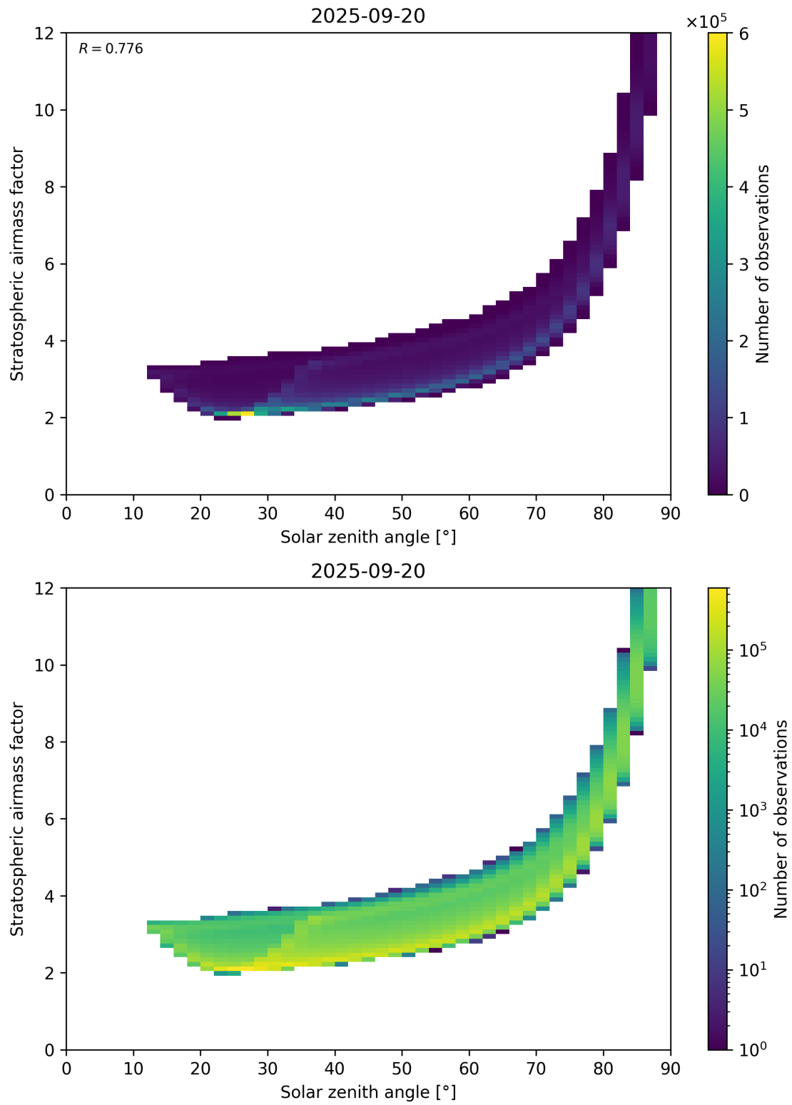
Figure 145: Scatter density plot of “Solar zenith angle” against “Stratospheric airmass factor” for 2025-09-20 to 2025-09-21.
