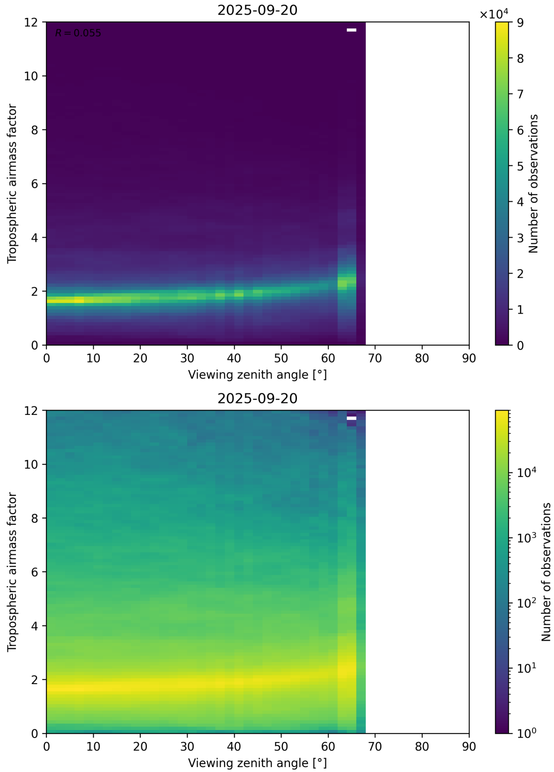
Figure 161: Scatter density plot of “Viewing zenith angle” against “Tropospheric airmass factor” for 2025-09-20 to 2025-09-21.
