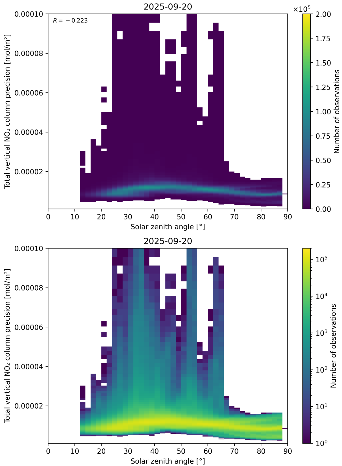
Figure 154: Scatter density plot of “Solar zenith angle” against “Total vertical NO 2 column precision” for 2025-09-20 to 2025-09-21.
