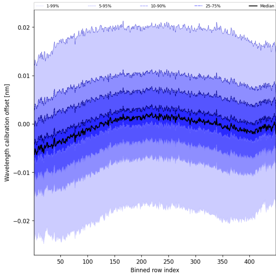
Figure 52: Along track statistics of “Wavelength calibration offset” for 2025-09-20 to 2025-09-21
