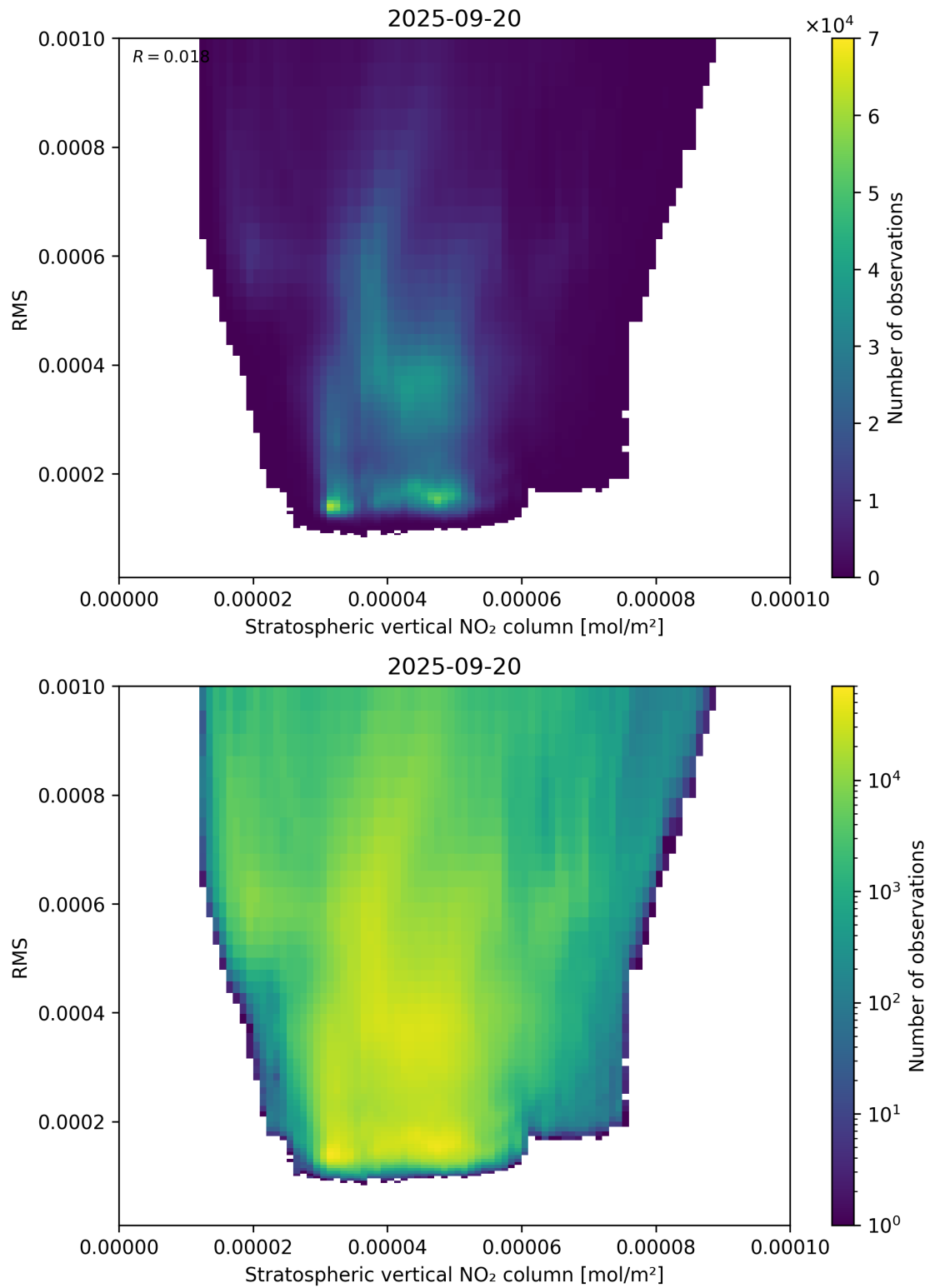
Figure 102: Scatter density plot of “Stratospheric vertical NO 2 column” against “RMS” for 2025-09-20 to 2025-09-21.
