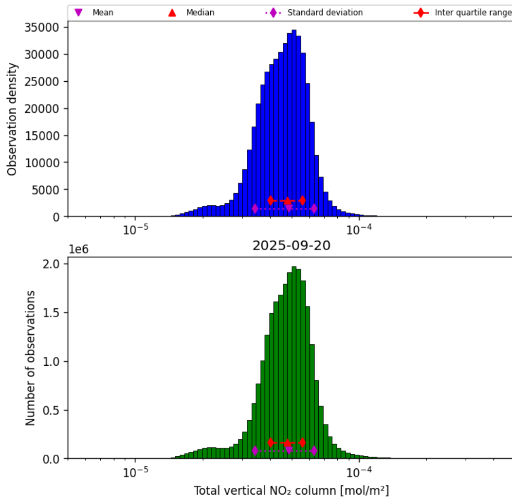
Figure 38: Histogram of “Total vertical NO 2 column” for 2025-09-20 to 2025-09-21
