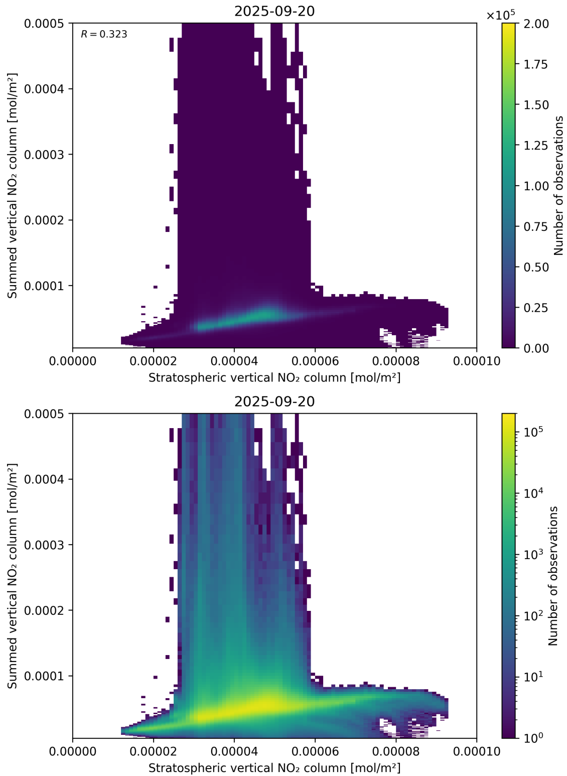
Figure 98: Scatter density plot of “Stratospheric vertical NO 2 column” against “Summed vertical NO 2 column” for 2025-09-20 to 2025-09-21.
