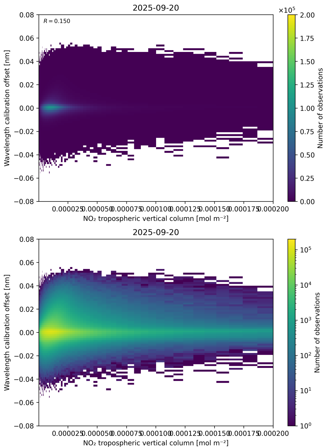
Figure 143: Scatter density plot of “NO 2 tropospheric vertical column” against “Wavelength calibration offset” for 2025-09-20 to 2025-09-21.
