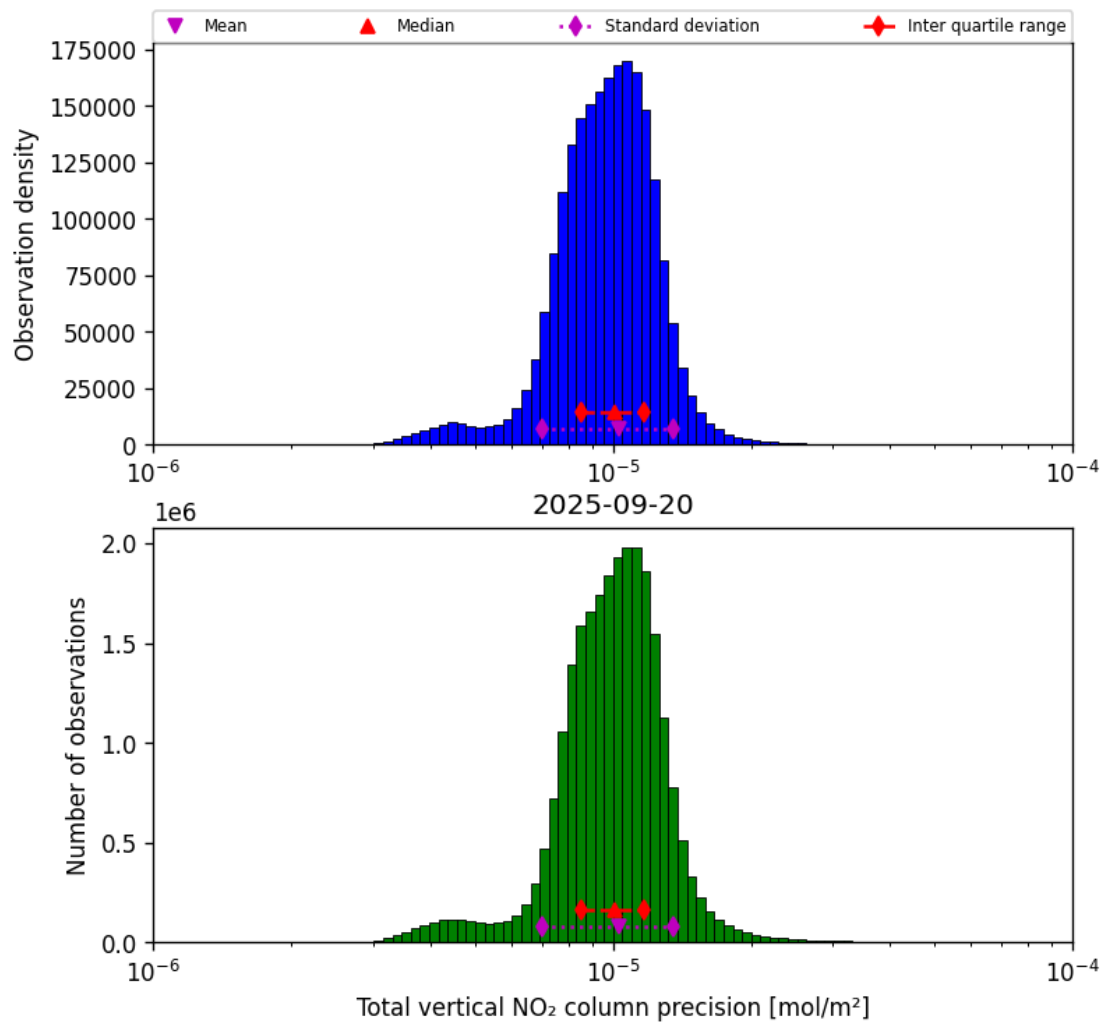
Figure 39: Histogram of “Total vertical NO 2 column precision” for 2025-09-20 to 2025-09-21
