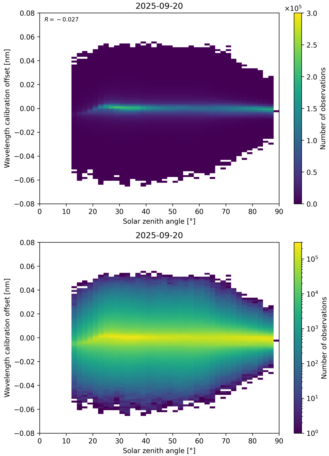
Figure 158: Scatter density plot of “Solar zenith angle” against “Wavelength calibration offset” for 2025-09-20 to 2025-09-21.
