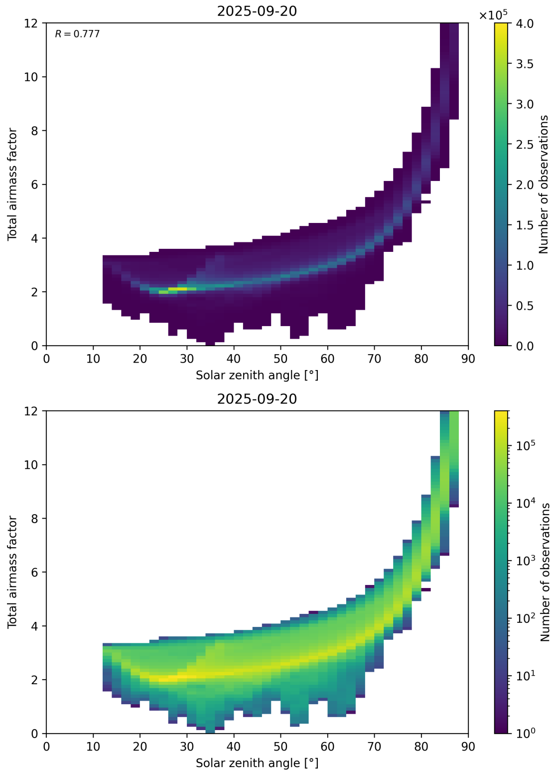
Figure 146: Scatter density plot of “Solar zenith angle” against “Total air mass factor” for 2025-09-20 to 2025-09-21.
