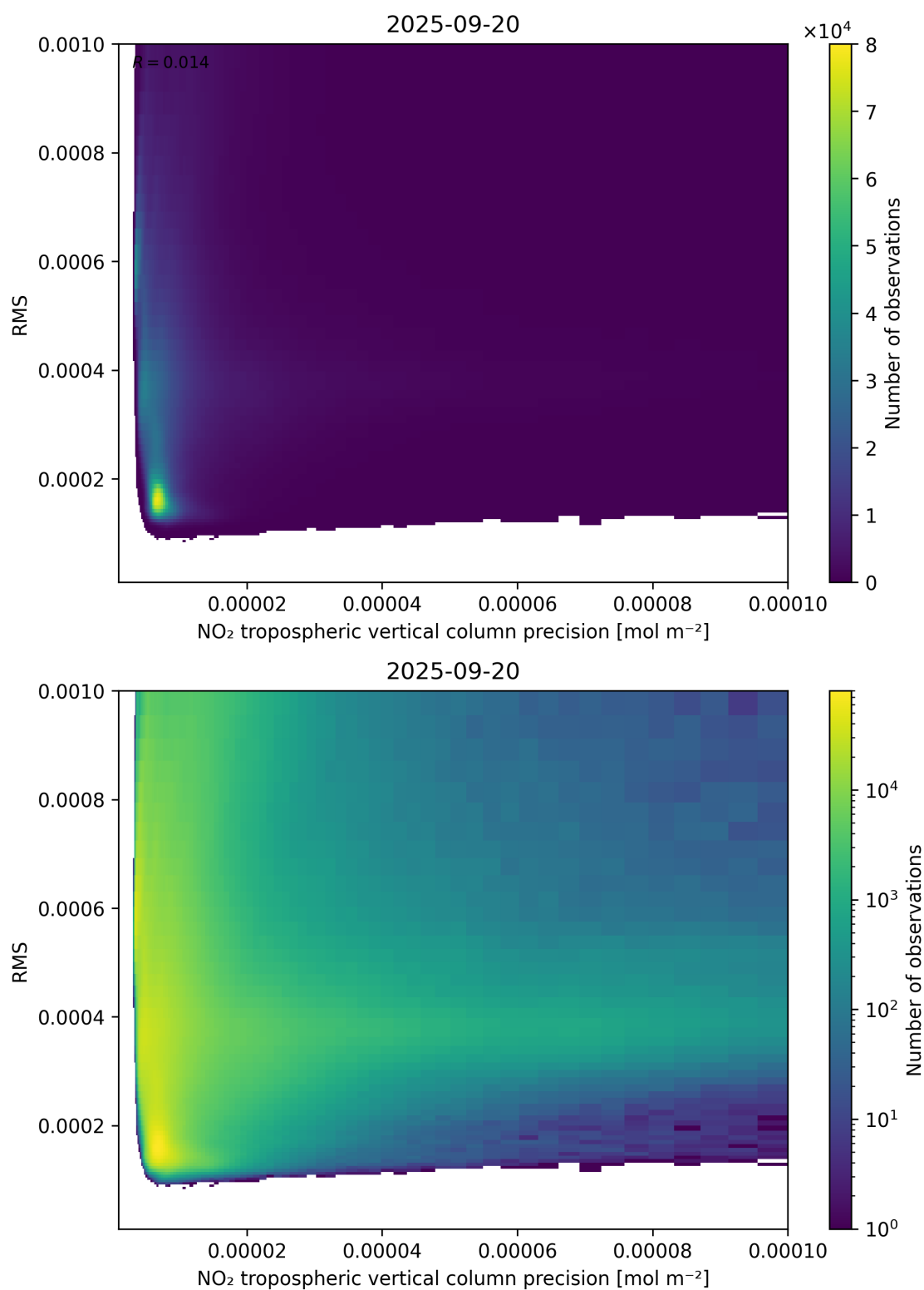
Figure 140: Scatter density plot of “NO 2 tropospheric vertical column precision” against “RMS” for 2025-09-20 to 2025-09-21.
