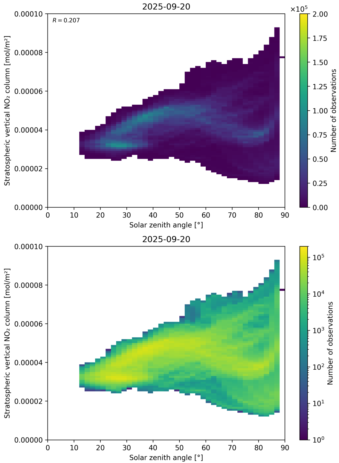
Figure 150: Scatter density plot of “Solar zenith angle” against “Stratospheric vertical NO 2 column” for 2025-09-20 to 2025-09-21.
