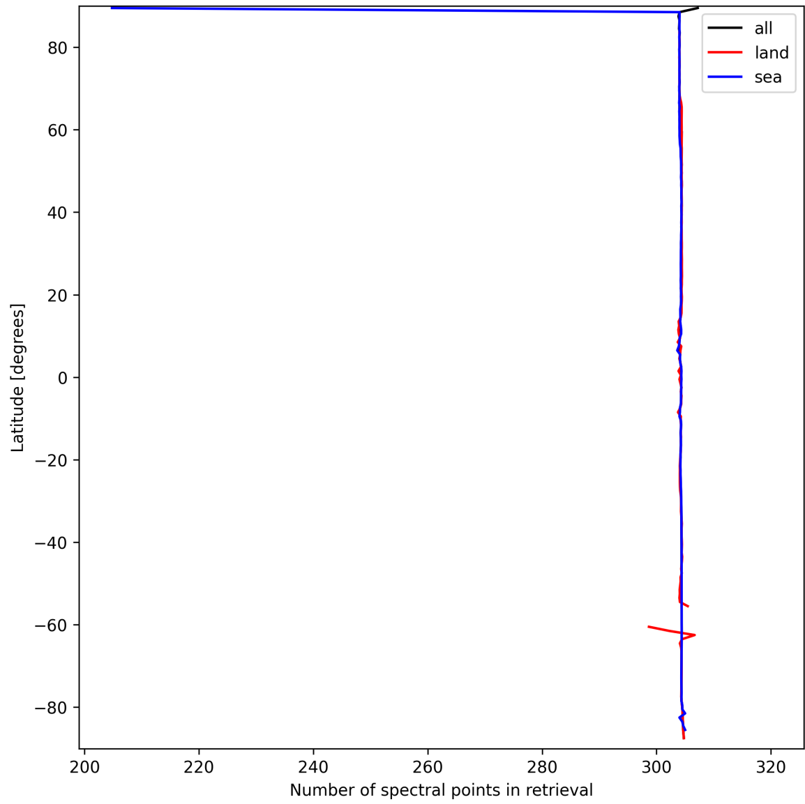
Figure 16: Zonal average of “Number of spectral points in retrieval” for 2025-09-20 to 2025-09-21.
