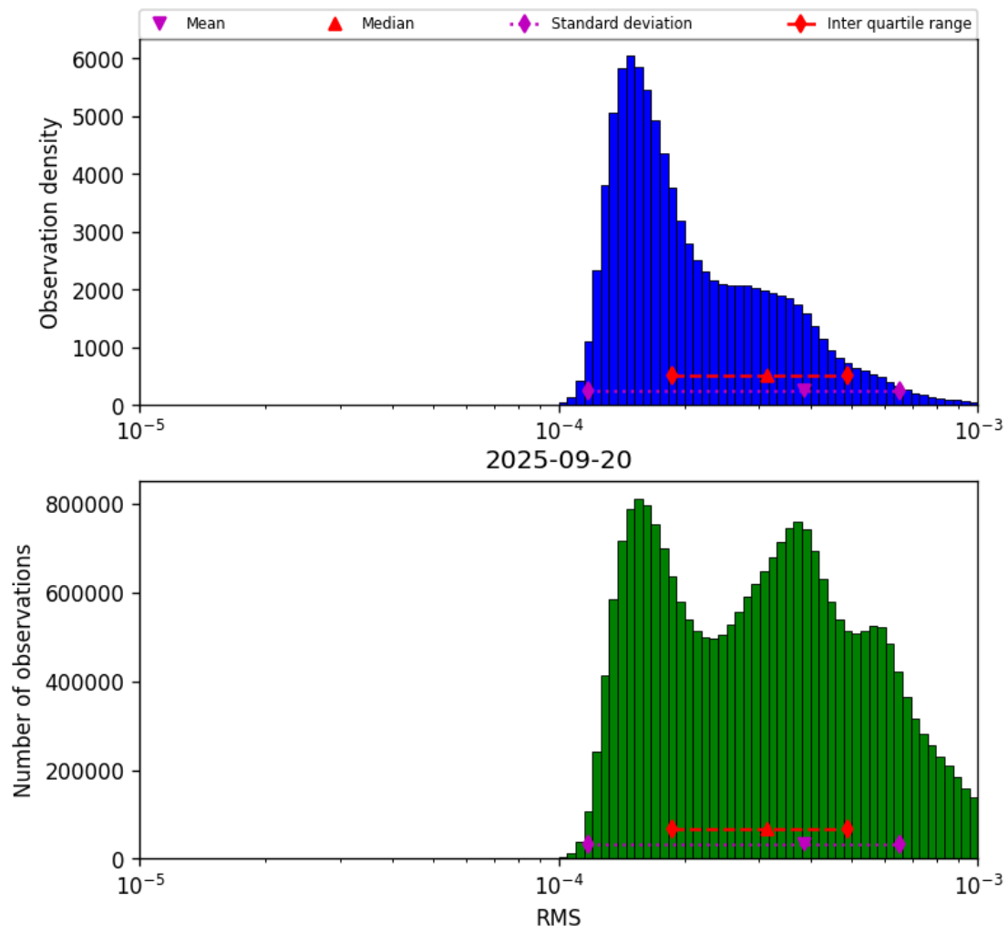
Figure 43: Histogram of “RMS” for 2025-09-20 to 2025-09-21
