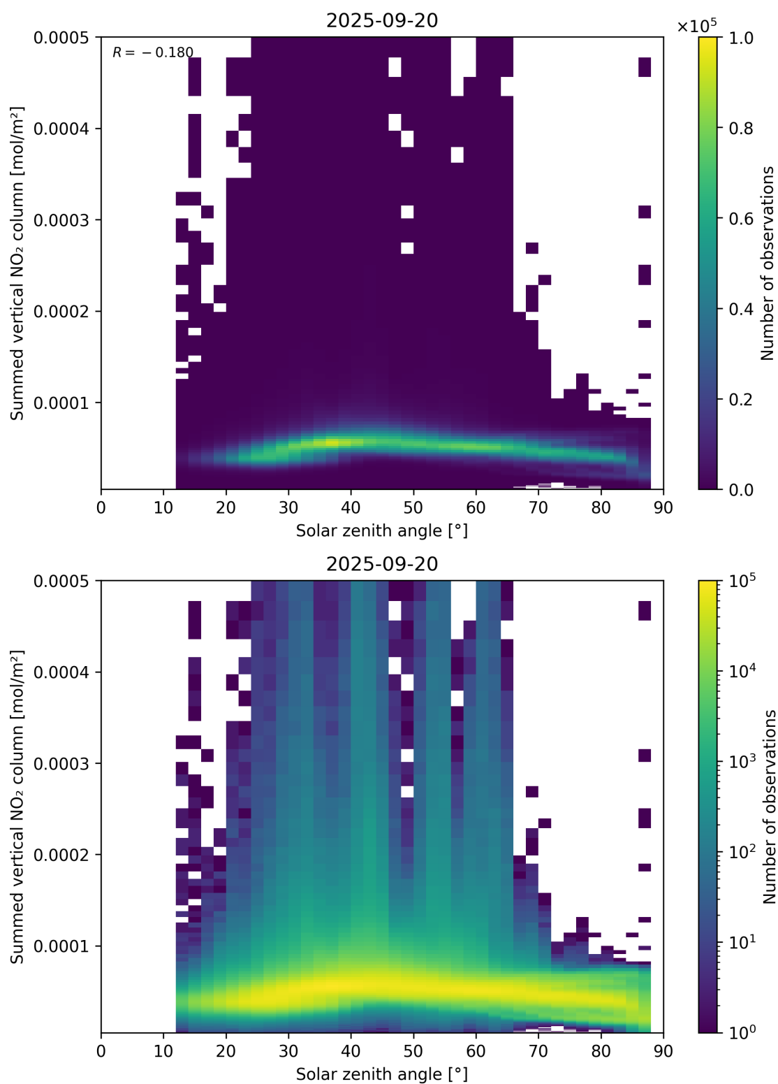
Figure 151: Scatter density plot of “Solar zenith angle” against “Summed vertical NO 2 column” for 2025-09-20 to 2025-09-21.
