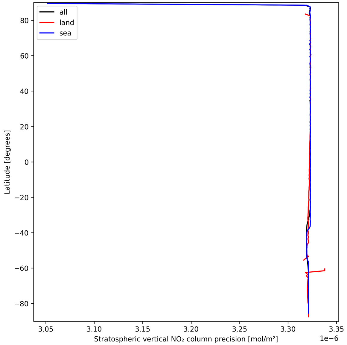
Figure 20: Zonal average of “Stratospheric vertical NO 2 column precision” for 2025-09-20 to 2025-09-21.
