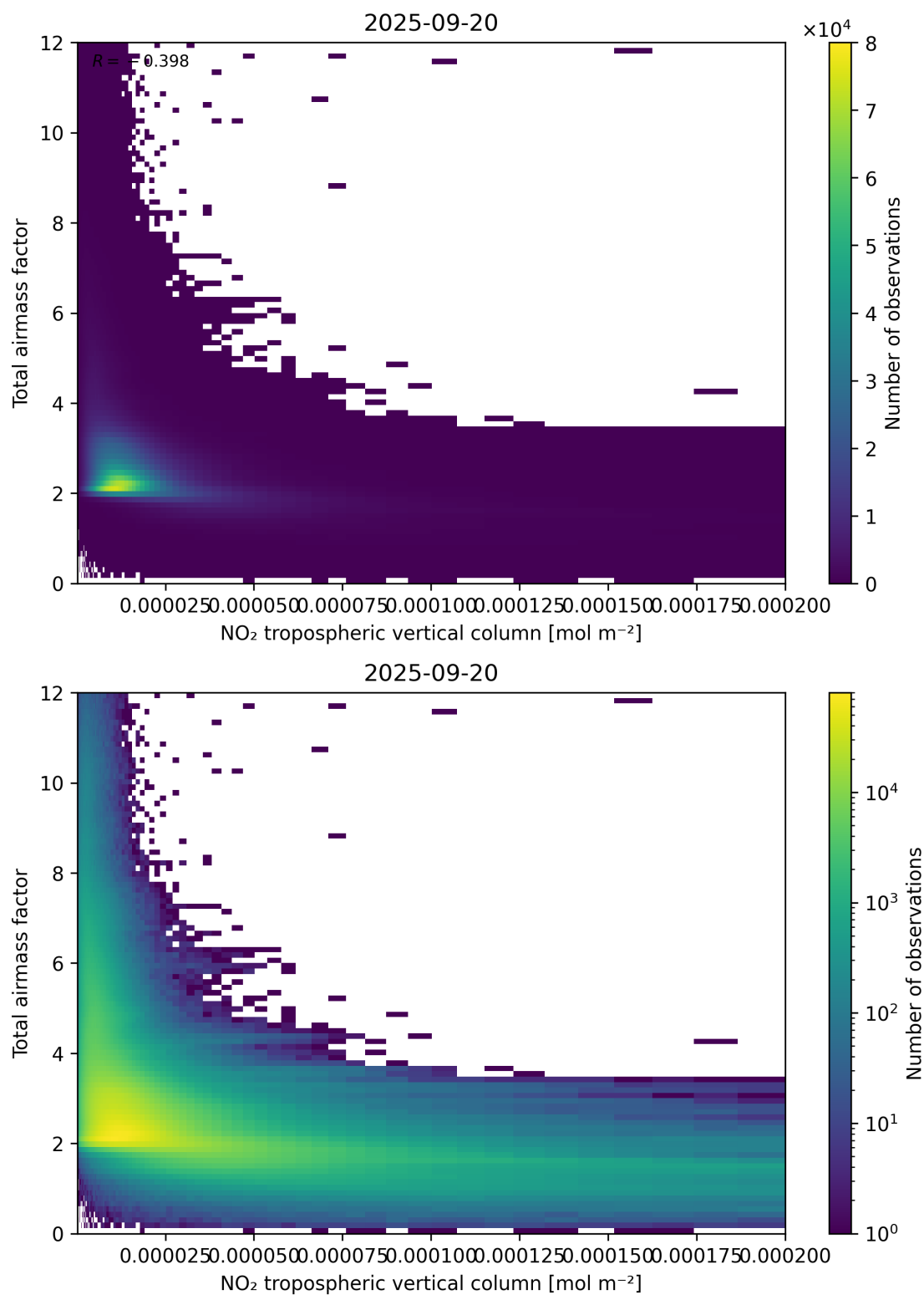
Figure 122: Scatter density plot of “NO 2 tropospheric vertical column” against “Total air mass factor” for 2025-09-20 to 2025-09-21.
