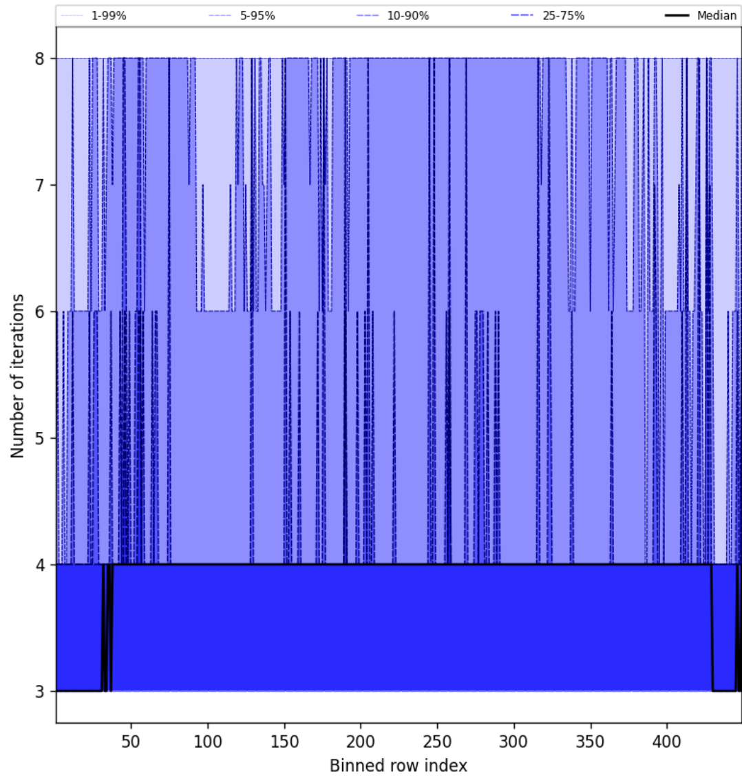
Figure 51: Along track statistics of “Number of iterations” for 2025-09-20 to 2025-09-21
