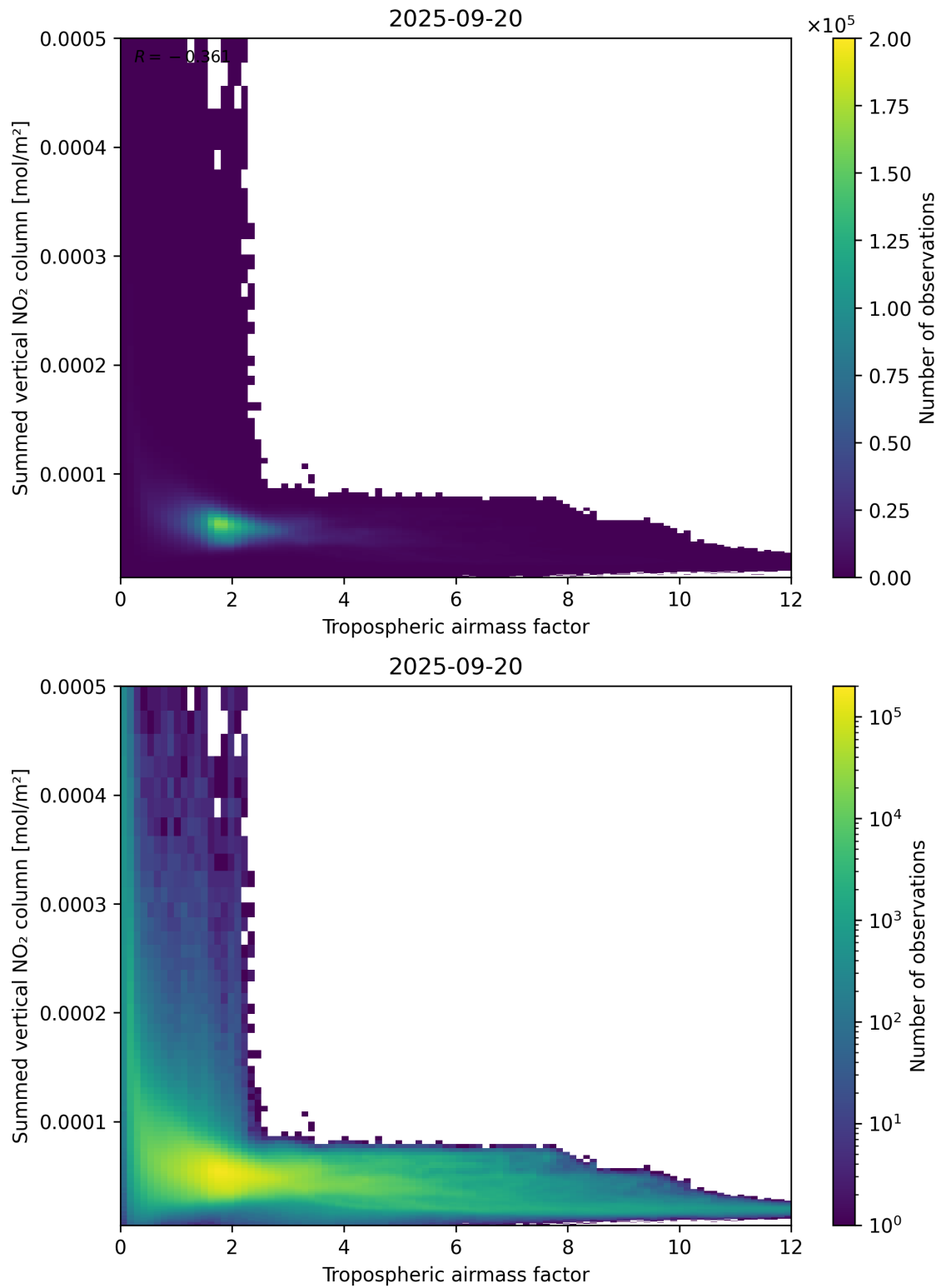
Figure 75: Scatter density plot of “Tropospheric air mass factor” against “Summed vertical NO 2 column” for 2025-09-20 to 2025-09-21.
