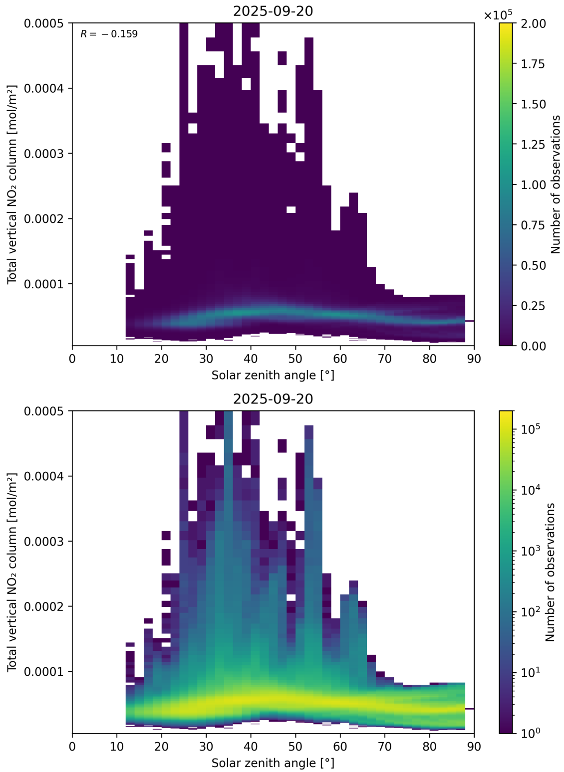
Figure 153: Scatter density plot of “Solar zenith angle” against “Total vertical NO 2 column” for 2025-09-20 to 2025-09-21.
