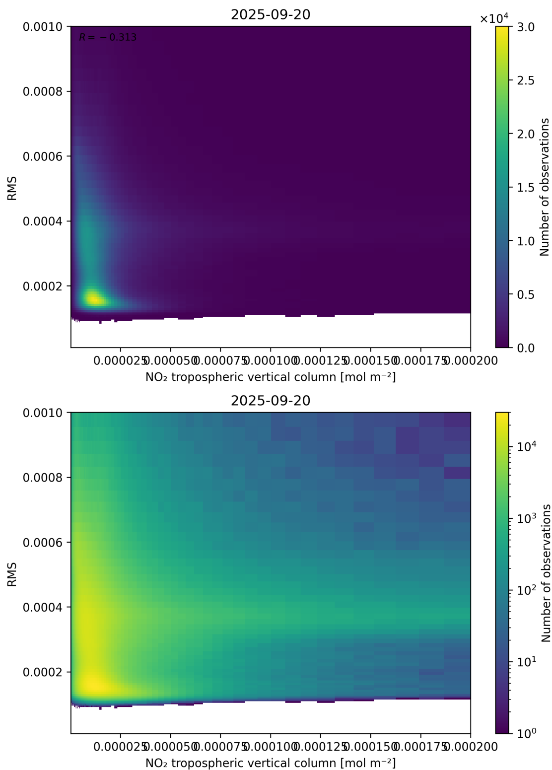
Figure 142: Scatter density plot of “NO 2 tropospheric vertical column” against “RMS” for 2025-09-20 to 2025-09-21.
