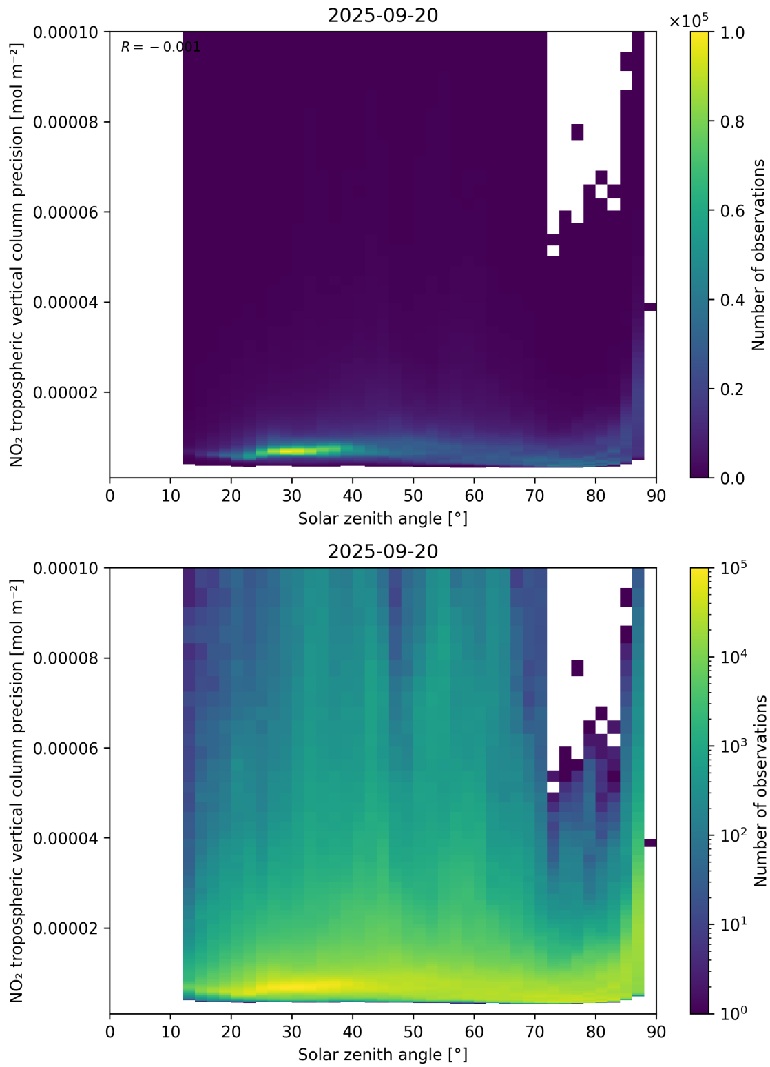
Figure 156: Scatter density plot of “Solar zenith angle” against “NO 2 tropospheric vertical column precision” for 2025-09-20 to 2025-09-21.
