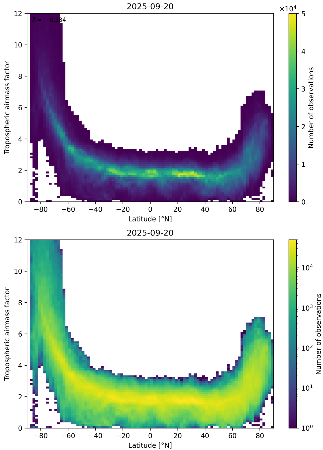
Figure 85: Scatter density plot of “Latitude” against “Tropospheric airmass factor” for 2025-09-20 to 2025-09-21.
