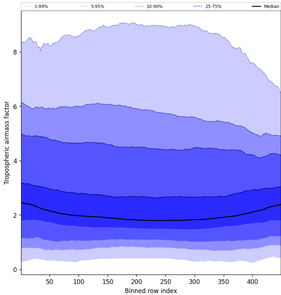
Figure 48: Along track statistics of “Tropospheric airmass factor” for 2025-09-20 to 2025-09-21
