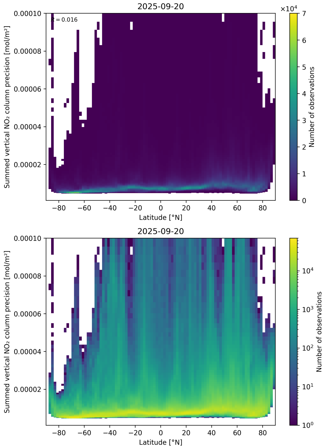
Figure 89: Scatter density plot of “Latitude” against “Summed vertical NO 2 column precision” for 2025-09-20 to 2025-09-21.
