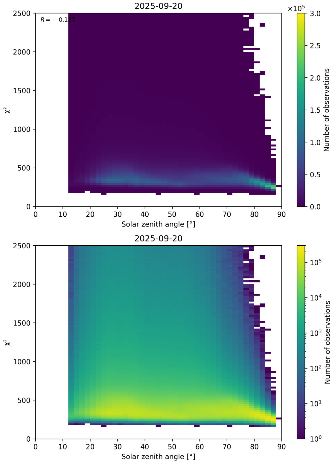
Figure 148: Scatter density plot of “Solar zenith angle” against “ \chi^2 ” for 2025-09-20 to 2025-09-21.
