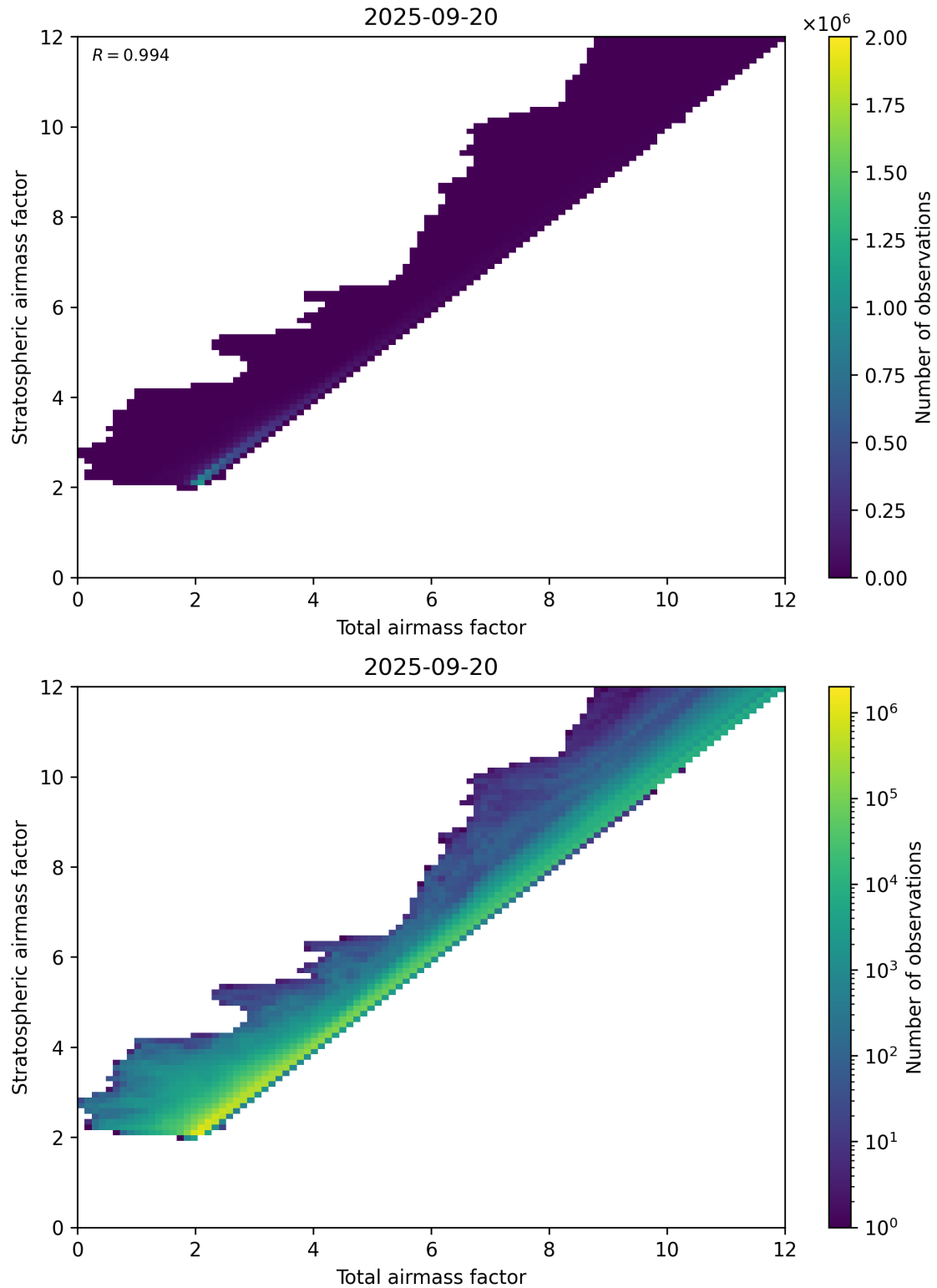
Figure 62: Scatter density plot of “Total airmass factor” against “Stratospheric airmass factor” for 2025-09-20 to 2025-09-21.
