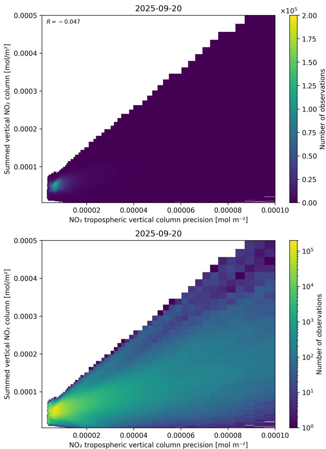
Figure 136: Scatter density plot of “NO 2 tropospheric vertical column precision” against “Summed vertical NO 2 column” for 2025-09-20 to 2025-09-21.
