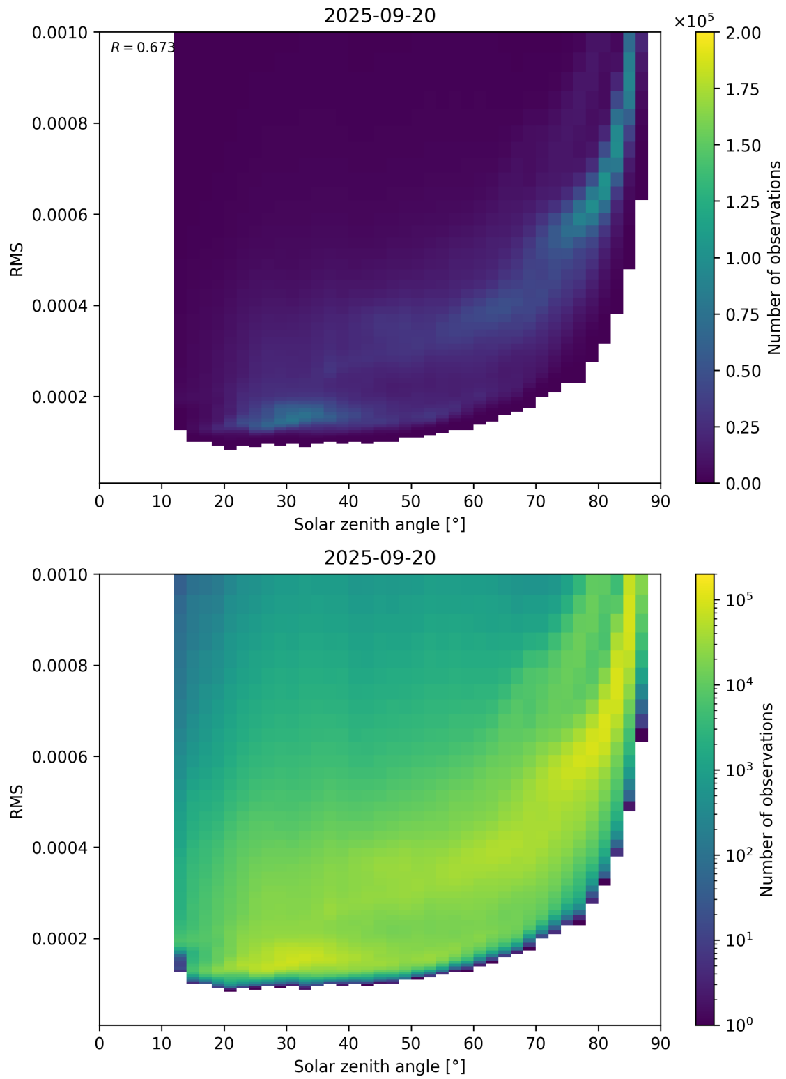
Figure 157: Scatter density plot of “Solar zenith angle” against “RMS” for 2025-09-20 to 2025-09-21.
