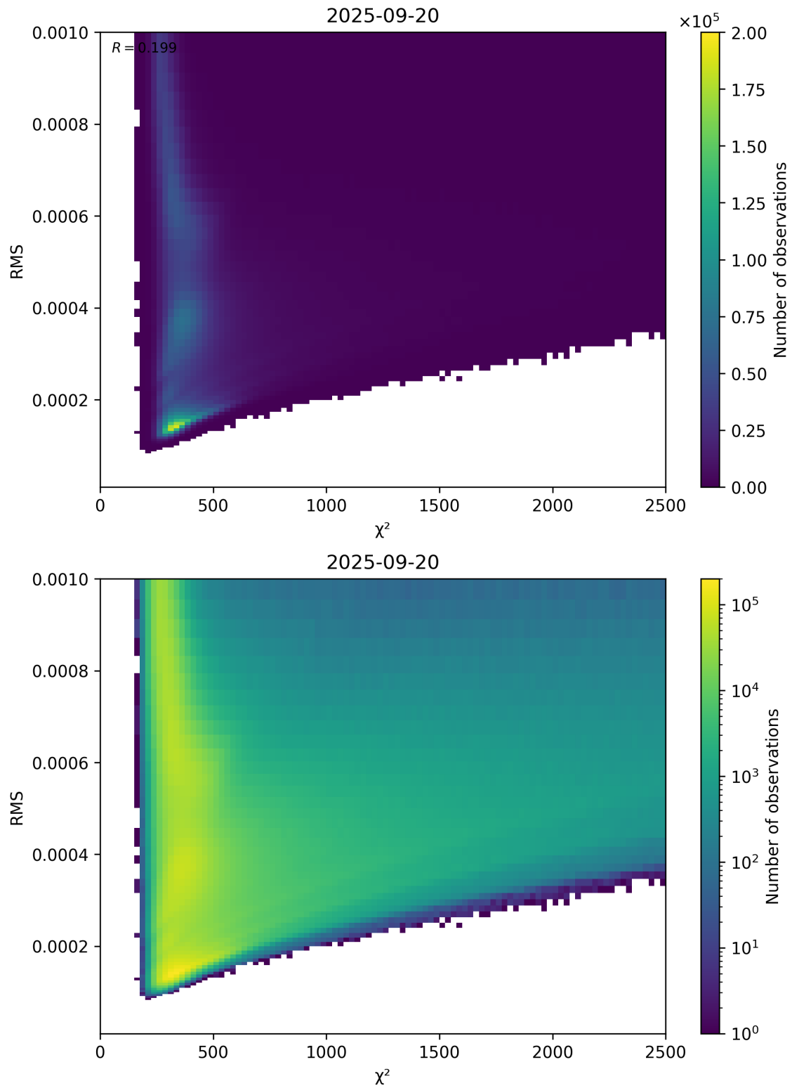
Figure 82: Scatter density plot of “ \chi^2 ” against “RMS” for 2025-09-20 to 2025-09-21.
