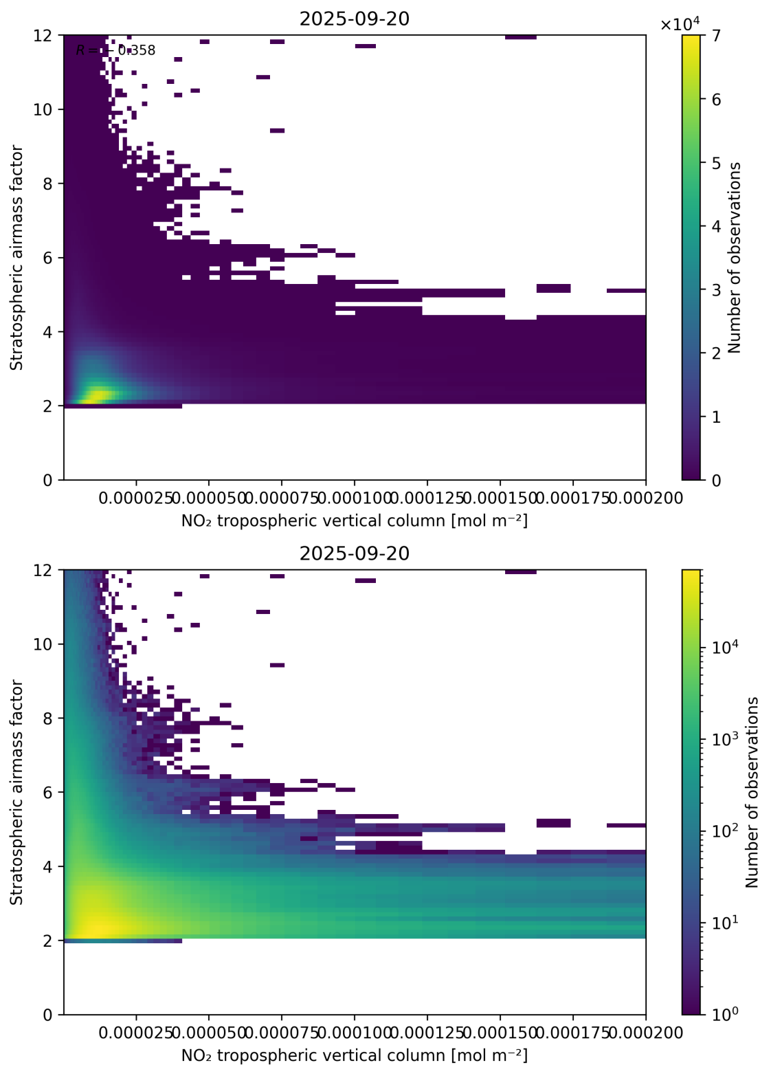
Figure 121: Scatter density plot of “NO 2 tropospheric vertical column” against “Stratospheric air mass factor” for 2025-09-20 to 2025-09-21.
