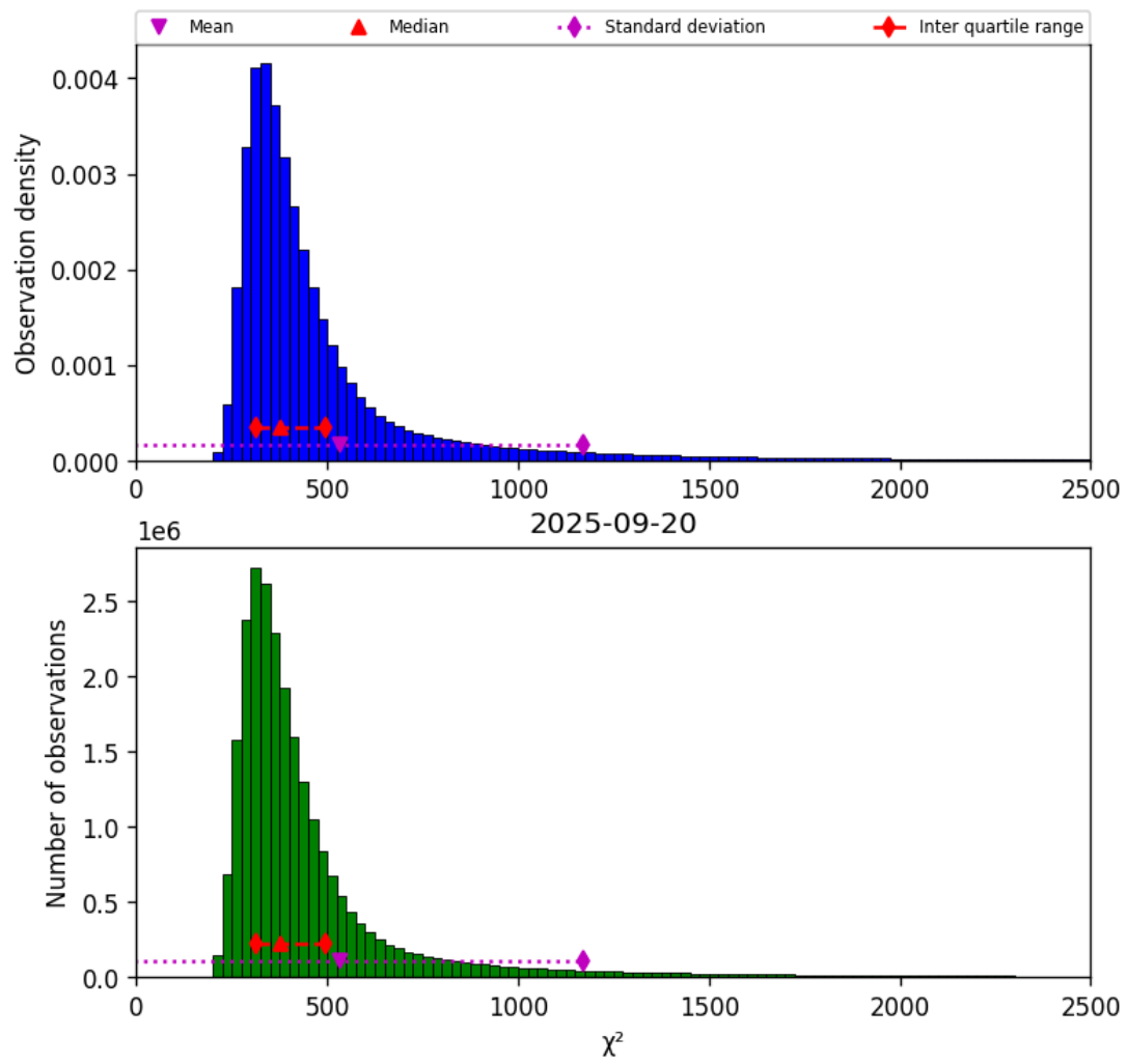
Figure 42: Histogram of “ \chi^2 ” for 2025-09-20 to 2025-09-21
