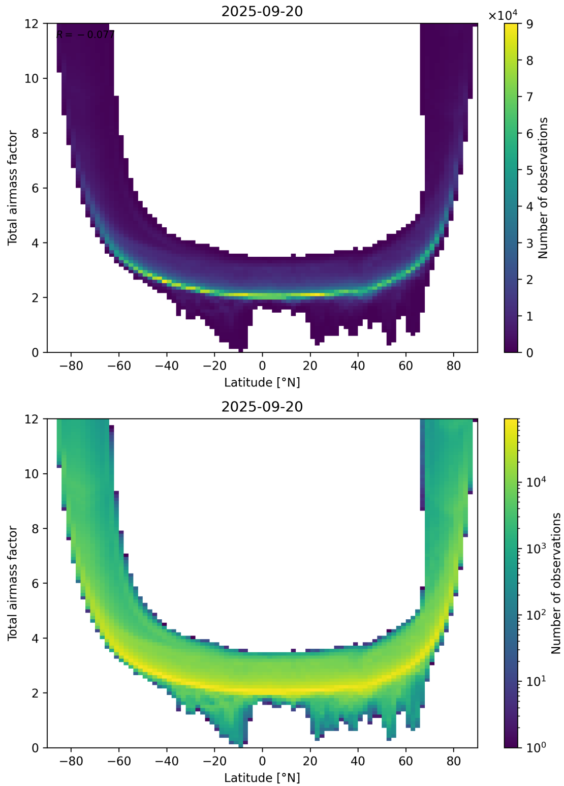
Figure 84: Scatter density plot of “Latitude” against “Total airmass factor” for 2025-09-20 to 2025-09-21.
