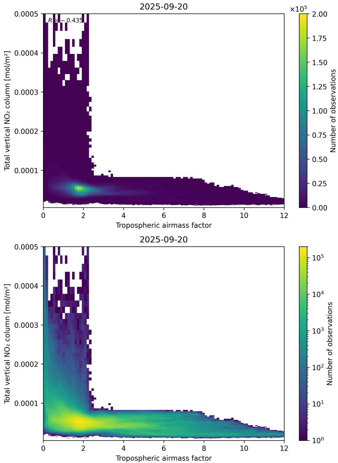
Figure 77: Scatter density plot of “Tropospheric airmass factor” against “Total vertical NO 2 column” for 2025-09-20 to 2025-09-21.
