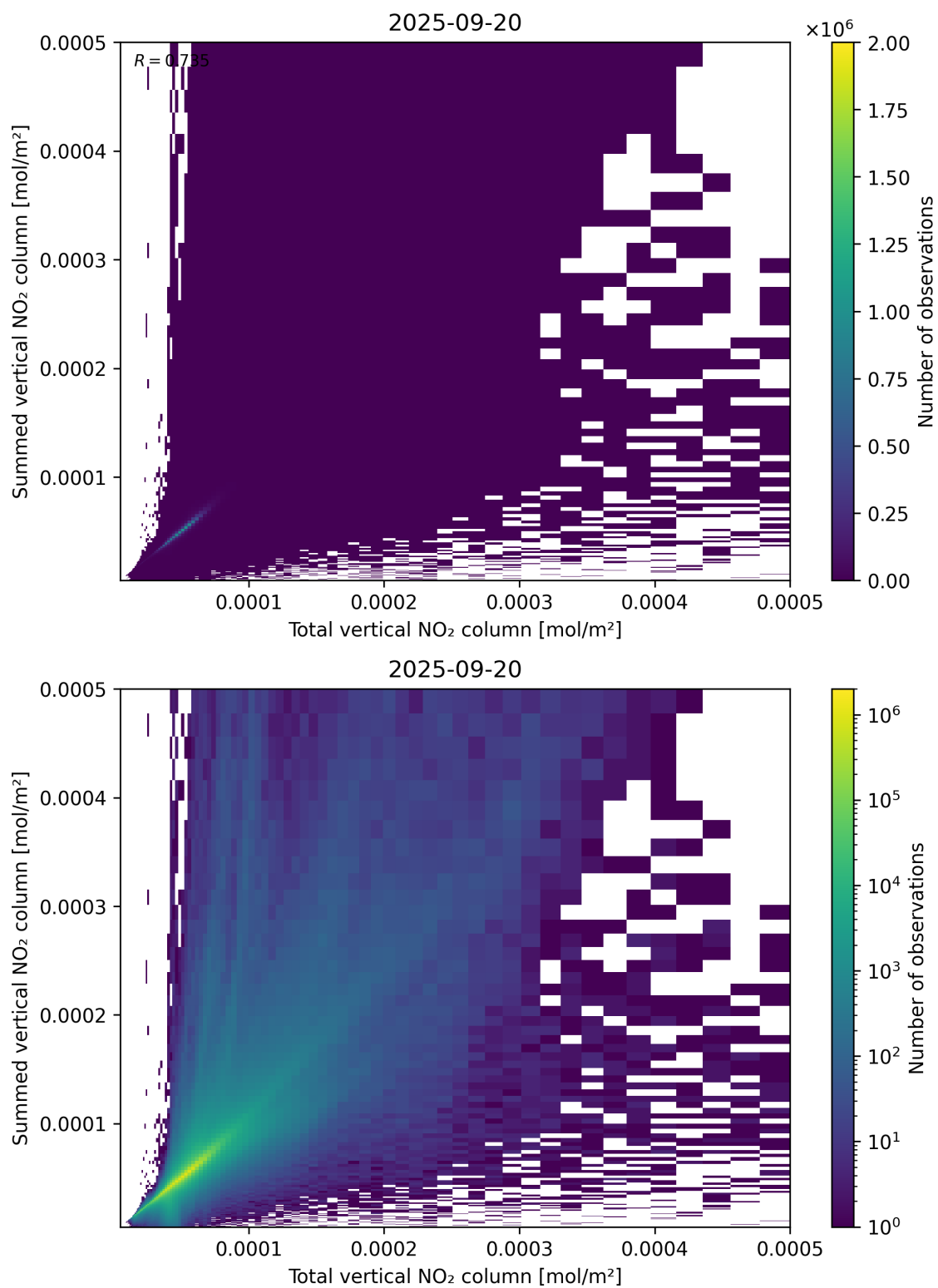
Figure 112: Scatter density plot of “Total vertical NO 2 column” against “Summed vertical NO 2 column” for 2025-09-20 to 2025-09-21.
