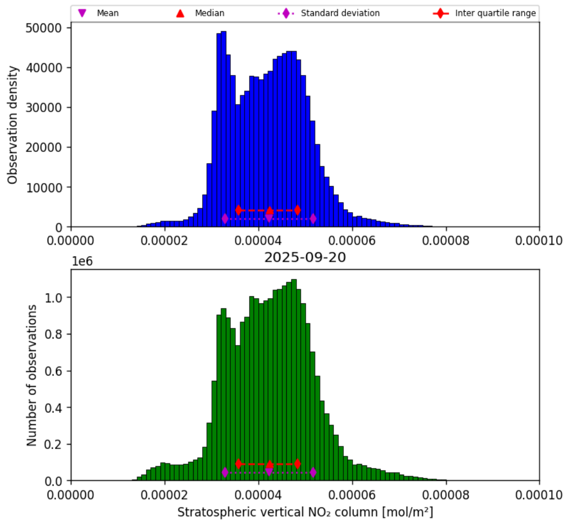
Figure 36: Histogram of “Stratospheric vertical NO 2 column” for 2025-09-20 to 2025-09-21
