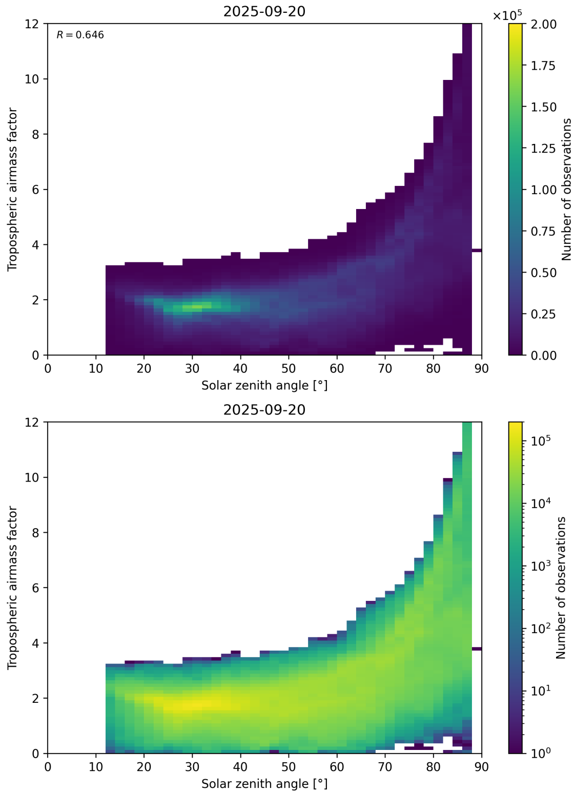
Figure 147: Scatter density plot of “Solar zenith angle” against “Tropospheric airmass factor” for 2025-09-20 to 2025-09-21.
