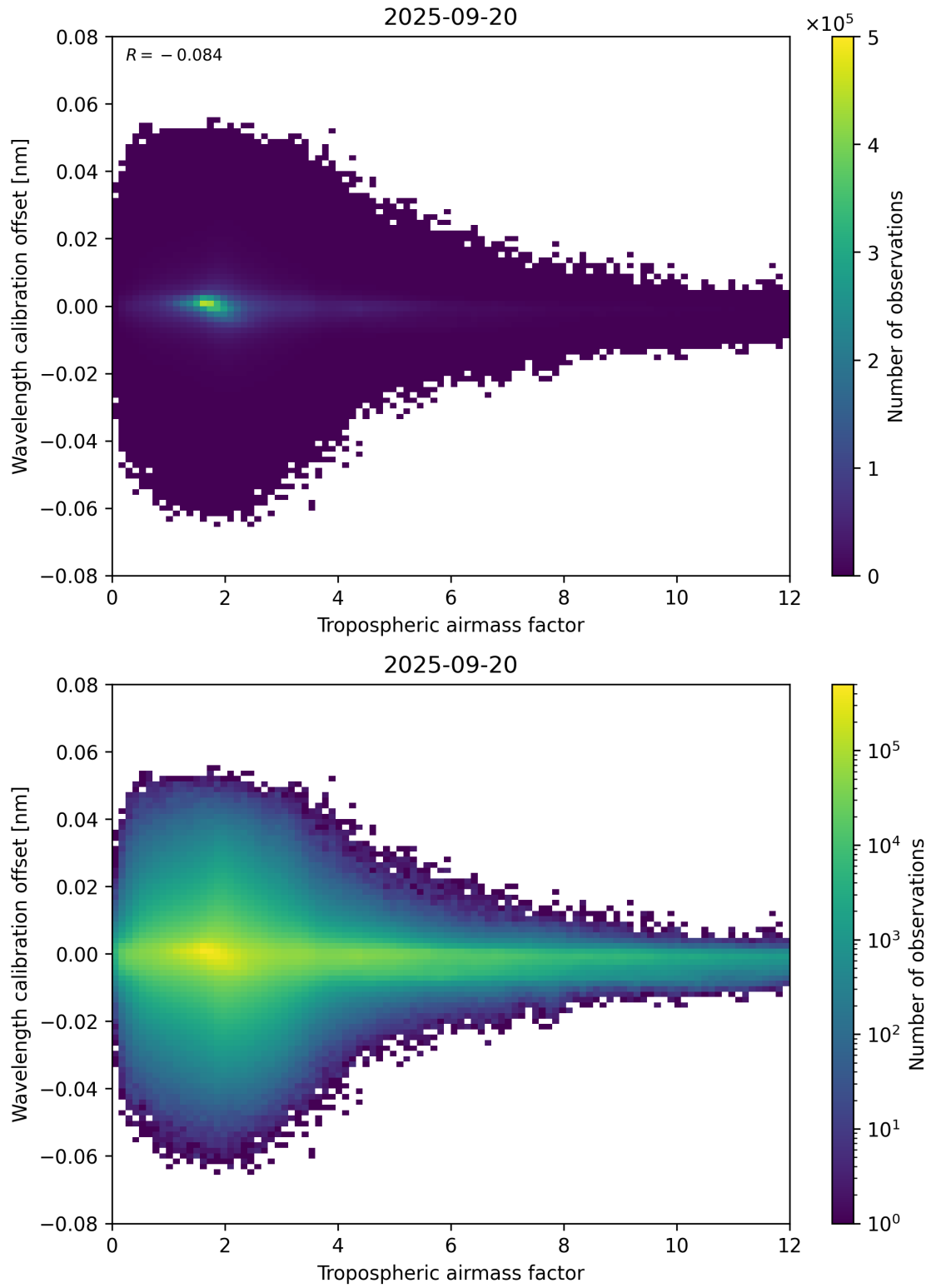
Figure 80: Scatter density plot of “Tropospheric airmass factor” against “Wavelength calibration offset” for 2025-09-20 to 2025-09-21.
