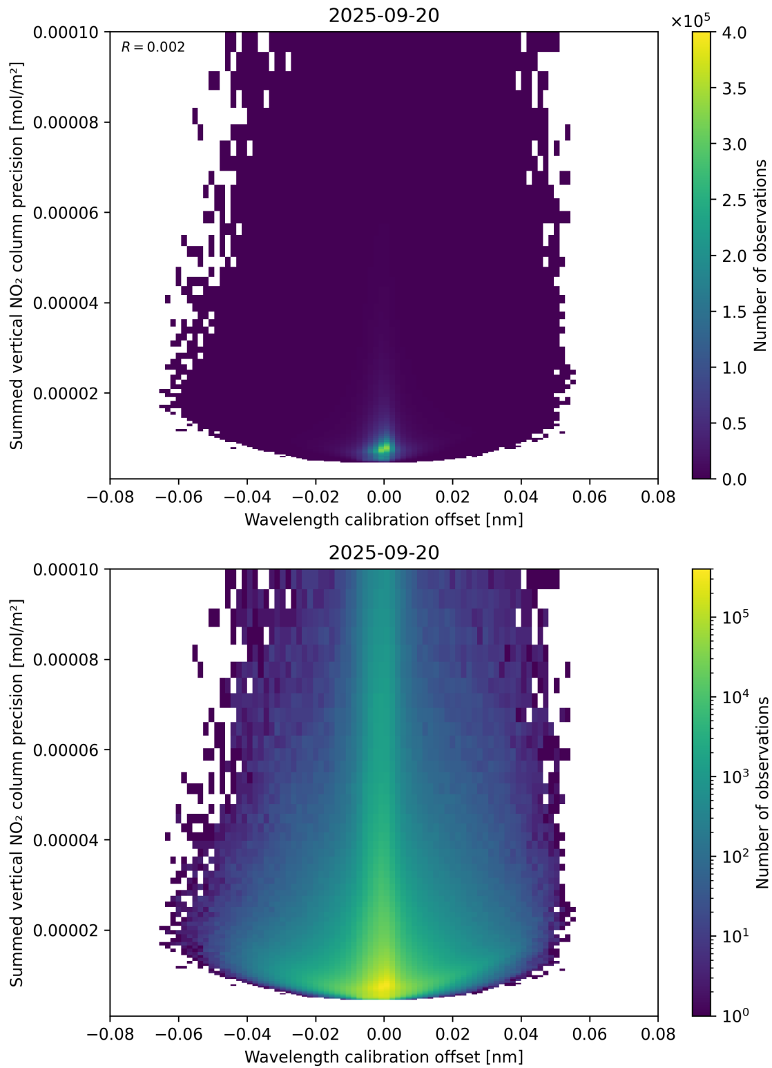
Figure 178: Scatter density plot of “Wavelength calibration offset” against “Summed vertical NO 2 column precision” for 2025-09-20 to 2025-09-21.
