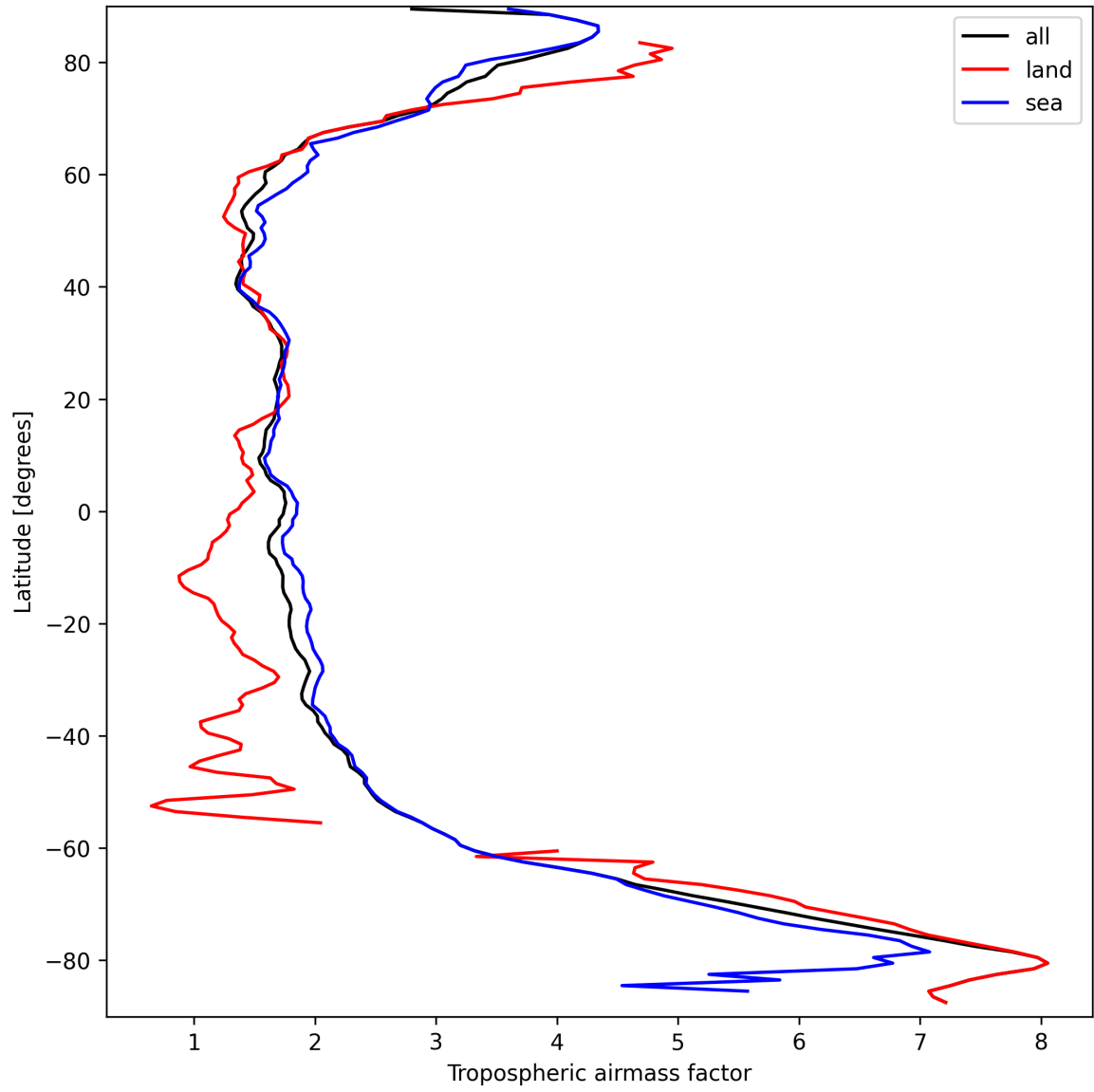
Figure 14: Zonal average of “Tropospheric airmass factor” for 2025-09-20 to 2025-09-21.
