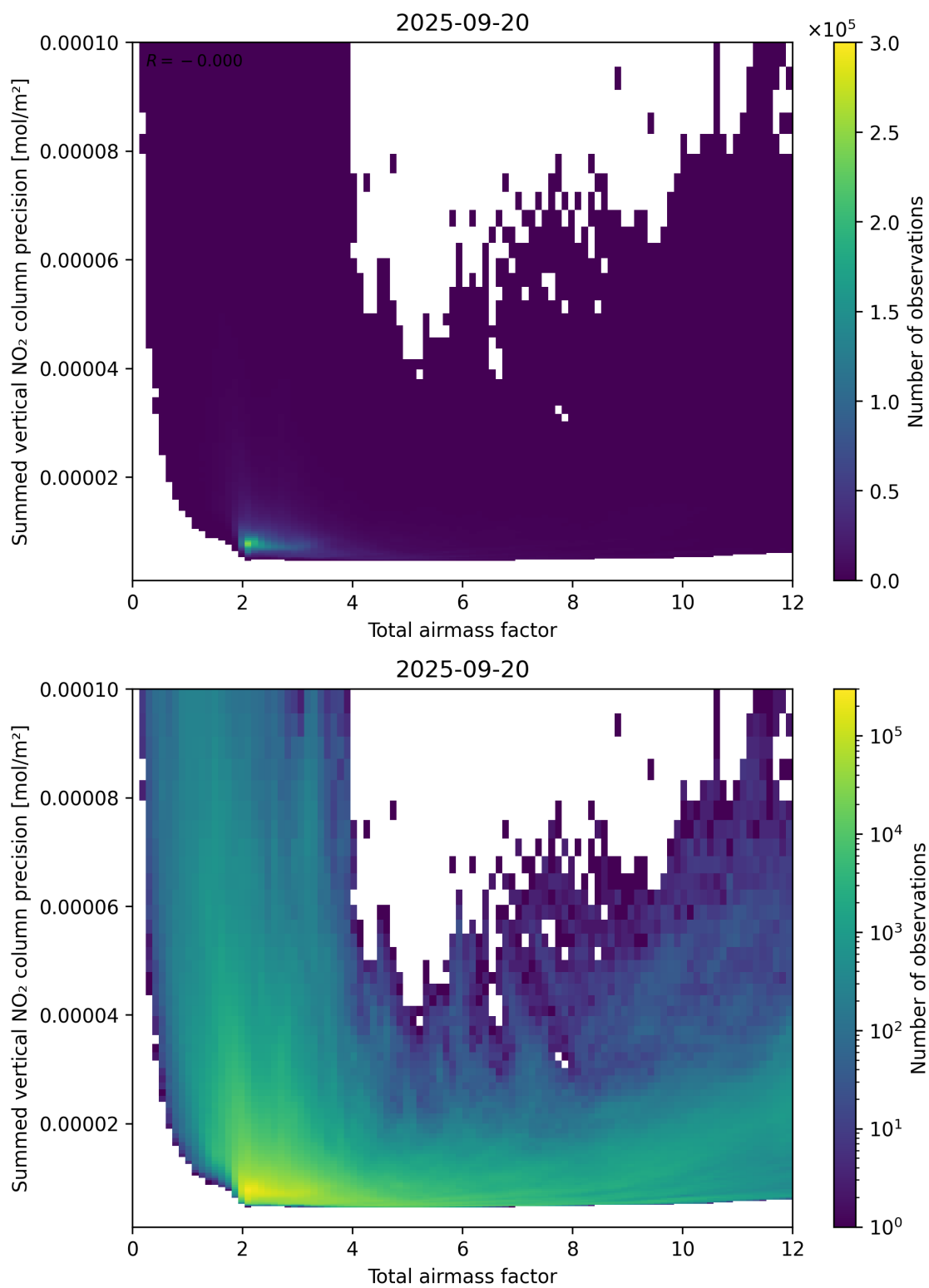
Figure 66: Scatter density plot of “Total airmass factor” against “Summed vertical NO 2 column precision” for 2025-09-20 to 2025-09-21.
