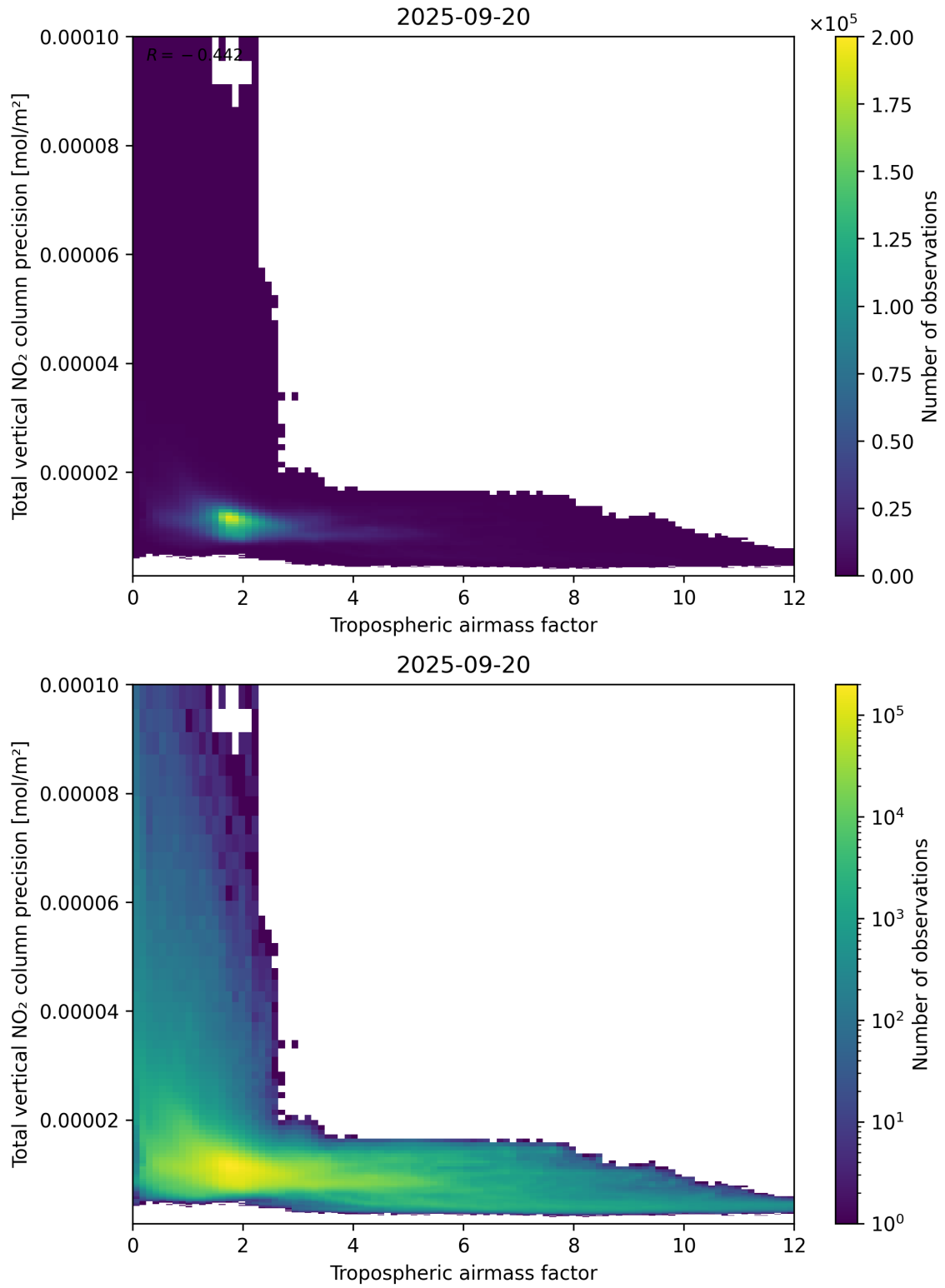
Figure 78: Scatter density plot of “Tropospheric air mass factor” against “Total vertical NO 2 column precision” for 2025-09-20 to 2025-09-21.
