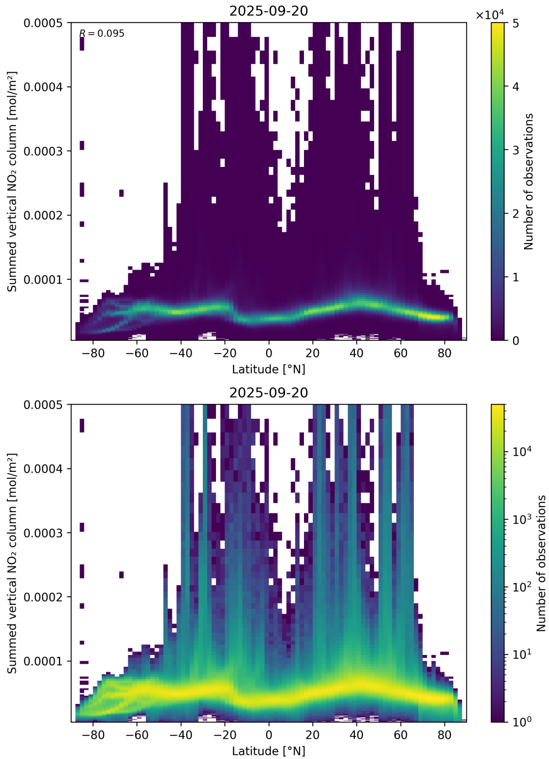
Figure 88: Scatter density plot of “Latitude” against “Summed vertical NO 2 column” for 2025-09-20 to 2025-09-21.
