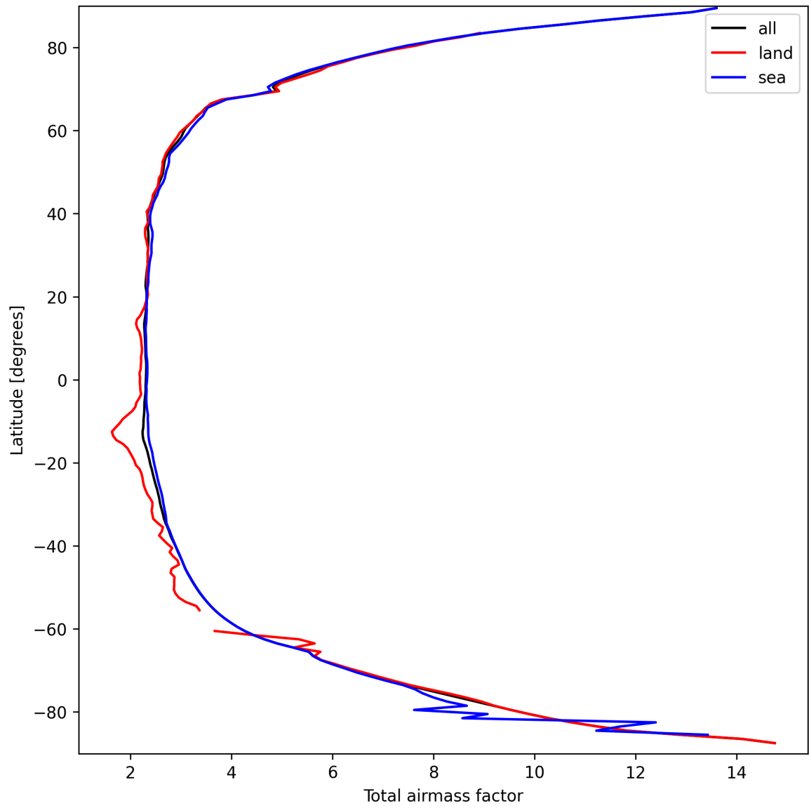
Figure 15: Zonal average of “Total airmass factor” for 2025-09-20 to 2025-09-21.
