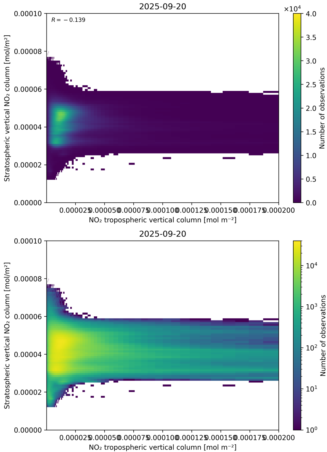
Figure 125: Scatter density plot of “NO 2 tropospheric vertical column” against “Stratospheric vertical NO 2 column” for 2025-09-20 to 2025-09-21.
