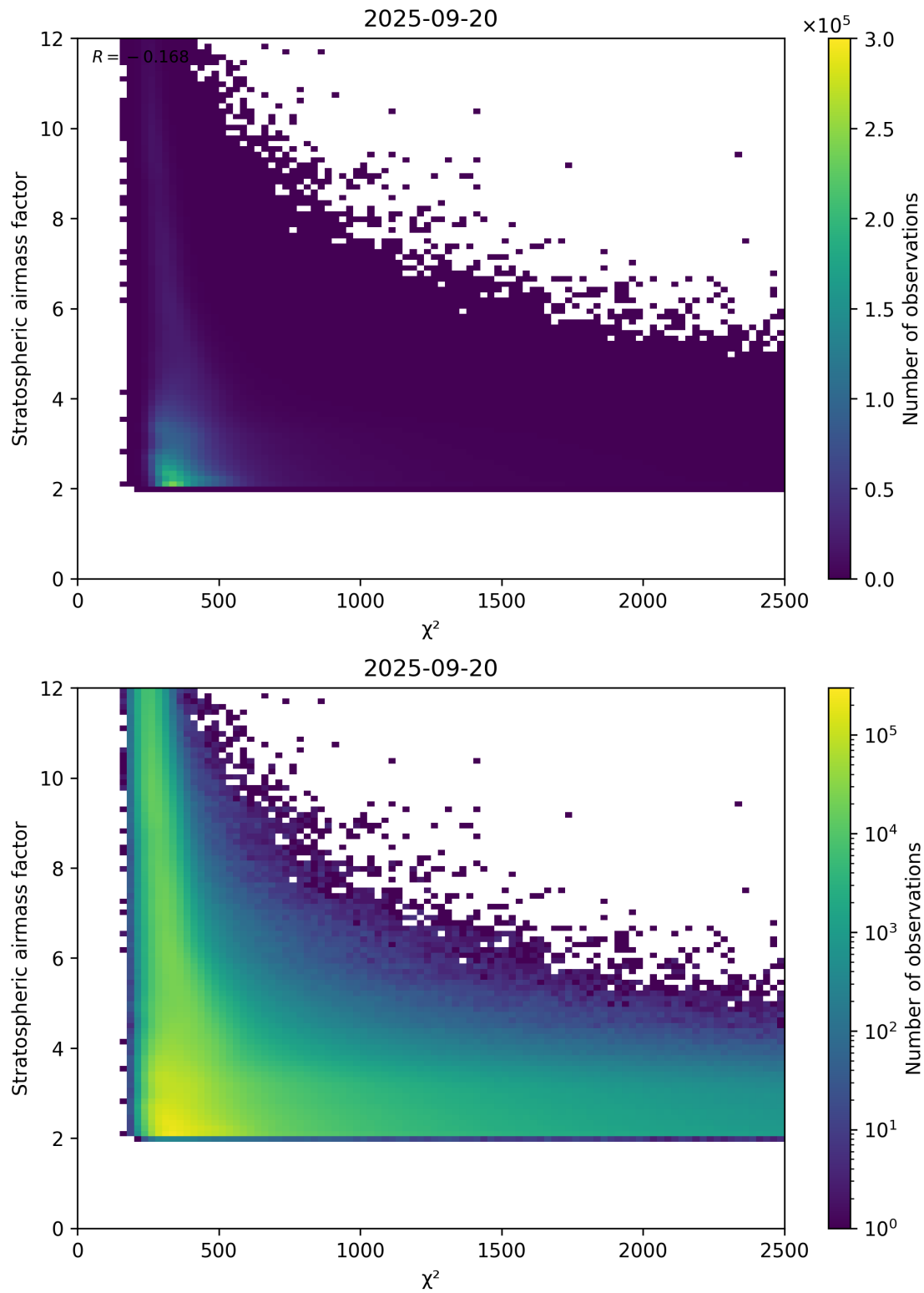
Figure 81: Scatter density plot of “ \chi^2 ” against “Stratospheric airmass factor” for 2025-09-20 to 2025-09-21.
