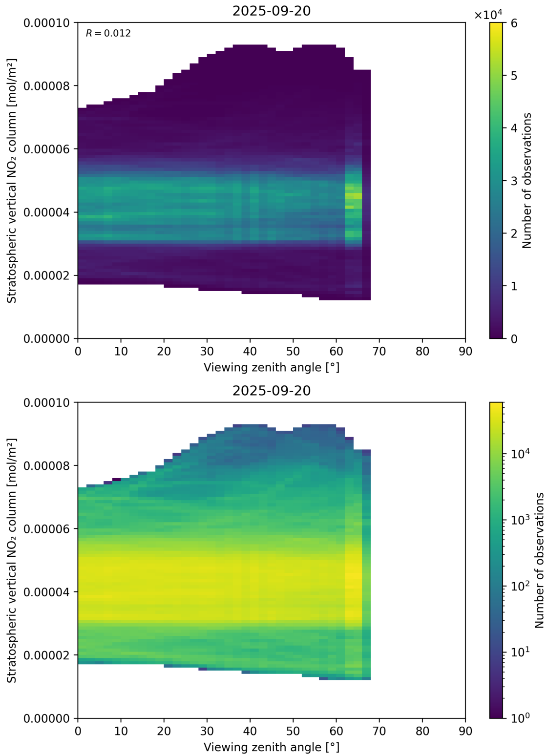
Figure 164: Scatter density plot of “Viewing zenith angle” against “Stratospheric vertical NO 2 column” for 2025-09-20 to 2025-09-21.
