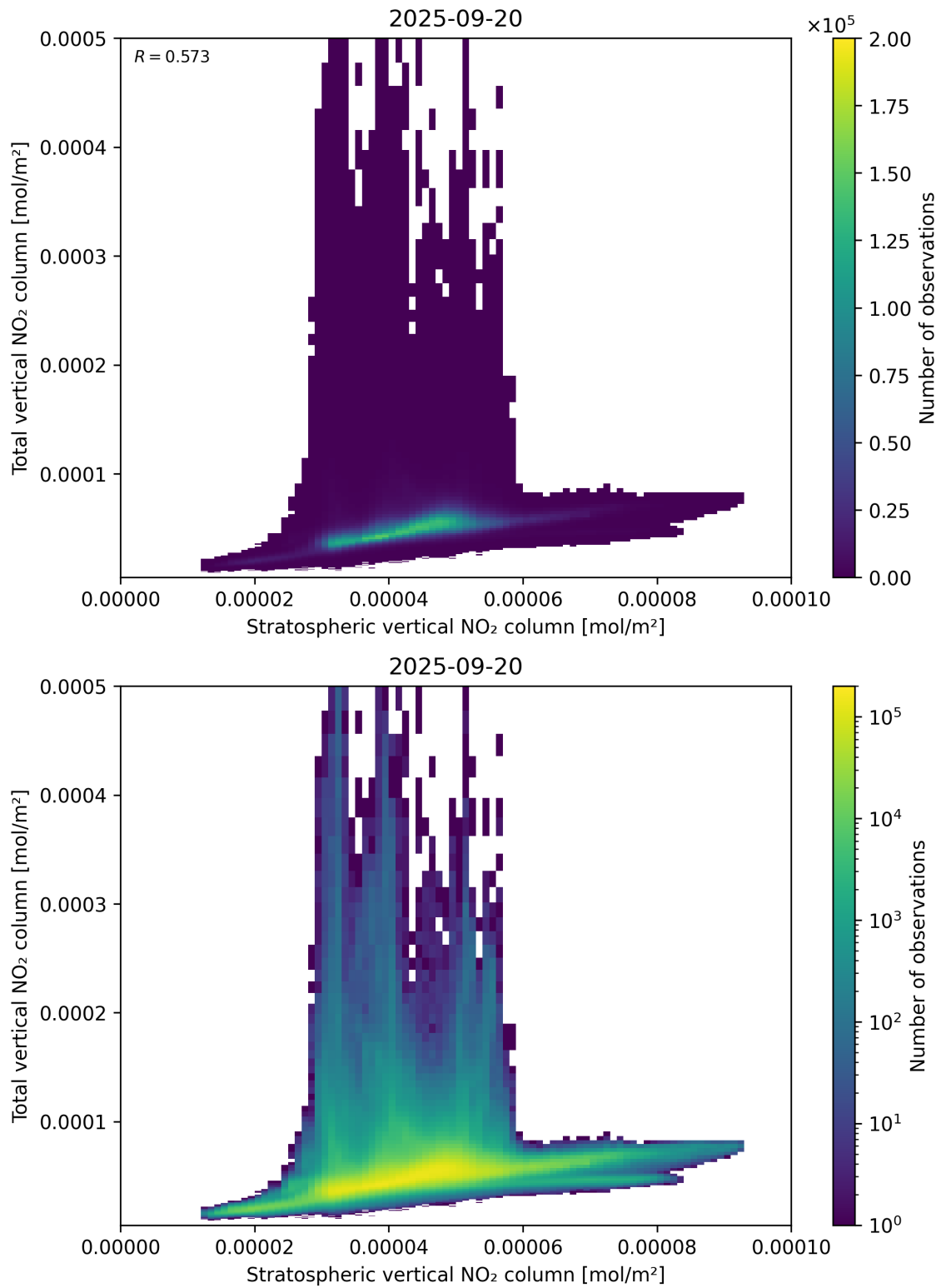
Figure 100: Scatter density plot of “Stratospheric vertical NO 2 column” against “Total vertical NO 2 column” for 2025-09-20 to 2025-09-21.
