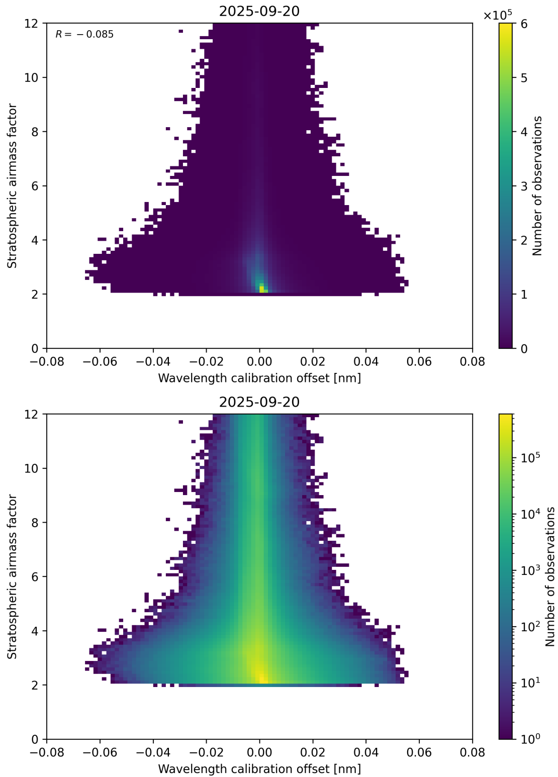
Figure 174: Scatter density plot of “Wavelength calibration offset” against “Stratospheric airmass factor” for 2025-09-20 to 2025-09-21.
