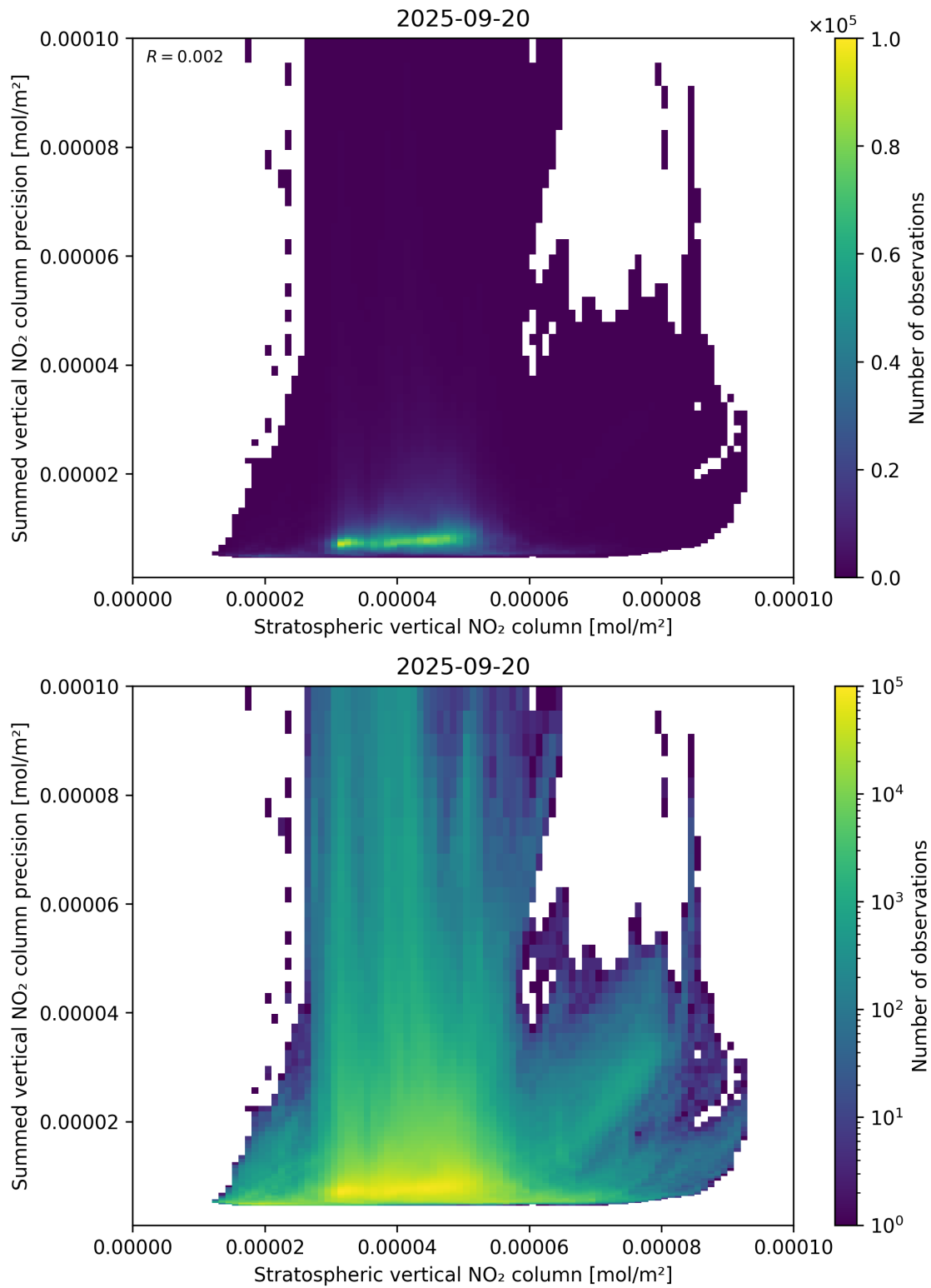
Figure 99: Scatter density plot of “Stratospheric vertical NO 2 column” against “Summed vertical NO 2 column precision” for 2025-09-20 to 2025-09-21.
