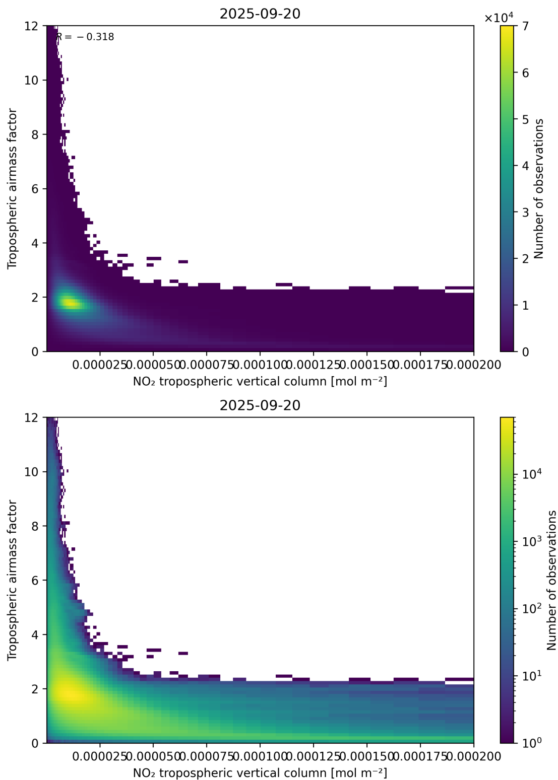
Figure 123: Scatter density plot of “NO 2 tropospheric vertical column” against “Tropospheric air mass factor” for 2025-09-20 to 2025-09-21.
