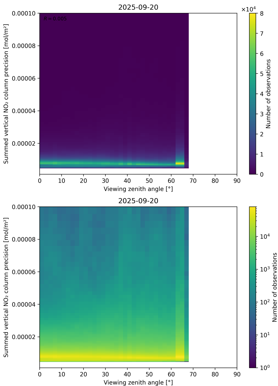
Figure 166: Scatter density plot of “Viewing zenith angle” against “Summed vertical NO 2 column precision” for 2025-09-20 to 2025-09-21.
