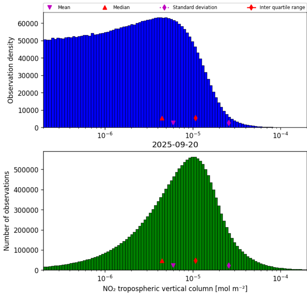
Figure 29: Histogram of “NO 2 tropospheric vertical column” for 2025-09-20 to 2025-09-21
