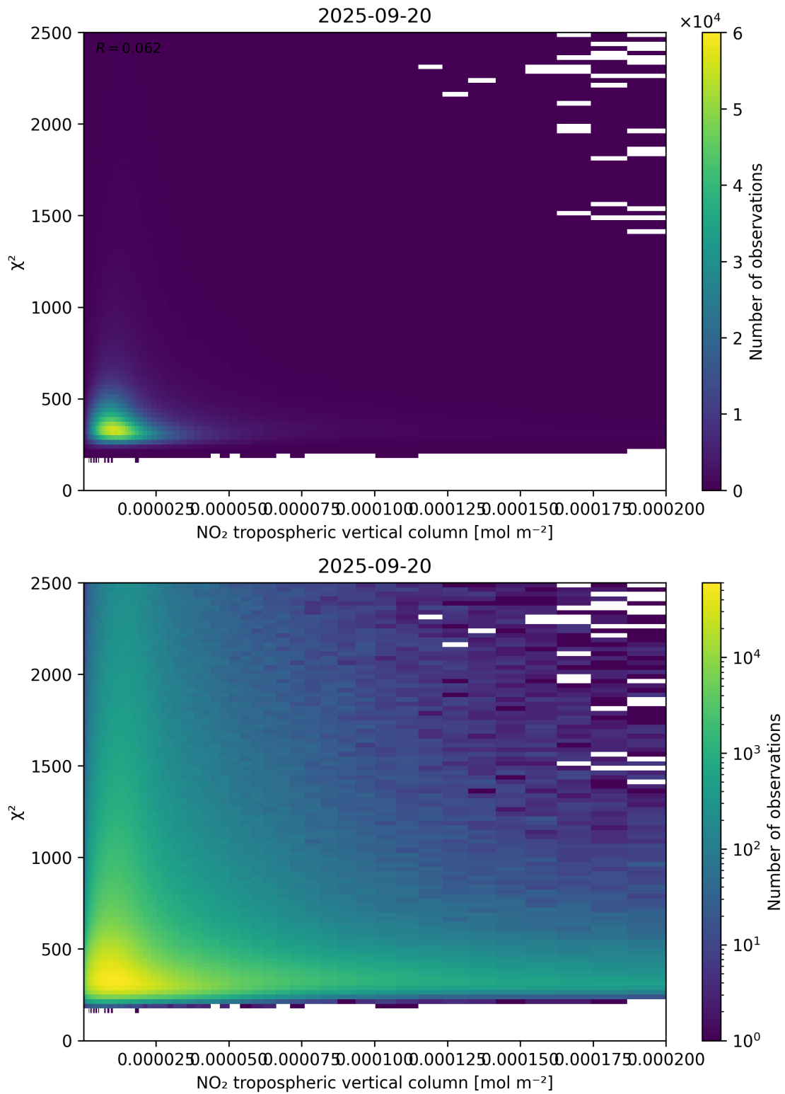
Figure 124: Scatter density plot of “NO 2 tropospheric vertical column” against “ \chi^2 ” for 2025-09-20 to 2025-09-21.
