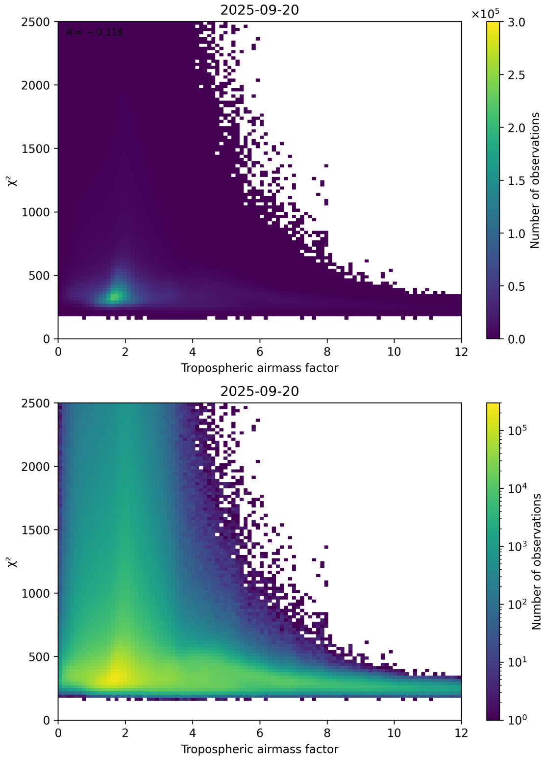
Figure 73: Scatter density plot of “Tropospheric airmass factor” against “ \chi^2 ” for 2025-09-20 to 2025-09-21.
