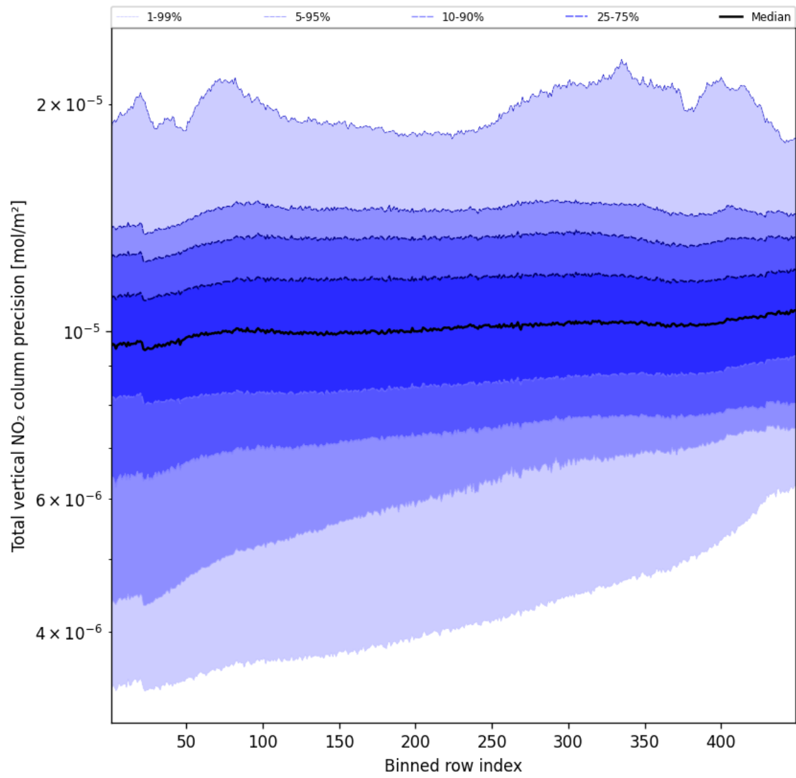
Figure 56: Along track statistics of “Total vertical NO 2 column precision” for 2025-09-20 to 2025-09-21
