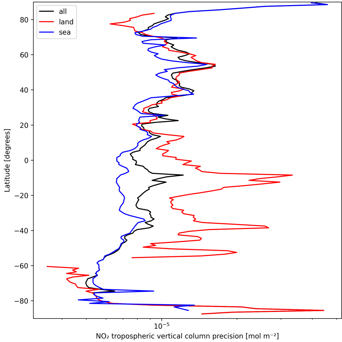
Figure 13: Zonal average of “NO 2 tropospheric vertical column precision” for 2025-09-20 to 2025-09-21.
