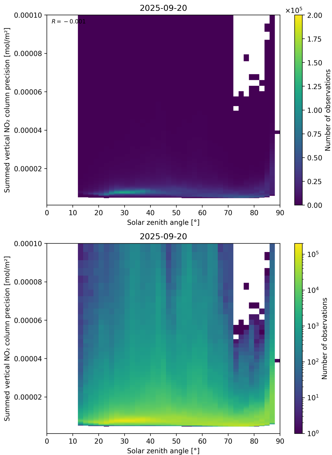
Figure 152: Scatter density plot of “Solar zenith angle” against “Summed vertical NO 2 column precision” for 2025-09-20 to 2025-09-21.
