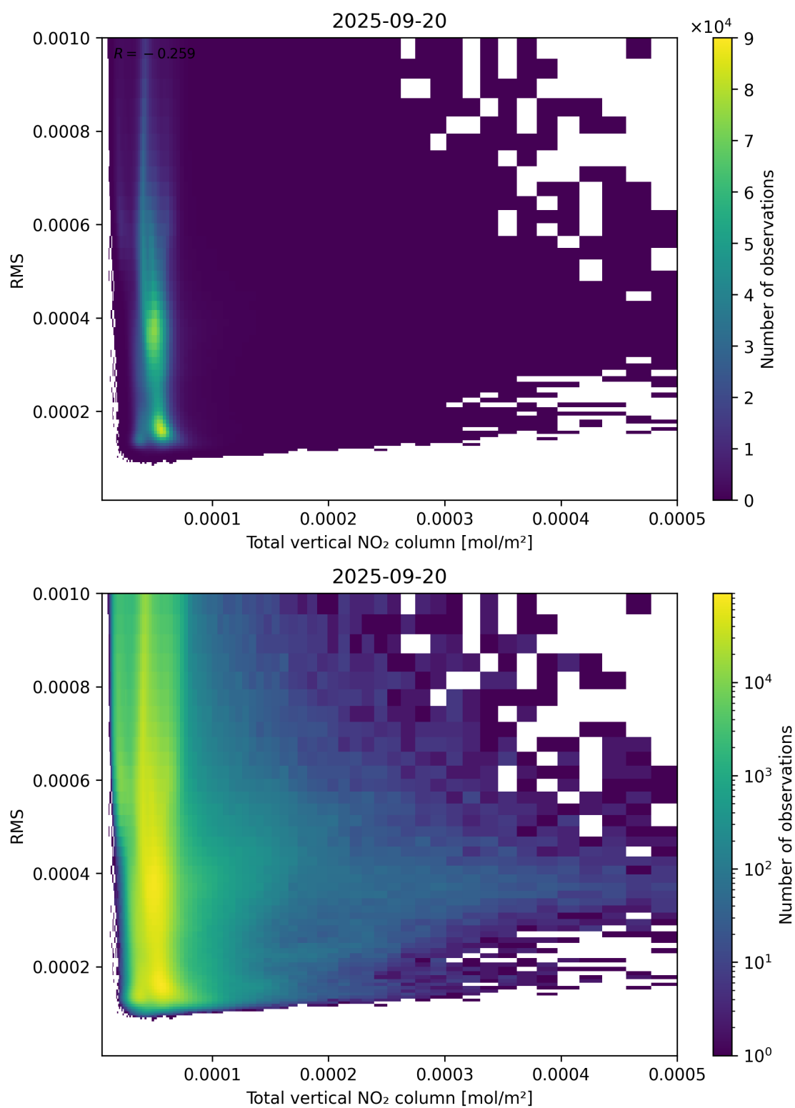
Figure 120: Scatter density plot of “Total vertical NO 2 column” against “RMS” for 2025-09-20 to 2025-09-21.
