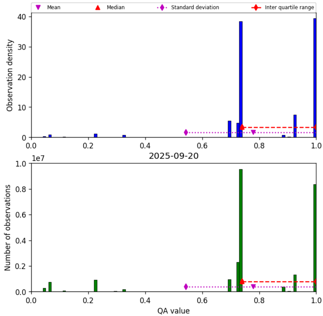
Figure 28: Histogram of “QA value” for 2025-09-20 to 2025-09-21
