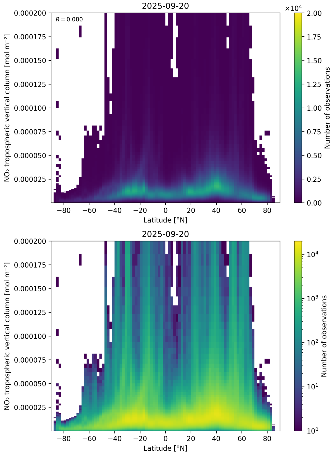
Figure 92: Scatter density plot of “Latitude” against “NO 2 tropospheric vertical column” for 2025-09-20 to 2025-09-21.
