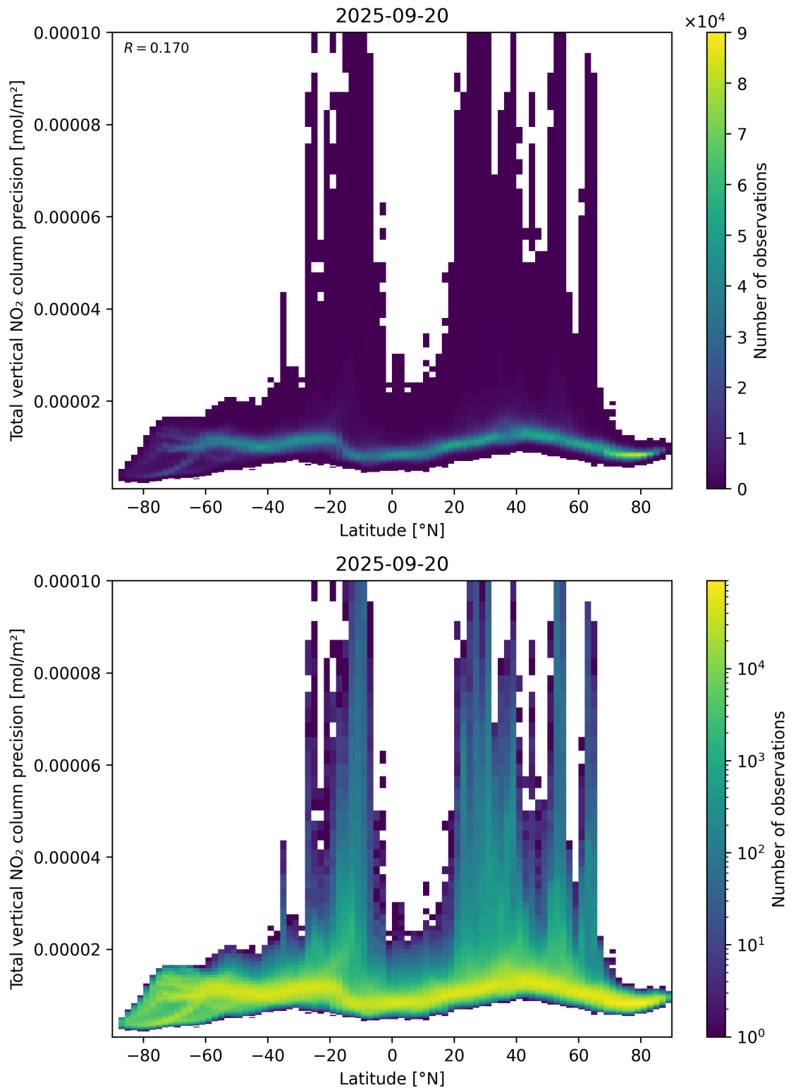
Figure 91: Scatter density plot of “Latitude” against “Total vertical NO 2 column precision” for 2025-09-20 to 2025-09-21.
