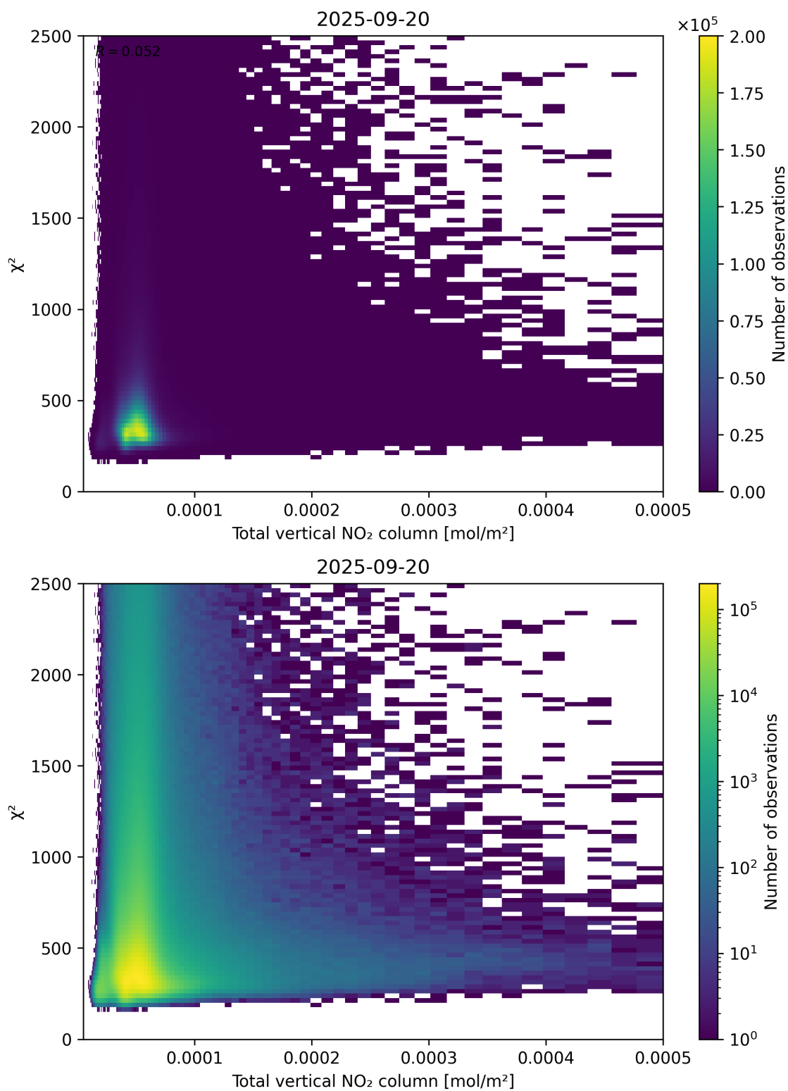
Figure 111: Scatter density plot of “Total vertical NO 2 column” against “ \chi^2 ” for 2025-09-20 to 2025-09-21.
