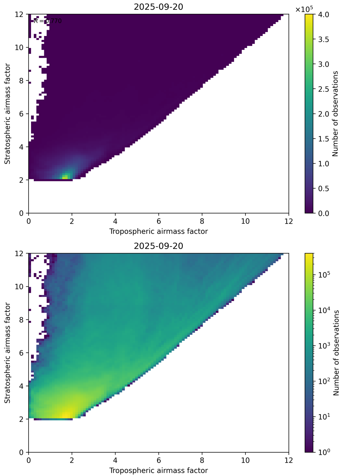
Figure 71: Scatter density plot of “Tropospheric airmass factor” against “Stratospheric airmass factor” for 2025-09-20 to 2025-09-21.
