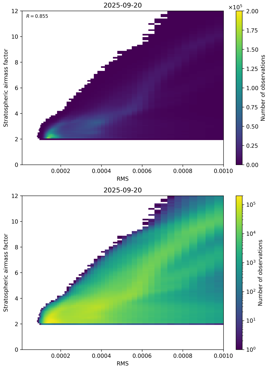
Figure 144: Scatter density plot of “RMS” against “Stratospheric airmass factor” for 2025-09-20 to 2025-09-21.
