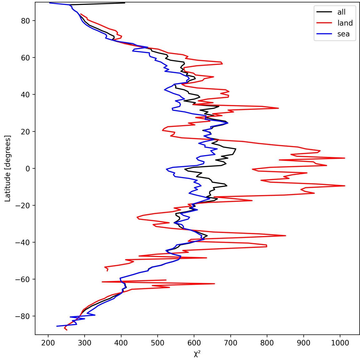
Figure 25: Zonal average of “ \chi^2 ” for 2025-09-20 to 2025-09-21.
