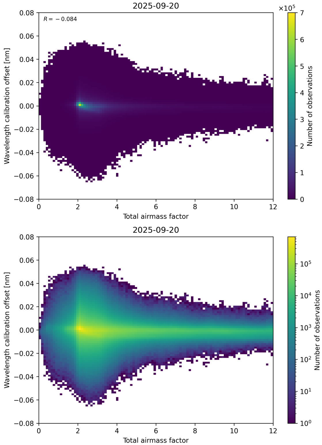
Figure 70: Scatter density plot of “Total airmass factor” against “Wavelength calibration offset” for 2025-09-20 to 2025-09-21.
