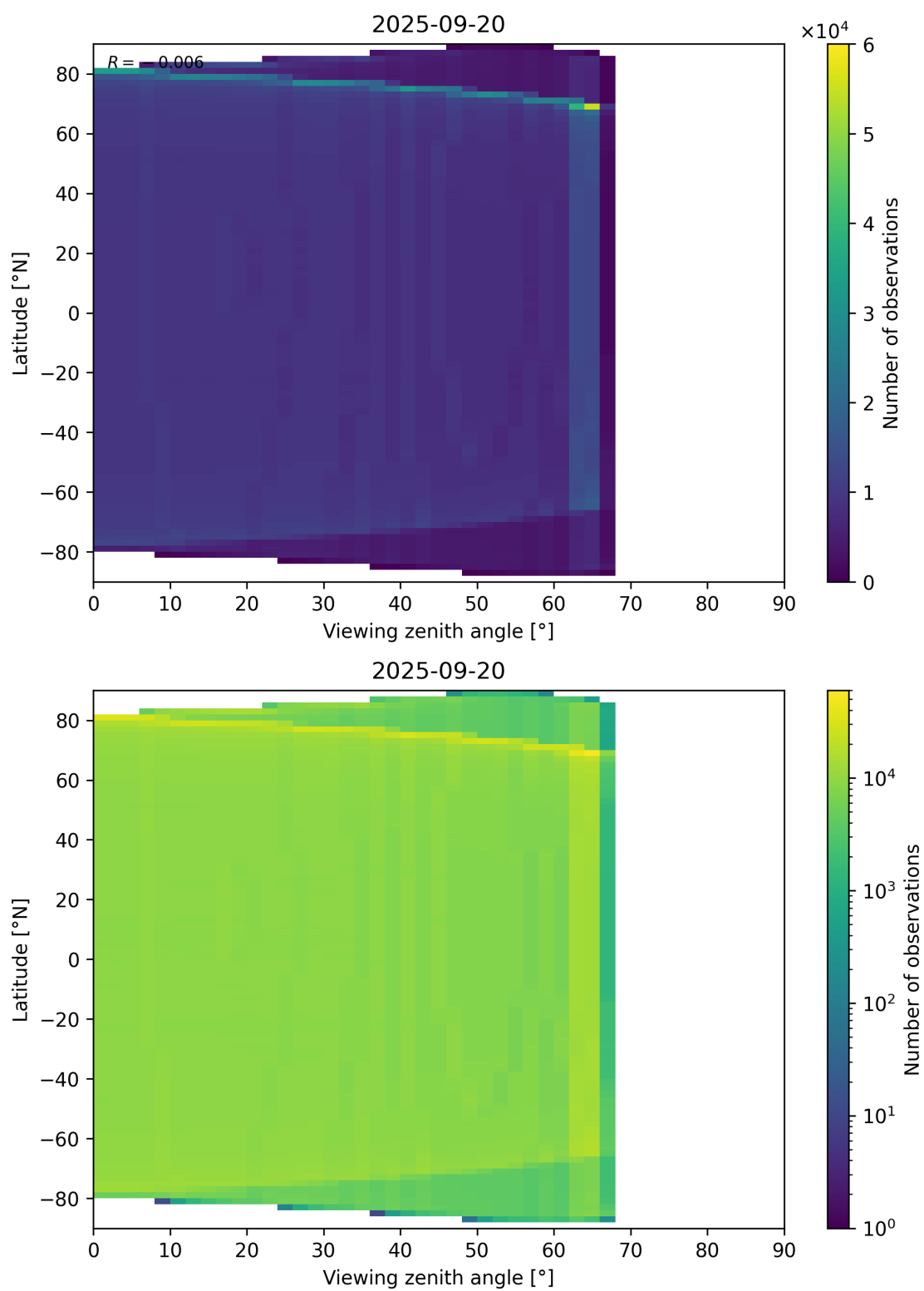
Figure 163: Scatter density plot of “Viewing zenith angle” against “Latitude” for 2025-09-20 to 2025-09-21.
