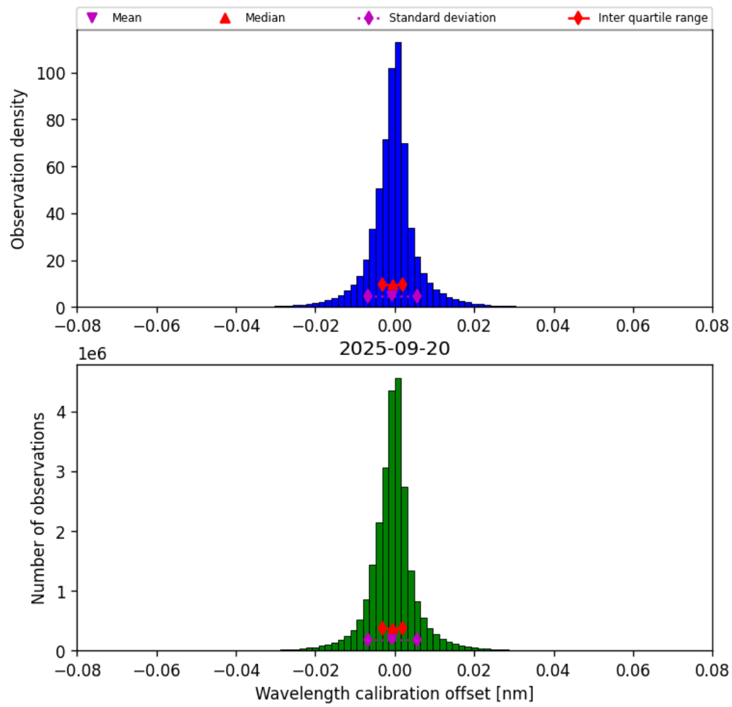
Figure 35: Histogram of “Wavelength calibration offset” for 2025-09-20 to 2025-09-21
