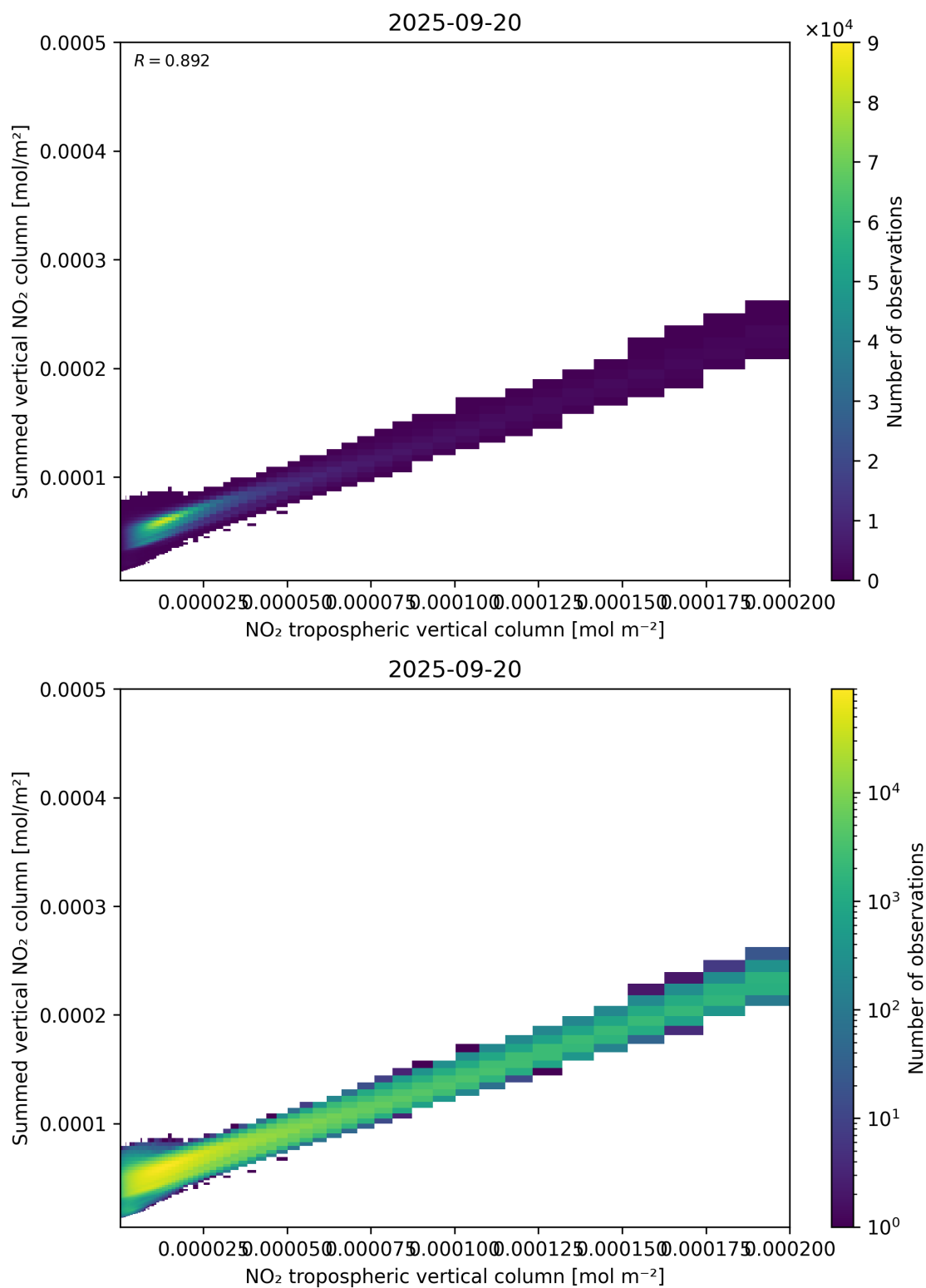
Figure 126: Scatter density plot of “NO 2 tropospheric vertical column” against “Summed vertical NO 2 column” for 2025-09-20 to 2025-09-21.
