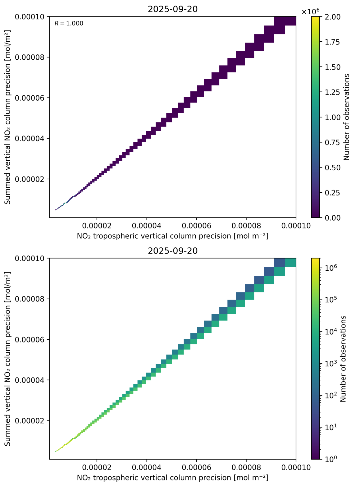
Figure 137: Scatter density plot of “NO 2 tropospheric vertical column precision” against “Summed vertical NO 2 column precision” for 2025-09-20 to 2025-09-21.
