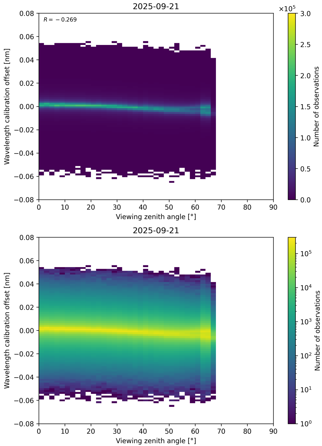
Figure 173: Scatter density plot of “Viewing zenith angle” against “Wavelength calibration offset” for 2025-09-20 to 2025-09-22.
