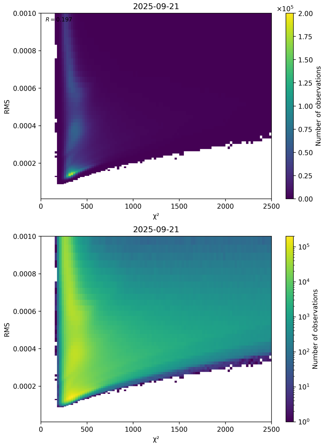
Figure 82: Scatter density plot of “ \chi^2 ” against “RMS” for 2025-09-20 to 2025-09-22.
