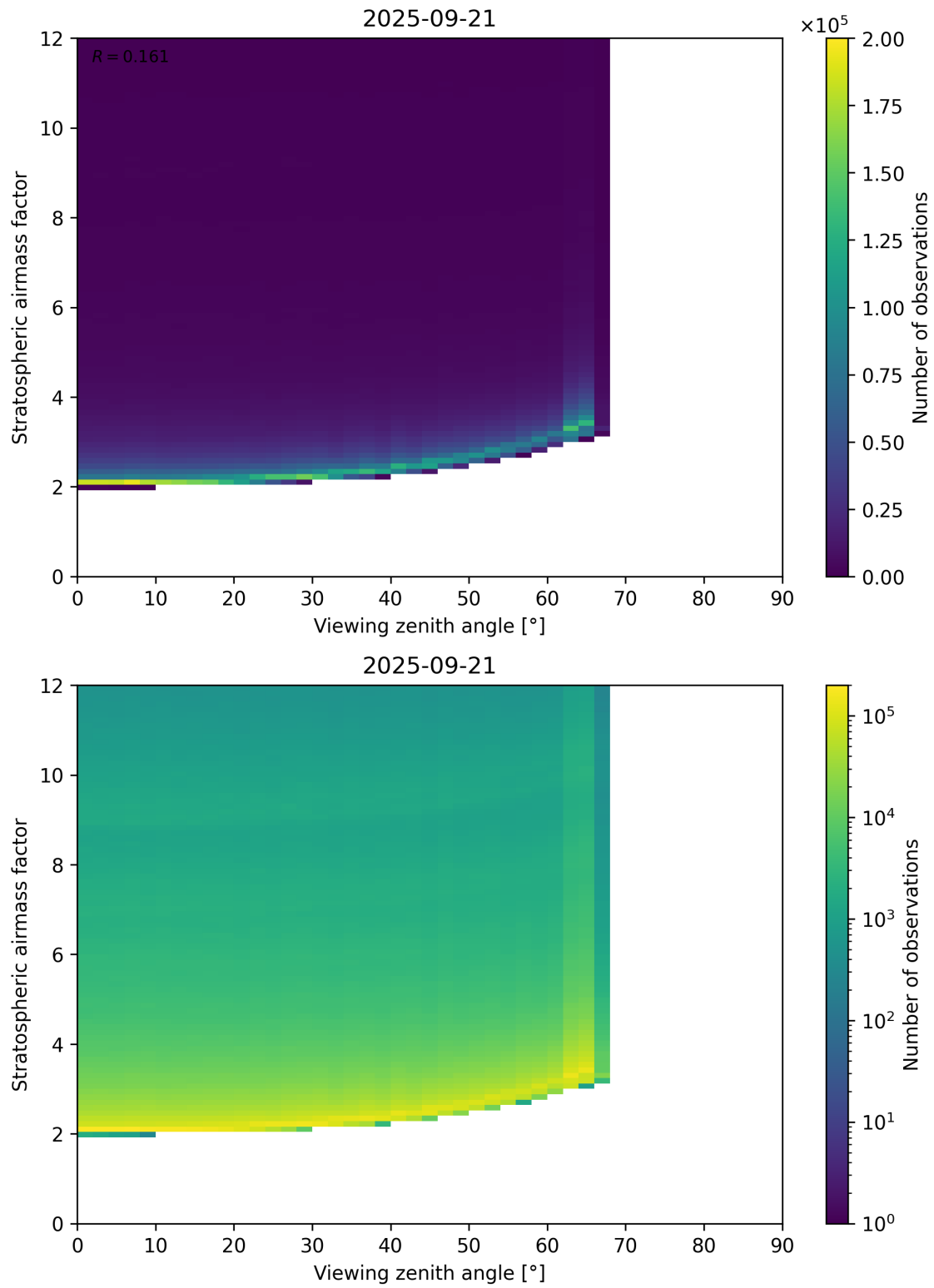
Figure 159: Scatter density plot of “Viewing zenith angle” against “Stratospheric airmass factor” for 2025-09-20 to 2025-09-22.
