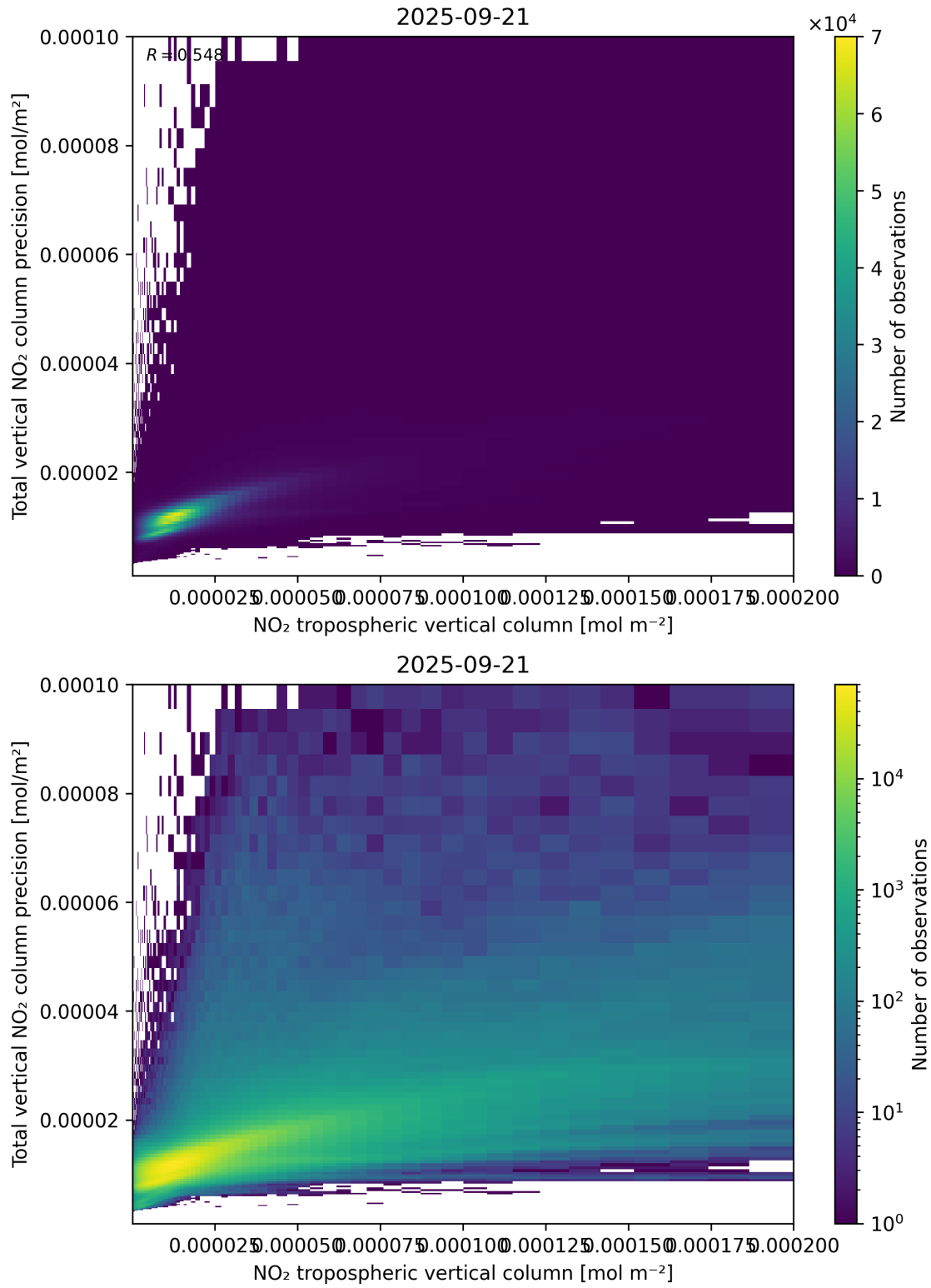
Figure 129: Scatter density plot of “NO 2 tropospheric vertical column” against “Total vertical NO 2 column precision” for 2025-09-20 to 2025-09-22.
