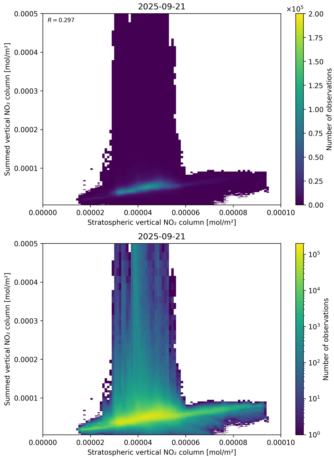
Figure 98: Scatter density plot of “Stratospheric vertical NO 2 column” against “Summed vertical NO 2 column” for 2025-09-20 to 2025-09-22.
