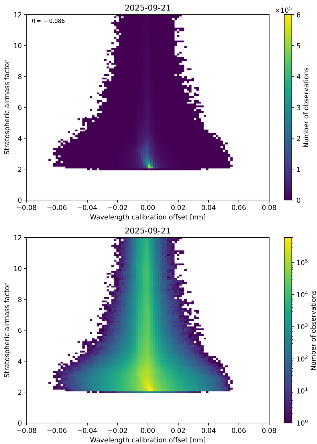
Figure 174: Scatter density plot of “Wavelength calibration offset” against “Stratospheric air mass factor” for 2025-09-20 to 2025-09-22.
