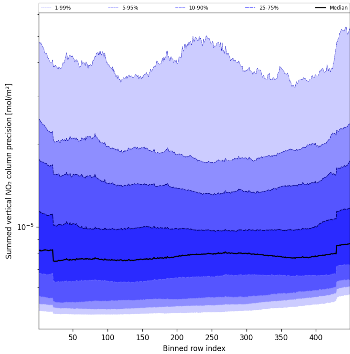
Figure 58: Along track statistics of “Summed vertical NO 2 column precision” for 2025-09-20 to 2025-09-22
