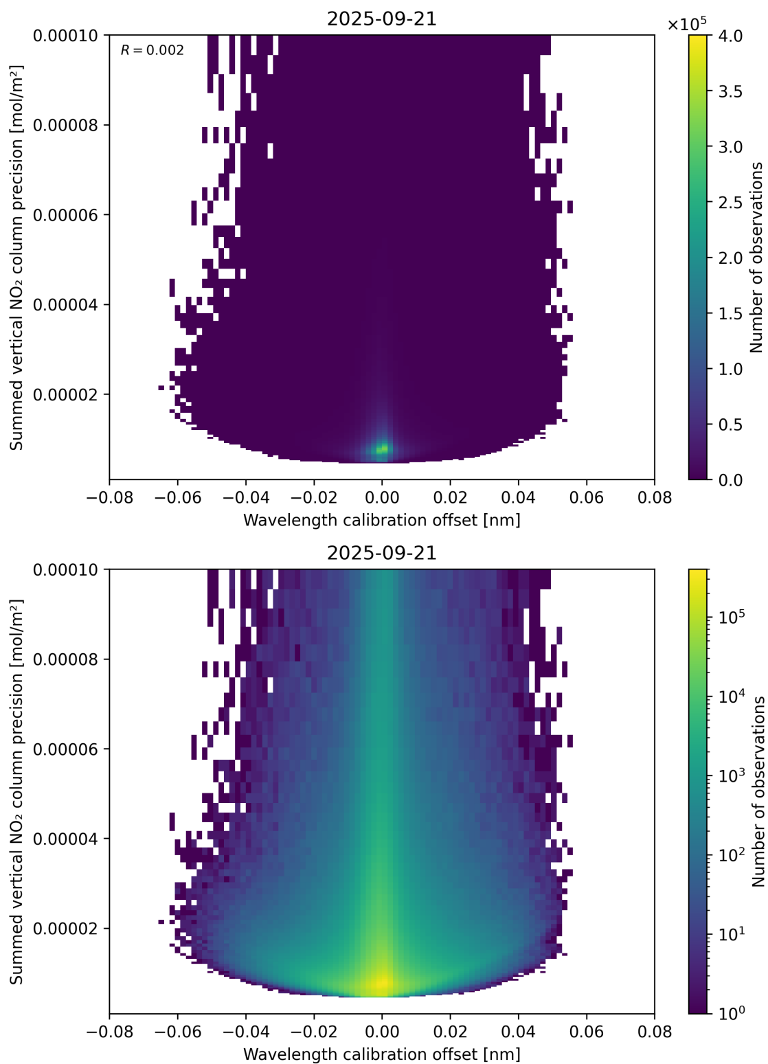
Figure 178: Scatter density plot of “Wavelength calibration offset” against “Summed vertical NO 2 column precision” for 2025-09-20 to 2025-09-22.
