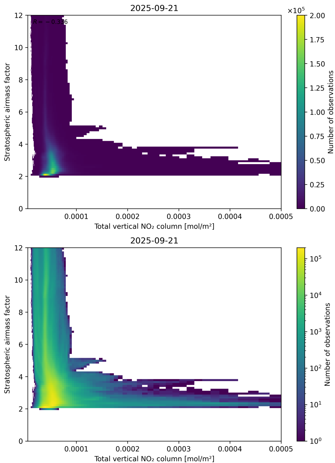
Figure 110: Scatter density plot of “Total vertical NO 2 column” against “Stratospheric airmass factor” for 2025-09-20 to 2025-09-22.
