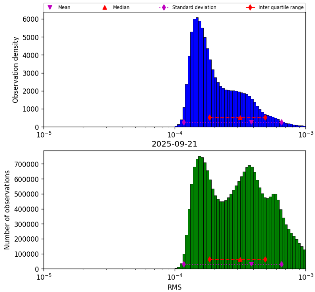
Figure 43: Histogram of “RMS” for 2025-09-20 to 2025-09-22
