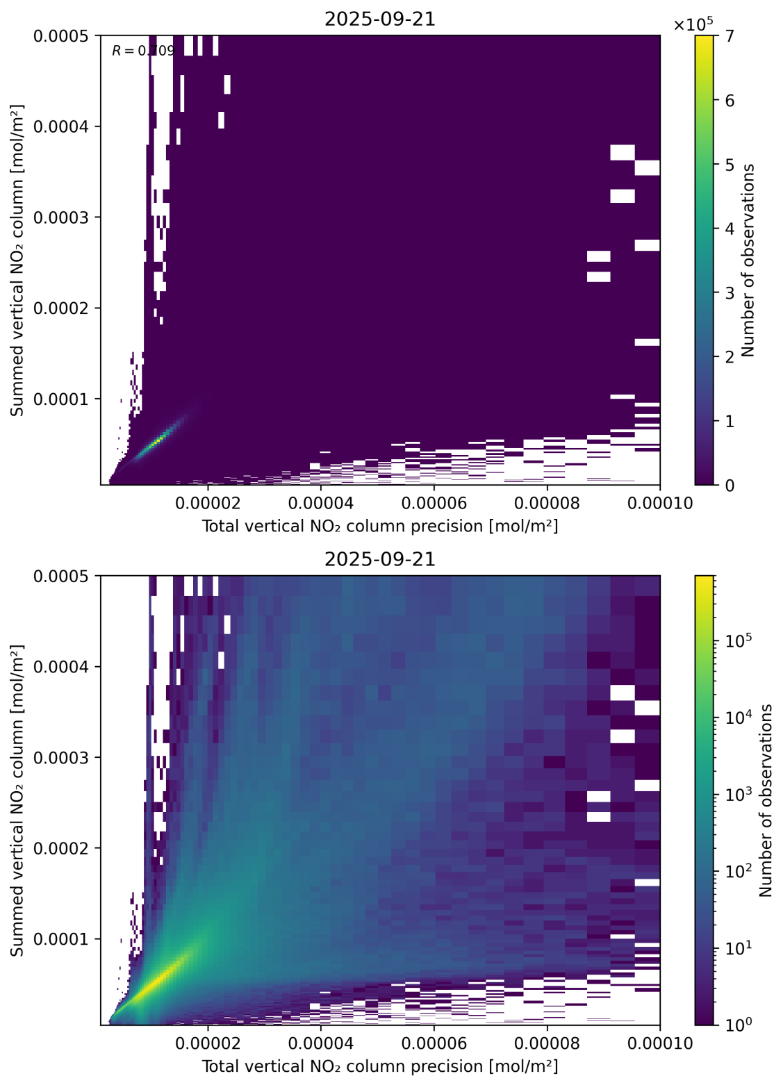
Figure 117: Scatter density plot of “Total vertical NO 2 column precision” against “Summed vertical NO 2 column” for 2025-09-20 to 2025-09-22.
