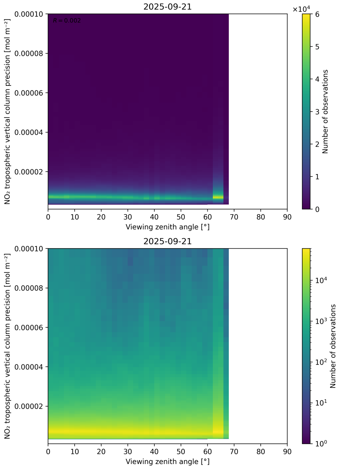
Figure 170: Scatter density plot of “Viewing zenith angle” against “NO 2 tropospheric vertical column precision” for 2025-09-20 to 2025-09-22.
