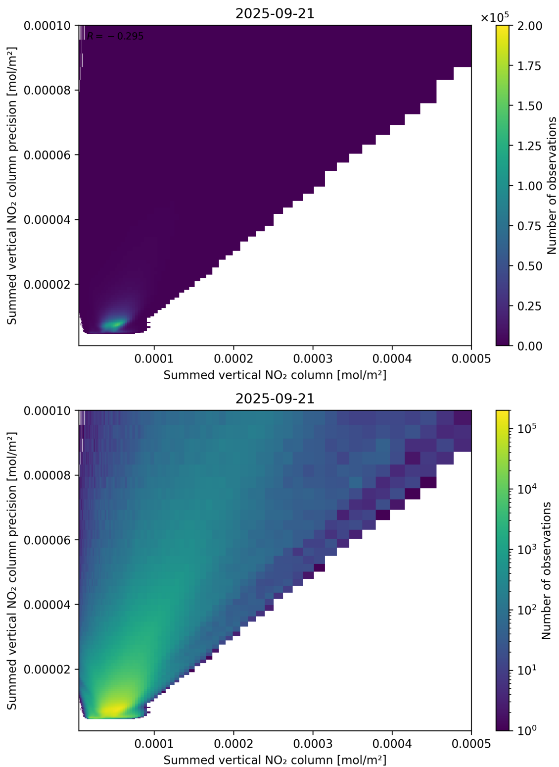
Figure 105: Scatter density plot of “Summed vertical NO 2 column” against “Summed vertical NO 2 column precision” for 2025-09-20 to 2025-09-22.
