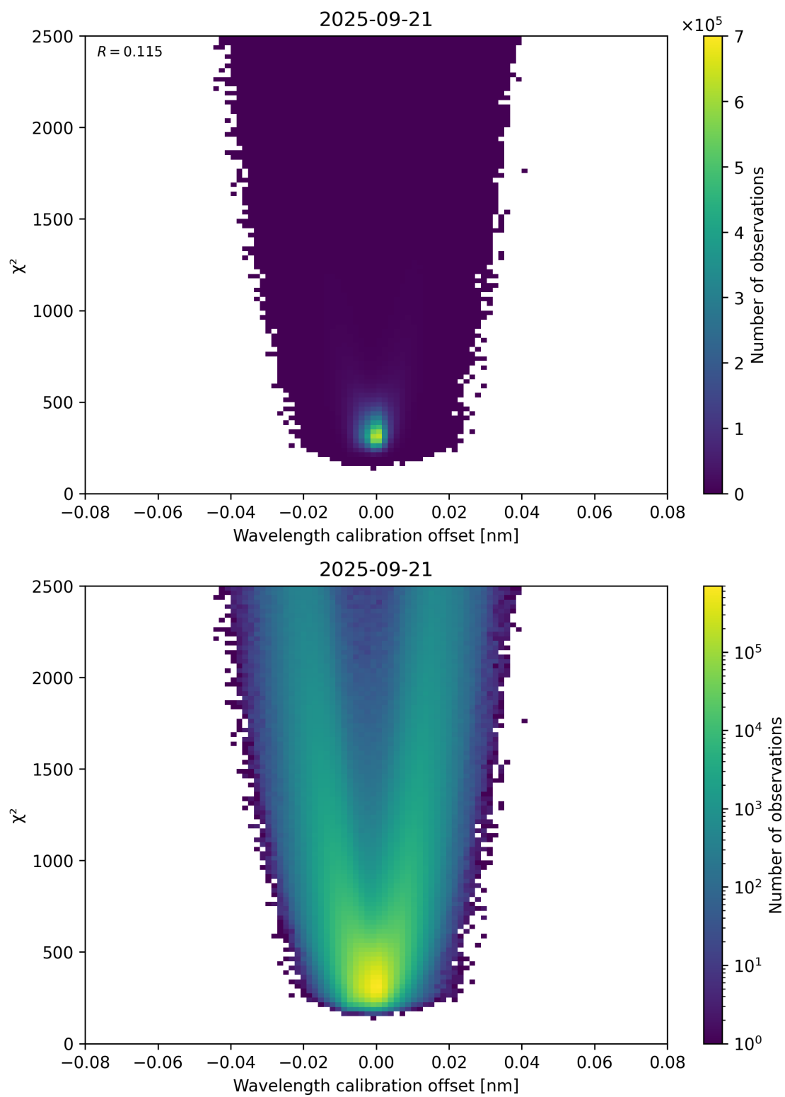
Figure 175: Scatter density plot of “Wavelength calibration offset” against “ \chi^2 ” for 2025-09-20 to 2025-09-22.
