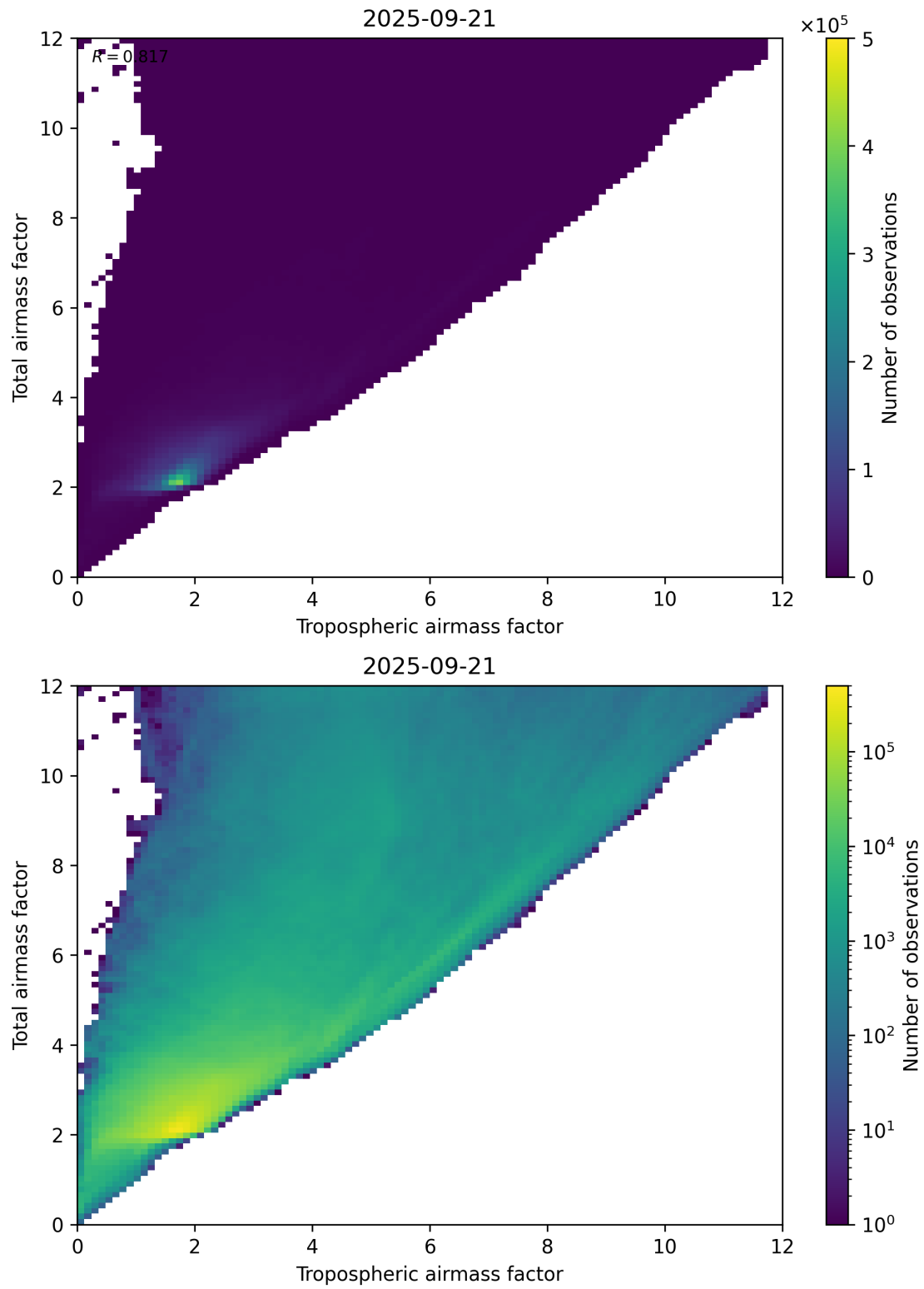
Figure 72: Scatter density plot of “Tropospheric airmass factor” against “Total airmass factor” for 2025-09-20 to 2025-09-22.
