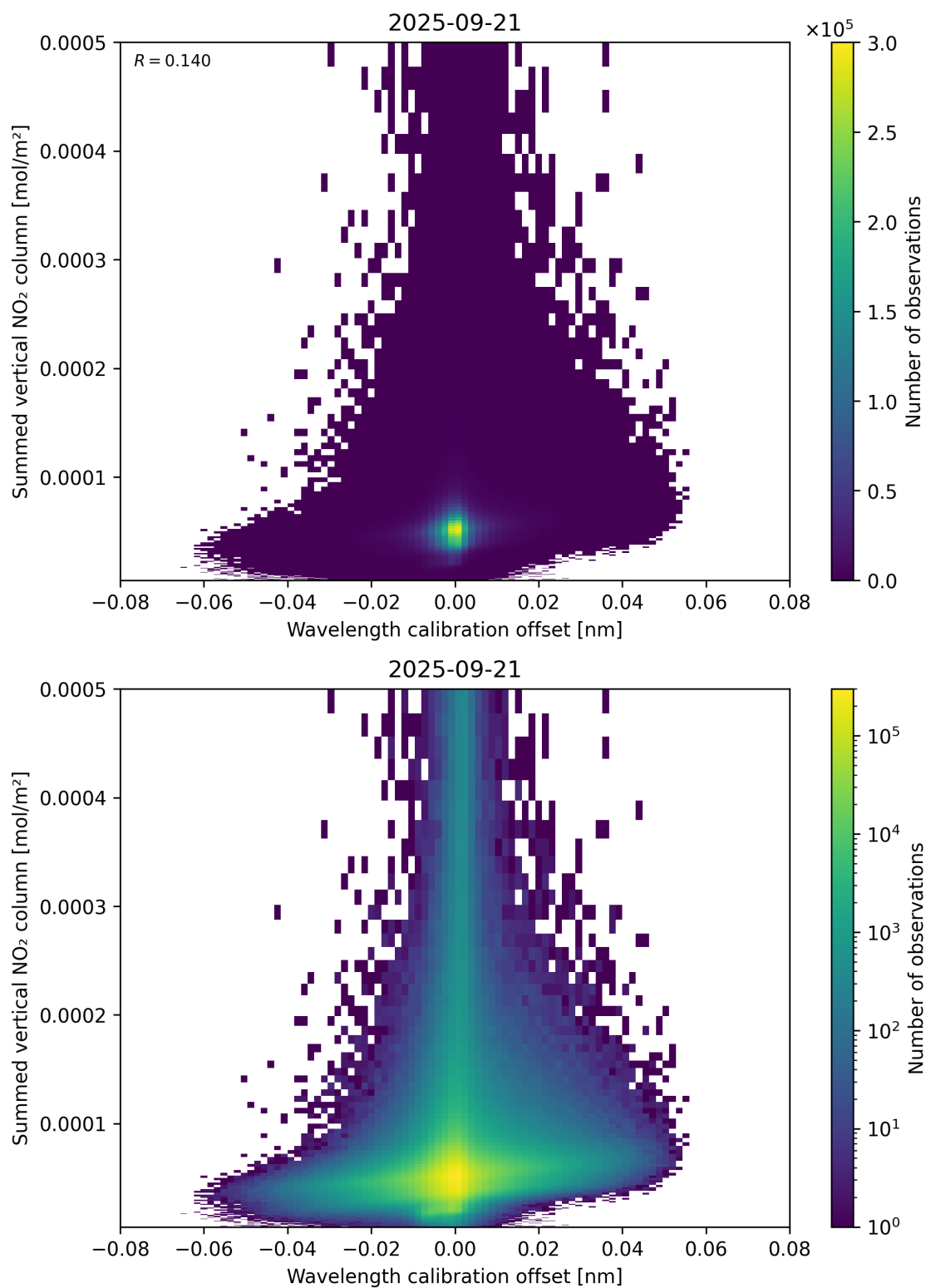
Figure 177: Scatter density plot of “Wavelength calibration offset” against “Summed vertical NO 2 column” for 2025-09-20 to 2025-09-22.
