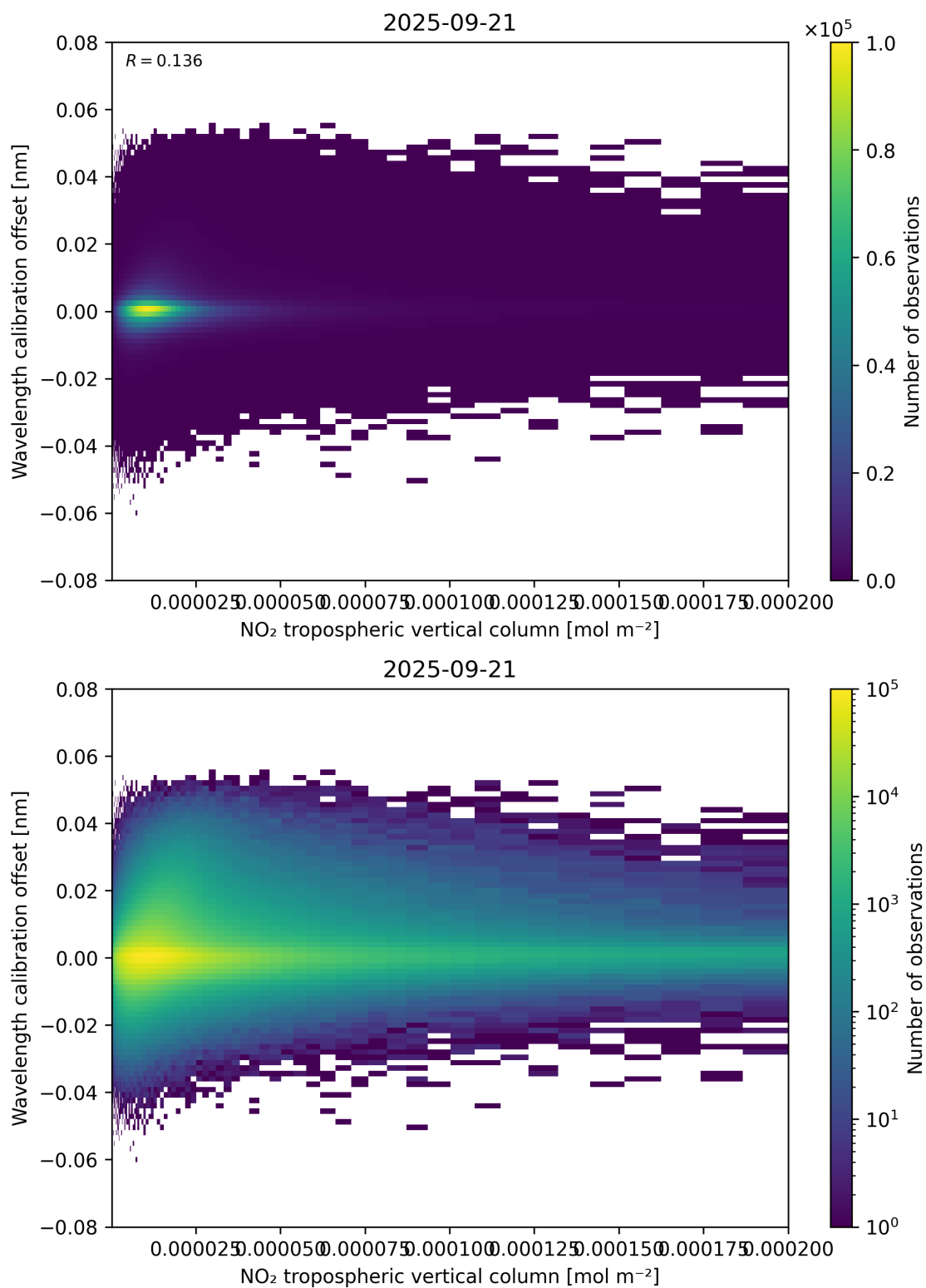
Figure 143: Scatter density plot of “NO 2 tropospheric vertical column” against “Wavelength calibration offset” for 2025-09-20 to 2025-09-22.
