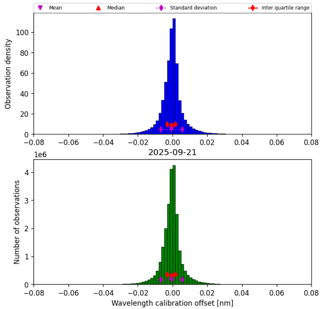
Figure 35: Histogram of “Wavelength calibration offset” for 2025-09-20 to 2025-09-22
