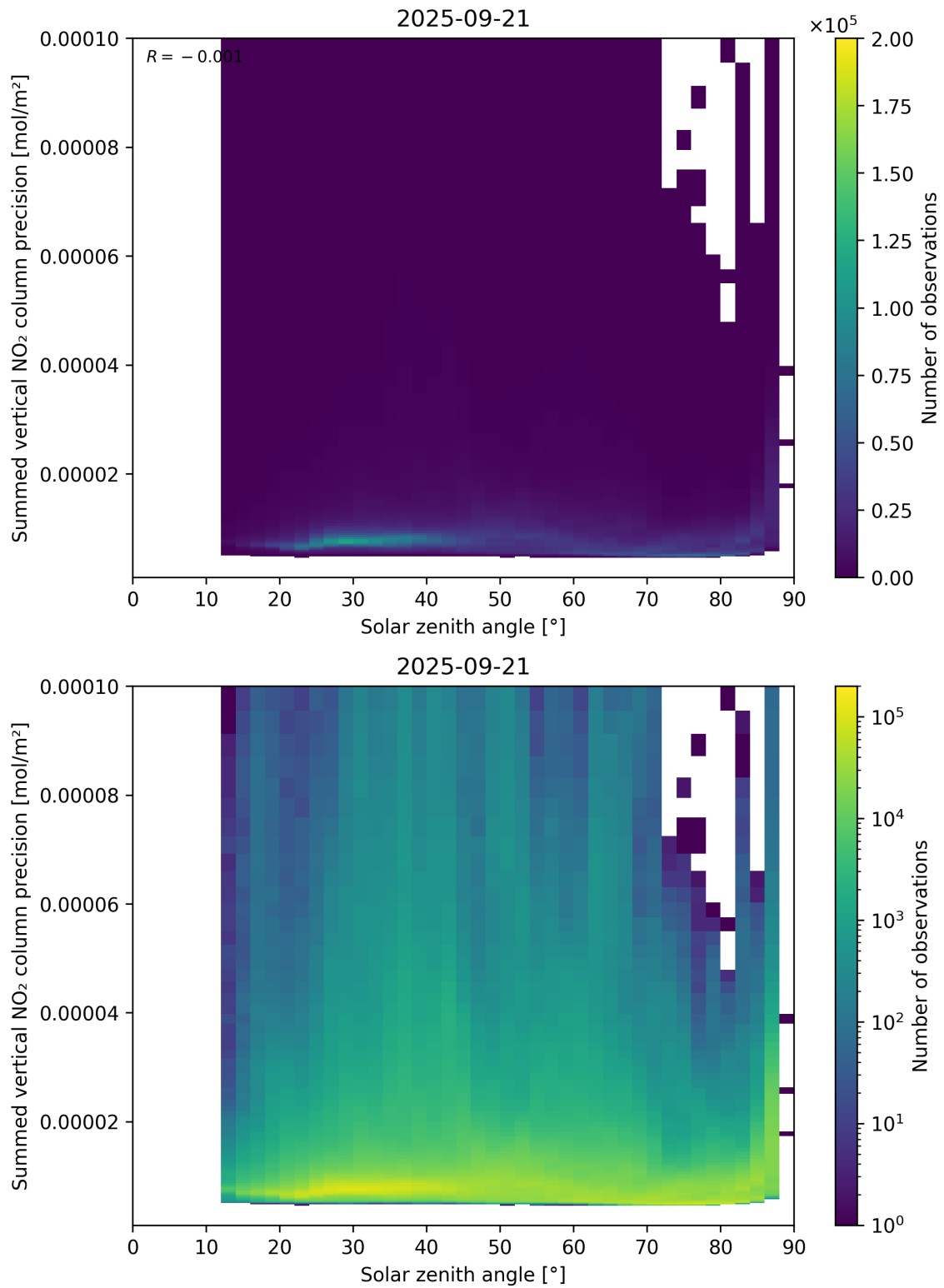
Figure 152: Scatter density plot of “Solar zenith angle” against “Summed vertical NO 2 column precision” for 2025-09-20 to 2025-09-22.
