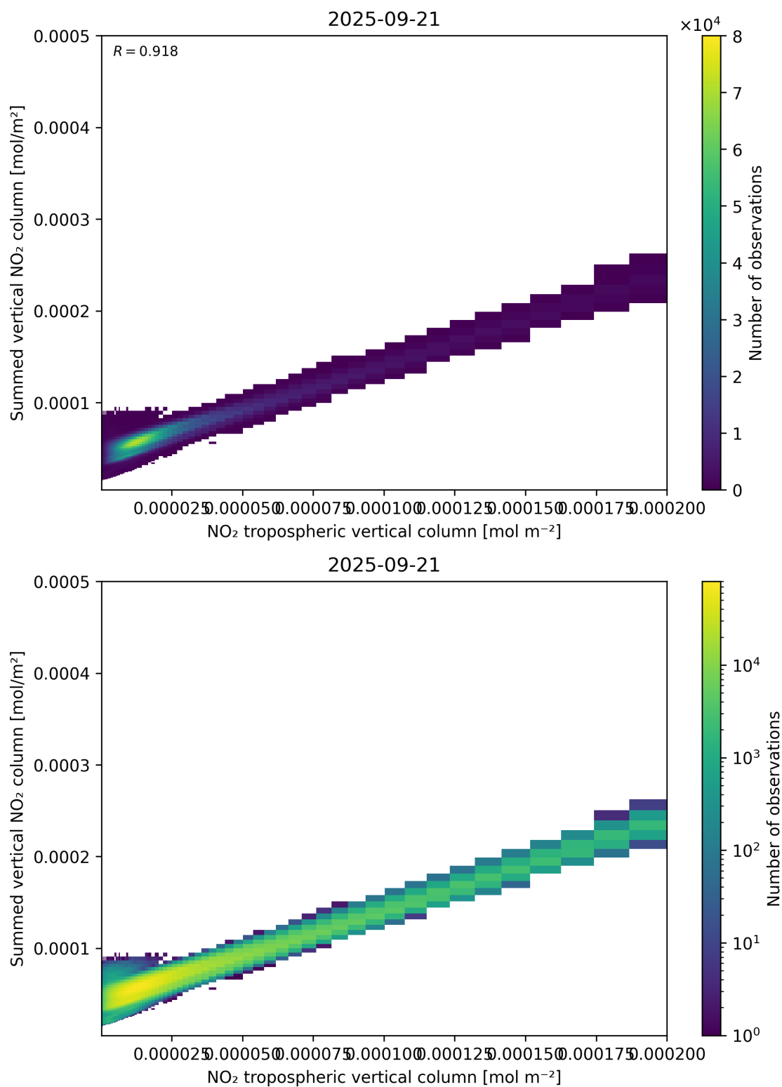
Figure 126: Scatter density plot of “NO 2 tropospheric vertical column” against “Summed vertical NO 2 column” for 2025-09-20 to 2025-09-22.
