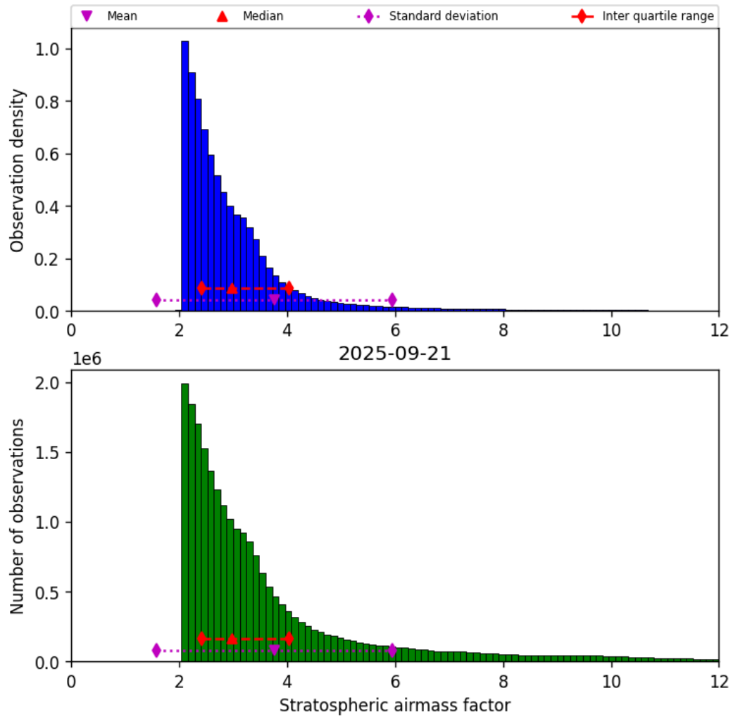
Figure 44: Histogram of “Stratospheric airmass factor” for 2025-09-20 to 2025-09-22
