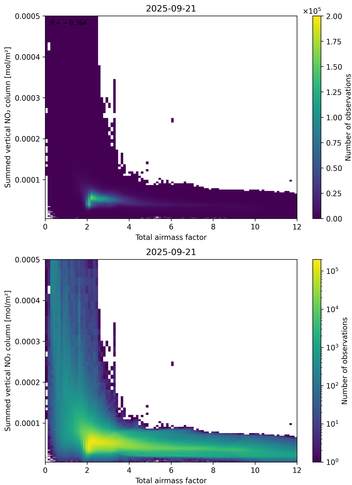
Figure 65: Scatter density plot of “Total airmass factor” against “Summed vertical NO 2 column” for 2025-09-20 to 2025-09-22.
