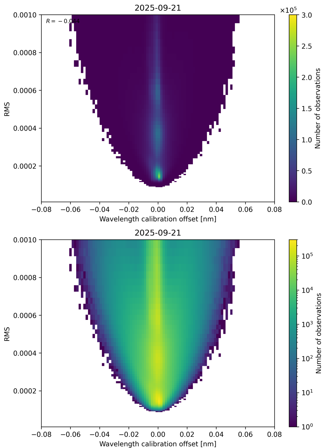
Figure 181: Scatter density plot of “Wavelength calibration offset” against “RMS” for 2025-09-20 to 2025-09-22.
