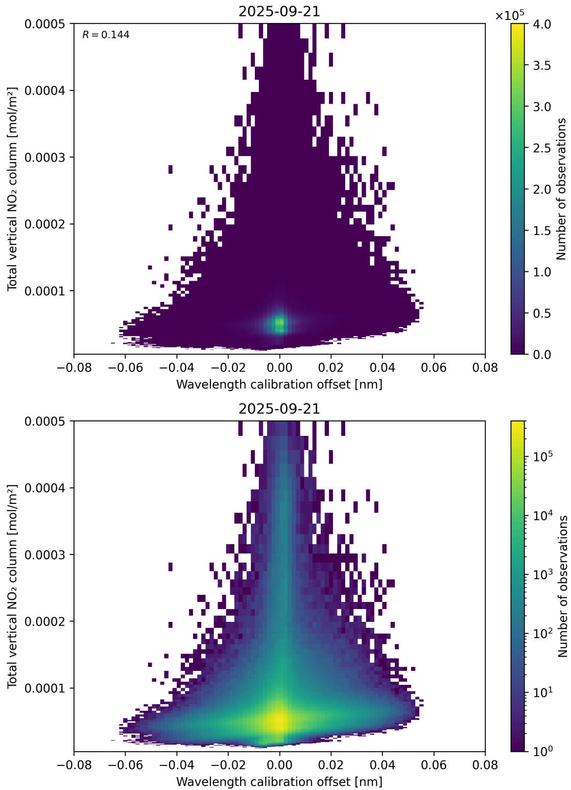
Figure 179: Scatter density plot of “Wavelength calibration offset” against “Total vertical NO 2 column” for 2025-09-20 to 2025-09-22.
