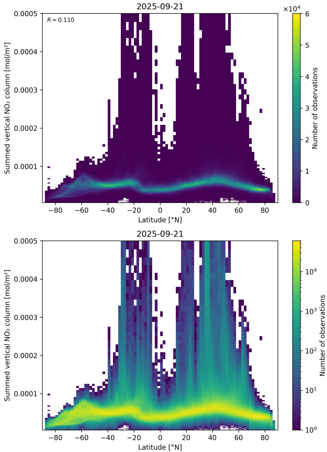
Figure 88: Scatter density plot of “Latitude” against “Summed vertical NO 2 column” for 2025-09-20 to 2025-09-22.
