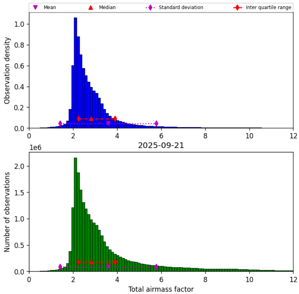
Figure 32: Histogram of “Total airmass factor” for 2025-09-20 to 2025-09-22
