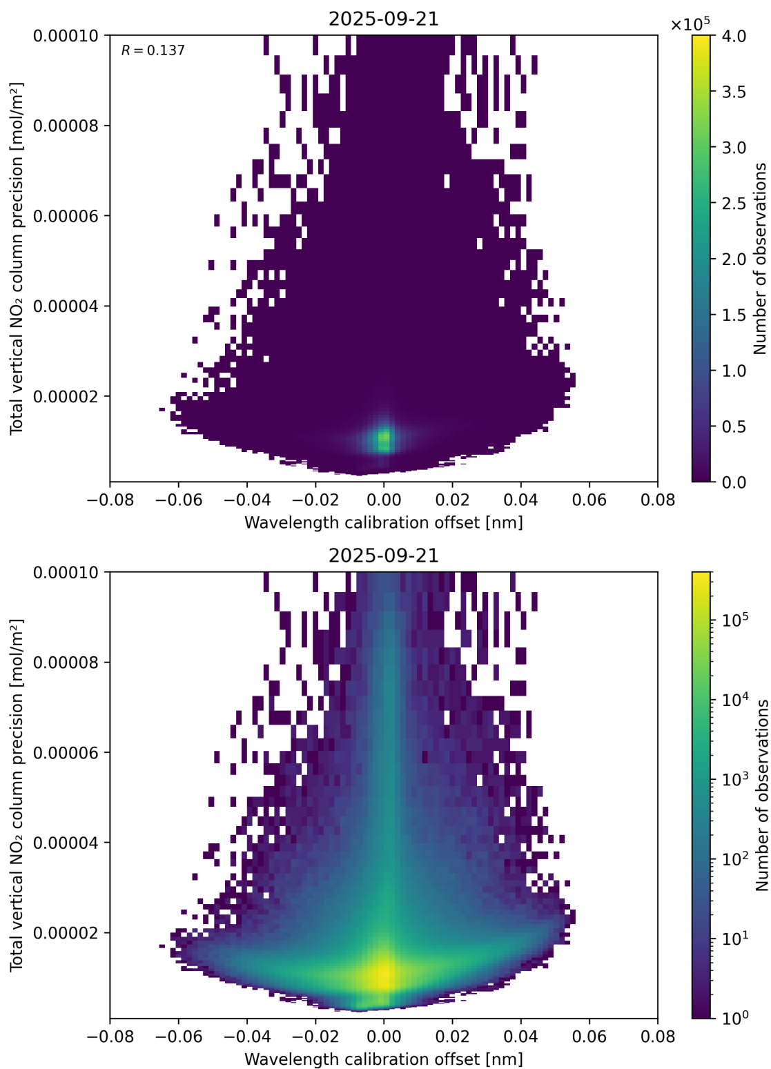
Figure 180: Scatter density plot of “Wavelength calibration offset” against “Total vertical NO 2 column precision” for 2025-09-20 to 2025-09-22.
