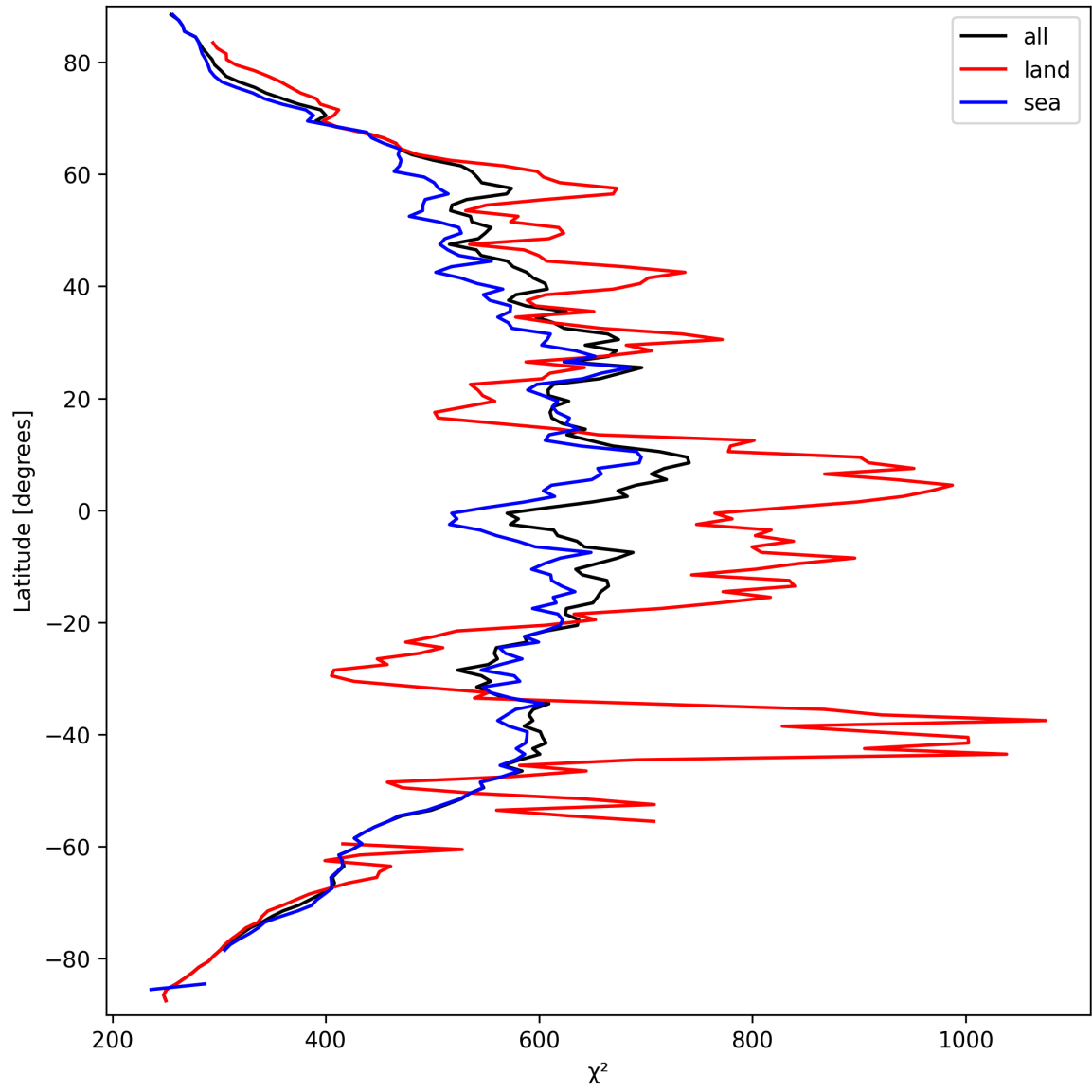
Figure 25: Zonal average of “ \chi^2 ” for 2025-09-20 to 2025-09-22.
