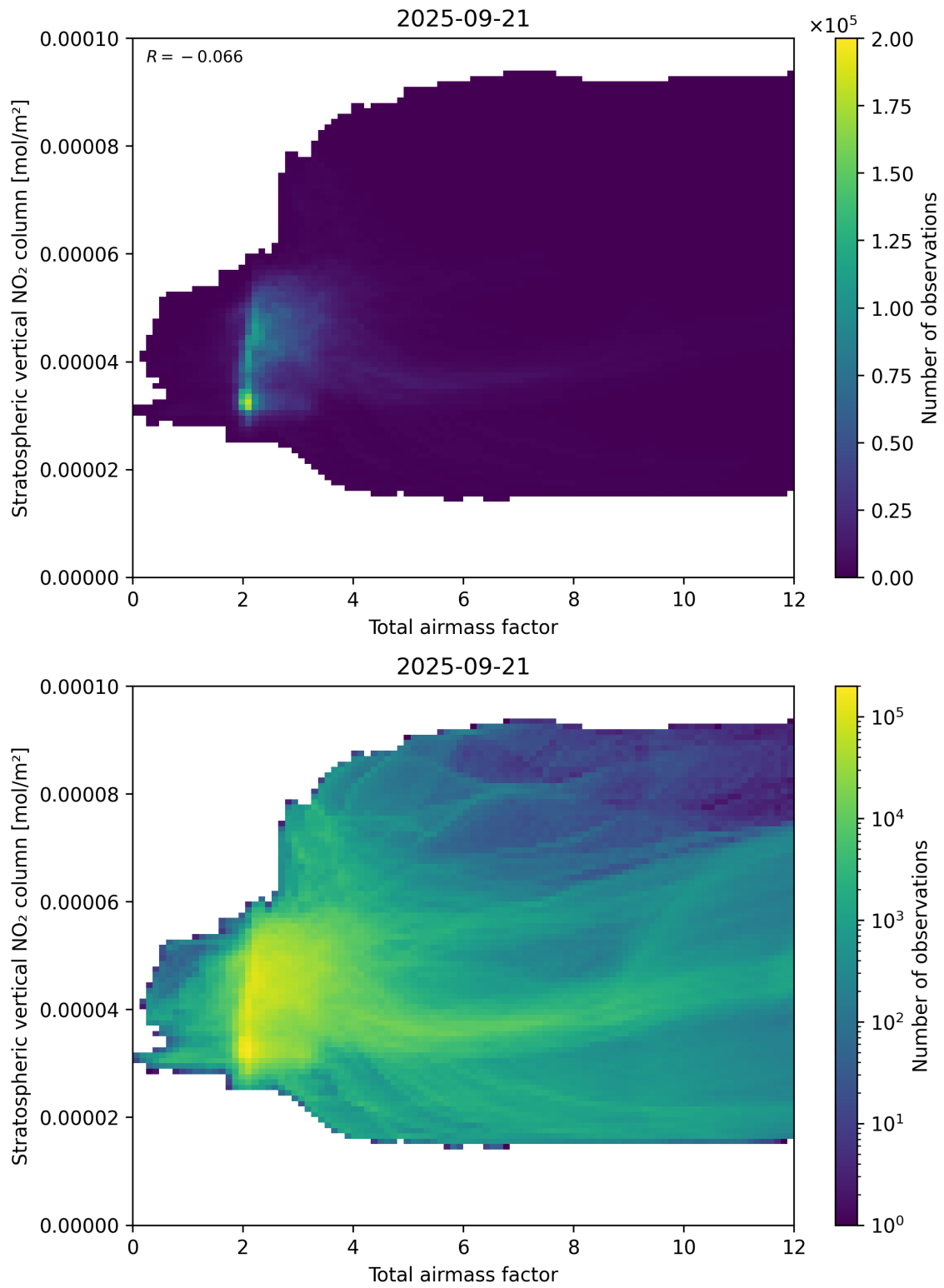
Figure 64: Scatter density plot of “Total airmass factor” against “Stratospheric vertical NO 2 column” for 2025-09-20 to 2025-09-22.
