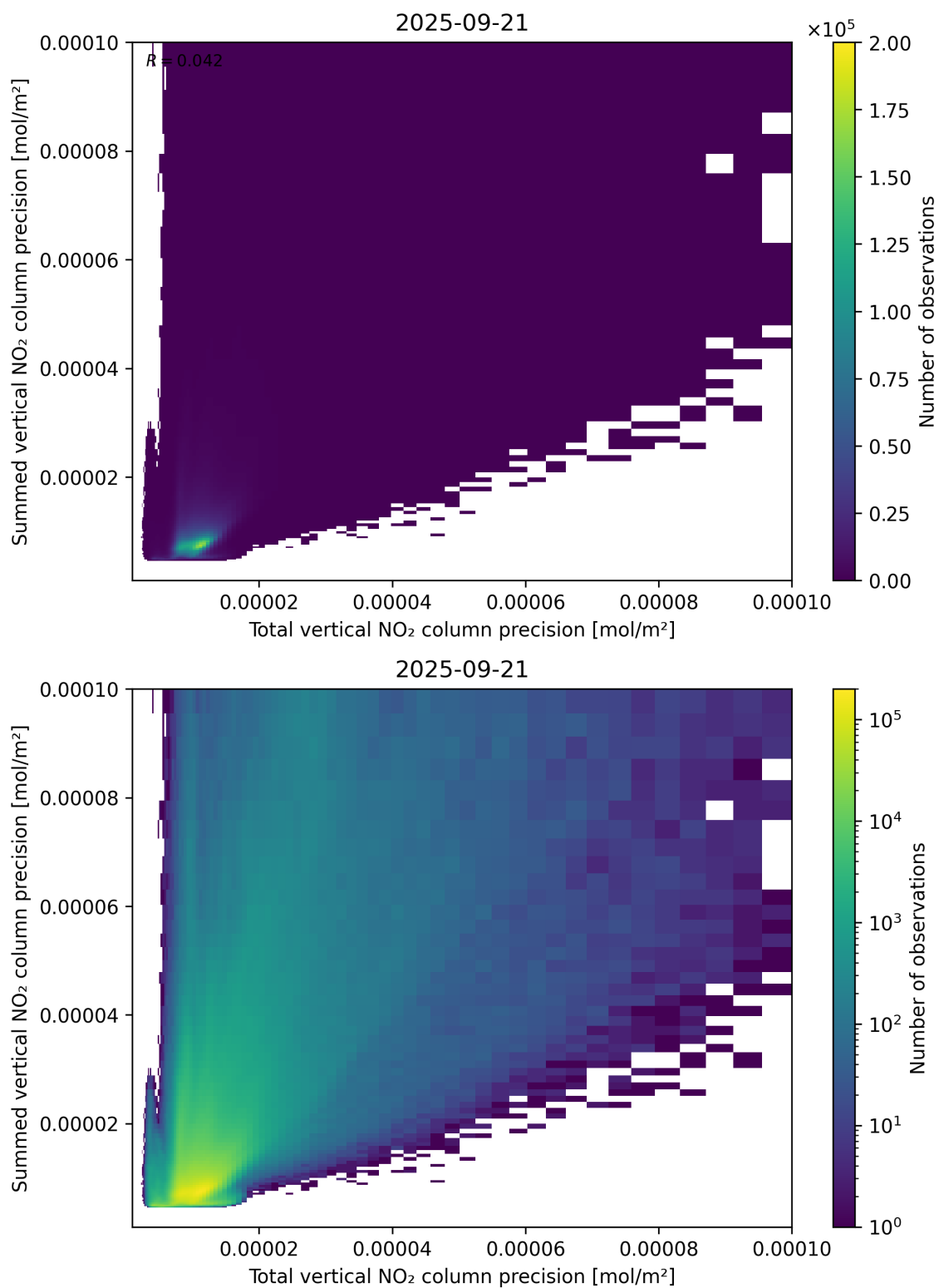
Figure 118: Scatter density plot of “Total vertical NO 2 column precision” against “Summed vertical NO 2 column precision” for 2025-09-20 to 2025-09-22.
