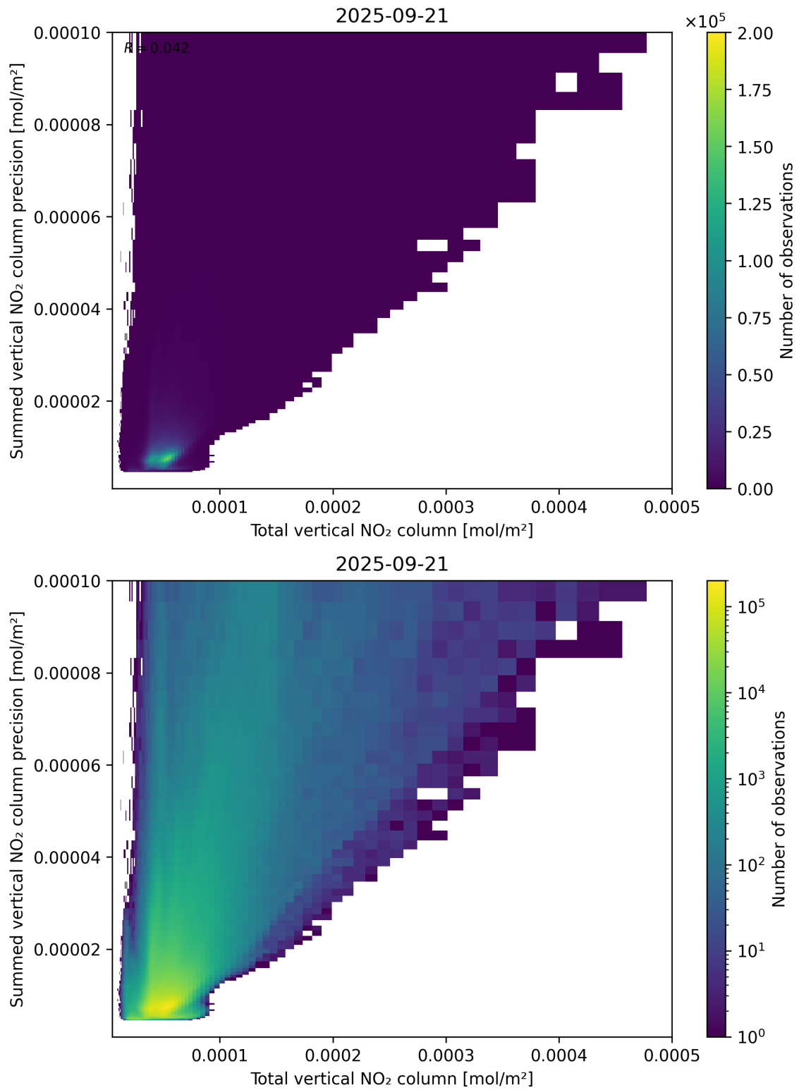
Figure 113: Scatter density plot of “Total vertical NO 2 column” against “Summed vertical NO 2 column precision” for 2025-09-20 to 2025-09-22.
