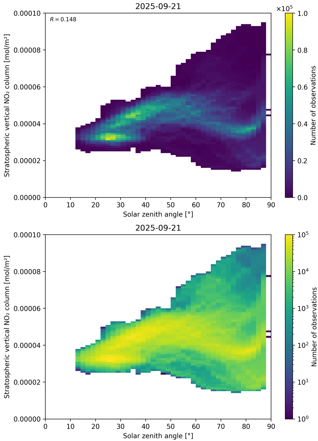
Figure 150: Scatter density plot of “Solar zenith angle” against “Stratospheric vertical \text{NO}_2 column” for 2025-09-20 to 2025-09-22.
