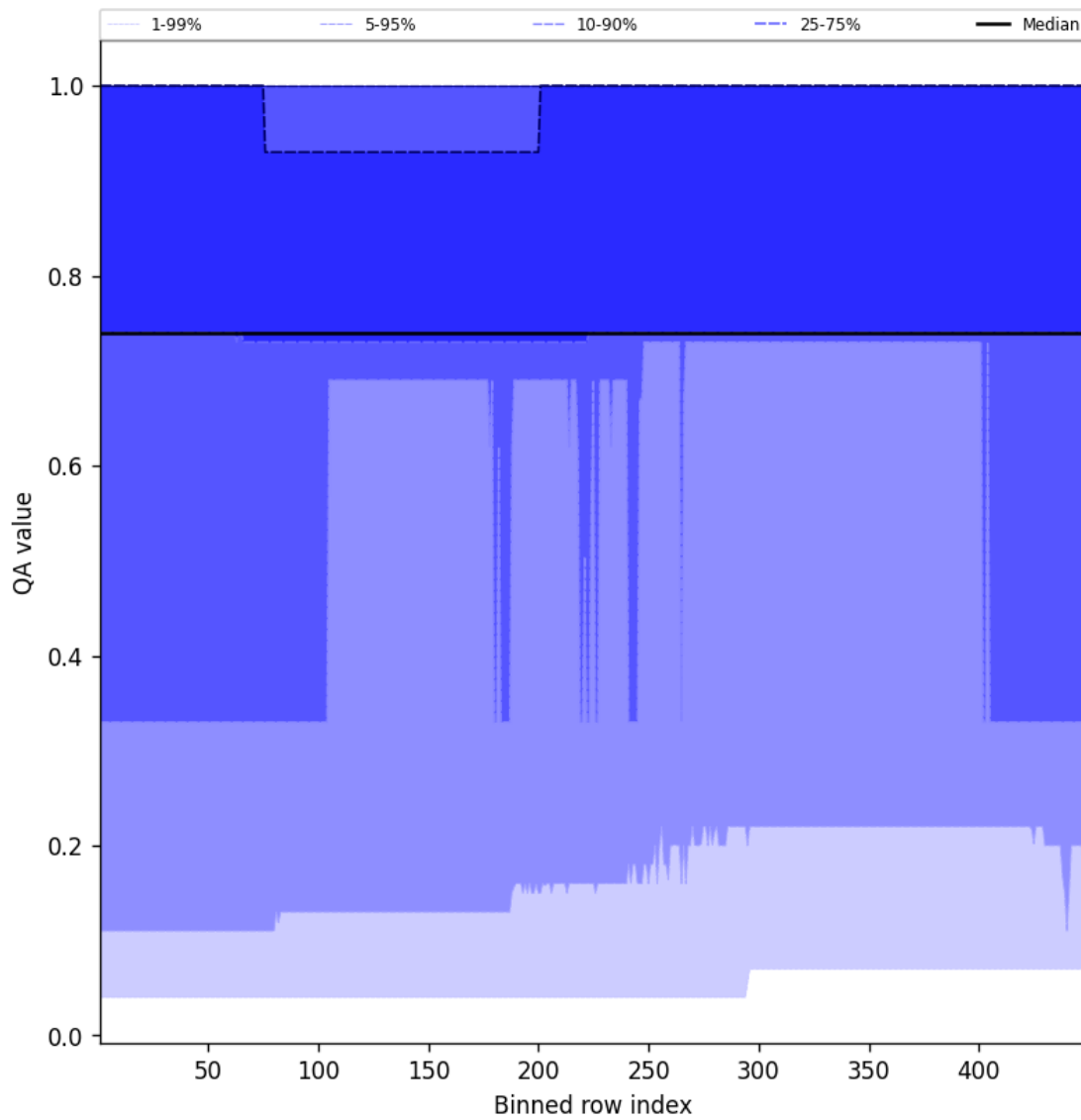
Figure 45: Along track statistics of “QA value” for 2025-09-20 to 2025-09-22
