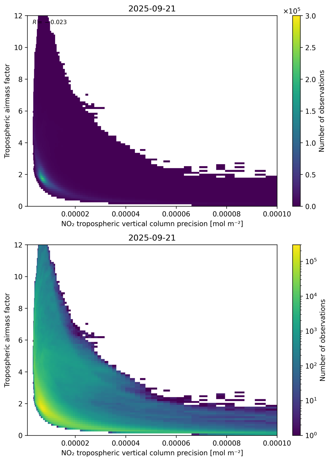
Figure 133: Scatter density plot of “NO 2 tropospheric vertical column precision” against “Tropospheric air mass factor” for 2025-09-20 to 2025-09-22.
