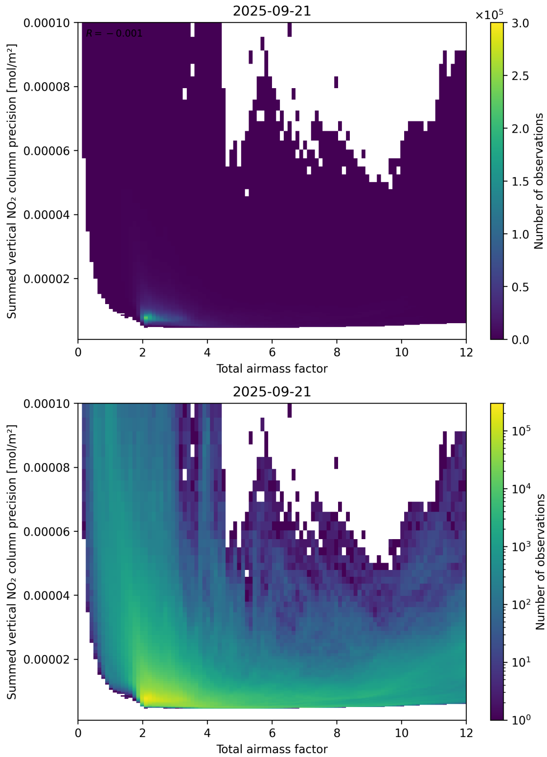
Figure 66: Scatter density plot of “Total airmass factor” against “Summed vertical NO 2 column precision” for 2025-09-20 to 2025-09-22.
