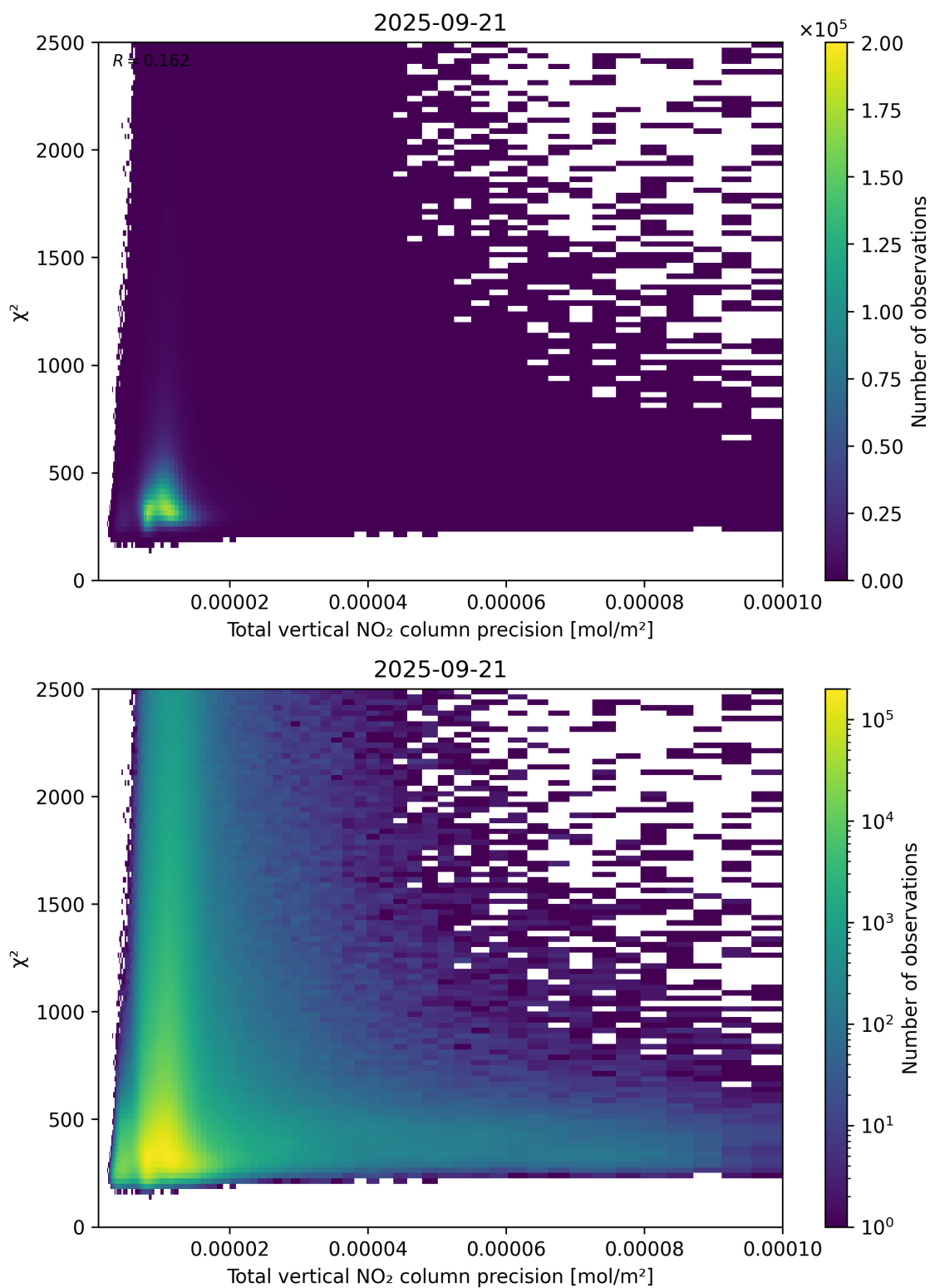
Figure 116: Scatter density plot of “Total vertical NO 2 column precision” against “ \chi^2 ” for 2025-09-20 to 2025-09-22.
