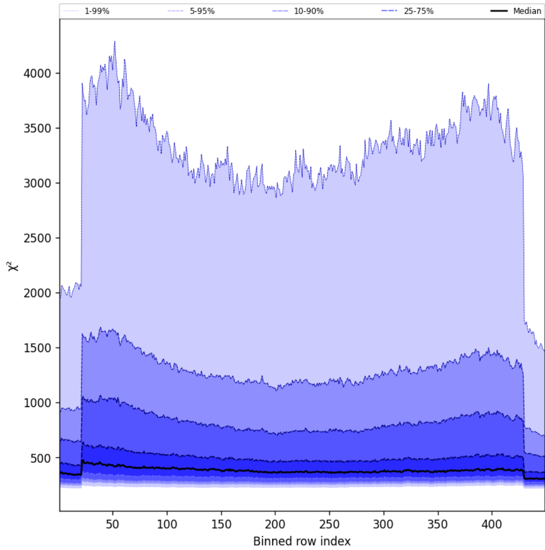
Figure 59: Along track statistics of “ \chi^2 ” for 2025-09-20 to 2025-09-22
