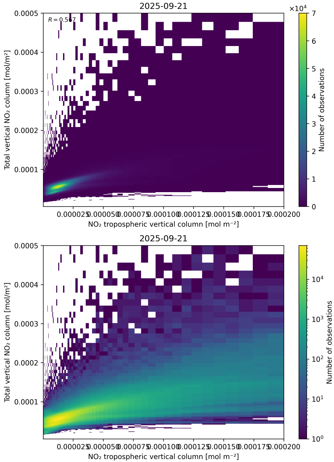
Figure 128: Scatter density plot of “NO 2 tropospheric vertical column” against “Total vertical NO 2 column” for 2025-09-20 to 2025-09-22.
