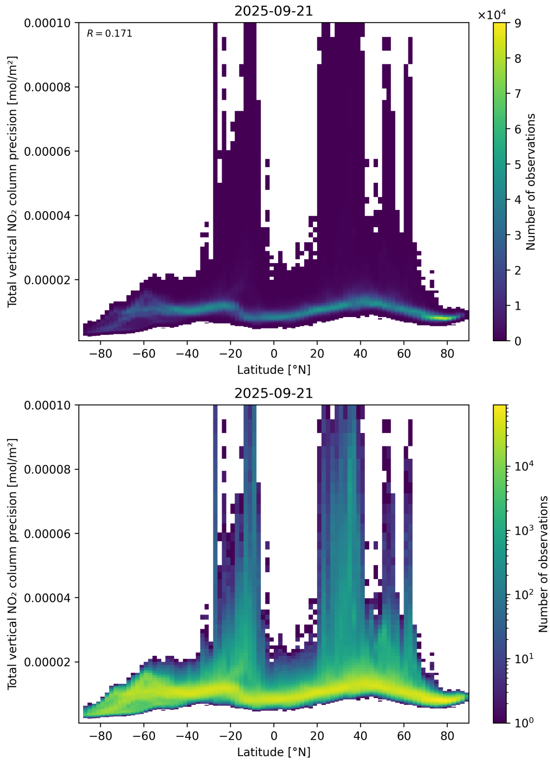
Figure 91: Scatter density plot of “Latitude” against “Total vertical NO 2 column precision” for 2025-09-20 to 2025-09-22.
