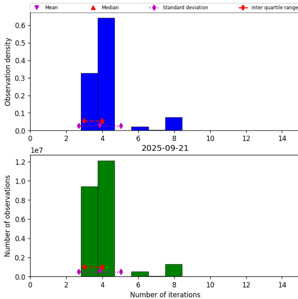
Figure 34: Histogram of “Number of iterations” for 2025-09-20 to 2025-09-22
