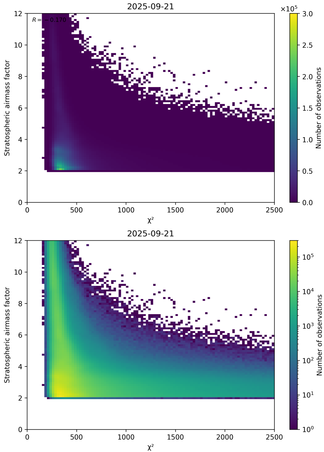
Figure 81: Scatter density plot of “ \chi^2 ” against “Stratospheric airmass factor” for 2025-09-20 to 2025-09-22.
