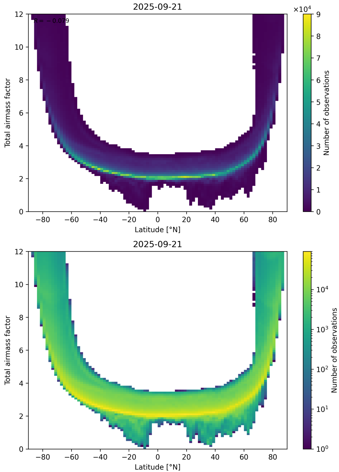
Figure 84: Scatter density plot of “Latitude” against “Total airmass factor” for 2025-09-20 to 2025-09-22.
