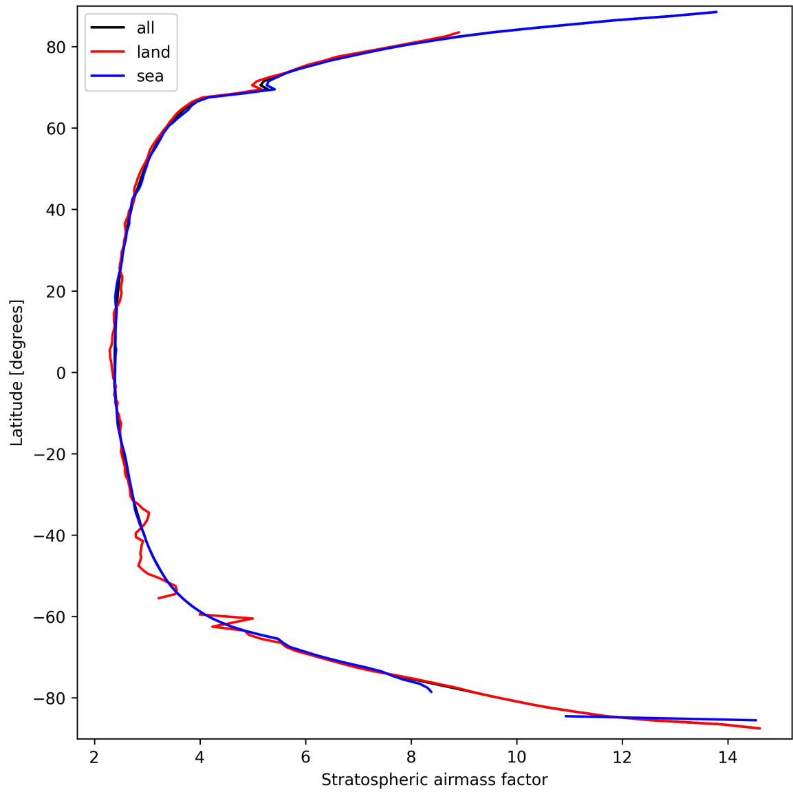
Figure 27: Zonal average of “Stratospheric air mass factor” for 2025-09-20 to 2025-09-22.
