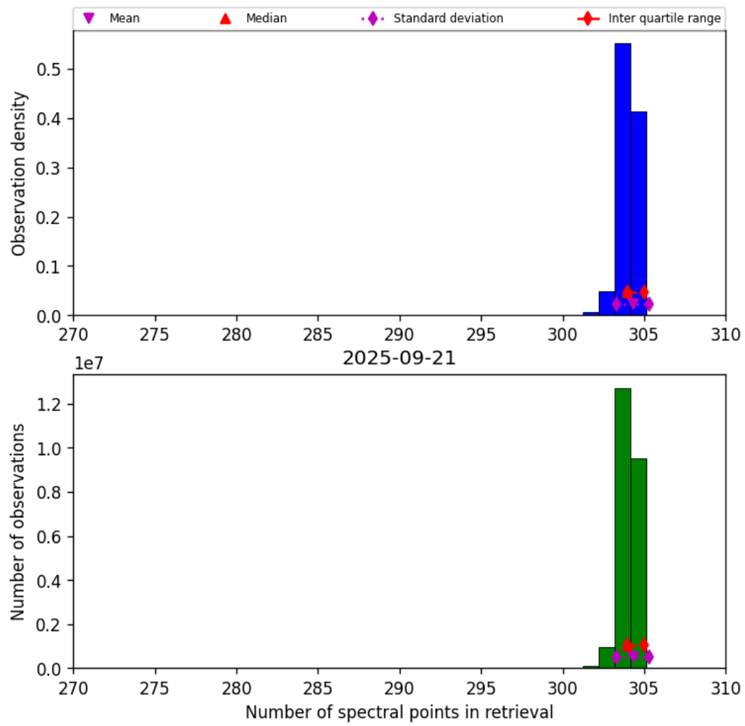
Figure 33: Histogram of “Number of spectral points in retrieval” for 2025-09-20 to 2025-09-22
