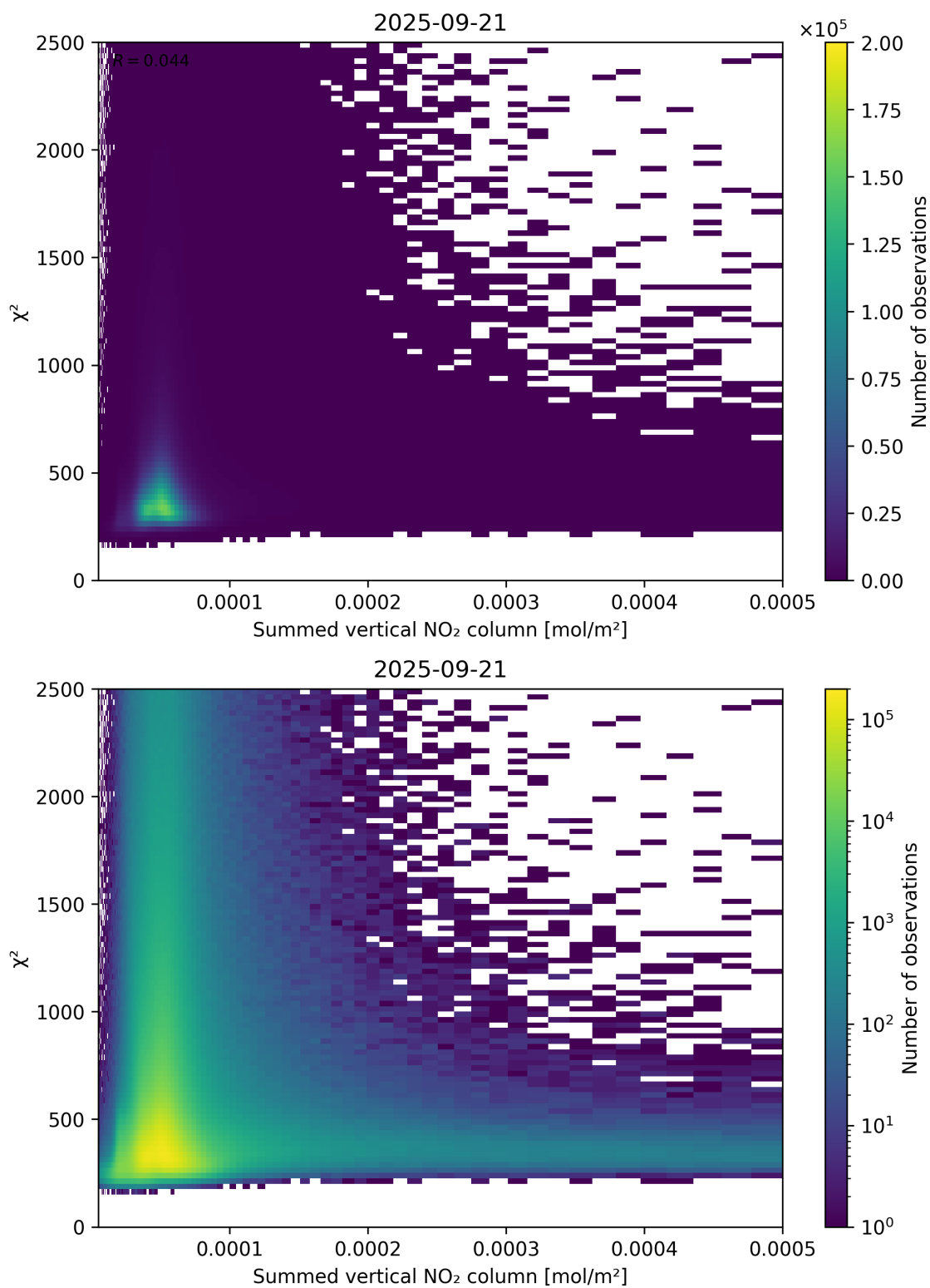
Figure 104: Scatter density plot of “Summed vertical NO 2 column” against “ \chi^2 ” for 2025-09-20 to 2025-09-22.
