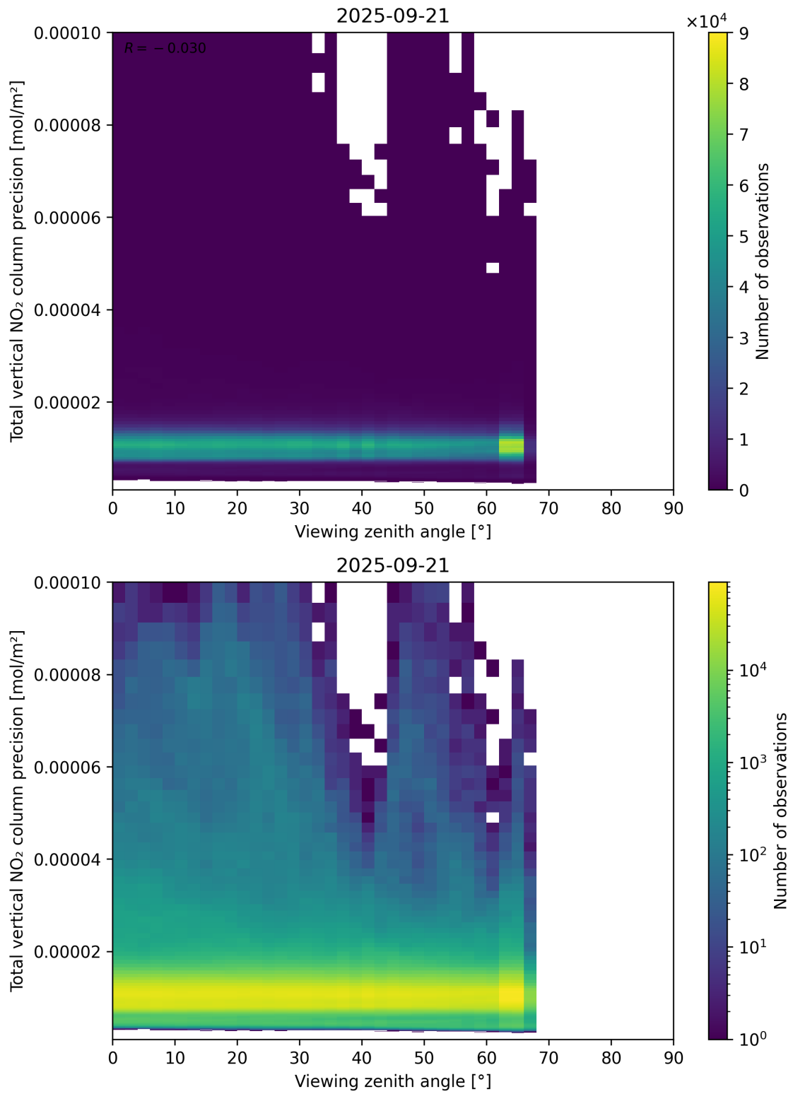
Figure 168: Scatter density plot of “Viewing zenith angle” against “Total vertical NO 2 column precision” for 2025-09-20 to 2025-09-22.
