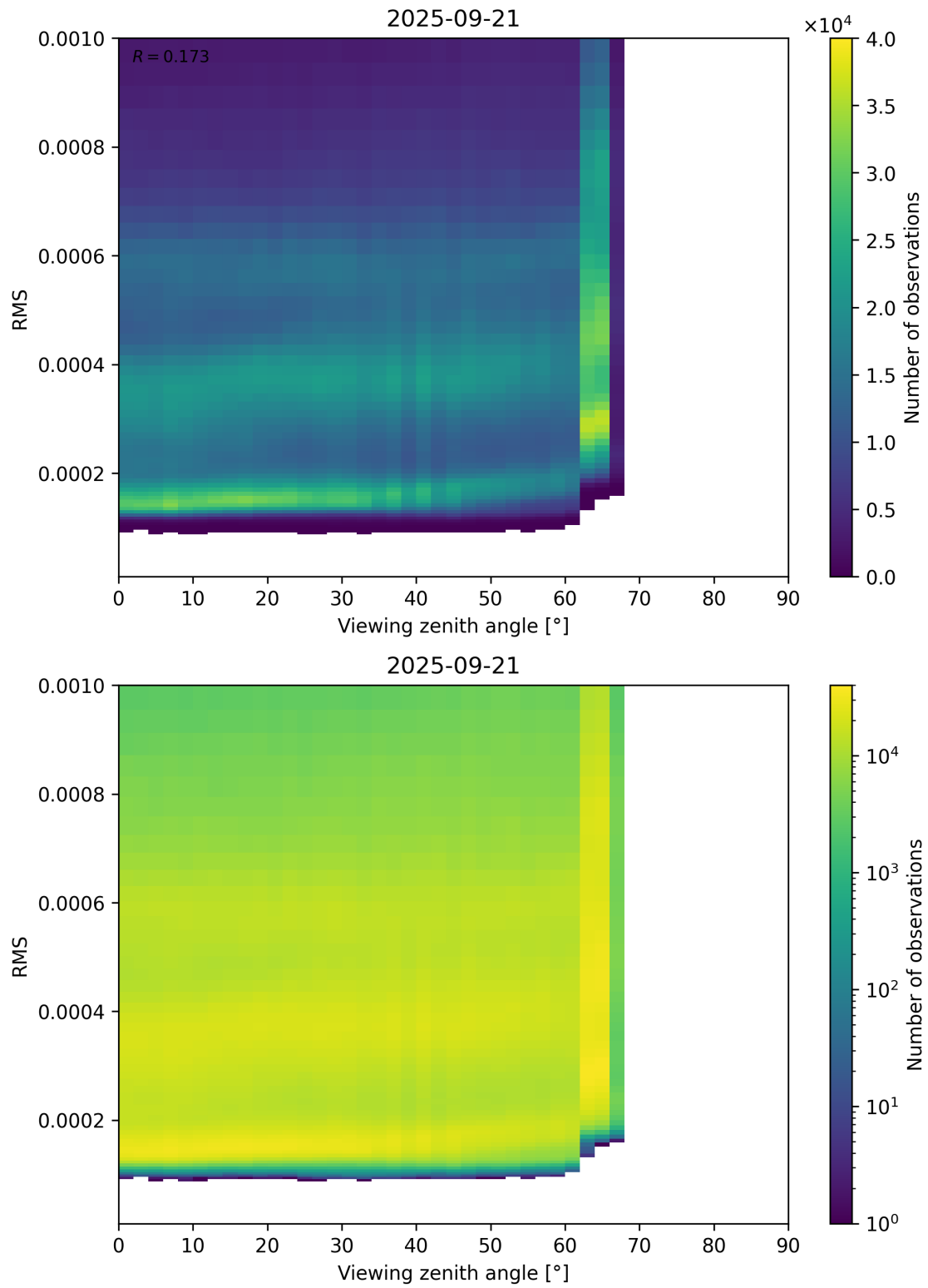
Figure 171: Scatter density plot of “Viewing zenith angle” against “RMS” for 2025-09-20 to 2025-09-22.
