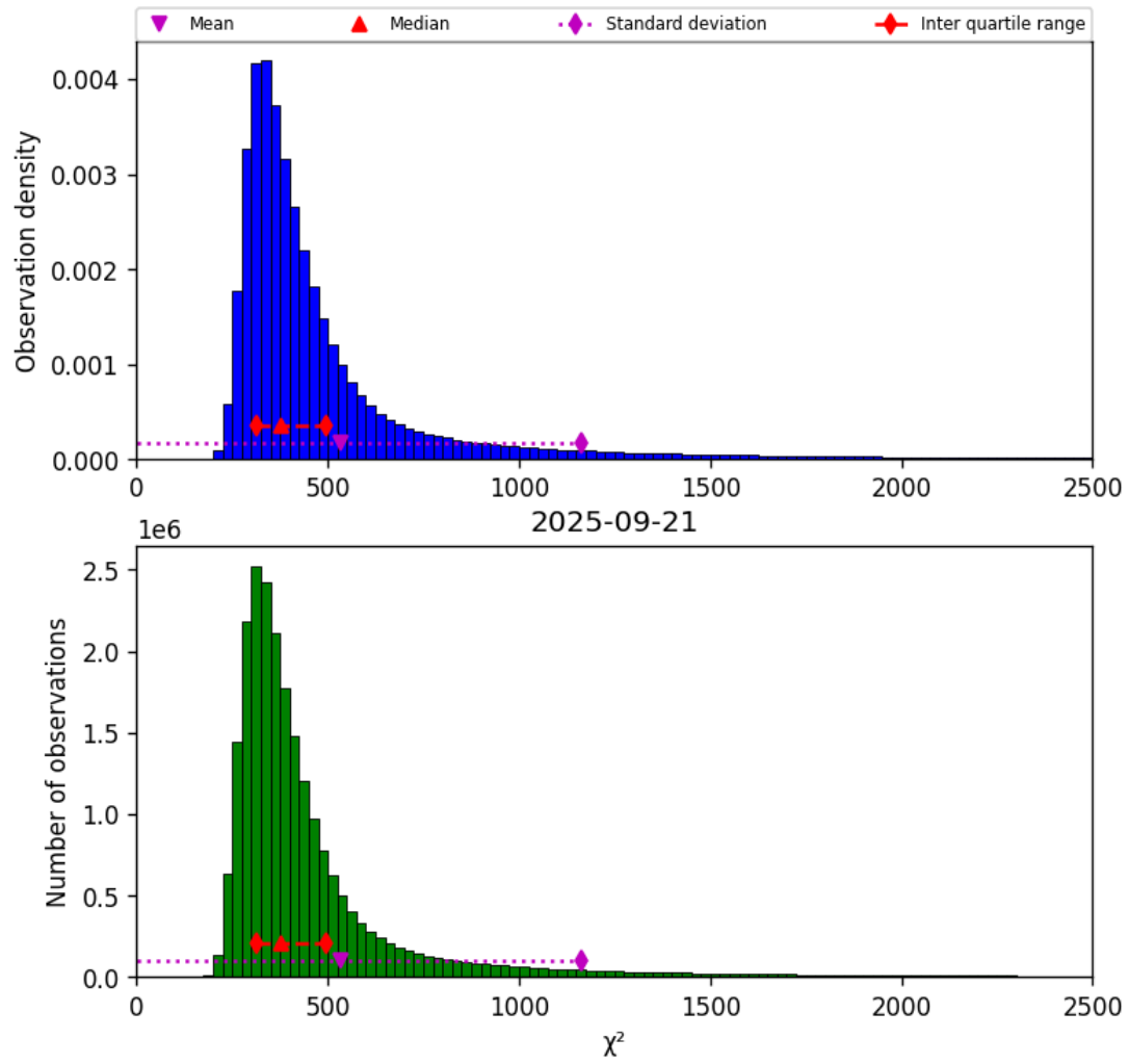
Figure 42: Histogram of “ \chi^2 ” for 2025-09-20 to 2025-09-22
