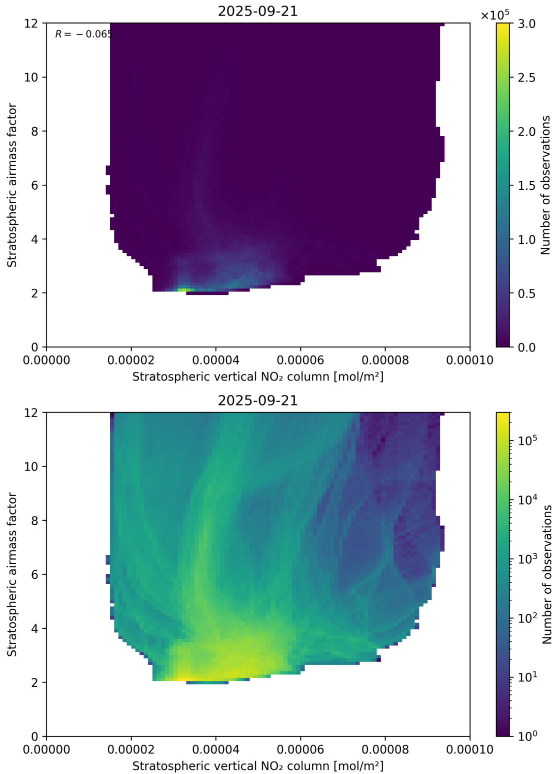
Figure 96: Scatter density plot of “Stratospheric vertical NO 2 column” against “Stratospheric airmass factor” for 2025-09-20 to 2025-09-22.
