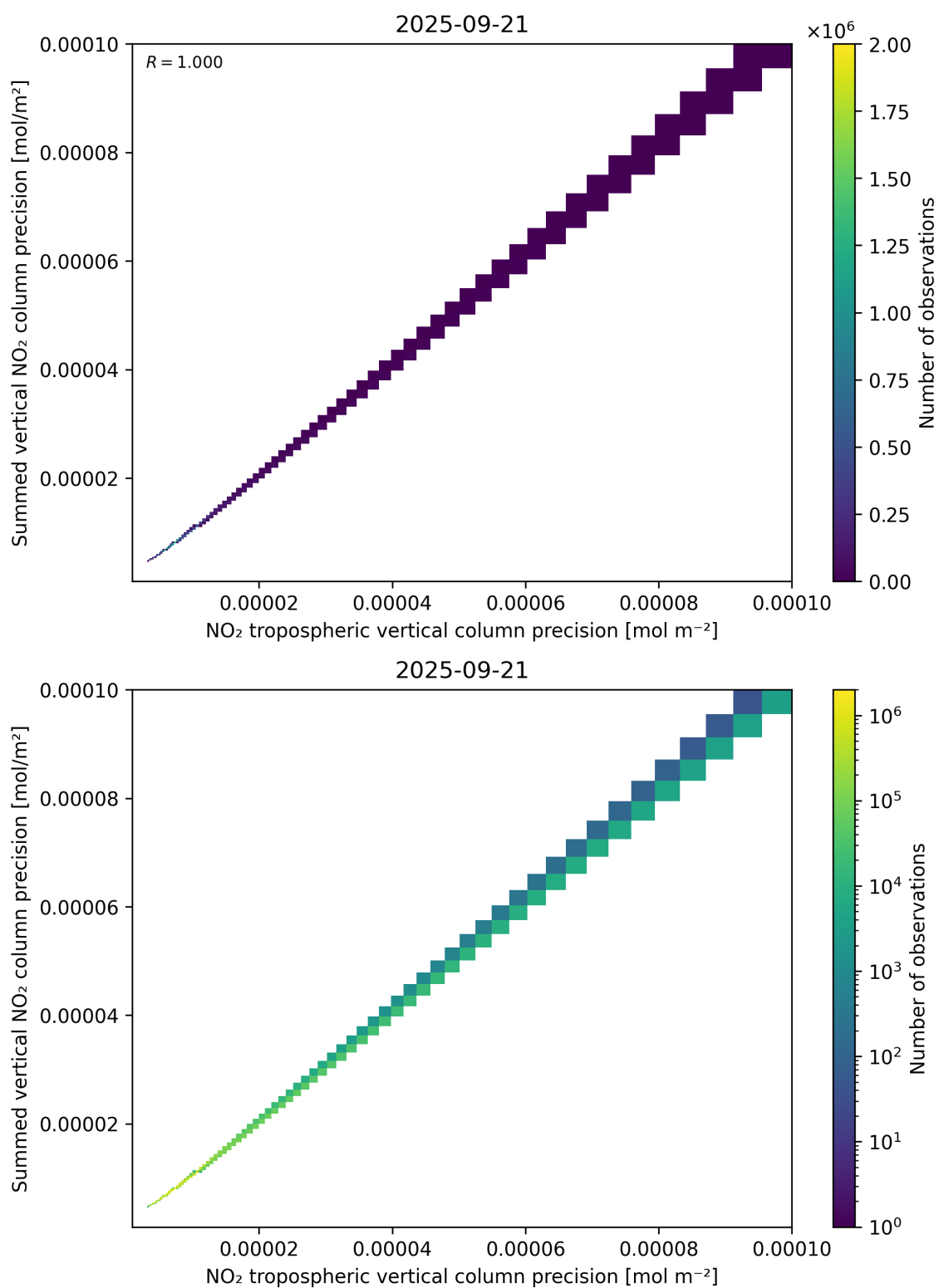
Figure 137: Scatter density plot of “NO 2 tropospheric vertical column precision” against “Summed vertical NO 2 column precision” for 2025-09-20 to 2025-09-22.
