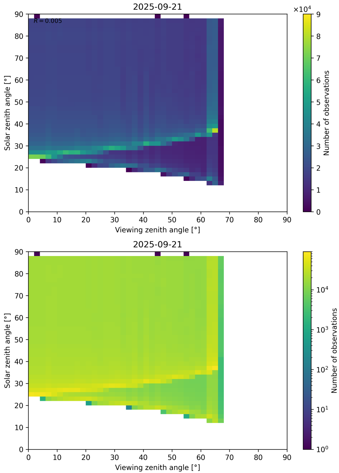
Figure 172: Scatter density plot of “Viewing zenith angle” against “Solar zenith angle” for 2025-09-20 to 2025-09-22.
