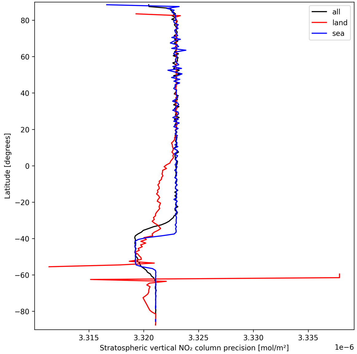
Figure 20: Zonal average of “Stratospheric vertical NO 2 column precision” for 2025-09-20 to 2025-09-22.
