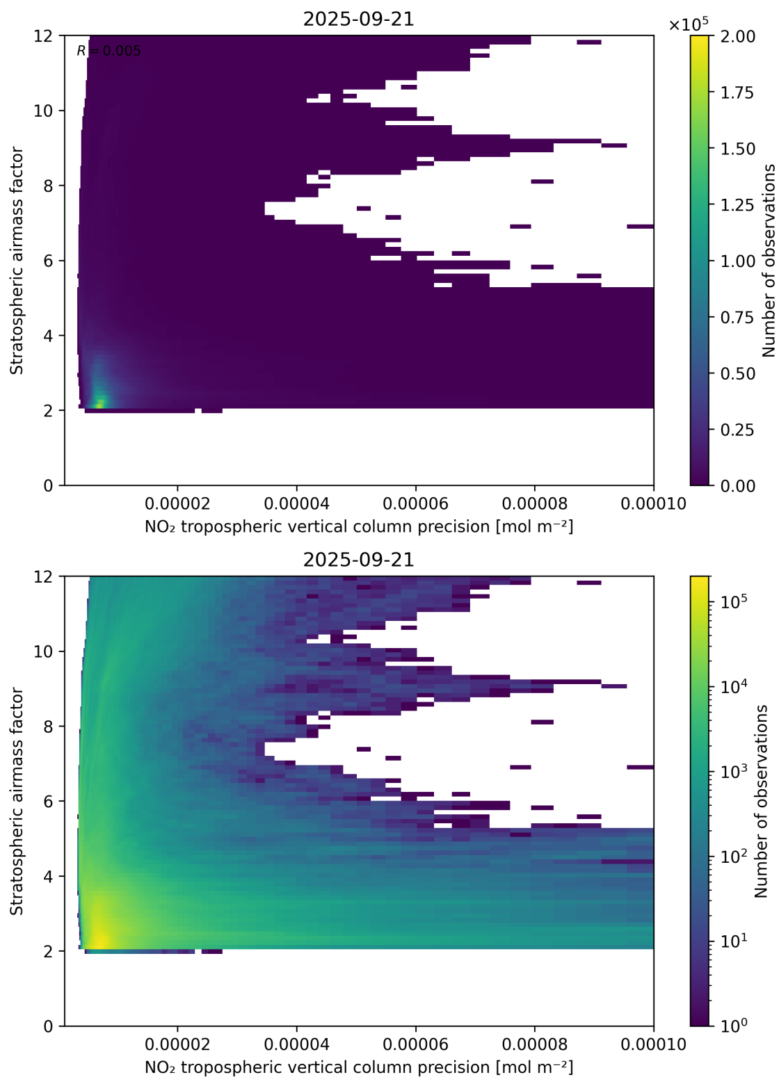
Figure 131: Scatter density plot of “NO 2 tropospheric vertical column precision” against “Stratospheric airmass factor” for 2025-09-20 to 2025-09-22.
