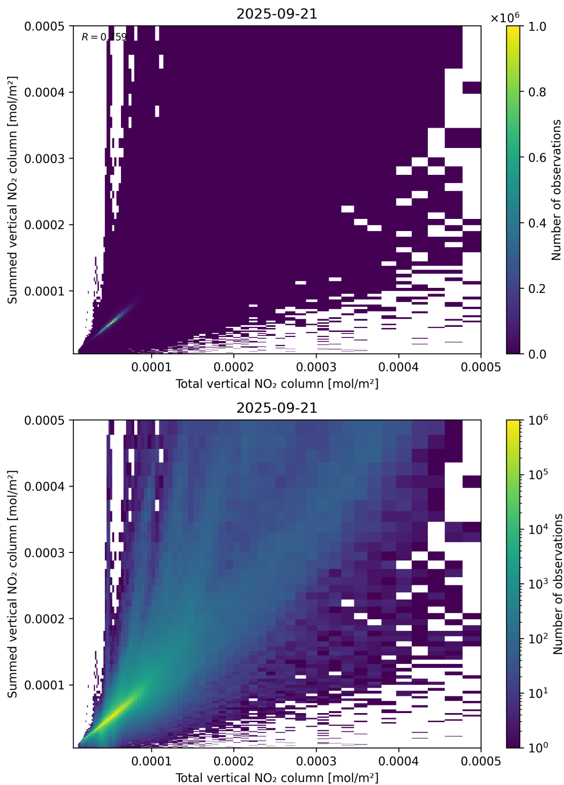
Figure 112: Scatter density plot of “Total vertical NO 2 column” against “Summed vertical NO 2 column” for 2025-09-20 to 2025-09-22.
