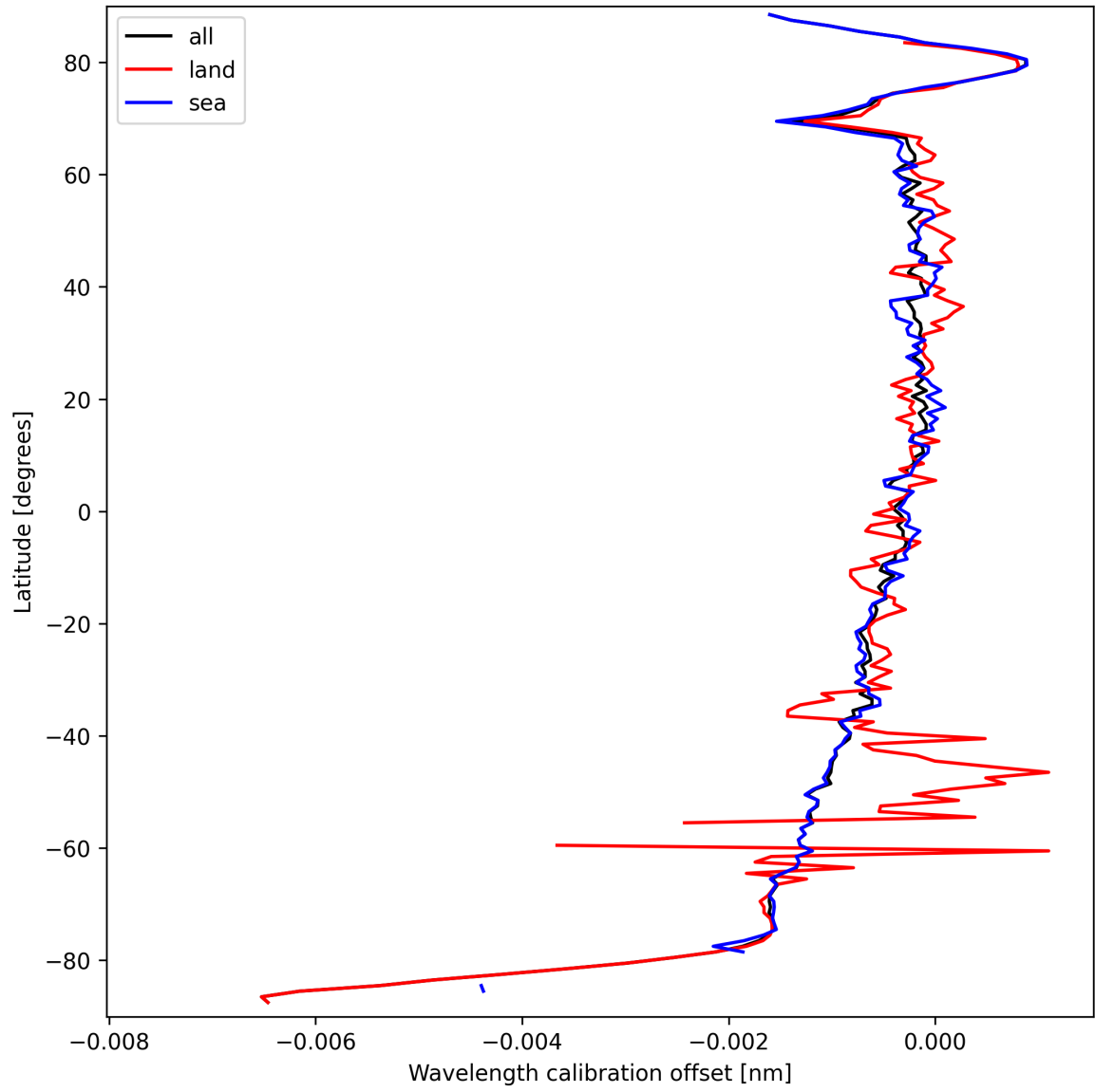
Figure 18: Zonal average of “Wavelength calibration offset” for 2025-09-20 to 2025-09-22.
