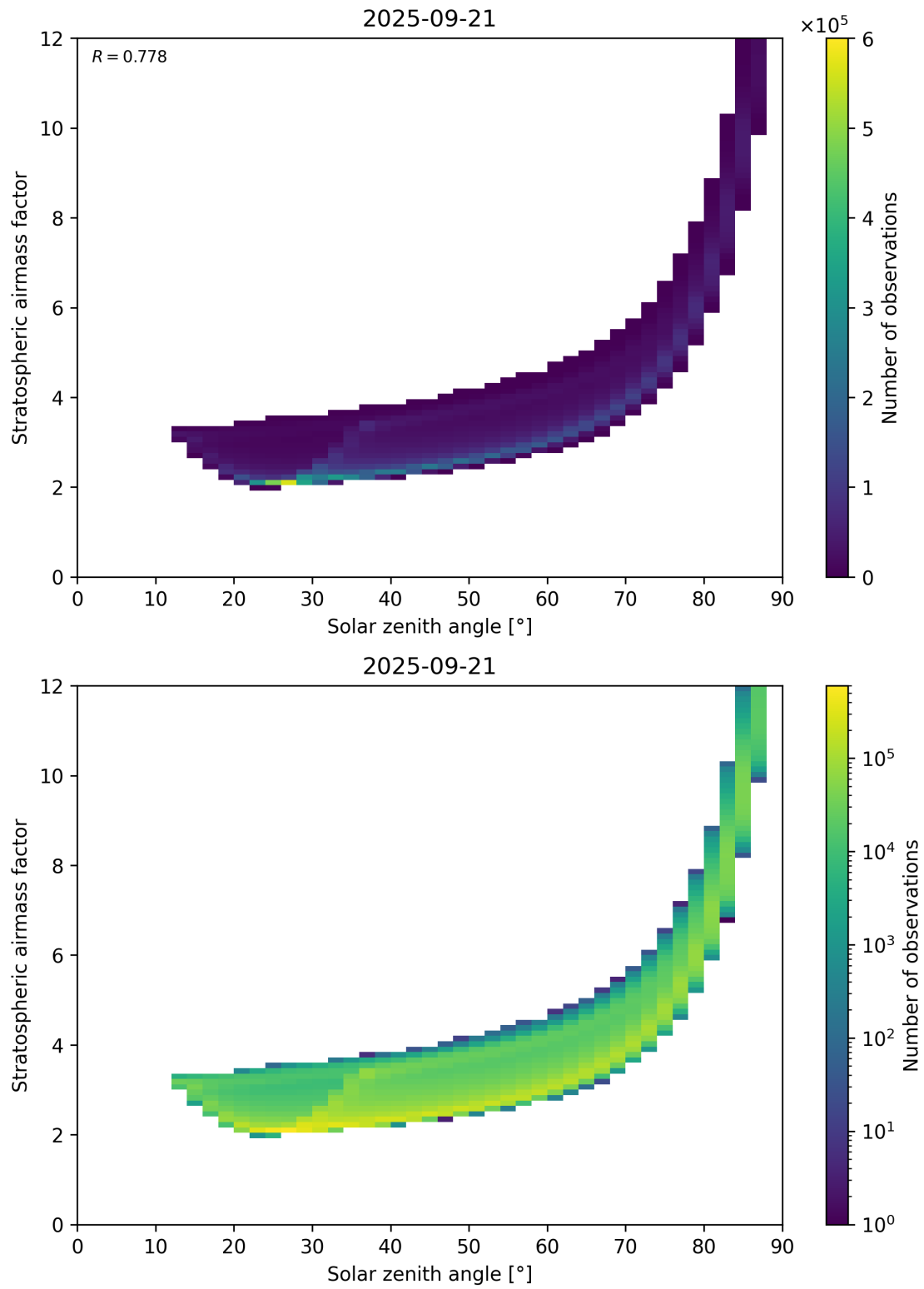
Figure 145: Scatter density plot of “Solar zenith angle” against “Stratospheric airmass factor” for 2025-09-20 to 2025-09-22.
