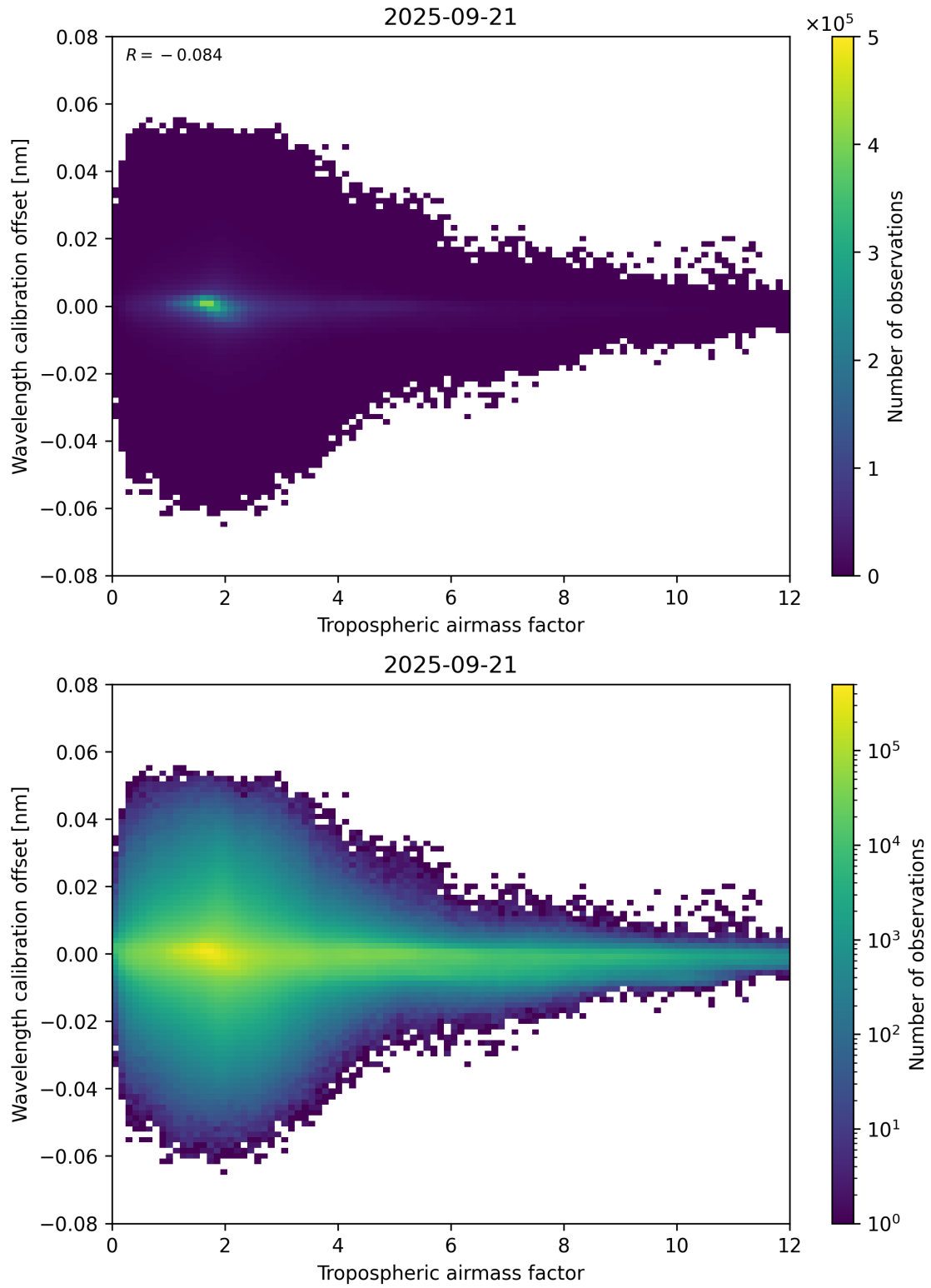
Figure 80: Scatter density plot of “Tropospheric airmass factor” against “Wavelength calibration offset” for 2025-09-20 to 2025-09-22.
