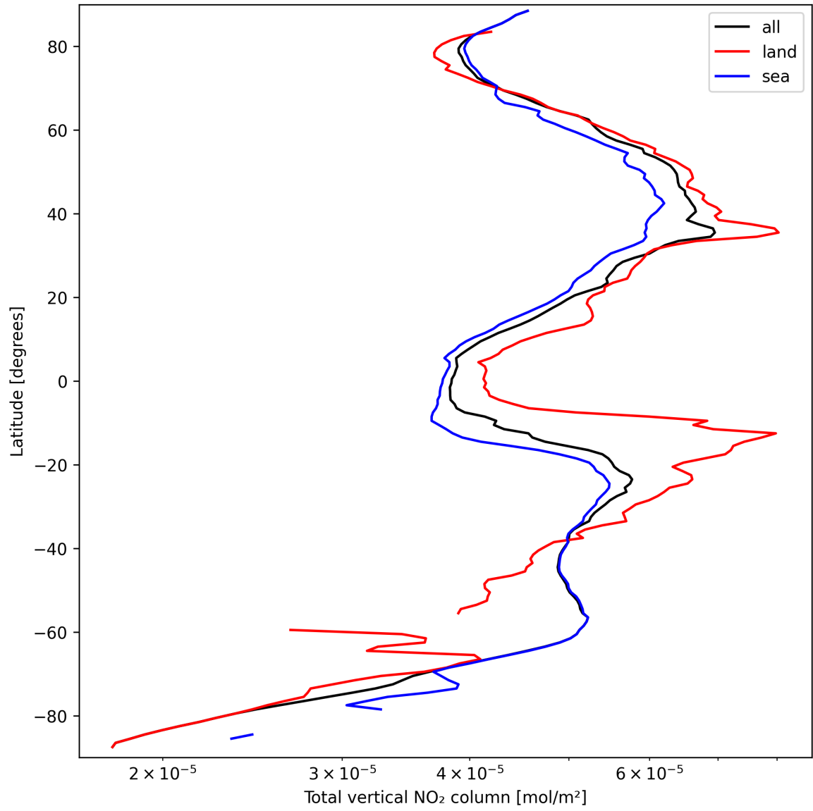
Figure 21: Zonal average of “Total vertical NO 2 column” for 2025-09-20 to 2025-09-22.
