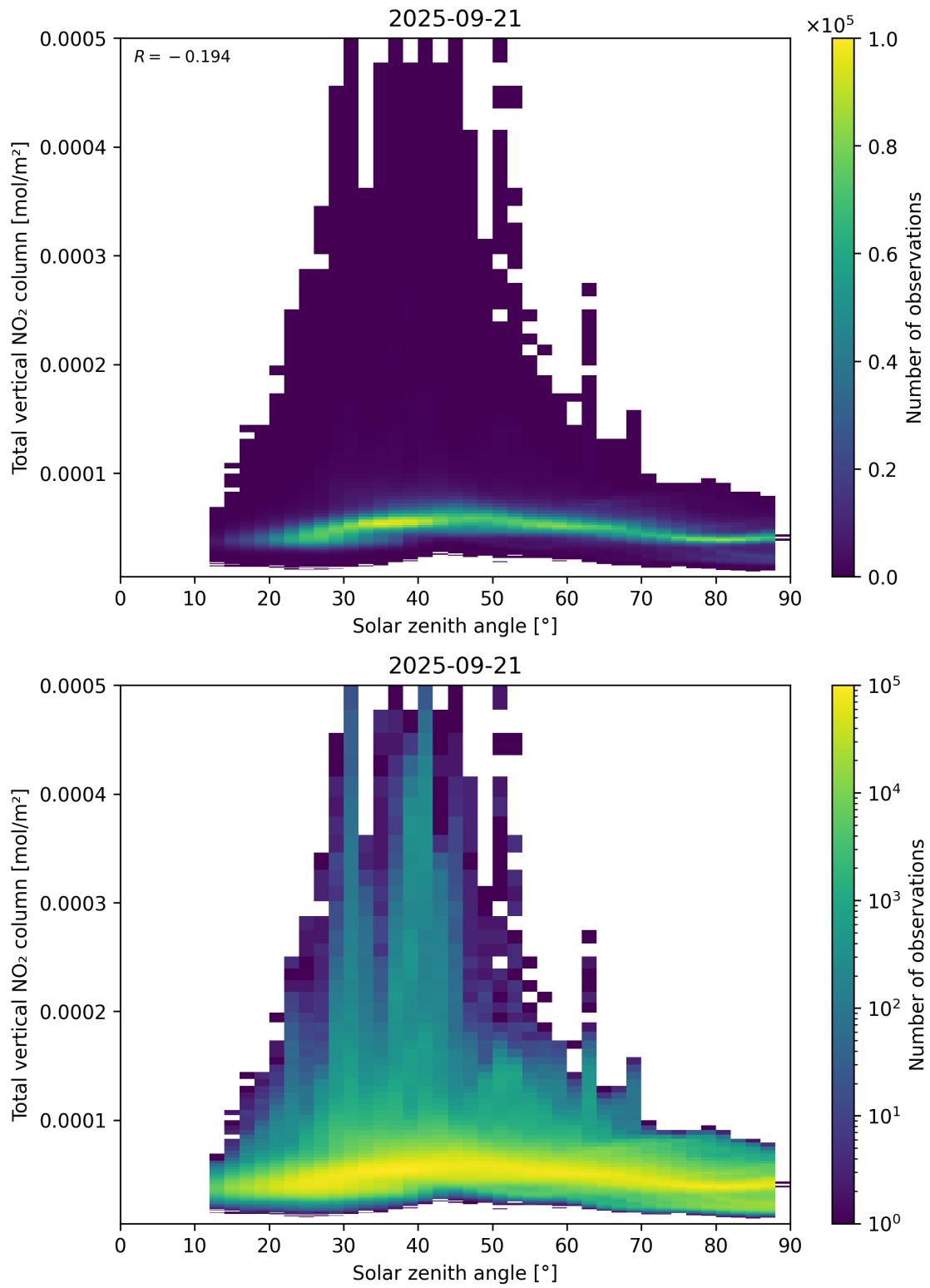
Figure 153: Scatter density plot of “Solar zenith angle” against “Total vertical NO 2 column” for 2025-09-20 to 2025-09-22.
