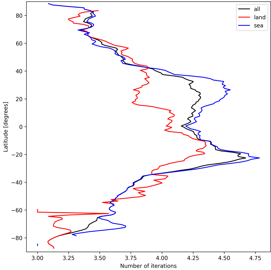
Figure 17: Zonal average of “Number of iterations” for 2025-09-20 to 2025-09-22.
