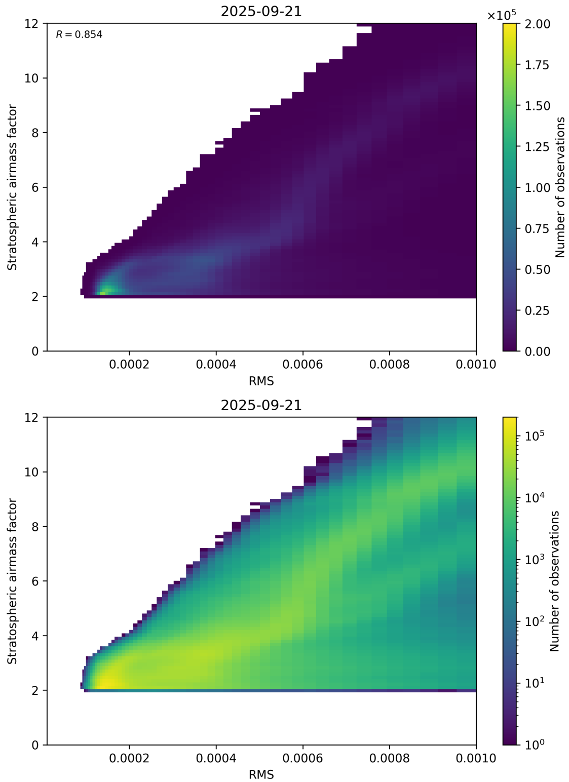
Figure 144: Scatter density plot of “RMS” against “Stratospheric airmass factor” for 2025-09-20 to 2025-09-22.
