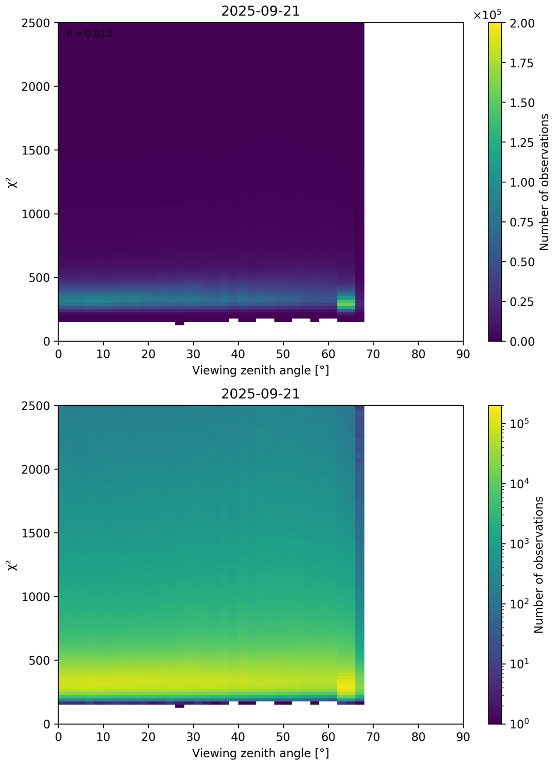
Figure 162: Scatter density plot of “Viewing zenith angle” against “ \chi^2 ” for 2025-09-20 to 2025-09-22.
