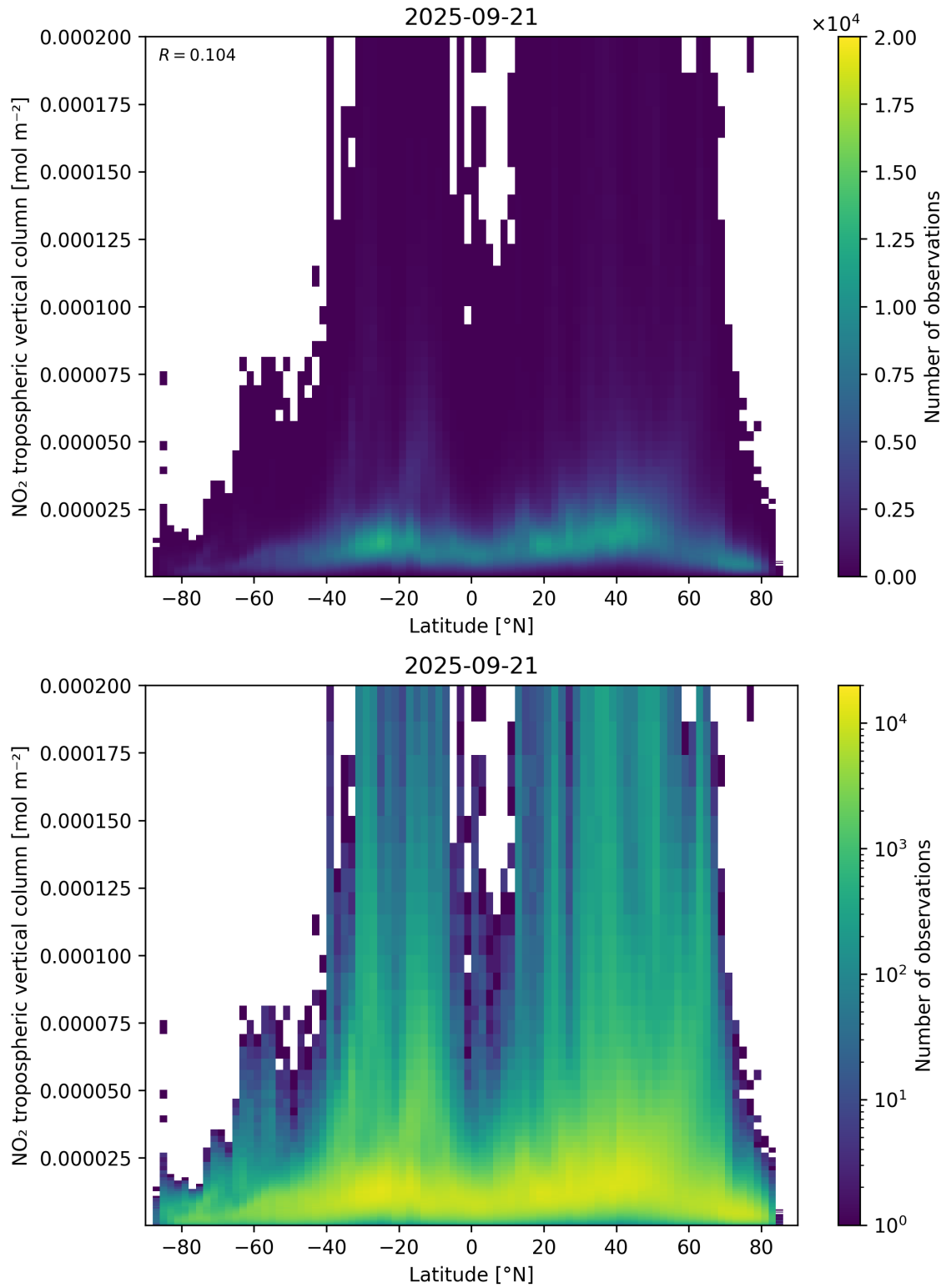
Figure 92: Scatter density plot of “Latitude” against “NO 2 tropospheric vertical column” for 2025-09-20 to 2025-09-22.
