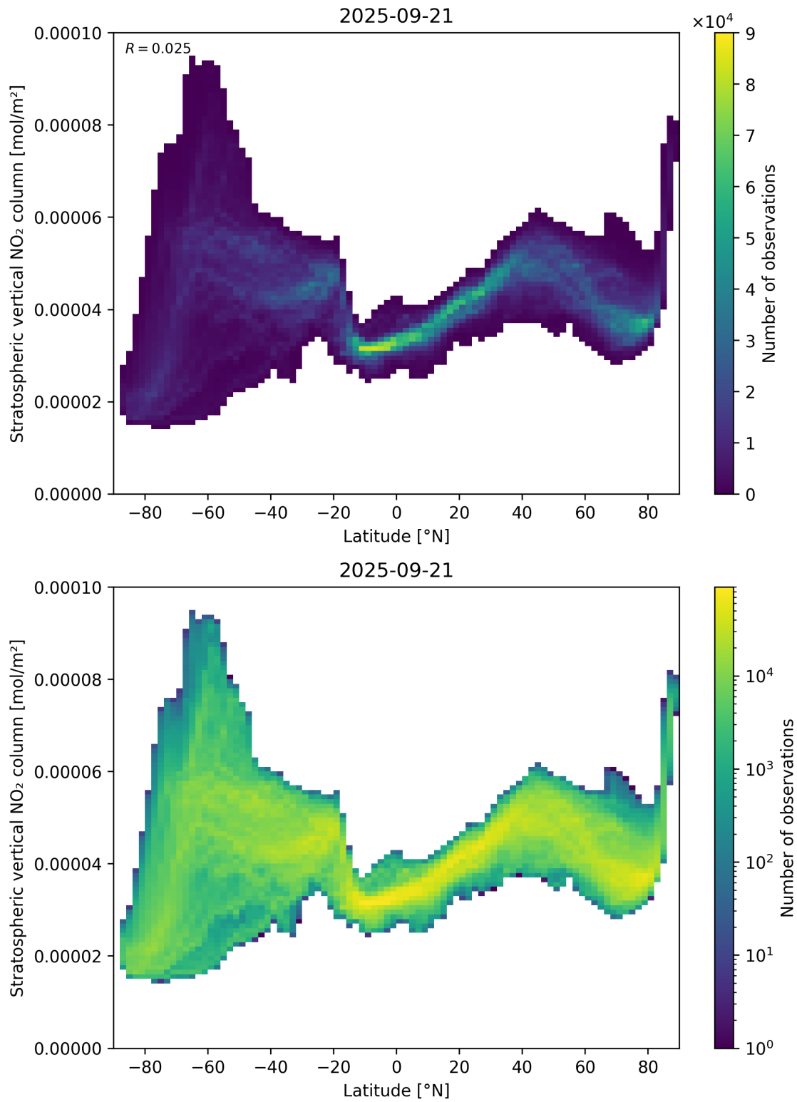
Figure 87: Scatter density plot of “Latitude” against “Stratospheric vertical NO 2 column” for 2025-09-20 to 2025-09-22.
