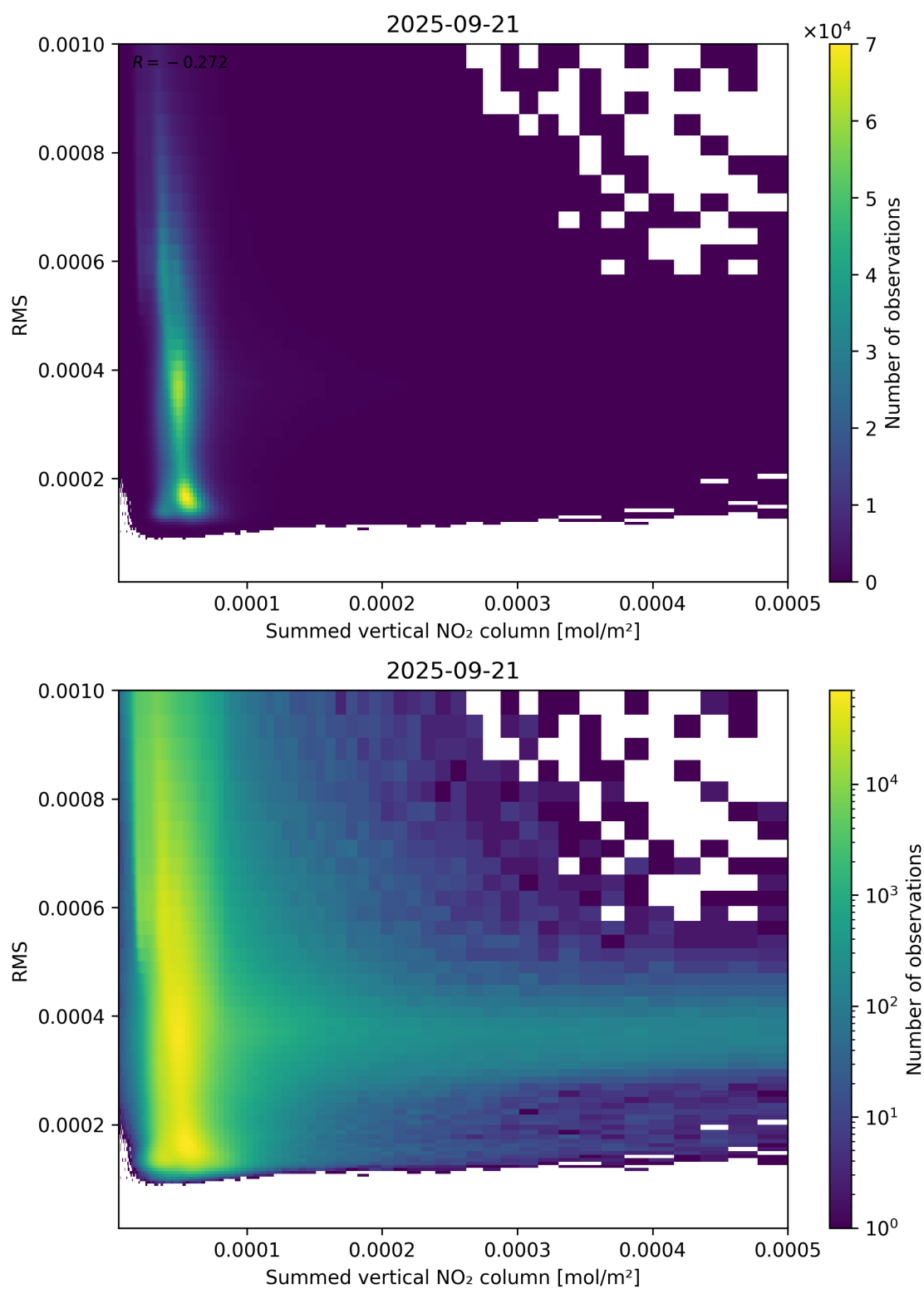
Figure 109: Scatter density plot of “Summed vertical NO 2 column” against “RMS” for 2025-09-20 to 2025-09-22.
