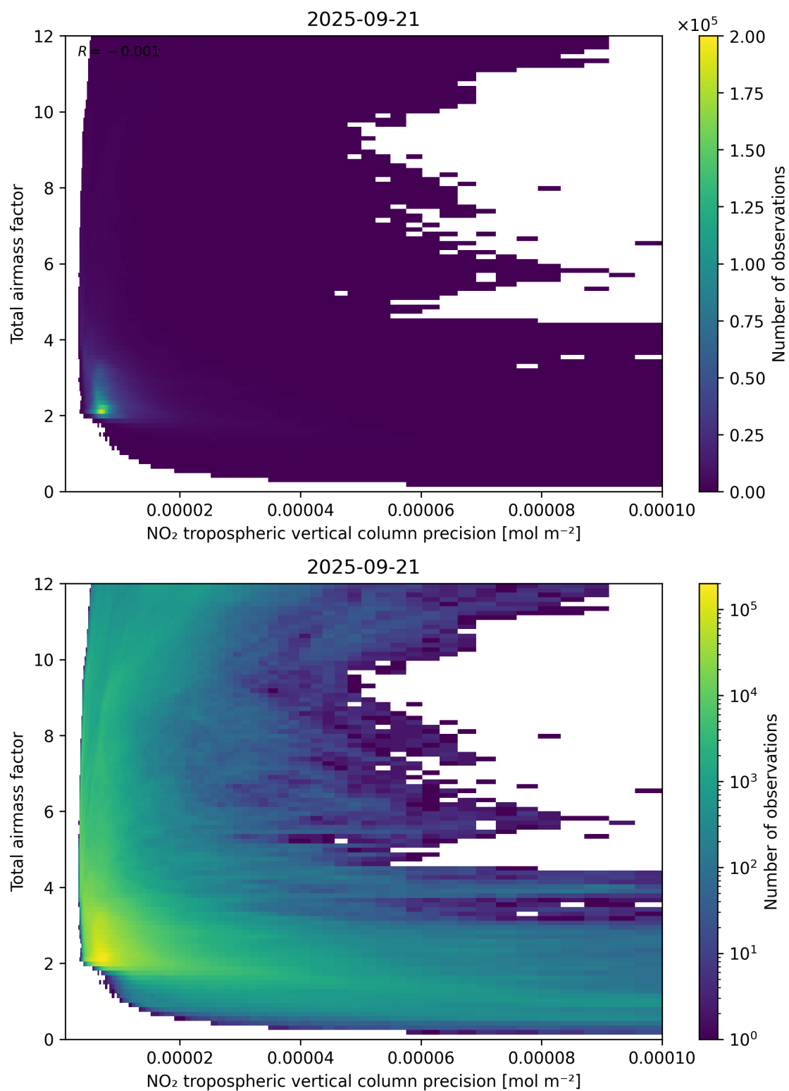
Figure 132: Scatter density plot of “NO 2 tropospheric vertical column precision” against “Total air mass factor” for 2025-09-20 to 2025-09-22.
