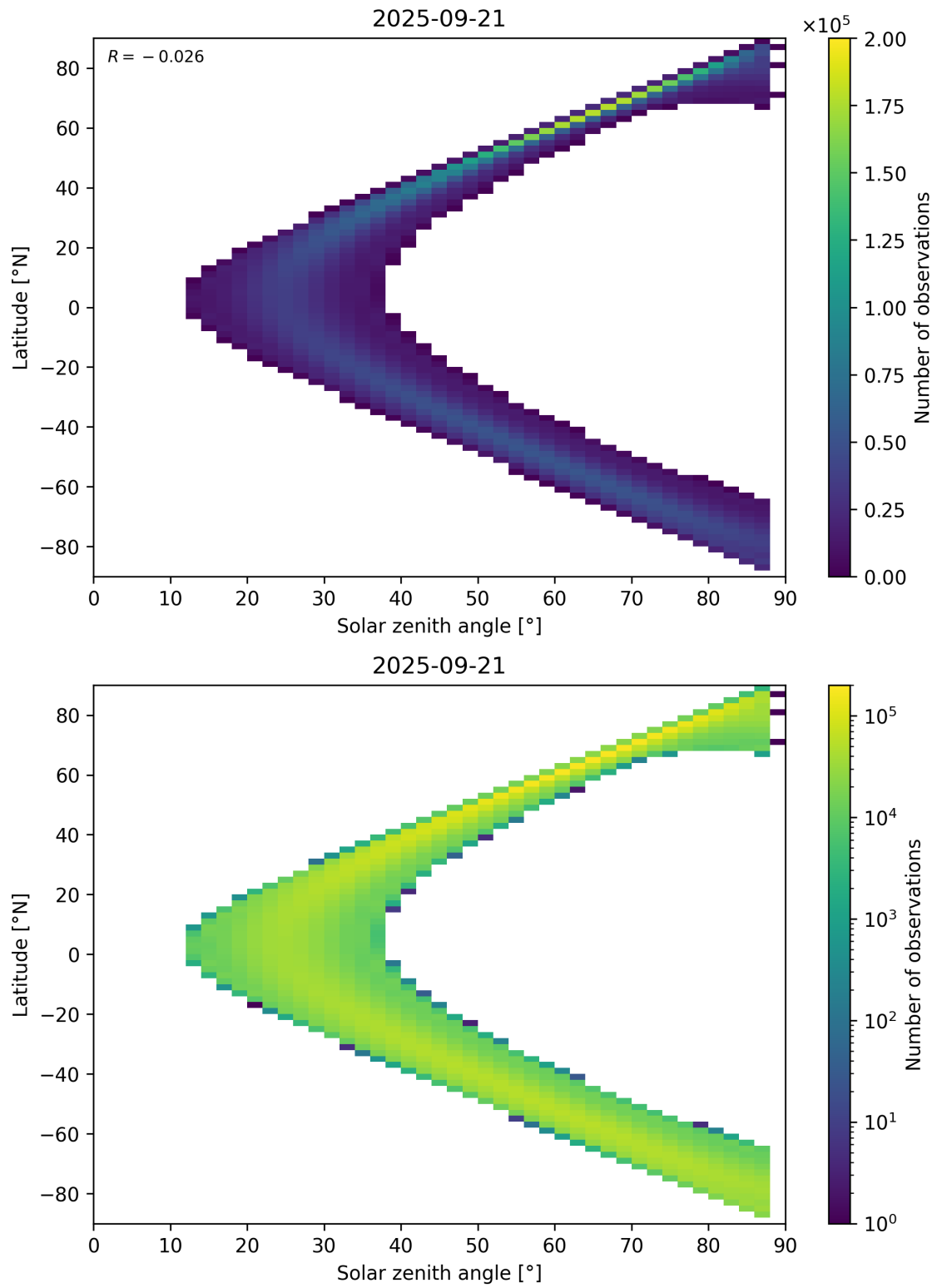
Figure 149: Scatter density plot of “Solar zenith angle” against “Latitude” for 2025-09-20 to 2025-09-22.
