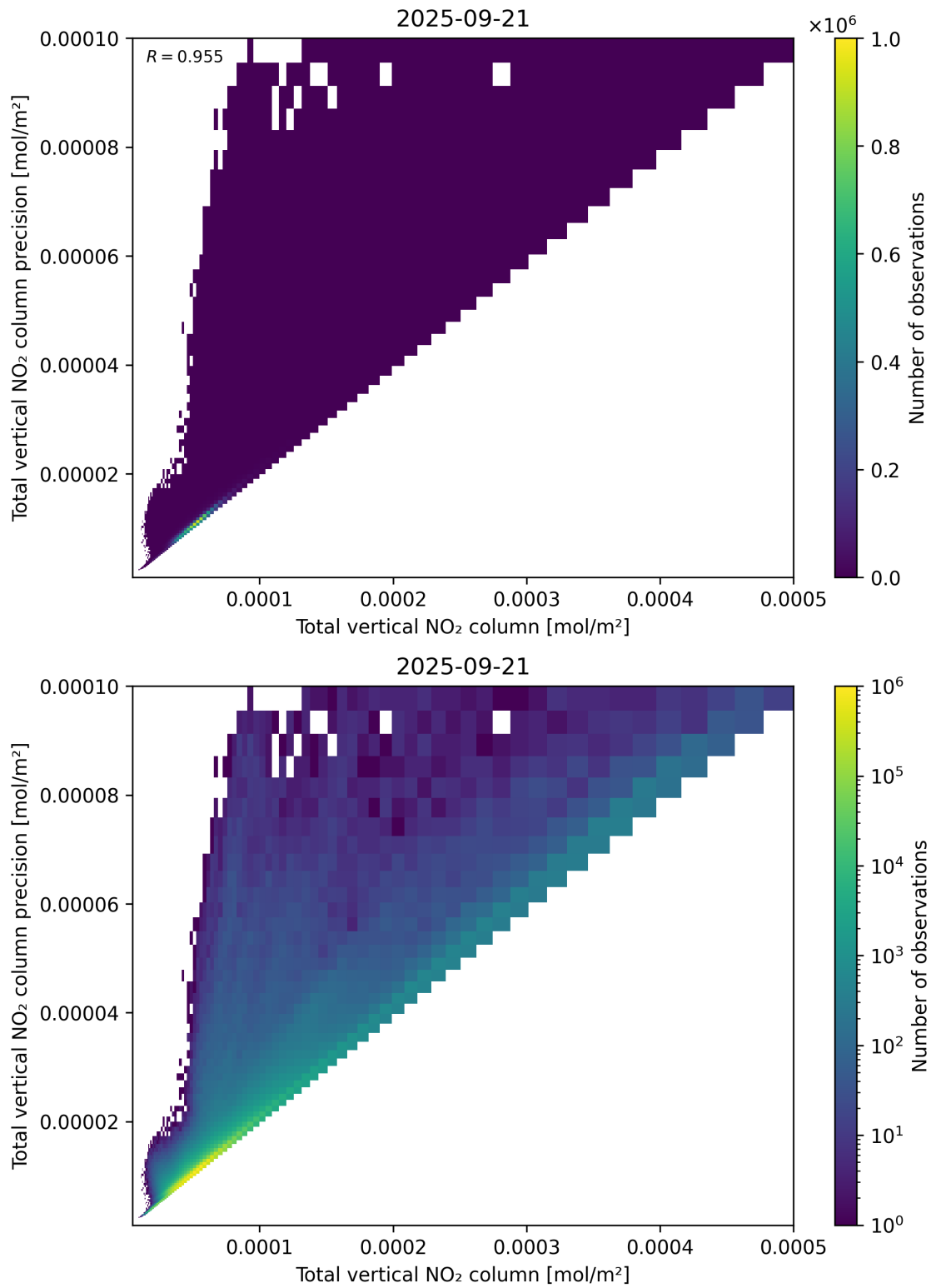
Figure 114: Scatter density plot of “Total vertical NO 2 column” against “Total vertical NO 2 column precision” for 2025-09-20 to 2025-09-22.
