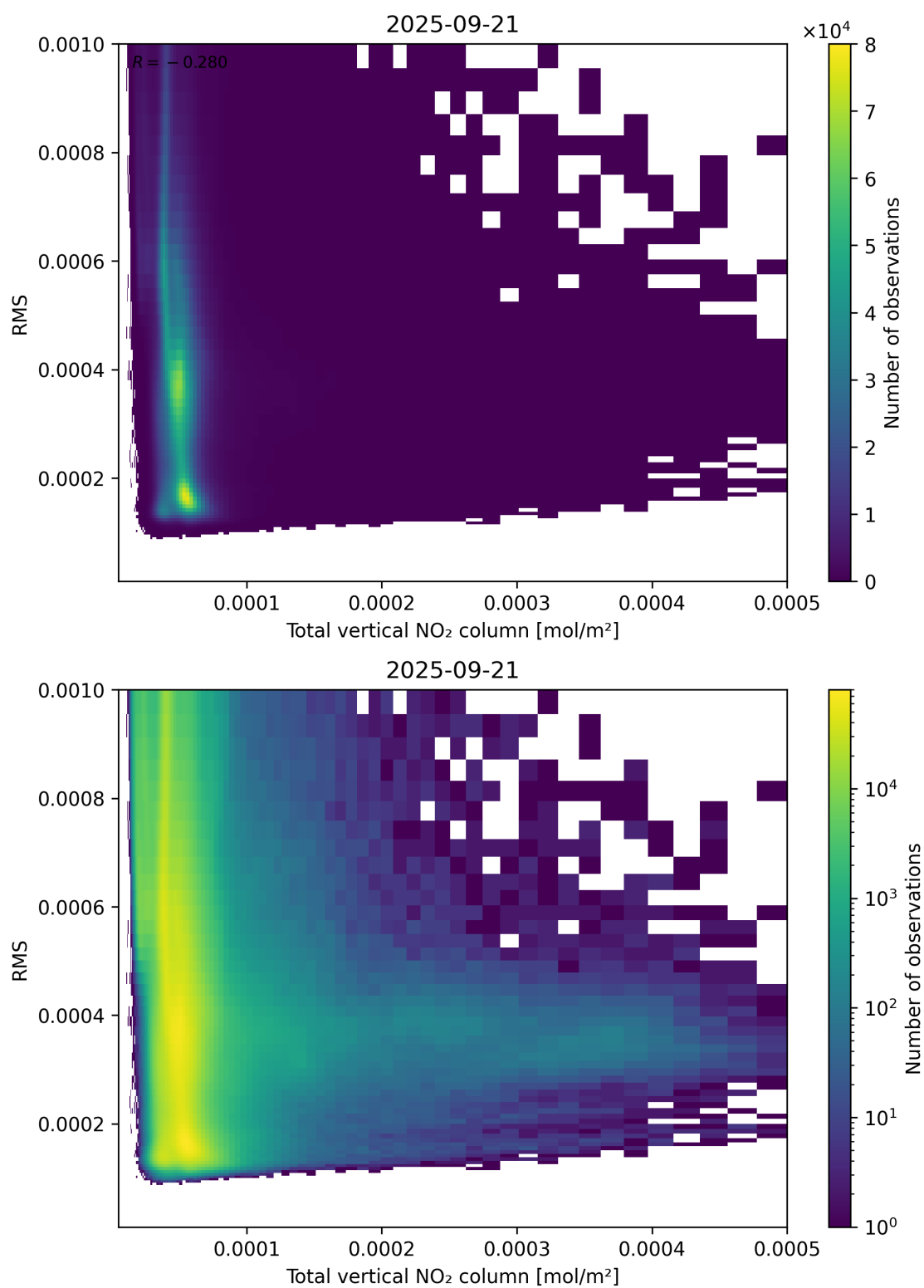
Figure 120: Scatter density plot of “Total vertical NO 2 column” against “RMS” for 2025-09-20 to 2025-09-22.
