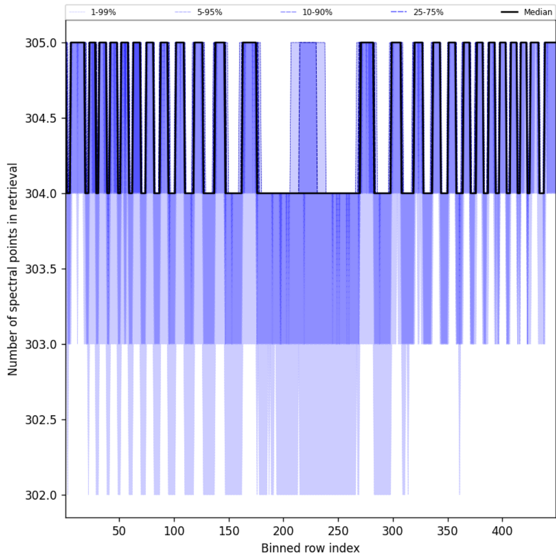
Figure 50: Along track statistics of “Number of spectral points in retrieval” for 2025-09-20 to 2025-09-22
