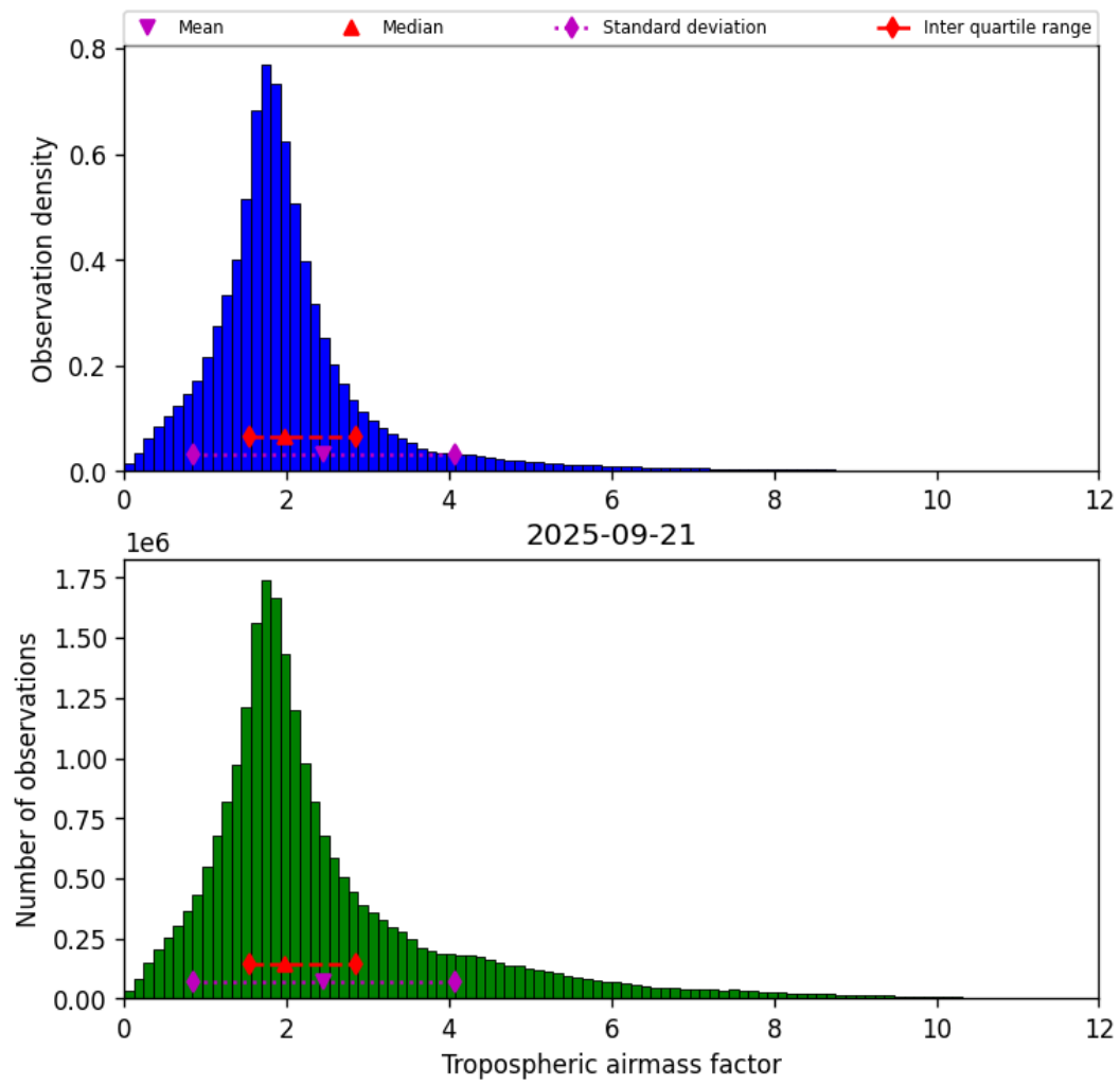
Figure 31: Histogram of “Tropospheric airmass factor” for 2025-09-20 to 2025-09-22
