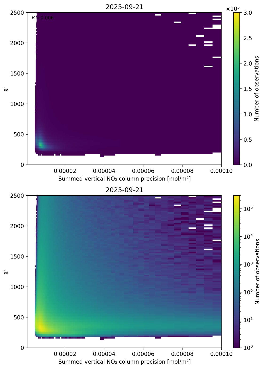
Figure 107: Scatter density plot of “Summed vertical NO 2 column precision” against “ \chi^2 ” for 2025-09-20 to 2025-09-22.
