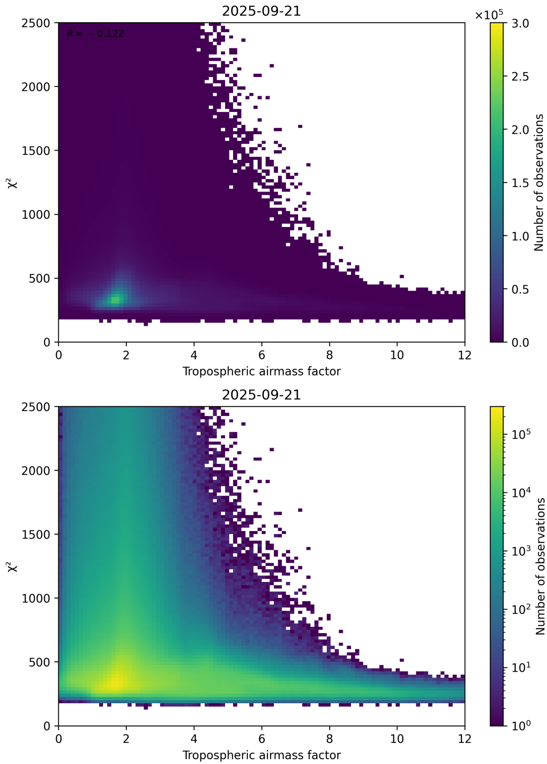
Figure 73: Scatter density plot of “Tropospheric airmass factor” against “ \chi^2 ” for 2025-09-20 to 2025-09-22.
