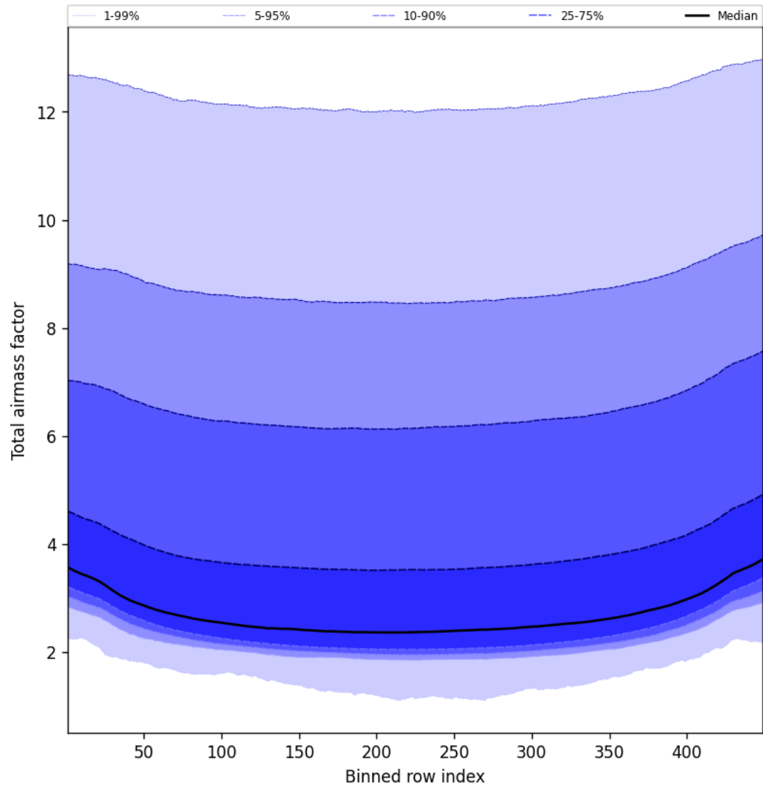
Figure 49: Along track statistics of “Total airmass factor” for 2025-09-20 to 2025-09-22
