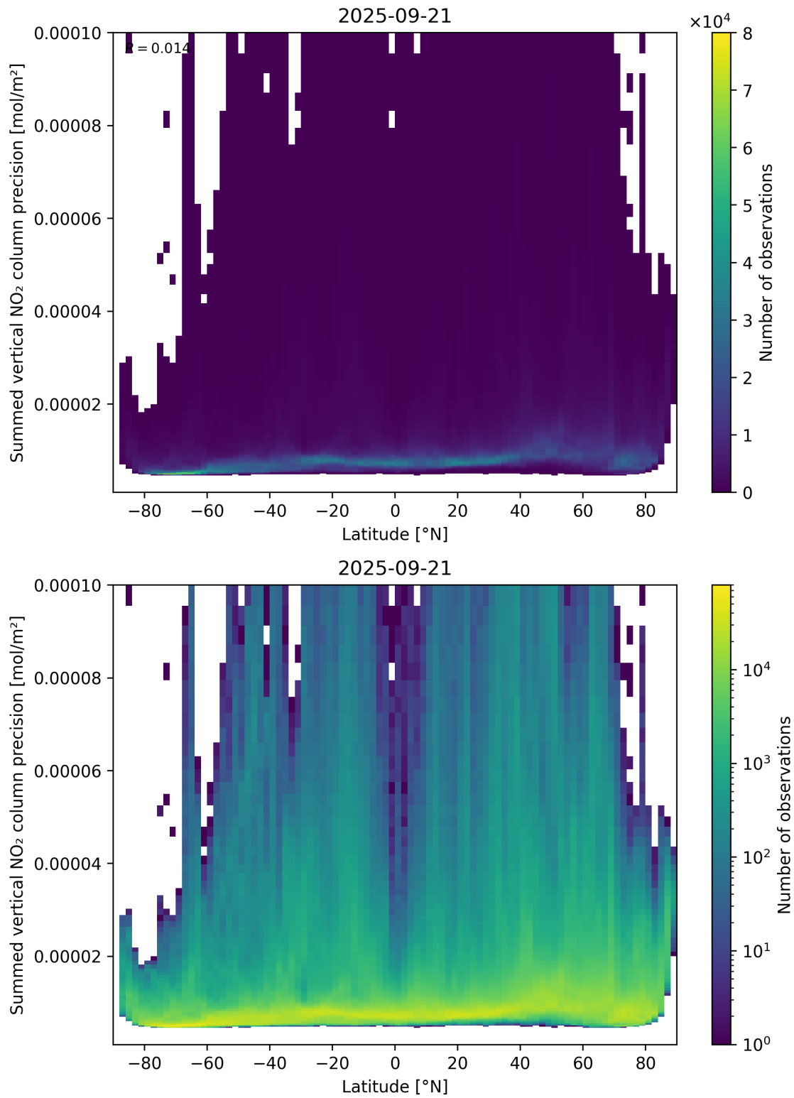
Figure 89: Scatter density plot of “Latitude” against “Summed vertical NO 2 column precision” for 2025-09-20 to 2025-09-22.
