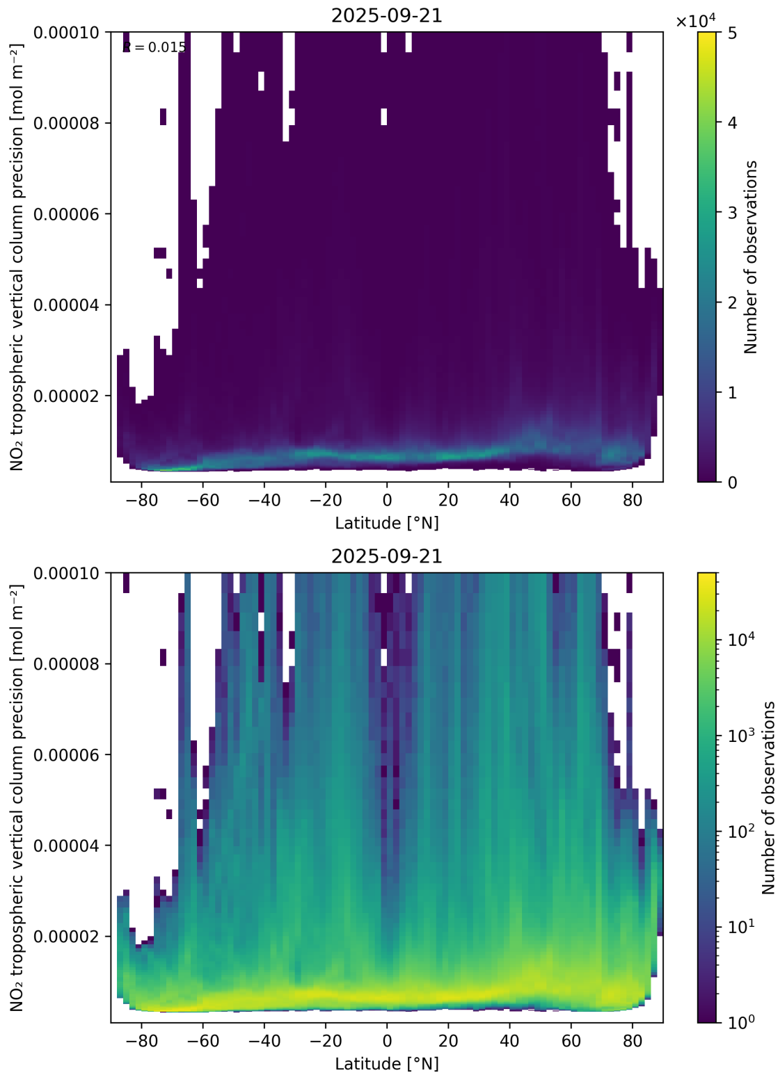
Figure 93: Scatter density plot of “Latitude” against “NO 2 tropospheric vertical column precision” for 2025-09-20 to 2025-09-22.
