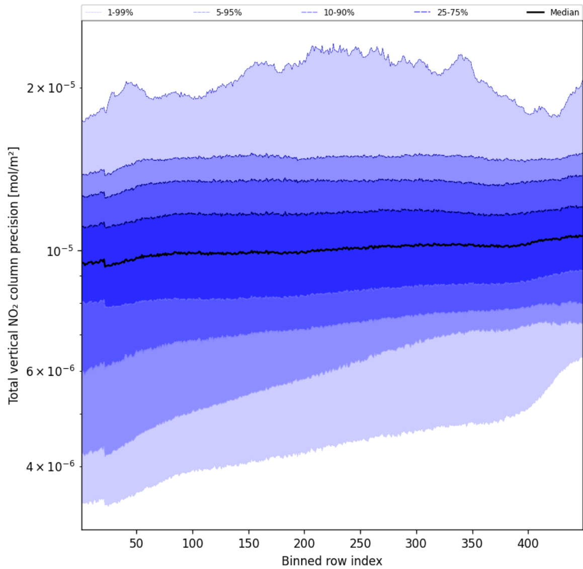
Figure 56: Along track statistics of “Total vertical NO 2 column precision” for 2025-09-20 to 2025-09-22
