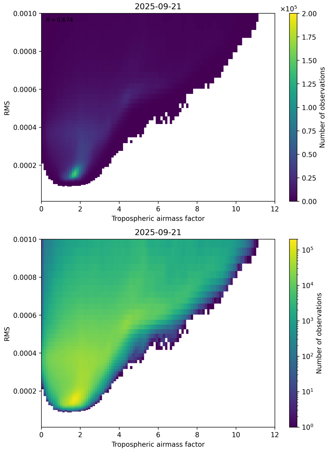
Figure 79: Scatter density plot of “Tropospheric airmass factor” against “RMS” for 2025-09-20 to 2025-09-22.
