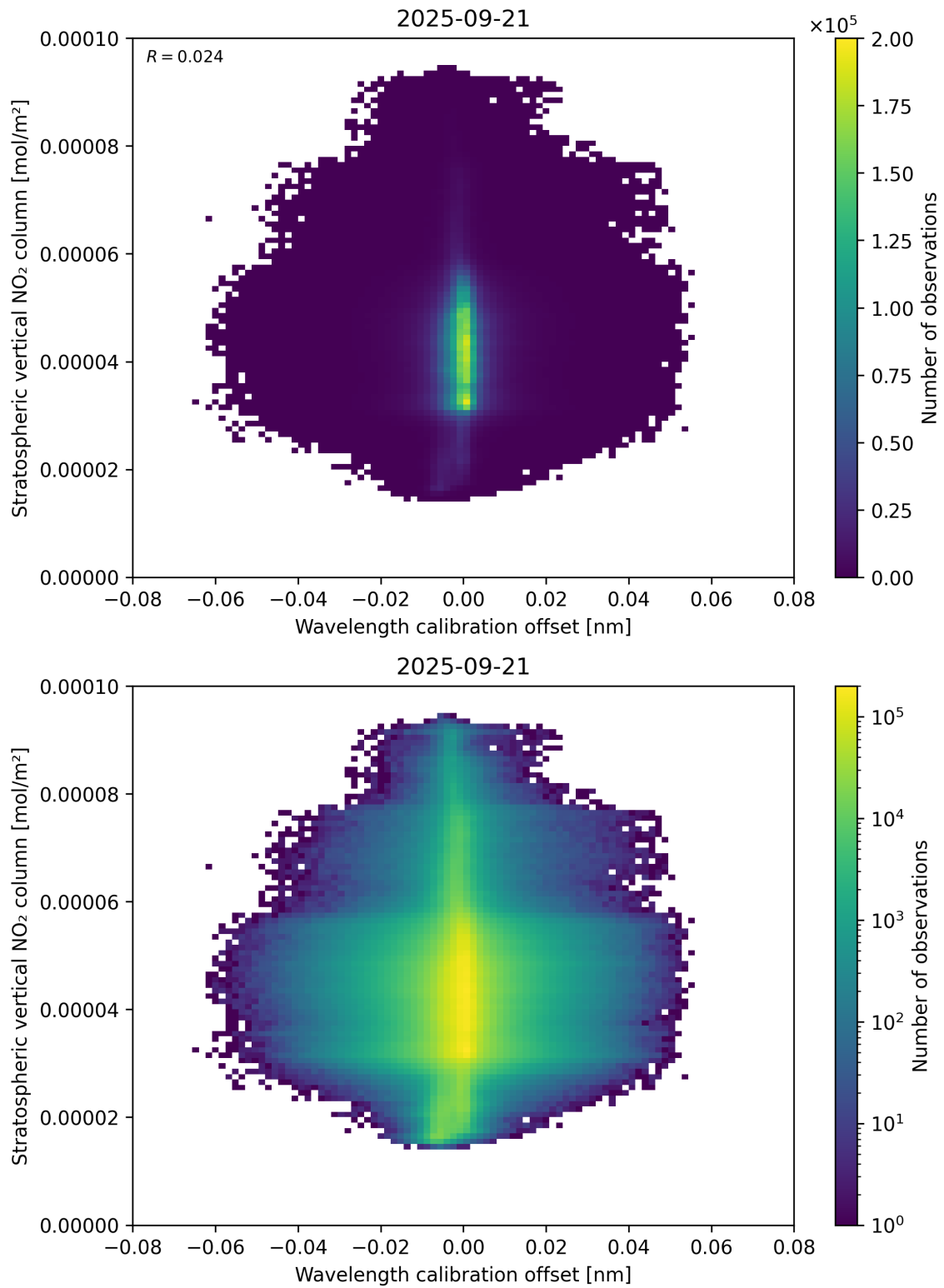
Figure 176: Scatter density plot of “Wavelength calibration offset” against “Stratospheric vertical NO 2 column” for 2025-09-20 to 2025-09-22.
