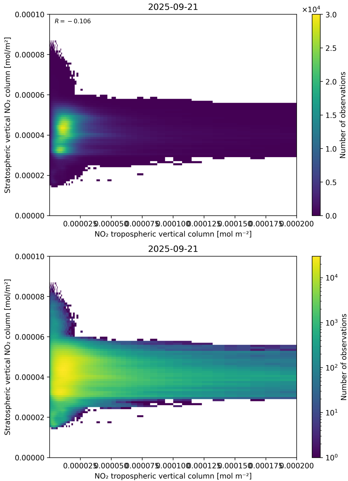
Figure 125: Scatter density plot of “NO 2 tropospheric vertical column” against “Stratospheric vertical NO 2 column” for 2025-09-20 to 2025-09-22.
