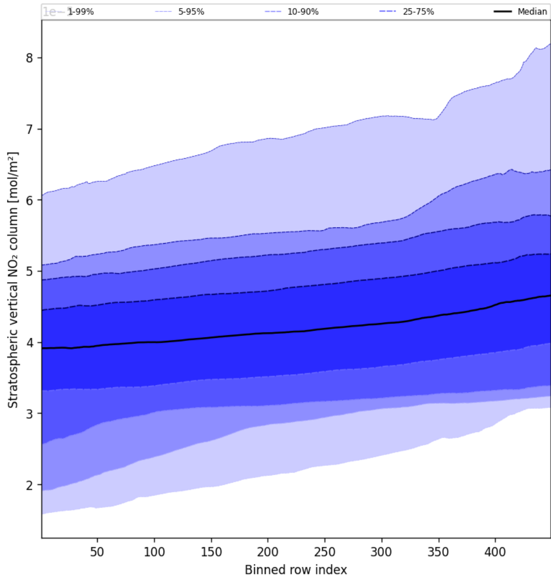
Figure 53: Along track statistics of “Stratospheric vertical NO 2 column” for 2025-09-20 to 2025-09-22
