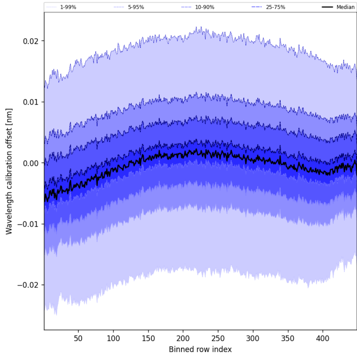
Figure 52: Along track statistics of “Wavelength calibration offset” for 2025-09-20 to 2025-09-22
