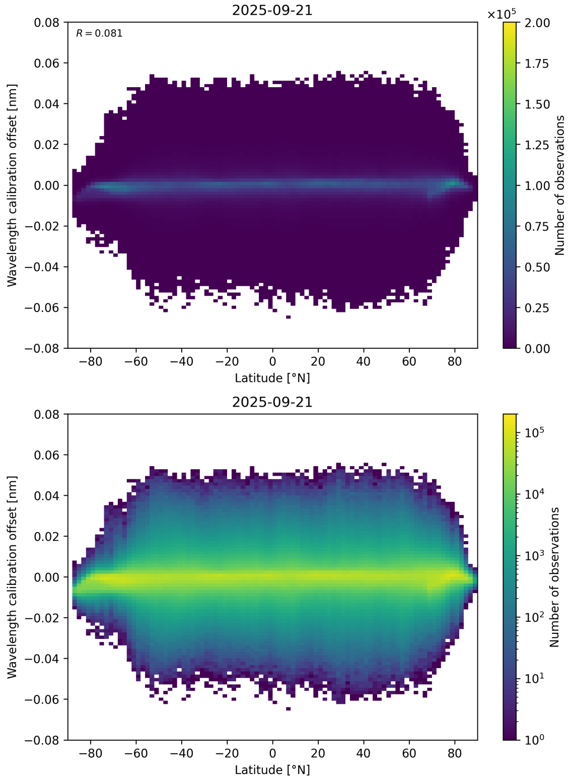
Figure 95: Scatter density plot of “Latitude” against “Wavelength calibration offset” for 2025-09-20 to 2025-09-22.
