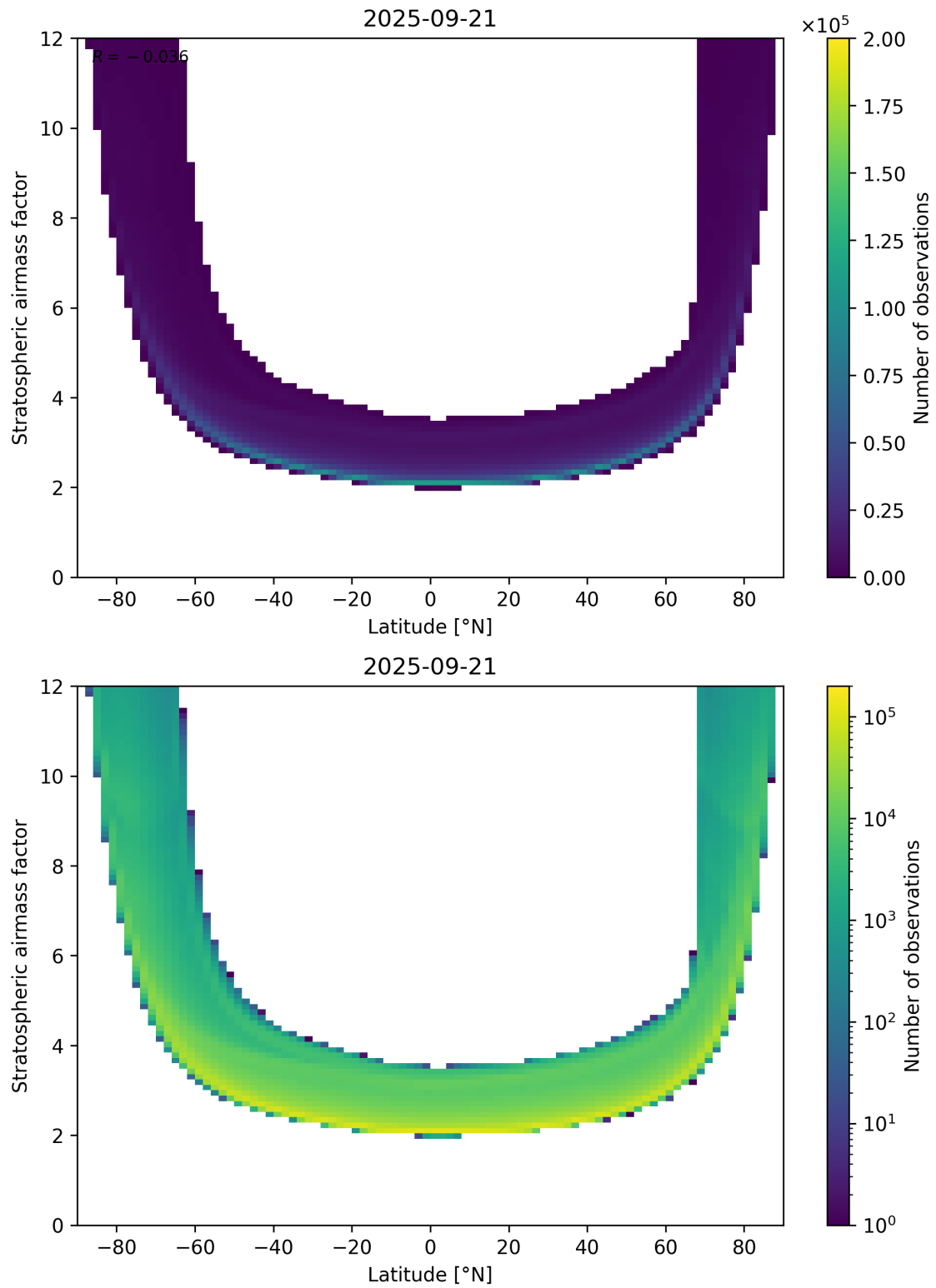
Figure 83: Scatter density plot of “Latitude” against “Stratospheric air mass factor” for 2025-09-20 to 2025-09-22.
