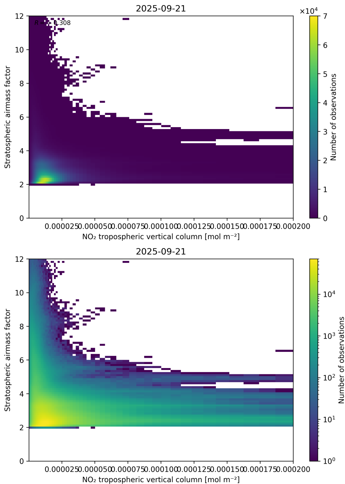
Figure 121: Scatter density plot of “NO 2 tropospheric vertical column” against “Stratospheric air mass factor” for 2025-09-20 to 2025-09-22.
