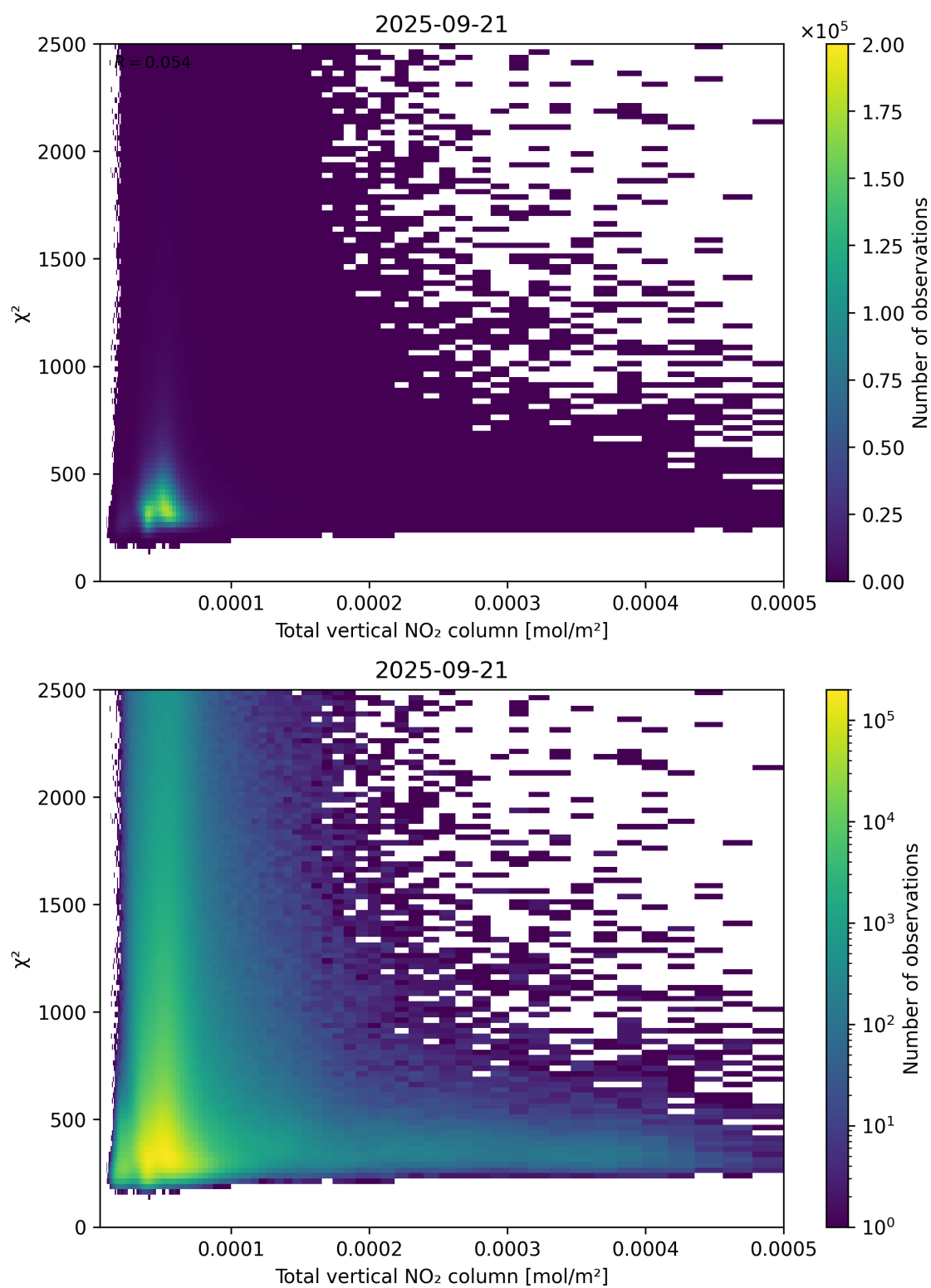
Figure 111: Scatter density plot of “Total vertical NO 2 column” against “ \chi^2 ” for 2025-09-20 to 2025-09-22.
