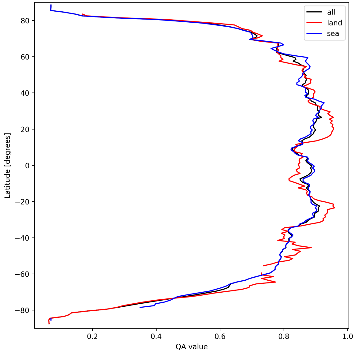
Figure 11: Zonal average of “QA value” for 2025-09-20 to 2025-09-22.
