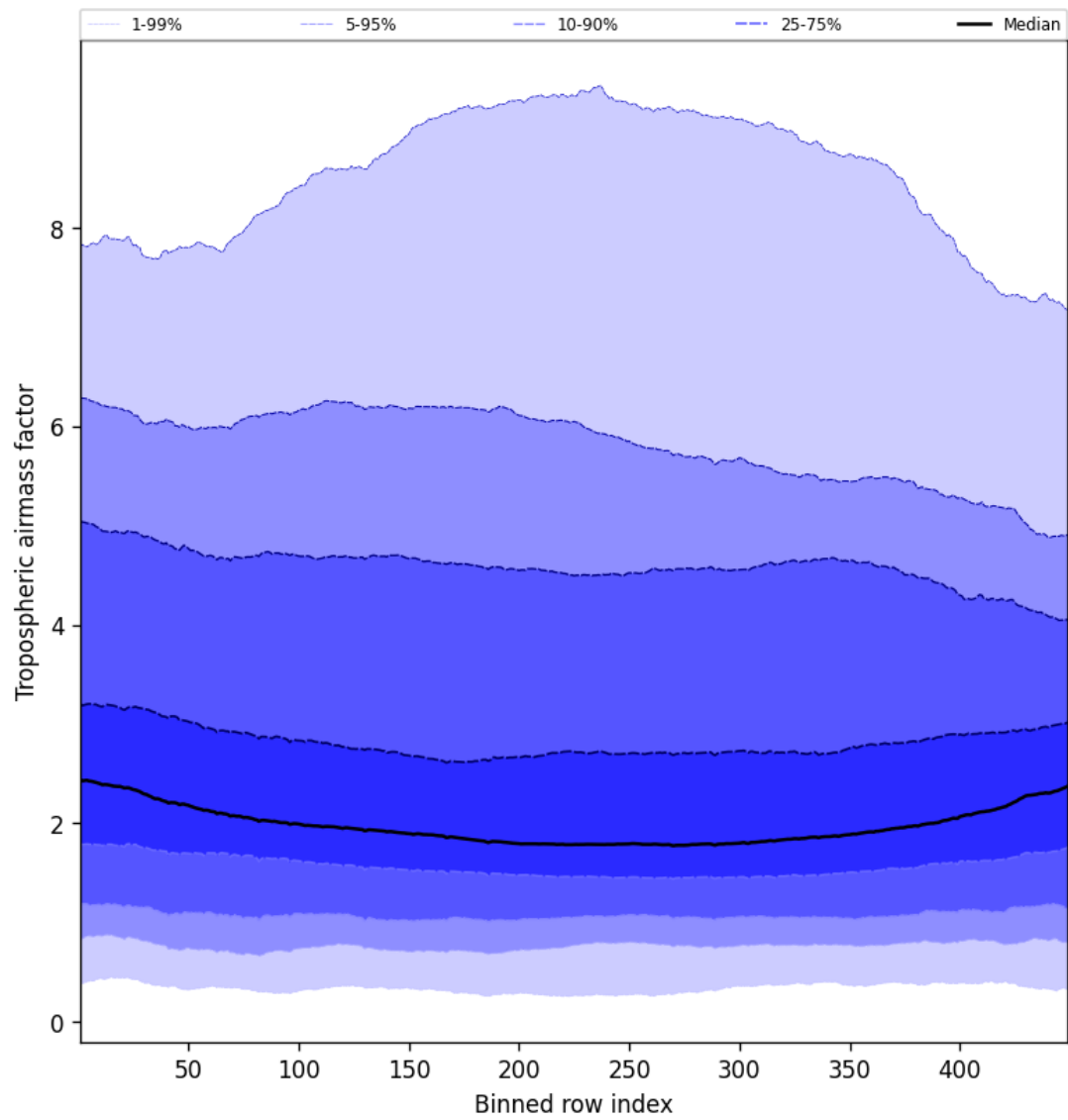
Figure 48: Along track statistics of “Tropospheric air mass factor” for 2025-09-20 to 2025-09-22
