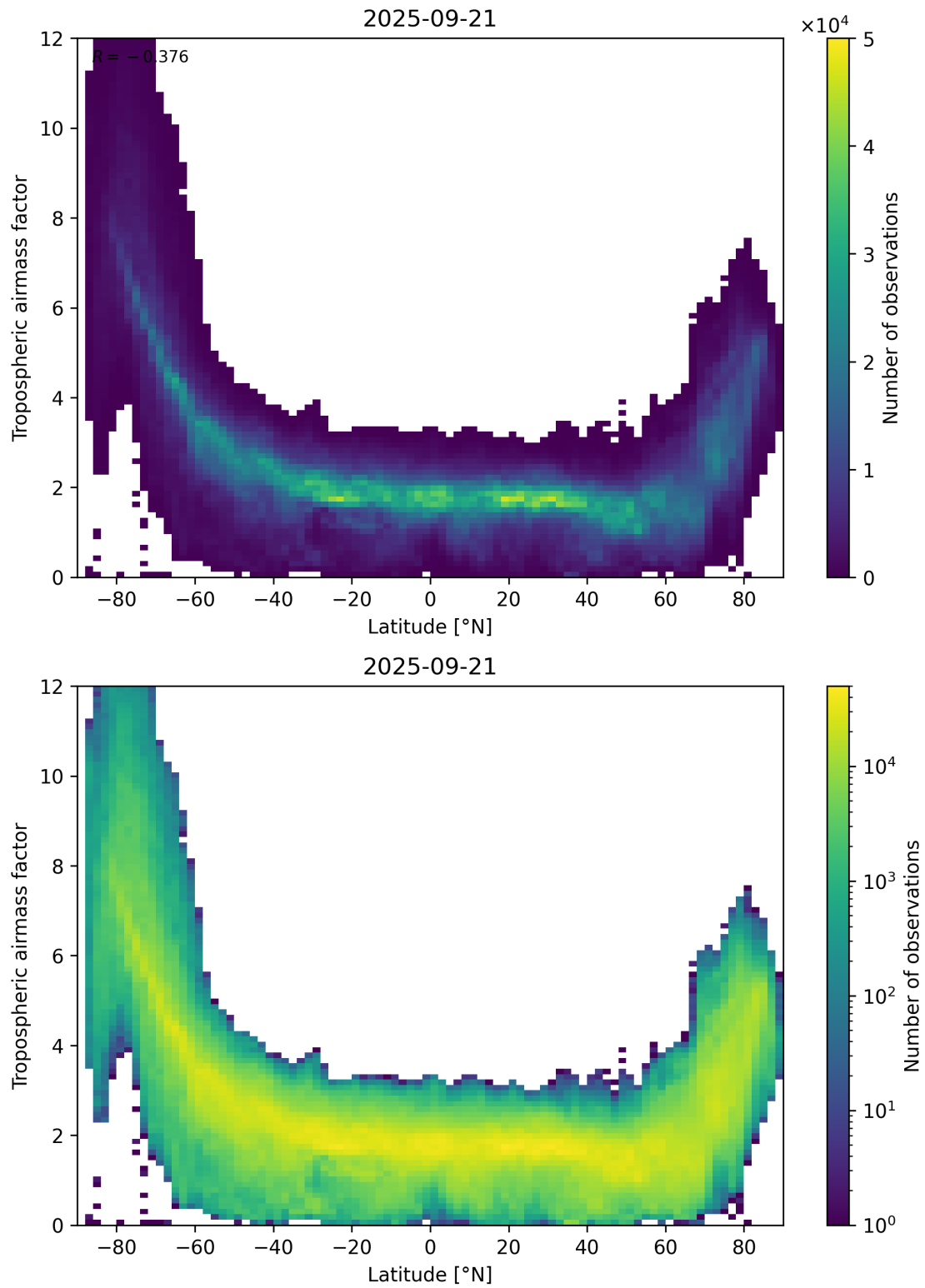
Figure 85: Scatter density plot of “Latitude” against “Tropospheric air mass factor” for 2025-09-20 to 2025-09-22.
