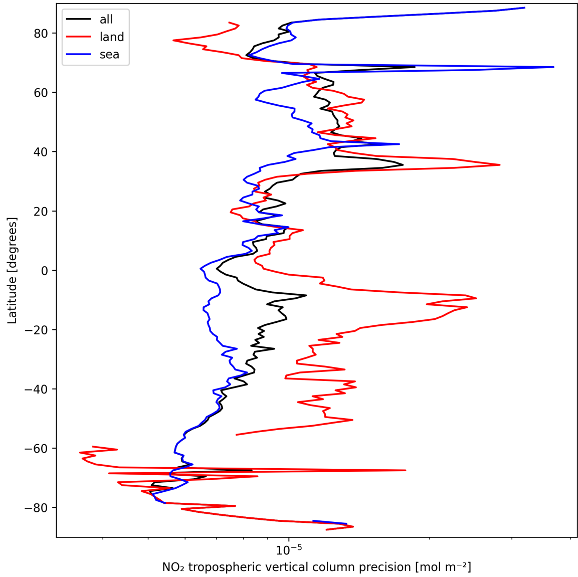
Figure 13: Zonal average of “NO 2 tropospheric vertical column precision” for 2025-09-20 to 2025-09-22.
