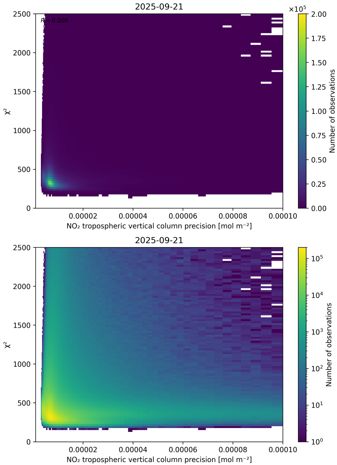
Figure 134: Scatter density plot of “NO 2 tropospheric vertical column precision” against “ \chi^2 ” for 2025-09-20 to 2025-09-22.
