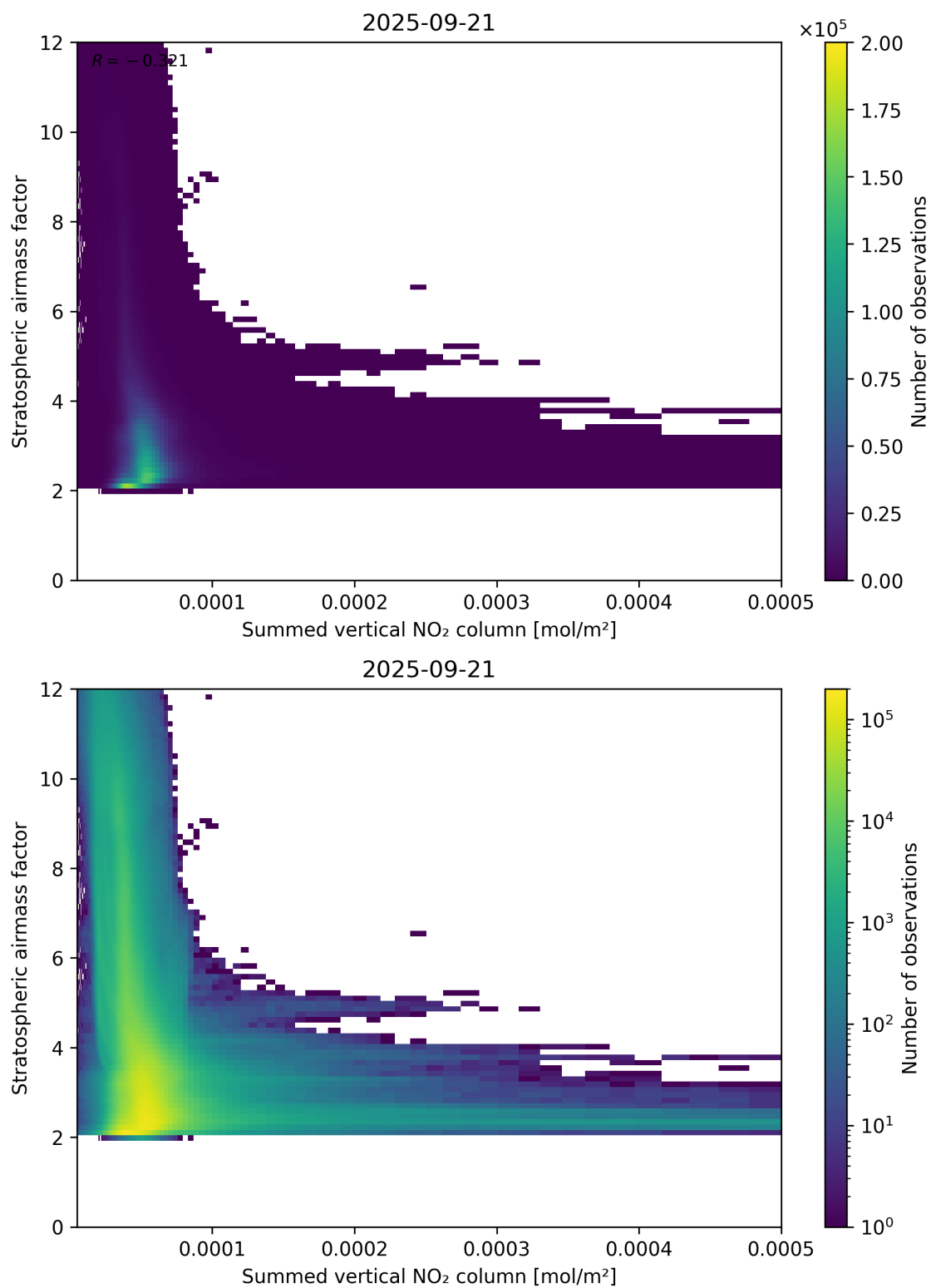
Figure 103: Scatter density plot of “Summed vertical NO 2 column” against “Stratospheric airmass factor” for 2025-09-20 to 2025-09-22.
