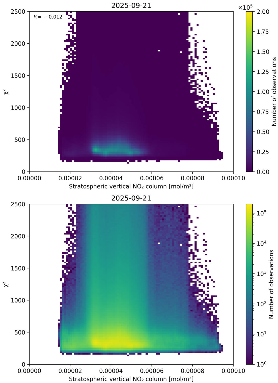
Figure 97: Scatter density plot of “Stratospheric vertical NO 2 column” against “ \chi^2 ” for 2025-09-20 to 2025-09-22.
