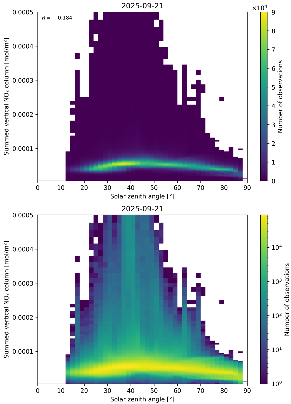
Figure 151: Scatter density plot of “Solar zenith angle” against “Summed vertical NO 2 column” for 2025-09-20 to 2025-09-22.
