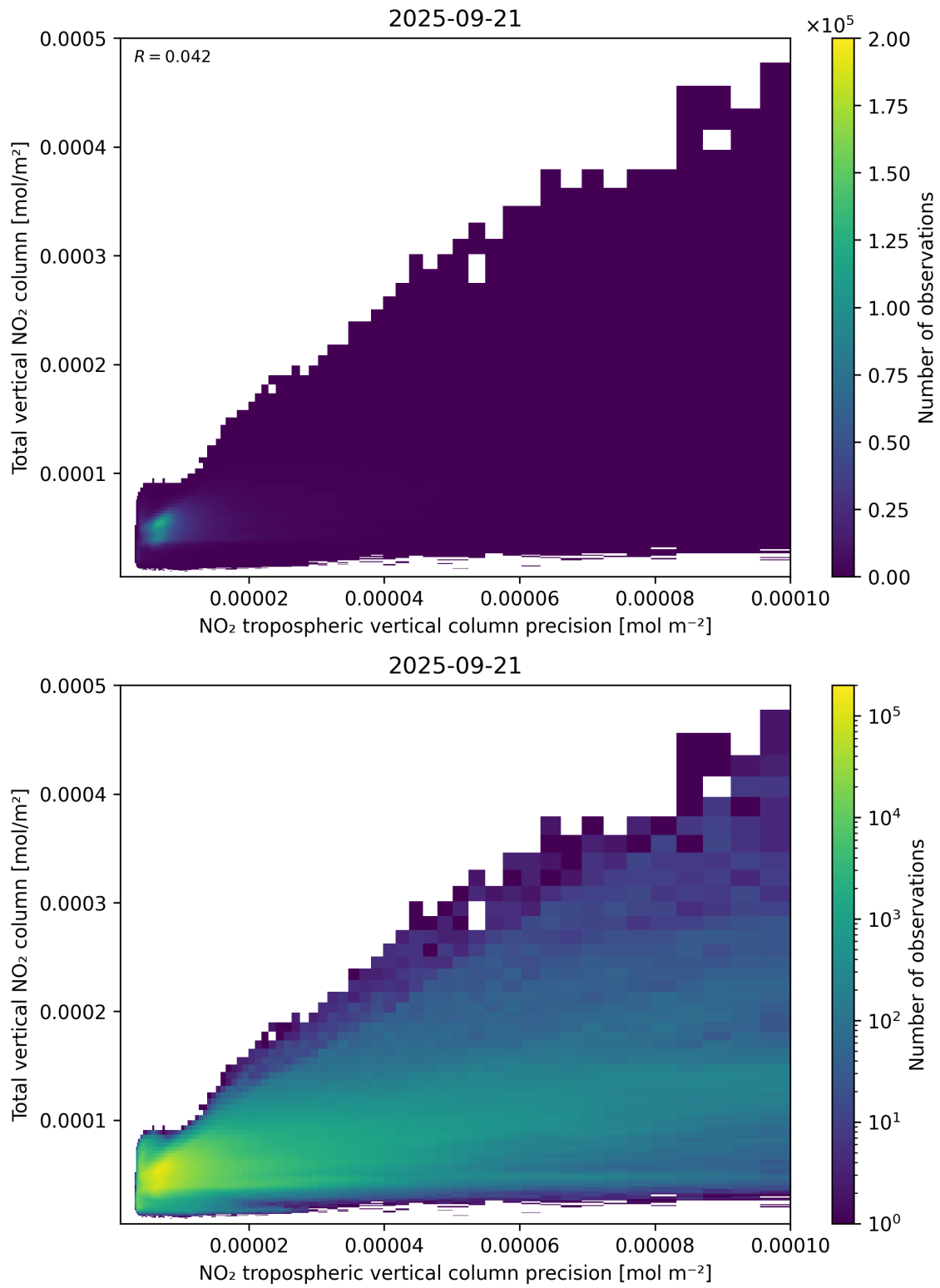
Figure 138: Scatter density plot of “NO 2 tropospheric vertical column precision” against “Total vertical NO 2 column” for 2025-09-20 to 2025-09-22.
