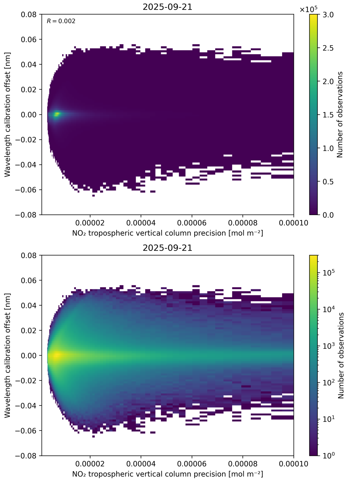
Figure 141: Scatter density plot of “NO 2 tropospheric vertical column precision” against “Wavelength calibration offset” for 2025-09-20 to 2025-09-22.
