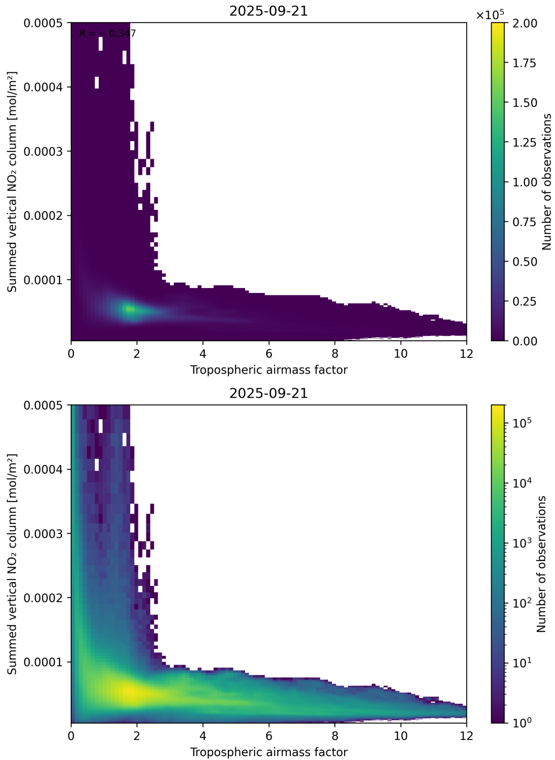
Figure 75: Scatter density plot of “Tropospheric airmass factor” against “Summed vertical NO 2 column” for 2025-09-20 to 2025-09-22.
