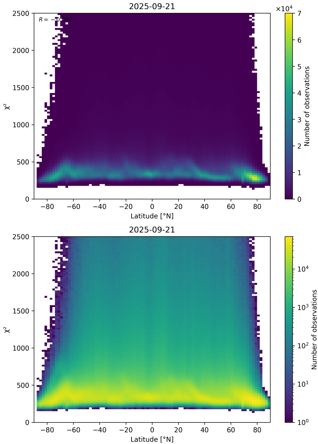
Figure 86: Scatter density plot of “Latitude” against “ \chi^2 ” for 2025-09-20 to 2025-09-22.
