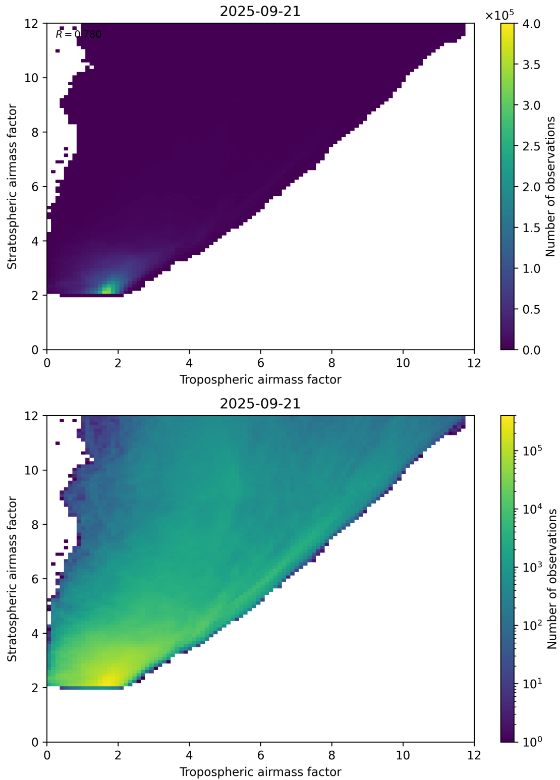
Figure 71: Scatter density plot of “Tropospheric airmass factor” against “Stratospheric airmass factor” for 2025-09-20 to 2025-09-22.
