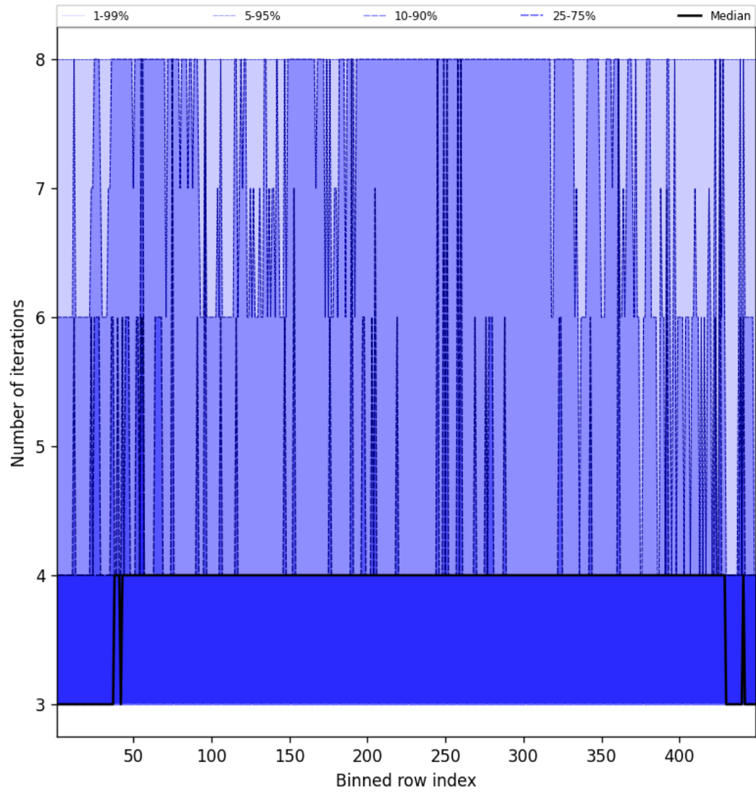
Figure 51: Along track statistics of “Number of iterations” for 2025-09-20 to 2025-09-22
