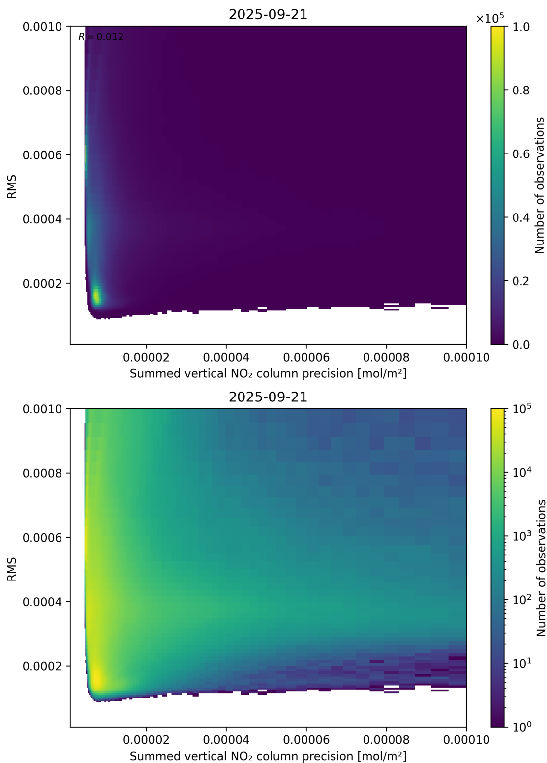
Figure 108: Scatter density plot of “Summed vertical NO 2 column precision” against “RMS” for 2025-09-20 to 2025-09-22.
