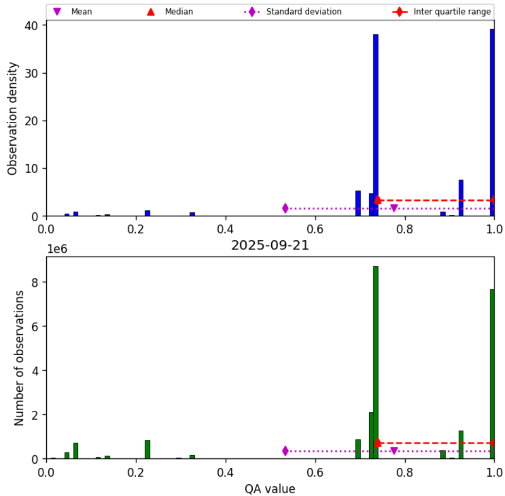
Figure 28: Histogram of “QA value” for 2025-09-20 to 2025-09-22
