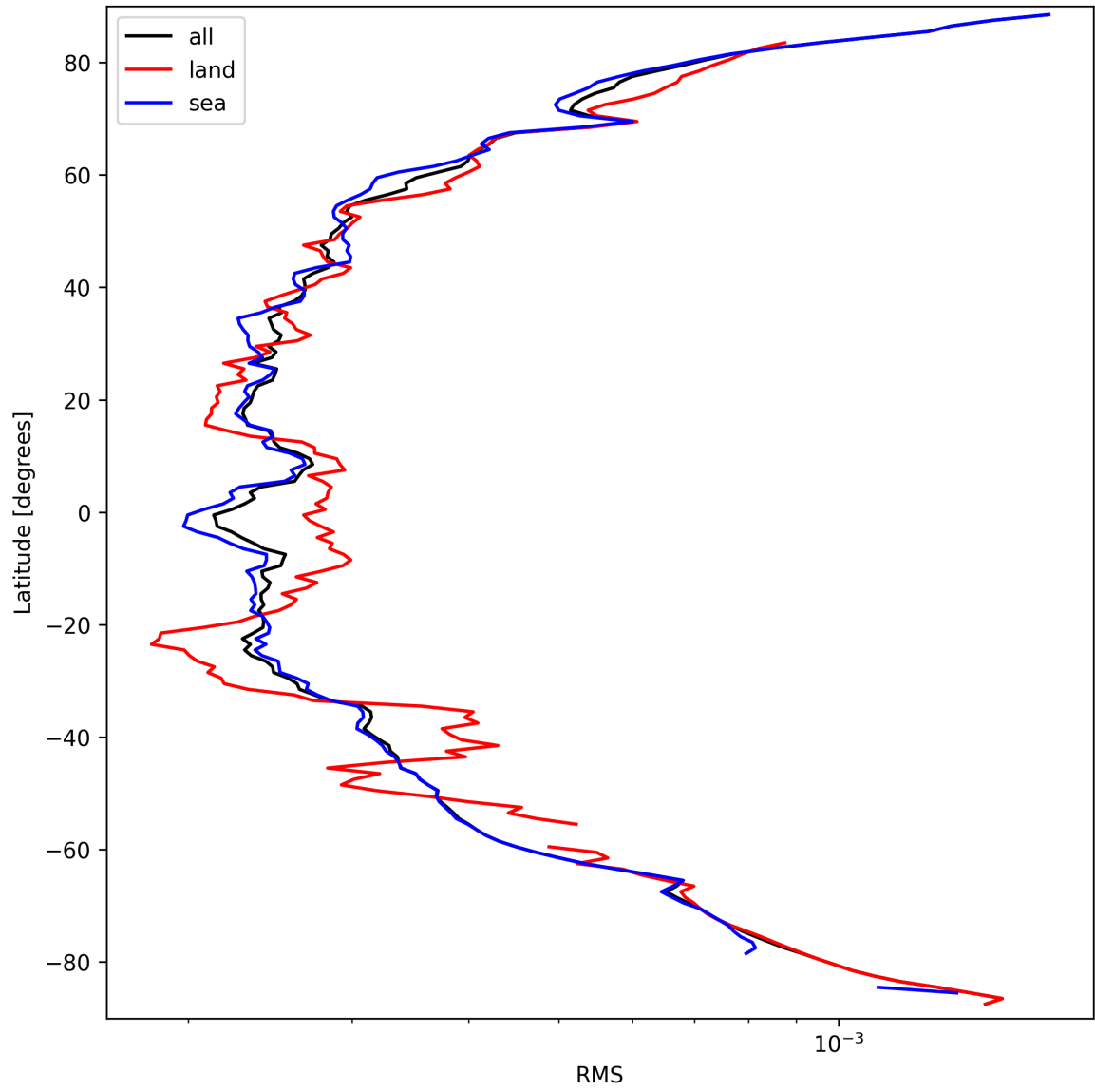
Figure 26: Zonal average of “RMS” for 2025-09-20 to 2025-09-22.
