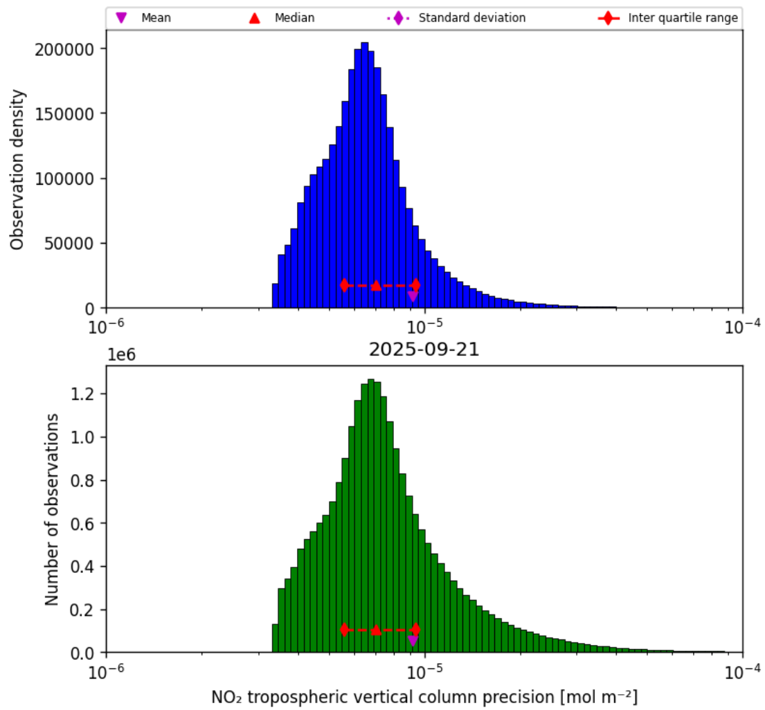
Figure 30: Histogram of “NO 2 tropospheric vertical column precision” for 2025-09-20 to 2025-09-22
