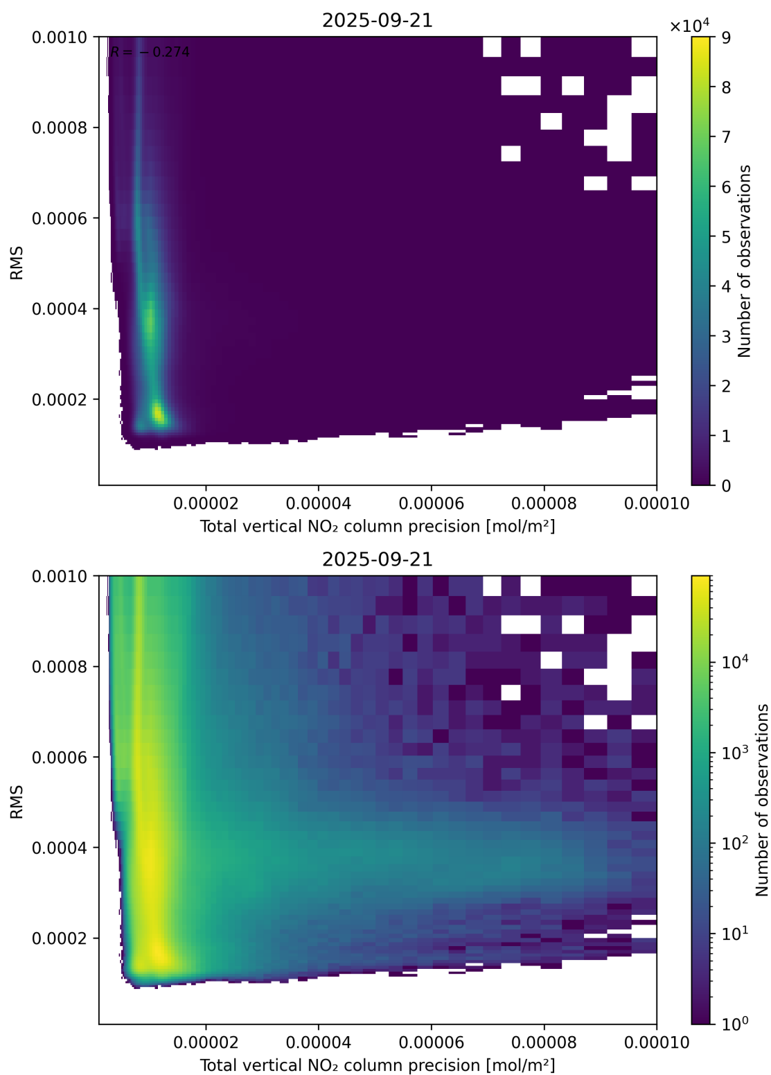
Figure 119: Scatter density plot of “Total vertical NO 2 column precision” against “RMS” for 2025-09-20 to 2025-09-22.
