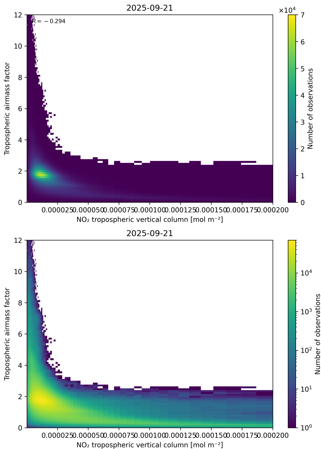
Figure 123: Scatter density plot of “NO 2 tropospheric vertical column” against “Tropospheric air mass factor” for 2025-09-20 to 2025-09-22.
