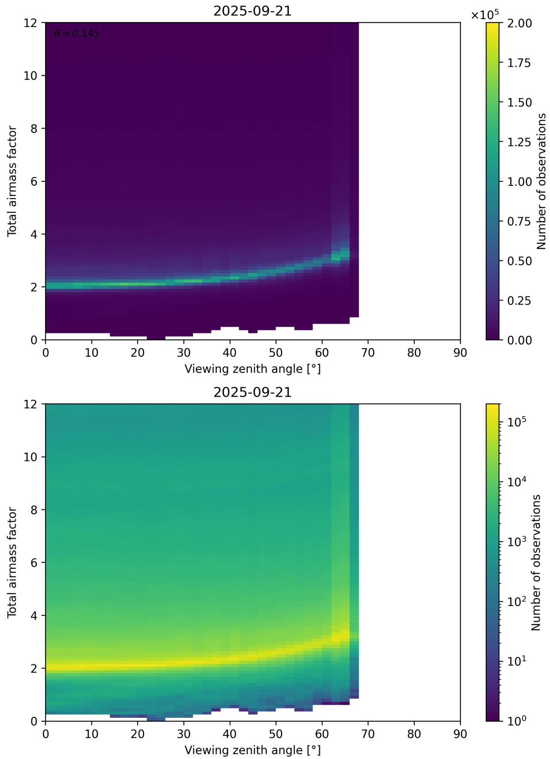
Figure 160: Scatter density plot of “Viewing zenith angle” against “Total airmass factor” for 2025-09-20 to 2025-09-22.
