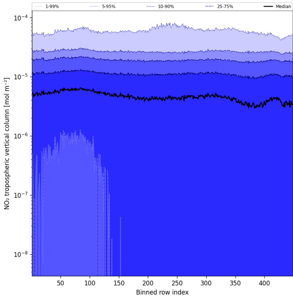
Figure 46: Along track statistics of “NO 2 tropospheric vertical column” for 2025-09-20 to 2025-09-22
