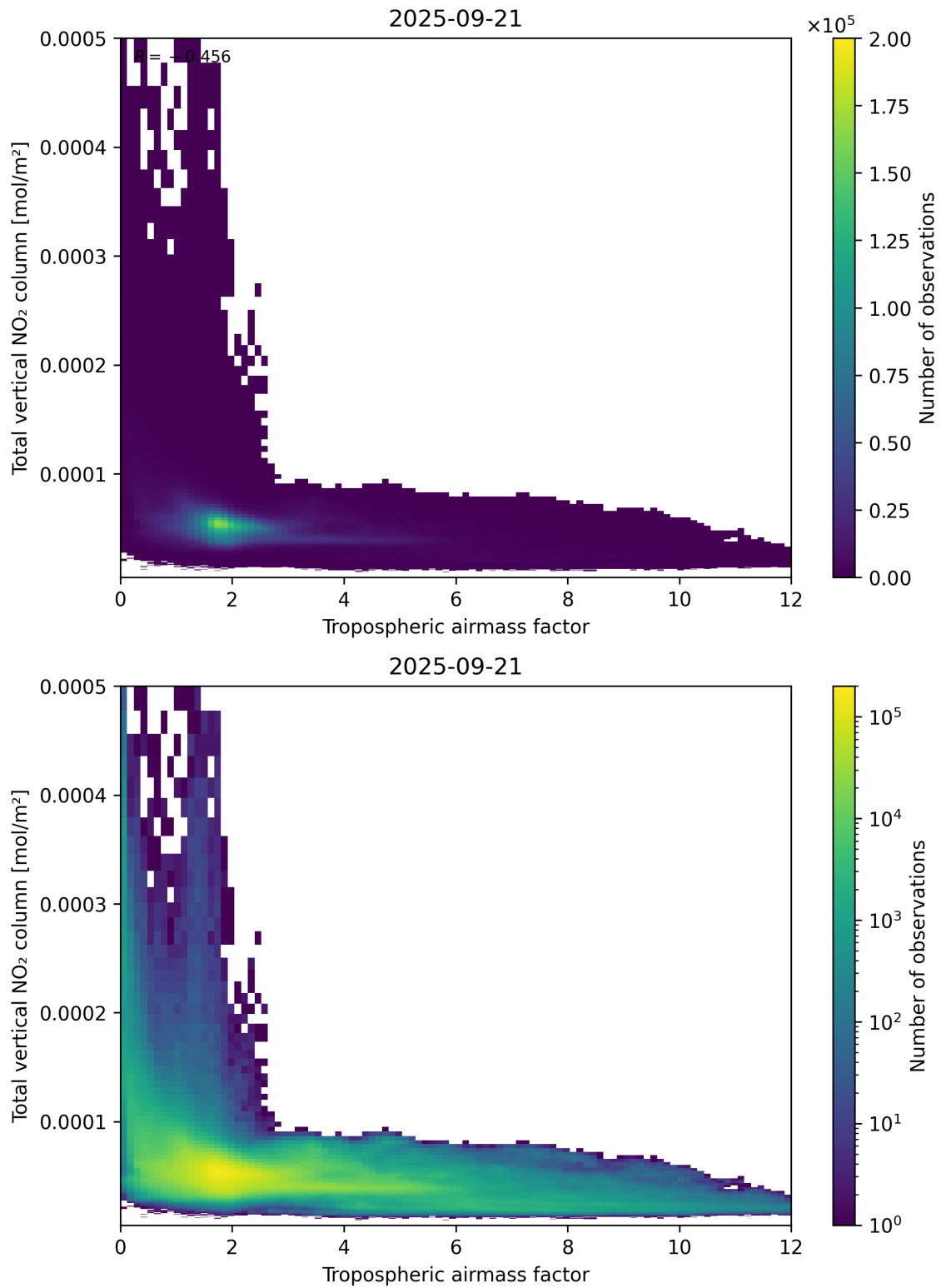
Figure 77: Scatter density plot of “Tropospheric airmass factor” against “Total vertical NO 2 column” for 2025-09-20 to 2025-09-22.
