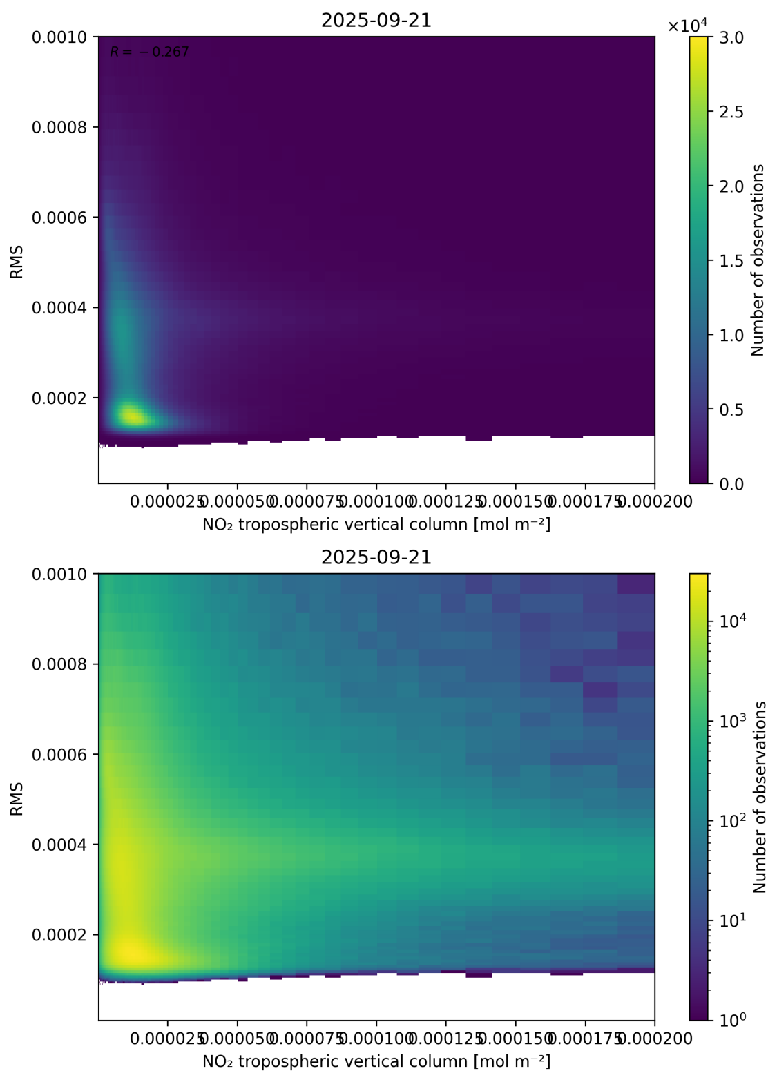
Figure 142: Scatter density plot of “NO 2 tropospheric vertical column” against “RMS” for 2025-09-20 to 2025-09-22.
