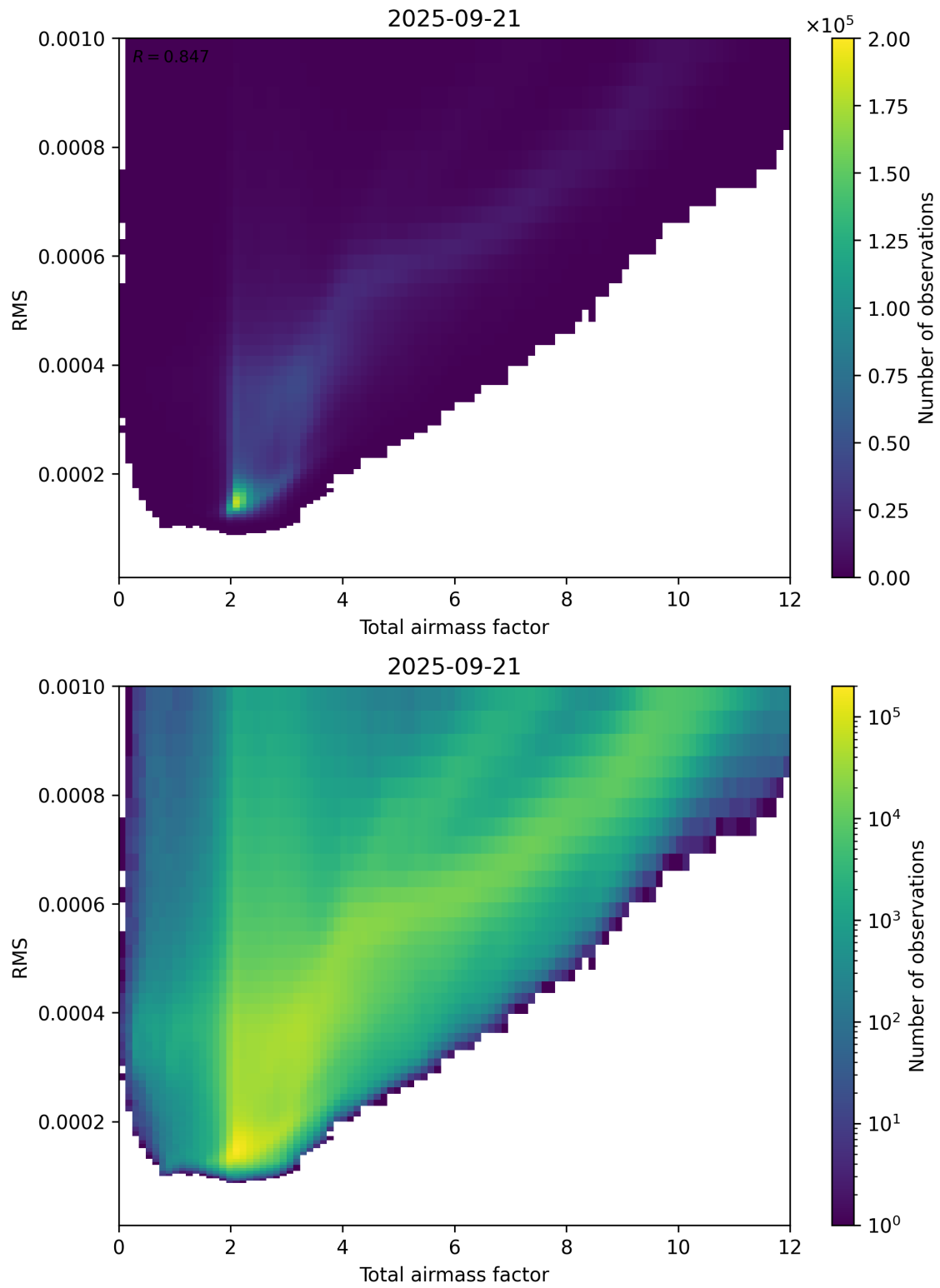
Figure 69: Scatter density plot of “Total airmass factor” against “RMS” for 2025-09-20 to 2025-09-22.
