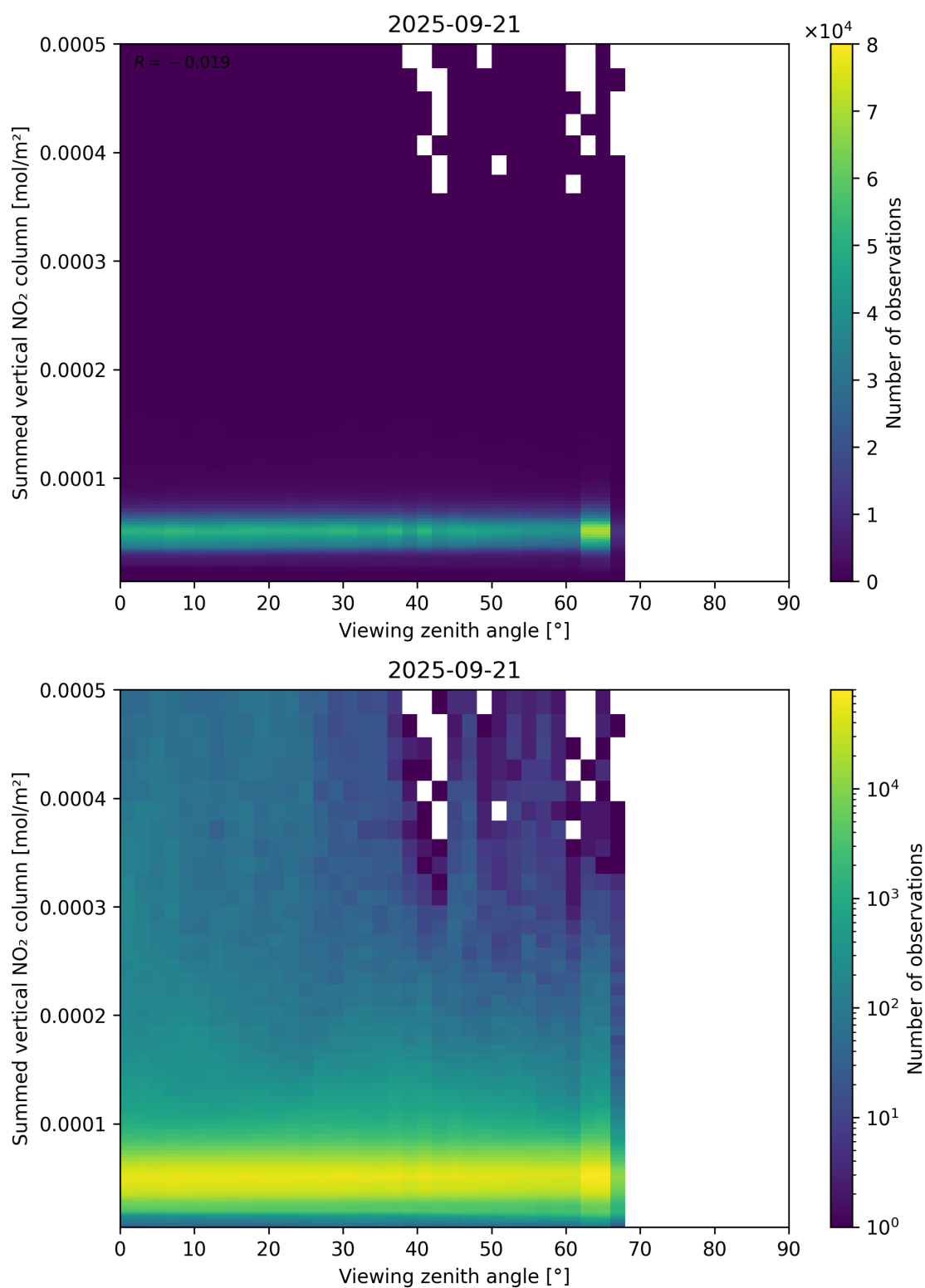
Figure 165: Scatter density plot of “Viewing zenith angle” against “Summed vertical NO 2 column” for 2025-09-20 to 2025-09-22.
