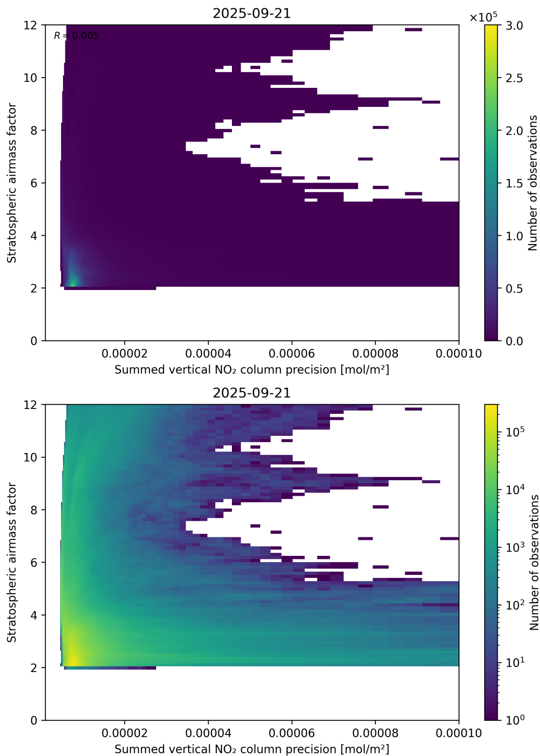
Figure 106: Scatter density plot of “Summed vertical NO 2 column precision” against “Stratospheric airmass factor” for 2025-09-20 to 2025-09-22.
