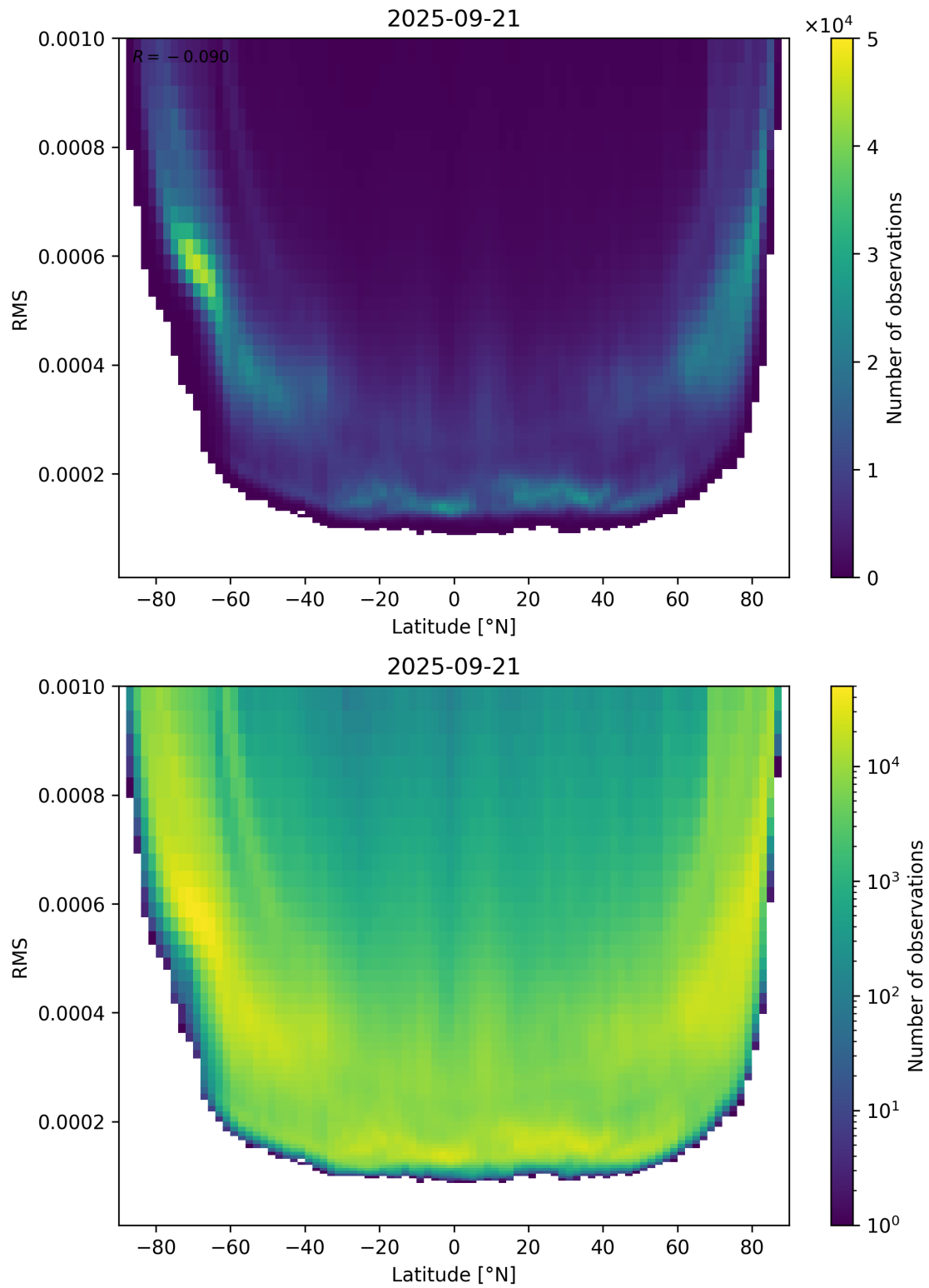
Figure 94: Scatter density plot of “Latitude” against “RMS” for 2025-09-20 to 2025-09-22.
