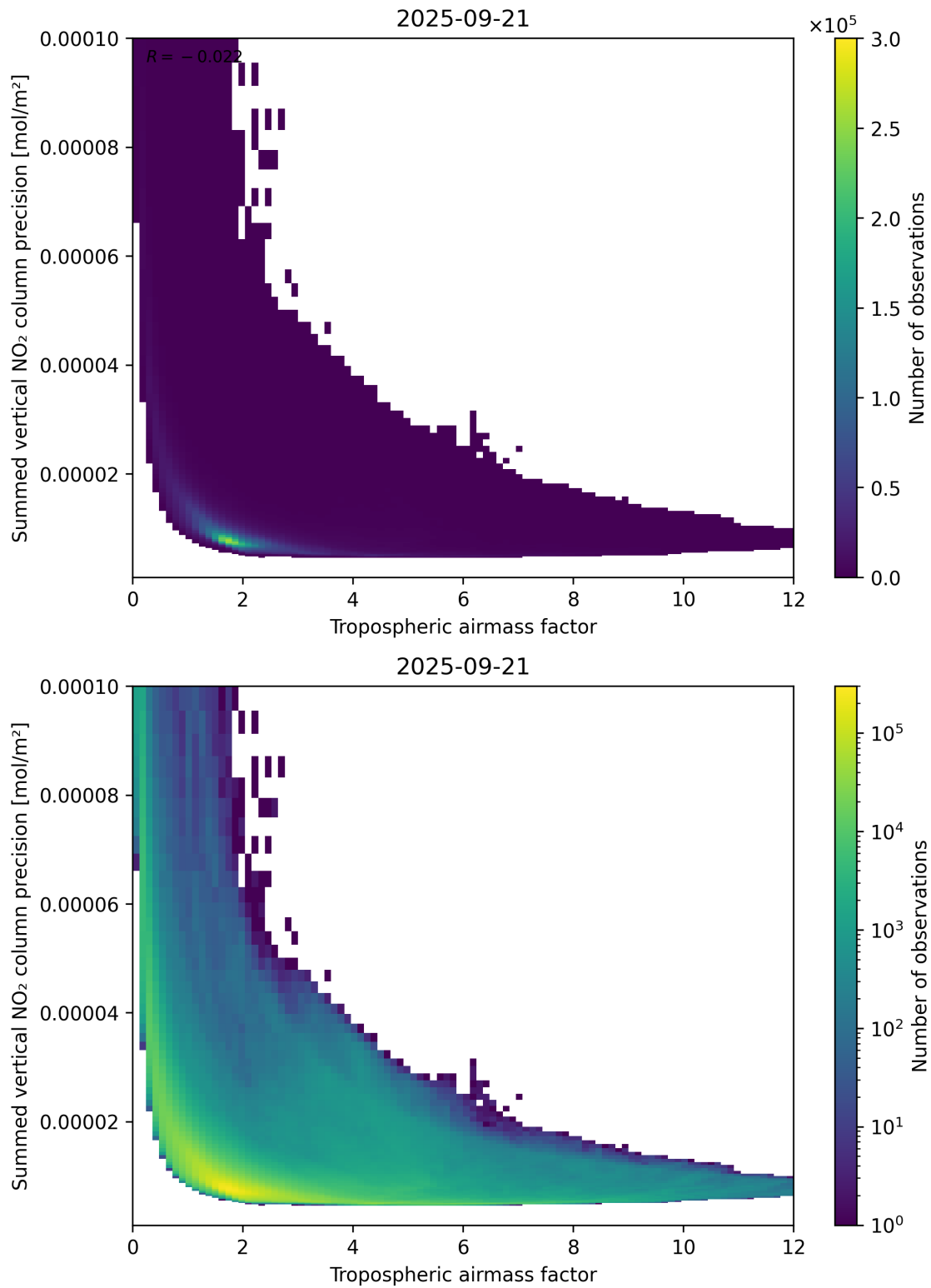
Figure 76: Scatter density plot of “Tropospheric air mass factor” against “Summed vertical NO 2 column precision” for 2025-09-20 to 2025-09-22.
