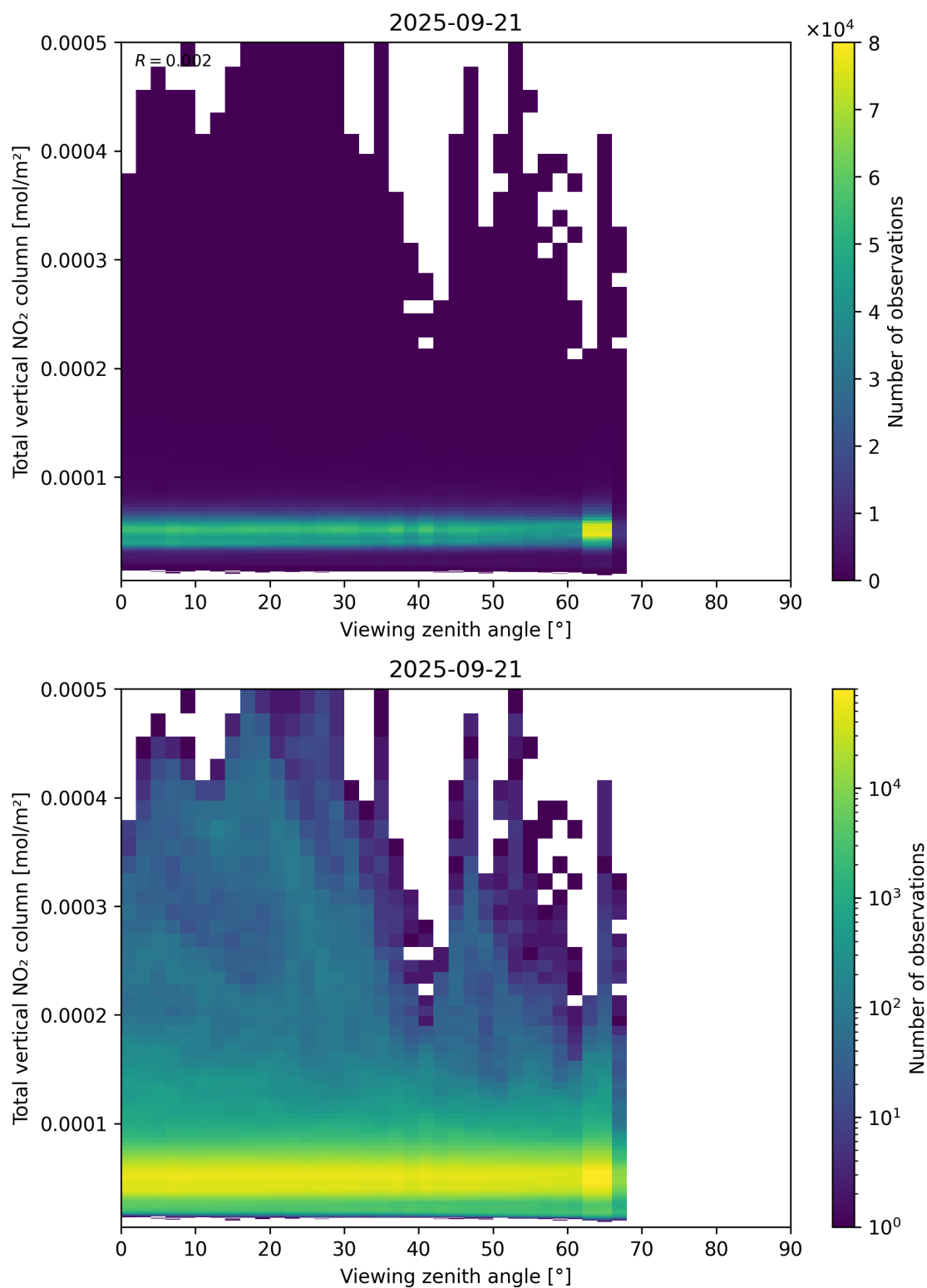
Figure 167: Scatter density plot of “Viewing zenith angle” against “Total vertical NO 2 column” for 2025-09-20 to 2025-09-22.
