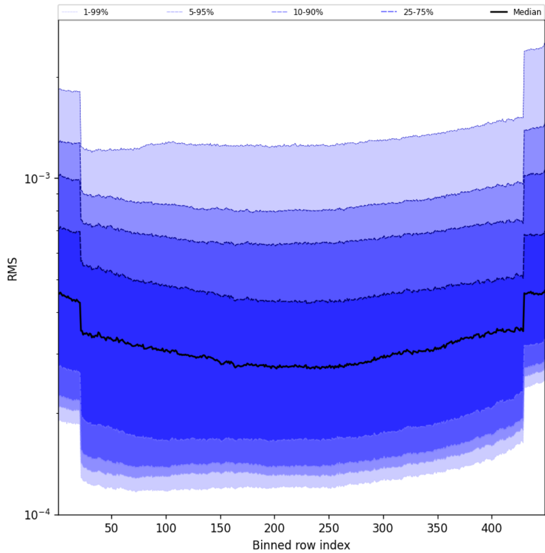
Figure 60: Along track statistics of “RMS” for 2025-09-20 to 2025-09-22
