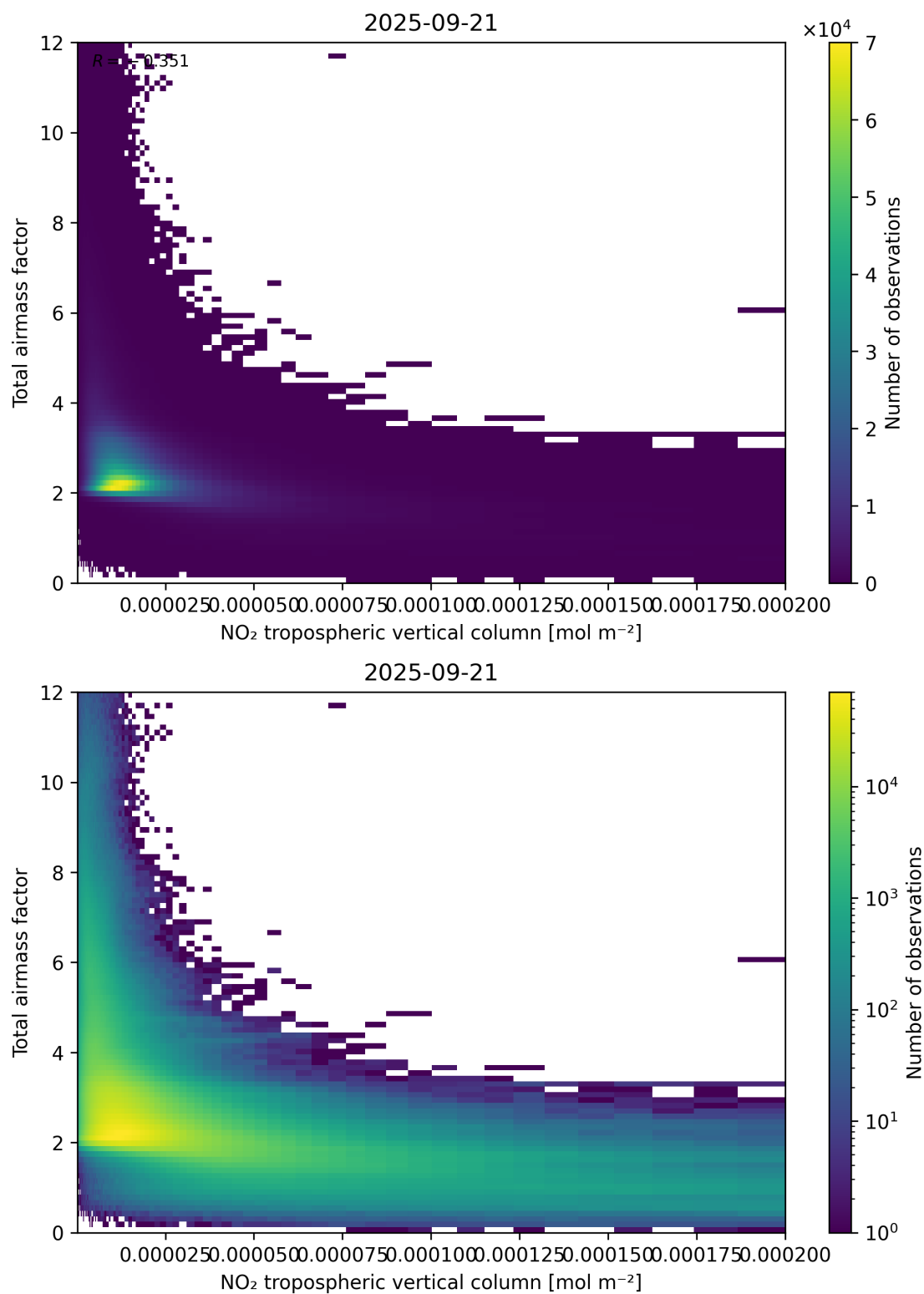
Figure 122: Scatter density plot of “NO 2 tropospheric vertical column” against “Total airmass factor” for 2025-09-20 to 2025-09-22.
