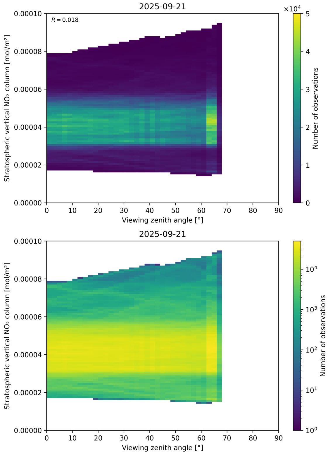
Figure 164: Scatter density plot of “Viewing zenith angle” against “Stratospheric vertical NO 2 column” for 2025-09-20 to 2025-09-22.
