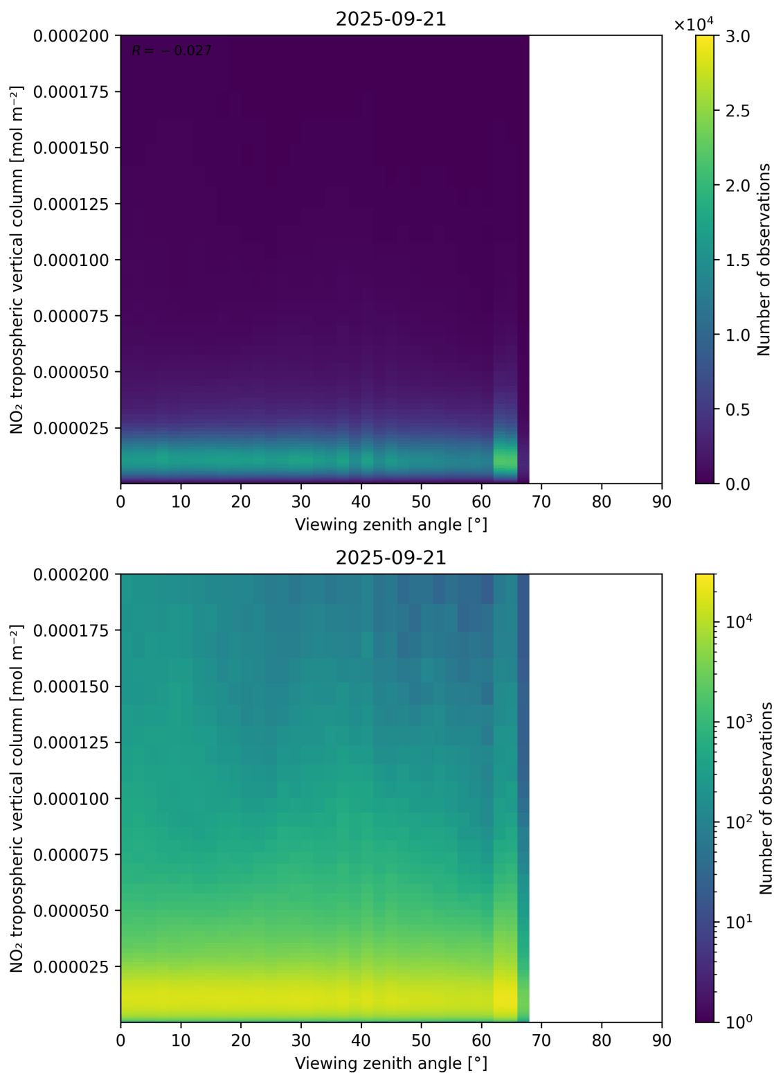
Figure 169: Scatter density plot of “Viewing zenith angle” against “NO 2 tropospheric vertical column” for 2025-09-20 to 2025-09-22.
