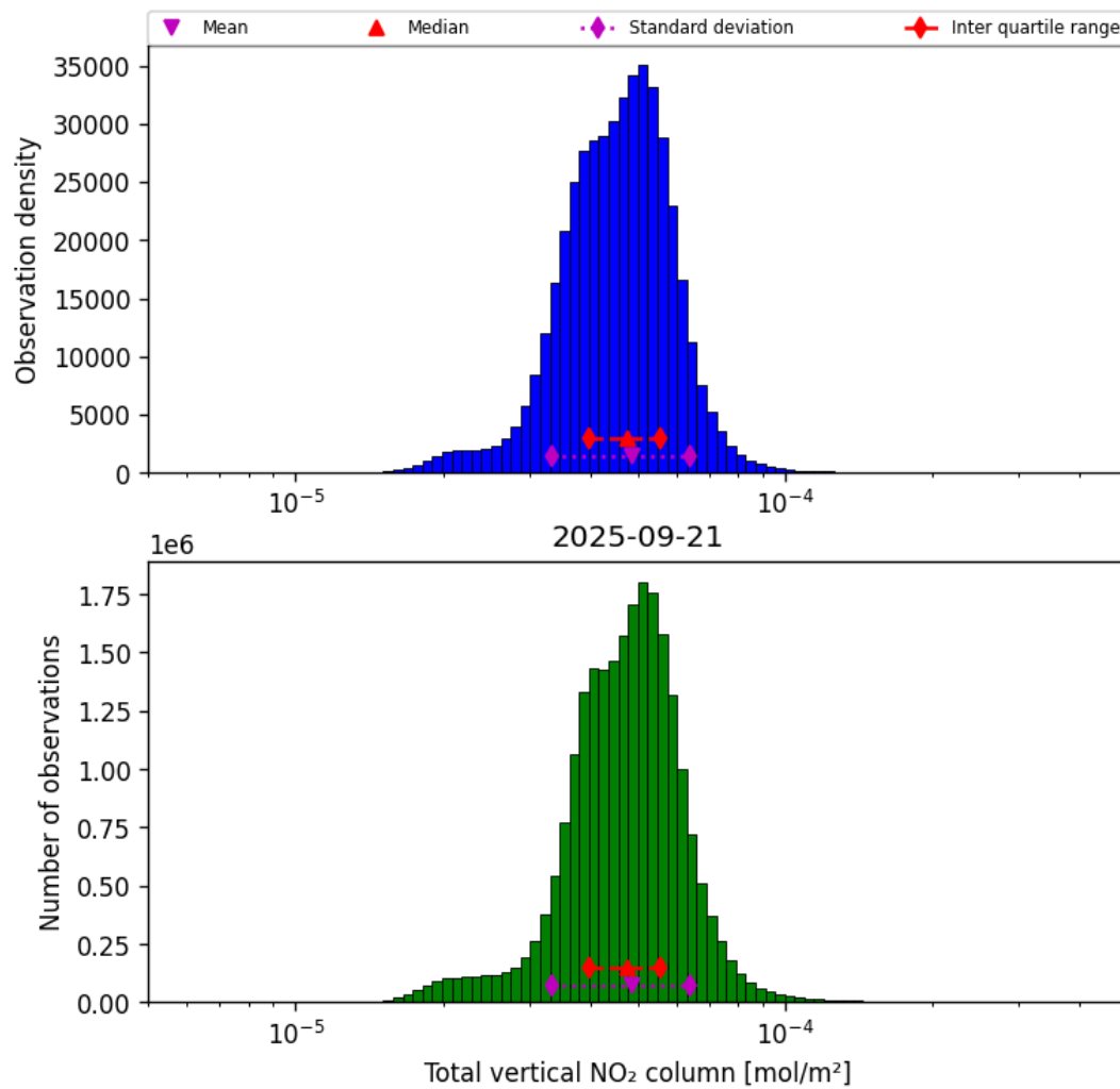
Figure 38: Histogram of “Total vertical NO 2 column” for 2025-09-20 to 2025-09-22
