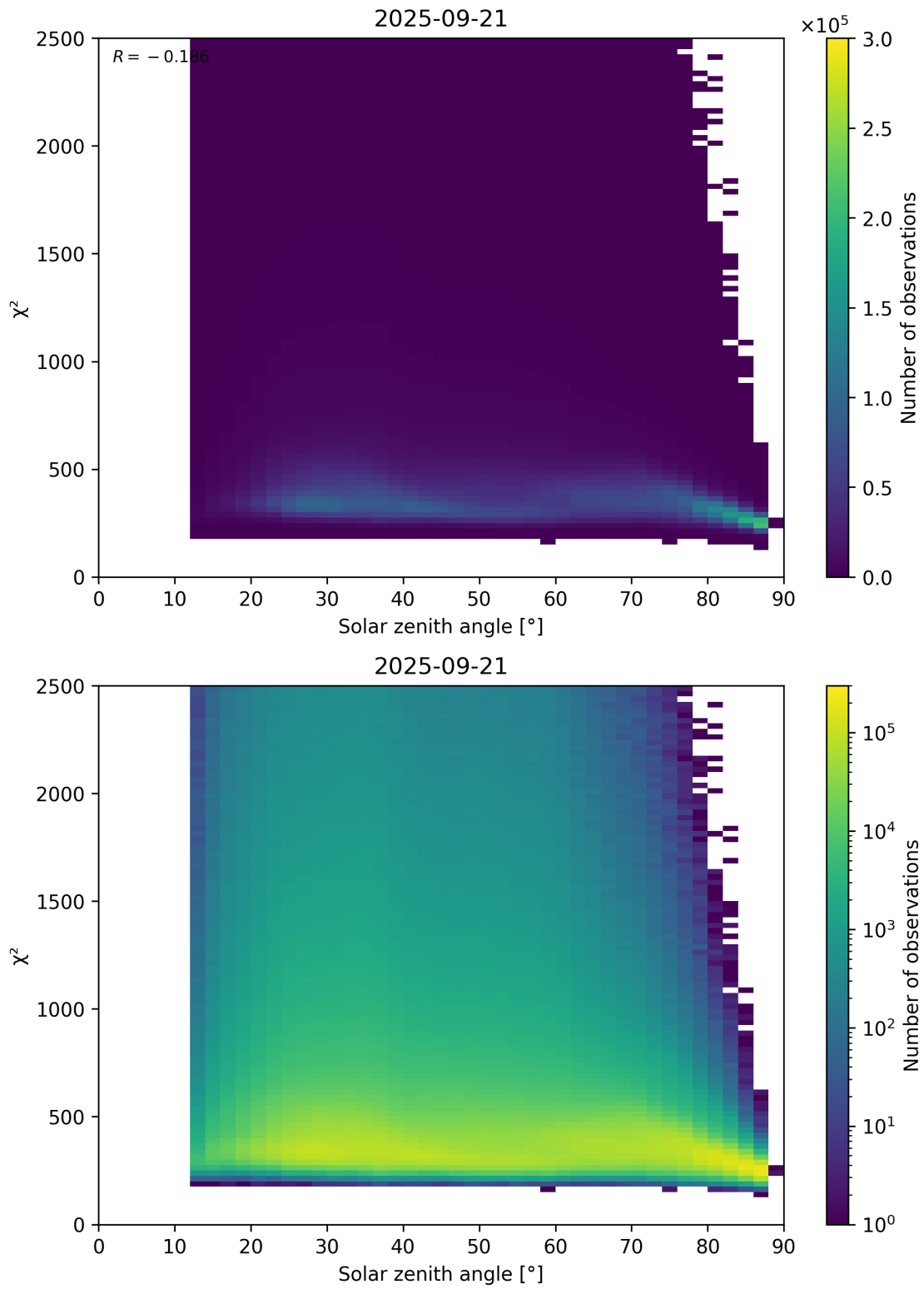
Figure 148: Scatter density plot of “Solar zenith angle” against “ \chi^2 ” for 2025-09-20 to 2025-09-22.
