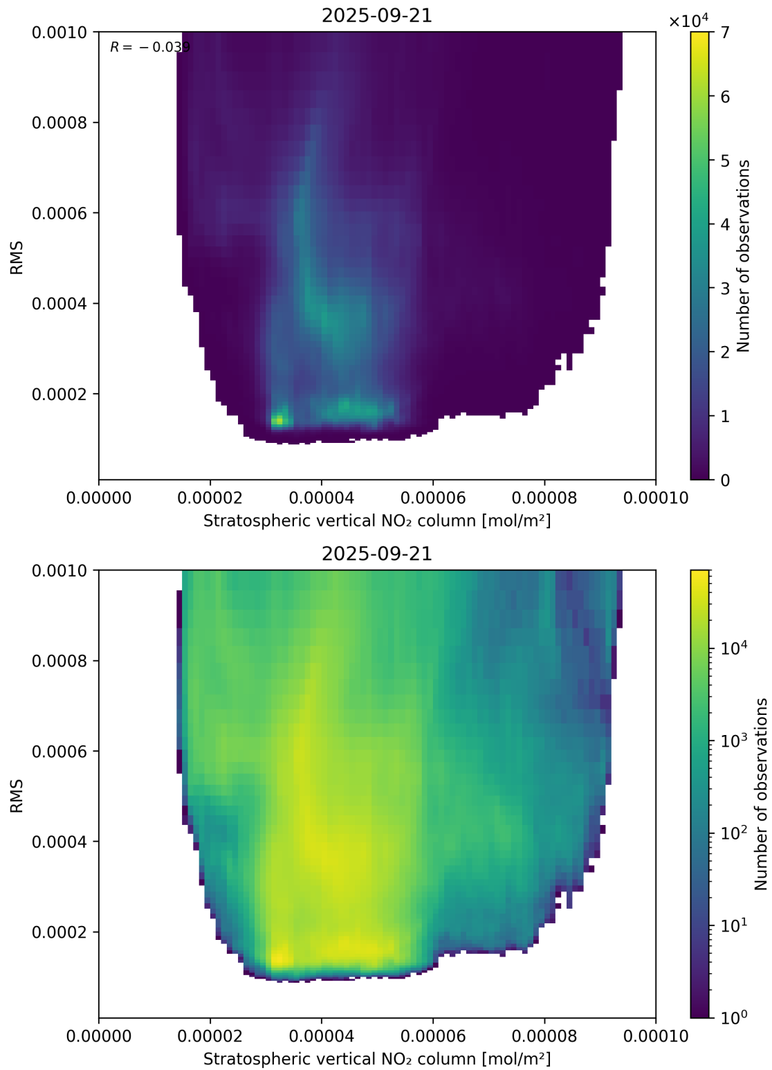
Figure 102: Scatter density plot of “Stratospheric vertical NO 2 column” against “RMS” for 2025-09-20 to 2025-09-22.
