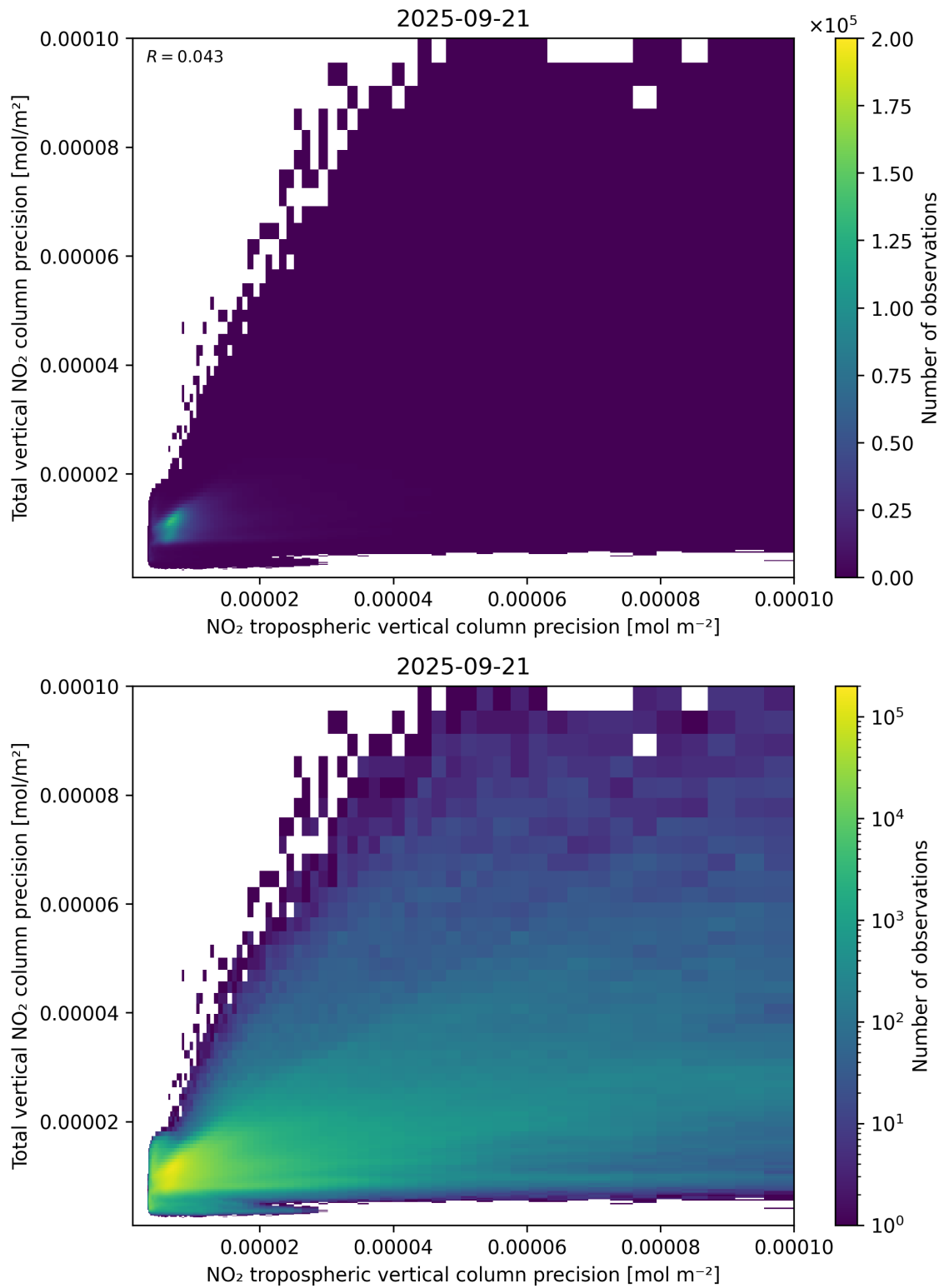
Figure 139: Scatter density plot of “NO 2 tropospheric vertical column precision” against “Total vertical NO 2 column precision” for 2025-09-20 to 2025-09-22.
