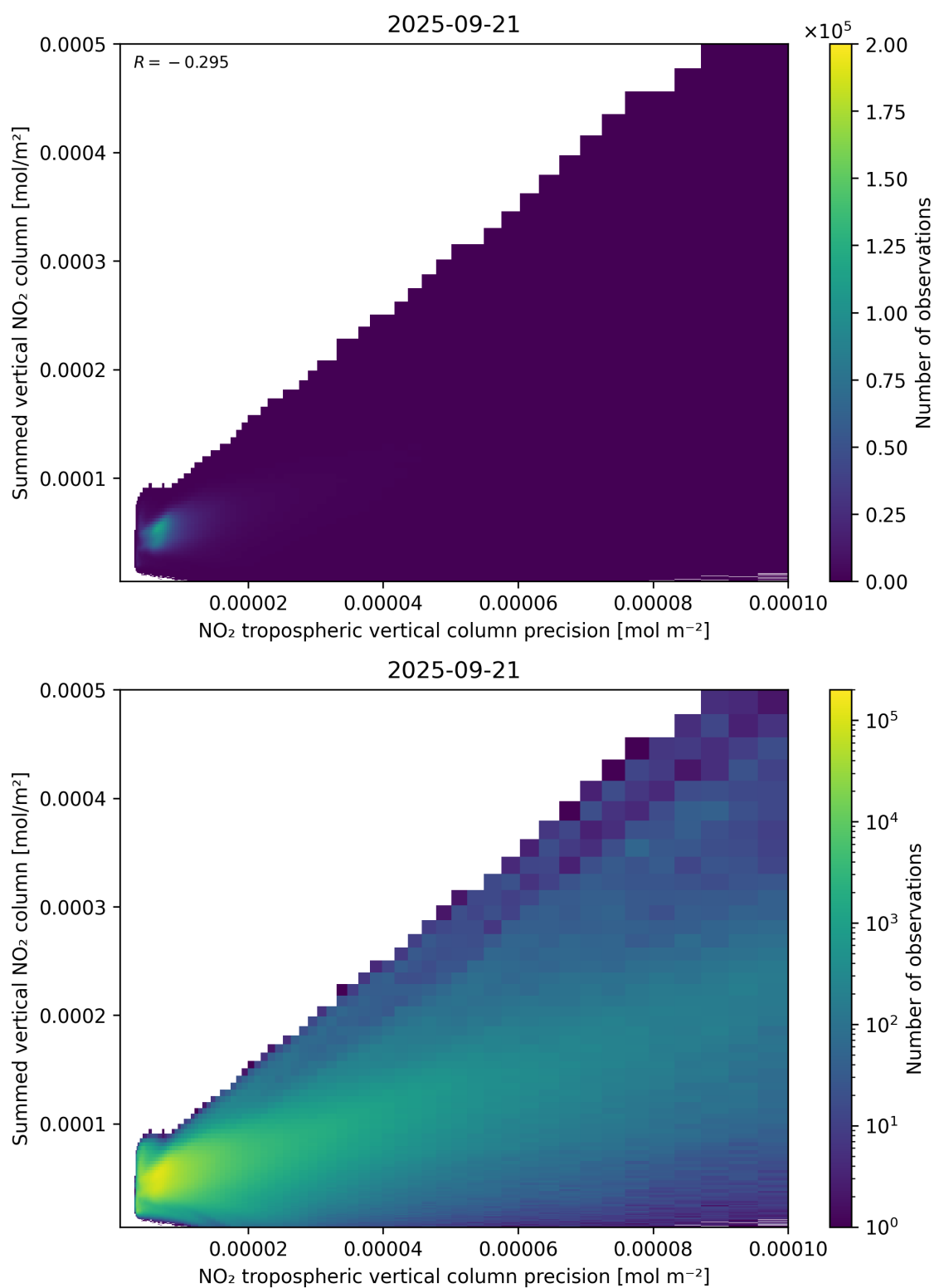
Figure 136: Scatter density plot of “NO 2 tropospheric vertical column precision” against “Summed vertical NO 2 column” for 2025-09-20 to 2025-09-22.
