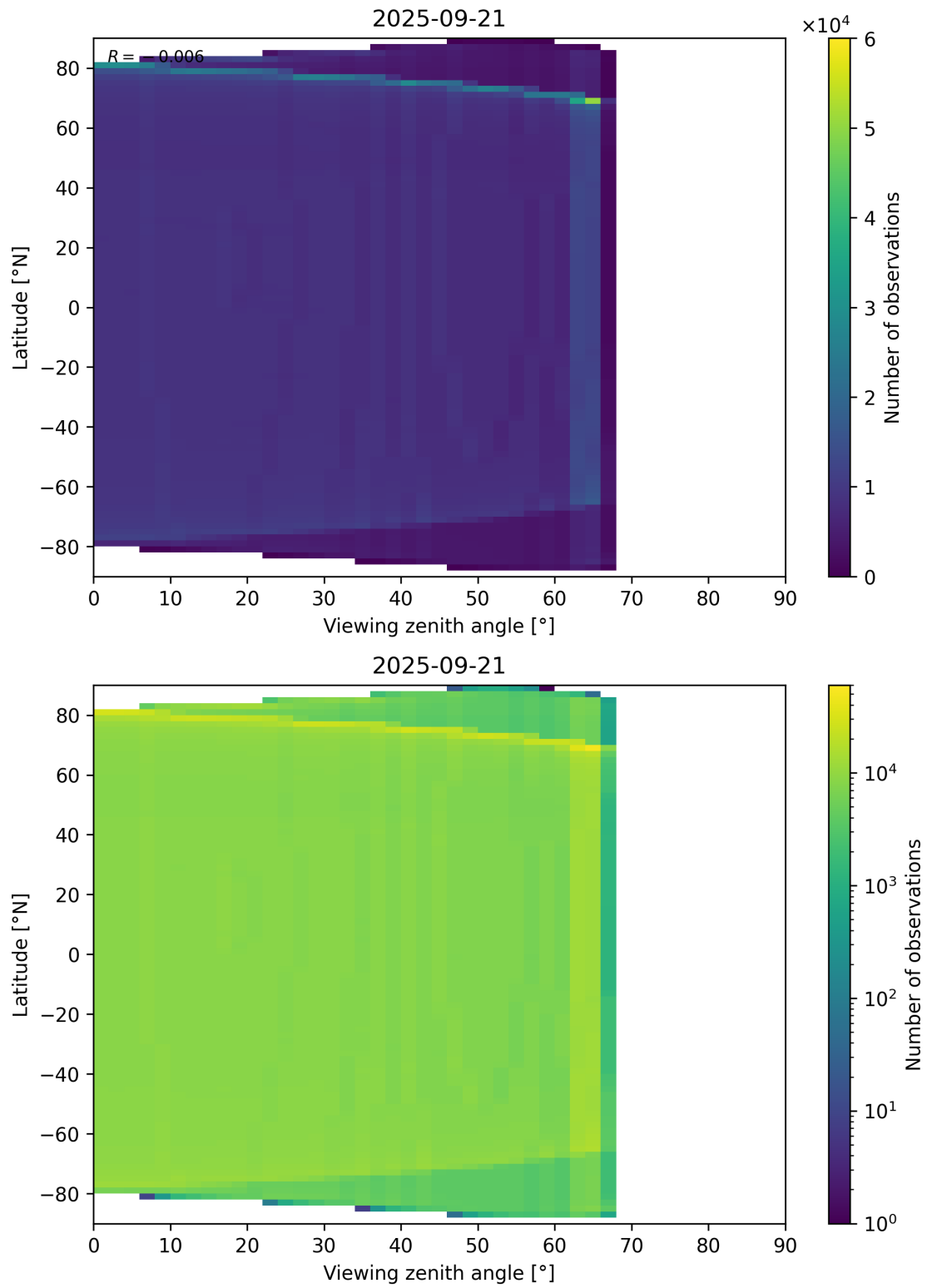
Figure 163: Scatter density plot of “Viewing zenith angle” against “Latitude” for 2025-09-20 to 2025-09-22.
