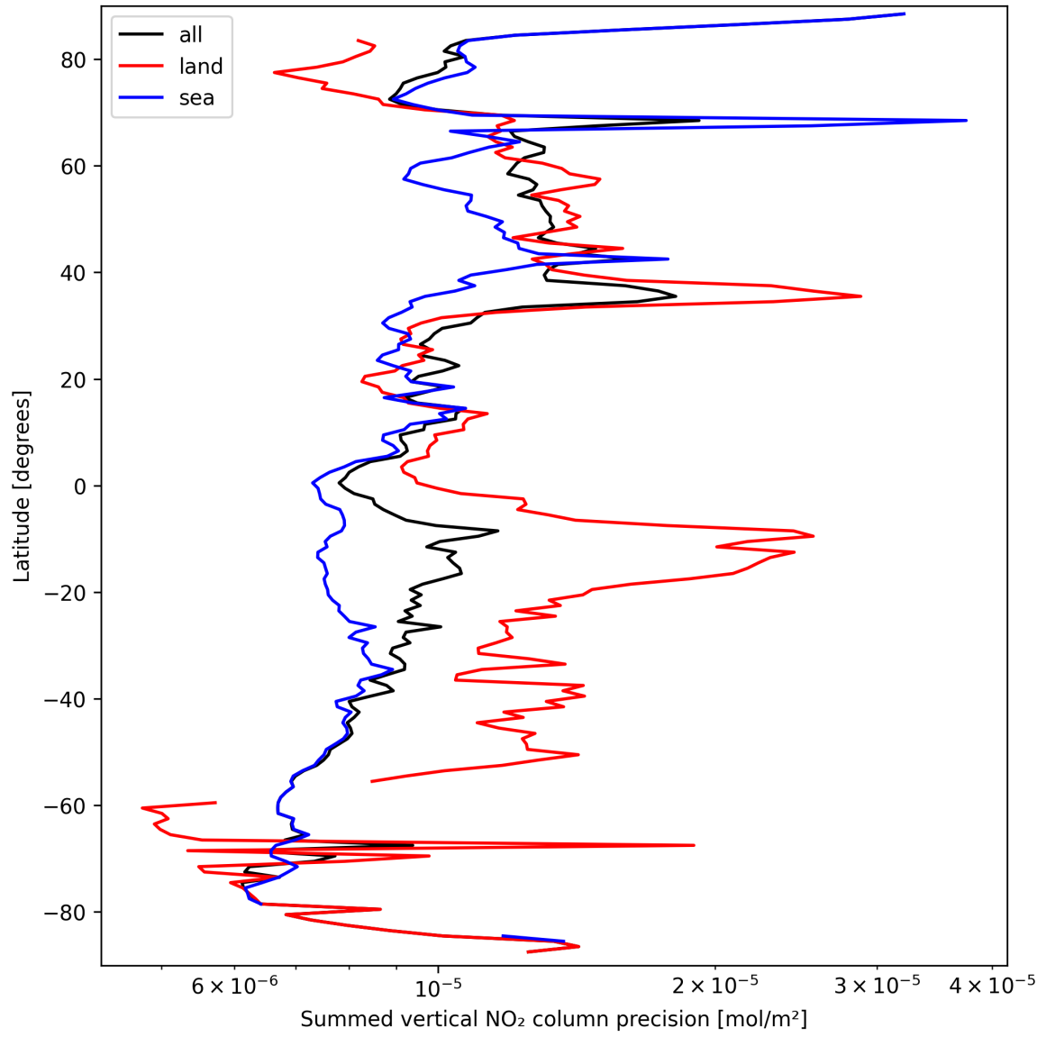
Figure 24: Zonal average of “Summed vertical NO 2 column precision” for 2025-09-20 to 2025-09-22.
