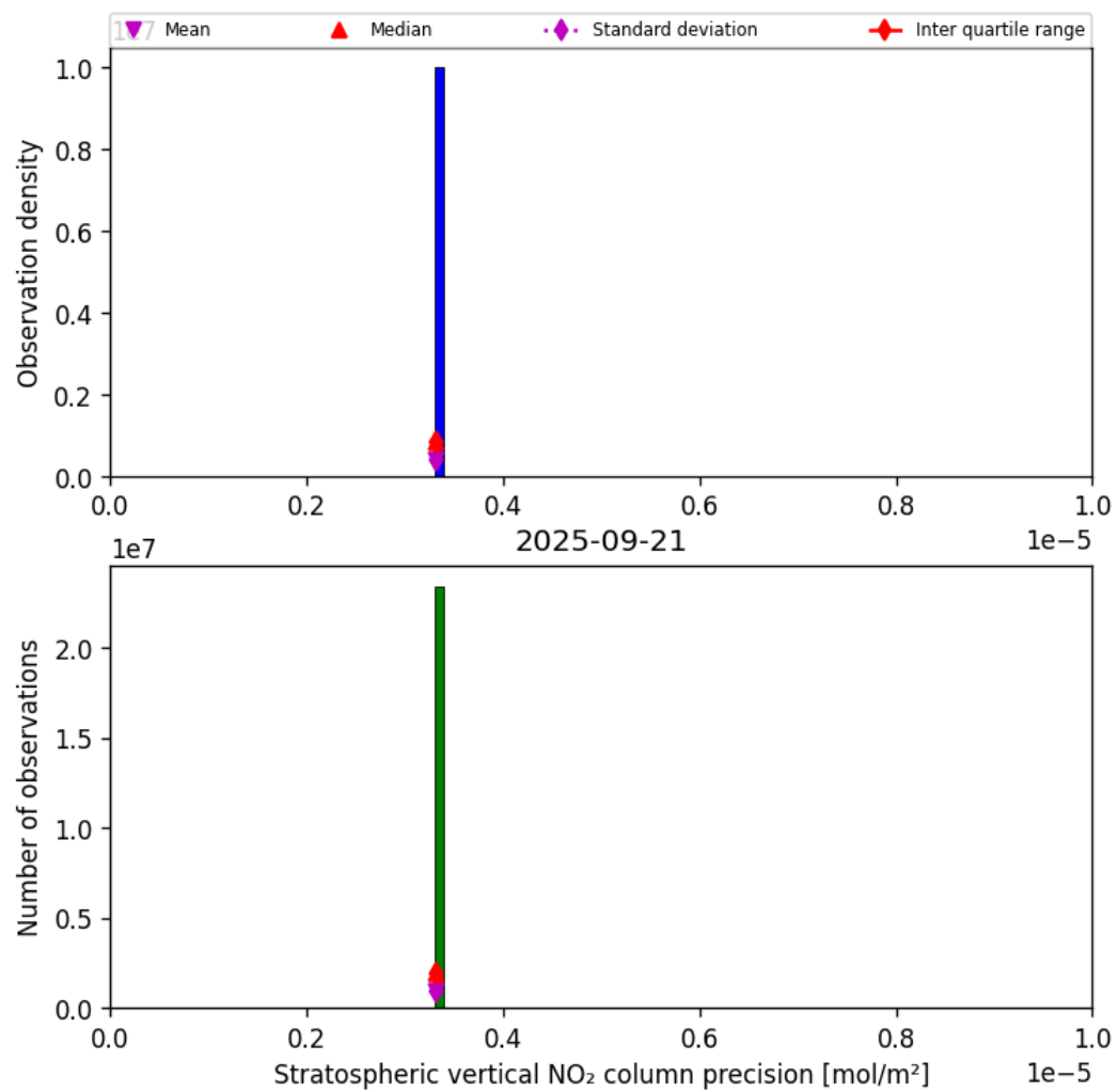
Figure 37: Histogram of “Stratospheric vertical NO 2 column precision” for 2025-09-20 to 2025-09-22
