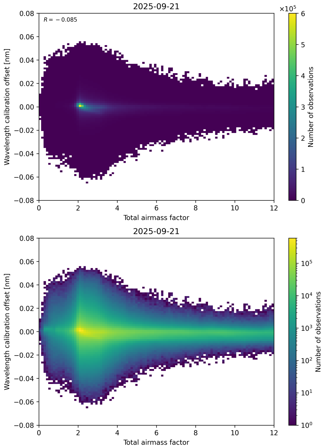
Figure 70: Scatter density plot of “Total airmass factor” against “Wavelength calibration offset” for 2025-09-20 to 2025-09-22.
