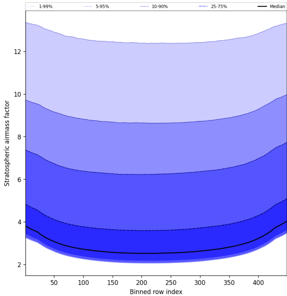
Figure 61: Along track statistics of “Stratospheric airmass factor” for 2025-09-20 to 2025-09-22
