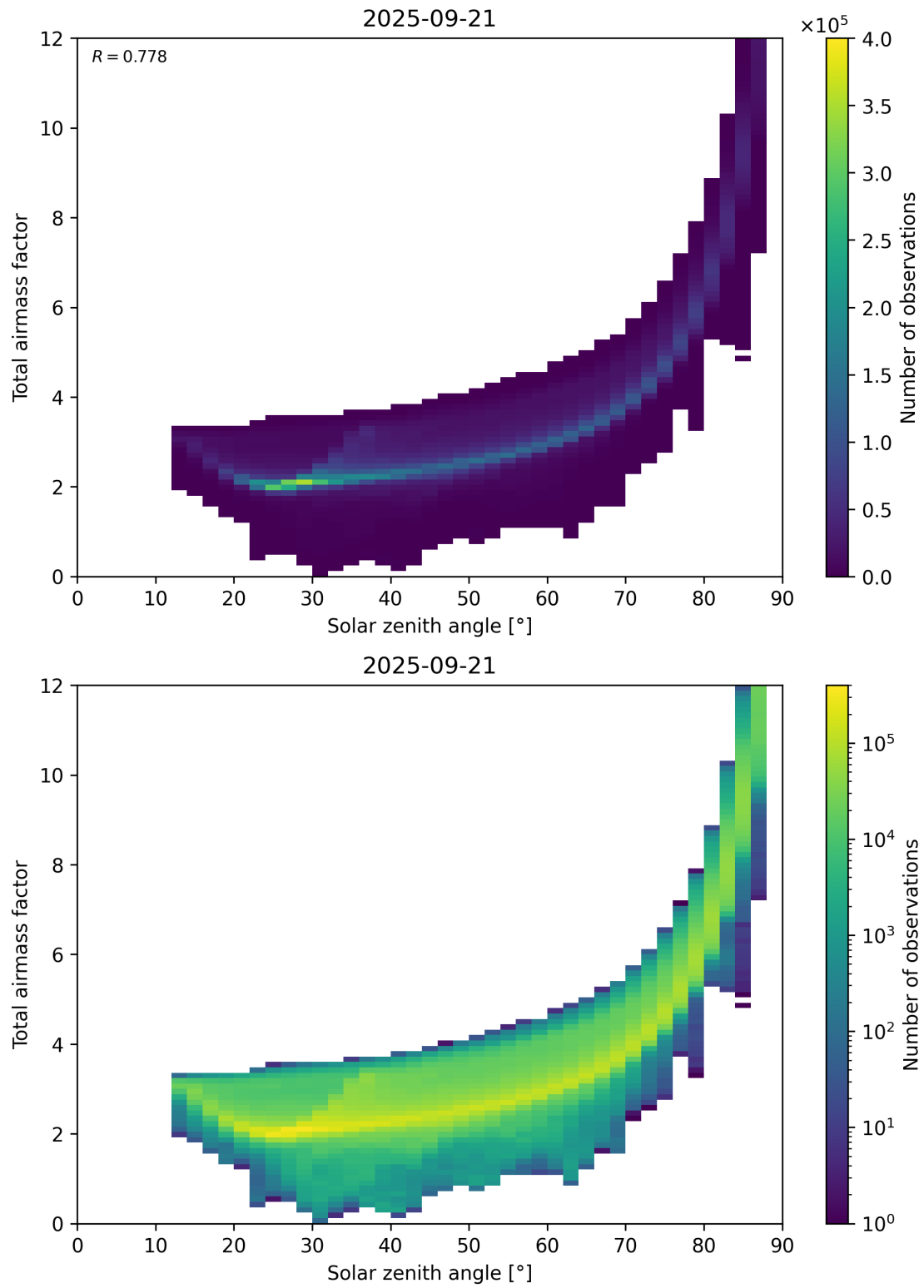
Figure 146: Scatter density plot of “Solar zenith angle” against “Total airmass factor” for 2025-09-20 to 2025-09-22.
