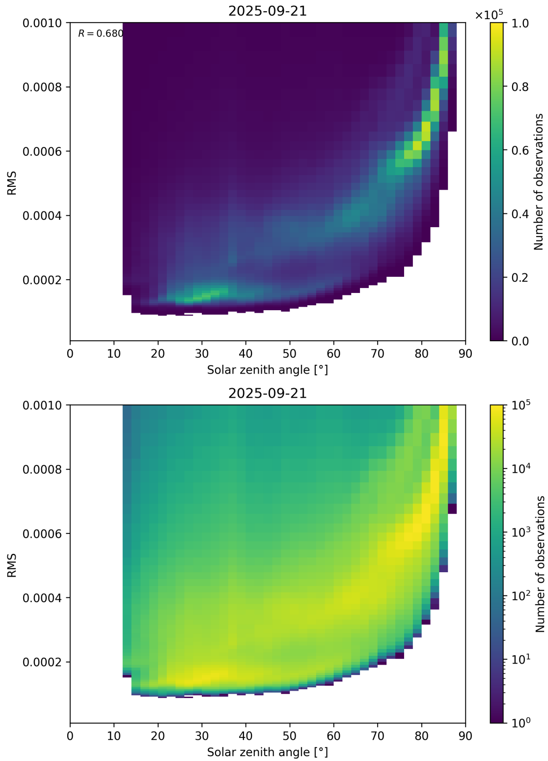
Figure 157: Scatter density plot of “Solar zenith angle” against “RMS” for 2025-09-20 to 2025-09-22.
