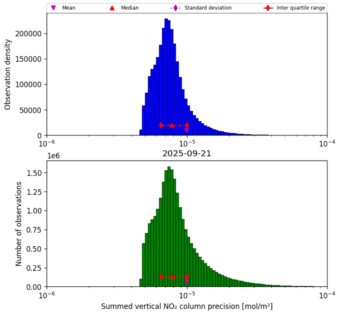
Figure 41: Histogram of “Summed vertical NO 2 column precision” for 2025-09-20 to 2025-09-22
