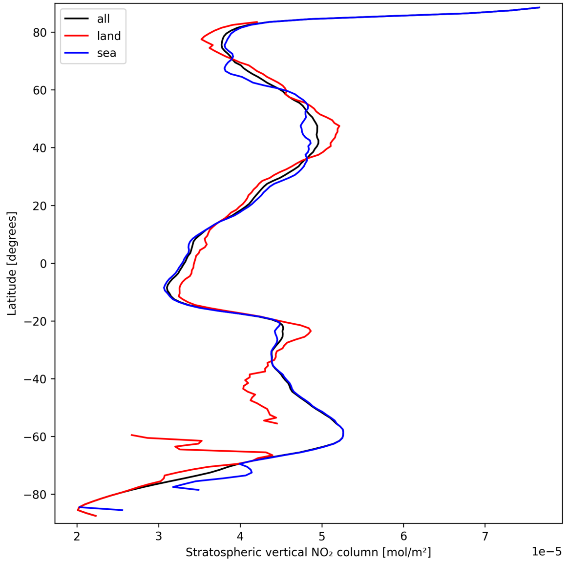
Figure 19: Zonal average of “Stratospheric vertical NO 2 column” for 2025-09-20 to 2025-09-22.
