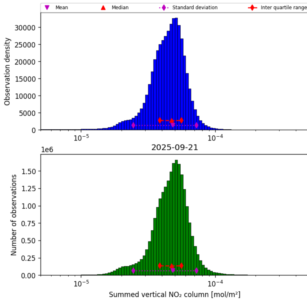
Figure 40: Histogram of “Summed vertical NO 2 column” for 2025-09-20 to 2025-09-22
