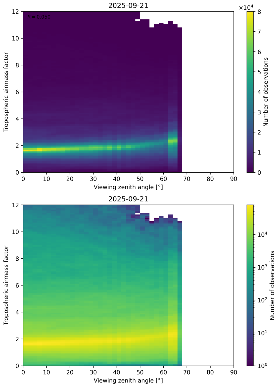
Figure 161: Scatter density plot of “Viewing zenith angle” against “Tropospheric airmass factor” for 2025-09-20 to 2025-09-22.
