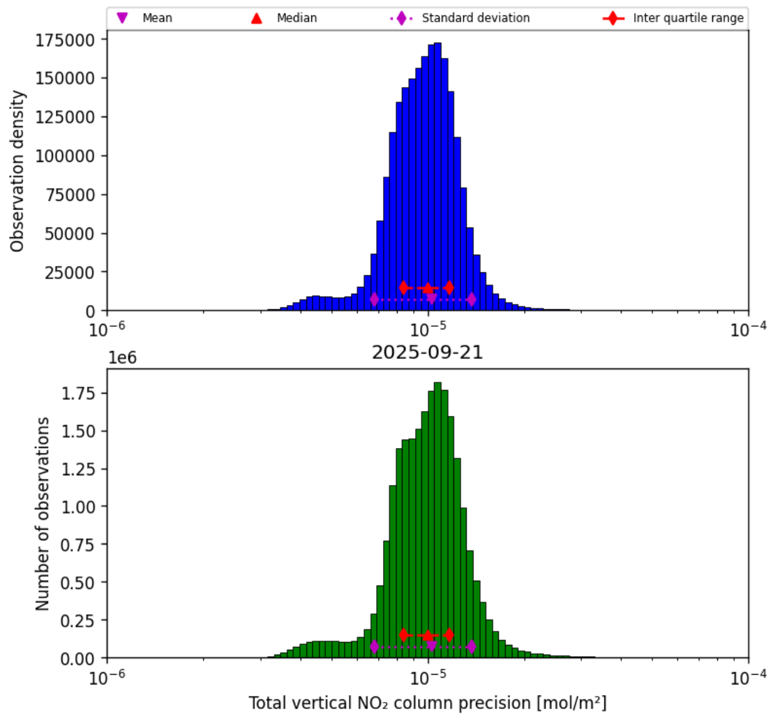
Figure 39: Histogram of "Total vertical NO 2 column precision" for 2025-09-20 to 2025-09-22
