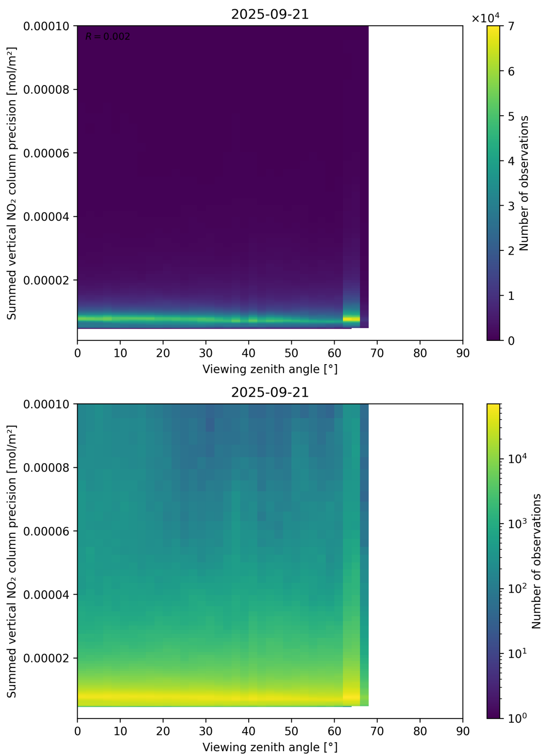
Figure 166: Scatter density plot of “Viewing zenith angle” against “Summed vertical NO 2 column precision” for 2025-09-20 to 2025-09-22.
