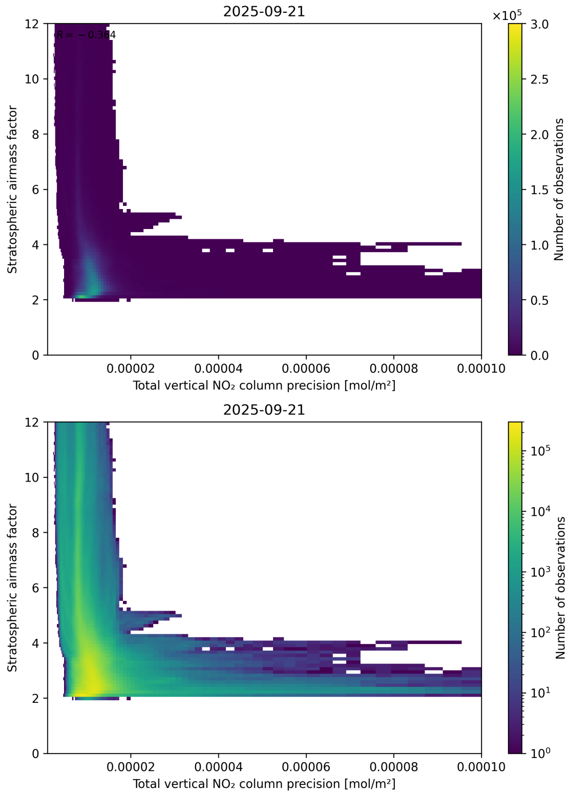
Figure 115: Scatter density plot of “Total vertical NO 2 column precision” against “Stratospheric air mass factor” for 2025-09-20 to 2025-09-22.
