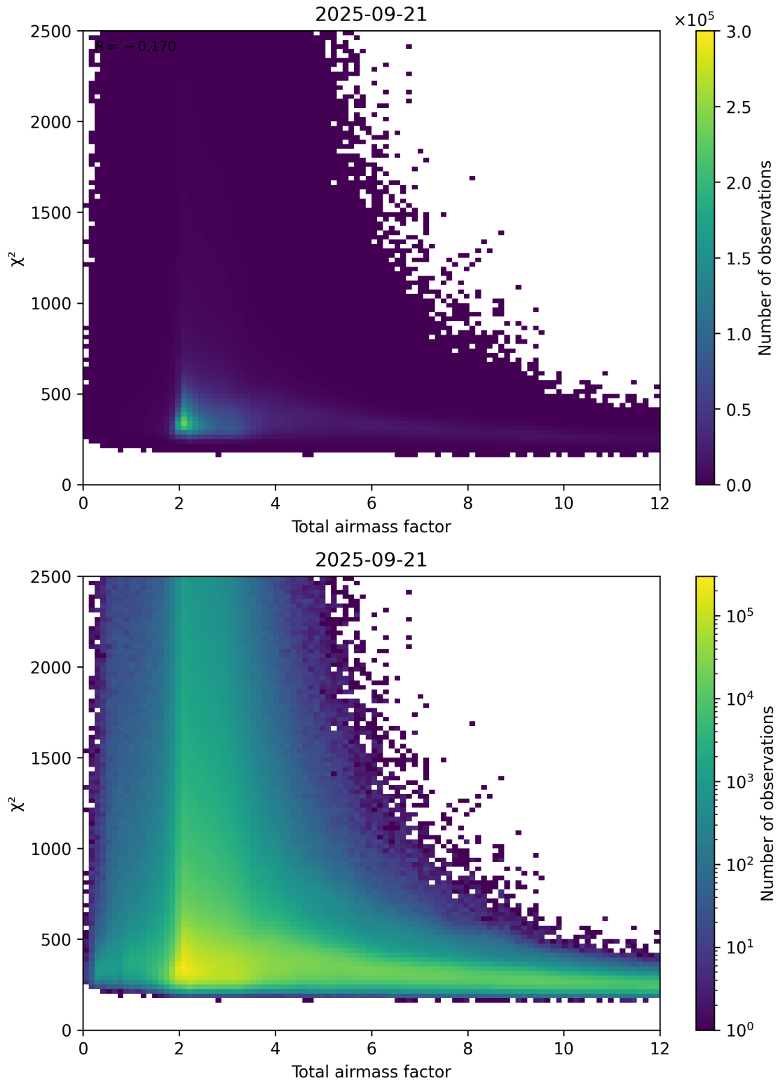
Figure 63: Scatter density plot of “Total airmass factor” against “ \chi^2 ” for 2025-09-20 to 2025-09-22.
