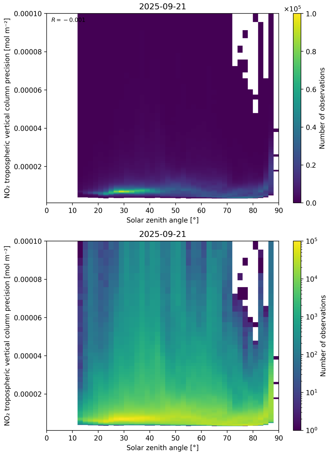
Figure 156: Scatter density plot of “Solar zenith angle” against “NO 2 tropospheric vertical column precision” for 2025-09-20 to 2025-09-22.
