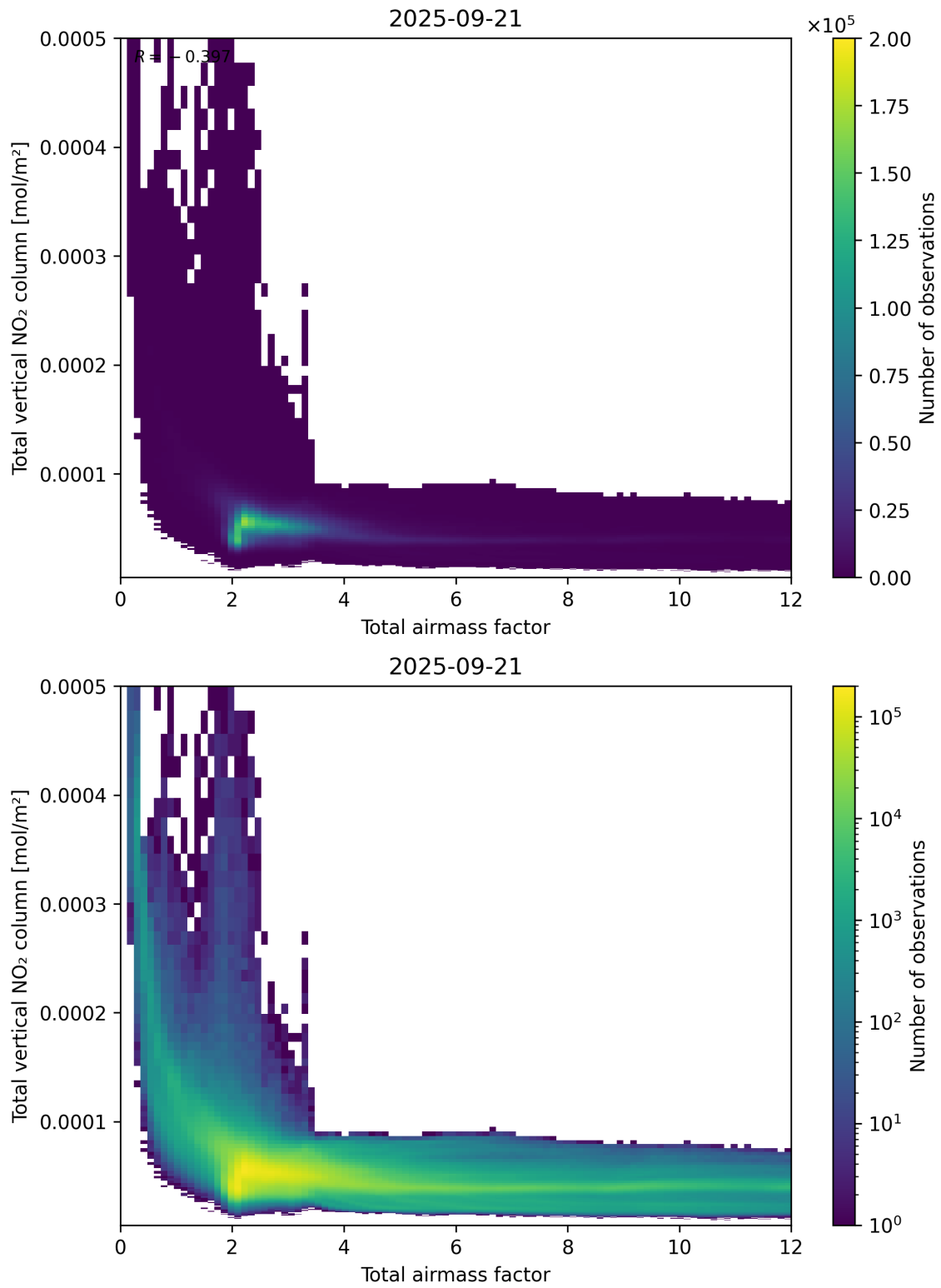
Figure 67: Scatter density plot of “Total airmass factor” against “Total vertical NO 2 column” for 2025-09-20 to 2025-09-22.
