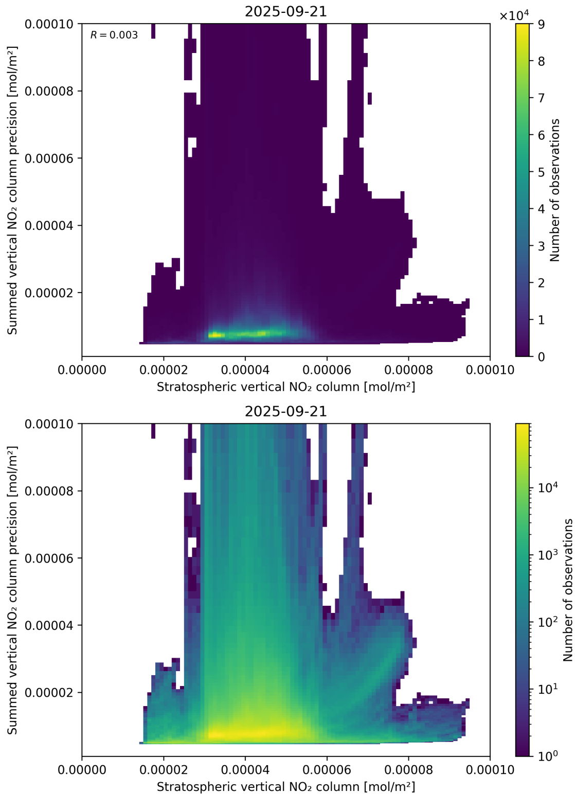
Figure 99: Scatter density plot of “Stratospheric vertical NO 2 column” against “Summed vertical NO 2 column precision” for 2025-09-20 to 2025-09-22.
