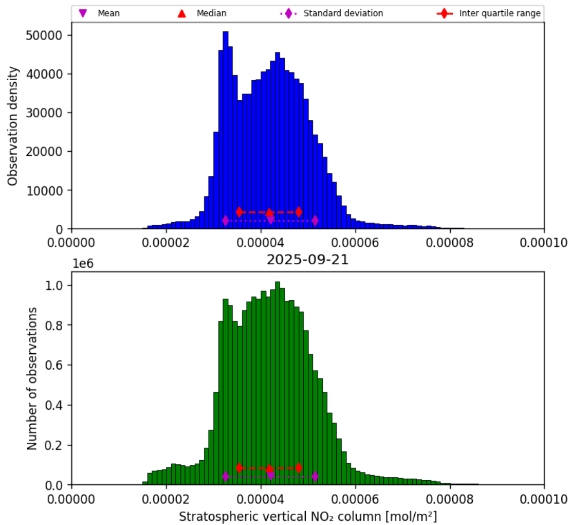
Figure 36: Histogram of “Stratospheric vertical NO 2 column” for 2025-09-20 to 2025-09-22
