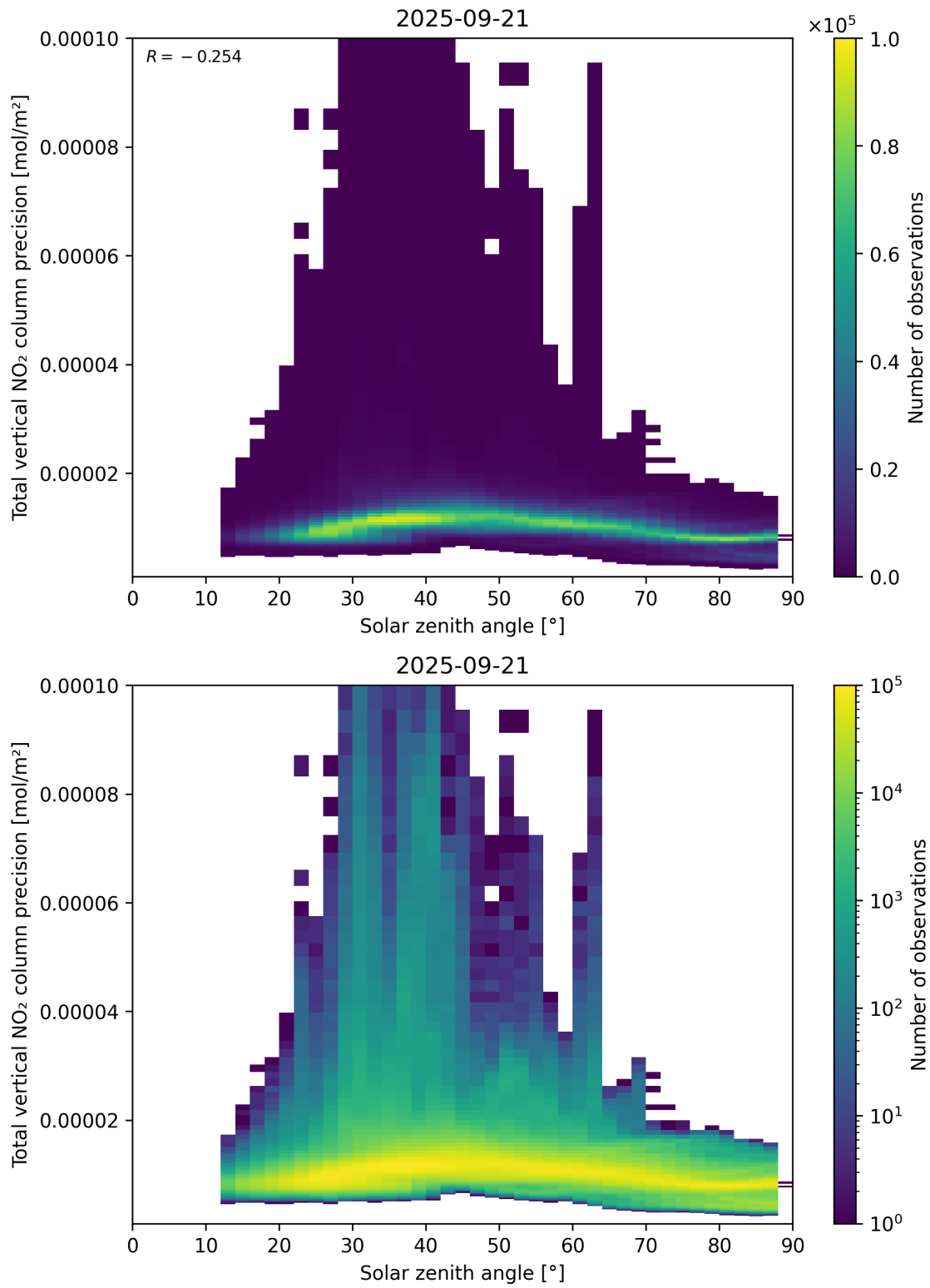
Figure 154: Scatter density plot of “Solar zenith angle” against “Total vertical NO 2 column precision” for 2025-09-20 to 2025-09-22.
