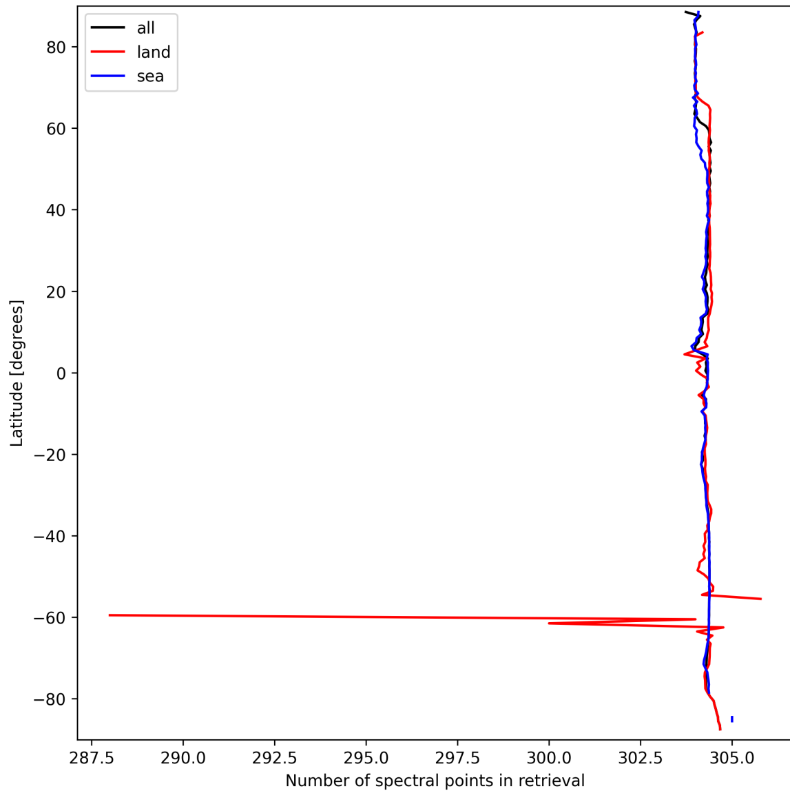
Figure 16: Zonal average of “Number of spectral points in retrieval” for 2025-09-20 to 2025-09-22.
