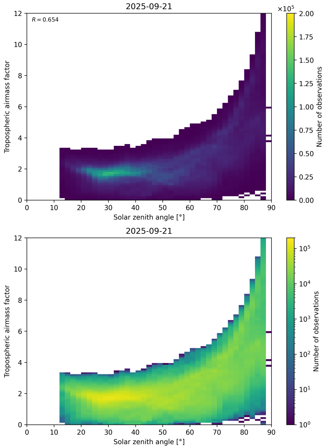
Figure 147: Scatter density plot of “Solar zenith angle” against “Tropospheric airmass factor” for 2025-09-20 to 2025-09-22.
