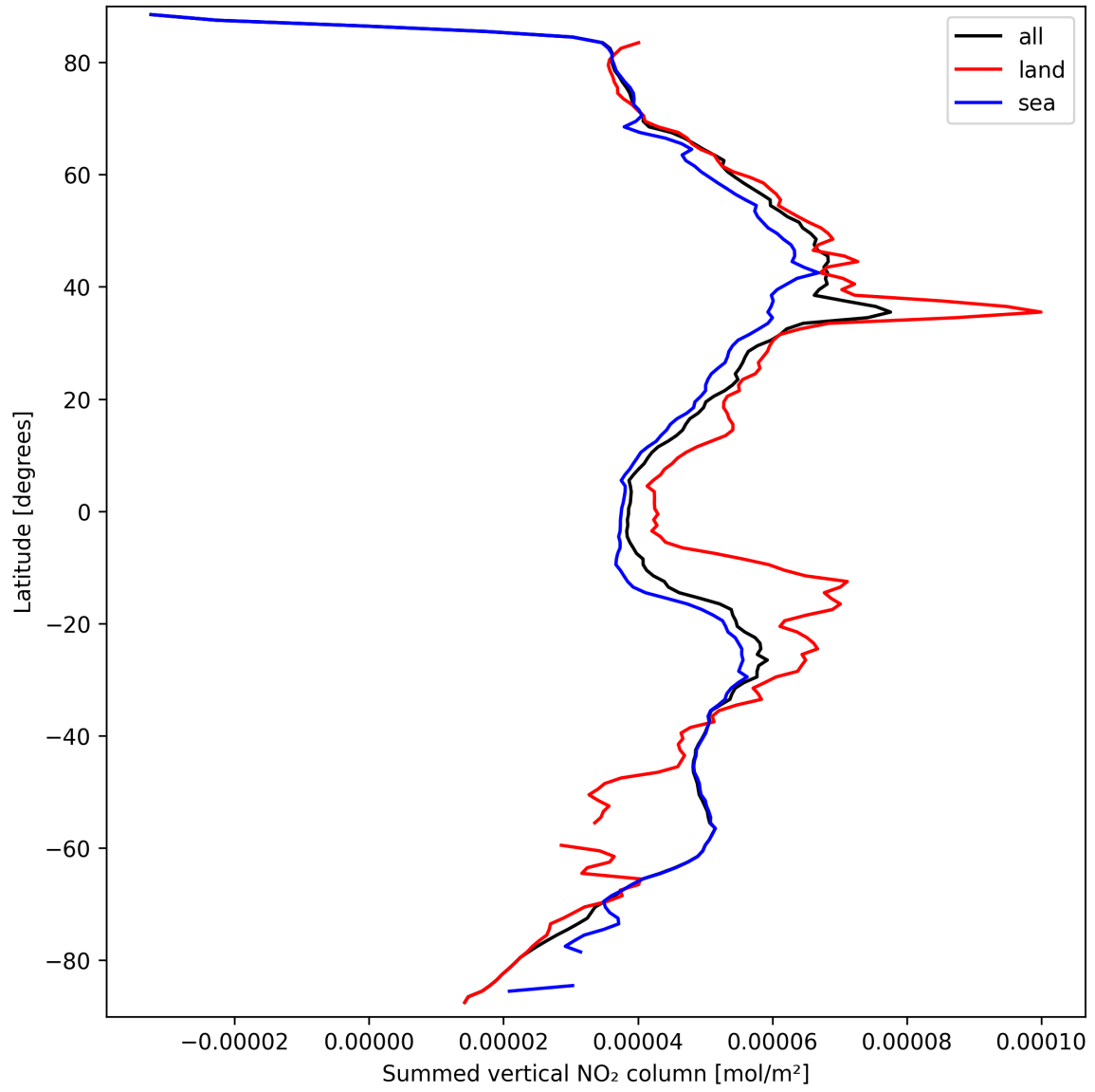
Figure 23: Zonal average of “Summed vertical NO 2 column” for 2025-09-20 to 2025-09-22.
