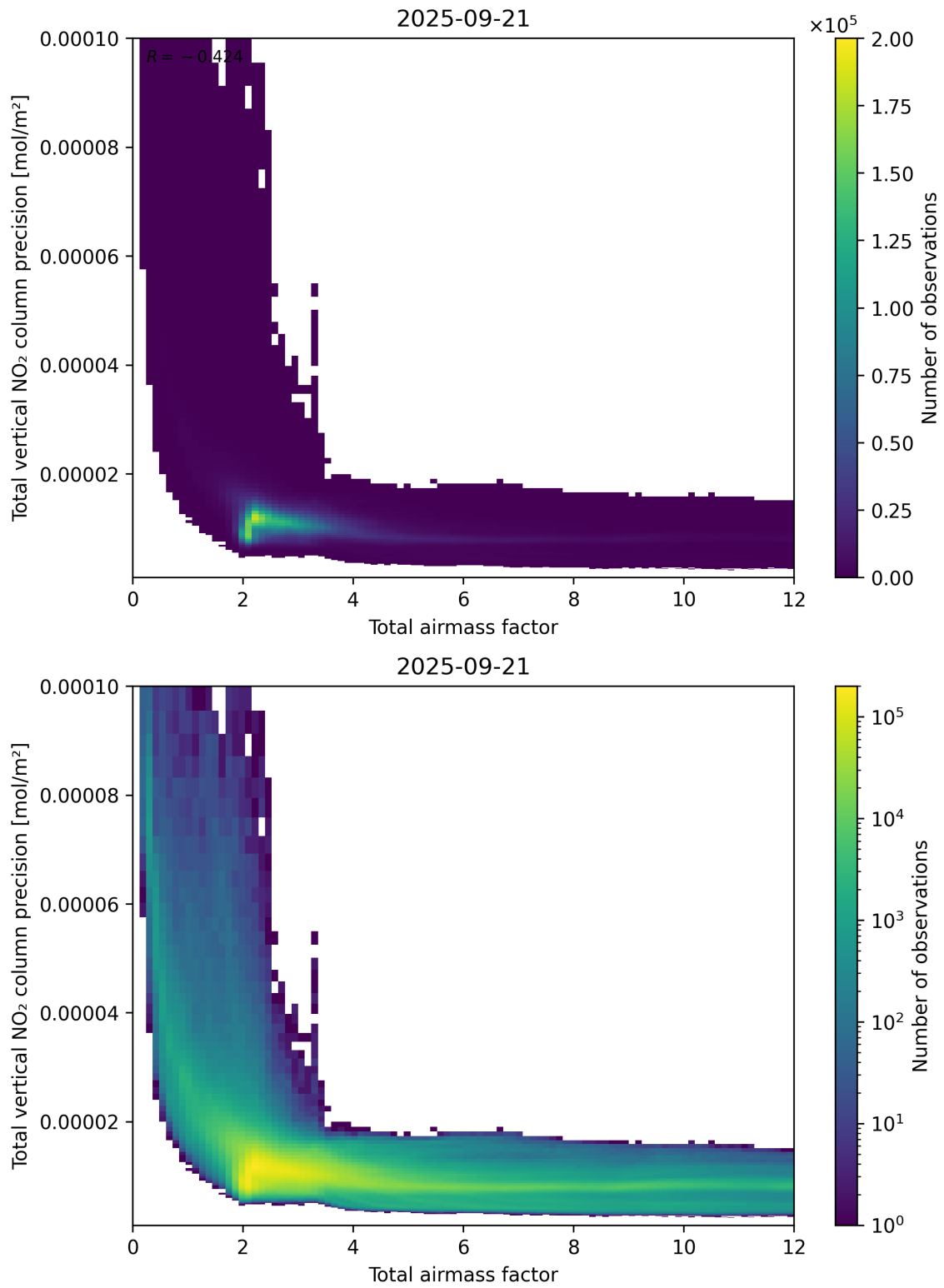
Figure 68: Scatter density plot of “Total airmass factor” against “Total vertical NO 2 column precision” for 2025-09-20 to 2025-09-22.
