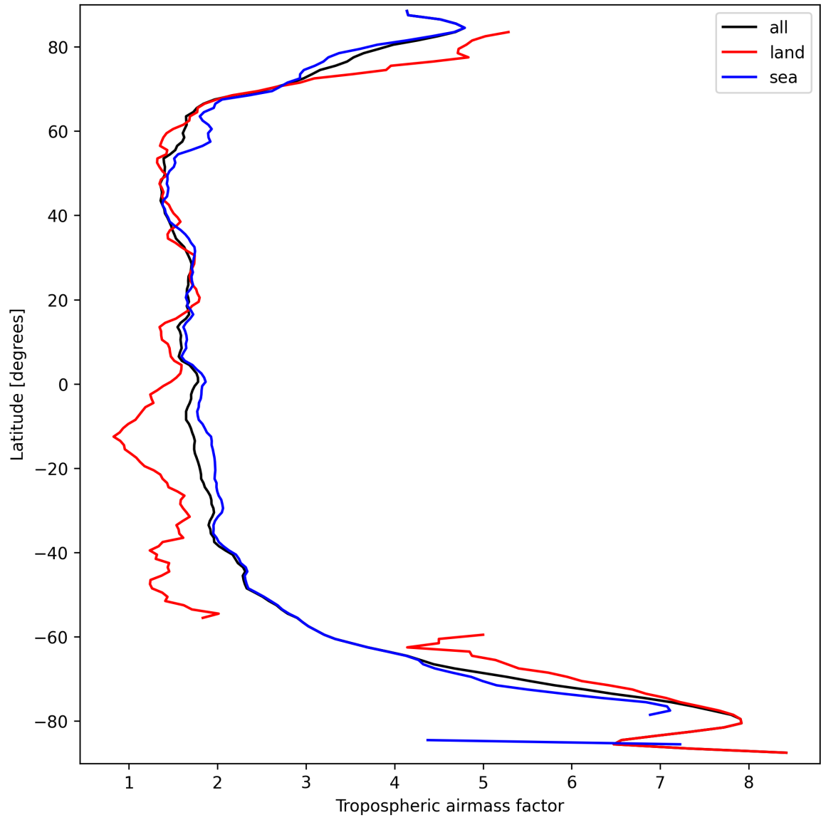
Figure 14: Zonal average of “Tropospheric airmass factor” for 2025-09-20 to 2025-09-22.
