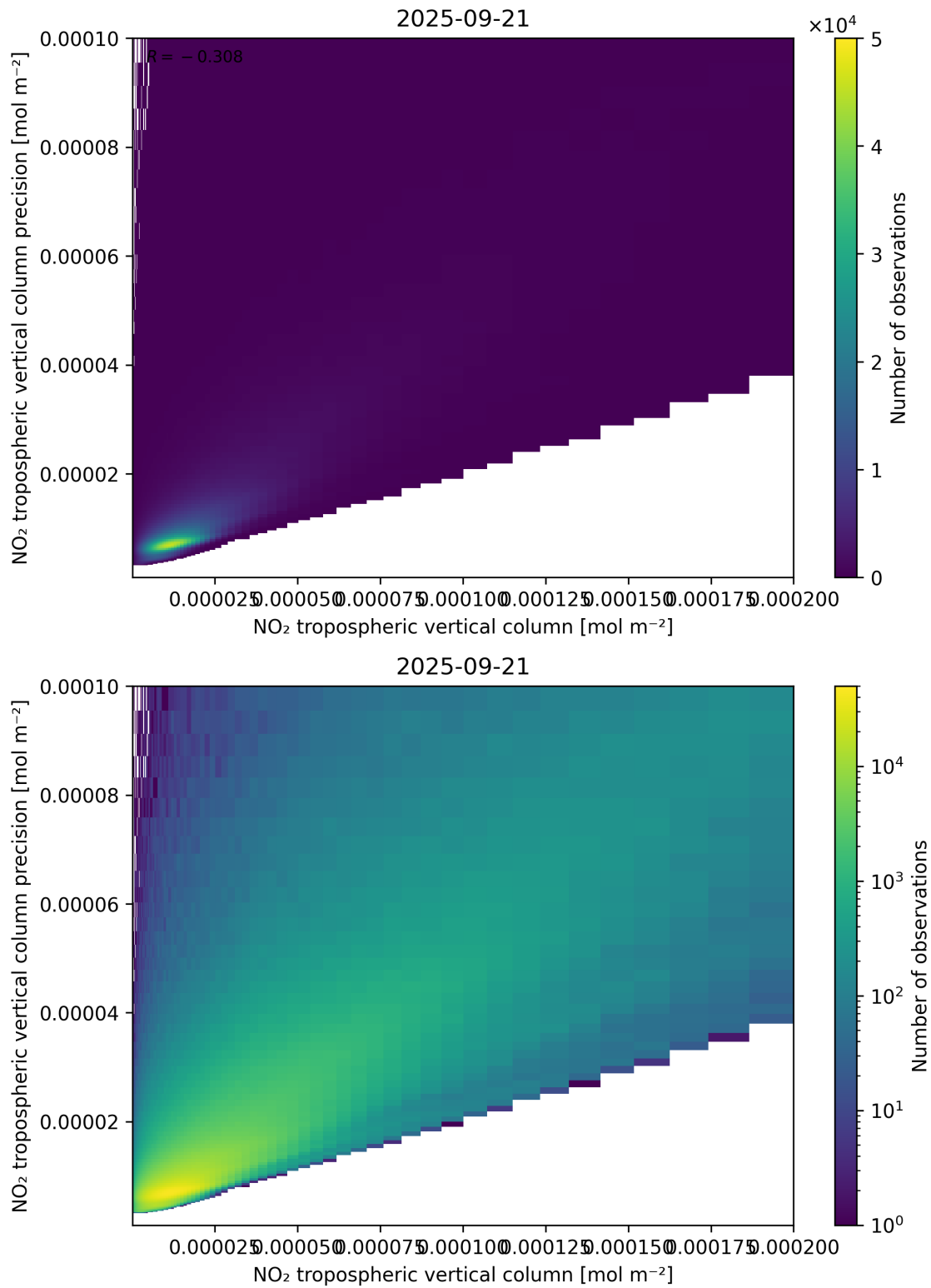
Figure 130: Scatter density plot of “NO 2 tropospheric vertical column” against “NO 2 tropospheric vertical column precision” for 2025-09-20 to 2025-09-22.
