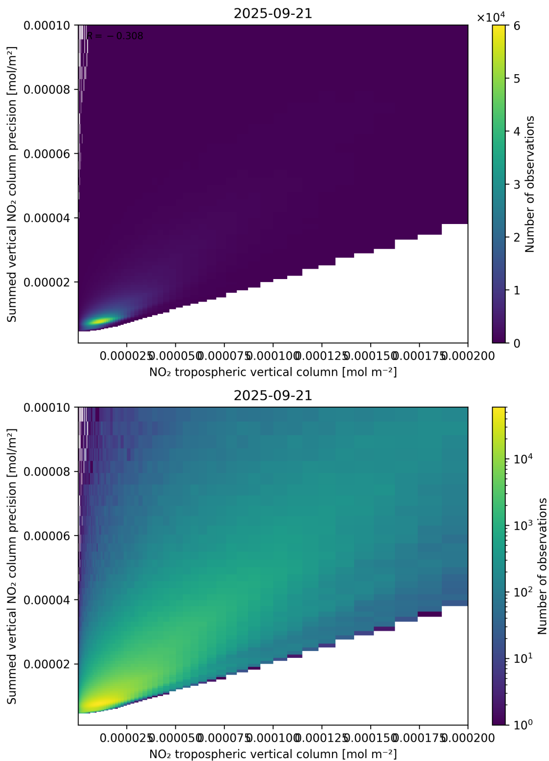
Figure 127: Scatter density plot of “NO 2 tropospheric vertical column” against “Summed vertical NO 2 column precision” for 2025-09-20 to 2025-09-22.
