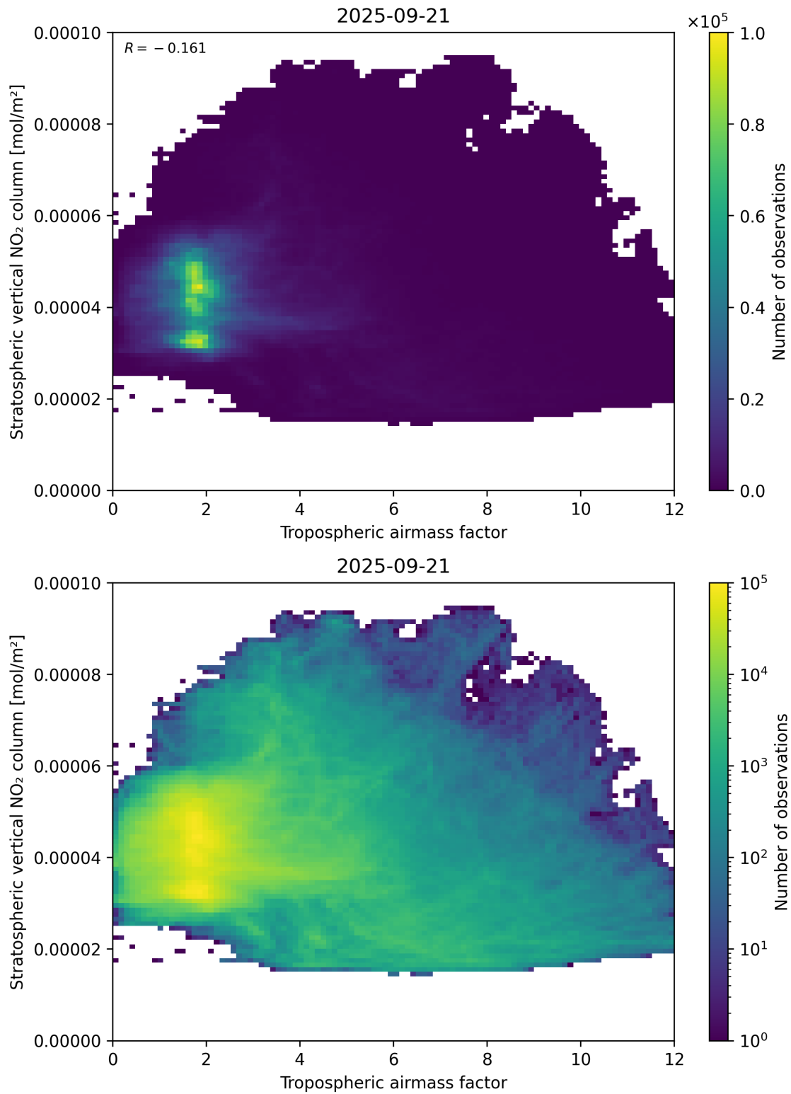
Figure 74: Scatter density plot of “Tropospheric airmass factor” against “Stratospheric vertical NO 2 column” for 2025-09-20 to 2025-09-22.
