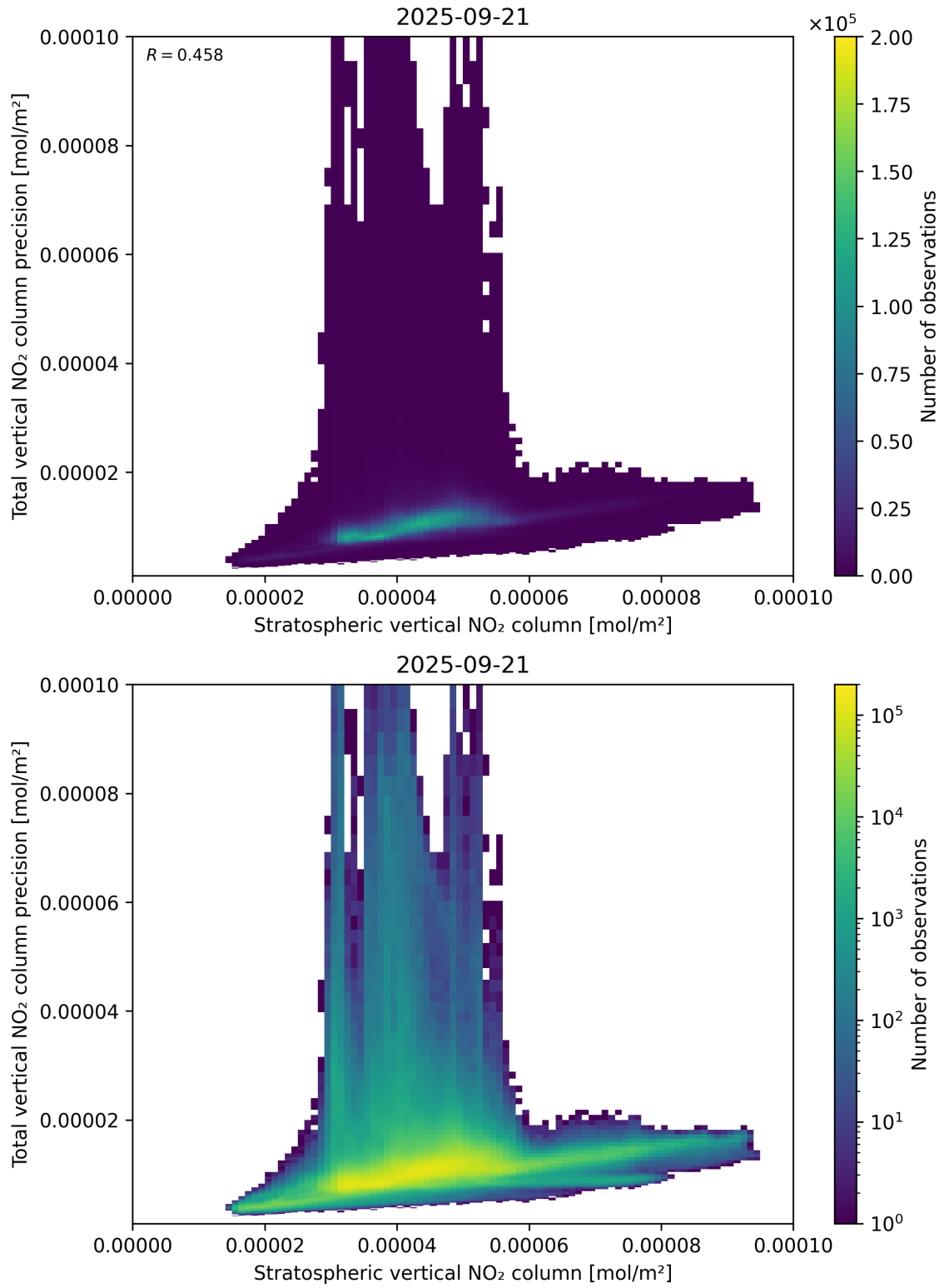
Figure 101: Scatter density plot of “Stratospheric vertical NO 2 column” against “Total vertical NO 2 column precision” for 2025-09-20 to 2025-09-22.
