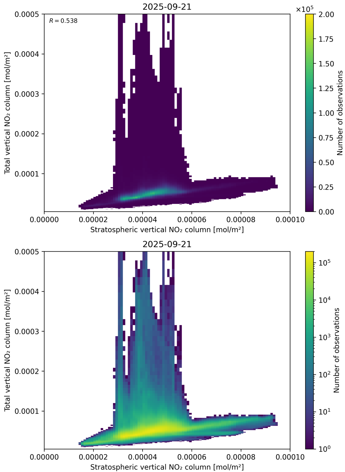
Figure 100: Scatter density plot of “Stratospheric vertical NO 2 column” against “Total vertical NO 2 column” for 2025-09-20 to 2025-09-22.
