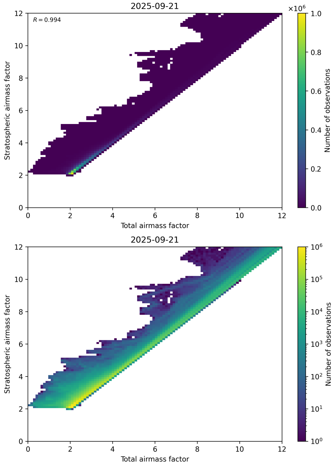
Figure 62: Scatter density plot of “Total airmass factor” against “Stratospheric airmass factor” for 2025-09-20 to 2025-09-22.
