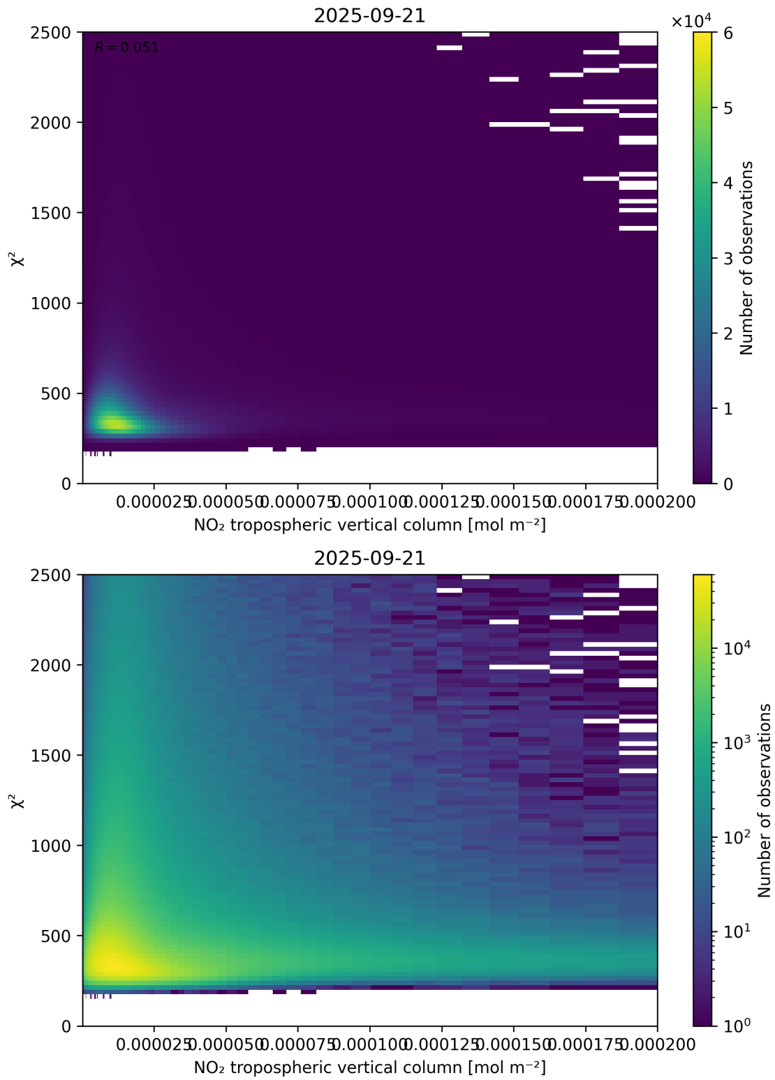
Figure 124: Scatter density plot of “NO 2 tropospheric vertical column” against “ \chi^2 ” for 2025-09-20 to 2025-09-22.
