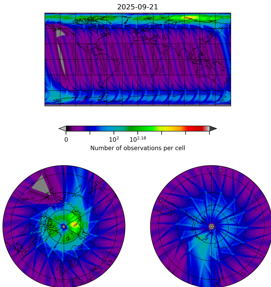
Figure 10: Map of the number of observations for 2025-09-20 to 2025-09-22
