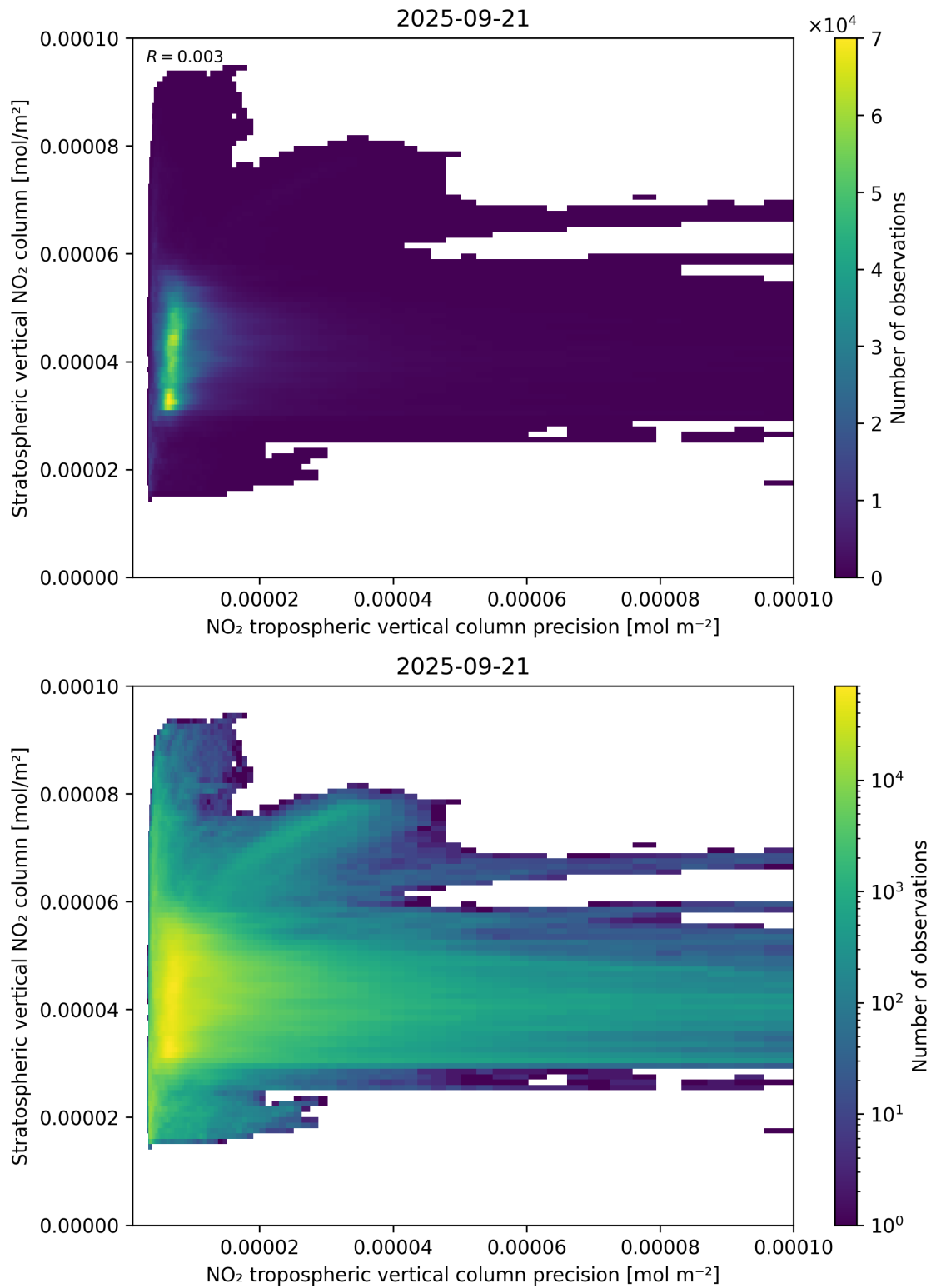
Figure 135: Scatter density plot of “NO 2 tropospheric vertical column precision” against “Stratospheric vertical NO 2 column” for 2025-09-20 to 2025-09-22.
