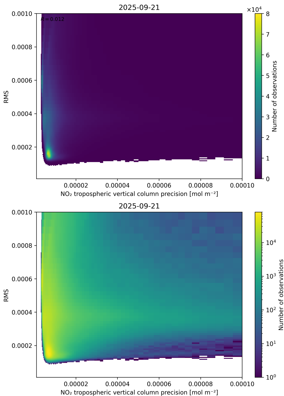
Figure 140: Scatter density plot of “NO 2 tropospheric vertical column precision” against “RMS” for 2025-09-20 to 2025-09-22.
