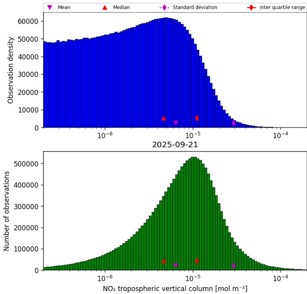
Figure 29: Histogram of “NO 2 tropospheric vertical column” for 2025-09-20 to 2025-09-22
