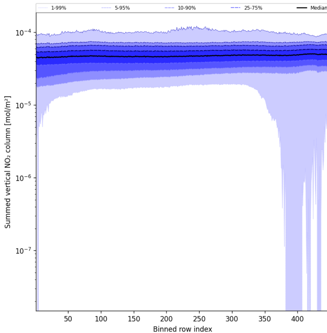
Figure 57: Along track statistics of “Summed vertical NO 2 column” for 2025-09-20 to 2025-09-22
