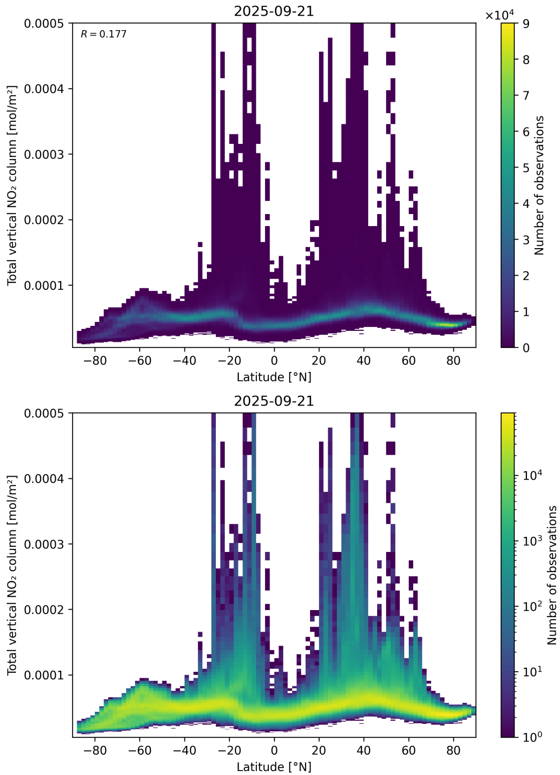
Figure 90: Scatter density plot of “Latitude” against “Total vertical NO 2 column” for 2025-09-20 to 2025-09-22.
