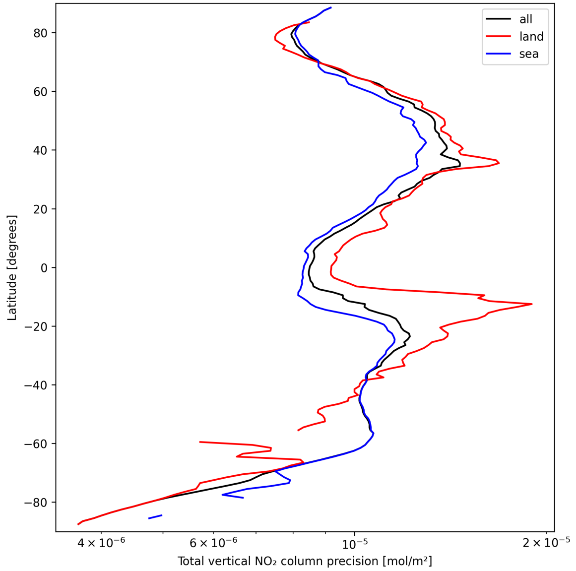
Figure 22: Zonal average of “Total vertical NO 2 column precision” for 2025-09-20 to 2025-09-22.
