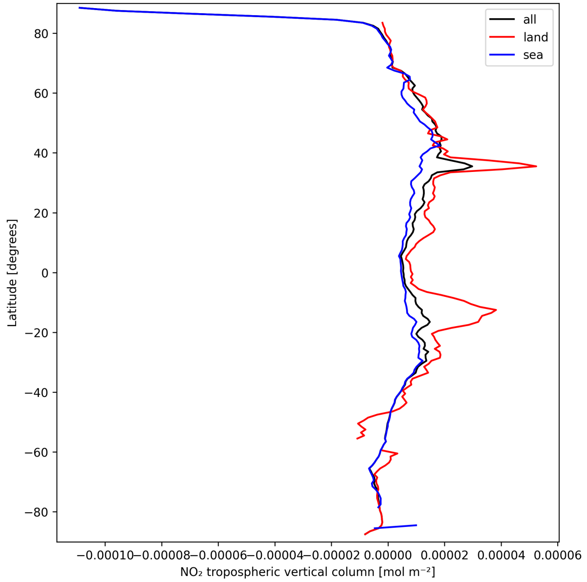
Figure 12: Zonal average of “NO 2 tropospheric vertical column” for 2025-09-20 to 2025-09-22.
