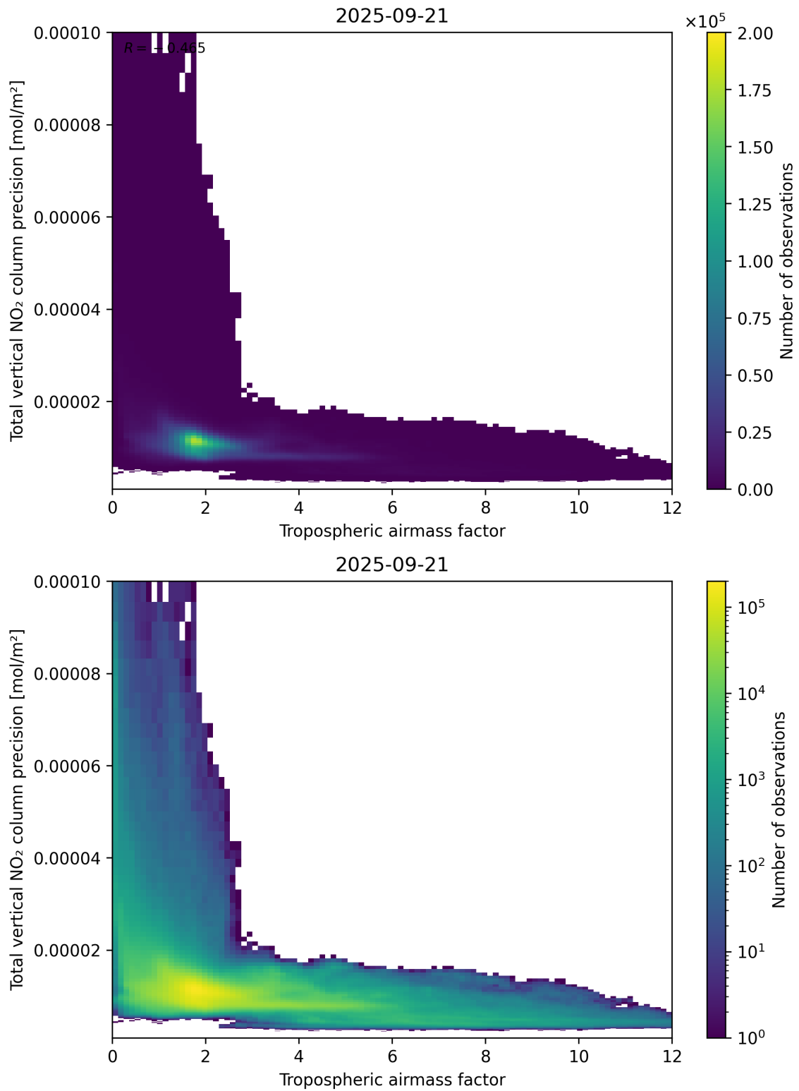
Figure 78: Scatter density plot of “Tropospheric airmass factor” against “Total vertical NO 2 column precision” for 2025-09-20 to 2025-09-22.
