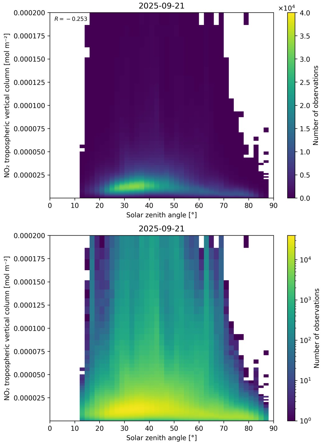
Figure 155: Scatter density plot of “Solar zenith angle” against “NO 2 tropospheric vertical column” for 2025-09-20 to 2025-09-22.
