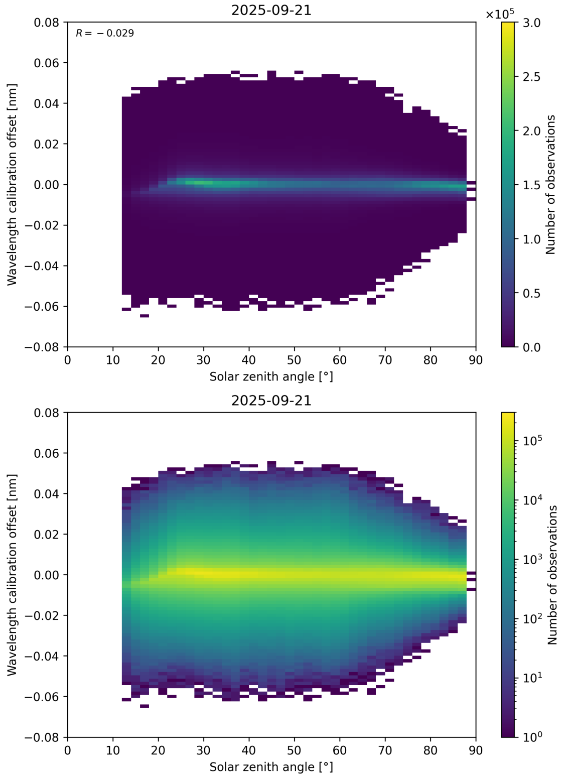
Figure 158: Scatter density plot of “Solar zenith angle” against “Wavelength calibration offset” for 2025-09-20 to 2025-09-22.
