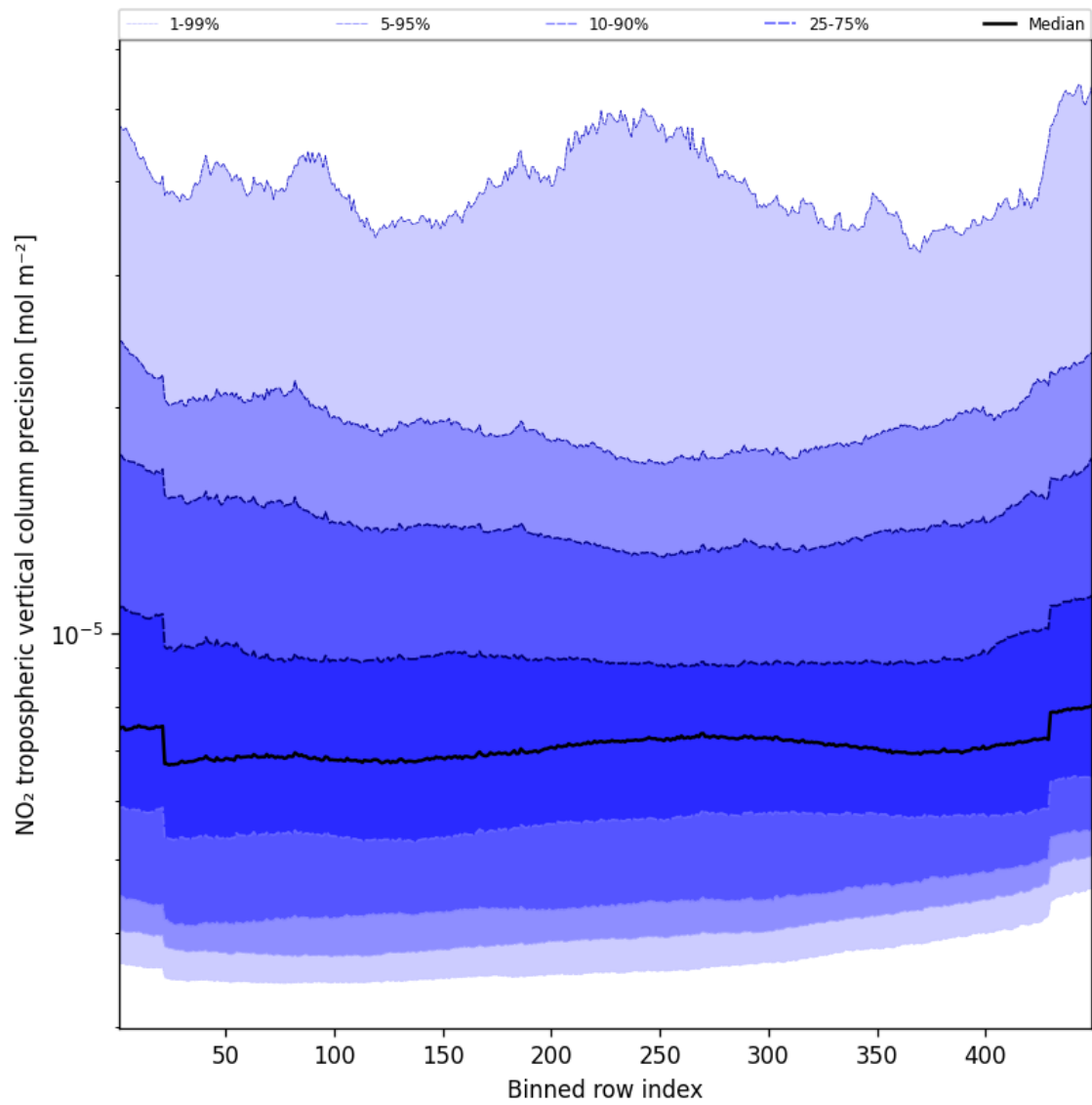
Figure 47: Along track statistics of “NO 2 tropospheric vertical column precision” for 2025-09-20 to 2025-09-22
