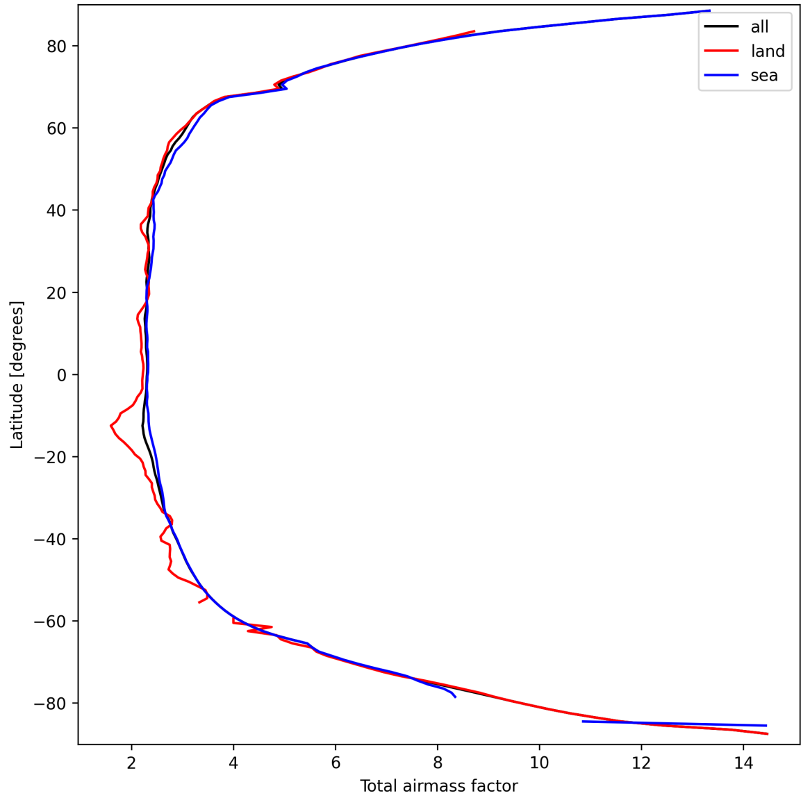
Figure 15: Zonal average of “Total airmass factor” for 2025-09-20 to 2025-09-22.
