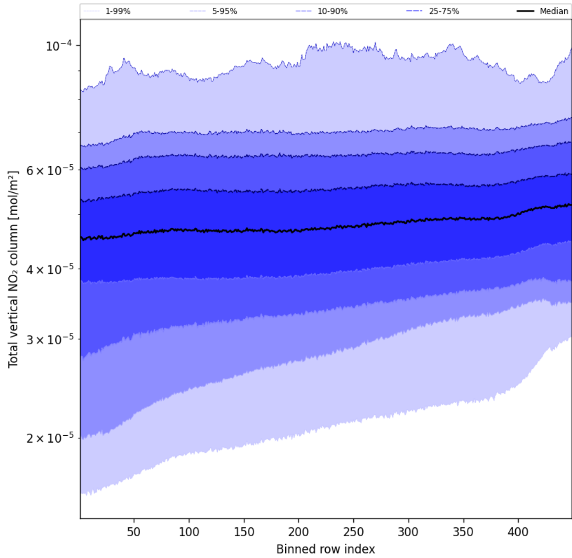
Figure 55: Along track statistics of “Total vertical NO 2 column” for 2025-09-20 to 2025-09-22
