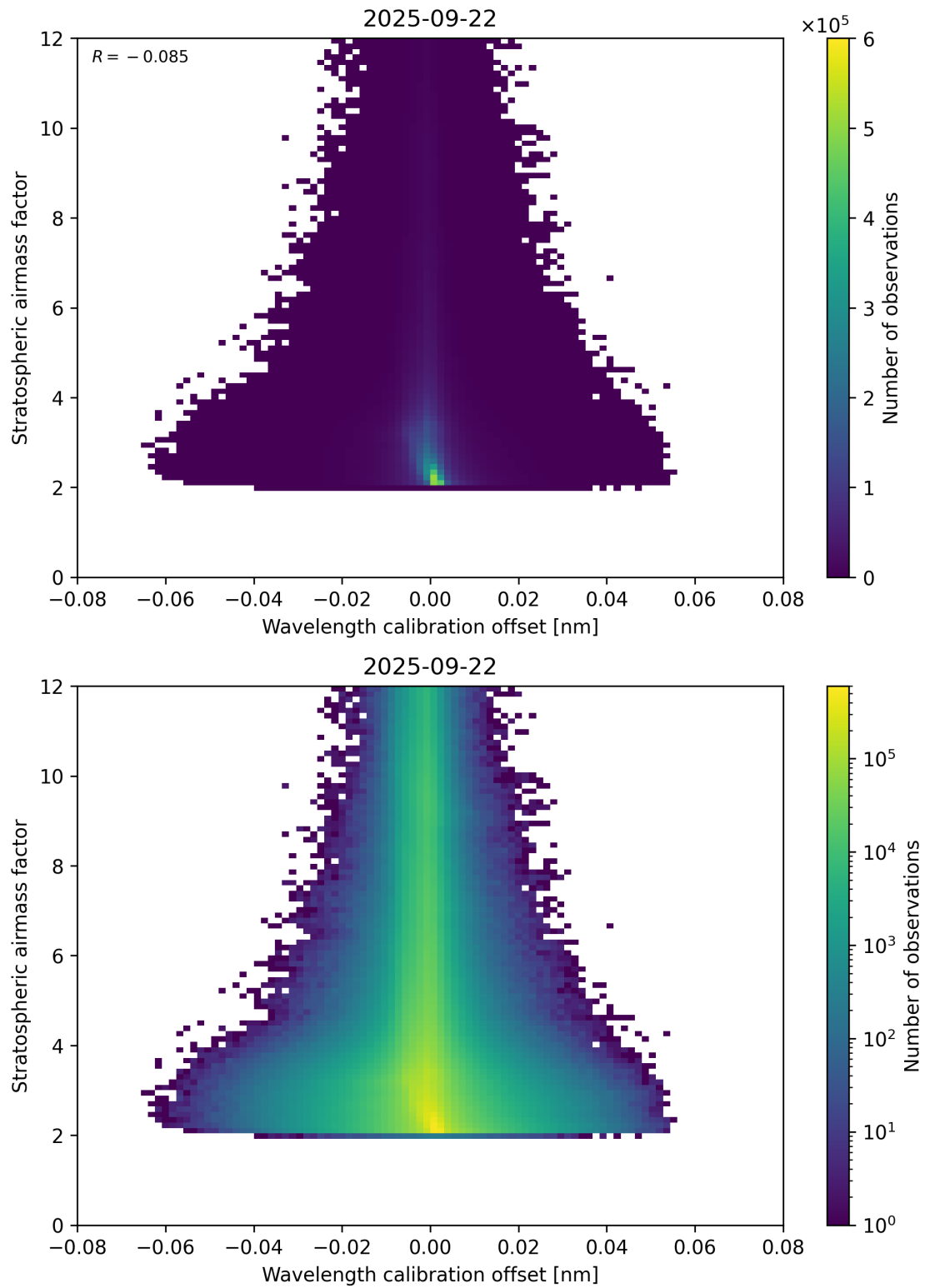
Figure 174: Scatter density plot of “Wavelength calibration offset” against “Stratospheric airmass factor” for 2025-09-22 to 2025-09-23.
