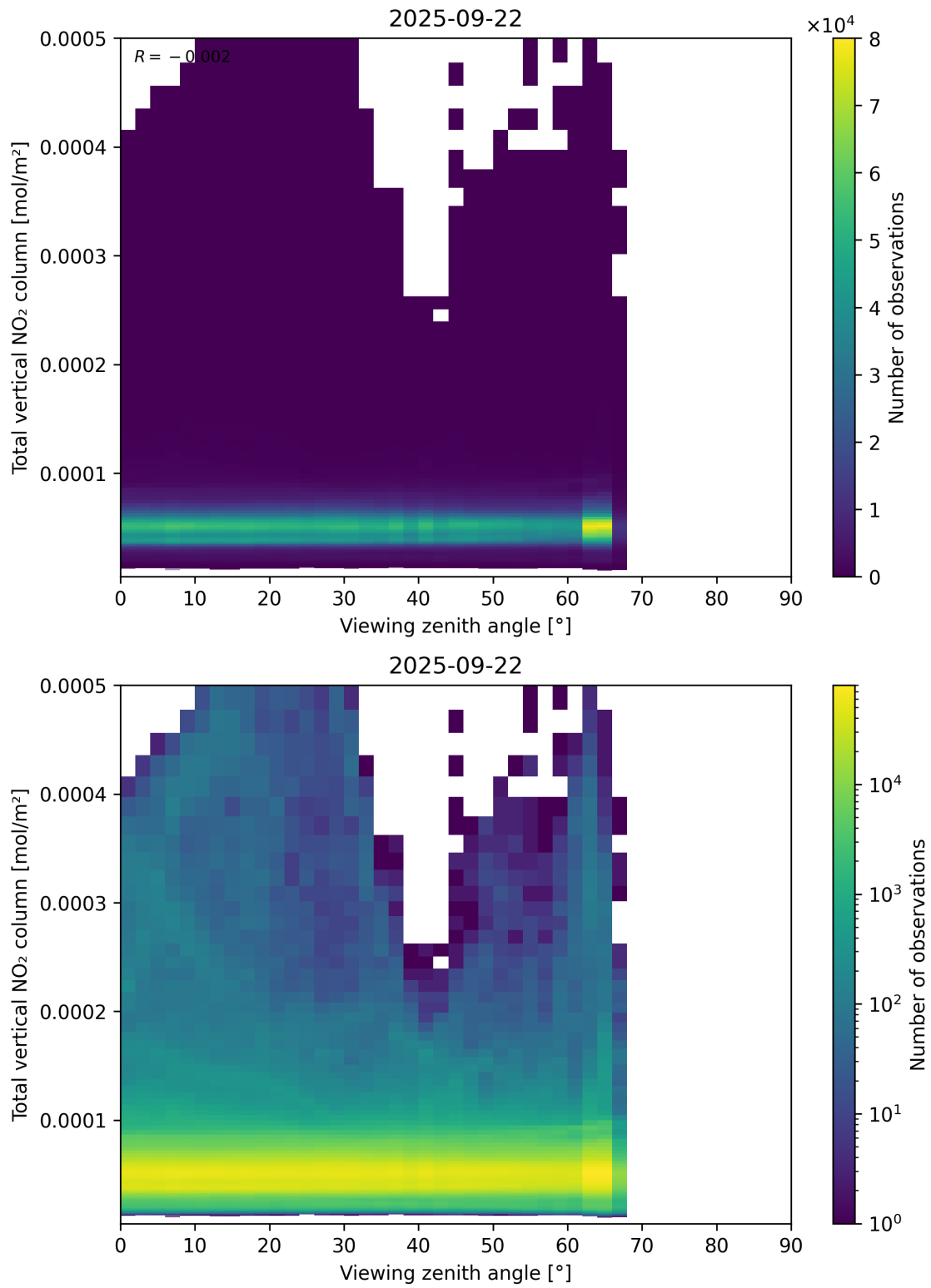
Figure 167: Scatter density plot of “Viewing zenith angle” against “Total vertical NO 2 column” for 2025-09-22 to 2025-09-23.
