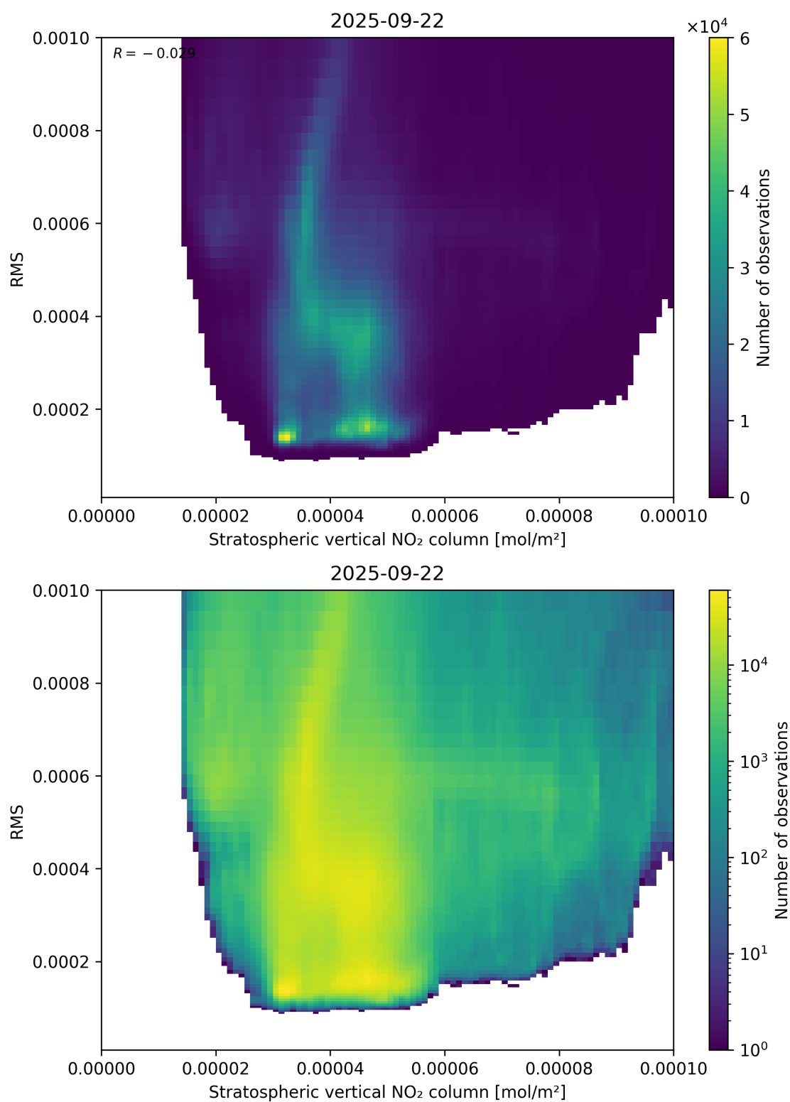
Figure 102: Scatter density plot of “Stratospheric vertical NO 2 column” against “RMS” for 2025-09-22 to 2025-09-23.
