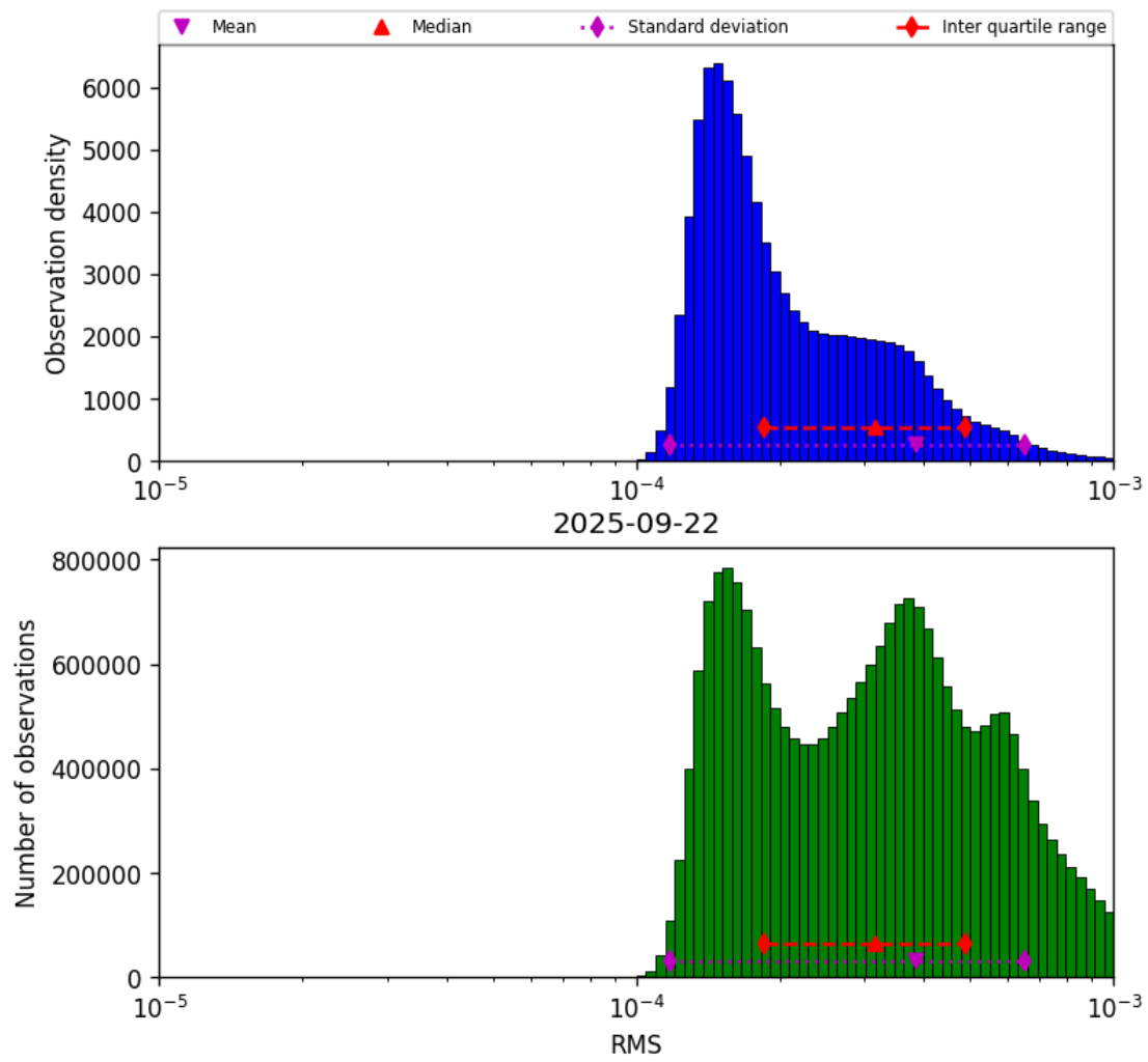
Figure 43: Histogram of “RMS” for 2025-09-22 to 2025-09-23
