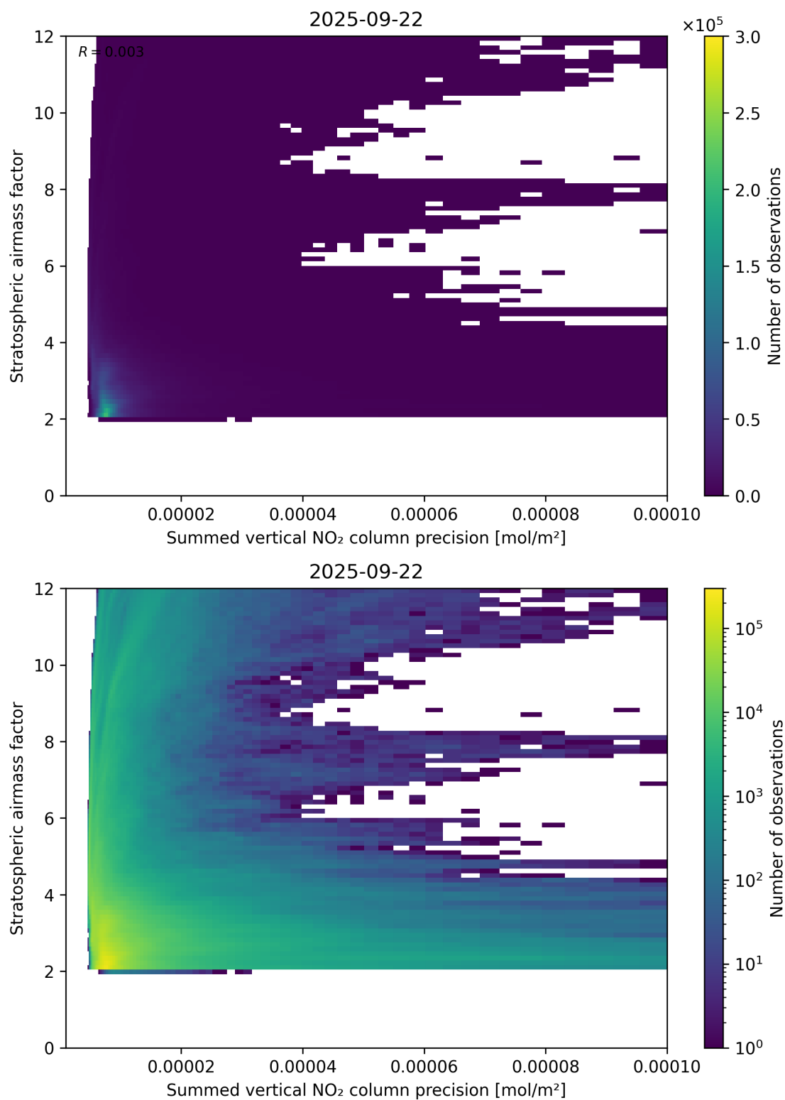
Figure 106: Scatter density plot of “Summed vertical NO 2 column precision” against “Stratospheric airmass factor” for 2025-09-22 to 2025-09-23.
