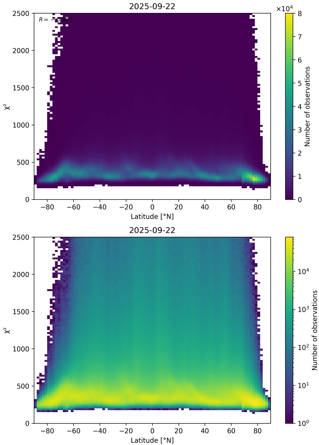
Figure 86: Scatter density plot of “Latitude” against “ \chi^2 ” for 2025-09-22 to 2025-09-23.
