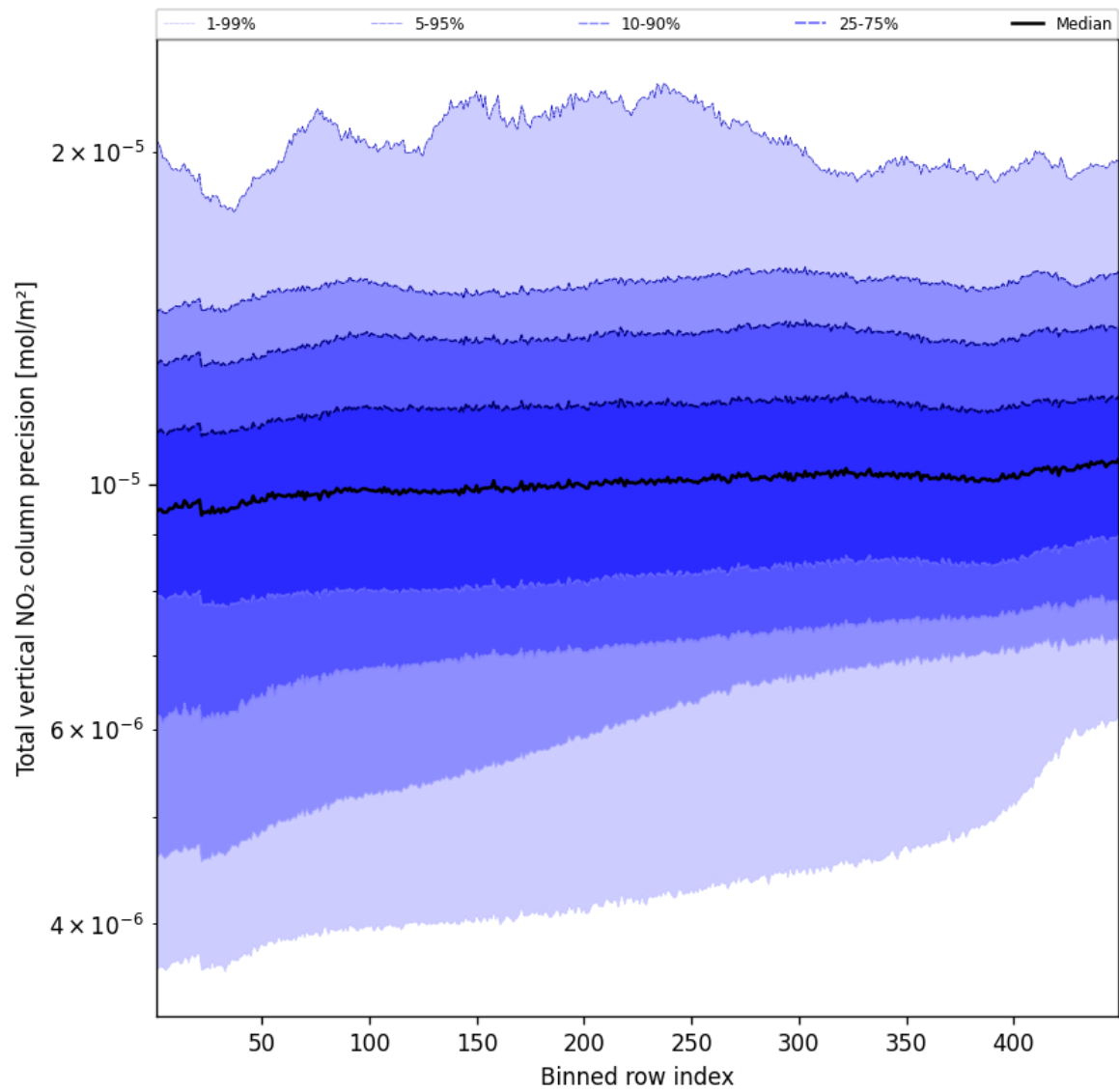
Figure 56: Along track statistics of "Total vertical NO 2 column precision" for 2025-09-22 to 2025-09-23
