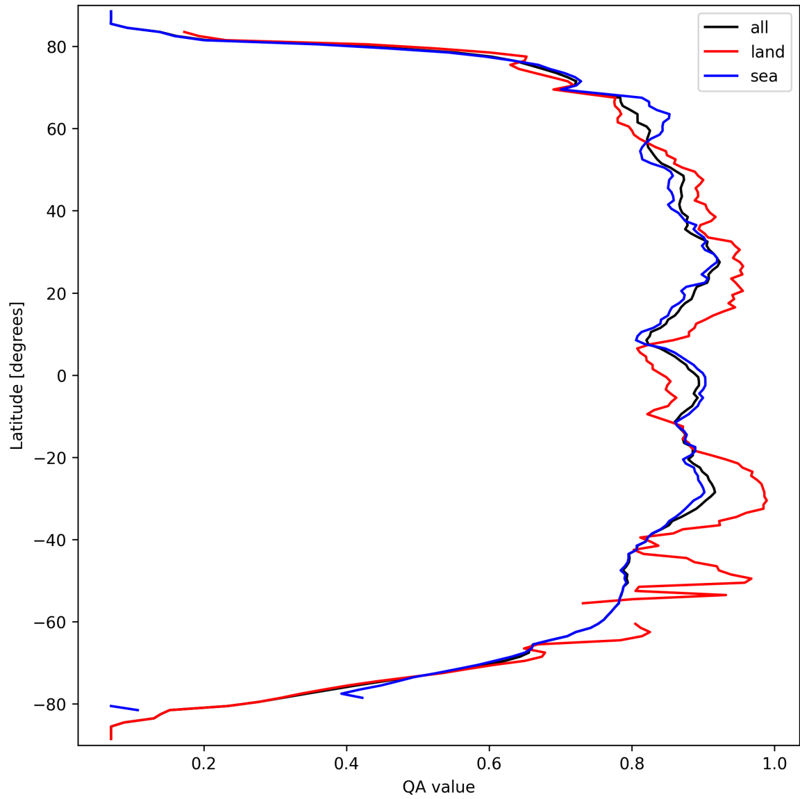
Figure 11: Zonal average of “QA value” for 2025-09-22 to 2025-09-23.
