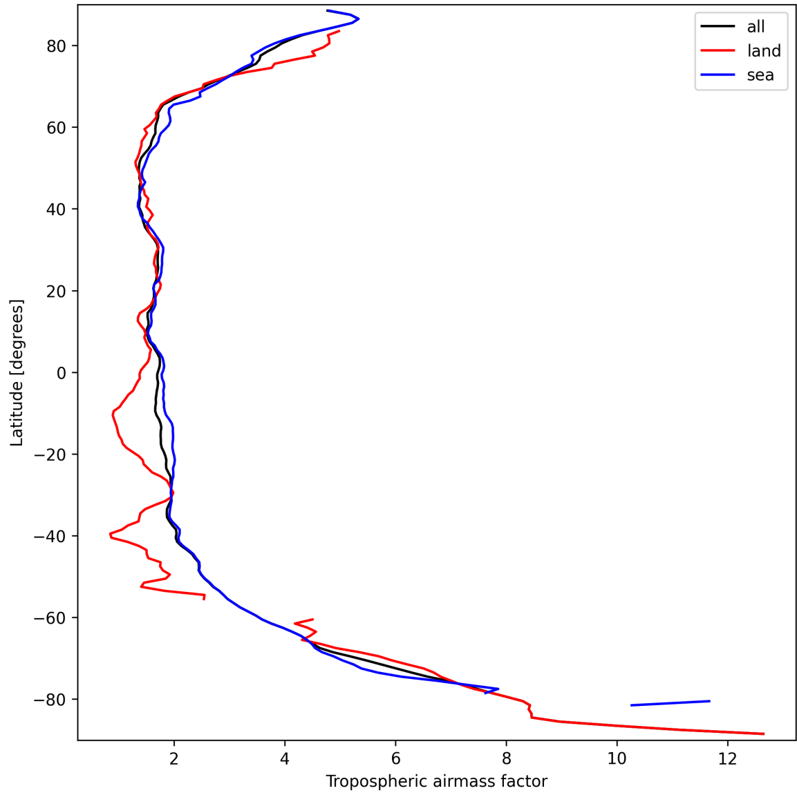
Figure 14: Zonal average of “Tropospheric airmass factor” for 2025-09-22 to 2025-09-23.
