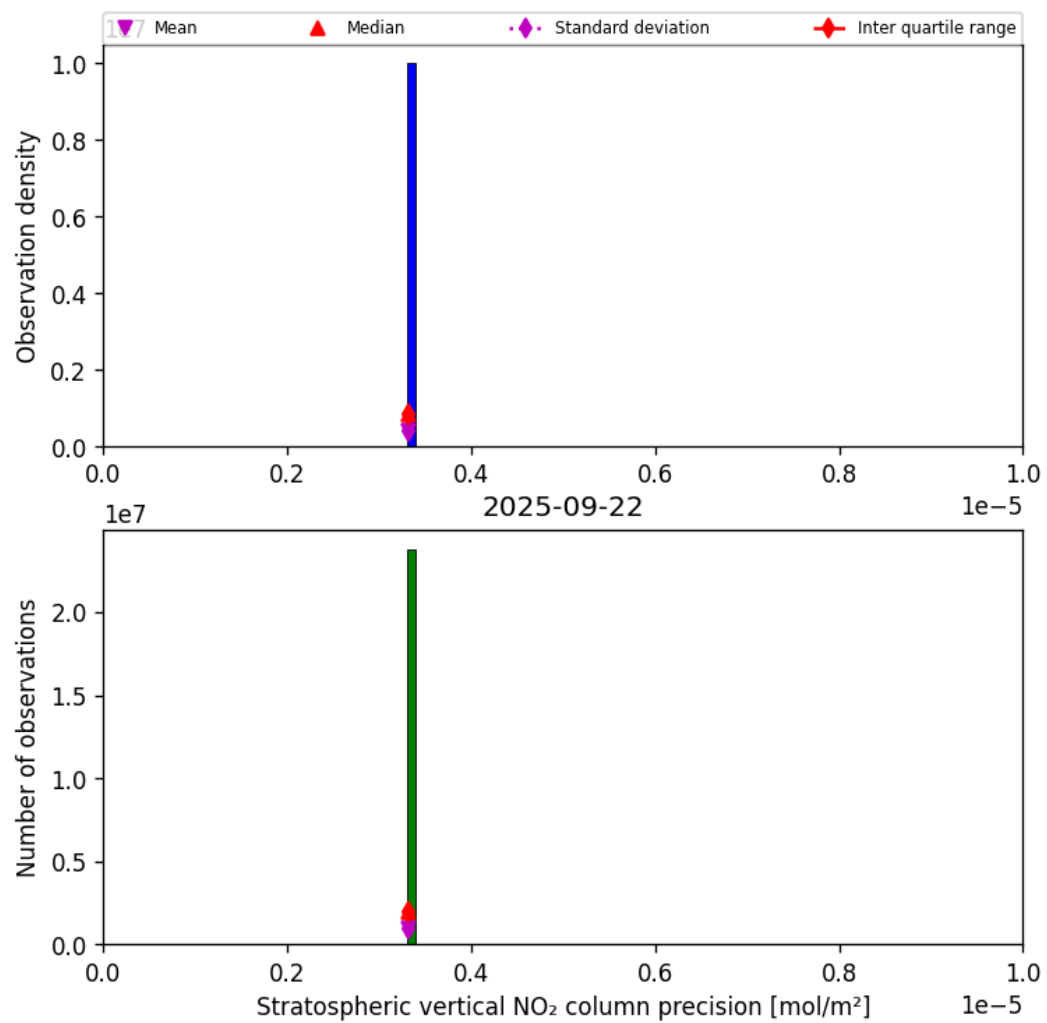
Figure 37: Histogram of “Stratospheric vertical NO 2 column precision” for 2025-09-22 to 2025-09-23
