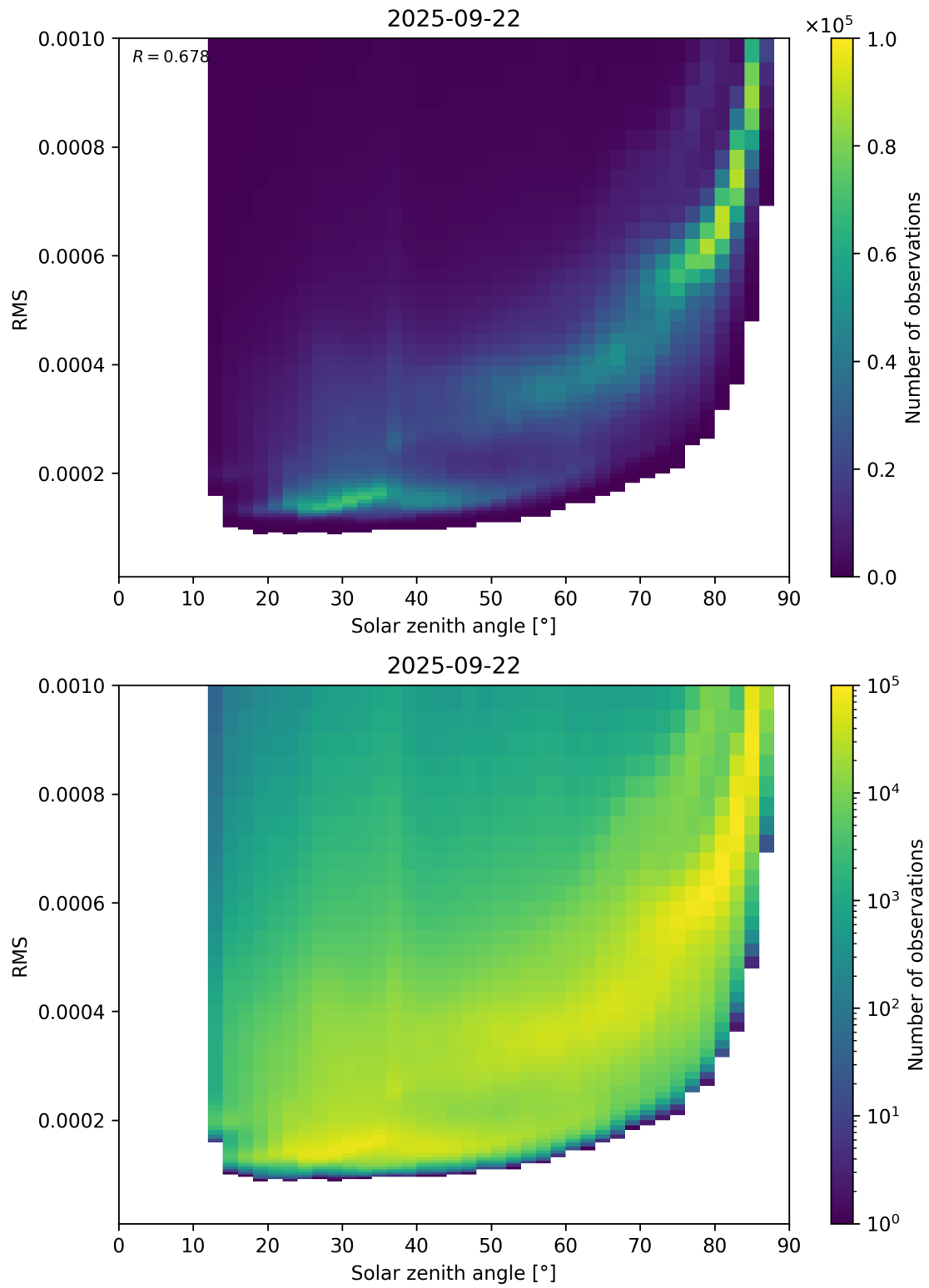
Figure 157: Scatter density plot of “Solar zenith angle” against “RMS” for 2025-09-22 to 2025-09-23.
