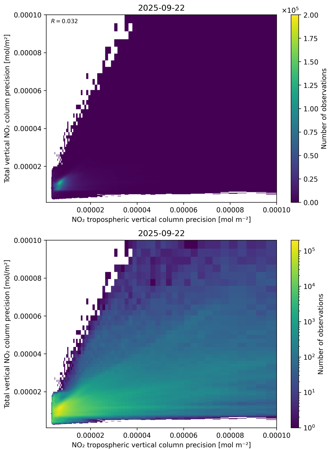
Figure 139: Scatter density plot of “NO 2 tropospheric vertical column precision” against “Total vertical NO 2 column precision” for 2025-09-22 to 2025-09-23.
