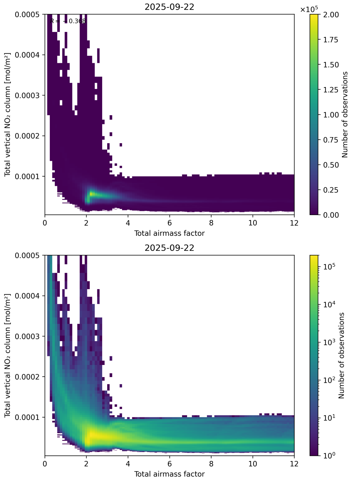
Figure 67: Scatter density plot of “Total airmass factor” against “Total vertical NO 2 column” for 2025-09-22 to 2025-09-23.
