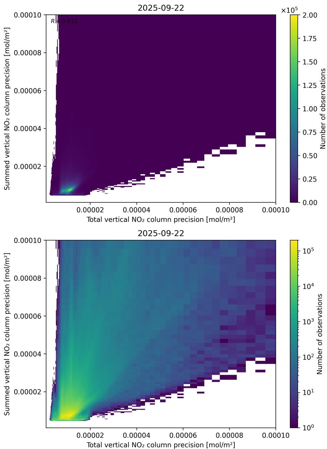
Figure 118: Scatter density plot of “Total vertical NO 2 column precision” against “Summed vertical NO 2 column precision” for 2025-09-22 to 2025-09-23.
