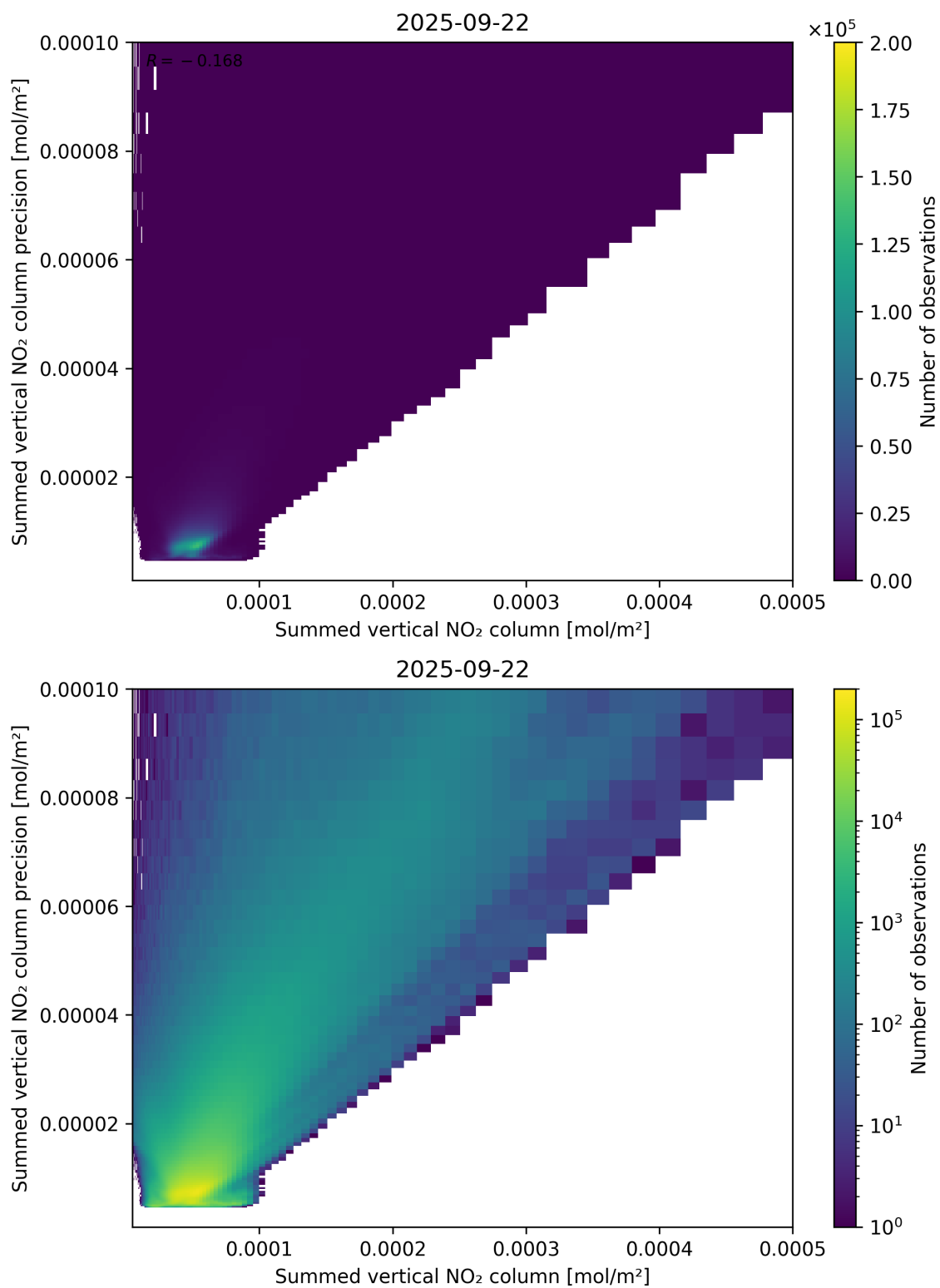
Figure 105: Scatter density plot of “Summed vertical NO 2 column” against “Summed vertical NO 2 column precision” for 2025-09-22 to 2025-09-23.
