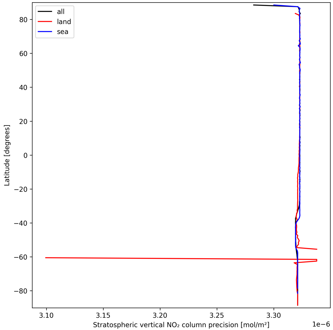
Figure 20: Zonal average of “Stratospheric vertical NO 2 column precision” for 2025-09-22 to 2025-09-23.
