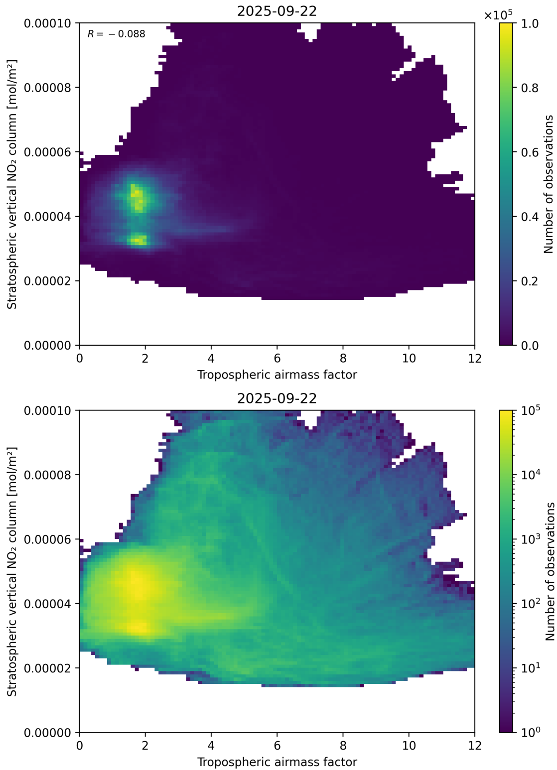
Figure 74: Scatter density plot of “Tropospheric air mass factor” against “Stratospheric vertical NO 2 column” for 2025-09-22 to 2025-09-23.
