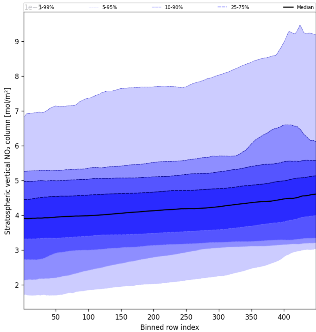
Figure 53: Along track statistics of “Stratospheric vertical NO 2 column” for 2025-09-22 to 2025-09-23
