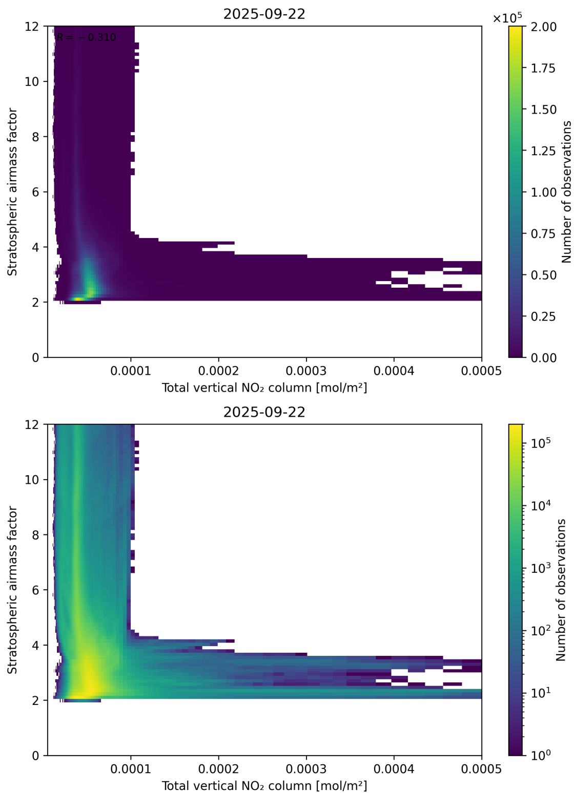
Figure 110: Scatter density plot of “Total vertical NO 2 column” against “Stratospheric air mass factor” for 2025-09-22 to 2025-09-23.
