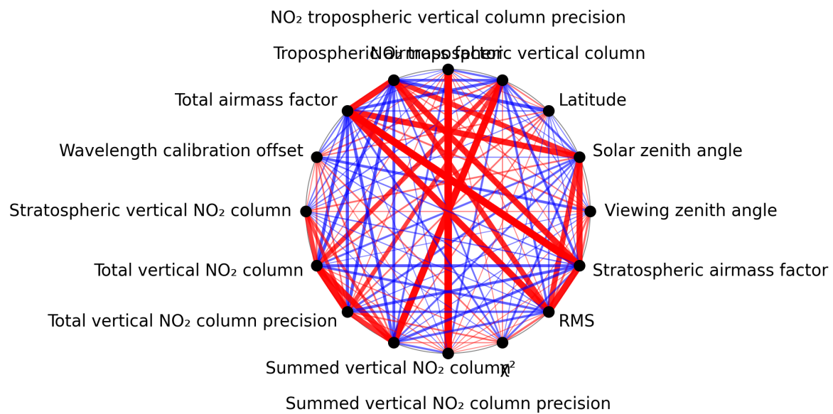
Figure 1: Map of correlation graph for 2025-09-22 to 2025-09-23.
