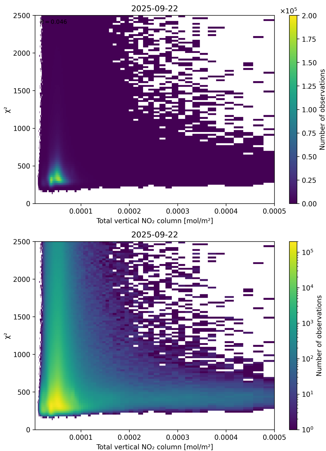
Figure 111: Scatter density plot of “Total vertical NO 2 column” against “ \chi^2 ” for 2025-09-22 to 2025-09-23.
