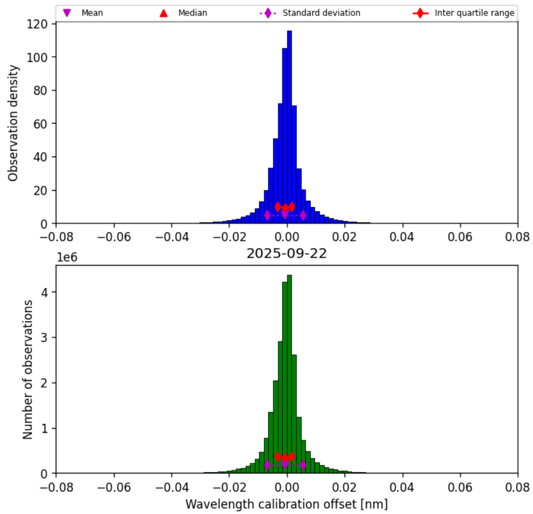
Figure 35: Histogram of “Wavelength calibration offset” for 2025-09-22 to 2025-09-23
