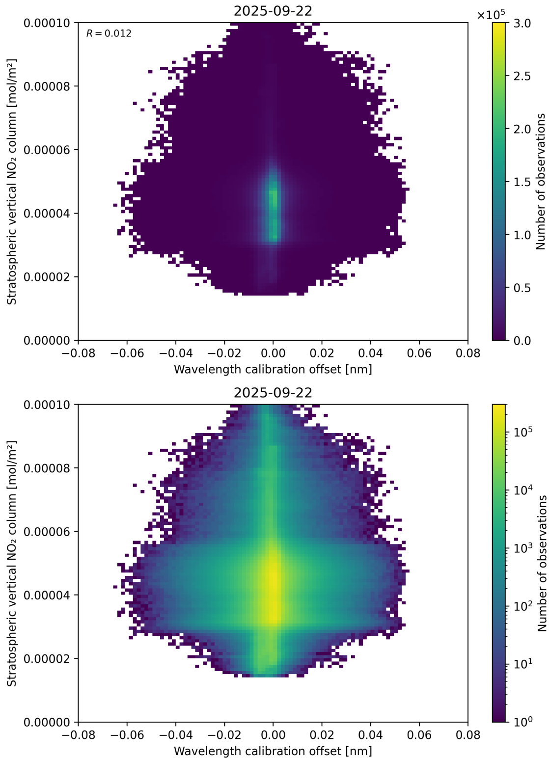
Figure 176: Scatter density plot of “Wavelength calibration offset” against “Stratospheric vertical NO 2 column” for 2025-09-22 to 2025-09-23.
