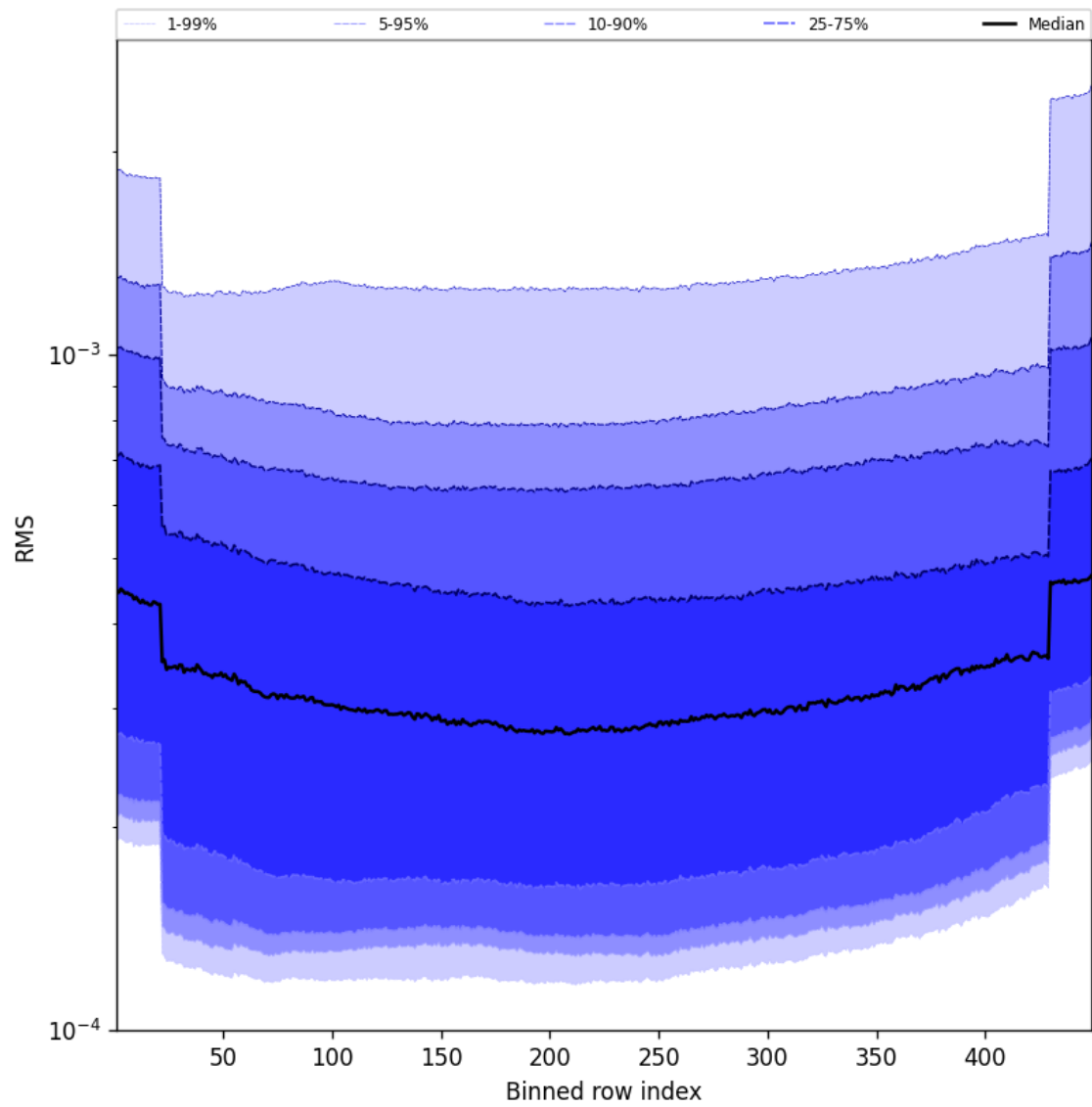
Figure 60: Along track statistics of “RMS” for 2025-09-22 to 2025-09-23
