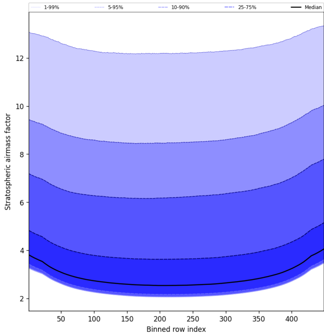
Figure 61: Along track statistics of “Stratospheric airmass factor” for 2025-09-22 to 2025-09-23
