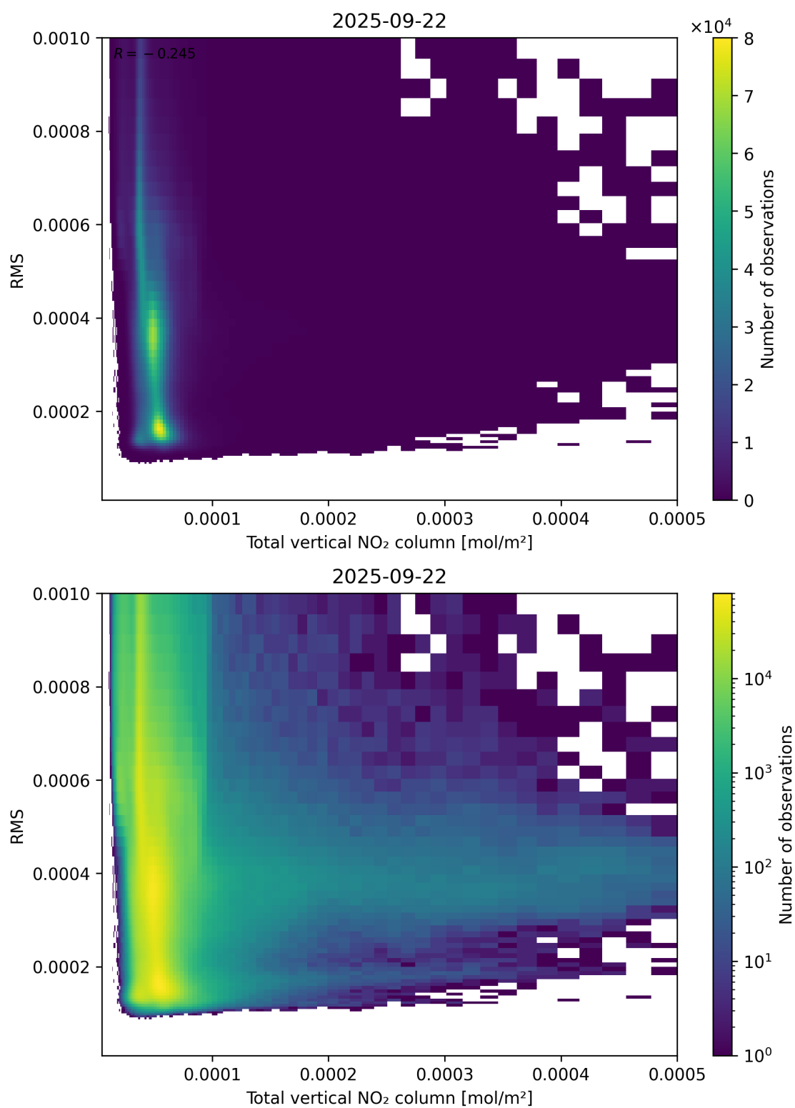
Figure 120: Scatter density plot of “Total vertical NO 2 column” against “RMS” for 2025-09-22 to 2025-09-23.
