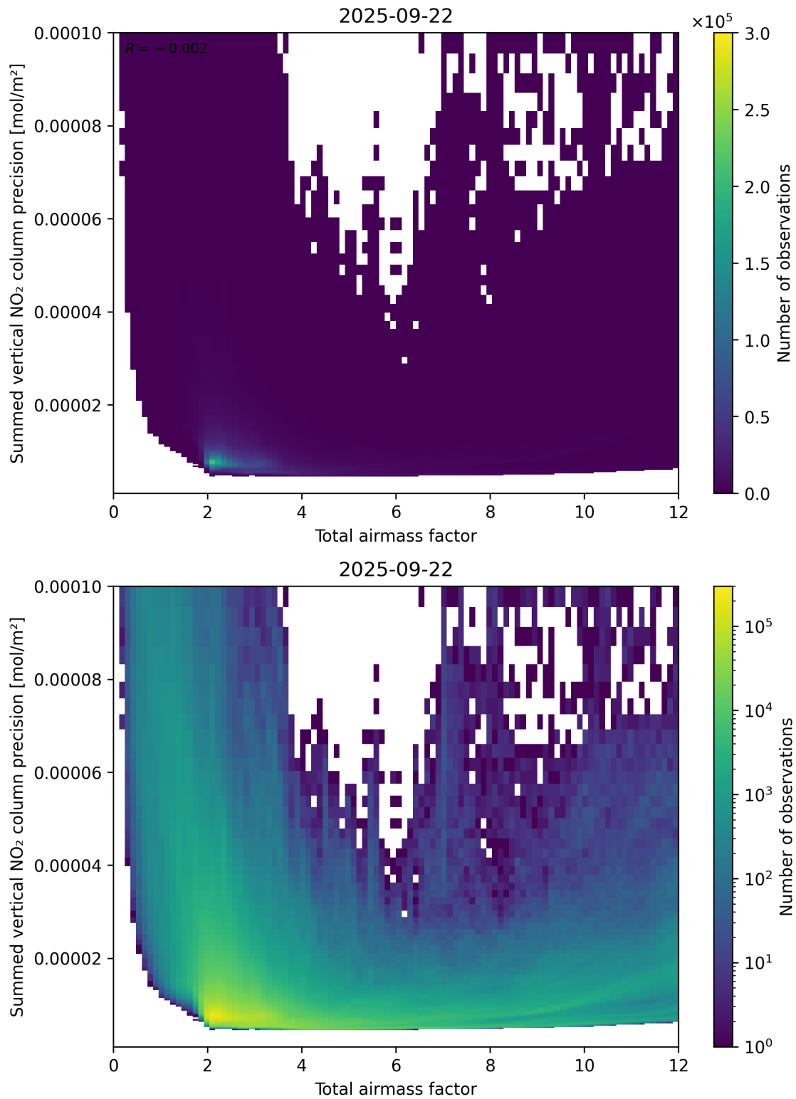
Figure 66: Scatter density plot of “Total airmass factor” against “Summed vertical NO 2 column precision” for 2025-09-22 to 2025-09-23.
