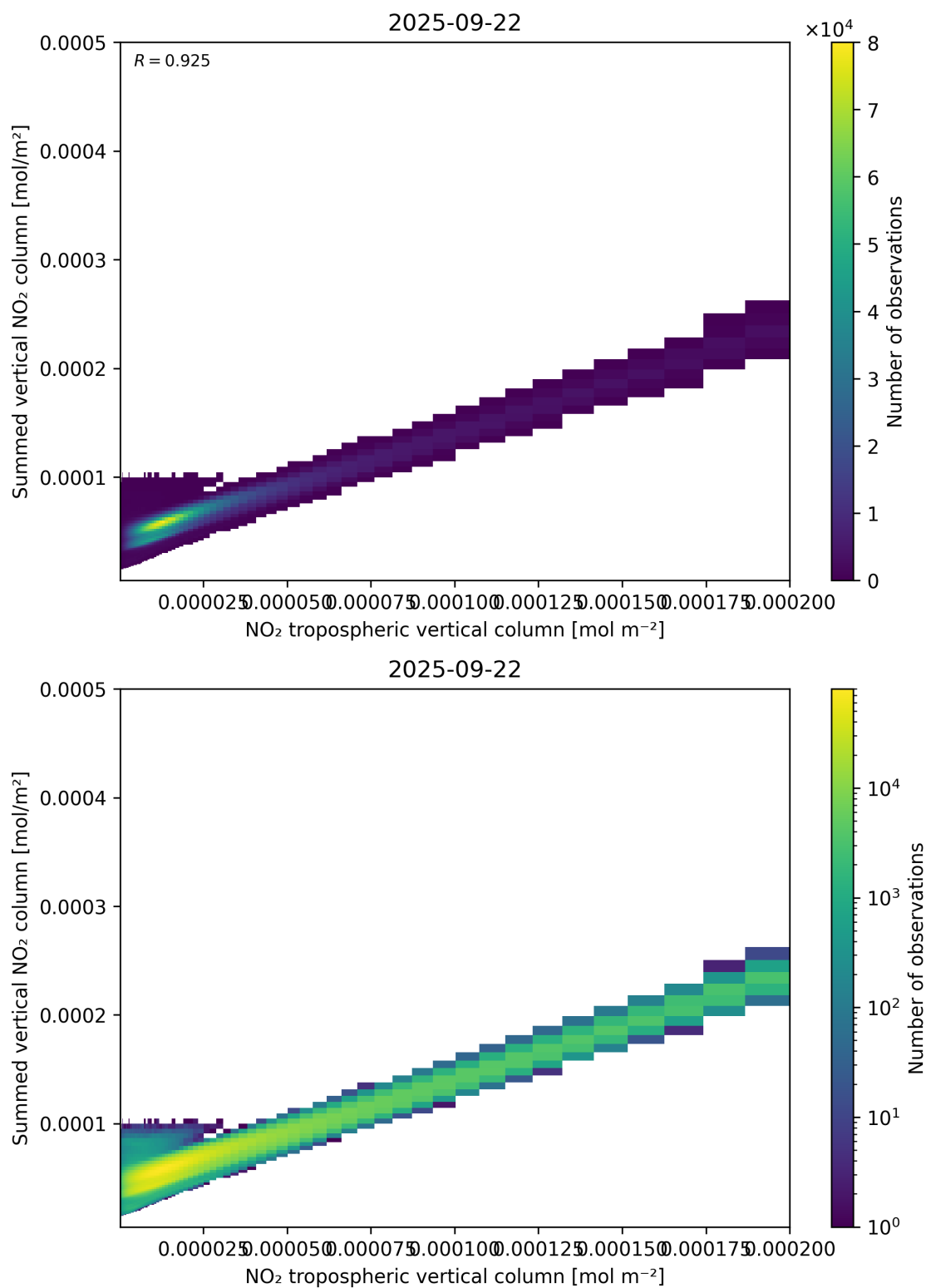
Figure 126: Scatter density plot of “NO 2 tropospheric vertical column” against “Summed vertical NO 2 column” for 2025-09-22 to 2025-09-23.
