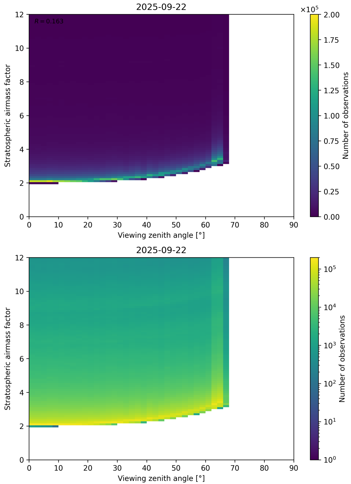
Figure 159: Scatter density plot of “Viewing zenith angle” against “Stratospheric airmass factor” for 2025-09-22 to 2025-09-23.
