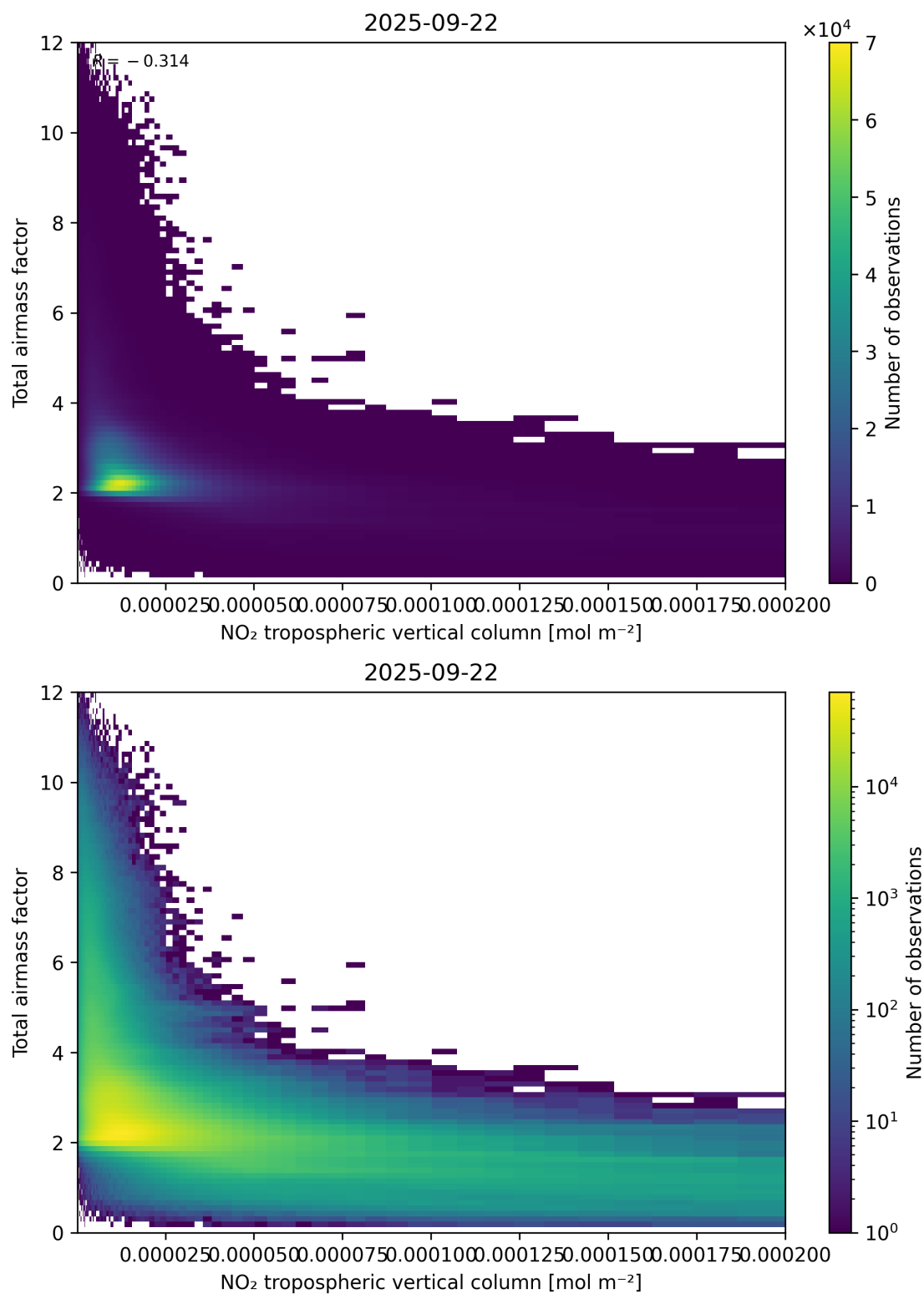
Figure 122: Scatter density plot of “NO 2 tropospheric vertical column” against “Total air mass factor” for 2025-09-22 to 2025-09-23.
