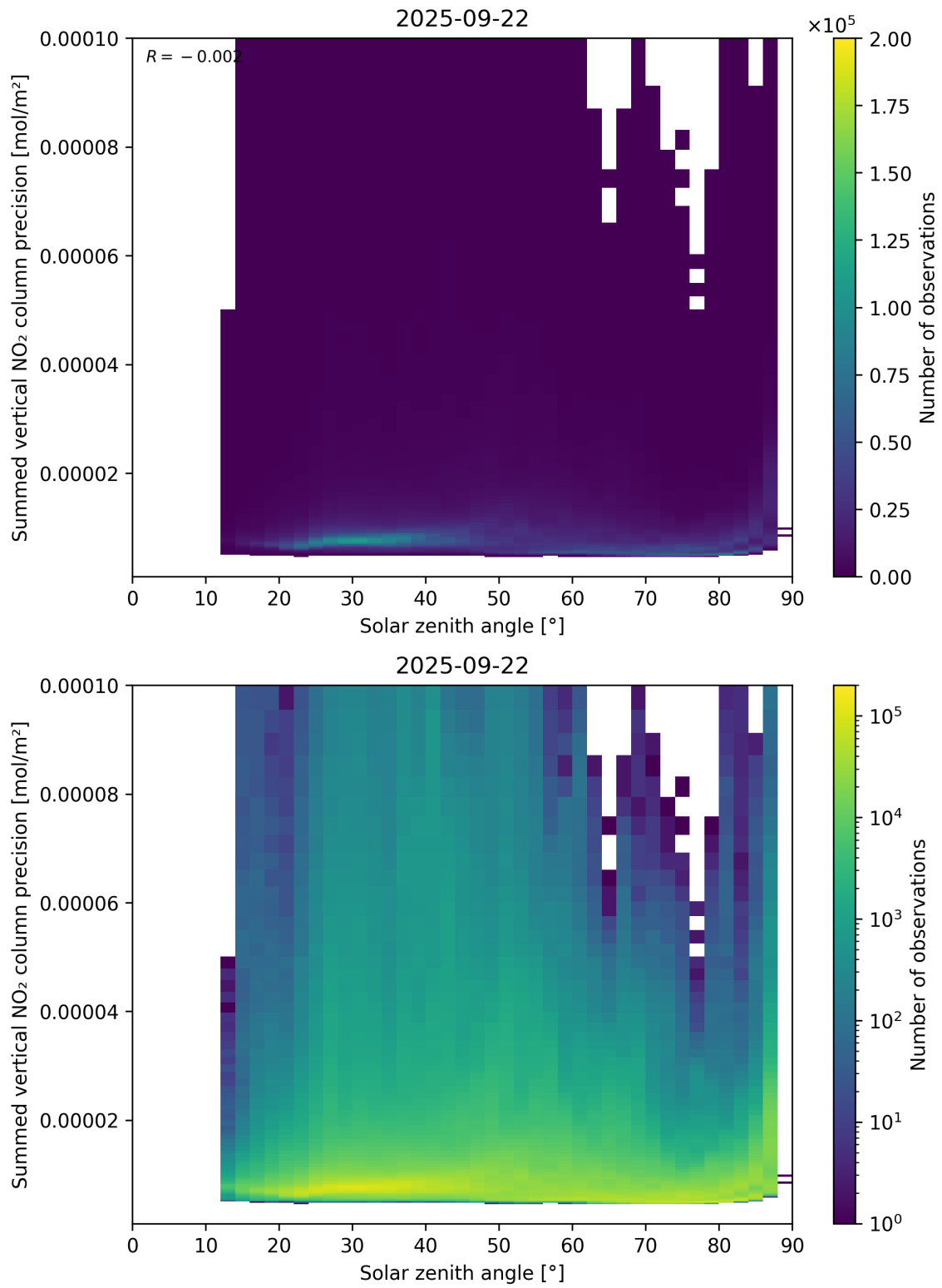
Figure 152: Scatter density plot of “Solar zenith angle” against “Summed vertical NO 2 column precision” for 2025-09-22 to 2025-09-23.
