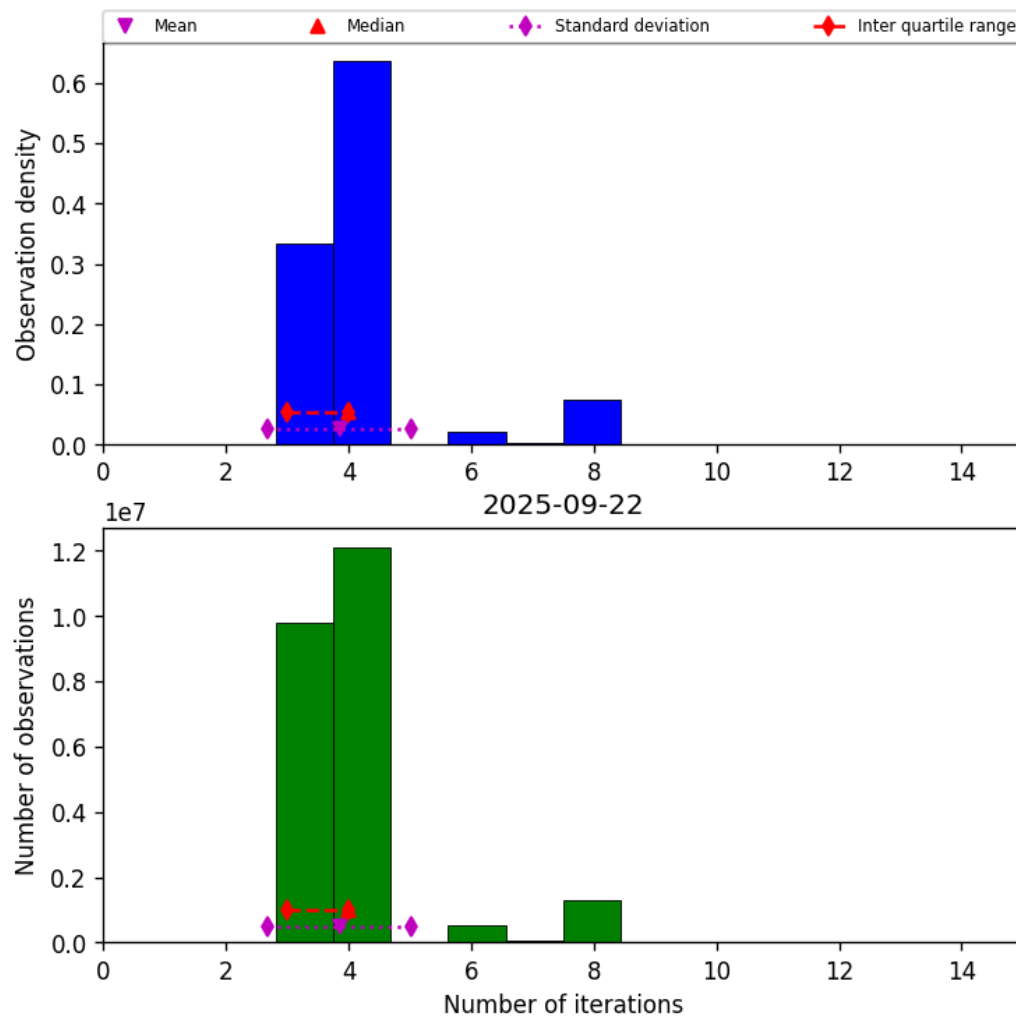
Figure 34: Histogram of “Number of iterations” for 2025-09-22 to 2025-09-23
