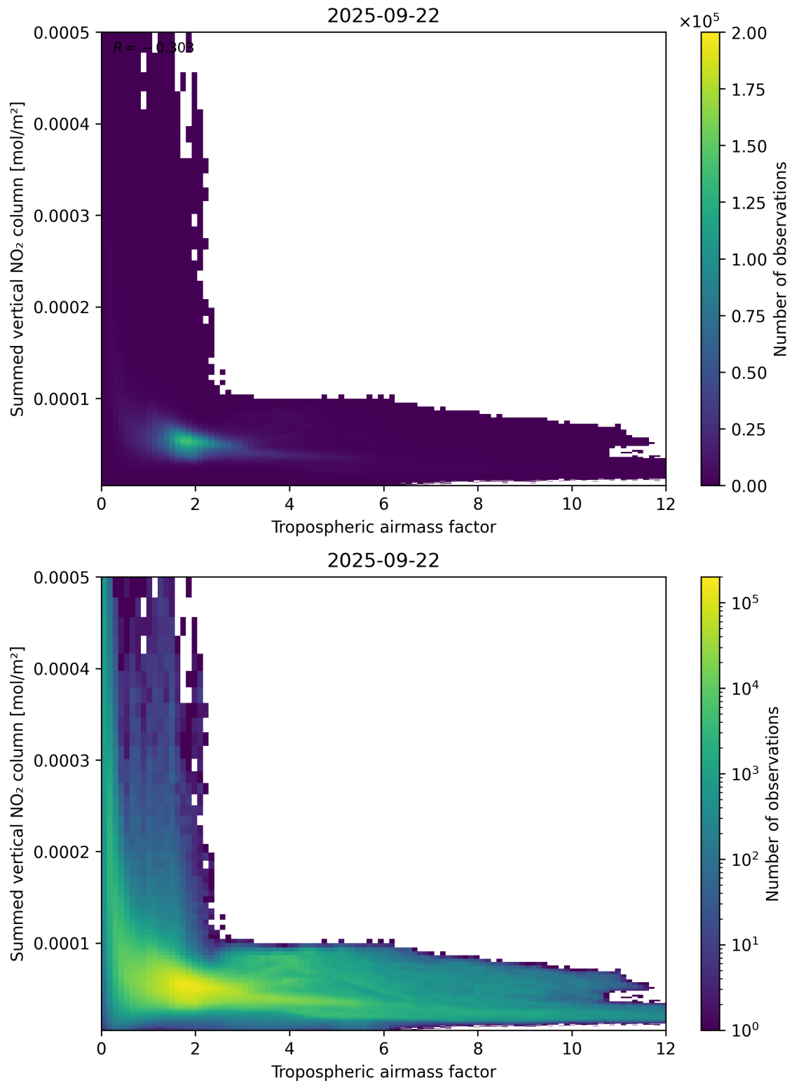
Figure 75: Scatter density plot of “Tropospheric air mass factor” against “Summed vertical NO 2 column” for 2025-09-22 to 2025-09-23.
