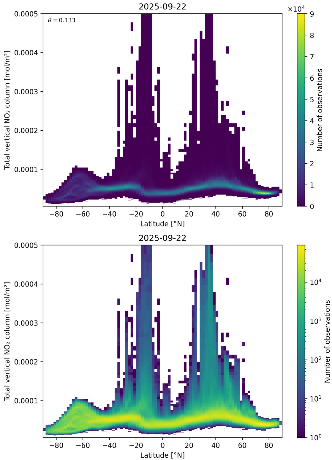
Figure 90: Scatter density plot of “Latitude” against “Total vertical NO 2 column” for 2025-09-22 to 2025-09-23.
