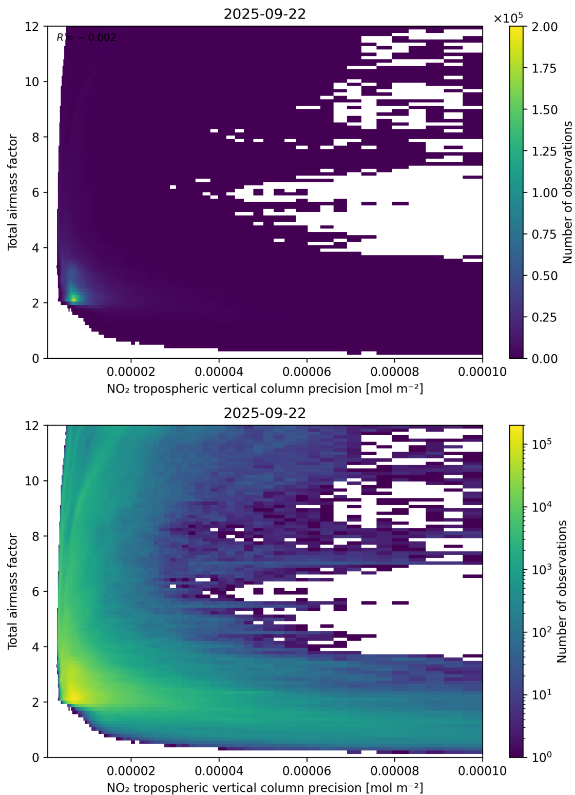
Figure 132: Scatter density plot of “NO 2 tropospheric vertical column precision” against “Total air mass factor” for 2025-09-22 to 2025-09-23.
