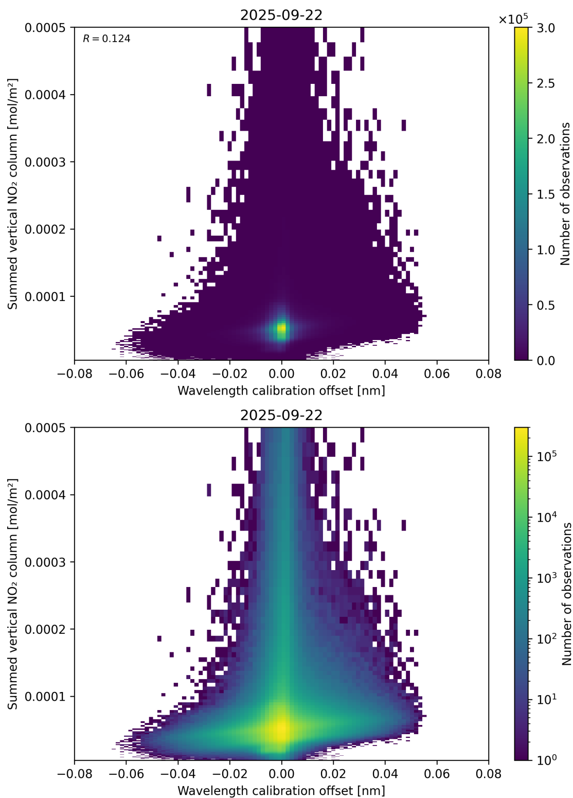
Figure 177: Scatter density plot of “Wavelength calibration offset” against “Summed vertical NO 2 column” for 2025-09-22 to 2025-09-23.
