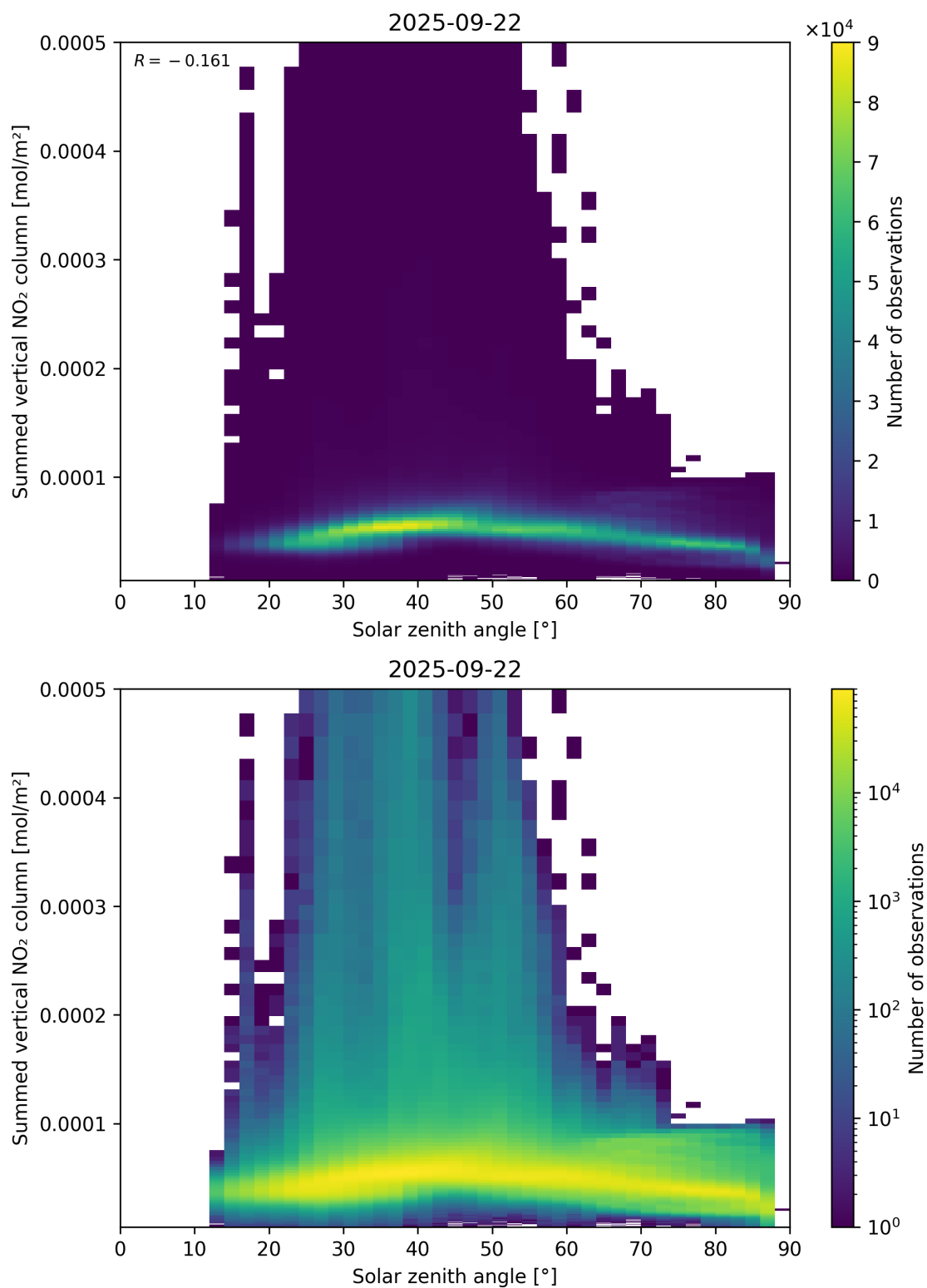
Figure 151: Scatter density plot of “Solar zenith angle” against “Summed vertical NO 2 column” for 2025-09-22 to 2025-09-23.
