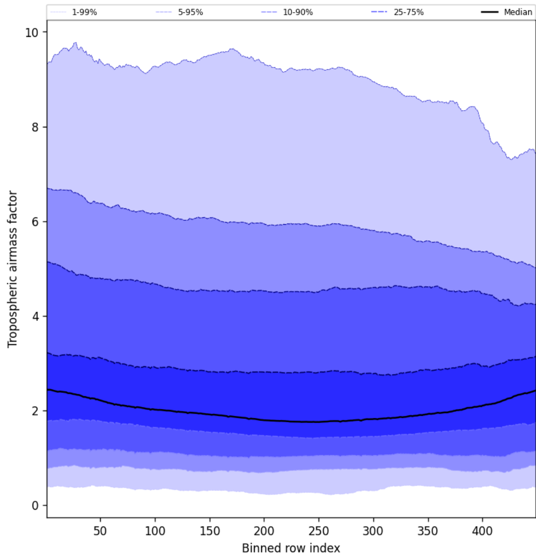
Figure 48: Along track statistics of “Tropospheric airmass factor” for 2025-09-22 to 2025-09-23
