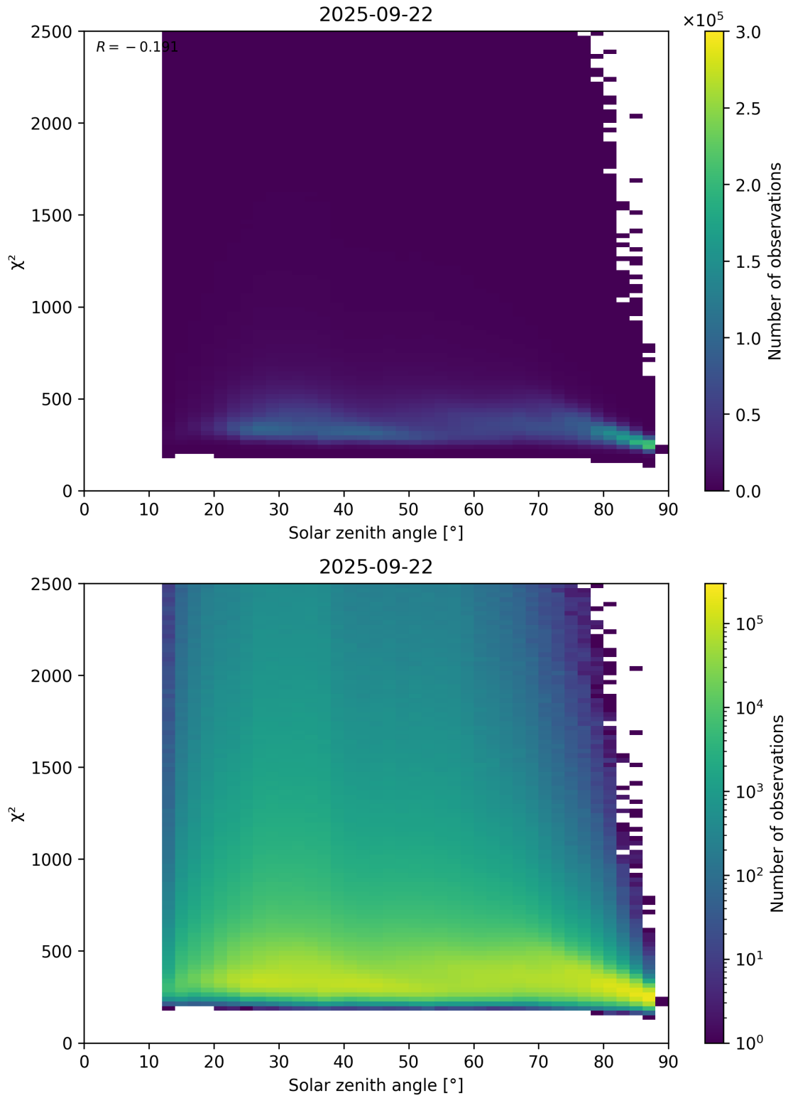
Figure 148: Scatter density plot of “Solar zenith angle” against “ \chi^2 ” for 2025-09-22 to 2025-09-23.
