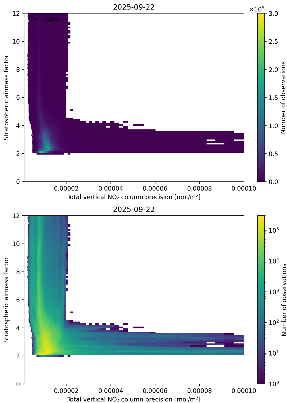
Figure 115: Scatter density plot of “Total vertical NO 2 column precision” against “Stratospheric air mass factor” for 2025-09-22 to 2025-09-23.
