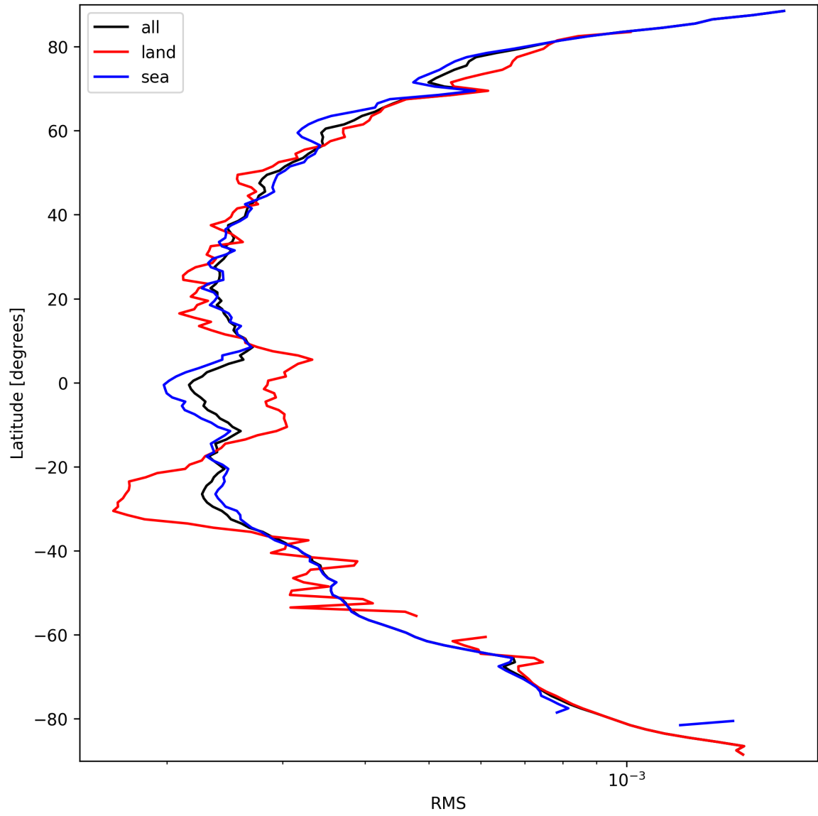
Figure 26: Zonal average of “RMS” for 2025-09-22 to 2025-09-23.
