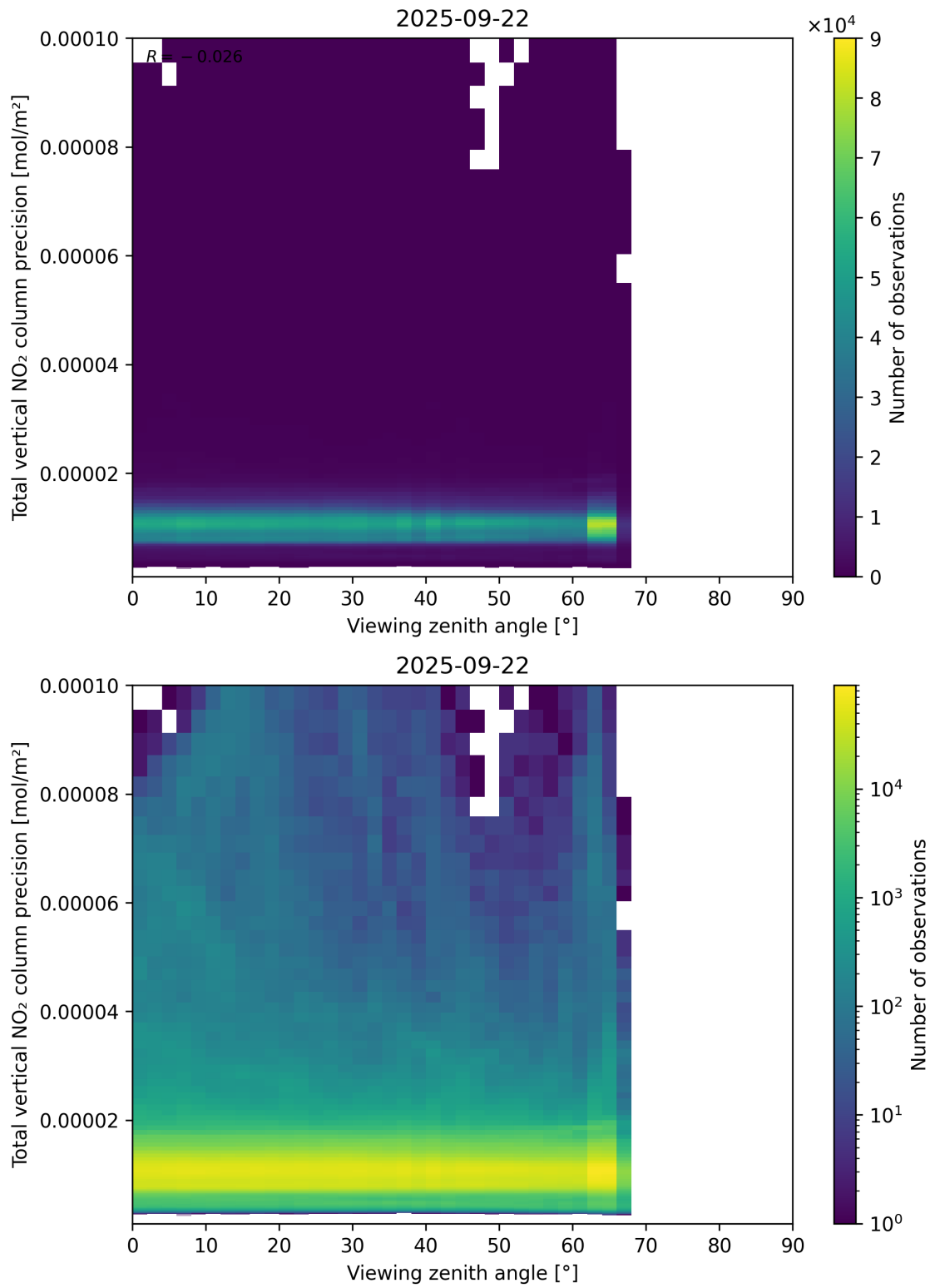
Figure 168: Scatter density plot of “Viewing zenith angle” against “Total vertical NO 2 column precision” for 2025-09-22 to 2025-09-23.
