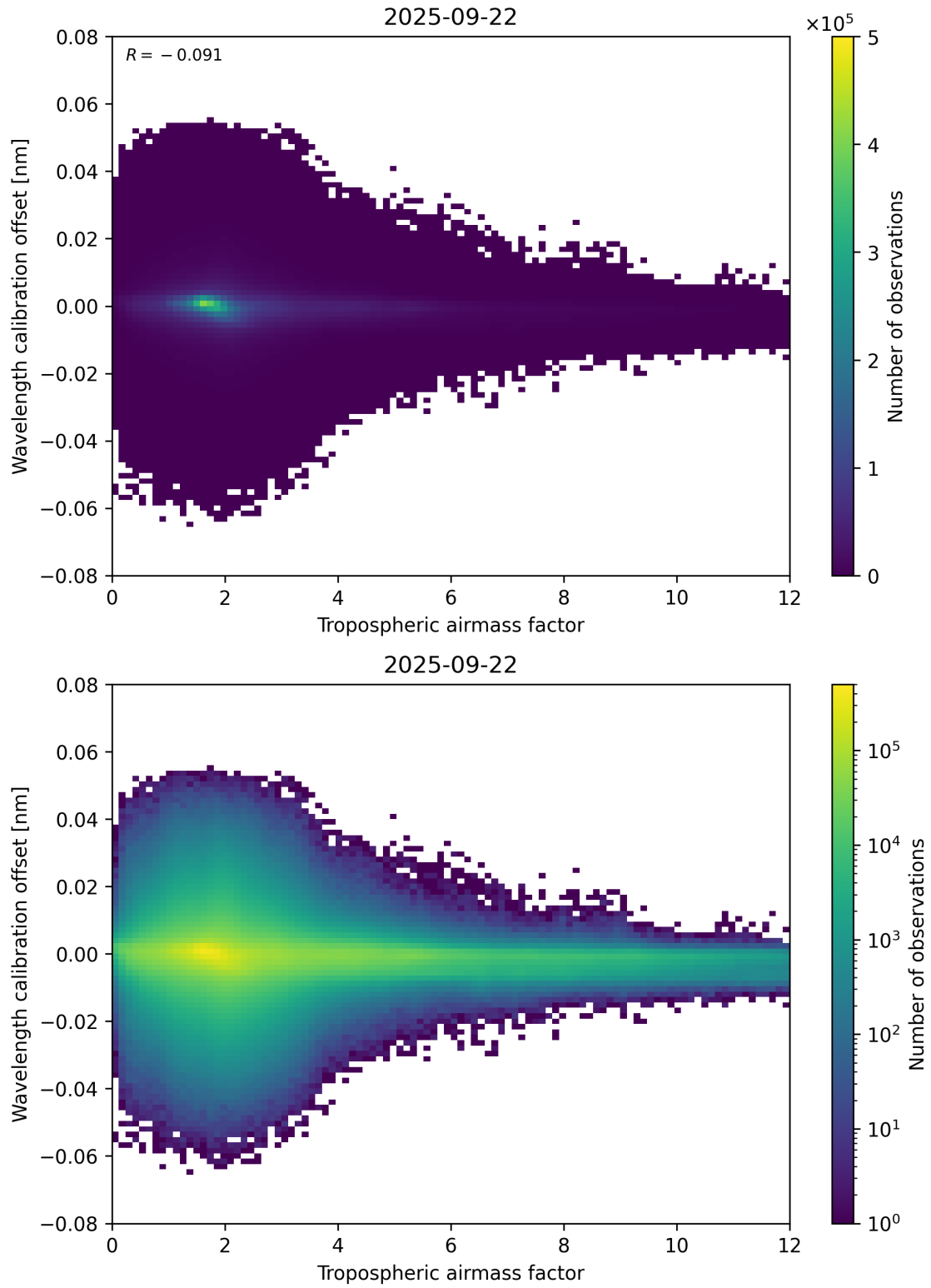
Figure 80: Scatter density plot of “Tropospheric airmass factor” against “Wavelength calibration offset” for 2025-09-22 to 2025-09-23.
