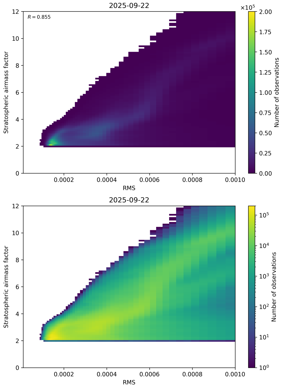
Figure 144: Scatter density plot of “RMS” against “Stratospheric airmass factor” for 2025-09-22 to 2025-09-23.
