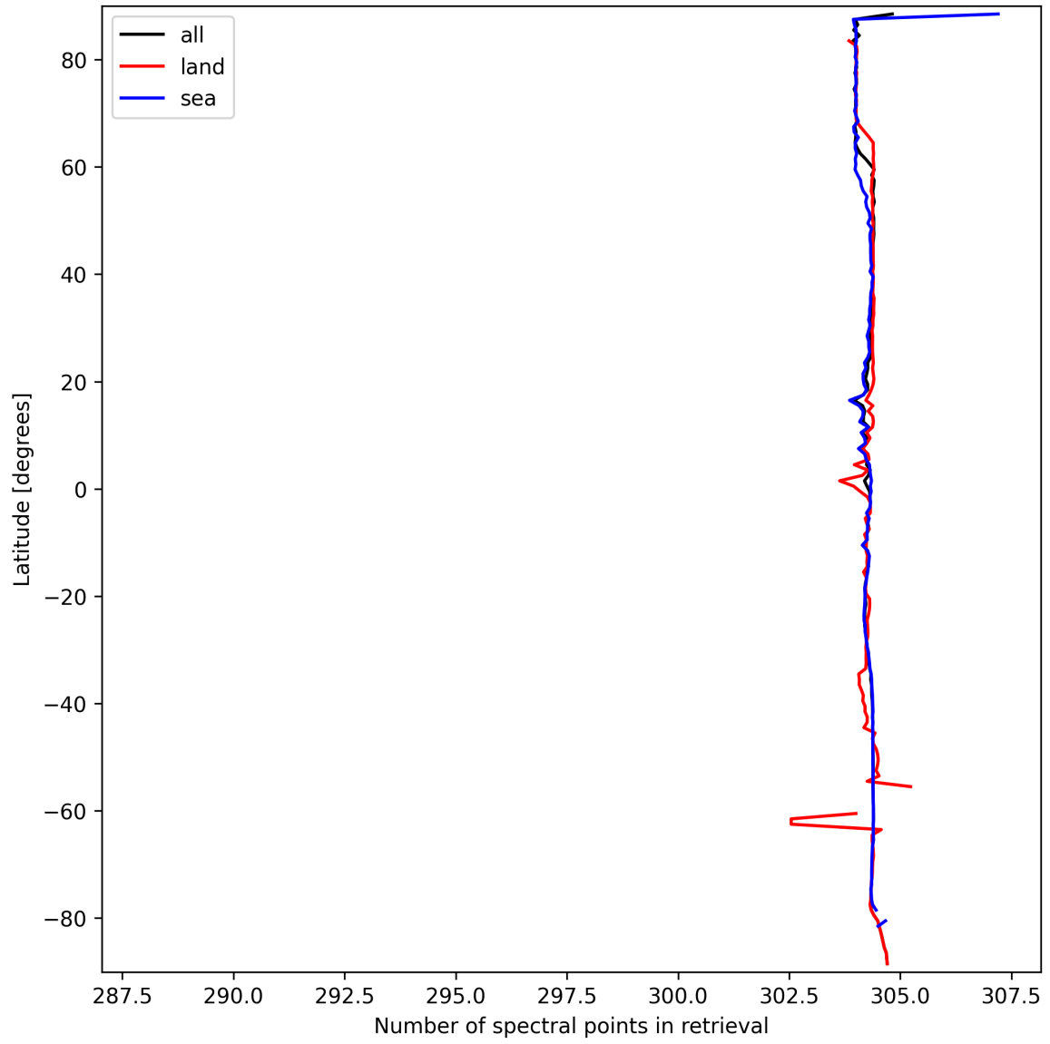
Figure 16: Zonal average of “Number of spectral points in retrieval” for 2025-09-22 to 2025-09-23.
