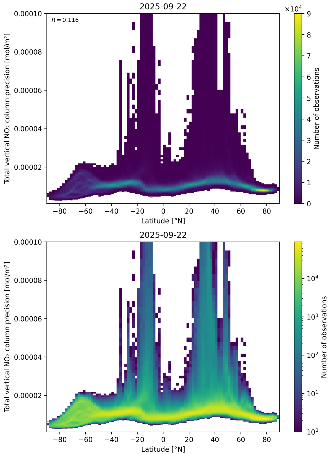
Figure 91: Scatter density plot of “Latitude” against “Total vertical NO 2 column precision” for 2025-09-22 to 2025-09-23.
