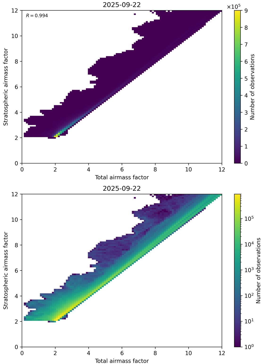
Figure 62: Scatter density plot of “Total airmass factor” against “Stratospheric airmass factor” for 2025-09-22 to 2025-09-23.
