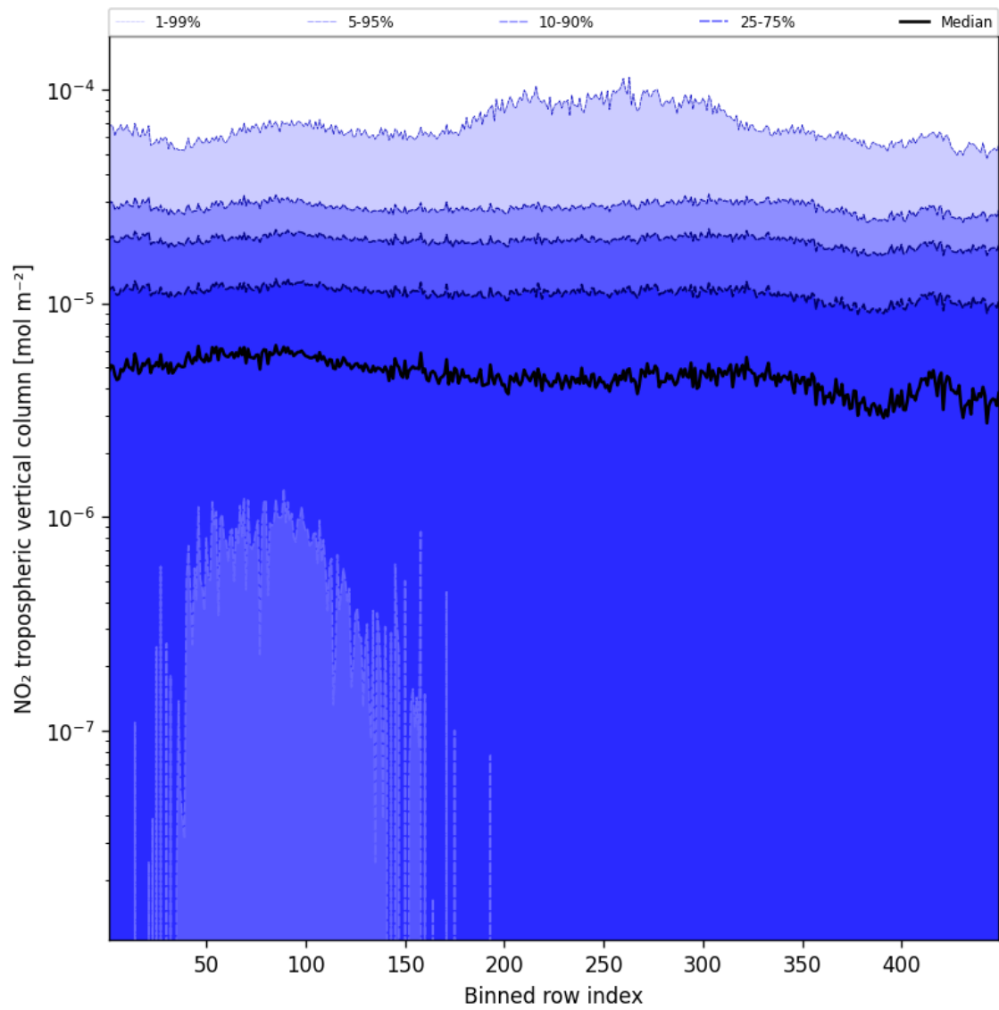
Figure 46: Along track statistics of “NO 2 tropospheric vertical column” for 2025-09-22 to 2025-09-23
