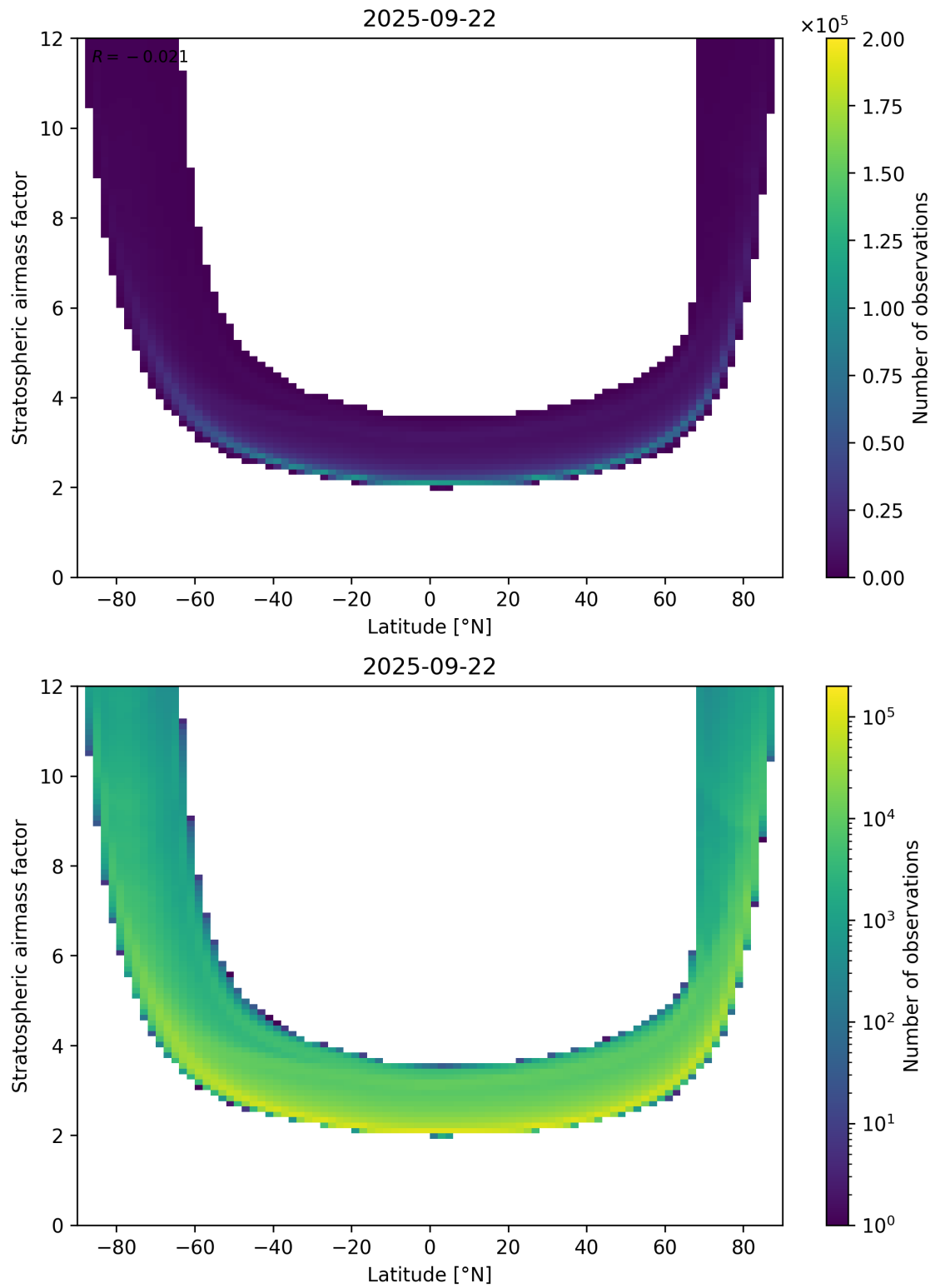
Figure 83: Scatter density plot of “Latitude” against “Stratospheric air mass factor” for 2025-09-22 to 2025-09-23.
