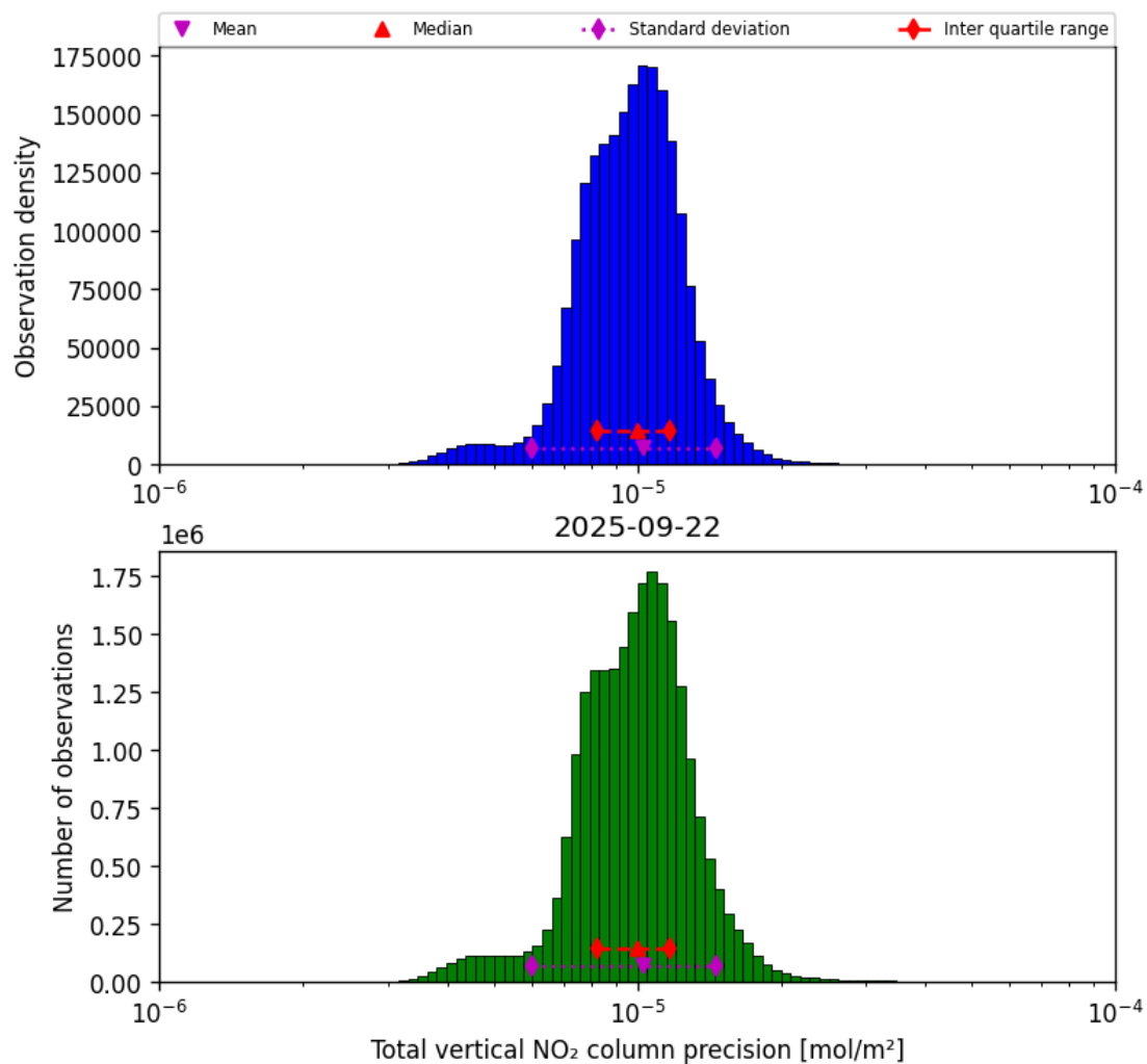
Figure 39: Histogram of “Total vertical NO 2 column precision” for 2025-09-22 to 2025-09-23
