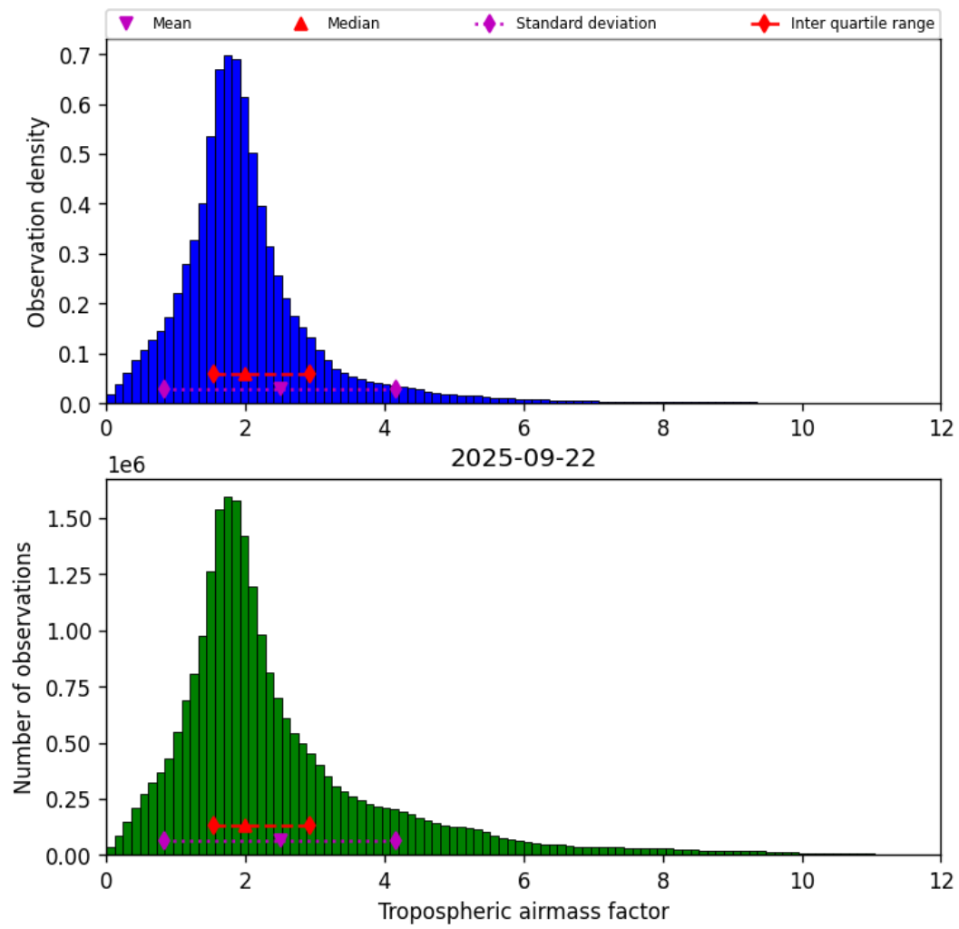
Figure 31: Histogram of “Tropospheric airmass factor” for 2025-09-22 to 2025-09-23
