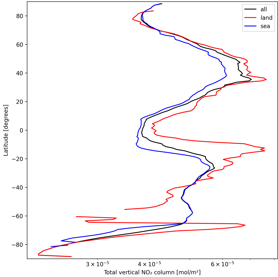
Figure 21: Zonal average of “Total vertical NO 2 column” for 2025-09-22 to 2025-09-23.
