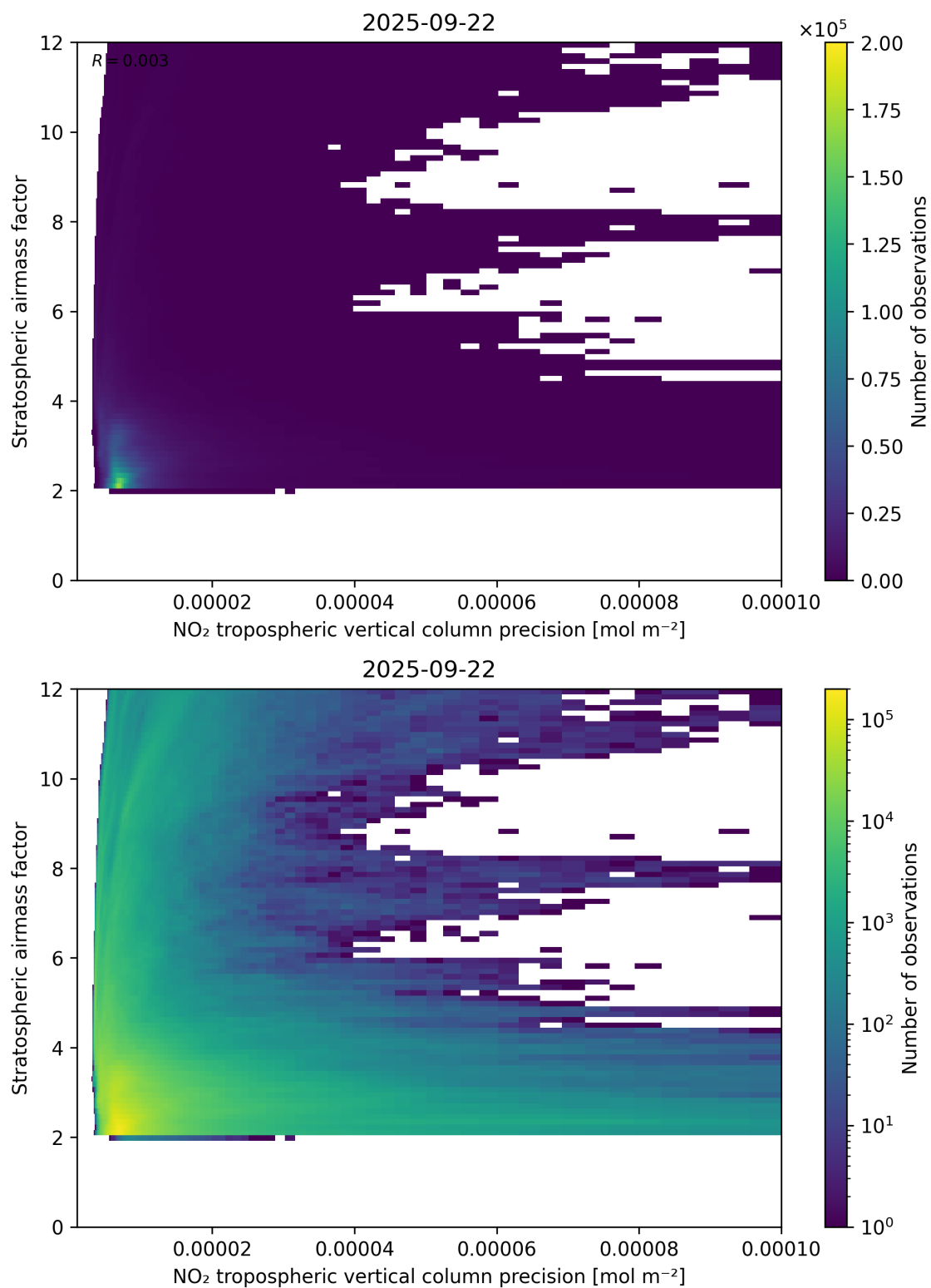
Figure 131: Scatter density plot of “NO 2 tropospheric vertical column precision” against “Stratospheric airmass factor” for 2025-09-22 to 2025-09-23.
