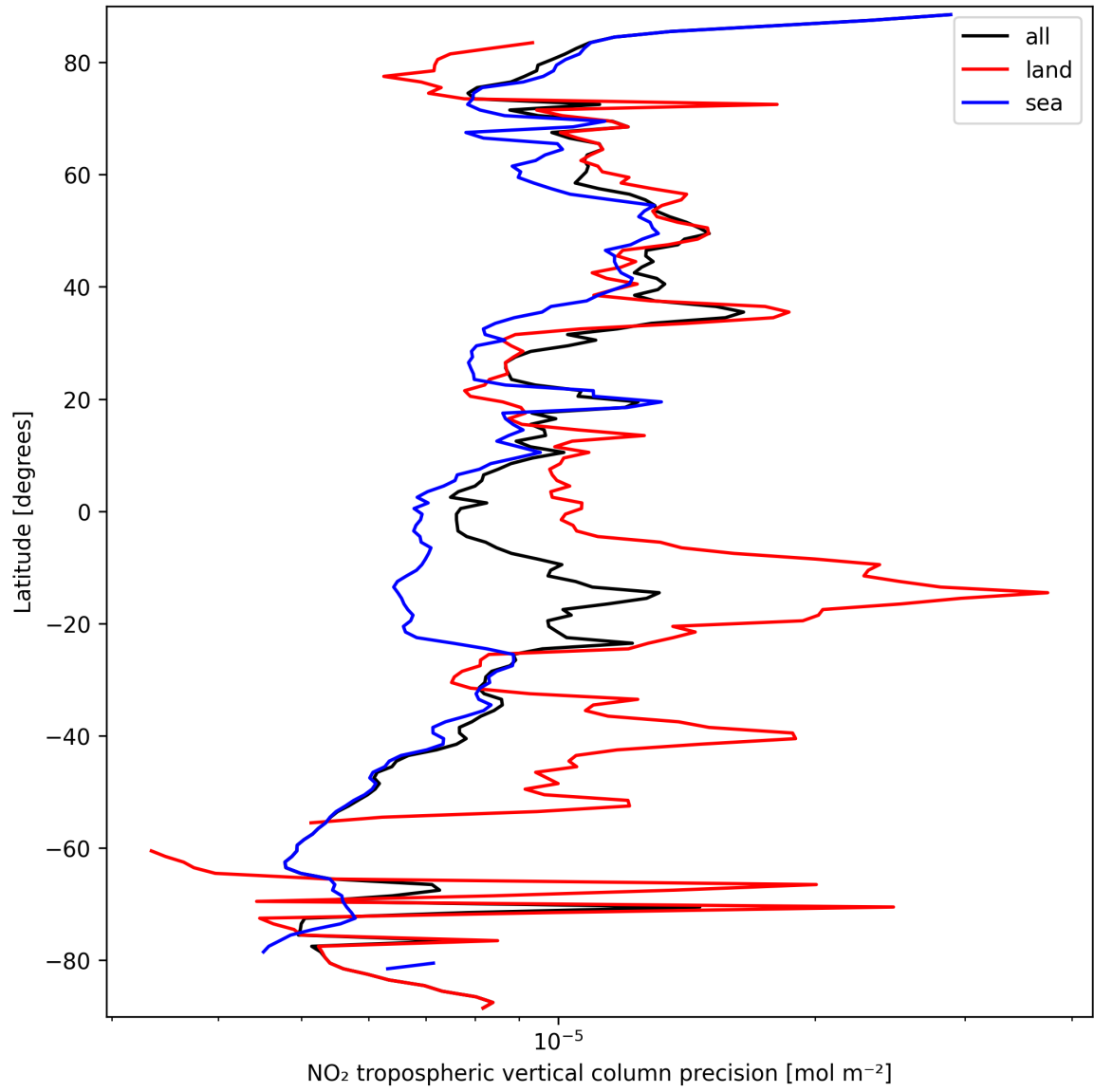
Figure 13: Zonal average of “NO 2 tropospheric vertical column precision” for 2025-09-22 to 2025-09-23.
