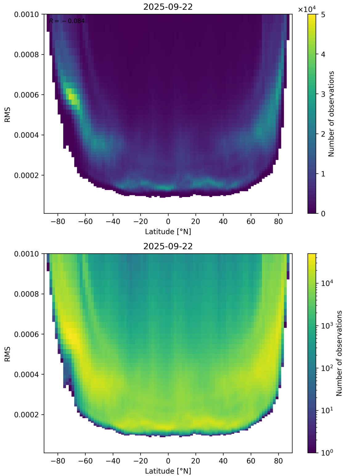
Figure 94: Scatter density plot of “Latitude” against “RMS” for 2025-09-22 to 2025-09-23.
