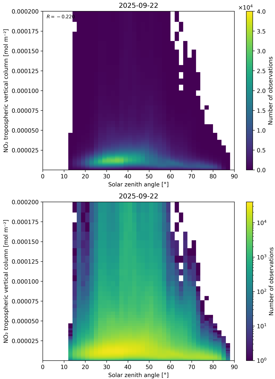
Figure 155: Scatter density plot of “Solar zenith angle” against “NO 2 tropospheric vertical column” for 2025-09-22 to 2025-09-23.
