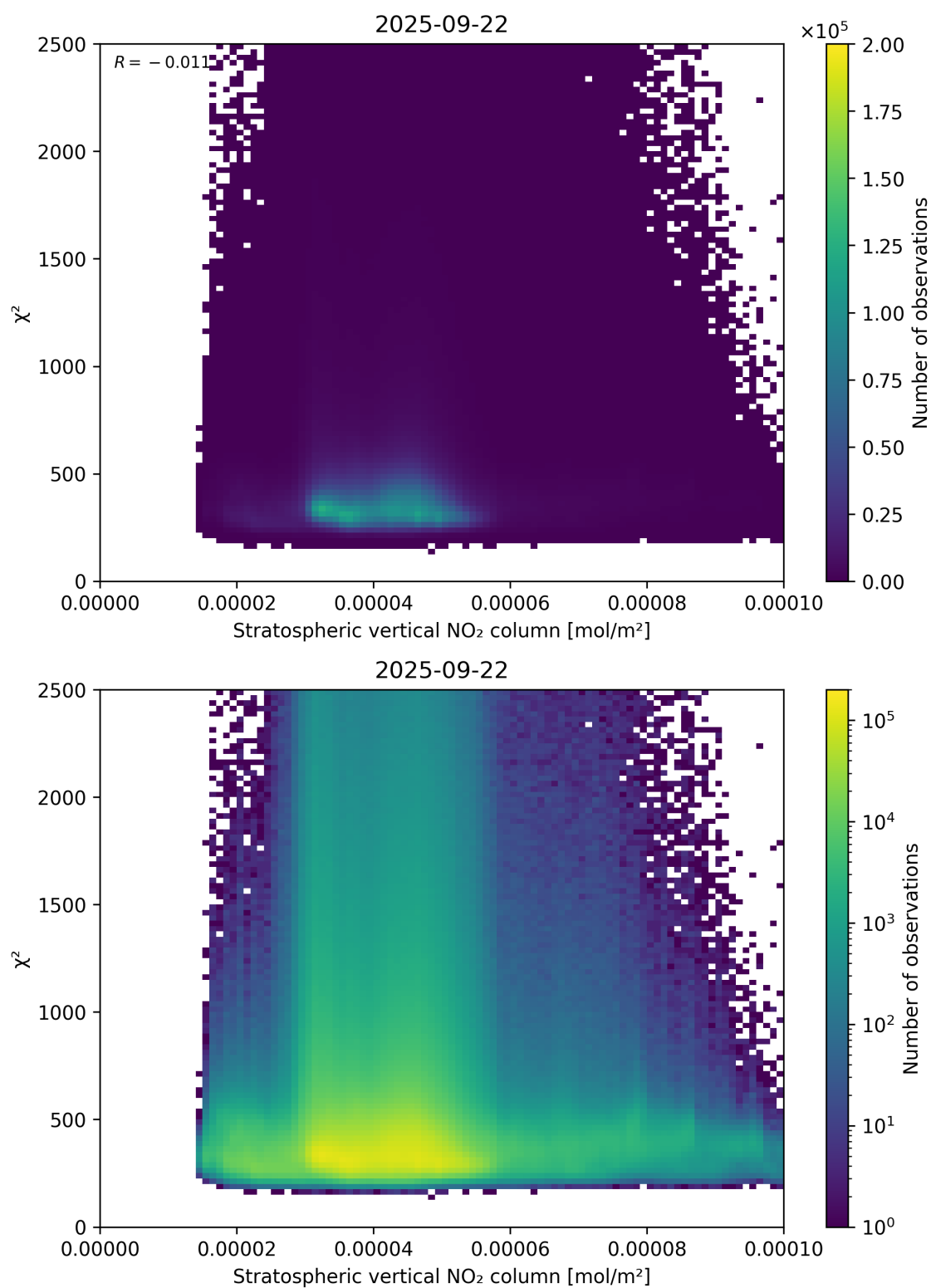
Figure 97: Scatter density plot of “Stratospheric vertical NO 2 column” against “ \chi^2 ” for 2025-09-22 to 2025-09-23.
