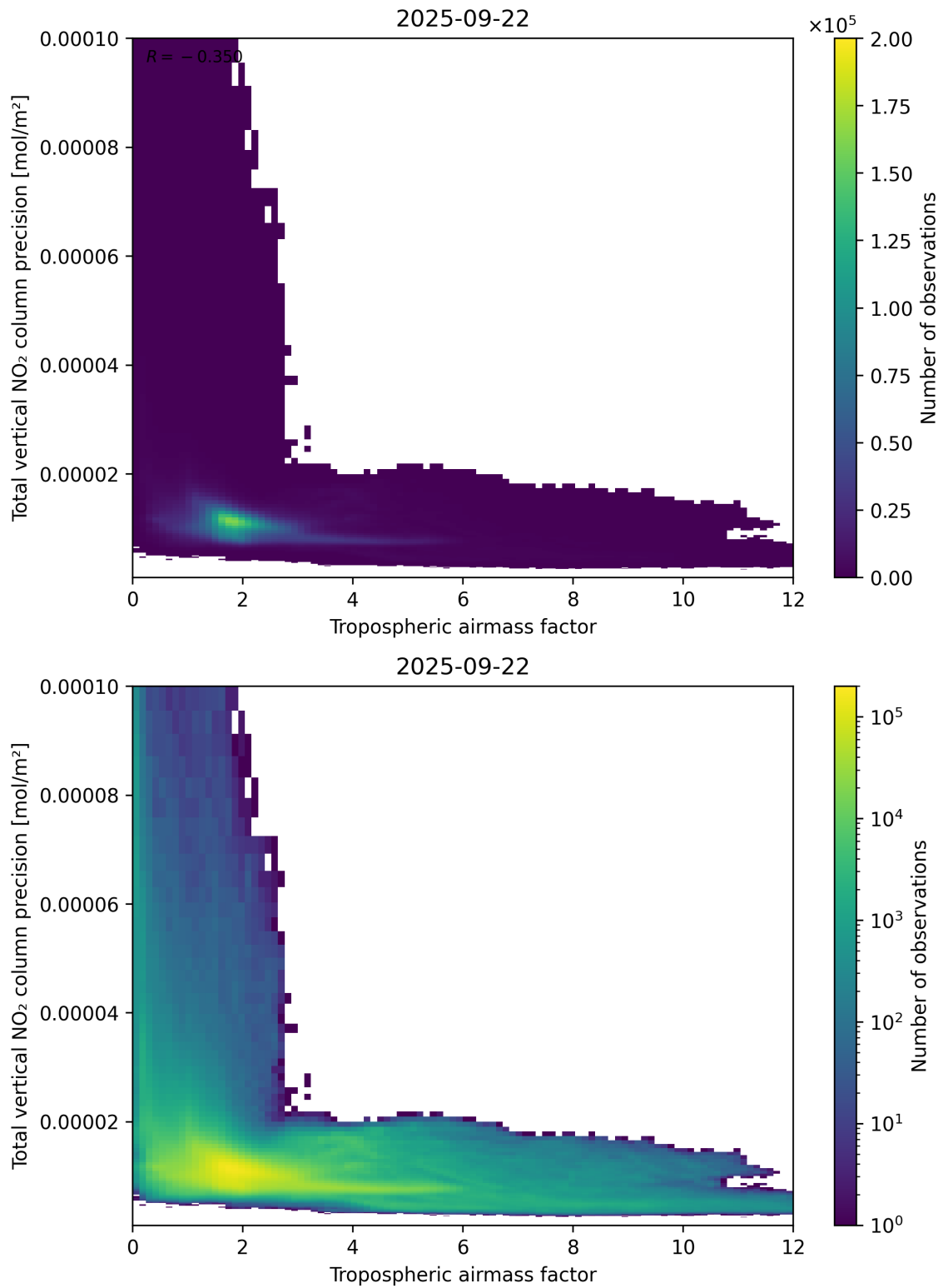
Figure 78: Scatter density plot of “Tropospheric airmass factor” against “Total vertical NO 2 column precision” for 2025-09-22 to 2025-09-23.
