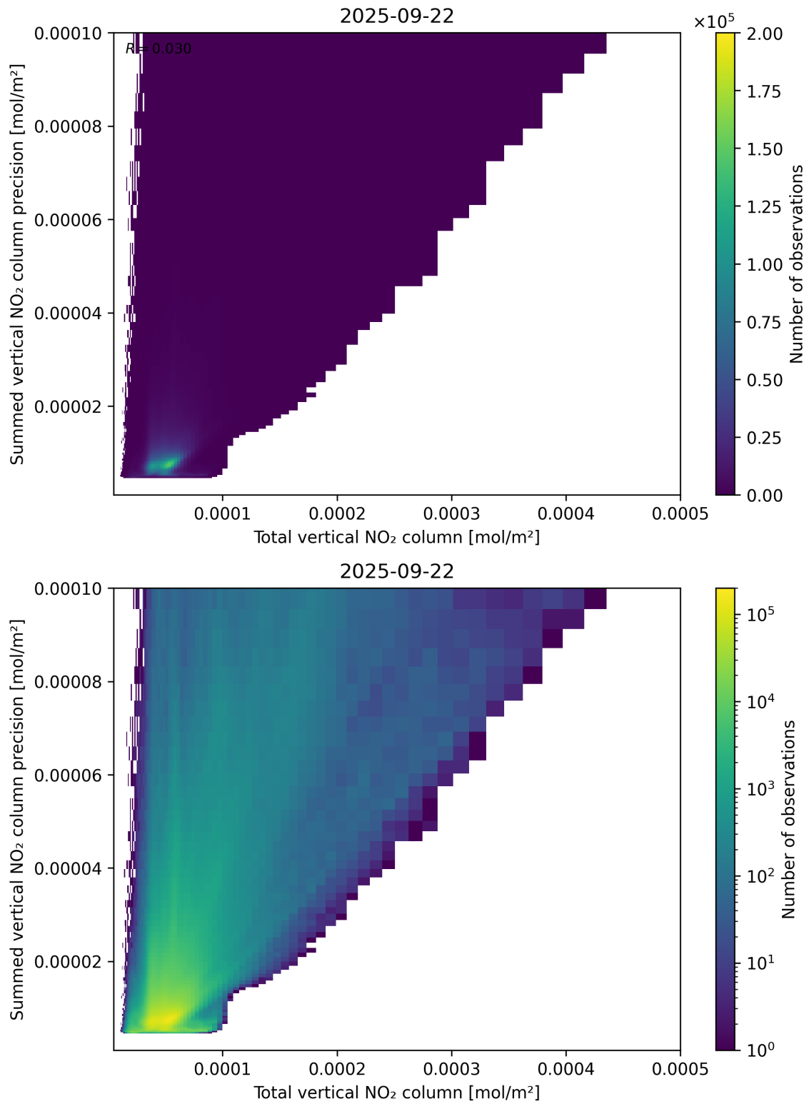
Figure 113: Scatter density plot of “Total vertical NO 2 column” against “Summed vertical NO 2 column precision” for 2025-09-22 to 2025-09-23.
