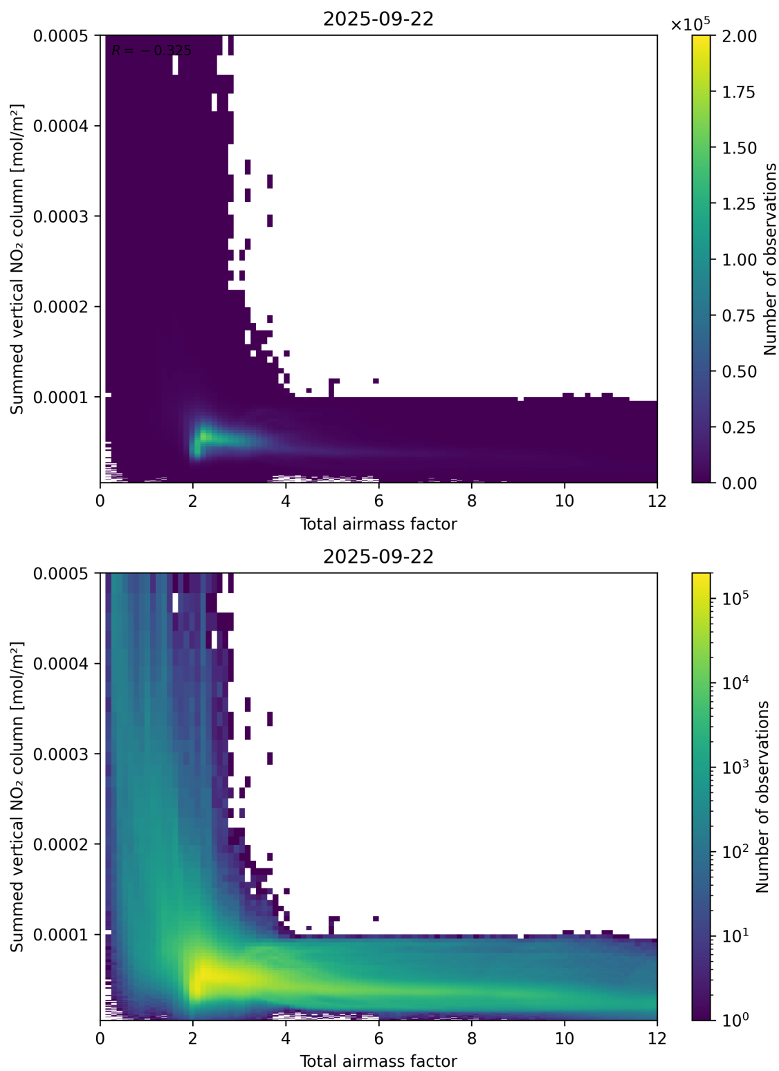
Figure 65: Scatter density plot of “Total airmass factor” against “Summed vertical NO 2 column” for 2025-09-22 to 2025-09-23.
