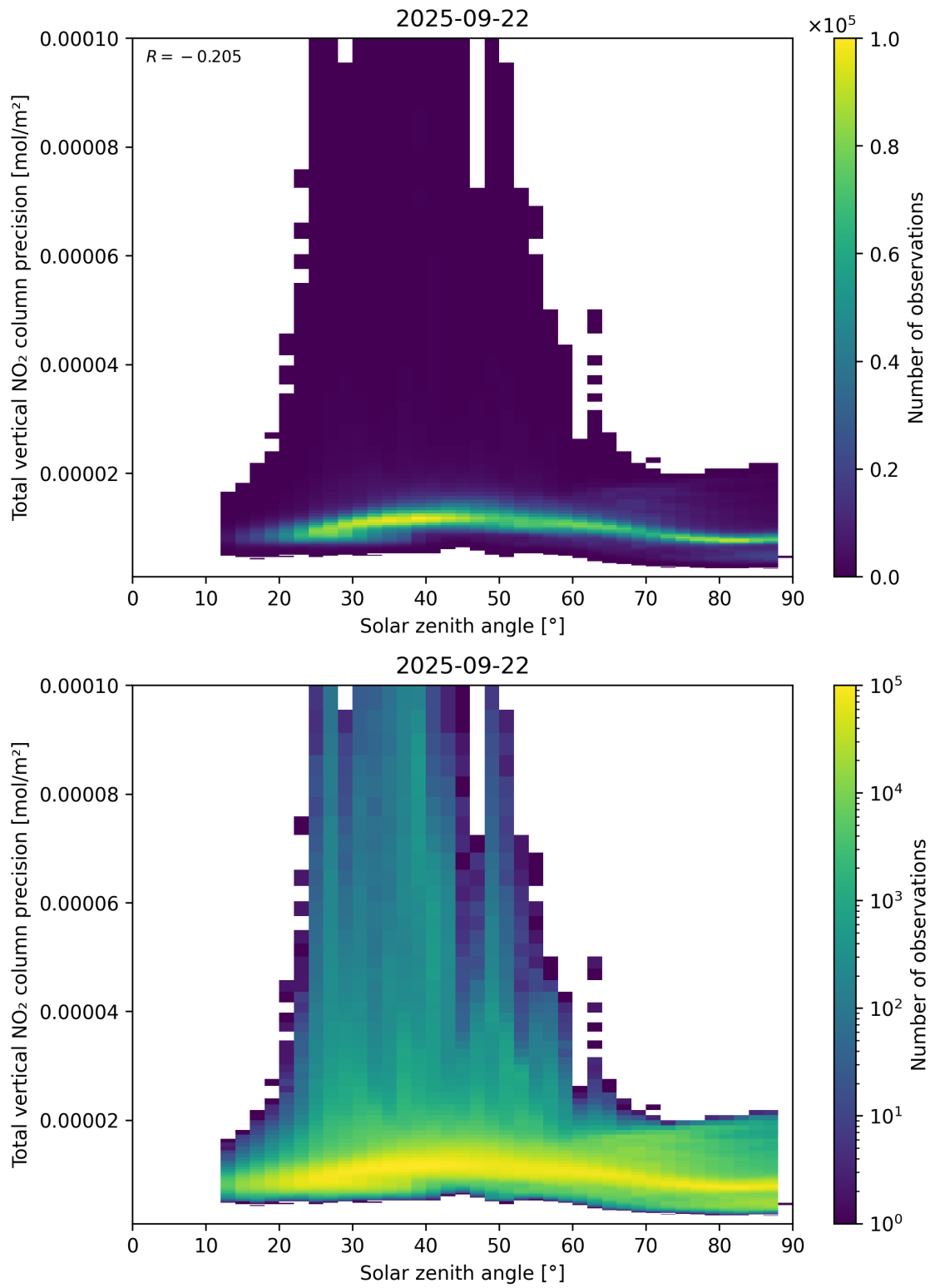
Figure 154: Scatter density plot of “Solar zenith angle” against “Total vertical NO 2 column precision” for 2025-09-22 to 2025-09-23.
