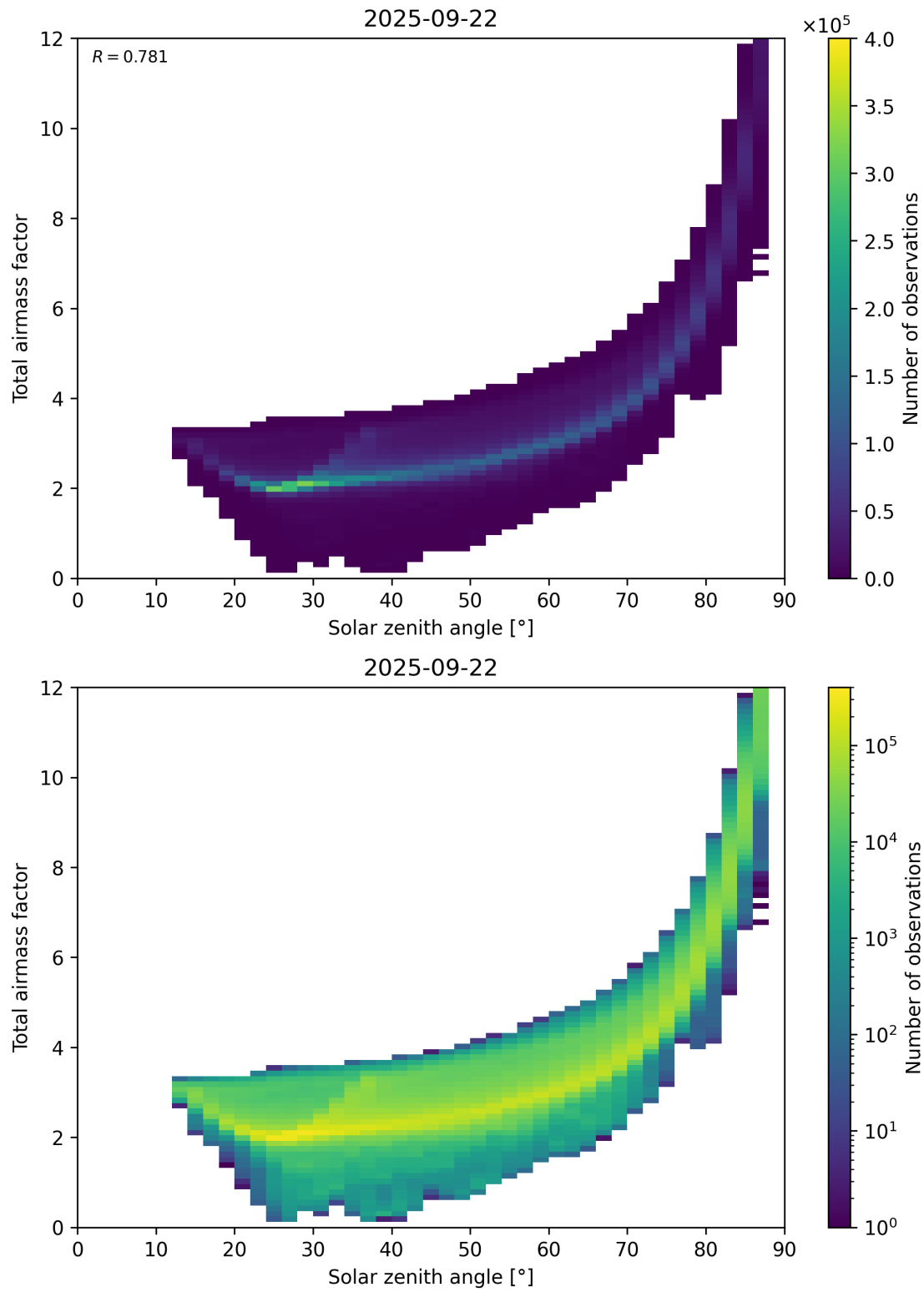
Figure 146: Scatter density plot of “Solar zenith angle” against “Total air mass factor” for 2025-09-22 to 2025-09-23.
