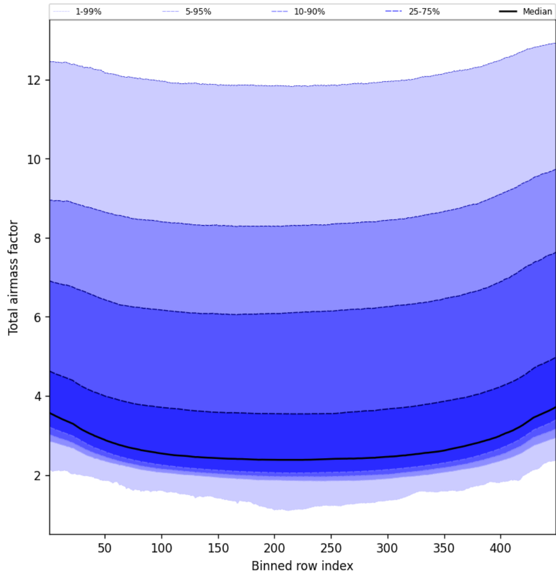
Figure 49: Along track statistics of “Total airmass factor” for 2025-09-22 to 2025-09-23
