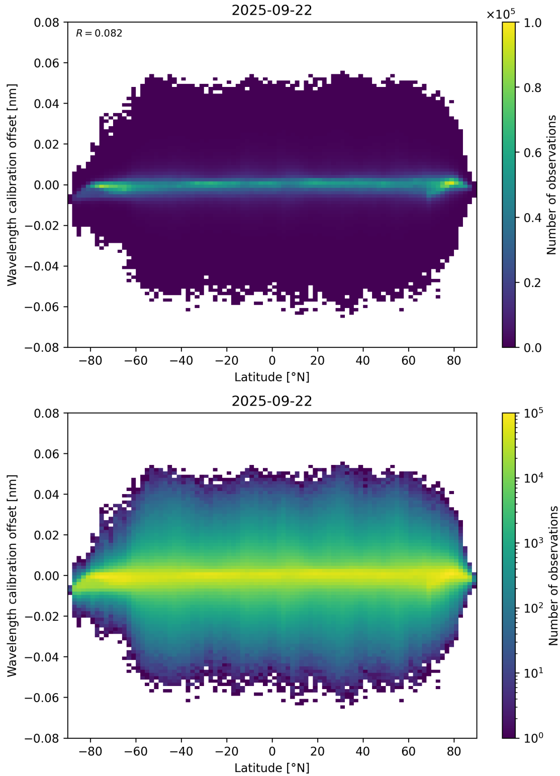
Figure 95: Scatter density plot of “Latitude” against “Wavelength calibration offset” for 2025-09-22 to 2025-09-23.
