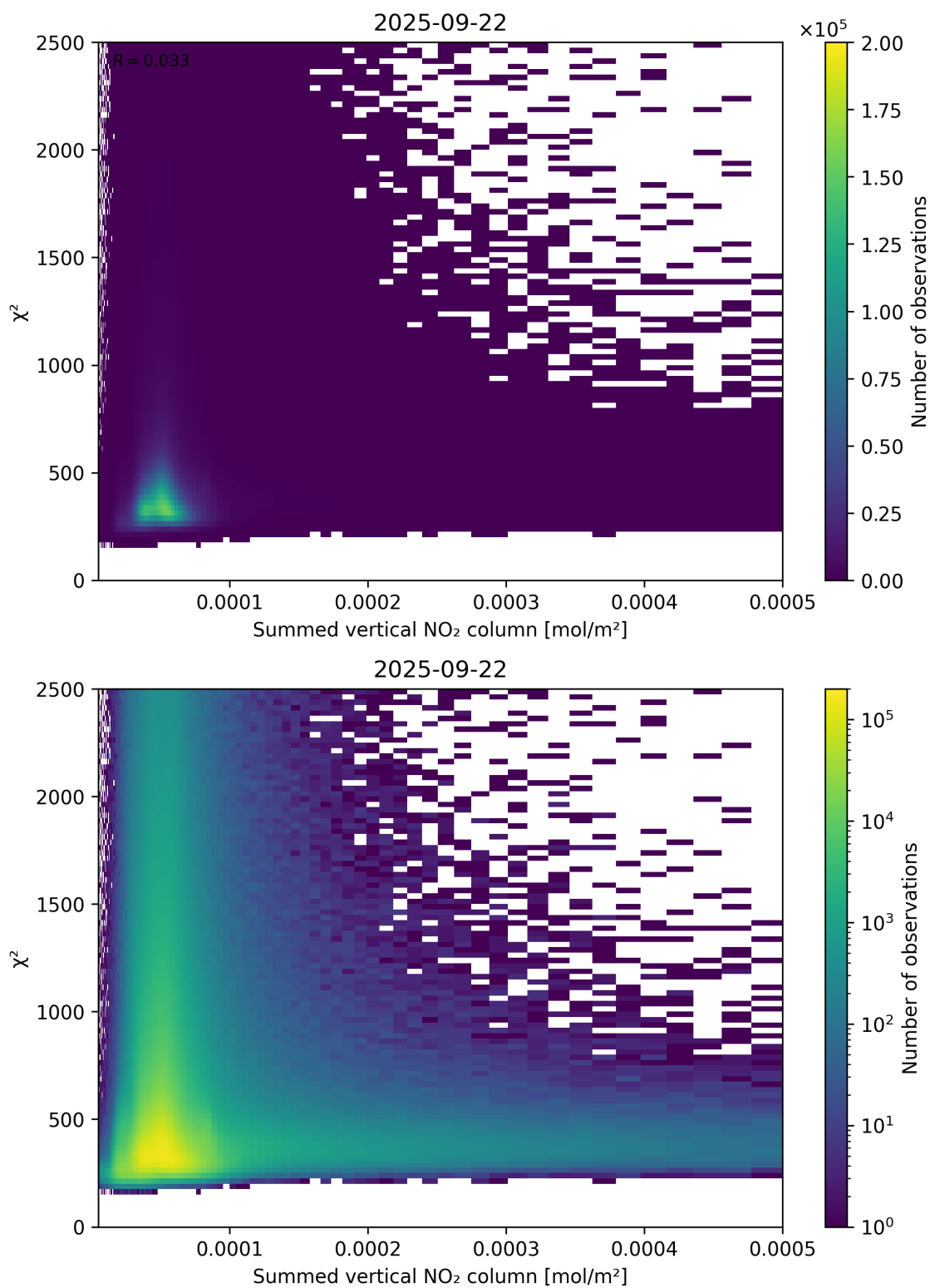
Figure 104: Scatter density plot of “Summed vertical NO 2 column” against “ \chi^2 ” for 2025-09-22 to 2025-09-23.
