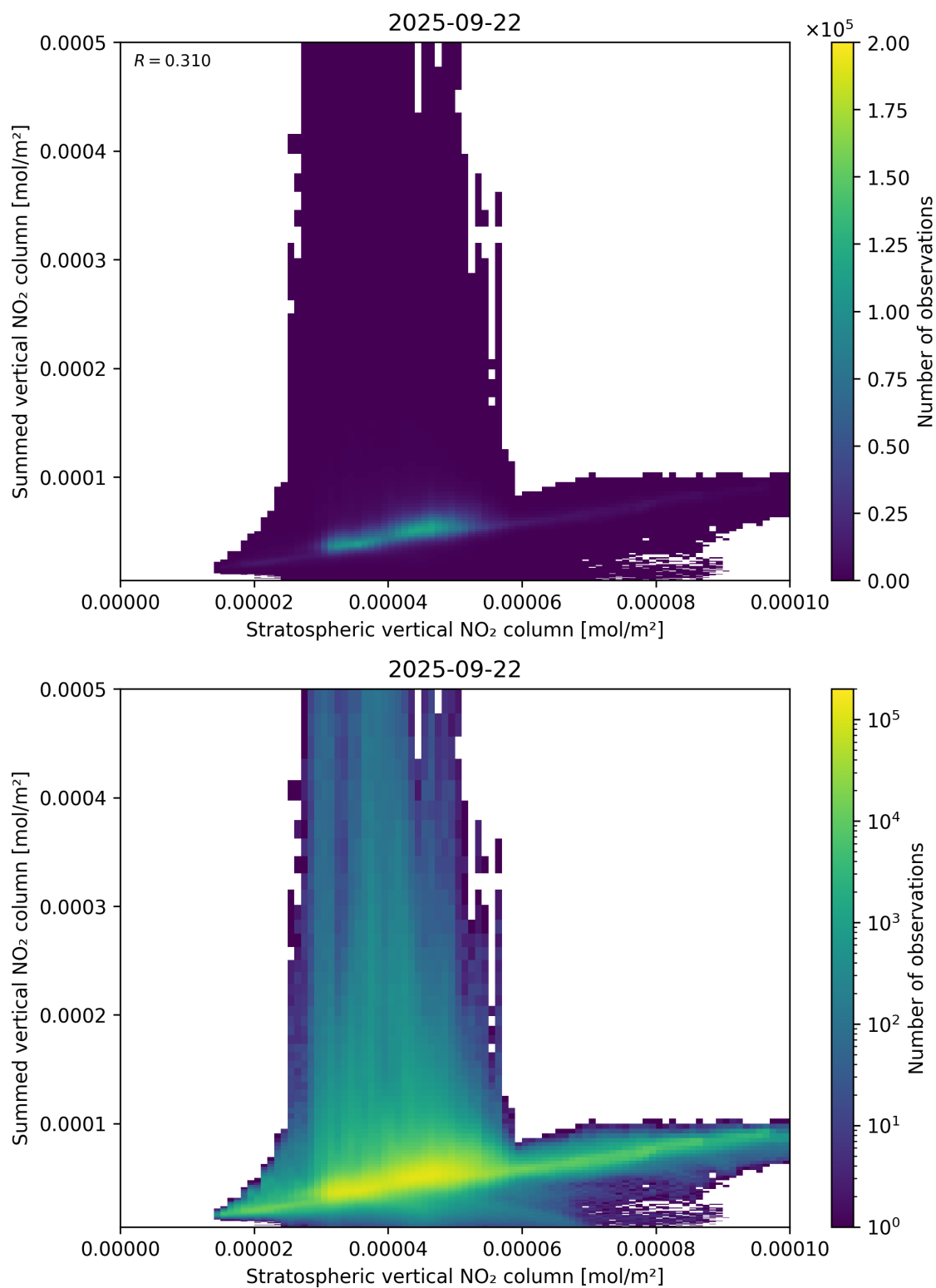
Figure 98: Scatter density plot of “Stratospheric vertical NO 2 column” against “Summed vertical NO 2 column” for 2025-09-22 to 2025-09-23.
