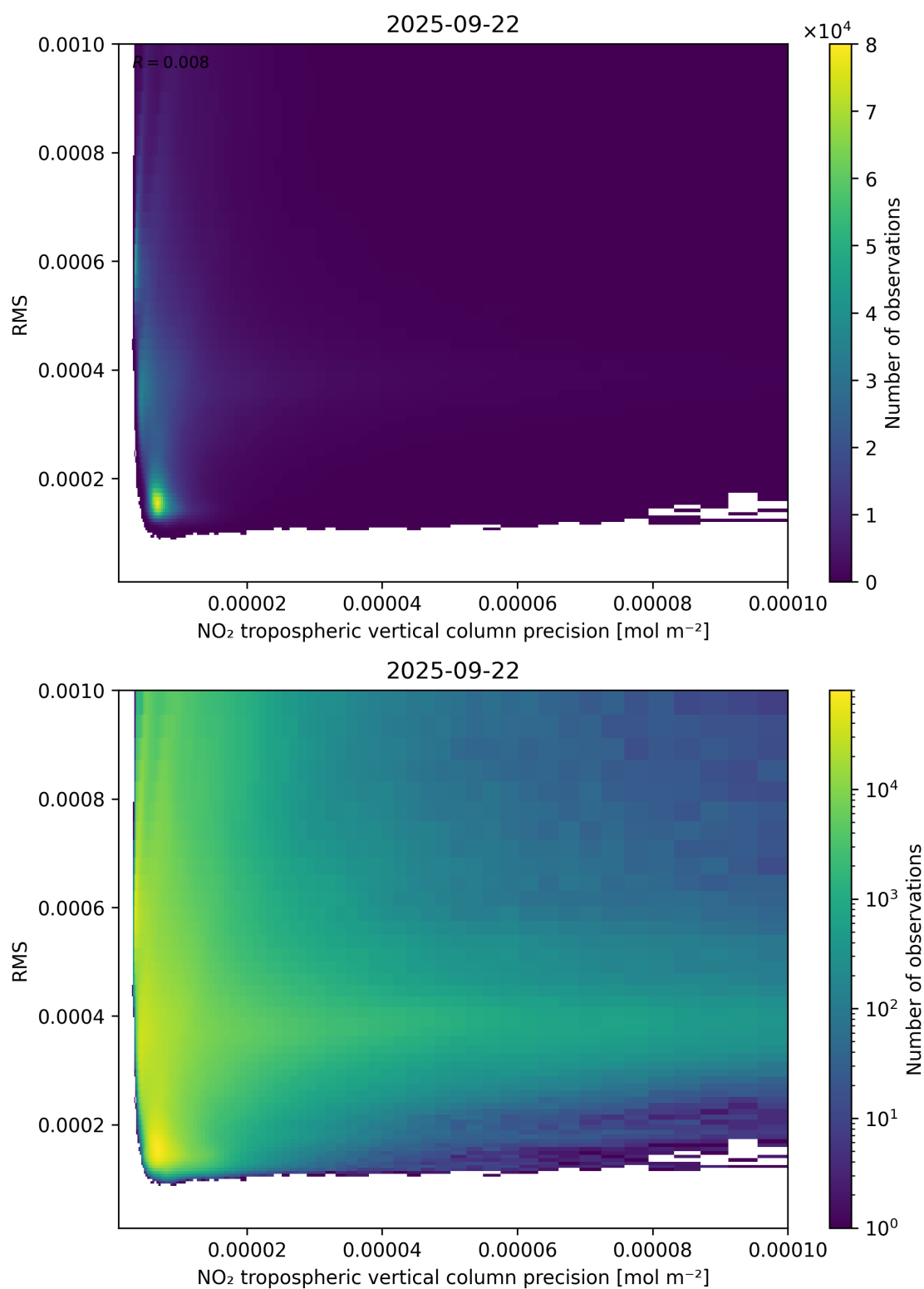
Figure 140: Scatter density plot of “NO 2 tropospheric vertical column precision” against “RMS” for 2025-09-22 to 2025-09-23.
