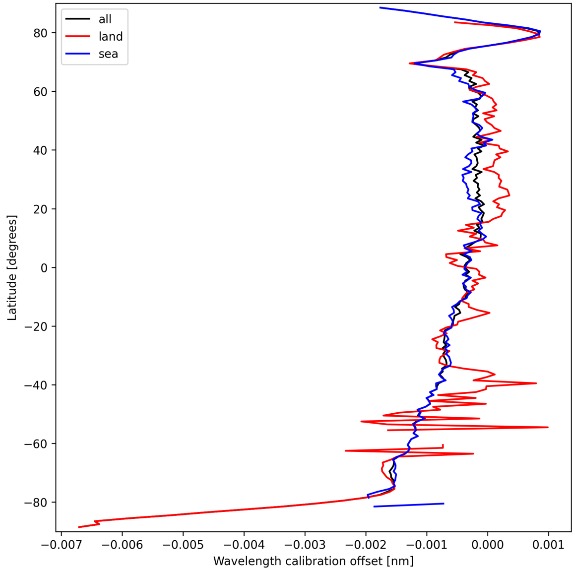
Figure 18: Zonal average of “Wavelength calibration offset” for 2025-09-22 to 2025-09-23.
