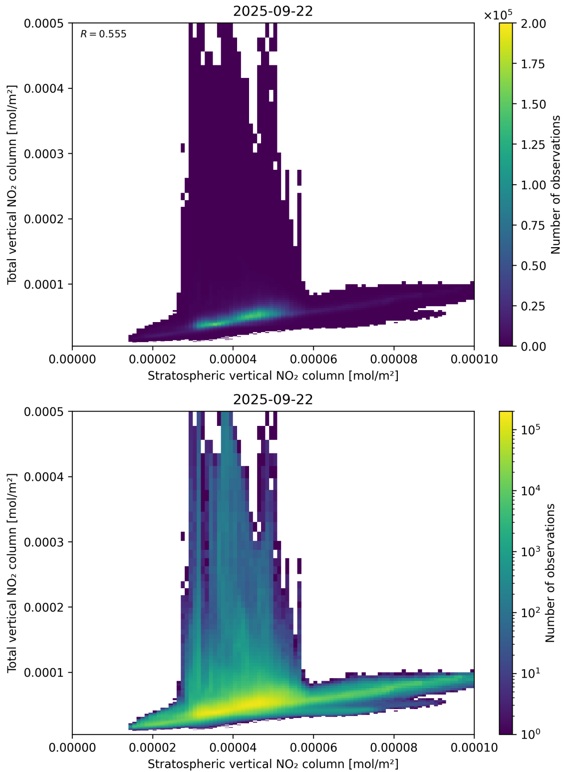
Figure 100: Scatter density plot of “Stratospheric vertical NO 2 column” against “Total vertical NO 2 column” for 2025-09-22 to 2025-09-23.
