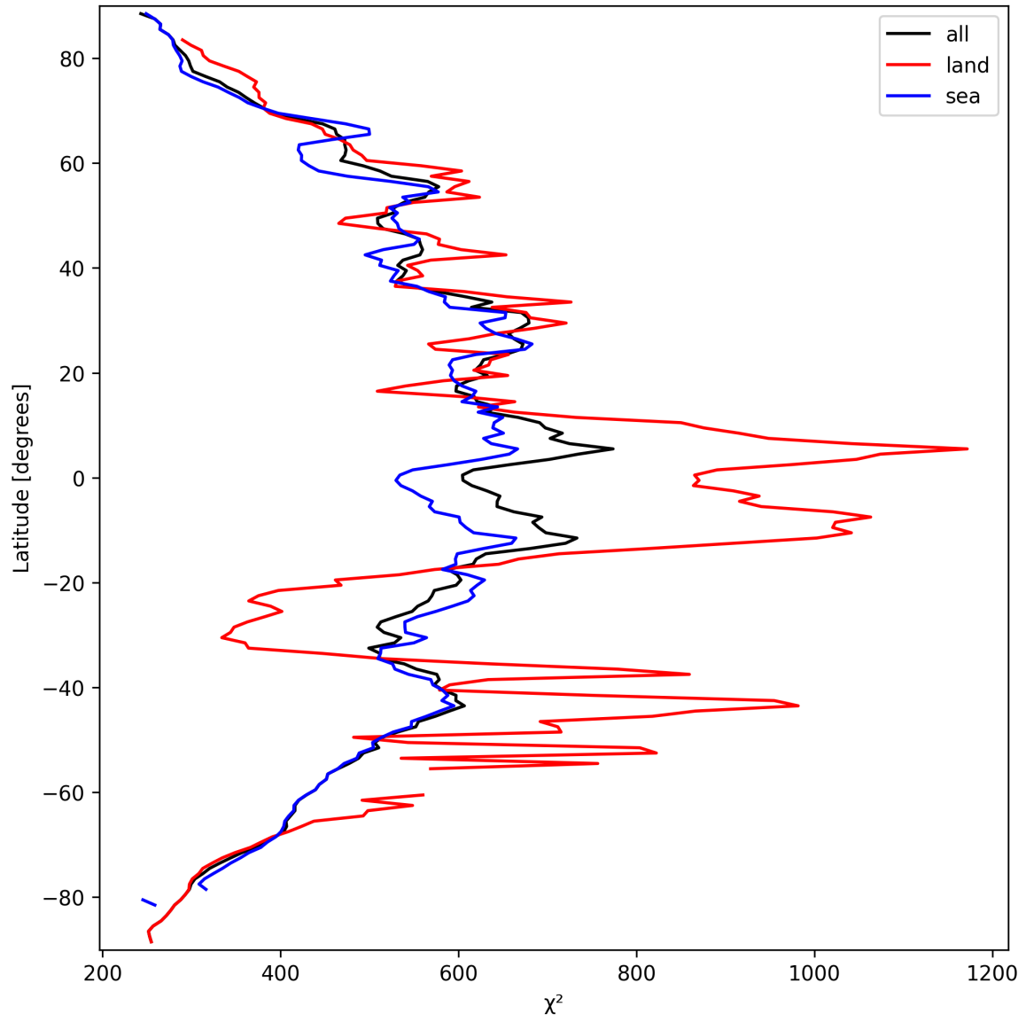
Figure 25: Zonal average of “ \chi^2 ” for 2025-09-22 to 2025-09-23.
