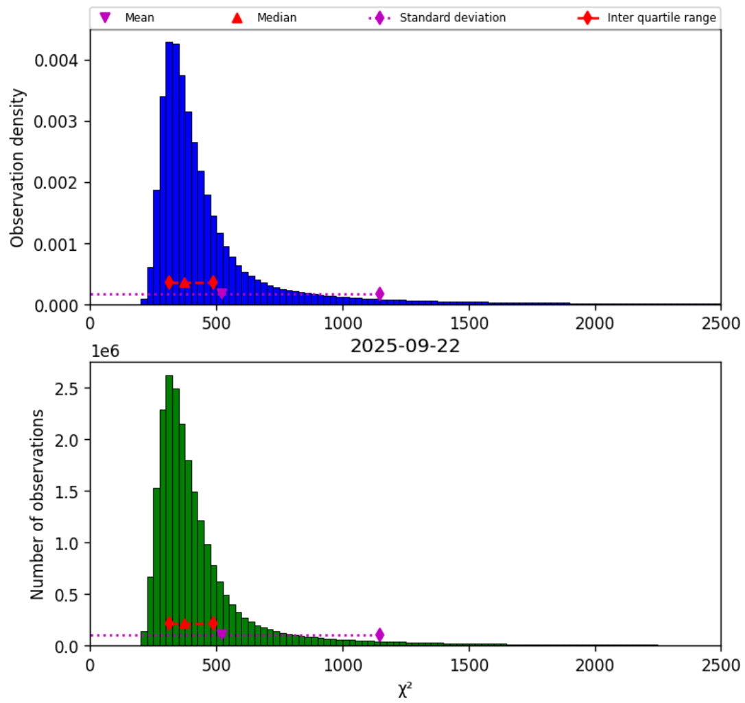
Figure 42: Histogram of “ \chi^2 ” for 2025-09-22 to 2025-09-23
