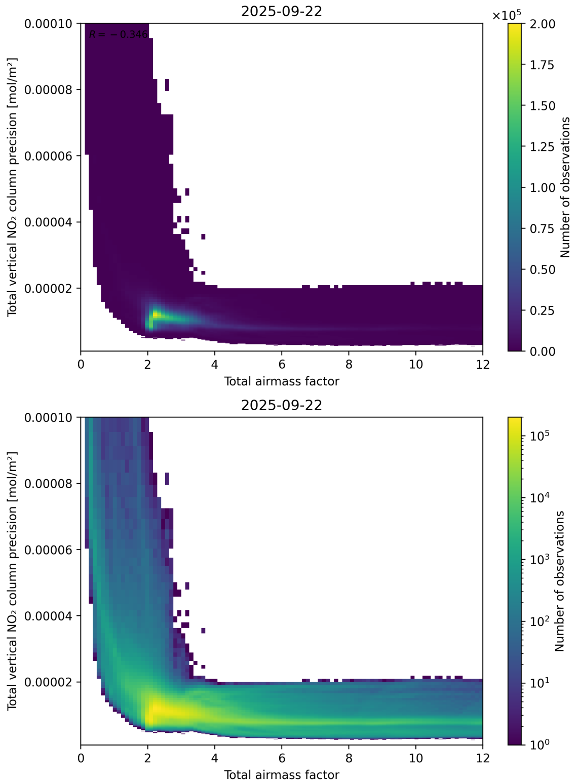
Figure 68: Scatter density plot of “Total airmass factor” against “Total vertical NO 2 column precision” for 2025-09-22 to 2025-09-23.
