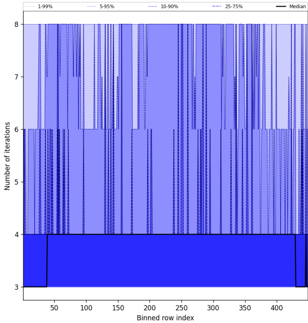
Figure 51: Along track statistics of “Number of iterations” for 2025-09-22 to 2025-09-23
