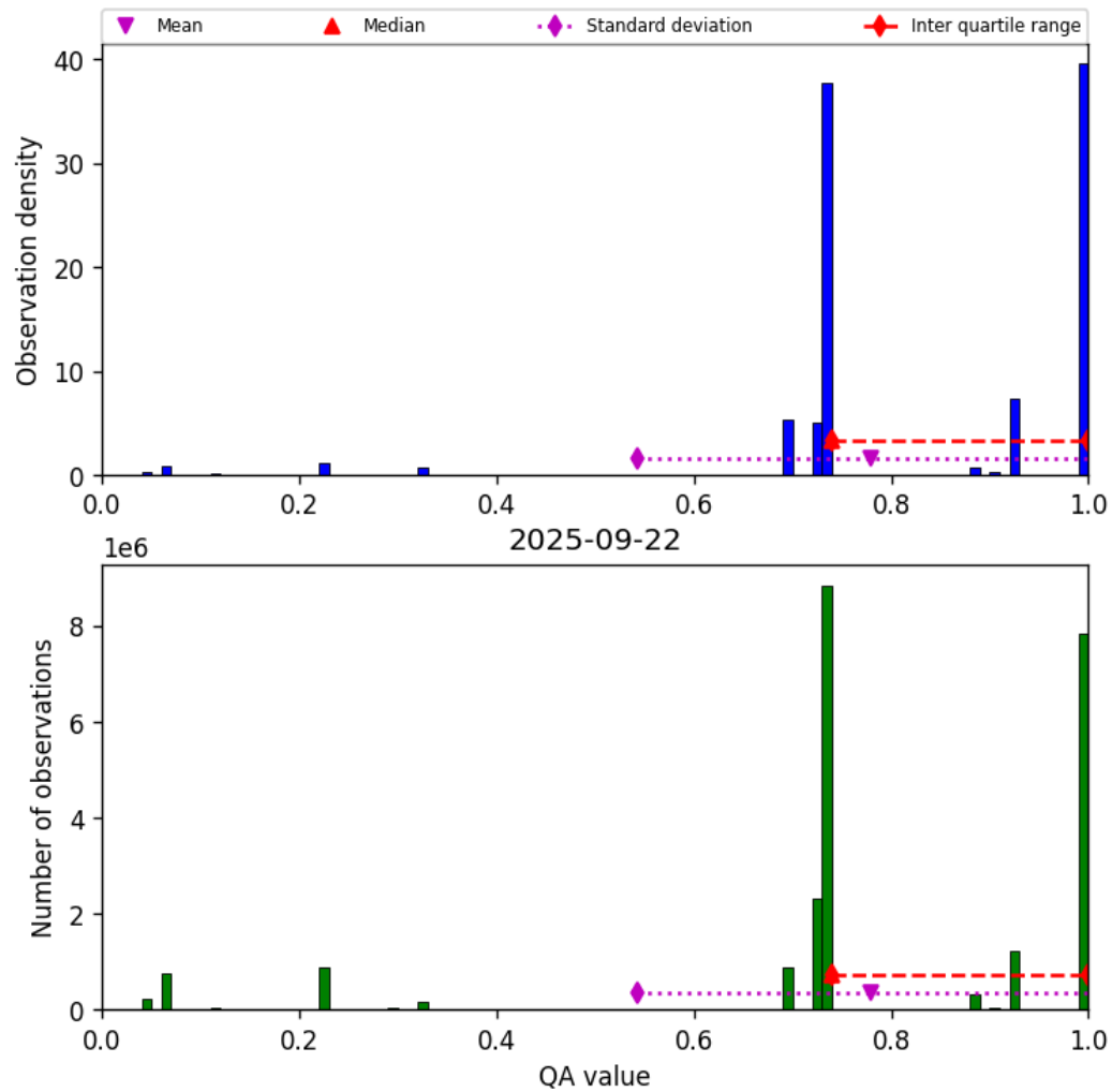
Figure 28: Histogram of “QA value” for 2025-09-22 to 2025-09-23
