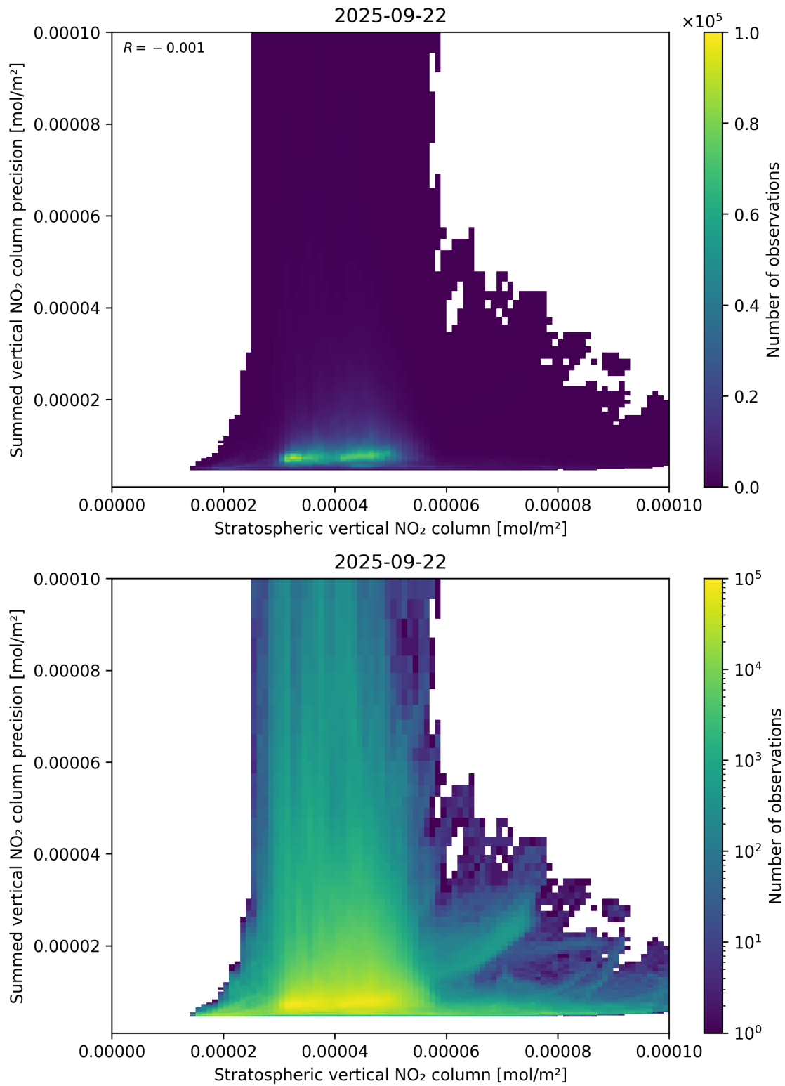
Figure 99: Scatter density plot of “Stratospheric vertical NO 2 column” against “Summed vertical NO 2 column precision” for 2025-09-22 to 2025-09-23.
