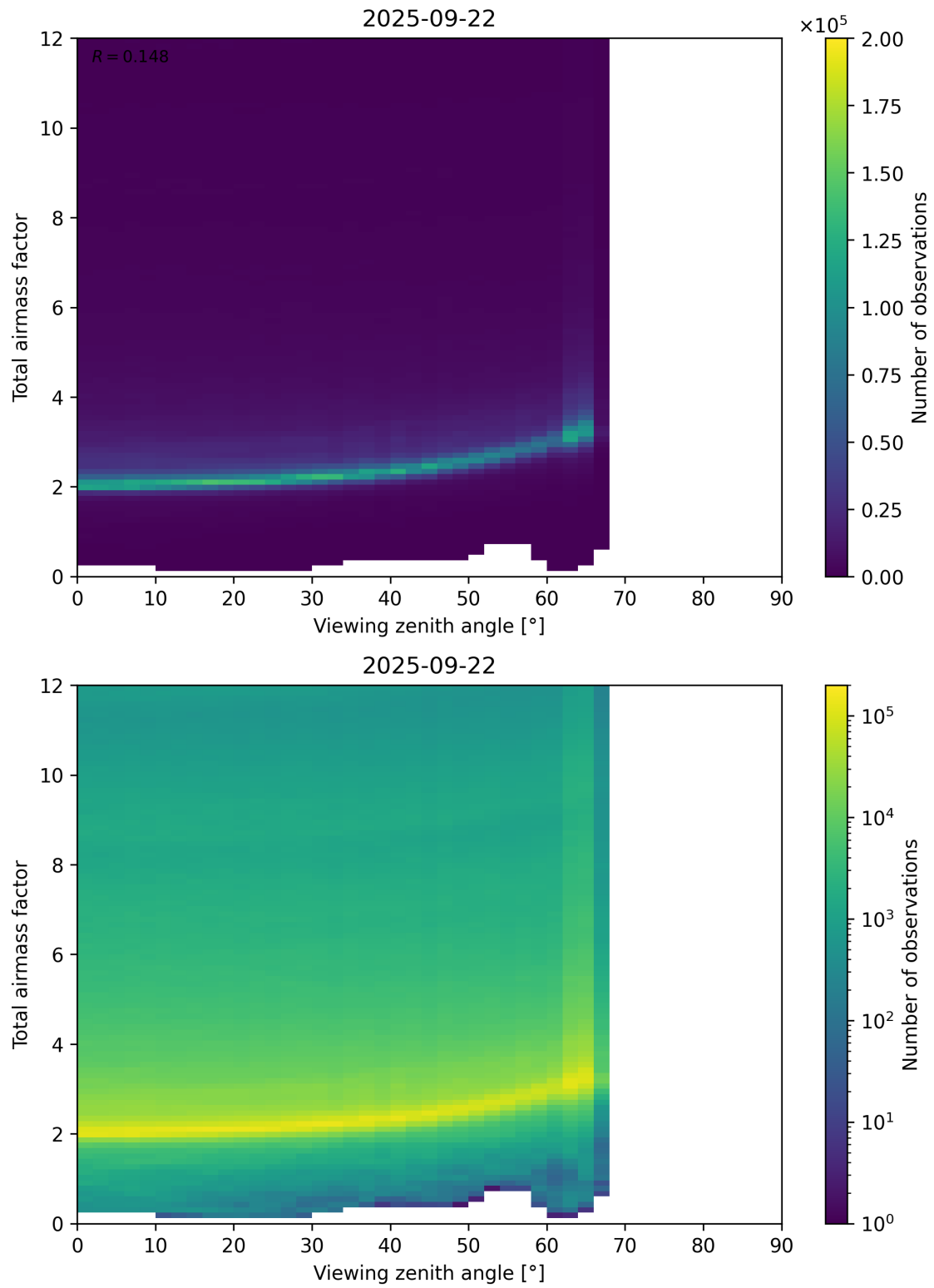
Figure 160: Scatter density plot of “Viewing zenith angle” against “Total airmass factor” for 2025-09-22 to 2025-09-23.
