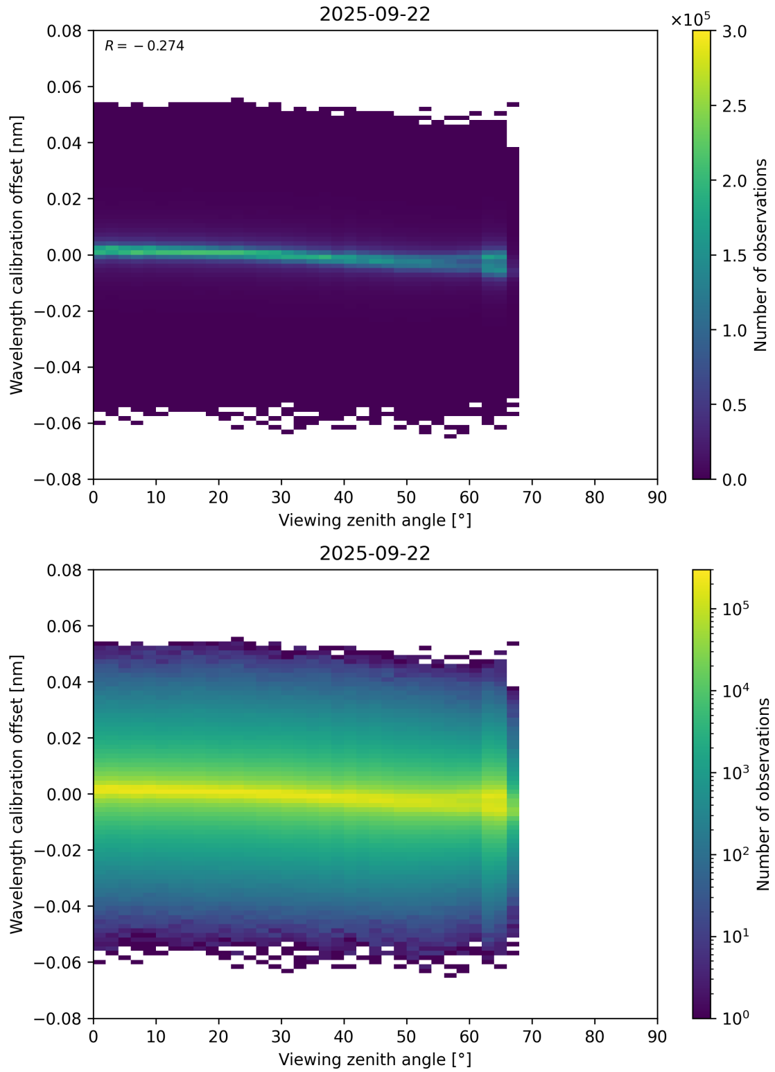
Figure 173: Scatter density plot of “Viewing zenith angle” against “Wavelength calibration offset” for 2025-09-22 to 2025-09-23.
