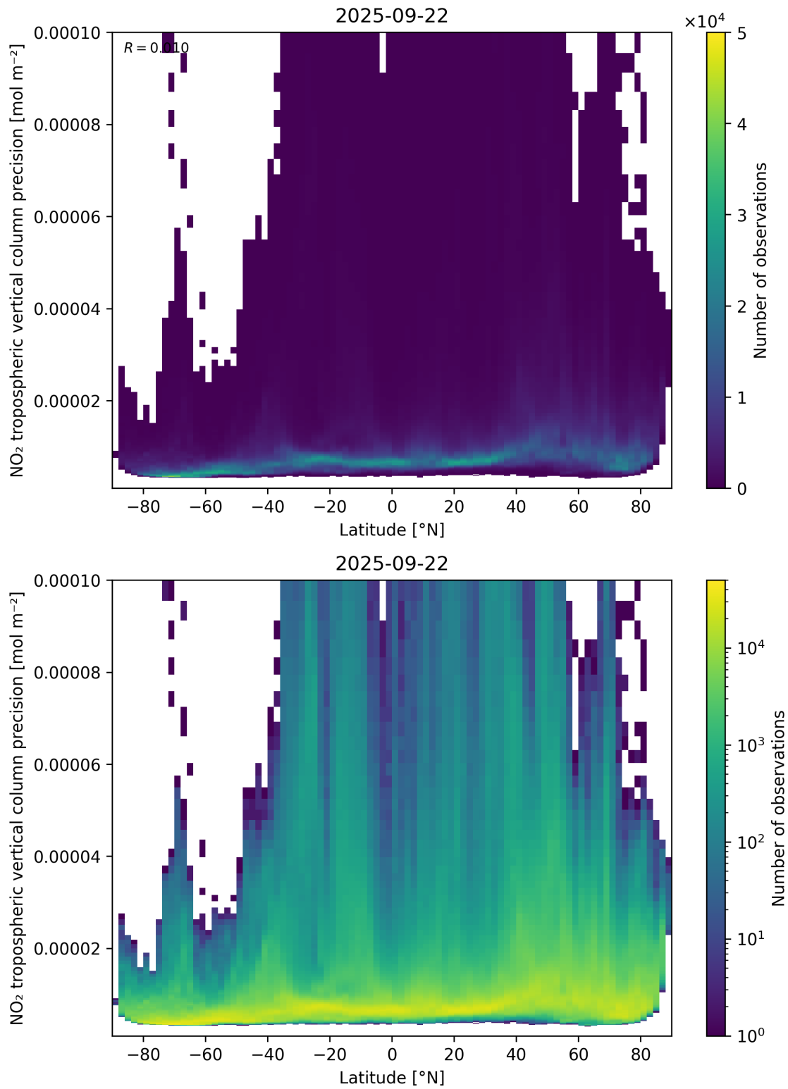
Figure 93: Scatter density plot of “Latitude” against “NO 2 tropospheric vertical column precision” for 2025-09-22 to 2025-09-23.
