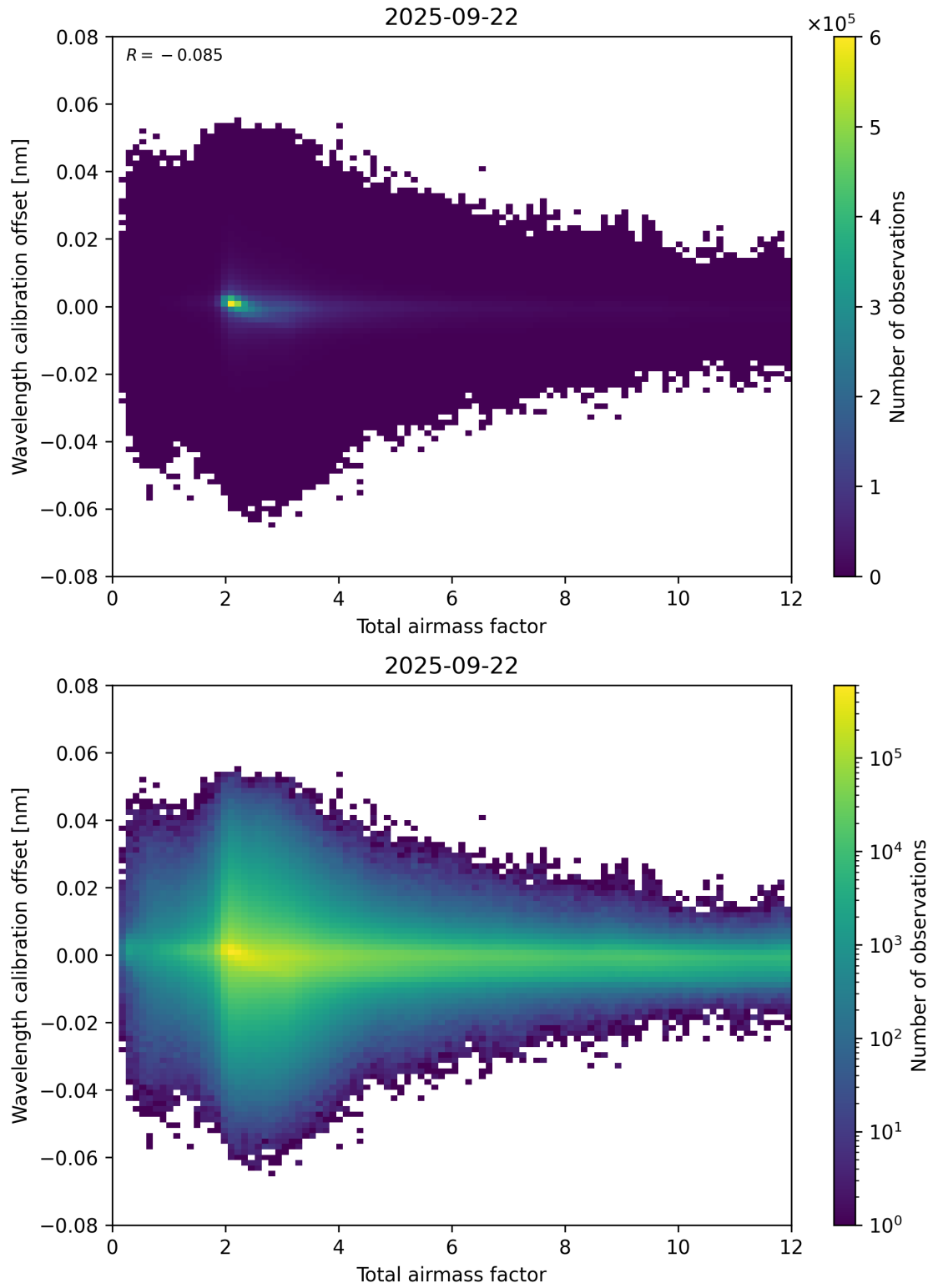
Figure 70: Scatter density plot of “Total airmass factor” against “Wavelength calibration offset” for 2025-09-22 to 2025-09-23.
