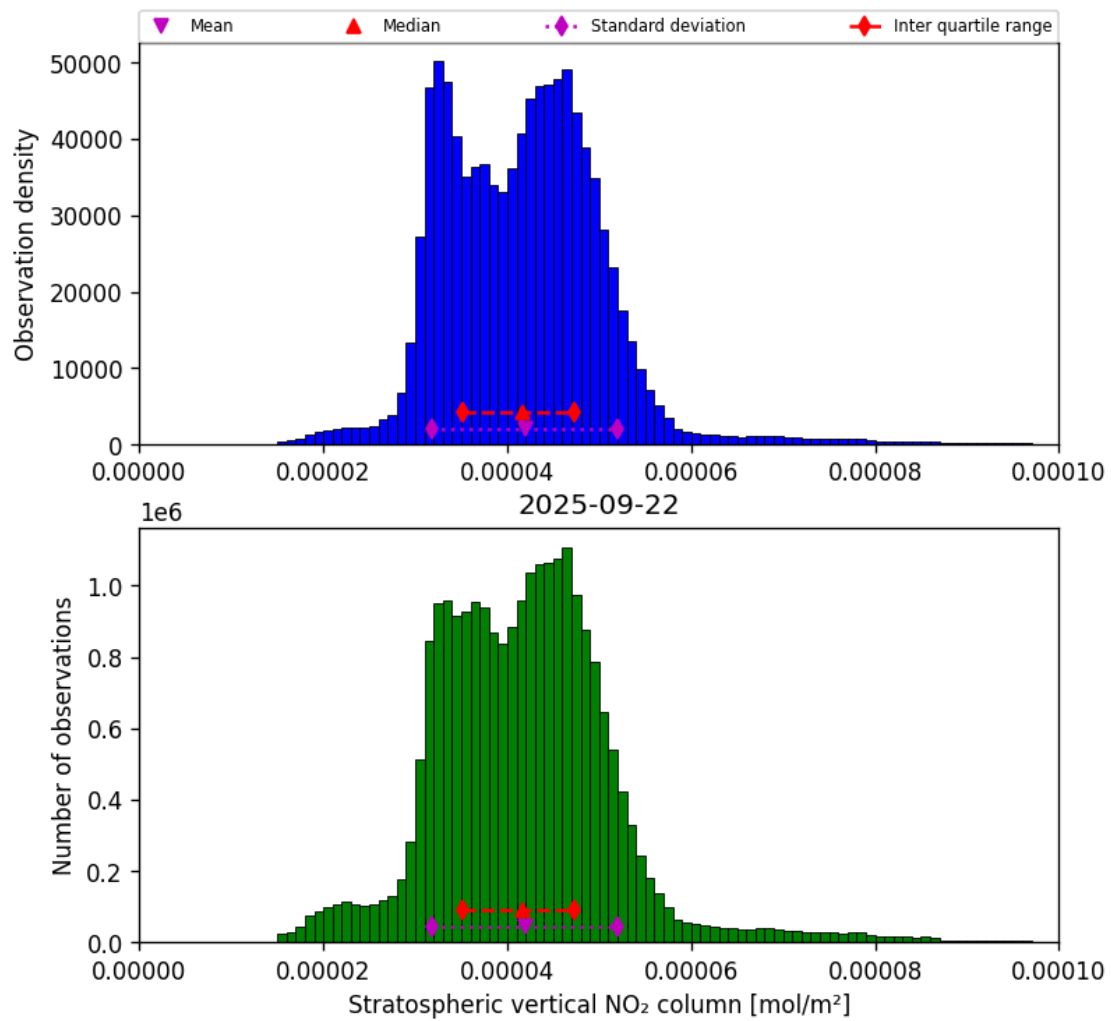
Figure 36: Histogram of “Stratospheric vertical NO 2 column” for 2025-09-22 to 2025-09-23
