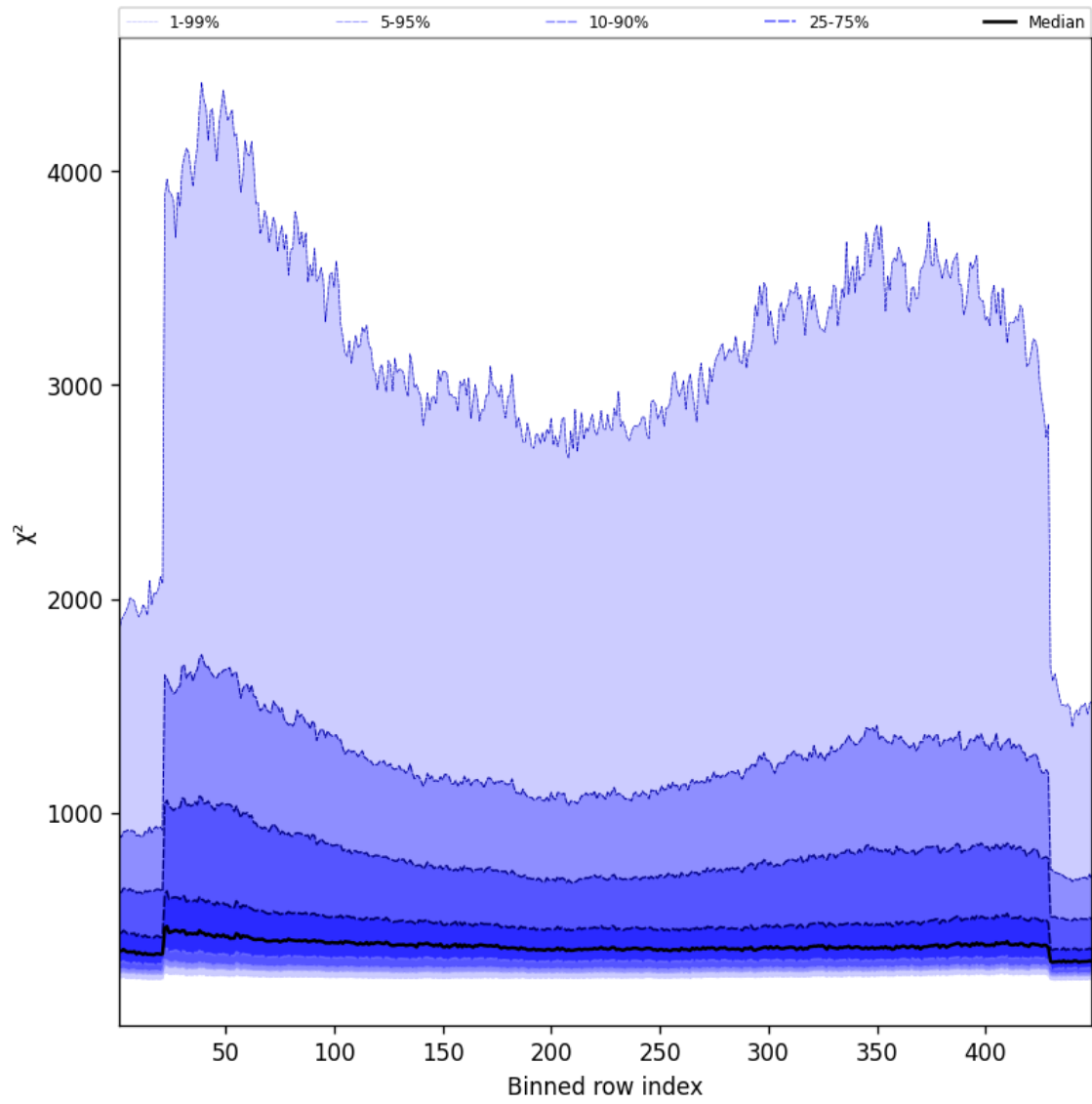
Figure 59: Along track statistics of “ \chi^2 ” for 2025-09-22 to 2025-09-23
