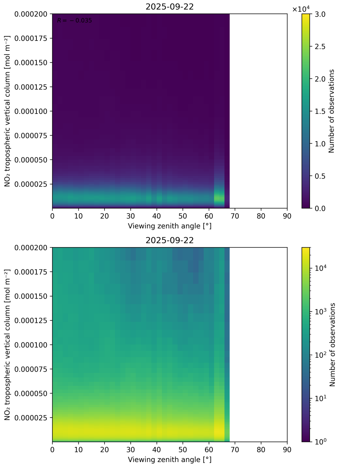
Figure 169: Scatter density plot of “Viewing zenith angle” against “NO 2 tropospheric vertical column” for 2025-09-22 to 2025-09-23.
