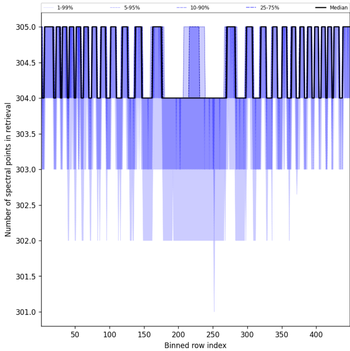
Figure 50: Along track statistics of “Number of spectral points in retrieval” for 2025-09-22 to 2025-09-23
