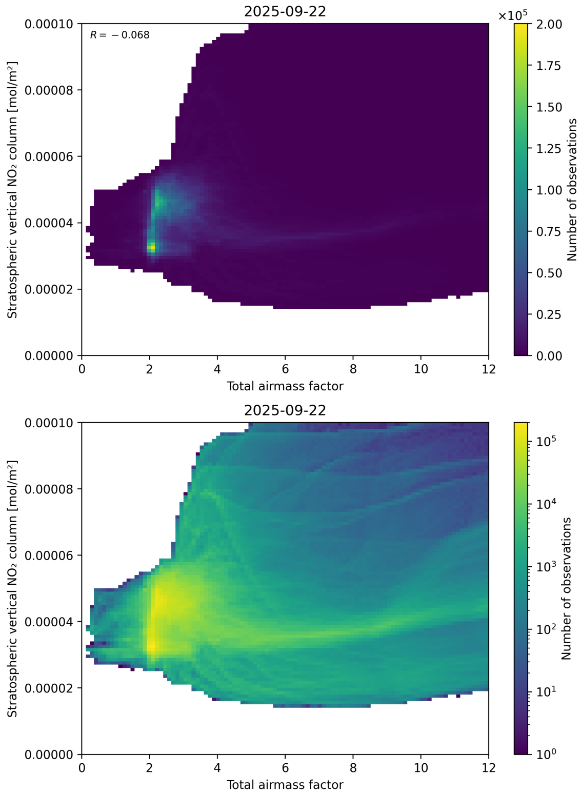
Figure 64: Scatter density plot of “Total airmass factor” against “Stratospheric vertical NO 2 column” for 2025-09-22 to 2025-09-23.
