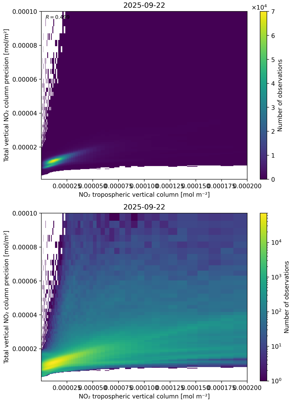
Figure 129: Scatter density plot of “NO 2 tropospheric vertical column” against “Total vertical NO 2 column precision” for 2025-09-22 to 2025-09-23.
