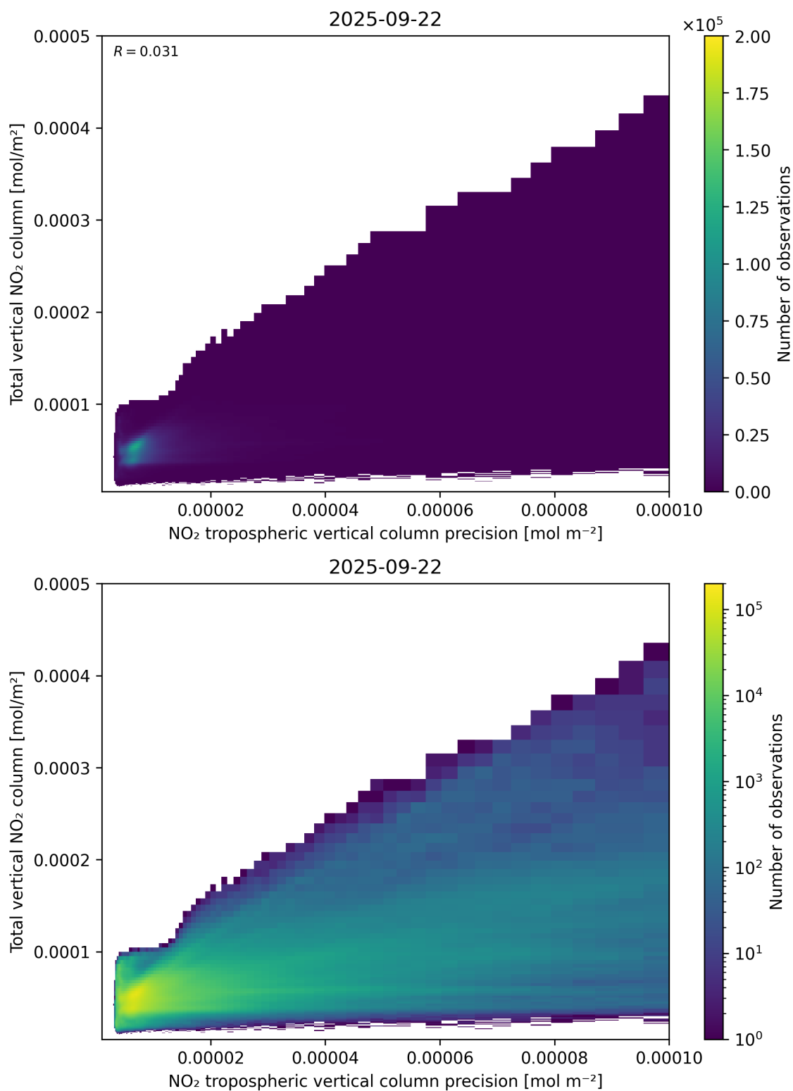
Figure 138: Scatter density plot of “NO 2 tropospheric vertical column precision” against “Total vertical NO 2 column” for 2025-09-22 to 2025-09-23.
