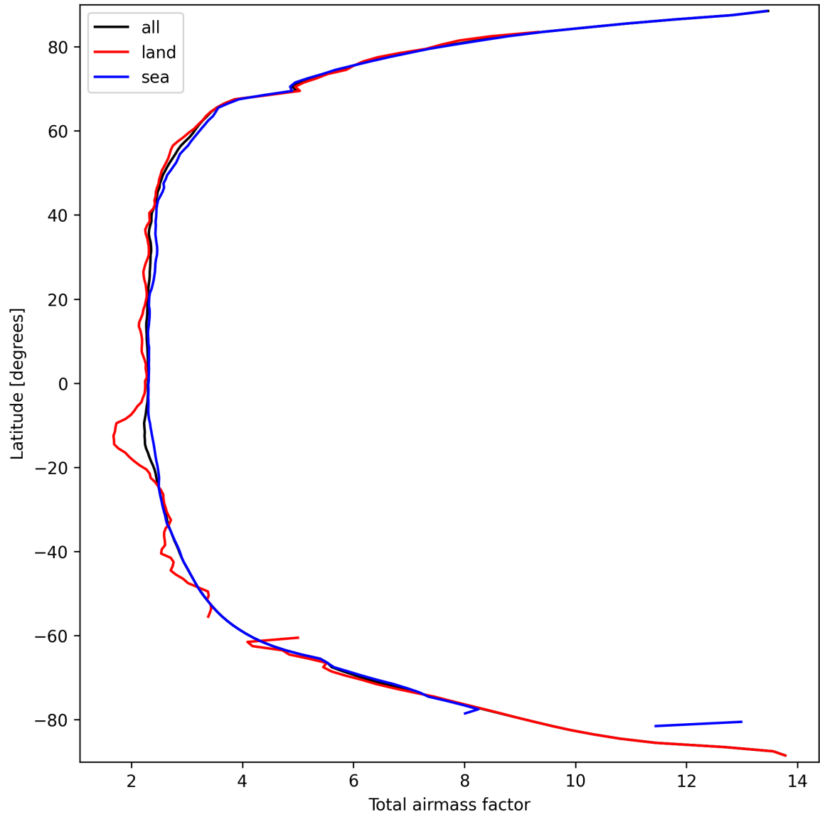
Figure 15: Zonal average of “Total airmass factor” for 2025-09-22 to 2025-09-23.
