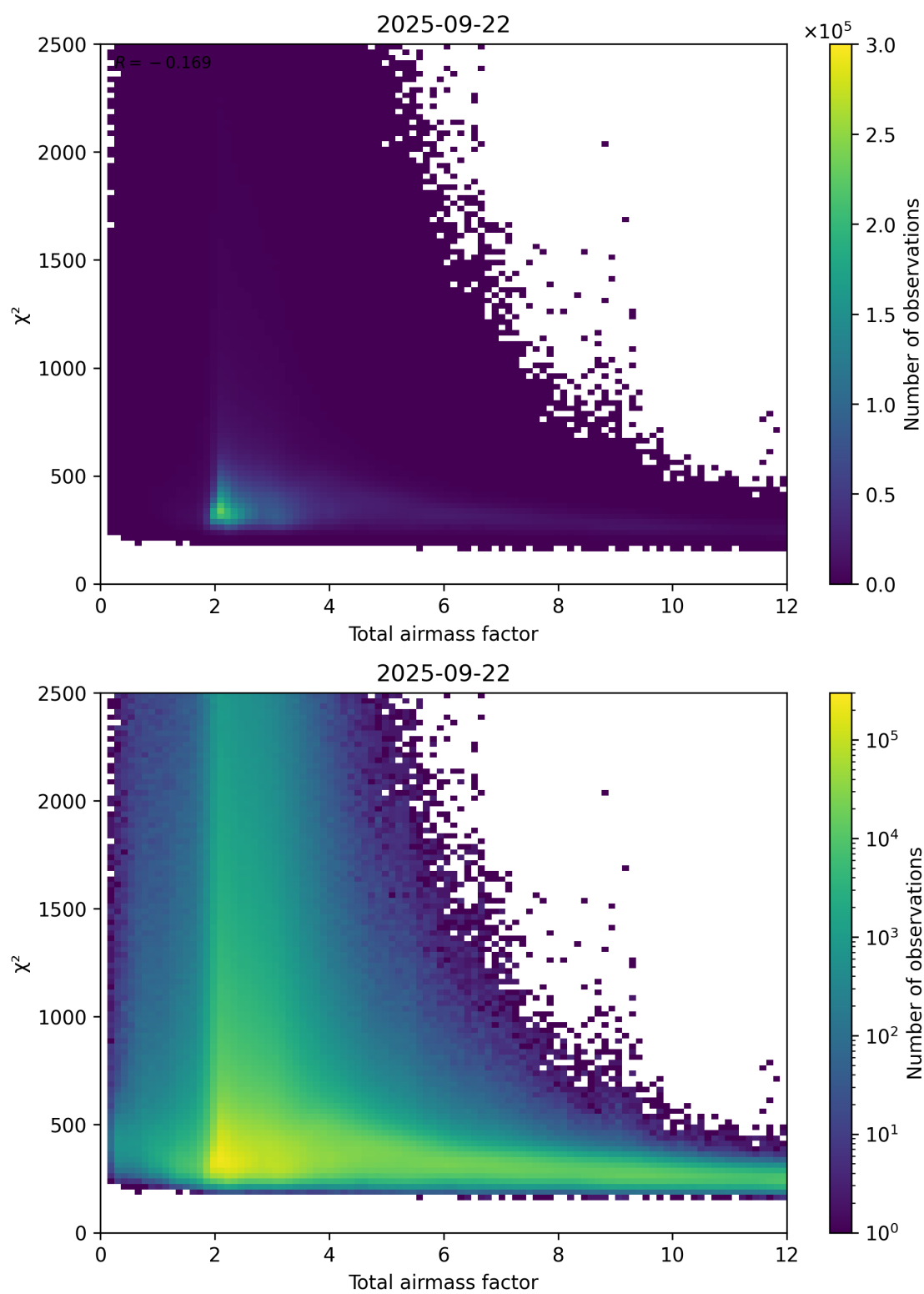
Figure 63: Scatter density plot of “Total airmass factor” against “ \chi^2 ” for 2025-09-22 to 2025-09-23.
