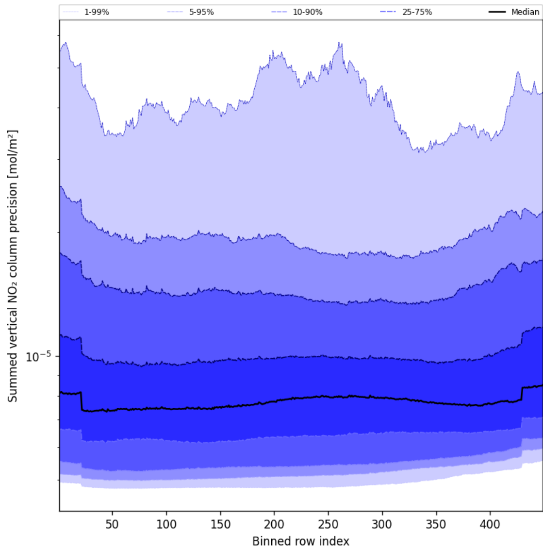
Figure 58: Along track statistics of “Summed vertical NO 2 column precision” for 2025-09-22 to 2025-09-23
