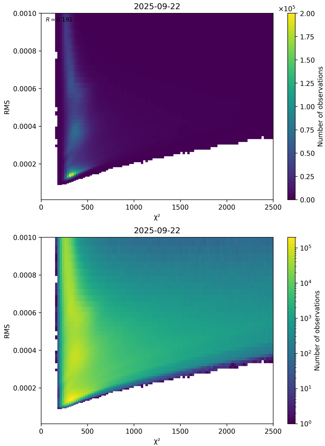
Figure 82: Scatter density plot of “ \chi^2 ” against “RMS” for 2025-09-22 to 2025-09-23.
