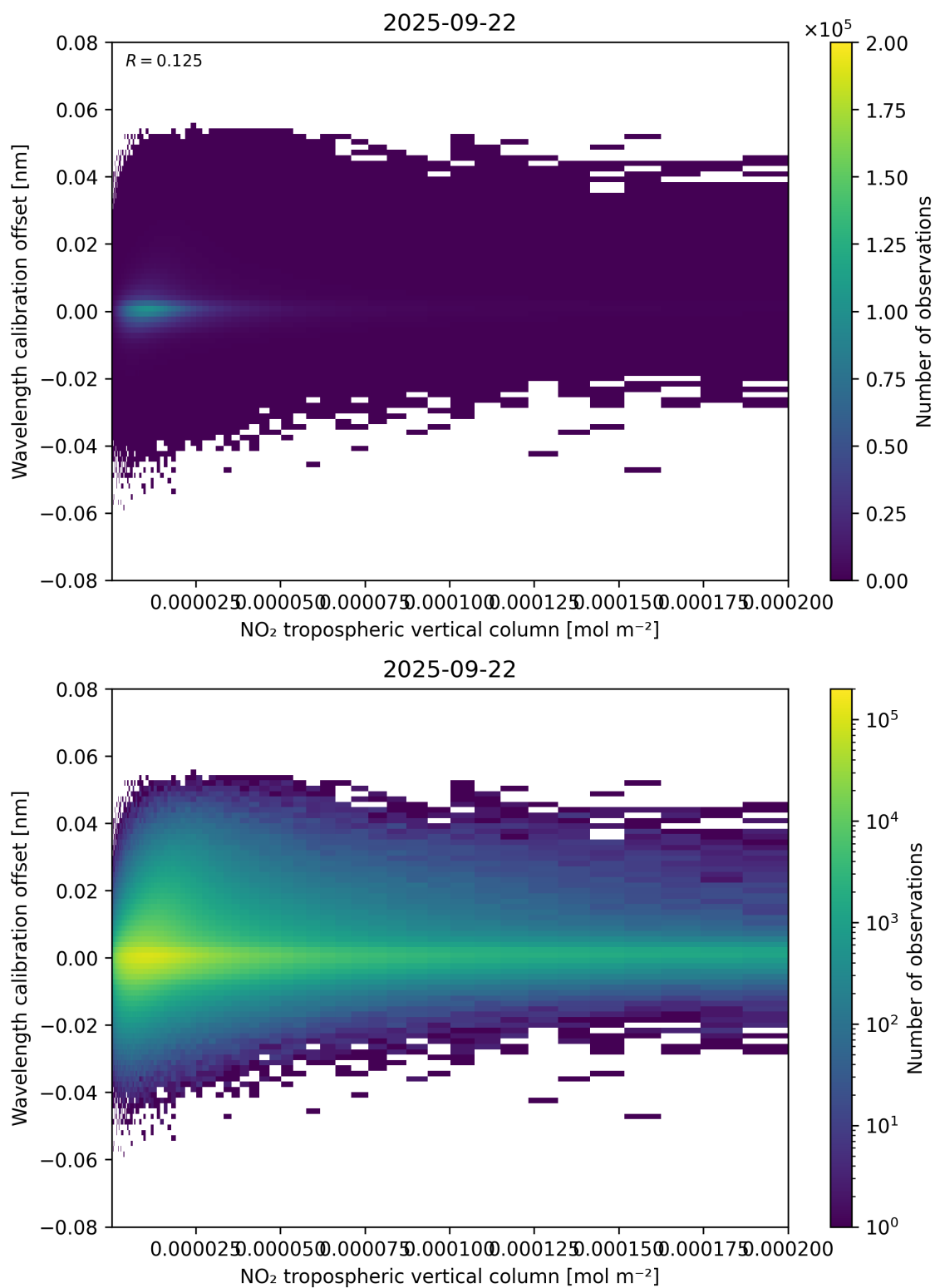
Figure 143: Scatter density plot of “NO 2 tropospheric vertical column” against “Wavelength calibration offset” for 2025-09-22 to 2025-09-23.
