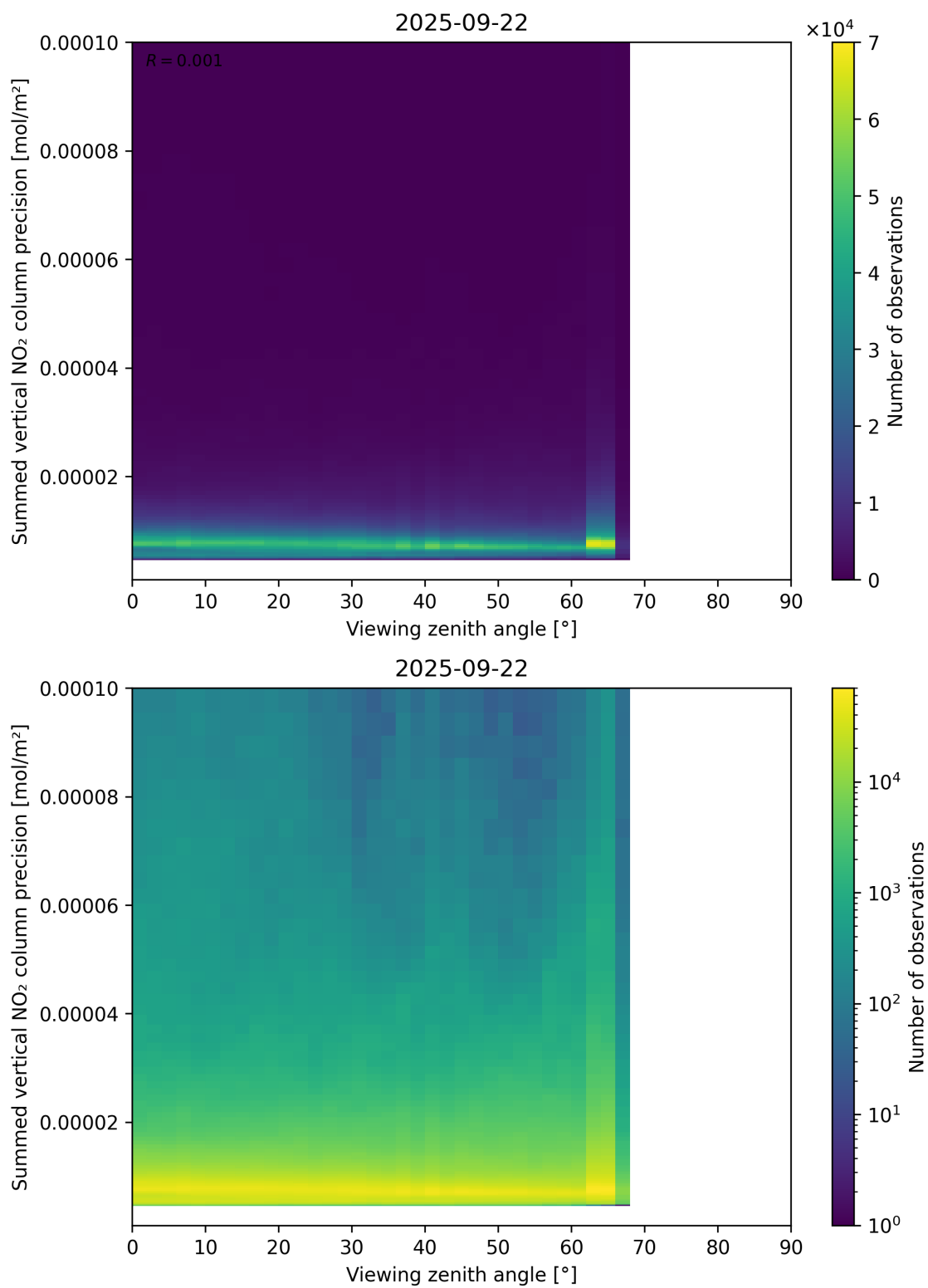
Figure 166: Scatter density plot of “Viewing zenith angle” against “Summed vertical NO 2 column precision” for 2025-09-22 to 2025-09-23.
