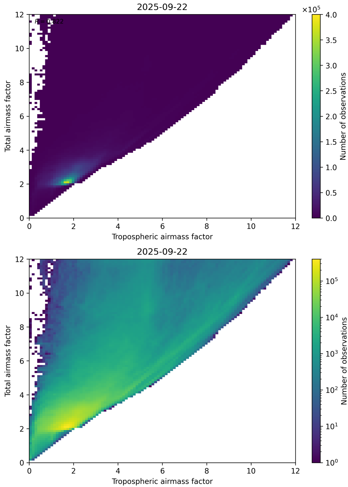
Figure 72: Scatter density plot of “Tropospheric airmass factor” against “Total airmass factor” for 2025-09-22 to 2025-09-23.
