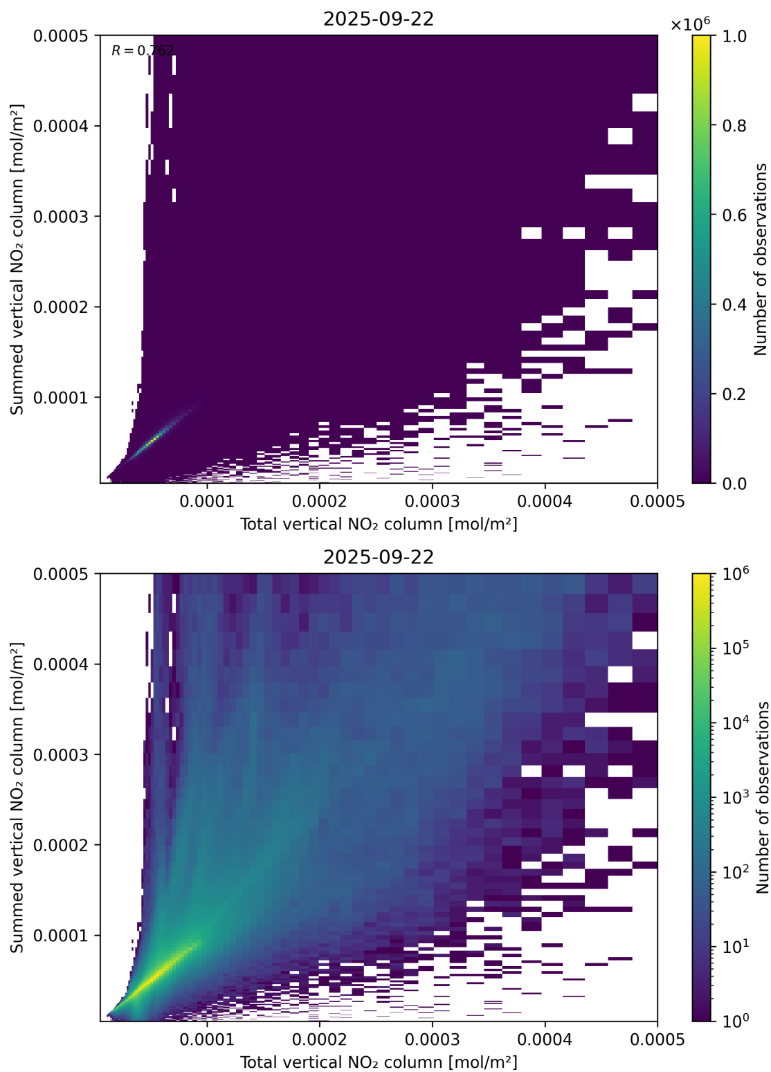
Figure 112: Scatter density plot of “Total vertical NO 2 column” against “Summed vertical NO 2 column” for 2025-09-22 to 2025-09-23.
