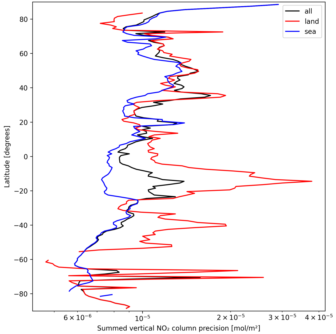
Figure 24: Zonal average of “Summed vertical NO 2 column precision” for 2025-09-22 to 2025-09-23.
