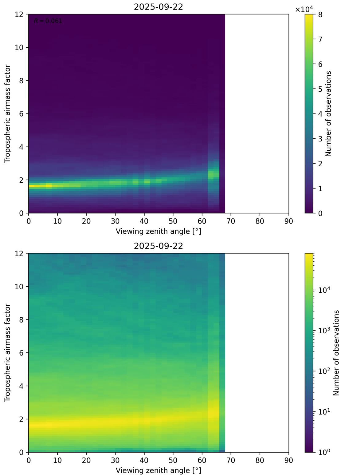
Figure 161: Scatter density plot of “Viewing zenith angle” against “Tropospheric airmass factor” for 2025-09-22 to 2025-09-23.
