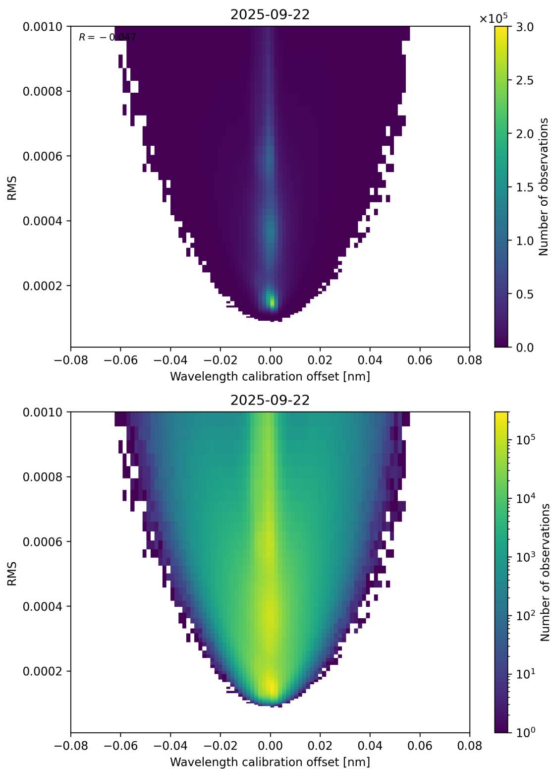
Figure 181: Scatter density plot of “Wavelength calibration offset” against “RMS” for 2025-09-22 to 2025-09-23.
