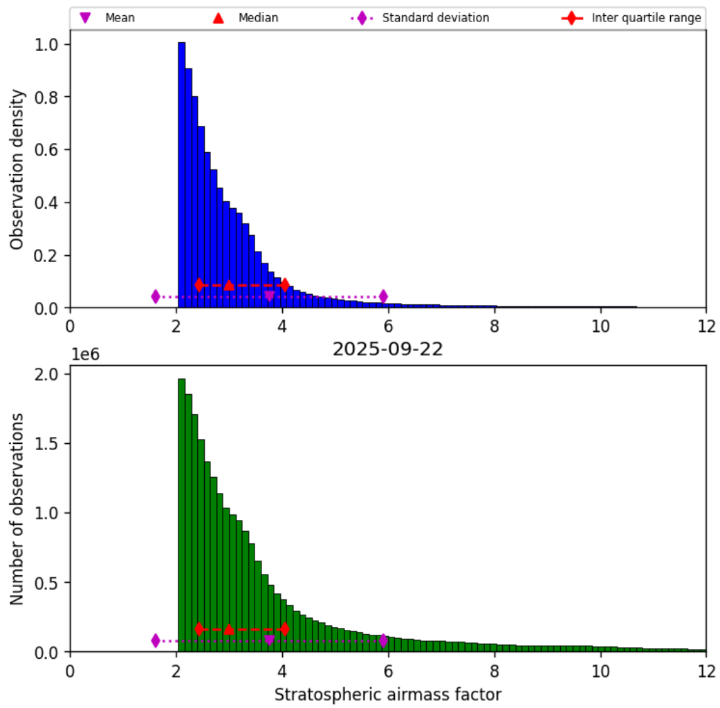
Figure 44: Histogram of “Stratospheric airmass factor” for 2025-09-22 to 2025-09-23
