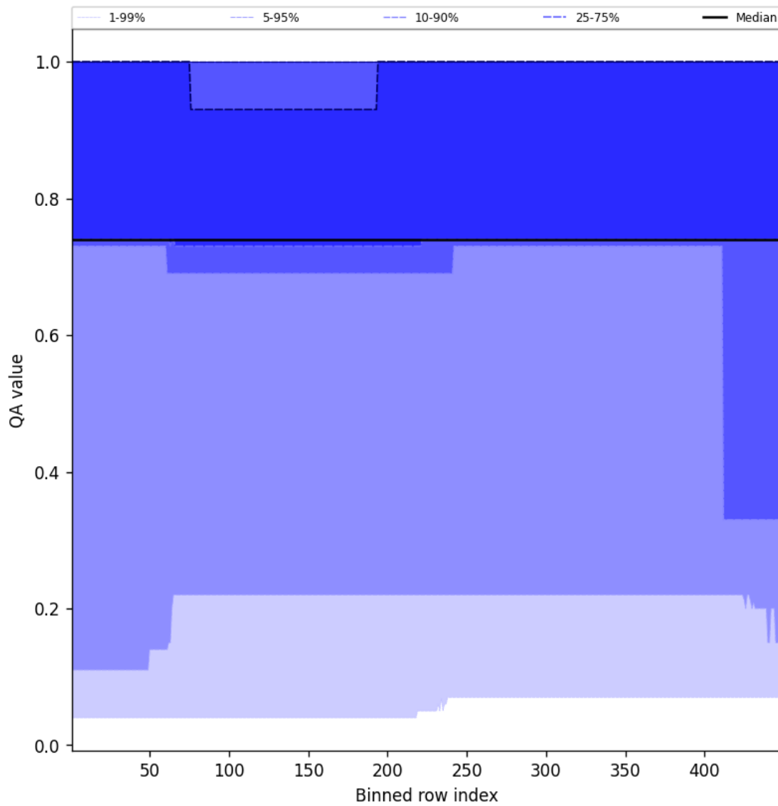
Figure 45: Along track statistics of “QA value” for 2025-09-22 to 2025-09-23
