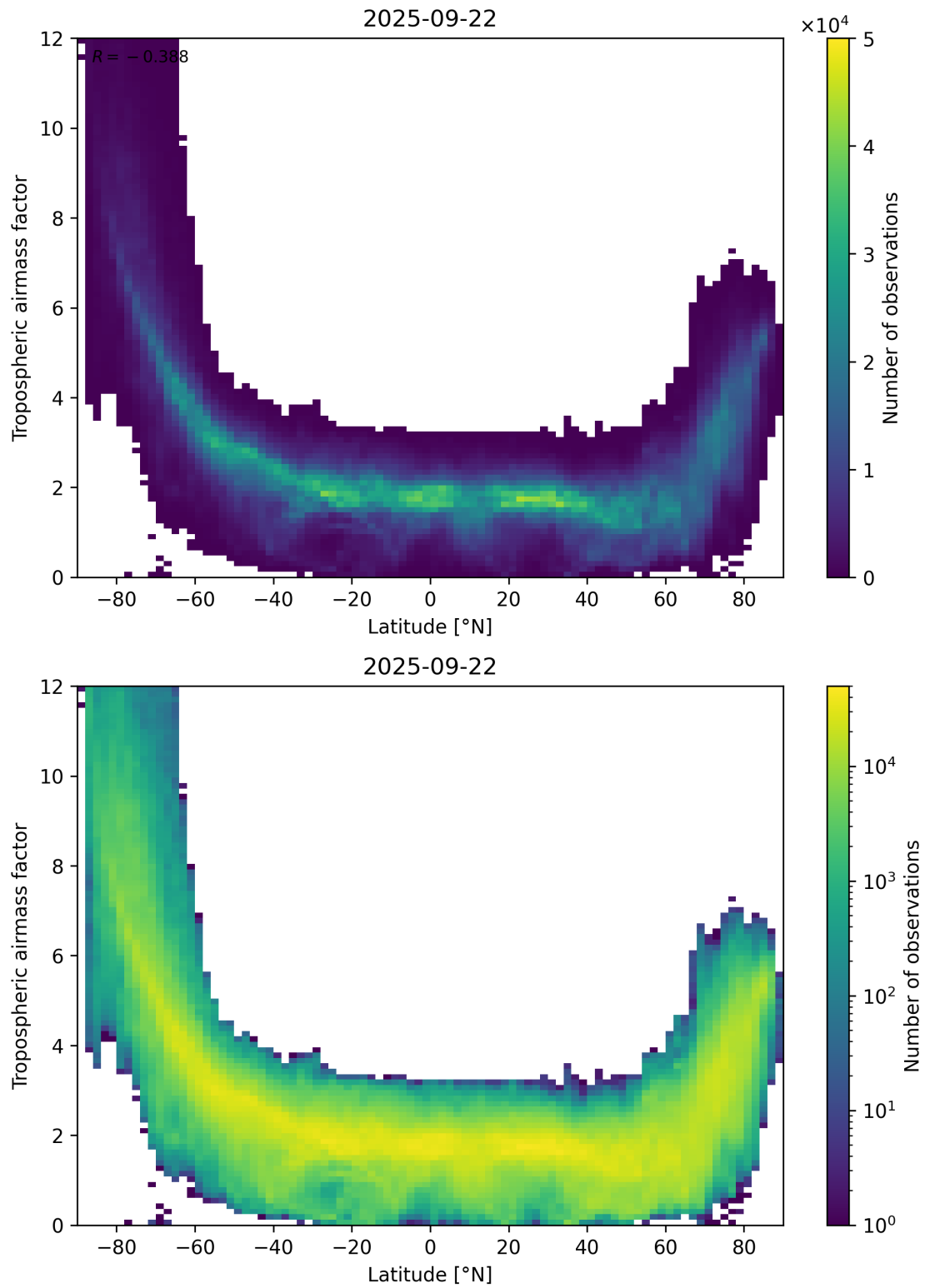
Figure 85: Scatter density plot of “Latitude” against “Tropospheric airmass factor” for 2025-09-22 to 2025-09-23.
