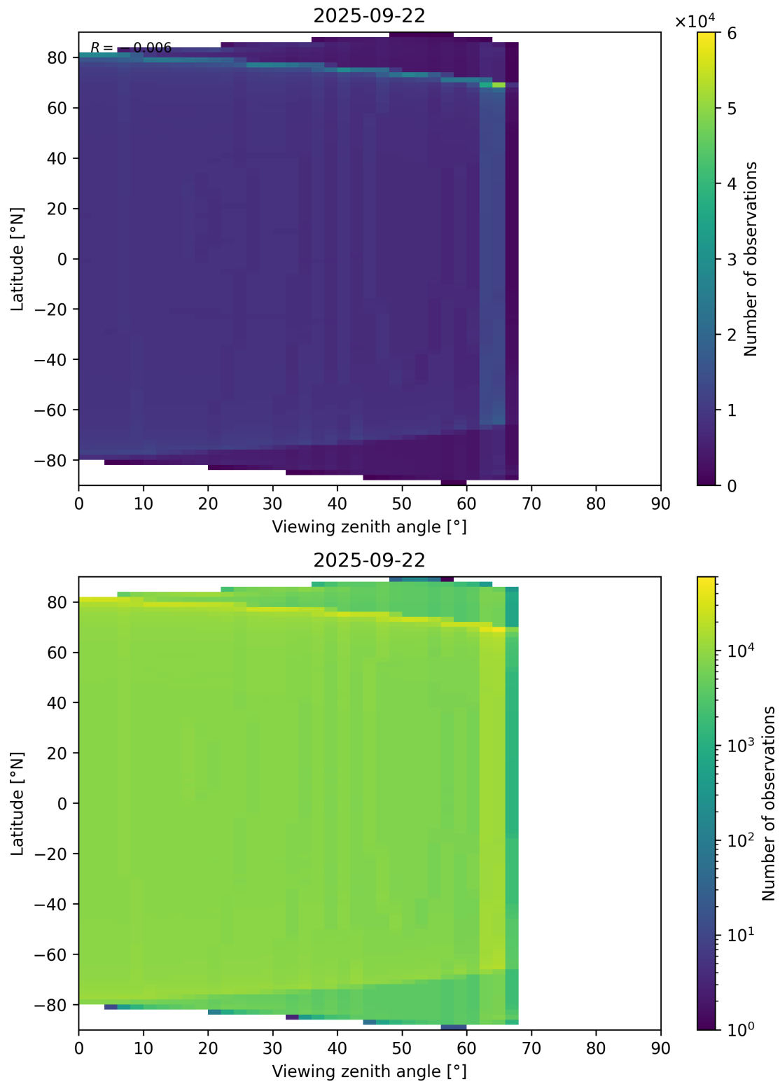
Figure 163: Scatter density plot of “Viewing zenith angle” against “Latitude” for 2025-09-22 to 2025-09-23.
