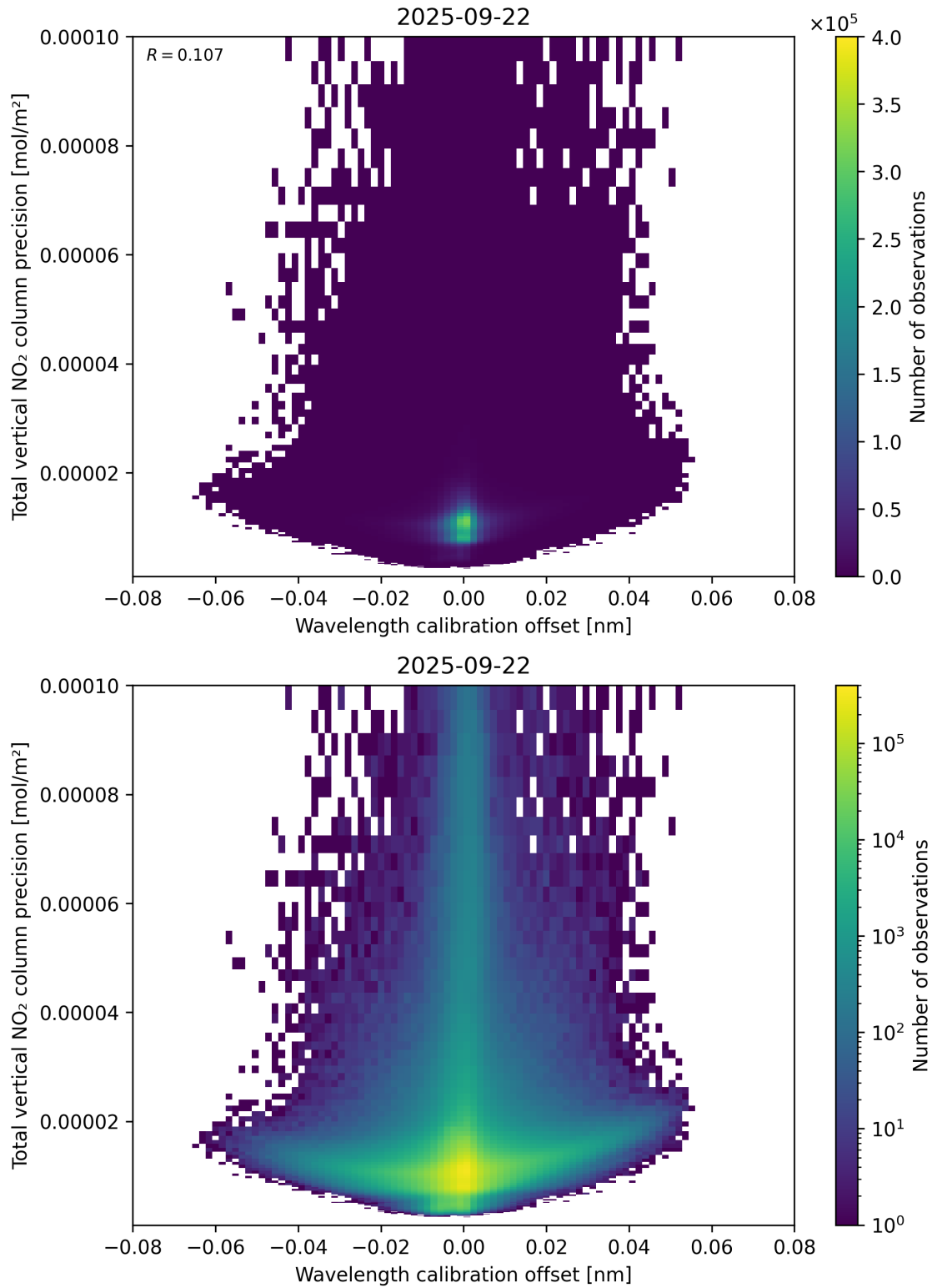
Figure 180: Scatter density plot of “Wavelength calibration offset” against “Total vertical NO 2 column precision” for 2025-09-22 to 2025-09-23.
