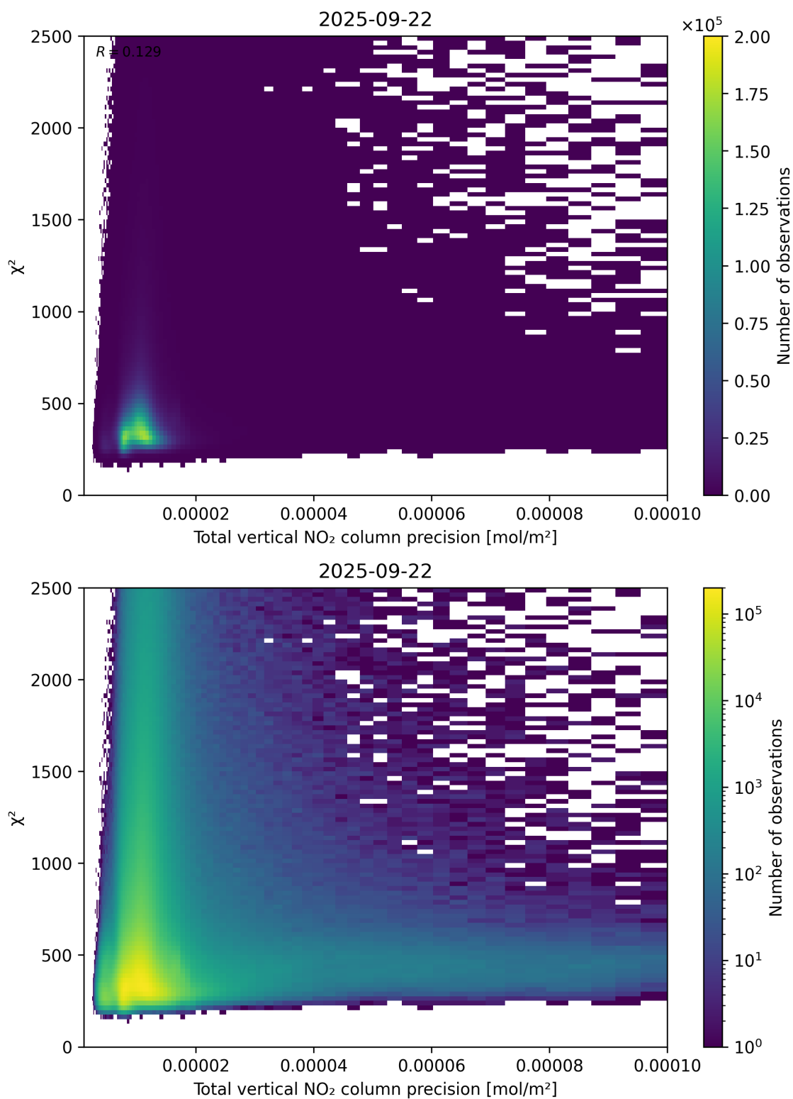
Figure 116: Scatter density plot of “Total vertical NO 2 column precision” against “ \chi^2 ” for 2025-09-22 to 2025-09-23.
