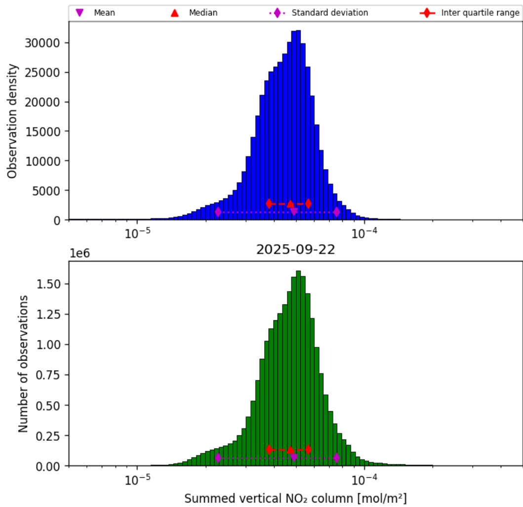
Figure 40: Histogram of “Summed vertical NO 2 column” for 2025-09-22 to 2025-09-23
