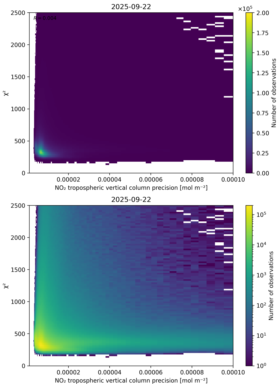
Figure 134: Scatter density plot of “NO 2 tropospheric vertical column precision” against “ \chi^2 ” for 2025-09-22 to 2025-09-23.
