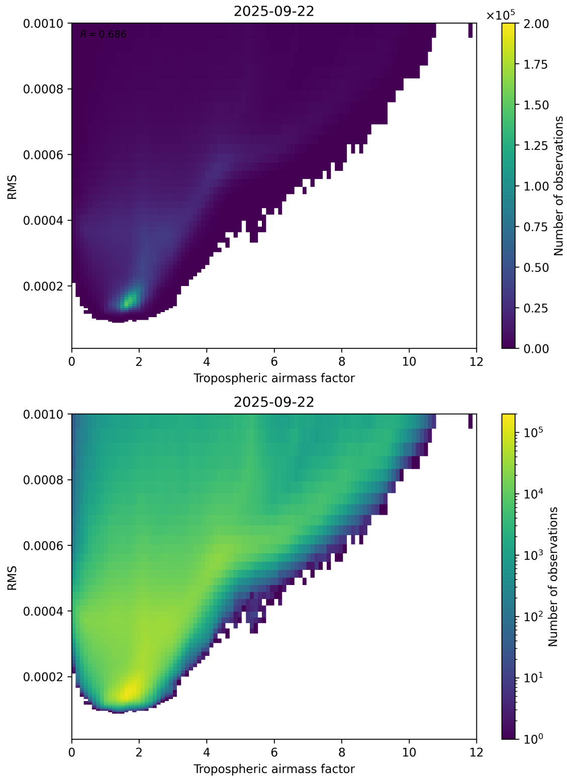
Figure 79: Scatter density plot of “Tropospheric airmass factor” against “RMS” for 2025-09-22 to 2025-09-23.
