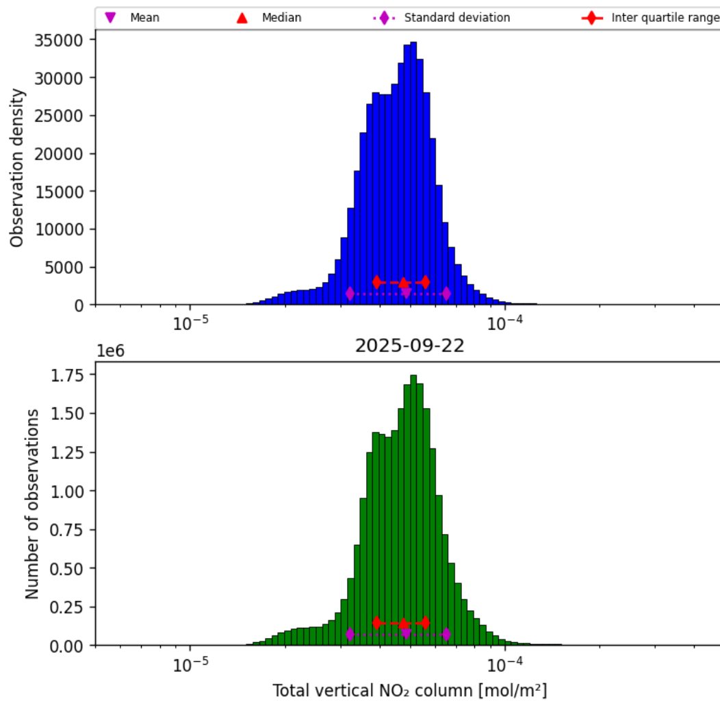
Figure 38: Histogram of “Total vertical NO 2 column” for 2025-09-22 to 2025-09-23
