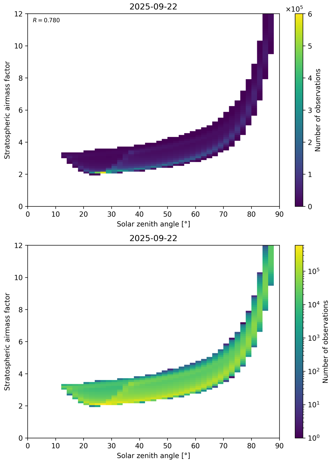
Figure 145: Scatter density plot of “Solar zenith angle” against “Stratospheric airmass factor” for 2025-09-22 to 2025-09-23.
