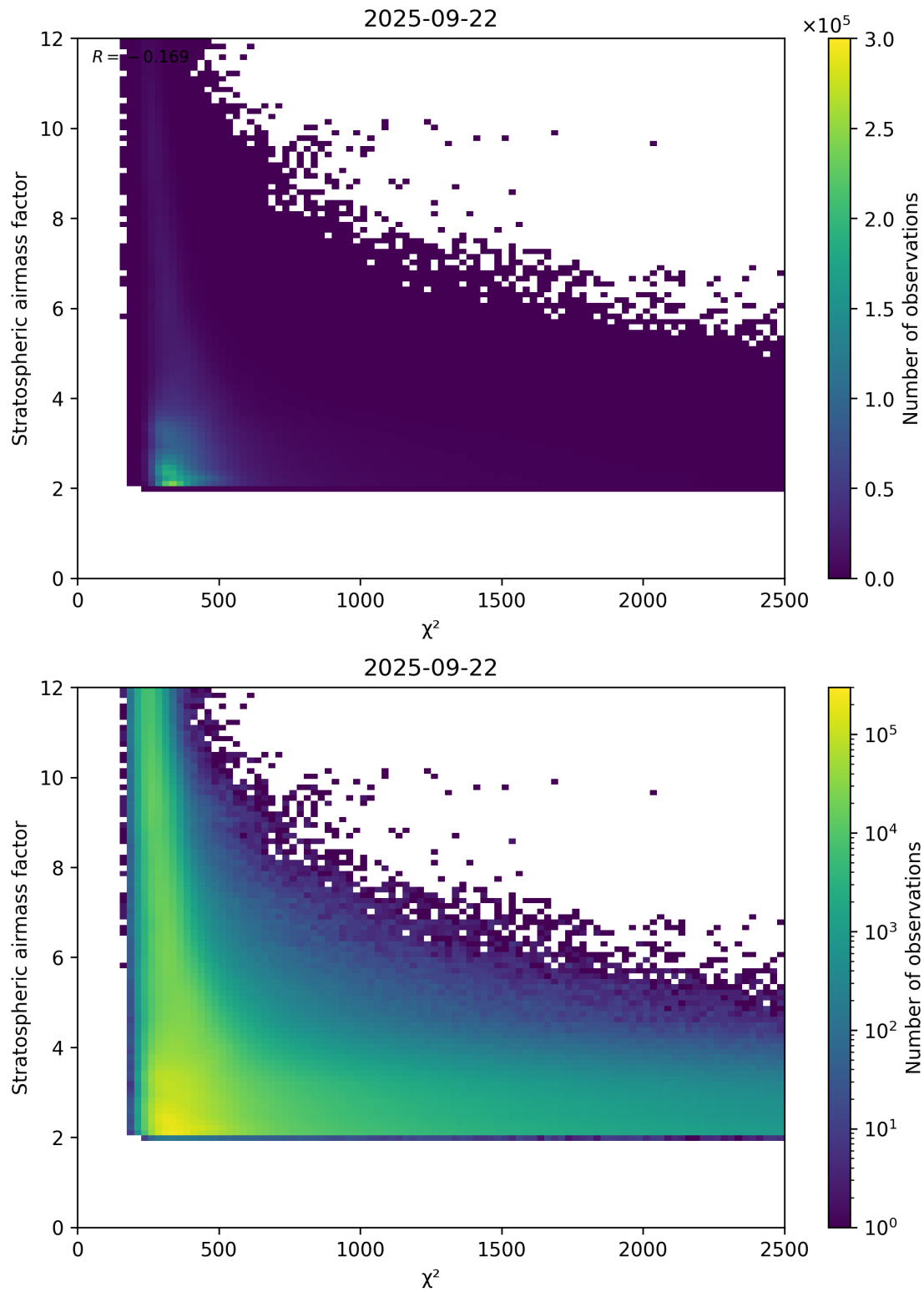
Figure 81: Scatter density plot of “ \chi^2 ” against “Stratospheric airmass factor” for 2025-09-22 to 2025-09-23.
