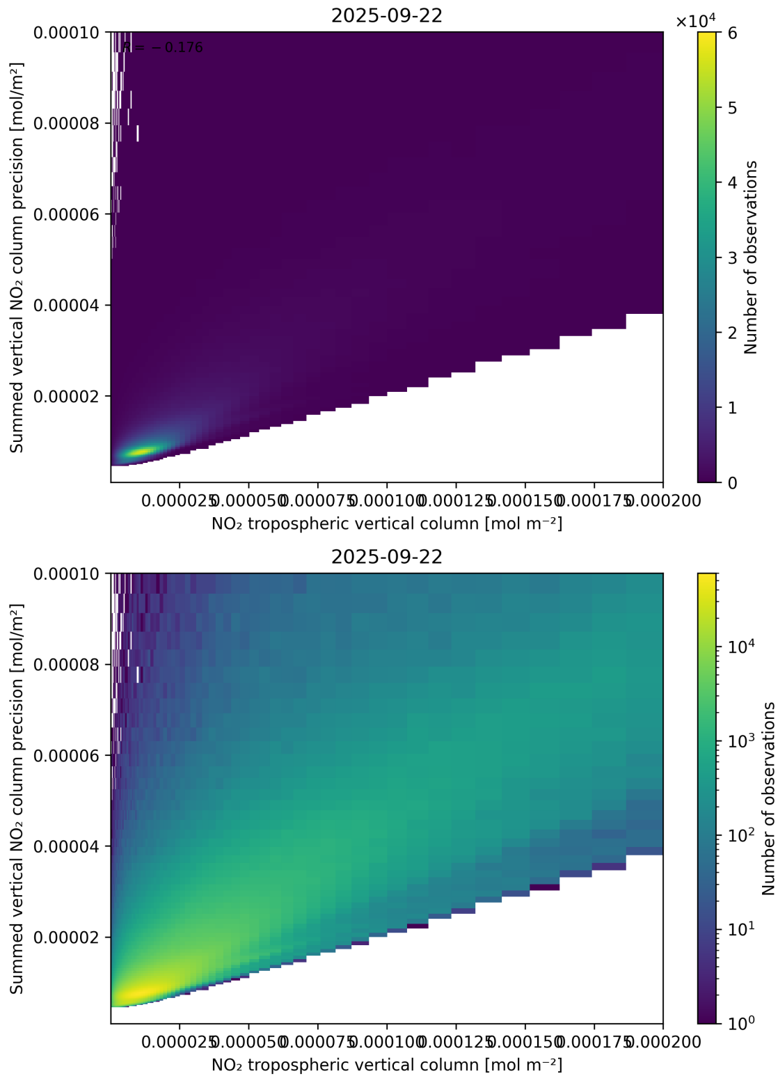
Figure 127: Scatter density plot of “NO 2 tropospheric vertical column” against “Summed vertical NO 2 column precision” for 2025-09-22 to 2025-09-23.
