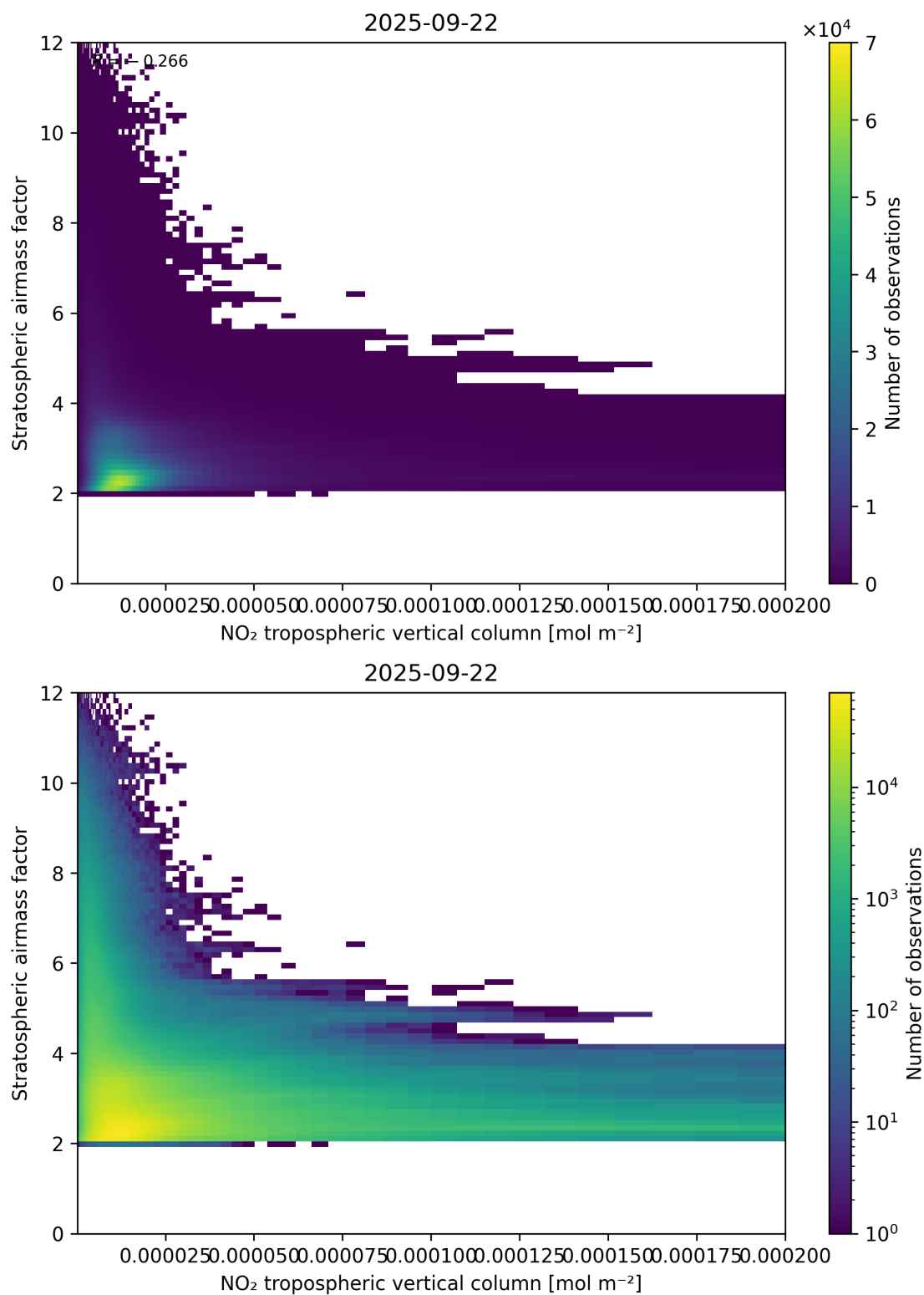
Figure 121: Scatter density plot of “ NO_2 tropospheric vertical column” against “Stratospheric air mass factor” for 2025-09-22 to 2025-09-23.
