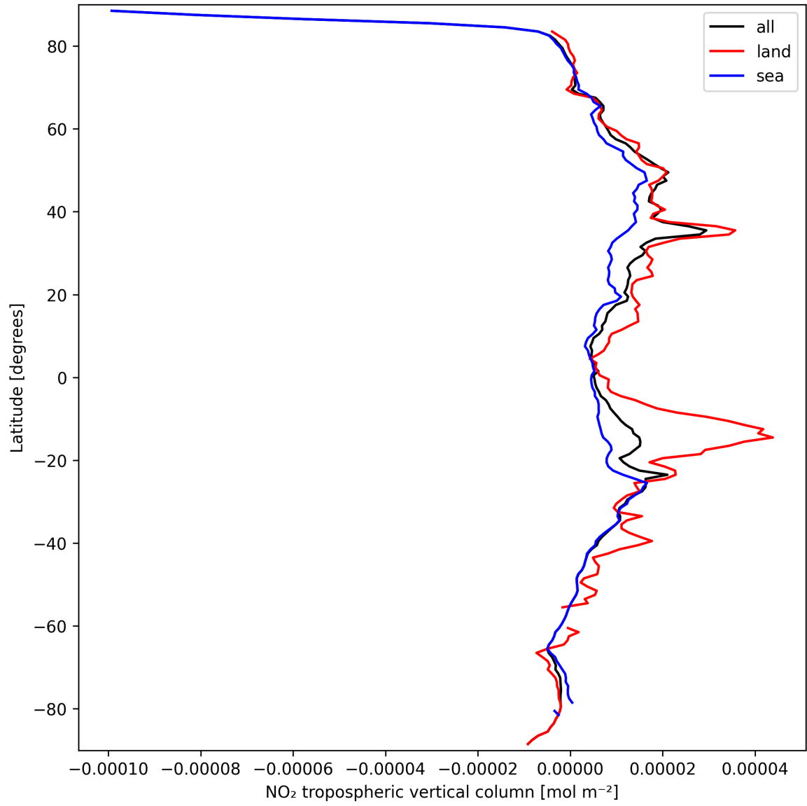
Figure 12: Zonal average of “NO 2 tropospheric vertical column” for 2025-09-22 to 2025-09-23.
