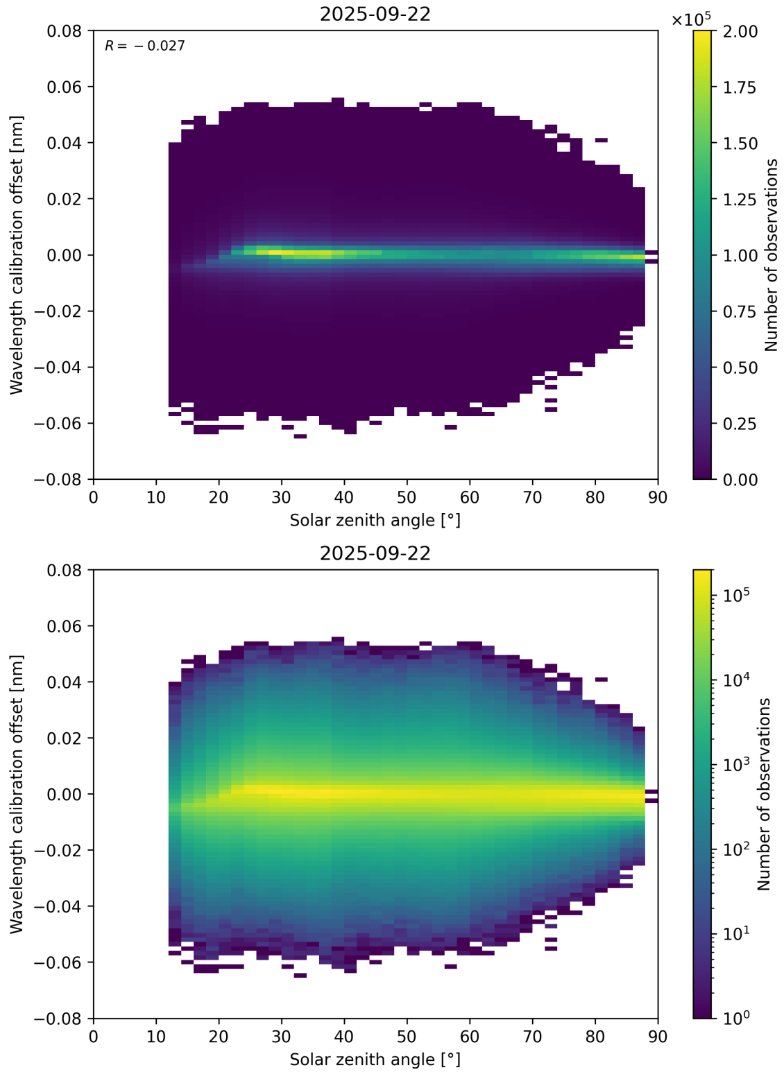
Figure 158: Scatter density plot of “Solar zenith angle” against “Wavelength calibration offset” for 2025-09-22 to 2025-09-23.
