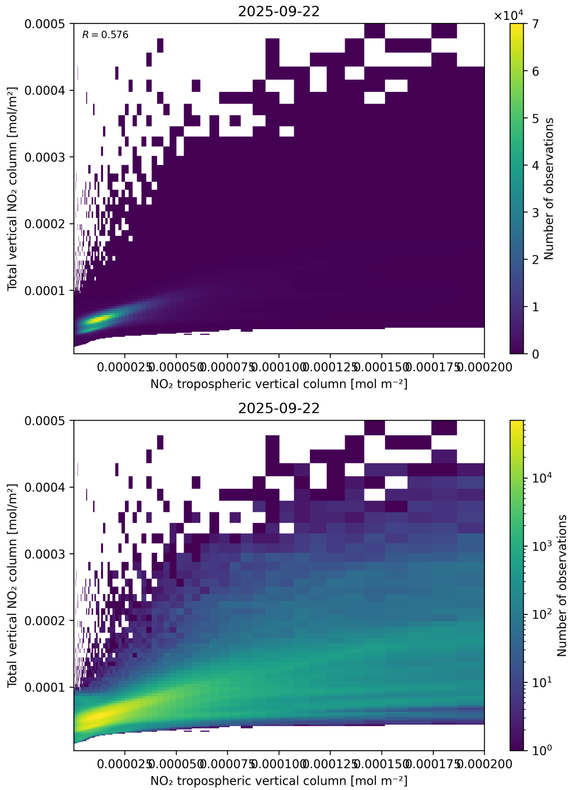
Figure 128: Scatter density plot of “NO 2 tropospheric vertical column” against “Total vertical NO 2 column” for 2025-09-22 to 2025-09-23.
