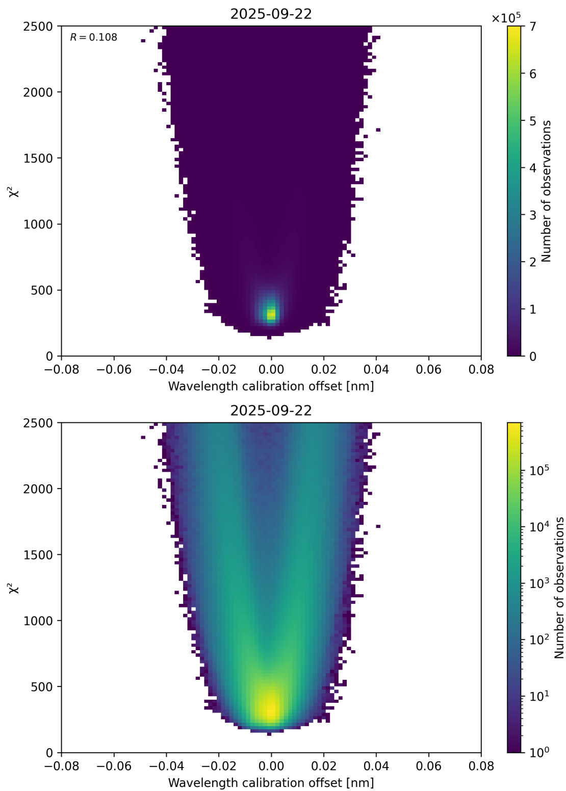
Figure 175: Scatter density plot of “Wavelength calibration offset” against “ \chi^2 ” for 2025-09-22 to 2025-09-23.
