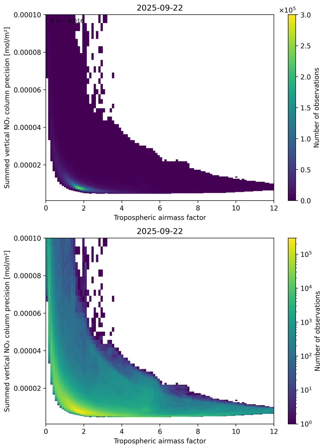
Figure 76: Scatter density plot of “Tropospheric air mass factor” against “Summed vertical NO 2 column precision” for 2025-09-22 to 2025-09-23.
