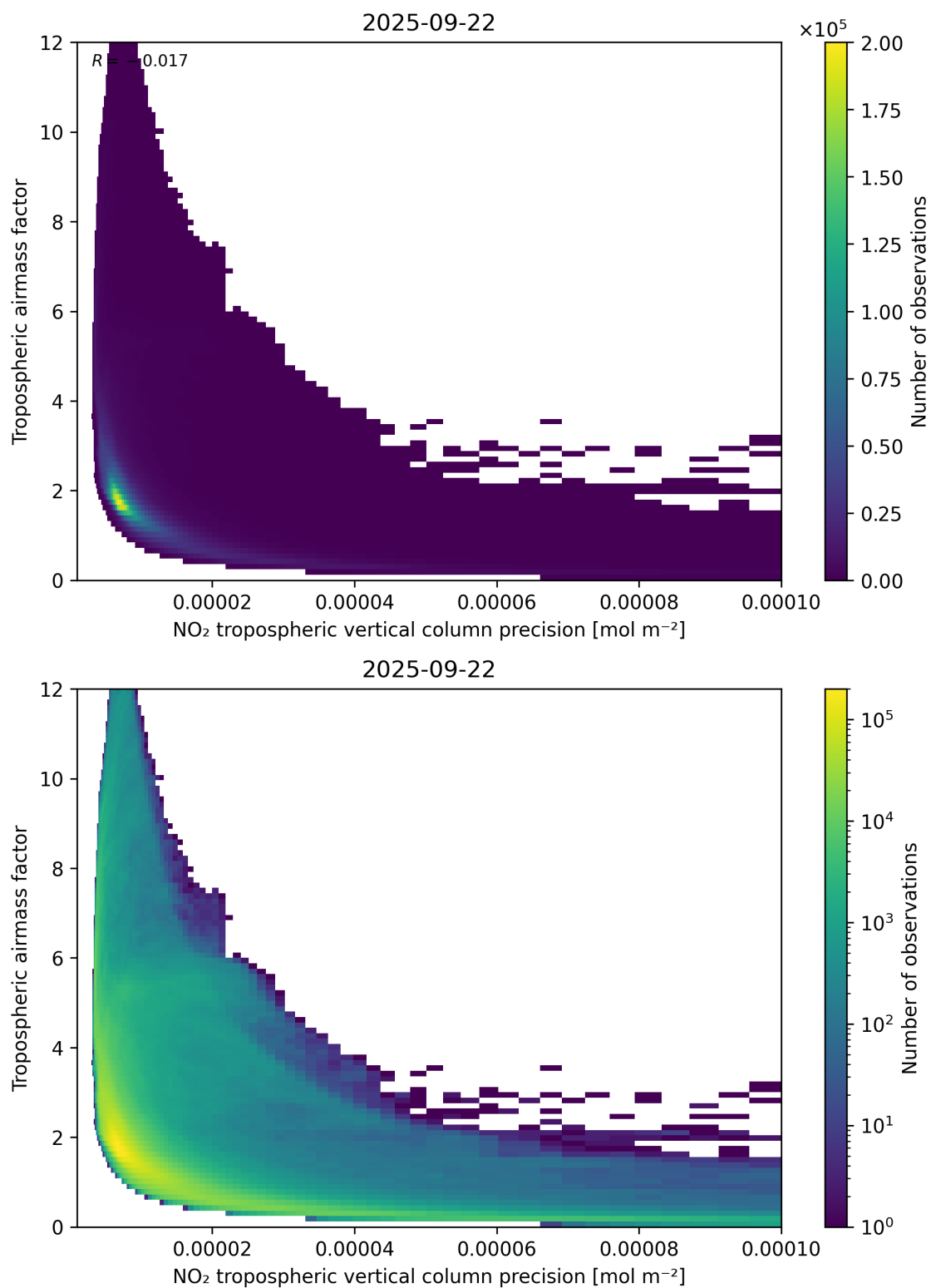
Figure 133: Scatter density plot of “NO 2 tropospheric vertical column precision” against “Tropospheric airmass factor” for 2025-09-22 to 2025-09-23.
