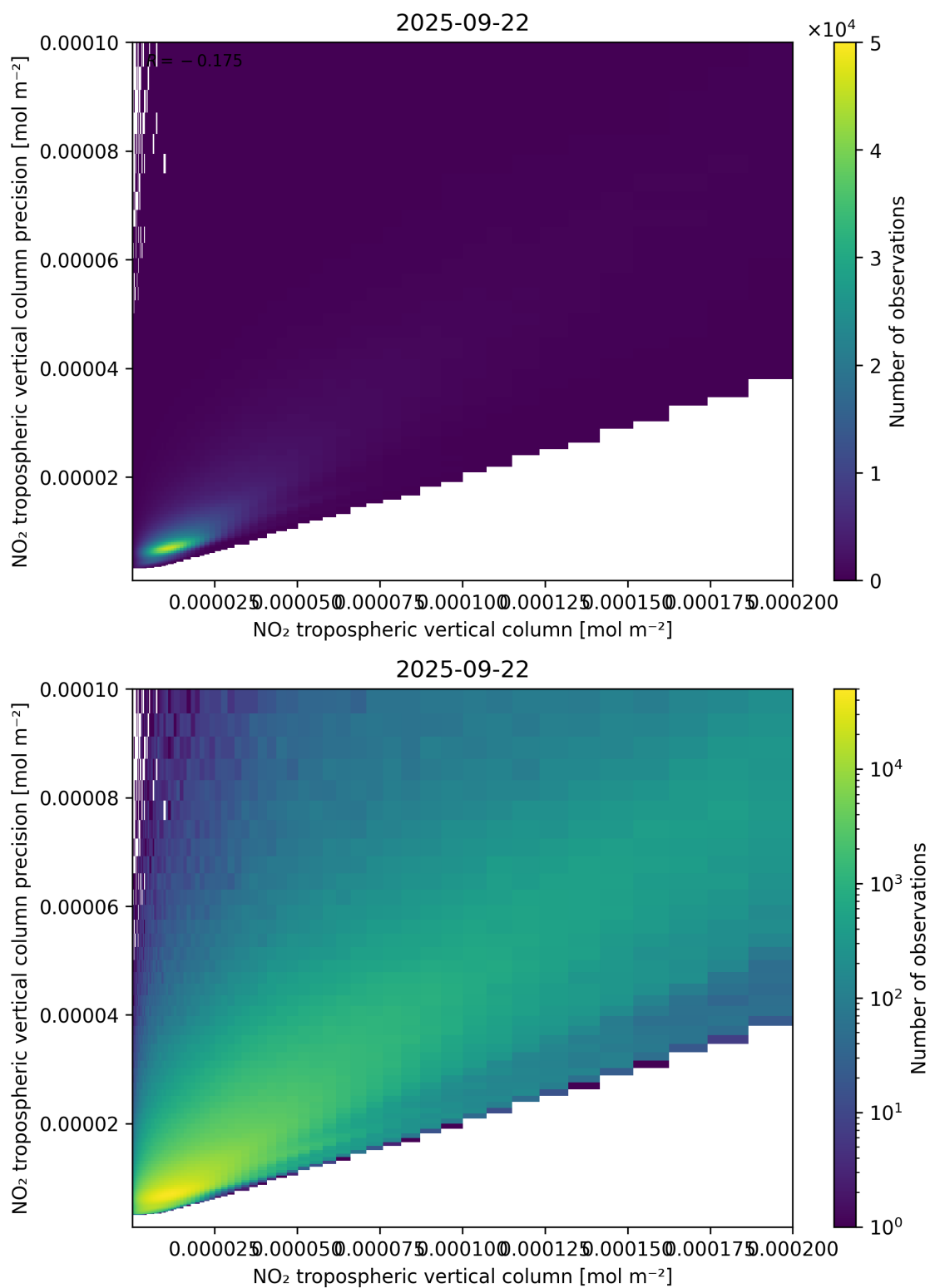
Figure 130: Scatter density plot of “NO 2 tropospheric vertical column” against “NO 2 tropospheric vertical column precision” for 2025-09-22 to 2025-09-23.
