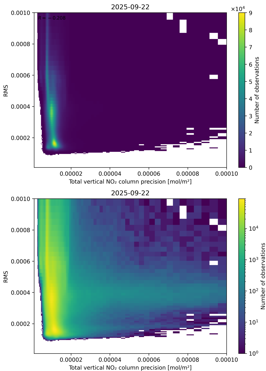
Figure 119: Scatter density plot of “Total vertical NO 2 column precision” against “RMS” for 2025-09-22 to 2025-09-23.
