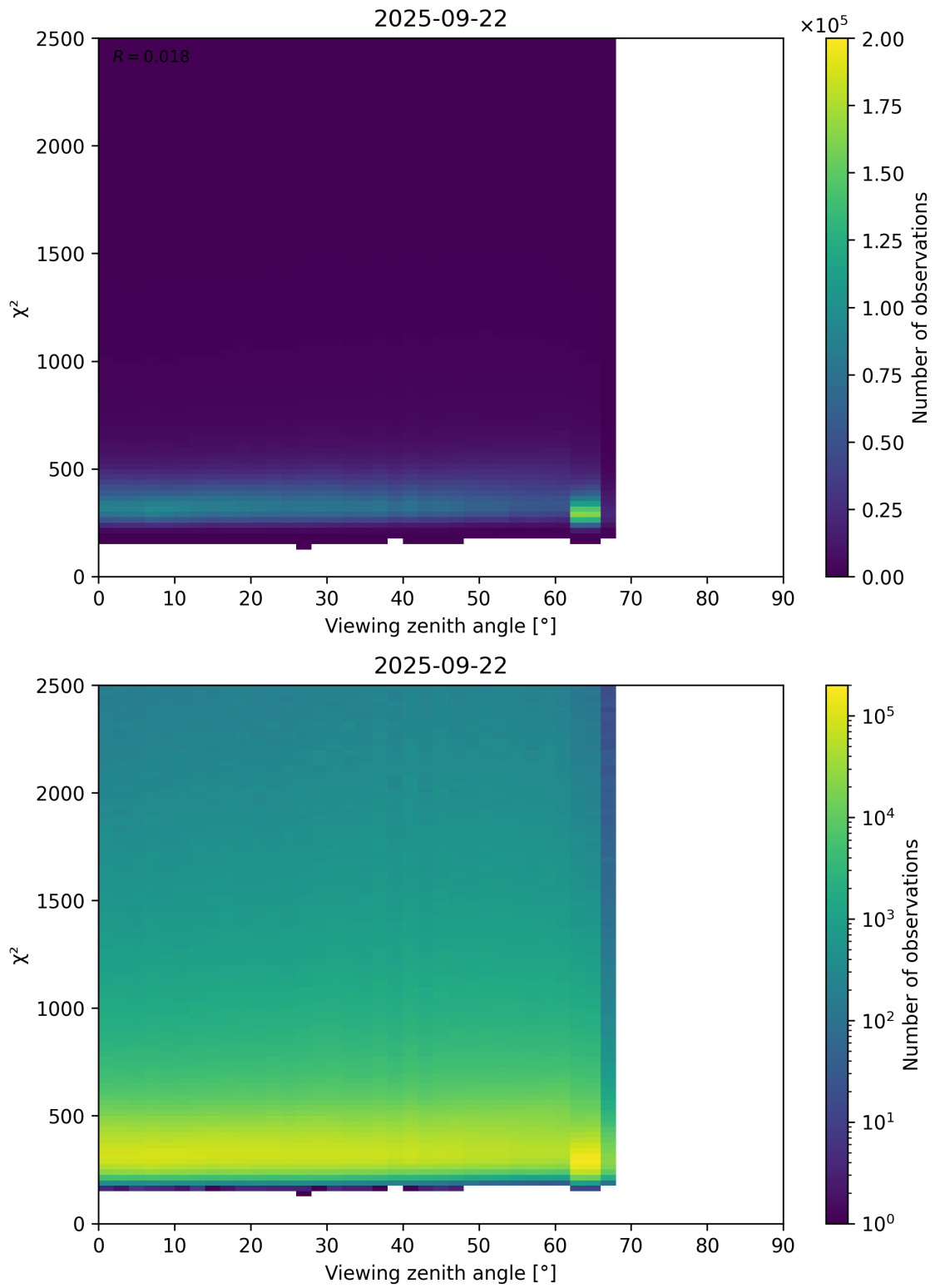
Figure 162: Scatter density plot of “Viewing zenith angle” against “ \chi^2 ” for 2025-09-22 to 2025-09-23.
