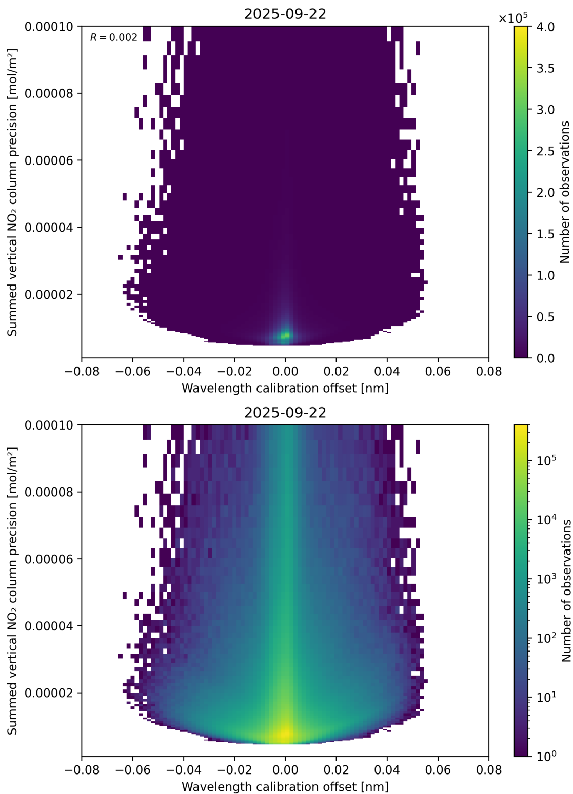
Figure 178: Scatter density plot of “Wavelength calibration offset” against “Summed vertical NO 2 column precision” for 2025-09-22 to 2025-09-23.
