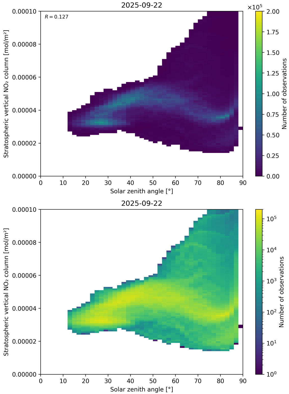
Figure 150: Scatter density plot of “Solar zenith angle” against “Stratospheric vertical NO 2 column” for 2025-09-22 to 2025-09-23.
