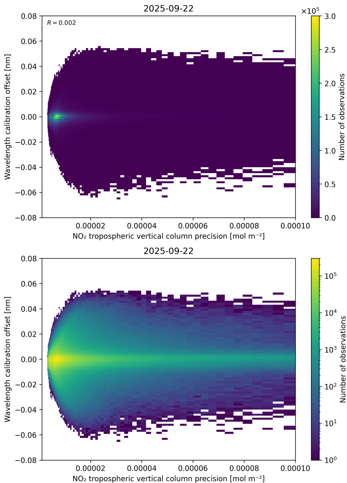
Figure 141: Scatter density plot of “NO 2 tropospheric vertical column precision” against “Wavelength calibration offset” for 2025-09-22 to 2025-09-23.
