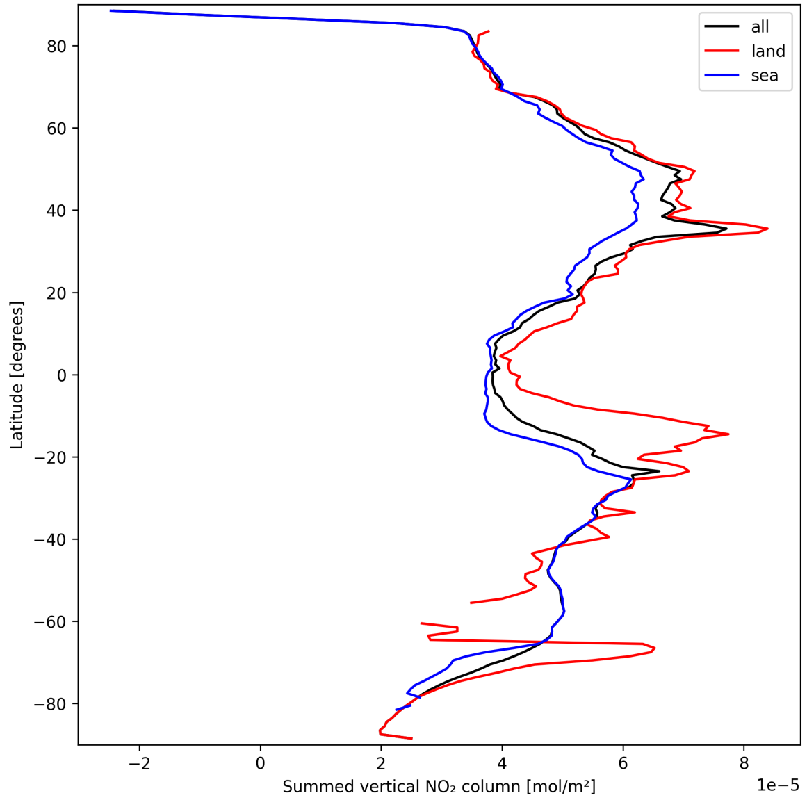
Figure 23: Zonal average of “Summed vertical NO 2 column” for 2025-09-22 to 2025-09-23.
