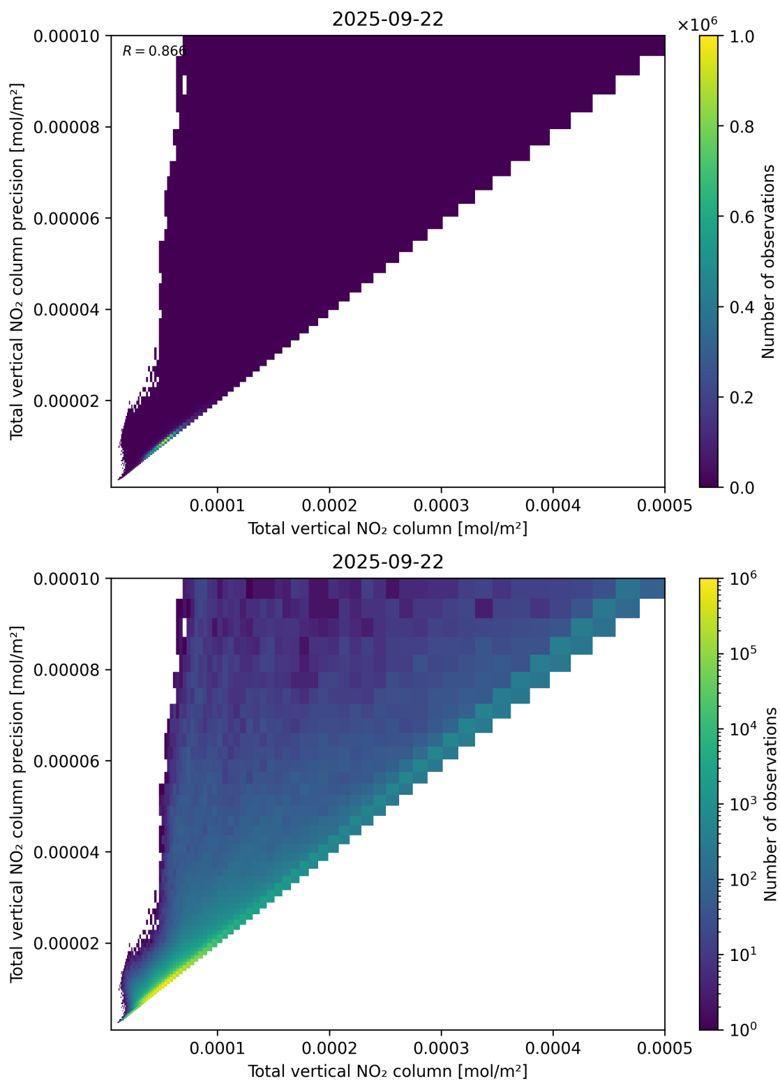
Figure 114: Scatter density plot of “Total vertical NO 2 column” against “Total vertical NO 2 column precision” for 2025-09-22 to 2025-09-23.
