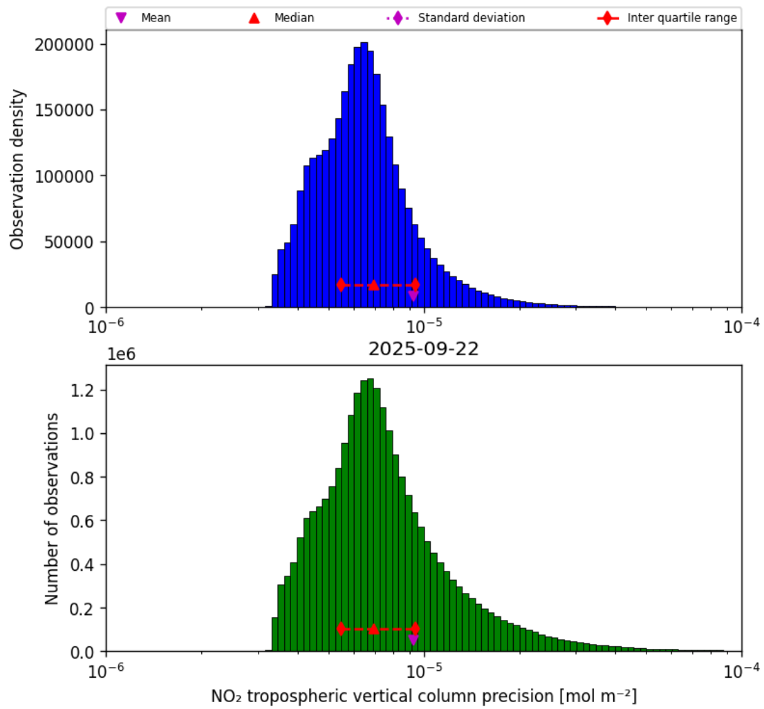
Figure 30: Histogram of “NO 2 tropospheric vertical column precision” for 2025-09-22 to 2025-09-23
