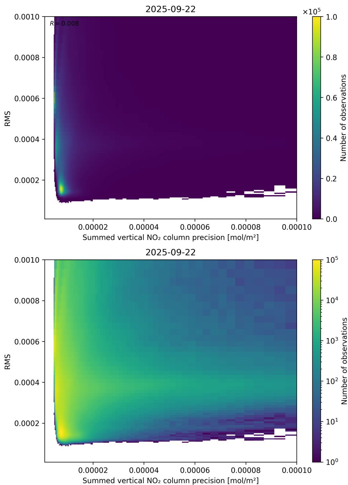
Figure 108: Scatter density plot of “Summed vertical NO 2 column precision” against “RMS” for 2025-09-22 to 2025-09-23.
