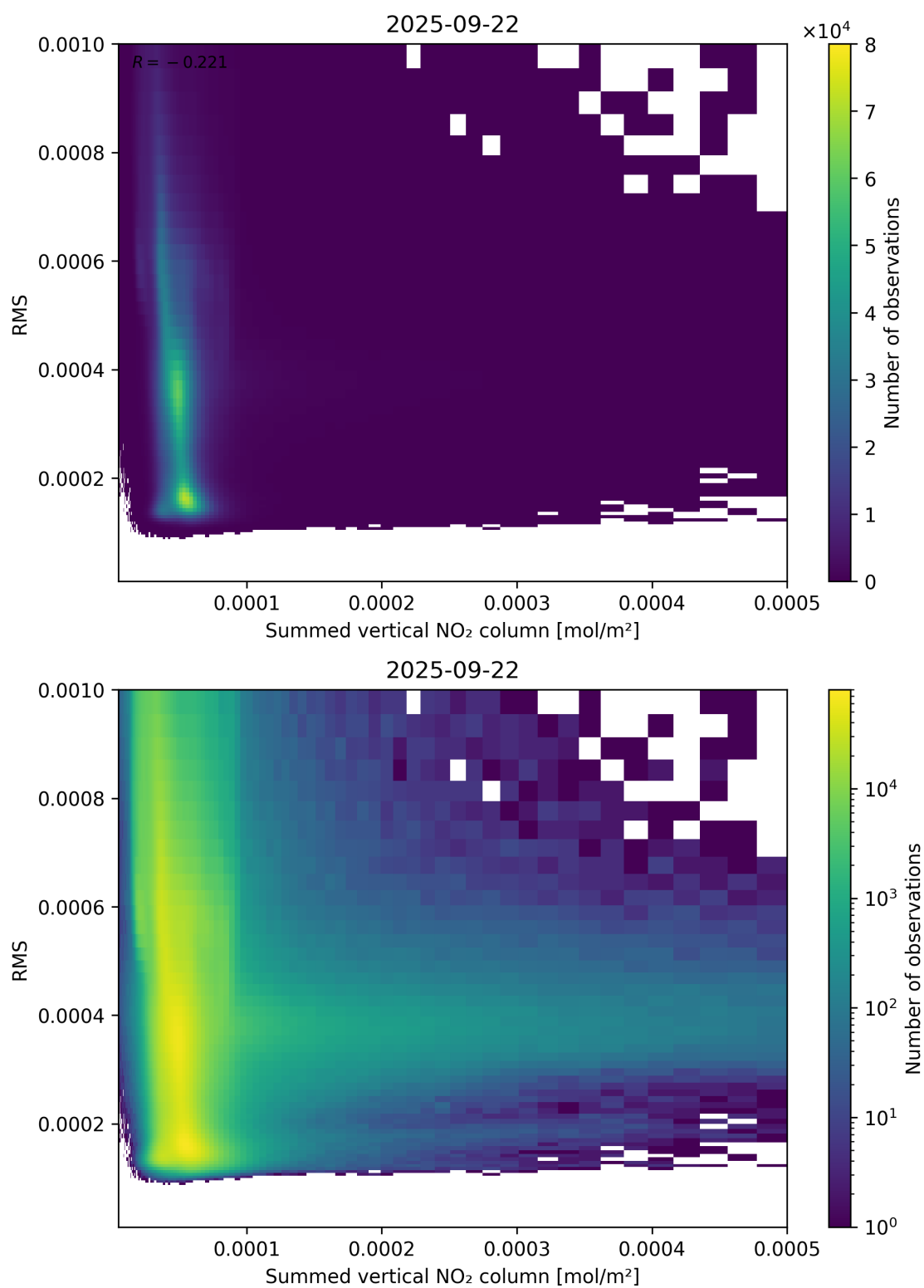
Figure 109: Scatter density plot of “Summed vertical NO 2 column” against “RMS” for 2025-09-22 to 2025-09-23.
