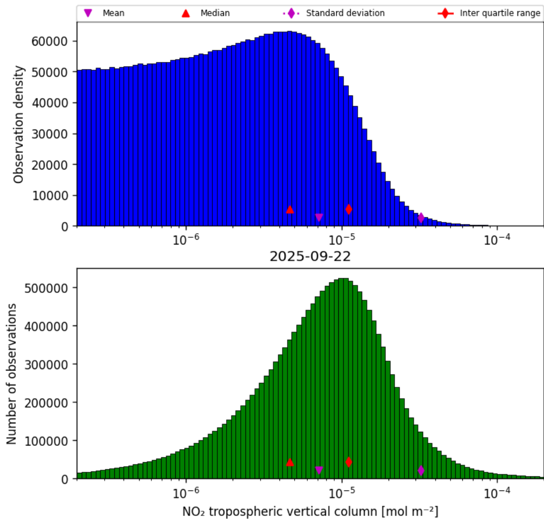
Figure 29: Histogram of “NO 2 tropospheric vertical column” for 2025-09-22 to 2025-09-23
