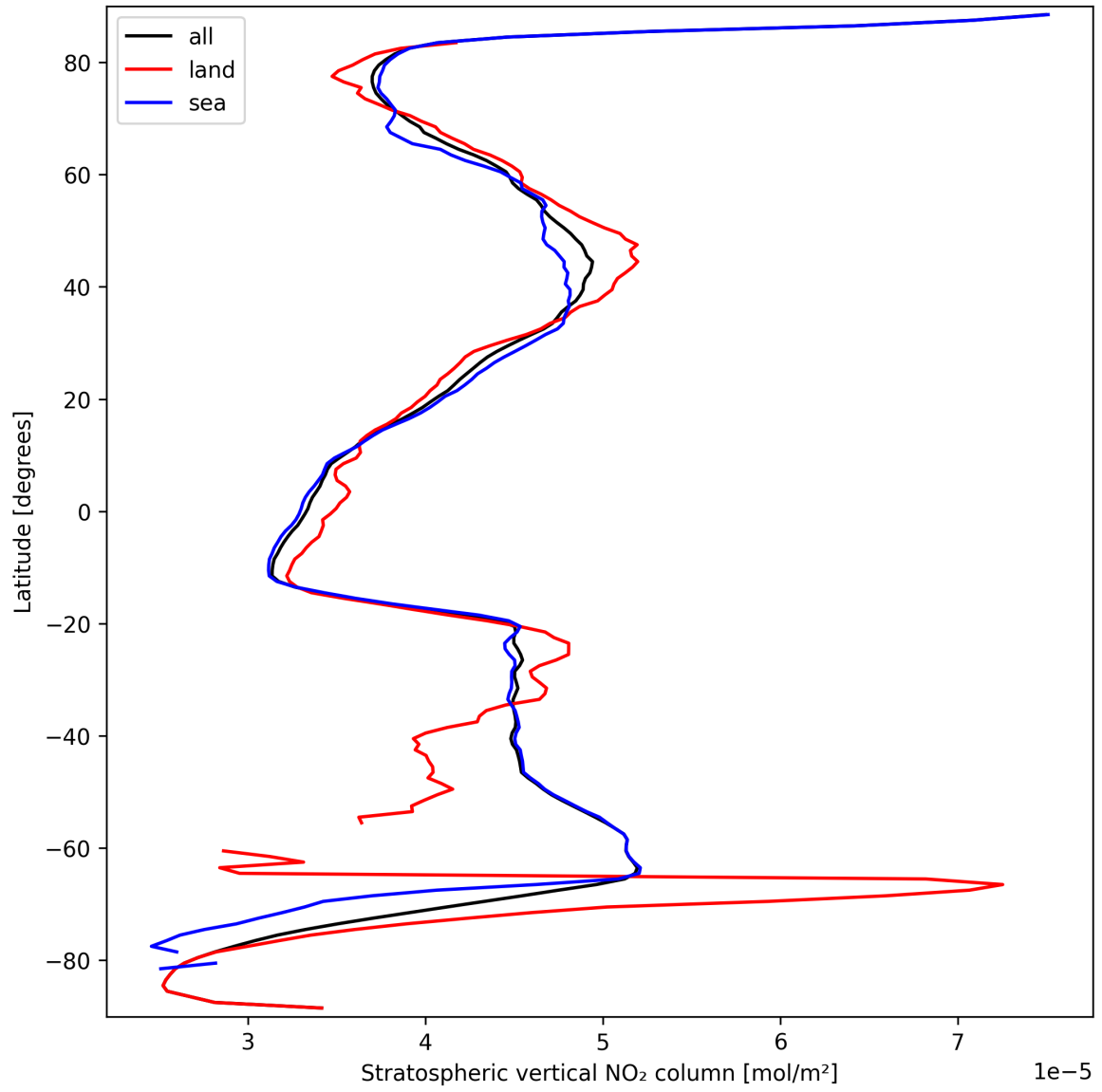
Figure 19: Zonal average of “Stratospheric vertical NO 2 column” for 2025-09-22 to 2025-09-23.
