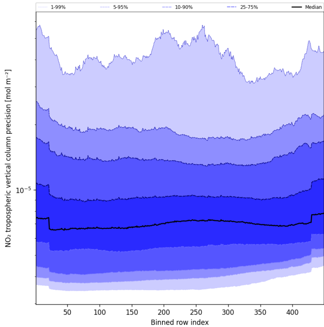
Figure 47: Along track statistics of “NO 2 tropospheric vertical column precision” for 2025-09-22 to 2025-09-23
