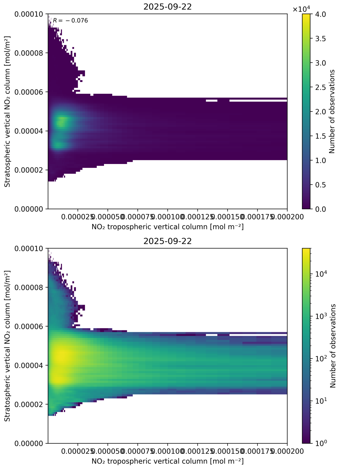
Figure 125: Scatter density plot of “NO 2 tropospheric vertical column” against “Stratospheric vertical NO 2 column” for 2025-09-22 to 2025-09-23.
