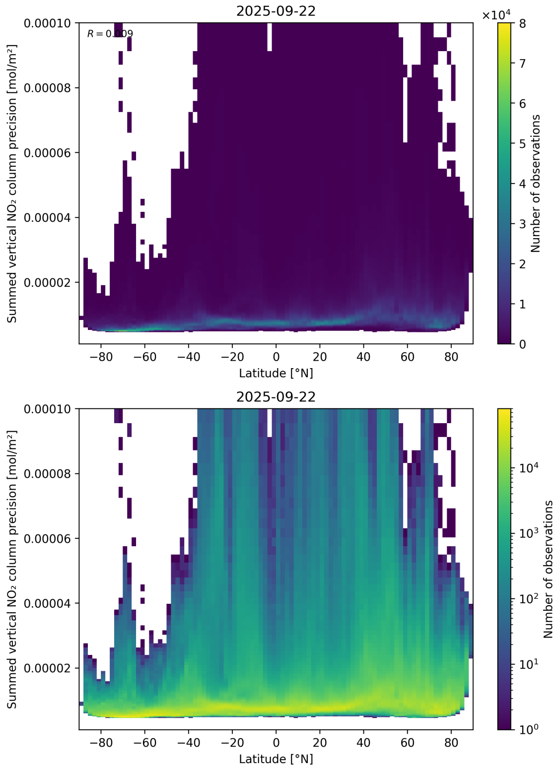
Figure 89: Scatter density plot of “Latitude” against “Summed vertical NO 2 column precision” for 2025-09-22 to 2025-09-23.
