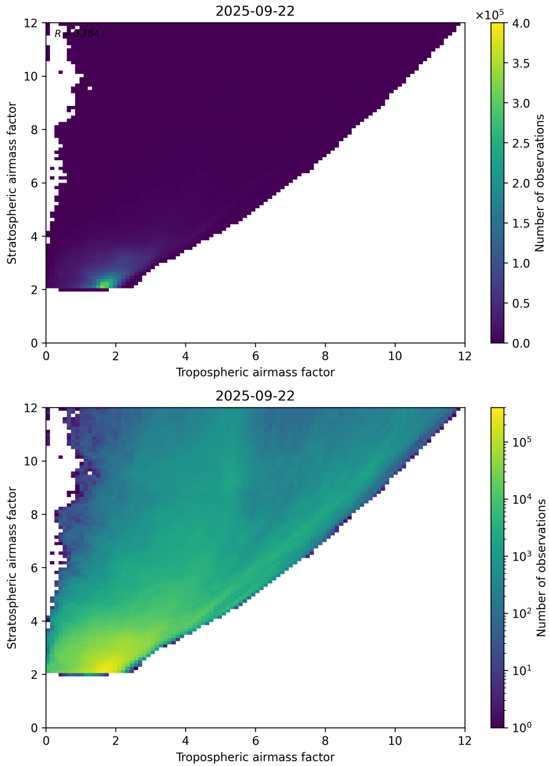
Figure 71: Scatter density plot of “Tropospheric airmass factor” against “Stratospheric airmass factor” for 2025-09-22 to 2025-09-23.
