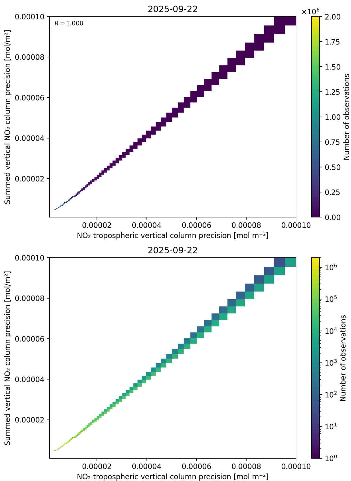
Figure 137: Scatter density plot of “NO 2 tropospheric vertical column precision” against “Summed vertical NO 2 column precision” for 2025-09-22 to 2025-09-23.
