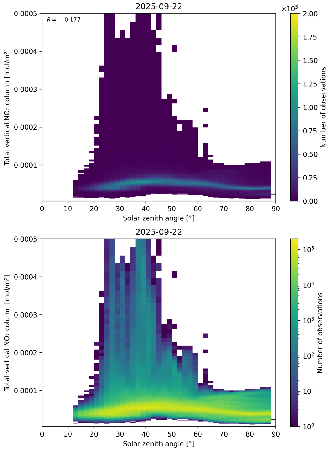
Figure 153: Scatter density plot of “Solar zenith angle” against “Total vertical NO 2 column” for 2025-09-22 to 2025-09-23.
