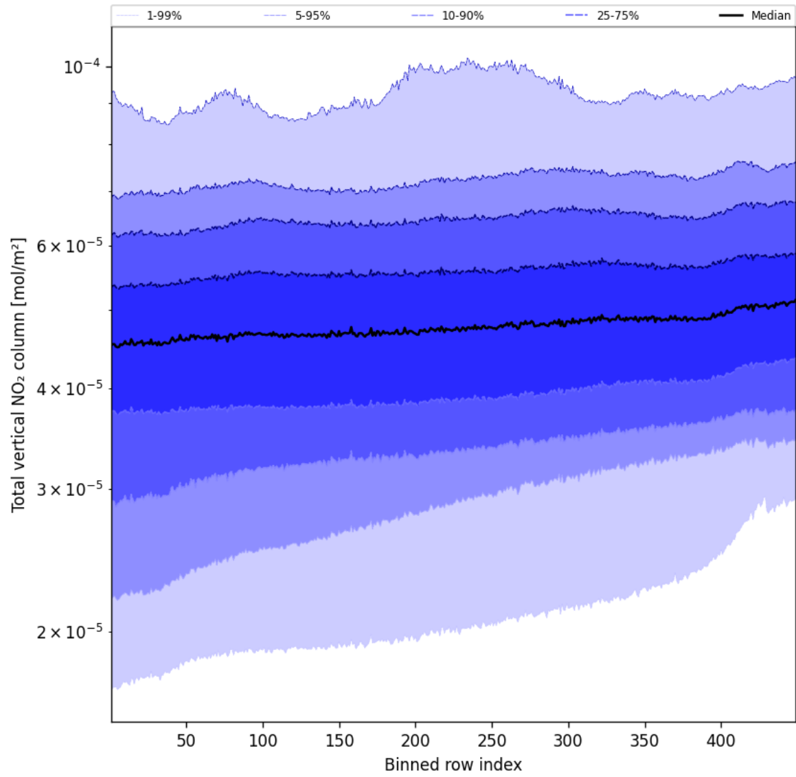
Figure 55: Along track statistics of “Total vertical NO 2 column” for 2025-09-22 to 2025-09-23
