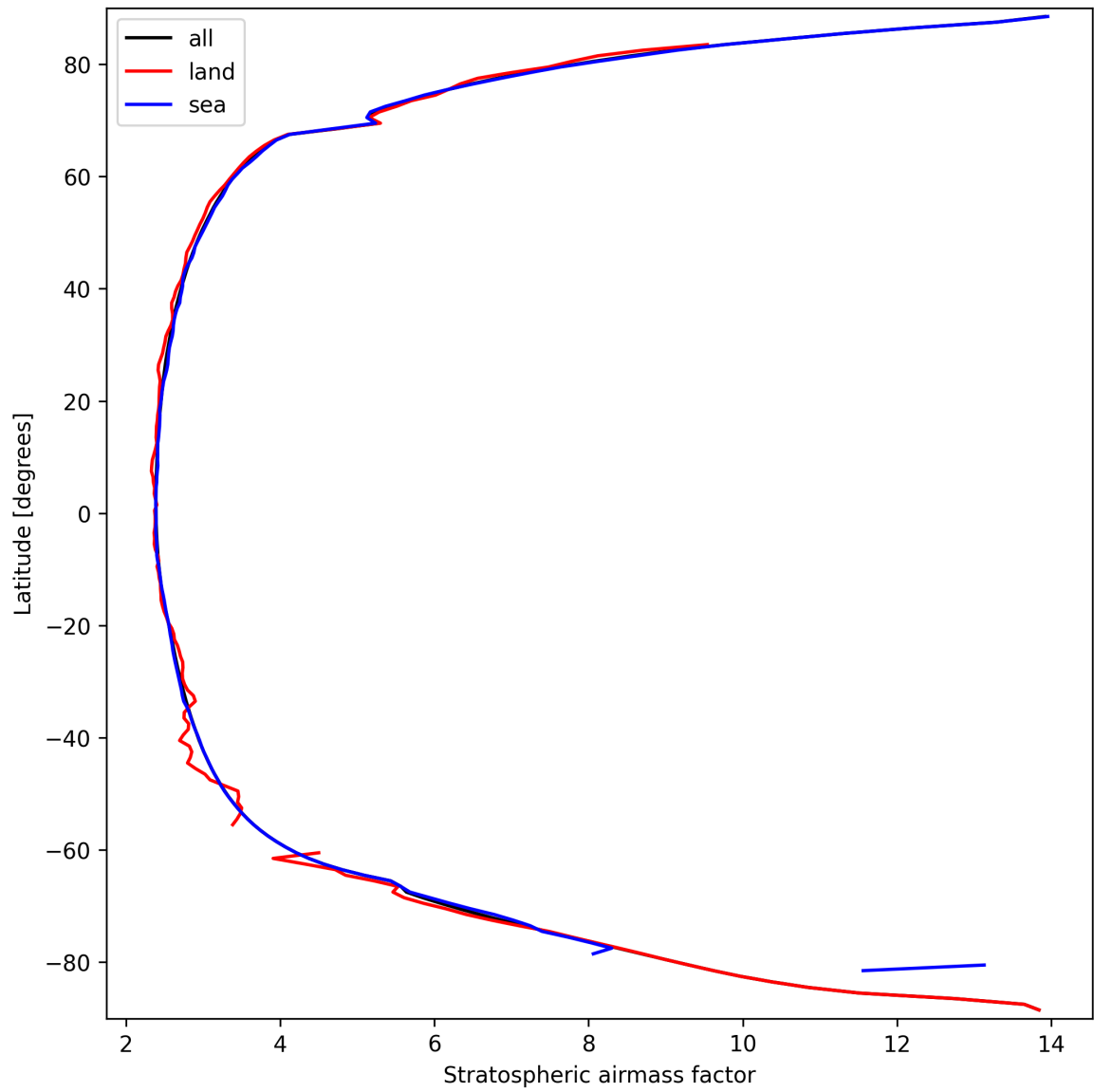
Figure 27: Zonal average of “Stratospheric airmass factor” for 2025-09-22 to 2025-09-23.
