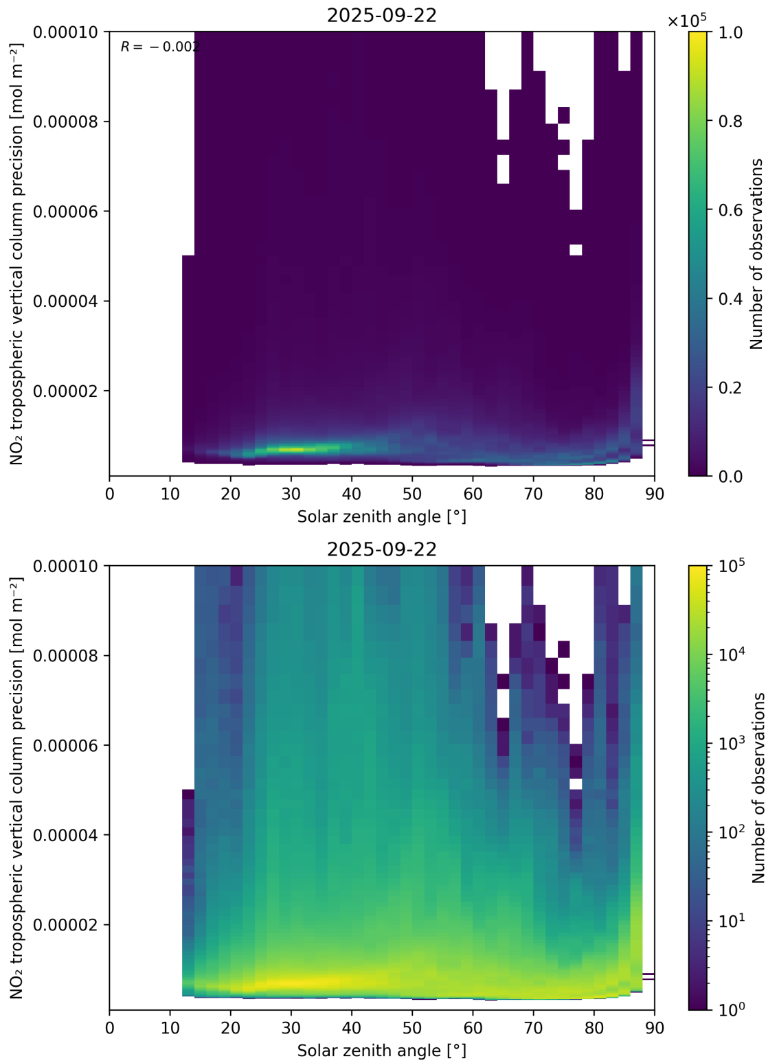
Figure 156: Scatter density plot of “Solar zenith angle” against “NO 2 tropospheric vertical column precision” for 2025-09-22 to 2025-09-23.
