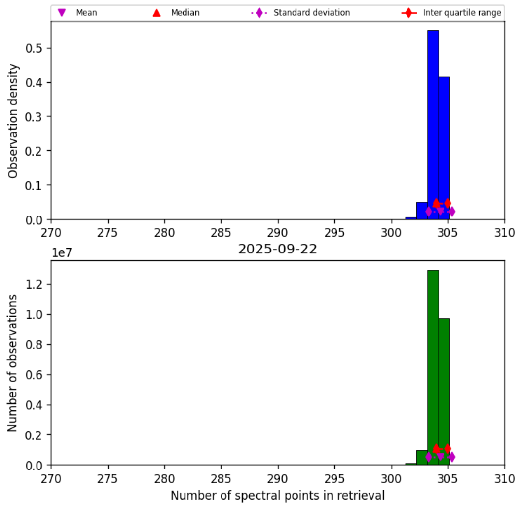
Figure 33: Histogram of “Number of spectral points in retrieval” for 2025-09-22 to 2025-09-23
