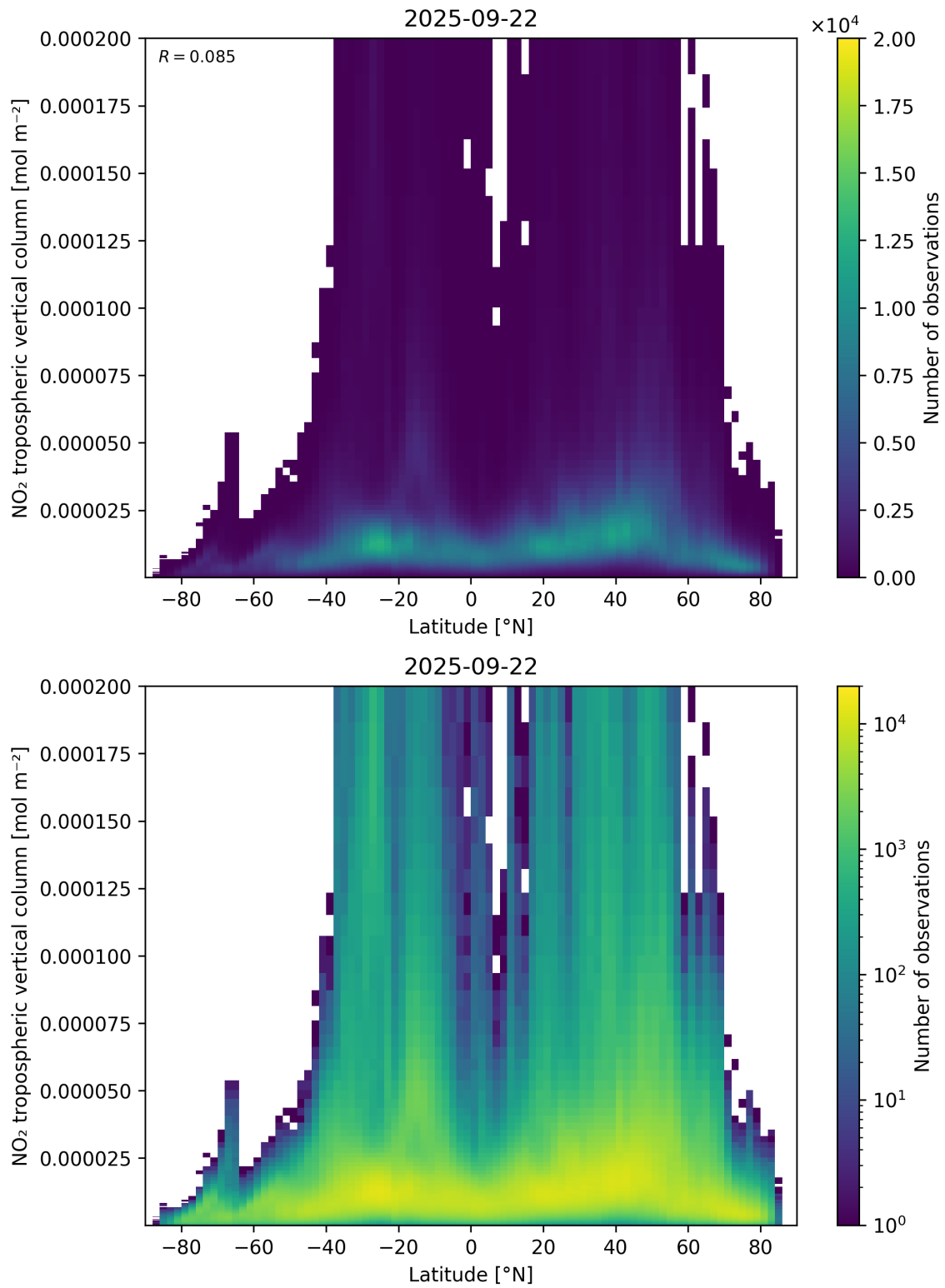
Figure 92: Scatter density plot of “Latitude” against “NO 2 tropospheric vertical column” for 2025-09-22 to 2025-09-23.
