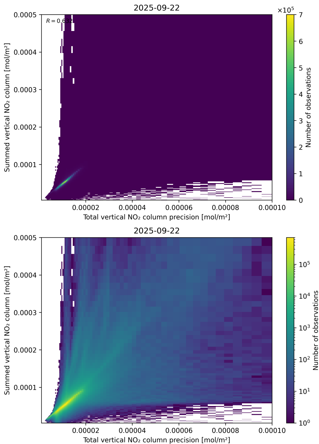
Figure 117: Scatter density plot of “Total vertical NO 2 column precision” against “Summed vertical NO 2 column” for 2025-09-22 to 2025-09-23.
