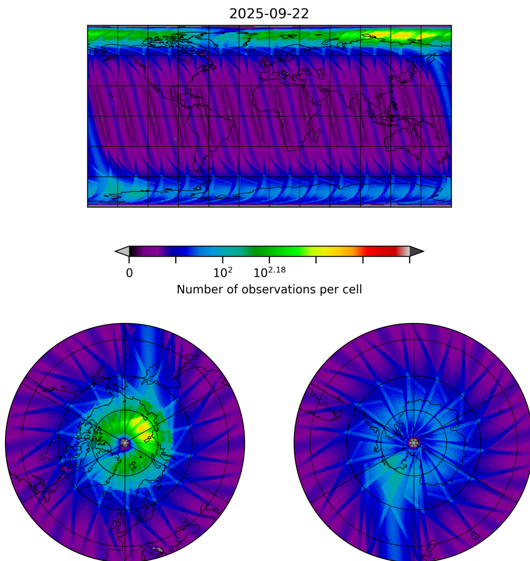
Figure 10: Map of the number of observations for 2025-09-22 to 2025-09-23
