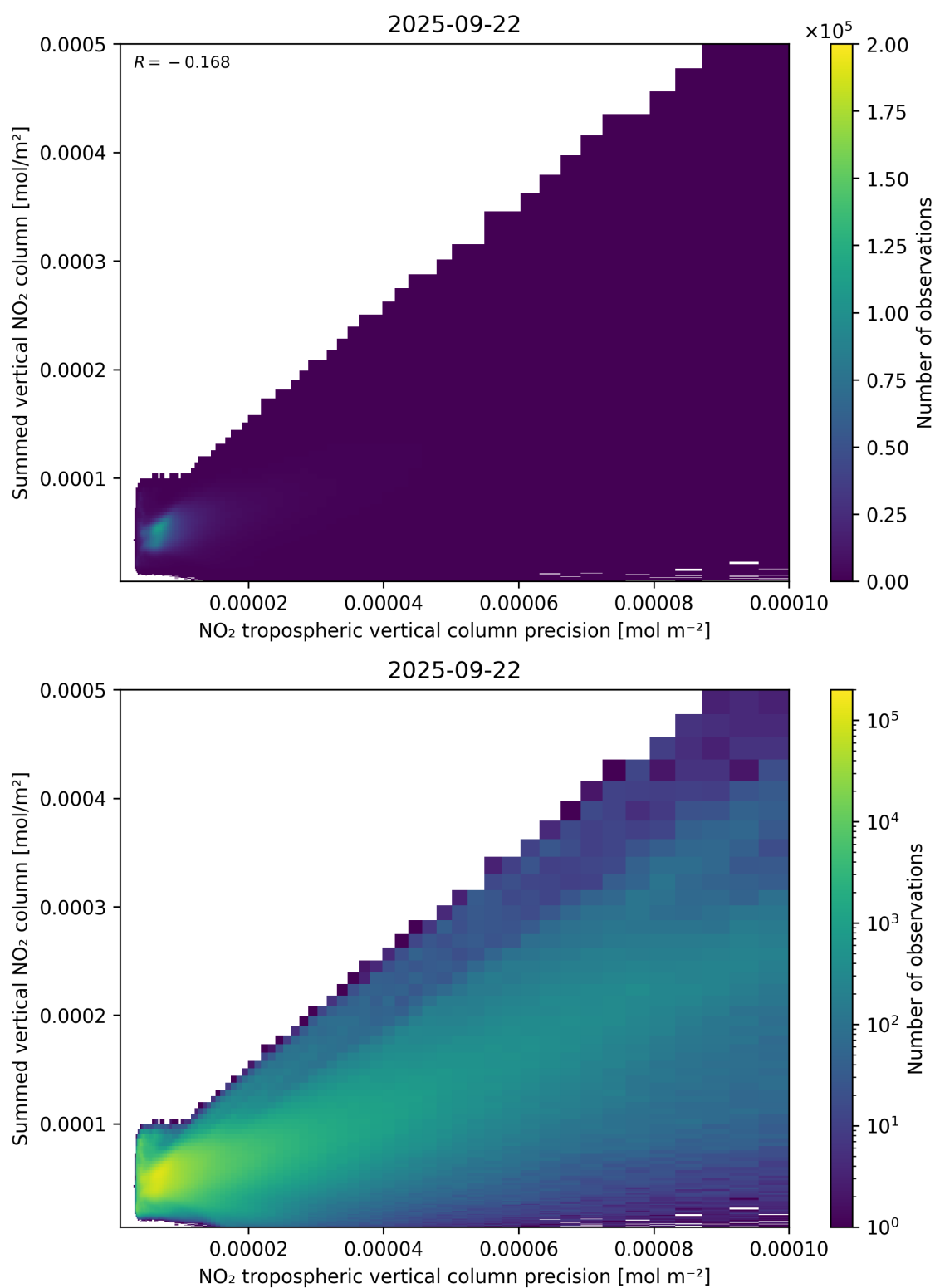
Figure 136: Scatter density plot of “NO 2 tropospheric vertical column precision” against “Summed vertical NO 2 column” for 2025-09-22 to 2025-09-23.
