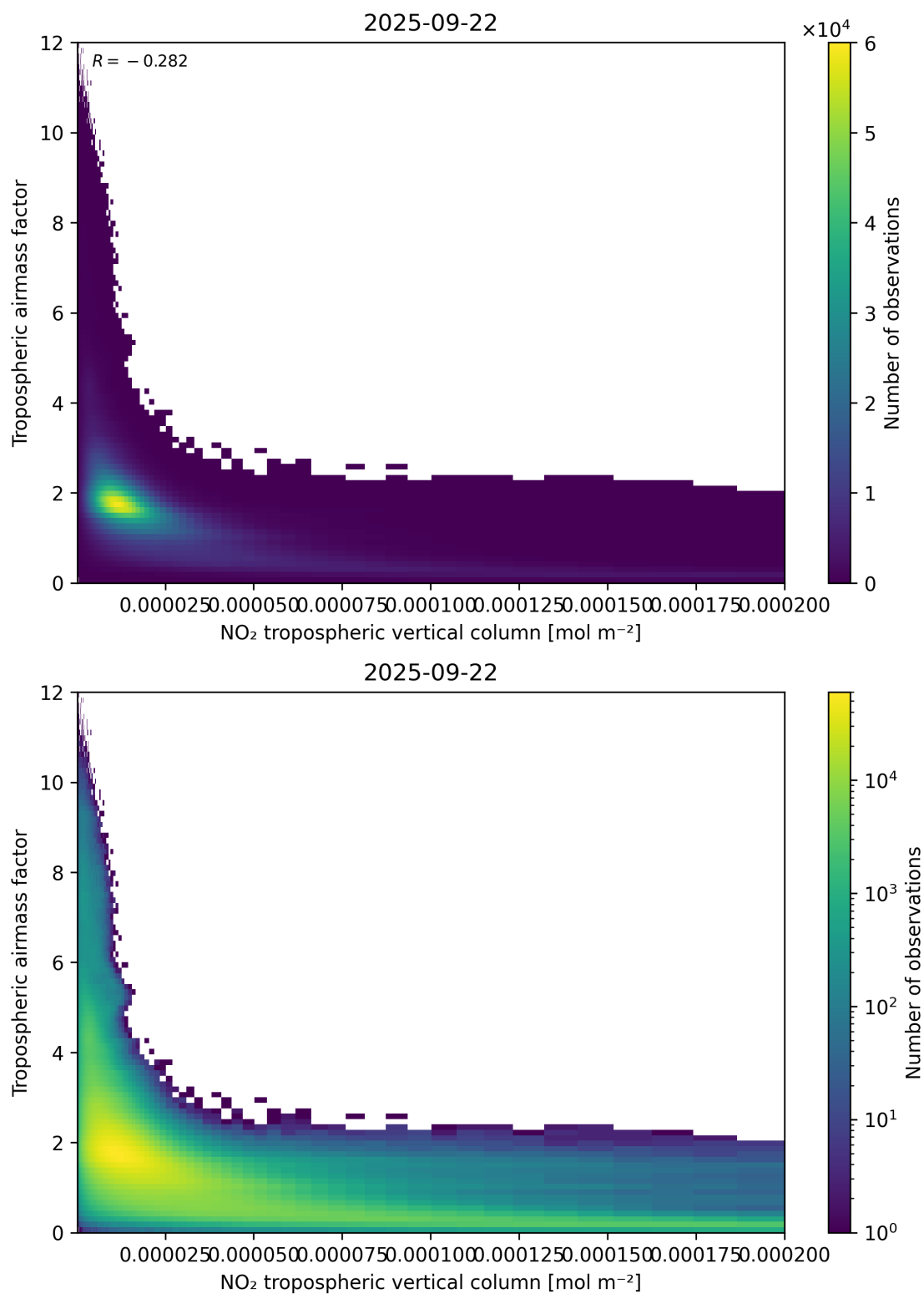
Figure 123: Scatter density plot of “NO 2 tropospheric vertical column” against “Tropospheric air mass factor” for 2025-09-22 to 2025-09-23.
