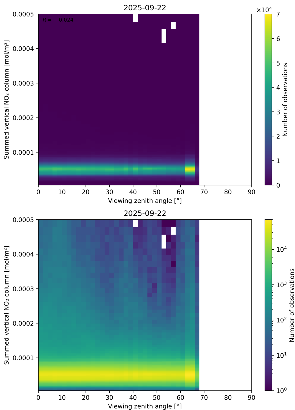
Figure 165: Scatter density plot of “Viewing zenith angle” against “Summed vertical NO 2 column” for 2025-09-22 to 2025-09-23.
