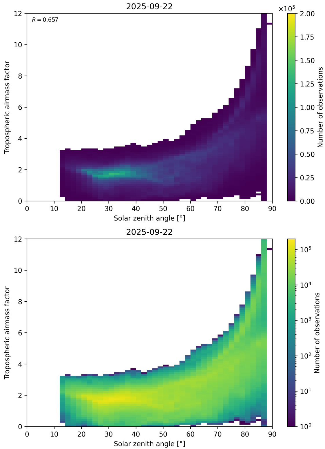
Figure 147: Scatter density plot of “Solar zenith angle” against “Tropospheric airmass factor” for 2025-09-22 to 2025-09-23.
