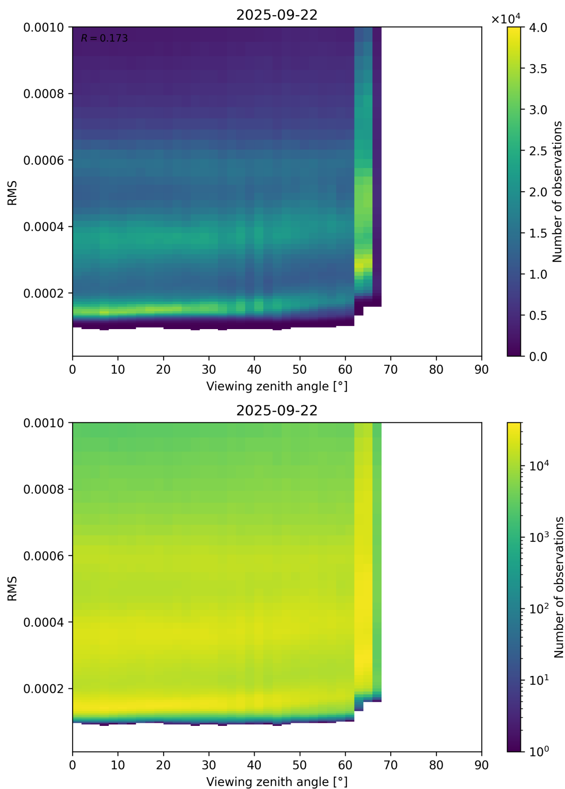
Figure 171: Scatter density plot of “Viewing zenith angle” against “RMS” for 2025-09-22 to 2025-09-23.
