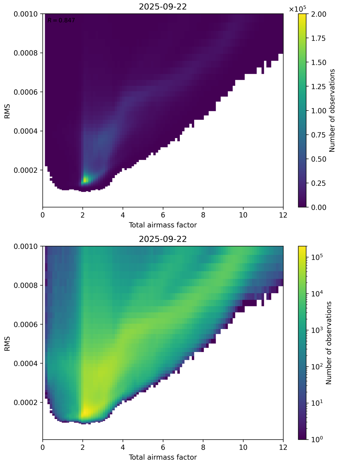
Figure 69: Scatter density plot of “Total airmass factor” against “RMS” for 2025-09-22 to 2025-09-23.
