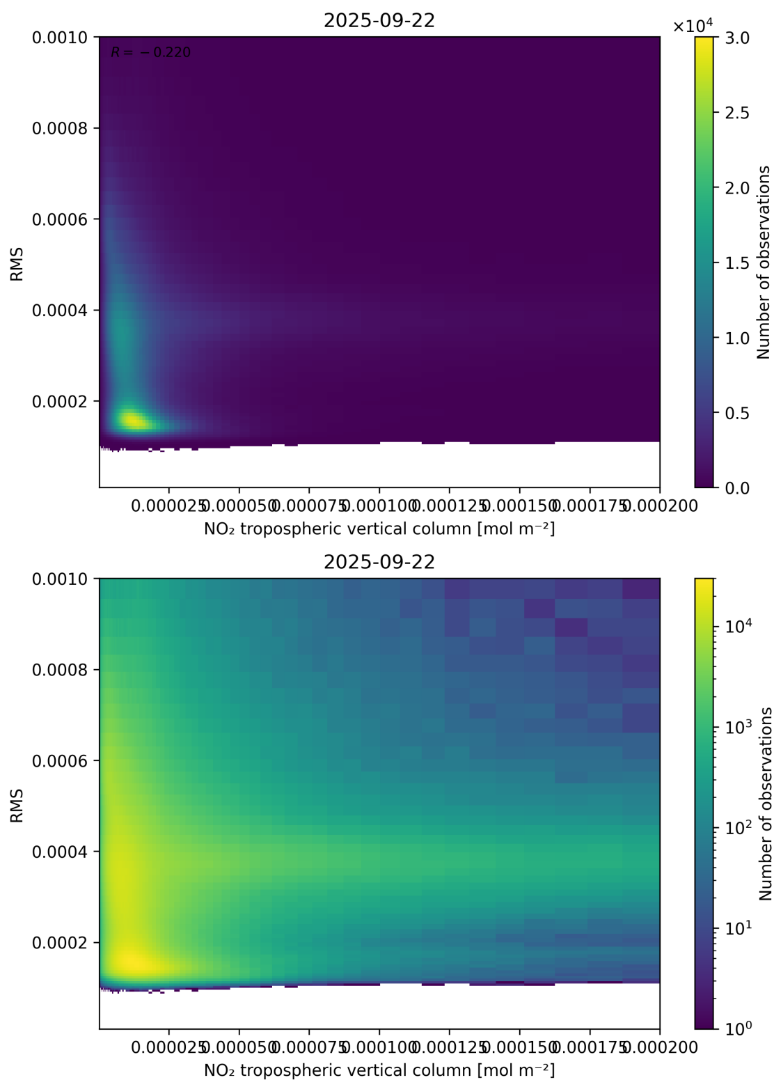
Figure 142: Scatter density plot of “NO 2 tropospheric vertical column” against “RMS” for 2025-09-22 to 2025-09-23.
