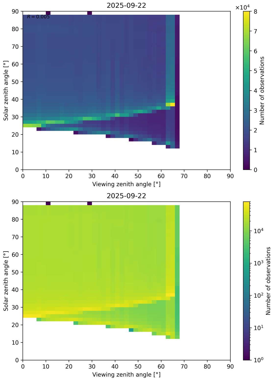
Figure 172: Scatter density plot of “Viewing zenith angle” against “Solar zenith angle” for 2025-09-22 to 2025-09-23.
