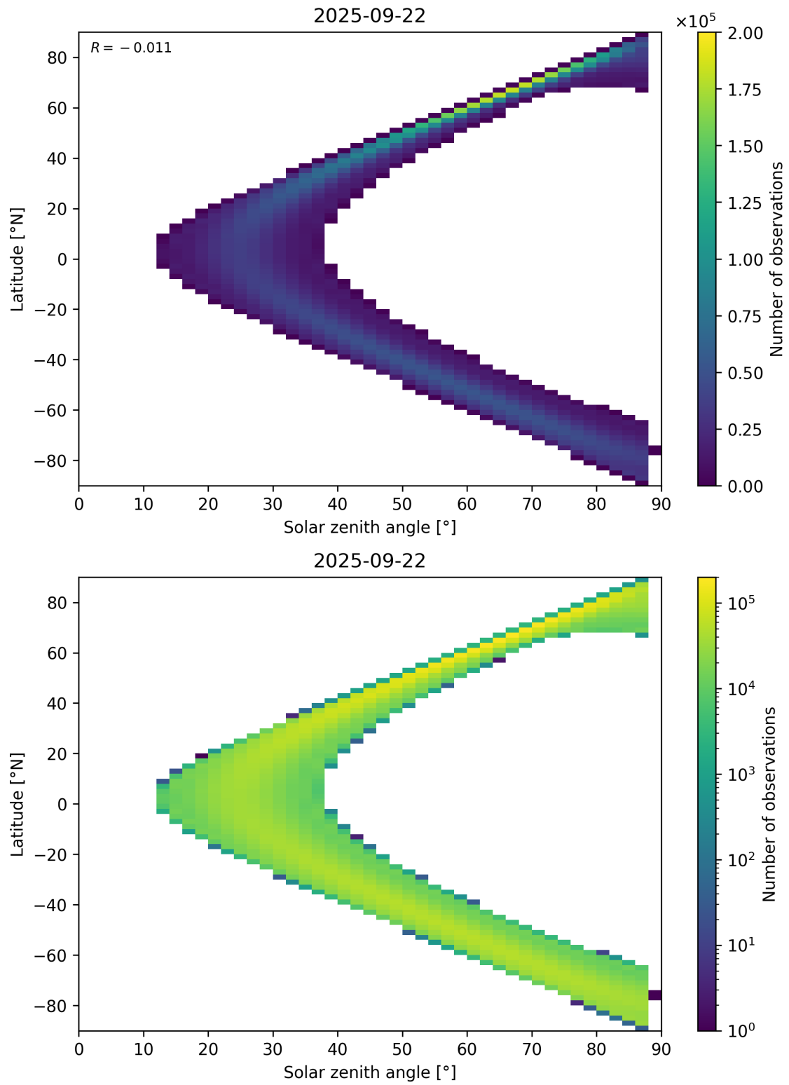
Figure 149: Scatter density plot of “Solar zenith angle” against “Latitude” for 2025-09-22 to 2025-09-23.
