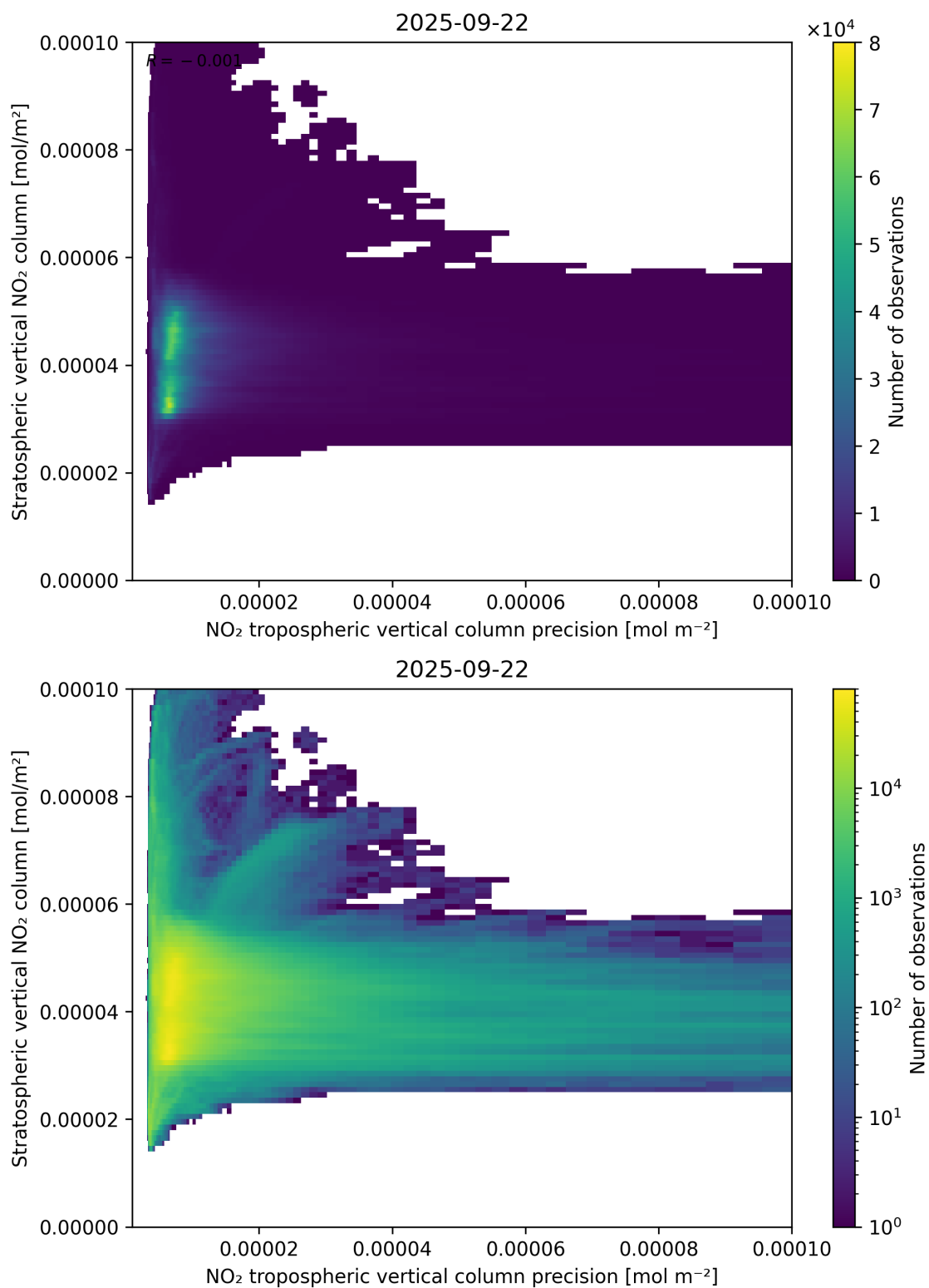
Figure 135: Scatter density plot of “NO 2 tropospheric vertical column precision” against “Stratospheric vertical NO 2 column” for 2025-09-22 to 2025-09-23.
