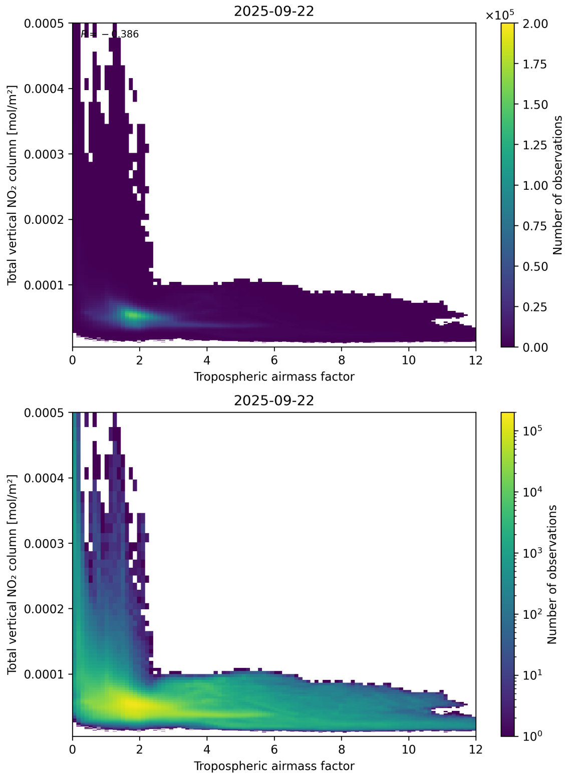
Figure 77: Scatter density plot of “Tropospheric airmass factor” against “Total vertical NO 2 column” for 2025-09-22 to 2025-09-23.
