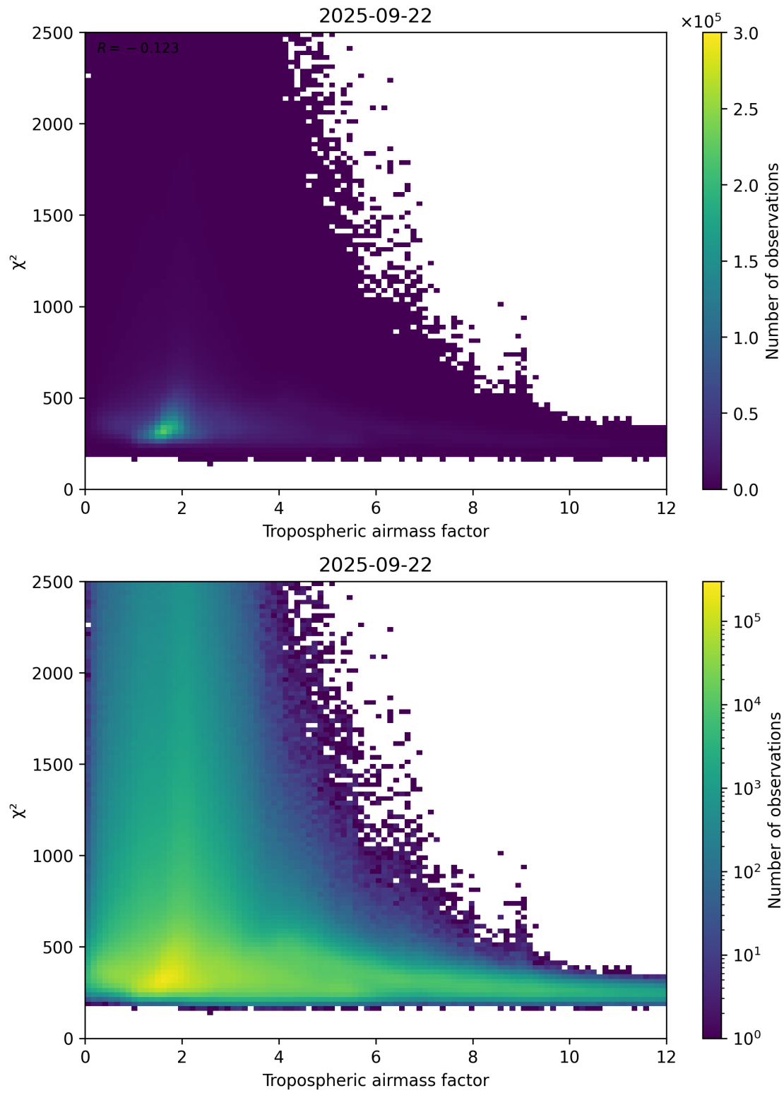
Figure 73: Scatter density plot of “Tropospheric airmass factor” against “ \chi^2 ” for 2025-09-22 to 2025-09-23.
