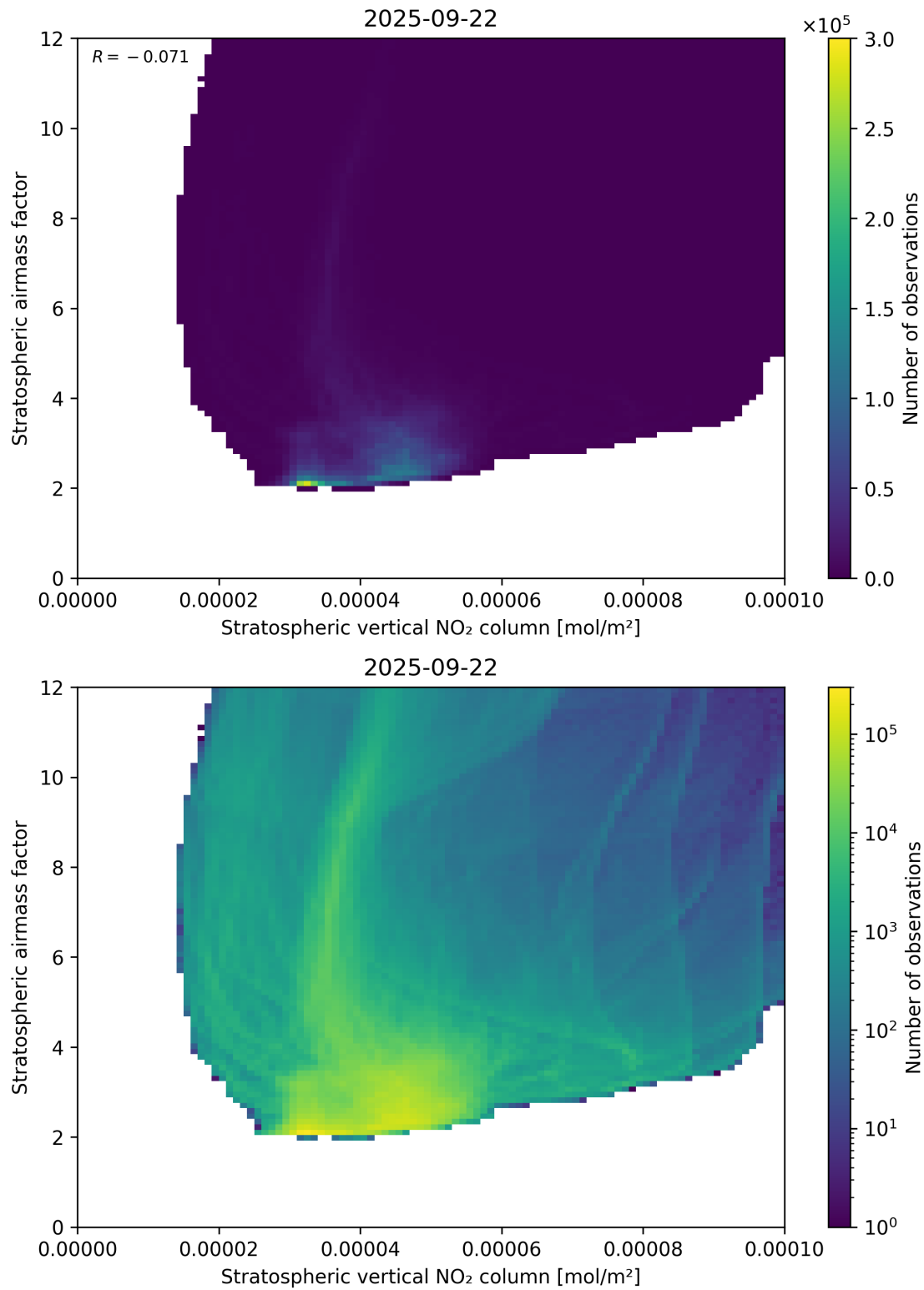
Figure 96: Scatter density plot of “Stratospheric vertical NO 2 column” against “Stratospheric airmass factor” for 2025-09-22 to 2025-09-23.
