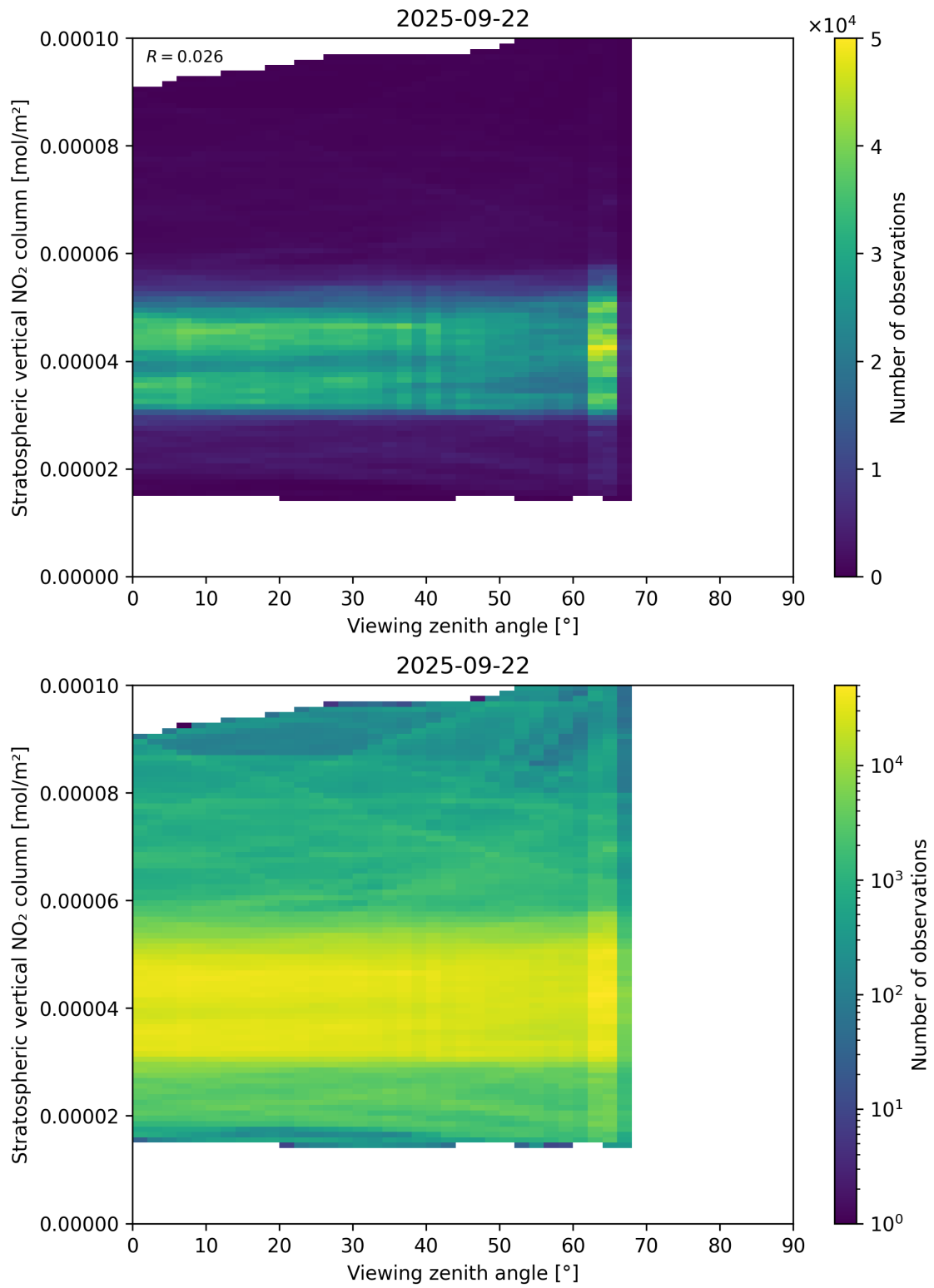
Figure 164: Scatter density plot of “Viewing zenith angle” against “Stratospheric vertical NO 2 column” for 2025-09-22 to 2025-09-23.
