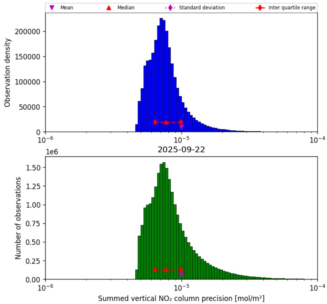
Figure 41: Histogram of “Summed vertical NO 2 column precision” for 2025-09-22 to 2025-09-23
