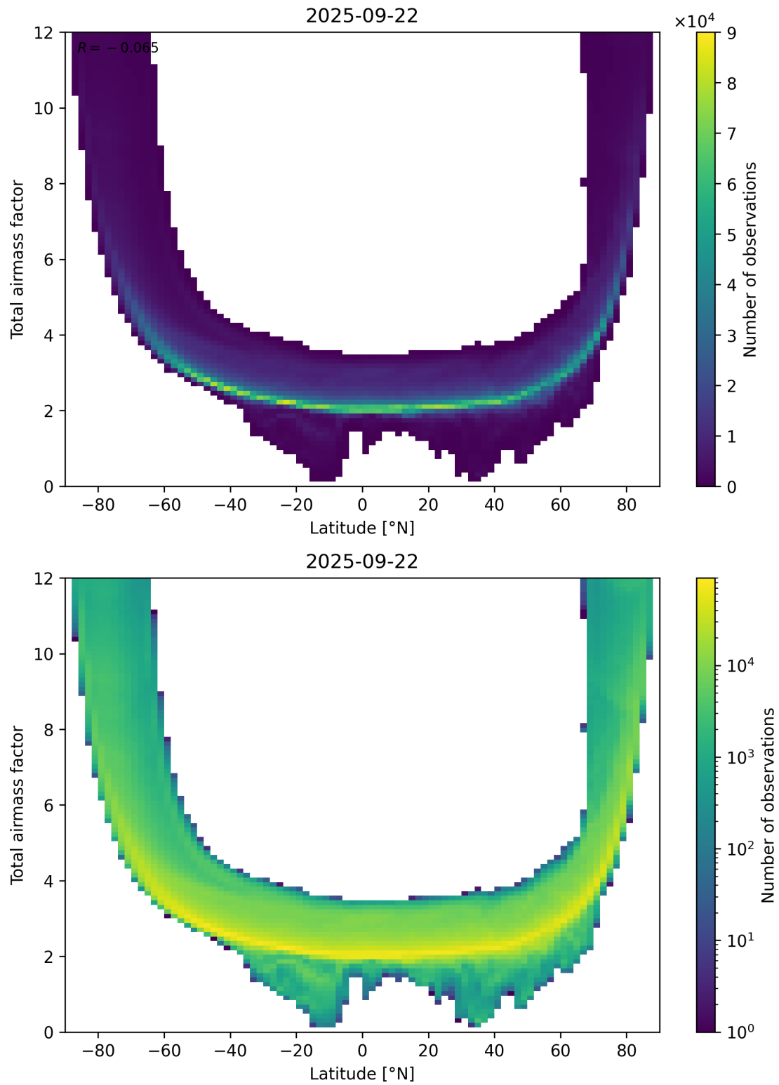
Figure 84: Scatter density plot of “Latitude” against “Total airmass factor” for 2025-09-22 to 2025-09-23.
