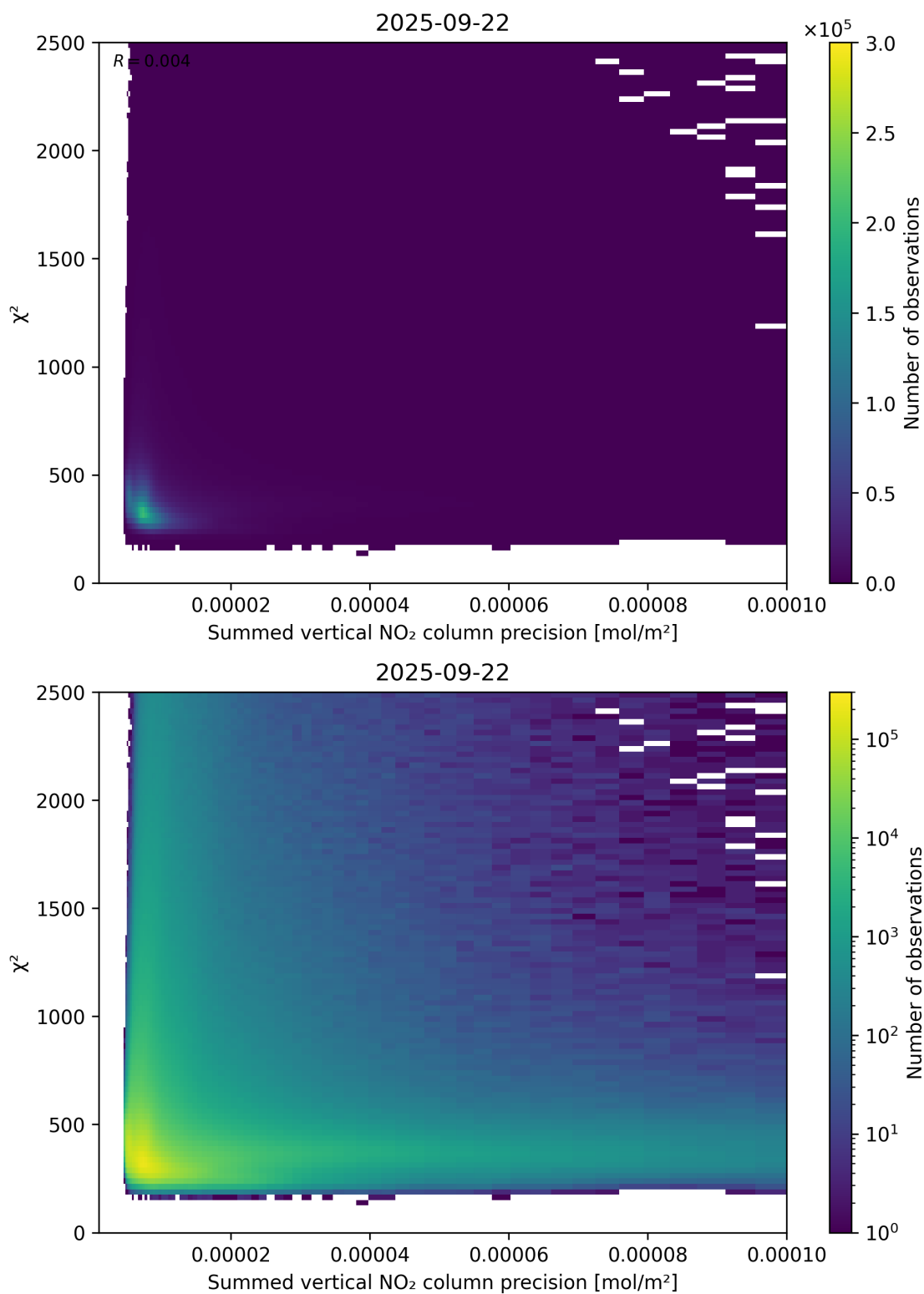
Figure 107: Scatter density plot of “Summed vertical NO 2 column precision” against “ \chi^2 ” for 2025-09-22 to 2025-09-23.
