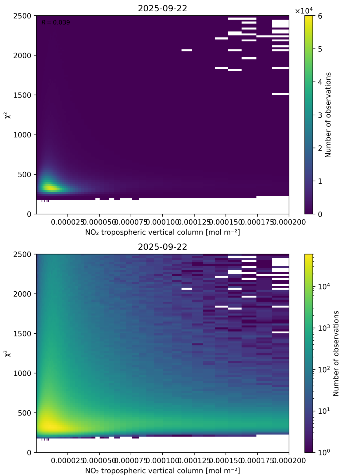
Figure 124: Scatter density plot of “NO 2 tropospheric vertical column” against “ \chi^2 ” for 2025-09-22 to 2025-09-23.
