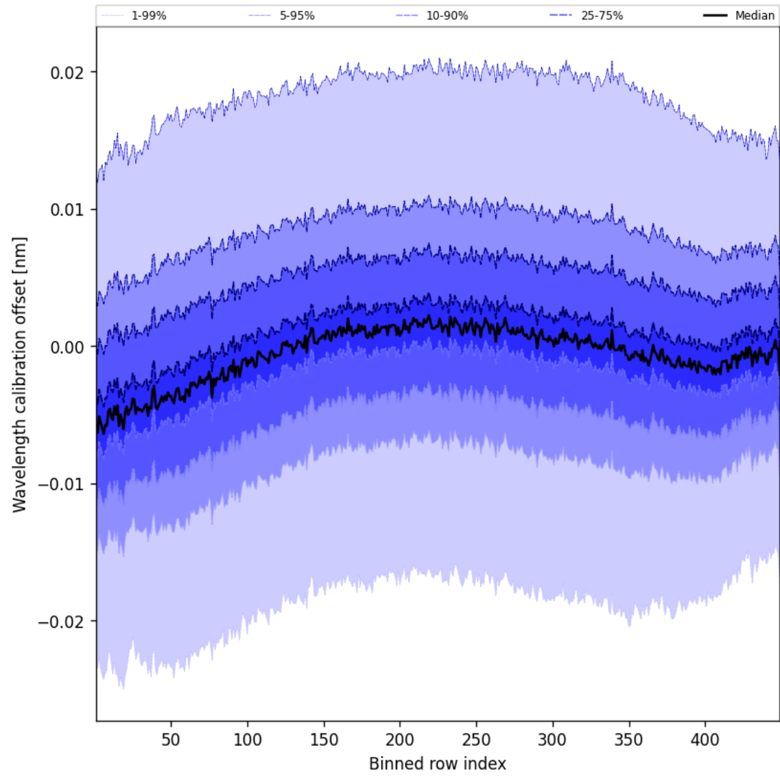
Figure 52: Along track statistics of “Wavelength calibration offset” for 2025-09-22 to 2025-09-23
