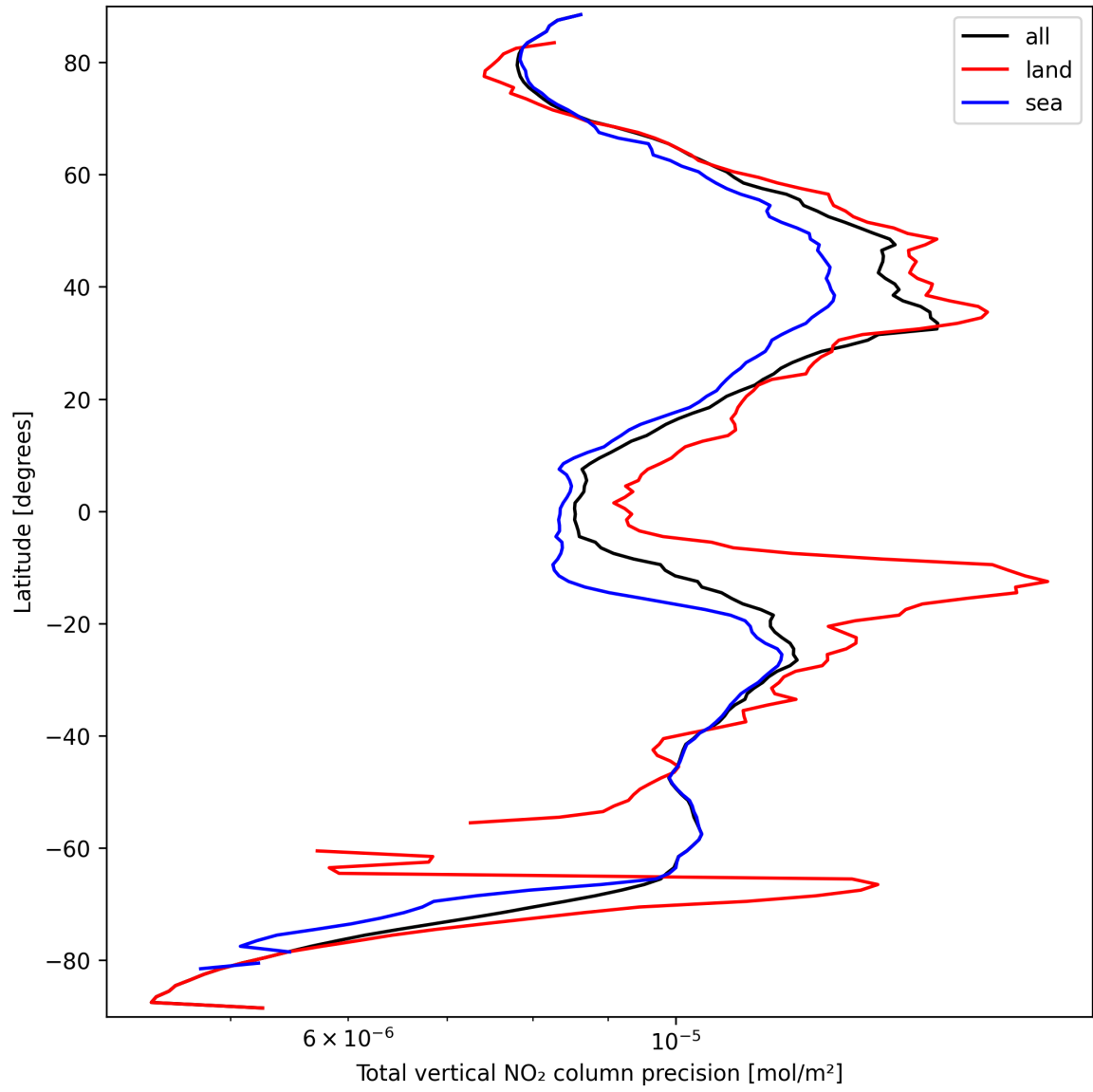
Figure 22: Zonal average of “Total vertical NO 2 column precision” for 2025-09-22 to 2025-09-23.
