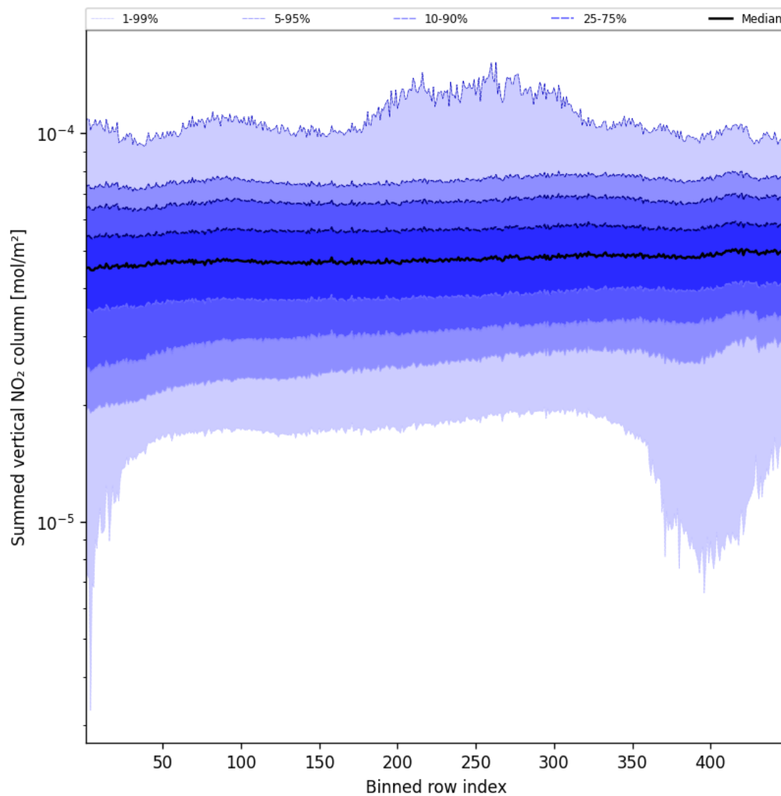
Figure 57: Along track statistics of “Summed vertical NO 2 column” for 2025-09-22 to 2025-09-23
