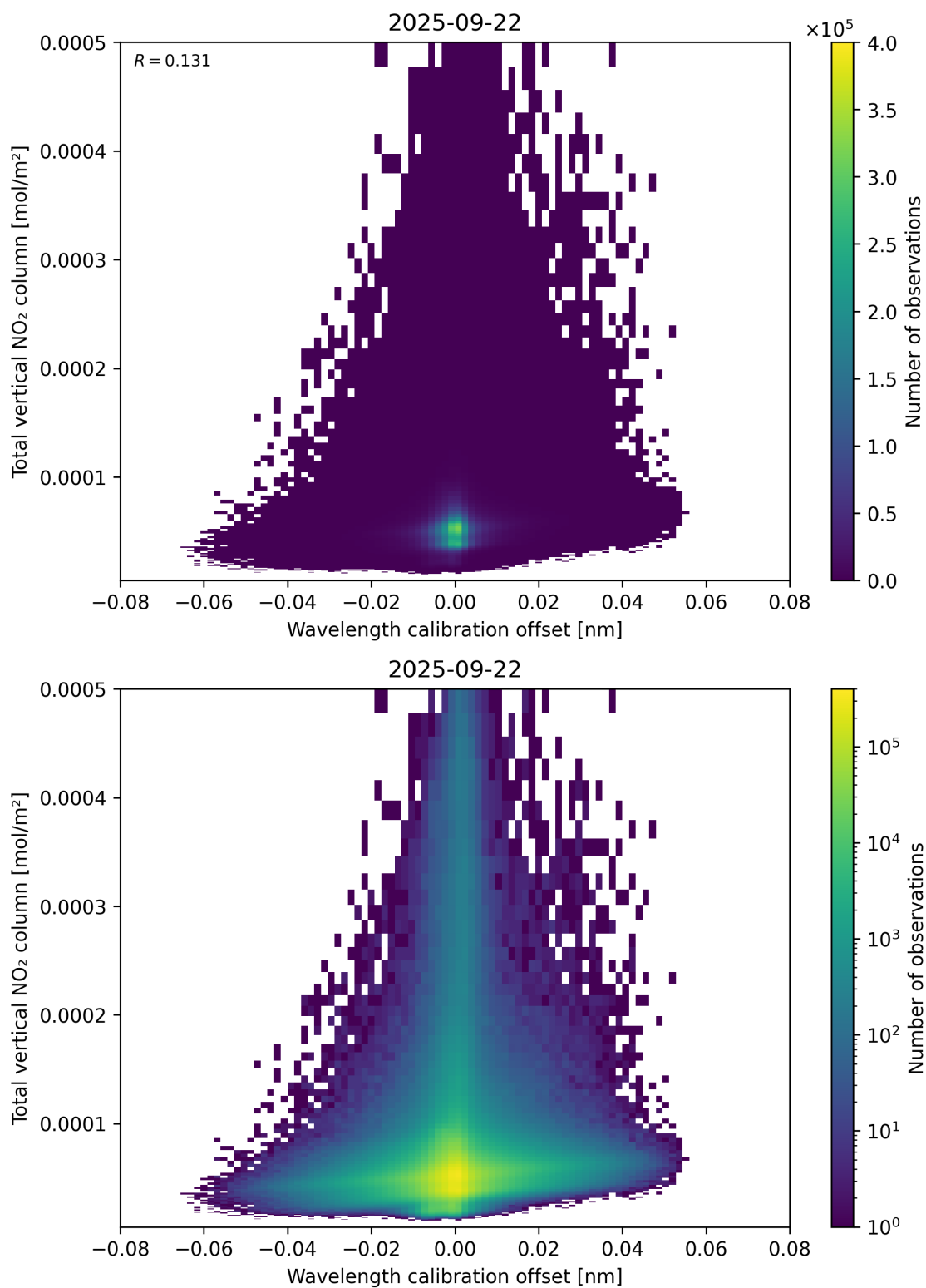
Figure 179: Scatter density plot of “Wavelength calibration offset” against “Total vertical NO 2 column” for 2025-09-22 to 2025-09-23.
