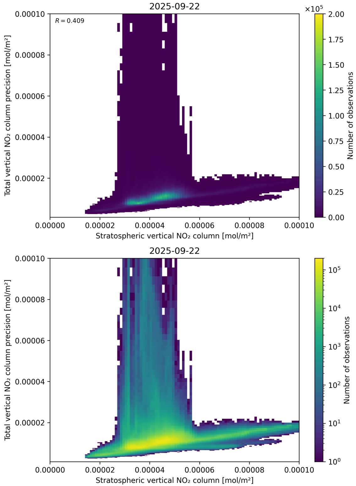
Figure 101: Scatter density plot of “Stratospheric vertical NO 2 column” against “Total vertical NO 2 column precision” for 2025-09-22 to 2025-09-23.
