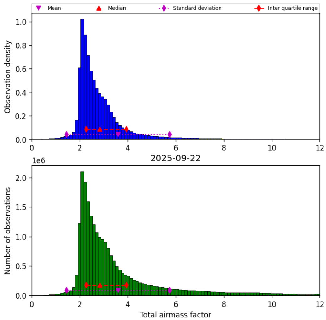
Figure 32: Histogram of “Total airmass factor” for 2025-09-22 to 2025-09-23
