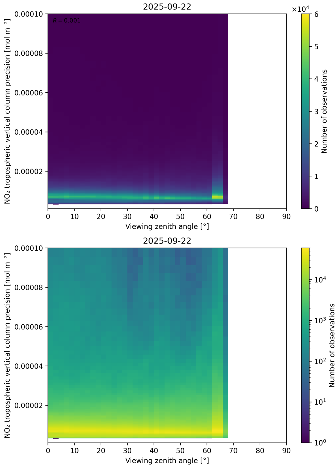
Figure 170: Scatter density plot of “Viewing zenith angle” against “NO 2 tropospheric vertical column precision” for 2025-09-22 to 2025-09-23.
