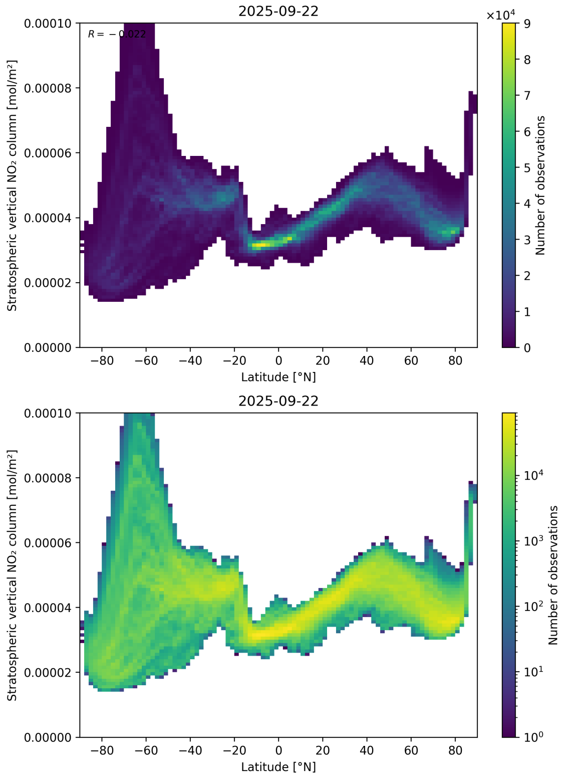
Figure 87: Scatter density plot of “Latitude” against “Stratospheric vertical NO 2 column” for 2025-09-22 to 2025-09-23.
