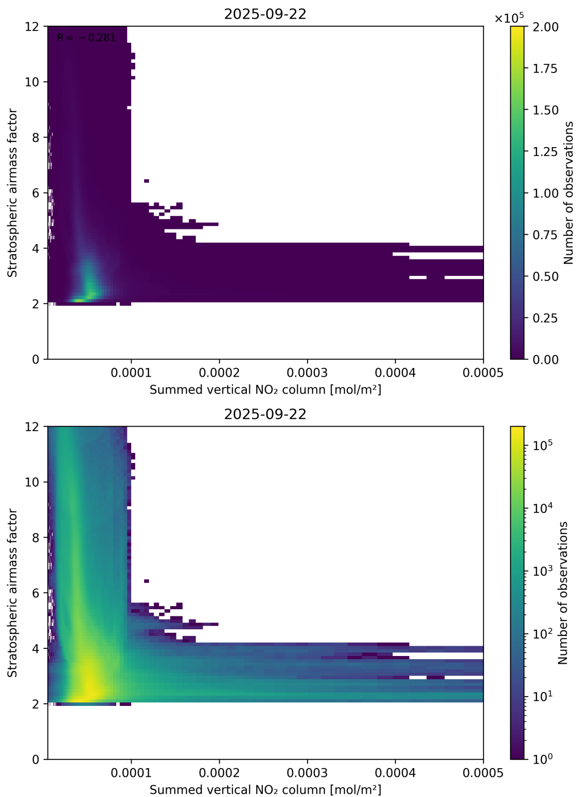
Figure 103: Scatter density plot of “Summed vertical NO 2 column” against “Stratospheric airmass factor” for 2025-09-22 to 2025-09-23.
