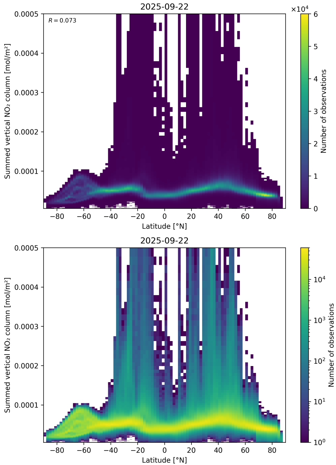
Figure 88: Scatter density plot of “Latitude” against “Summed vertical NO 2 column” for 2025-09-22 to 2025-09-23.
