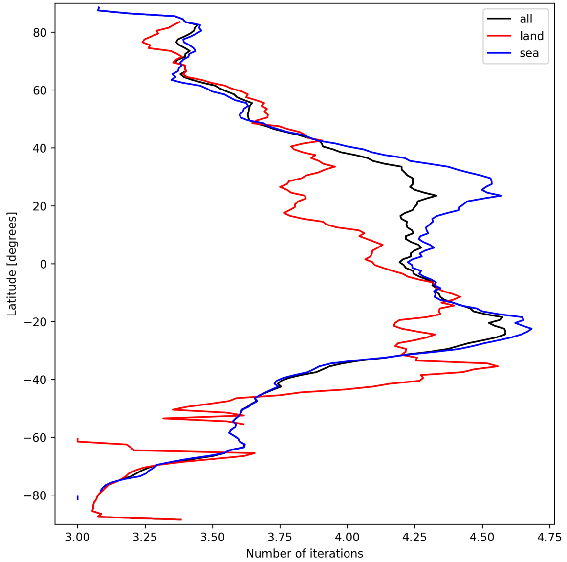
Figure 17: Zonal average of “Number of iterations” for 2025-09-22 to 2025-09-23.
