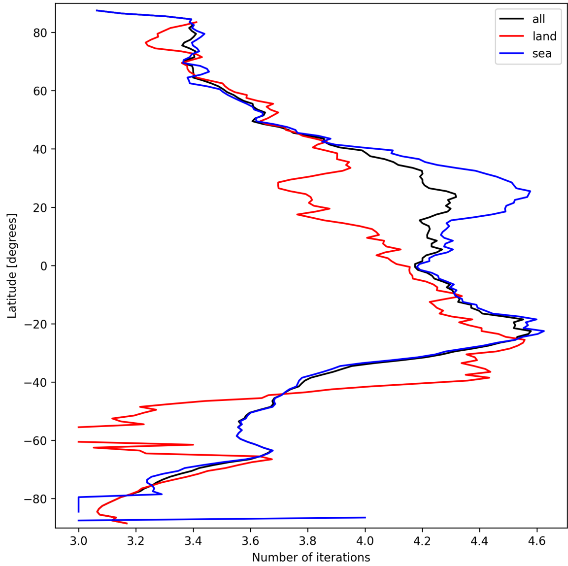
Figure 17: Zonal average of “Number of iterations” for 2025-09-22 to 2025-09-24.
