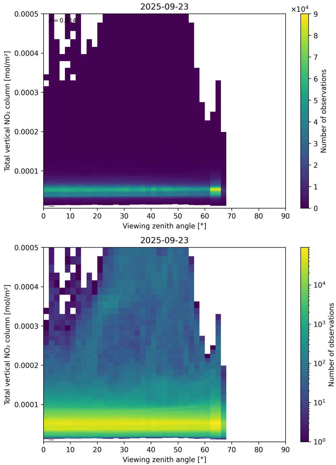
Figure 167: Scatter density plot of “Viewing zenith angle” against “Total vertical NO 2 column” for 2025-09-22 to 2025-09-24.
