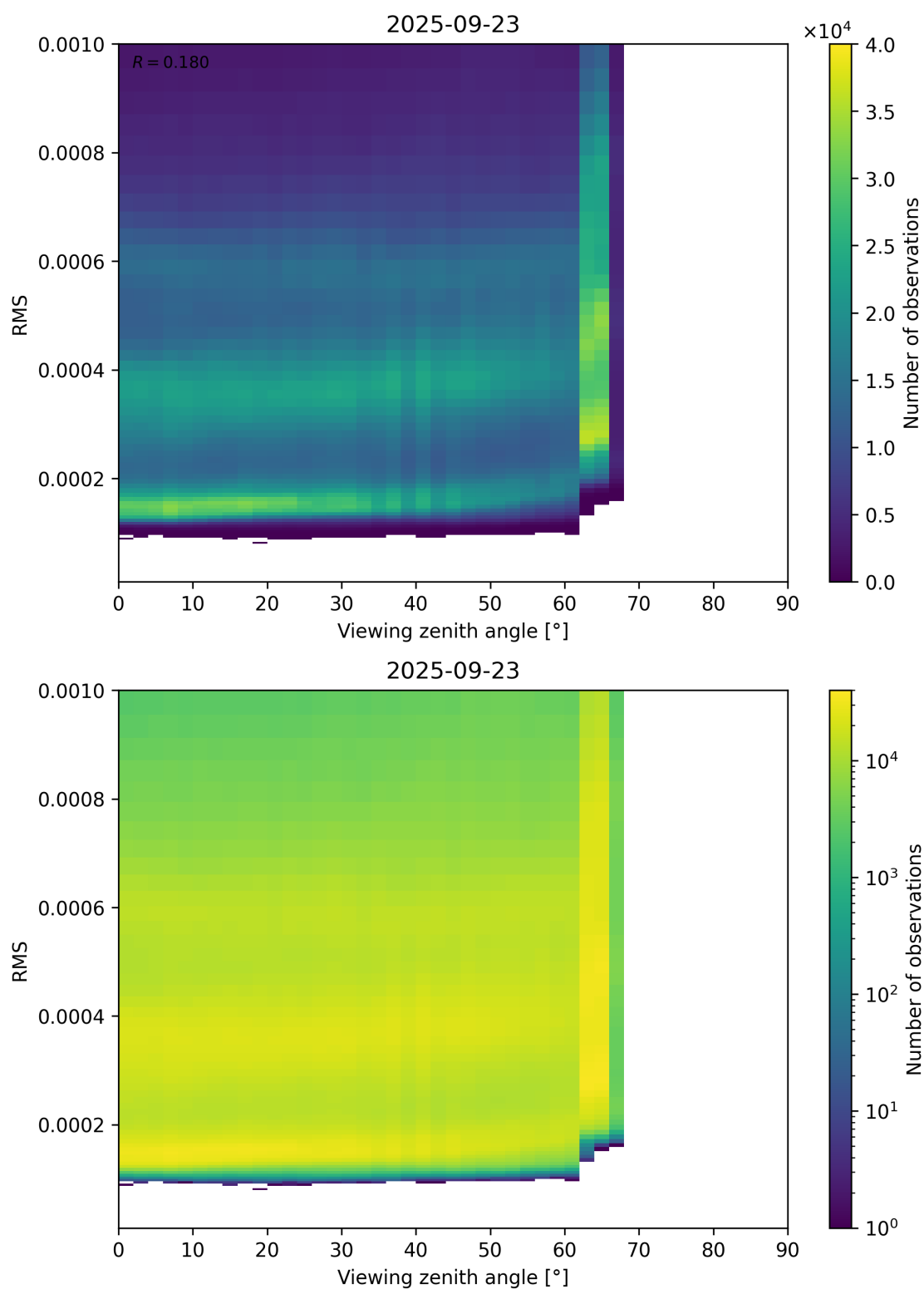
Figure 171: Scatter density plot of “Viewing zenith angle” against “RMS” for 2025-09-22 to 2025-09-24.
