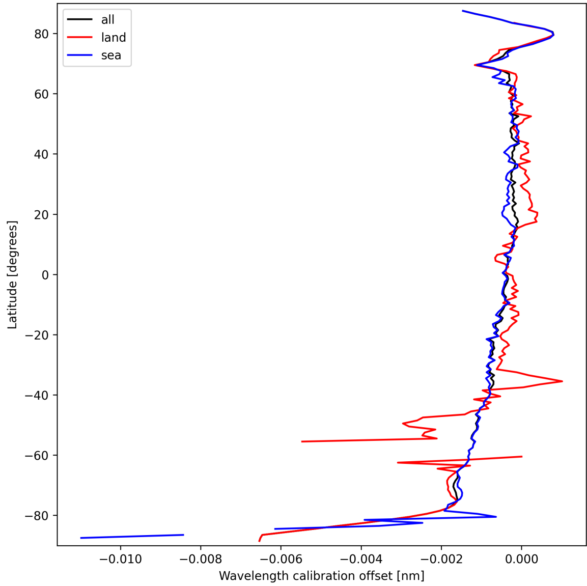
Figure 18: Zonal average of “Wavelength calibration offset” for 2025-09-22 to 2025-09-24.
