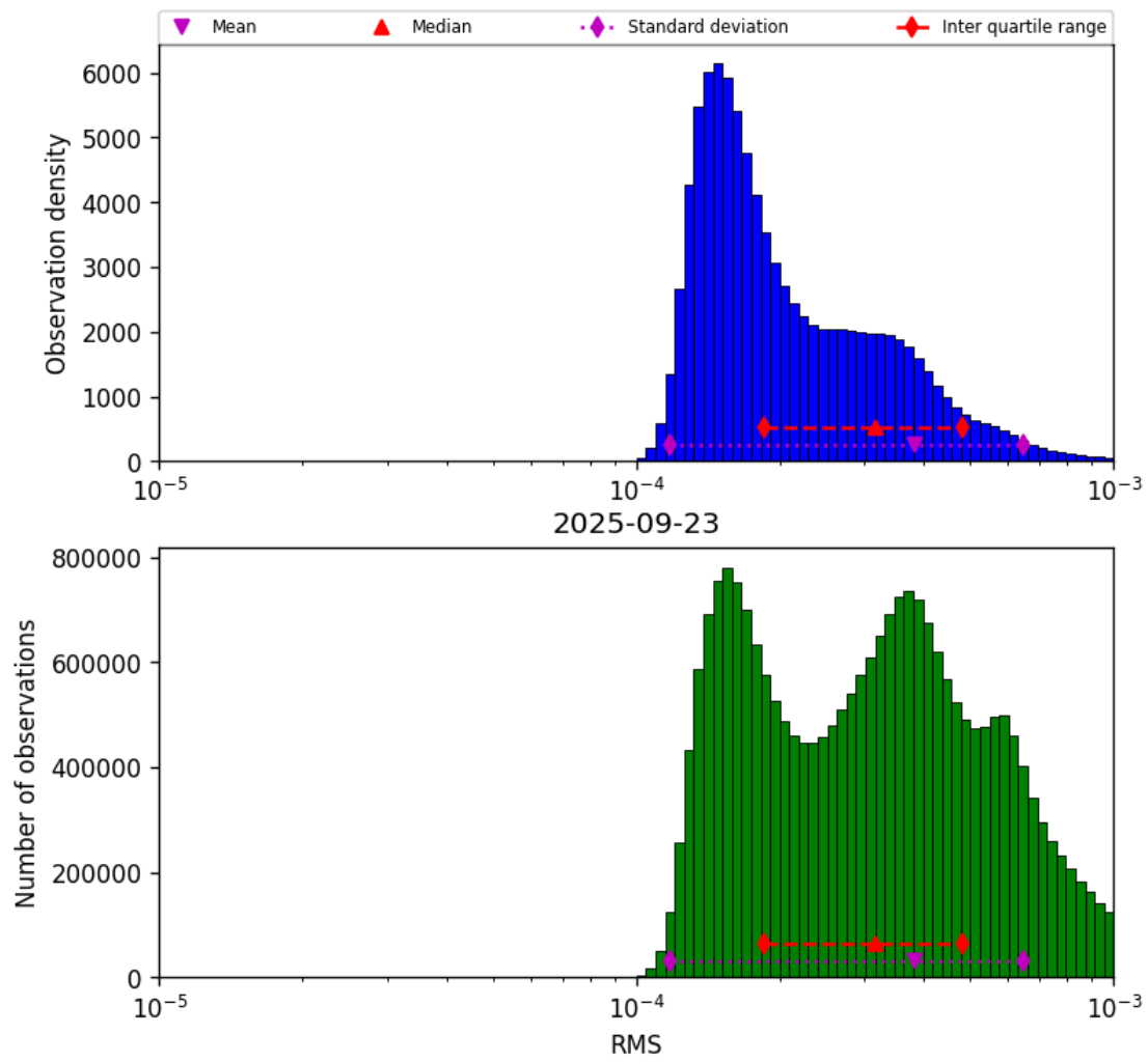
Figure 43: Histogram of “RMS” for 2025-09-22 to 2025-09-24
