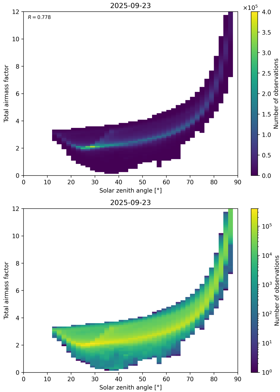
Figure 146: Scatter density plot of “Solar zenith angle” against “Total air mass factor” for 2025-09-22 to 2025-09-24.
