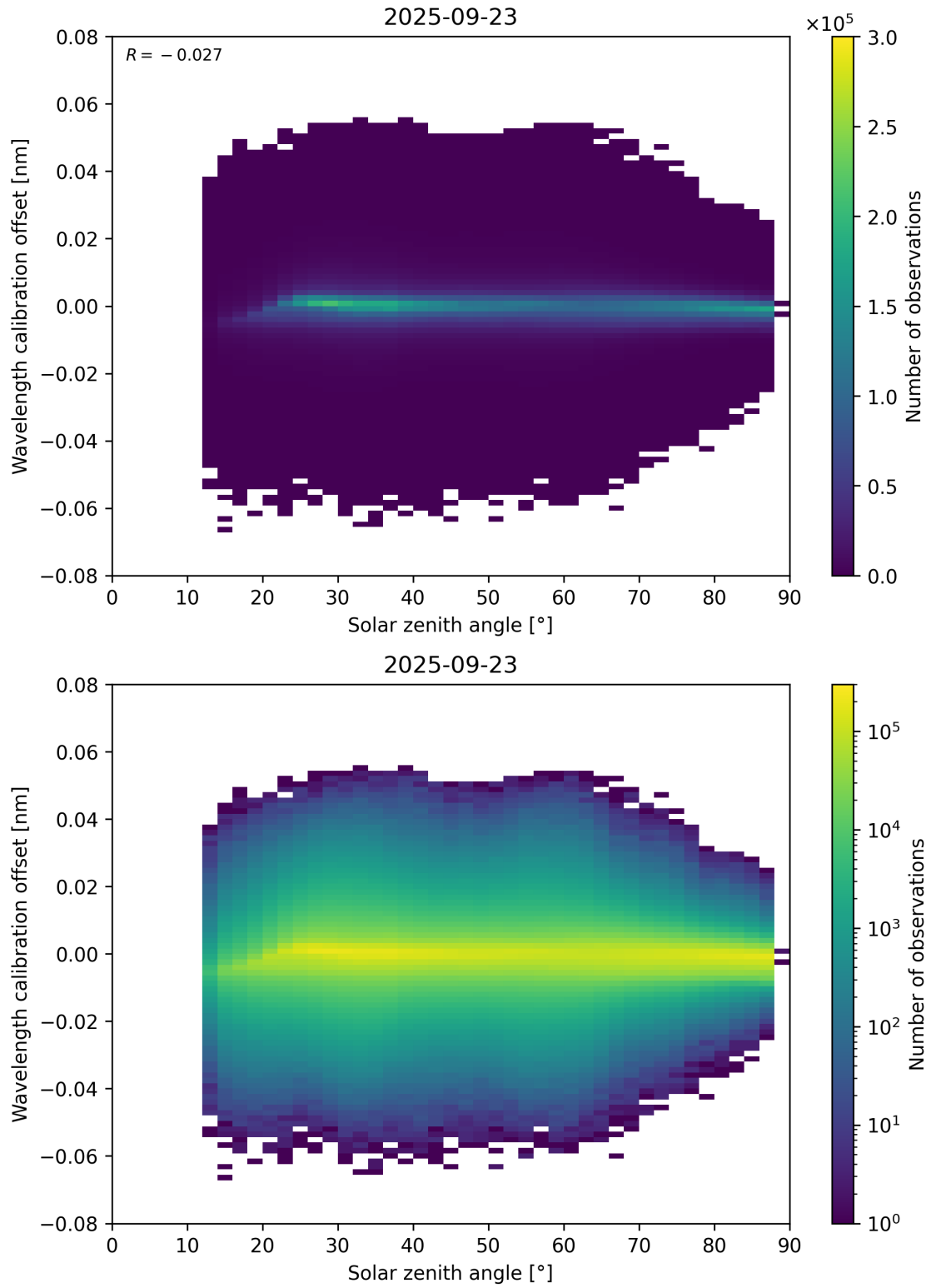
Figure 158: Scatter density plot of “Solar zenith angle” against “Wavelength calibration offset” for 2025-09-22 to 2025-09-24.
