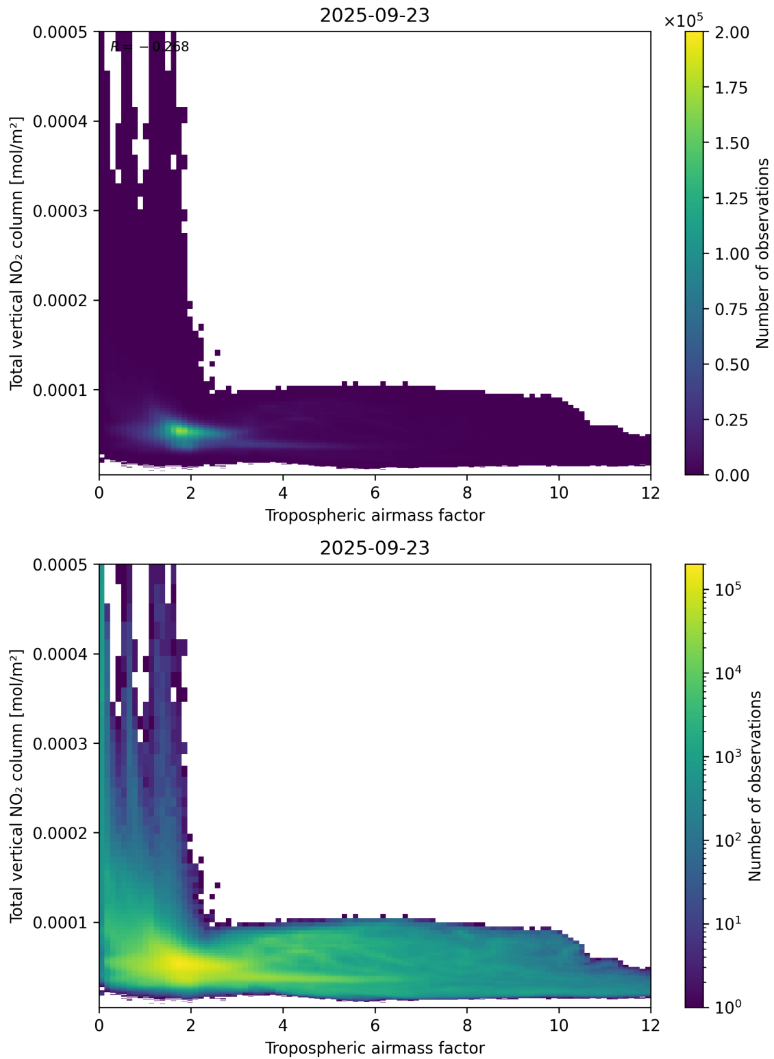
Figure 77: Scatter density plot of “Tropospheric airmass factor” against “Total vertical NO 2 column” for 2025-09-22 to 2025-09-24.
