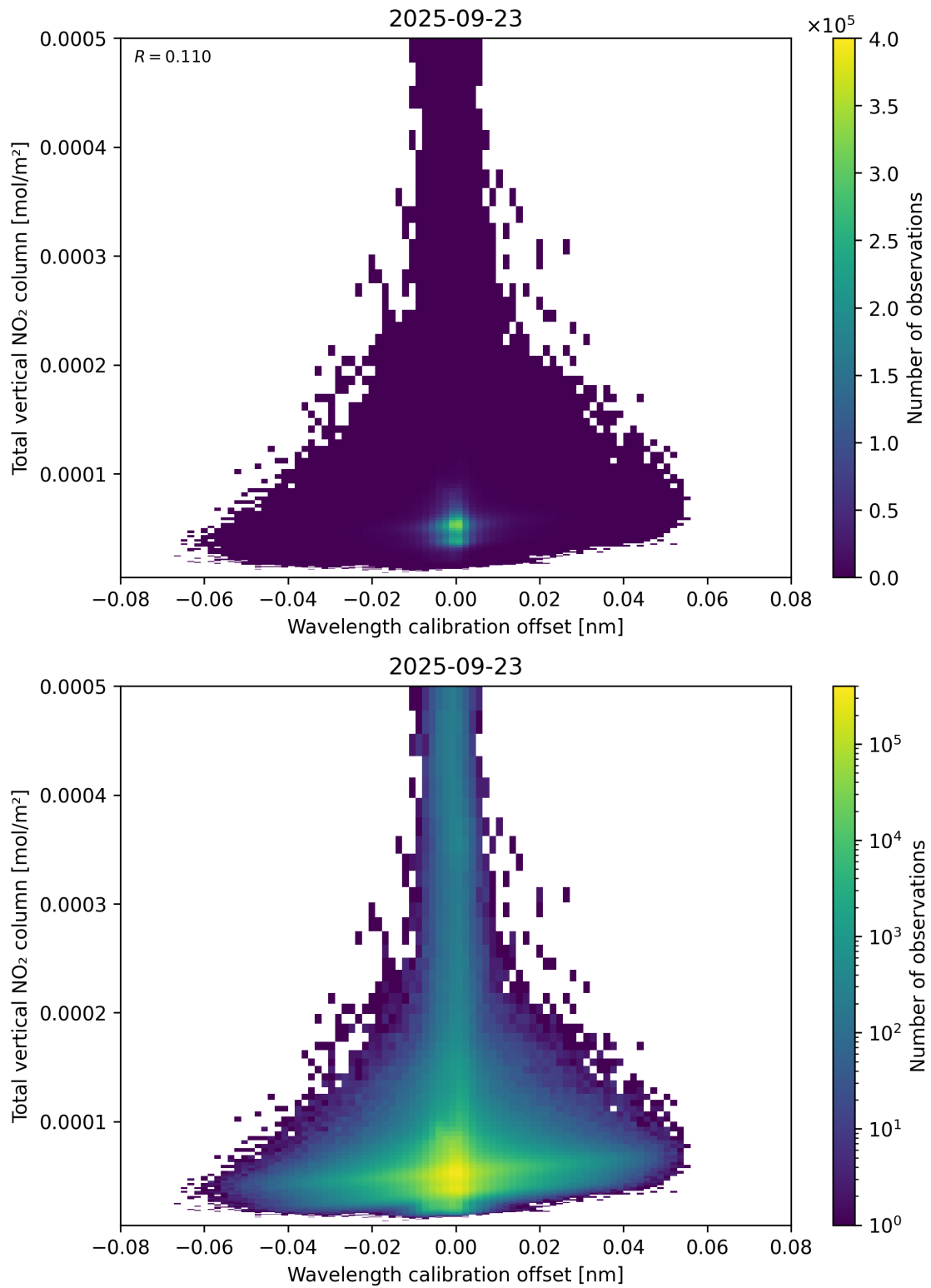
Figure 179: Scatter density plot of “Wavelength calibration offset” against “Total vertical NO 2 column” for 2025-09-22 to 2025-09-24.
