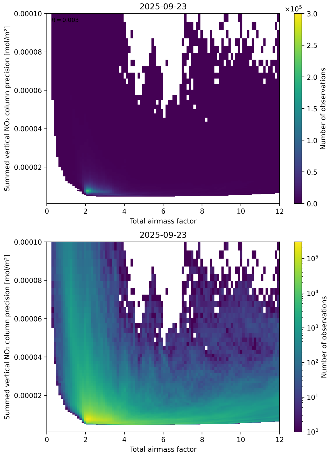
Figure 66: Scatter density plot of “Total airmass factor” against “Summed vertical NO 2 column precision” for 2025-09-22 to 2025-09-24.
