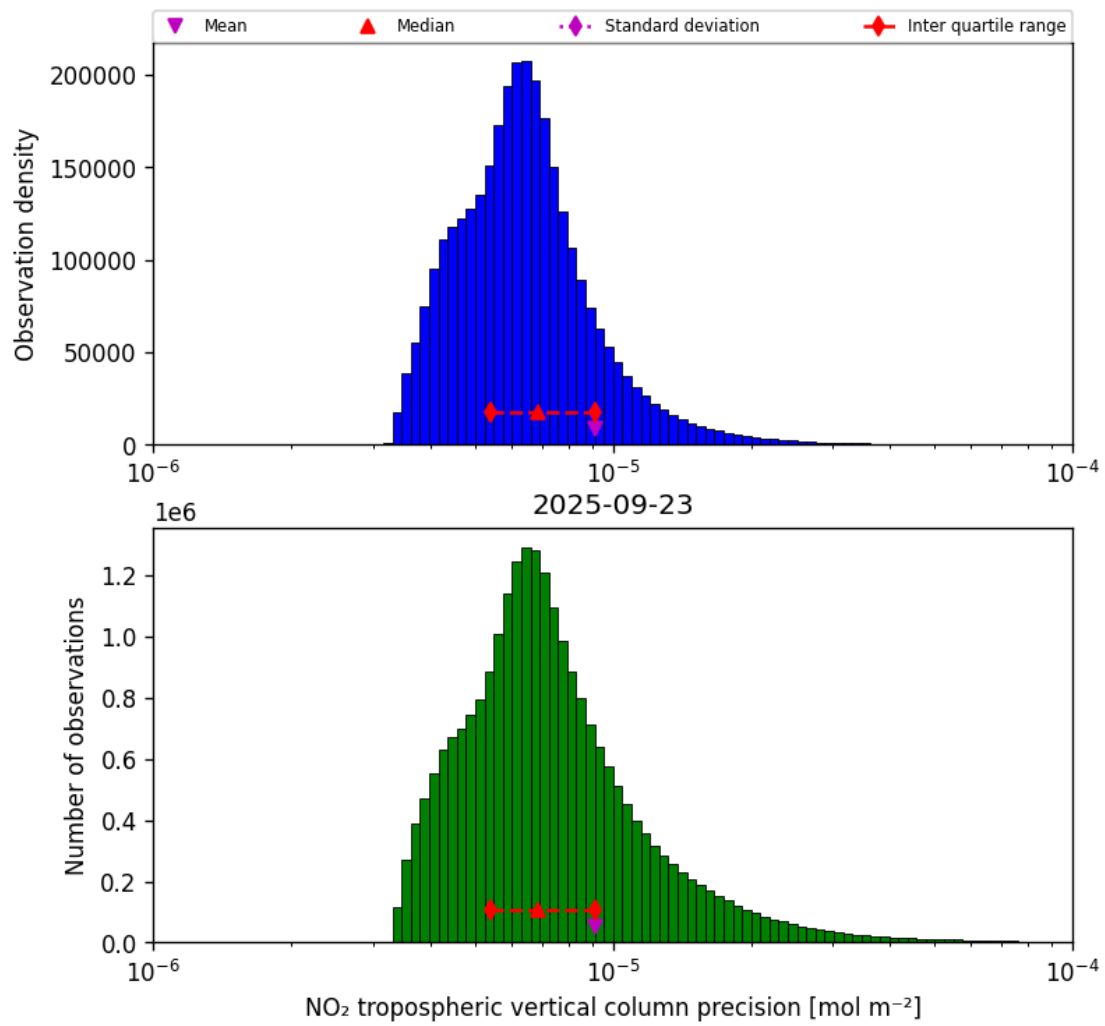
Figure 30: Histogram of “NO 2 tropospheric vertical column precision” for 2025-09-22 to 2025-09-24
