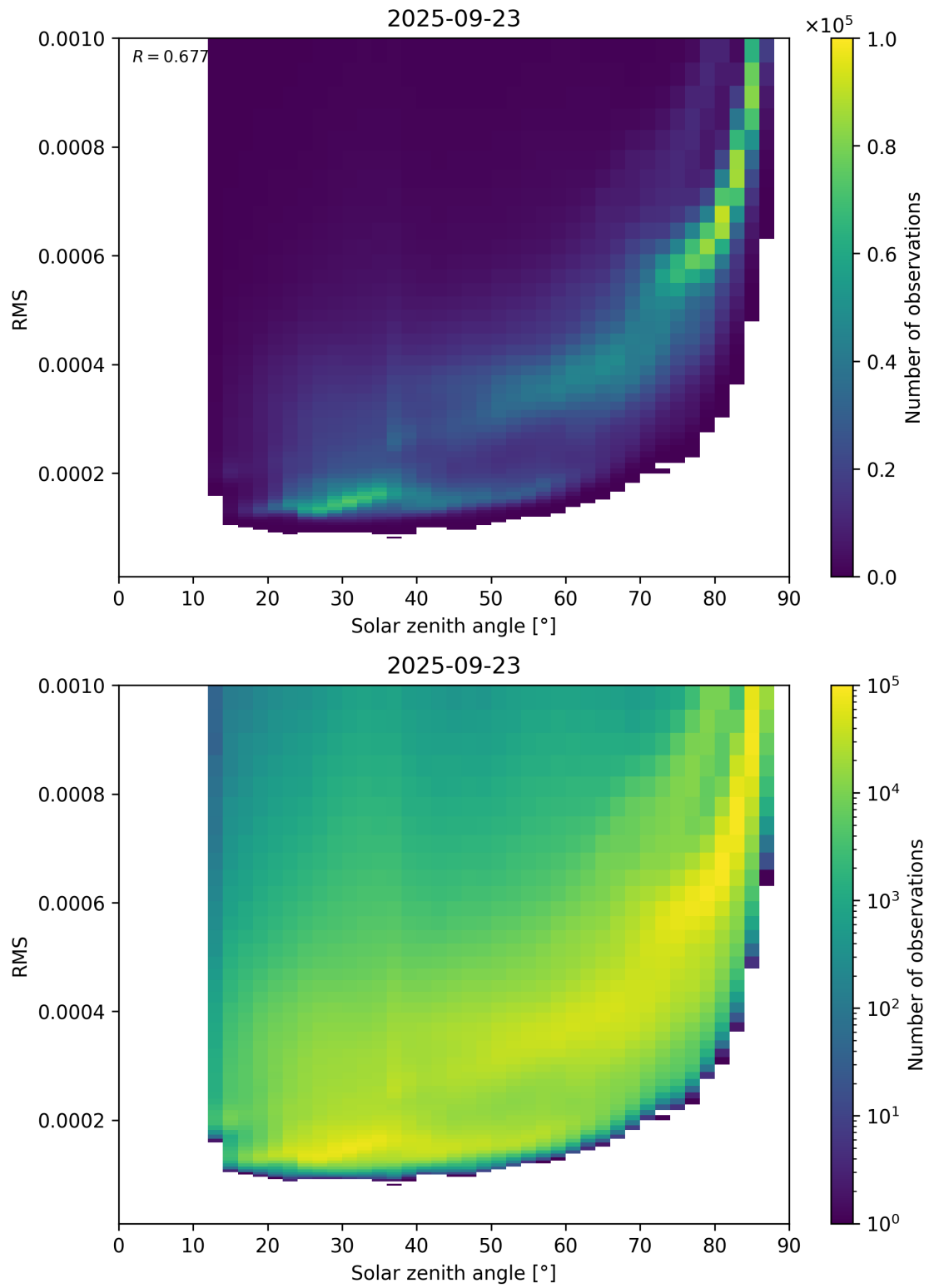
Figure 157: Scatter density plot of “Solar zenith angle” against “RMS” for 2025-09-22 to 2025-09-24.
