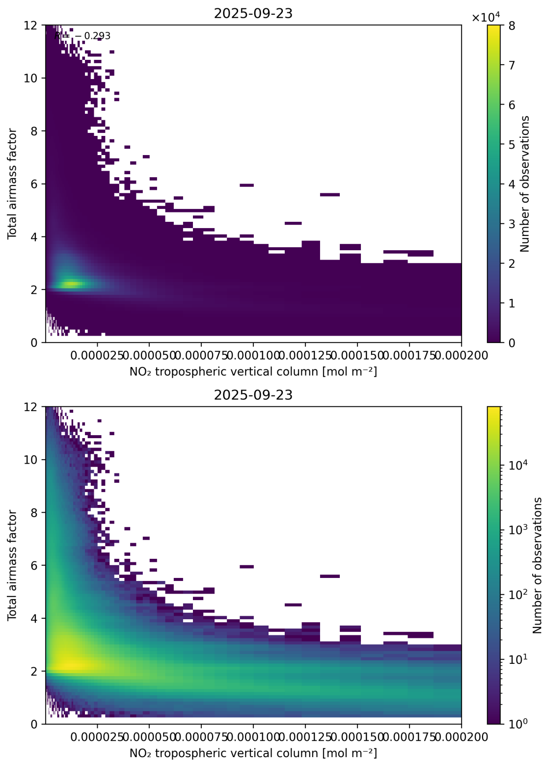
Figure 122: Scatter density plot of “NO 2 tropospheric vertical column” against “Total air mass factor” for 2025-09-22 to 2025-09-24.
