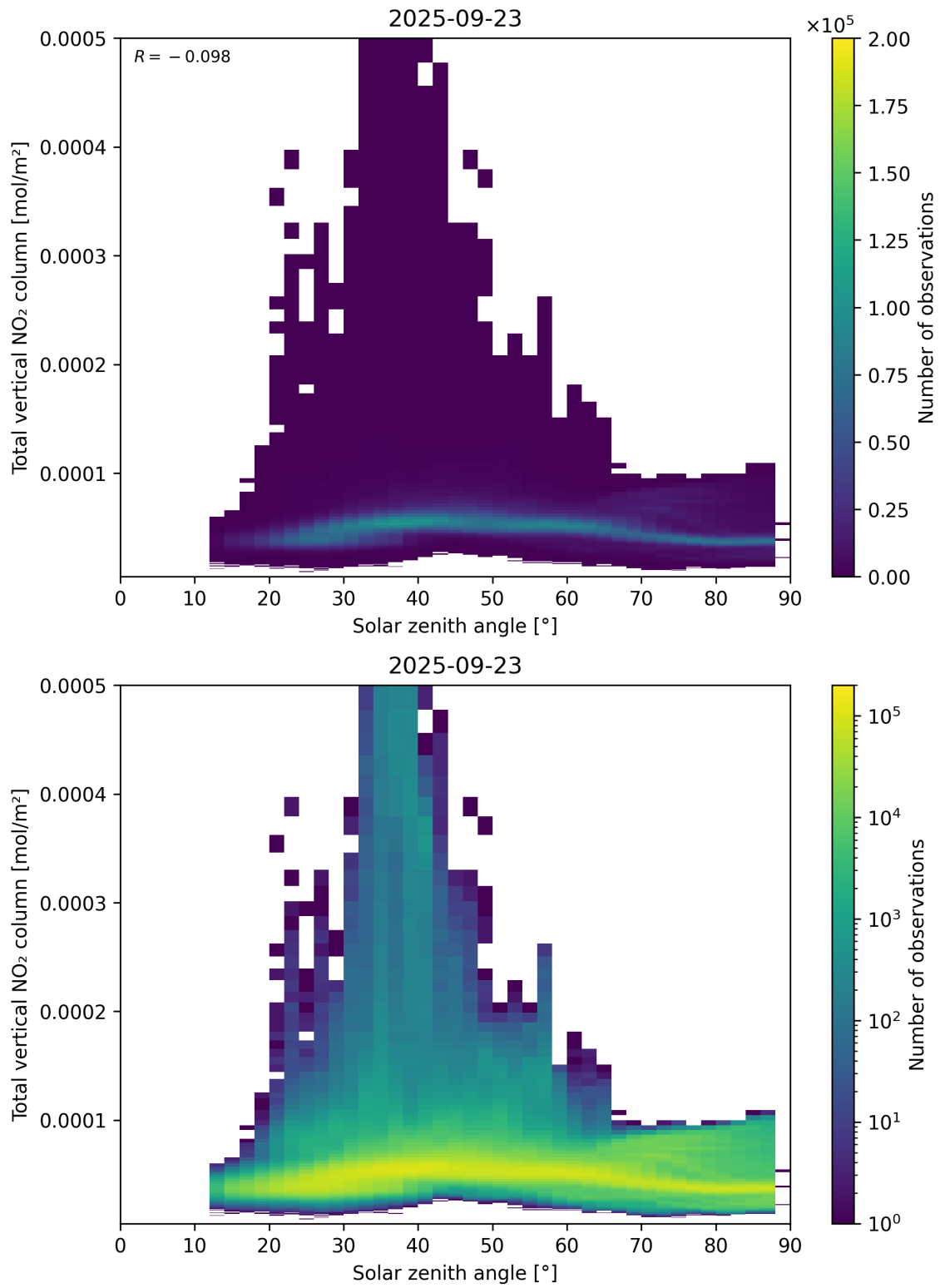
Figure 153: Scatter density plot of “Solar zenith angle” against “Total vertical NO 2 column” for 2025-09-22 to 2025-09-24.
