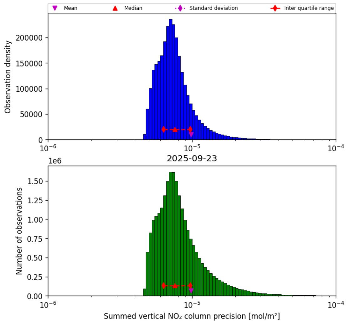
Figure 41: Histogram of “Summed vertical NO 2 column precision” for 2025-09-22 to 2025-09-24
