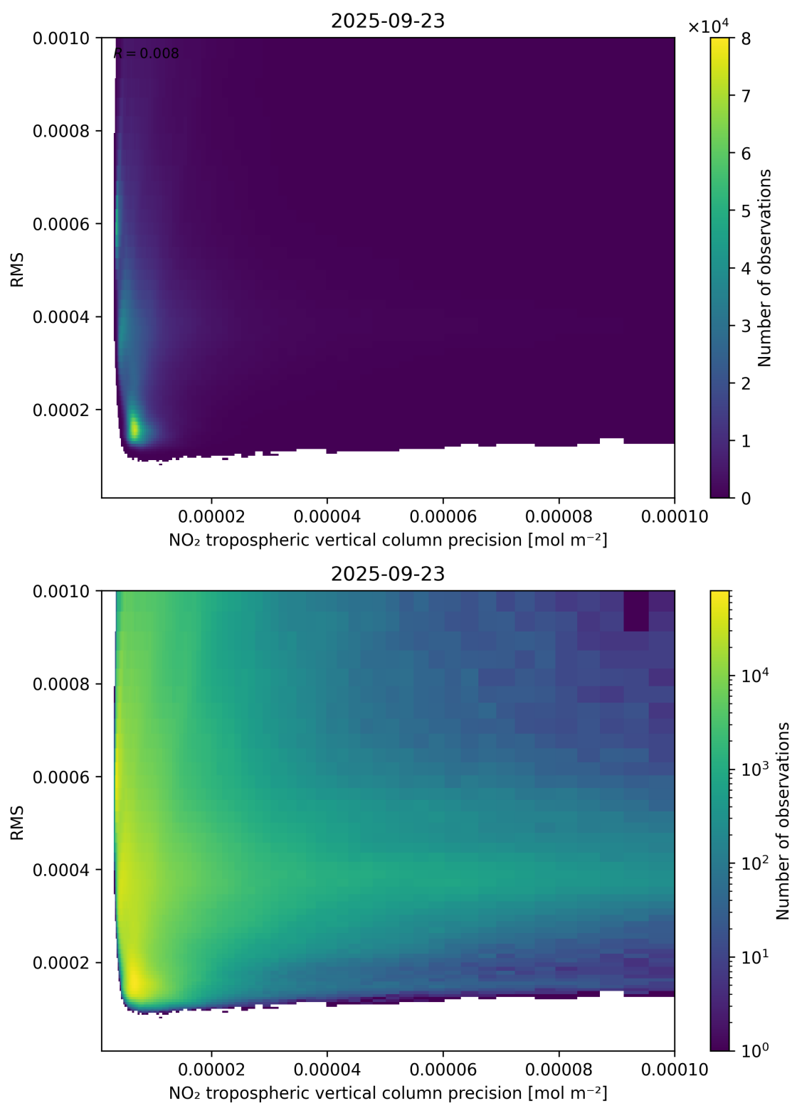
Figure 140: Scatter density plot of “NO 2 tropospheric vertical column precision” against “RMS” for 2025-09-22 to 2025-09-24.
