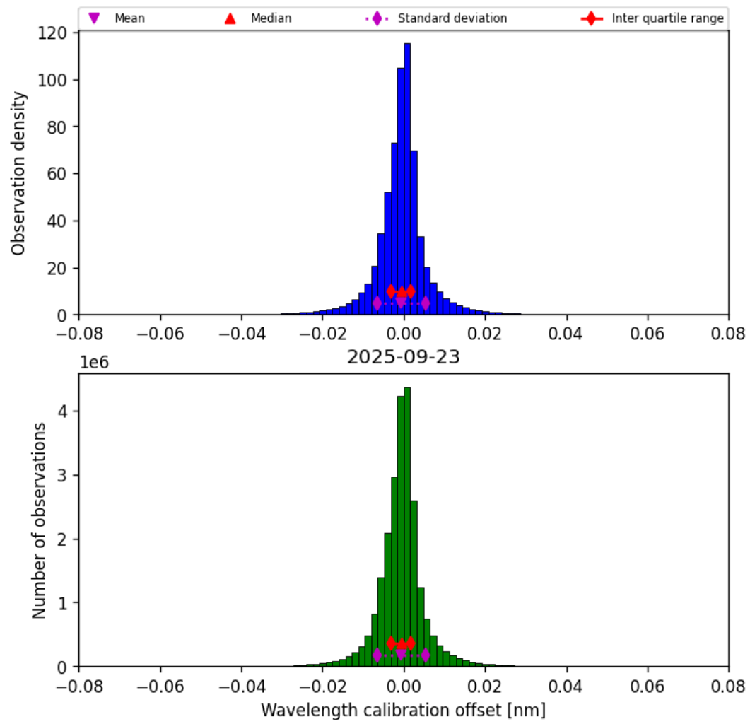
Figure 35: Histogram of “Wavelength calibration offset” for 2025-09-22 to 2025-09-24
