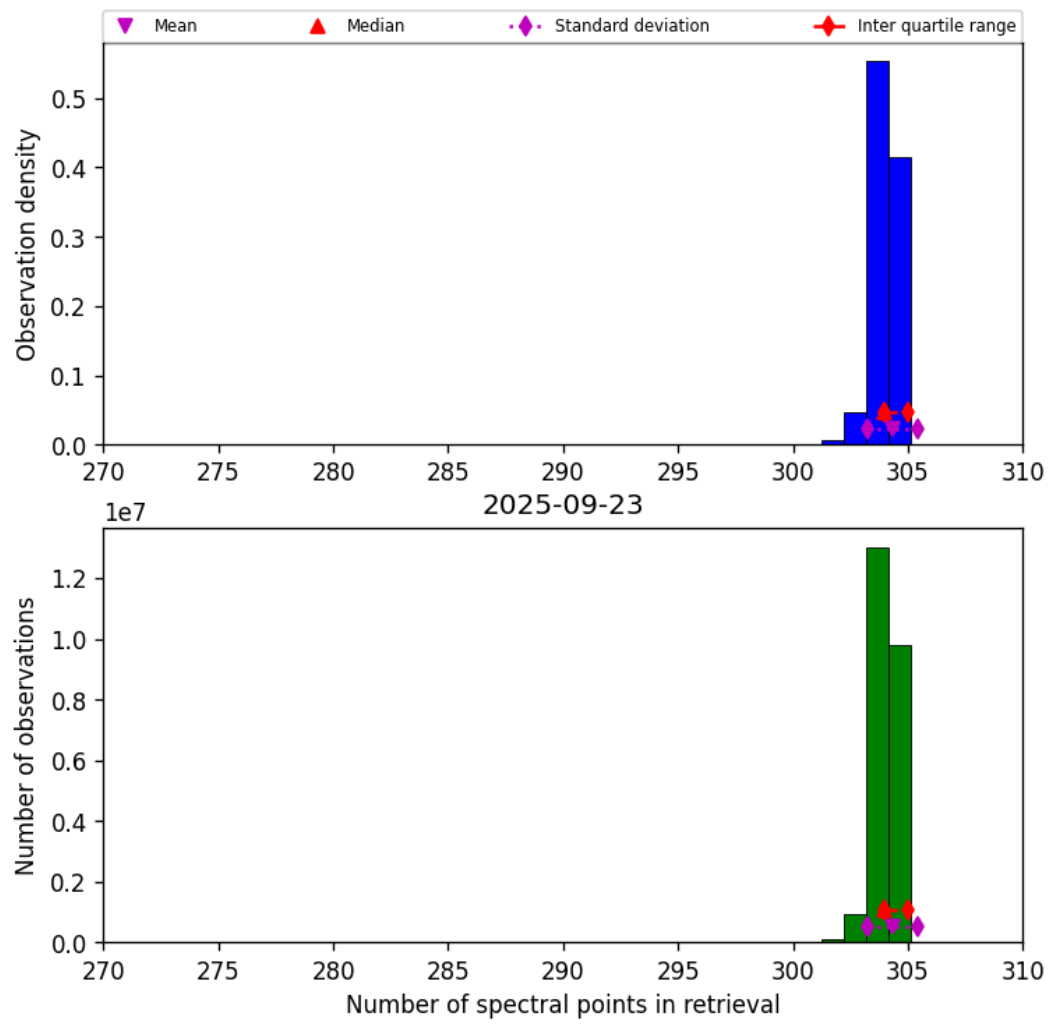
Figure 33: Histogram of “Number of spectral points in retrieval” for 2025-09-22 to 2025-09-24
