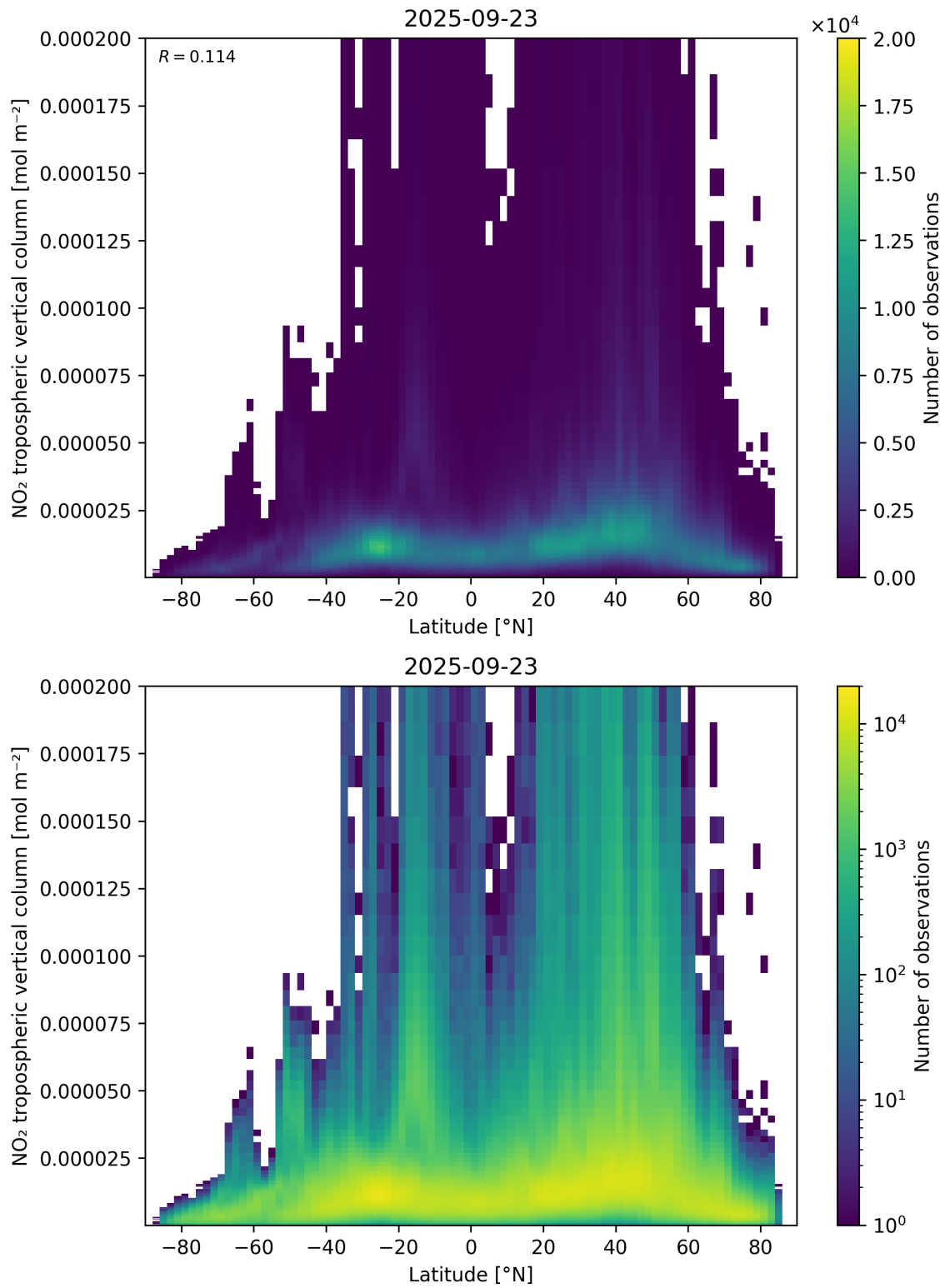
Figure 92: Scatter density plot of “Latitude” against “NO 2 tropospheric vertical column” for 2025-09-22 to 2025-09-24.
