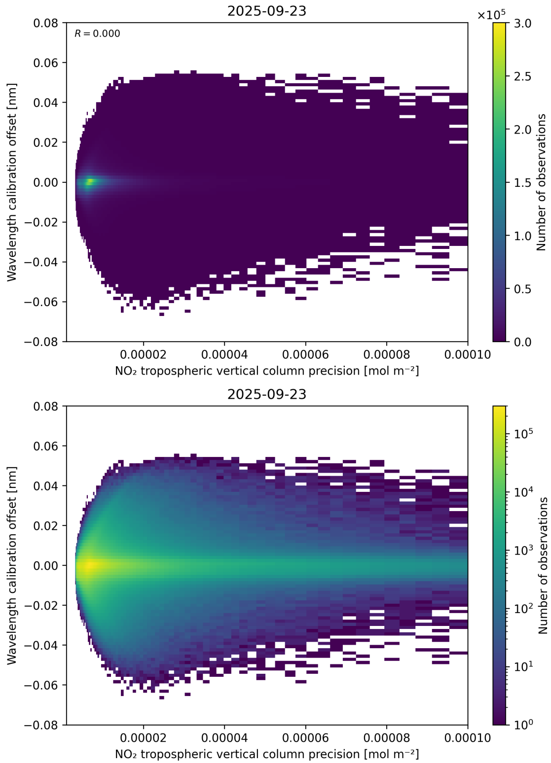
Figure 141: Scatter density plot of “NO 2 tropospheric vertical column precision” against “Wavelength calibration offset” for 2025-09-22 to 2025-09-24.
