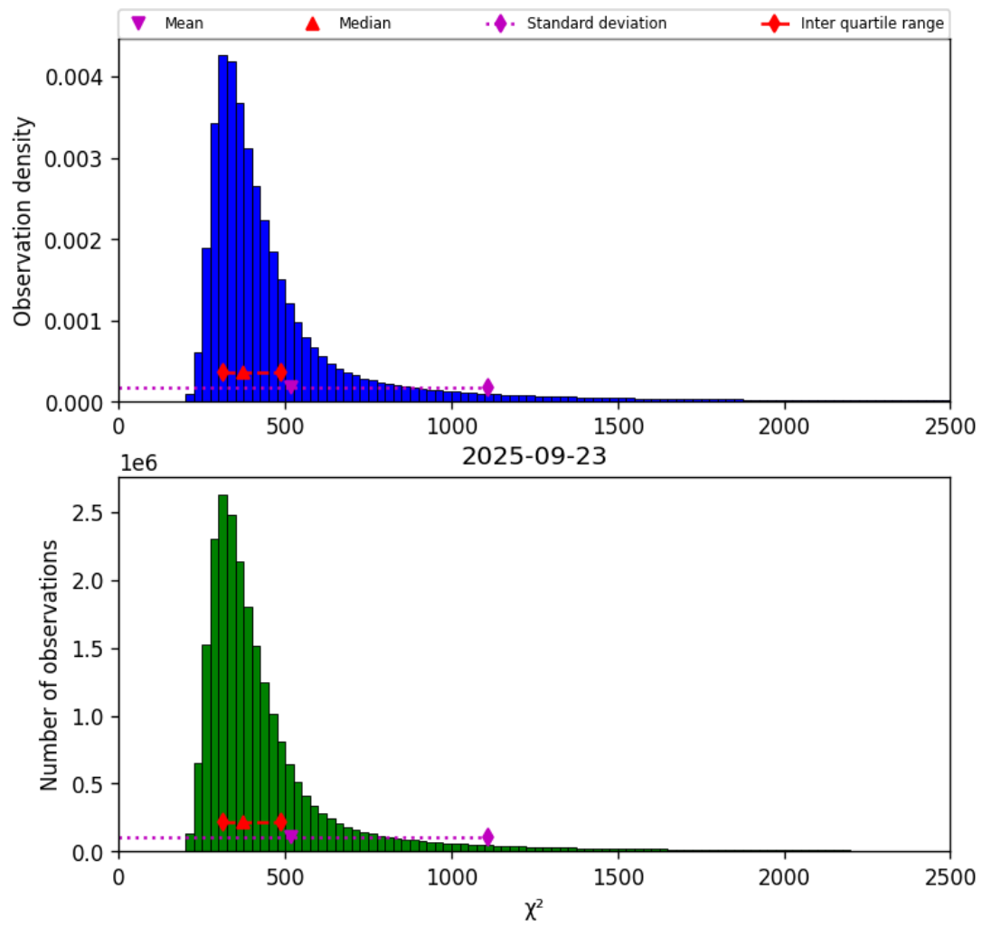
Figure 42: Histogram of “ \chi^2 ” for 2025-09-22 to 2025-09-24
