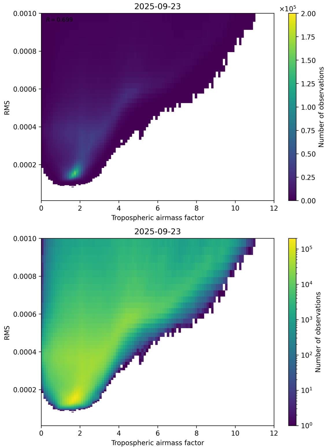
Figure 79: Scatter density plot of “Tropospheric airmass factor” against “RMS” for 2025-09-22 to 2025-09-24.
