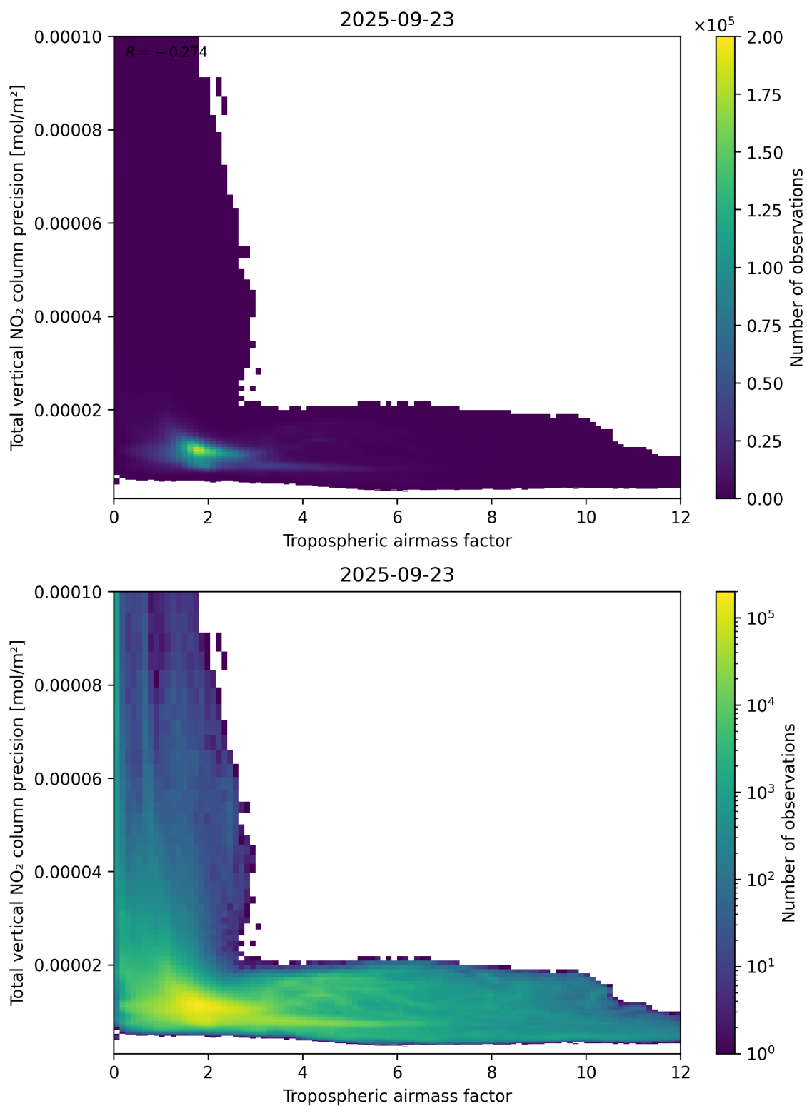
Figure 78: Scatter density plot of “Tropospheric airmass factor” against “Total vertical NO 2 column precision” for 2025-09-22 to 2025-09-24.
