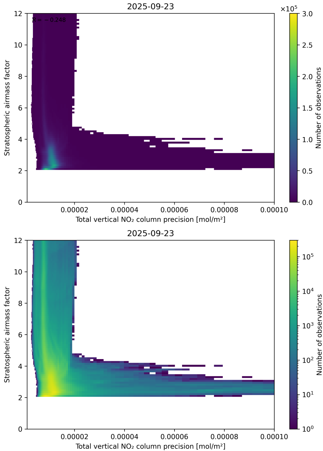
Figure 115: Scatter density plot of “Total vertical NO 2 column precision” against “Stratospheric air mass factor” for 2025-09-22 to 2025-09-24.
