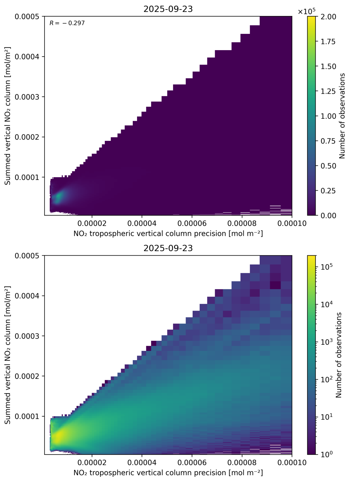
Figure 136: Scatter density plot of “NO 2 tropospheric vertical column precision” against “Summed vertical NO 2 column” for 2025-09-22 to 2025-09-24.
