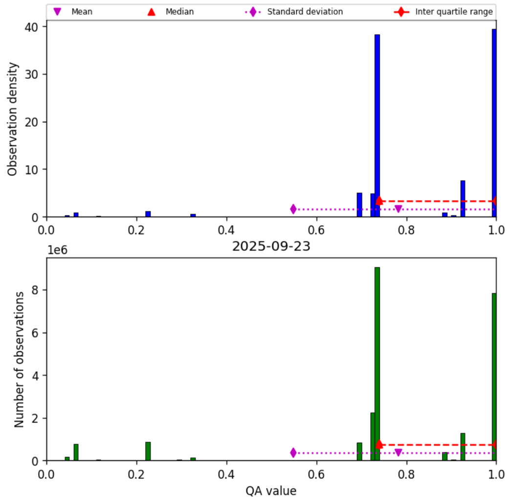
Figure 28: Histogram of “QA value” for 2025-09-22 to 2025-09-24
