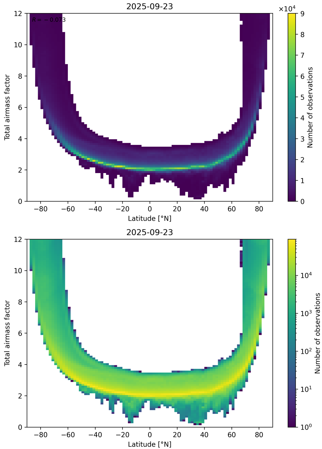
Figure 84: Scatter density plot of “Latitude” against “Total airmass factor” for 2025-09-22 to 2025-09-24.
