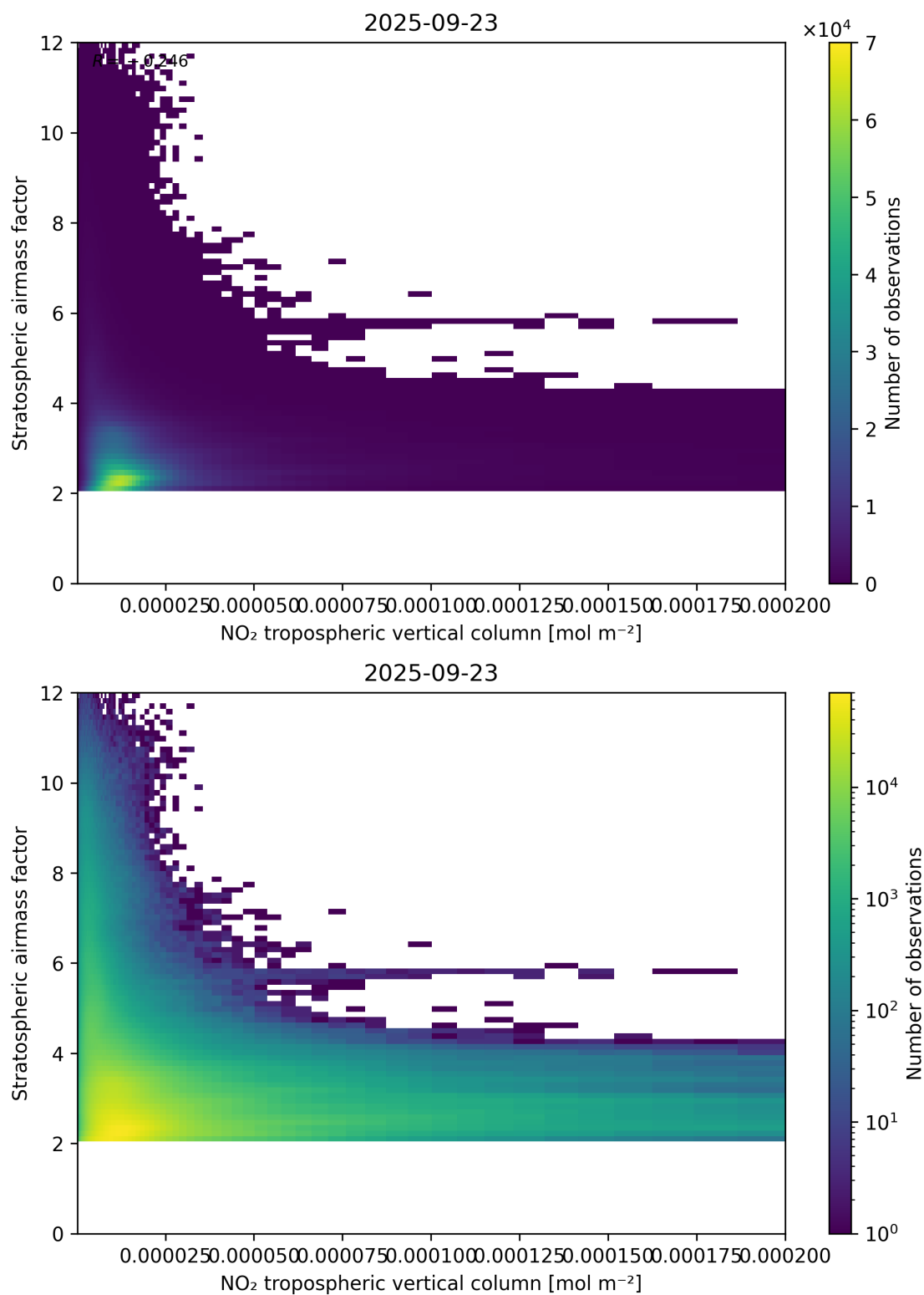
Figure 121: Scatter density plot of “NO 2 tropospheric vertical column” against “Stratospheric air mass factor” for 2025-09-22 to 2025-09-24.
