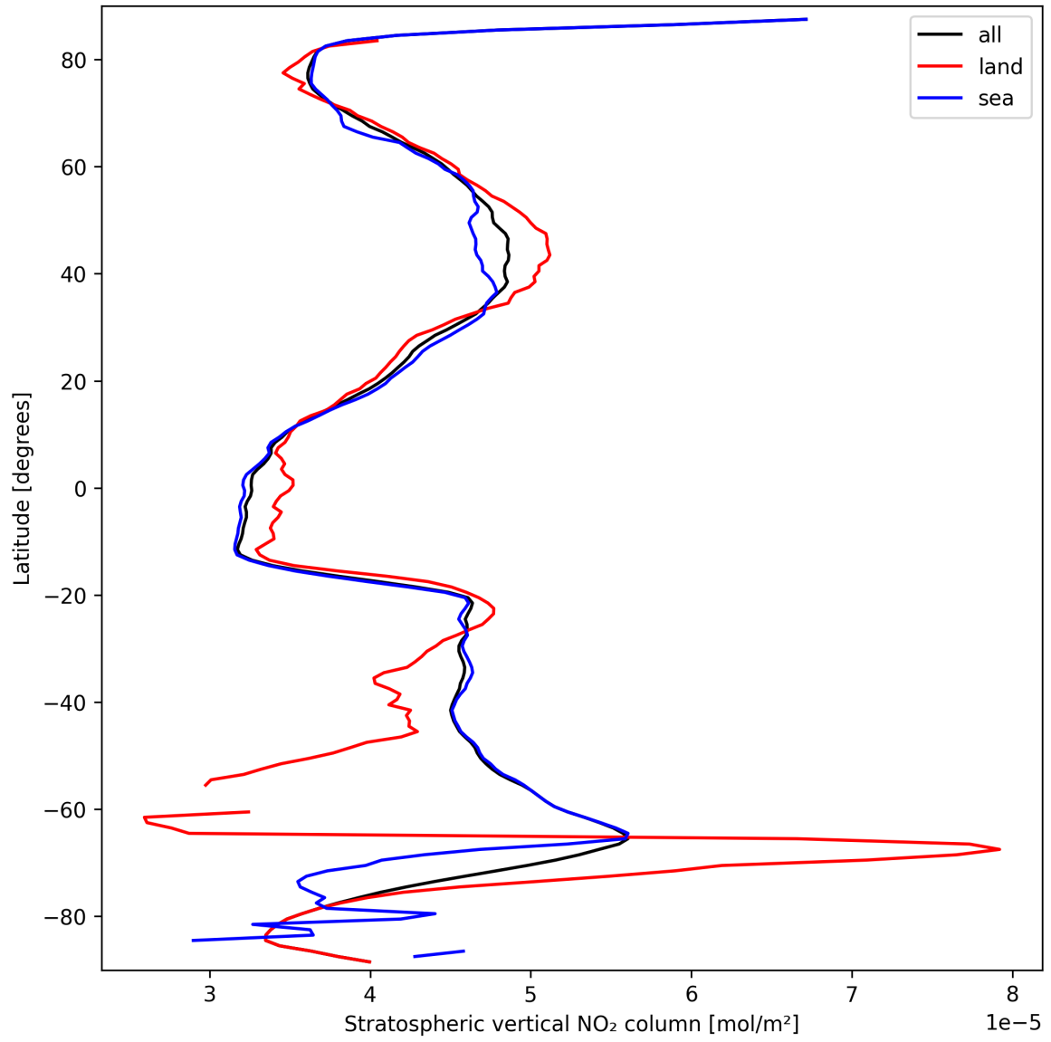
Figure 19: Zonal average of “Stratospheric vertical NO 2 column” for 2025-09-22 to 2025-09-24.
