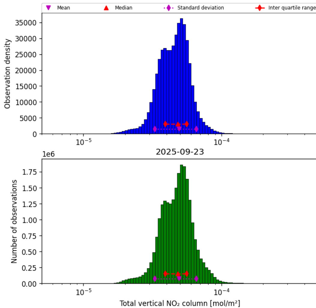
Figure 38: Histogram of “Total vertical NO 2 column” for 2025-09-22 to 2025-09-24
