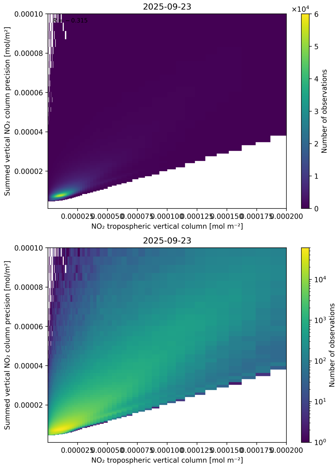
Figure 127: Scatter density plot of “NO 2 tropospheric vertical column” against “Summed vertical NO 2 column precision” for 2025-09-22 to 2025-09-24.
