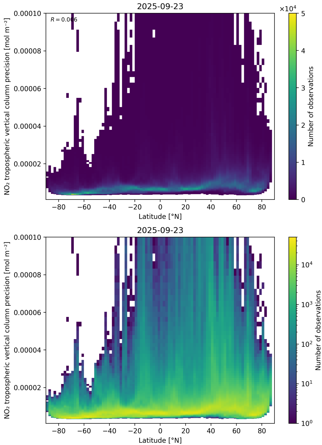
Figure 93: Scatter density plot of “Latitude” against “NO 2 tropospheric vertical column precision” for 2025-09-22 to 2025-09-24.
