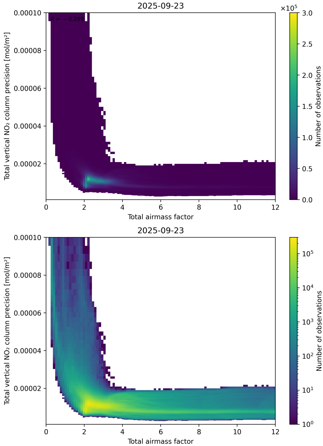
Figure 68: Scatter density plot of “Total airmass factor” against “Total vertical NO 2 column precision” for 2025-09-22 to 2025-09-24.
