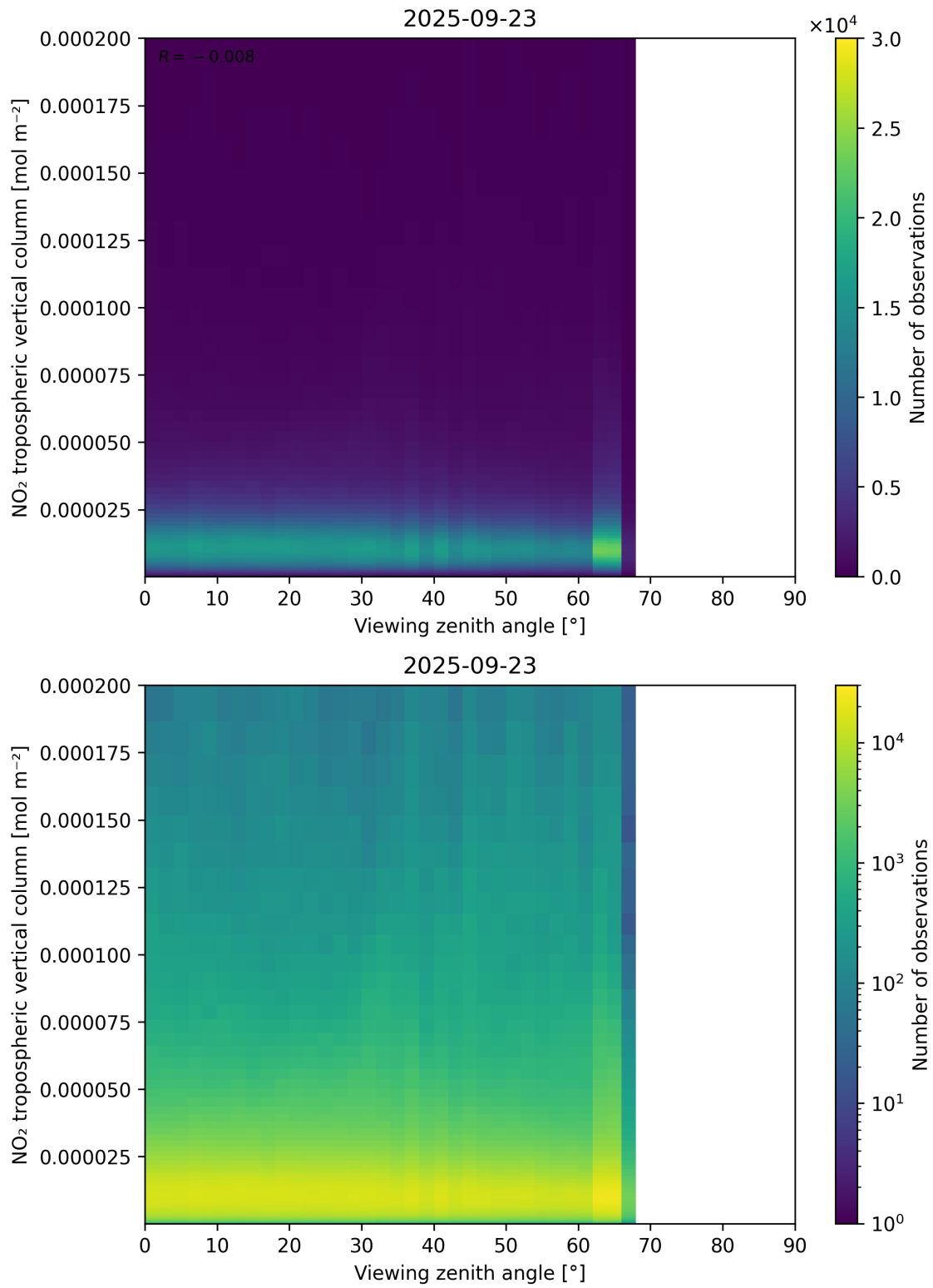
Figure 169: Scatter density plot of “Viewing zenith angle” against “NO 2 tropospheric vertical column” for 2025-09-22 to 2025-09-24.
