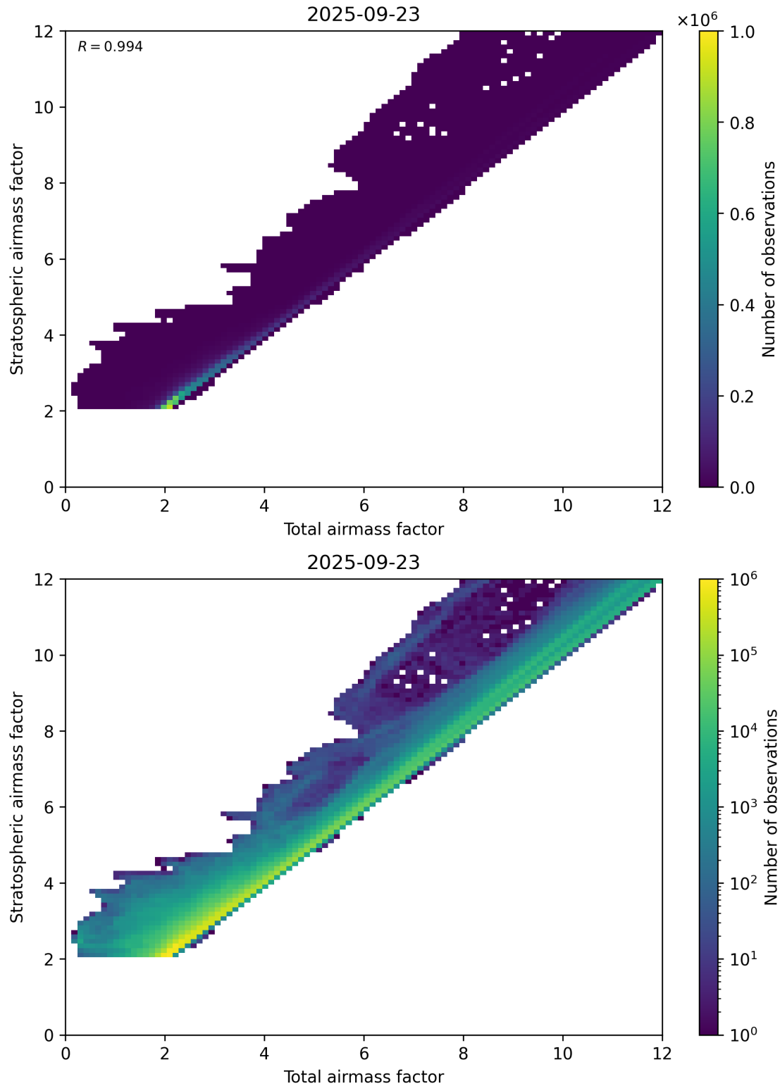
Figure 62: Scatter density plot of “Total airmass factor” against “Stratospheric airmass factor” for 2025-09-22 to 2025-09-24.
