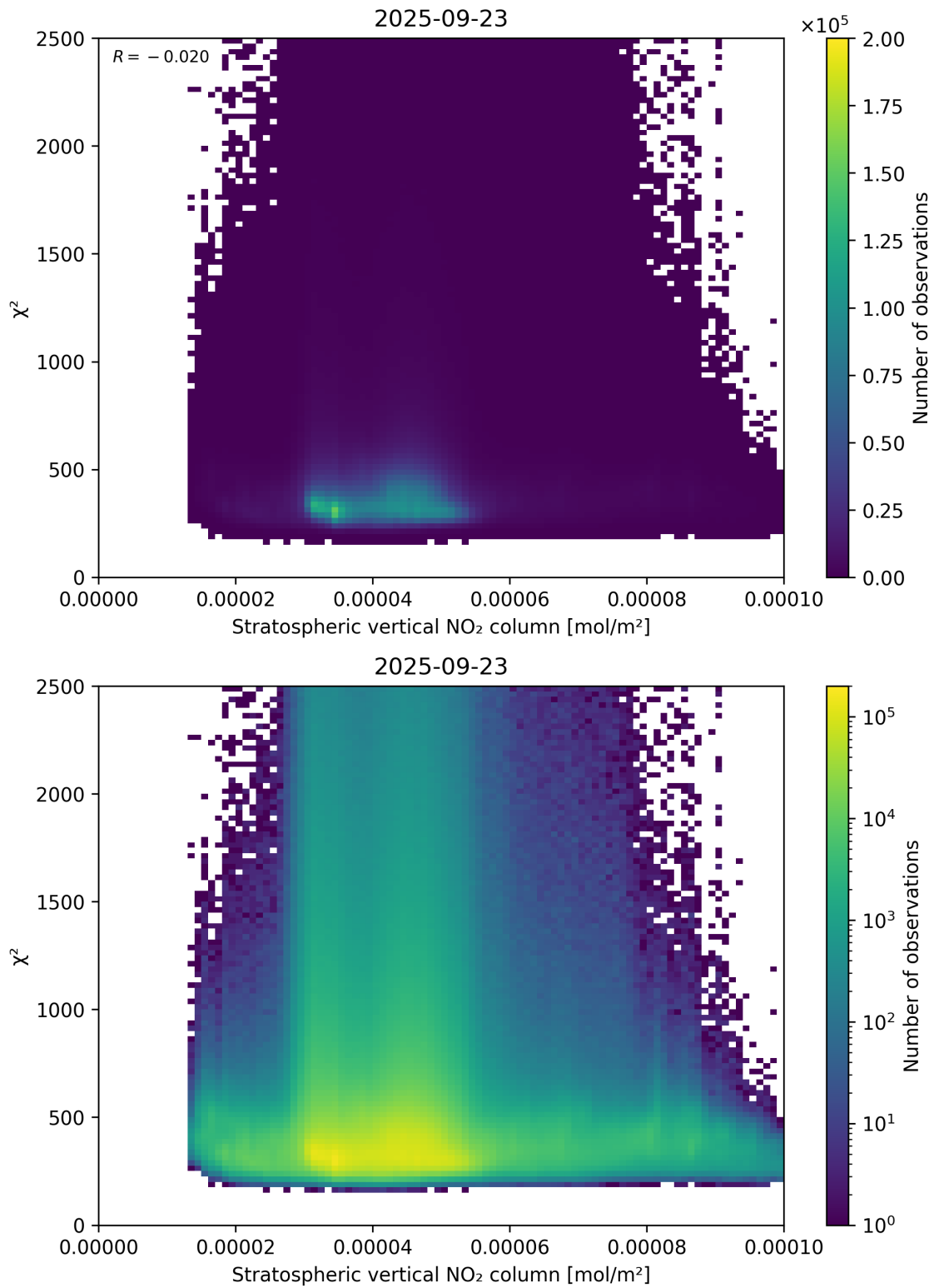
Figure 97: Scatter density plot of “Stratospheric vertical NO 2 column” against “ \chi^2 ” for 2025-09-22 to 2025-09-24.
