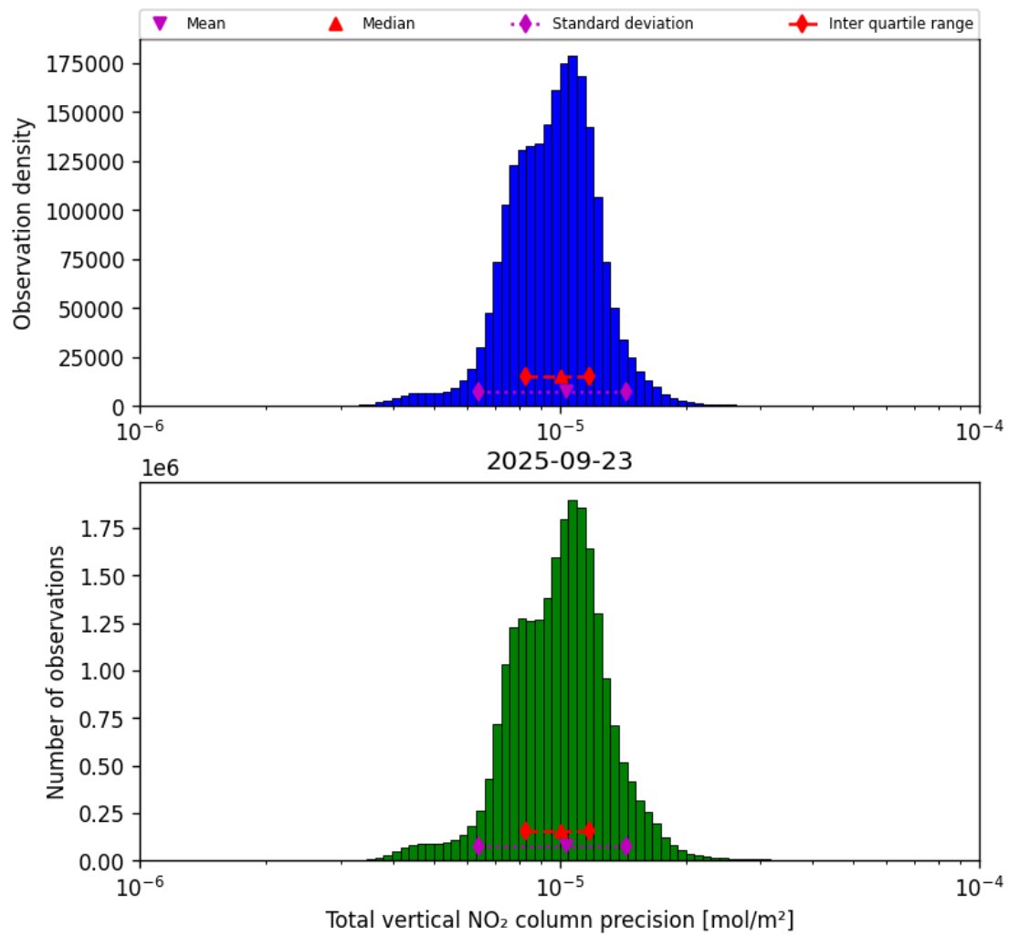
Figure 39: Histogram of "Total vertical NO 2 column precision" for 2025-09-22 to 2025-09-24
