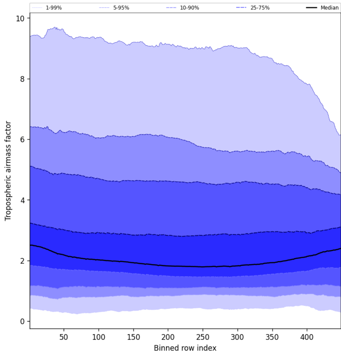
Figure 48: Along track statistics of “Tropospheric air mass factor” for 2025-09-22 to 2025-09-24
