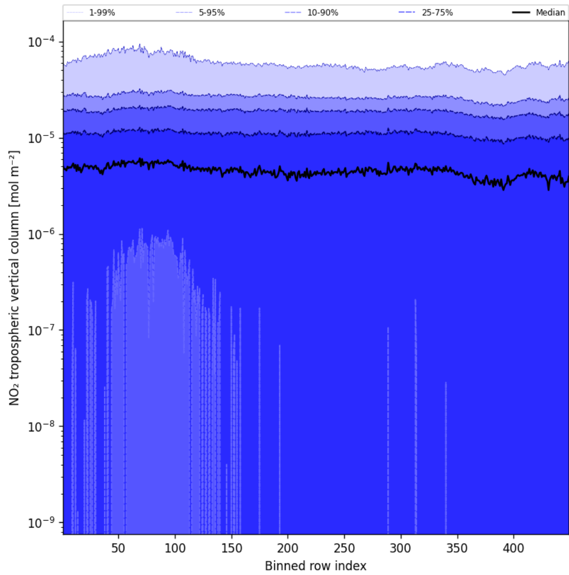
Figure 46: Along track statistics of “NO 2 tropospheric vertical column” for 2025-09-22 to 2025-09-24
