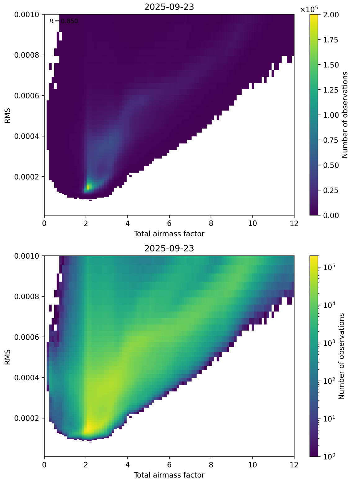
Figure 69: Scatter density plot of “Total airmass factor” against “RMS” for 2025-09-22 to 2025-09-24.
