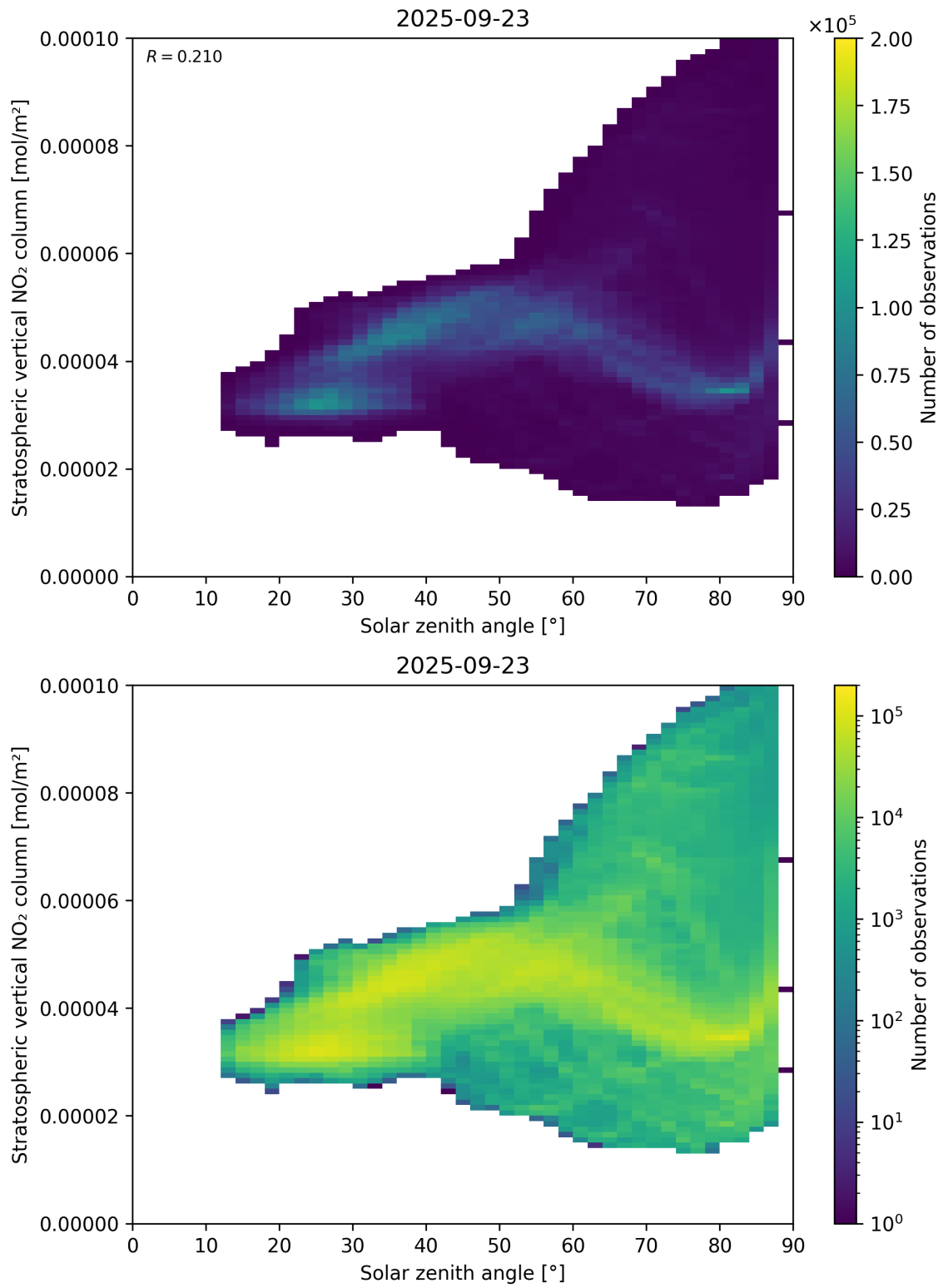
Figure 150: Scatter density plot of “Solar zenith angle” against “Stratospheric vertical NO 2 column” for 2025-09-22 to 2025-09-24.
