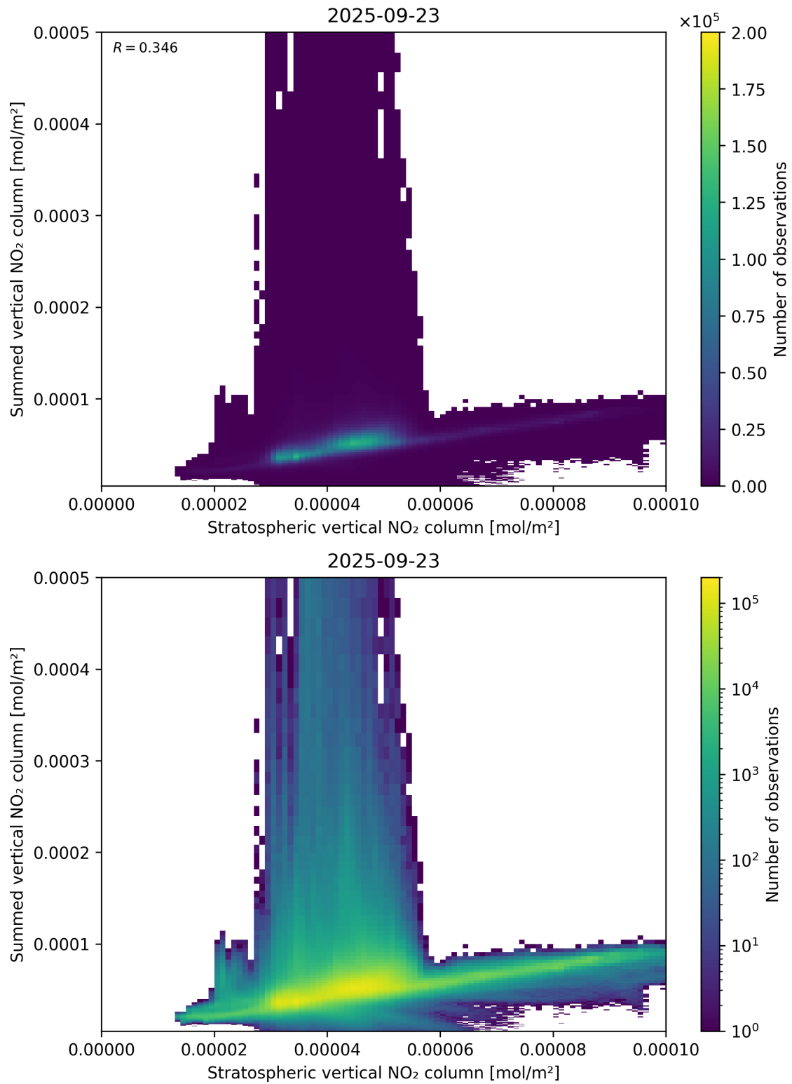
Figure 98: Scatter density plot of “Stratospheric vertical NO 2 column” against “Summed vertical NO 2 column” for 2025-09-22 to 2025-09-24.
