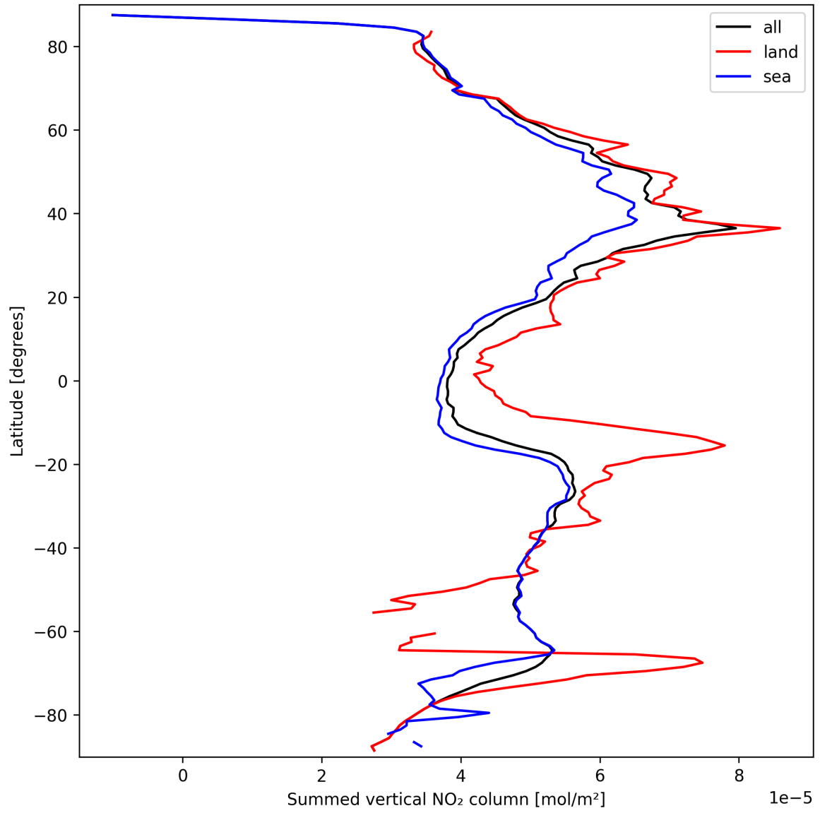
Figure 23: Zonal average of “Summed vertical NO 2 column” for 2025-09-22 to 2025-09-24.
