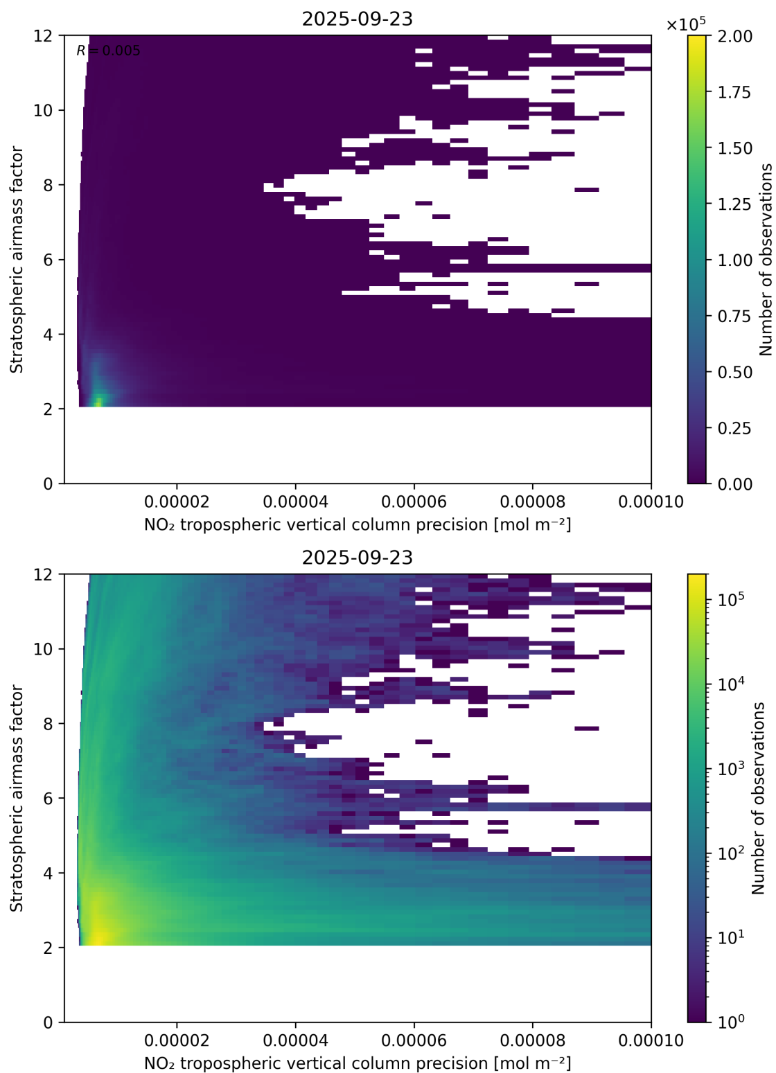
Figure 131: Scatter density plot of “NO 2 tropospheric vertical column precision” against “Stratospheric airmass factor” for 2025-09-22 to 2025-09-24.
