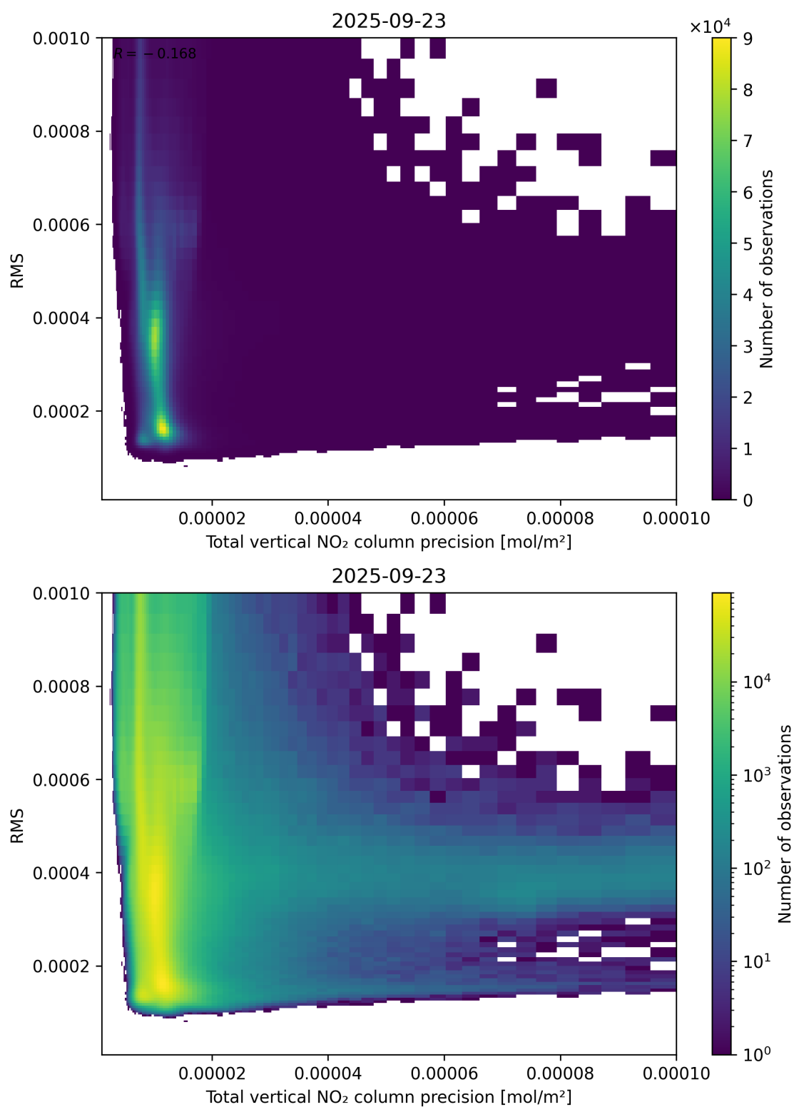
Figure 119: Scatter density plot of “Total vertical NO 2 column precision” against “RMS” for 2025-09-22 to 2025-09-24.
