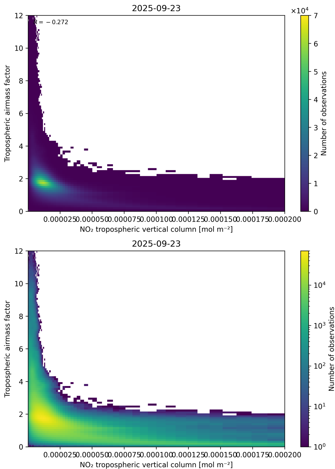
Figure 123: Scatter density plot of “NO 2 tropospheric vertical column” against “Tropospheric air mass factor” for 2025-09-22 to 2025-09-24.
