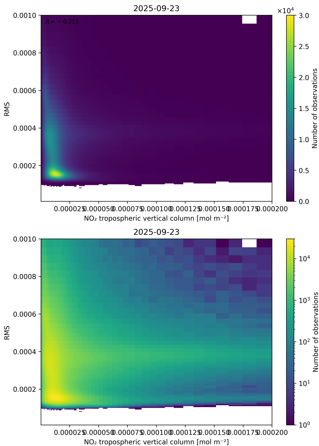
Figure 142: Scatter density plot of “NO 2 tropospheric vertical column” against “RMS” for 2025-09-22 to 2025-09-24.
