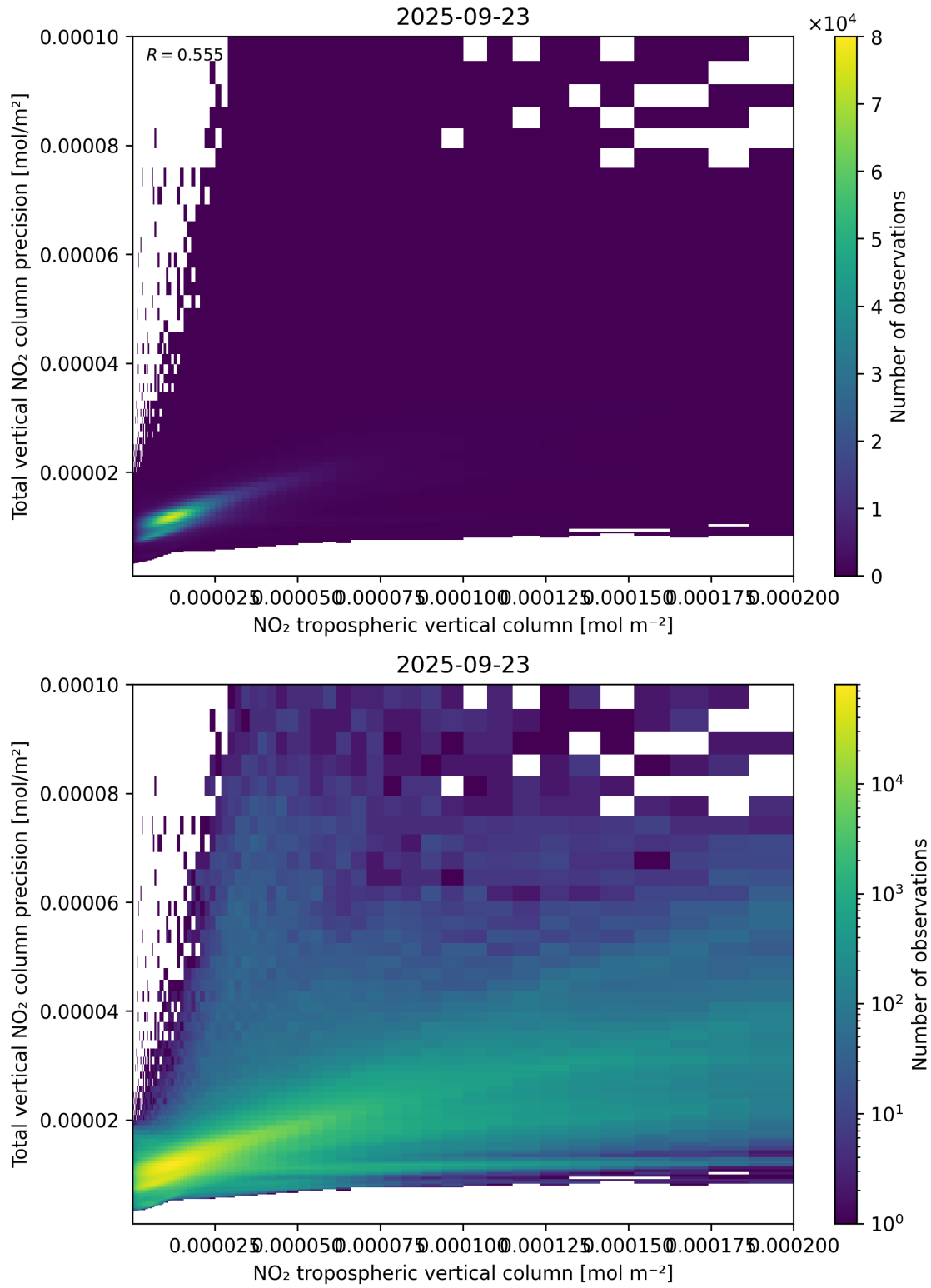
Figure 129: Scatter density plot of “NO 2 tropospheric vertical column” against “Total vertical NO 2 column precision” for 2025-09-22 to 2025-09-24.
