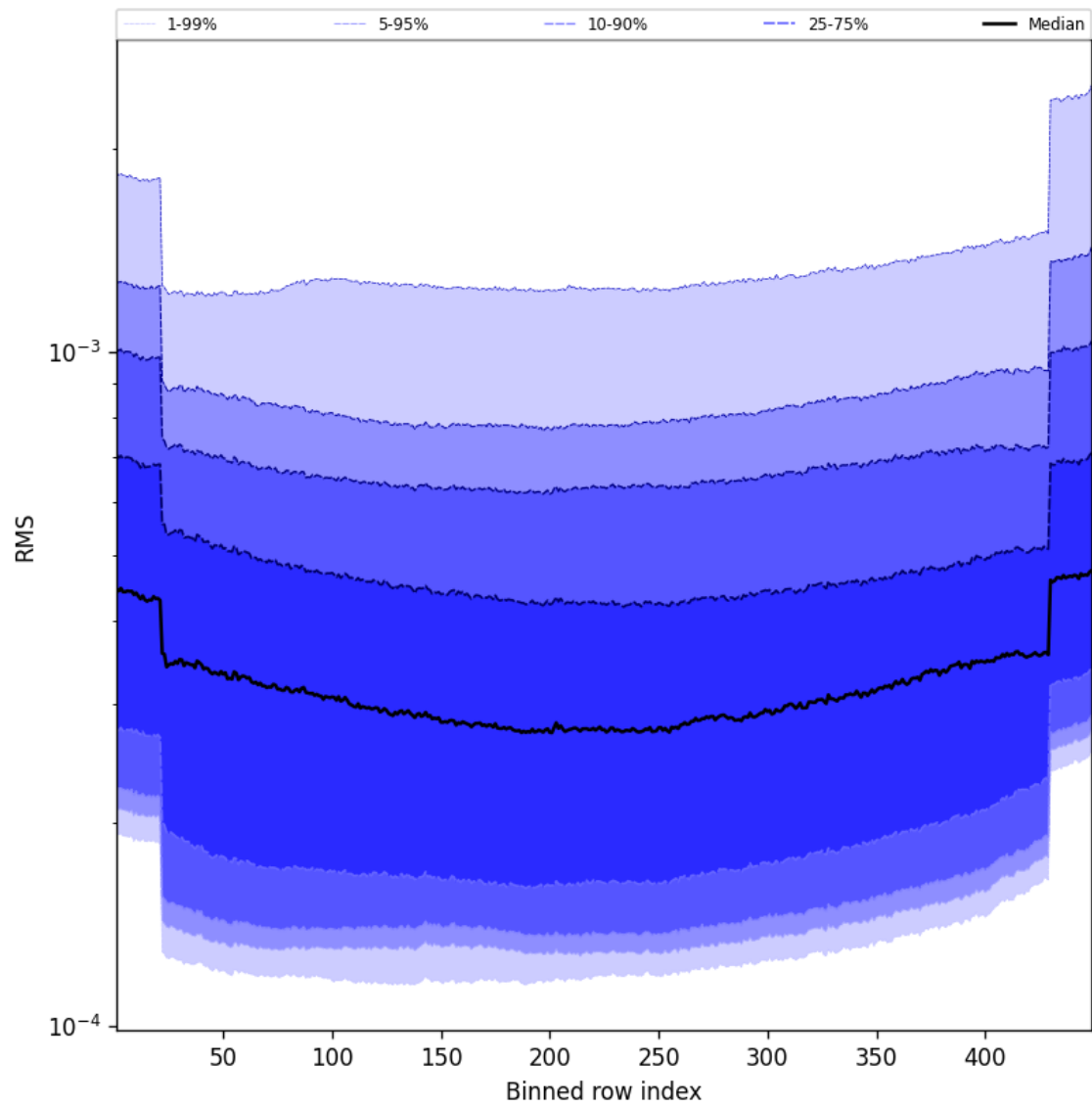
Figure 60: Along track statistics of “RMS” for 2025-09-22 to 2025-09-24
