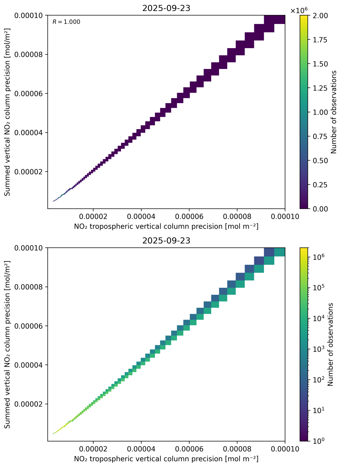
Figure 137: Scatter density plot of “NO 2 tropospheric vertical column precision” against “Summed vertical NO 2 column precision” for 2025-09-22 to 2025-09-24.
