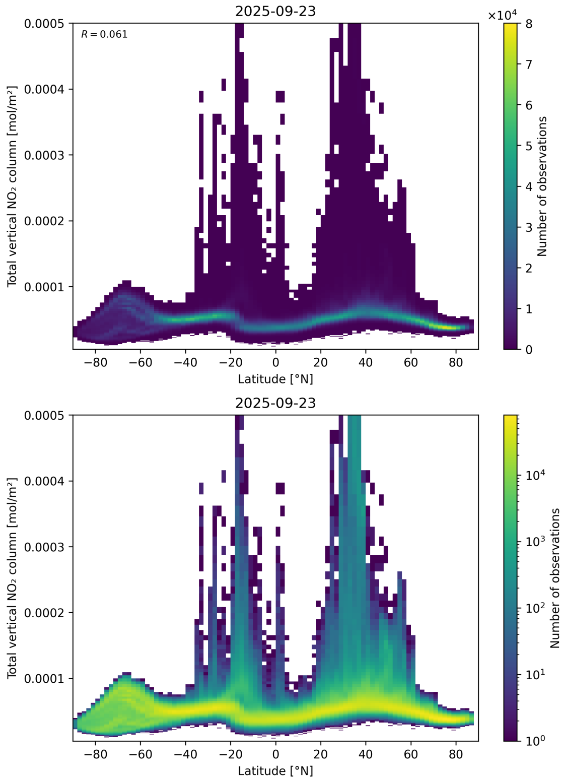
Figure 90: Scatter density plot of “Latitude” against “Total vertical NO 2 column” for 2025-09-22 to 2025-09-24.
