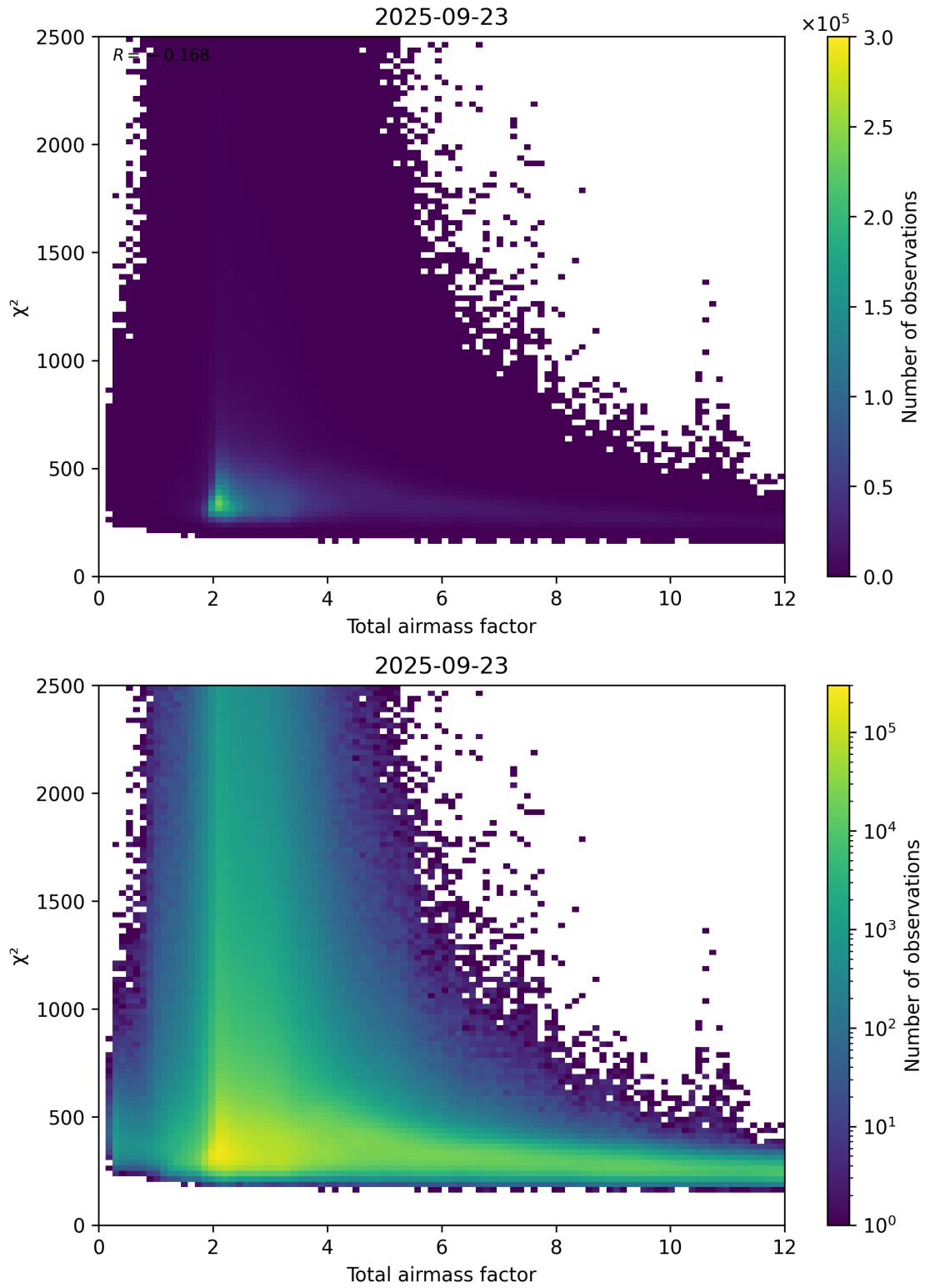
Figure 63: Scatter density plot of “Total airmass factor” against “ \chi^2 ” for 2025-09-22 to 2025-09-24.
