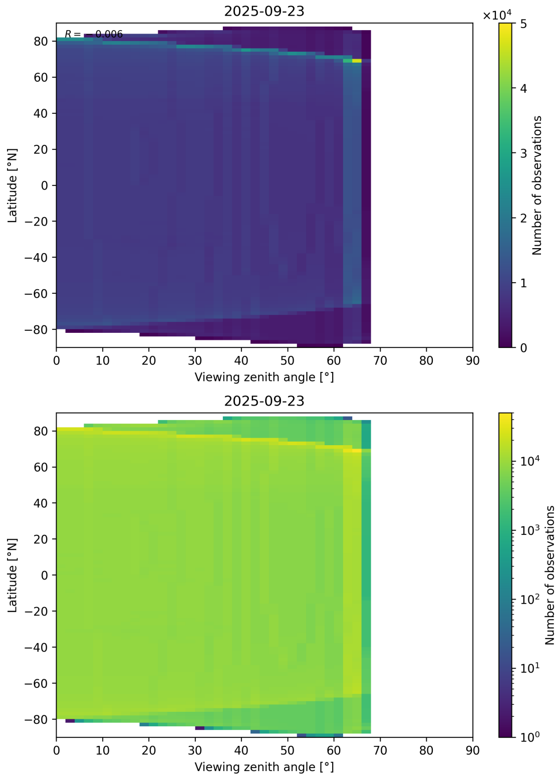
Figure 163: Scatter density plot of “Viewing zenith angle” against “Latitude” for 2025-09-22 to 2025-09-24.
