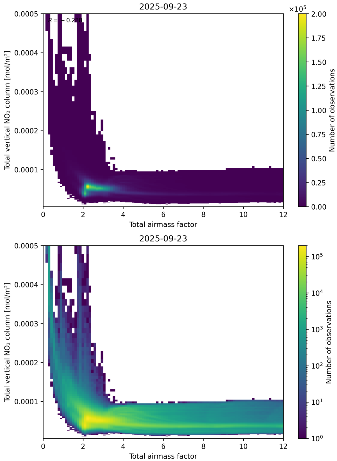
Figure 67: Scatter density plot of “Total airmass factor” against “Total vertical NO 2 column” for 2025-09-22 to 2025-09-24.
