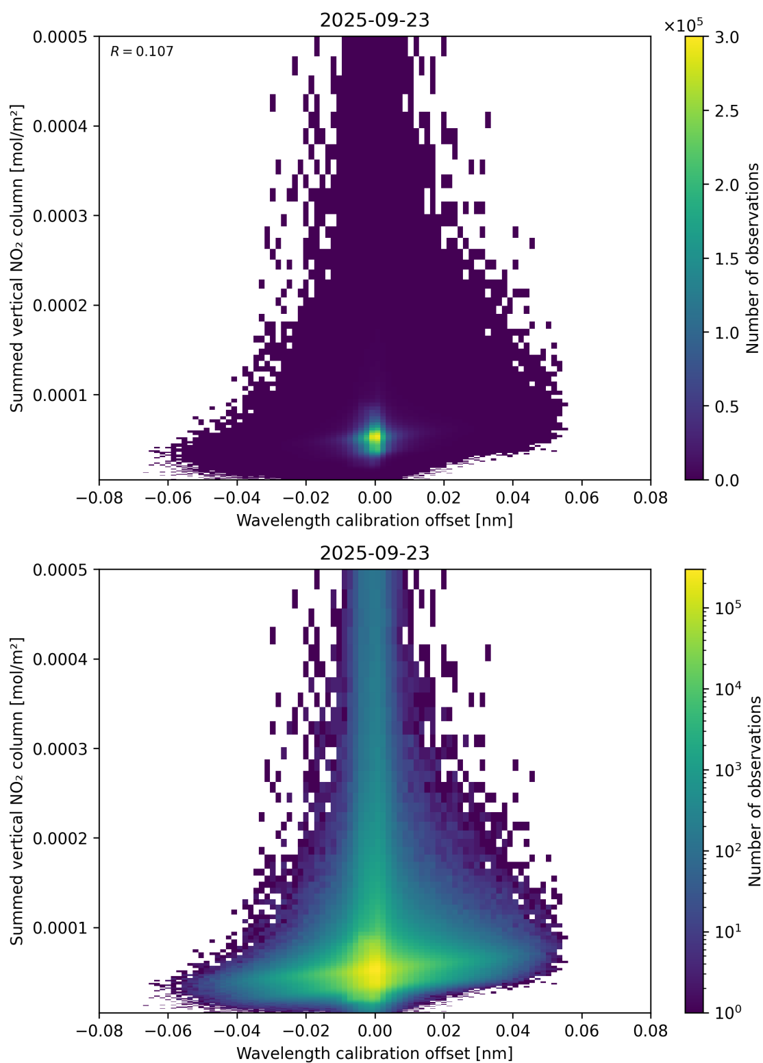
Figure 177: Scatter density plot of “Wavelength calibration offset” against “Summed vertical NO 2 column” for 2025-09-22 to 2025-09-24.
