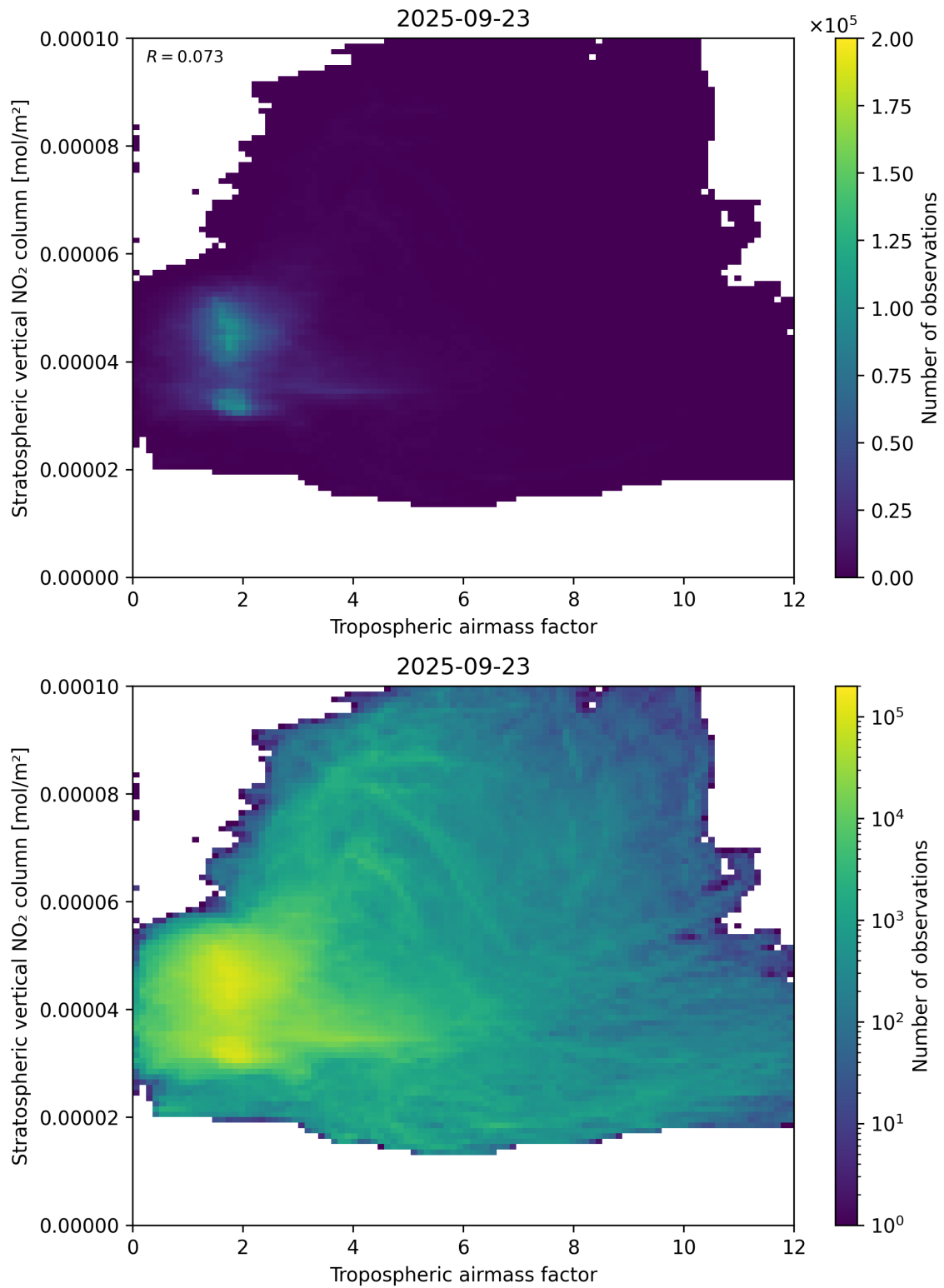
Figure 74: Scatter density plot of “Tropospheric air mass factor” against “Stratospheric vertical NO 2 column” for 2025-09-22 to 2025-09-24.
