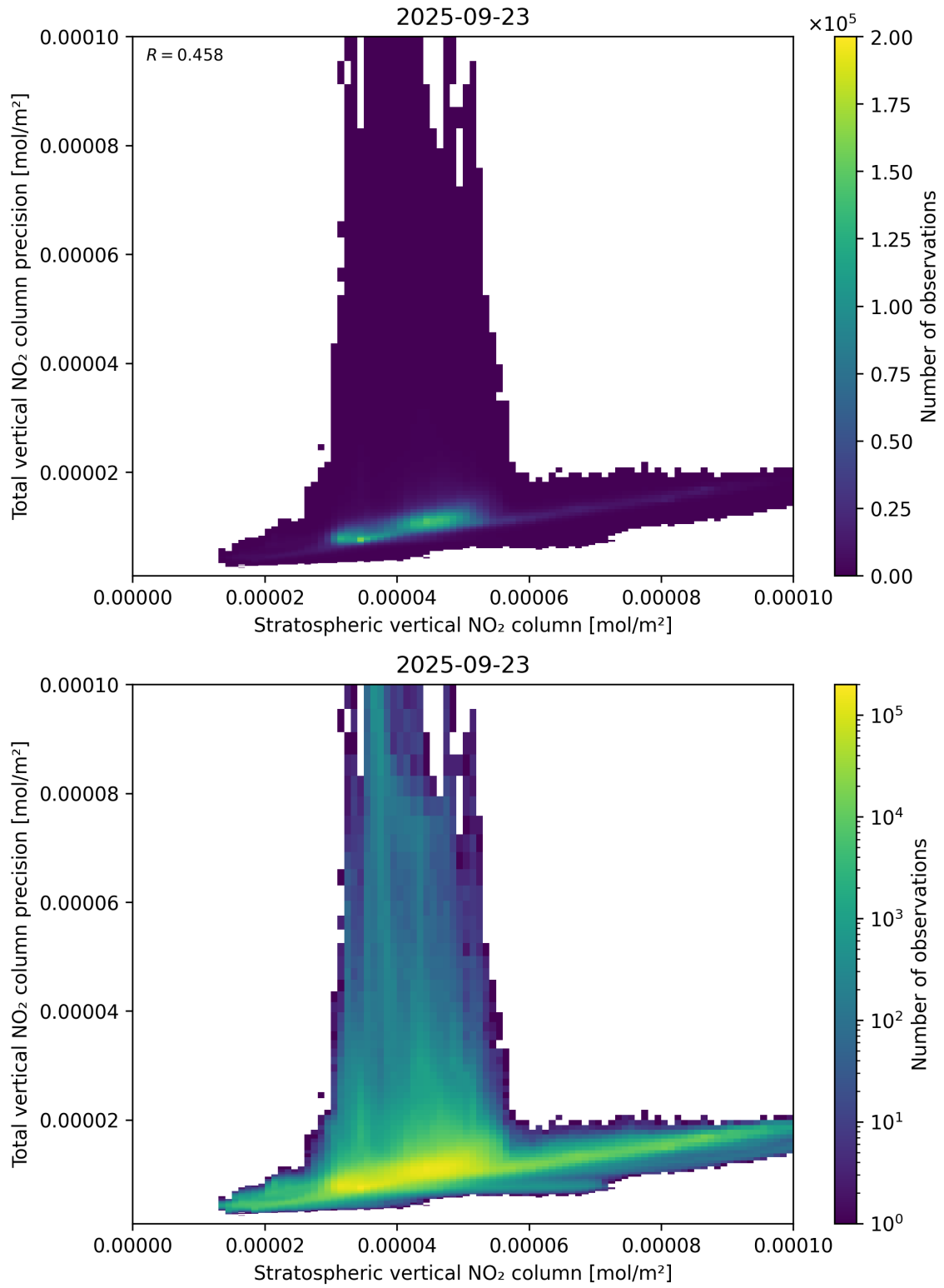
Figure 101: Scatter density plot of “Stratospheric vertical NO 2 column” against “Total vertical NO 2 column precision” for 2025-09-22 to 2025-09-24.
