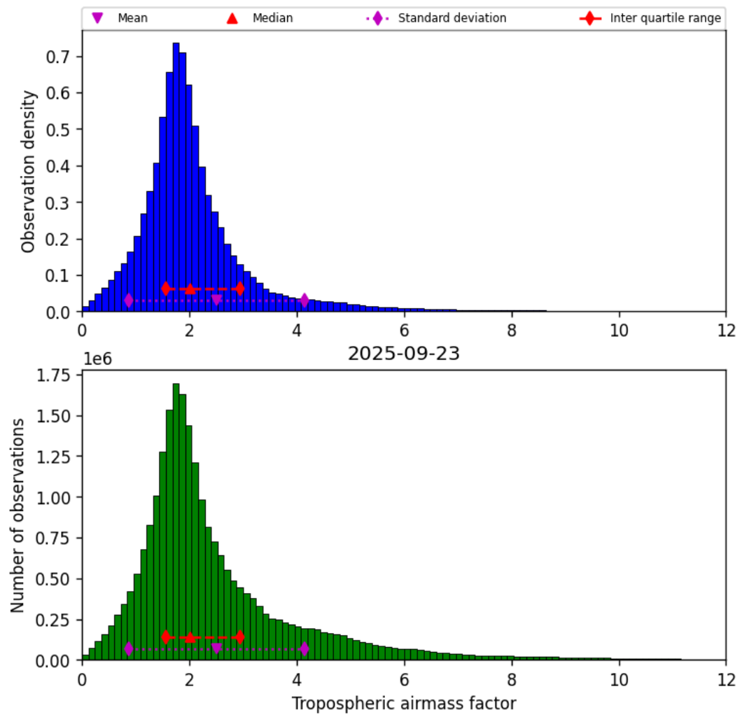
Figure 31: Histogram of “Tropospheric airmass factor” for 2025-09-22 to 2025-09-24
