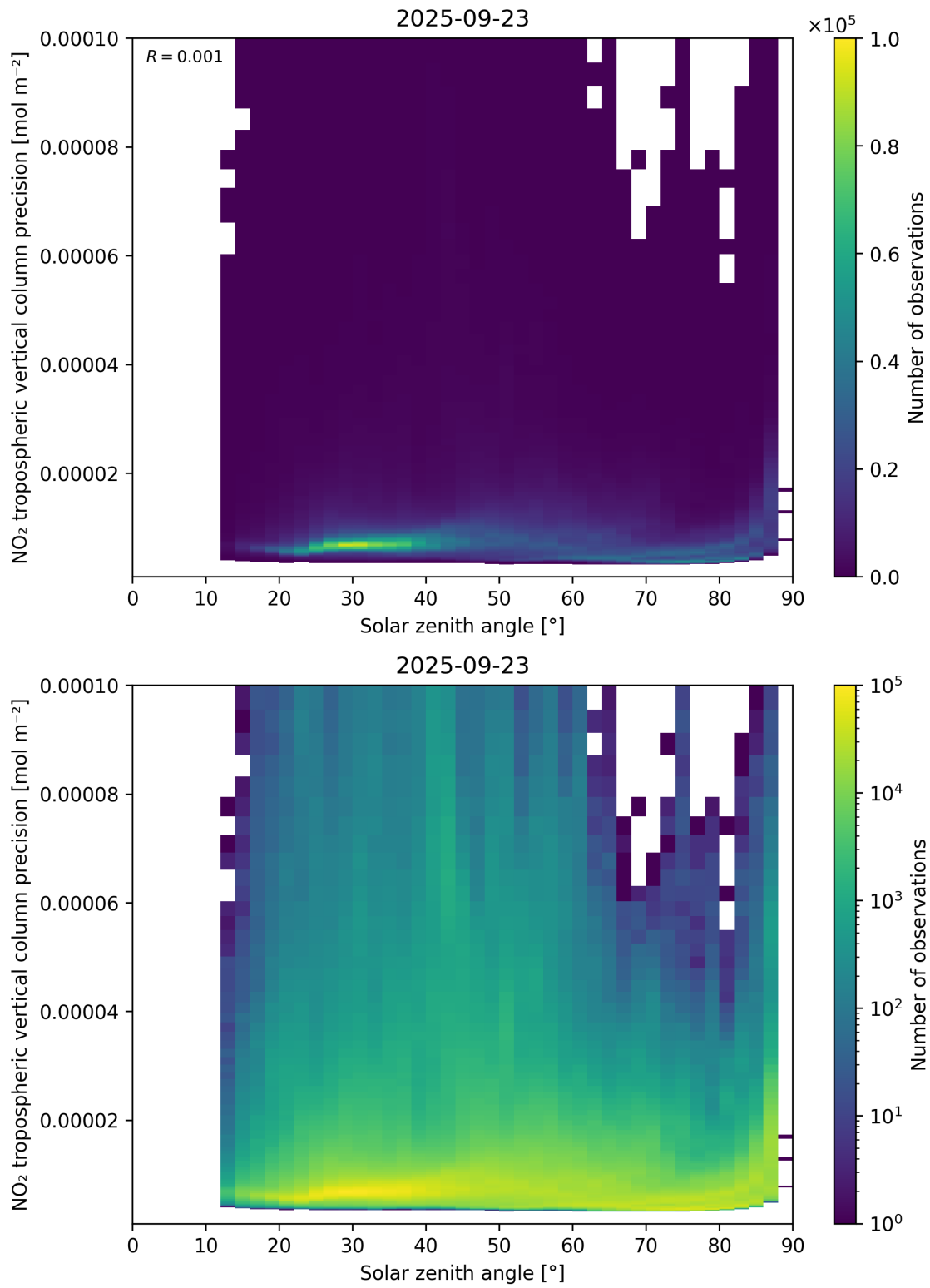
Figure 156: Scatter density plot of “Solar zenith angle” against “NO 2 tropospheric vertical column precision” for 2025-09-22 to 2025-09-24.
