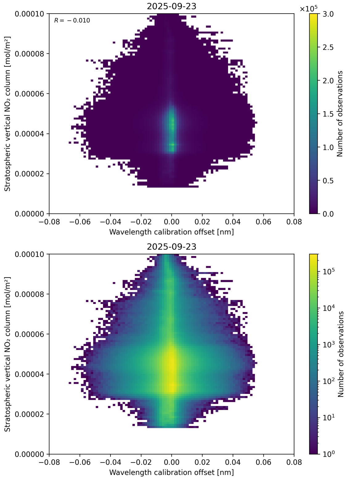
Figure 176: Scatter density plot of “Wavelength calibration offset” against “Stratospheric vertical NO 2 column” for 2025-09-22 to 2025-09-24.
