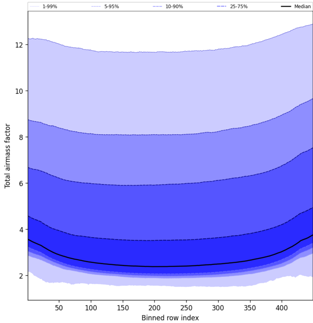
Figure 49: Along track statistics of “Total airmass factor” for 2025-09-22 to 2025-09-24
