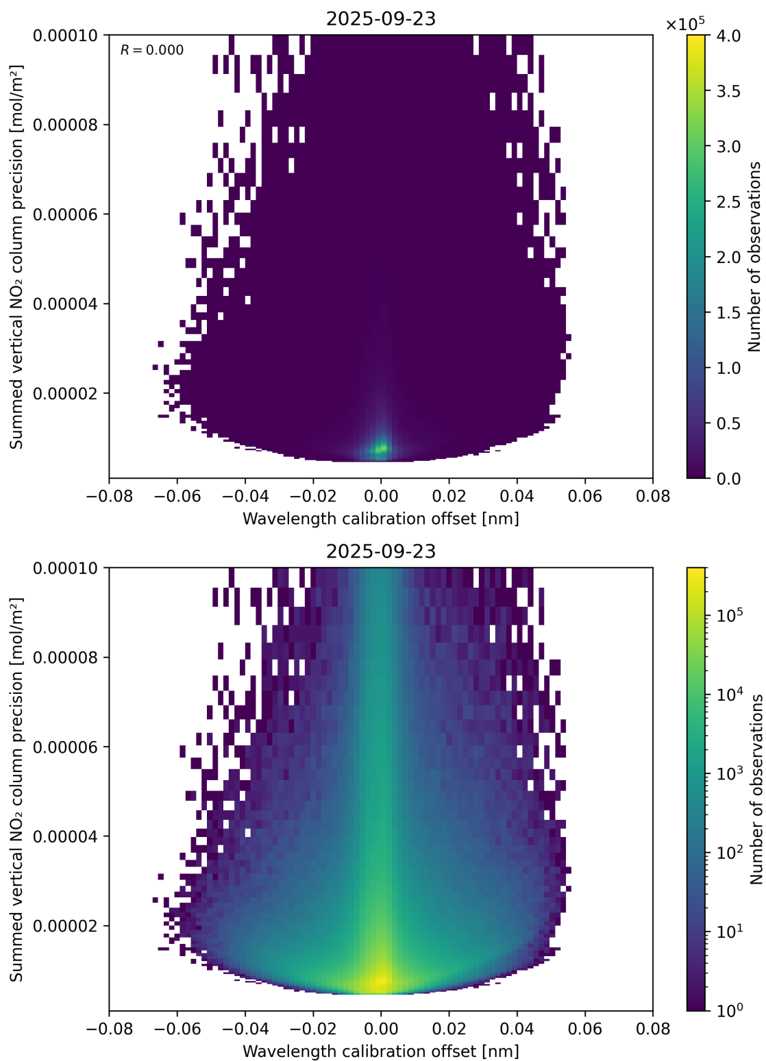
Figure 178: Scatter density plot of “Wavelength calibration offset” against “Summed vertical NO 2 column precision” for 2025-09-22 to 2025-09-24.
