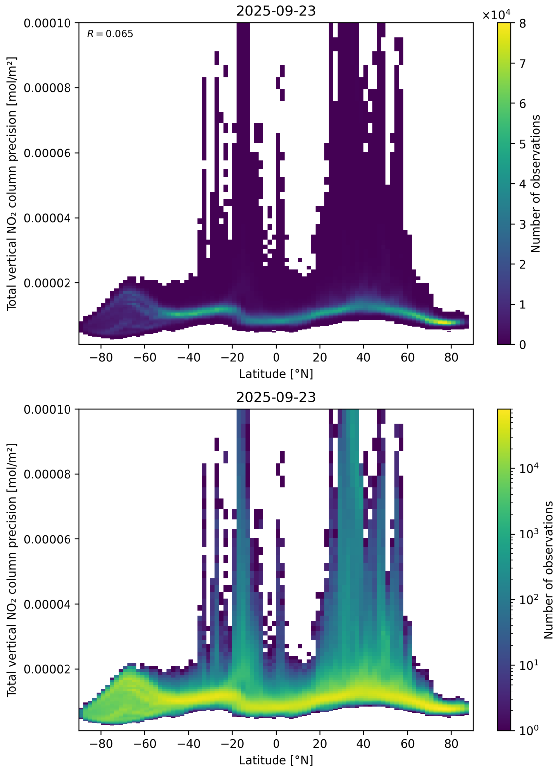
Figure 91: Scatter density plot of “Latitude” against “Total vertical NO 2 column precision” for 2025-09-22 to 2025-09-24.
