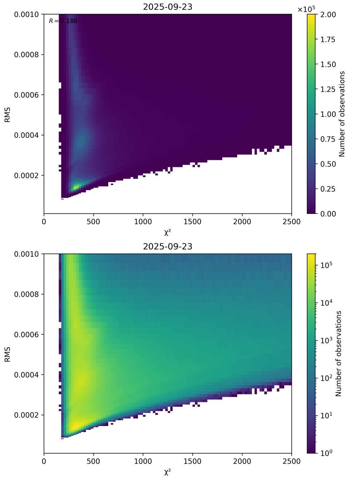
Figure 82: Scatter density plot of “ \chi^2 ” against “RMS” for 2025-09-22 to 2025-09-24.
