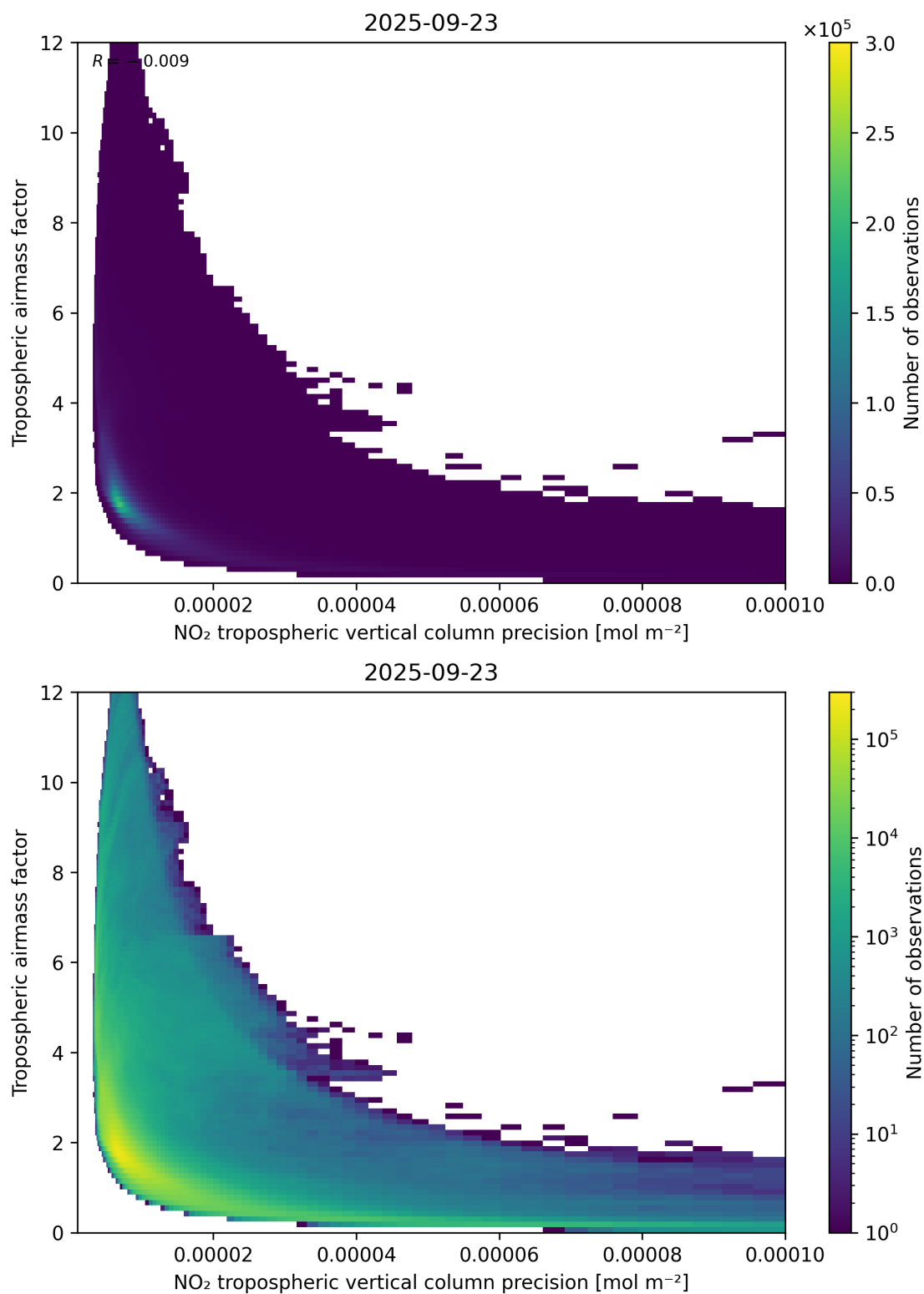
Figure 133: Scatter density plot of “NO 2 tropospheric vertical column precision” against “Tropospheric air mass factor” for 2025-09-22 to 2025-09-24.
