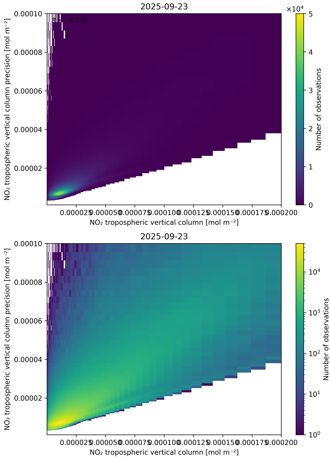
Figure 130: Scatter density plot of “NO 2 tropospheric vertical column” against “NO 2 tropospheric vertical column precision” for 2025-09-22 to 2025-09-24.
