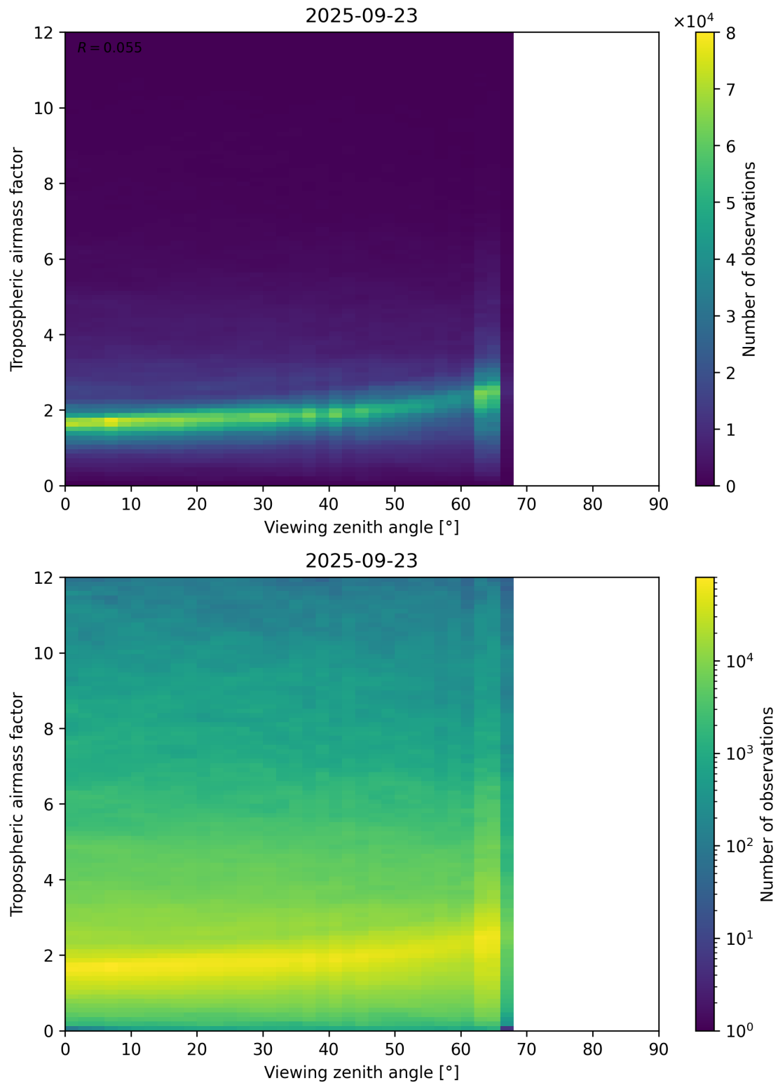
Figure 161: Scatter density plot of “Viewing zenith angle” against “Tropospheric airmass factor” for 2025-09-22 to 2025-09-24.
