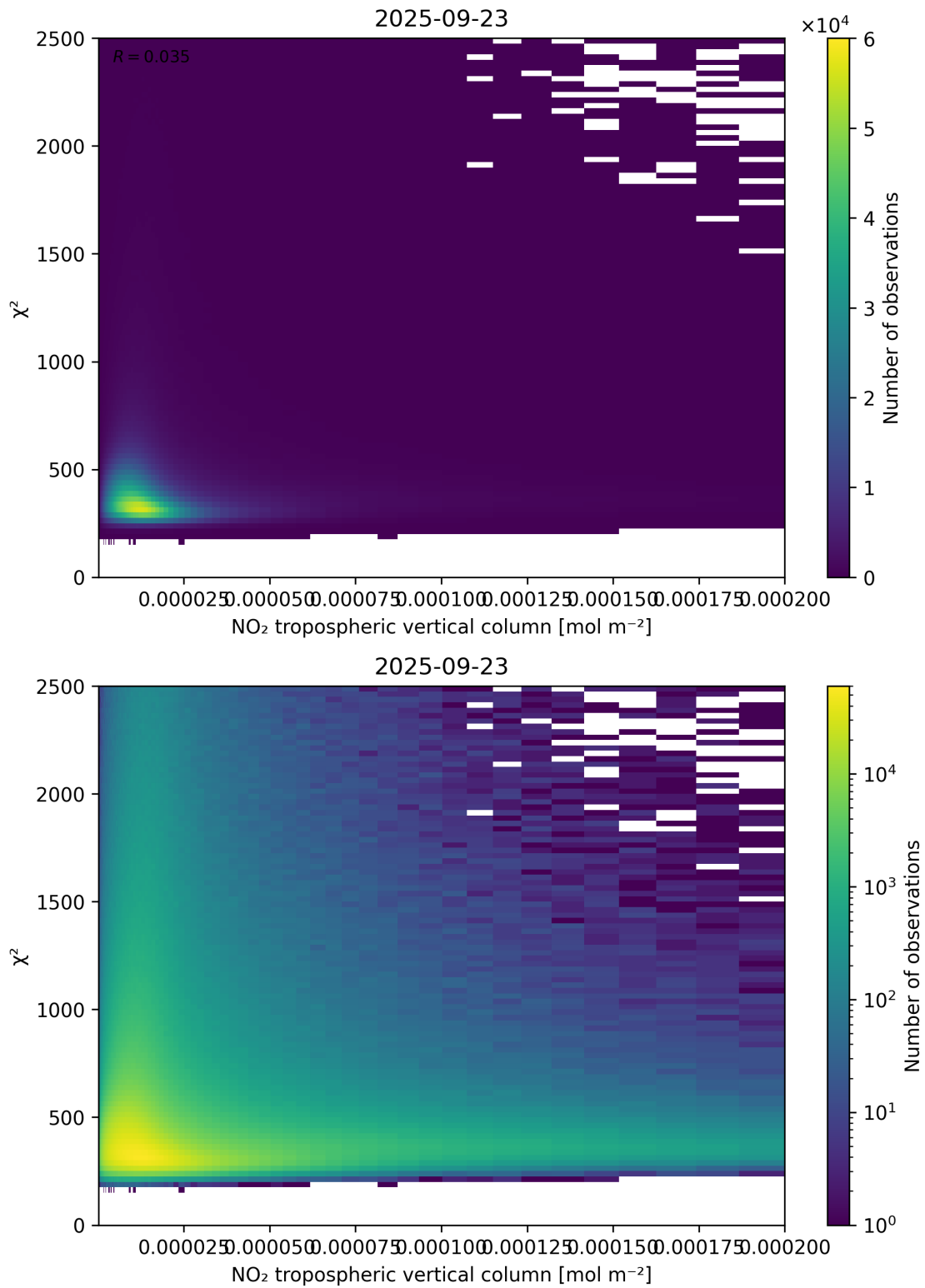
Figure 124: Scatter density plot of “NO 2 tropospheric vertical column” against “ \chi^2 ” for 2025-09-22 to 2025-09-24.
