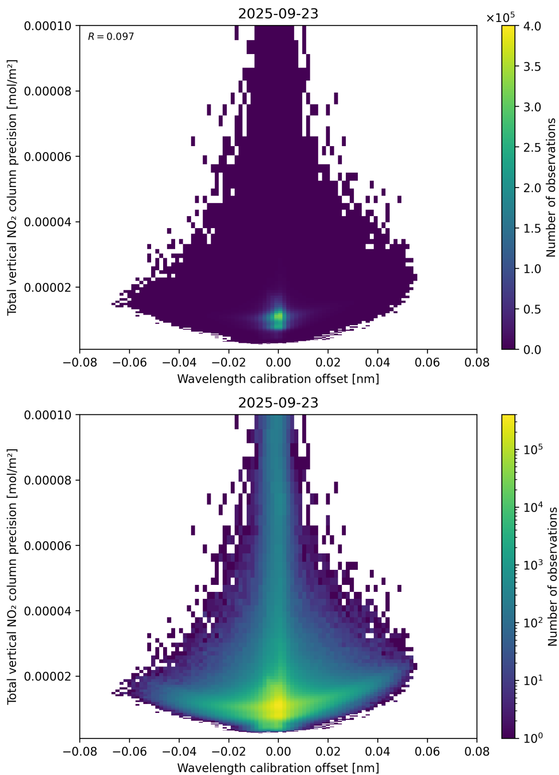
Figure 180: Scatter density plot of “Wavelength calibration offset” against “Total vertical NO 2 column precision” for 2025-09-22 to 2025-09-24.
