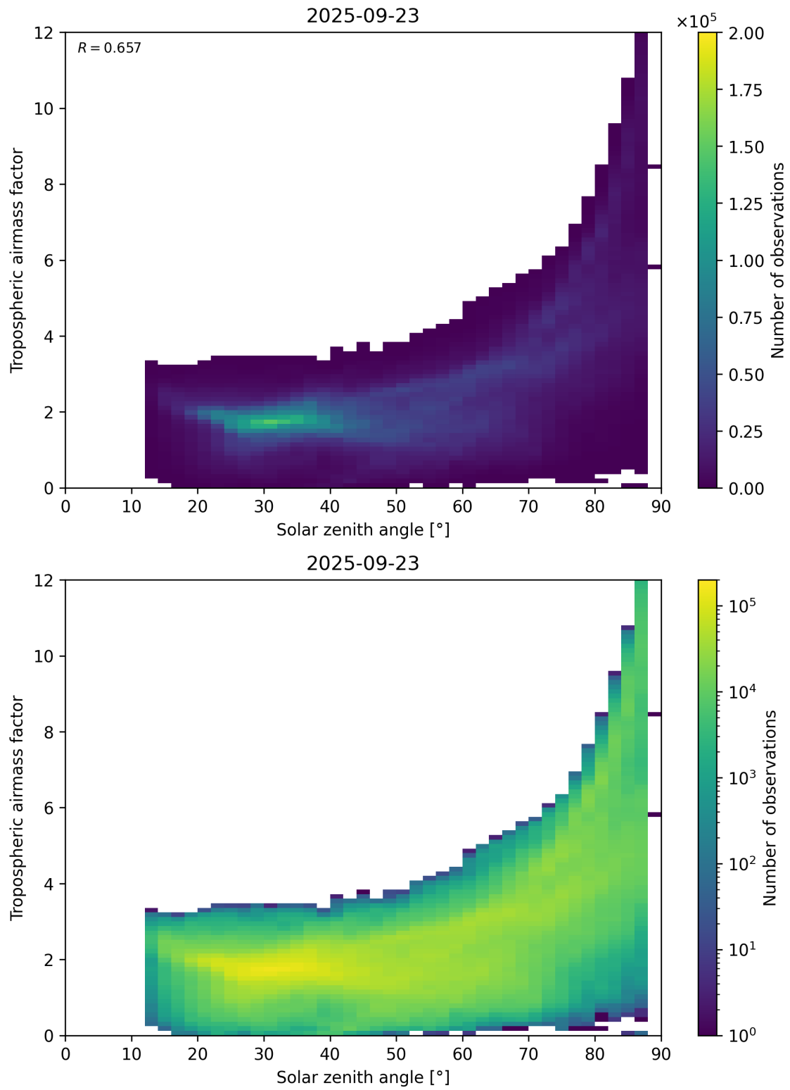
Figure 147: Scatter density plot of “Solar zenith angle” against “Tropospheric airmass factor” for 2025-09-22 to 2025-09-24.
