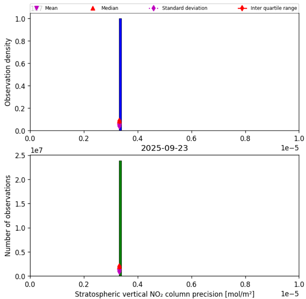
Figure 37: Histogram of “Stratospheric vertical NO 2 column precision” for 2025-09-22 to 2025-09-24
