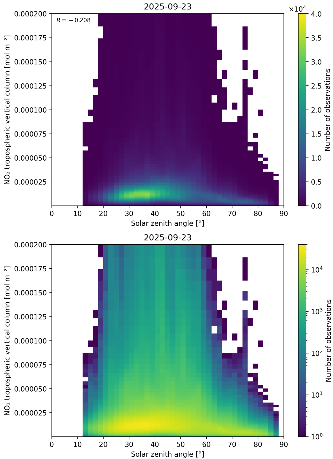
Figure 155: Scatter density plot of “Solar zenith angle” against “NO 2 tropospheric vertical column” for 2025-09-22 to 2025-09-24.
