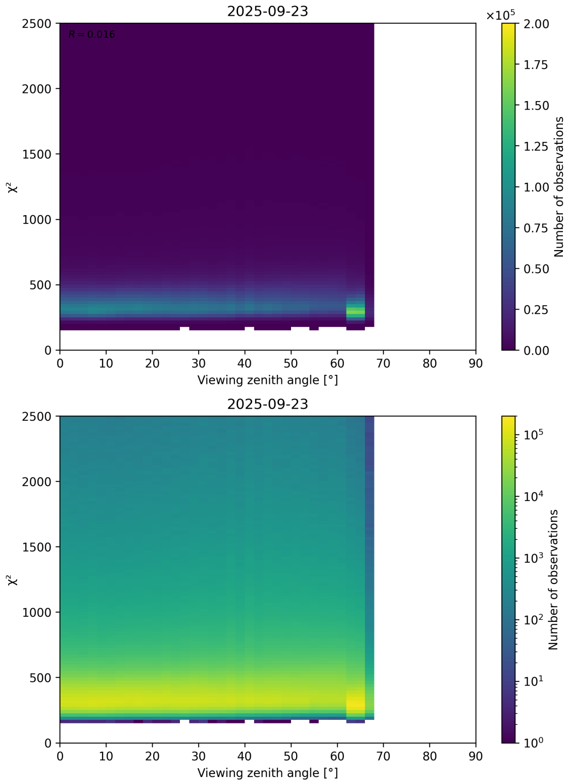
Figure 162: Scatter density plot of “Viewing zenith angle” against “ \chi^2 ” for 2025-09-22 to 2025-09-24.
