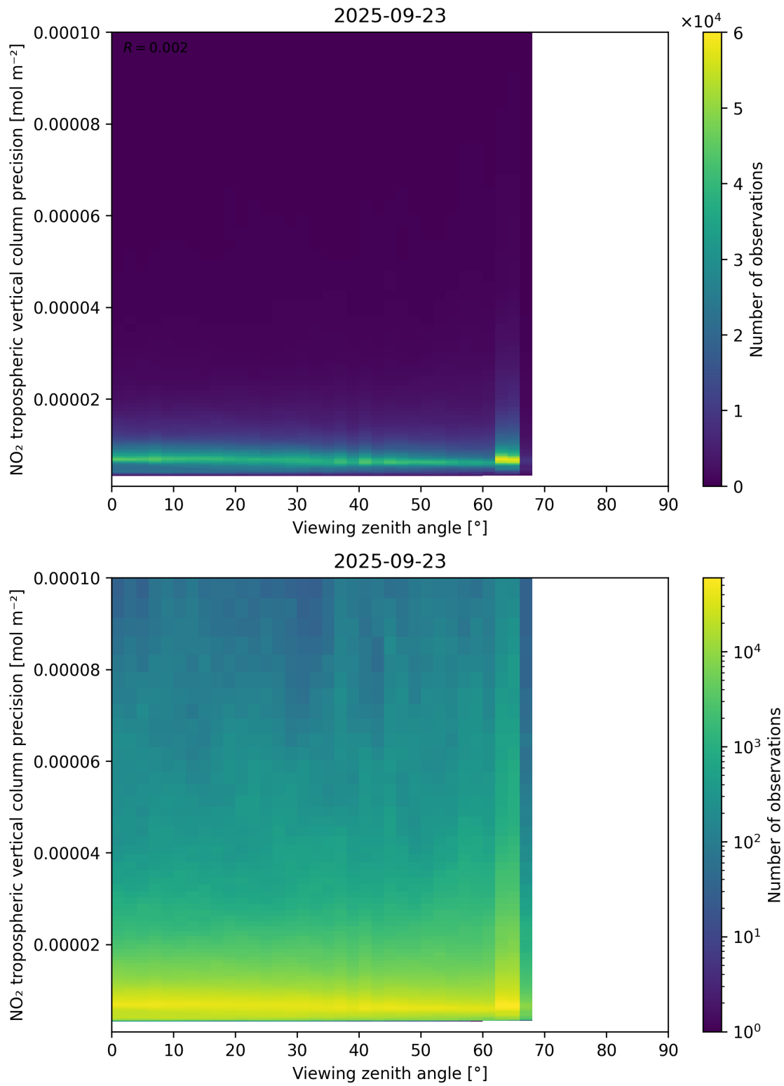
Figure 170: Scatter density plot of “Viewing zenith angle” against “NO 2 tropospheric vertical column precision” for 2025-09-22 to 2025-09-24.
