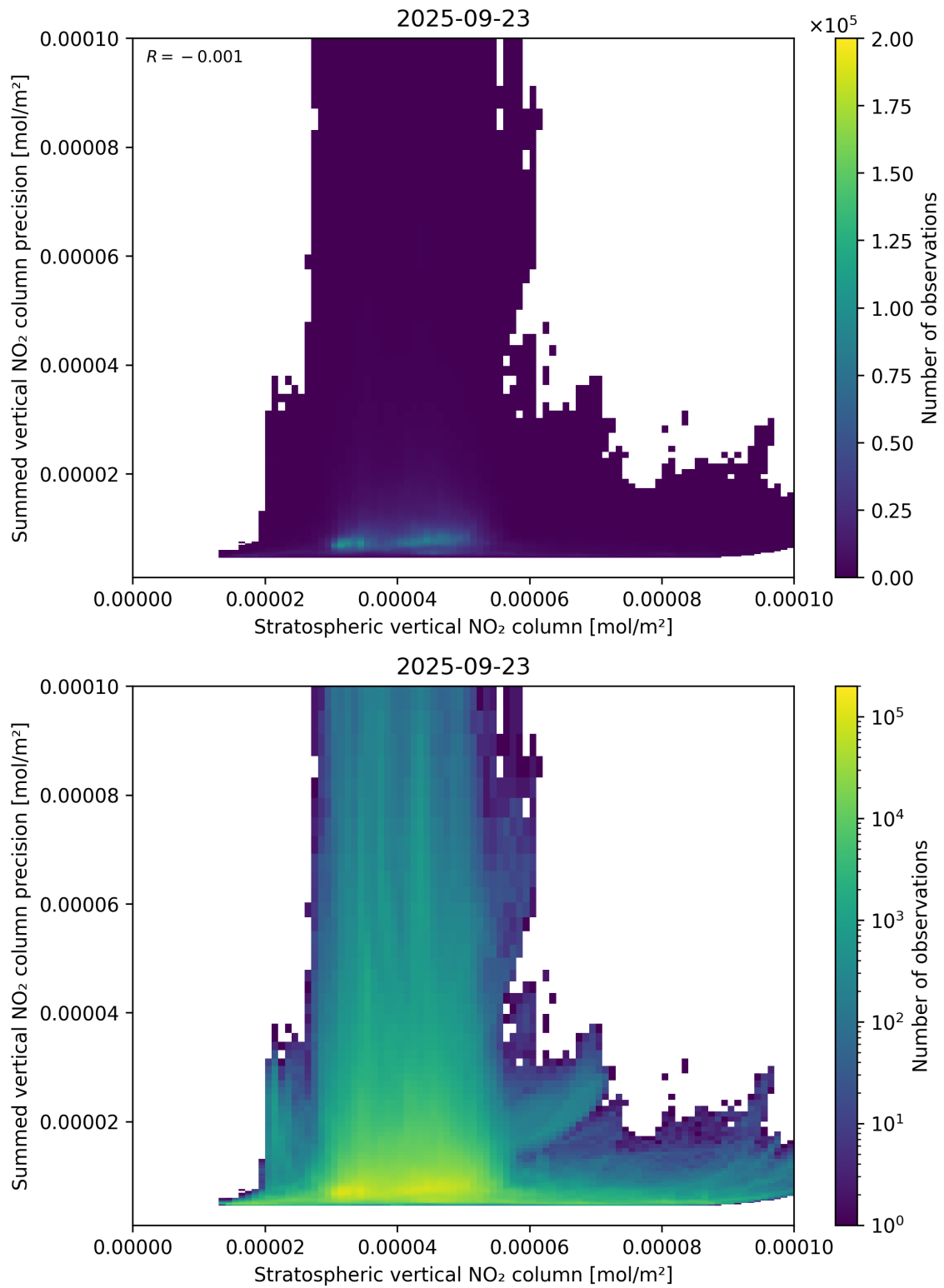
Figure 99: Scatter density plot of “Stratospheric vertical NO 2 column” against “Summed vertical NO 2 column precision” for 2025-09-22 to 2025-09-24.
