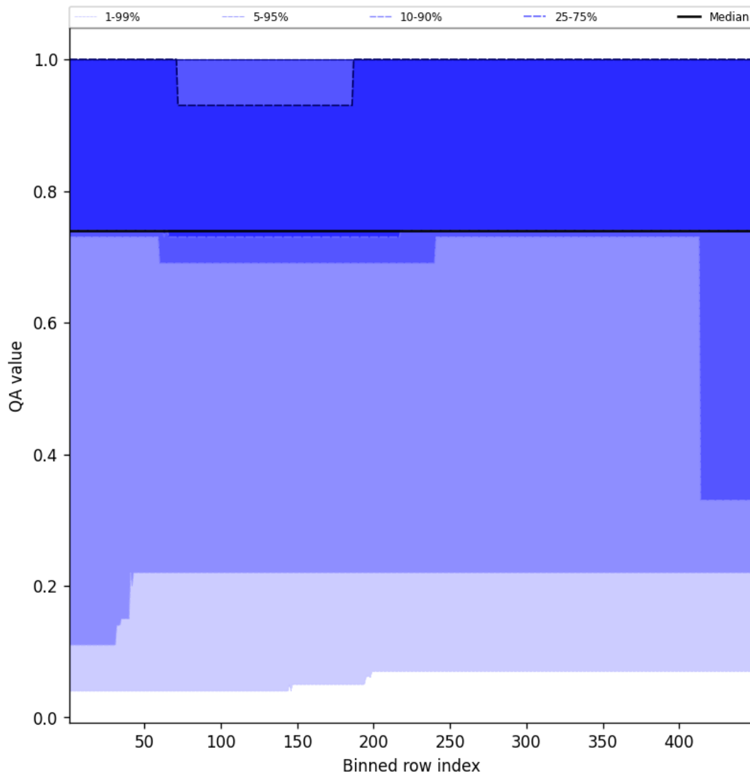
Figure 45: Along track statistics of “QA value” for 2025-09-22 to 2025-09-24
