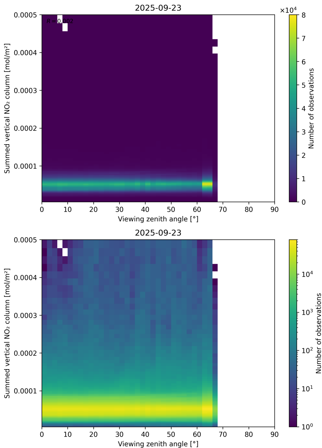
Figure 165: Scatter density plot of “Viewing zenith angle” against “Summed vertical NO 2 column” for 2025-09-22 to 2025-09-24.
