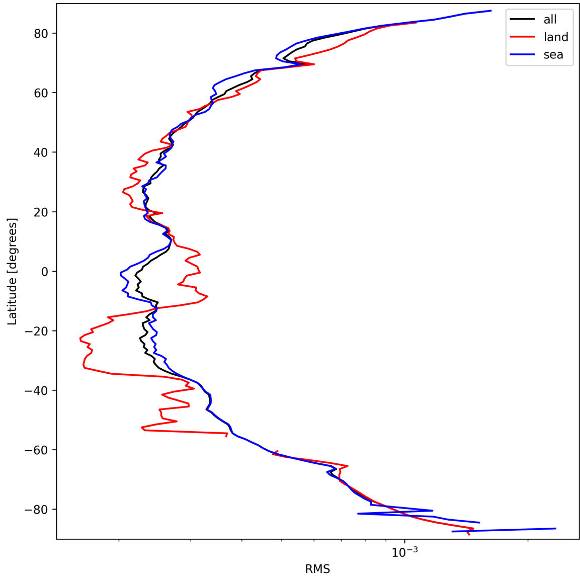
Figure 26: Zonal average of “RMS” for 2025-09-22 to 2025-09-24.
