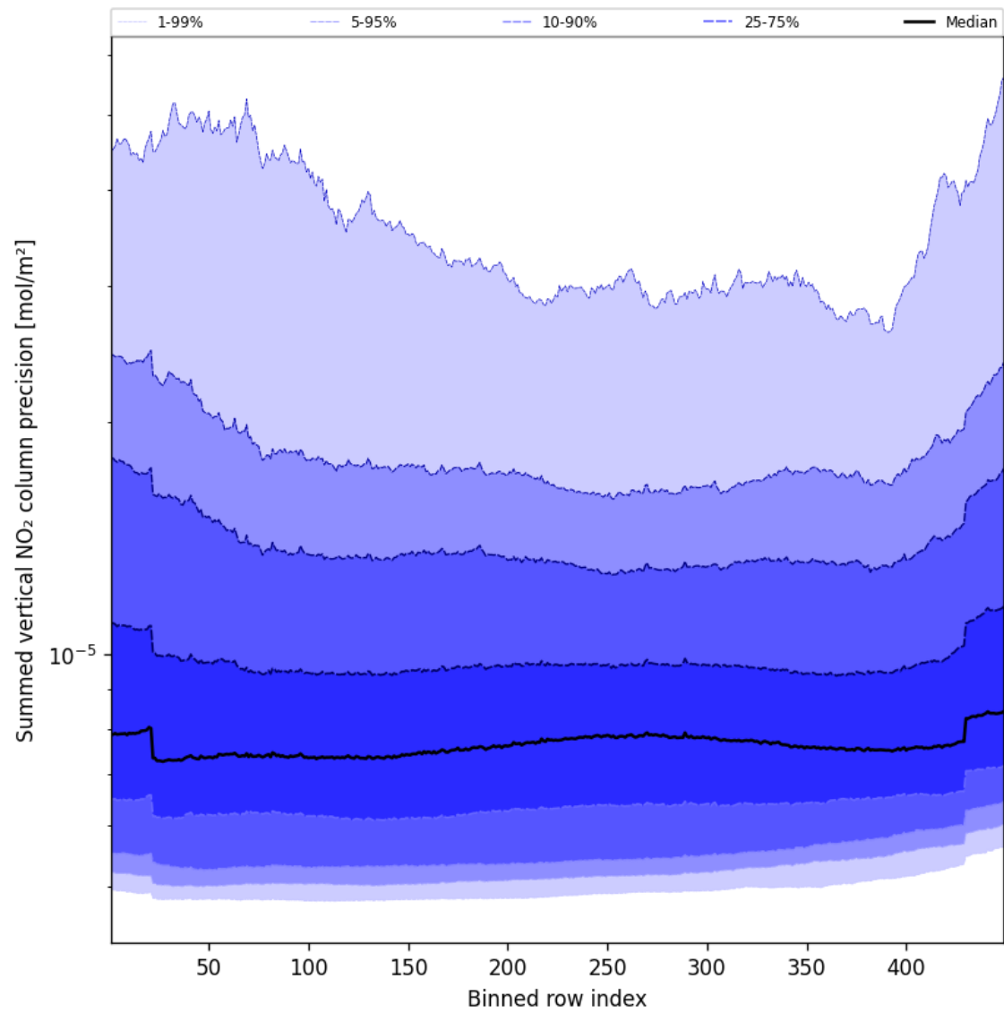
Figure 58: Along track statistics of “Summed vertical NO 2 column precision” for 2025-09-22 to 2025-09-24
