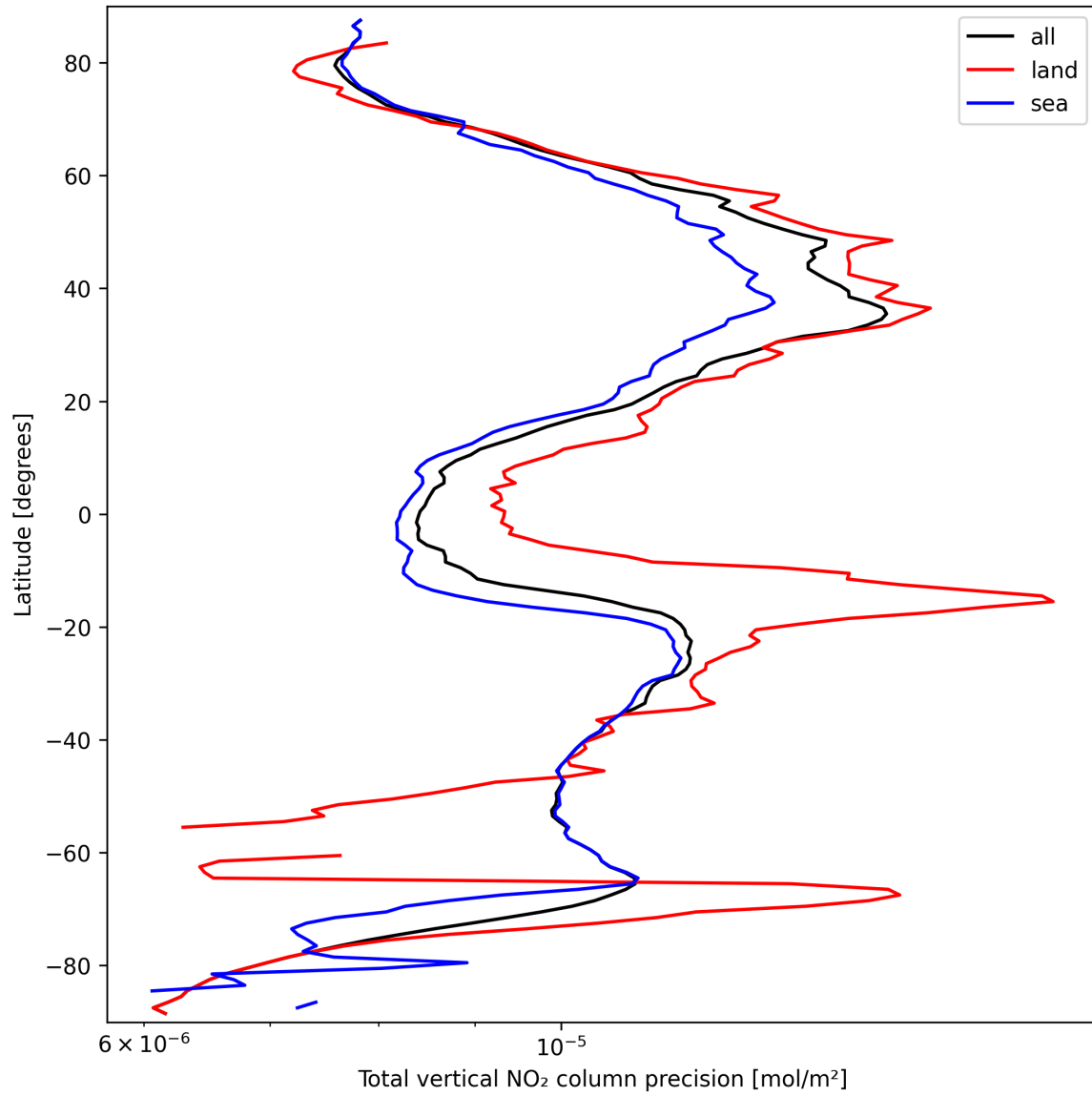
Figure 22: Zonal average of “Total vertical NO 2 column precision” for 2025-09-22 to 2025-09-24.
