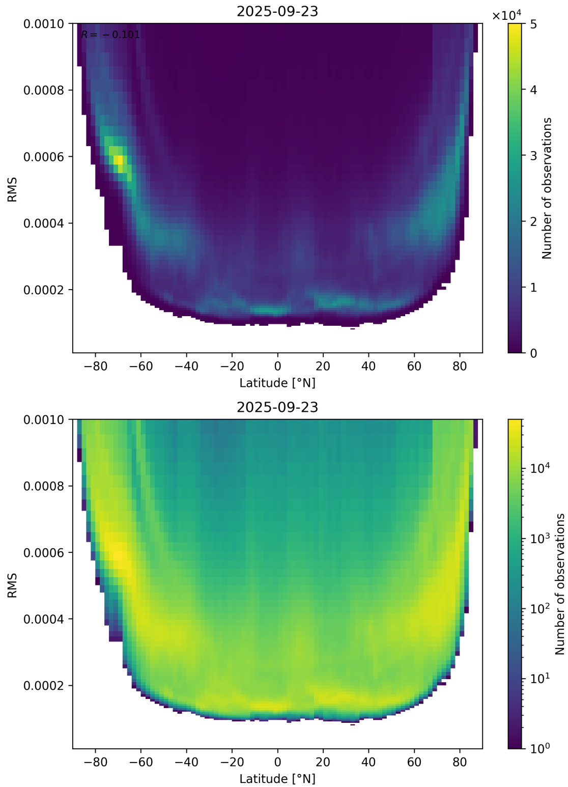
Figure 94: Scatter density plot of “Latitude” against “RMS” for 2025-09-22 to 2025-09-24.
