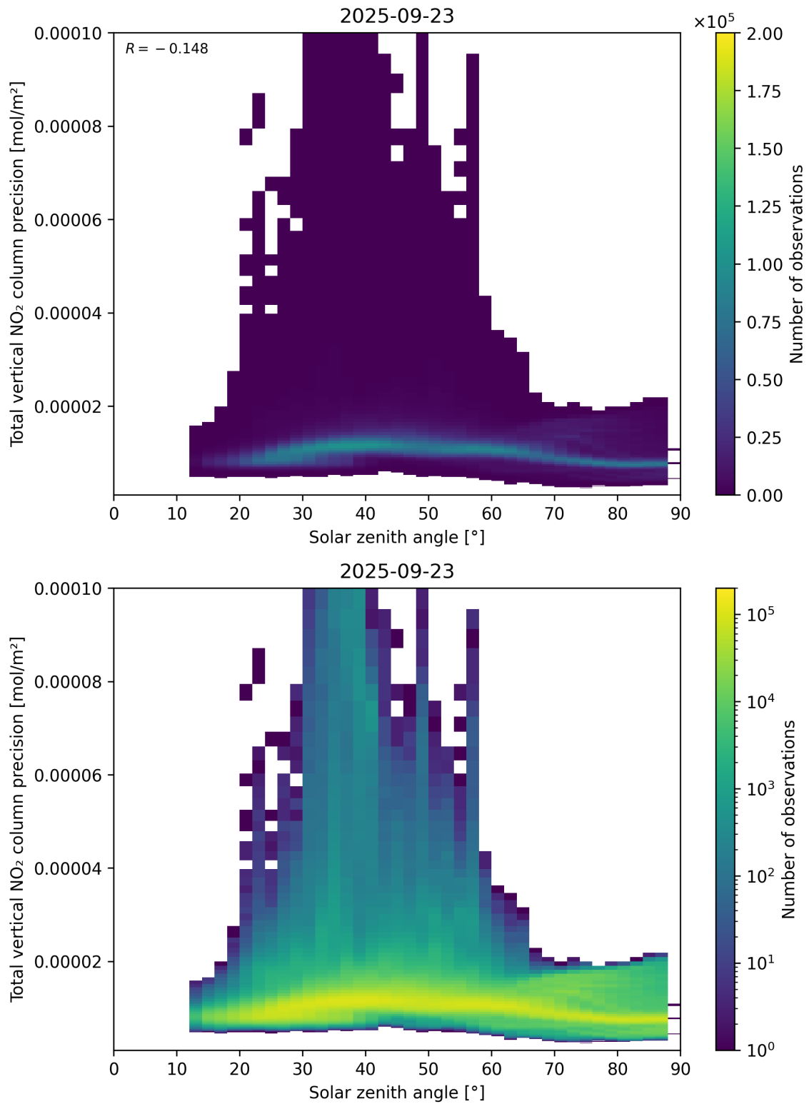
Figure 154: Scatter density plot of “Solar zenith angle” against “Total vertical NO 2 column precision” for 2025-09-22 to 2025-09-24.
