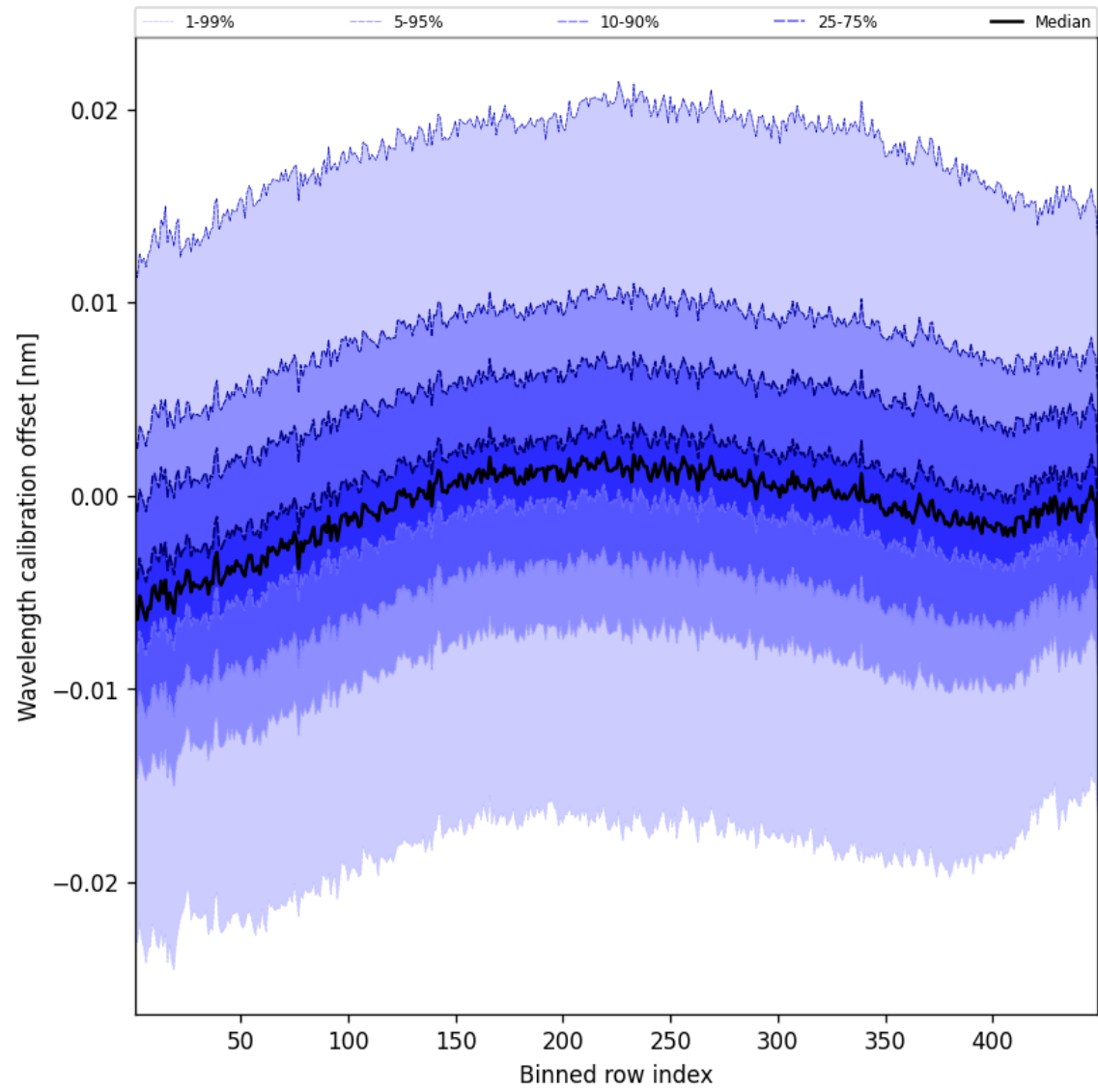
Figure 52: Along track statistics of “Wavelength calibration offset” for 2025-09-22 to 2025-09-24
