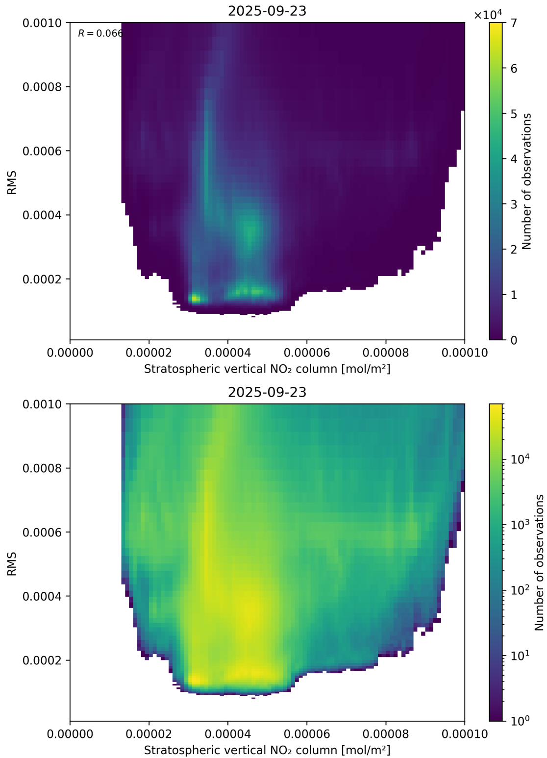
Figure 102: Scatter density plot of “Stratospheric vertical NO 2 column” against “RMS” for 2025-09-22 to 2025-09-24.
