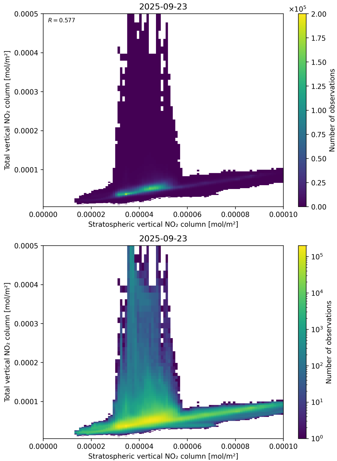
Figure 100: Scatter density plot of “Stratospheric vertical NO 2 column” against “Total vertical NO 2 column” for 2025-09-22 to 2025-09-24.
