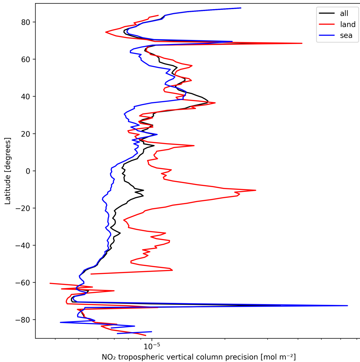
Figure 13: Zonal average of “NO 2 tropospheric vertical column precision” for 2025-09-22 to 2025-09-24.
