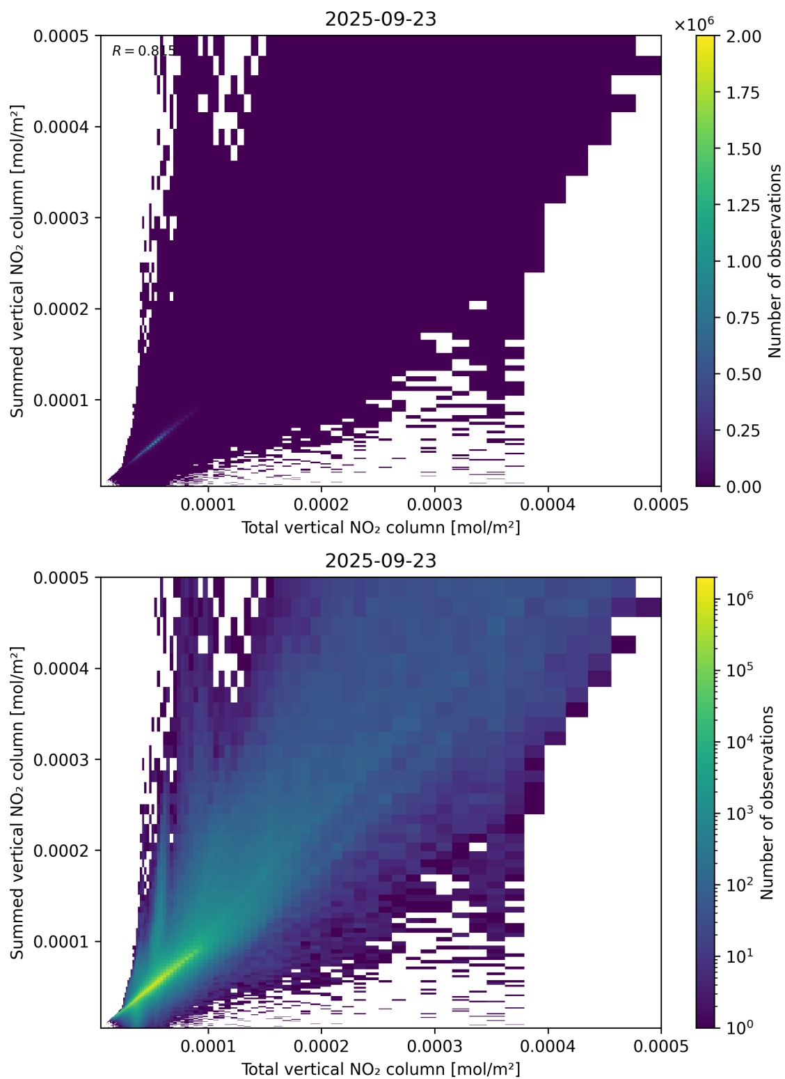
Figure 112: Scatter density plot of “Total vertical NO 2 column” against “Summed vertical NO 2 column” for 2025-09-22 to 2025-09-24.
