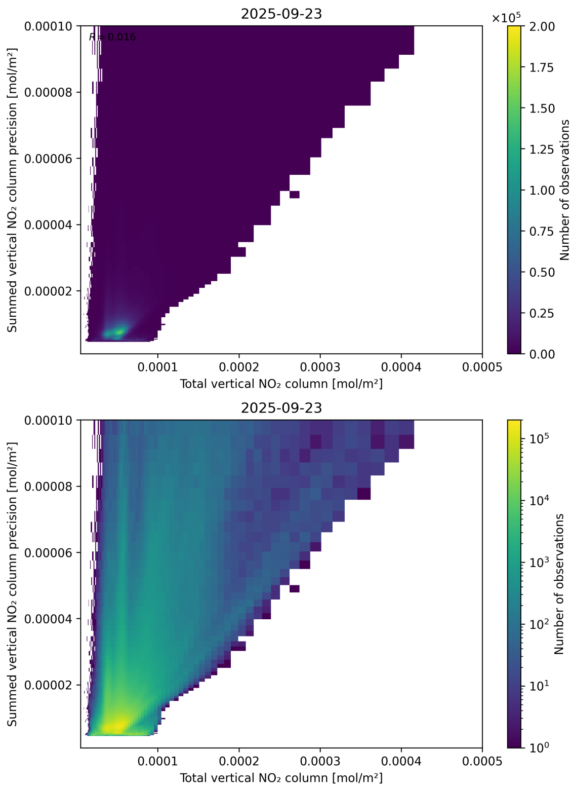
Figure 113: Scatter density plot of “Total vertical NO 2 column” against “Summed vertical NO 2 column precision” for 2025-09-22 to 2025-09-24.
