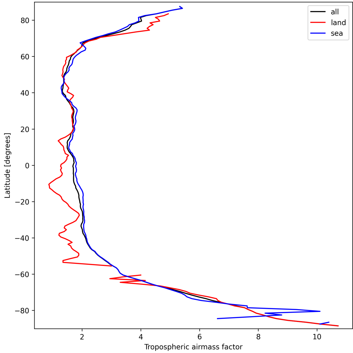
Figure 14: Zonal average of “Tropospheric air mass factor” for 2025-09-22 to 2025-09-24.
