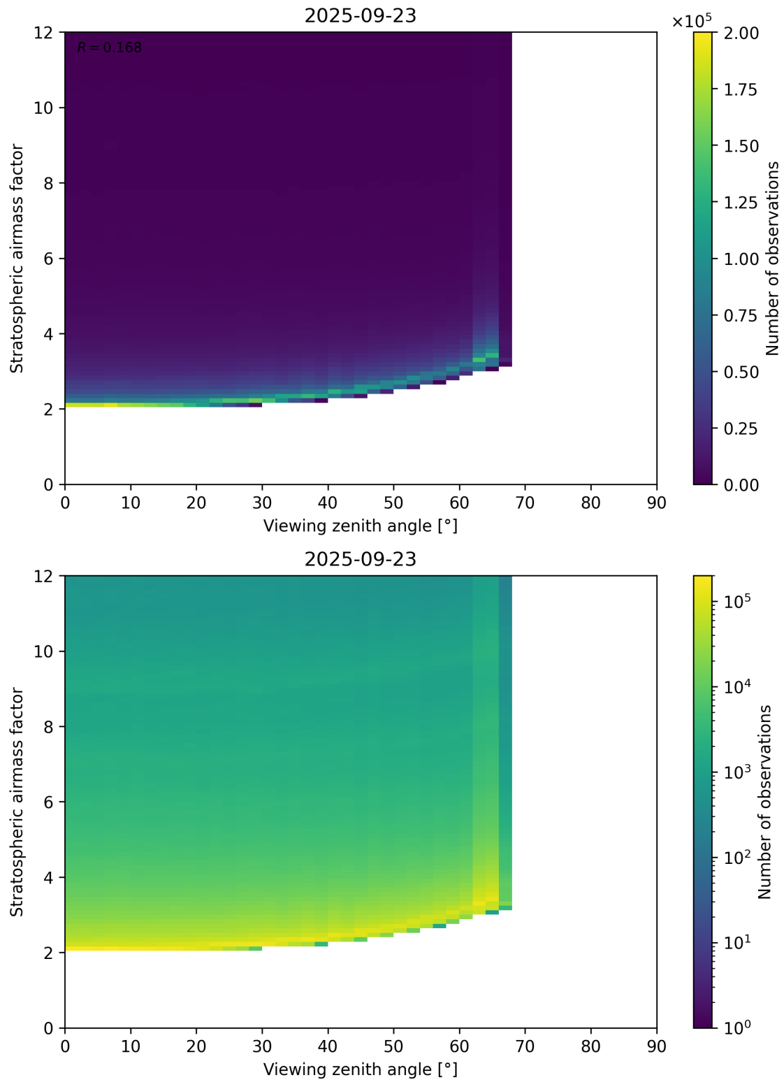
Figure 159: Scatter density plot of “Viewing zenith angle” against “Stratospheric airmass factor” for 2025-09-22 to 2025-09-24.
