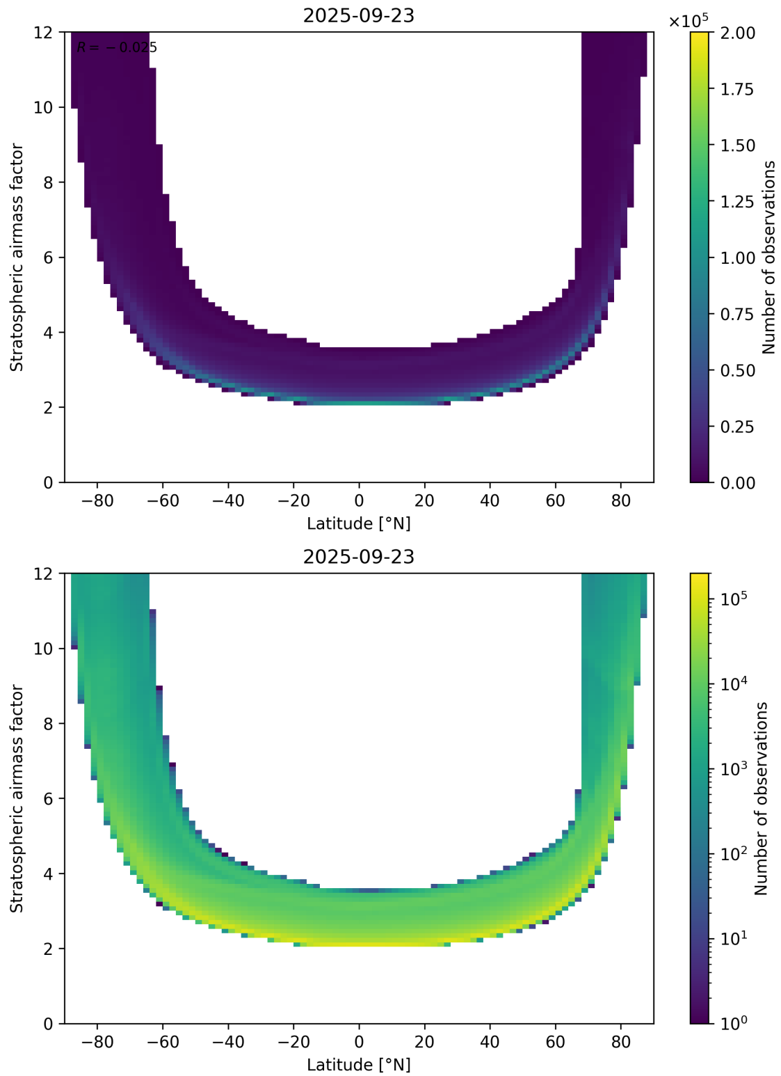
Figure 83: Scatter density plot of “Latitude” against “Stratospheric airmass factor” for 2025-09-22 to 2025-09-24.
