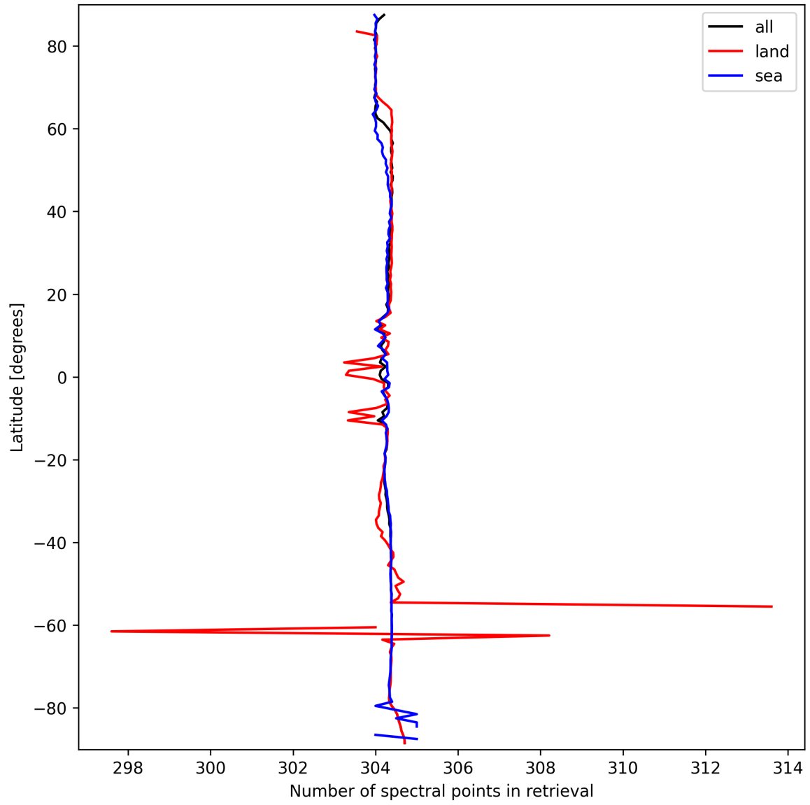
Figure 16: Zonal average of “Number of spectral points in retrieval” for 2025-09-22 to 2025-09-24.
