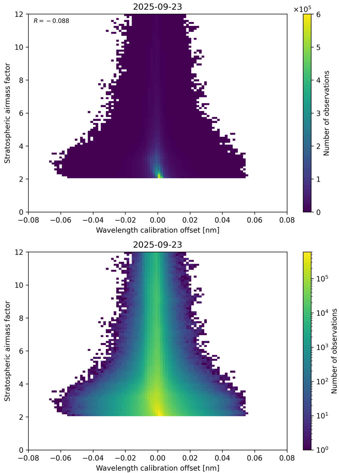
Figure 174: Scatter density plot of “Wavelength calibration offset” against “Stratospheric air mass factor” for 2025-09-22 to 2025-09-24.
