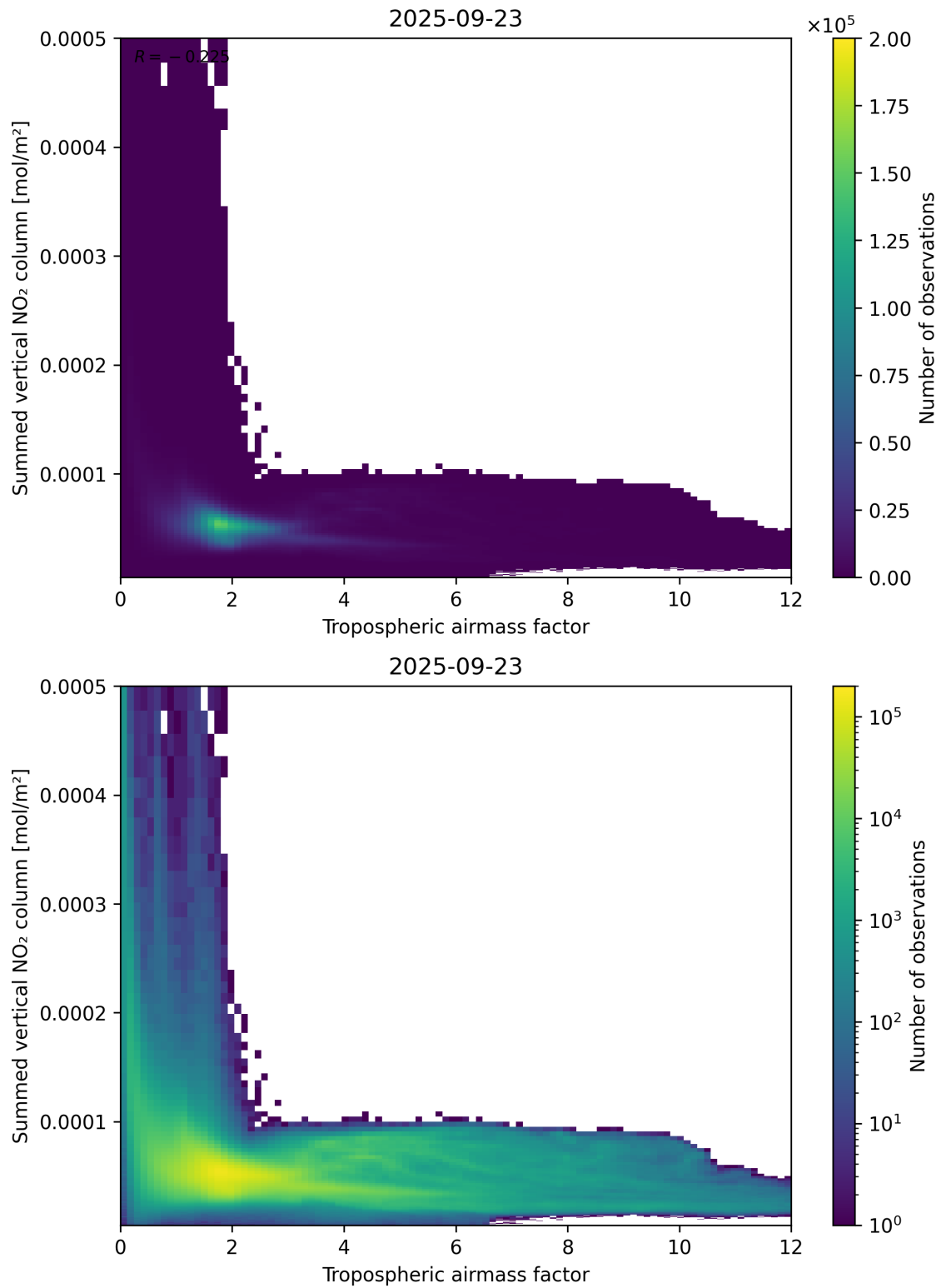
Figure 75: Scatter density plot of “Tropospheric airmass factor” against “Summed vertical NO 2 column” for 2025-09-22 to 2025-09-24.
