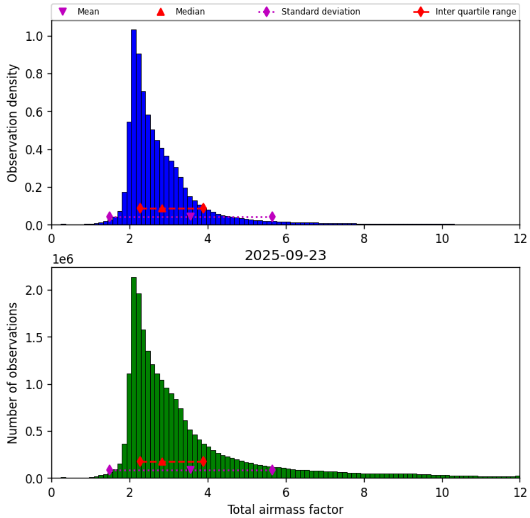
Figure 32: Histogram of “Total airmass factor” for 2025-09-22 to 2025-09-24
