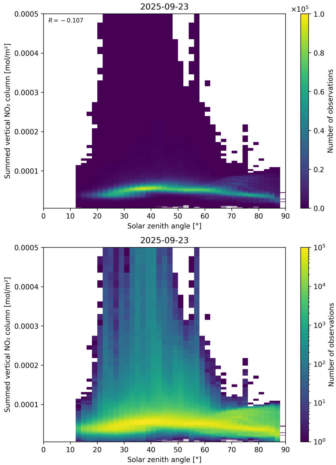
Figure 151: Scatter density plot of “Solar zenith angle” against “Summed vertical NO 2 column” for 2025-09-22 to 2025-09-24.
