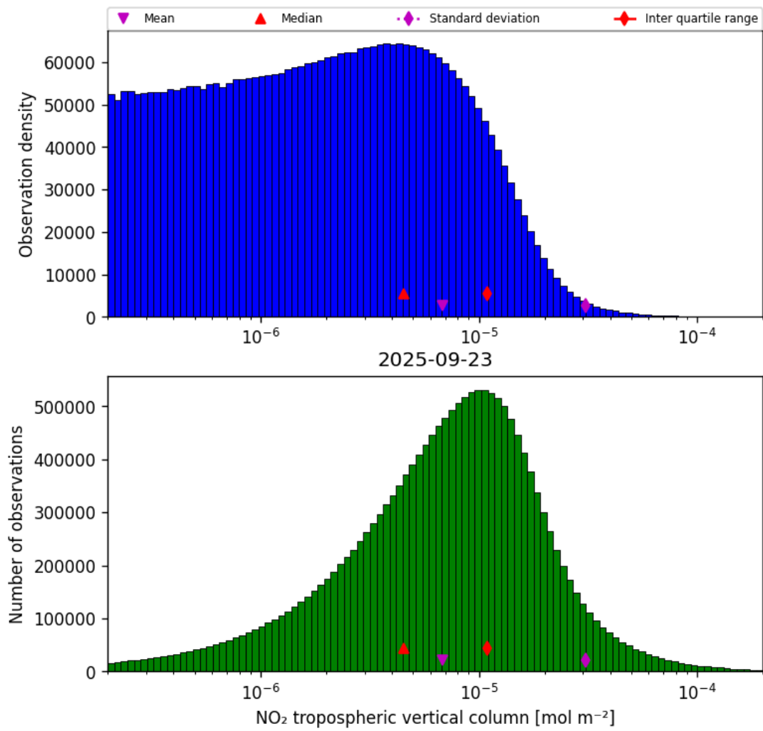
Figure 29: Histogram of “NO 2 tropospheric vertical column” for 2025-09-22 to 2025-09-24
