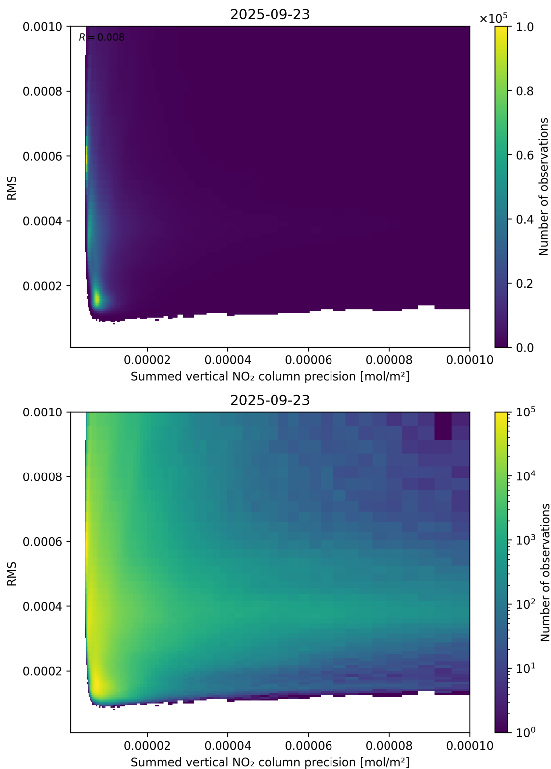
Figure 108: Scatter density plot of “Summed vertical NO 2 column precision” against “RMS” for 2025-09-22 to 2025-09-24.
