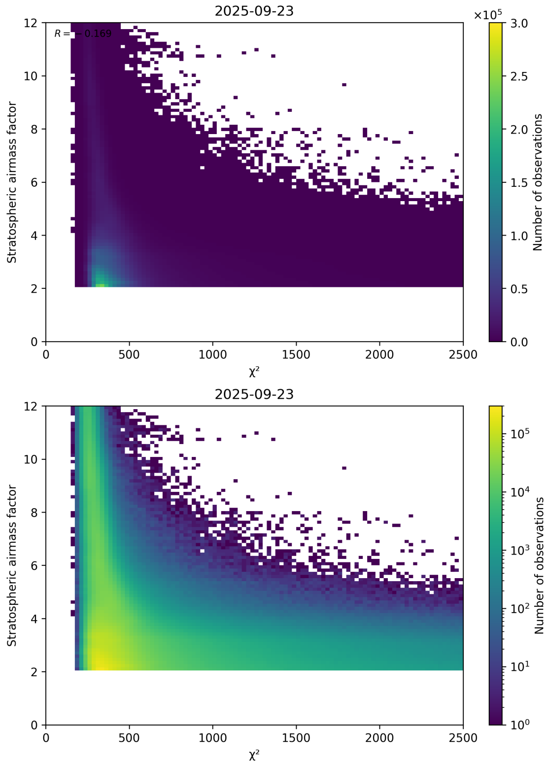
Figure 81: Scatter density plot of “ \chi^2 ” against “Stratospheric airmass factor” for 2025-09-22 to 2025-09-24.
