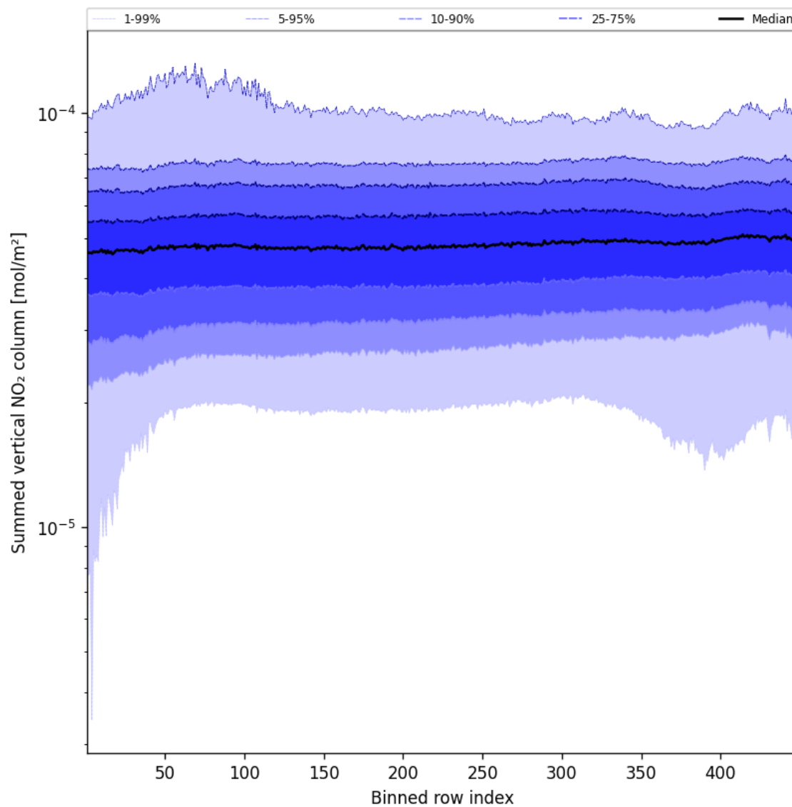
Figure 57: Along track statistics of “Summed vertical NO 2 column” for 2025-09-22 to 2025-09-24
