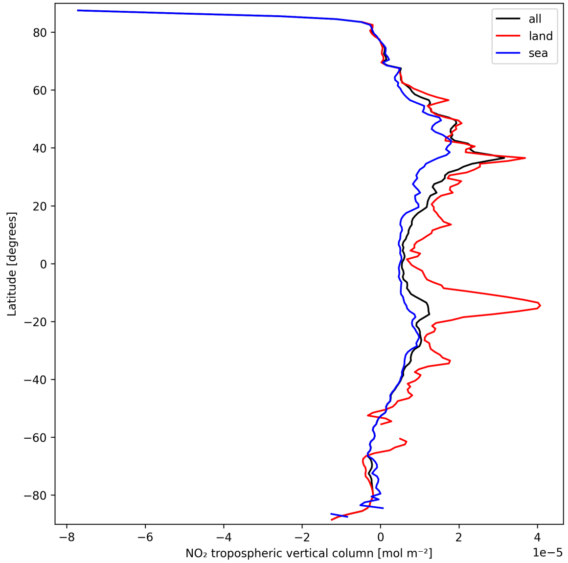
Figure 12: Zonal average of “NO 2 tropospheric vertical column” for 2025-09-22 to 2025-09-24.
