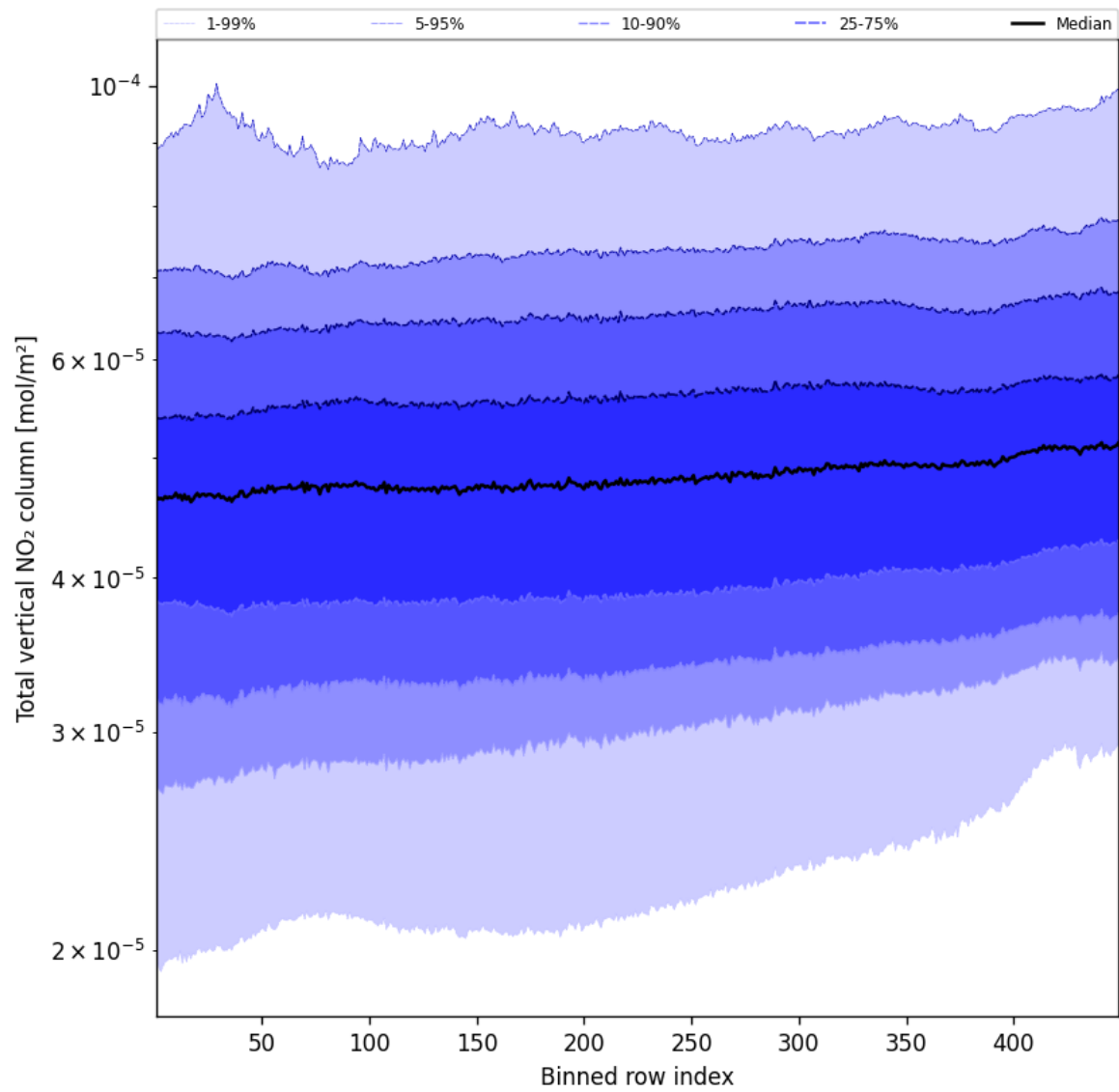
Figure 55: Along track statistics of “Total vertical NO 2 column” for 2025-09-22 to 2025-09-24
