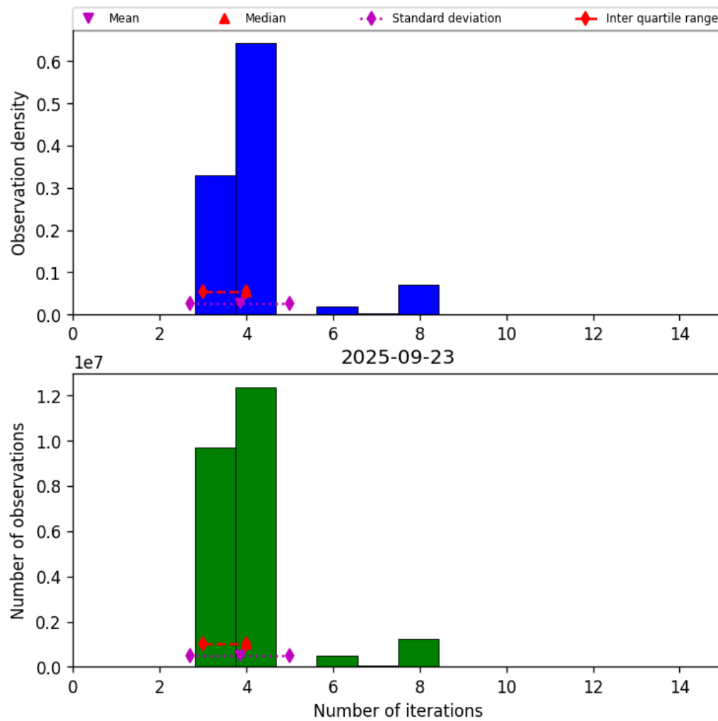
Figure 34: Histogram of “Number of iterations” for 2025-09-22 to 2025-09-24
