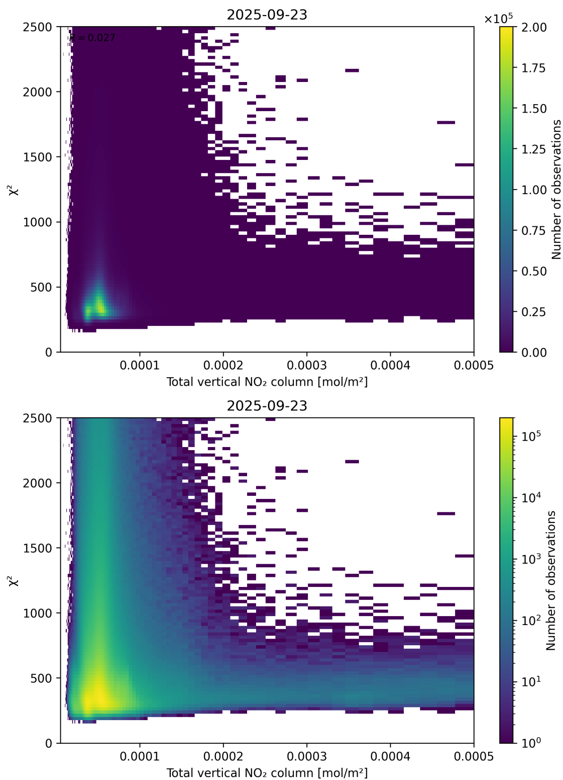
Figure 111: Scatter density plot of “Total vertical NO 2 column” against “ \chi^2 ” for 2025-09-22 to 2025-09-24.
