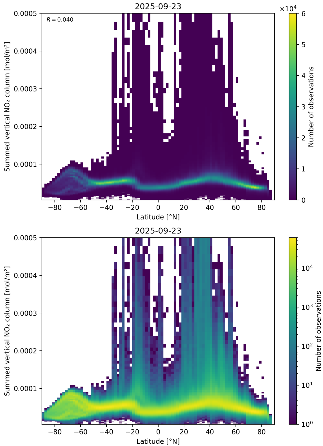
Figure 88: Scatter density plot of “Latitude” against “Summed vertical NO 2 column” for 2025-09-22 to 2025-09-24.
