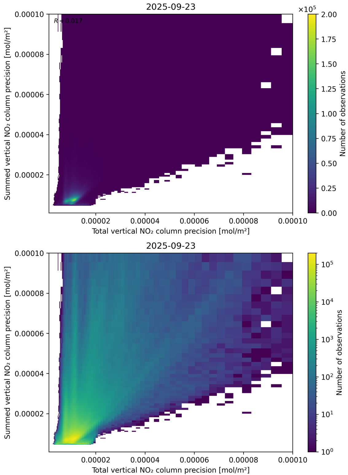
Figure 118: Scatter density plot of “Total vertical NO 2 column precision” against “Summed vertical NO 2 column precision” for 2025-09-22 to 2025-09-24.
