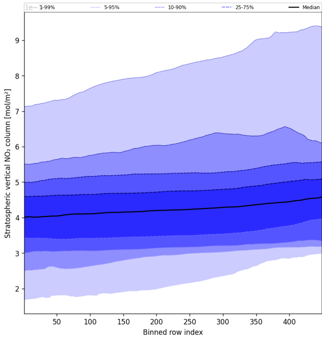
Figure 53: Along track statistics of “Stratospheric vertical NO 2 column” for 2025-09-22 to 2025-09-24
