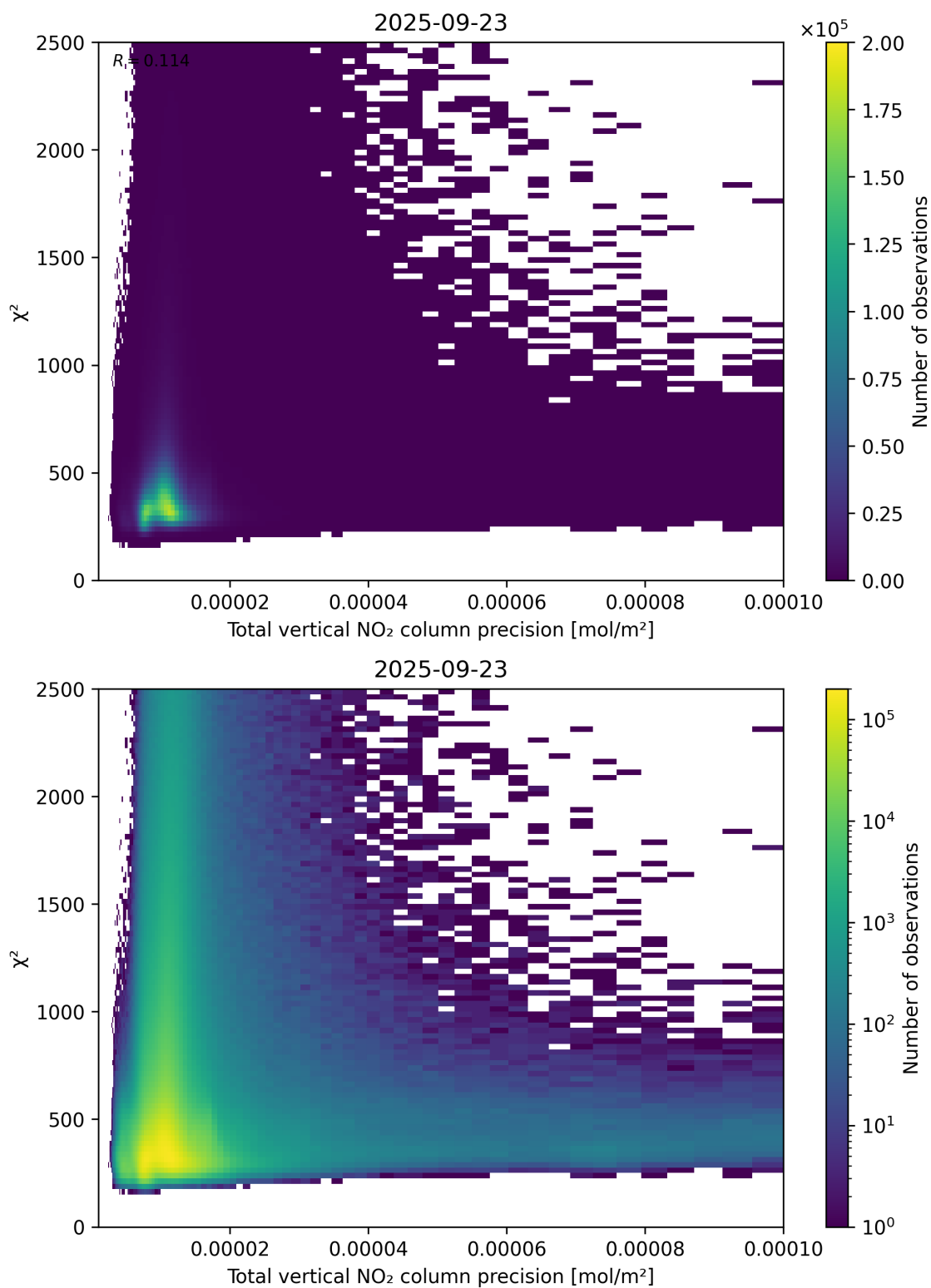
Figure 116: Scatter density plot of “Total vertical NO 2 column precision” against “ \chi^2 ” for 2025-09-22 to 2025-09-24.
