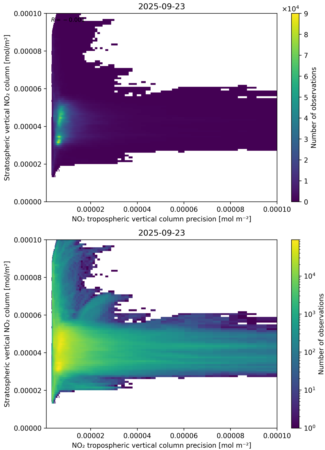
Figure 135: Scatter density plot of “NO 2 tropospheric vertical column precision” against “Stratospheric vertical NO 2 column” for 2025-09-22 to 2025-09-24.
