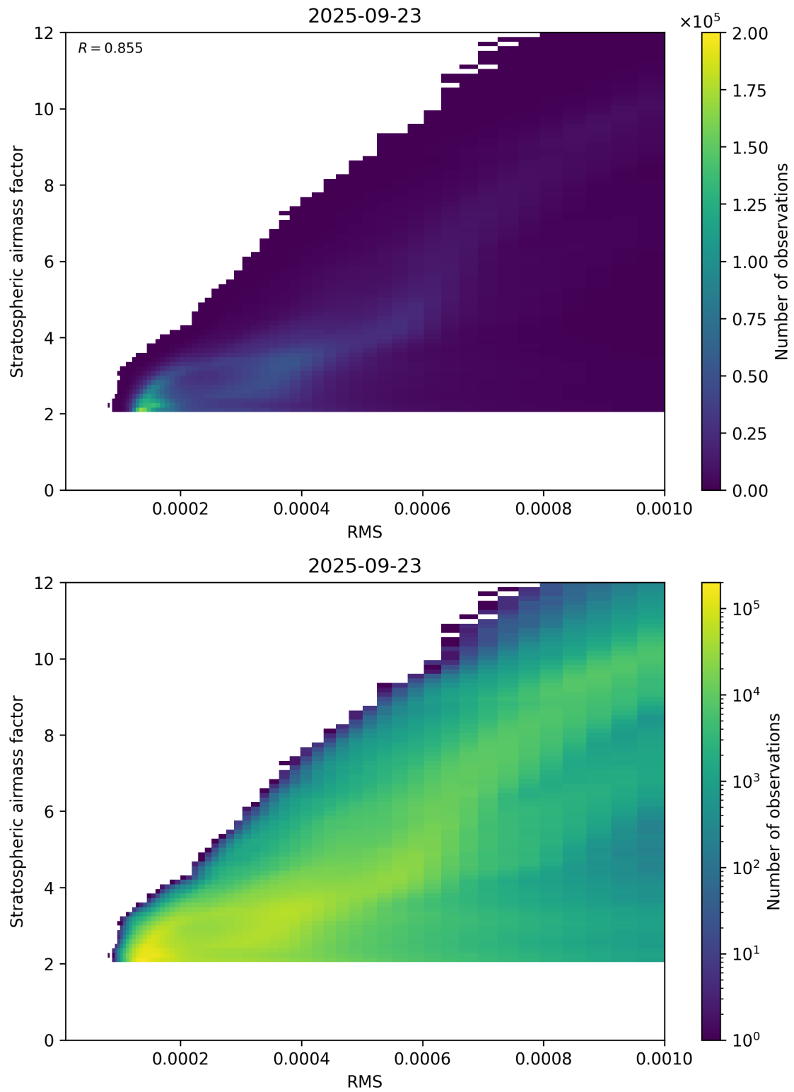
Figure 144: Scatter density plot of “RMS” against “Stratospheric airmass factor” for 2025-09-22 to 2025-09-24.
