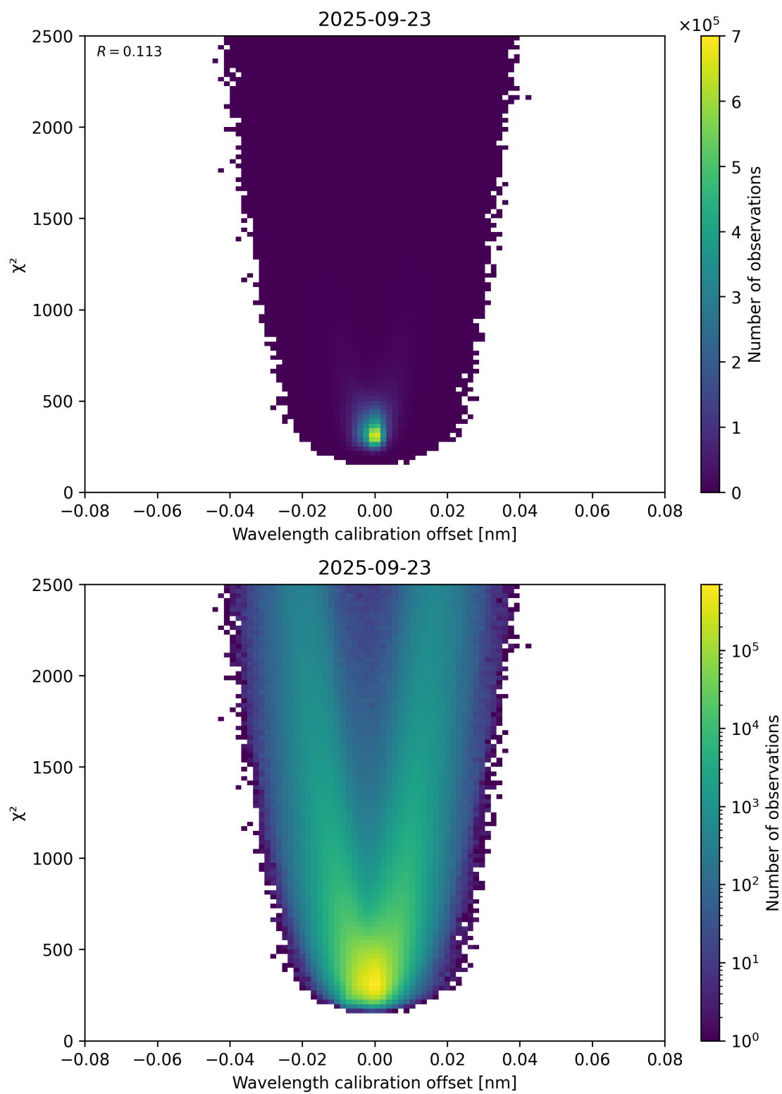
Figure 175: Scatter density plot of “Wavelength calibration offset” against “ \chi^2 ” for 2025-09-22 to 2025-09-24.
