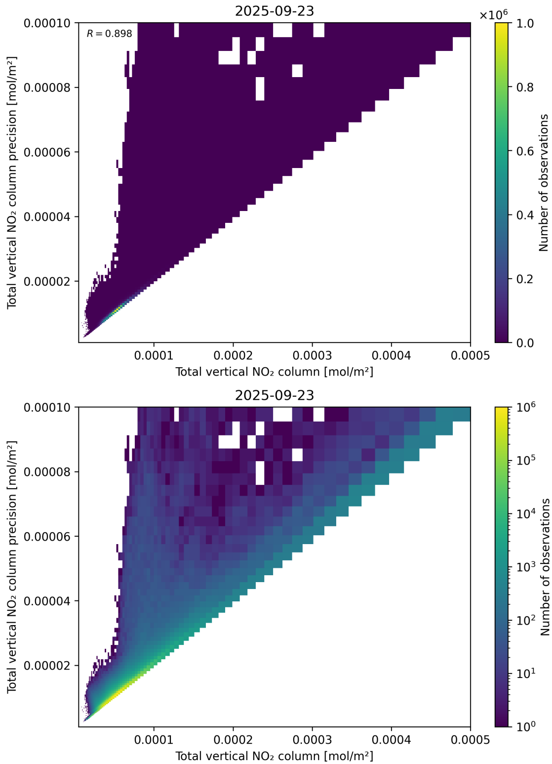
Figure 114: Scatter density plot of “Total vertical NO 2 column” against “Total vertical NO 2 column precision” for 2025-09-22 to 2025-09-24.
