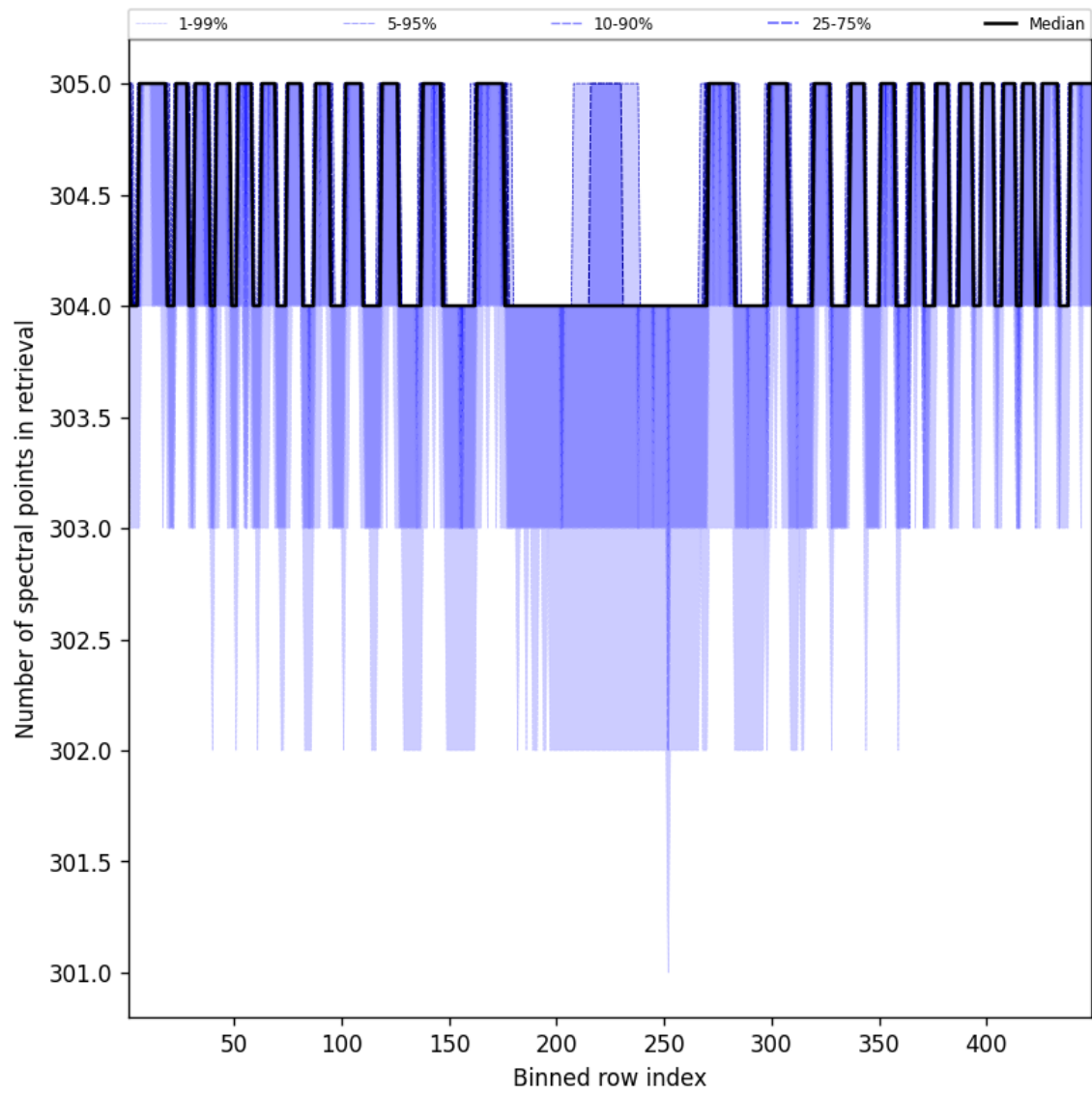
Figure 50: Along track statistics of “Number of spectral points in retrieval” for 2025-09-22 to 2025-09-24
