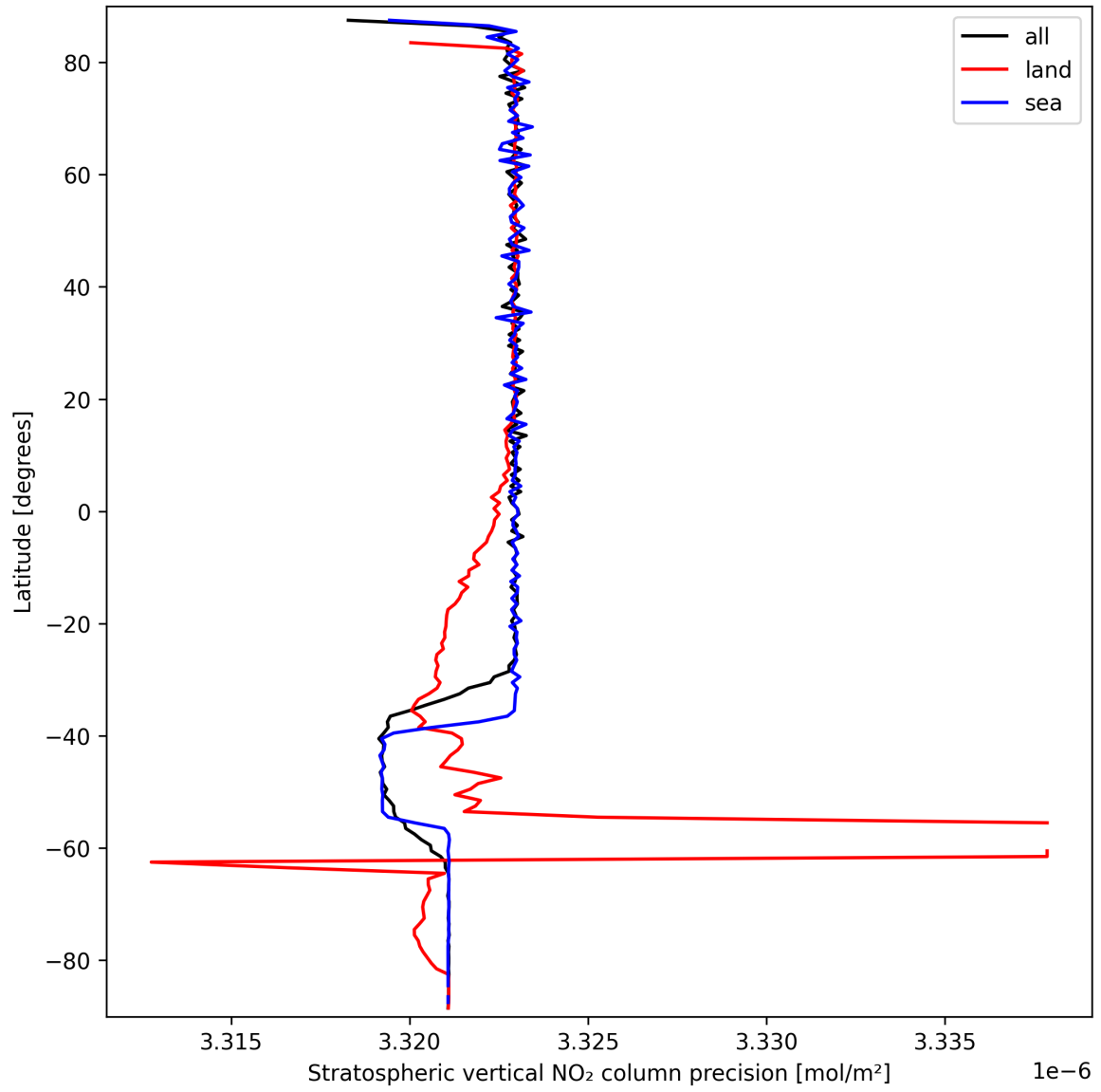
Figure 20: Zonal average of “Stratospheric vertical NO 2 column precision” for 2025-09-22 to 2025-09-24.
