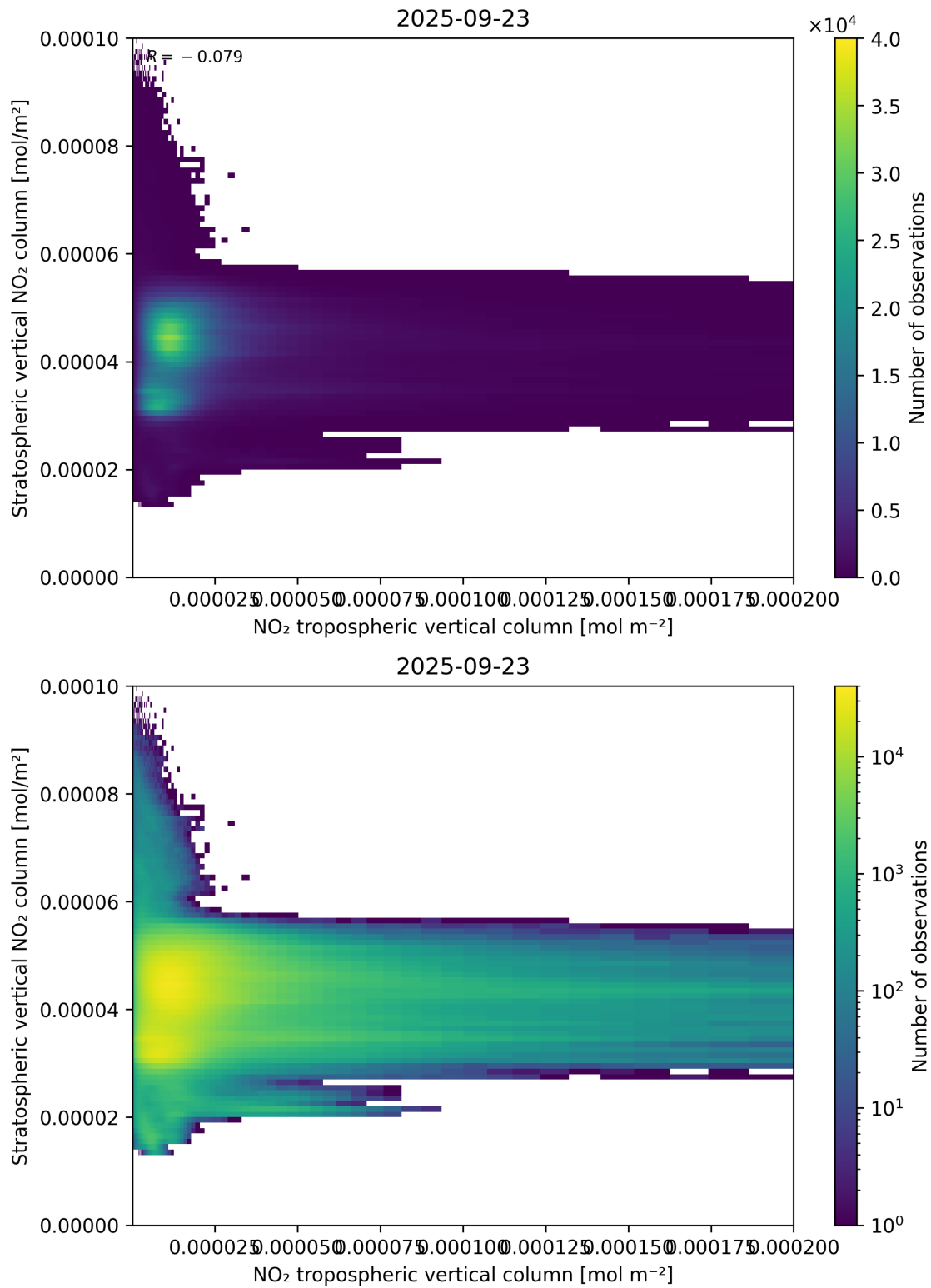
Figure 125: Scatter density plot of “NO 2 tropospheric vertical column” against “Stratospheric vertical NO 2 column” for 2025-09-22 to 2025-09-24.
