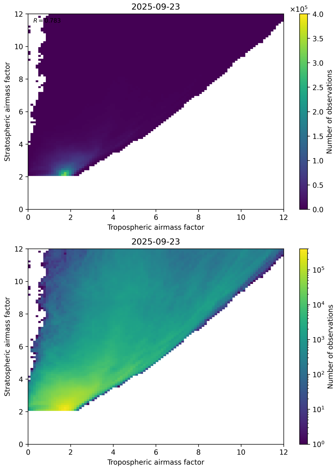
Figure 71: Scatter density plot of “Tropospheric airmass factor” against “Stratospheric airmass factor” for 2025-09-22 to 2025-09-24.
