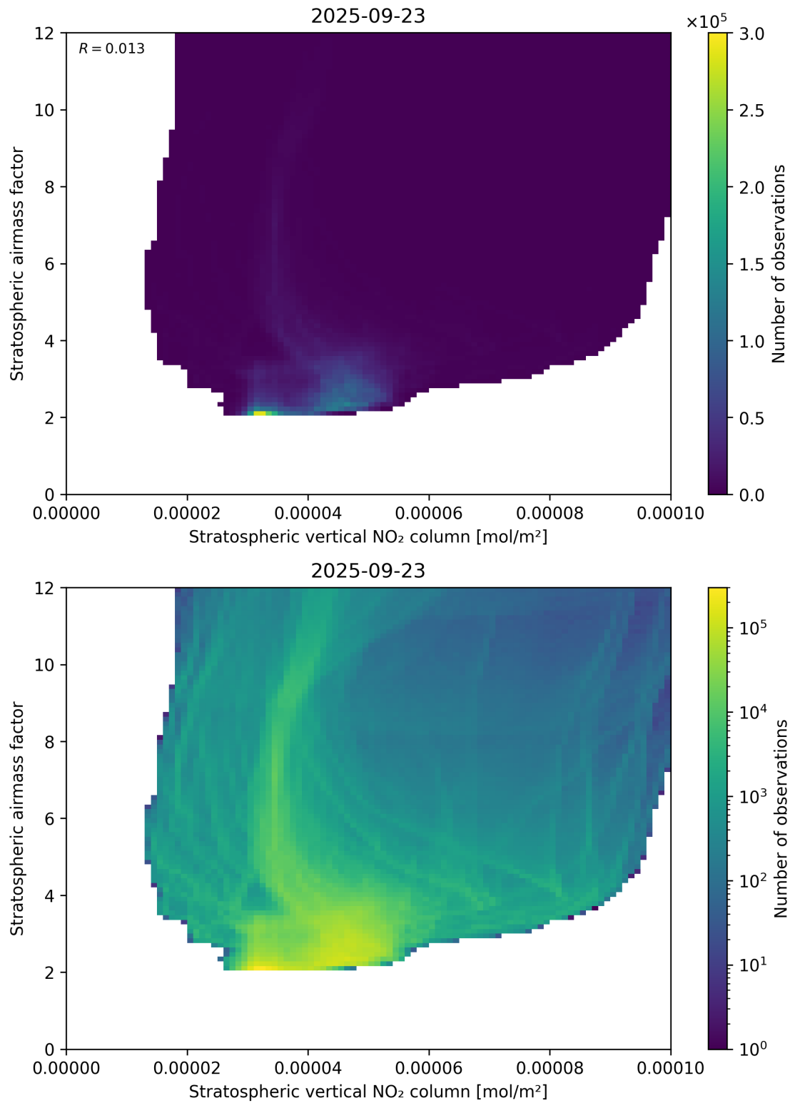
Figure 96: Scatter density plot of “Stratospheric vertical NO 2 column” against “Stratospheric airmass factor” for 2025-09-22 to 2025-09-24.
