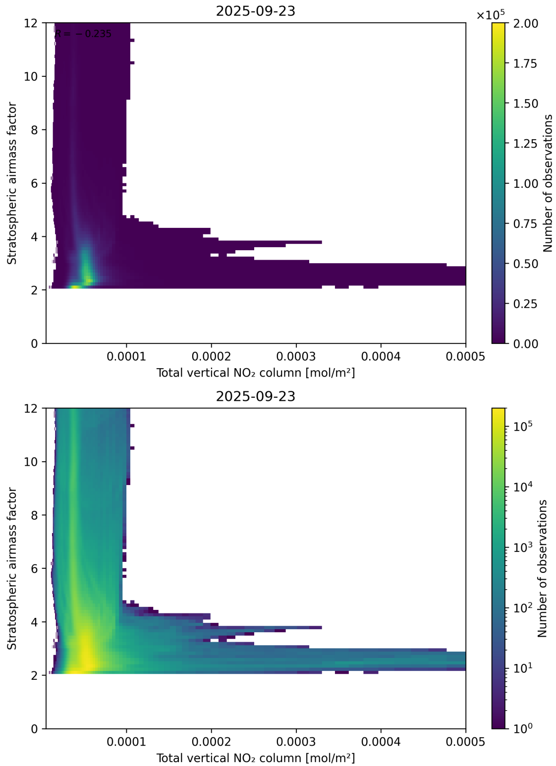
Figure 110: Scatter density plot of “Total vertical NO 2 column” against “Stratospheric airmass factor” for 2025-09-22 to 2025-09-24.
