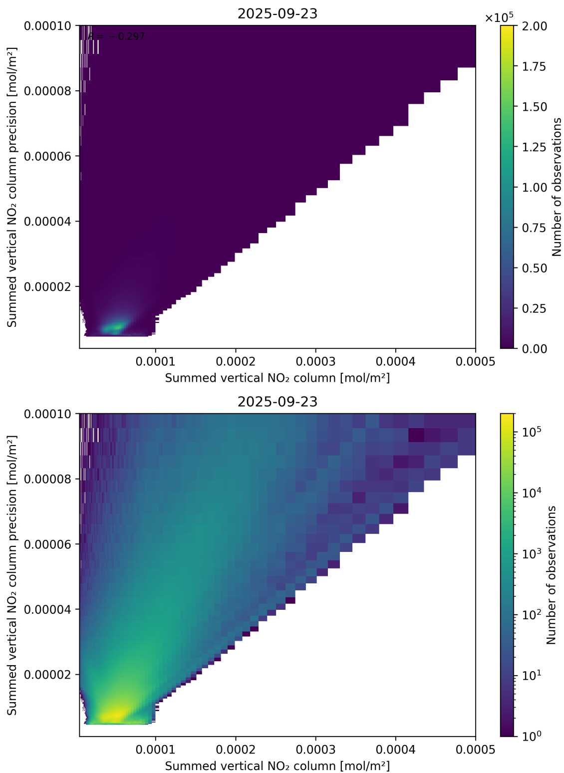
Figure 105: Scatter density plot of “Summed vertical NO 2 column” against “Summed vertical NO 2 column precision” for 2025-09-22 to 2025-09-24.
