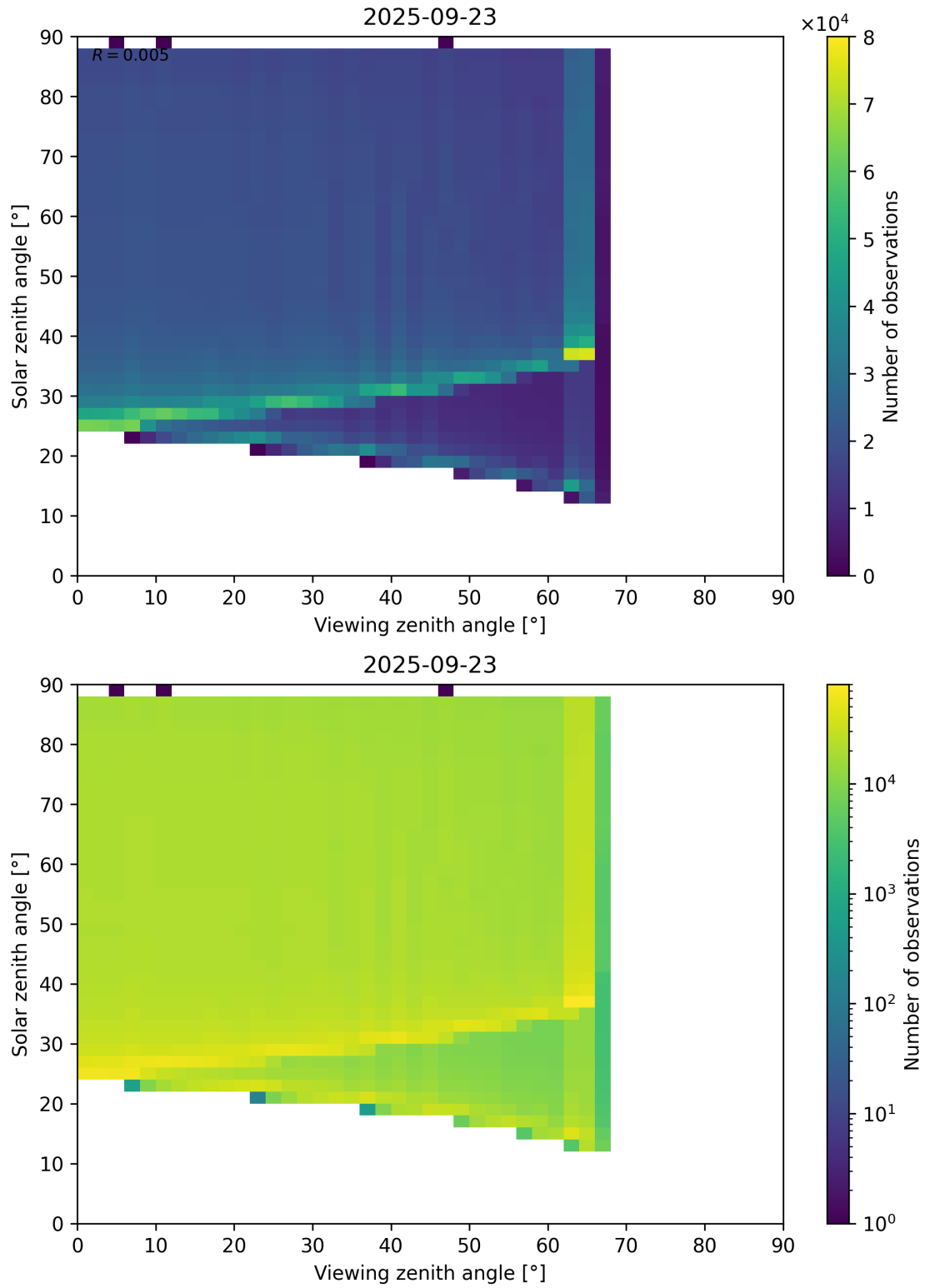
Figure 172: Scatter density plot of “Viewing zenith angle” against “Solar zenith angle” for 2025-09-22 to 2025-09-24.
