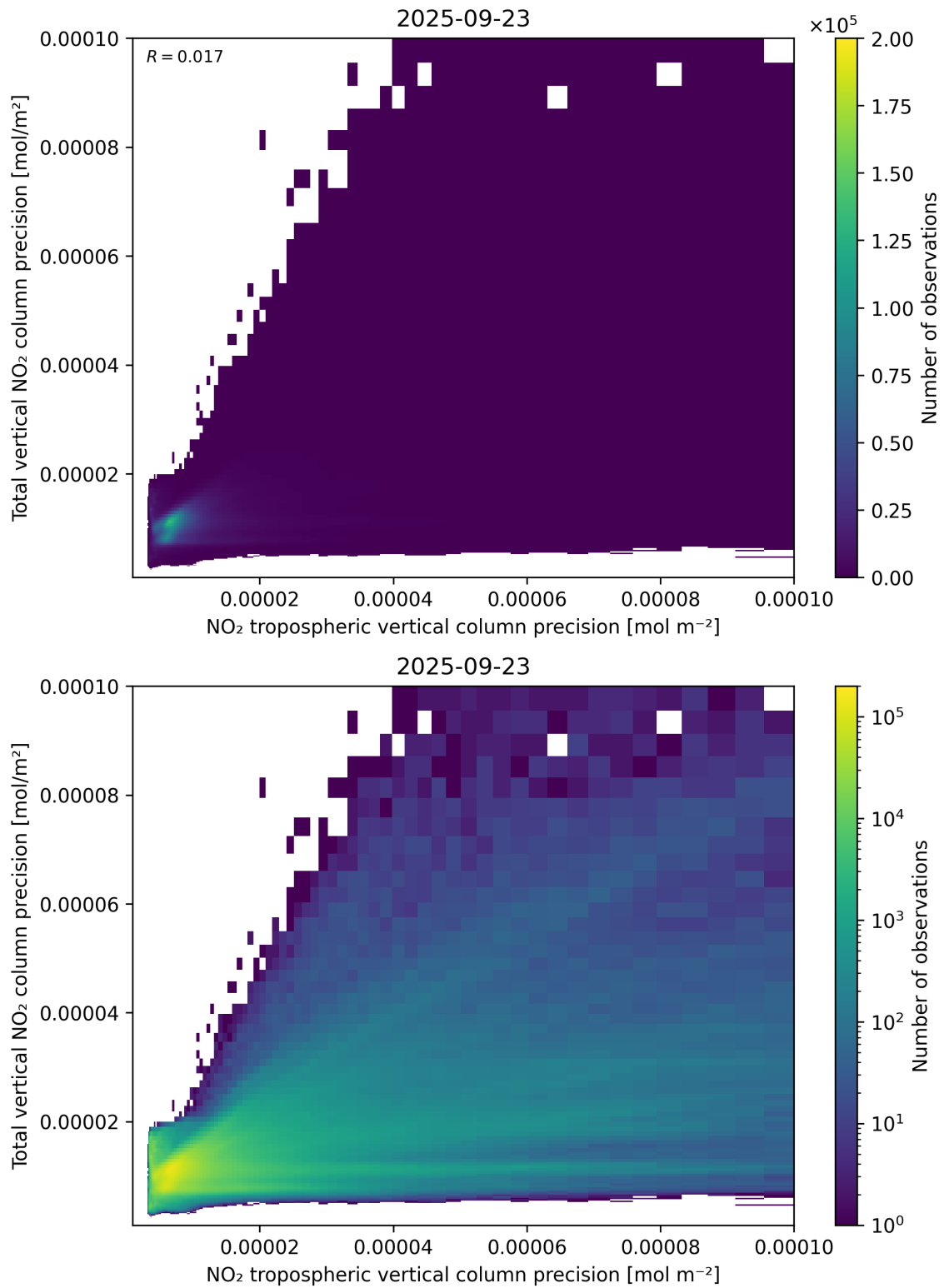
Figure 139: Scatter density plot of “NO 2 tropospheric vertical column precision” against “Total vertical NO 2 column precision” for 2025-09-22 to 2025-09-24.
