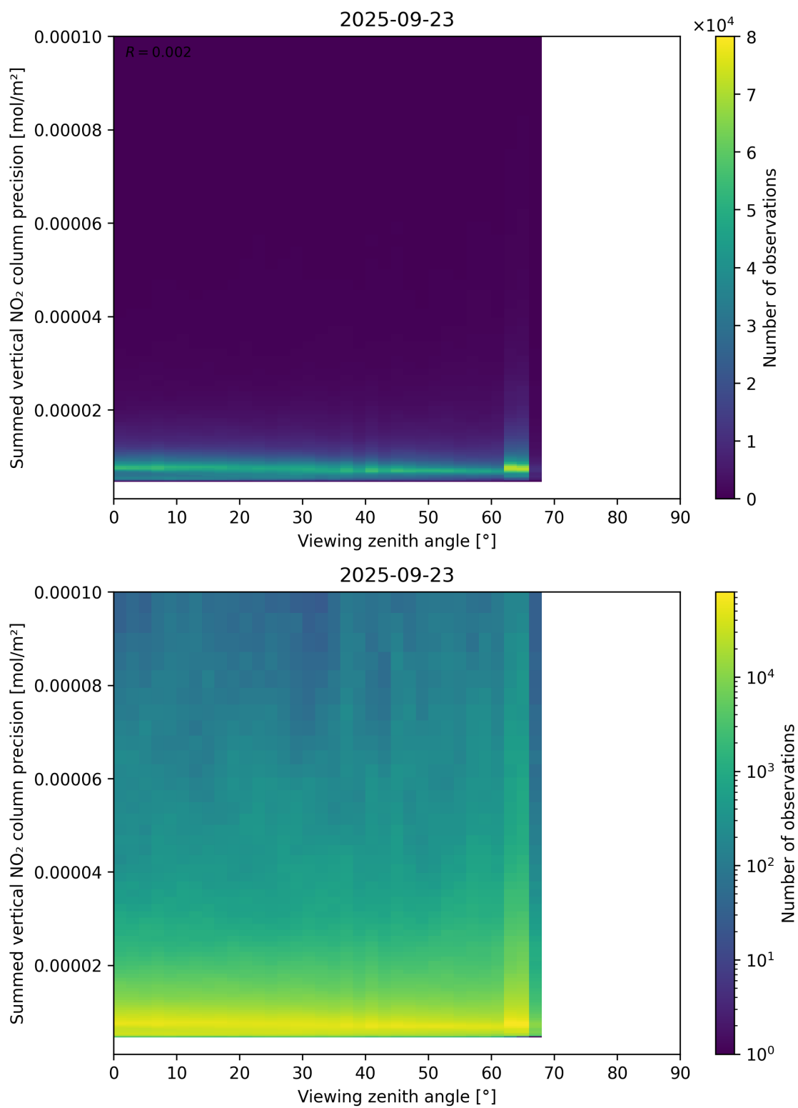
Figure 166: Scatter density plot of “Viewing zenith angle” against “Summed vertical NO 2 column precision” for 2025-09-22 to 2025-09-24.
