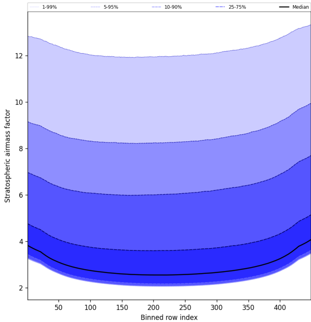
Figure 61: Along track statistics of “Stratospheric airmass factor” for 2025-09-22 to 2025-09-24
