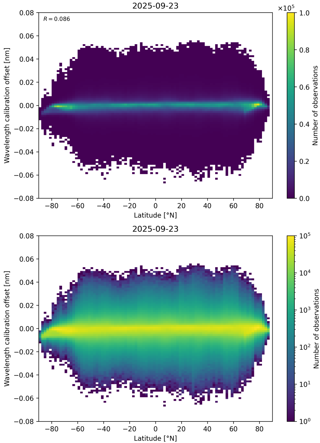
Figure 95: Scatter density plot of “Latitude” against “Wavelength calibration offset” for 2025-09-22 to 2025-09-24.
