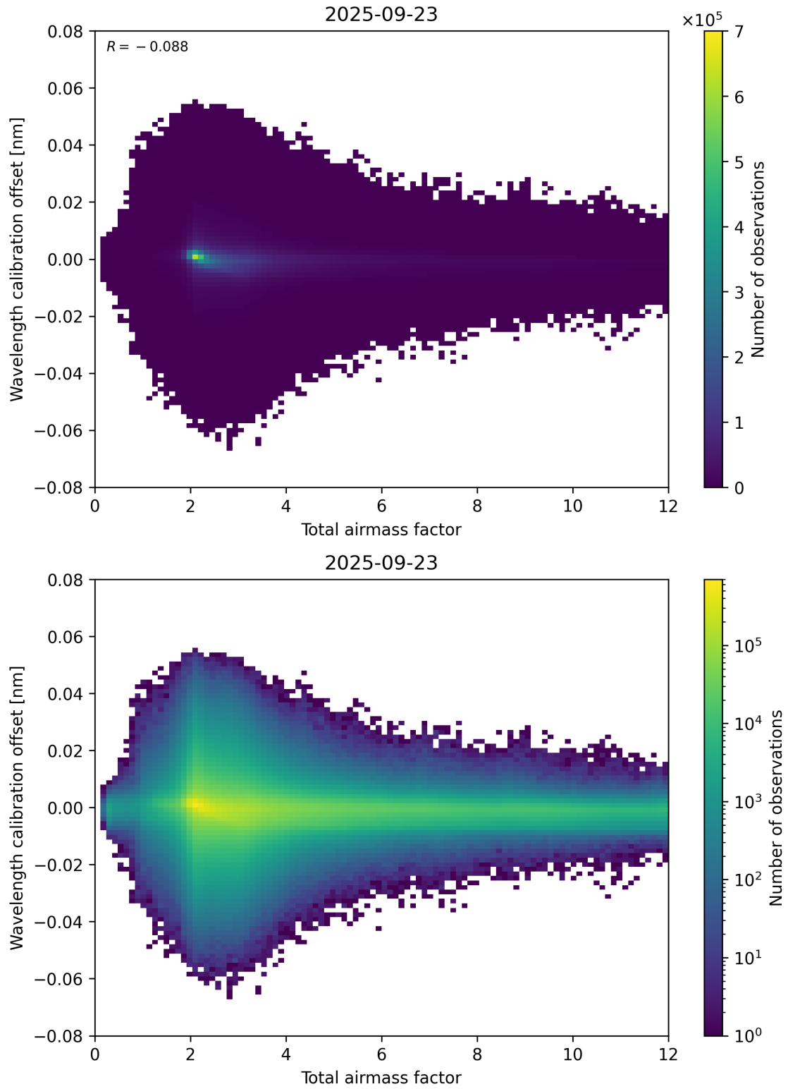
Figure 70: Scatter density plot of “Total airmass factor” against “Wavelength calibration offset” for 2025-09-22 to 2025-09-24.
