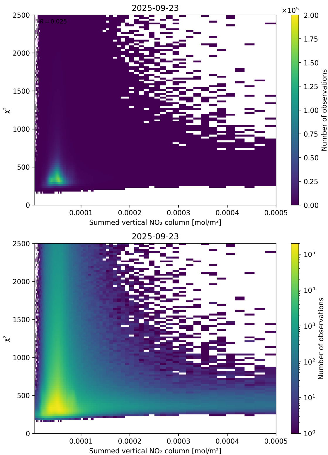
Figure 104: Scatter density plot of “Summed vertical NO 2 column” against “ \chi^2 ” for 2025-09-22 to 2025-09-24.
