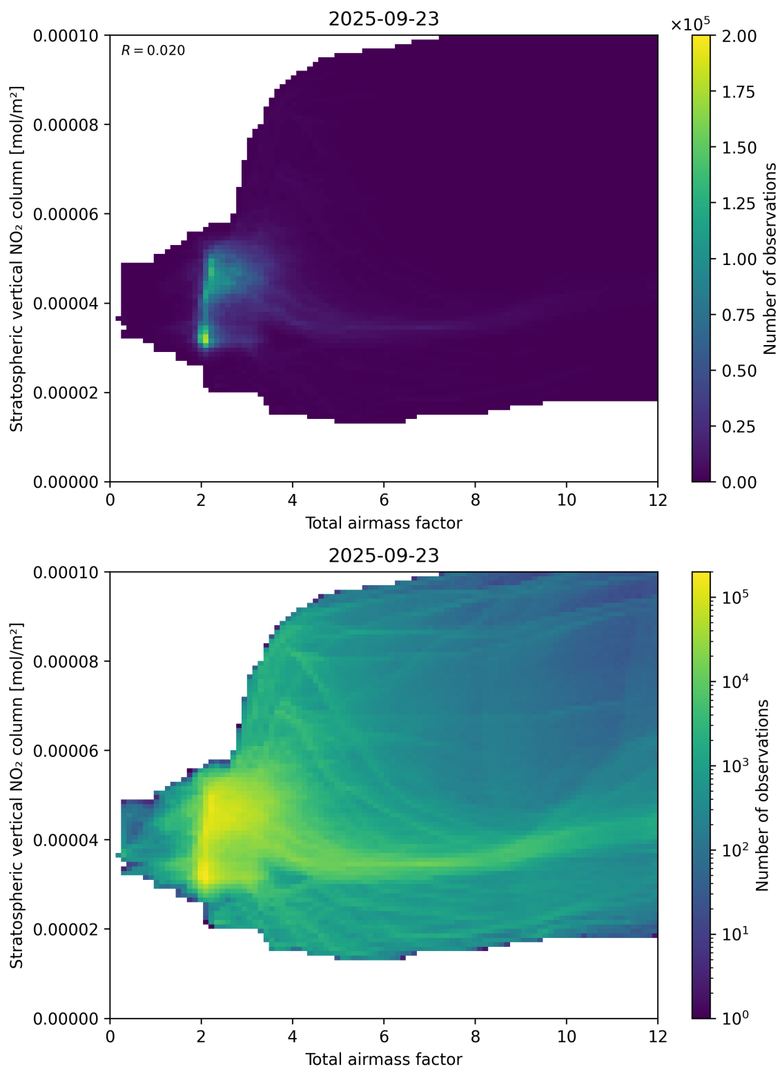
Figure 64: Scatter density plot of “Total airmass factor” against “Stratospheric vertical \text{NO}_2 column” for 2025-09-22 to 2025-09-24.
