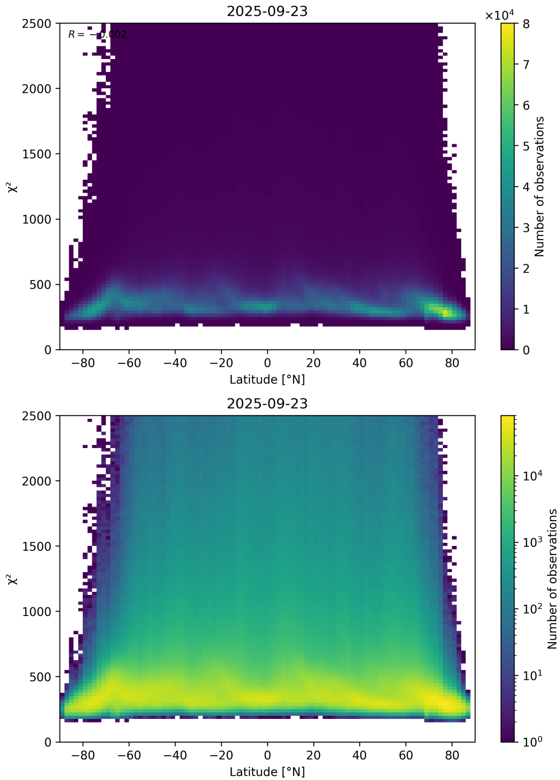
Figure 86: Scatter density plot of “Latitude” against “ \chi^2 ” for 2025-09-22 to 2025-09-24.
