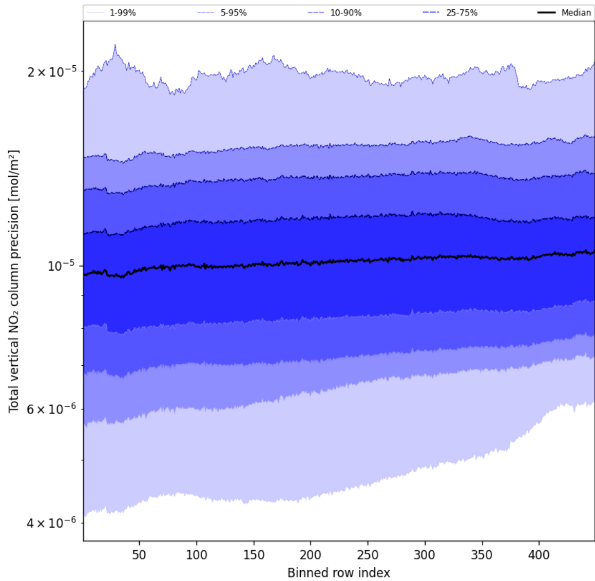
Figure 56: Along track statistics of "Total vertical NO 2 column precision" for 2025-09-22 to 2025-09-24
