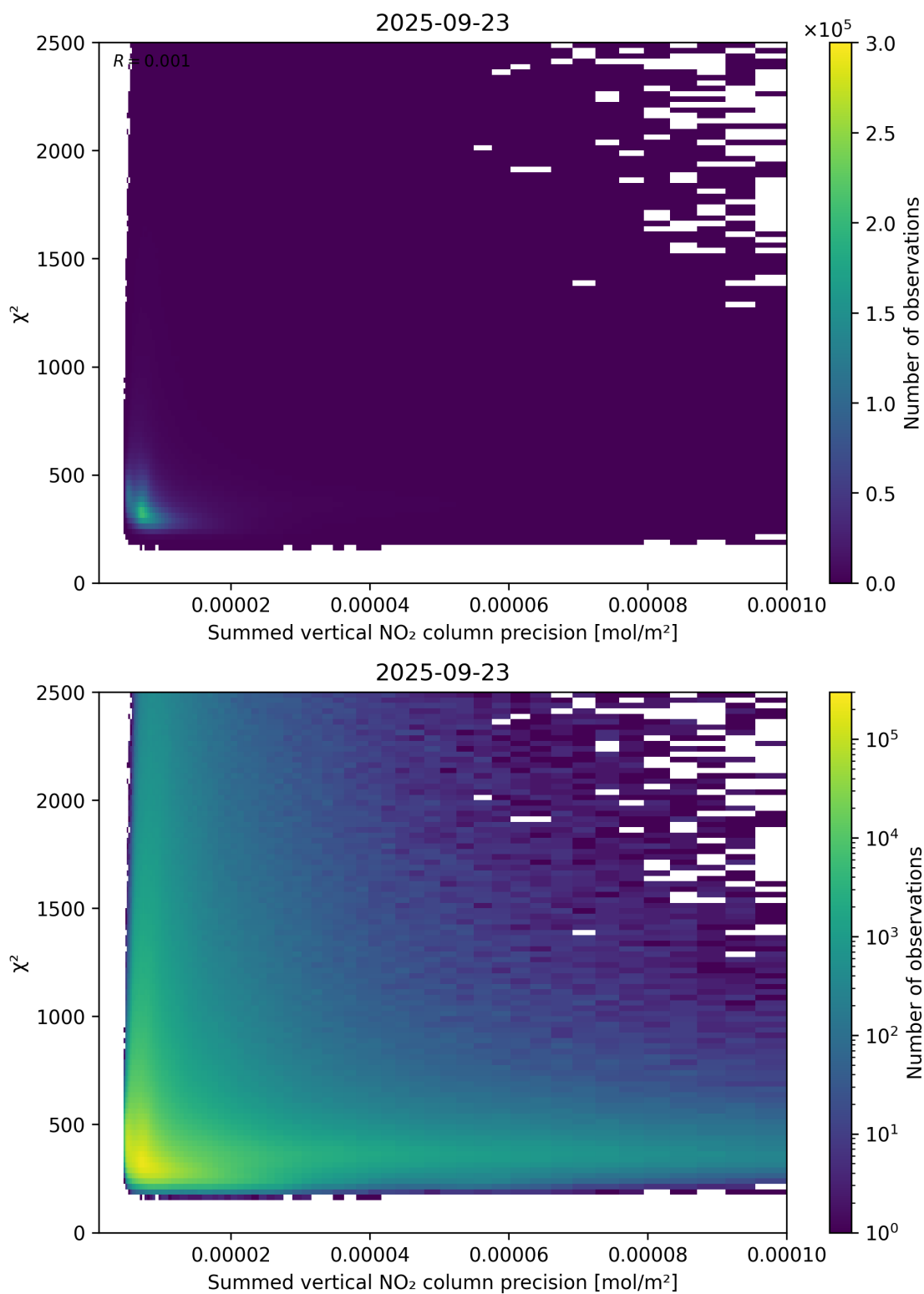
Figure 107: Scatter density plot of “Summed vertical NO 2 column precision” against “ \chi^2 ” for 2025-09-22 to 2025-09-24.
