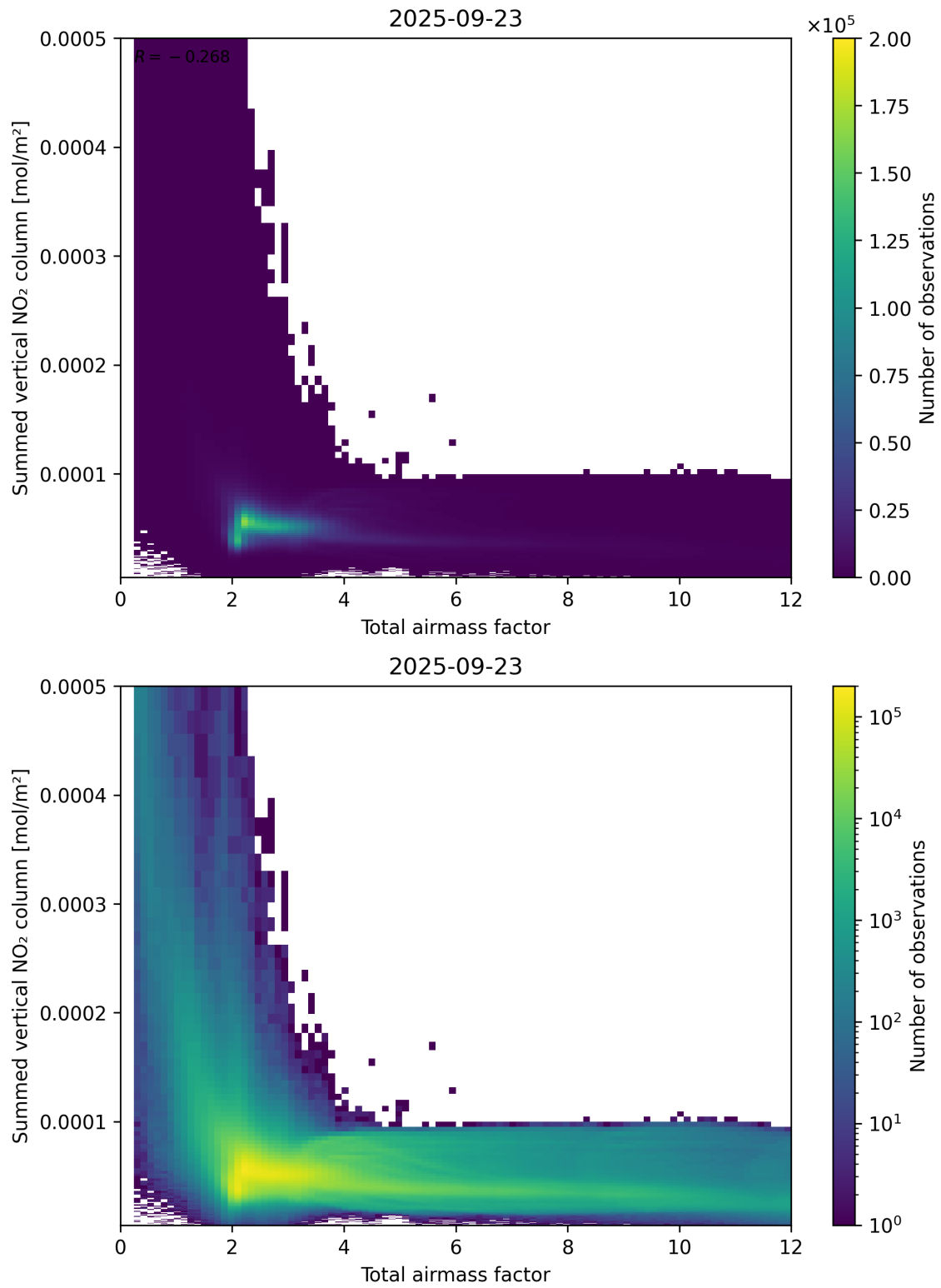
Figure 65: Scatter density plot of “Total airmass factor” against “Summed vertical NO 2 column” for 2025-09-22 to 2025-09-24.
