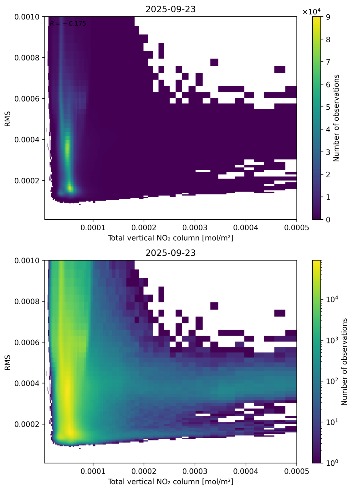
Figure 120: Scatter density plot of “Total vertical NO 2 column” against “RMS” for 2025-09-22 to 2025-09-24.
