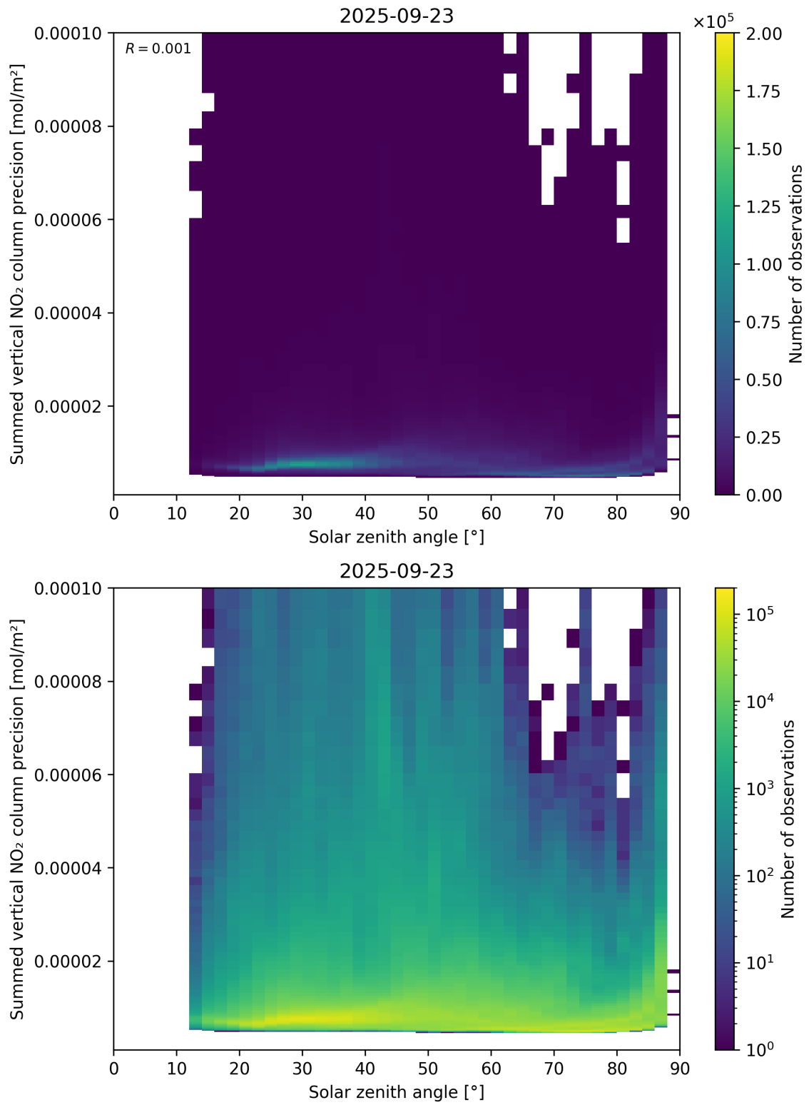
Figure 152: Scatter density plot of “Solar zenith angle” against “Summed vertical NO 2 column precision” for 2025-09-22 to 2025-09-24.
