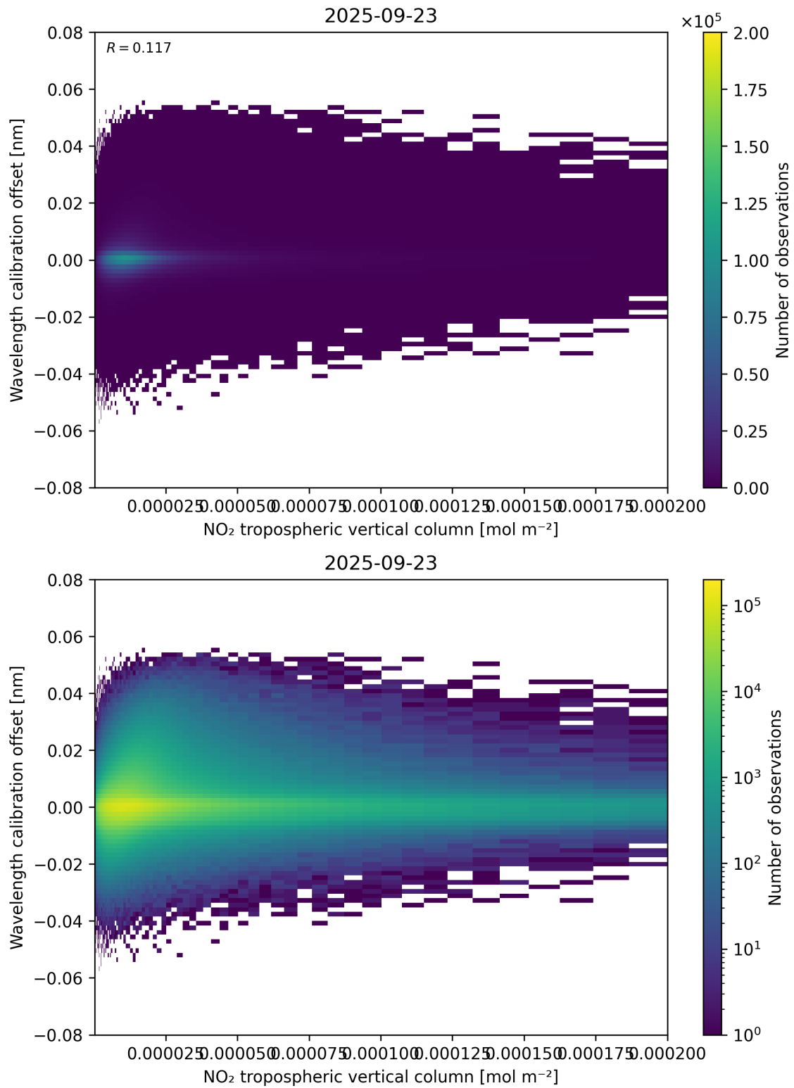
Figure 143: Scatter density plot of “NO 2 tropospheric vertical column” against “Wavelength calibration offset” for 2025-09-22 to 2025-09-24.
