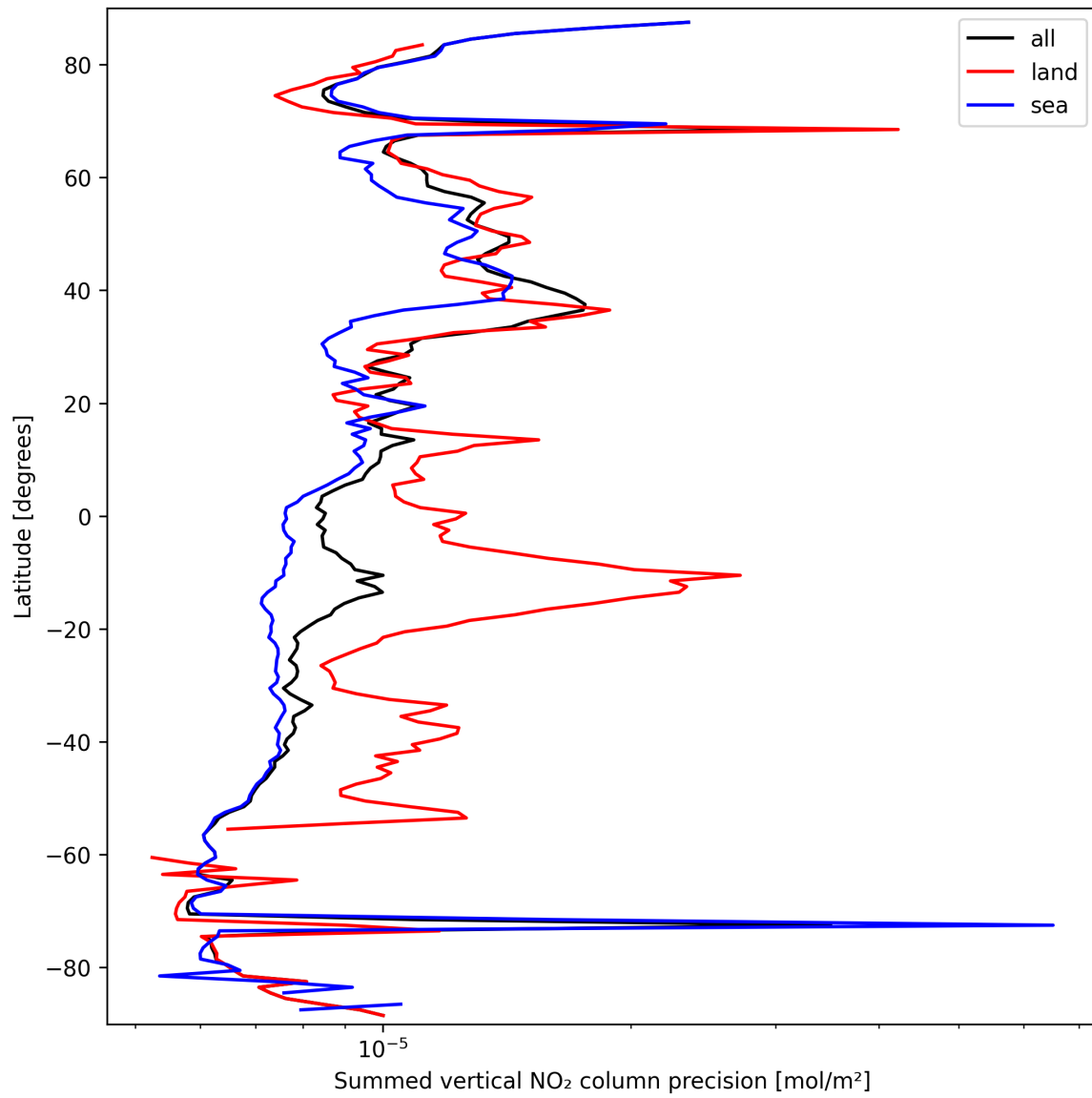
Figure 24: Zonal average of “Summed vertical NO 2 column precision” for 2025-09-22 to 2025-09-24.
