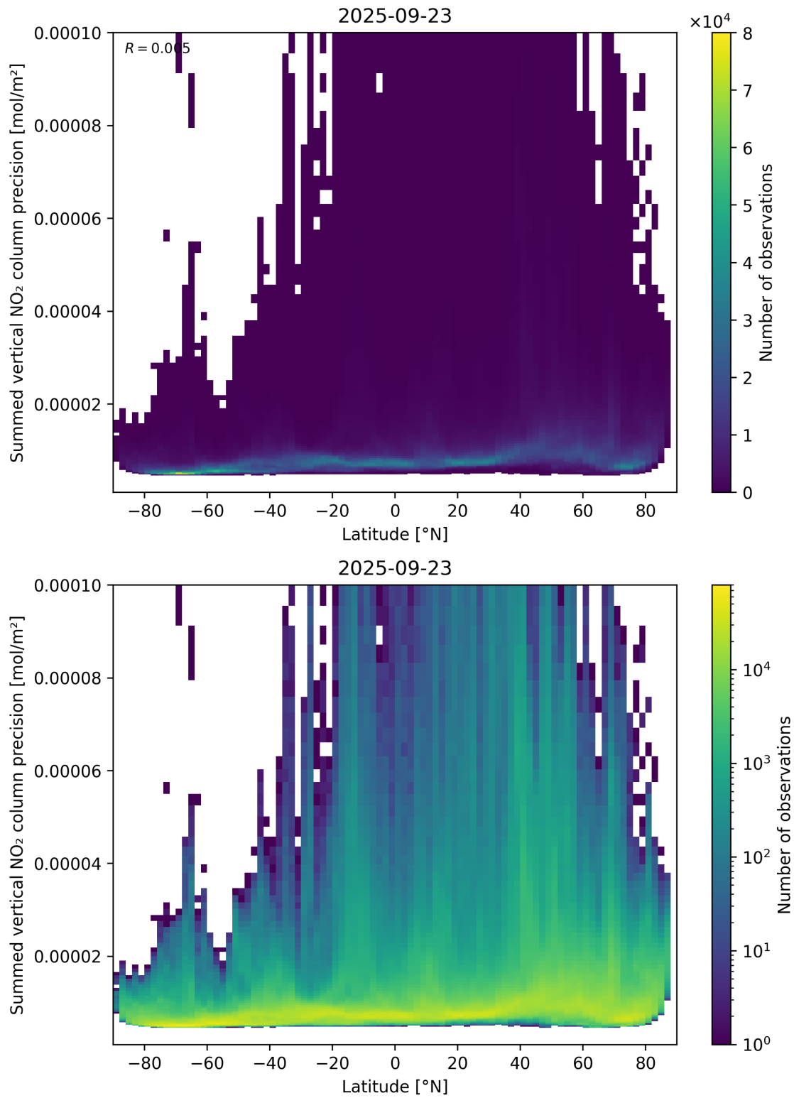
Figure 89: Scatter density plot of “Latitude” against “Summed vertical NO 2 column precision” for 2025-09-22 to 2025-09-24.
