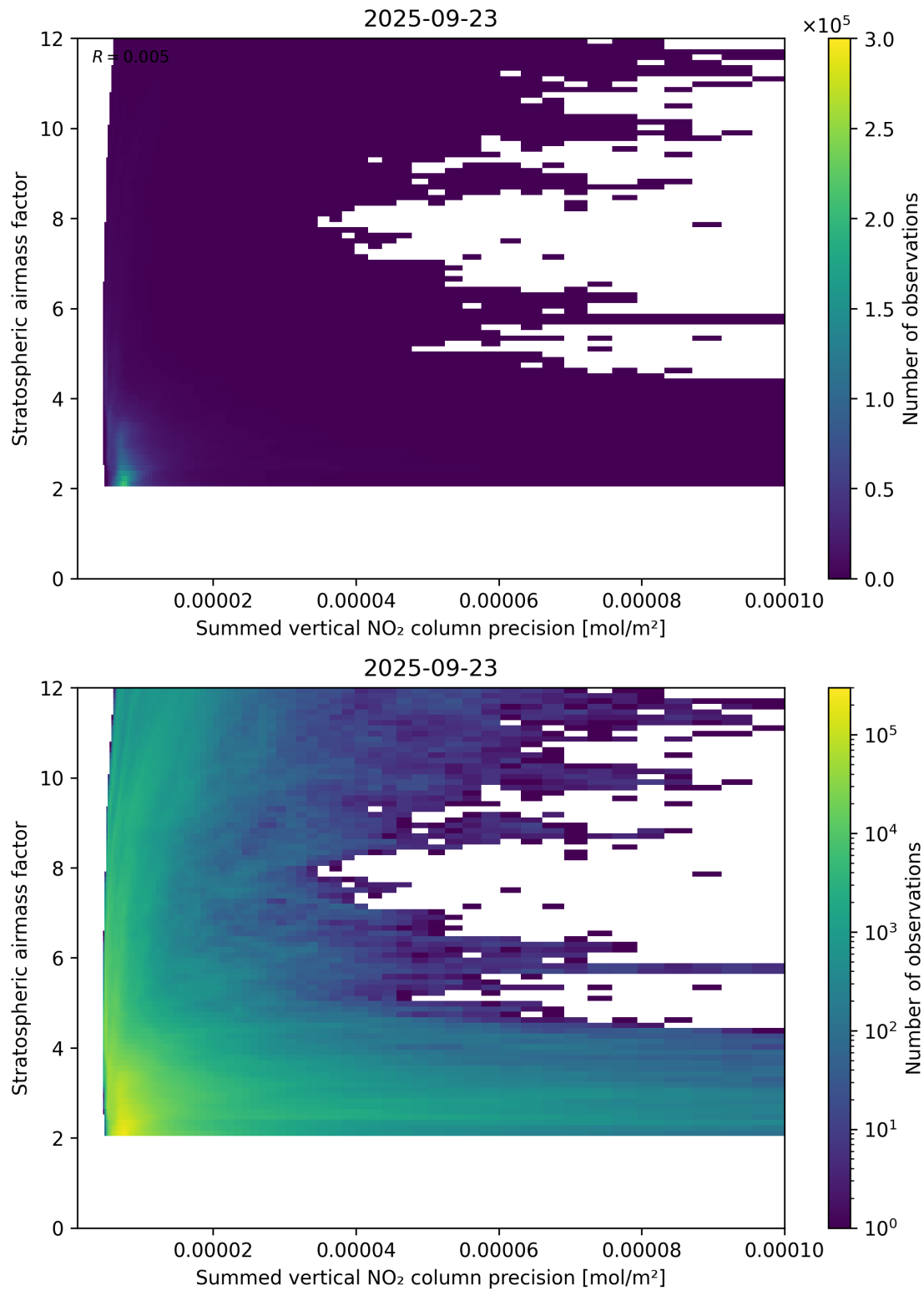
Figure 106: Scatter density plot of “Summed vertical NO 2 column precision” against “Stratospheric airmass factor” for 2025-09-22 to 2025-09-24.
