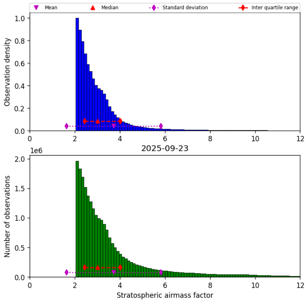
Figure 44: Histogram of “Stratospheric airmass factor” for 2025-09-22 to 2025-09-24
