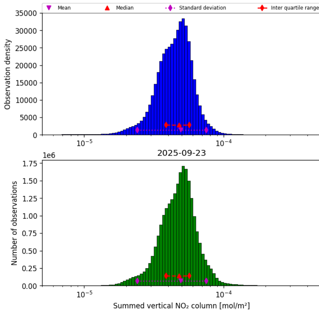
Figure 40: Histogram of “Summed vertical NO 2 column” for 2025-09-22 to 2025-09-24
