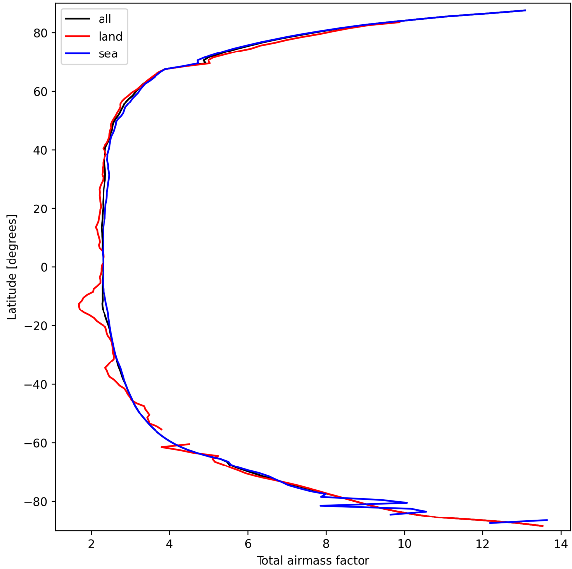
Figure 15: Zonal average of “Total airmass factor” for 2025-09-22 to 2025-09-24.
