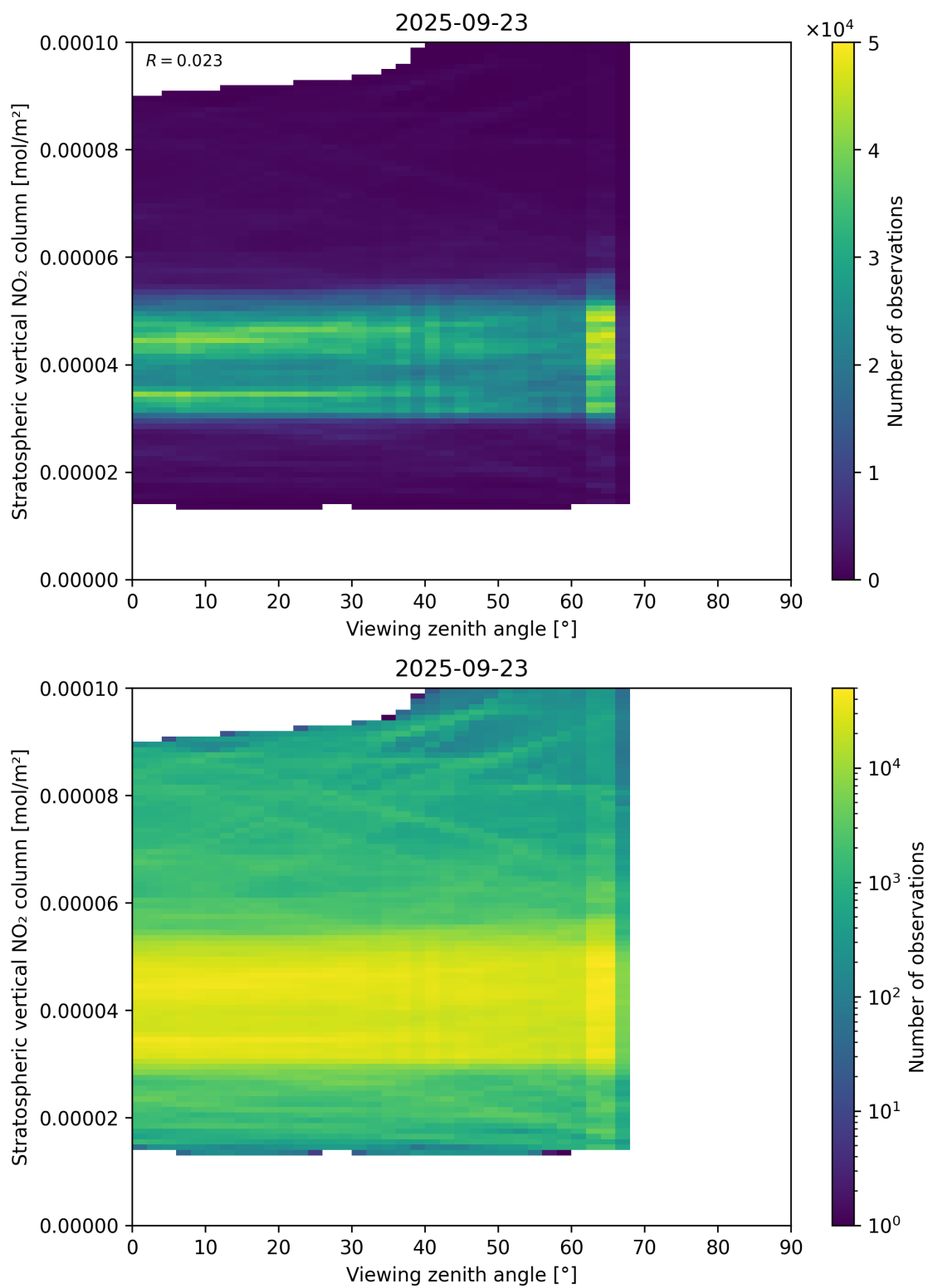
Figure 164: Scatter density plot of “Viewing zenith angle” against “Stratospheric vertical NO 2 column” for 2025-09-22 to 2025-09-24.
