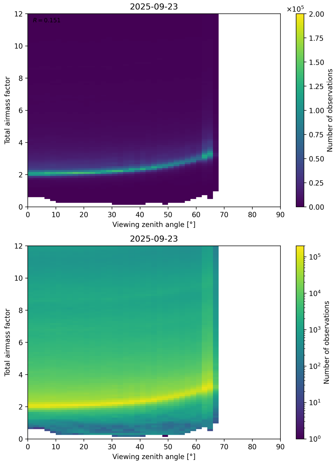
Figure 160: Scatter density plot of “Viewing zenith angle” against “Total airmass factor” for 2025-09-22 to 2025-09-24.
