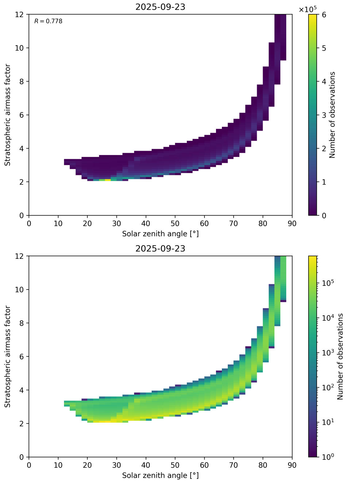
Figure 145: Scatter density plot of “Solar zenith angle” against “Stratospheric airmass factor” for 2025-09-22 to 2025-09-24.
