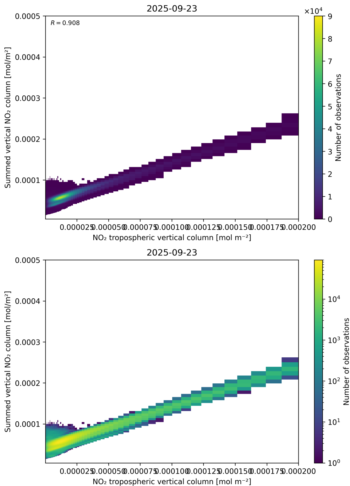
Figure 126: Scatter density plot of “NO 2 tropospheric vertical column” against “Summed vertical NO 2 column” for 2025-09-22 to 2025-09-24.
