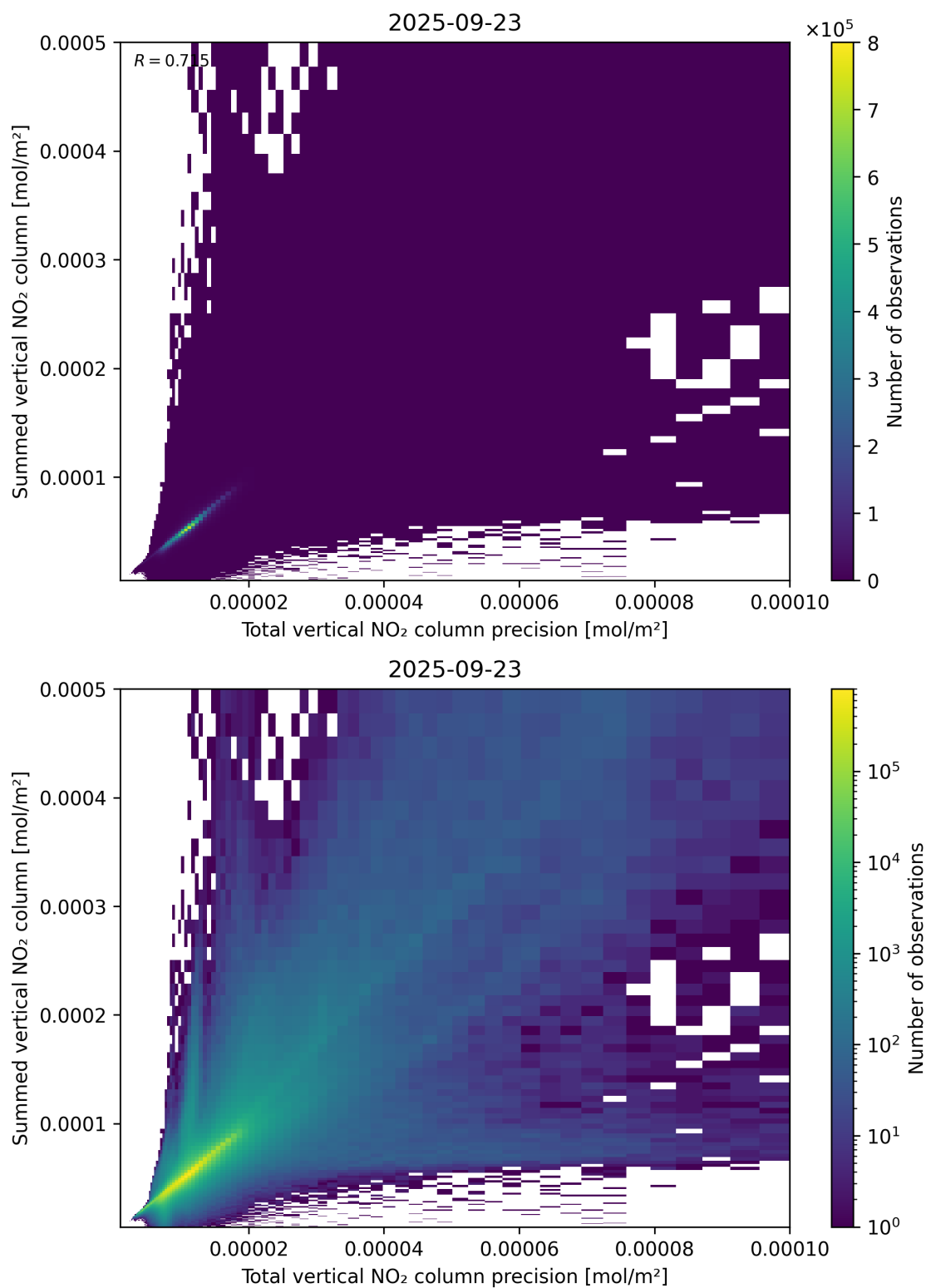
Figure 117: Scatter density plot of “Total vertical NO 2 column precision” against “Summed vertical NO 2 column” for 2025-09-22 to 2025-09-24.
