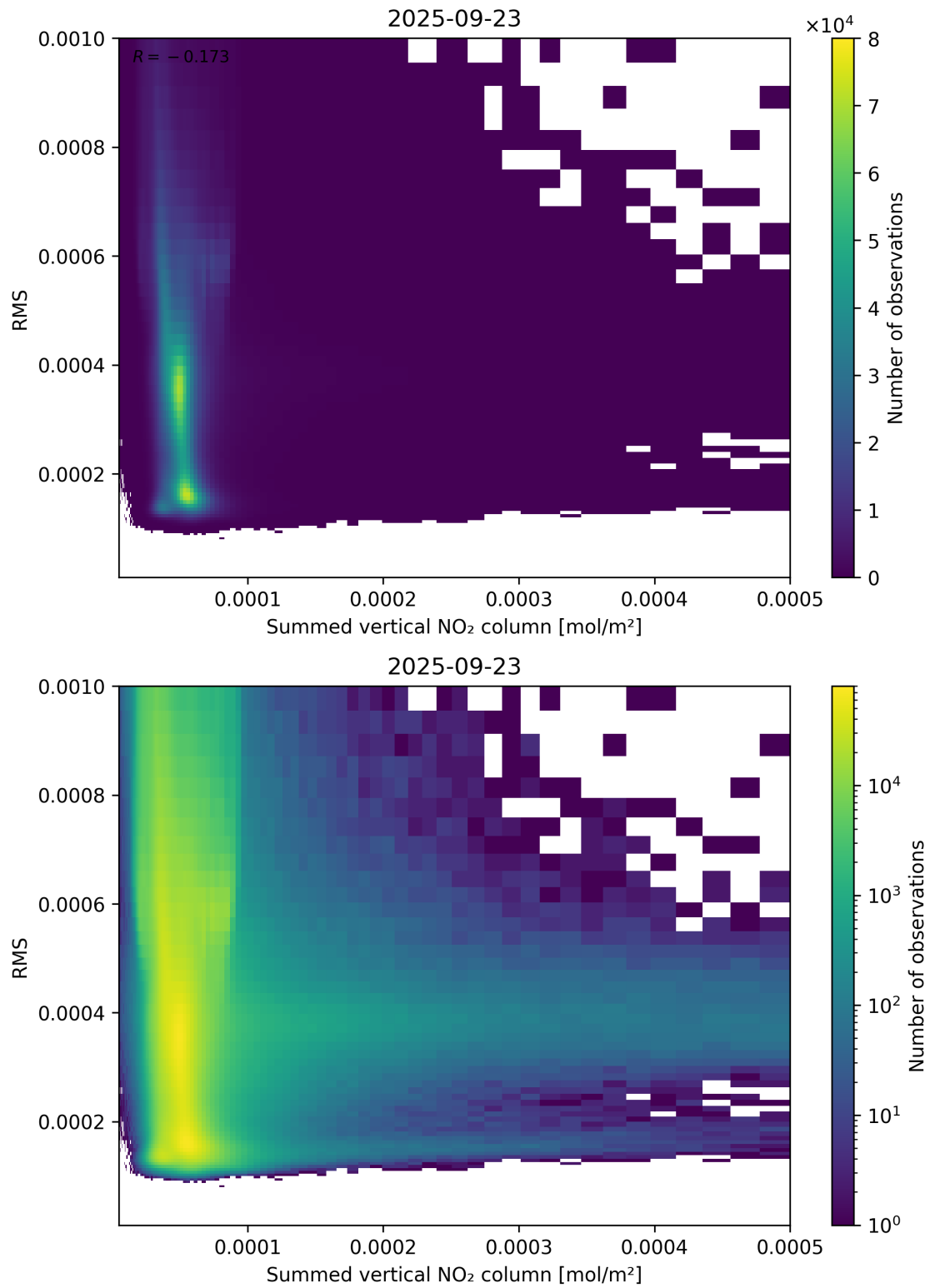
Figure 109: Scatter density plot of “Summed vertical NO 2 column” against “RMS” for 2025-09-22 to 2025-09-24.
