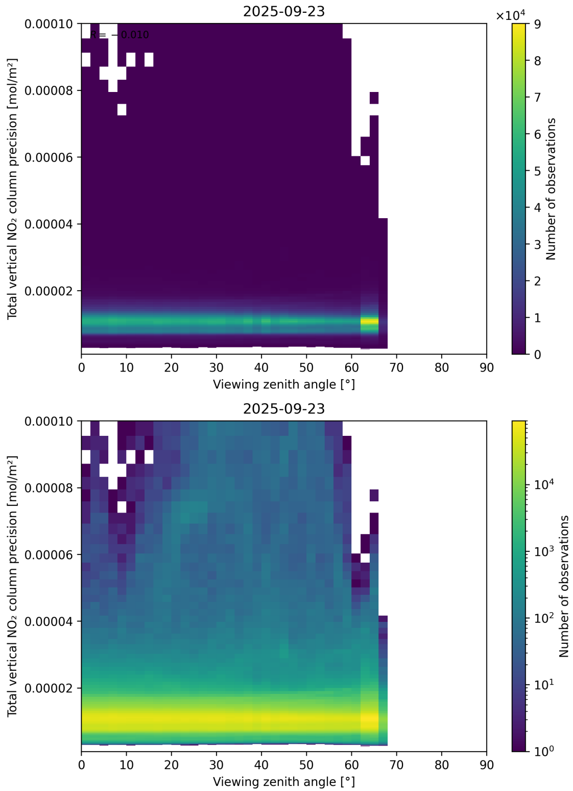
Figure 168: Scatter density plot of “Viewing zenith angle” against “Total vertical NO 2 column precision” for 2025-09-22 to 2025-09-24.
