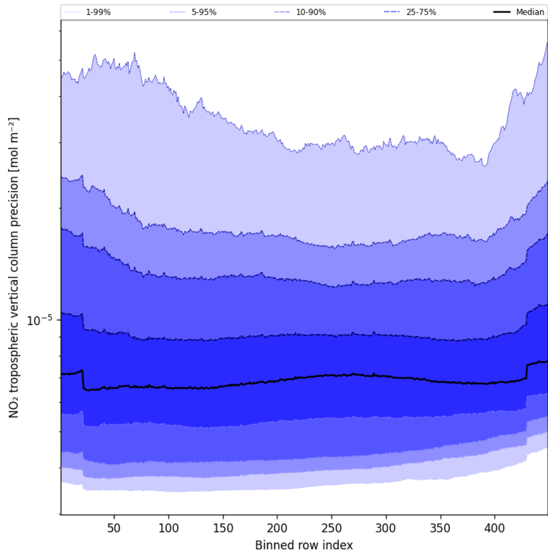
Figure 47: Along track statistics of “NO 2 tropospheric vertical column precision” for 2025-09-22 to 2025-09-24
