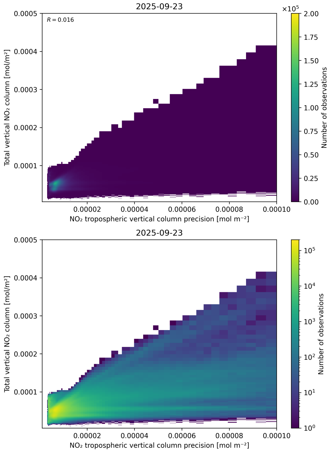
Figure 138: Scatter density plot of “NO 2 tropospheric vertical column precision” against “Total vertical NO 2 column” for 2025-09-22 to 2025-09-24.
