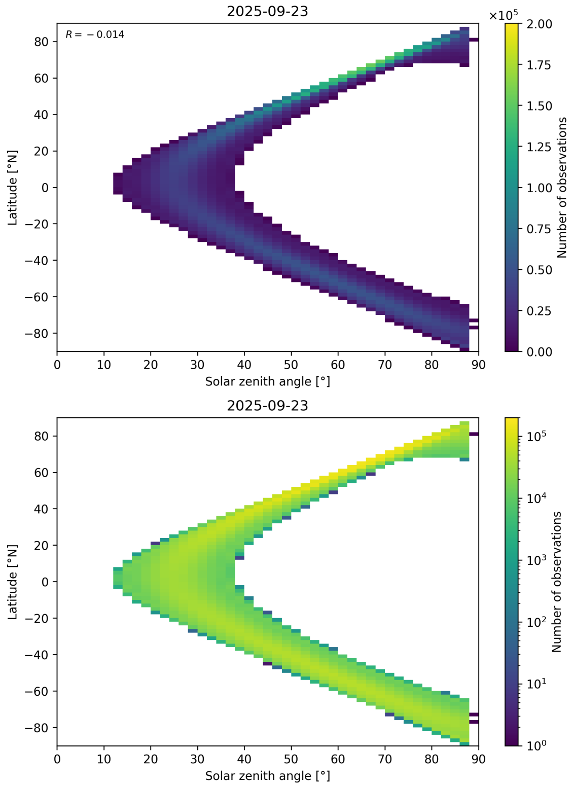
Figure 149: Scatter density plot of “Solar zenith angle” against “Latitude” for 2025-09-22 to 2025-09-24.
