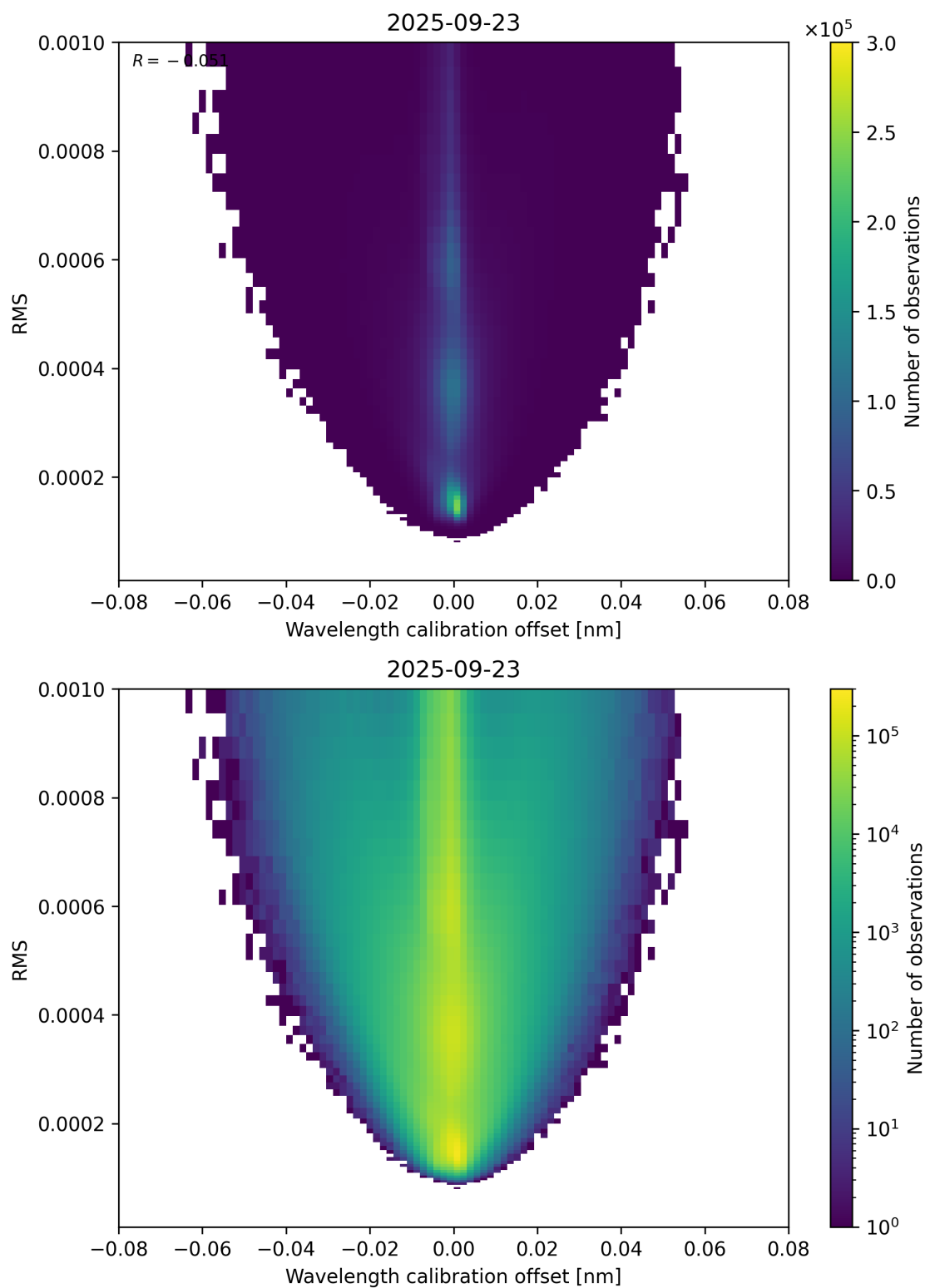
Figure 181: Scatter density plot of “Wavelength calibration offset” against “RMS” for 2025-09-22 to 2025-09-24.
