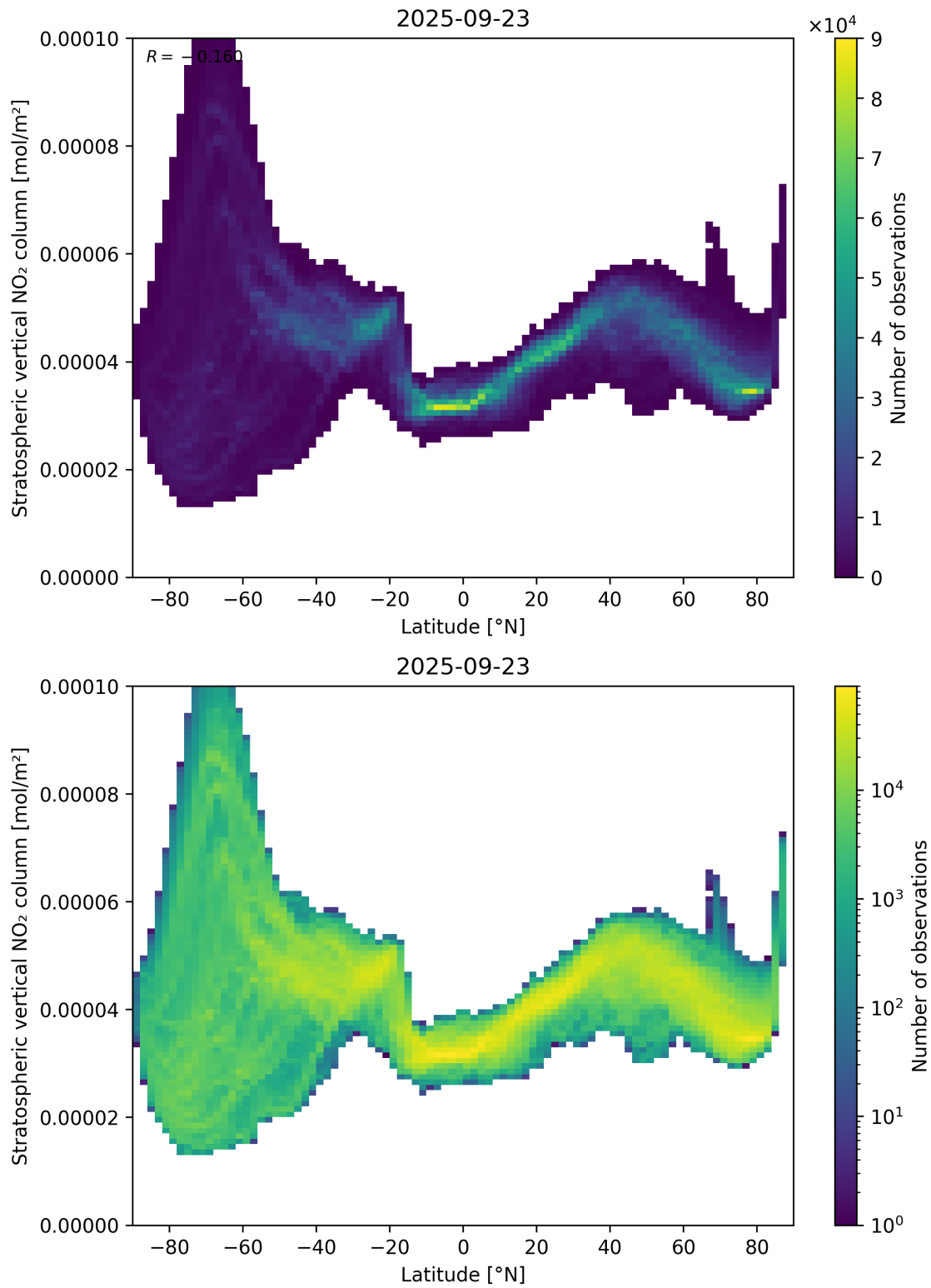
Figure 87: Scatter density plot of “Latitude” against “Stratospheric vertical NO 2 column” for 2025-09-22 to 2025-09-24.
