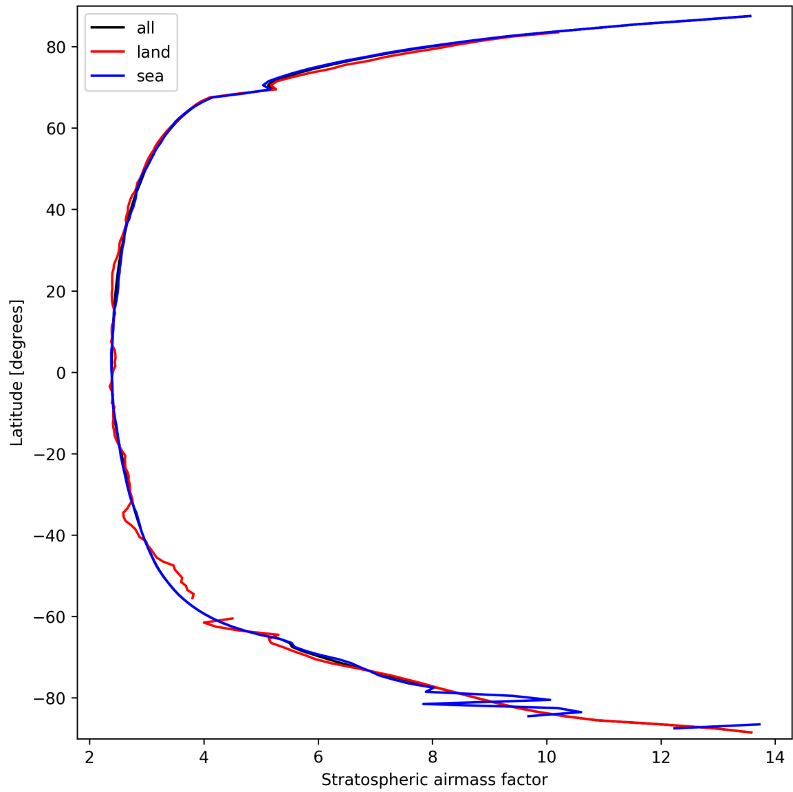
Figure 27: Zonal average of “Stratospheric air mass factor” for 2025-09-22 to 2025-09-24.
