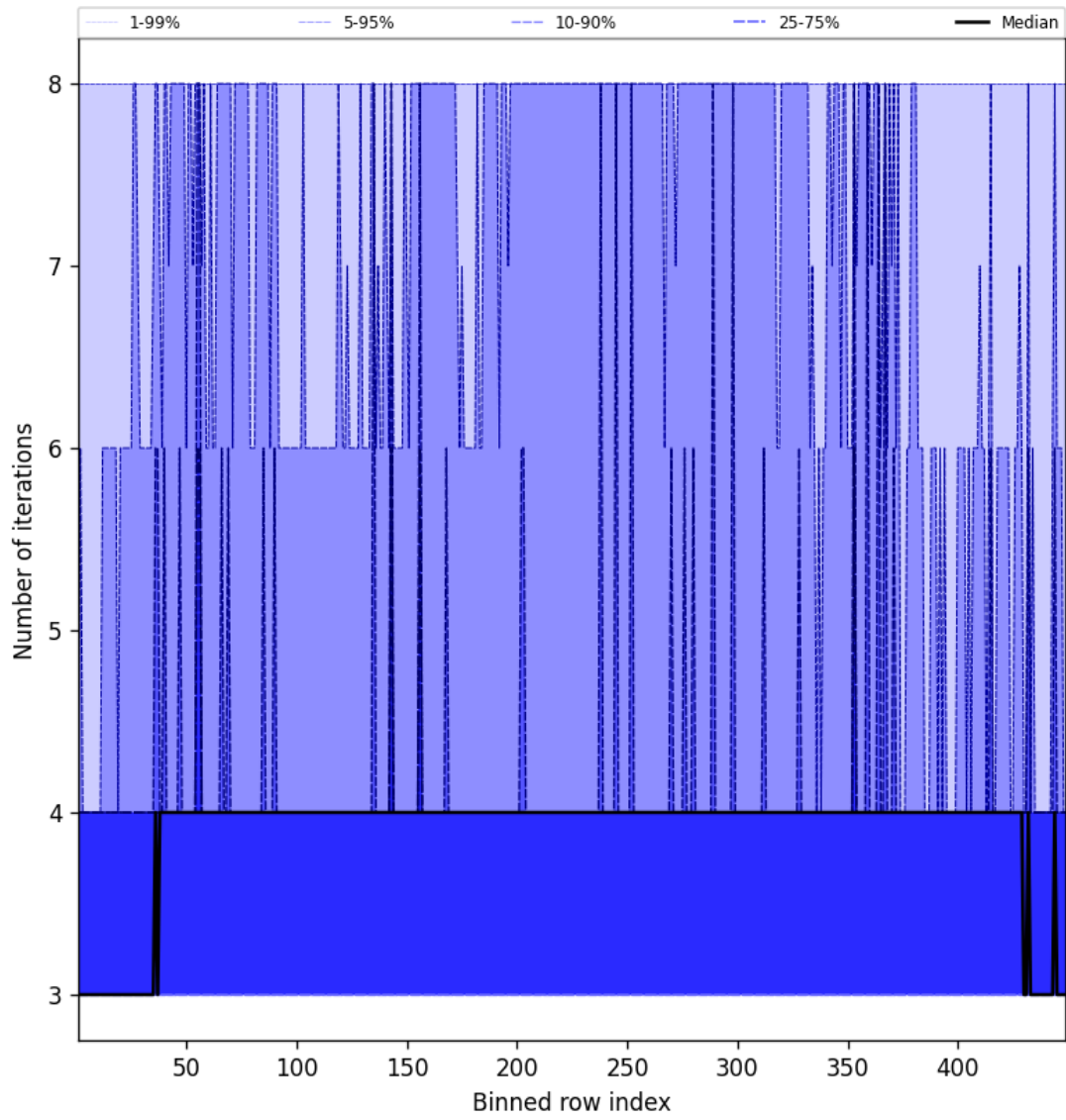
Figure 51: Along track statistics of “Number of iterations” for 2025-09-22 to 2025-09-24
