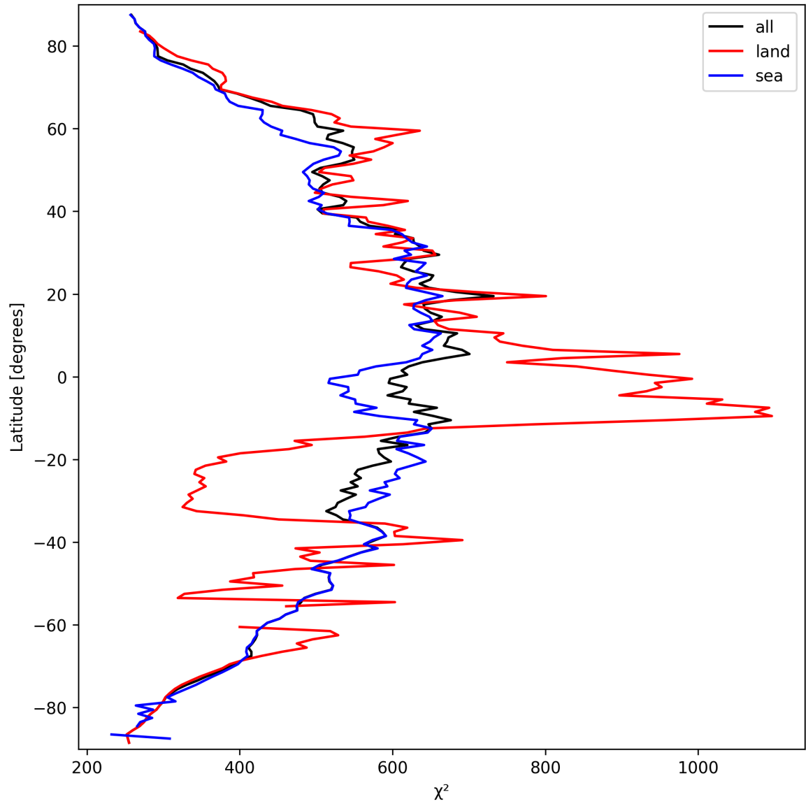
Figure 25: Zonal average of “ \chi^2 ” for 2025-09-22 to 2025-09-24.
