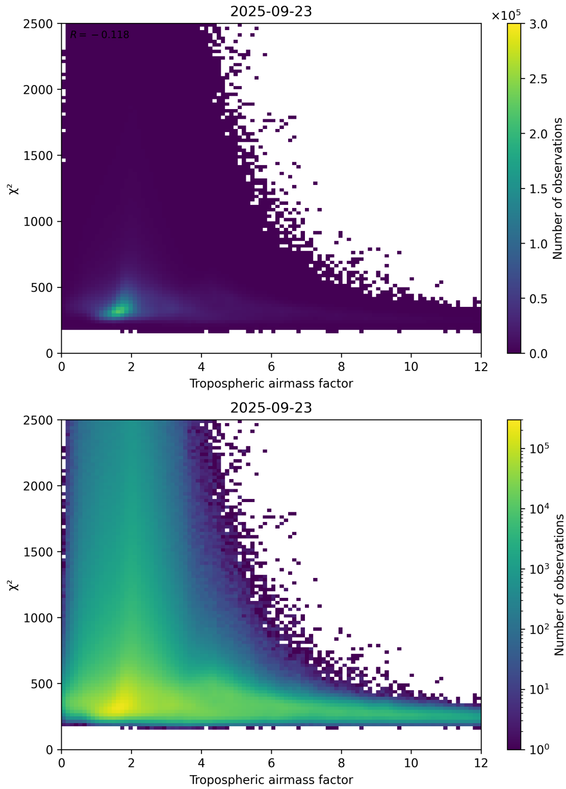
Figure 73: Scatter density plot of “Tropospheric airmass factor” against “ \chi^2 ” for 2025-09-22 to 2025-09-24.
