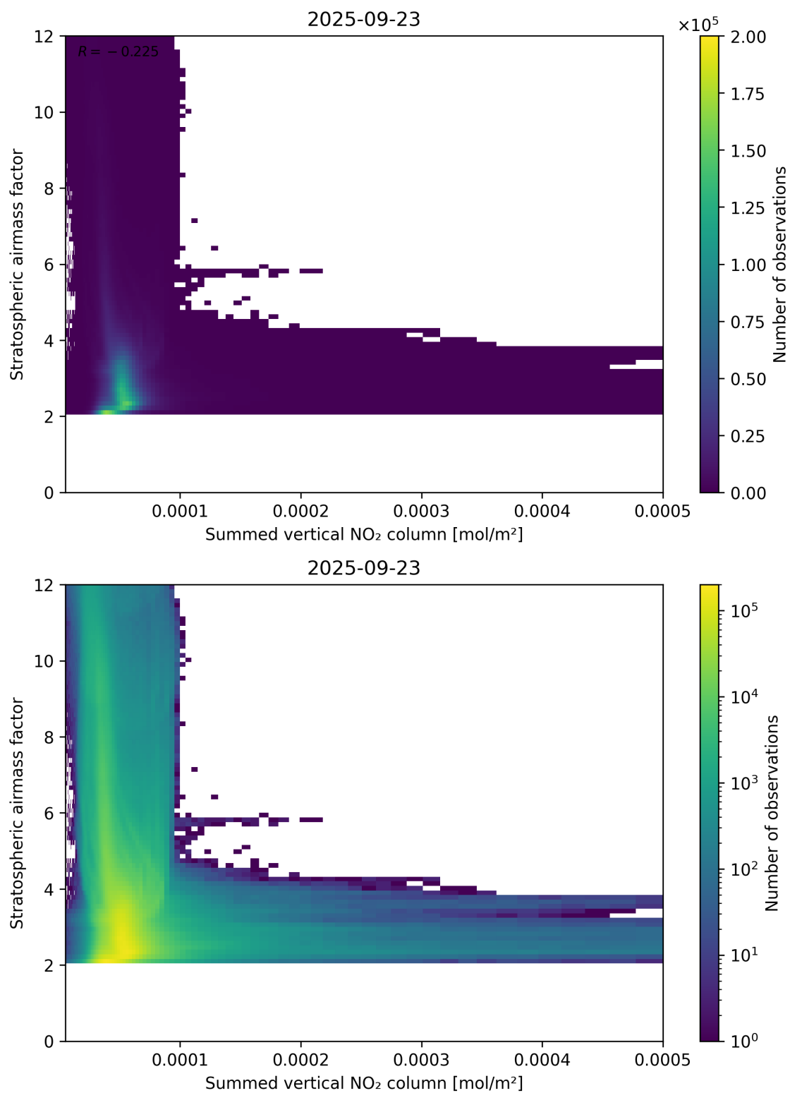
Figure 103: Scatter density plot of “Summed vertical NO 2 column” against “Stratospheric airmass factor” for 2025-09-22 to 2025-09-24.
