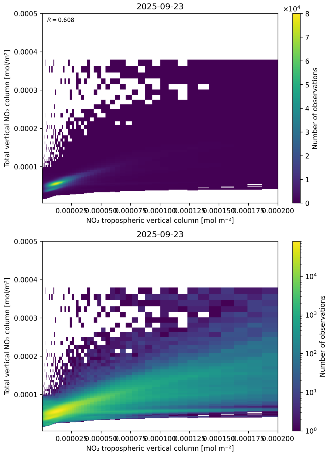
Figure 128: Scatter density plot of “NO 2 tropospheric vertical column” against “Total vertical NO 2 column” for 2025-09-22 to 2025-09-24.
