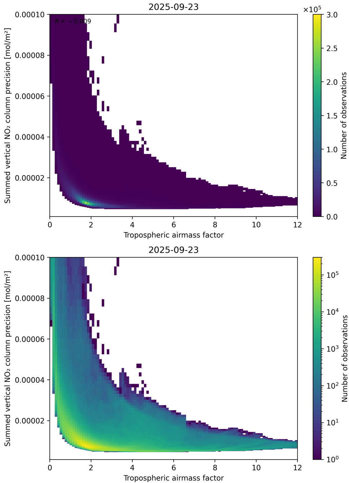
Figure 76: Scatter density plot of “Tropospheric airmass factor” against “Summed vertical NO 2 column precision” for 2025-09-22 to 2025-09-24.
