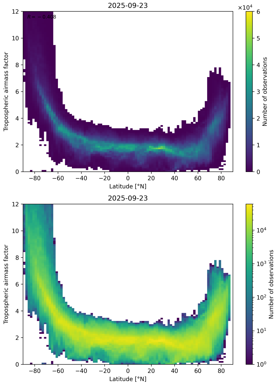
Figure 85: Scatter density plot of “Latitude” against “Tropospheric airmass factor” for 2025-09-22 to 2025-09-24.
