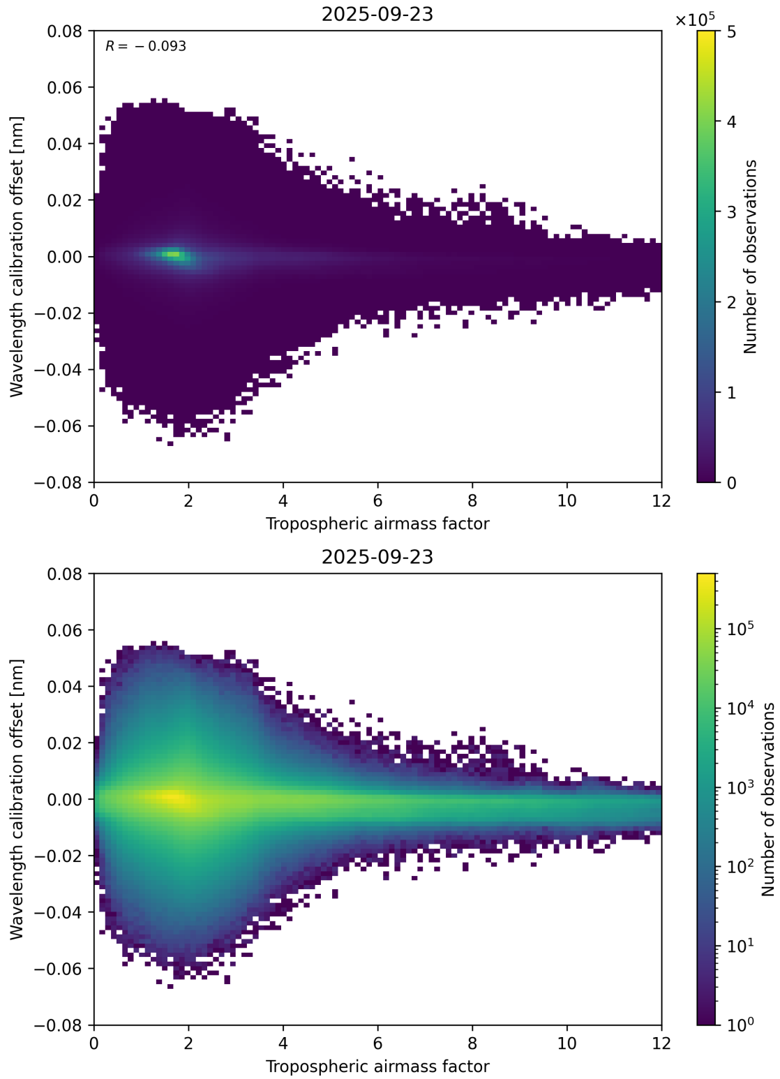
Figure 80: Scatter density plot of “Tropospheric airmass factor” against “Wavelength calibration offset” for 2025-09-22 to 2025-09-24.
