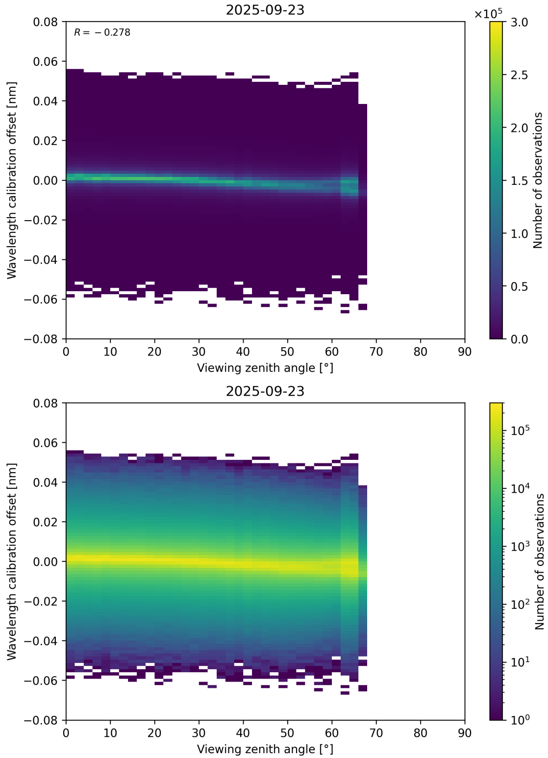
Figure 173: Scatter density plot of “Viewing zenith angle” against “Wavelength calibration offset” for 2025-09-22 to 2025-09-24.
