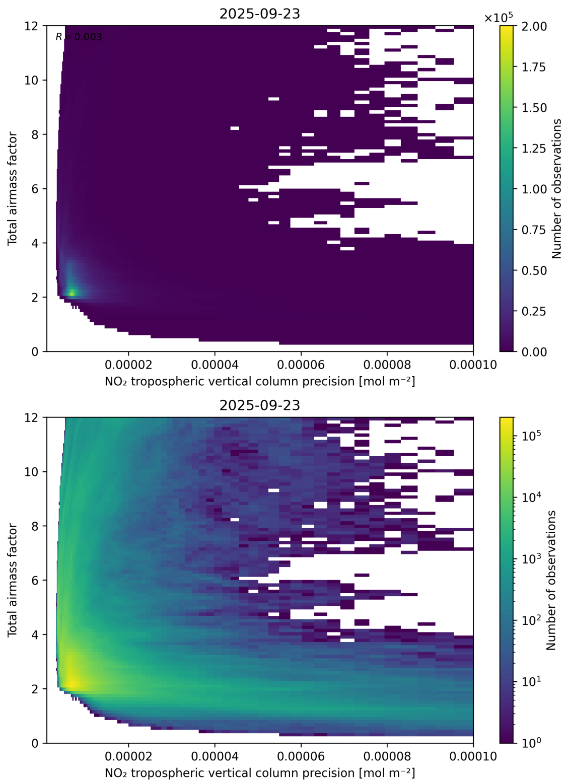
Figure 132: Scatter density plot of “NO 2 tropospheric vertical column precision” against “Total air mass factor” for 2025-09-22 to 2025-09-24.
