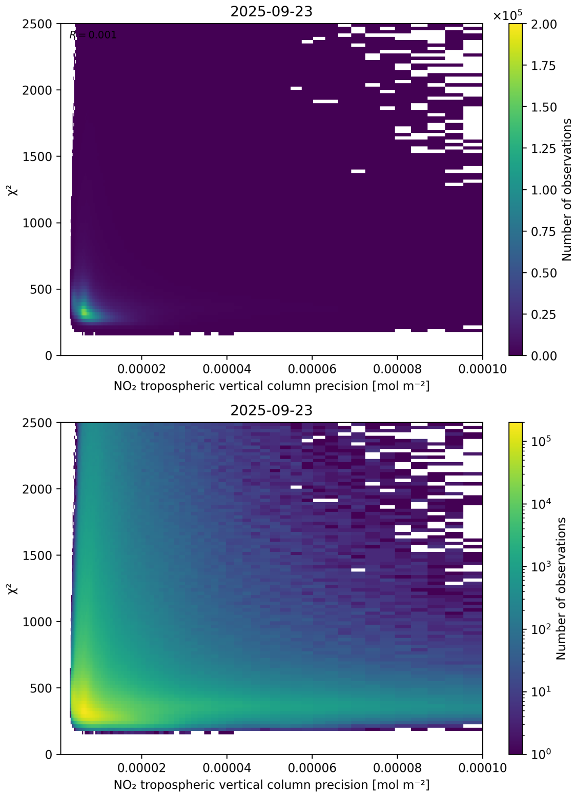
Figure 134: Scatter density plot of “NO 2 tropospheric vertical column precision” against “ \chi^2 ” for 2025-09-22 to 2025-09-24.
