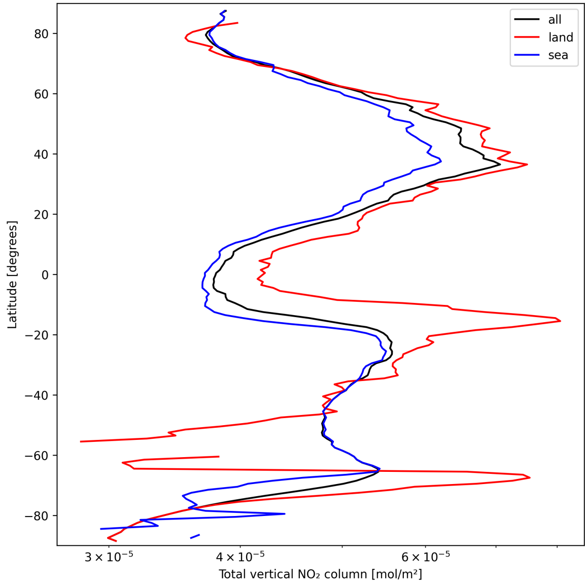
Figure 21: Zonal average of “Total vertical NO 2 column” for 2025-09-22 to 2025-09-24.
