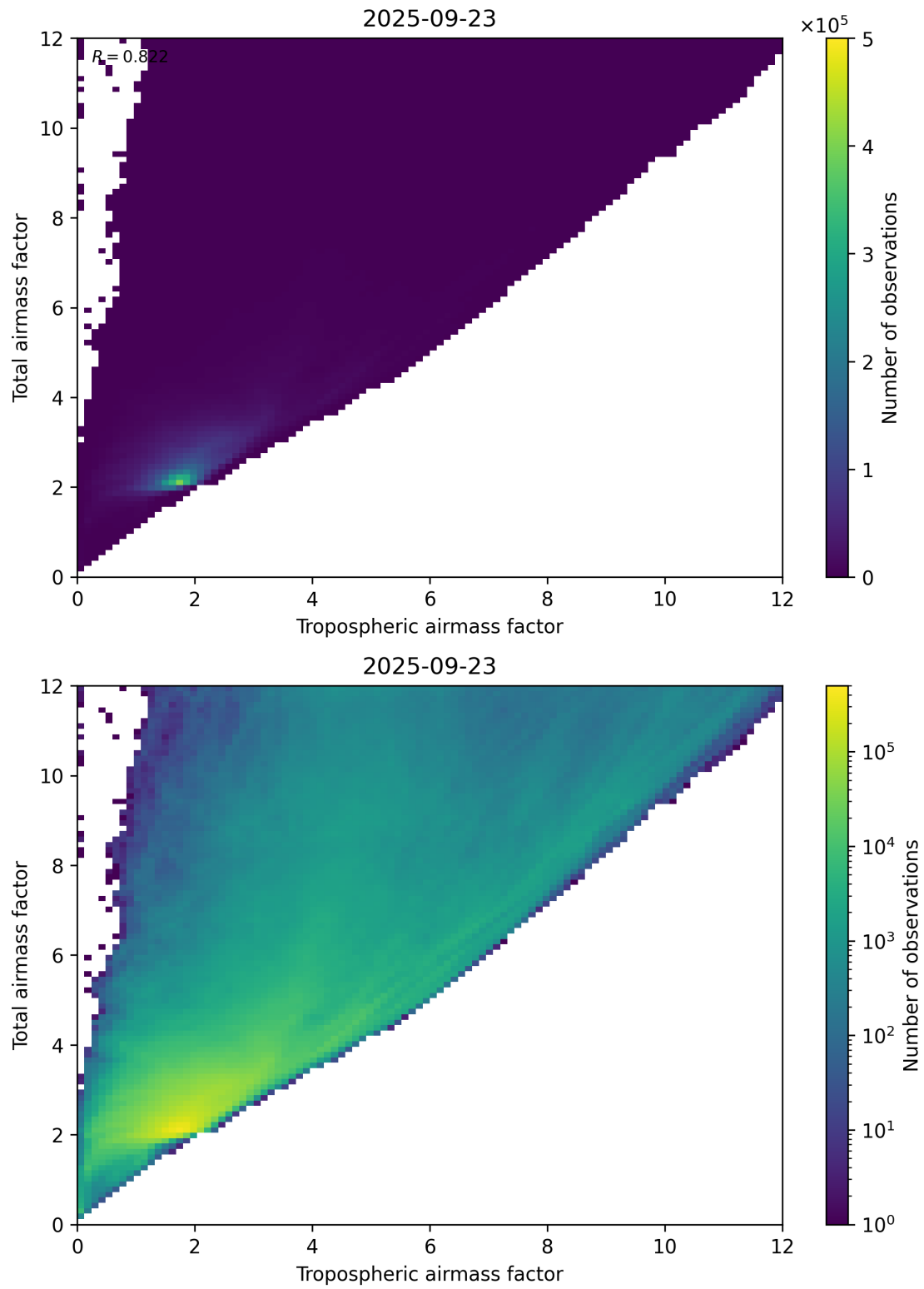
Figure 72: Scatter density plot of “Tropospheric airmass factor” against “Total airmass factor” for 2025-09-22 to 2025-09-24.
