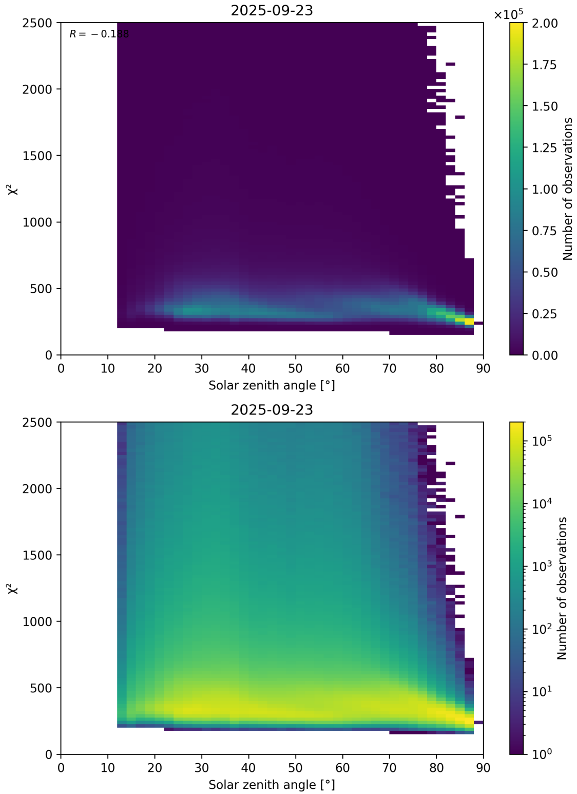
Figure 148: Scatter density plot of “Solar zenith angle” against “ \chi^2 ” for 2025-09-22 to 2025-09-24.
