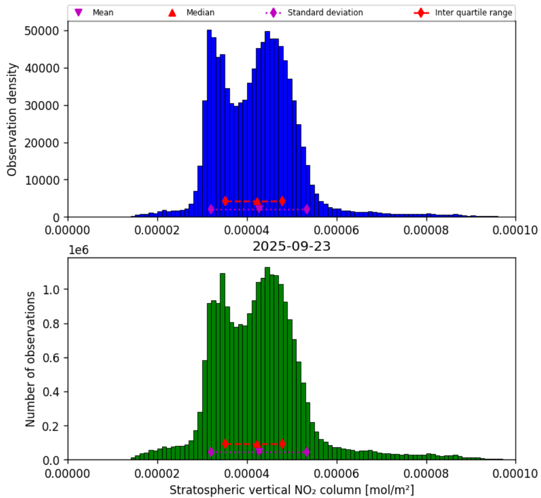
Figure 36: Histogram of “Stratospheric vertical NO 2 column” for 2025-09-22 to 2025-09-24
