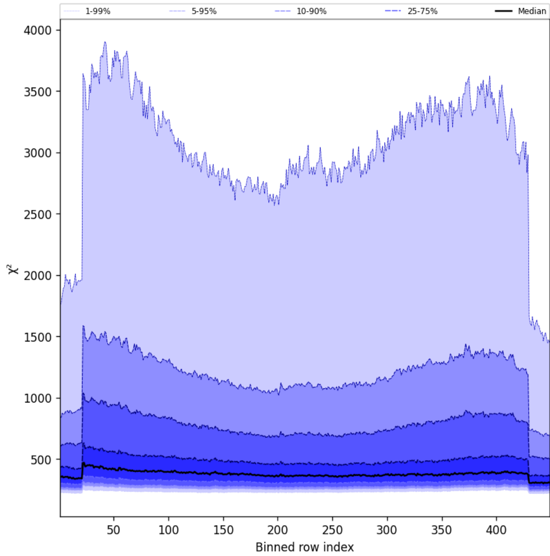
Figure 59: Along track statistics of “ \chi^2 ” for 2025-09-22 to 2025-09-24
