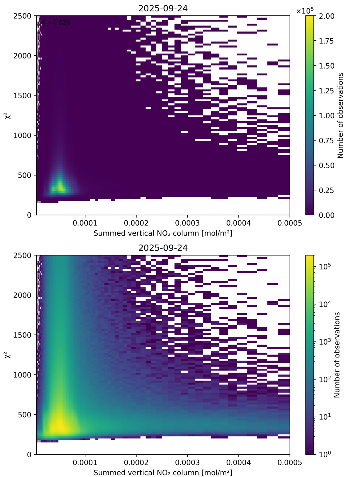
Figure 104: Scatter density plot of “Summed vertical NO 2 column” against “ \chi^2 ” for 2025-09-23 to 2025-09-25.
