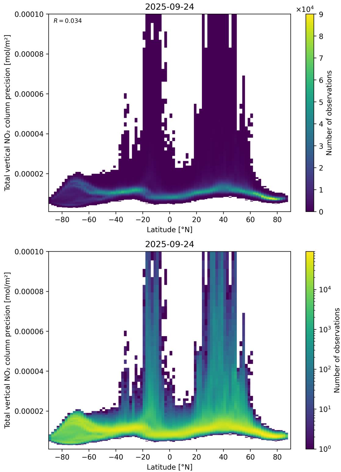
Figure 91: Scatter density plot of “Latitude” against “Total vertical NO 2 column precision” for 2025-09-23 to 2025-09-25.
