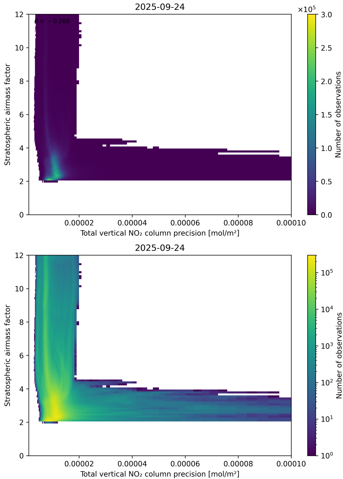
Figure 115: Scatter density plot of “Total vertical NO 2 column precision” against “Stratospheric air mass factor” for 2025-09-23 to 2025-09-25.
