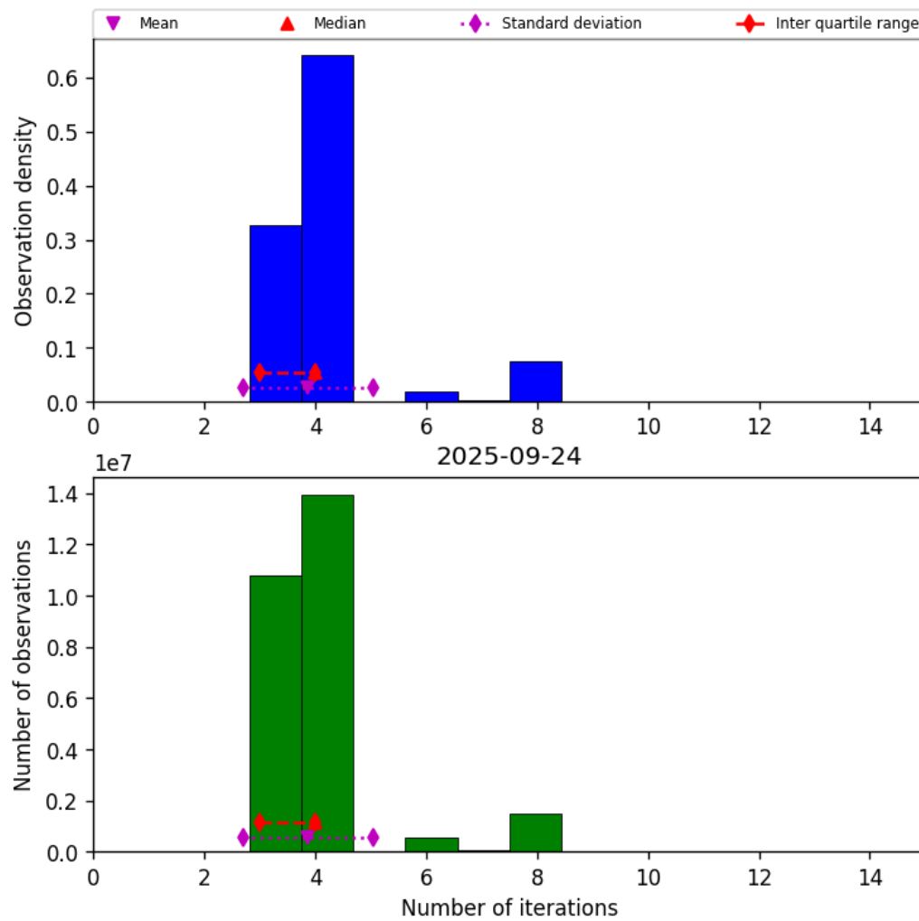
Figure 34: Histogram of “Number of iterations” for 2025-09-23 to 2025-09-25
