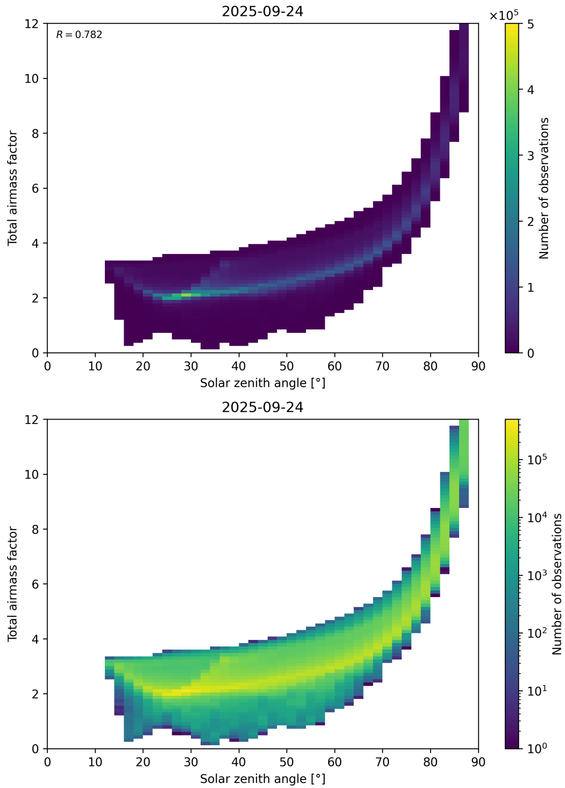
Figure 146: Scatter density plot of “Solar zenith angle” against “Total airmass factor” for 2025-09-23 to 2025-09-25.
