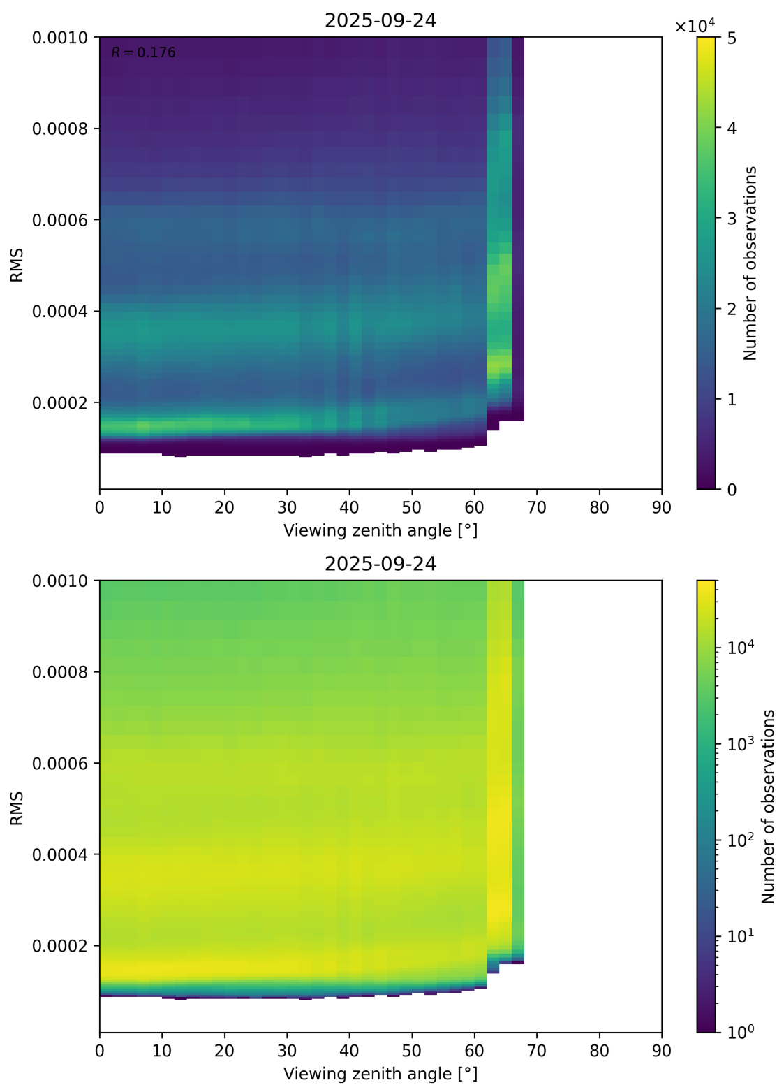
Figure 171: Scatter density plot of “Viewing zenith angle” against “RMS” for 2025-09-23 to 2025-09-25.
