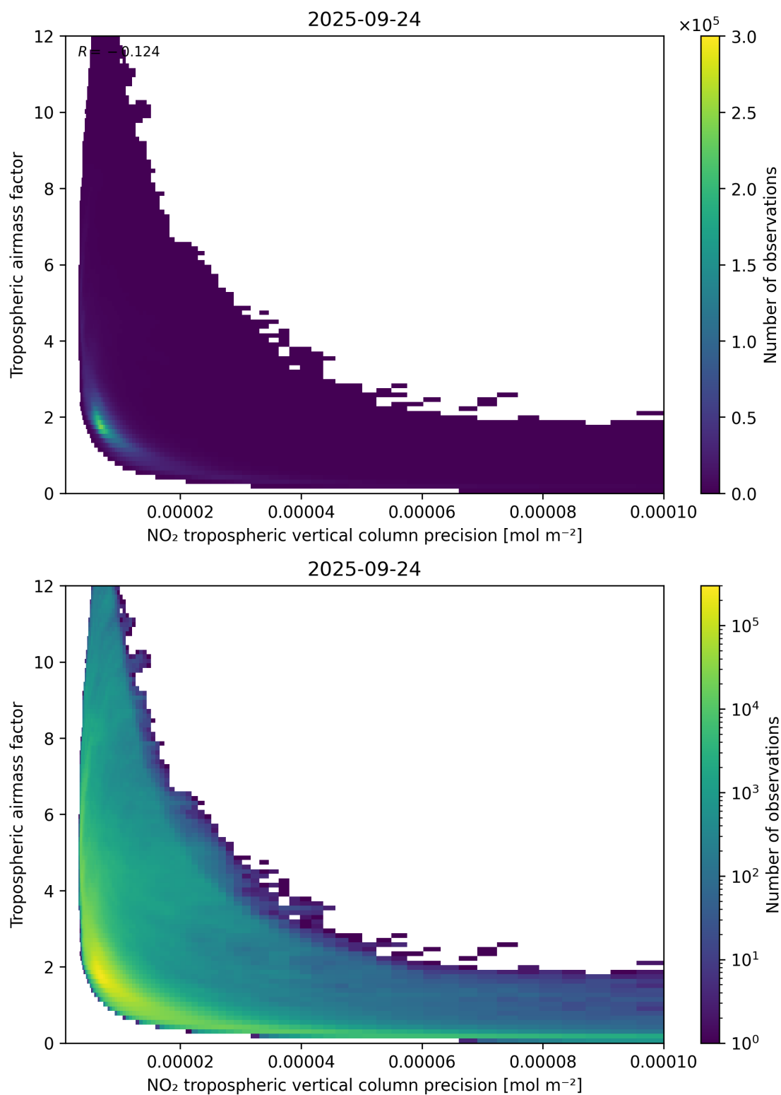
Figure 133: Scatter density plot of “NO 2 tropospheric vertical column precision” against “Tropospheric airmass factor” for 2025-09-23 to 2025-09-25.
