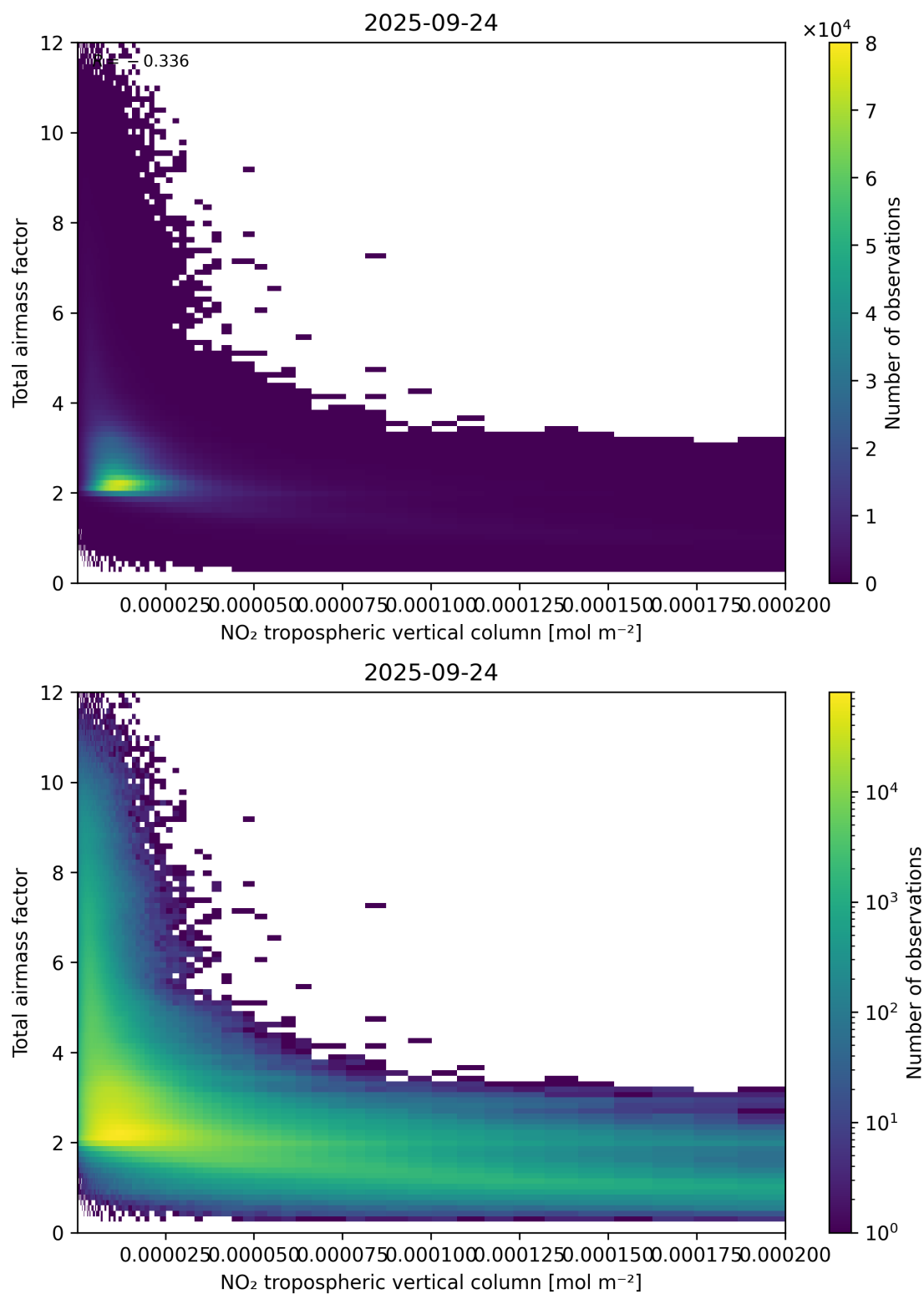
Figure 122: Scatter density plot of “NO 2 tropospheric vertical column” against “Total airmass factor” for 2025-09-23 to 2025-09-25.
