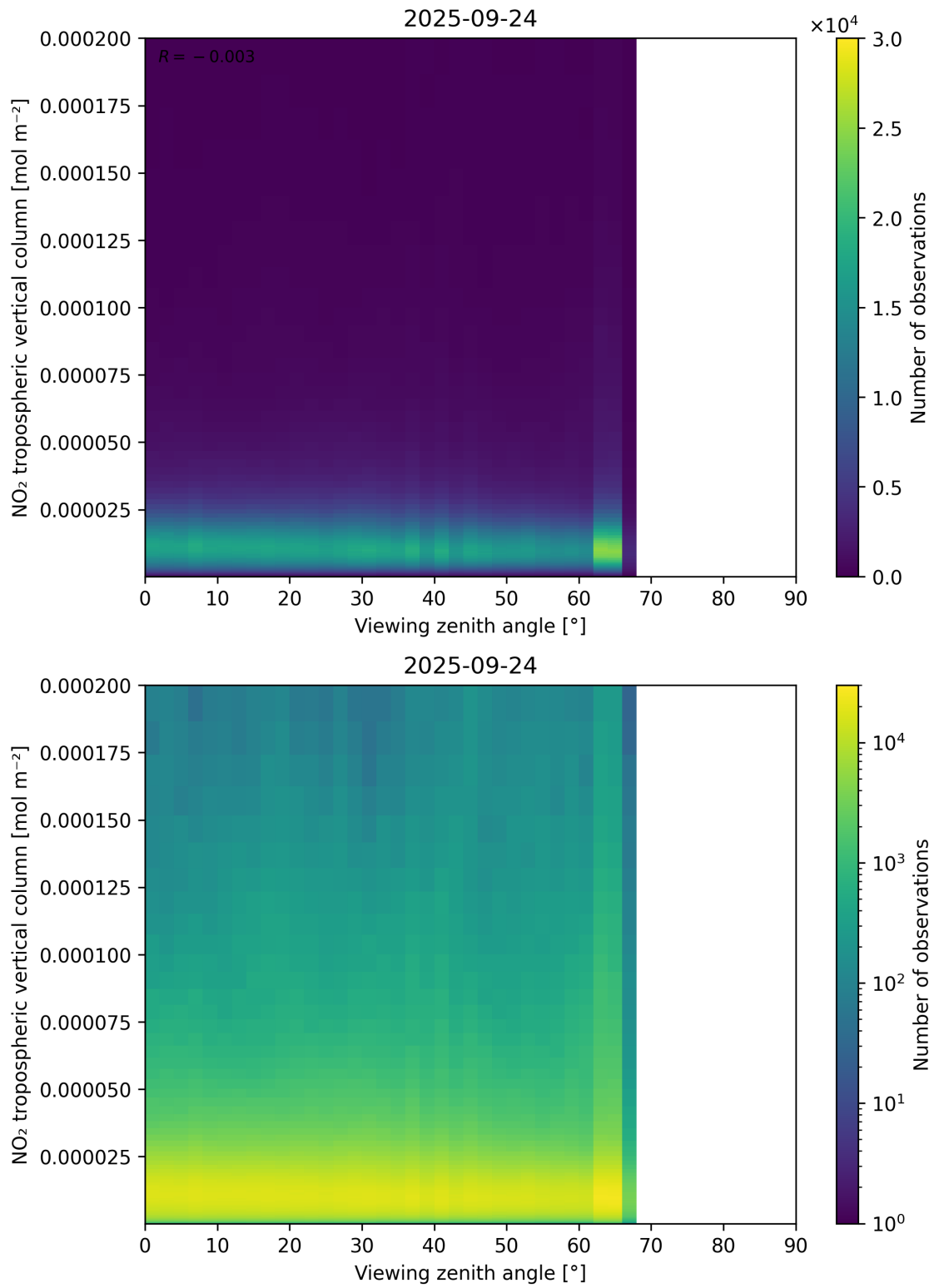
Figure 169: Scatter density plot of “Viewing zenith angle” against “NO 2 tropospheric vertical column” for 2025-09-23 to 2025-09-25.
