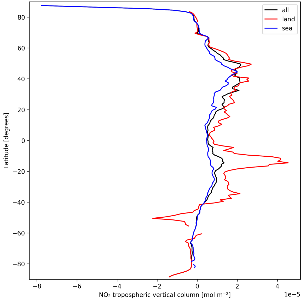
Figure 12: Zonal average of “NO 2 tropospheric vertical column” for 2025-09-23 to 2025-09-25.
