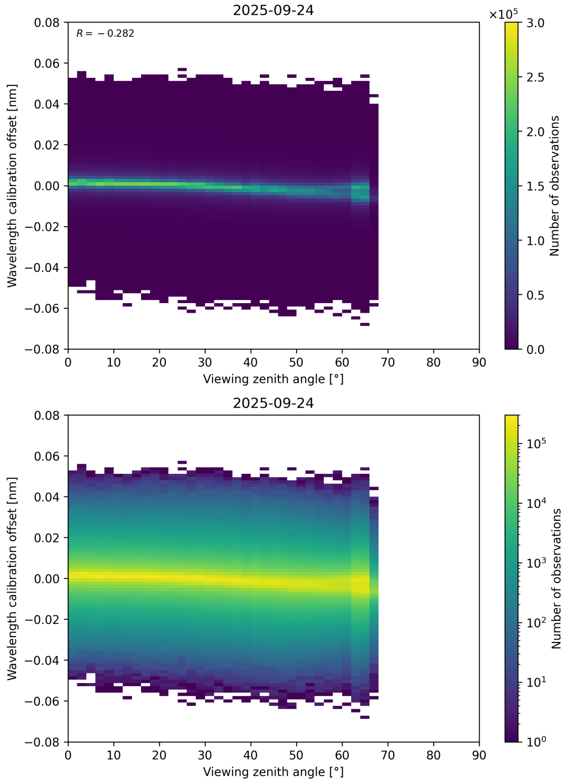
Figure 173: Scatter density plot of “Viewing zenith angle” against “Wavelength calibration offset” for 2025-09-23 to 2025-09-25.
