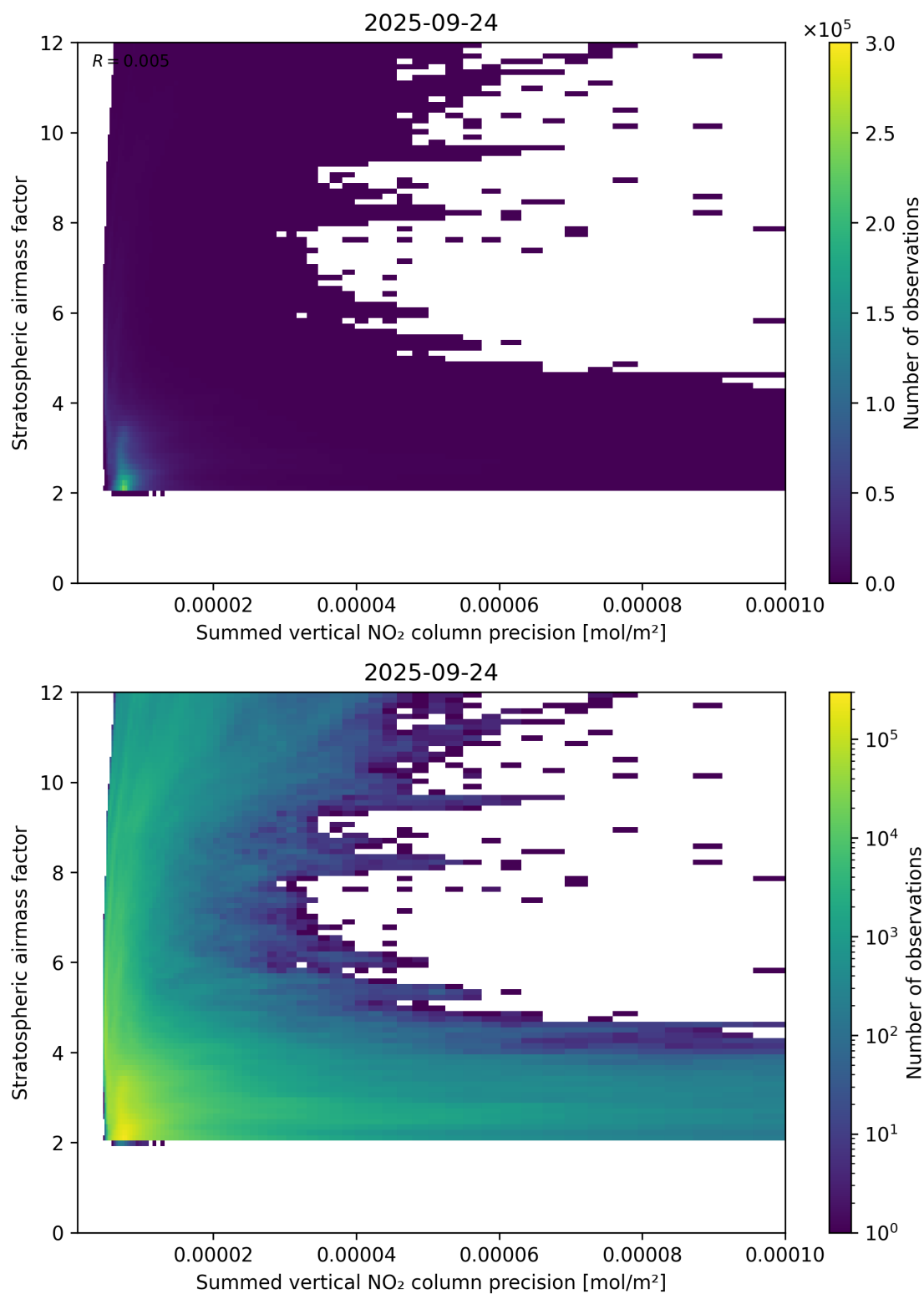
Figure 106: Scatter density plot of “Summed vertical NO 2 column precision” against “Stratospheric airmass factor” for 2025-09-23 to 2025-09-25.
