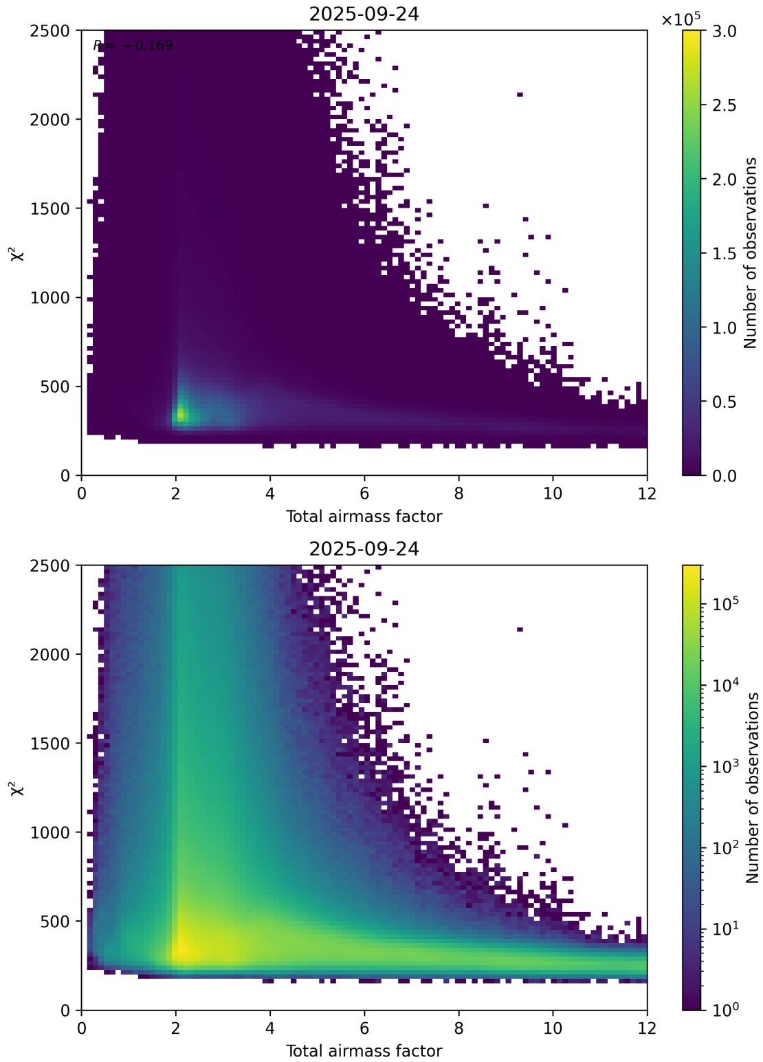
Figure 63: Scatter density plot of “Total airmass factor” against “ \chi^2 ” for 2025-09-23 to 2025-09-25.
