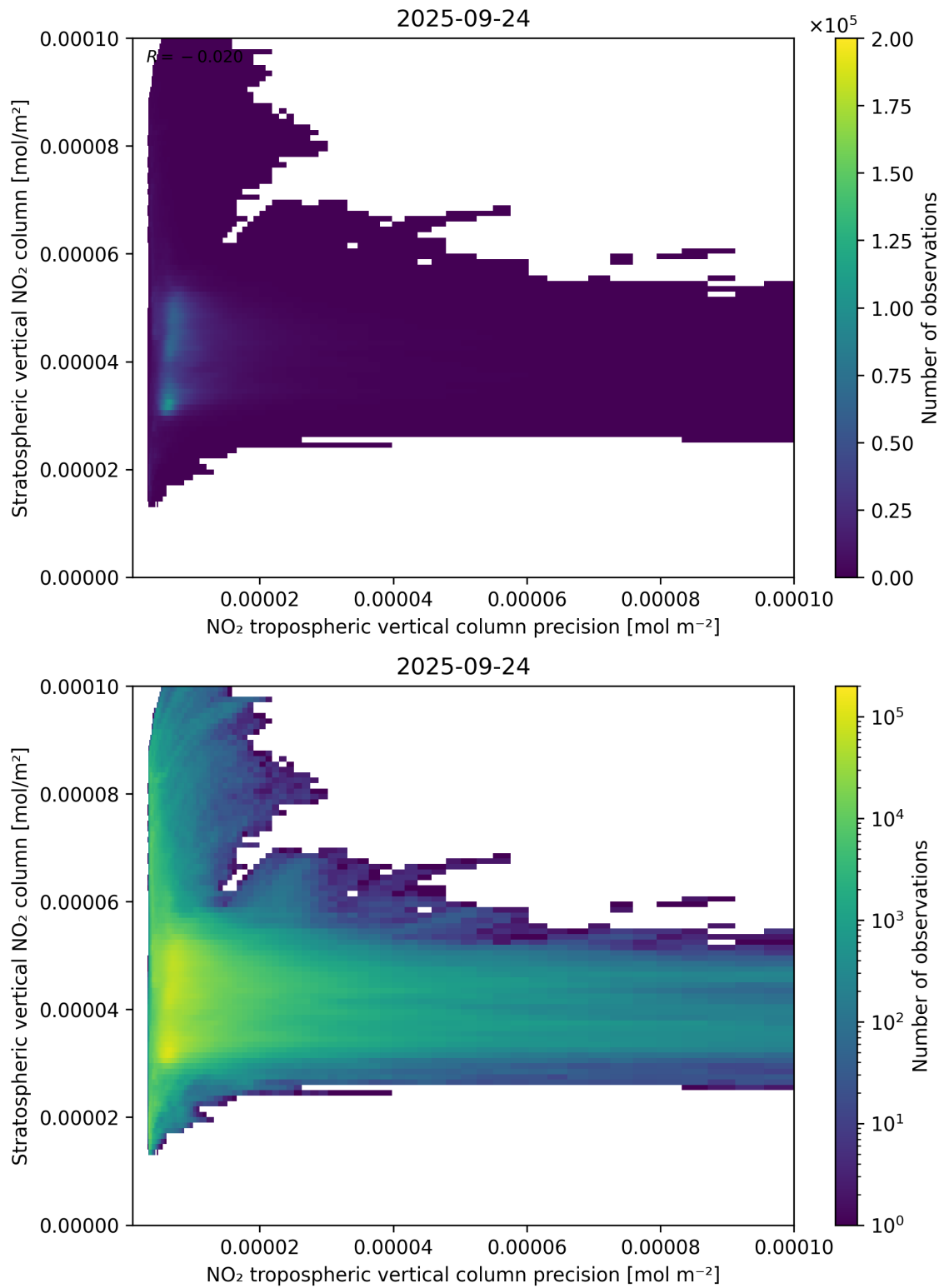
Figure 135: Scatter density plot of “NO 2 tropospheric vertical column precision” against “Stratospheric vertical NO 2 column” for 2025-09-23 to 2025-09-25.
