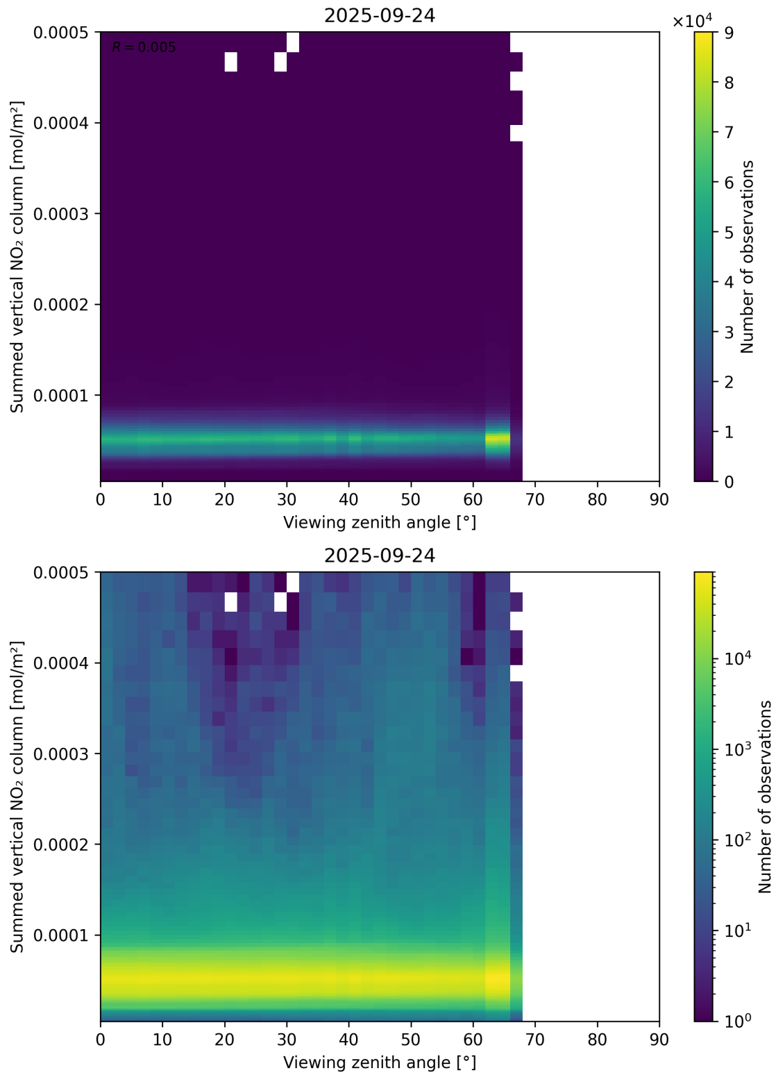
Figure 165: Scatter density plot of “Viewing zenith angle” against “Summed vertical NO 2 column” for 2025-09-23 to 2025-09-25.
