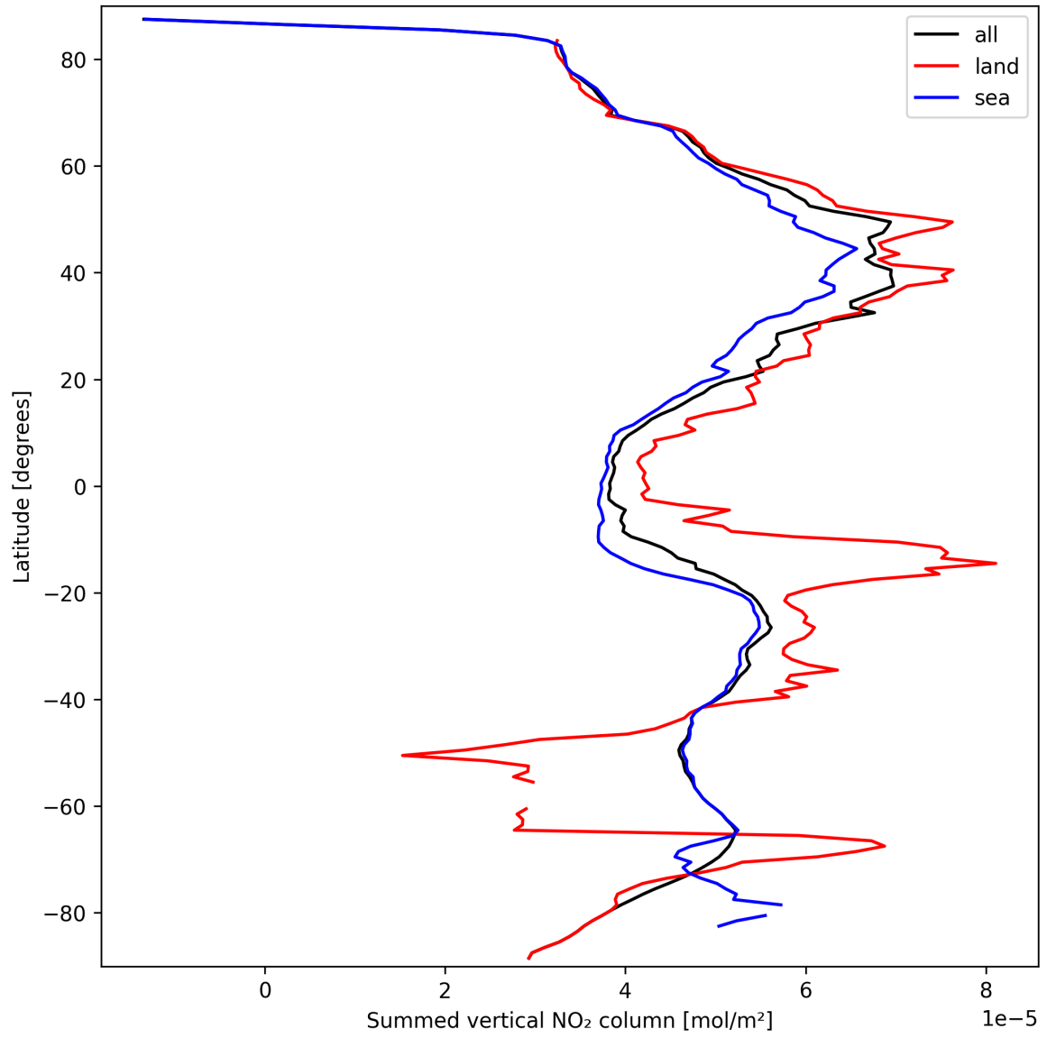
Figure 23: Zonal average of “Summed vertical NO 2 column” for 2025-09-23 to 2025-09-25.
