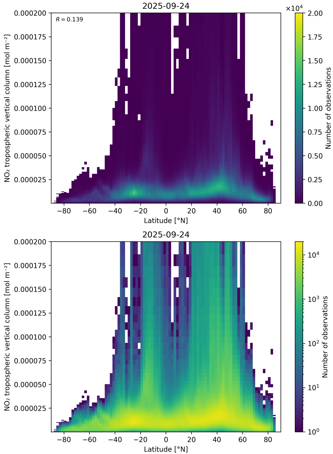
Figure 92: Scatter density plot of “Latitude” against “NO 2 tropospheric vertical column” for 2025-09-23 to 2025-09-25.
