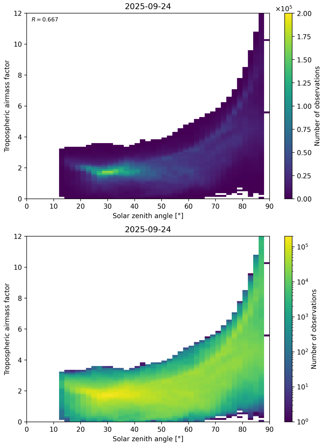
Figure 147: Scatter density plot of “Solar zenith angle” against “Tropospheric airmass factor” for 2025-09-23 to 2025-09-25.
