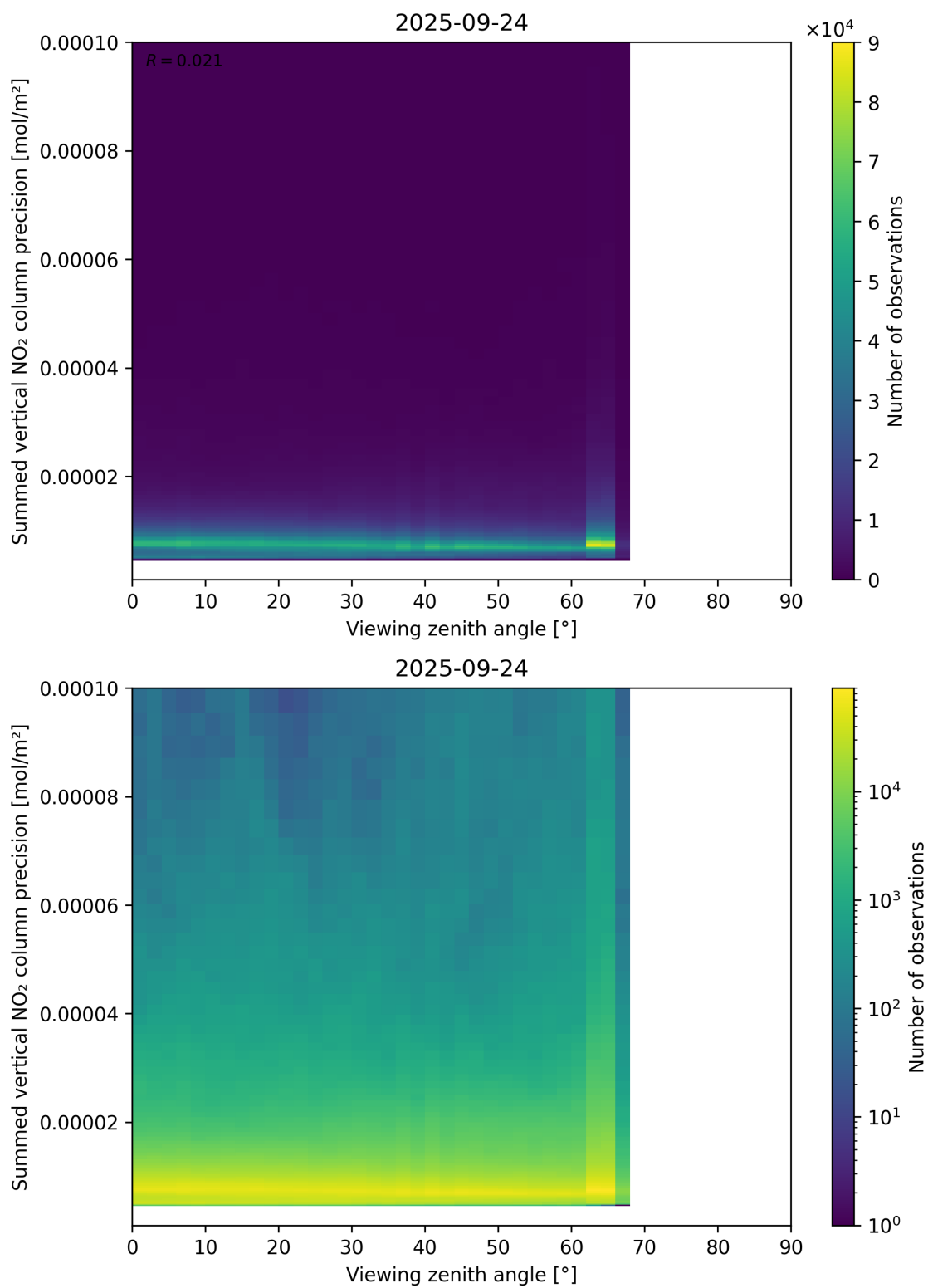
Figure 166: Scatter density plot of “Viewing zenith angle” against “Summed vertical NO 2 column precision” for 2025-09-23 to 2025-09-25.
