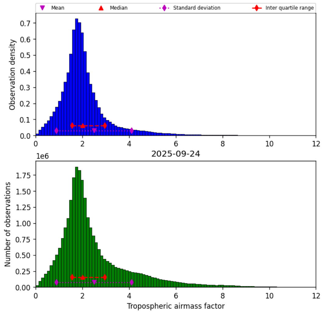
Figure 31: Histogram of “Tropospheric airmass factor” for 2025-09-23 to 2025-09-25
