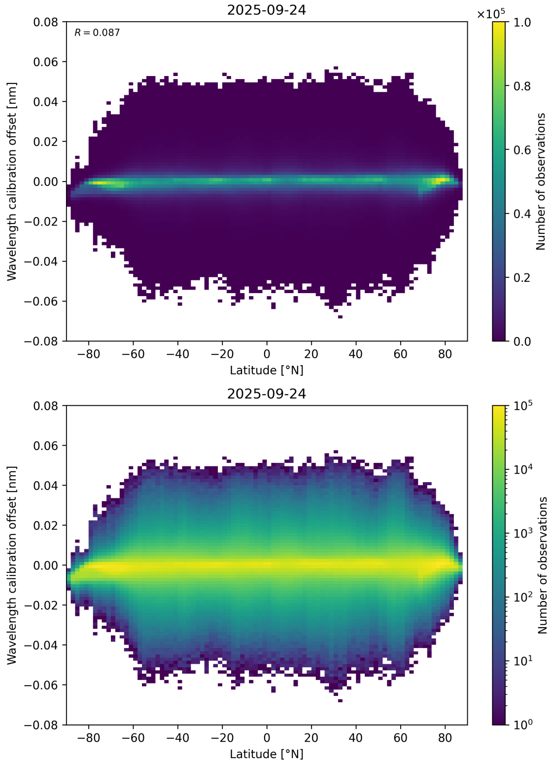
Figure 95: Scatter density plot of “Latitude” against “Wavelength calibration offset” for 2025-09-23 to 2025-09-25.
