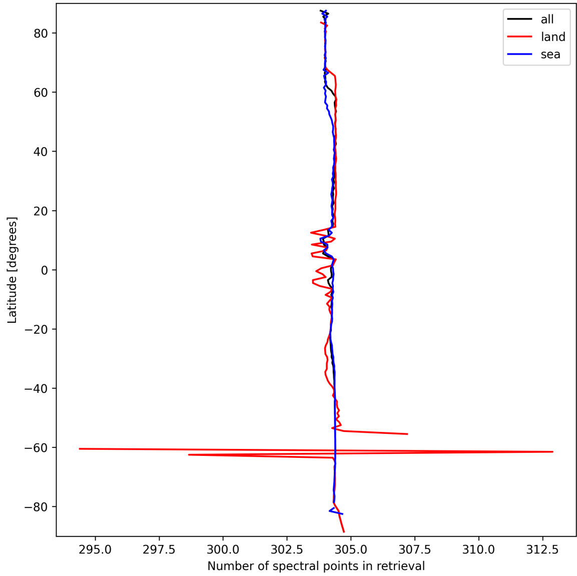
Figure 16: Zonal average of “Number of spectral points in retrieval” for 2025-09-23 to 2025-09-25.
