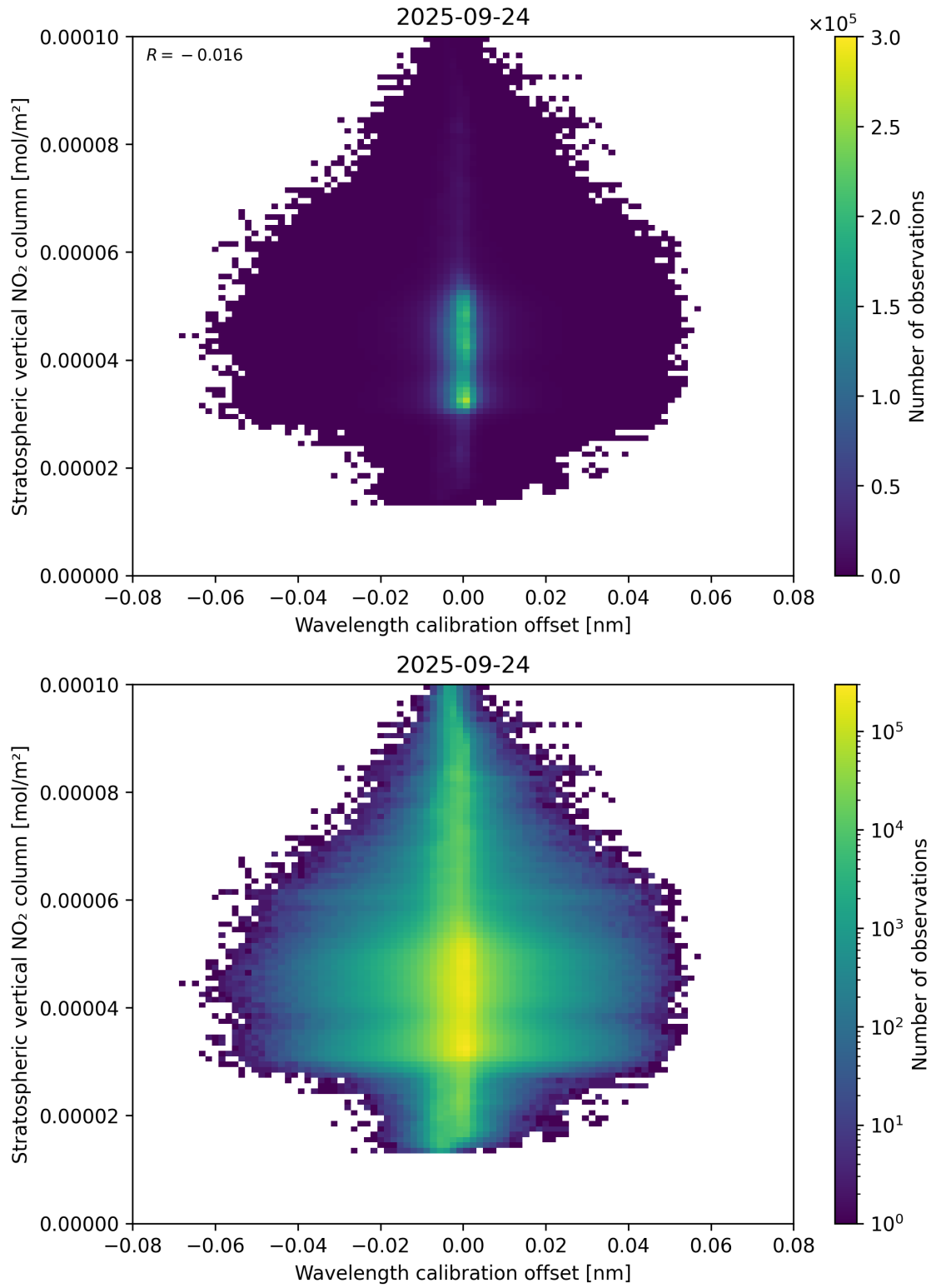
Figure 176: Scatter density plot of “Wavelength calibration offset” against “Stratospheric vertical NO 2 column” for 2025-09-23 to 2025-09-25.
