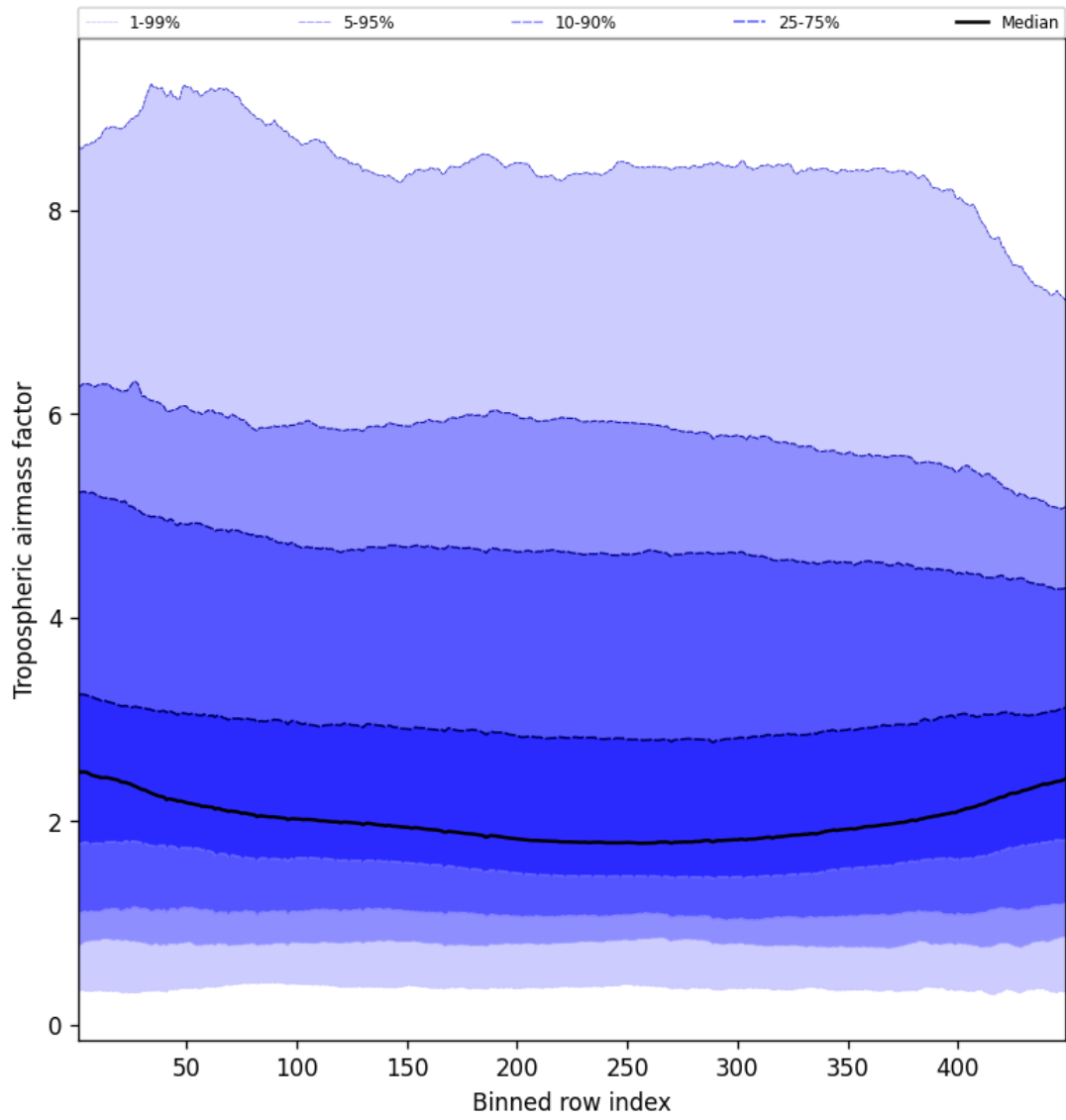
Figure 48: Along track statistics of “Tropospheric air mass factor” for 2025-09-23 to 2025-09-25
