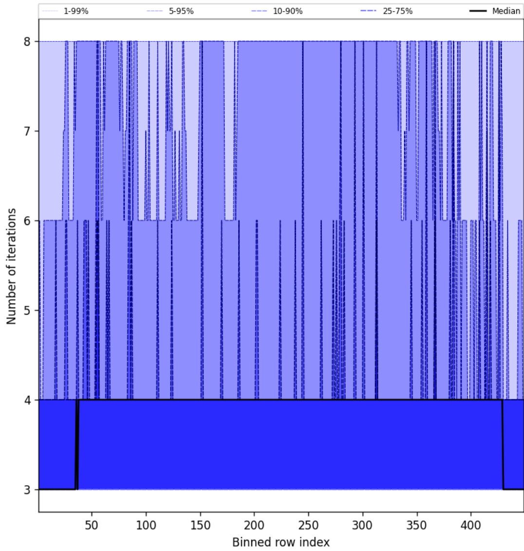
Figure 51: Along track statistics of “Number of iterations” for 2025-09-23 to 2025-09-25
