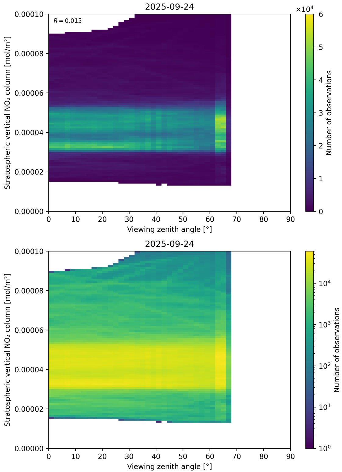
Figure 164: Scatter density plot of “Viewing zenith angle” against “Stratospheric vertical NO 2 column” for 2025-09-23 to 2025-09-25.
