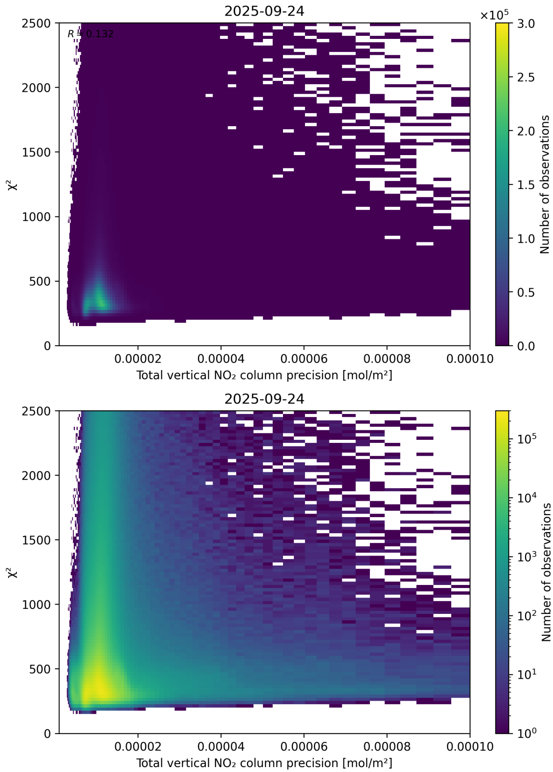
Figure 116: Scatter density plot of “Total vertical NO 2 column precision” against “ \chi^2 ” for 2025-09-23 to 2025-09-25.
