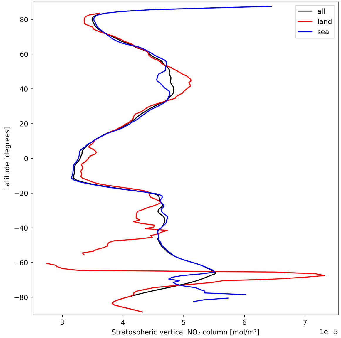
Figure 19: Zonal average of “Stratospheric vertical NO 2 column” for 2025-09-23 to 2025-09-25.
