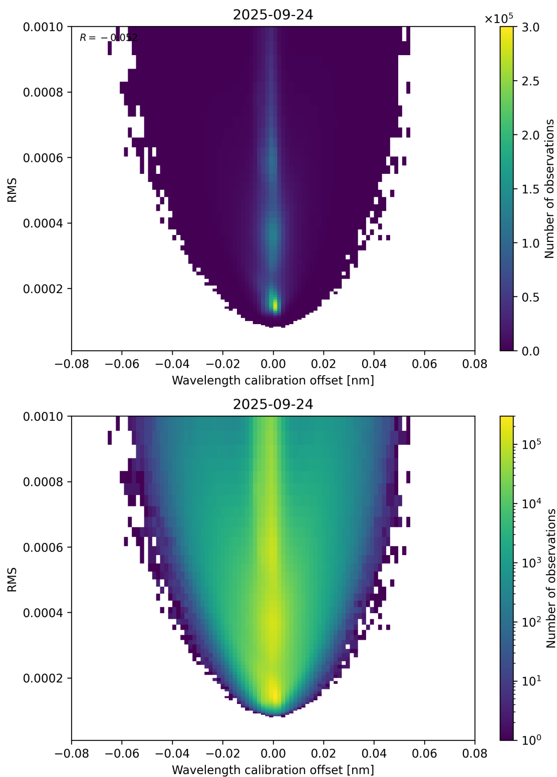
Figure 181: Scatter density plot of “Wavelength calibration offset” against “RMS” for 2025-09-23 to 2025-09-25.
