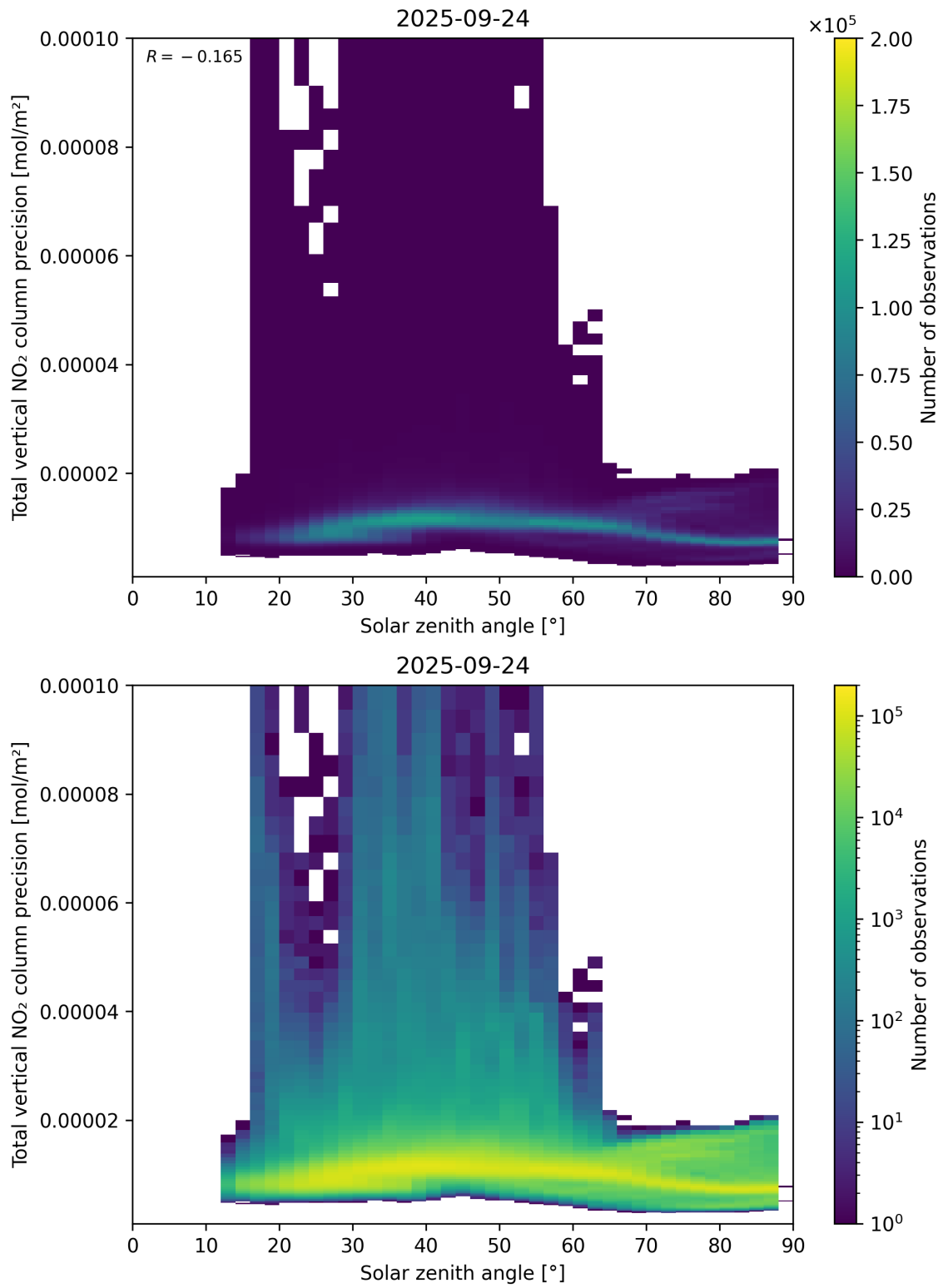
Figure 154: Scatter density plot of “Solar zenith angle” against “Total vertical NO 2 column precision” for 2025-09-23 to 2025-09-25.
