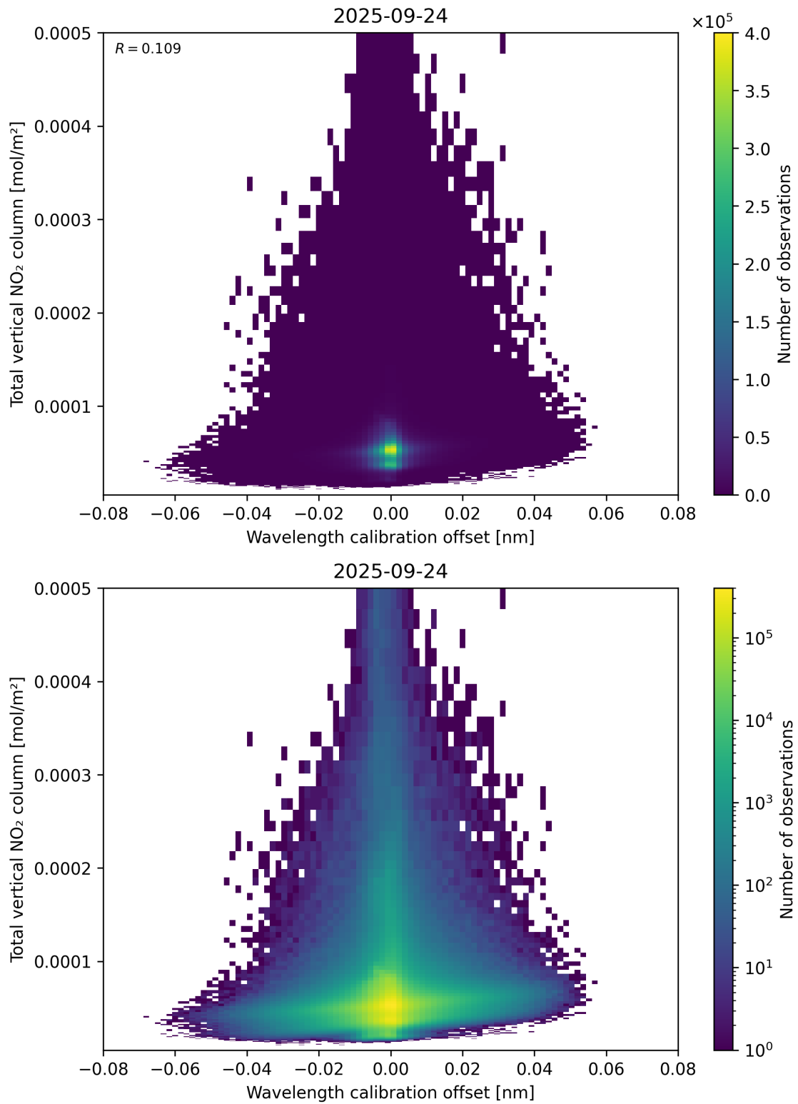
Figure 179: Scatter density plot of “Wavelength calibration offset” against “Total vertical NO 2 column” for 2025-09-23 to 2025-09-25.
