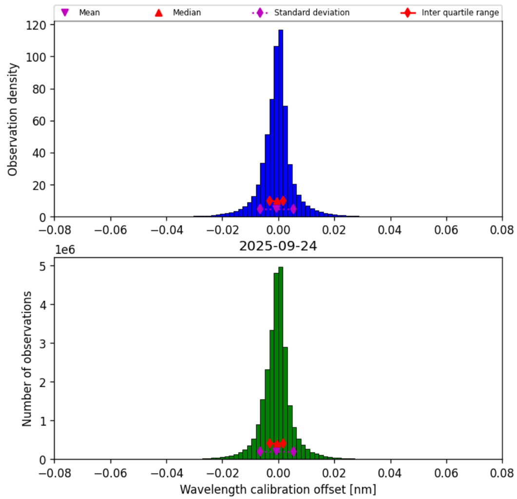
Figure 35: Histogram of “Wavelength calibration offset” for 2025-09-23 to 2025-09-25
