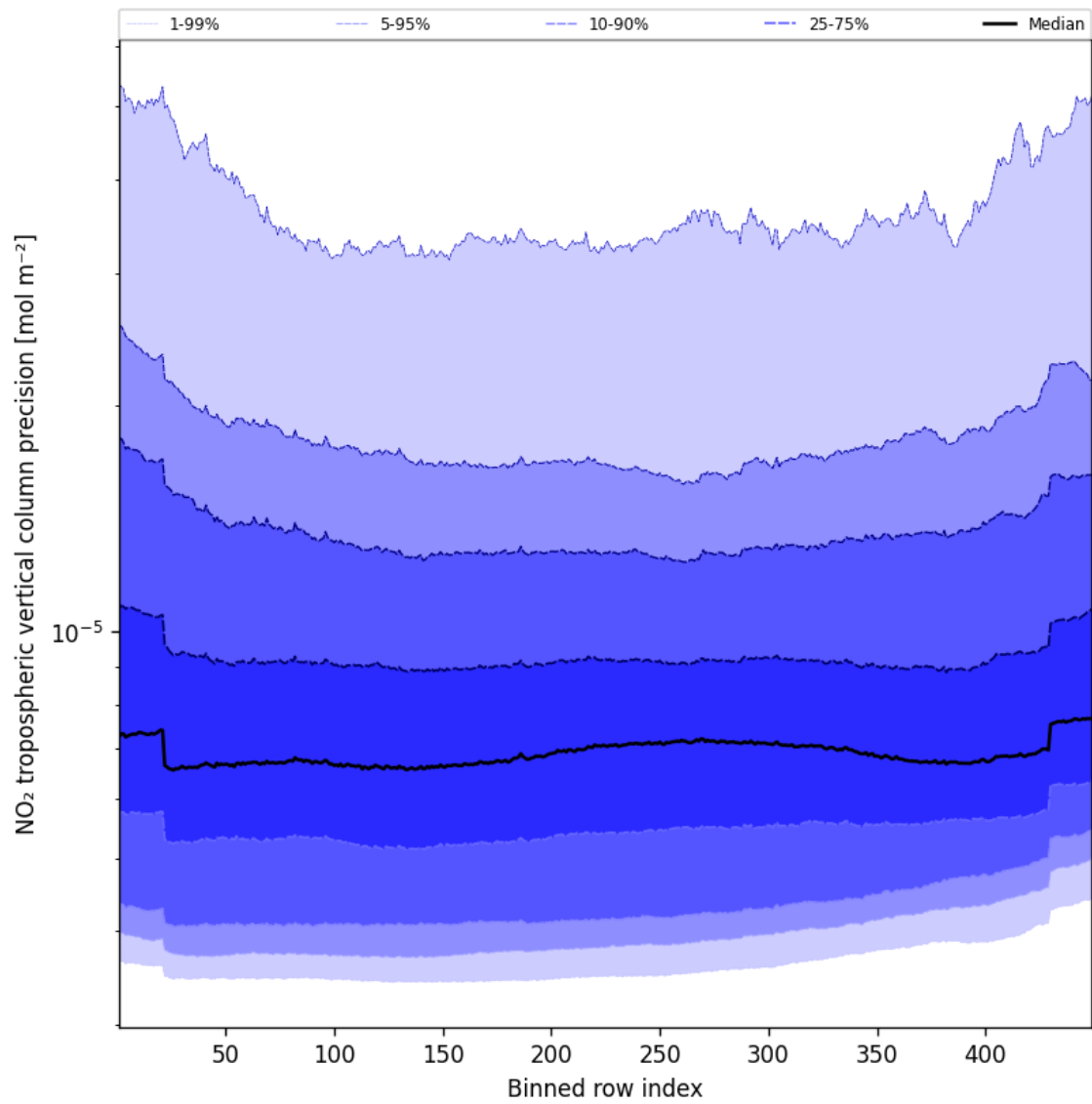
Figure 47: Along track statistics of “NO 2 tropospheric vertical column precision” for 2025-09-23 to 2025-09-25
