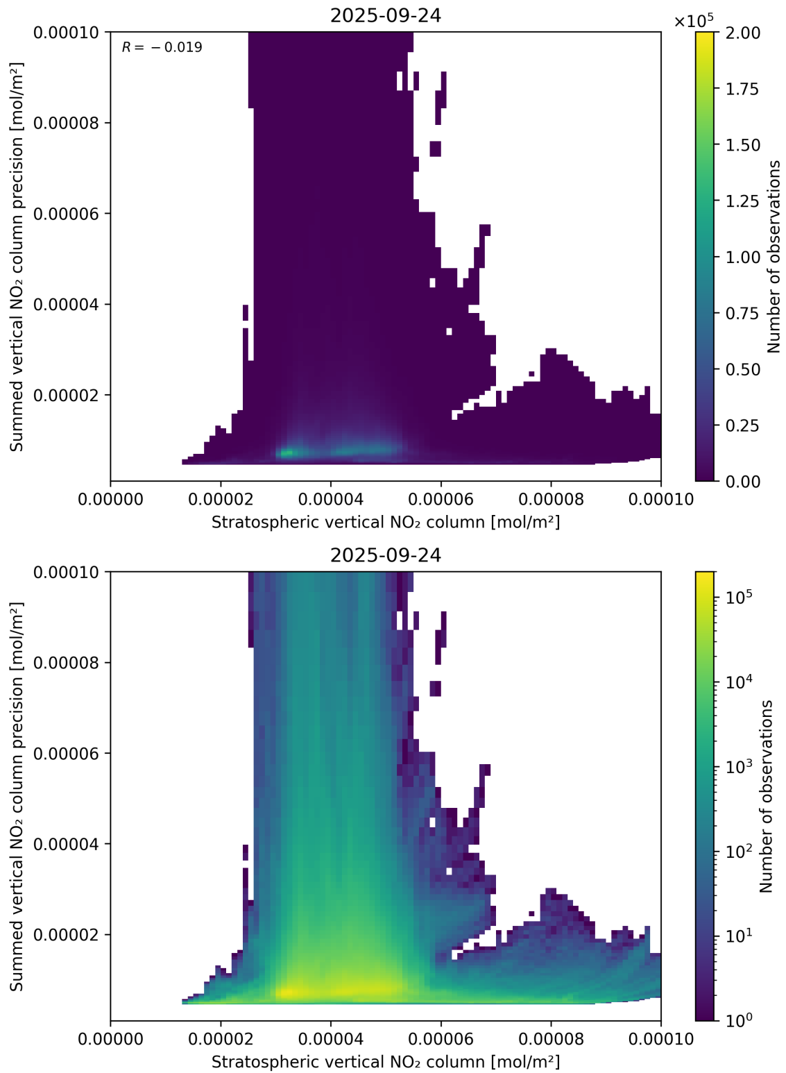
Figure 99: Scatter density plot of “Stratospheric vertical NO 2 column” against “Summed vertical NO 2 column precision” for 2025-09-23 to 2025-09-25.
