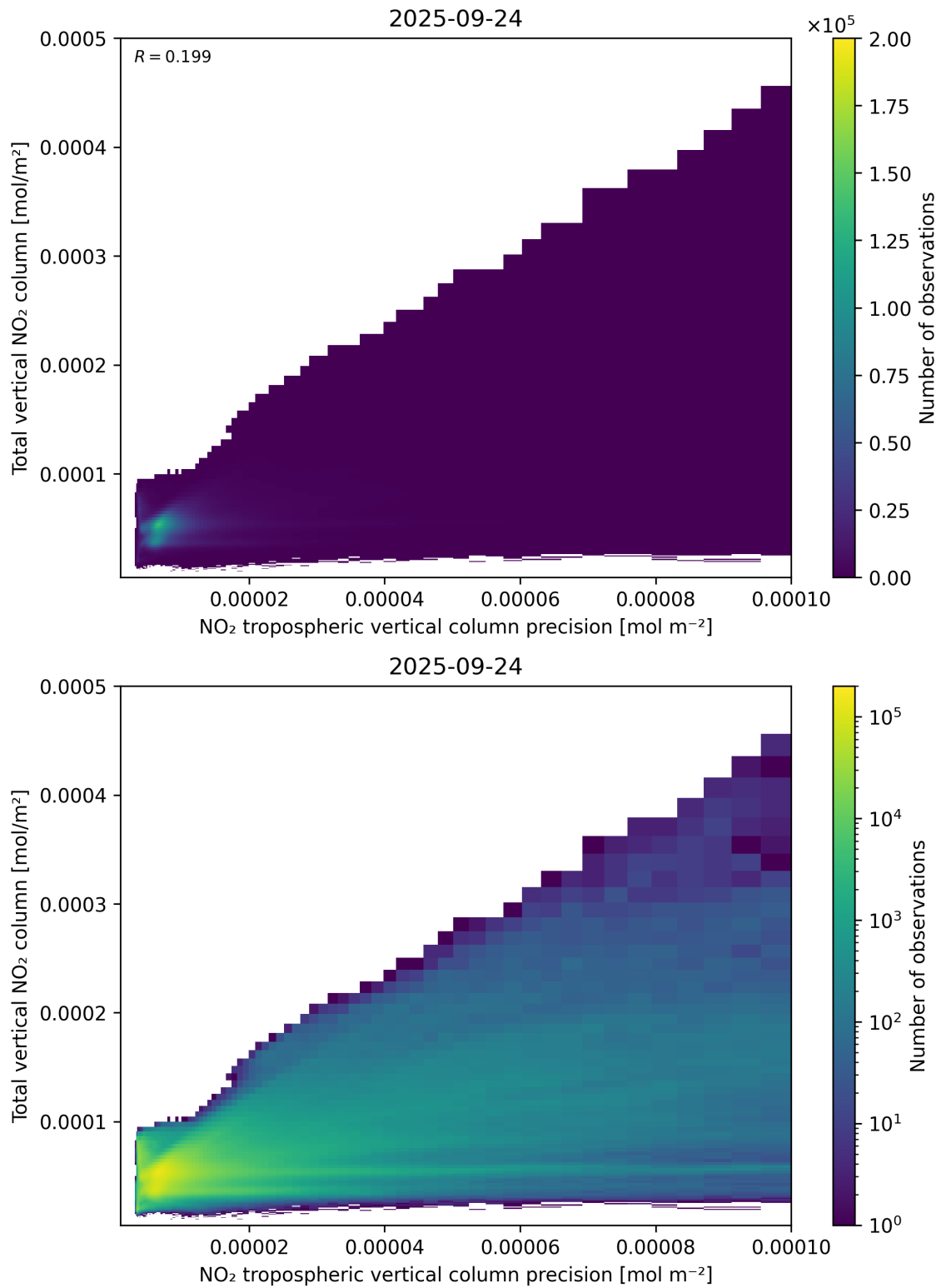
Figure 138: Scatter density plot of “NO 2 tropospheric vertical column precision” against “Total vertical NO 2 column” for 2025-09-23 to 2025-09-25.
