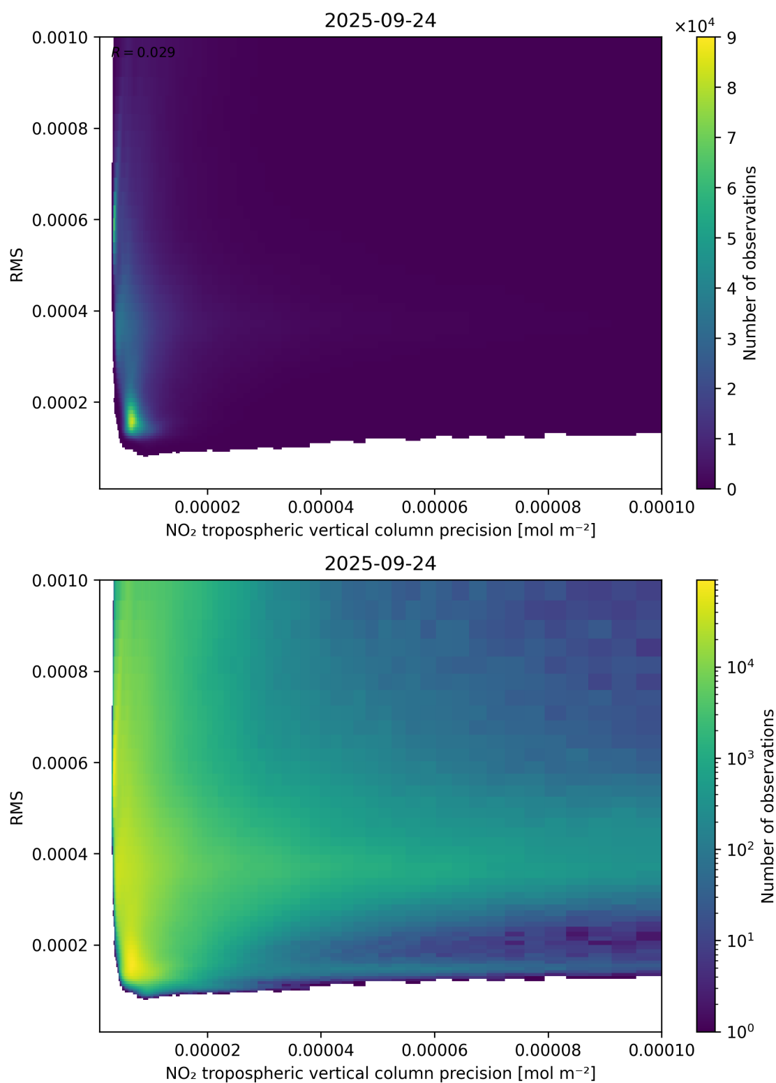
Figure 140: Scatter density plot of “NO 2 tropospheric vertical column precision” against “RMS” for 2025-09-23 to 2025-09-25.
