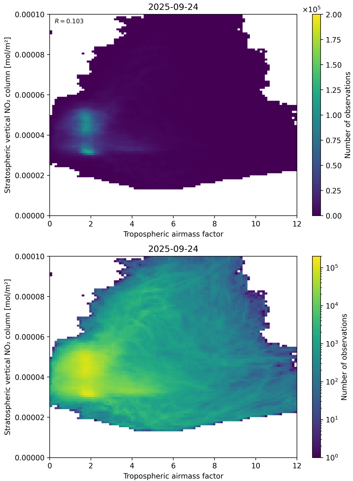
Figure 74: Scatter density plot of “Tropospheric air mass factor” against “Stratospheric vertical NO 2 column” for 2025-09-23 to 2025-09-25.
