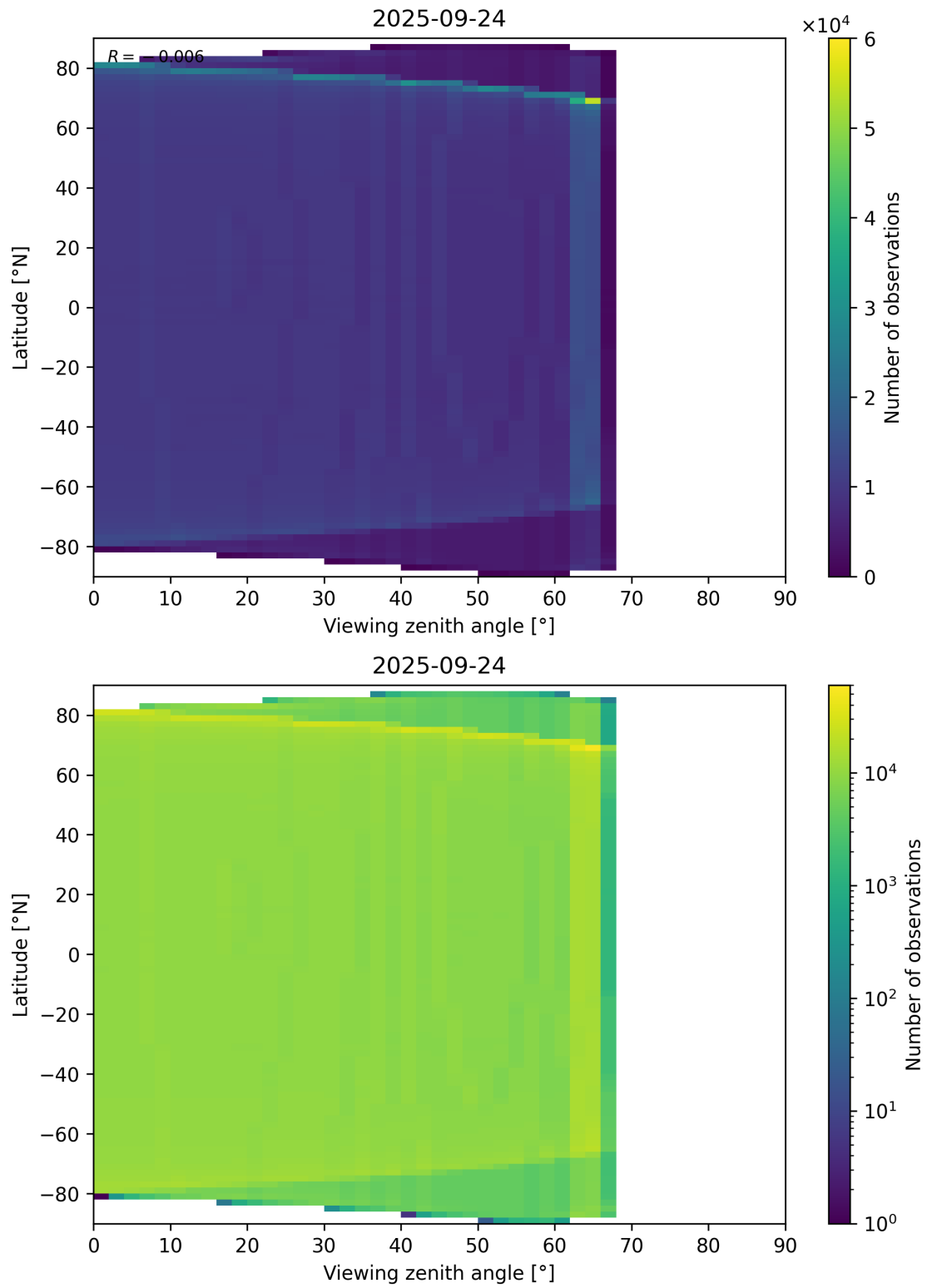
Figure 163: Scatter density plot of “Viewing zenith angle” against “Latitude” for 2025-09-23 to 2025-09-25.
