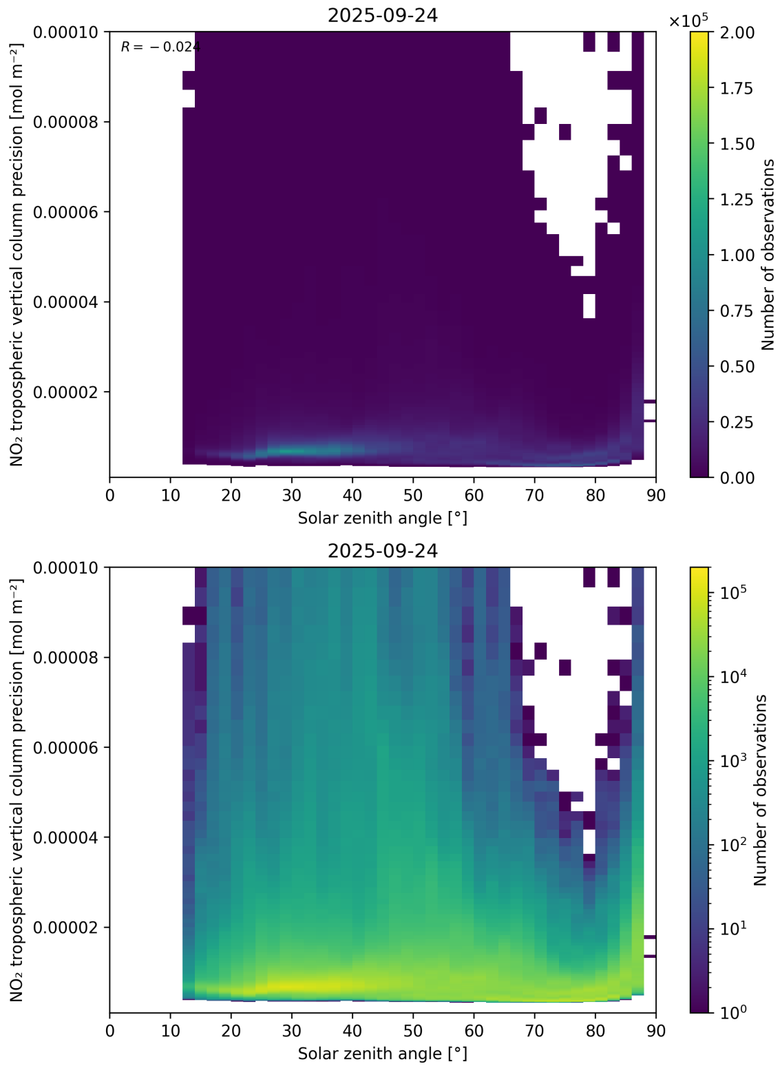
Figure 156: Scatter density plot of “Solar zenith angle” against “NO 2 tropospheric vertical column precision” for 2025-09-23 to 2025-09-25.
