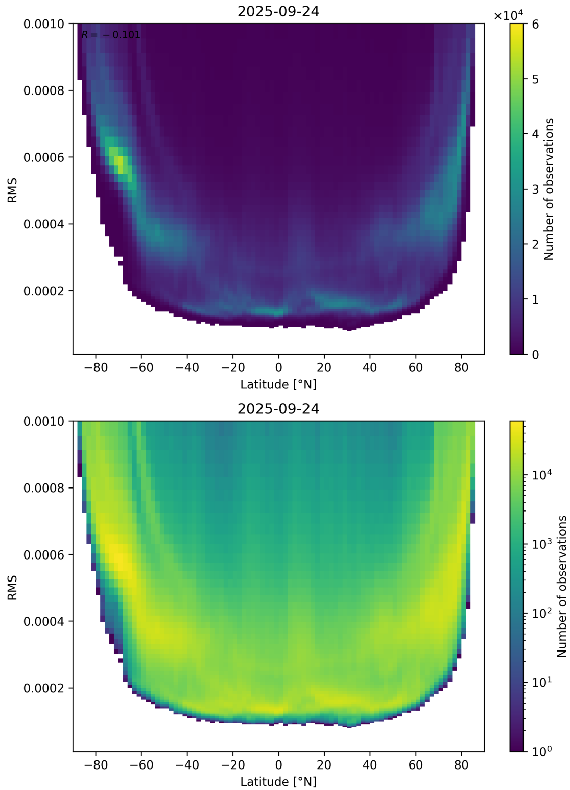
Figure 94: Scatter density plot of “Latitude” against “RMS” for 2025-09-23 to 2025-09-25.
