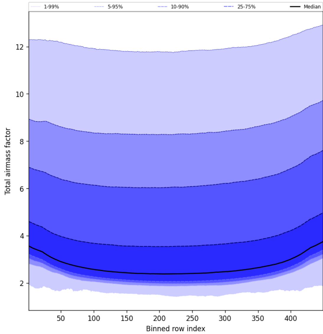
Figure 49: Along track statistics of “Total airmass factor” for 2025-09-23 to 2025-09-25
