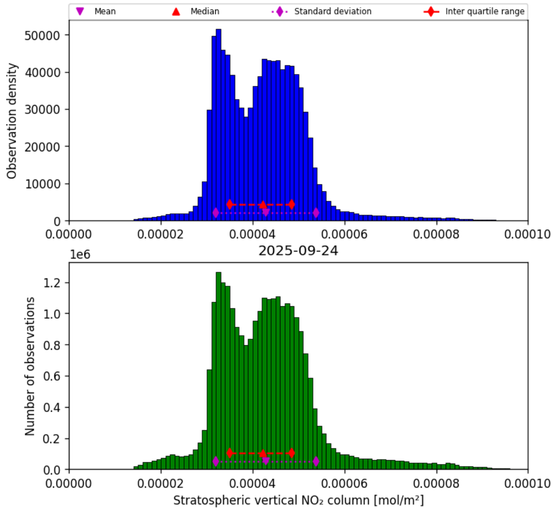
Figure 36: Histogram of “Stratospheric vertical NO 2 column” for 2025-09-23 to 2025-09-25
