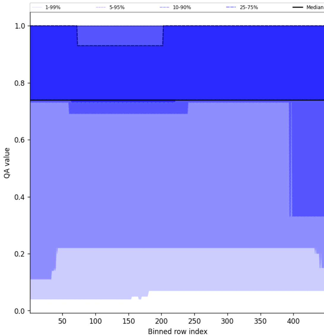
Figure 45: Along track statistics of "QA value" for 2025-09-23 to 2025-09-25
