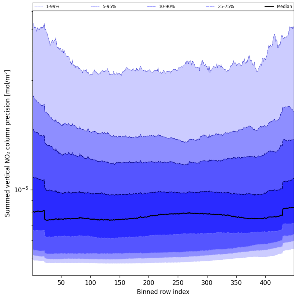
Figure 58: Along track statistics of “Summed vertical NO 2 column precision” for 2025-09-23 to 2025-09-25
