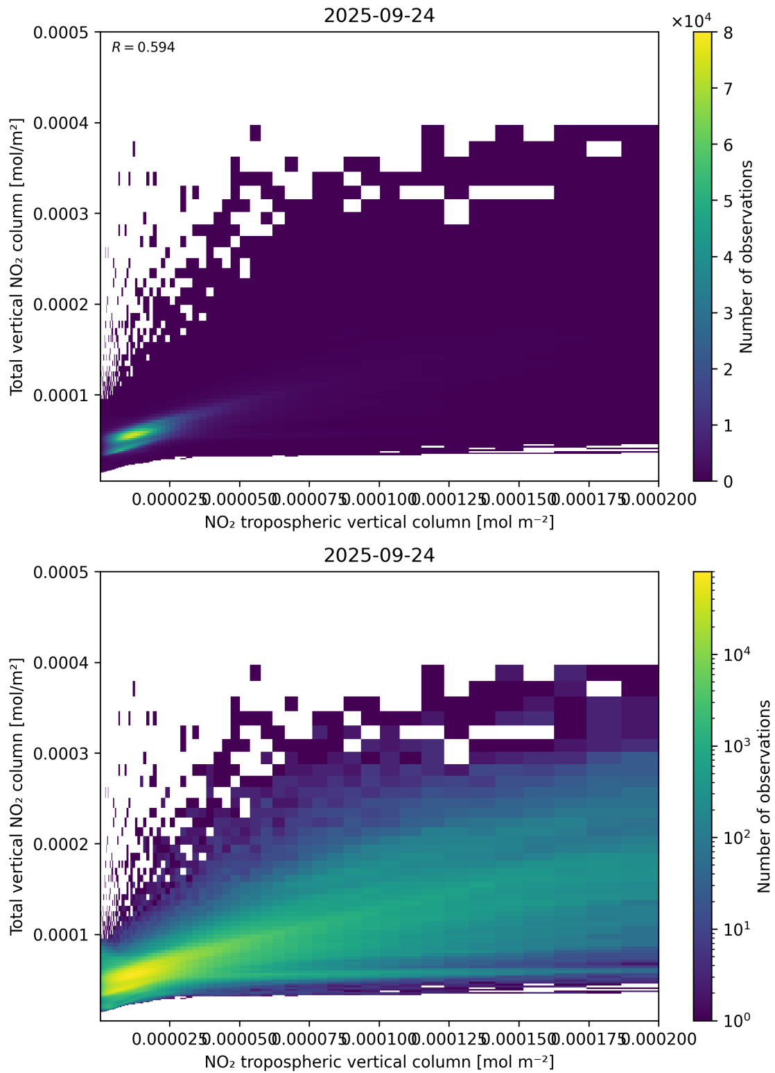
Figure 128: Scatter density plot of “NO 2 tropospheric vertical column” against “Total vertical NO 2 column” for 2025-09-23 to 2025-09-25.
