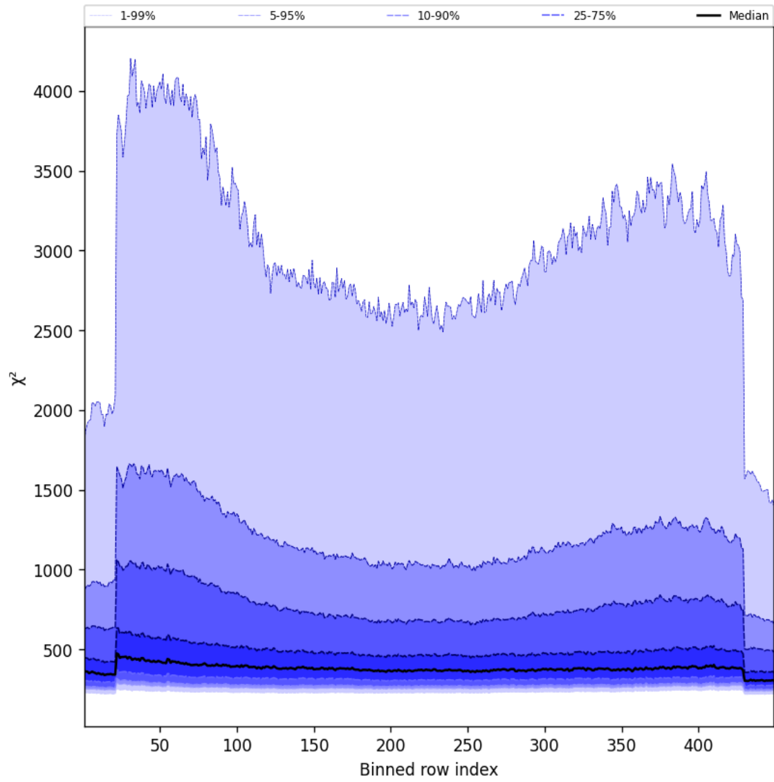
Figure 59: Along track statistics of “ \chi^2 ” for 2025-09-23 to 2025-09-25
