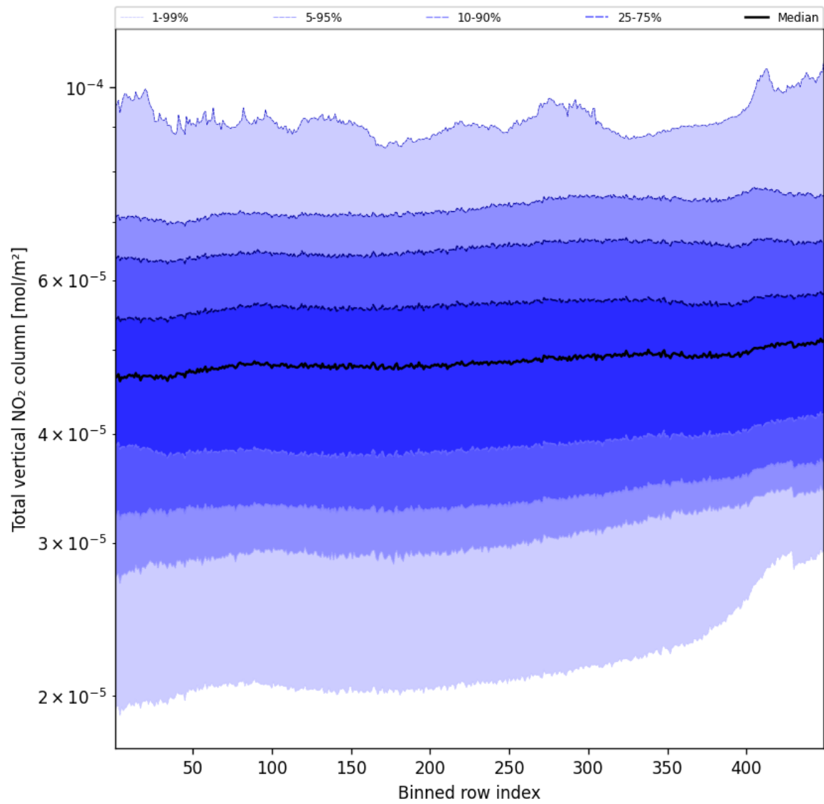
Figure 55: Along track statistics of “Total vertical NO 2 column” for 2025-09-23 to 2025-09-25
