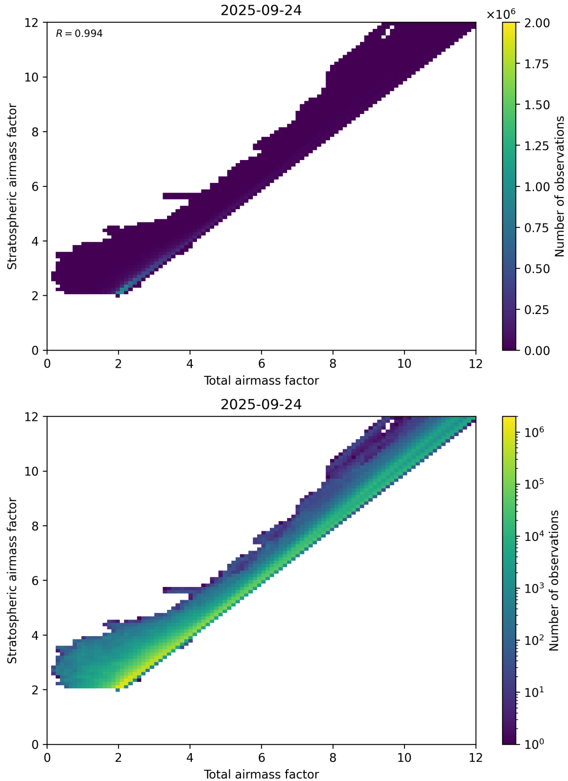
Figure 62: Scatter density plot of “Total airmass factor” against “Stratospheric airmass factor” for 2025-09-23 to 2025-09-25.
