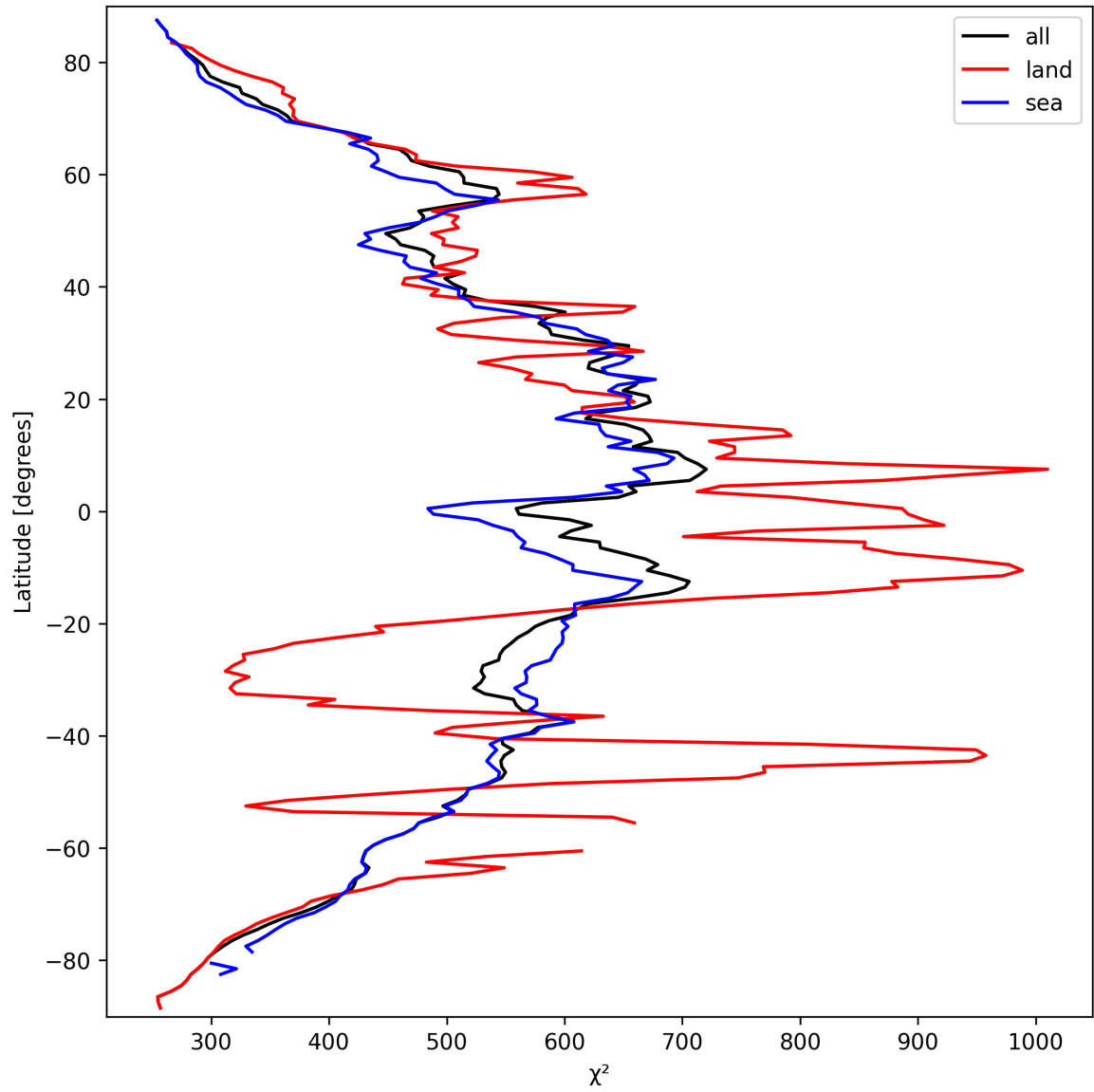
Figure 25: Zonal average of “ \chi^2 ” for 2025-09-23 to 2025-09-25.
