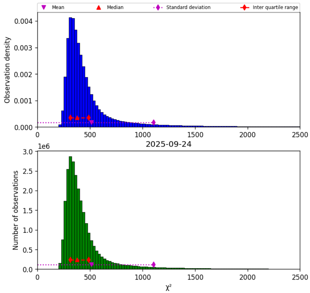
Figure 42: Histogram of " \chi^2 " for 2025-09-23 to 2025-09-25
