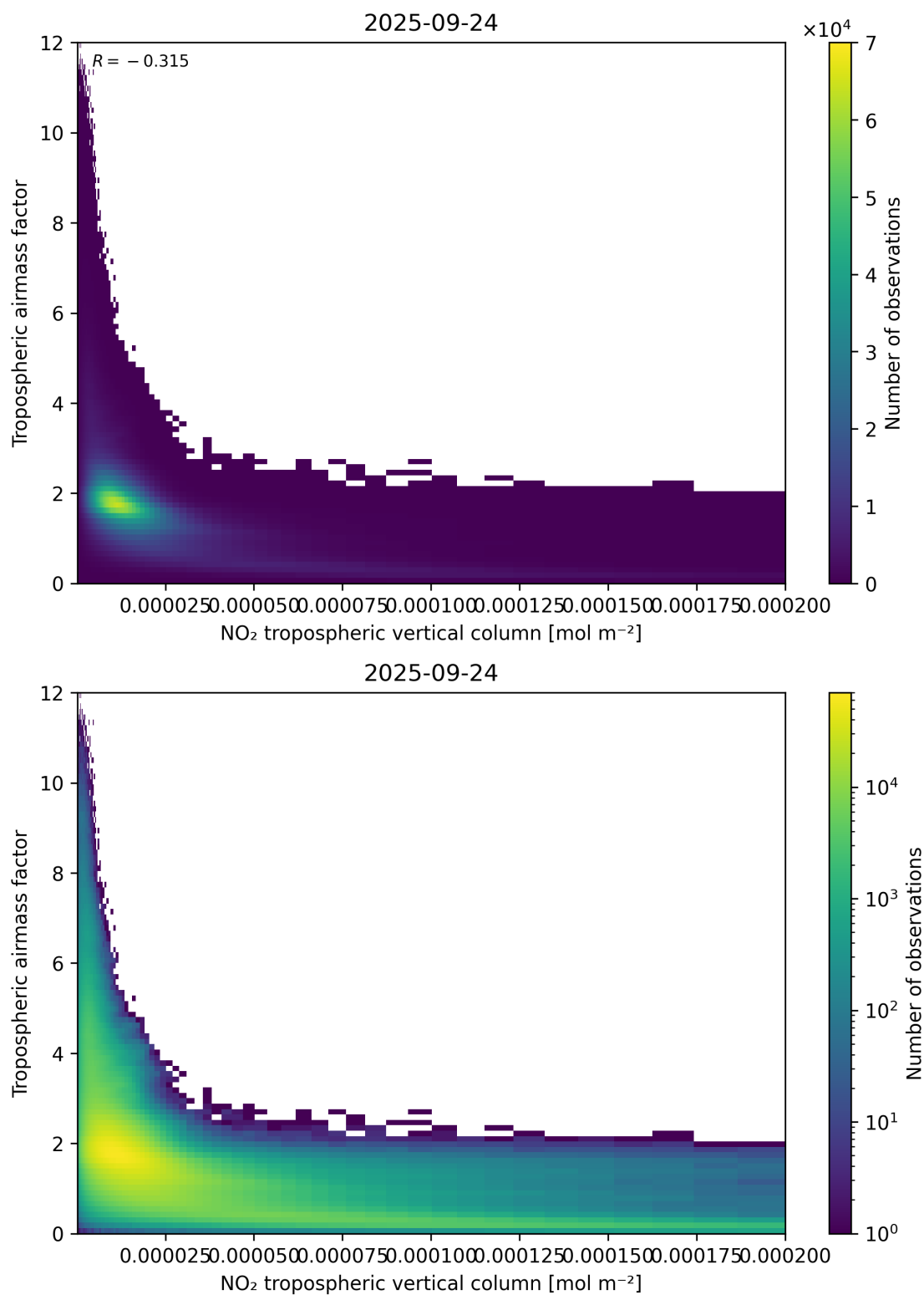
Figure 123: Scatter density plot of “NO 2 tropospheric vertical column” against “Tropospheric air mass factor” for 2025-09-23 to 2025-09-25.
