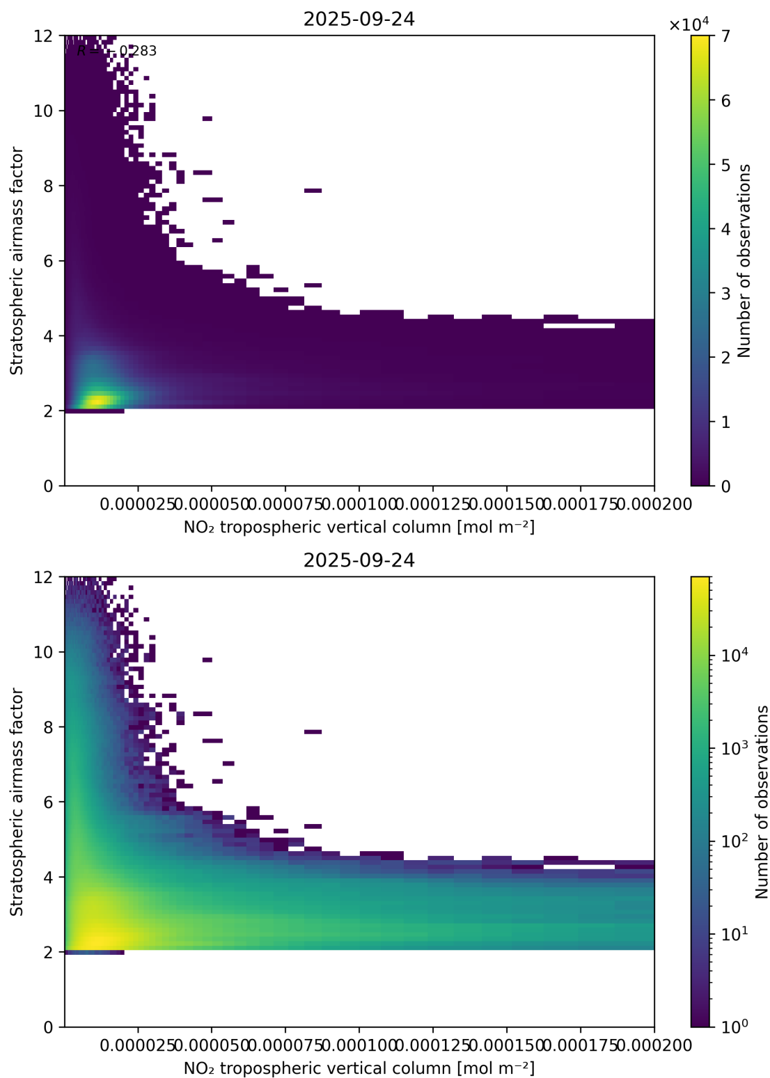
Figure 121: Scatter density plot of “NO 2 tropospheric vertical column” against “Stratospheric air mass factor” for 2025-09-23 to 2025-09-25.
