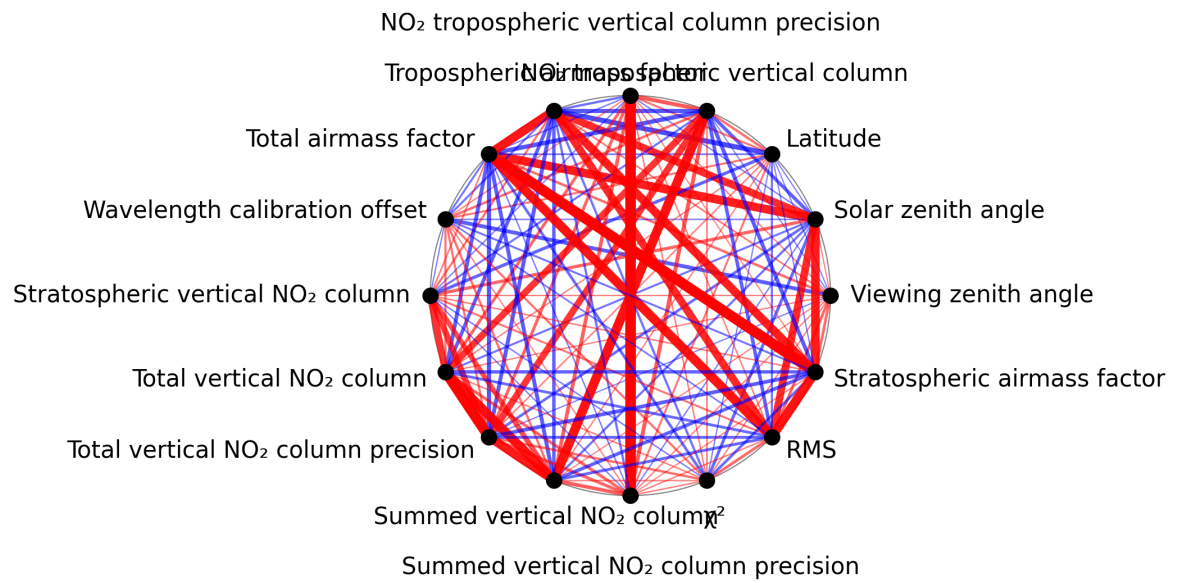
Figure 1: Map of correlation graph for 2025-09-23 to 2025-09-25.
