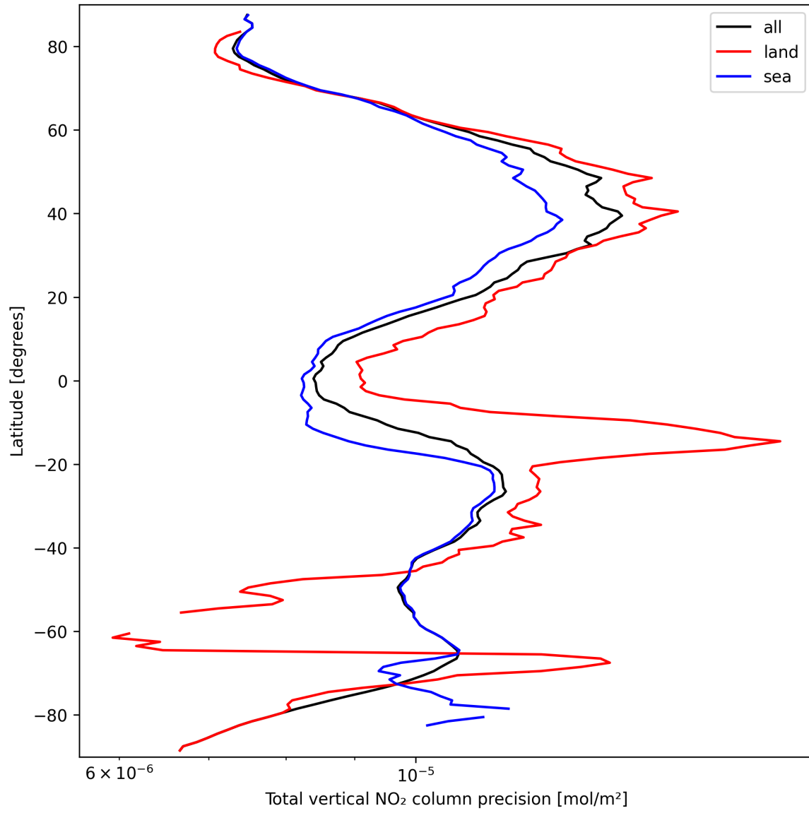
Figure 22: Zonal average of “Total vertical NO 2 column precision” for 2025-09-23 to 2025-09-25.
