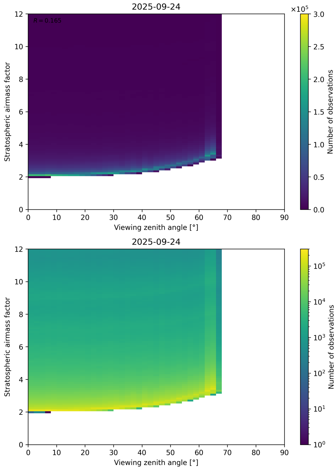
Figure 159: Scatter density plot of “Viewing zenith angle” against “Stratospheric airmass factor” for 2025-09-23 to 2025-09-25.
