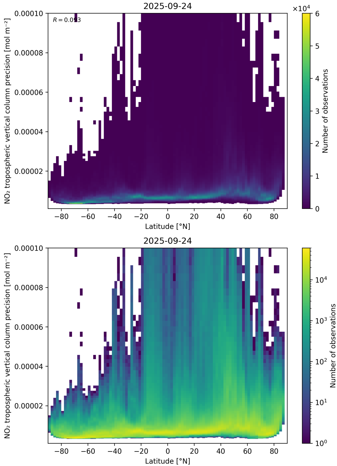
Figure 93: Scatter density plot of “Latitude” against “NO 2 tropospheric vertical column precision” for 2025-09-23 to 2025-09-25.
