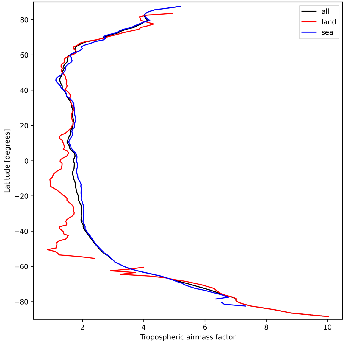
Figure 14: Zonal average of “Tropospheric airmass factor” for 2025-09-23 to 2025-09-25.
