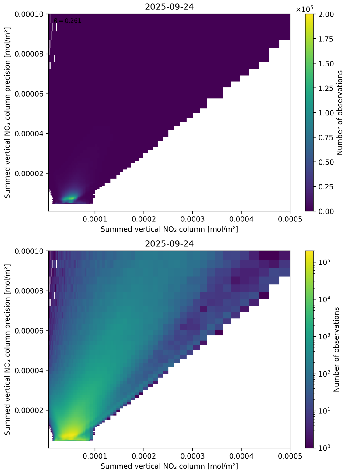
Figure 105: Scatter density plot of “Summed vertical NO 2 column” against “Summed vertical NO 2 column precision” for 2025-09-23 to 2025-09-25.
