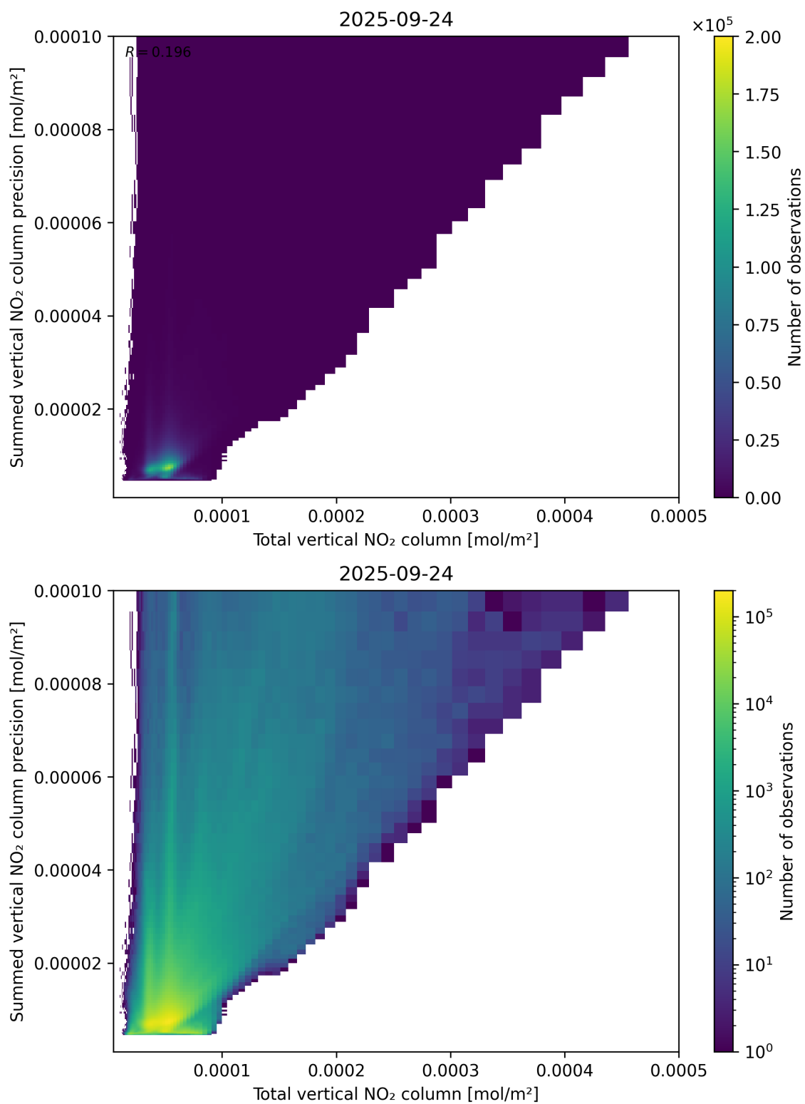
Figure 113: Scatter density plot of “Total vertical NO 2 column” against “Summed vertical NO 2 column precision” for 2025-09-23 to 2025-09-25.
