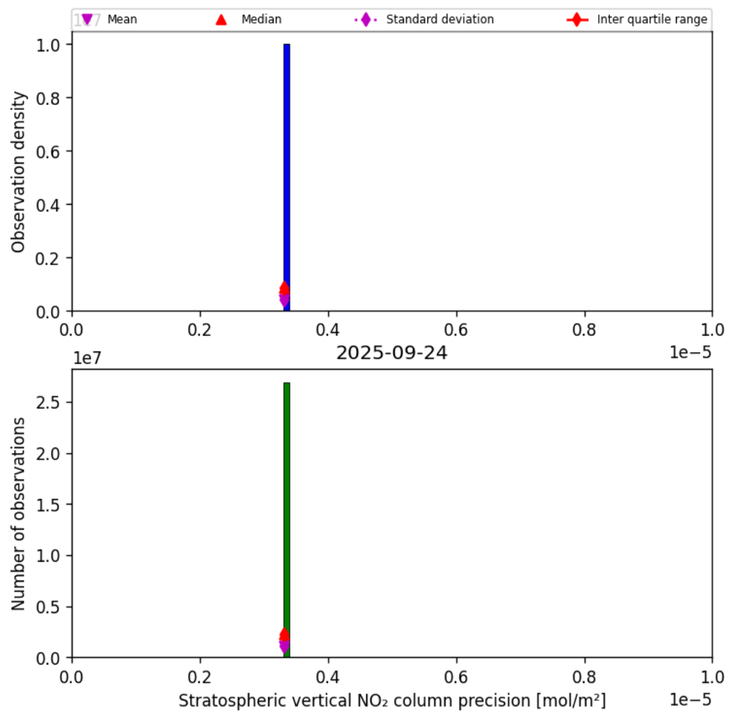
Figure 37: Histogram of “Stratospheric vertical NO 2 column precision” for 2025-09-23 to 2025-09-25
