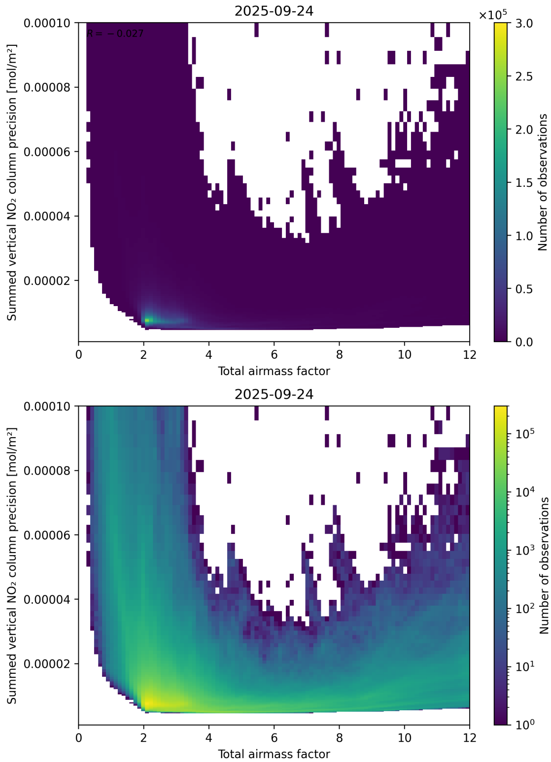
Figure 66: Scatter density plot of “Total airmass factor” against “Summed vertical NO 2 column precision” for 2025-09-23 to 2025-09-25.
