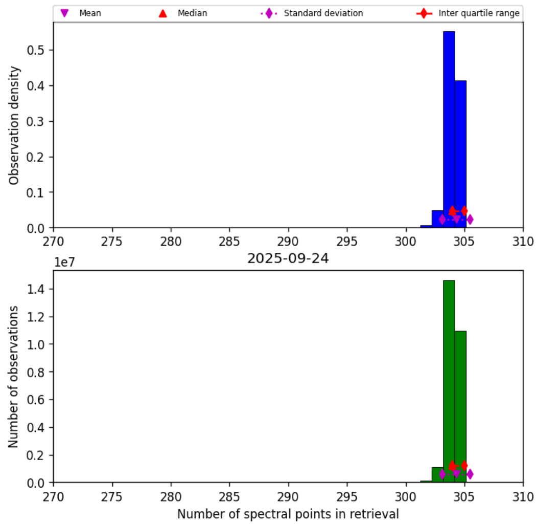
Figure 33: Histogram of “Number of spectral points in retrieval” for 2025-09-23 to 2025-09-25
