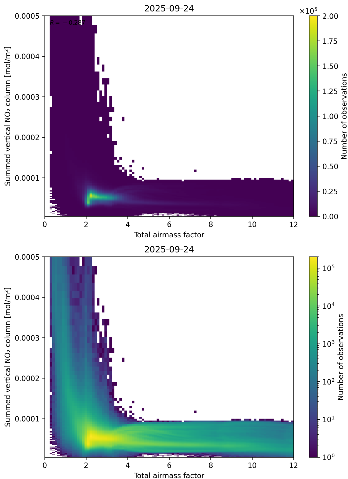
Figure 65: Scatter density plot of “Total airmass factor” against “Summed vertical NO 2 column” for 2025-09-23 to 2025-09-25.
