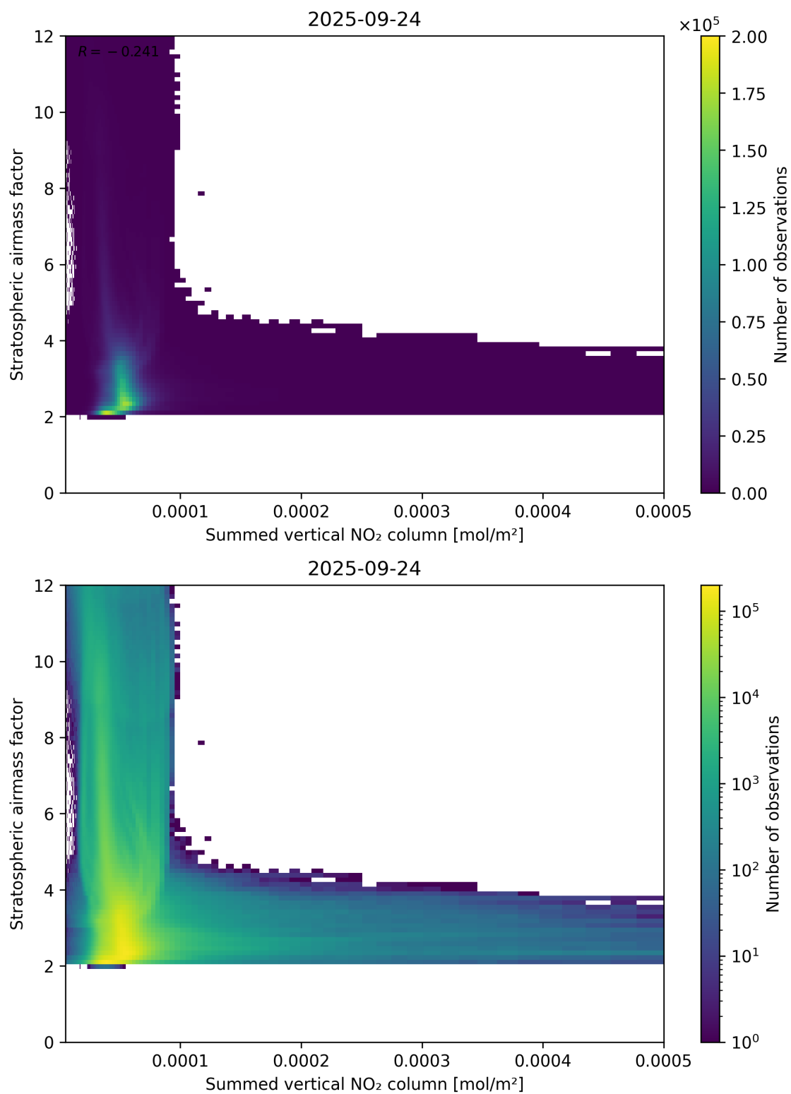
Figure 103: Scatter density plot of “Summed vertical NO 2 column” against “Stratospheric airmass factor” for 2025-09-23 to 2025-09-25.
