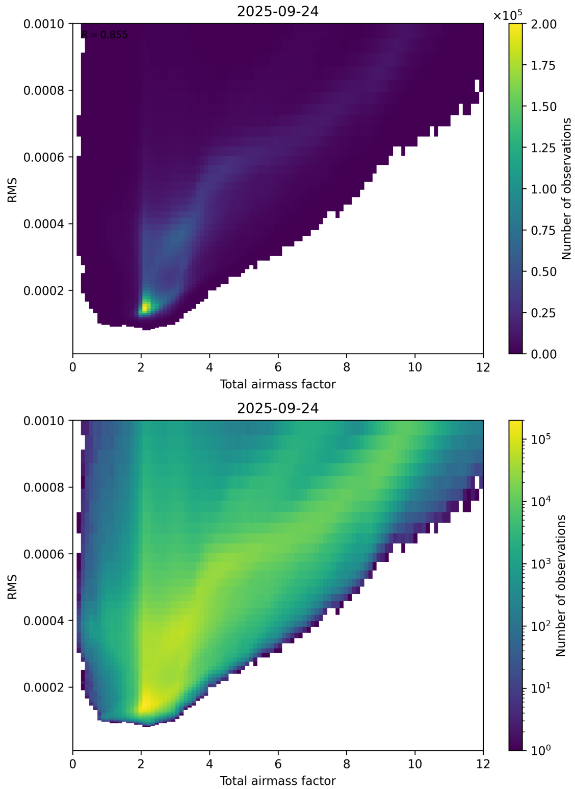
Figure 69: Scatter density plot of “Total airmass factor” against “RMS” for 2025-09-23 to 2025-09-25.
