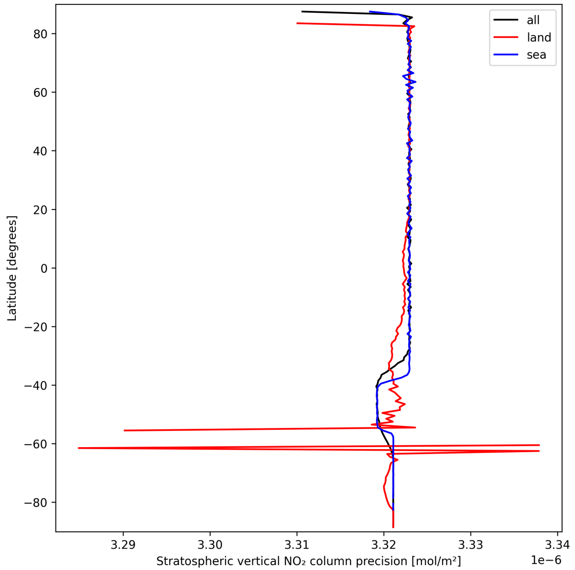
Figure 20: Zonal average of “Stratospheric vertical NO 2 column precision” for 2025-09-23 to 2025-09-25.
