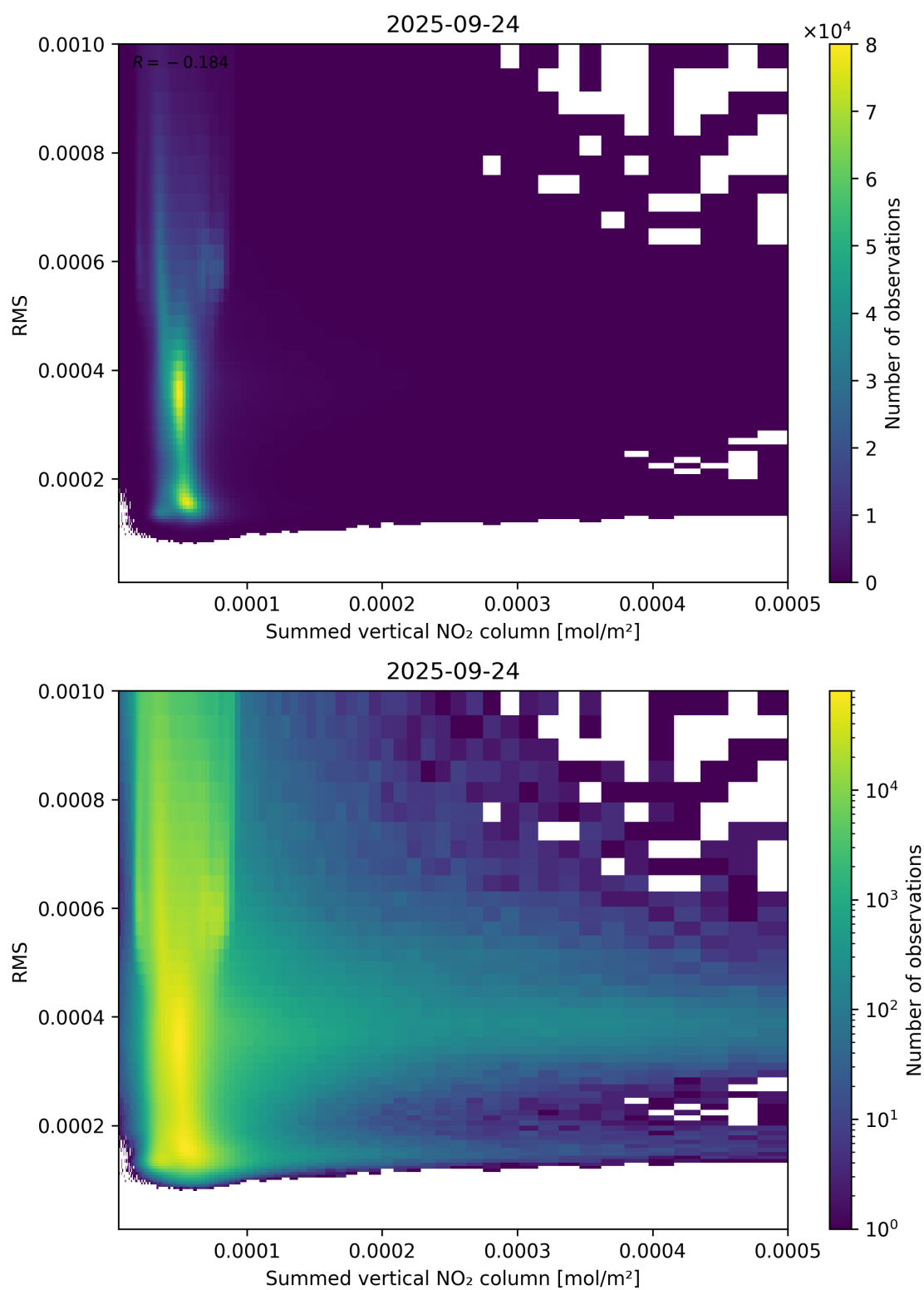
Figure 109: Scatter density plot of “Summed vertical NO 2 column” against “RMS” for 2025-09-23 to 2025-09-25.
