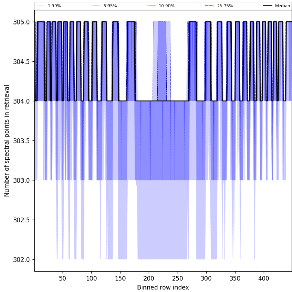
Figure 50: Along track statistics of “Number of spectral points in retrieval” for 2025-09-23 to 2025-09-25
