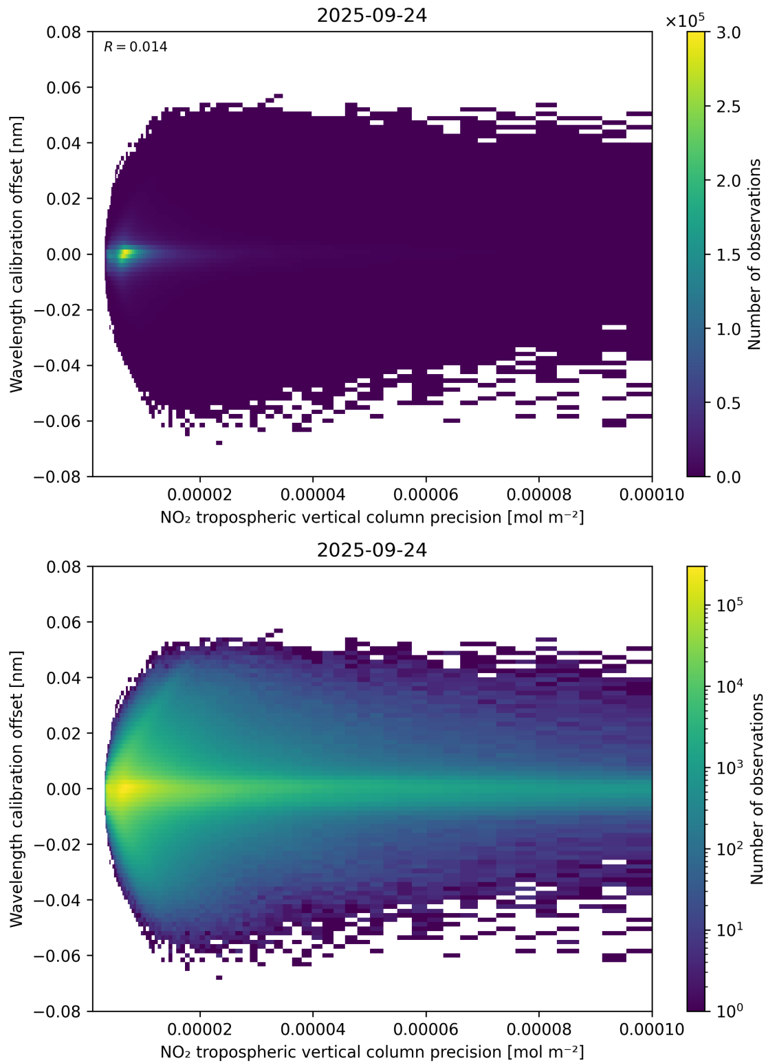
Figure 141: Scatter density plot of “NO 2 tropospheric vertical column precision” against “Wavelength calibration offset” for 2025-09-23 to 2025-09-25.
