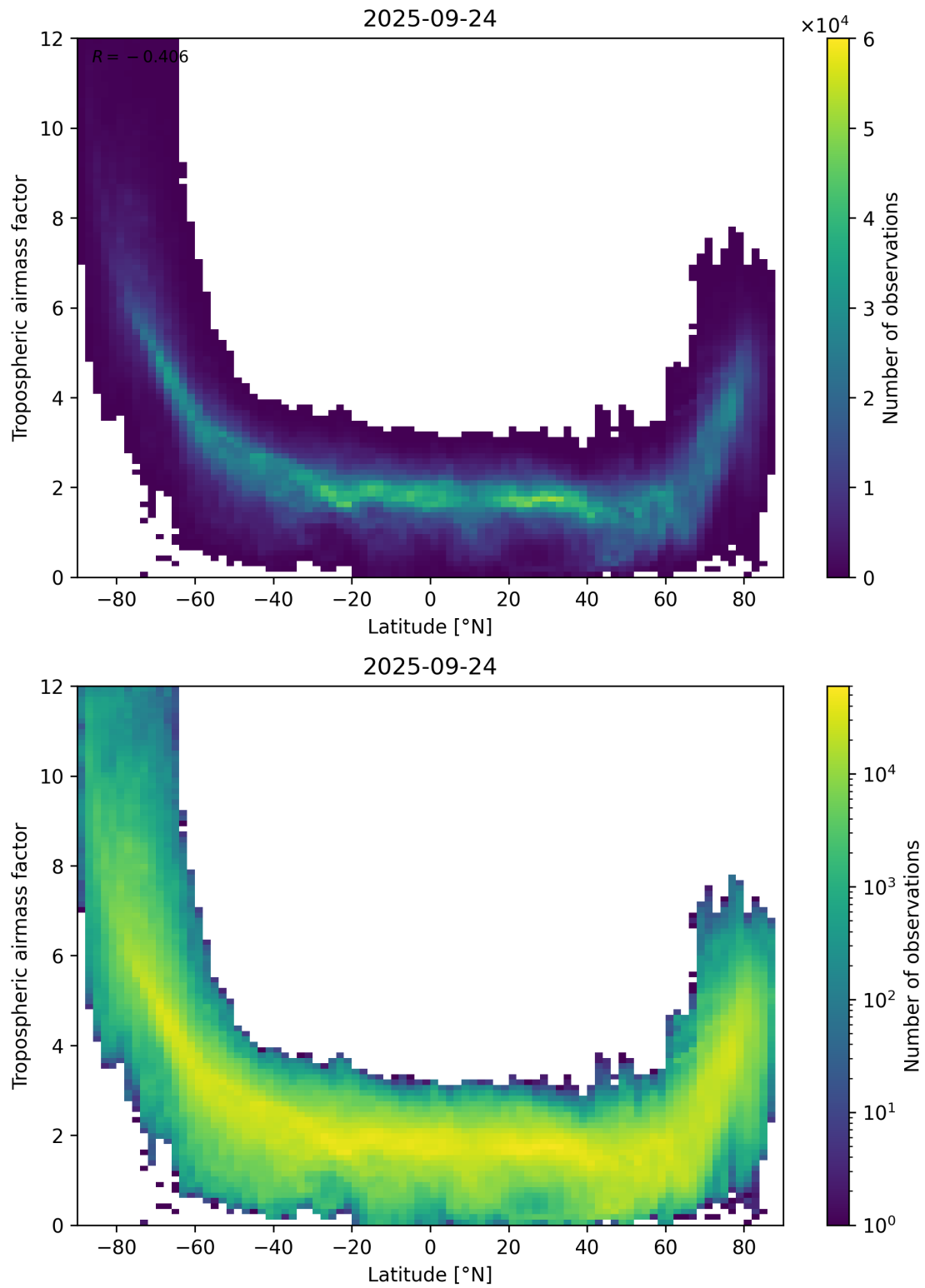
Figure 85: Scatter density plot of “Latitude” against “Tropospheric airmass factor” for 2025-09-23 to 2025-09-25.
