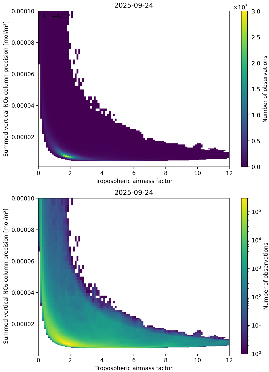
Figure 76: Scatter density plot of “Tropospheric air mass factor” against “Summed vertical NO 2 column precision” for 2025-09-23 to 2025-09-25.
