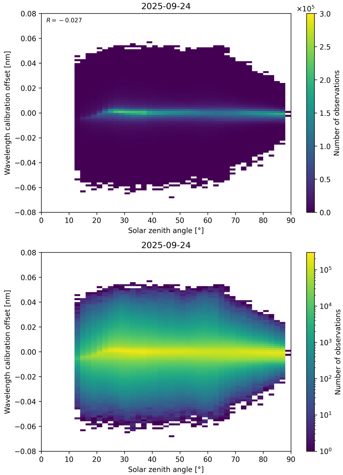
Figure 158: Scatter density plot of “Solar zenith angle” against “Wavelength calibration offset” for 2025-09-23 to 2025-09-25.
