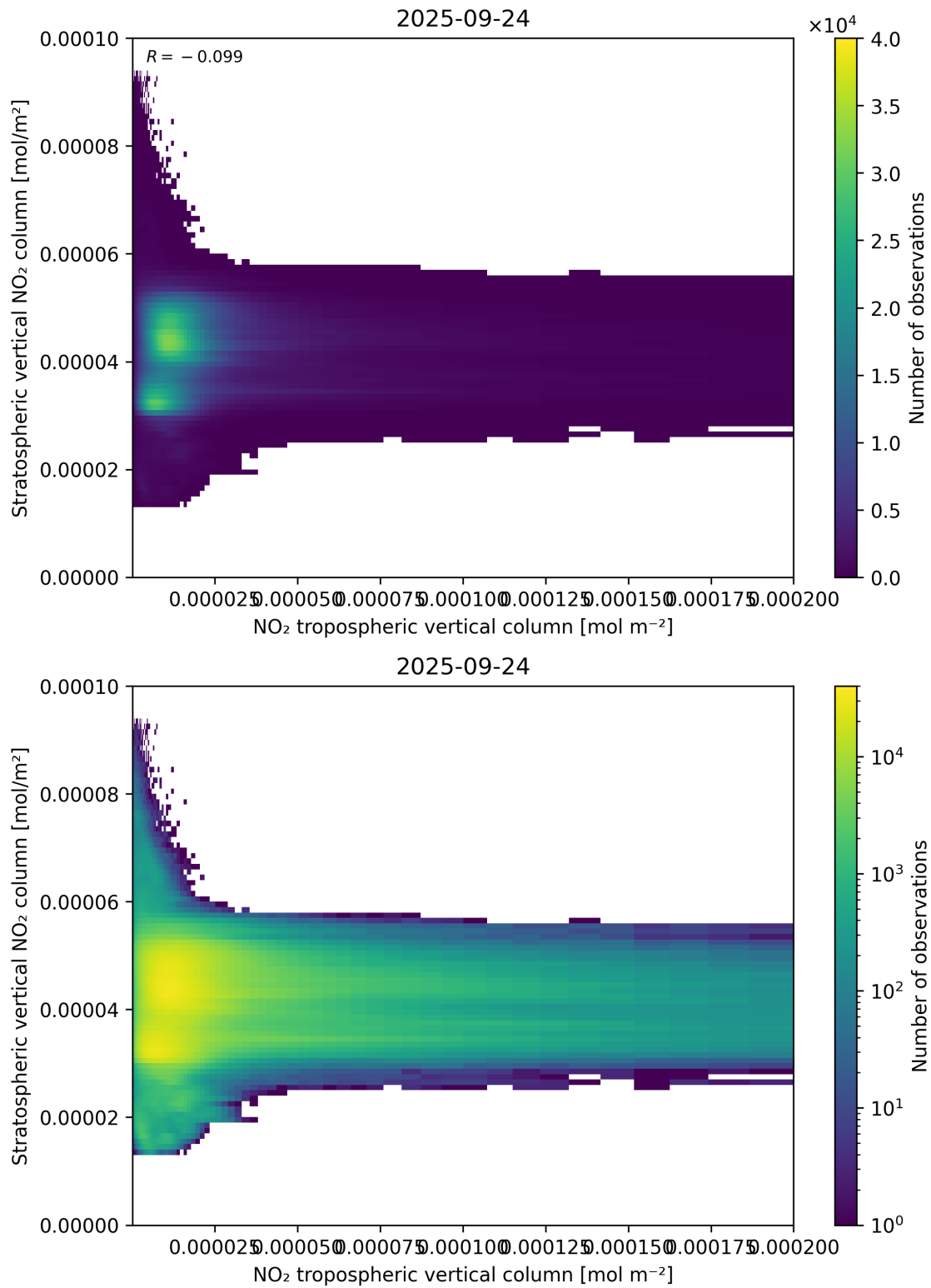
Figure 125: Scatter density plot of “NO 2 tropospheric vertical column” against “Stratospheric vertical NO 2 column” for 2025-09-23 to 2025-09-25.
