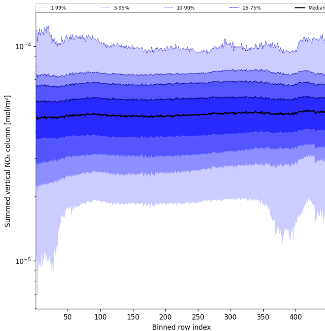
Figure 57: Along track statistics of “Summed vertical NO 2 column” for 2025-09-23 to 2025-09-25
