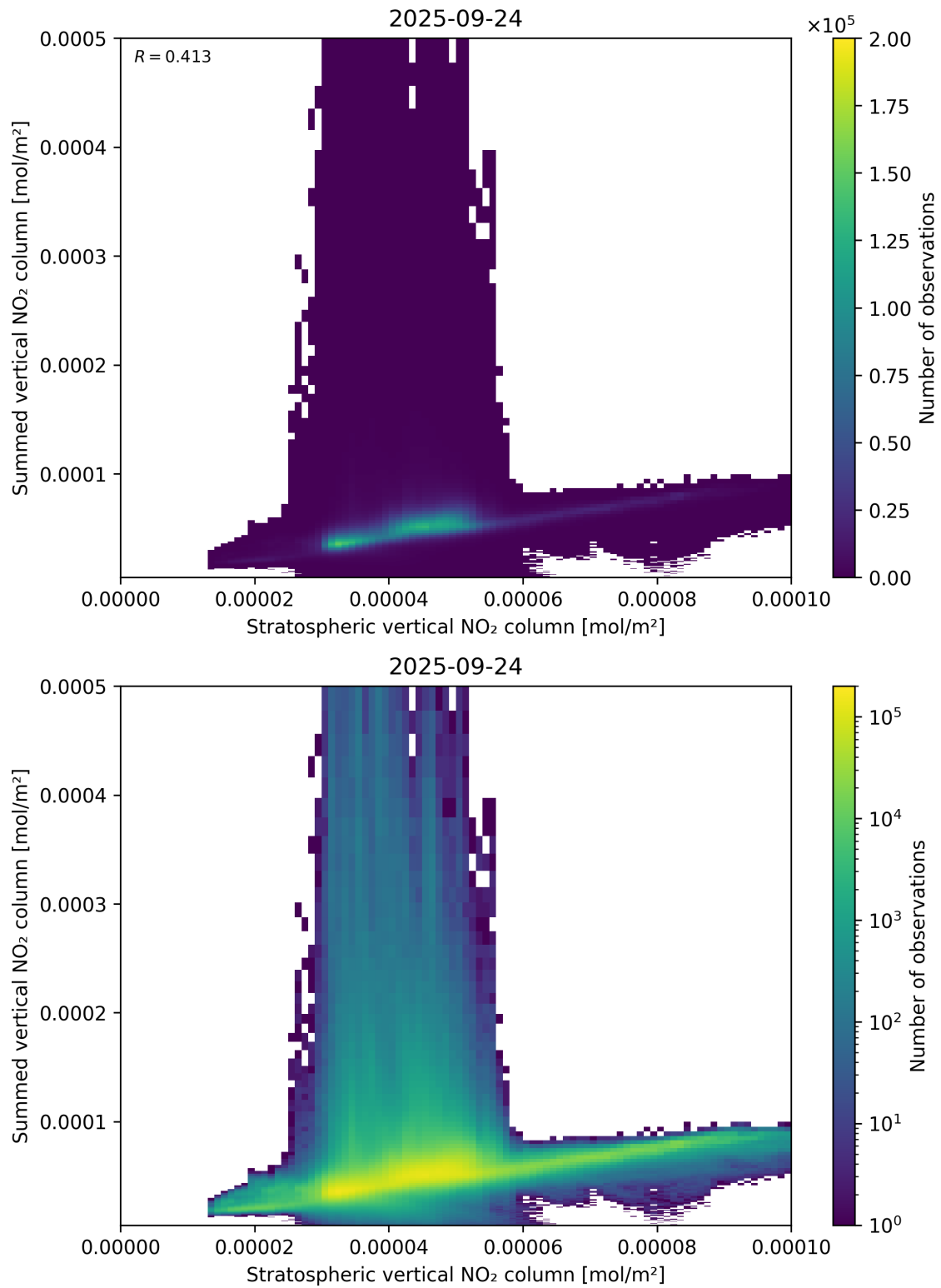
Figure 98: Scatter density plot of “Stratospheric vertical NO 2 column” against “Summed vertical NO 2 column” for 2025-09-23 to 2025-09-25.
