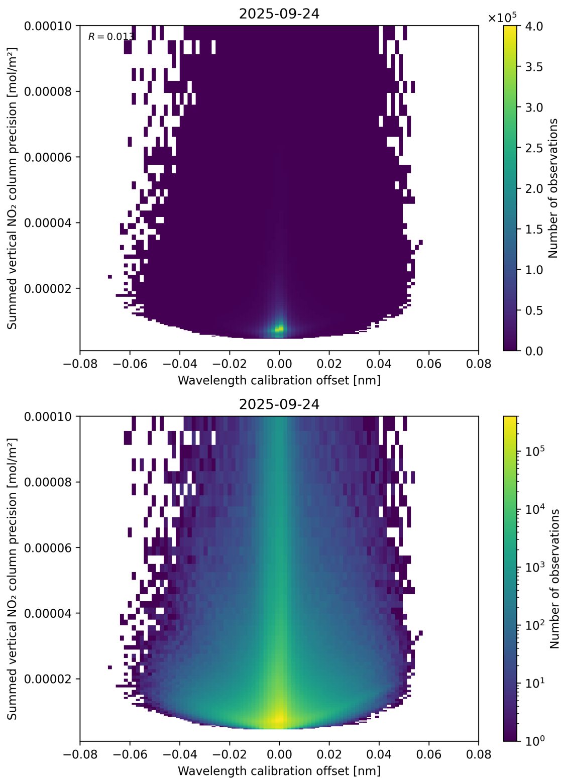
Figure 178: Scatter density plot of “Wavelength calibration offset” against “Summed vertical NO 2 column precision” for 2025-09-23 to 2025-09-25.
