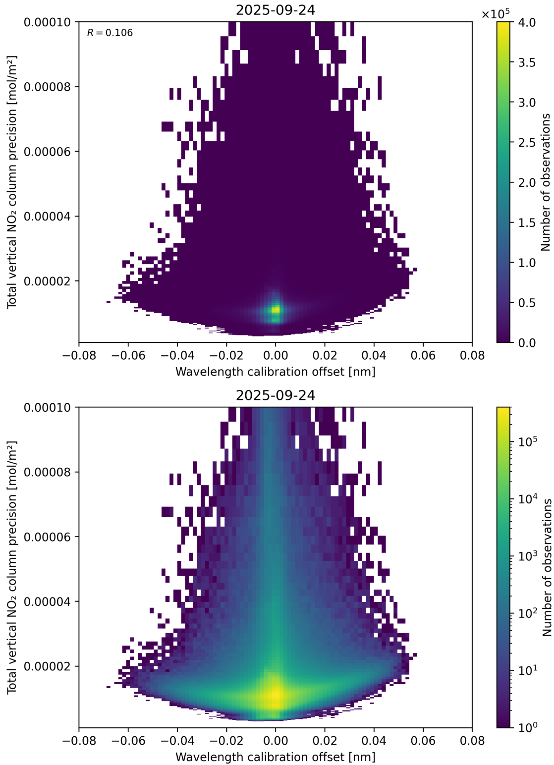
Figure 180: Scatter density plot of “Wavelength calibration offset” against “Total vertical NO 2 column precision” for 2025-09-23 to 2025-09-25.
