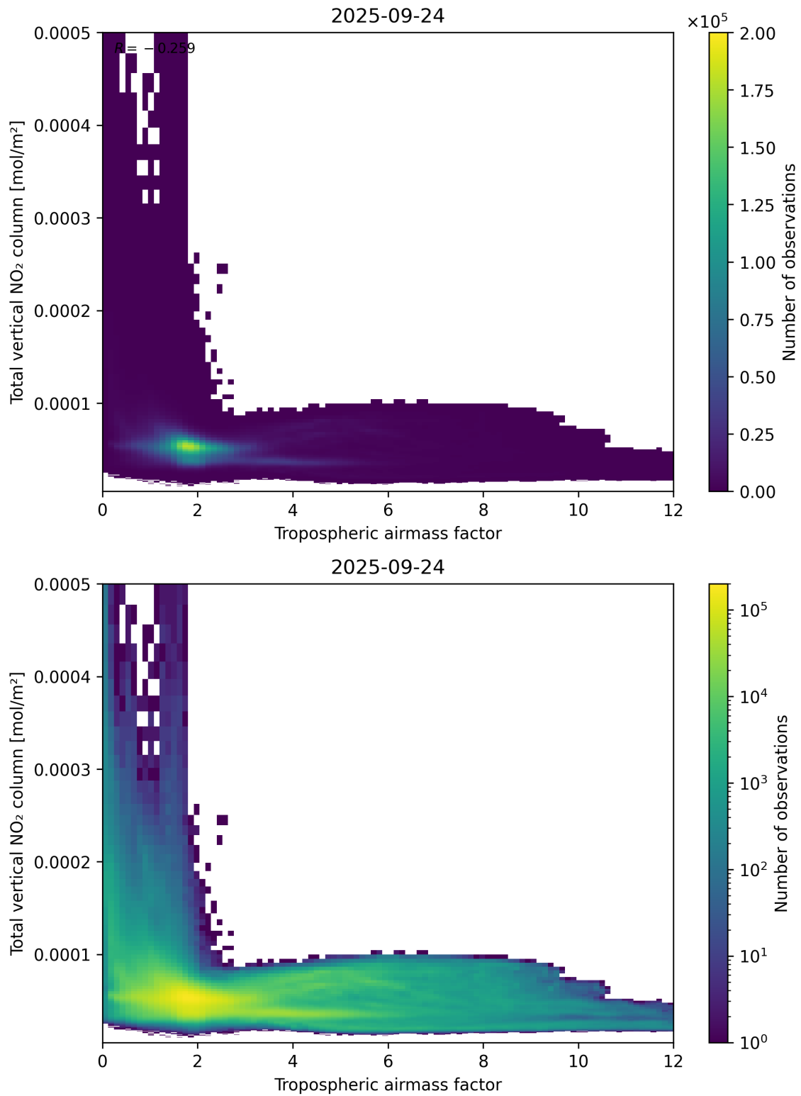
Figure 77: Scatter density plot of “Tropospheric airmass factor” against “Total vertical NO 2 column” for 2025-09-23 to 2025-09-25.
