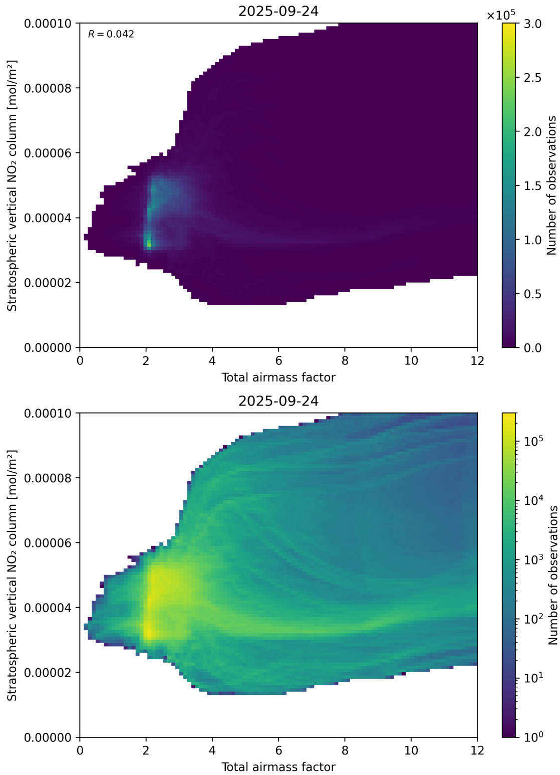
Figure 64: Scatter density plot of “Total airmass factor” against “Stratospheric vertical \text{NO}_2 column” for 2025-09-23 to 2025-09-25.
