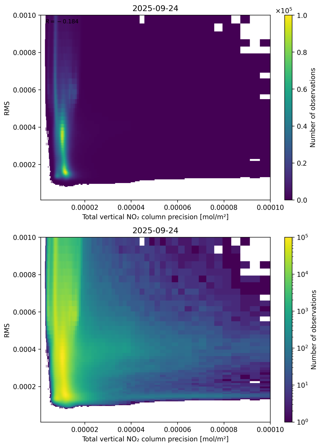
Figure 119: Scatter density plot of “Total vertical NO 2 column precision” against “RMS” for 2025-09-23 to 2025-09-25.
