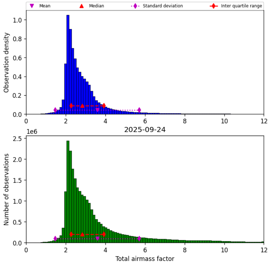
Figure 32: Histogram of “Total airmass factor” for 2025-09-23 to 2025-09-25
