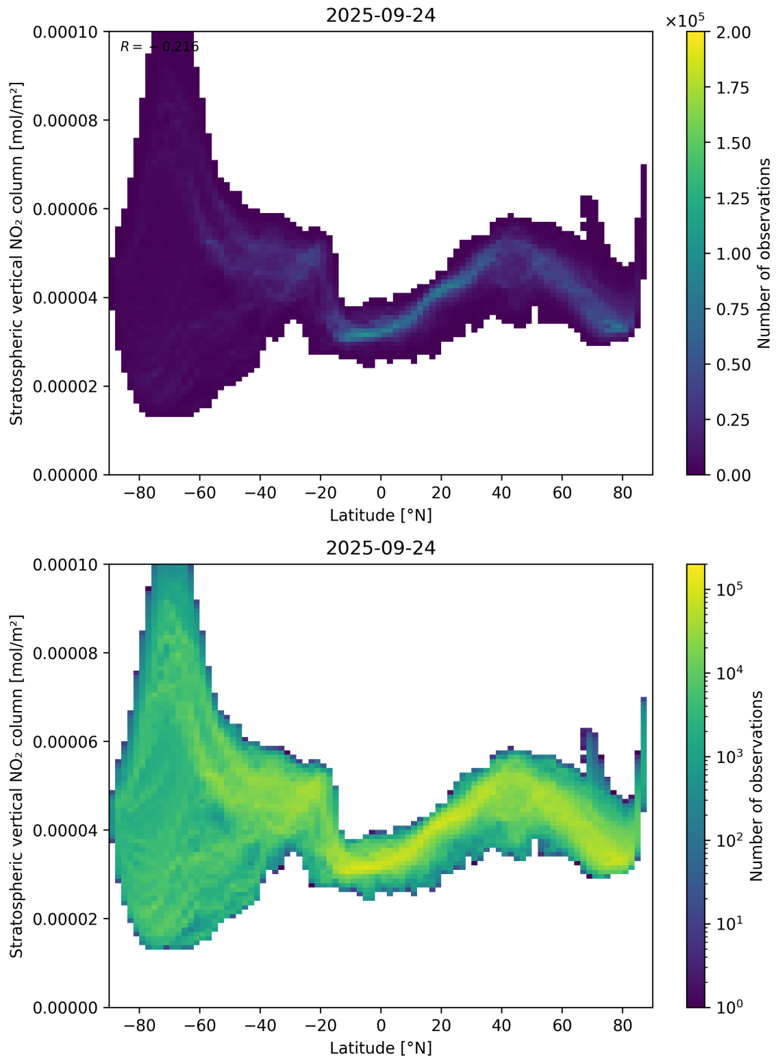
Figure 87: Scatter density plot of “Latitude” against “Stratospheric vertical NO 2 column” for 2025-09-23 to 2025-09-25.
