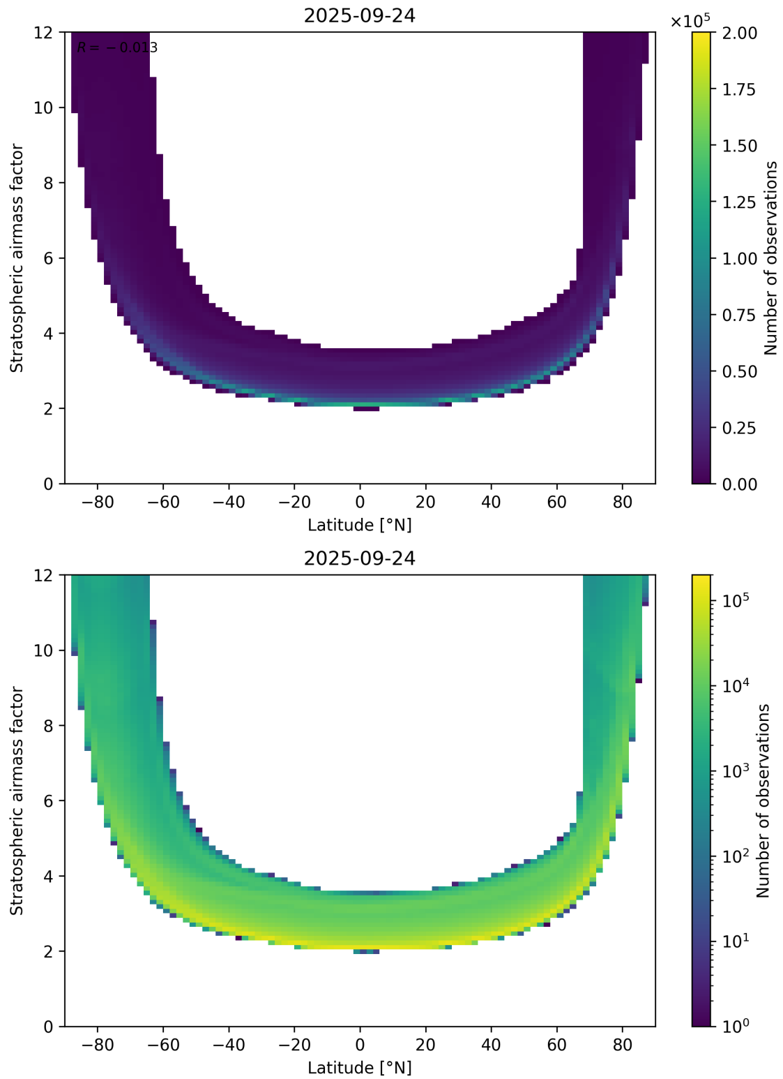
Figure 83: Scatter density plot of “Latitude” against “Stratospheric air mass factor” for 2025-09-23 to 2025-09-25.
