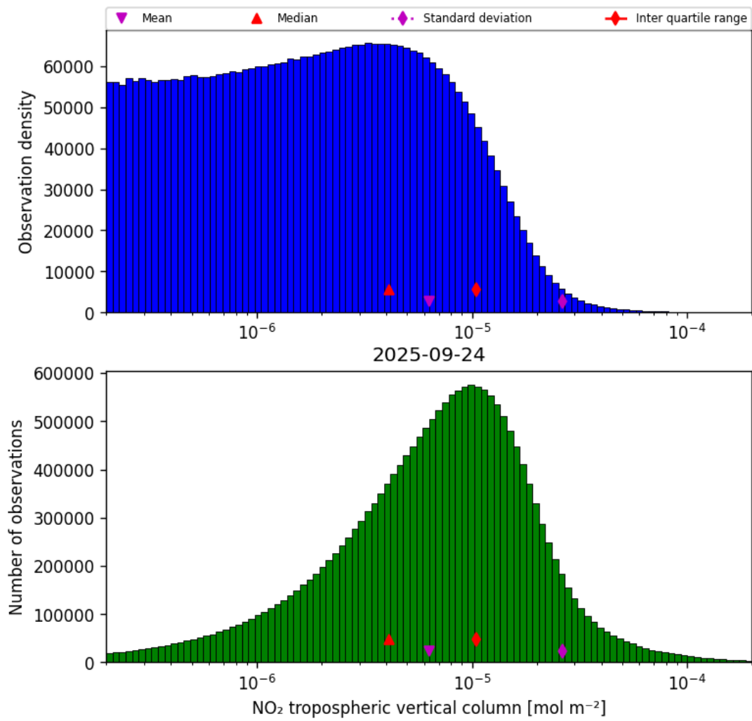
Figure 29: Histogram of “NO 2 tropospheric vertical column” for 2025-09-23 to 2025-09-25
