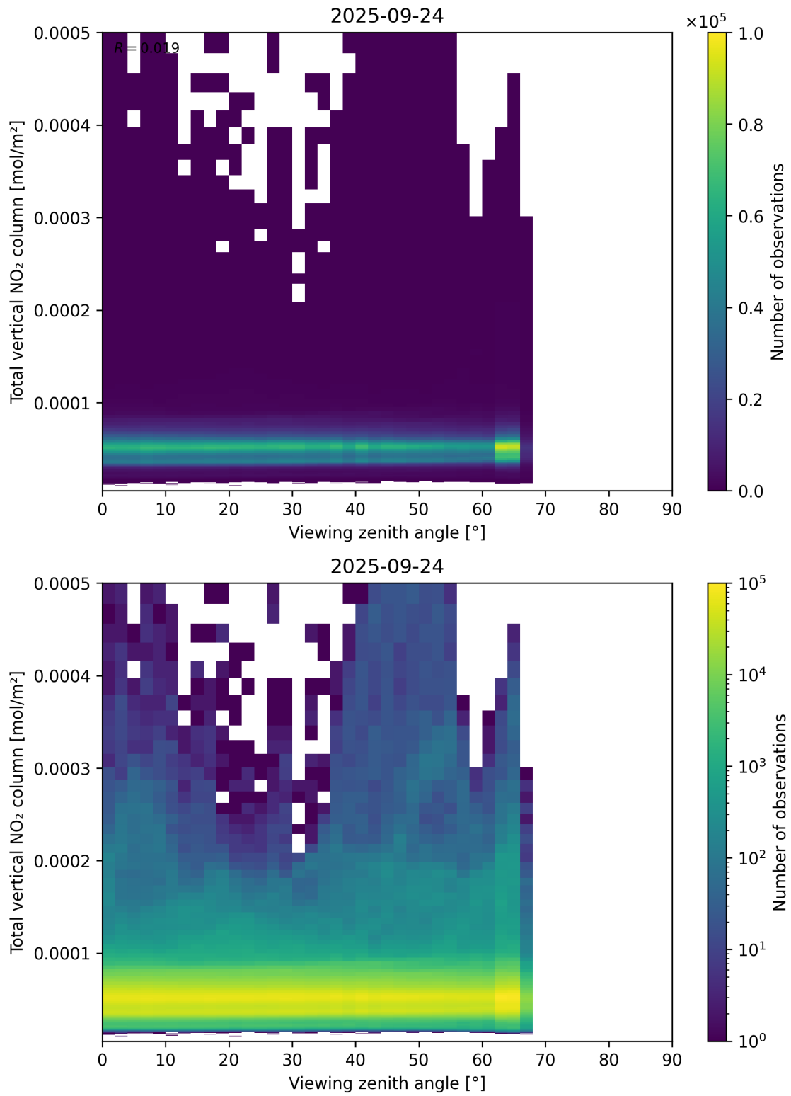
Figure 167: Scatter density plot of “Viewing zenith angle” against “Total vertical NO 2 column” for 2025-09-23 to 2025-09-25.
