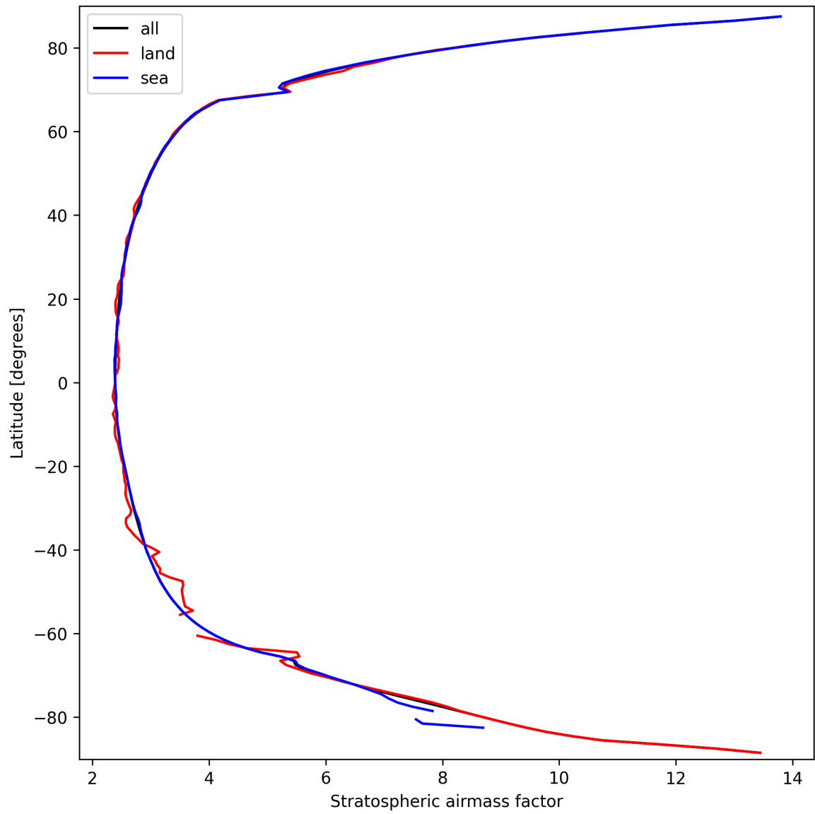
Figure 27: Zonal average of “Stratospheric airmass factor” for 2025-09-23 to 2025-09-25.
