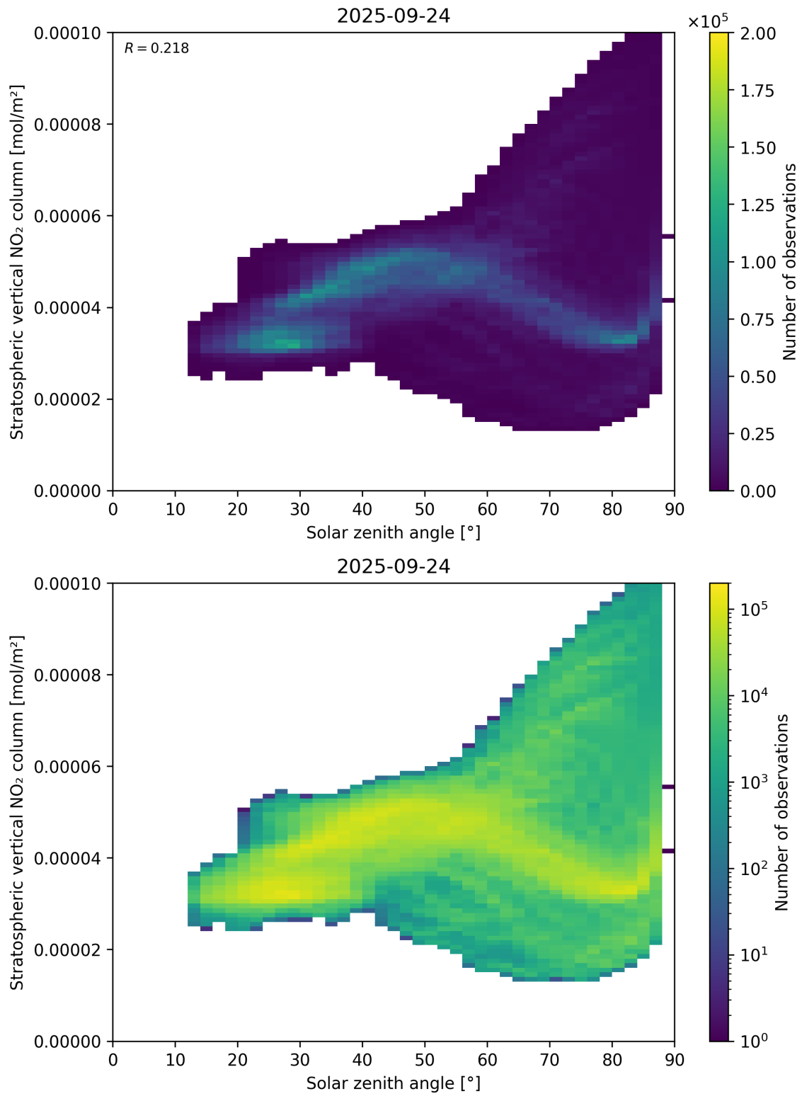
Figure 150: Scatter density plot of “Solar zenith angle” against “Stratospheric vertical NO 2 column” for 2025-09-23 to 2025-09-25.
