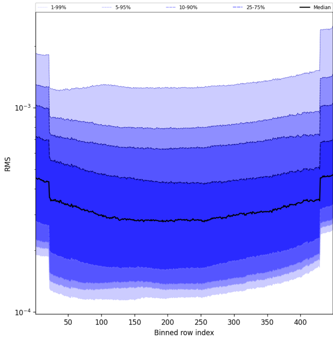
Figure 60: Along track statistics of “RMS” for 2025-09-23 to 2025-09-25
