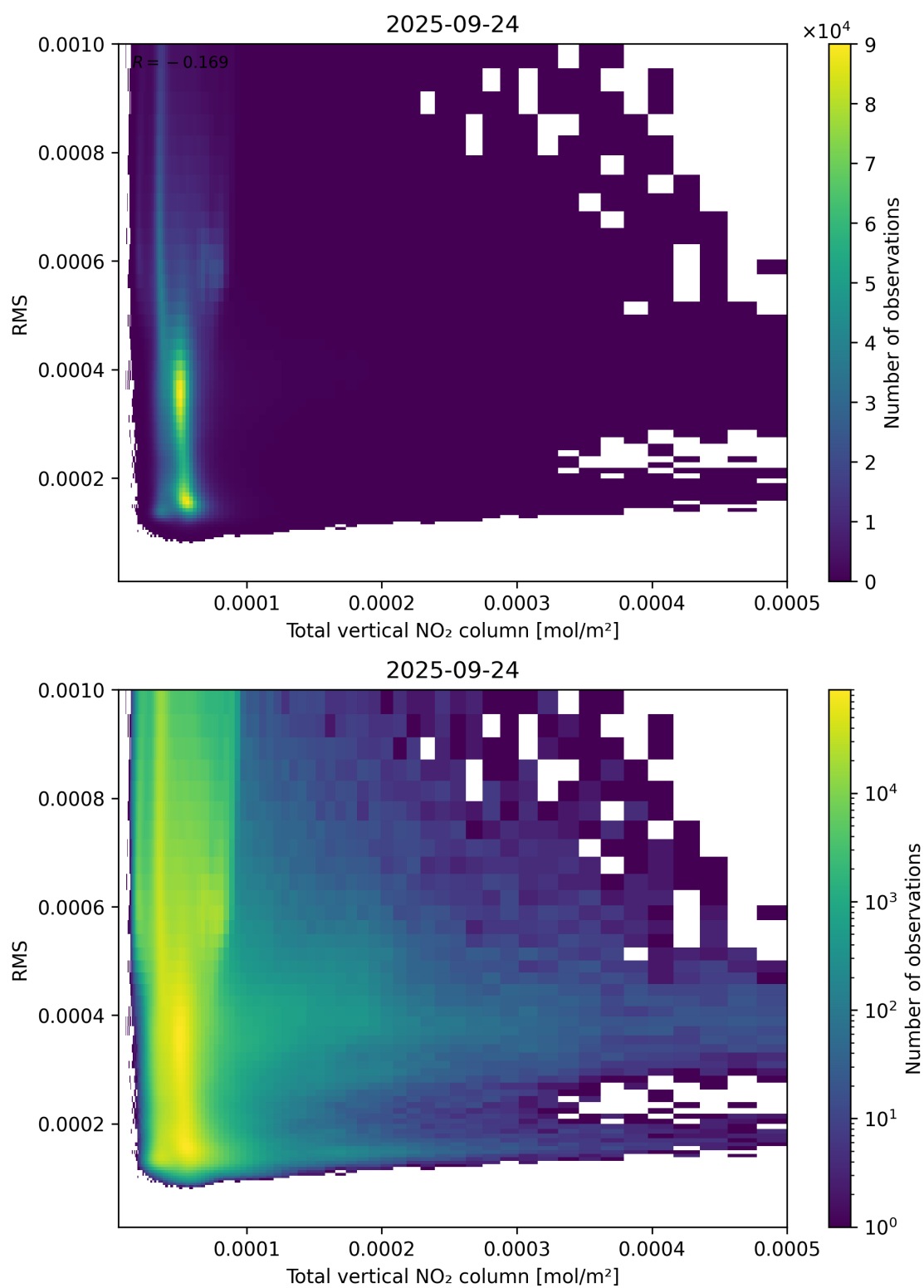
Figure 120: Scatter density plot of “Total vertical NO 2 column” against “RMS” for 2025-09-23 to 2025-09-25.
