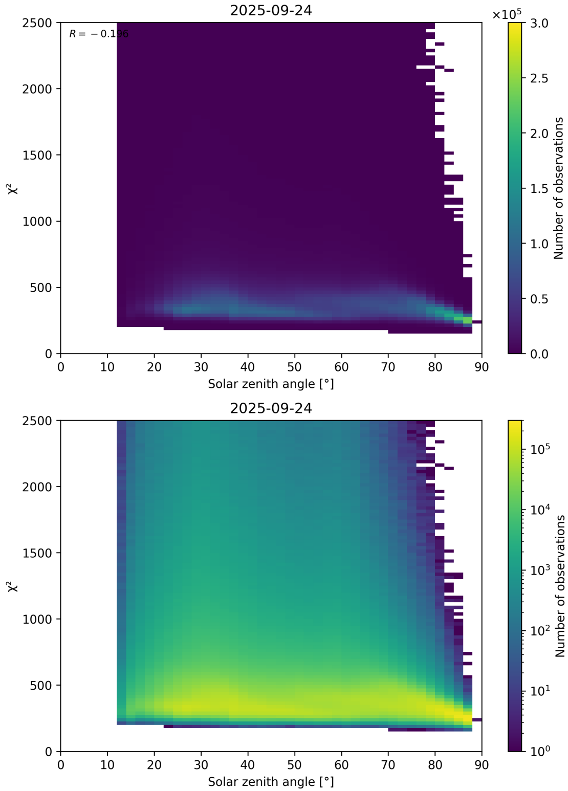
Figure 148: Scatter density plot of “Solar zenith angle” against “ \chi^2 ” for 2025-09-23 to 2025-09-25.
