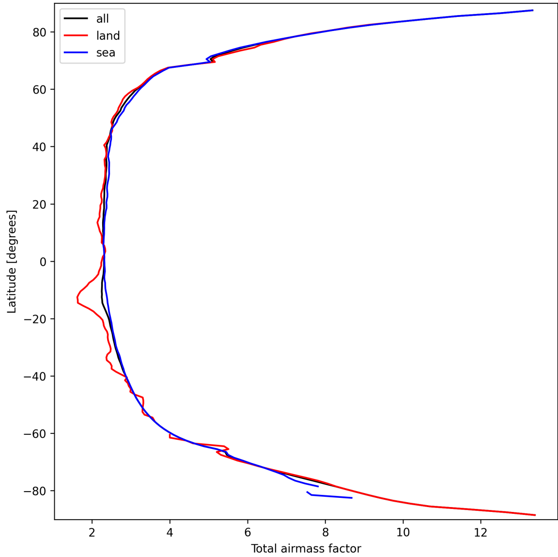
Figure 15: Zonal average of “Total airmass factor” for 2025-09-23 to 2025-09-25.
