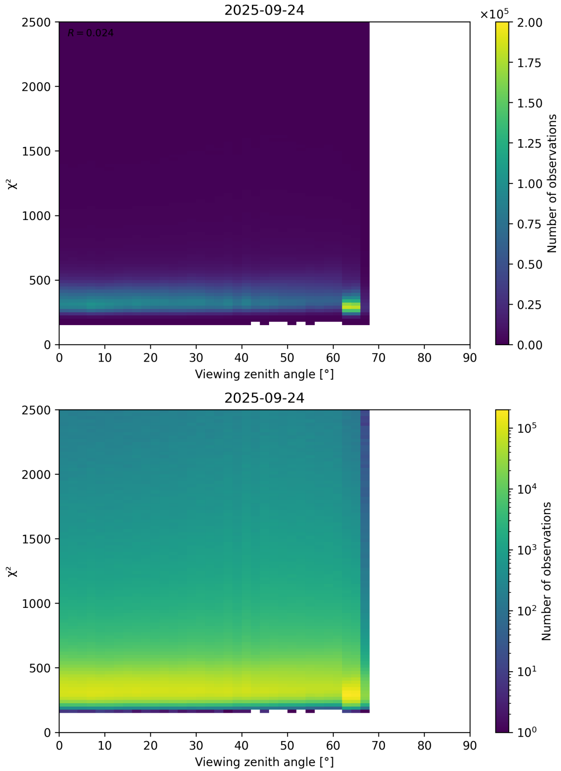
Figure 162: Scatter density plot of “Viewing zenith angle” against “ \chi^2 ” for 2025-09-23 to 2025-09-25.
