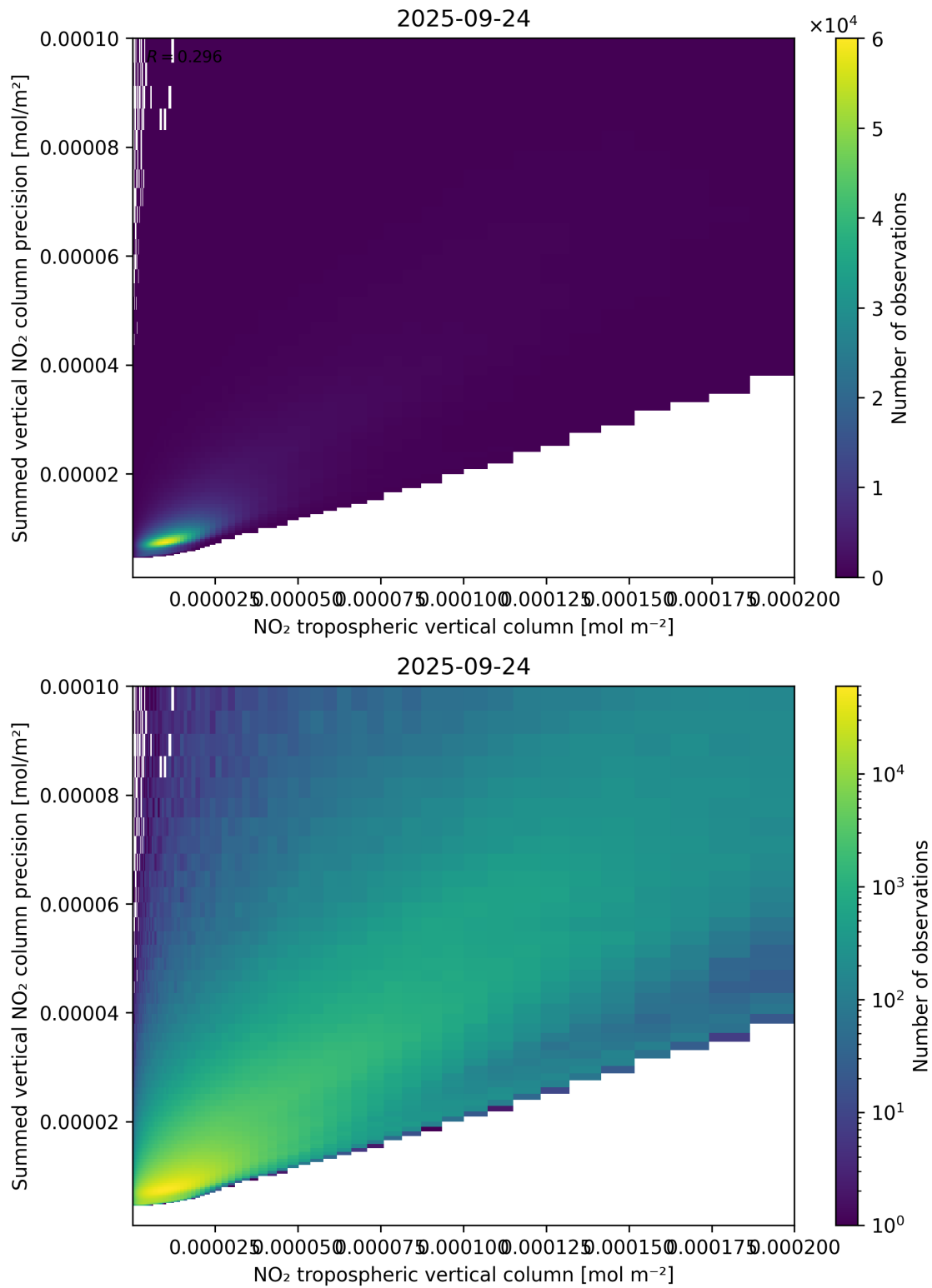
Figure 127: Scatter density plot of “NO 2 tropospheric vertical column” against “Summed vertical NO 2 column precision” for 2025-09-23 to 2025-09-25.
