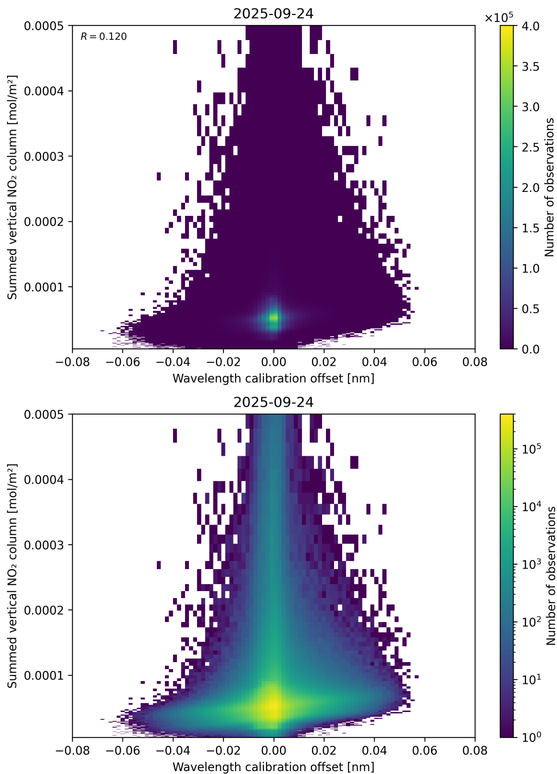
Figure 177: Scatter density plot of “Wavelength calibration offset” against “Summed vertical NO 2 column” for 2025-09-23 to 2025-09-25.
