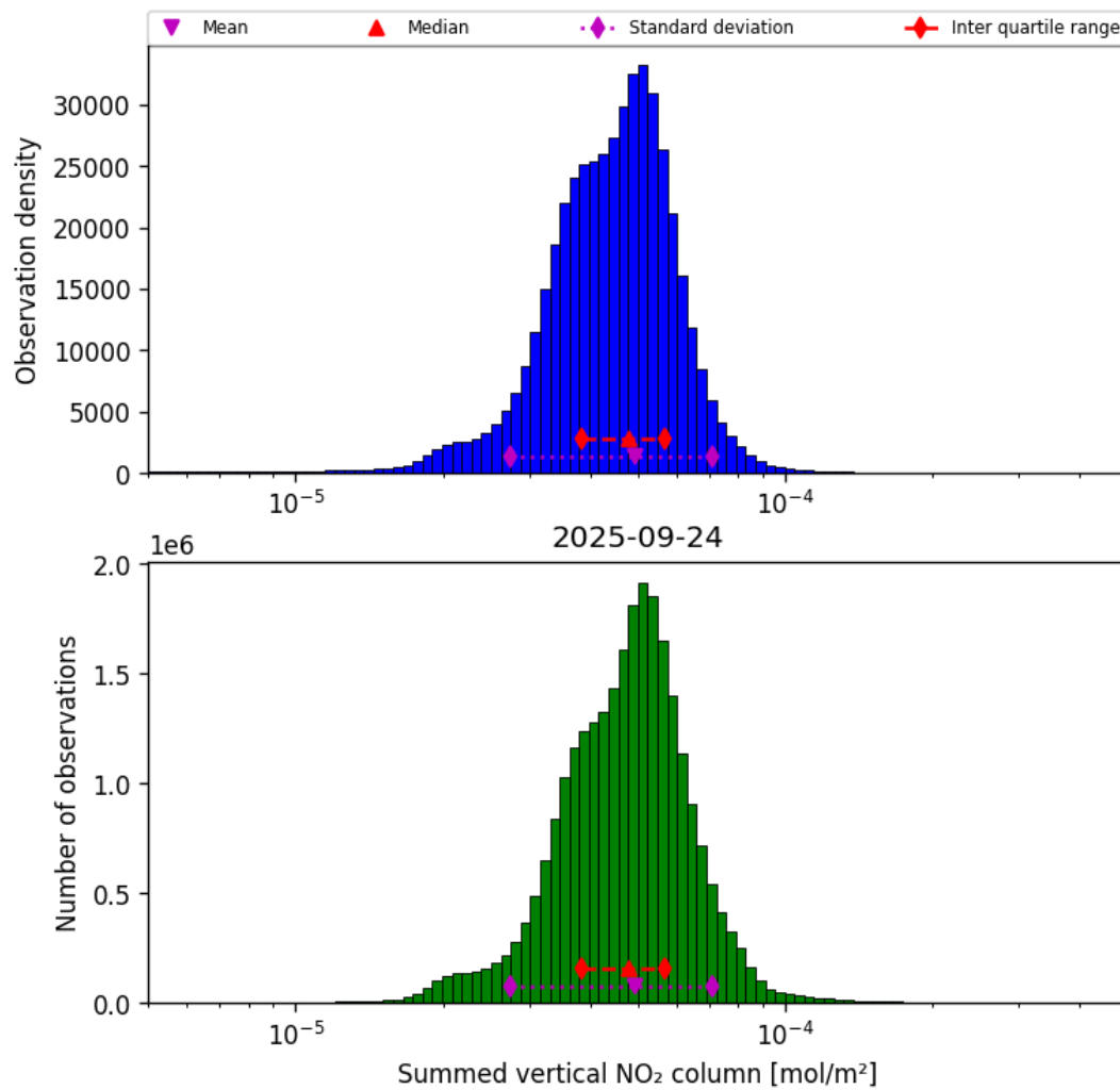
Figure 40: Histogram of “Summed vertical NO 2 column” for 2025-09-23 to 2025-09-25
