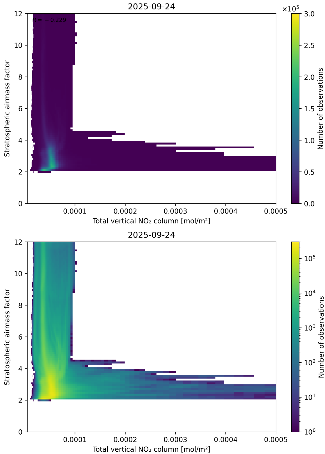
Figure 110: Scatter density plot of “Total vertical NO 2 column” against “Stratospheric airmass factor” for 2025-09-23 to 2025-09-25.
