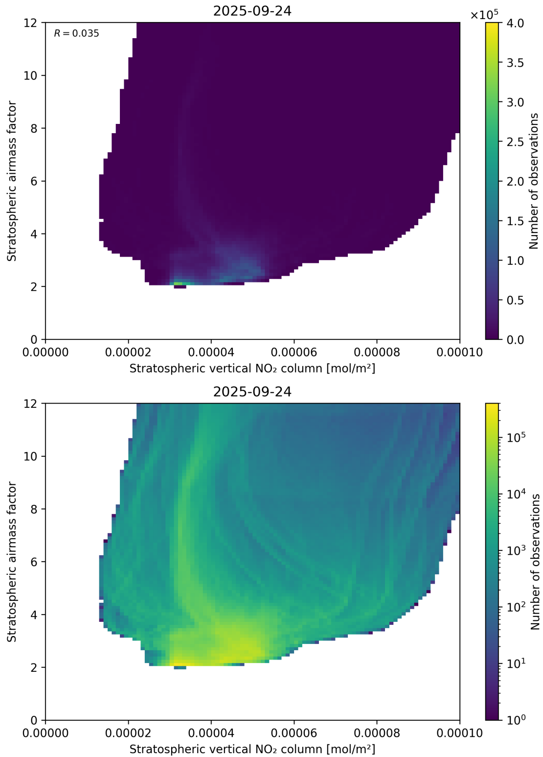
Figure 96: Scatter density plot of “Stratospheric vertical NO 2 column” against “Stratospheric airmass factor” for 2025-09-23 to 2025-09-25.
