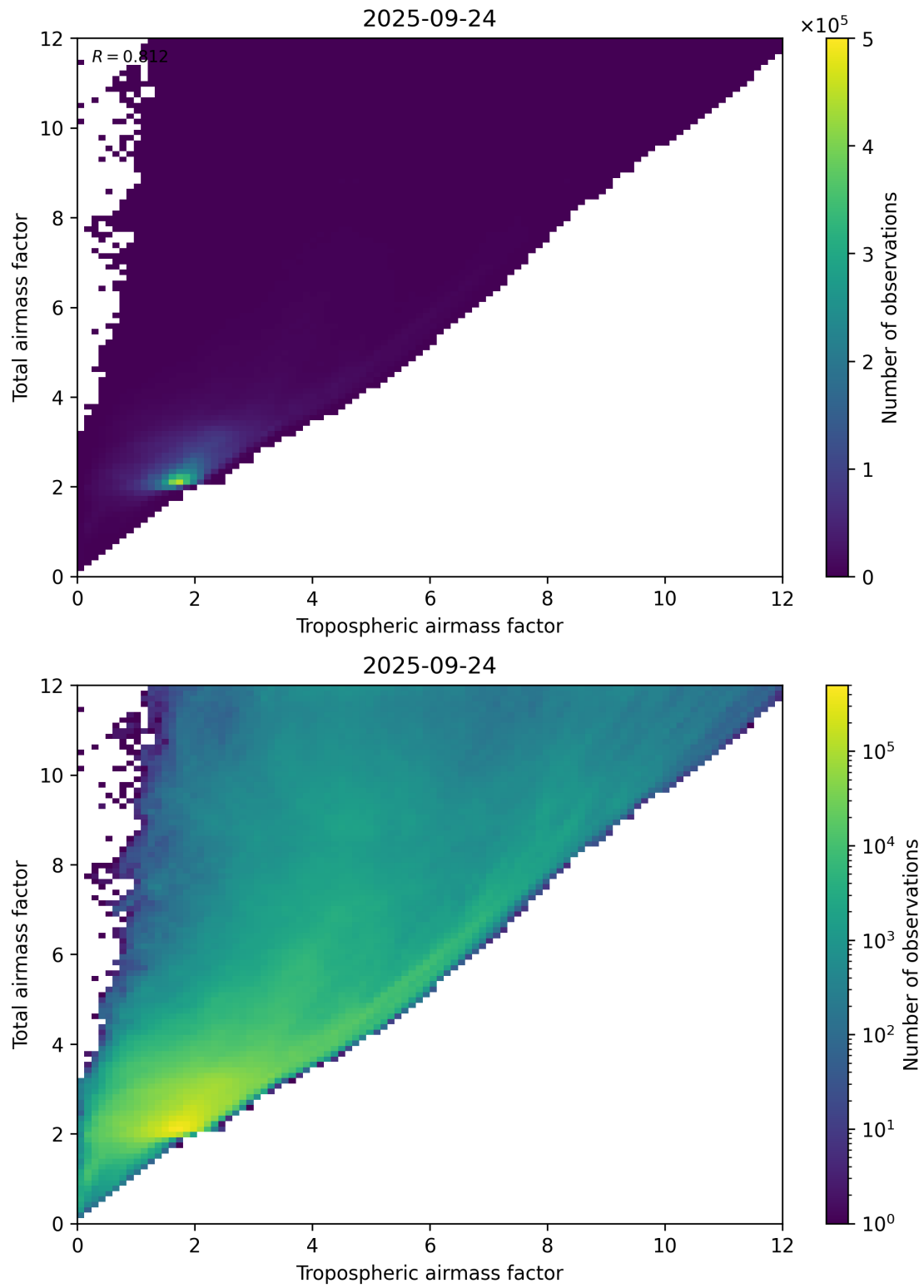
Figure 72: Scatter density plot of “Tropospheric airmass factor” against “Total airmass factor” for 2025-09-23 to 2025-09-25.
