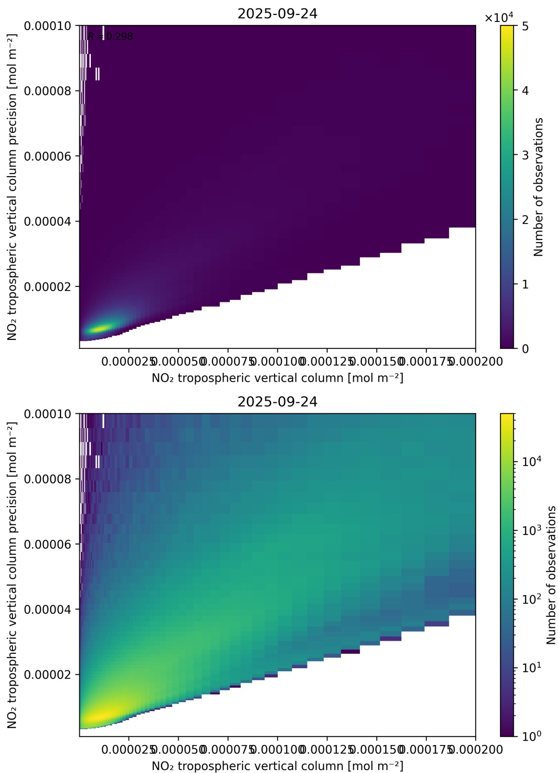
Figure 130: Scatter density plot of “NO 2 tropospheric vertical column” against “NO 2 tropospheric vertical column precision” for 2025-09-23 to 2025-09-25.
