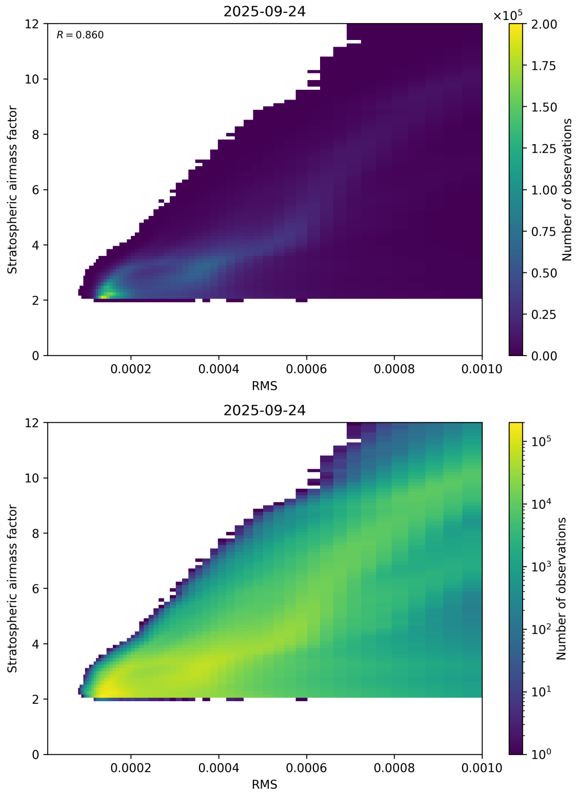
Figure 144: Scatter density plot of “RMS” against “Stratospheric airmass factor” for 2025-09-23 to 2025-09-25.
