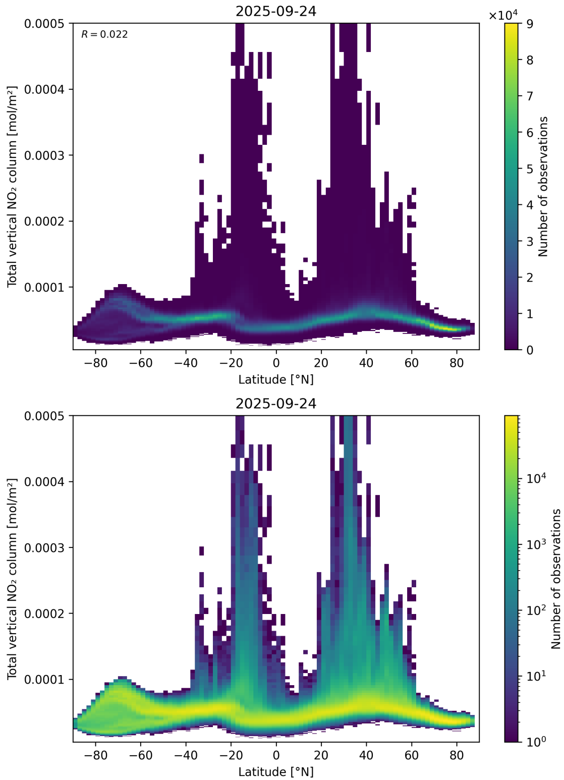
Figure 90: Scatter density plot of “Latitude” against “Total vertical NO 2 column” for 2025-09-23 to 2025-09-25.
