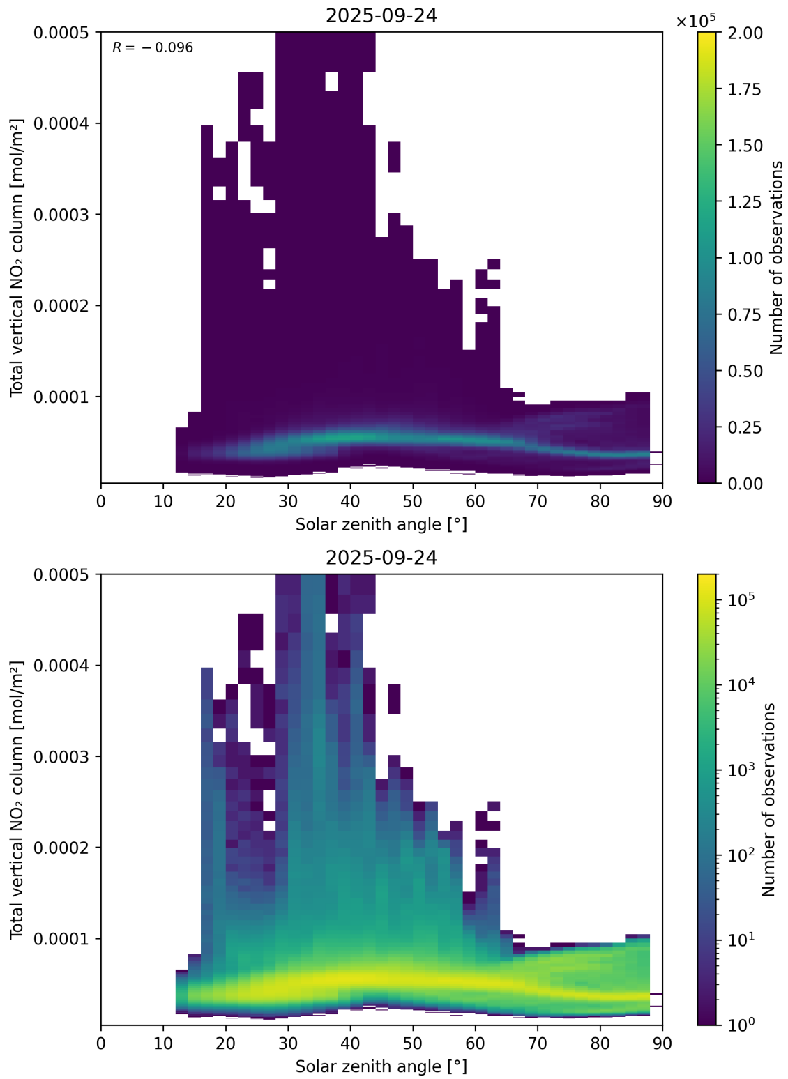
Figure 153: Scatter density plot of “Solar zenith angle” against “Total vertical NO 2 column” for 2025-09-23 to 2025-09-25.
