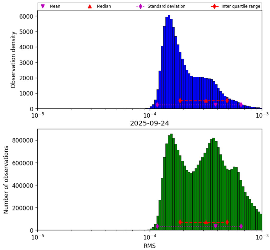
Figure 43: Histogram of “RMS” for 2025-09-23 to 2025-09-25
