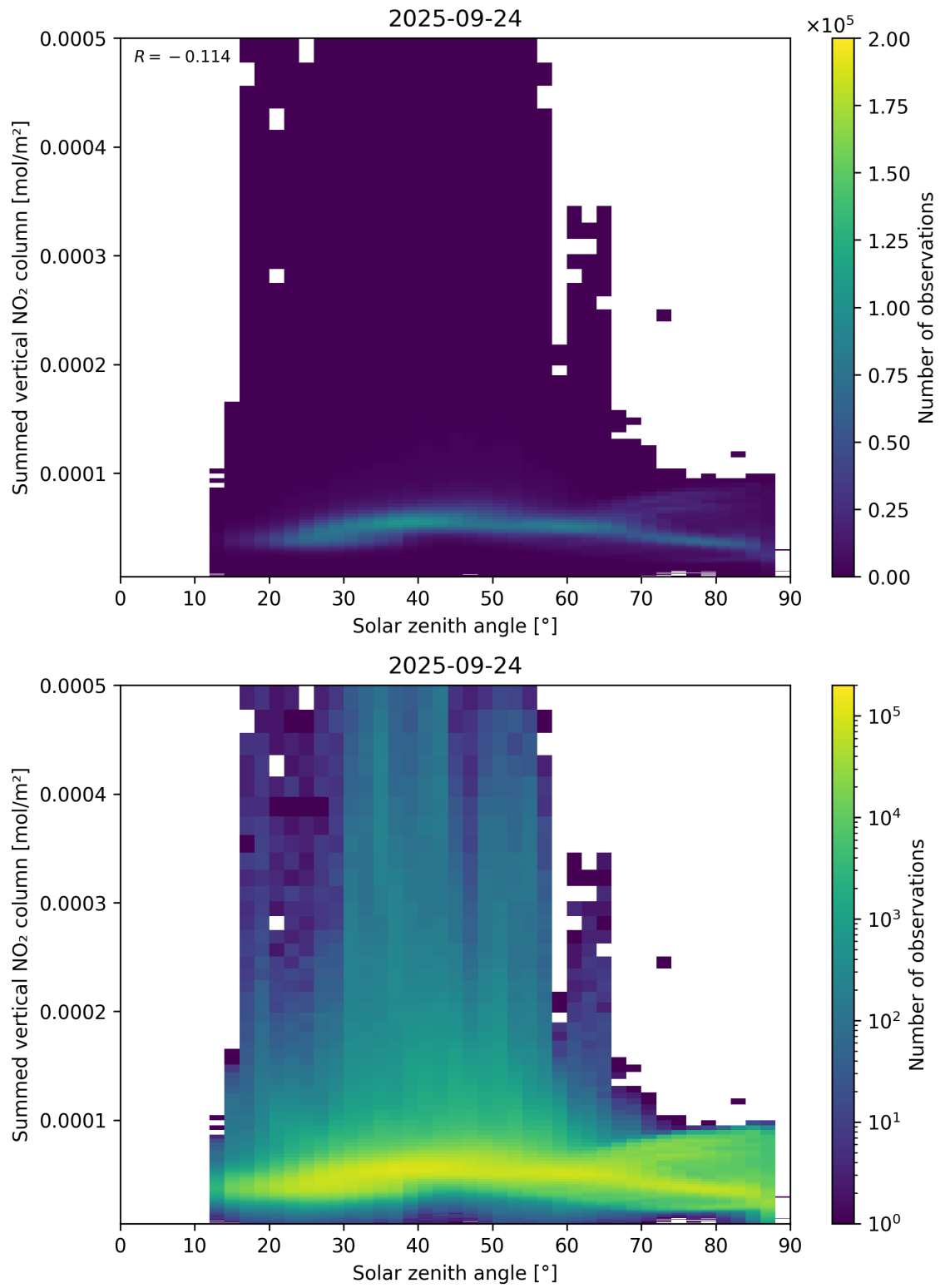
Figure 151: Scatter density plot of “Solar zenith angle” against “Summed vertical NO 2 column” for 2025-09-23 to 2025-09-25.
