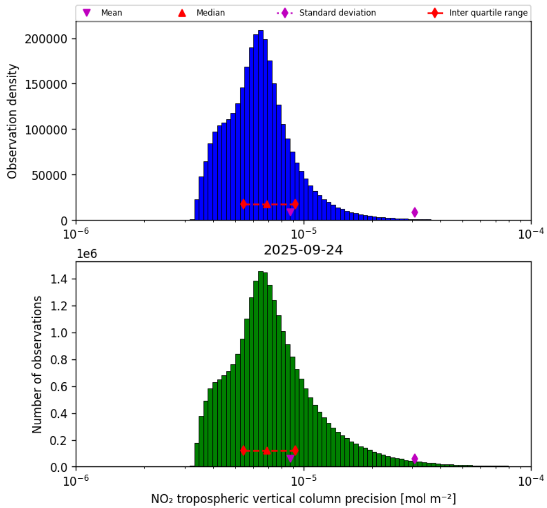
Figure 30: Histogram of “NO 2 tropospheric vertical column precision” for 2025-09-23 to 2025-09-25
