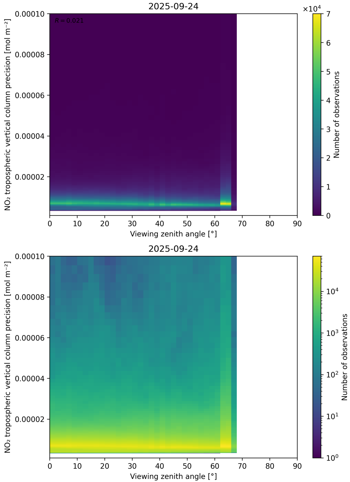
Figure 170: Scatter density plot of “Viewing zenith angle” against “NO 2 tropospheric vertical column precision” for 2025-09-23 to 2025-09-25.
