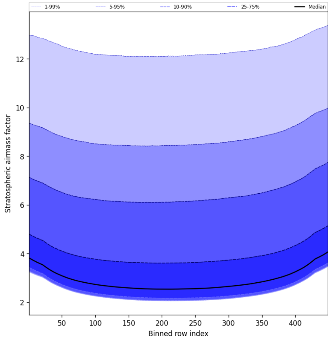
Figure 61: Along track statistics of “Stratospheric airmass factor” for 2025-09-23 to 2025-09-25
