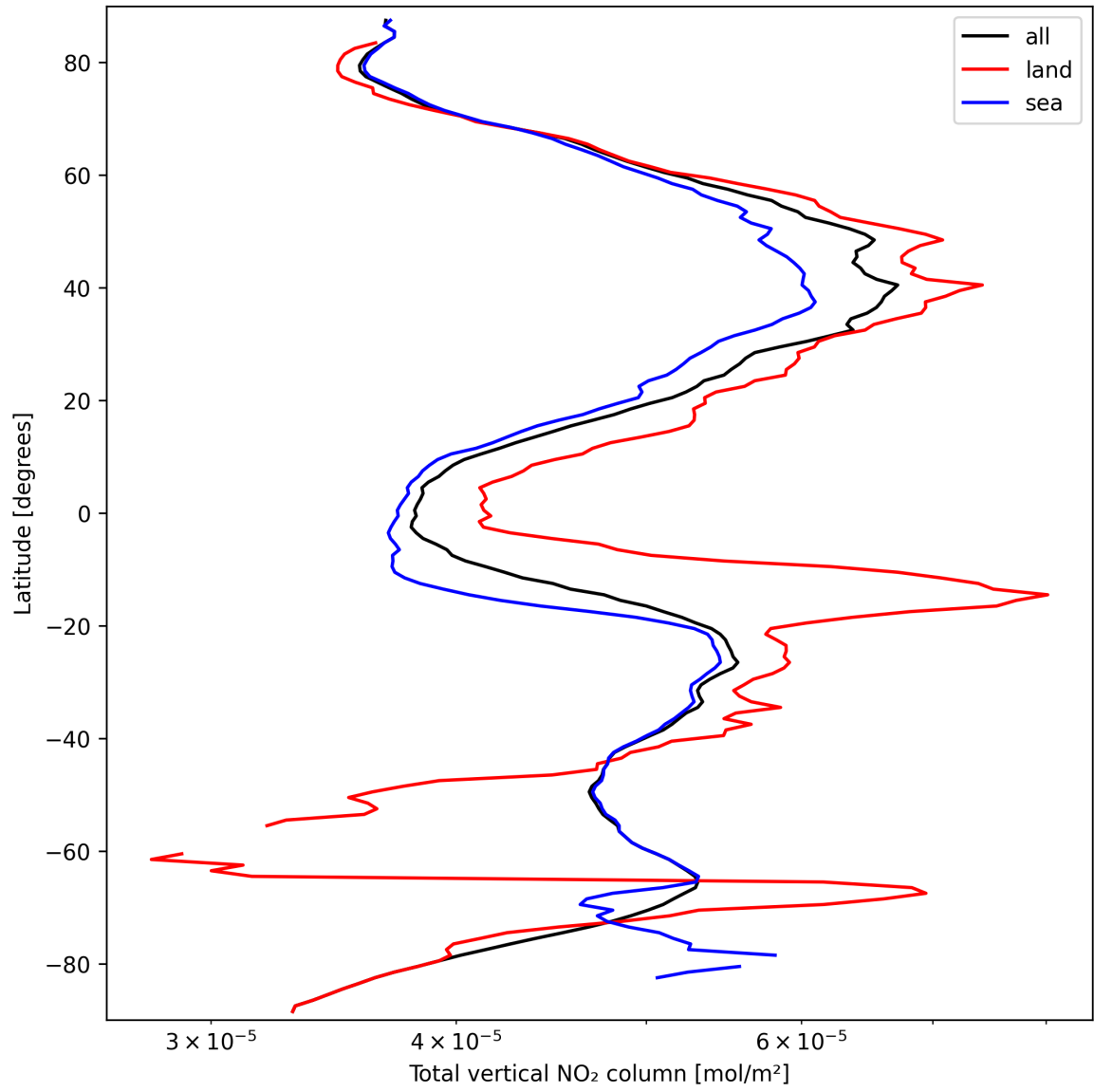
Figure 21: Zonal average of “Total vertical NO 2 column” for 2025-09-23 to 2025-09-25.
