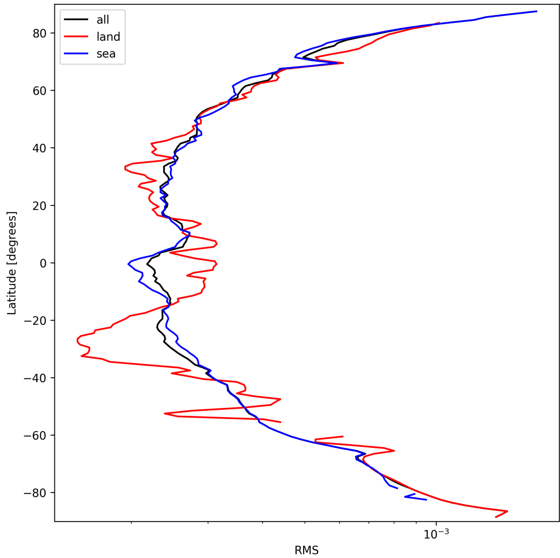
Figure 26: Zonal average of “RMS” for 2025-09-23 to 2025-09-25.
