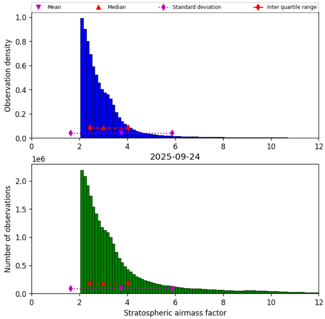
Figure 44: Histogram of “Stratospheric airmass factor” for 2025-09-23 to 2025-09-25
