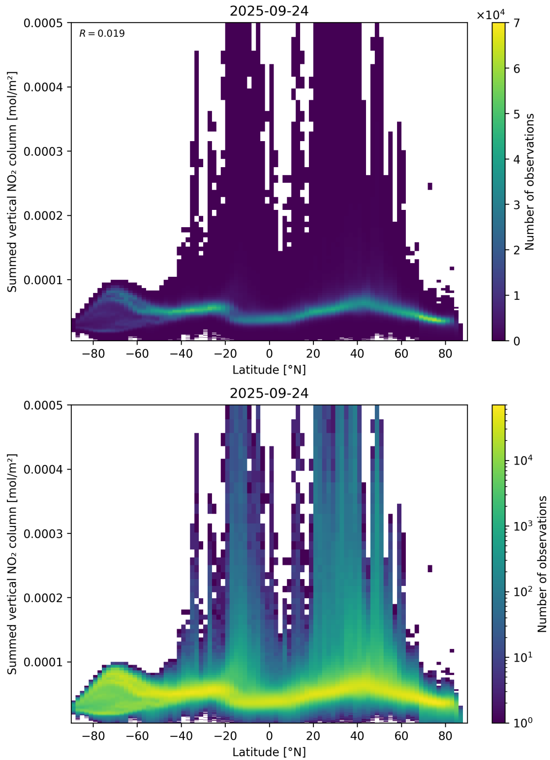
Figure 88: Scatter density plot of “Latitude” against “Summed vertical NO 2 column” for 2025-09-23 to 2025-09-25.
