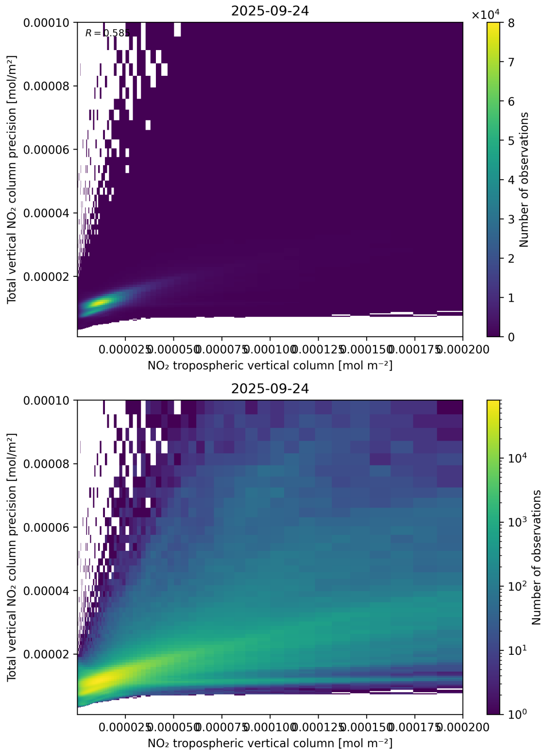
Figure 129: Scatter density plot of “NO 2 tropospheric vertical column” against “Total vertical NO 2 column precision” for 2025-09-23 to 2025-09-25.
