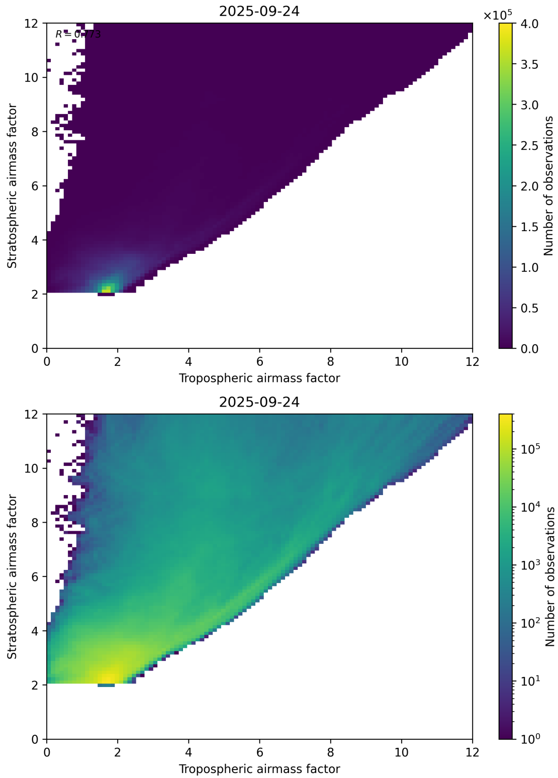
Figure 71: Scatter density plot of “Tropospheric airmass factor” against “Stratospheric airmass factor” for 2025-09-23 to 2025-09-25.
