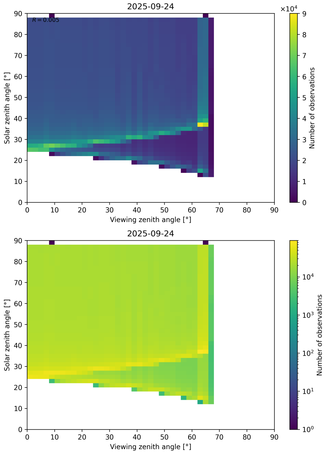
Figure 172: Scatter density plot of “Viewing zenith angle” against “Solar zenith angle” for 2025-09-23 to 2025-09-25.
