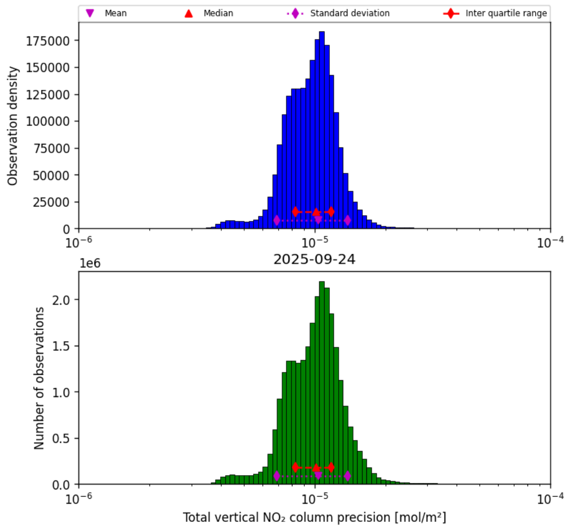
Figure 39: Histogram of “Total vertical NO 2 column precision” for 2025-09-23 to 2025-09-25
