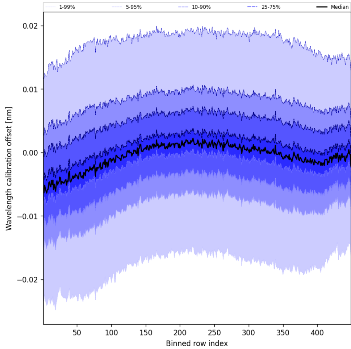
Figure 52: Along track statistics of “Wavelength calibration offset” for 2025-09-23 to 2025-09-25
