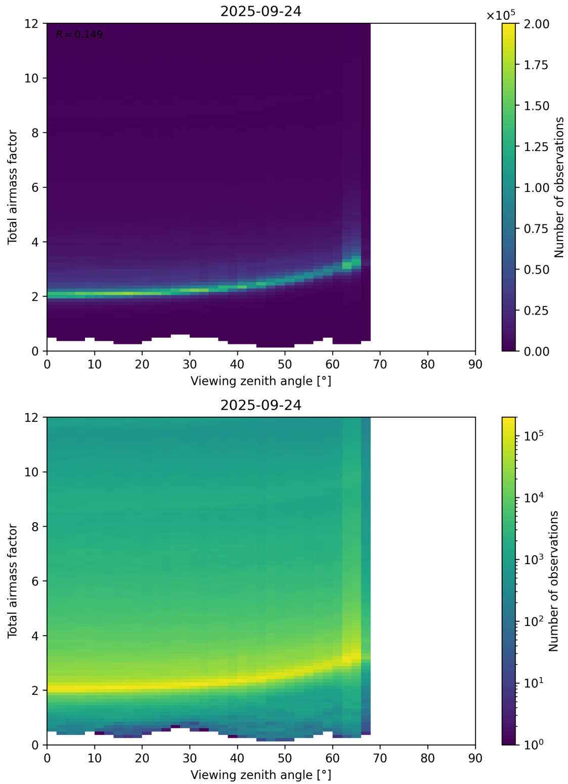
Figure 160: Scatter density plot of “Viewing zenith angle” against “Total airmass factor” for 2025-09-23 to 2025-09-25.
