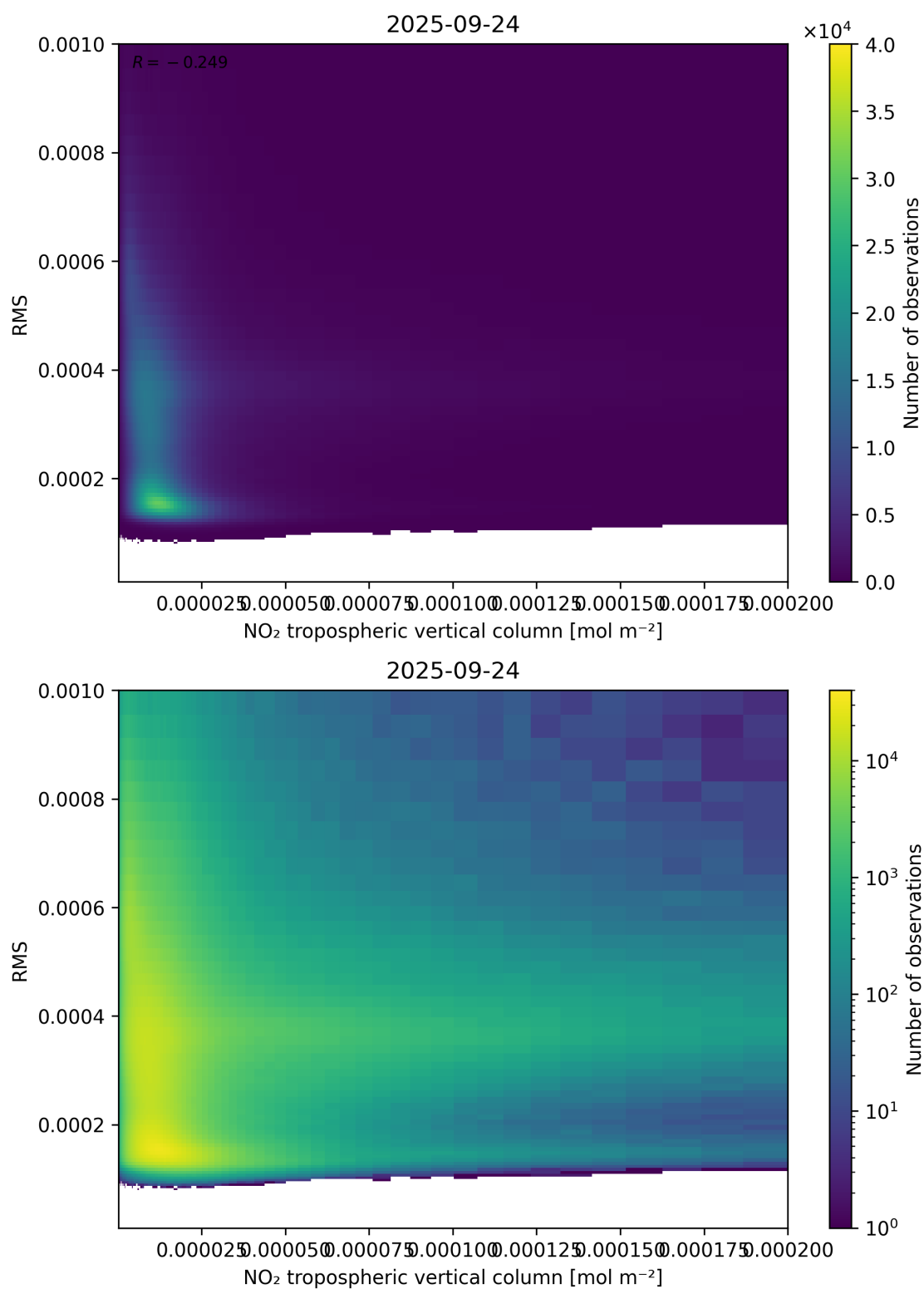
Figure 142: Scatter density plot of “NO 2 tropospheric vertical column” against “RMS” for 2025-09-23 to 2025-09-25.
