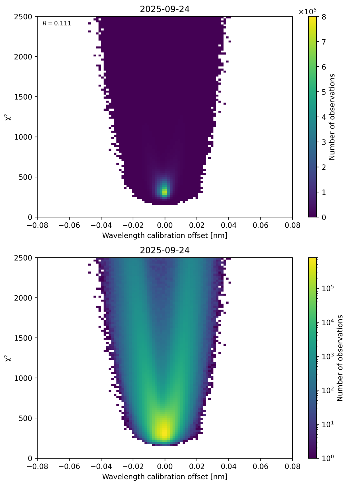
Figure 175: Scatter density plot of “Wavelength calibration offset” against “ \chi^2 ” for 2025-09-23 to 2025-09-25.
