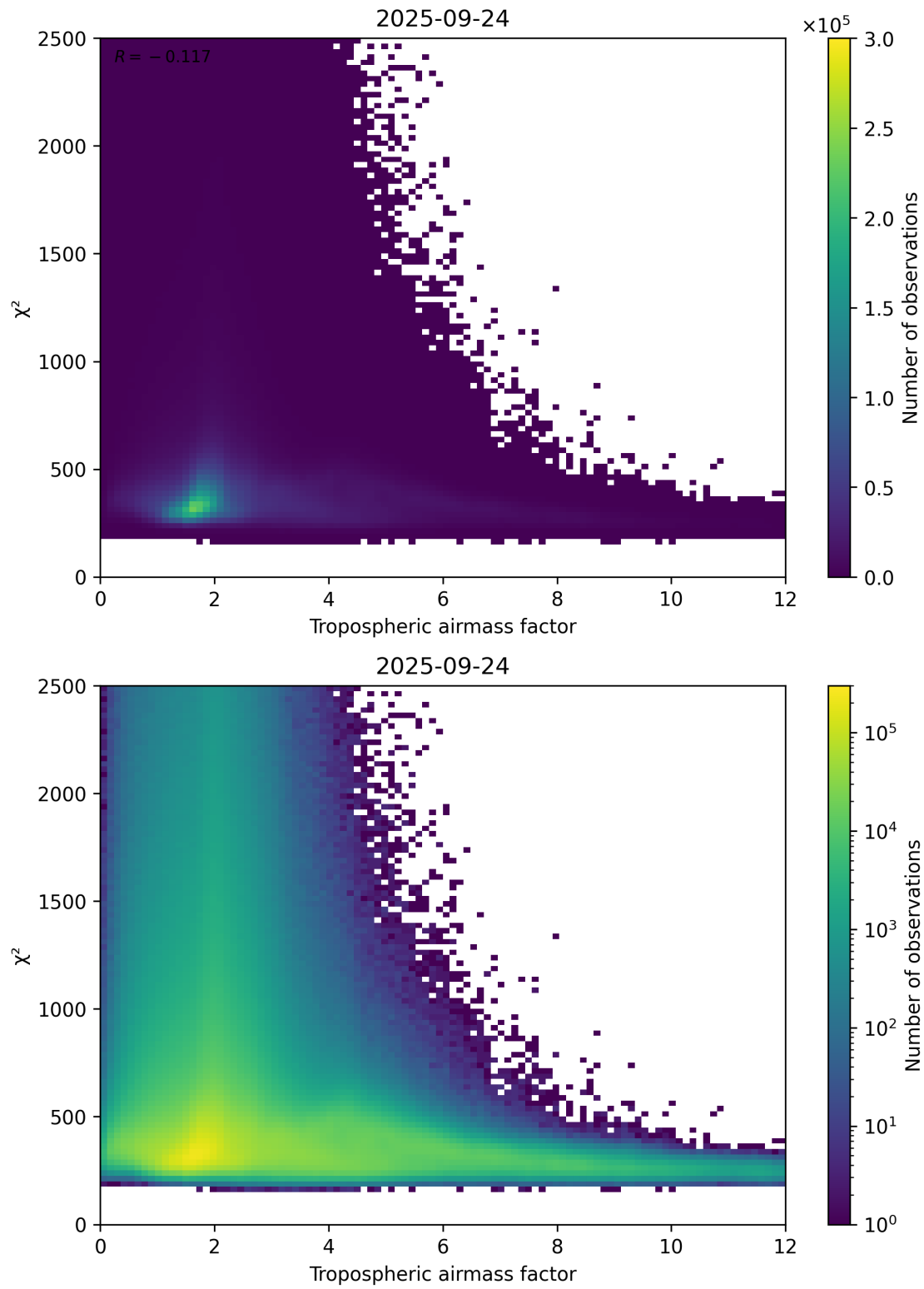
Figure 73: Scatter density plot of “Tropospheric airmass factor” against “ \chi^2 ” for 2025-09-23 to 2025-09-25.
