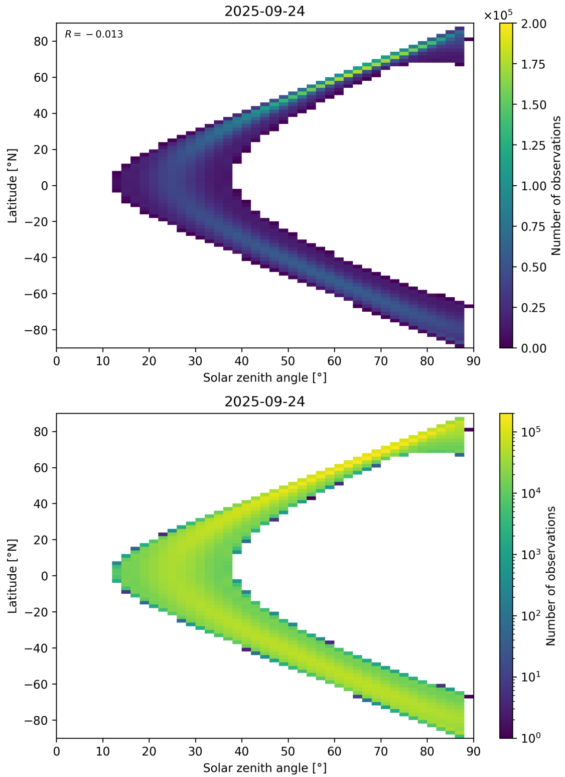
Figure 149: Scatter density plot of “Solar zenith angle” against “Latitude” for 2025-09-23 to 2025-09-25.
