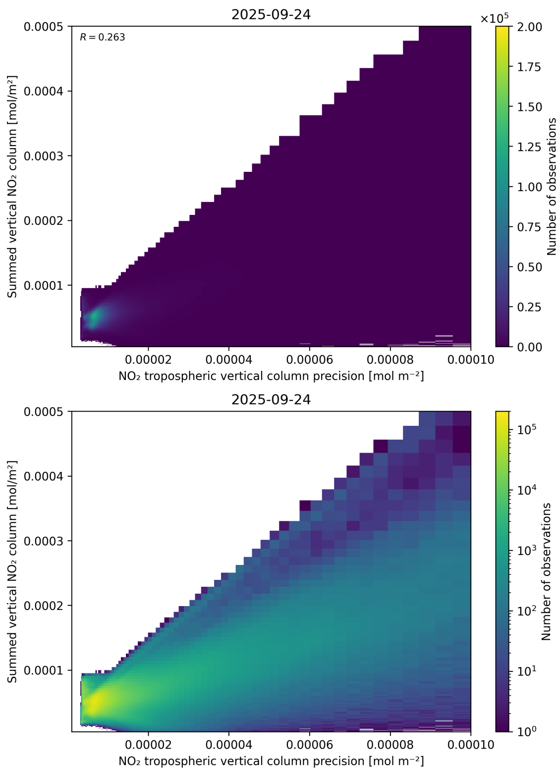
Figure 136: Scatter density plot of “NO 2 tropospheric vertical column precision” against “Summed vertical NO 2 column” for 2025-09-23 to 2025-09-25.
