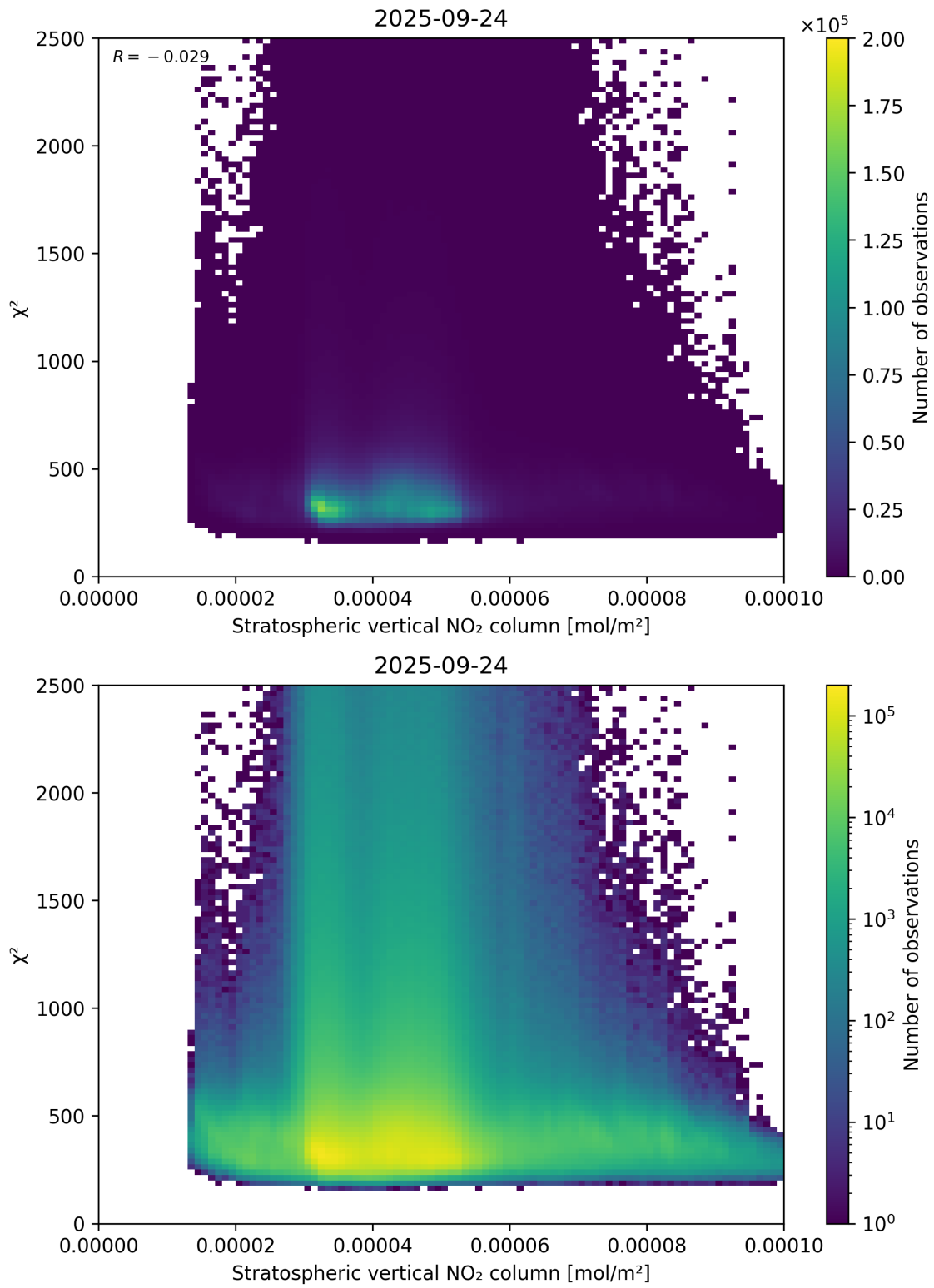
Figure 97: Scatter density plot of “Stratospheric vertical NO 2 column” against “ \chi^2 ” for 2025-09-23 to 2025-09-25.
