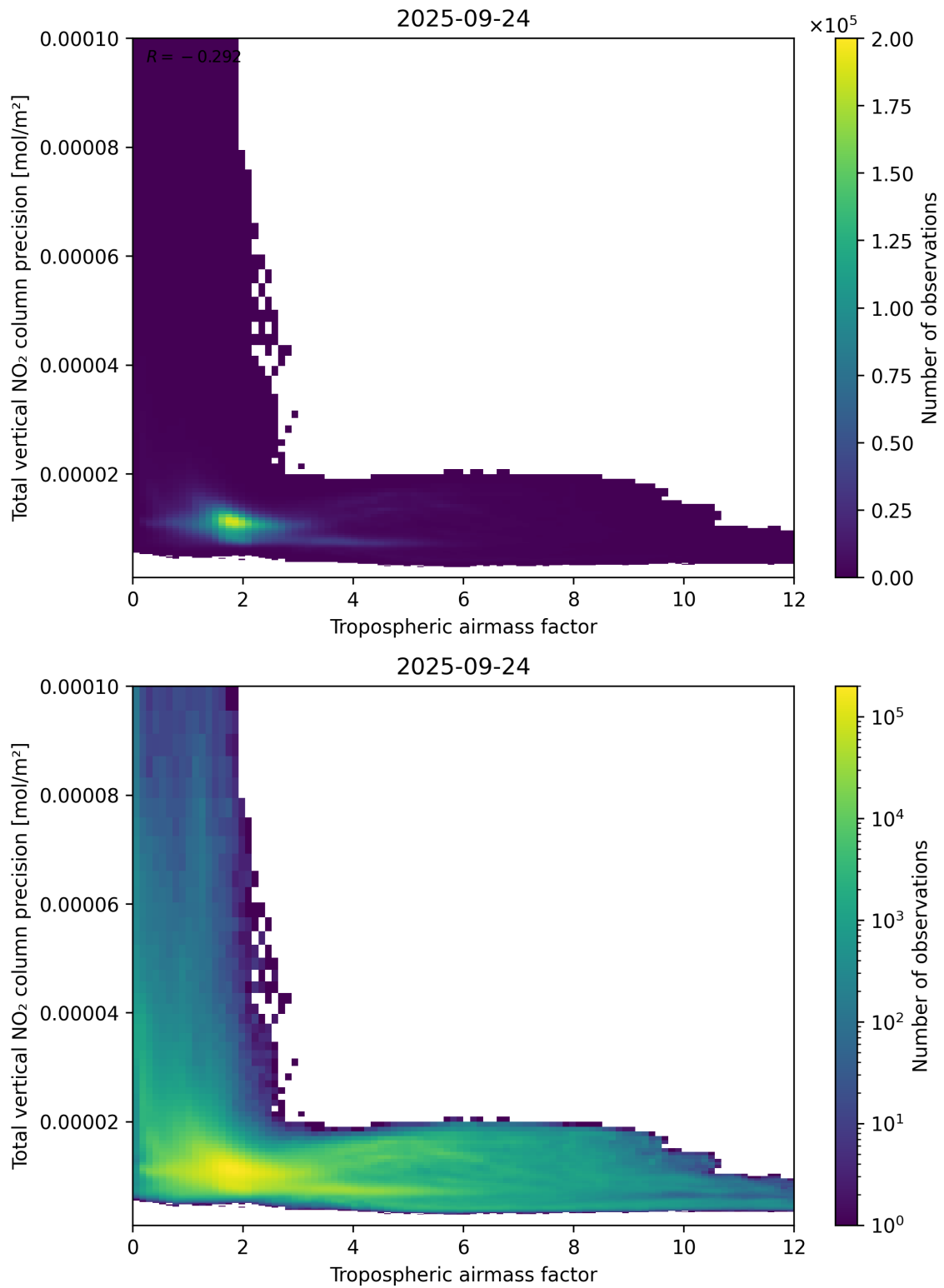
Figure 78: Scatter density plot of “Tropospheric air mass factor” against “Total vertical NO 2 column precision” for 2025-09-23 to 2025-09-25.
