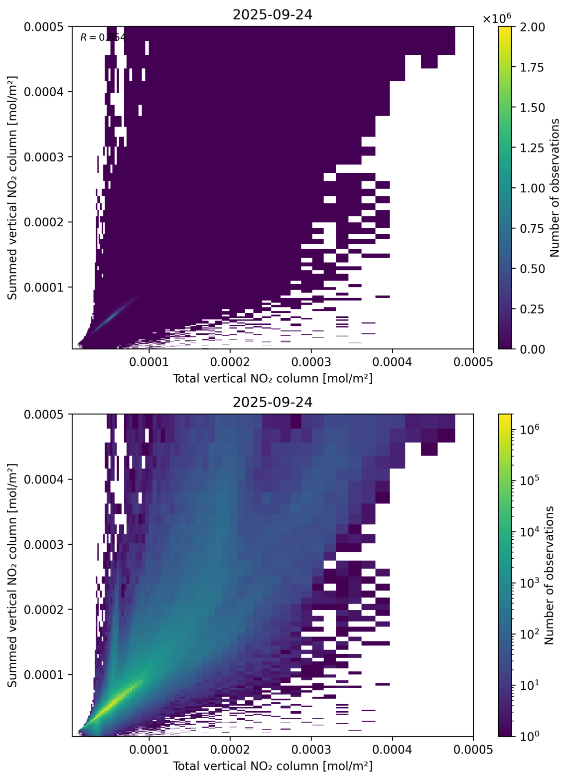
Figure 112: Scatter density plot of “Total vertical NO 2 column” against “Summed vertical NO 2 column” for 2025-09-23 to 2025-09-25.
