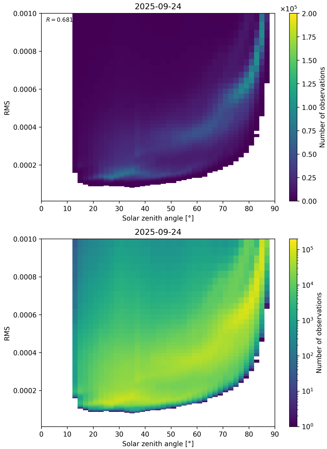
Figure 157: Scatter density plot of “Solar zenith angle” against “RMS” for 2025-09-23 to 2025-09-25.
