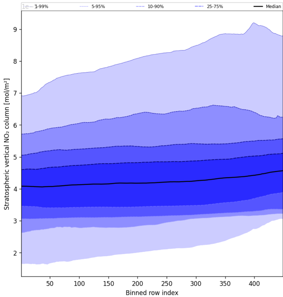
Figure 53: Along track statistics of “Stratospheric vertical NO 2 column” for 2025-09-23 to 2025-09-25
