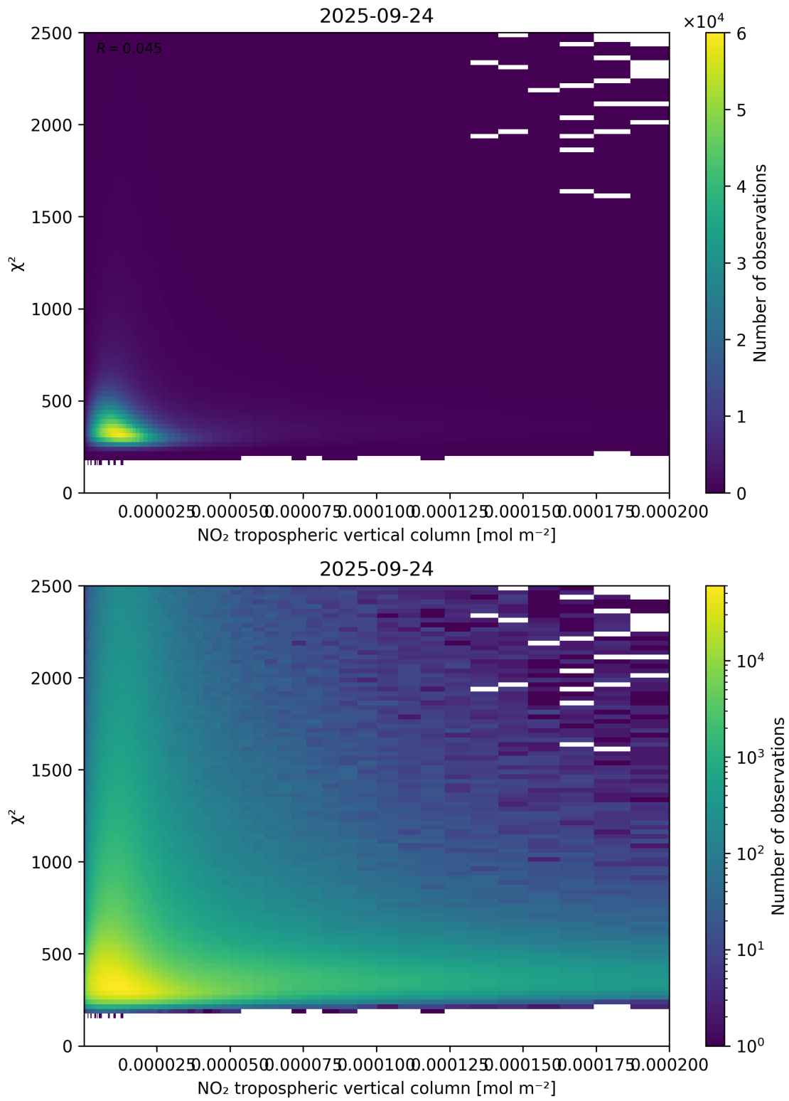
Figure 124: Scatter density plot of “NO 2 tropospheric vertical column” against “ \chi^2 ” for 2025-09-23 to 2025-09-25.
