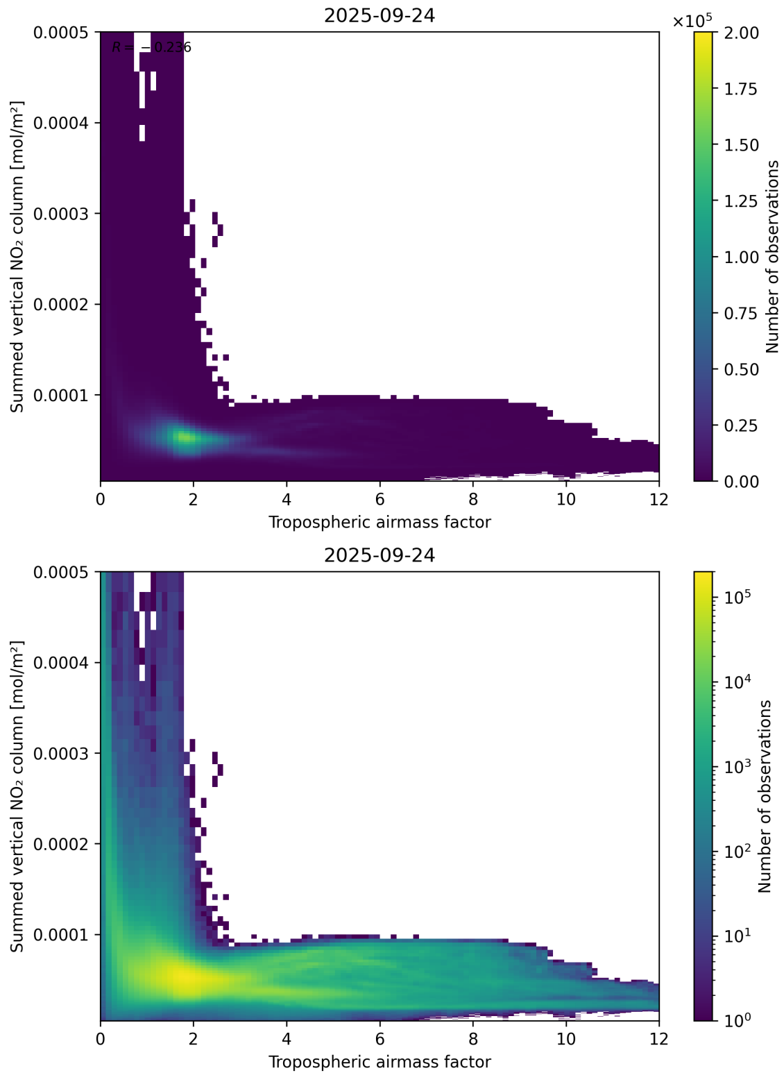
Figure 75: Scatter density plot of “Tropospheric air mass factor” against “Summed vertical NO 2 column” for 2025-09-23 to 2025-09-25.
