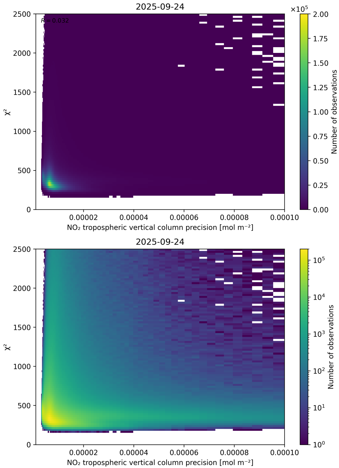
Figure 134: Scatter density plot of “NO 2 tropospheric vertical column precision” against “ \chi^2 ” for 2025-09-23 to 2025-09-25.
