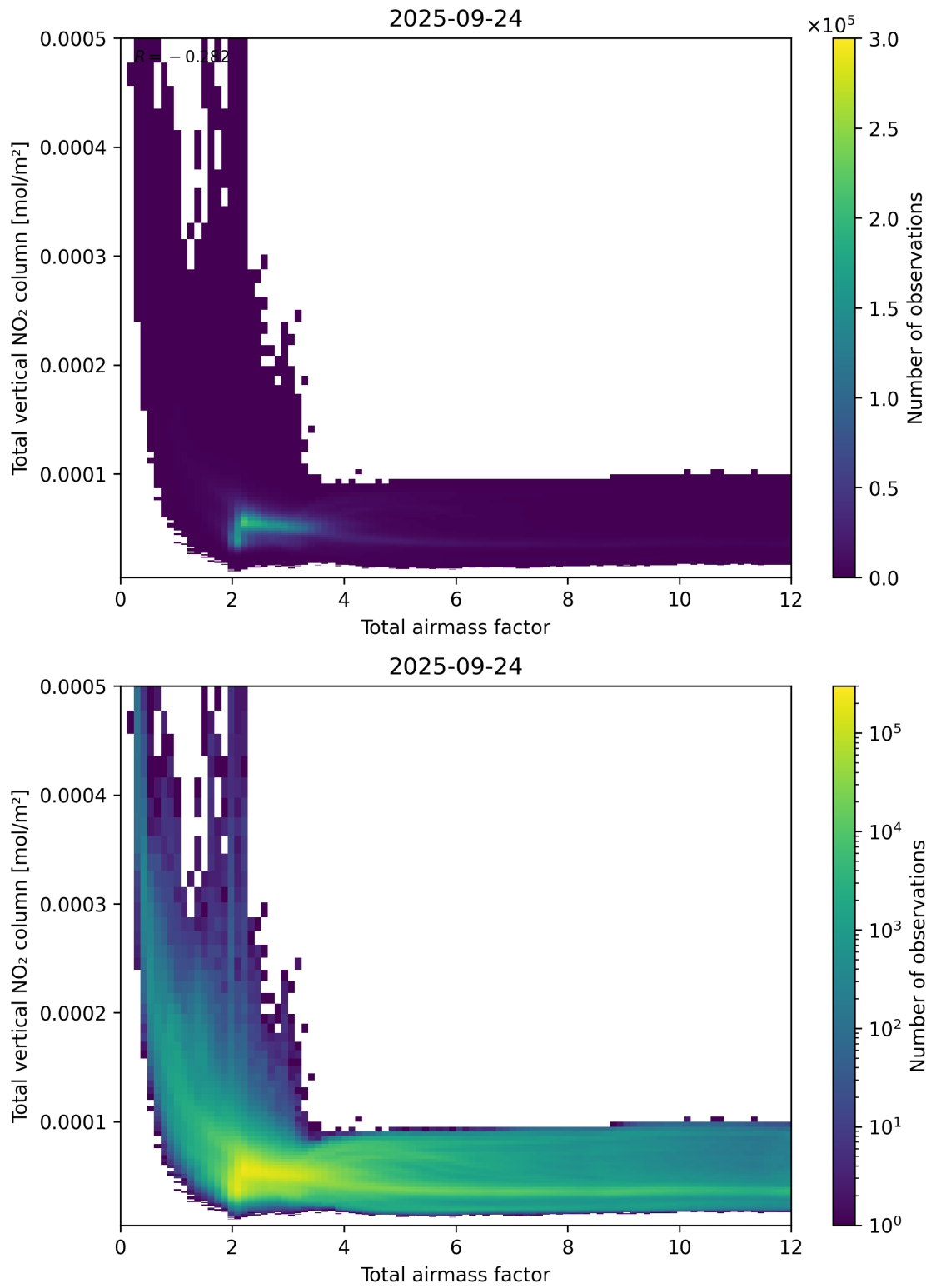
Figure 67: Scatter density plot of “Total airmass factor” against “Total vertical NO 2 column” for 2025-09-23 to 2025-09-25.
