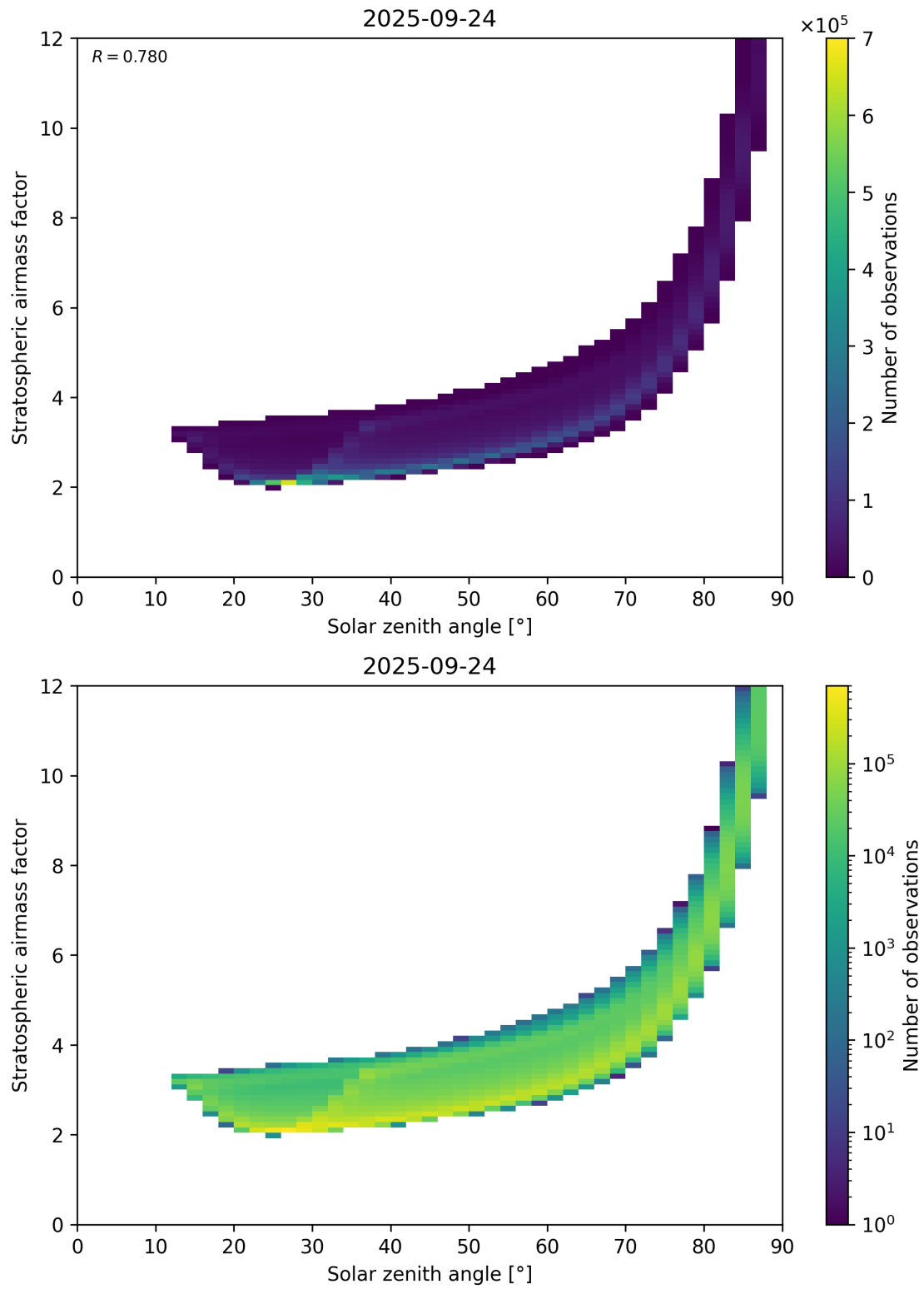
Figure 145: Scatter density plot of “Solar zenith angle” against “Stratospheric airmass factor” for 2025-09-23 to 2025-09-25.
