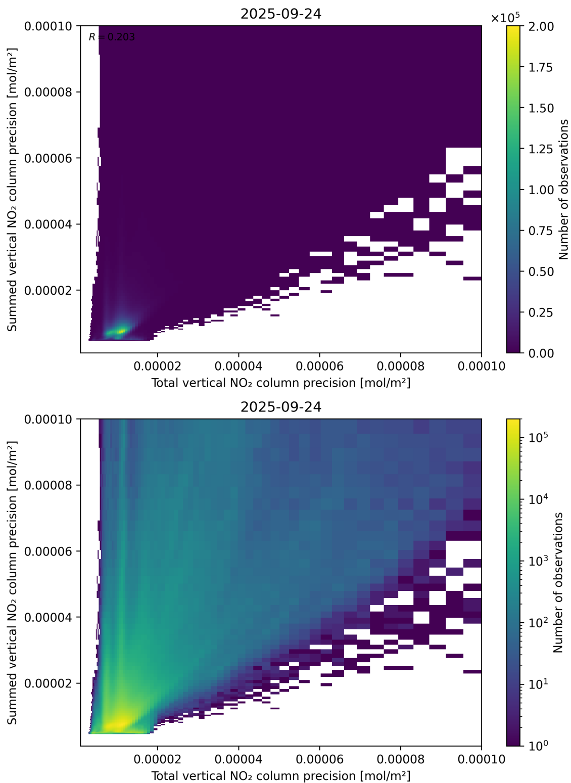
Figure 118: Scatter density plot of “Total vertical NO 2 column precision” against “Summed vertical NO 2 column precision” for 2025-09-23 to 2025-09-25.
