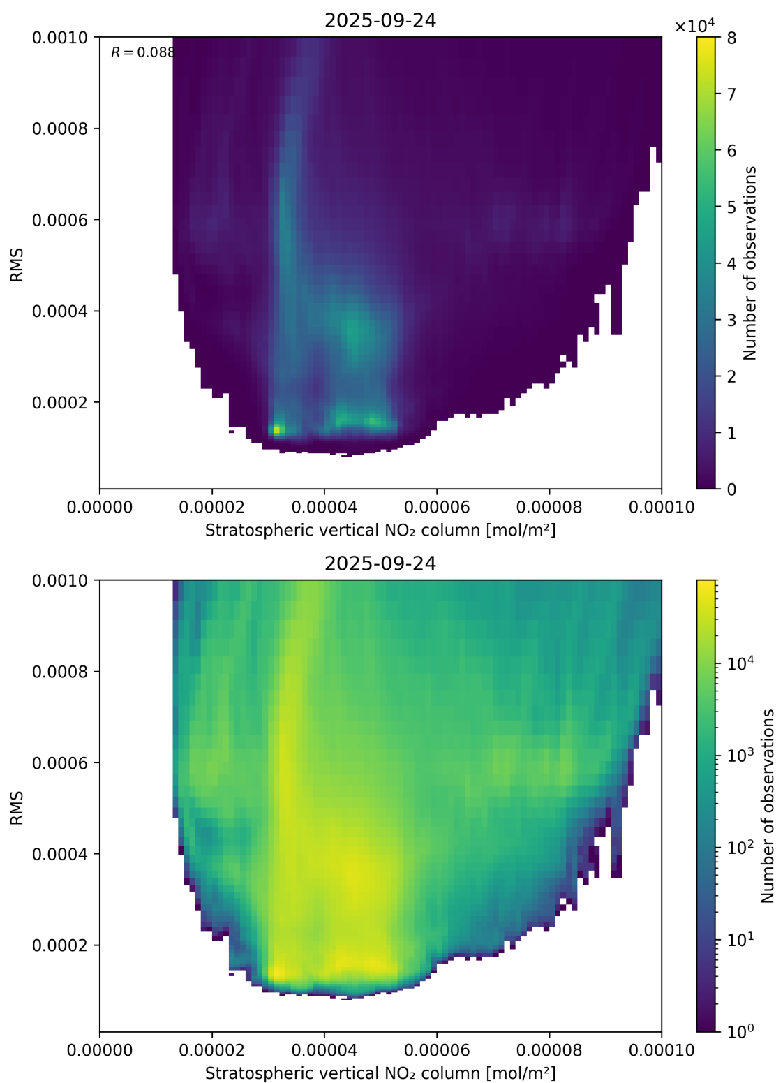
Figure 102: Scatter density plot of “Stratospheric vertical NO 2 column” against “RMS” for 2025-09-23 to 2025-09-25.
