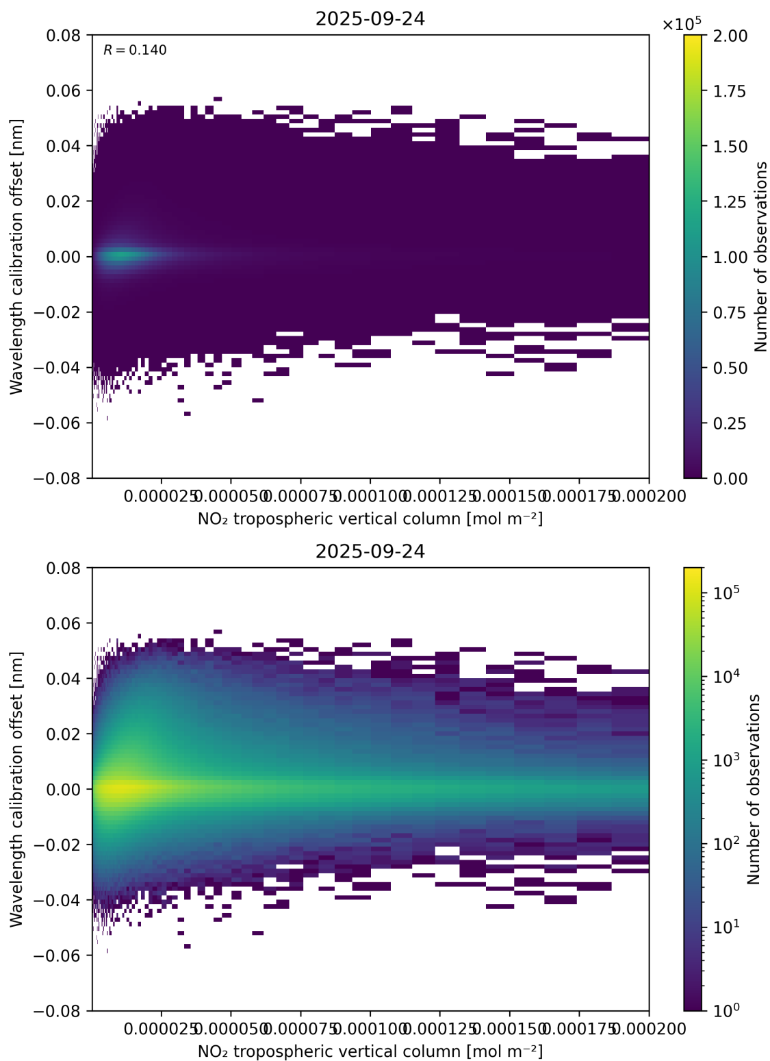
Figure 143: Scatter density plot of “NO 2 tropospheric vertical column” against “Wavelength calibration offset” for 2025-09-23 to 2025-09-25.
