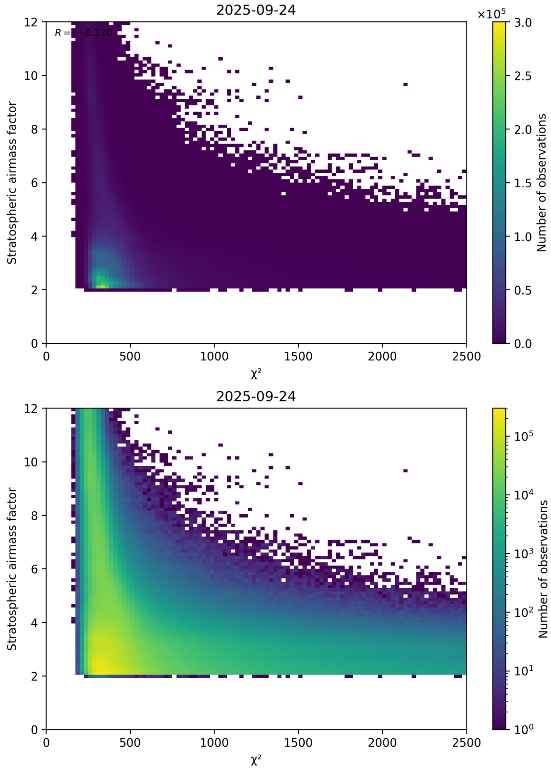
Figure 81: Scatter density plot of “ \chi^2 ” against “Stratospheric airmass factor” for 2025-09-23 to 2025-09-25.
