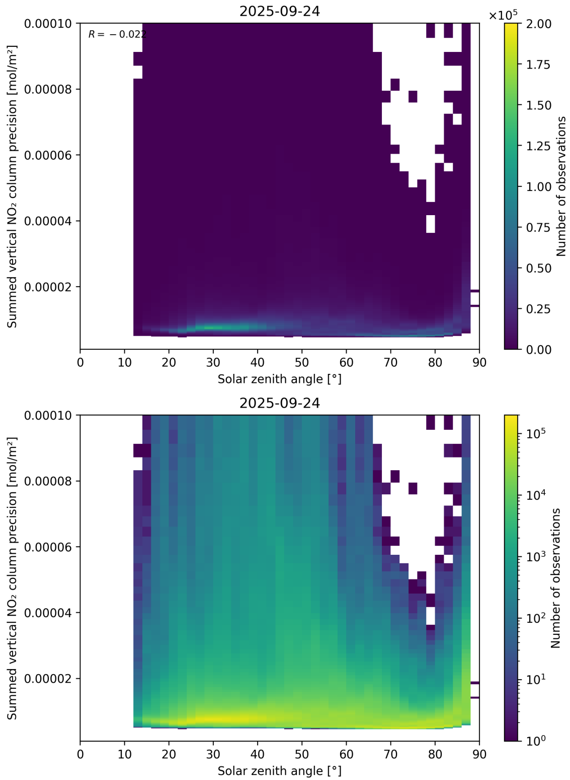
Figure 152: Scatter density plot of “Solar zenith angle” against “Summed vertical NO 2 column precision” for 2025-09-23 to 2025-09-25.
