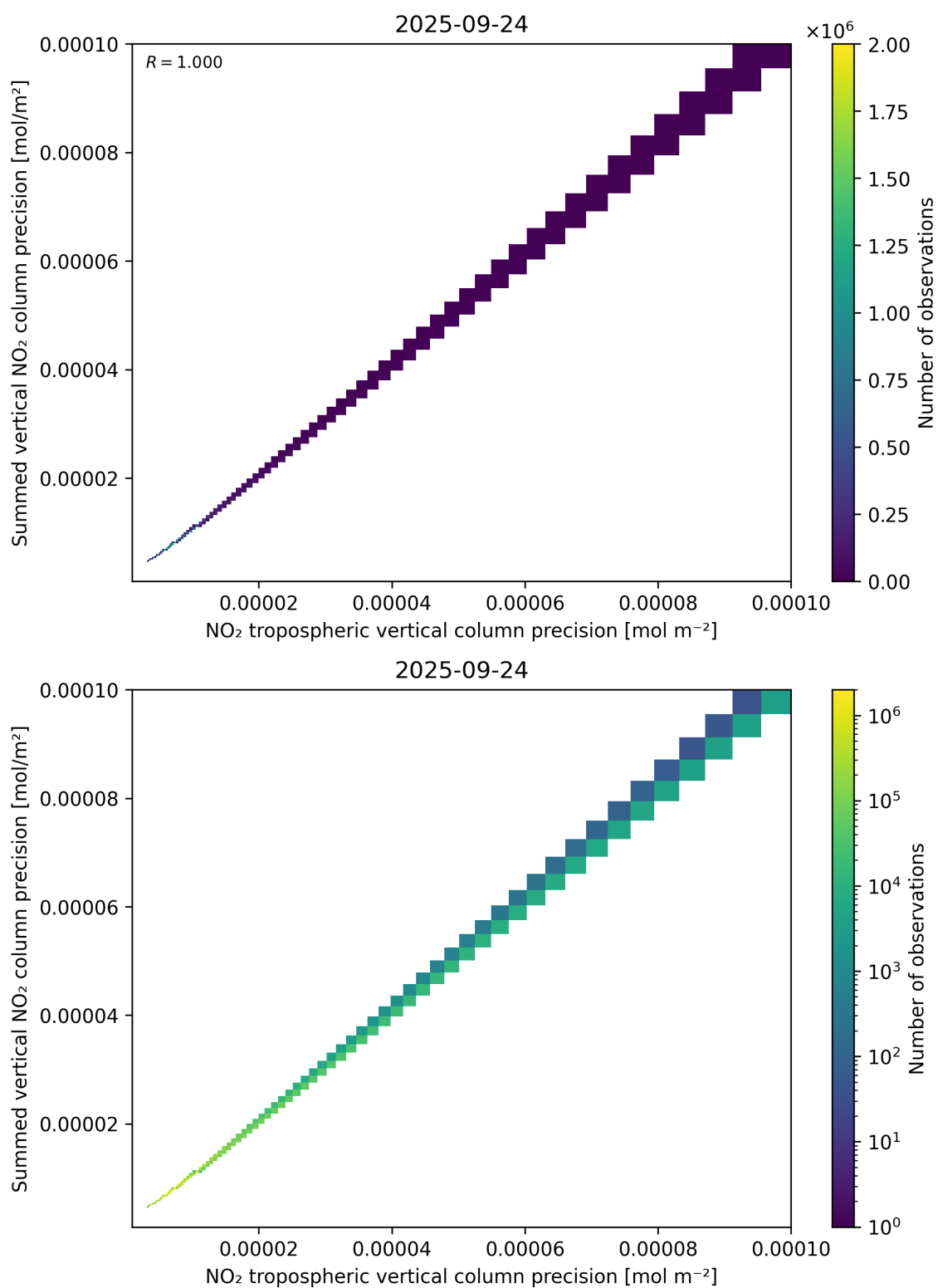
Figure 137: Scatter density plot of “NO 2 tropospheric vertical column precision” against “Summed vertical NO 2 column precision” for 2025-09-23 to 2025-09-25.
