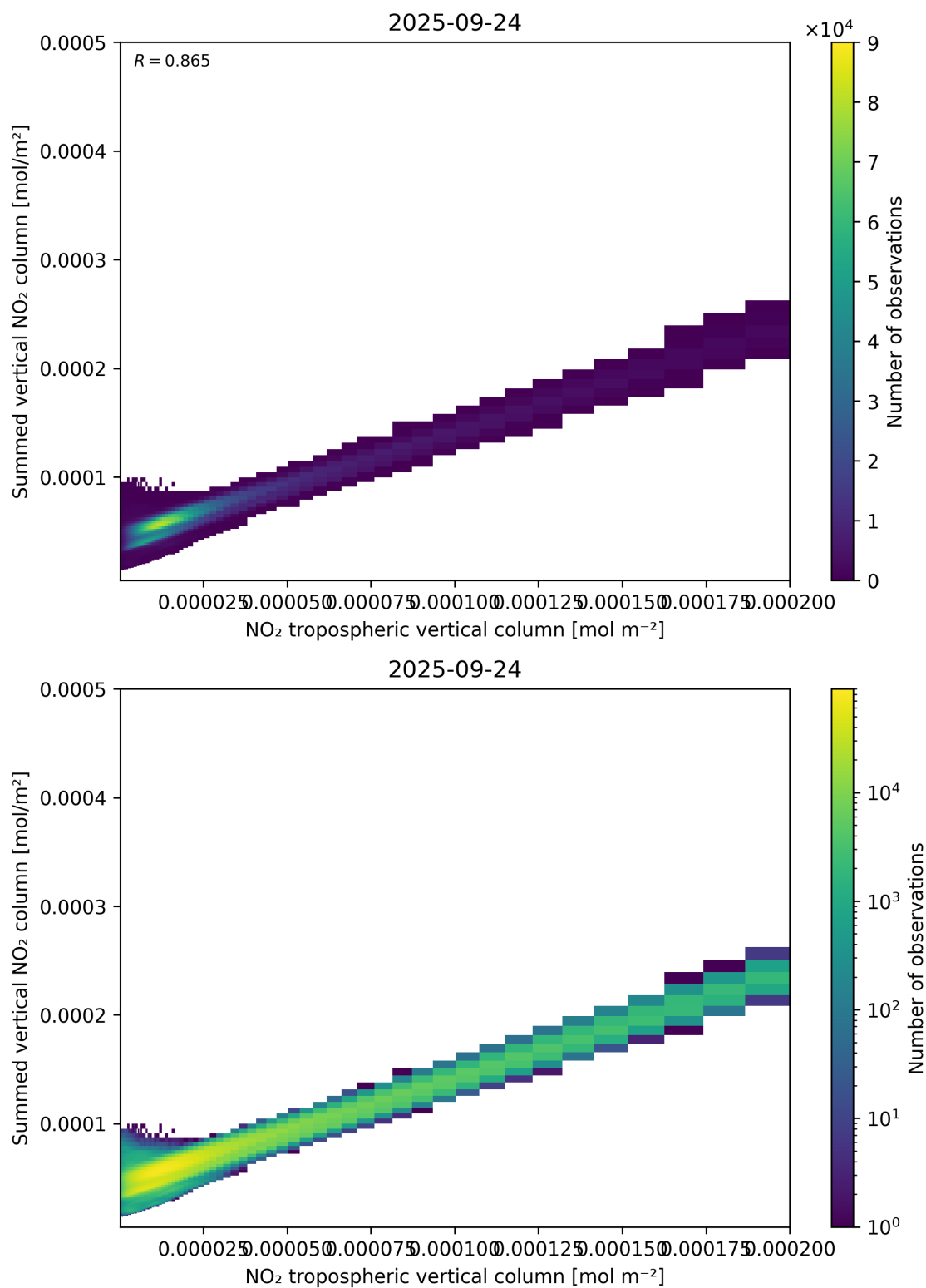
Figure 126: Scatter density plot of “NO 2 tropospheric vertical column” against “Summed vertical NO 2 column” for 2025-09-23 to 2025-09-25.
