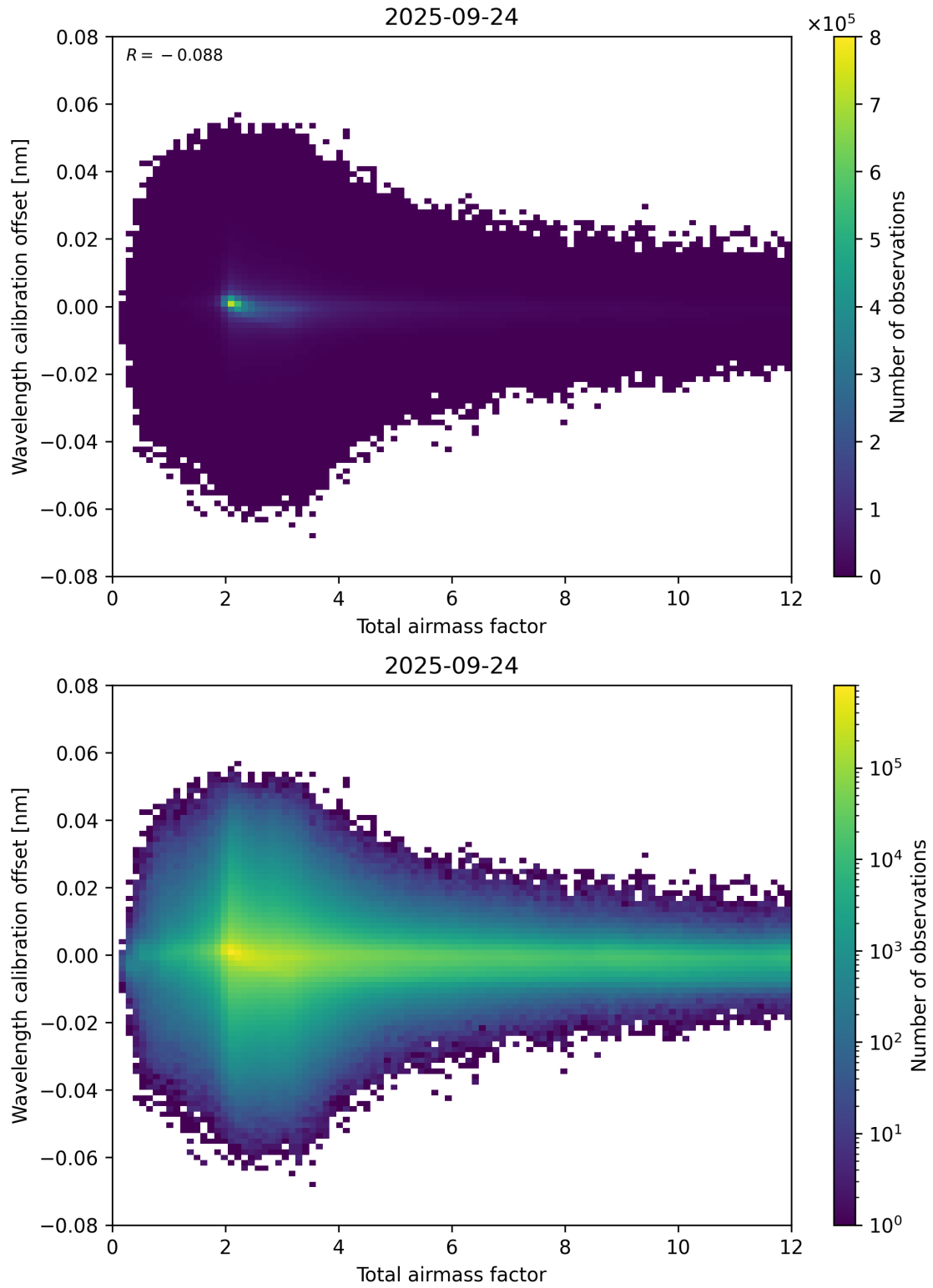
Figure 70: Scatter density plot of “Total airmass factor” against “Wavelength calibration offset” for 2025-09-23 to 2025-09-25.
