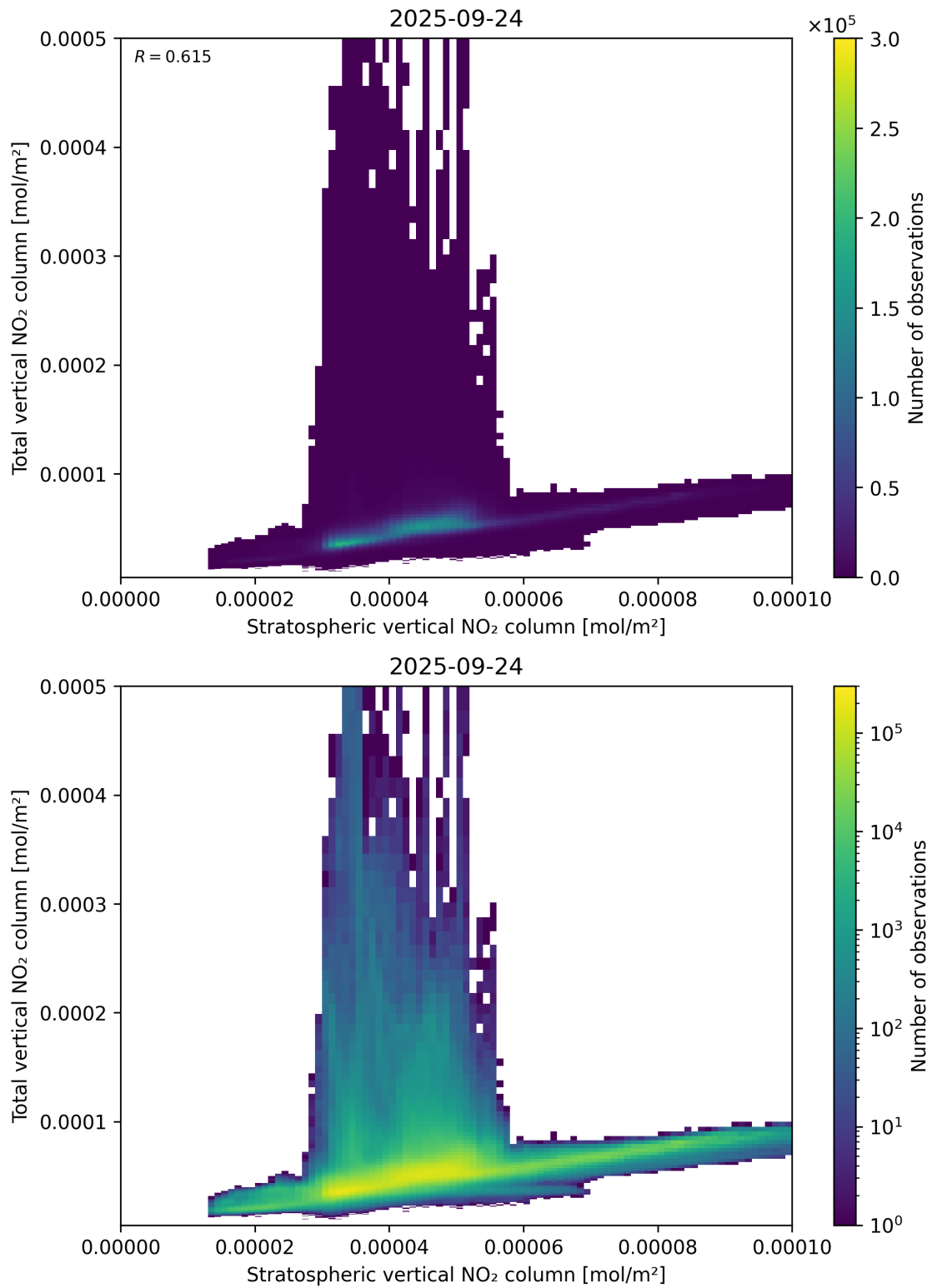
Figure 100: Scatter density plot of “Stratospheric vertical NO 2 column” against “Total vertical NO 2 column” for 2025-09-23 to 2025-09-25.
