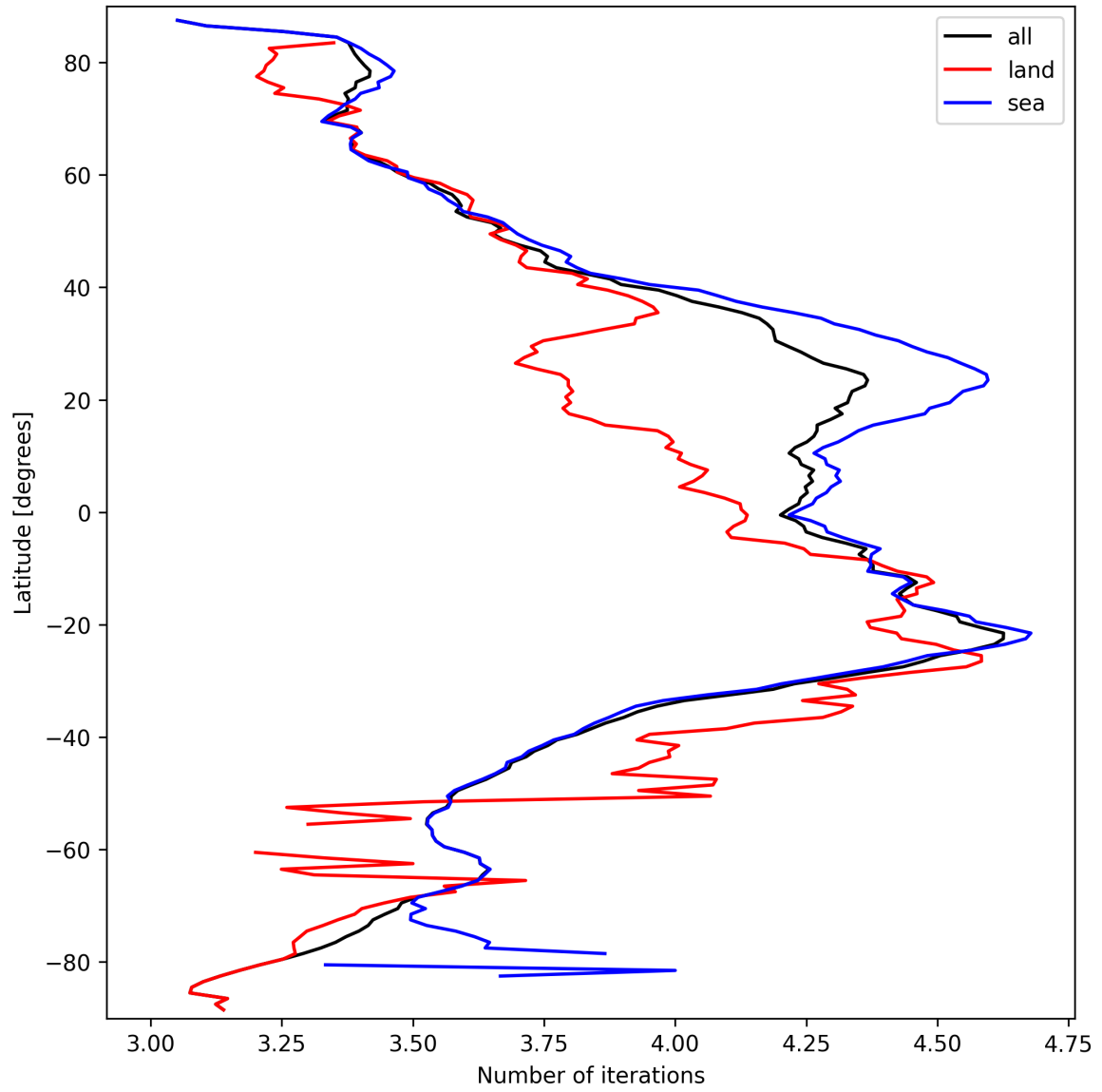
Figure 17: Zonal average of “Number of iterations” for 2025-09-23 to 2025-09-25.
