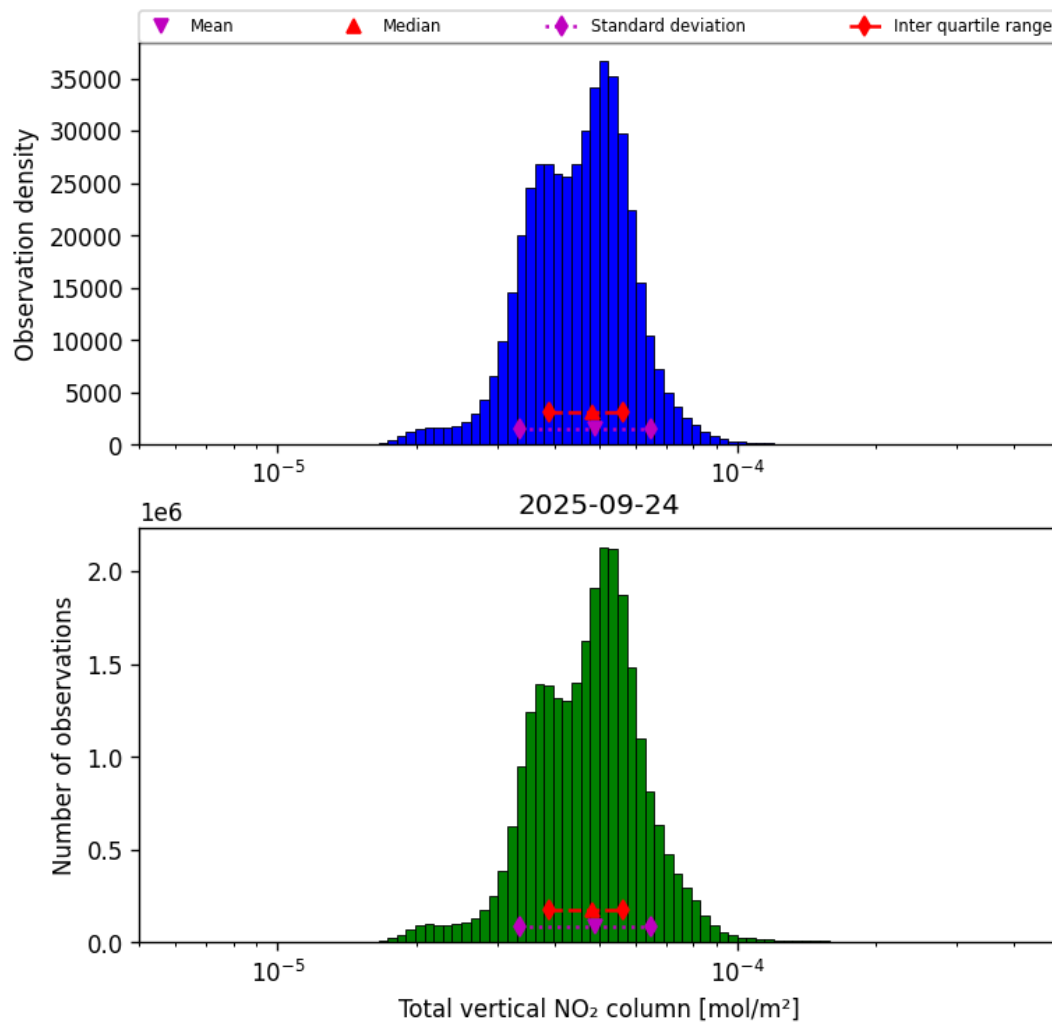
Figure 38: Histogram of “Total vertical NO 2 column” for 2025-09-23 to 2025-09-25
