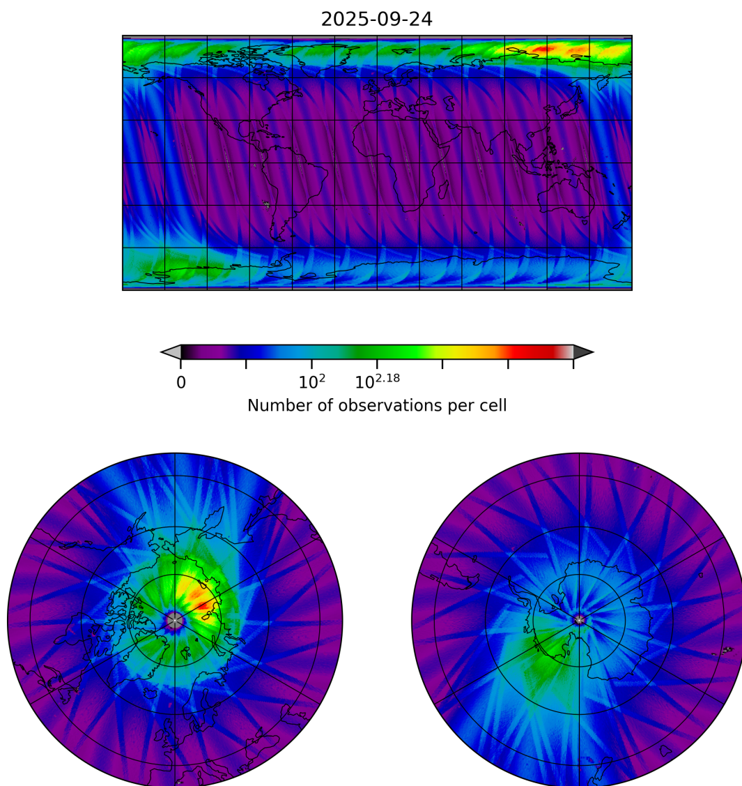
Figure 10: Map of the number of observations for 2025-09-23 to 2025-09-25
