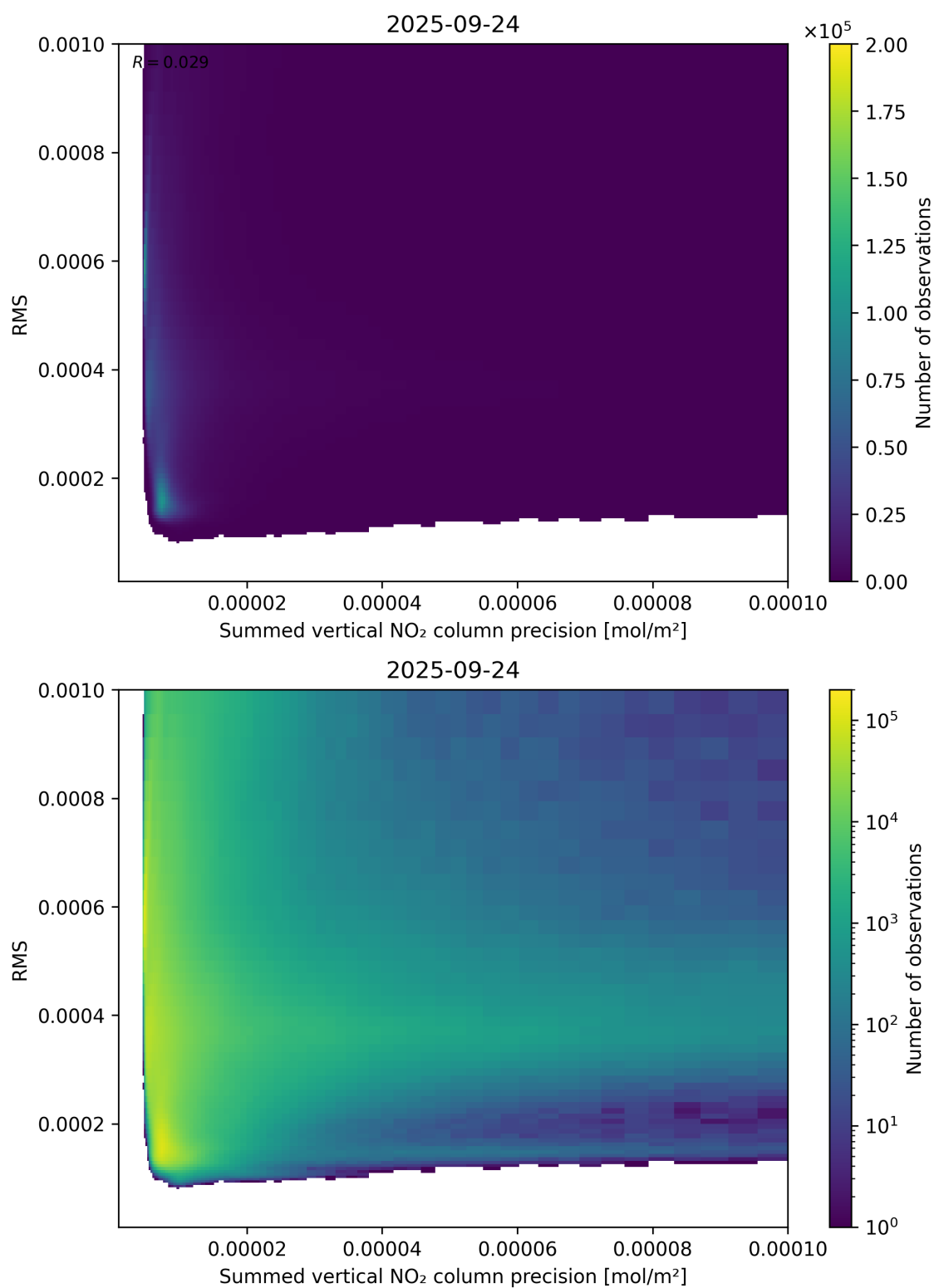
Figure 108: Scatter density plot of “Summed vertical NO 2 column precision” against “RMS” for 2025-09-23 to 2025-09-25.
