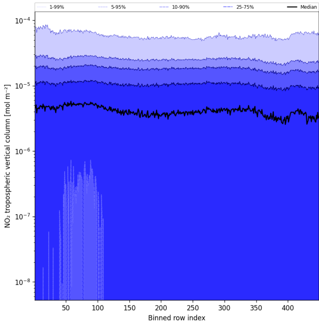
Figure 46: Along track statistics of “NO 2 tropospheric vertical column” for 2025-09-23 to 2025-09-25
