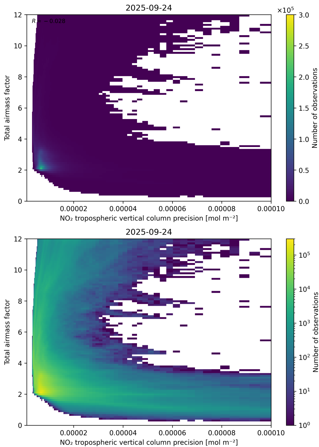
Figure 132: Scatter density plot of “NO 2 tropospheric vertical column precision” against “Total air mass factor” for 2025-09-23 to 2025-09-25.
