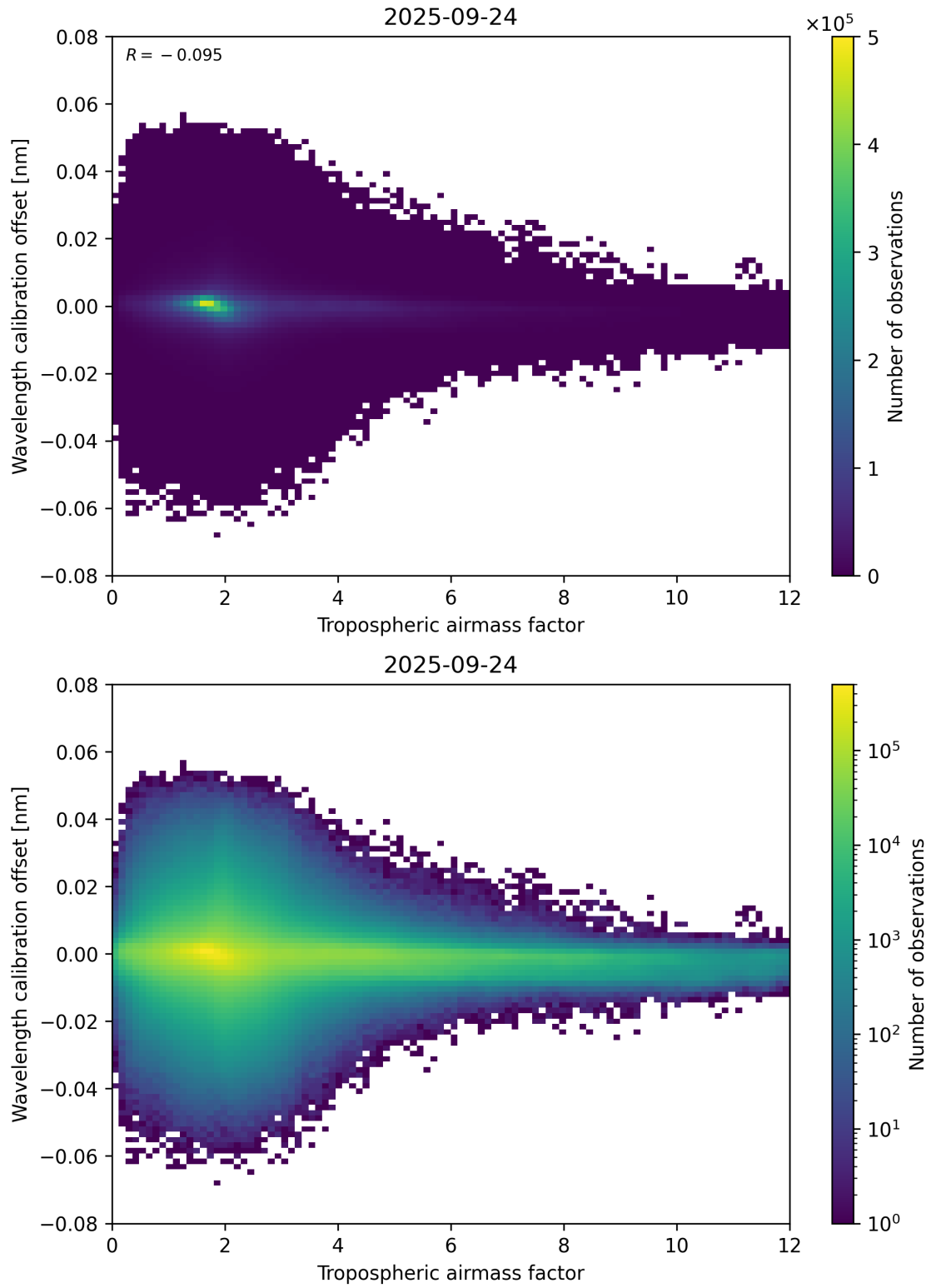
Figure 80: Scatter density plot of “Tropospheric airmass factor” against “Wavelength calibration offset” for 2025-09-23 to 2025-09-25.
