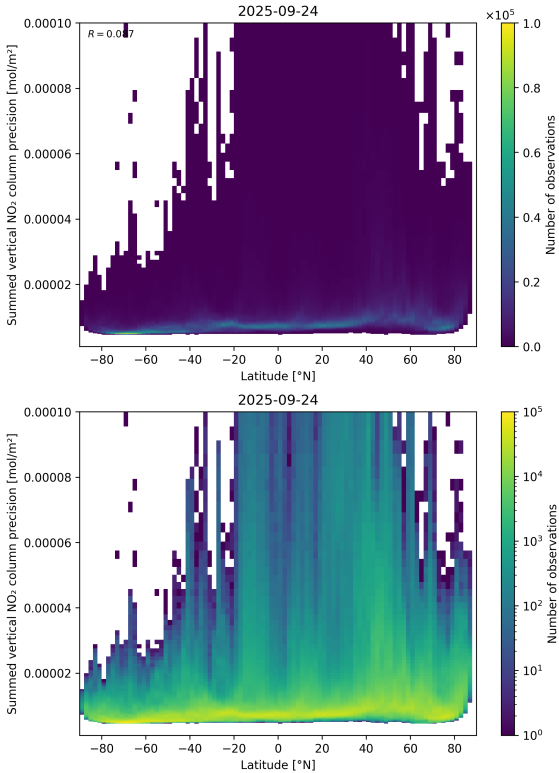
Figure 89: Scatter density plot of “Latitude” against “Summed vertical NO 2 column precision” for 2025-09-23 to 2025-09-25.
