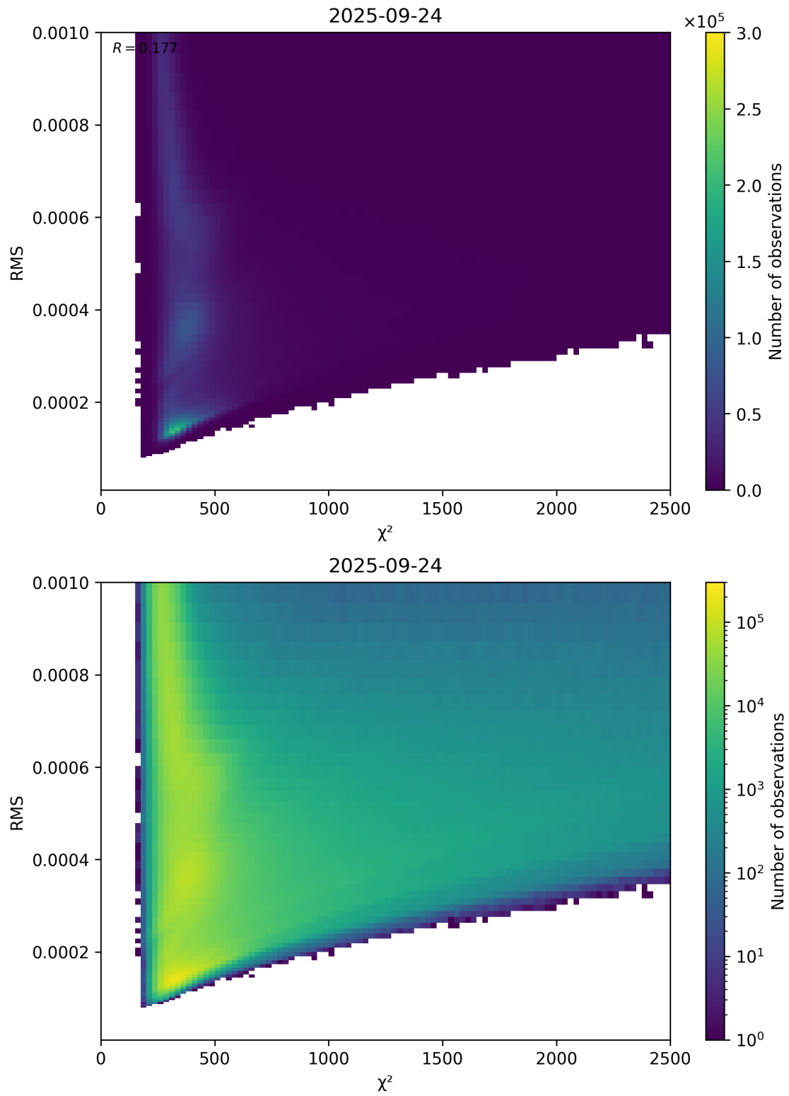
Figure 82: Scatter density plot of “ \chi^2 ” against “RMS” for 2025-09-23 to 2025-09-25.
