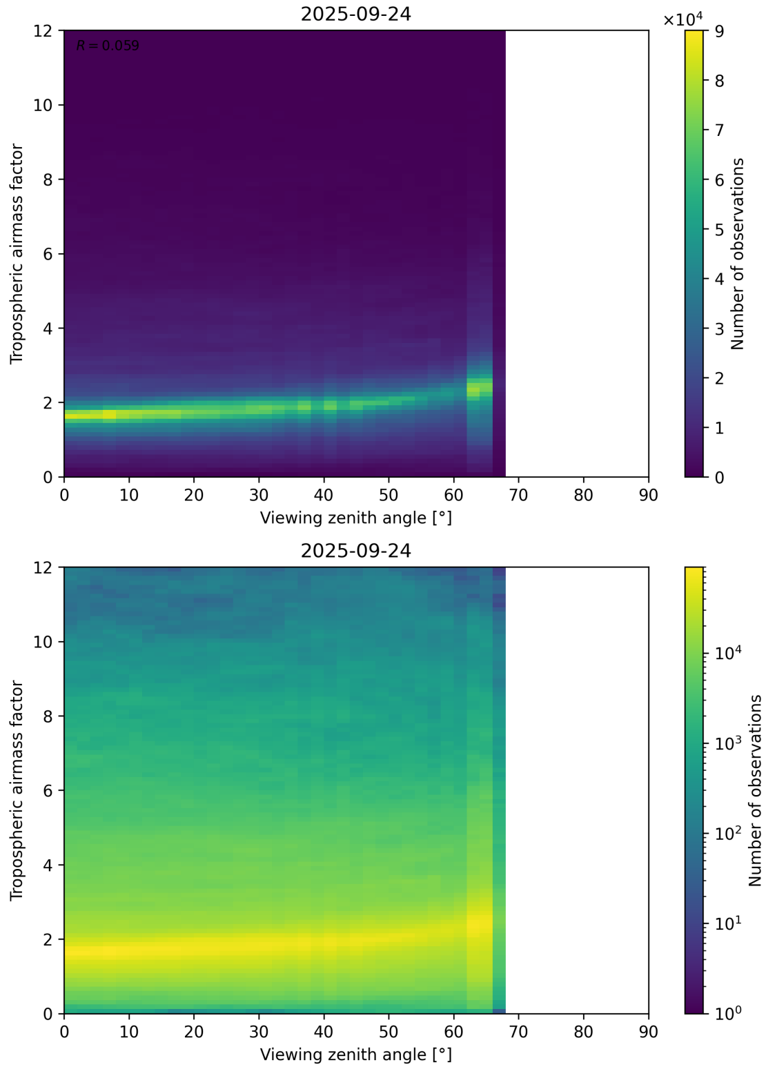
Figure 161: Scatter density plot of “Viewing zenith angle” against “Tropospheric airmass factor” for 2025-09-23 to 2025-09-25.
