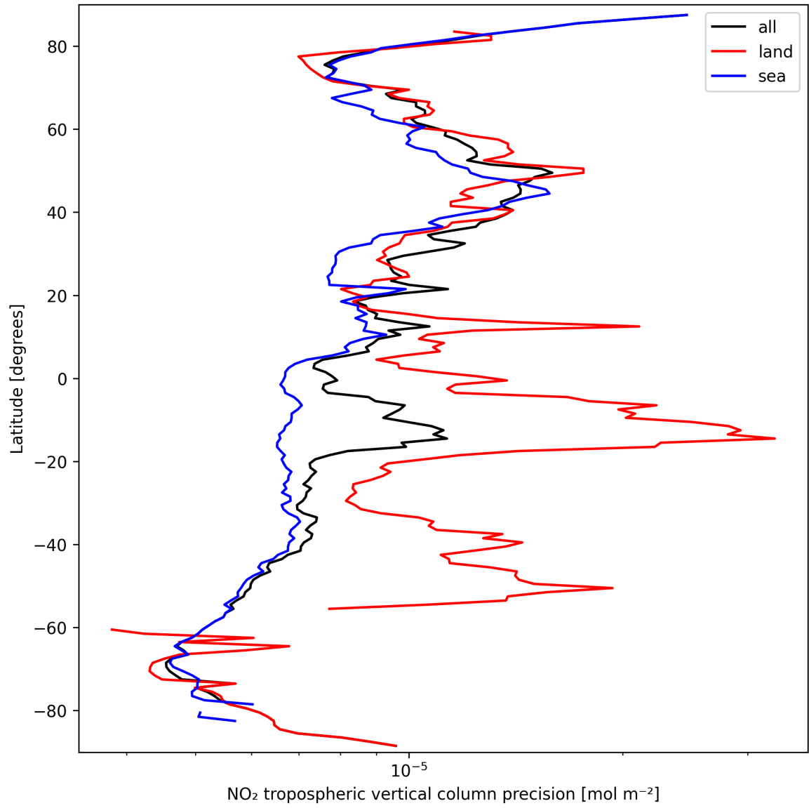
Figure 13: Zonal average of “NO 2 tropospheric vertical column precision” for 2025-09-23 to 2025-09-25.
