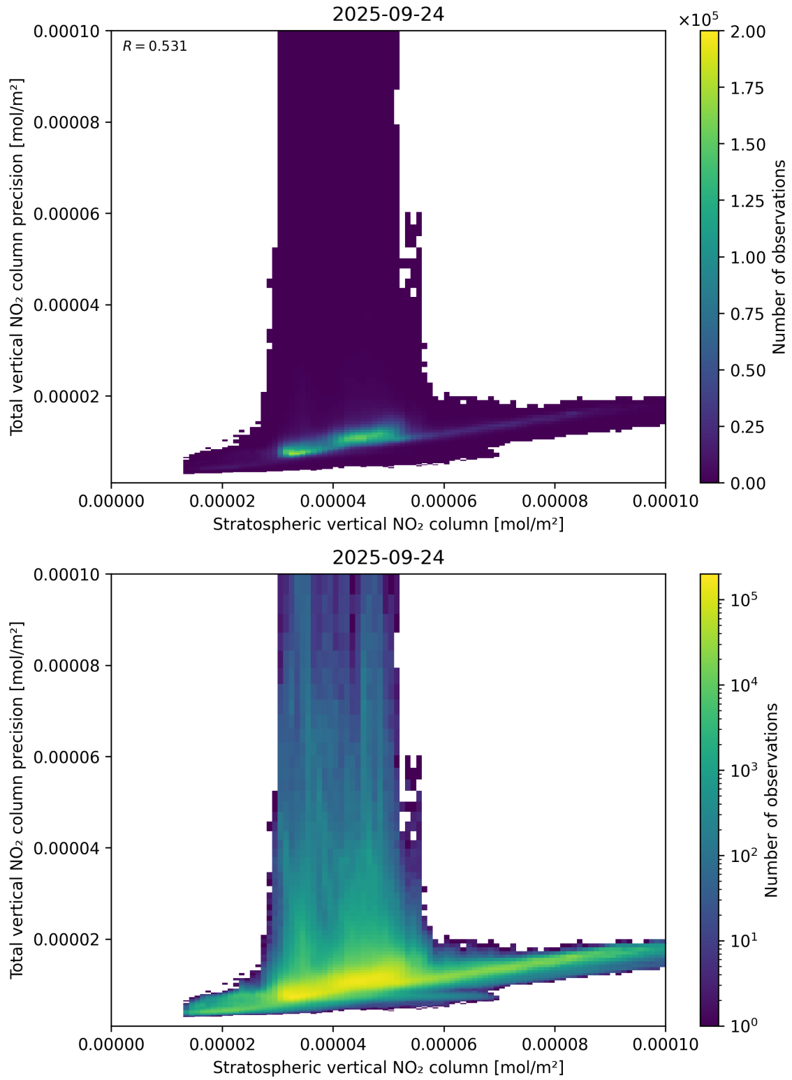
Figure 101: Scatter density plot of “Stratospheric vertical NO 2 column” against “Total vertical NO 2 column precision” for 2025-09-23 to 2025-09-25.
