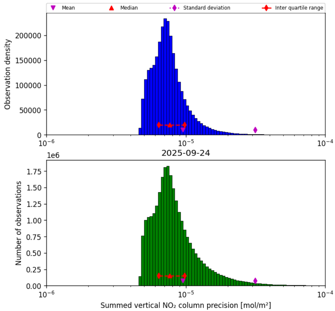
Figure 41: Histogram of “Summed vertical NO 2 column precision” for 2025-09-23 to 2025-09-25
