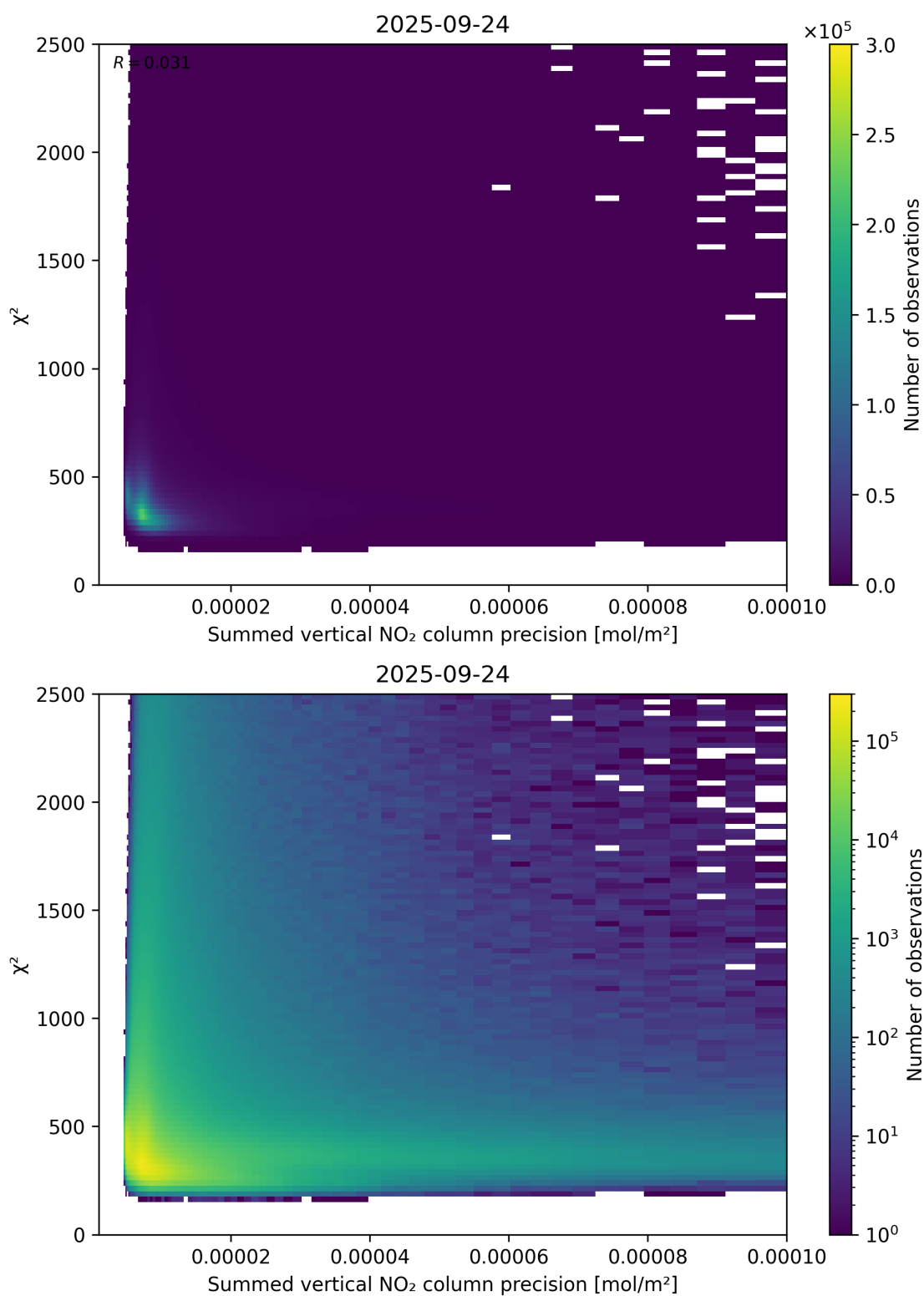
Figure 107: Scatter density plot of “Summed vertical NO 2 column precision” against “ \chi^2 ” for 2025-09-23 to 2025-09-25.
