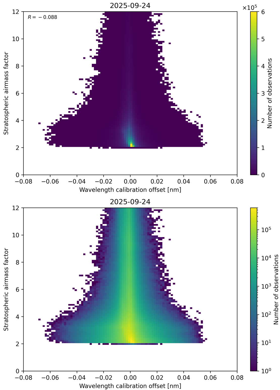
Figure 174: Scatter density plot of “Wavelength calibration offset” against “Stratospheric airmass factor” for 2025-09-23 to 2025-09-25.
