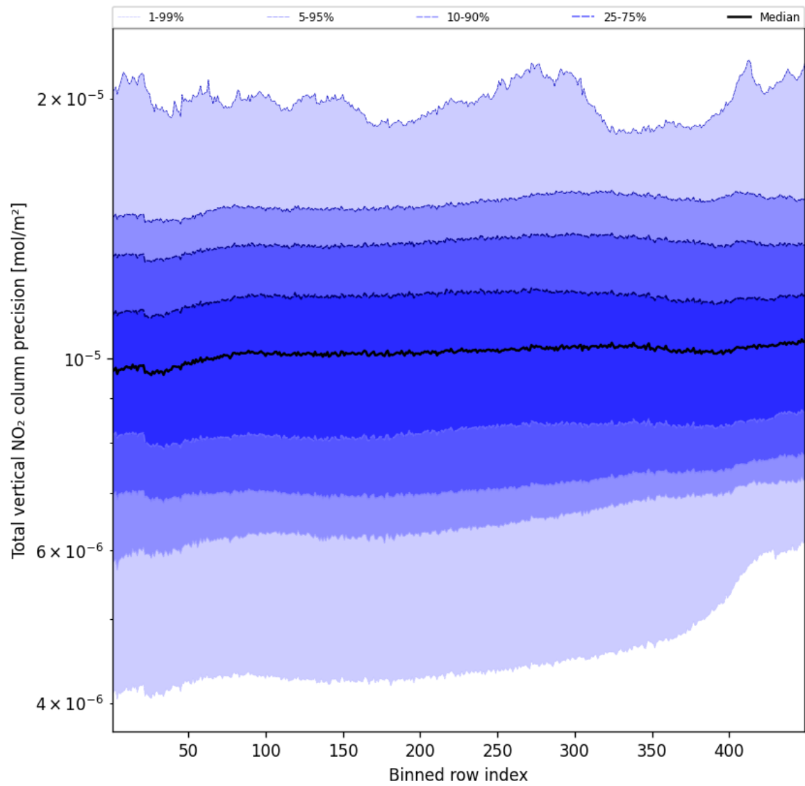
Figure 56: Along track statistics of “Total vertical NO 2 column precision” for 2025-09-23 to 2025-09-25
