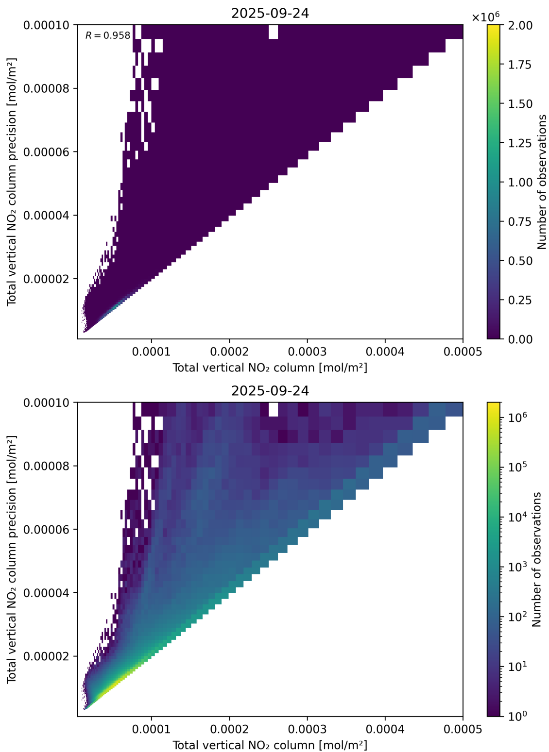
Figure 114: Scatter density plot of “Total vertical NO 2 column” against “Total vertical NO 2 column precision” for 2025-09-23 to 2025-09-25.
