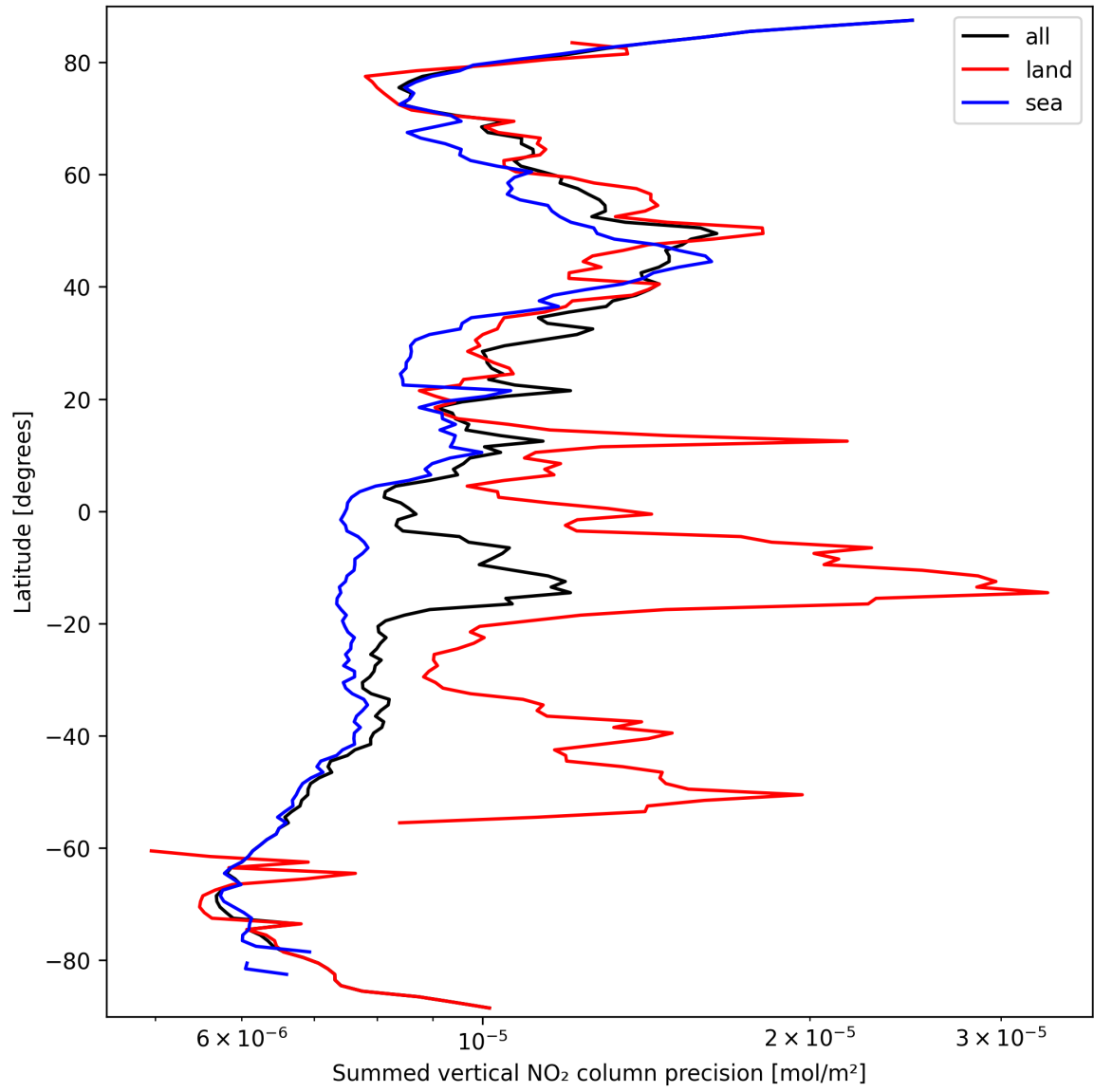
Figure 24: Zonal average of “Summed vertical NO 2 column precision” for 2025-09-23 to 2025-09-25.
