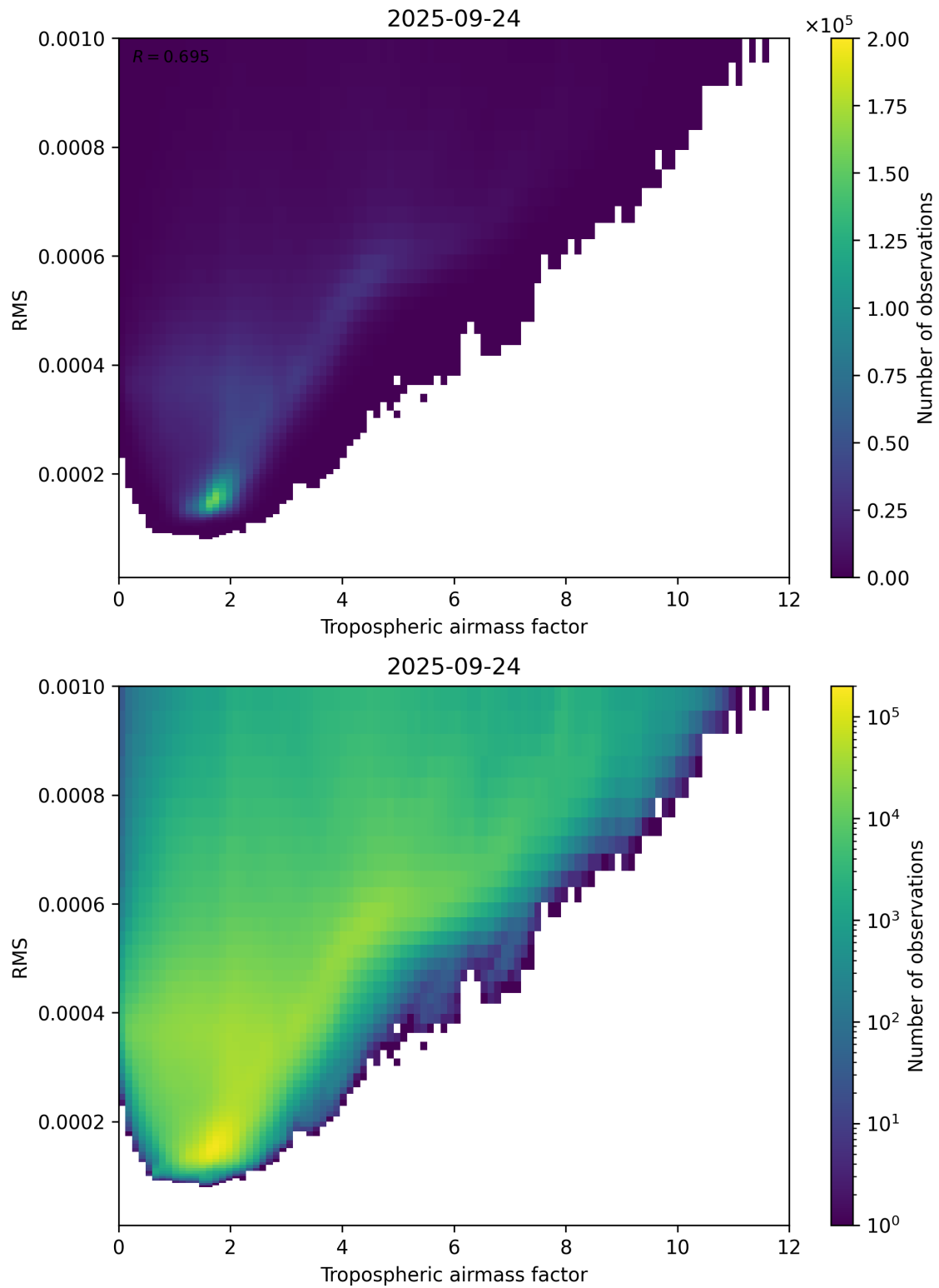
Figure 79: Scatter density plot of “Tropospheric airmass factor” against “RMS” for 2025-09-23 to 2025-09-25.
