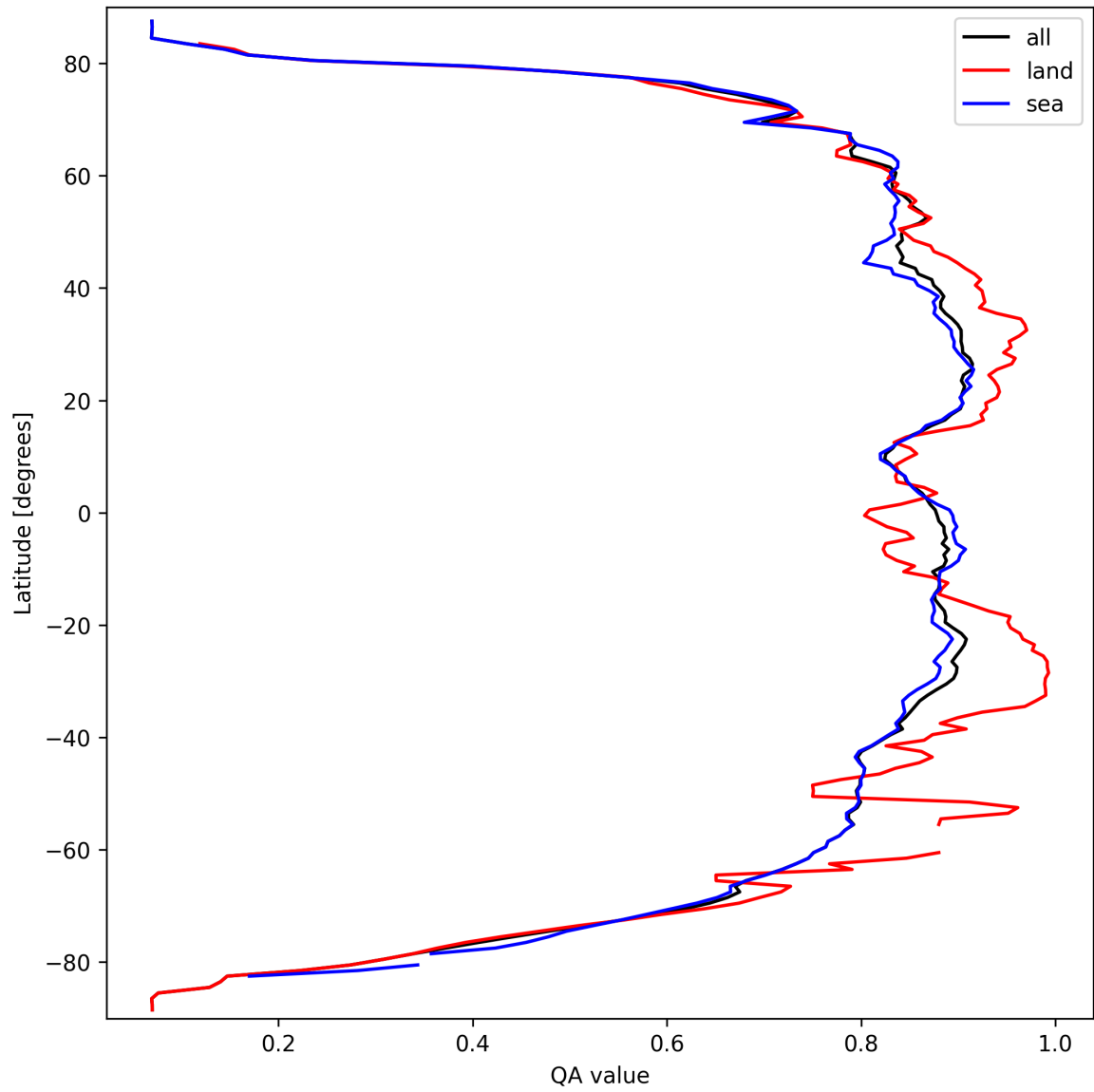
Figure 11: Zonal average of “QA value” for 2025-09-23 to 2025-09-25.
