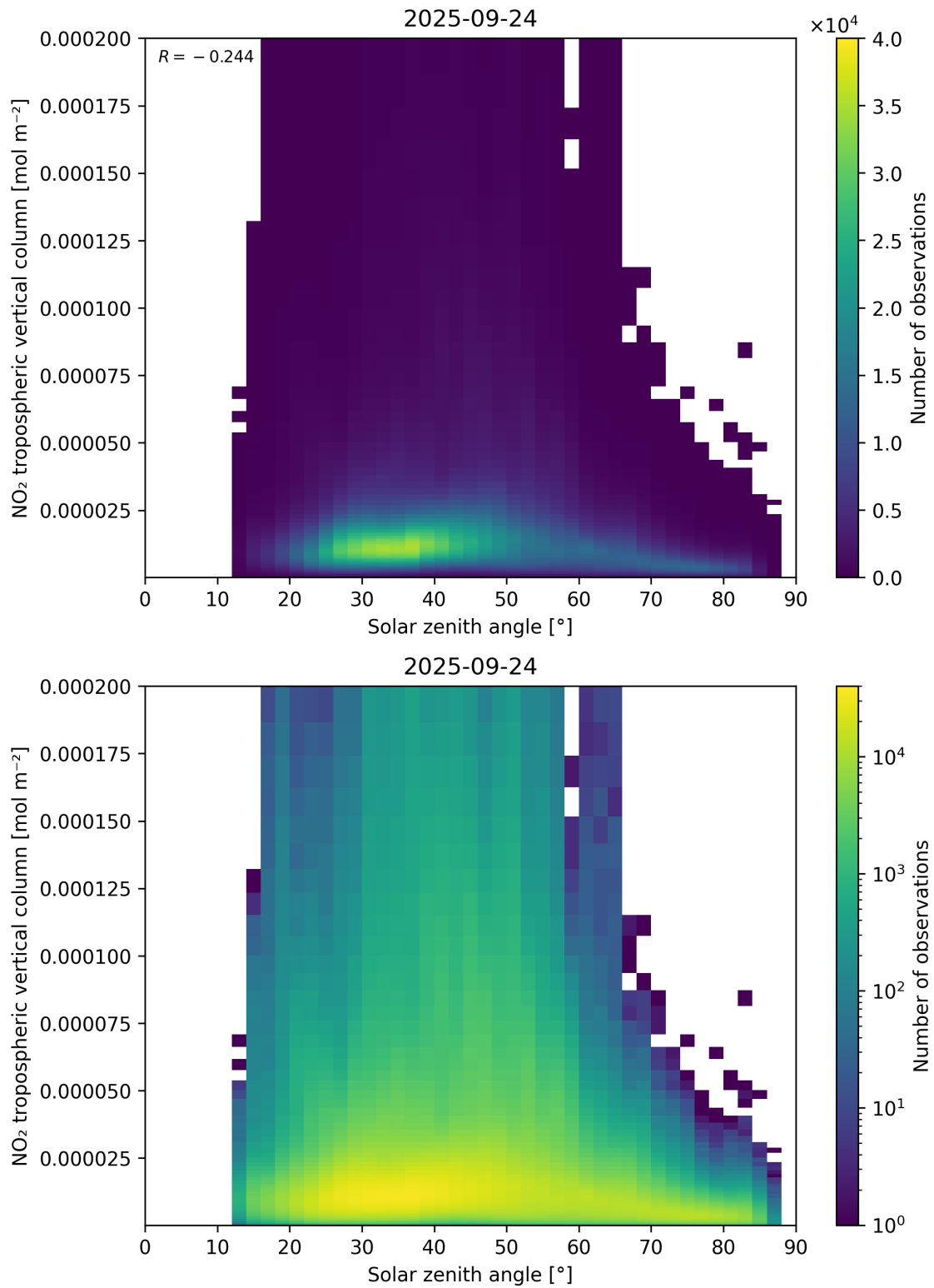
Figure 155: Scatter density plot of “Solar zenith angle” against “NO 2 tropospheric vertical column” for 2025-09-23 to 2025-09-25.
