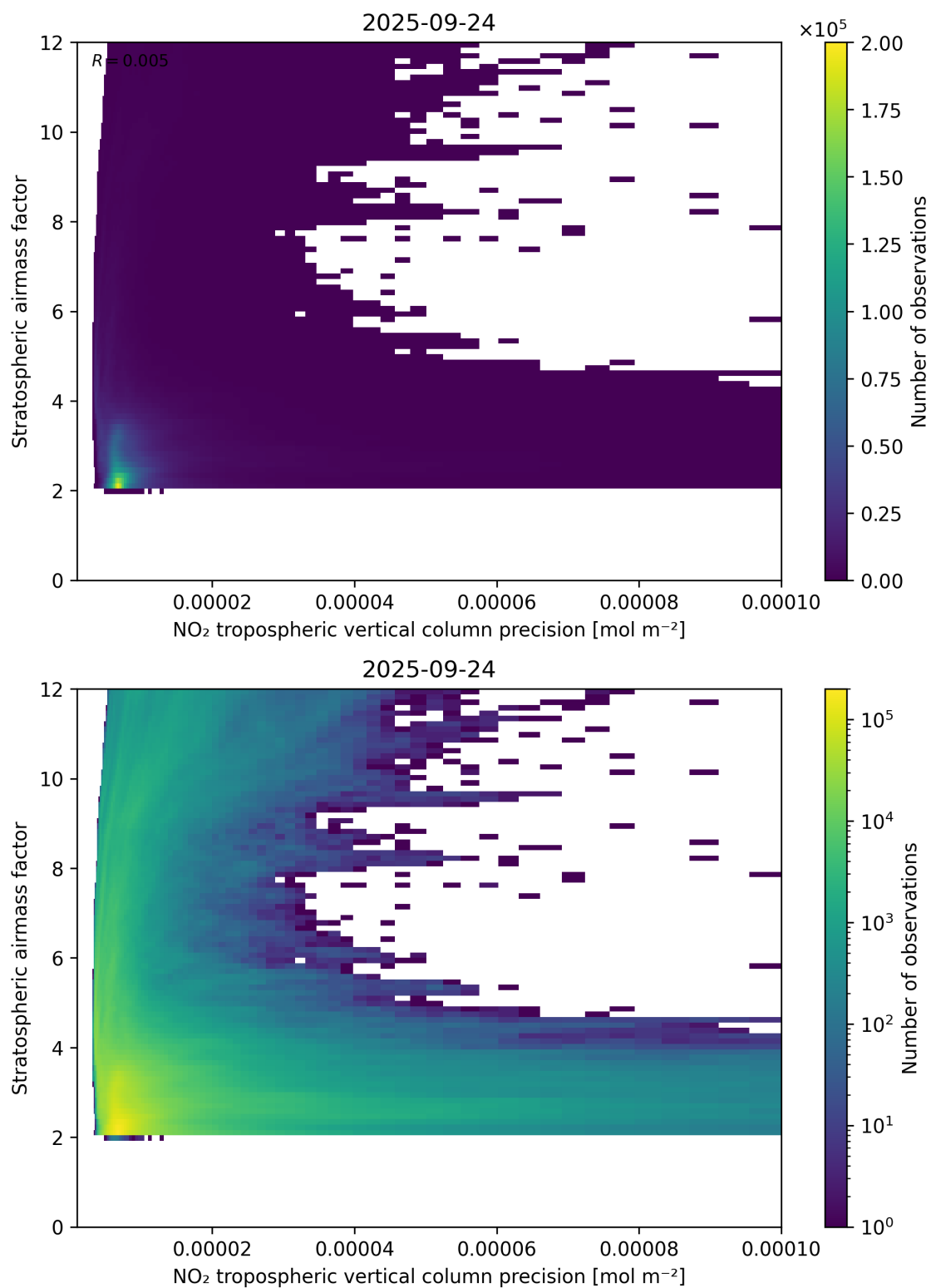
Figure 131: Scatter density plot of “NO 2 tropospheric vertical column precision” against “Stratospheric airmass factor” for 2025-09-23 to 2025-09-25.
