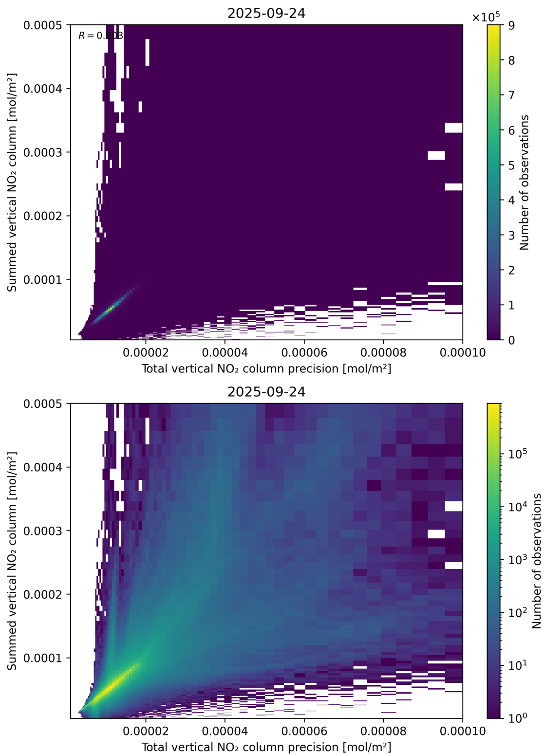
Figure 117: Scatter density plot of “Total vertical NO 2 column precision” against “Summed vertical NO 2 column” for 2025-09-23 to 2025-09-25.
