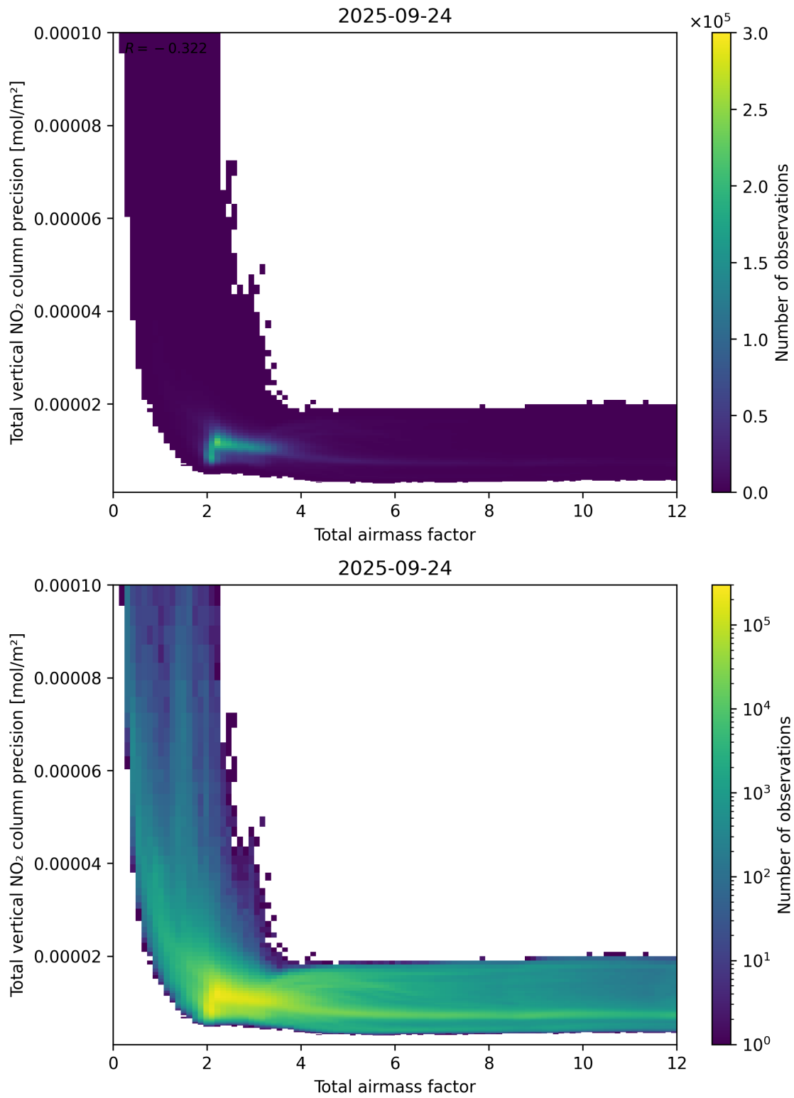
Figure 68: Scatter density plot of “Total airmass factor” against “Total vertical NO 2 column precision” for 2025-09-23 to 2025-09-25.
