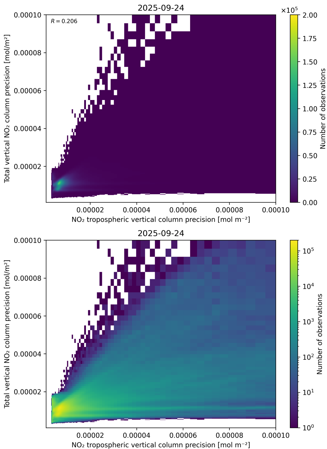
Figure 139: Scatter density plot of “NO 2 tropospheric vertical column precision” against “Total vertical NO 2 column precision” for 2025-09-23 to 2025-09-25.
