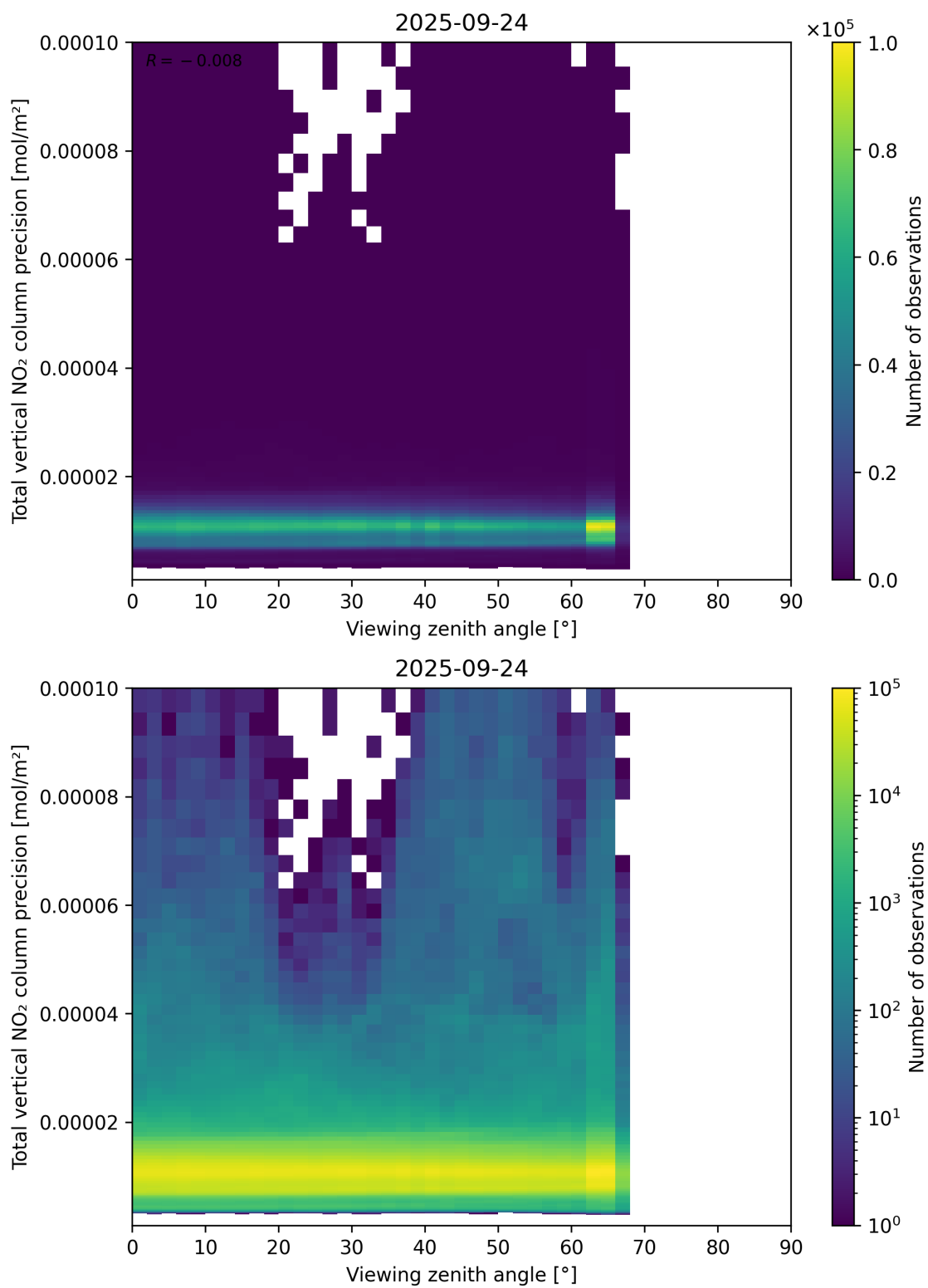
Figure 168: Scatter density plot of “Viewing zenith angle” against “Total vertical NO 2 column precision” for 2025-09-23 to 2025-09-25.
