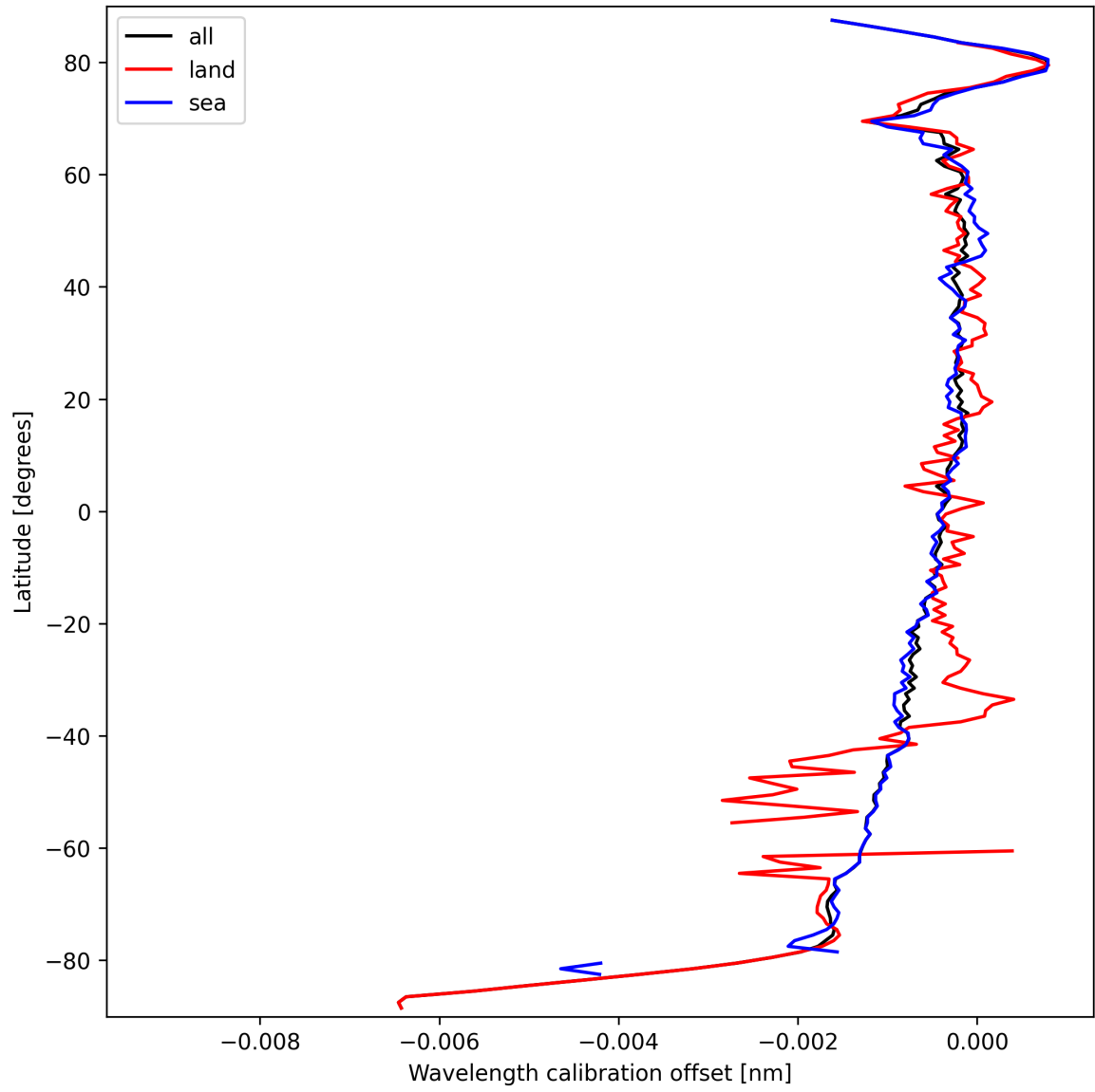
Figure 18: Zonal average of “Wavelength calibration offset” for 2025-09-23 to 2025-09-25.
