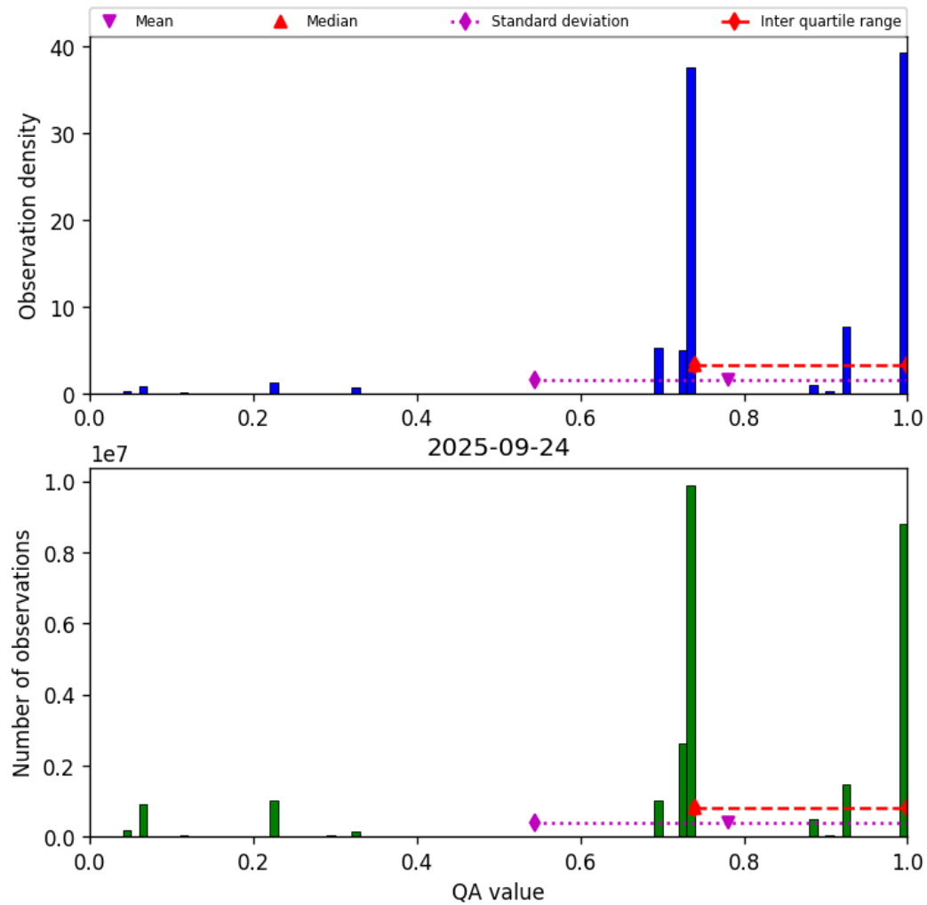
Figure 28: Histogram of “QA value” for 2025-09-23 to 2025-09-25
