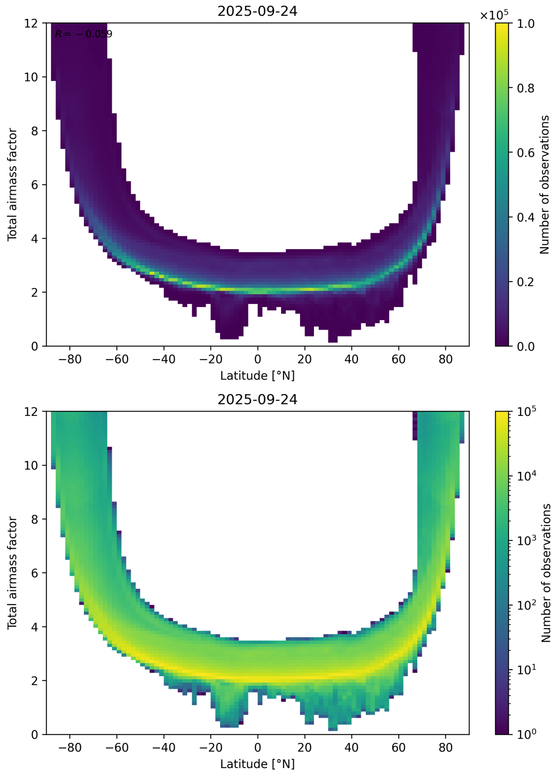
Figure 84: Scatter density plot of “Latitude” against “Total airmass factor” for 2025-09-23 to 2025-09-25.
