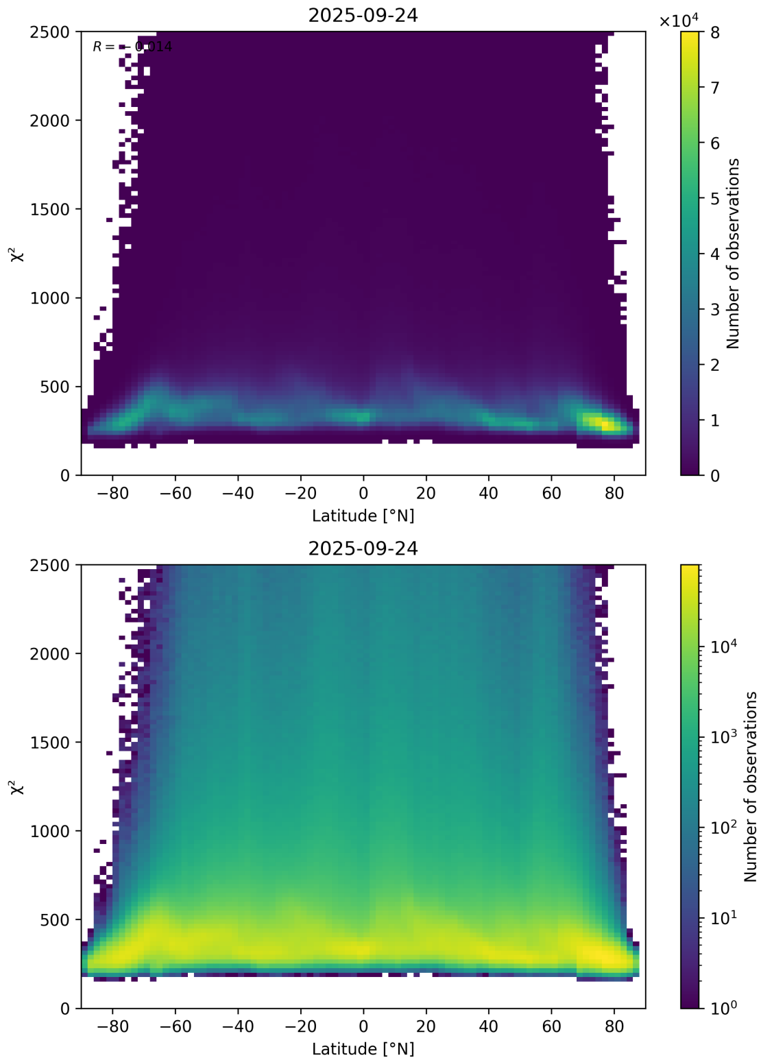
Figure 86: Scatter density plot of “Latitude” against “ \chi^2 ” for 2025-09-23 to 2025-09-25.
