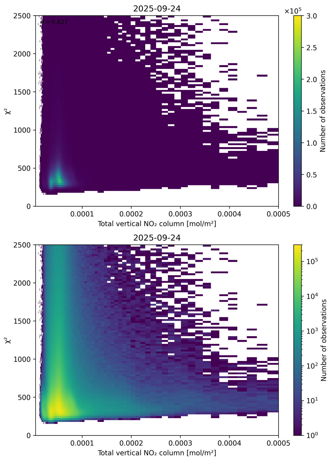
Figure 111: Scatter density plot of “Total vertical NO 2 column” against “ \chi^2 ” for 2025-09-23 to 2025-09-25.
