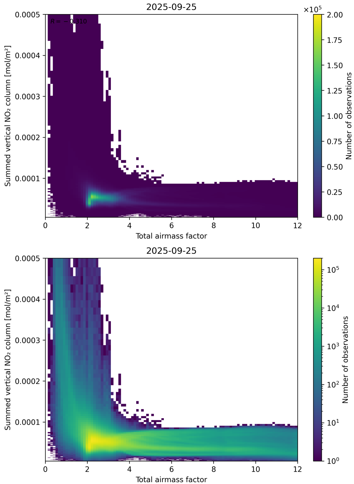
Figure 65: Scatter density plot of “Total airmass factor” against “Summed vertical NO 2 column” for 2025-09-25 to 2025-09-26.
