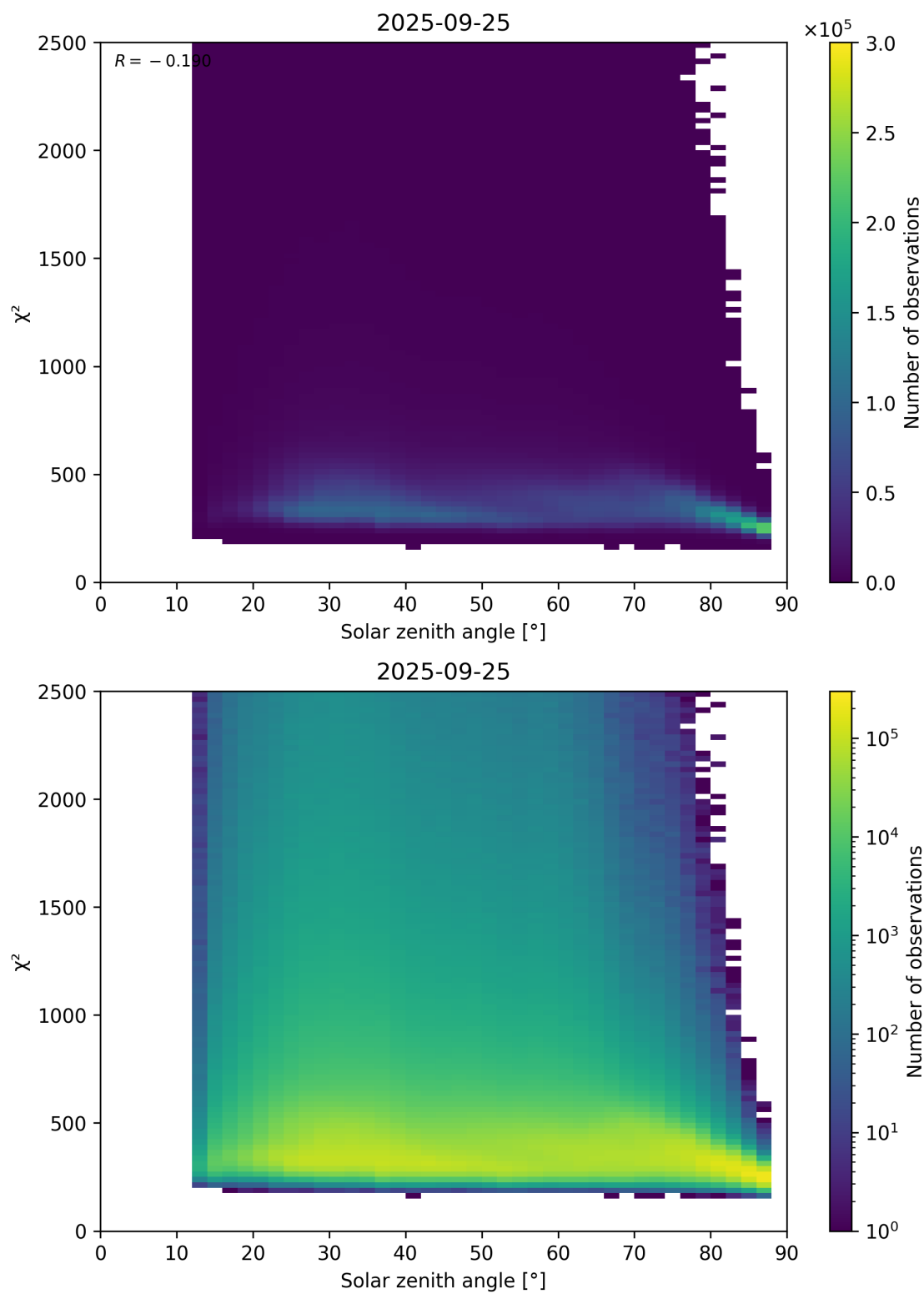
Figure 148: Scatter density plot of “Solar zenith angle” against “ \chi^2 ” for 2025-09-25 to 2025-09-26.
