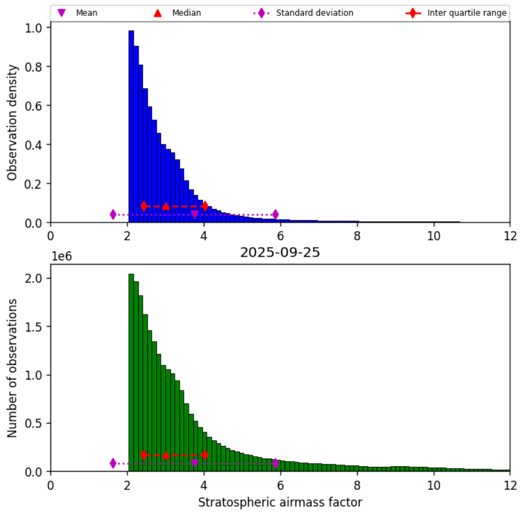
Figure 44: Histogram of “Stratospheric airmass factor” for 2025-09-25 to 2025-09-26
