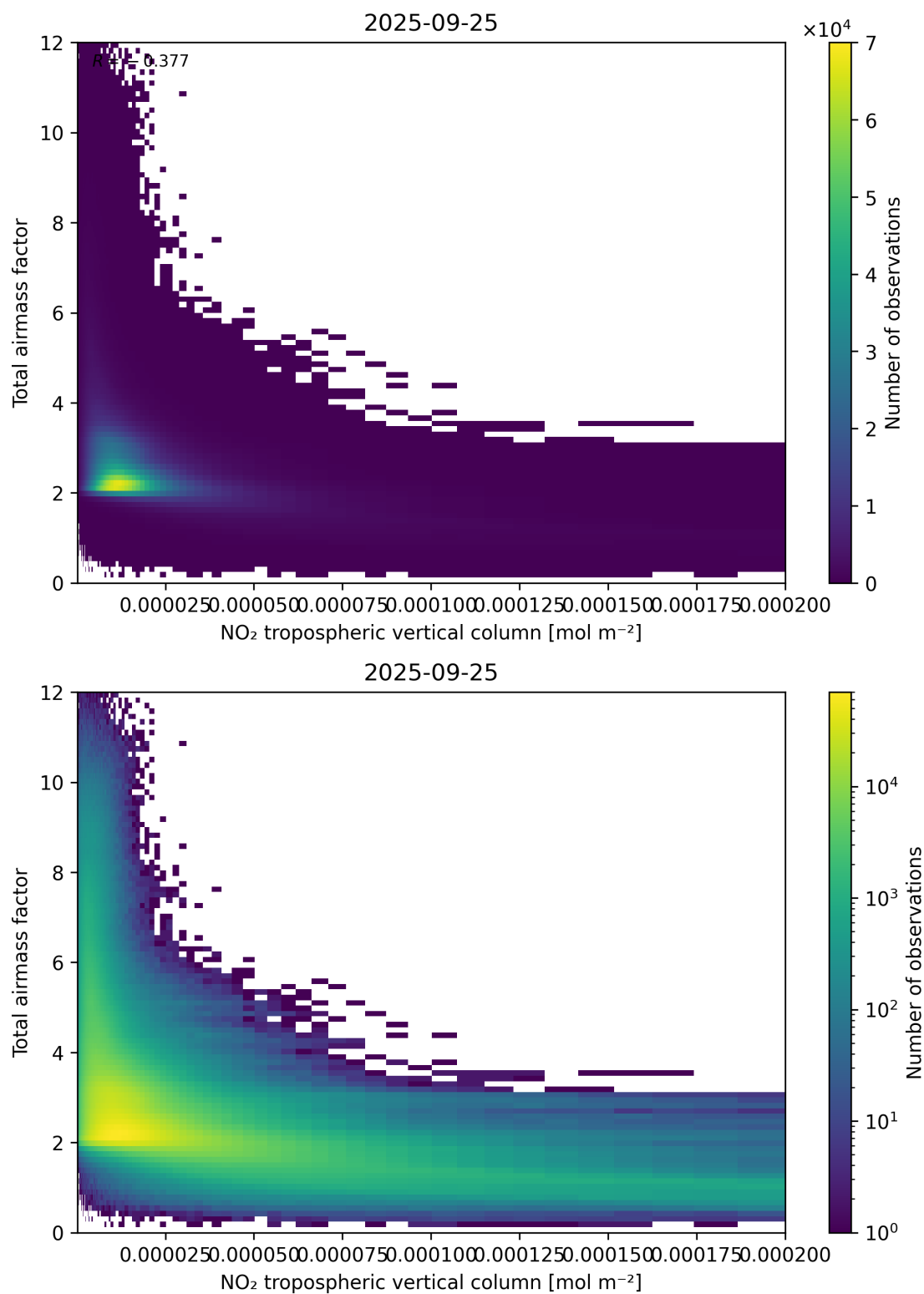
Figure 122: Scatter density plot of “NO 2 tropospheric vertical column” against “Total air mass factor” for 2025-09-25 to 2025-09-26.
