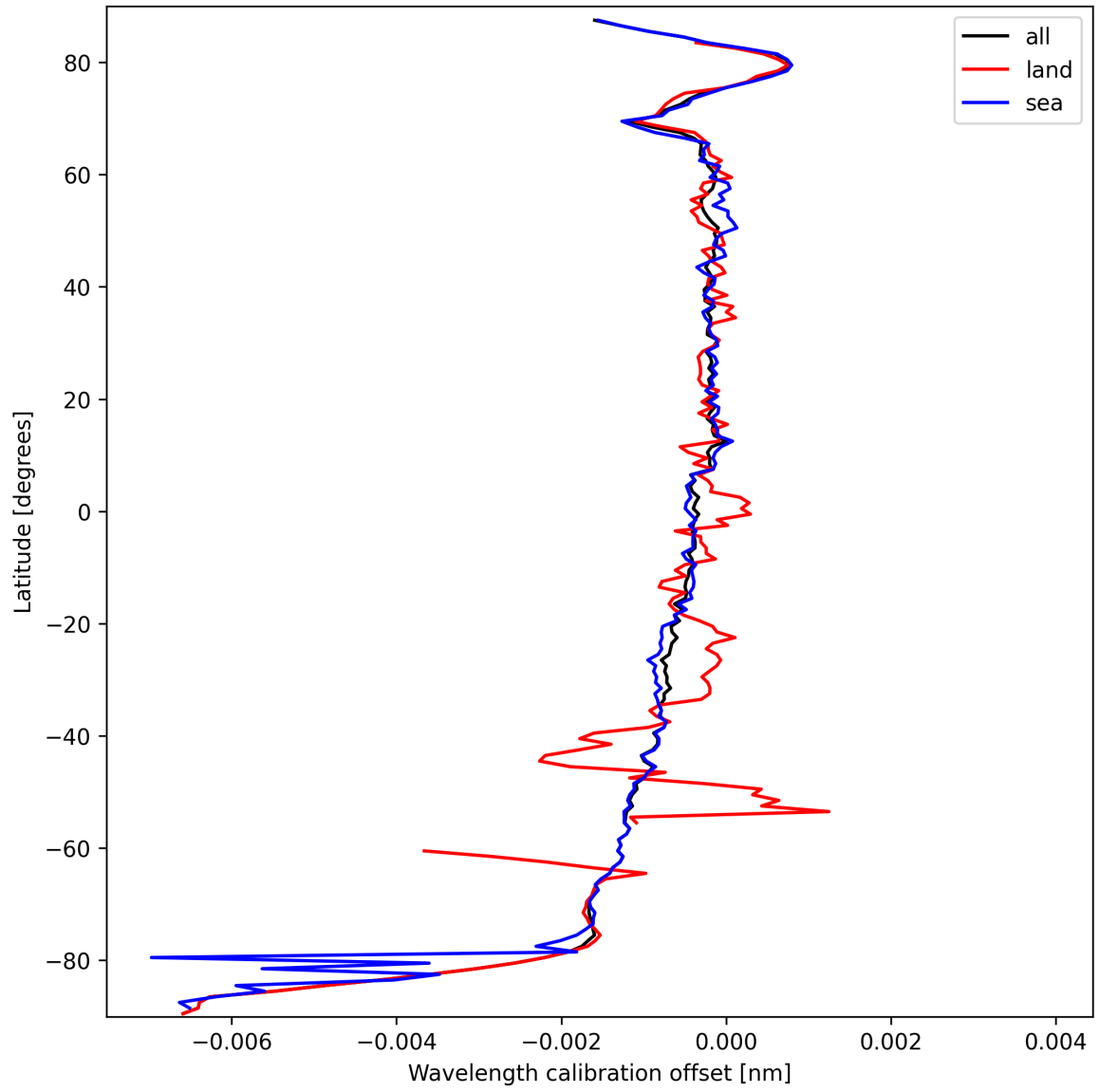
Figure 18: Zonal average of “Wavelength calibration offset” for 2025-09-25 to 2025-09-26.
