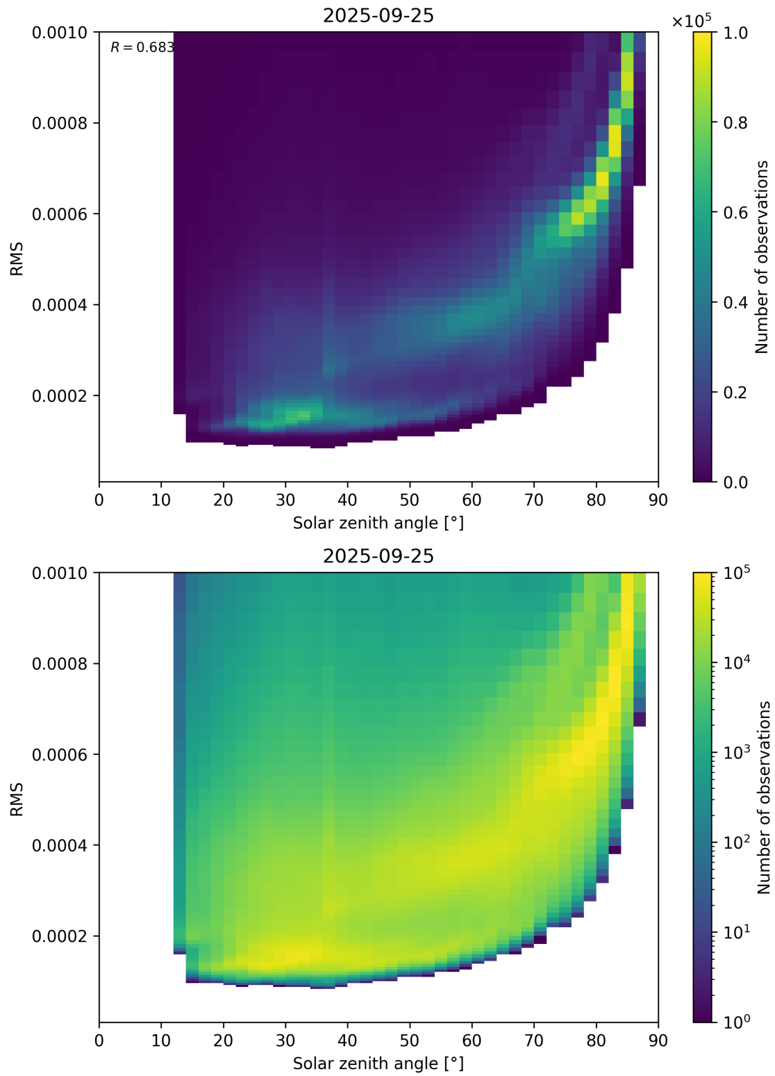
Figure 157: Scatter density plot of “Solar zenith angle” against “RMS” for 2025-09-25 to 2025-09-26.
