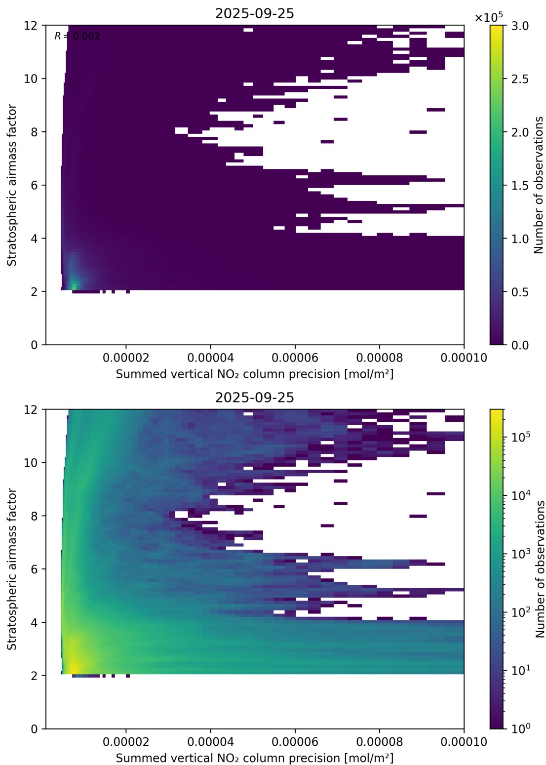
Figure 106: Scatter density plot of “Summed vertical NO 2 column precision” against “Stratospheric airmass factor” for 2025-09-25 to 2025-09-26.
