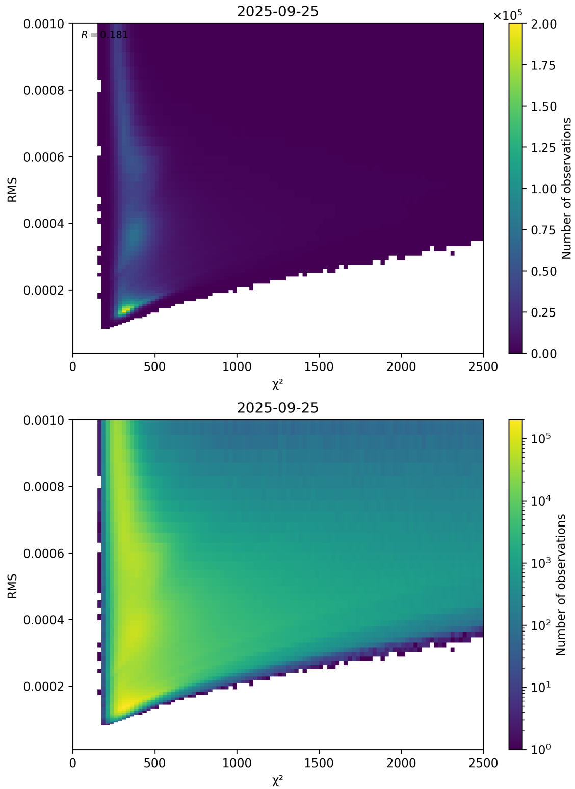
Figure 82: Scatter density plot of “ \chi^2 ” against “RMS” for 2025-09-25 to 2025-09-26.
