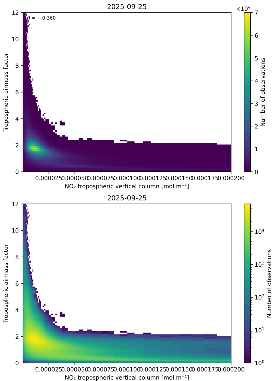
Figure 123: Scatter density plot of “NO 2 tropospheric vertical column” against “Tropospheric air mass factor” for 2025-09-25 to 2025-09-26.
