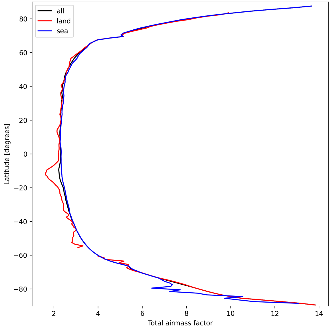
Figure 15: Zonal average of “Total airmass factor” for 2025-09-25 to 2025-09-26.
