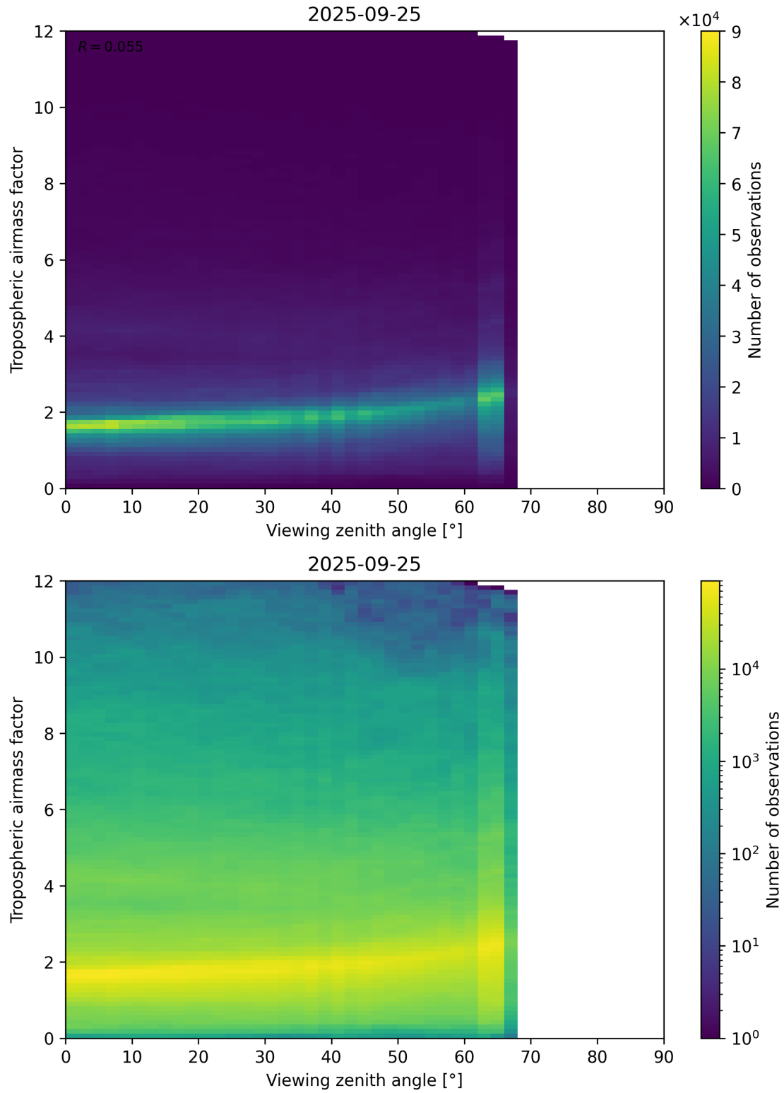
Figure 161: Scatter density plot of “Viewing zenith angle” against “Tropospheric airmass factor” for 2025-09-25 to 2025-09-26.
