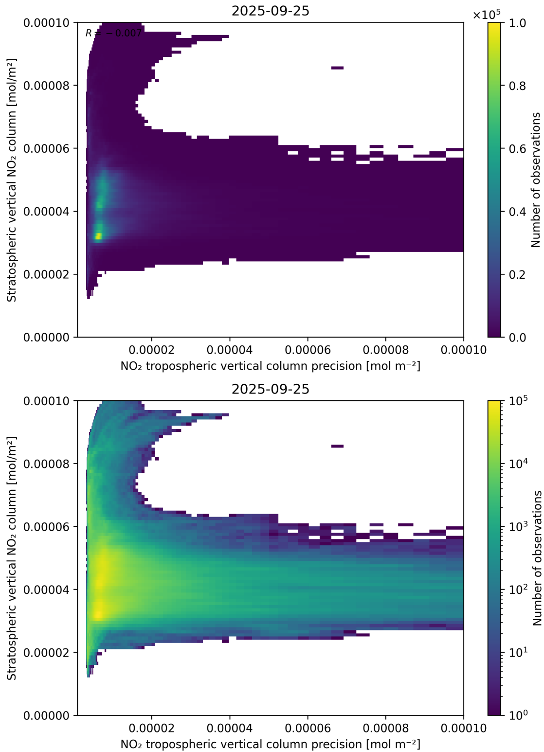
Figure 135: Scatter density plot of “NO 2 tropospheric vertical column precision” against “Stratospheric vertical NO 2 column” for 2025-09-25 to 2025-09-26.
