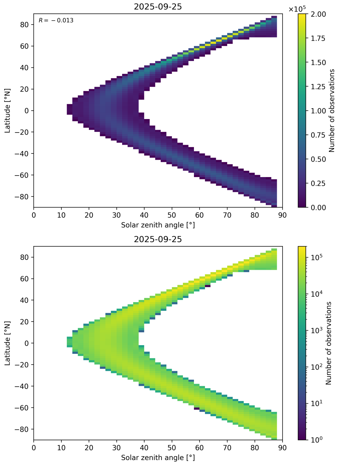
Figure 149: Scatter density plot of “Solar zenith angle” against “Latitude” for 2025-09-25 to 2025-09-26.
