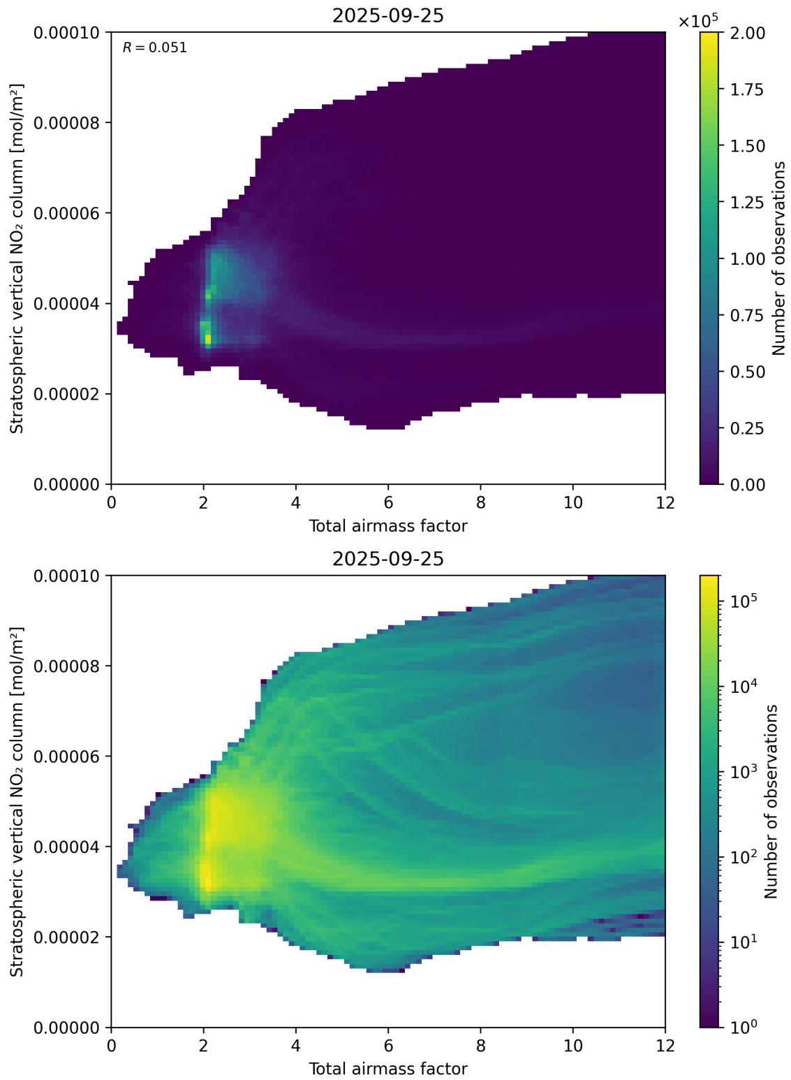
Figure 64: Scatter density plot of “Total airmass factor” against “Stratospheric vertical NO 2 column” for 2025-09-25 to 2025-09-26.
