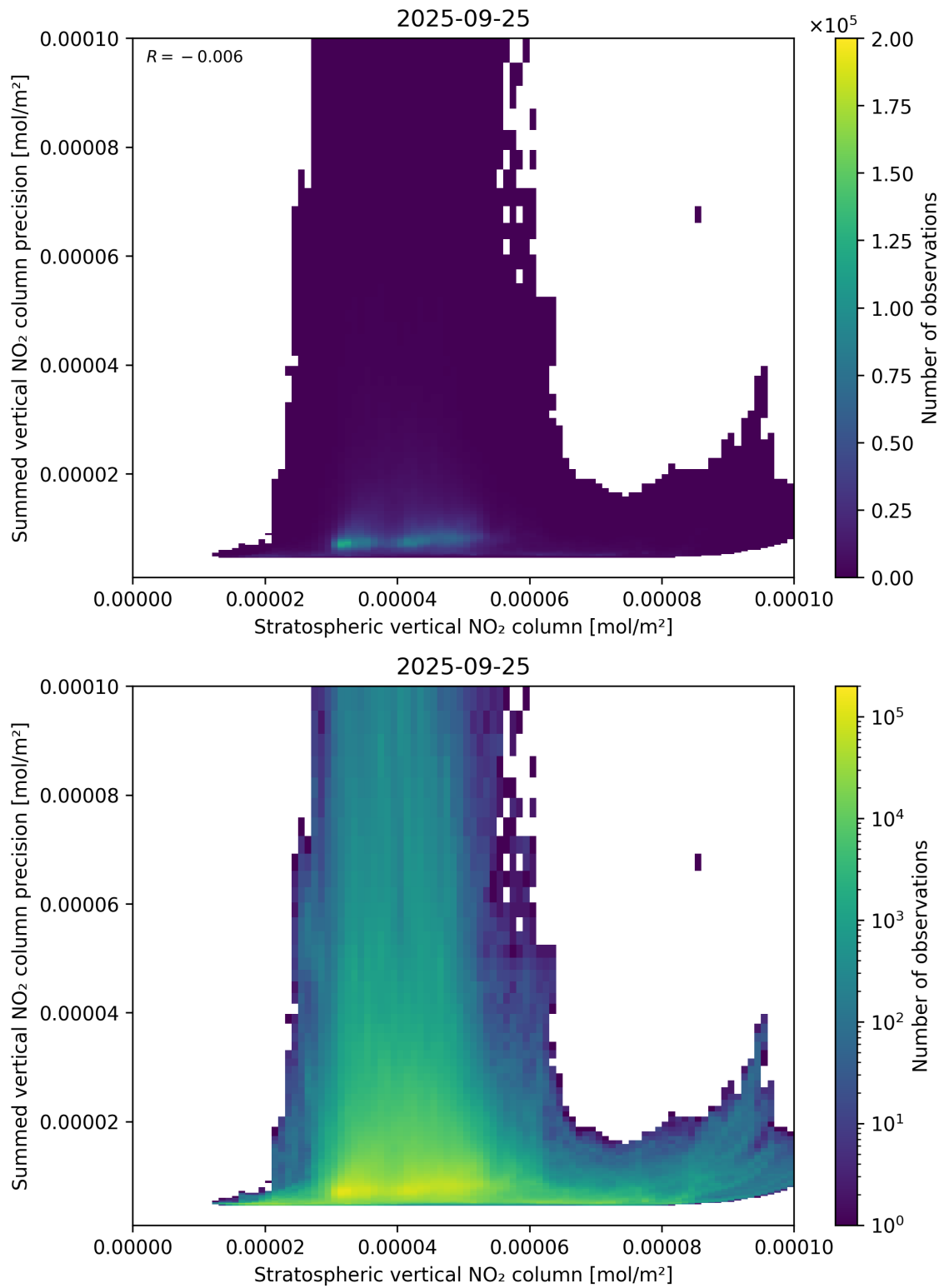
Figure 99: Scatter density plot of “Stratospheric vertical NO 2 column” against “Summed vertical NO 2 column precision” for 2025-09-25 to 2025-09-26.
