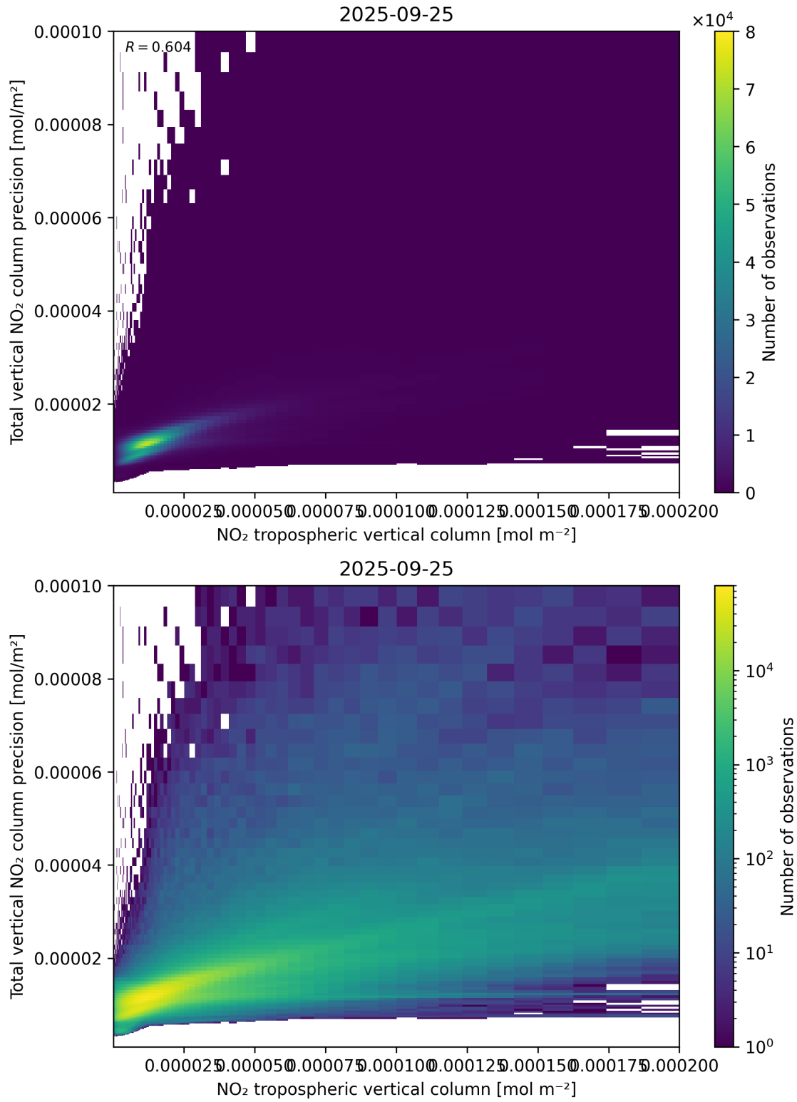
Figure 129: Scatter density plot of “NO 2 tropospheric vertical column” against “Total vertical NO 2 column precision” for 2025-09-25 to 2025-09-26.
