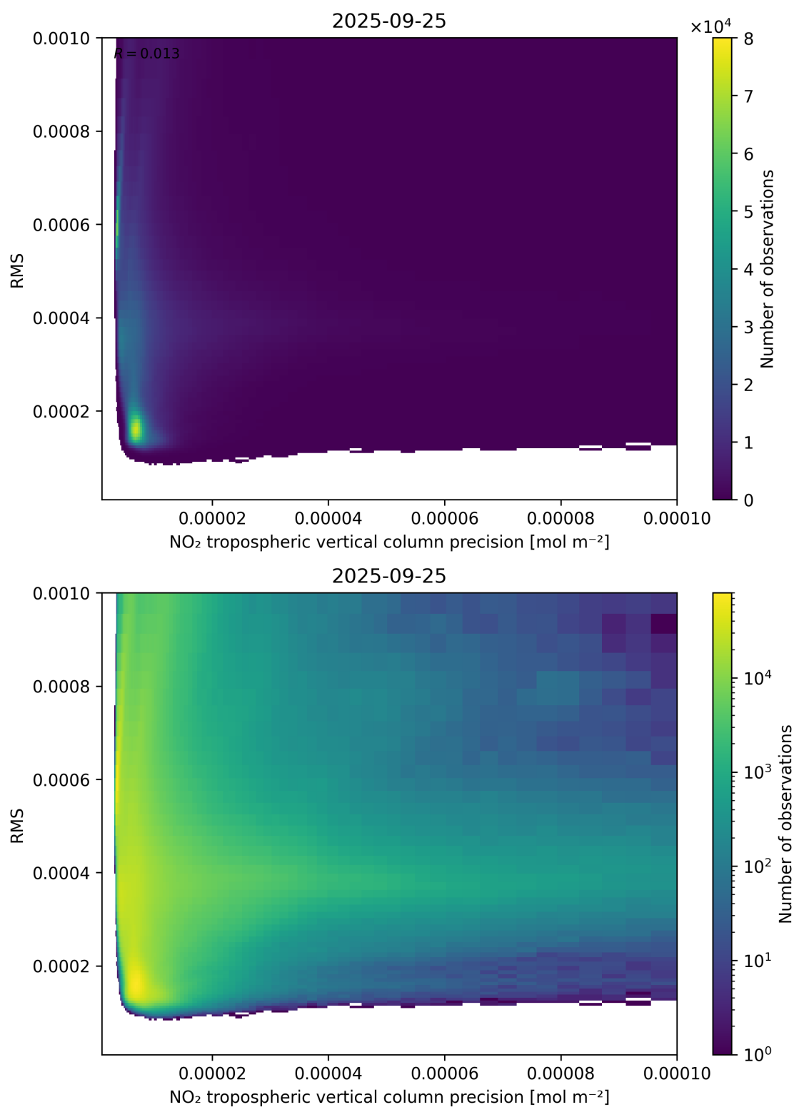
Figure 140: Scatter density plot of “NO 2 tropospheric vertical column precision” against “RMS” for 2025-09-25 to 2025-09-26.
