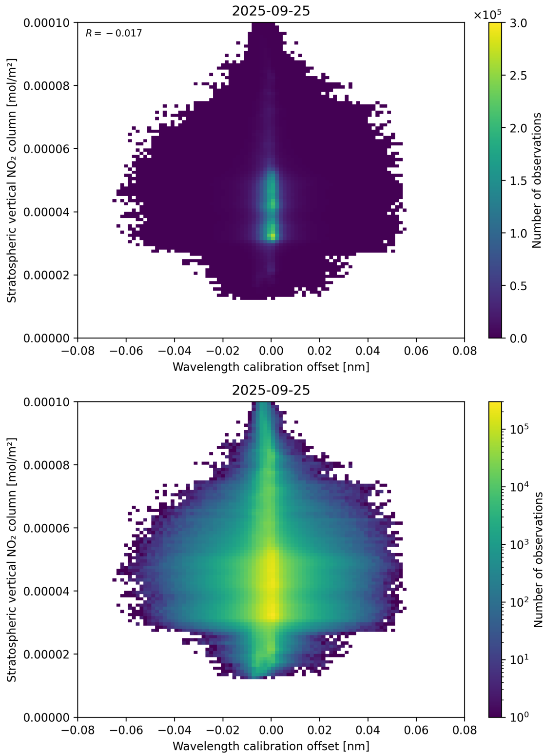
Figure 176: Scatter density plot of “Wavelength calibration offset” against “Stratospheric vertical NO 2 column” for 2025-09-25 to 2025-09-26.
