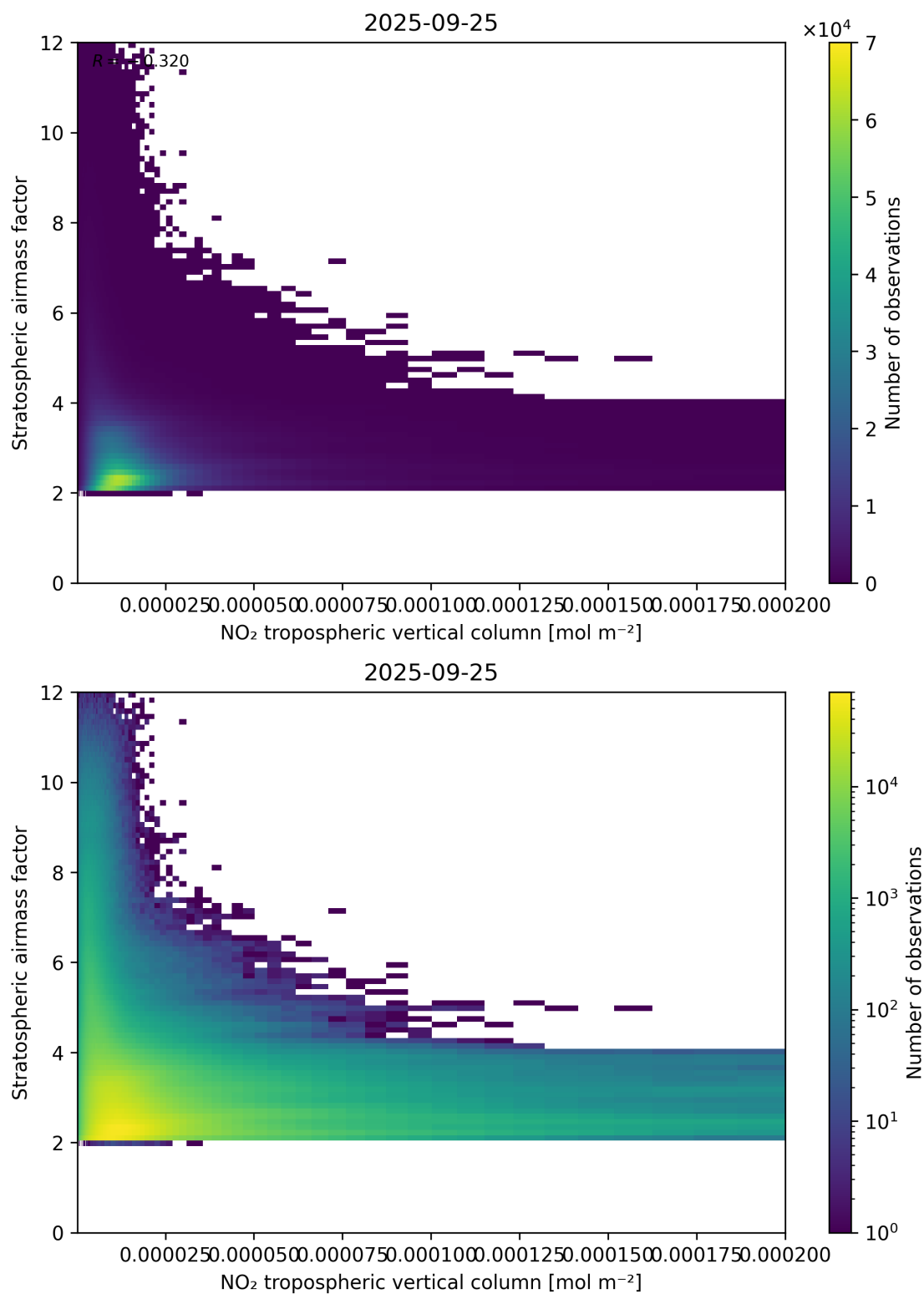
Figure 121: Scatter density plot of “NO 2 tropospheric vertical column” against “Stratospheric air mass factor” for 2025-09-25 to 2025-09-26.
