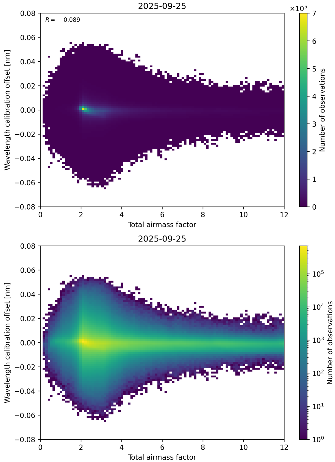
Figure 70: Scatter density plot of “Total airmass factor” against “Wavelength calibration offset” for 2025-09-25 to 2025-09-26.
