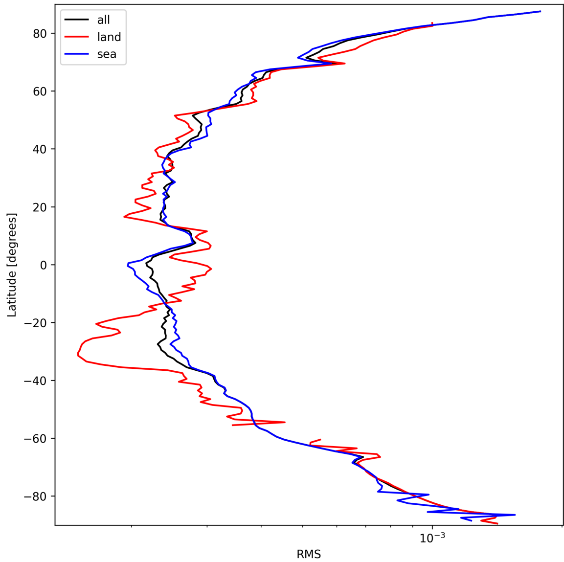
Figure 26: Zonal average of “RMS” for 2025-09-25 to 2025-09-26.
