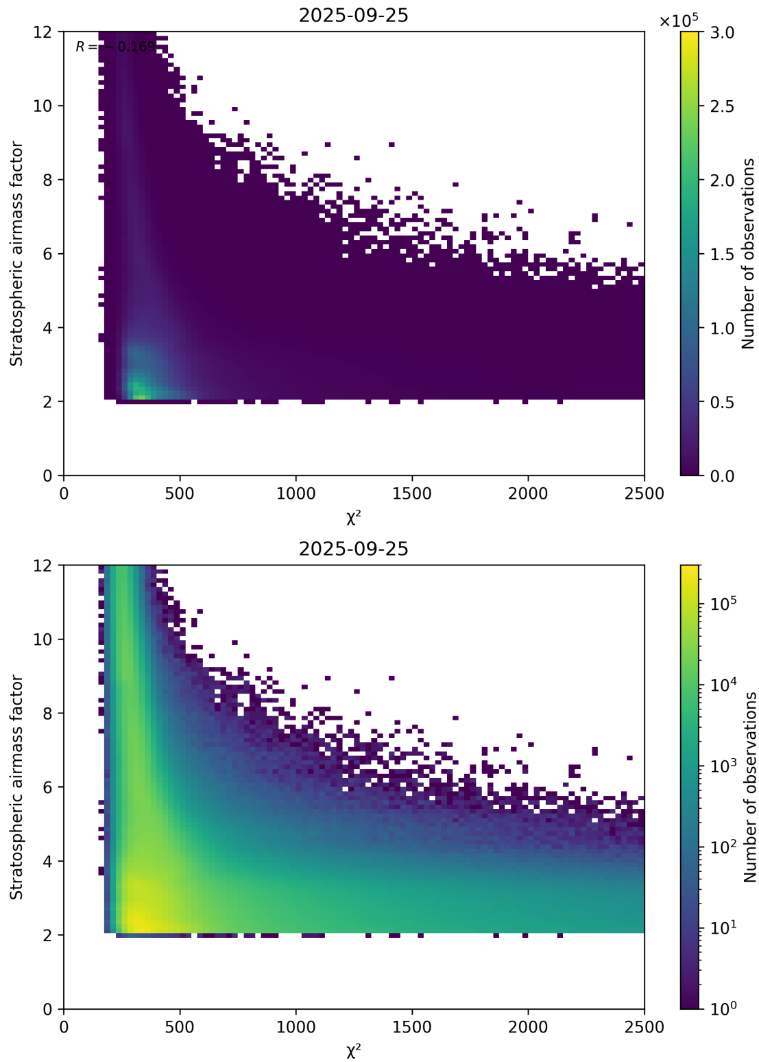
Figure 81: Scatter density plot of “ \chi^2 ” against “Stratospheric airmass factor” for 2025-09-25 to 2025-09-26.
