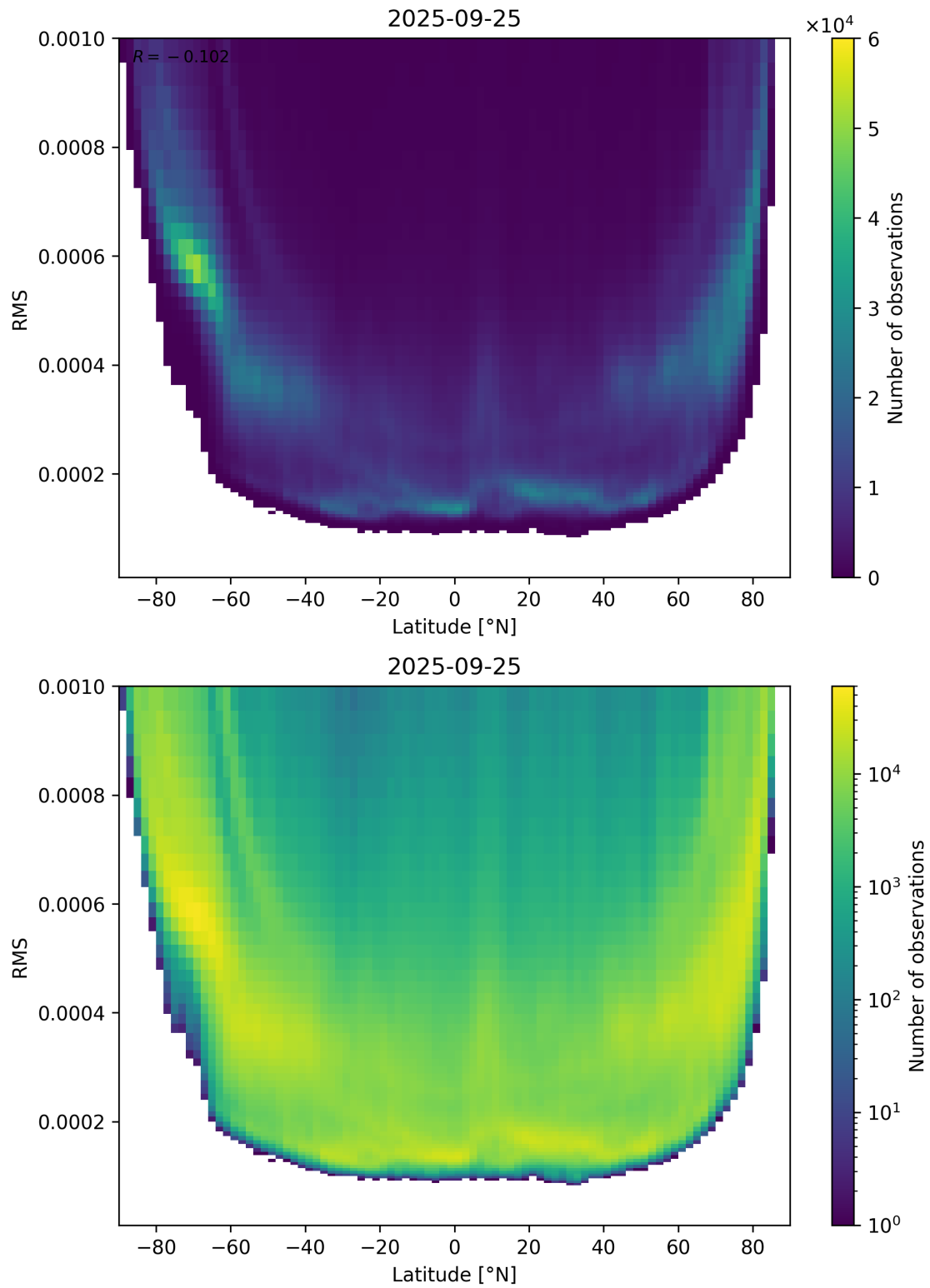
Figure 94: Scatter density plot of “Latitude” against “RMS” for 2025-09-25 to 2025-09-26.
