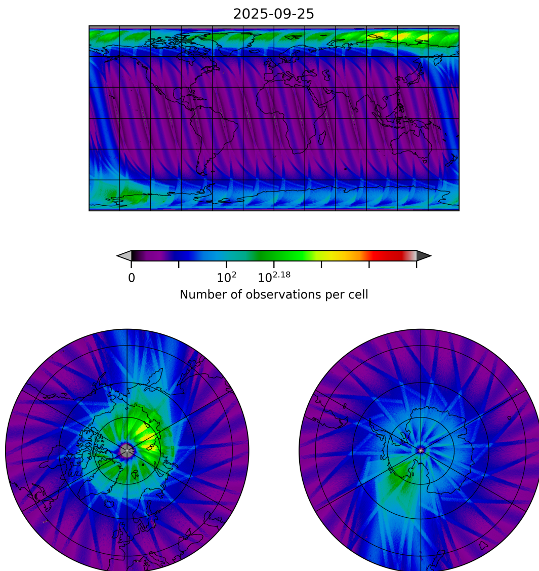
Figure 10: Map of the number of observations for 2025-09-25 to 2025-09-26
