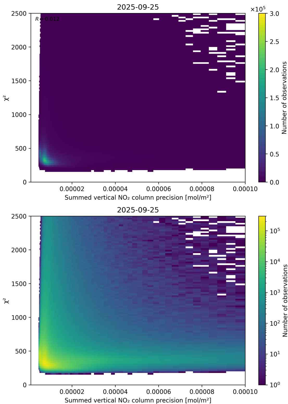
Figure 107: Scatter density plot of “Summed vertical NO 2 column precision” against “ \chi^2 ” for 2025-09-25 to 2025-09-26.
