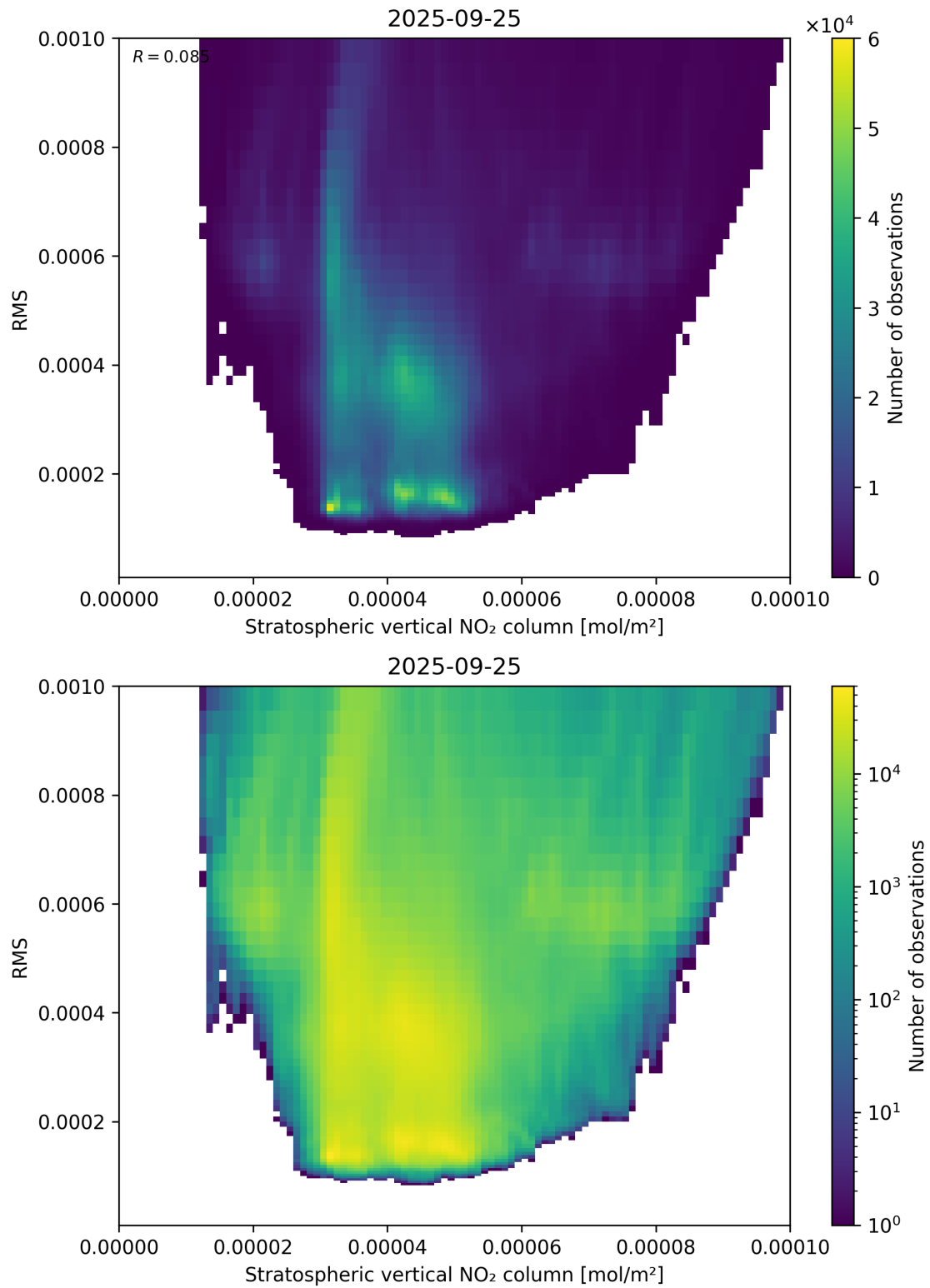
Figure 102: Scatter density plot of “Stratospheric vertical NO 2 column” against “RMS” for 2025-09-25 to 2025-09-26.
