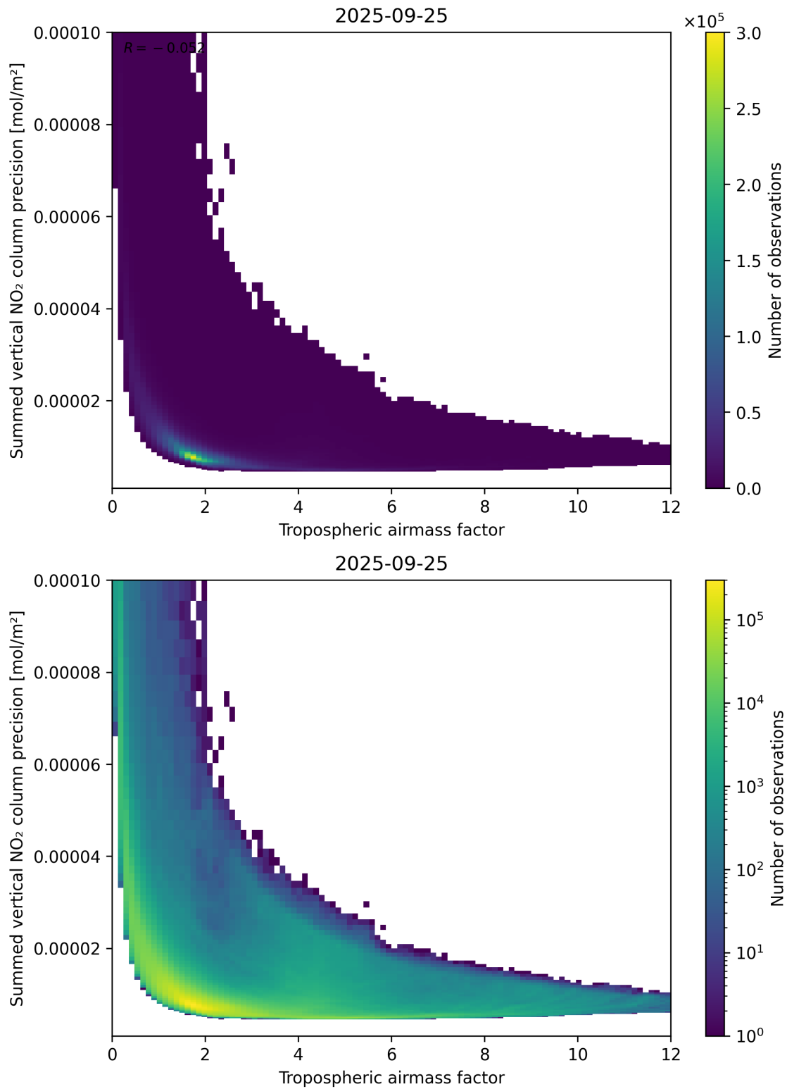
Figure 76: Scatter density plot of “Tropospheric air mass factor” against “Summed vertical NO 2 column precision” for 2025-09-25 to 2025-09-26.
