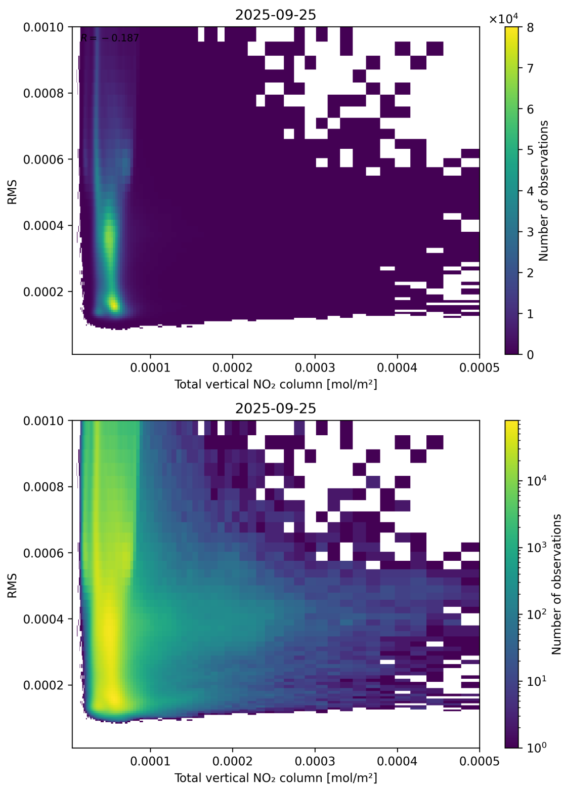
Figure 120: Scatter density plot of “Total vertical NO 2 column” against “RMS” for 2025-09-25 to 2025-09-26.
