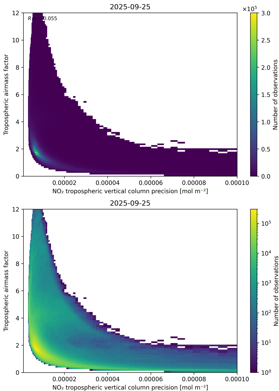
Figure 133: Scatter density plot of “NO 2 tropospheric vertical column precision” against “Tropospheric airmass factor” for 2025-09-25 to 2025-09-26.
