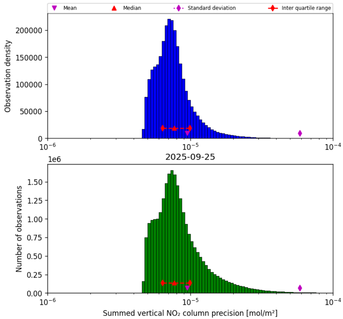
Figure 41: Histogram of "Summed vertical NO 2 column precision" for 2025-09-25 to 2025-09-26
