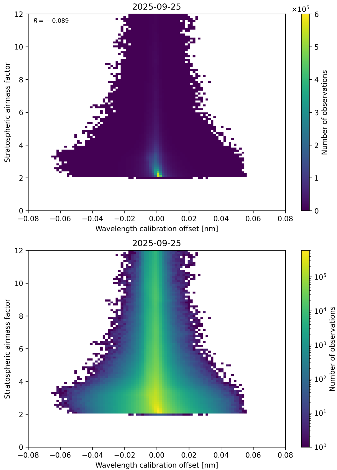
Figure 174: Scatter density plot of “Wavelength calibration offset” against “Stratospheric airmass factor” for 2025-09-25 to 2025-09-26.
