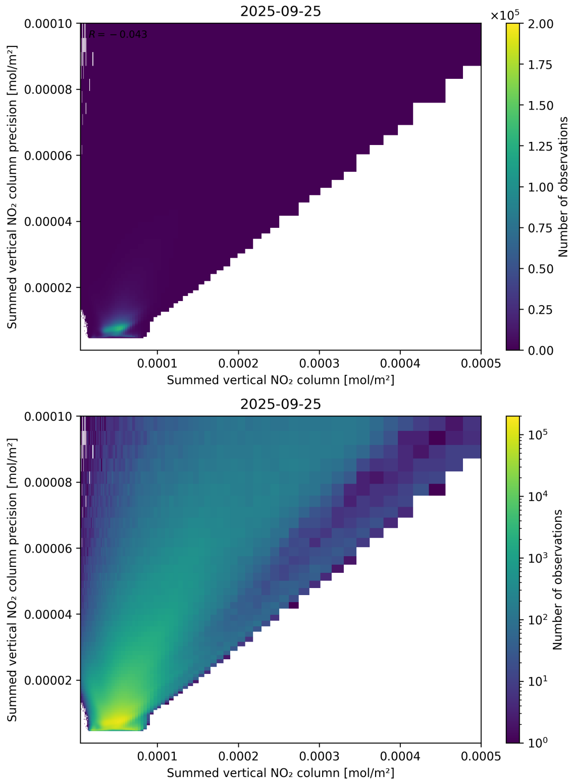
Figure 105: Scatter density plot of “Summed vertical NO 2 column” against “Summed vertical NO 2 column precision” for 2025-09-25 to 2025-09-26.
