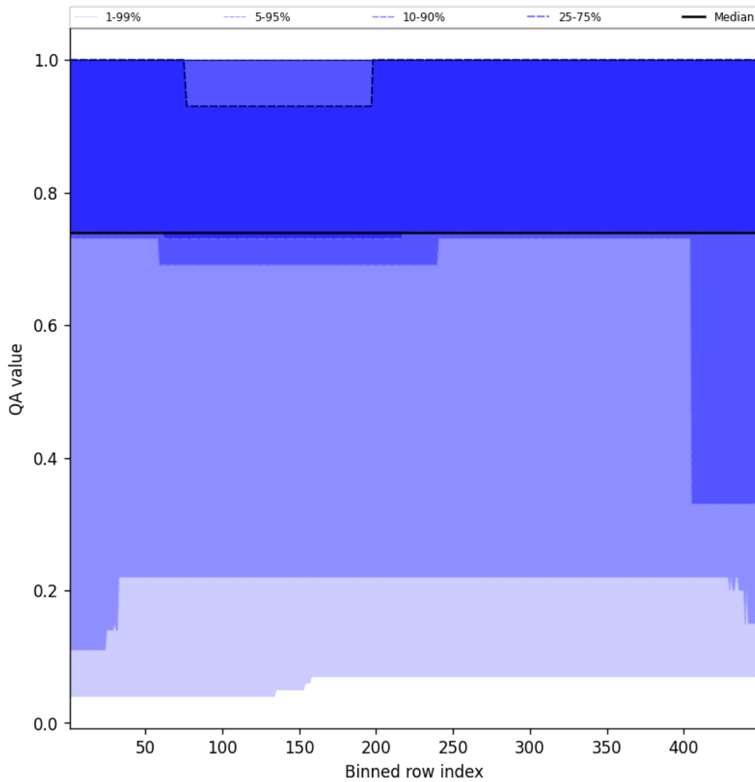
Figure 45: Along track statistics of “QA value” for 2025-09-25 to 2025-09-26
