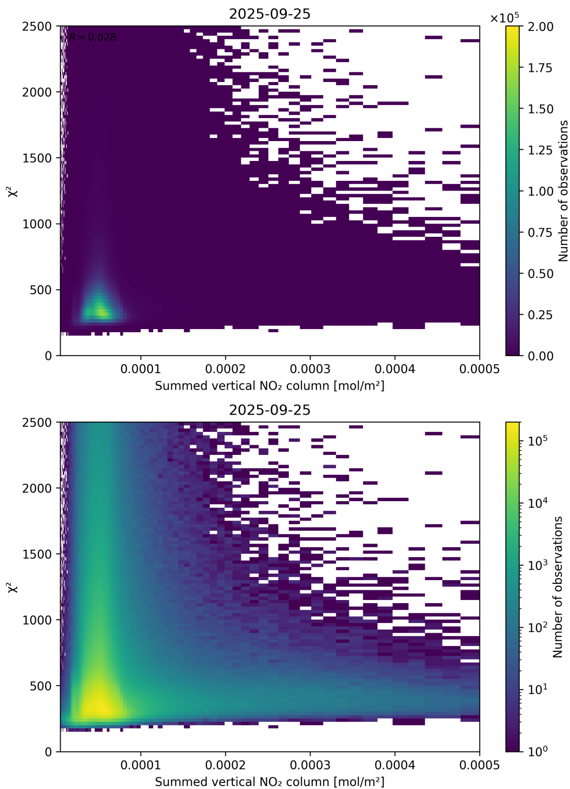
Figure 104: Scatter density plot of “Summed vertical NO 2 column” against “ \chi^2 ” for 2025-09-25 to 2025-09-26.
