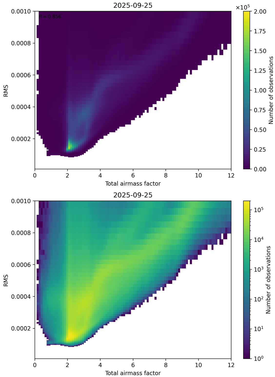
Figure 69: Scatter density plot of “Total airmass factor” against “RMS” for 2025-09-25 to 2025-09-26.
