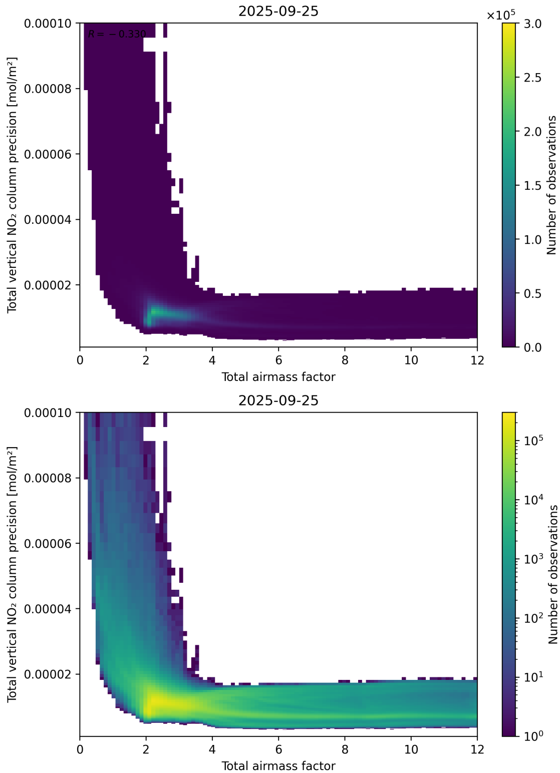
Figure 68: Scatter density plot of “Total airmass factor” against “Total vertical NO 2 column precision” for 2025-09-25 to 2025-09-26.
