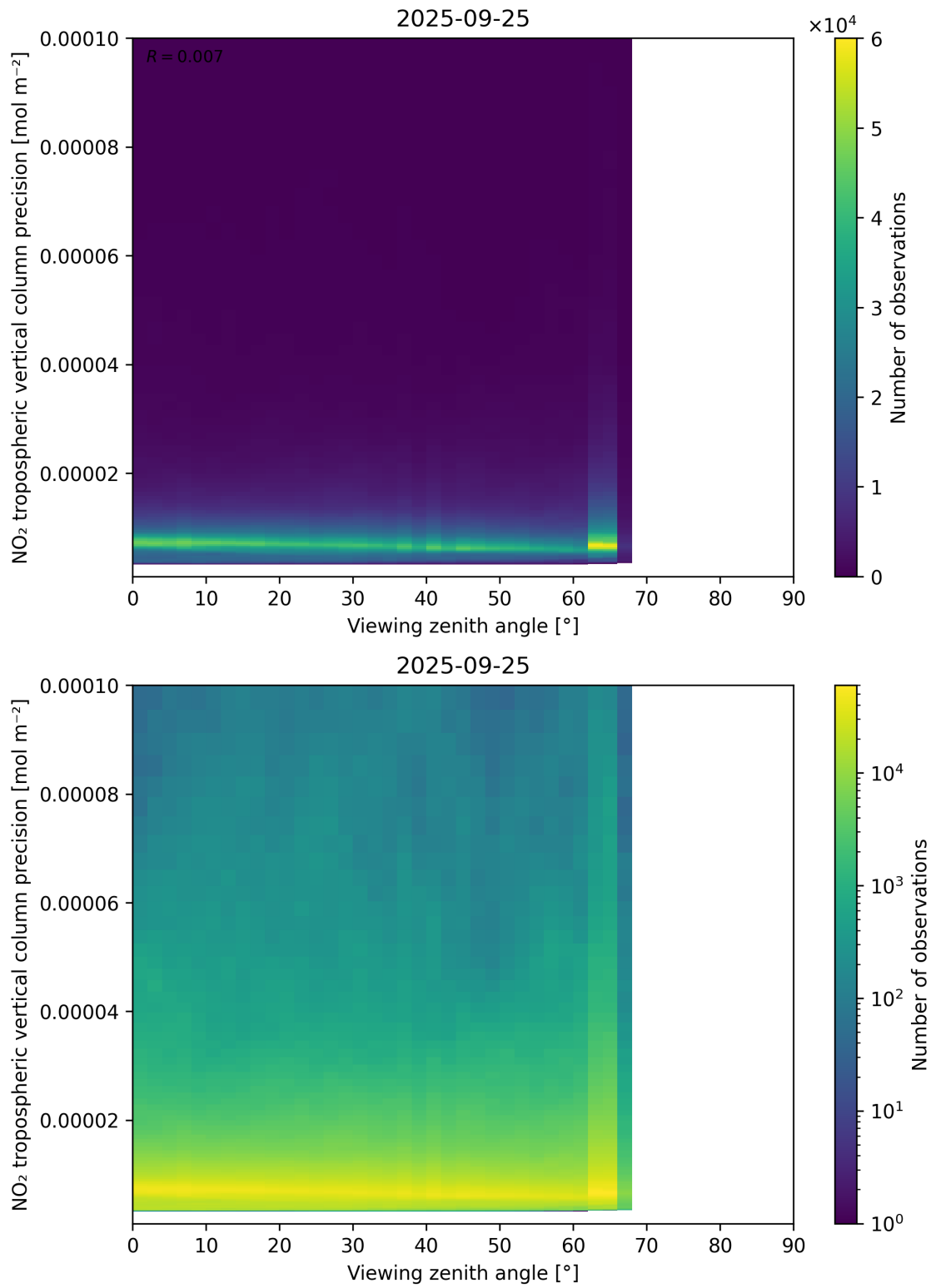
Figure 170: Scatter density plot of “Viewing zenith angle” against “NO 2 tropospheric vertical column precision” for 2025-09-25 to 2025-09-26.
