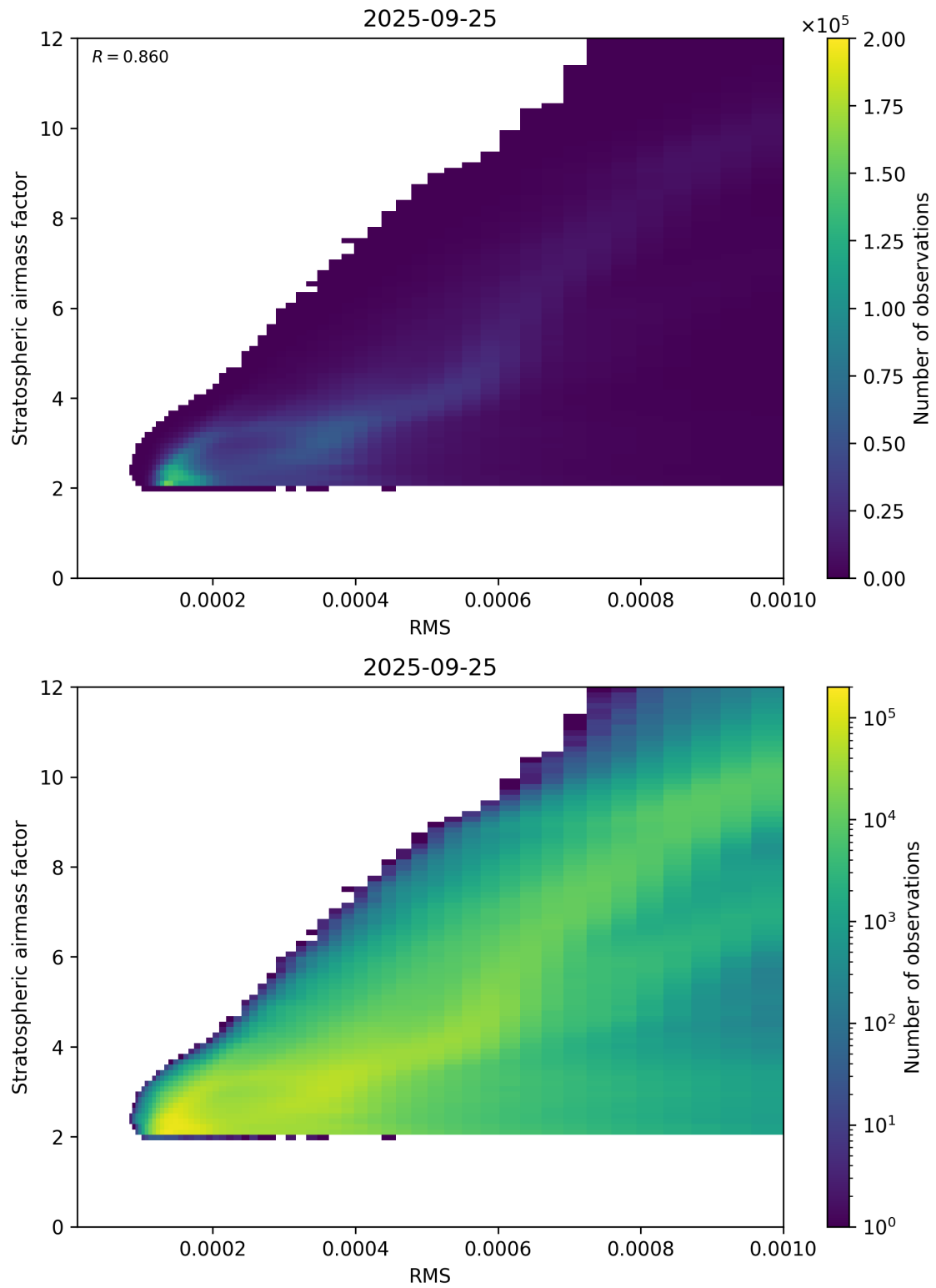
Figure 144: Scatter density plot of “RMS” against “Stratospheric airmass factor” for 2025-09-25 to 2025-09-26.
