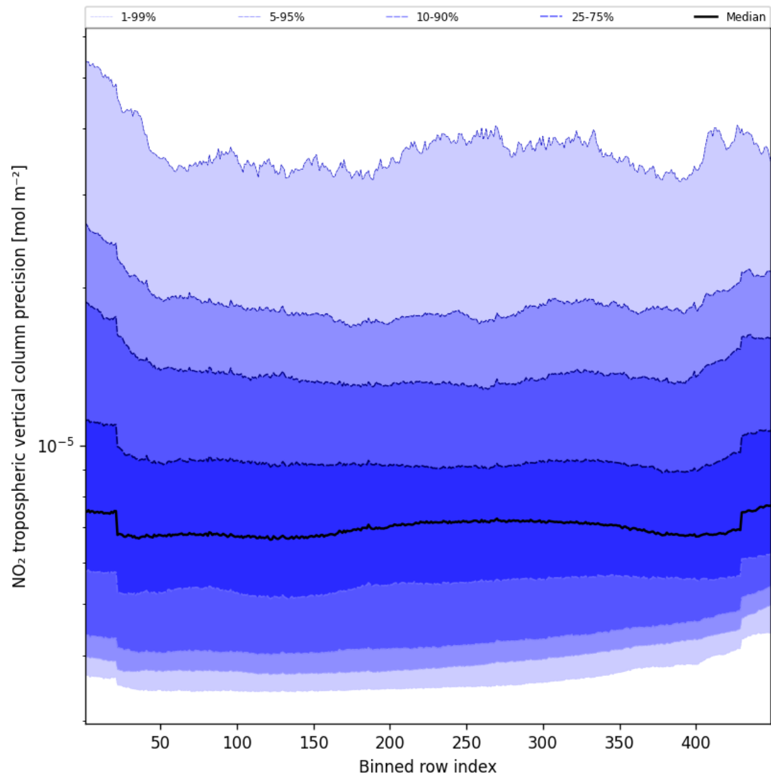
Figure 47: Along track statistics of “NO 2 tropospheric vertical column precision” for 2025-09-25 to 2025-09-26
