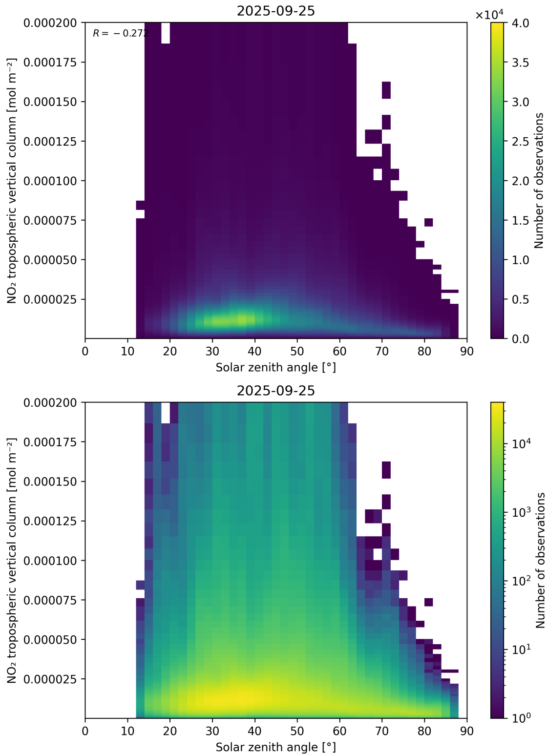
Figure 155: Scatter density plot of “Solar zenith angle” against “NO 2 tropospheric vertical column” for 2025-09-25 to 2025-09-26.
