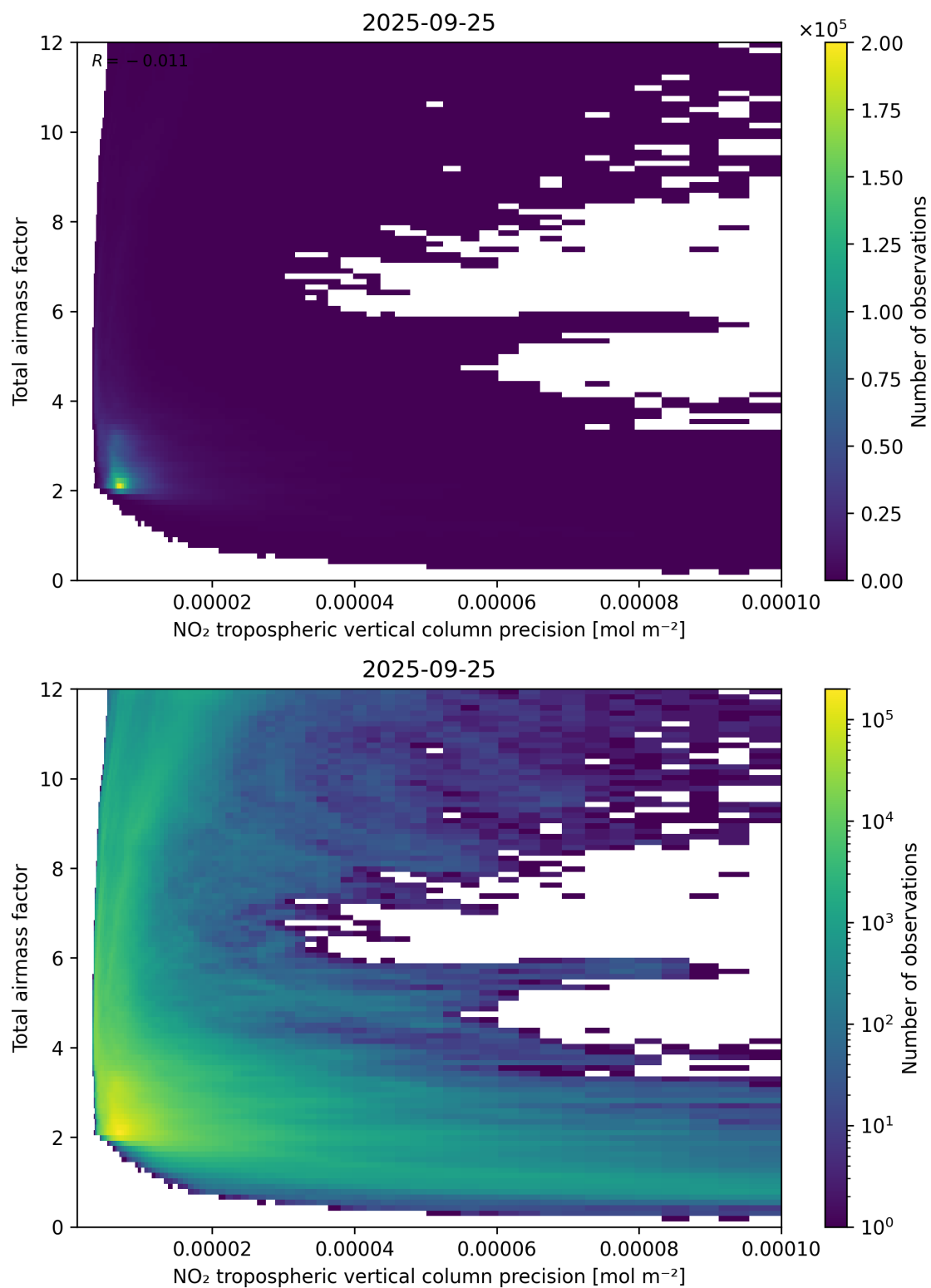
Figure 132: Scatter density plot of “NO 2 tropospheric vertical column precision” against “Total air mass factor” for 2025-09-25 to 2025-09-26.
