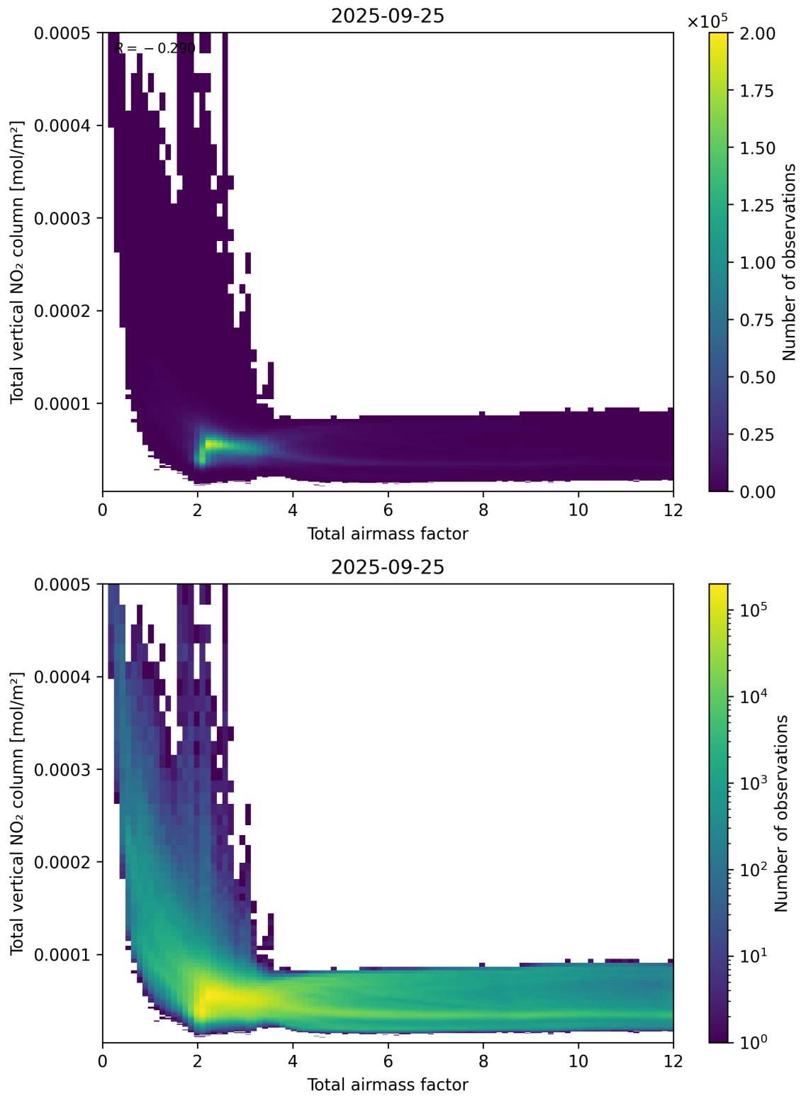
Figure 67: Scatter density plot of “Total airmass factor” against “Total vertical NO 2 column” for 2025-09-25 to 2025-09-26.
