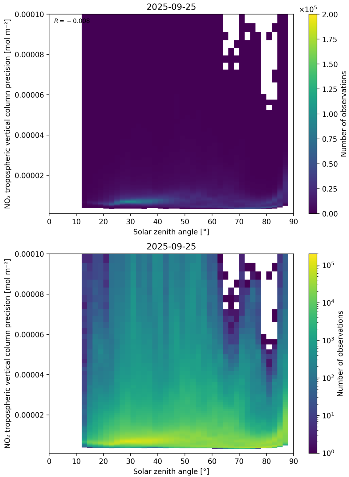
Figure 156: Scatter density plot of “Solar zenith angle” against “NO 2 tropospheric vertical column precision” for 2025-09-25 to 2025-09-26.
