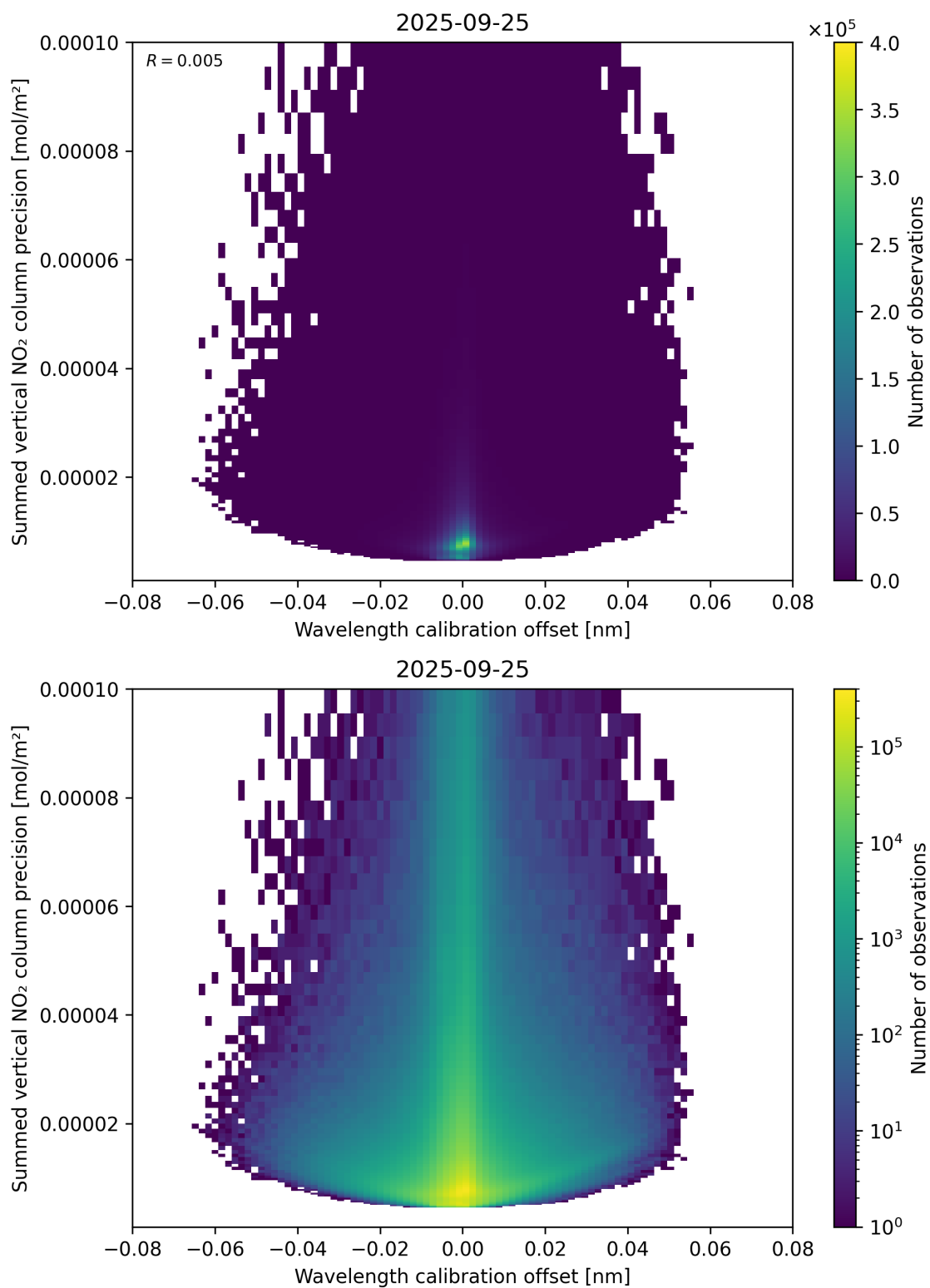
Figure 178: Scatter density plot of “Wavelength calibration offset” against “Summed vertical NO 2 column precision” for 2025-09-25 to 2025-09-26.
