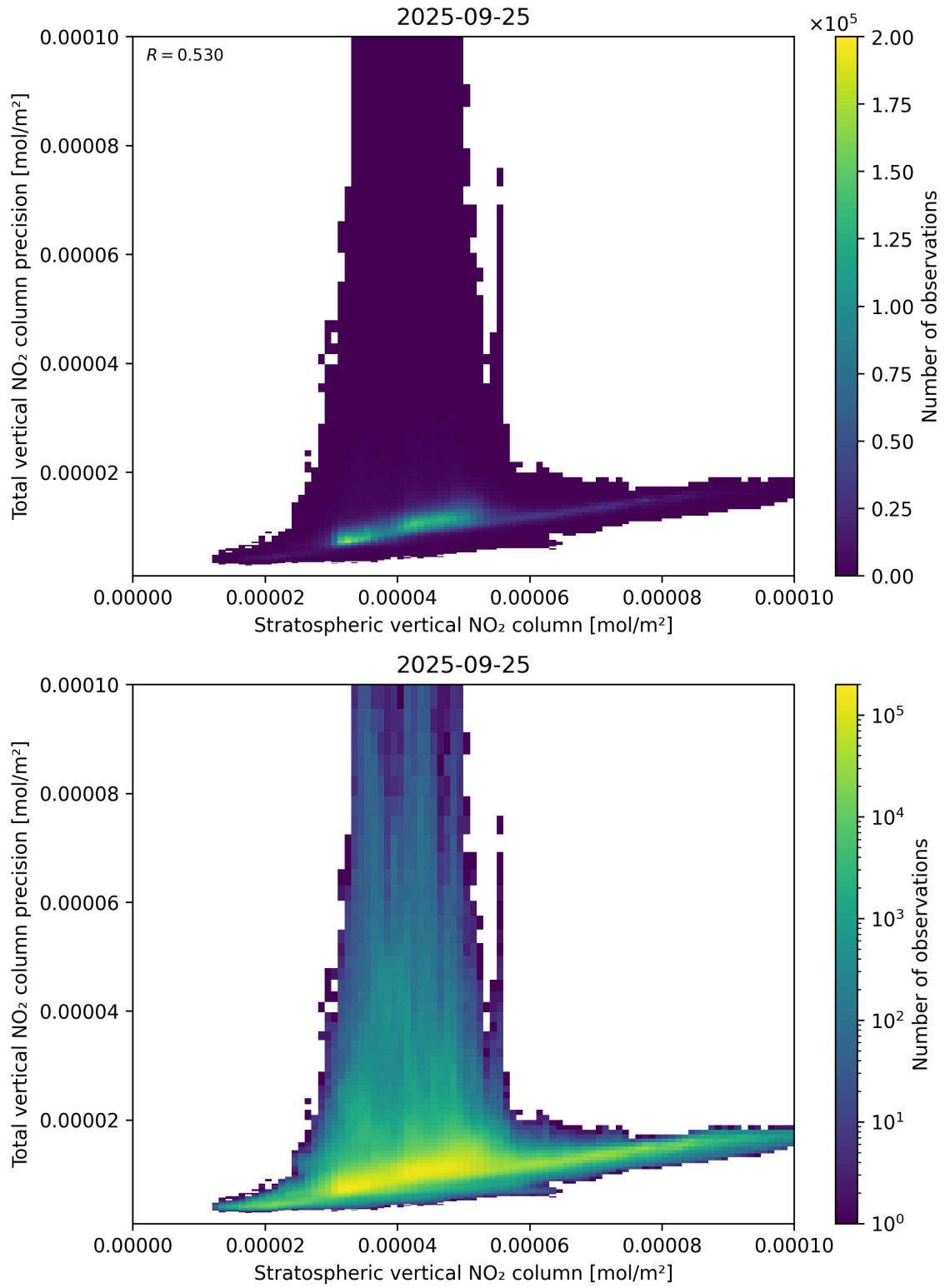
Figure 101: Scatter density plot of “Stratospheric vertical NO 2 column” against “Total vertical NO 2 column precision” for 2025-09-25 to 2025-09-26.
