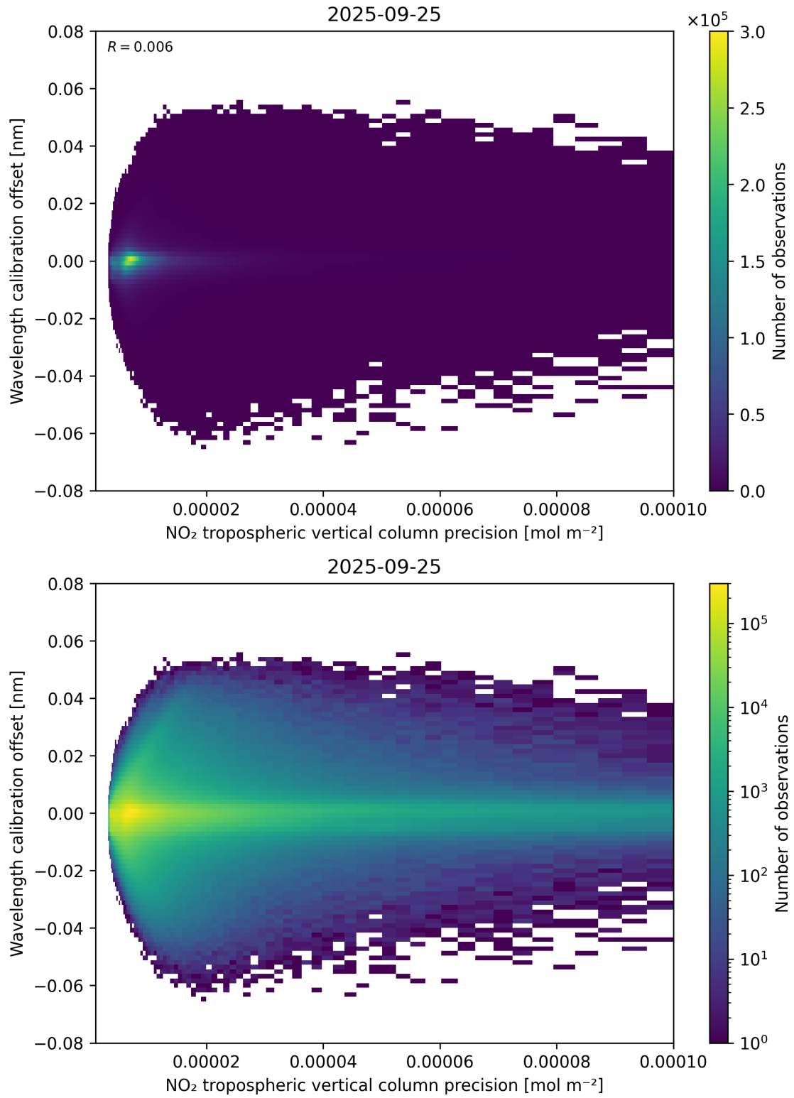
Figure 141: Scatter density plot of “NO 2 tropospheric vertical column precision” against “Wavelength calibration offset” for 2025-09-25 to 2025-09-26.
