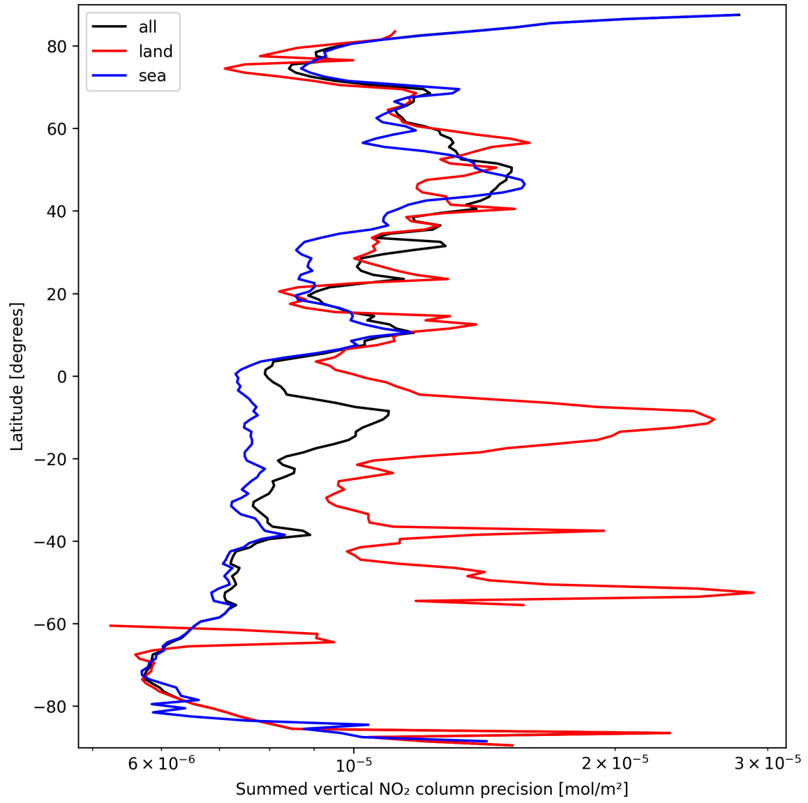
Figure 24: Zonal average of “Summed vertical NO 2 column precision” for 2025-09-25 to 2025-09-26.
