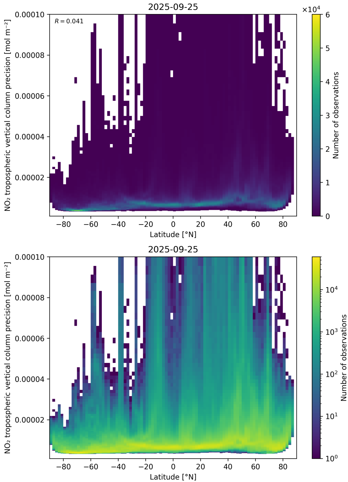
Figure 93: Scatter density plot of “Latitude” against “NO 2 tropospheric vertical column precision” for 2025-09-25 to 2025-09-26.
