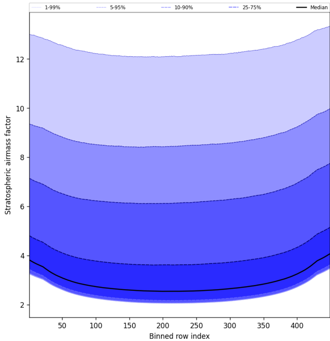
Figure 61: Along track statistics of “Stratospheric airmass factor” for 2025-09-25 to 2025-09-26
