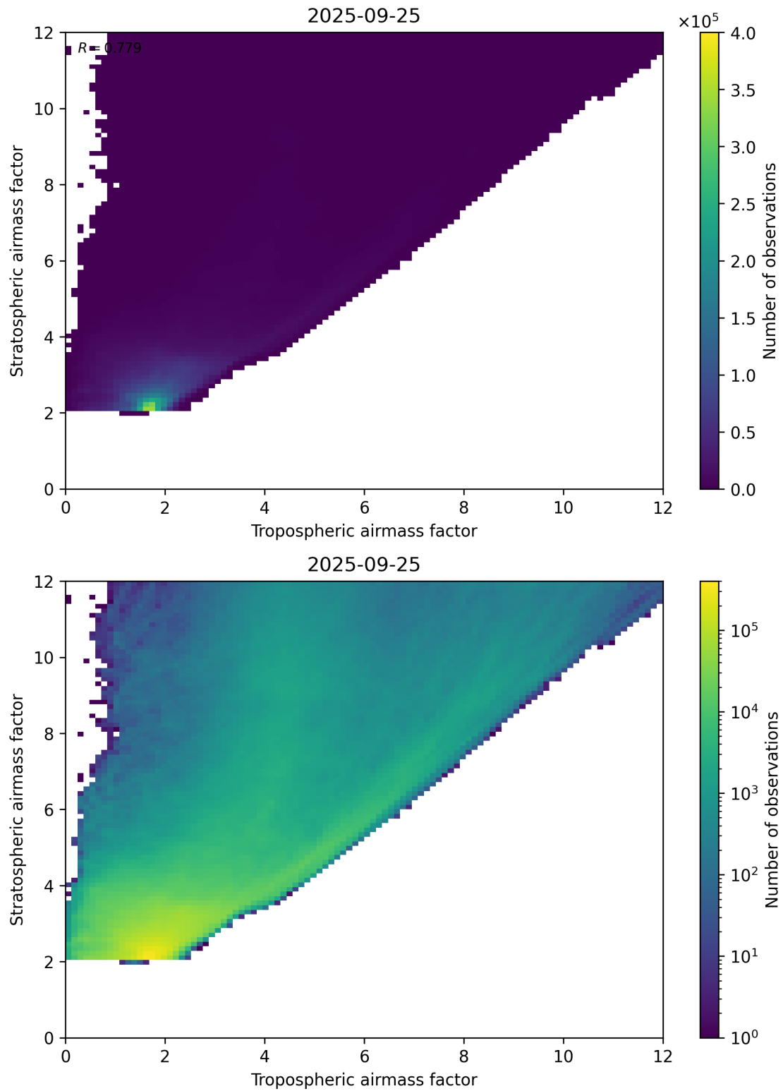
Figure 71: Scatter density plot of “Tropospheric airmass factor” against “Stratospheric airmass factor” for 2025-09-25 to 2025-09-26.
