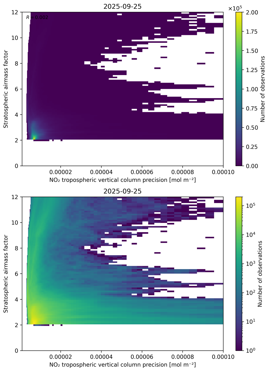
Figure 131: Scatter density plot of “NO 2 tropospheric vertical column precision” against “Stratospheric airmass factor” for 2025-09-25 to 2025-09-26.
