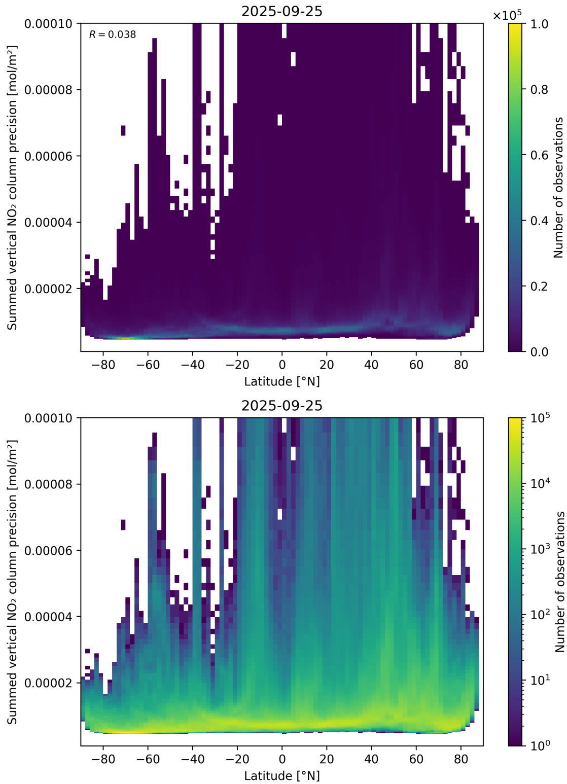
Figure 89: Scatter density plot of “Latitude” against “Summed vertical NO 2 column precision” for 2025-09-25 to 2025-09-26.
