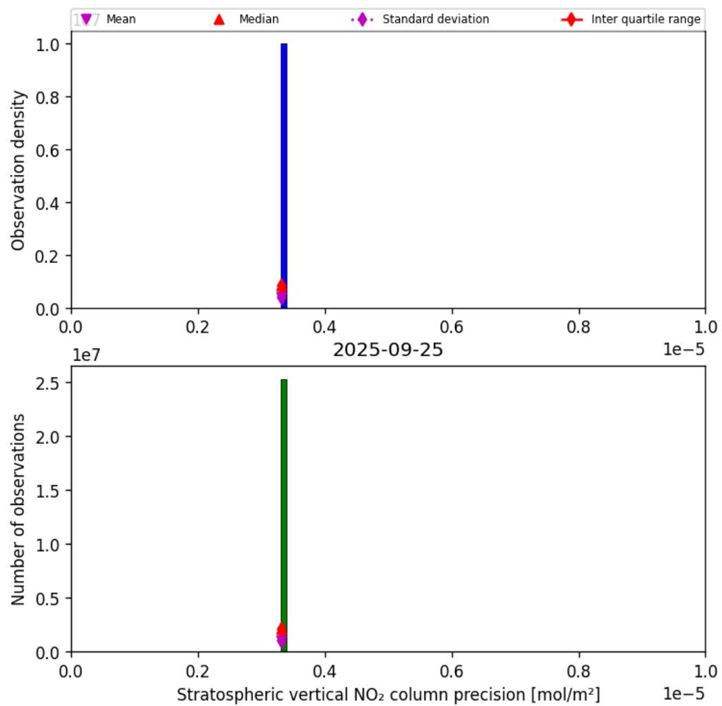
Figure 37: Histogram of “Stratospheric vertical NO 2 column precision” for 2025-09-25 to 2025-09-26
