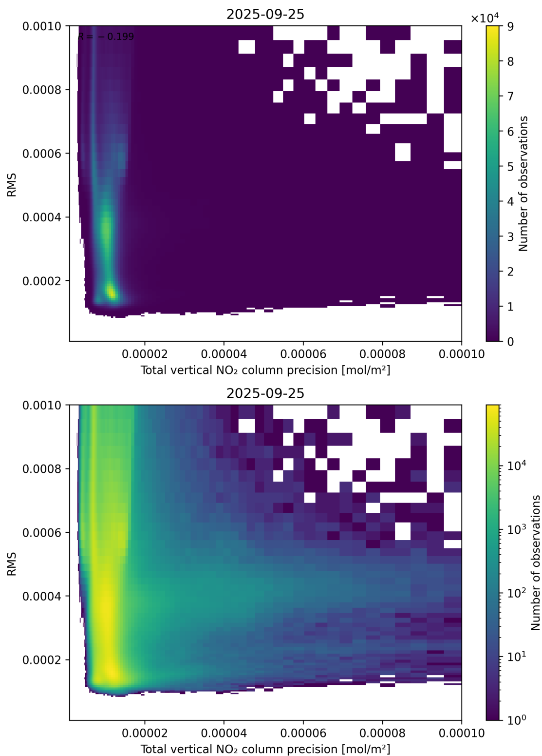
Figure 119: Scatter density plot of “Total vertical NO 2 column precision” against “RMS” for 2025-09-25 to 2025-09-26.
