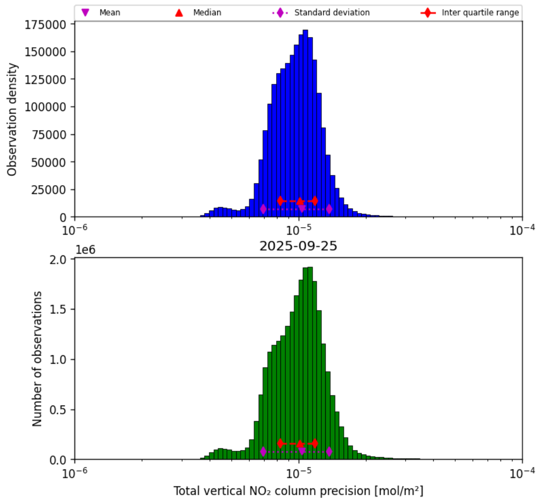
Figure 39: Histogram of "Total vertical NO 2 column precision" for 2025-09-25 to 2025-09-26
