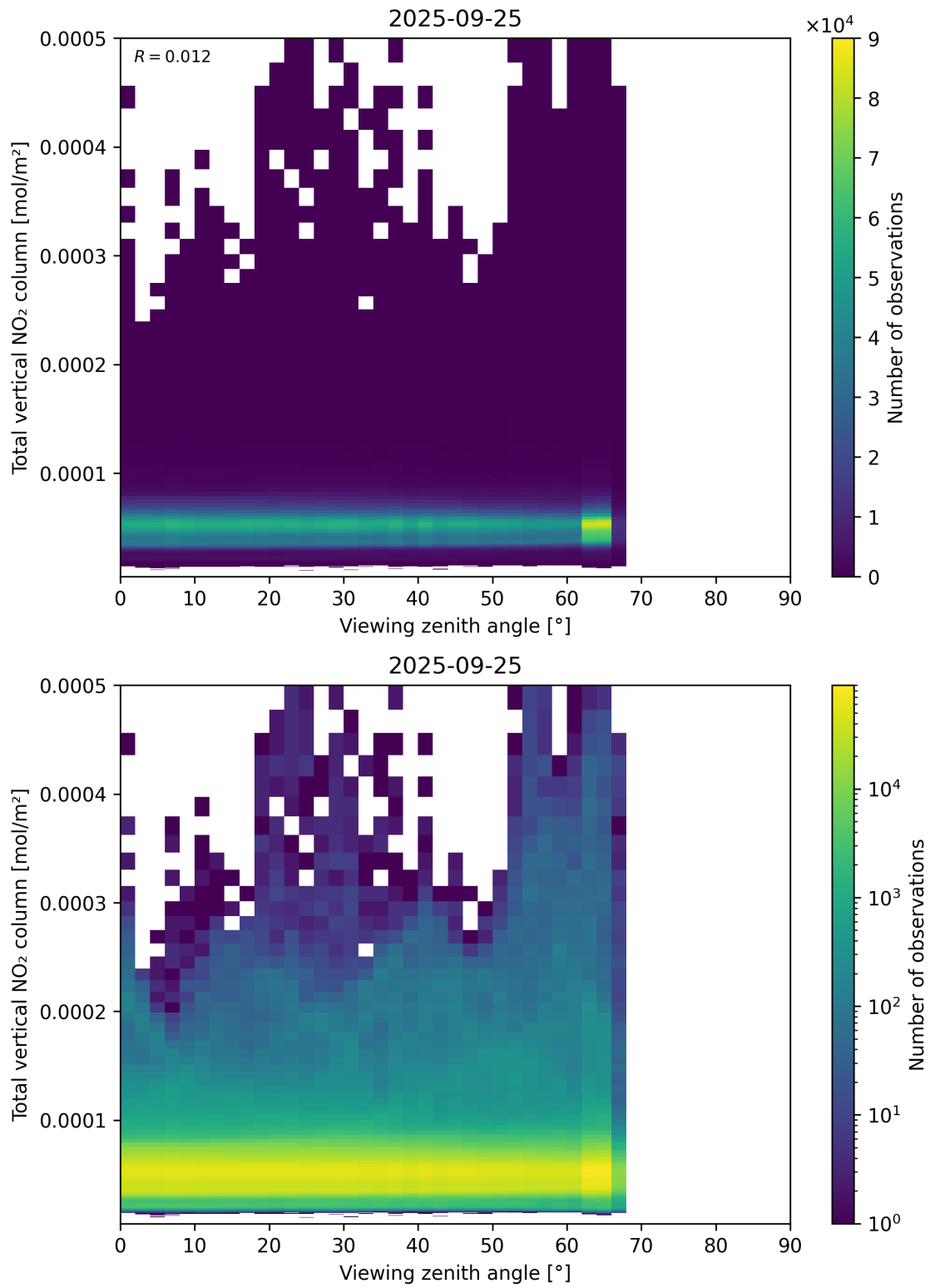
Figure 167: Scatter density plot of “Viewing zenith angle” against “Total vertical NO 2 column” for 2025-09-25 to 2025-09-26.
