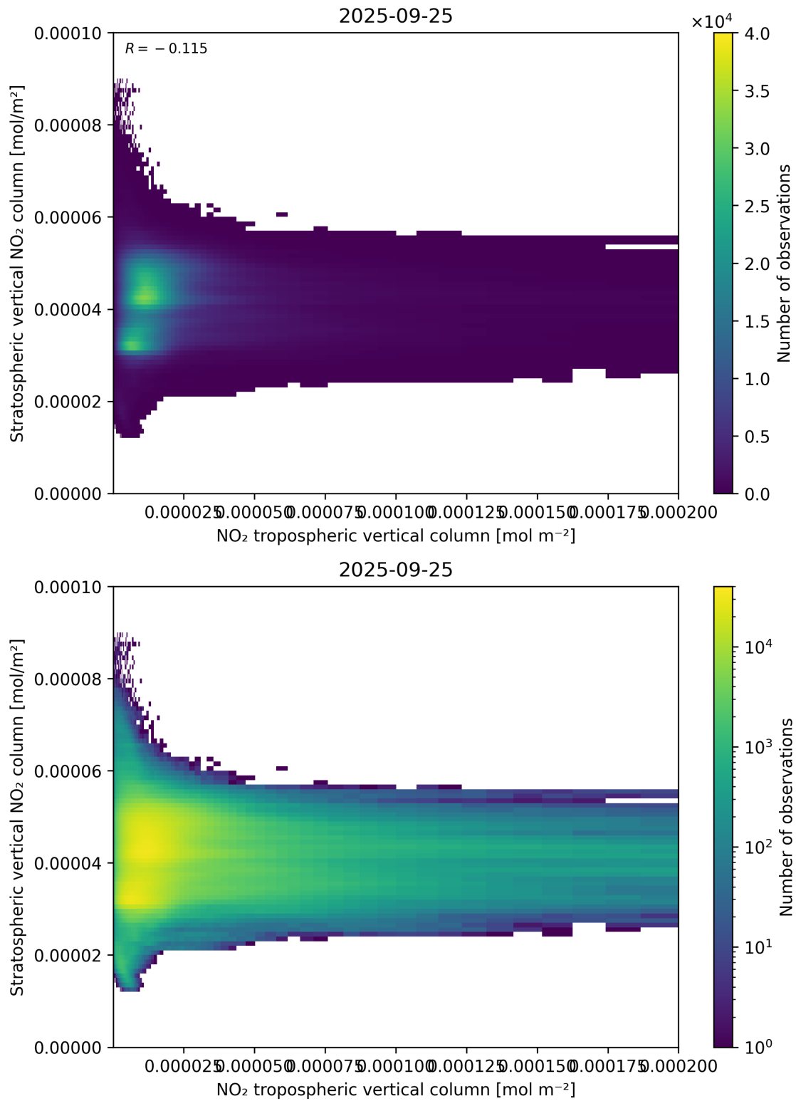
Figure 125: Scatter density plot of “NO 2 tropospheric vertical column” against “Stratospheric vertical NO 2 column” for 2025-09-25 to 2025-09-26.
