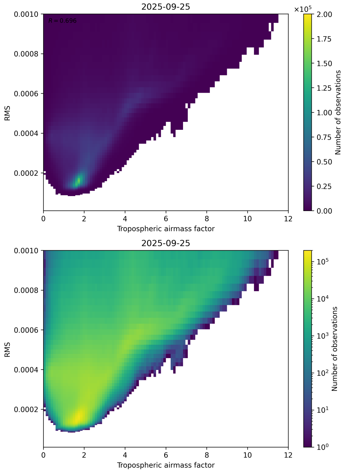
Figure 79: Scatter density plot of “Tropospheric airmass factor” against “RMS” for 2025-09-25 to 2025-09-26.
