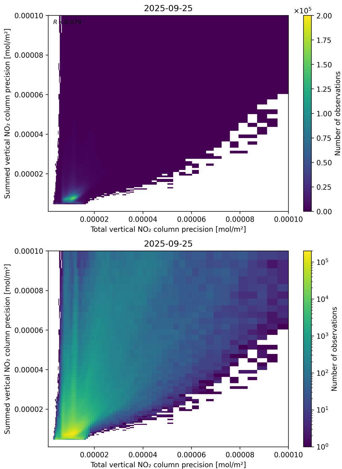
Figure 118: Scatter density plot of “Total vertical NO 2 column precision” against “Summed vertical NO 2 column precision” for 2025-09-25 to 2025-09-26.
