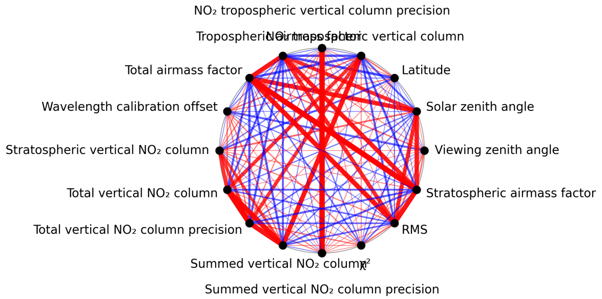
Figure 1: Map of correlation graph for 2025-09-25 to 2025-09-26.
