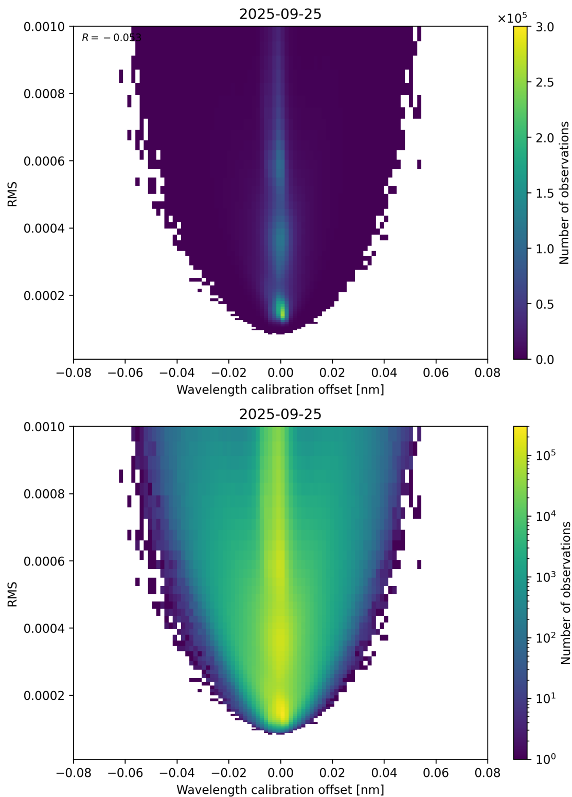
Figure 181: Scatter density plot of “Wavelength calibration offset” against “RMS” for 2025-09-25 to 2025-09-26.
