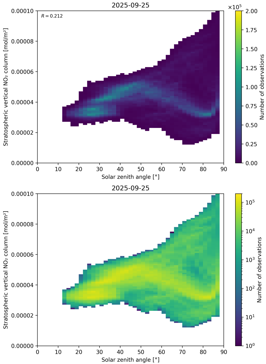
Figure 150: Scatter density plot of “Solar zenith angle” against “Stratospheric vertical NO 2 column” for 2025-09-25 to 2025-09-26.
