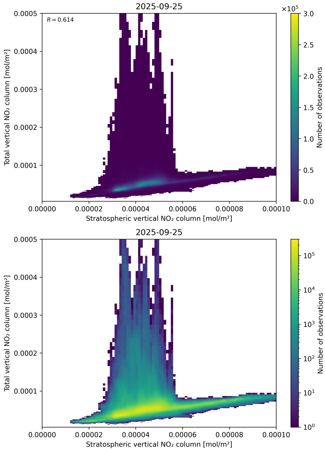
Figure 100: Scatter density plot of “Stratospheric vertical NO 2 column” against “Total vertical NO 2 column” for 2025-09-25 to 2025-09-26.
