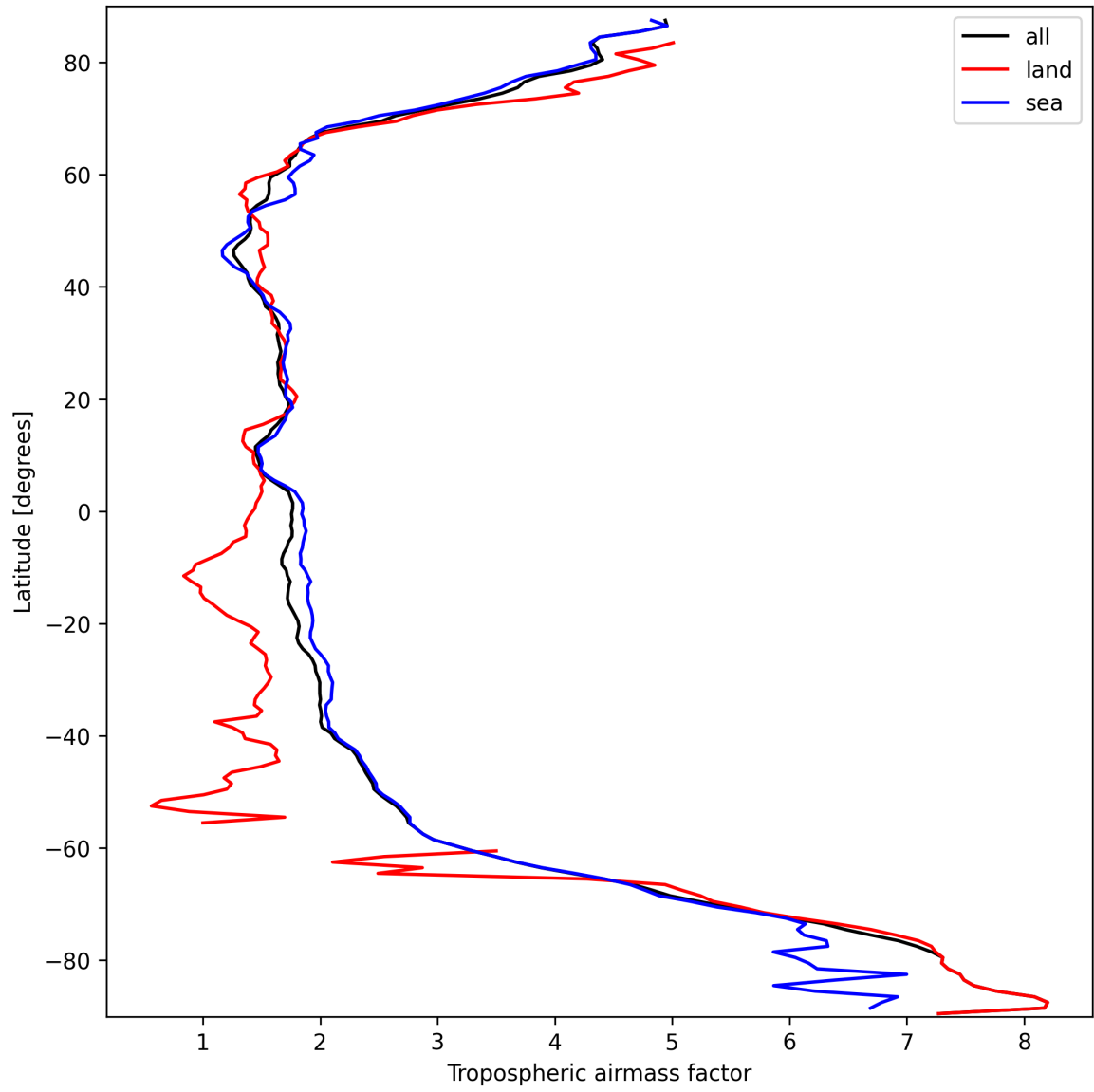
Figure 14: Zonal average of “Tropospheric airmass factor” for 2025-09-25 to 2025-09-26.
