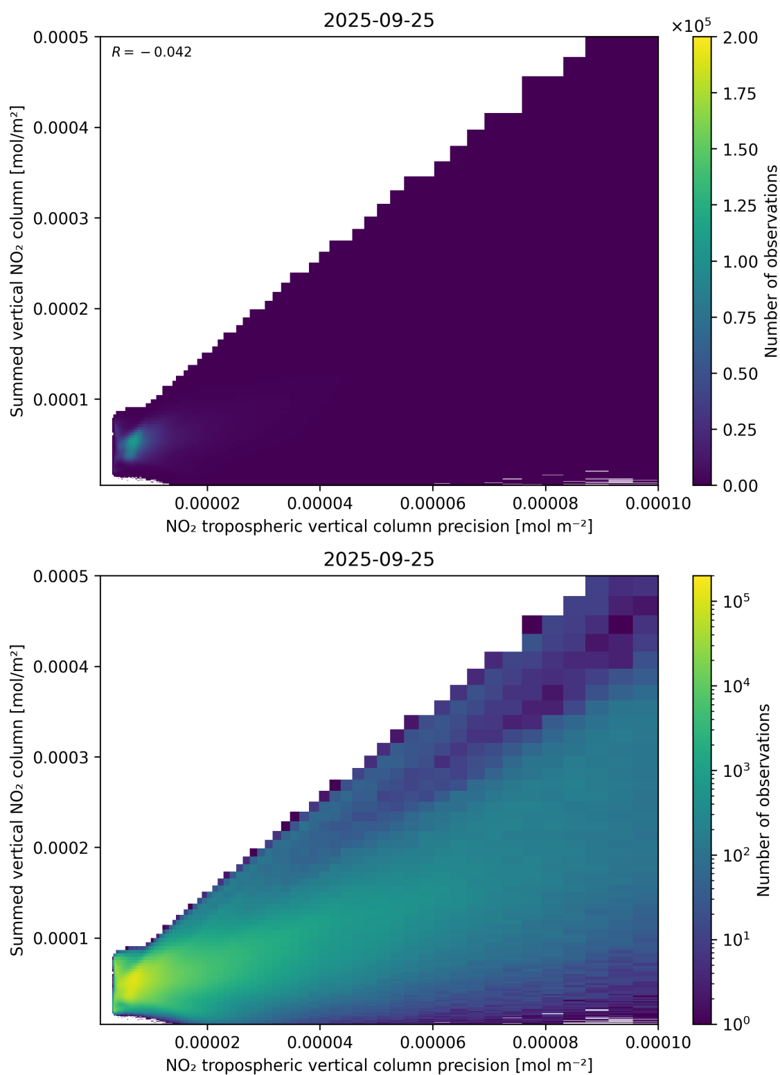
Figure 136: Scatter density plot of “NO 2 tropospheric vertical column precision” against “Summed vertical NO 2 column” for 2025-09-25 to 2025-09-26.
