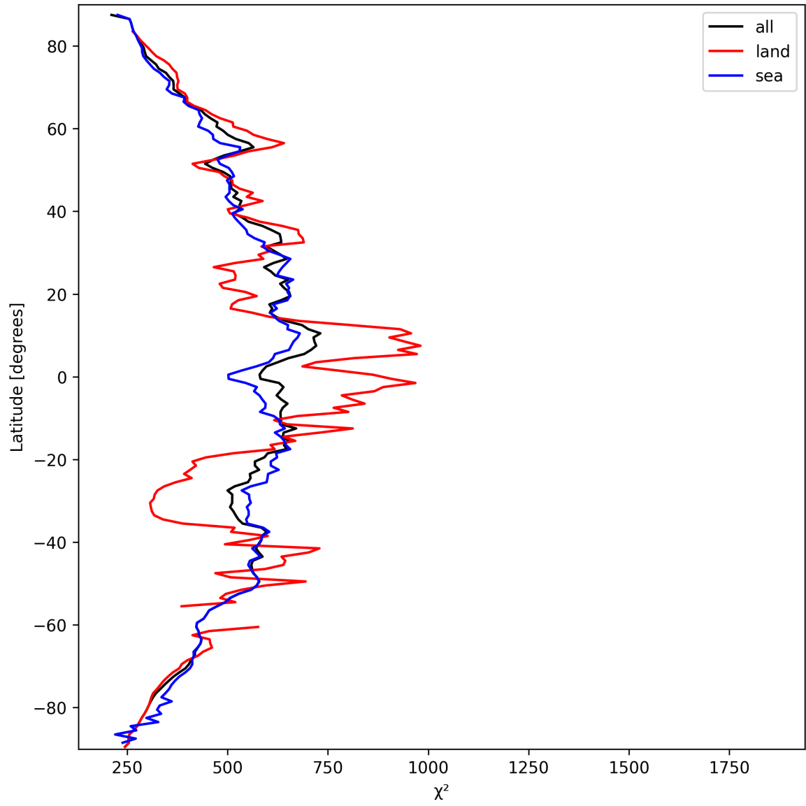
Figure 25: Zonal average of “ \chi^2 ” for 2025-09-25 to 2025-09-26.
