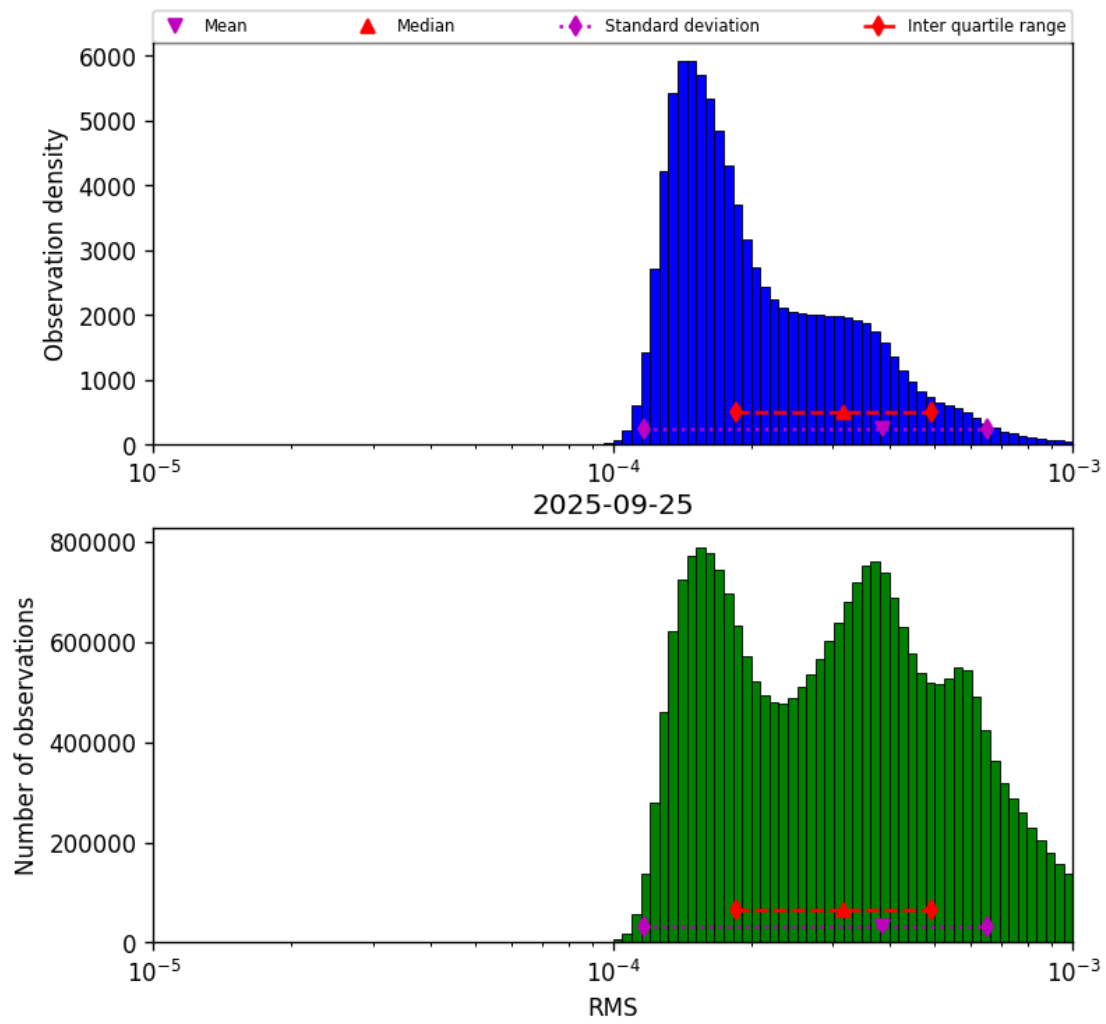
Figure 43: Histogram of “RMS” for 2025-09-25 to 2025-09-26
