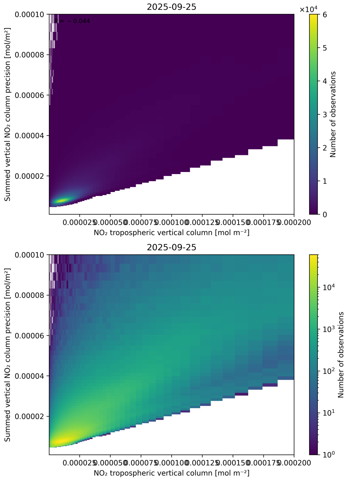
Figure 127: Scatter density plot of “NO 2 tropospheric vertical column” against “Summed vertical NO 2 column precision” for 2025-09-25 to 2025-09-26.
