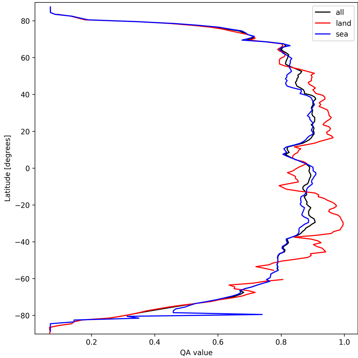
Figure 11: Zonal average of “QA value” for 2025-09-25 to 2025-09-26.
