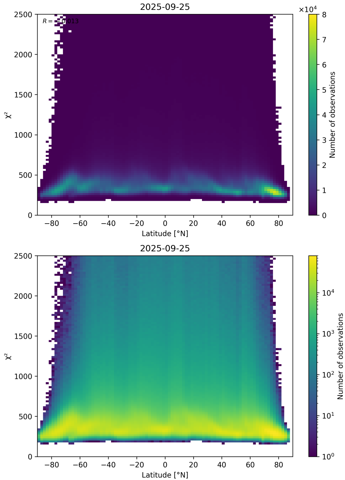
Figure 86: Scatter density plot of “Latitude” against “ \chi^2 ” for 2025-09-25 to 2025-09-26.
