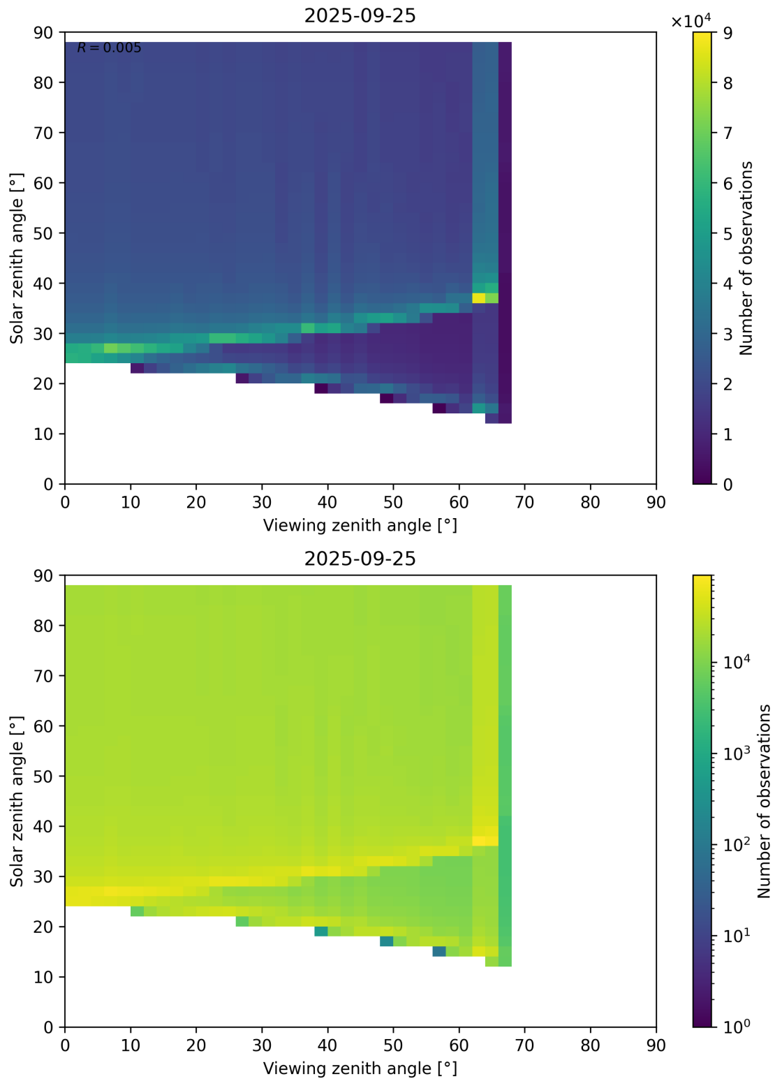
Figure 172: Scatter density plot of “Viewing zenith angle” against “Solar zenith angle” for 2025-09-25 to 2025-09-26.
