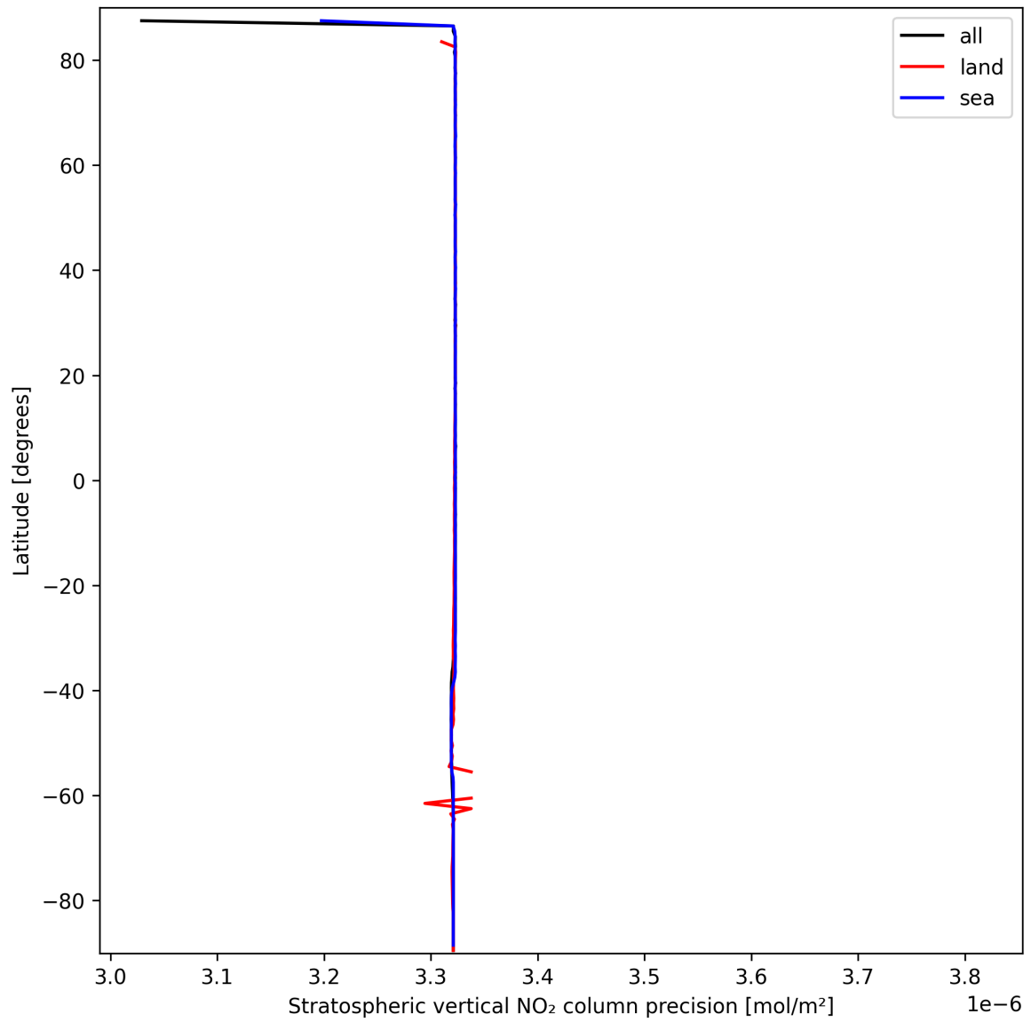
Figure 20: Zonal average of "Stratospheric vertical NO 2 column precision" for 2025-09-25 to 2025-09-26.
