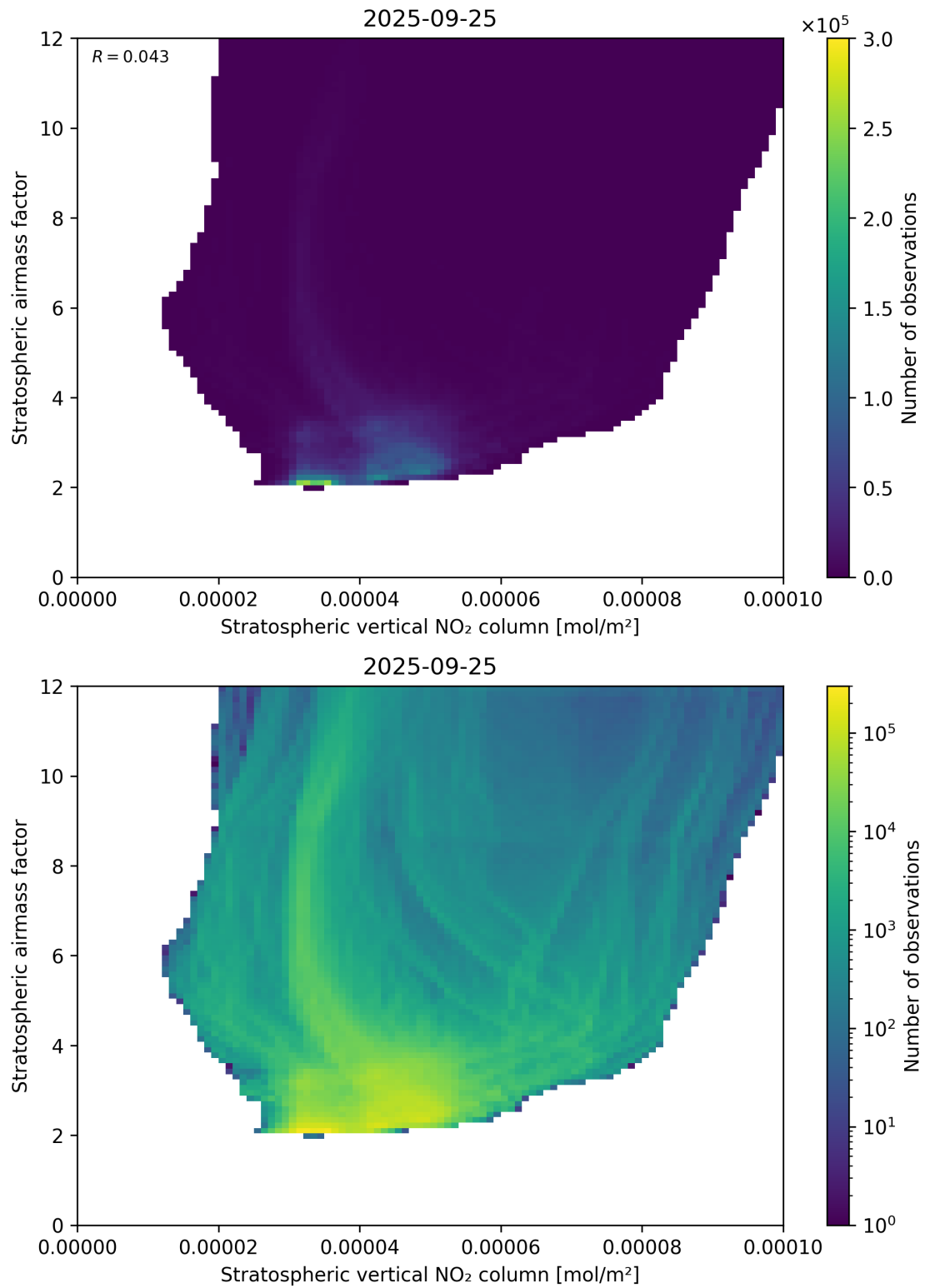
Figure 96: Scatter density plot of “Stratospheric vertical NO 2 column” against “Stratospheric airmass factor” for 2025-09-25 to 2025-09-26.
