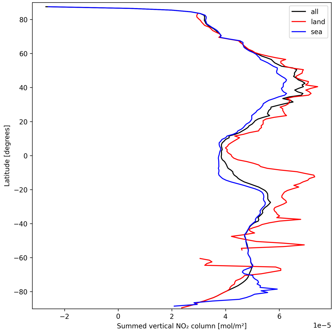
Figure 23: Zonal average of “Summed vertical NO 2 column” for 2025-09-25 to 2025-09-26.
