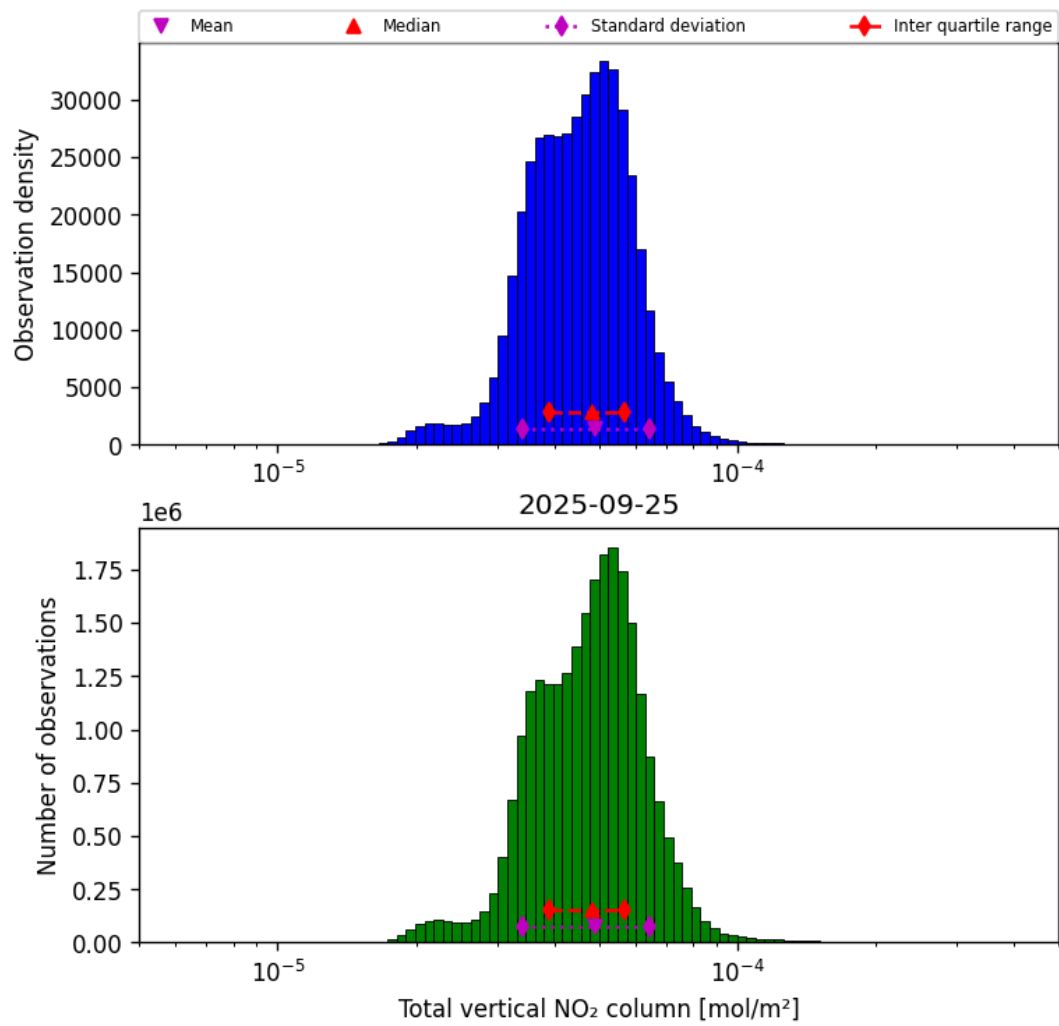
Figure 38: Histogram of “Total vertical NO 2 column” for 2025-09-25 to 2025-09-26
