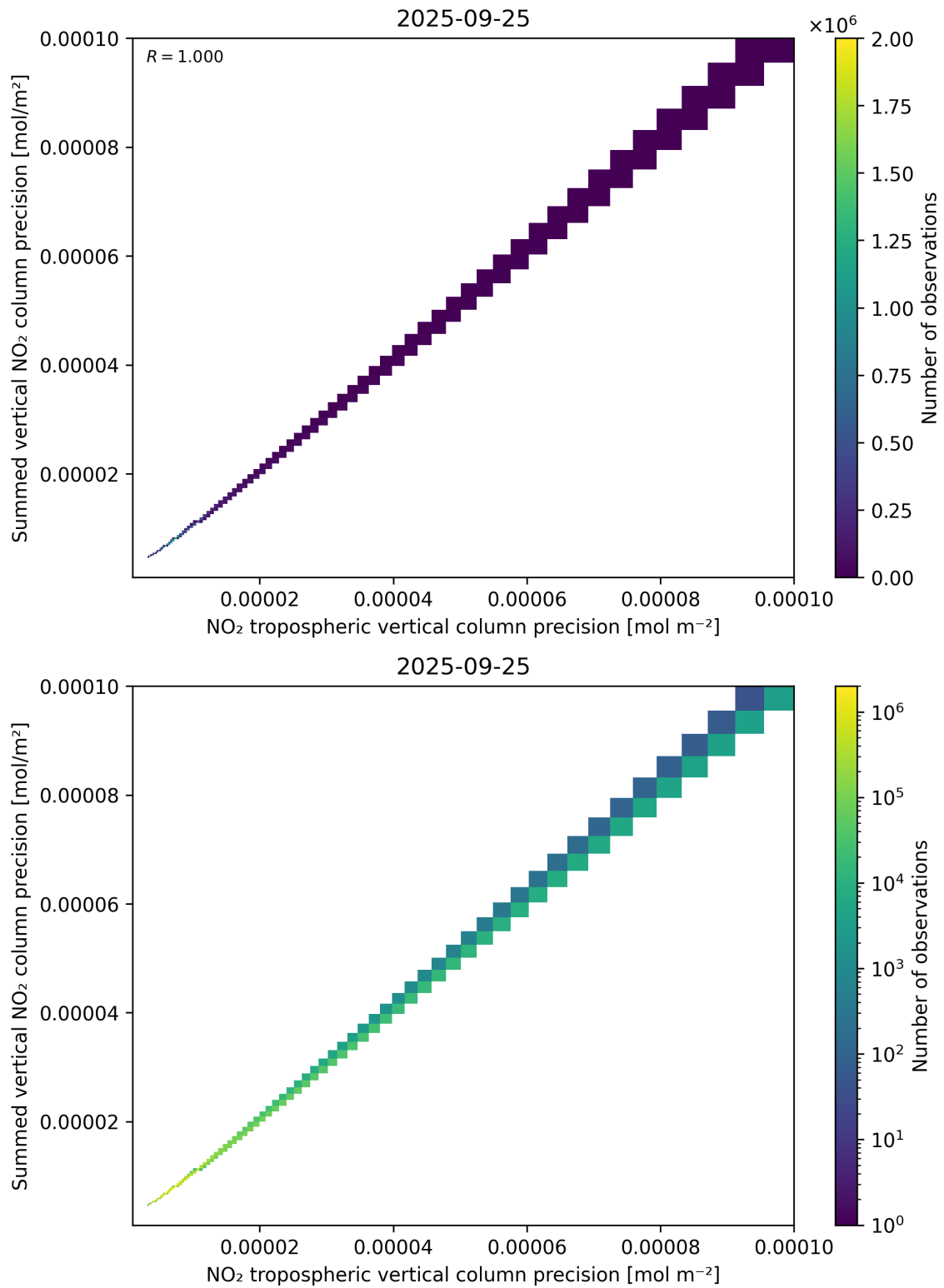
Figure 137: Scatter density plot of “NO 2 tropospheric vertical column precision” against “Summed vertical NO 2 column precision” for 2025-09-25 to 2025-09-26.
