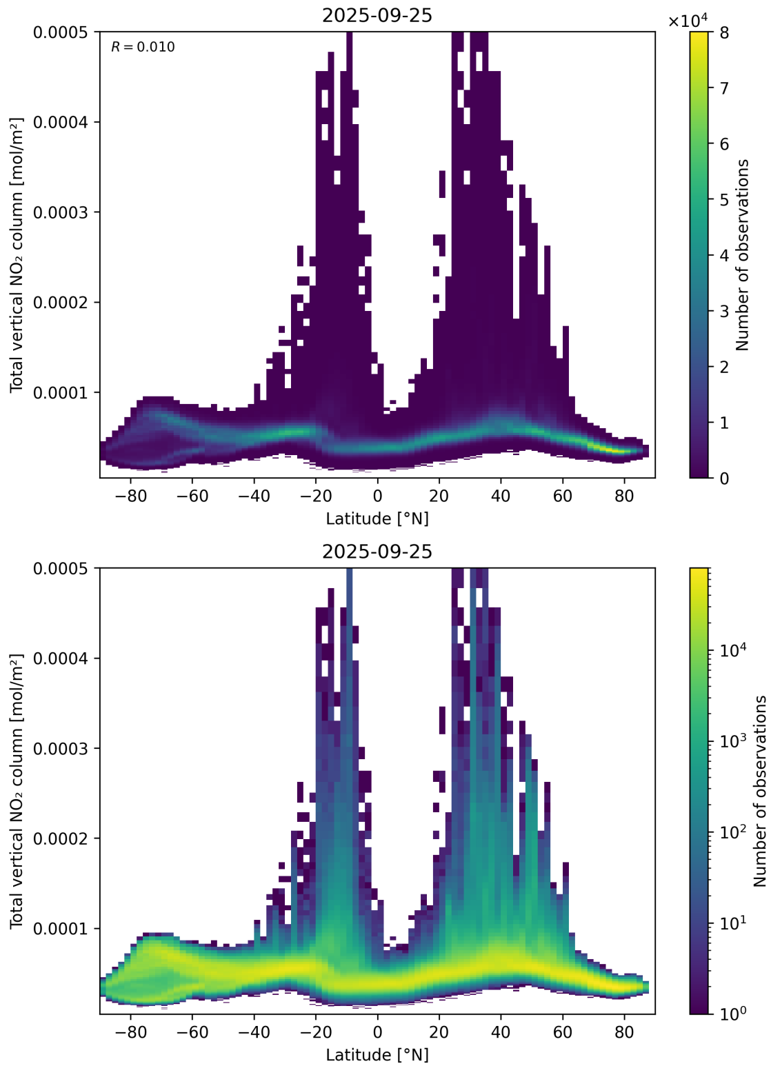
Figure 90: Scatter density plot of “Latitude” against “Total vertical NO 2 column” for 2025-09-25 to 2025-09-26.
