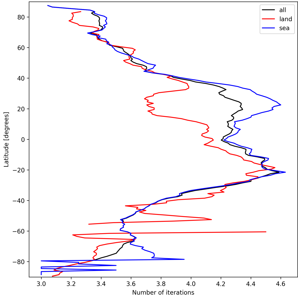
Figure 17: Zonal average of “Number of iterations” for 2025-09-25 to 2025-09-26.
