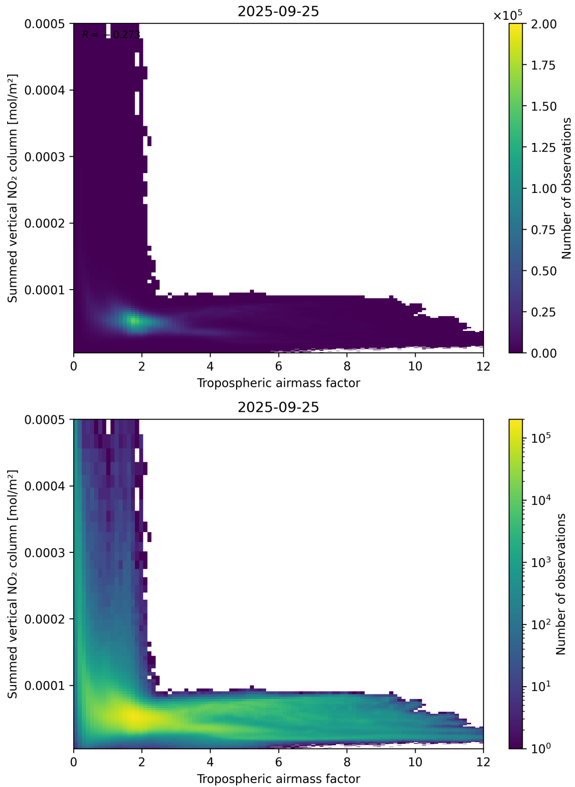
Figure 75: Scatter density plot of “Tropospheric air mass factor” against “Summed vertical NO 2 column” for 2025-09-25 to 2025-09-26.
