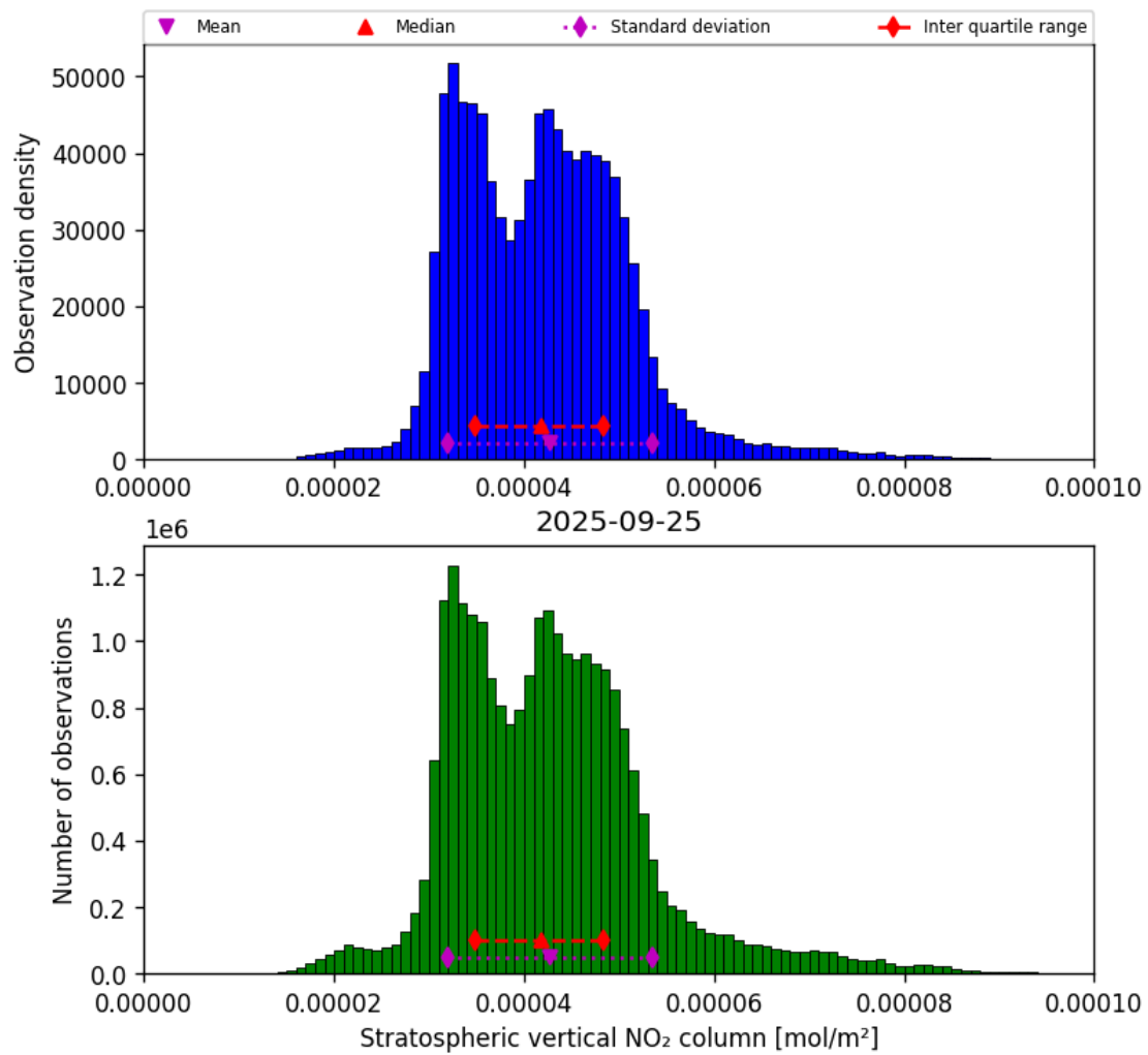
Figure 36: Histogram of “Stratospheric vertical NO 2 column” for 2025-09-25 to 2025-09-26
