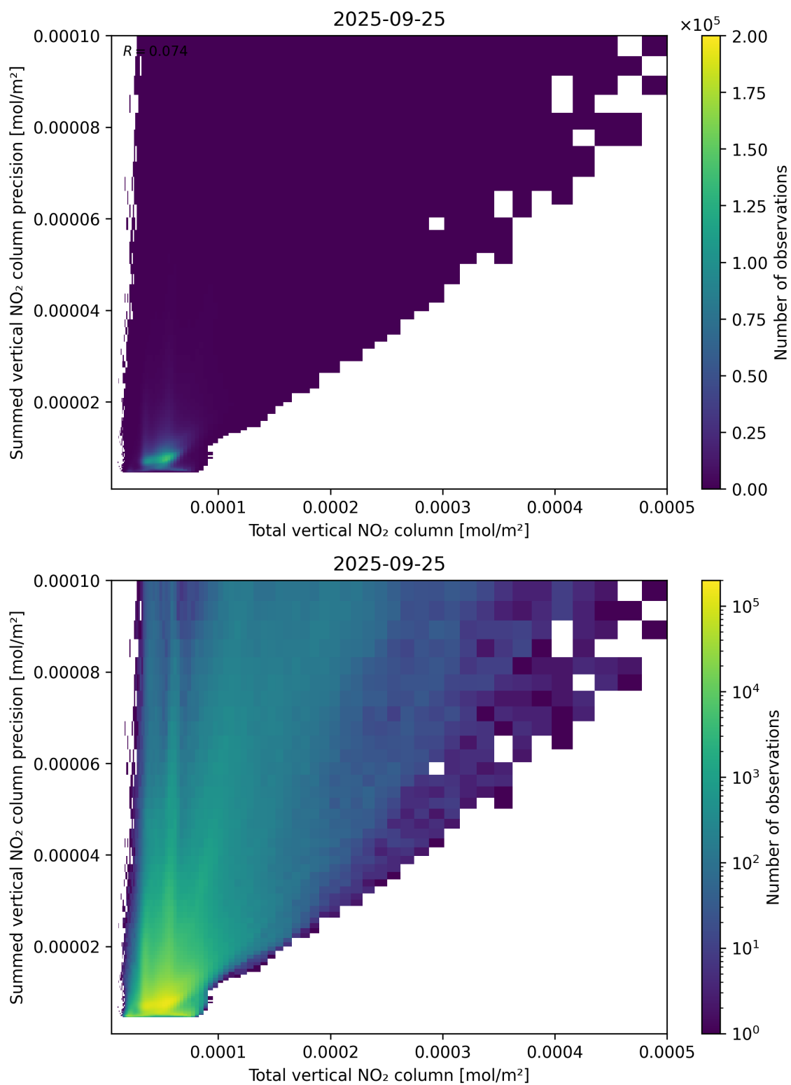
Figure 113: Scatter density plot of “Total vertical NO 2 column” against “Summed vertical NO 2 column precision” for 2025-09-25 to 2025-09-26.
