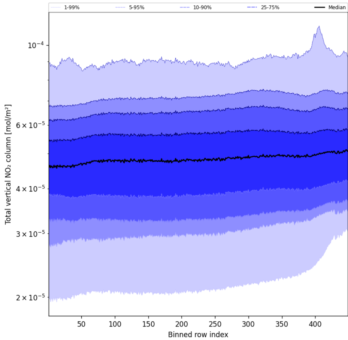
Figure 55: Along track statistics of “Total vertical NO 2 column” for 2025-09-25 to 2025-09-26
