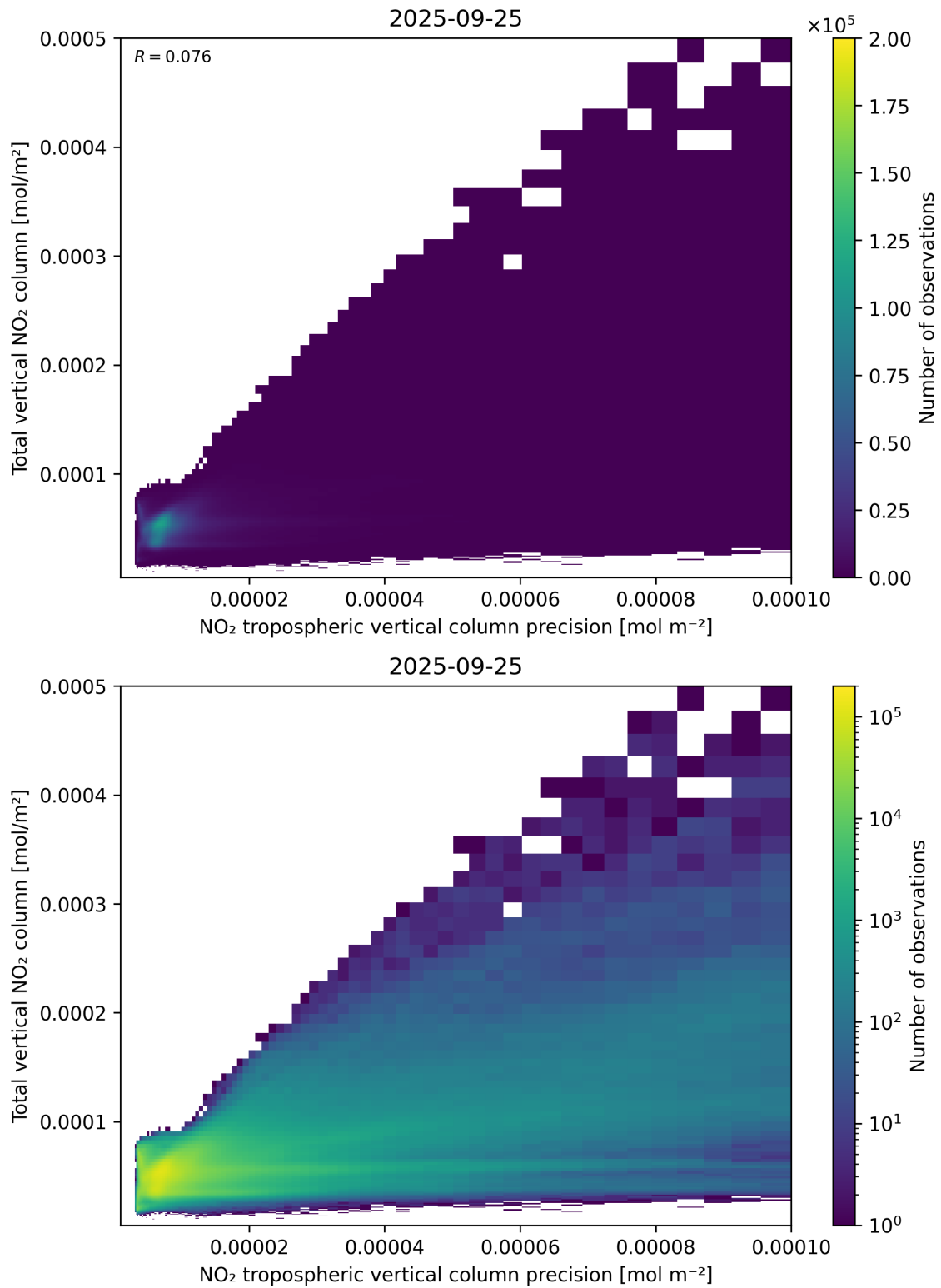
Figure 138: Scatter density plot of “NO 2 tropospheric vertical column precision” against “Total vertical NO 2 column” for 2025-09-25 to 2025-09-26.
