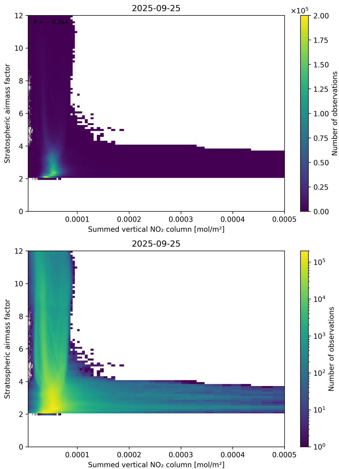
Figure 103: Scatter density plot of “Summed vertical NO 2 column” against “Stratospheric airmass factor” for 2025-09-25 to 2025-09-26.
