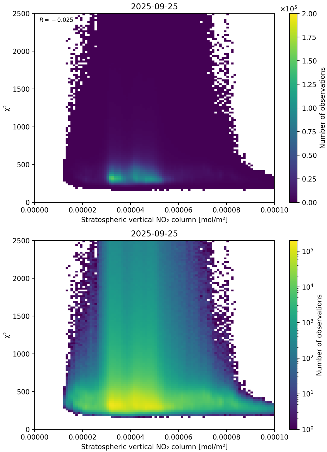
Figure 97: Scatter density plot of “Stratospheric vertical NO 2 column” against “ \chi^2 ” for 2025-09-25 to 2025-09-26.
