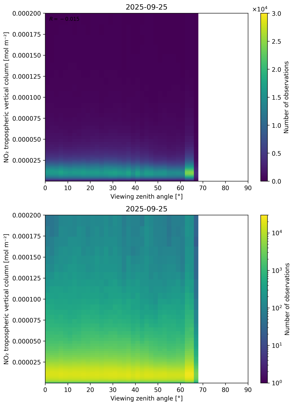
Figure 169: Scatter density plot of “Viewing zenith angle” against “NO 2 tropospheric vertical column” for 2025-09-25 to 2025-09-26.
