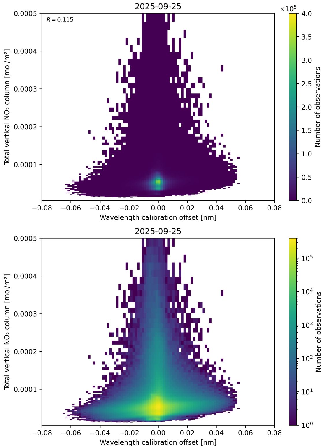
Figure 179: Scatter density plot of “Wavelength calibration offset” against “Total vertical NO 2 column” for 2025-09-25 to 2025-09-26.
