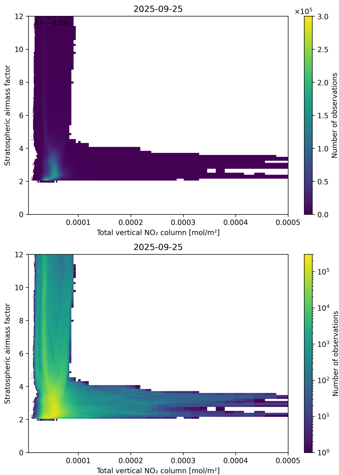
Figure 110: Scatter density plot of “Total vertical NO 2 column” against “Stratospheric airmass factor” for 2025-09-25 to 2025-09-26.
