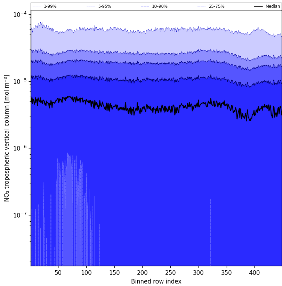
Figure 46: Along track statistics of “NO 2 tropospheric vertical column” for 2025-09-25 to 2025-09-26
