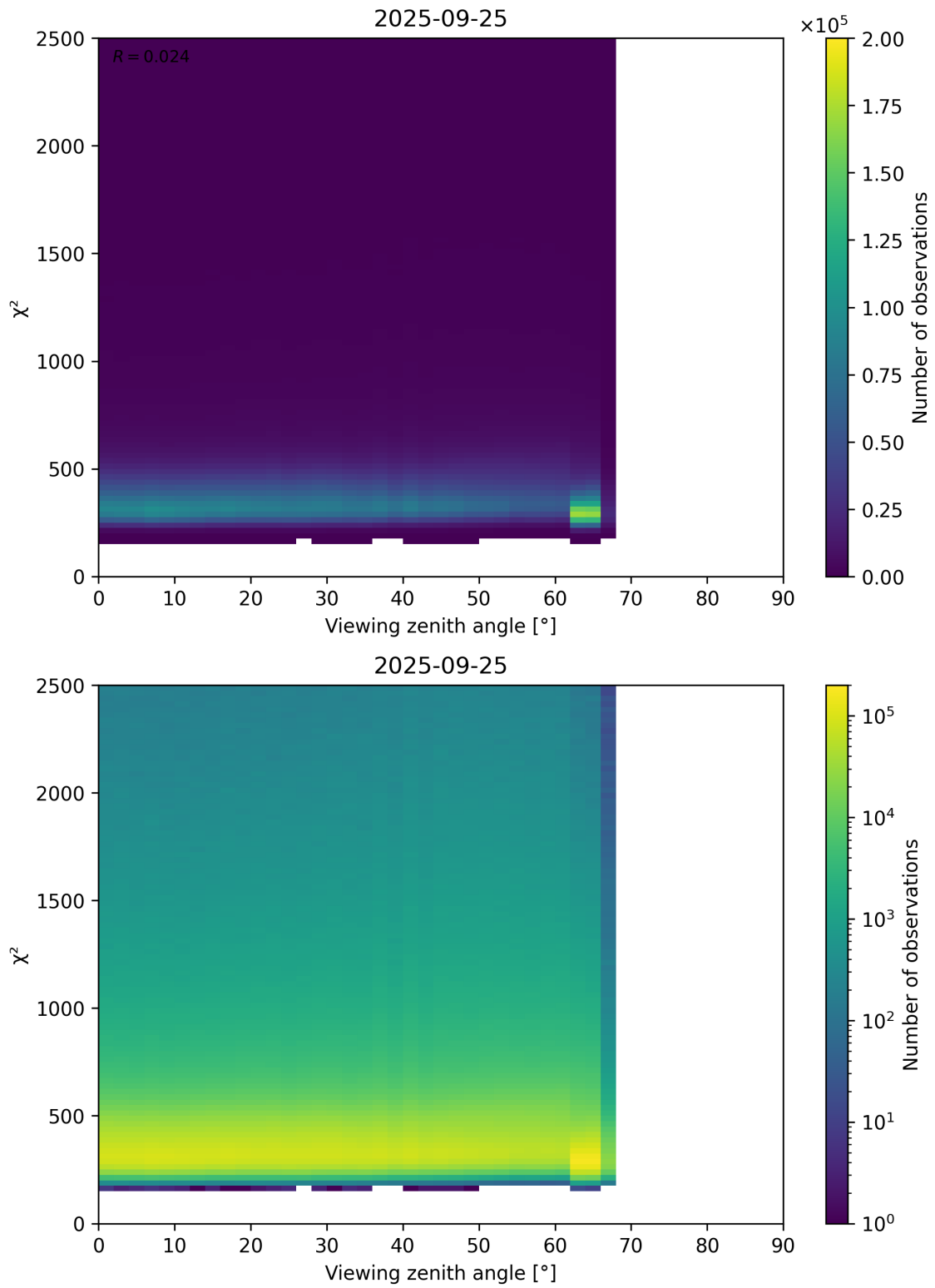
Figure 162: Scatter density plot of “Viewing zenith angle” against “ \chi^2 ” for 2025-09-25 to 2025-09-26.
