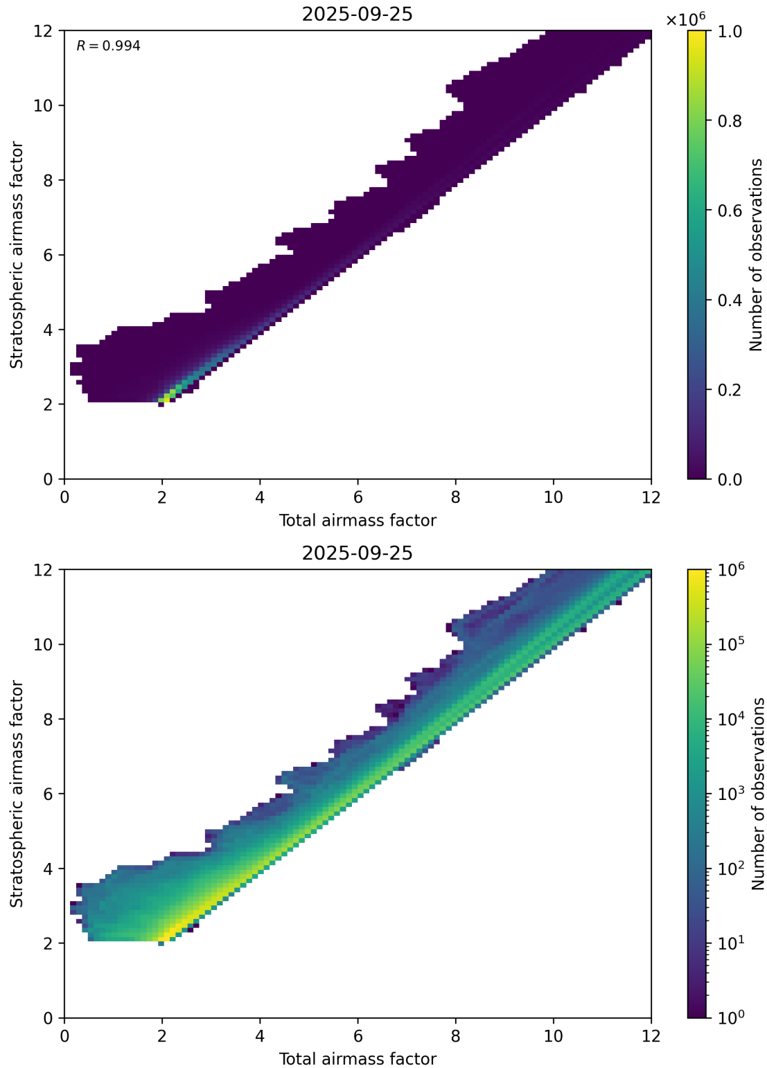
Figure 62: Scatter density plot of “Total airmass factor” against “Stratospheric airmass factor” for 2025-09-25 to 2025-09-26.
