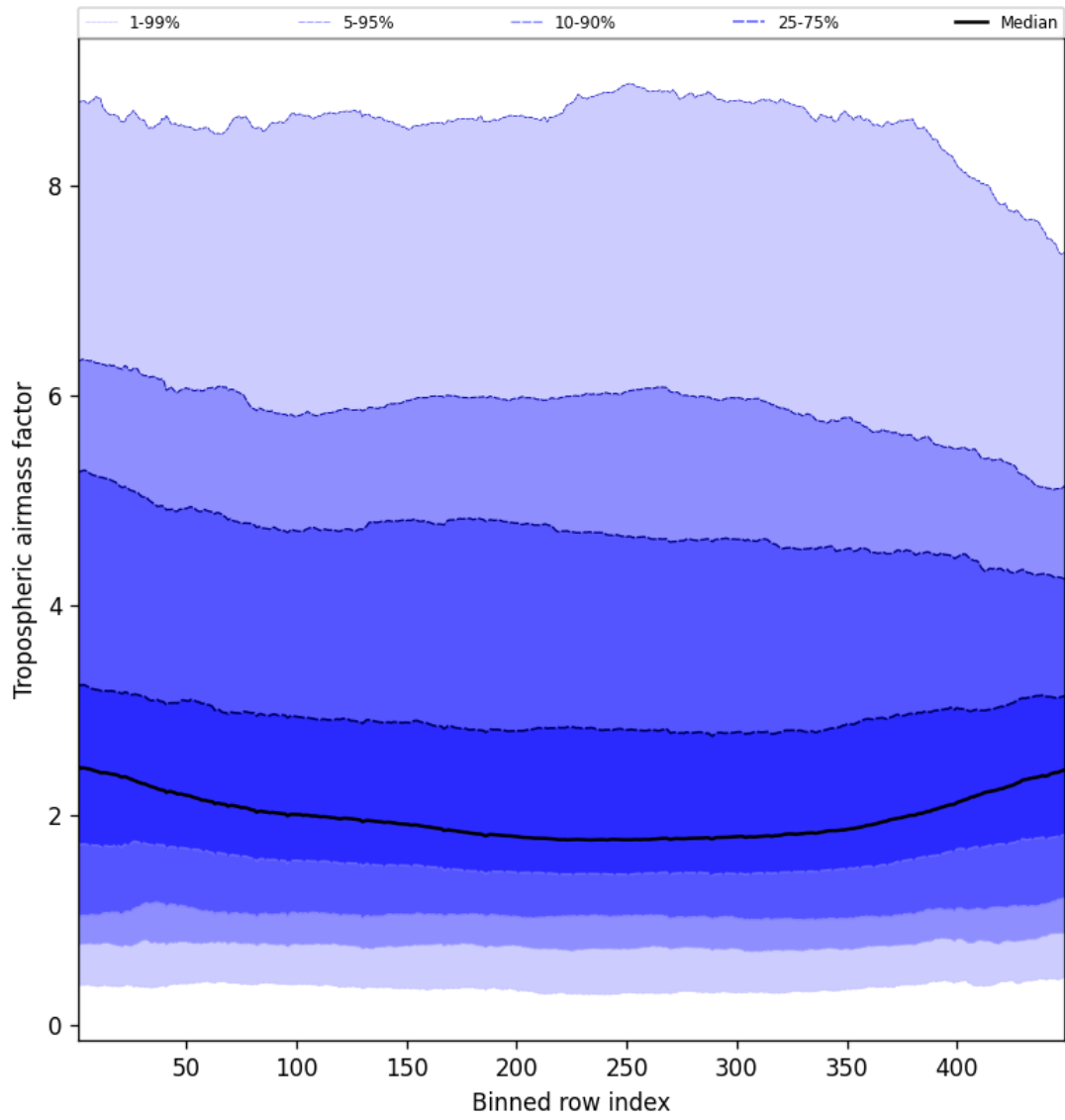
Figure 48: Along track statistics of “Tropospheric air mass factor” for 2025-09-25 to 2025-09-26
