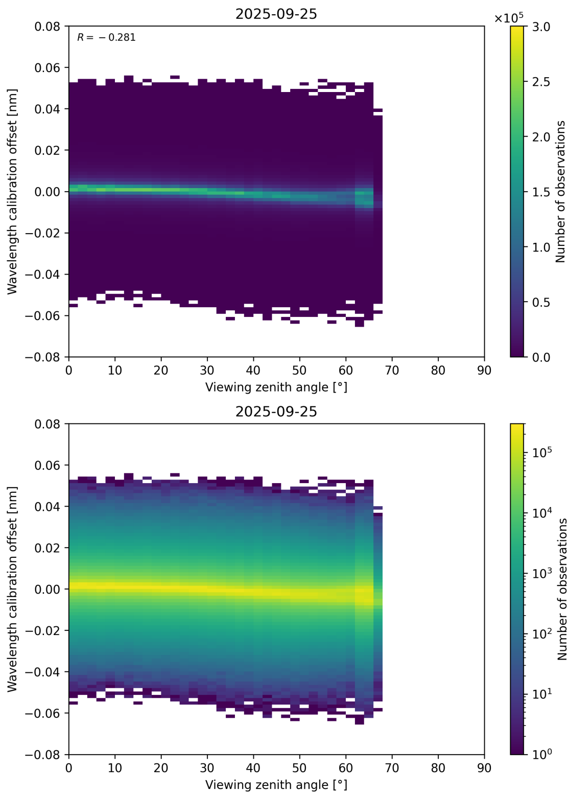
Figure 173: Scatter density plot of “Viewing zenith angle” against “Wavelength calibration offset” for 2025-09-25 to 2025-09-26.
