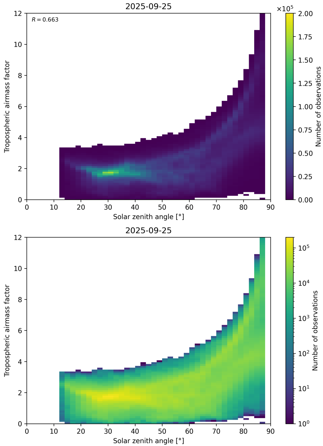
Figure 147: Scatter density plot of “Solar zenith angle” against “Tropospheric airmass factor” for 2025-09-25 to 2025-09-26.
