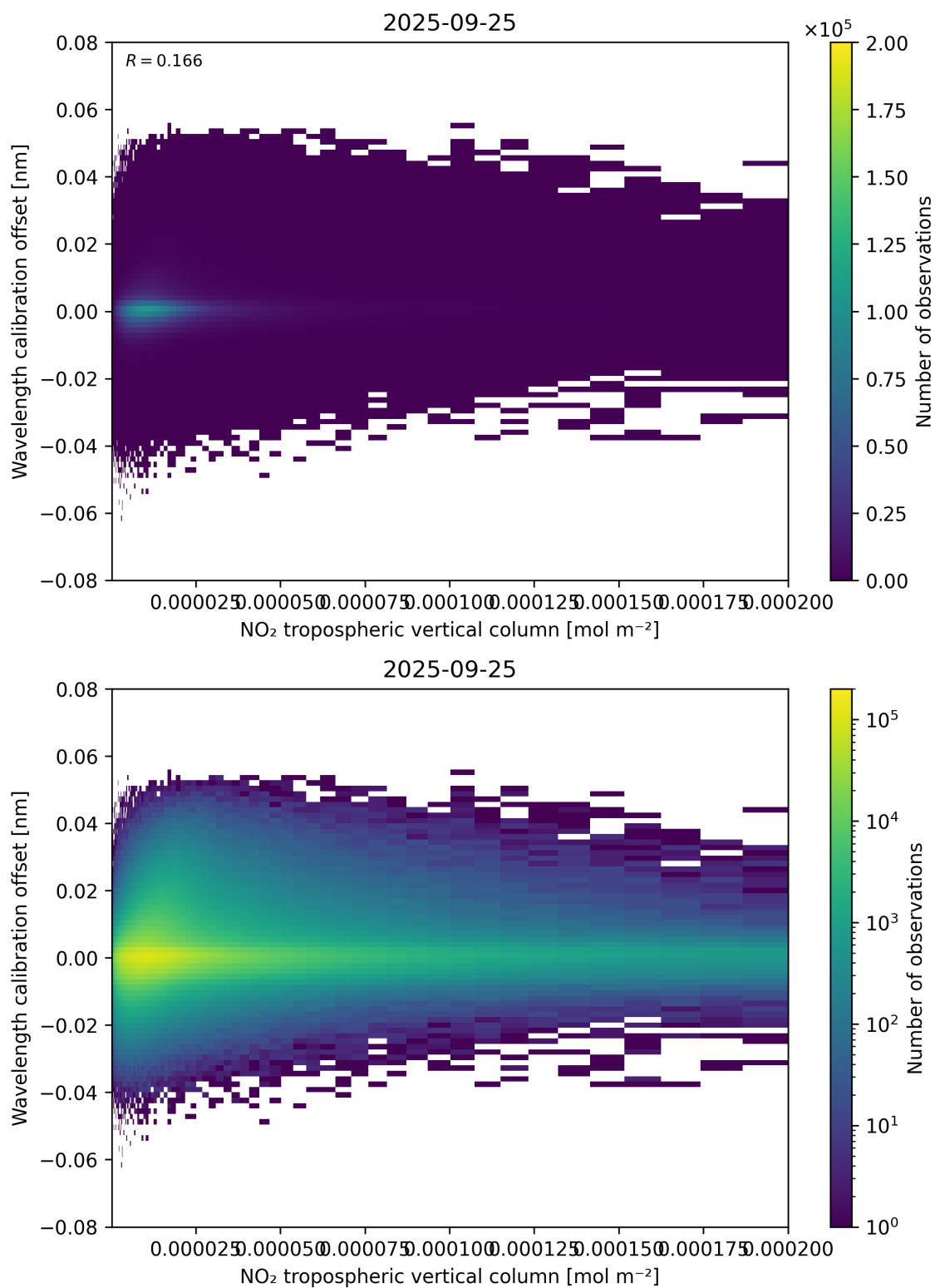
Figure 143: Scatter density plot of “NO 2 tropospheric vertical column” against “Wavelength calibration offset” for 2025-09-25 to 2025-09-26.
