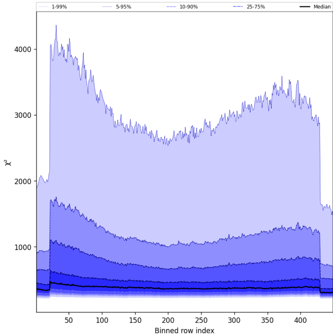
Figure 59: Along track statistics of “ \chi^2 ” for 2025-09-25 to 2025-09-26
