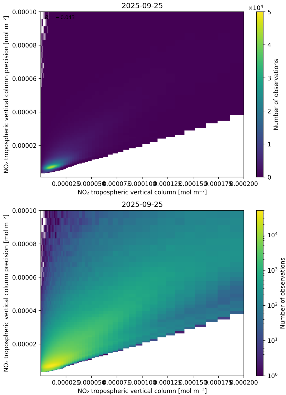
Figure 130: Scatter density plot of “NO 2 tropospheric vertical column” against “NO 2 tropospheric vertical column precision” for 2025-09-25 to 2025-09-26.
