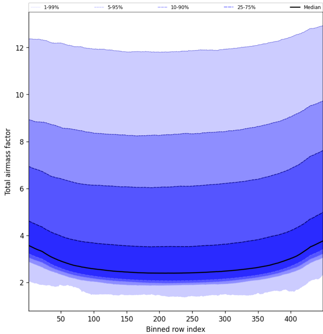
Figure 49: Along track statistics of “Total airmass factor” for 2025-09-25 to 2025-09-26
