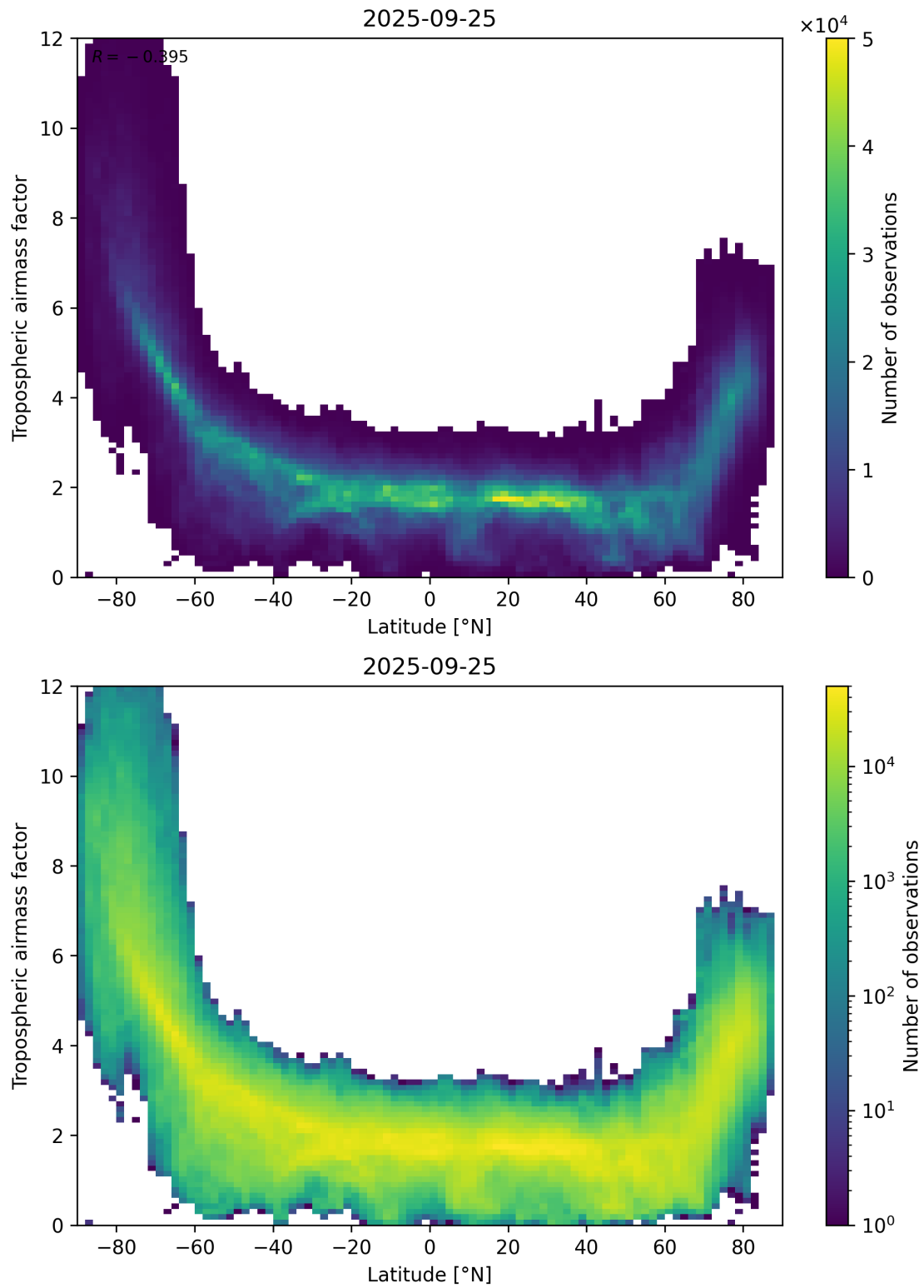
Figure 85: Scatter density plot of “Latitude” against “Tropospheric airmass factor” for 2025-09-25 to 2025-09-26.
