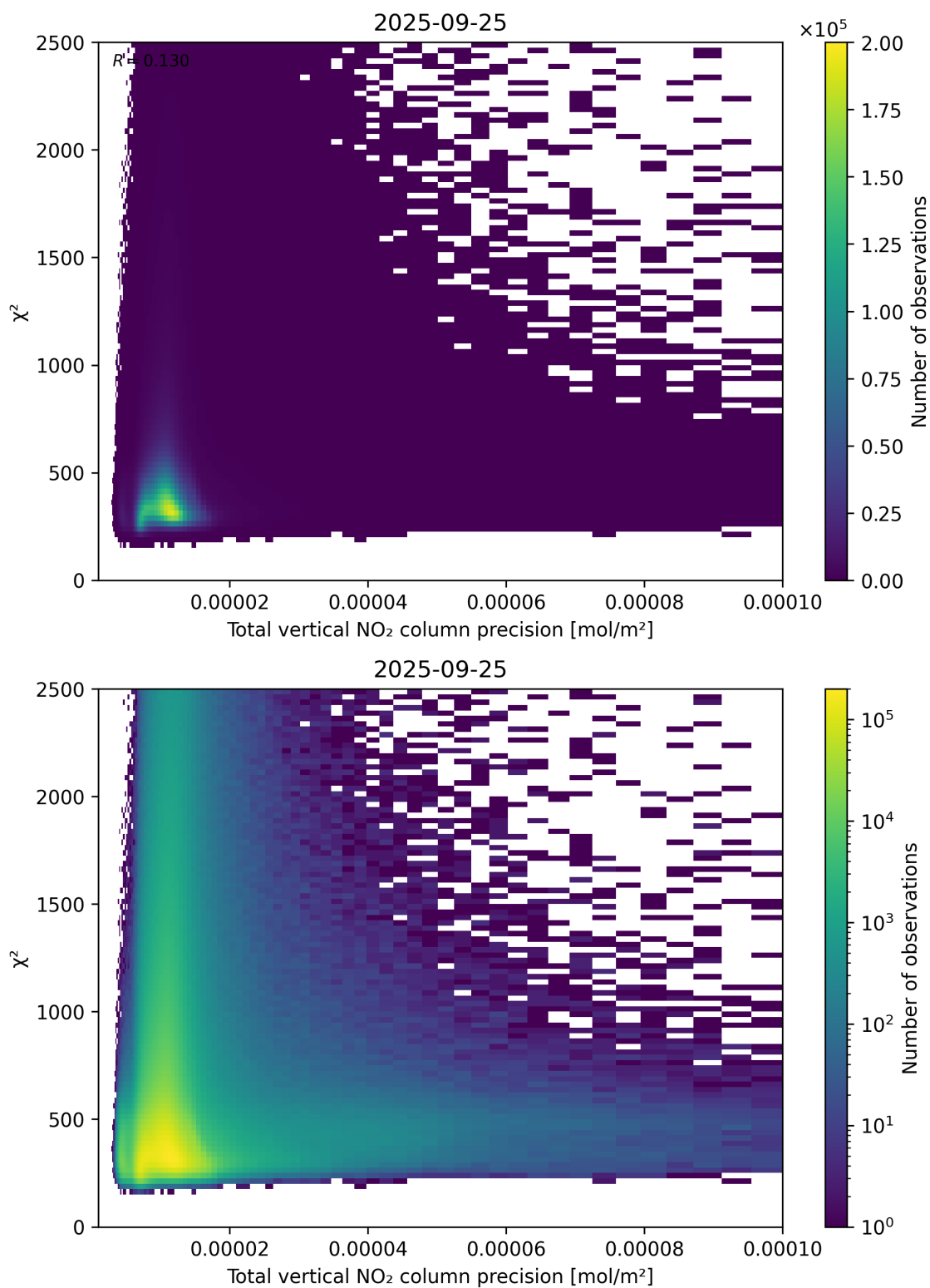
Figure 116: Scatter density plot of “Total vertical NO 2 column precision” against “ \chi^2 ” for 2025-09-25 to 2025-09-26.
