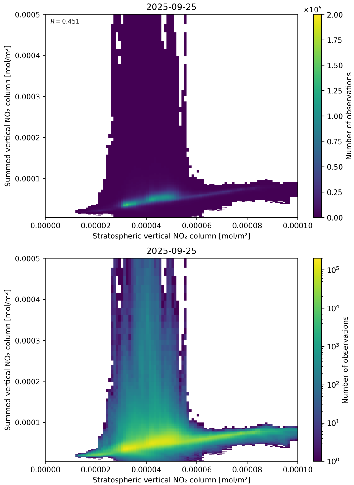
Figure 98: Scatter density plot of “Stratospheric vertical NO 2 column” against “Summed vertical NO 2 column” for 2025-09-25 to 2025-09-26.
