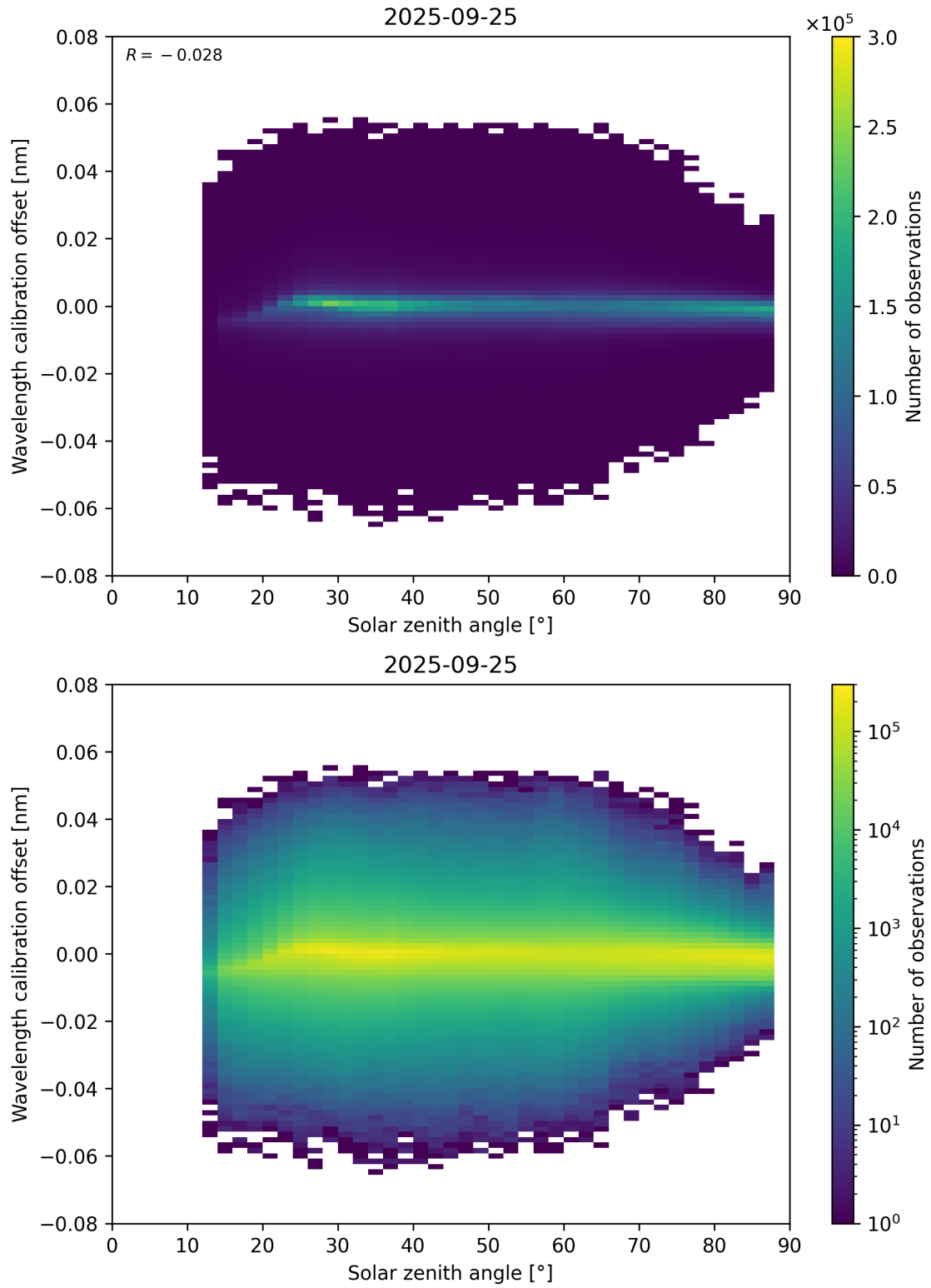
Figure 158: Scatter density plot of “Solar zenith angle” against “Wavelength calibration offset” for 2025-09-25 to 2025-09-26.
