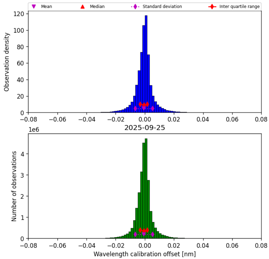
Figure 35: Histogram of “Wavelength calibration offset” for 2025-09-25 to 2025-09-26
