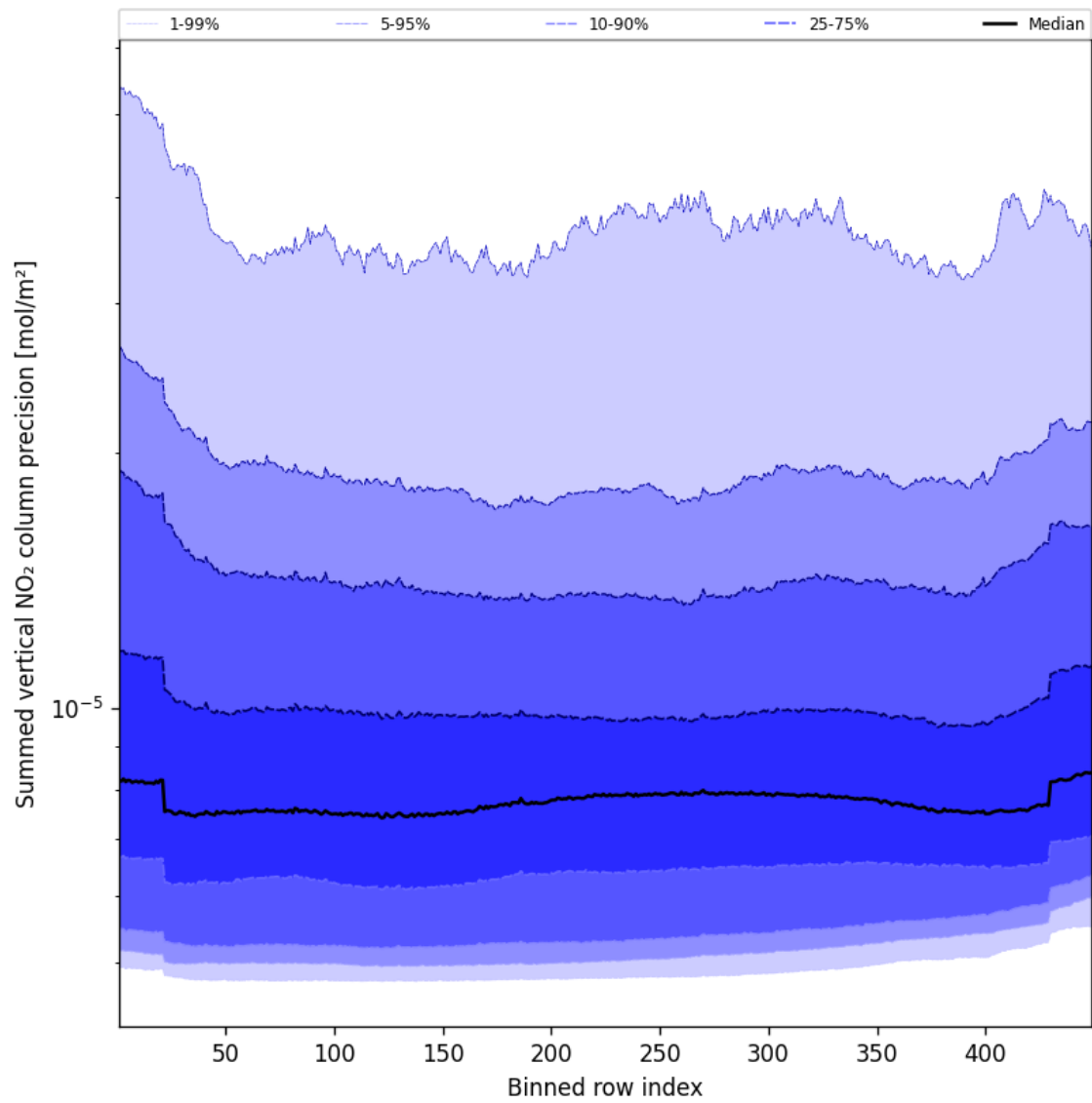
Figure 58: Along track statistics of “Summed vertical NO 2 column precision” for 2025-09-25 to 2025-09-26
