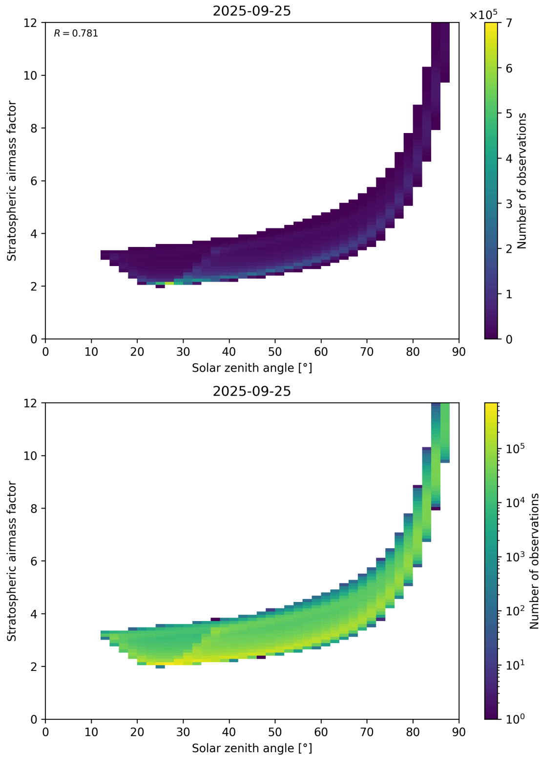
Figure 145: Scatter density plot of “Solar zenith angle” against “Stratospheric airmass factor” for 2025-09-25 to 2025-09-26.
