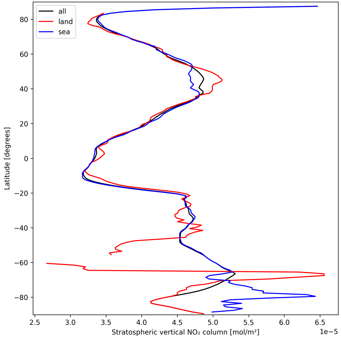
Figure 19: Zonal average of “Stratospheric vertical NO 2 column” for 2025-09-25 to 2025-09-26.
