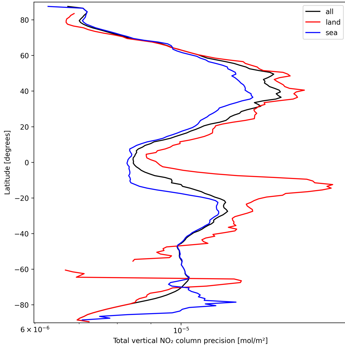
Figure 22: Zonal average of “Total vertical NO 2 column precision” for 2025-09-25 to 2025-09-26.
