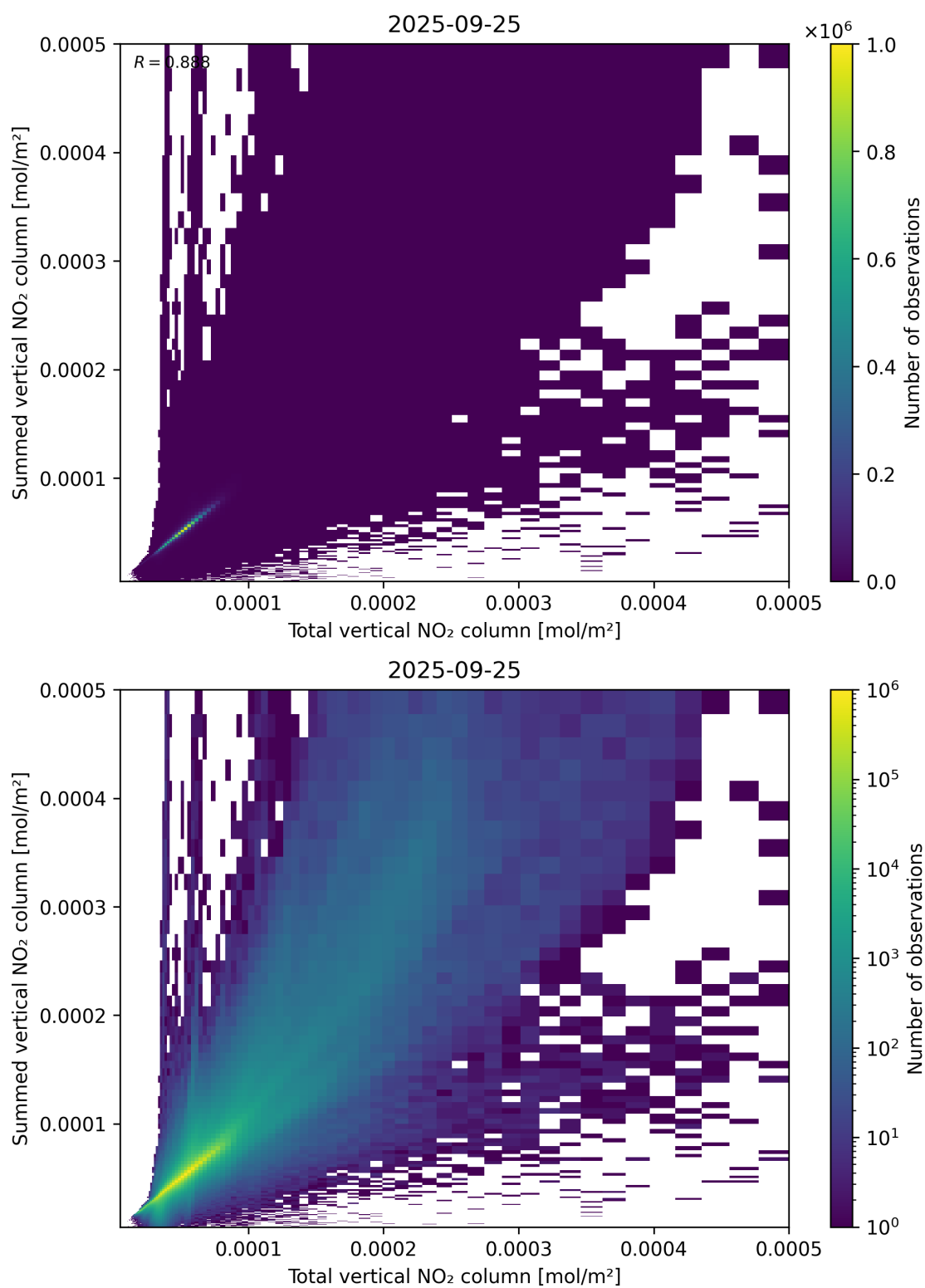
Figure 112: Scatter density plot of “Total vertical NO 2 column” against “Summed vertical NO 2 column” for 2025-09-25 to 2025-09-26.
