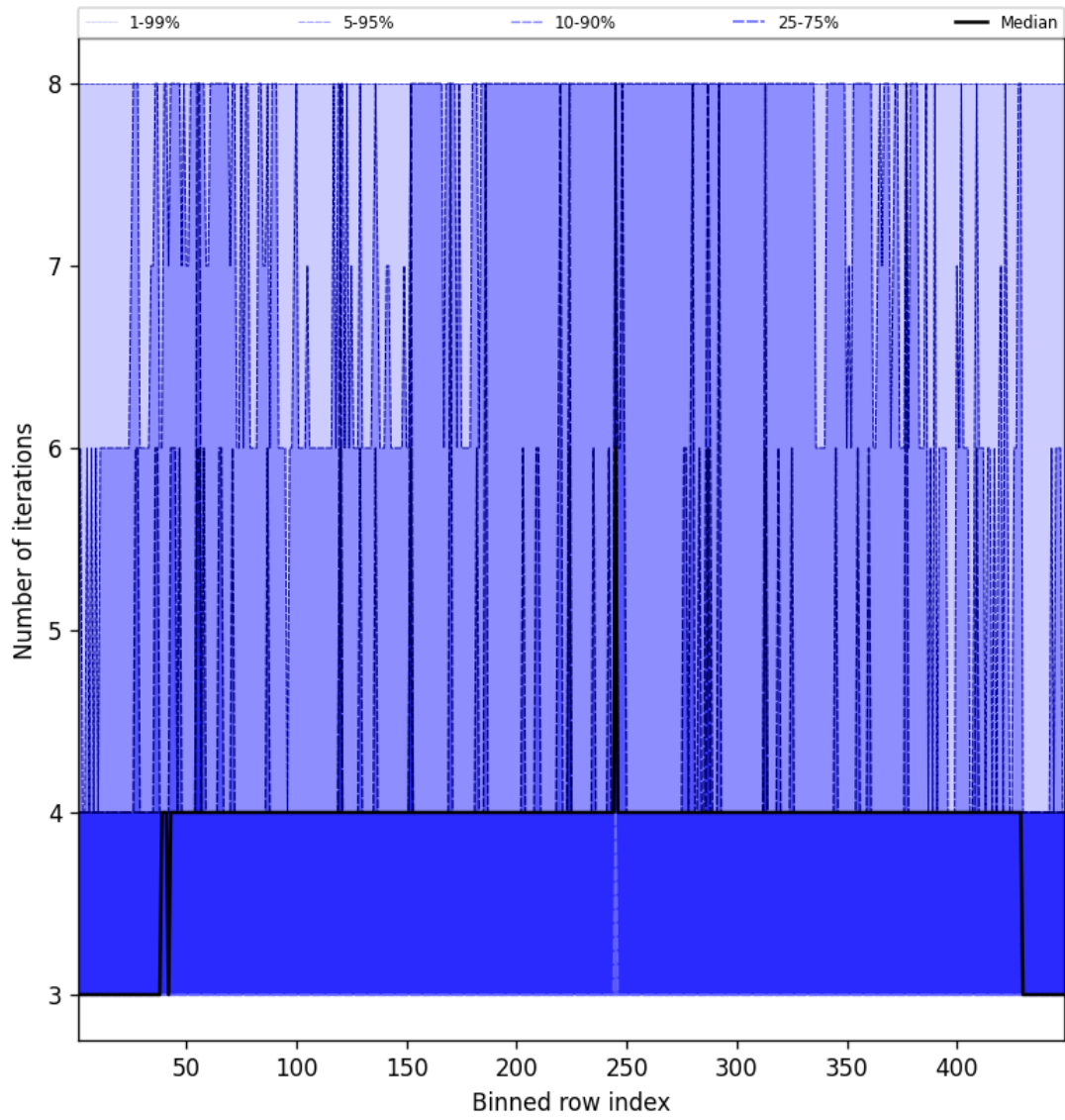
Figure 51: Along track statistics of “Number of iterations” for 2025-09-25 to 2025-09-26
