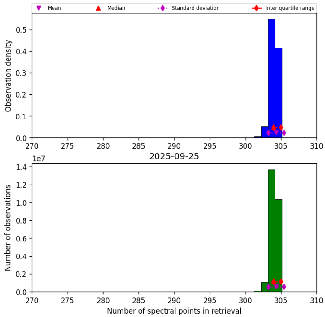
Figure 33: Histogram of “Number of spectral points in retrieval” for 2025-09-25 to 2025-09-26
