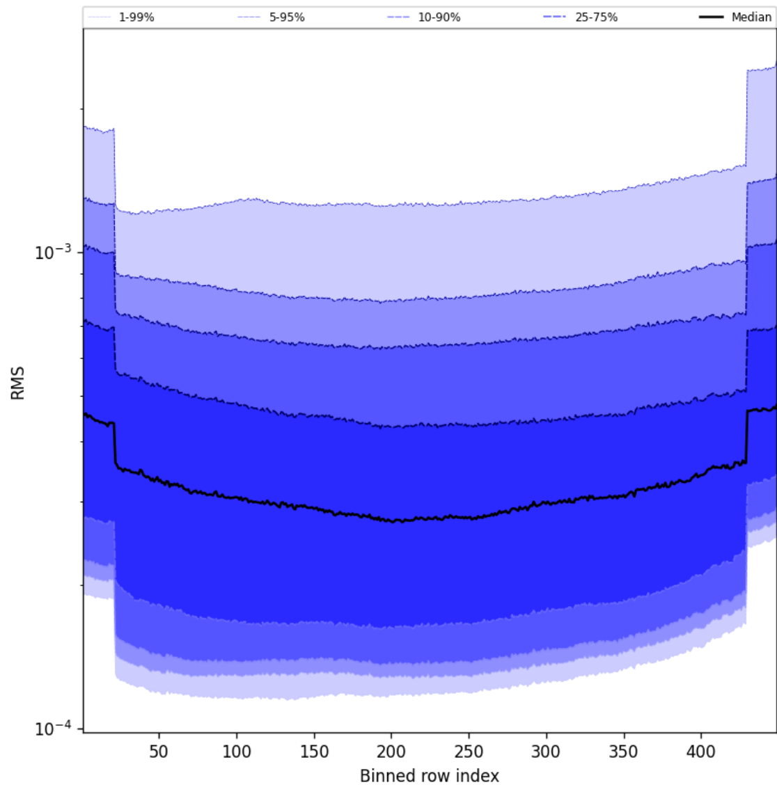
Figure 60: Along track statistics of “RMS” for 2025-09-25 to 2025-09-26
