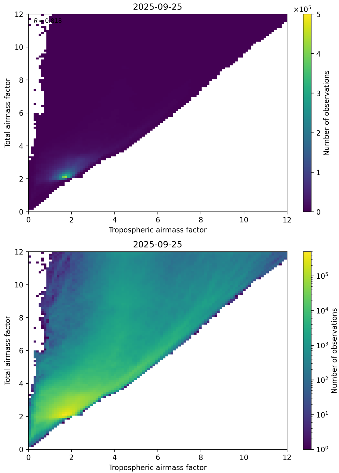
Figure 72: Scatter density plot of “Tropospheric airmass factor” against “Total airmass factor” for 2025-09-25 to 2025-09-26.
