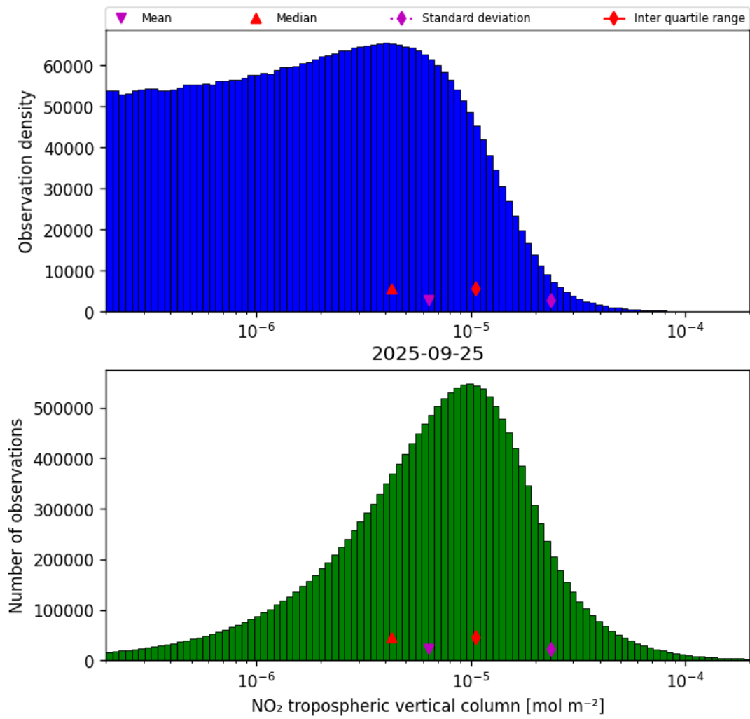
Figure 29: Histogram of “NO 2 tropospheric vertical column” for 2025-09-25 to 2025-09-26
