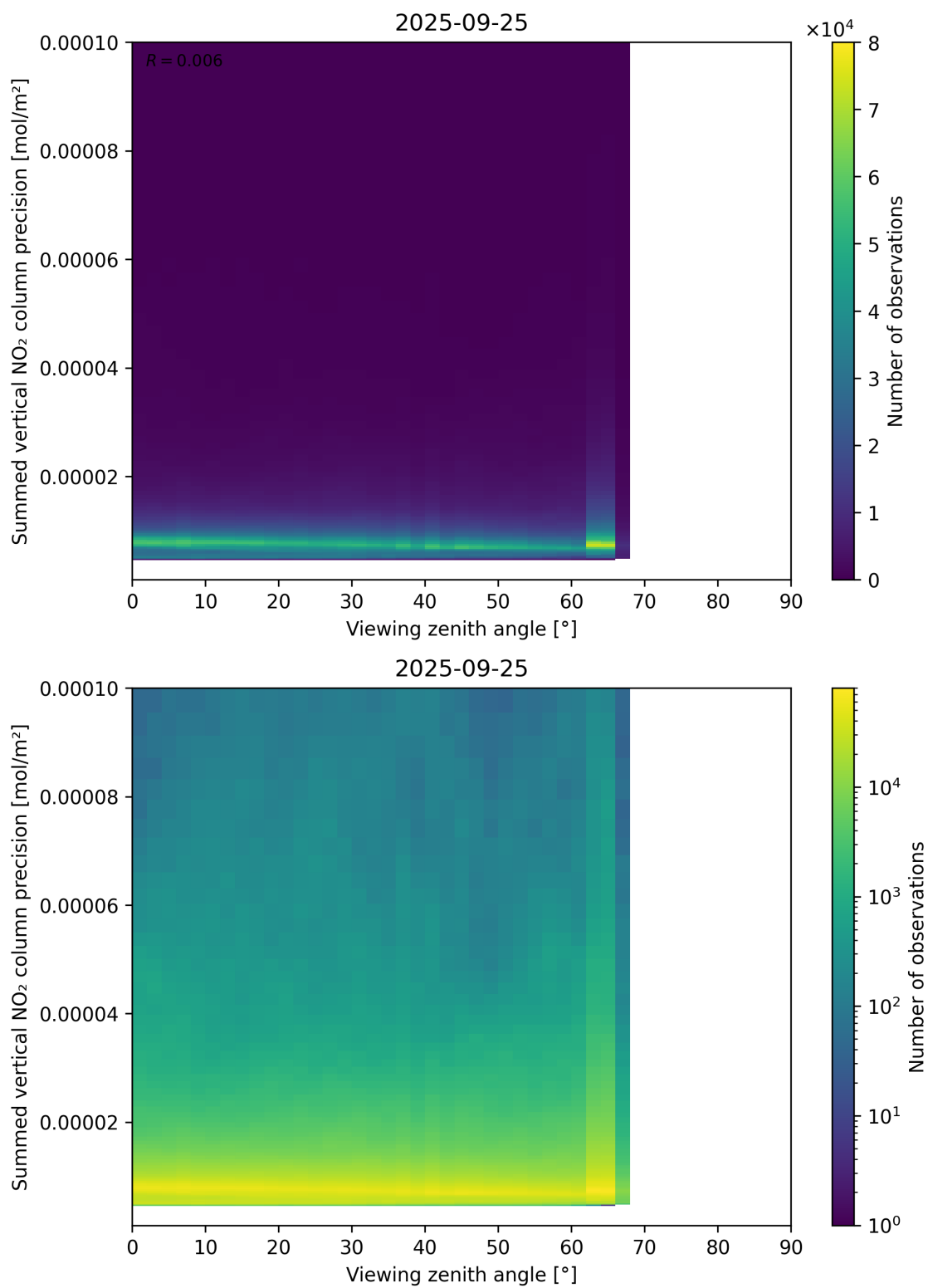
Figure 166: Scatter density plot of “Viewing zenith angle” against “Summed vertical NO 2 column precision” for 2025-09-25 to 2025-09-26.
