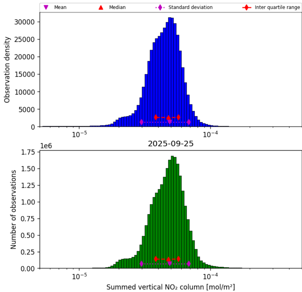
Figure 40: Histogram of “Summed vertical NO 2 column” for 2025-09-25 to 2025-09-26
