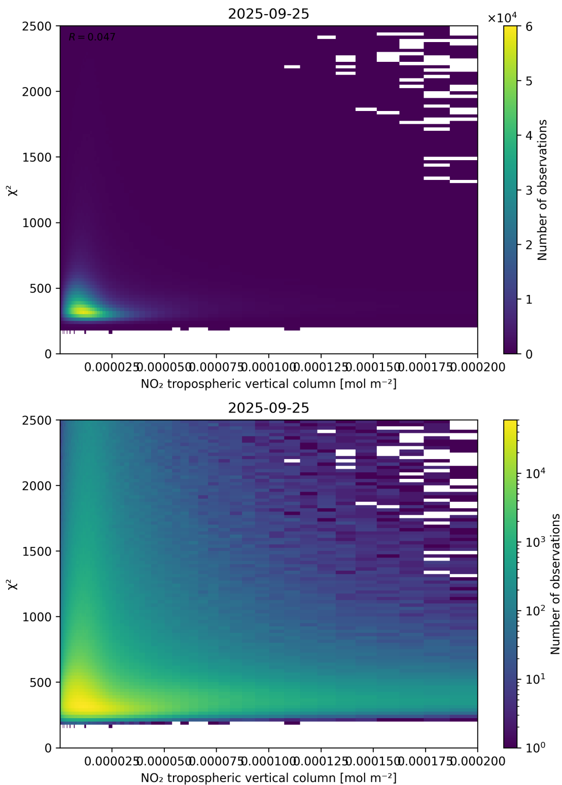
Figure 124: Scatter density plot of “NO 2 tropospheric vertical column” against “ \chi^2 ” for 2025-09-25 to 2025-09-26.
