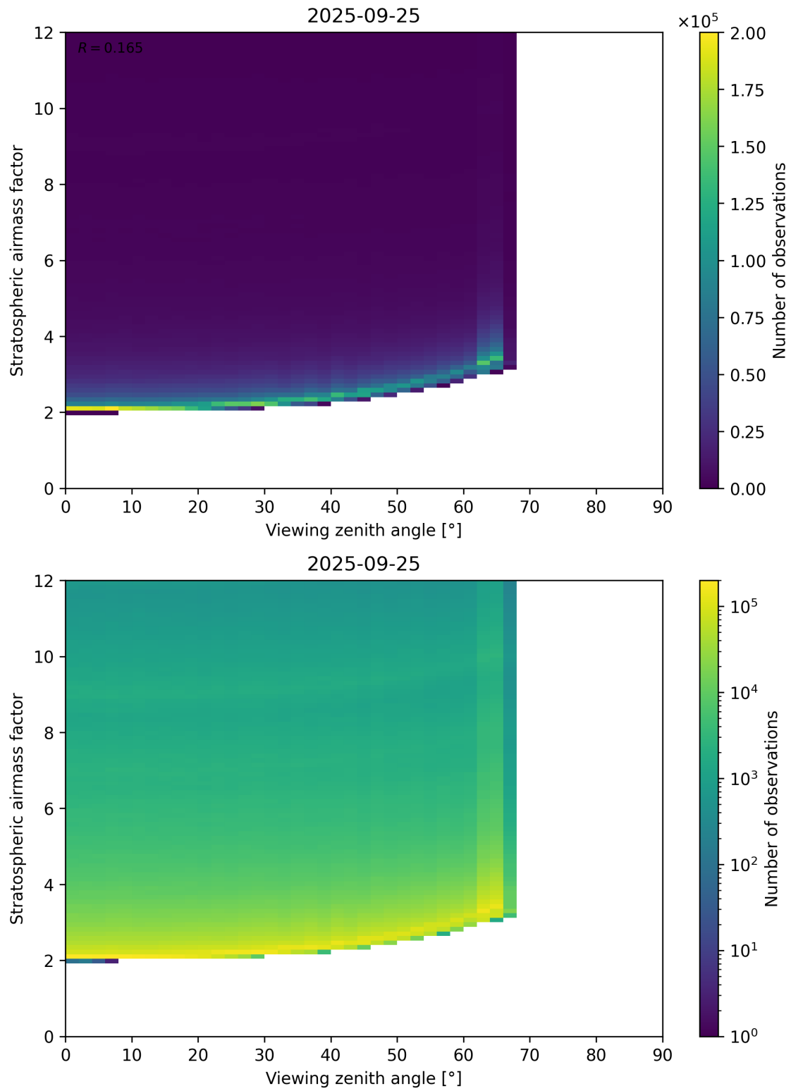
Figure 159: Scatter density plot of “Viewing zenith angle” against “Stratospheric airmass factor” for 2025-09-25 to 2025-09-26.
