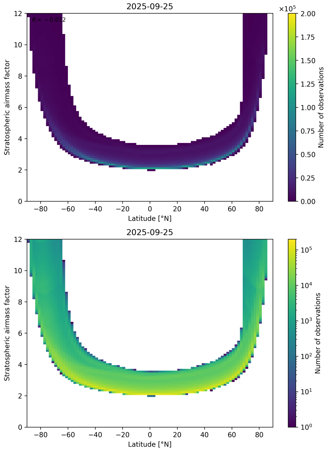
Figure 83: Scatter density plot of “Latitude” against “Stratospheric air mass factor” for 2025-09-25 to 2025-09-26.
