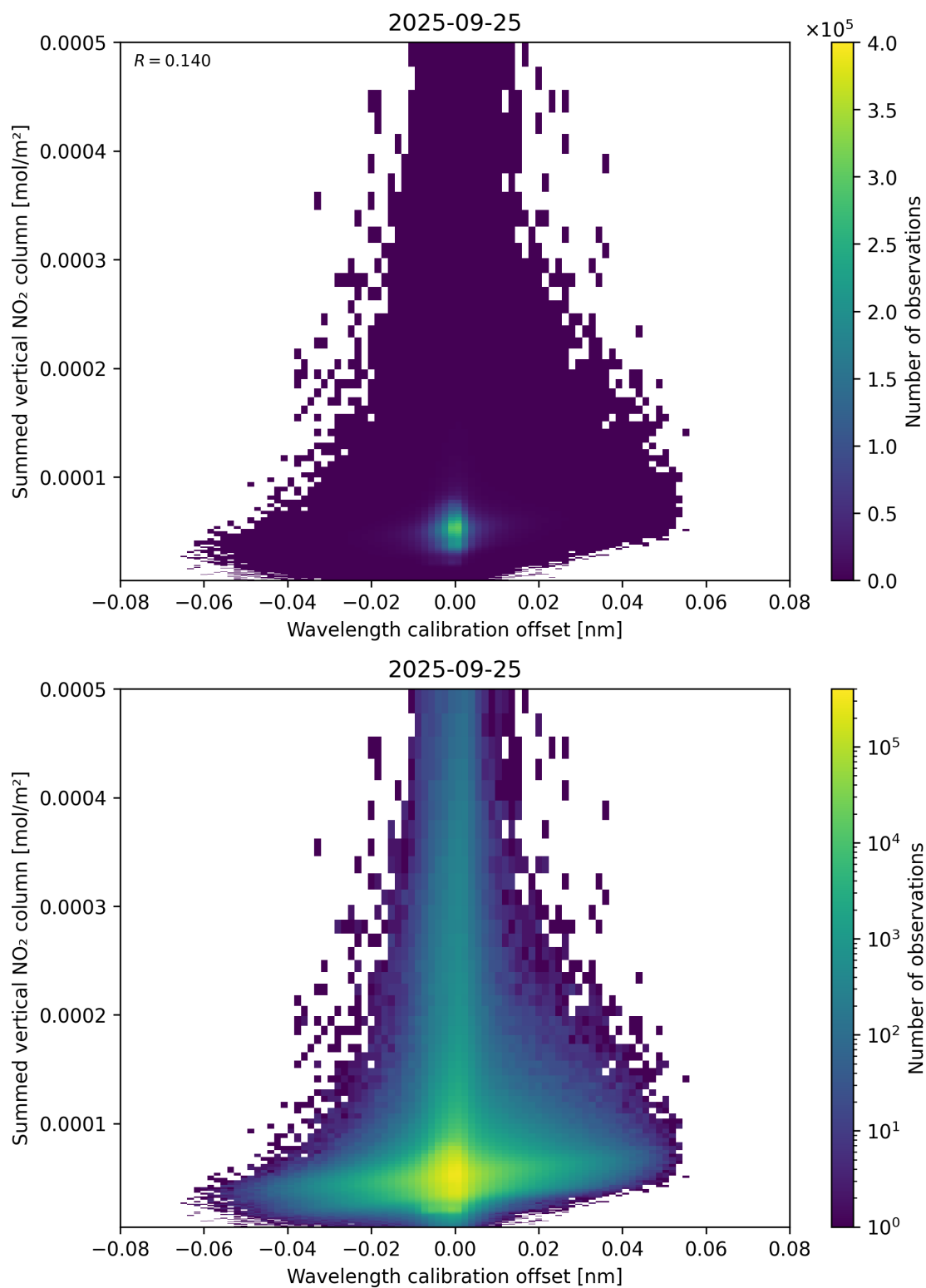
Figure 177: Scatter density plot of “Wavelength calibration offset” against “Summed vertical NO 2 column” for 2025-09-25 to 2025-09-26.
