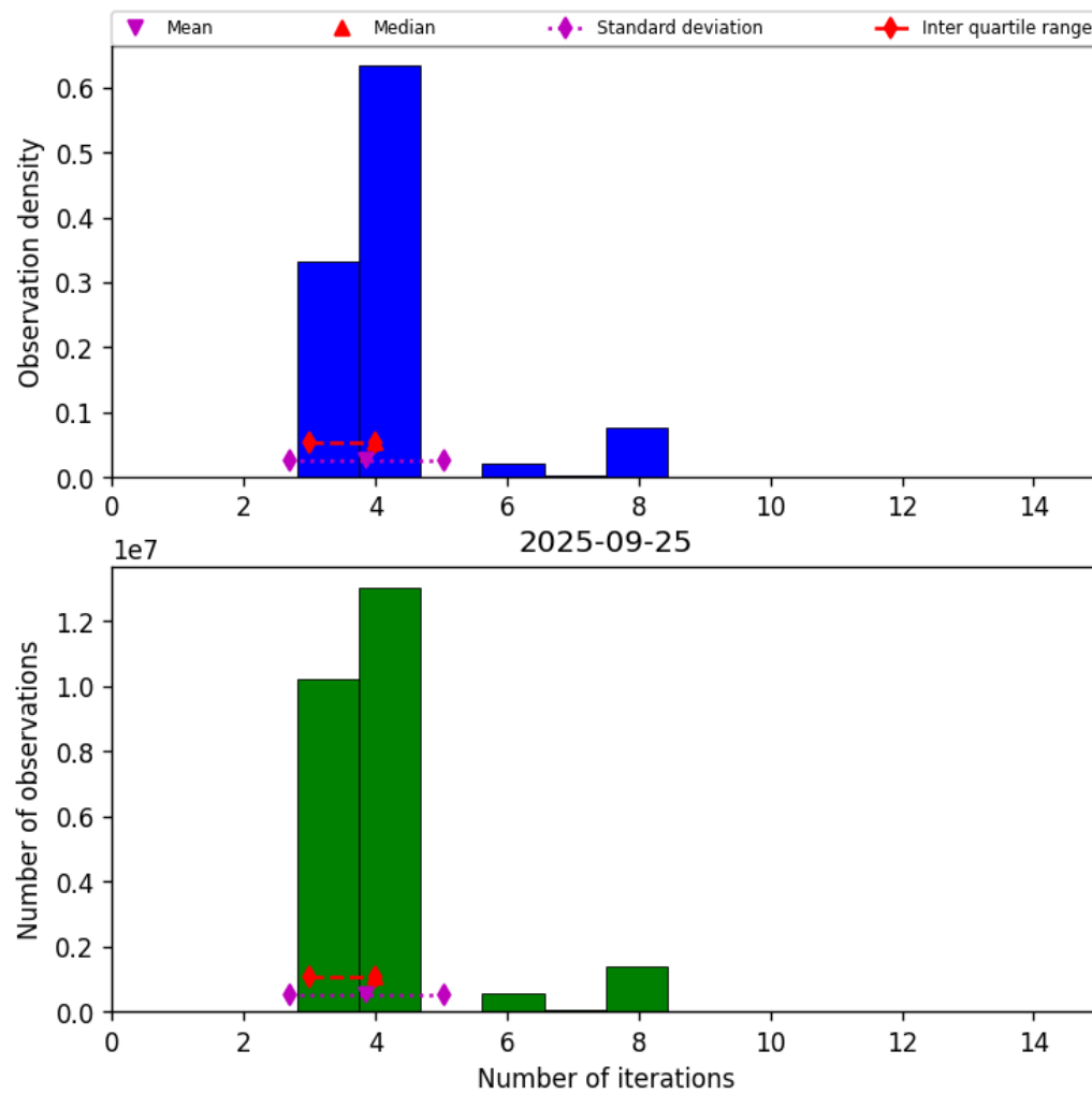
Figure 34: Histogram of “Number of iterations” for 2025-09-25 to 2025-09-26
