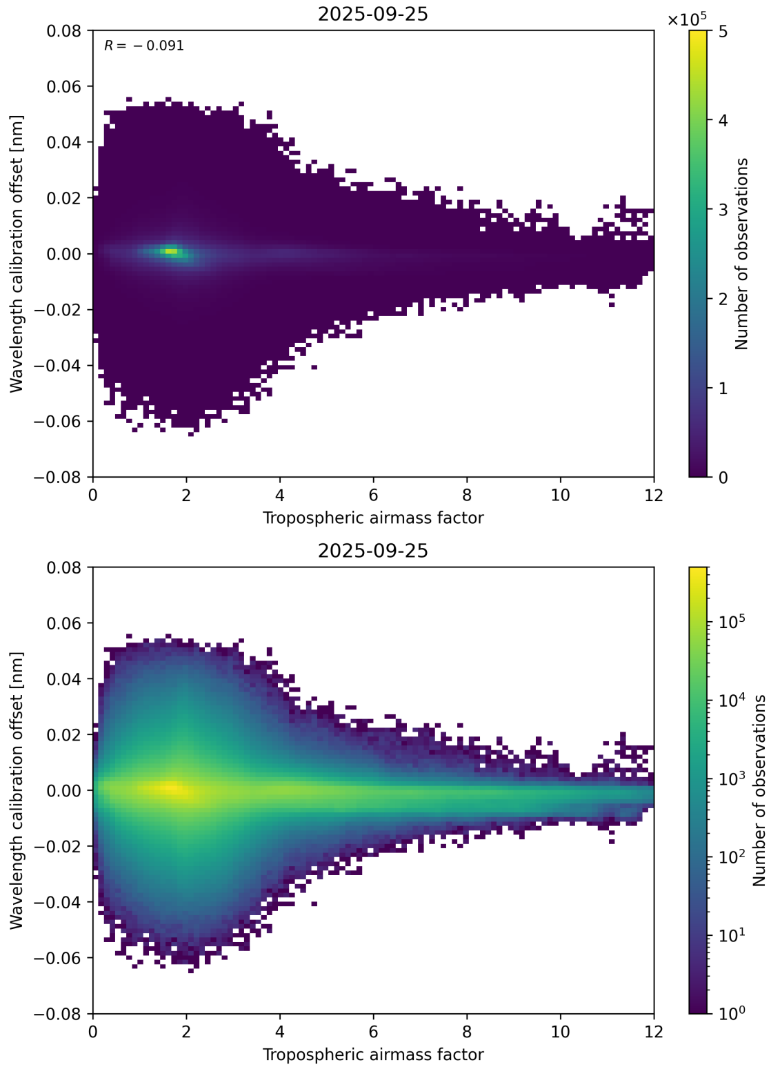
Figure 80: Scatter density plot of “Tropospheric airmass factor” against “Wavelength calibration offset” for 2025-09-25 to 2025-09-26.
