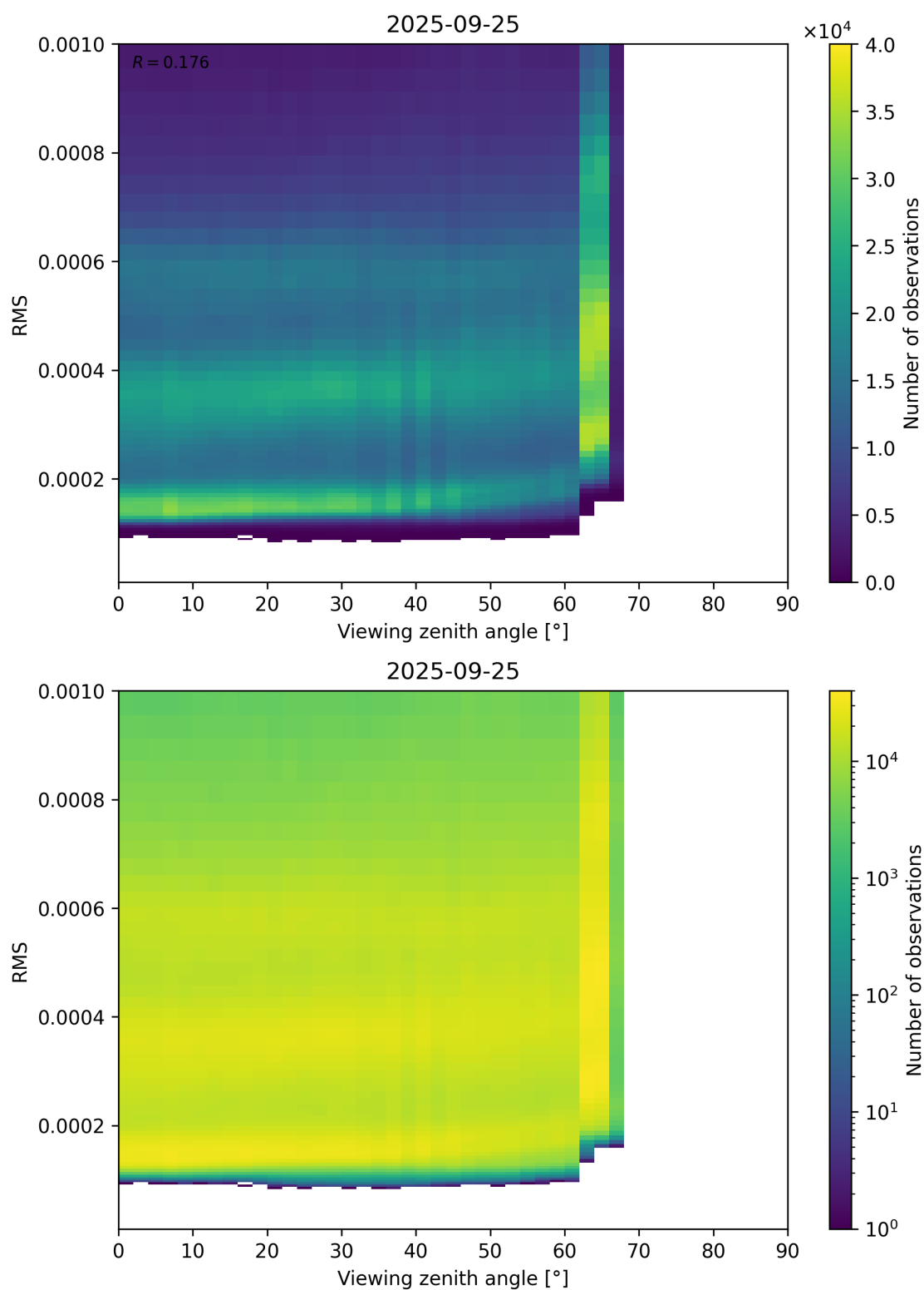
Figure 171: Scatter density plot of “Viewing zenith angle” against “RMS” for 2025-09-25 to 2025-09-26.
