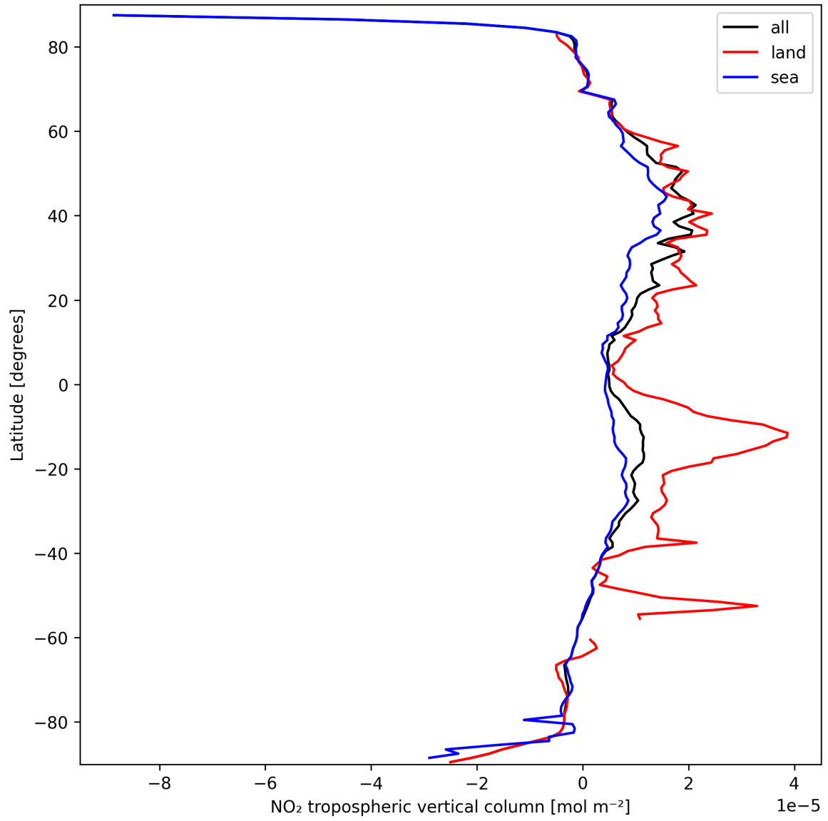
Figure 12: Zonal average of “NO 2 tropospheric vertical column” for 2025-09-25 to 2025-09-26.
