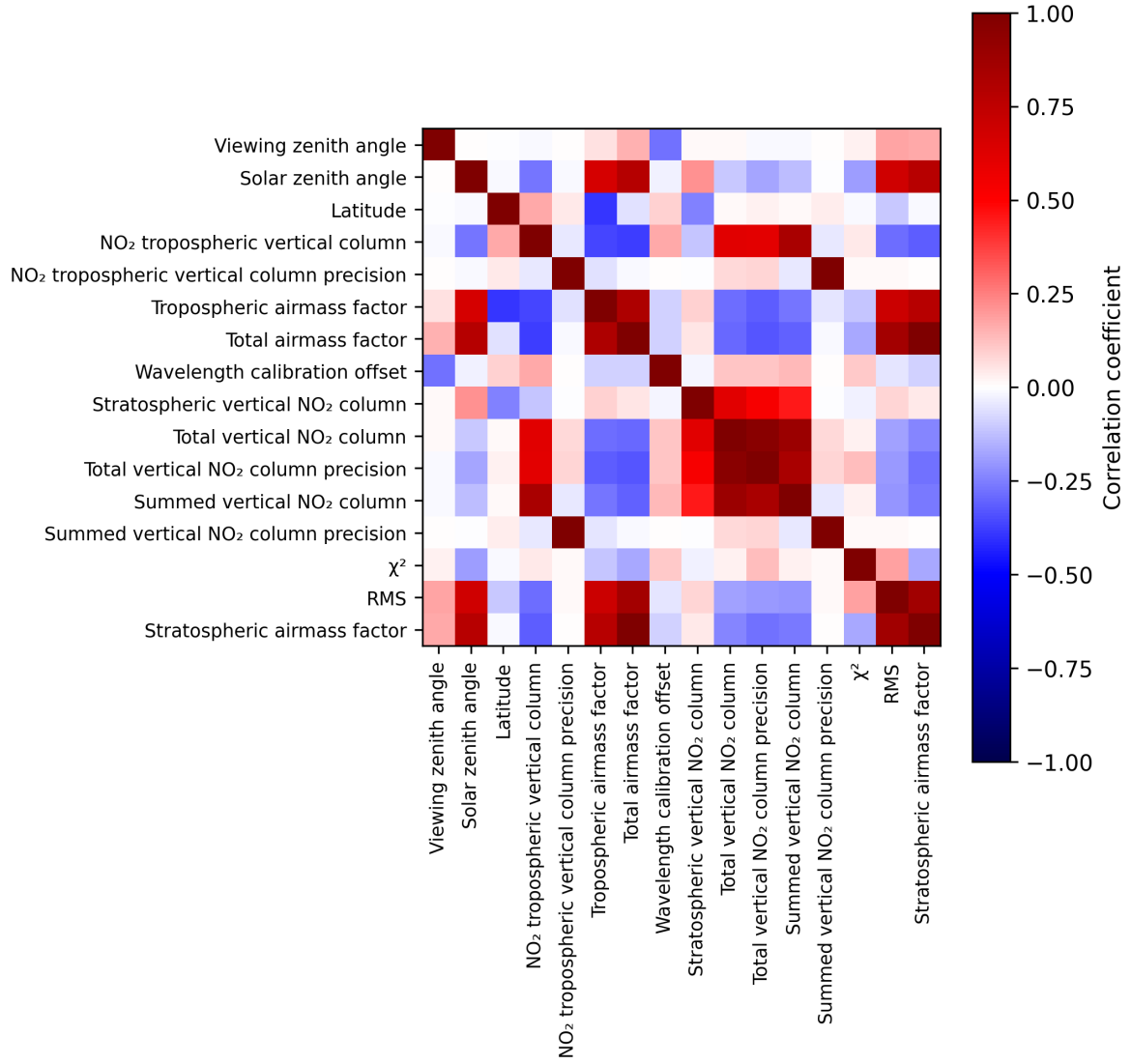
Figure 2: Map of correlation matrix for 2025-09-25 to 2025-09-26.
