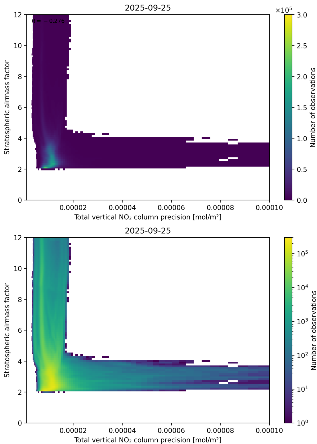
Figure 115: Scatter density plot of “Total vertical NO 2 column precision” against “Stratospheric airmass factor” for 2025-09-25 to 2025-09-26.
