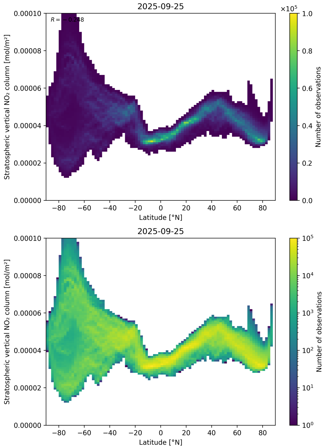
Figure 87: Scatter density plot of “Latitude” against “Stratospheric vertical NO 2 column” for 2025-09-25 to 2025-09-26.
