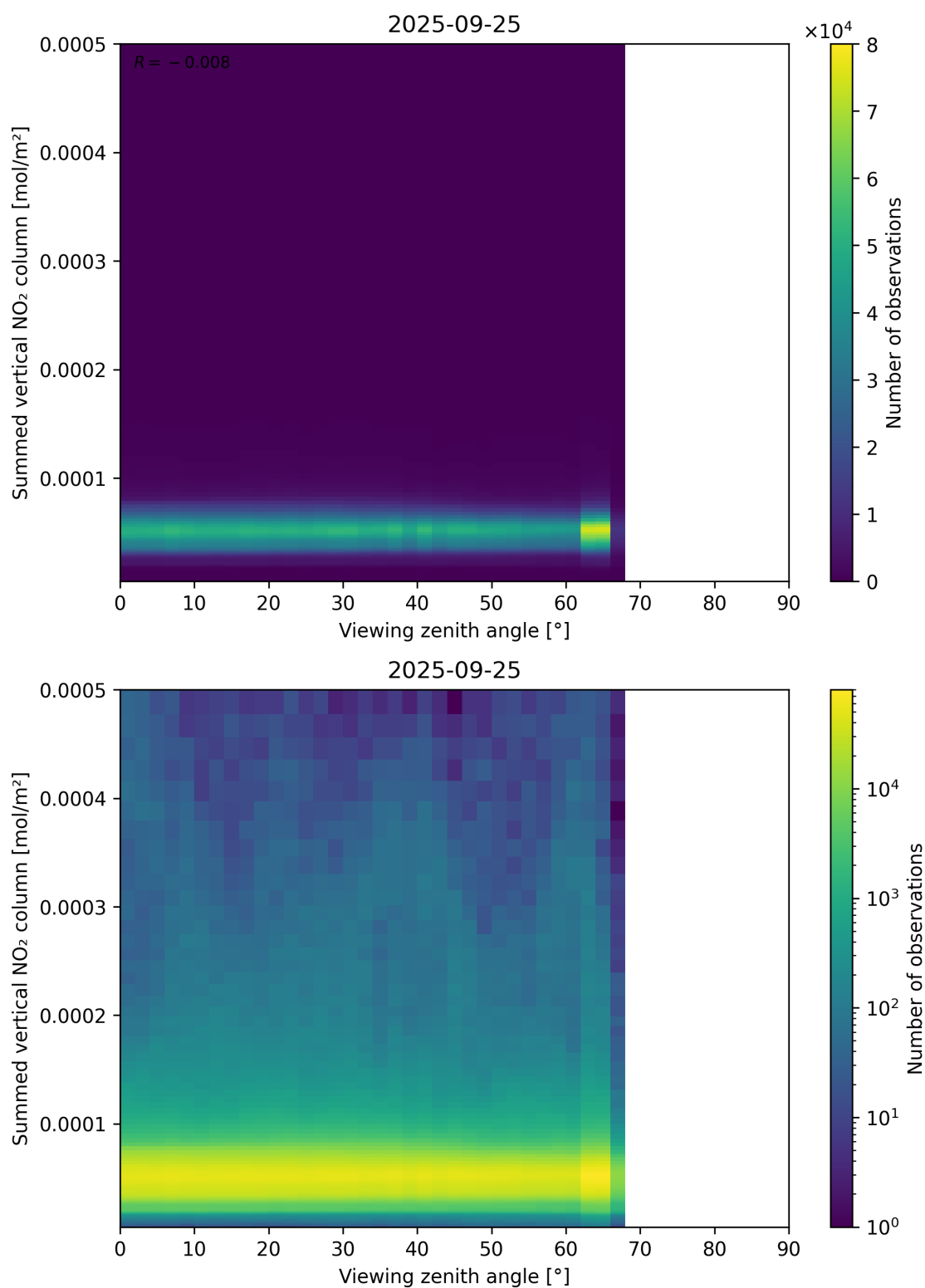
Figure 165: Scatter density plot of “Viewing zenith angle” against “Summed vertical NO 2 column” for 2025-09-25 to 2025-09-26.
