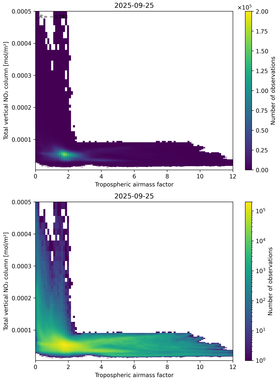
Figure 77: Scatter density plot of “Tropospheric airmass factor” against “Total vertical NO 2 column” for 2025-09-25 to 2025-09-26.
