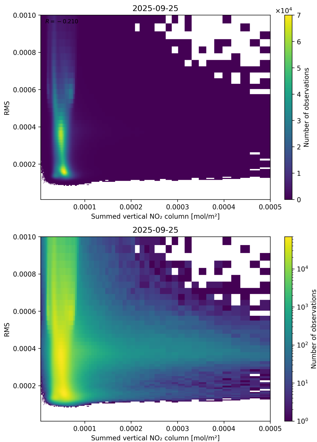
Figure 109: Scatter density plot of “Summed vertical NO 2 column” against “RMS” for 2025-09-25 to 2025-09-26.
