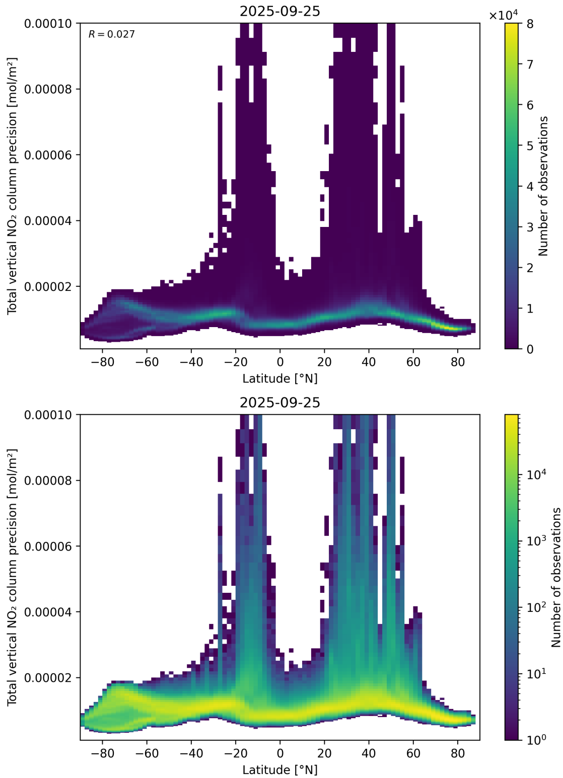
Figure 91: Scatter density plot of “Latitude” against “Total vertical NO 2 column precision” for 2025-09-25 to 2025-09-26.
