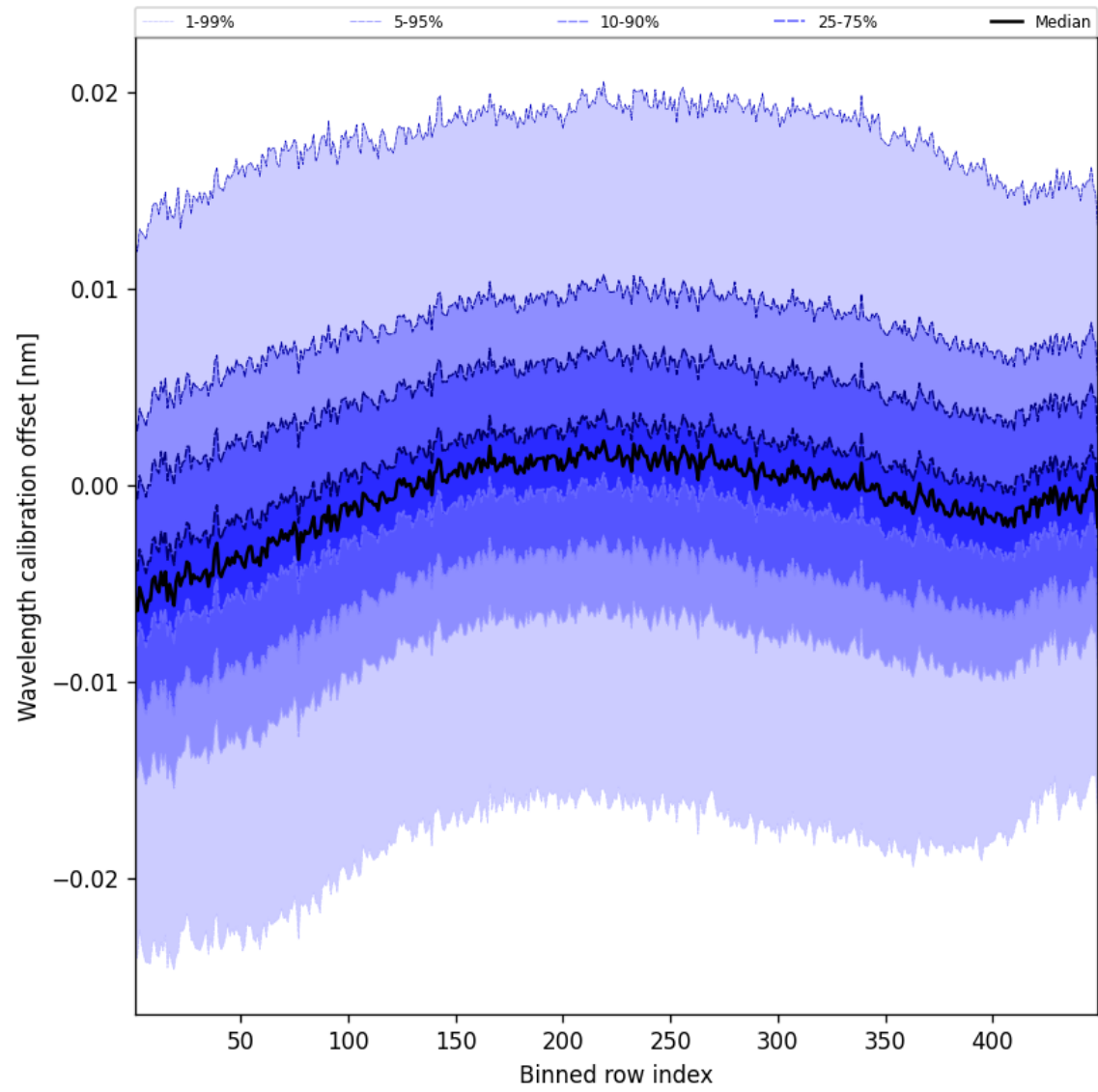
Figure 52: Along track statistics of “Wavelength calibration offset” for 2025-09-25 to 2025-09-26
