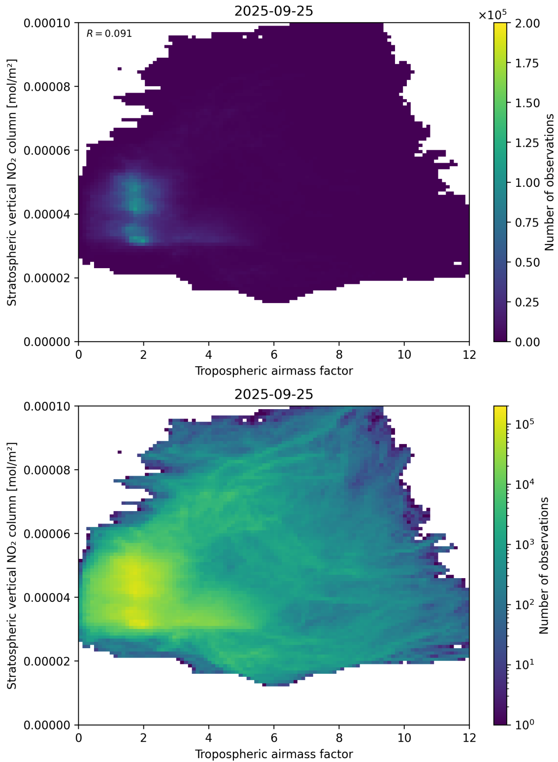
Figure 74: Scatter density plot of “Tropospheric air mass factor” against “Stratospheric vertical NO 2 column” for 2025-09-25 to 2025-09-26.
