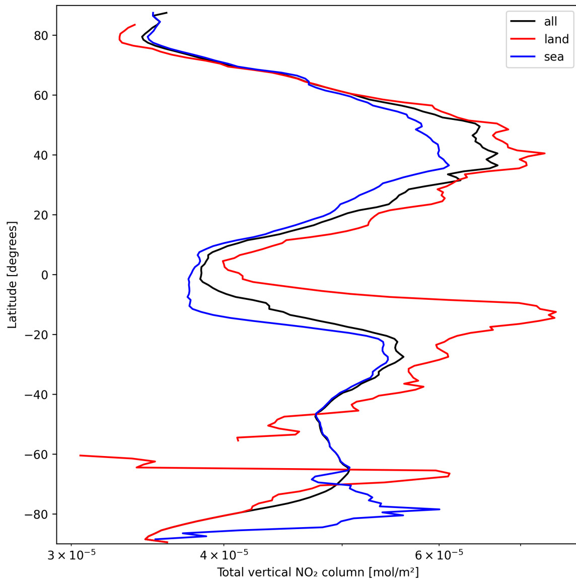
Figure 21: Zonal average of “Total vertical NO 2 column” for 2025-09-25 to 2025-09-26.
