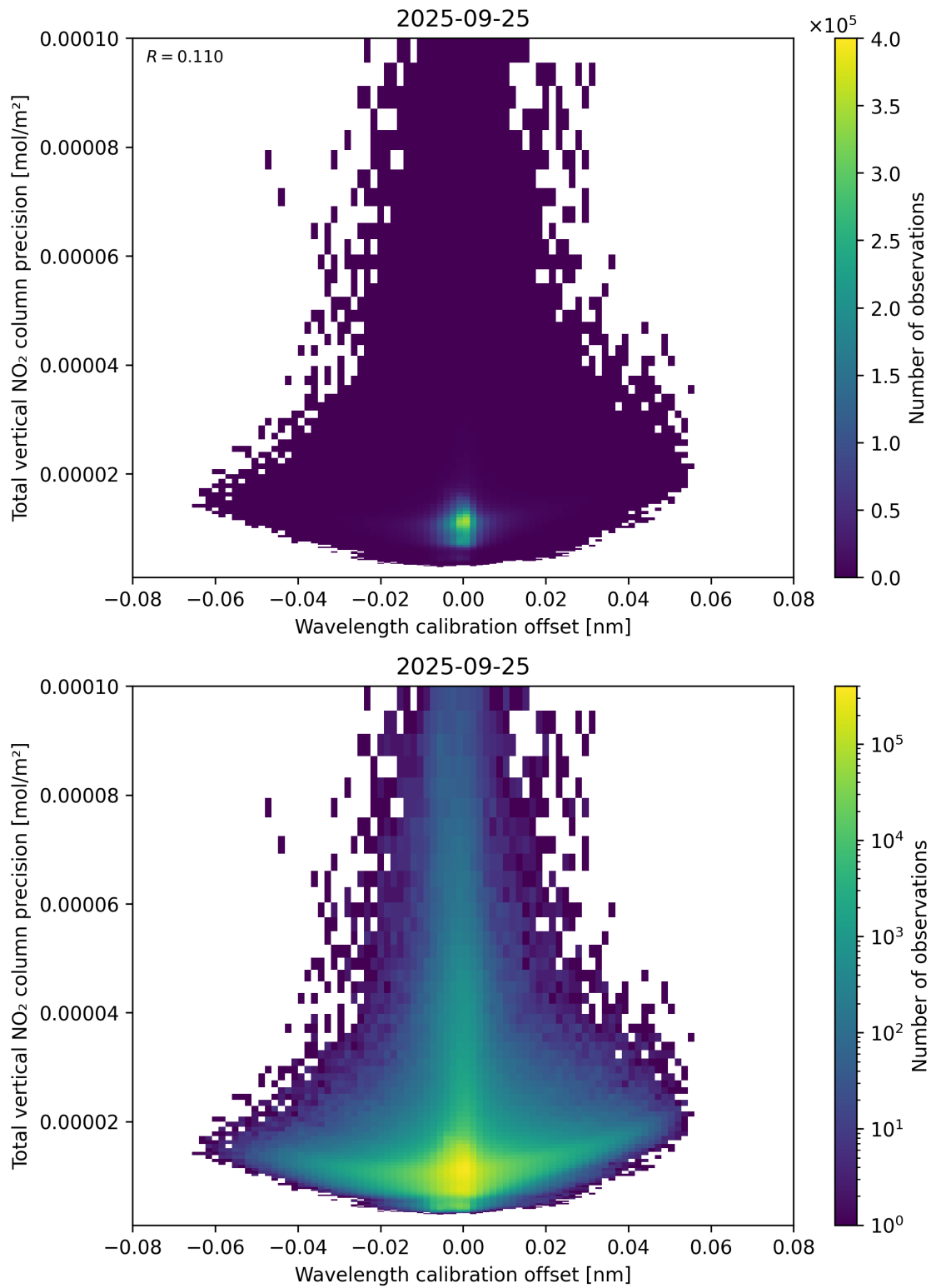
Figure 180: Scatter density plot of “Wavelength calibration offset” against “Total vertical NO 2 column precision” for 2025-09-25 to 2025-09-26.
