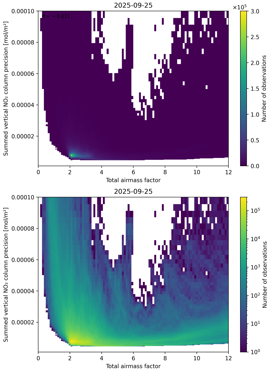
Figure 66: Scatter density plot of “Total airmass factor” against “Summed vertical NO 2 column precision” for 2025-09-25 to 2025-09-26.
