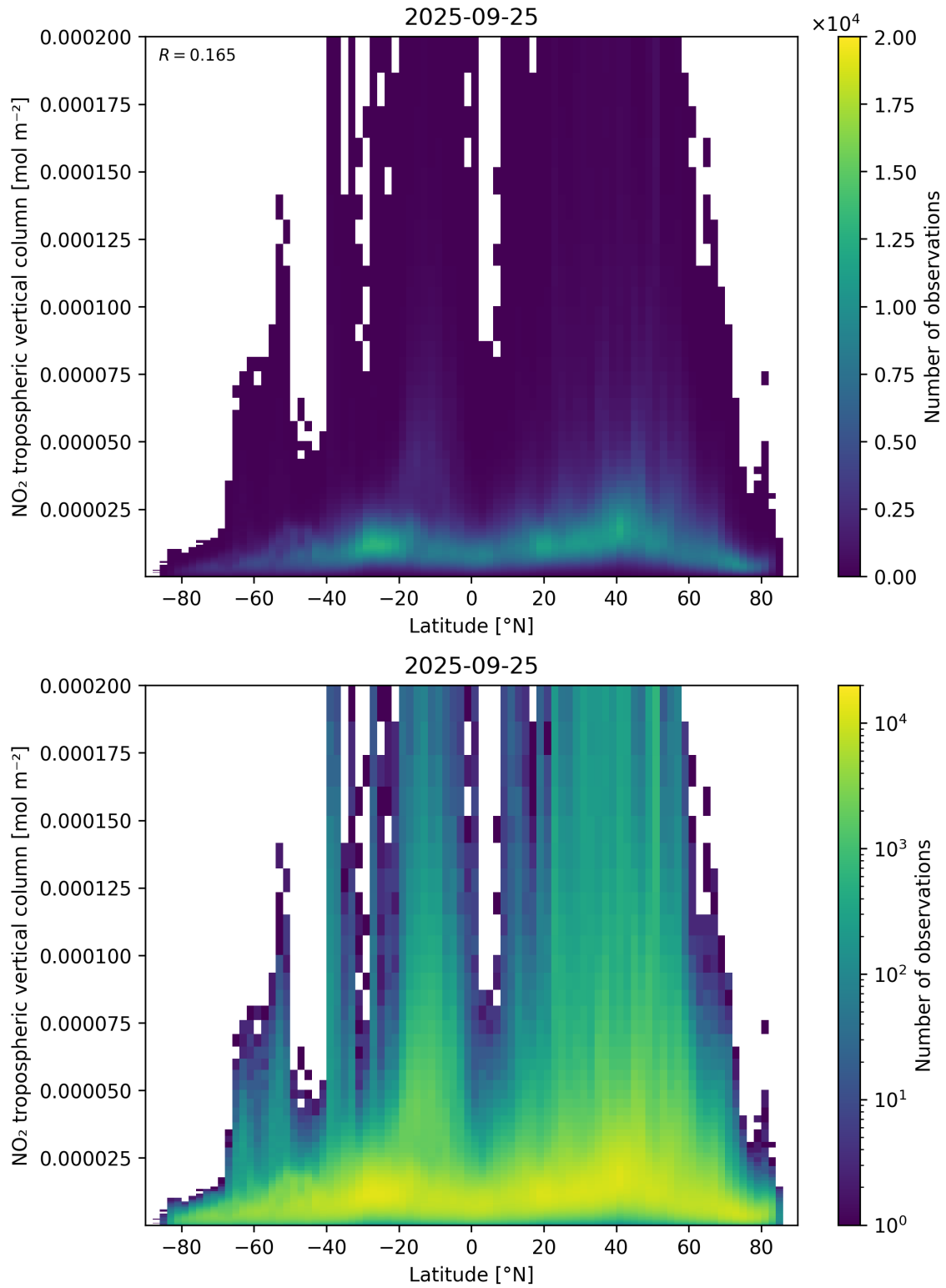
Figure 92: Scatter density plot of “Latitude” against “NO 2 tropospheric vertical column” for 2025-09-25 to 2025-09-26.
