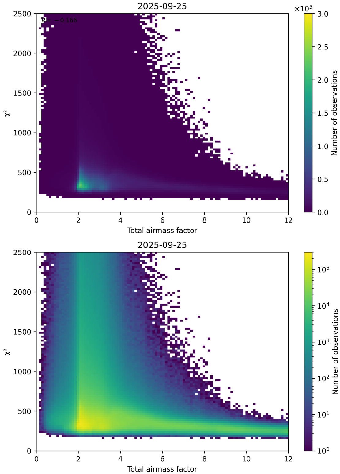
Figure 63: Scatter density plot of “Total airmass factor” against “ \chi^2 ” for 2025-09-25 to 2025-09-26.
