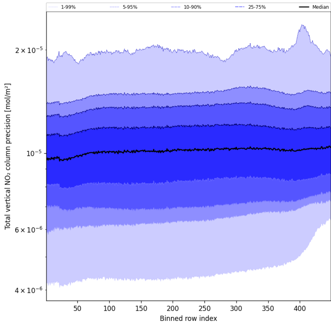
Figure 56: Along track statistics of “Total vertical NO 2 column precision” for 2025-09-25 to 2025-09-26
