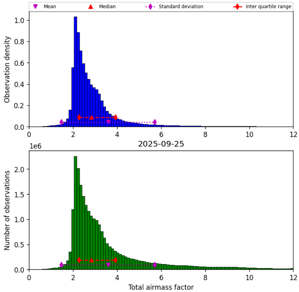
Figure 32: Histogram of “Total airmass factor” for 2025-09-25 to 2025-09-26
