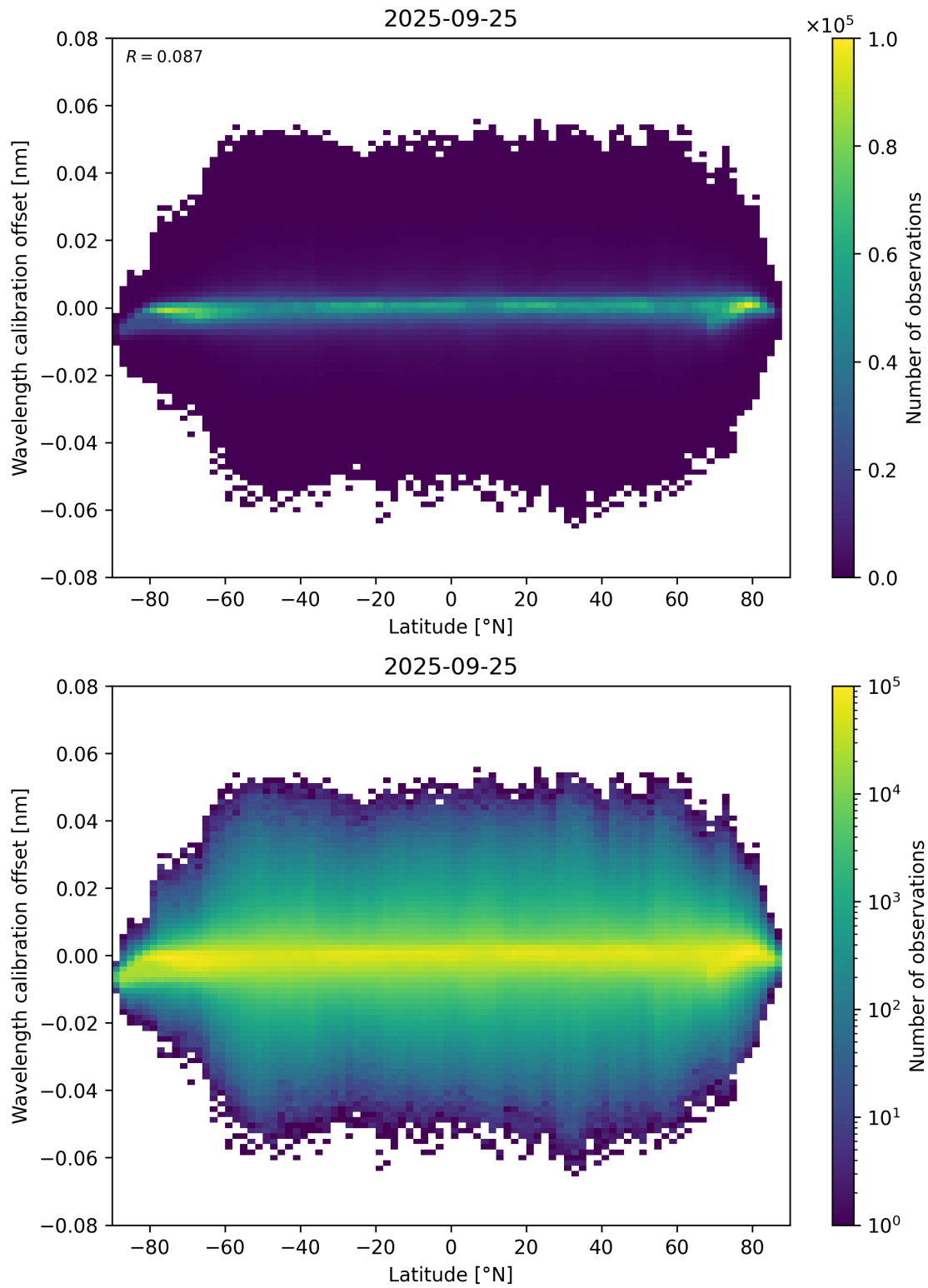
Figure 95: Scatter density plot of “Latitude” against “Wavelength calibration offset” for 2025-09-25 to 2025-09-26.
