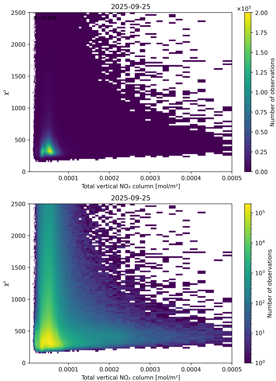
Figure 111: Scatter density plot of “Total vertical NO 2 column” against “ \chi^2 ” for 2025-09-25 to 2025-09-26.
