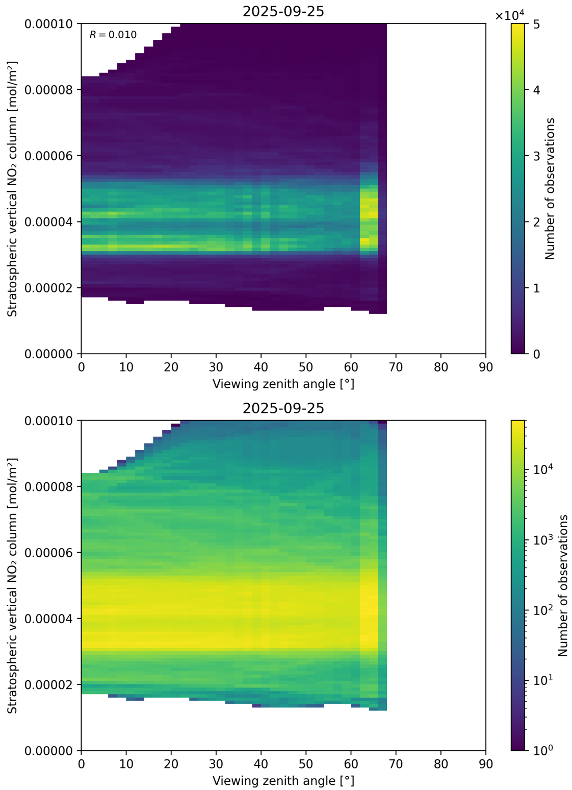
Figure 164: Scatter density plot of “Viewing zenith angle” against “Stratospheric vertical NO 2 column” for 2025-09-25 to 2025-09-26.
