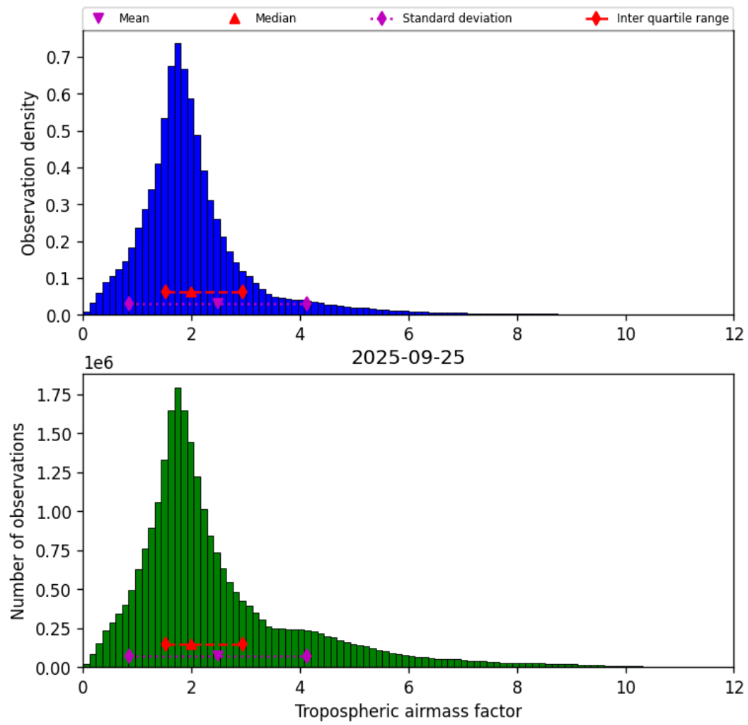
Figure 31: Histogram of “Tropospheric airmass factor” for 2025-09-25 to 2025-09-26
