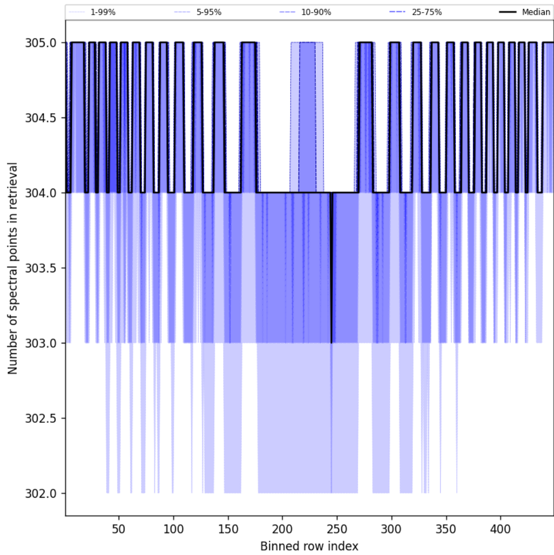
Figure 50: Along track statistics of “Number of spectral points in retrieval” for 2025-09-25 to 2025-09-26
