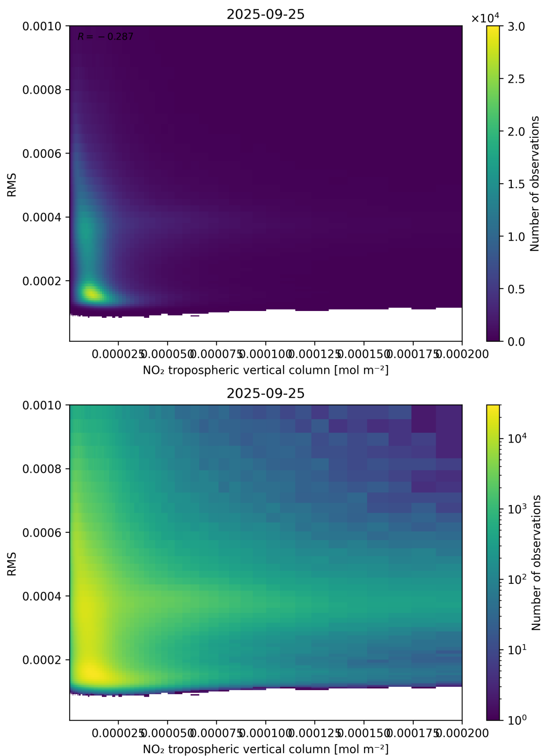
Figure 142: Scatter density plot of “NO 2 tropospheric vertical column” against “RMS” for 2025-09-25 to 2025-09-26.
