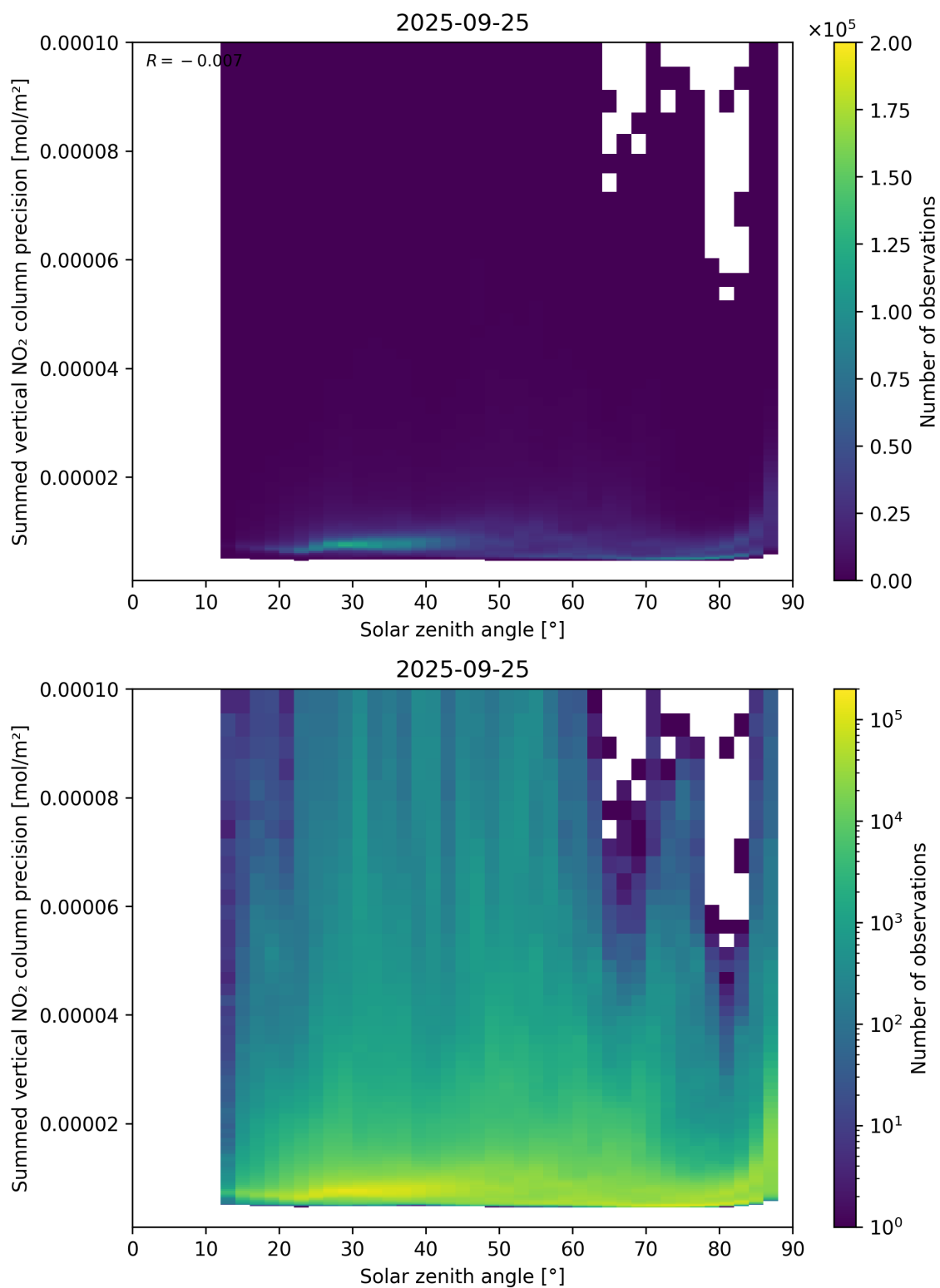
Figure 152: Scatter density plot of “Solar zenith angle” against “Summed vertical NO 2 column precision” for 2025-09-25 to 2025-09-26.
