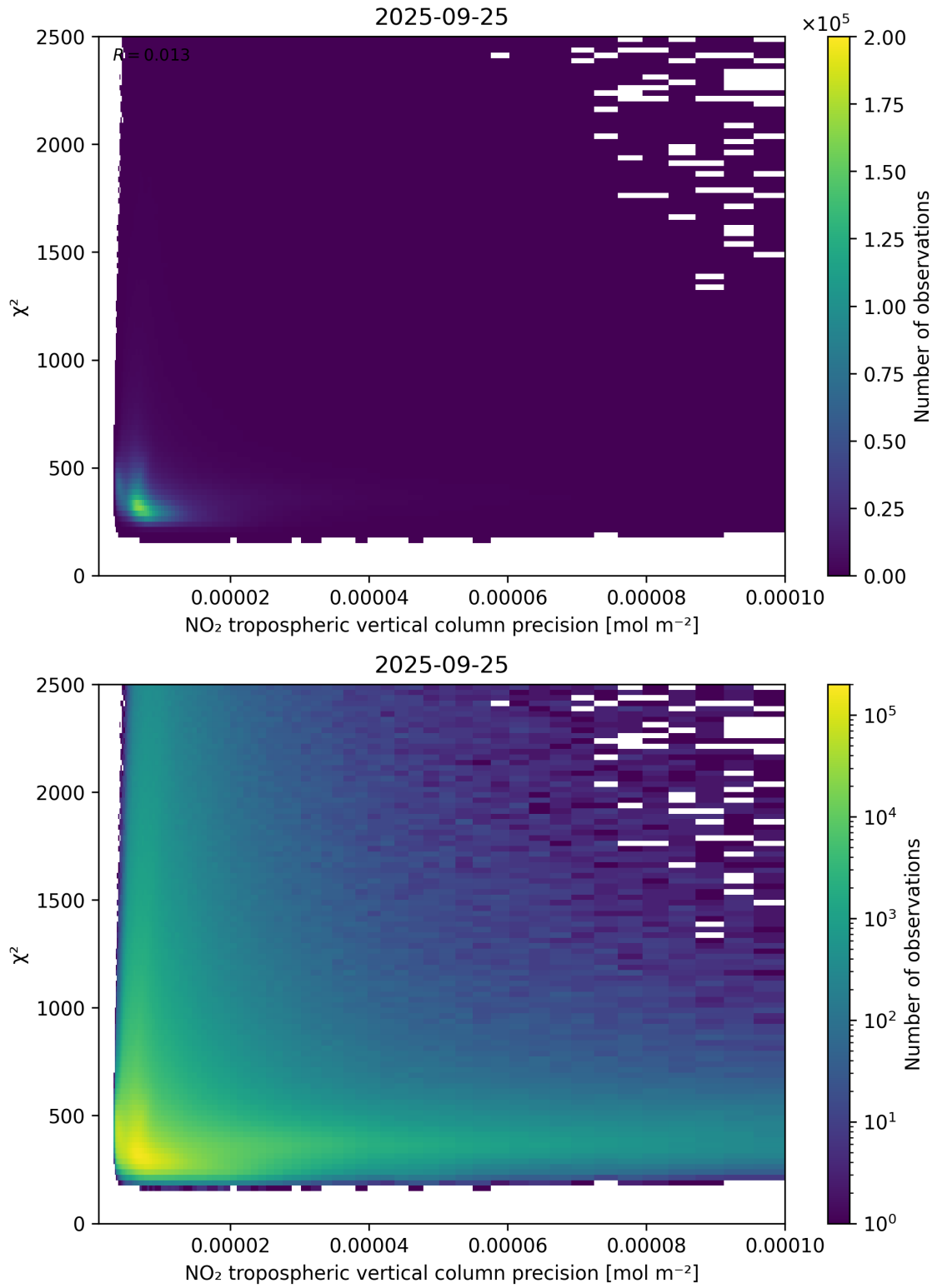
Figure 134: Scatter density plot of “NO 2 tropospheric vertical column precision” against “ \chi^2 ” for 2025-09-25 to 2025-09-26.
