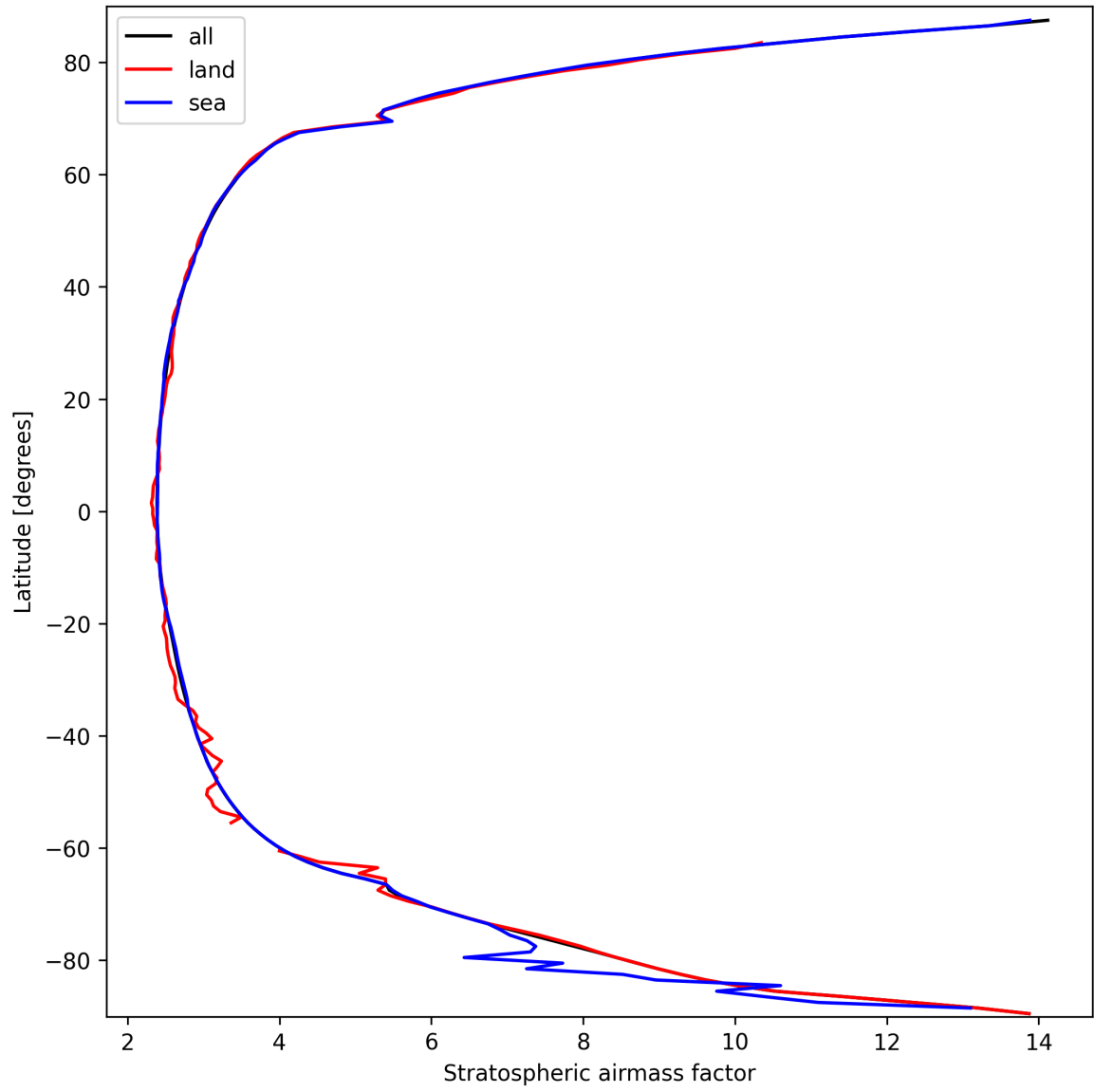
Figure 27: Zonal average of “Stratospheric air mass factor” for 2025-09-25 to 2025-09-26.
