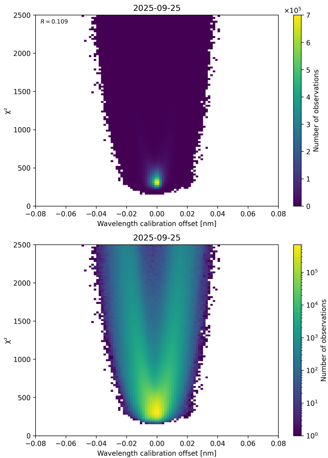
Figure 175: Scatter density plot of “Wavelength calibration offset” against “ \chi^2 ” for 2025-09-25 to 2025-09-26.
