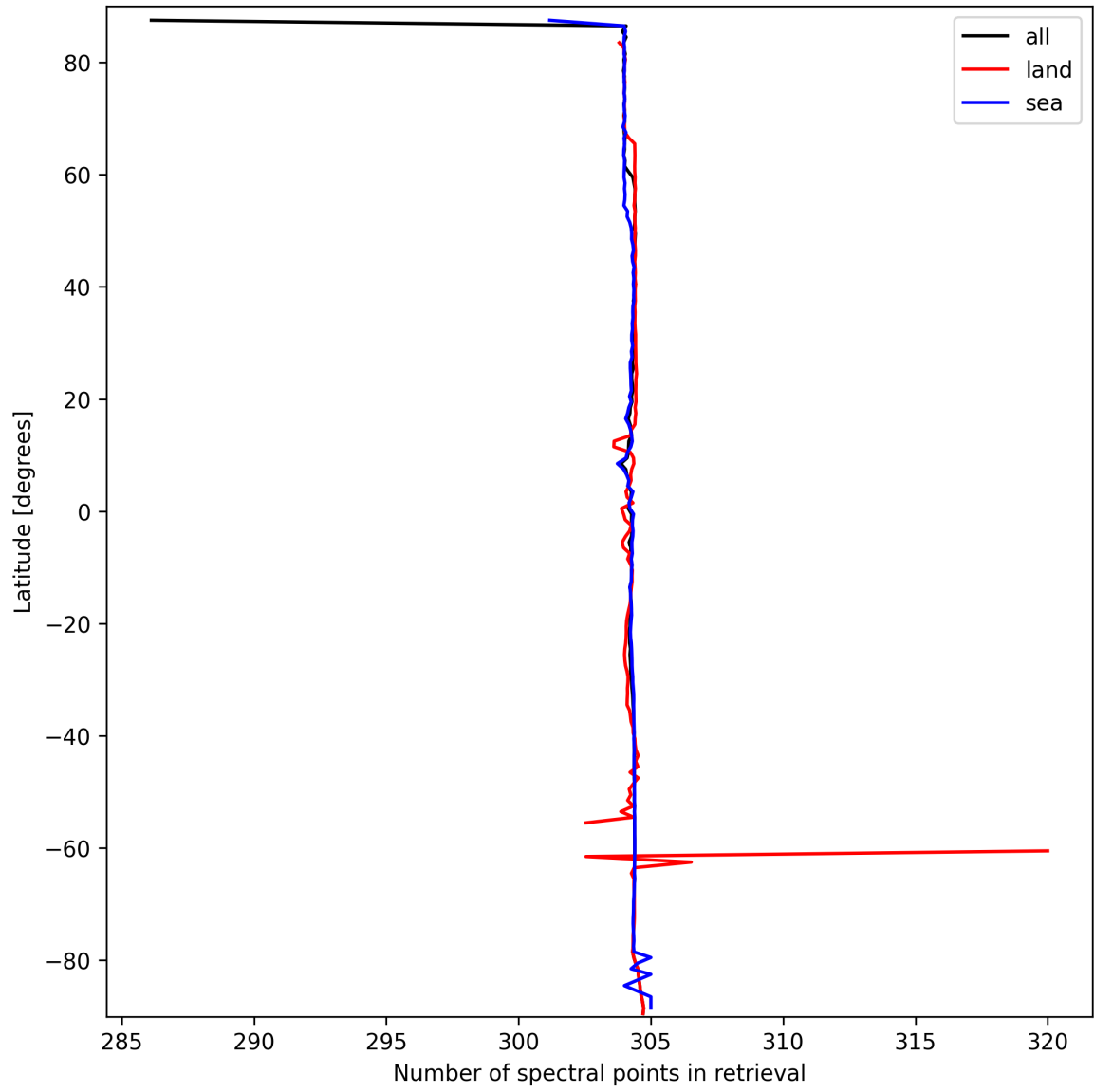
Figure 16: Zonal average of “Number of spectral points in retrieval” for 2025-09-25 to 2025-09-26.
