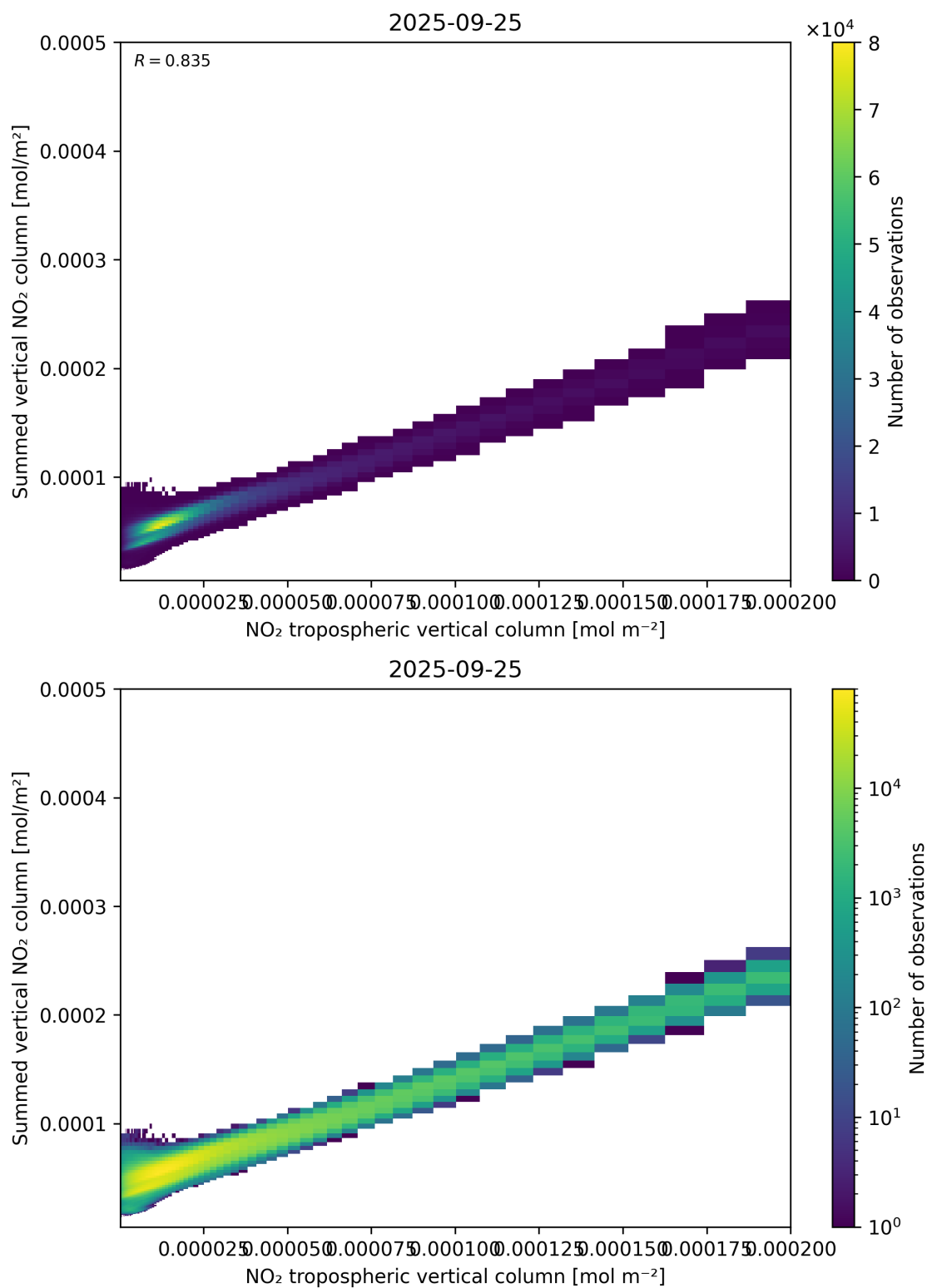
Figure 126: Scatter density plot of “NO 2 tropospheric vertical column” against “Summed vertical NO 2 column” for 2025-09-25 to 2025-09-26.
