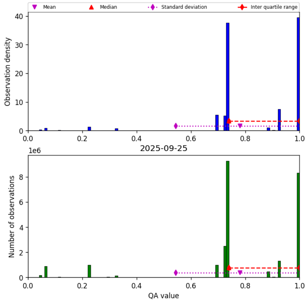
Figure 28: Histogram of “QA value” for 2025-09-25 to 2025-09-26
