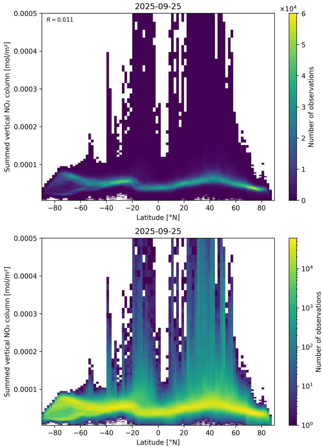
Figure 88: Scatter density plot of “Latitude” against “Summed vertical NO 2 column” for 2025-09-25 to 2025-09-26.
