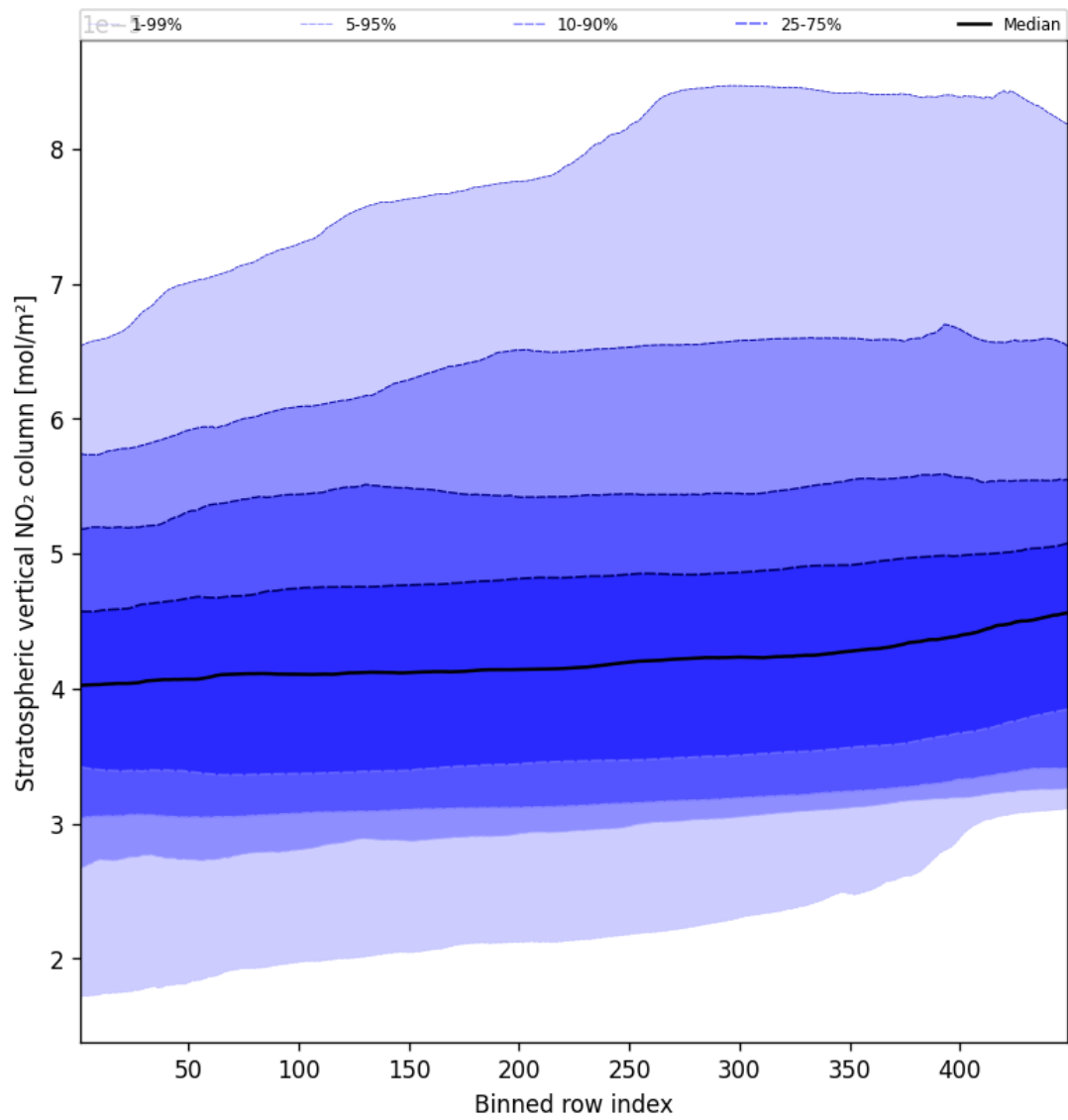
Figure 53: Along track statistics of “Stratospheric vertical NO 2 column” for 2025-09-25 to 2025-09-26
