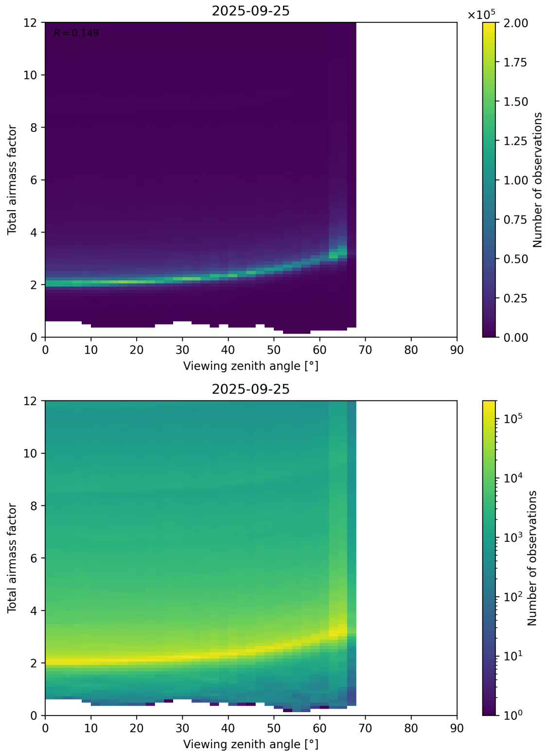
Figure 160: Scatter density plot of “Viewing zenith angle” against “Total airmass factor” for 2025-09-25 to 2025-09-26.
