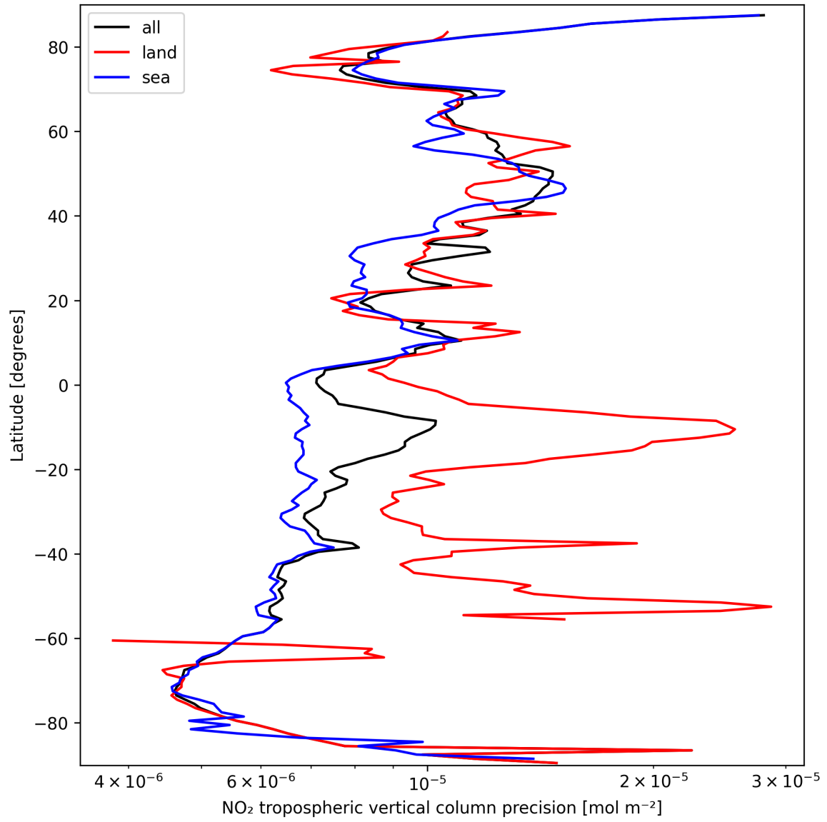
Figure 13: Zonal average of “NO 2 tropospheric vertical column precision” for 2025-09-25 to 2025-09-26.
