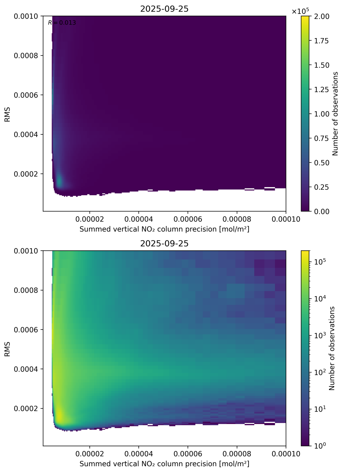
Figure 108: Scatter density plot of “Summed vertical NO 2 column precision” against “RMS” for 2025-09-25 to 2025-09-26.
