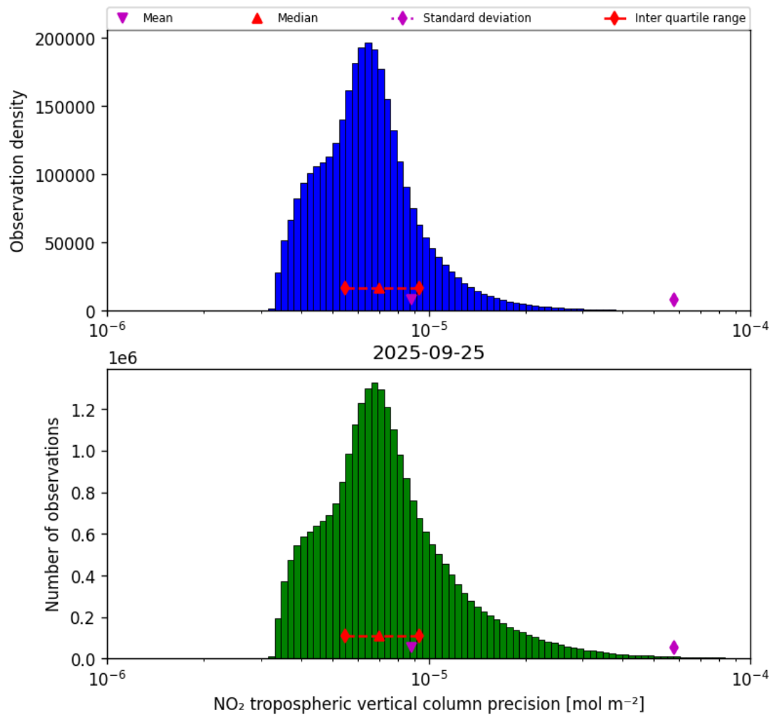
Figure 30: Histogram of “NO 2 tropospheric vertical column precision” for 2025-09-25 to 2025-09-26
