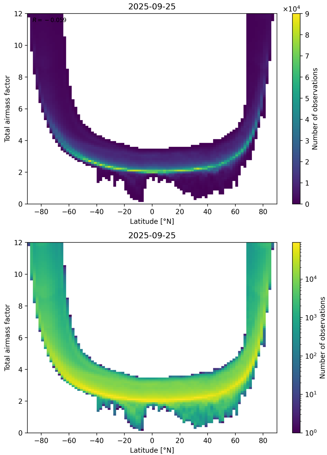
Figure 84: Scatter density plot of “Latitude” against “Total airmass factor” for 2025-09-25 to 2025-09-26.
