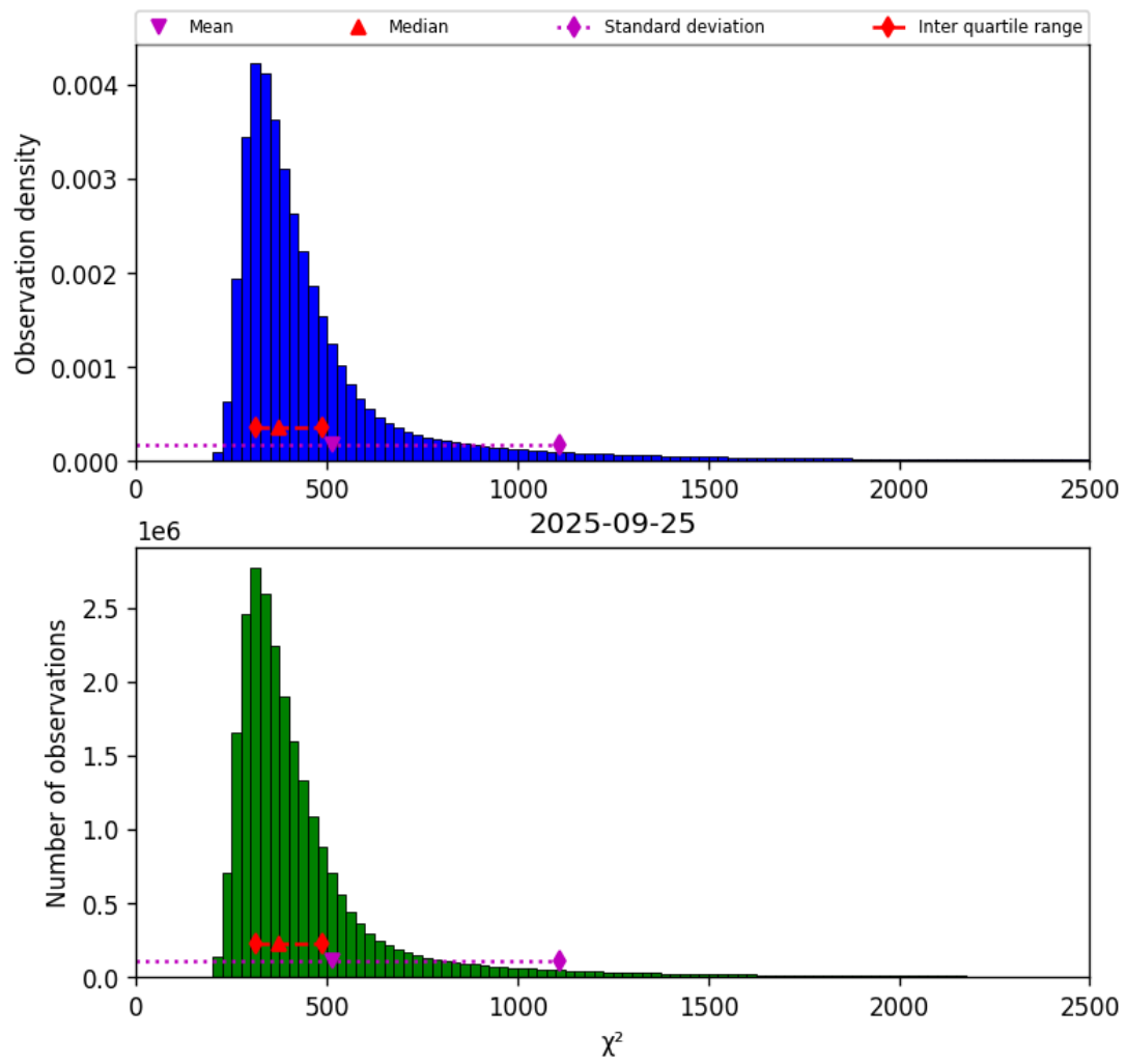
Figure 42: Histogram of “ \chi^2 ” for 2025-09-25 to 2025-09-26
