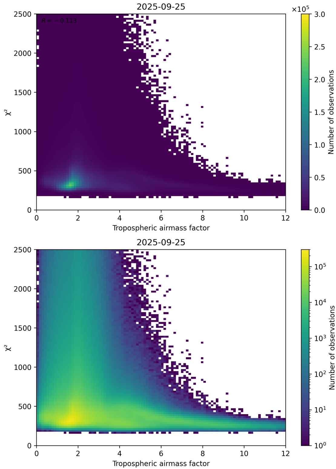
Figure 73: Scatter density plot of “Tropospheric airmass factor” against “ \chi^2 ” for 2025-09-25 to 2025-09-26.
