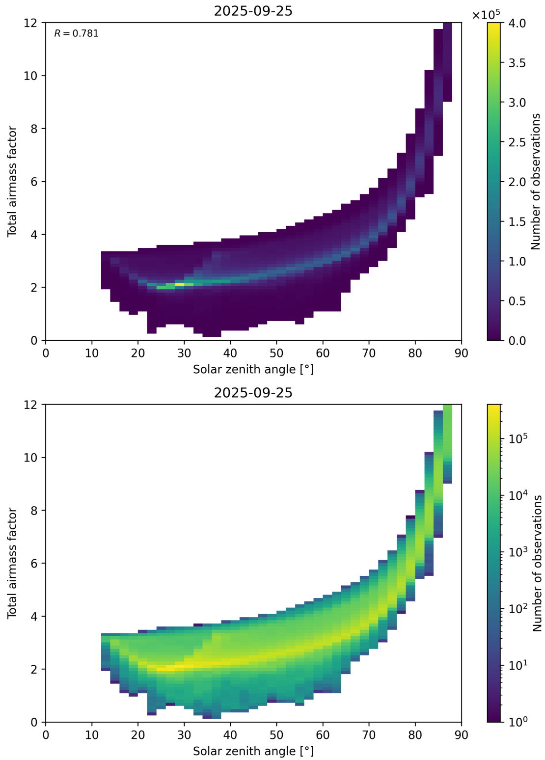
Figure 146: Scatter density plot of “Solar zenith angle” against “Total air mass factor” for 2025-09-25 to 2025-09-26.
