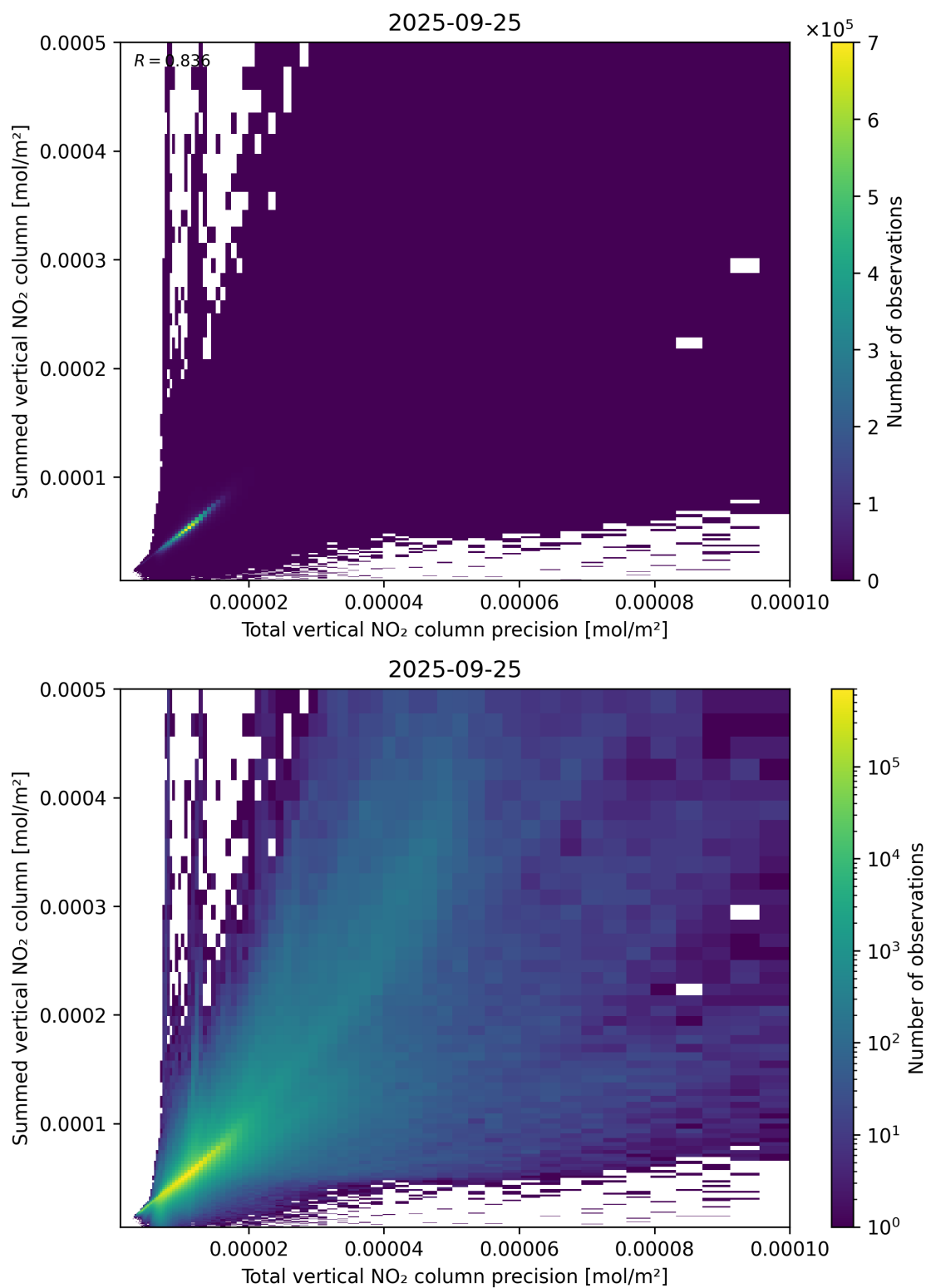
Figure 117: Scatter density plot of “Total vertical NO 2 column precision” against “Summed vertical NO 2 column” for 2025-09-25 to 2025-09-26.
