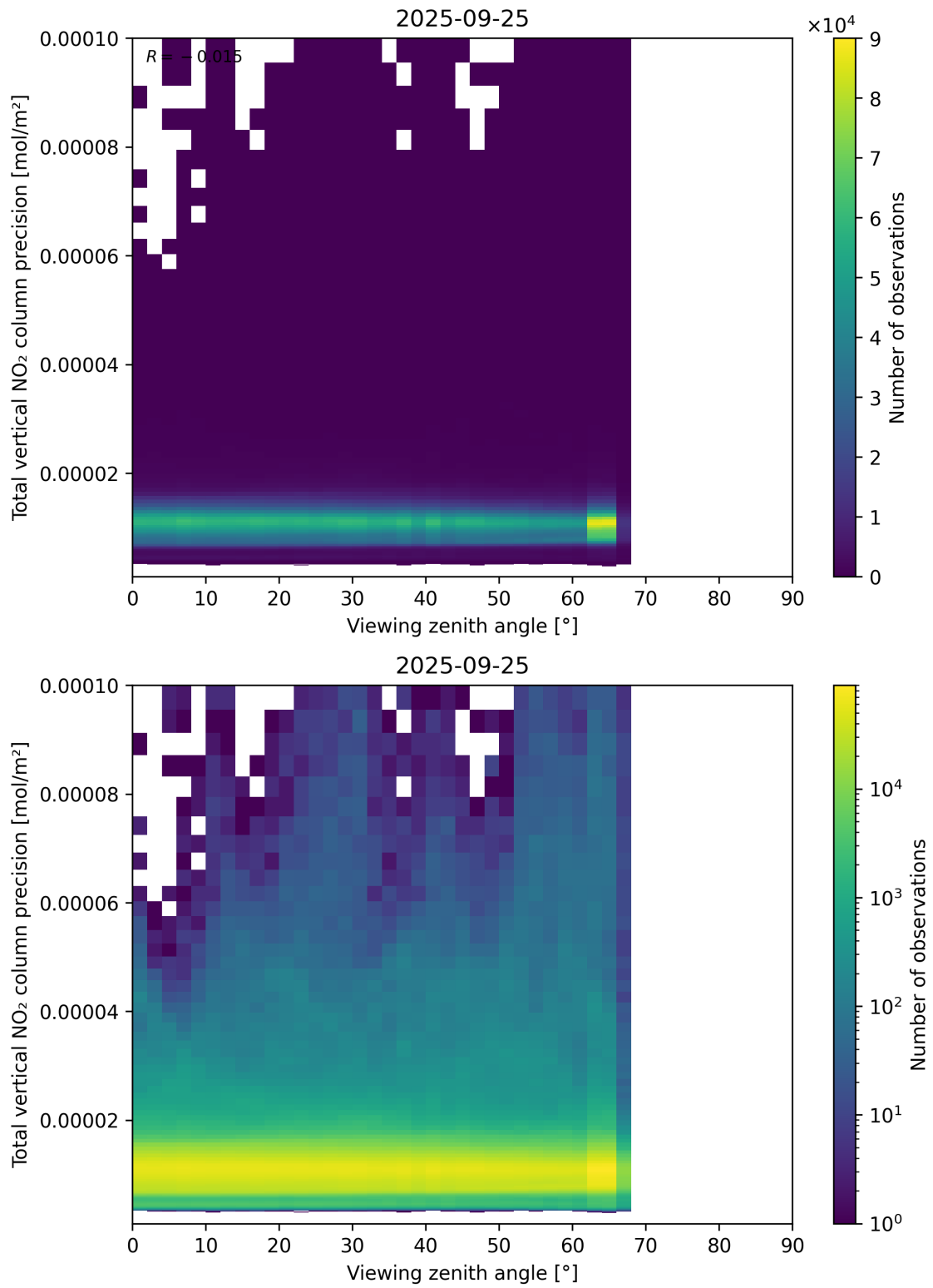
Figure 168: Scatter density plot of “Viewing zenith angle” against “Total vertical NO 2 column precision” for 2025-09-25 to 2025-09-26.
