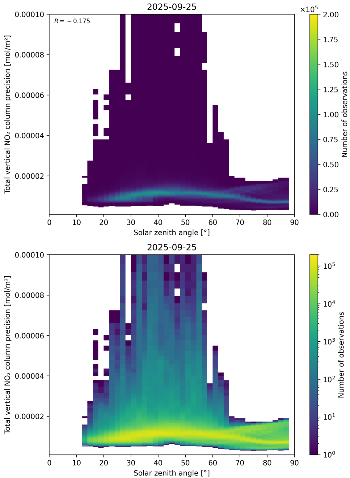
Figure 154: Scatter density plot of “Solar zenith angle” against “Total vertical NO 2 column precision” for 2025-09-25 to 2025-09-26.
