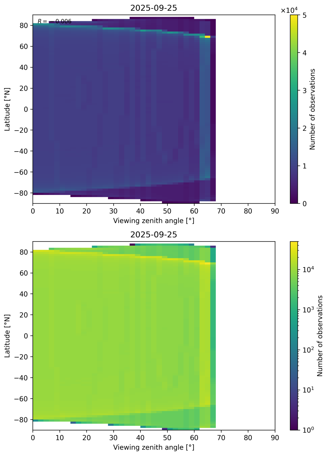
Figure 163: Scatter density plot of “Viewing zenith angle” against “Latitude” for 2025-09-25 to 2025-09-26.
