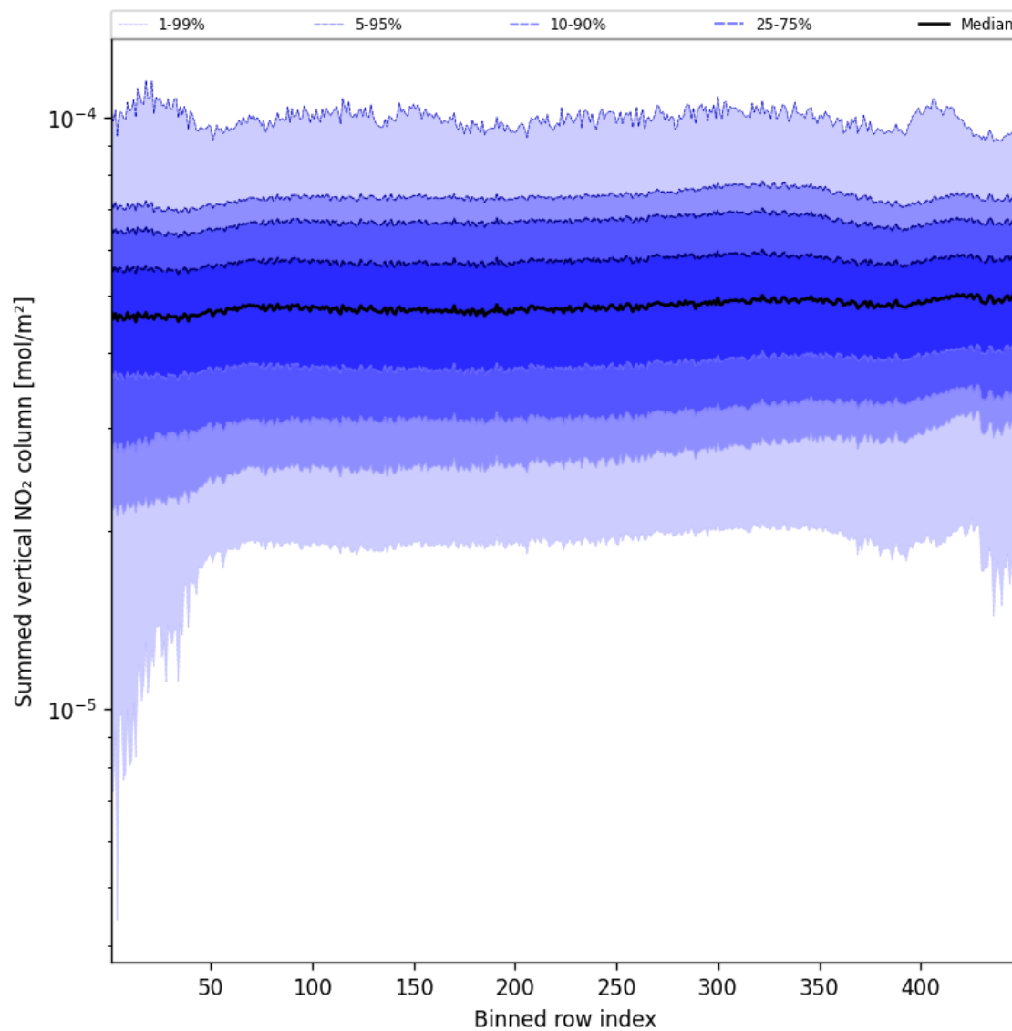
Figure 57: Along track statistics of “Summed vertical NO 2 column” for 2025-09-25 to 2025-09-26
