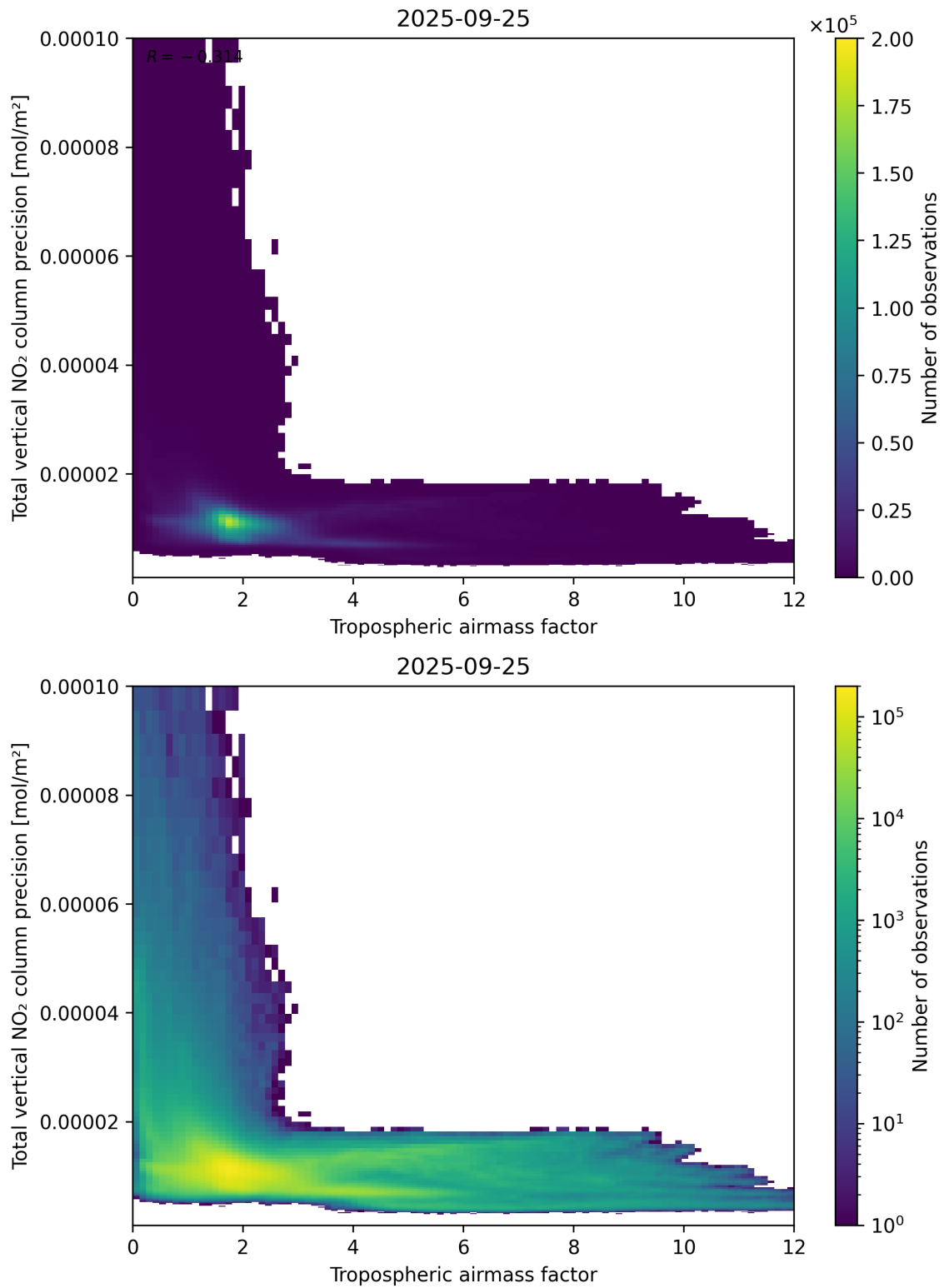
Figure 78: Scatter density plot of “Tropospheric air mass factor” against “Total vertical NO 2 column precision” for 2025-09-25 to 2025-09-26.
