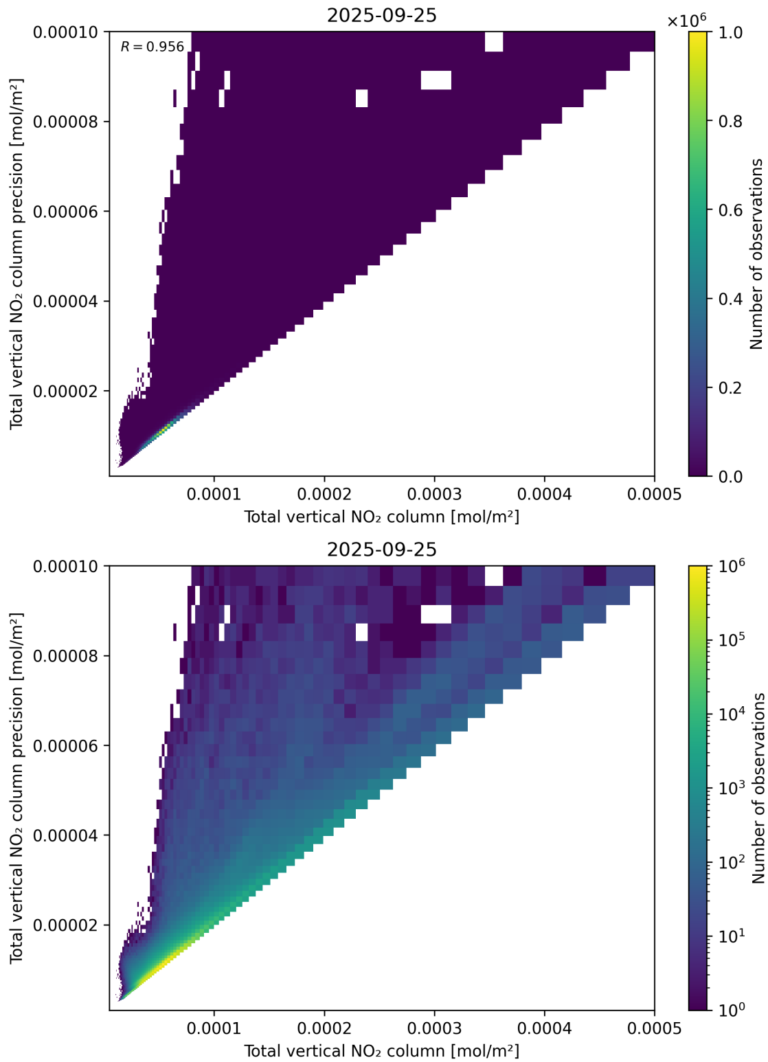
Figure 114: Scatter density plot of “Total vertical NO 2 column” against “Total vertical NO 2 column precision” for 2025-09-25 to 2025-09-26.
