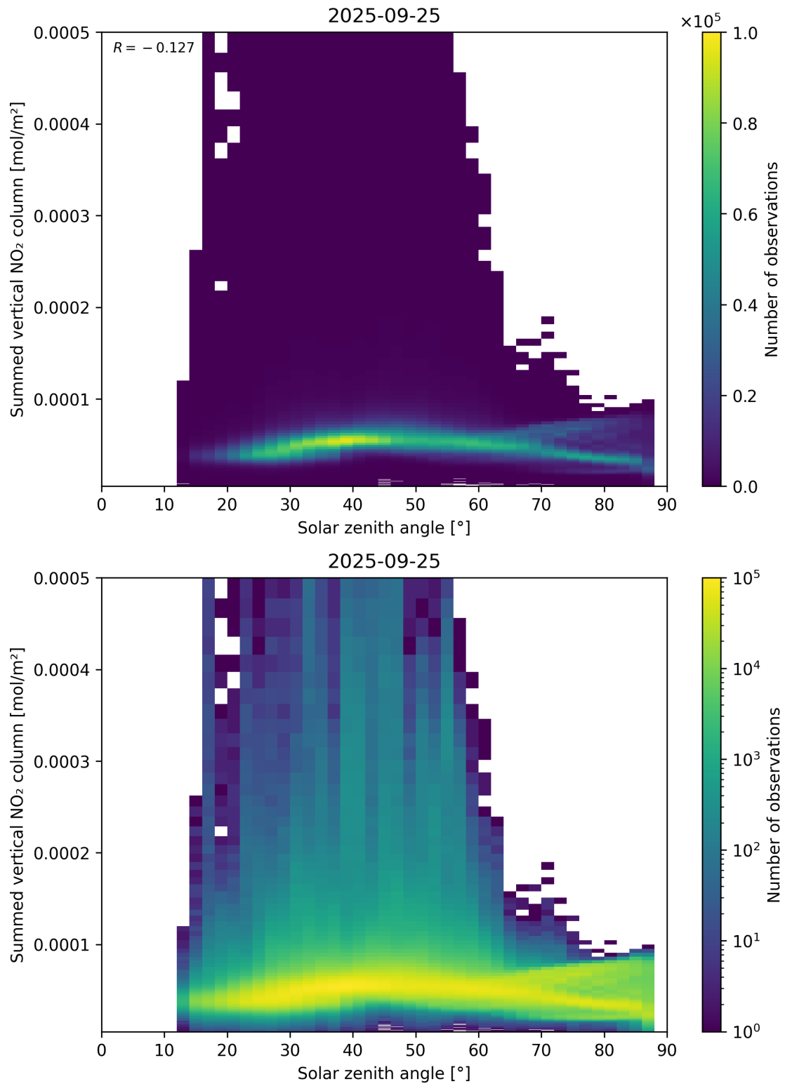
Figure 151: Scatter density plot of “Solar zenith angle” against “Summed vertical NO 2 column” for 2025-09-25 to 2025-09-26.
