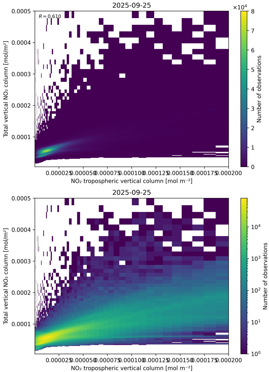
Figure 128: Scatter density plot of “NO 2 tropospheric vertical column” against “Total vertical NO 2 column” for 2025-09-25 to 2025-09-26.
