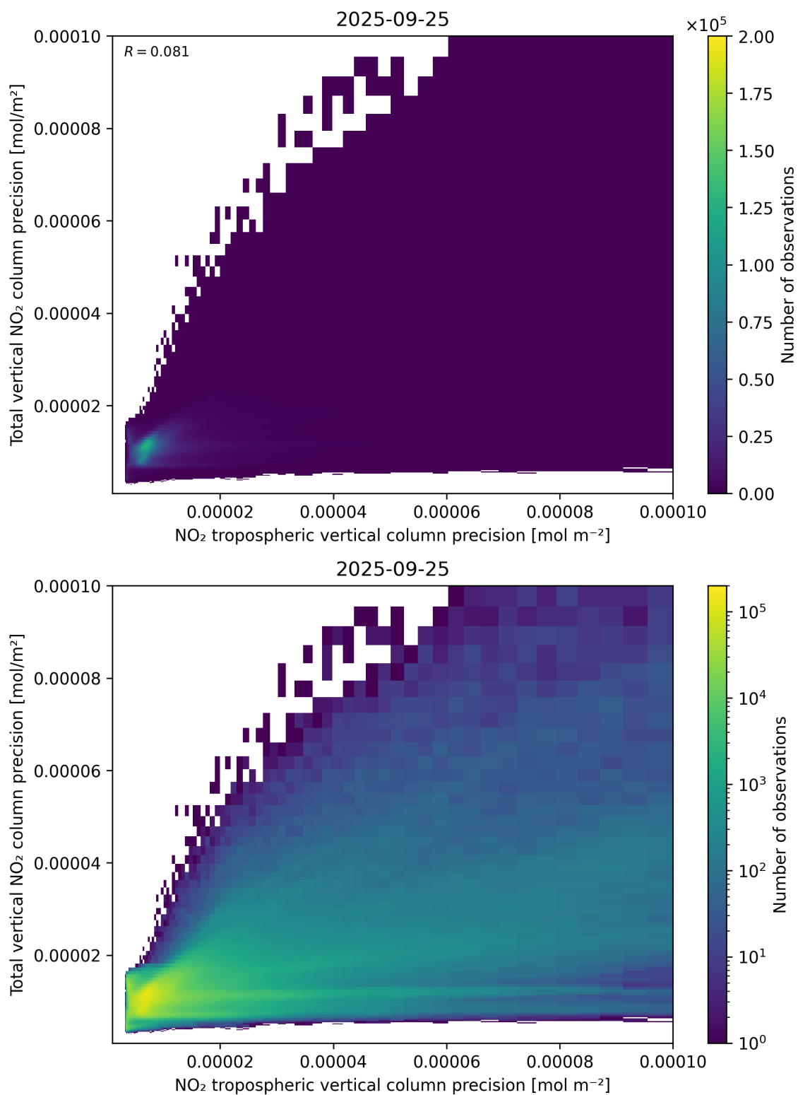
Figure 139: Scatter density plot of “NO 2 tropospheric vertical column precision” against “Total vertical NO 2 column precision” for 2025-09-25 to 2025-09-26.
