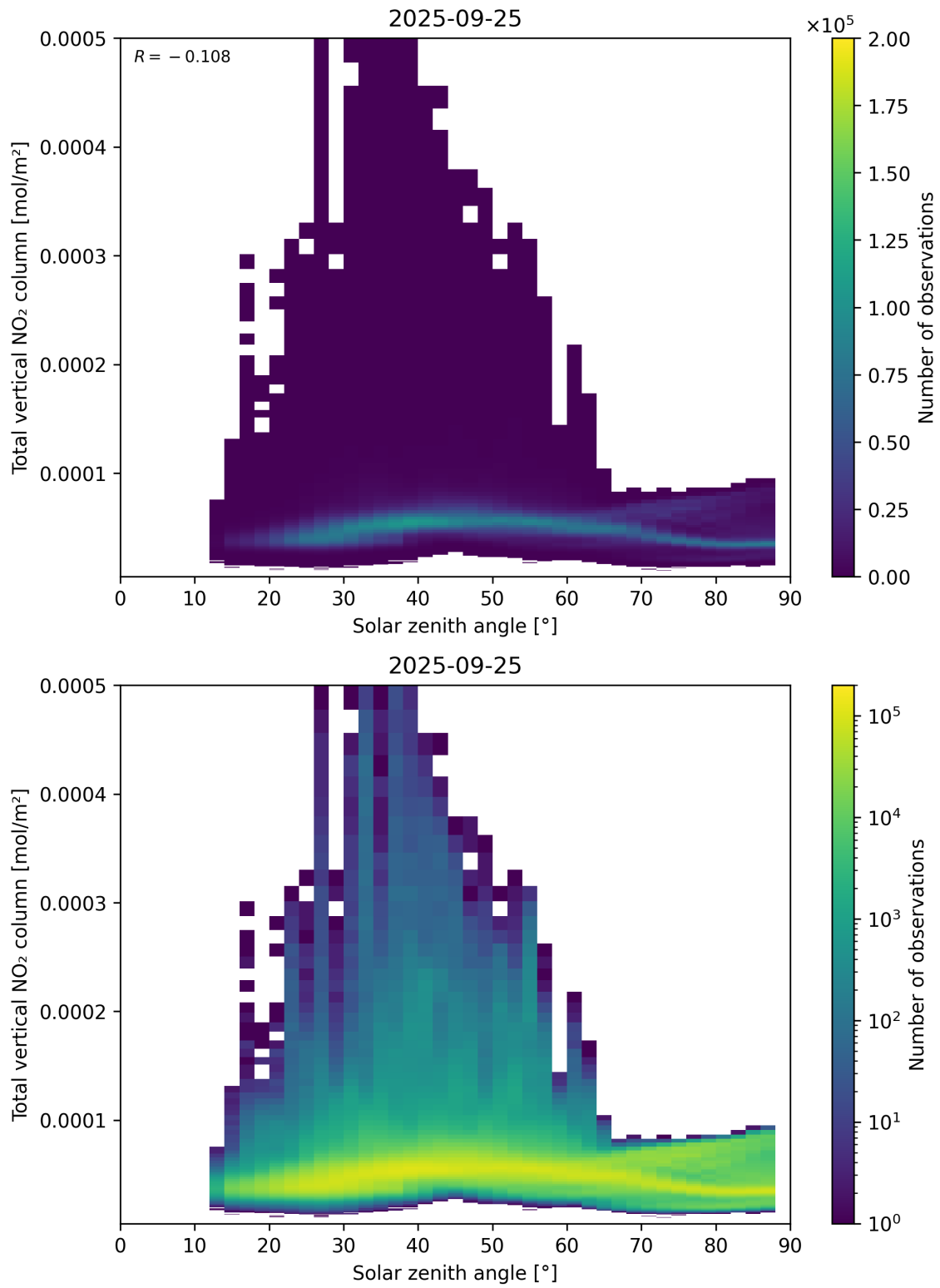
Figure 153: Scatter density plot of “Solar zenith angle” against “Total vertical NO 2 column” for 2025-09-25 to 2025-09-26.
