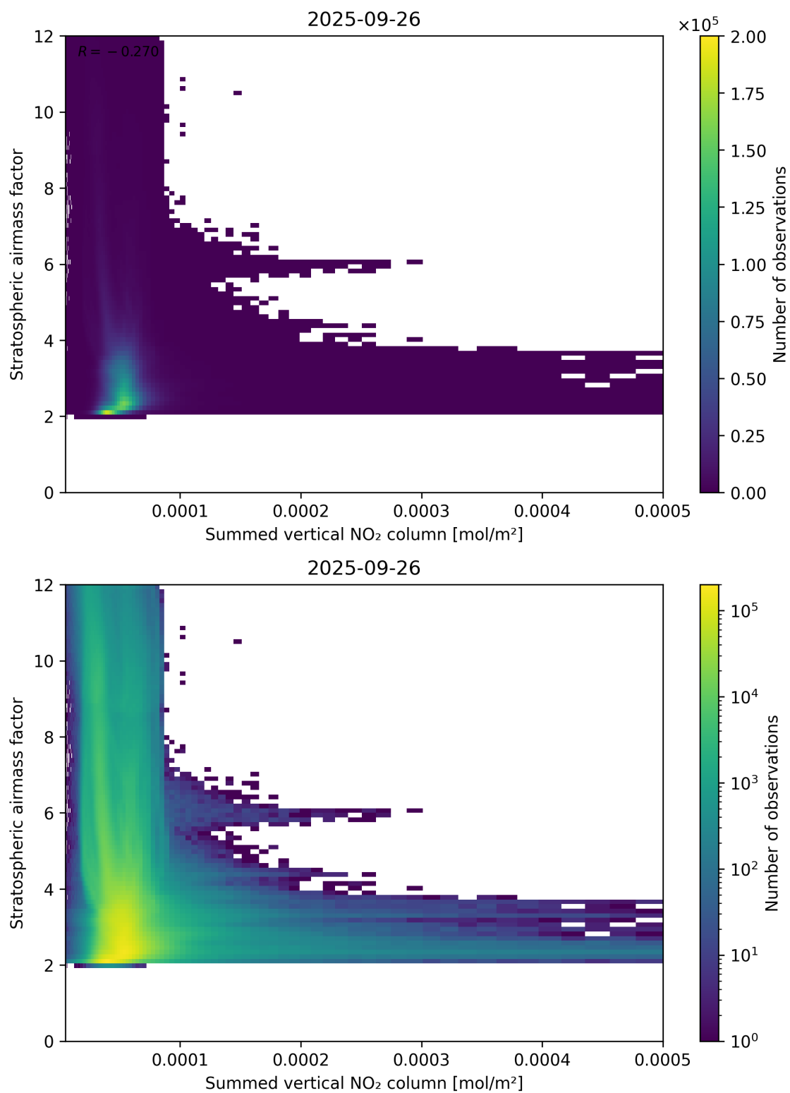
Figure 103: Scatter density plot of “Summed vertical NO 2 column” against “Stratospheric air mass factor” for 2025-09-26 to 2025-09-27.
