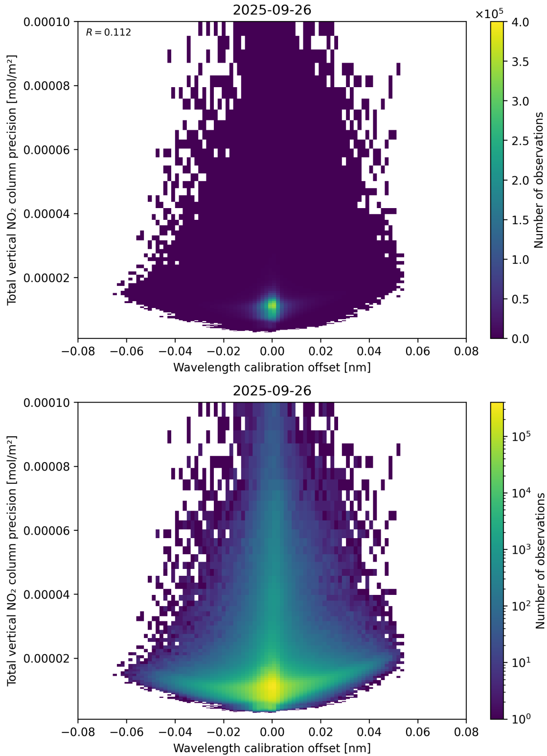
Figure 180: Scatter density plot of “Wavelength calibration offset” against “Total vertical NO 2 column precision” for 2025-09-26 to 2025-09-27.
