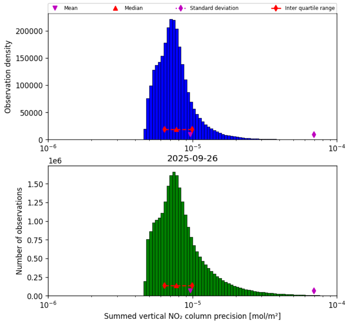
Figure 41: Histogram of “Summed vertical NO 2 column precision” for 2025-09-26 to 2025-09-27
