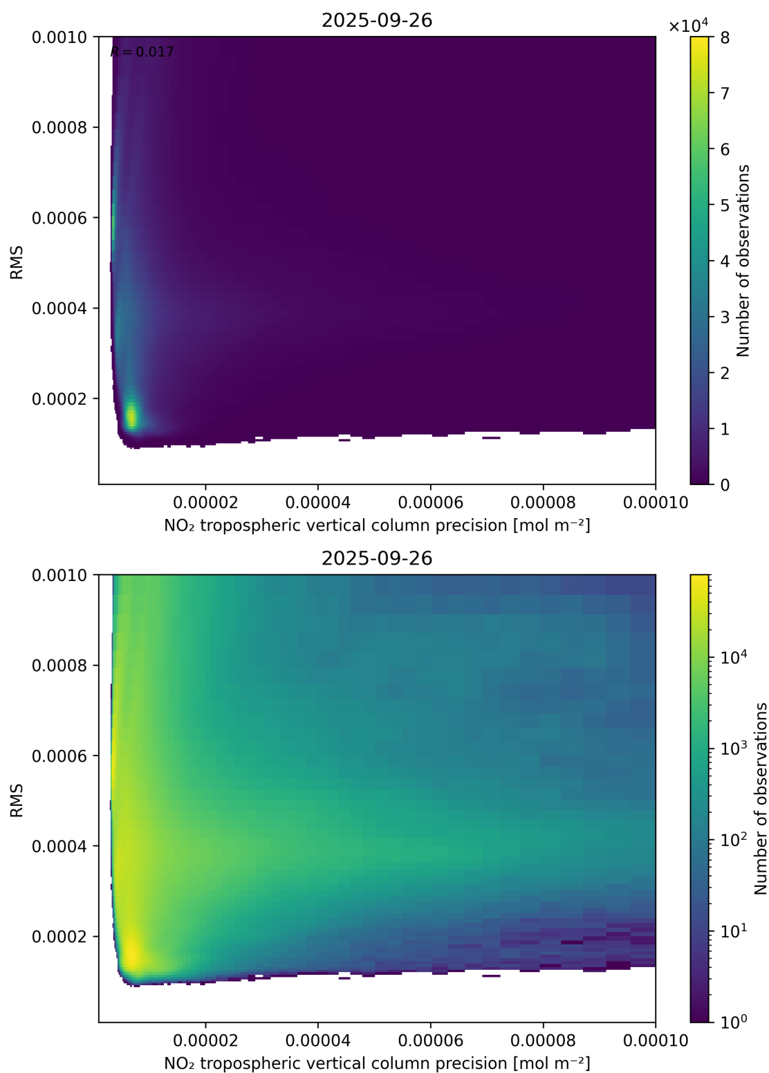
Figure 140: Scatter density plot of “NO 2 tropospheric vertical column precision” against “RMS” for 2025-09-26 to 2025-09-27.
