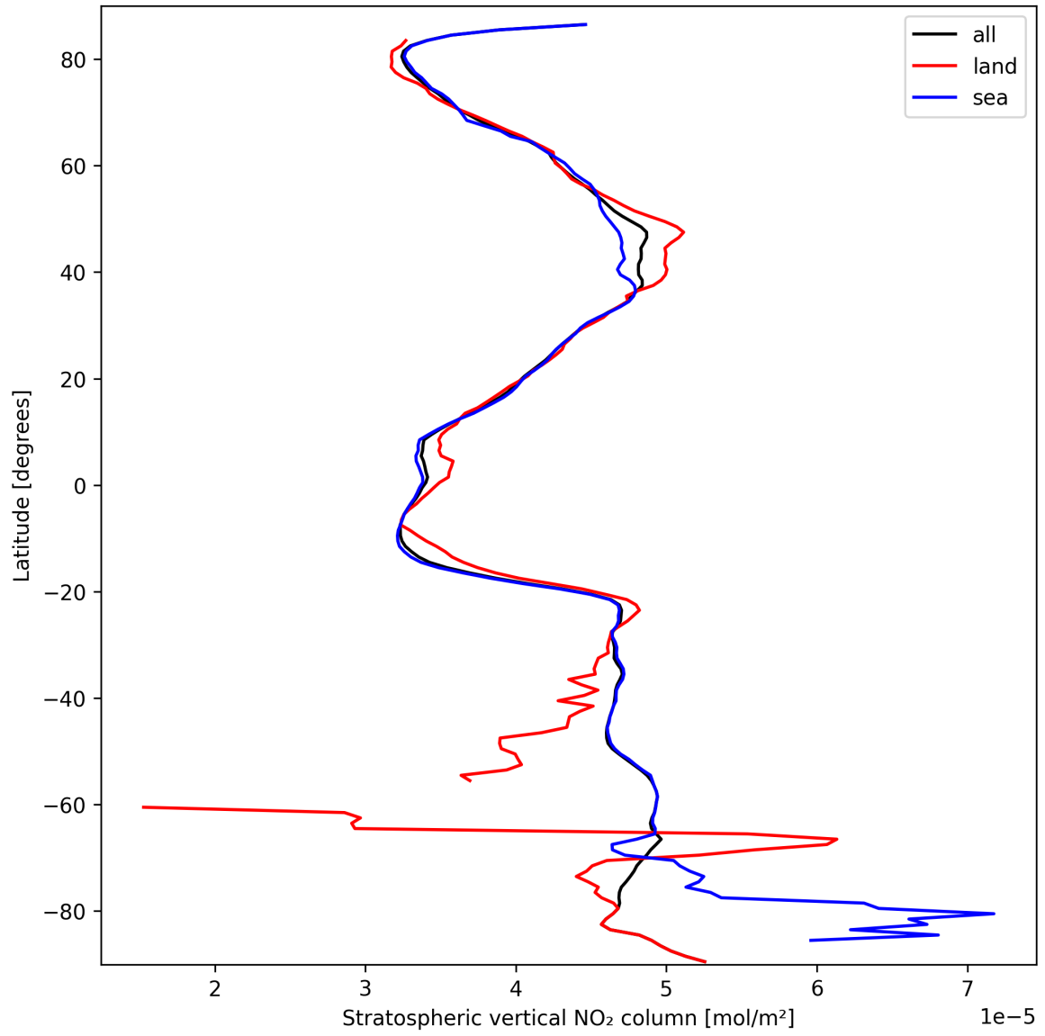
Figure 19: Zonal average of “Stratospheric vertical NO 2 column” for 2025-09-26 to 2025-09-27.
