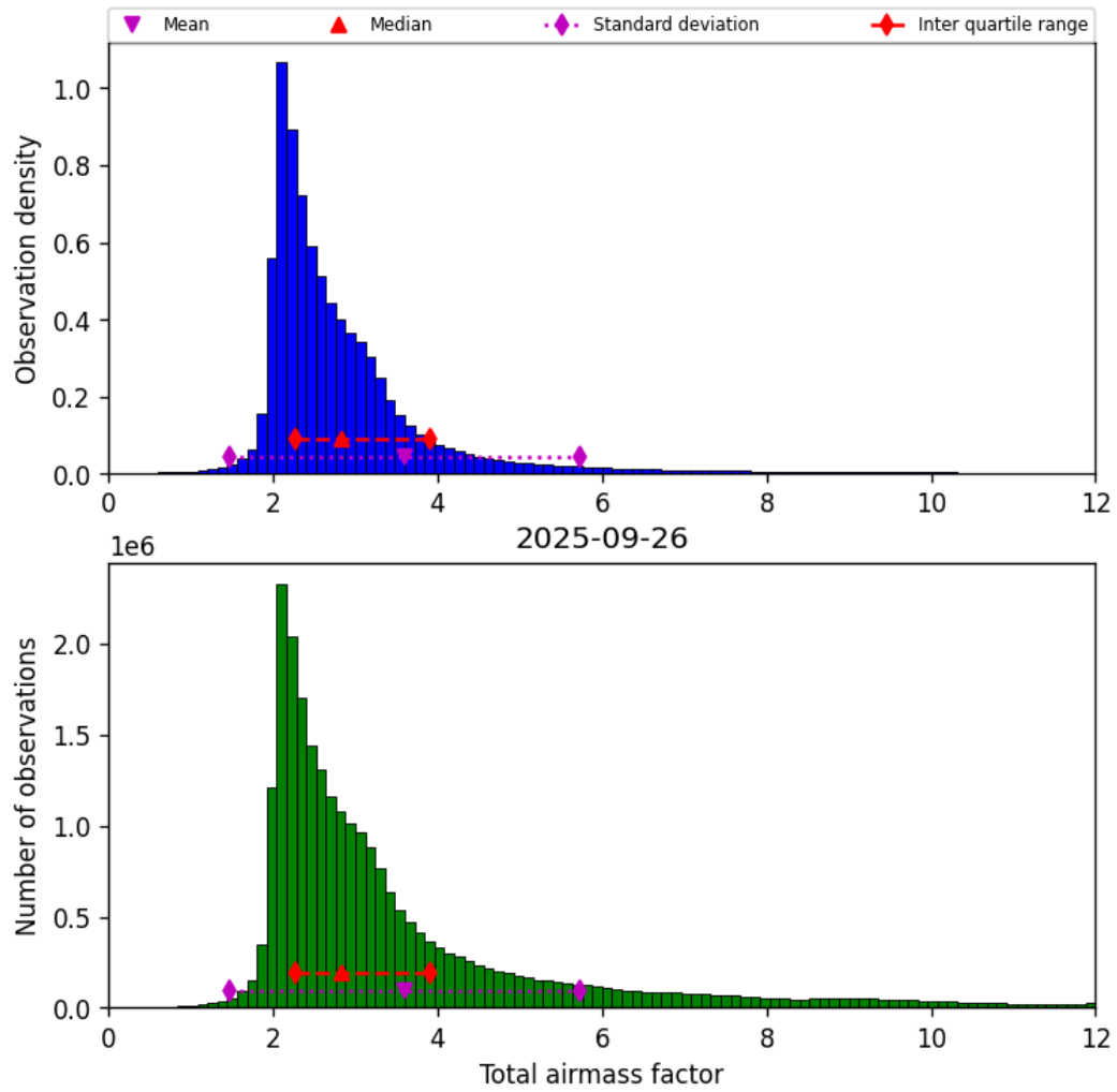
Figure 32: Histogram of “Total airmass factor” for 2025-09-26 to 2025-09-27
