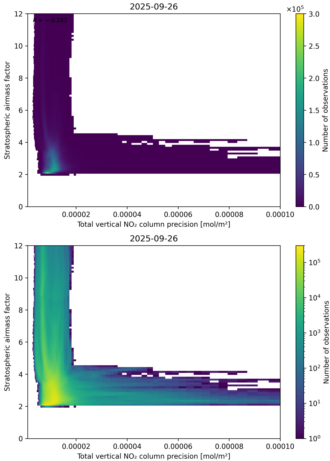
Figure 115: Scatter density plot of “Total vertical NO 2 column precision” against “Stratospheric air mass factor” for 2025-09-26 to 2025-09-27.
