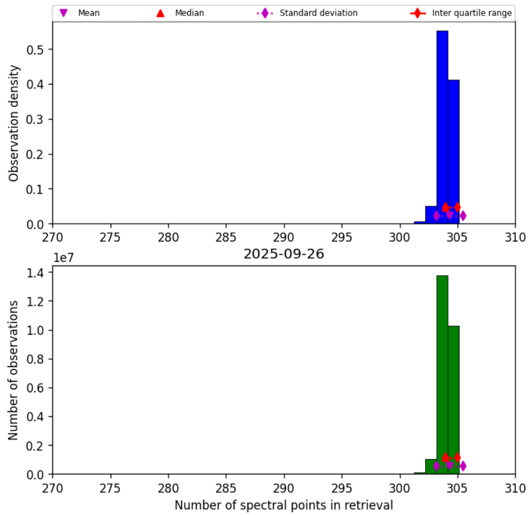
Figure 33: Histogram of “Number of spectral points in retrieval” for 2025-09-26 to 2025-09-27
