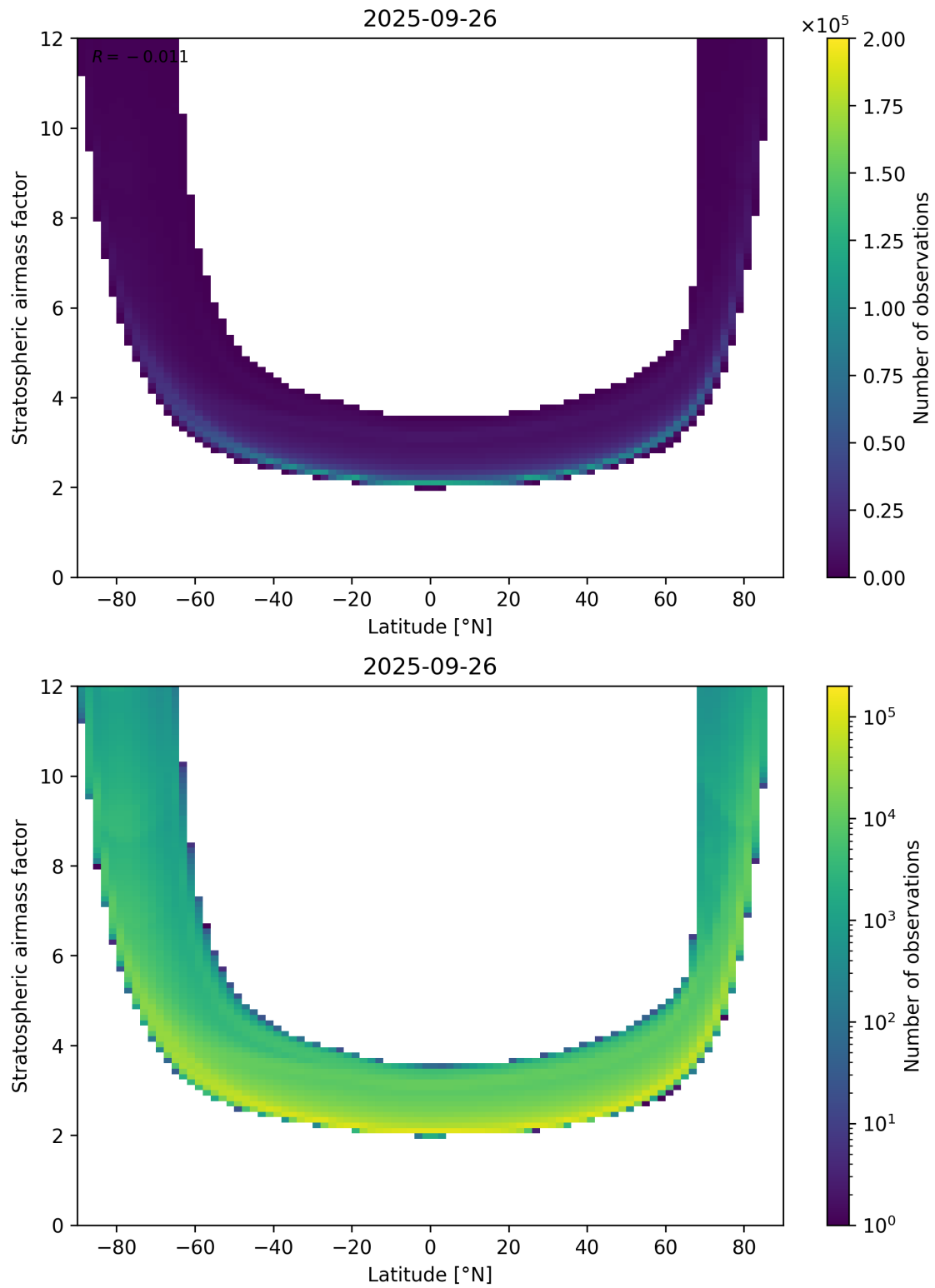
Figure 83: Scatter density plot of “Latitude” against “Stratospheric air mass factor” for 2025-09-26 to 2025-09-27.
