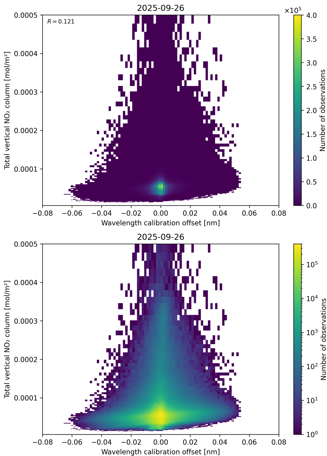
Figure 179: Scatter density plot of “Wavelength calibration offset” against “Total vertical NO 2 column” for 2025-09-26 to 2025-09-27.
