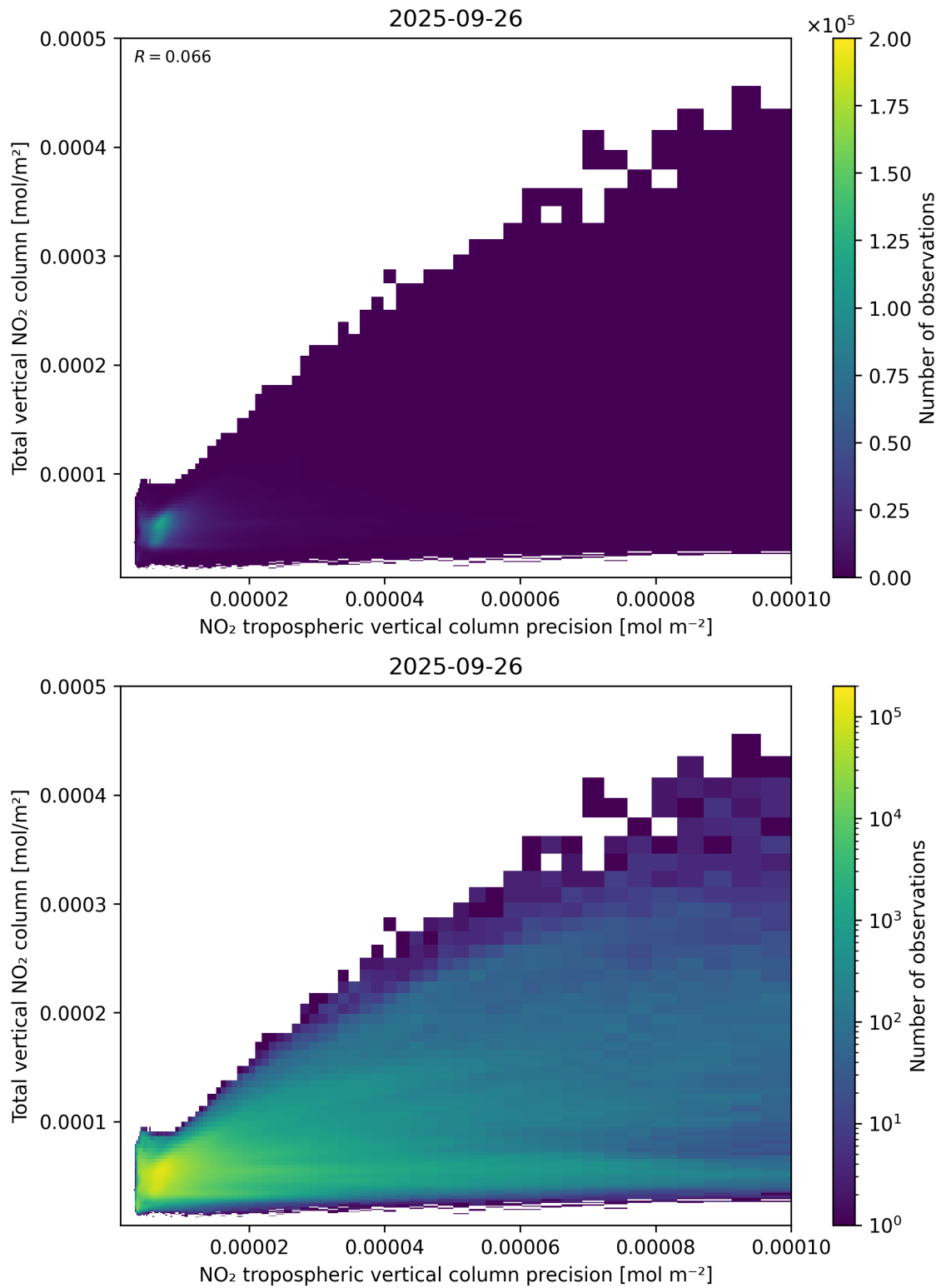
Figure 138: Scatter density plot of “NO 2 tropospheric vertical column precision” against “Total vertical NO 2 column” for 2025-09-26 to 2025-09-27.
