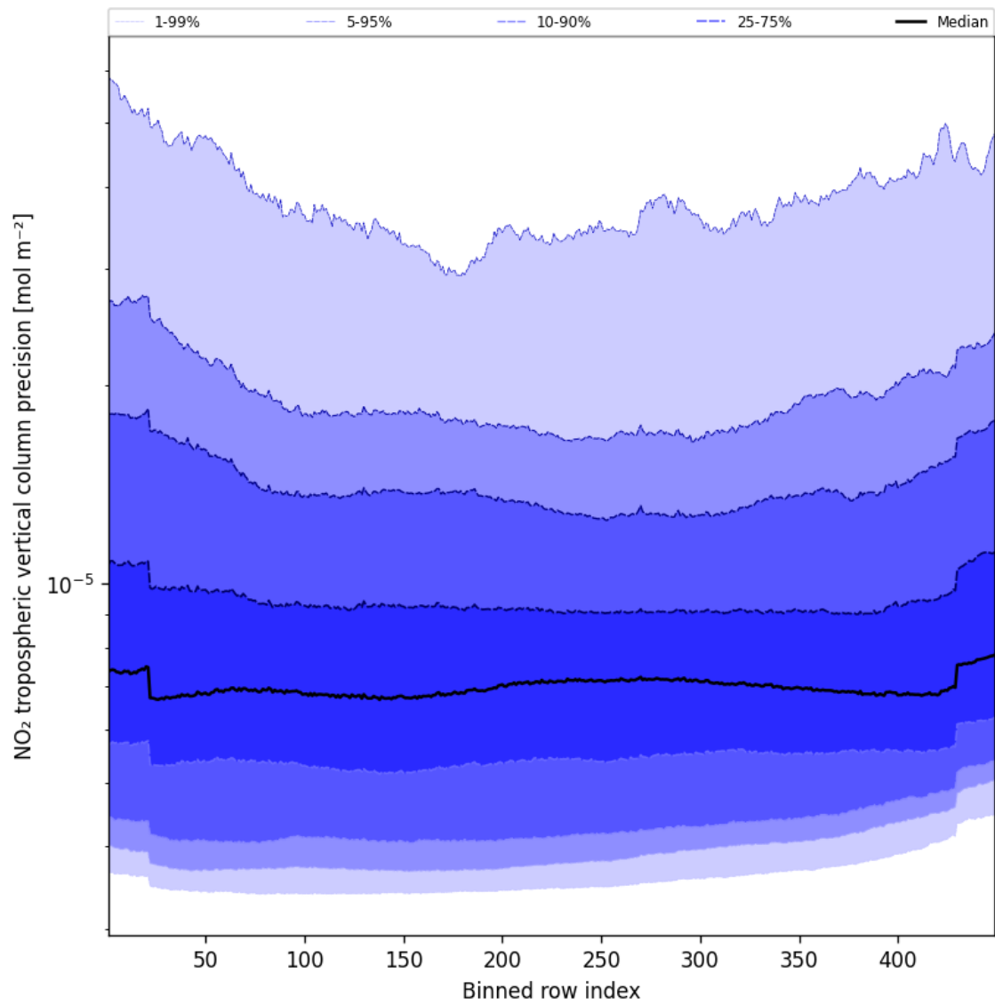
Figure 47: Along track statistics of “NO 2 tropospheric vertical column precision” for 2025-09-26 to 2025-09-27
