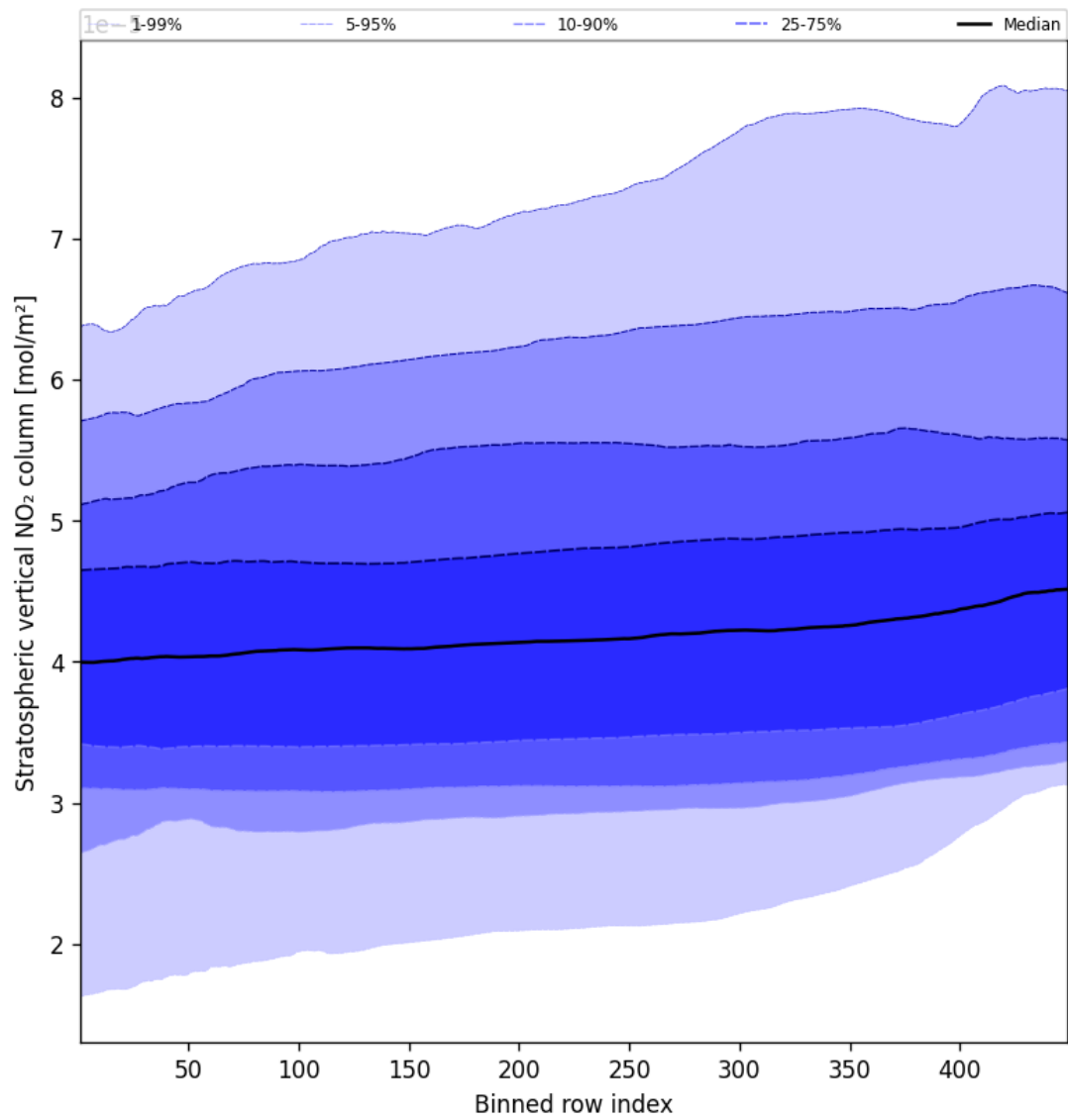
Figure 53: Along track statistics of "Stratospheric vertical NO 2 column" for 2025-09-26 to 2025-09-27
