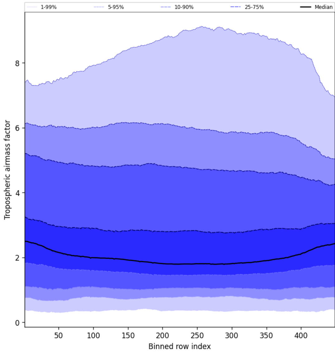
Figure 48: Along track statistics of “Tropospheric air mass factor” for 2025-09-26 to 2025-09-27
