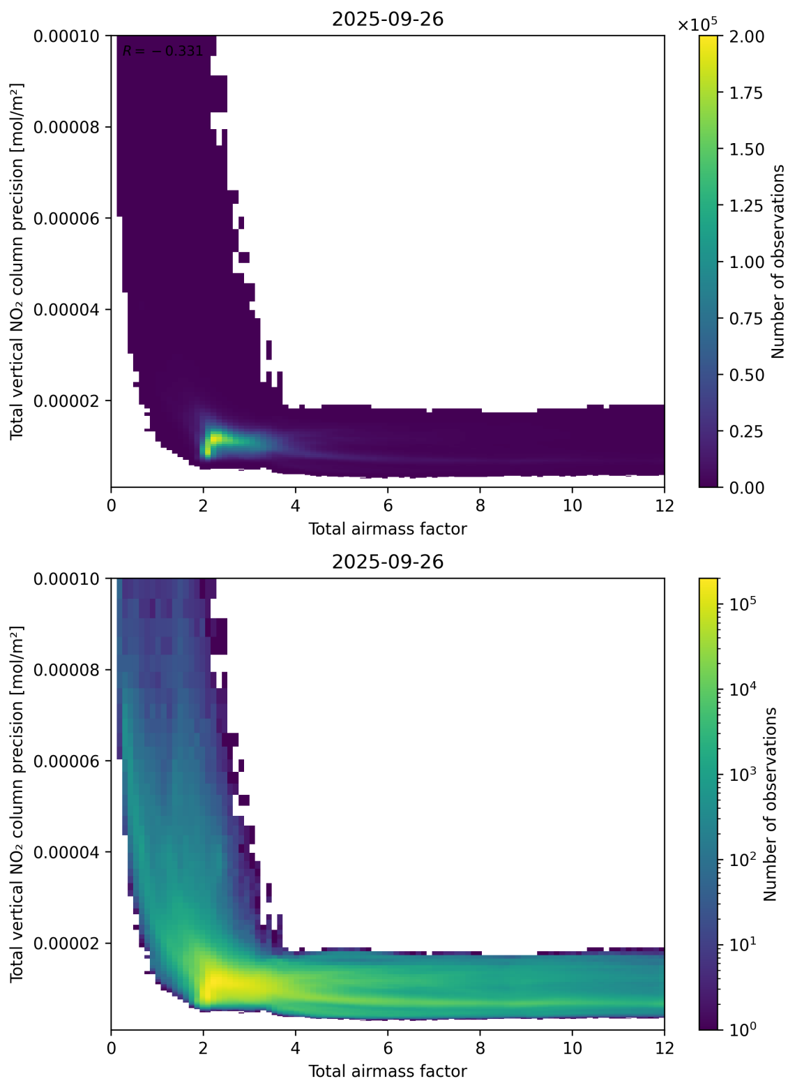
Figure 68: Scatter density plot of “Total airmass factor” against “Total vertical NO 2 column precision” for 2025-09-26 to 2025-09-27.
