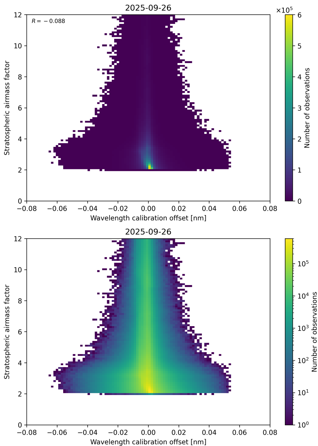
Figure 174: Scatter density plot of “Wavelength calibration offset” against “Stratospheric air mass factor” for 2025-09-26 to 2025-09-27.
