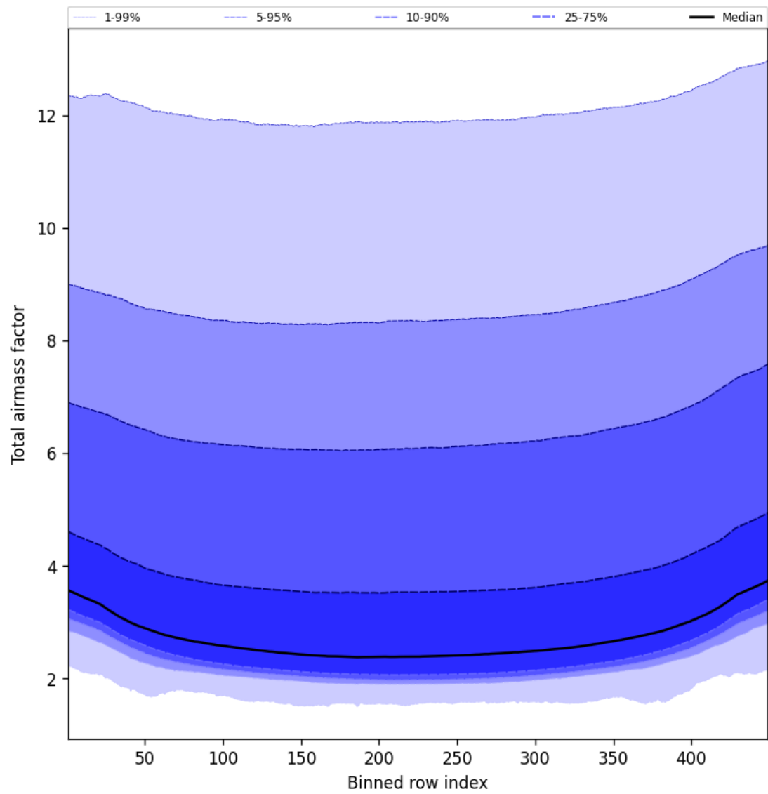
Figure 49: Along track statistics of “Total airmass factor” for 2025-09-26 to 2025-09-27
