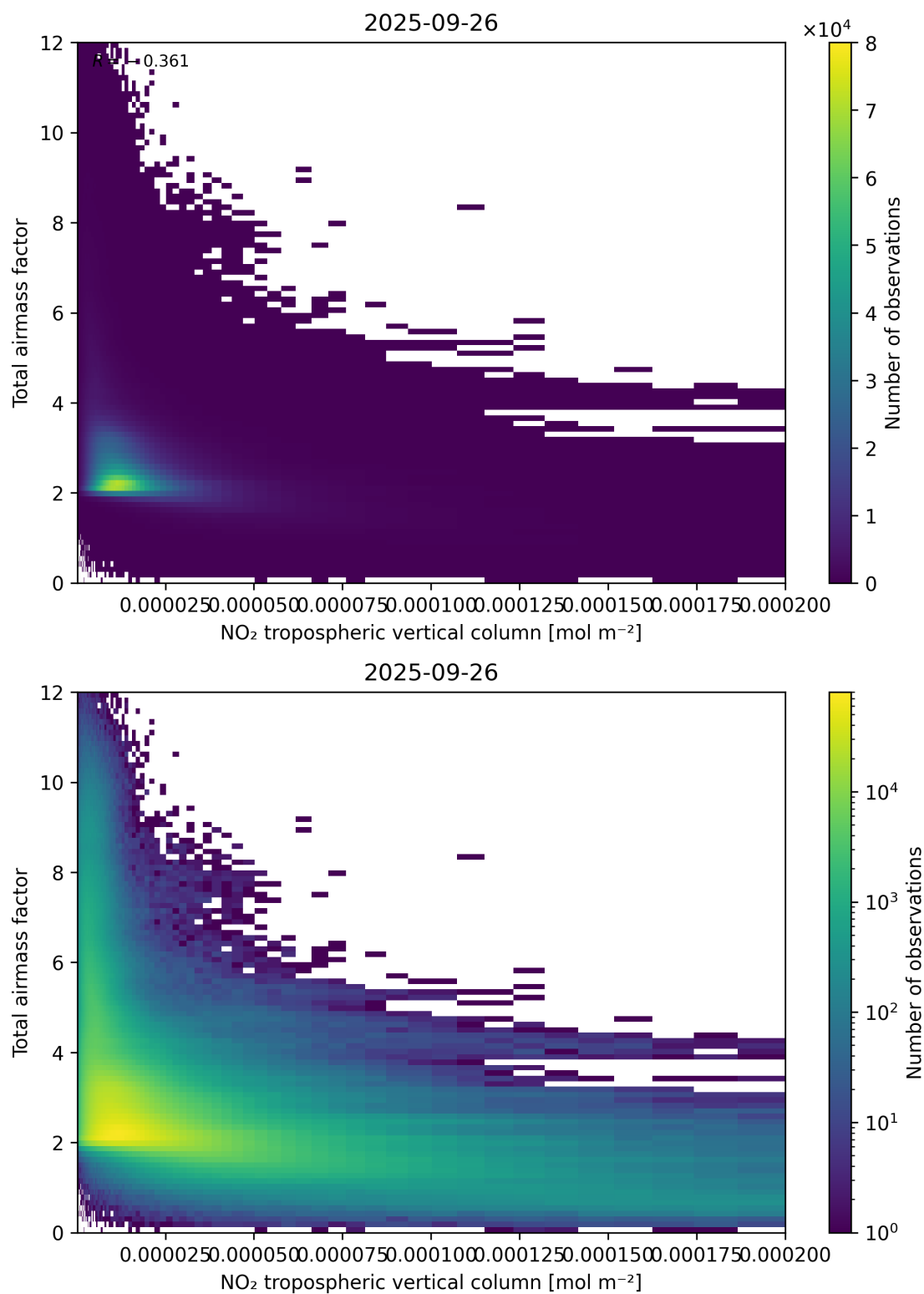
Figure 122: Scatter density plot of “NO 2 tropospheric vertical column” against “Total air mass factor” for 2025-09-26 to 2025-09-27.
