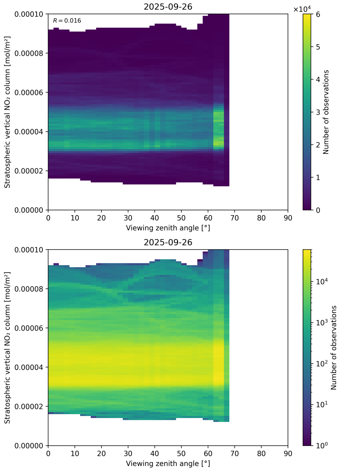
Figure 164: Scatter density plot of “Viewing zenith angle” against “Stratospheric vertical NO 2 column” for 2025-09-26 to 2025-09-27.
