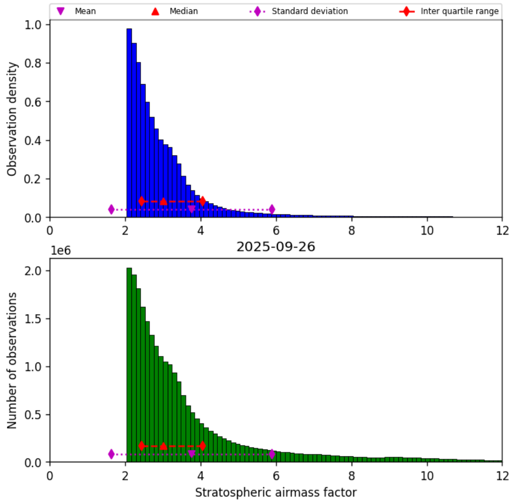
Figure 44: Histogram of “Stratospheric airmass factor” for 2025-09-26 to 2025-09-27
