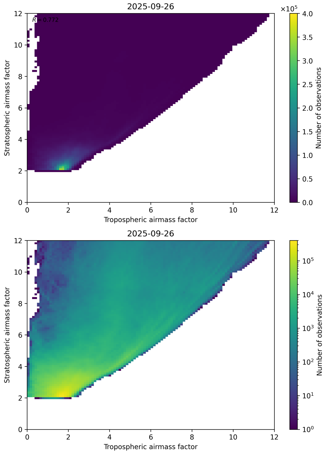
Figure 71: Scatter density plot of “Tropospheric airmass factor” against “Stratospheric airmass factor” for 2025-09-26 to 2025-09-27.
