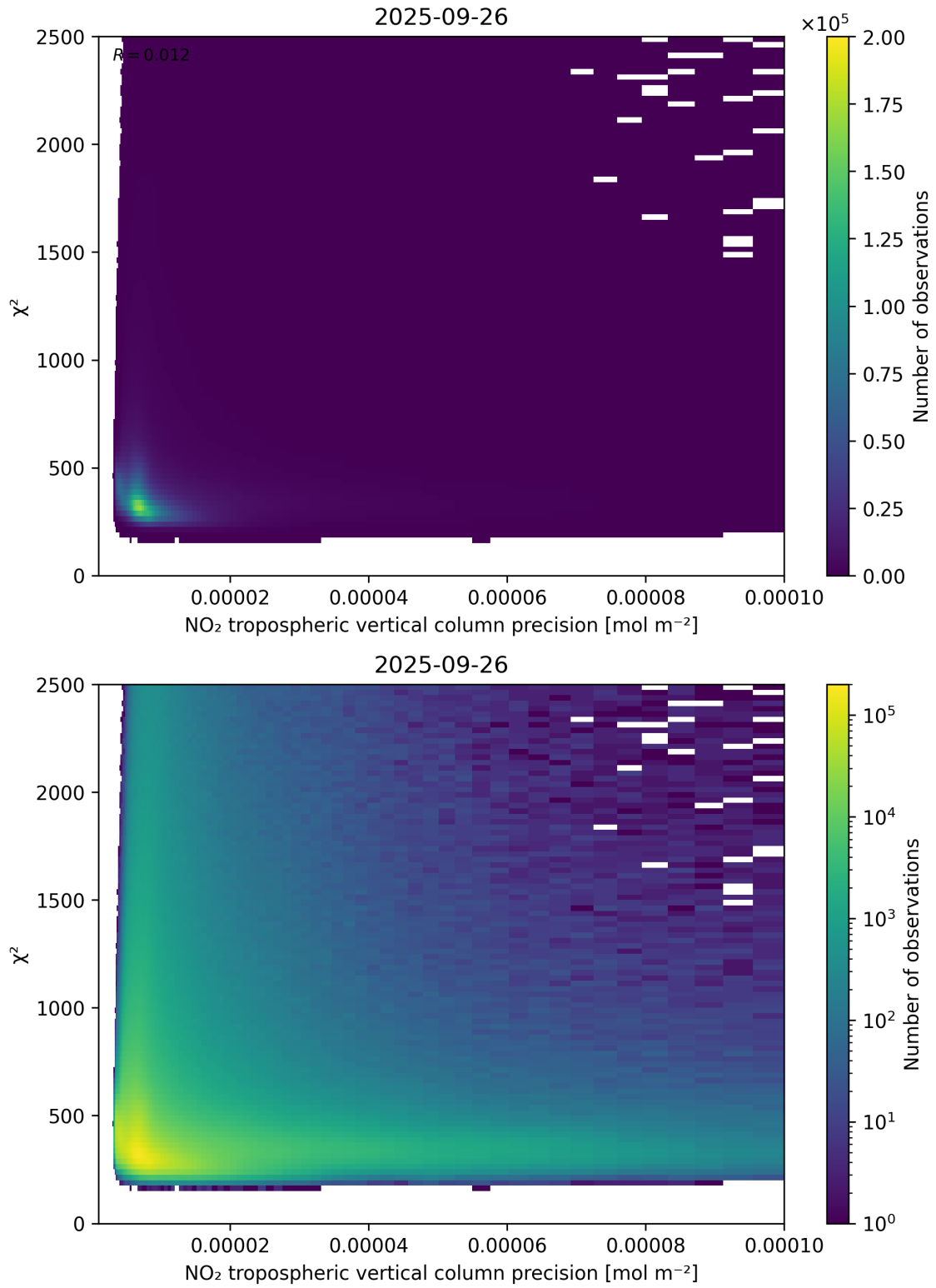
Figure 134: Scatter density plot of “NO 2 tropospheric vertical column precision” against “ \chi^2 ” for 2025-09-26 to 2025-09-27.
