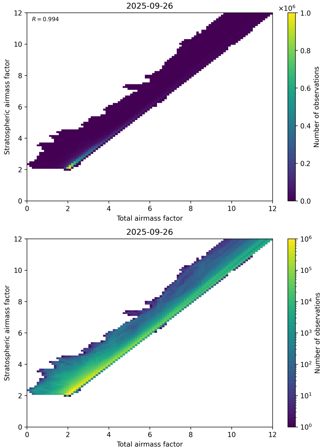
Figure 62: Scatter density plot of “Total airmass factor” against “Stratospheric airmass factor” for 2025-09-26 to 2025-09-27.
