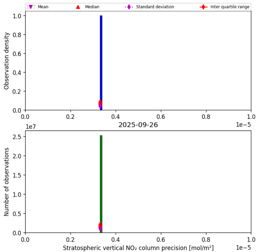
Figure 37: Histogram of “Stratospheric vertical NO 2 column precision” for 2025-09-26 to 2025-09-27
