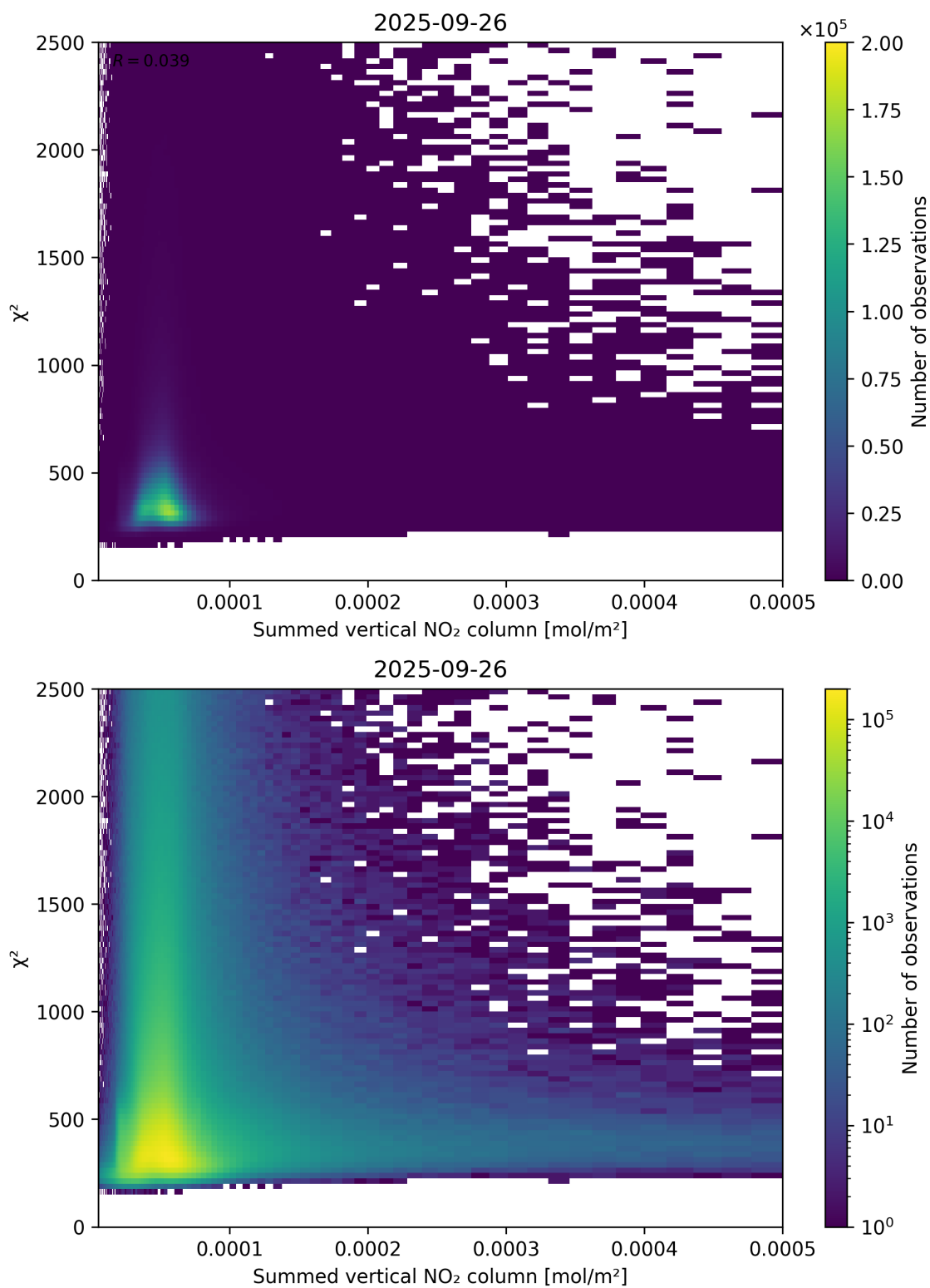
Figure 104: Scatter density plot of “Summed vertical NO 2 column” against “ \chi^2 ” for 2025-09-26 to 2025-09-27.
