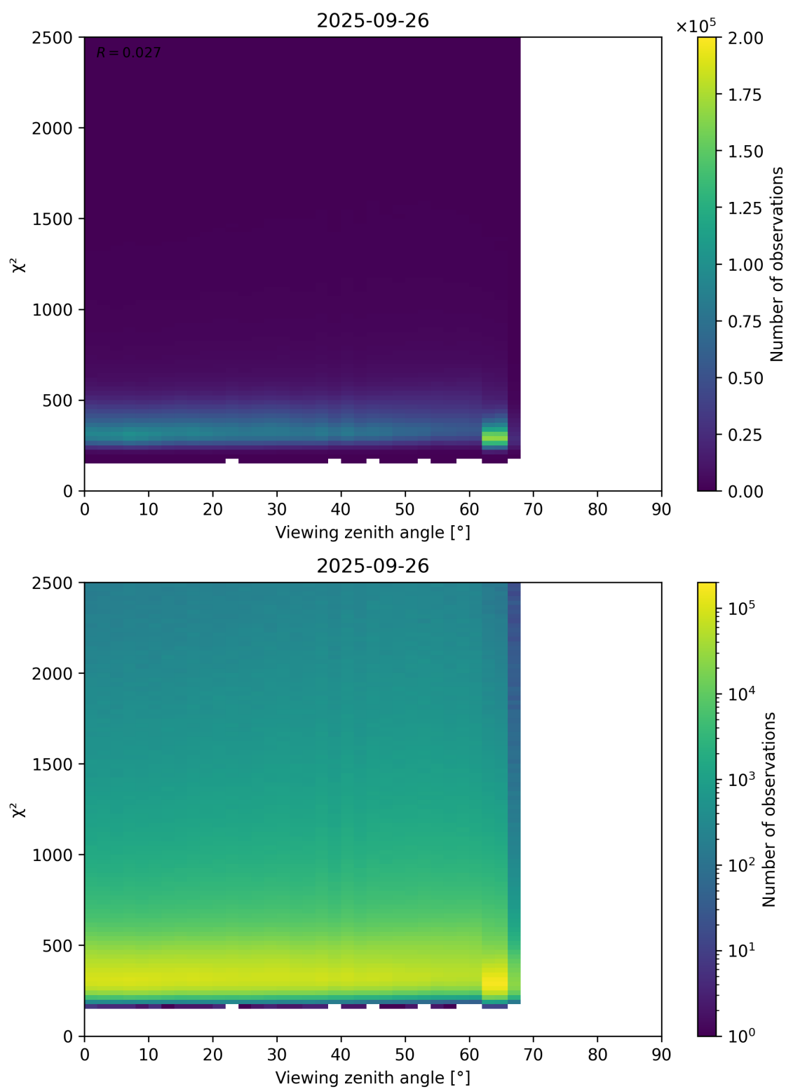
Figure 162: Scatter density plot of “Viewing zenith angle” against “ \chi^2 ” for 2025-09-26 to 2025-09-27.
