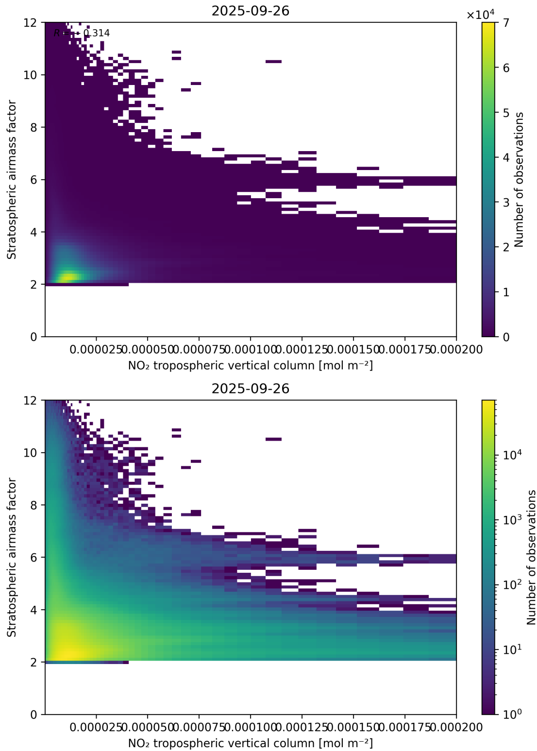
Figure 121: Scatter density plot of “NO 2 tropospheric vertical column” against “Stratospheric air mass factor” for 2025-09-26 to 2025-09-27.
