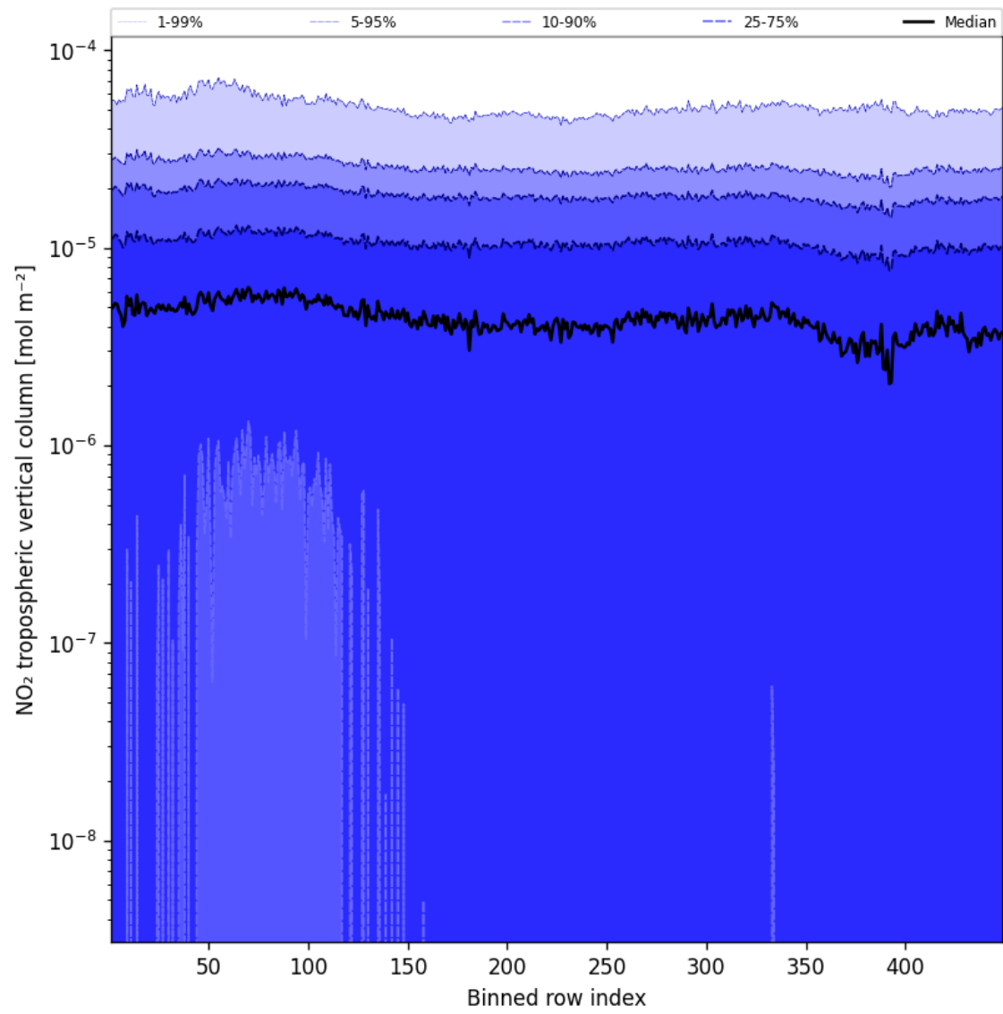
Figure 46: Along track statistics of “NO 2 tropospheric vertical column” for 2025-09-26 to 2025-09-27
