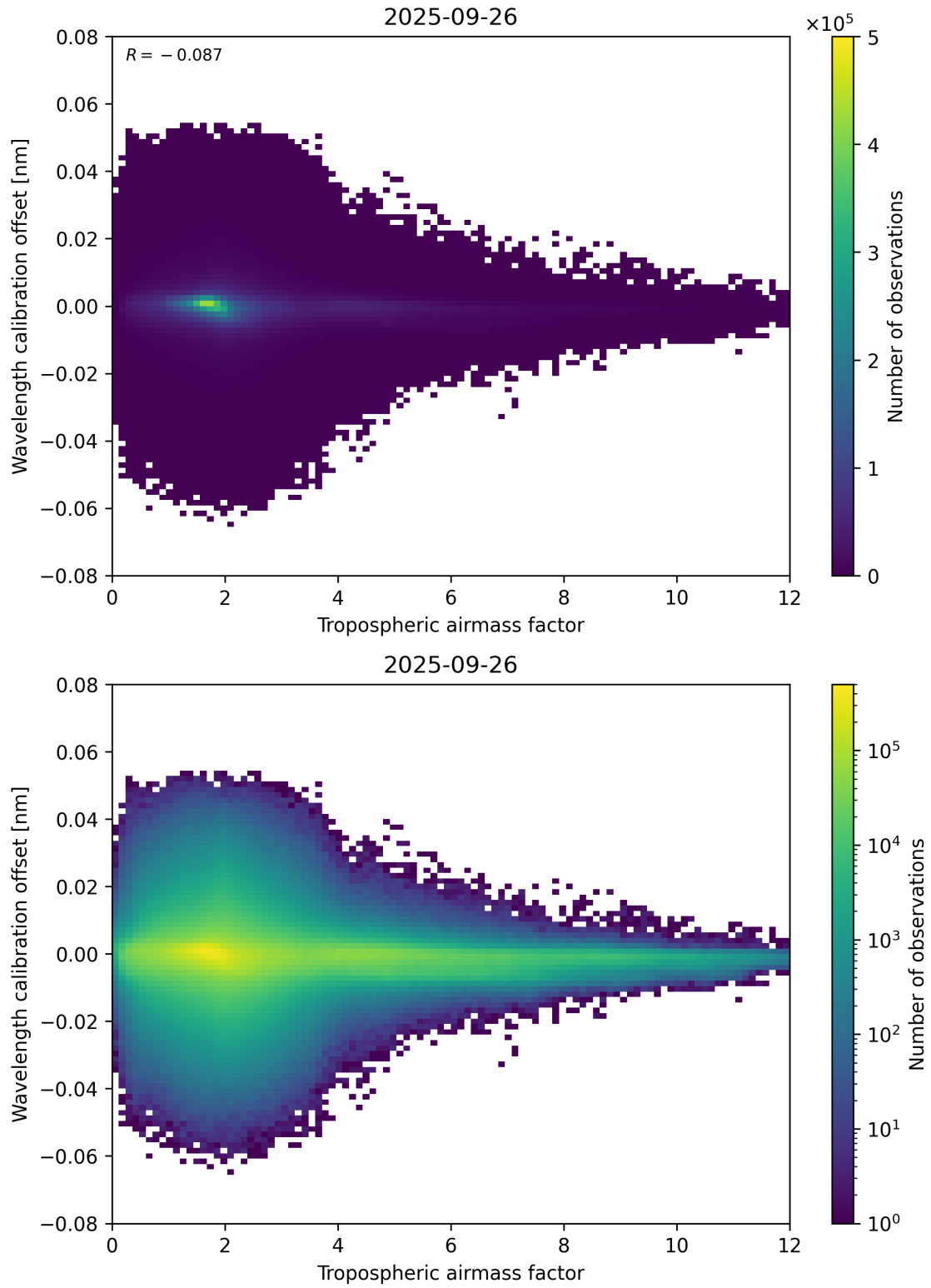
Figure 80: Scatter density plot of “Tropospheric airmass factor” against “Wavelength calibration offset” for 2025-09-26 to 2025-09-27.
