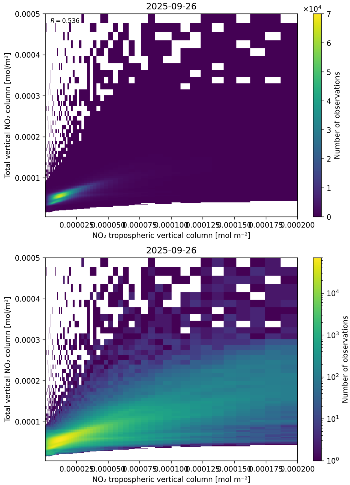
Figure 128: Scatter density plot of “NO 2 tropospheric vertical column” against “Total vertical NO 2 column” for 2025-09-26 to 2025-09-27.
