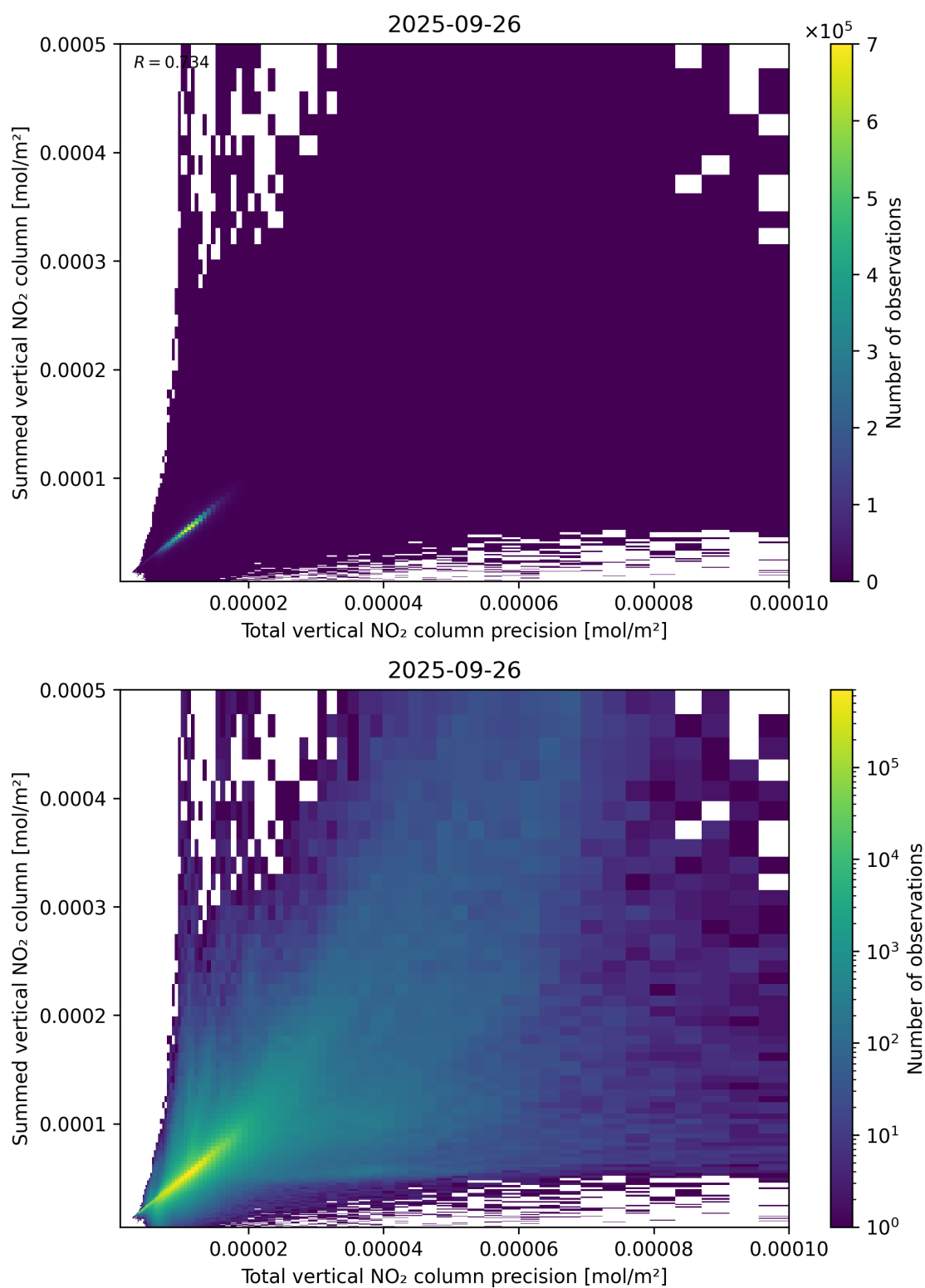
Figure 117: Scatter density plot of “Total vertical NO 2 column precision” against “Summed vertical NO 2 column” for 2025-09-26 to 2025-09-27.
