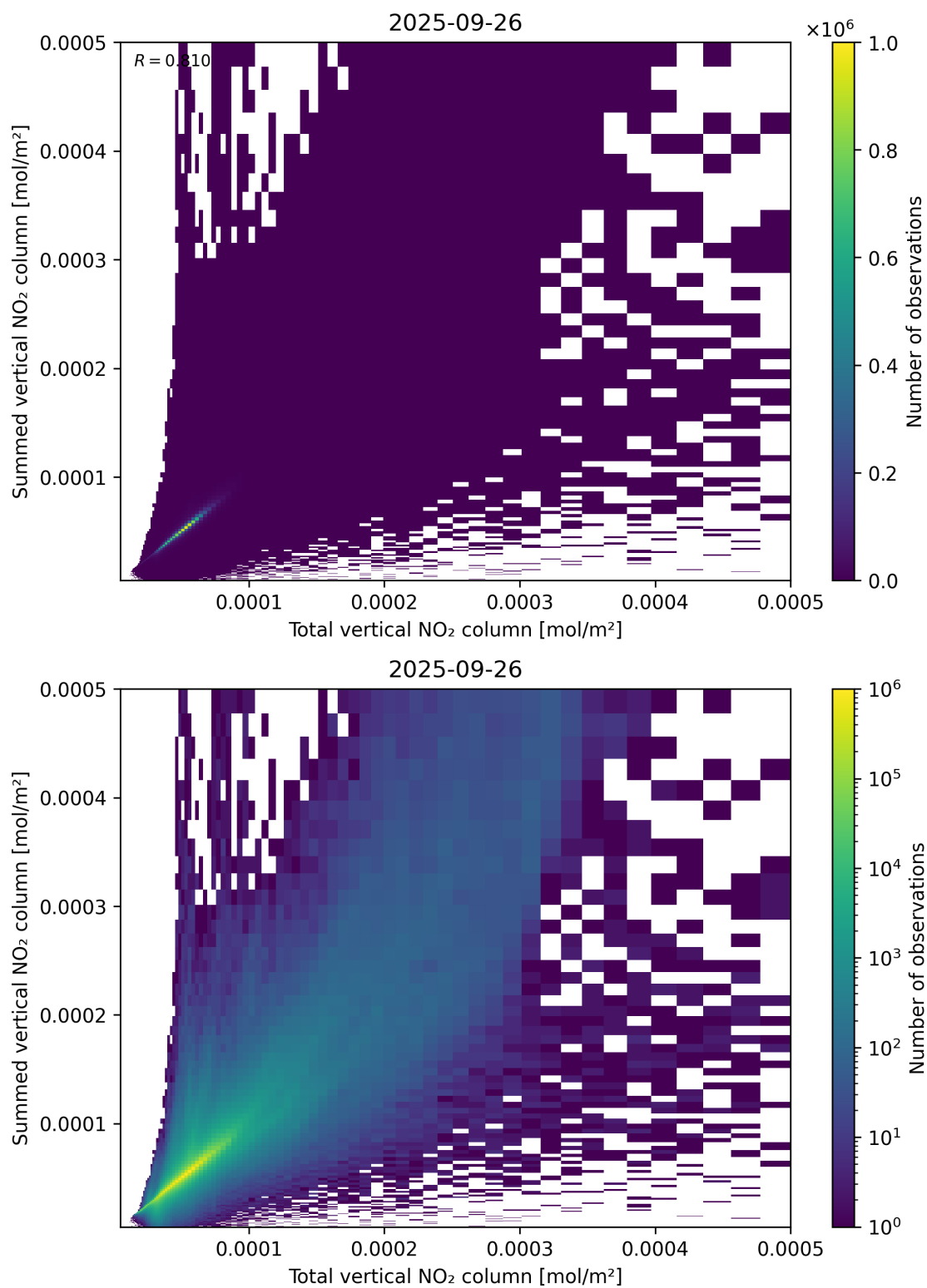
Figure 112: Scatter density plot of “Total vertical NO 2 column” against “Summed vertical NO 2 column” for 2025-09-26 to 2025-09-27.
