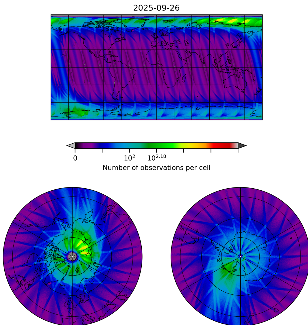
Figure 10: Map of the number of observations for 2025-09-26 to 2025-09-27
