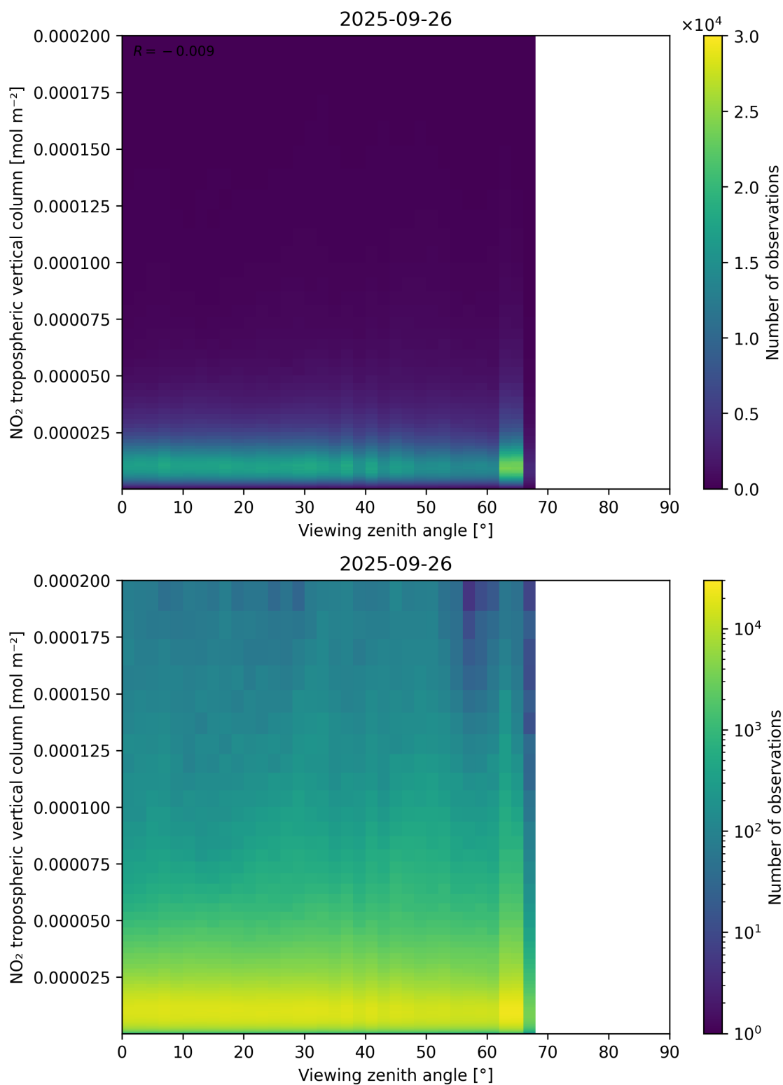
Figure 169: Scatter density plot of “Viewing zenith angle” against “NO 2 tropospheric vertical column” for 2025-09-26 to 2025-09-27.
