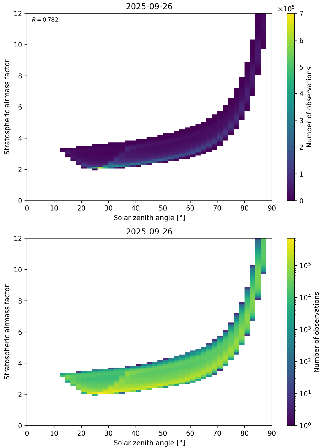
Figure 145: Scatter density plot of “Solar zenith angle” against “Stratospheric airmass factor” for 2025-09-26 to 2025-09-27.
