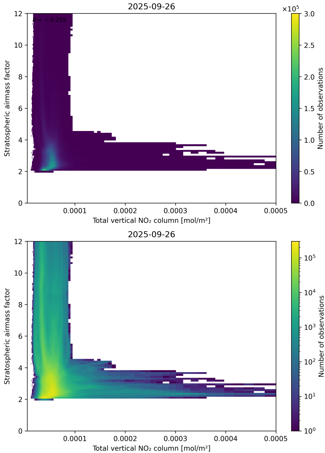
Figure 110: Scatter density plot of “Total vertical NO 2 column” against “Stratospheric airmass factor” for 2025-09-26 to 2025-09-27.
