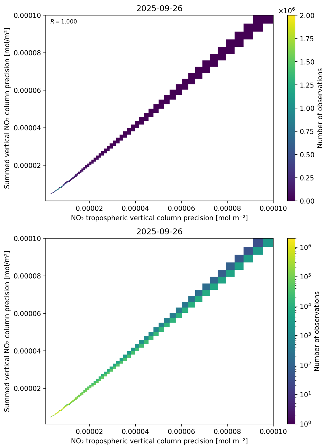
Figure 137: Scatter density plot of “NO 2 tropospheric vertical column precision” against “Summed vertical NO 2 column precision” for 2025-09-26 to 2025-09-27.
