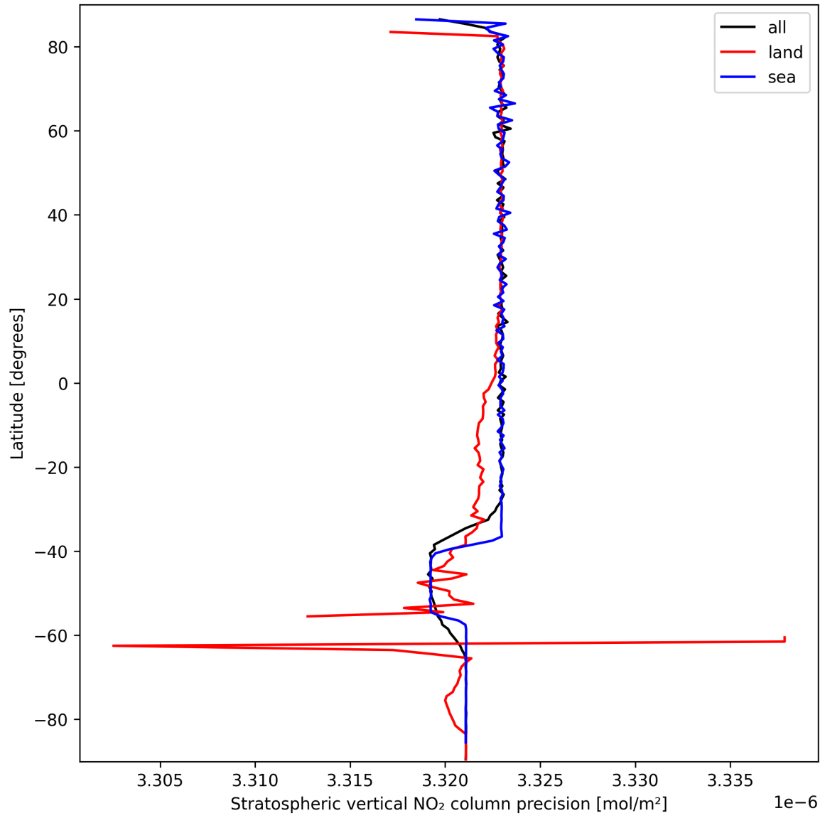
Figure 20: Zonal average of "Stratospheric vertical NO 2 column precision" for 2025-09-26 to 2025-09-27.
