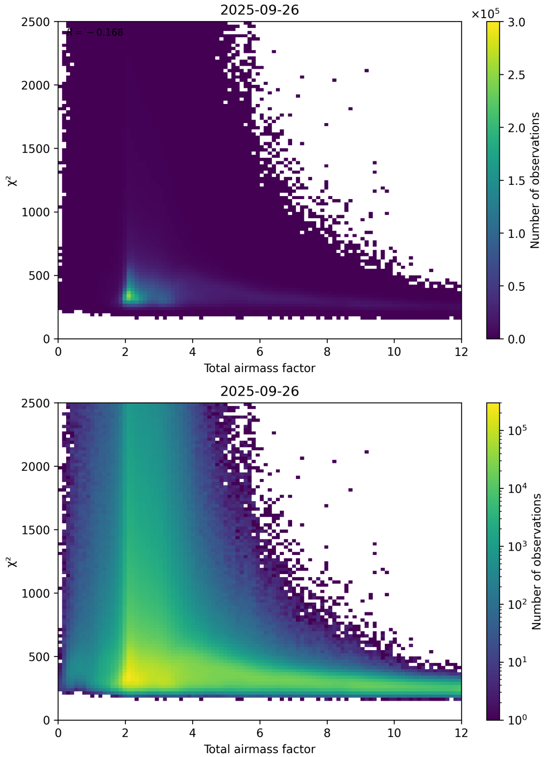
Figure 63: Scatter density plot of “Total airmass factor” against “ \chi^2 ” for 2025-09-26 to 2025-09-27.
