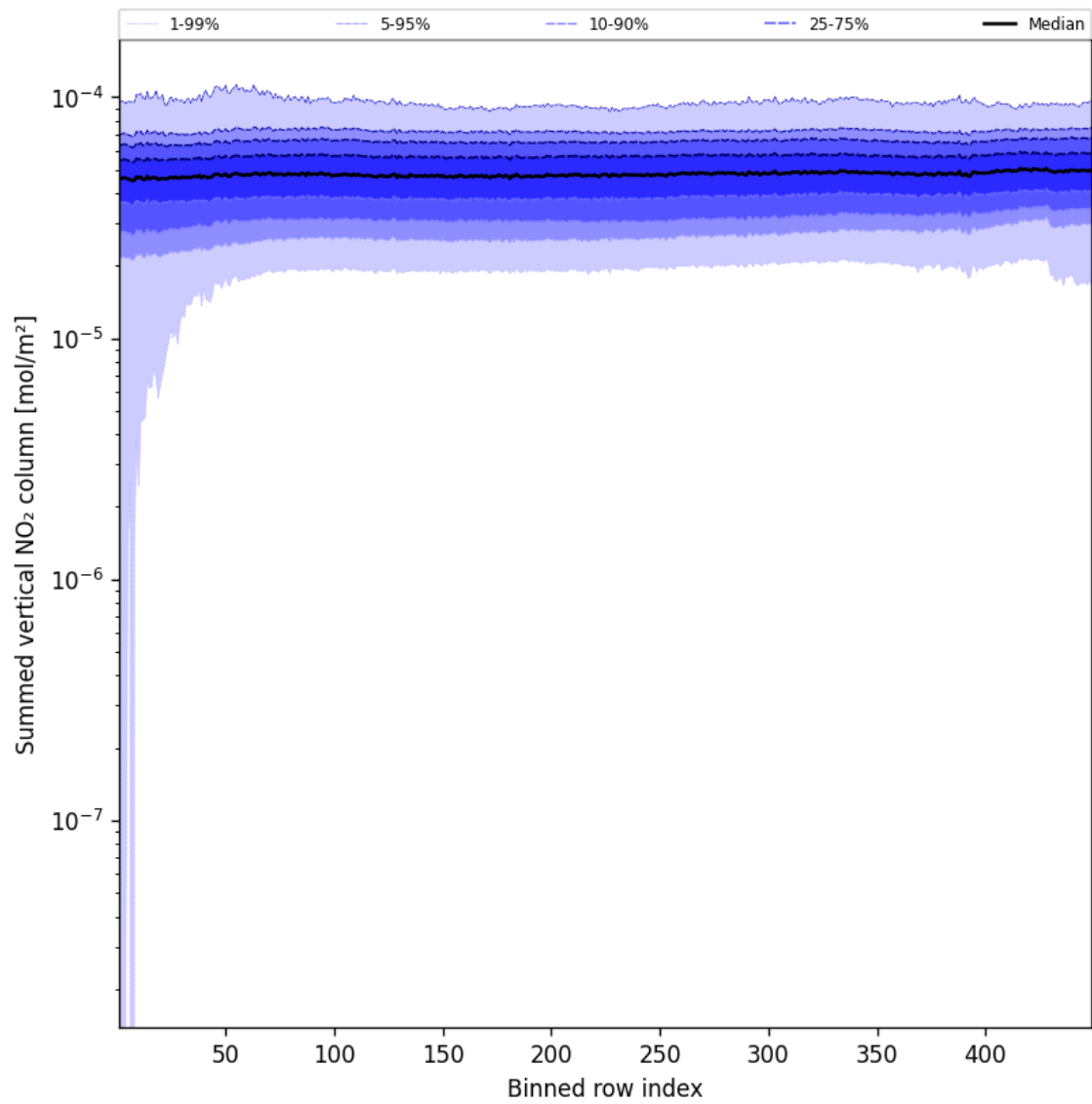
Figure 57: Along track statistics of “Summed vertical NO 2 column” for 2025-09-26 to 2025-09-27
