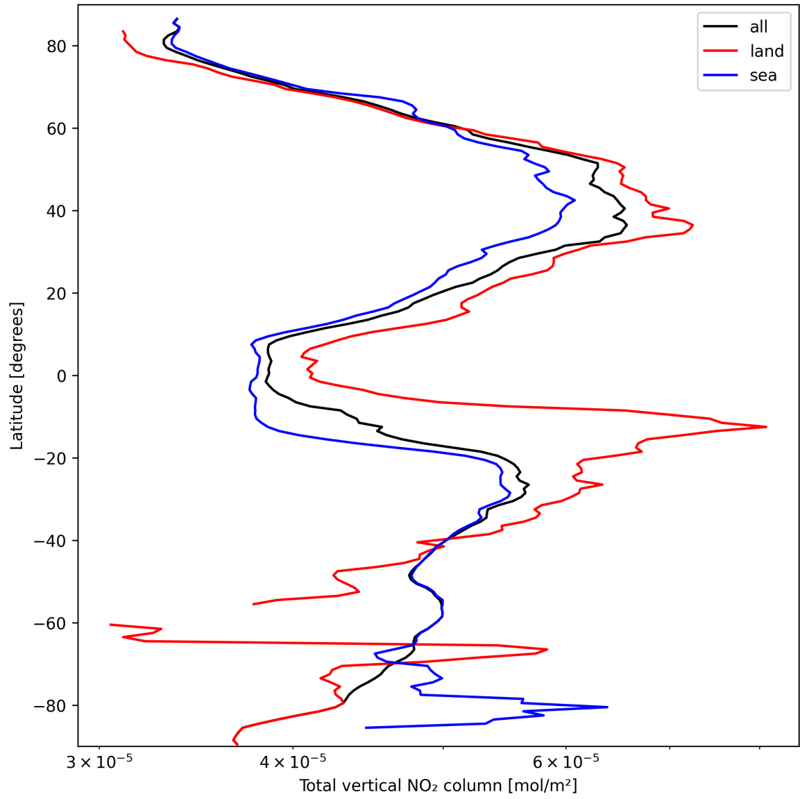
Figure 21: Zonal average of “Total vertical NO 2 column” for 2025-09-26 to 2025-09-27.
