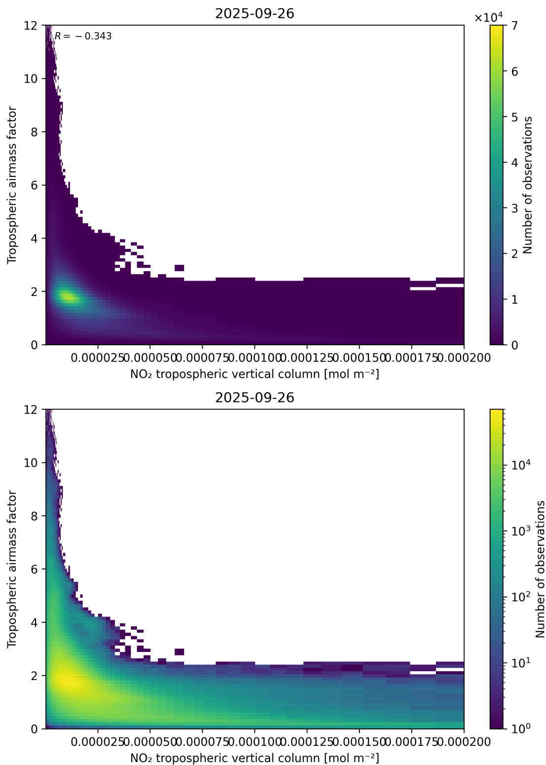
Figure 123: Scatter density plot of “NO 2 tropospheric vertical column” against “Tropospheric air mass factor” for 2025-09-26 to 2025-09-27.
