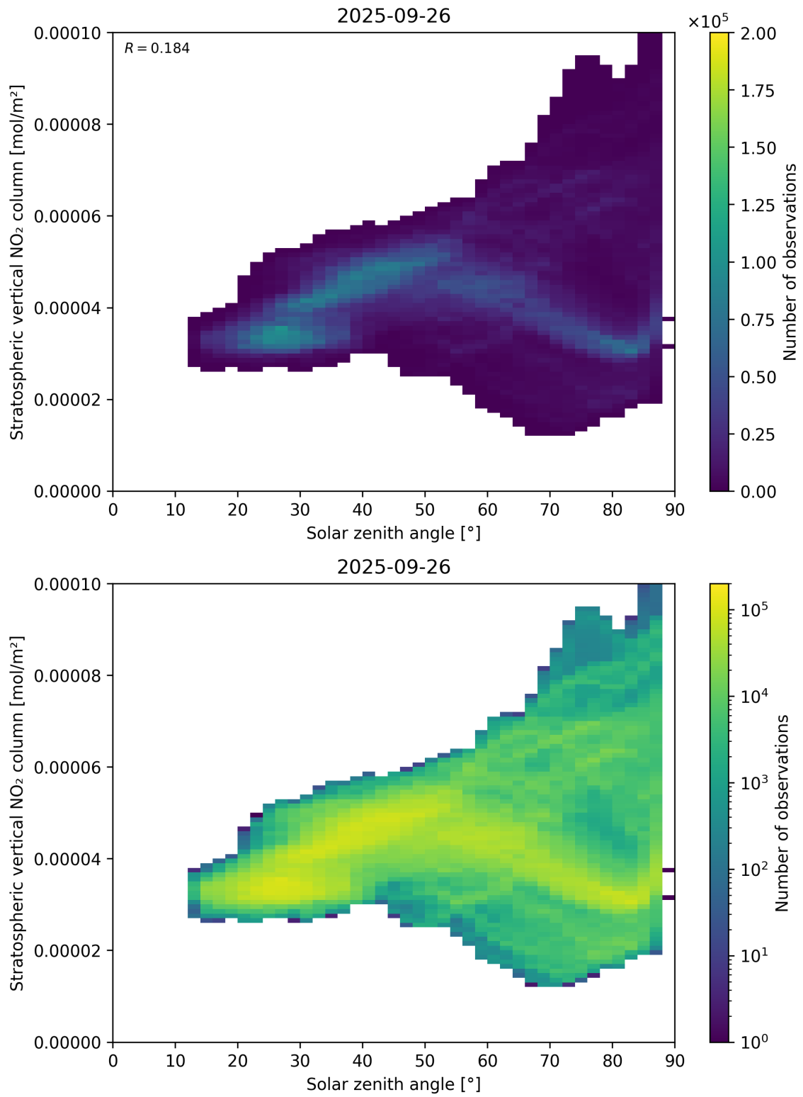
Figure 150: Scatter density plot of “Solar zenith angle” against “Stratospheric vertical \text{NO}_2 column” for 2025-09-26 to 2025-09-27.
