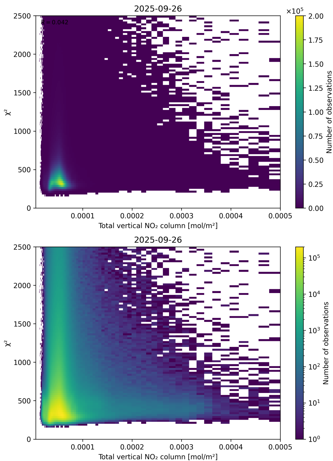
Figure 111: Scatter density plot of “Total vertical NO 2 column” against “ \chi^2 ” for 2025-09-26 to 2025-09-27.
