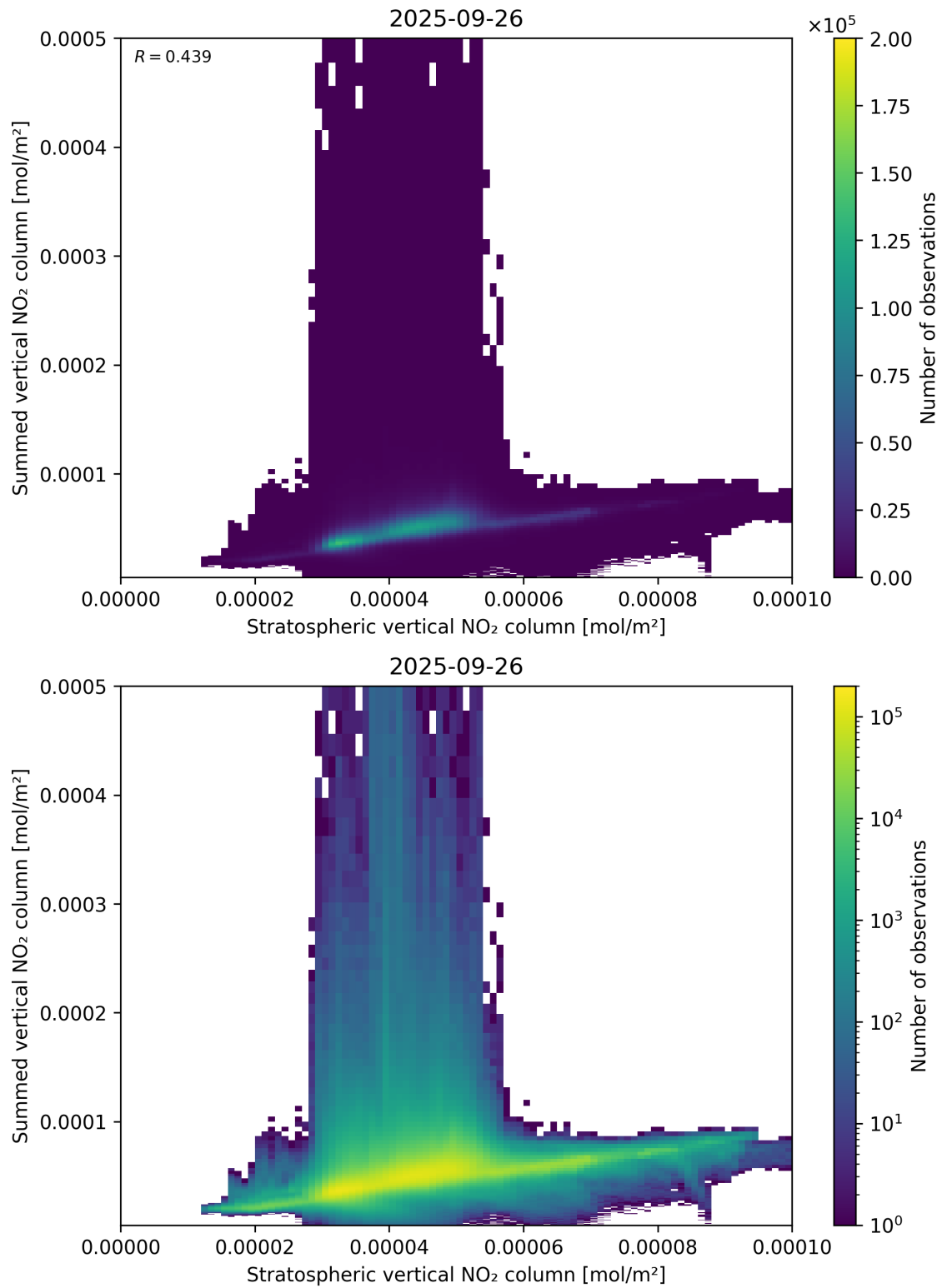
Figure 98: Scatter density plot of “Stratospheric vertical NO 2 column” against “Summed vertical NO 2 column” for 2025-09-26 to 2025-09-27.
