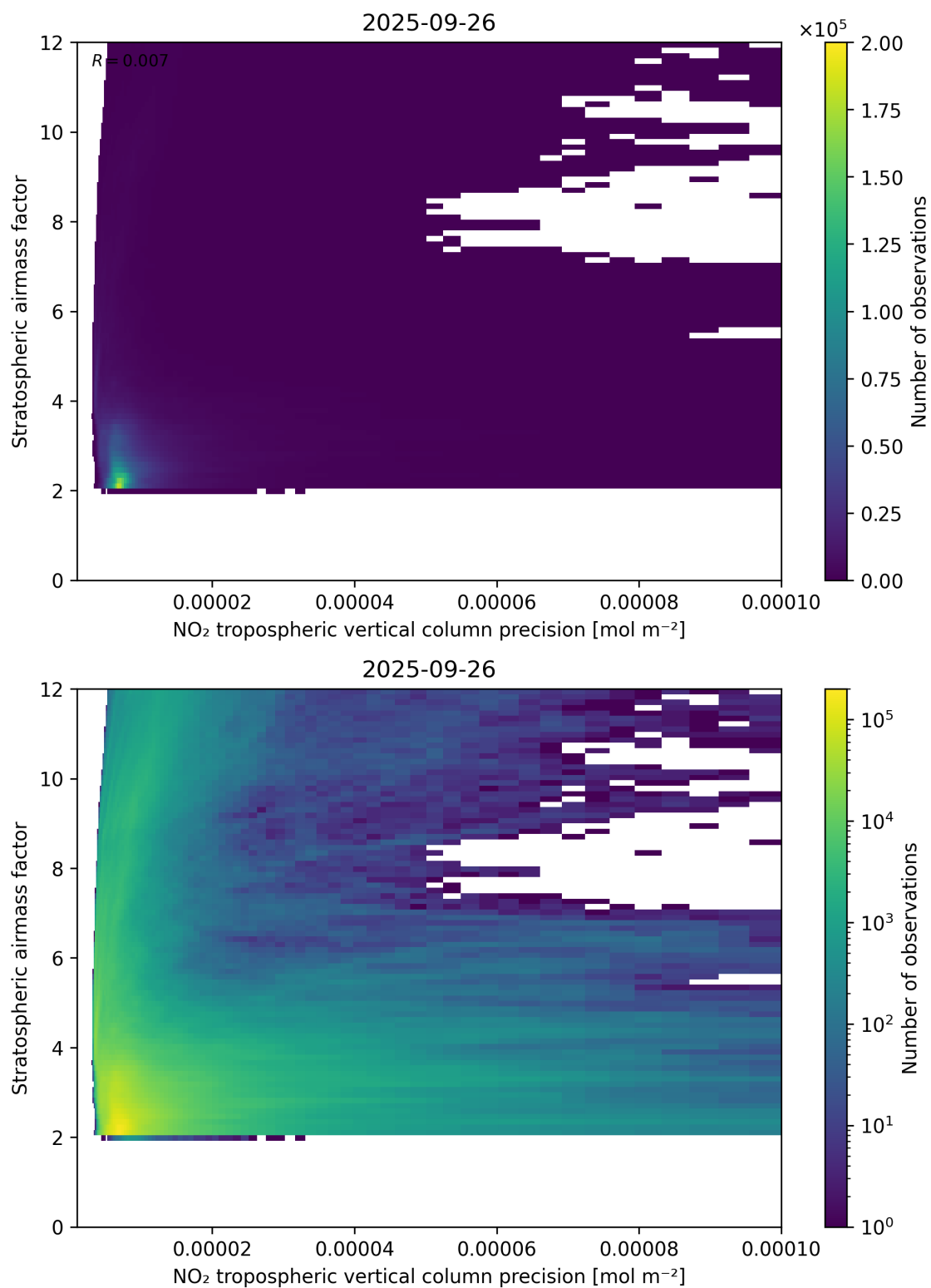
Figure 131: Scatter density plot of “NO 2 tropospheric vertical column precision” against “Stratospheric airmass factor” for 2025-09-26 to 2025-09-27.
