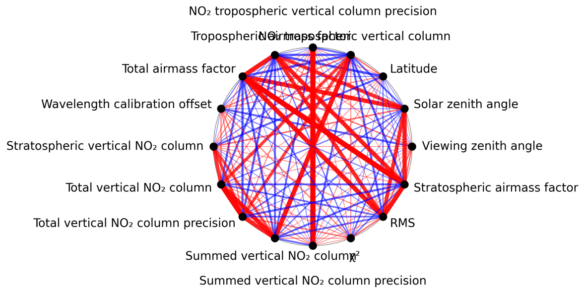
Figure 1: Map of correlation graph for 2025-09-26 to 2025-09-27.
