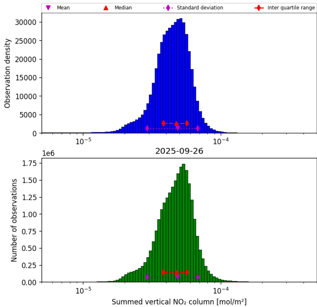
Figure 40: Histogram of "Summed vertical NO 2 column" for 2025-09-26 to 2025-09-27
