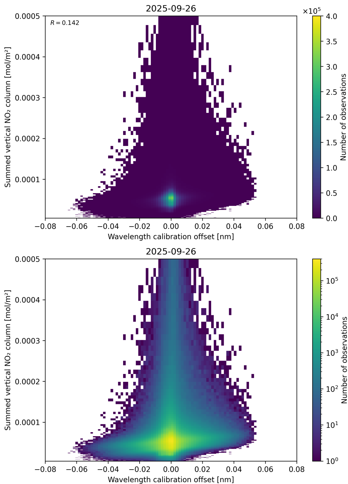
Figure 177: Scatter density plot of “Wavelength calibration offset” against “Summed vertical NO 2 column” for 2025-09-26 to 2025-09-27.
