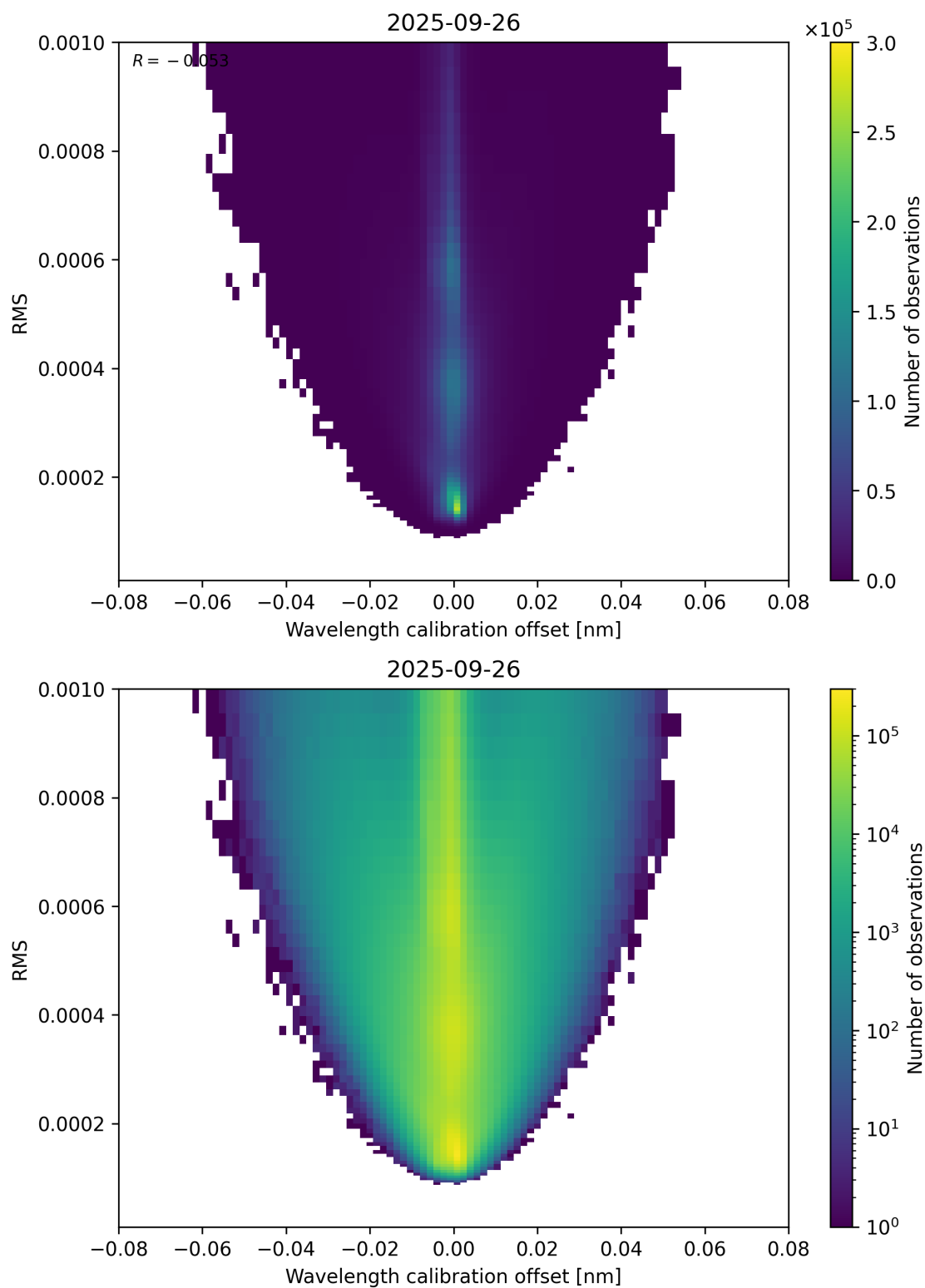
Figure 181: Scatter density plot of “Wavelength calibration offset” against “RMS” for 2025-09-26 to 2025-09-27.
