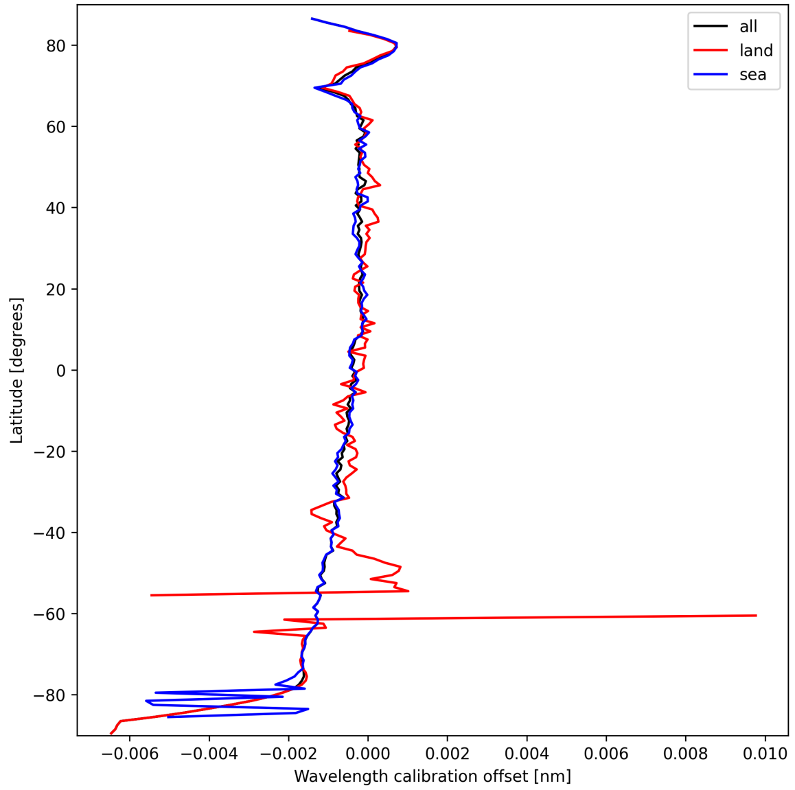
Figure 18: Zonal average of “Wavelength calibration offset” for 2025-09-26 to 2025-09-27.
