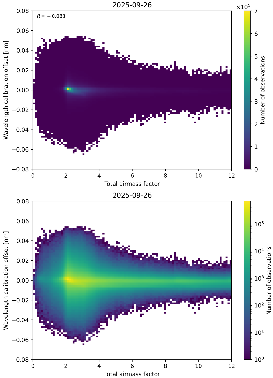
Figure 70: Scatter density plot of “Total airmass factor” against “Wavelength calibration offset” for 2025-09-26 to 2025-09-27.
