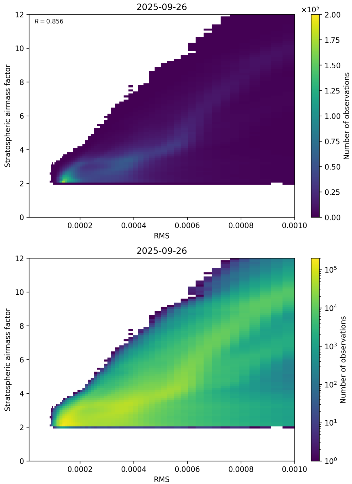
Figure 144: Scatter density plot of “RMS” against “Stratospheric airmass factor” for 2025-09-26 to 2025-09-27.
