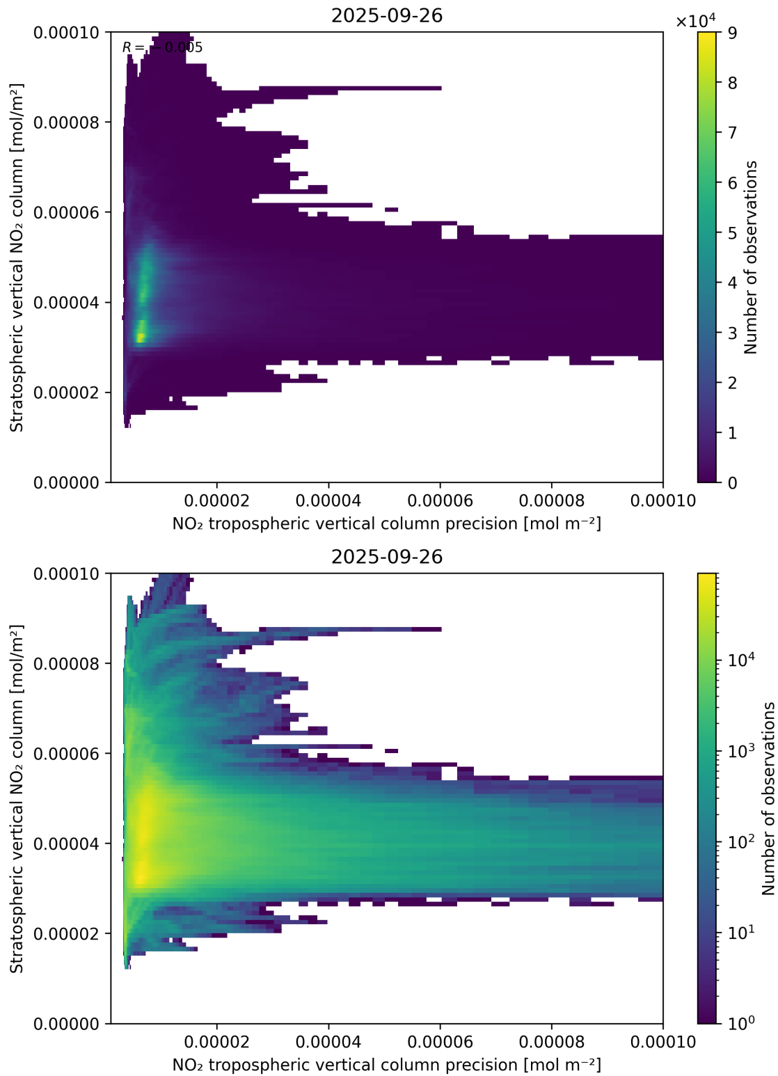
Figure 135: Scatter density plot of “NO 2 tropospheric vertical column precision” against “Stratospheric vertical NO 2 column” for 2025-09-26 to 2025-09-27.
