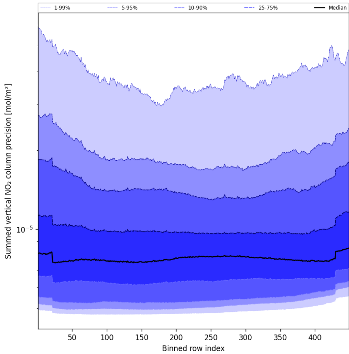
Figure 58: Along track statistics of “Summed vertical NO 2 column precision” for 2025-09-26 to 2025-09-27
