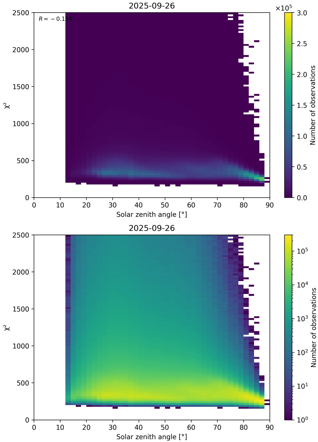
Figure 148: Scatter density plot of “Solar zenith angle” against “ \chi^2 ” for 2025-09-26 to 2025-09-27.
