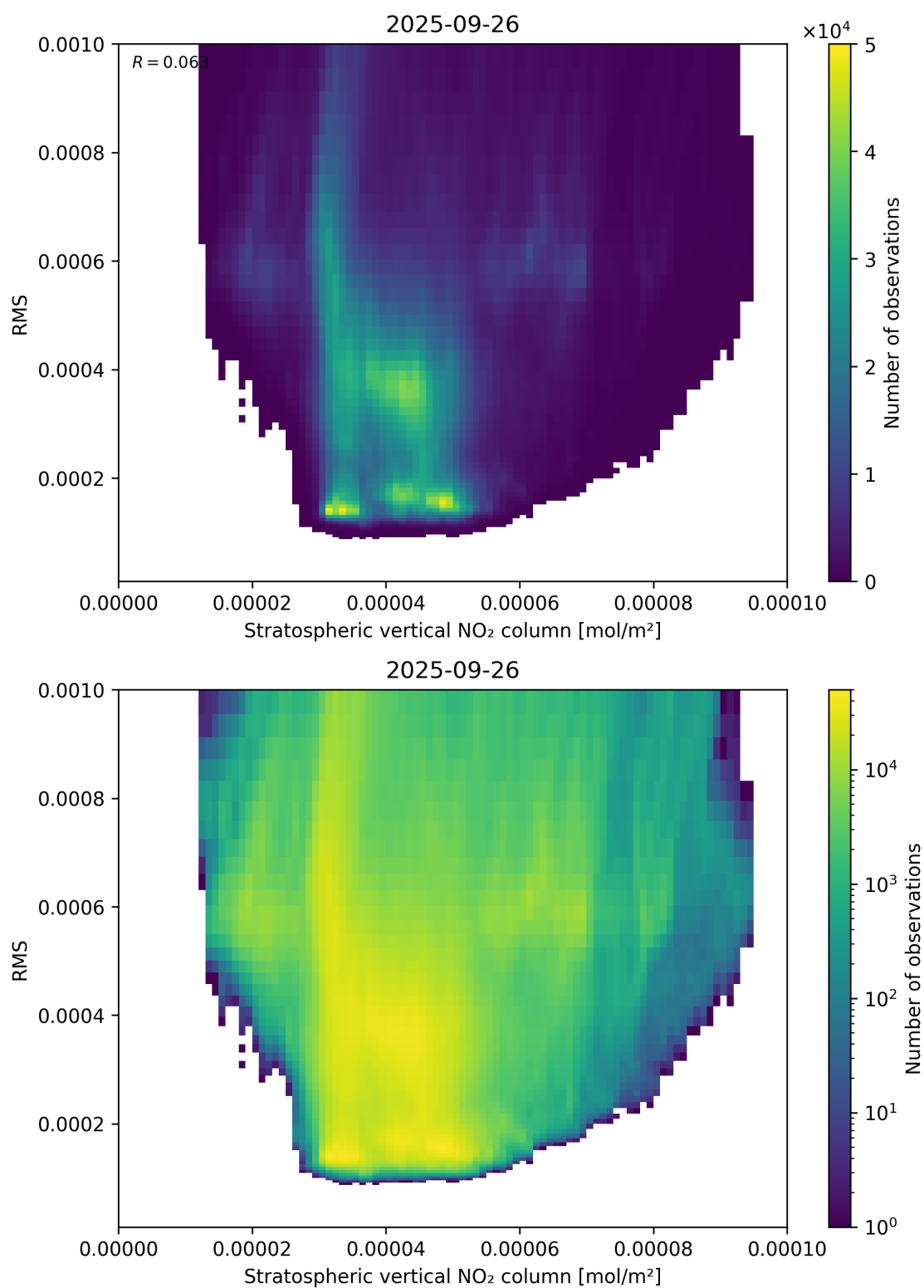
Figure 102: Scatter density plot of “Stratospheric vertical NO 2 column” against “RMS” for 2025-09-26 to 2025-09-27.
