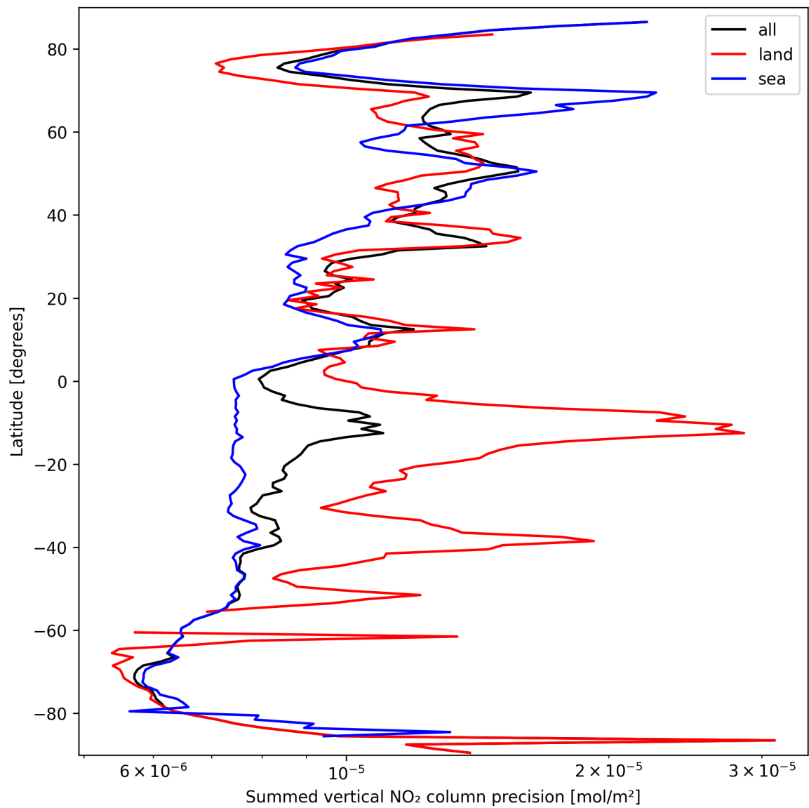
Figure 24: Zonal average of “Summed vertical NO 2 column precision” for 2025-09-26 to 2025-09-27.
