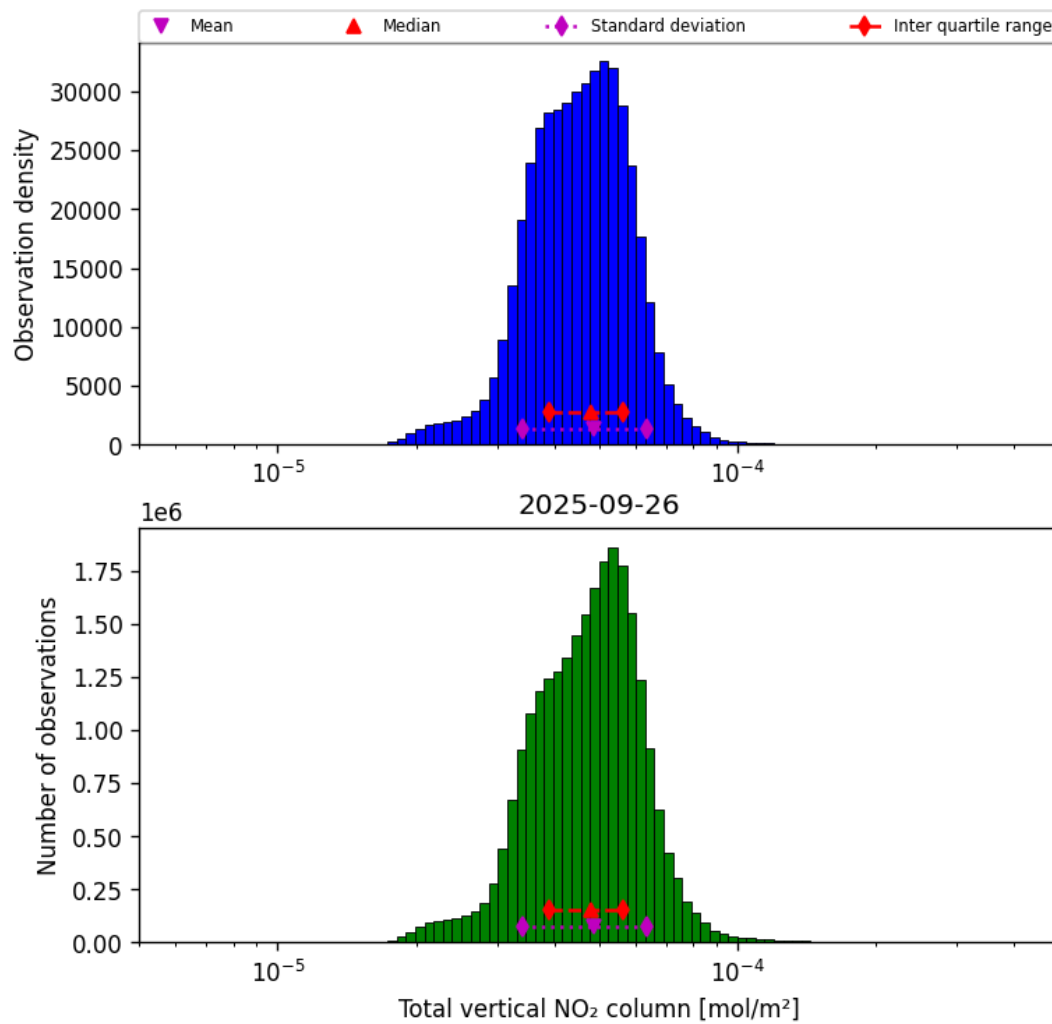
Figure 38: Histogram of “Total vertical NO 2 column” for 2025-09-26 to 2025-09-27
