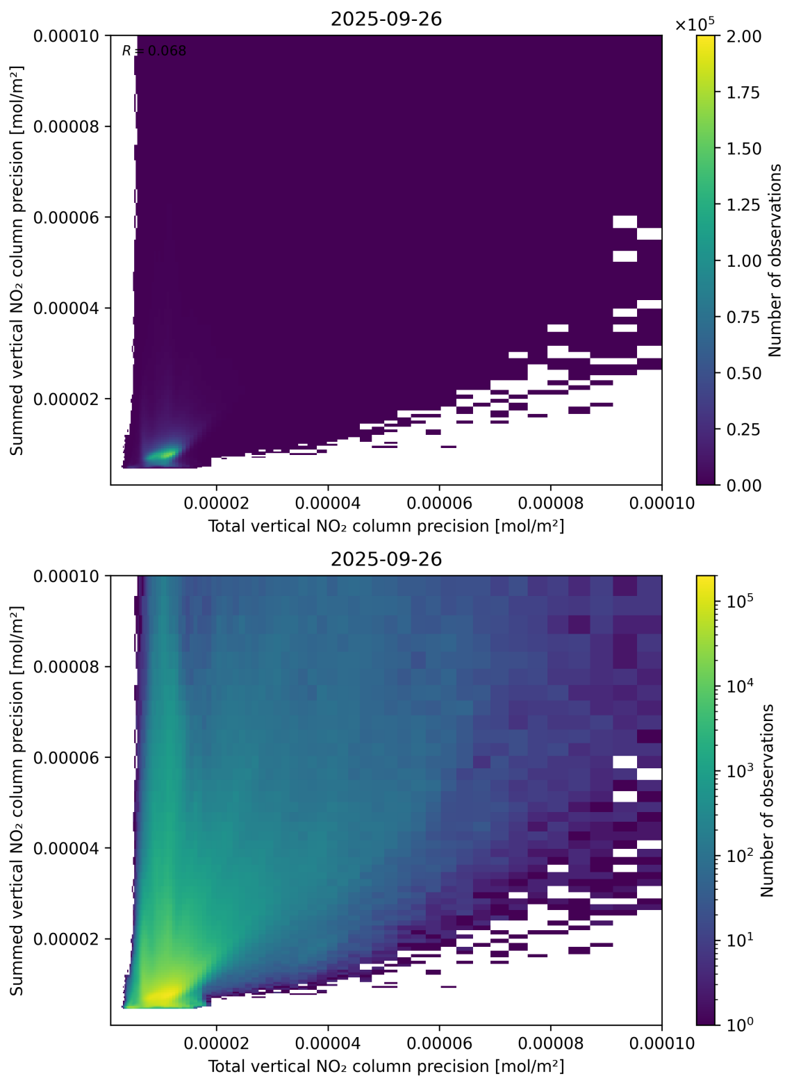
Figure 118: Scatter density plot of “Total vertical NO 2 column precision” against “Summed vertical NO 2 column precision” for 2025-09-26 to 2025-09-27.
