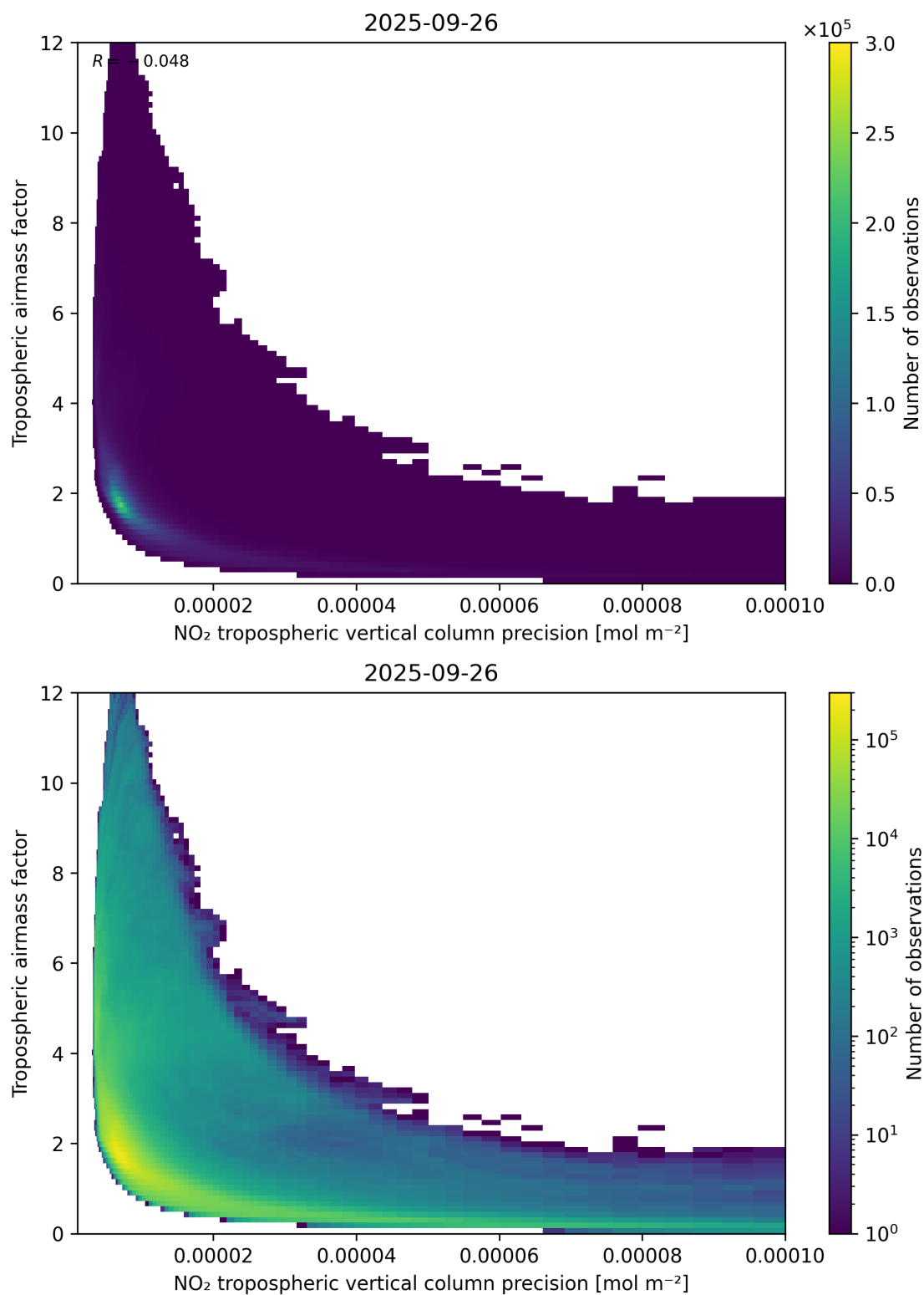
Figure 133: Scatter density plot of “NO 2 tropospheric vertical column precision” against “Tropospheric airmass factor” for 2025-09-26 to 2025-09-27.
