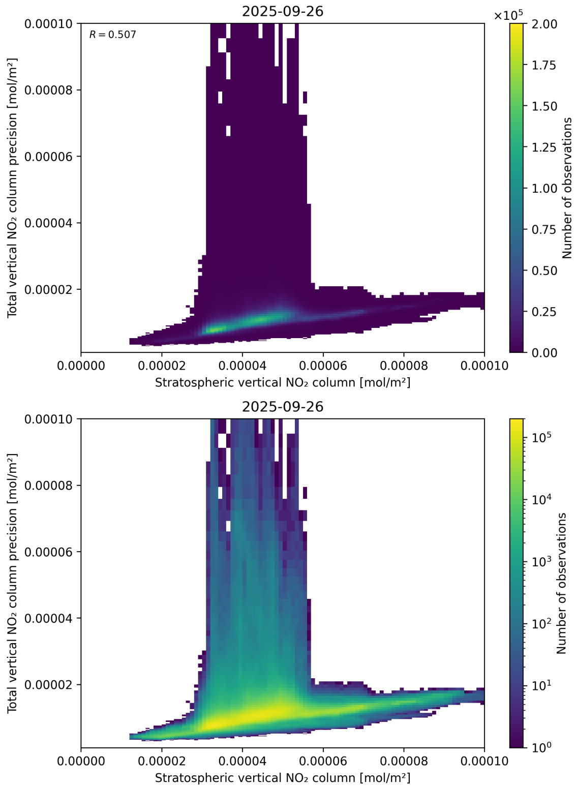
Figure 101: Scatter density plot of “Stratospheric vertical NO 2 column” against “Total vertical NO 2 column precision” for 2025-09-26 to 2025-09-27.
