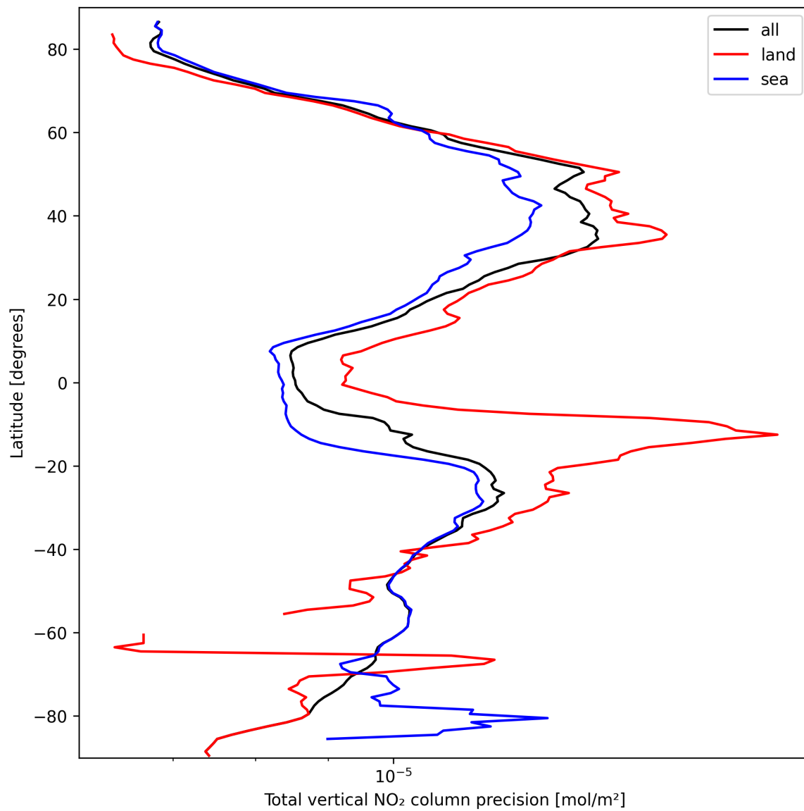
Figure 22: Zonal average of “Total vertical NO 2 column precision” for 2025-09-26 to 2025-09-27.
