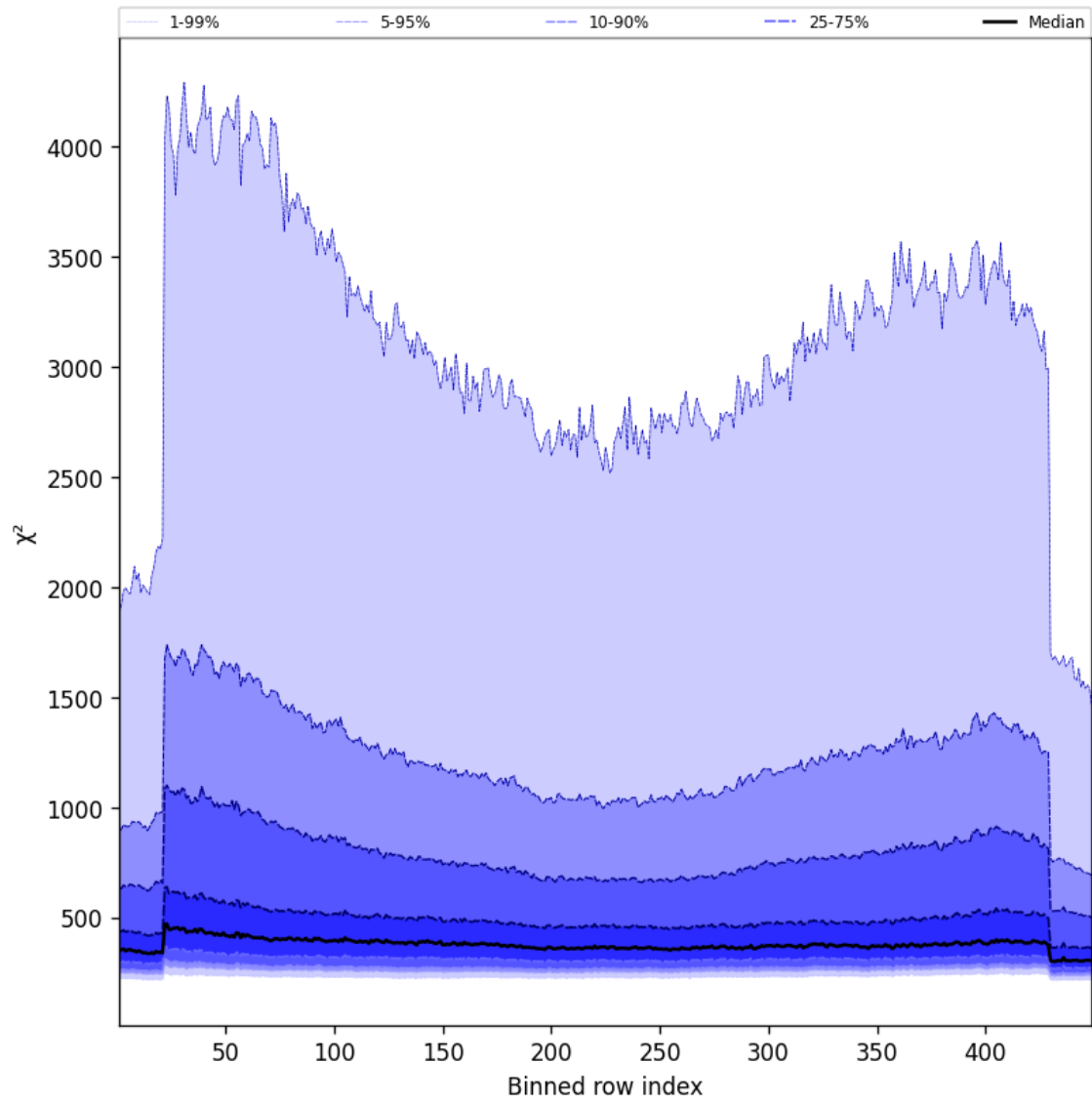
Figure 59: Along track statistics of “ \chi^2 ” for 2025-09-26 to 2025-09-27
