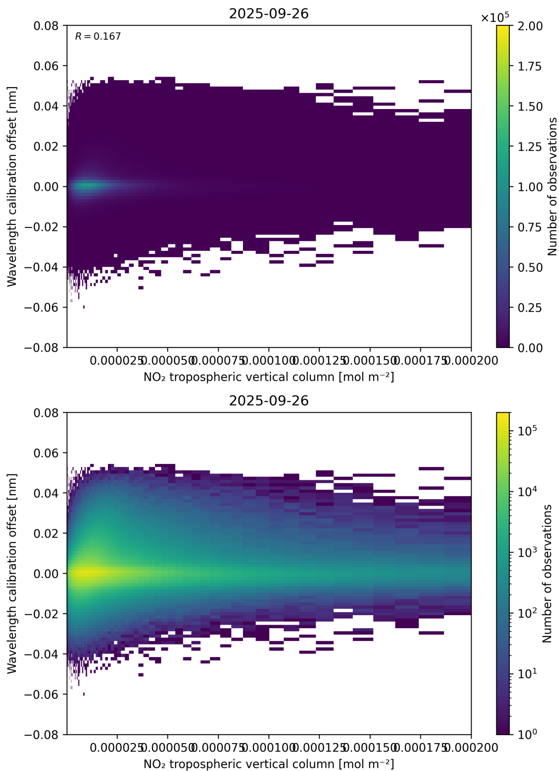
Figure 143: Scatter density plot of “NO 2 tropospheric vertical column” against “Wavelength calibration offset” for 2025-09-26 to 2025-09-27.
