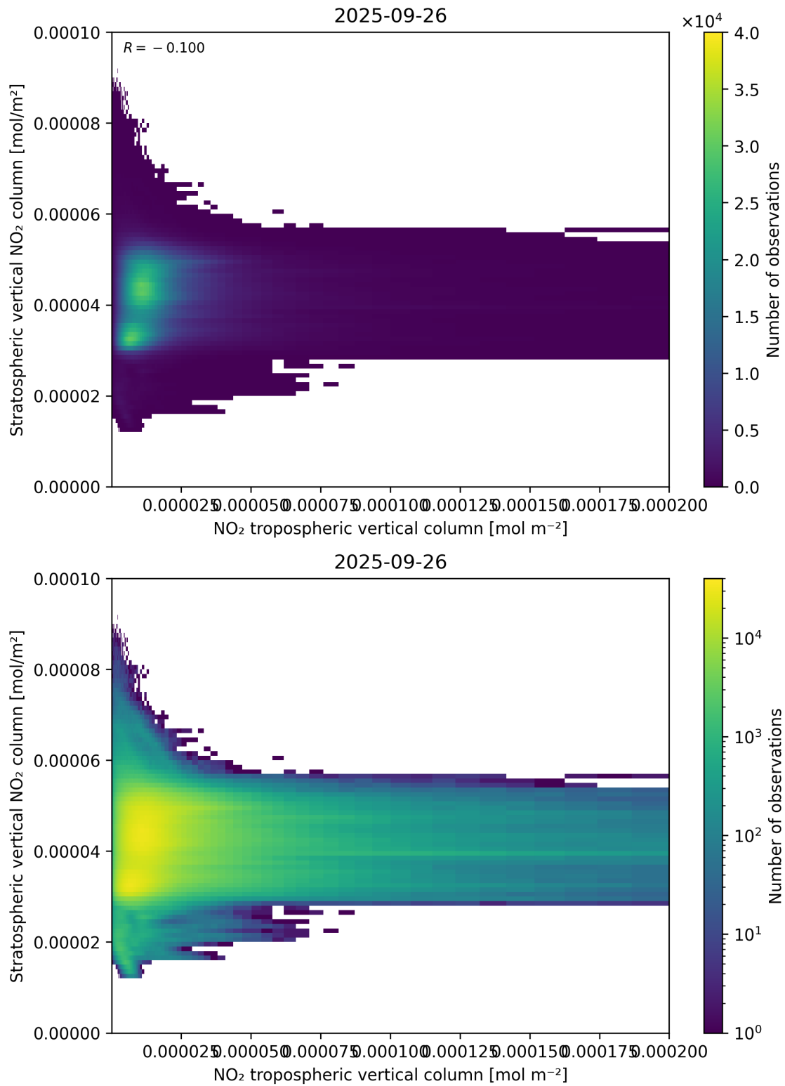
Figure 125: Scatter density plot of “NO 2 tropospheric vertical column” against “Stratospheric vertical NO 2 column” for 2025-09-26 to 2025-09-27.
