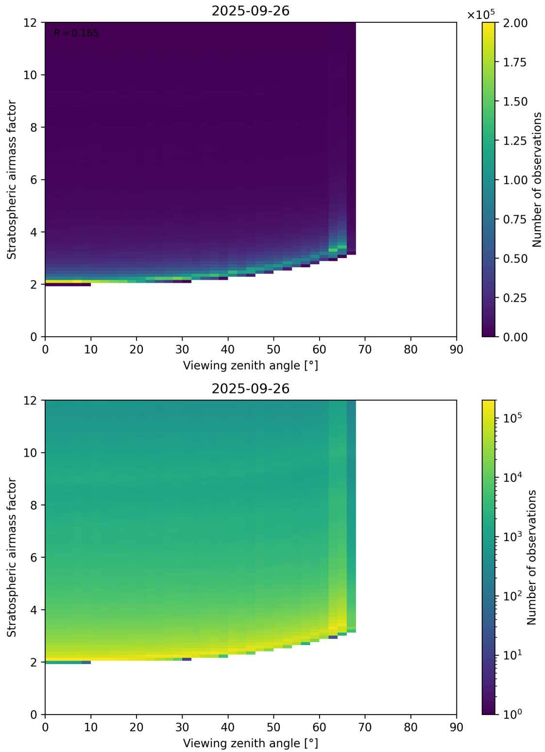
Figure 159: Scatter density plot of “Viewing zenith angle” against “Stratospheric airmass factor” for 2025-09-26 to 2025-09-27.
