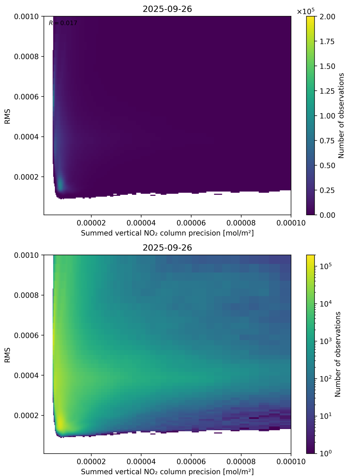
Figure 108: Scatter density plot of “Summed vertical NO 2 column precision” against “RMS” for 2025-09-26 to 2025-09-27.
