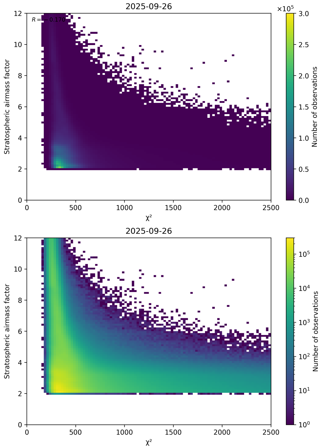
Figure 81: Scatter density plot of “ \chi^2 ” against “Stratospheric airmass factor” for 2025-09-26 to 2025-09-27.
