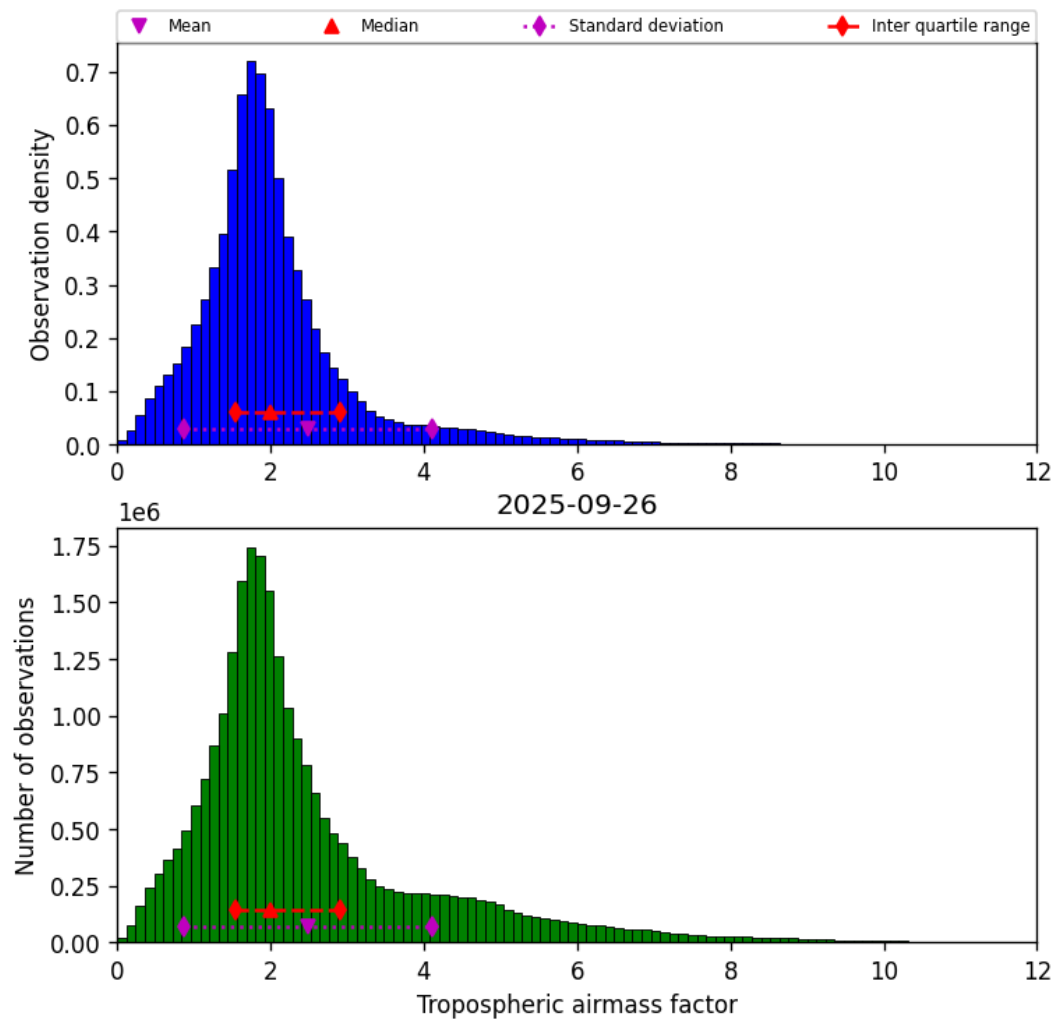
Figure 31: Histogram of “Tropospheric airmass factor” for 2025-09-26 to 2025-09-27
