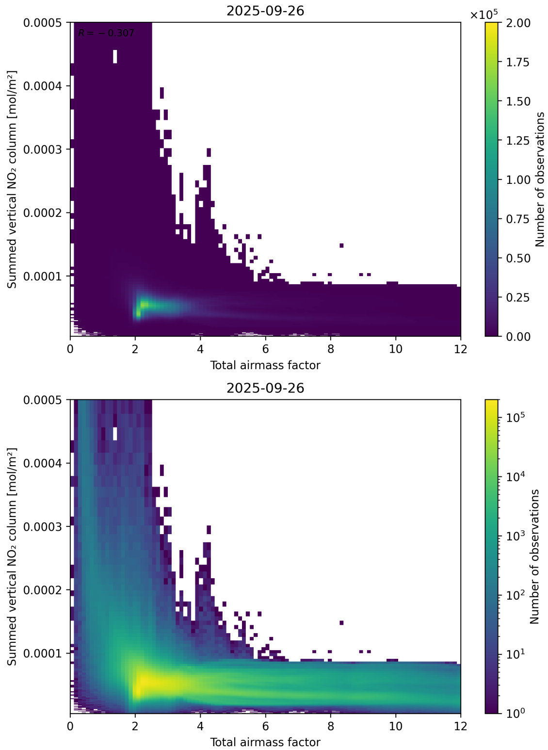
Figure 65: Scatter density plot of “Total airmass factor” against “Summed vertical NO 2 column” for 2025-09-26 to 2025-09-27.
