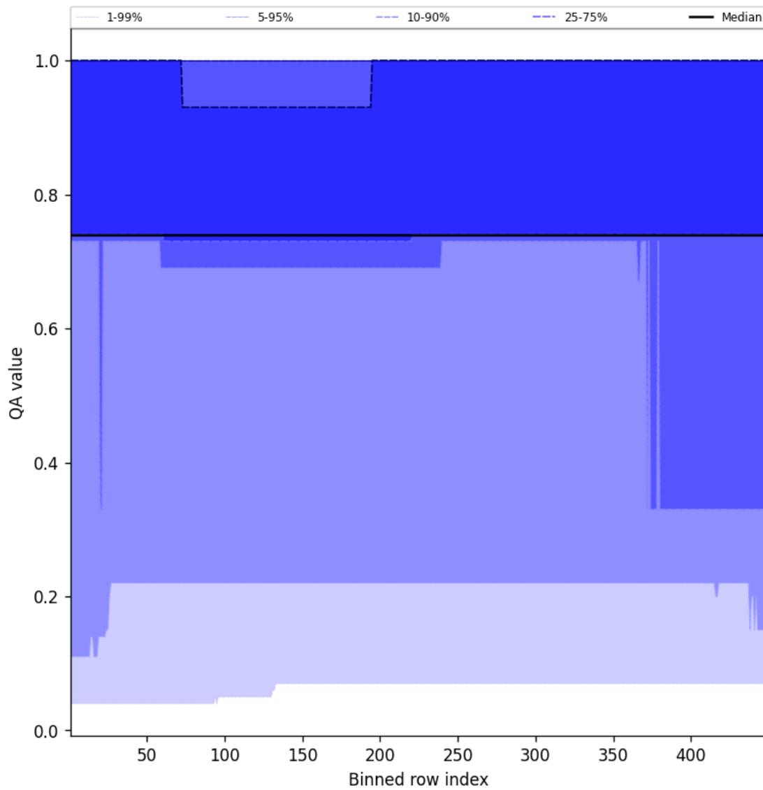
Figure 45: Along track statistics of “QA value” for 2025-09-26 to 2025-09-27
