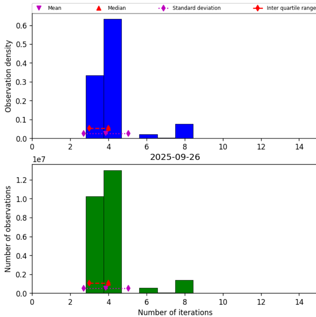
Figure 34: Histogram of “Number of iterations” for 2025-09-26 to 2025-09-27
