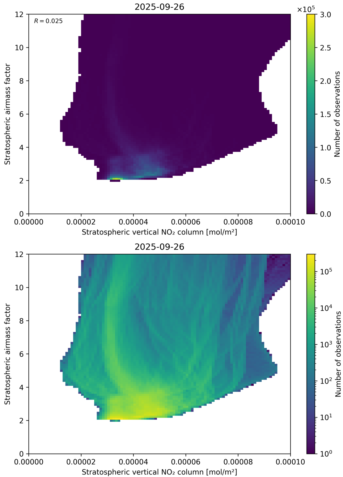
Figure 96: Scatter density plot of “Stratospheric vertical NO 2 column” against “Stratospheric airmass factor” for 2025-09-26 to 2025-09-27.
