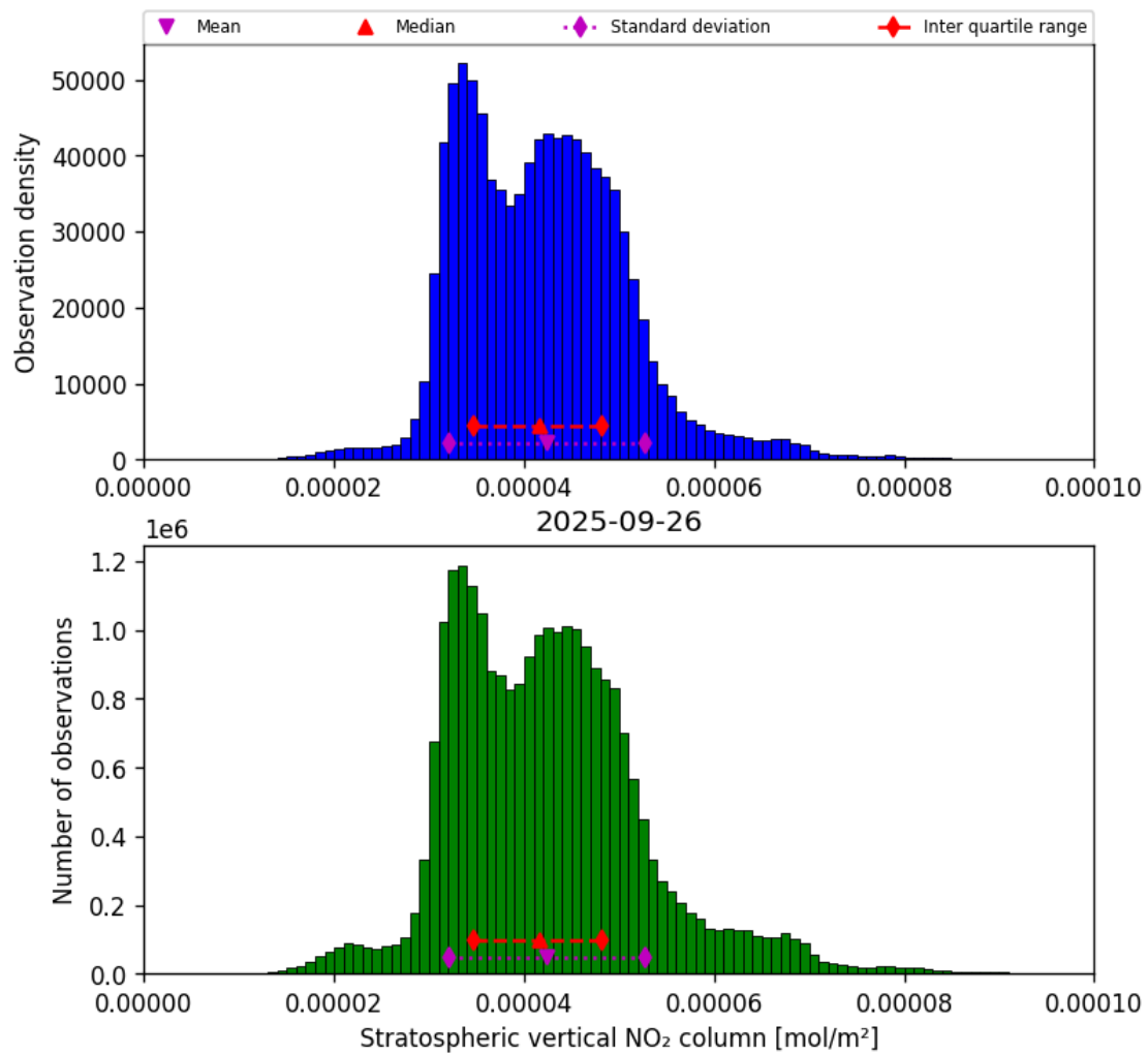
Figure 36: Histogram of “Stratospheric vertical NO 2 column” for 2025-09-26 to 2025-09-27
