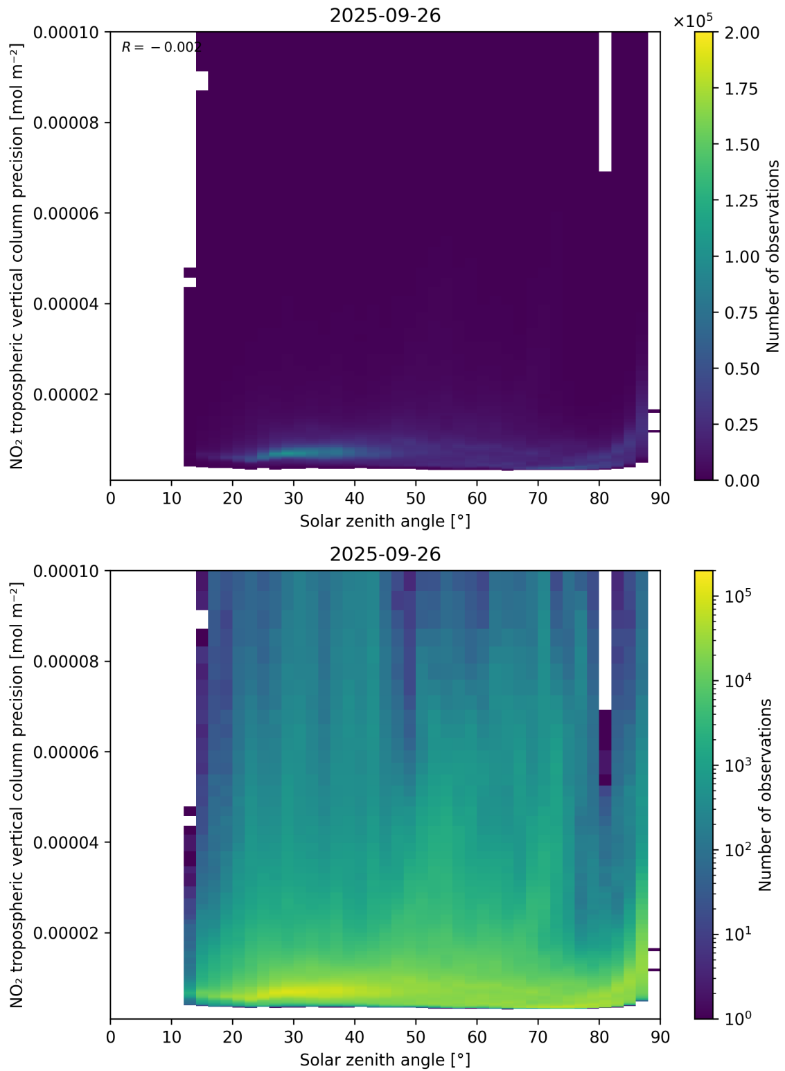
Figure 156: Scatter density plot of “Solar zenith angle” against “NO 2 tropospheric vertical column precision” for 2025-09-26 to 2025-09-27.
