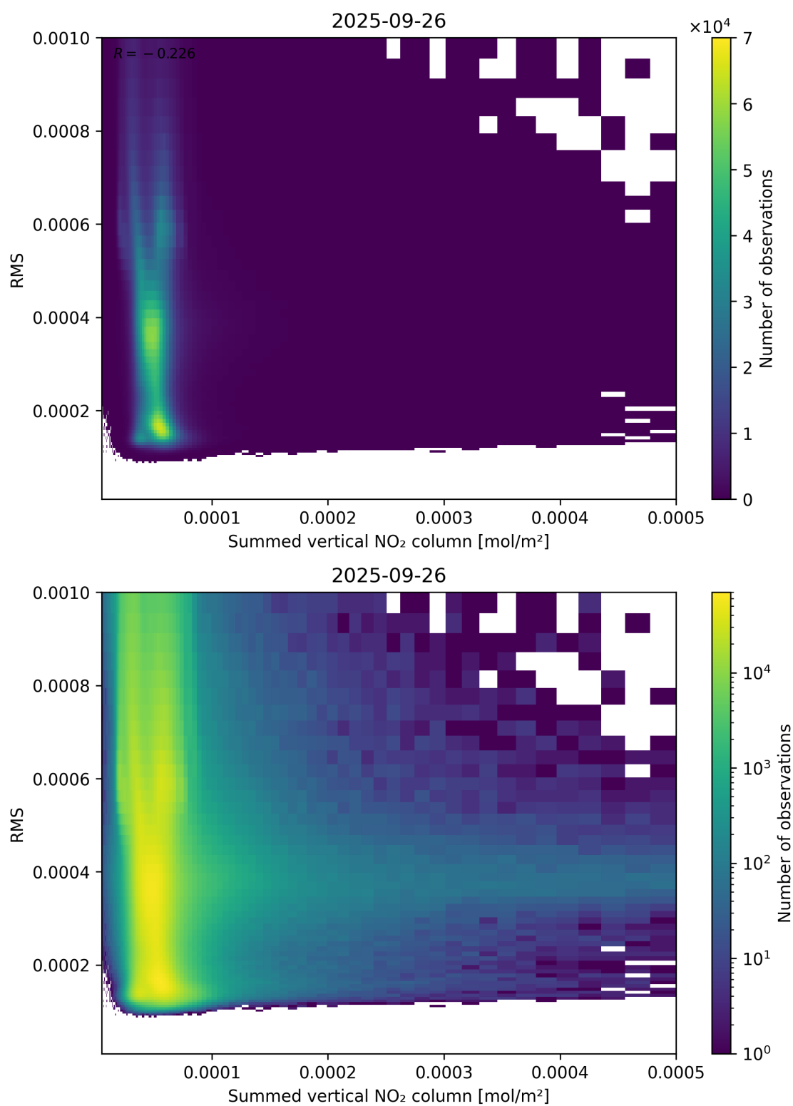
Figure 109: Scatter density plot of “Summed vertical NO 2 column” against “RMS” for 2025-09-26 to 2025-09-27.
