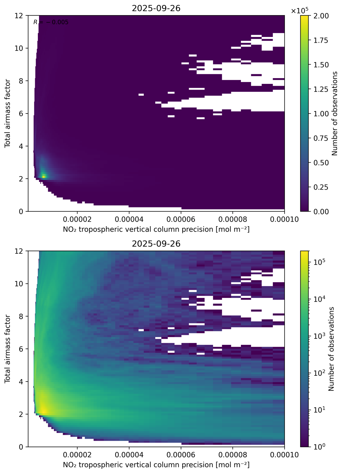
Figure 132: Scatter density plot of “NO 2 tropospheric vertical column precision” against “Total air mass factor” for 2025-09-26 to 2025-09-27.
