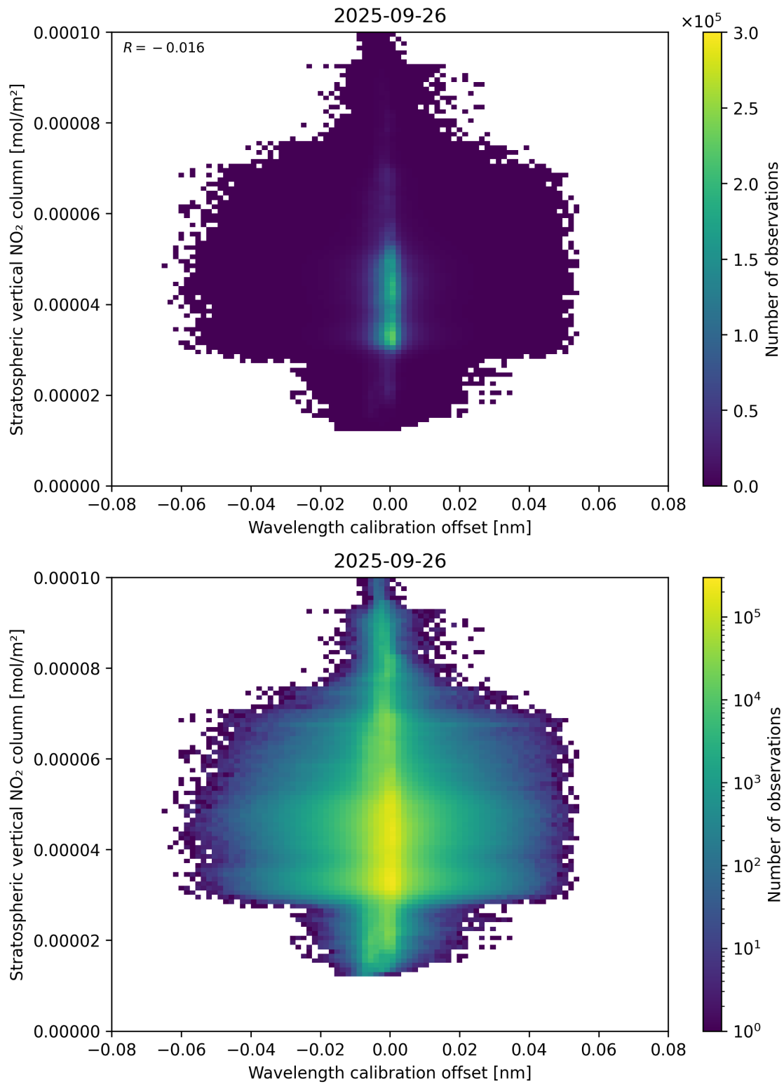
Figure 176: Scatter density plot of “Wavelength calibration offset” against “Stratospheric vertical NO 2 column” for 2025-09-26 to 2025-09-27.
