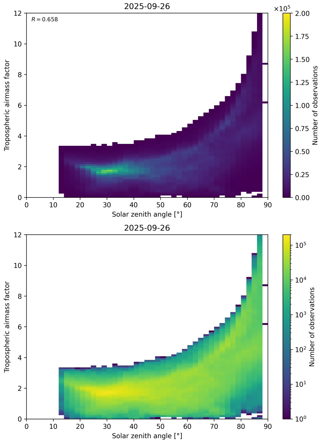
Figure 147: Scatter density plot of “Solar zenith angle” against “Tropospheric airmass factor” for 2025-09-26 to 2025-09-27.
