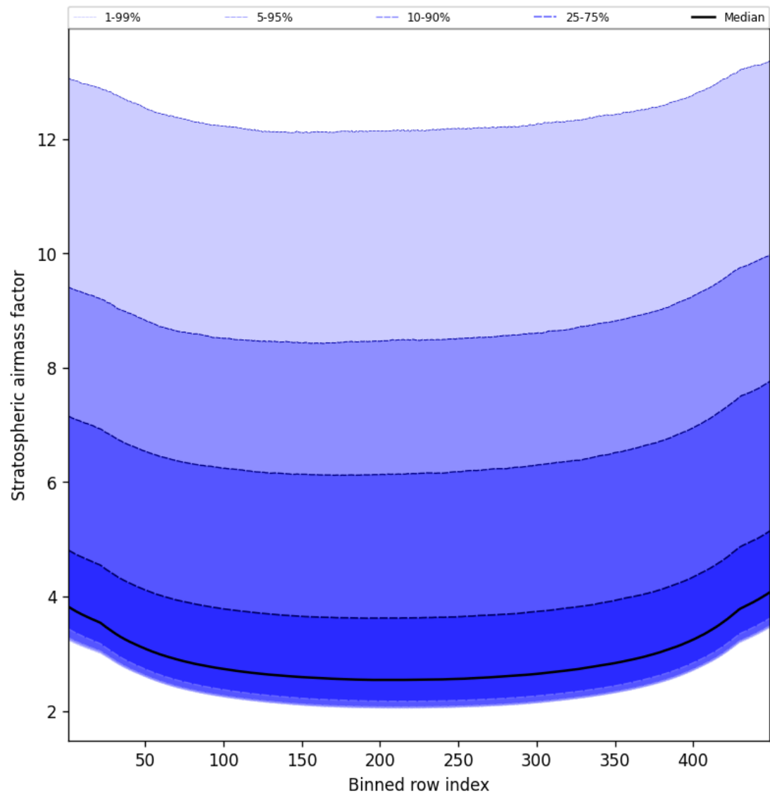
Figure 61: Along track statistics of “Stratospheric air mass factor” for 2025-09-26 to 2025-09-27
