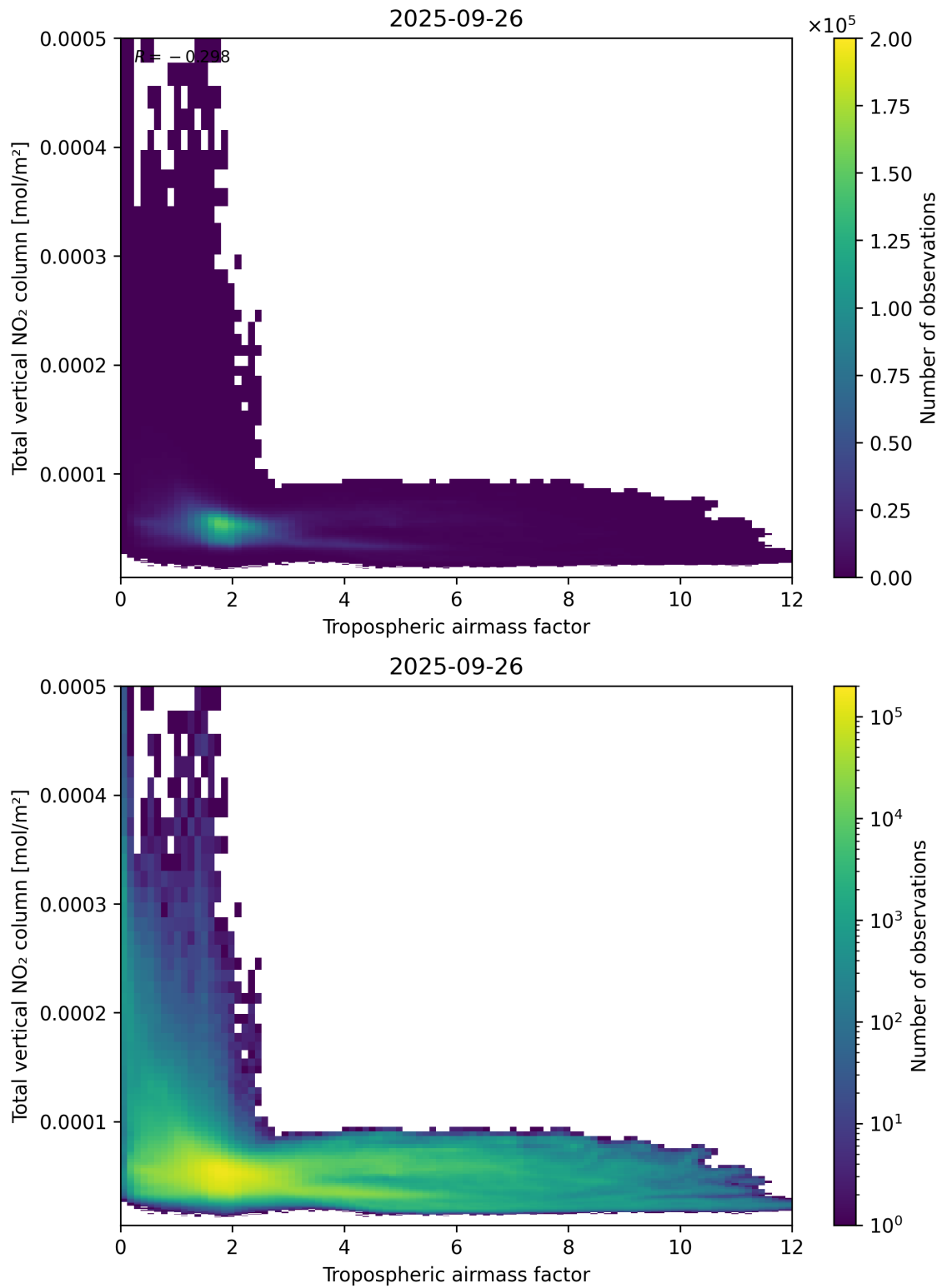
Figure 77: Scatter density plot of “Tropospheric airmass factor” against “Total vertical NO 2 column” for 2025-09-26 to 2025-09-27.
