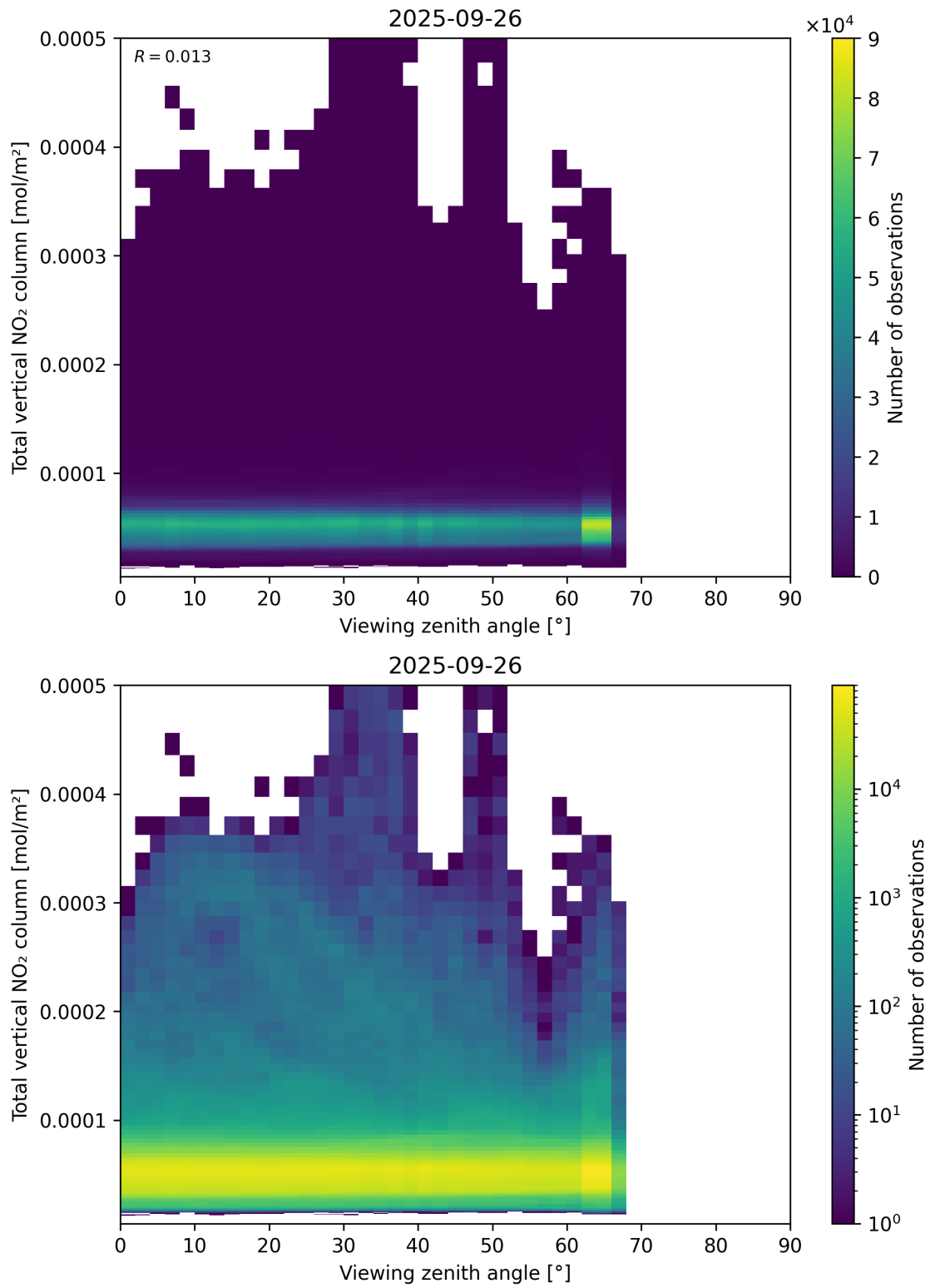
Figure 167: Scatter density plot of “Viewing zenith angle” against “Total vertical NO 2 column” for 2025-09-26 to 2025-09-27.
