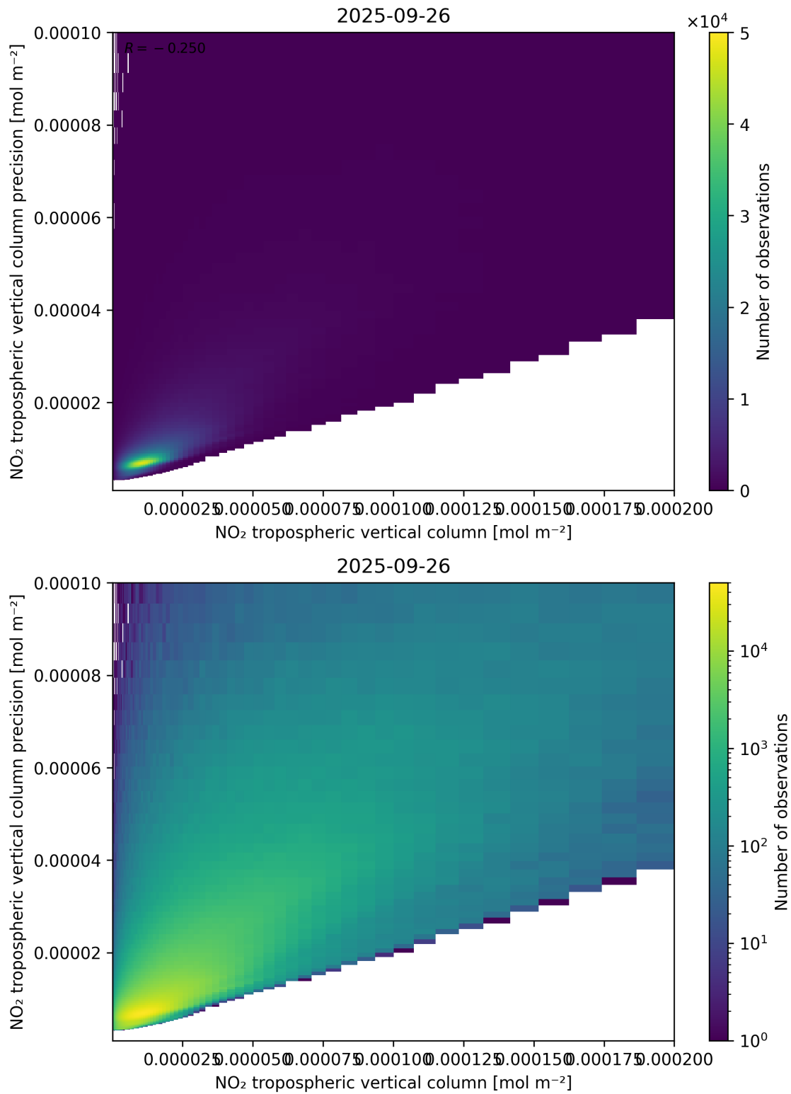
Figure 130: Scatter density plot of “NO 2 tropospheric vertical column” against “NO 2 tropospheric vertical column precision” for 2025-09-26 to 2025-09-27.
