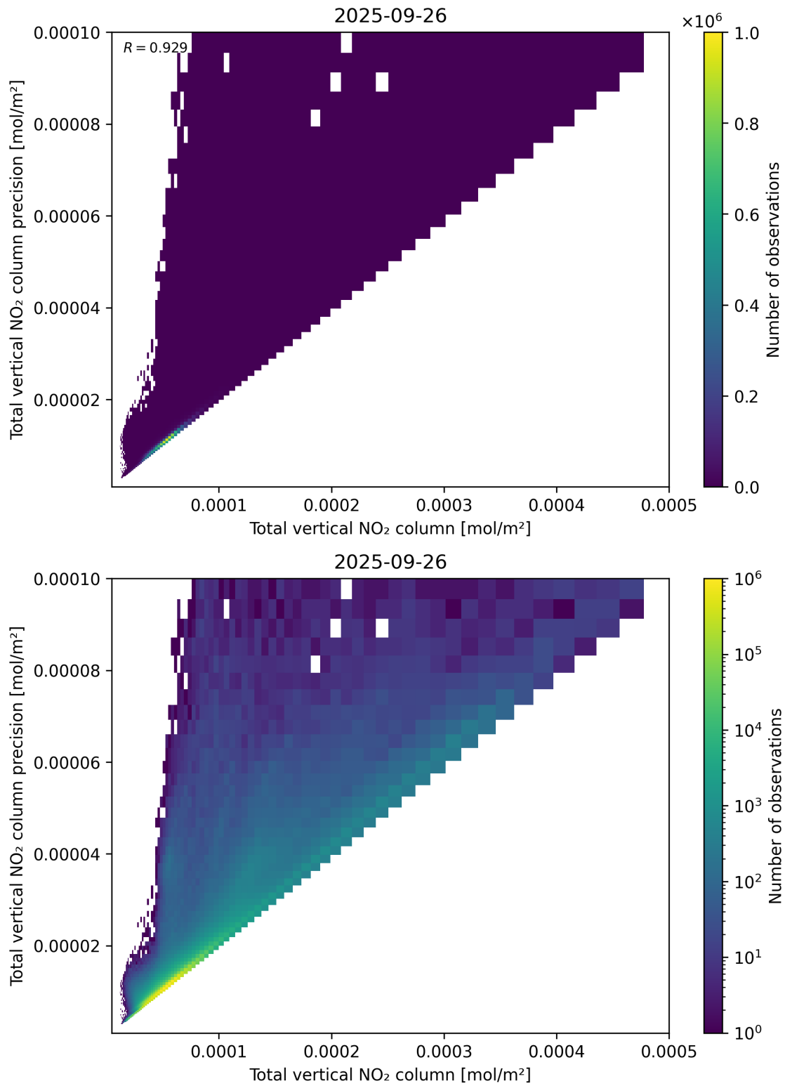
Figure 114: Scatter density plot of “Total vertical NO 2 column” against “Total vertical NO 2 column precision” for 2025-09-26 to 2025-09-27.
