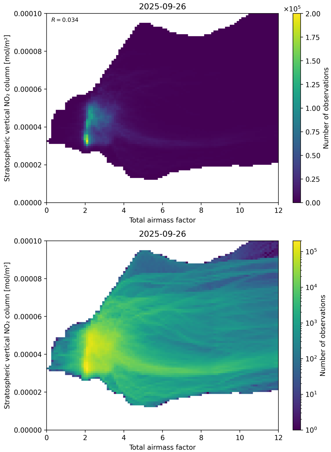
Figure 64: Scatter density plot of “Total airmass factor” against “Stratospheric vertical NO 2 column” for 2025-09-26 to 2025-09-27.
