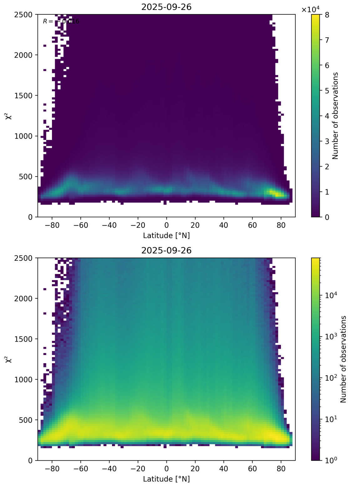
Figure 86: Scatter density plot of “Latitude” against “ \chi^2 ” for 2025-09-26 to 2025-09-27.
