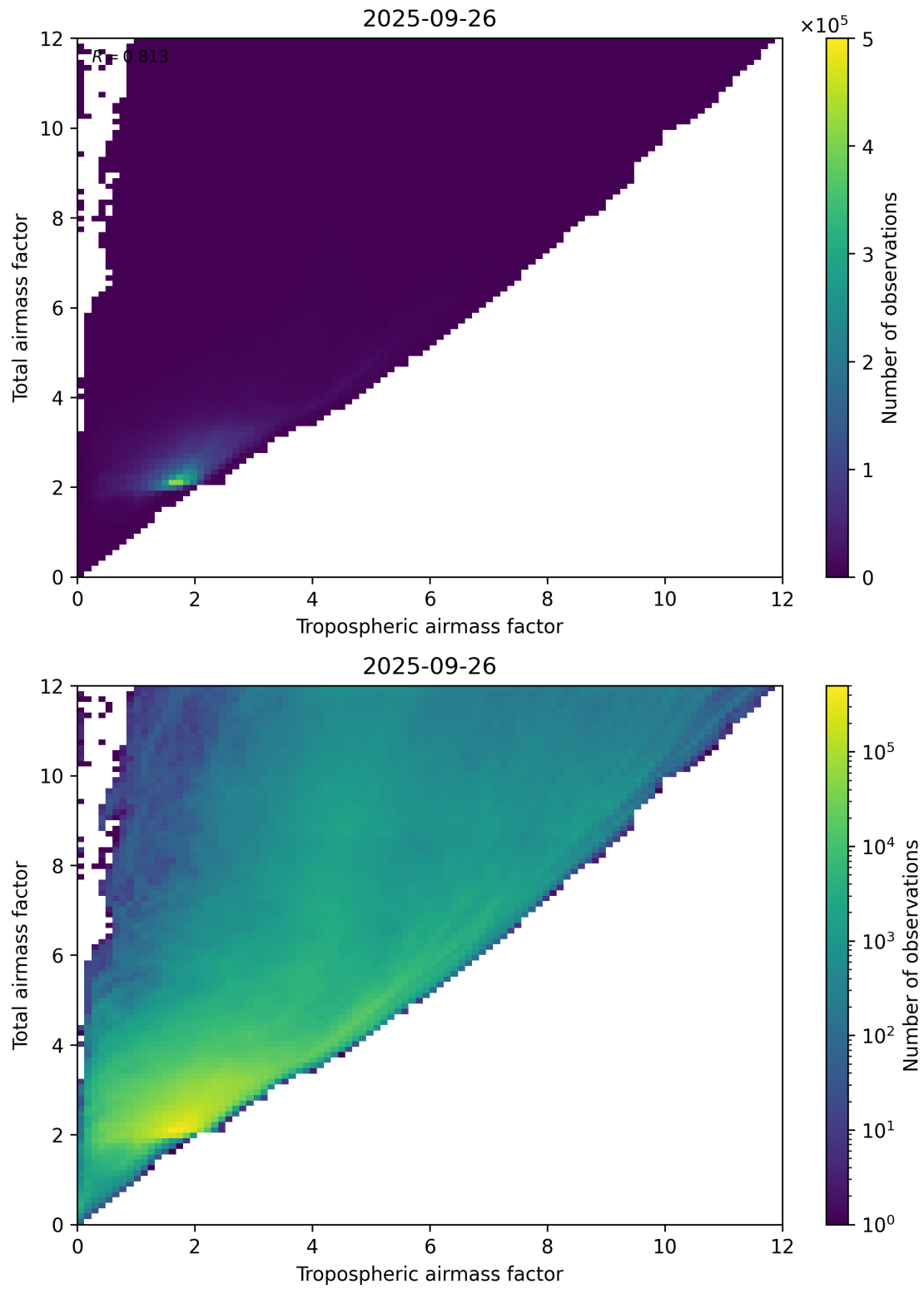
Figure 72: Scatter density plot of “Tropospheric airmass factor” against “Total airmass factor” for 2025-09-26 to 2025-09-27.
