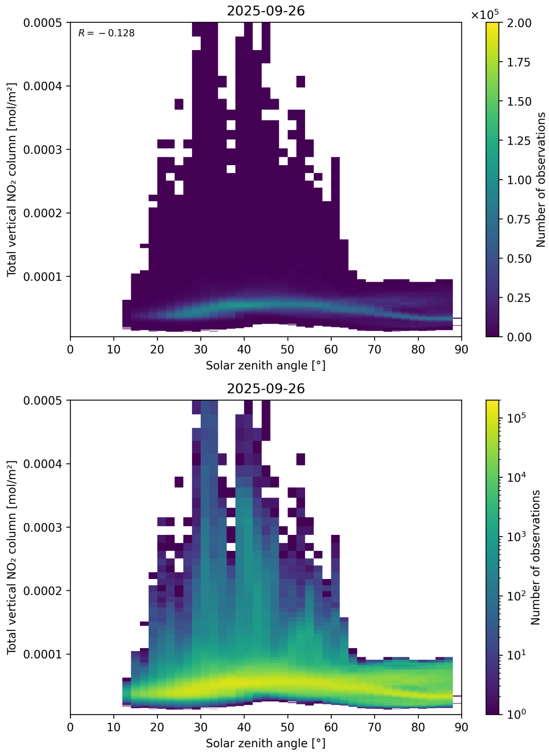
Figure 153: Scatter density plot of “Solar zenith angle” against “Total vertical NO 2 column” for 2025-09-26 to 2025-09-27.
