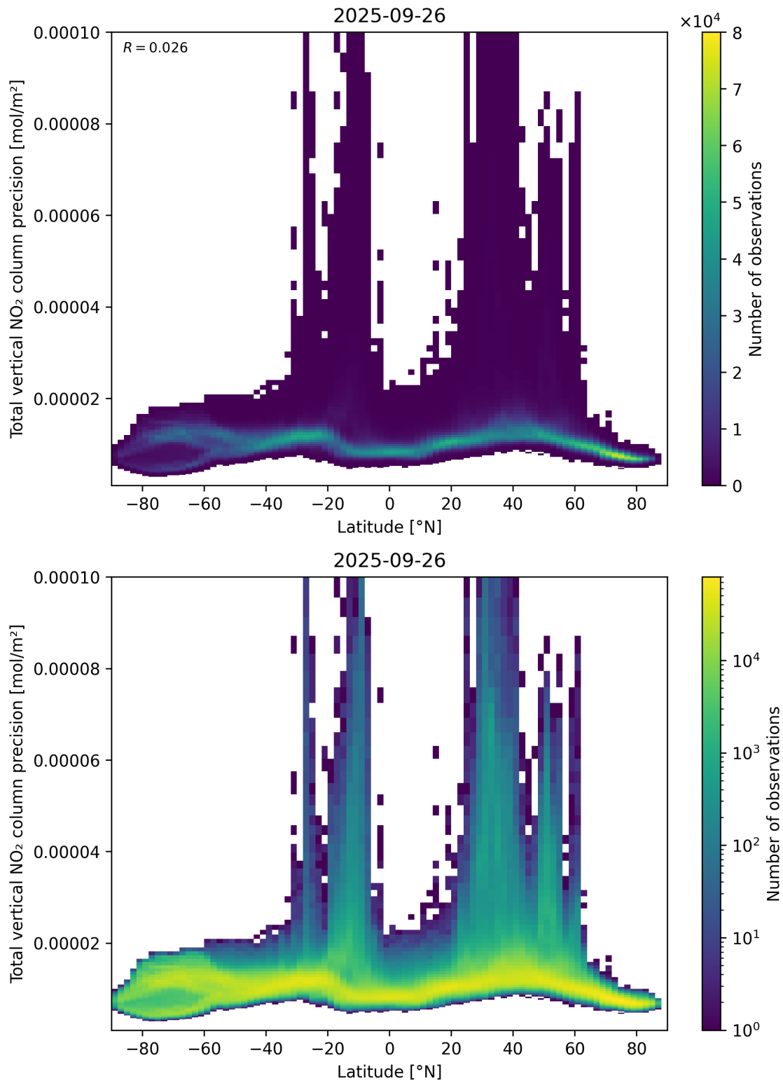
Figure 91: Scatter density plot of “Latitude” against “Total vertical NO 2 column precision” for 2025-09-26 to 2025-09-27.
