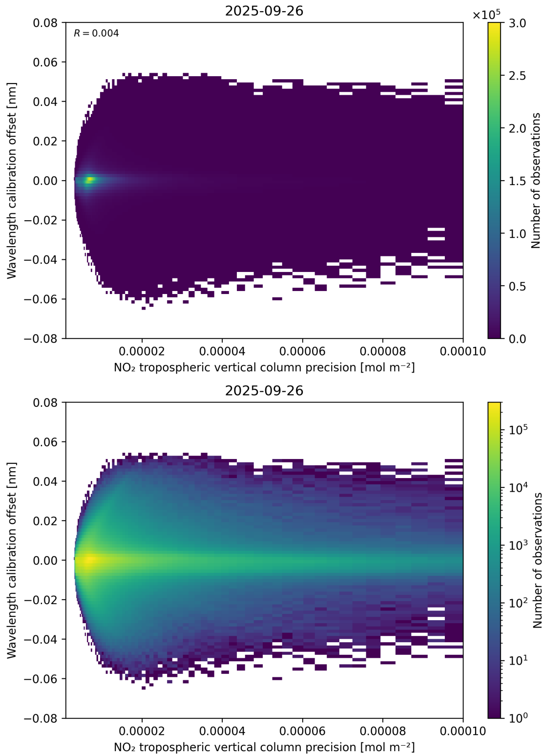
Figure 141: Scatter density plot of “NO 2 tropospheric vertical column precision” against “Wavelength calibration offset” for 2025-09-26 to 2025-09-27.
