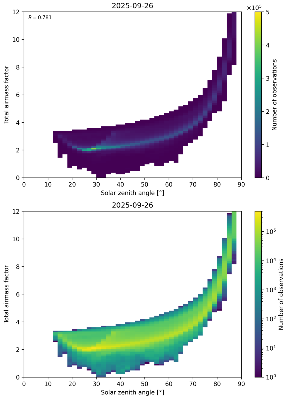
Figure 146: Scatter density plot of “Solar zenith angle” against “Total airmass factor” for 2025-09-26 to 2025-09-27.
