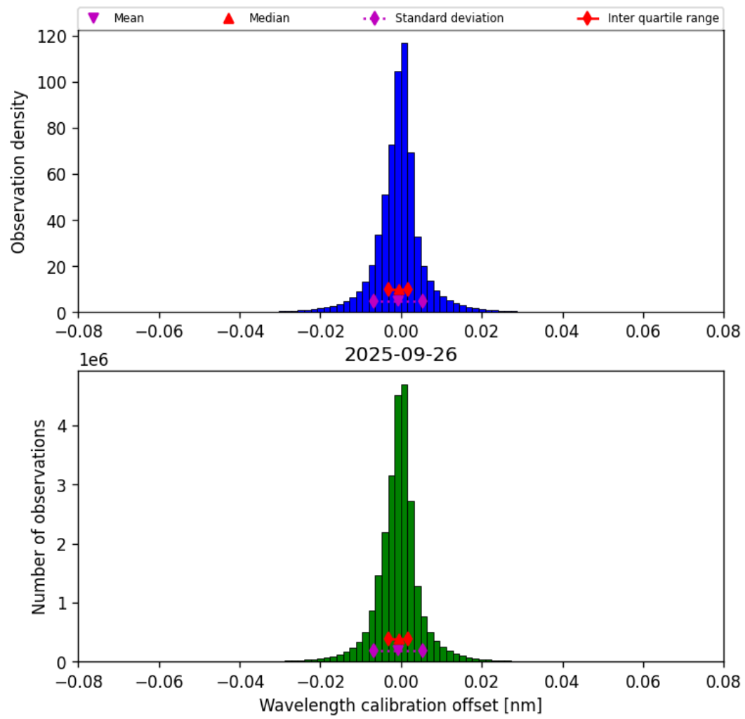
Figure 35: Histogram of “Wavelength calibration offset” for 2025-09-26 to 2025-09-27
