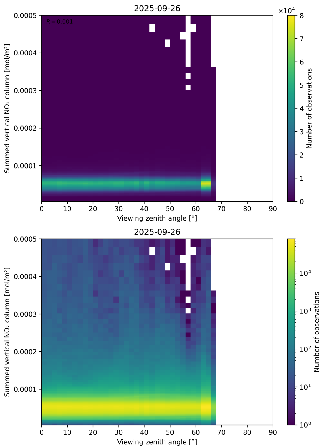
Figure 165: Scatter density plot of “Viewing zenith angle” against “Summed vertical NO 2 column” for 2025-09-26 to 2025-09-27.
