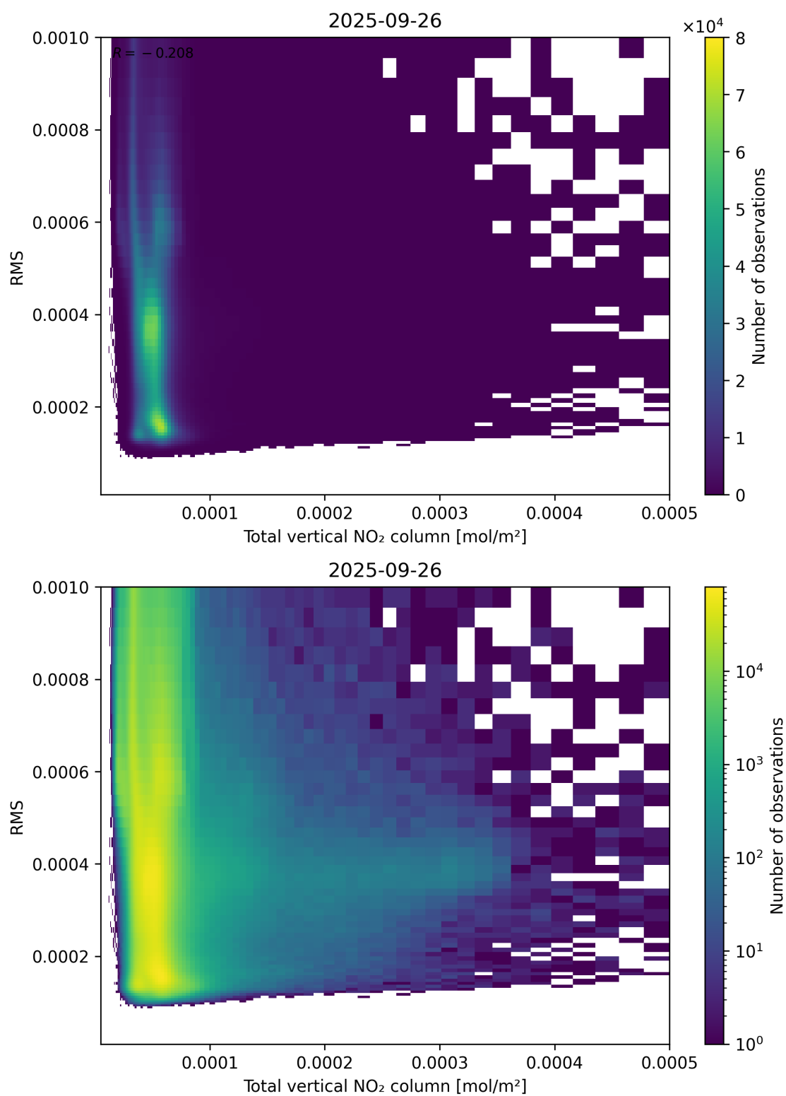
Figure 120: Scatter density plot of “Total vertical NO 2 column” against “RMS” for 2025-09-26 to 2025-09-27.
