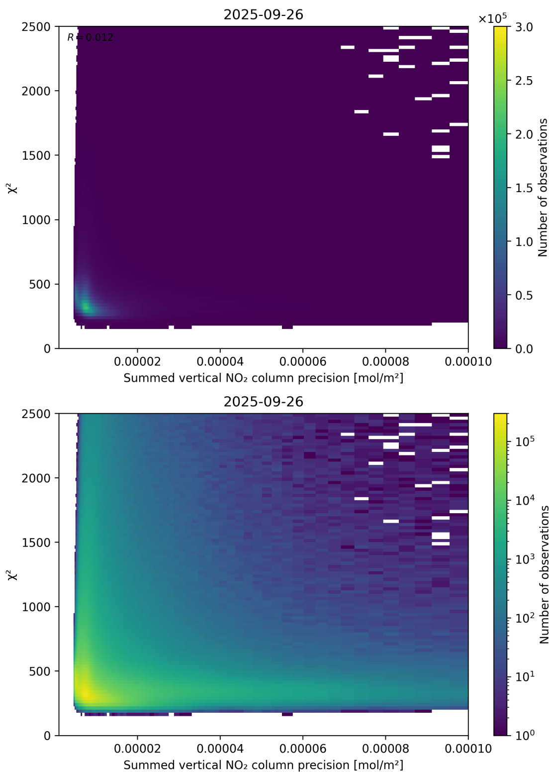
Figure 107: Scatter density plot of “Summed vertical NO 2 column precision” against “ \chi^2 ” for 2025-09-26 to 2025-09-27.
