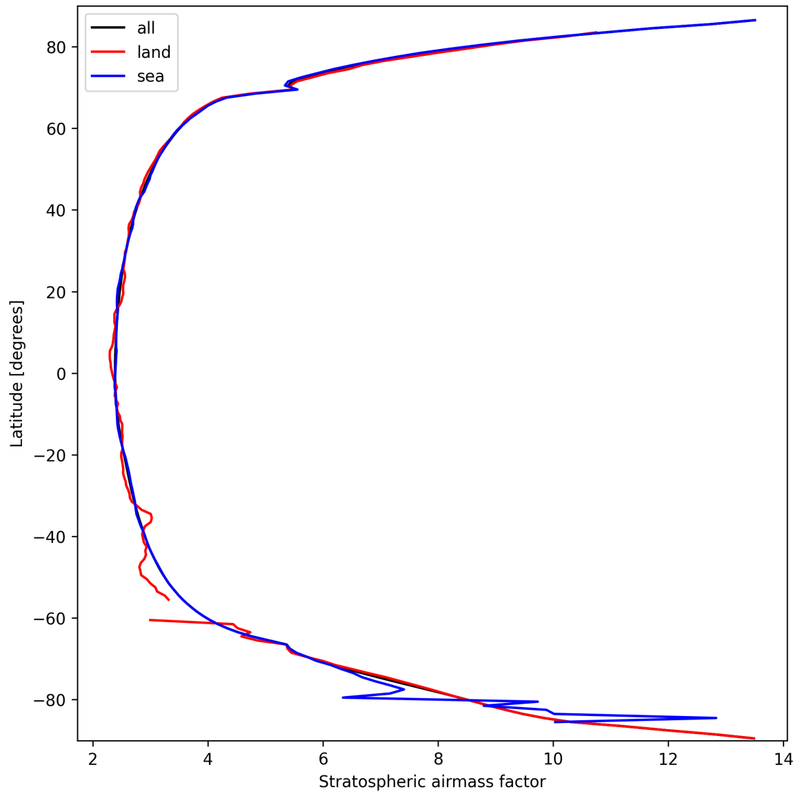
Figure 27: Zonal average of “Stratospheric air mass factor” for 2025-09-26 to 2025-09-27.
