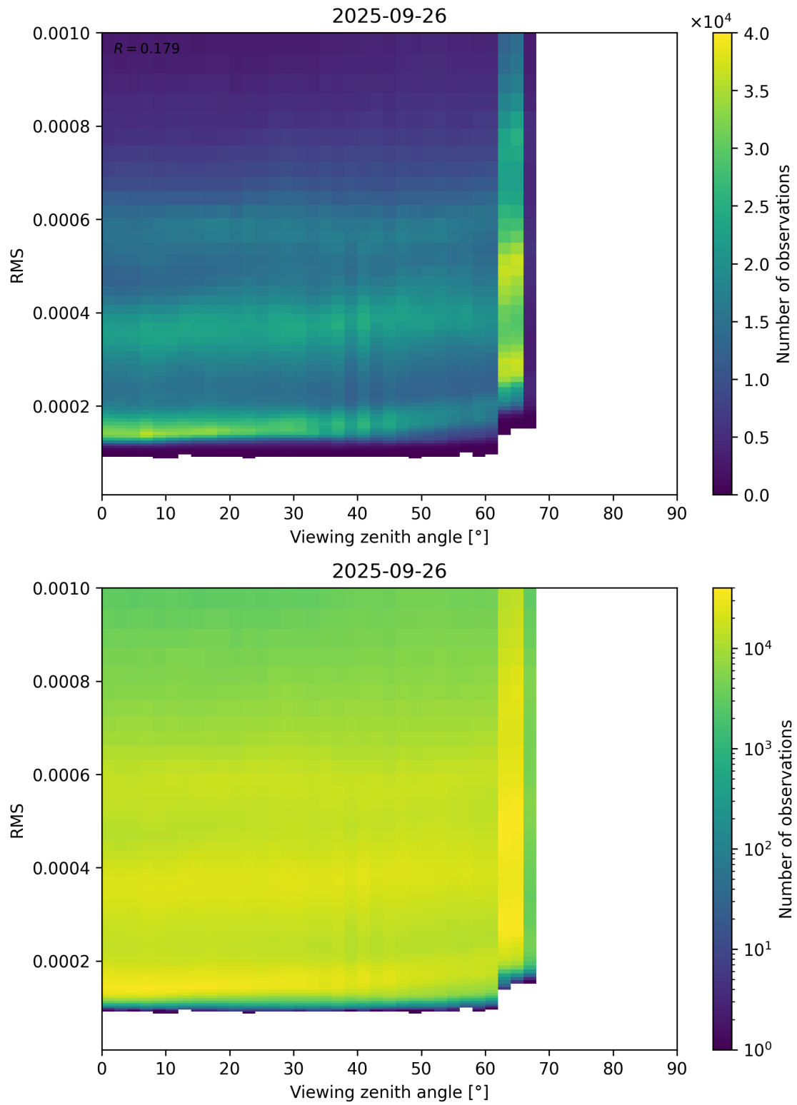
Figure 171: Scatter density plot of “Viewing zenith angle” against “RMS” for 2025-09-26 to 2025-09-27.
