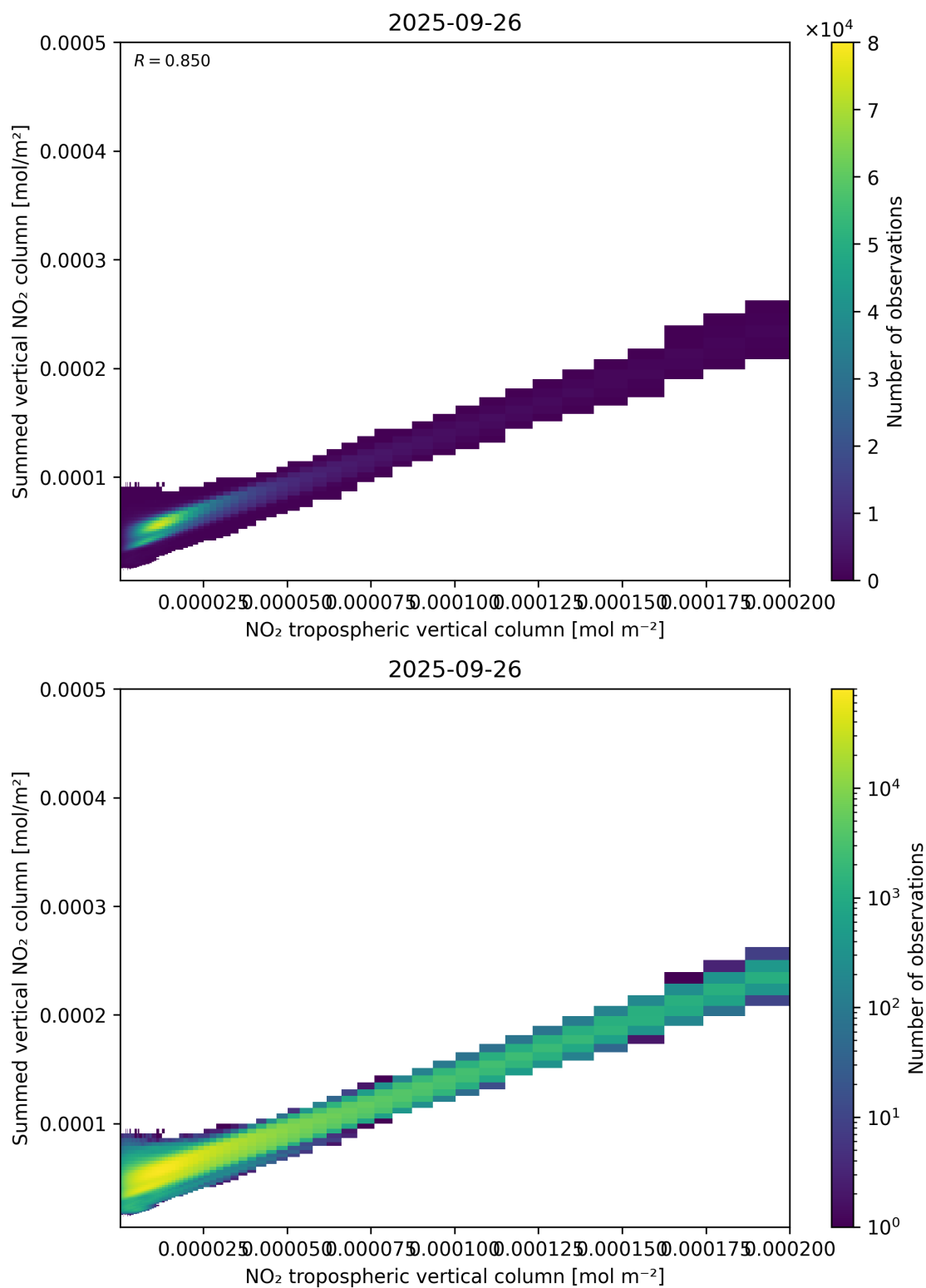
Figure 126: Scatter density plot of “NO 2 tropospheric vertical column” against “Summed vertical NO 2 column” for 2025-09-26 to 2025-09-27.
