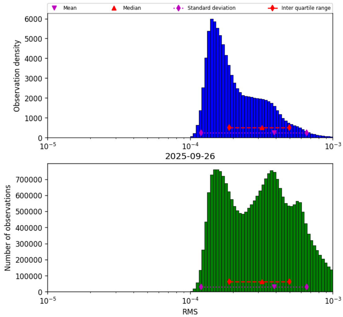
Figure 43: Histogram of “RMS” for 2025-09-26 to 2025-09-27
