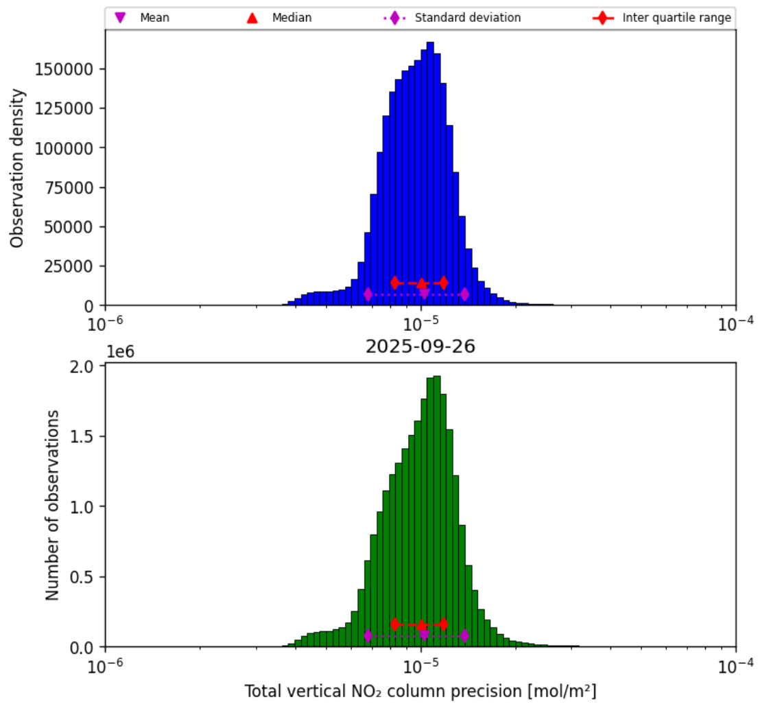
Figure 39: Histogram of “Total vertical NO 2 column precision” for 2025-09-26 to 2025-09-27
