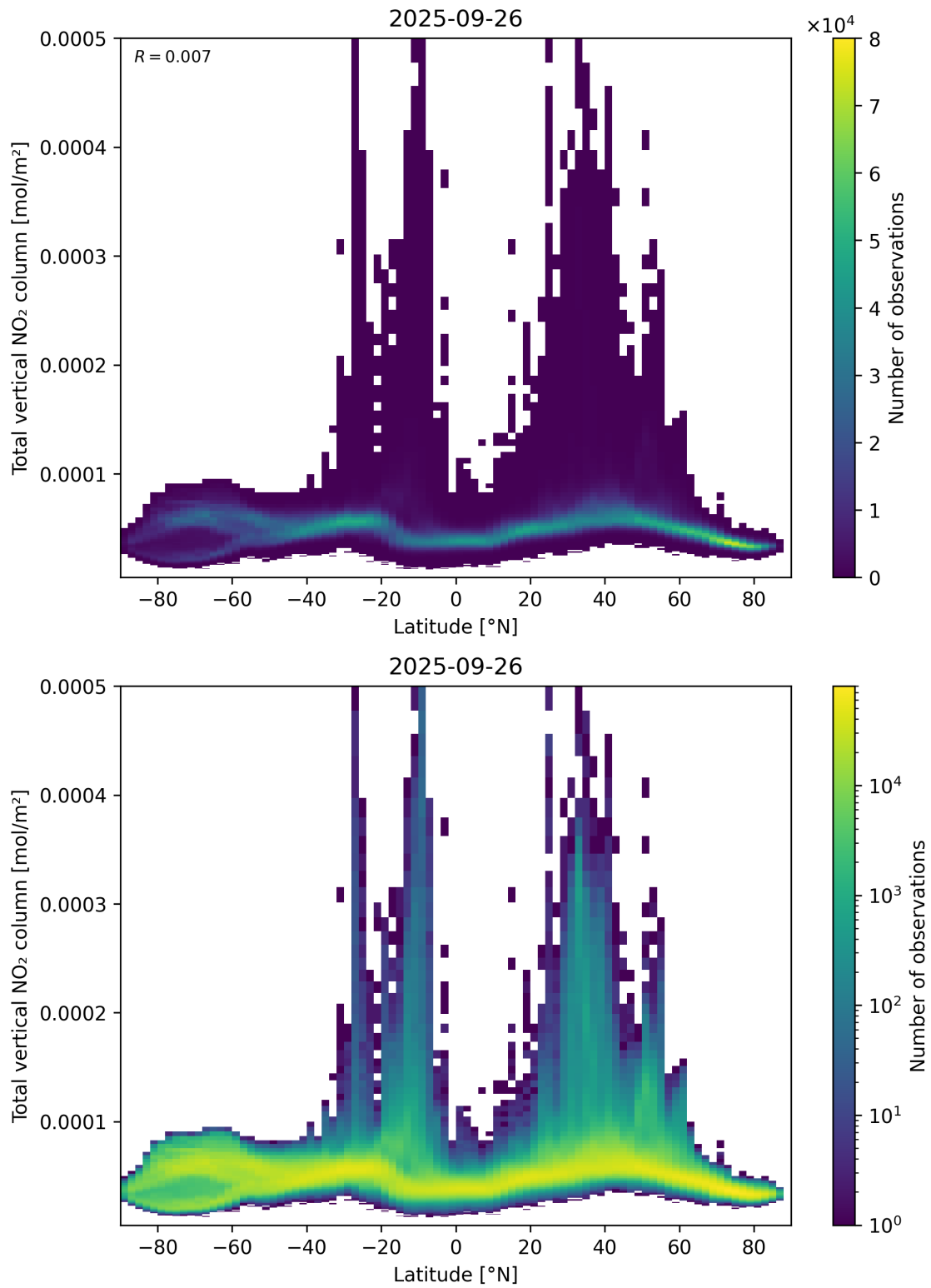
Figure 90: Scatter density plot of “Latitude” against “Total vertical NO 2 column” for 2025-09-26 to 2025-09-27.
