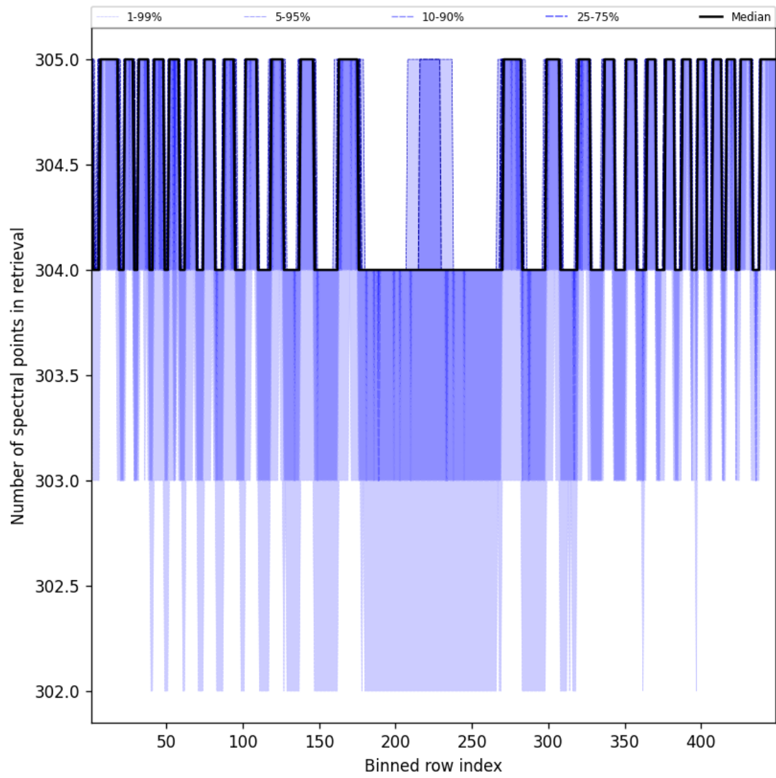
Figure 50: Along track statistics of “Number of spectral points in retrieval” for 2025-09-26 to 2025-09-27
