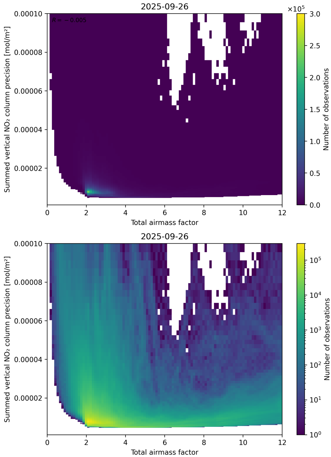
Figure 66: Scatter density plot of “Total airmass factor” against “Summed vertical NO 2 column precision” for 2025-09-26 to 2025-09-27.
