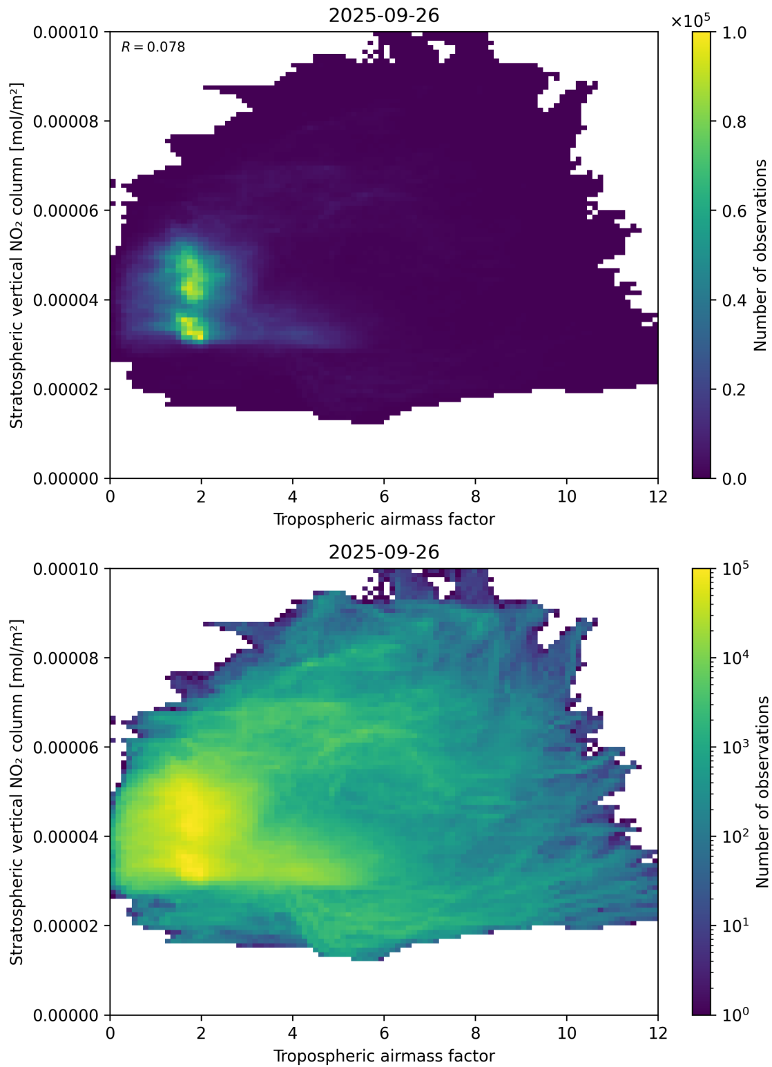
Figure 74: Scatter density plot of “Tropospheric airmass factor” against “Stratospheric vertical NO 2 column” for 2025-09-26 to 2025-09-27.
