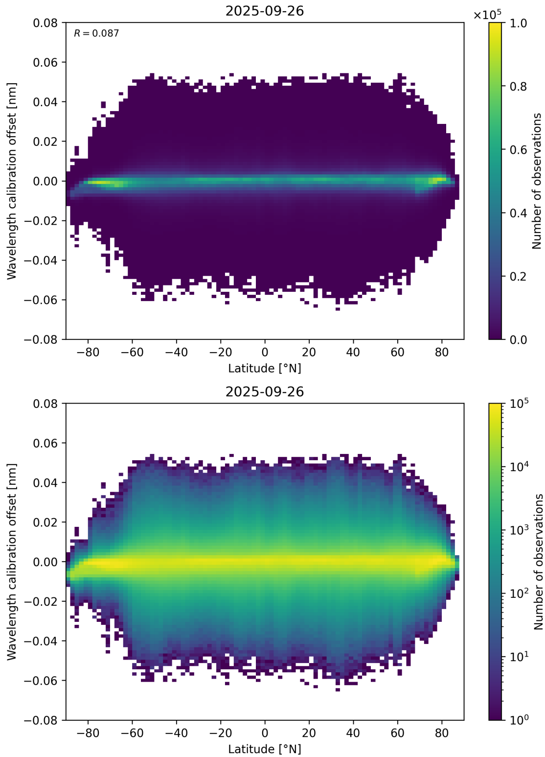
Figure 95: Scatter density plot of “Latitude” against “Wavelength calibration offset” for 2025-09-26 to 2025-09-27.
