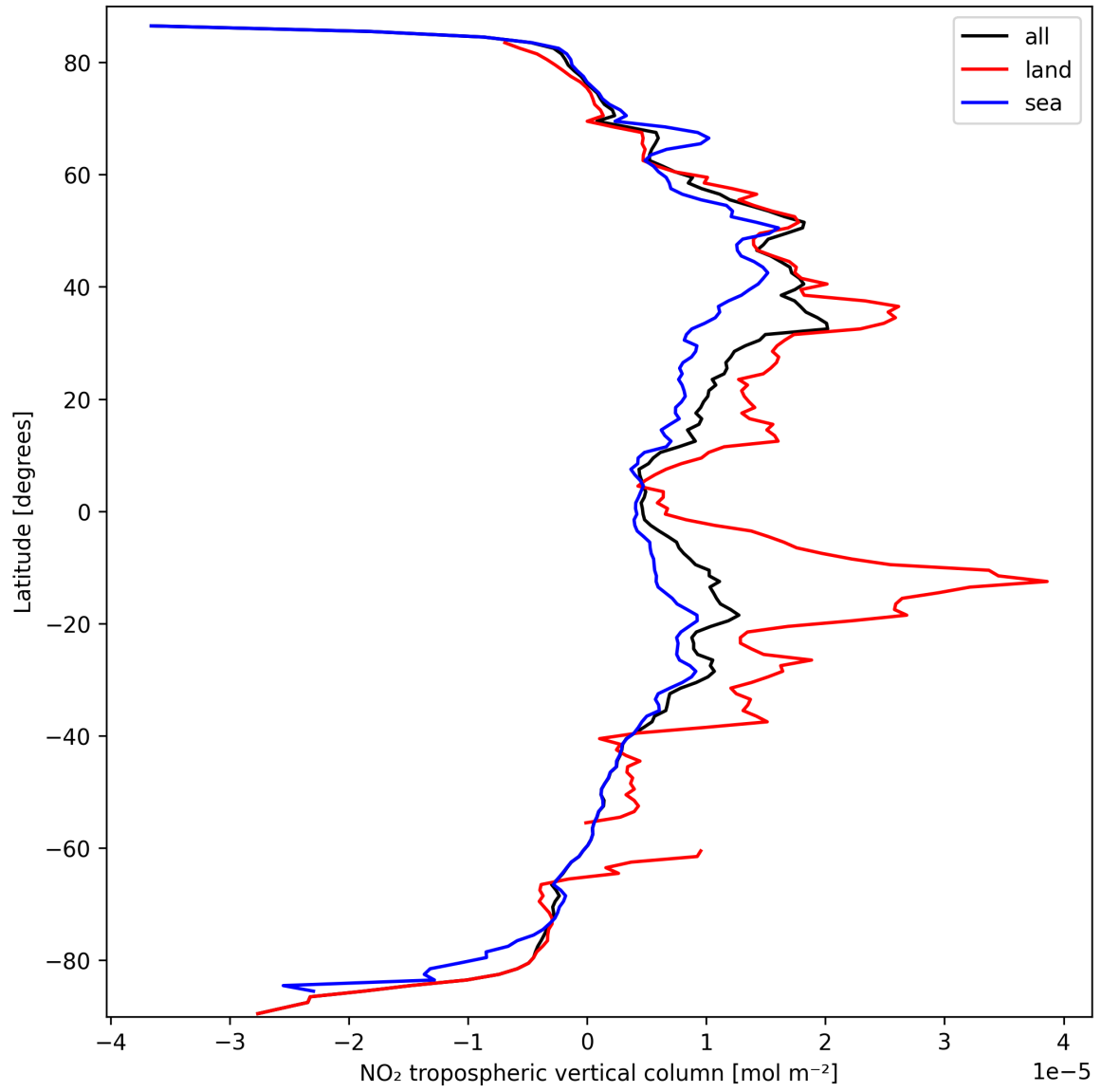
Figure 12: Zonal average of “NO 2 tropospheric vertical column” for 2025-09-26 to 2025-09-27.
