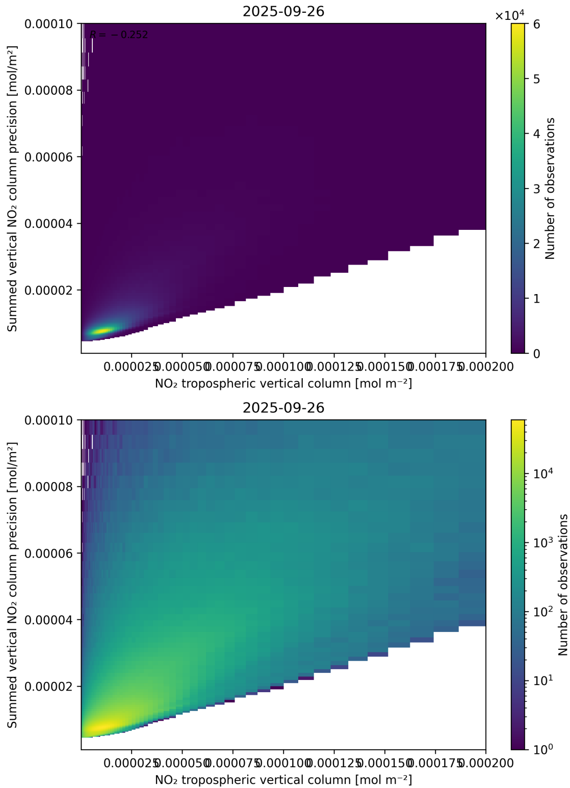
Figure 127: Scatter density plot of “NO 2 tropospheric vertical column” against “Summed vertical NO 2 column precision” for 2025-09-26 to 2025-09-27.
