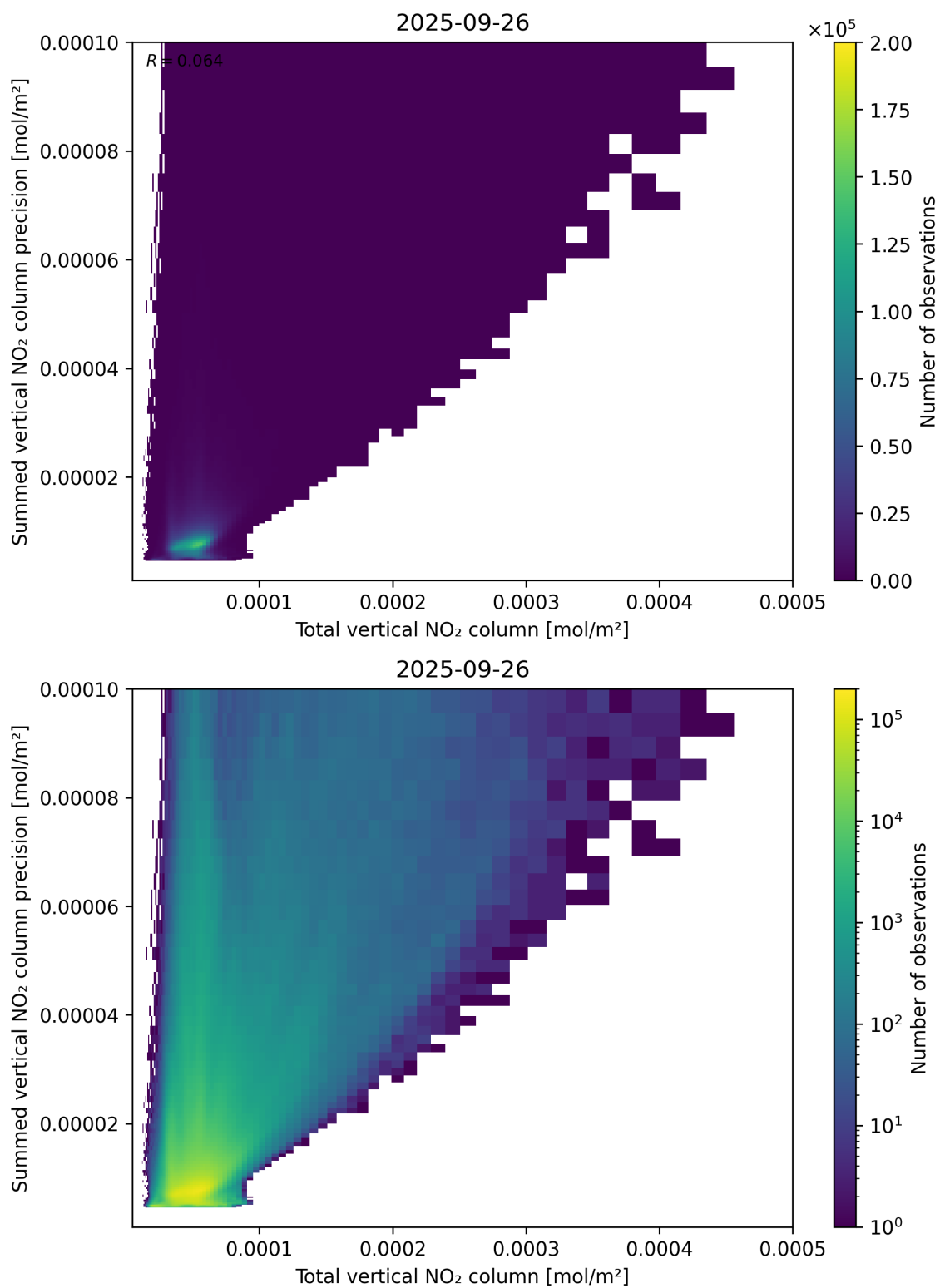
Figure 113: Scatter density plot of “Total vertical NO 2 column” against “Summed vertical NO 2 column precision” for 2025-09-26 to 2025-09-27.
