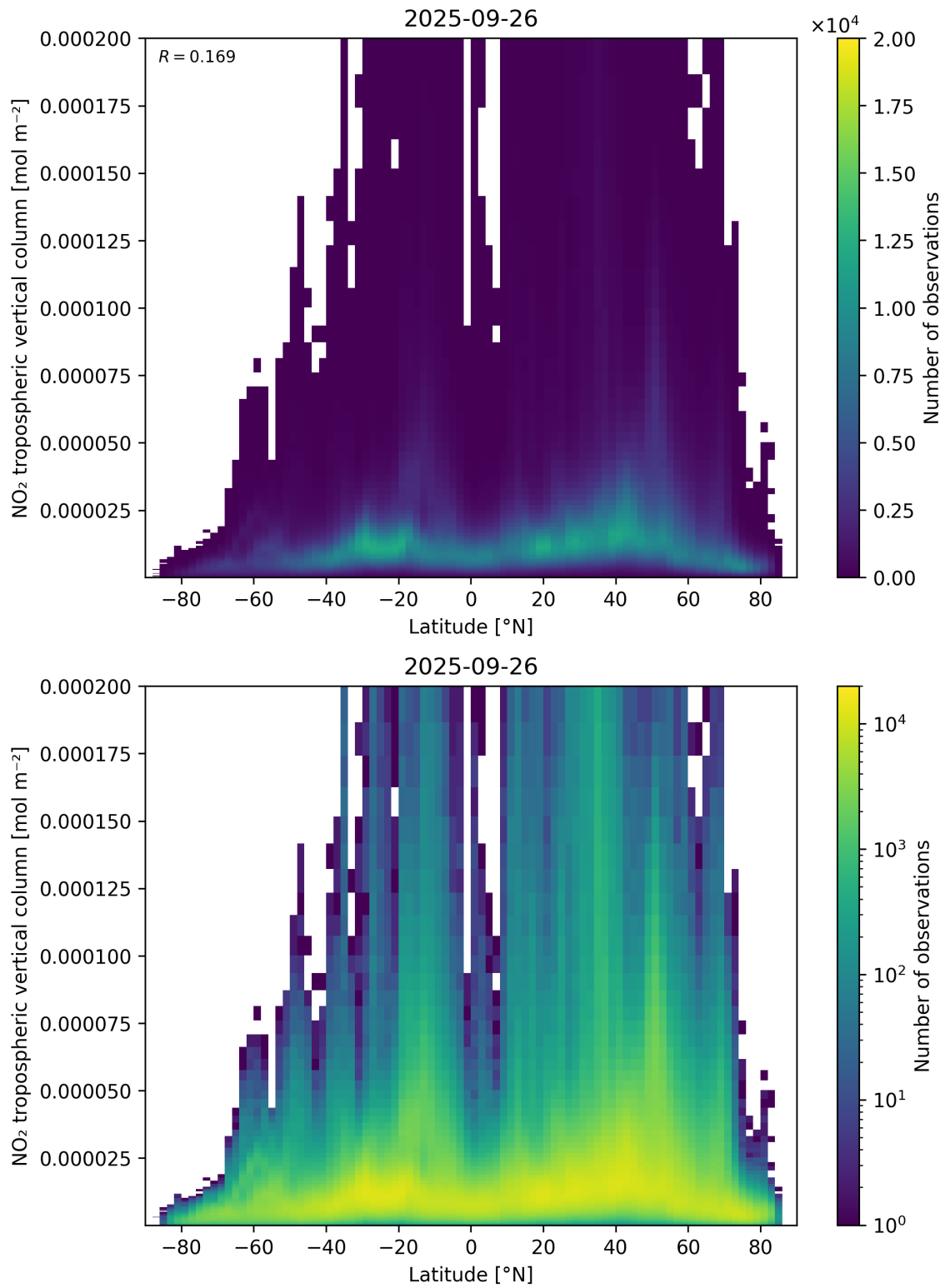
Figure 92: Scatter density plot of “Latitude” against “NO 2 tropospheric vertical column” for 2025-09-26 to 2025-09-27.
