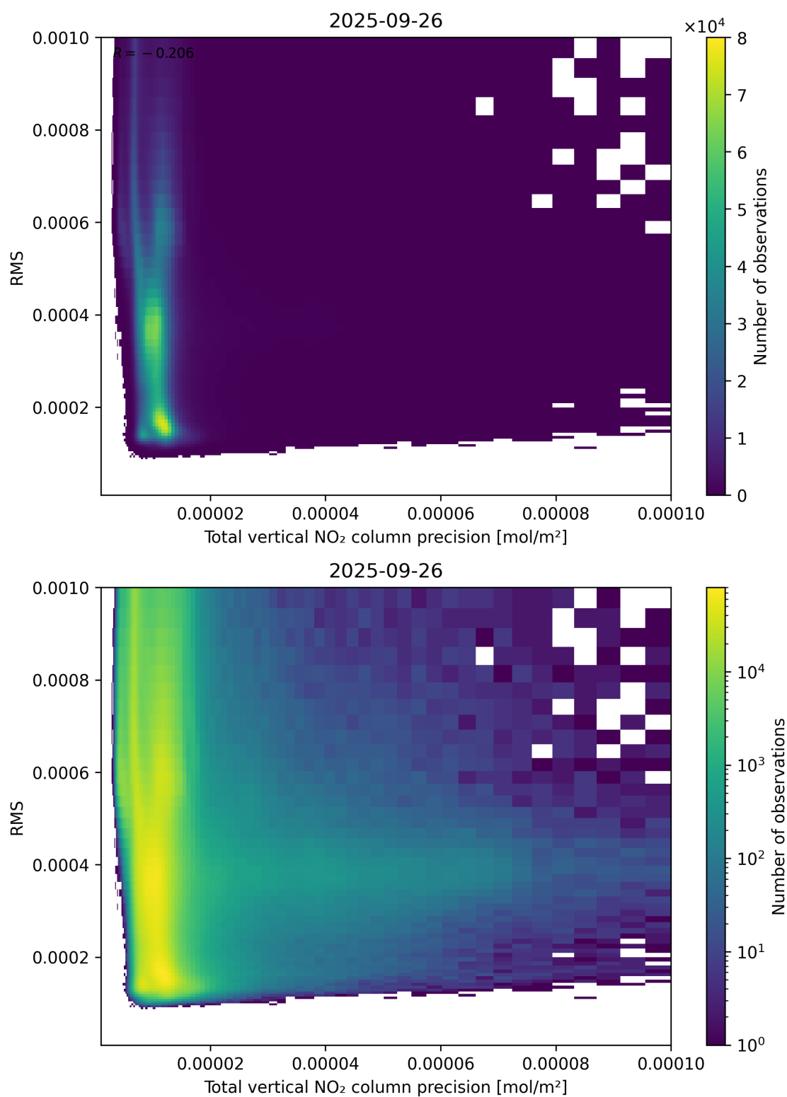
Figure 119: Scatter density plot of “Total vertical NO 2 column precision” against “RMS” for 2025-09-26 to 2025-09-27.
