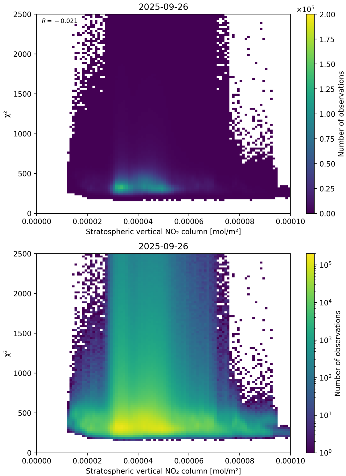
Figure 97: Scatter density plot of “Stratospheric vertical NO 2 column” against “ \chi^2 ” for 2025-09-26 to 2025-09-27.
