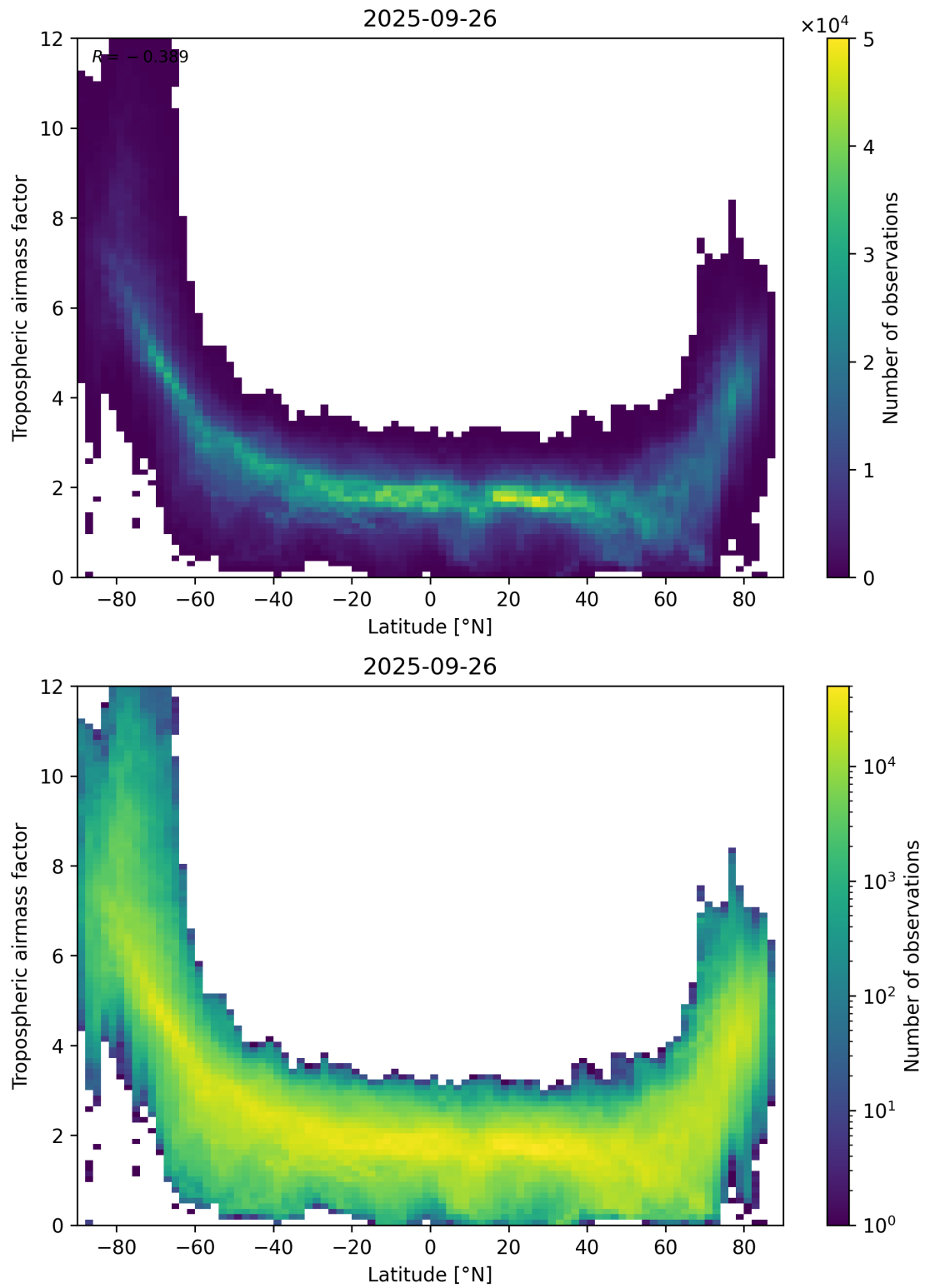
Figure 85: Scatter density plot of “Latitude” against “Tropospheric airmass factor” for 2025-09-26 to 2025-09-27.
