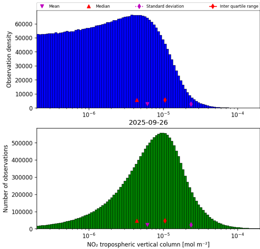
Figure 29: Histogram of “NO 2 tropospheric vertical column” for 2025-09-26 to 2025-09-27
