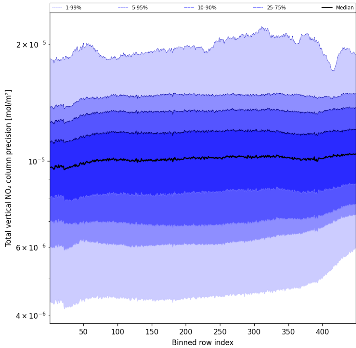
Figure 56: Along track statistics of “Total vertical NO 2 column precision” for 2025-09-26 to 2025-09-27
