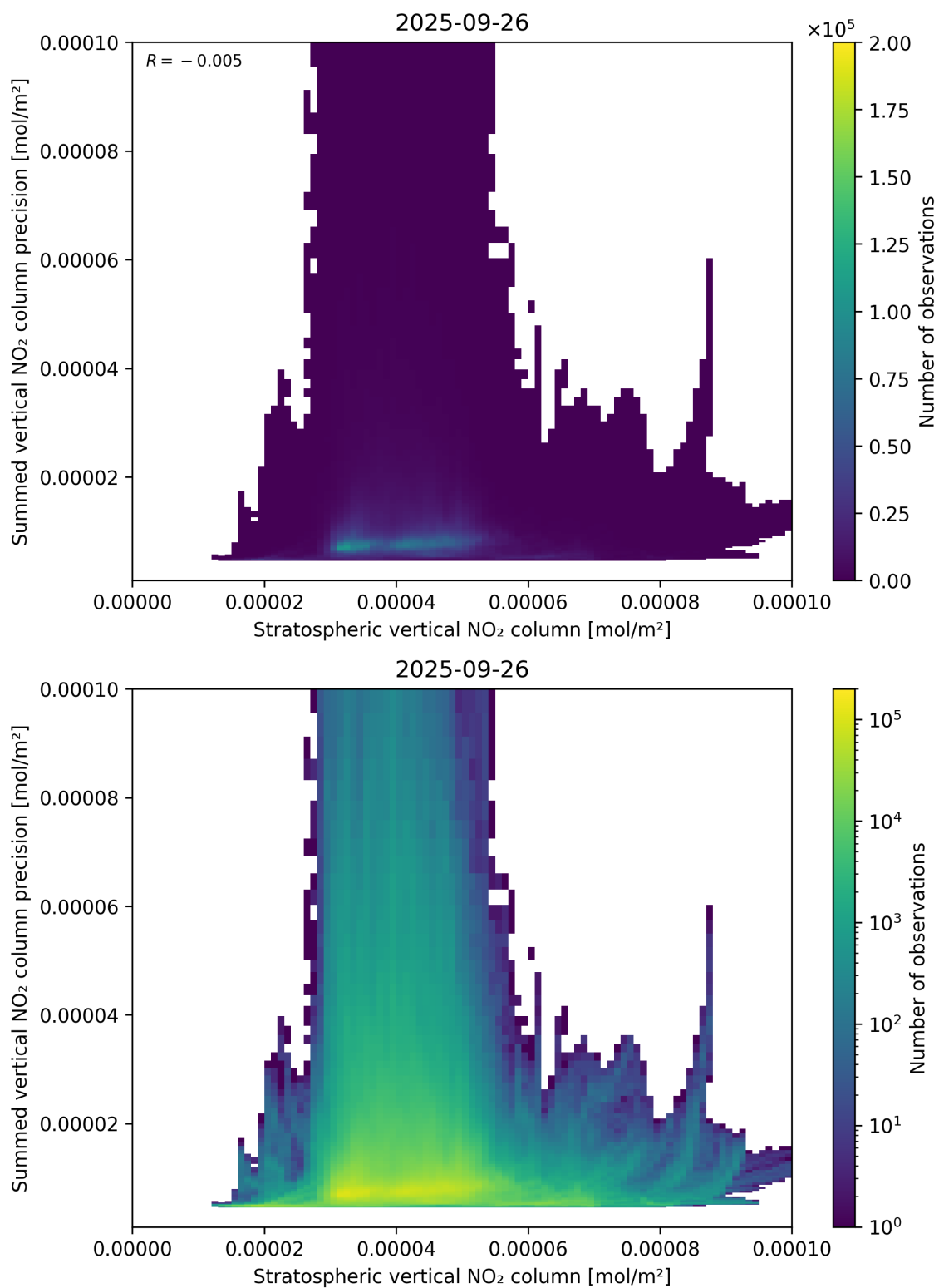
Figure 99: Scatter density plot of “Stratospheric vertical NO 2 column” against “Summed vertical NO 2 column precision” for 2025-09-26 to 2025-09-27.
