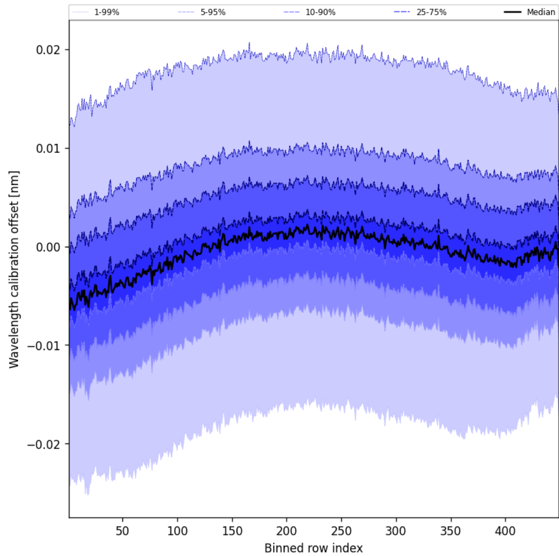
Figure 52: Along track statistics of “Wavelength calibration offset” for 2025-09-26 to 2025-09-27
