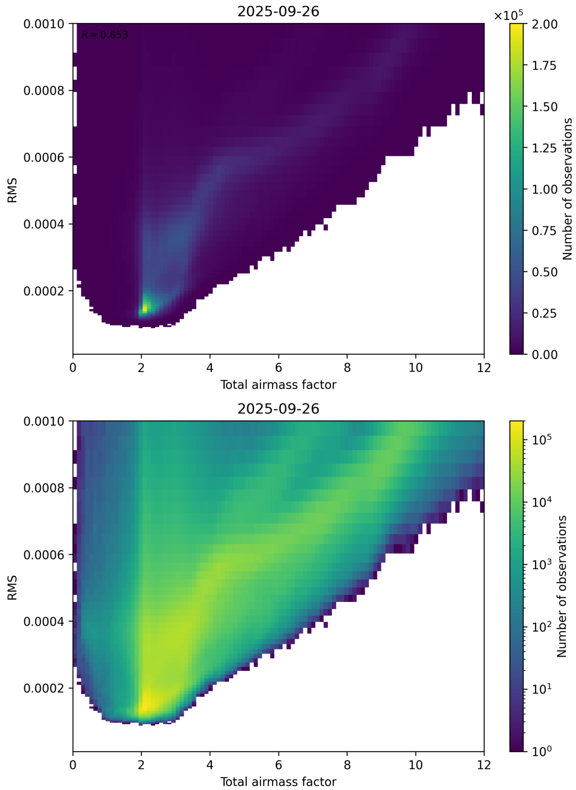
Figure 69: Scatter density plot of “Total airmass factor” against “RMS” for 2025-09-26 to 2025-09-27.
