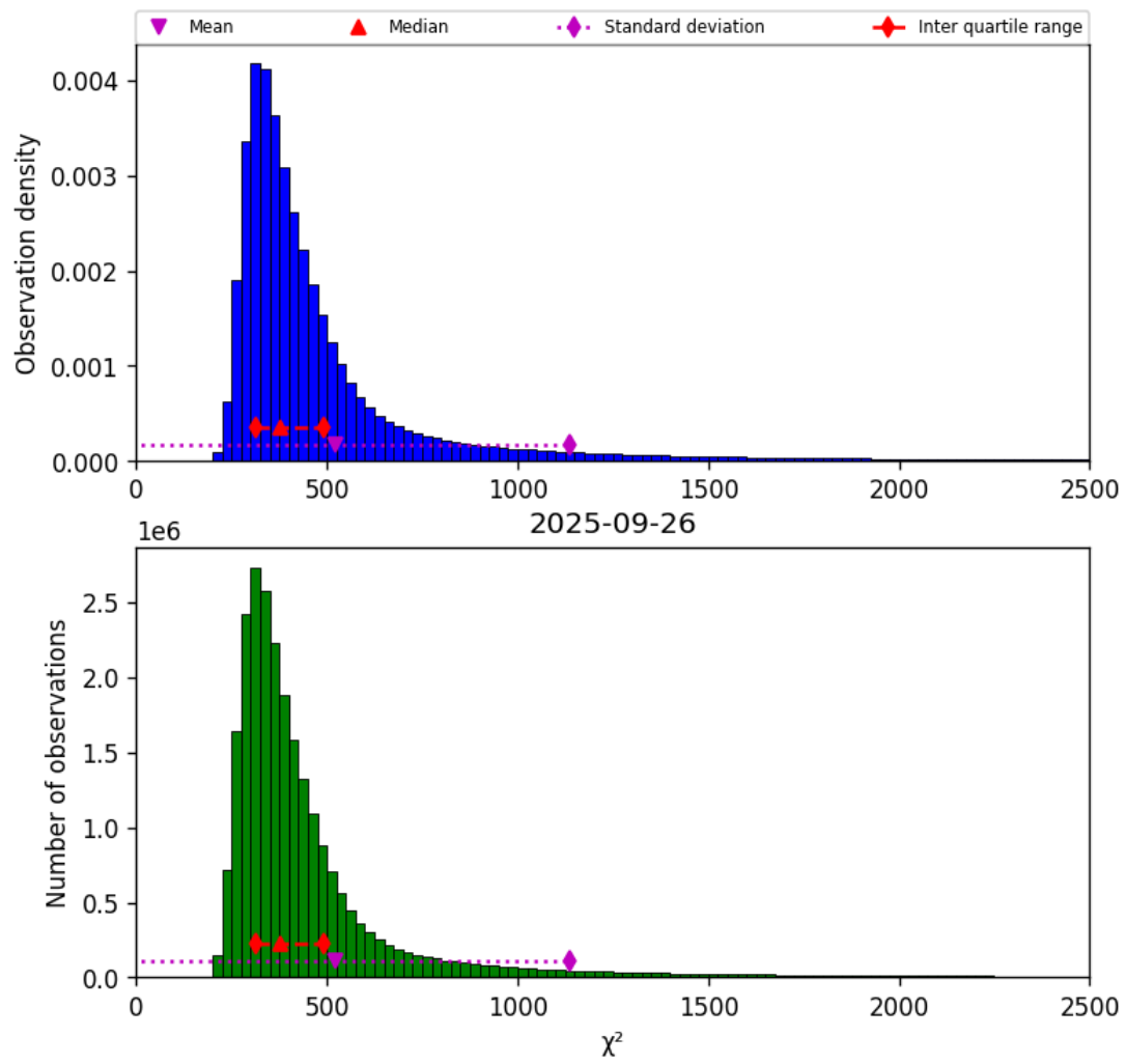
Figure 42: Histogram of " \chi^2 " for 2025-09-26 to 2025-09-27
