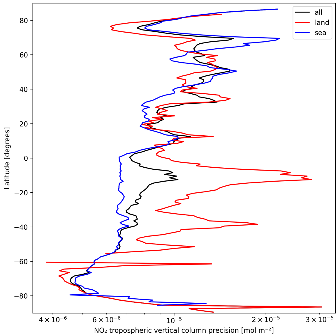
Figure 13: Zonal average of “NO 2 tropospheric vertical column precision” for 2025-09-26 to 2025-09-27.
