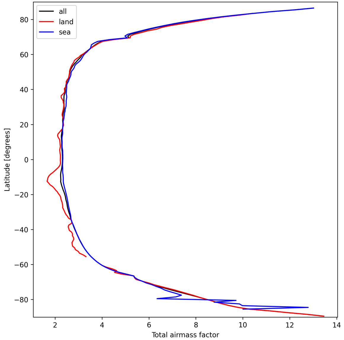
Figure 15: Zonal average of “Total airmass factor” for 2025-09-26 to 2025-09-27.
