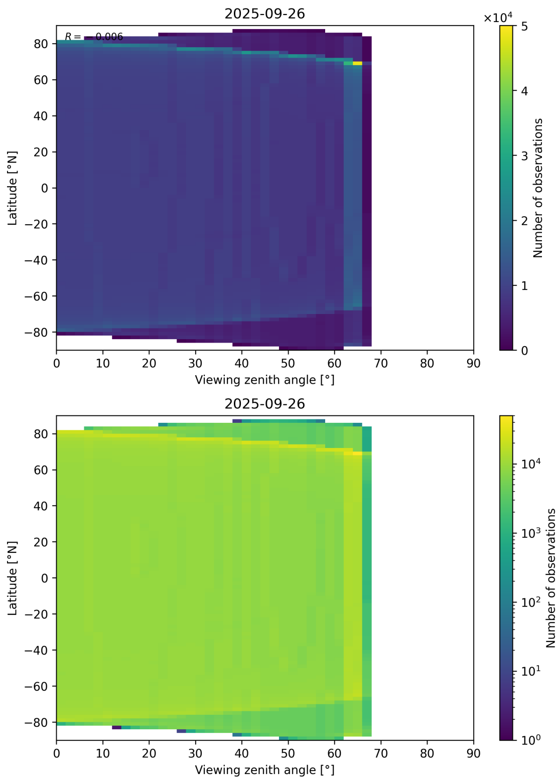
Figure 163: Scatter density plot of “Viewing zenith angle” against “Latitude” for 2025-09-26 to 2025-09-27.
