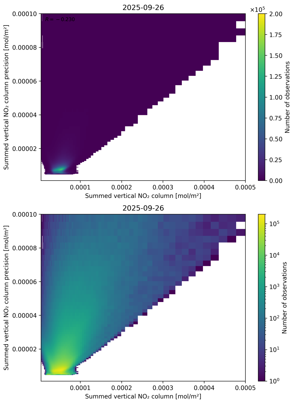
Figure 105: Scatter density plot of “Summed vertical NO 2 column” against “Summed vertical NO 2 column precision” for 2025-09-26 to 2025-09-27.
