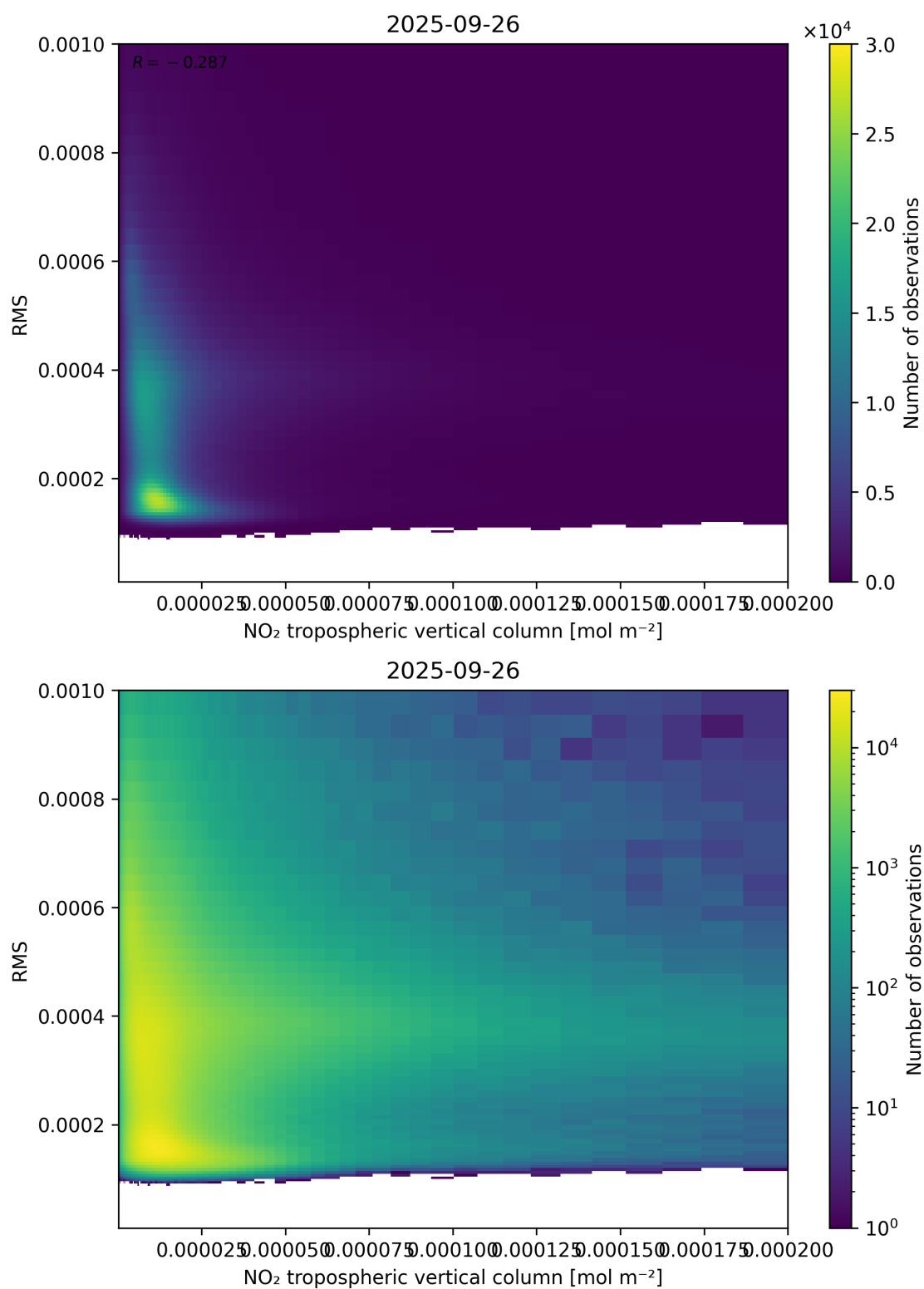
Figure 142: Scatter density plot of “NO 2 tropospheric vertical column” against “RMS” for 2025-09-26 to 2025-09-27.
