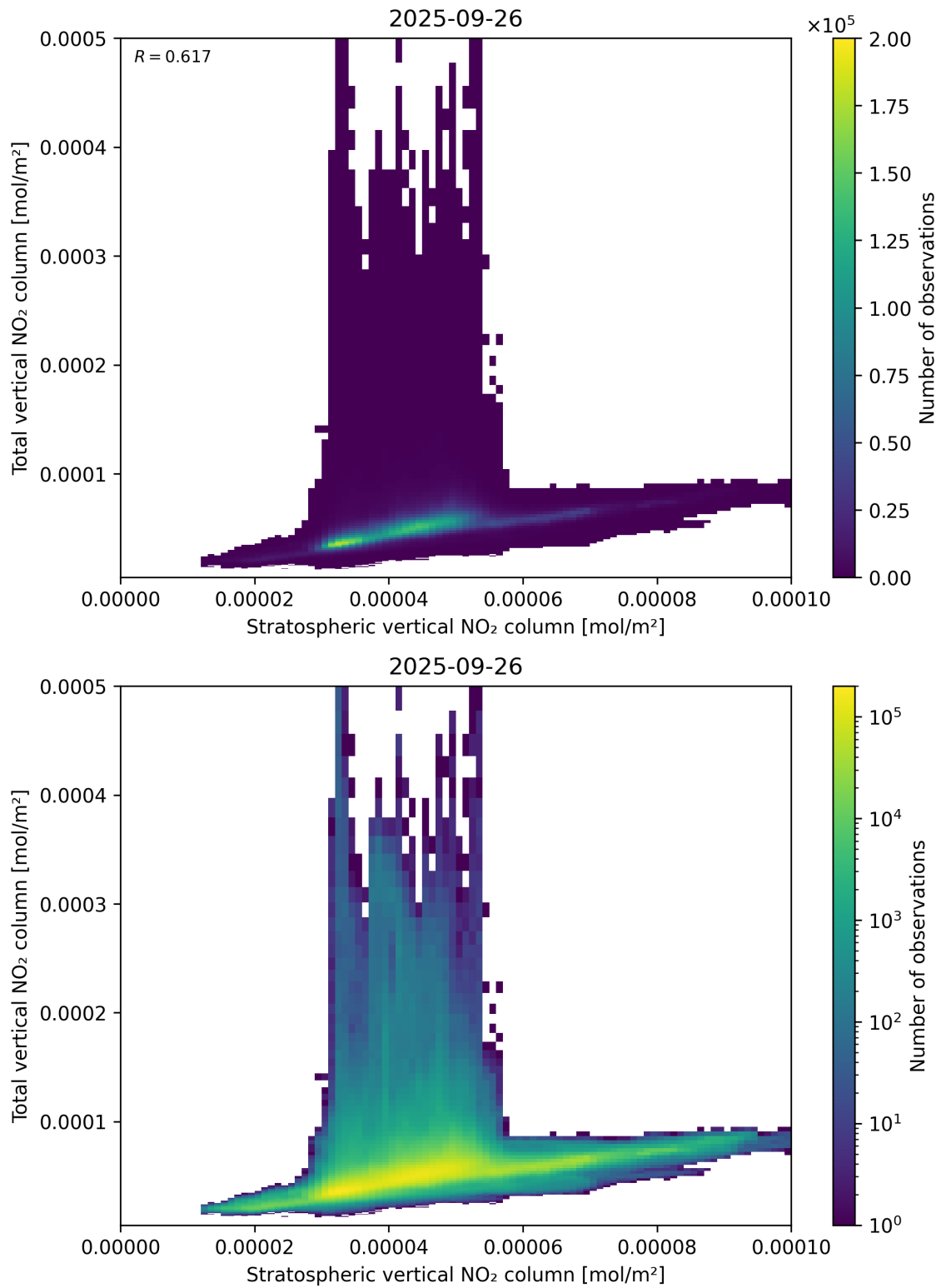
Figure 100: Scatter density plot of “Stratospheric vertical NO 2 column” against “Total vertical NO 2 column” for 2025-09-26 to 2025-09-27.
