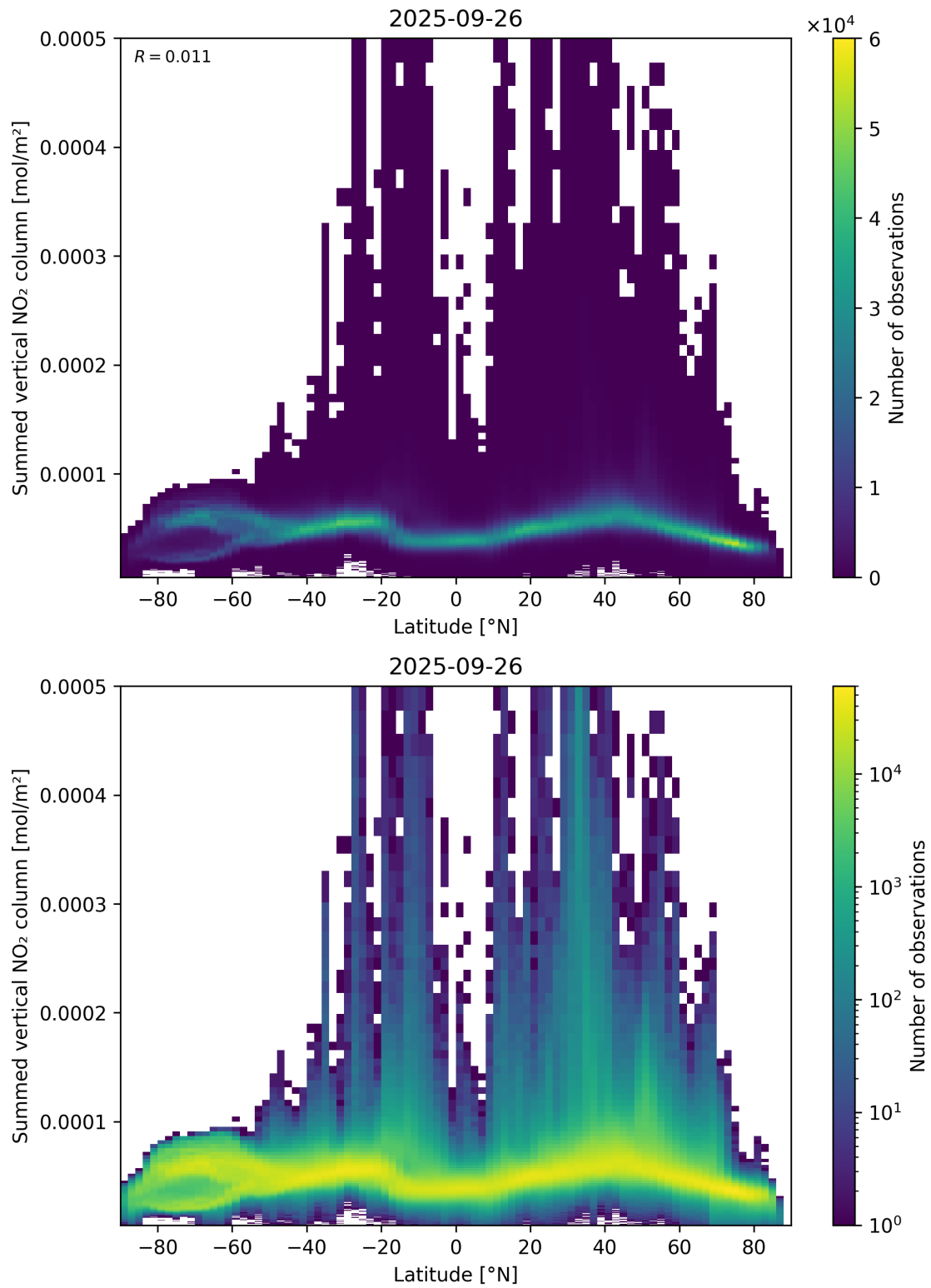
Figure 88: Scatter density plot of “Latitude” against “Summed vertical NO 2 column” for 2025-09-26 to 2025-09-27.
