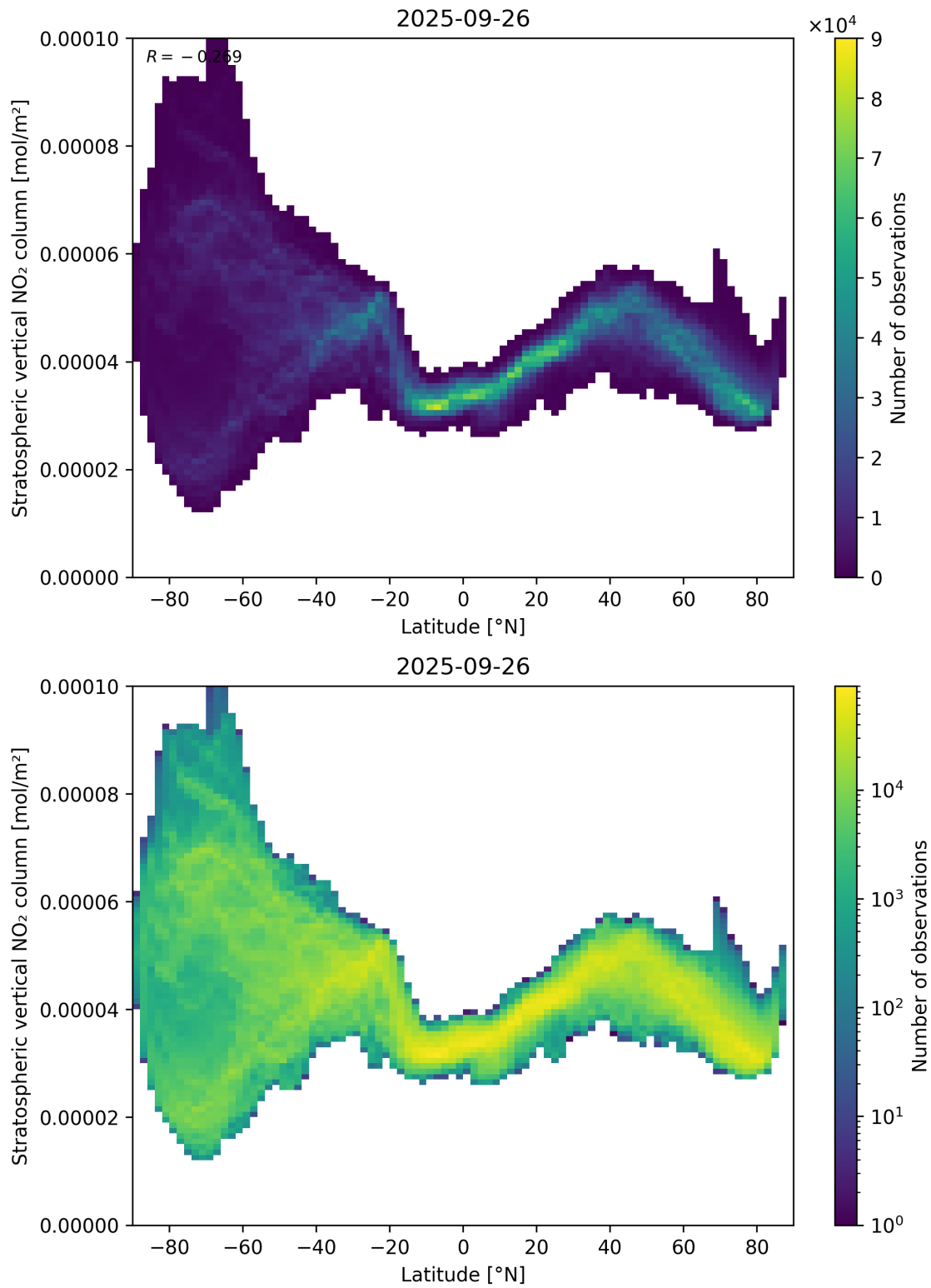
Figure 87: Scatter density plot of “Latitude” against “Stratospheric vertical NO 2 column” for 2025-09-26 to 2025-09-27.
