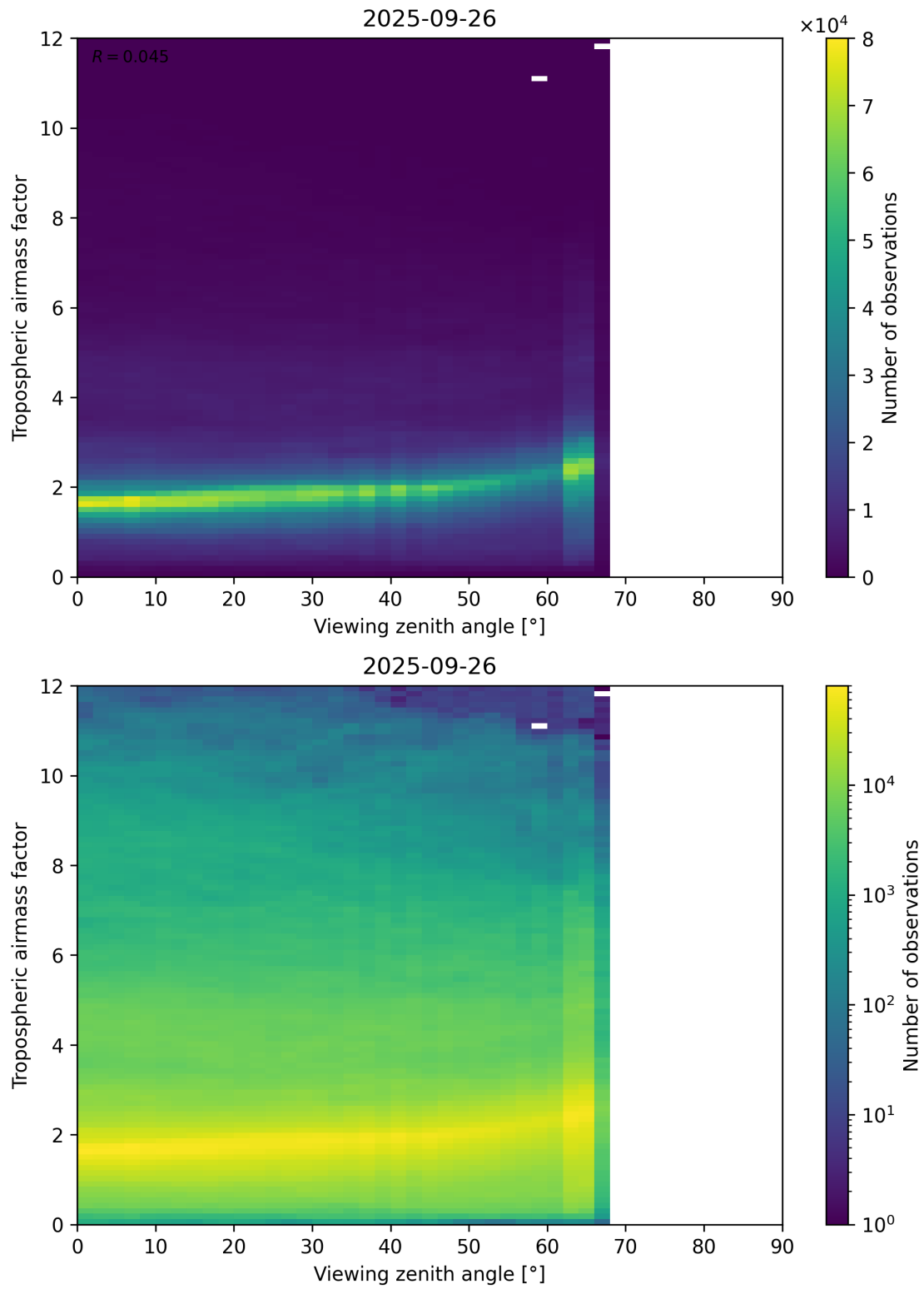
Figure 161: Scatter density plot of “Viewing zenith angle” against “Tropospheric airmass factor” for 2025-09-26 to 2025-09-27.
