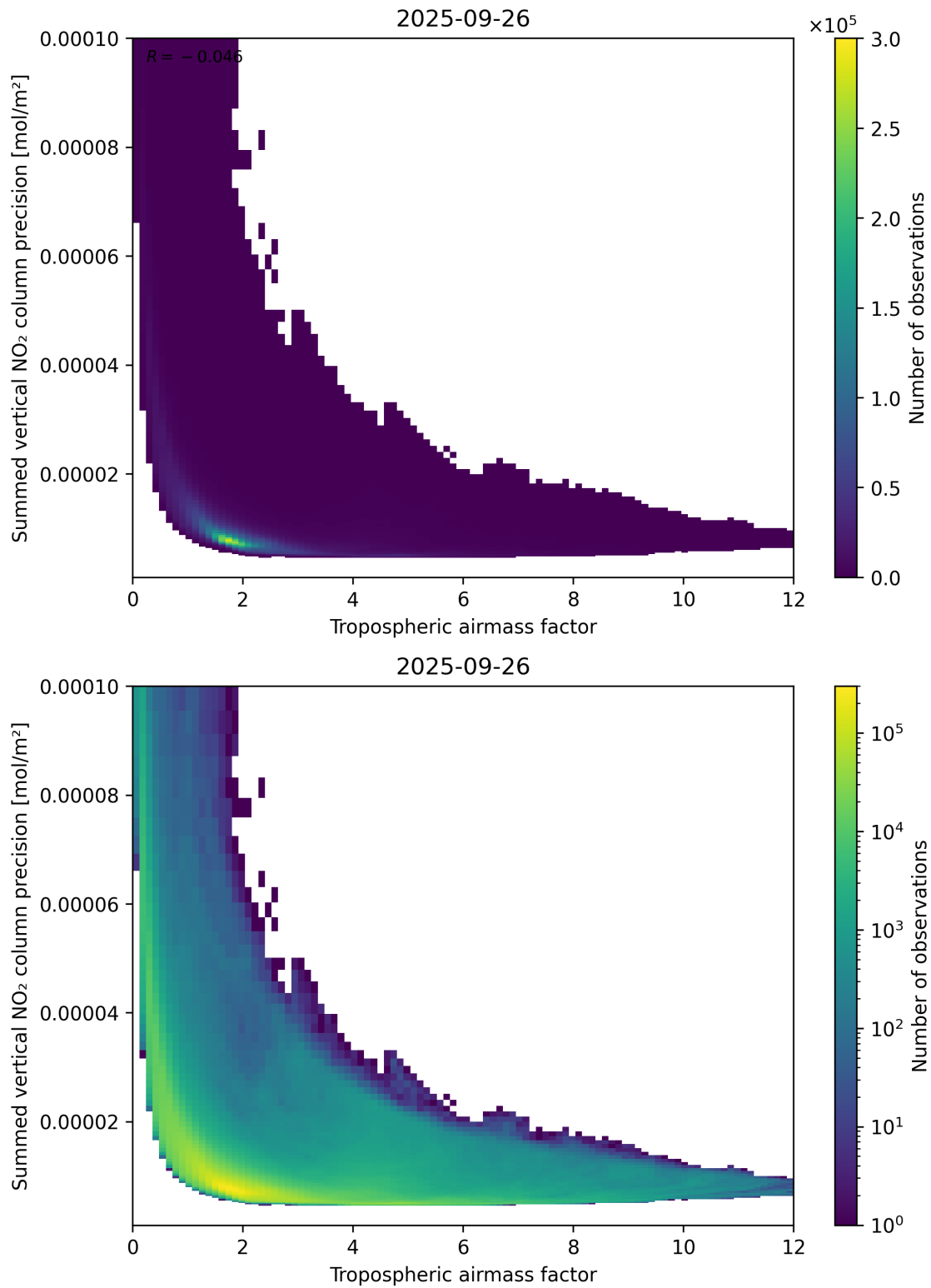
Figure 76: Scatter density plot of “Tropospheric air mass factor” against “Summed vertical NO 2 column precision” for 2025-09-26 to 2025-09-27.
