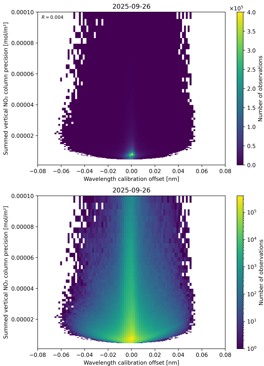
Figure 178: Scatter density plot of “Wavelength calibration offset” against “Summed vertical NO 2 column precision” for 2025-09-26 to 2025-09-27.
