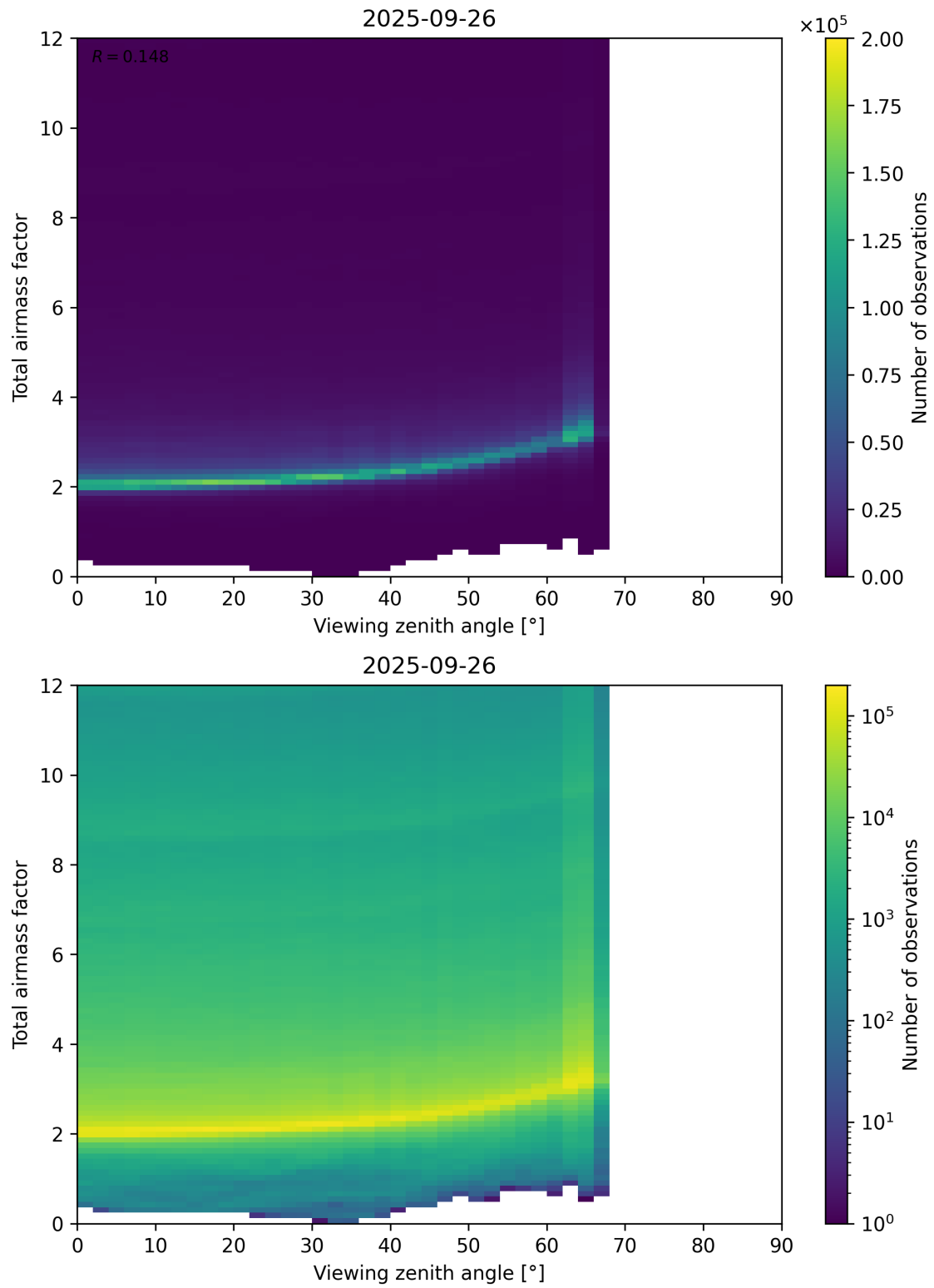
Figure 160: Scatter density plot of “Viewing zenith angle” against “Total airmass factor” for 2025-09-26 to 2025-09-27.
