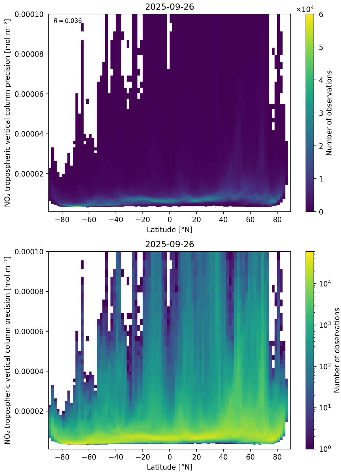
Figure 93: Scatter density plot of “Latitude” against “NO 2 tropospheric vertical column precision” for 2025-09-26 to 2025-09-27.
