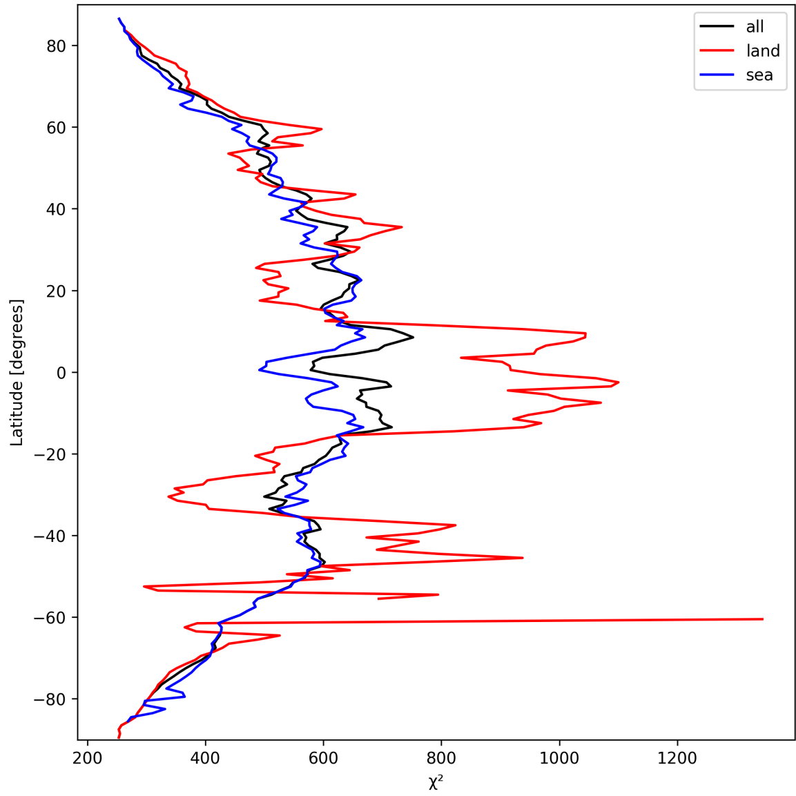
Figure 25: Zonal average of “ \chi^2 ” for 2025-09-26 to 2025-09-27.
