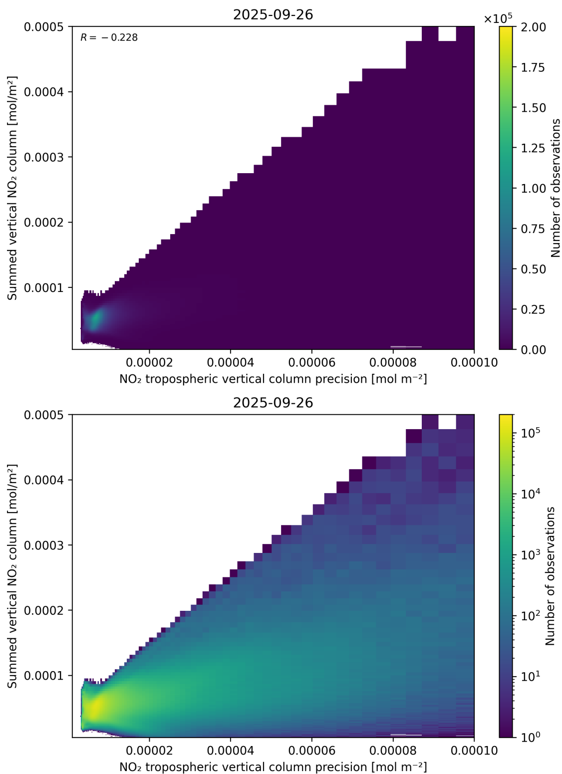
Figure 136: Scatter density plot of “NO 2 tropospheric vertical column precision” against “Summed vertical NO 2 column” for 2025-09-26 to 2025-09-27.
