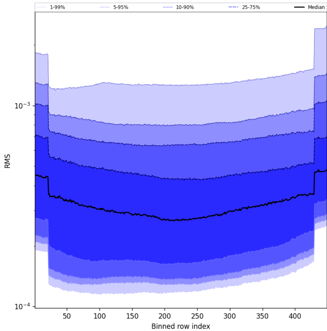
Figure 60: Along track statistics of “RMS” for 2025-09-26 to 2025-09-27
