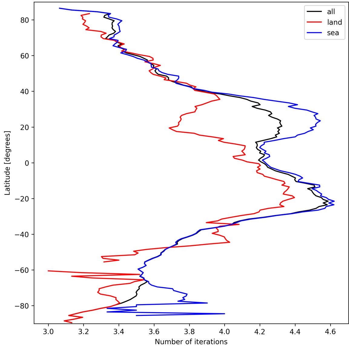
Figure 17: Zonal average of “Number of iterations” for 2025-09-26 to 2025-09-27.
