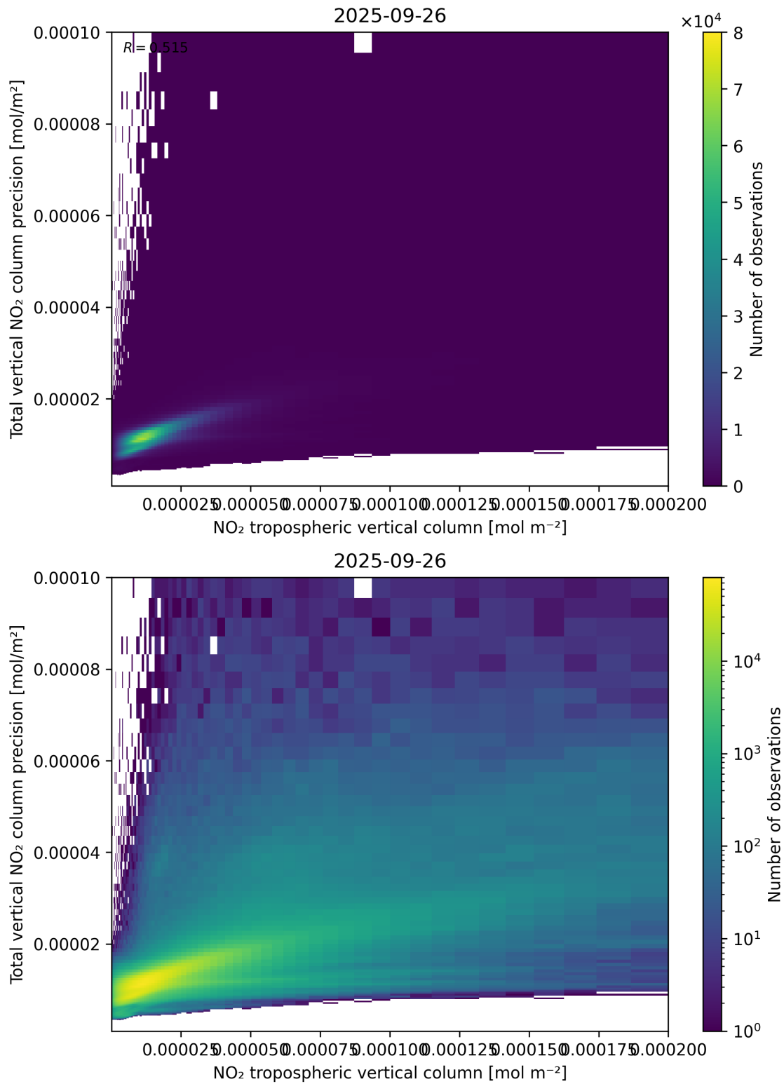
Figure 129: Scatter density plot of “NO 2 tropospheric vertical column” against “Total vertical NO 2 column precision” for 2025-09-26 to 2025-09-27.
