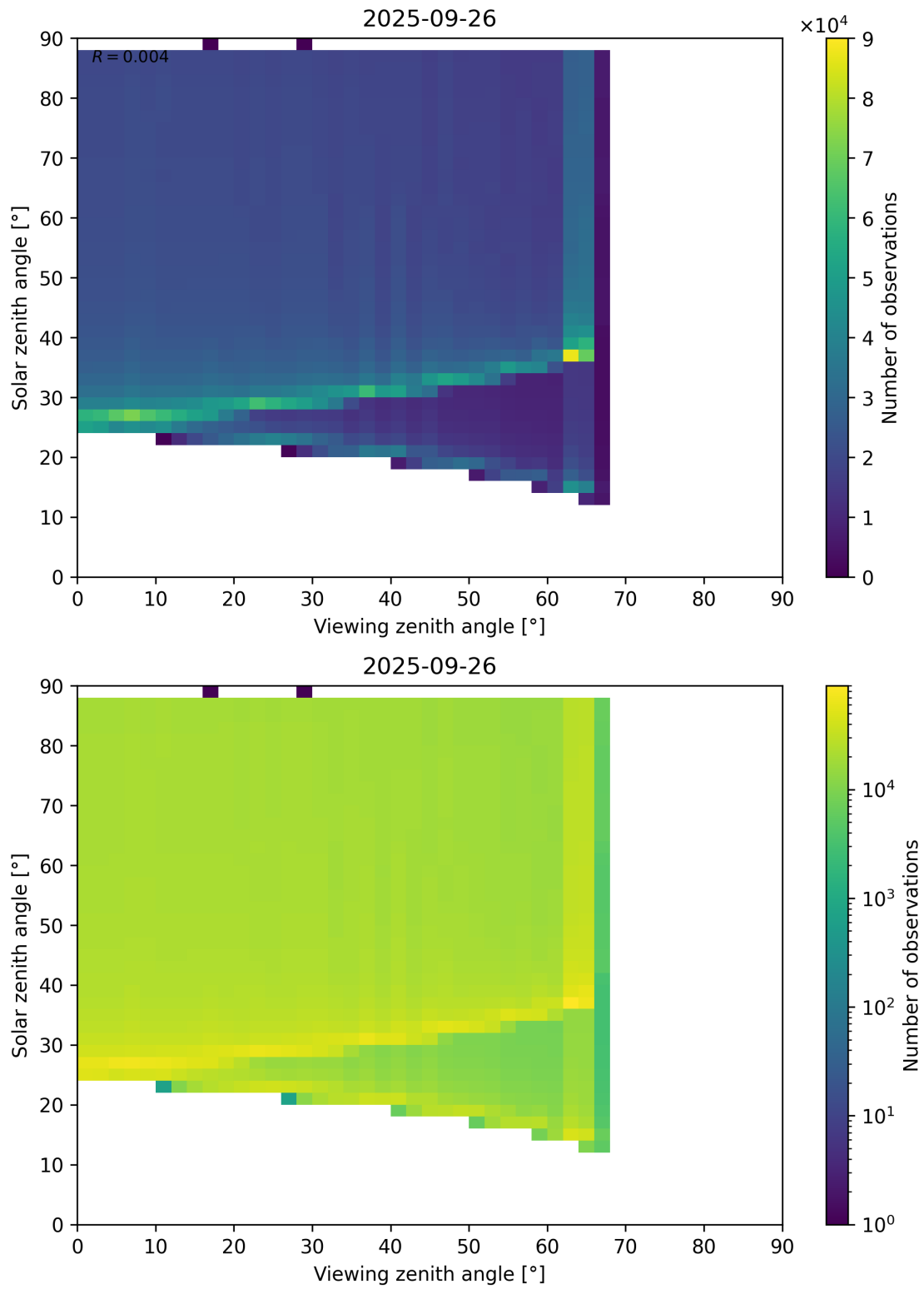
Figure 172: Scatter density plot of “Viewing zenith angle” against “Solar zenith angle” for 2025-09-26 to 2025-09-27.
