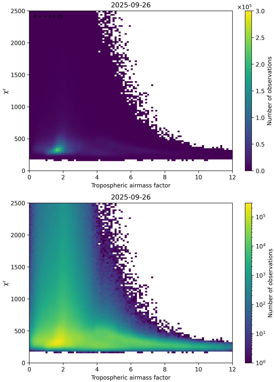
Figure 73: Scatter density plot of “Tropospheric airmass factor” against “ \chi^2 ” for 2025-09-26 to 2025-09-27.
