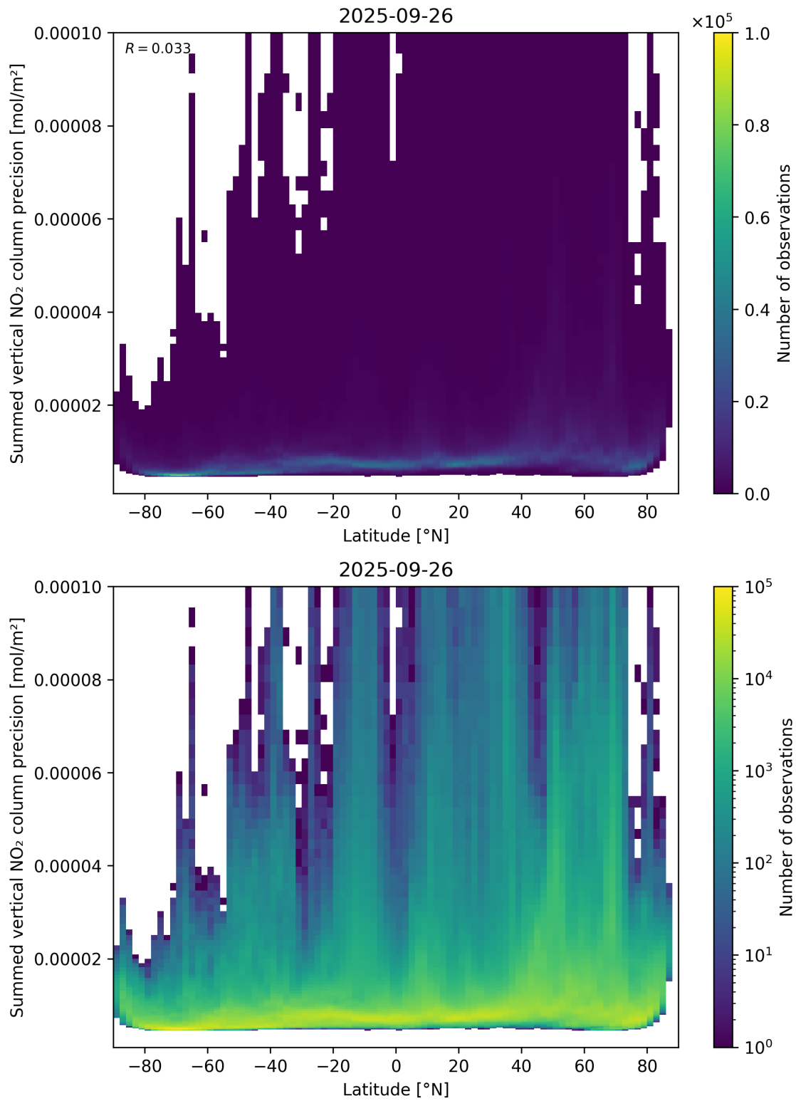
Figure 89: Scatter density plot of “Latitude” against “Summed vertical NO 2 column precision” for 2025-09-26 to 2025-09-27.
