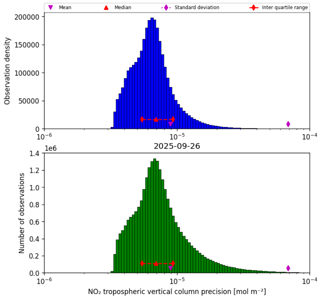
Figure 30: Histogram of “NO 2 tropospheric vertical column precision” for 2025-09-26 to 2025-09-27
