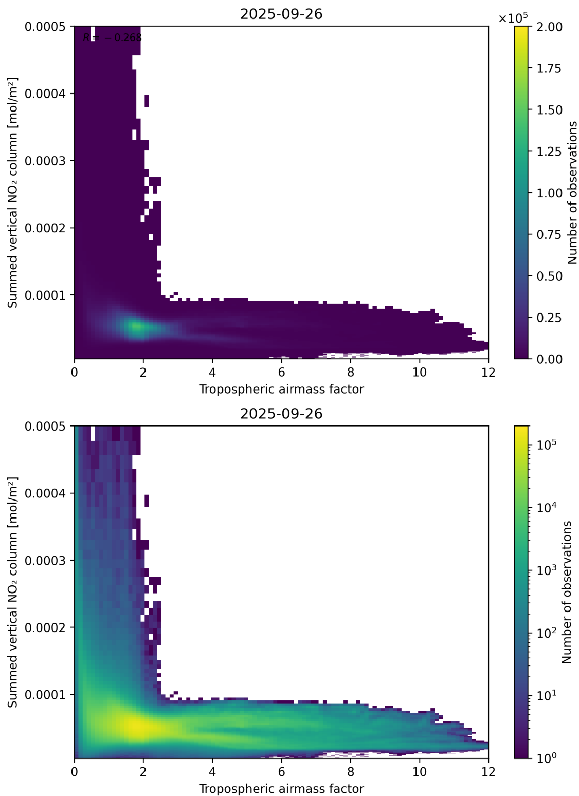
Figure 75: Scatter density plot of “Tropospheric air mass factor” against “Summed vertical NO 2 column” for 2025-09-26 to 2025-09-27.
