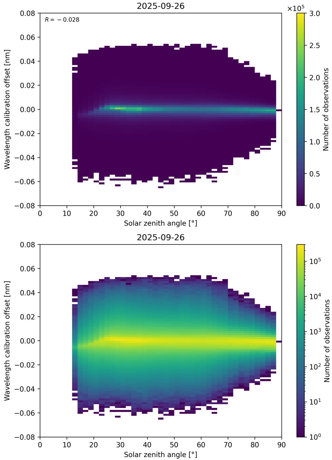
Figure 158: Scatter density plot of “Solar zenith angle” against “Wavelength calibration offset” for 2025-09-26 to 2025-09-27.
