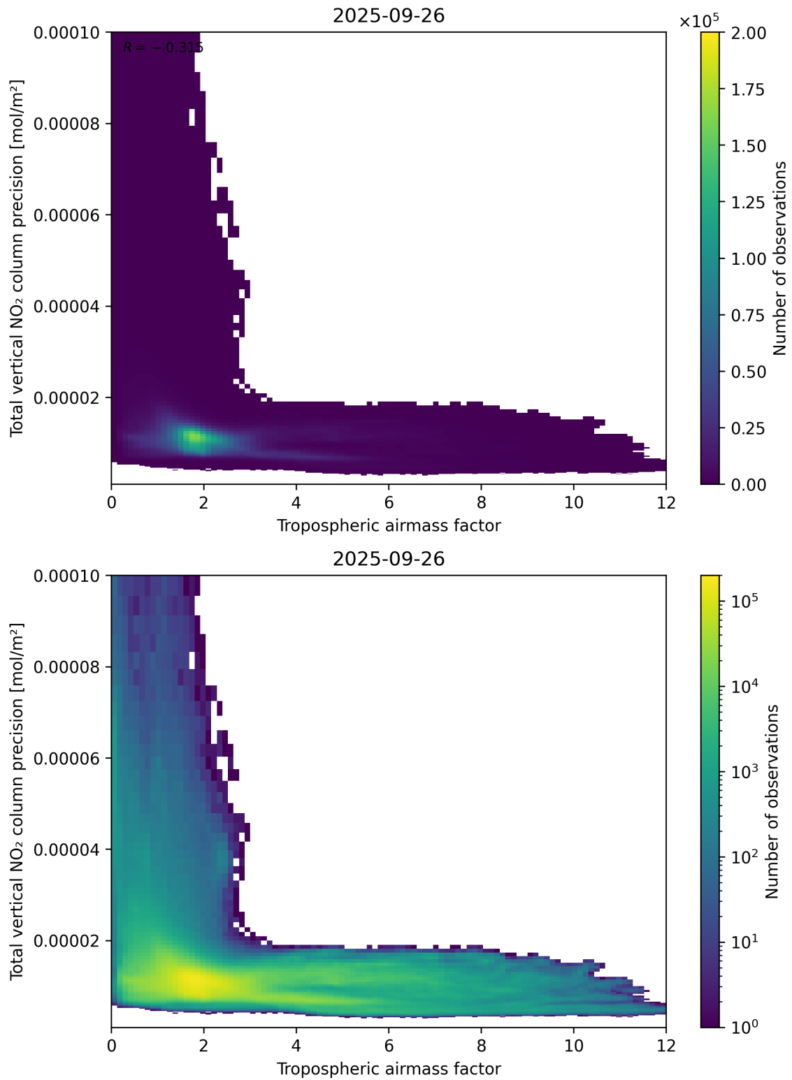
Figure 78: Scatter density plot of “Tropospheric air mass factor” against “Total vertical NO 2 column precision” for 2025-09-26 to 2025-09-27.
