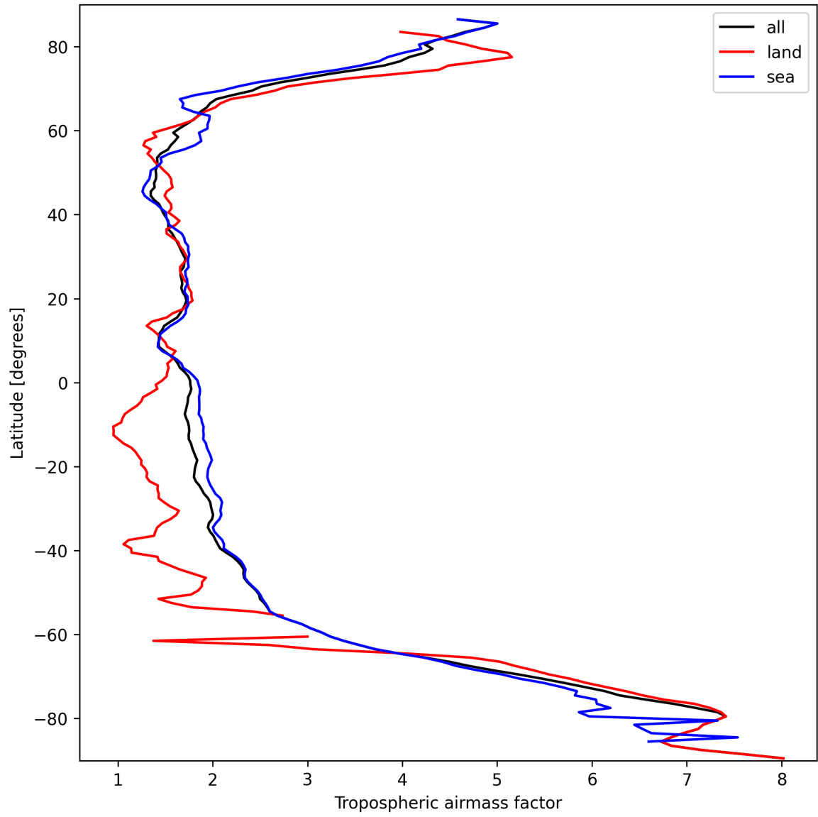
Figure 14: Zonal average of “Tropospheric airmass factor” for 2025-09-26 to 2025-09-27.
