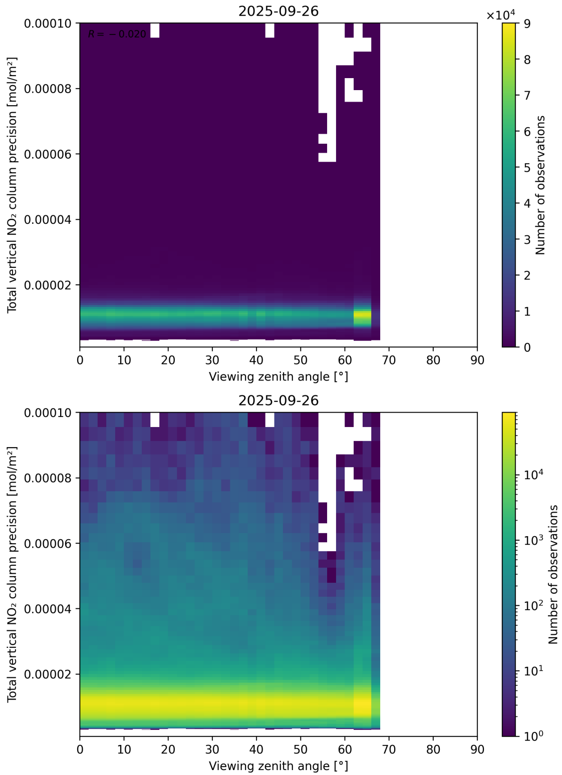
Figure 168: Scatter density plot of “Viewing zenith angle” against “Total vertical NO 2 column precision” for 2025-09-26 to 2025-09-27.
