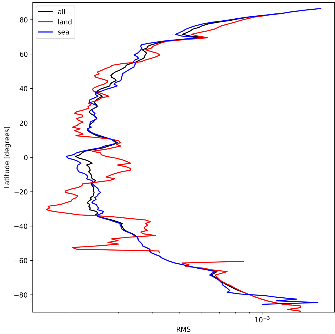
Figure 26: Zonal average of “RMS” for 2025-09-26 to 2025-09-27.
