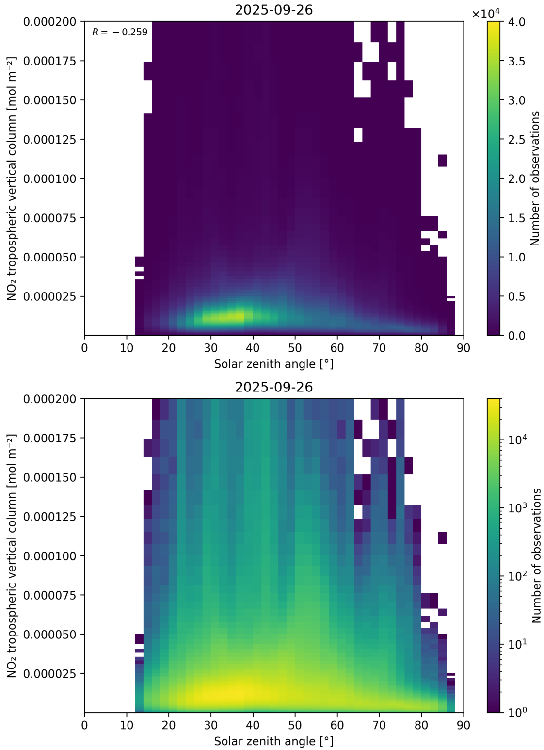
Figure 155: Scatter density plot of “Solar zenith angle” against “NO 2 tropospheric vertical column” for 2025-09-26 to 2025-09-27.
