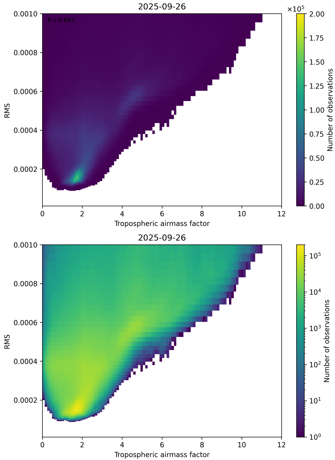
Figure 79: Scatter density plot of “Tropospheric airmass factor” against “RMS” for 2025-09-26 to 2025-09-27.
