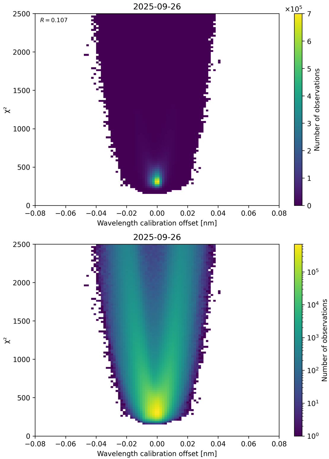
Figure 175: Scatter density plot of “Wavelength calibration offset” against “ \chi^2 ” for 2025-09-26 to 2025-09-27.
