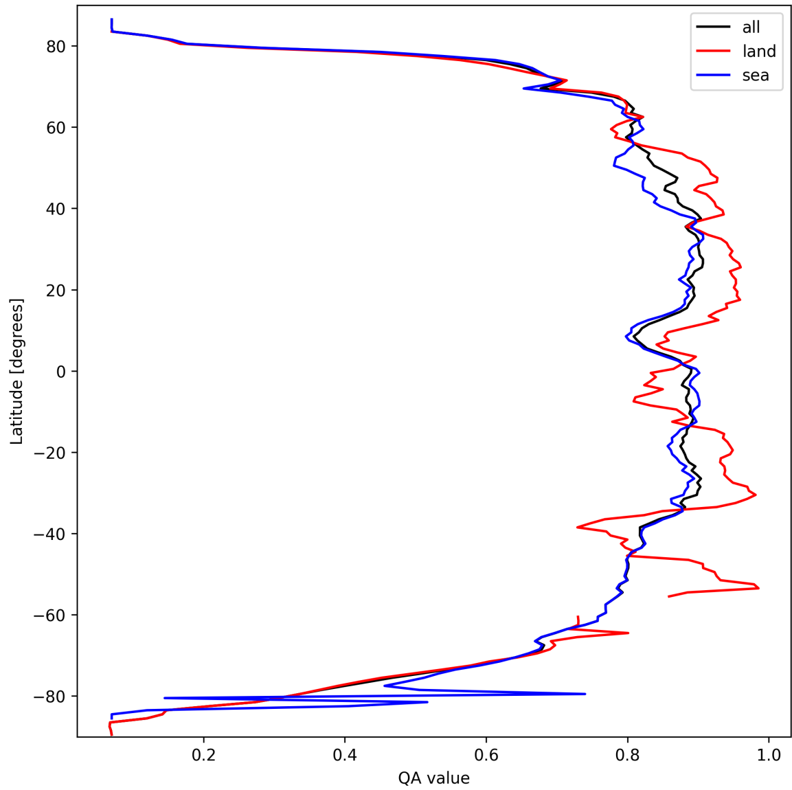
Figure 11: Zonal average of “QA value” for 2025-09-26 to 2025-09-27.
