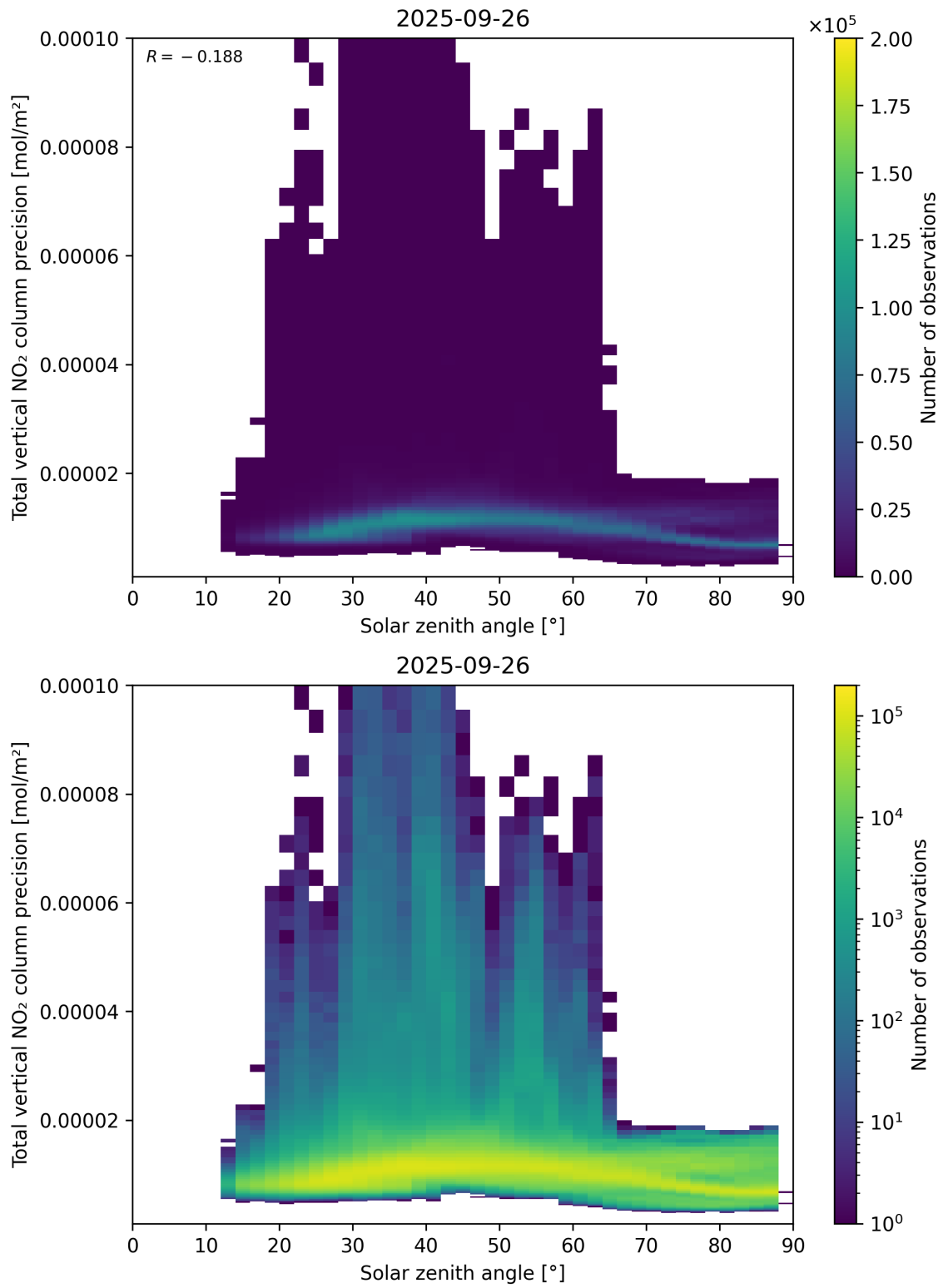
Figure 154: Scatter density plot of “Solar zenith angle” against “Total vertical NO 2 column precision” for 2025-09-26 to 2025-09-27.
