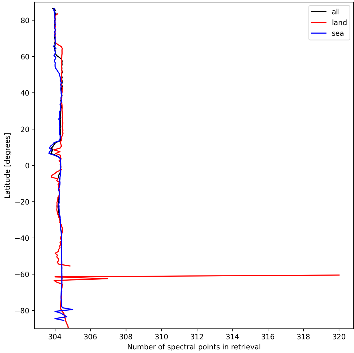
Figure 16: Zonal average of “Number of spectral points in retrieval” for 2025-09-26 to 2025-09-27.
