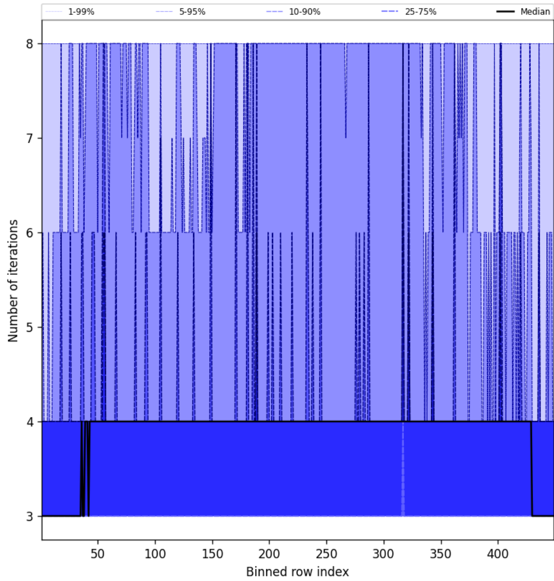
Figure 51: Along track statistics of “Number of iterations” for 2025-09-26 to 2025-09-27
