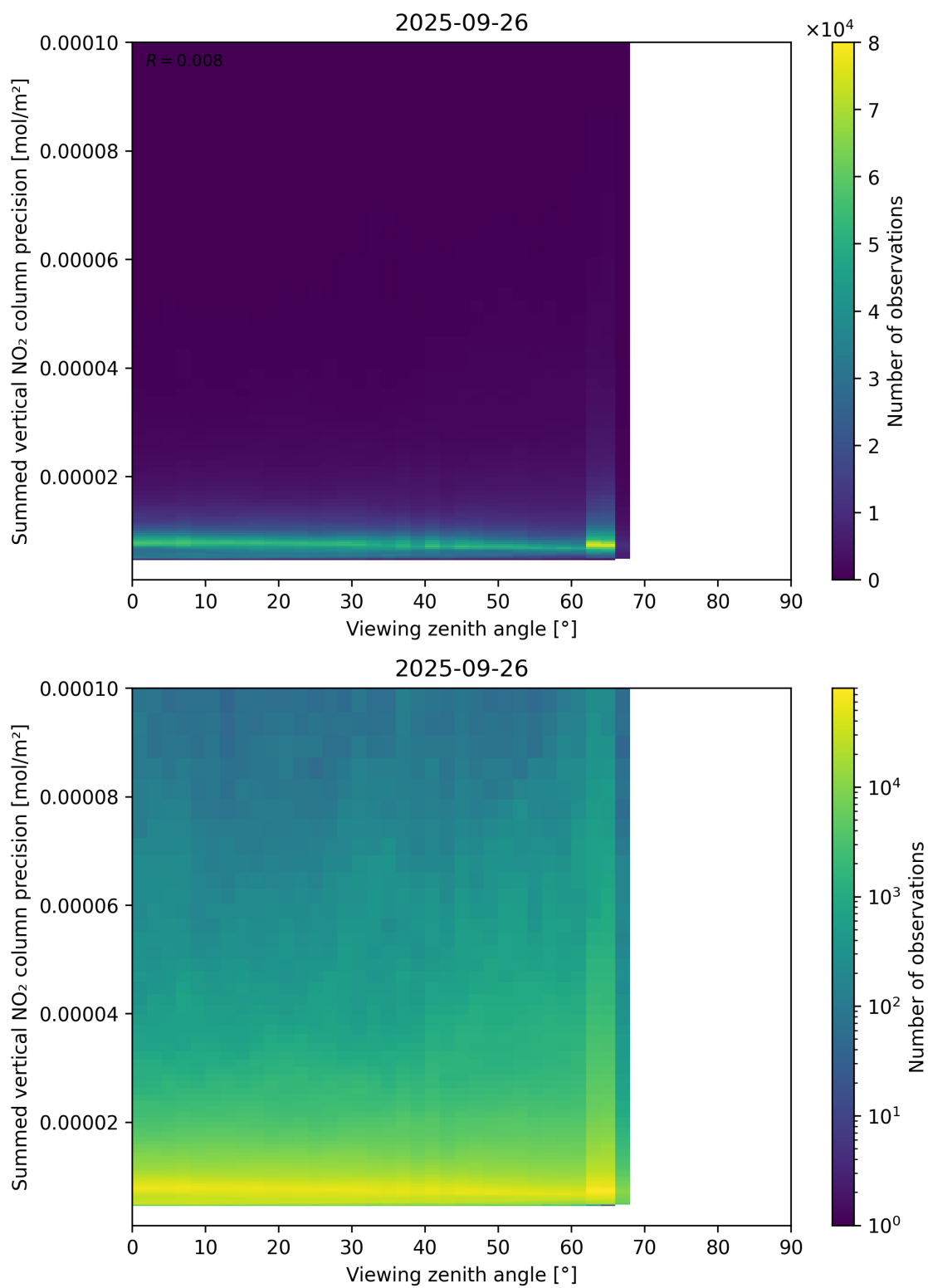
Figure 166: Scatter density plot of “Viewing zenith angle” against “Summed vertical NO 2 column precision” for 2025-09-26 to 2025-09-27.
