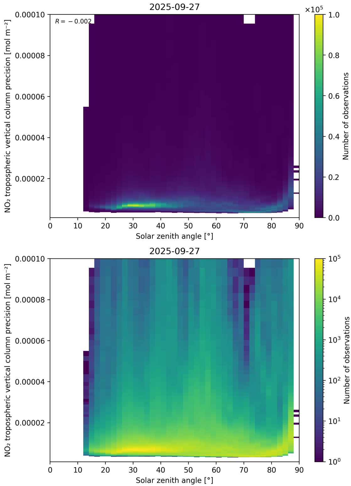
Figure 156: Scatter density plot of “Solar zenith angle” against “NO 2 tropospheric vertical column precision” for 2025-09-26 to 2025-09-28.
