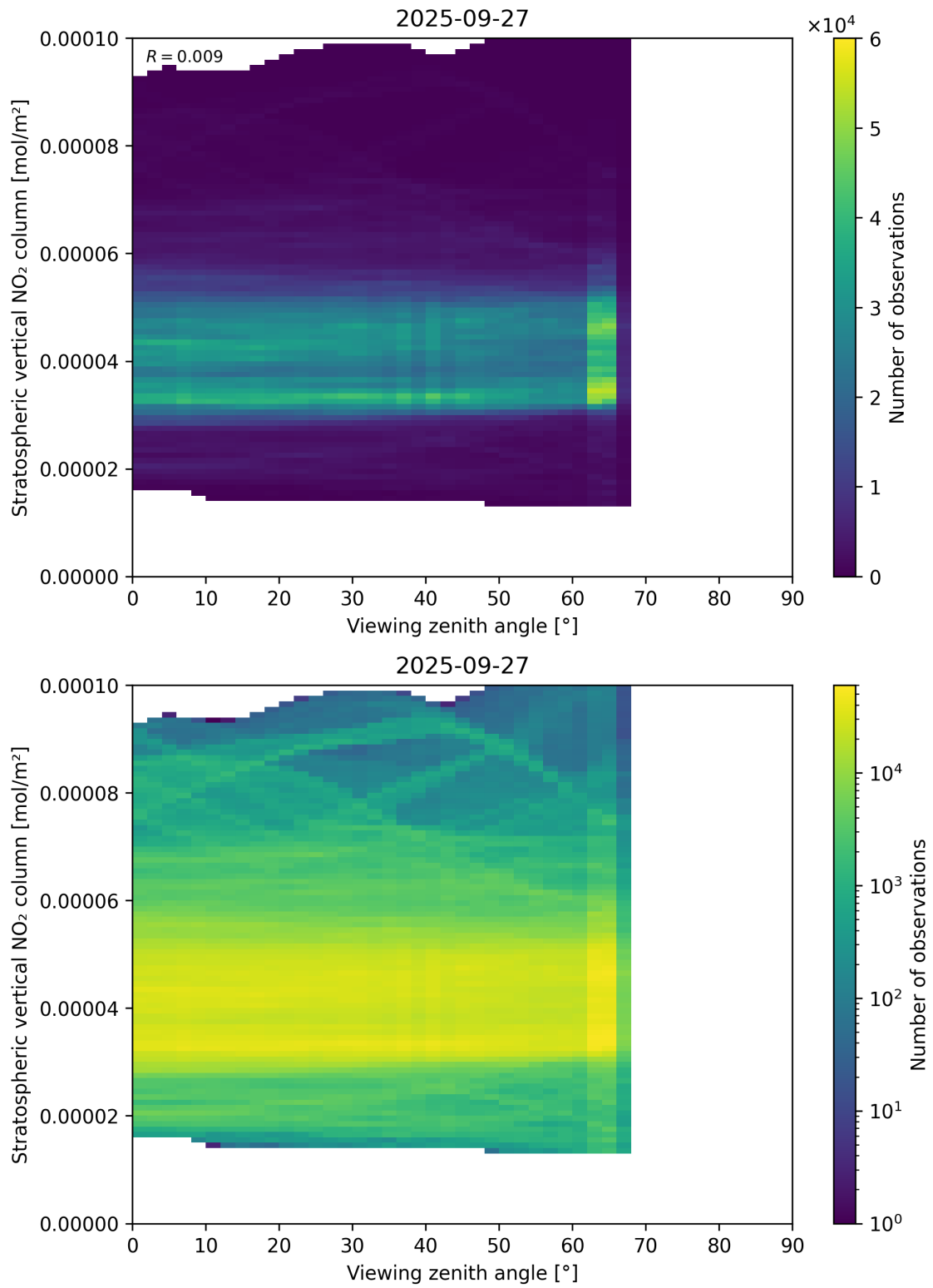
Figure 164: Scatter density plot of “Viewing zenith angle” against “Stratospheric vertical NO 2 column” for 2025-09-26 to 2025-09-28.
