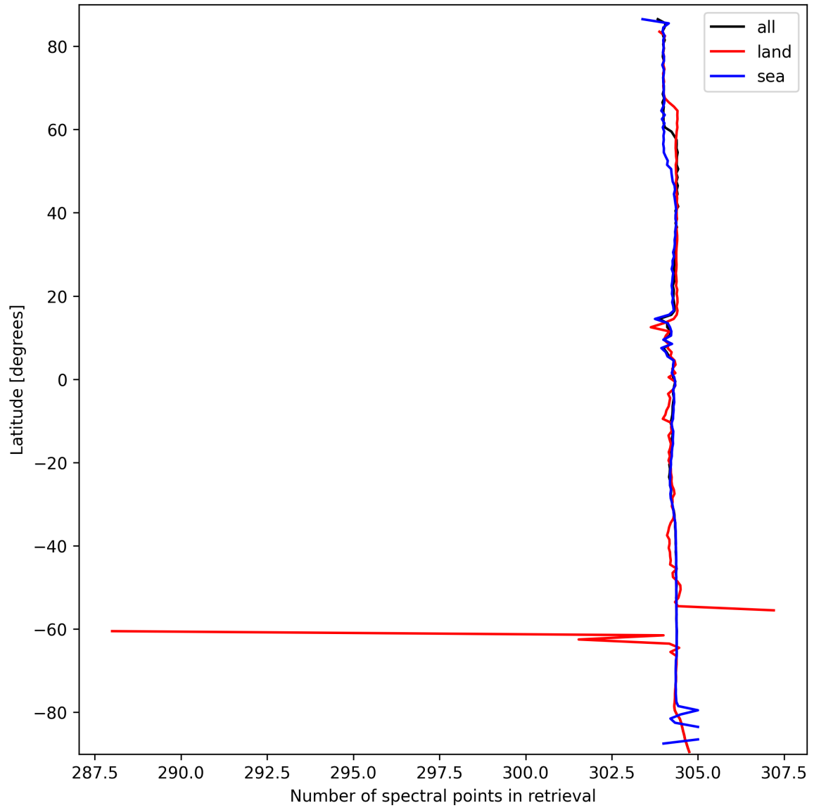
Figure 16: Zonal average of “Number of spectral points in retrieval” for 2025-09-26 to 2025-09-28.
