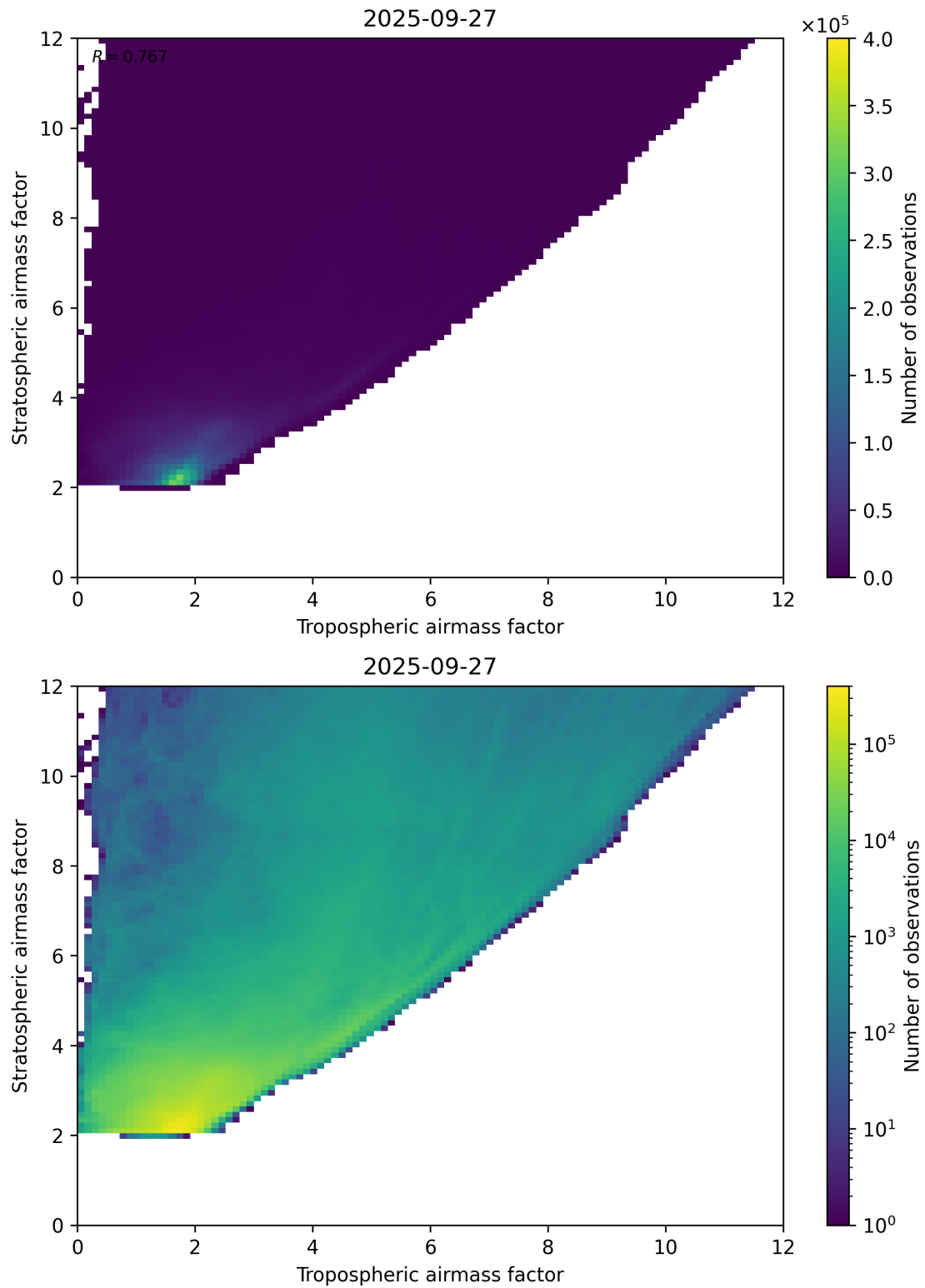
Figure 71: Scatter density plot of “Tropospheric airmass factor” against “Stratospheric airmass factor” for 2025-09-26 to 2025-09-28.
