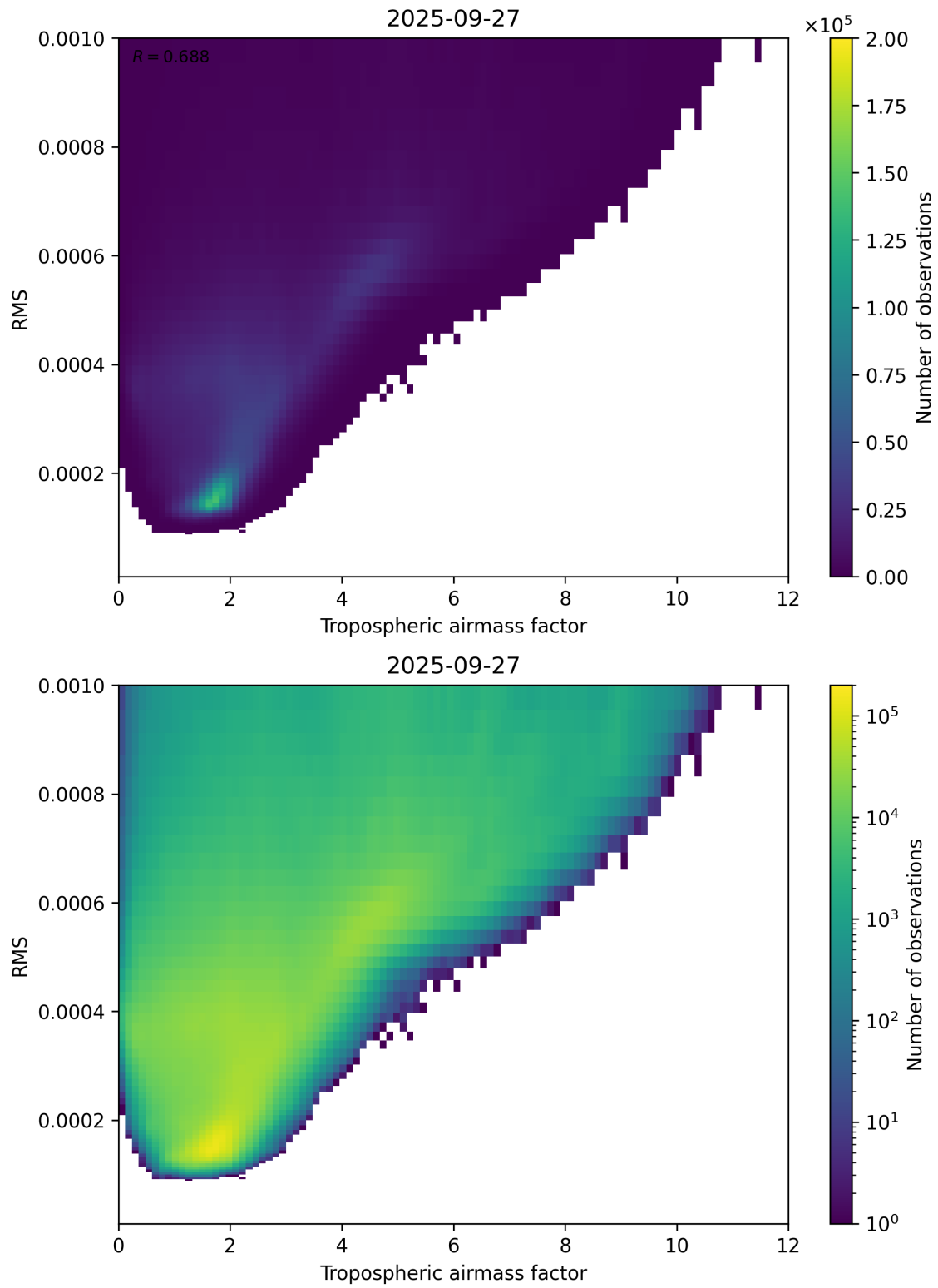
Figure 79: Scatter density plot of “Tropospheric airmass factor” against “RMS” for 2025-09-26 to 2025-09-28.
