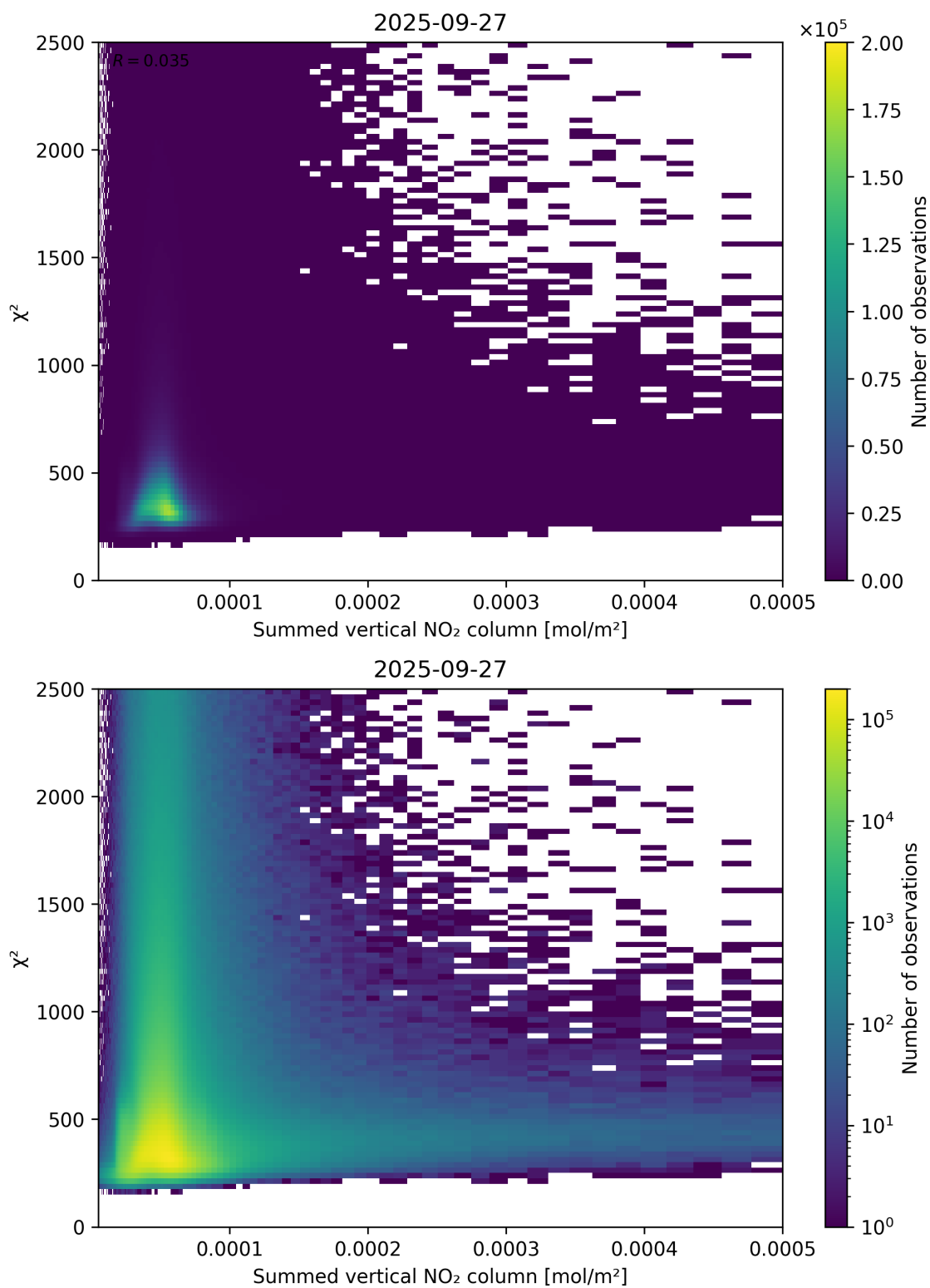
Figure 104: Scatter density plot of “Summed vertical NO 2 column” against “ \chi^2 ” for 2025-09-26 to 2025-09-28.
