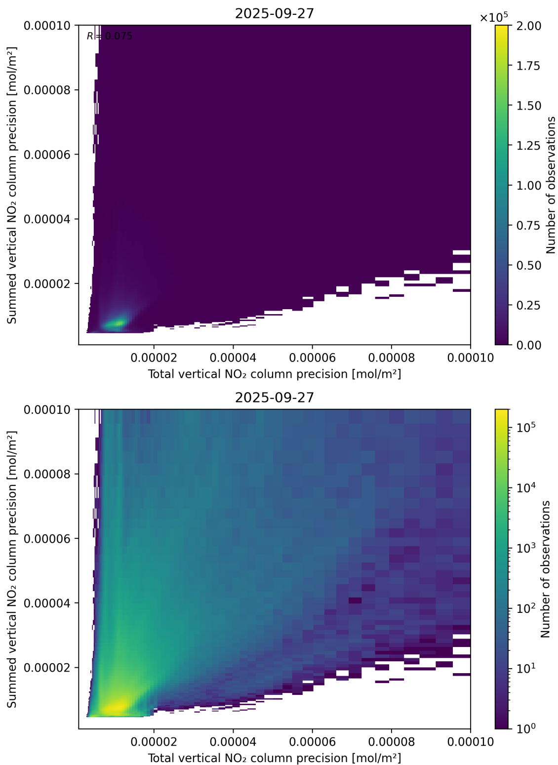
Figure 118: Scatter density plot of “Total vertical NO 2 column precision” against “Summed vertical NO 2 column precision” for 2025-09-26 to 2025-09-28.
