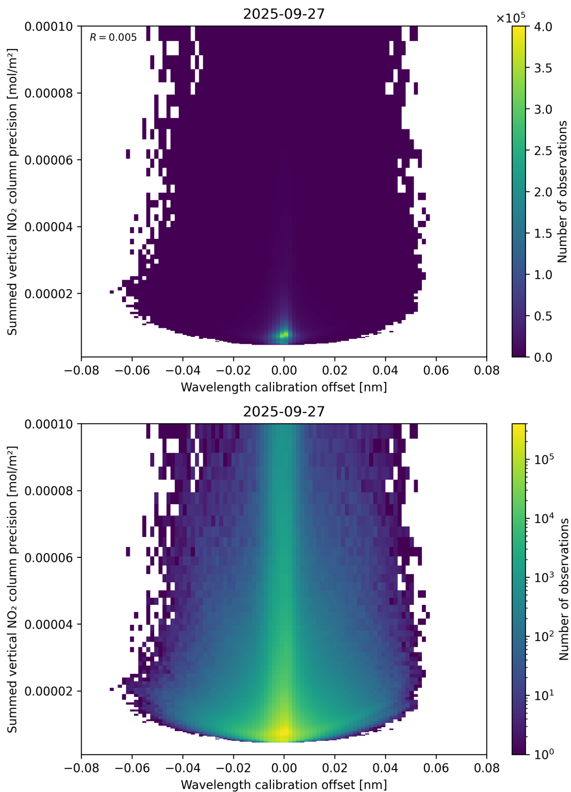
Figure 178: Scatter density plot of “Wavelength calibration offset” against “Summed vertical NO 2 column precision” for 2025-09-26 to 2025-09-28.
