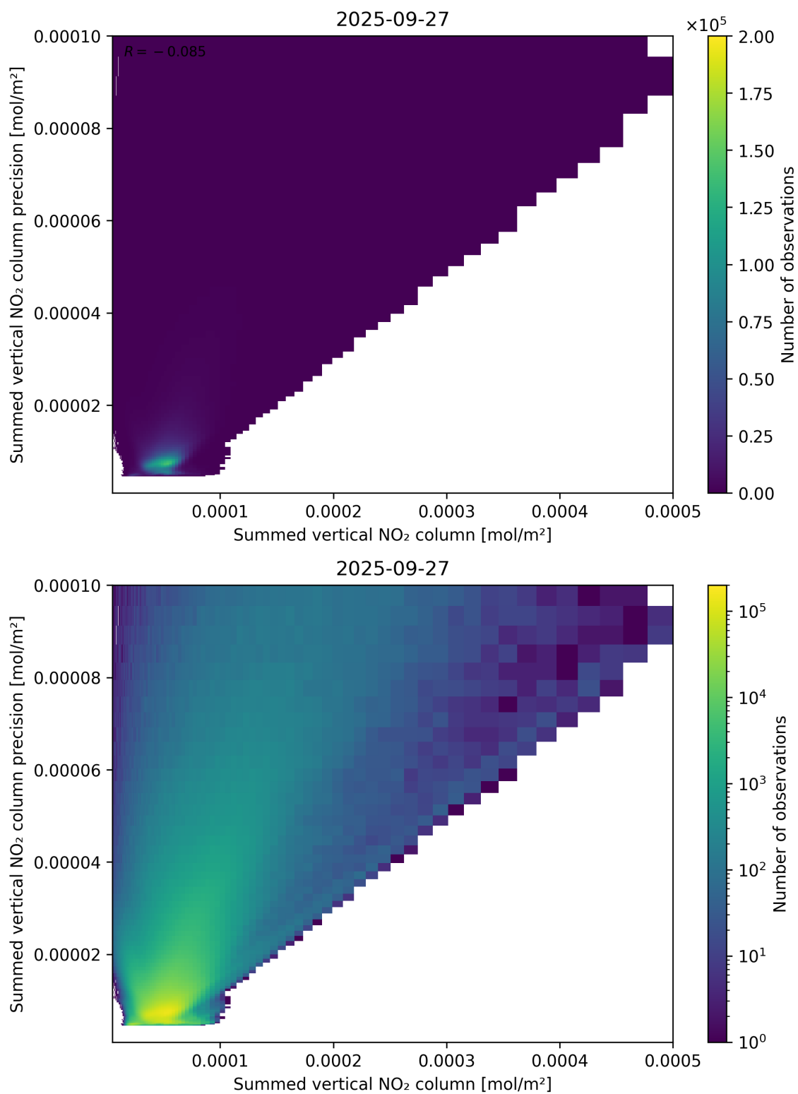
Figure 105: Scatter density plot of “Summed vertical NO 2 column” against “Summed vertical NO 2 column precision” for 2025-09-26 to 2025-09-28.
