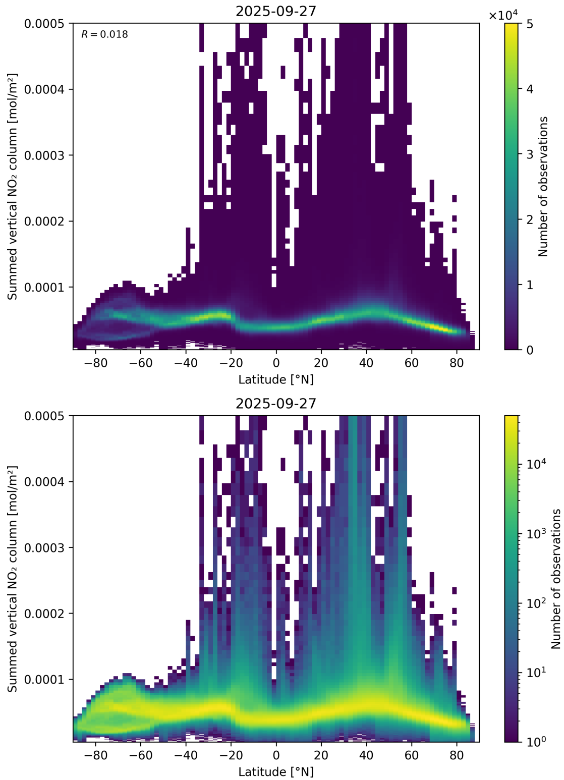
Figure 88: Scatter density plot of “Latitude” against “Summed vertical NO 2 column” for 2025-09-26 to 2025-09-28.
