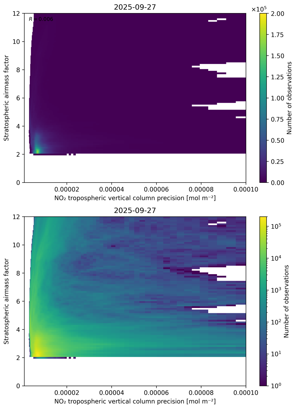
Figure 131: Scatter density plot of “NO 2 tropospheric vertical column precision” against “Stratospheric airmass factor” for 2025-09-26 to 2025-09-28.
