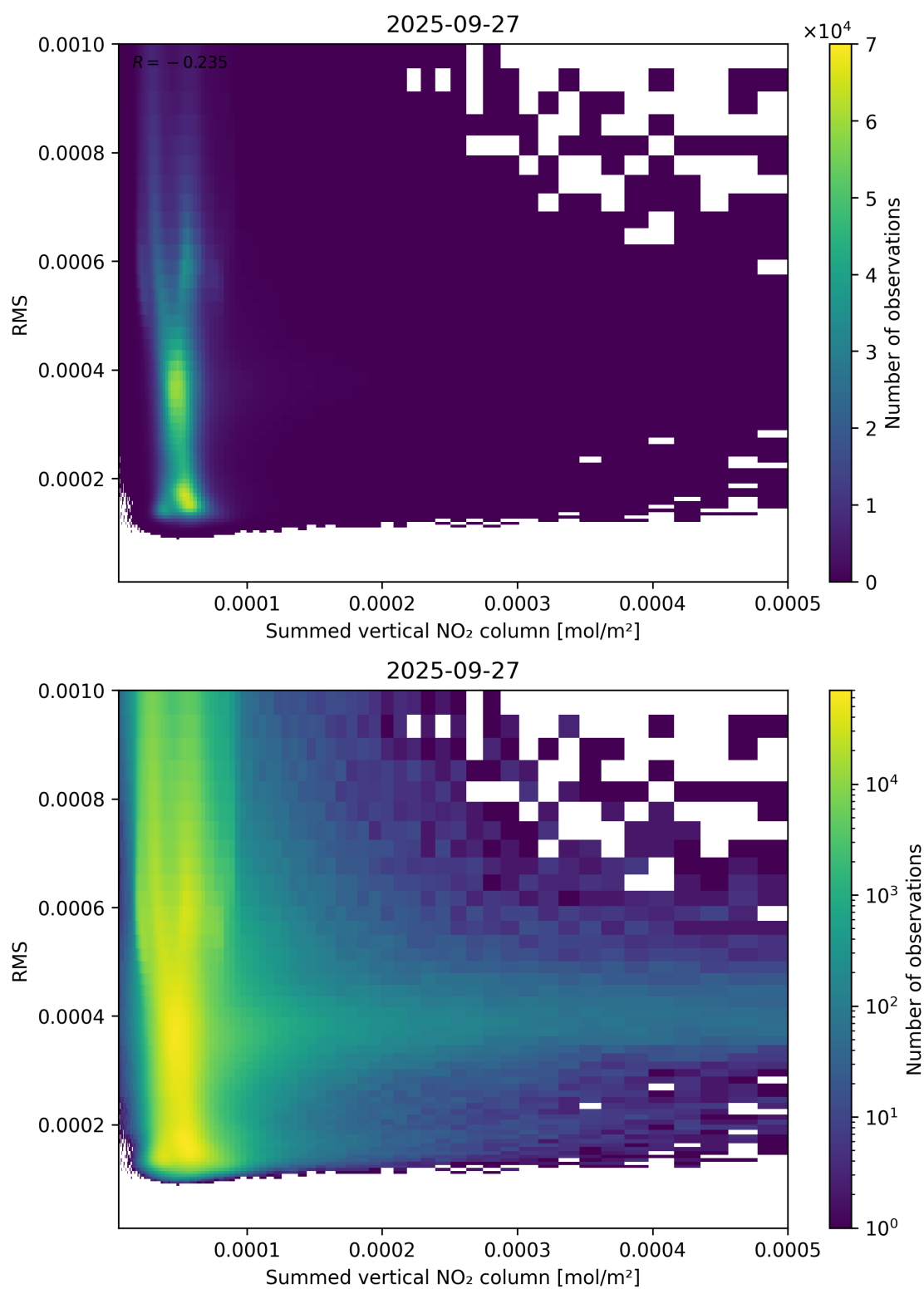
Figure 109: Scatter density plot of “Summed vertical NO 2 column” against “RMS” for 2025-09-26 to 2025-09-28.
