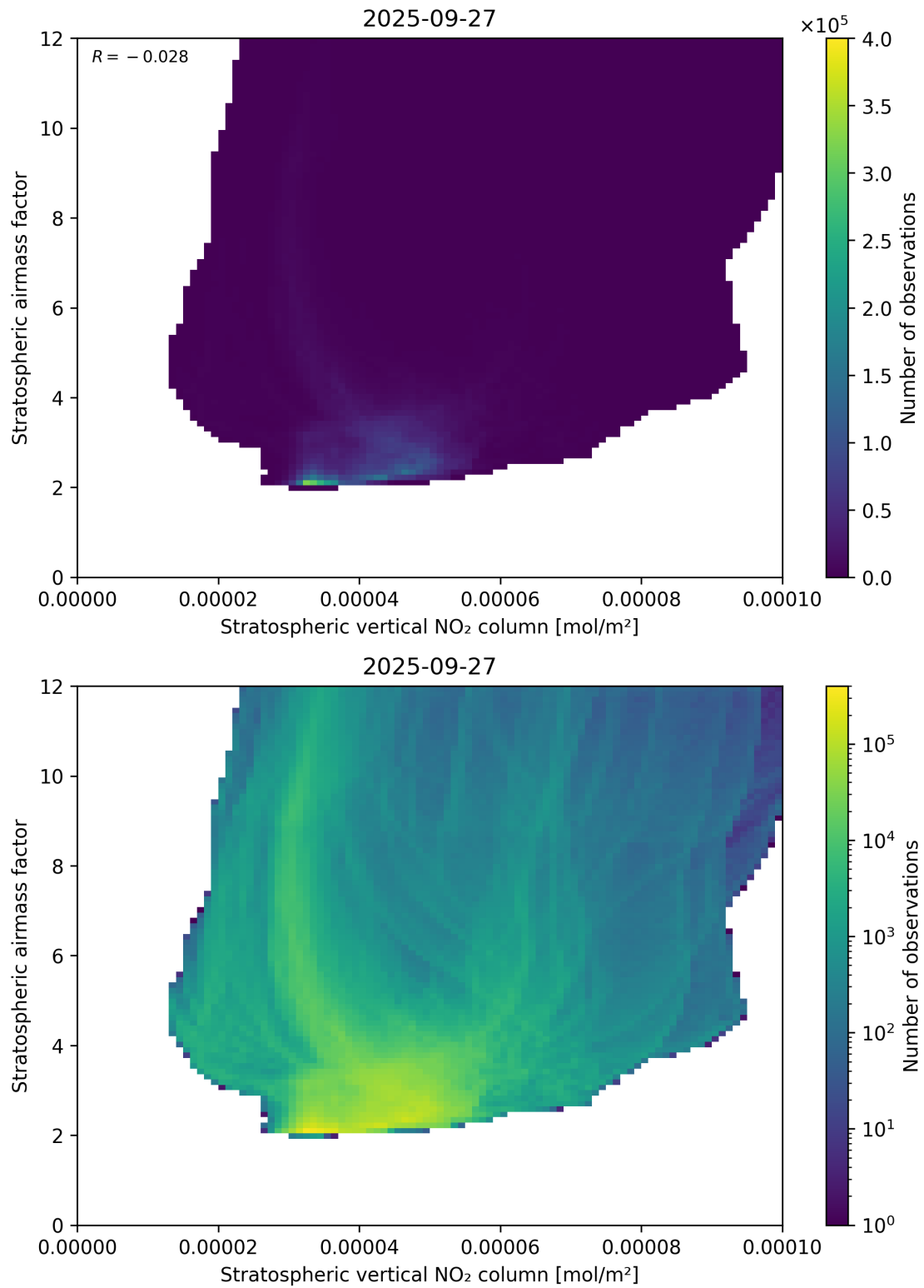
Figure 96: Scatter density plot of “Stratospheric vertical NO 2 column” against “Stratospheric airmass factor” for 2025-09-26 to 2025-09-28.
