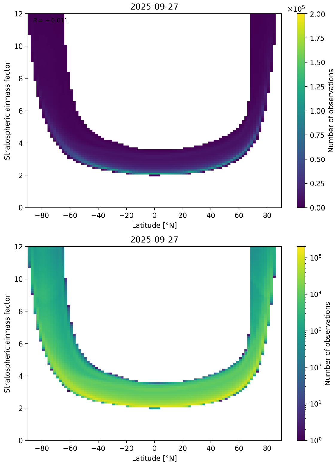
Figure 83: Scatter density plot of “Latitude” against “Stratospheric air mass factor” for 2025-09-26 to 2025-09-28.
