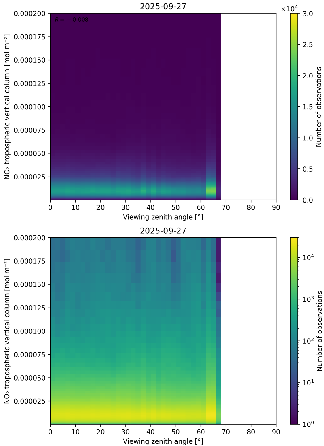
Figure 169: Scatter density plot of “Viewing zenith angle” against “NO 2 tropospheric vertical column” for 2025-09-26 to 2025-09-28.
