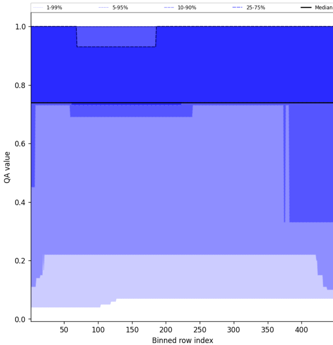
Figure 45: Along track statistics of “QA value” for 2025-09-26 to 2025-09-28
