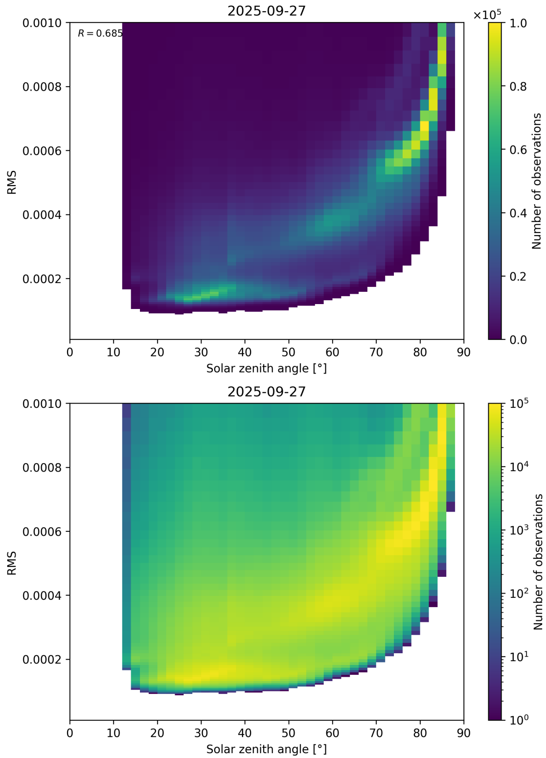
Figure 157: Scatter density plot of “Solar zenith angle” against “RMS” for 2025-09-26 to 2025-09-28.
