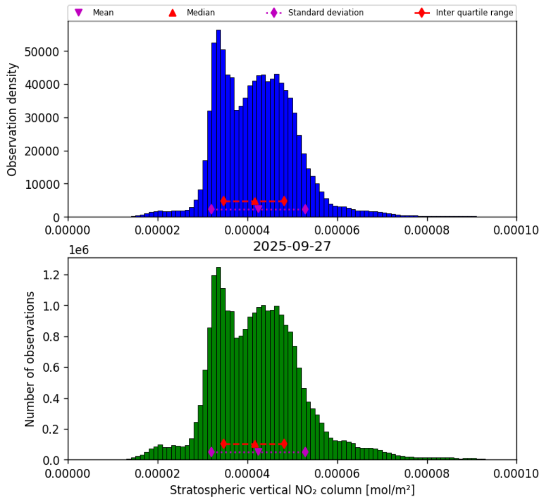
Figure 36: Histogram of “Stratospheric vertical NO 2 column” for 2025-09-26 to 2025-09-28
