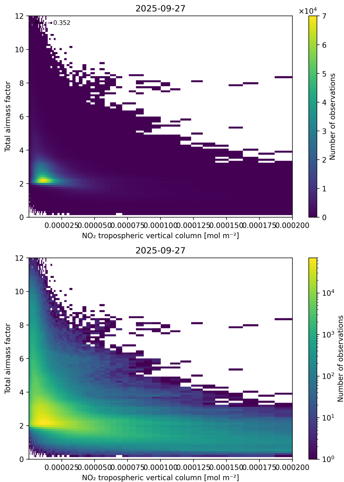
Figure 122: Scatter density plot of “NO 2 tropospheric vertical column” against “Total air mass factor” for 2025-09-26 to 2025-09-28.
