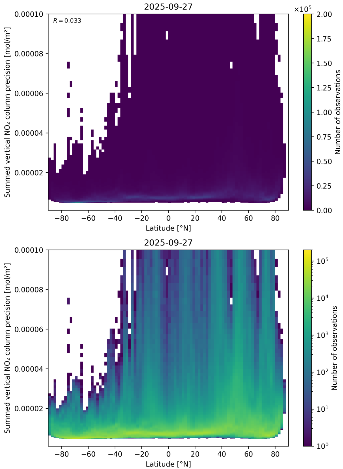
Figure 89: Scatter density plot of “Latitude” against “Summed vertical NO 2 column precision” for 2025-09-26 to 2025-09-28.
