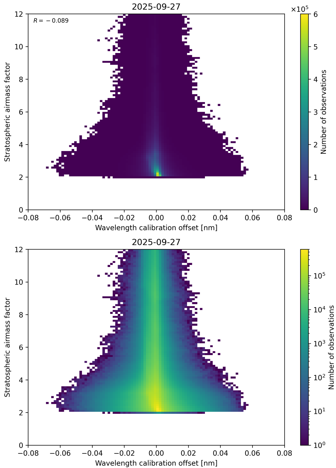
Figure 174: Scatter density plot of “Wavelength calibration offset” against “Stratospheric air mass factor” for 2025-09-26 to 2025-09-28.
