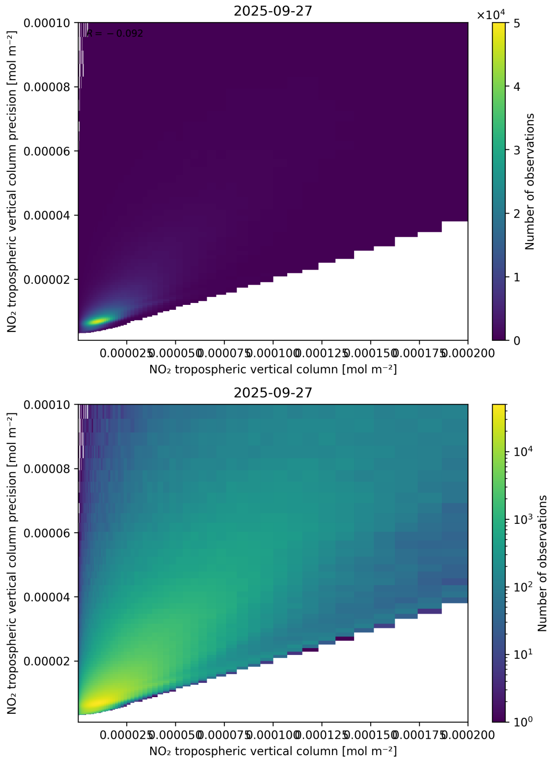
Figure 130: Scatter density plot of “NO 2 tropospheric vertical column” against “NO 2 tropospheric vertical column precision” for 2025-09-26 to 2025-09-28.
