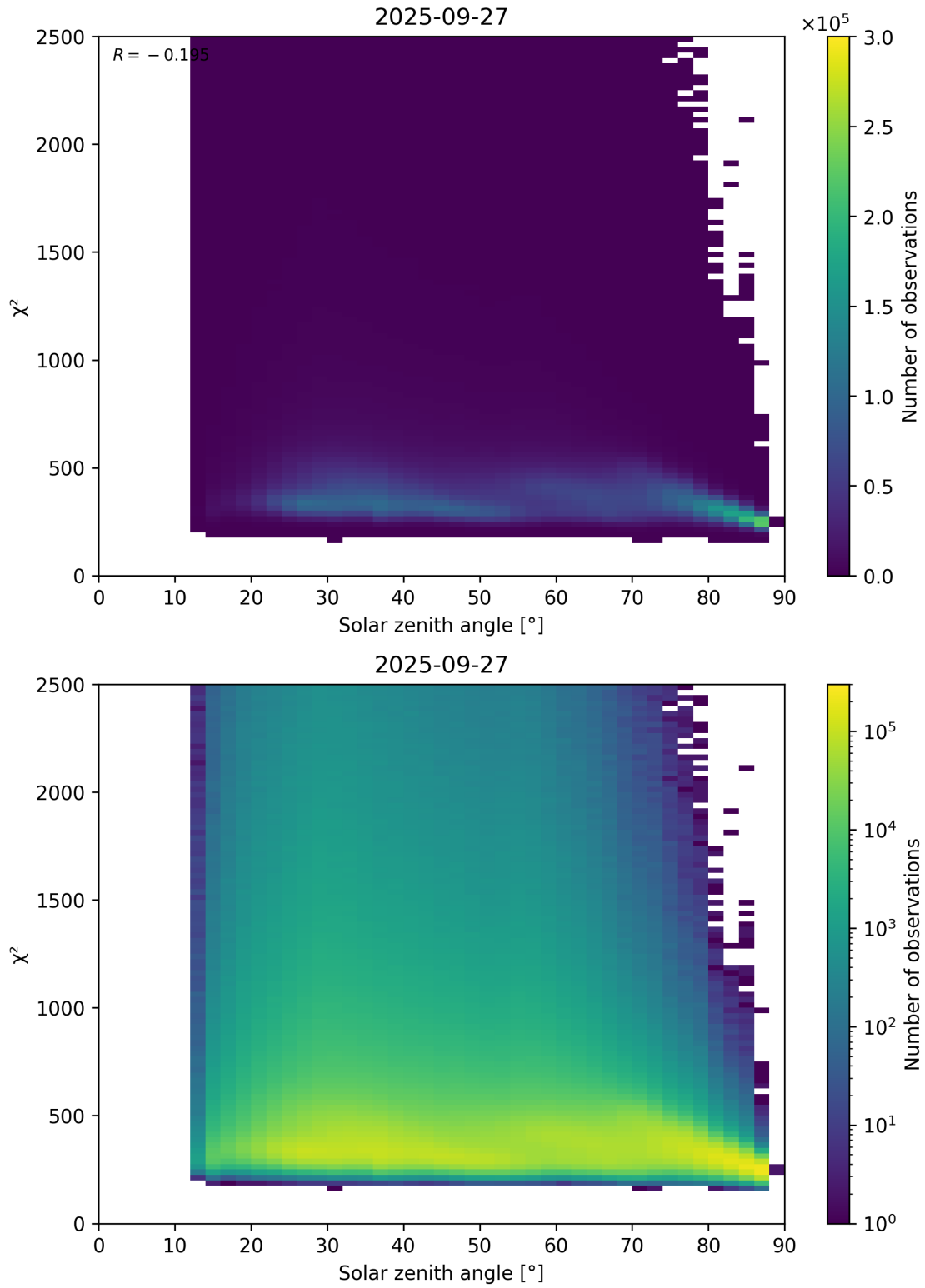
Figure 148: Scatter density plot of “Solar zenith angle” against “ \chi^2 ” for 2025-09-26 to 2025-09-28.
