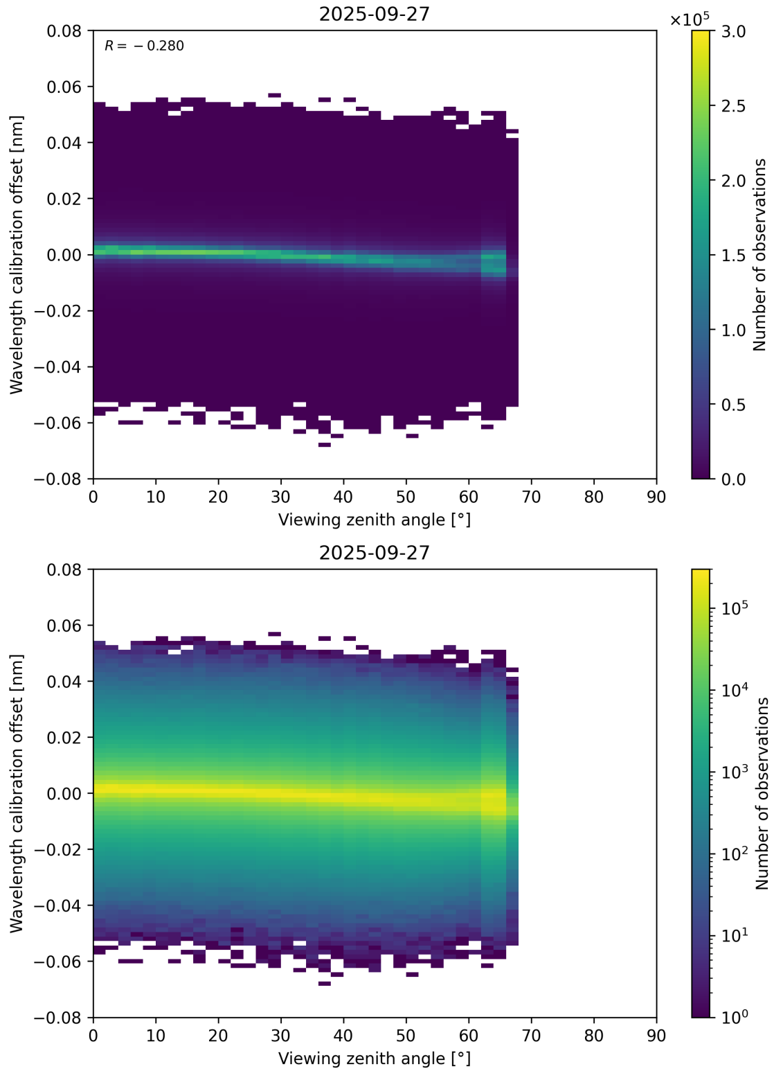
Figure 173: Scatter density plot of “Viewing zenith angle” against “Wavelength calibration offset” for 2025-09-26 to 2025-09-28.
