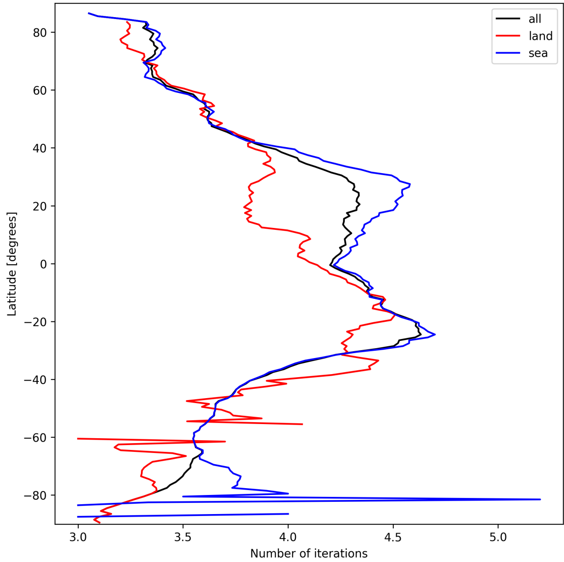
Figure 17: Zonal average of “Number of iterations” for 2025-09-26 to 2025-09-28.
