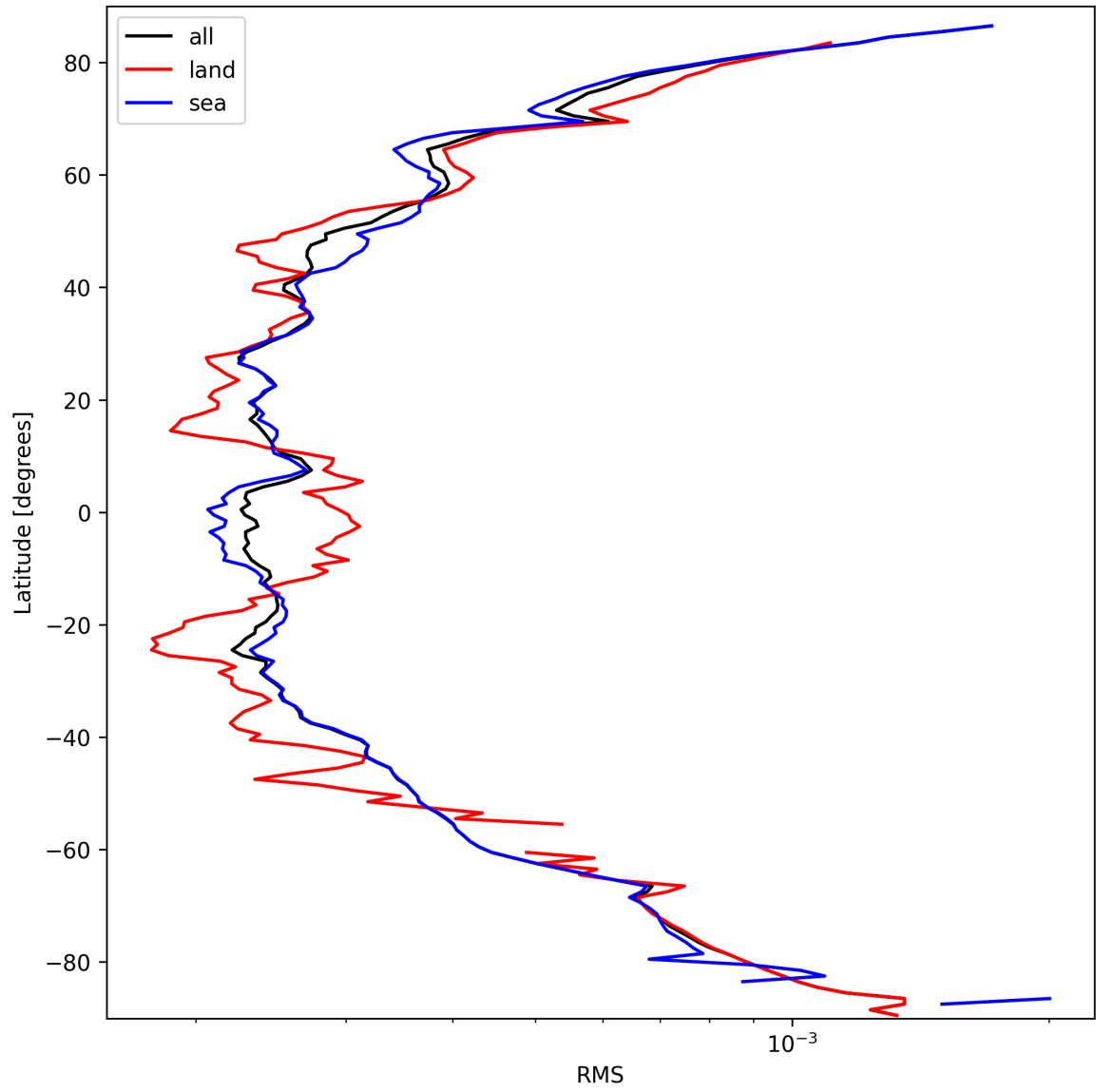
Figure 26: Zonal average of “RMS” for 2025-09-26 to 2025-09-28.
