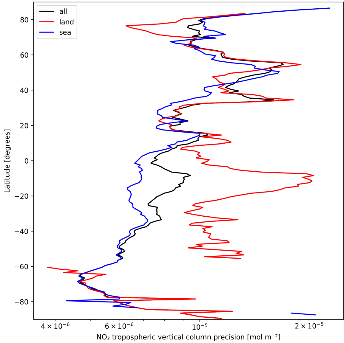
Figure 13: Zonal average of “NO 2 tropospheric vertical column precision” for 2025-09-26 to 2025-09-28.
