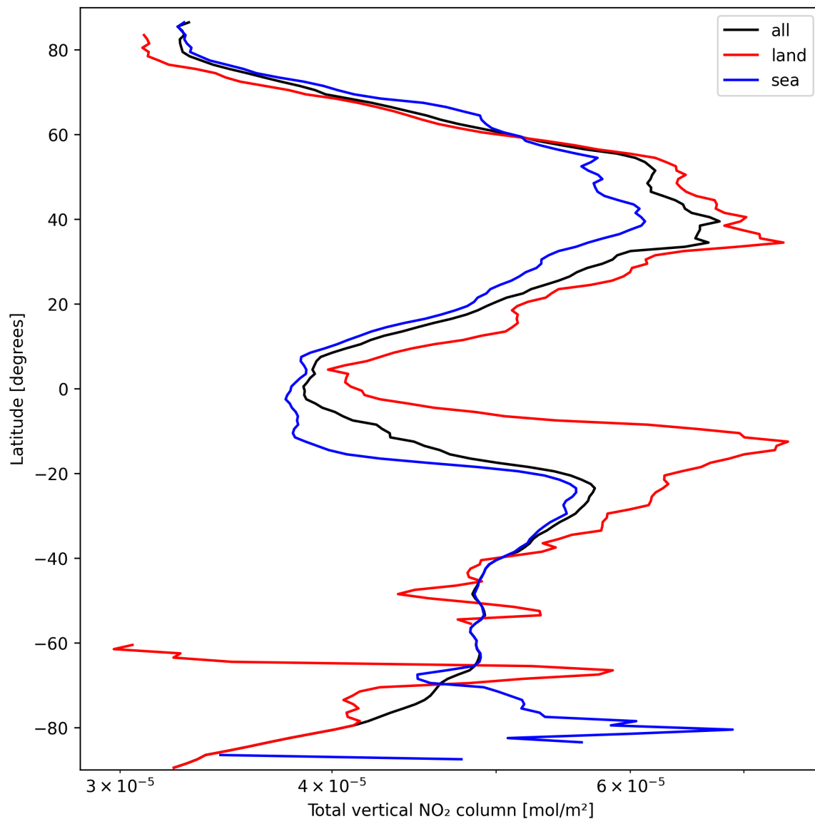
Figure 21: Zonal average of “Total vertical NO 2 column” for 2025-09-26 to 2025-09-28.
