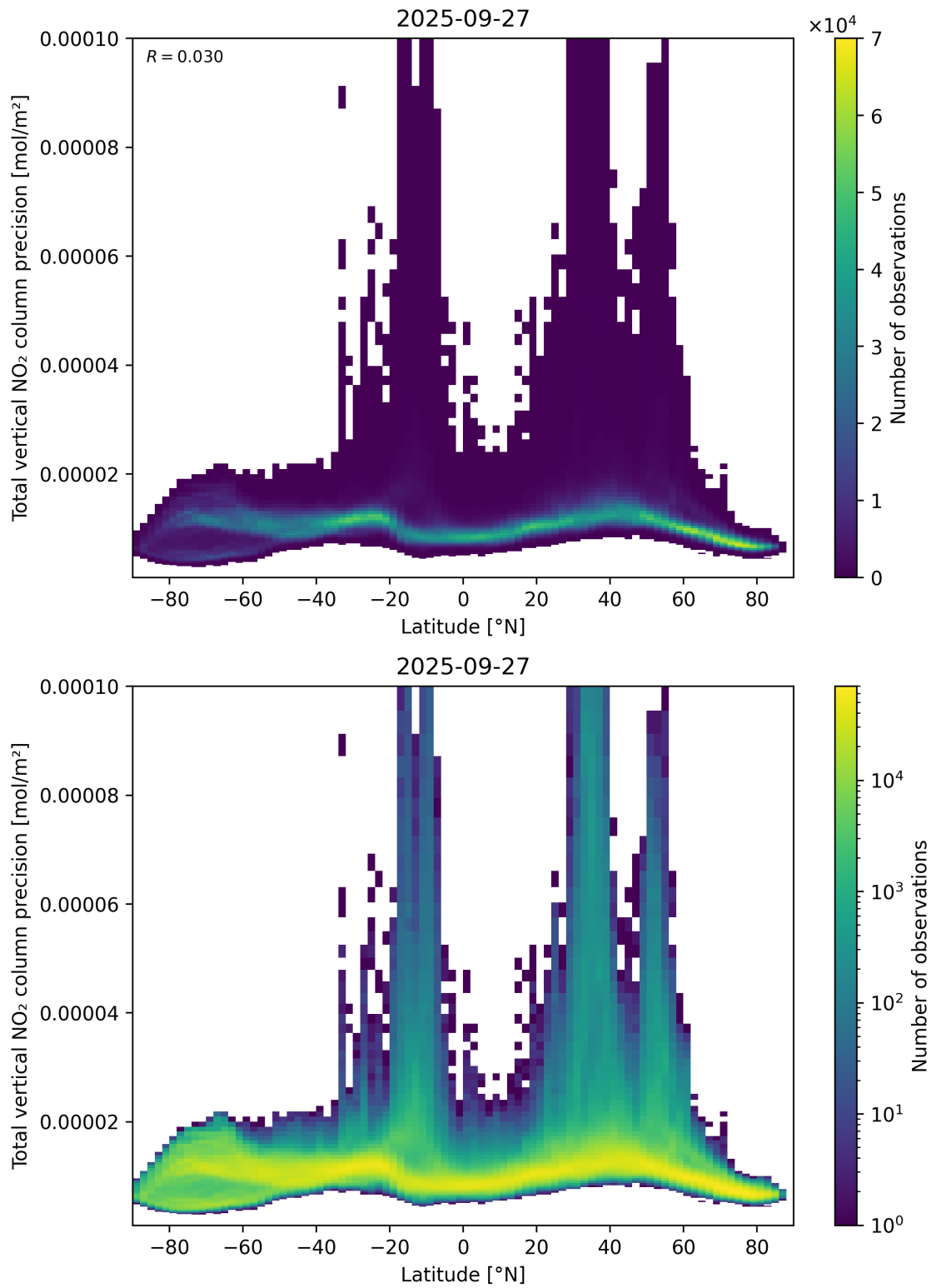
Figure 91: Scatter density plot of “Latitude” against “Total vertical NO 2 column precision” for 2025-09-26 to 2025-09-28.
