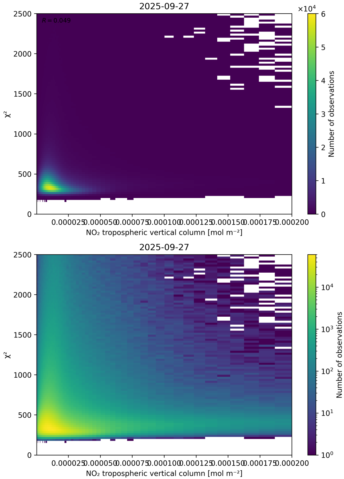
Figure 124: Scatter density plot of “NO 2 tropospheric vertical column” against “ \chi^2 ” for 2025-09-26 to 2025-09-28.
