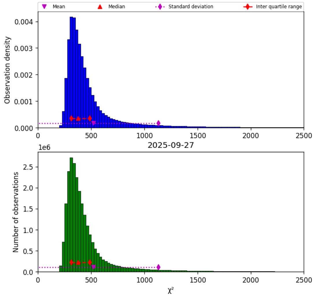
Figure 42: Histogram of “ \chi^2 ” for 2025-09-26 to 2025-09-28
