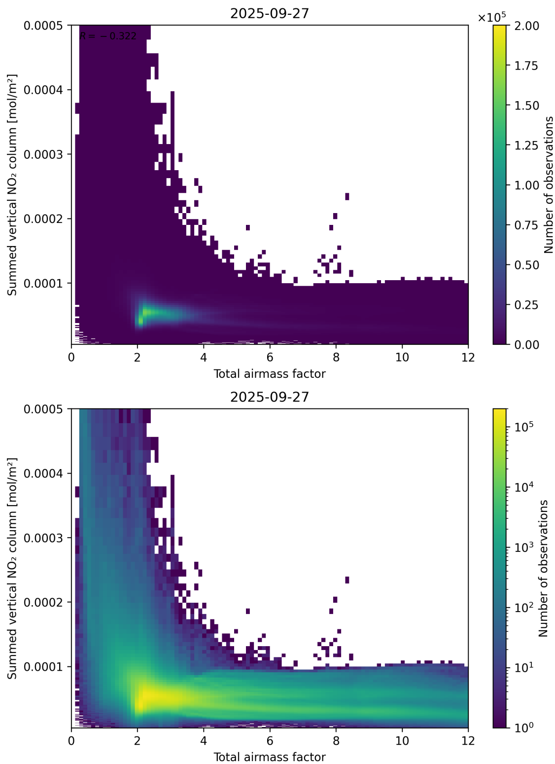
Figure 65: Scatter density plot of “Total airmass factor” against “Summed vertical NO 2 column” for 2025-09-26 to 2025-09-28.
