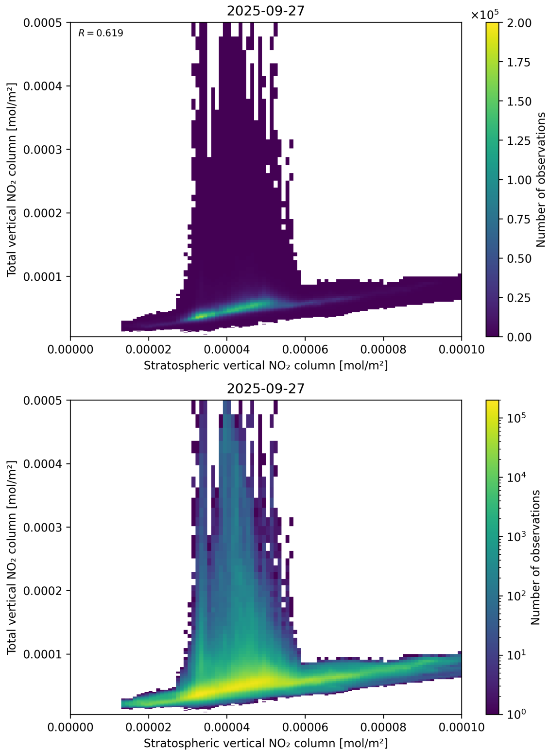
Figure 100: Scatter density plot of “Stratospheric vertical NO 2 column” against “Total vertical NO 2 column” for 2025-09-26 to 2025-09-28.
