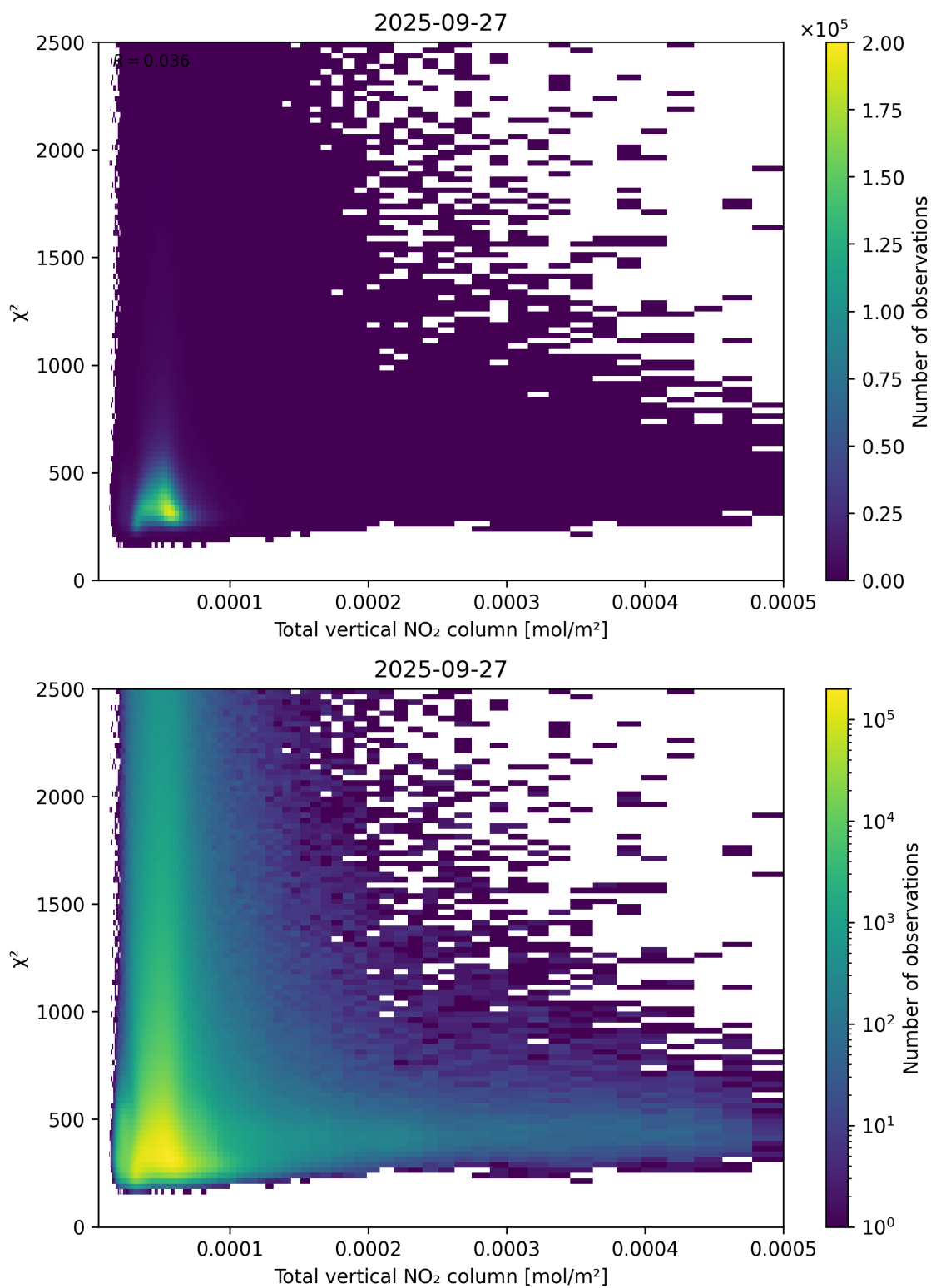
Figure 111: Scatter density plot of “Total vertical NO 2 column” against “ \chi^2 ” for 2025-09-26 to 2025-09-28.
