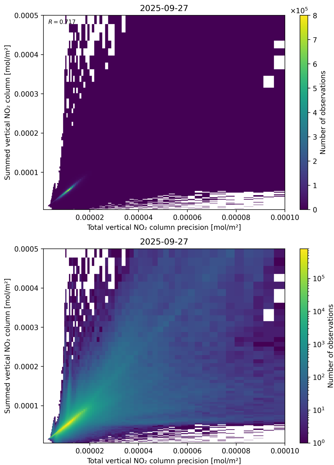
Figure 117: Scatter density plot of “Total vertical NO 2 column precision” against “Summed vertical NO 2 column” for 2025-09-26 to 2025-09-28.
