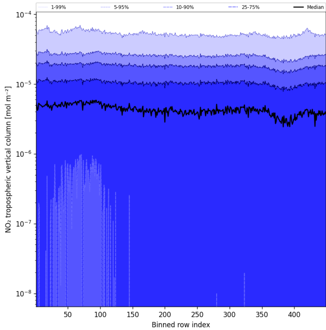
Figure 46: Along track statistics of “NO 2 tropospheric vertical column” for 2025-09-26 to 2025-09-28
