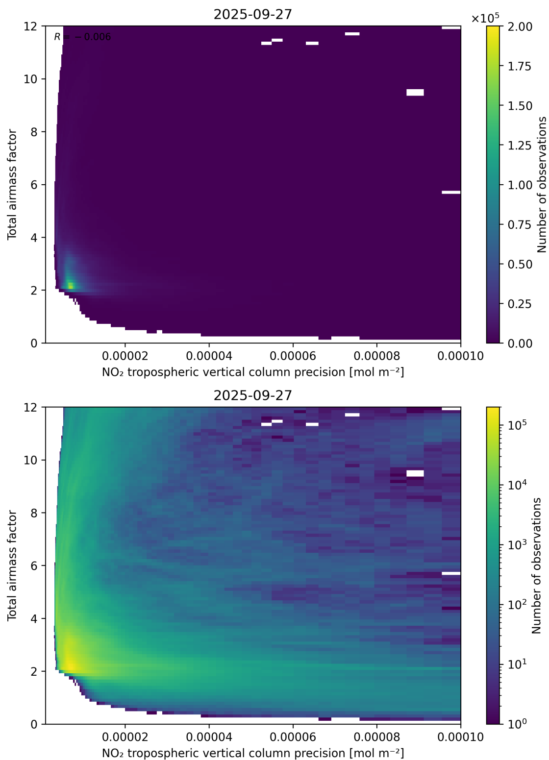
Figure 132: Scatter density plot of “NO 2 tropospheric vertical column precision” against “Total air mass factor” for 2025-09-26 to 2025-09-28.
