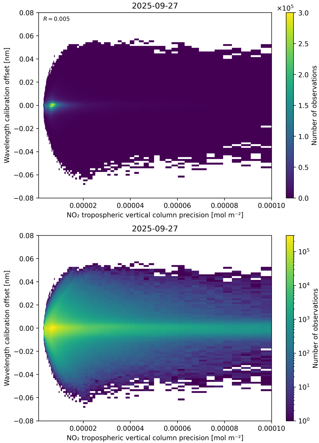
Figure 141: Scatter density plot of “NO 2 tropospheric vertical column precision” against “Wavelength calibration offset” for 2025-09-26 to 2025-09-28.
