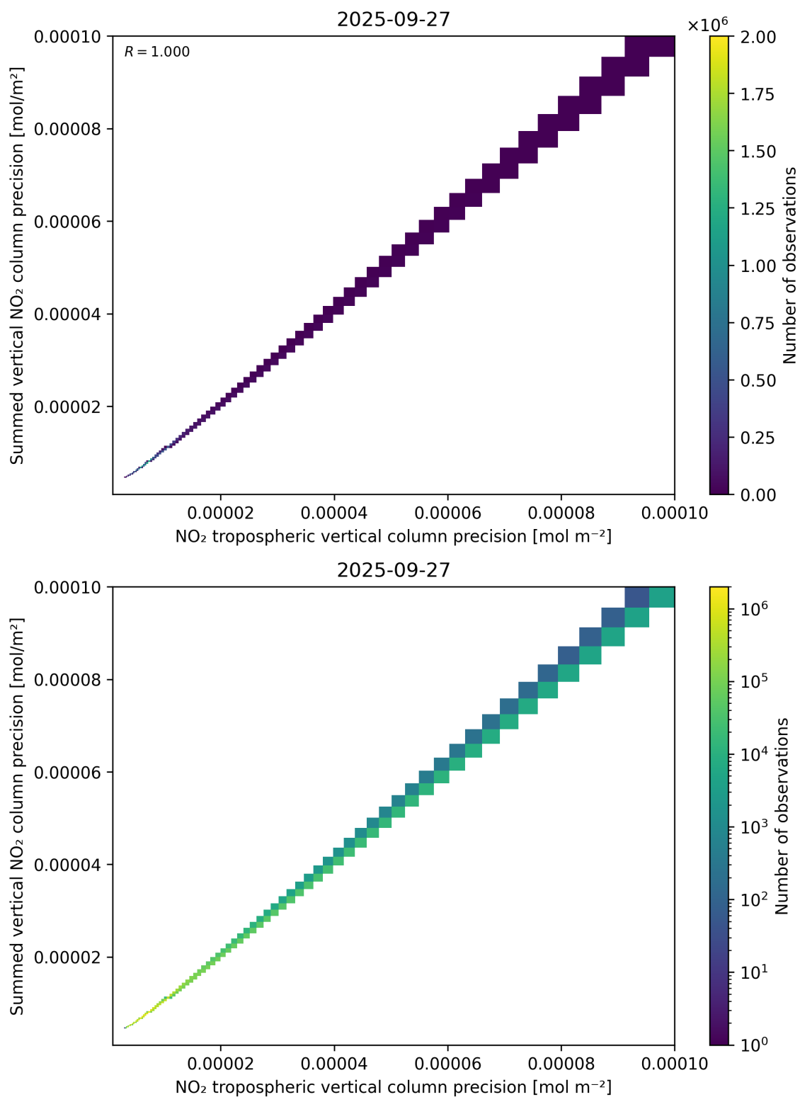
Figure 137: Scatter density plot of “NO 2 tropospheric vertical column precision” against “Summed vertical NO 2 column precision” for 2025-09-26 to 2025-09-28.
