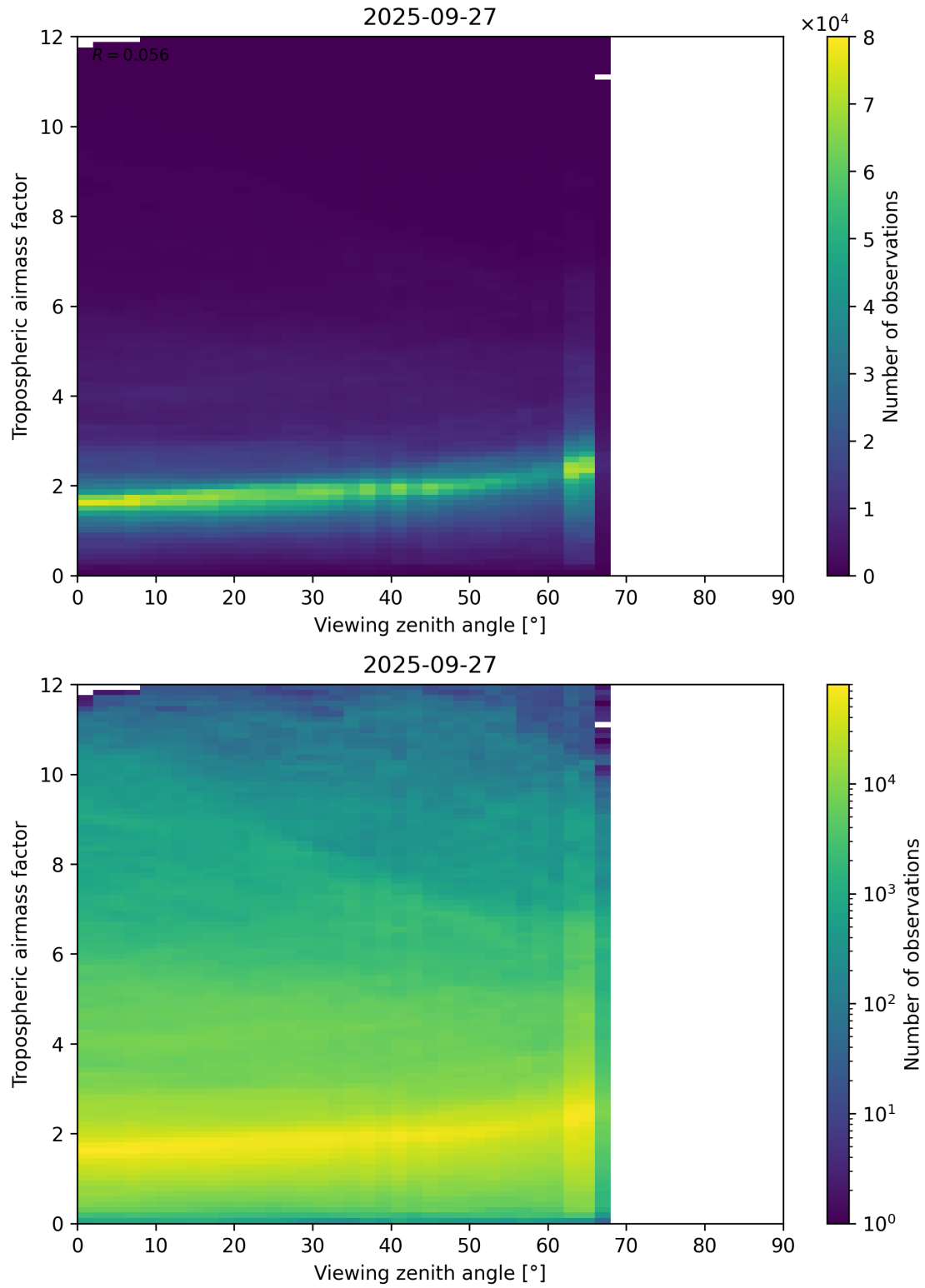
Figure 161: Scatter density plot of “Viewing zenith angle” against “Tropospheric airmass factor” for 2025-09-26 to 2025-09-28.
