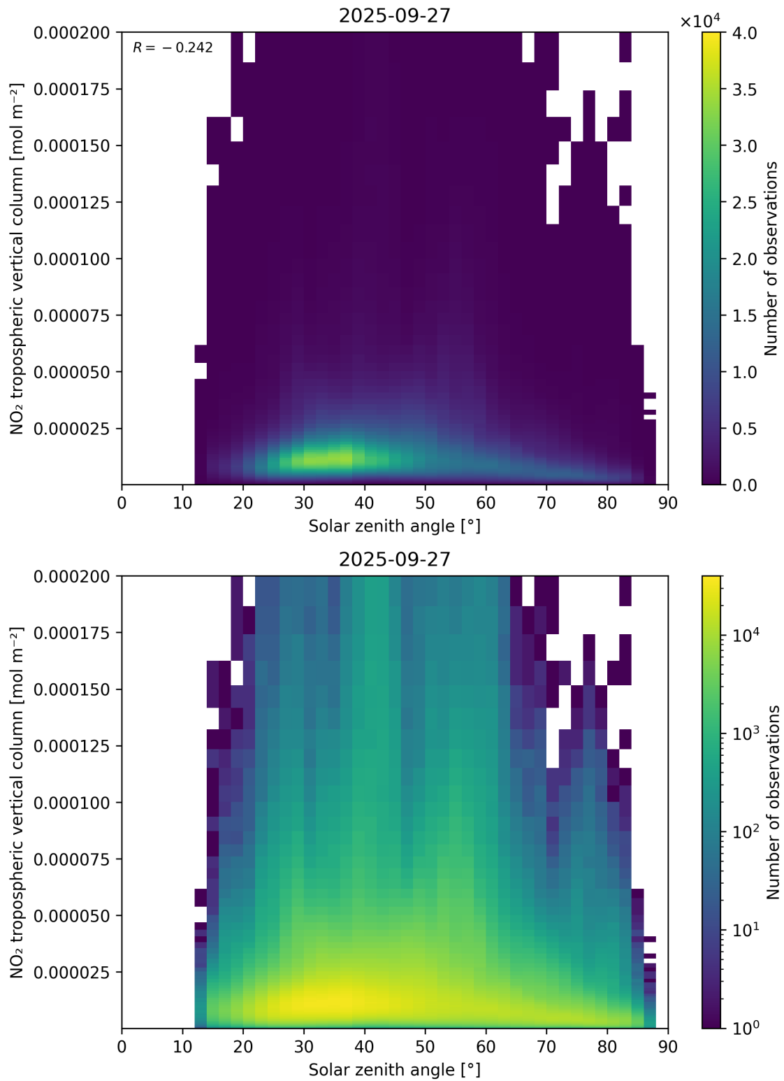
Figure 155: Scatter density plot of “Solar zenith angle” against “NO 2 tropospheric vertical column” for 2025-09-26 to 2025-09-28.
