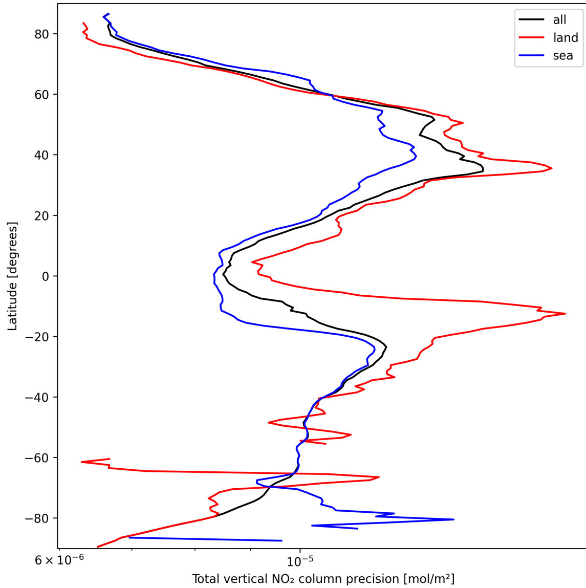
Figure 22: Zonal average of “Total vertical NO 2 column precision” for 2025-09-26 to 2025-09-28.
