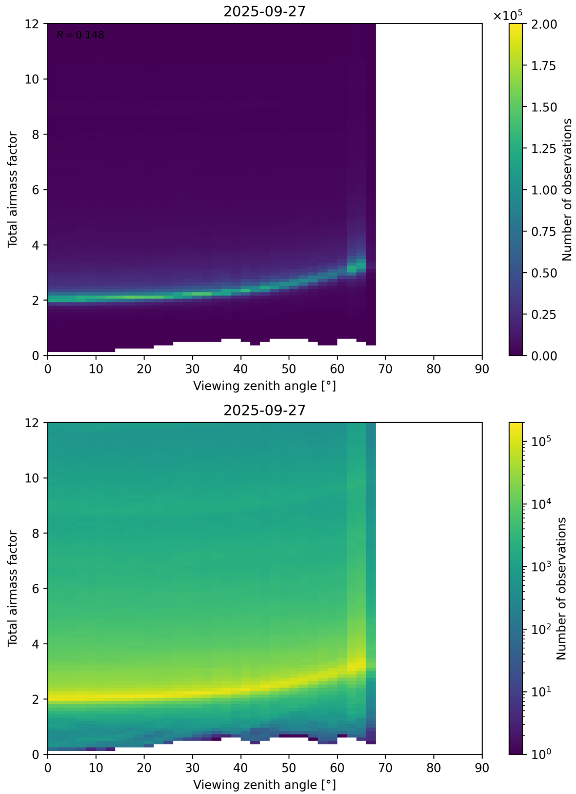
Figure 160: Scatter density plot of “Viewing zenith angle” against “Total airmass factor” for 2025-09-26 to 2025-09-28.
