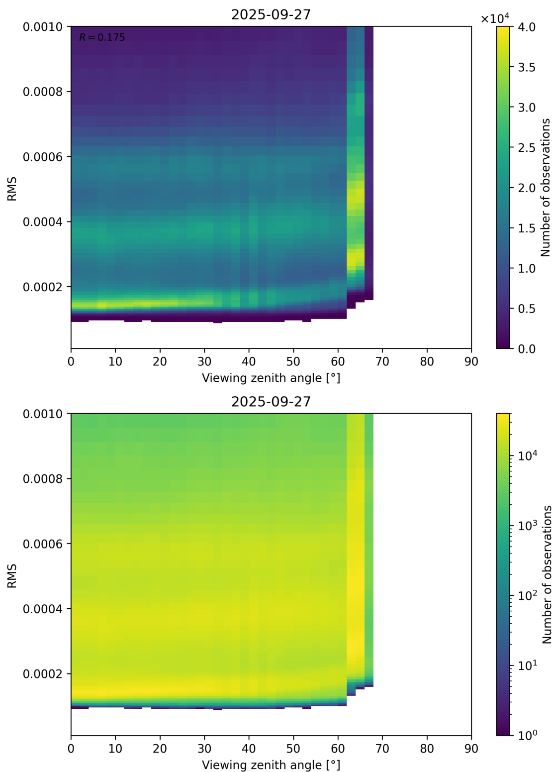
Figure 171: Scatter density plot of “Viewing zenith angle” against “RMS” for 2025-09-26 to 2025-09-28.
