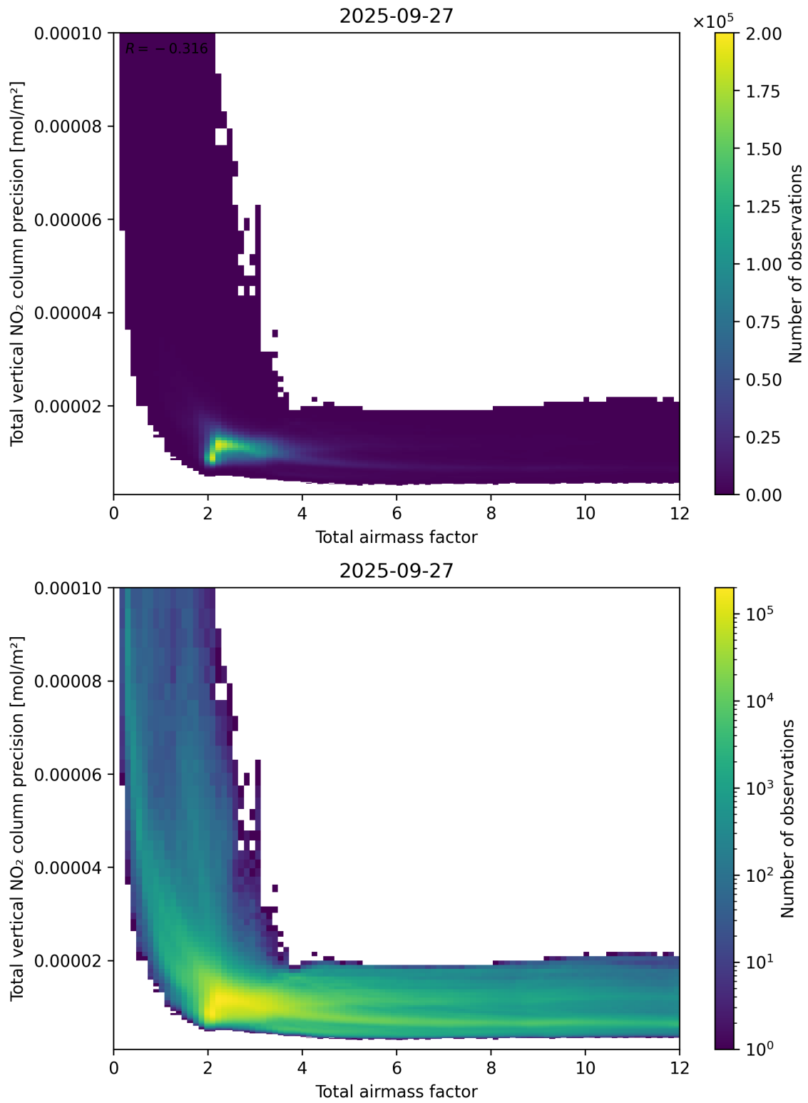
Figure 68: Scatter density plot of “Total airmass factor” against “Total vertical NO 2 column precision” for 2025-09-26 to 2025-09-28.
