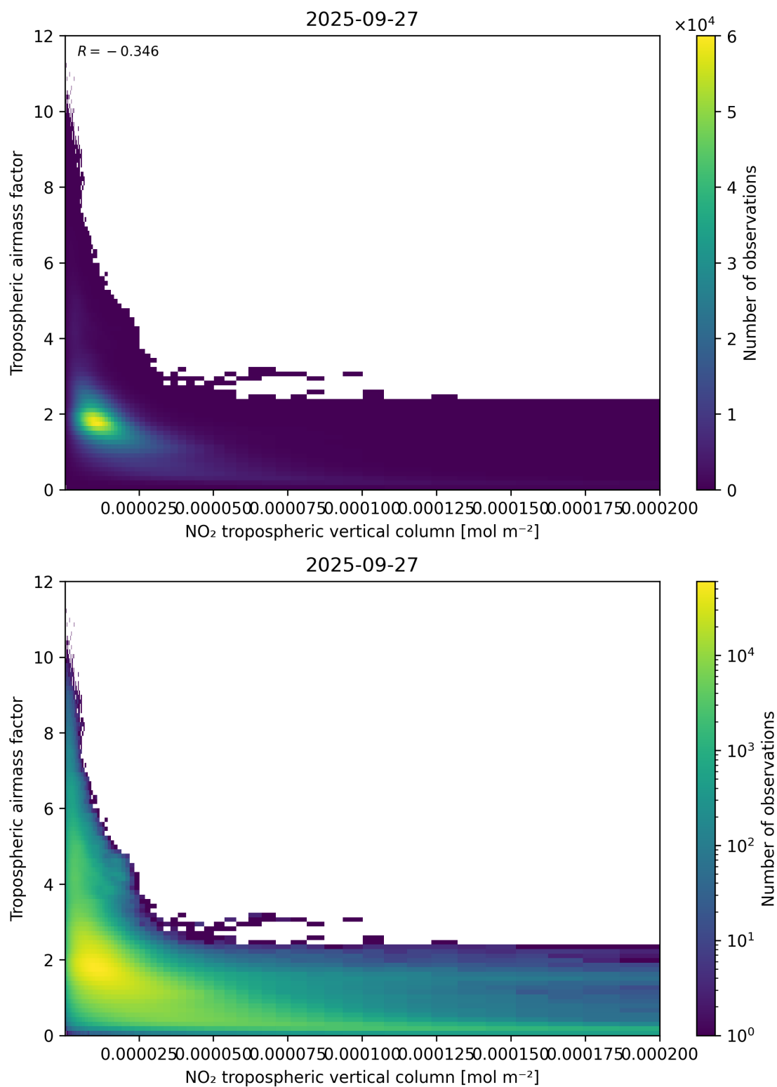
Figure 123: Scatter density plot of “NO 2 tropospheric vertical column” against “Tropospheric air mass factor” for 2025-09-26 to 2025-09-28.
