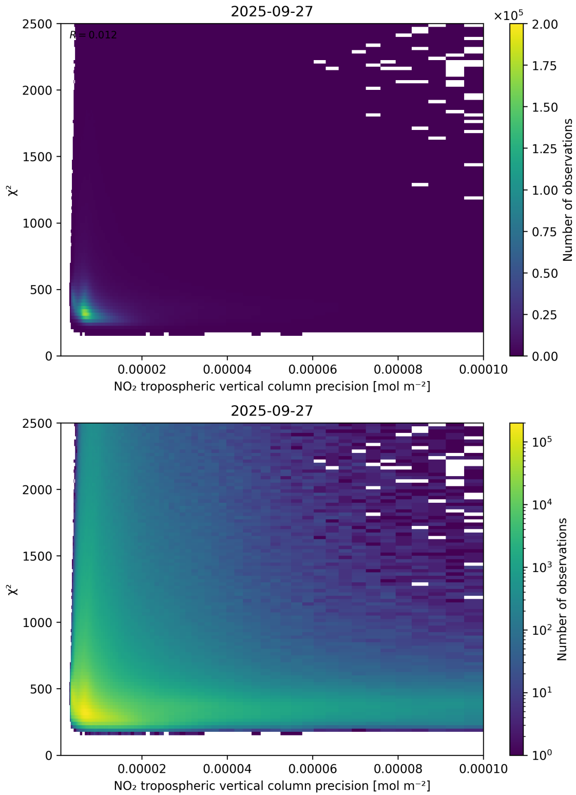
Figure 134: Scatter density plot of “NO 2 tropospheric vertical column precision” against “ \chi^2 ” for 2025-09-26 to 2025-09-28.
