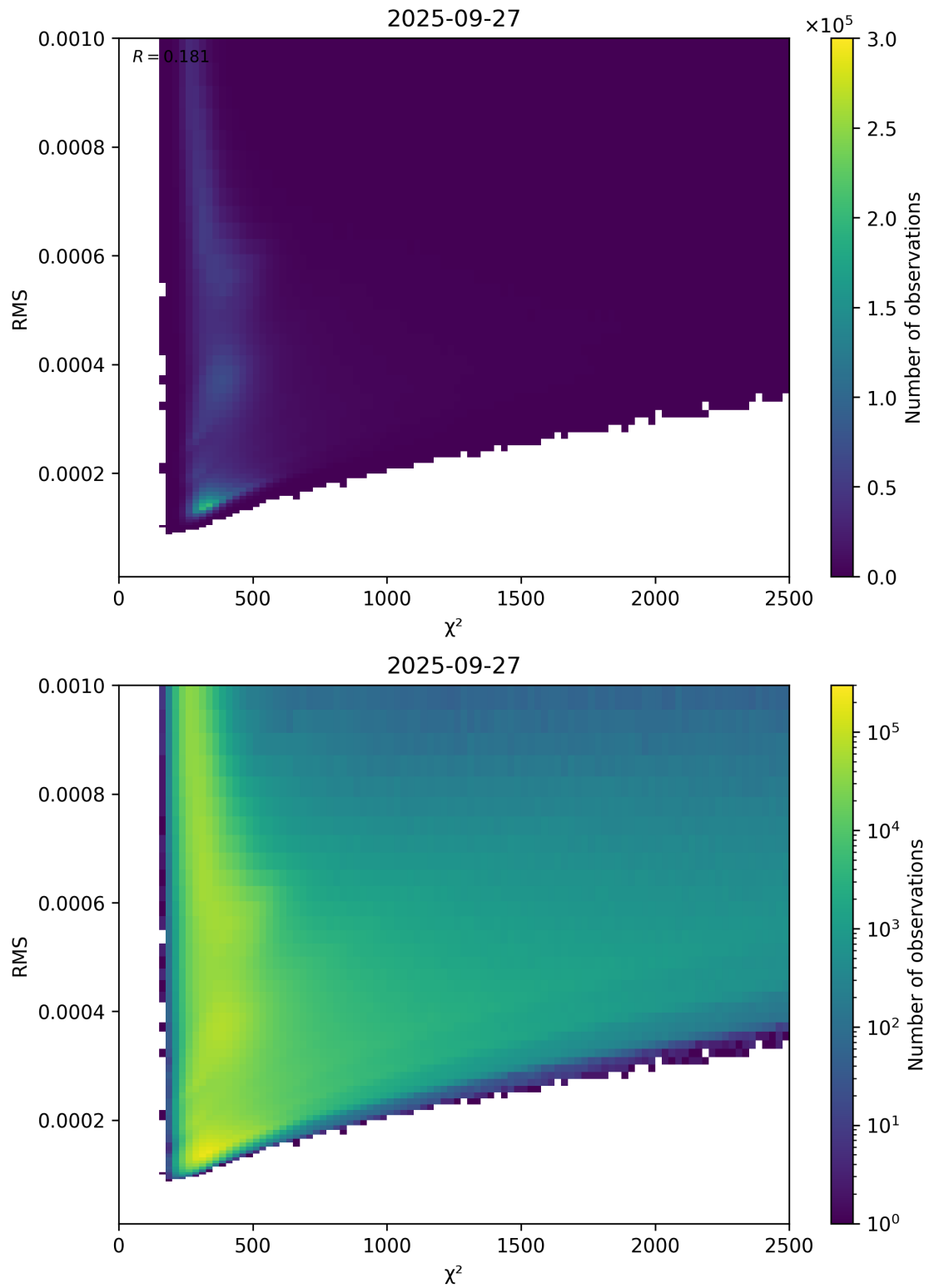
Figure 82: Scatter density plot of “ \chi^2 ” against “RMS” for 2025-09-26 to 2025-09-28.
