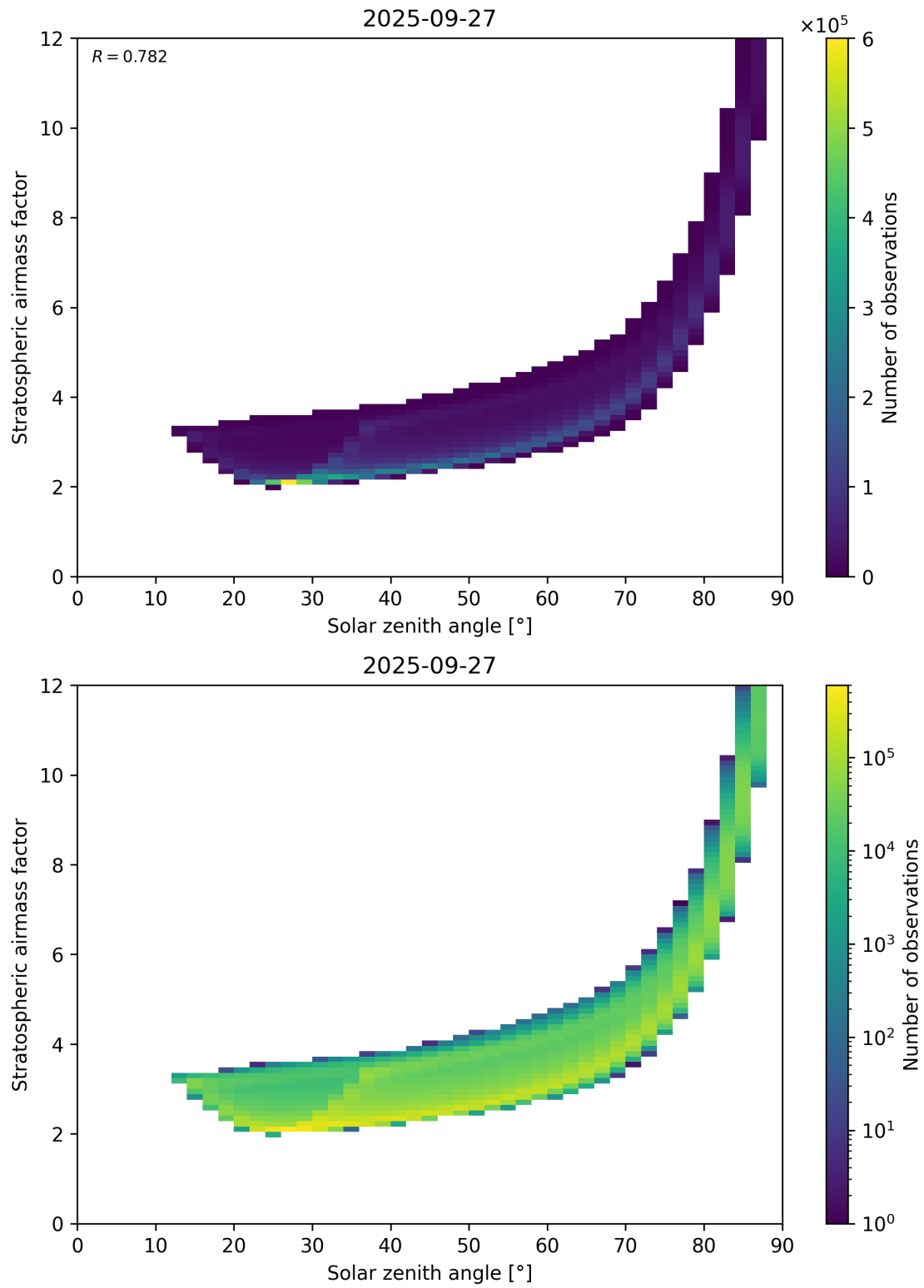
Figure 145: Scatter density plot of “Solar zenith angle” against “Stratospheric airmass factor” for 2025-09-26 to 2025-09-28.
