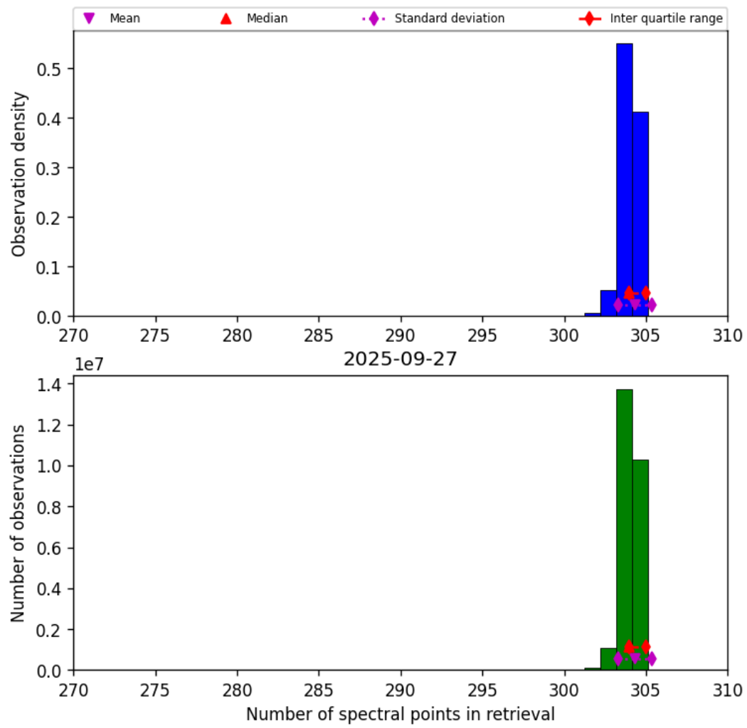
Figure 33: Histogram of “Number of spectral points in retrieval” for 2025-09-26 to 2025-09-28
