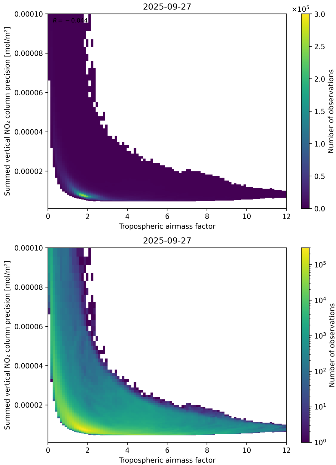
Figure 76: Scatter density plot of “Tropospheric air mass factor” against “Summed vertical NO 2 column precision” for 2025-09-26 to 2025-09-28.
