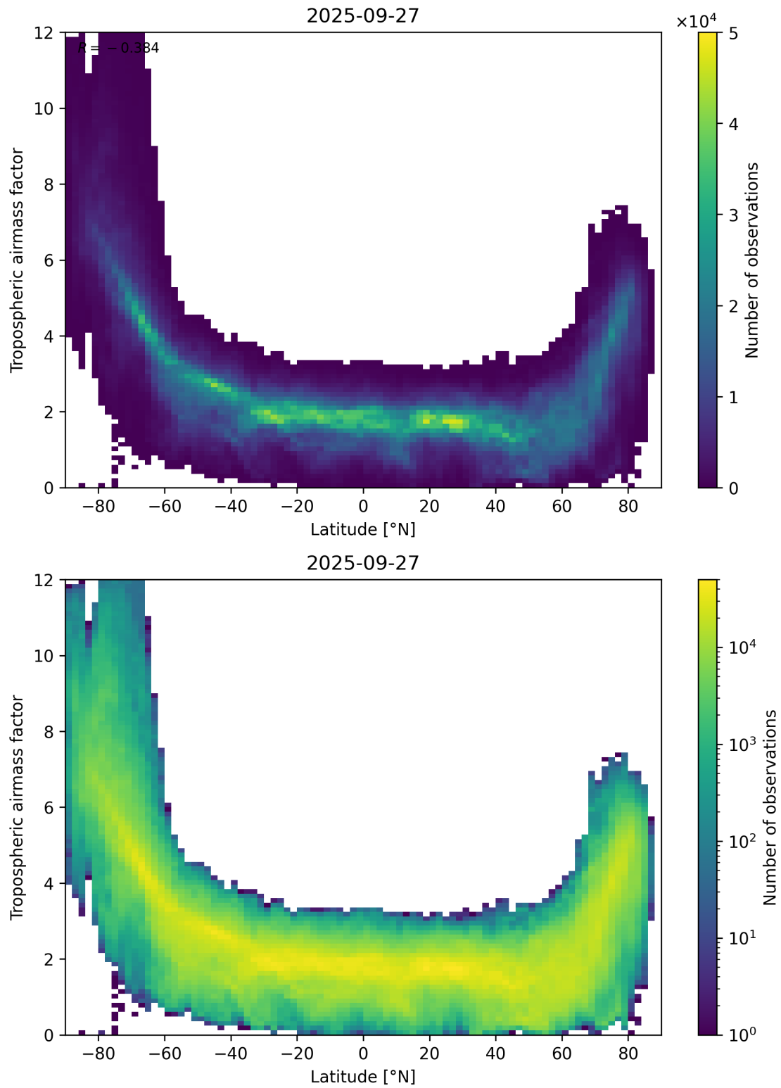
Figure 85: Scatter density plot of “Latitude” against “Tropospheric airmass factor” for 2025-09-26 to 2025-09-28.
