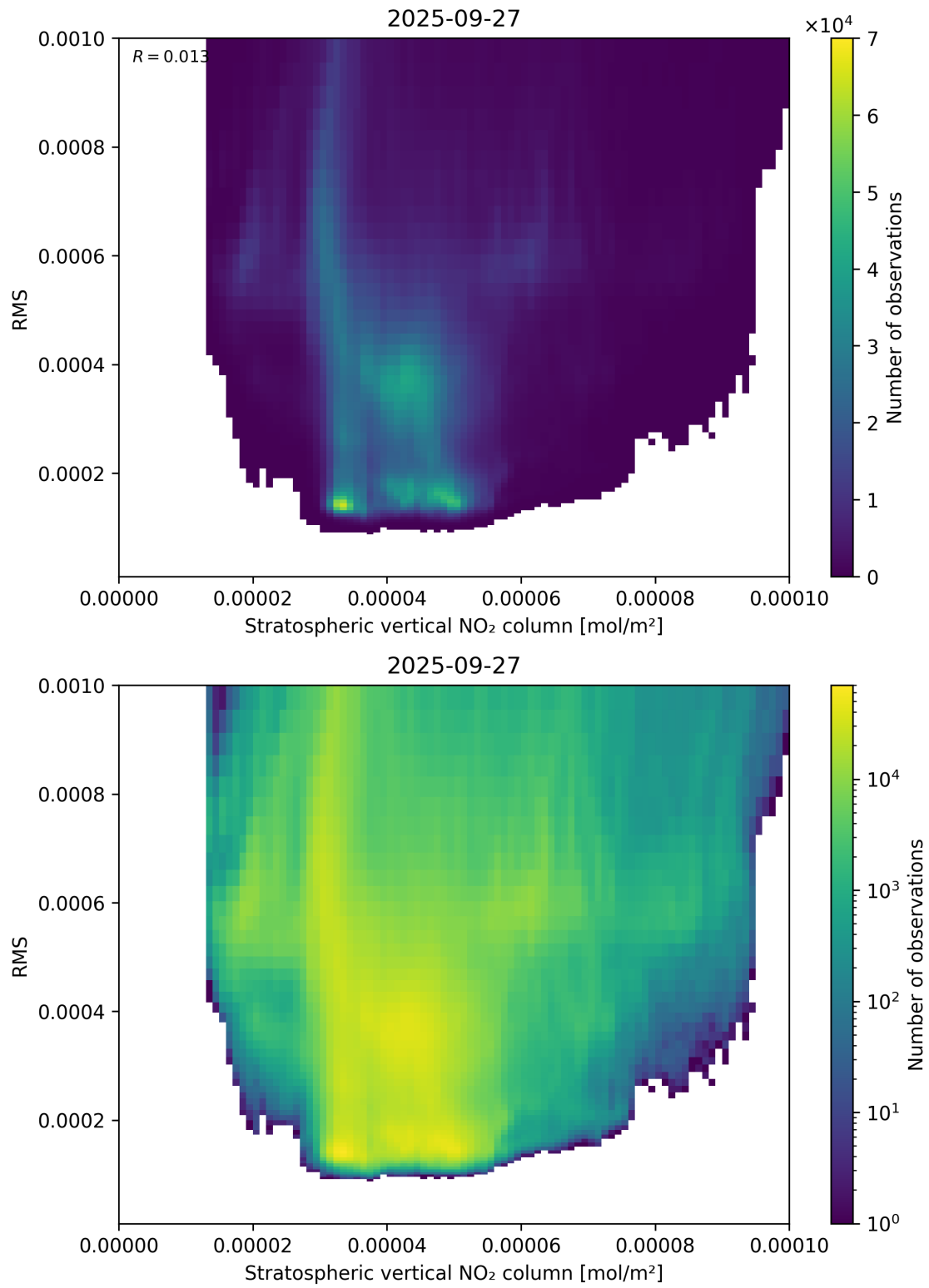
Figure 102: Scatter density plot of “Stratospheric vertical NO 2 column” against “RMS” for 2025-09-26 to 2025-09-28.
