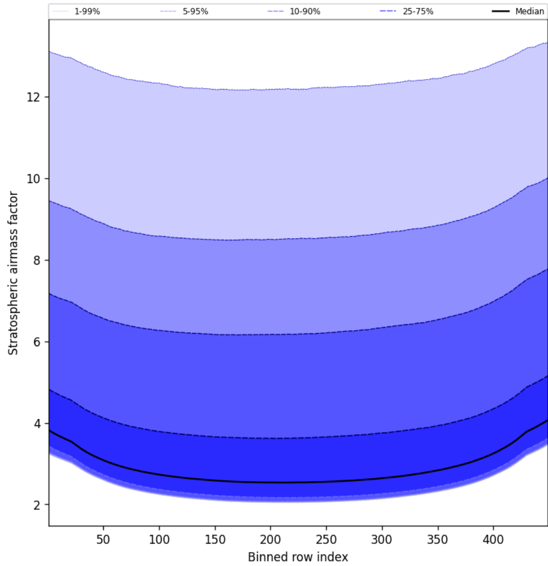
Figure 61: Along track statistics of “Stratospheric airmass factor” for 2025-09-26 to 2025-09-28
