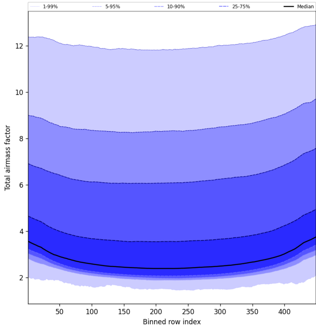
Figure 49: Along track statistics of “Total airmass factor” for 2025-09-26 to 2025-09-28
