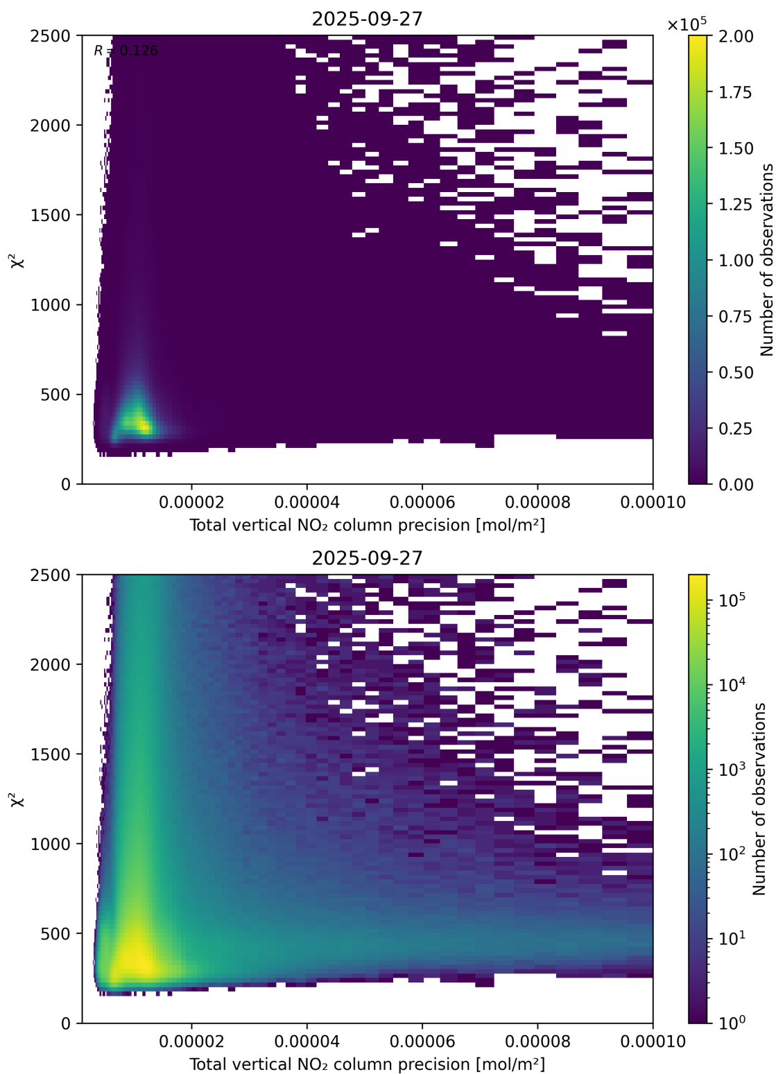
Figure 116: Scatter density plot of “Total vertical NO 2 column precision” against “ \chi^2 ” for 2025-09-26 to 2025-09-28.
