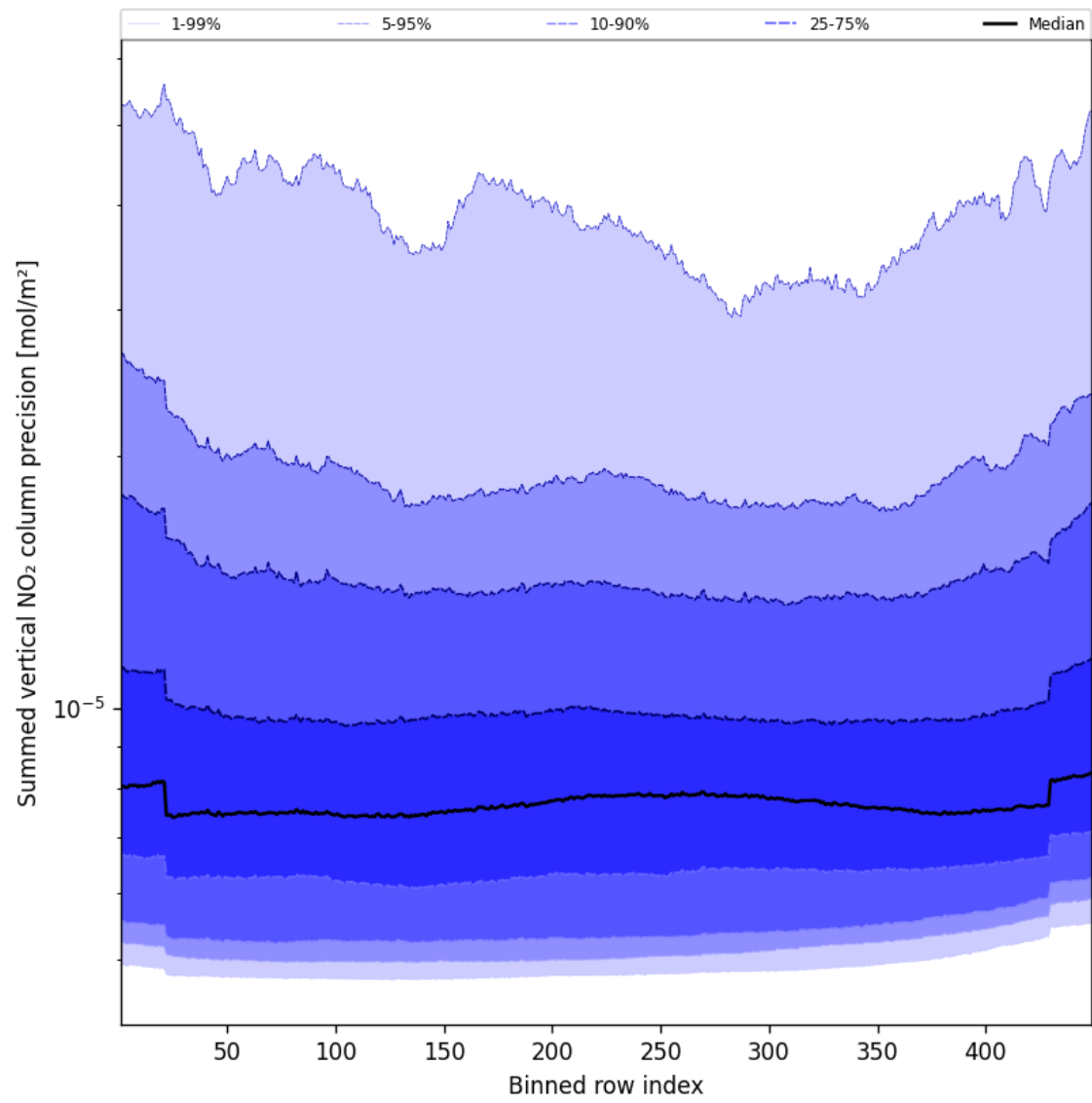
Figure 58: Along track statistics of “Summed vertical NO 2 column precision” for 2025-09-26 to 2025-09-28
