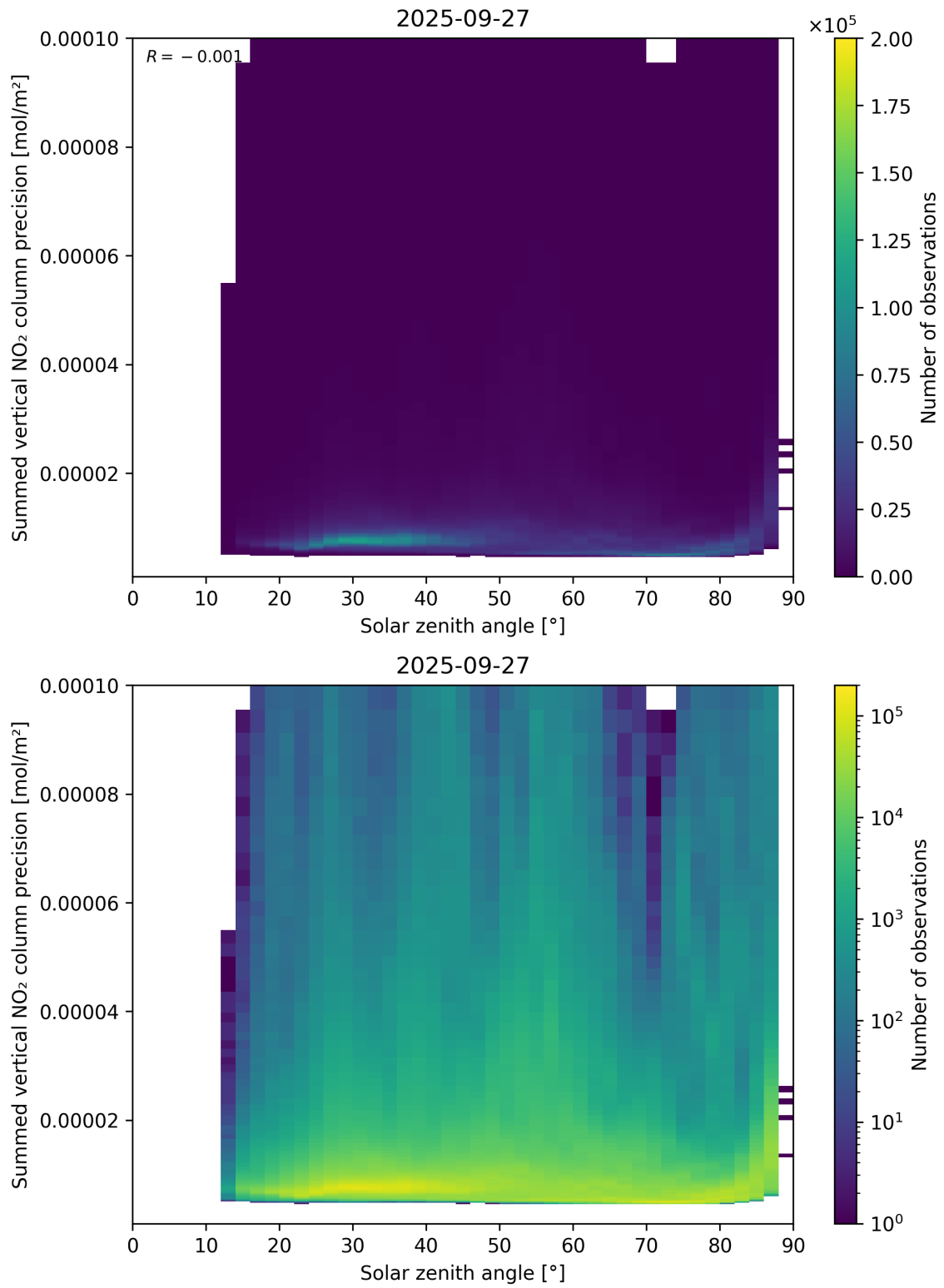
Figure 152: Scatter density plot of “Solar zenith angle” against “Summed vertical NO 2 column precision” for 2025-09-26 to 2025-09-28.
