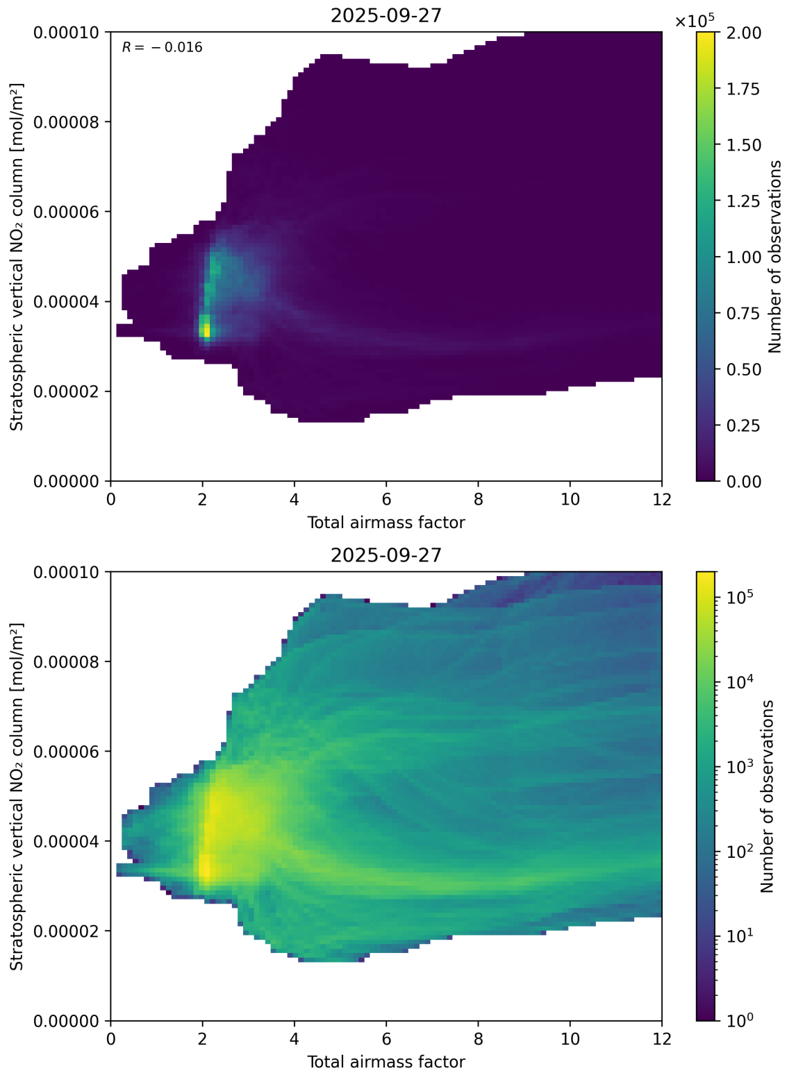
Figure 64: Scatter density plot of “Total airmass factor” against “Stratospheric vertical NO 2 column” for 2025-09-26 to 2025-09-28.
