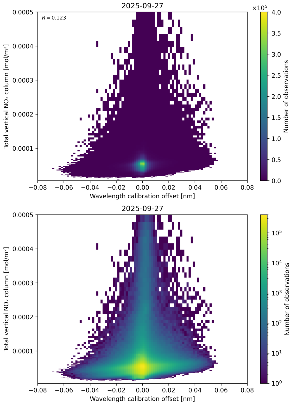
Figure 179: Scatter density plot of “Wavelength calibration offset” against “Total vertical NO 2 column” for 2025-09-26 to 2025-09-28.
