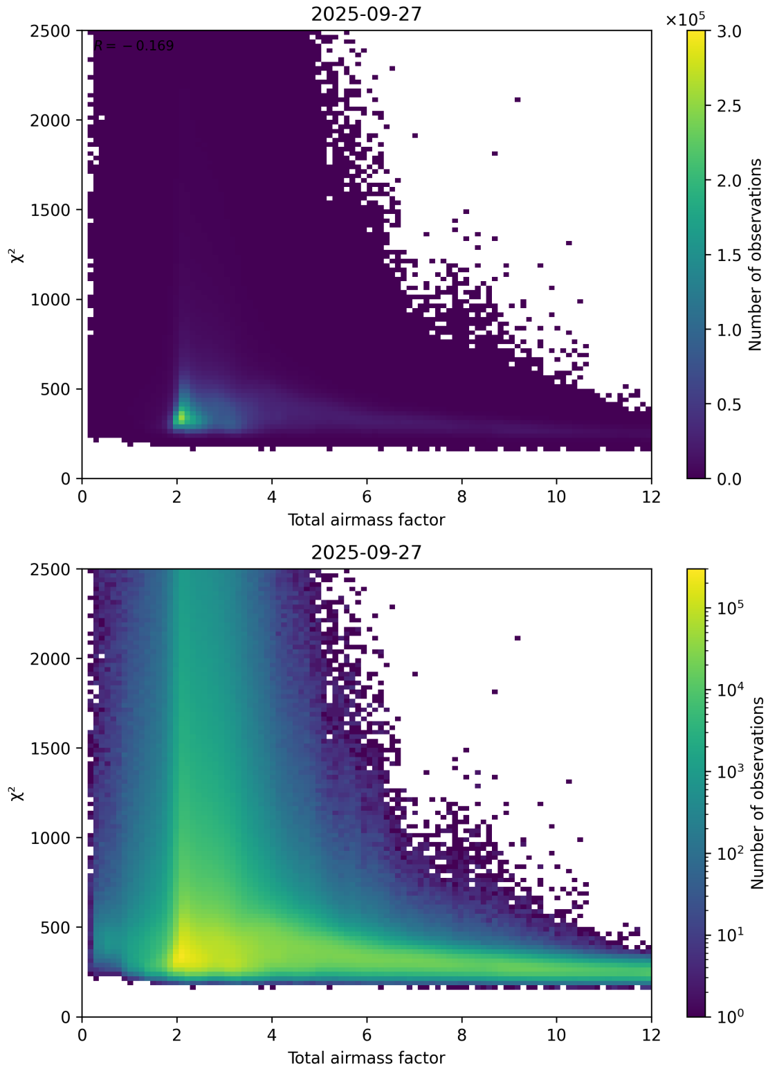
Figure 63: Scatter density plot of “Total airmass factor” against “ \chi^2 ” for 2025-09-26 to 2025-09-28.
