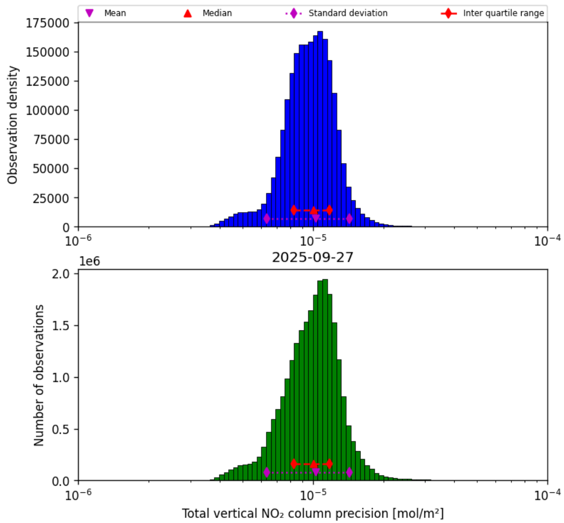
Figure 39: Histogram of "Total vertical NO 2 column precision" for 2025-09-26 to 2025-09-28
