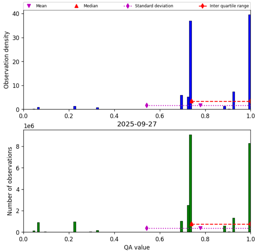
Figure 28: Histogram of “QA value” for 2025-09-26 to 2025-09-28
