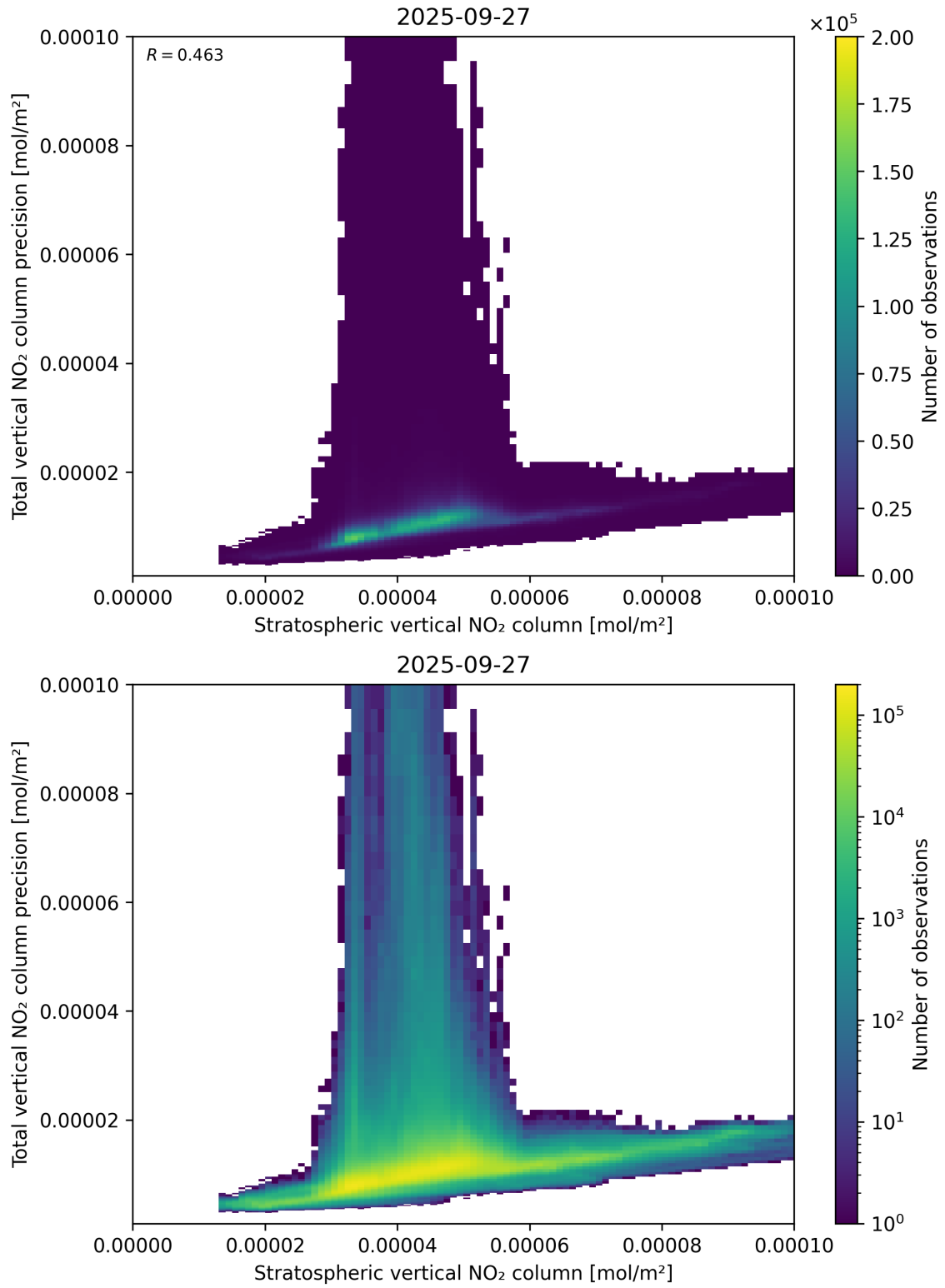
Figure 101: Scatter density plot of “Stratospheric vertical NO 2 column” against “Total vertical NO 2 column precision” for 2025-09-26 to 2025-09-28.
