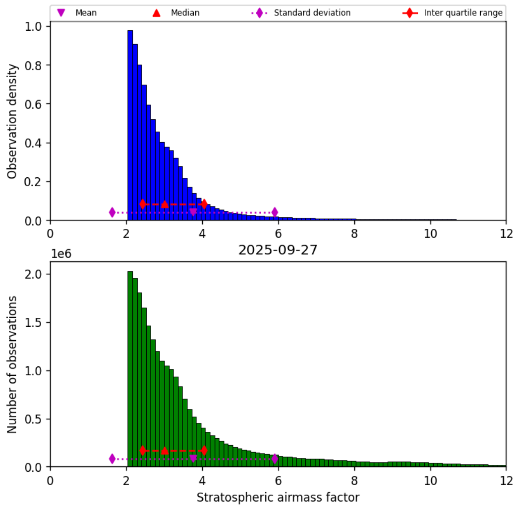
Figure 44: Histogram of “Stratospheric airmass factor” for 2025-09-26 to 2025-09-28
