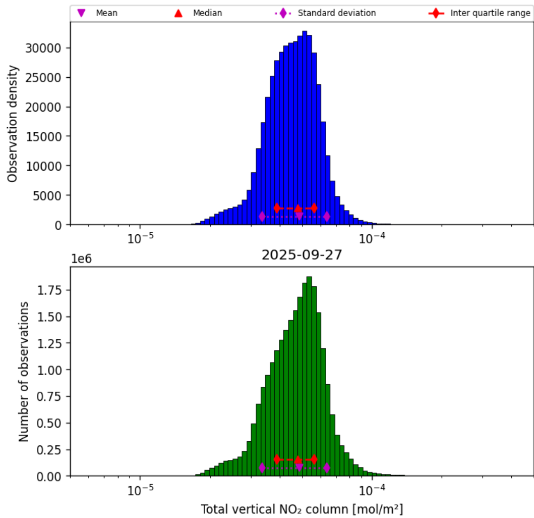
Figure 38: Histogram of “Total vertical NO 2 column” for 2025-09-26 to 2025-09-28
