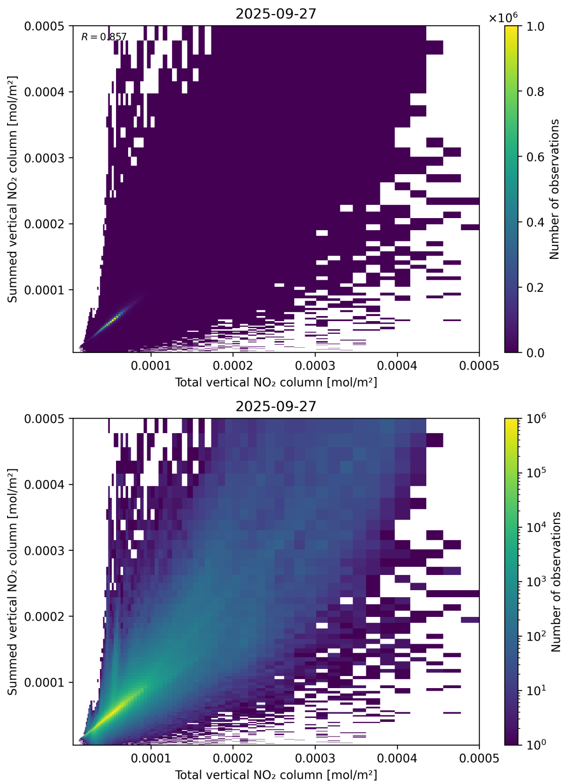
Figure 112: Scatter density plot of “Total vertical NO 2 column” against “Summed vertical NO 2 column” for 2025-09-26 to 2025-09-28.
