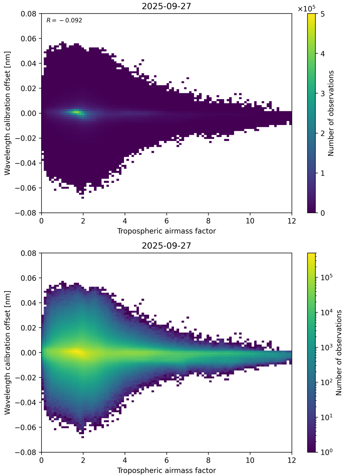
Figure 80: Scatter density plot of “Tropospheric airmass factor” against “Wavelength calibration offset” for 2025-09-26 to 2025-09-28.
