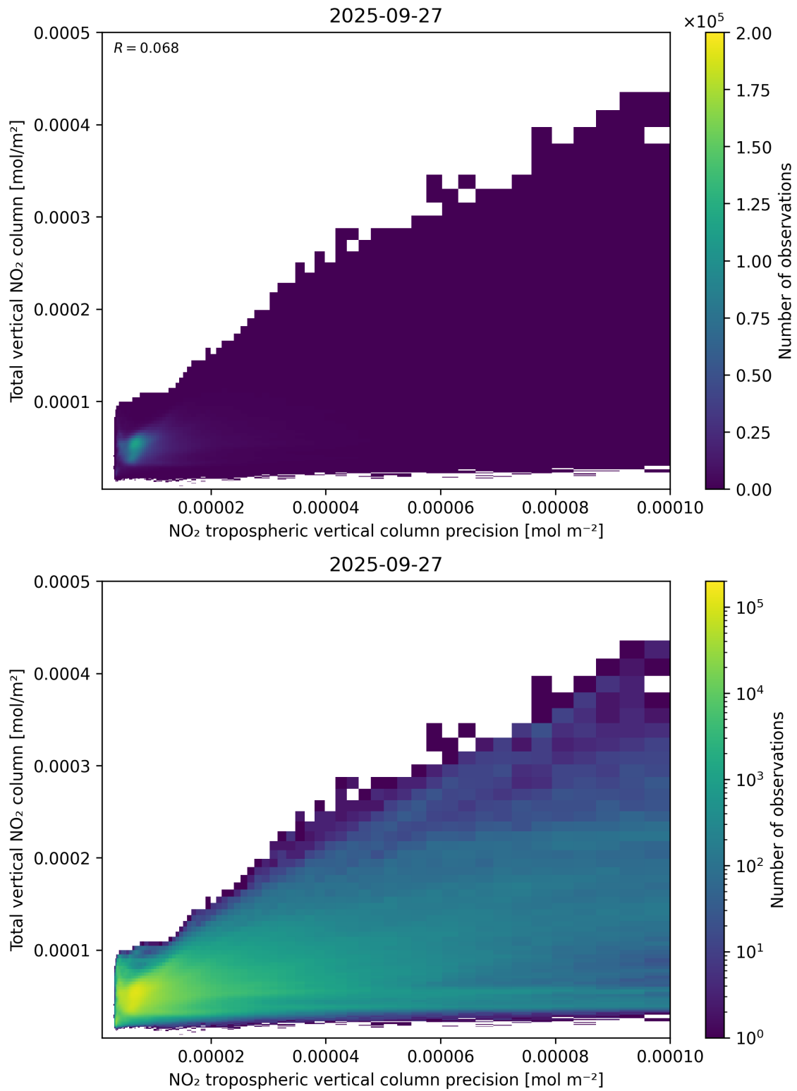
Figure 138: Scatter density plot of “NO 2 tropospheric vertical column precision” against “Total vertical NO 2 column” for 2025-09-26 to 2025-09-28.
