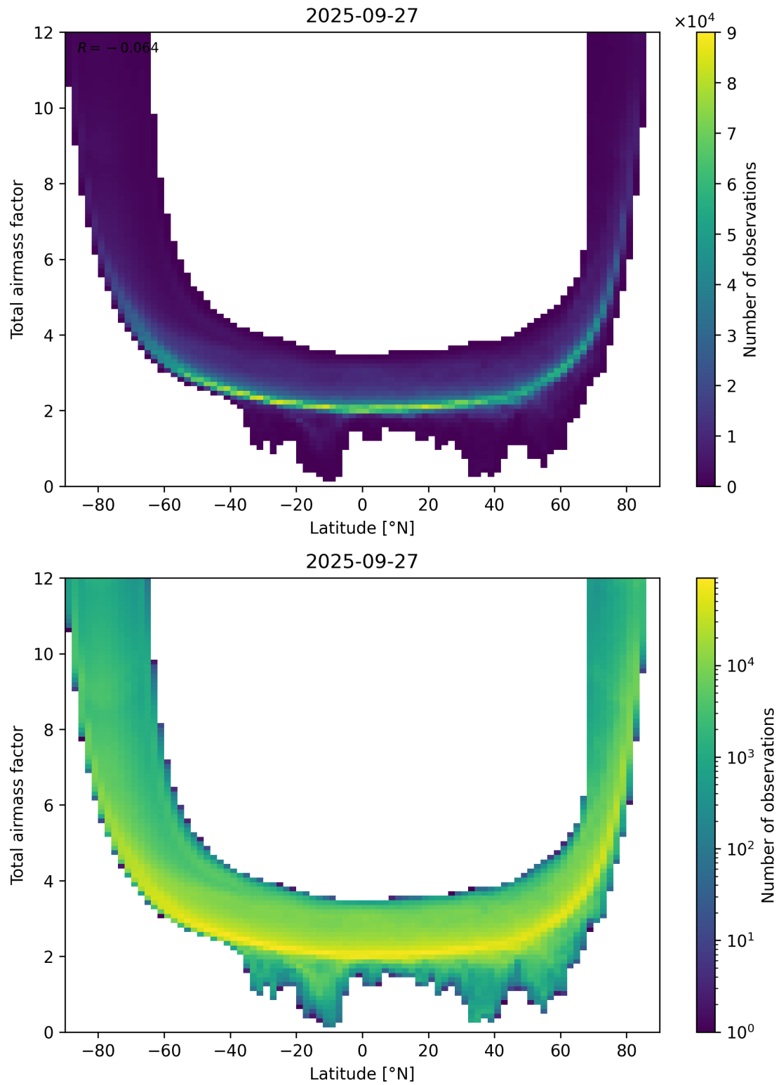
Figure 84: Scatter density plot of “Latitude” against “Total airmass factor” for 2025-09-26 to 2025-09-28.
