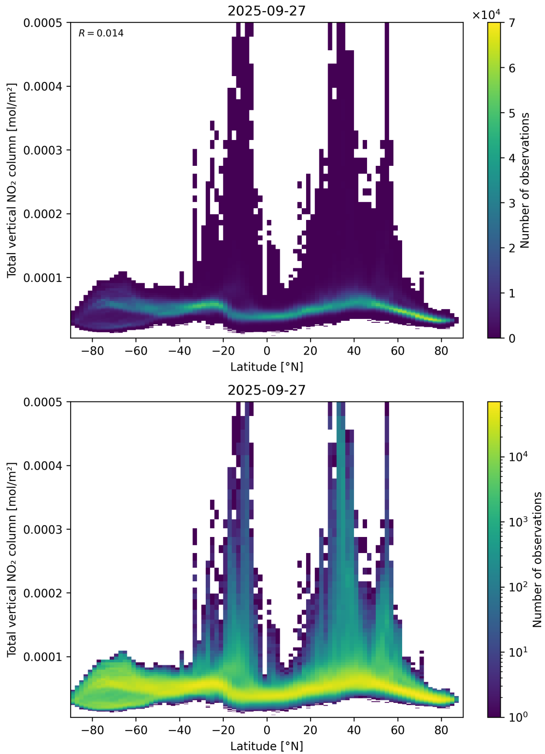
Figure 90: Scatter density plot of “Latitude” against “Total vertical NO 2 column” for 2025-09-26 to 2025-09-28.
