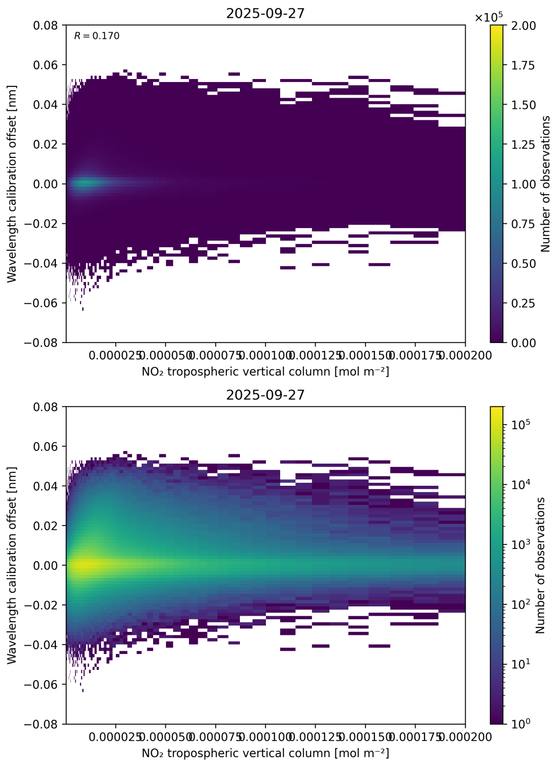
Figure 143: Scatter density plot of “NO 2 tropospheric vertical column” against “Wavelength calibration offset” for 2025-09-26 to 2025-09-28.
