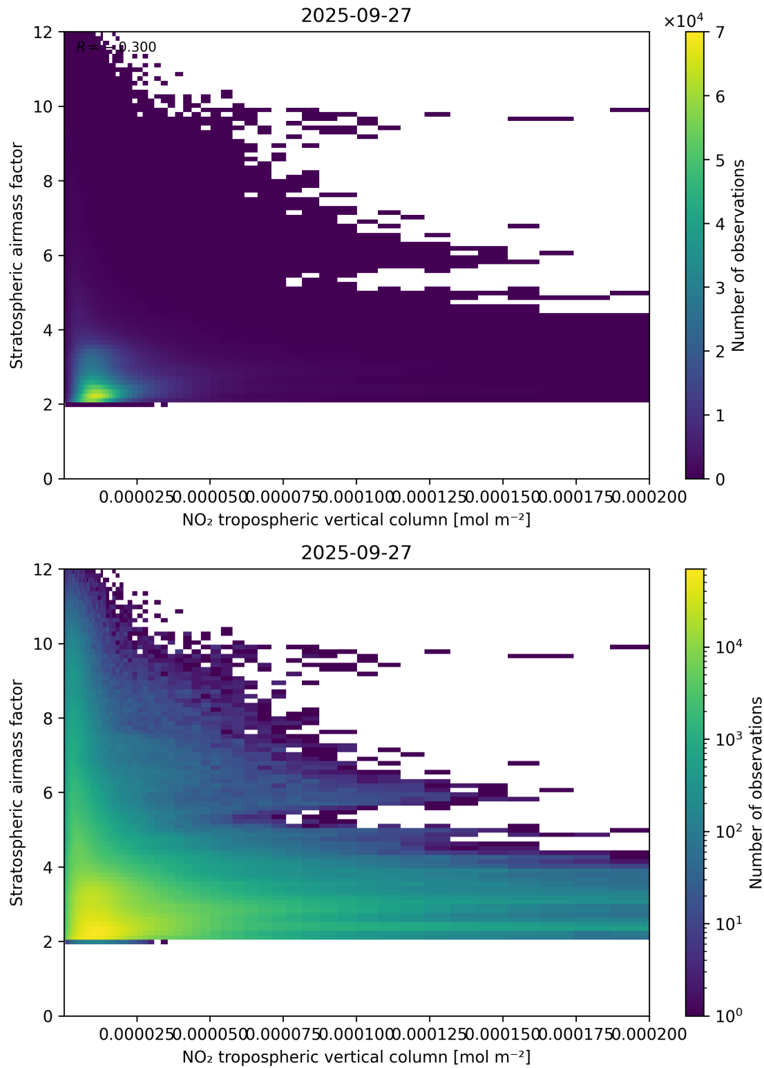
Figure 121: Scatter density plot of “NO 2 tropospheric vertical column” against “Stratospheric air mass factor” for 2025-09-26 to 2025-09-28.
