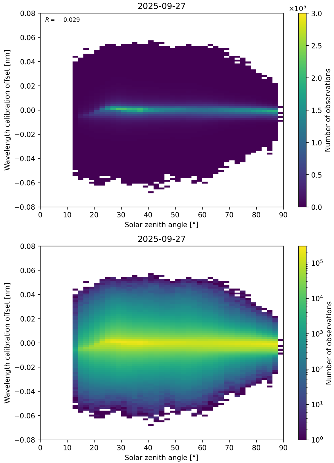
Figure 158: Scatter density plot of “Solar zenith angle” against “Wavelength calibration offset” for 2025-09-26 to 2025-09-28.
