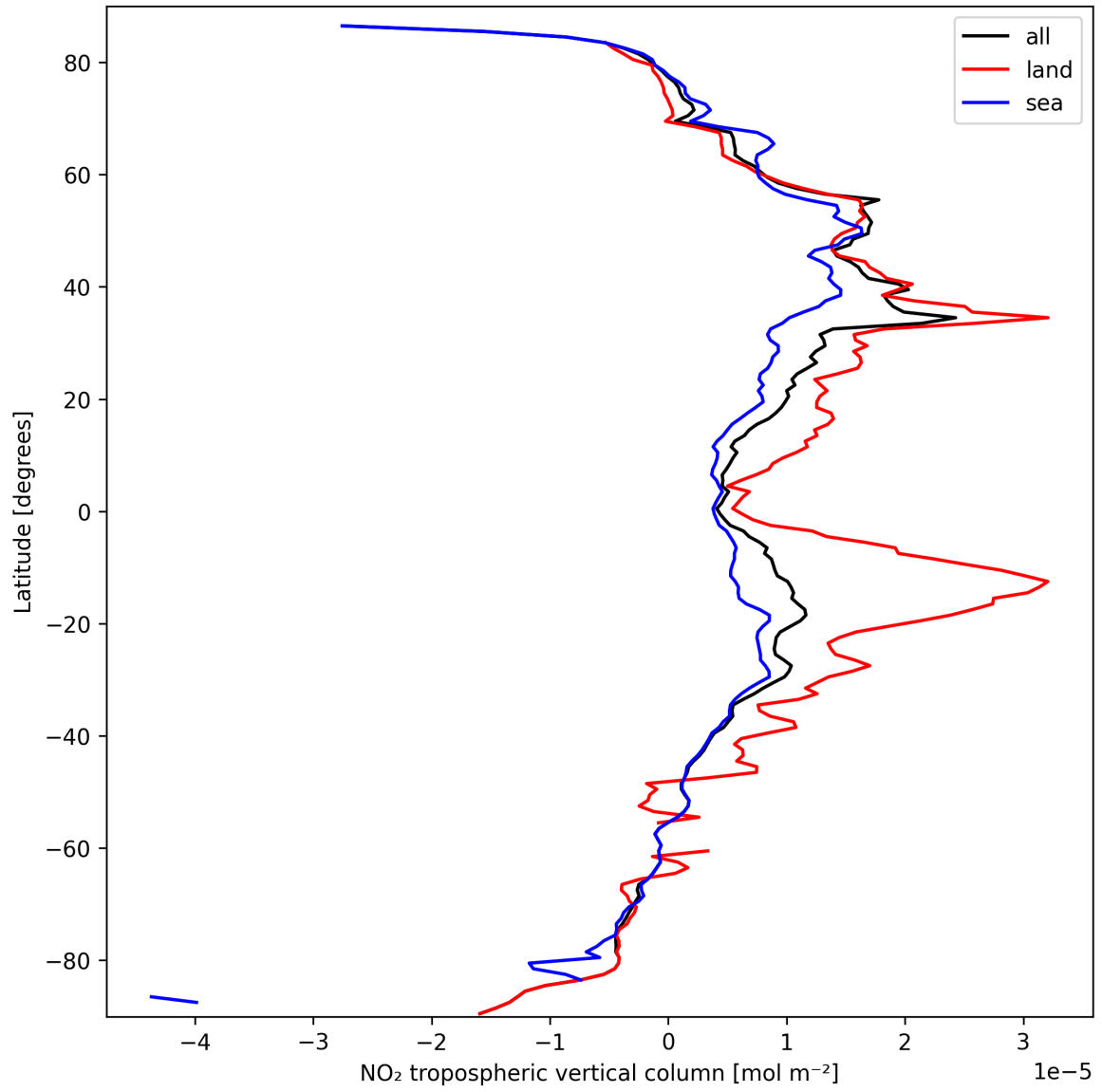
Figure 12: Zonal average of “NO 2 tropospheric vertical column” for 2025-09-26 to 2025-09-28.
