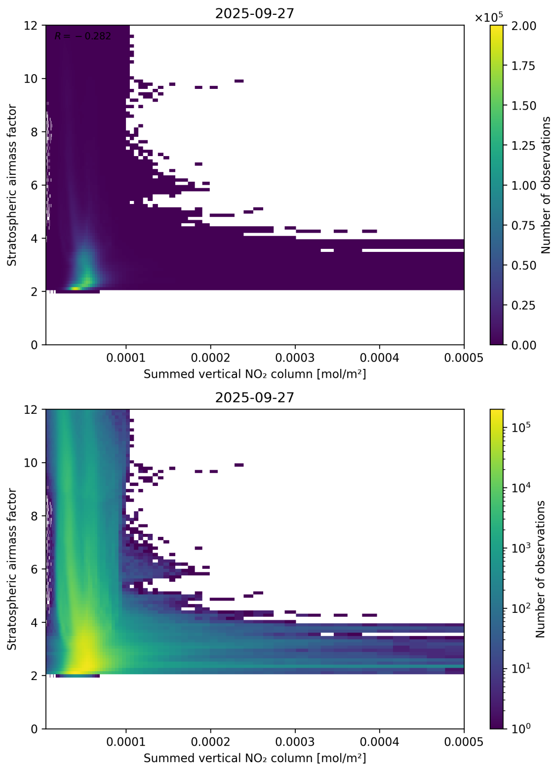
Figure 103: Scatter density plot of “Summed vertical NO 2 column” against “Stratospheric air mass factor” for 2025-09-26 to 2025-09-28.
