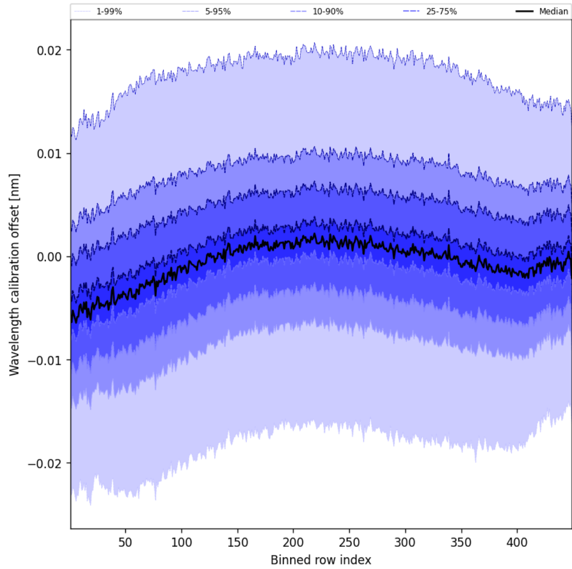
Figure 52: Along track statistics of “Wavelength calibration offset” for 2025-09-26 to 2025-09-28
