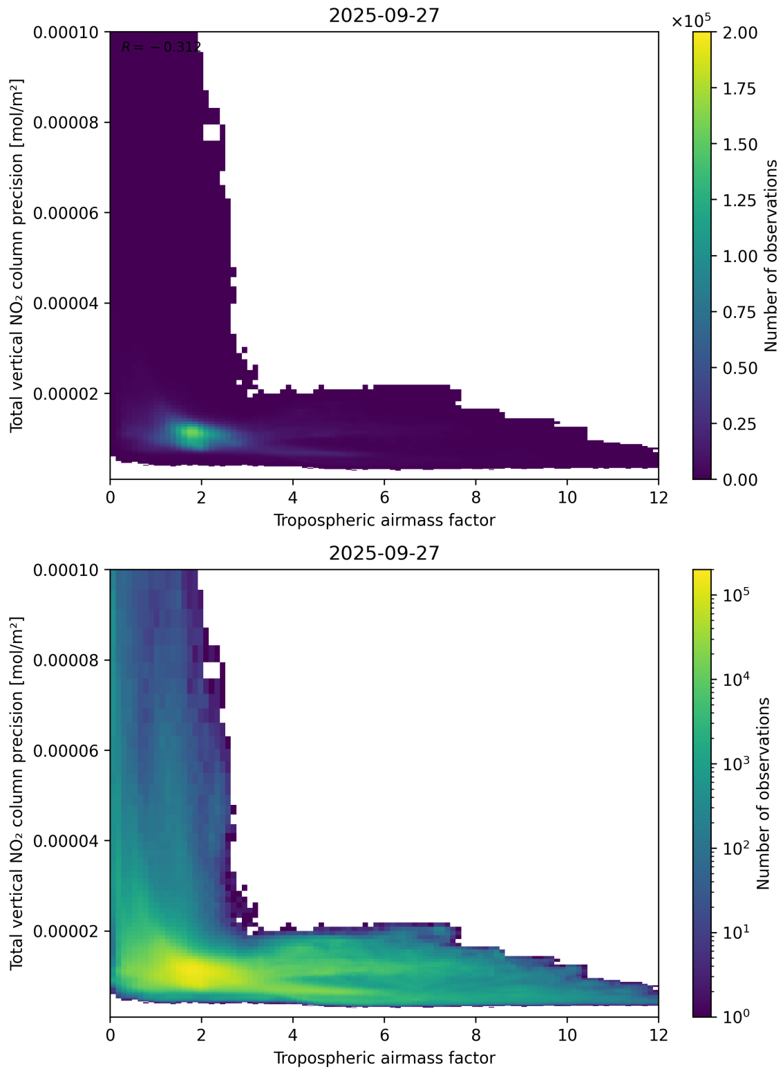
Figure 78: Scatter density plot of “Tropospheric air mass factor” against “Total vertical NO 2 column precision” for 2025-09-26 to 2025-09-28.
