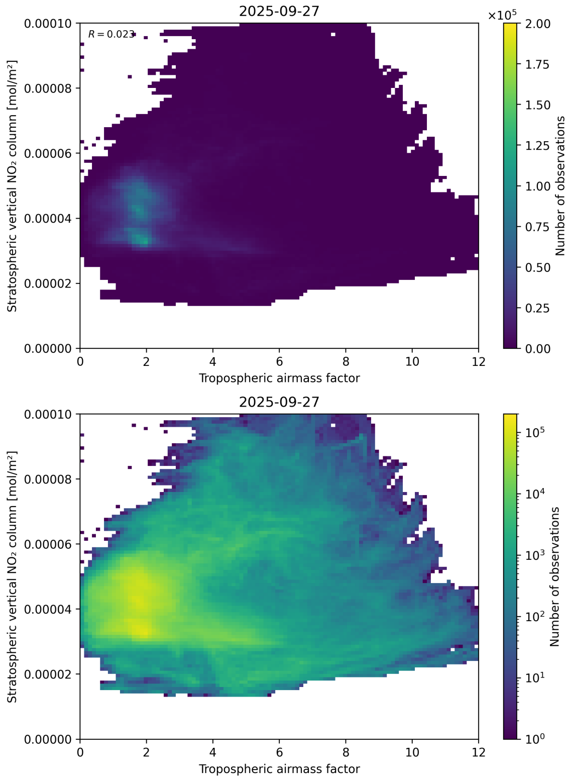
Figure 74: Scatter density plot of “Tropospheric airmass factor” against “Stratospheric vertical NO 2 column” for 2025-09-26 to 2025-09-28.
