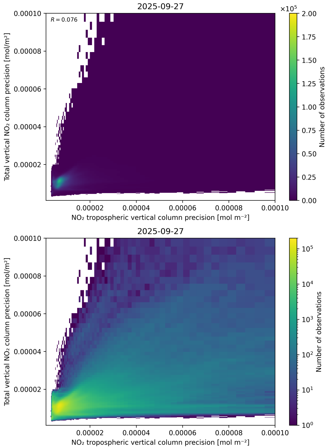
Figure 139: Scatter density plot of “NO 2 tropospheric vertical column precision” against “Total vertical NO 2 column precision” for 2025-09-26 to 2025-09-28.
