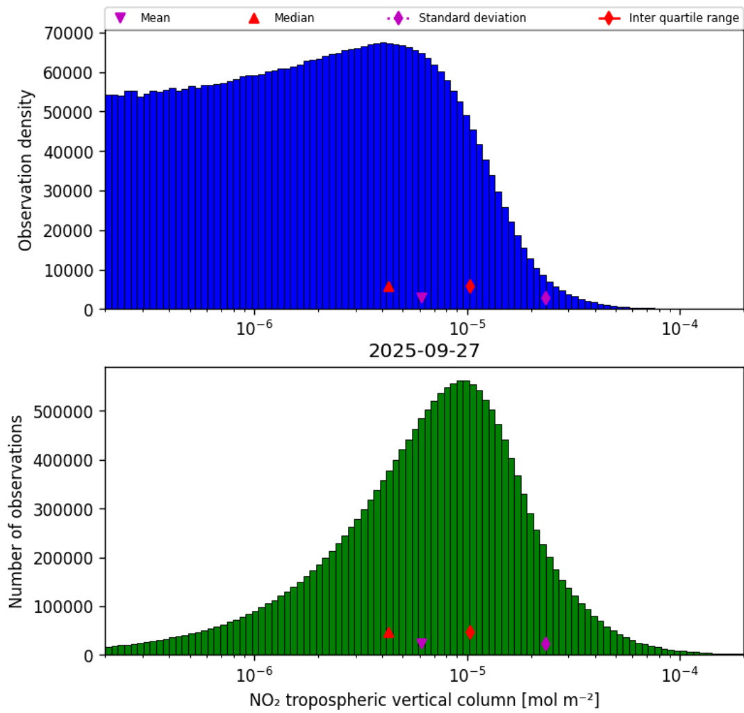
Figure 29: Histogram of “NO 2 tropospheric vertical column” for 2025-09-26 to 2025-09-28
