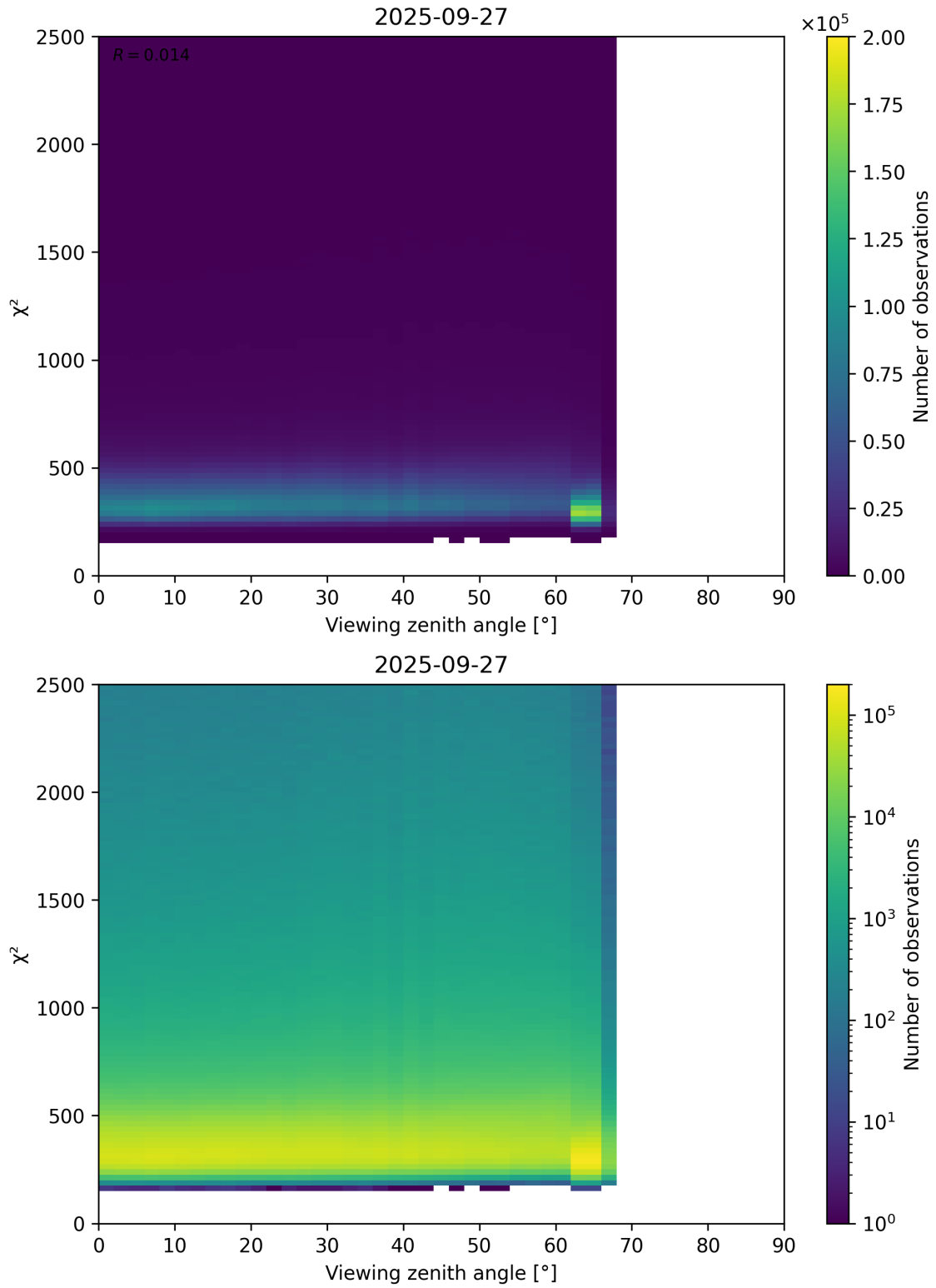
Figure 162: Scatter density plot of “Viewing zenith angle” against “ \chi^2 ” for 2025-09-26 to 2025-09-28.
