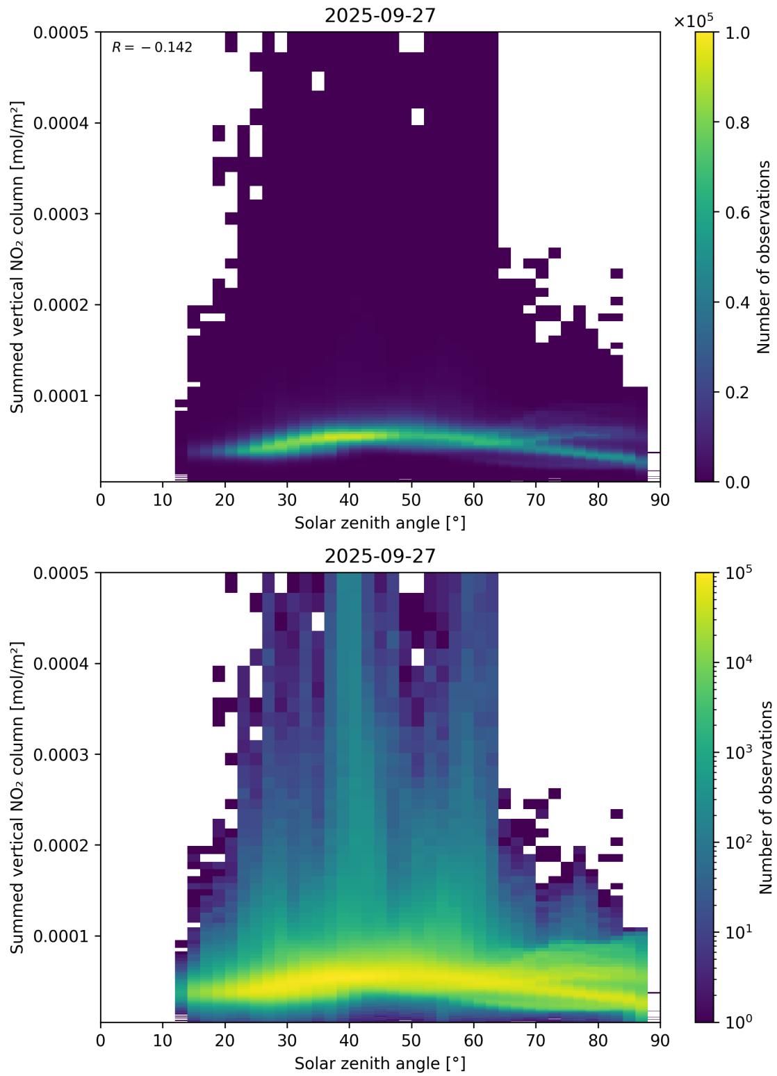
Figure 151: Scatter density plot of “Solar zenith angle” against “Summed vertical NO 2 column” for 2025-09-26 to 2025-09-28.
