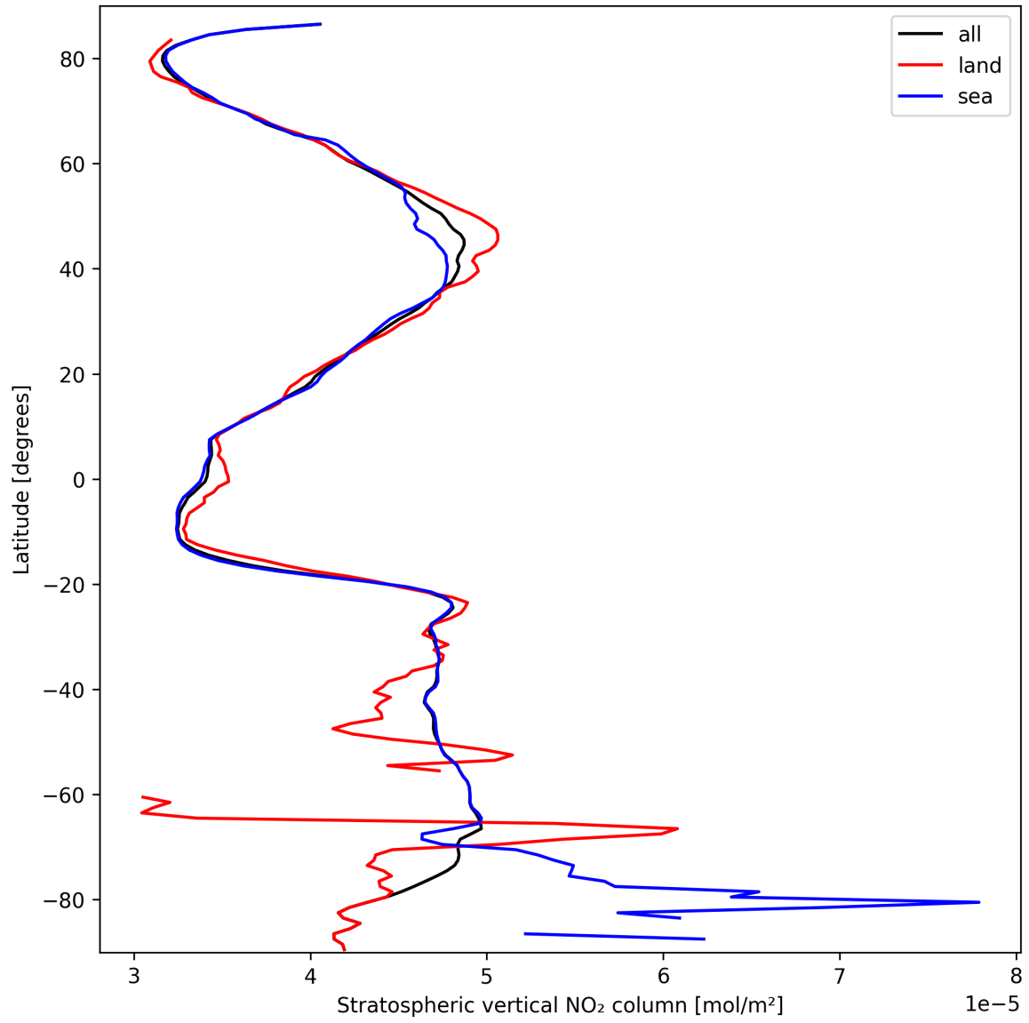
Figure 19: Zonal average of “Stratospheric vertical NO 2 column” for 2025-09-26 to 2025-09-28.
