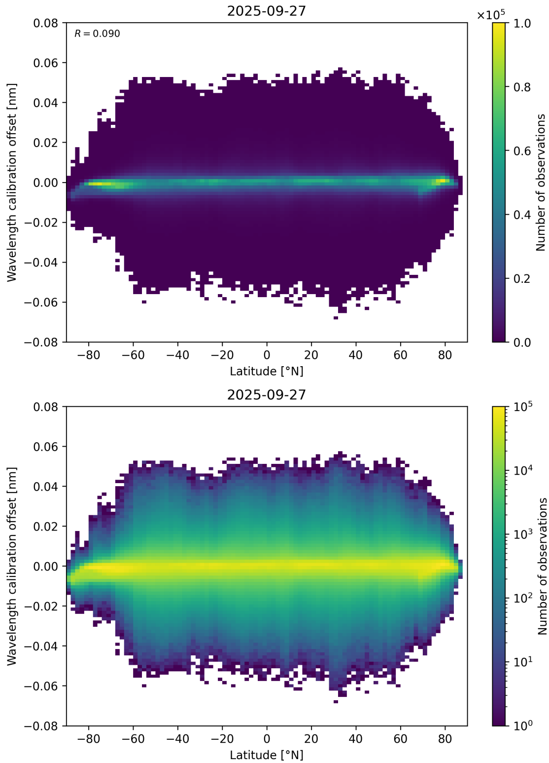
Figure 95: Scatter density plot of “Latitude” against “Wavelength calibration offset” for 2025-09-26 to 2025-09-28.
