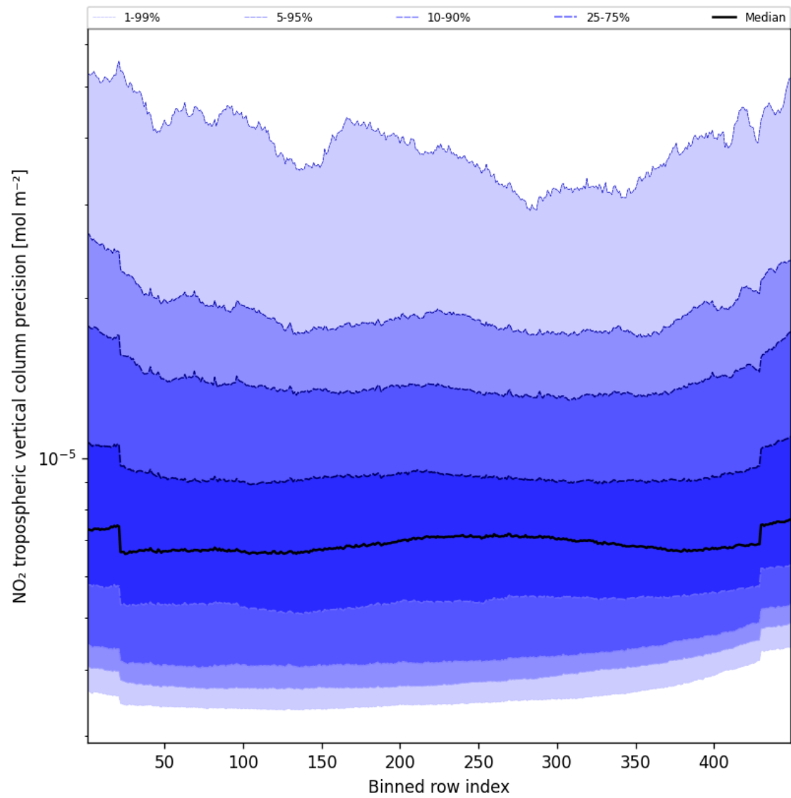
Figure 47: Along track statistics of “NO 2 tropospheric vertical column precision” for 2025-09-26 to 2025-09-28
