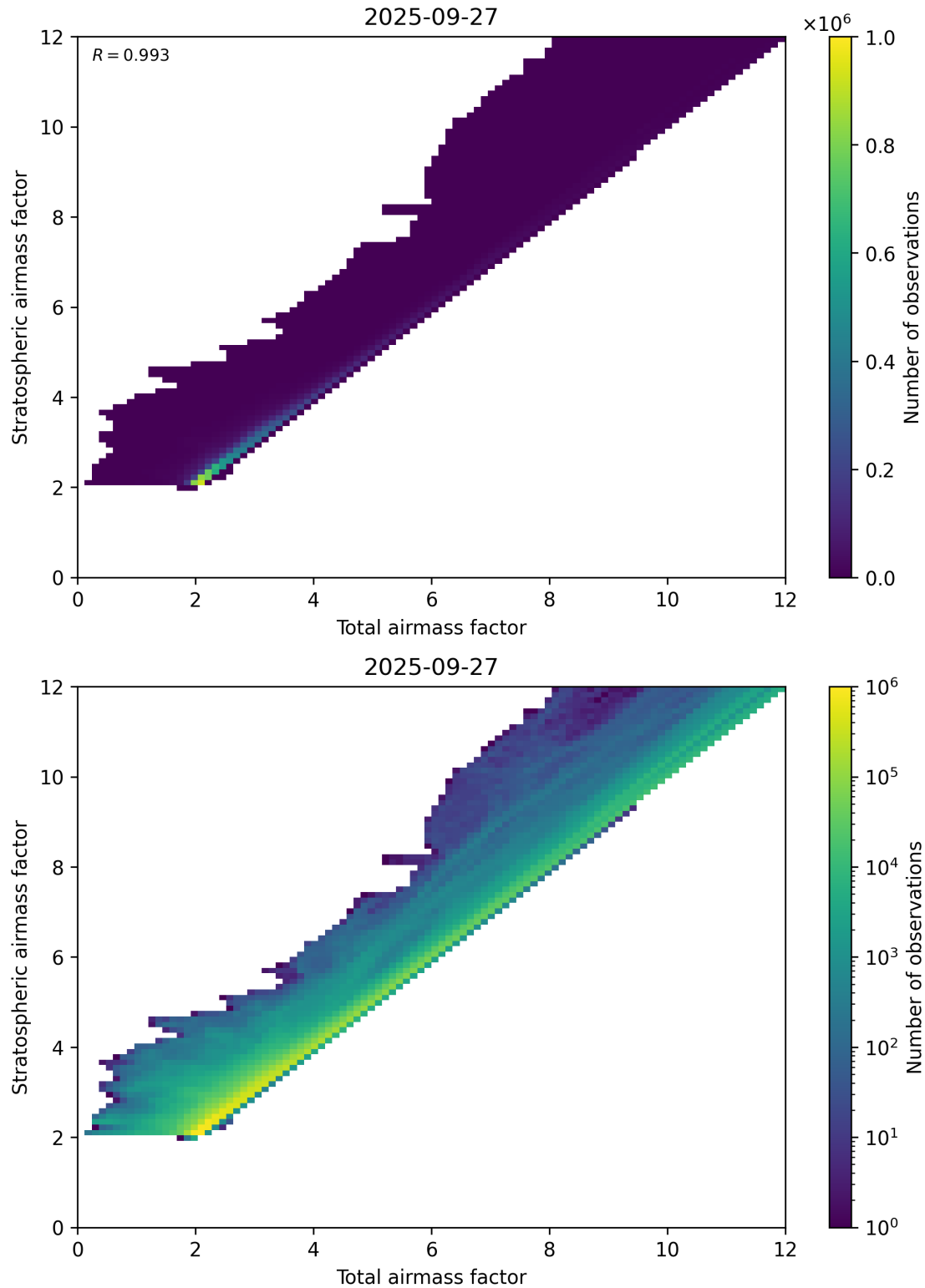
Figure 62: Scatter density plot of “Total airmass factor” against “Stratospheric airmass factor” for 2025-09-26 to 2025-09-28.
