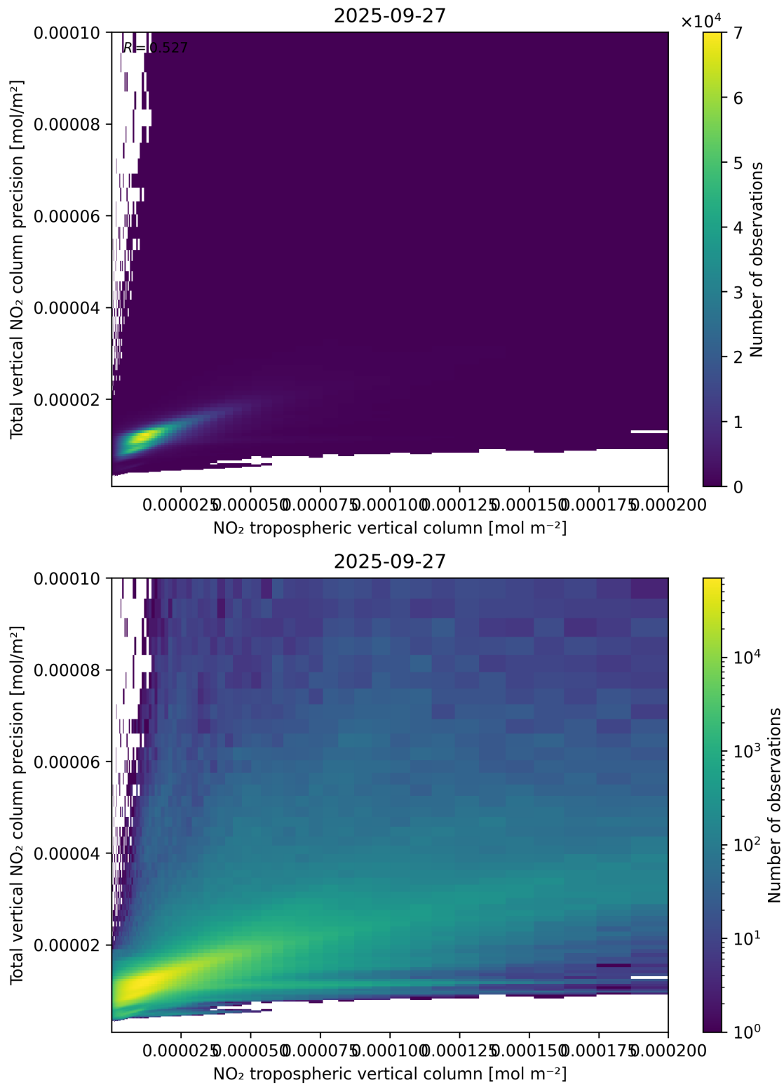
Figure 129: Scatter density plot of “NO 2 tropospheric vertical column” against “Total vertical NO 2 column precision” for 2025-09-26 to 2025-09-28.
