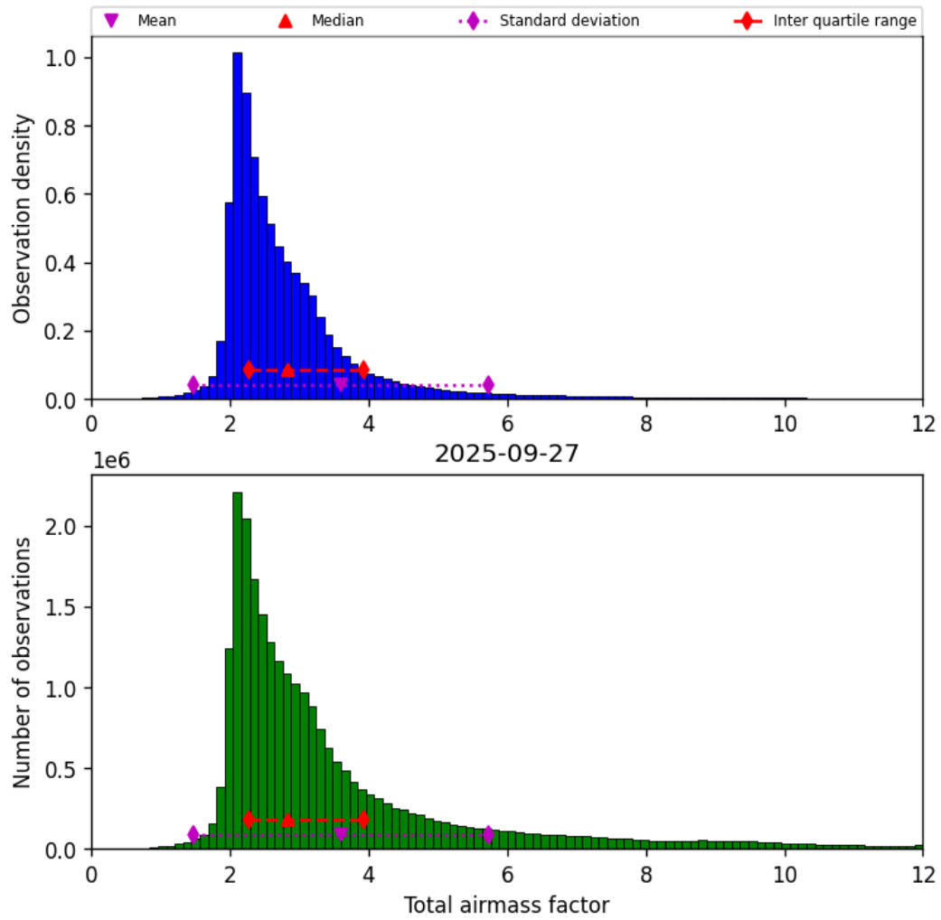
Figure 32: Histogram of “Total airmass factor” for 2025-09-26 to 2025-09-28
