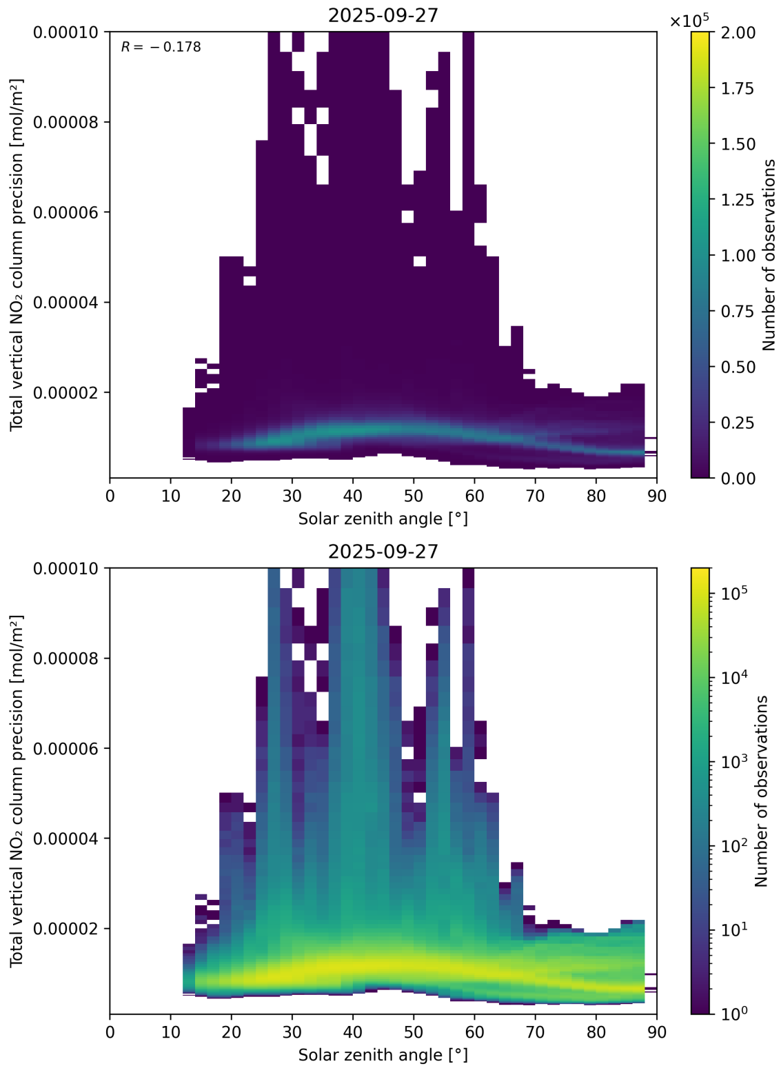
Figure 154: Scatter density plot of “Solar zenith angle” against “Total vertical NO 2 column precision” for 2025-09-26 to 2025-09-28.
