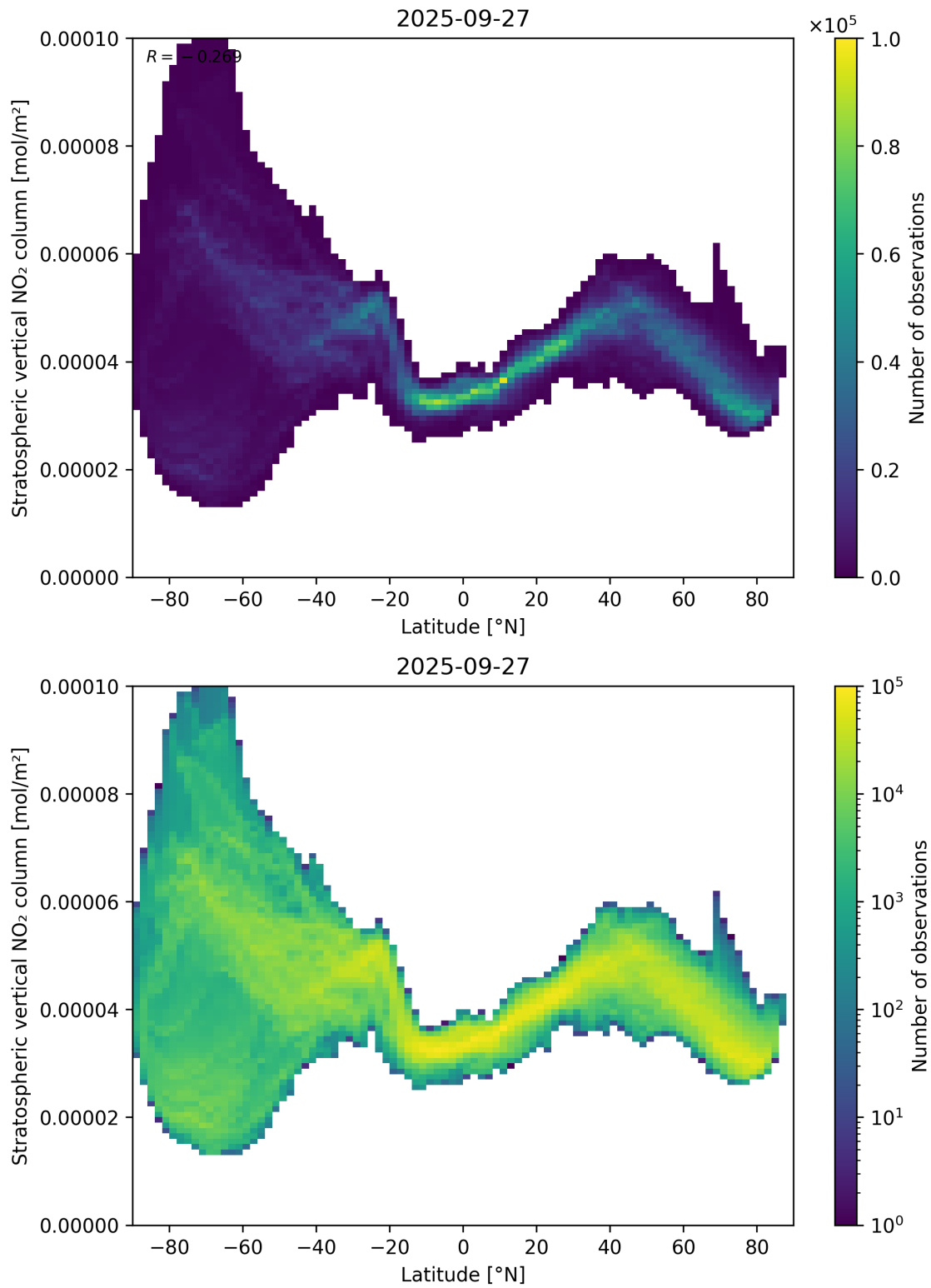
Figure 87: Scatter density plot of “Latitude” against “Stratospheric vertical NO 2 column” for 2025-09-26 to 2025-09-28.
