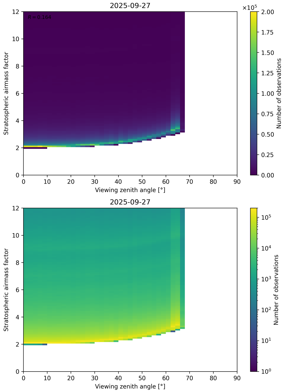
Figure 159: Scatter density plot of “Viewing zenith angle” against “Stratospheric airmass factor” for 2025-09-26 to 2025-09-28.
