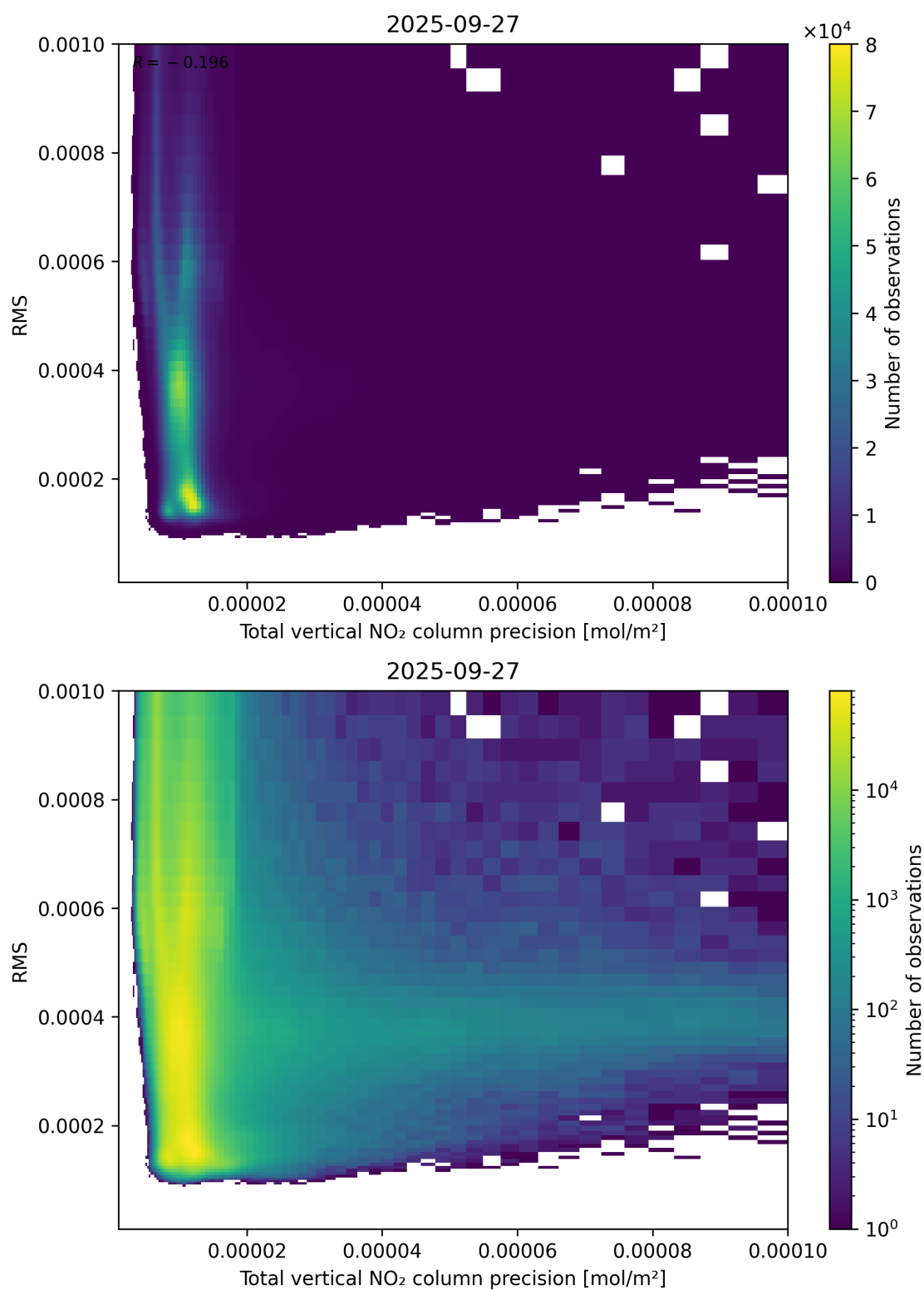
Figure 119: Scatter density plot of “Total vertical NO 2 column precision” against “RMS” for 2025-09-26 to 2025-09-28.
