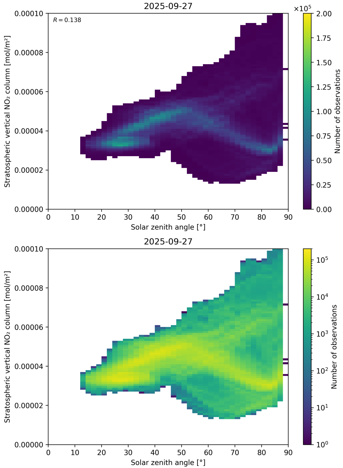
Figure 150: Scatter density plot of “Solar zenith angle” against “Stratospheric vertical NO 2 column” for 2025-09-26 to 2025-09-28.
