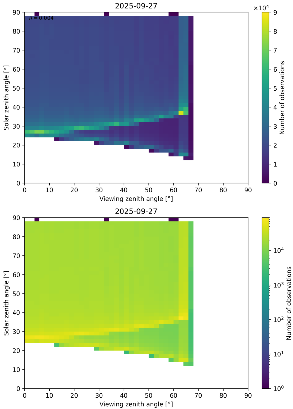
Figure 172: Scatter density plot of “Viewing zenith angle” against “Solar zenith angle” for 2025-09-26 to 2025-09-28.
