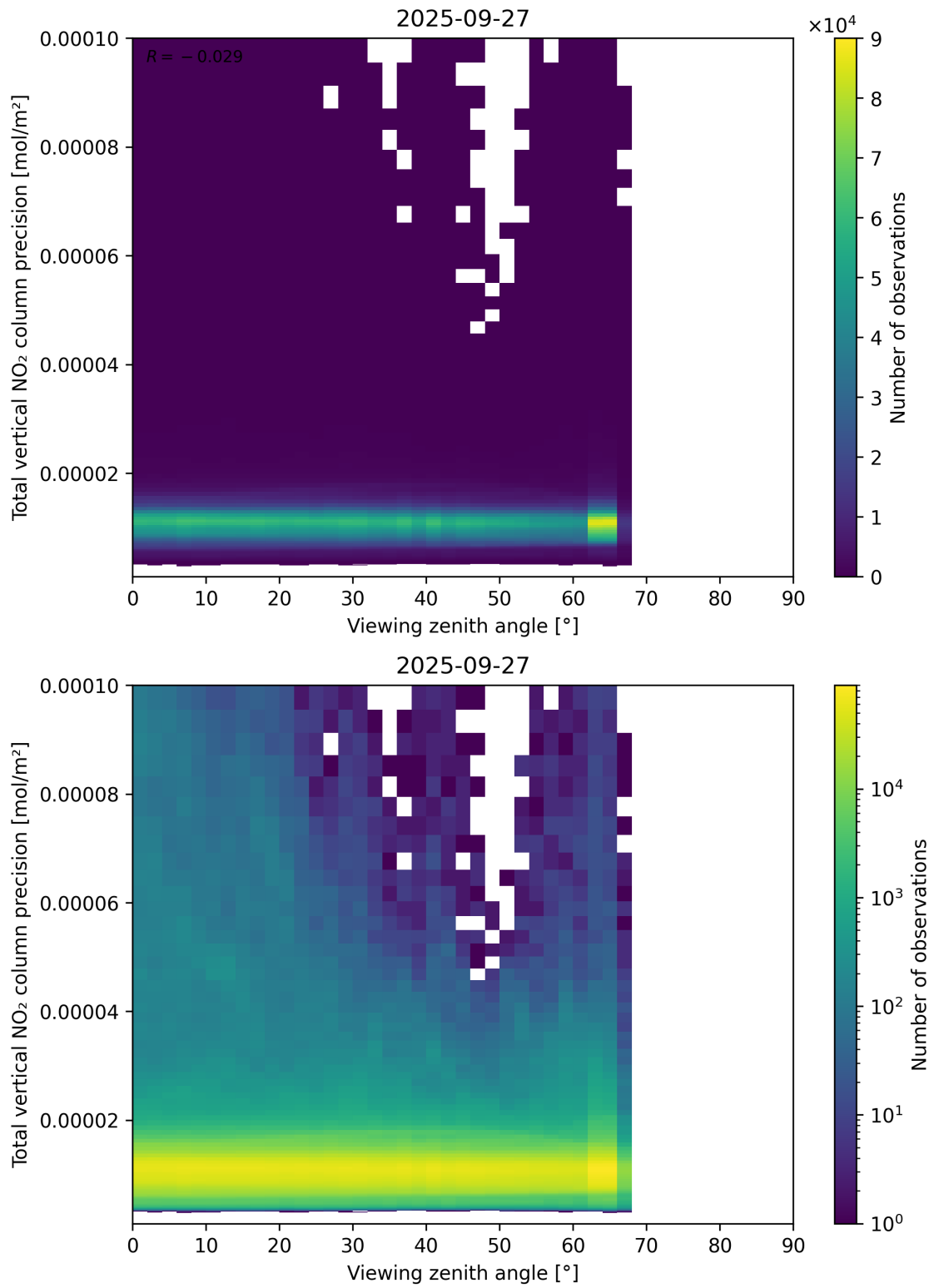
Figure 168: Scatter density plot of “Viewing zenith angle” against “Total vertical NO 2 column precision” for 2025-09-26 to 2025-09-28.
