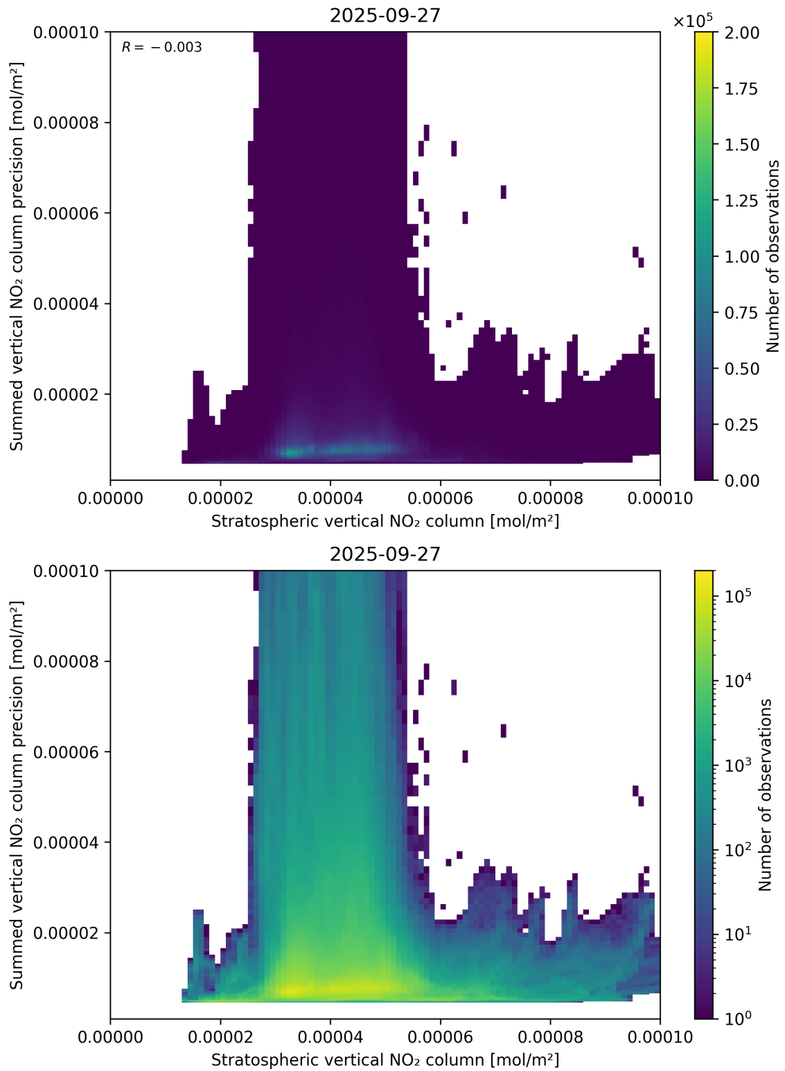
Figure 99: Scatter density plot of “Stratospheric vertical NO 2 column” against “Summed vertical NO 2 column precision” for 2025-09-26 to 2025-09-28.
