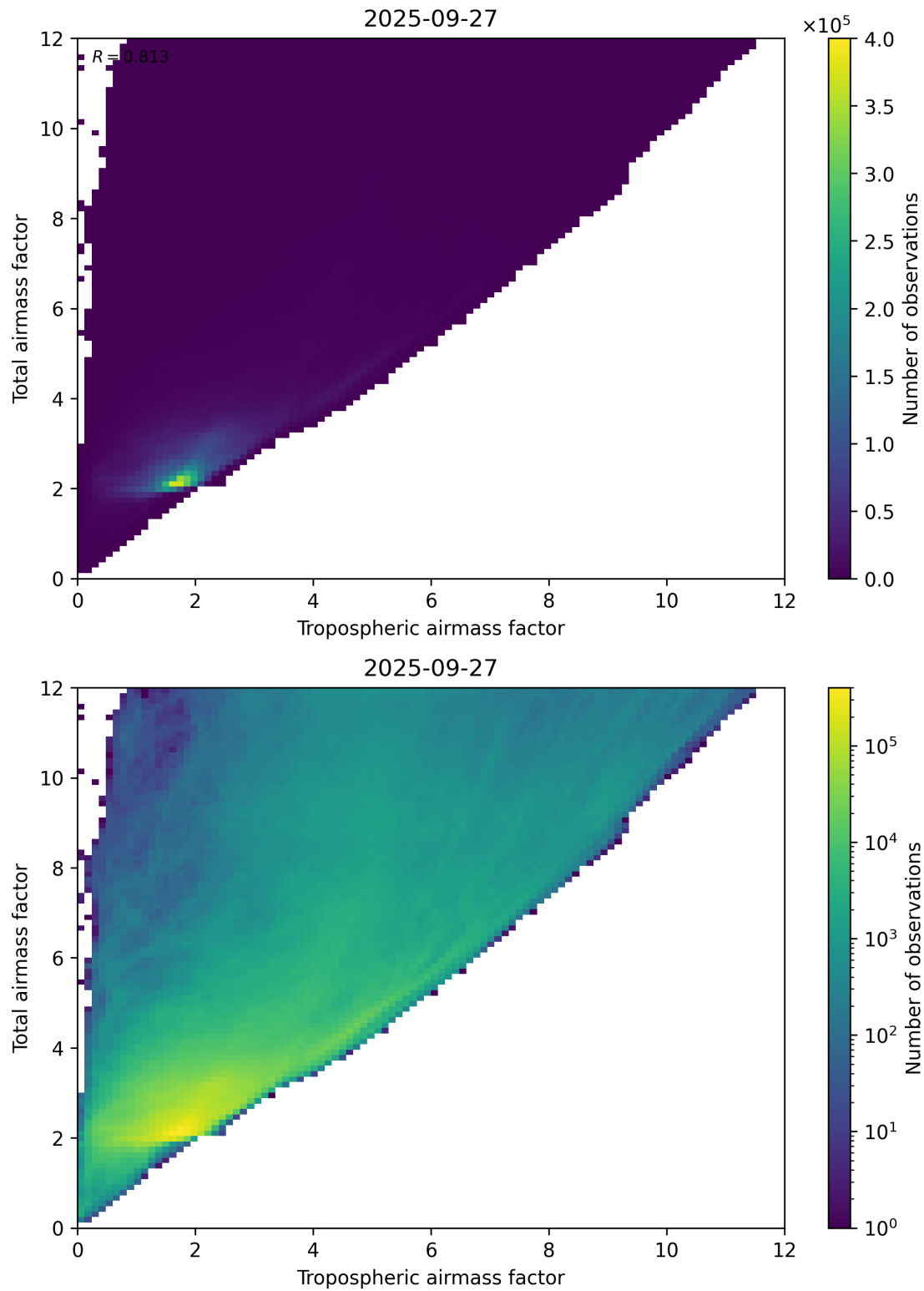
Figure 72: Scatter density plot of “Tropospheric airmass factor” against “Total airmass factor” for 2025-09-26 to 2025-09-28.
