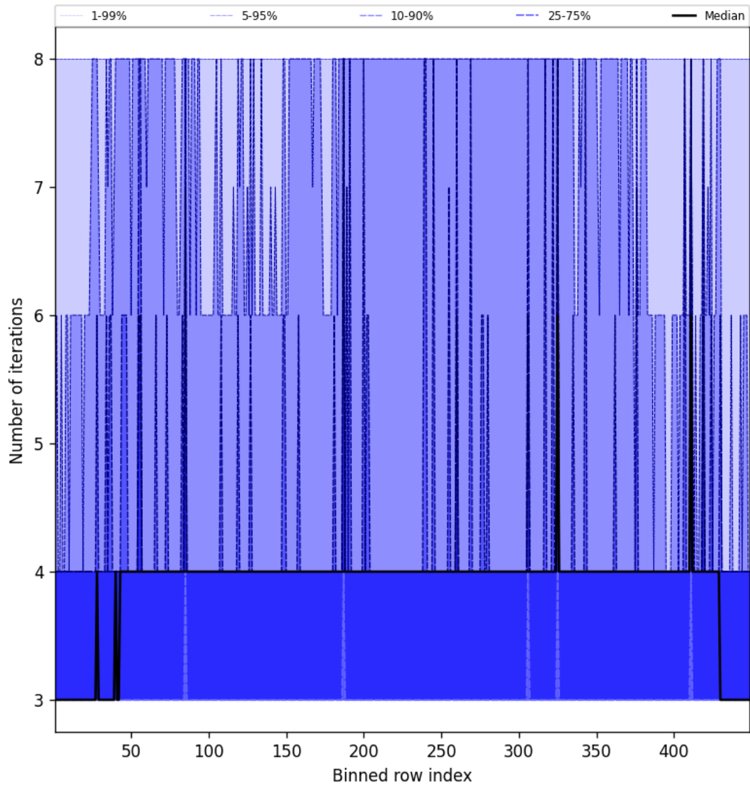
Figure 51: Along track statistics of “Number of iterations” for 2025-09-26 to 2025-09-28
