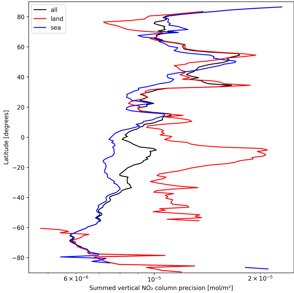
Figure 24: Zonal average of “Summed vertical NO 2 column precision” for 2025-09-26 to 2025-09-28.
