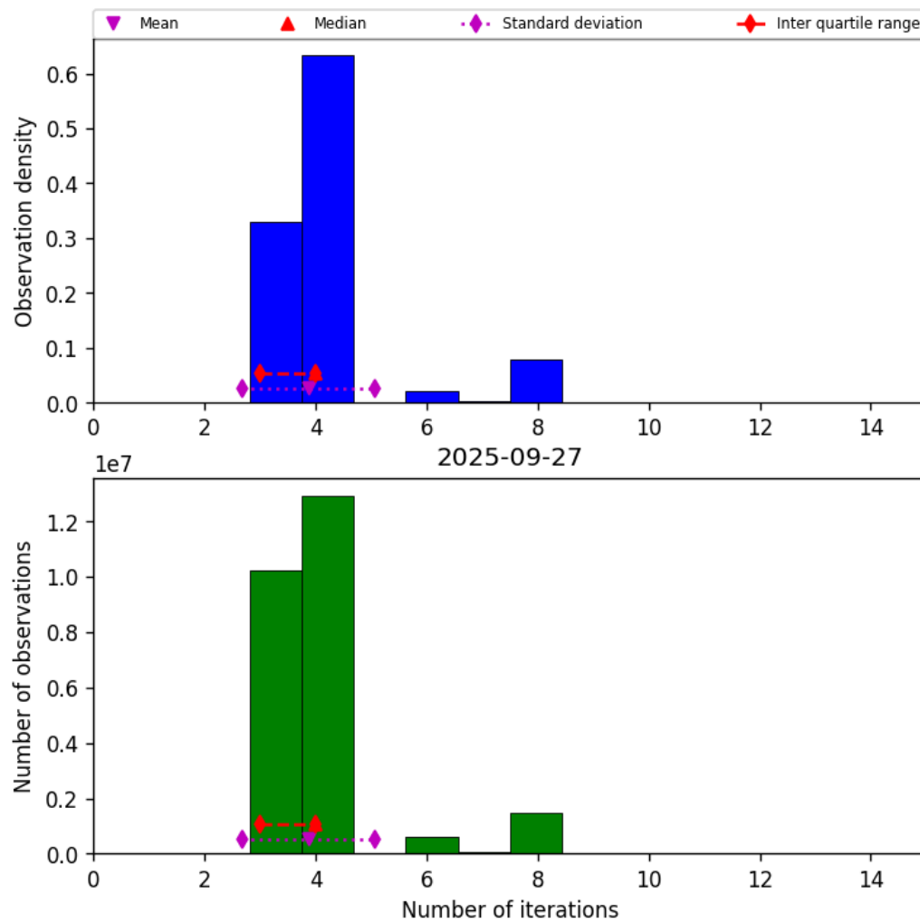
Figure 34: Histogram of “Number of iterations” for 2025-09-26 to 2025-09-28
