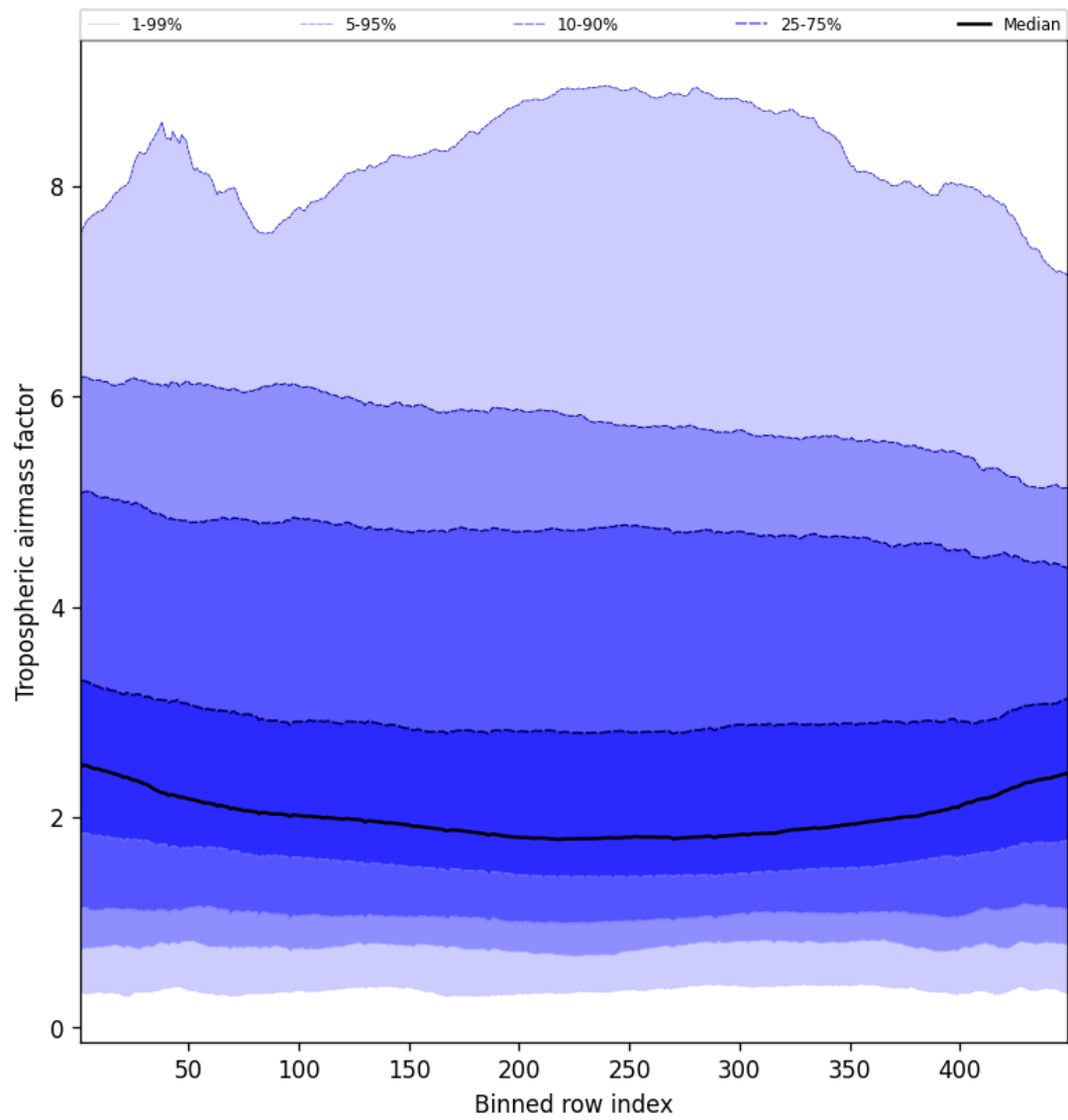
Figure 48: Along track statistics of “Tropospheric airmass factor” for 2025-09-26 to 2025-09-28
