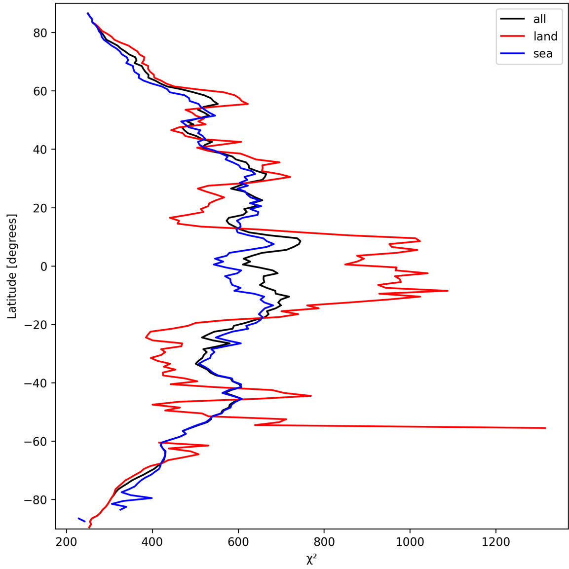
Figure 25: Zonal average of “ \chi^2 ” for 2025-09-26 to 2025-09-28.
