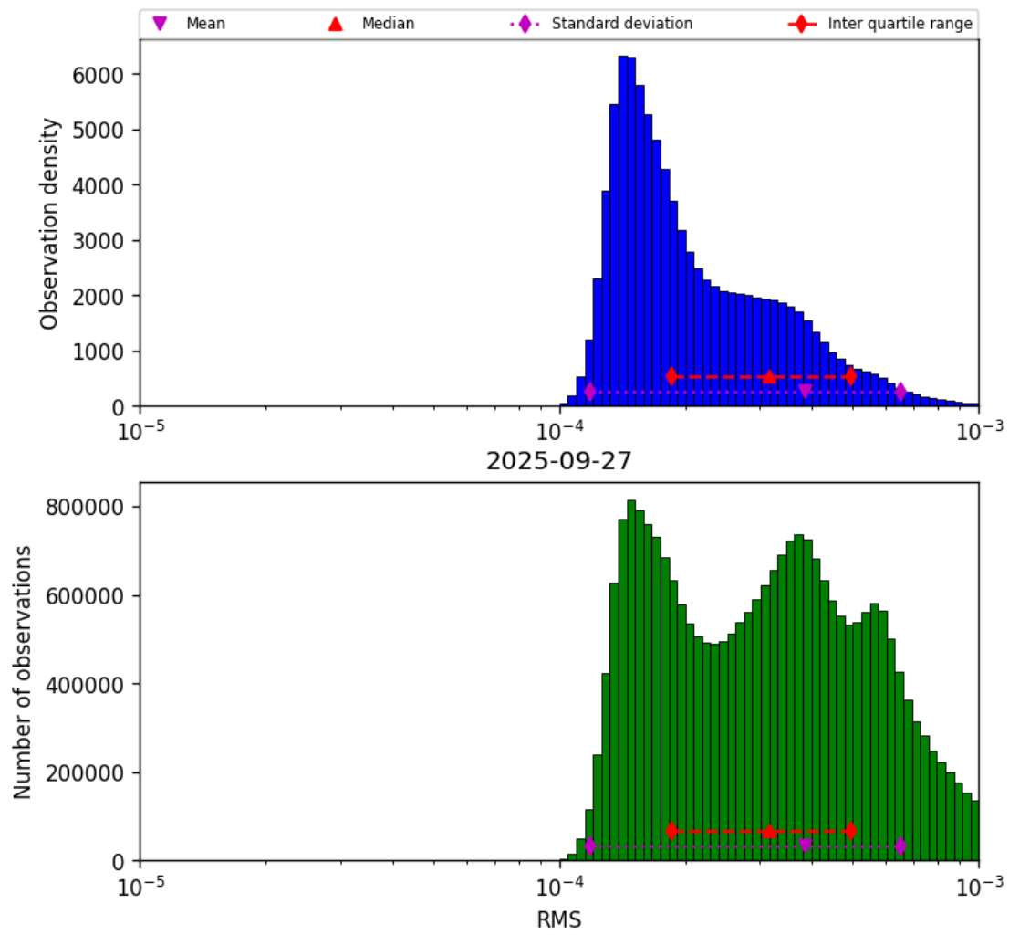
Figure 43: Histogram of “RMS” for 2025-09-26 to 2025-09-28
