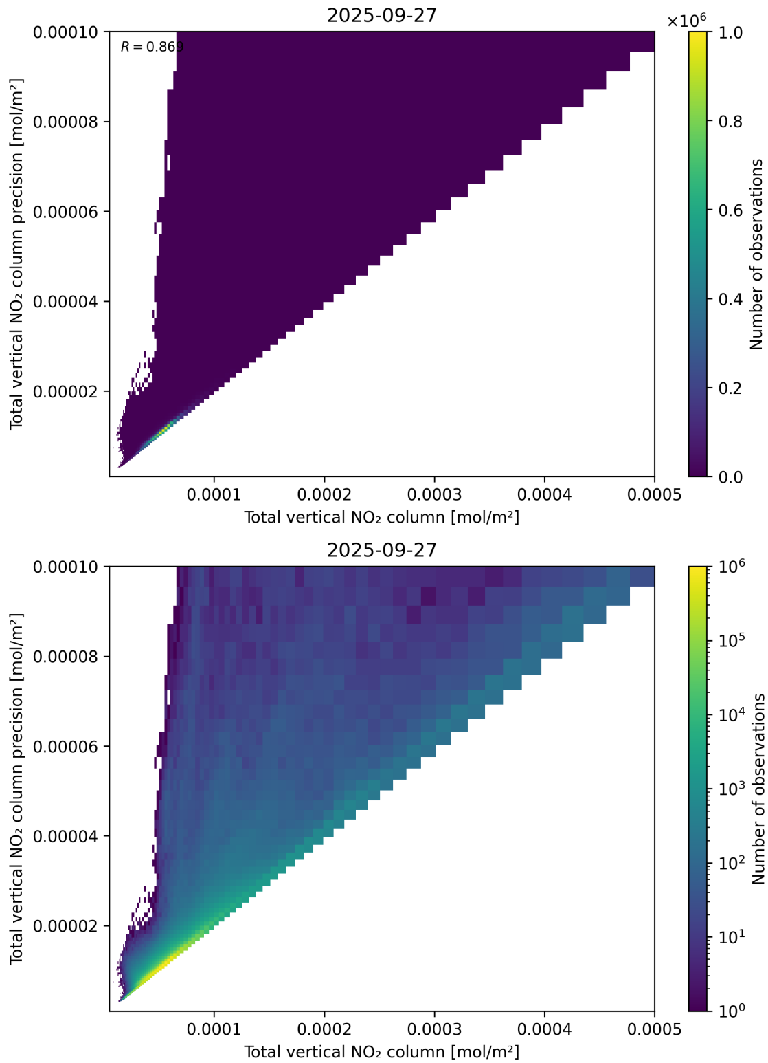
Figure 114: Scatter density plot of “Total vertical NO 2 column” against “Total vertical NO 2 column precision” for 2025-09-26 to 2025-09-28.
