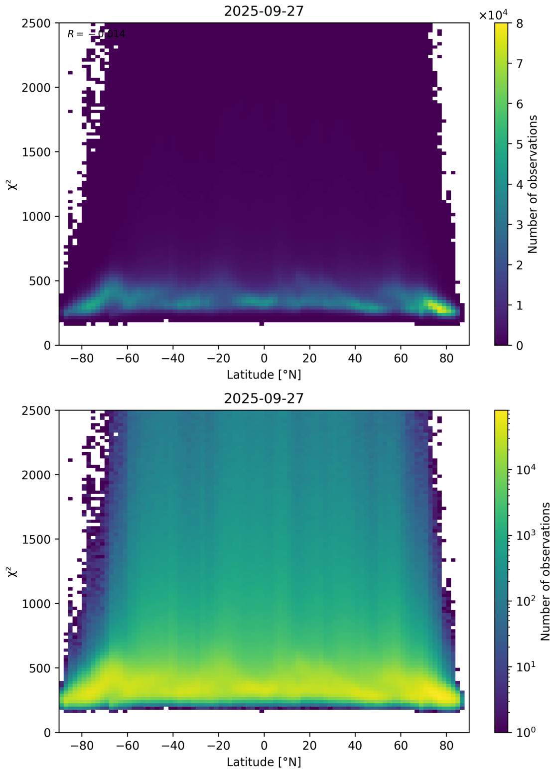
Figure 86: Scatter density plot of “Latitude” against “ \chi^2 ” for 2025-09-26 to 2025-09-28.
