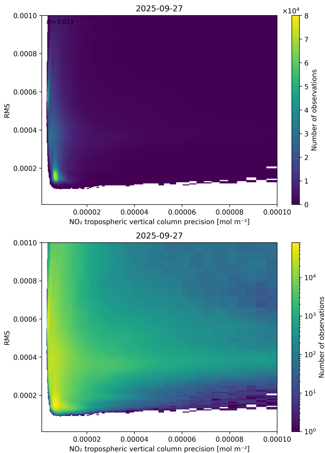
Figure 140: Scatter density plot of “NO 2 tropospheric vertical column precision” against “RMS” for 2025-09-26 to 2025-09-28.
