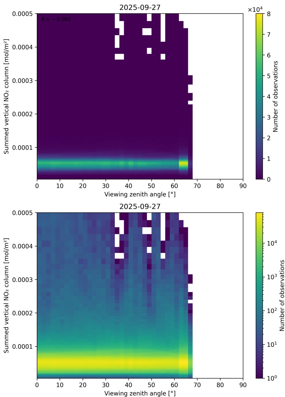
Figure 165: Scatter density plot of “Viewing zenith angle” against “Summed vertical NO 2 column” for 2025-09-26 to 2025-09-28.
