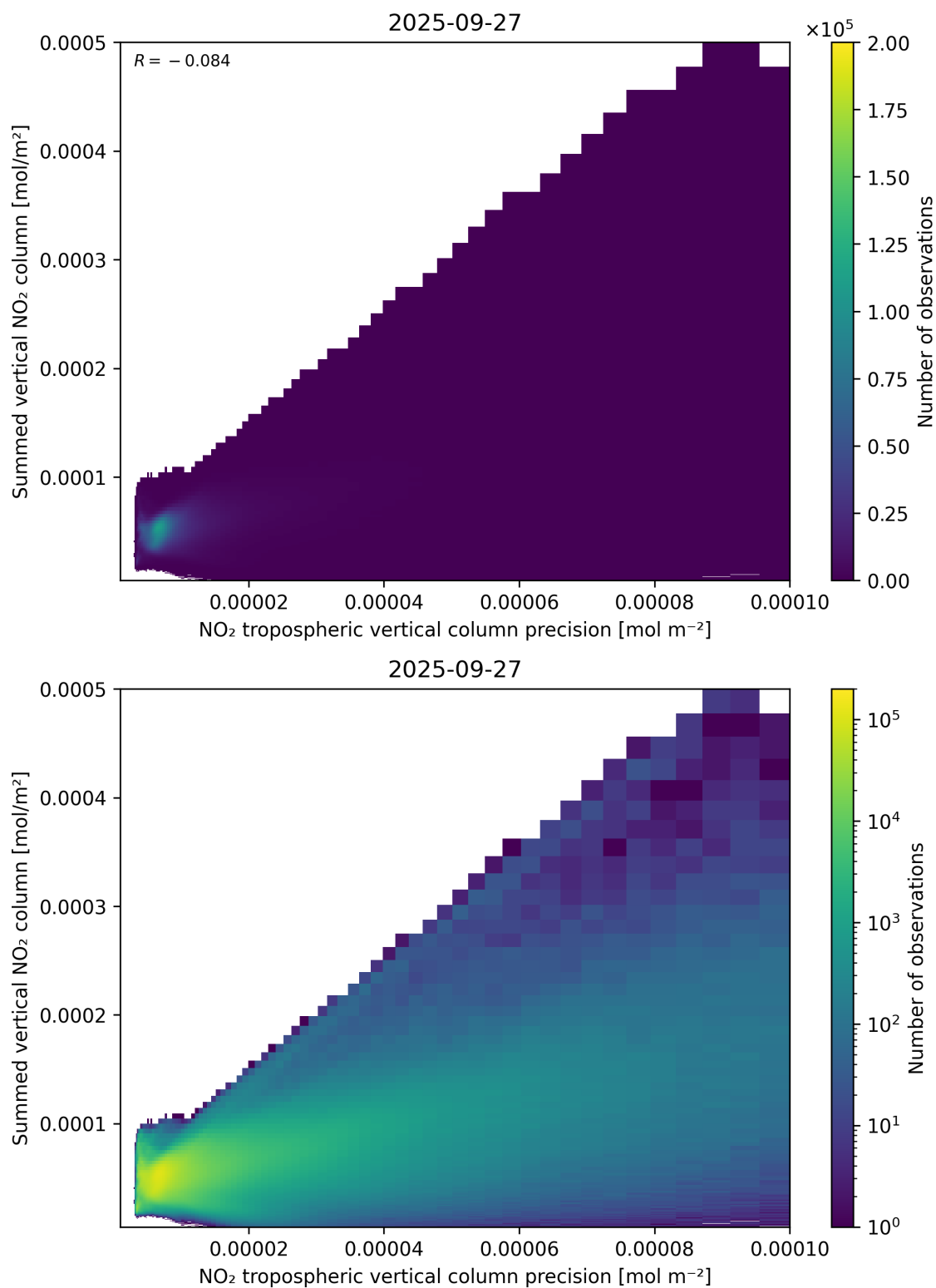
Figure 136: Scatter density plot of “NO 2 tropospheric vertical column precision” against “Summed vertical NO 2 column” for 2025-09-26 to 2025-09-28.
