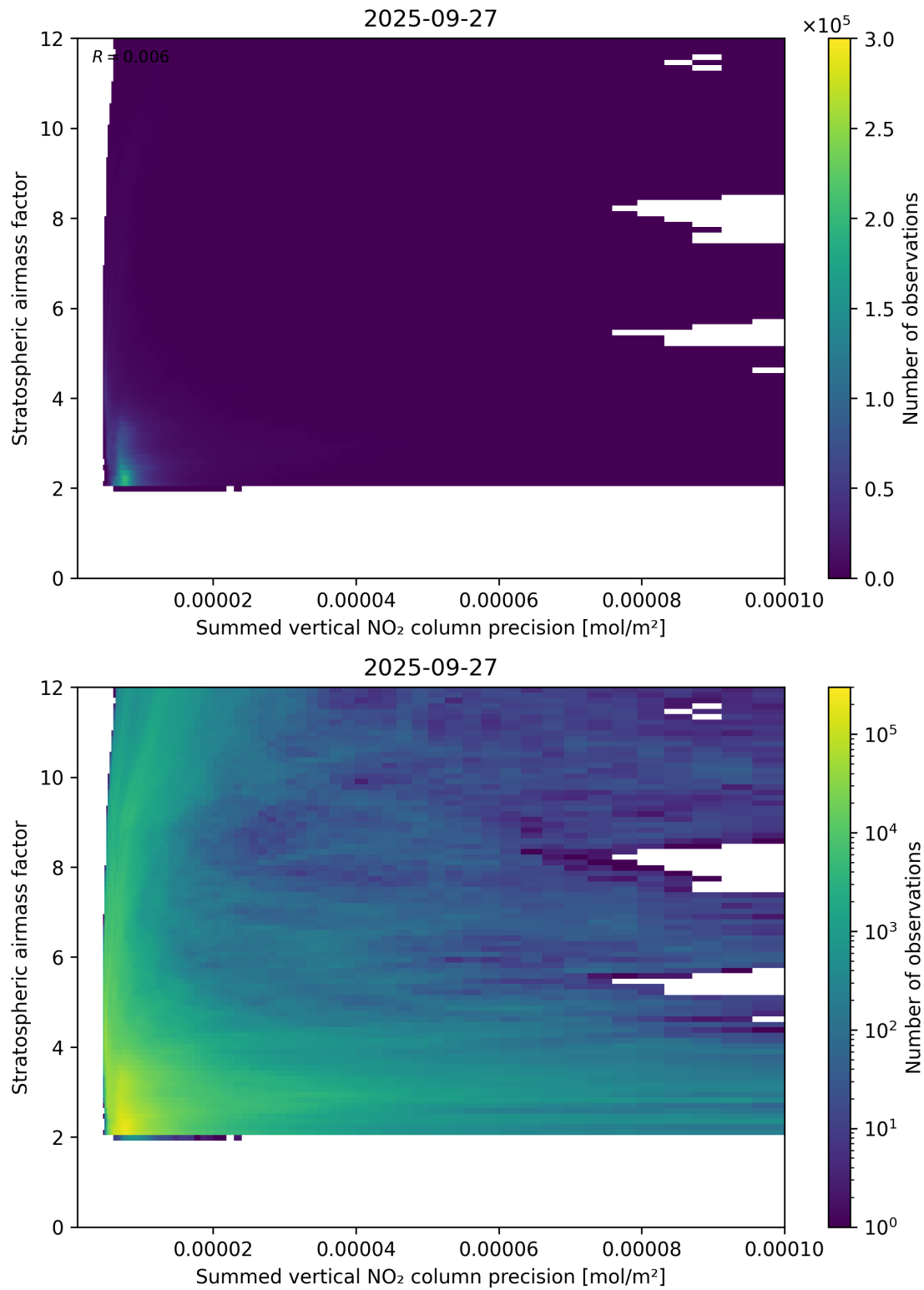
Figure 106: Scatter density plot of “Summed vertical NO 2 column precision” against “Stratospheric airmass factor” for 2025-09-26 to 2025-09-28.
