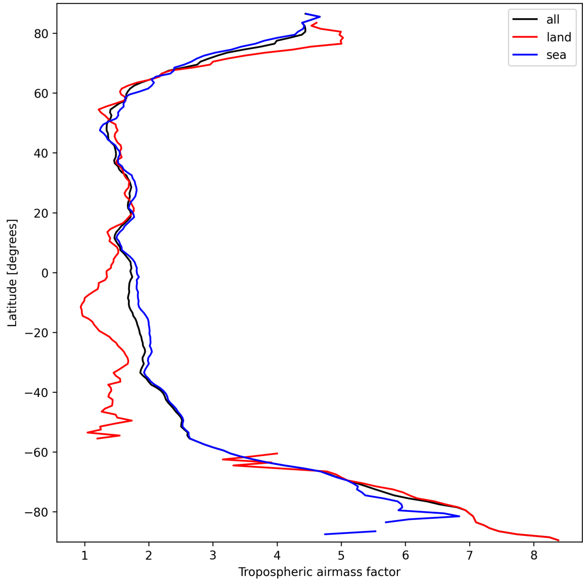
Figure 14: Zonal average of “Tropospheric airmass factor” for 2025-09-26 to 2025-09-28.
