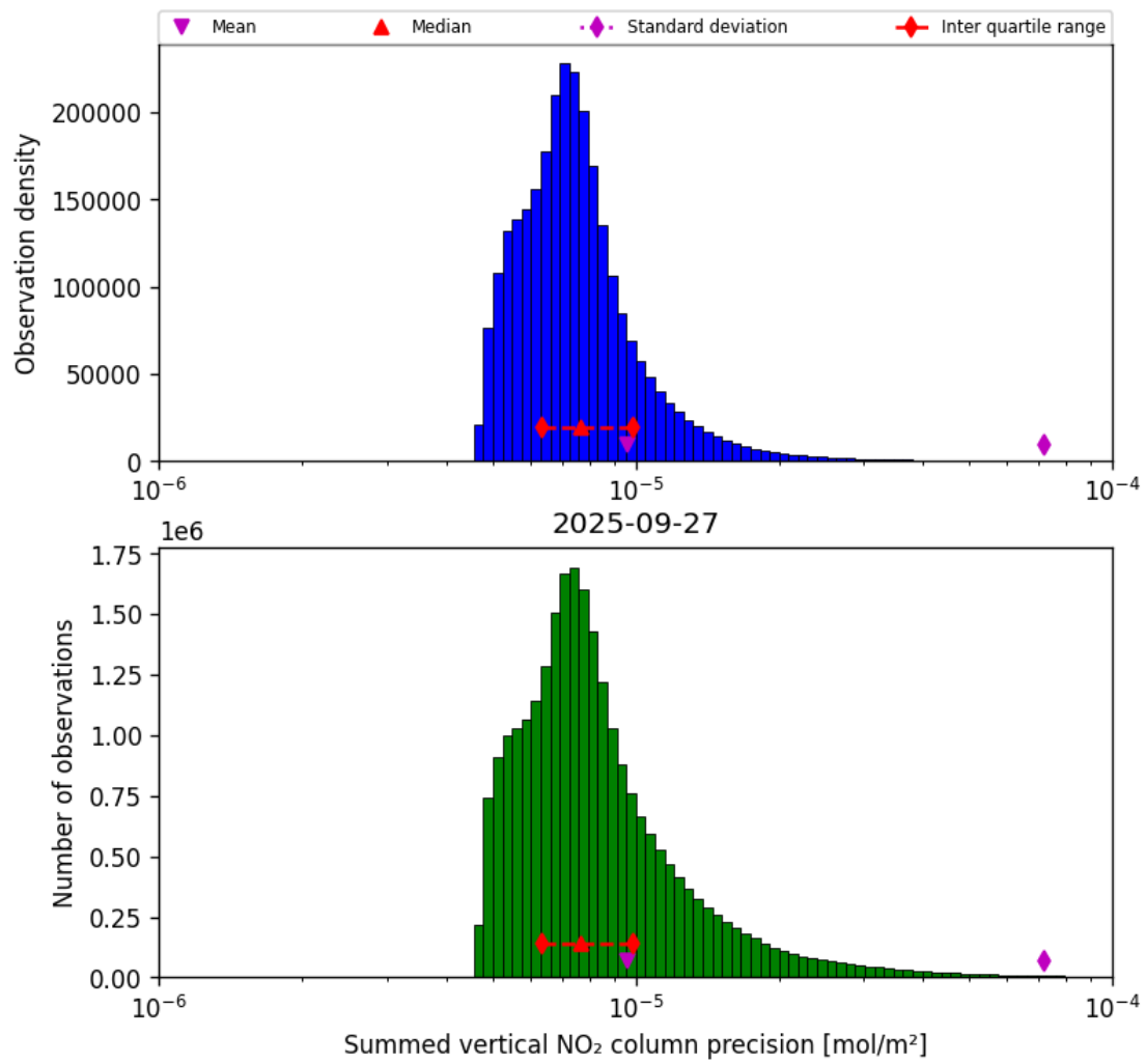
Figure 41: Histogram of “Summed vertical NO 2 column precision” for 2025-09-26 to 2025-09-28
