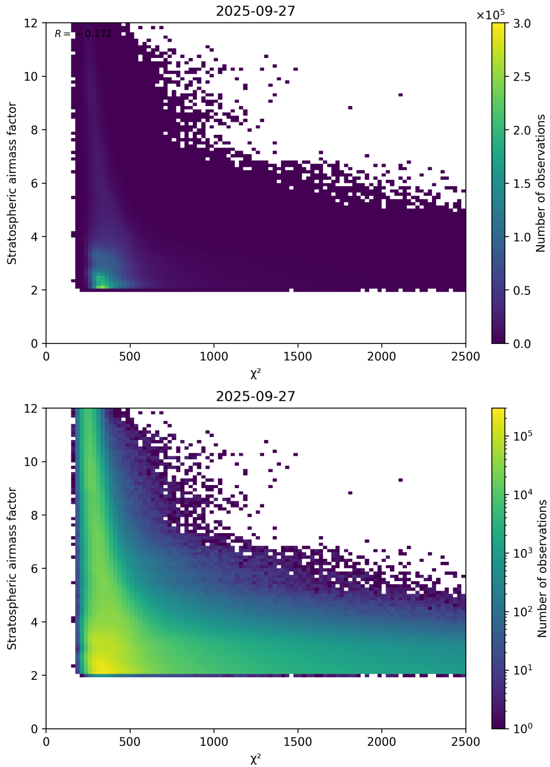
Figure 81: Scatter density plot of “ \chi^2 ” against “Stratospheric airmass factor” for 2025-09-26 to 2025-09-28.
