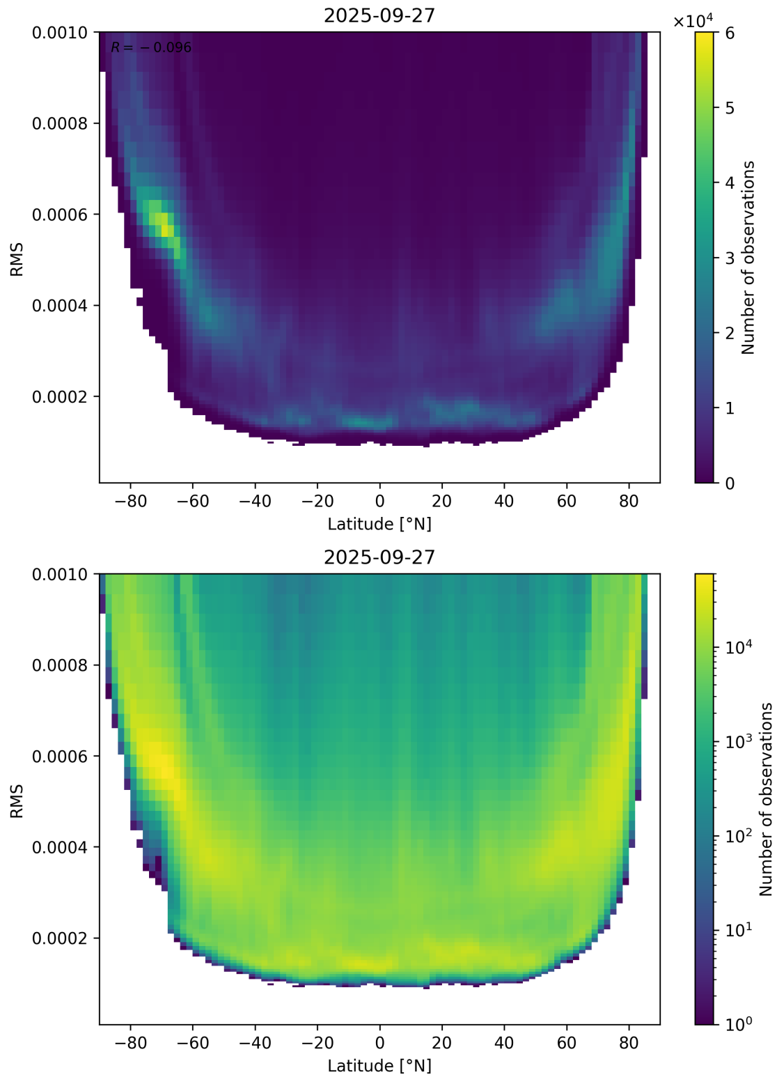
Figure 94: Scatter density plot of “Latitude” against “RMS” for 2025-09-26 to 2025-09-28.
