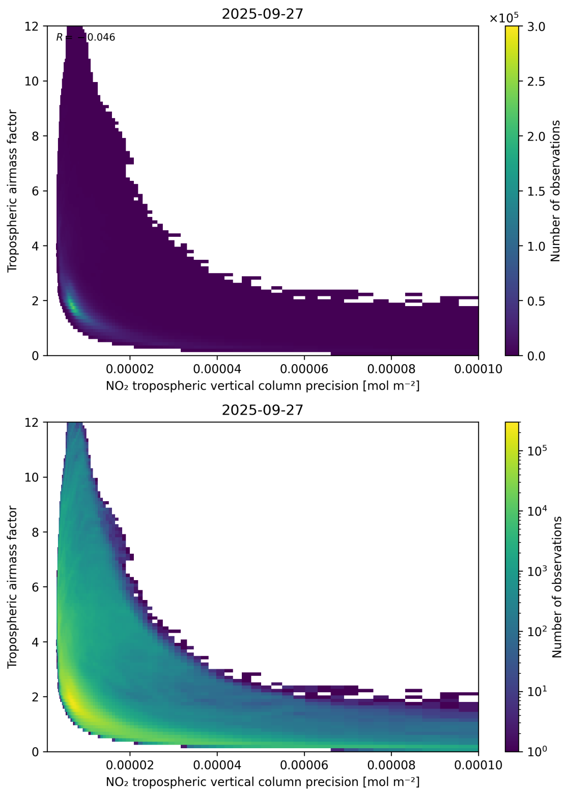
Figure 133: Scatter density plot of “NO 2 tropospheric vertical column precision” against “Tropospheric airmass factor” for 2025-09-26 to 2025-09-28.
