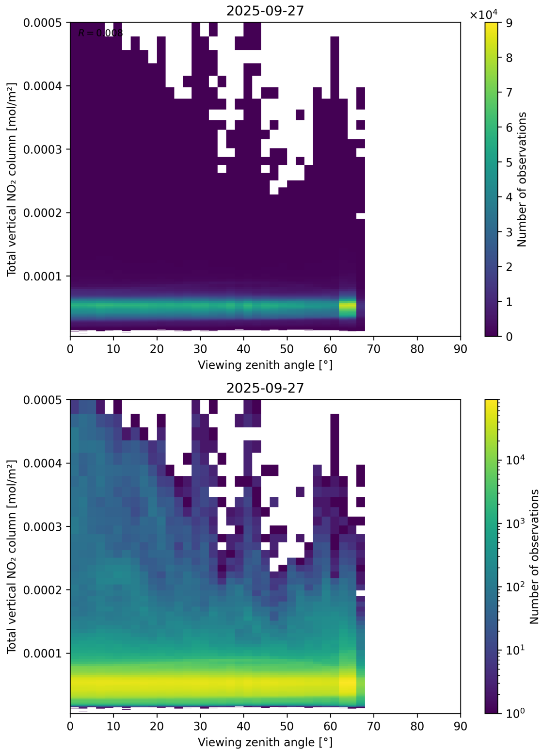
Figure 167: Scatter density plot of “Viewing zenith angle” against “Total vertical NO 2 column” for 2025-09-26 to 2025-09-28.
