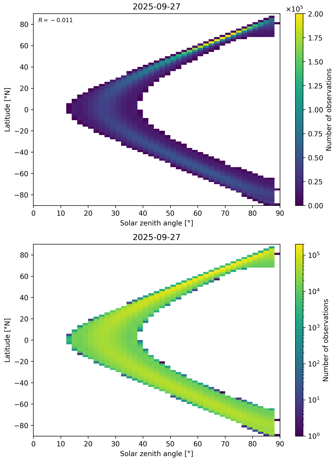
Figure 149: Scatter density plot of “Solar zenith angle” against “Latitude” for 2025-09-26 to 2025-09-28.
