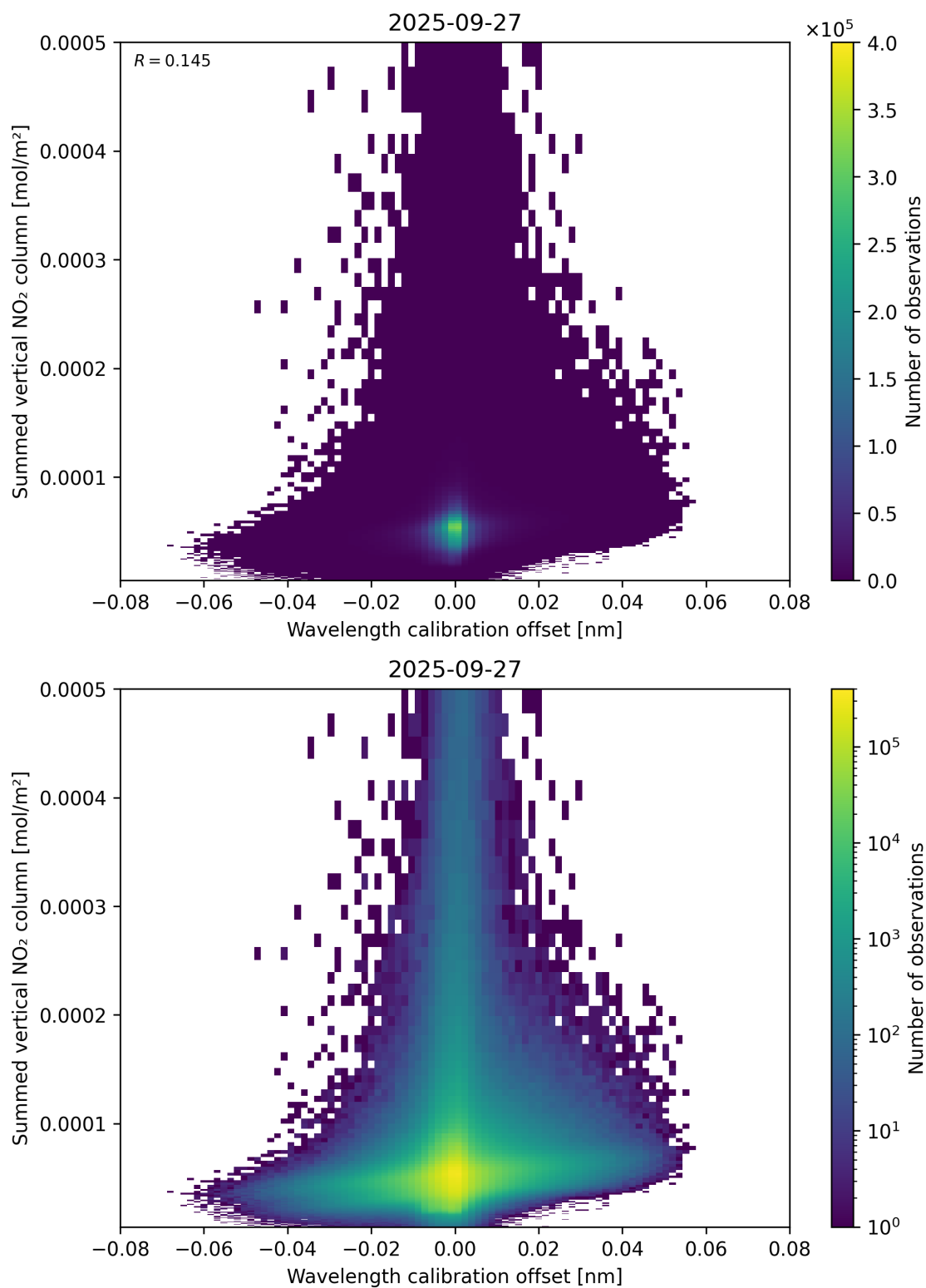
Figure 177: Scatter density plot of “Wavelength calibration offset” against “Summed vertical NO 2 column” for 2025-09-26 to 2025-09-28.
