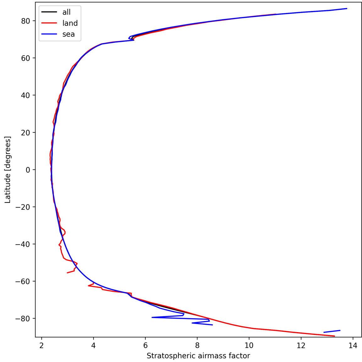
Figure 27: Zonal average of “Stratospheric air mass factor” for 2025-09-26 to 2025-09-28.
