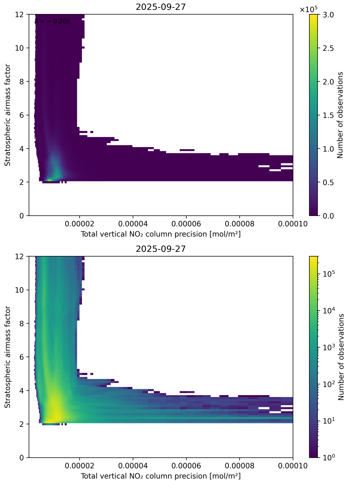
Figure 115: Scatter density plot of “Total vertical NO 2 column precision” against “Stratospheric airmass factor” for 2025-09-26 to 2025-09-28.
