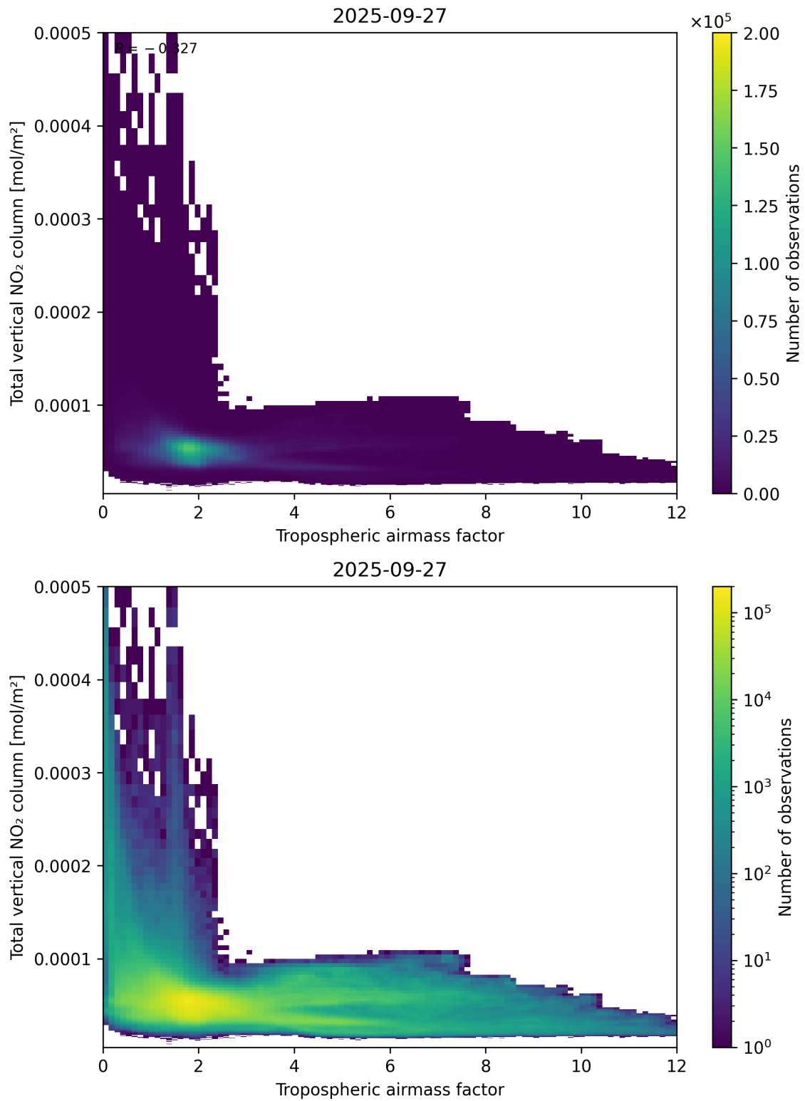
Figure 77: Scatter density plot of “Tropospheric airmass factor” against “Total vertical NO 2 column” for 2025-09-26 to 2025-09-28.
