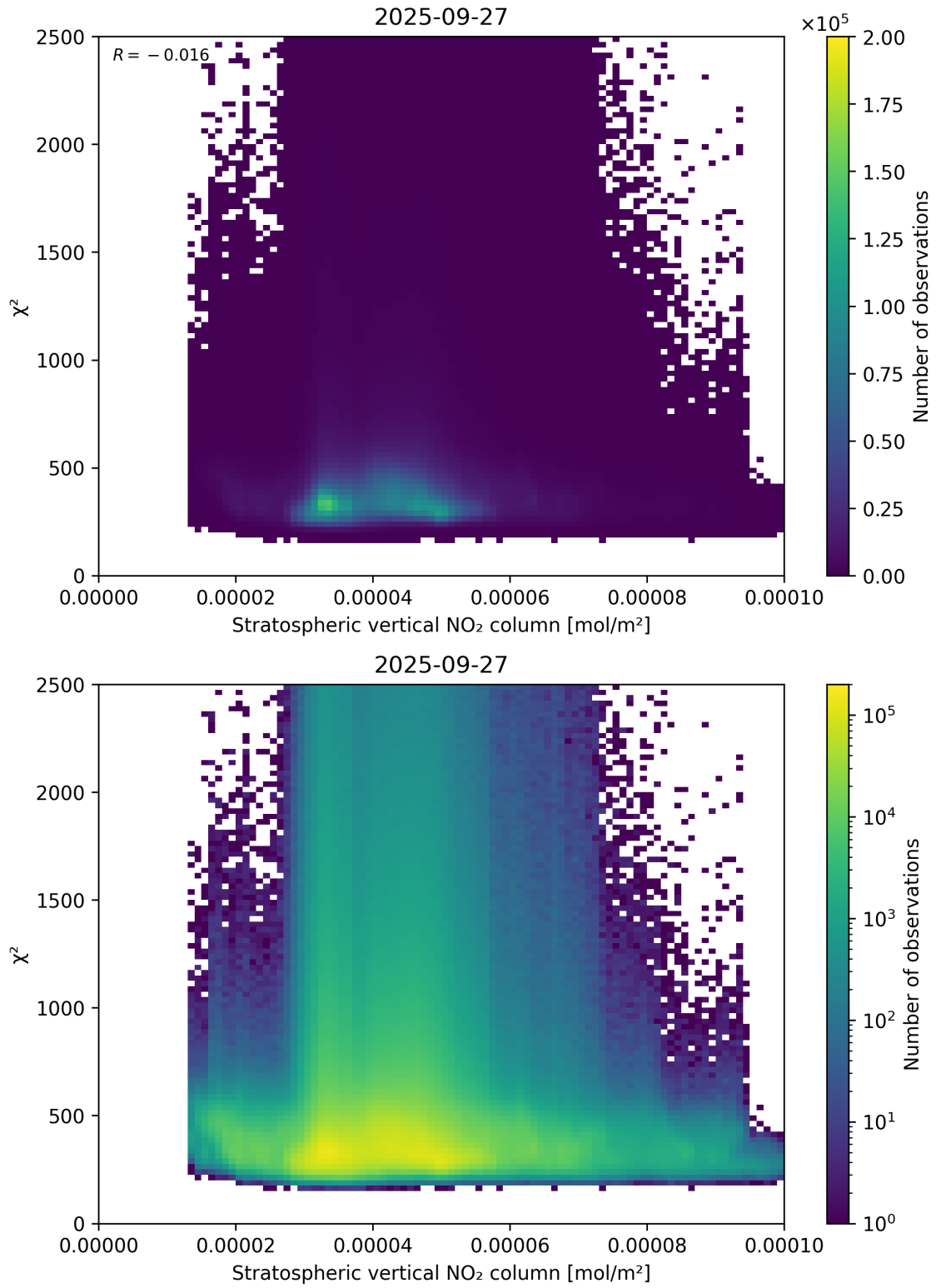
Figure 97: Scatter density plot of “Stratospheric vertical NO 2 column” against “ \chi^2 ” for 2025-09-26 to 2025-09-28.
