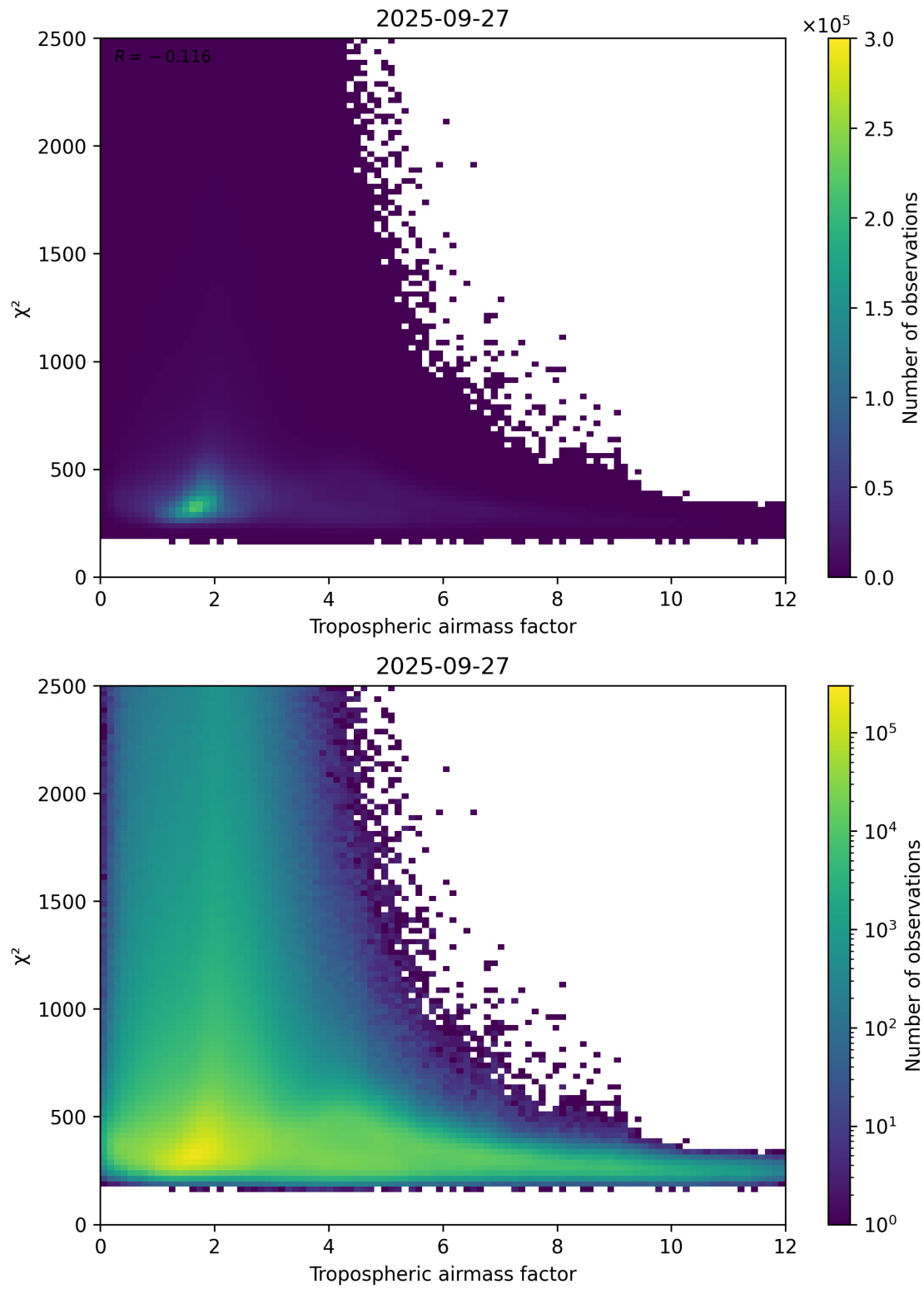
Figure 73: Scatter density plot of “Tropospheric airmass factor” against “ \chi^2 ” for 2025-09-26 to 2025-09-28.
