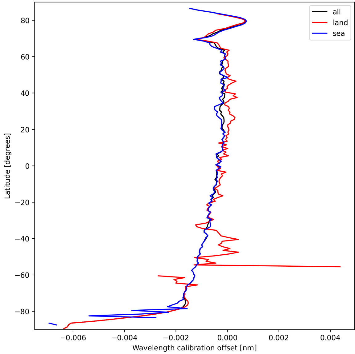
Figure 18: Zonal average of “Wavelength calibration offset” for 2025-09-26 to 2025-09-28.
