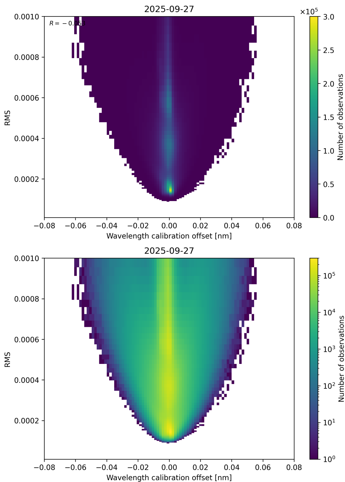
Figure 181: Scatter density plot of “Wavelength calibration offset” against “RMS” for 2025-09-26 to 2025-09-28.
