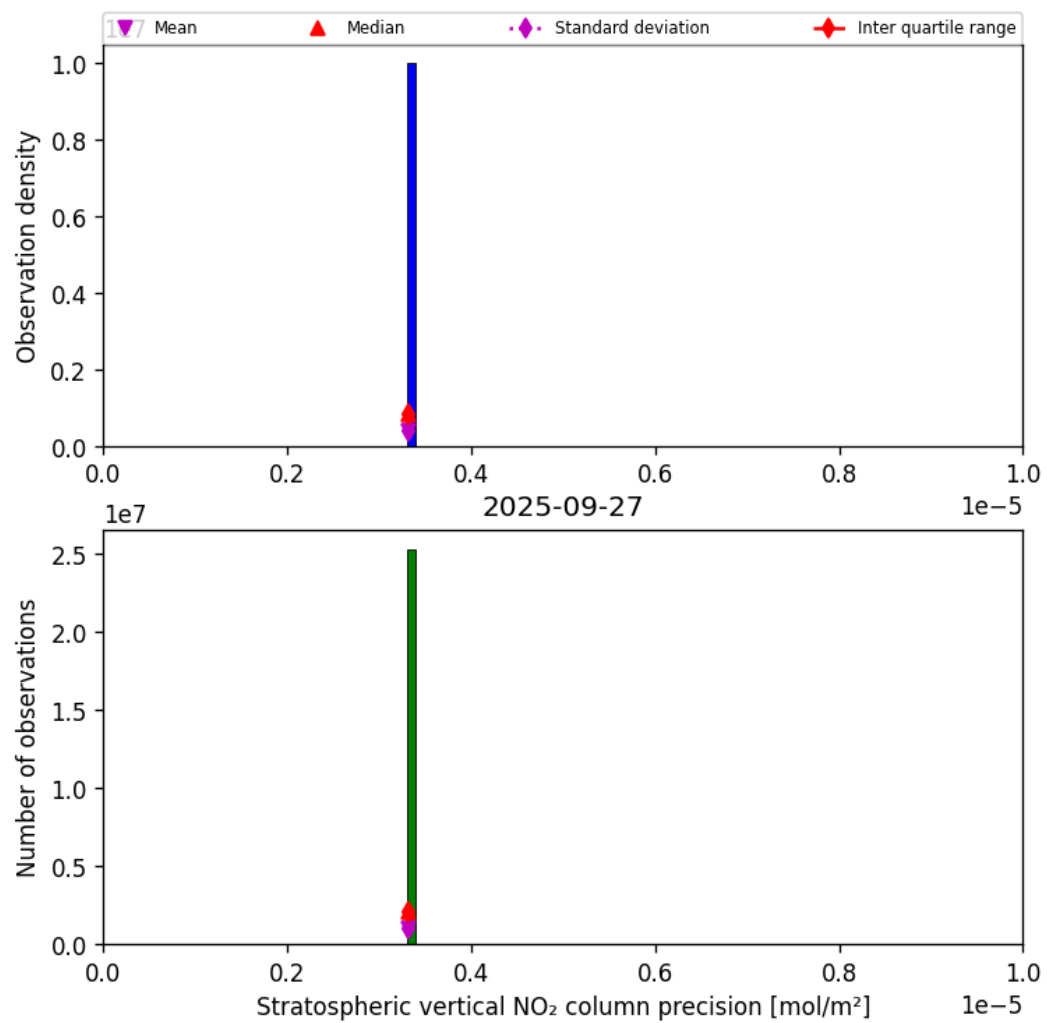
Figure 37: Histogram of “Stratospheric vertical NO 2 column precision” for 2025-09-26 to 2025-09-28
