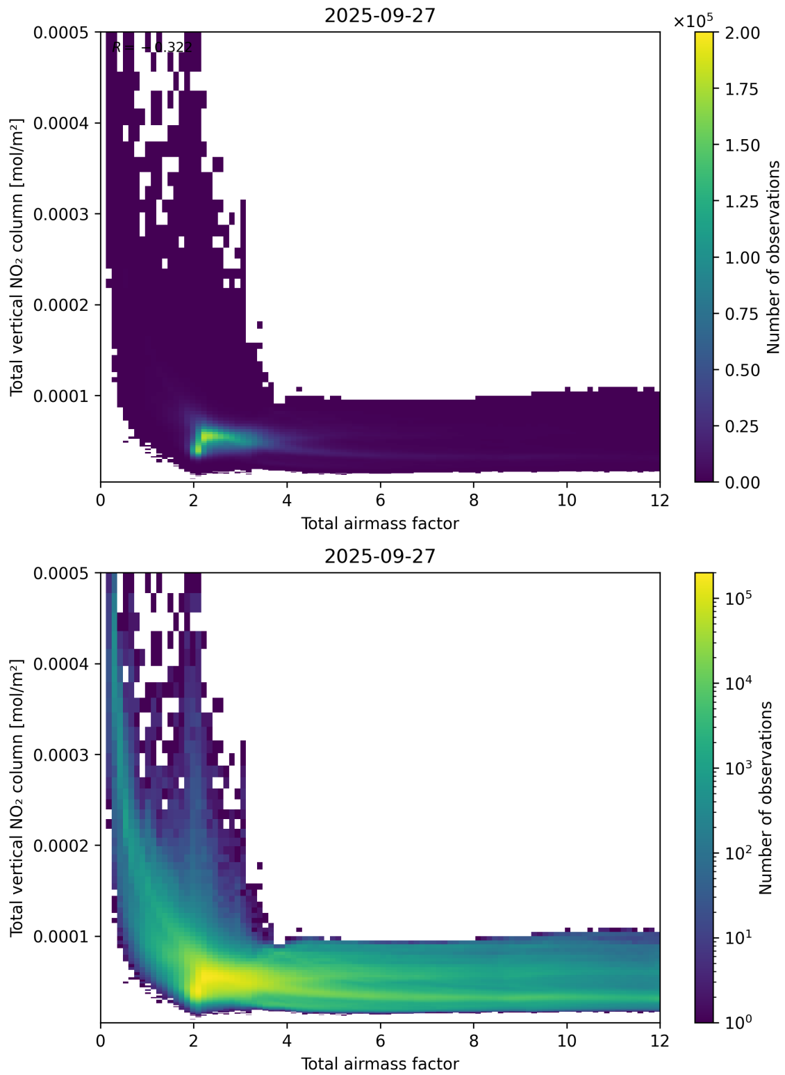
Figure 67: Scatter density plot of “Total airmass factor” against “Total vertical NO 2 column” for 2025-09-26 to 2025-09-28.
