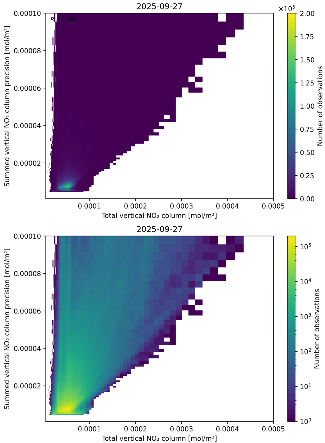
Figure 113: Scatter density plot of “Total vertical NO 2 column” against “Summed vertical NO 2 column precision” for 2025-09-26 to 2025-09-28.
