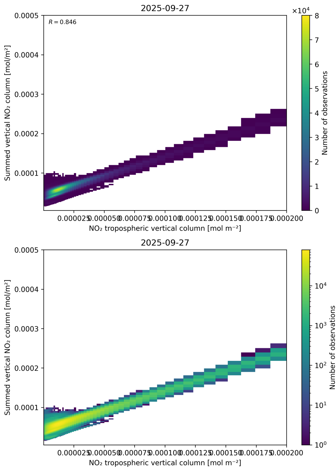
Figure 126: Scatter density plot of “NO 2 tropospheric vertical column” against “Summed vertical NO 2 column” for 2025-09-26 to 2025-09-28.
