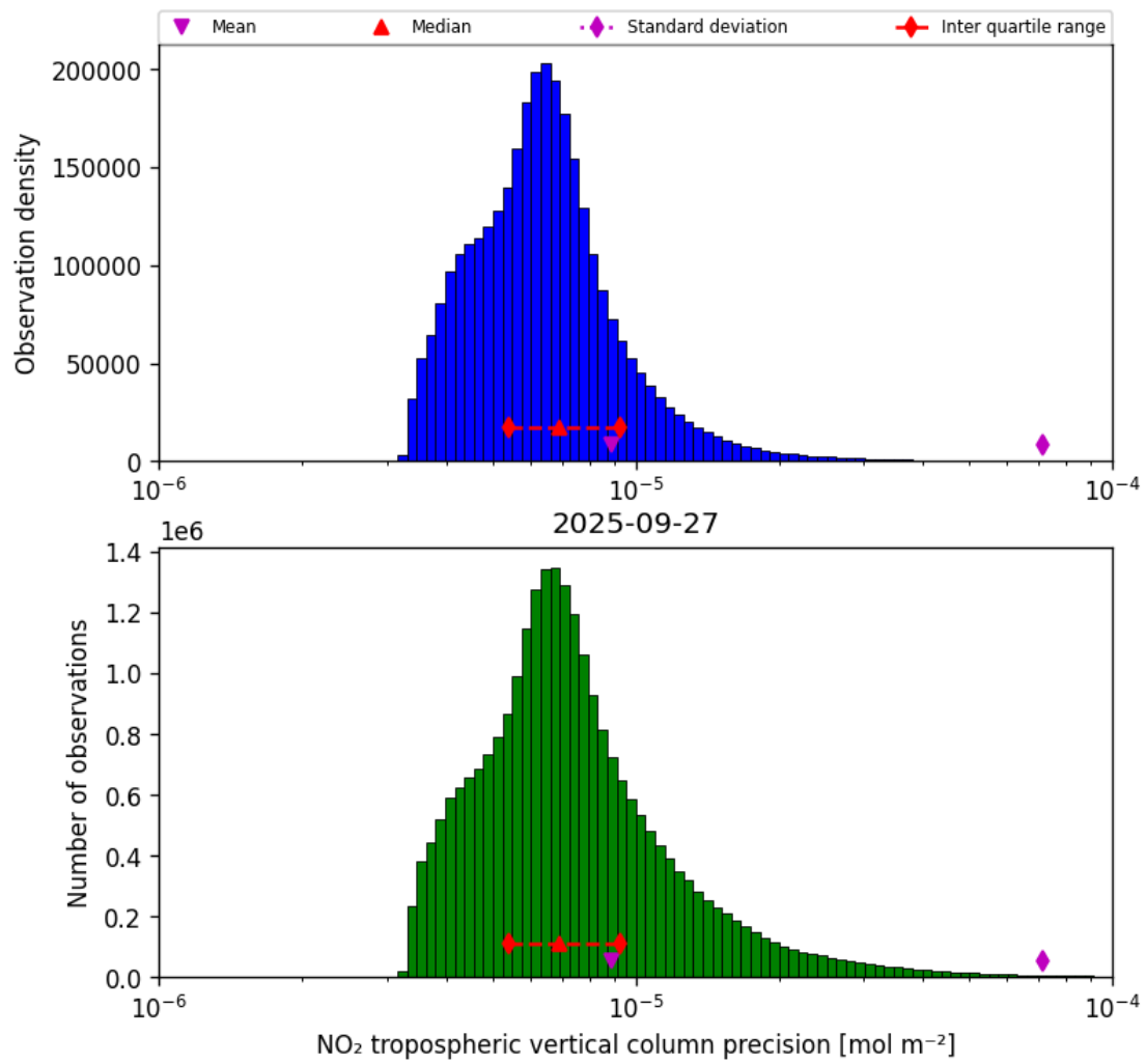
Figure 30: Histogram of “NO 2 tropospheric vertical column precision” for 2025-09-26 to 2025-09-28
