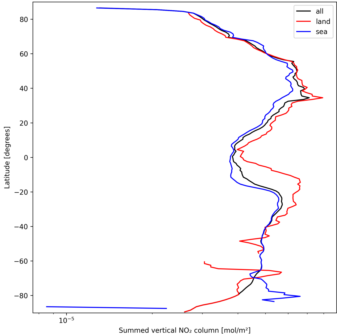
Figure 23: Zonal average of “Summed vertical NO 2 column” for 2025-09-26 to 2025-09-28.
