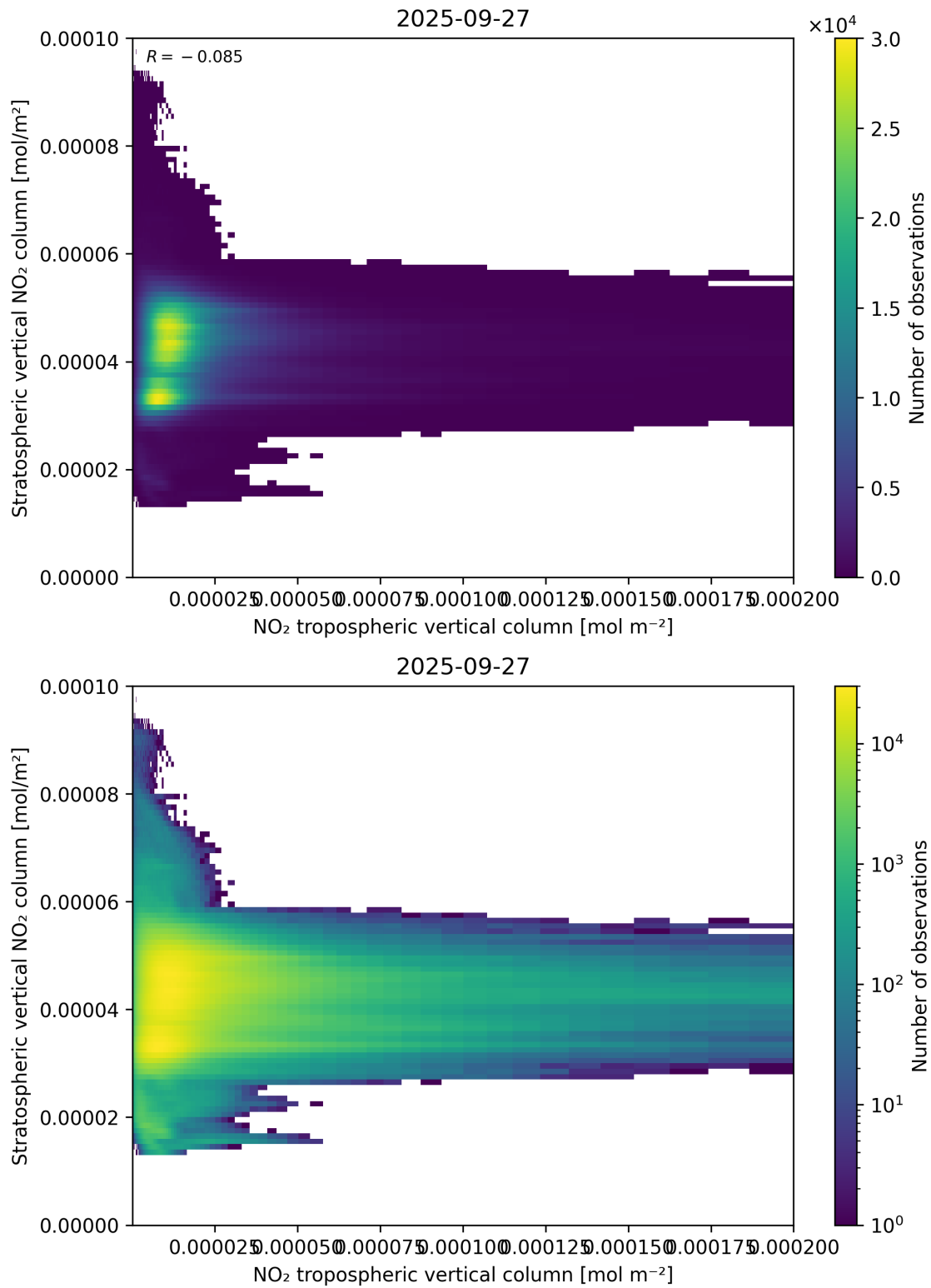
Figure 125: Scatter density plot of “NO 2 tropospheric vertical column” against “Stratospheric vertical NO 2 column” for 2025-09-26 to 2025-09-28.
