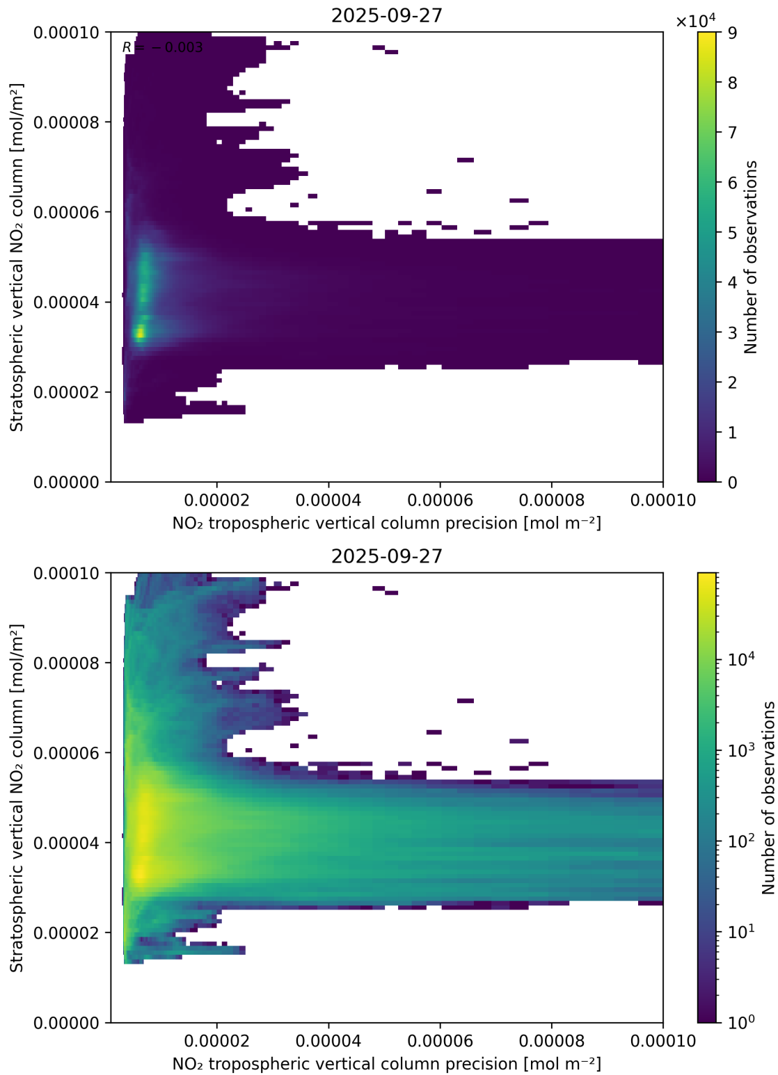
Figure 135: Scatter density plot of “NO 2 tropospheric vertical column precision” against “Stratospheric vertical NO 2 column” for 2025-09-26 to 2025-09-28.
