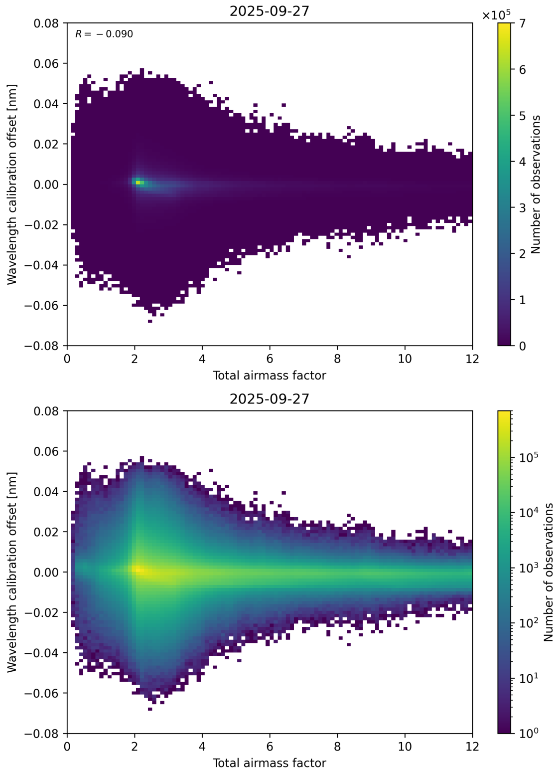
Figure 70: Scatter density plot of “Total airmass factor” against “Wavelength calibration offset” for 2025-09-26 to 2025-09-28.
