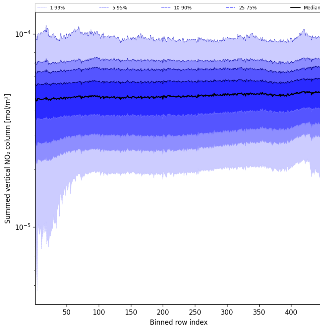
Figure 57: Along track statistics of “Summed vertical NO 2 column” for 2025-09-26 to 2025-09-28
