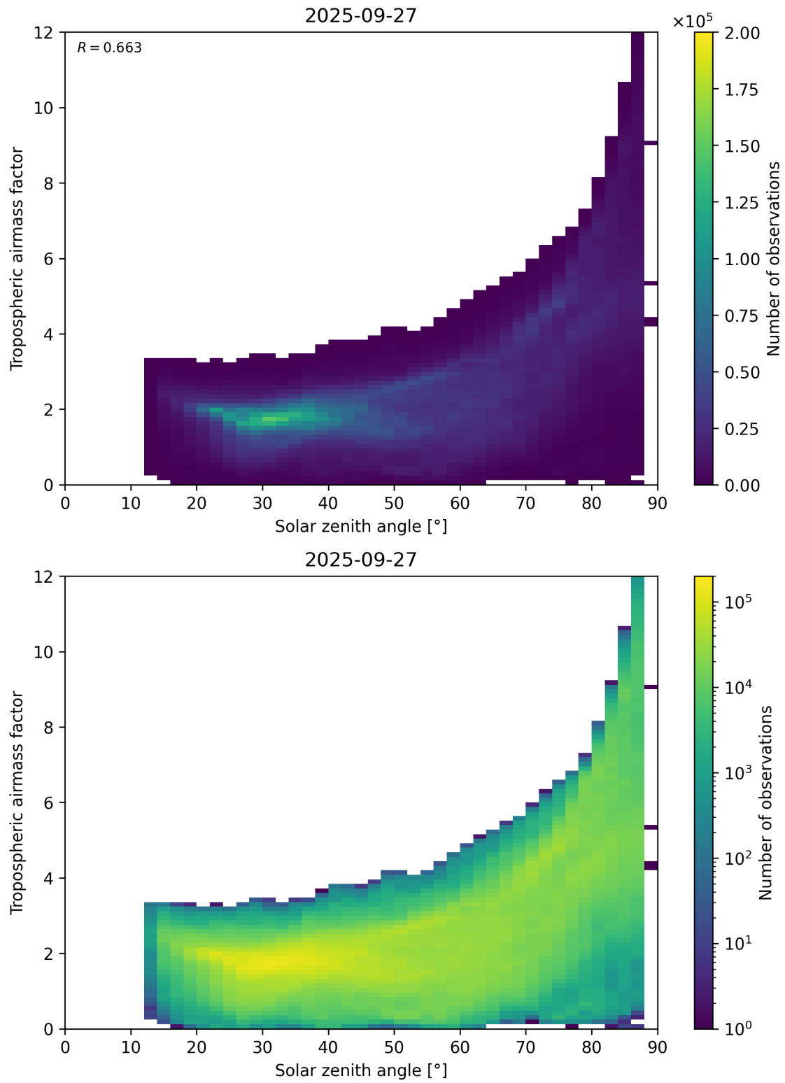
Figure 147: Scatter density plot of “Solar zenith angle” against “Tropospheric airmass factor” for 2025-09-26 to 2025-09-28.
