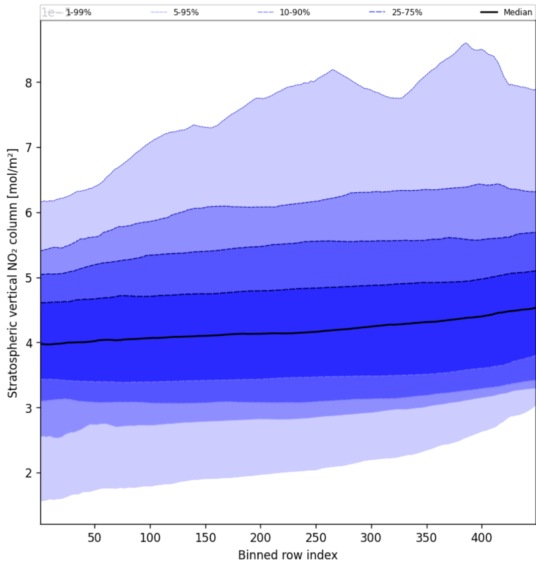
Figure 53: Along track statistics of “Stratospheric vertical NO 2 column” for 2025-09-26 to 2025-09-28
