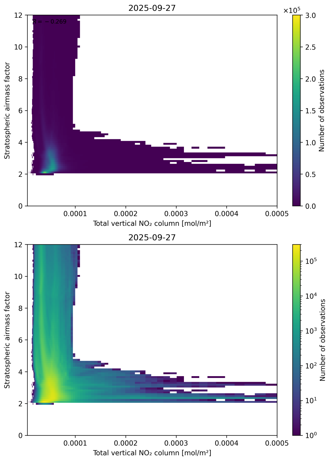
Figure 110: Scatter density plot of “Total vertical NO 2 column” against “Stratospheric airmass factor” for 2025-09-26 to 2025-09-28.
