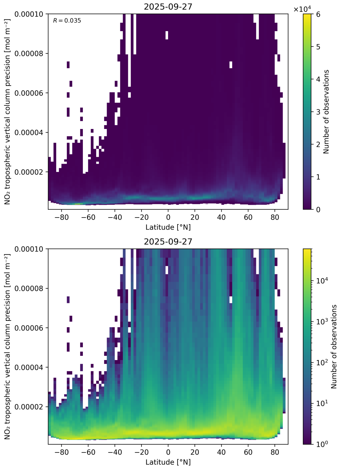
Figure 93: Scatter density plot of “Latitude” against “NO 2 tropospheric vertical column precision” for 2025-09-26 to 2025-09-28.
