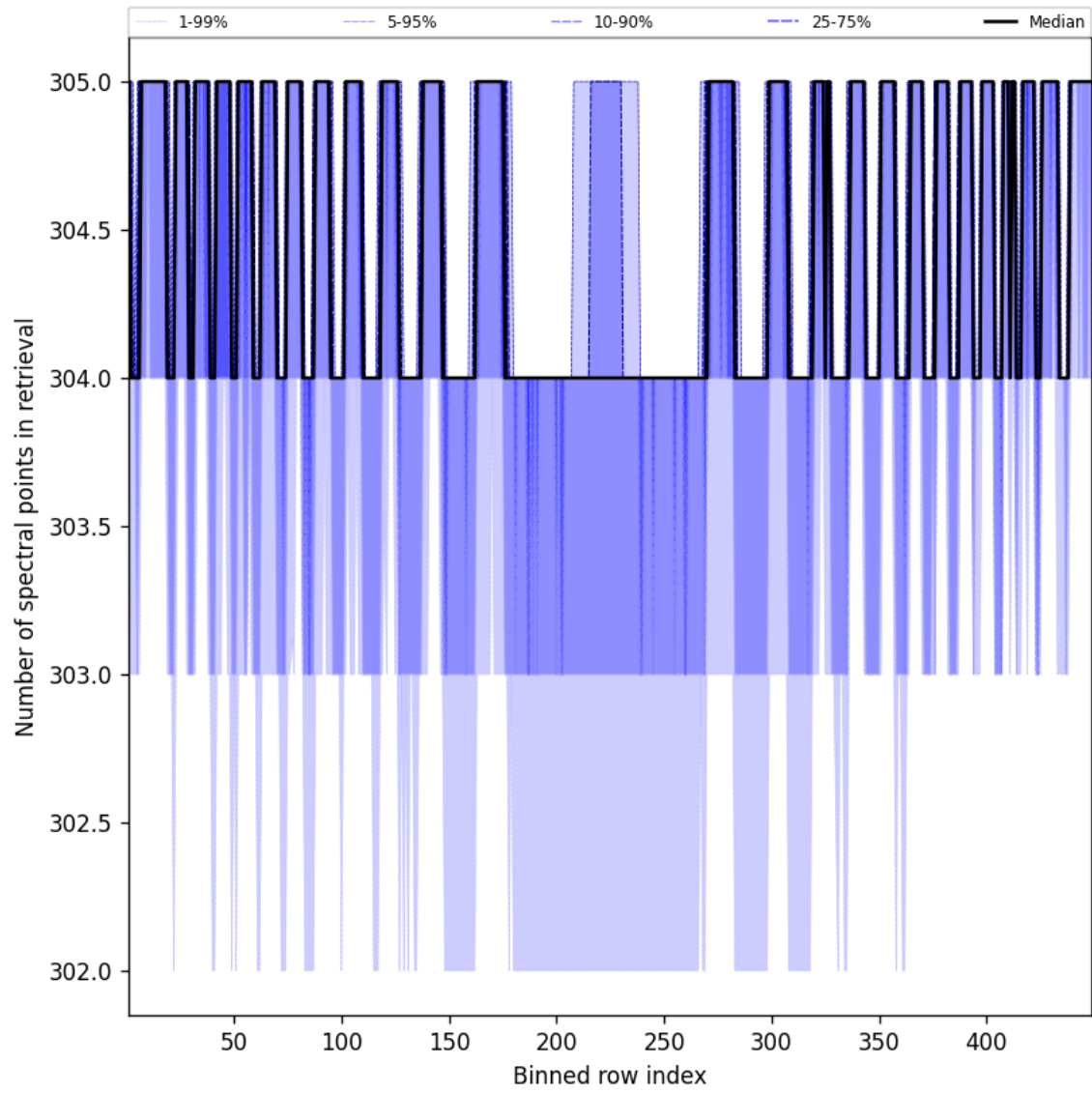
Figure 50: Along track statistics of “Number of spectral points in retrieval” for 2025-09-26 to 2025-09-28
