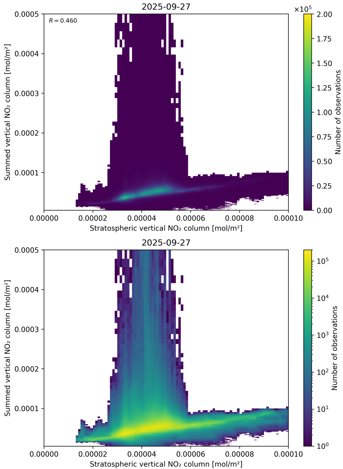
Figure 98: Scatter density plot of “Stratospheric vertical NO 2 column” against “Summed vertical NO 2 column” for 2025-09-26 to 2025-09-28.
