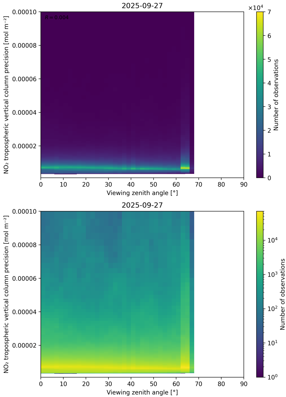
Figure 170: Scatter density plot of “Viewing zenith angle” against “NO 2 tropospheric vertical column precision” for 2025-09-26 to 2025-09-28.
