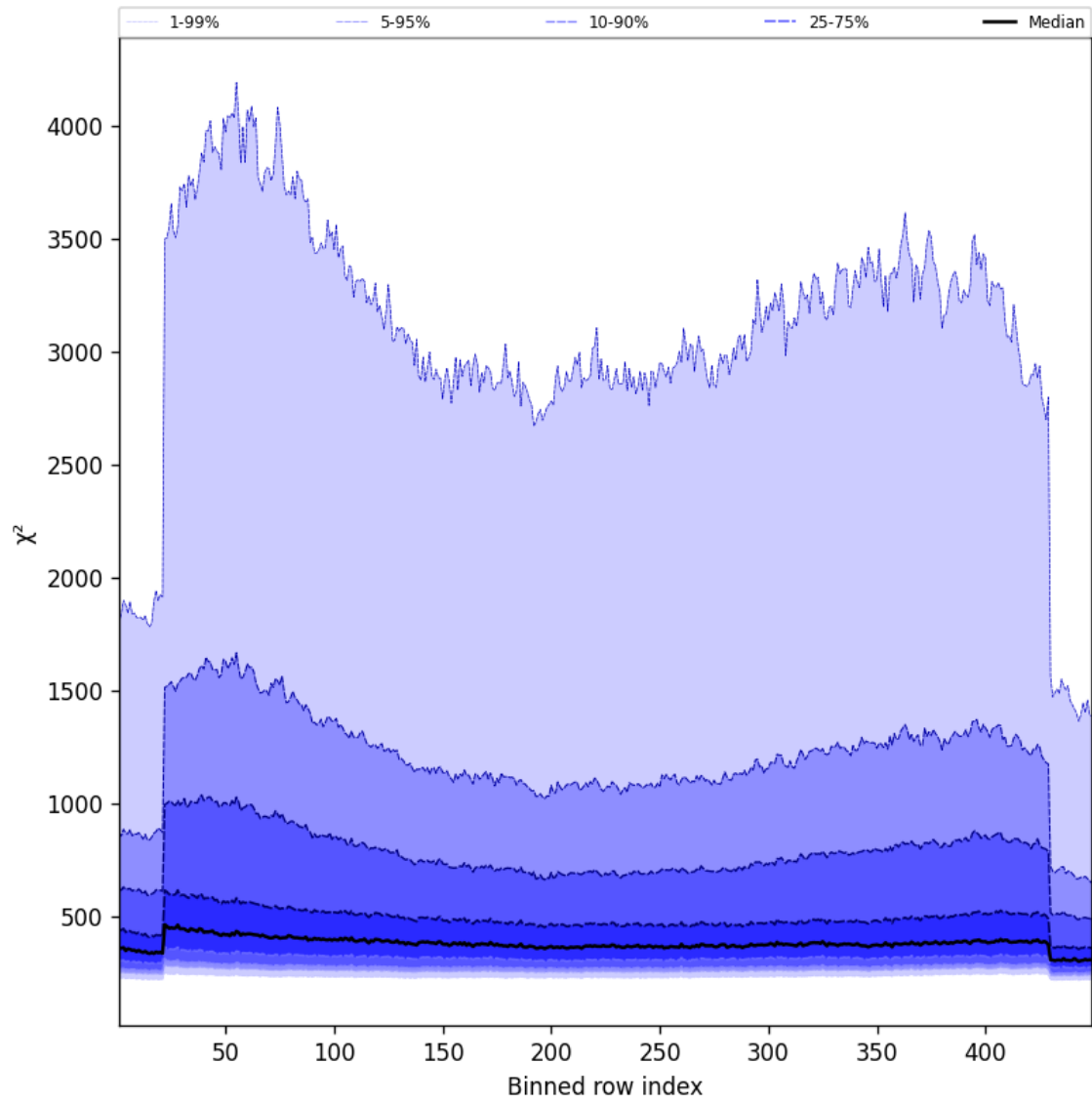
Figure 59: Along track statistics of “ \chi^2 ” for 2025-09-26 to 2025-09-28
