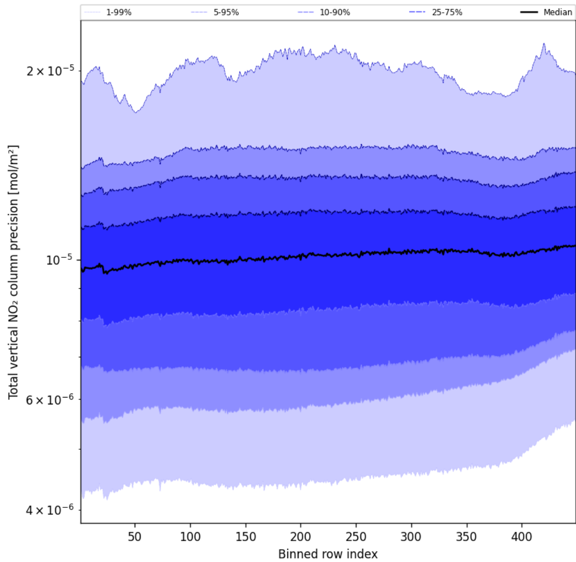
Figure 56: Along track statistics of “Total vertical NO 2 column precision” for 2025-09-26 to 2025-09-28
