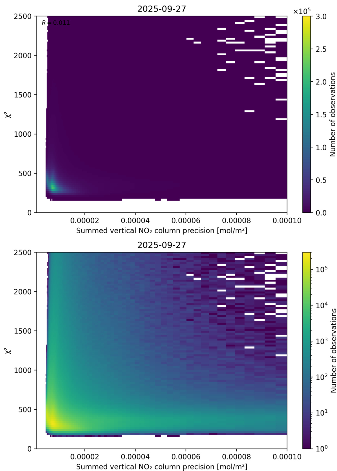
Figure 107: Scatter density plot of “Summed vertical NO 2 column precision” against “ \chi^2 ” for 2025-09-26 to 2025-09-28.
