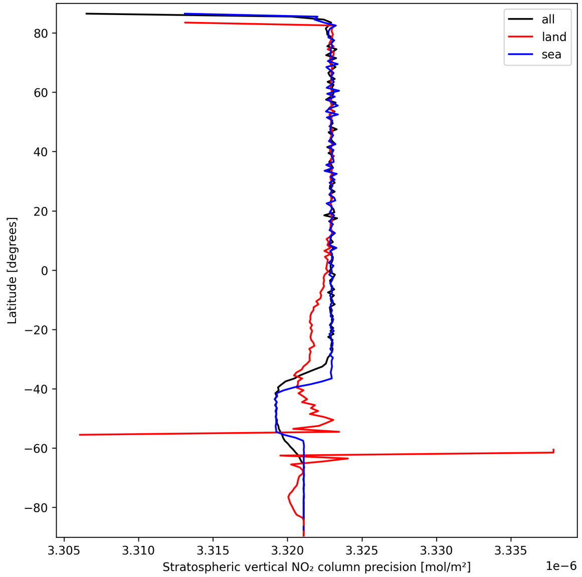
Figure 20: Zonal average of “Stratospheric vertical NO 2 column precision” for 2025-09-26 to 2025-09-28.
