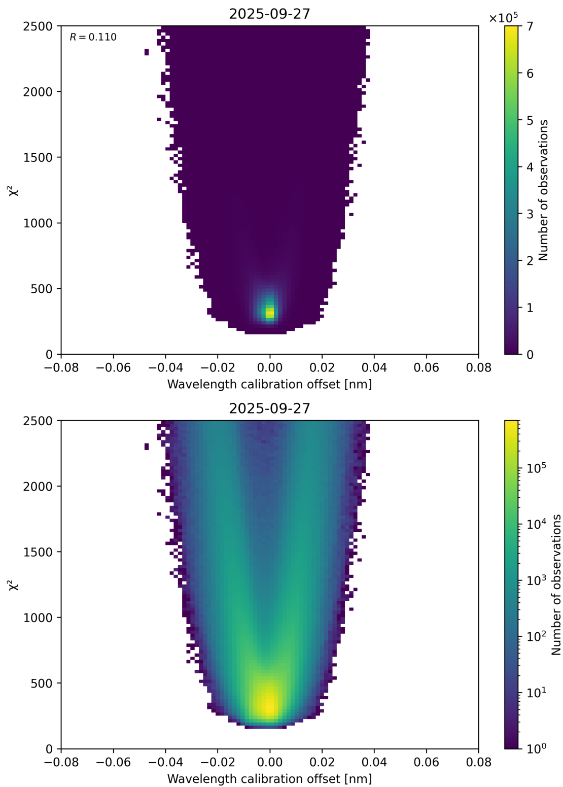
Figure 175: Scatter density plot of “Wavelength calibration offset” against “ \chi^2 ” for 2025-09-26 to 2025-09-28.
