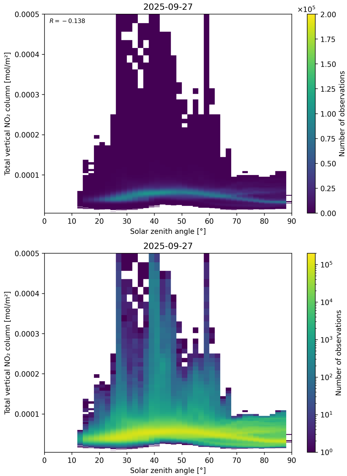
Figure 153: Scatter density plot of “Solar zenith angle” against “Total vertical NO 2 column” for 2025-09-26 to 2025-09-28.
