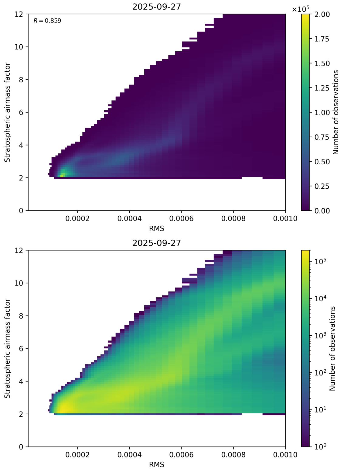
Figure 144: Scatter density plot of “RMS” against “Stratospheric airmass factor” for 2025-09-26 to 2025-09-28.
