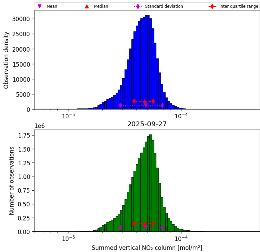
Figure 40: Histogram of “Summed vertical NO 2 column” for 2025-09-26 to 2025-09-28
