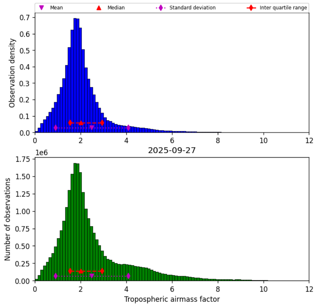
Figure 31: Histogram of “Tropospheric airmass factor” for 2025-09-26 to 2025-09-28
