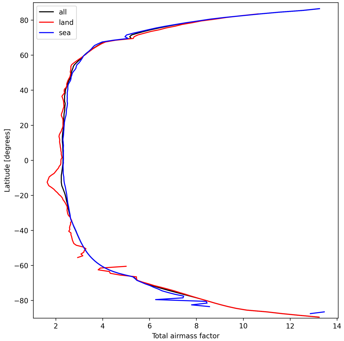
Figure 15: Zonal average of “Total airmass factor” for 2025-09-26 to 2025-09-28.
