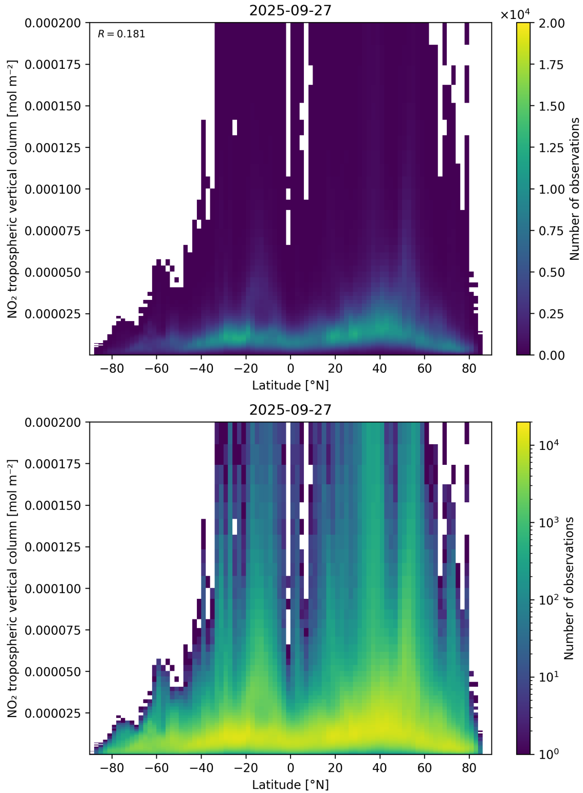
Figure 92: Scatter density plot of “Latitude” against “NO 2 tropospheric vertical column” for 2025-09-26 to 2025-09-28.
