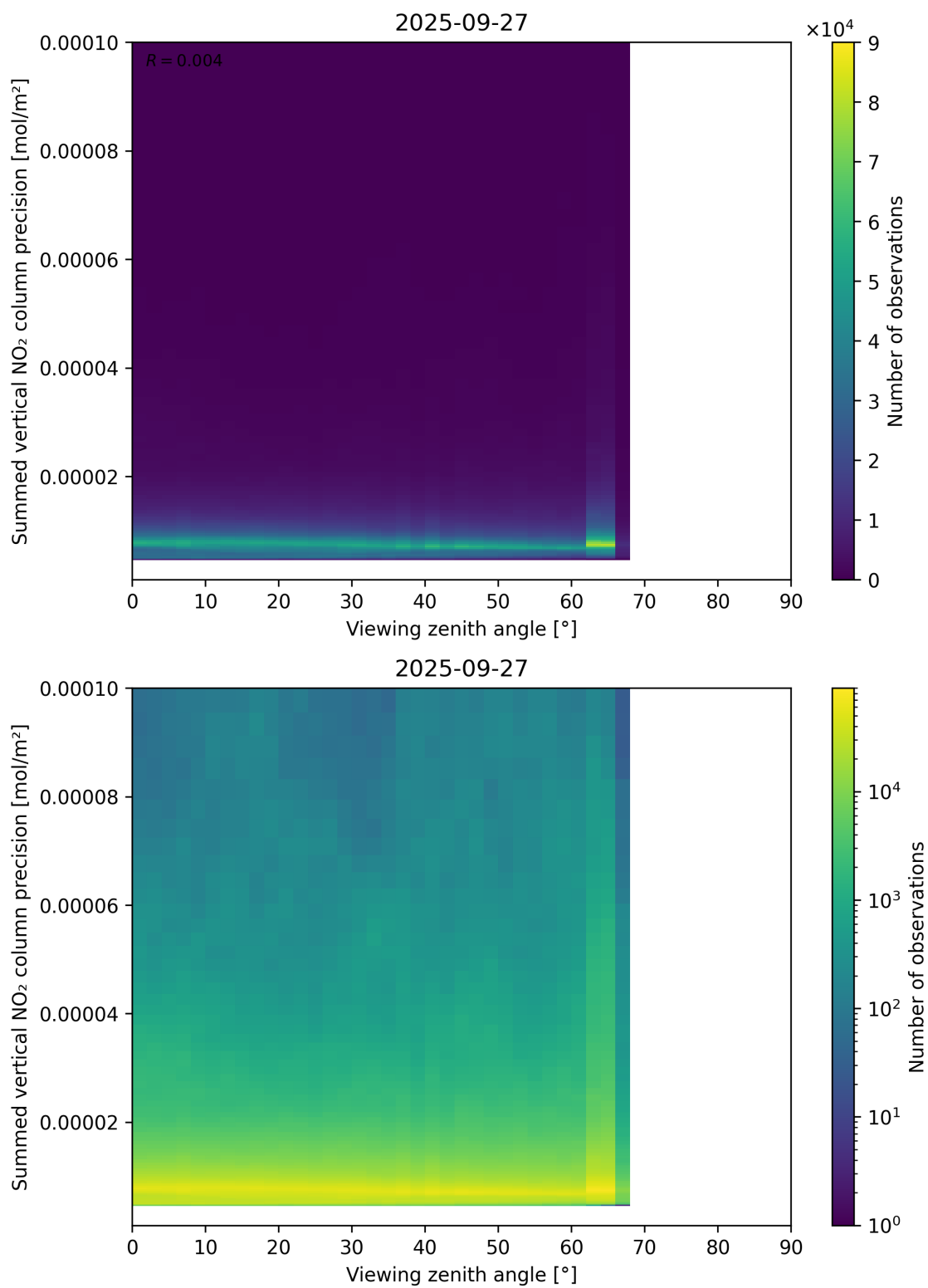
Figure 166: Scatter density plot of “Viewing zenith angle” against “Summed vertical NO 2 column precision” for 2025-09-26 to 2025-09-28.
