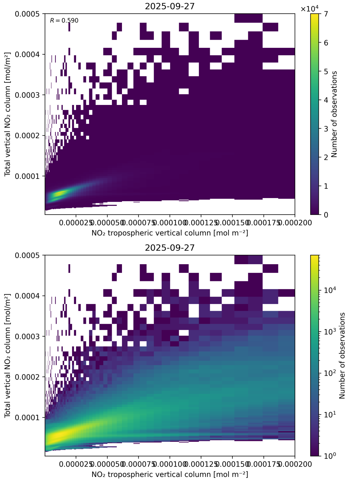
Figure 128: Scatter density plot of “NO 2 tropospheric vertical column” against “Total vertical NO 2 column” for 2025-09-26 to 2025-09-28.
