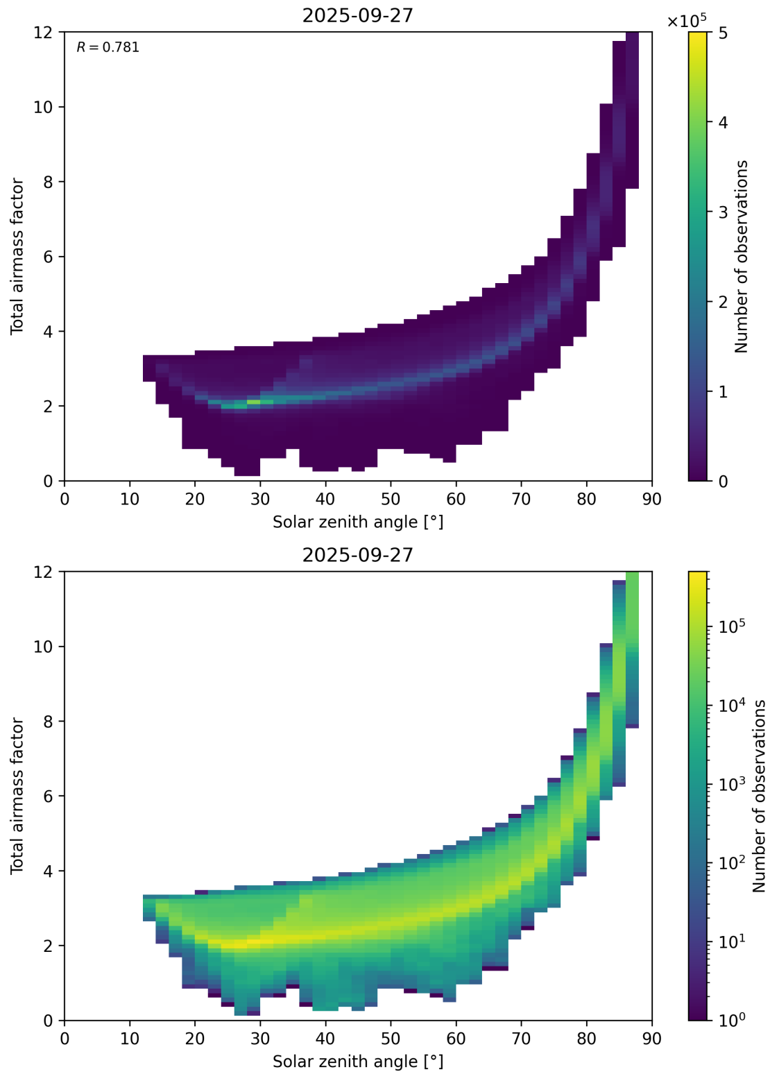
Figure 146: Scatter density plot of “Solar zenith angle” against “Total air mass factor” for 2025-09-26 to 2025-09-28.
