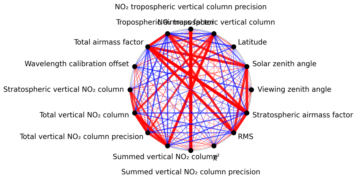
Figure 1: Map of correlation graph for 2025-09-26 to 2025-09-28.
