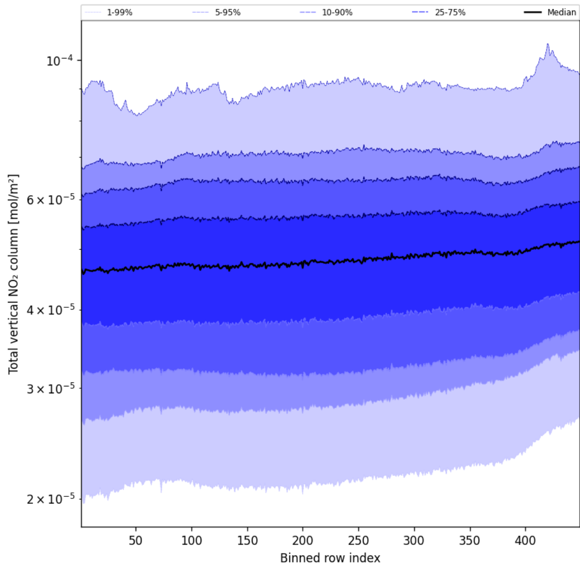
Figure 55: Along track statistics of “Total vertical NO 2 column” for 2025-09-26 to 2025-09-28
