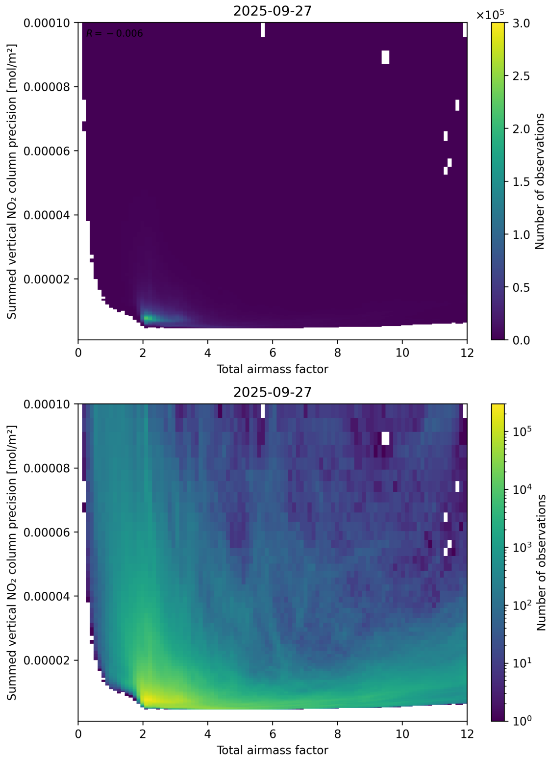
Figure 66: Scatter density plot of “Total airmass factor” against “Summed vertical NO 2 column precision” for 2025-09-26 to 2025-09-28.
