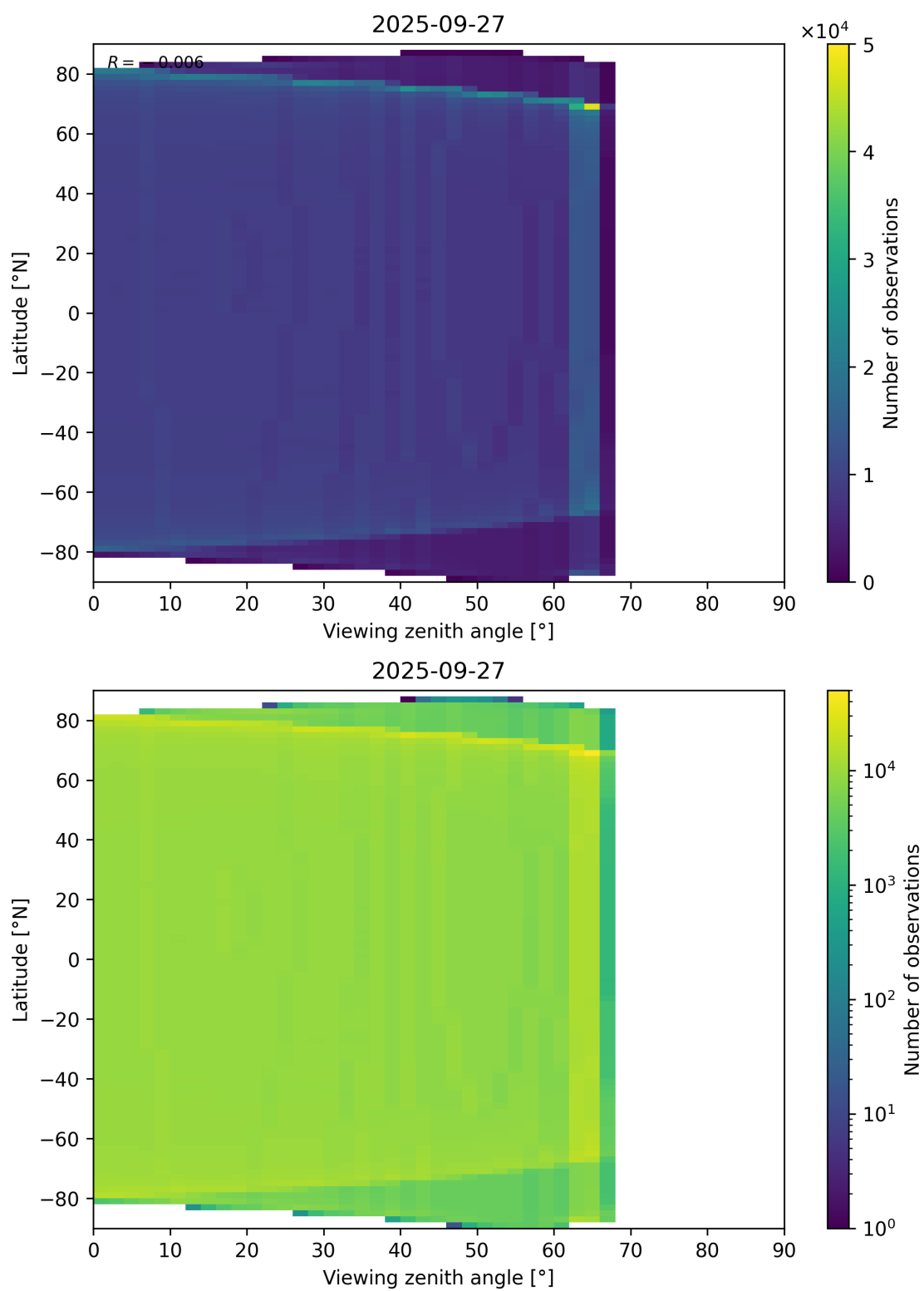
Figure 163: Scatter density plot of “Viewing zenith angle” against “Latitude” for 2025-09-26 to 2025-09-28.
