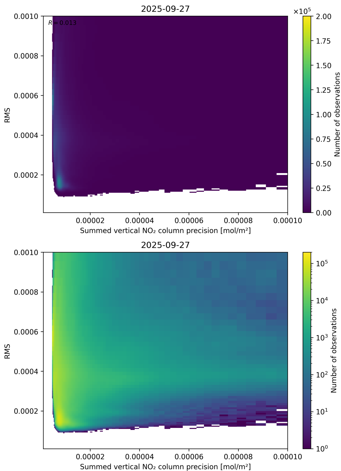
Figure 108: Scatter density plot of “Summed vertical NO 2 column precision” against “RMS” for 2025-09-26 to 2025-09-28.
