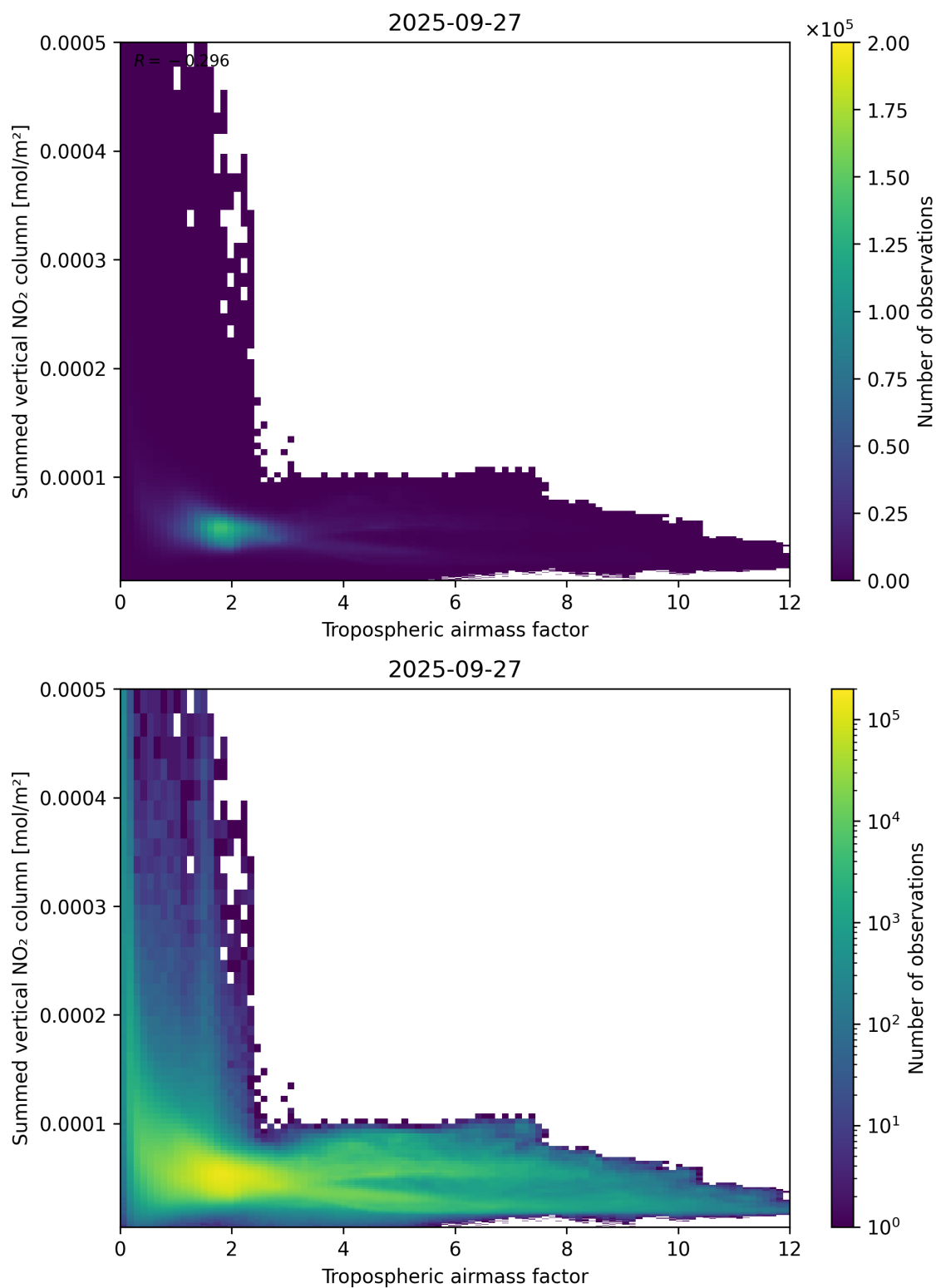
Figure 75: Scatter density plot of “Tropospheric air mass factor” against “Summed vertical NO 2 column” for 2025-09-26 to 2025-09-28.
