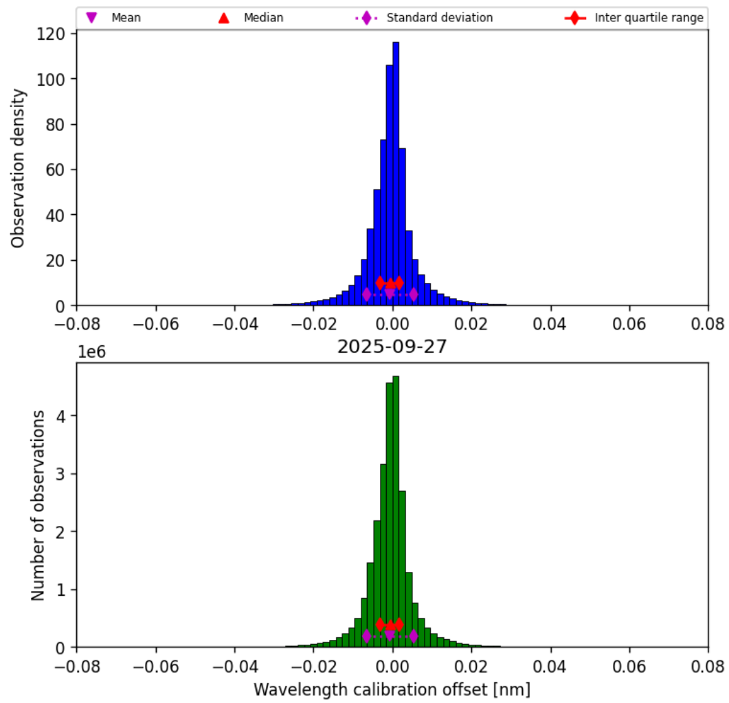
Figure 35: Histogram of “Wavelength calibration offset” for 2025-09-26 to 2025-09-28
