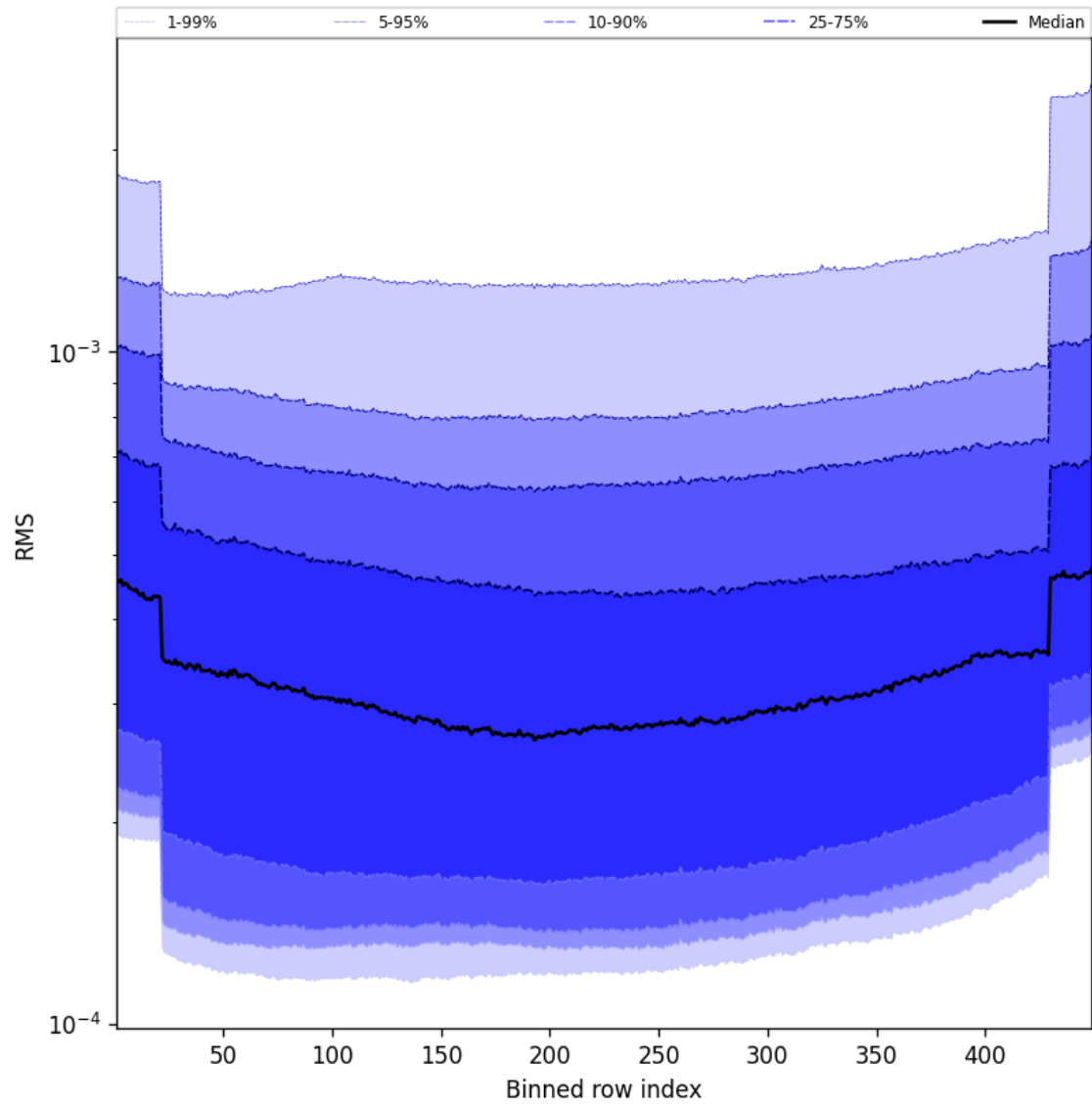
Figure 60: Along track statistics of “RMS” for 2025-09-26 to 2025-09-28
