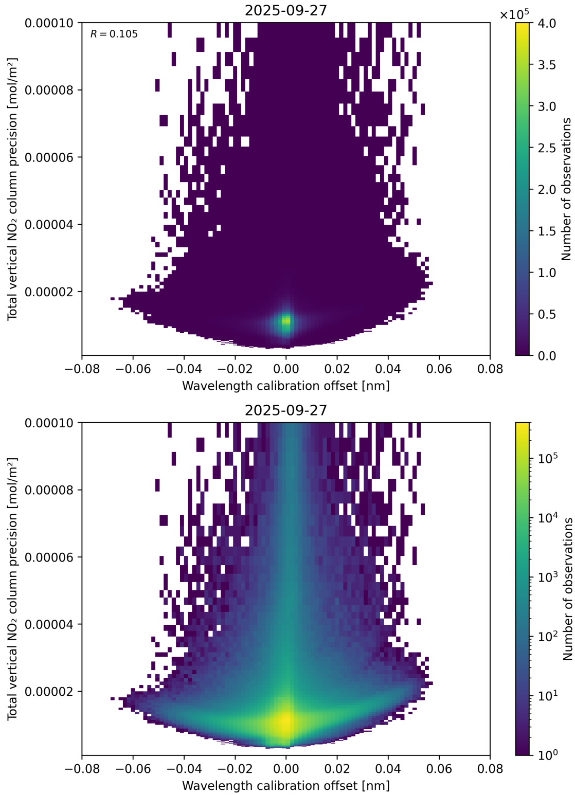
Figure 180: Scatter density plot of “Wavelength calibration offset” against “Total vertical NO 2 column precision” for 2025-09-26 to 2025-09-28.
