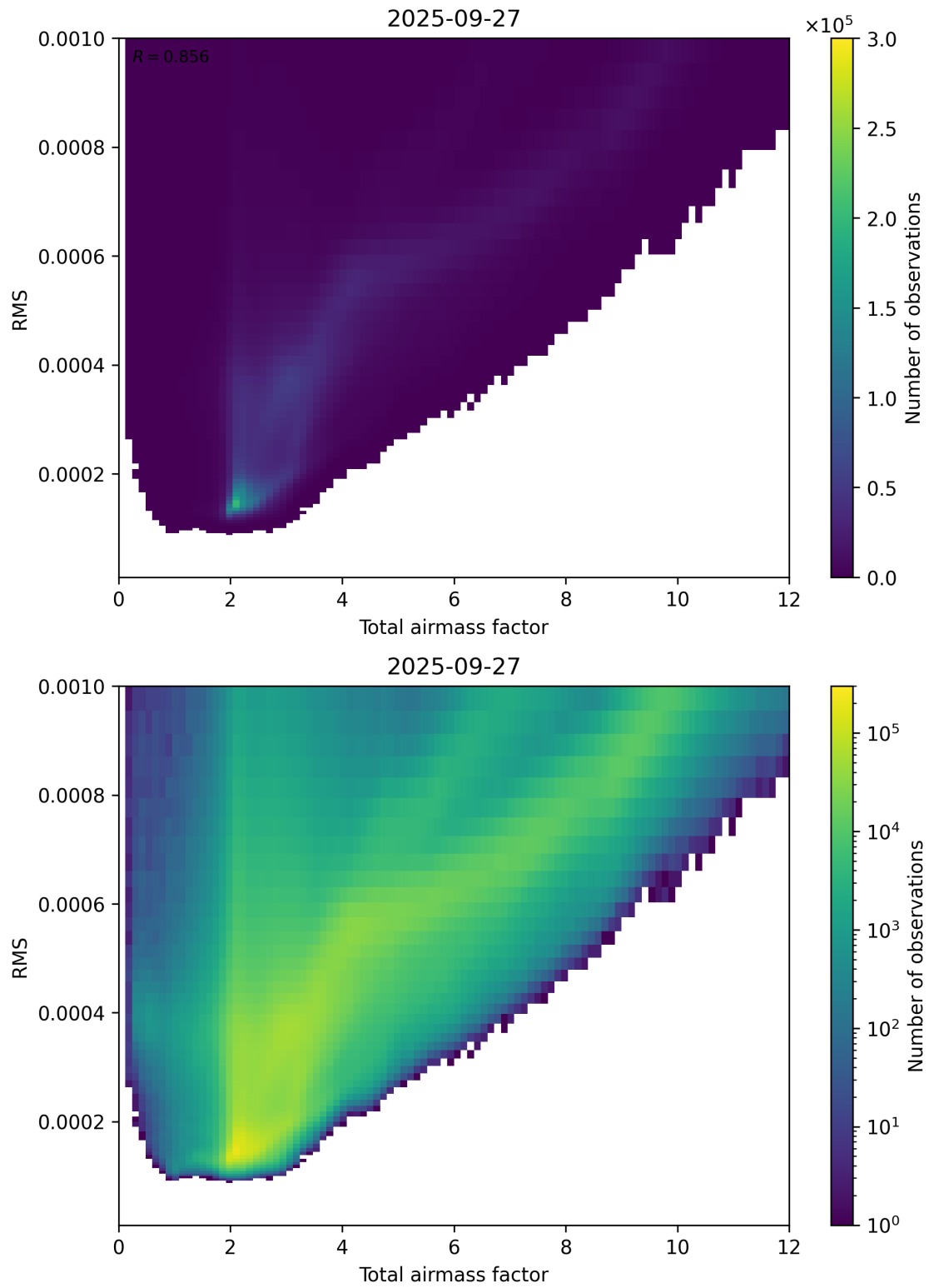
Figure 69: Scatter density plot of “Total airmass factor” against “RMS” for 2025-09-26 to 2025-09-28.
