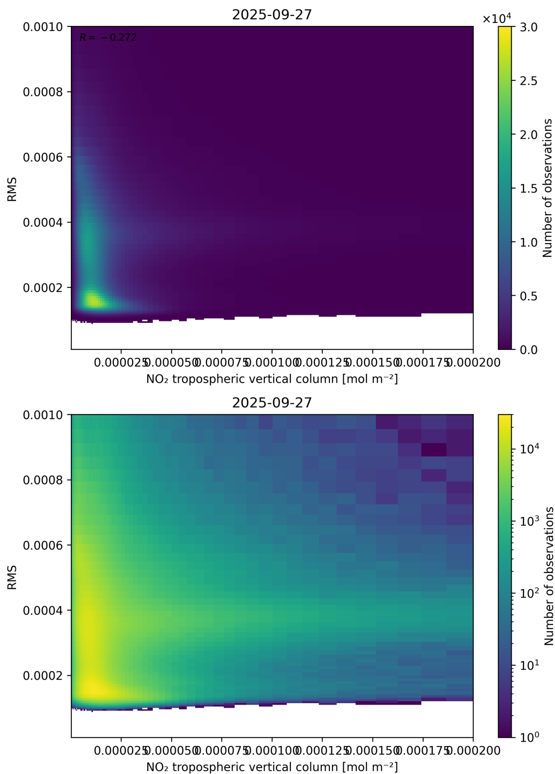
Figure 142: Scatter density plot of “NO 2 tropospheric vertical column” against “RMS” for 2025-09-26 to 2025-09-28.
