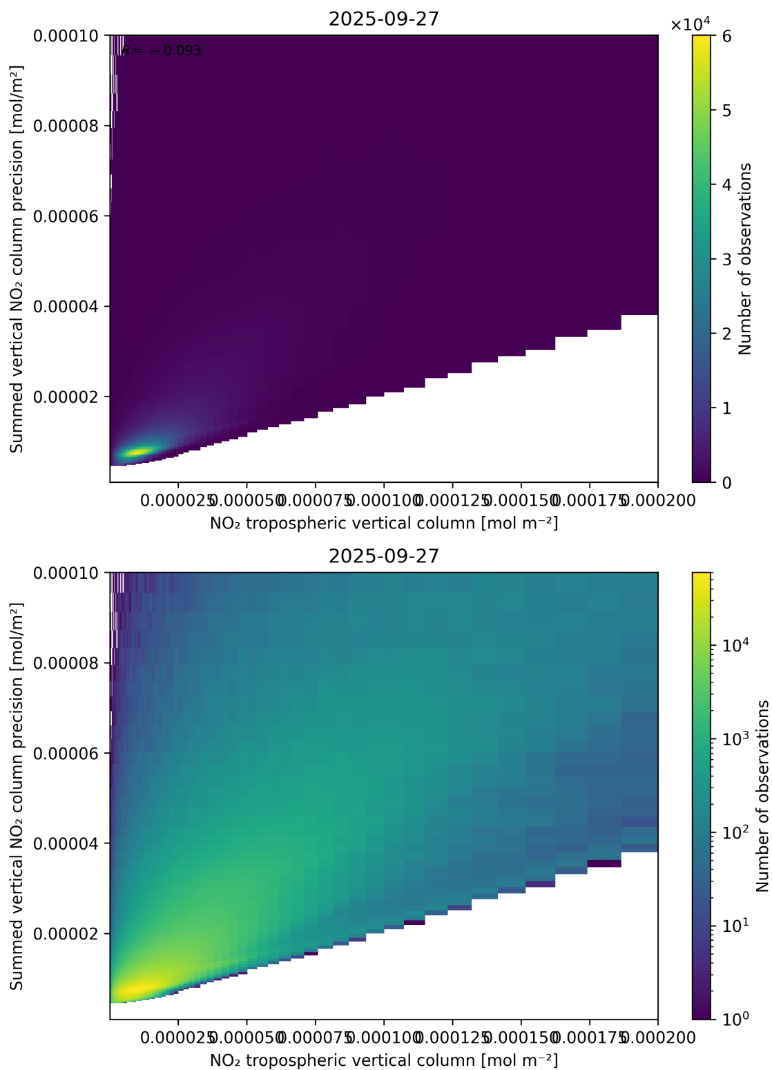
Figure 127: Scatter density plot of “NO 2 tropospheric vertical column” against “Summed vertical NO 2 column precision” for 2025-09-26 to 2025-09-28.
