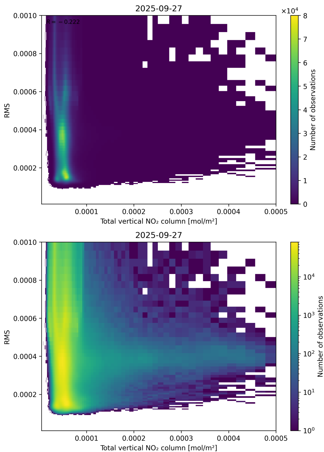
Figure 120: Scatter density plot of “Total vertical NO 2 column” against “RMS” for 2025-09-26 to 2025-09-28.
