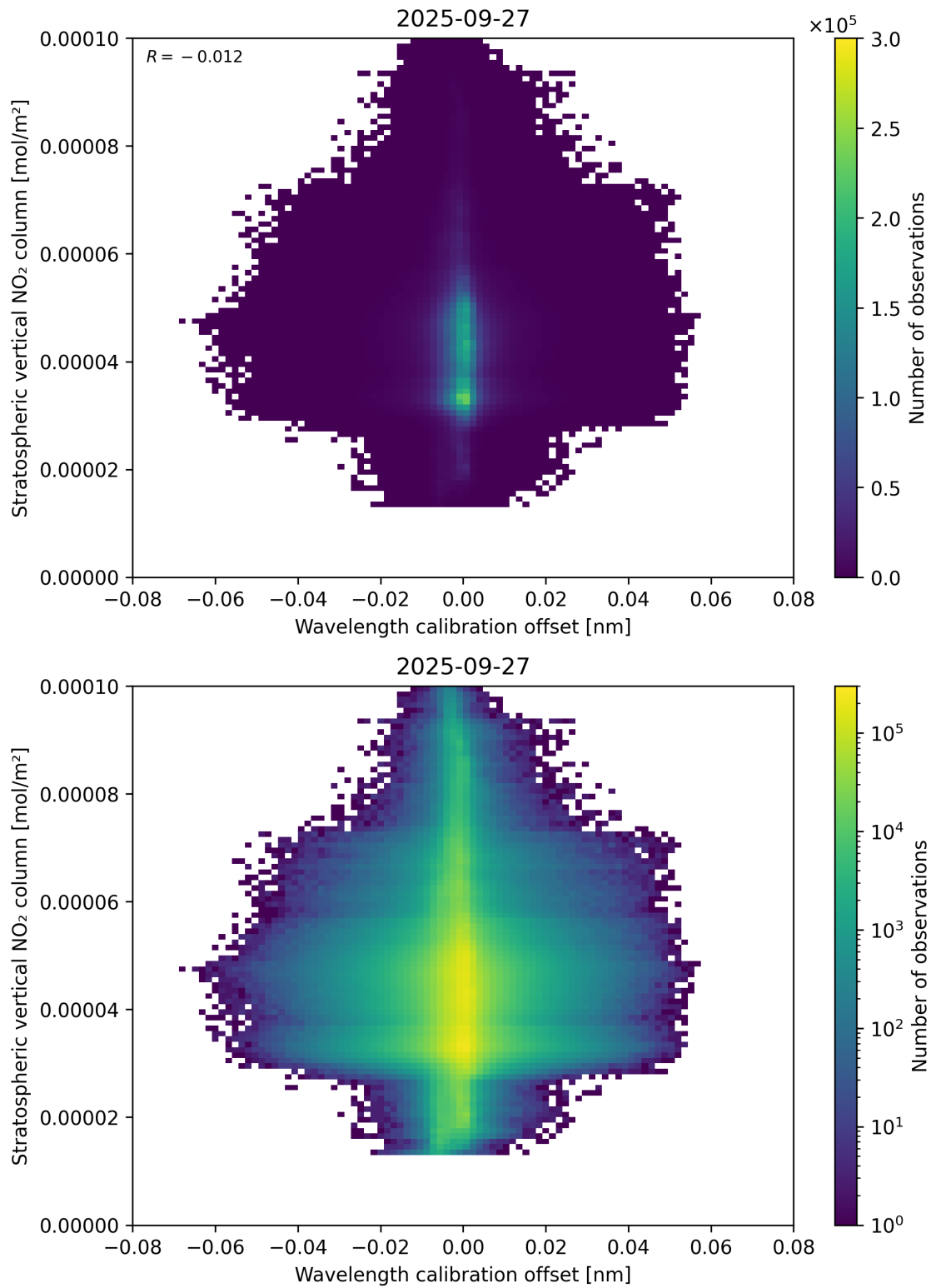
Figure 176: Scatter density plot of “Wavelength calibration offset” against “Stratospheric vertical NO 2 column” for 2025-09-26 to 2025-09-28.
