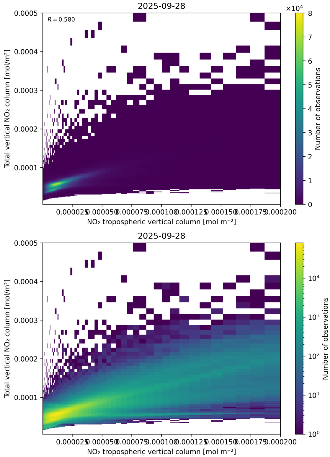
Figure 128: Scatter density plot of “NO 2 tropospheric vertical column” against “Total vertical NO 2 column” for 2025-09-27 to 2025-09-29.
