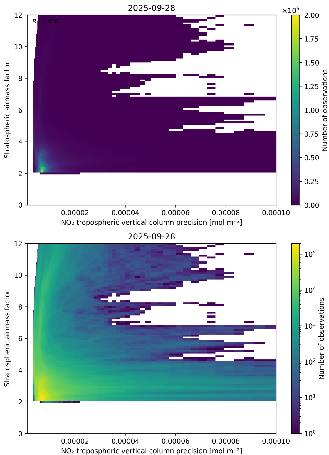
Figure 131: Scatter density plot of “NO 2 tropospheric vertical column precision” against “Stratospheric airmass factor” for 2025-09-27 to 2025-09-29.
