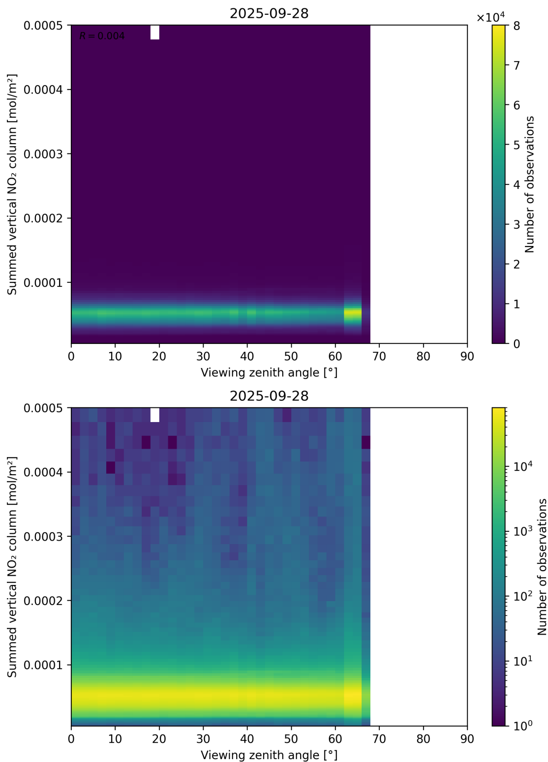
Figure 165: Scatter density plot of “Viewing zenith angle” against “Summed vertical NO 2 column” for 2025-09-27 to 2025-09-29.
