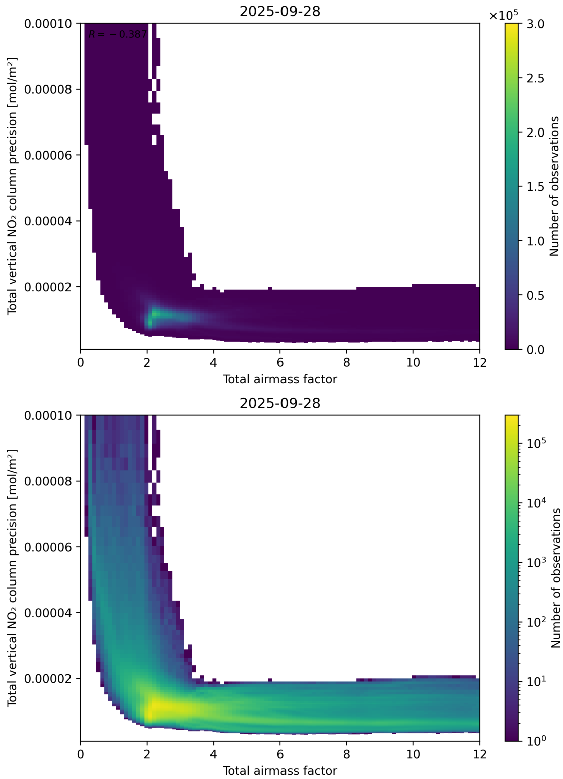
Figure 68: Scatter density plot of “Total airmass factor” against “Total vertical NO 2 column precision” for 2025-09-27 to 2025-09-29.
