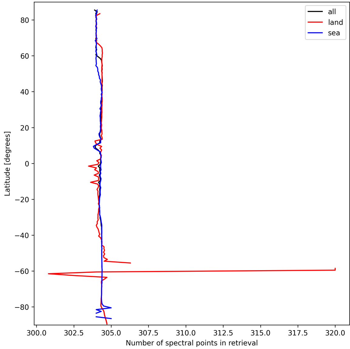
Figure 16: Zonal average of “Number of spectral points in retrieval” for 2025-09-27 to 2025-09-29.
