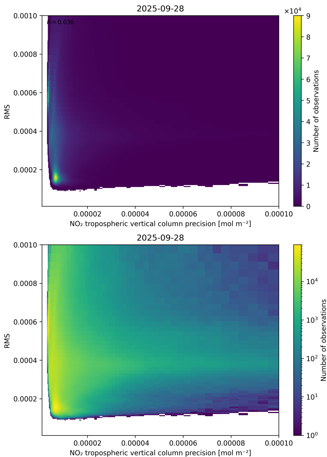
Figure 140: Scatter density plot of “NO 2 tropospheric vertical column precision” against “RMS” for 2025-09-27 to 2025-09-29.
