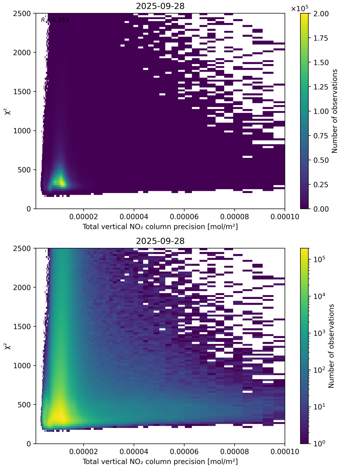
Figure 116: Scatter density plot of “Total vertical NO 2 column precision” against “ \chi^2 ” for 2025-09-27 to 2025-09-29.
