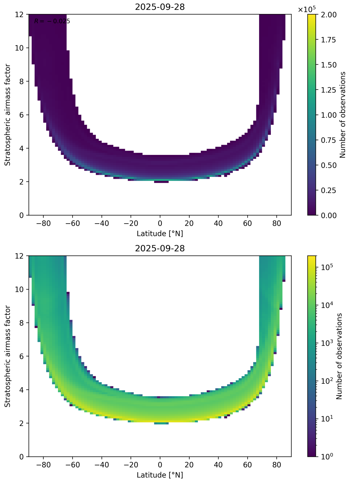
Figure 83: Scatter density plot of “Latitude” against “Stratospheric air mass factor” for 2025-09-27 to 2025-09-29.
