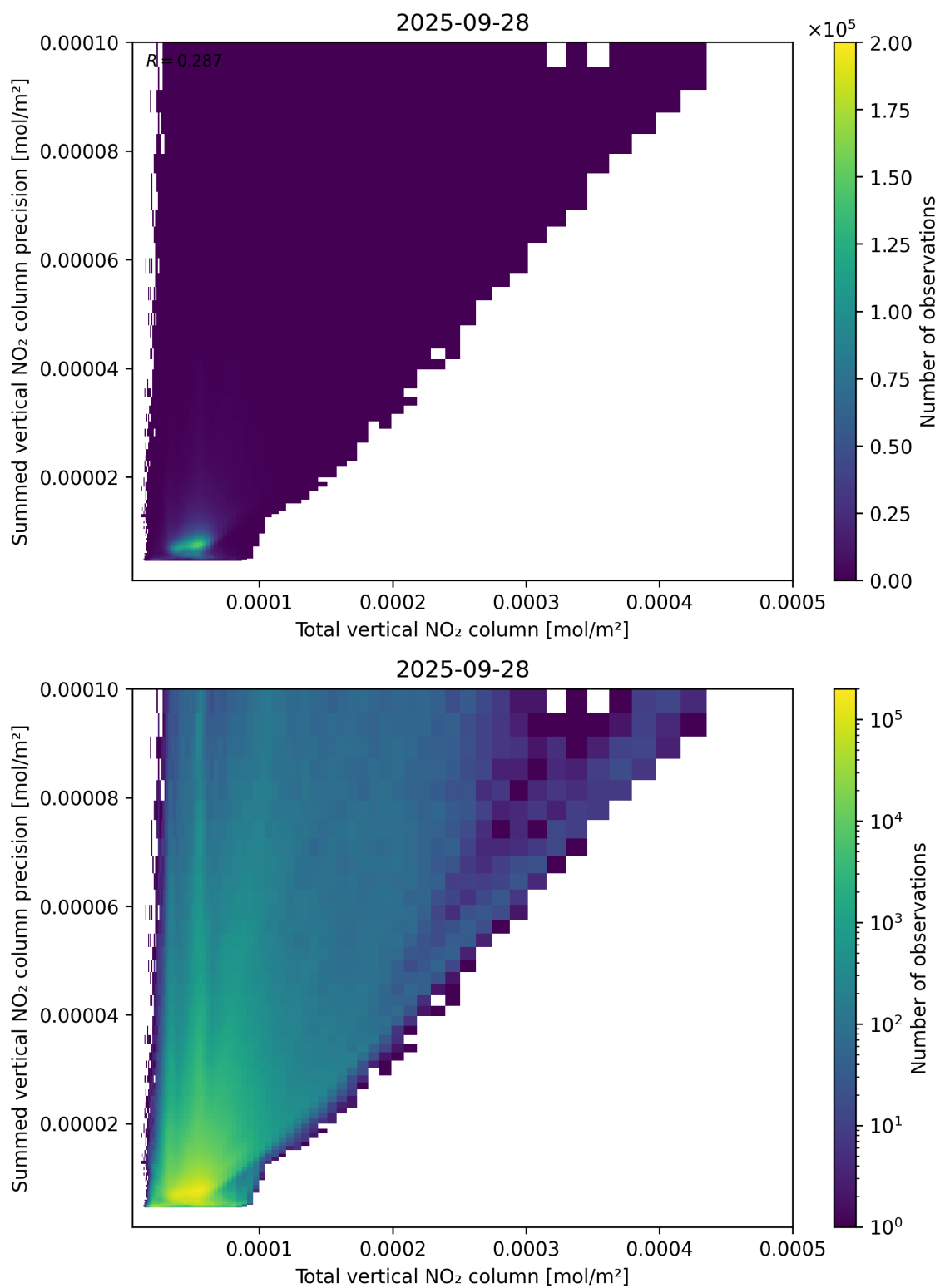
Figure 113: Scatter density plot of “Total vertical NO 2 column” against “Summed vertical NO 2 column precision” for 2025-09-27 to 2025-09-29.
