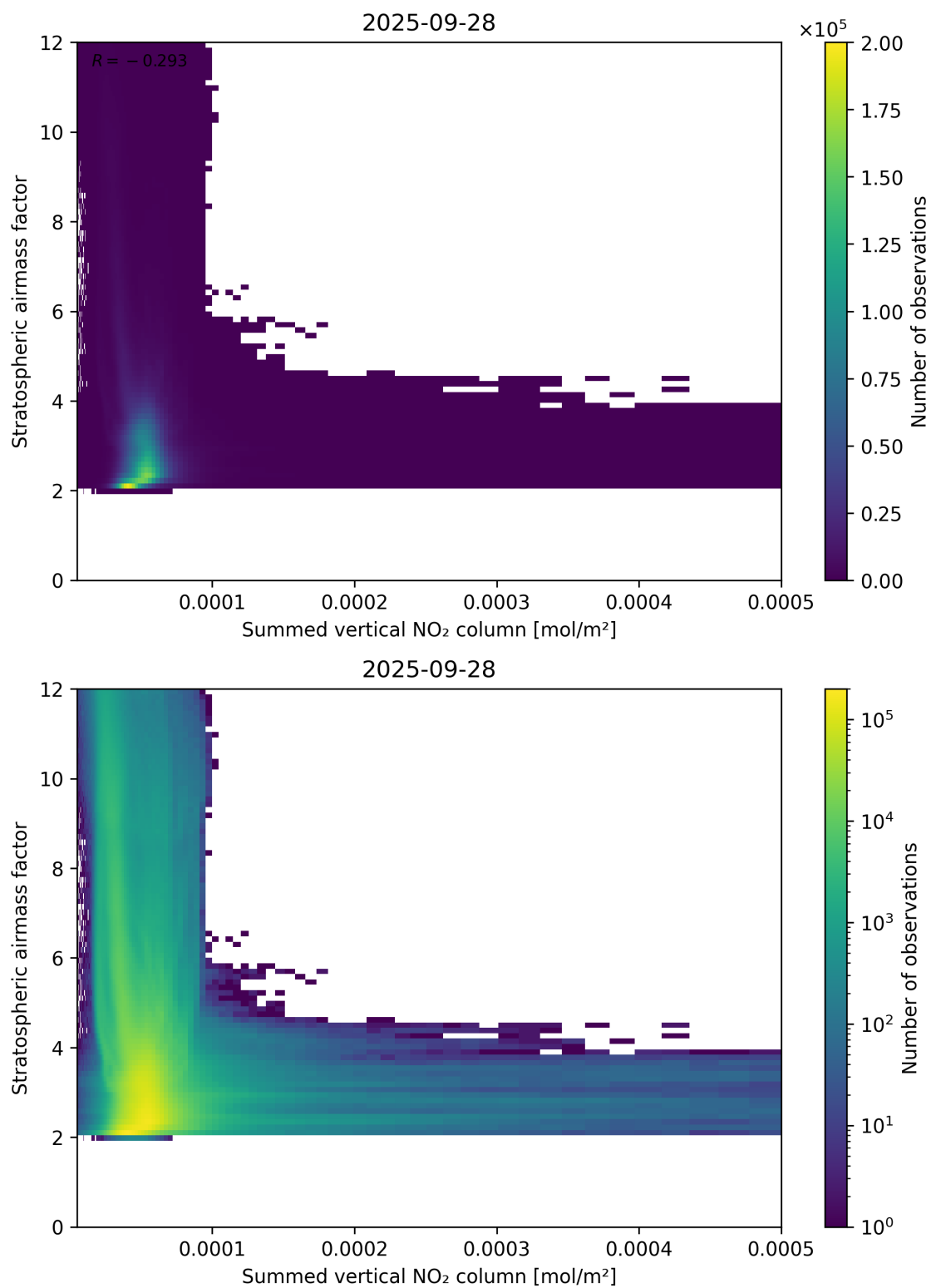
Figure 103: Scatter density plot of “Summed vertical NO 2 column” against “Stratospheric airmass factor” for 2025-09-27 to 2025-09-29.
