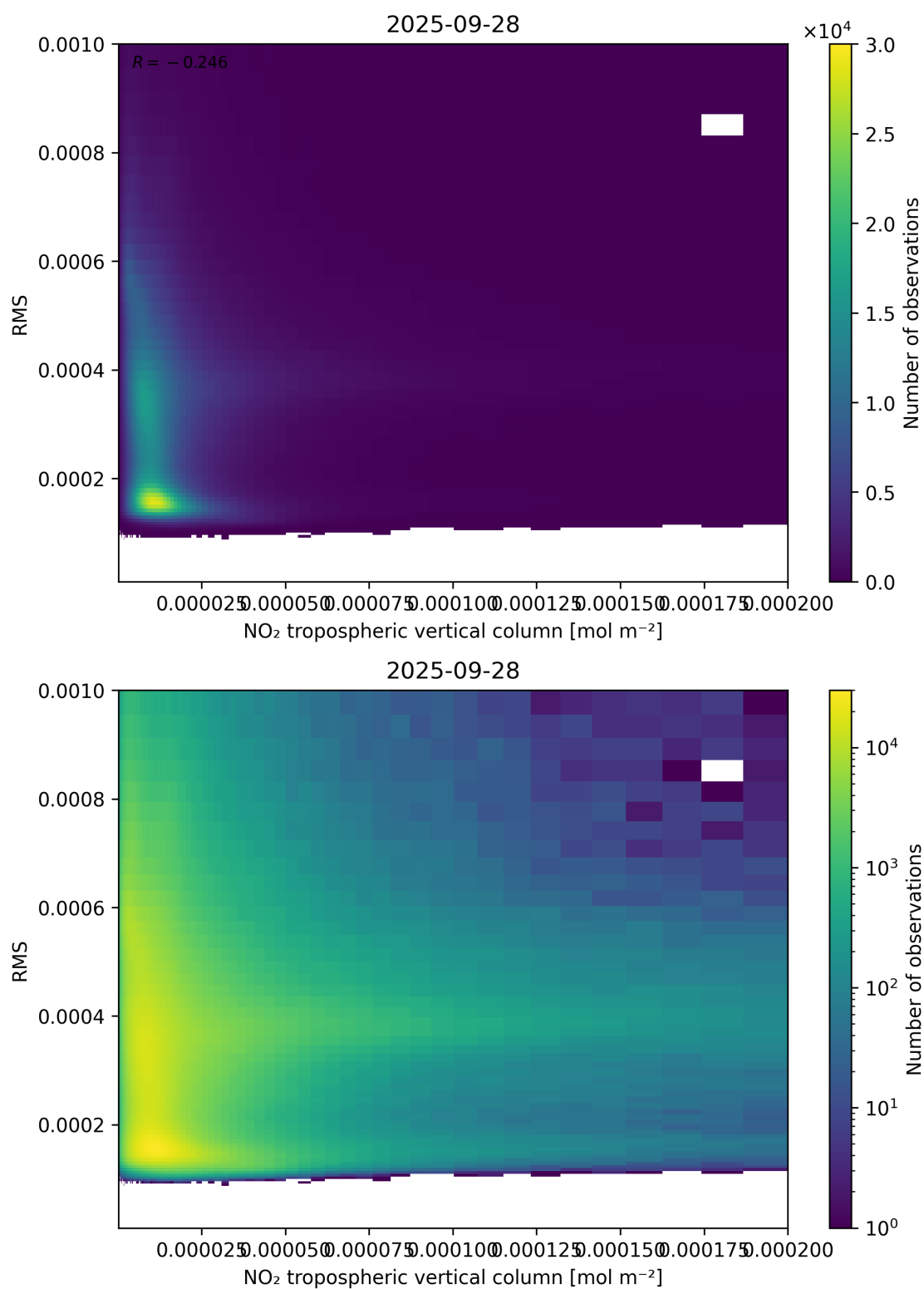
Figure 142: Scatter density plot of “NO 2 tropospheric vertical column” against “RMS” for 2025-09-27 to 2025-09-29.
