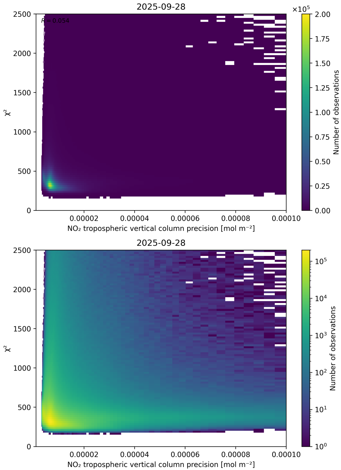
Figure 134: Scatter density plot of “NO 2 tropospheric vertical column precision” against “ \chi^2 ” for 2025-09-27 to 2025-09-29.
