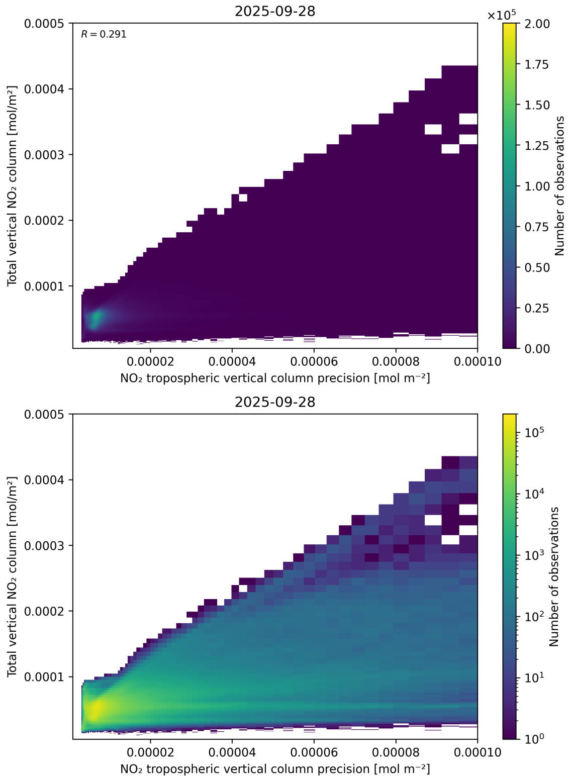
Figure 138: Scatter density plot of “NO 2 tropospheric vertical column precision” against “Total vertical NO 2 column” for 2025-09-27 to 2025-09-29.
