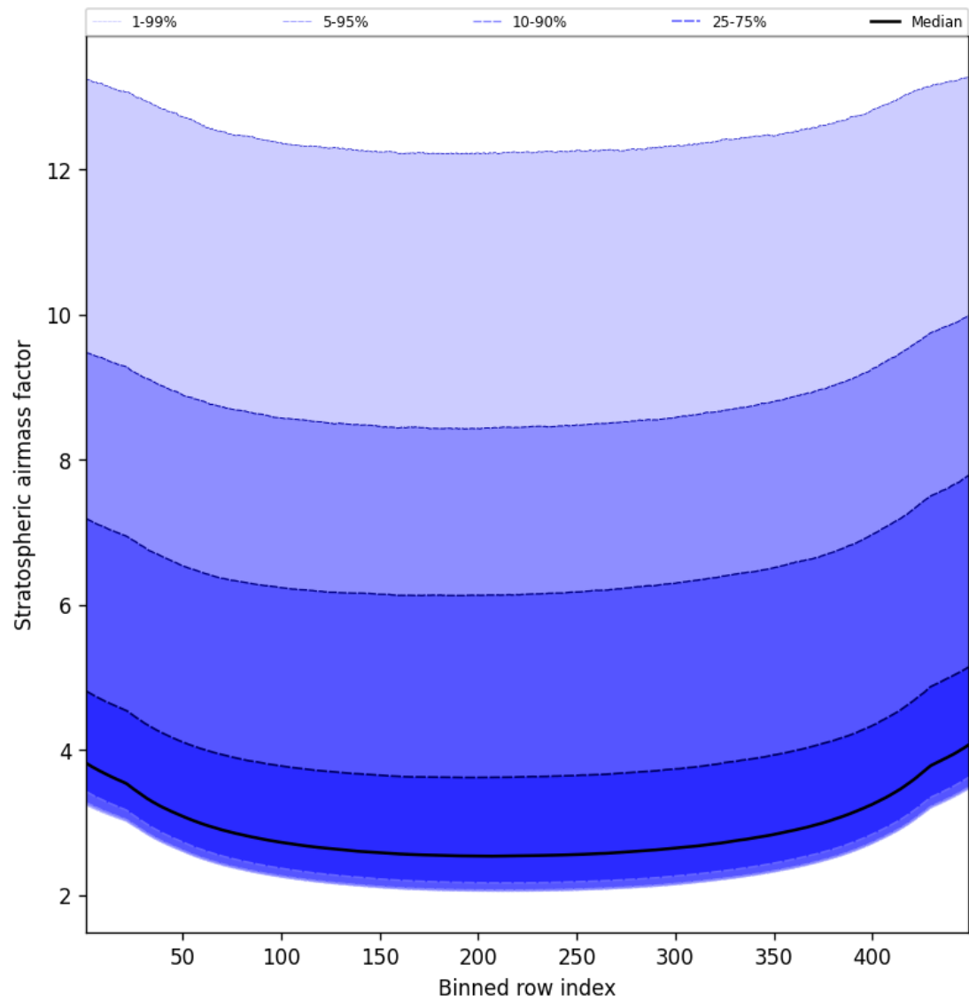
Figure 61: Along track statistics of “Stratospheric airmass factor” for 2025-09-27 to 2025-09-29
