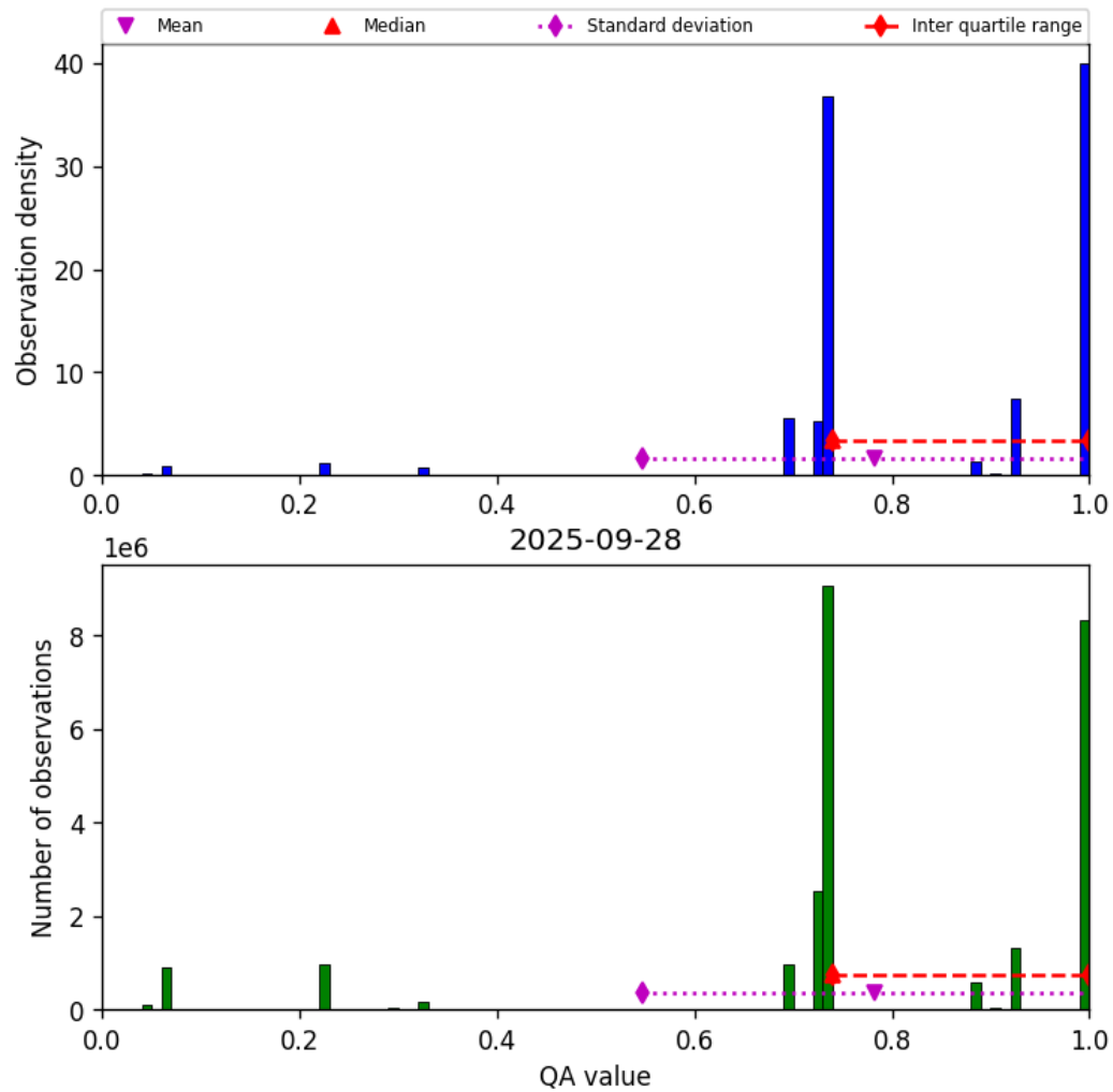
Figure 28: Histogram of “QA value” for 2025-09-27 to 2025-09-29
