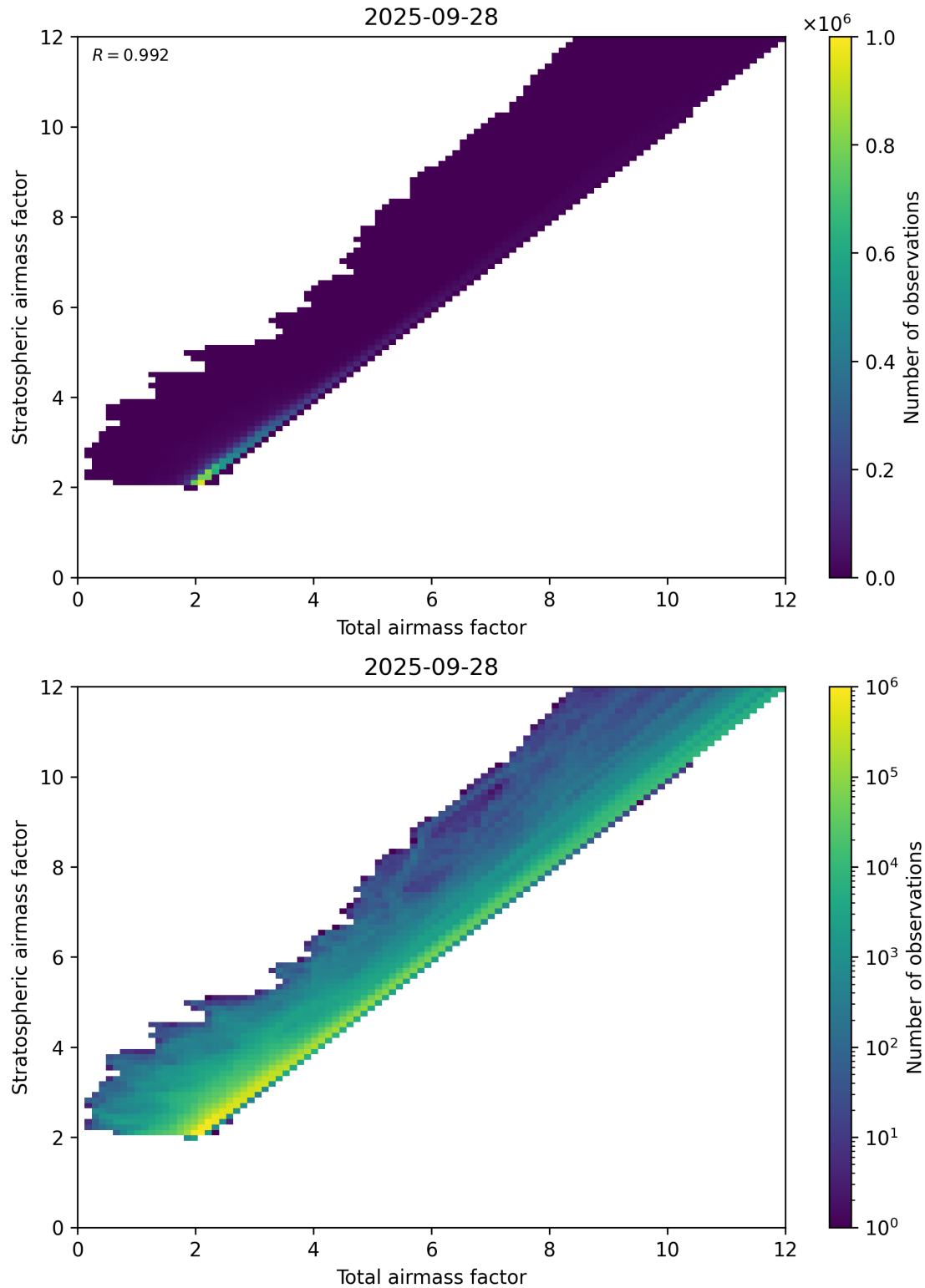
Figure 62: Scatter density plot of “Total airmass factor” against “Stratospheric airmass factor” for 2025-09-27 to 2025-09-29.
