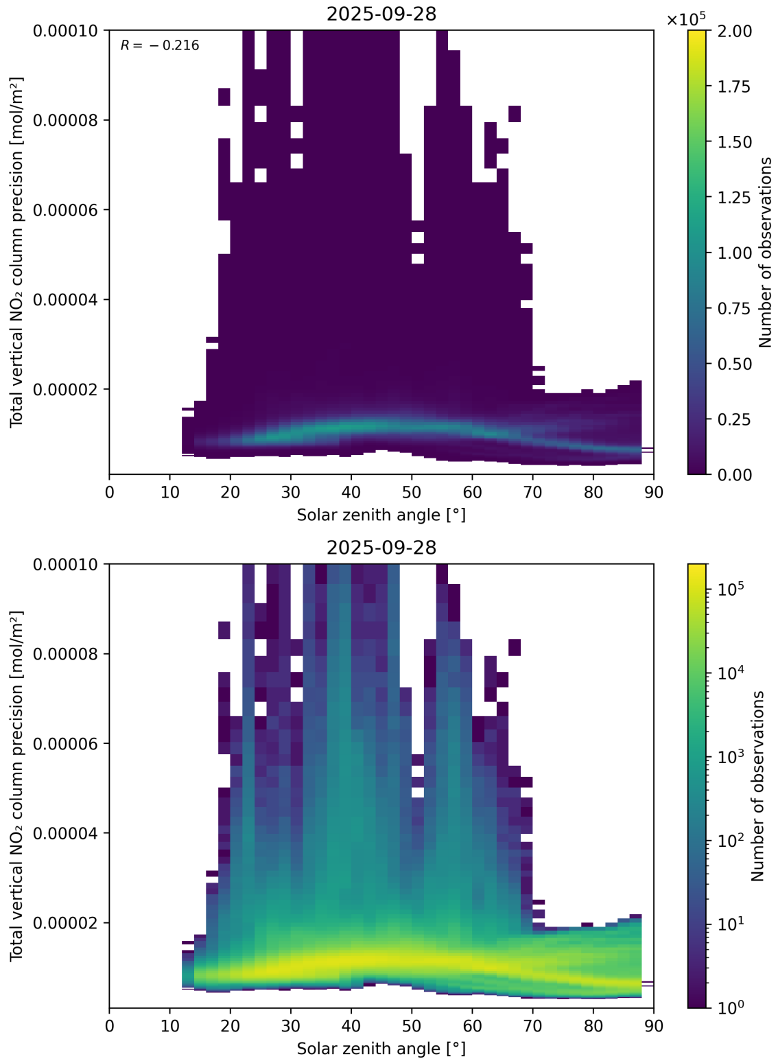
Figure 154: Scatter density plot of “Solar zenith angle” against “Total vertical NO 2 column precision” for 2025-09-27 to 2025-09-29.
