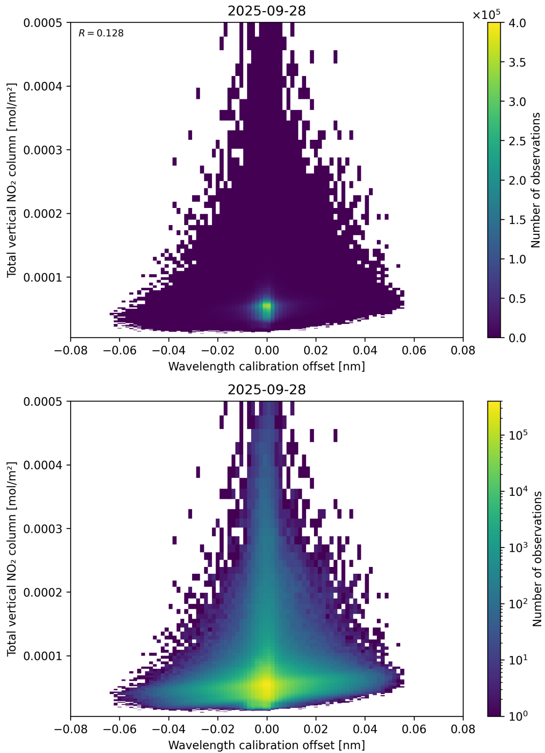
Figure 179: Scatter density plot of “Wavelength calibration offset” against “Total vertical NO 2 column” for 2025-09-27 to 2025-09-29.
