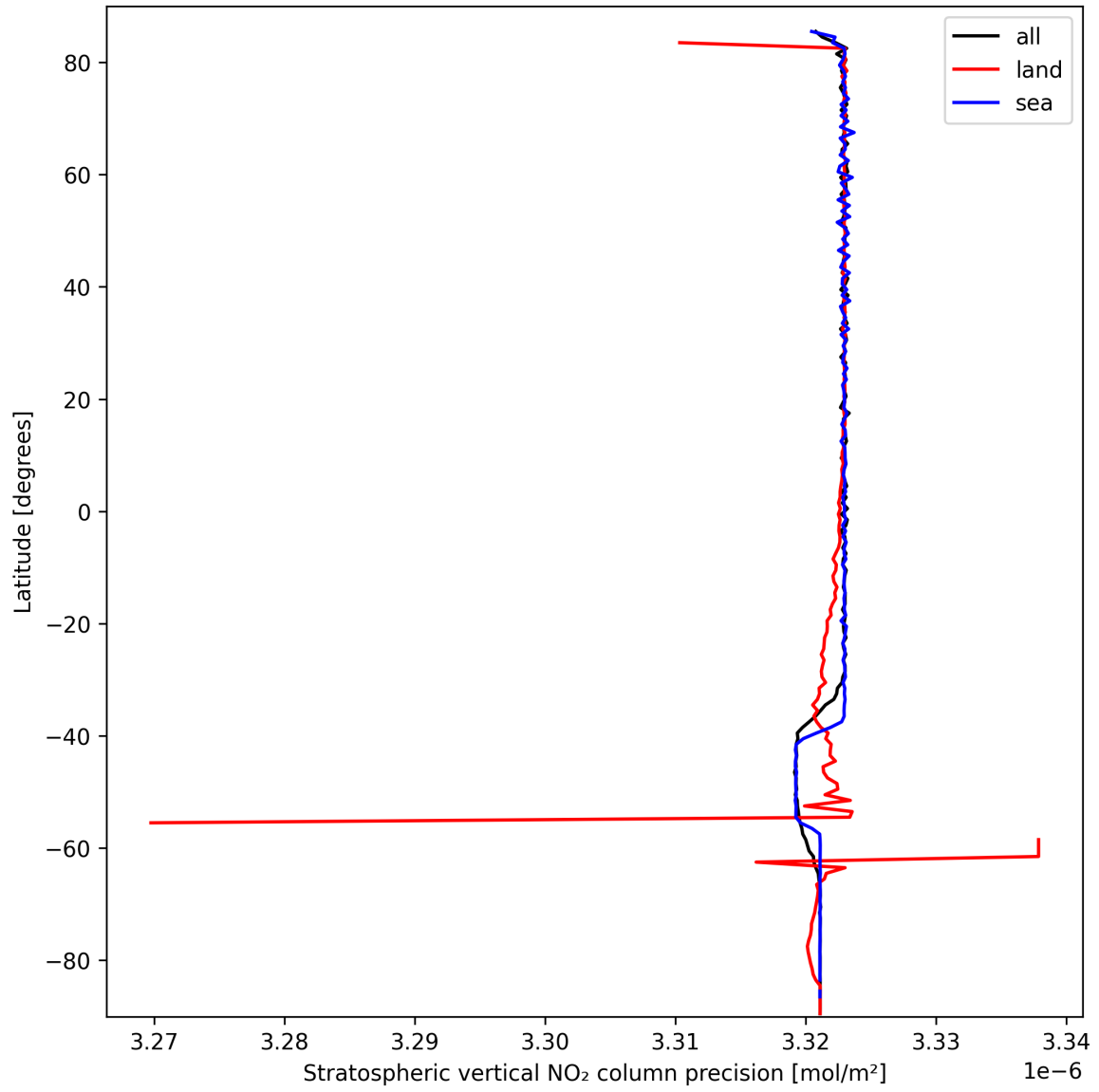
Figure 20: Zonal average of “Stratospheric vertical NO 2 column precision” for 2025-09-27 to 2025-09-29.
