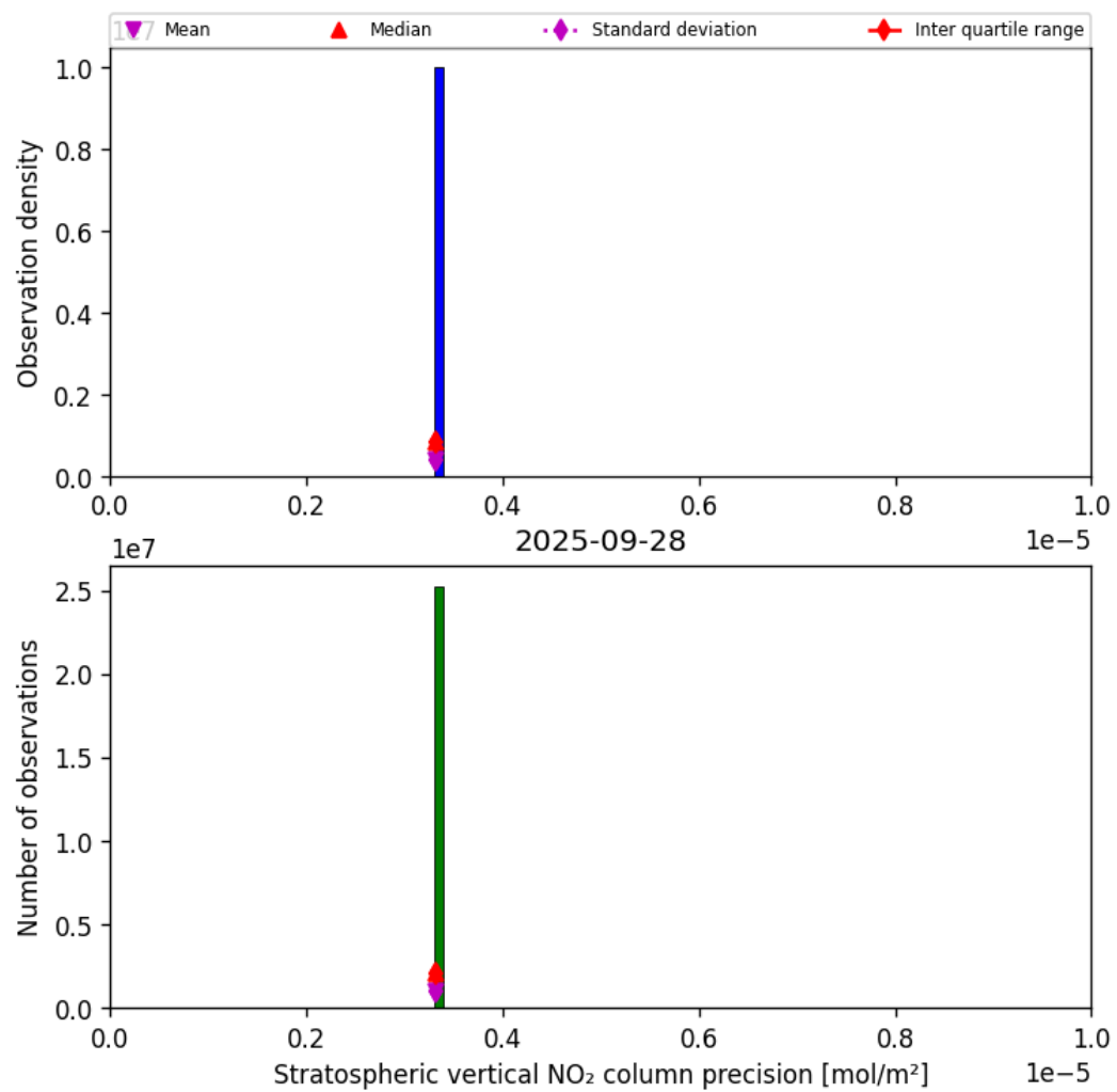
Figure 37: Histogram of “Stratospheric vertical NO 2 column precision” for 2025-09-27 to 2025-09-29
