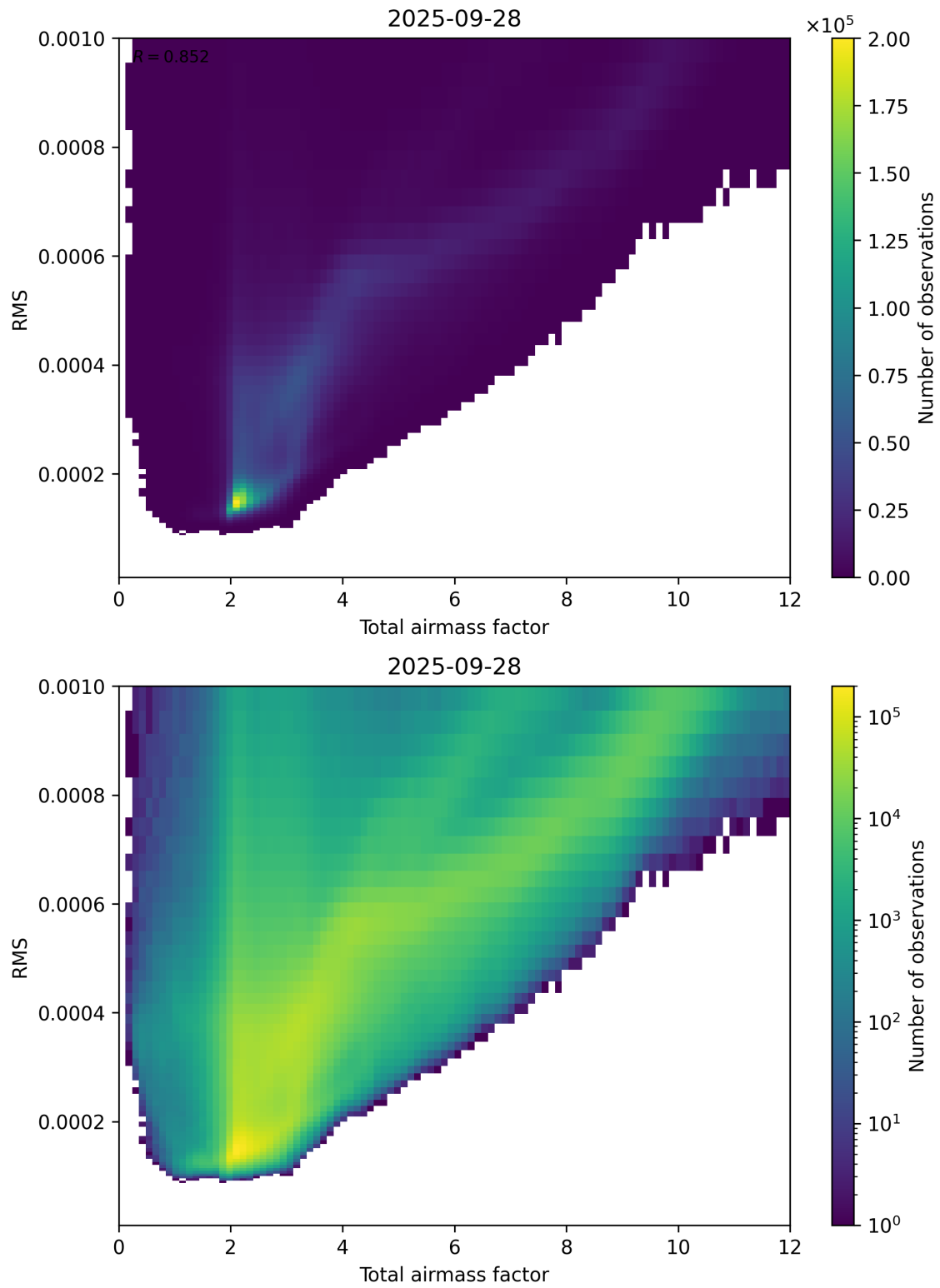
Figure 69: Scatter density plot of “Total airmass factor” against “RMS” for 2025-09-27 to 2025-09-29.
