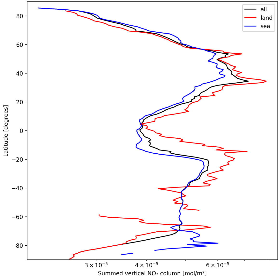
Figure 23: Zonal average of “Summed vertical NO 2 column” for 2025-09-27 to 2025-09-29.
