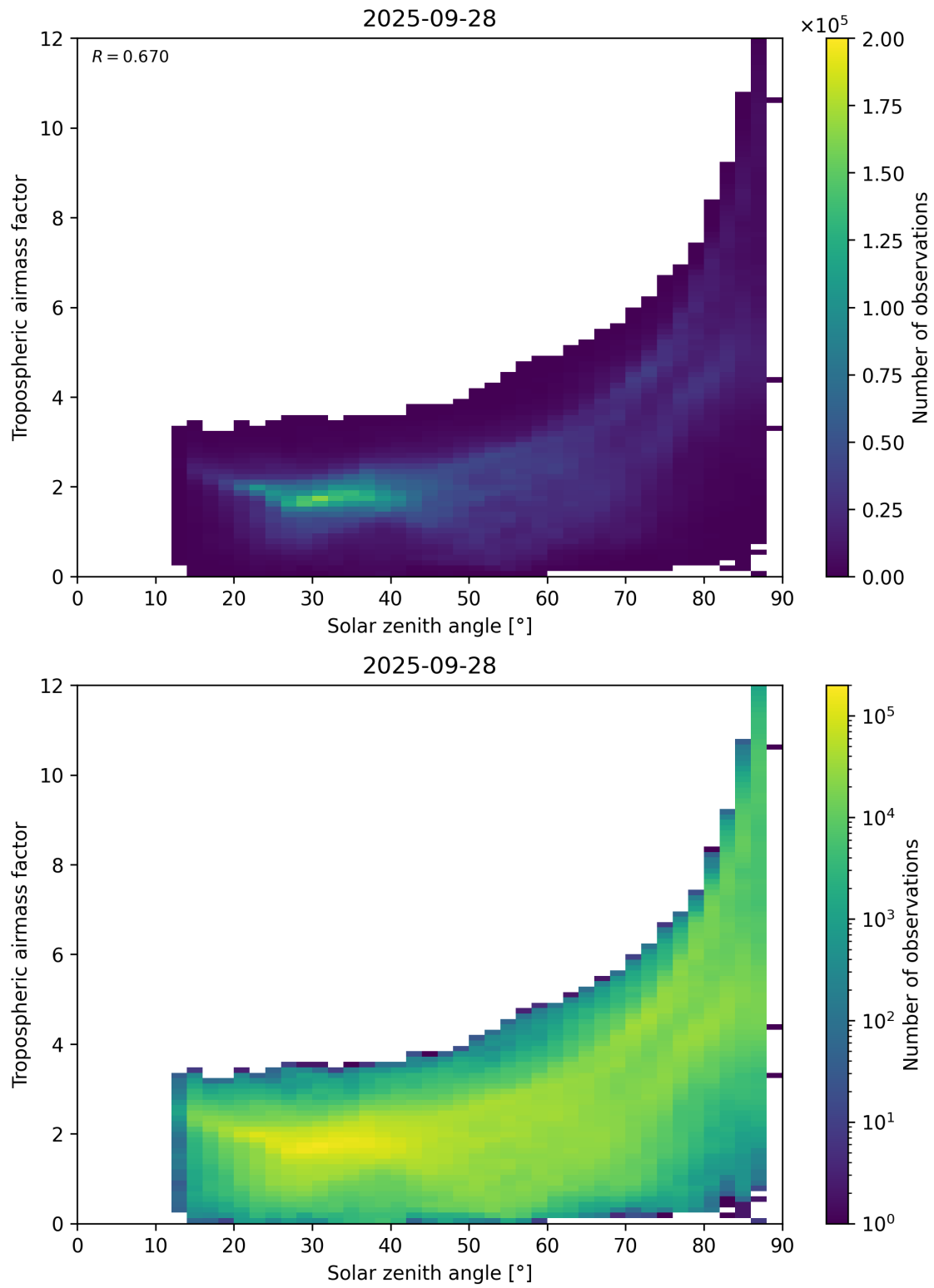
Figure 147: Scatter density plot of “Solar zenith angle” against “Tropospheric airmass factor” for 2025-09-27 to 2025-09-29.
