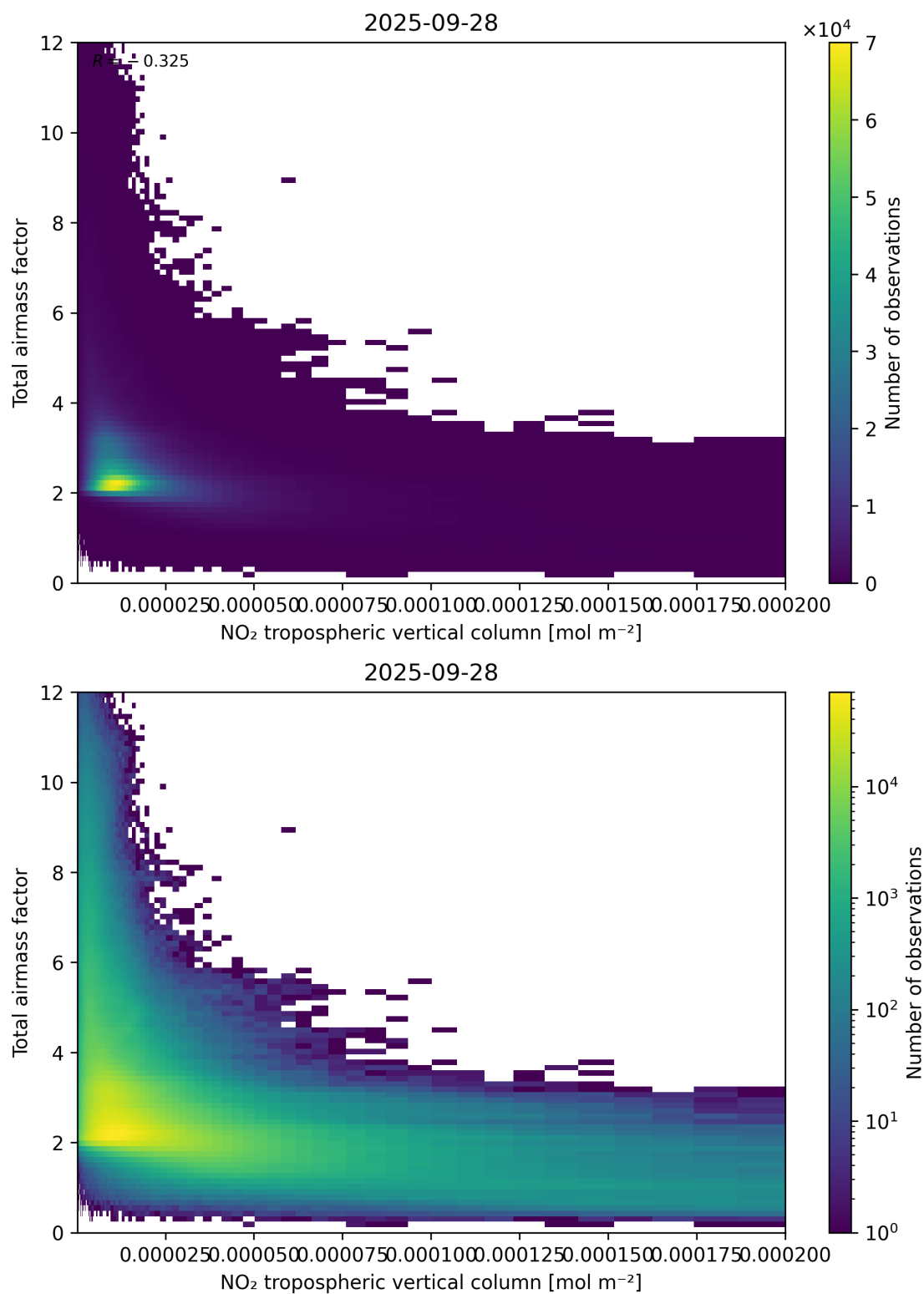
Figure 122: Scatter density plot of “NO 2 tropospheric vertical column” against “Total air mass factor” for 2025-09-27 to 2025-09-29.
