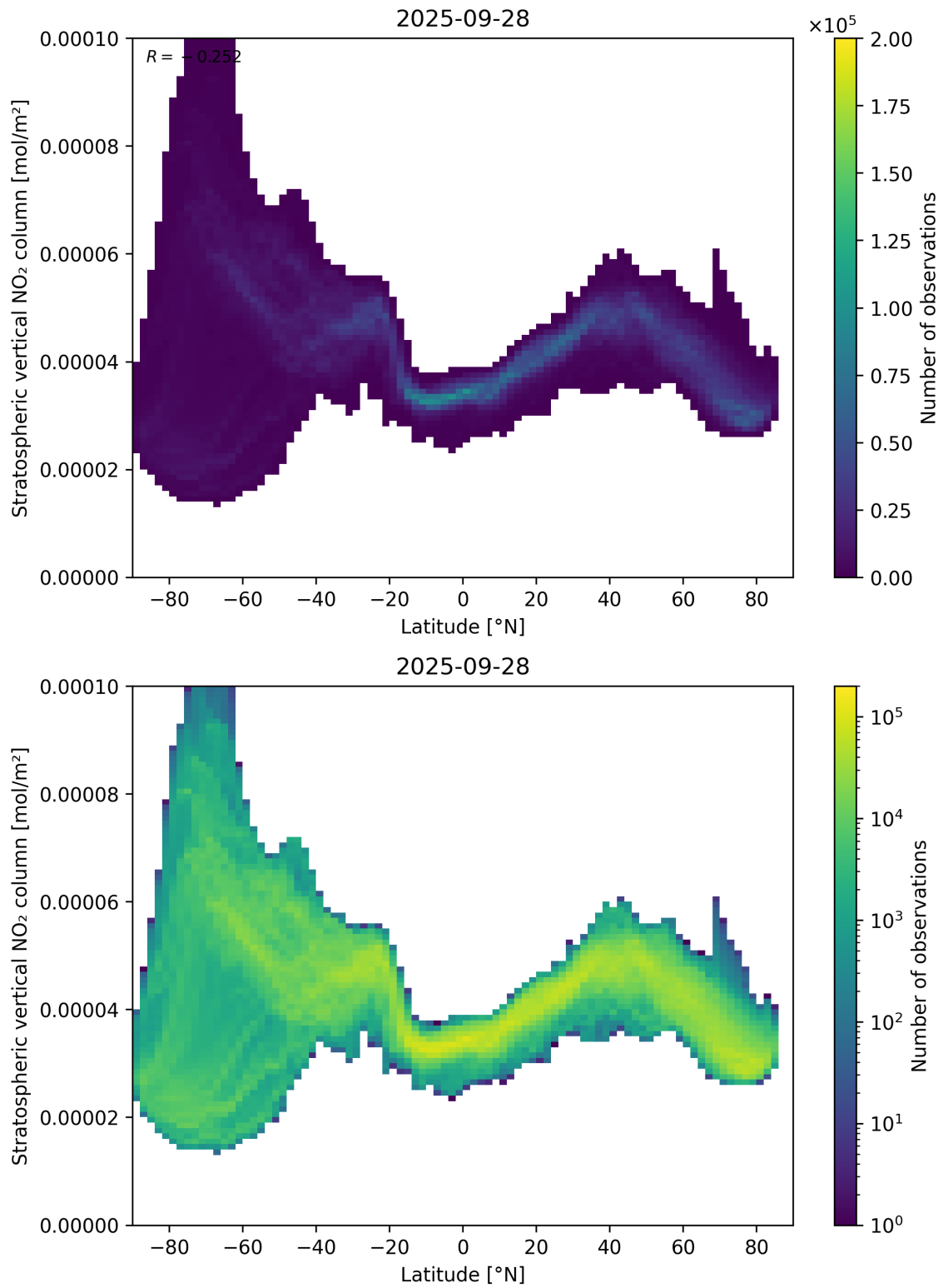
Figure 87: Scatter density plot of “Latitude” against “Stratospheric vertical NO 2 column” for 2025-09-27 to 2025-09-29.
