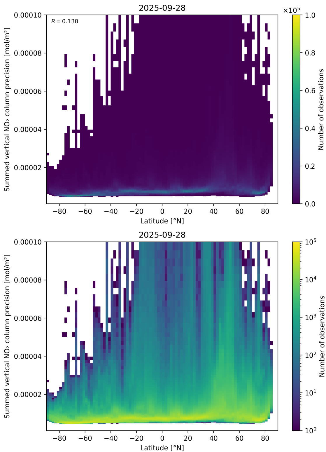
Figure 89: Scatter density plot of “Latitude” against “Summed vertical NO 2 column precision” for 2025-09-27 to 2025-09-29.
