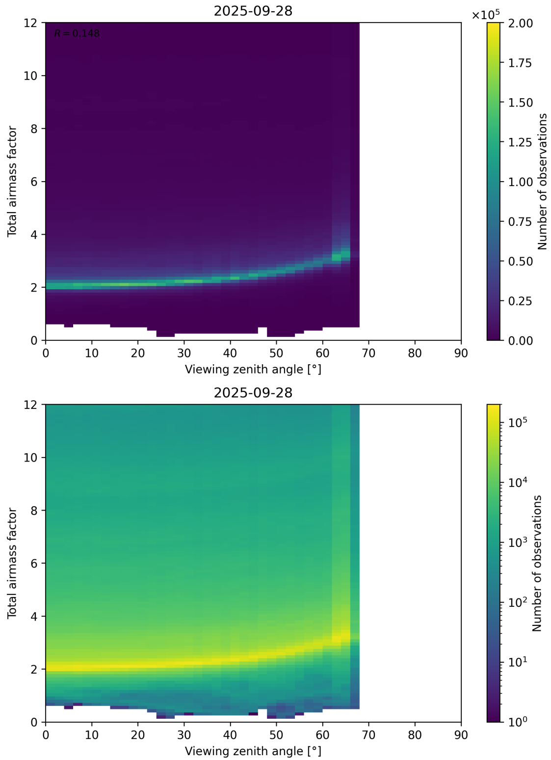
Figure 160: Scatter density plot of “Viewing zenith angle” against “Total airmass factor” for 2025-09-27 to 2025-09-29.
