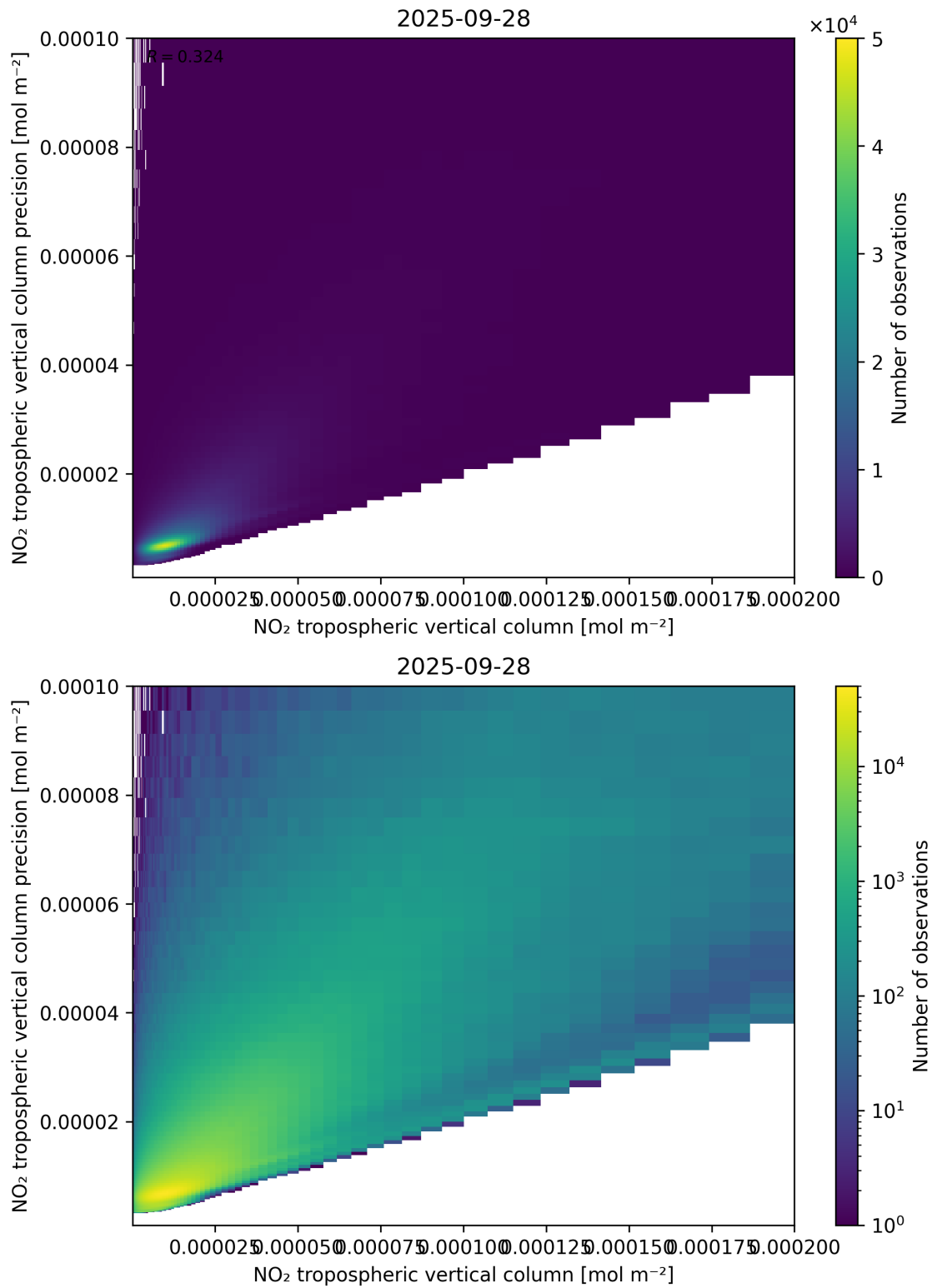
Figure 130: Scatter density plot of “NO 2 tropospheric vertical column” against “NO 2 tropospheric vertical column precision” for 2025-09-27 to 2025-09-29.
