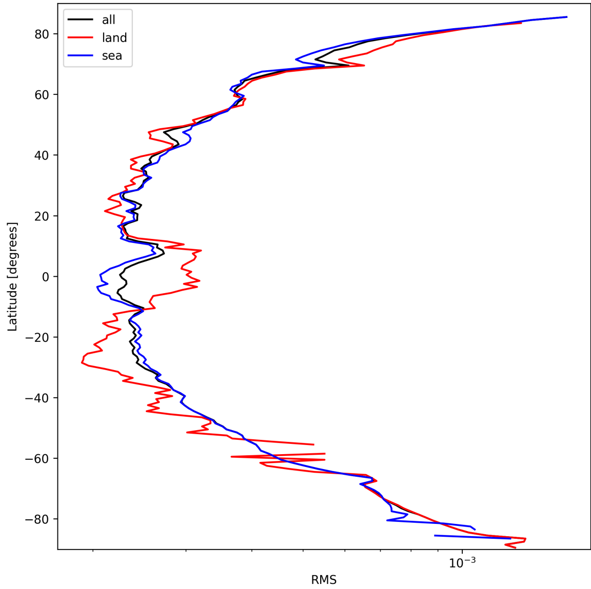
Figure 26: Zonal average of “RMS” for 2025-09-27 to 2025-09-29.
