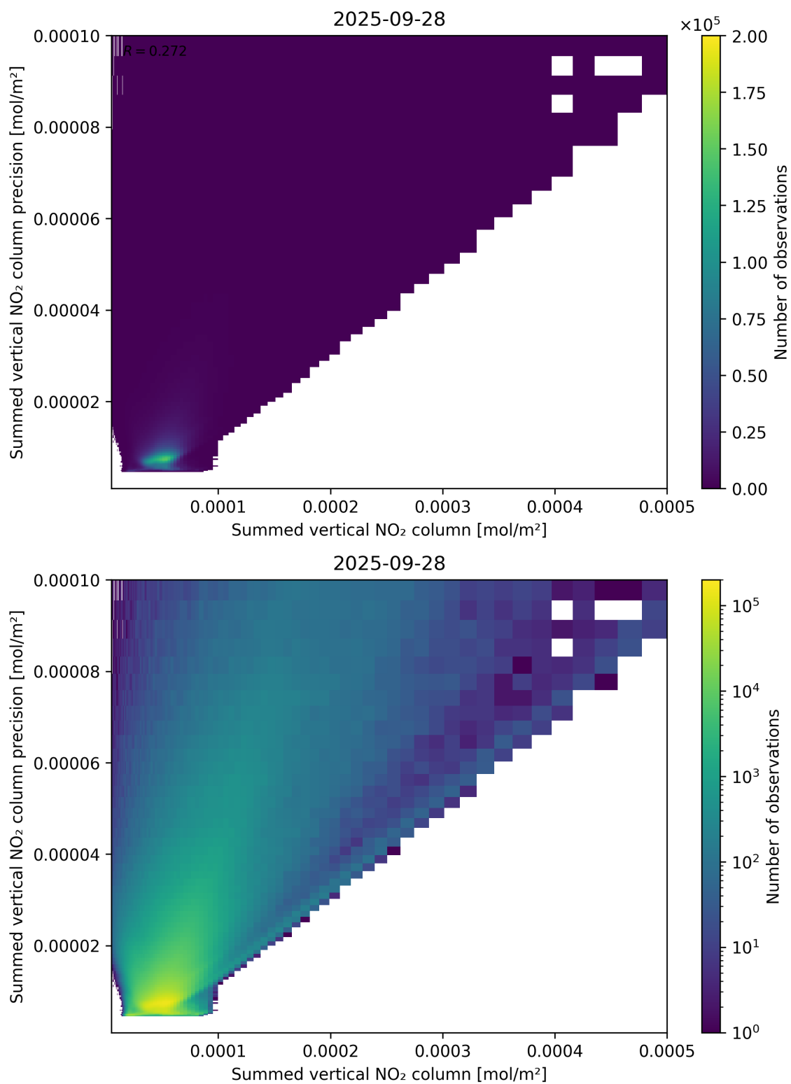
Figure 105: Scatter density plot of “Summed vertical NO 2 column” against “Summed vertical NO 2 column precision” for 2025-09-27 to 2025-09-29.
