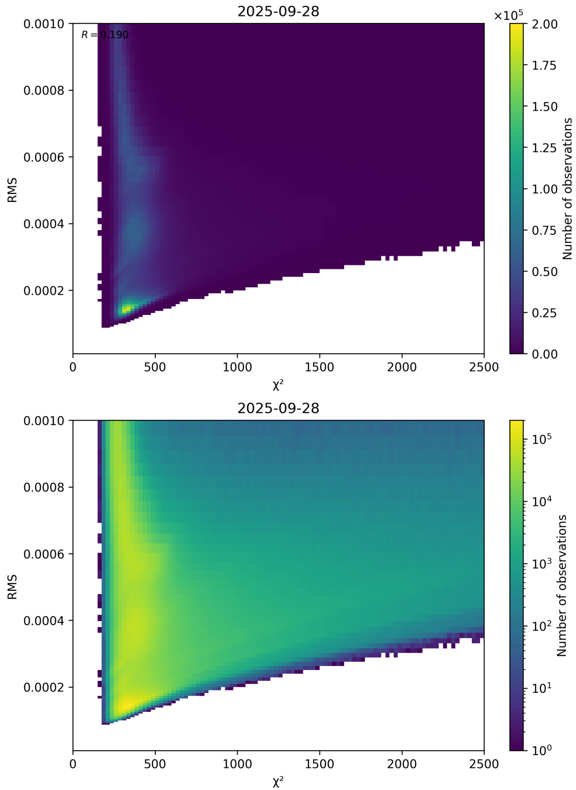
Figure 82: Scatter density plot of “ \chi^2 ” against “RMS” for 2025-09-27 to 2025-09-29.
