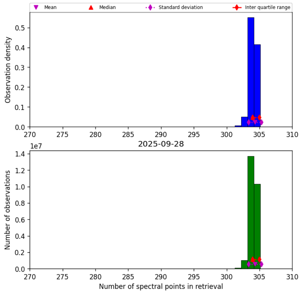
Figure 33: Histogram of “Number of spectral points in retrieval” for 2025-09-27 to 2025-09-29
