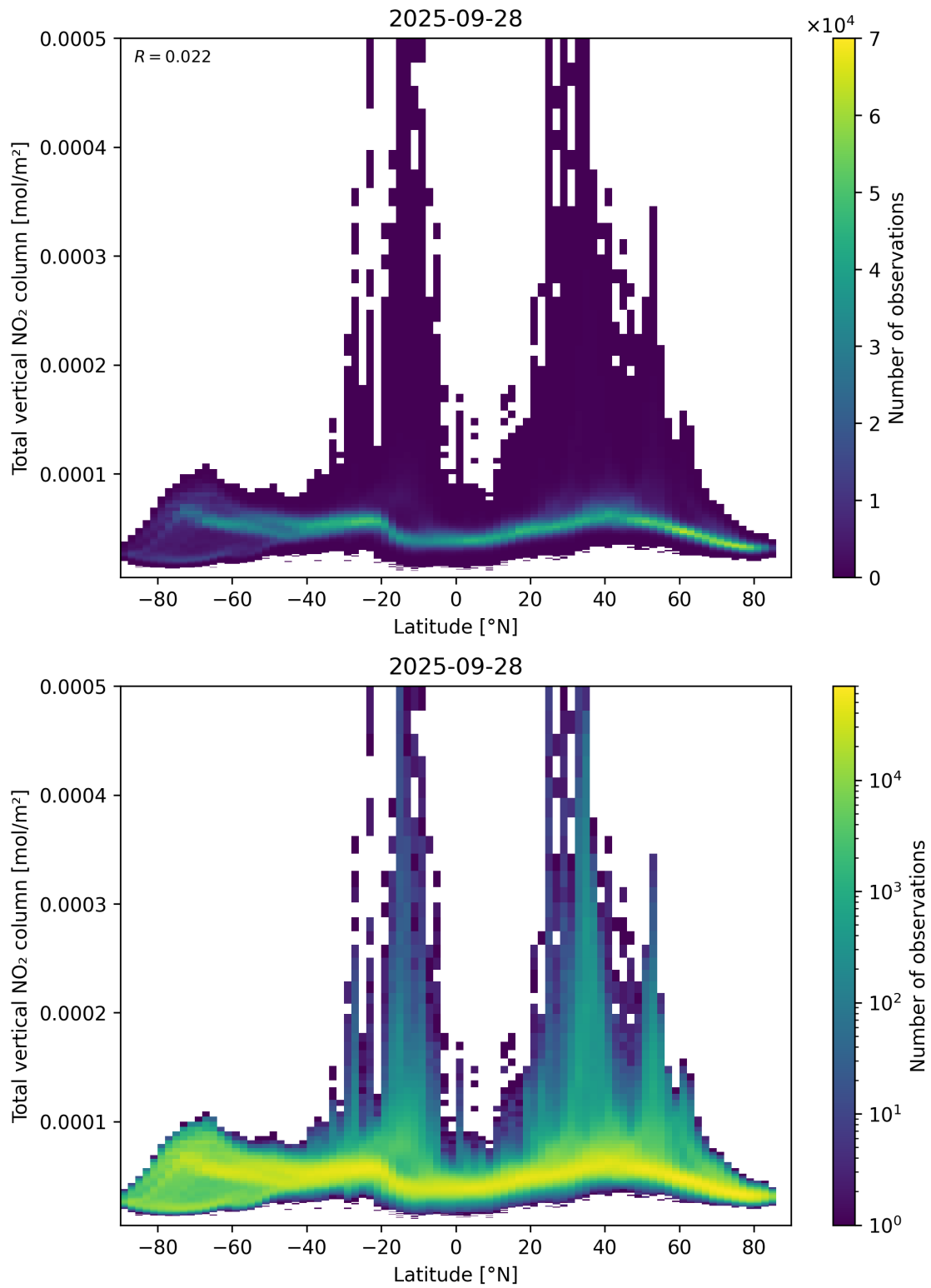
Figure 90: Scatter density plot of “Latitude” against “Total vertical NO 2 column” for 2025-09-27 to 2025-09-29.
