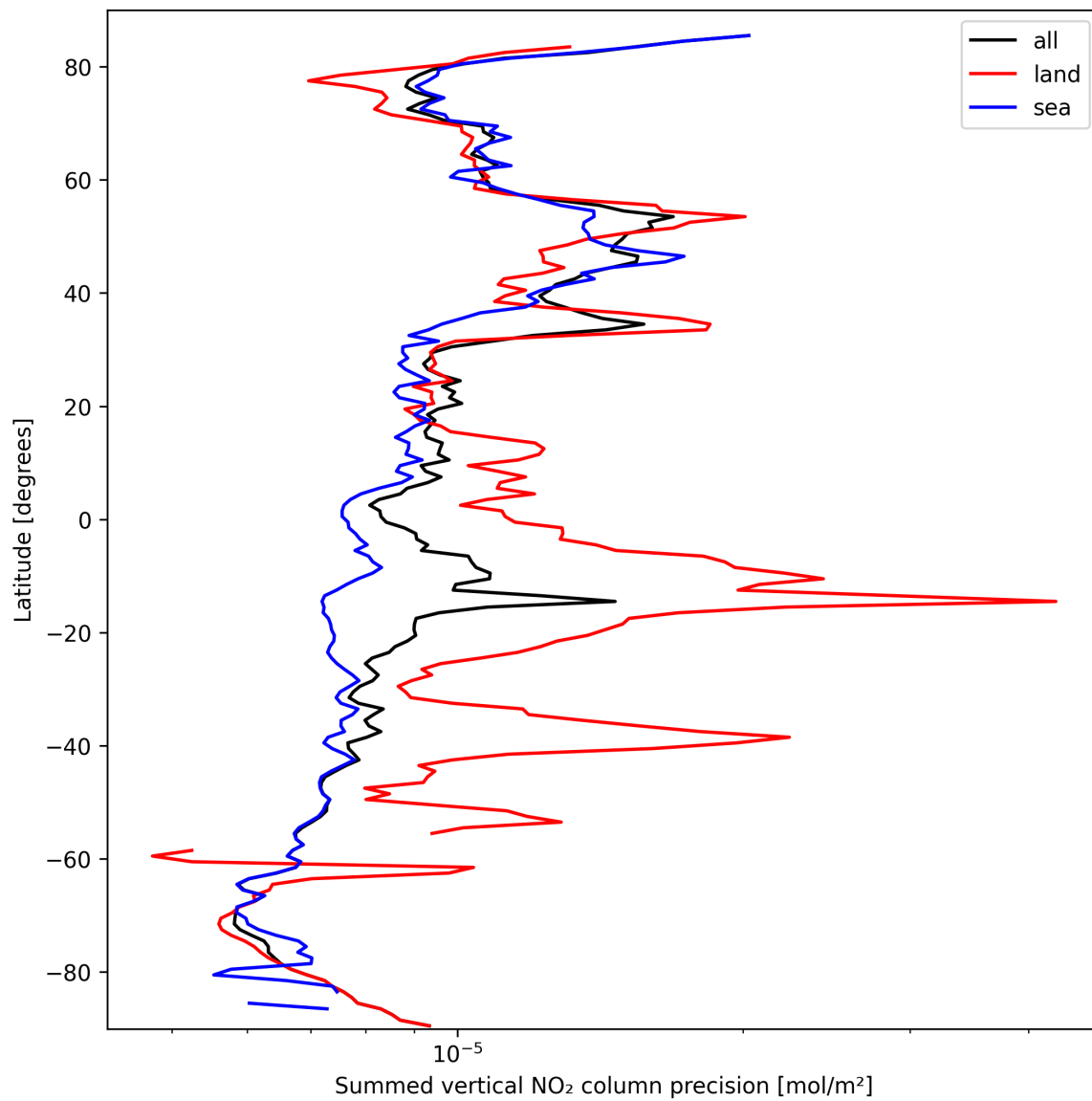
Figure 24: Zonal average of “Summed vertical NO 2 column precision” for 2025-09-27 to 2025-09-29.
