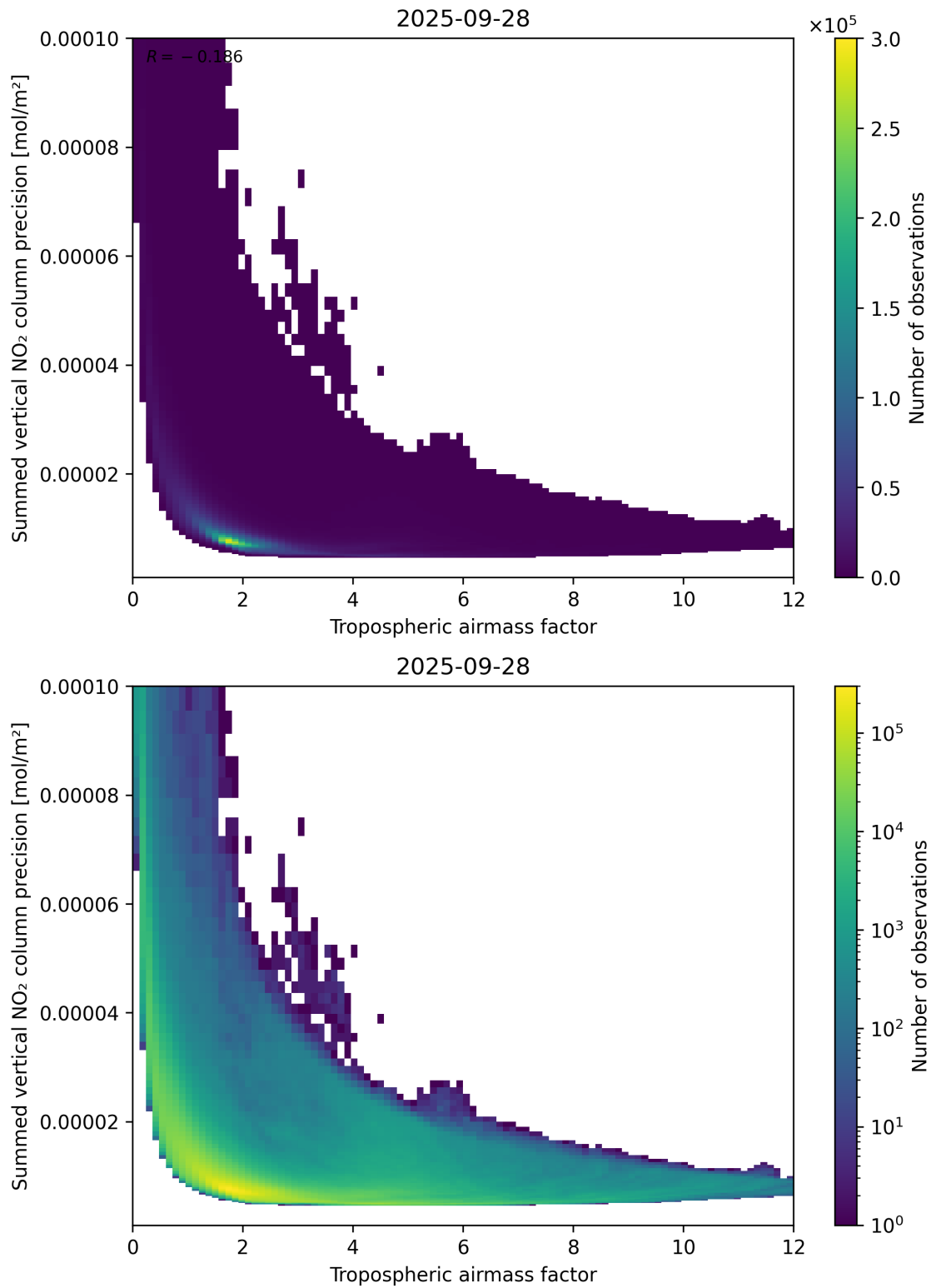
Figure 76: Scatter density plot of “Tropospheric air mass factor” against “Summed vertical NO 2 column precision” for 2025-09-27 to 2025-09-29.
