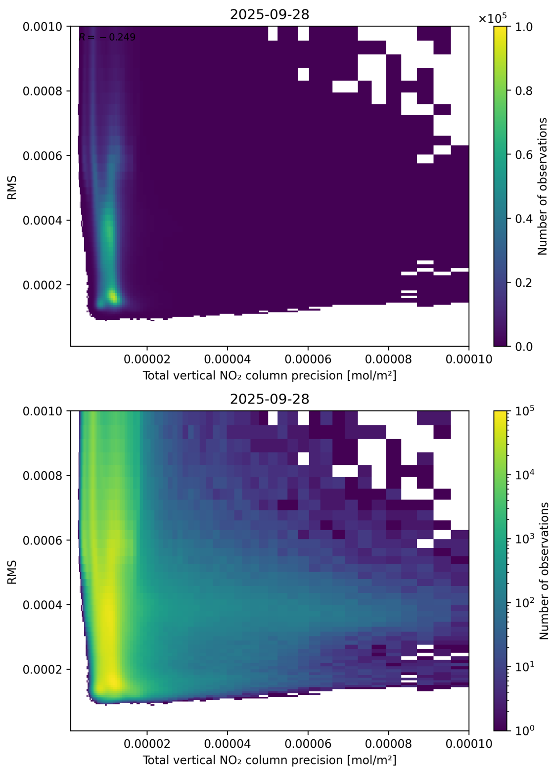
Figure 119: Scatter density plot of “Total vertical NO 2 column precision” against “RMS” for 2025-09-27 to 2025-09-29.
