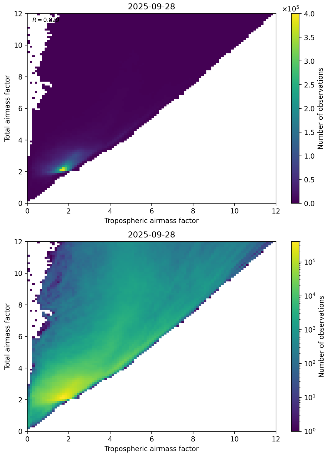
Figure 72: Scatter density plot of “Tropospheric airmass factor” against “Total airmass factor” for 2025-09-27 to 2025-09-29.
