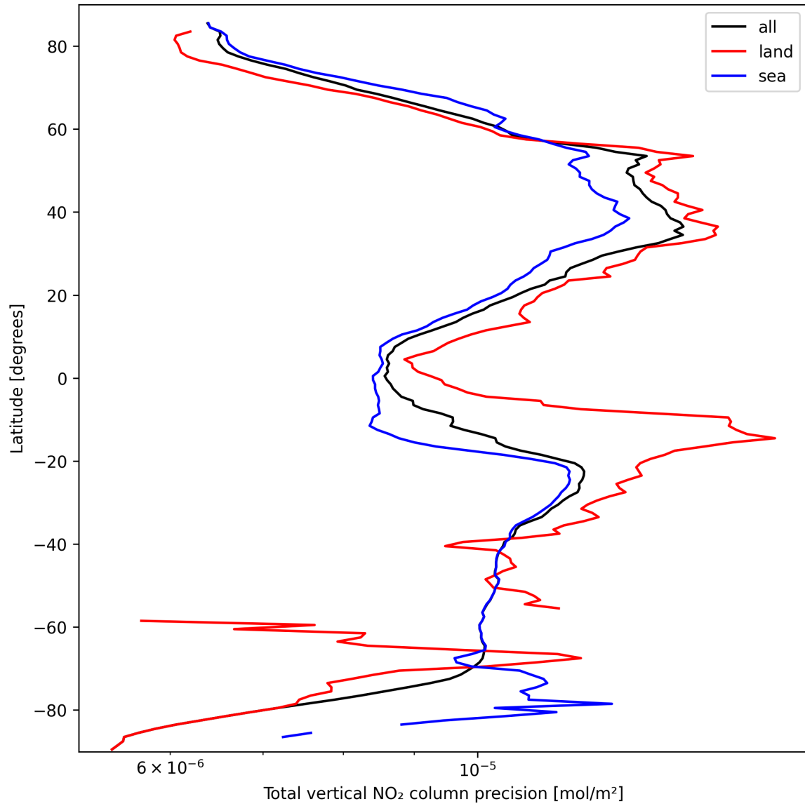
Figure 22: Zonal average of “Total vertical NO 2 column precision” for 2025-09-27 to 2025-09-29.
