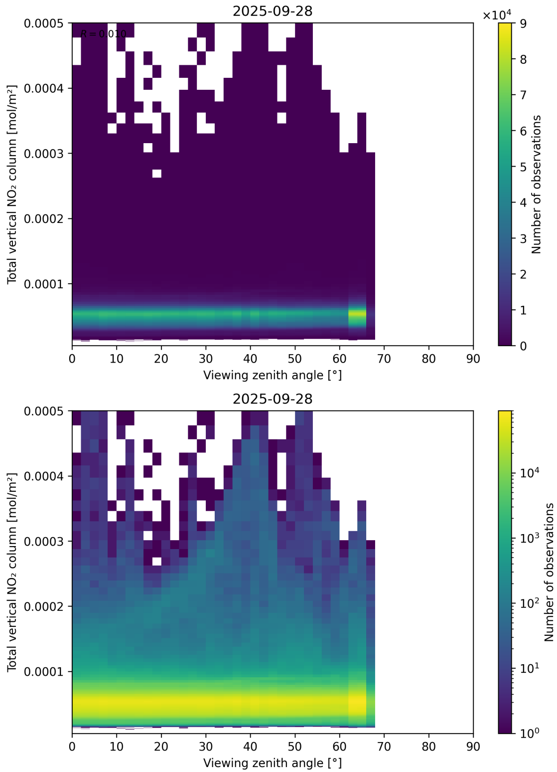
Figure 167: Scatter density plot of “Viewing zenith angle” against “Total vertical NO 2 column” for 2025-09-27 to 2025-09-29.
