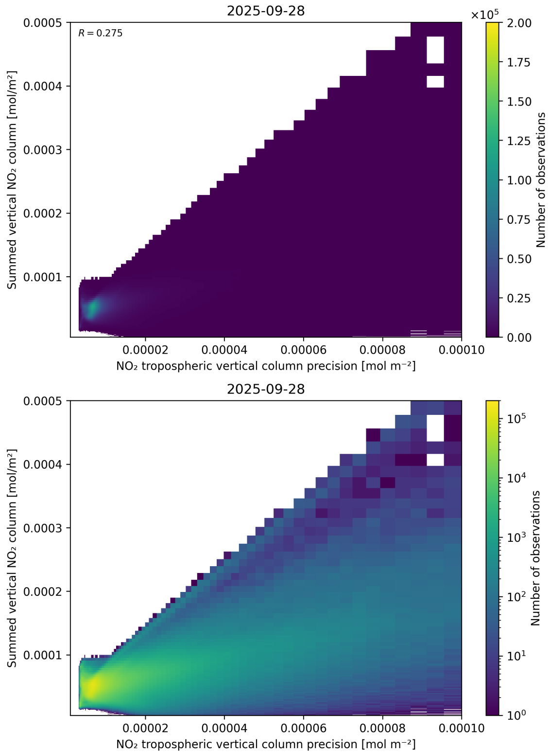
Figure 136: Scatter density plot of “NO 2 tropospheric vertical column precision” against “Summed vertical NO 2 column” for 2025-09-27 to 2025-09-29.
