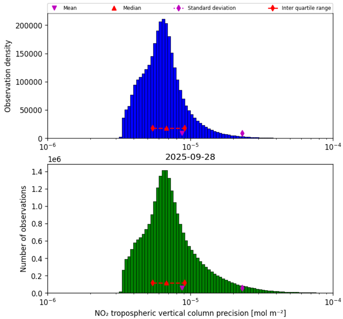
Figure 30: Histogram of “NO 2 tropospheric vertical column precision” for 2025-09-27 to 2025-09-29
