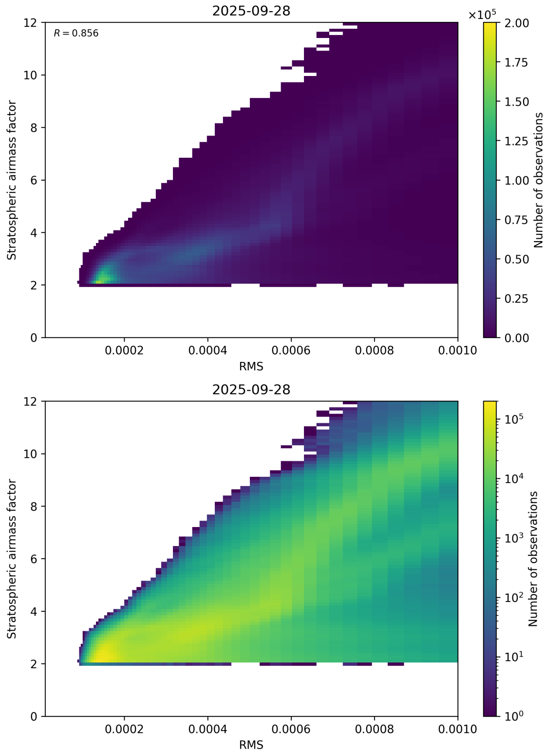
Figure 144: Scatter density plot of “RMS” against “Stratospheric airmass factor” for 2025-09-27 to 2025-09-29.
