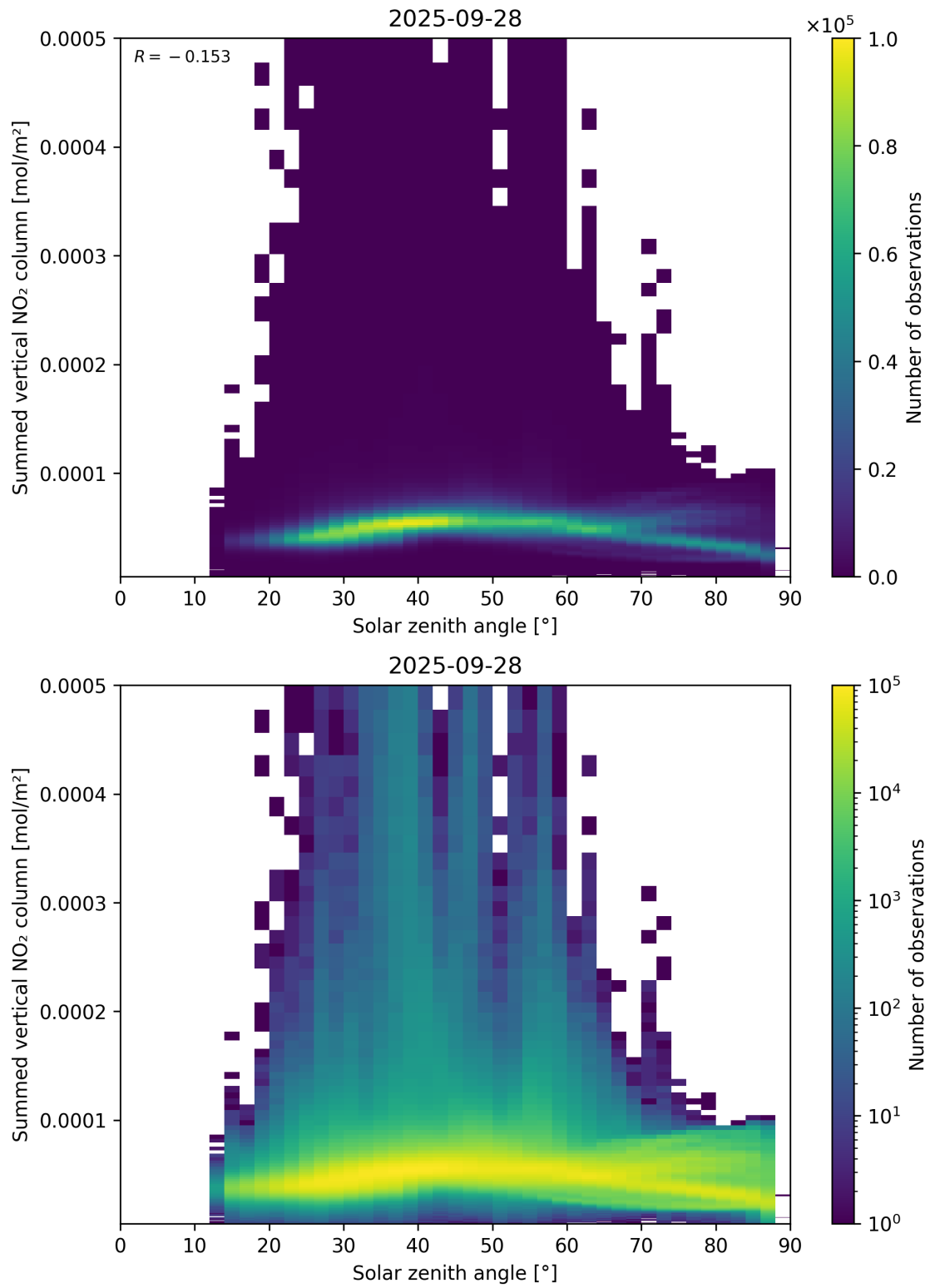
Figure 151: Scatter density plot of “Solar zenith angle” against “Summed vertical NO 2 column” for 2025-09-27 to 2025-09-29.
