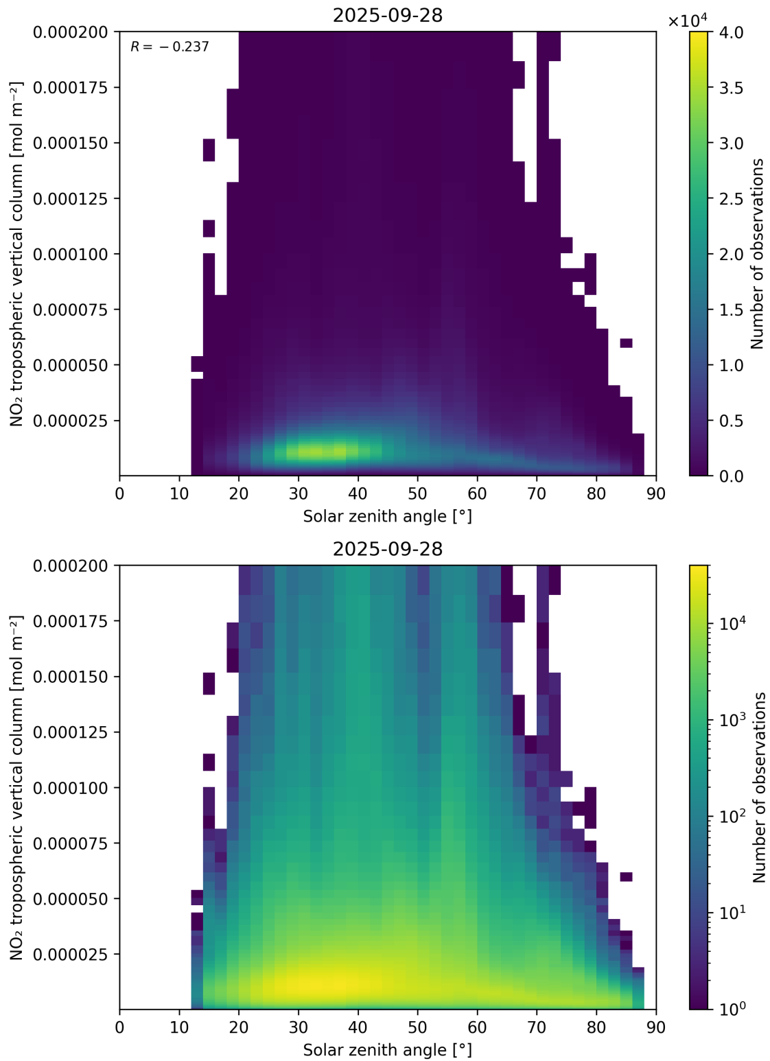
Figure 155: Scatter density plot of “Solar zenith angle” against “NO 2 tropospheric vertical column” for 2025-09-27 to 2025-09-29.
