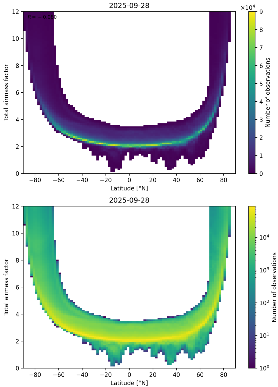
Figure 84: Scatter density plot of “Latitude” against “Total airmass factor” for 2025-09-27 to 2025-09-29.
