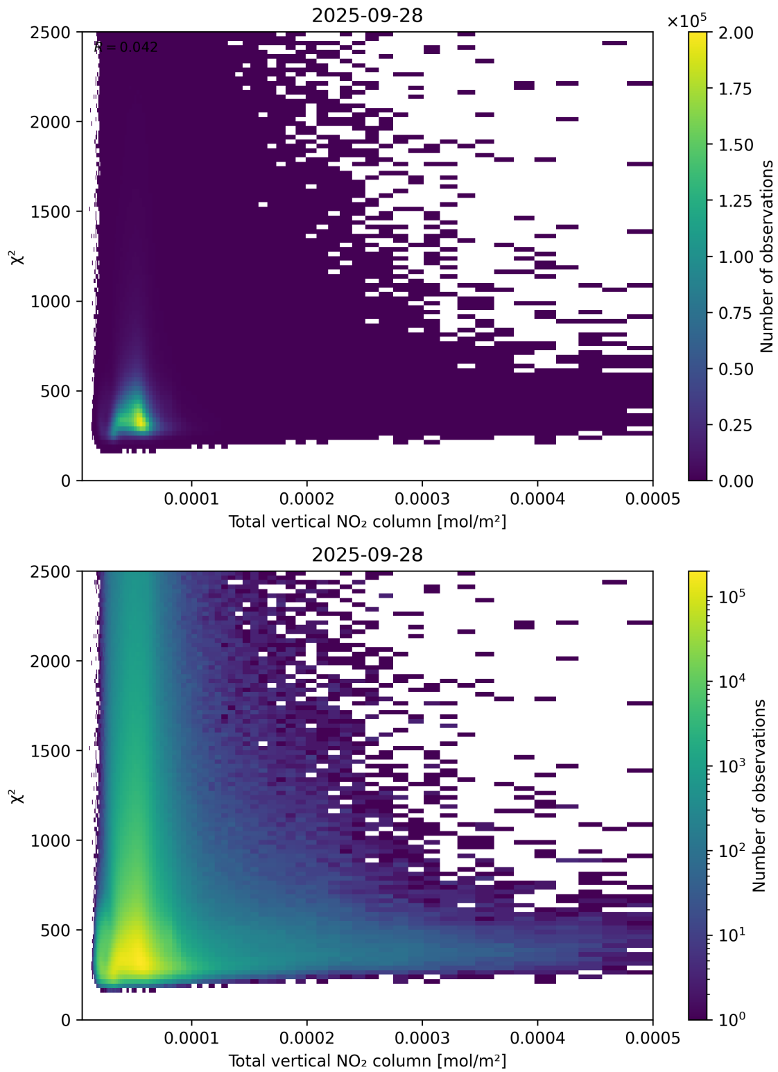
Figure 111: Scatter density plot of “Total vertical NO 2 column” against “ \chi^2 ” for 2025-09-27 to 2025-09-29.
