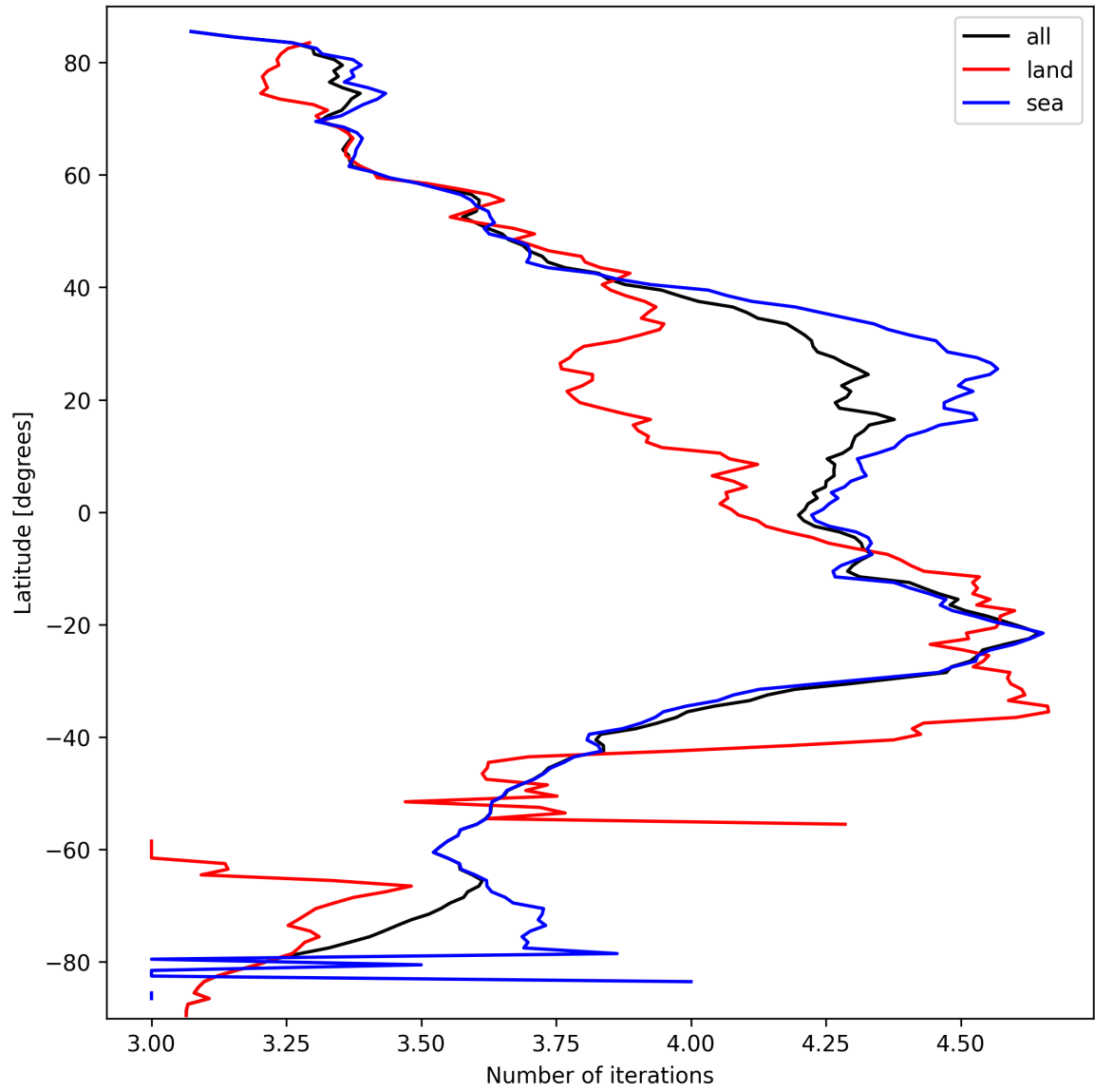
Figure 17: Zonal average of “Number of iterations” for 2025-09-27 to 2025-09-29.
