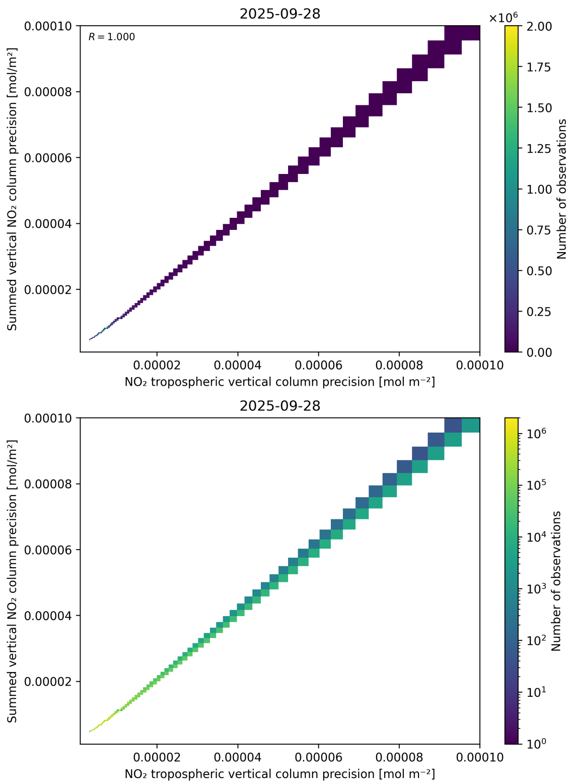
Figure 137: Scatter density plot of “NO 2 tropospheric vertical column precision” against “Summed vertical NO 2 column precision” for 2025-09-27 to 2025-09-29.
