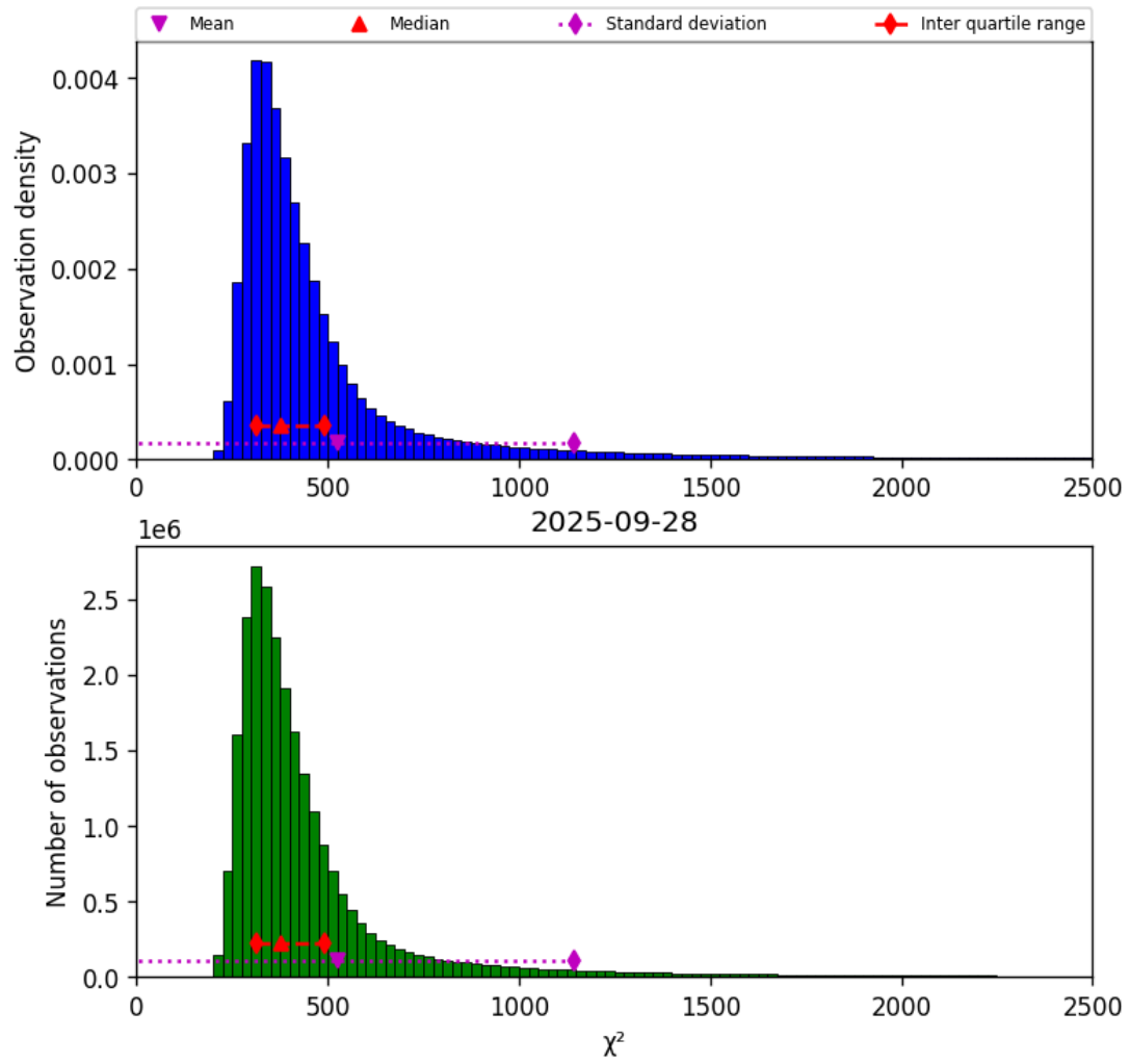
Figure 42: Histogram of “ \chi^2 ” for 2025-09-27 to 2025-09-29
