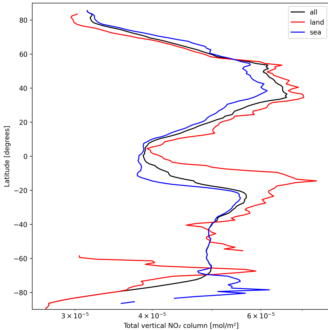
Figure 21: Zonal average of “Total vertical NO 2 column” for 2025-09-27 to 2025-09-29.
