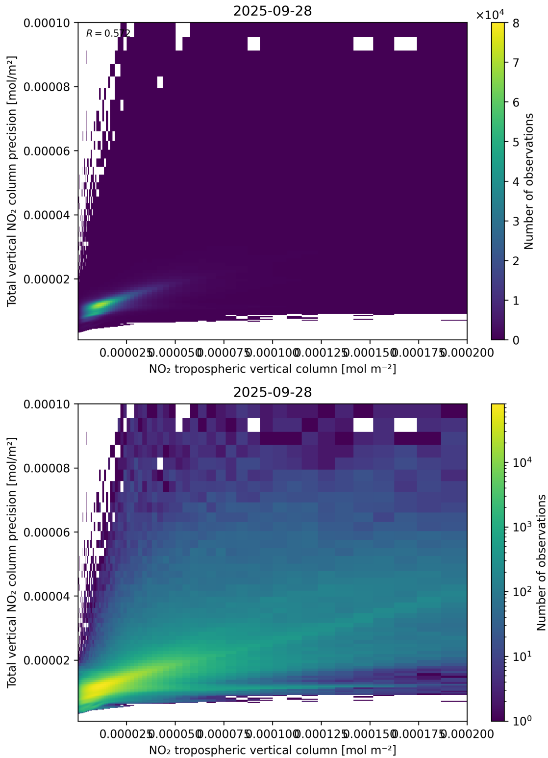
Figure 129: Scatter density plot of “NO 2 tropospheric vertical column” against “Total vertical NO 2 column precision” for 2025-09-27 to 2025-09-29.
