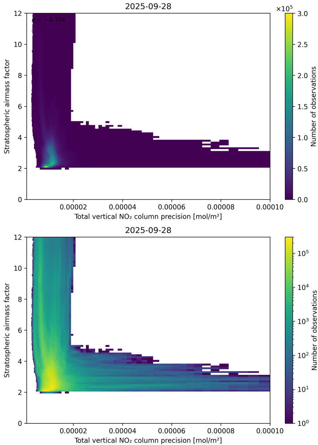
Figure 115: Scatter density plot of “Total vertical NO 2 column precision” against “Stratospheric airmass factor” for 2025-09-27 to 2025-09-29.
