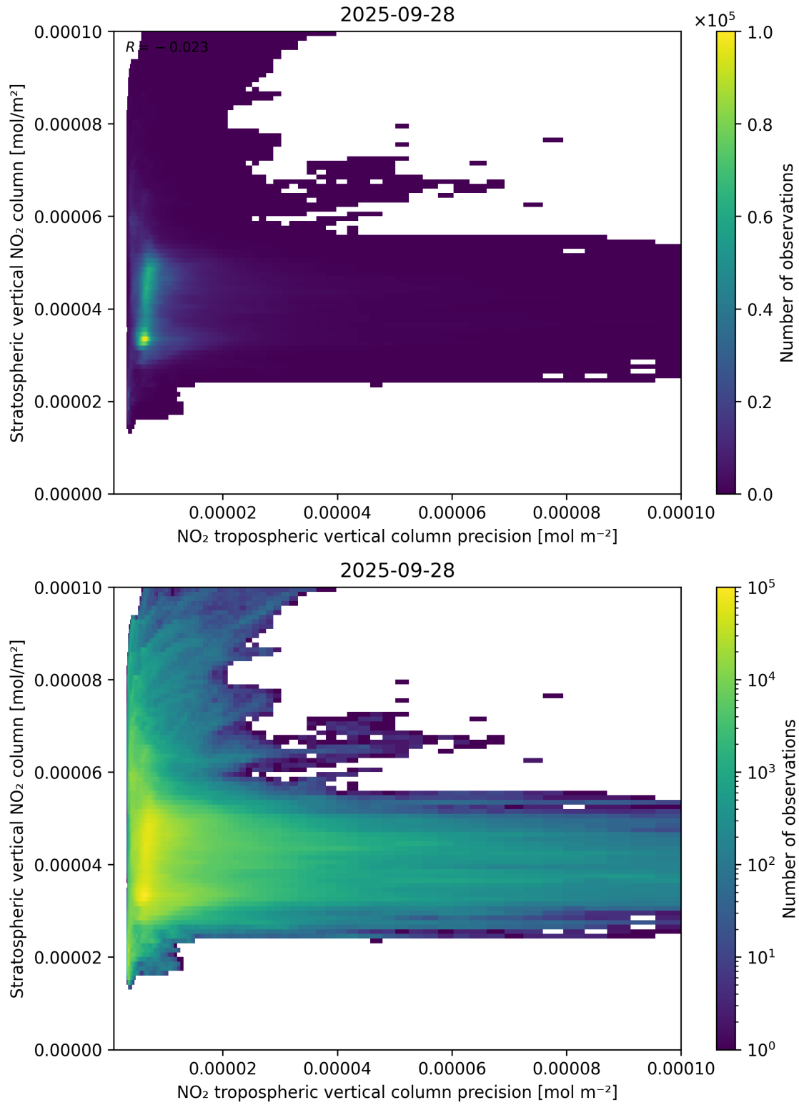
Figure 135: Scatter density plot of “NO 2 tropospheric vertical column precision” against “Stratospheric vertical NO 2 column” for 2025-09-27 to 2025-09-29.
