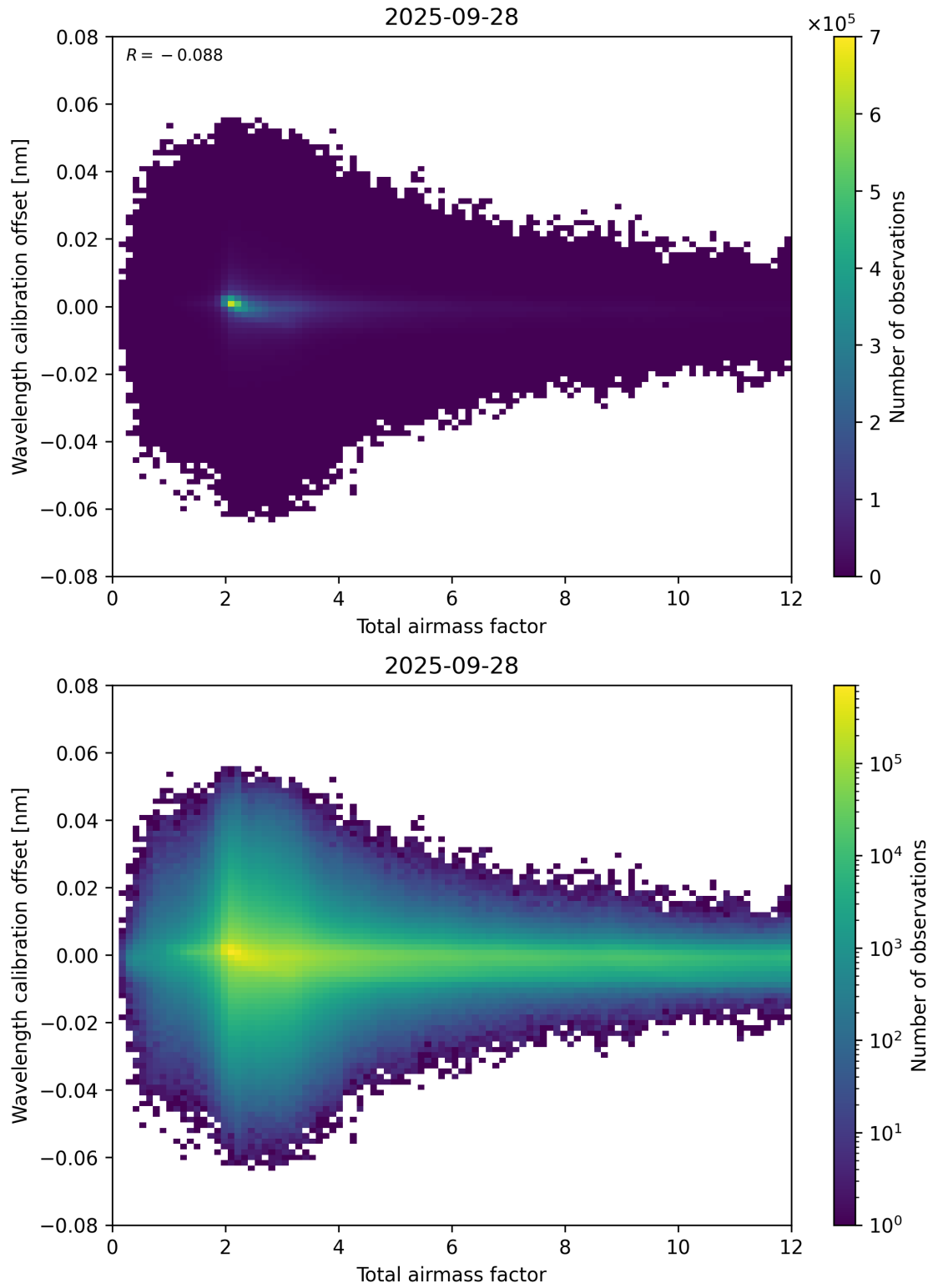
Figure 70: Scatter density plot of “Total airmass factor” against “Wavelength calibration offset” for 2025-09-27 to 2025-09-29.
