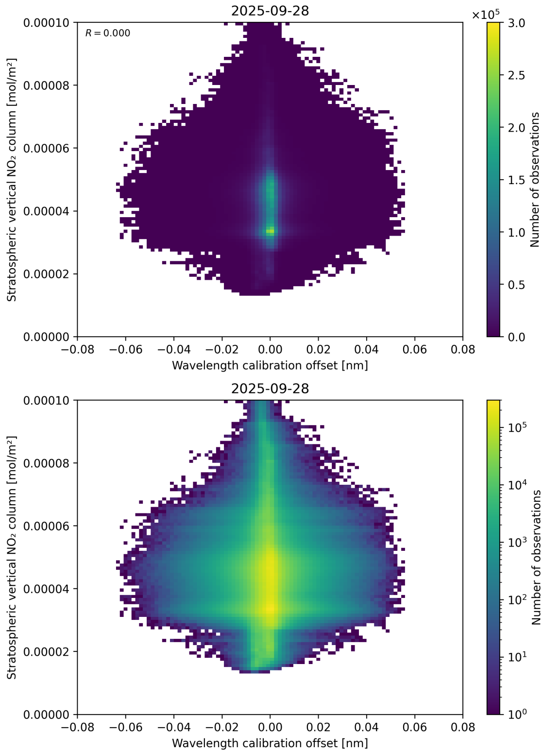
Figure 176: Scatter density plot of “Wavelength calibration offset” against “Stratospheric vertical NO 2 column” for 2025-09-27 to 2025-09-29.
