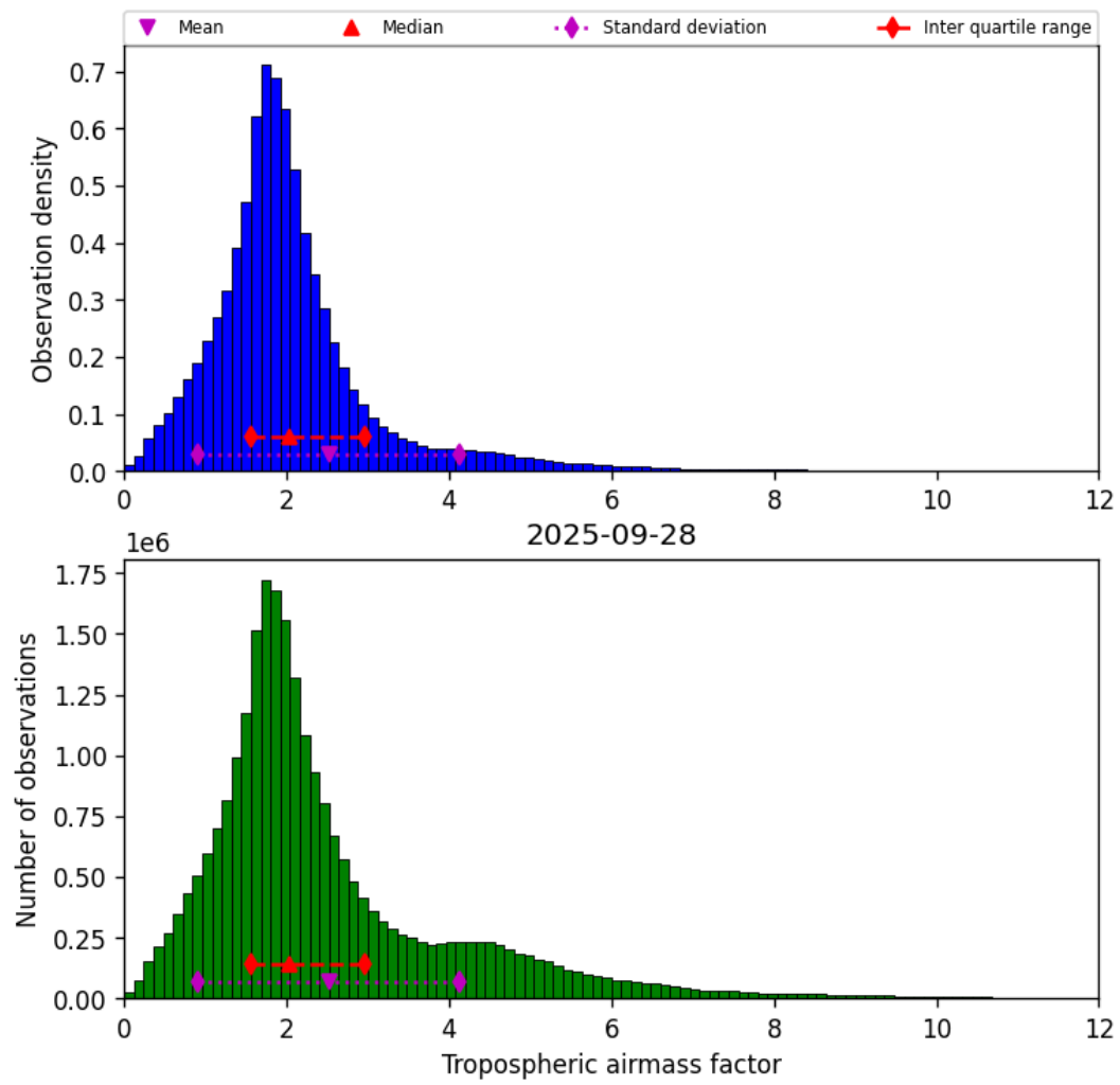
Figure 31: Histogram of “Tropospheric airmass factor” for 2025-09-27 to 2025-09-29
