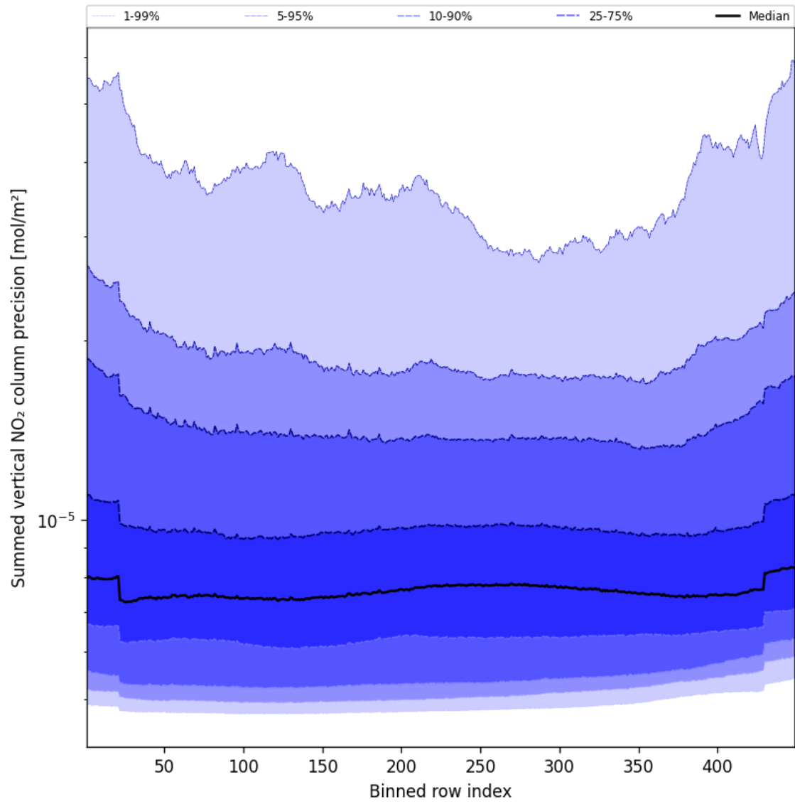
Figure 58: Along track statistics of “Summed vertical NO 2 column precision” for 2025-09-27 to 2025-09-29
