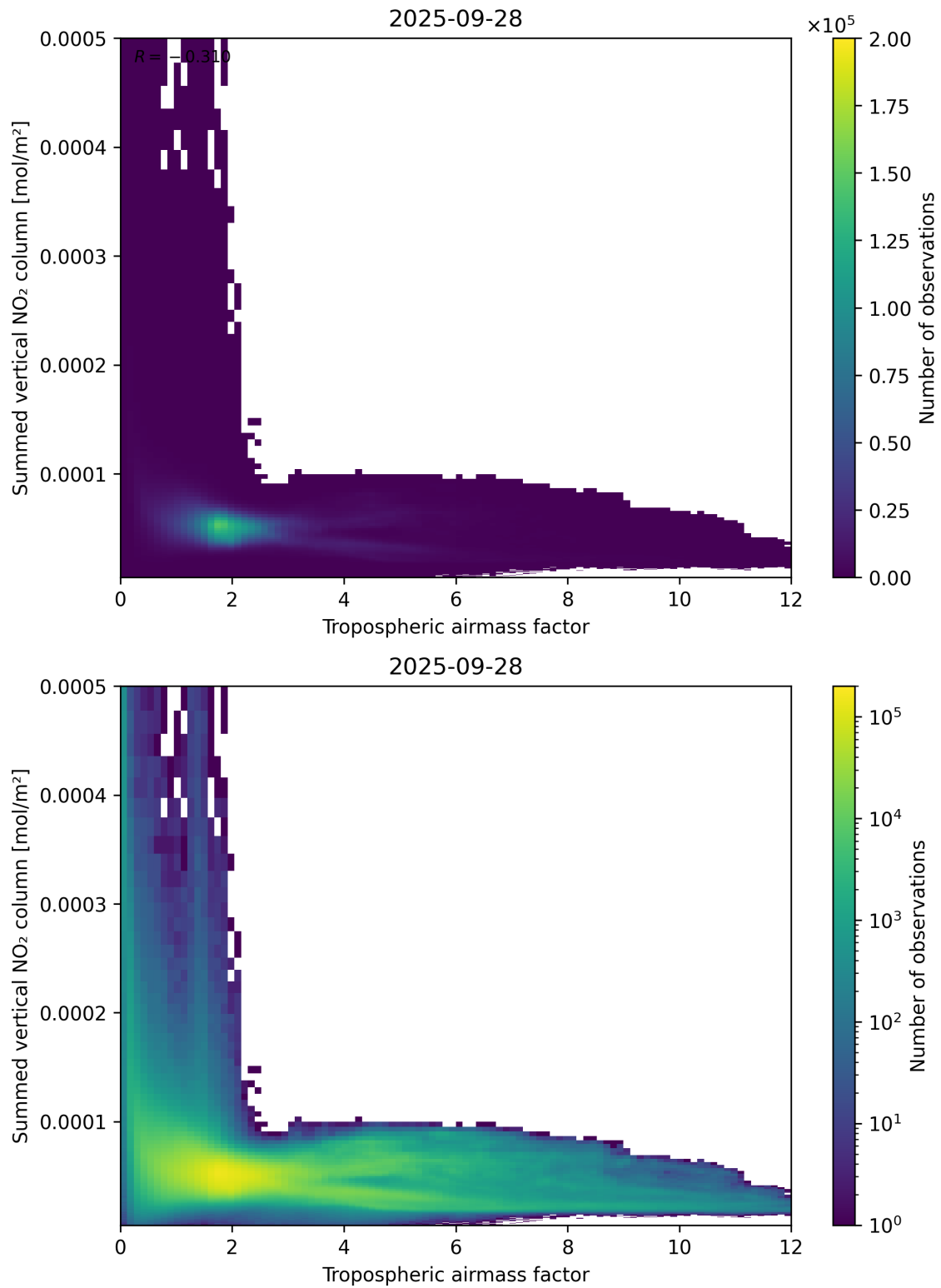
Figure 75: Scatter density plot of “Tropospheric air mass factor” against “Summed vertical NO 2 column” for 2025-09-27 to 2025-09-29.
