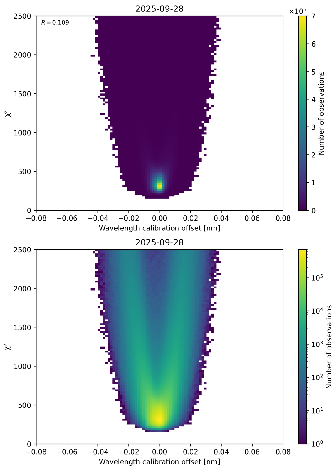
Figure 175: Scatter density plot of “Wavelength calibration offset” against “ \chi^2 ” for 2025-09-27 to 2025-09-29.
