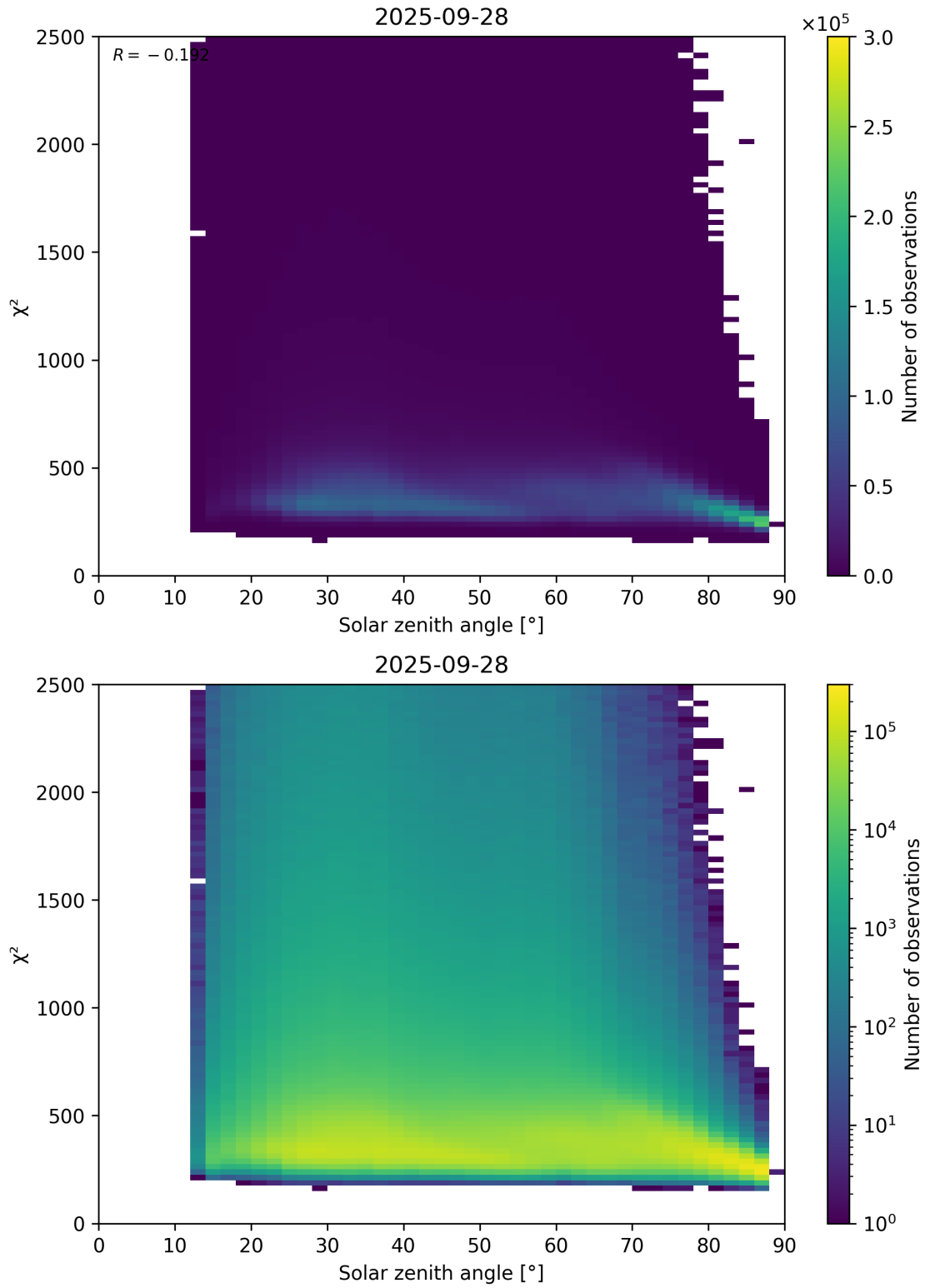
Figure 148: Scatter density plot of “Solar zenith angle” against “ \chi^2 ” for 2025-09-27 to 2025-09-29.
