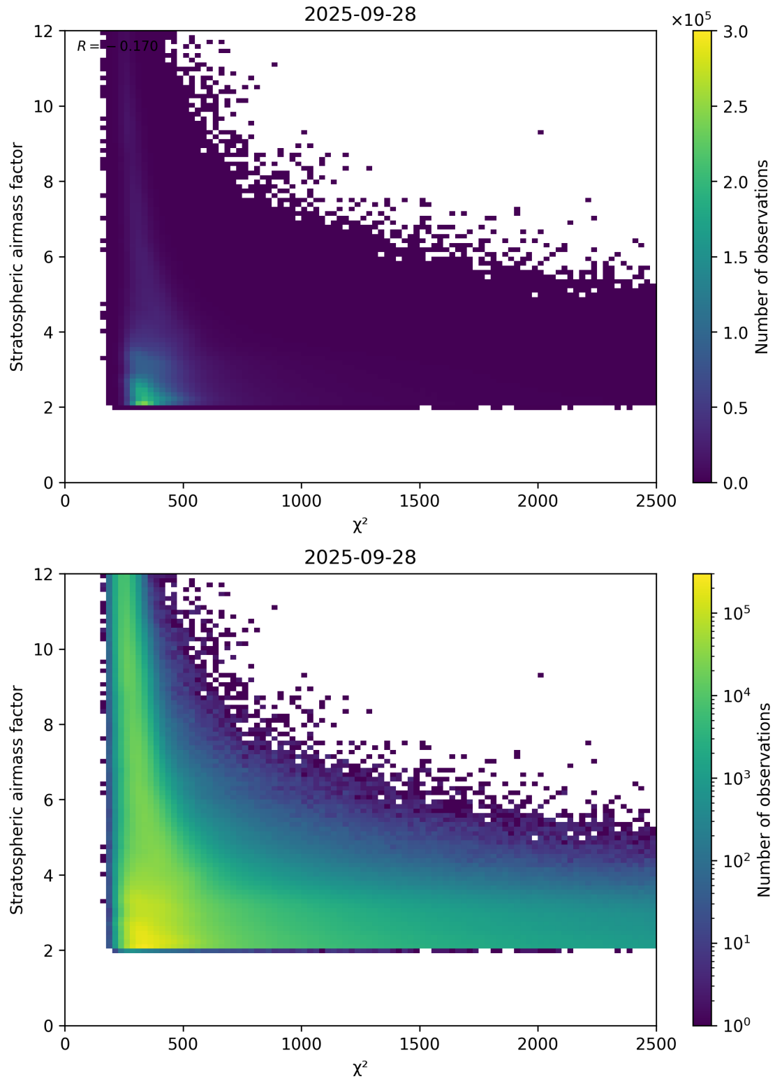
Figure 81: Scatter density plot of “ \chi^2 ” against “Stratospheric airmass factor” for 2025-09-27 to 2025-09-29.
