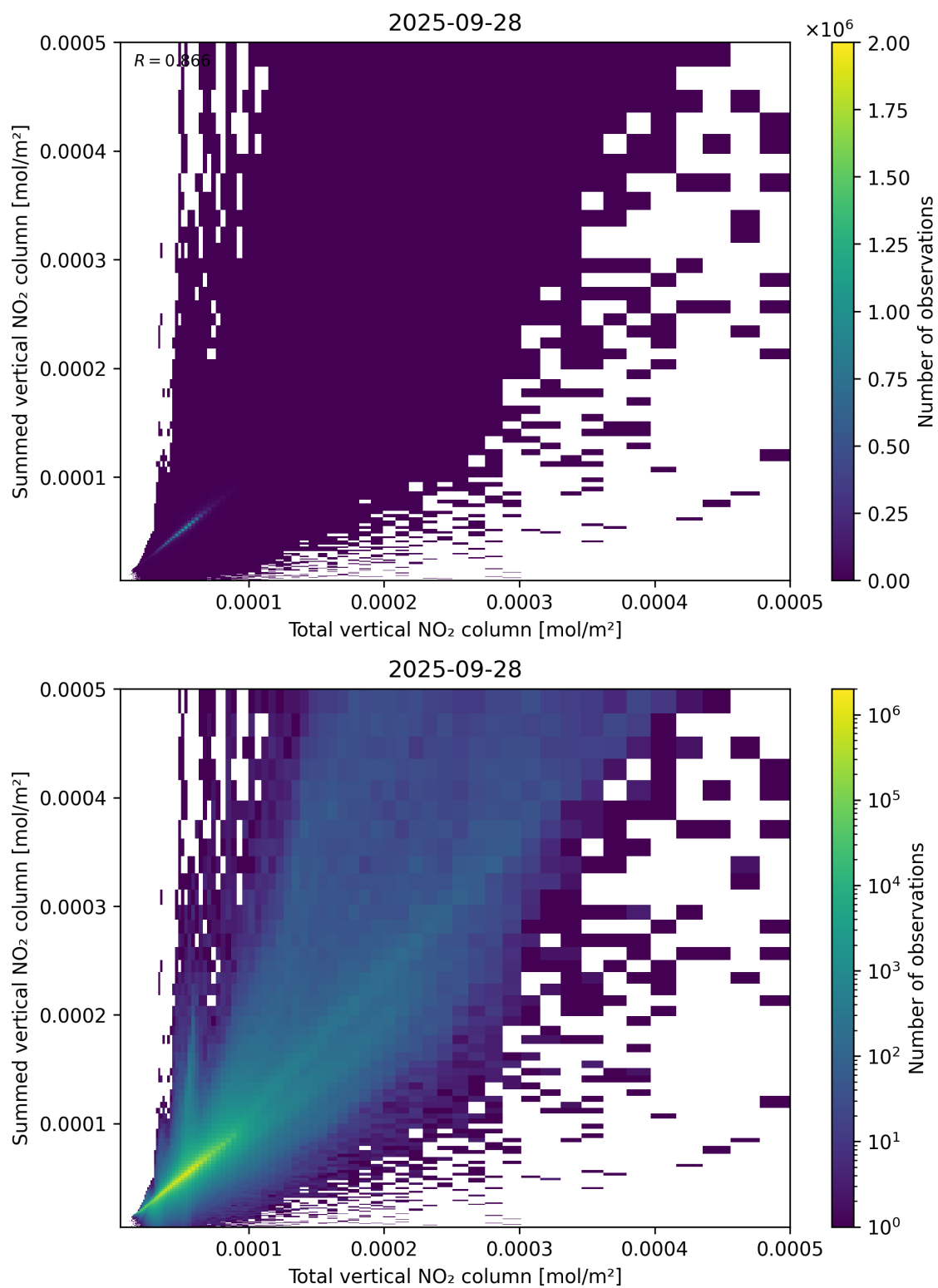
Figure 112: Scatter density plot of “Total vertical NO 2 column” against “Summed vertical NO 2 column” for 2025-09-27 to 2025-09-29.
