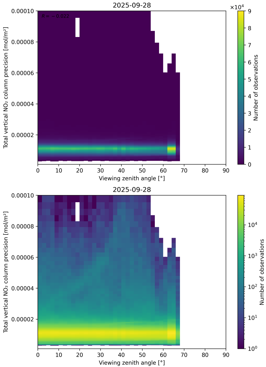
Figure 168: Scatter density plot of “Viewing zenith angle” against “Total vertical NO 2 column precision” for 2025-09-27 to 2025-09-29.
