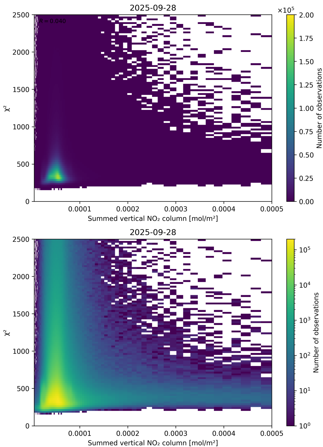
Figure 104: Scatter density plot of “Summed vertical NO 2 column” against “ \chi^2 ” for 2025-09-27 to 2025-09-29.
