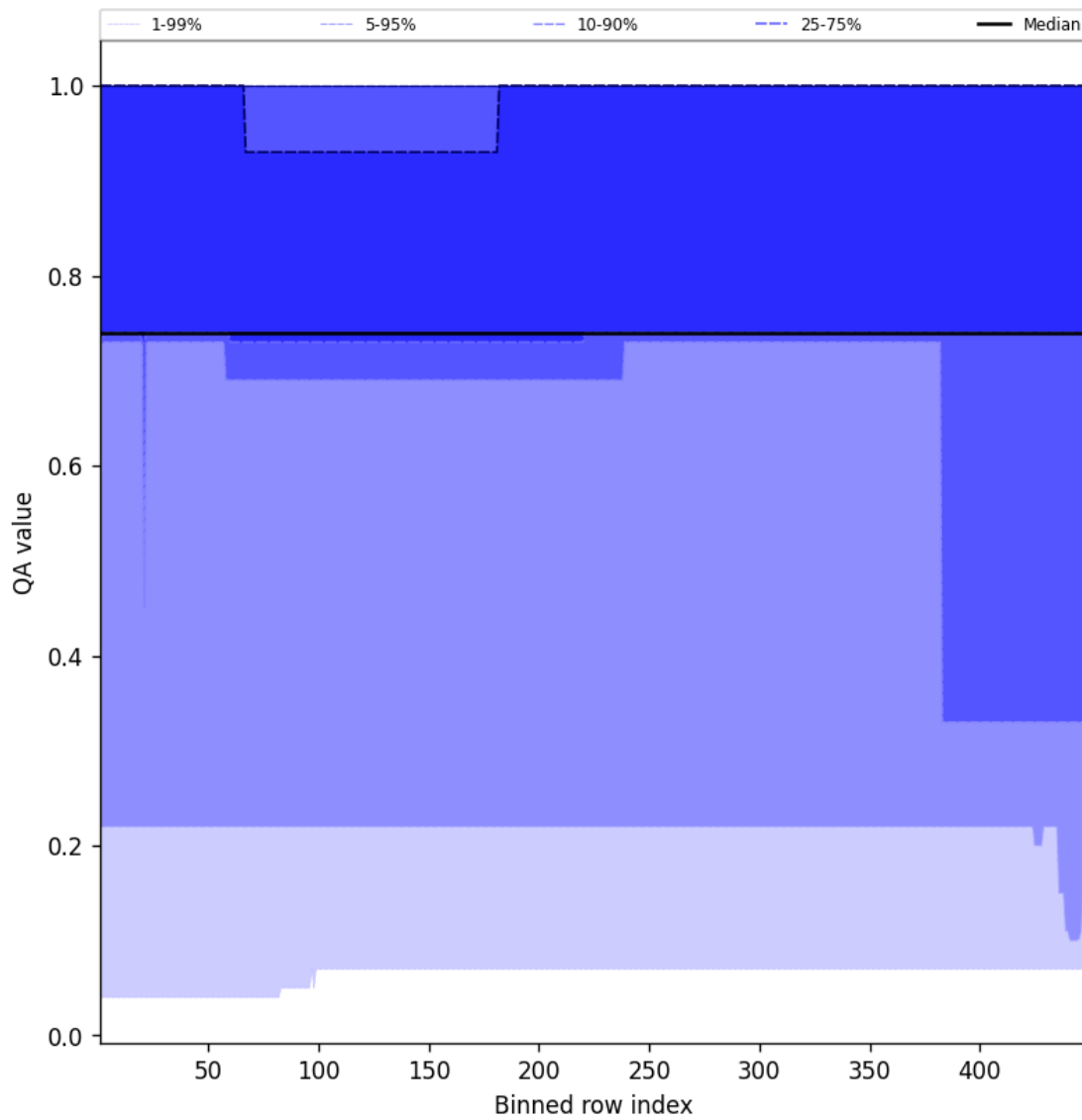
Figure 45: Along track statistics of “QA value” for 2025-09-27 to 2025-09-29
