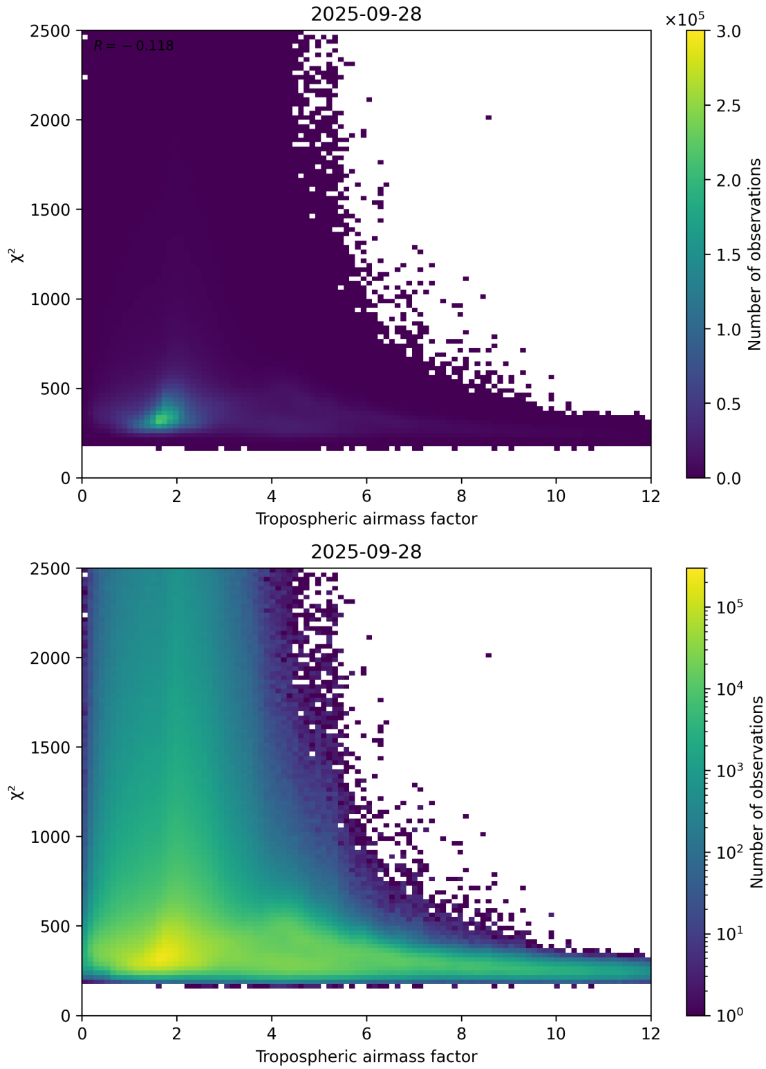
Figure 73: Scatter density plot of “Tropospheric airmass factor” against “ \chi^2 ” for 2025-09-27 to 2025-09-29.
