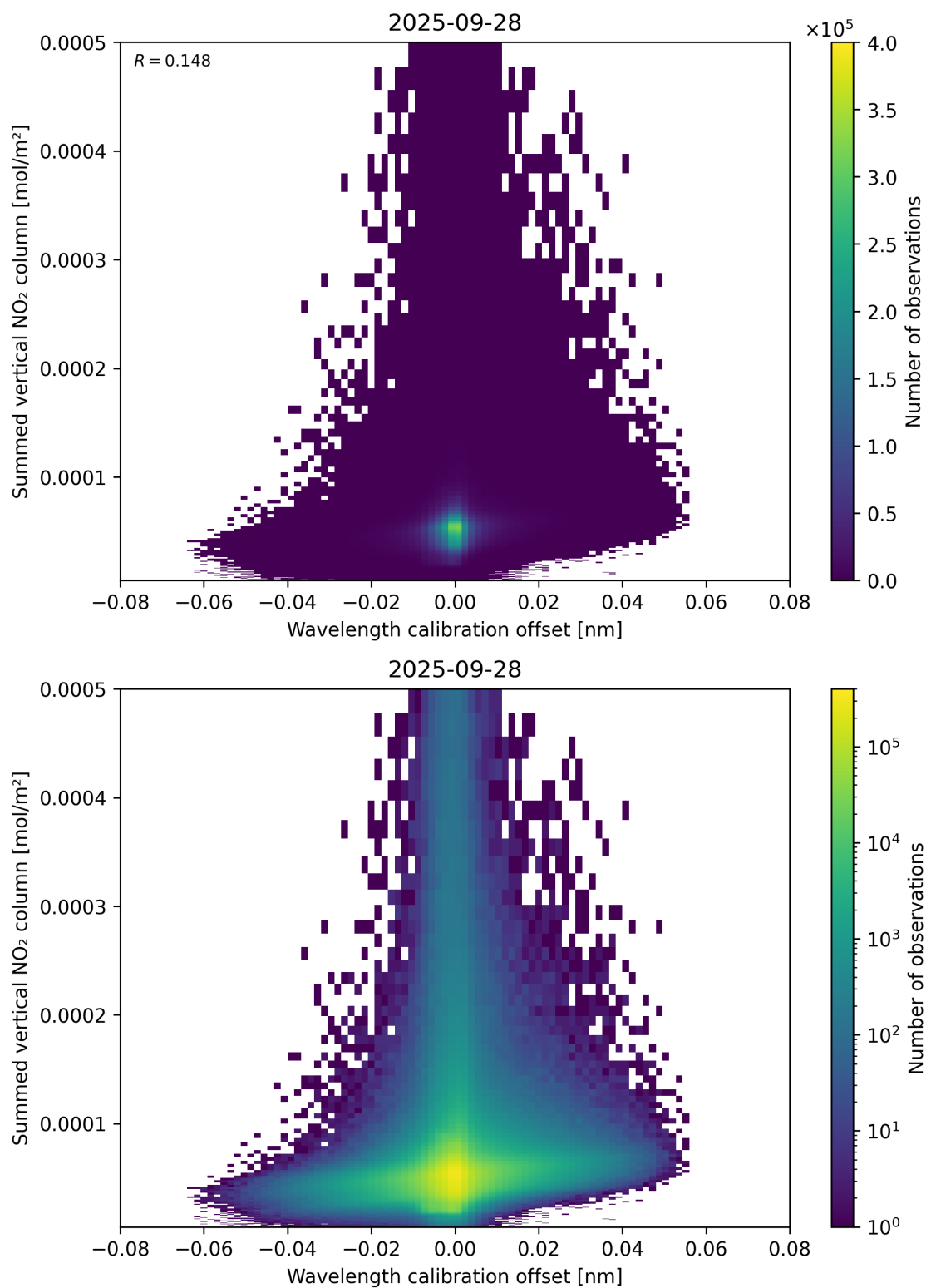
Figure 177: Scatter density plot of “Wavelength calibration offset” against “Summed vertical NO 2 column” for 2025-09-27 to 2025-09-29.
