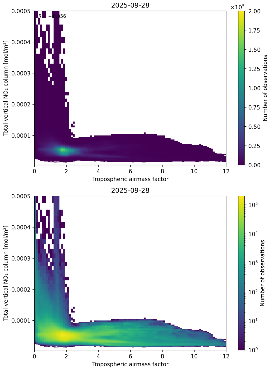
Figure 77: Scatter density plot of “Tropospheric airmass factor” against “Total vertical NO 2 column” for 2025-09-27 to 2025-09-29.
