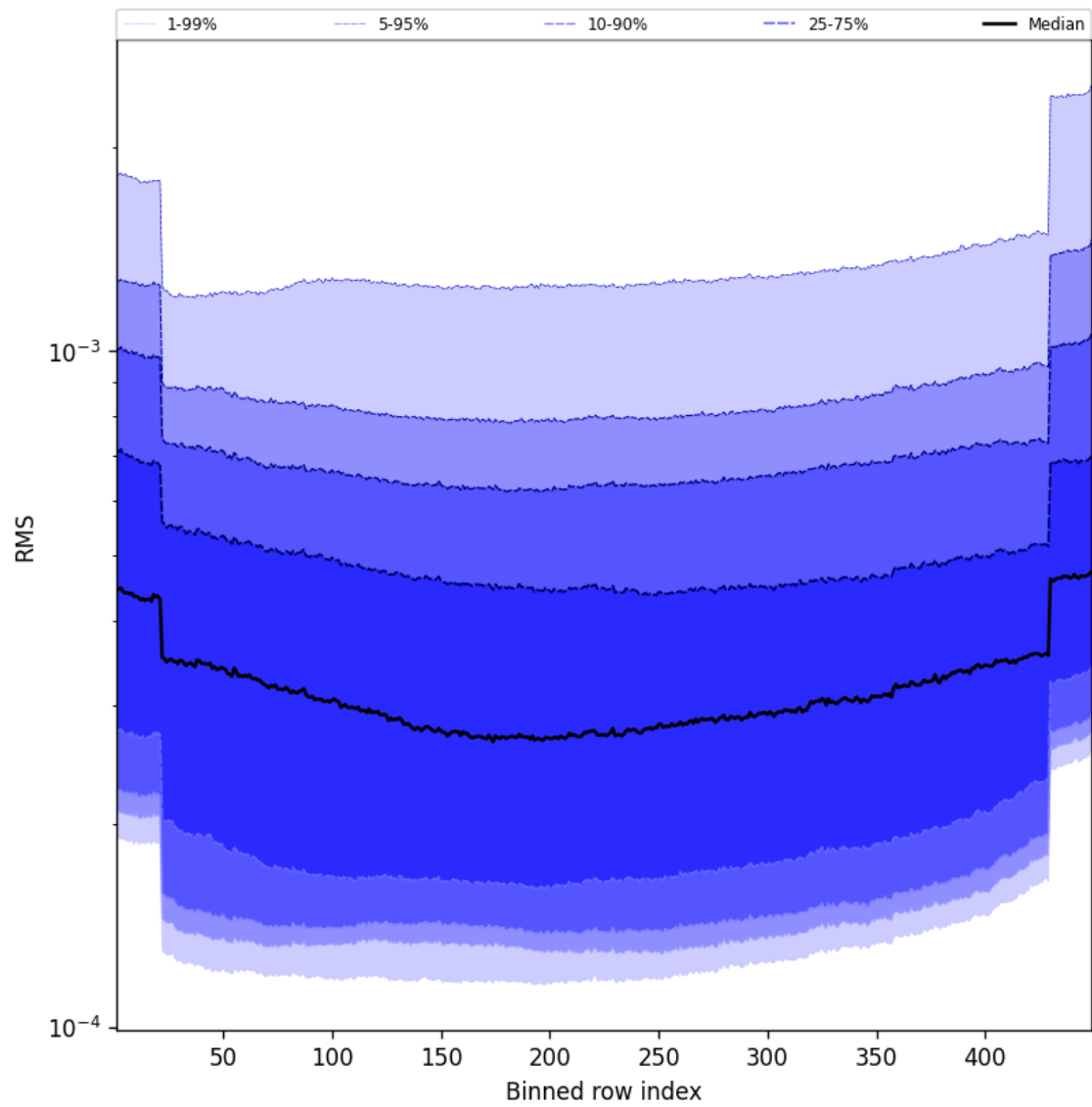
Figure 60: Along track statistics of “RMS” for 2025-09-27 to 2025-09-29
