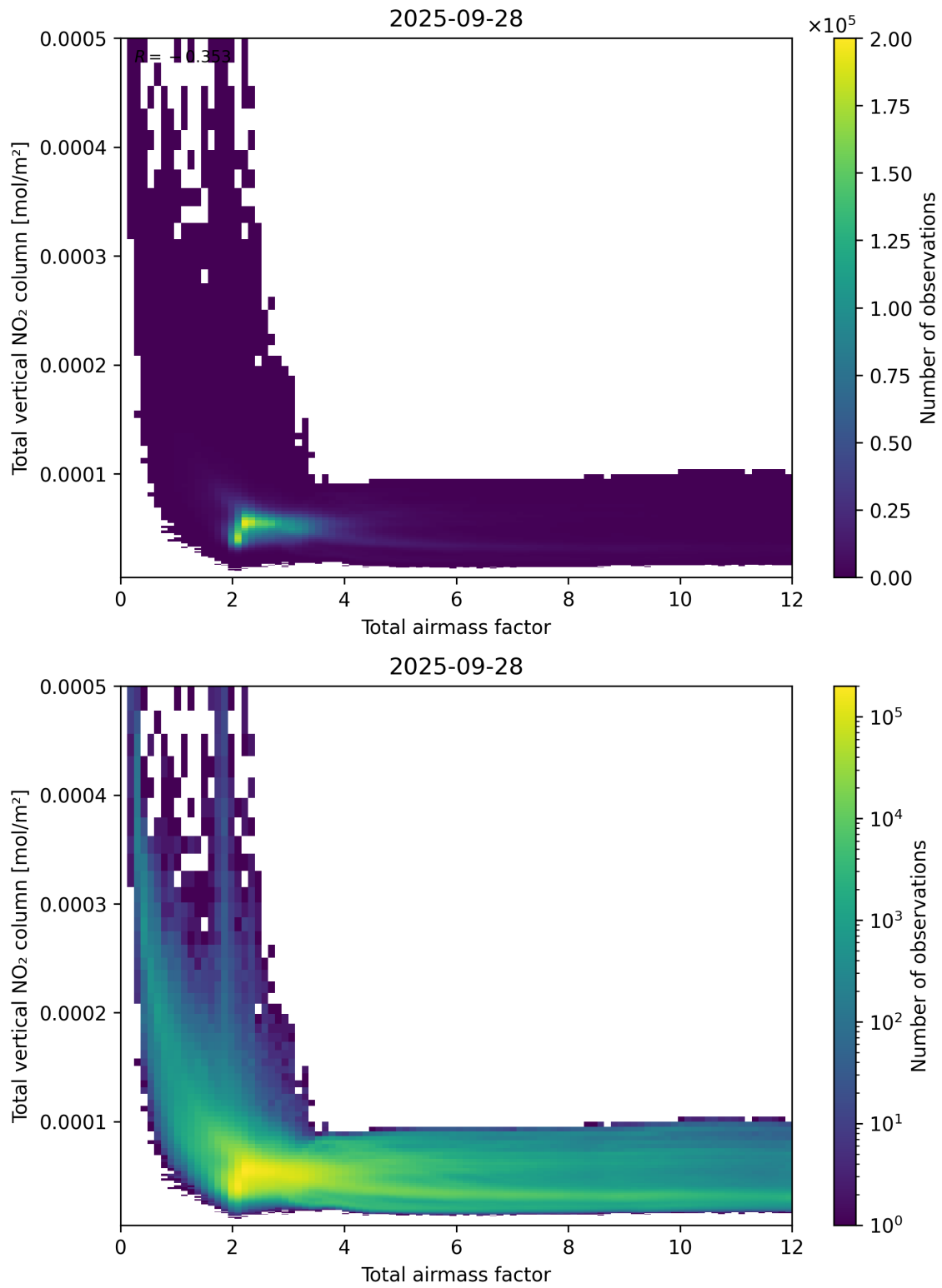
Figure 67: Scatter density plot of “Total air mass factor” against “Total vertical NO 2 column” for 2025-09-27 to 2025-09-29.
