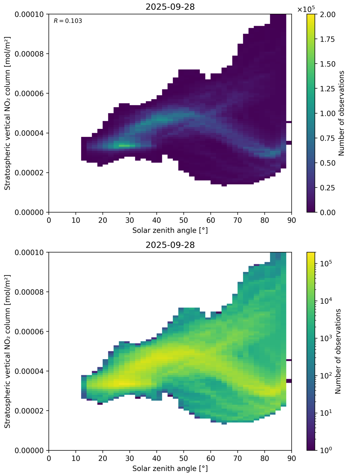
Figure 150: Scatter density plot of “Solar zenith angle” against “Stratospheric vertical \text{NO}_2 column” for 2025-09-27 to 2025-09-29.
