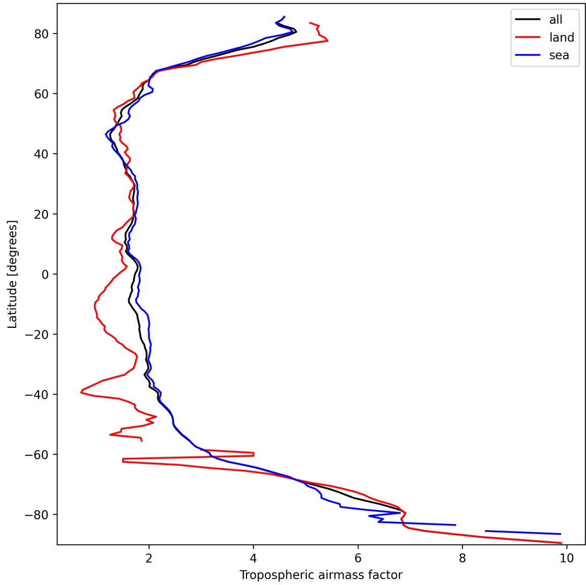
Figure 14: Zonal average of “Tropospheric airmass factor” for 2025-09-27 to 2025-09-29.
