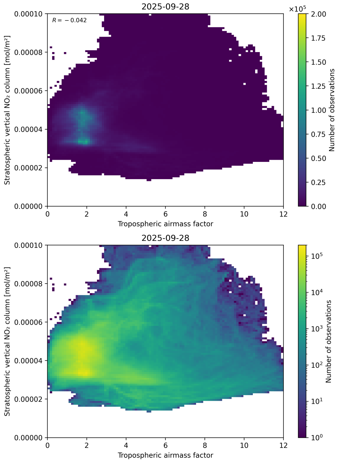
Figure 74: Scatter density plot of “Tropospheric air mass factor” against “Stratospheric vertical NO 2 column” for 2025-09-27 to 2025-09-29.
