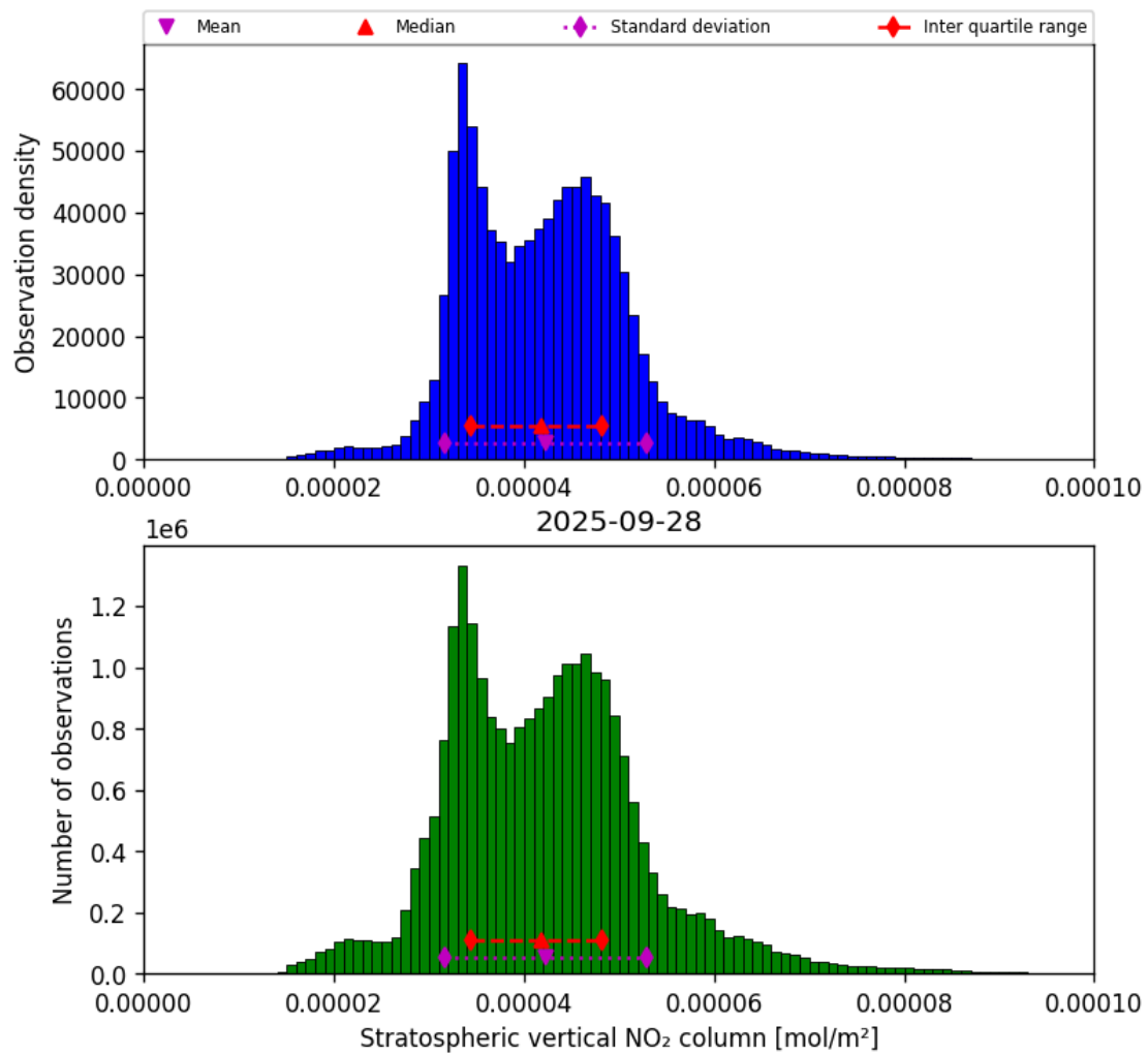
Figure 36: Histogram of “Stratospheric vertical NO 2 column” for 2025-09-27 to 2025-09-29
