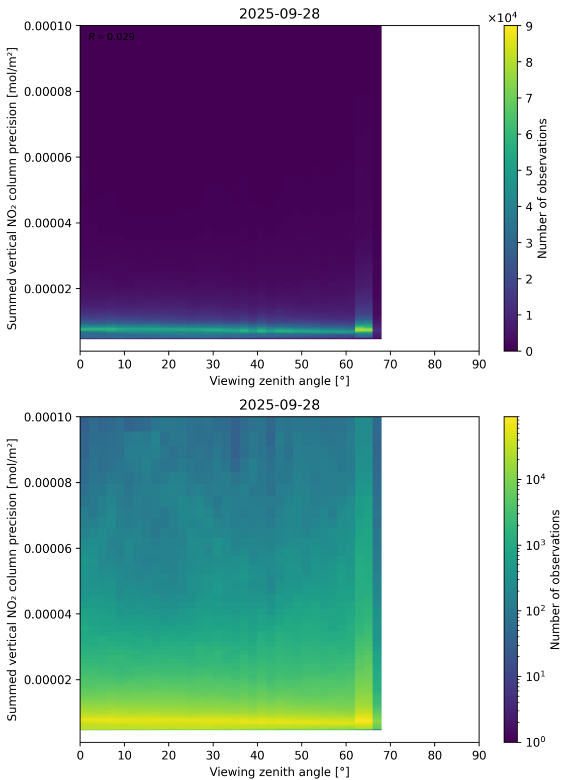
Figure 166: Scatter density plot of “Viewing zenith angle” against “Summed vertical NO 2 column precision” for 2025-09-27 to 2025-09-29.
