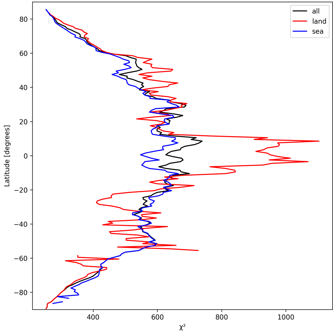
Figure 25: Zonal average of “ \chi^2 ” for 2025-09-27 to 2025-09-29.
