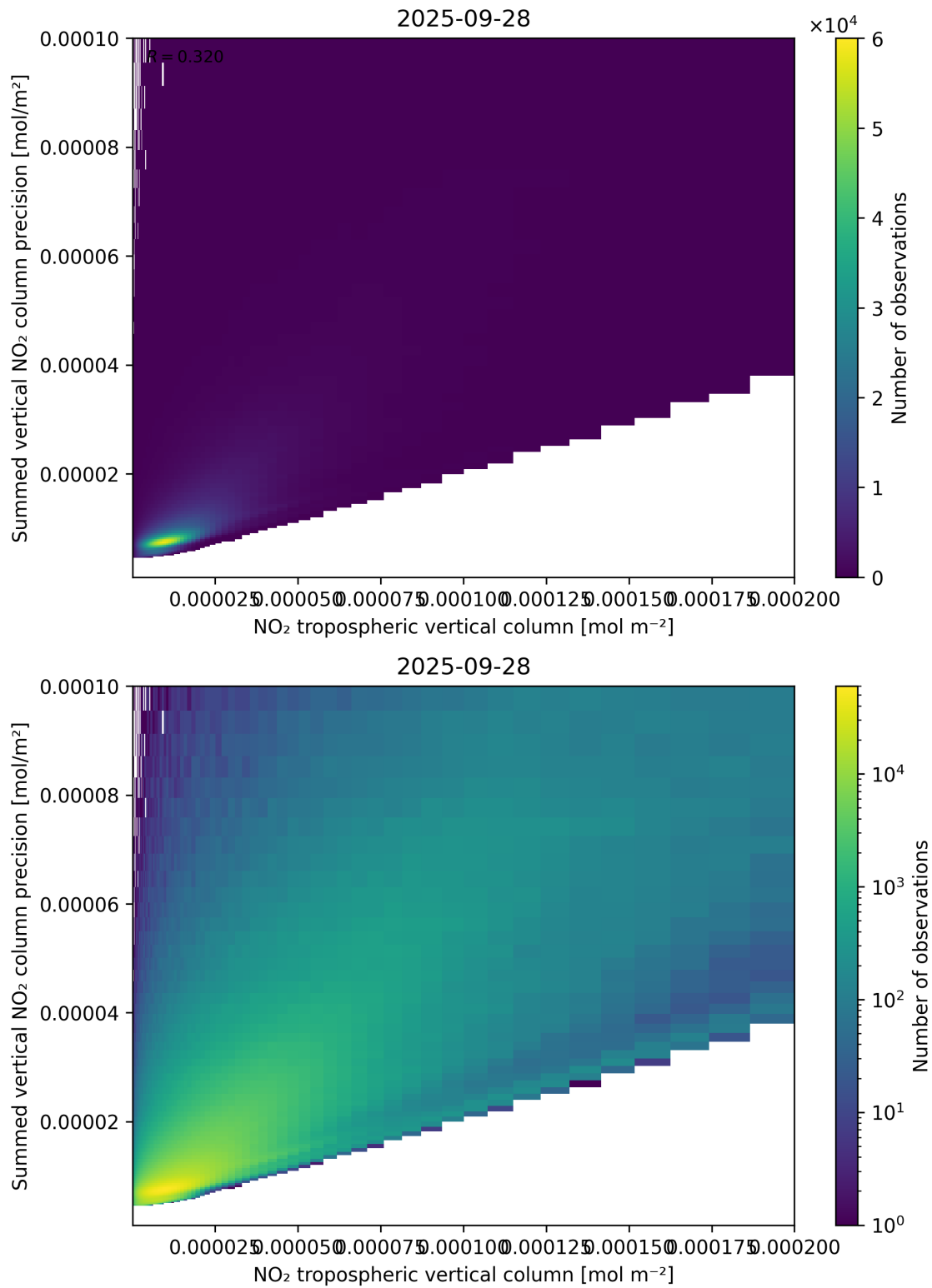
Figure 127: Scatter density plot of “NO 2 tropospheric vertical column” against “Summed vertical NO 2 column precision” for 2025-09-27 to 2025-09-29.
