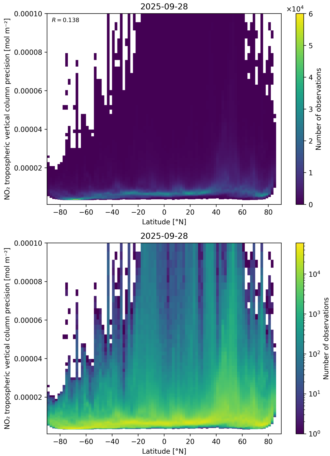
Figure 93: Scatter density plot of “Latitude” against “NO 2 tropospheric vertical column precision” for 2025-09-27 to 2025-09-29.
