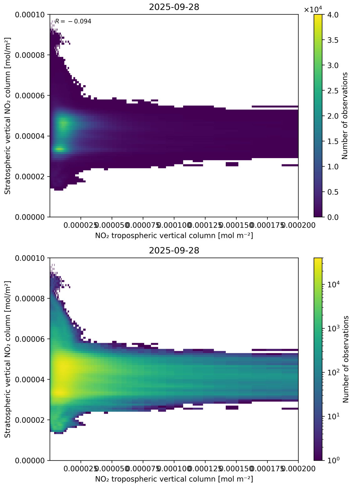
Figure 125: Scatter density plot of “NO 2 tropospheric vertical column” against “Stratospheric vertical NO 2 column” for 2025-09-27 to 2025-09-29.
