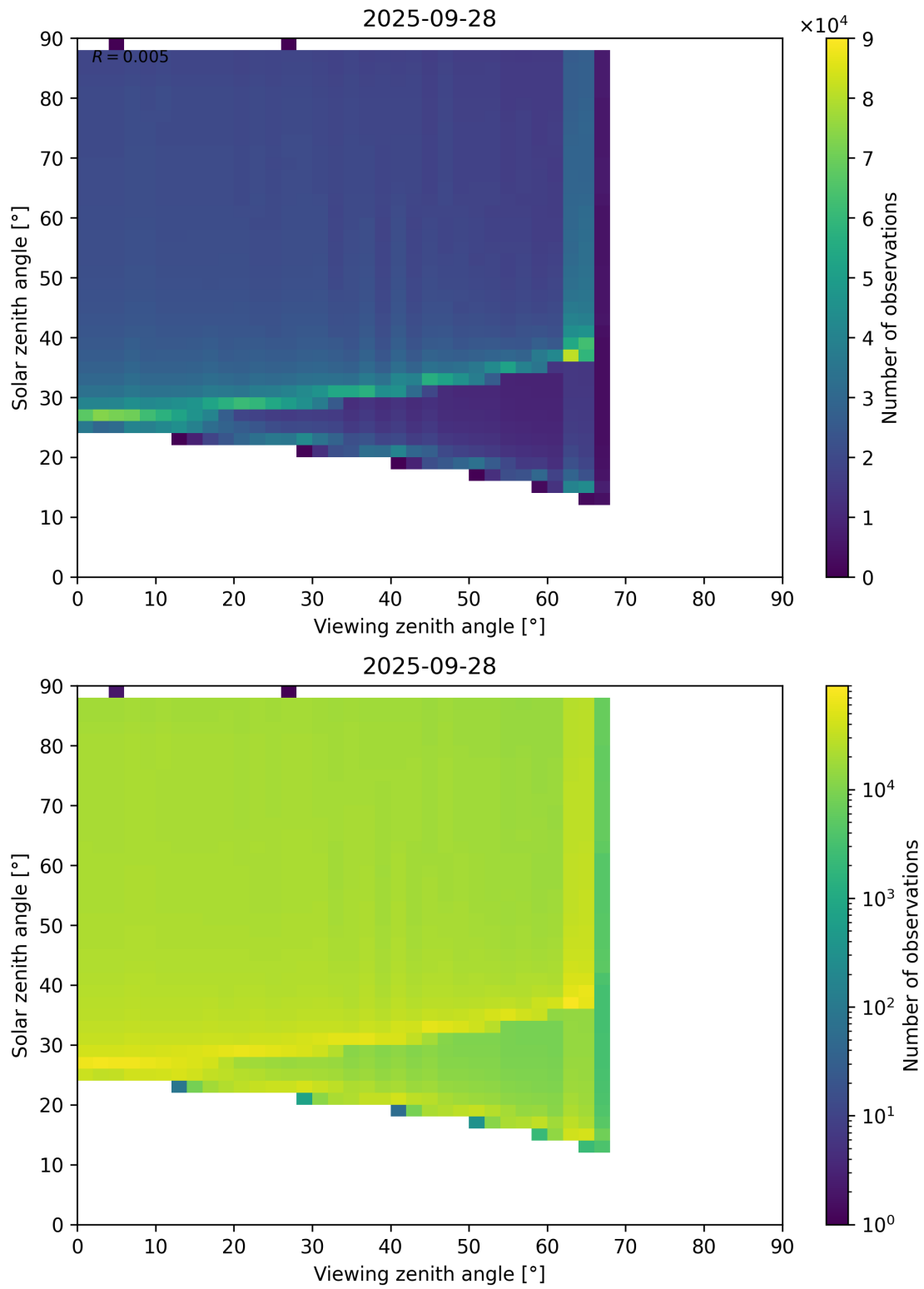
Figure 172: Scatter density plot of “Viewing zenith angle” against “Solar zenith angle” for 2025-09-27 to 2025-09-29.
