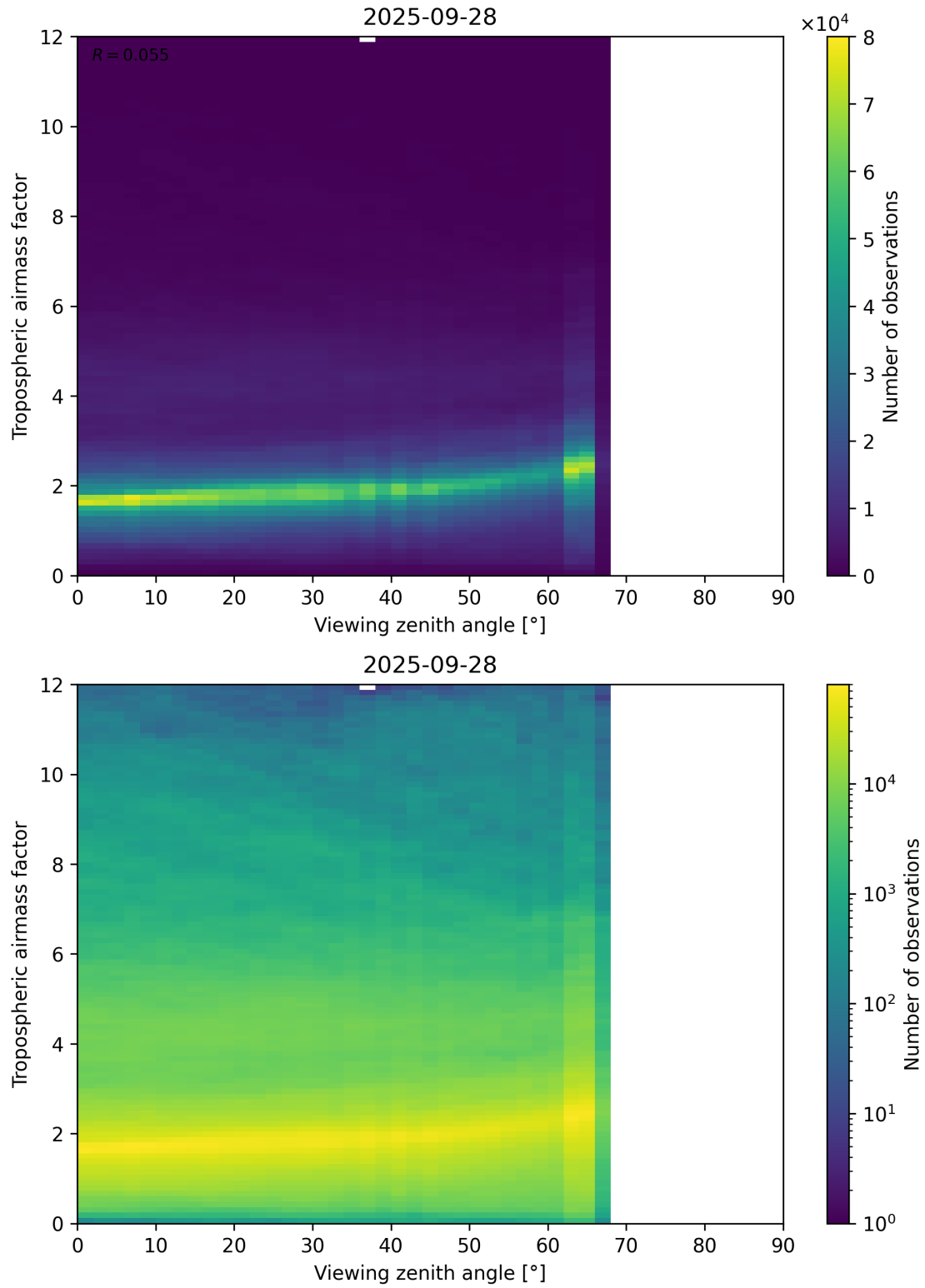
Figure 161: Scatter density plot of “Viewing zenith angle” against “Tropospheric airmass factor” for 2025-09-27 to 2025-09-29.
