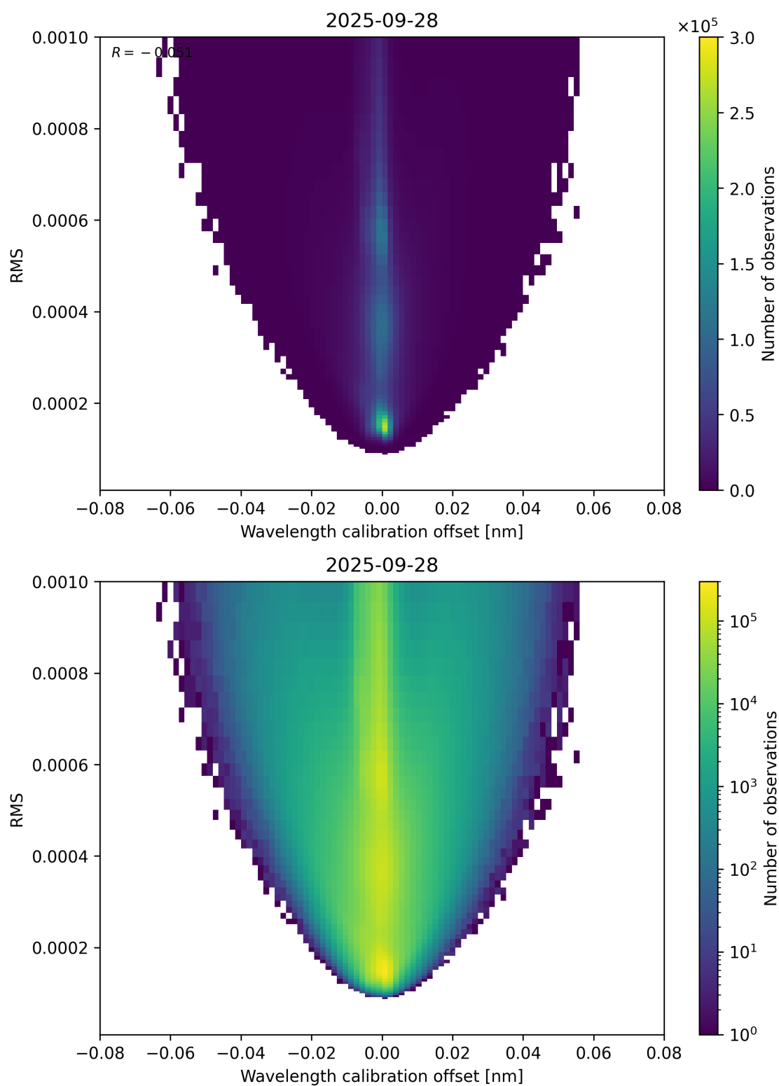
Figure 181: Scatter density plot of “Wavelength calibration offset” against “RMS” for 2025-09-27 to 2025-09-29.
