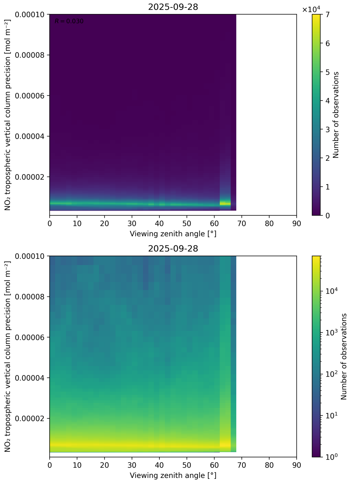
Figure 170: Scatter density plot of “Viewing zenith angle” against “NO 2 tropospheric vertical column precision” for 2025-09-27 to 2025-09-29.
