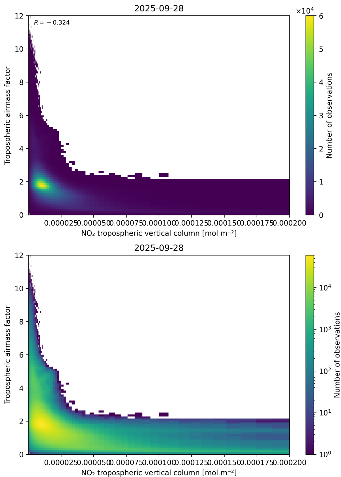
Figure 123: Scatter density plot of “NO 2 tropospheric vertical column” against “Tropospheric air mass factor” for 2025-09-27 to 2025-09-29.
