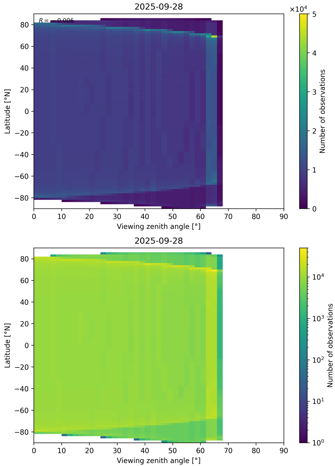
Figure 163: Scatter density plot of “Viewing zenith angle” against “Latitude” for 2025-09-27 to 2025-09-29.
