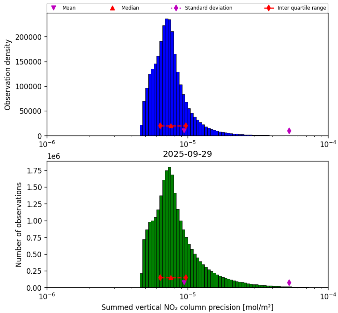
Figure 41: Histogram of “Summed vertical NO 2 column precision” for 2025-09-28 to 2025-09-30
