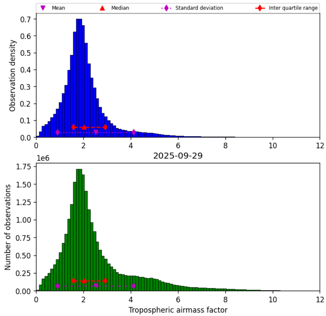
Figure 31: Histogram of “Tropospheric airmass factor” for 2025-09-28 to 2025-09-30
