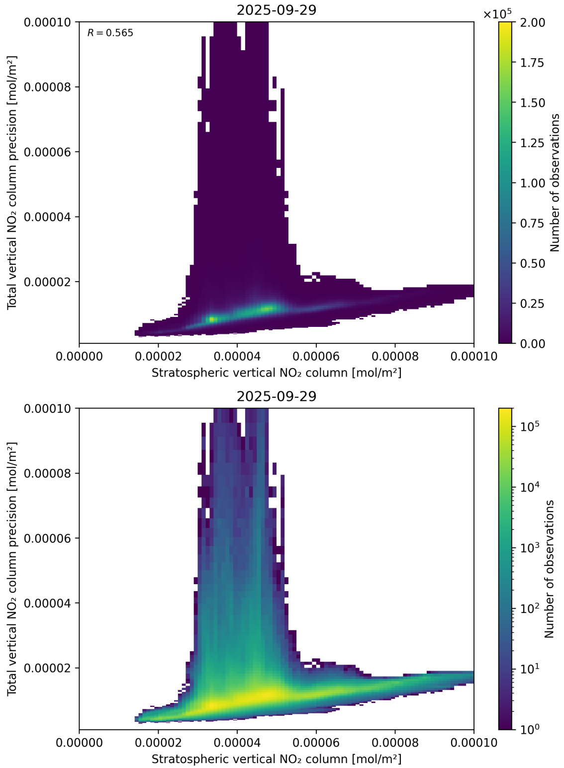
Figure 101: Scatter density plot of “Stratospheric vertical NO 2 column” against “Total vertical NO 2 column precision” for 2025-09-28 to 2025-09-30.
