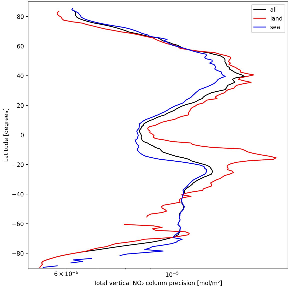
Figure 22: Zonal average of “Total vertical NO 2 column precision” for 2025-09-28 to 2025-09-30.
