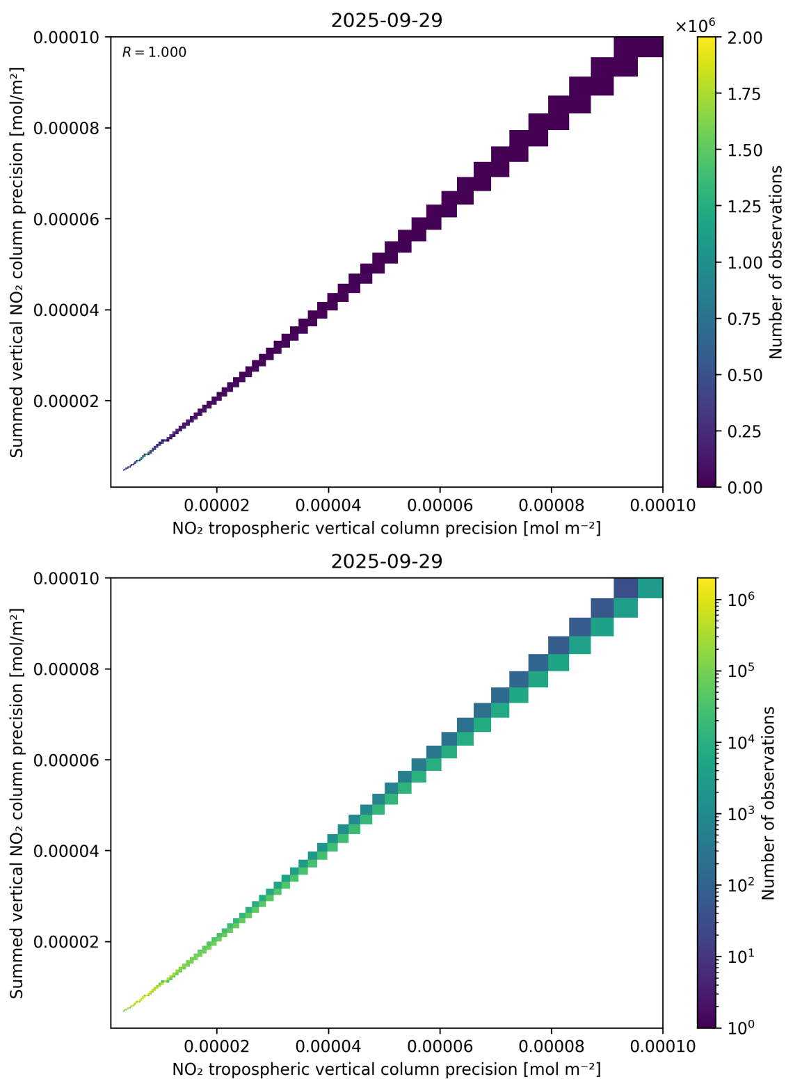
Figure 137: Scatter density plot of “NO 2 tropospheric vertical column precision” against “Summed vertical NO 2 column precision” for 2025-09-28 to 2025-09-30.
