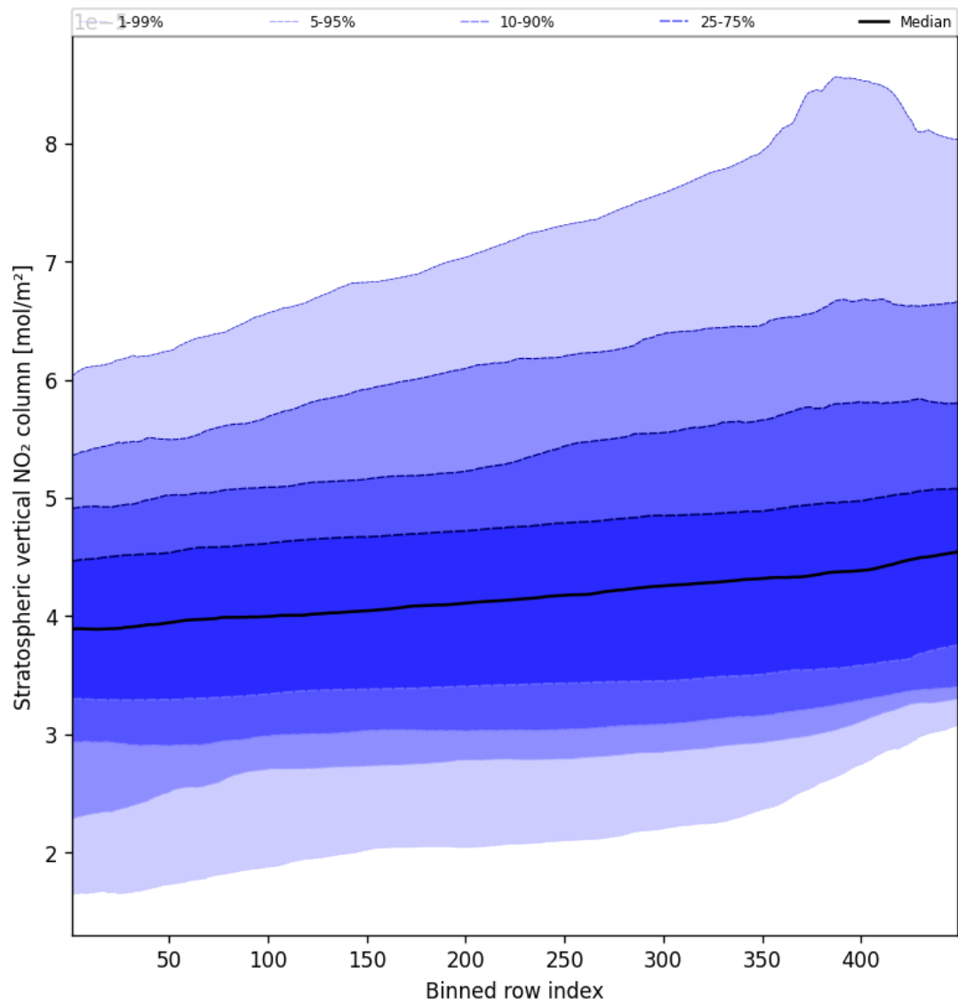
Figure 53: Along track statistics of “Stratospheric vertical NO 2 column” for 2025-09-28 to 2025-09-30
