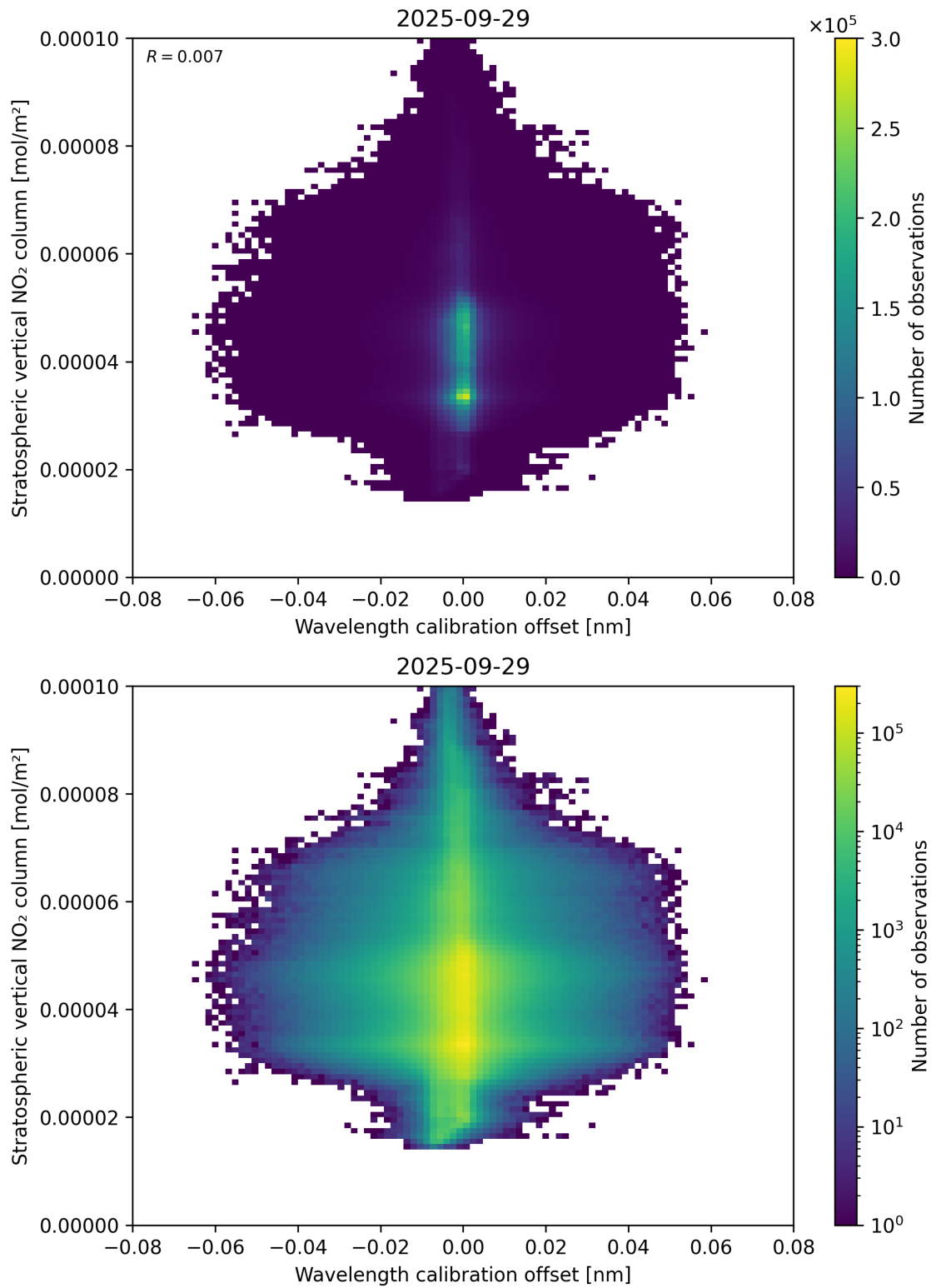
Figure 176: Scatter density plot of “Wavelength calibration offset” against “Stratospheric vertical NO 2 column” for 2025-09-28 to 2025-09-30.
