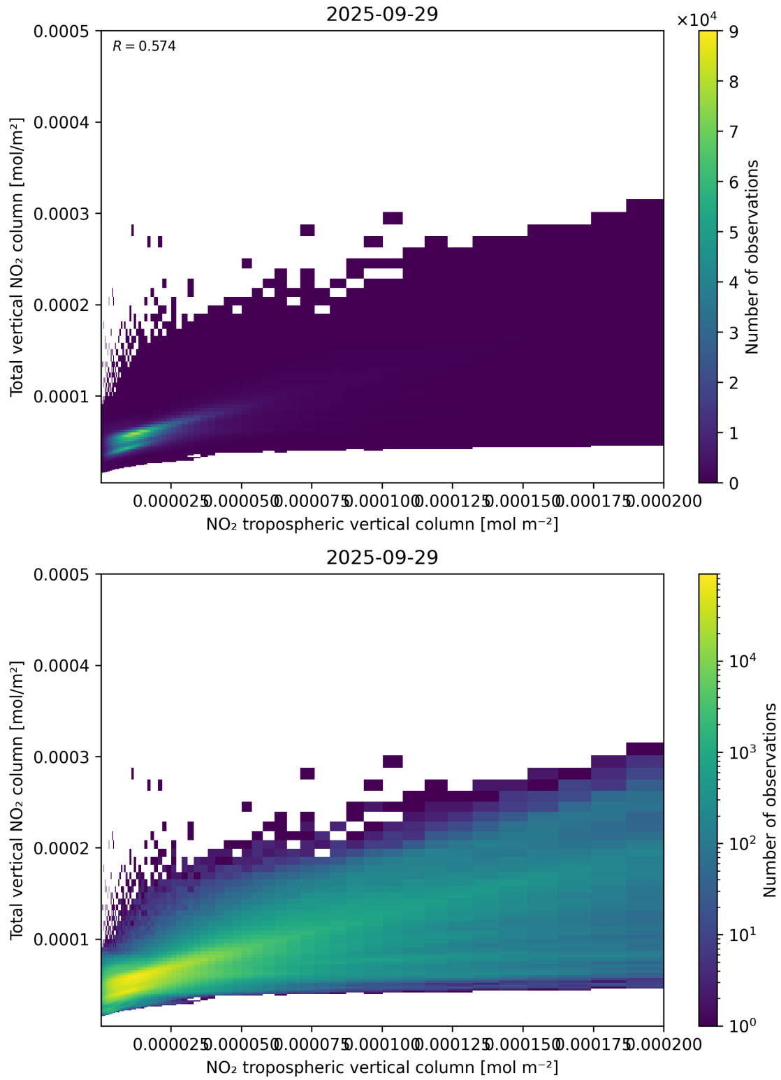
Figure 128: Scatter density plot of “NO 2 tropospheric vertical column” against “Total vertical NO 2 column” for 2025-09-28 to 2025-09-30.
