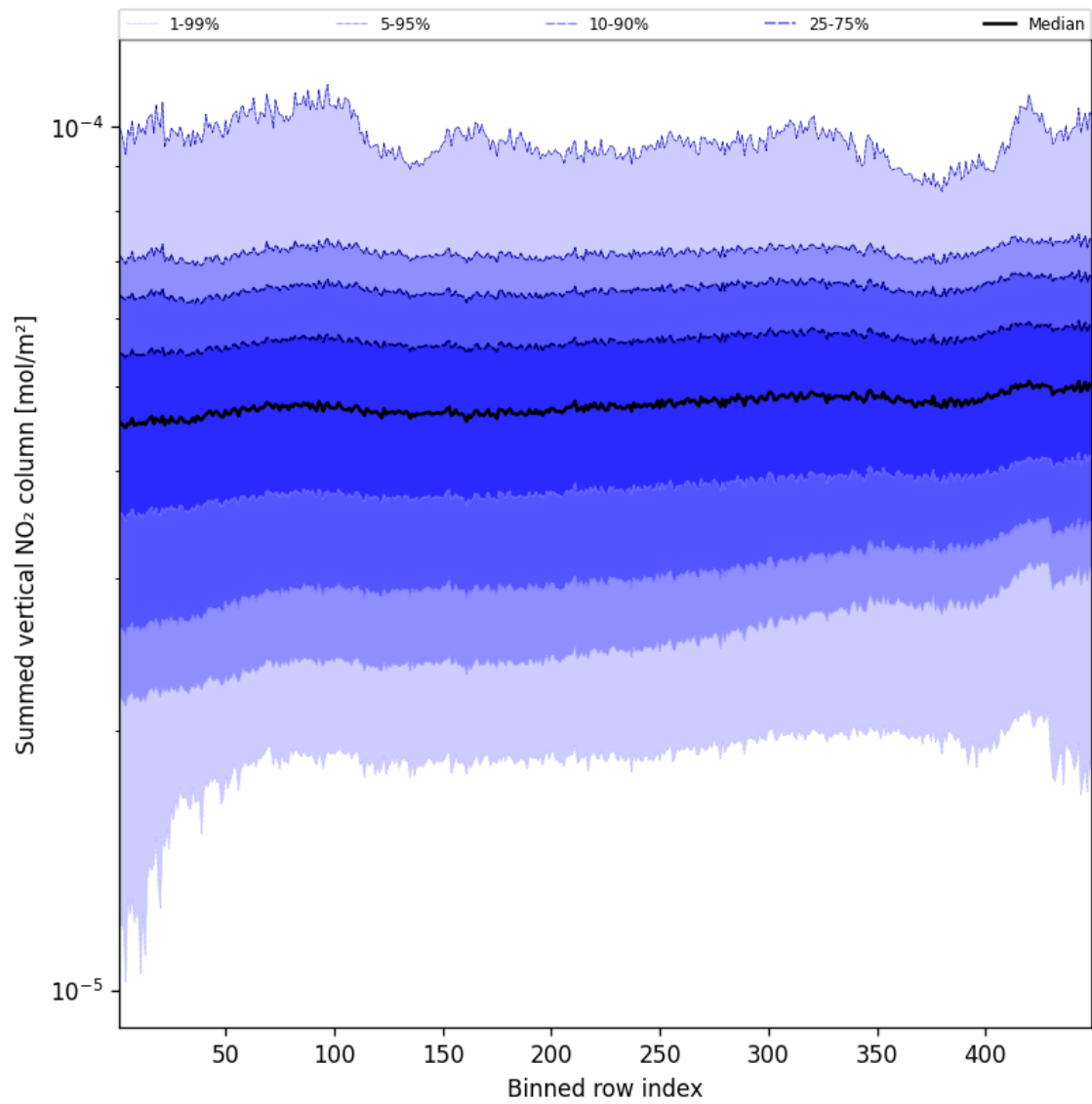
Figure 57: Along track statistics of “Summed vertical NO 2 column” for 2025-09-28 to 2025-09-30
