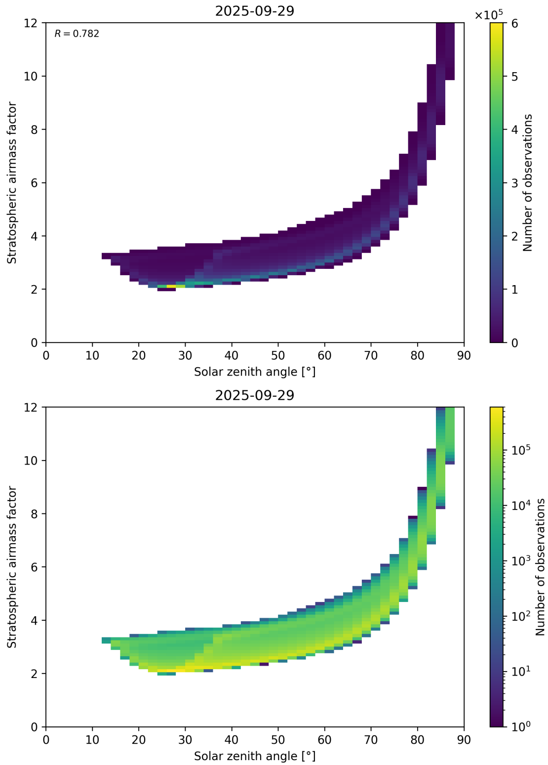
Figure 145: Scatter density plot of “Solar zenith angle” against “Stratospheric airmass factor” for 2025-09-28 to 2025-09-30.
