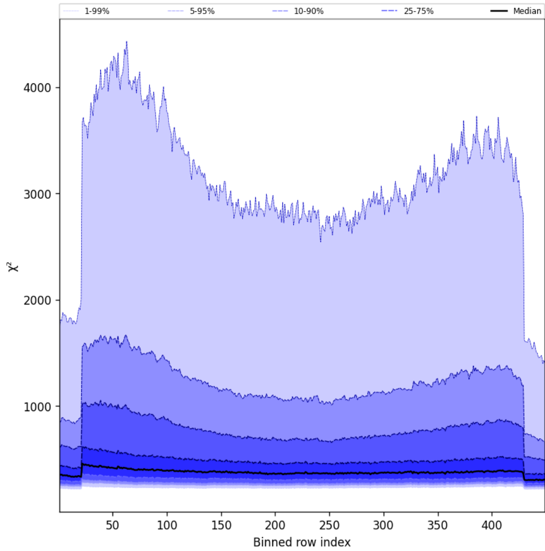
Figure 59: Along track statistics of “ \chi^2 ” for 2025-09-28 to 2025-09-30
