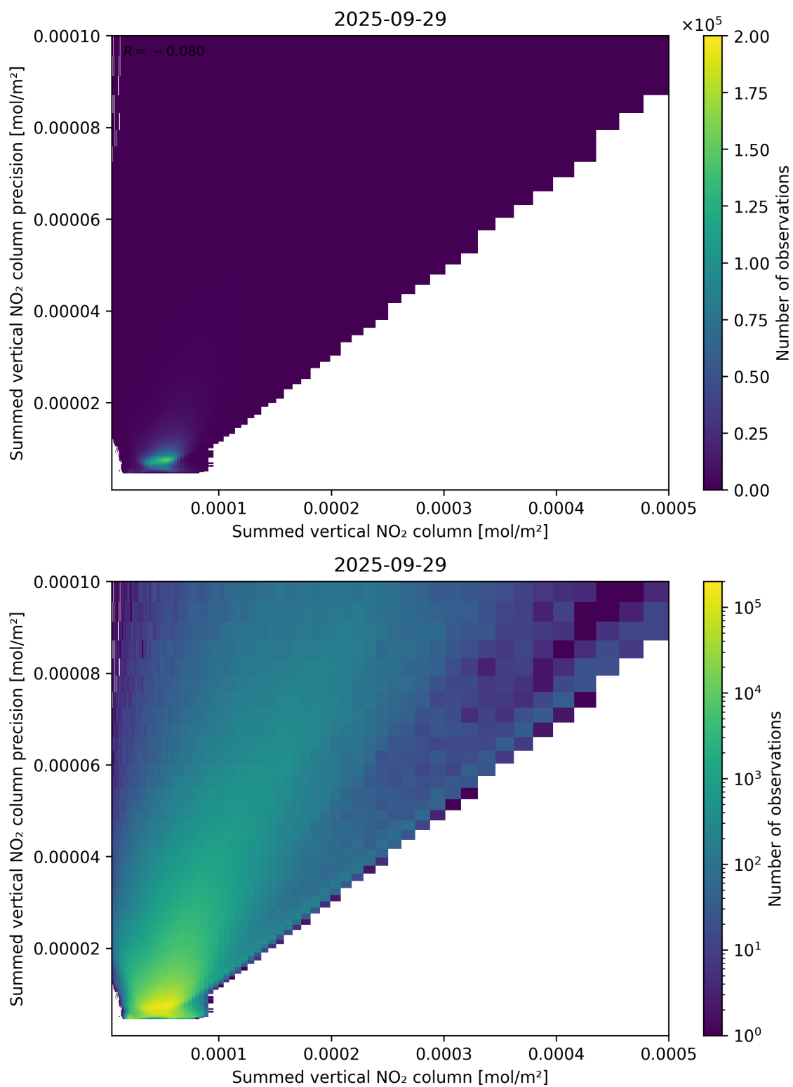
Figure 105: Scatter density plot of “Summed vertical NO 2 column” against “Summed vertical NO 2 column precision” for 2025-09-28 to 2025-09-30.
