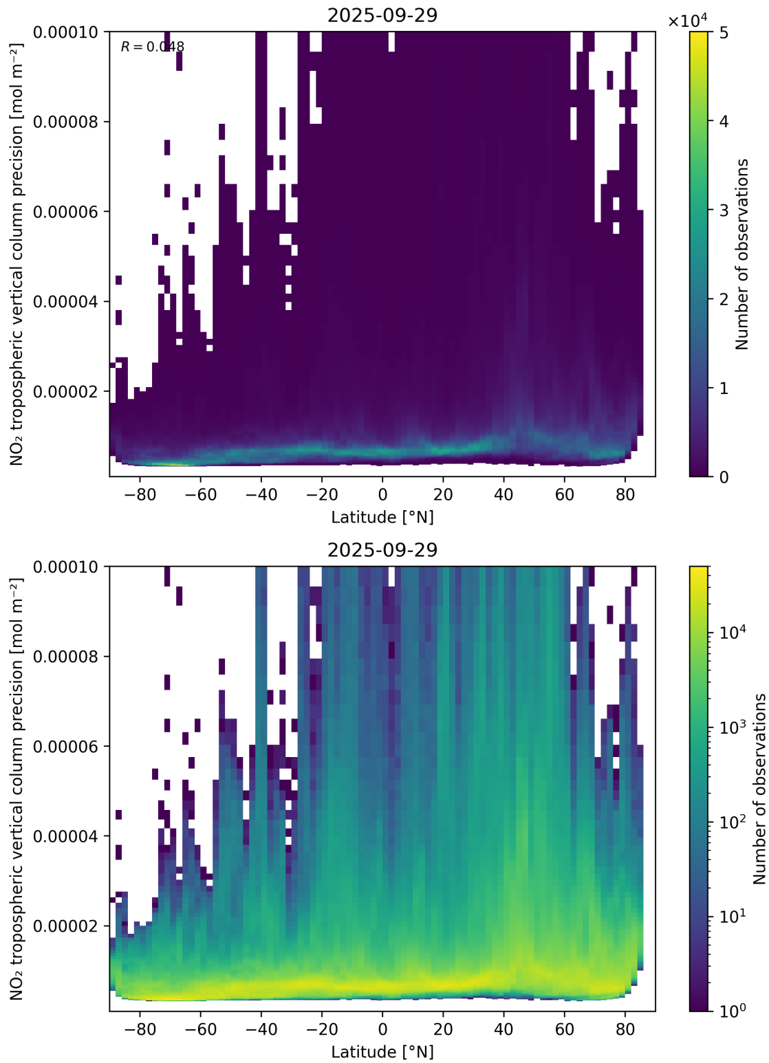
Figure 93: Scatter density plot of “Latitude” against “NO 2 tropospheric vertical column precision” for 2025-09-28 to 2025-09-30.
