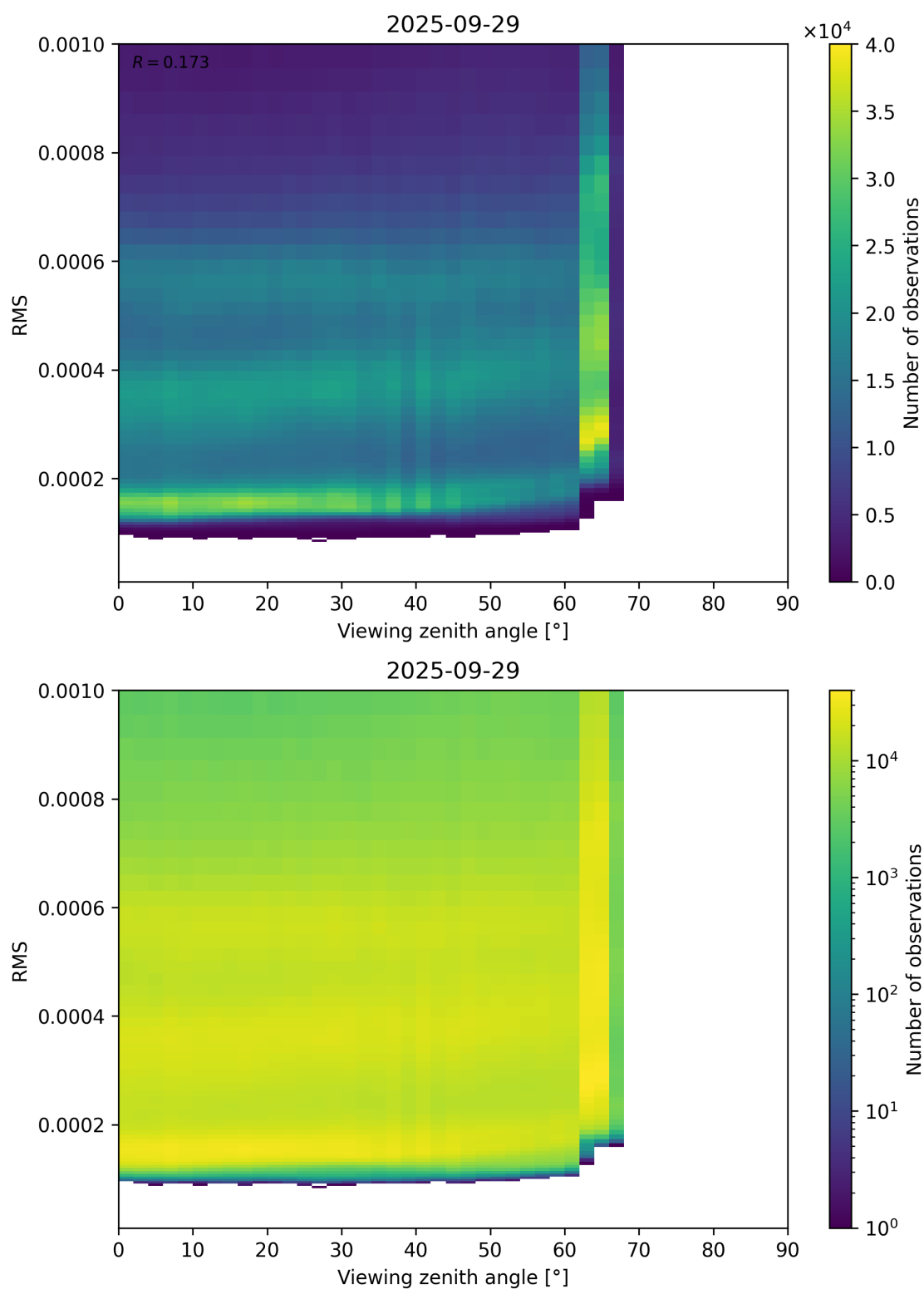
Figure 171: Scatter density plot of “Viewing zenith angle” against “RMS” for 2025-09-28 to 2025-09-30.
