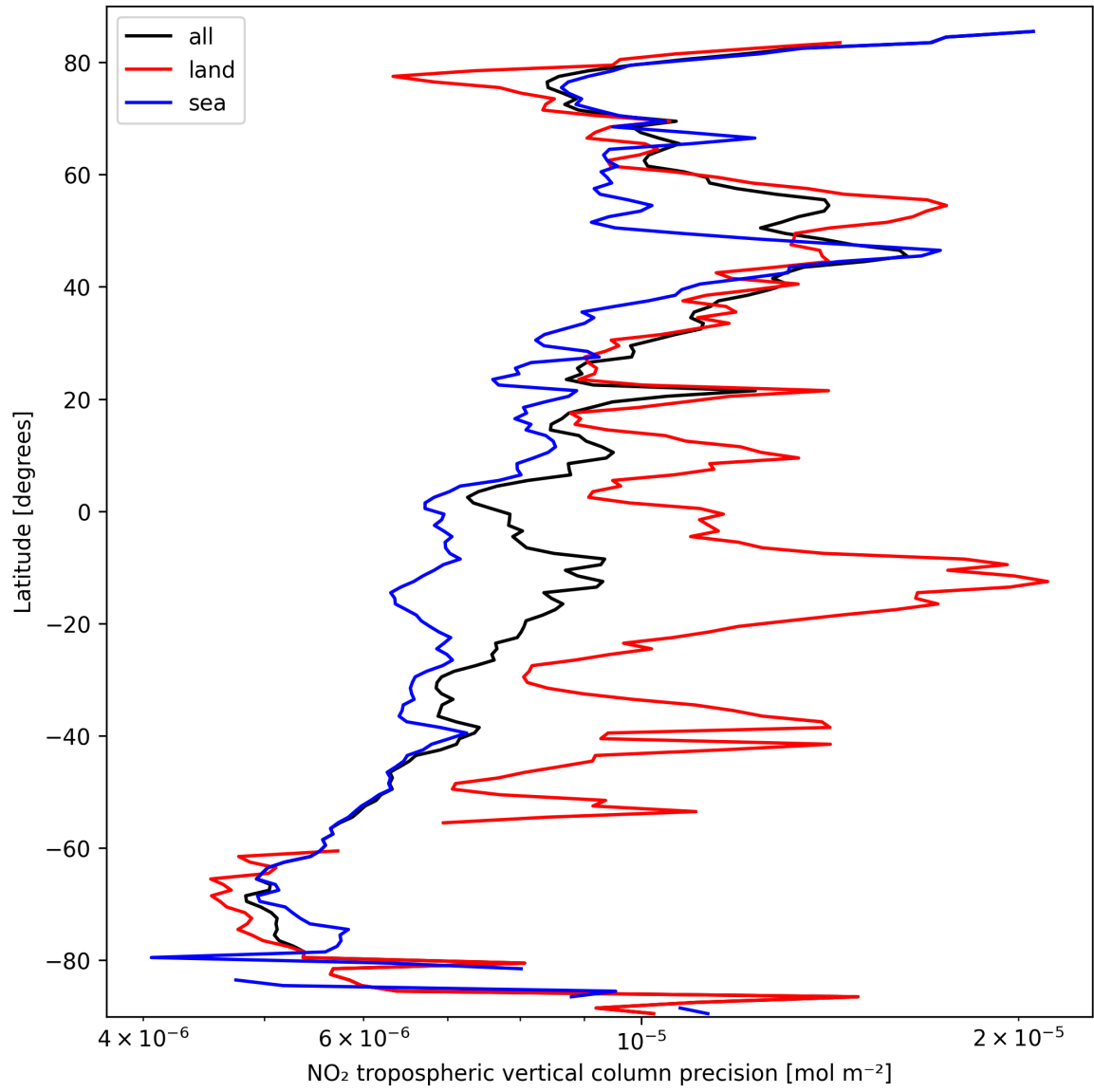
Figure 13: Zonal average of “NO 2 tropospheric vertical column precision” for 2025-09-28 to 2025-09-30.
