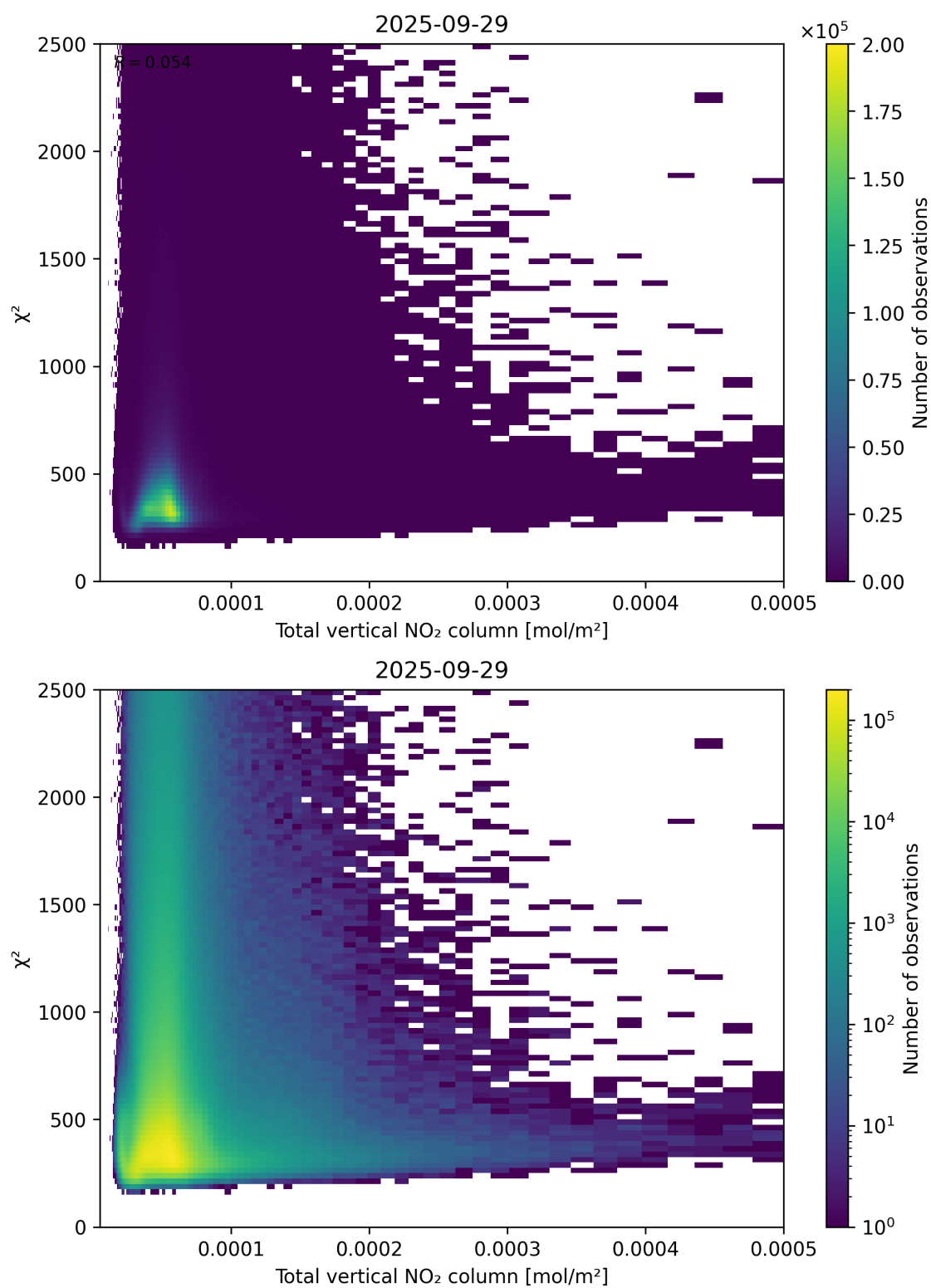
Figure 111: Scatter density plot of “Total vertical NO 2 column” against “ \chi^2 ” for 2025-09-28 to 2025-09-30.
