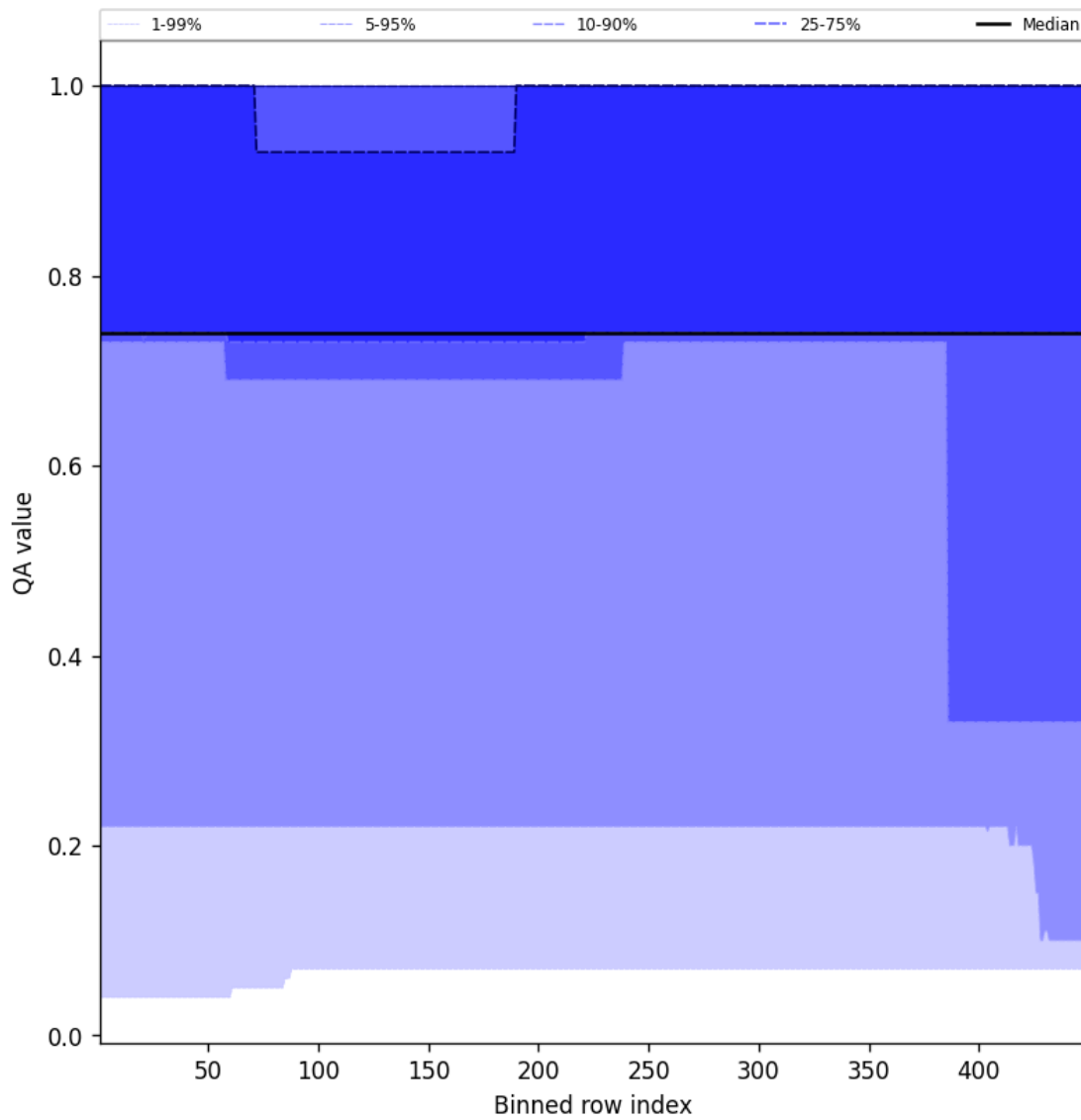
Figure 45: Along track statistics of "QA value" for 2025-09-28 to 2025-09-30
