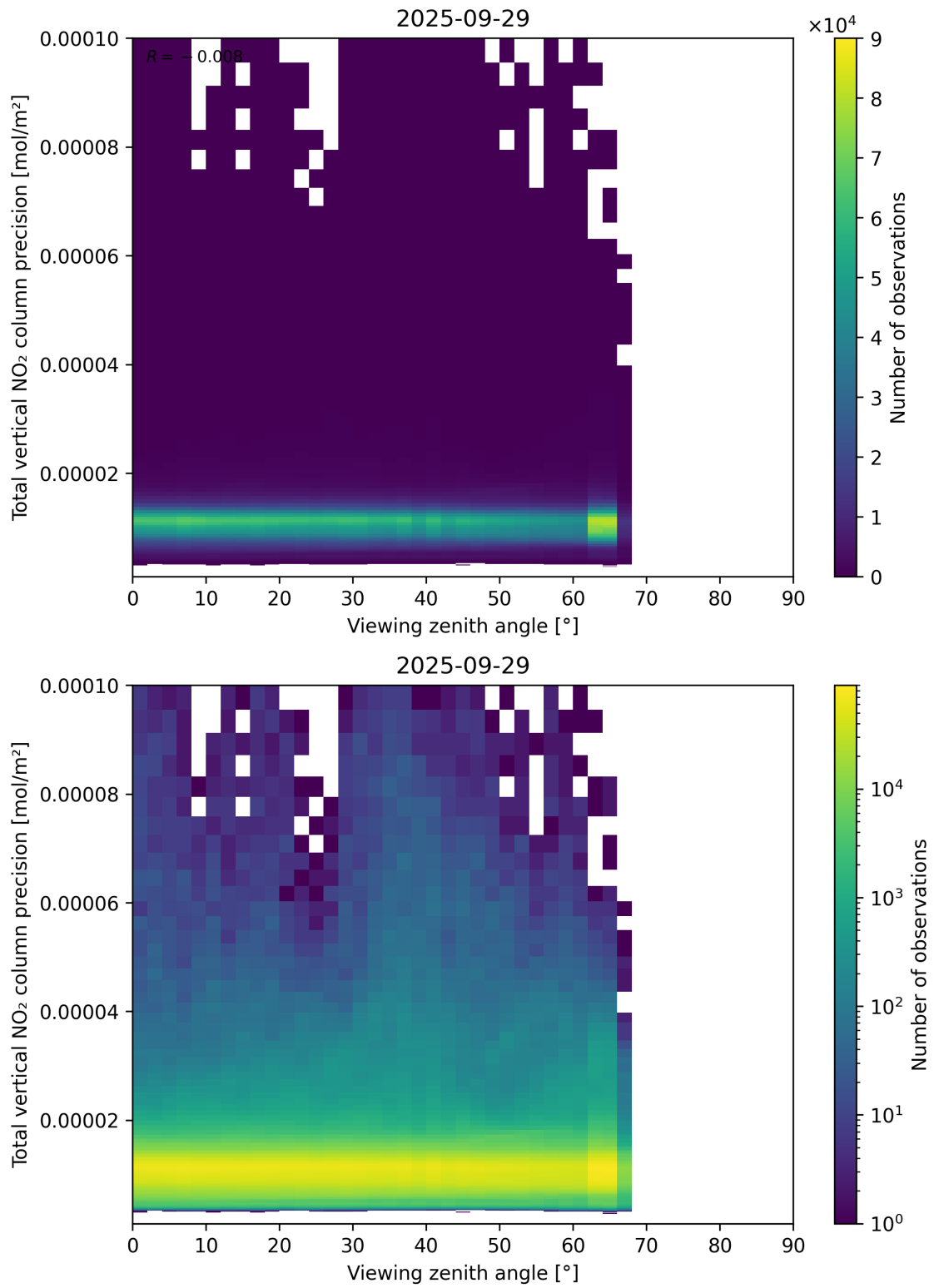
Figure 168: Scatter density plot of “Viewing zenith angle” against “Total vertical NO 2 column precision” for 2025-09-28 to 2025-09-30.
