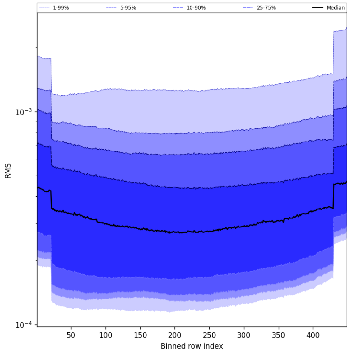
Figure 60: Along track statistics of “RMS” for 2025-09-28 to 2025-09-30
