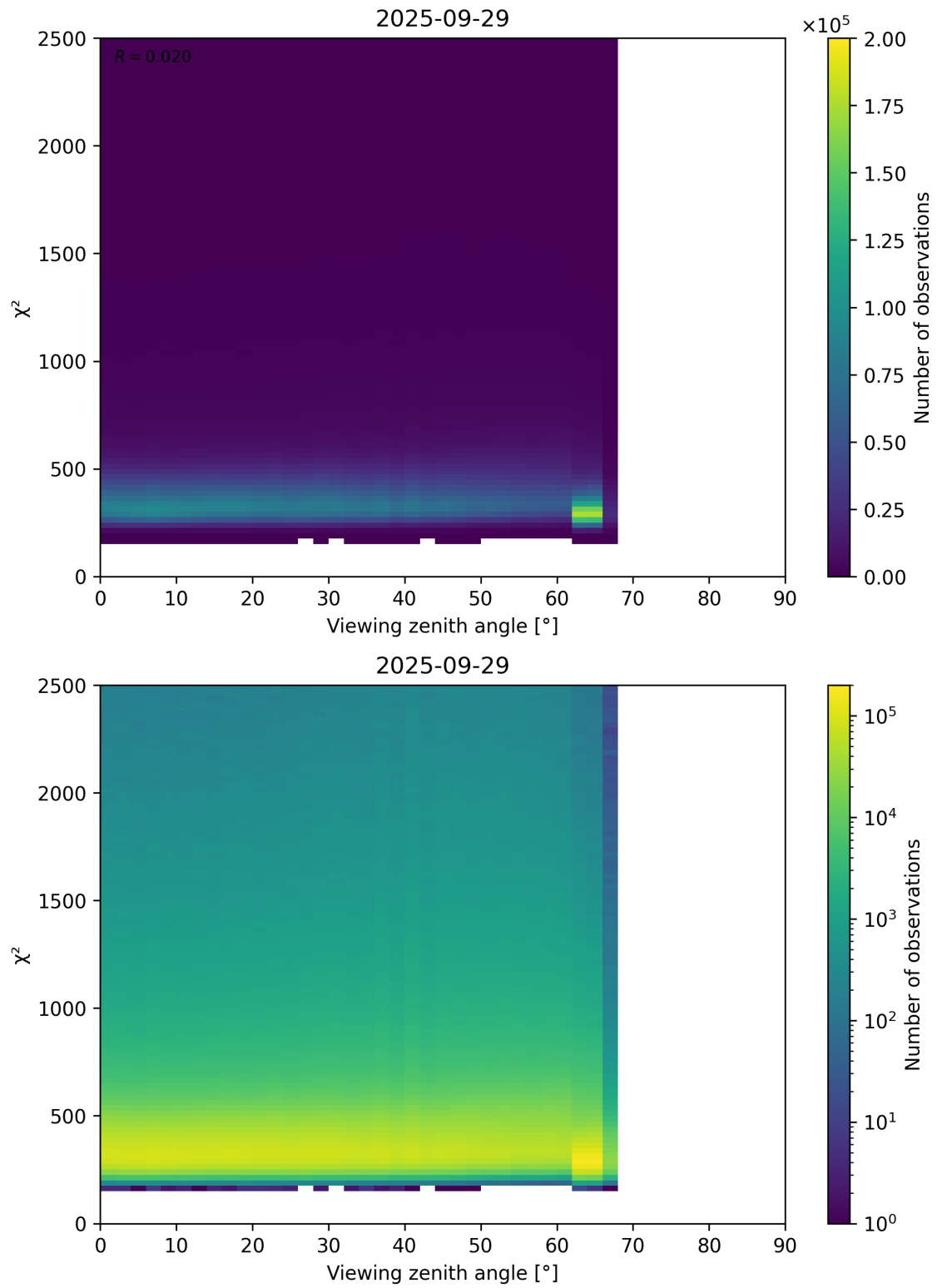
Figure 162: Scatter density plot of “Viewing zenith angle” against “ \chi^2 ” for 2025-09-28 to 2025-09-30.
