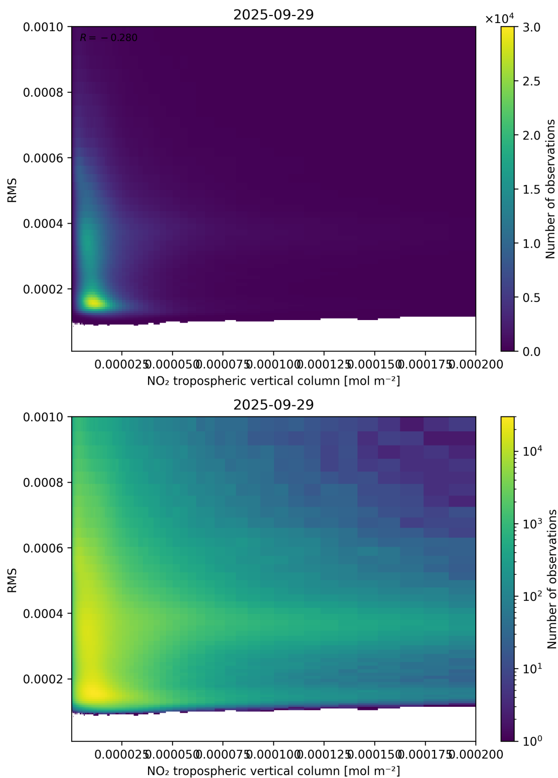
Figure 142: Scatter density plot of “NO 2 tropospheric vertical column” against “RMS” for 2025-09-28 to 2025-09-30.
