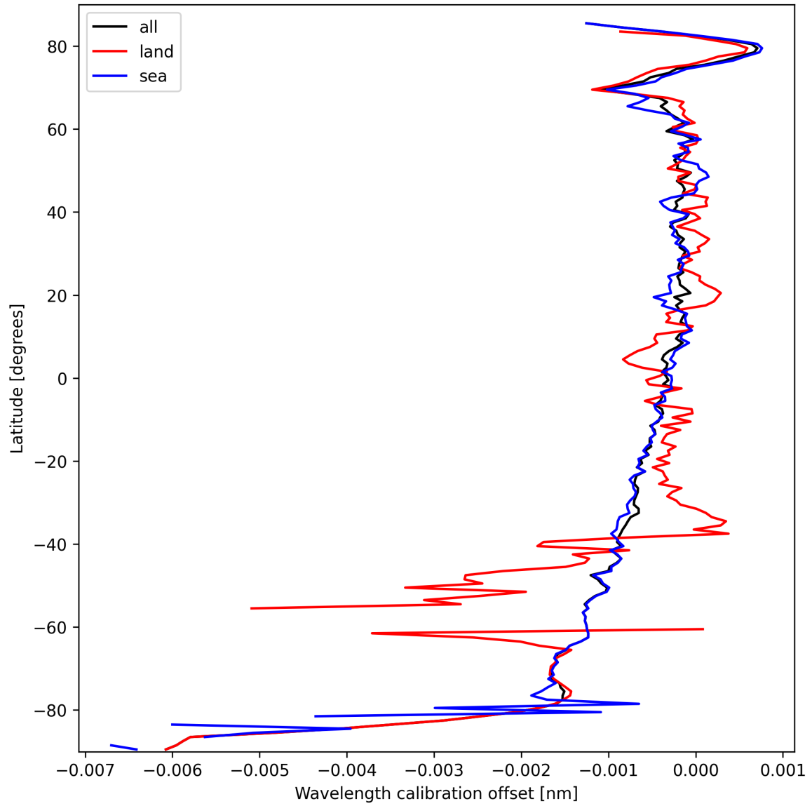
Figure 18: Zonal average of “Wavelength calibration offset” for 2025-09-28 to 2025-09-30.
