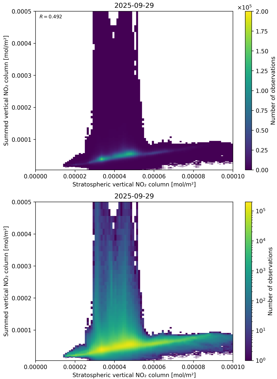
Figure 98: Scatter density plot of “Stratospheric vertical NO 2 column” against “Summed vertical NO 2 column” for 2025-09-28 to 2025-09-30.
