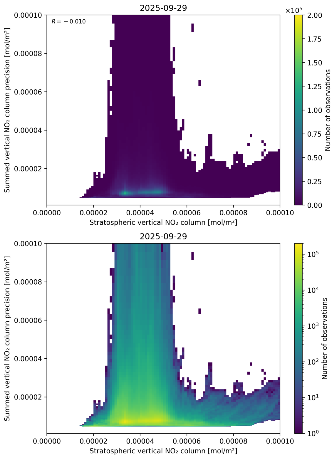
Figure 99: Scatter density plot of “Stratospheric vertical NO 2 column” against “Summed vertical NO 2 column precision” for 2025-09-28 to 2025-09-30.
