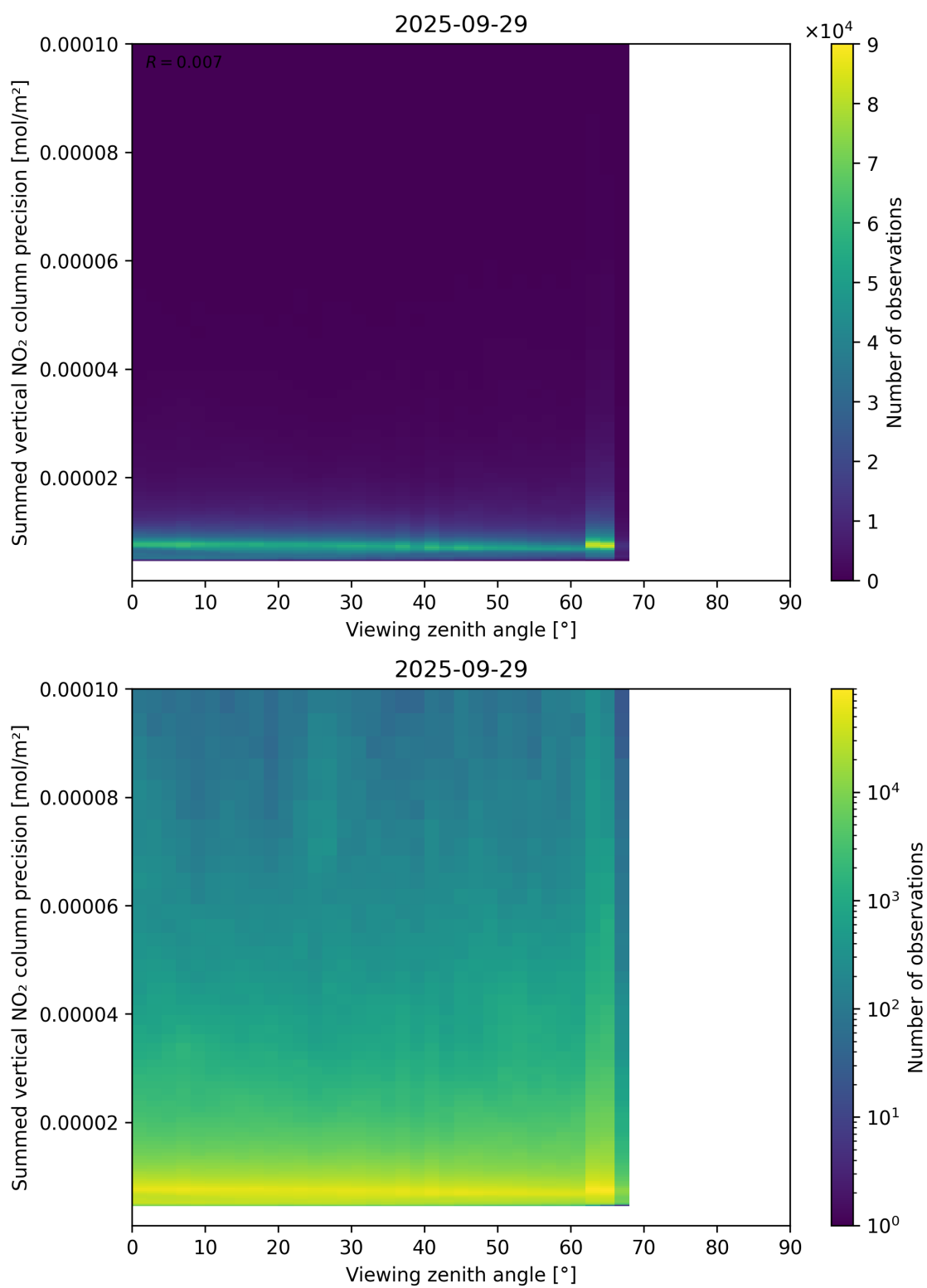
Figure 166: Scatter density plot of “Viewing zenith angle” against “Summed vertical NO 2 column precision” for 2025-09-28 to 2025-09-30.
