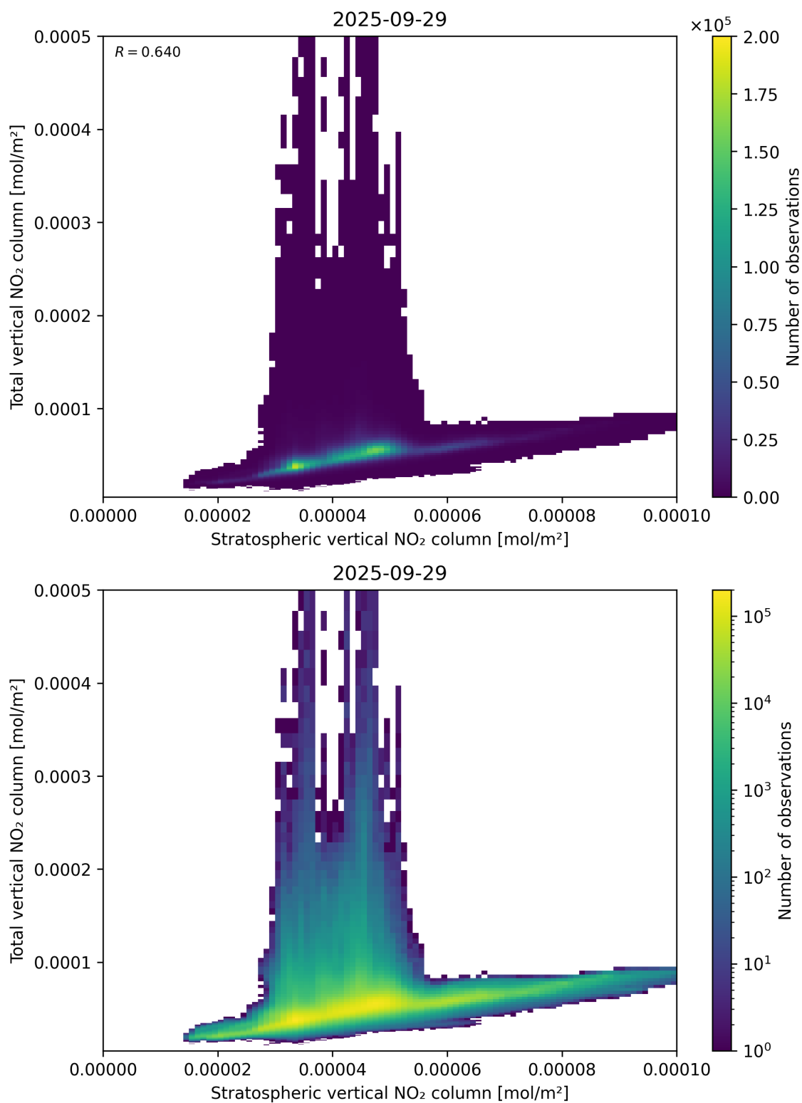
Figure 100: Scatter density plot of “Stratospheric vertical NO 2 column” against “Total vertical NO 2 column” for 2025-09-28 to 2025-09-30.
