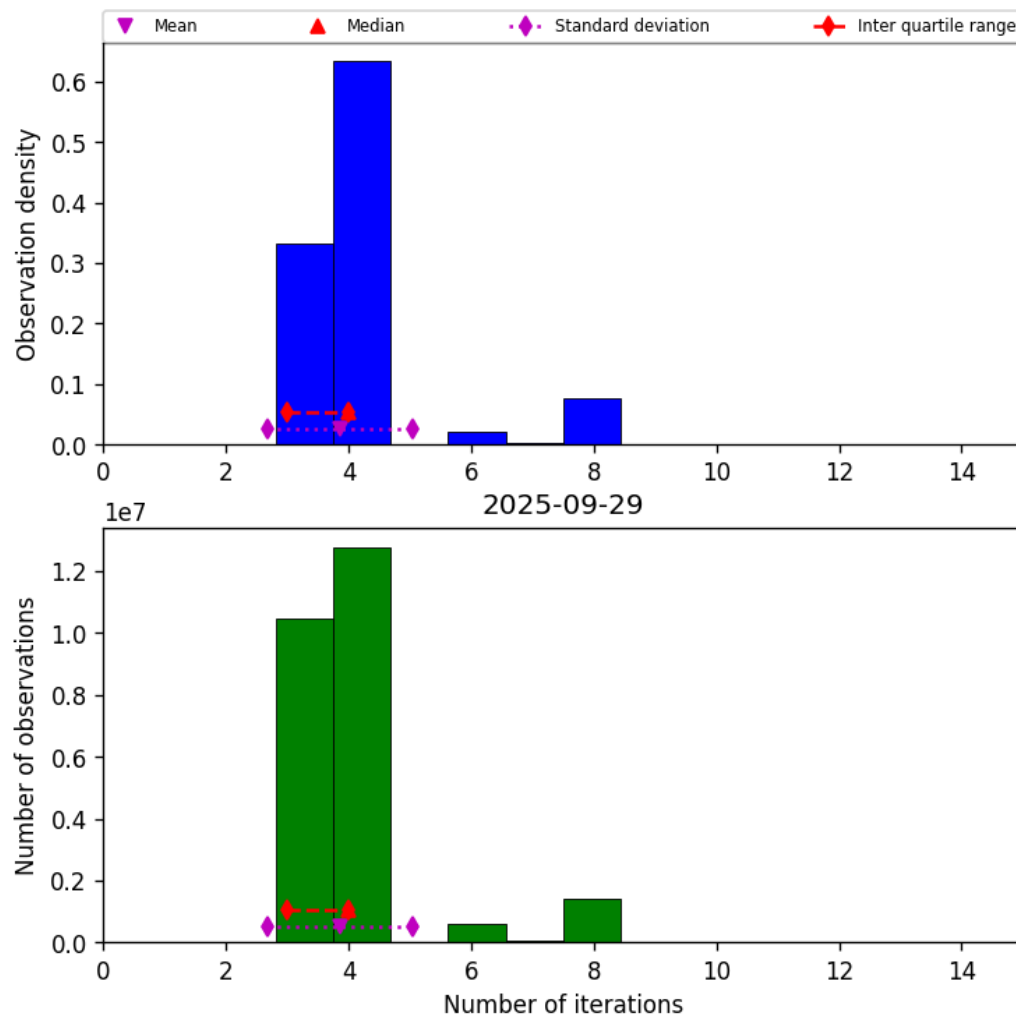
Figure 34: Histogram of “Number of iterations” for 2025-09-28 to 2025-09-30
