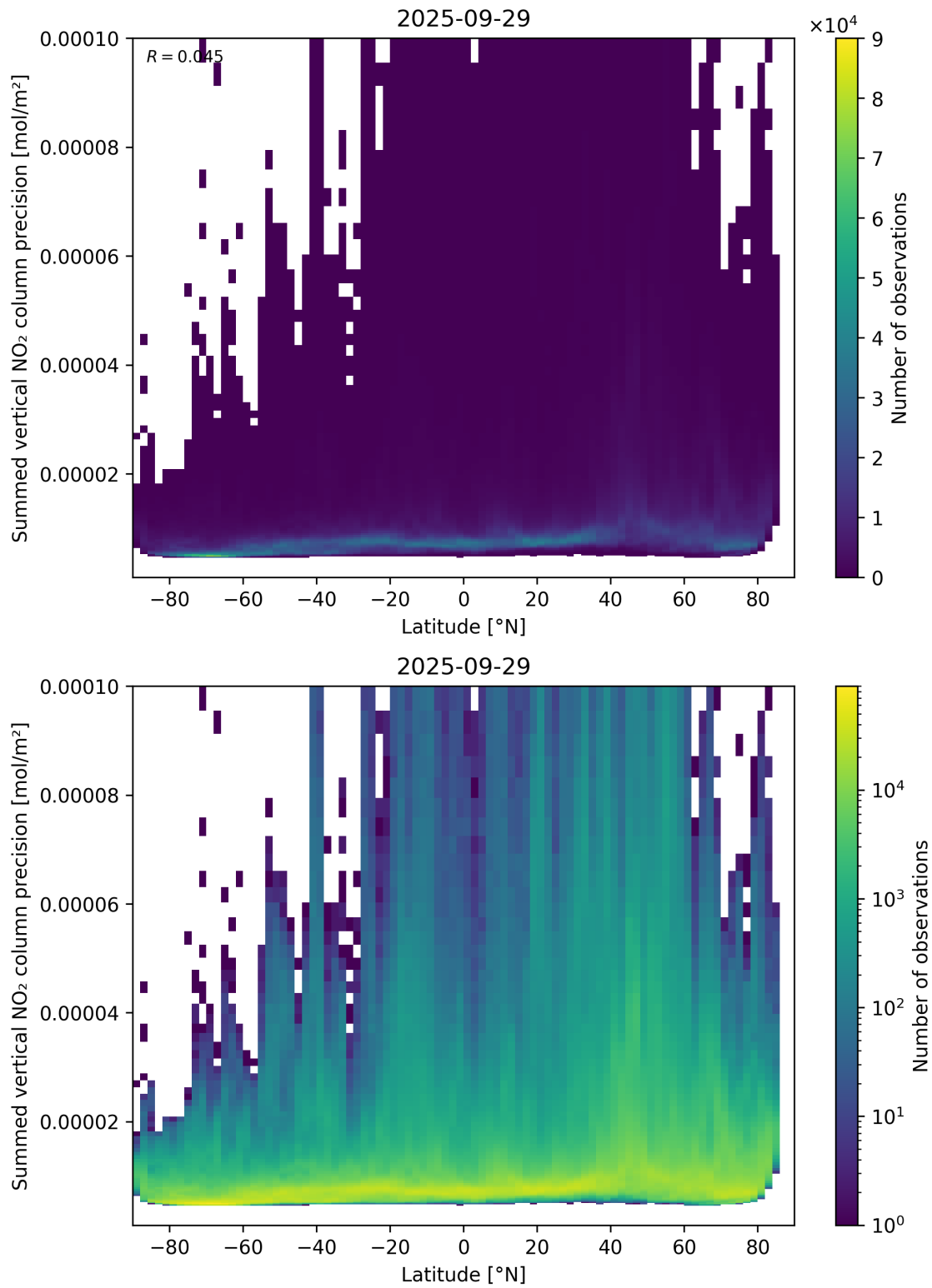
Figure 89: Scatter density plot of “Latitude” against “Summed vertical NO 2 column precision” for 2025-09-28 to 2025-09-30.
