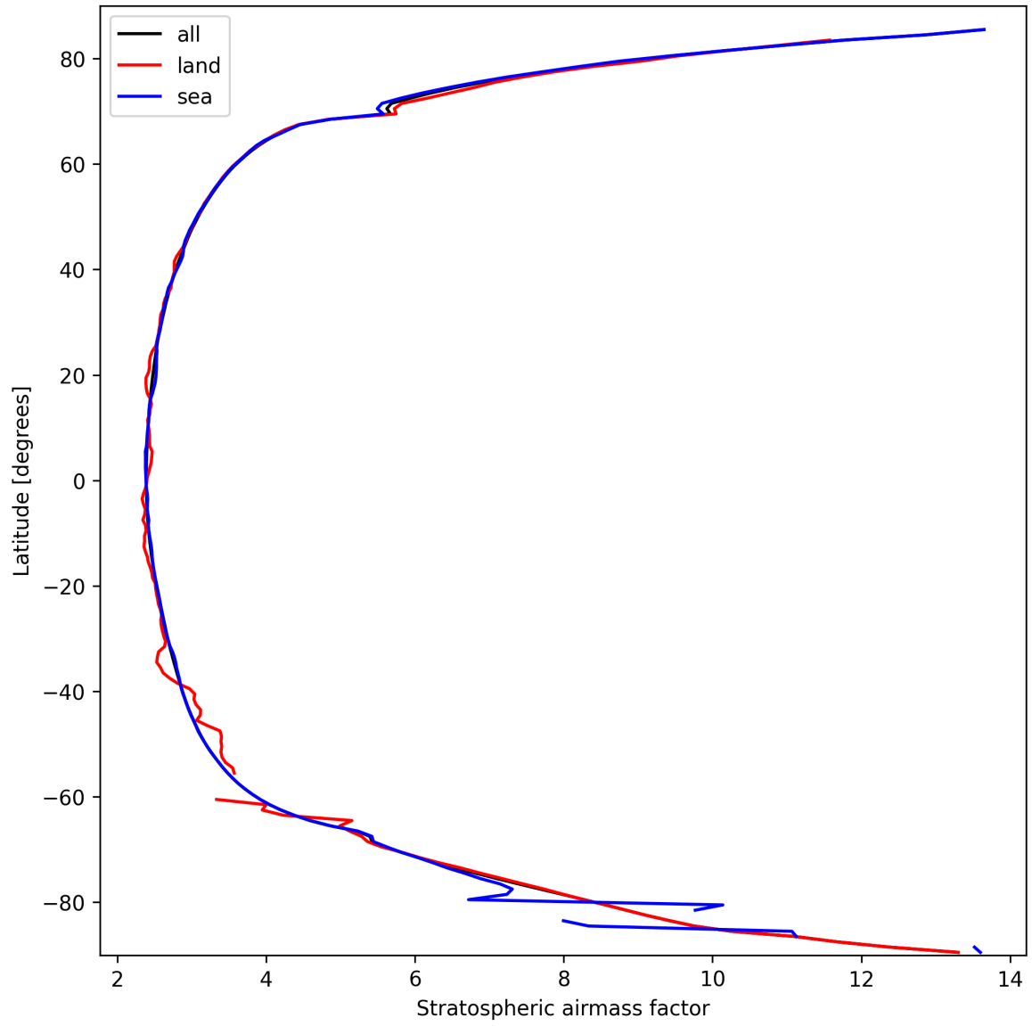
Figure 27: Zonal average of “Stratospheric air mass factor” for 2025-09-28 to 2025-09-30.
