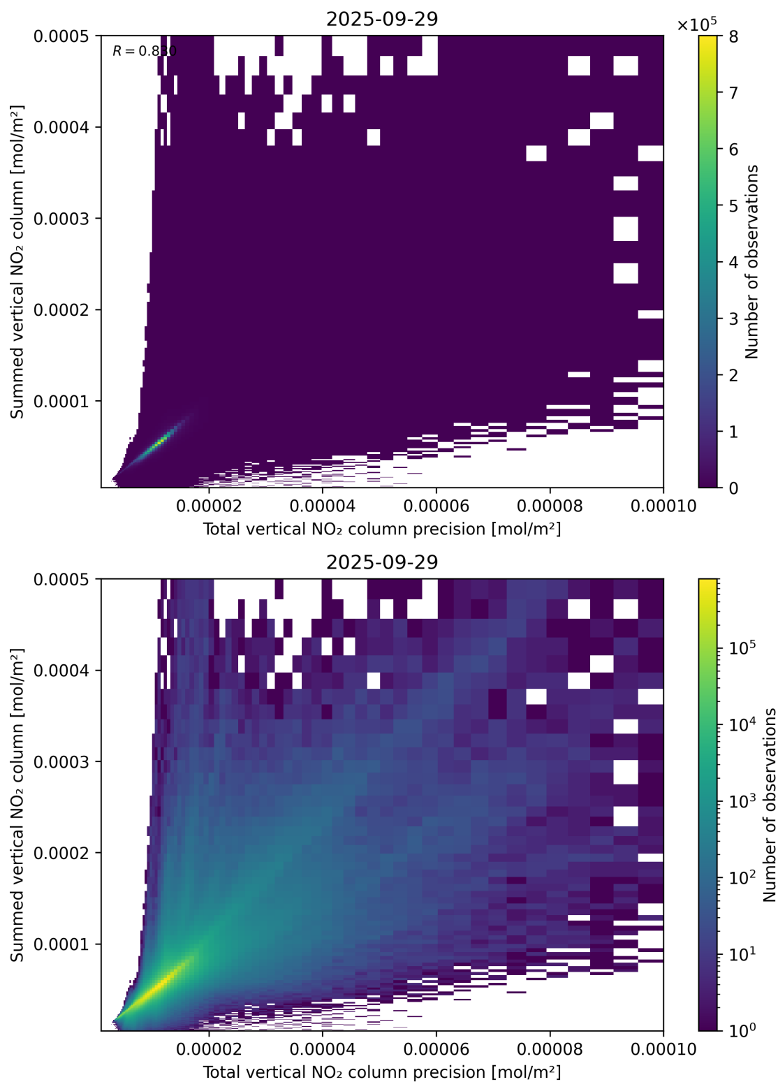
Figure 117: Scatter density plot of “Total vertical NO 2 column precision” against “Summed vertical NO 2 column” for 2025-09-28 to 2025-09-30.
