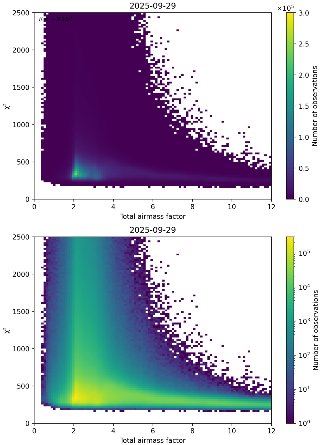
Figure 63: Scatter density plot of “Total airmass factor” against “ \chi^2 ” for 2025-09-28 to 2025-09-30.
