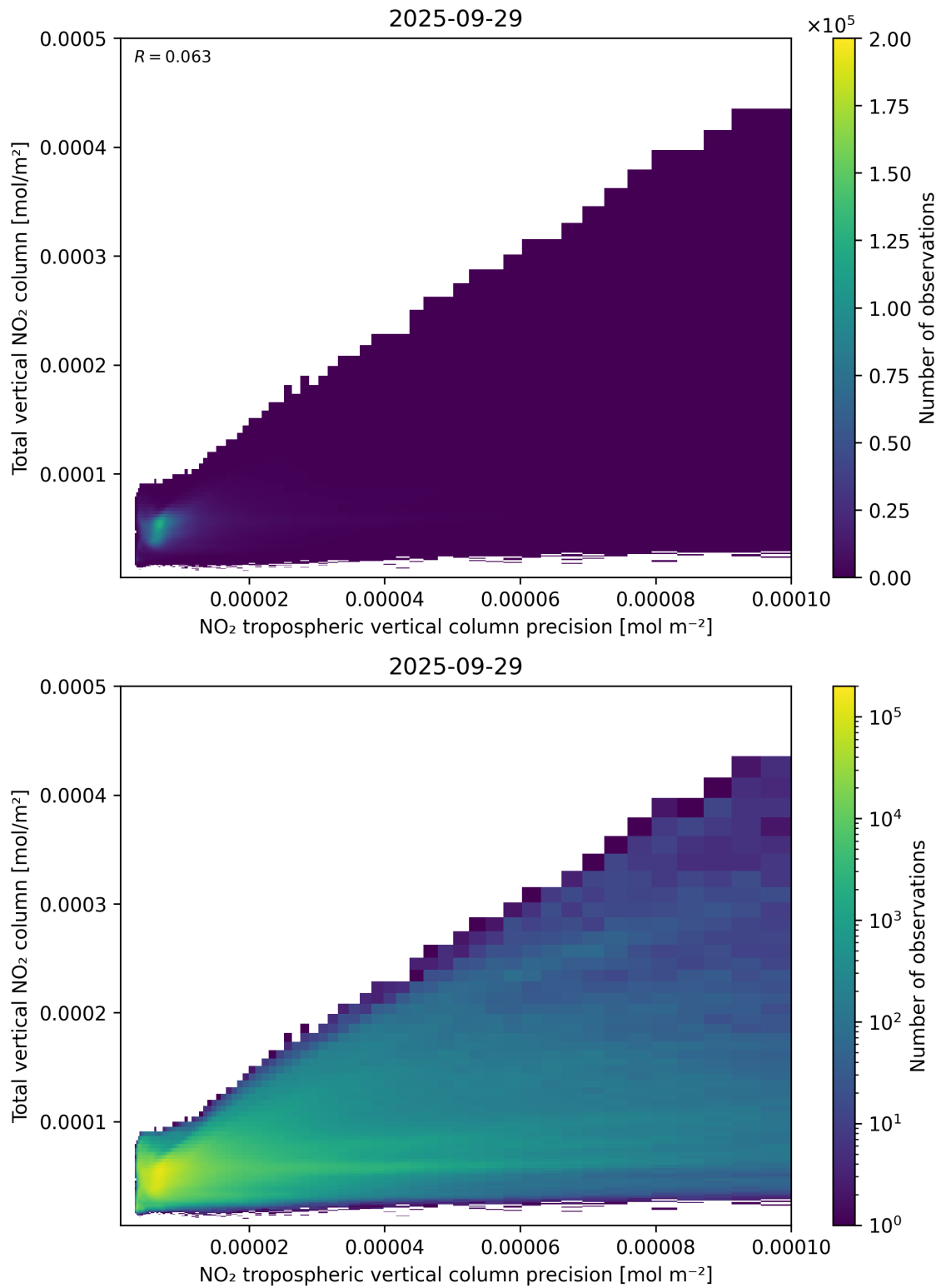
Figure 138: Scatter density plot of “NO 2 tropospheric vertical column precision” against “Total vertical NO 2 column” for 2025-09-28 to 2025-09-30.
