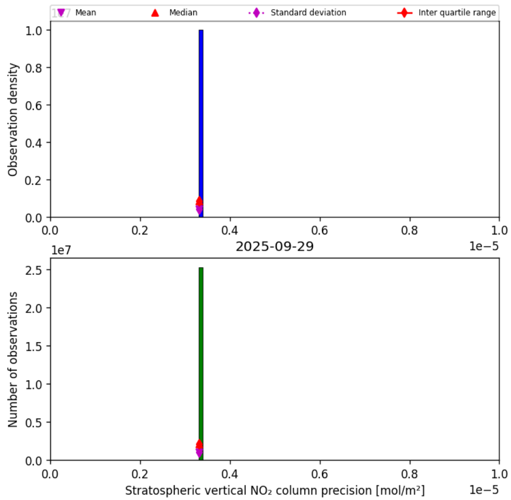
Figure 37: Histogram of “Stratospheric vertical NO 2 column precision” for 2025-09-28 to 2025-09-30
