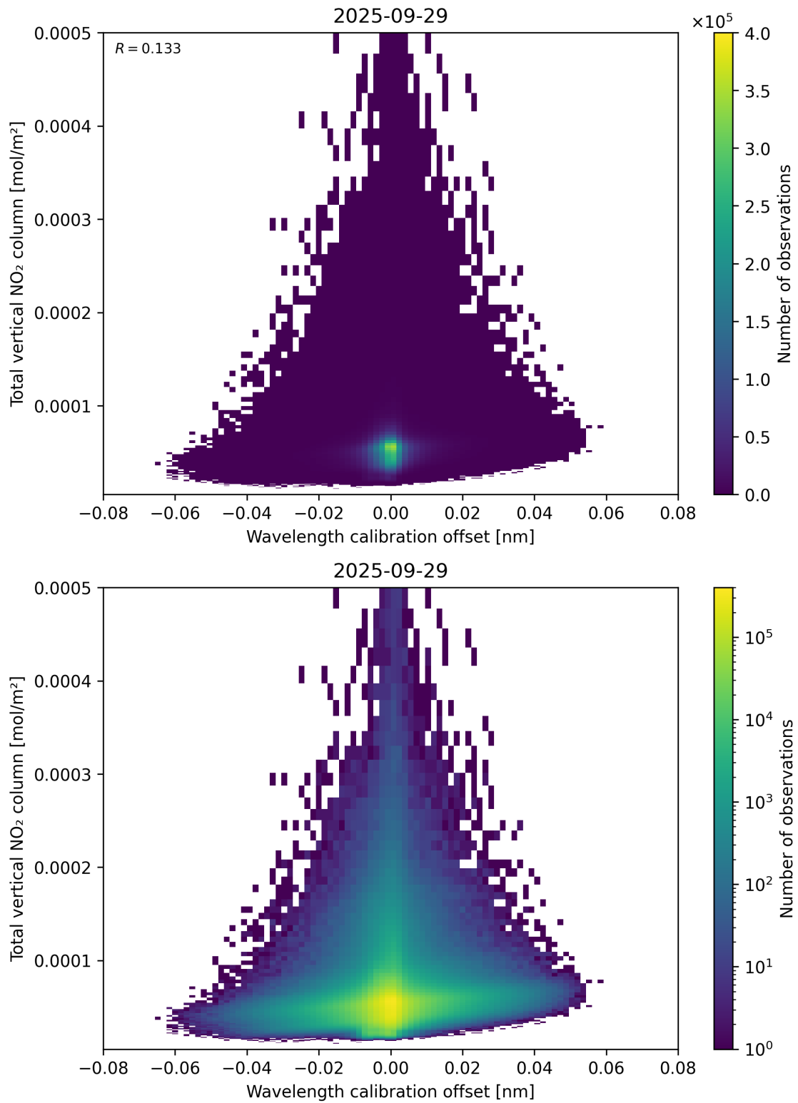
Figure 179: Scatter density plot of “Wavelength calibration offset” against “Total vertical NO 2 column” for 2025-09-28 to 2025-09-30.
