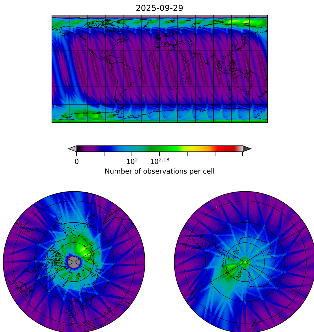
Figure 10: Map of the number of observations for 2025-09-28 to 2025-09-30
