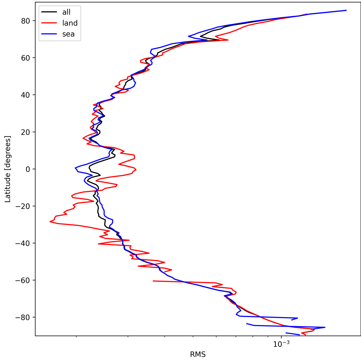
Figure 26: Zonal average of “RMS” for 2025-09-28 to 2025-09-30.
