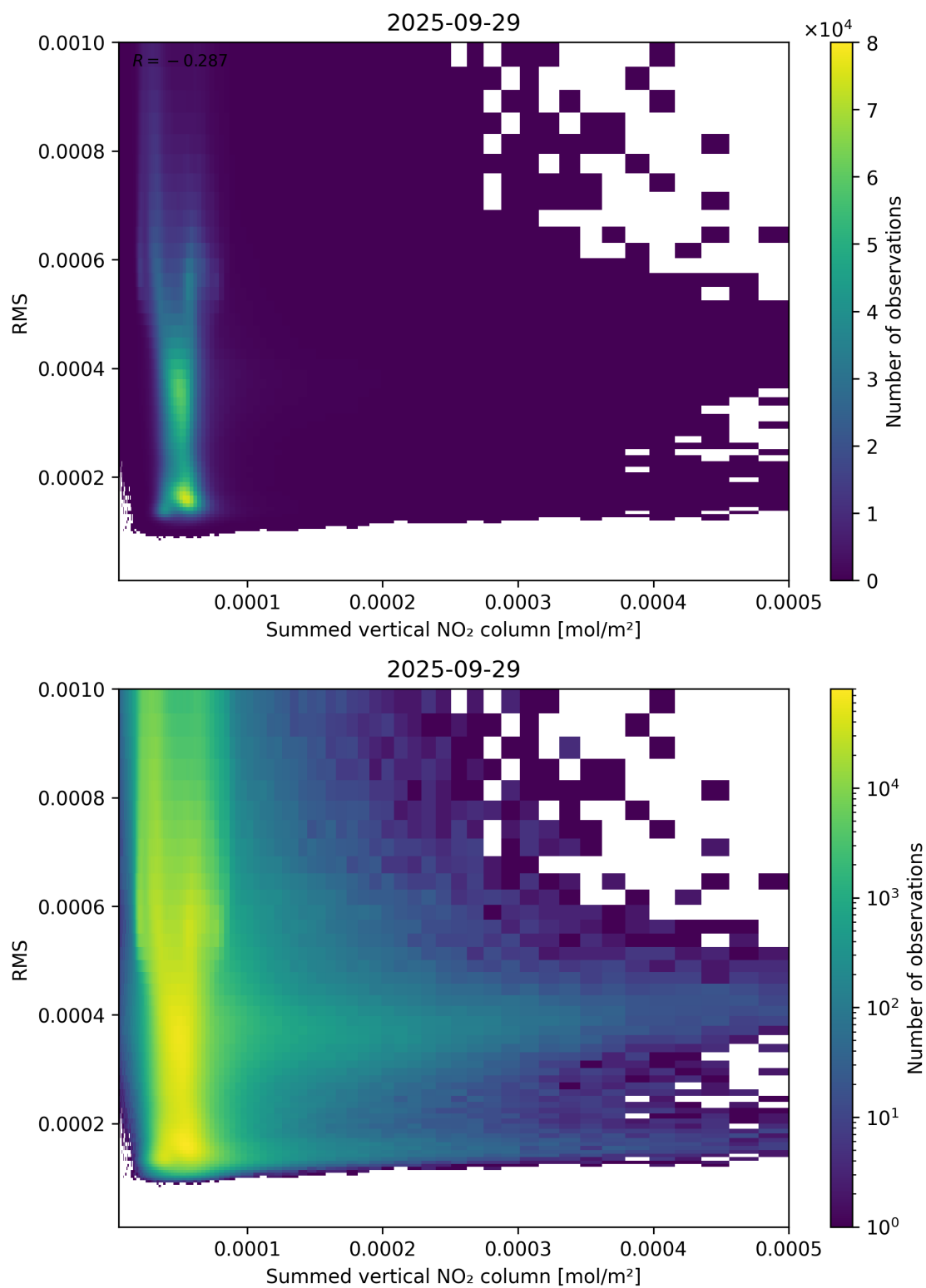
Figure 109: Scatter density plot of “Summed vertical NO 2 column” against “RMS” for 2025-09-28 to 2025-09-30.
