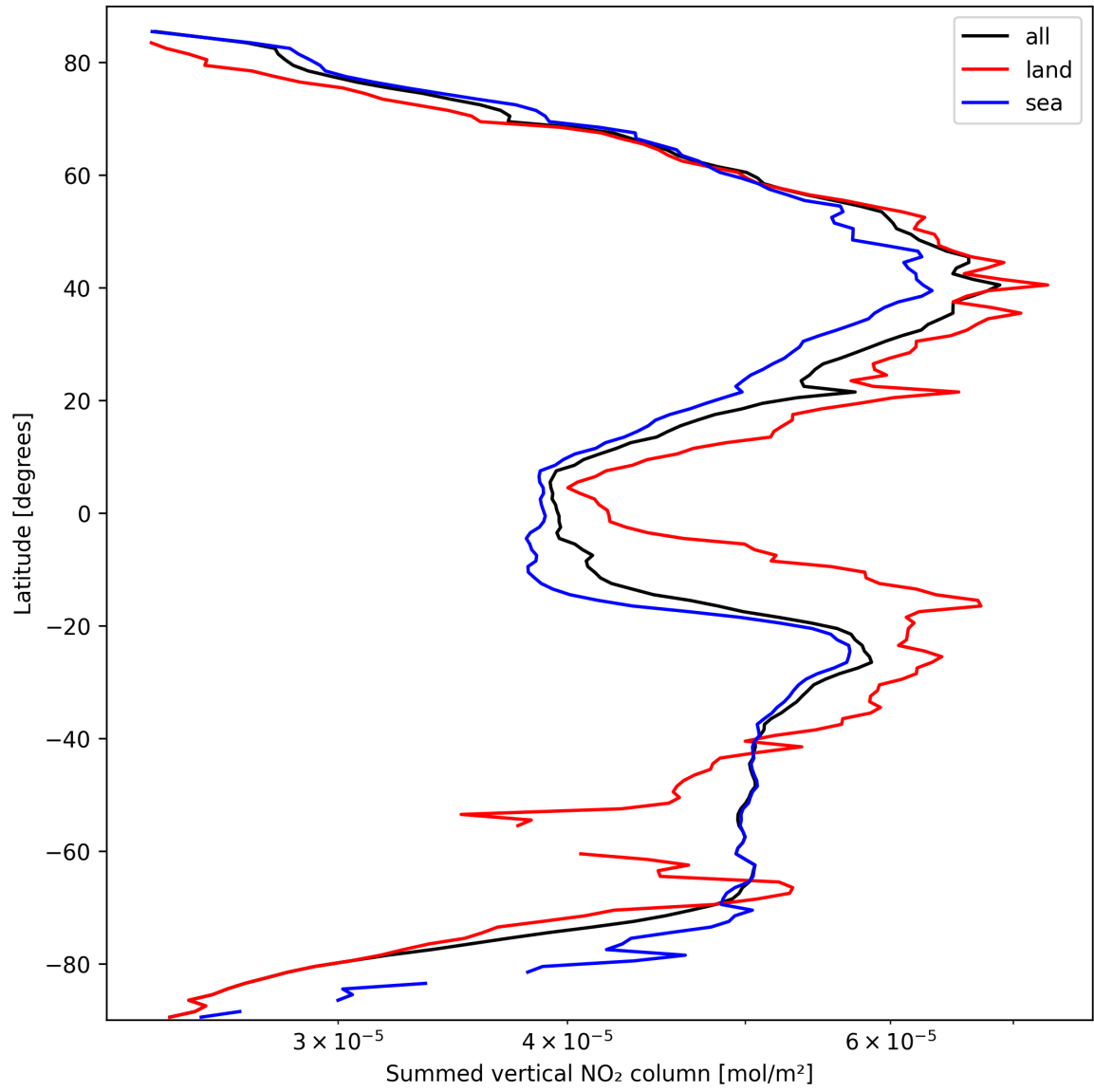
Figure 23: Zonal average of “Summed vertical NO 2 column” for 2025-09-28 to 2025-09-30.
