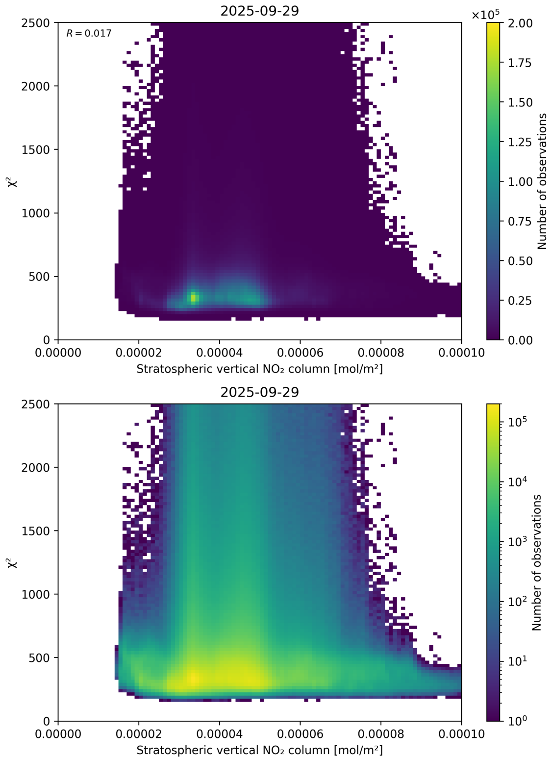
Figure 97: Scatter density plot of “Stratospheric vertical NO 2 column” against “ \chi^2 ” for 2025-09-28 to 2025-09-30.
