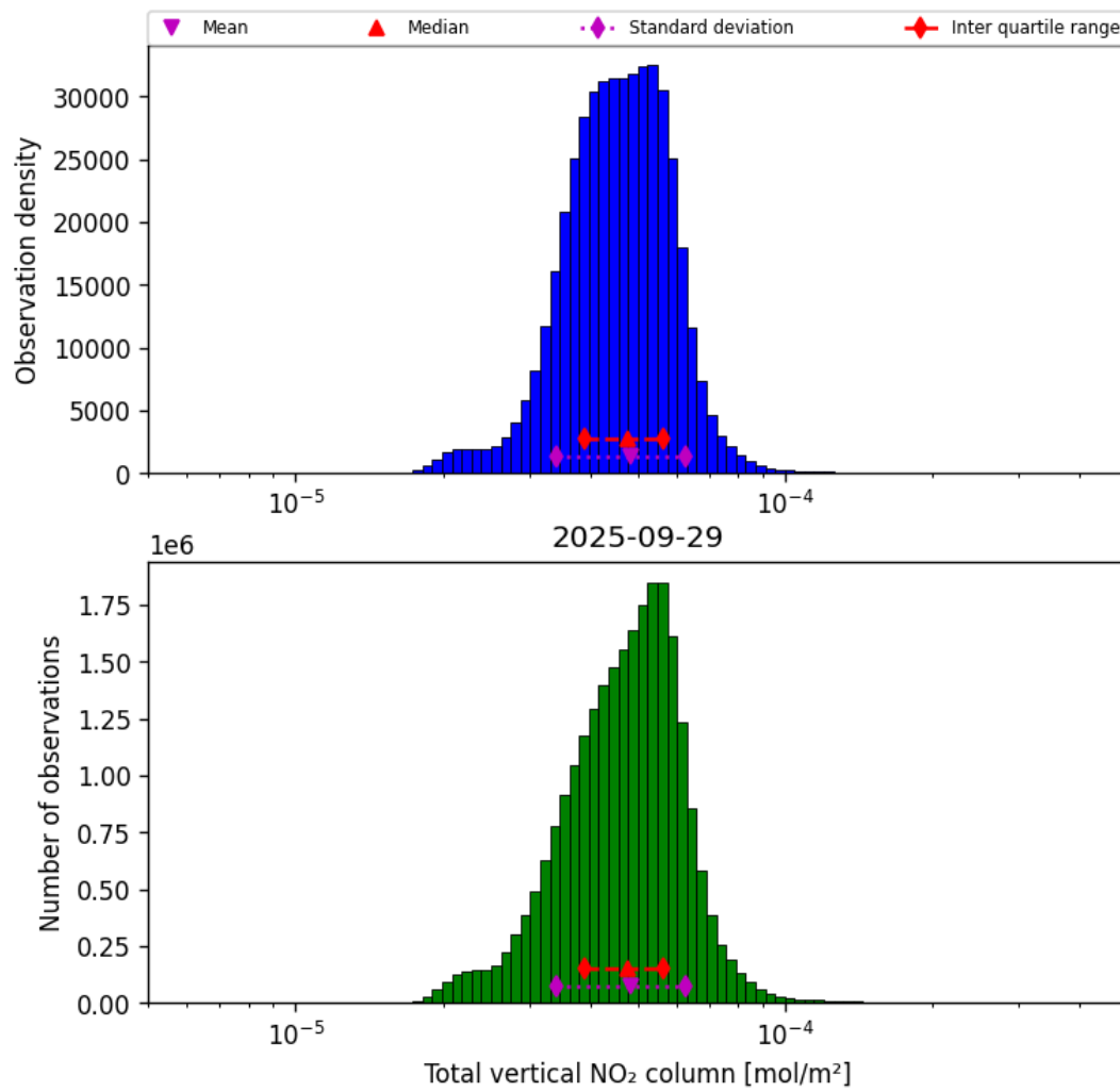
Figure 38: Histogram of “Total vertical NO 2 column” for 2025-09-28 to 2025-09-30
