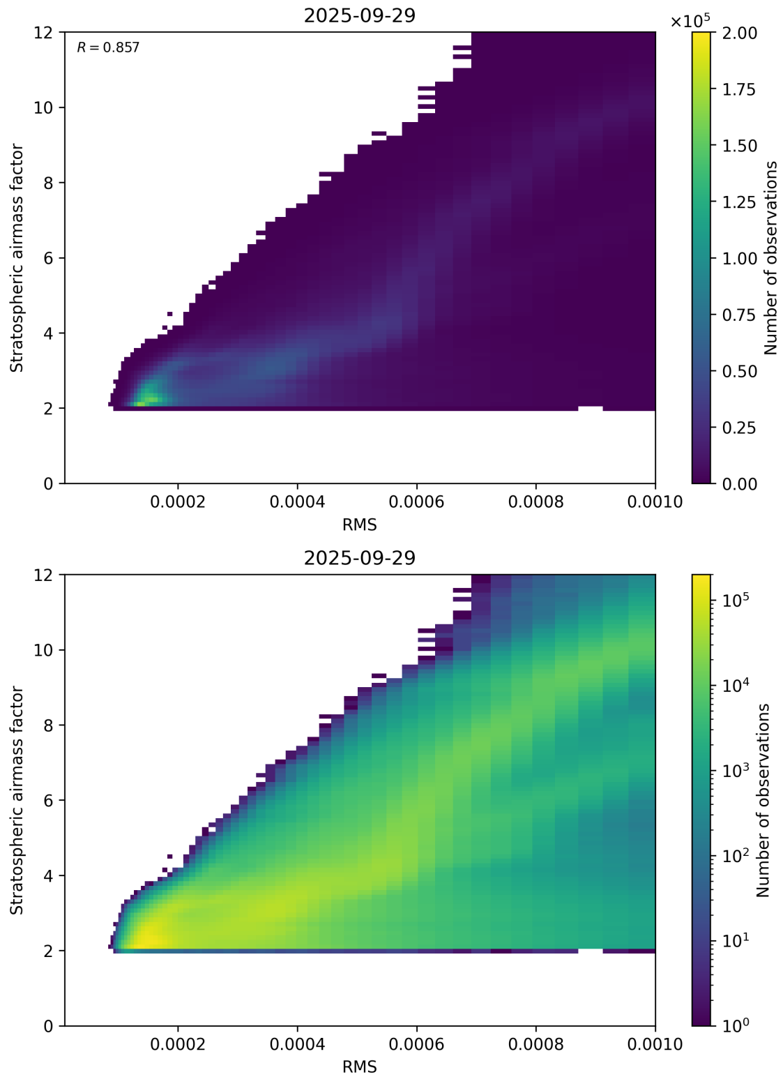
Figure 144: Scatter density plot of “RMS” against “Stratospheric airmass factor” for 2025-09-28 to 2025-09-30.
