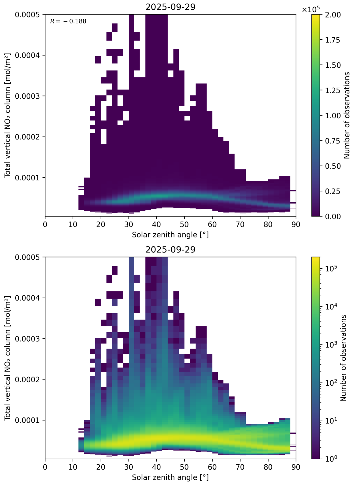
Figure 153: Scatter density plot of “Solar zenith angle” against “Total vertical NO 2 column” for 2025-09-28 to 2025-09-30.
