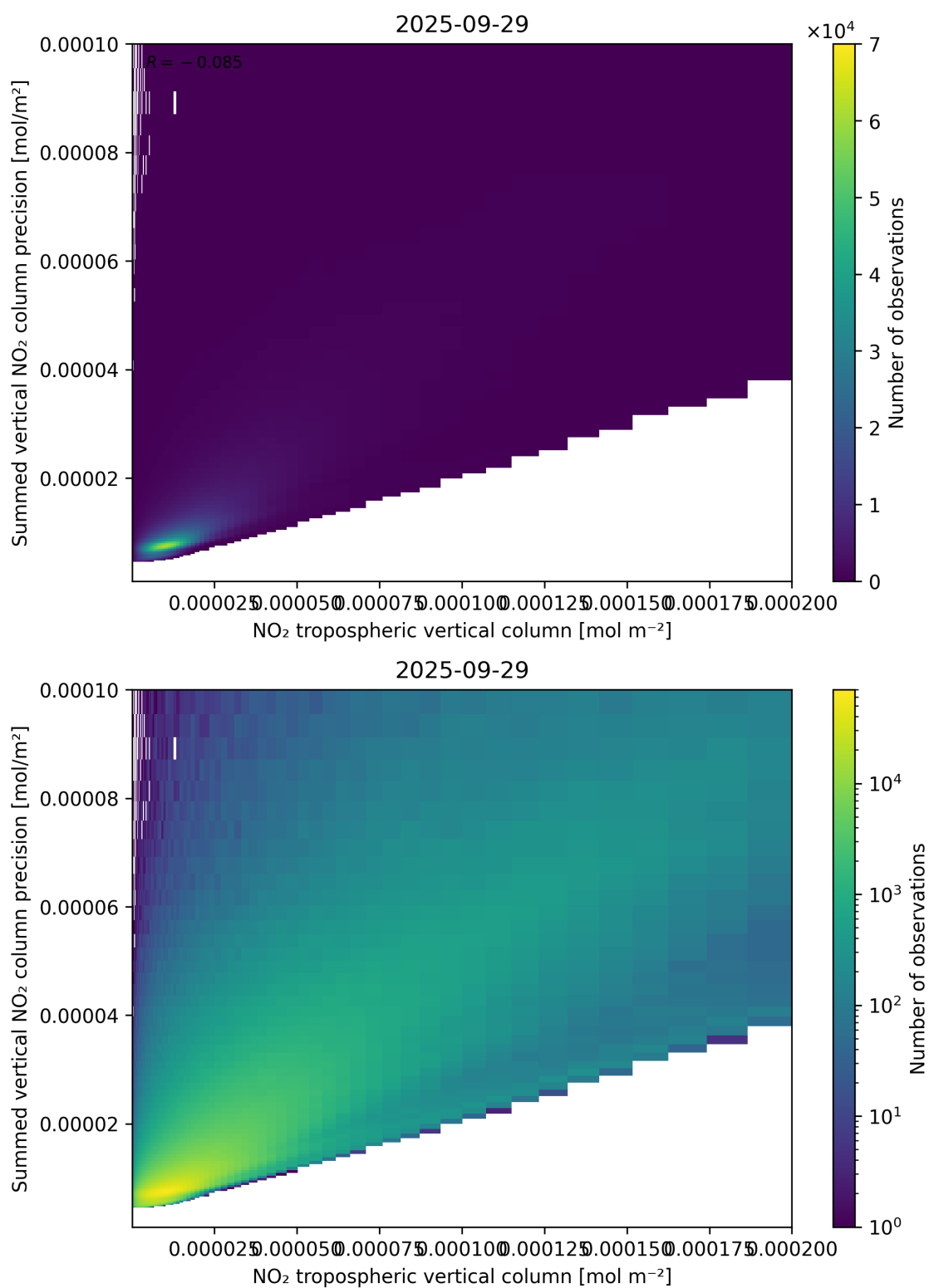
Figure 127: Scatter density plot of “NO 2 tropospheric vertical column” against “Summed vertical NO 2 column precision” for 2025-09-28 to 2025-09-30.
