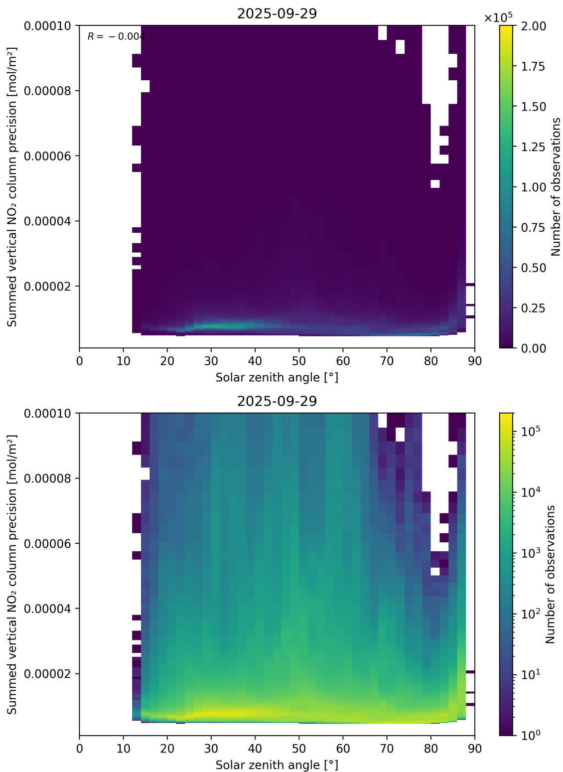
Figure 152: Scatter density plot of “Solar zenith angle” against “Summed vertical NO 2 column precision” for 2025-09-28 to 2025-09-30.
