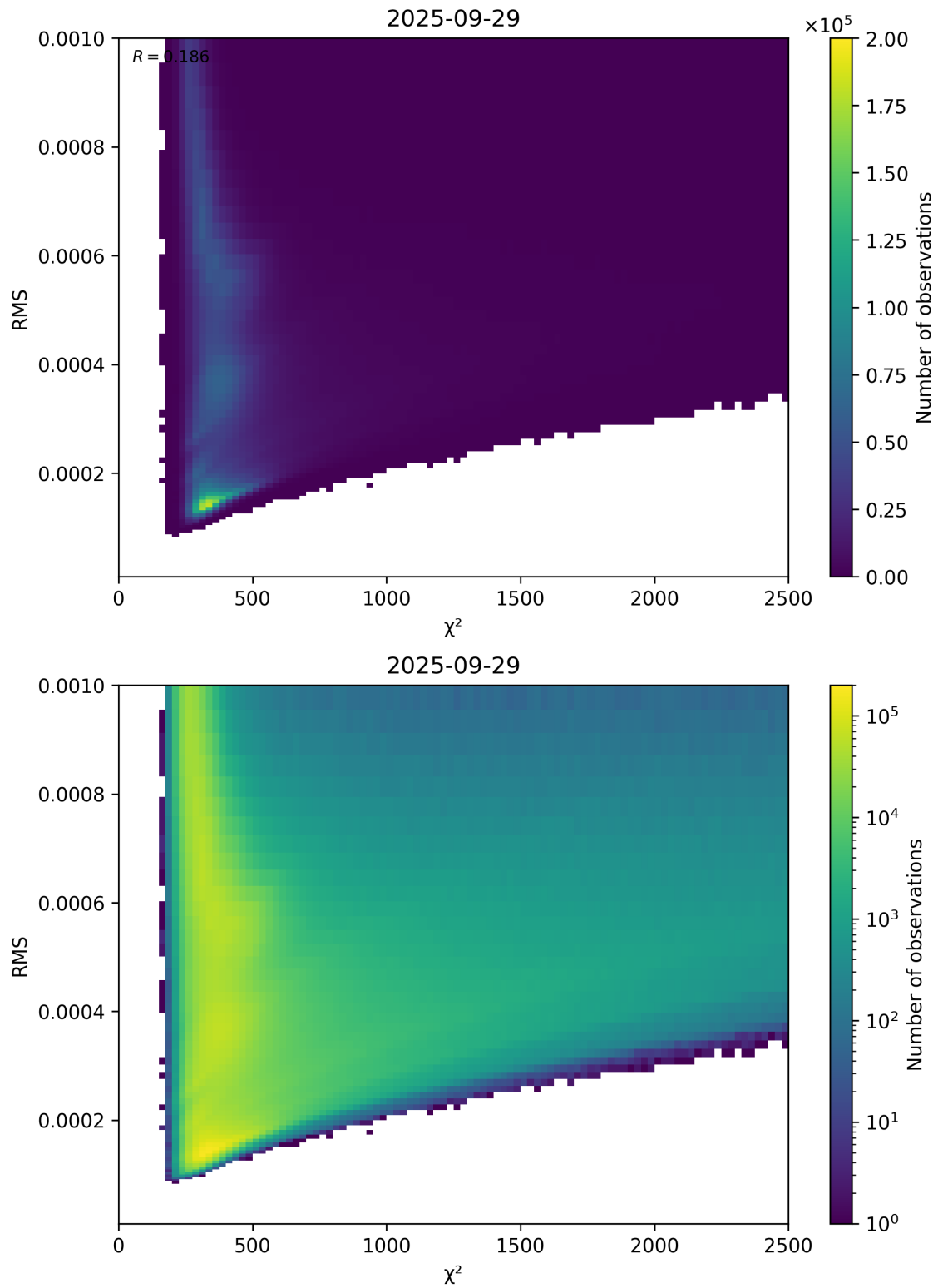
Figure 82: Scatter density plot of “ \chi^2 ” against “RMS” for 2025-09-28 to 2025-09-30.
