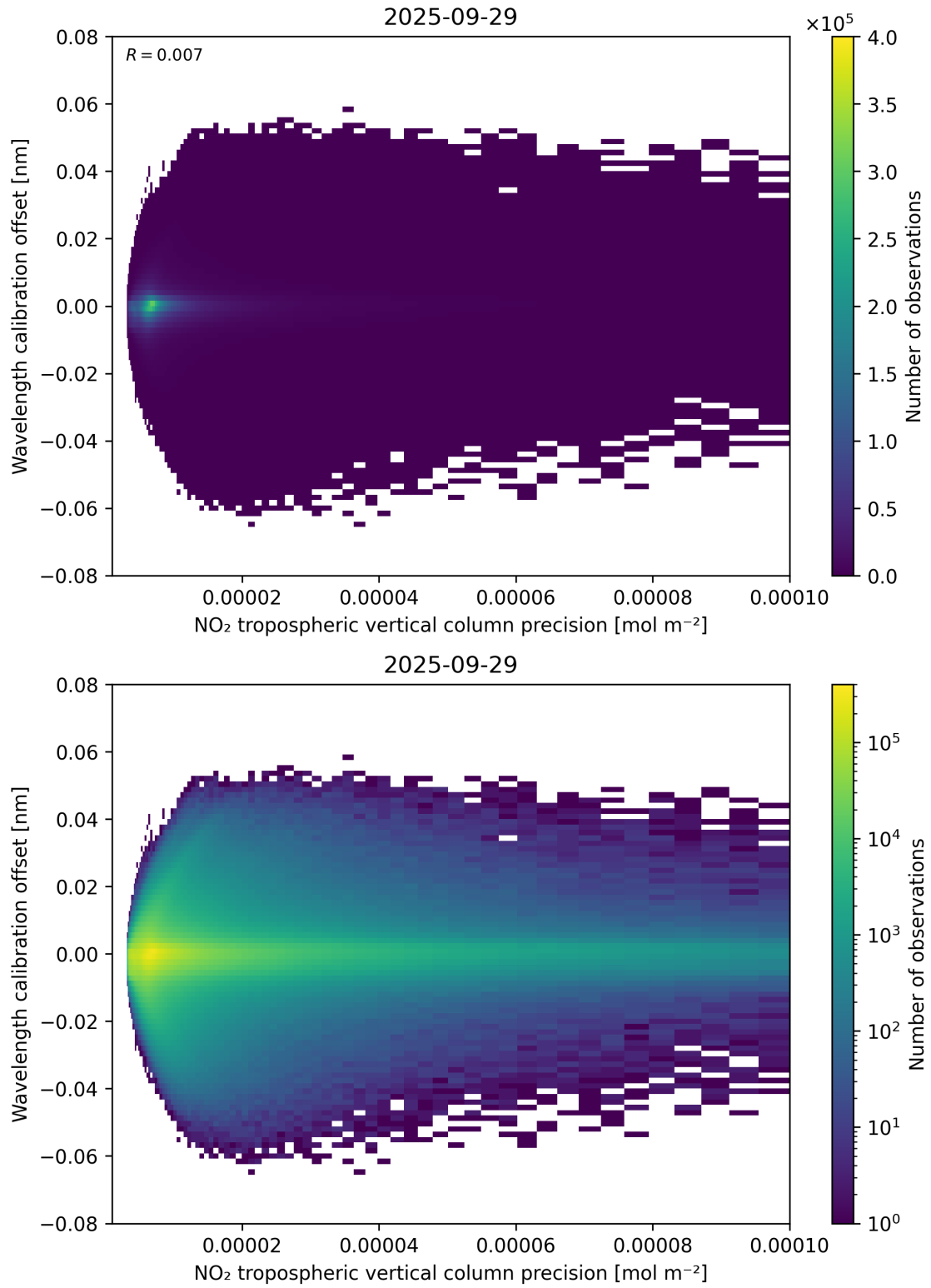
Figure 141: Scatter density plot of “NO 2 tropospheric vertical column precision” against “Wavelength calibration offset” for 2025-09-28 to 2025-09-30.
