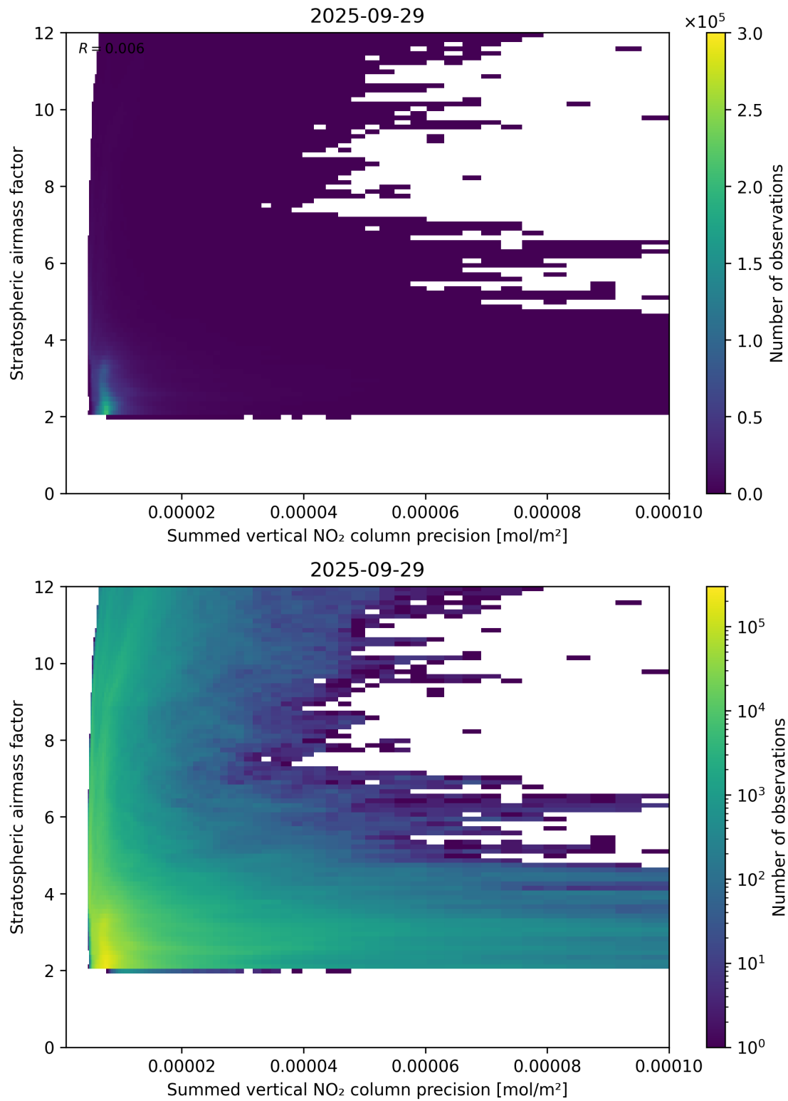
Figure 106: Scatter density plot of “Summed vertical NO 2 column precision” against “Stratospheric airmass factor” for 2025-09-28 to 2025-09-30.
