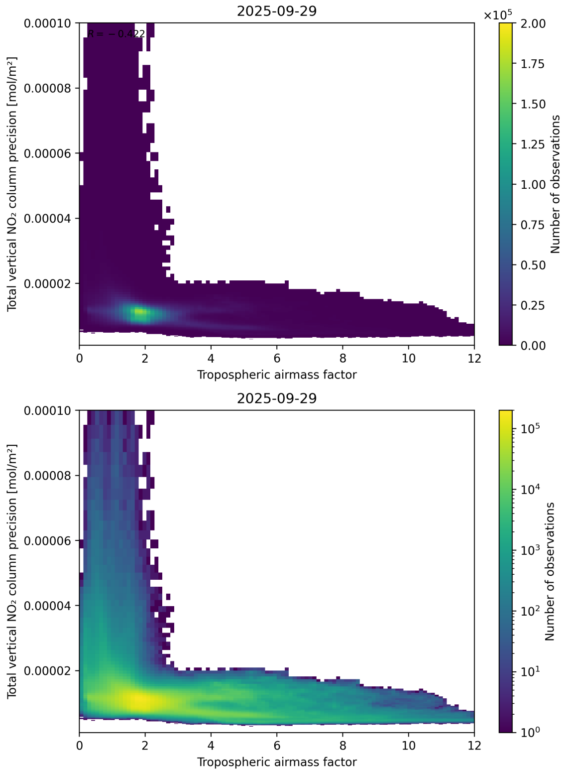
Figure 78: Scatter density plot of “Tropospheric air mass factor” against “Total vertical NO 2 column precision” for 2025-09-28 to 2025-09-30.
