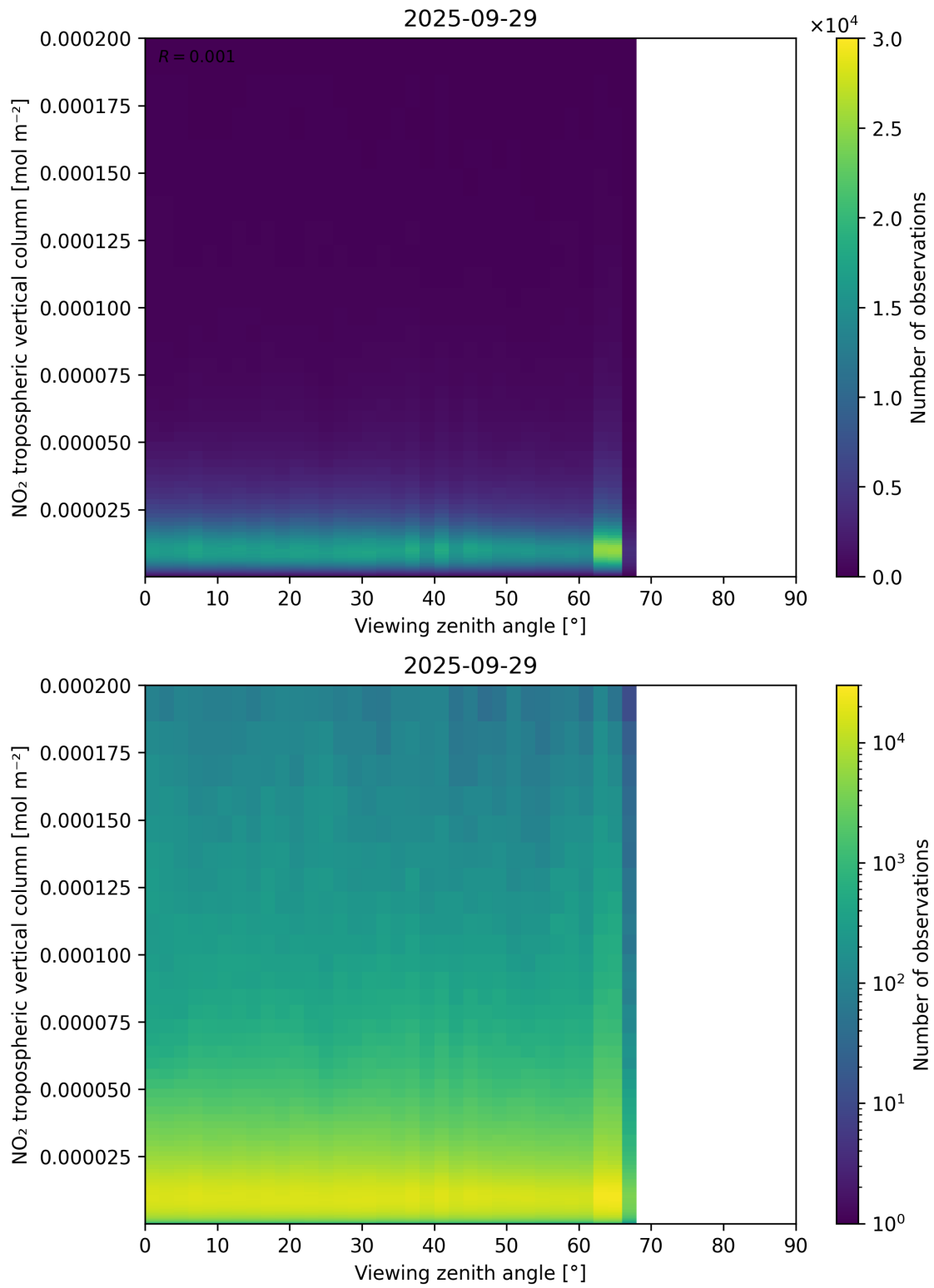
Figure 169: Scatter density plot of “Viewing zenith angle” against “NO 2 tropospheric vertical column” for 2025-09-28 to 2025-09-30.
