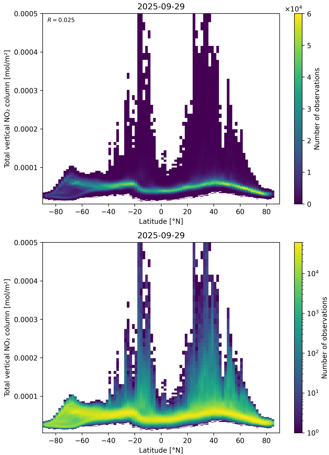
Figure 90: Scatter density plot of “Latitude” against “Total vertical NO 2 column” for 2025-09-28 to 2025-09-30.
