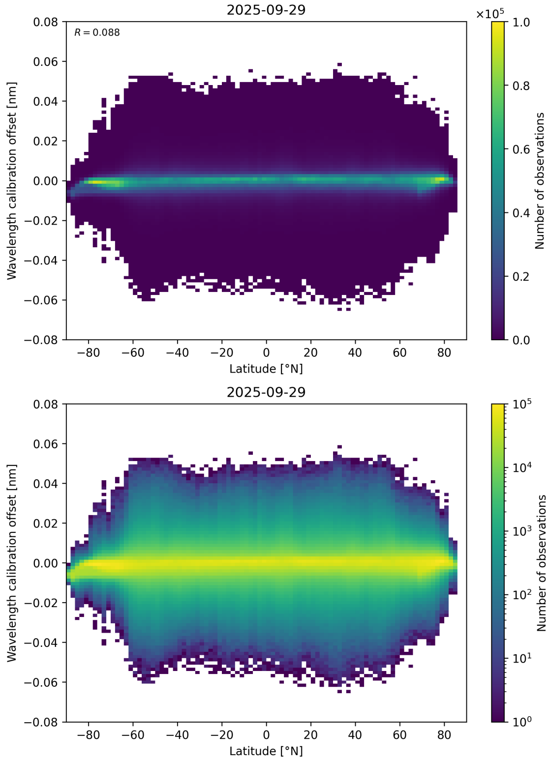
Figure 95: Scatter density plot of “Latitude” against “Wavelength calibration offset” for 2025-09-28 to 2025-09-30.
