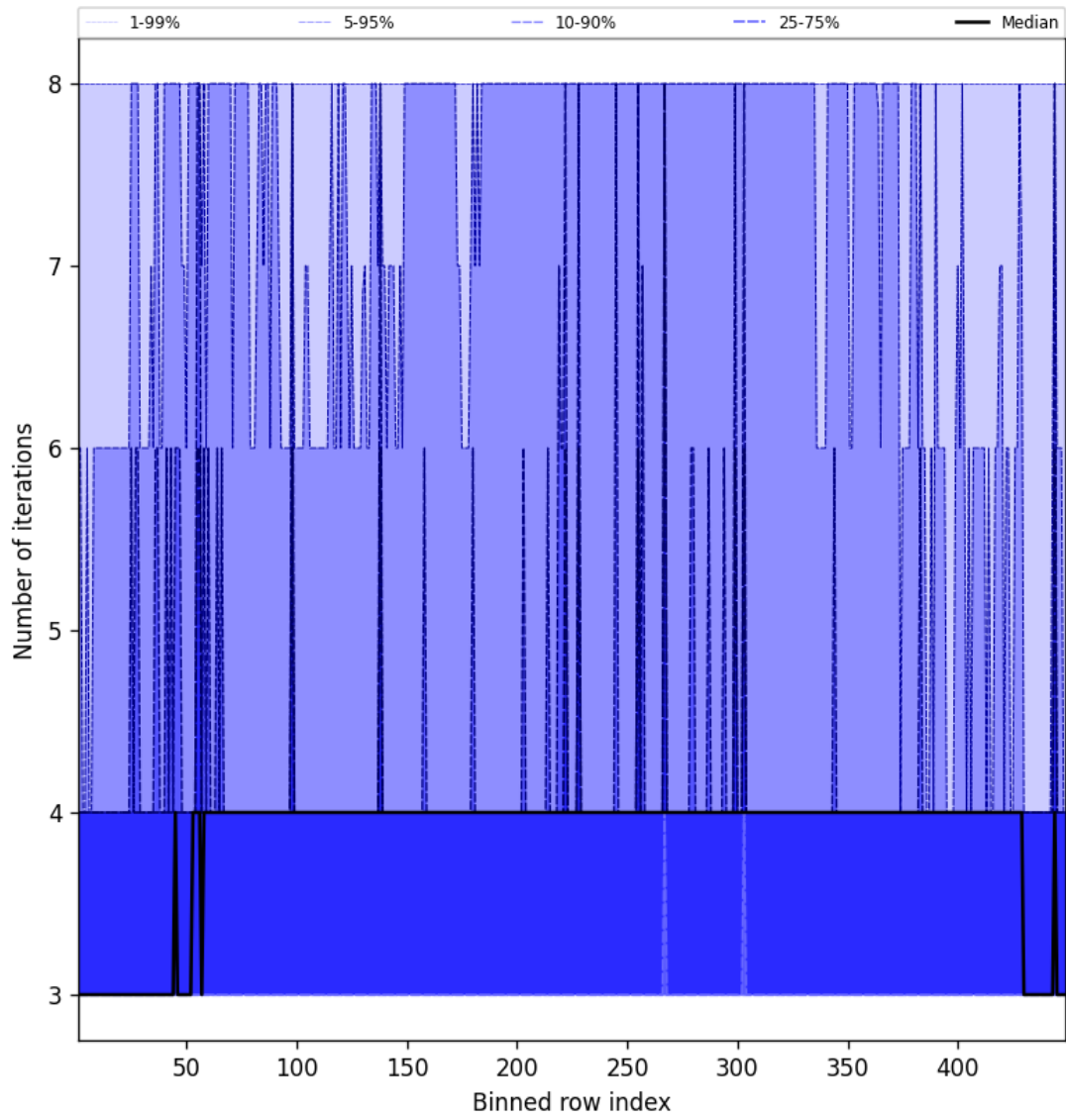
Figure 51: Along track statistics of “Number of iterations” for 2025-09-28 to 2025-09-30
