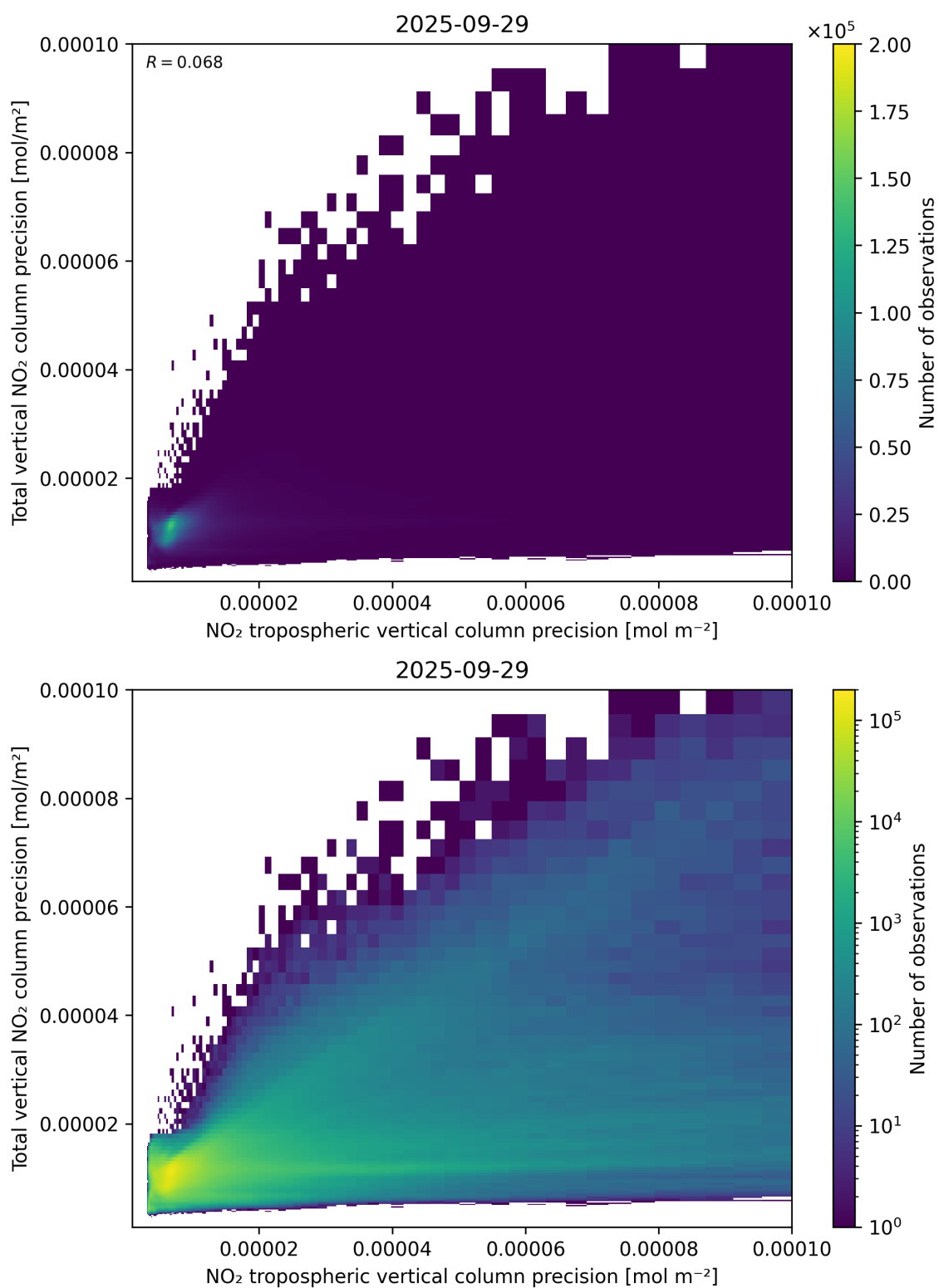
Figure 139: Scatter density plot of “NO 2 tropospheric vertical column precision” against “Total vertical NO 2 column precision” for 2025-09-28 to 2025-09-30.
