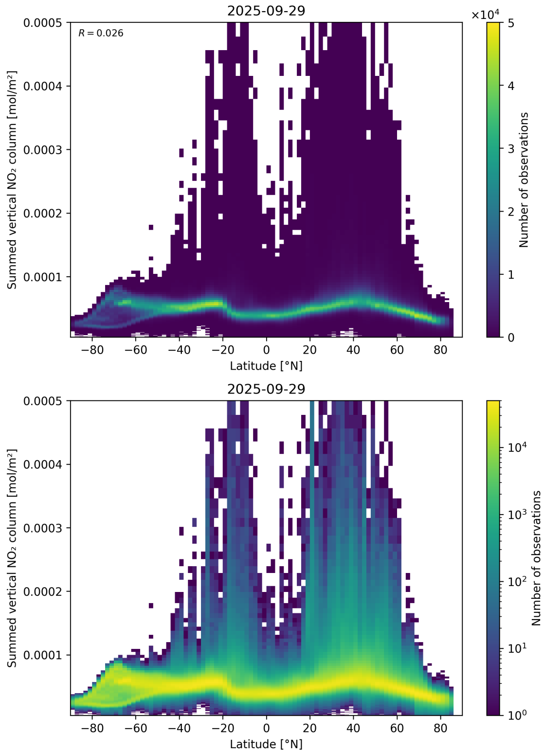
Figure 88: Scatter density plot of “Latitude” against “Summed vertical NO 2 column” for 2025-09-28 to 2025-09-30.
