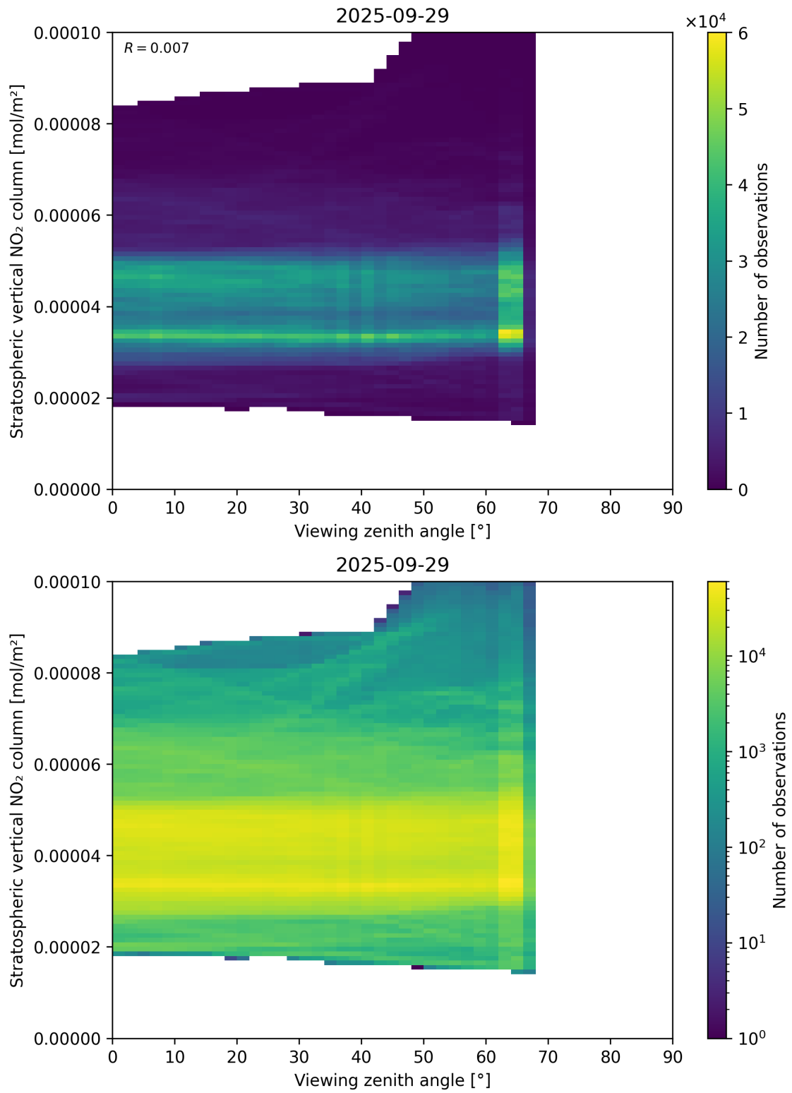
Figure 164: Scatter density plot of “Viewing zenith angle” against “Stratospheric vertical NO 2 column” for 2025-09-28 to 2025-09-30.
