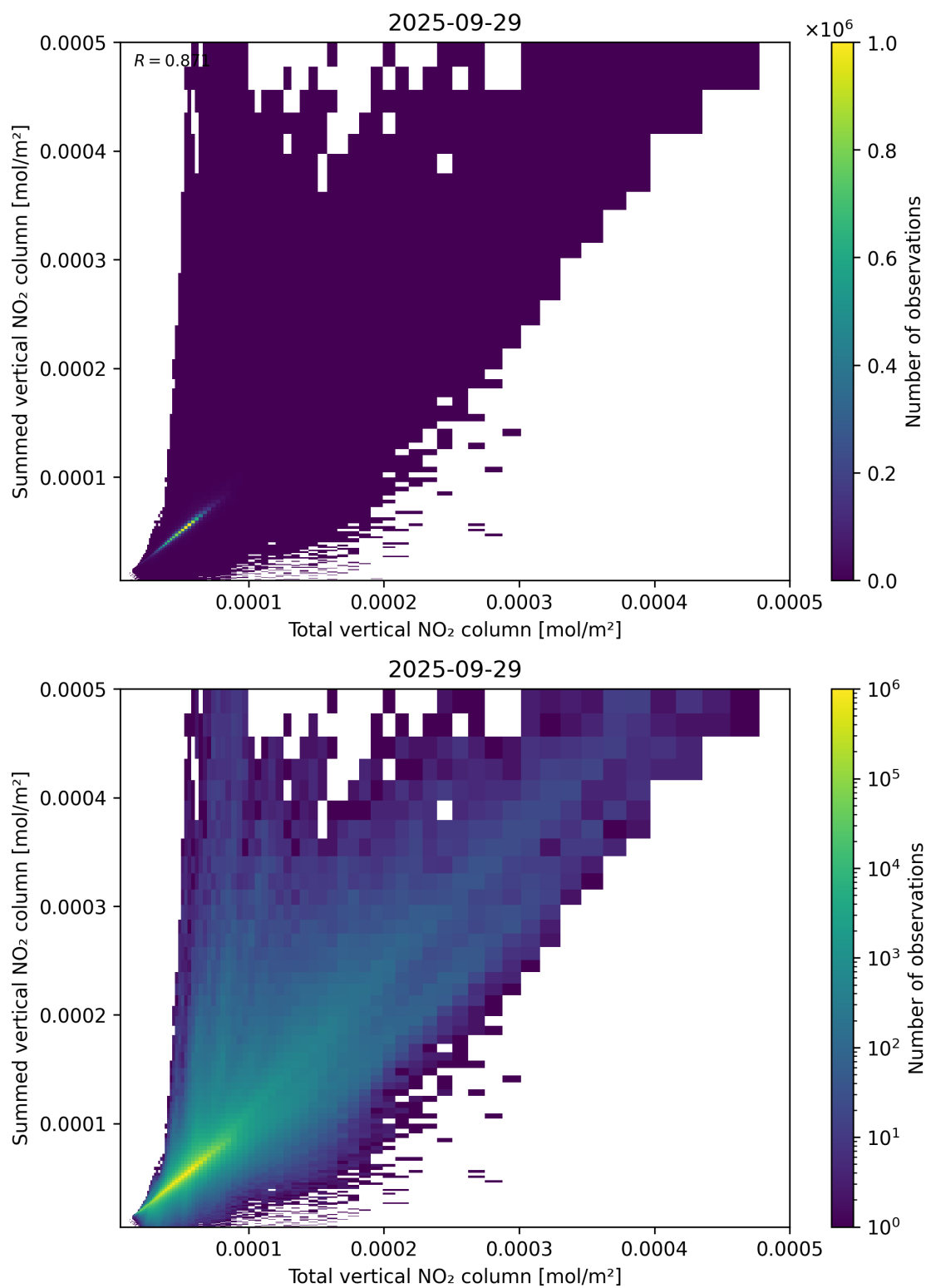
Figure 112: Scatter density plot of “Total vertical NO 2 column” against “Summed vertical NO 2 column” for 2025-09-28 to 2025-09-30.
