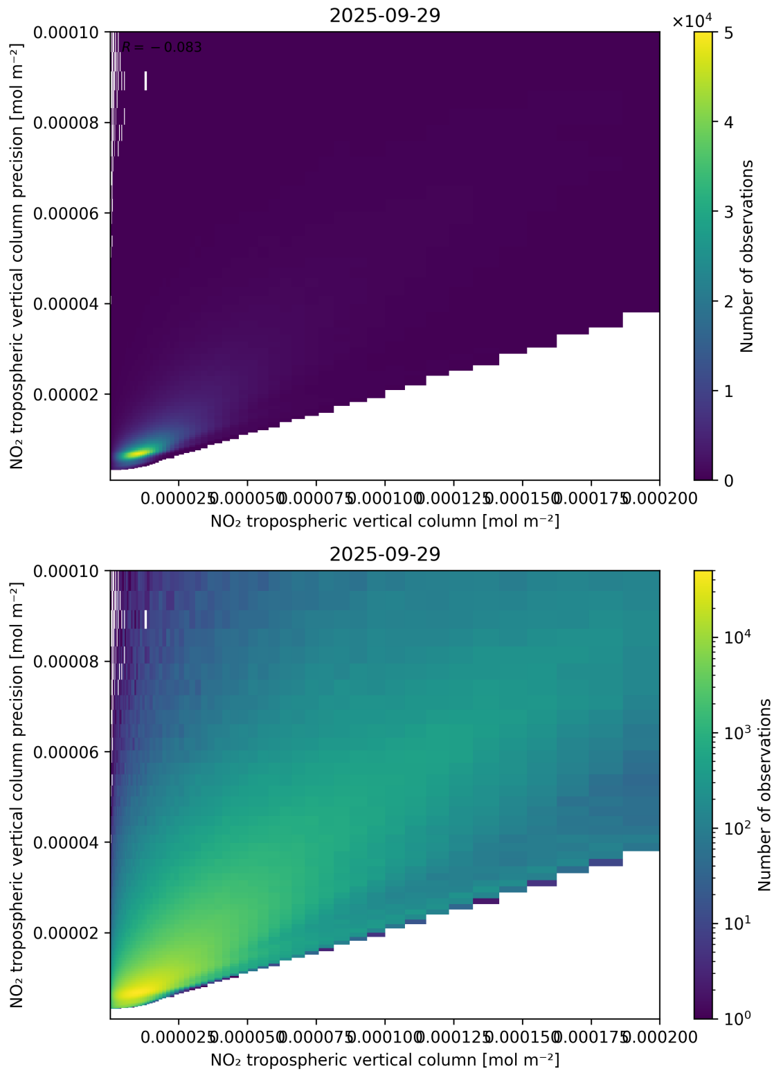
Figure 130: Scatter density plot of “NO 2 tropospheric vertical column” against “NO 2 tropospheric vertical column precision” for 2025-09-28 to 2025-09-30.
