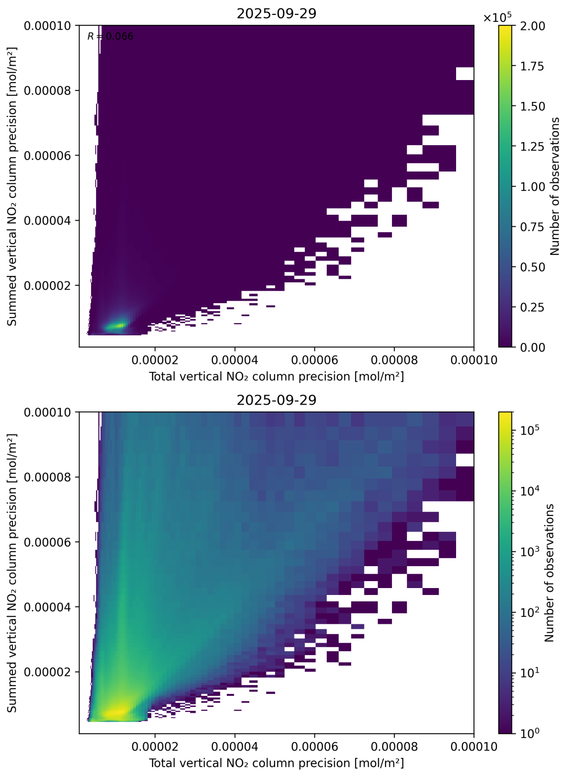
Figure 118: Scatter density plot of “Total vertical NO 2 column precision” against “Summed vertical NO 2 column precision” for 2025-09-28 to 2025-09-30.
