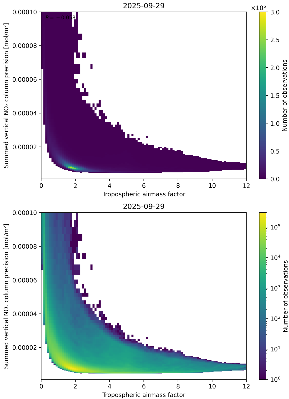
Figure 76: Scatter density plot of “Tropospheric airmass factor” against “Summed vertical NO 2 column precision” for 2025-09-28 to 2025-09-30.
