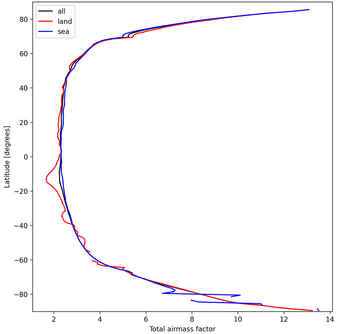
Figure 15: Zonal average of “Total airmass factor” for 2025-09-28 to 2025-09-30.
