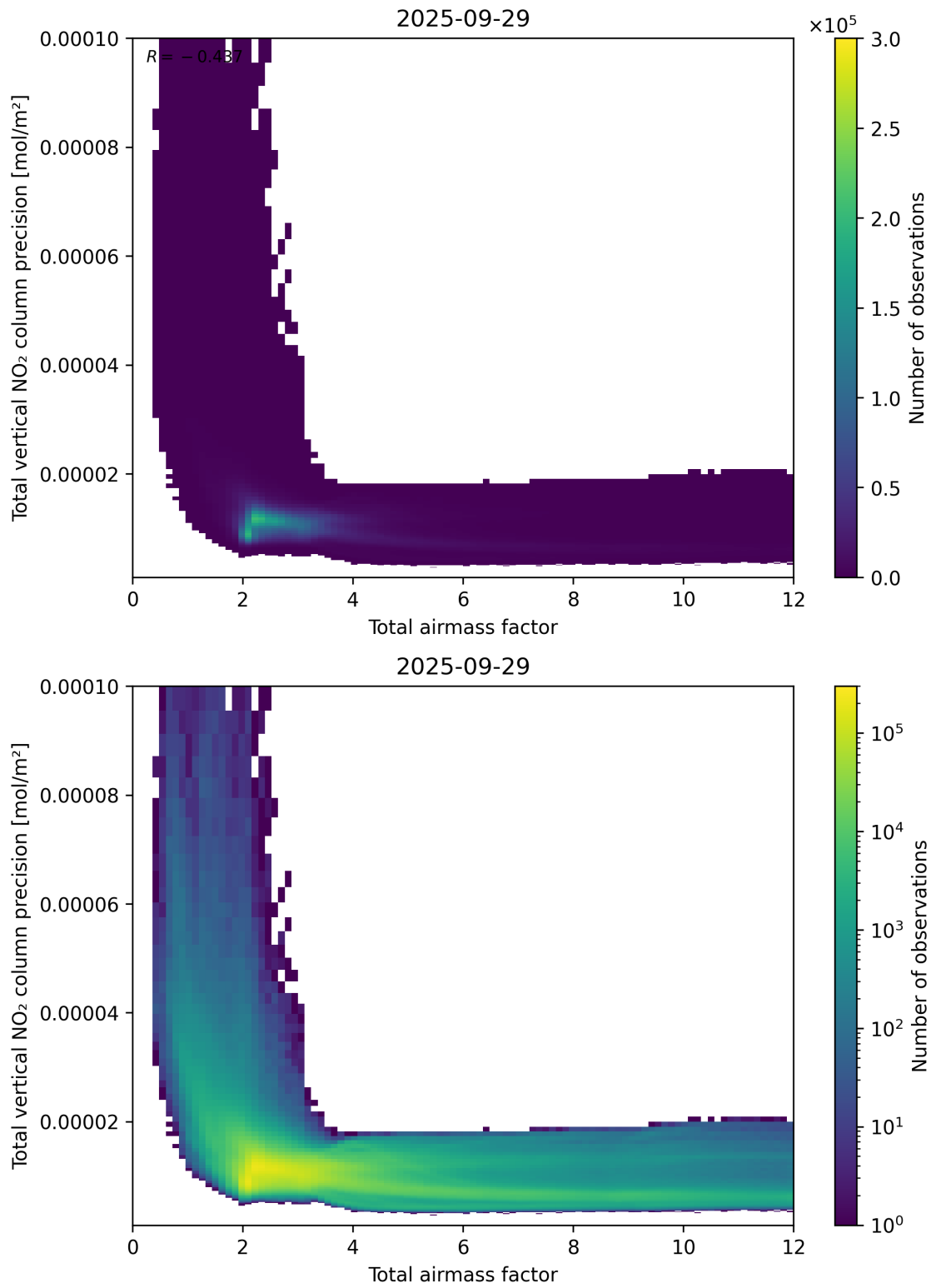
Figure 68: Scatter density plot of “Total airmass factor” against “Total vertical NO 2 column precision” for 2025-09-28 to 2025-09-30.
