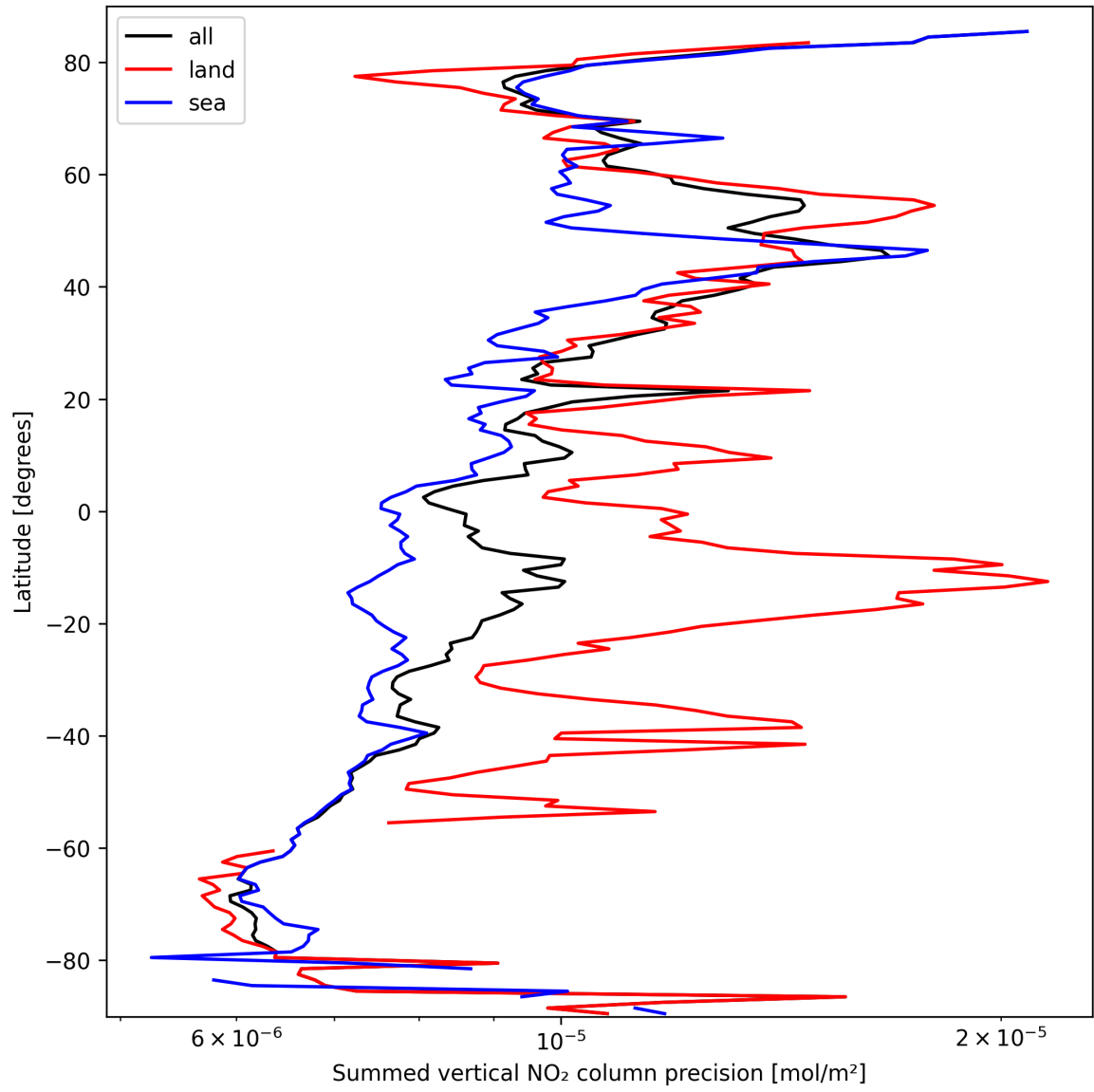
Figure 24: Zonal average of “Summed vertical NO 2 column precision” for 2025-09-28 to 2025-09-30.
