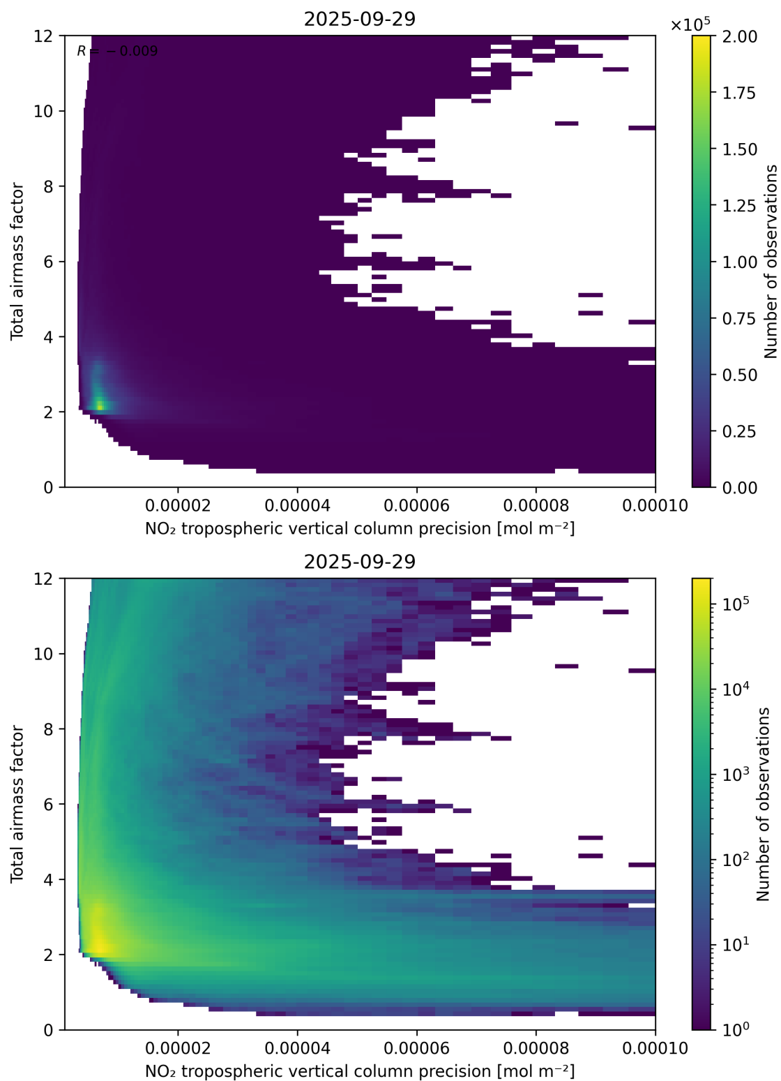
Figure 132: Scatter density plot of “NO 2 tropospheric vertical column precision” against “Total air mass factor” for 2025-09-28 to 2025-09-30.
