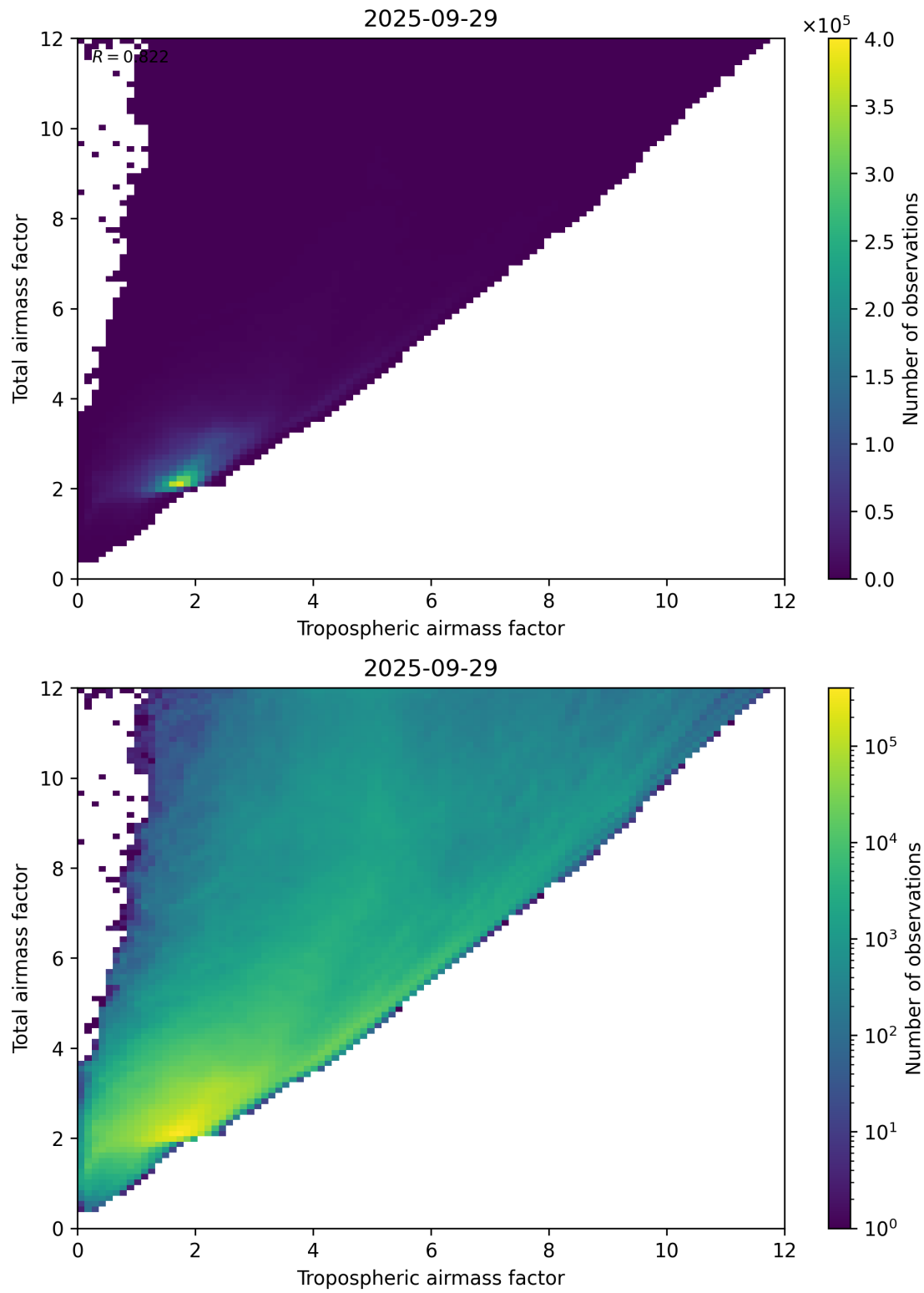
Figure 72: Scatter density plot of “Tropospheric airmass factor” against “Total airmass factor” for 2025-09-28 to 2025-09-30.
