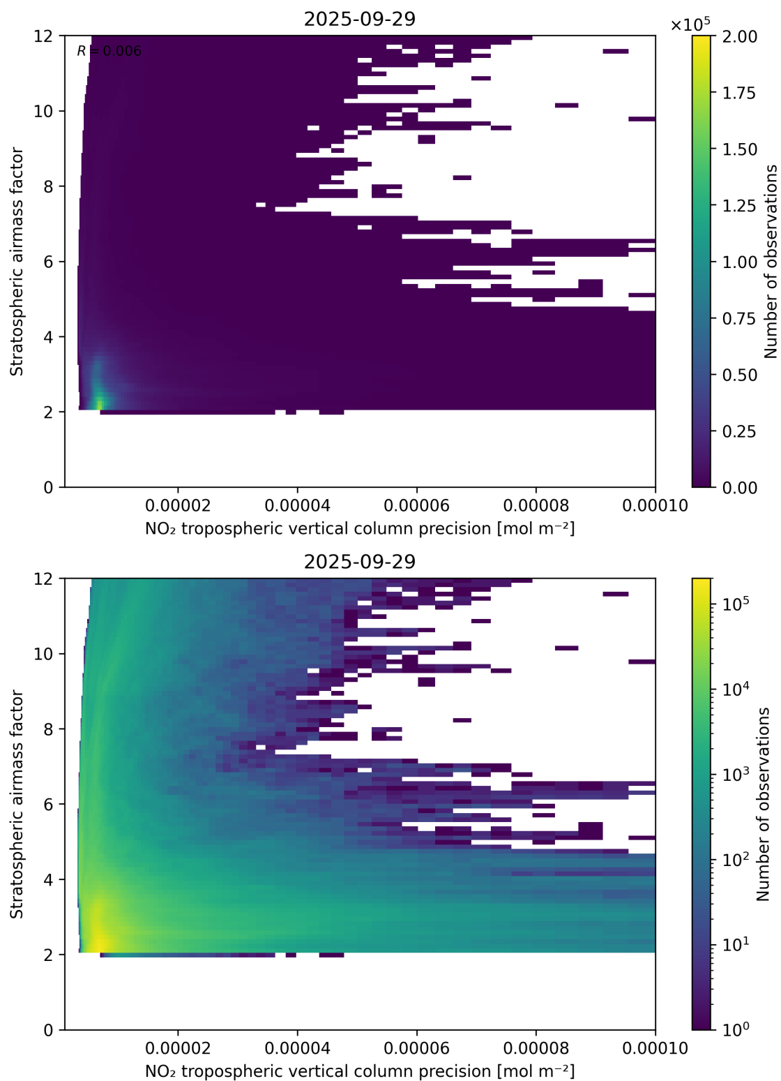
Figure 131: Scatter density plot of “NO 2 tropospheric vertical column precision” against “Stratospheric airmass factor” for 2025-09-28 to 2025-09-30.
