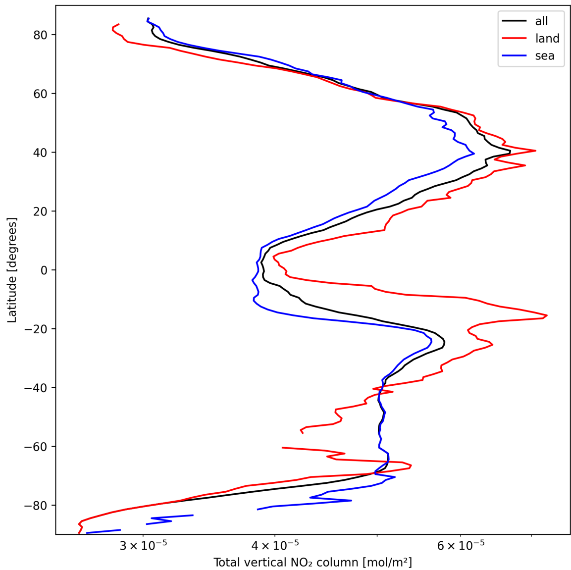
Figure 21: Zonal average of “Total vertical NO 2 column” for 2025-09-28 to 2025-09-30.
