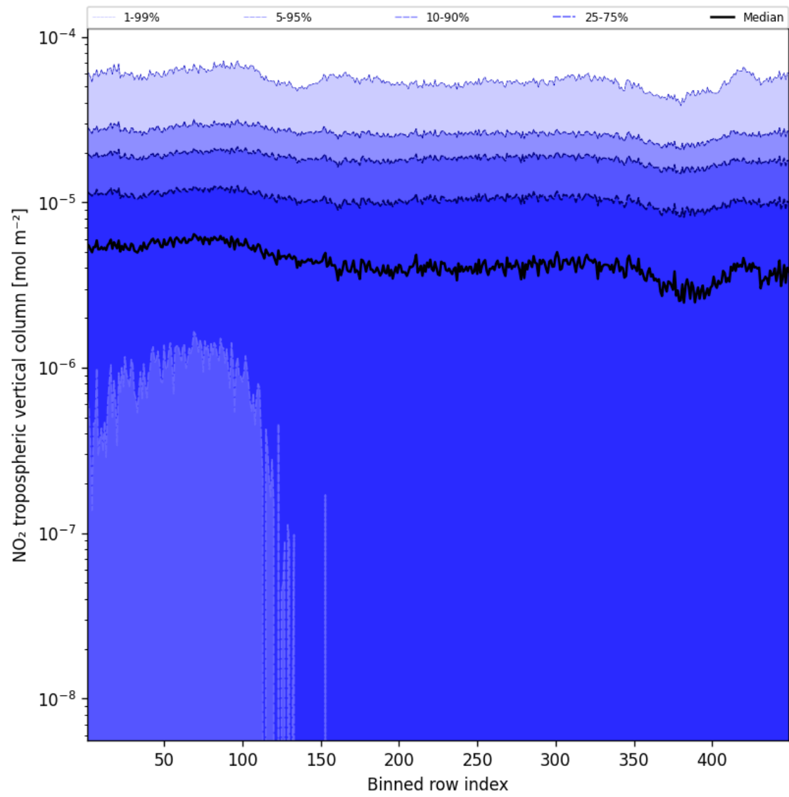
Figure 46: Along track statistics of “ \text{NO}_2 tropospheric vertical column” for 2025-09-28 to 2025-09-30
