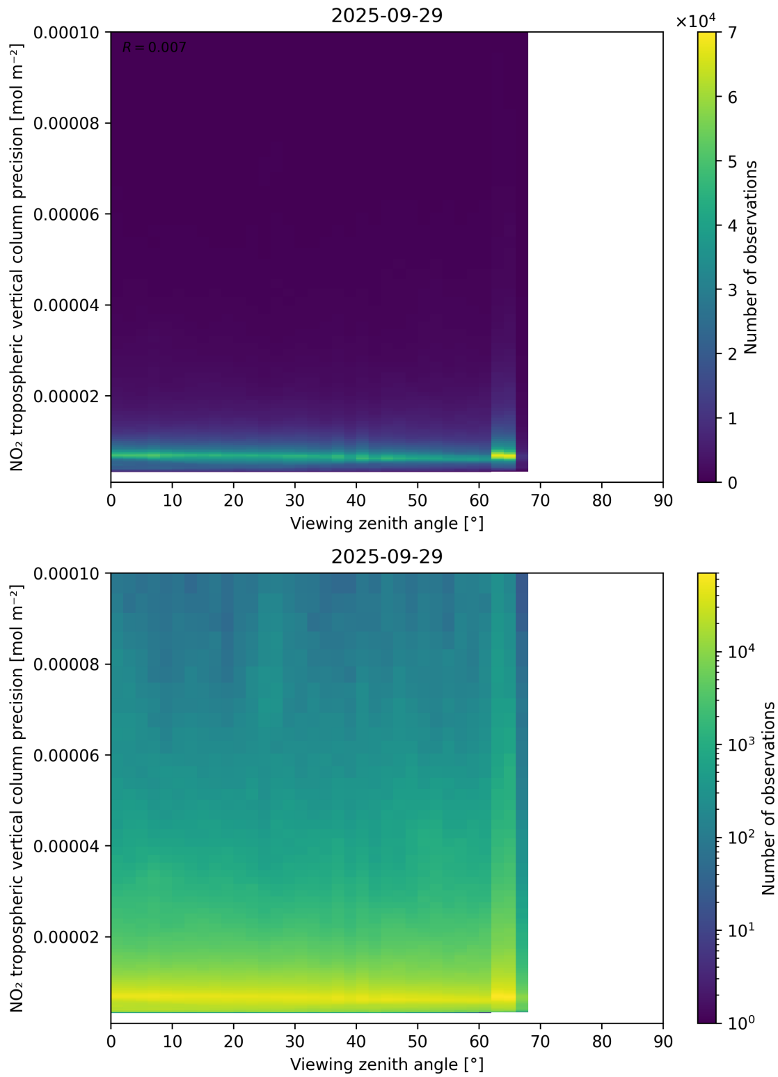
Figure 170: Scatter density plot of “Viewing zenith angle” against “NO 2 tropospheric vertical column precision” for 2025-09-28 to 2025-09-30.
