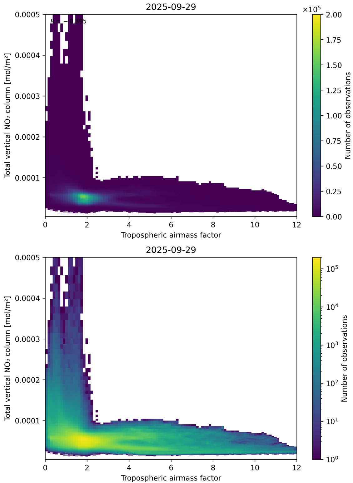
Figure 77: Scatter density plot of “Tropospheric airmass factor” against “Total vertical NO 2 column” for 2025-09-28 to 2025-09-30.
