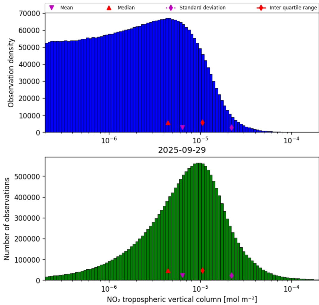
Figure 29: Histogram of “NO 2 tropospheric vertical column” for 2025-09-28 to 2025-09-30
