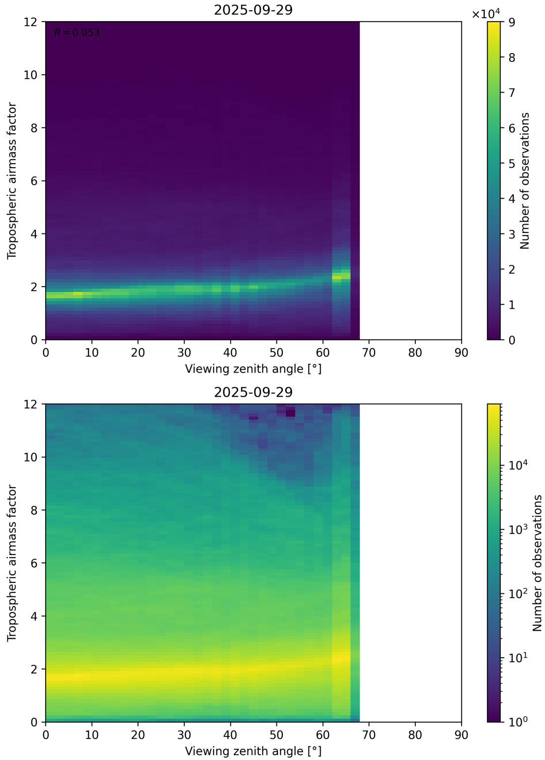
Figure 161: Scatter density plot of “Viewing zenith angle” against “Tropospheric airmass factor” for 2025-09-28 to 2025-09-30.
