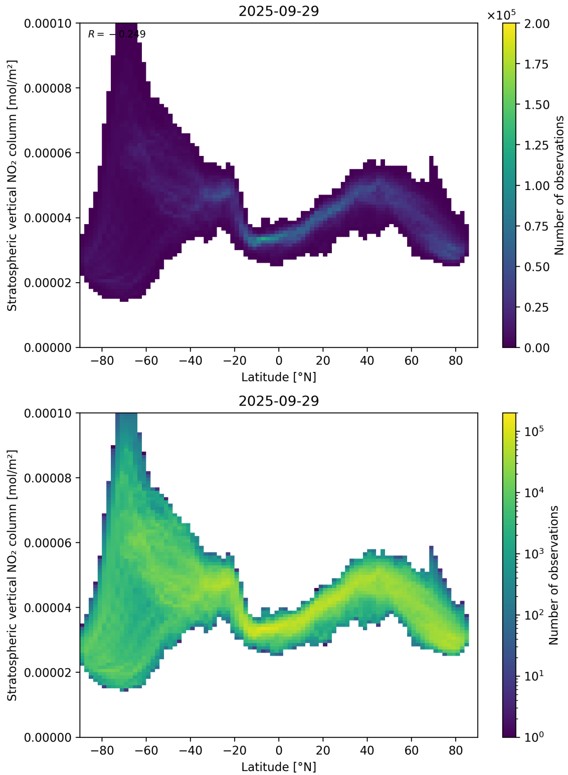
Figure 87: Scatter density plot of “Latitude” against “Stratospheric vertical NO 2 column” for 2025-09-28 to 2025-09-30.
