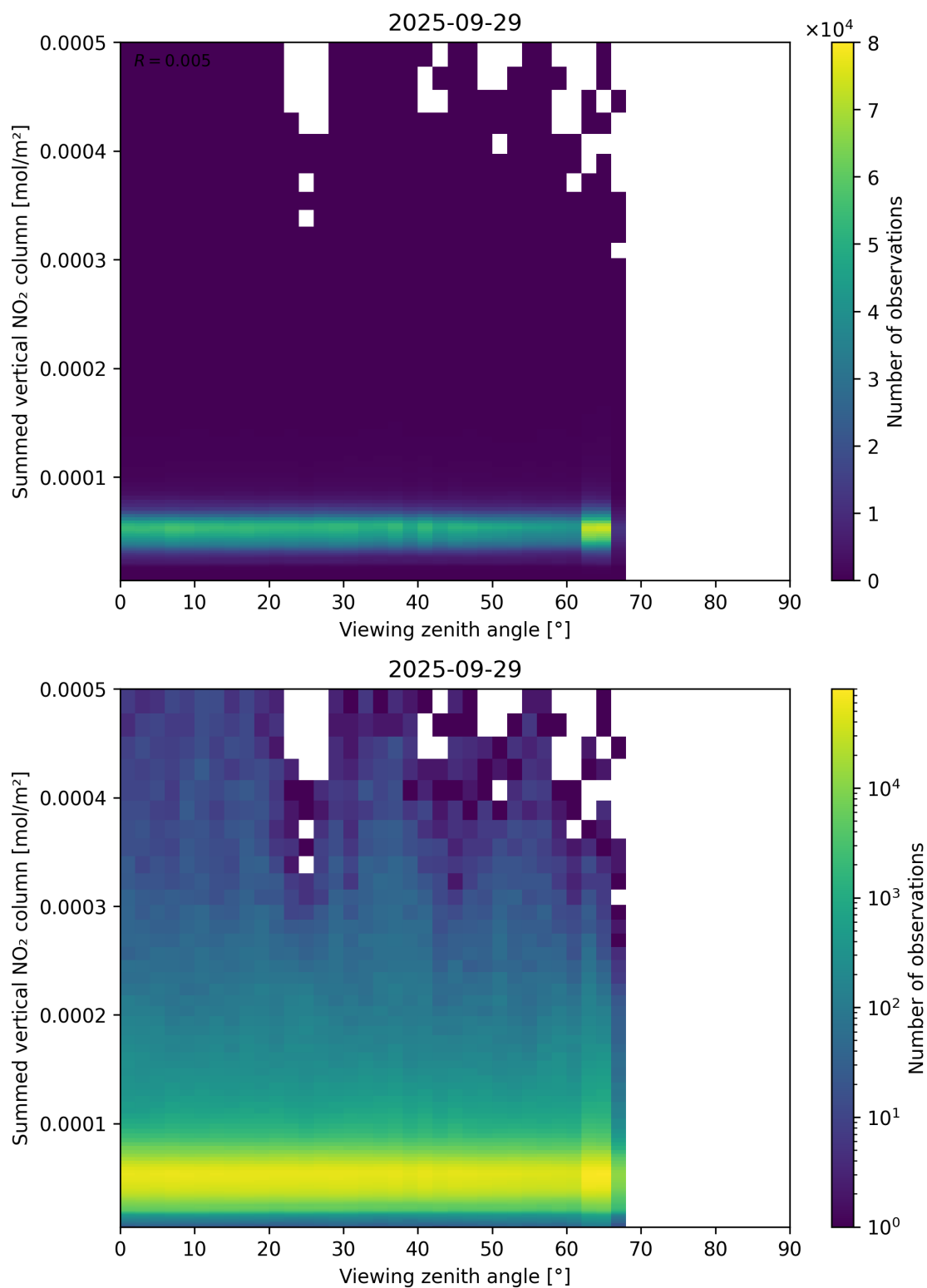
Figure 165: Scatter density plot of “Viewing zenith angle” against “Summed vertical NO 2 column” for 2025-09-28 to 2025-09-30.
