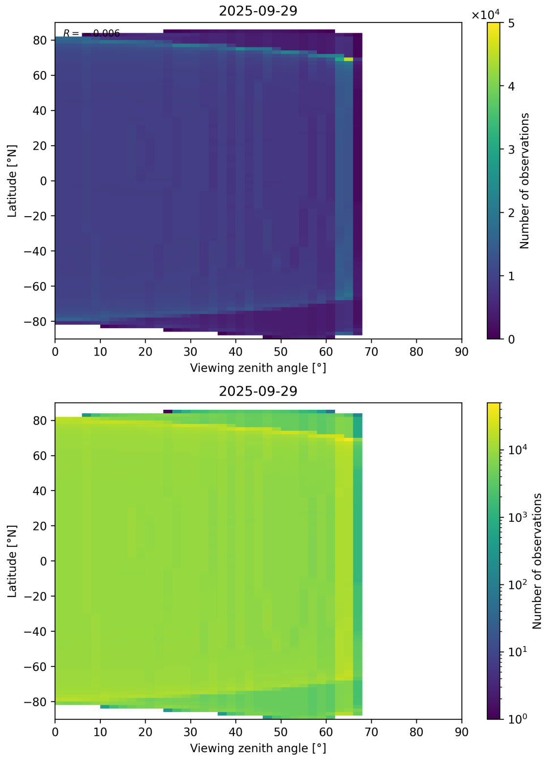
Figure 163: Scatter density plot of “Viewing zenith angle” against “Latitude” for 2025-09-28 to 2025-09-30.
