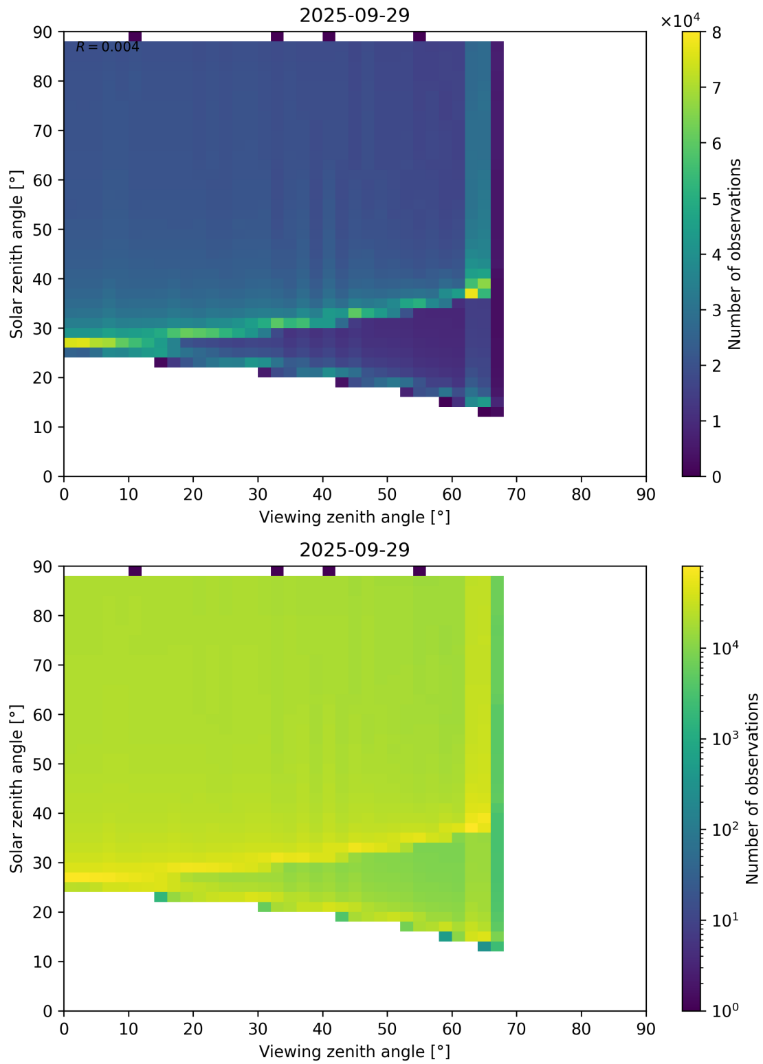
Figure 172: Scatter density plot of “Viewing zenith angle” against “Solar zenith angle” for 2025-09-28 to 2025-09-30.
