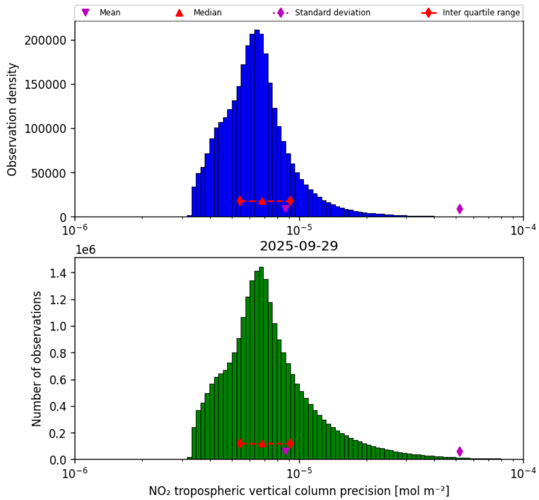
Figure 30: Histogram of “NO 2 tropospheric vertical column precision” for 2025-09-28 to 2025-09-30
