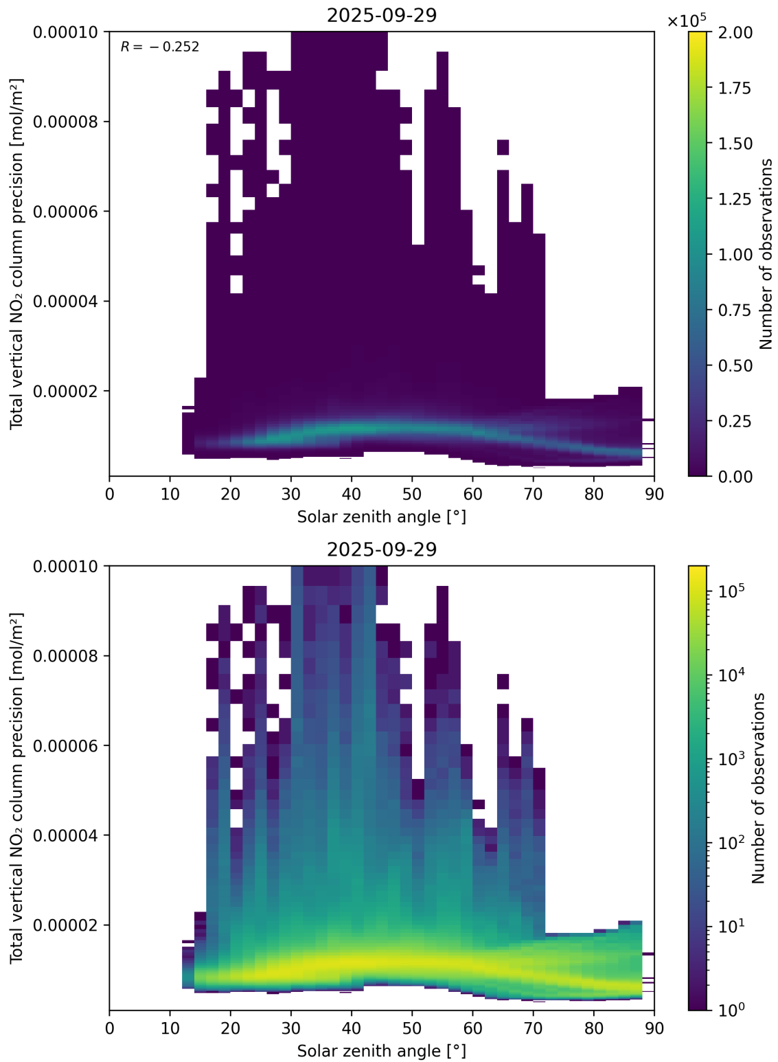
Figure 154: Scatter density plot of “Solar zenith angle” against “Total vertical NO 2 column precision” for 2025-09-28 to 2025-09-30.
