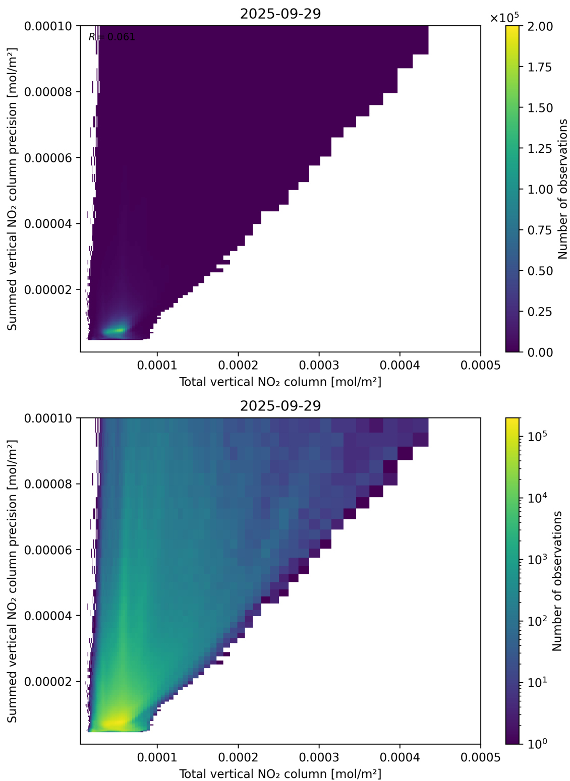
Figure 113: Scatter density plot of “Total vertical NO 2 column” against “Summed vertical NO 2 column precision” for 2025-09-28 to 2025-09-30.
