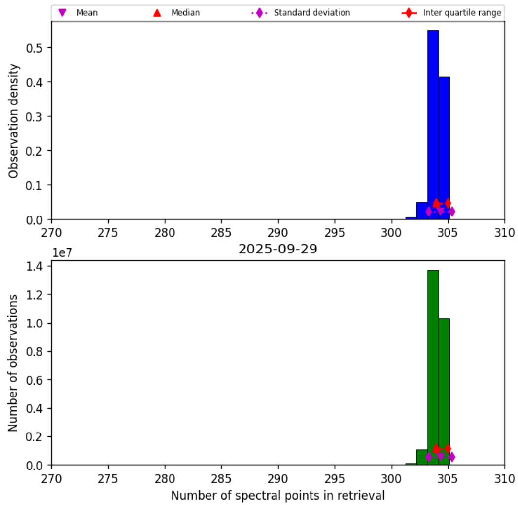
Figure 33: Histogram of “Number of spectral points in retrieval” for 2025-09-28 to 2025-09-30
