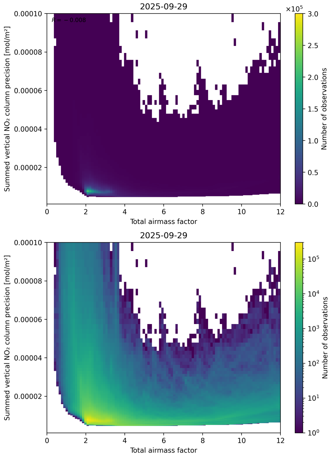
Figure 66: Scatter density plot of “Total airmass factor” against “Summed vertical NO 2 column precision” for 2025-09-28 to 2025-09-30.
