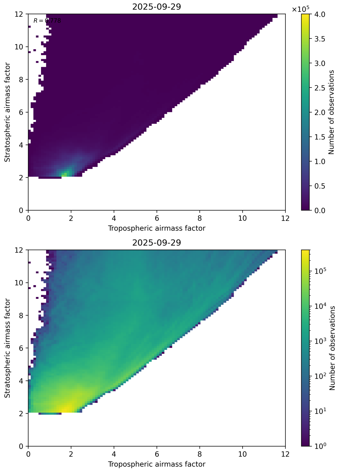
Figure 71: Scatter density plot of “Tropospheric airmass factor” against “Stratospheric airmass factor” for 2025-09-28 to 2025-09-30.
