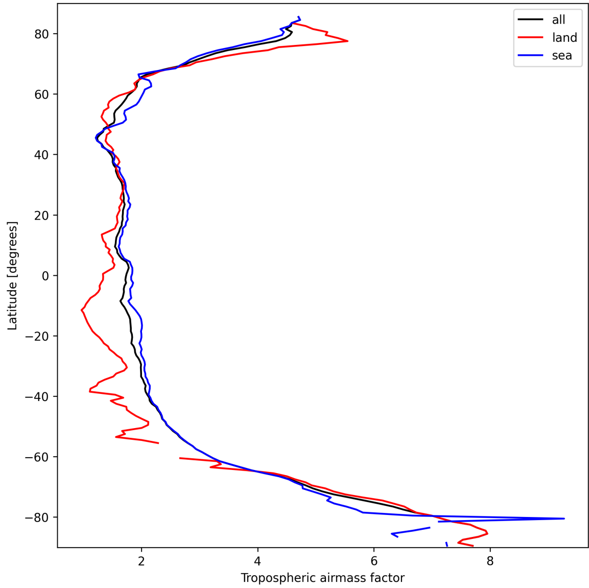
Figure 14: Zonal average of “Tropospheric airmass factor” for 2025-09-28 to 2025-09-30.
