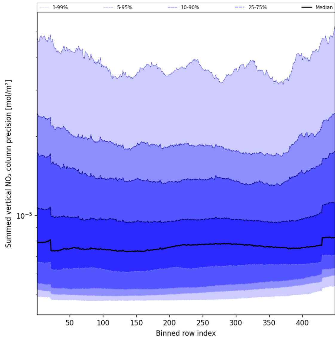
Figure 58: Along track statistics of “Summed vertical NO 2 column precision” for 2025-09-28 to 2025-09-30
