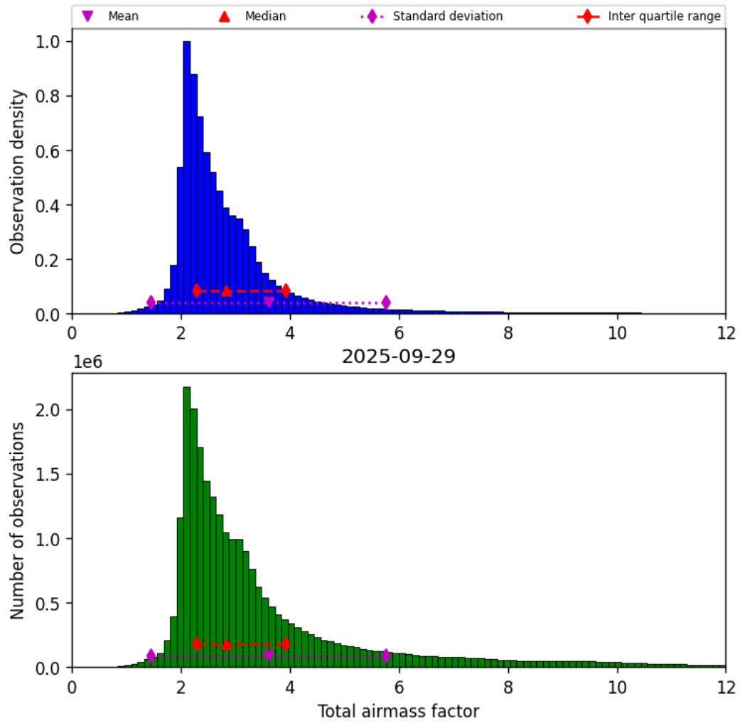
Figure 32: Histogram of “Total airmass factor” for 2025-09-28 to 2025-09-30
