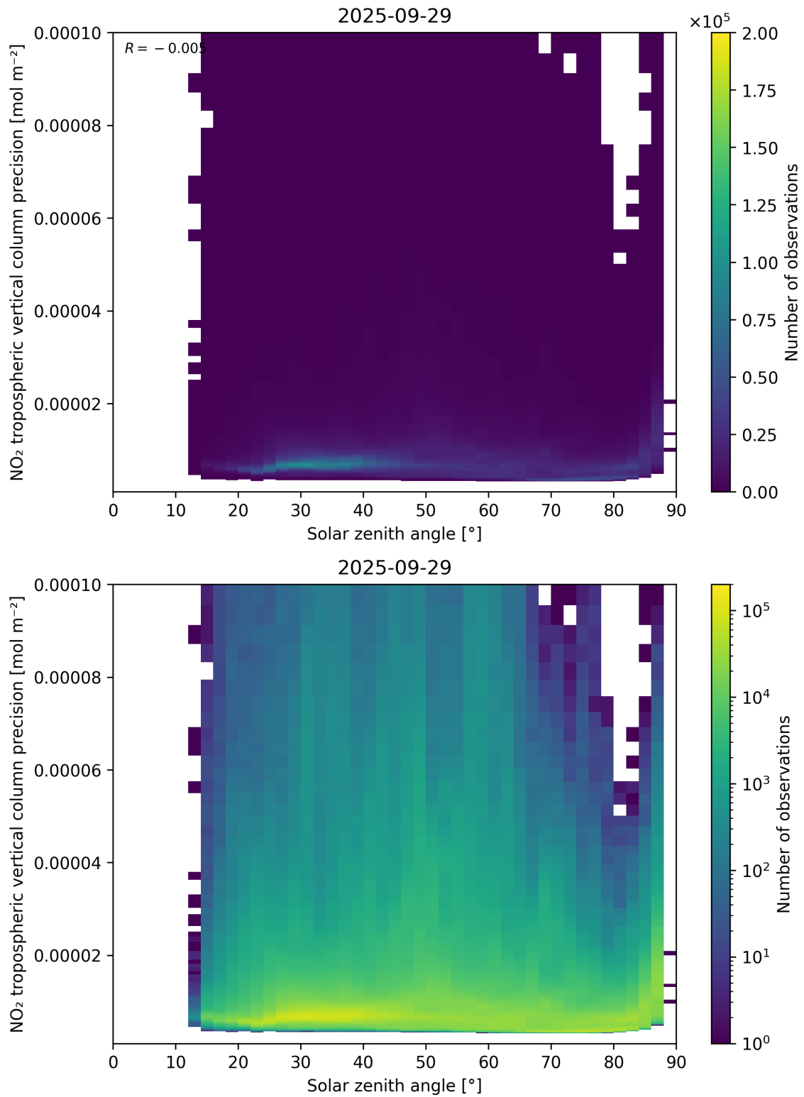
Figure 156: Scatter density plot of “Solar zenith angle” against “NO 2 tropospheric vertical column precision” for 2025-09-28 to 2025-09-30.
