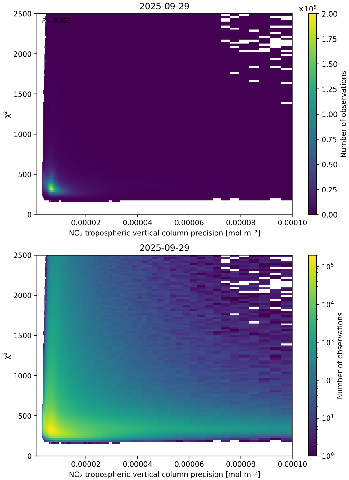
Figure 134: Scatter density plot of “NO 2 tropospheric vertical column precision” against “ \chi^2 ” for 2025-09-28 to 2025-09-30.
