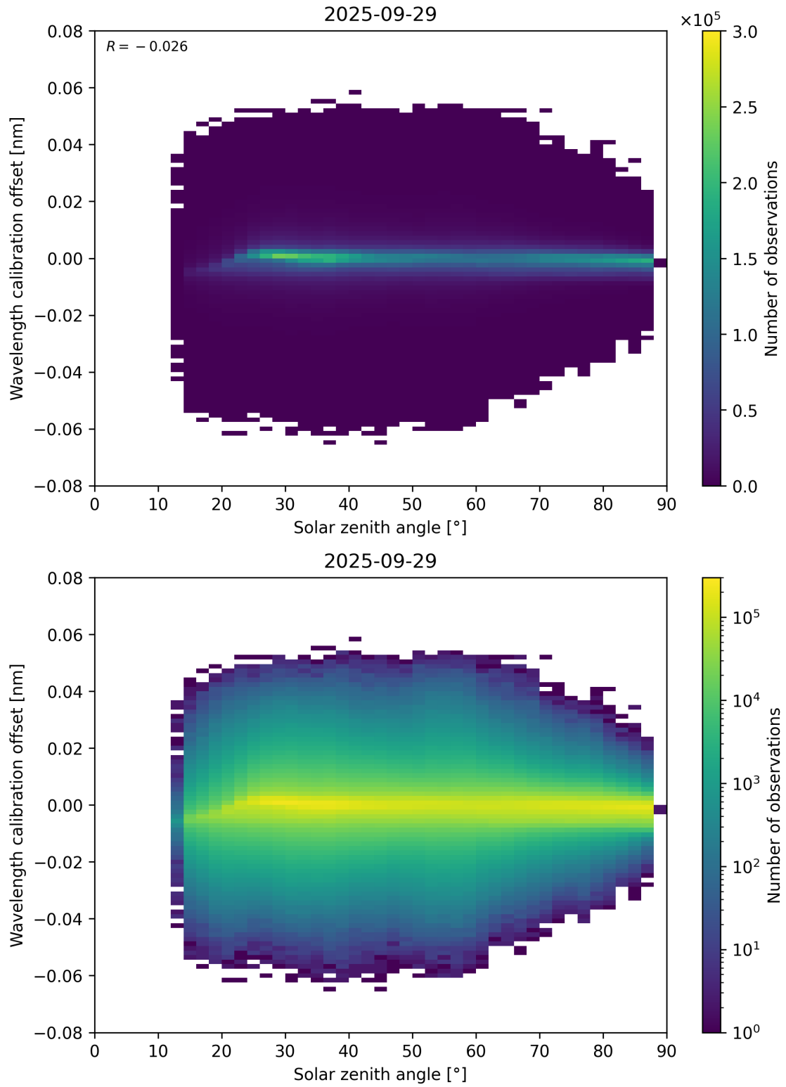
Figure 158: Scatter density plot of “Solar zenith angle” against “Wavelength calibration offset” for 2025-09-28 to 2025-09-30.
