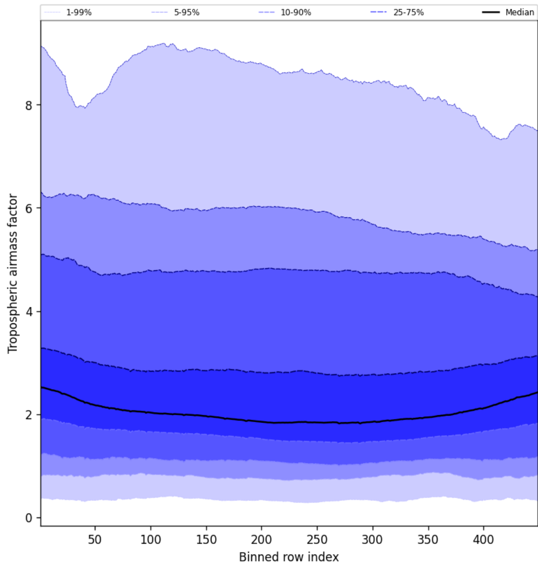
Figure 48: Along track statistics of “Tropospheric air mass factor” for 2025-09-28 to 2025-09-30
