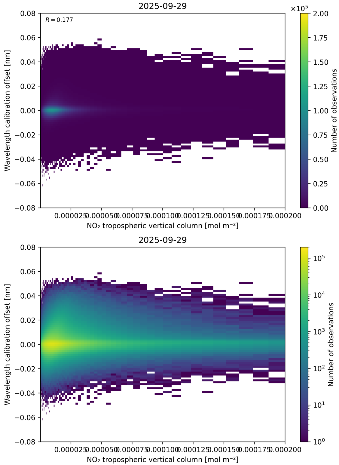
Figure 143: Scatter density plot of “NO 2 tropospheric vertical column” against “Wavelength calibration offset” for 2025-09-28 to 2025-09-30.
