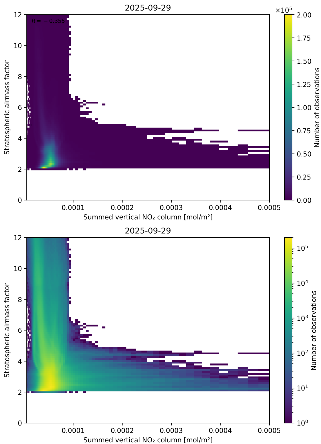
Figure 103: Scatter density plot of “Summed vertical NO 2 column” against “Stratospheric airmass factor” for 2025-09-28 to 2025-09-30.
