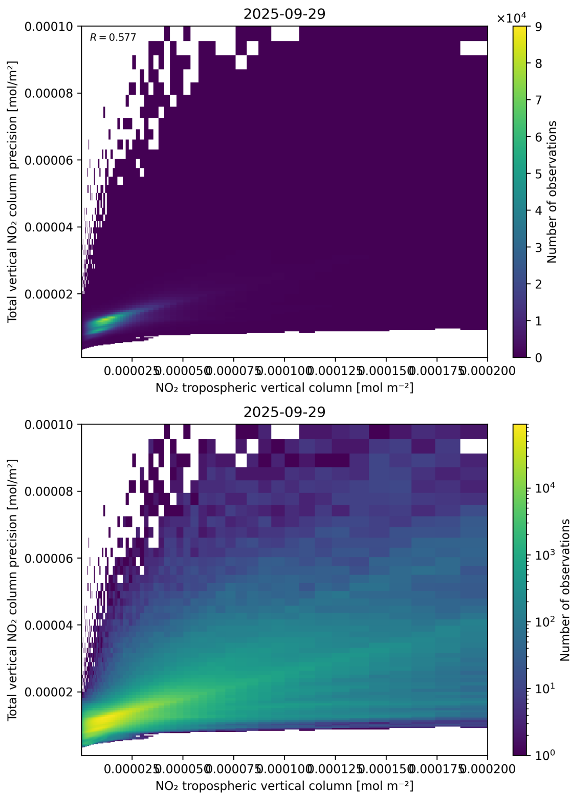
Figure 129: Scatter density plot of “NO 2 tropospheric vertical column” against “Total vertical NO 2 column precision” for 2025-09-28 to 2025-09-30.
