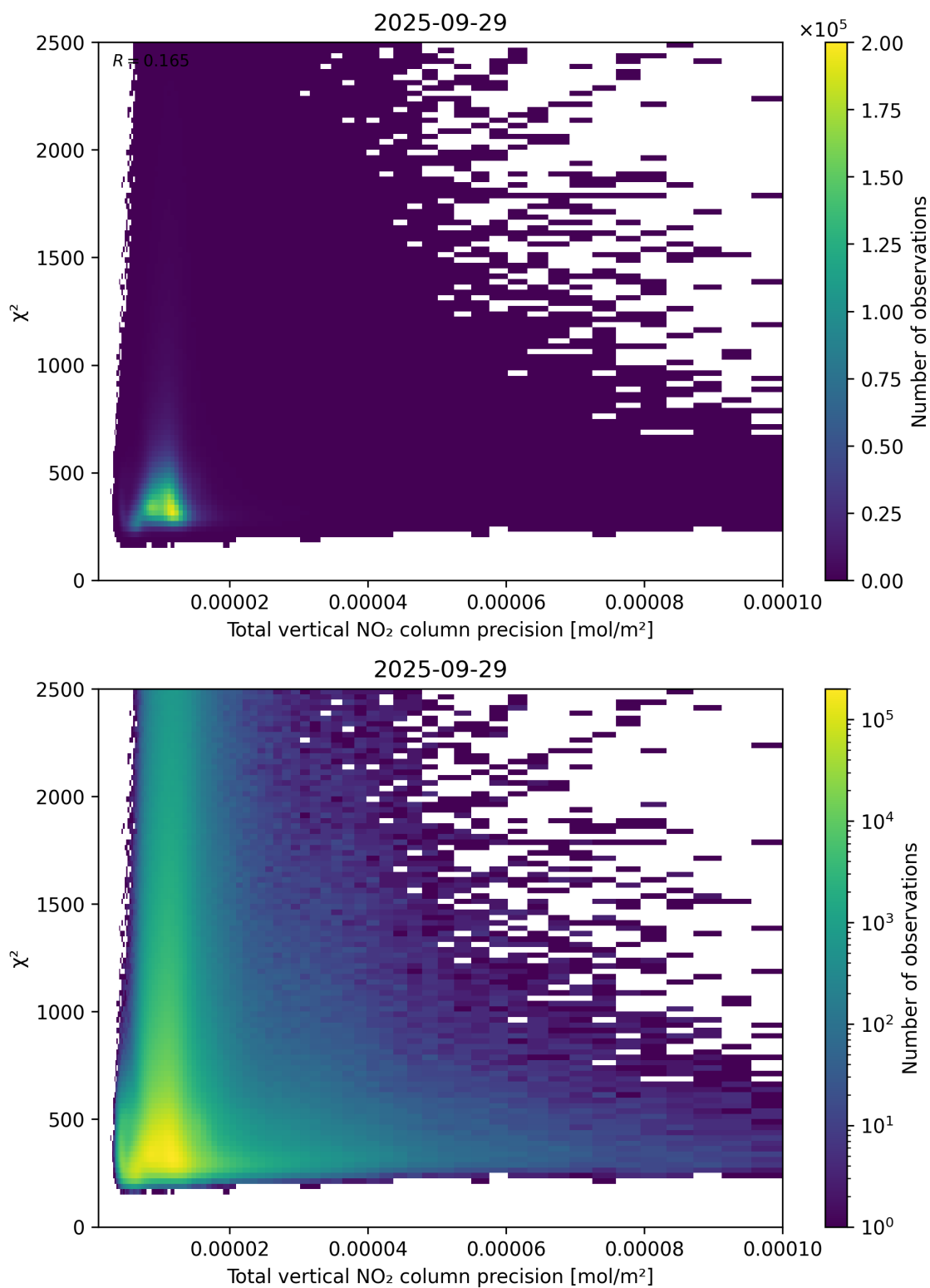
Figure 116: Scatter density plot of “Total vertical NO 2 column precision” against “ \chi^2 ” for 2025-09-28 to 2025-09-30.
