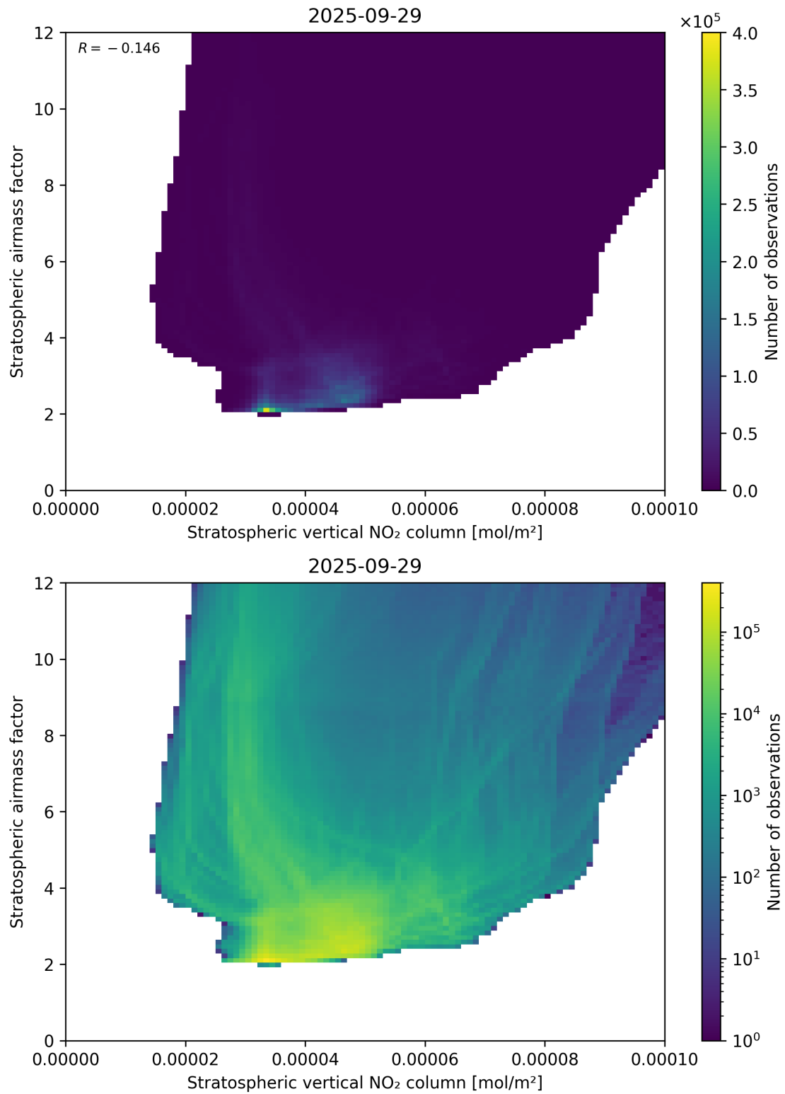
Figure 96: Scatter density plot of “Stratospheric vertical NO 2 column” against “Stratospheric airmass factor” for 2025-09-28 to 2025-09-30.
