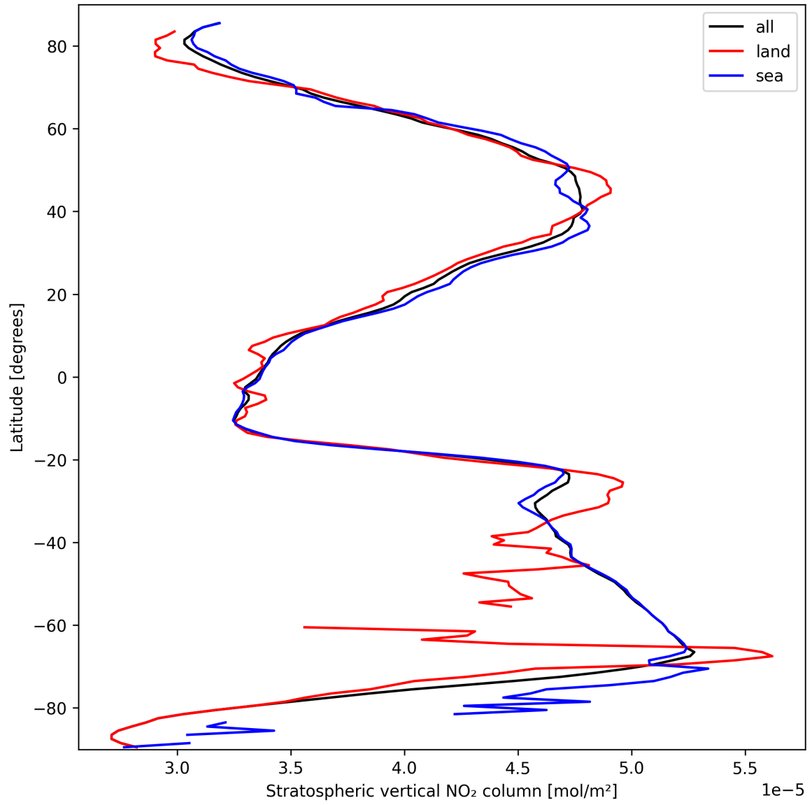
Figure 19: Zonal average of “Stratospheric vertical NO 2 column” for 2025-09-28 to 2025-09-30.
