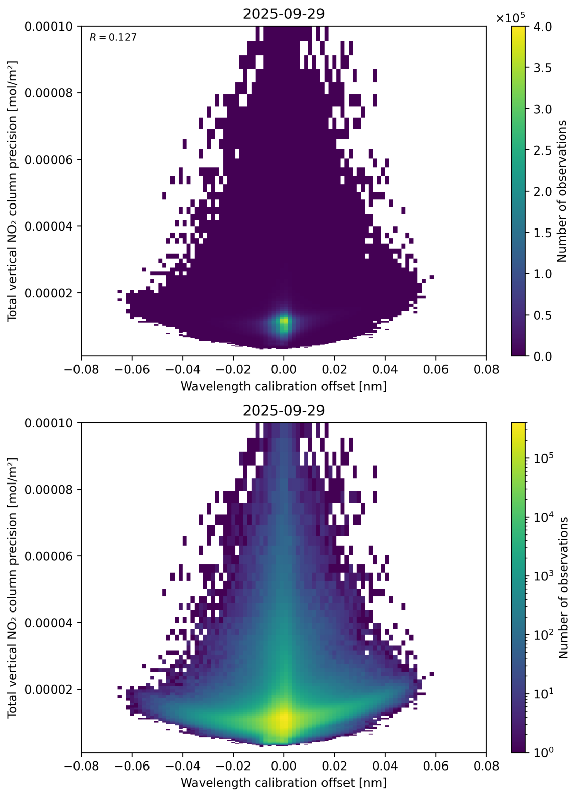
Figure 180: Scatter density plot of “Wavelength calibration offset” against “Total vertical NO 2 column precision” for 2025-09-28 to 2025-09-30.
