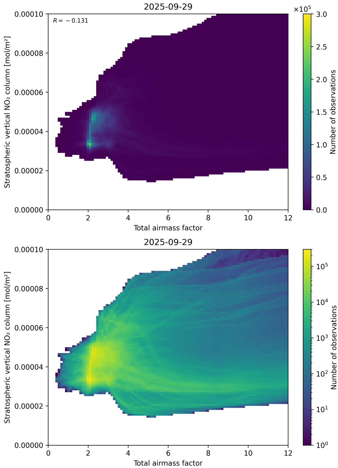
Figure 64: Scatter density plot of “Total airmass factor” against “Stratospheric vertical \text{NO}_2 column” for 2025-09-28 to 2025-09-30.
