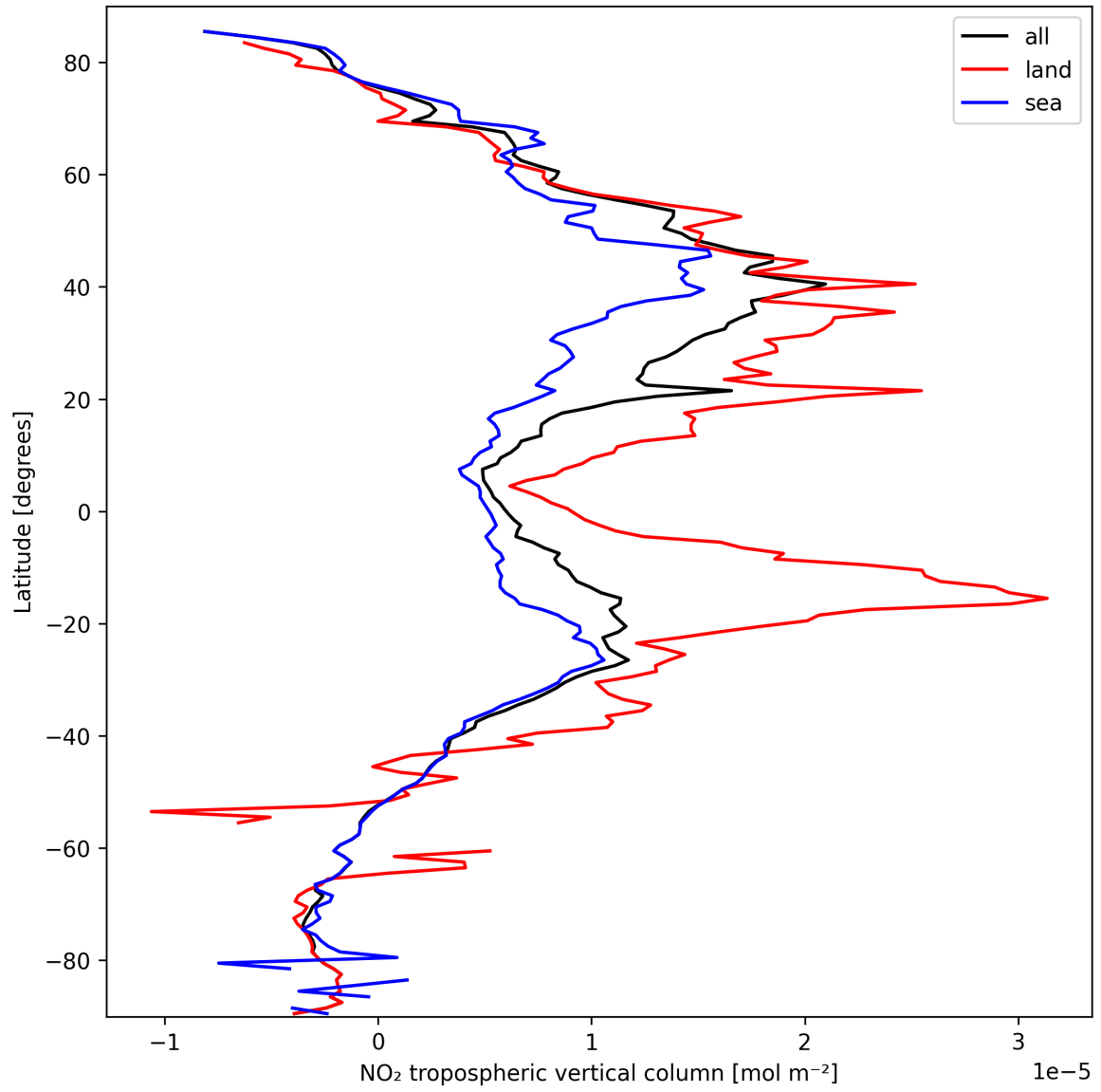
Figure 12: Zonal average of “NO 2 tropospheric vertical column” for 2025-09-28 to 2025-09-30.
