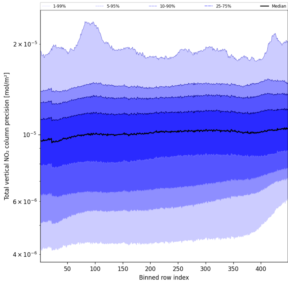
Figure 56: Along track statistics of “Total vertical NO 2 column precision” for 2025-09-28 to 2025-09-30
