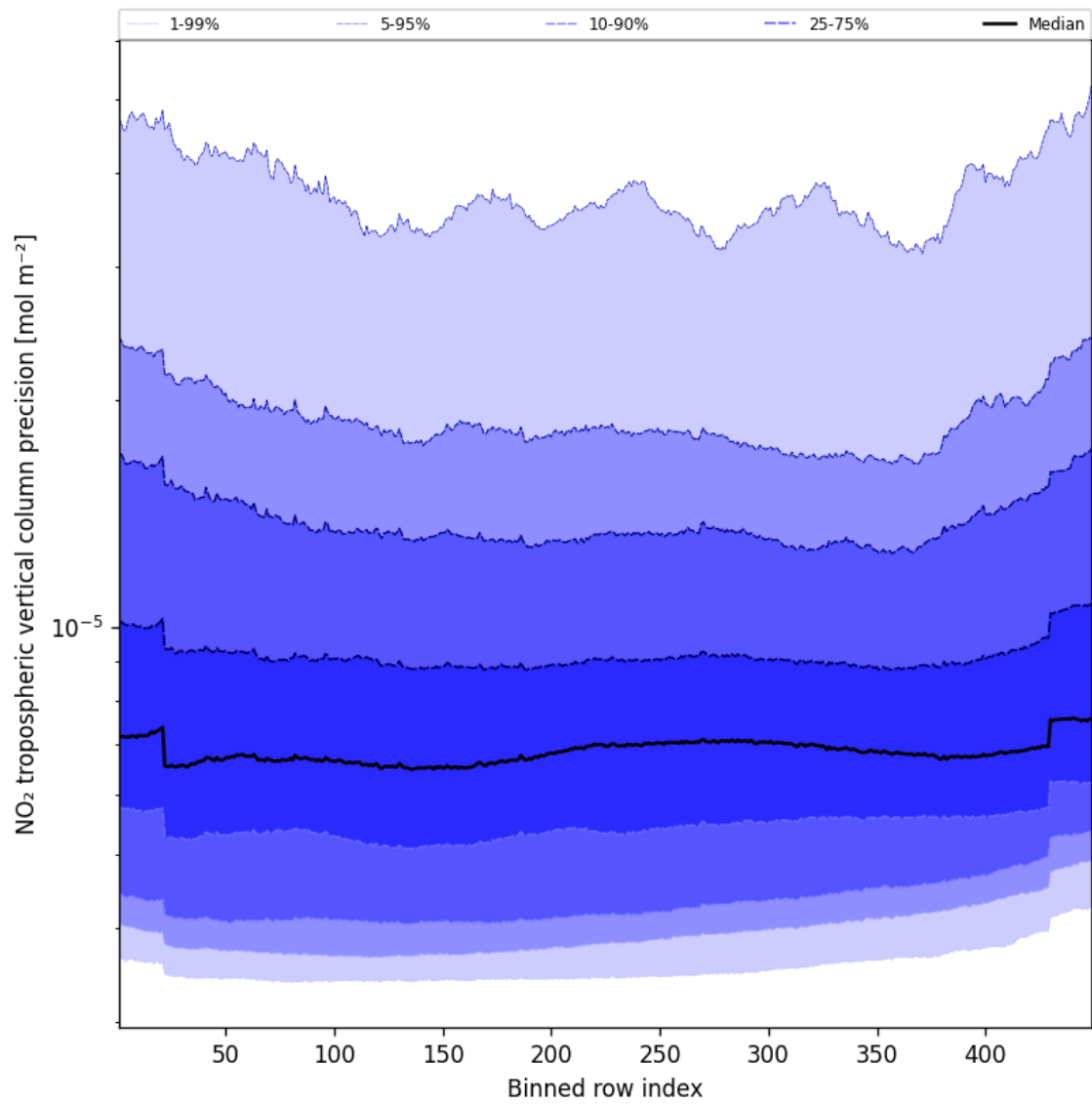
Figure 47: Along track statistics of “NO 2 tropospheric vertical column precision” for 2025-09-28 to 2025-09-30
