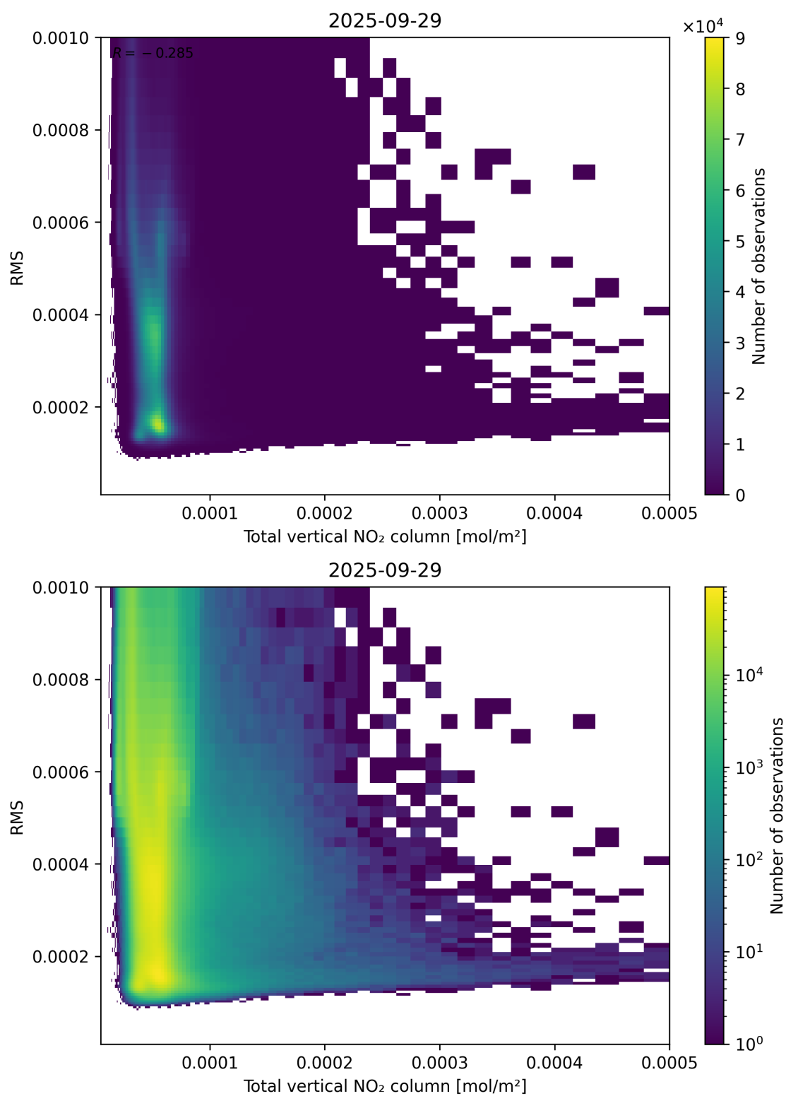
Figure 120: Scatter density plot of “Total vertical NO 2 column” against “RMS” for 2025-09-28 to 2025-09-30.
