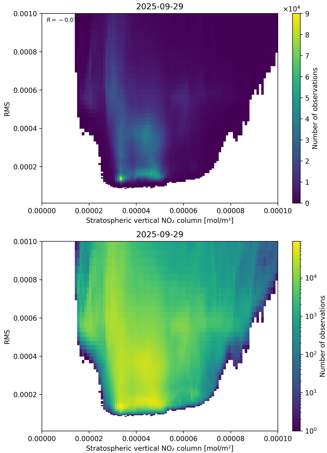
Figure 102: Scatter density plot of “Stratospheric vertical NO 2 column” against “RMS” for 2025-09-28 to 2025-09-30.
