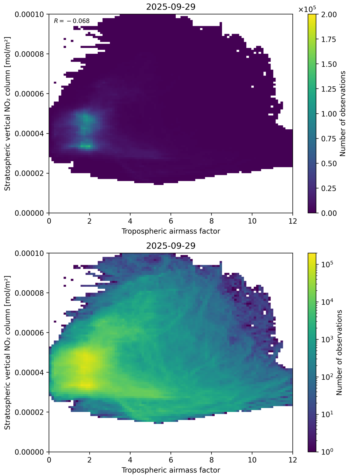
Figure 74: Scatter density plot of “Tropospheric air mass factor” against “Stratospheric vertical NO 2 column” for 2025-09-28 to 2025-09-30.
