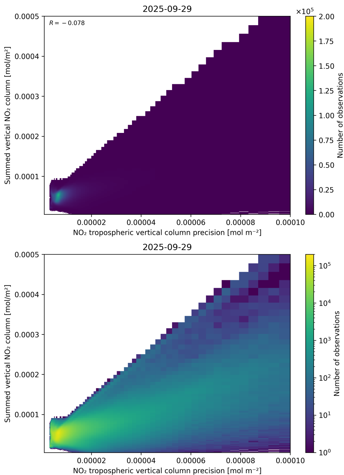
Figure 136: Scatter density plot of “NO 2 tropospheric vertical column precision” against “Summed vertical NO 2 column” for 2025-09-28 to 2025-09-30.
