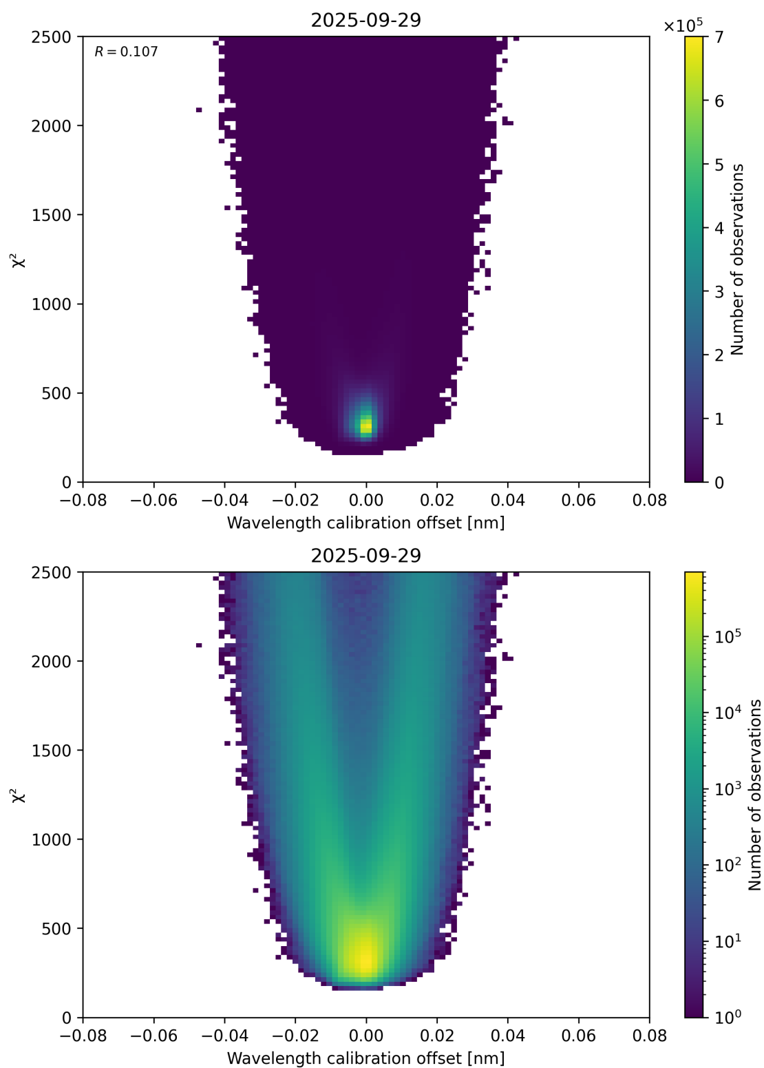
Figure 175: Scatter density plot of “Wavelength calibration offset” against “ \chi^2 ” for 2025-09-28 to 2025-09-30.
