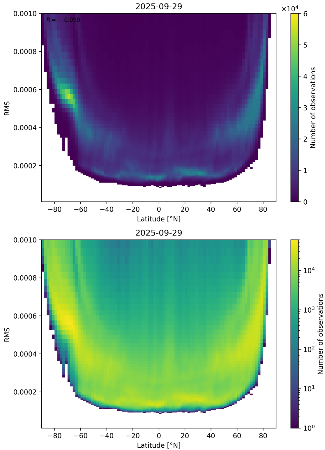
Figure 94: Scatter density plot of “Latitude” against “RMS” for 2025-09-28 to 2025-09-30.
