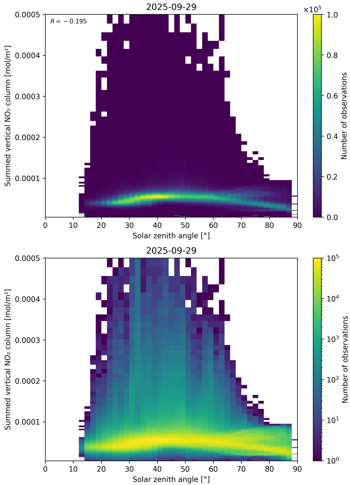
Figure 151: Scatter density plot of “Solar zenith angle” against “Summed vertical NO 2 column” for 2025-09-28 to 2025-09-30.
