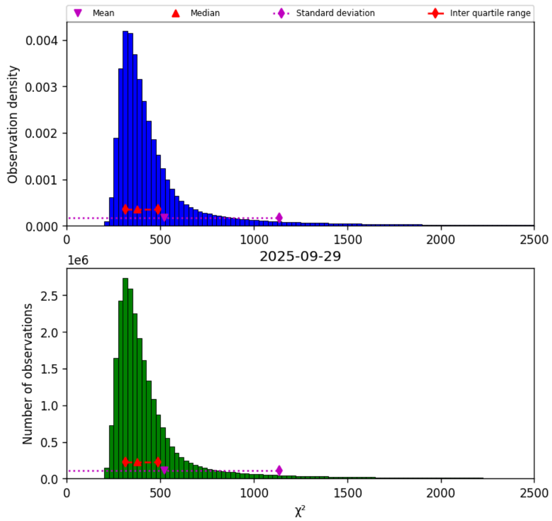
Figure 42: Histogram of “ \chi^2 ” for 2025-09-28 to 2025-09-30
