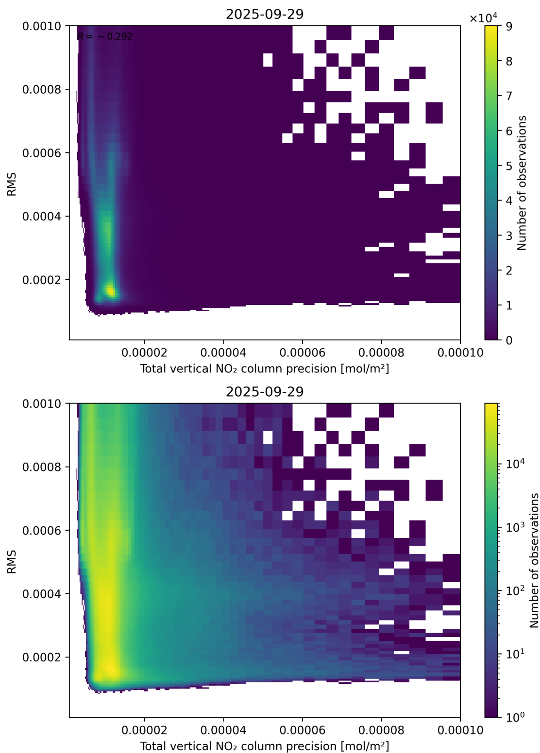
Figure 119: Scatter density plot of “Total vertical NO 2 column precision” against “RMS” for 2025-09-28 to 2025-09-30.
