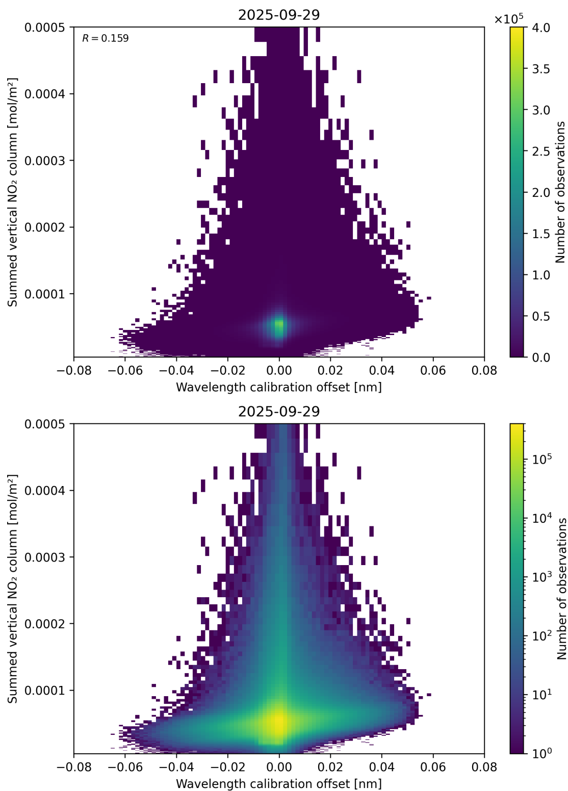
Figure 177: Scatter density plot of “Wavelength calibration offset” against “Summed vertical NO 2 column” for 2025-09-28 to 2025-09-30.
