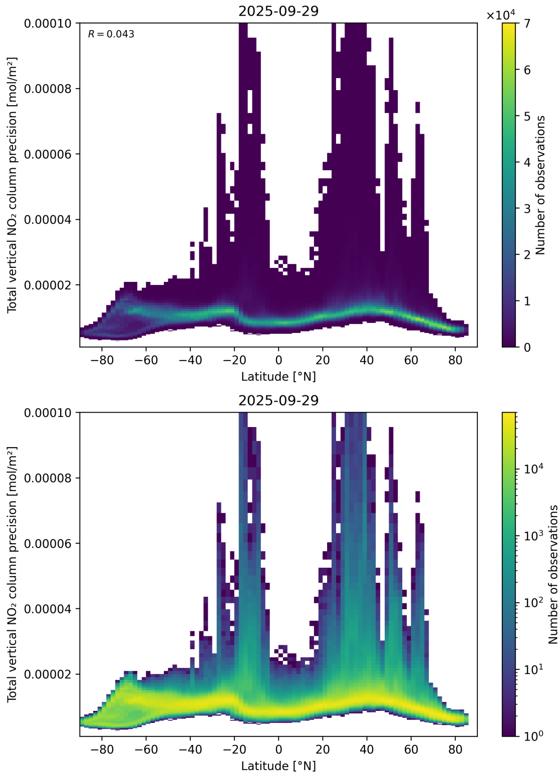
Figure 91: Scatter density plot of “Latitude” against “Total vertical NO 2 column precision” for 2025-09-28 to 2025-09-30.
