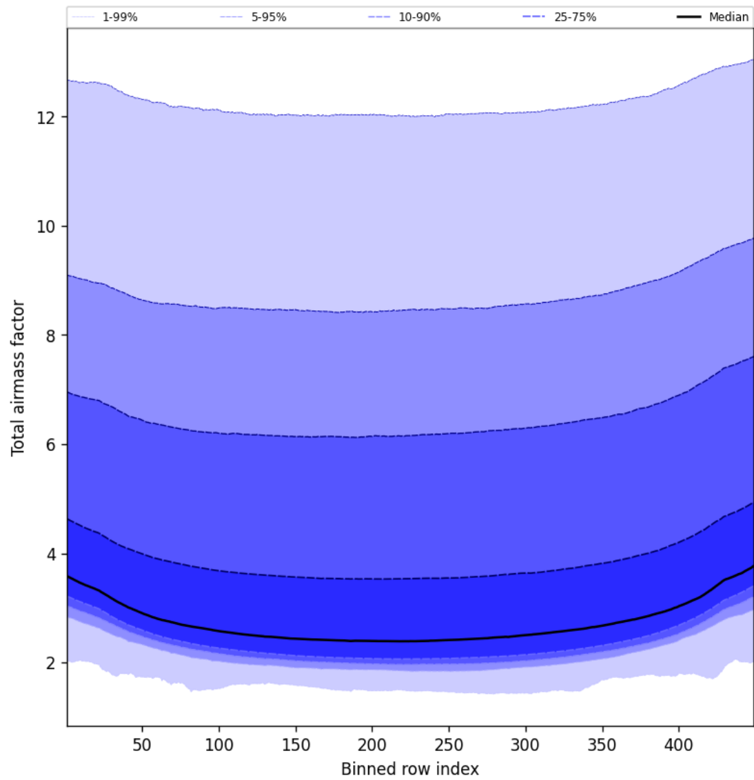
Figure 49: Along track statistics of “Total airmass factor” for 2025-09-28 to 2025-09-30
