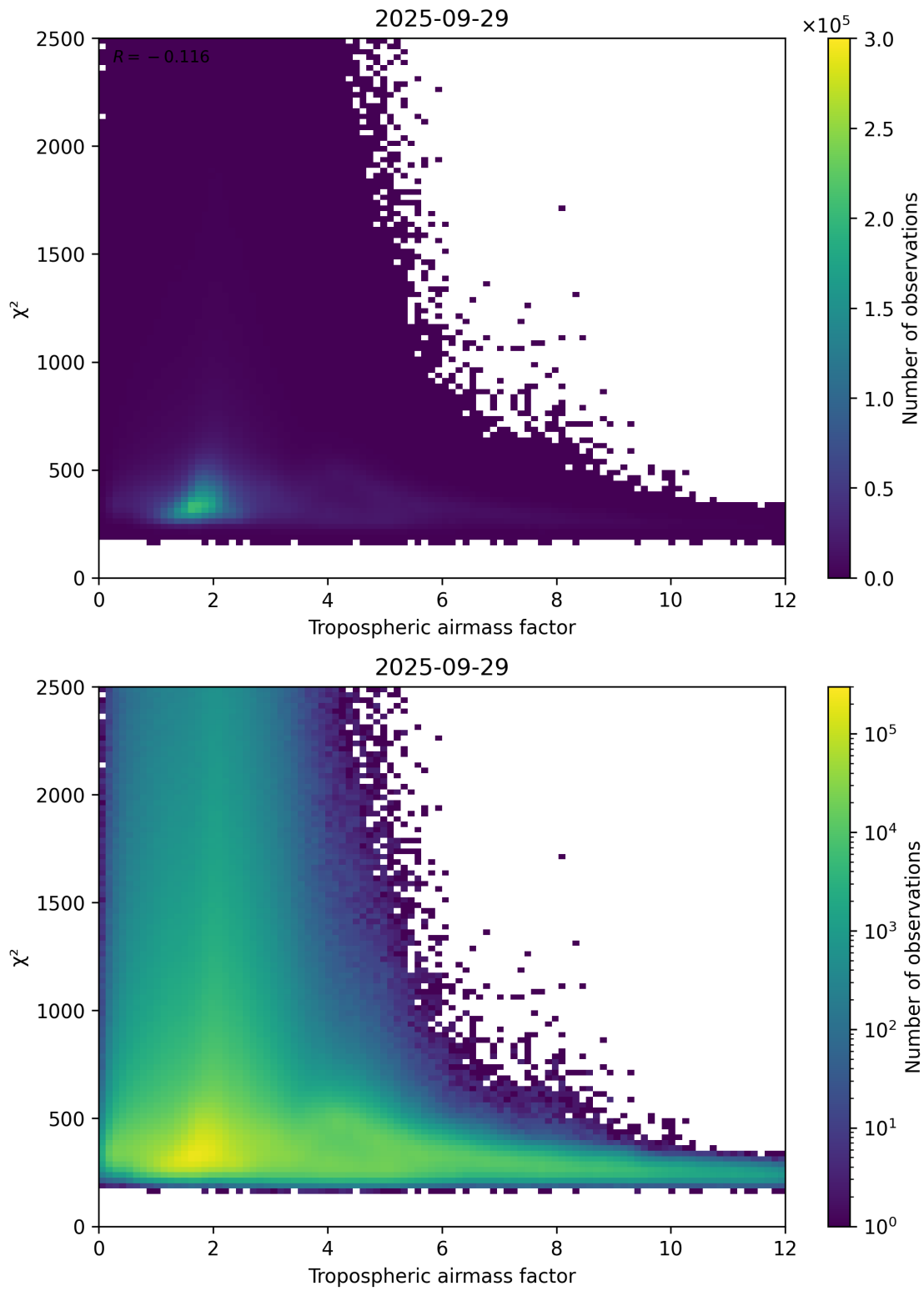
Figure 73: Scatter density plot of “Tropospheric airmass factor” against “ \chi^2 ” for 2025-09-28 to 2025-09-30.
