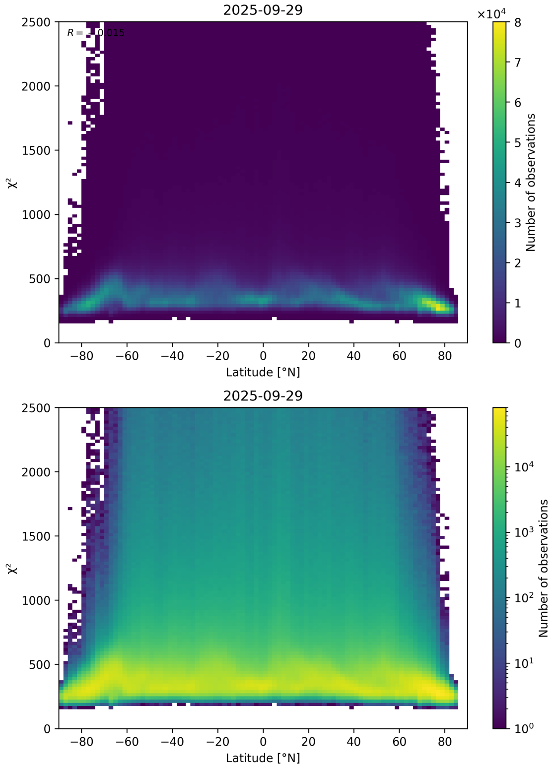
Figure 86: Scatter density plot of “Latitude” against “ \chi^2 ” for 2025-09-28 to 2025-09-30.
