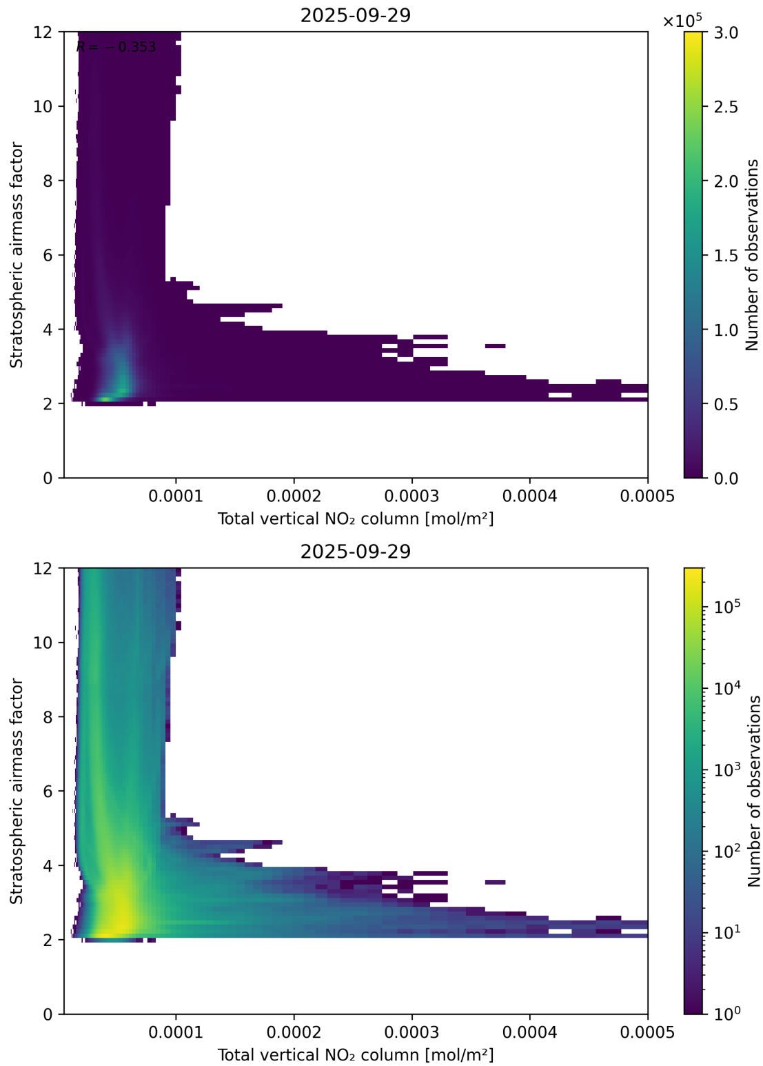
Figure 110: Scatter density plot of “Total vertical NO 2 column” against “Stratospheric airmass factor” for 2025-09-28 to 2025-09-30.
