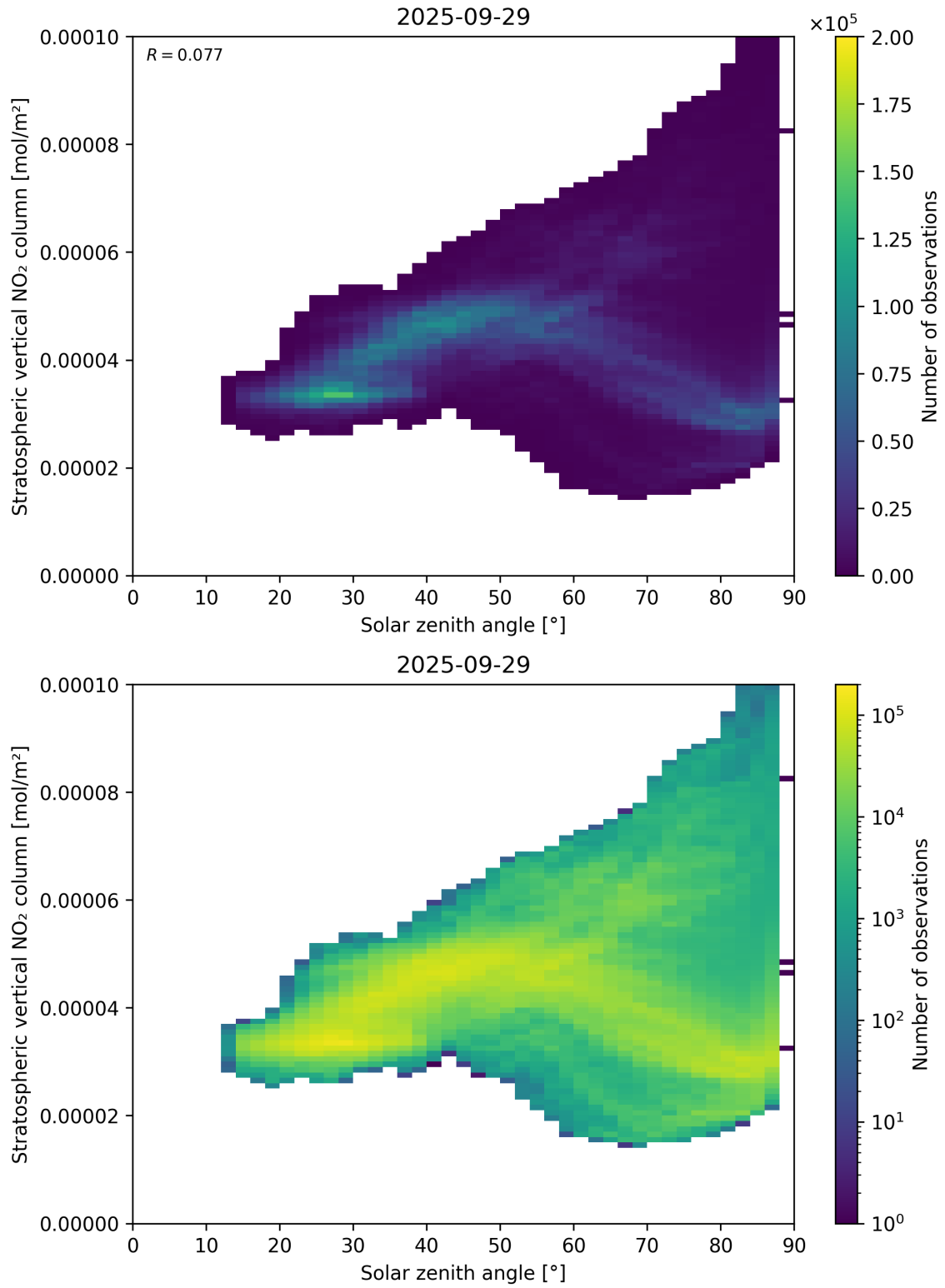
Figure 150: Scatter density plot of “Solar zenith angle” against “Stratospheric vertical \text{NO}_2 column” for 2025-09-28 to 2025-09-30.
