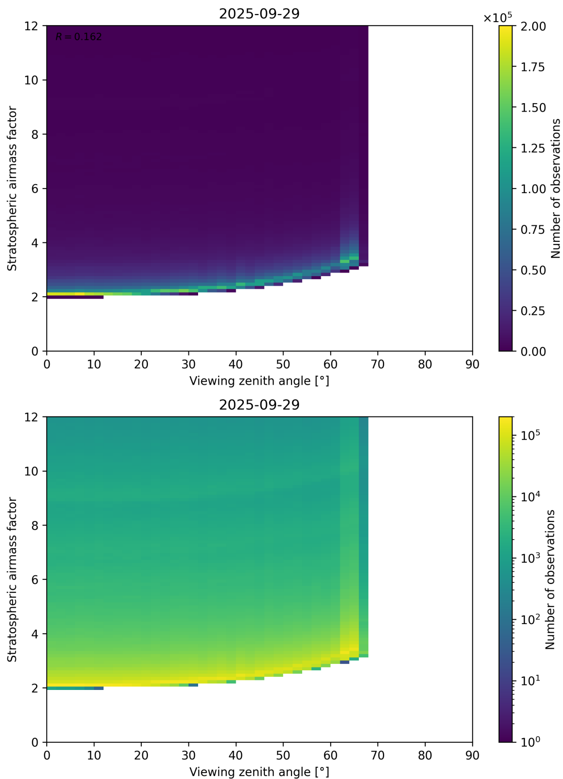
Figure 159: Scatter density plot of “Viewing zenith angle” against “Stratospheric airmass factor” for 2025-09-28 to 2025-09-30.
