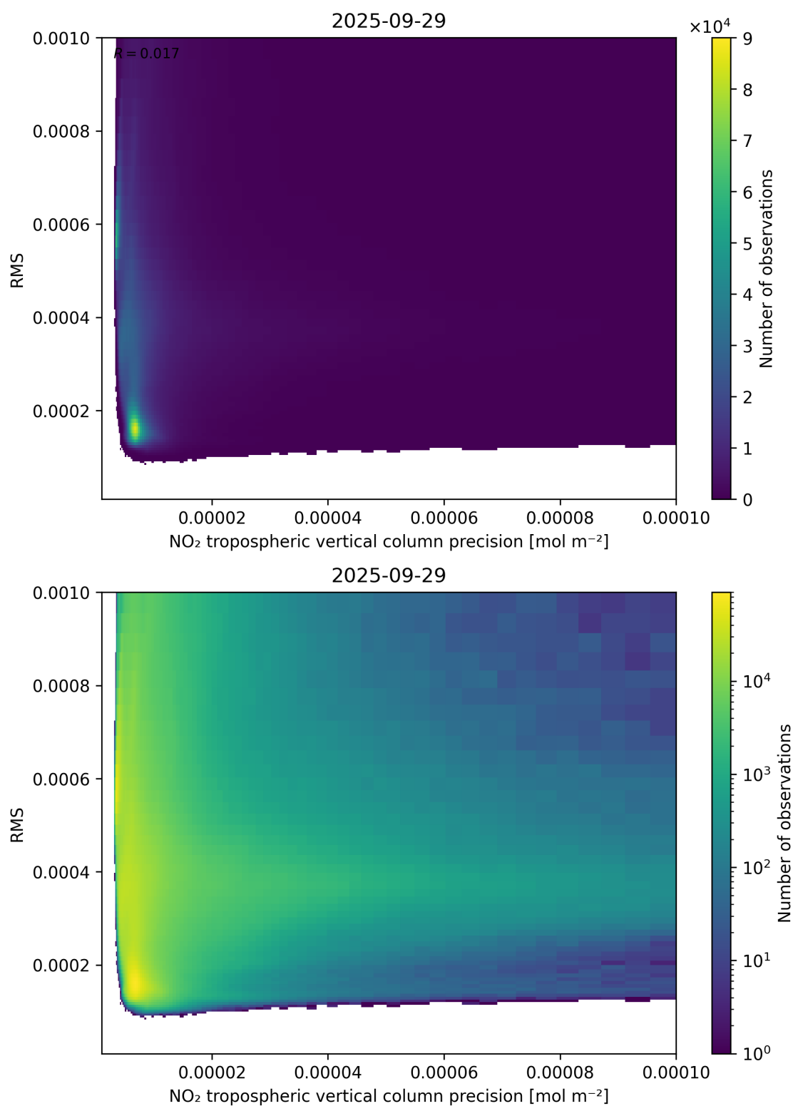
Figure 140: Scatter density plot of “NO 2 tropospheric vertical column precision” against “RMS” for 2025-09-28 to 2025-09-30.
