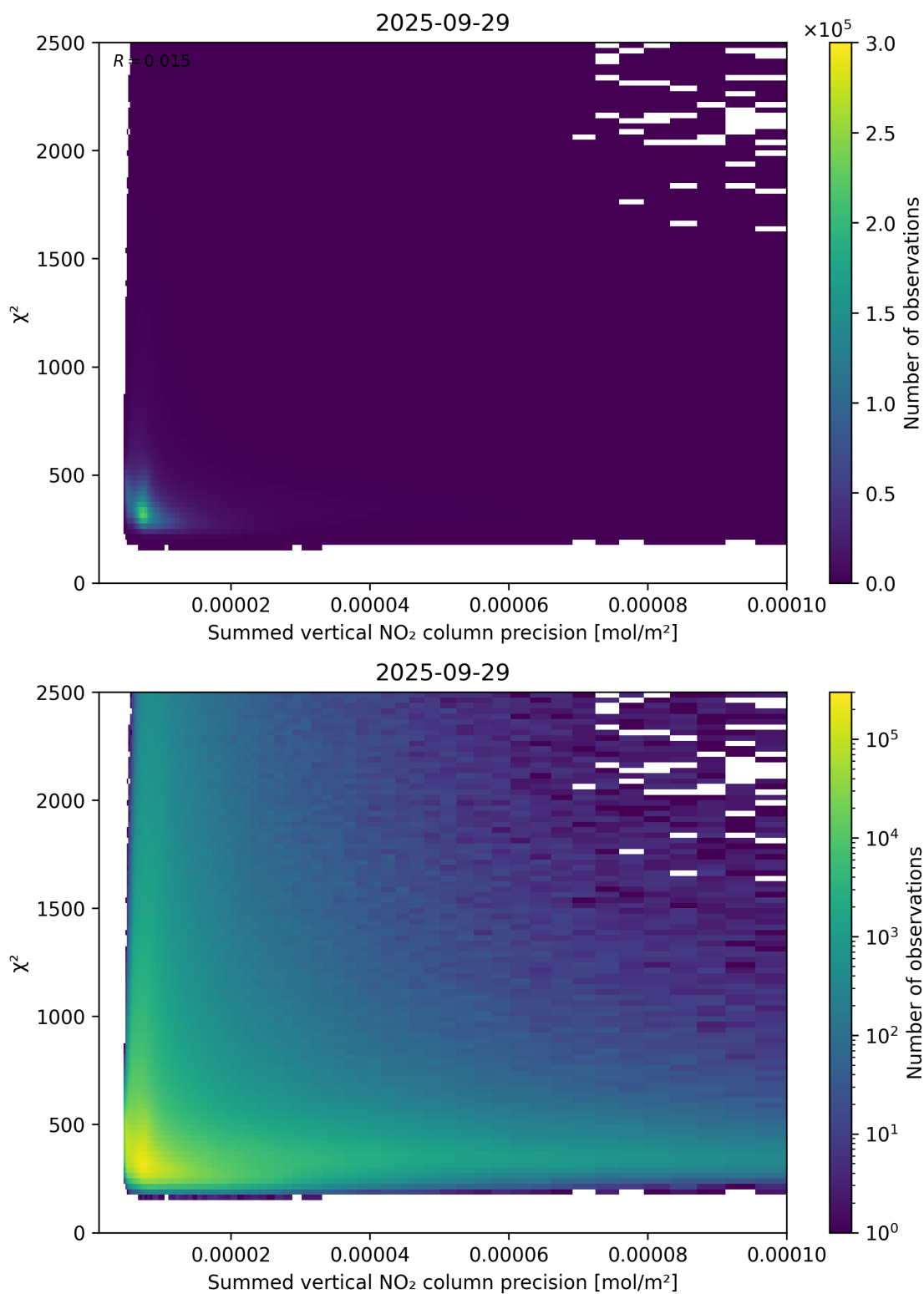
Figure 107: Scatter density plot of “Summed vertical NO 2 column precision” against “ \chi^2 ” for 2025-09-28 to 2025-09-30.
