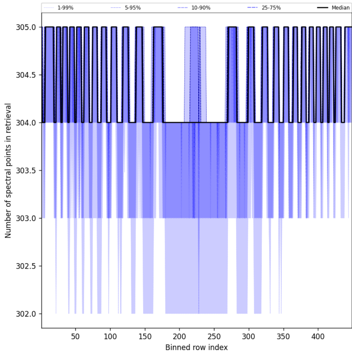
Figure 50: Along track statistics of “Number of spectral points in retrieval” for 2025-09-28 to 2025-09-30
