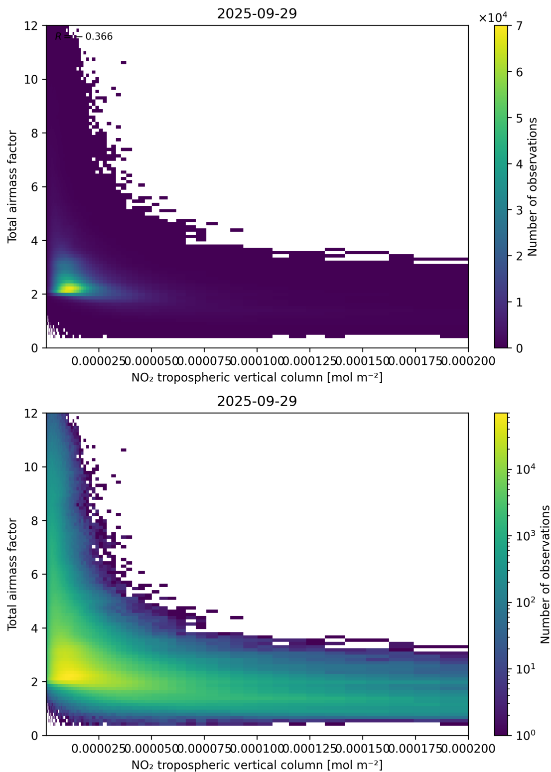
Figure 122: Scatter density plot of “NO 2 tropospheric vertical column” against “Total airmass factor” for 2025-09-28 to 2025-09-30.
