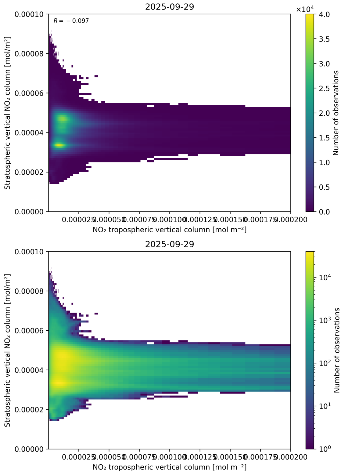
Figure 125: Scatter density plot of “NO 2 tropospheric vertical column” against “Stratospheric vertical NO 2 column” for 2025-09-28 to 2025-09-30.
