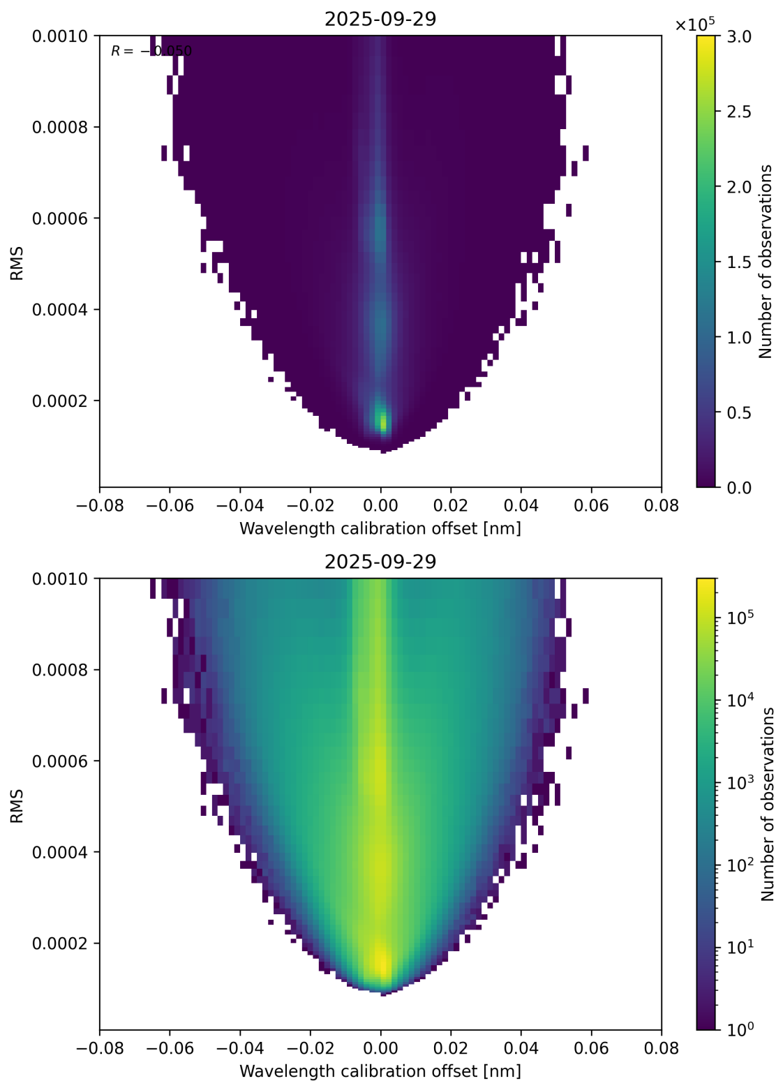
Figure 181: Scatter density plot of “Wavelength calibration offset” against “RMS” for 2025-09-28 to 2025-09-30.
