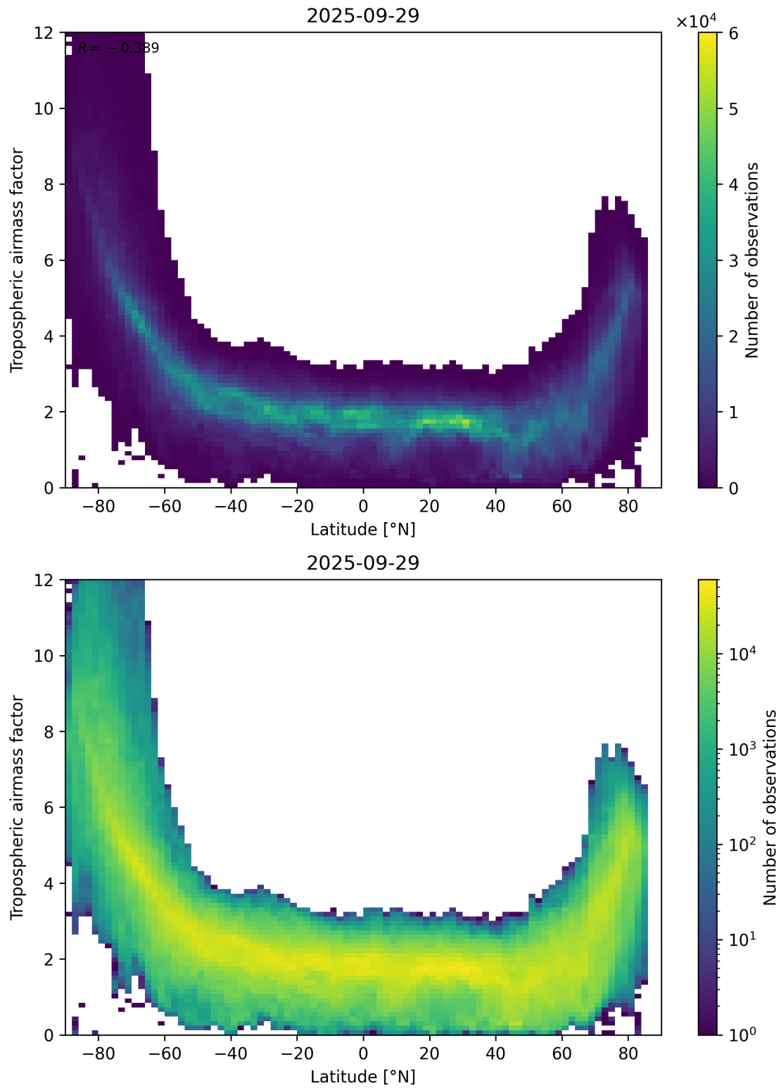
Figure 85: Scatter density plot of “Latitude” against “Tropospheric airmass factor” for 2025-09-28 to 2025-09-30.
