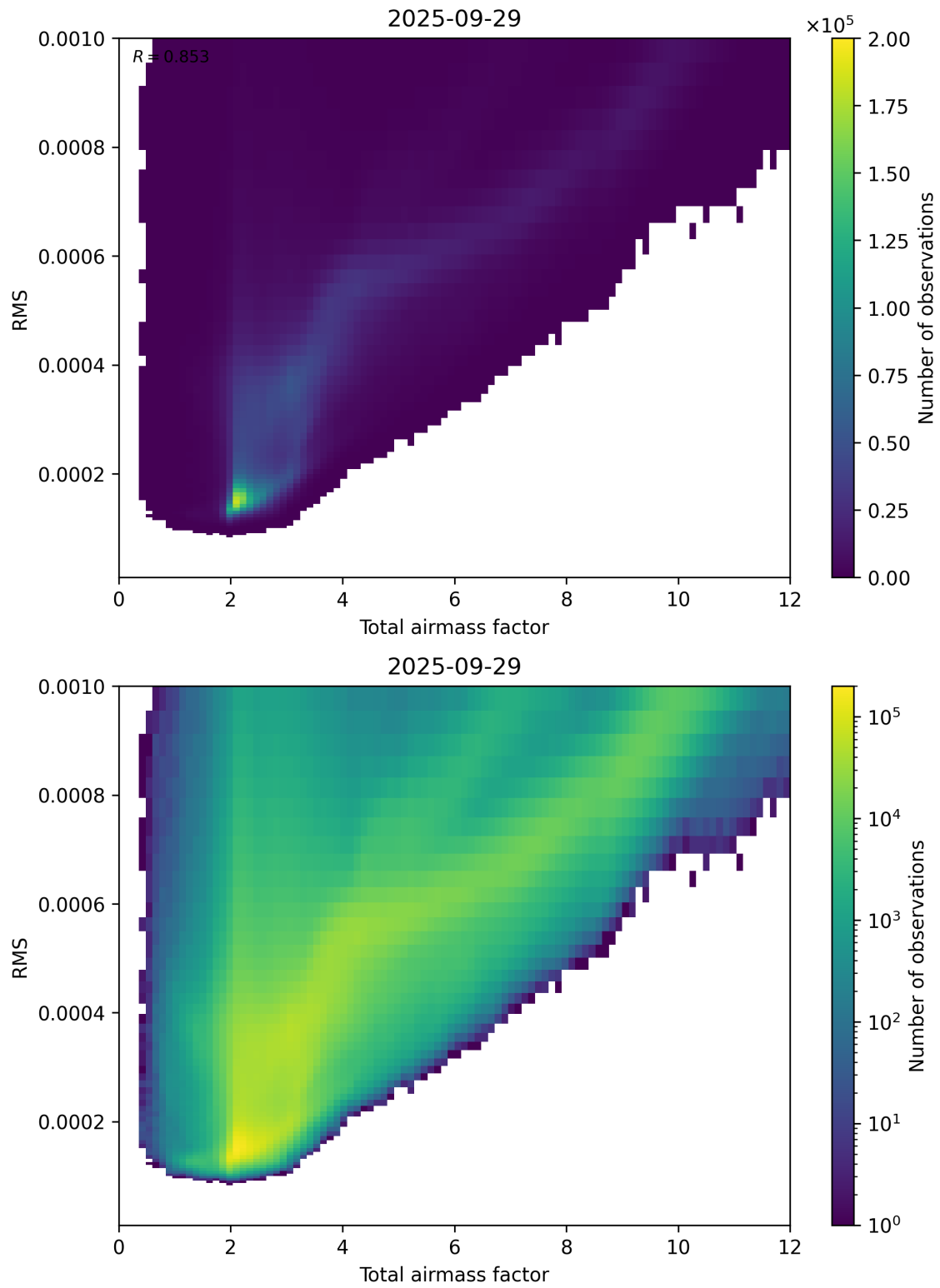
Figure 69: Scatter density plot of “Total airmass factor” against “RMS” for 2025-09-28 to 2025-09-30.
