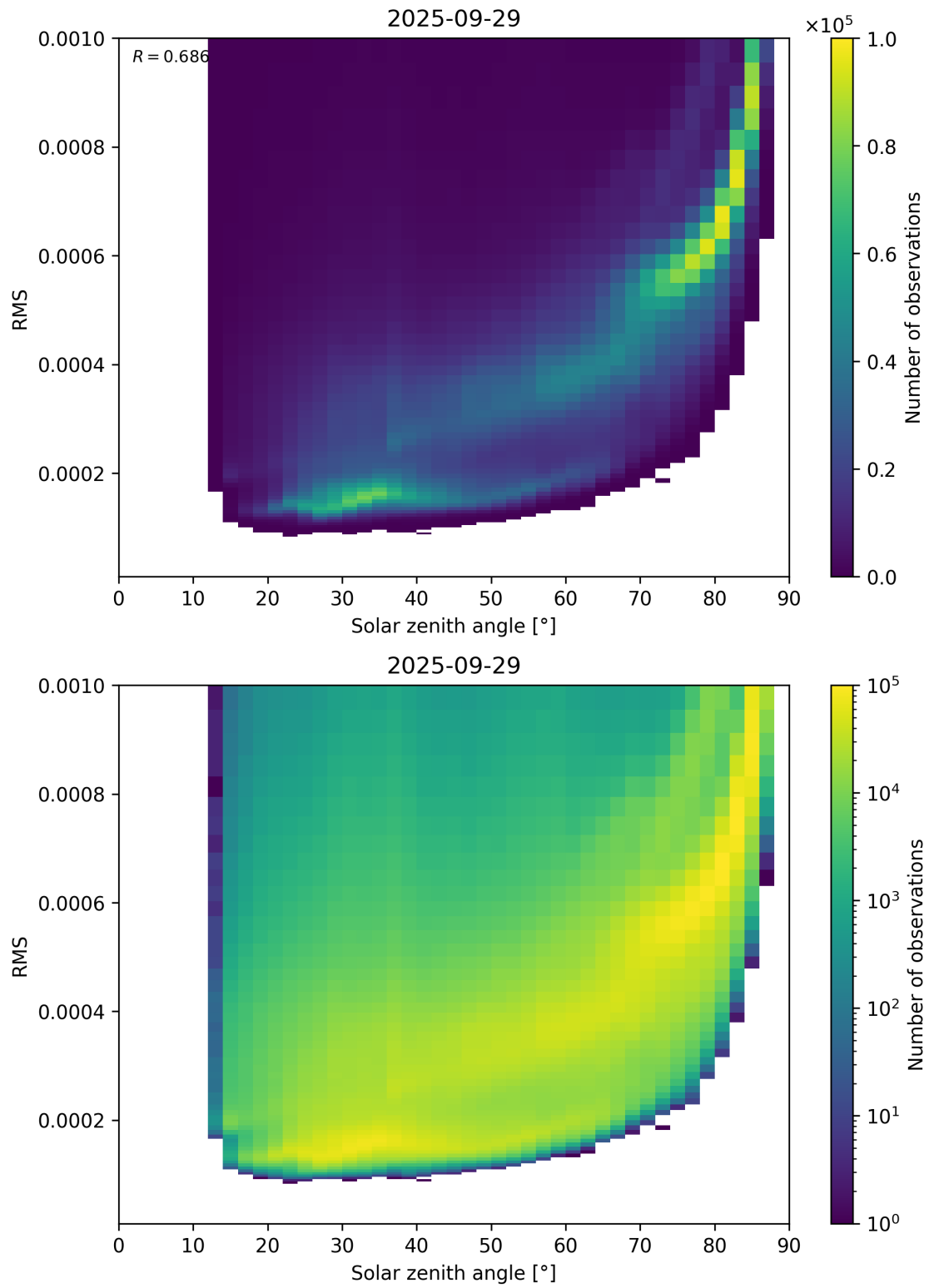
Figure 157: Scatter density plot of “Solar zenith angle” against “RMS” for 2025-09-28 to 2025-09-30.
