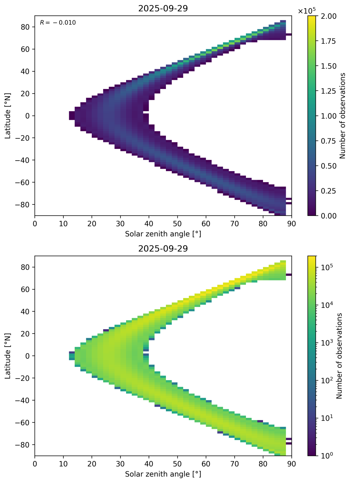
Figure 149: Scatter density plot of “Solar zenith angle” against “Latitude” for 2025-09-28 to 2025-09-30.
