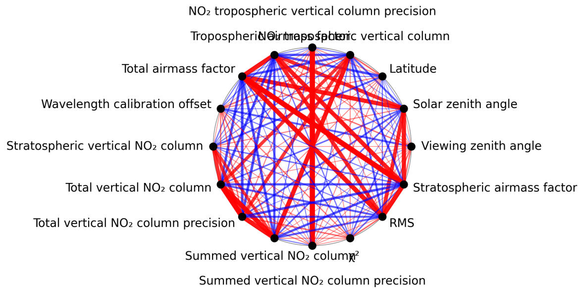
Figure 1: Map of correlation graph for 2025-09-28 to 2025-09-30.
