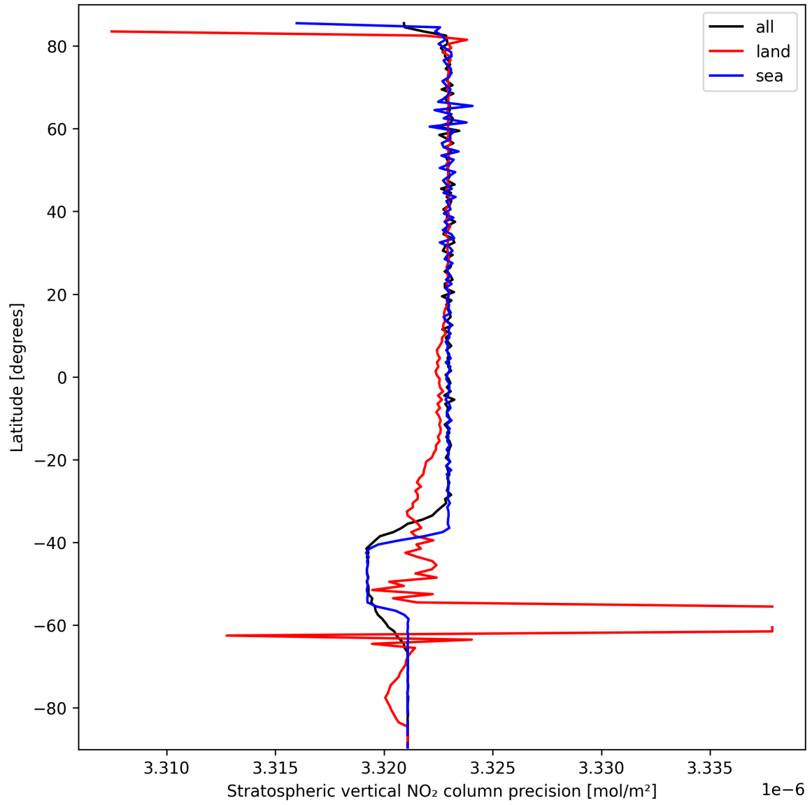
Figure 20: Zonal average of “Stratospheric vertical NO 2 column precision” for 2025-09-28 to 2025-09-30.
