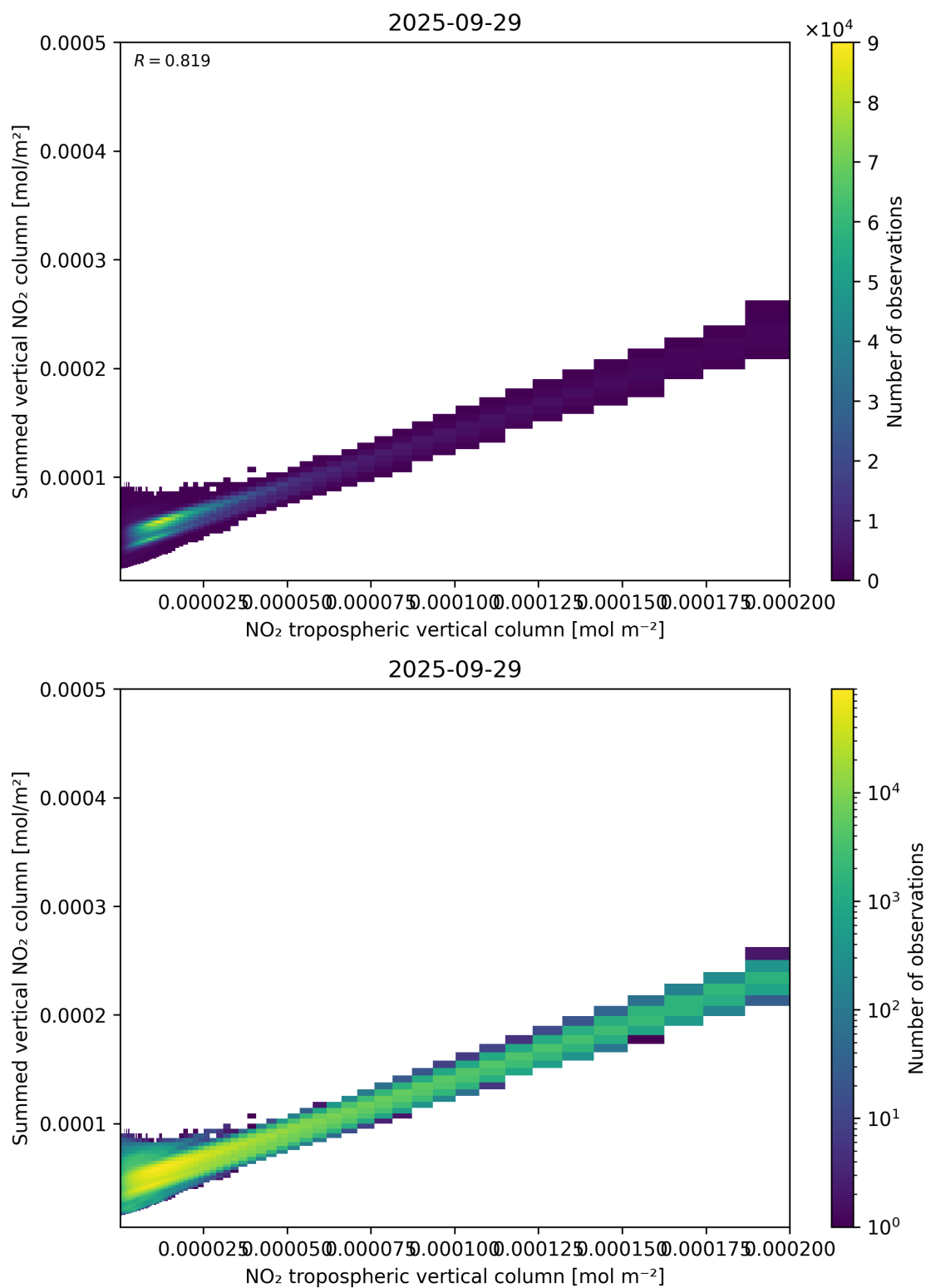
Figure 126: Scatter density plot of “NO 2 tropospheric vertical column” against “Summed vertical NO 2 column” for 2025-09-28 to 2025-09-30.
