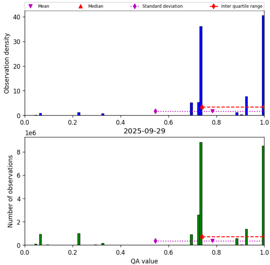
Figure 28: Histogram of “QA value” for 2025-09-28 to 2025-09-30
