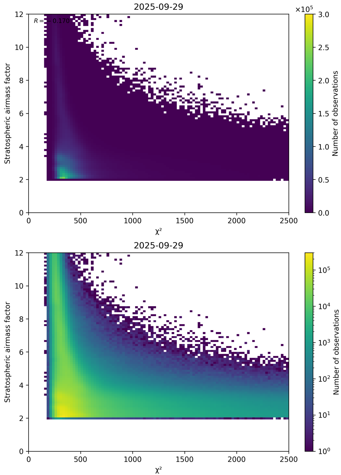
Figure 81: Scatter density plot of “ \chi^2 ” against “Stratospheric airmass factor” for 2025-09-28 to 2025-09-30.
