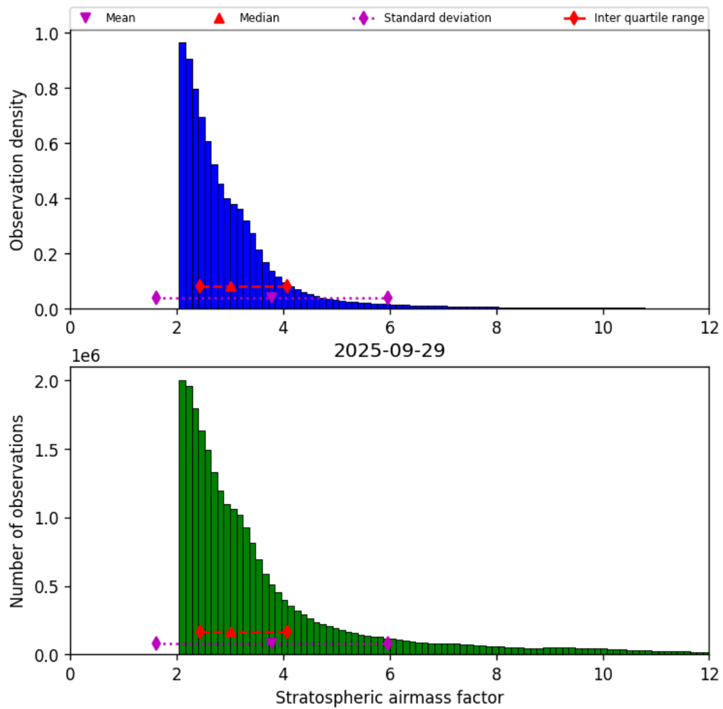
Figure 44: Histogram of “Stratospheric airmass factor” for 2025-09-28 to 2025-09-30
