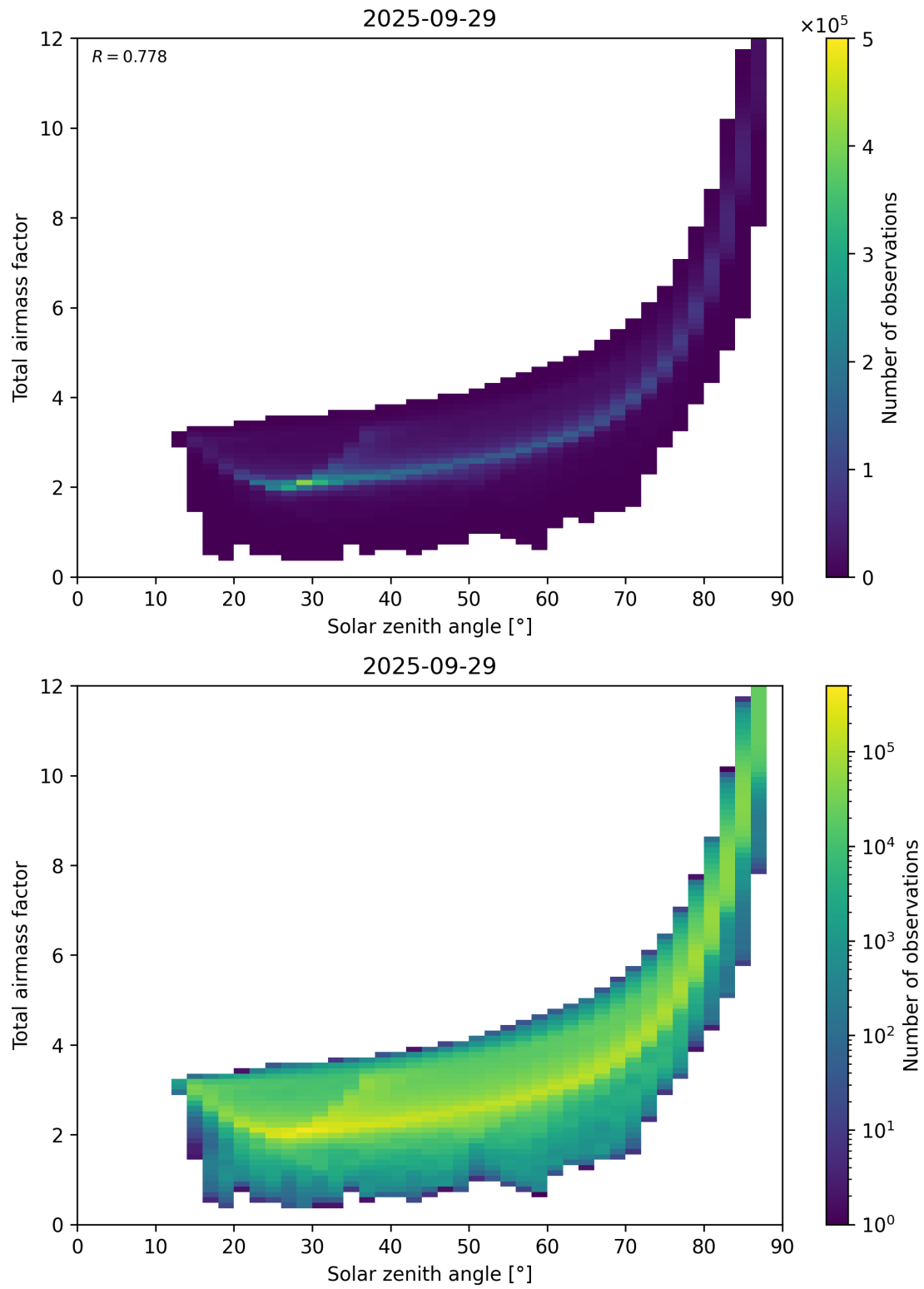
Figure 146: Scatter density plot of “Solar zenith angle” against “Total airmass factor” for 2025-09-28 to 2025-09-30.
