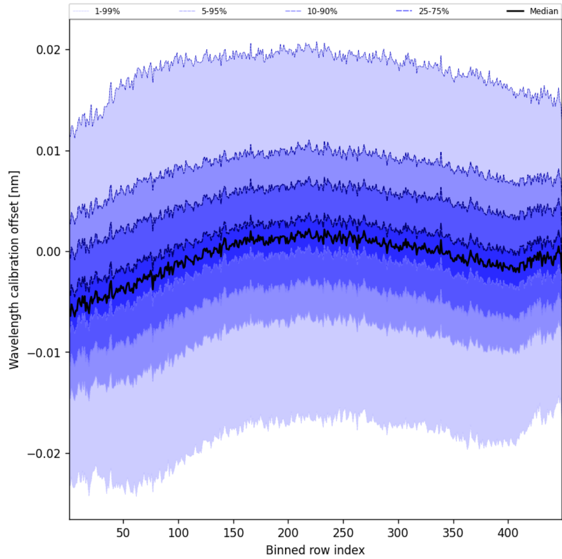
Figure 52: Along track statistics of “Wavelength calibration offset” for 2025-09-28 to 2025-09-30
