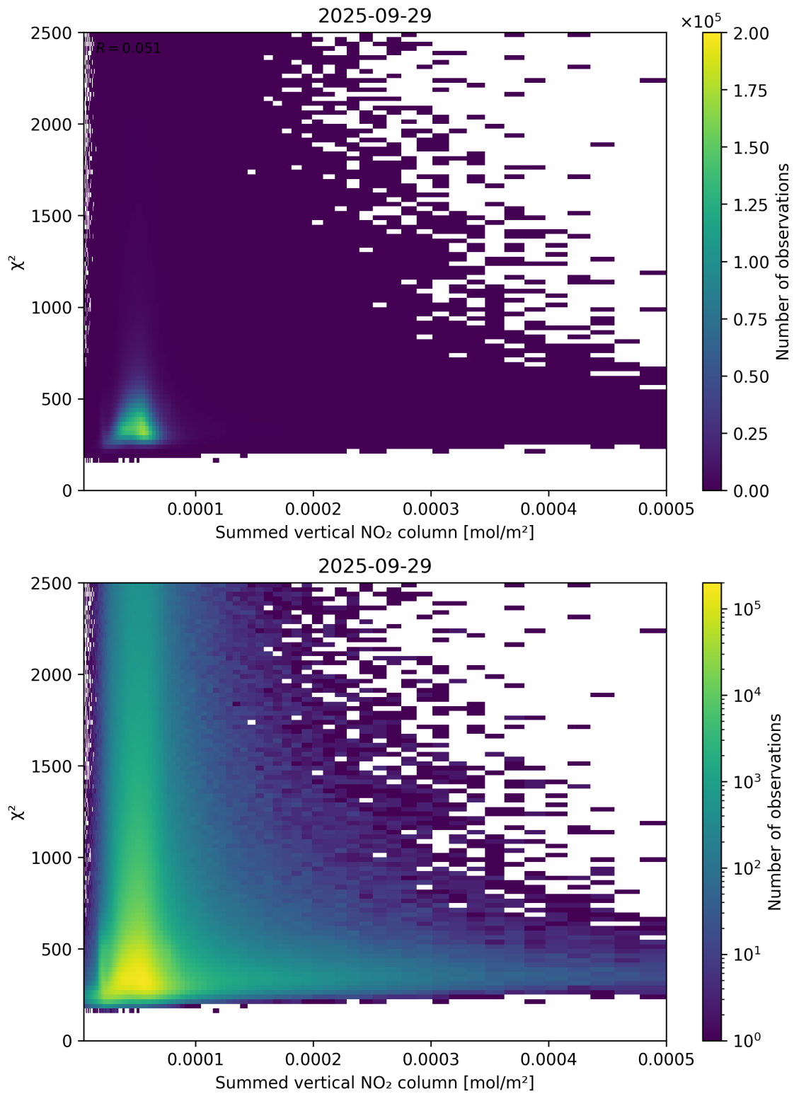
Figure 104: Scatter density plot of “Summed vertical NO 2 column” against “ \chi^2 ” for 2025-09-28 to 2025-09-30.
