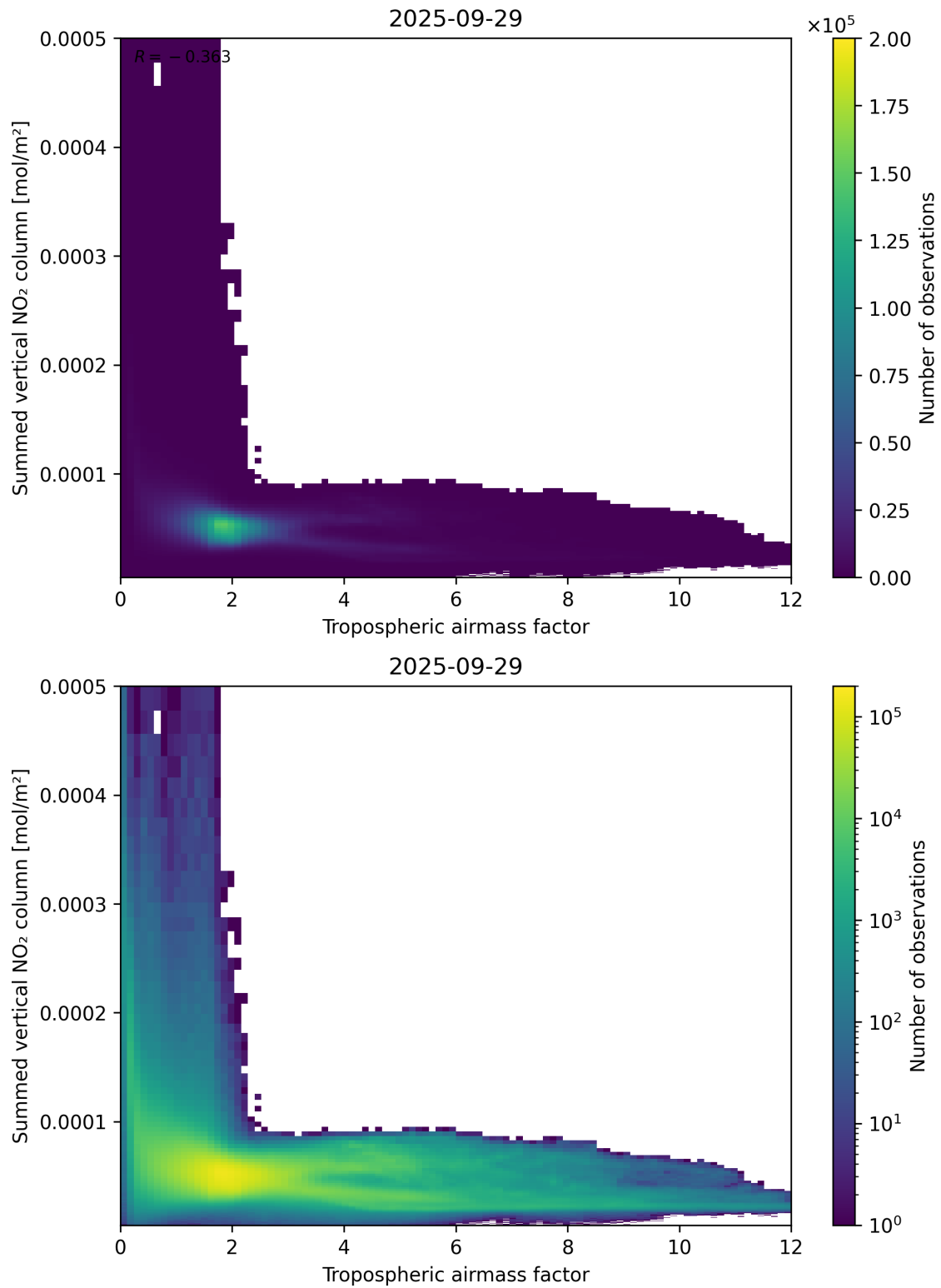
Figure 75: Scatter density plot of “Tropospheric air mass factor” against “Summed vertical NO 2 column” for 2025-09-28 to 2025-09-30.
