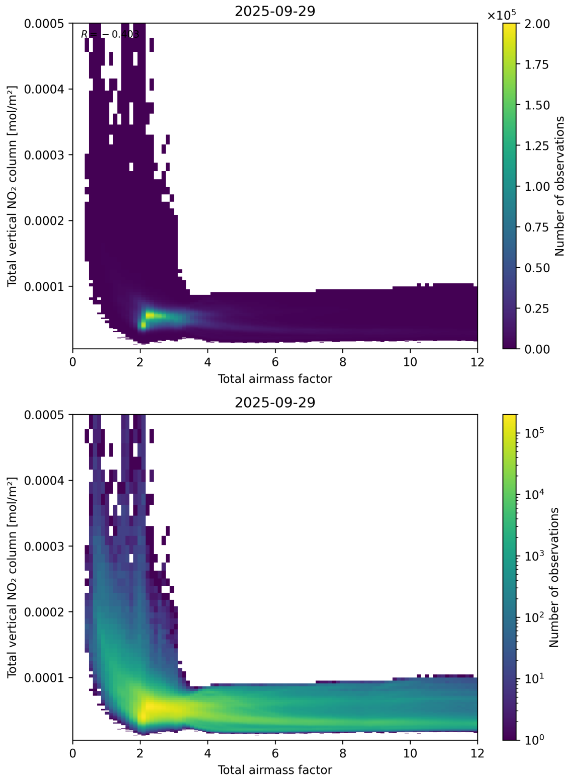
Figure 67: Scatter density plot of “Total airmass factor” against “Total vertical NO 2 column” for 2025-09-28 to 2025-09-30.
