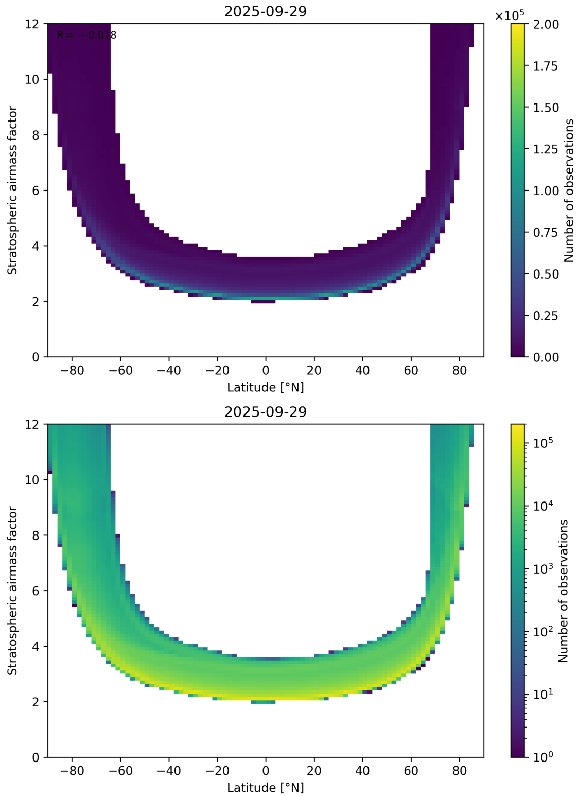
Figure 83: Scatter density plot of “Latitude” against “Stratospheric air mass factor” for 2025-09-28 to 2025-09-30.
