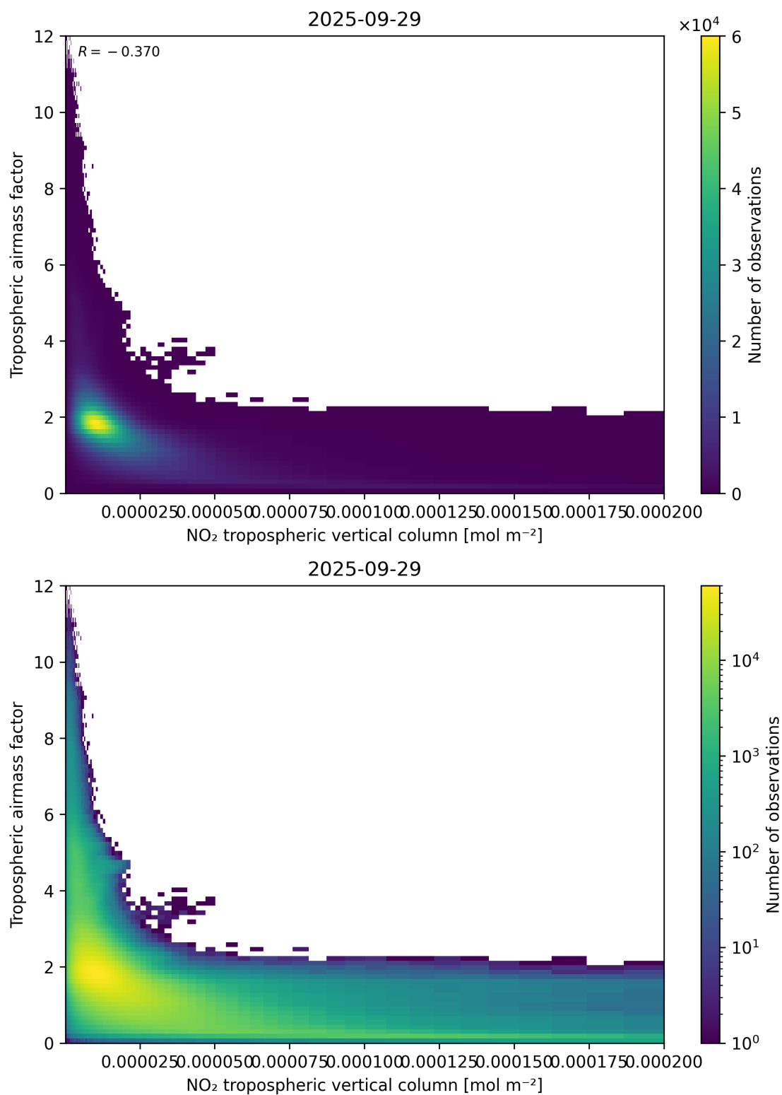
Figure 123: Scatter density plot of “NO 2 tropospheric vertical column” against “Tropospheric air mass factor” for 2025-09-28 to 2025-09-30.
