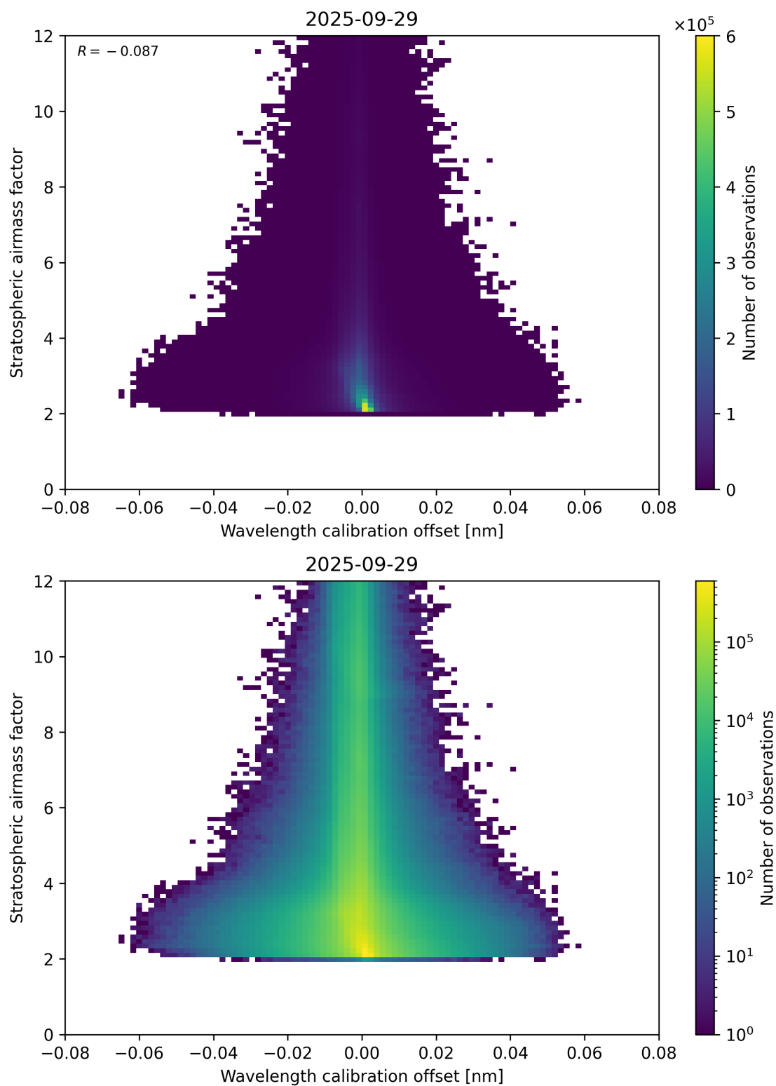
Figure 174: Scatter density plot of “Wavelength calibration offset” against “Stratospheric air mass factor” for 2025-09-28 to 2025-09-30.
