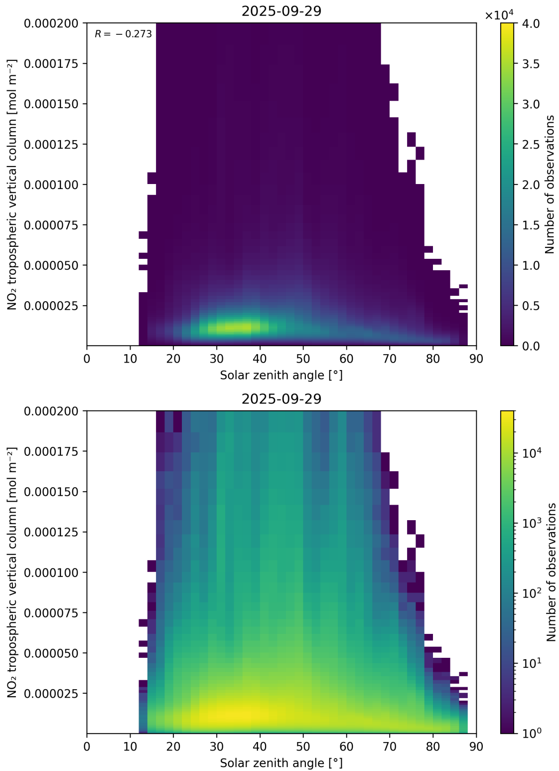
Figure 155: Scatter density plot of “Solar zenith angle” against “NO 2 tropospheric vertical column” for 2025-09-28 to 2025-09-30.
