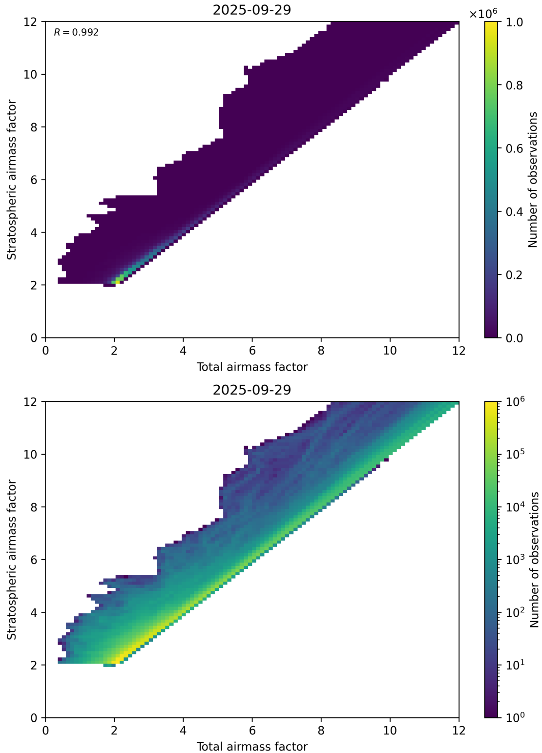
Figure 62: Scatter density plot of “Total airmass factor” against “Stratospheric airmass factor” for 2025-09-28 to 2025-09-30.
