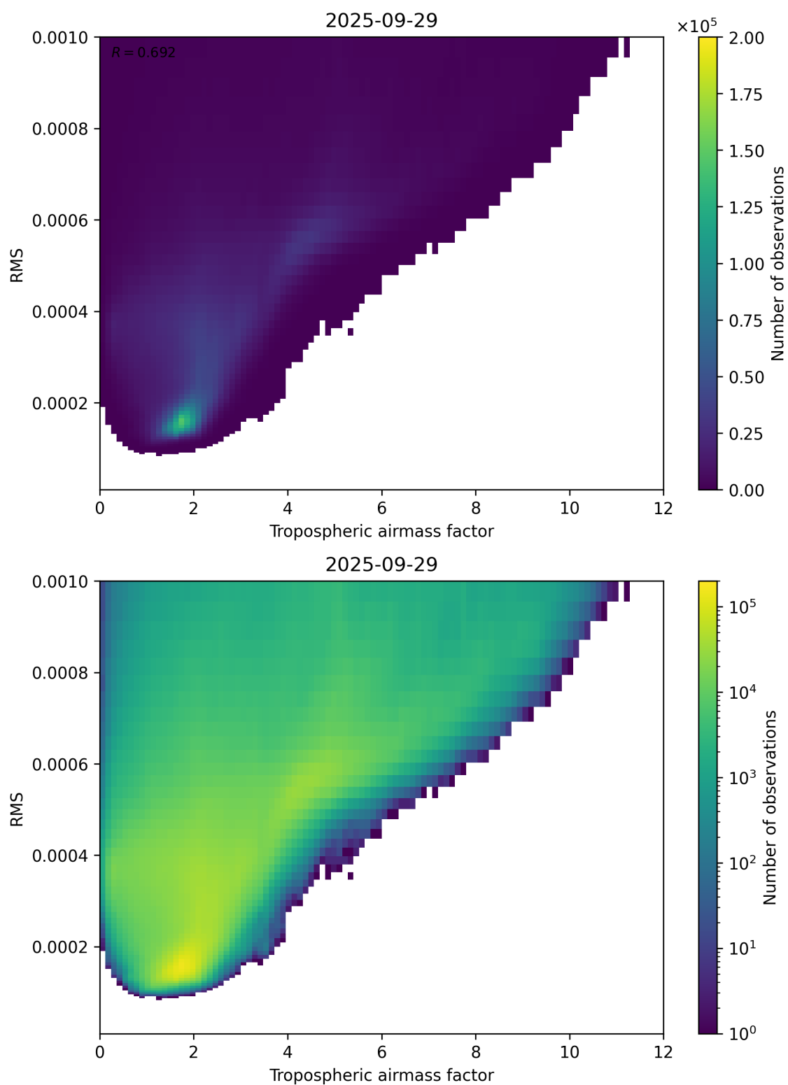
Figure 79: Scatter density plot of “Tropospheric airmass factor” against “RMS” for 2025-09-28 to 2025-09-30.
