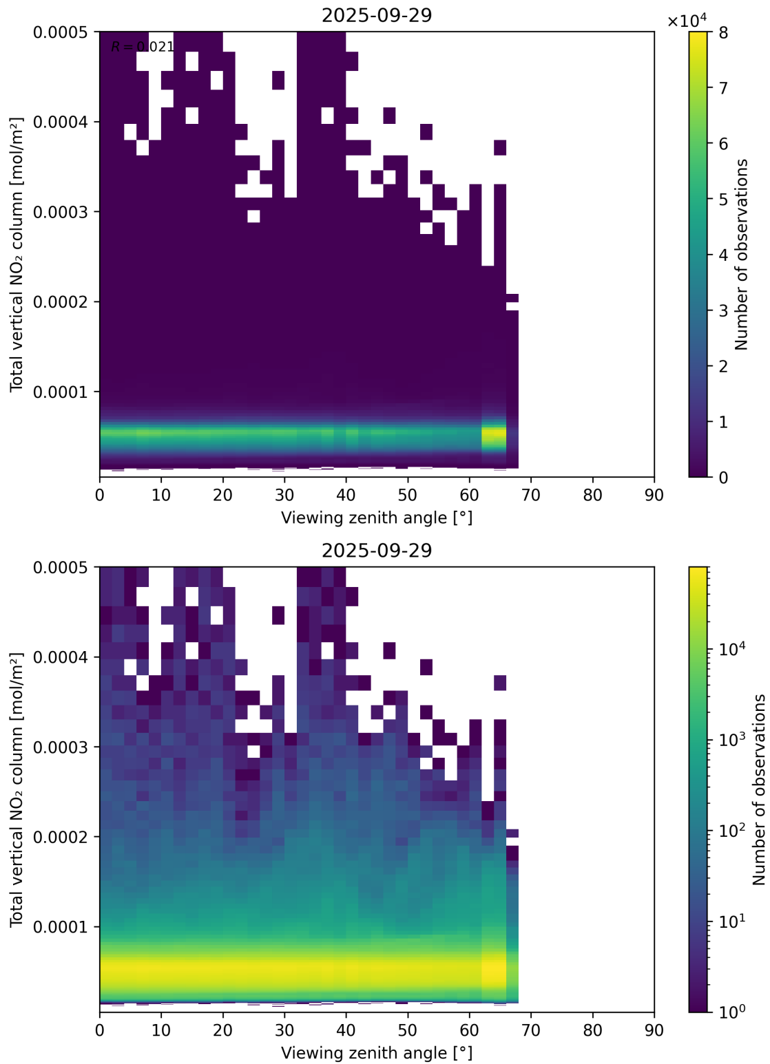
Figure 167: Scatter density plot of “Viewing zenith angle” against “Total vertical NO 2 column” for 2025-09-28 to 2025-09-30.
