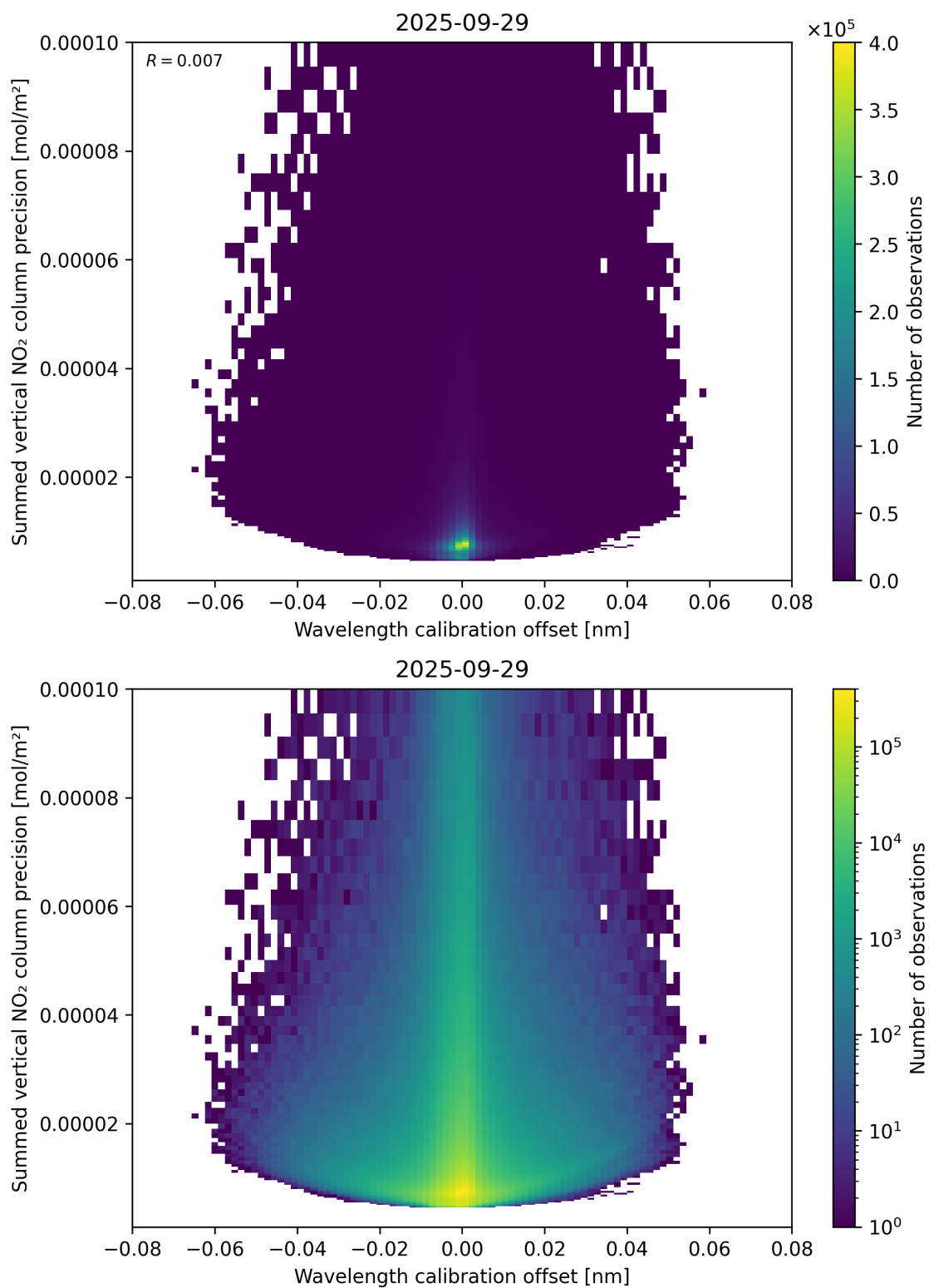
Figure 178: Scatter density plot of “Wavelength calibration offset” against “Summed vertical NO 2 column precision” for 2025-09-28 to 2025-09-30.
