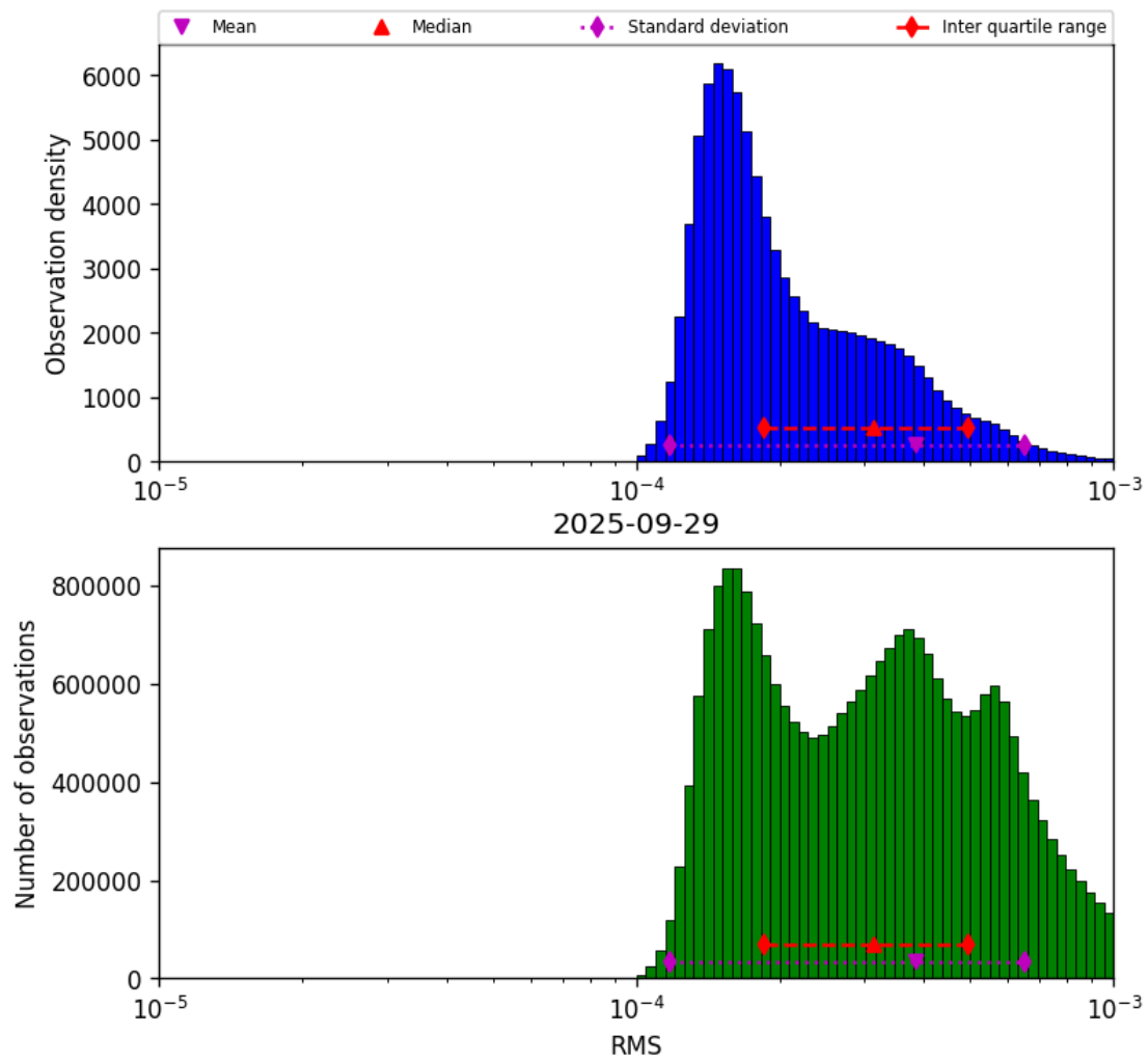
Figure 43: Histogram of “RMS” for 2025-09-28 to 2025-09-30
