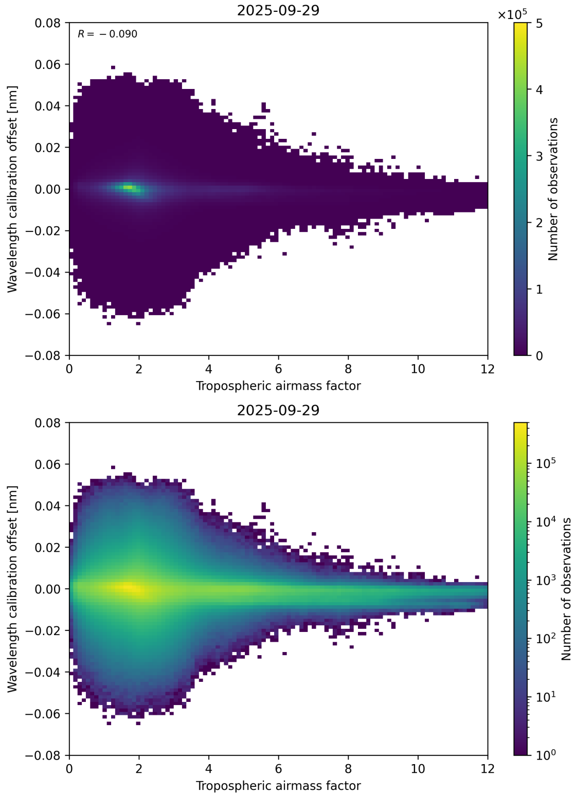
Figure 80: Scatter density plot of “Tropospheric airmass factor” against “Wavelength calibration offset” for 2025-09-28 to 2025-09-30.
