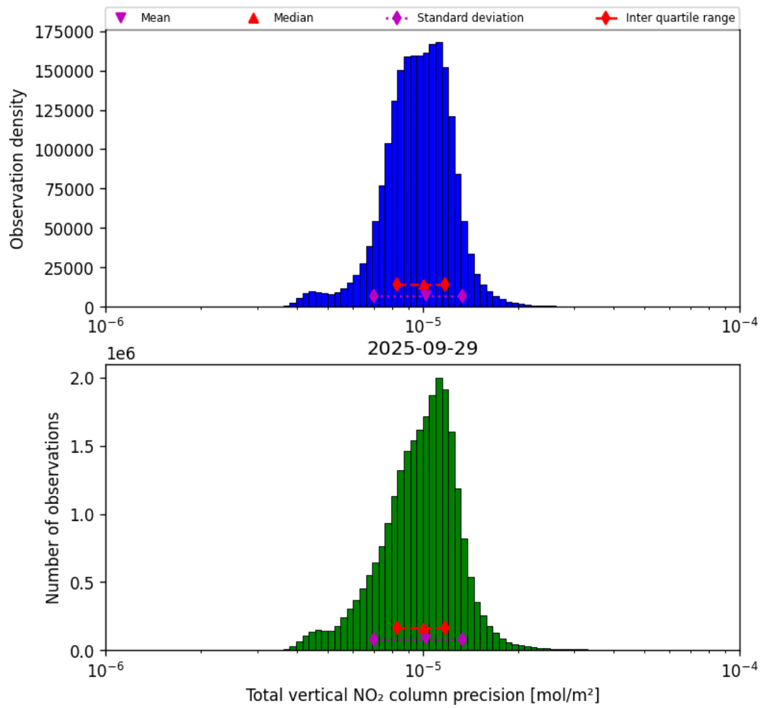
Figure 39: Histogram of “Total vertical NO 2 column precision” for 2025-09-28 to 2025-09-30
