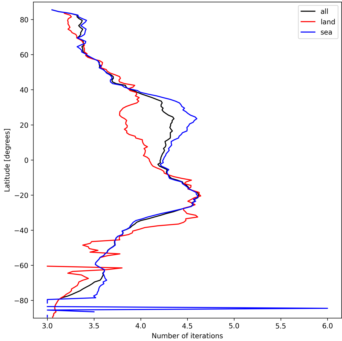
Figure 17: Zonal average of “Number of iterations” for 2025-09-28 to 2025-09-30.
