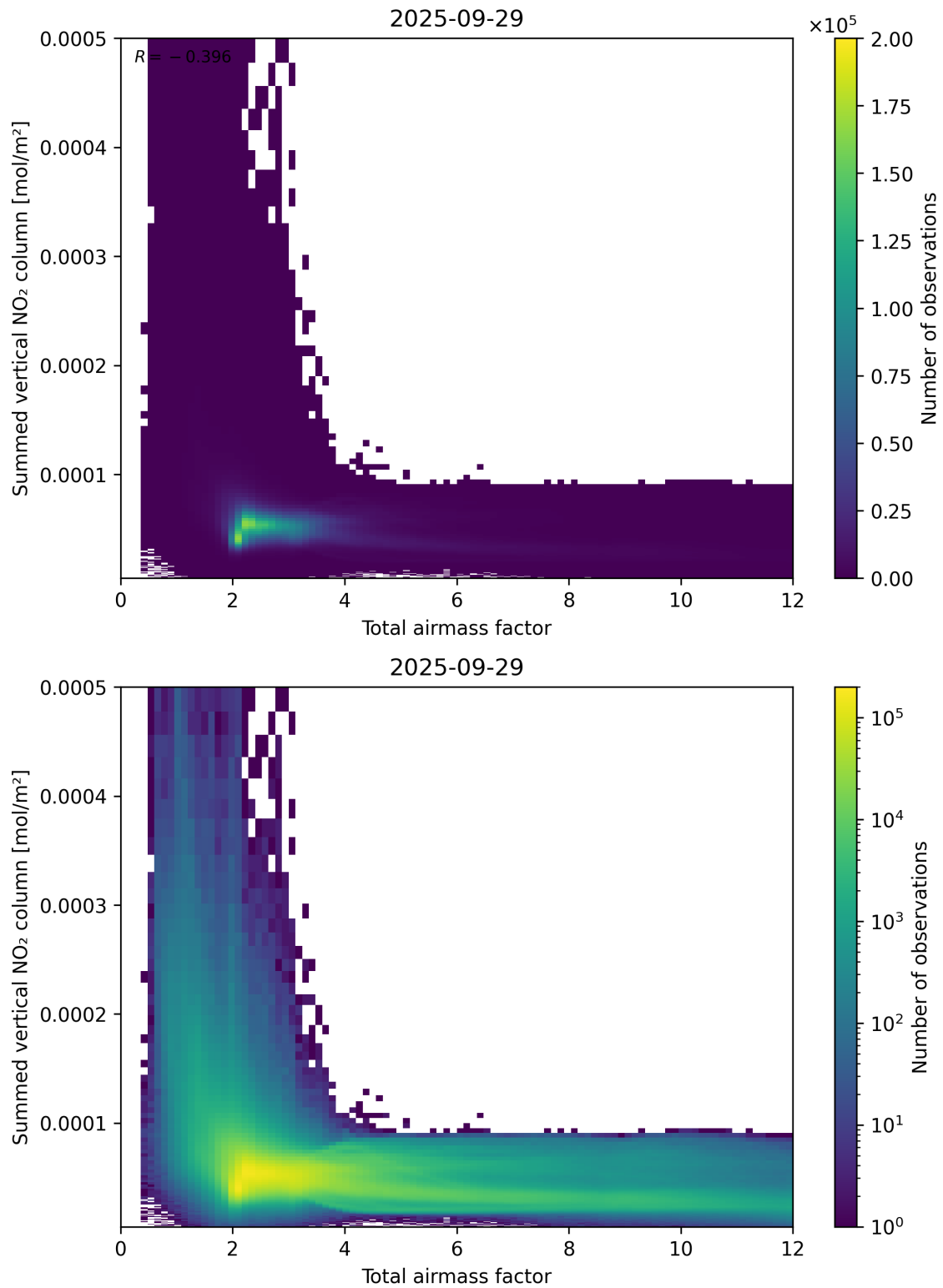
Figure 65: Scatter density plot of “Total airmass factor” against “Summed vertical NO 2 column” for 2025-09-28 to 2025-09-30.
