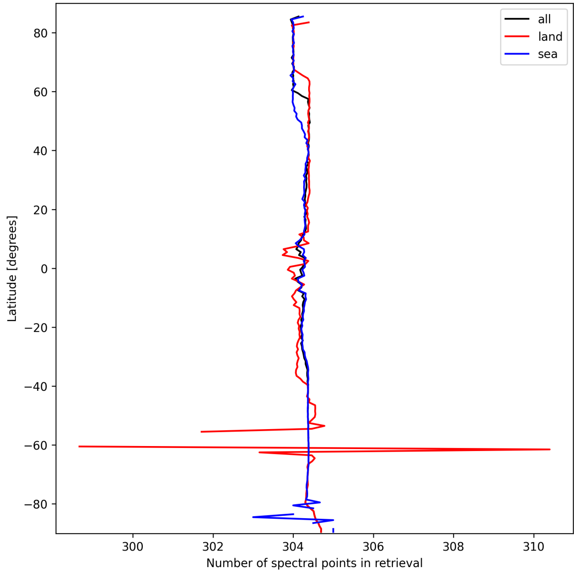
Figure 16: Zonal average of “Number of spectral points in retrieval” for 2025-09-28 to 2025-09-30.
