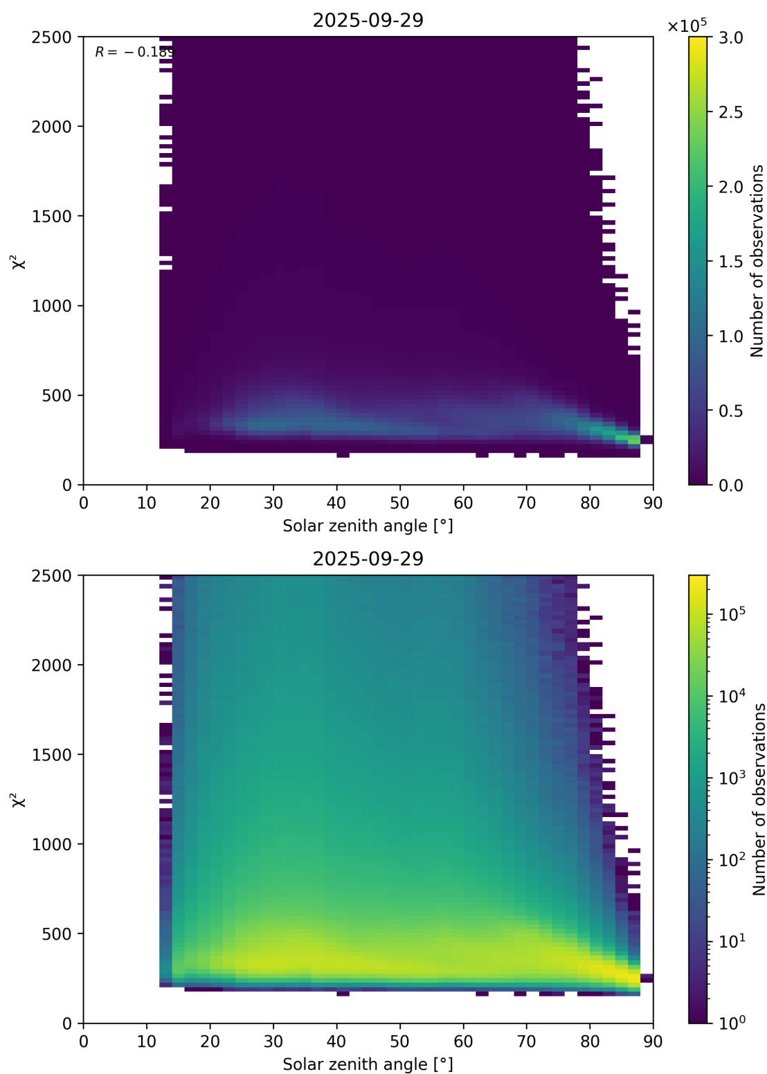
Figure 148: Scatter density plot of “Solar zenith angle” against “ \chi^2 ” for 2025-09-28 to 2025-09-30.
