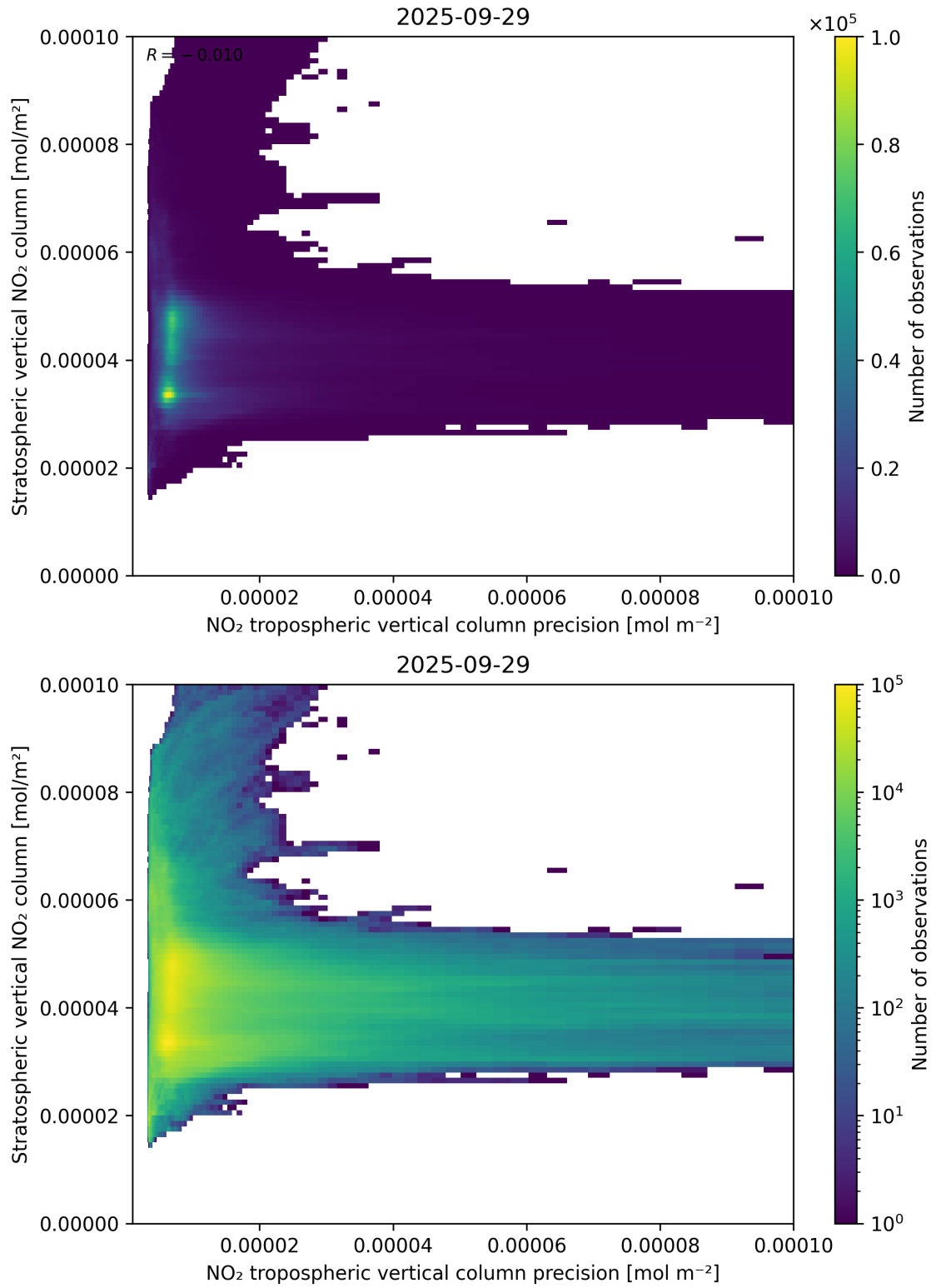
Figure 135: Scatter density plot of “NO 2 tropospheric vertical column precision” against “Stratospheric vertical NO 2 column” for 2025-09-28 to 2025-09-30.
