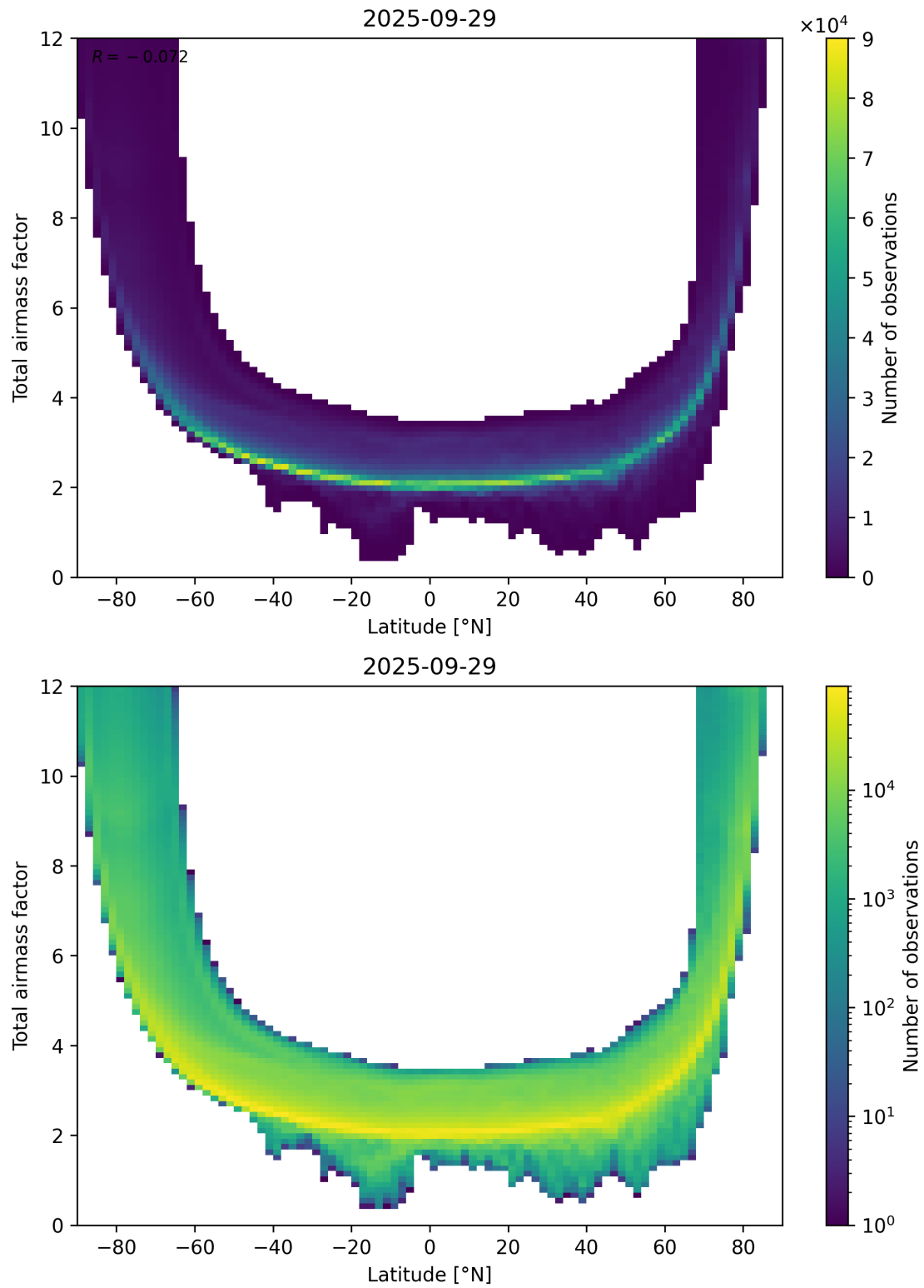
Figure 84: Scatter density plot of “Latitude” against “Total airmass factor” for 2025-09-28 to 2025-09-30.
