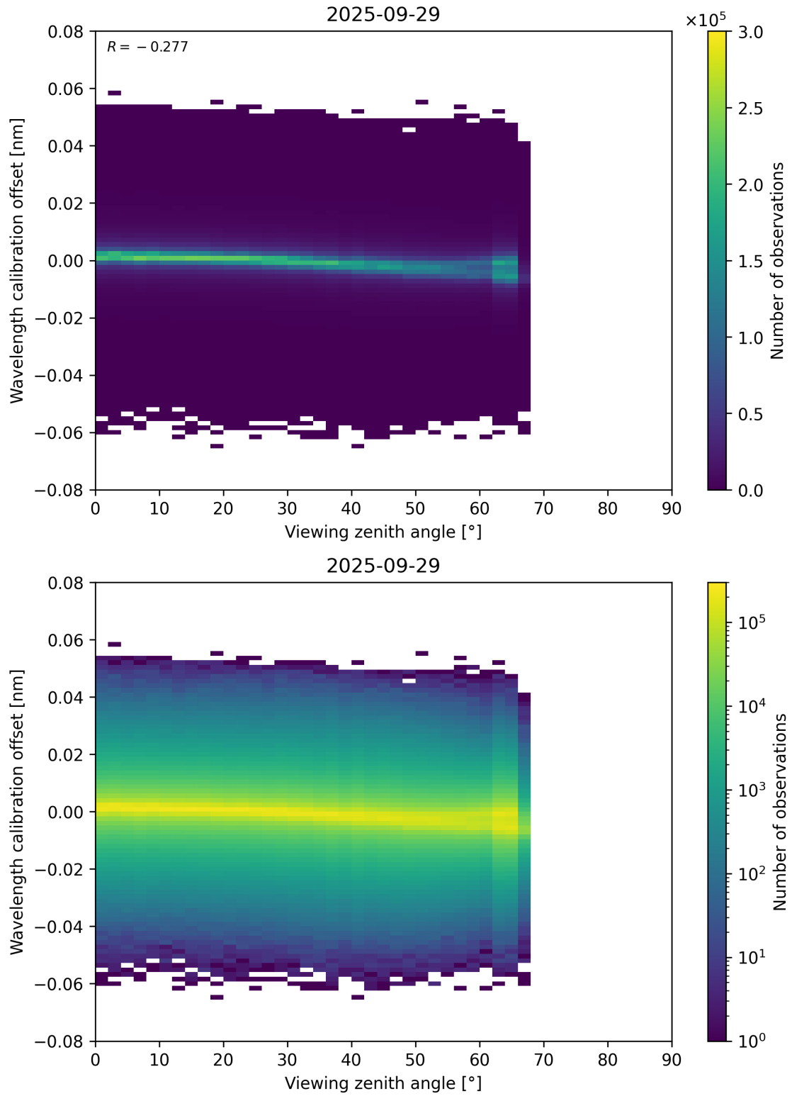
Figure 173: Scatter density plot of “Viewing zenith angle” against “Wavelength calibration offset” for 2025-09-28 to 2025-09-30.
