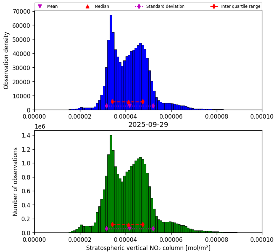
Figure 36: Histogram of “Stratospheric vertical NO 2 column” for 2025-09-28 to 2025-09-30
