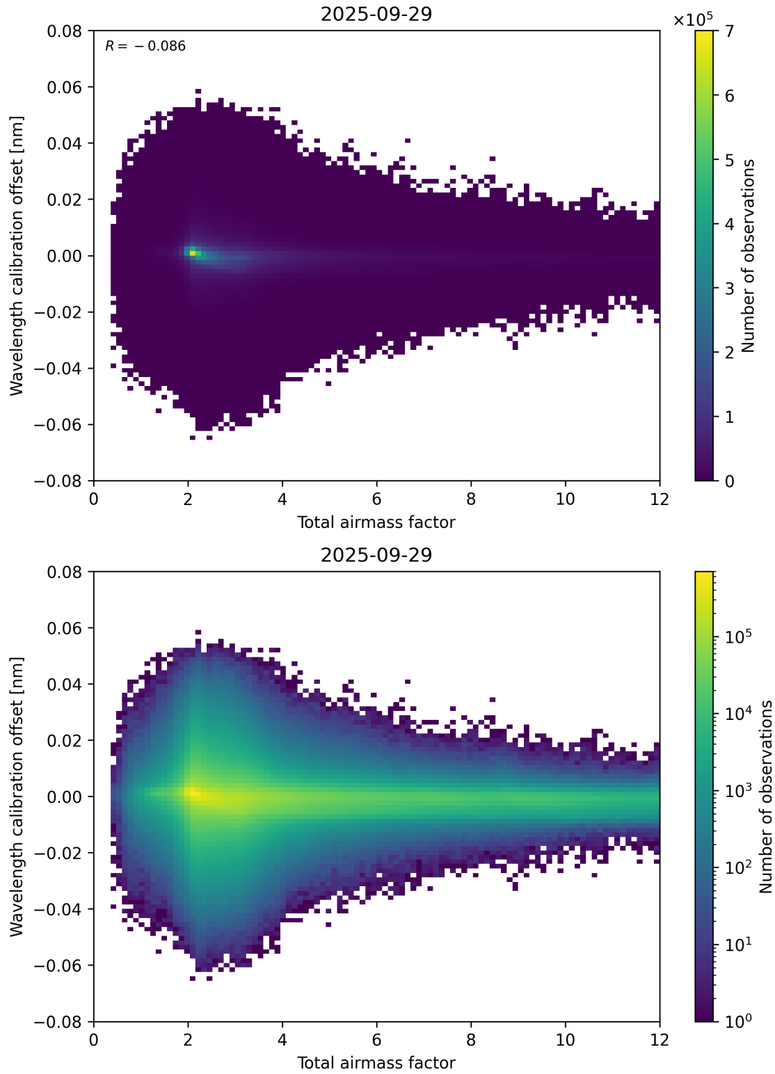
Figure 70: Scatter density plot of “Total airmass factor” against “Wavelength calibration offset” for 2025-09-28 to 2025-09-30.
