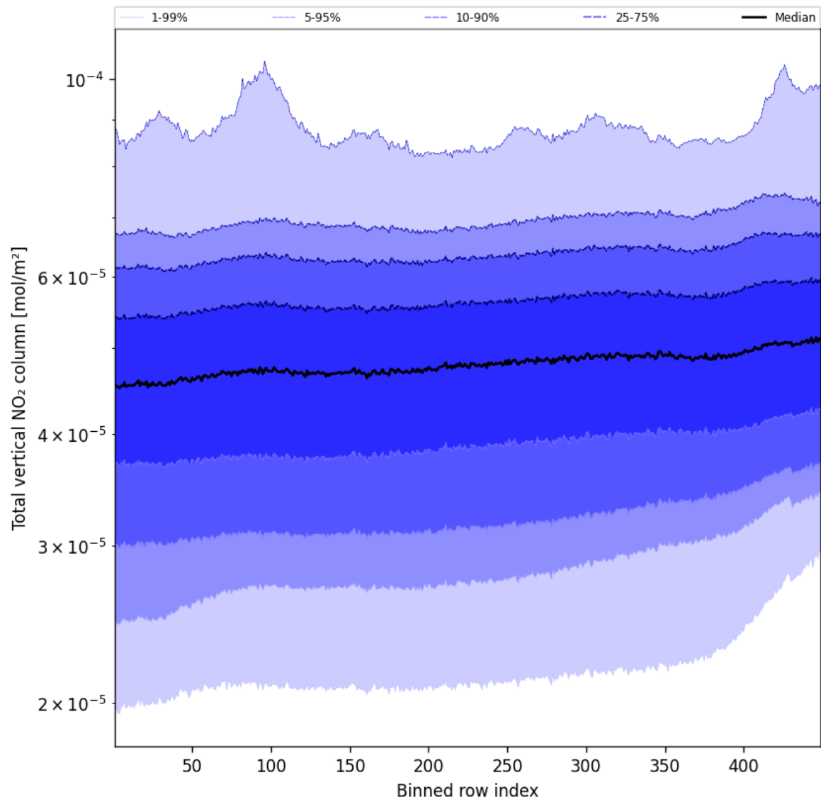
Figure 55: Along track statistics of “Total vertical NO 2 column” for 2025-09-28 to 2025-09-30
