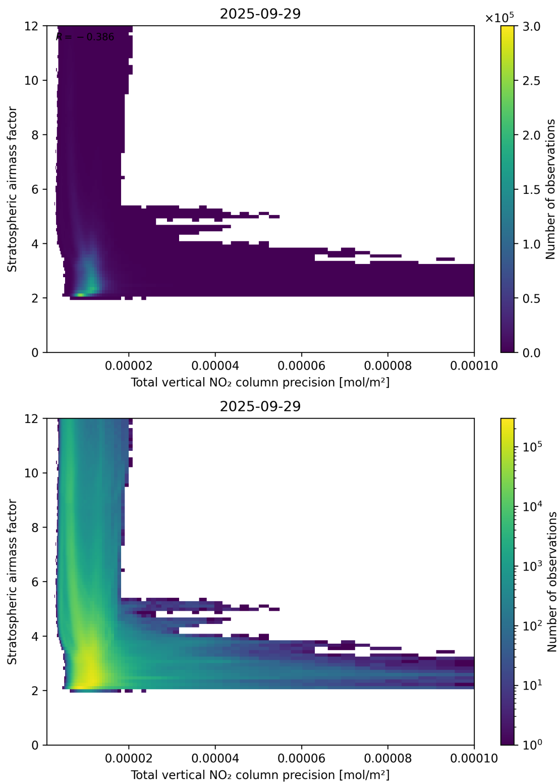
Figure 115: Scatter density plot of “Total vertical NO 2 column precision” against “Stratospheric air mass factor” for 2025-09-28 to 2025-09-30.
