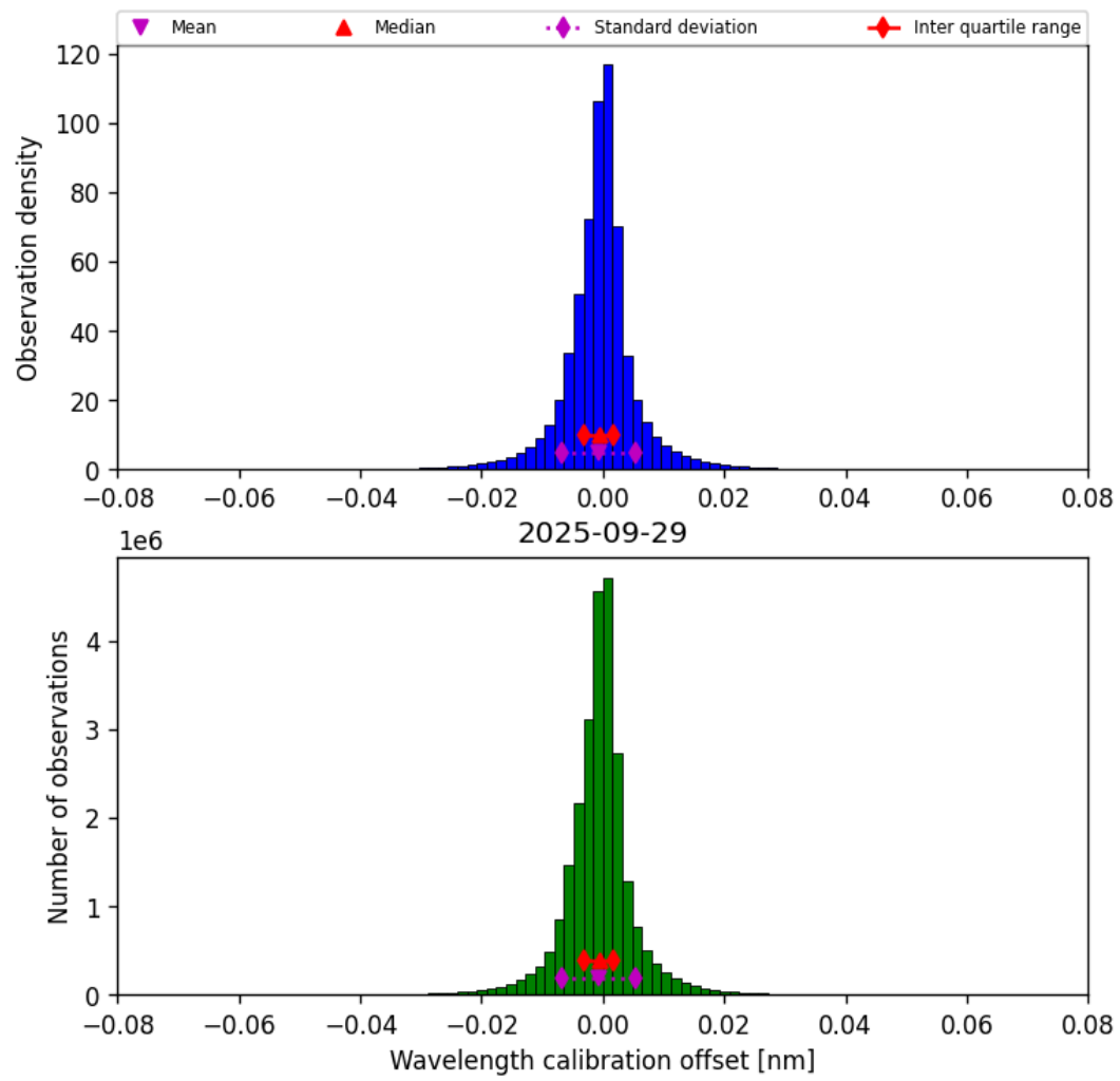
Figure 35: Histogram of “Wavelength calibration offset” for 2025-09-28 to 2025-09-30
