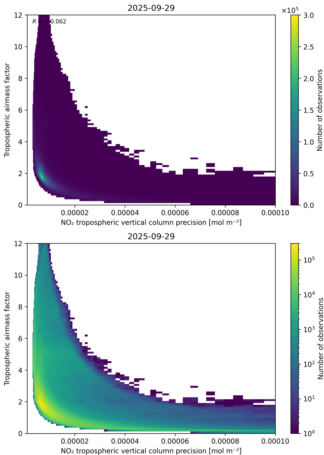
Figure 133: Scatter density plot of “NO 2 tropospheric vertical column precision” against “Tropospheric airmass factor” for 2025-09-28 to 2025-09-30.
