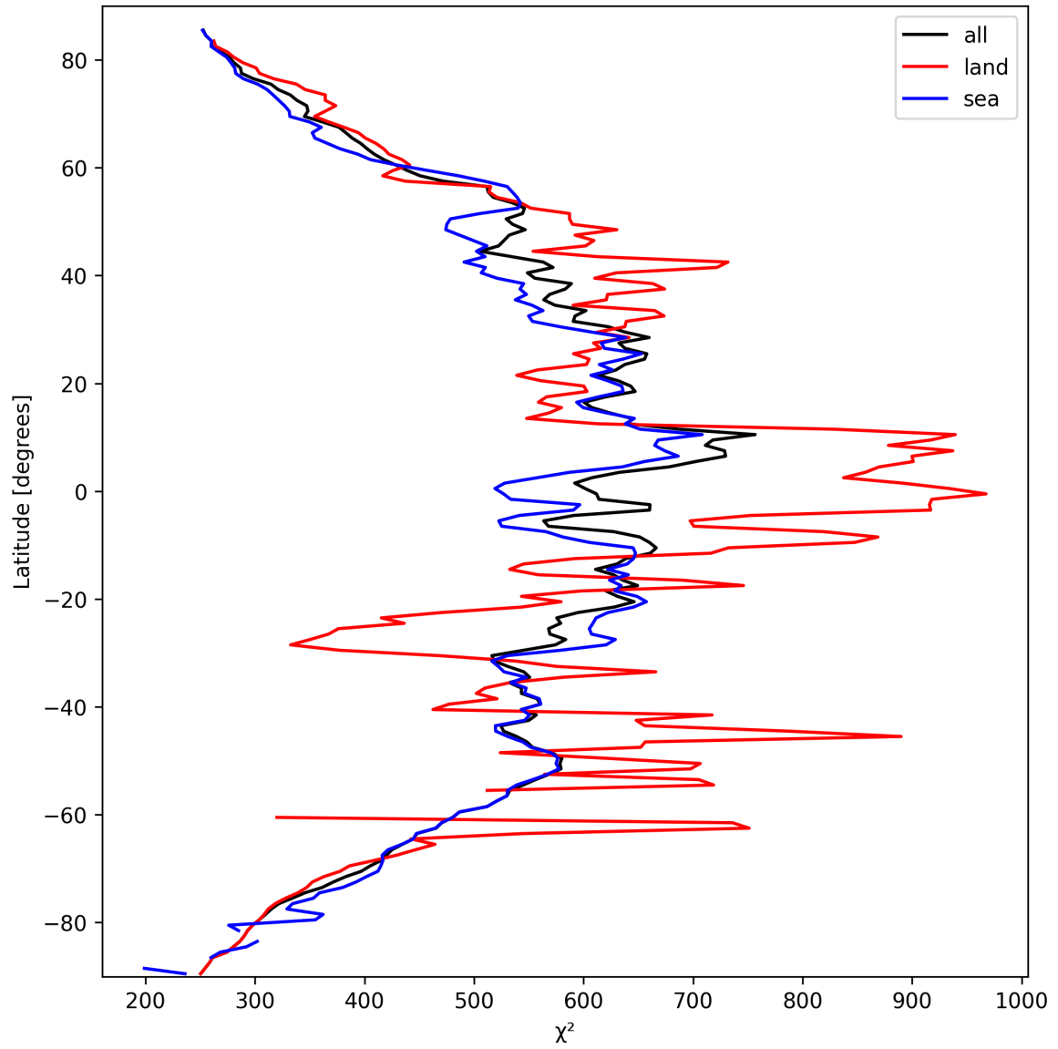
Figure 25: Zonal average of “ \chi^2 ” for 2025-09-28 to 2025-09-30.
