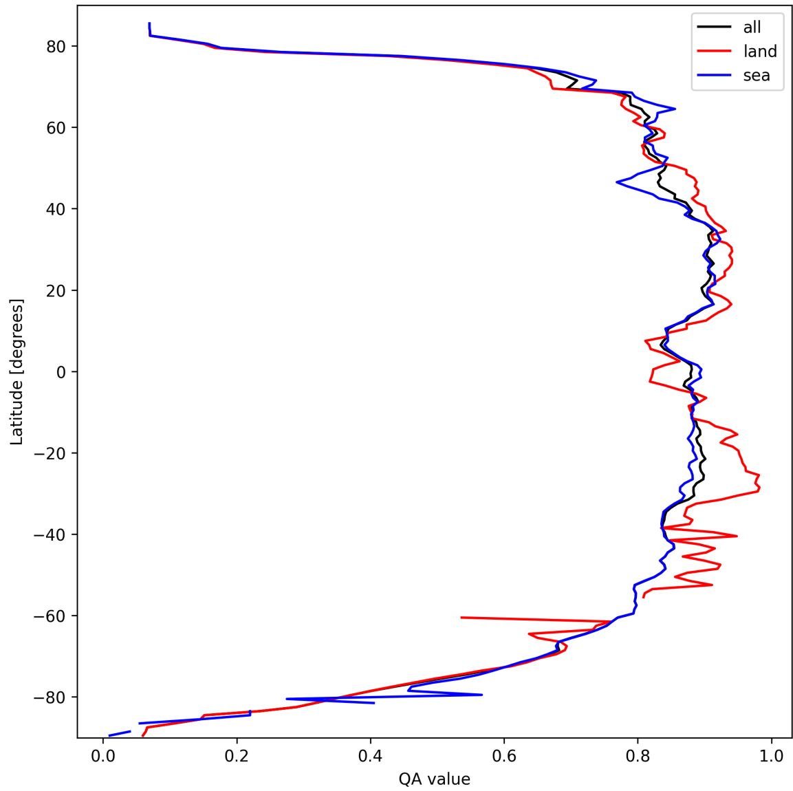
Figure 11: Zonal average of “QA value” for 2025-09-28 to 2025-09-30.
