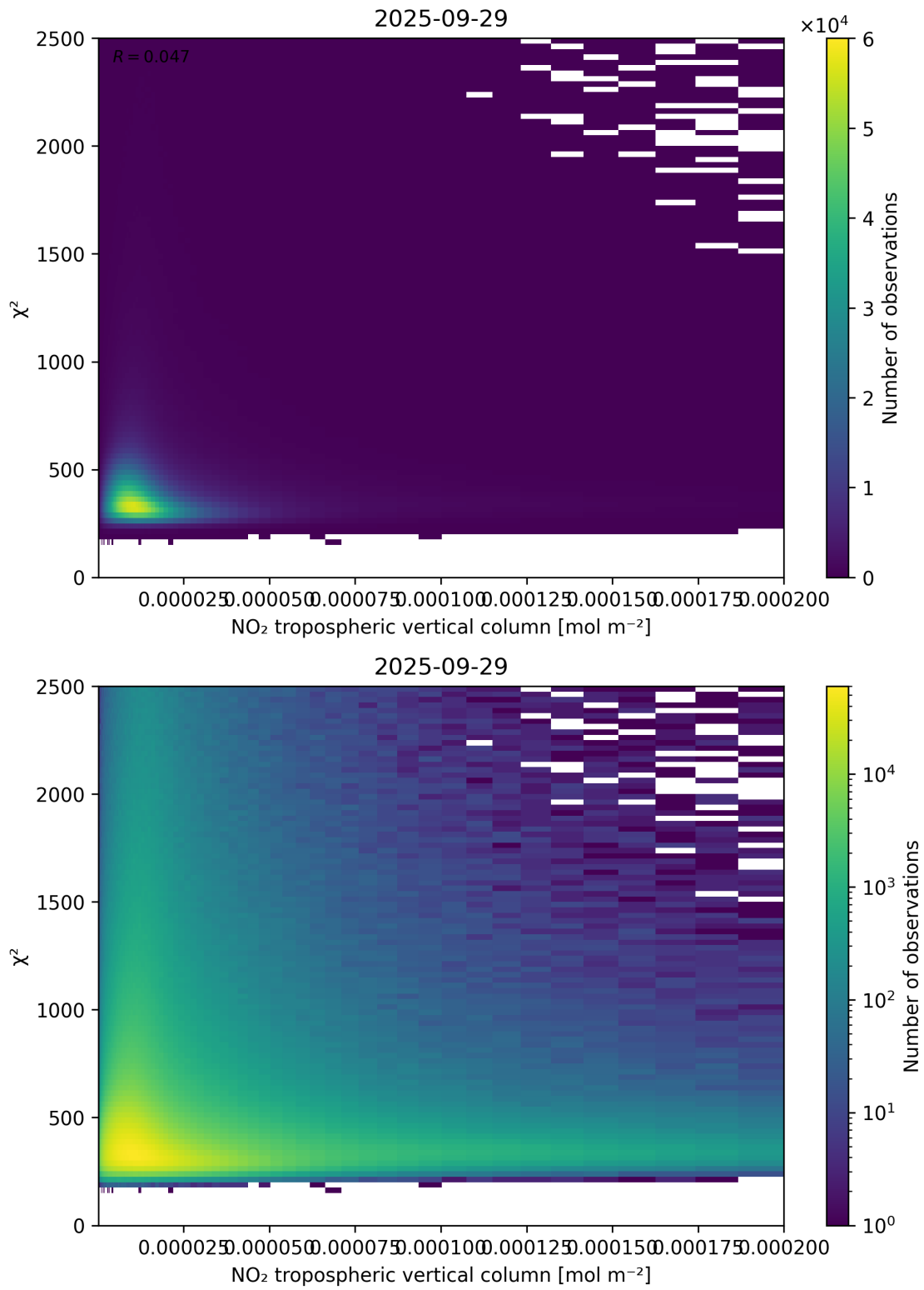
Figure 124: Scatter density plot of “NO 2 tropospheric vertical column” against “ \chi^2 ” for 2025-09-28 to 2025-09-30.
