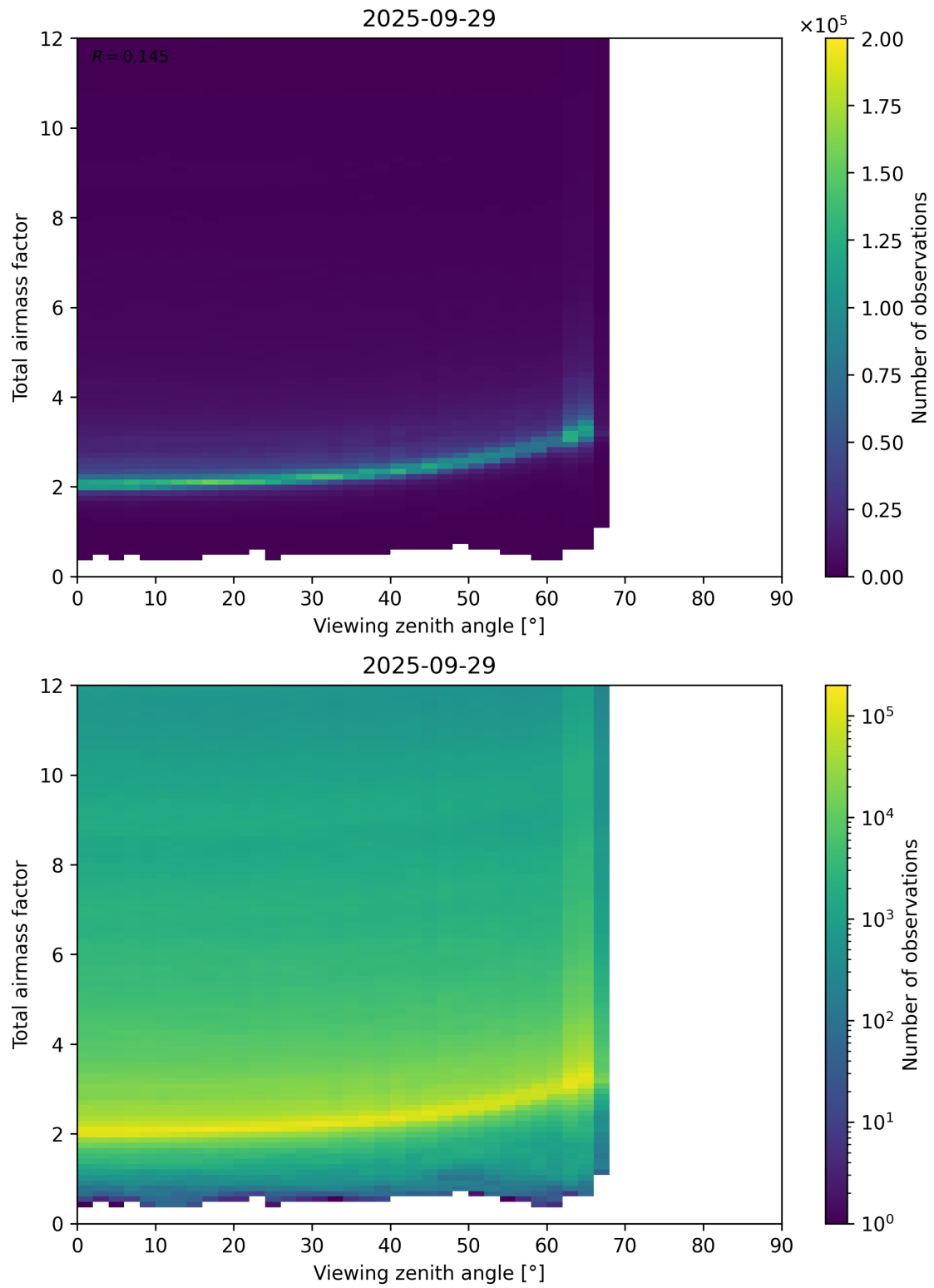
Figure 160: Scatter density plot of “Viewing zenith angle” against “Total airmass factor” for 2025-09-28 to 2025-09-30.
