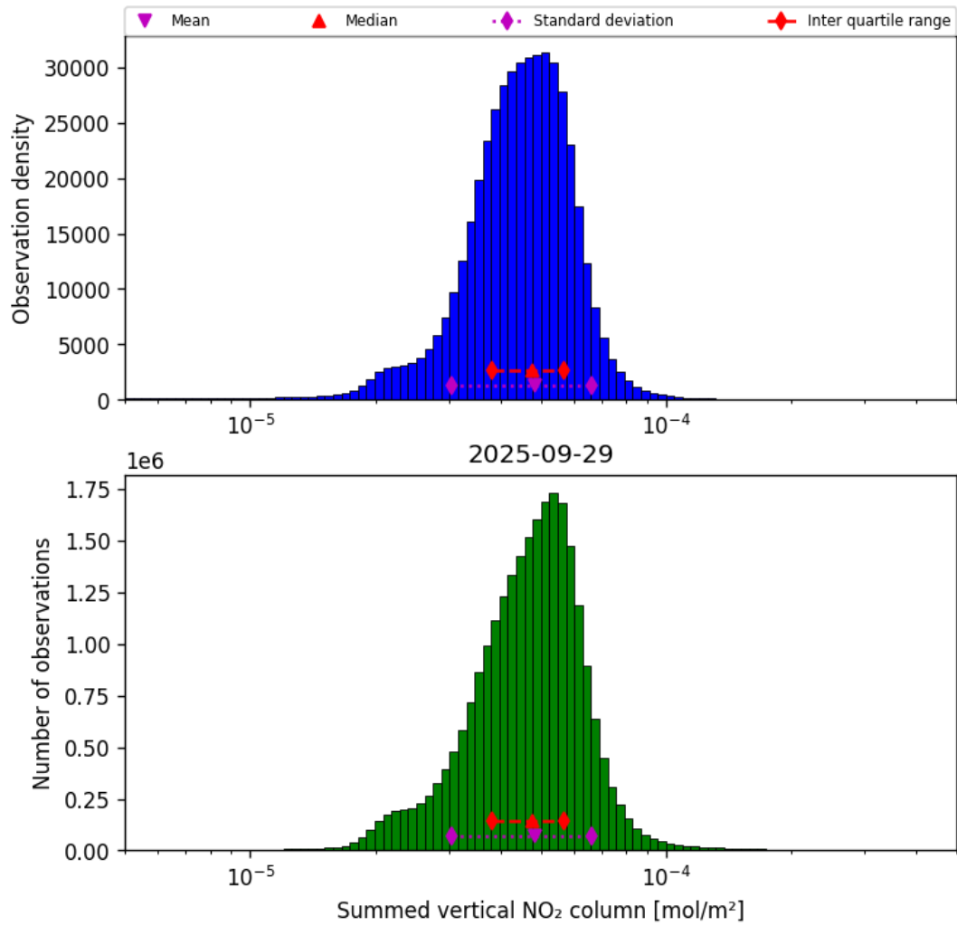
Figure 40: Histogram of “Summed vertical NO 2 column” for 2025-09-28 to 2025-09-30
