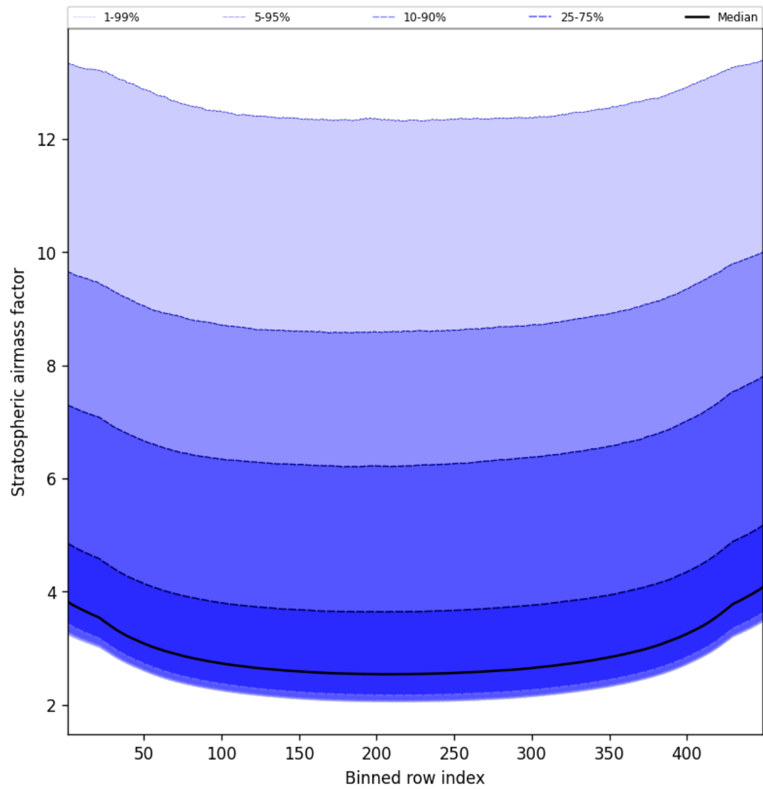
Figure 61: Along track statistics of “Stratospheric airmass factor” for 2025-09-28 to 2025-09-30
