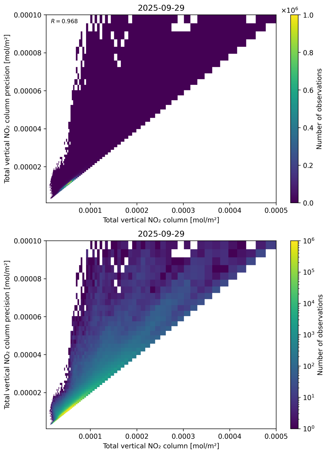
Figure 114: Scatter density plot of “Total vertical NO 2 column” against “Total vertical NO 2 column precision” for 2025-09-28 to 2025-09-30.
