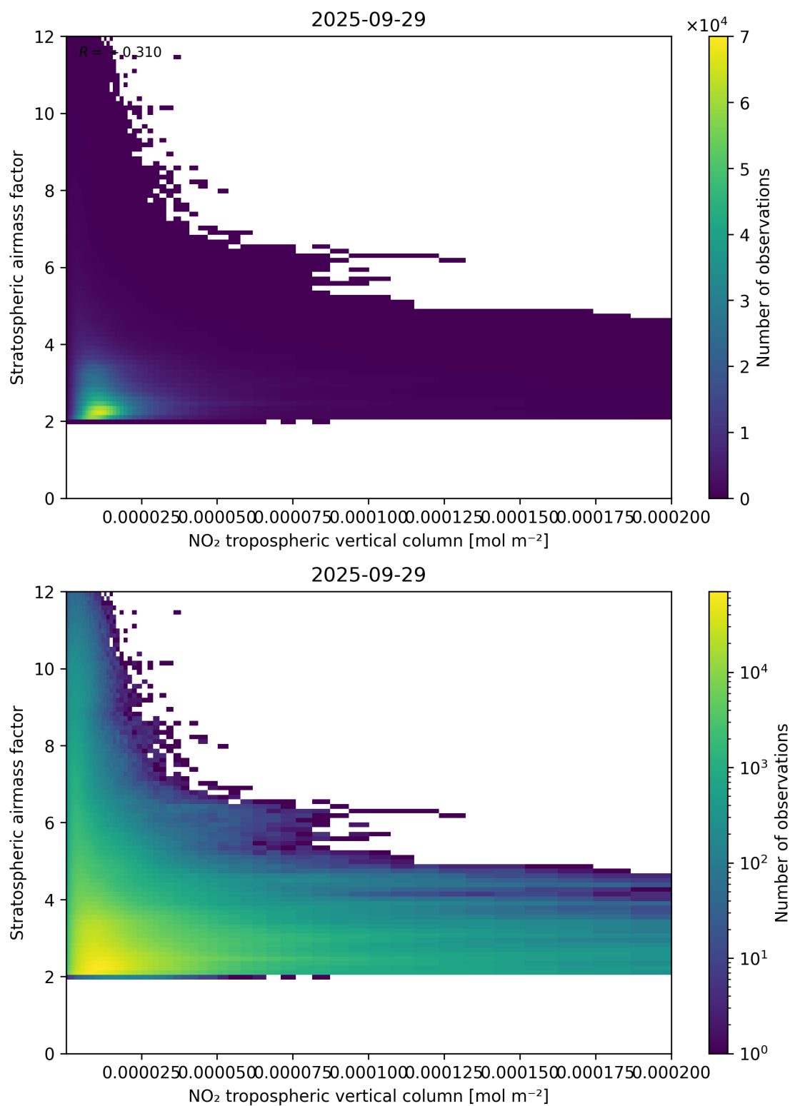
Figure 121: Scatter density plot of “NO 2 tropospheric vertical column” against “Stratospheric air mass factor” for 2025-09-28 to 2025-09-30.
