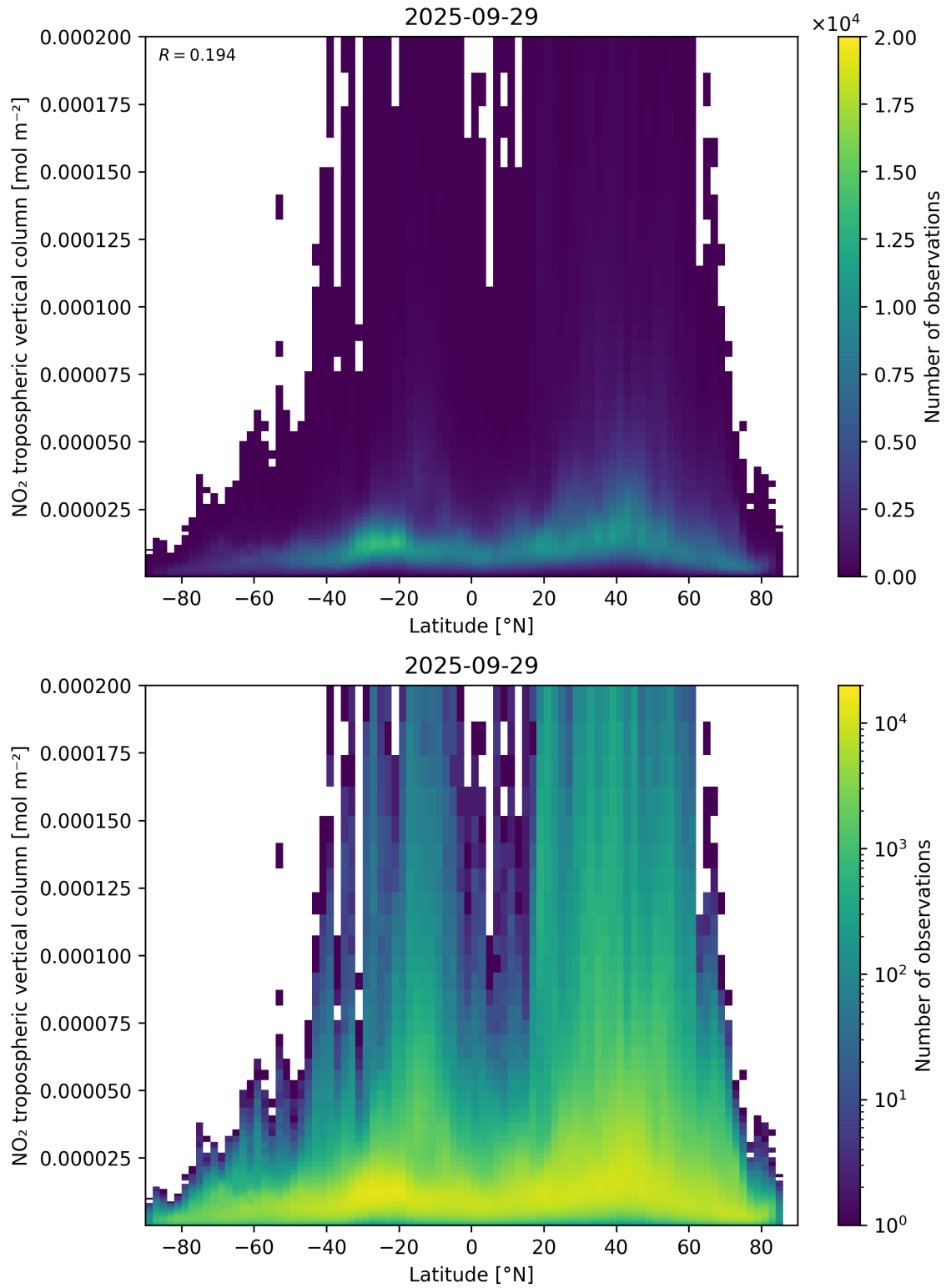
Figure 92: Scatter density plot of “Latitude” against “NO 2 tropospheric vertical column” for 2025-09-28 to 2025-09-30.
