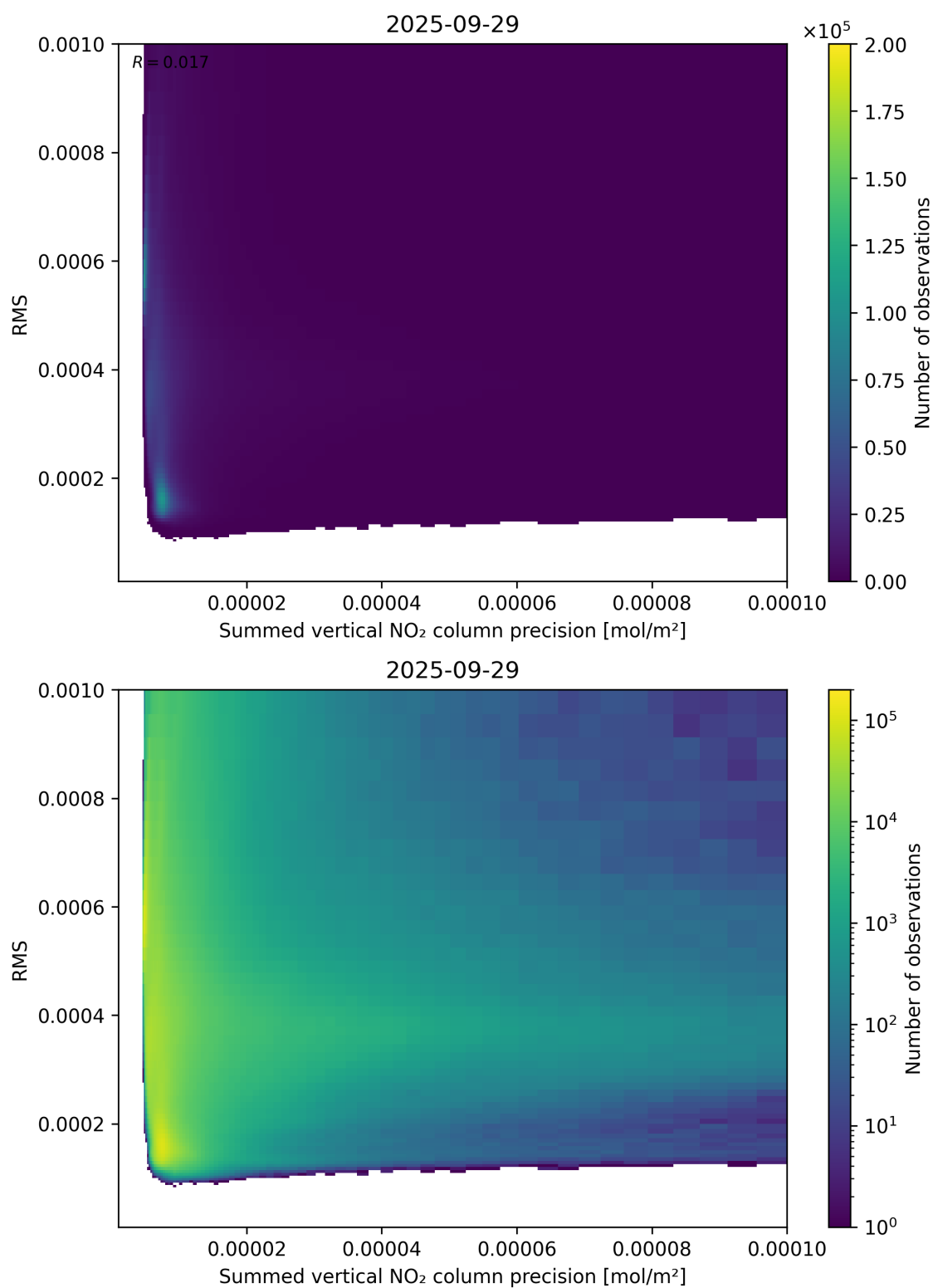
Figure 108: Scatter density plot of “Summed vertical NO 2 column precision” against “RMS” for 2025-09-28 to 2025-09-30.
