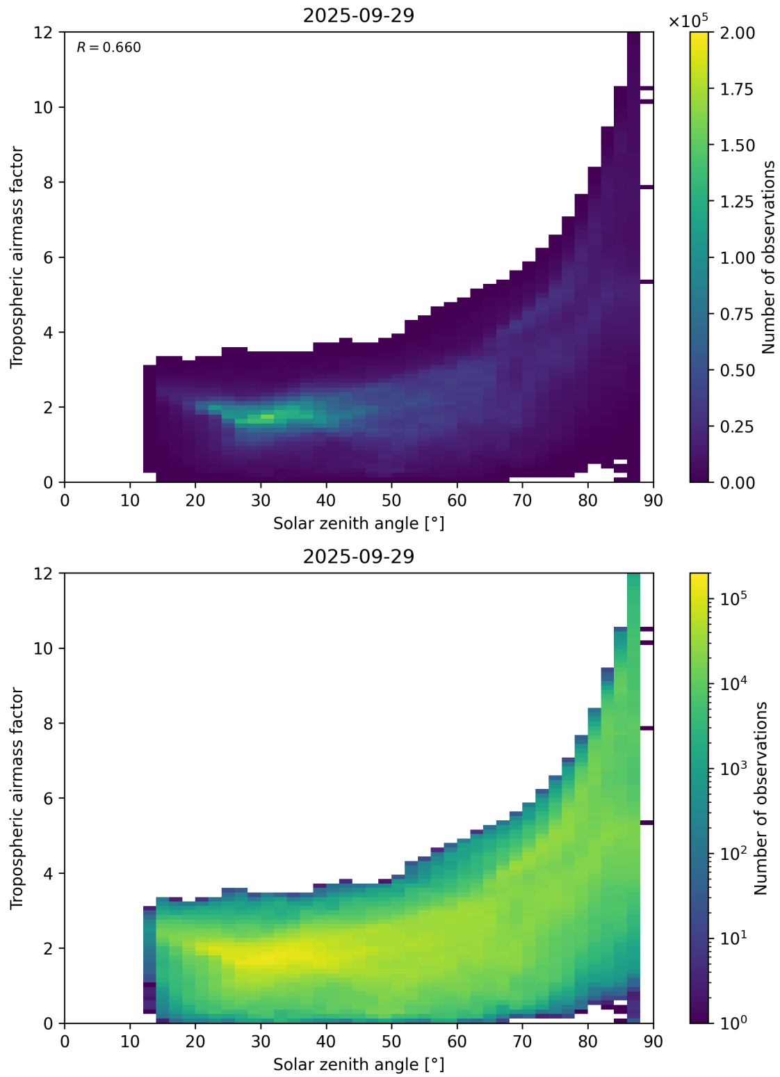
Figure 147: Scatter density plot of “Solar zenith angle” against “Tropospheric airmass factor” for 2025-09-28 to 2025-09-30.
