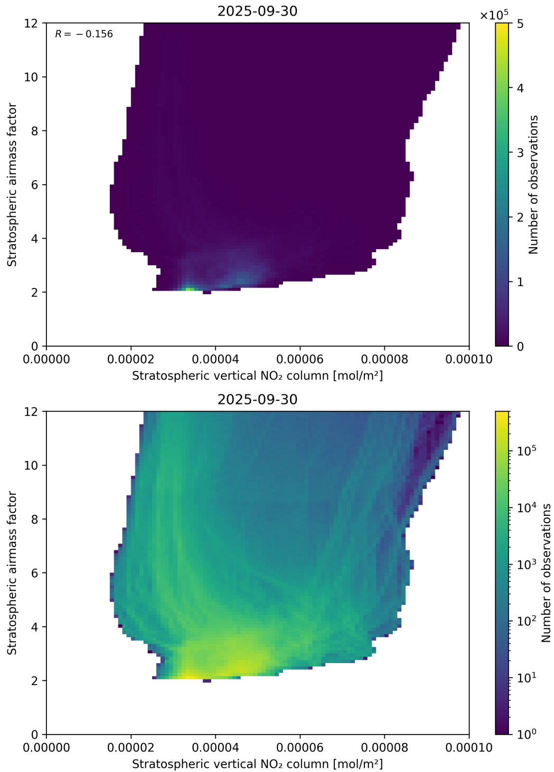
Figure 96: Scatter density plot of “Stratospheric vertical NO 2 column” against “Stratospheric airmass factor” for 2025-09-29 to 2025-10-01.
