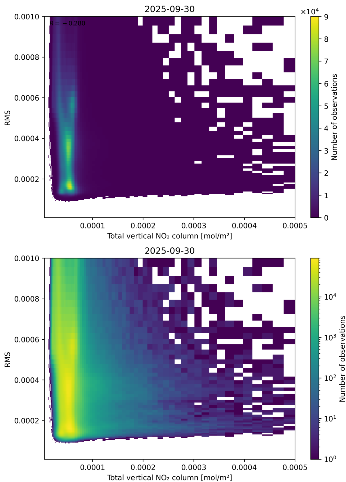
Figure 120: Scatter density plot of “Total vertical NO 2 column” against “RMS” for 2025-09-29 to 2025-10-01.
