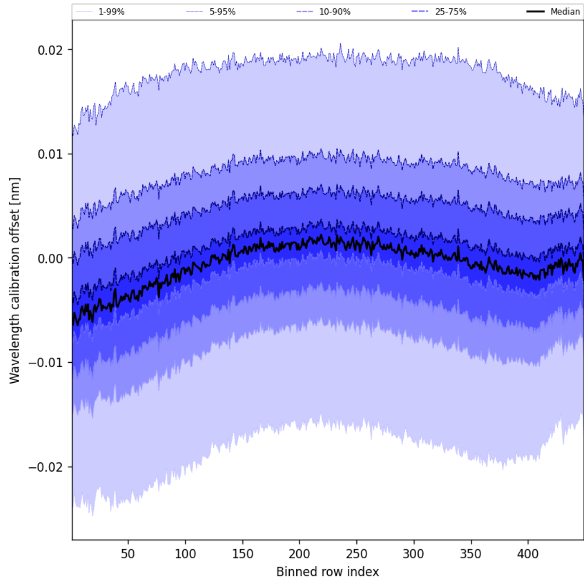
Figure 52: Along track statistics of “Wavelength calibration offset” for 2025-09-29 to 2025-10-01
