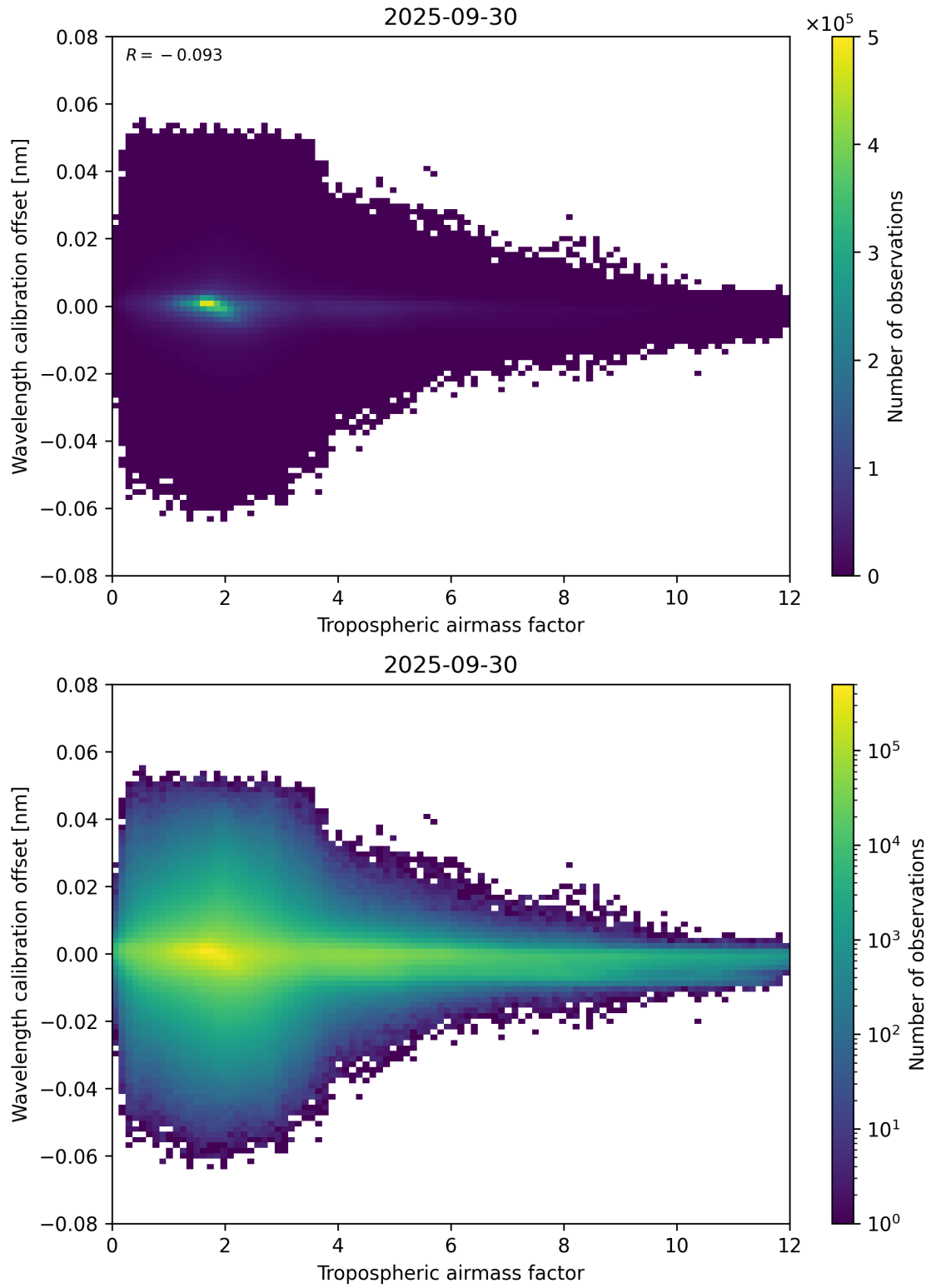
Figure 80: Scatter density plot of “Tropospheric airmass factor” against “Wavelength calibration offset” for 2025-09-29 to 2025-10-01.
