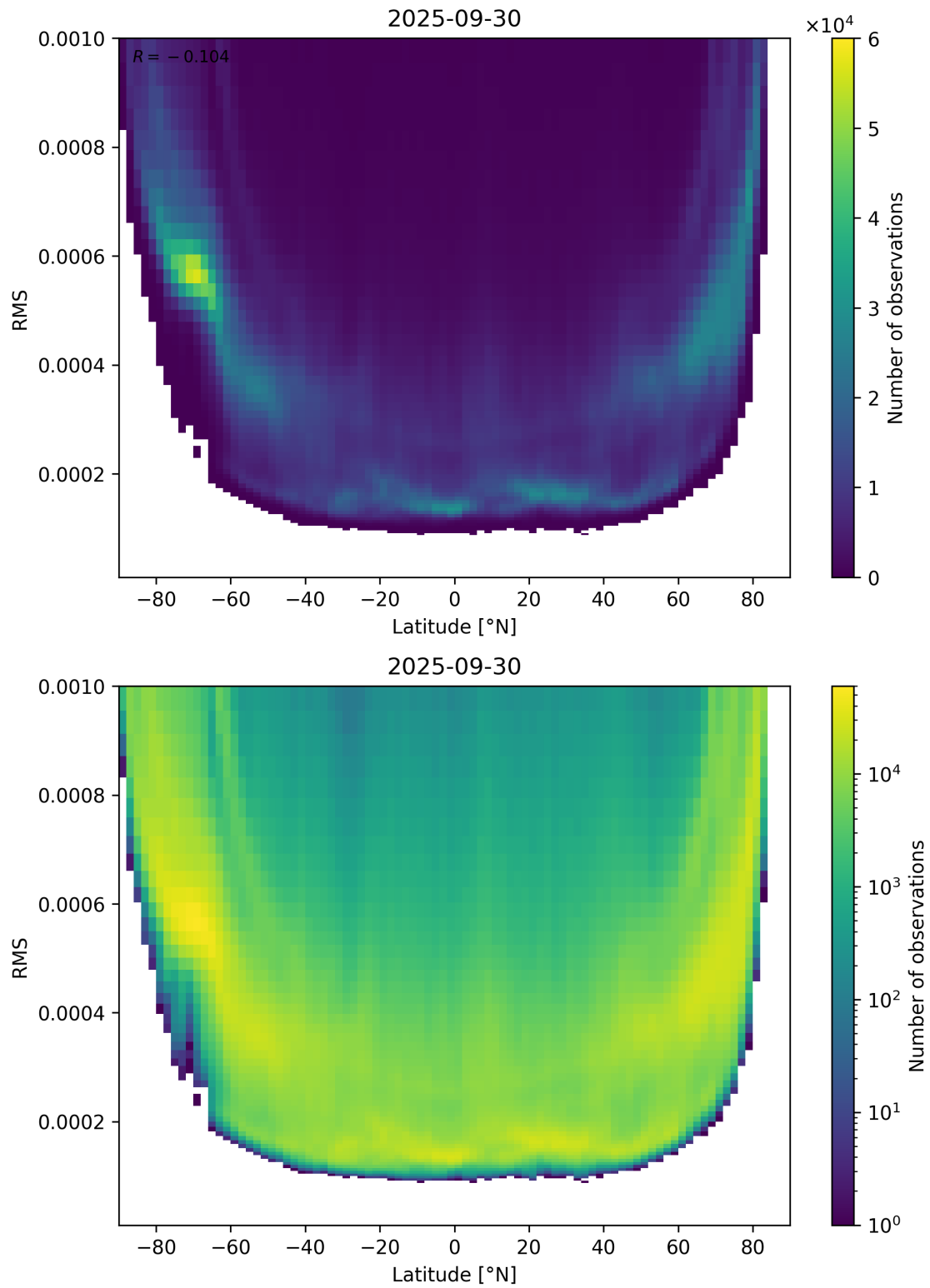
Figure 94: Scatter density plot of “Latitude” against “RMS” for 2025-09-29 to 2025-10-01.
