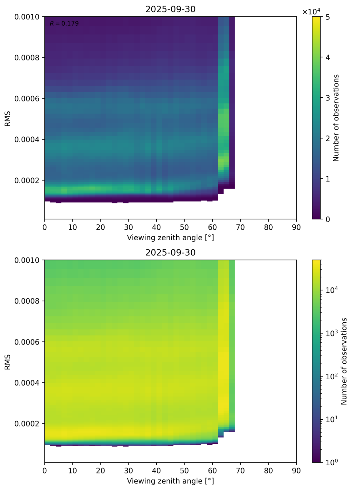
Figure 171: Scatter density plot of “Viewing zenith angle” against “RMS” for 2025-09-29 to 2025-10-01.
