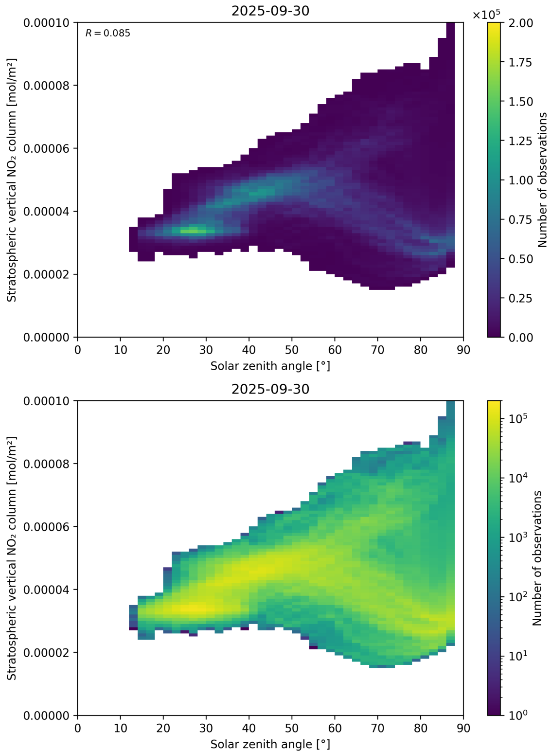
Figure 150: Scatter density plot of “Solar zenith angle” against “Stratospheric vertical NO 2 column” for 2025-09-29 to 2025-10-01.
