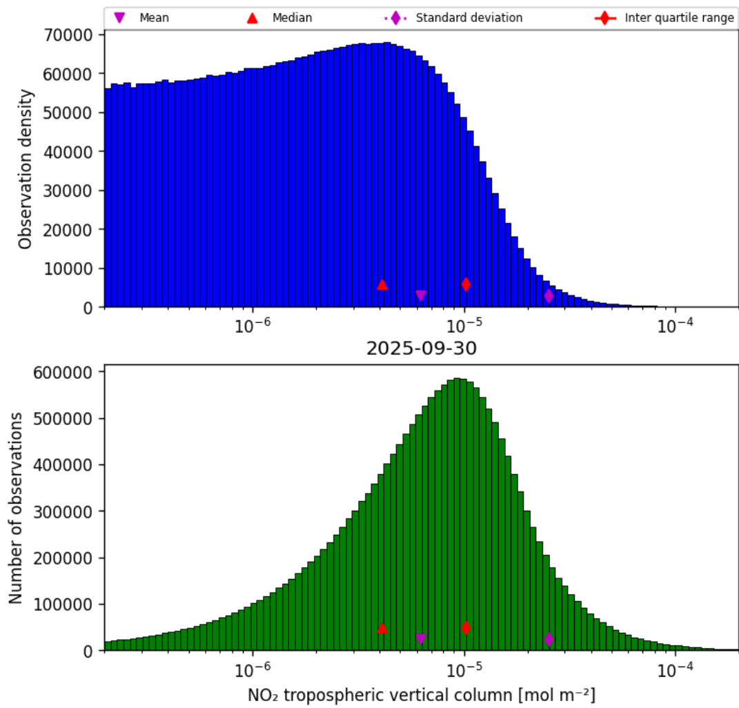
Figure 29: Histogram of “NO 2 tropospheric vertical column” for 2025-09-29 to 2025-10-01
