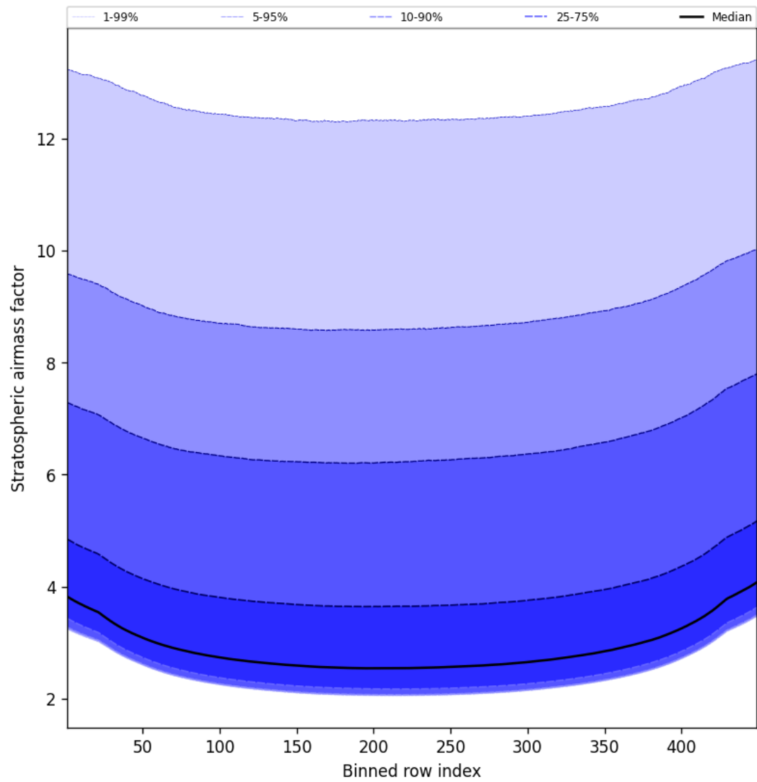
Figure 61: Along track statistics of “Stratospheric airmass factor” for 2025-09-29 to 2025-10-01
