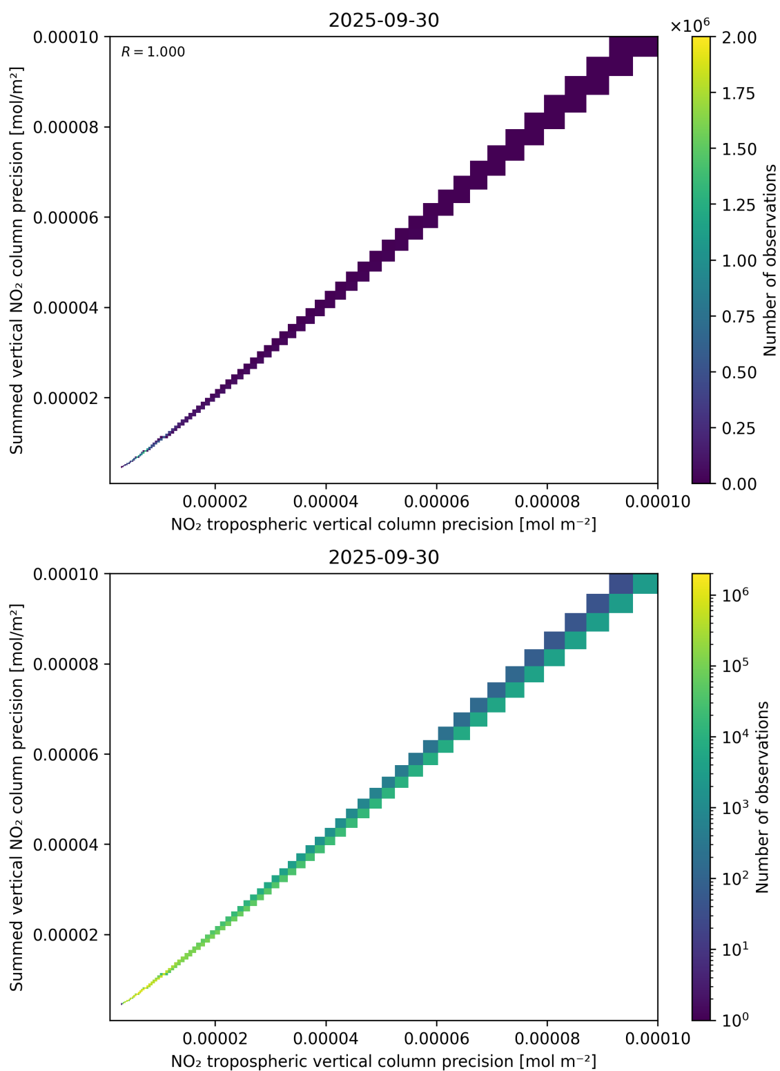
Figure 137: Scatter density plot of “NO 2 tropospheric vertical column precision” against “Summed vertical NO 2 column precision” for 2025-09-29 to 2025-10-01.
