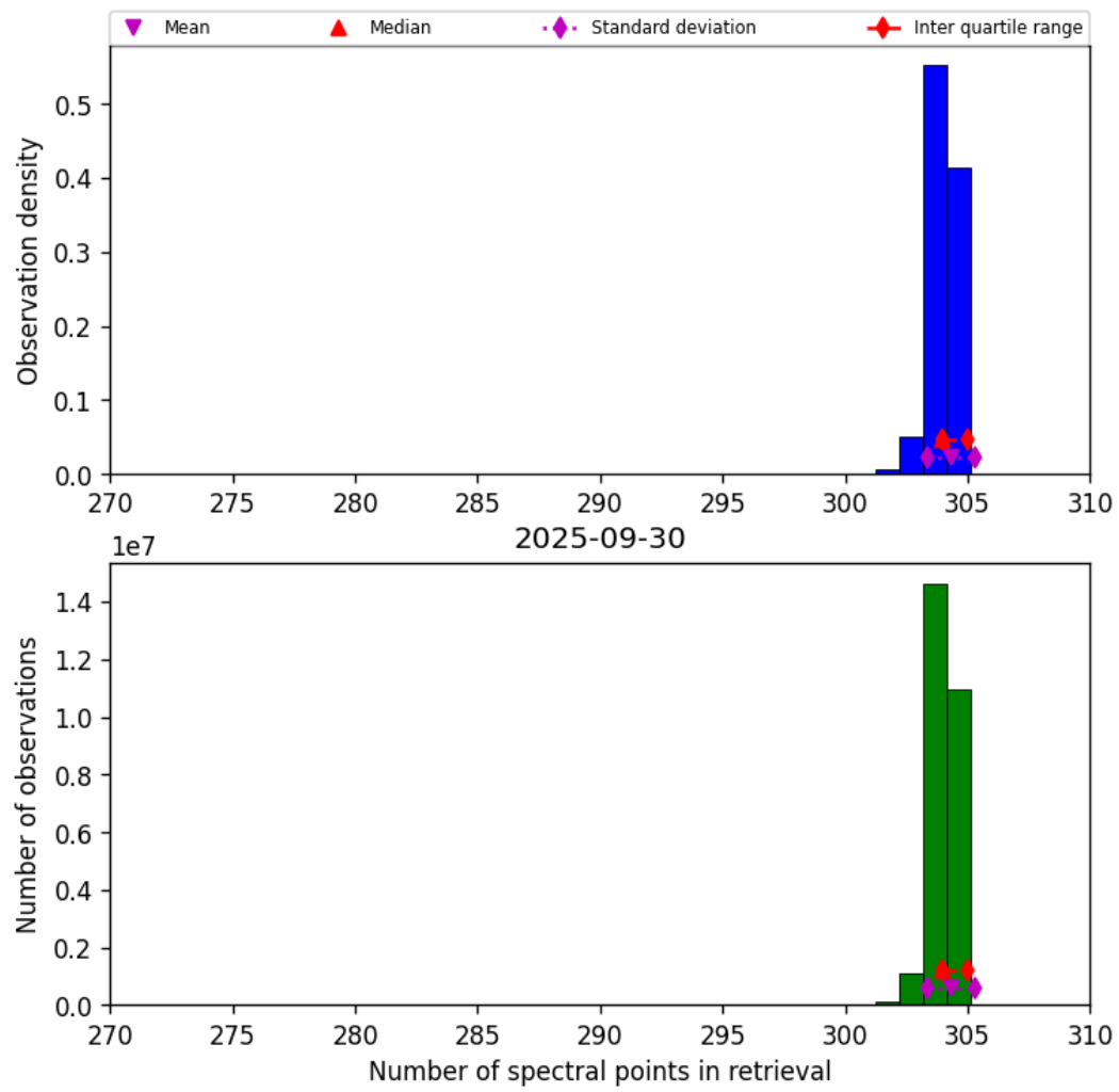
Figure 33: Histogram of “Number of spectral points in retrieval” for 2025-09-29 to 2025-10-01
