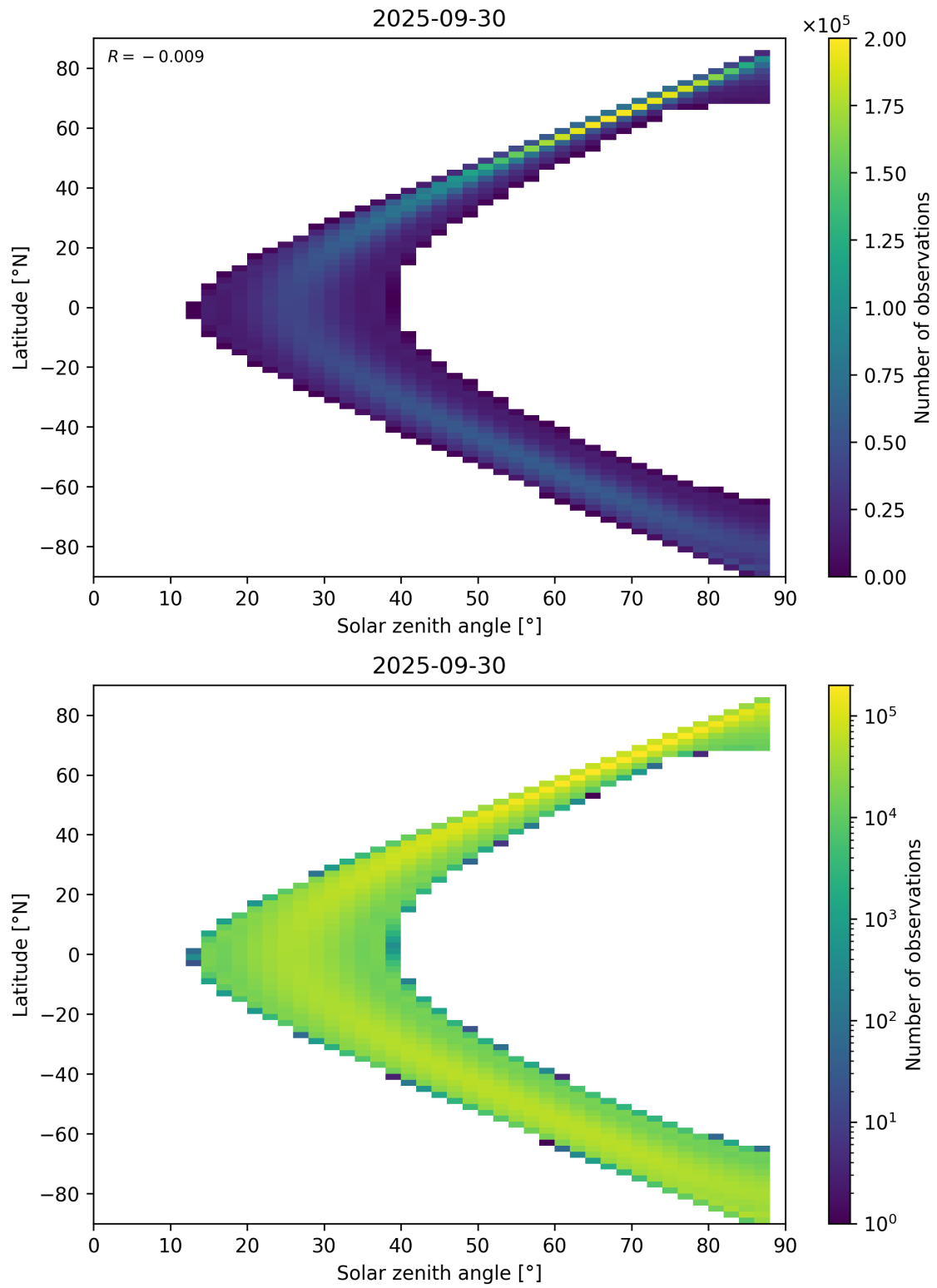
Figure 149: Scatter density plot of “Solar zenith angle” against “Latitude” for 2025-09-29 to 2025-10-01.
