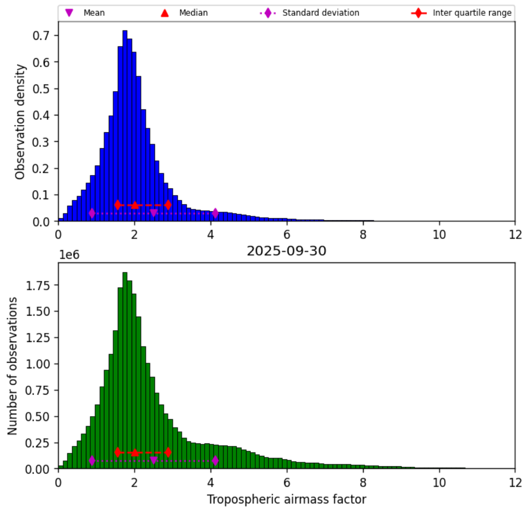
Figure 31: Histogram of “Tropospheric airmass factor” for 2025-09-29 to 2025-10-01
