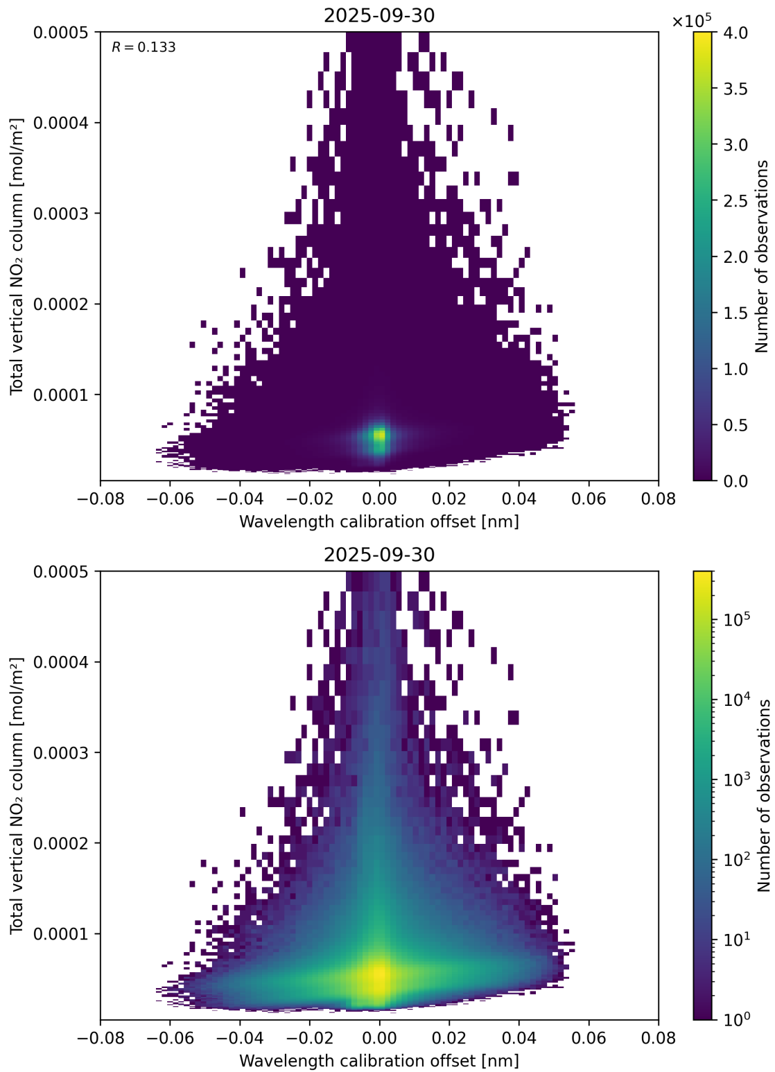
Figure 179: Scatter density plot of “Wavelength calibration offset” against “Total vertical NO 2 column” for 2025-09-29 to 2025-10-01.
