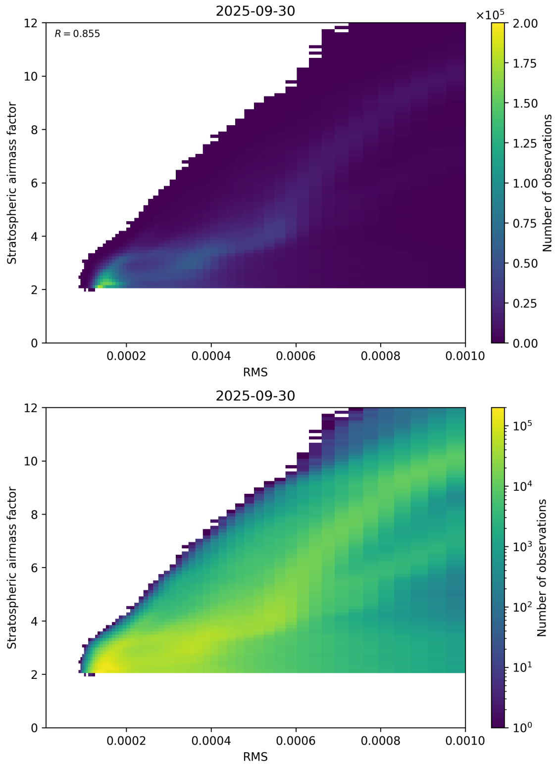
Figure 144: Scatter density plot of “RMS” against “Stratospheric airmass factor” for 2025-09-29 to 2025-10-01.
