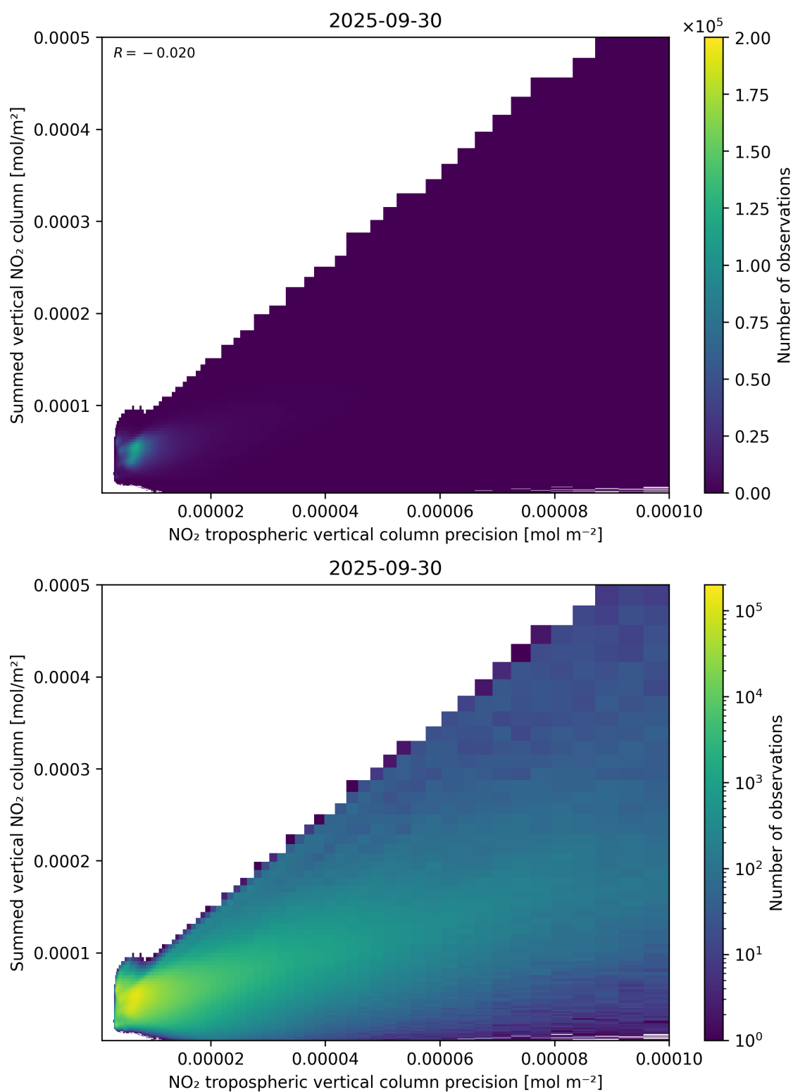
Figure 136: Scatter density plot of “NO 2 tropospheric vertical column precision” against “Summed vertical NO 2 column” for 2025-09-29 to 2025-10-01.
