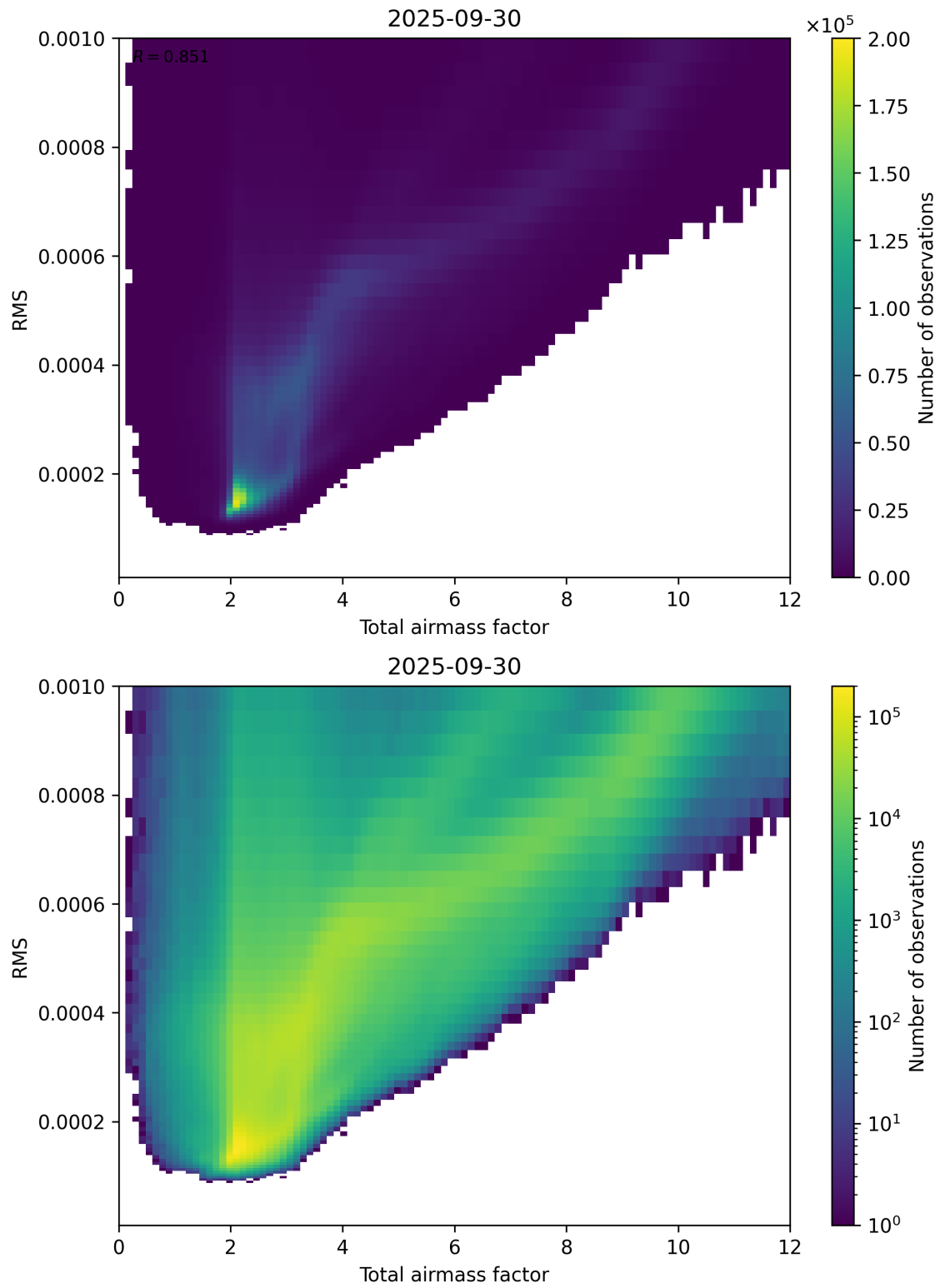
Figure 69: Scatter density plot of “Total airmass factor” against “RMS” for 2025-09-29 to 2025-10-01.
