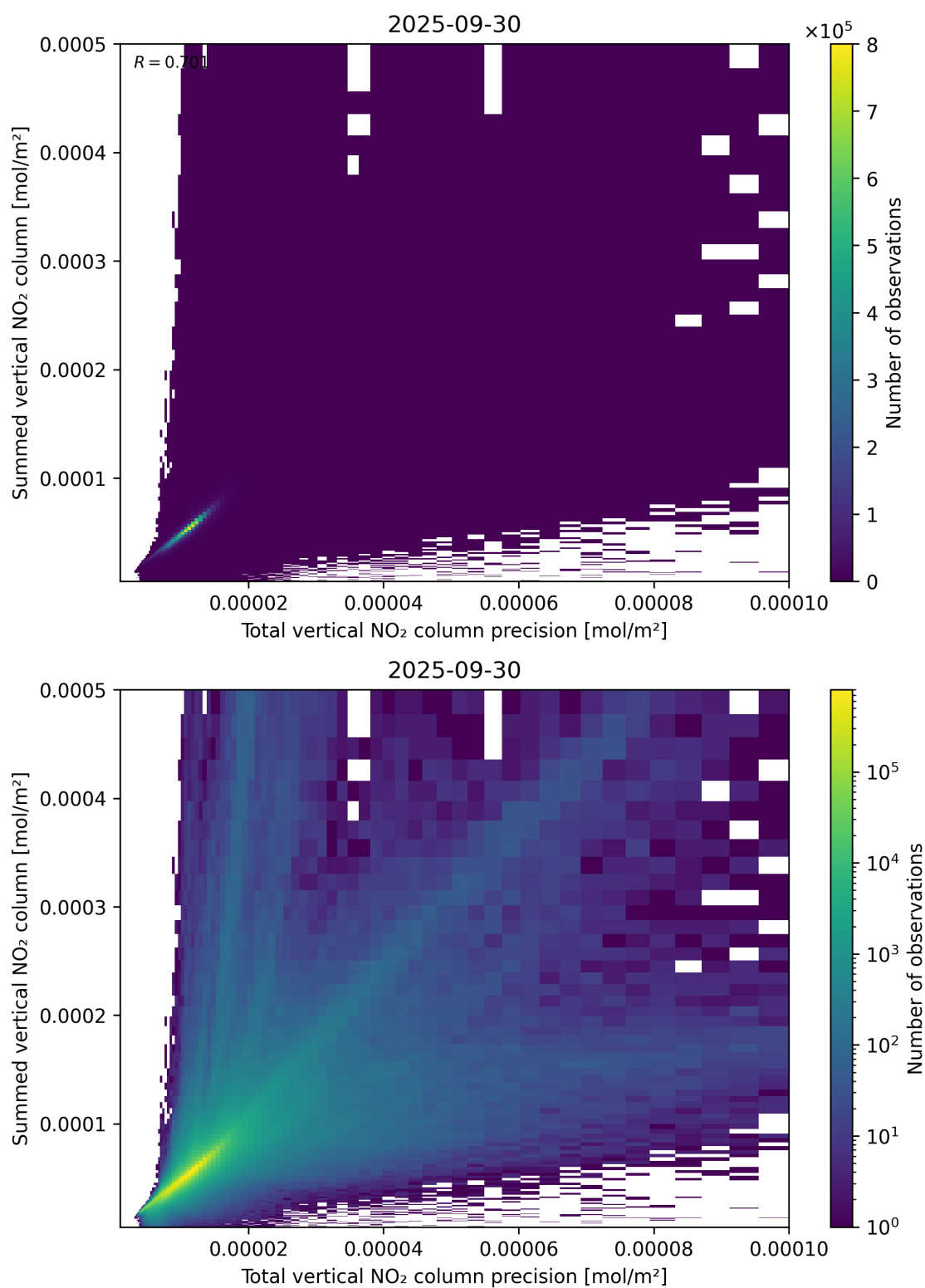
Figure 117: Scatter density plot of “Total vertical NO 2 column precision” against “Summed vertical NO 2 column” for 2025-09-29 to 2025-10-01.
