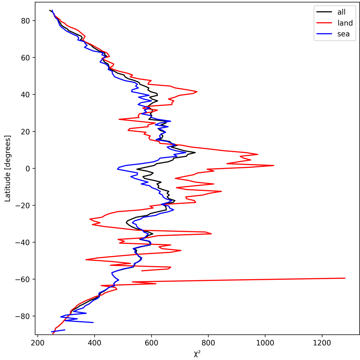
Figure 25: Zonal average of “ \chi^2 ” for 2025-09-29 to 2025-10-01.
