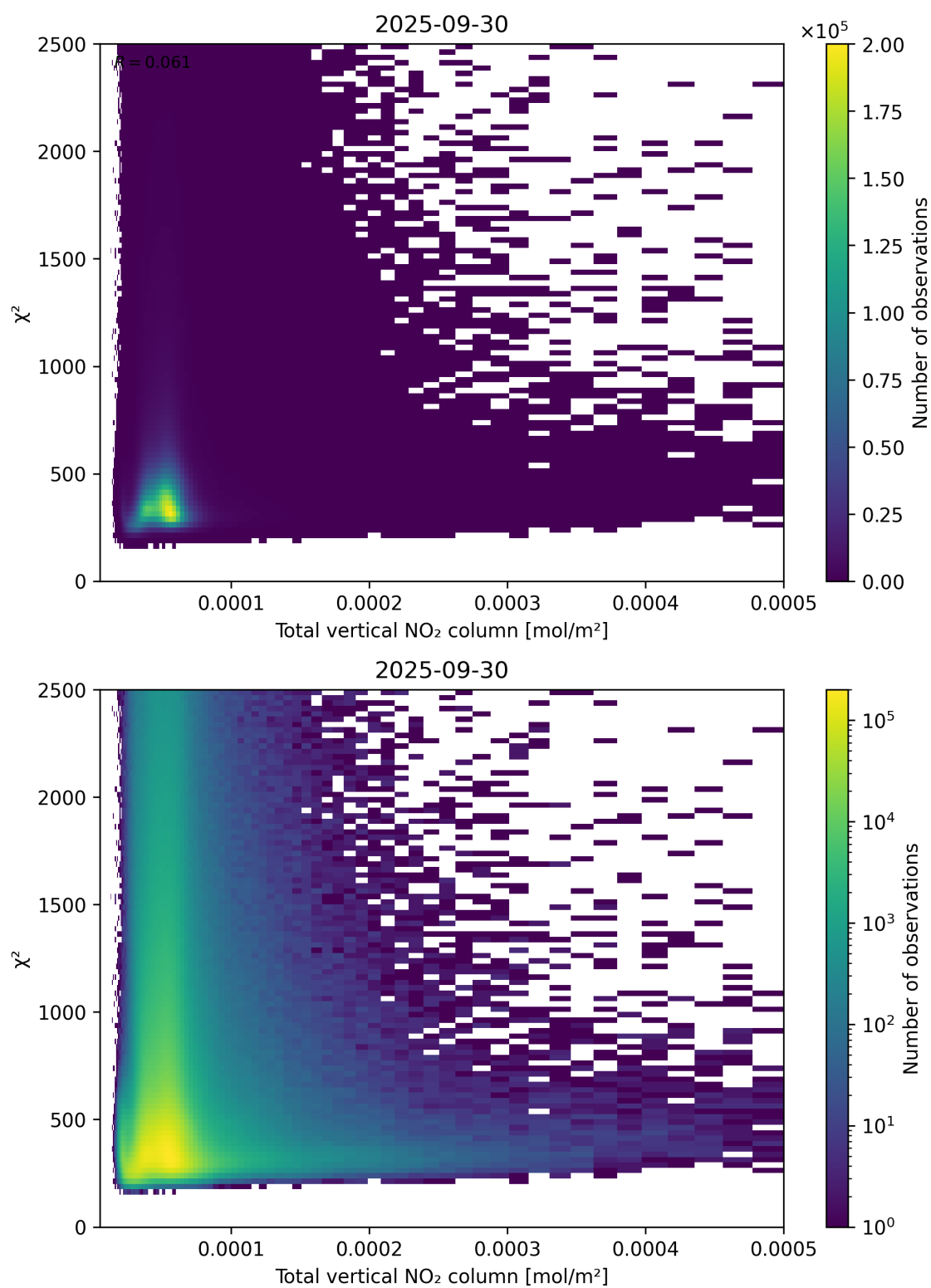
Figure 111: Scatter density plot of “Total vertical NO 2 column” against “ \chi^2 ” for 2025-09-29 to 2025-10-01.
