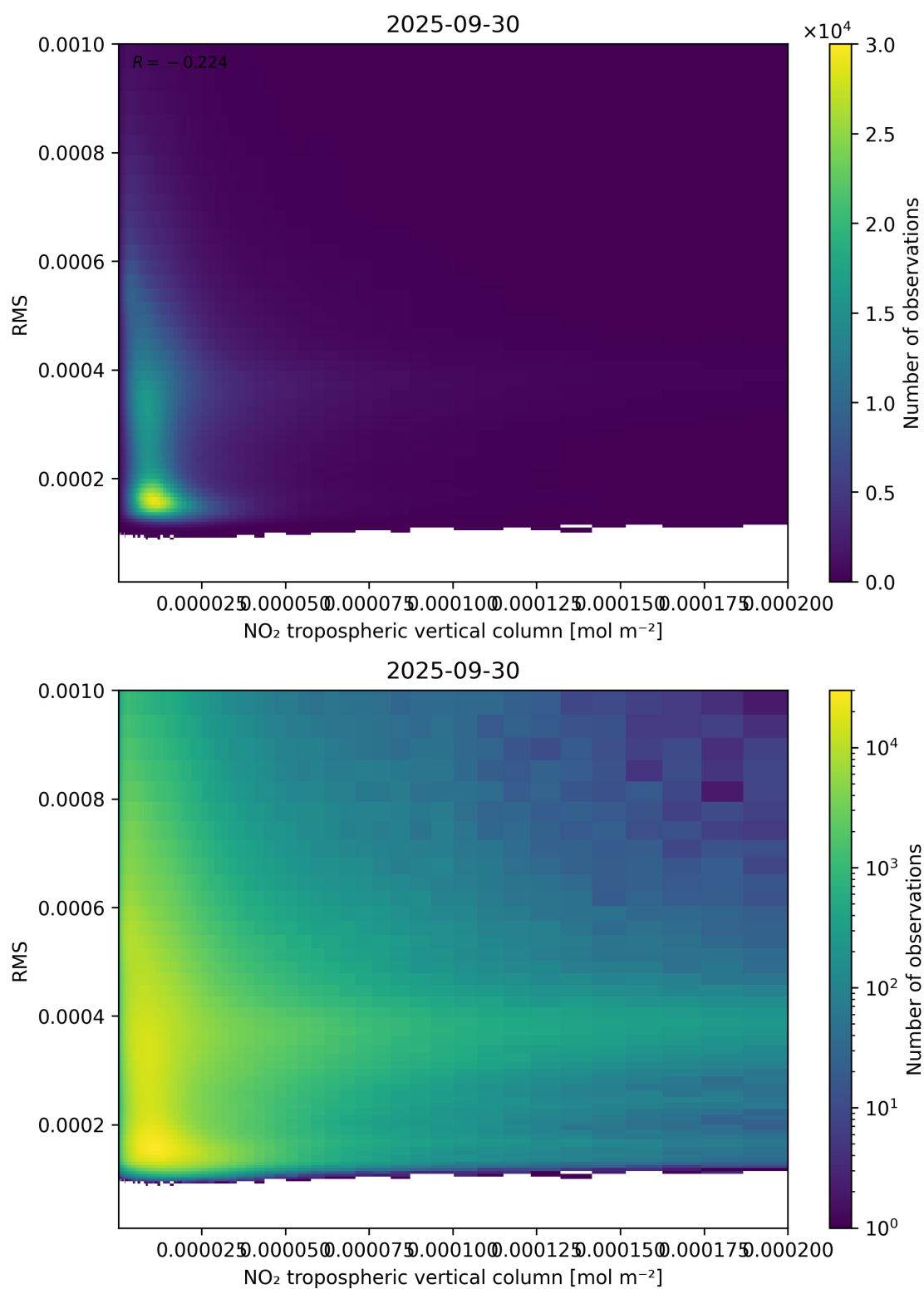
Figure 142: Scatter density plot of “NO 2 tropospheric vertical column” against “RMS” for 2025-09-29 to 2025-10-01.
