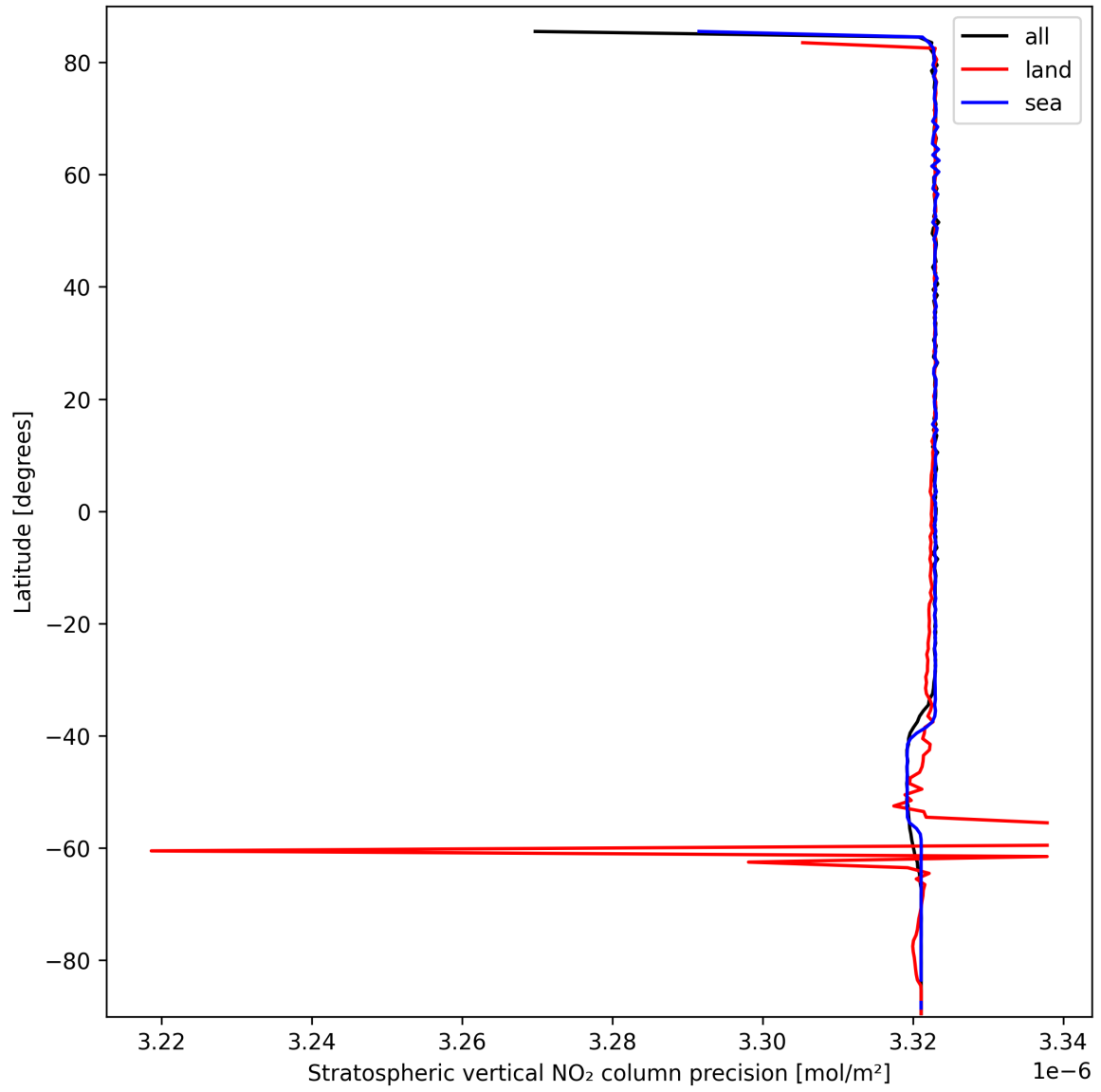
Figure 20: Zonal average of “Stratospheric vertical NO 2 column precision” for 2025-09-29 to 2025-10-01.
