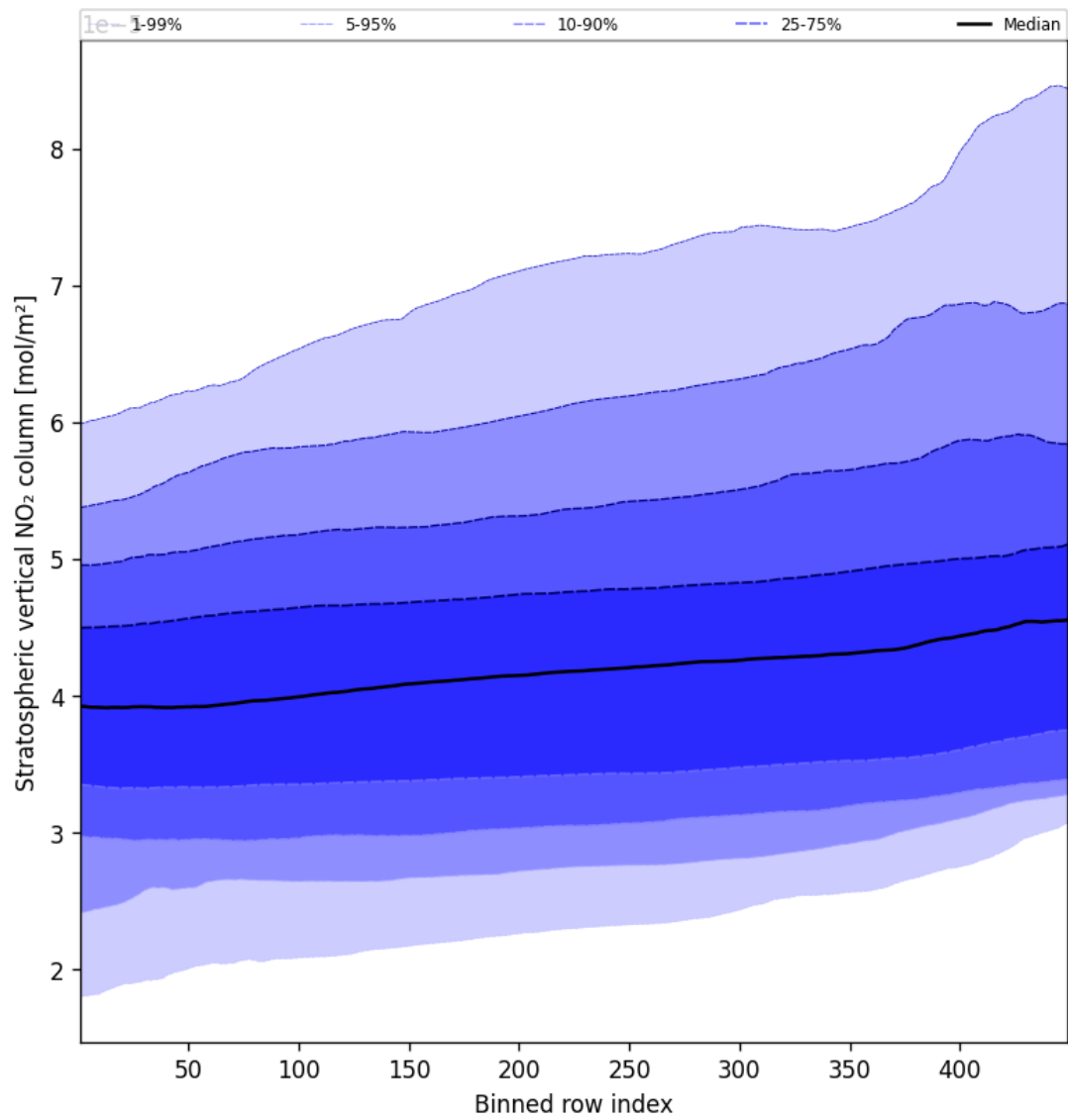
Figure 53: Along track statistics of “Stratospheric vertical NO 2 column” for 2025-09-29 to 2025-10-01
