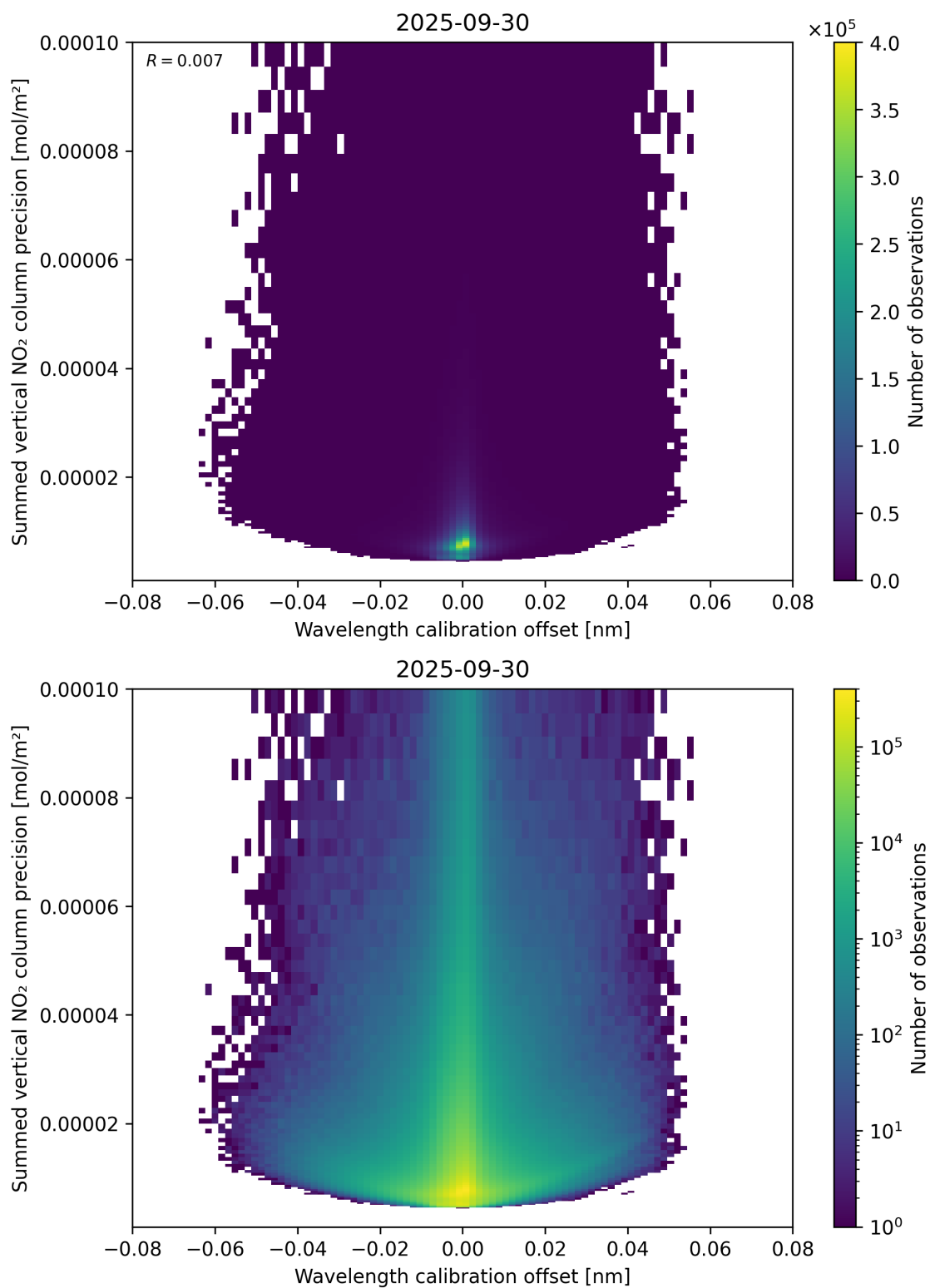
Figure 178: Scatter density plot of “Wavelength calibration offset” against “Summed vertical NO 2 column precision” for 2025-09-29 to 2025-10-01.
