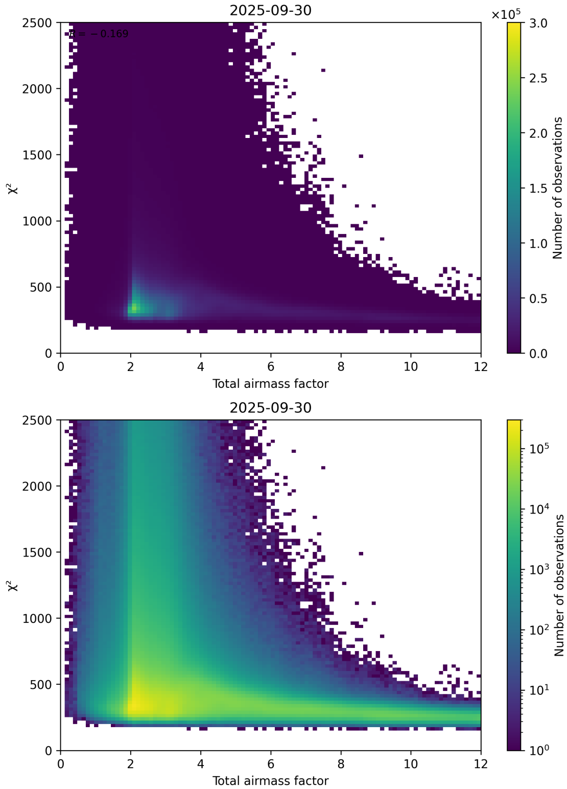
Figure 63: Scatter density plot of “Total airmass factor” against “ \chi^2 ” for 2025-09-29 to 2025-10-01.
