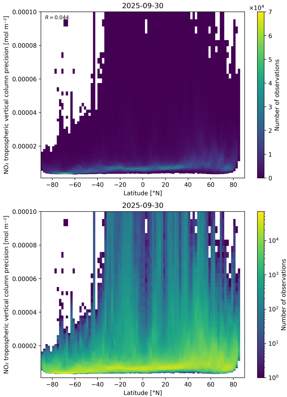
Figure 93: Scatter density plot of “Latitude” against “NO 2 tropospheric vertical column precision” for 2025-09-29 to 2025-10-01.
