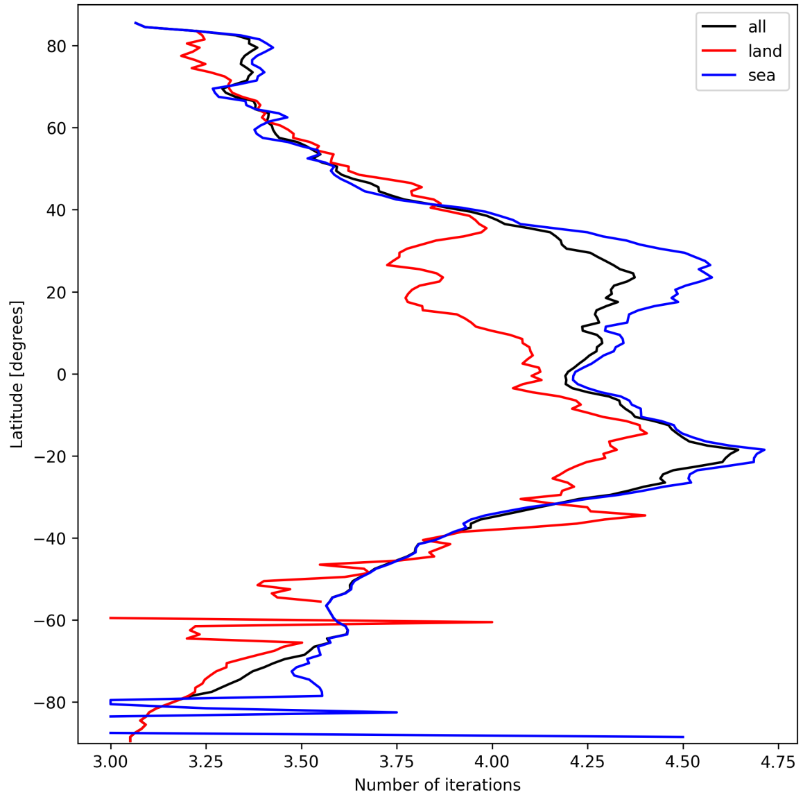
Figure 17: Zonal average of “Number of iterations” for 2025-09-29 to 2025-10-01.
