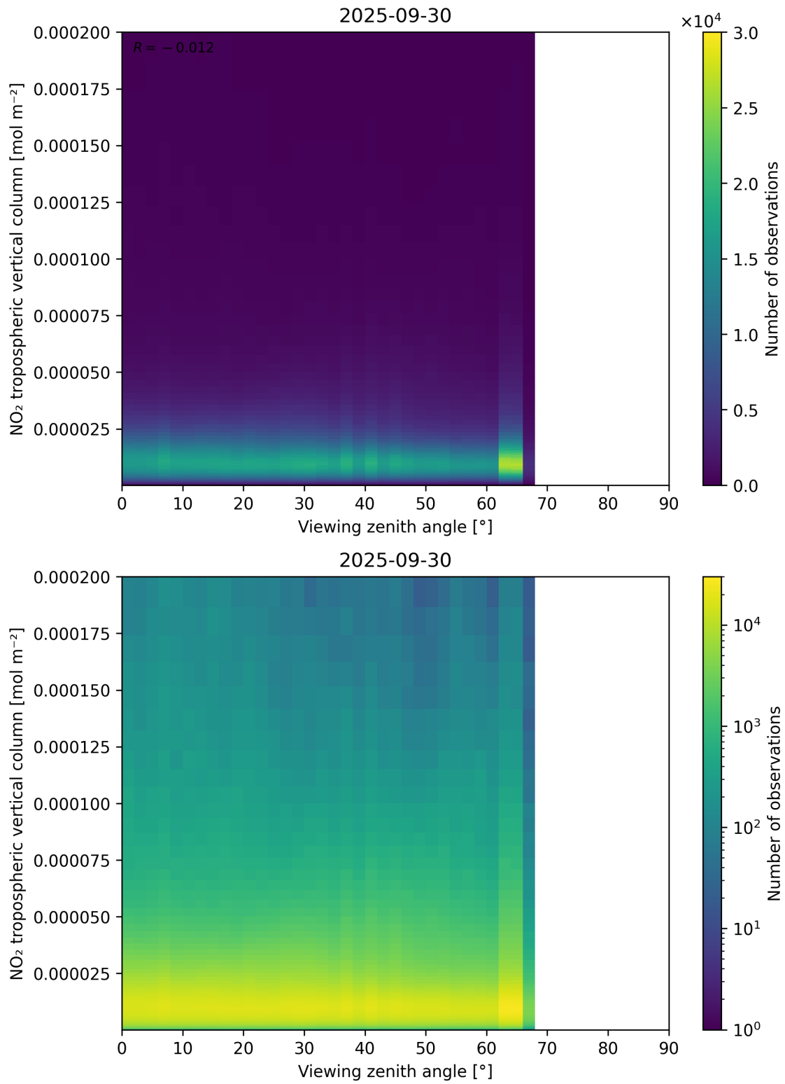
Figure 169: Scatter density plot of “Viewing zenith angle” against “NO 2 tropospheric vertical column” for 2025-09-29 to 2025-10-01.
