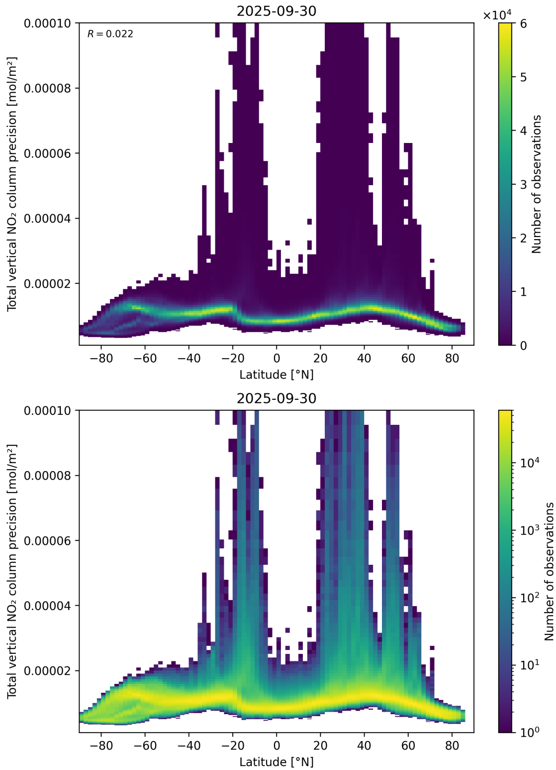
Figure 91: Scatter density plot of “Latitude” against “Total vertical NO 2 column precision” for 2025-09-29 to 2025-10-01.
