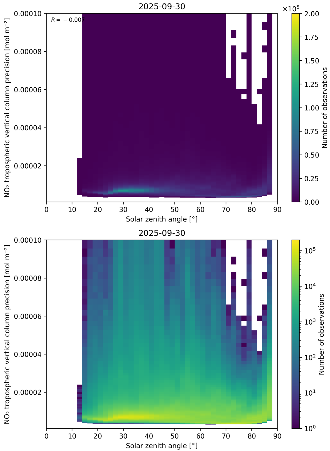
Figure 156: Scatter density plot of “Solar zenith angle” against “NO 2 tropospheric vertical column precision” for 2025-09-29 to 2025-10-01.
