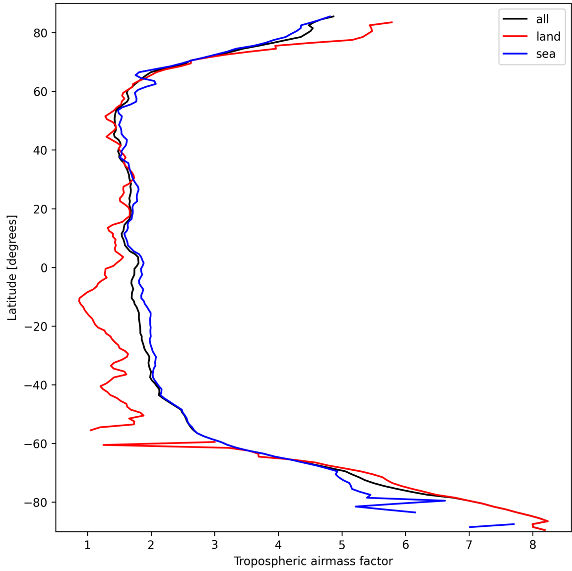
Figure 14: Zonal average of “Tropospheric airmass factor” for 2025-09-29 to 2025-10-01.
