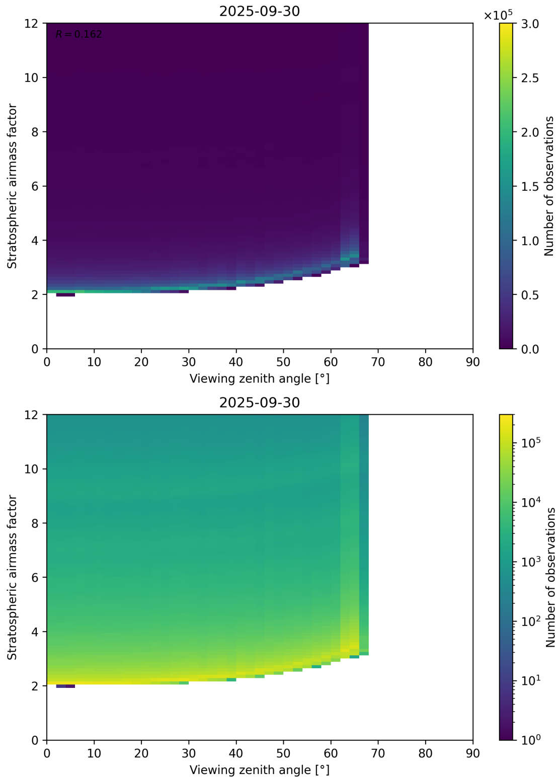
Figure 159: Scatter density plot of “Viewing zenith angle” against “Stratospheric airmass factor” for 2025-09-29 to 2025-10-01.
