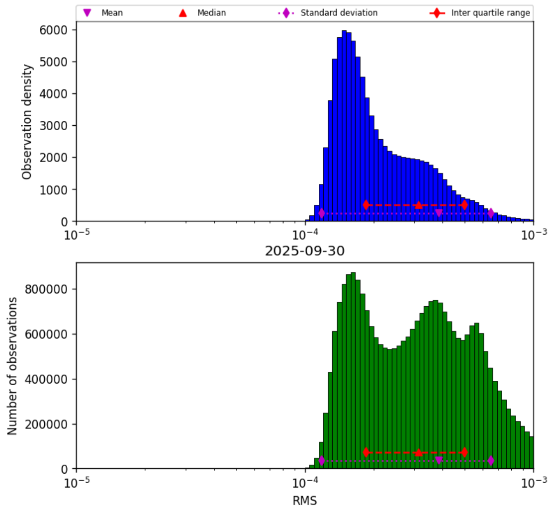
Figure 43: Histogram of “RMS” for 2025-09-29 to 2025-10-01
