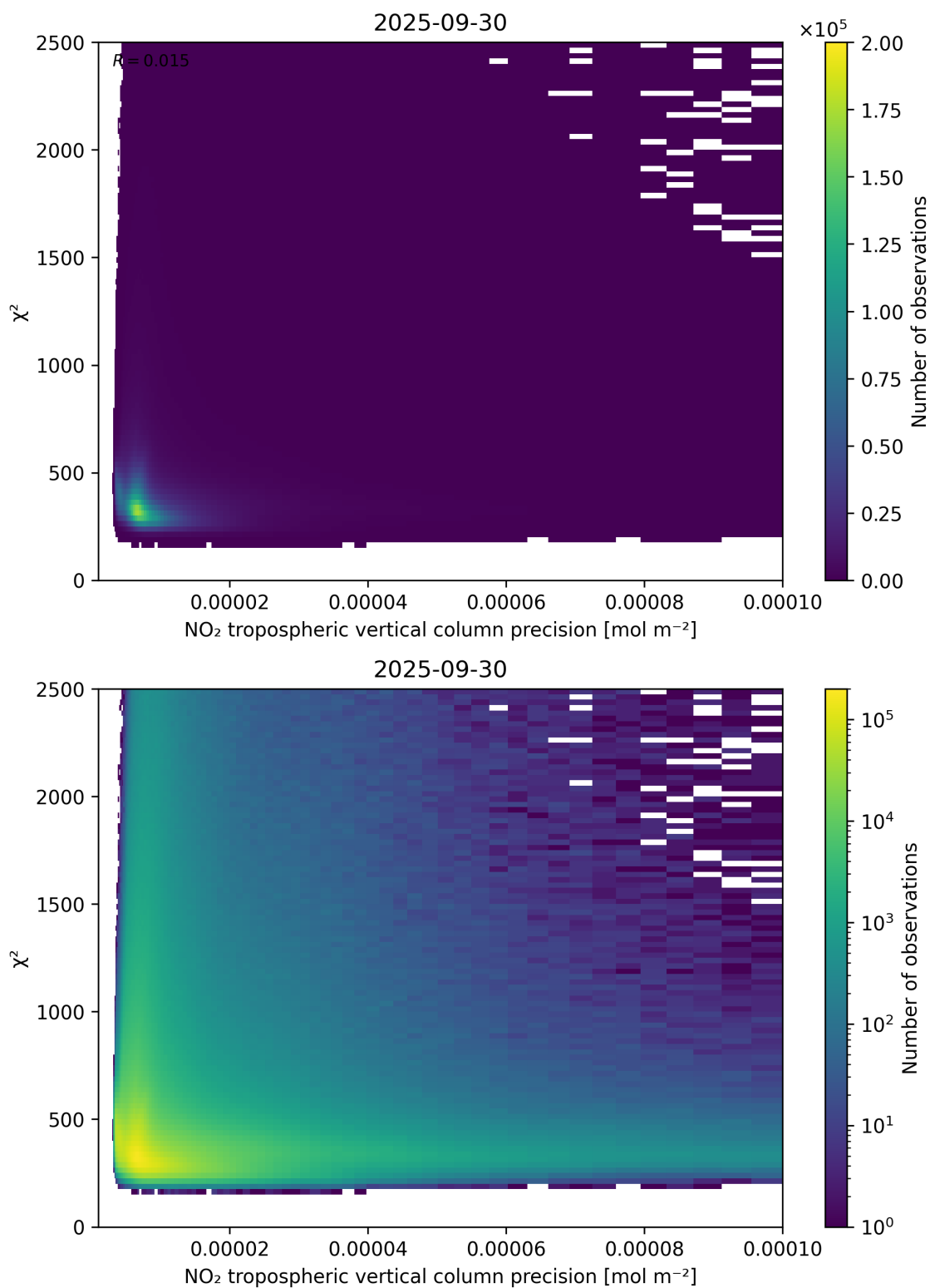
Figure 134: Scatter density plot of “NO 2 tropospheric vertical column precision” against “ \chi^2 ” for 2025-09-29 to 2025-10-01.
