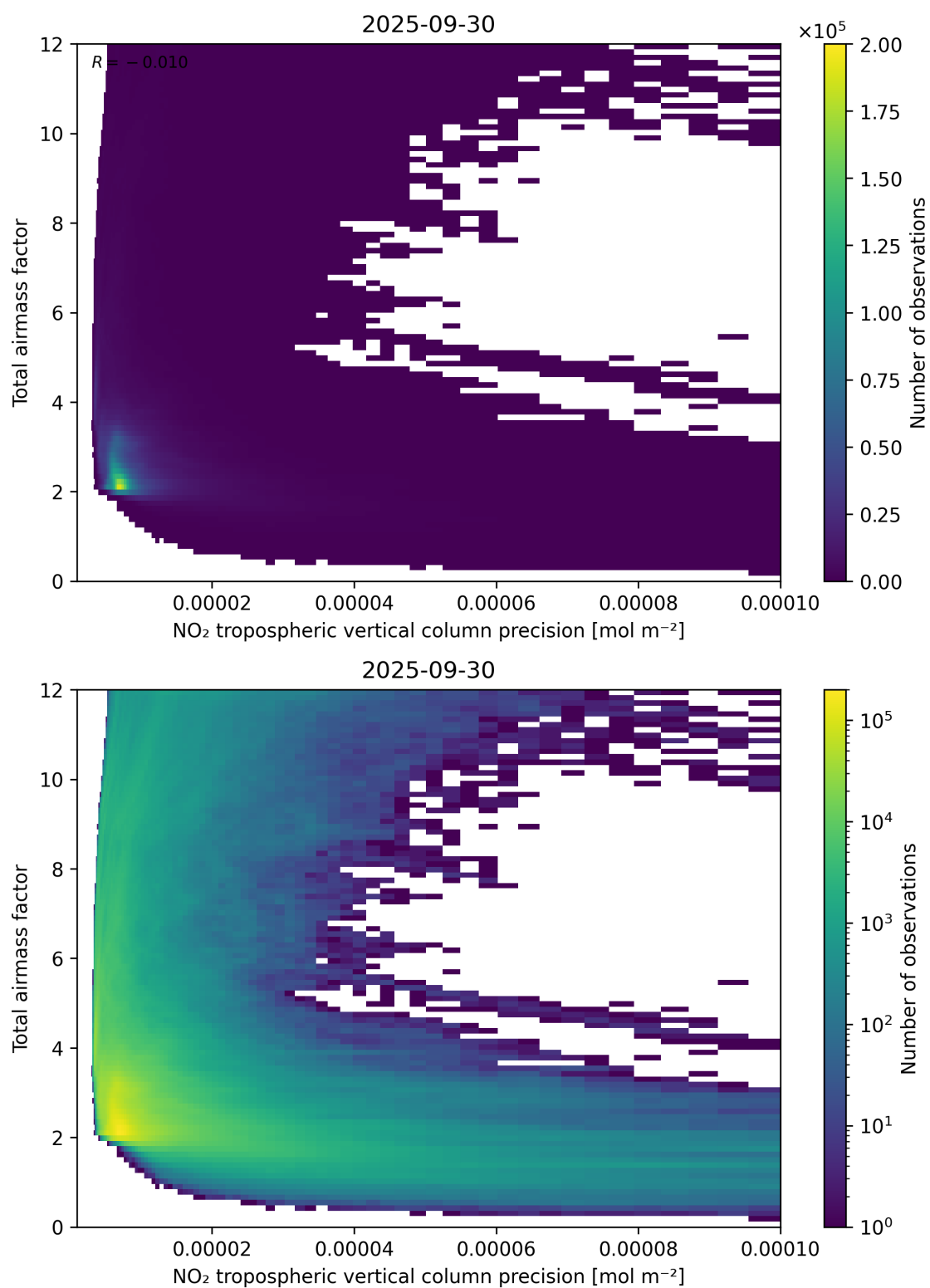
Figure 132: Scatter density plot of “NO 2 tropospheric vertical column precision” against “Total air mass factor” for 2025-09-29 to 2025-10-01.
