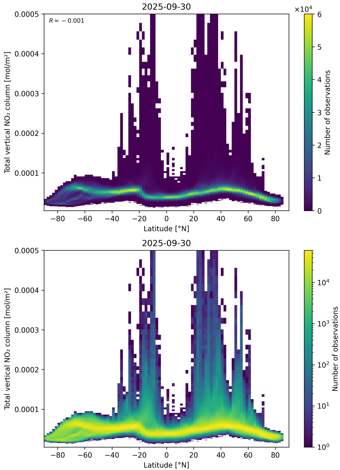
Figure 90: Scatter density plot of “Latitude” against “Total vertical NO 2 column” for 2025-09-29 to 2025-10-01.
