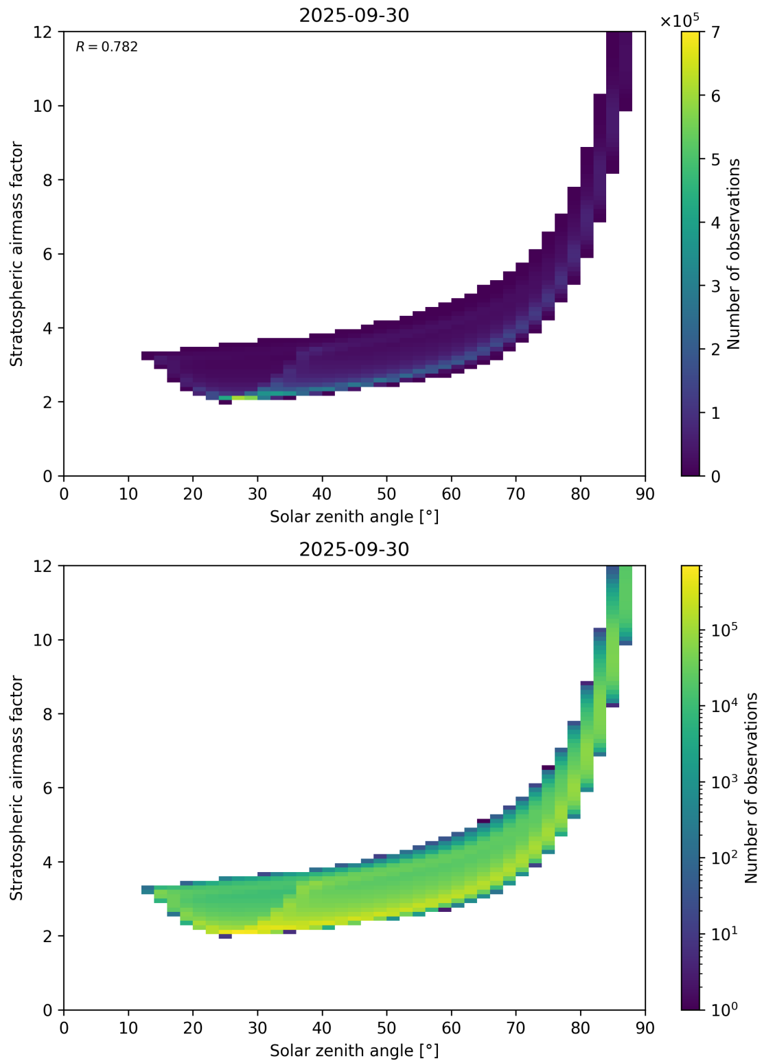
Figure 145: Scatter density plot of “Solar zenith angle” against “Stratospheric airmass factor” for 2025-09-29 to 2025-10-01.
