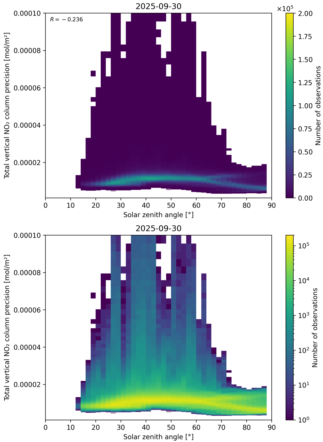
Figure 154: Scatter density plot of “Solar zenith angle” against “Total vertical NO 2 column precision” for 2025-09-29 to 2025-10-01.
