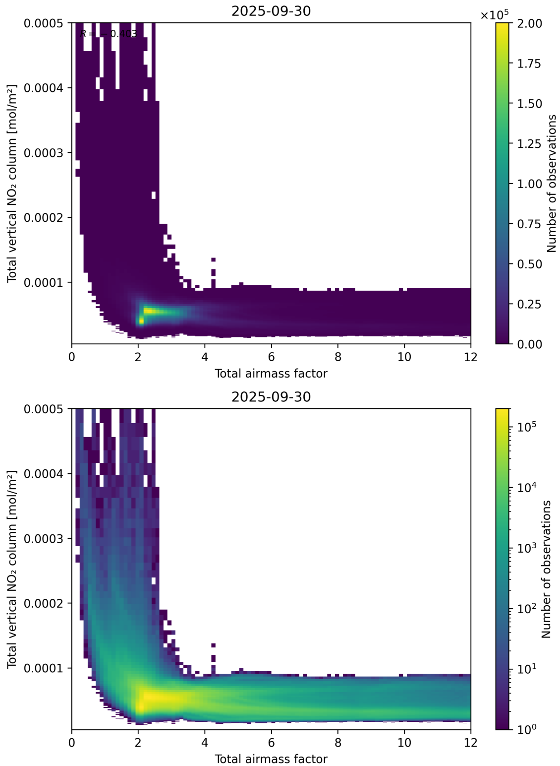
Figure 67: Scatter density plot of “Total airmass factor” against “Total vertical NO 2 column” for 2025-09-29 to 2025-10-01.
