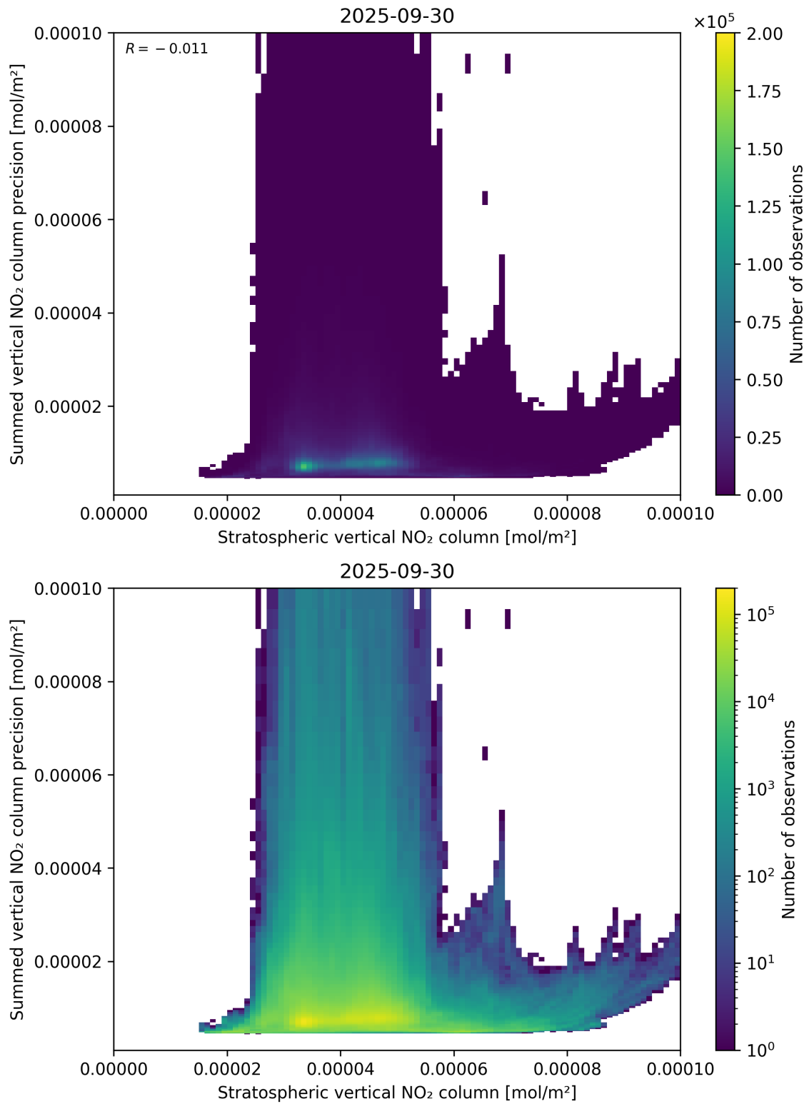
Figure 99: Scatter density plot of “Stratospheric vertical NO 2 column” against “Summed vertical NO 2 column precision” for 2025-09-29 to 2025-10-01.
