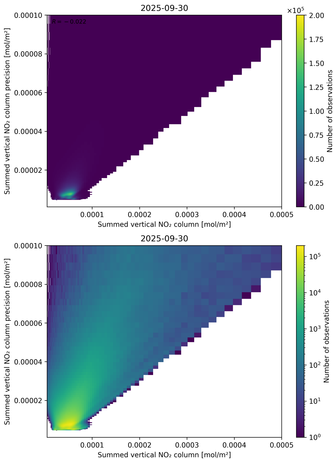
Figure 105: Scatter density plot of “Summed vertical NO 2 column” against “Summed vertical NO 2 column precision” for 2025-09-29 to 2025-10-01.
