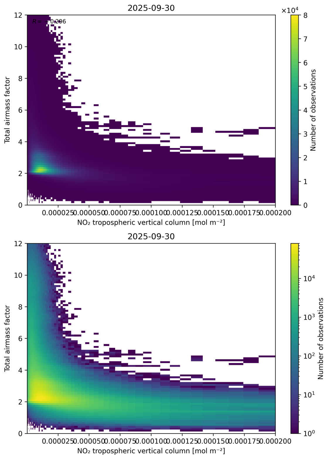
Figure 122: Scatter density plot of “NO 2 tropospheric vertical column” against “Total air mass factor” for 2025-09-29 to 2025-10-01.
