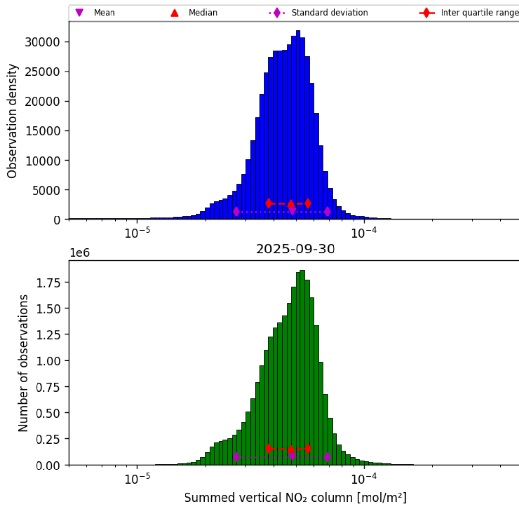
Figure 40: Histogram of “Summed vertical NO 2 column” for 2025-09-29 to 2025-10-01
