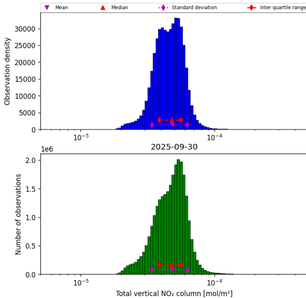
Figure 38: Histogram of “Total vertical NO 2 column” for 2025-09-29 to 2025-10-01
