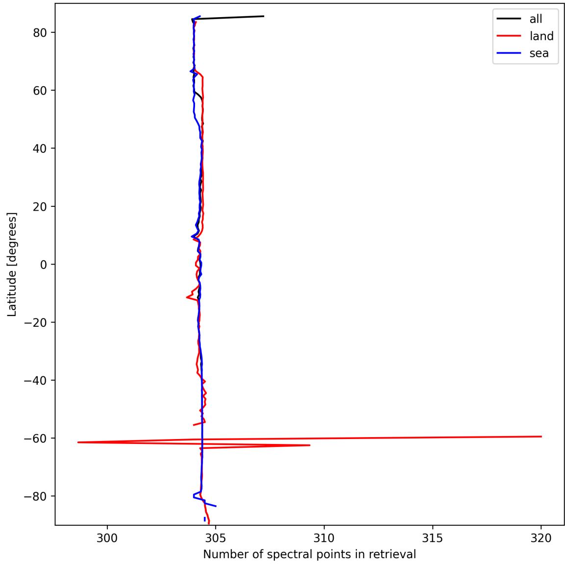
Figure 16: Zonal average of “Number of spectral points in retrieval” for 2025-09-29 to 2025-10-01.
