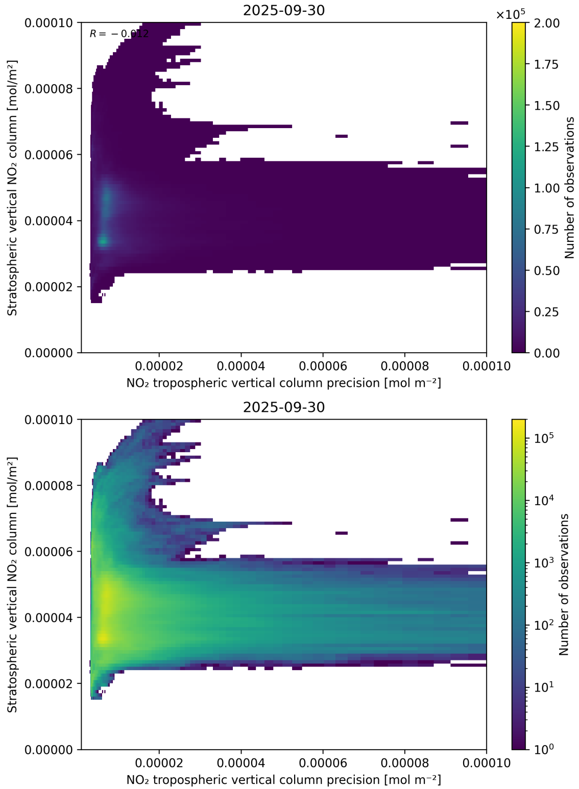
Figure 135: Scatter density plot of “NO 2 tropospheric vertical column precision” against “Stratospheric vertical NO 2 column” for 2025-09-29 to 2025-10-01.
