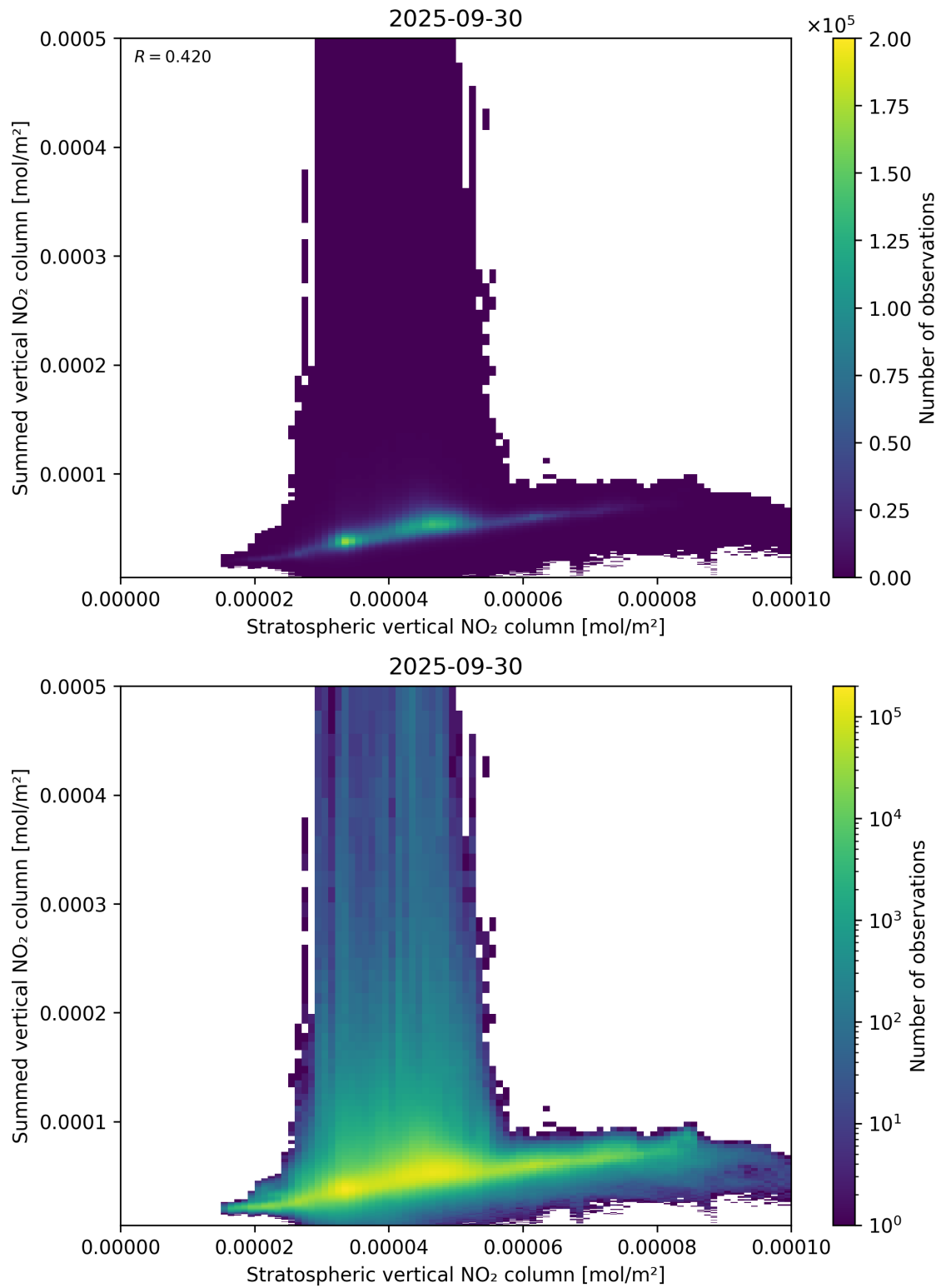
Figure 98: Scatter density plot of “Stratospheric vertical NO 2 column” against “Summed vertical NO 2 column” for 2025-09-29 to 2025-10-01.
