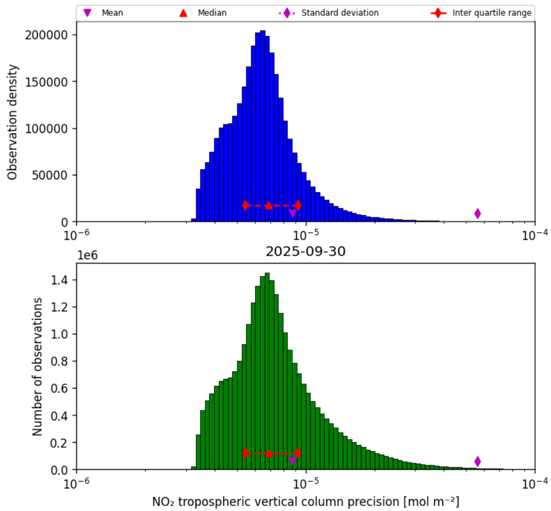
Figure 30: Histogram of “NO 2 tropospheric vertical column precision” for 2025-09-29 to 2025-10-01
