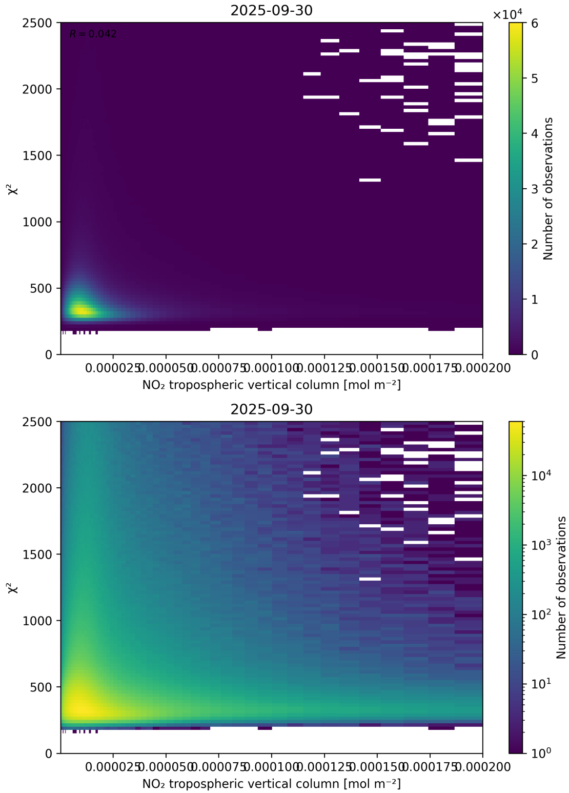
Figure 124: Scatter density plot of “NO 2 tropospheric vertical column” against “ \chi^2 ” for 2025-09-29 to 2025-10-01.
