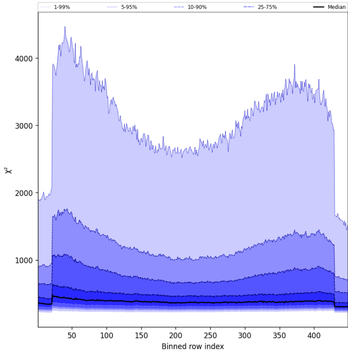
Figure 59: Along track statistics of “ \chi^2 ” for 2025-09-29 to 2025-10-01
