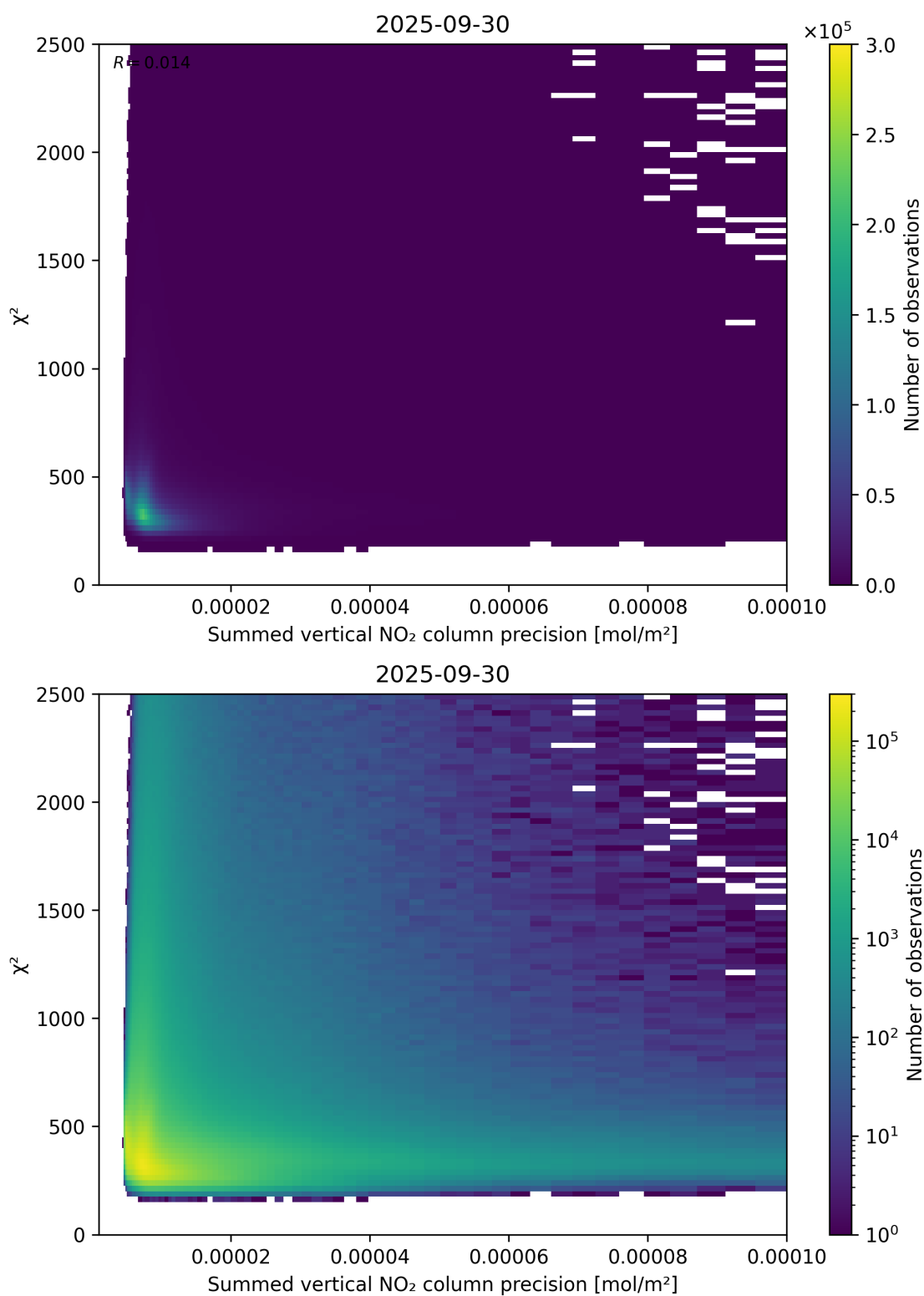
Figure 107: Scatter density plot of “Summed vertical NO 2 column precision” against “ \chi^2 ” for 2025-09-29 to 2025-10-01.
