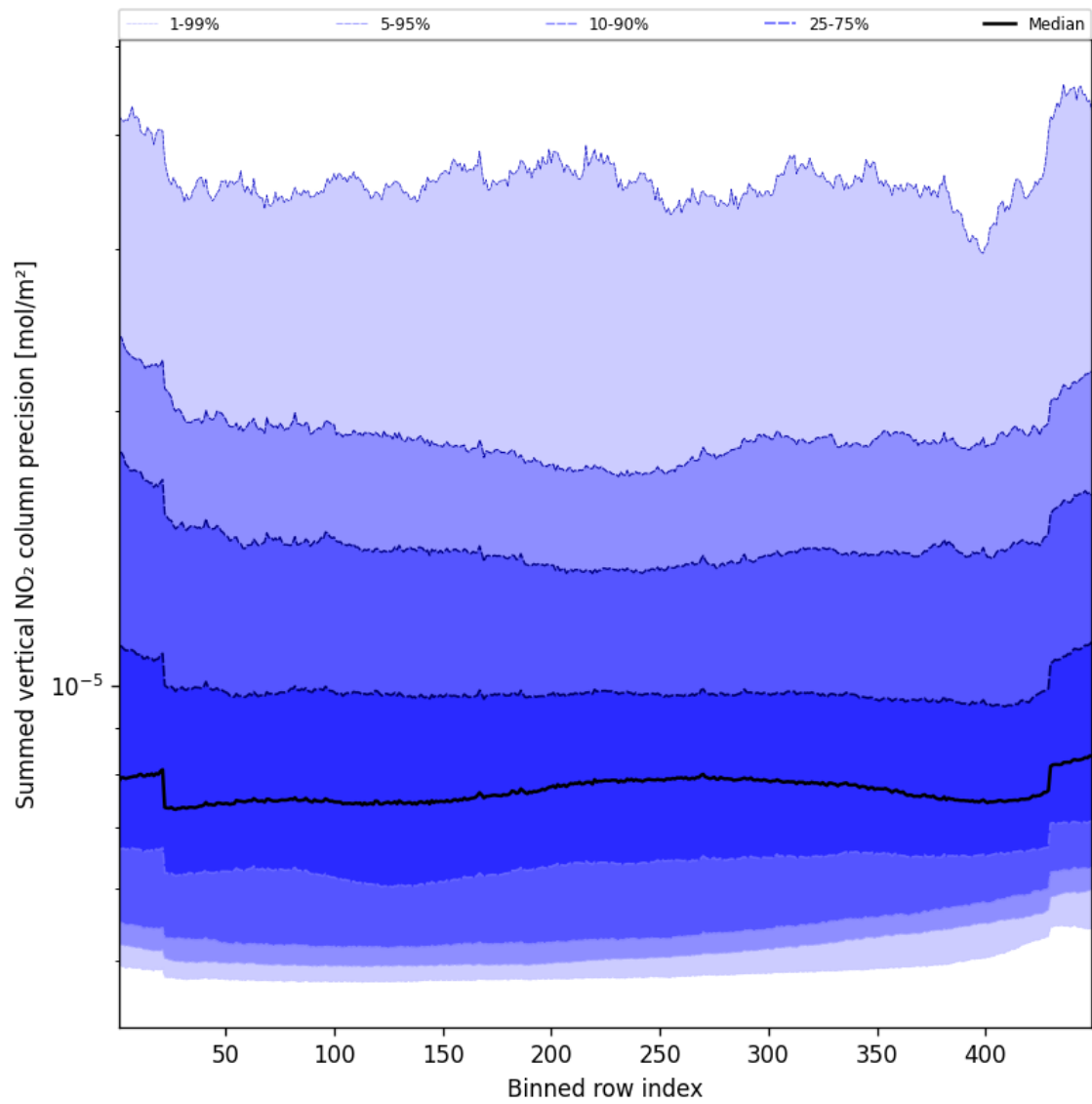
Figure 58: Along track statistics of “Summed vertical NO 2 column precision” for 2025-09-29 to 2025-10-01
