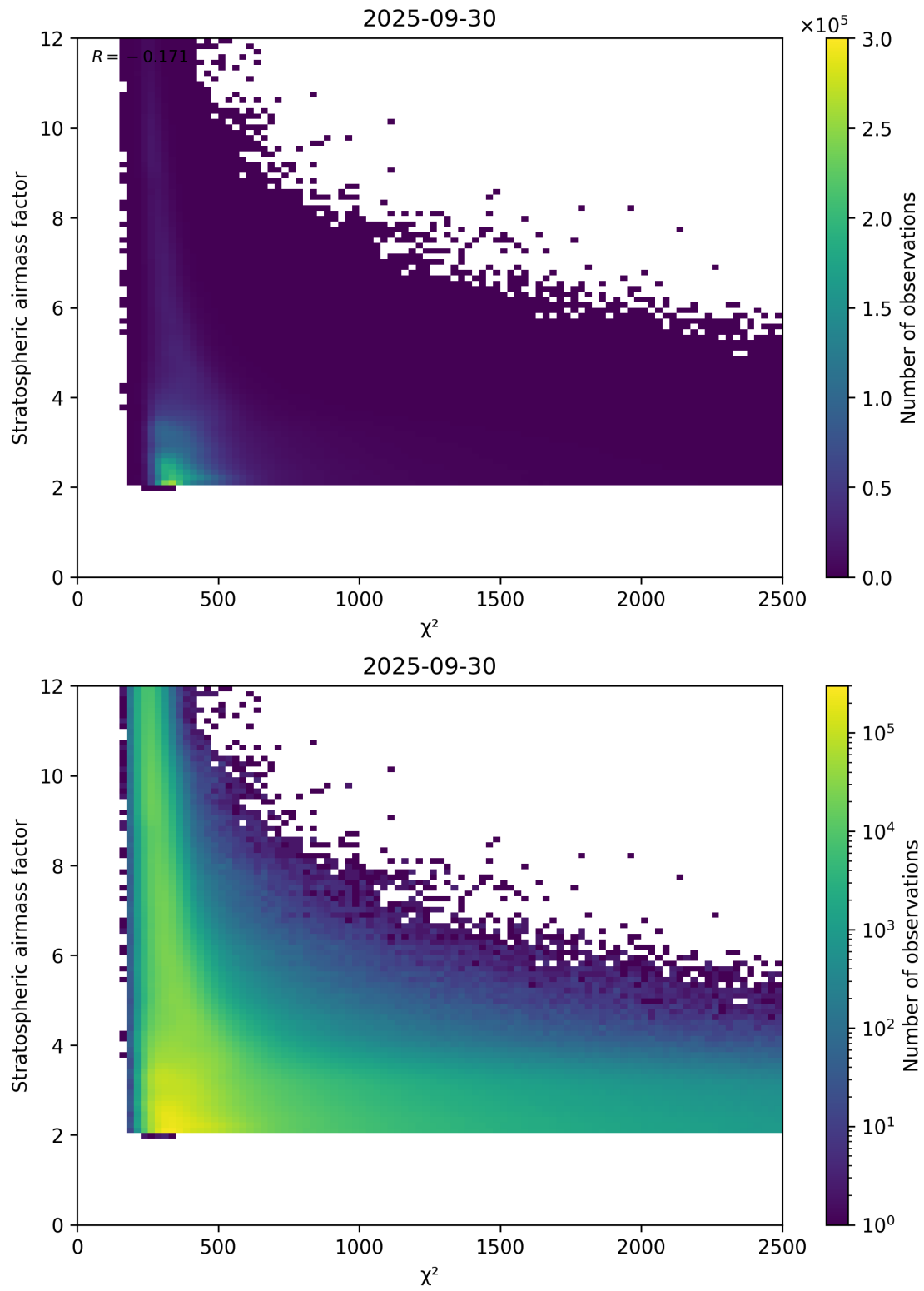
Figure 81: Scatter density plot of “ \chi^2 ” against “Stratospheric airmass factor” for 2025-09-29 to 2025-10-01.
