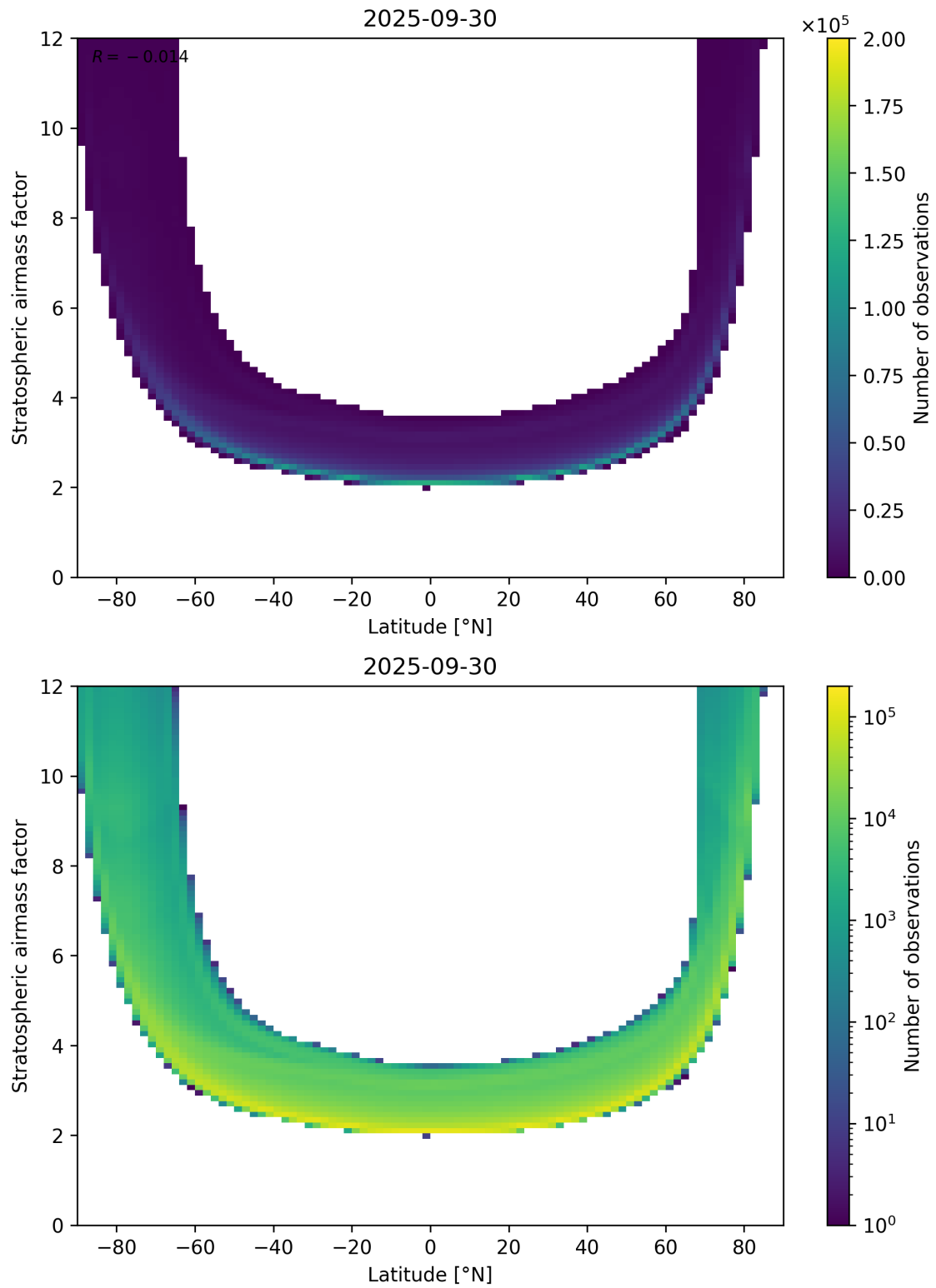
Figure 83: Scatter density plot of “Latitude” against “Stratospheric airmass factor” for 2025-09-29 to 2025-10-01.
