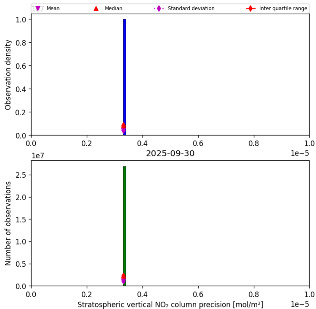
Figure 37: Histogram of “Stratospheric vertical NO 2 column precision” for 2025-09-29 to 2025-10-01
