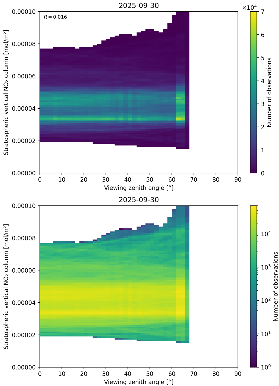
Figure 164: Scatter density plot of “Viewing zenith angle” against “Stratospheric vertical NO 2 column” for 2025-09-29 to 2025-10-01.
