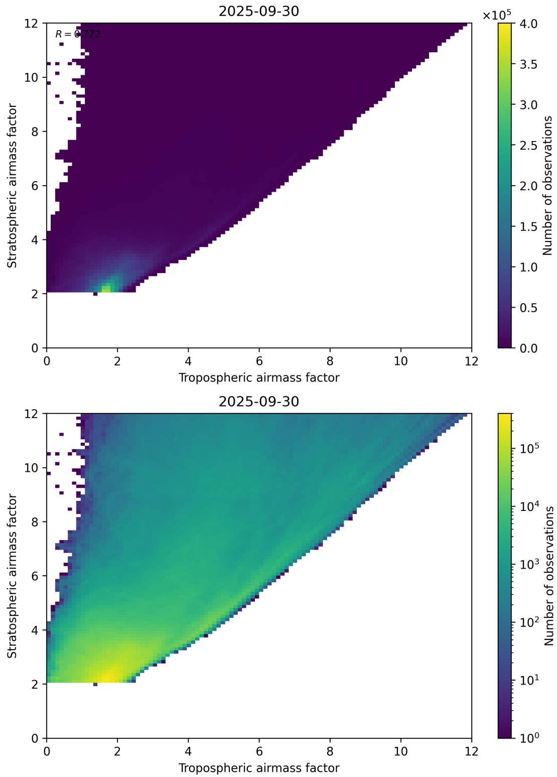
Figure 71: Scatter density plot of “Tropospheric airmass factor” against “Stratospheric airmass factor” for 2025-09-29 to 2025-10-01.
