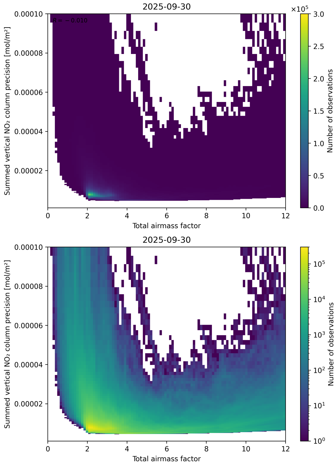
Figure 66: Scatter density plot of “Total airmass factor” against “Summed vertical NO 2 column precision” for 2025-09-29 to 2025-10-01.
