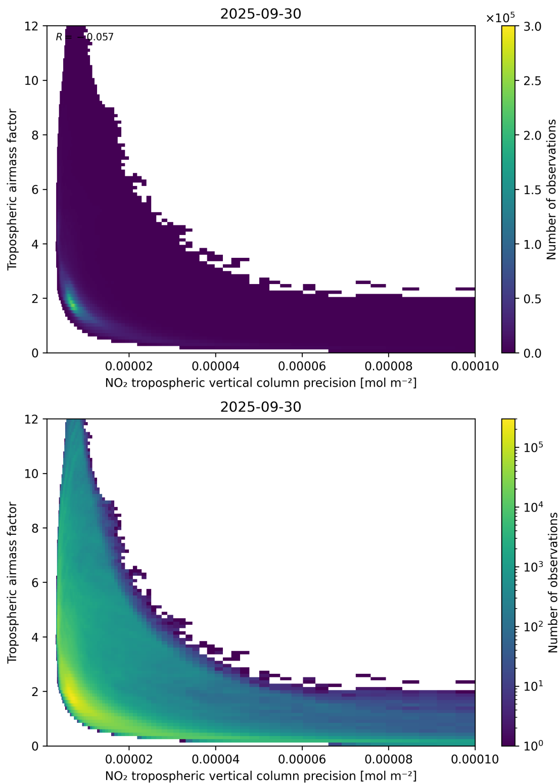
Figure 133: Scatter density plot of “NO 2 tropospheric vertical column precision” against “Tropospheric air mass factor” for 2025-09-29 to 2025-10-01.
