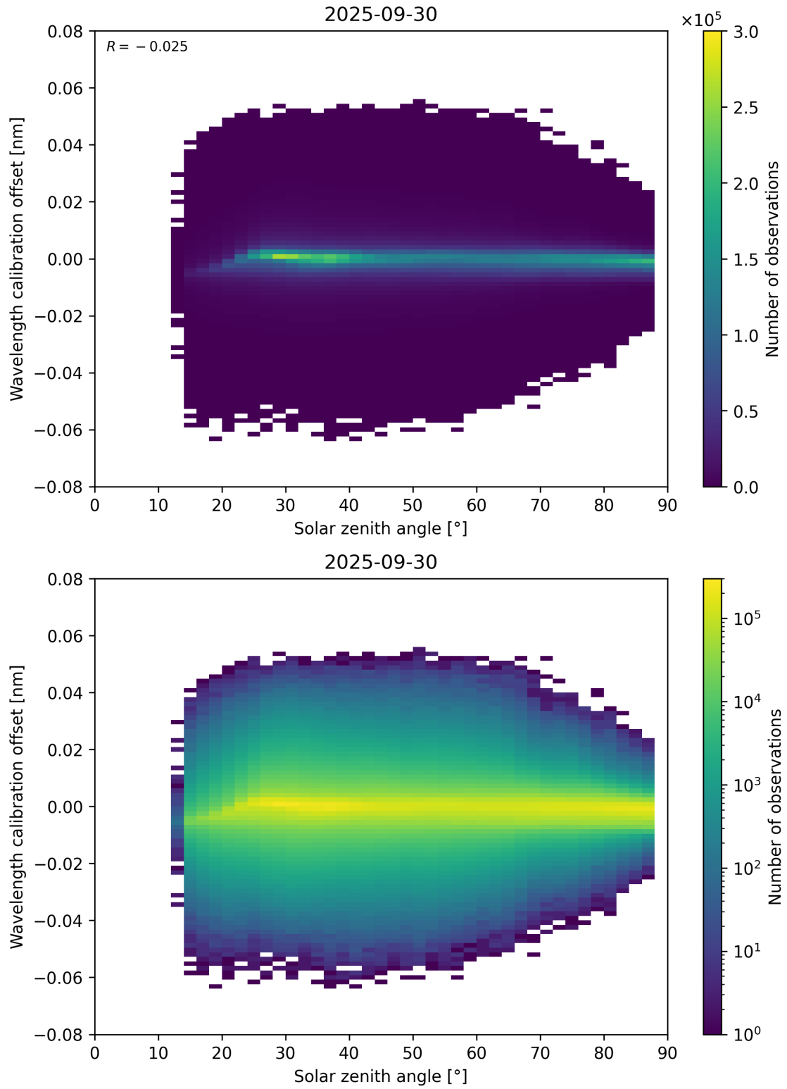
Figure 158: Scatter density plot of “Solar zenith angle” against “Wavelength calibration offset” for 2025-09-29 to 2025-10-01.
