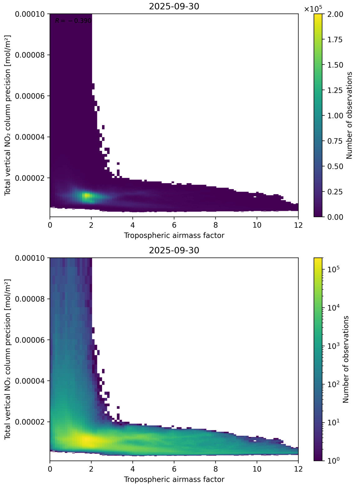
Figure 78: Scatter density plot of “Tropospheric air mass factor” against “Total vertical NO 2 column precision” for 2025-09-29 to 2025-10-01.
