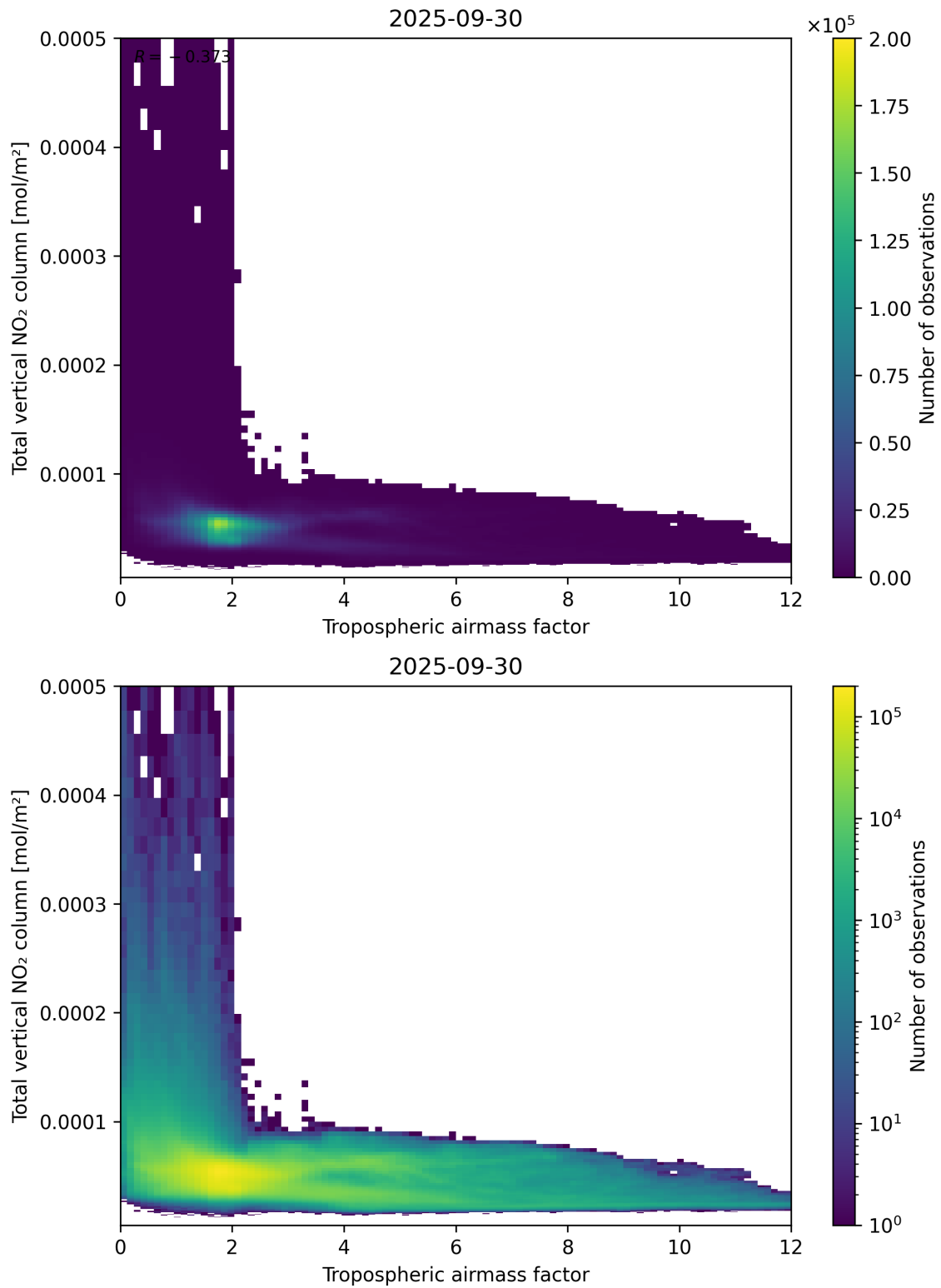
Figure 77: Scatter density plot of “Tropospheric airmass factor” against “Total vertical NO 2 column” for 2025-09-29 to 2025-10-01.
