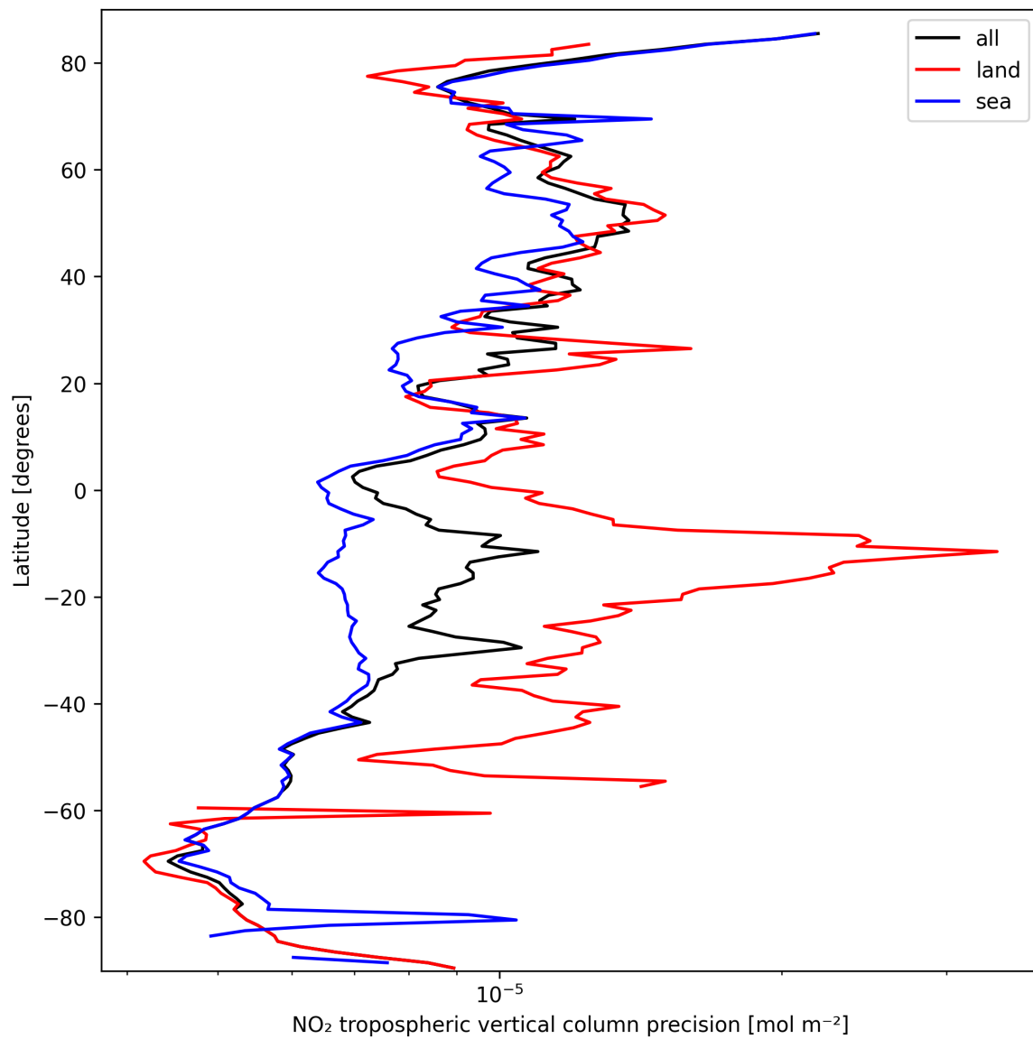
Figure 13: Zonal average of “NO 2 tropospheric vertical column precision” for 2025-09-29 to 2025-10-01.
