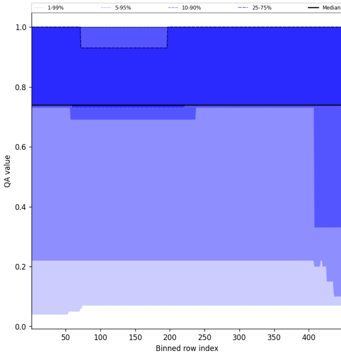
Figure 45: Along track statistics of “QA value” for 2025-09-29 to 2025-10-01
