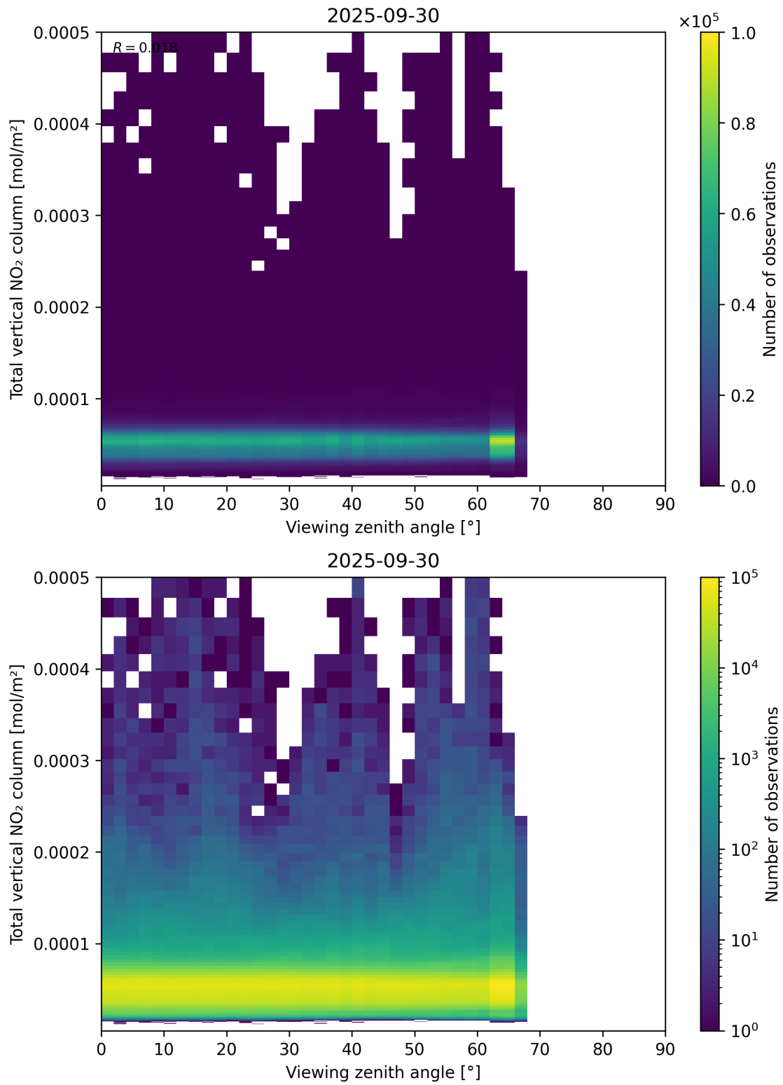
Figure 167: Scatter density plot of “Viewing zenith angle” against “Total vertical NO 2 column” for 2025-09-29 to 2025-10-01.
