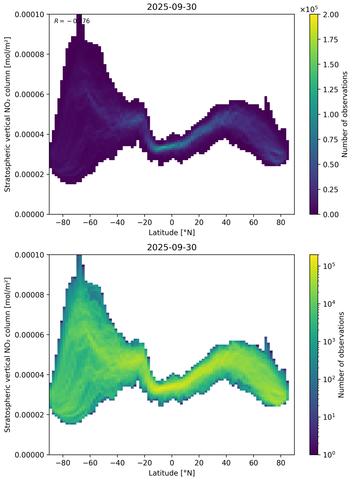
Figure 87: Scatter density plot of “Latitude” against “Stratospheric vertical NO 2 column” for 2025-09-29 to 2025-10-01.
