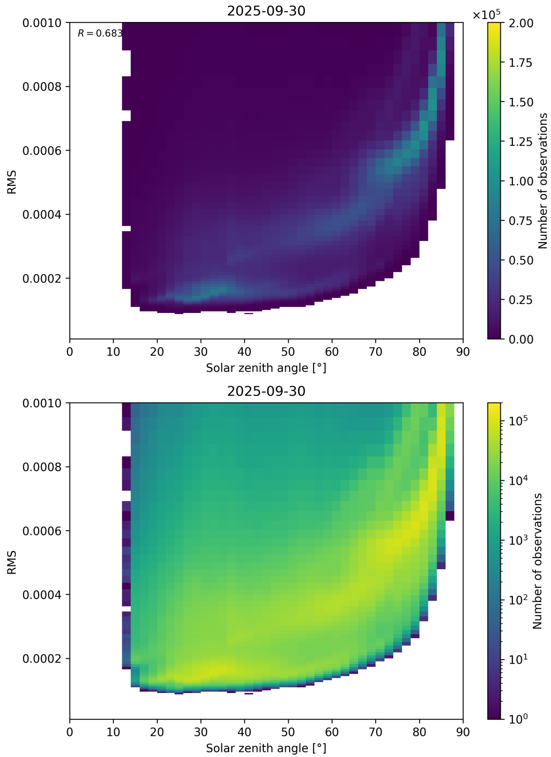
Figure 157: Scatter density plot of “Solar zenith angle” against “RMS” for 2025-09-29 to 2025-10-01.
