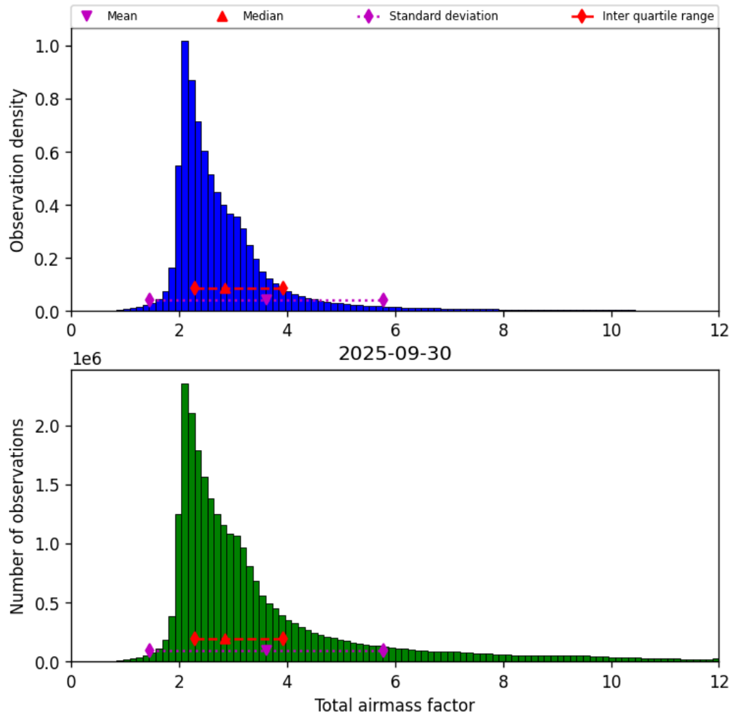
Figure 32: Histogram of “Total airmass factor” for 2025-09-29 to 2025-10-01
