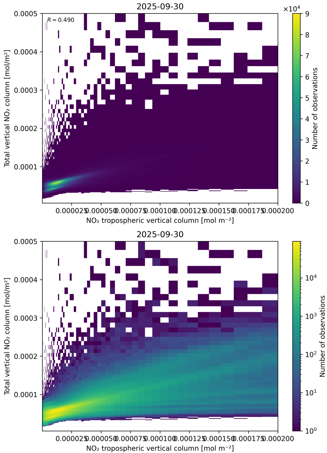
Figure 128: Scatter density plot of “NO 2 tropospheric vertical column” against “Total vertical NO 2 column” for 2025-09-29 to 2025-10-01.
