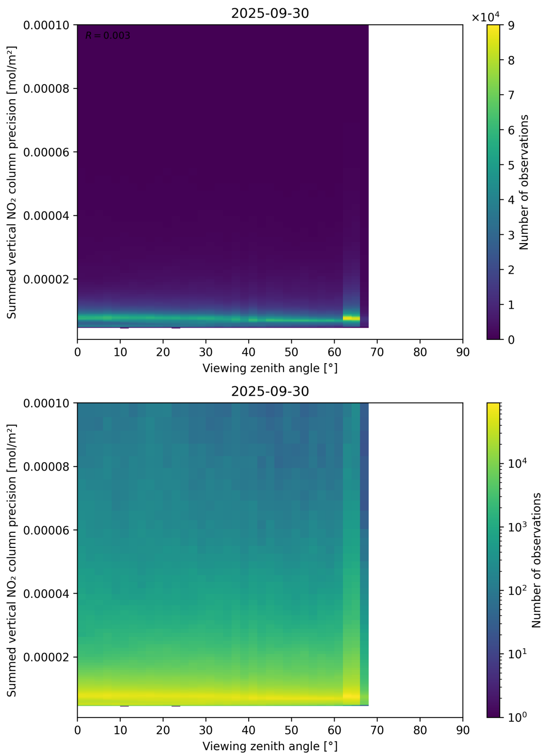
Figure 166: Scatter density plot of “Viewing zenith angle” against “Summed vertical NO 2 column precision” for 2025-09-29 to 2025-10-01.
