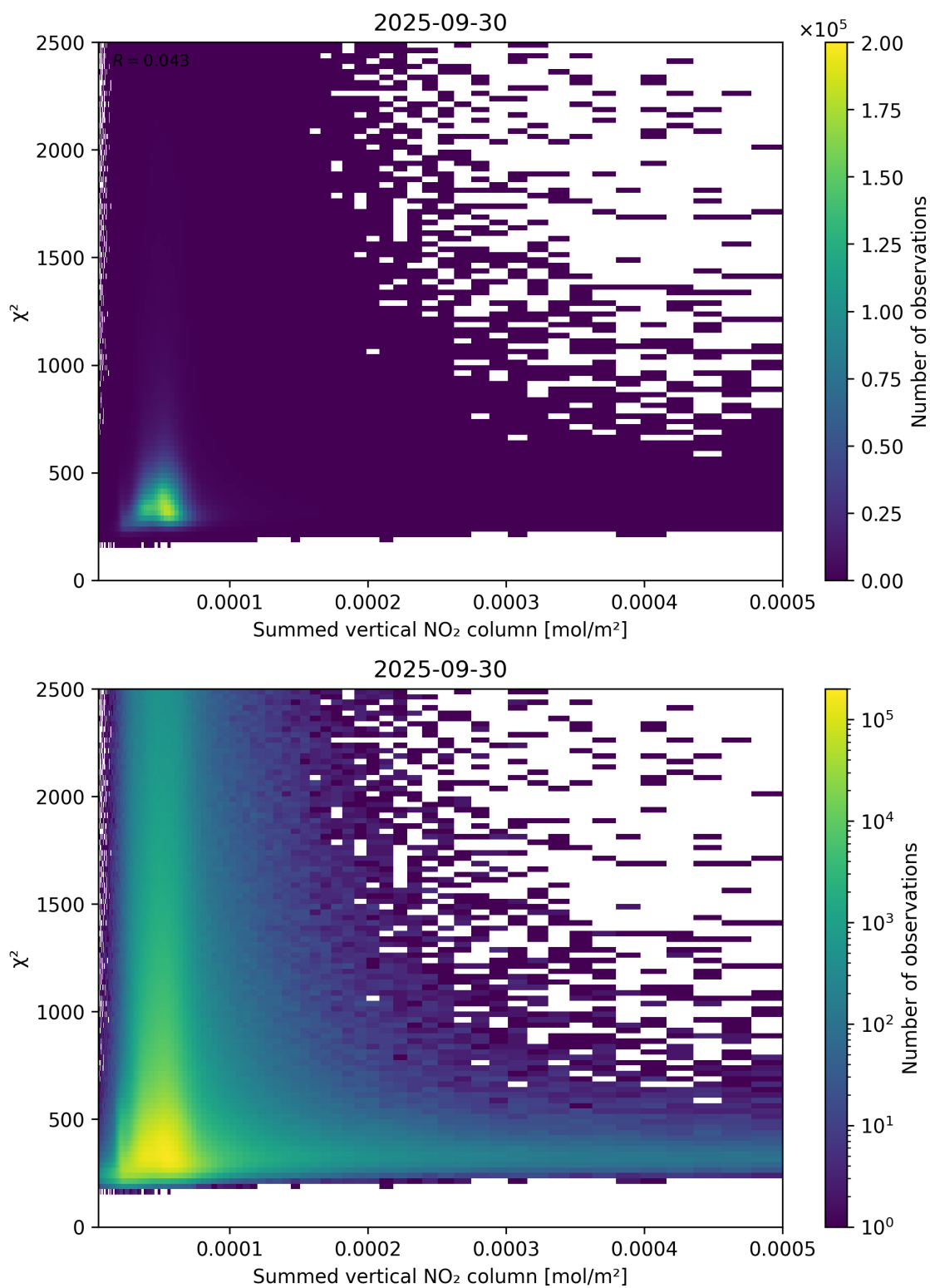
Figure 104: Scatter density plot of “Summed vertical NO 2 column” against “ \chi^2 ” for 2025-09-29 to 2025-10-01.
