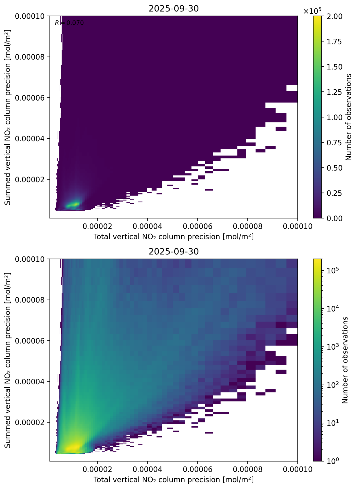
Figure 118: Scatter density plot of “Total vertical NO 2 column precision” against “Summed vertical NO 2 column precision” for 2025-09-29 to 2025-10-01.
