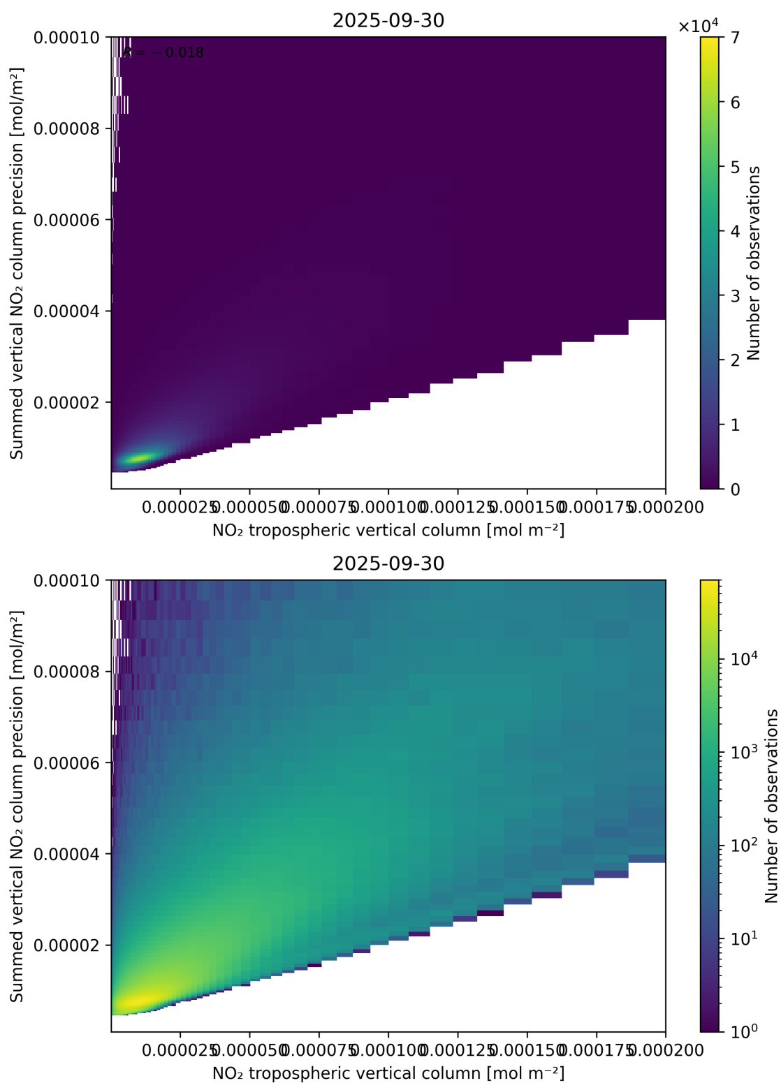
Figure 127: Scatter density plot of “NO 2 tropospheric vertical column” against “Summed vertical NO 2 column precision” for 2025-09-29 to 2025-10-01.
