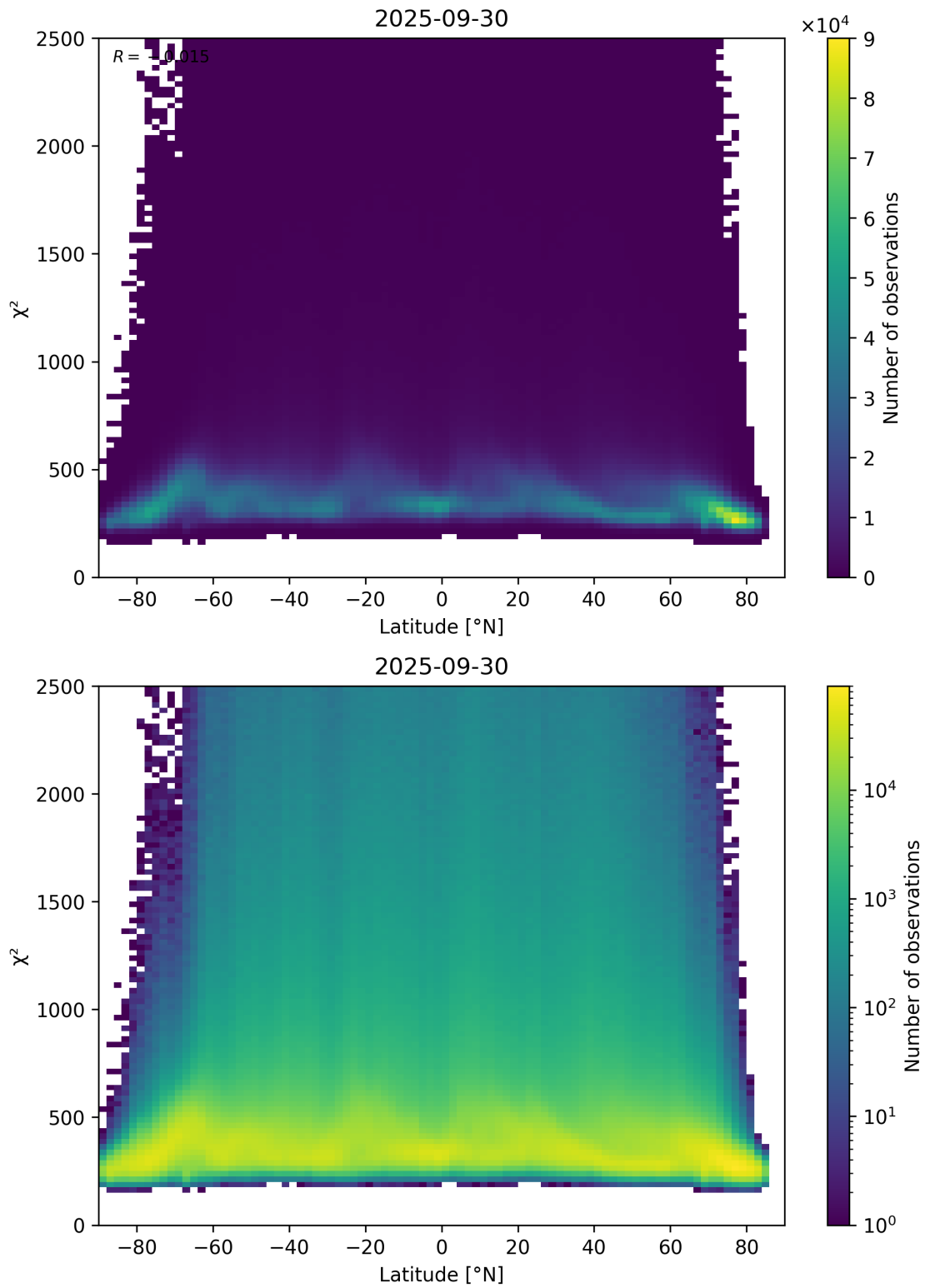
Figure 86: Scatter density plot of “Latitude” against “ \chi^2 ” for 2025-09-29 to 2025-10-01.
