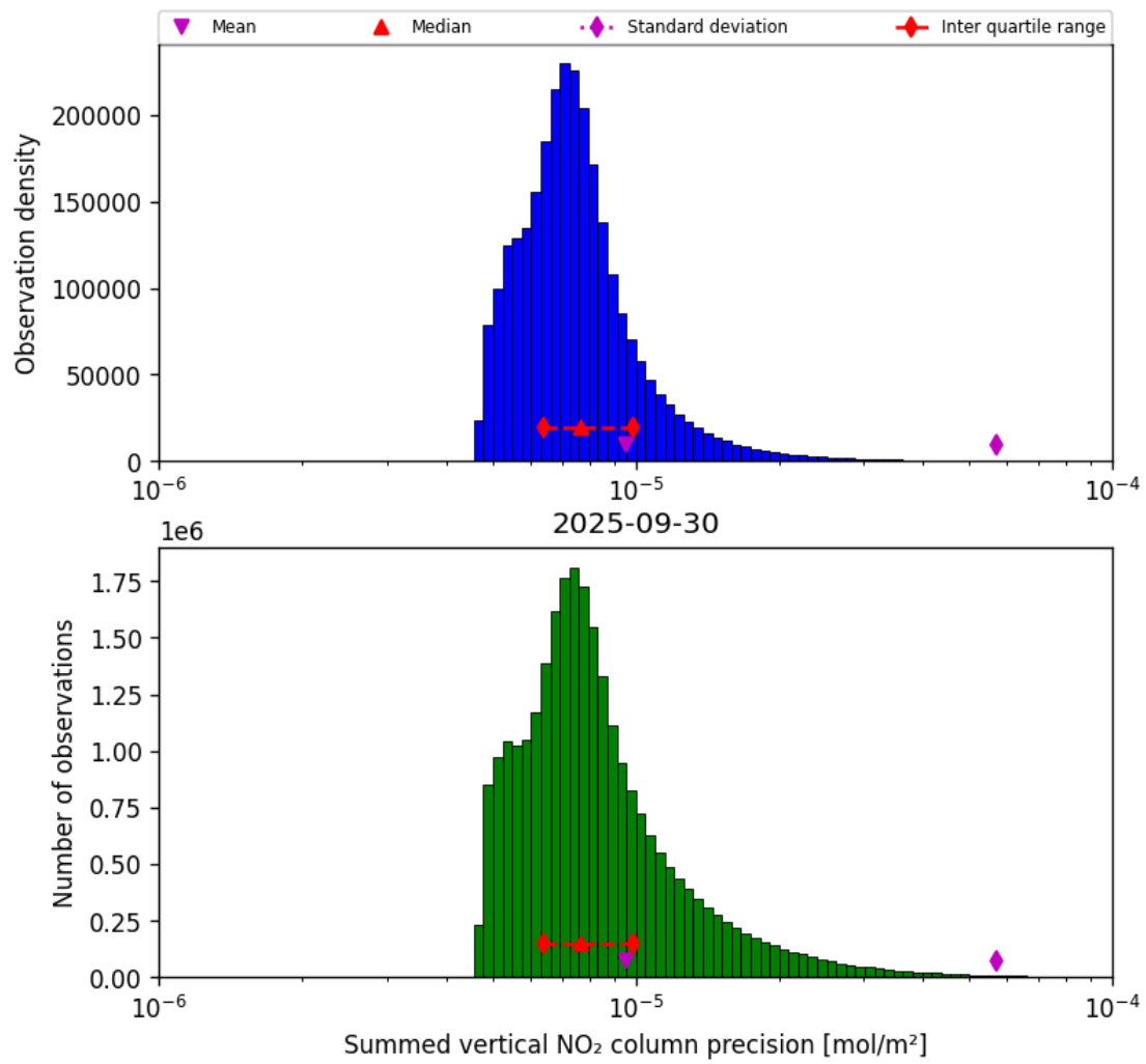
Figure 41: Histogram of “Summed vertical NO 2 column precision” for 2025-09-29 to 2025-10-01
