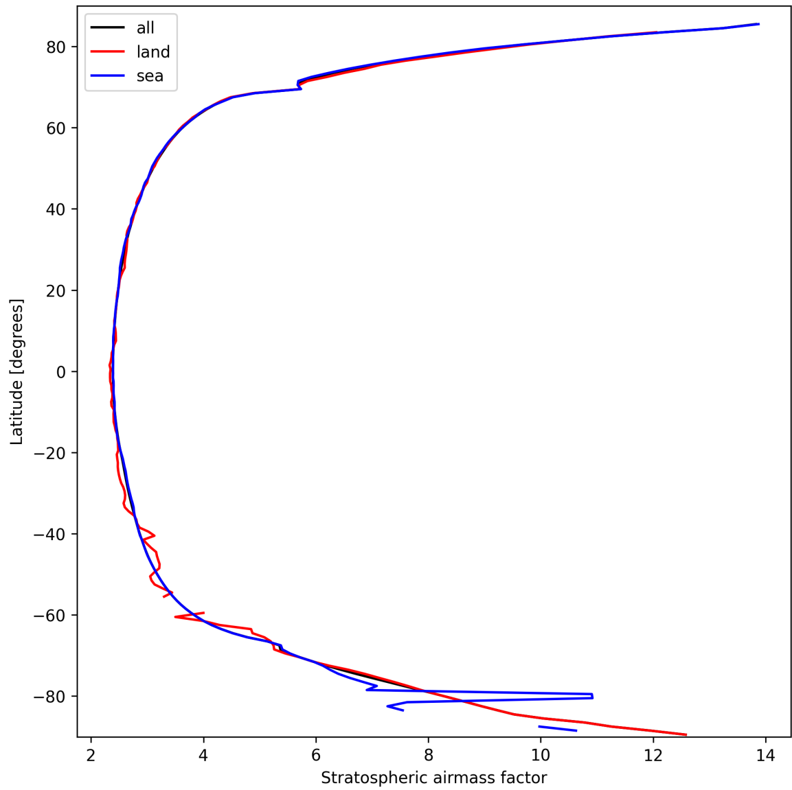
Figure 27: Zonal average of “Stratospheric airmass factor” for 2025-09-29 to 2025-10-01.
