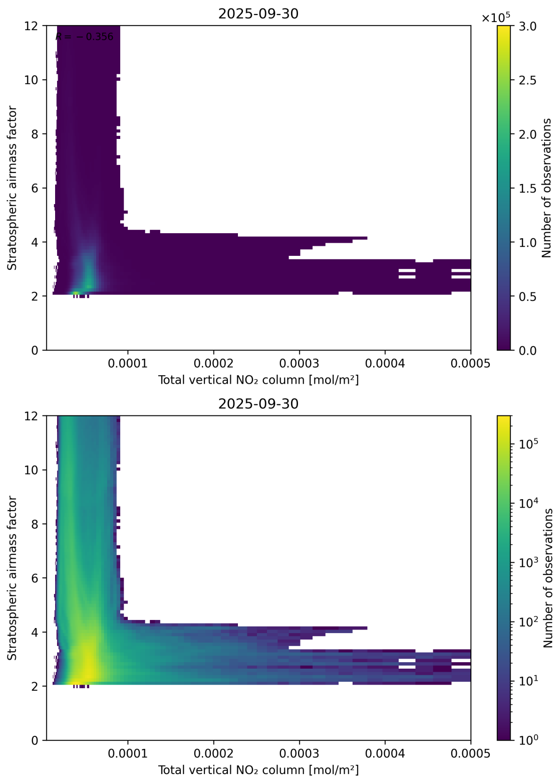
Figure 110: Scatter density plot of “Total vertical NO 2 column” against “Stratospheric airmass factor” for 2025-09-29 to 2025-10-01.
