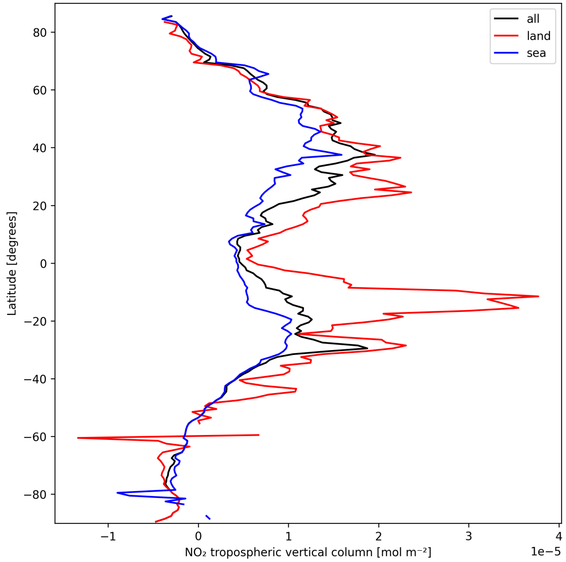
Figure 12: Zonal average of “NO 2 tropospheric vertical column” for 2025-09-29 to 2025-10-01.
