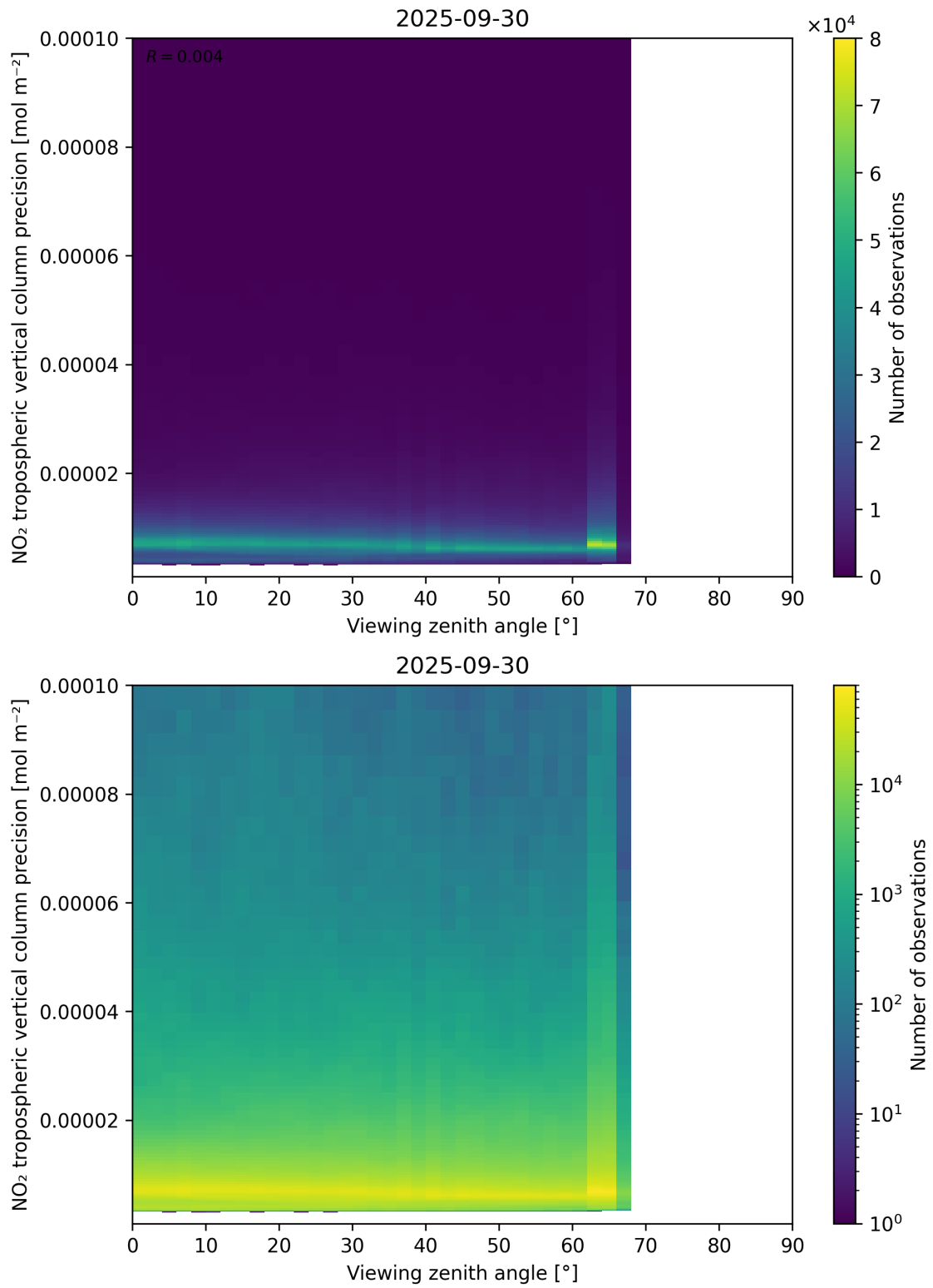
Figure 170: Scatter density plot of “Viewing zenith angle” against “NO 2 tropospheric vertical column precision” for 2025-09-29 to 2025-10-01.
