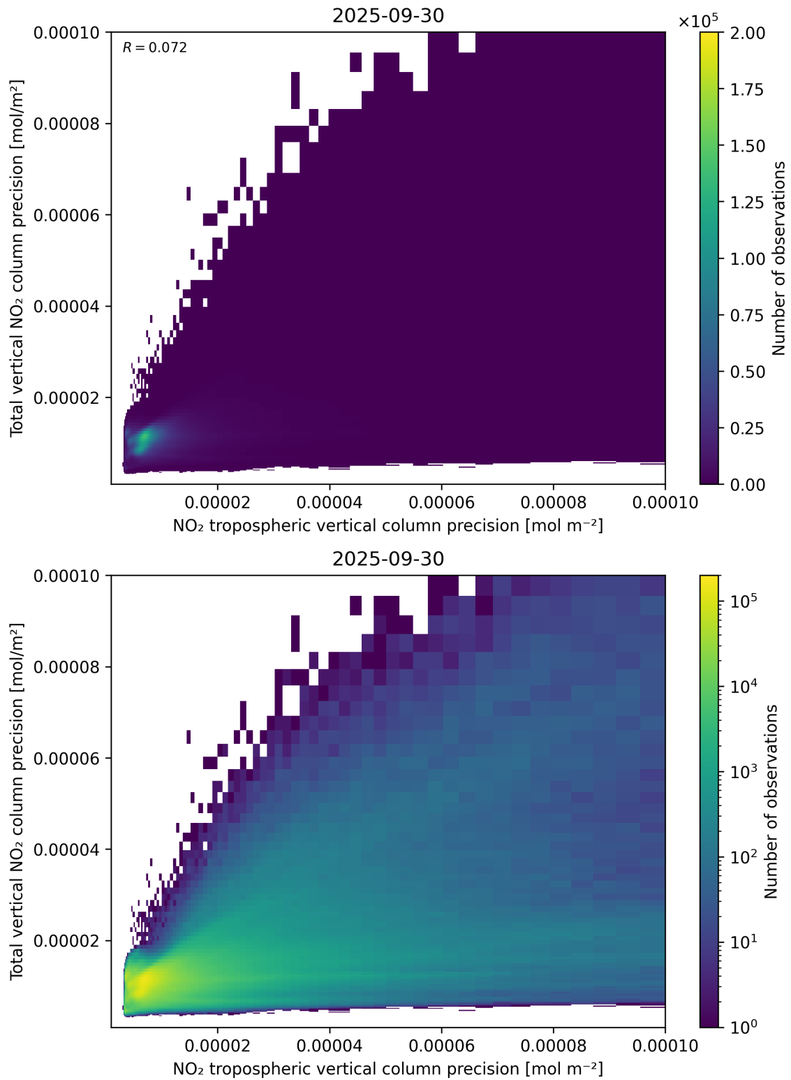
Figure 139: Scatter density plot of “NO 2 tropospheric vertical column precision” against “Total vertical NO 2 column precision” for 2025-09-29 to 2025-10-01.
