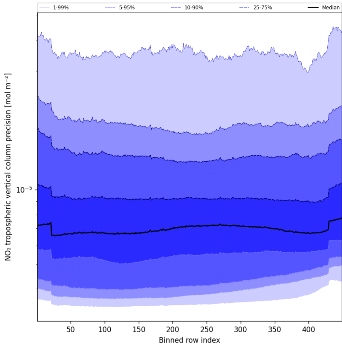
Figure 47: Along track statistics of “NO 2 tropospheric vertical column precision” for 2025-09-29 to 2025-10-01
