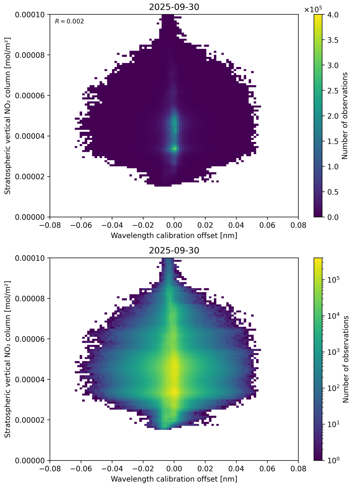
Figure 176: Scatter density plot of “Wavelength calibration offset” against “Stratospheric vertical NO 2 column” for 2025-09-29 to 2025-10-01.
