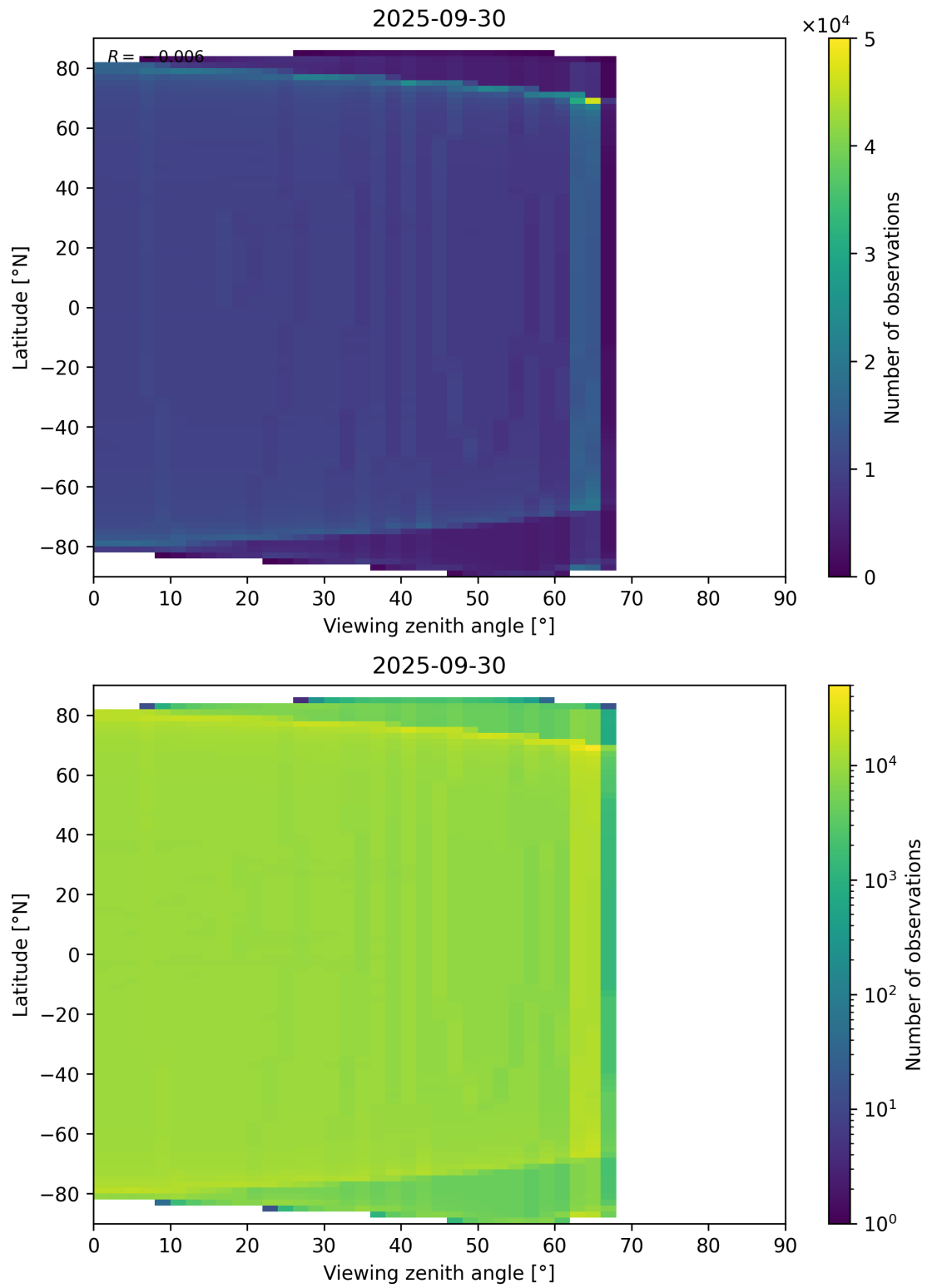
Figure 163: Scatter density plot of “Viewing zenith angle” against “Latitude” for 2025-09-29 to 2025-10-01.
