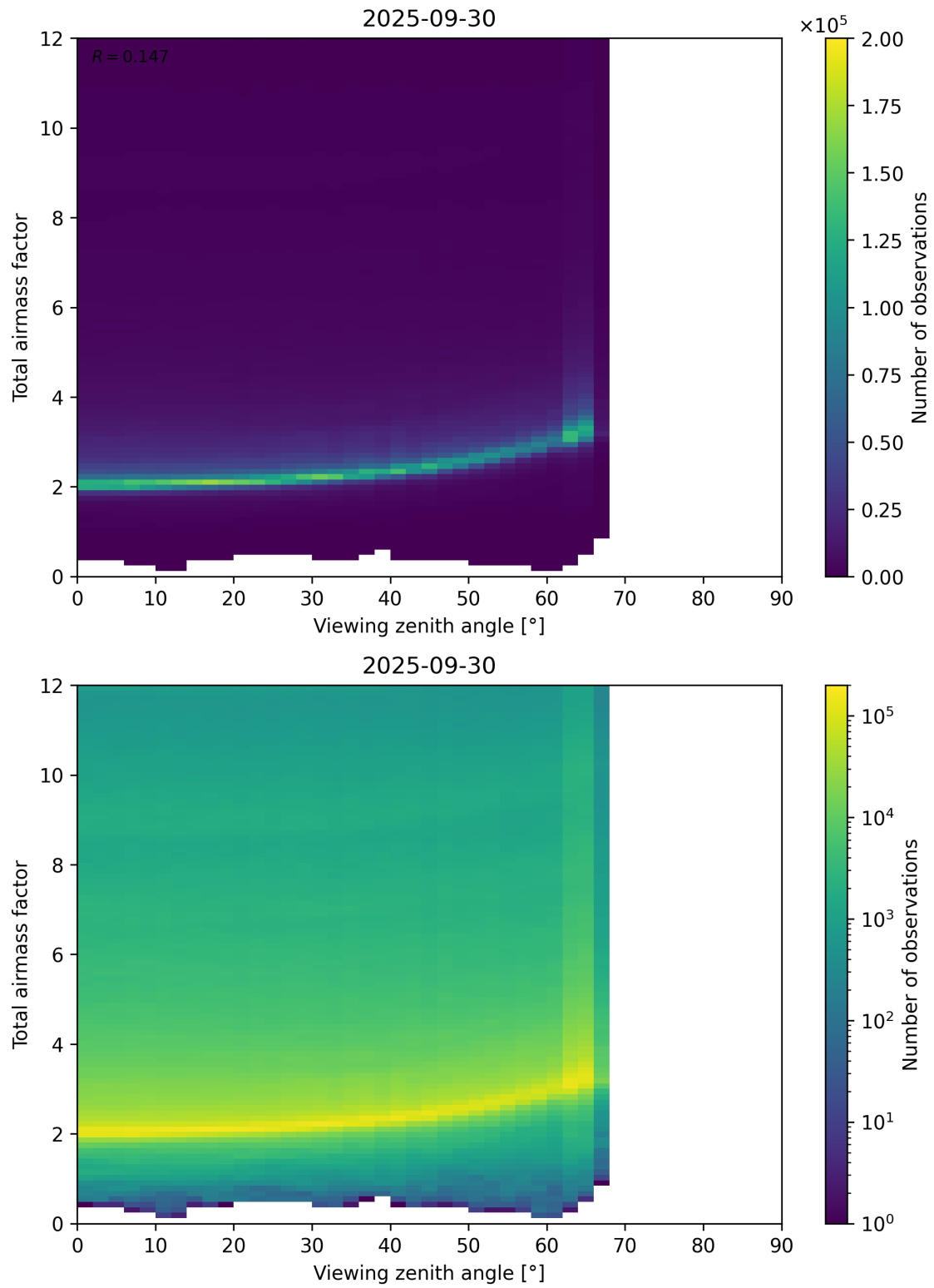
Figure 160: Scatter density plot of “Viewing zenith angle” against “Total airmass factor” for 2025-09-29 to 2025-10-01.
