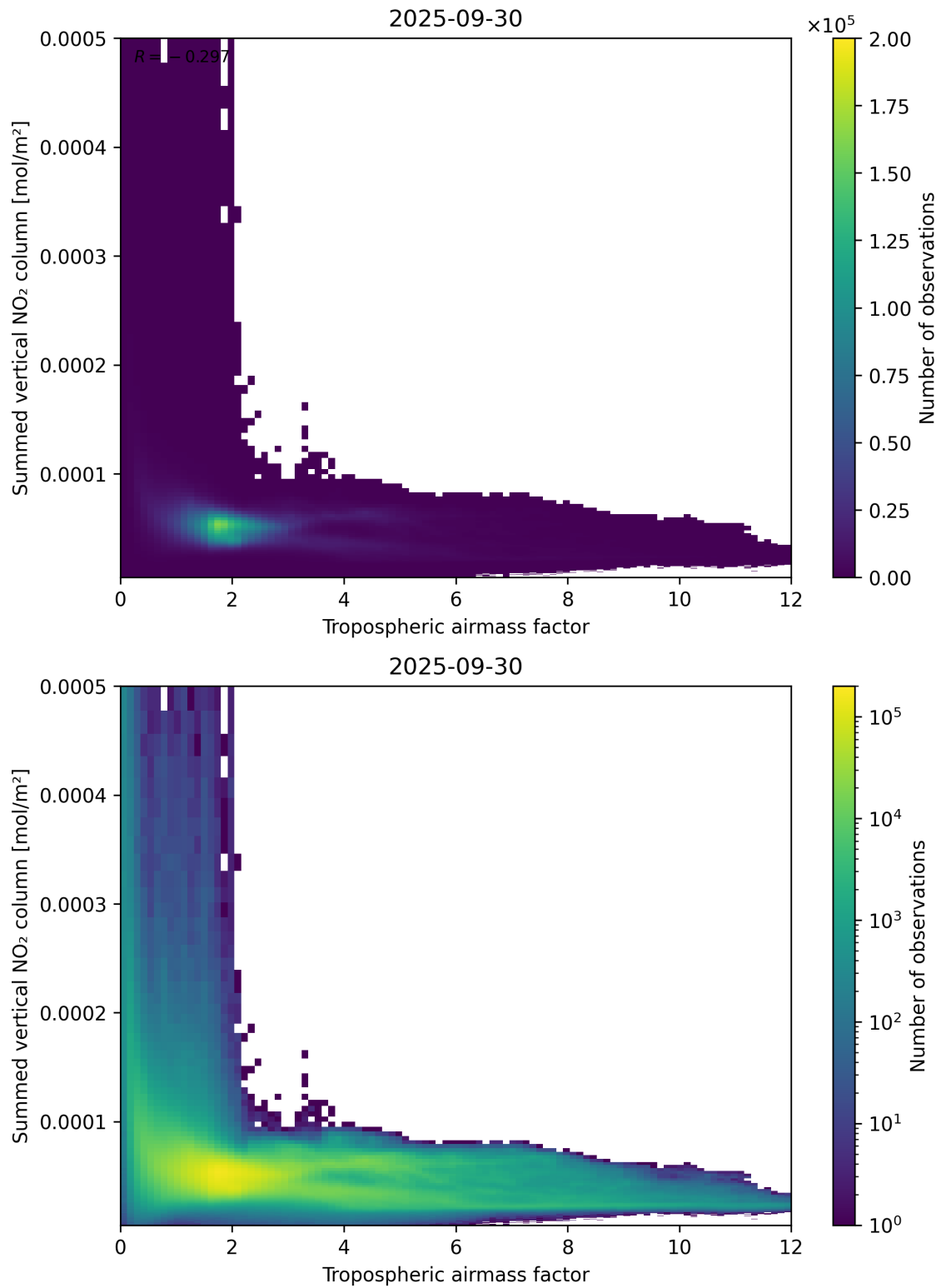
Figure 75: Scatter density plot of “Tropospheric airmass factor” against “Summed vertical NO 2 column” for 2025-09-29 to 2025-10-01.
