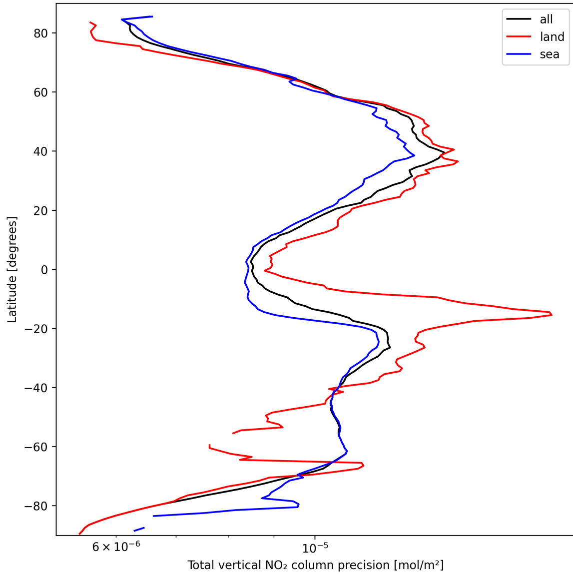
Figure 22: Zonal average of “Total vertical NO 2 column precision” for 2025-09-29 to 2025-10-01.
