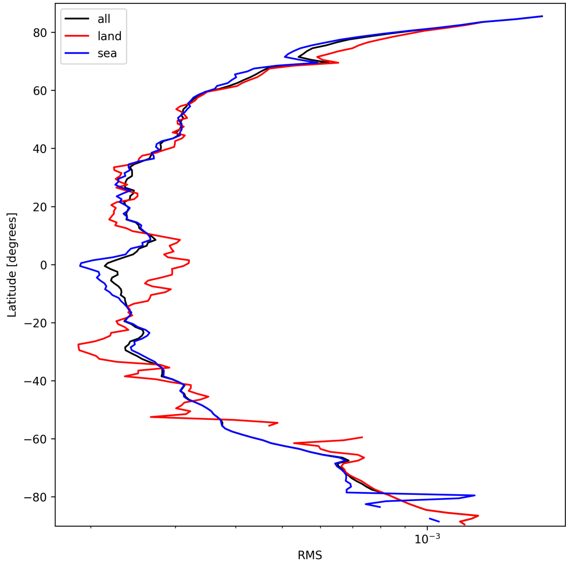
Figure 26: Zonal average of “RMS” for 2025-09-29 to 2025-10-01.
