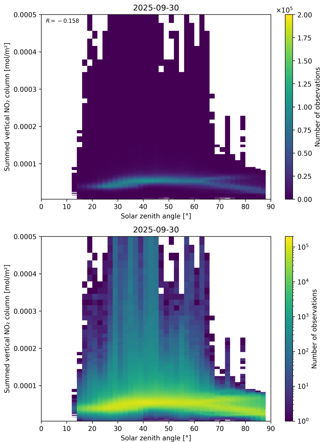
Figure 151: Scatter density plot of “Solar zenith angle” against “Summed vertical NO 2 column” for 2025-09-29 to 2025-10-01.
