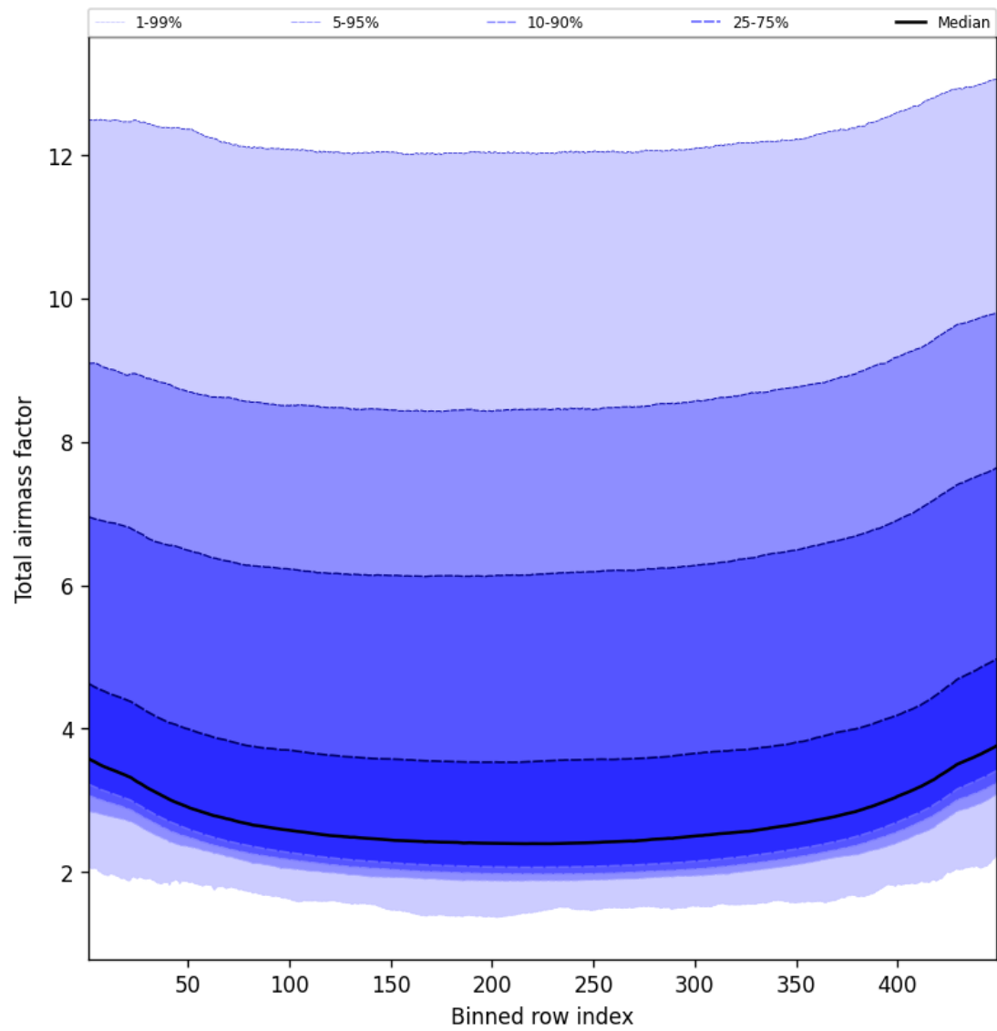
Figure 49: Along track statistics of “Total airmass factor” for 2025-09-29 to 2025-10-01
