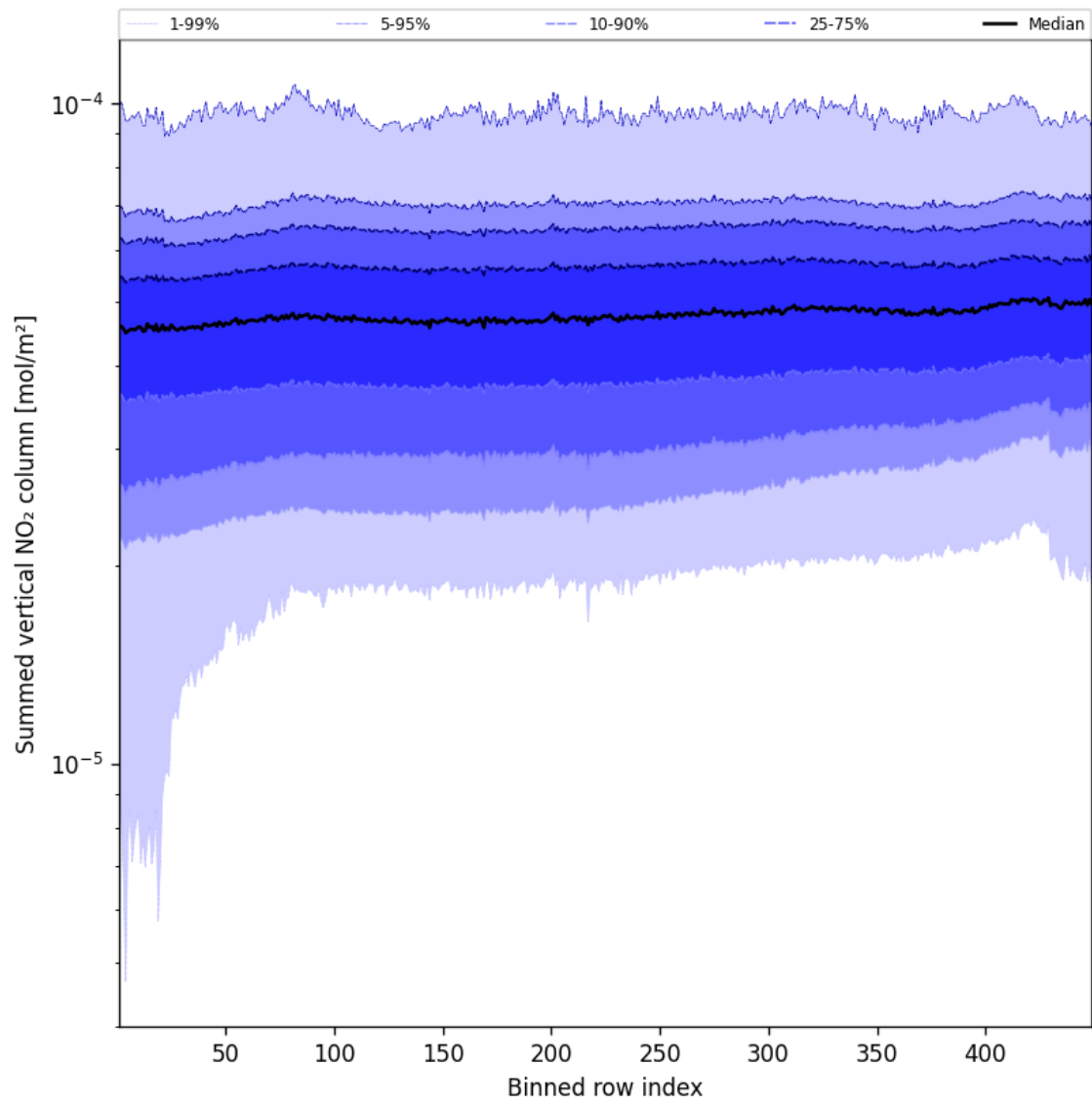
Figure 57: Along track statistics of “Summed vertical NO 2 column” for 2025-09-29 to 2025-10-01
