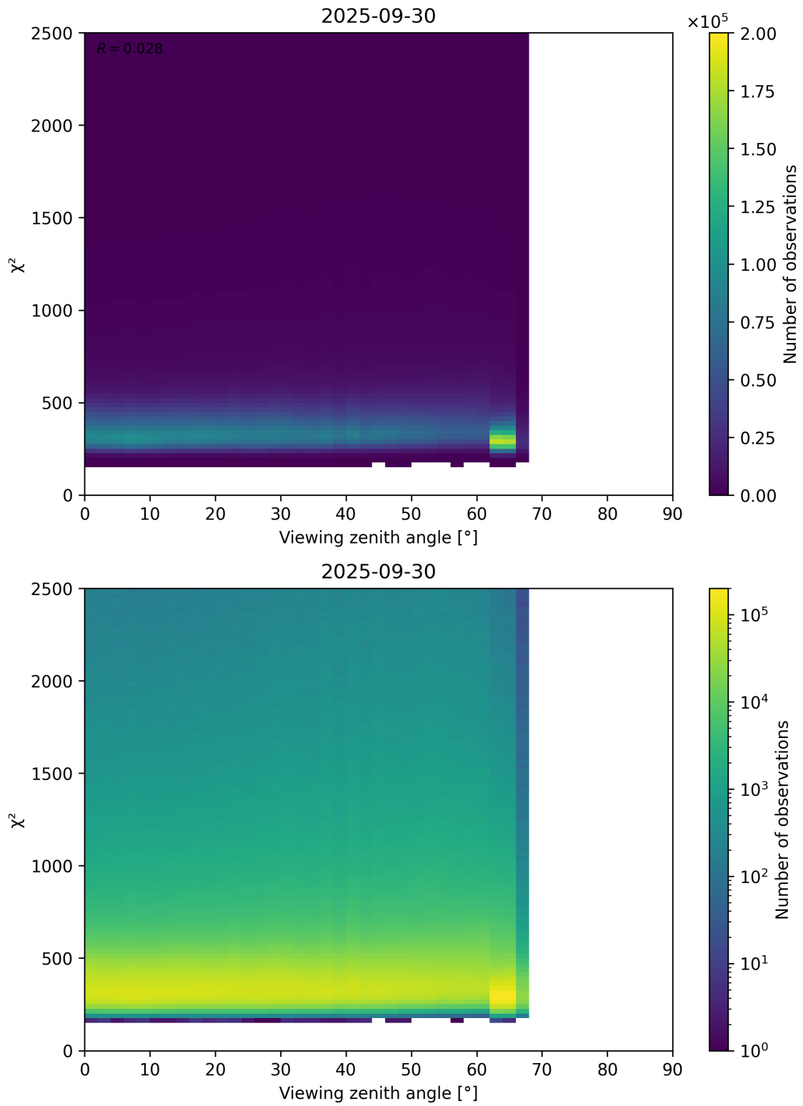
Figure 162: Scatter density plot of “Viewing zenith angle” against “ \chi^2 ” for 2025-09-29 to 2025-10-01.
