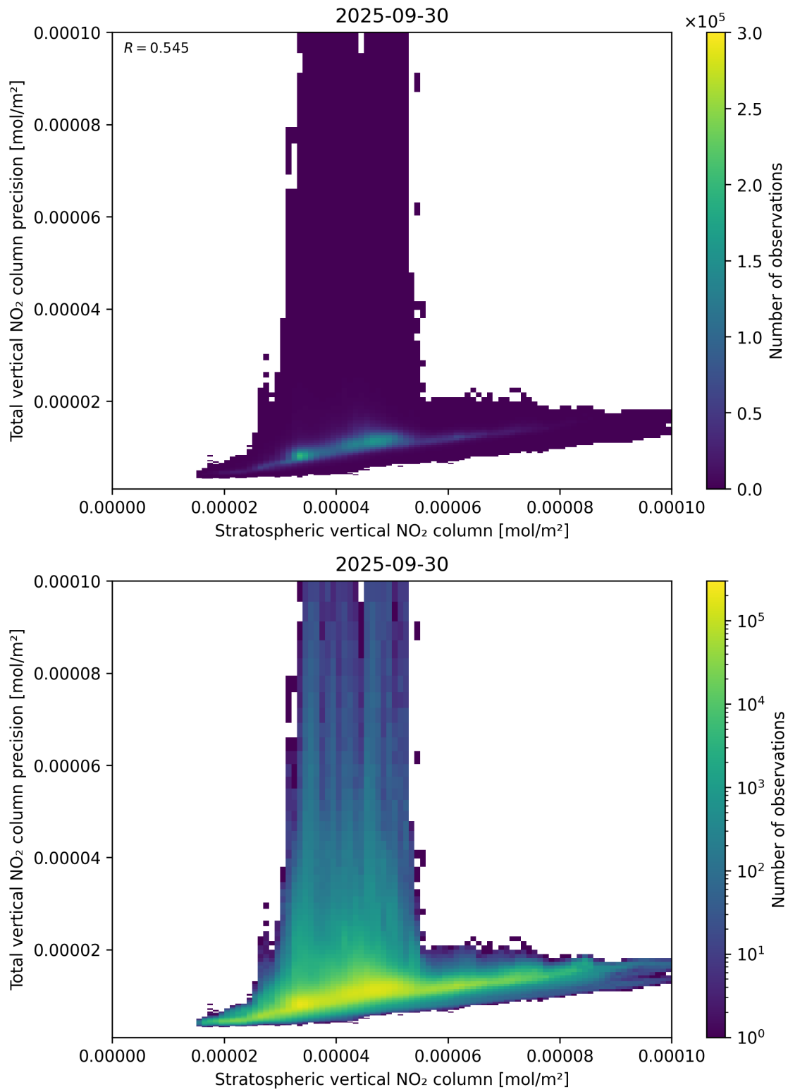
Figure 101: Scatter density plot of “Stratospheric vertical NO 2 column” against “Total vertical NO 2 column precision” for 2025-09-29 to 2025-10-01.
