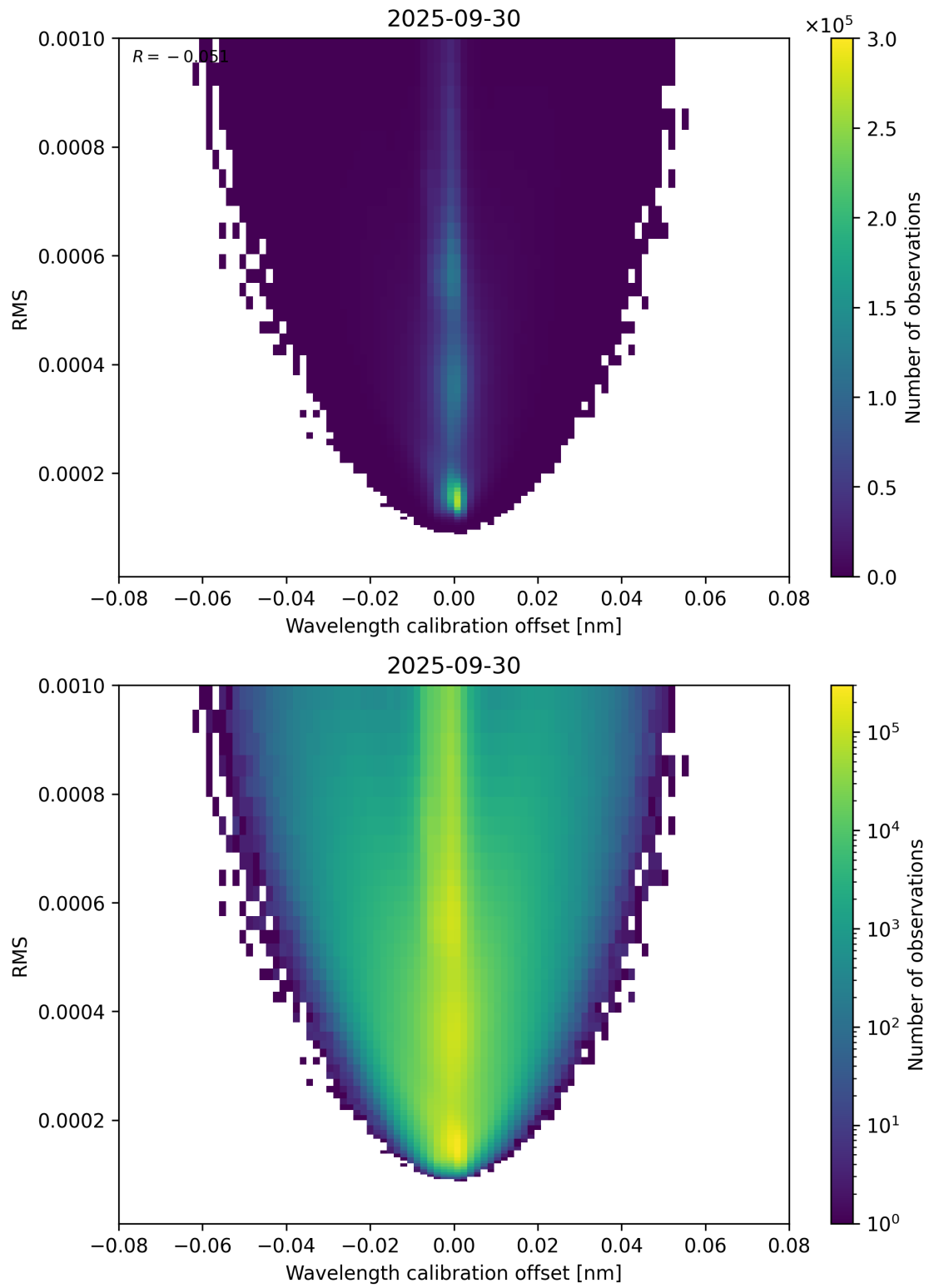
Figure 181: Scatter density plot of “Wavelength calibration offset” against “RMS” for 2025-09-29 to 2025-10-01.
