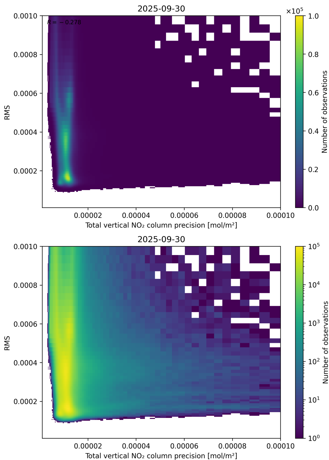
Figure 119: Scatter density plot of “Total vertical NO 2 column precision” against “RMS” for 2025-09-29 to 2025-10-01.
