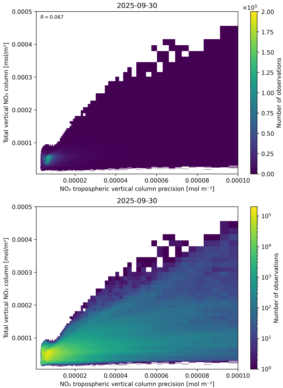
Figure 138: Scatter density plot of “NO 2 tropospheric vertical column precision” against “Total vertical NO 2 column” for 2025-09-29 to 2025-10-01.
