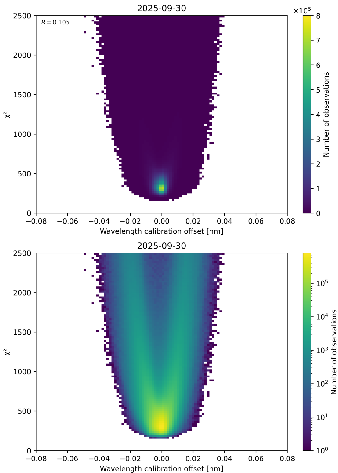
Figure 175: Scatter density plot of “Wavelength calibration offset” against “ \chi^2 ” for 2025-09-29 to 2025-10-01.
