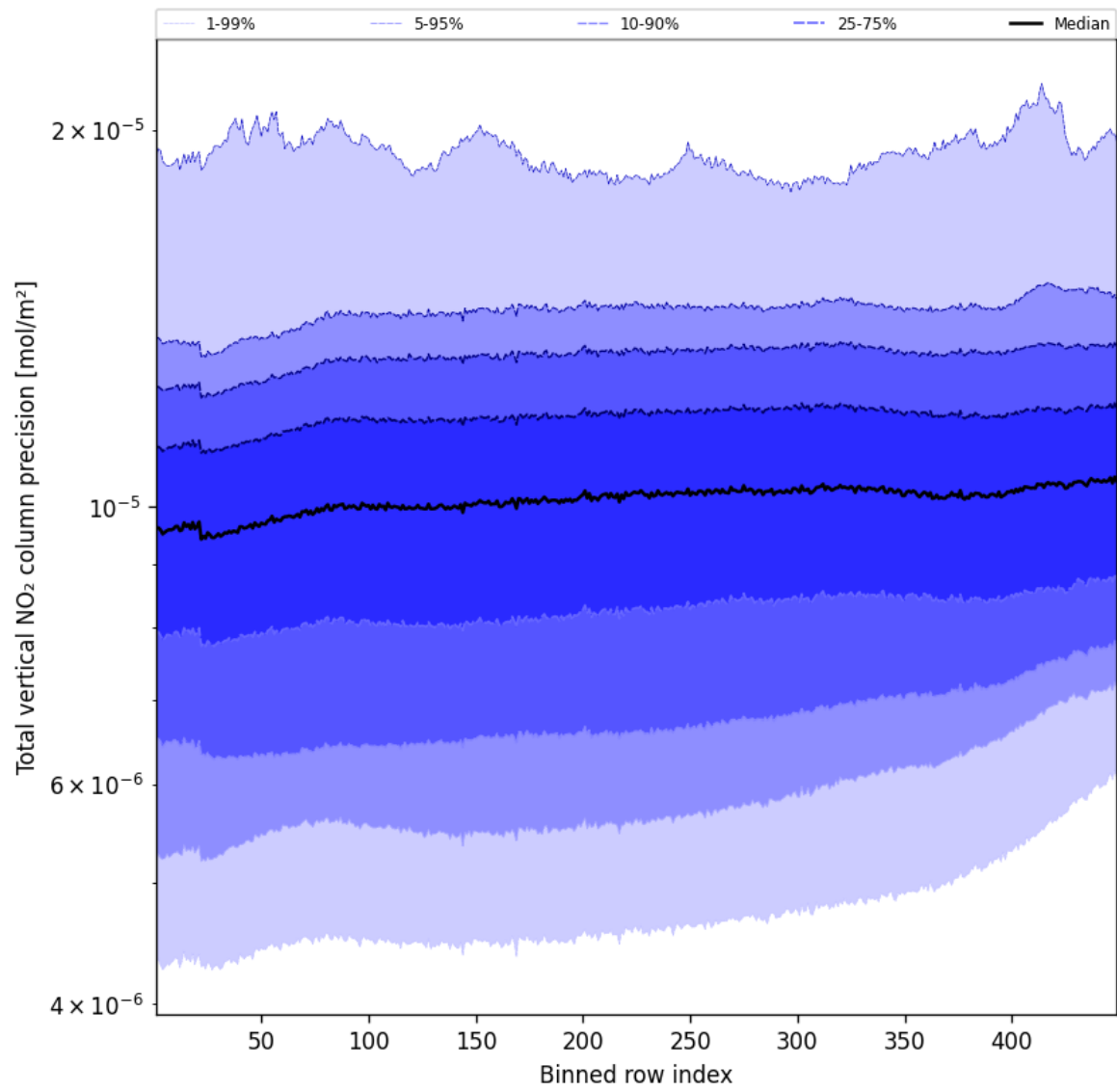
Figure 56: Along track statistics of "Total vertical NO 2 column precision" for 2025-09-29 to 2025-10-01
