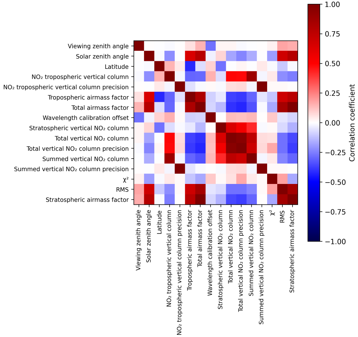
Figure 2: Map of correlation matrix for 2025-09-29 to 2025-10-01.
