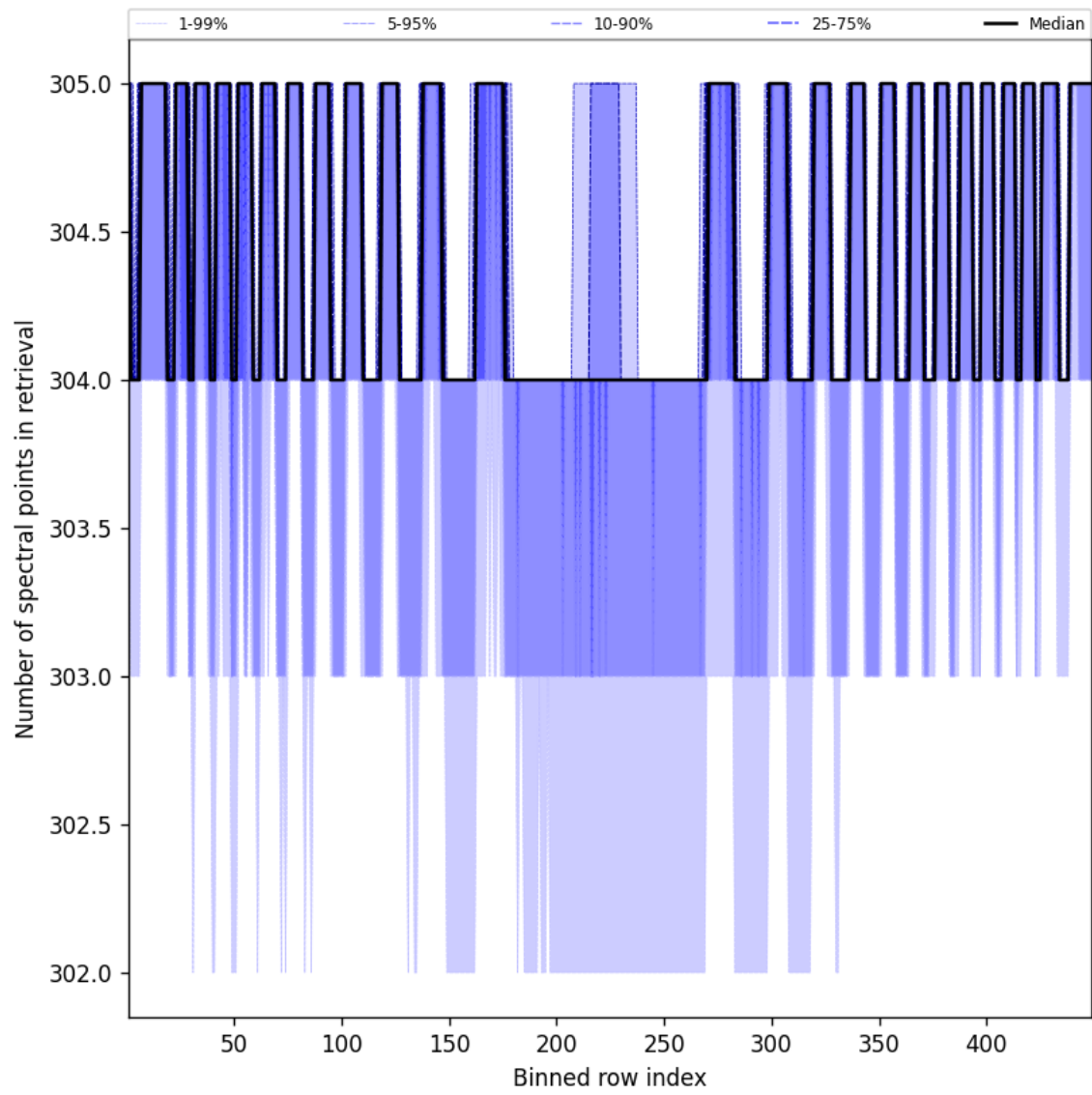
Figure 50: Along track statistics of “Number of spectral points in retrieval” for 2025-09-29 to 2025-10-01
