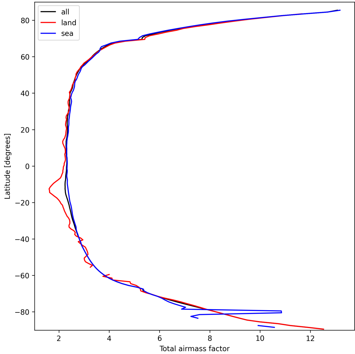
Figure 15: Zonal average of “Total airmass factor” for 2025-09-29 to 2025-10-01.
