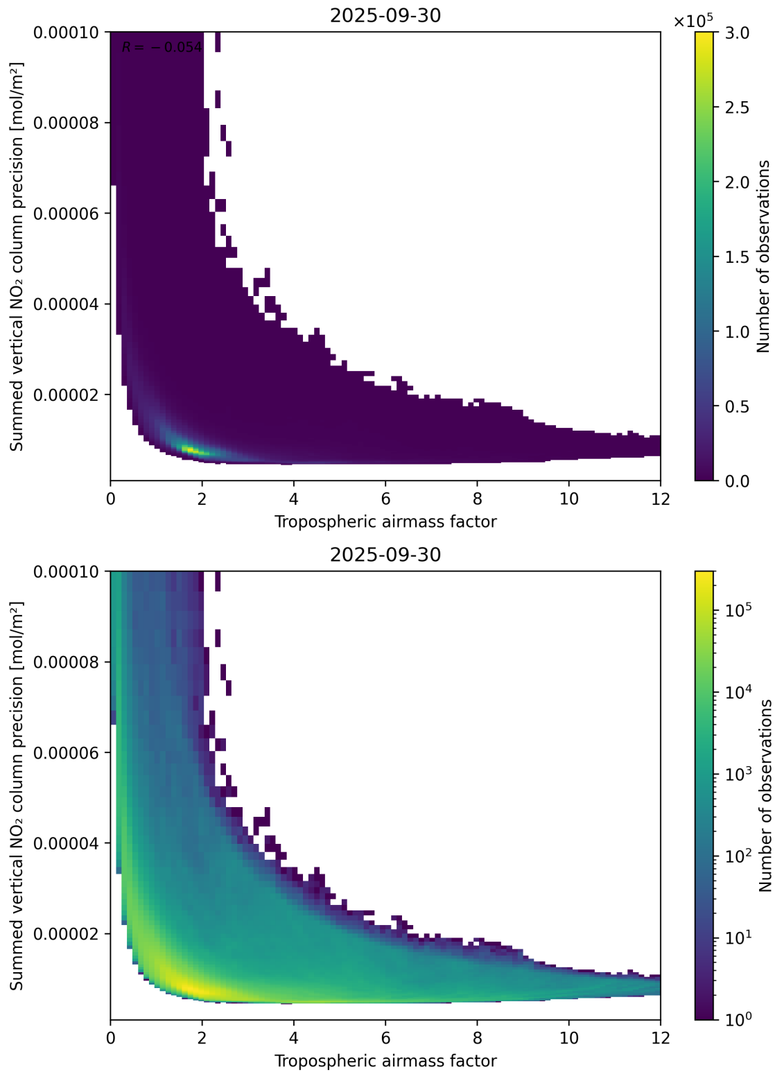
Figure 76: Scatter density plot of “Tropospheric air mass factor” against “Summed vertical NO 2 column precision” for 2025-09-29 to 2025-10-01.
