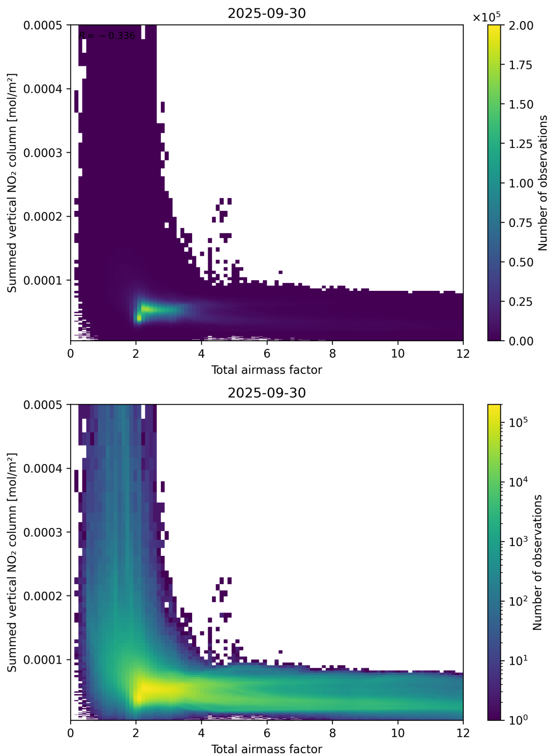
Figure 65: Scatter density plot of “Total airmass factor” against “Summed vertical NO 2 column” for 2025-09-29 to 2025-10-01.
