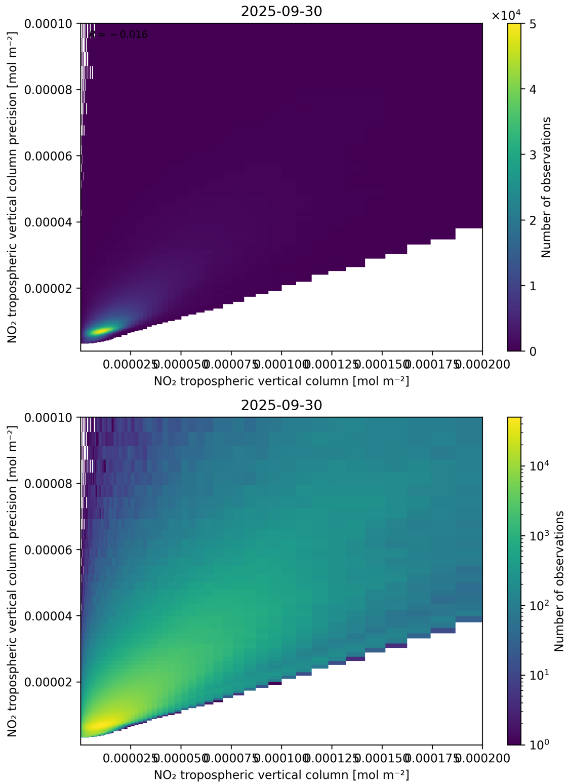
Figure 130: Scatter density plot of “NO 2 tropospheric vertical column” against “NO 2 tropospheric vertical column precision” for 2025-09-29 to 2025-10-01.
