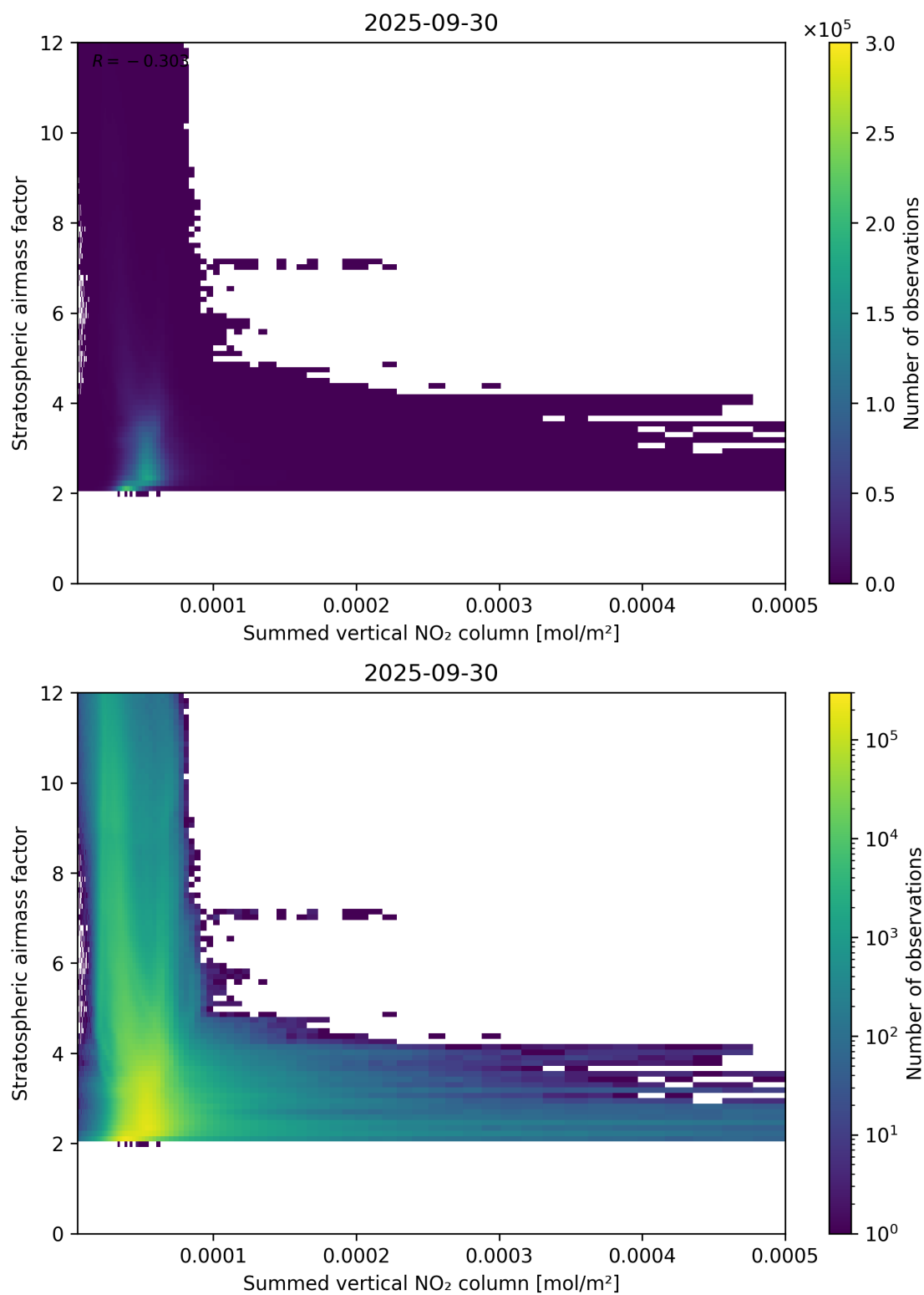
Figure 103: Scatter density plot of “Summed vertical NO 2 column” against “Stratospheric airmass factor” for 2025-09-29 to 2025-10-01.
