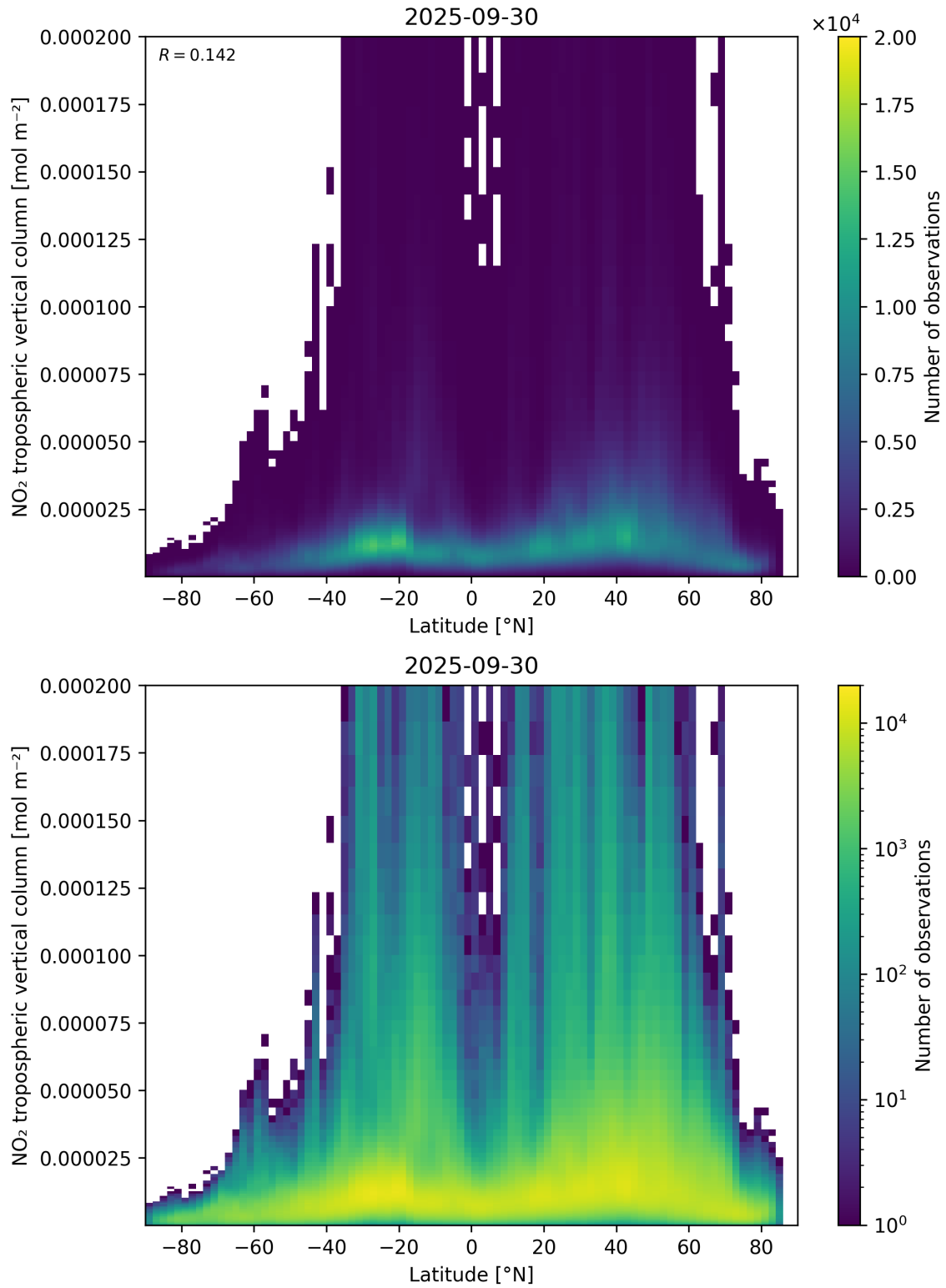
Figure 92: Scatter density plot of “Latitude” against “NO 2 tropospheric vertical column” for 2025-09-29 to 2025-10-01.
