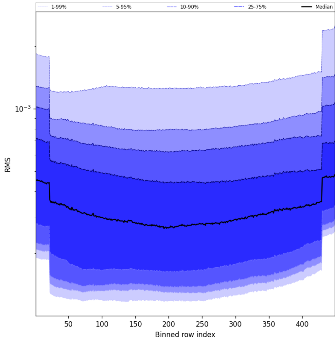
Figure 60: Along track statistics of “RMS” for 2025-09-29 to 2025-10-01
