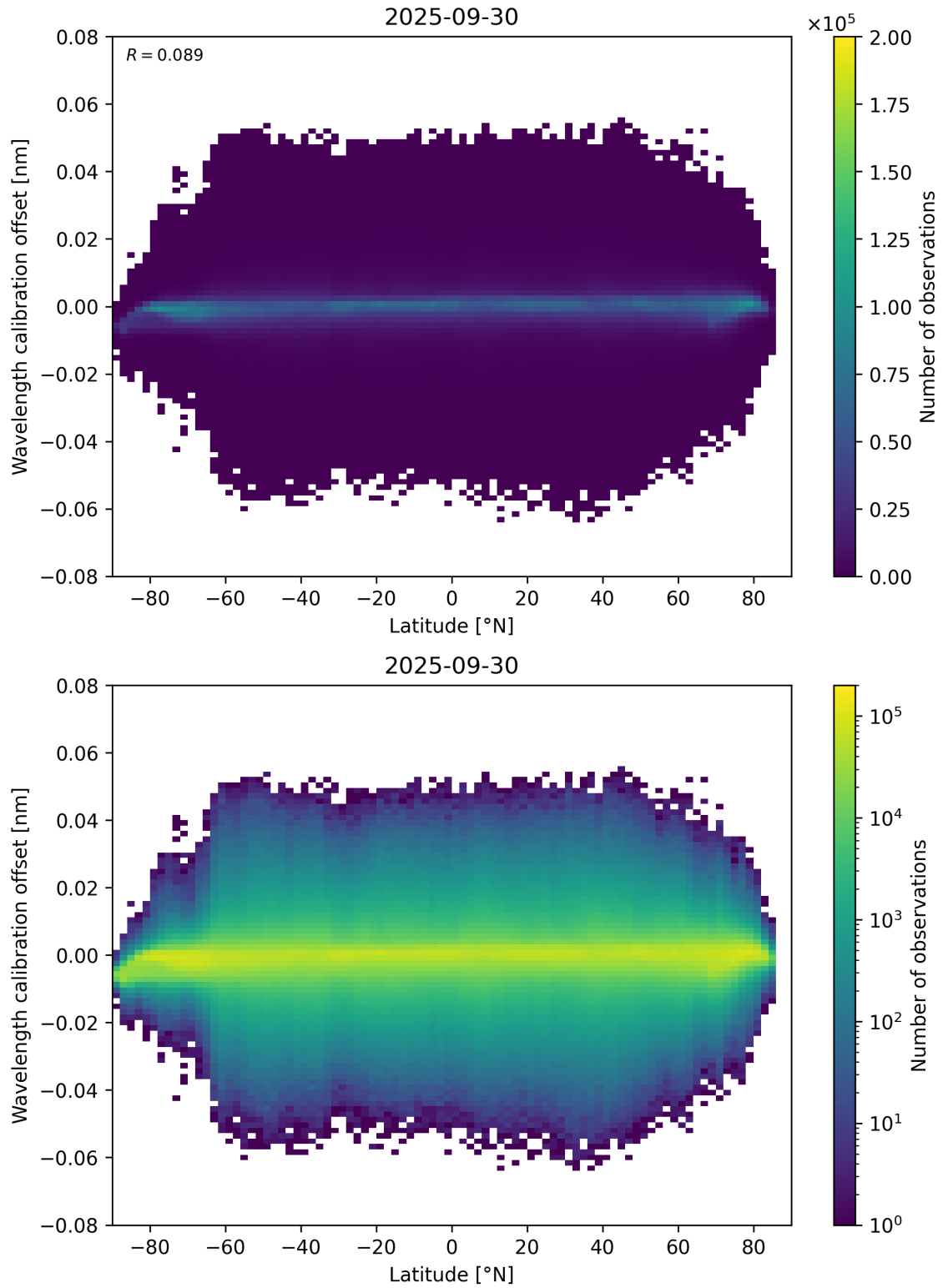
Figure 95: Scatter density plot of “Latitude” against “Wavelength calibration offset” for 2025-09-29 to 2025-10-01.
