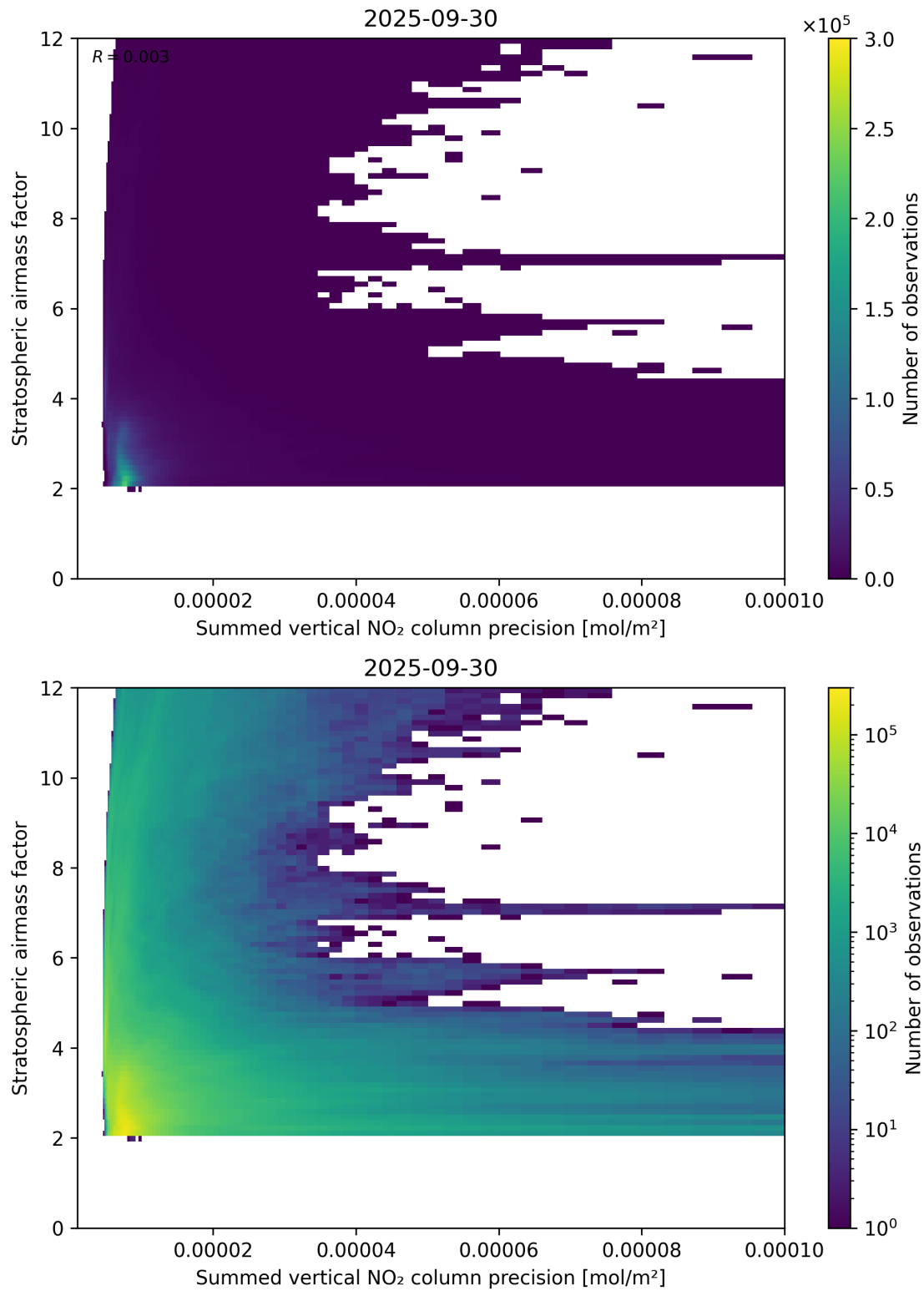
Figure 106: Scatter density plot of “Summed vertical NO 2 column precision” against “Stratospheric airmass factor” for 2025-09-29 to 2025-10-01.
