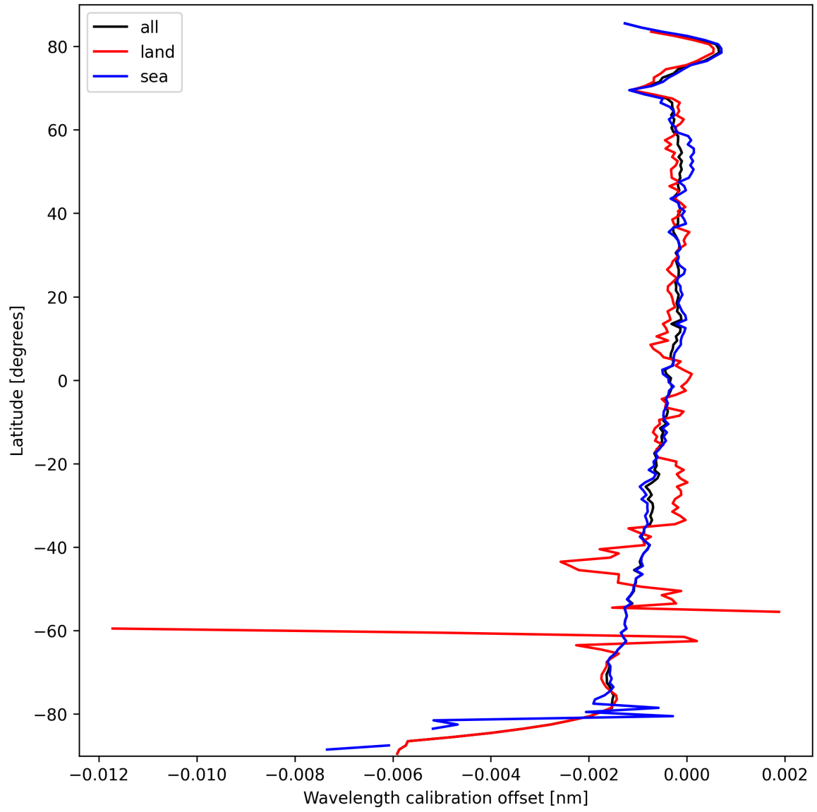
Figure 18: Zonal average of “Wavelength calibration offset” for 2025-09-29 to 2025-10-01.
