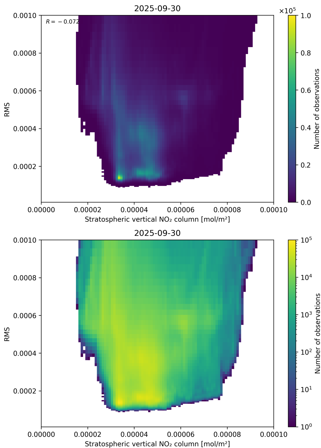
Figure 102: Scatter density plot of “Stratospheric vertical NO 2 column” against “RMS” for 2025-09-29 to 2025-10-01.
