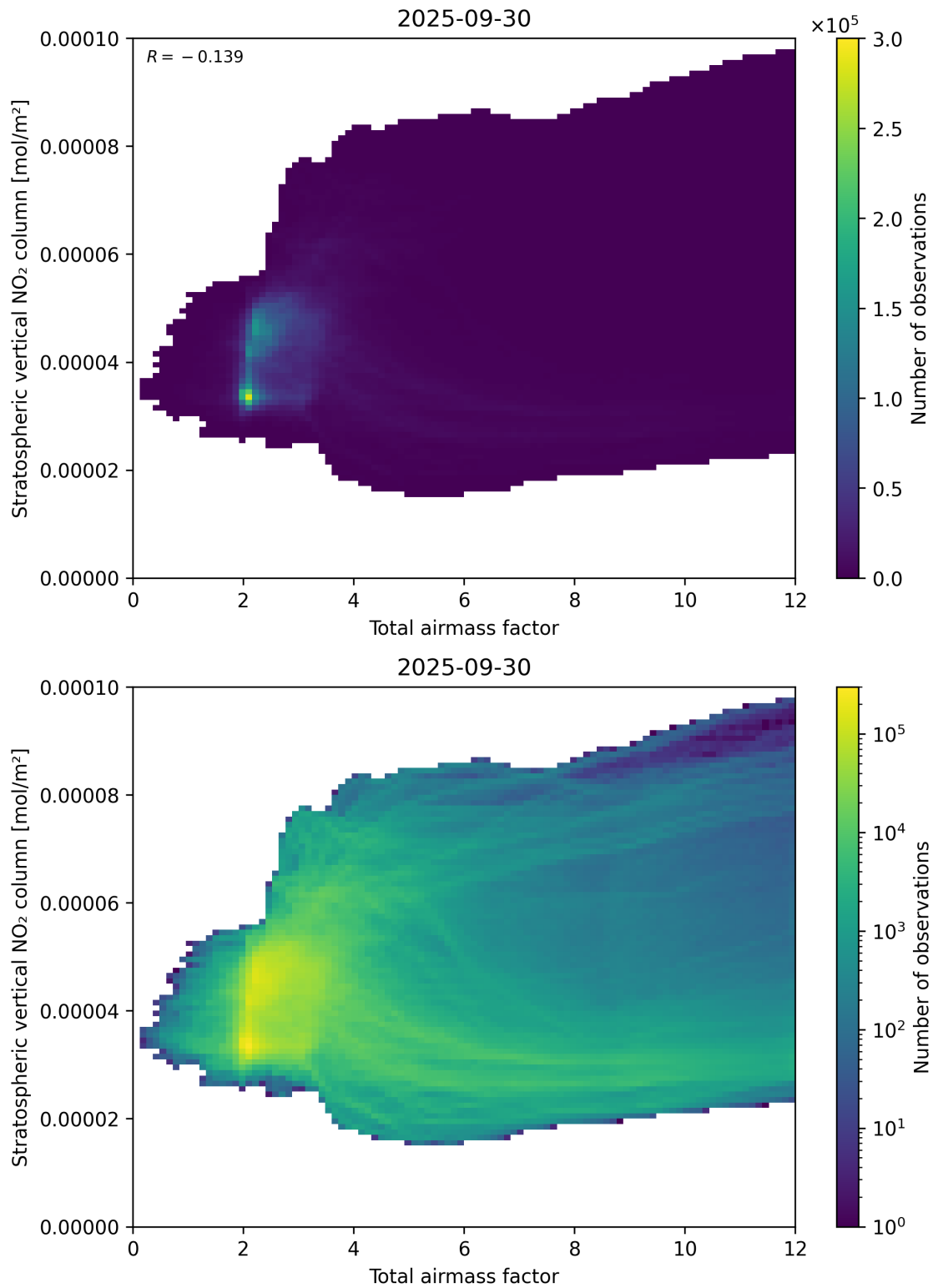
Figure 64: Scatter density plot of “Total airmass factor” against “Stratospheric vertical \text{NO}_2 column” for 2025-09-29 to 2025-10-01.
