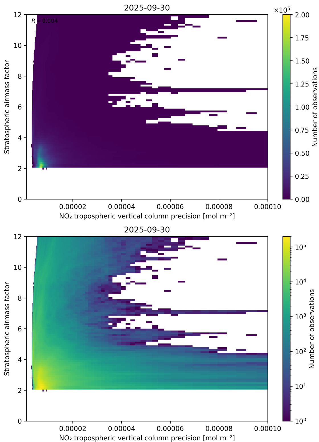
Figure 131: Scatter density plot of “NO 2 tropospheric vertical column precision” against “Stratospheric air mass factor” for 2025-09-29 to 2025-10-01.
