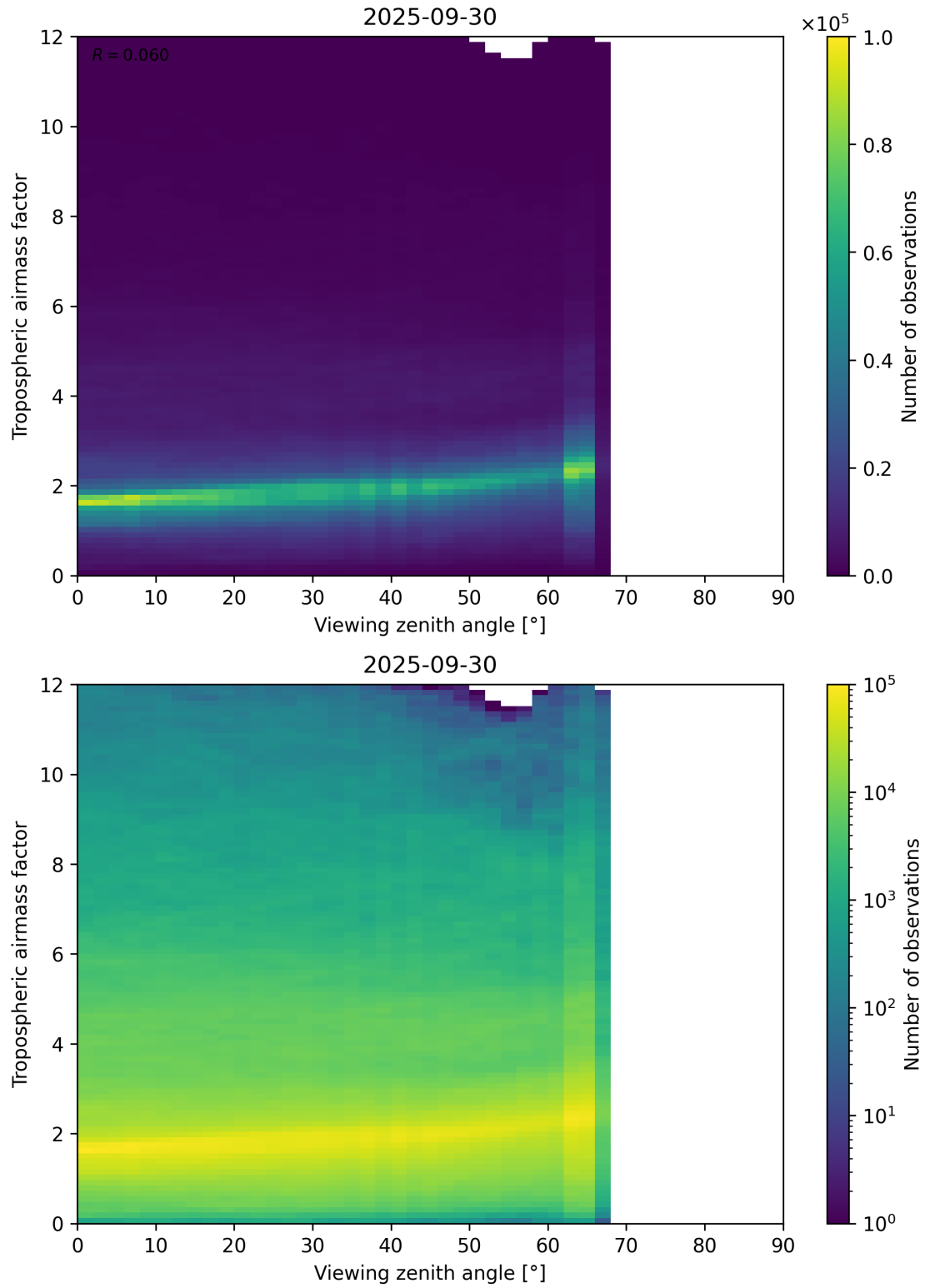
Figure 161: Scatter density plot of “Viewing zenith angle” against “Tropospheric airmass factor” for 2025-09-29 to 2025-10-01.
