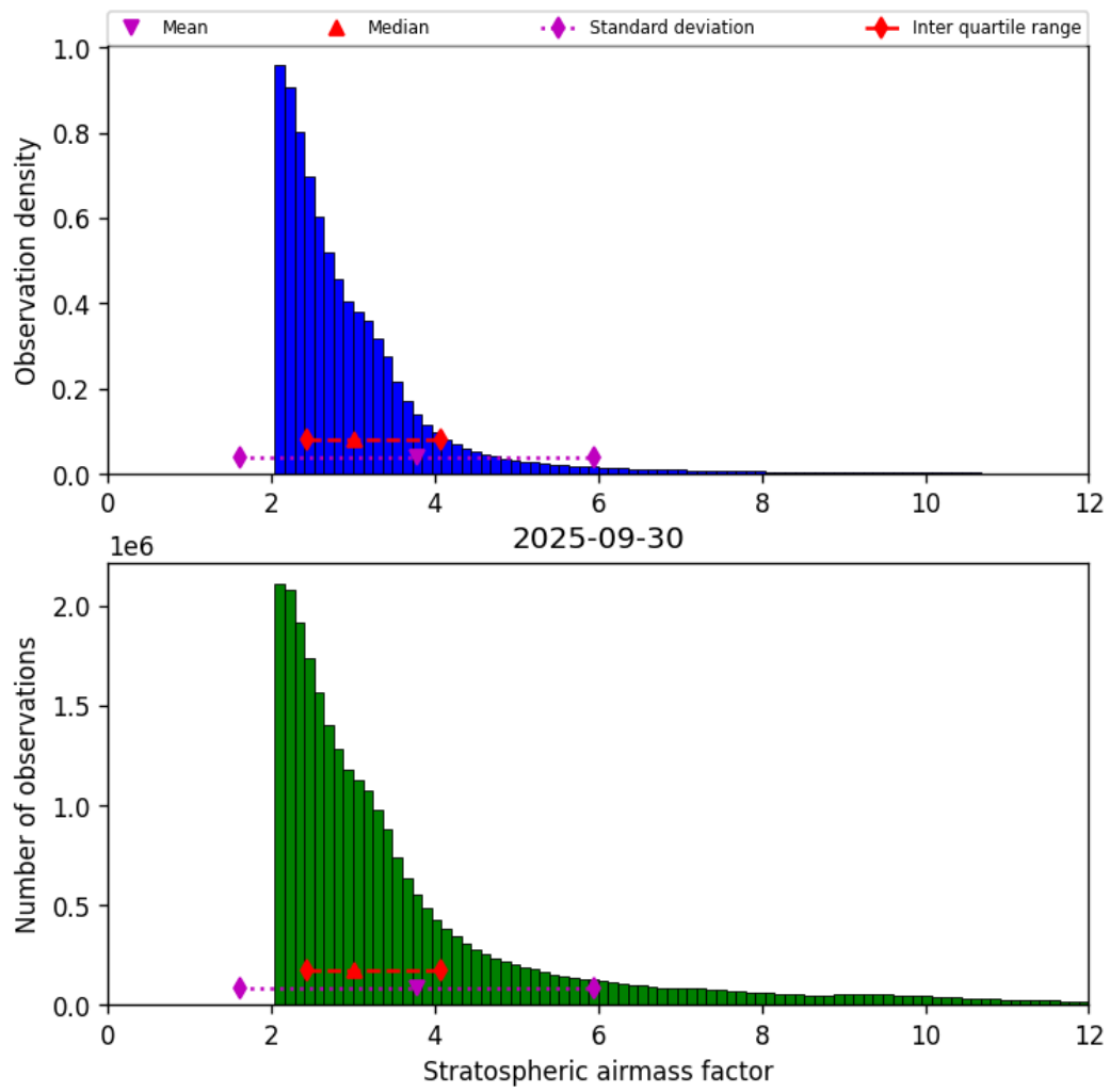
Figure 44: Histogram of “Stratospheric airmass factor” for 2025-09-29 to 2025-10-01
