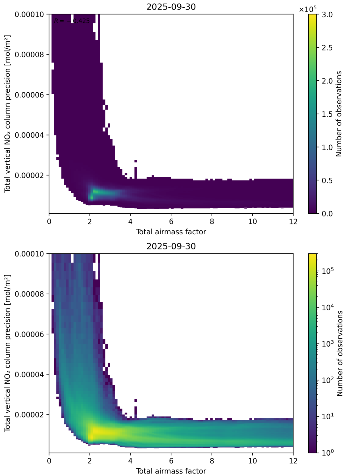
Figure 68: Scatter density plot of “Total airmass factor” against “Total vertical NO 2 column precision” for 2025-09-29 to 2025-10-01.
