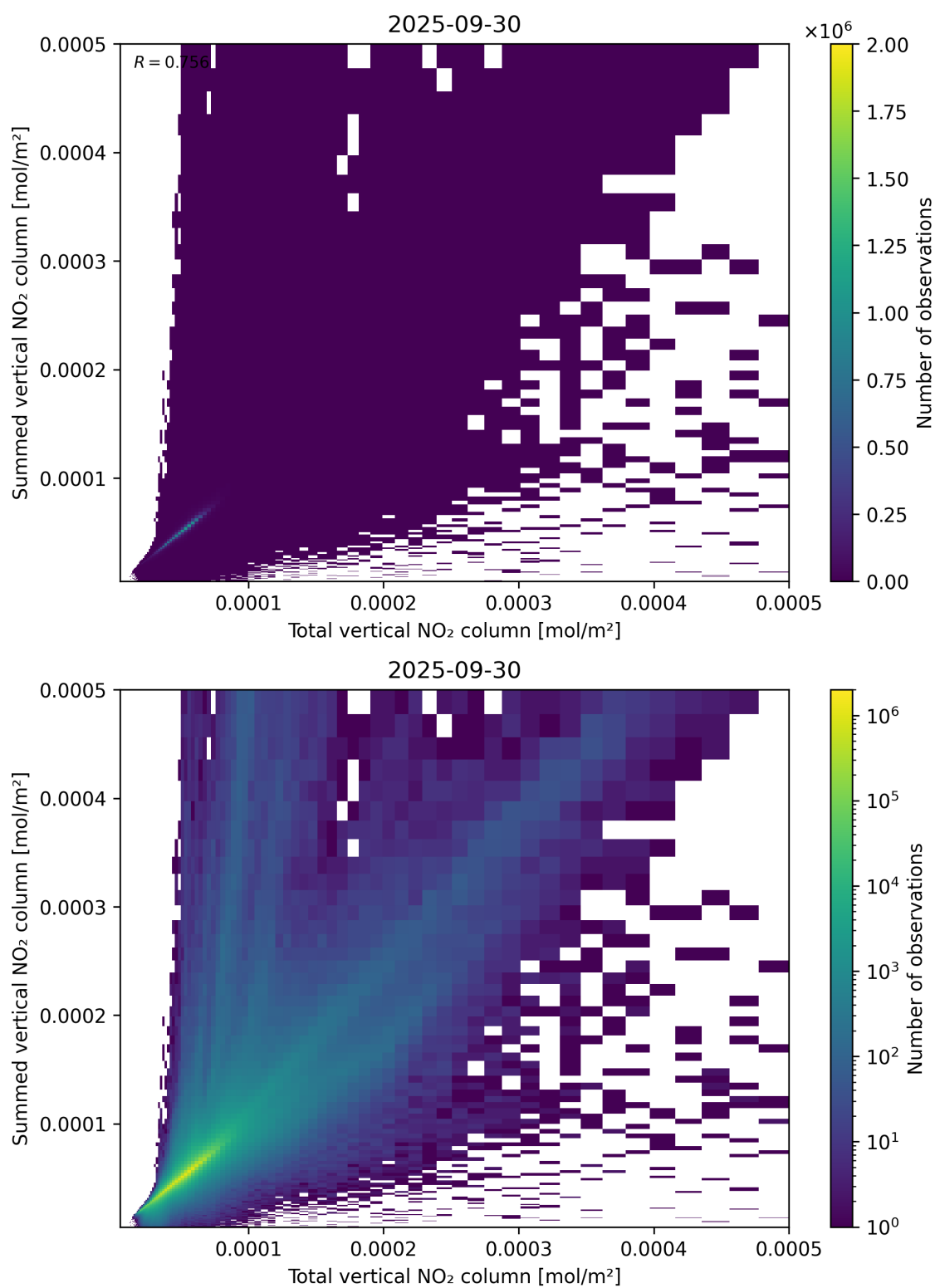
Figure 112: Scatter density plot of “Total vertical NO 2 column” against “Summed vertical NO 2 column” for 2025-09-29 to 2025-10-01.
