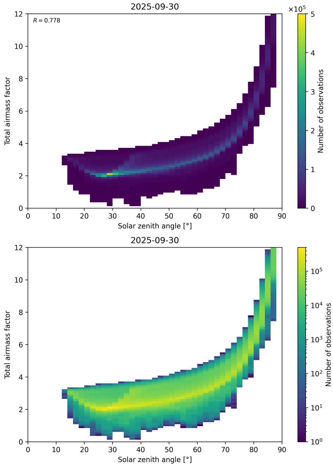
Figure 146: Scatter density plot of “Solar zenith angle” against “Total air mass factor” for 2025-09-29 to 2025-10-01.
