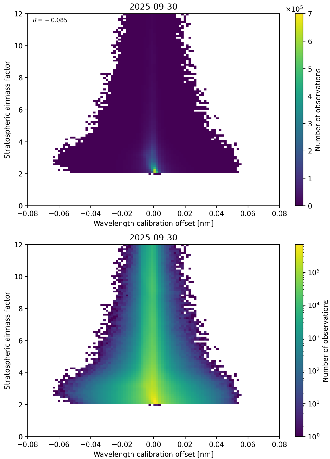
Figure 174: Scatter density plot of “Wavelength calibration offset” against “Stratospheric airmass factor” for 2025-09-29 to 2025-10-01.
