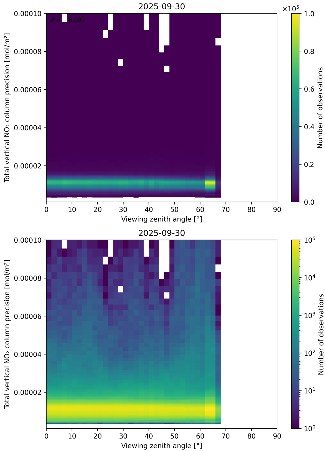
Figure 168: Scatter density plot of “Viewing zenith angle” against “Total vertical NO 2 column precision” for 2025-09-29 to 2025-10-01.
