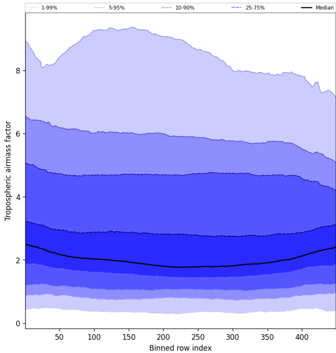
Figure 48: Along track statistics of “Tropospheric air mass factor” for 2025-09-29 to 2025-10-01
