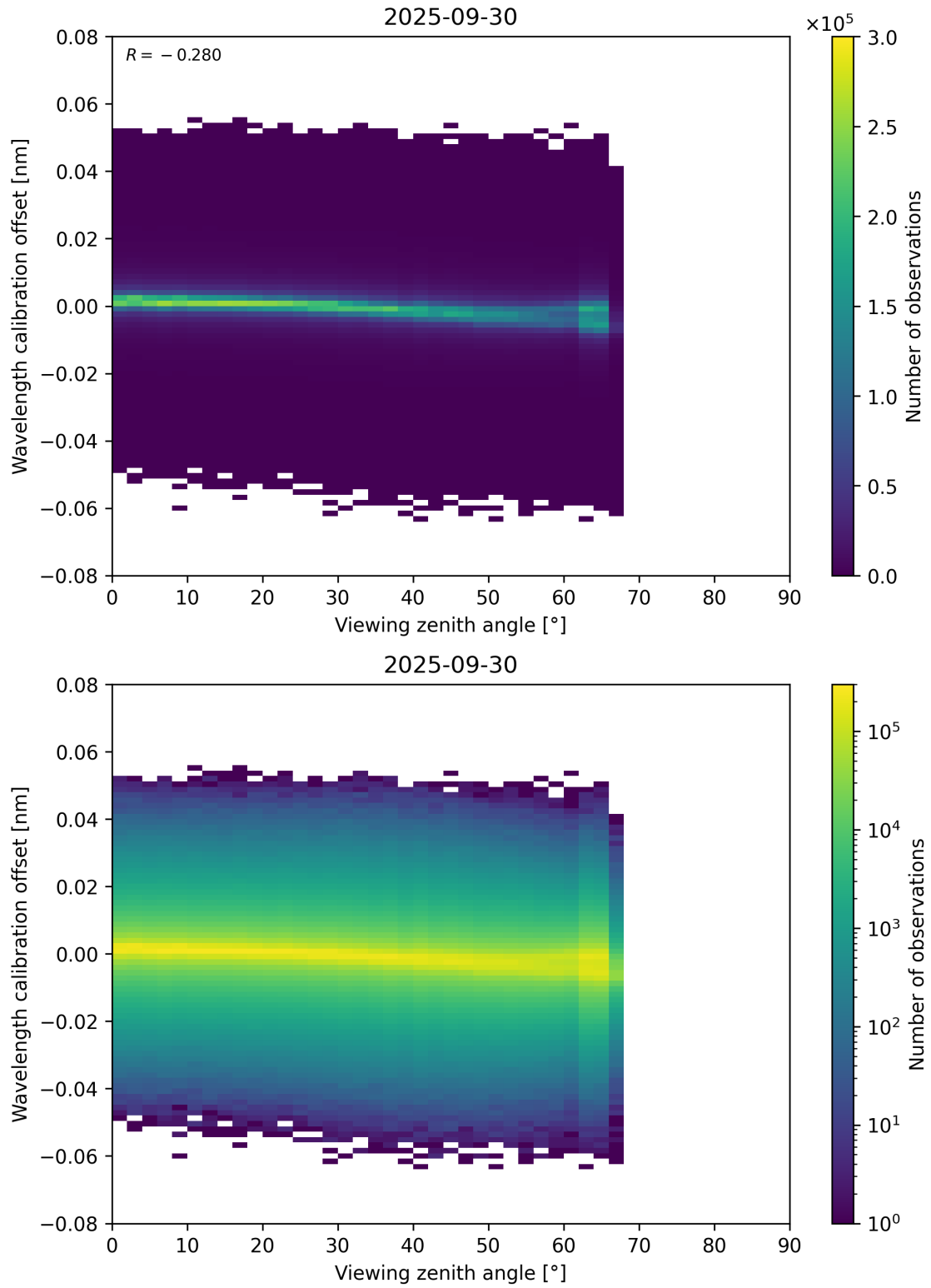
Figure 173: Scatter density plot of “Viewing zenith angle” against “Wavelength calibration offset” for 2025-09-29 to 2025-10-01.
