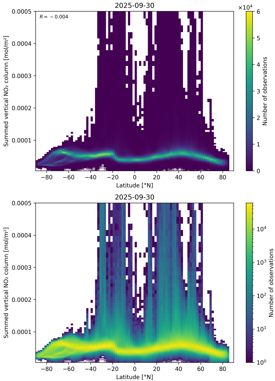
Figure 88: Scatter density plot of “Latitude” against “Summed vertical NO 2 column” for 2025-09-29 to 2025-10-01.
