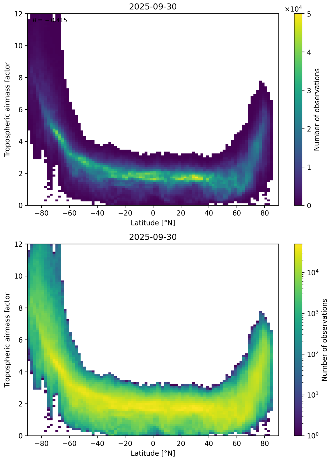
Figure 85: Scatter density plot of “Latitude” against “Tropospheric airmass factor” for 2025-09-29 to 2025-10-01.
