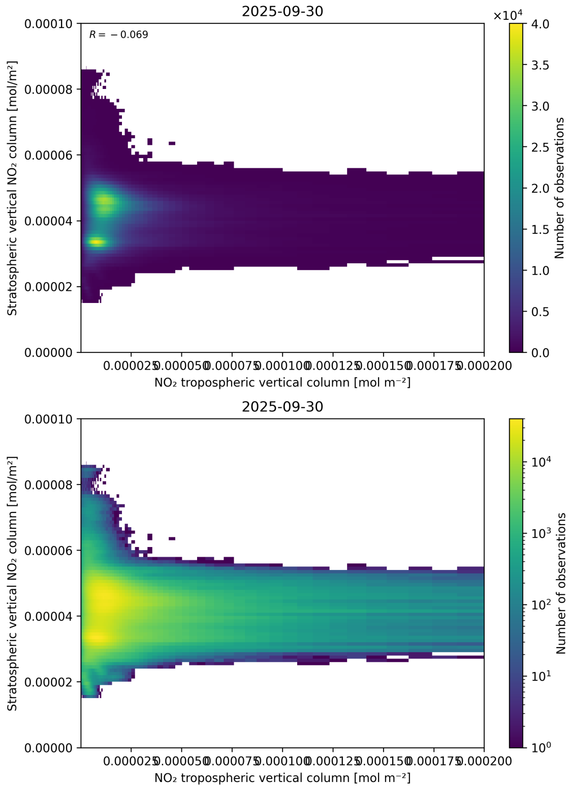
Figure 125: Scatter density plot of “NO 2 tropospheric vertical column” against “Stratospheric vertical NO 2 column” for 2025-09-29 to 2025-10-01.
