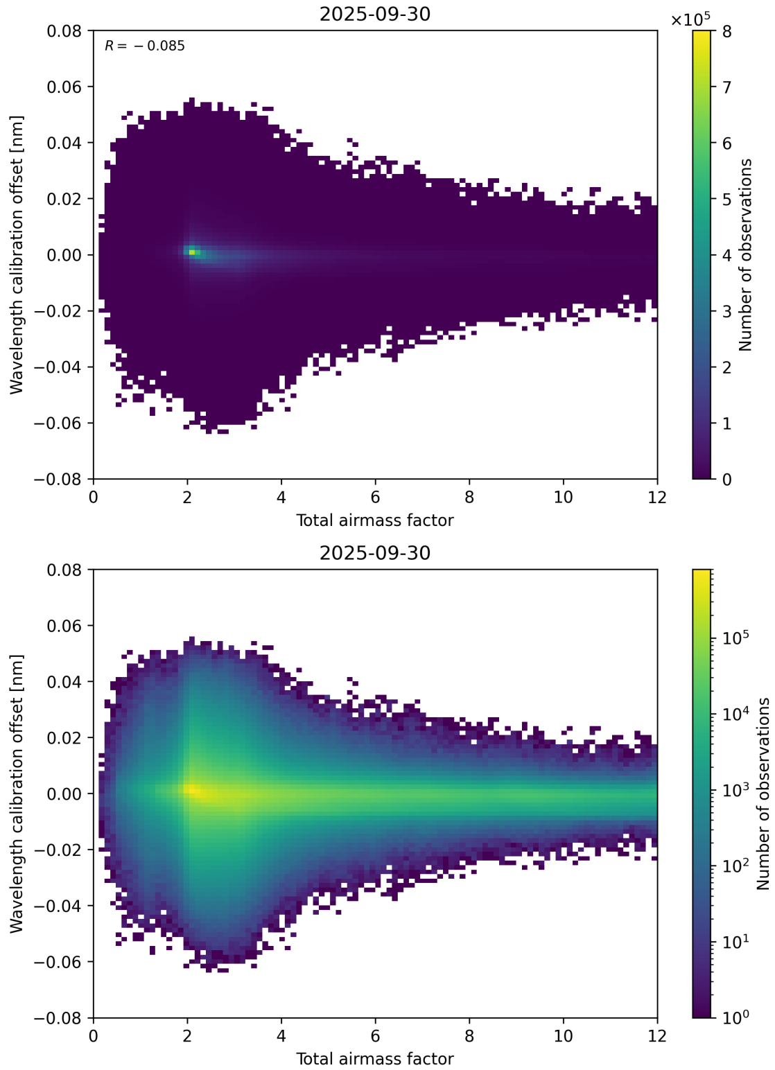
Figure 70: Scatter density plot of “Total airmass factor” against “Wavelength calibration offset” for 2025-09-29 to 2025-10-01.
