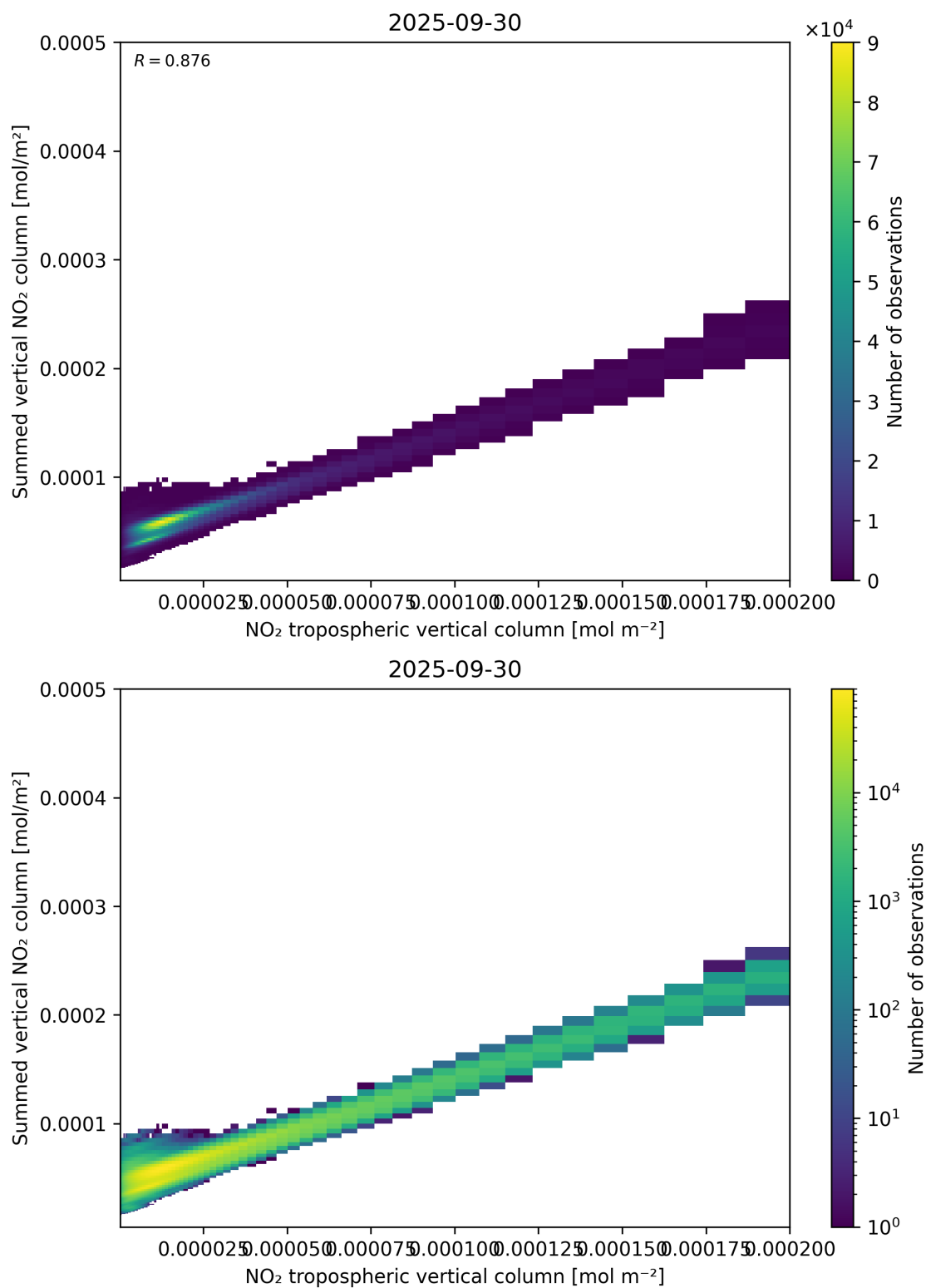
Figure 126: Scatter density plot of “NO 2 tropospheric vertical column” against “Summed vertical NO 2 column” for 2025-09-29 to 2025-10-01.
