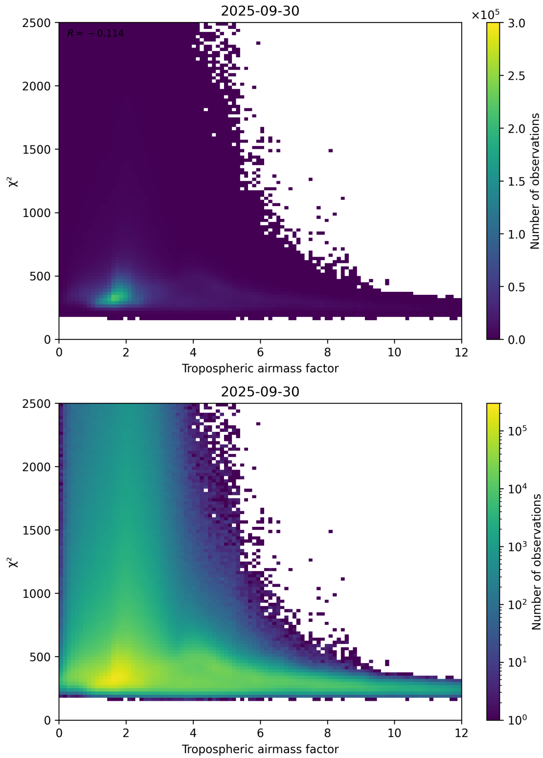
Figure 73: Scatter density plot of “Tropospheric airmass factor” against “ \chi^2 ” for 2025-09-29 to 2025-10-01.
