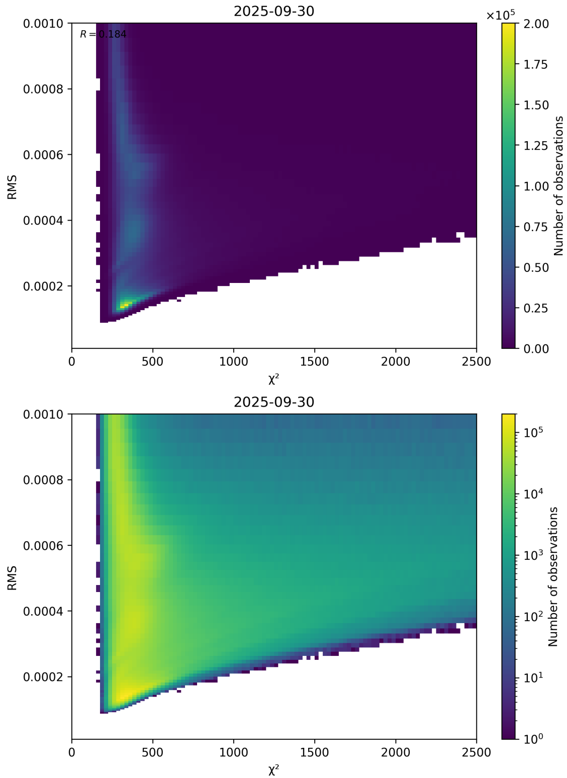
Figure 82: Scatter density plot of “ \chi^2 ” against “RMS” for 2025-09-29 to 2025-10-01.
