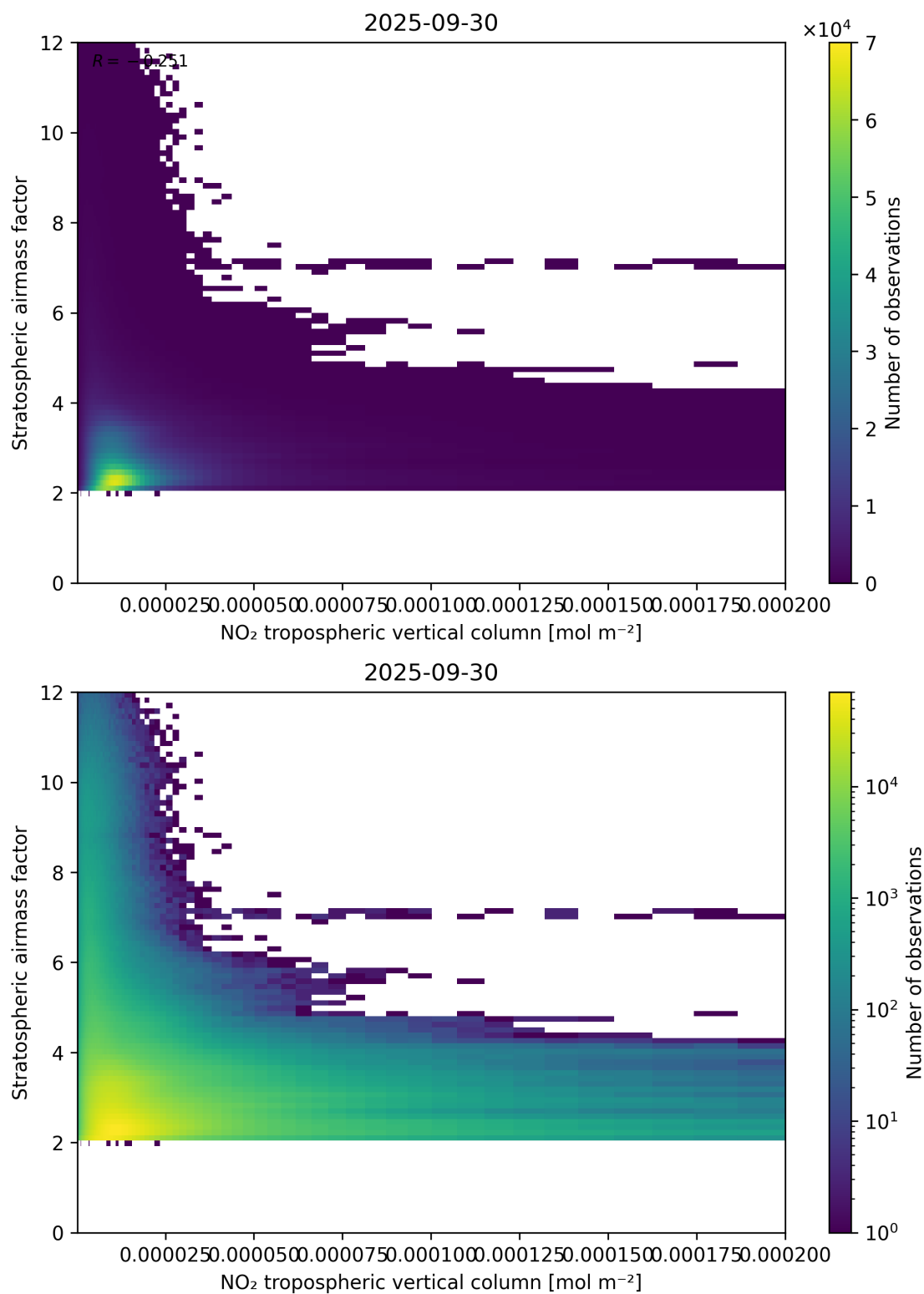
Figure 121: Scatter density plot of “NO 2 tropospheric vertical column” against “Stratospheric air mass factor” for 2025-09-29 to 2025-10-01.
