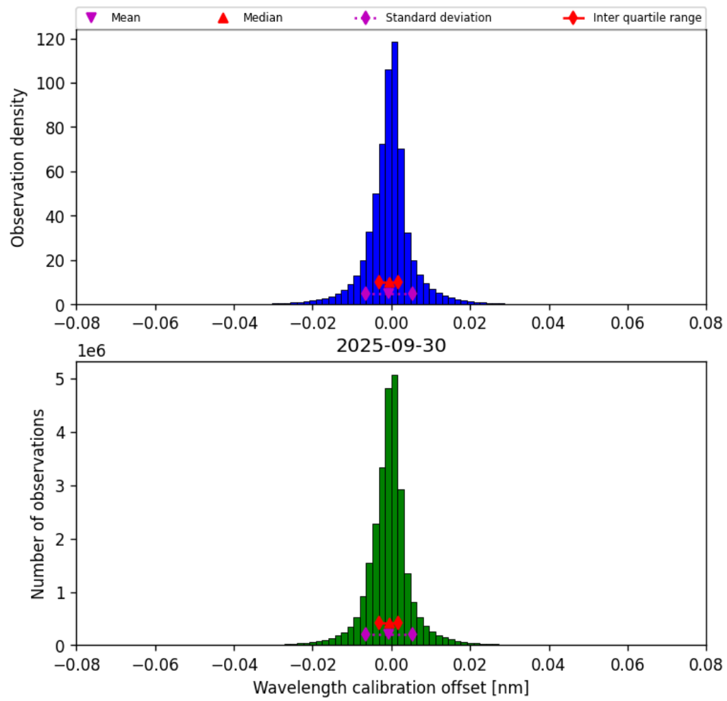
Figure 35: Histogram of “Wavelength calibration offset” for 2025-09-29 to 2025-10-01
