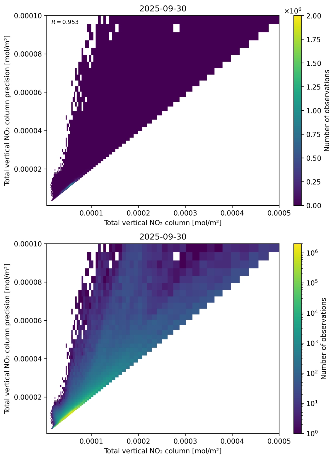
Figure 114: Scatter density plot of “Total vertical NO 2 column” against “Total vertical NO 2 column precision” for 2025-09-29 to 2025-10-01.
