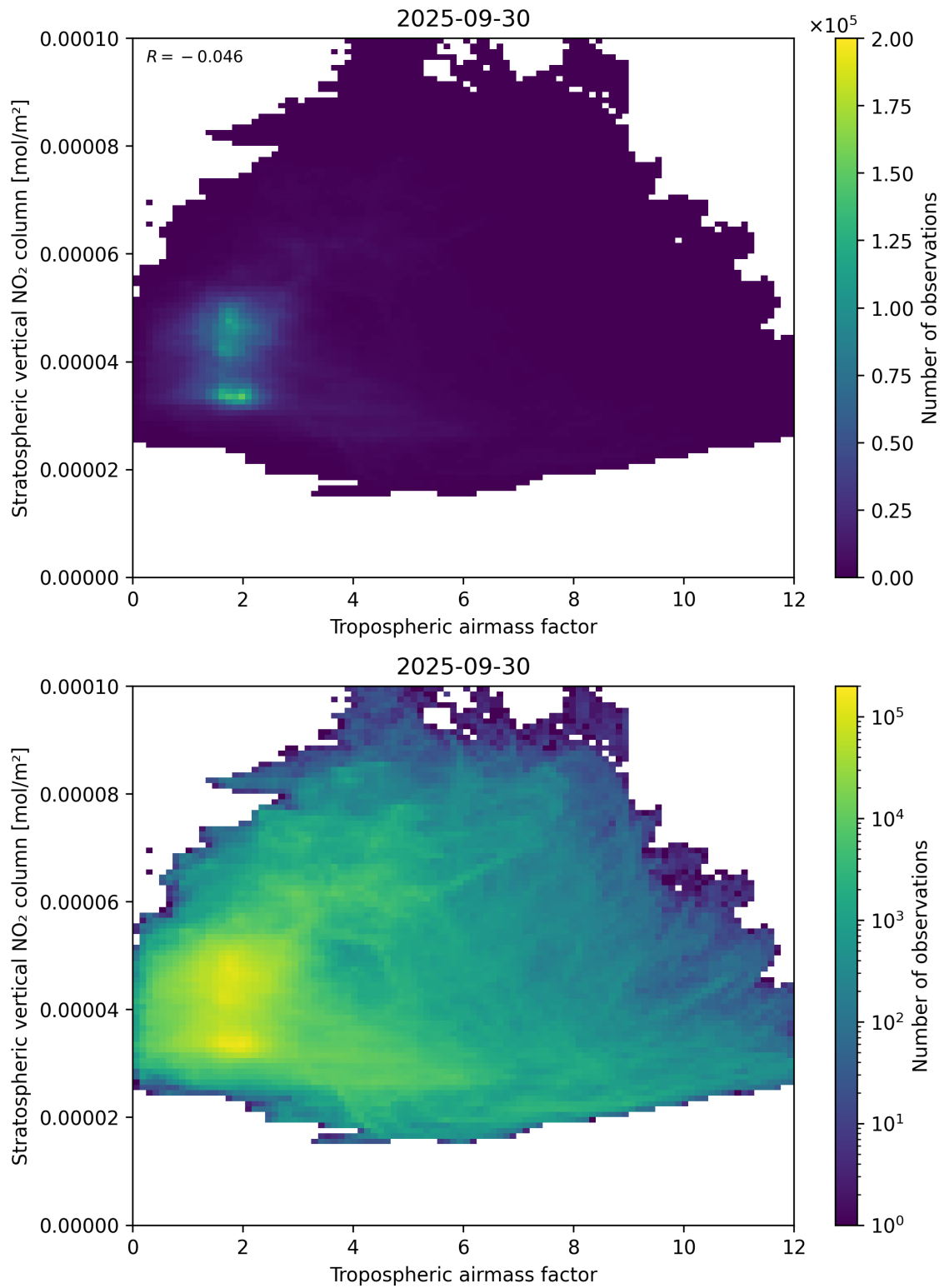
Figure 74: Scatter density plot of “Tropospheric air mass factor” against “Stratospheric vertical NO 2 column” for 2025-09-29 to 2025-10-01.
