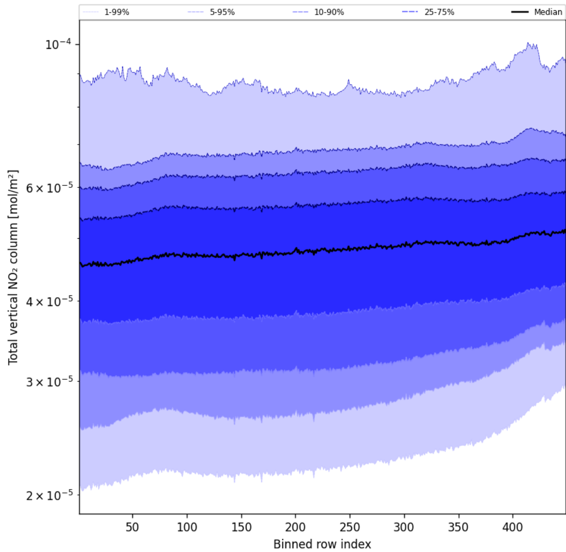
Figure 55: Along track statistics of “Total vertical NO 2 column” for 2025-09-29 to 2025-10-01
