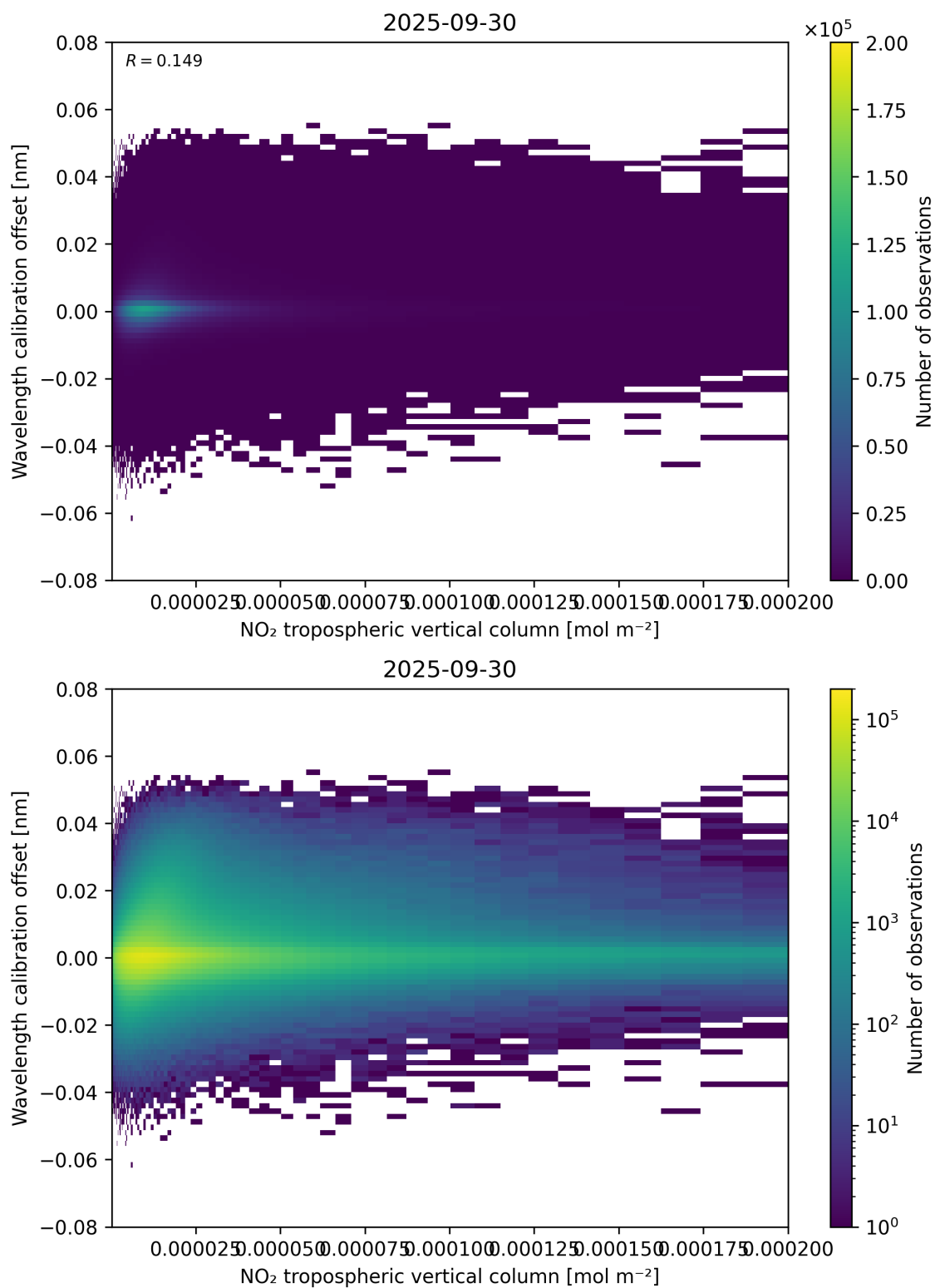
Figure 143: Scatter density plot of “NO 2 tropospheric vertical column” against “Wavelength calibration offset” for 2025-09-29 to 2025-10-01.
