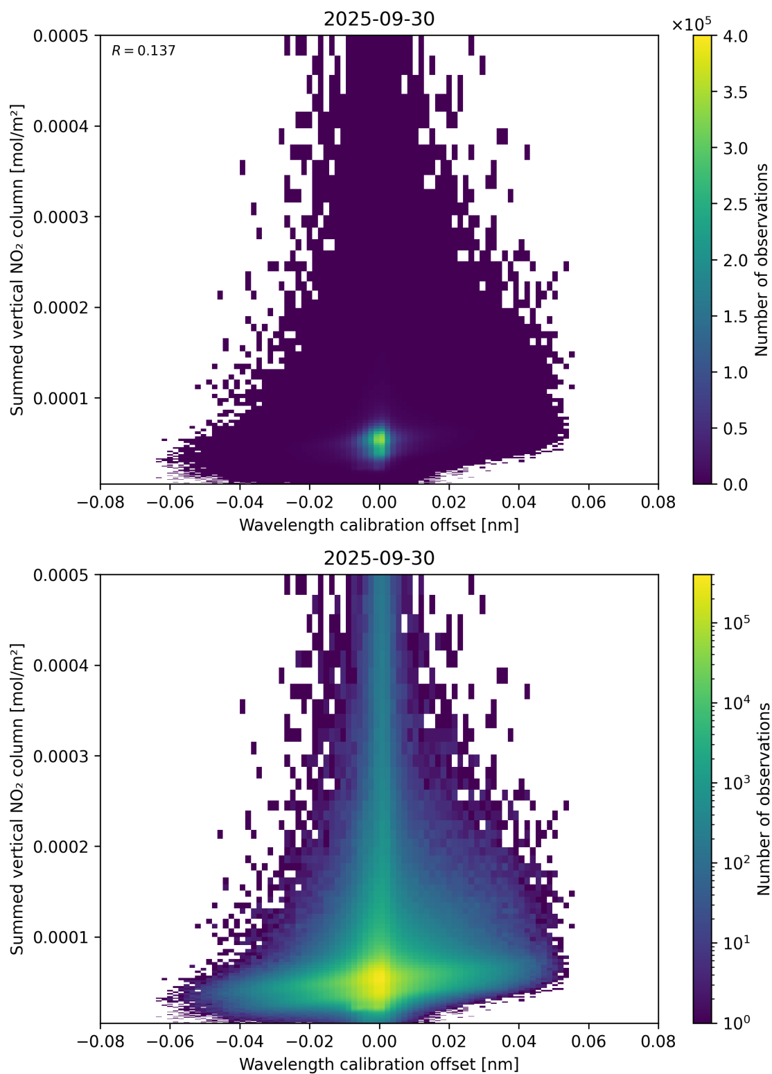
Figure 177: Scatter density plot of “Wavelength calibration offset” against “Summed vertical NO 2 column” for 2025-09-29 to 2025-10-01.
