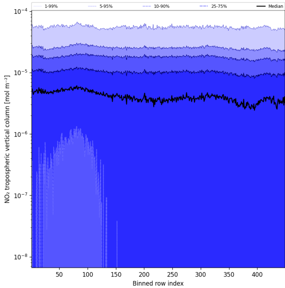
Figure 46: Along track statistics of “NO 2 tropospheric vertical column” for 2025-09-29 to 2025-10-01
