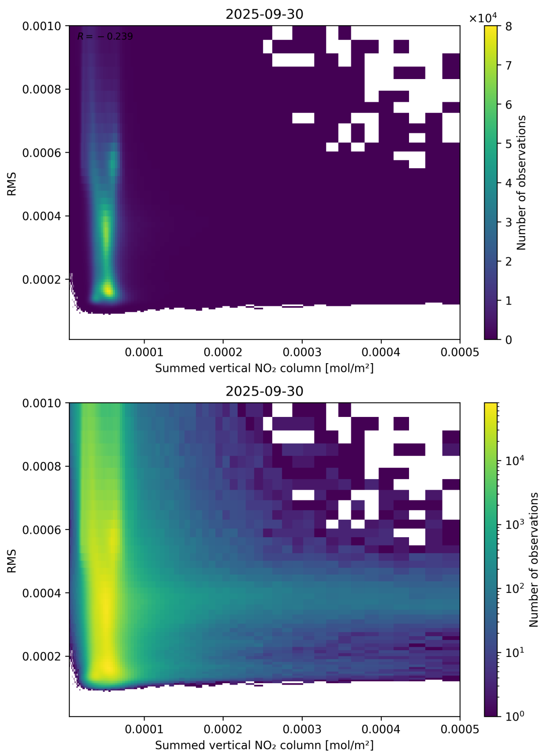
Figure 109: Scatter density plot of “Summed vertical NO 2 column” against “RMS” for 2025-09-29 to 2025-10-01.
