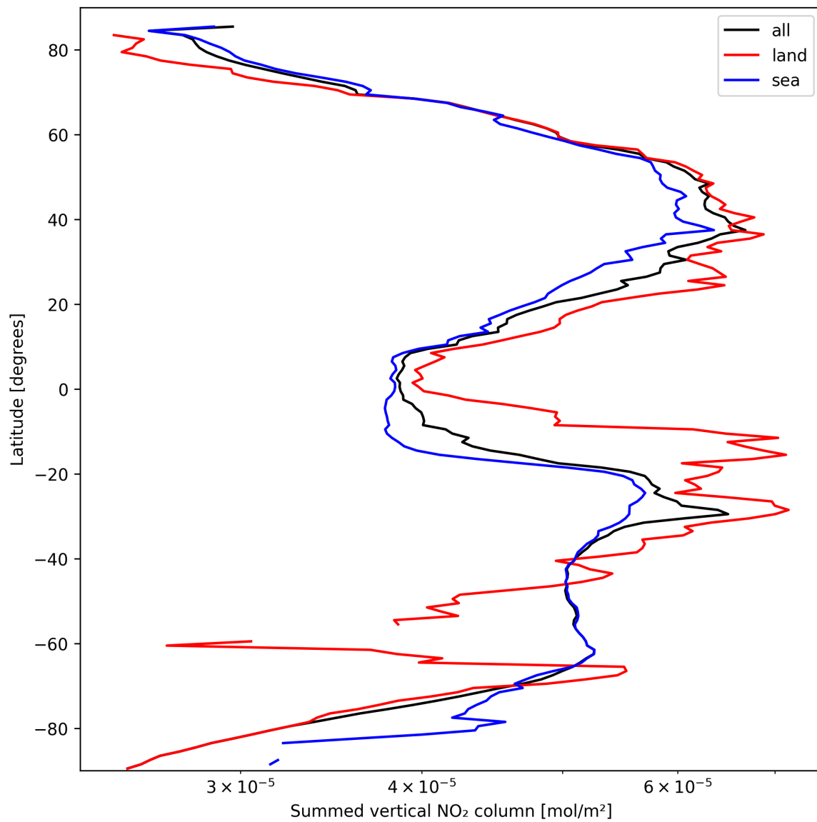
Figure 23: Zonal average of “Summed vertical NO 2 column” for 2025-09-29 to 2025-10-01.
