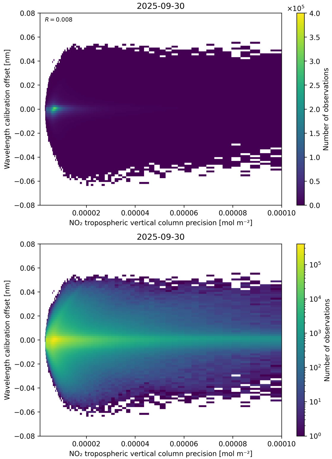
Figure 141: Scatter density plot of “NO 2 tropospheric vertical column precision” against “Wavelength calibration offset” for 2025-09-29 to 2025-10-01.
