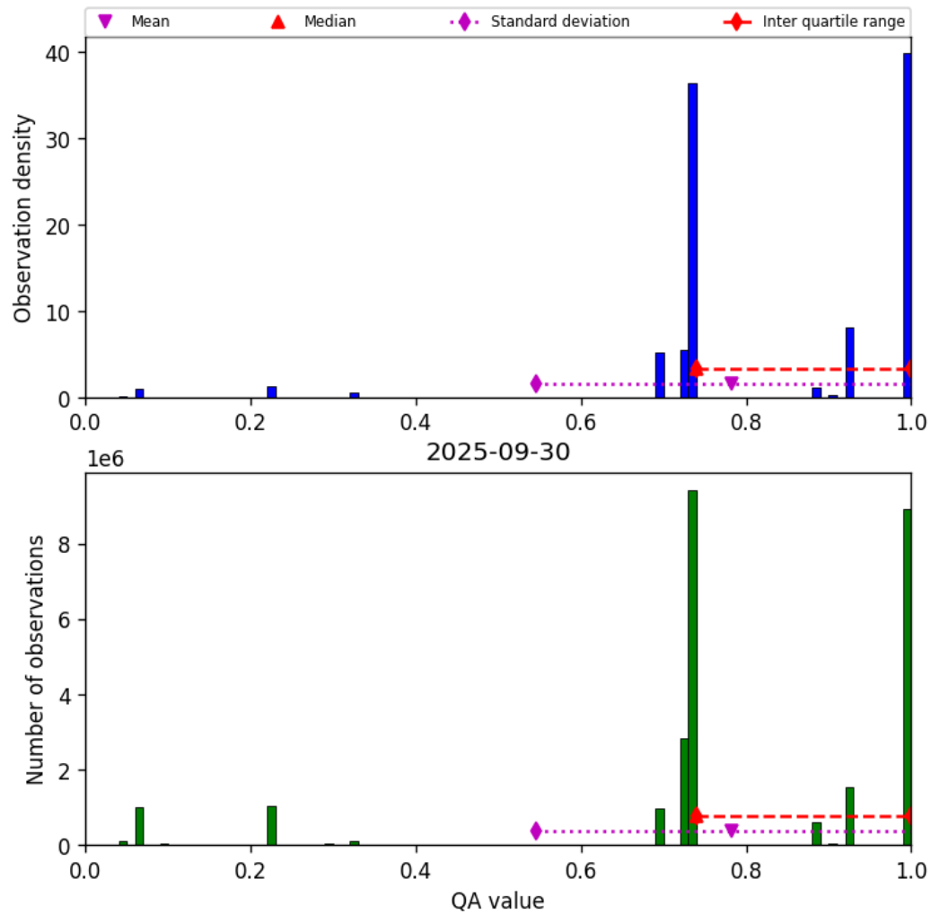
Figure 28: Histogram of “QA value” for 2025-09-29 to 2025-10-01
