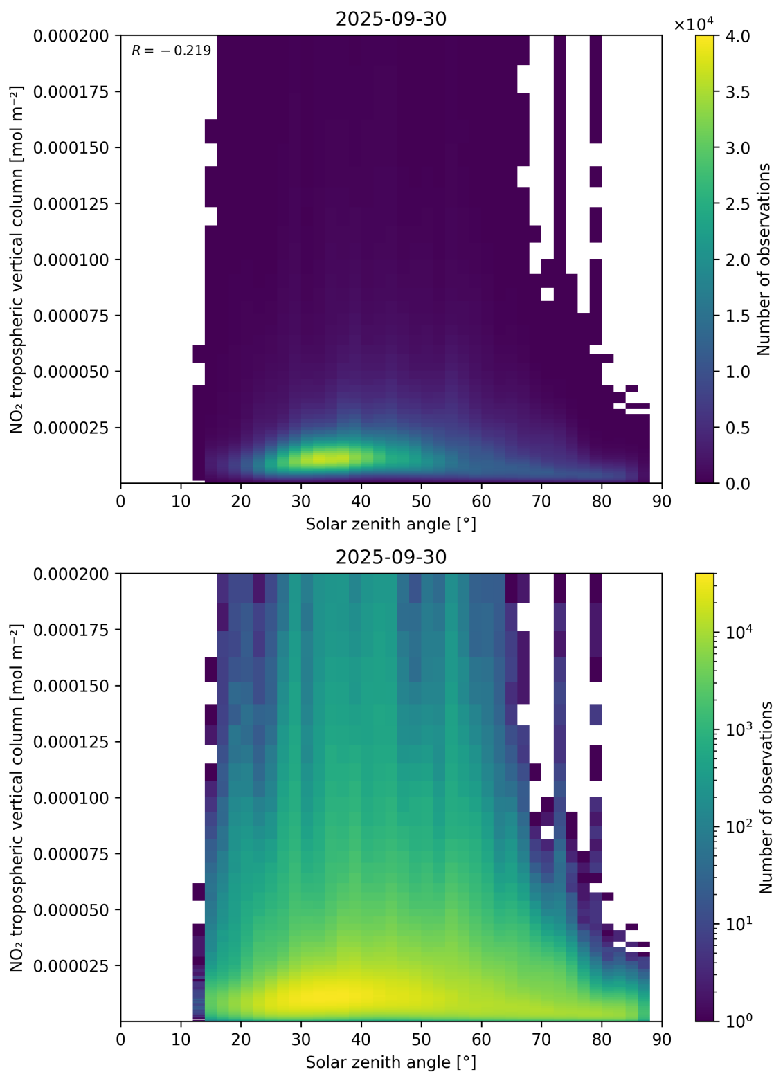
Figure 155: Scatter density plot of “Solar zenith angle” against “NO 2 tropospheric vertical column” for 2025-09-29 to 2025-10-01.
