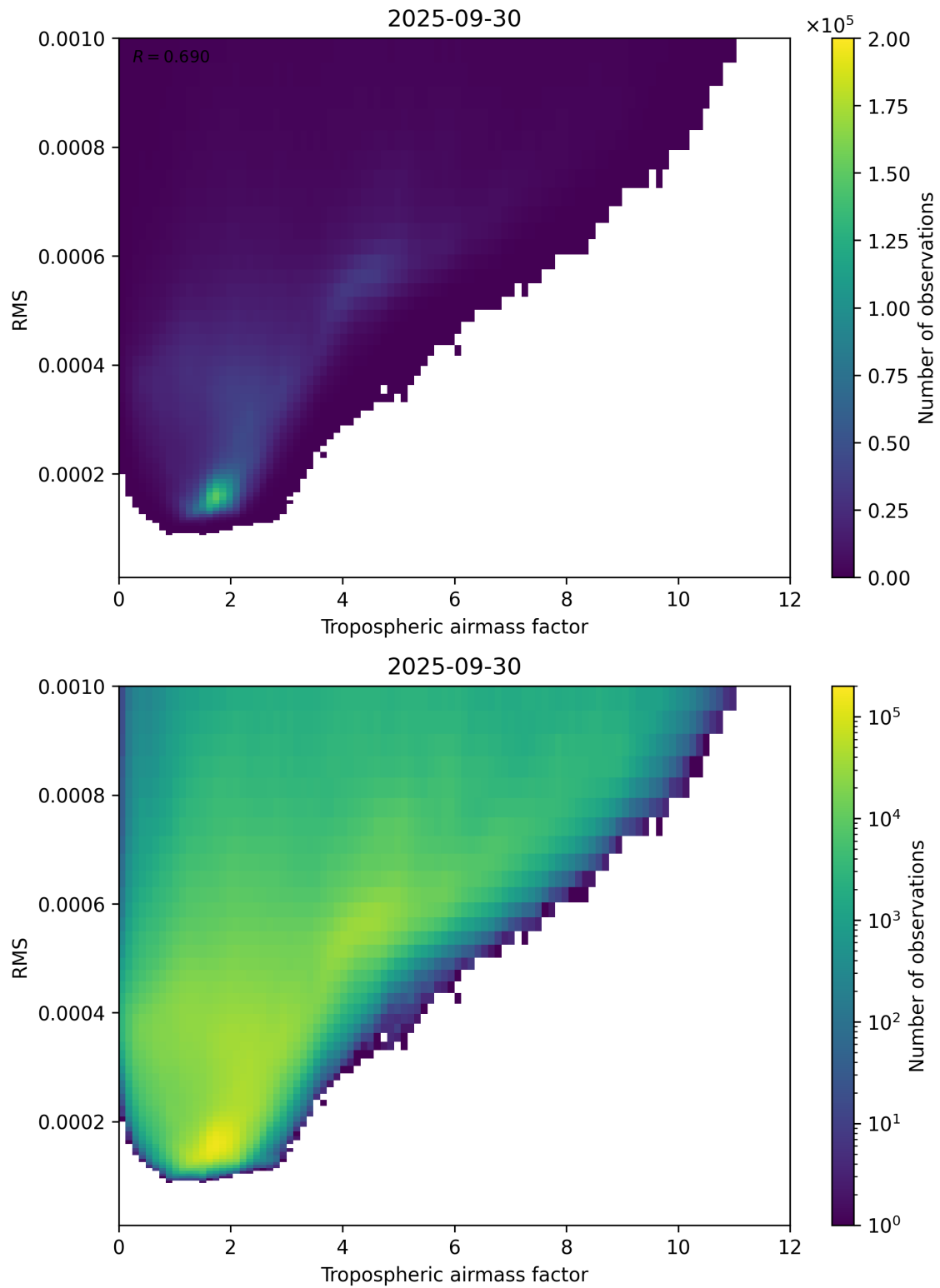
Figure 79: Scatter density plot of “Tropospheric airmass factor” against “RMS” for 2025-09-29 to 2025-10-01.
