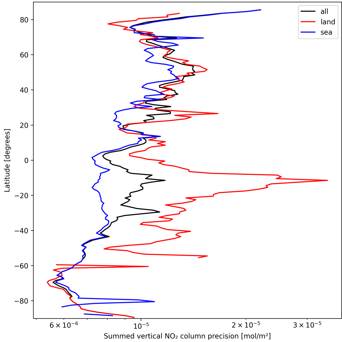
Figure 24: Zonal average of “Summed vertical NO 2 column precision” for 2025-09-29 to 2025-10-01.
