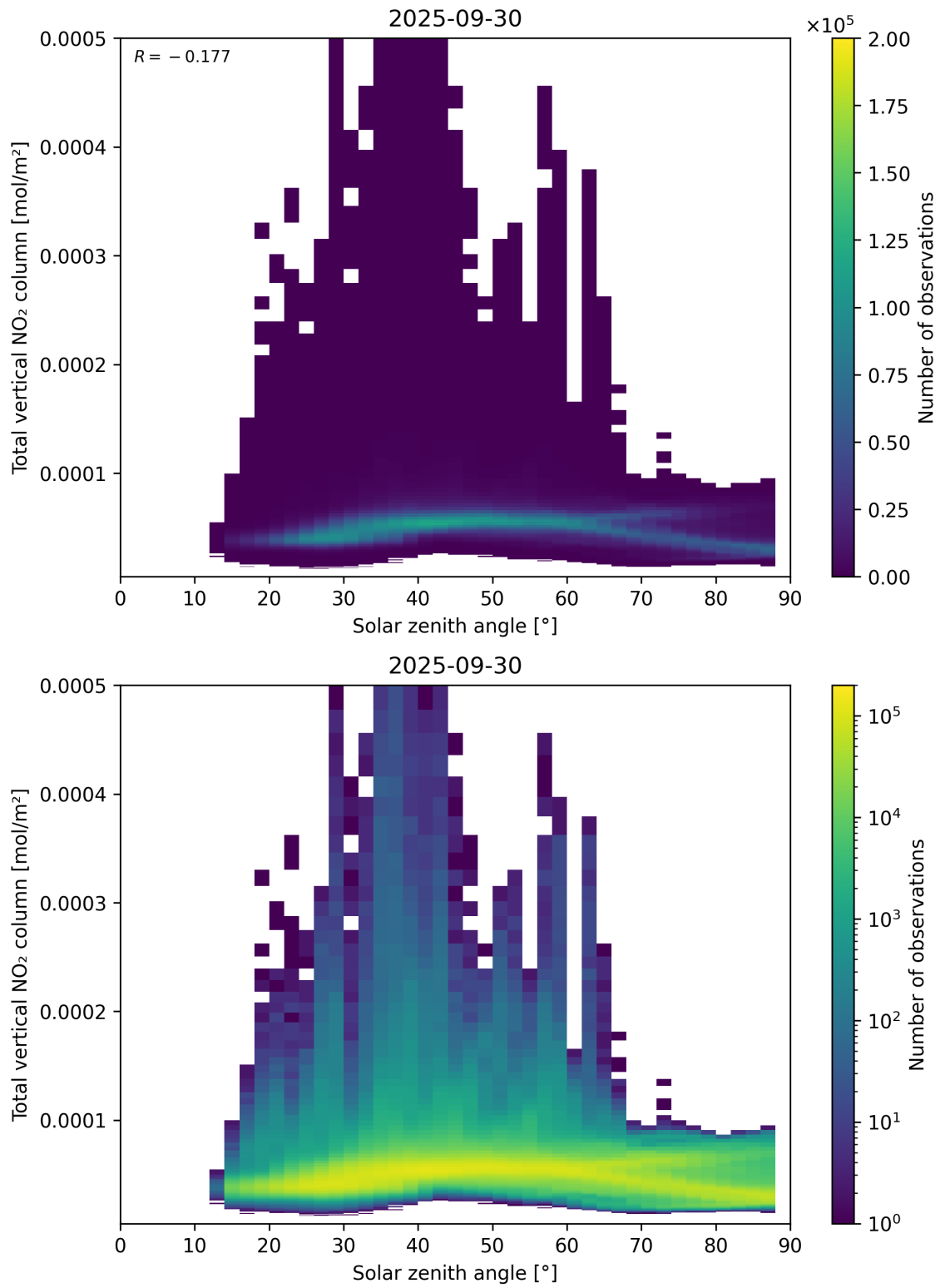
Figure 153: Scatter density plot of “Solar zenith angle” against “Total vertical NO 2 column” for 2025-09-29 to 2025-10-01.
