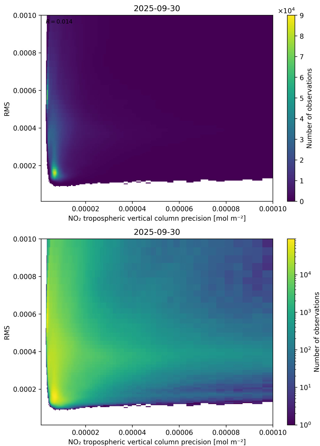
Figure 140: Scatter density plot of “NO 2 tropospheric vertical column precision” against “RMS” for 2025-09-29 to 2025-10-01.
