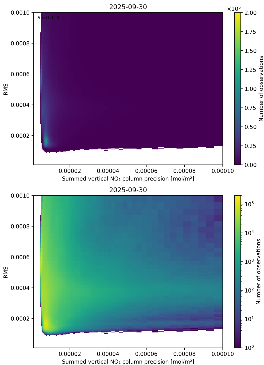
Figure 108: Scatter density plot of “Summed vertical NO 2 column precision” against “RMS” for 2025-09-29 to 2025-10-01.
