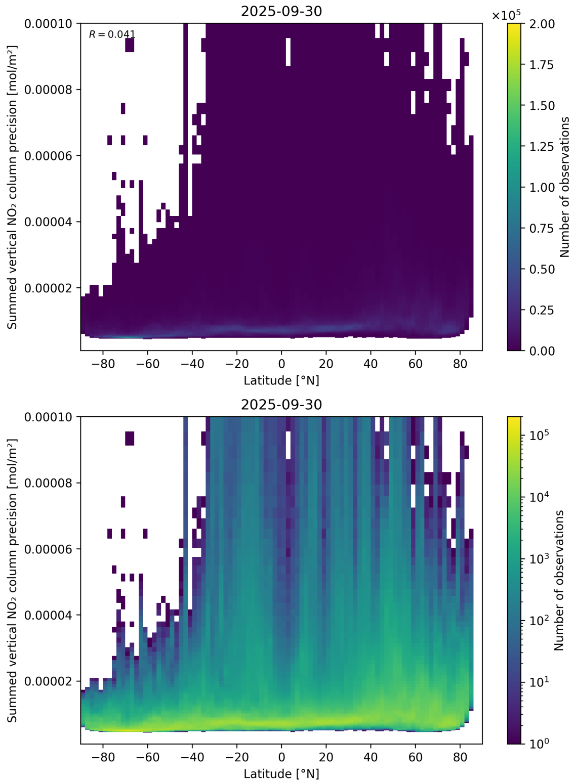
Figure 89: Scatter density plot of “Latitude” against “Summed vertical NO 2 column precision” for 2025-09-29 to 2025-10-01.
