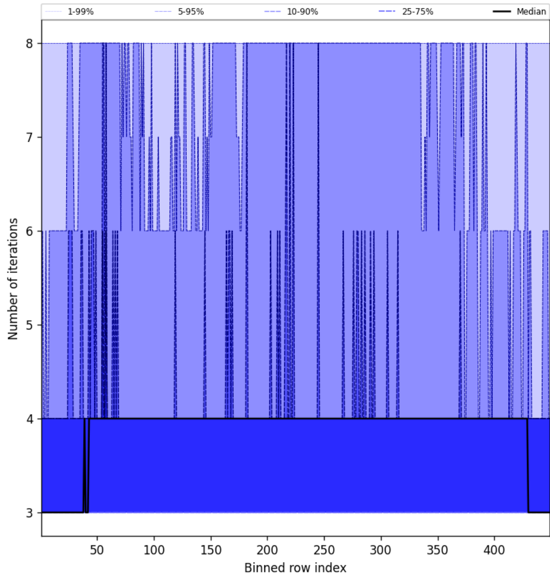
Figure 51: Along track statistics of “Number of iterations” for 2025-09-29 to 2025-10-01
