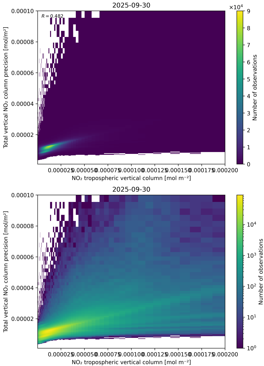
Figure 129: Scatter density plot of “NO 2 tropospheric vertical column” against “Total vertical NO 2 column precision” for 2025-09-29 to 2025-10-01.
