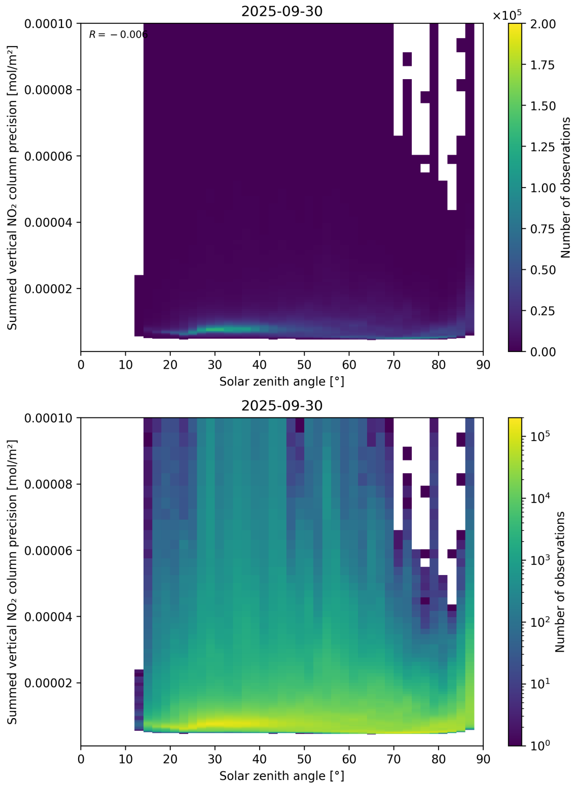
Figure 152: Scatter density plot of “Solar zenith angle” against “Summed vertical NO 2 column precision” for 2025-09-29 to 2025-10-01.
