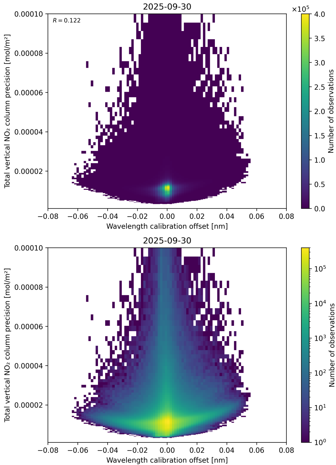
Figure 180: Scatter density plot of “Wavelength calibration offset” against “Total vertical NO 2 column precision” for 2025-09-29 to 2025-10-01.
