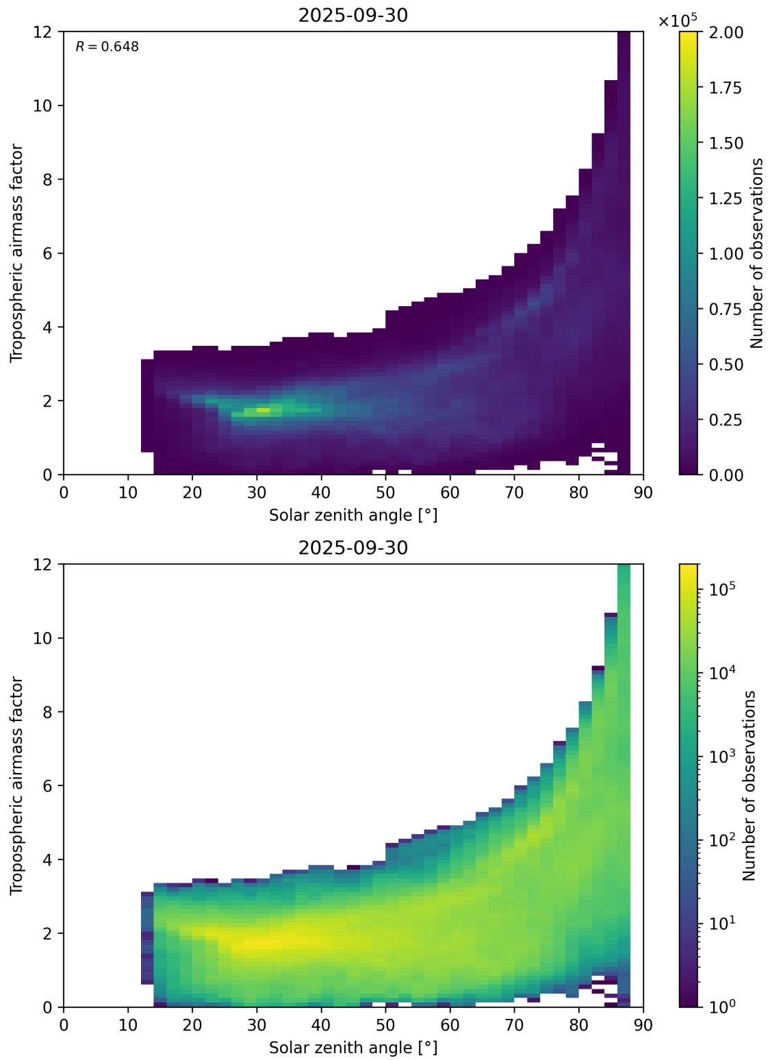
Figure 147: Scatter density plot of “Solar zenith angle” against “Tropospheric airmass factor” for 2025-09-29 to 2025-10-01.
