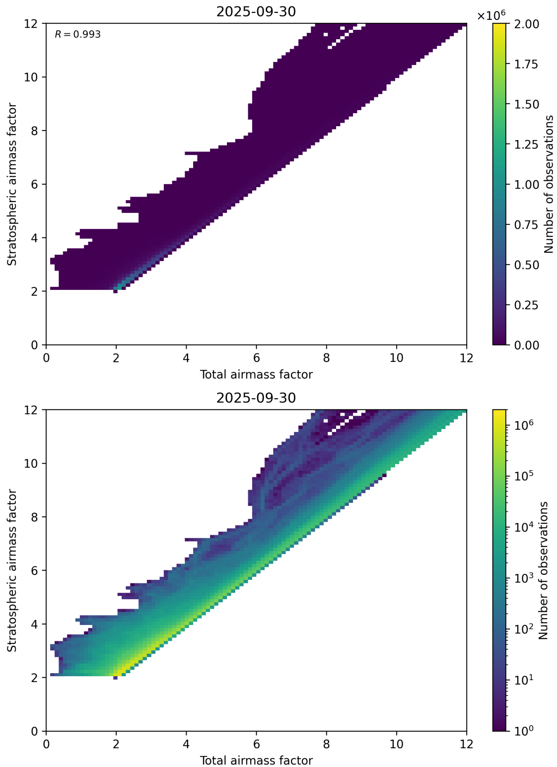
Figure 62: Scatter density plot of “Total airmass factor” against “Stratospheric airmass factor” for 2025-09-29 to 2025-10-01.
