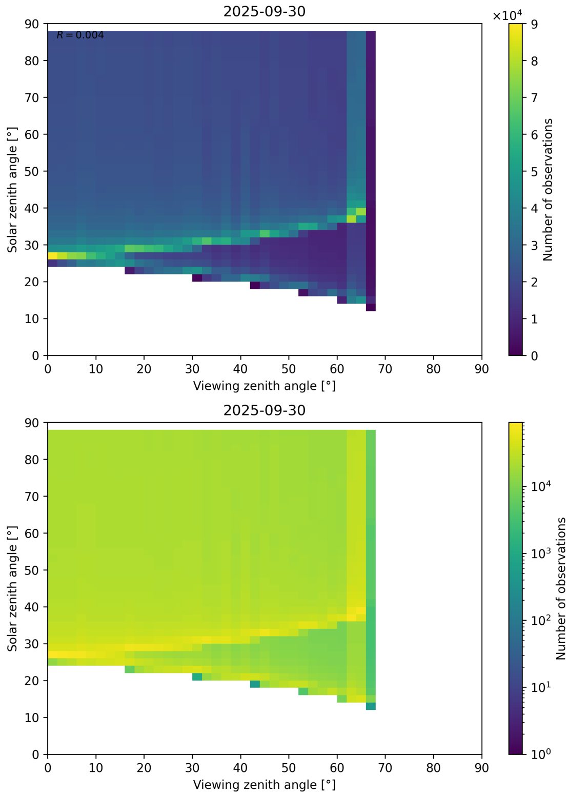
Figure 172: Scatter density plot of “Viewing zenith angle” against “Solar zenith angle” for 2025-09-29 to 2025-10-01.
