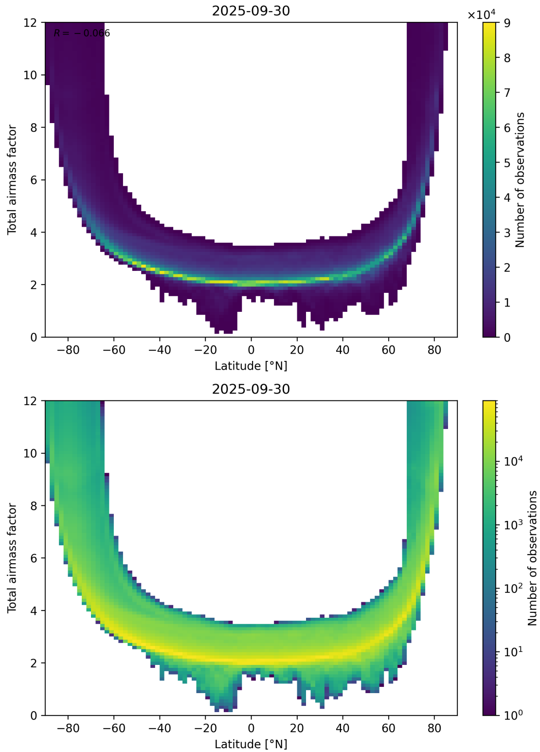
Figure 84: Scatter density plot of “Latitude” against “Total airmass factor” for 2025-09-29 to 2025-10-01.
