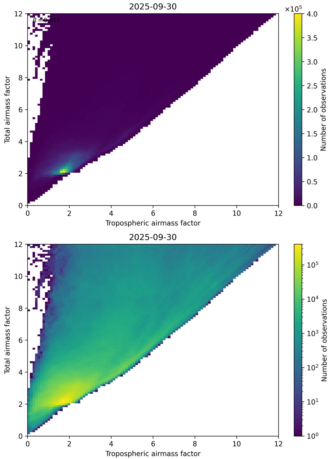
Figure 72: Scatter density plot of “Tropospheric airmass factor” against “Total airmass factor” for 2025-09-29 to 2025-10-01.
