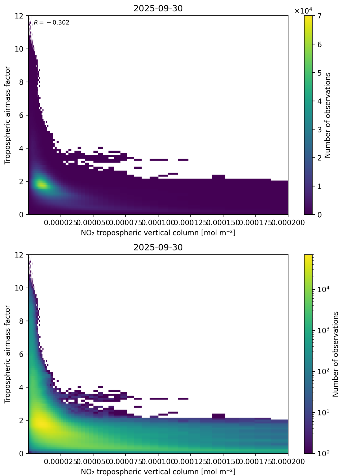
Figure 123: Scatter density plot of “NO 2 tropospheric vertical column” against “Tropospheric air mass factor” for 2025-09-29 to 2025-10-01.
