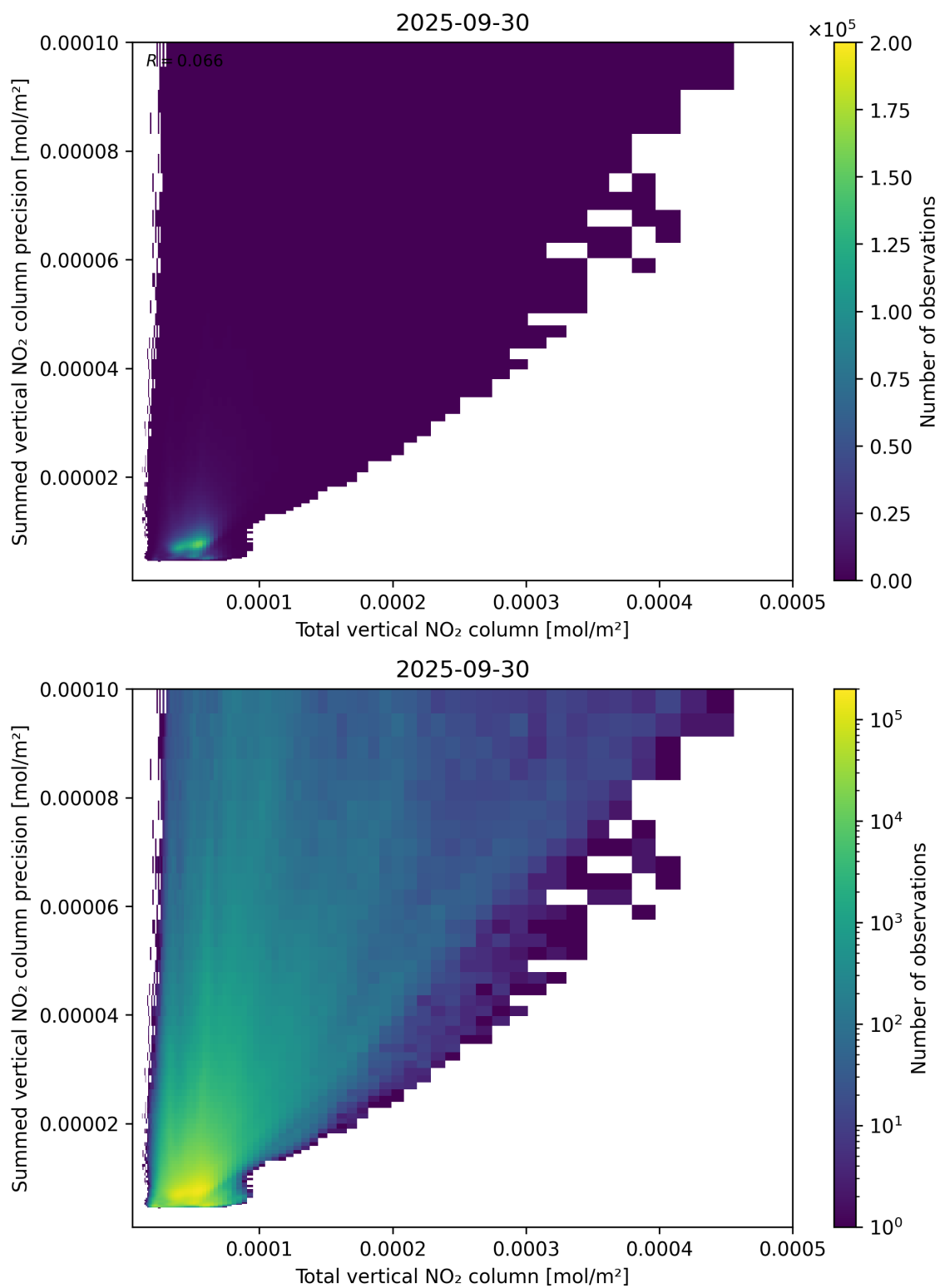
Figure 113: Scatter density plot of “Total vertical NO 2 column” against “Summed vertical NO 2 column precision” for 2025-09-29 to 2025-10-01.
