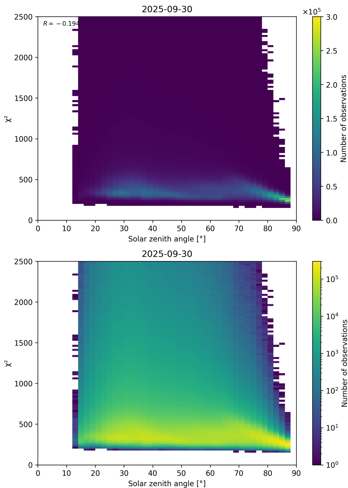
Figure 148: Scatter density plot of “Solar zenith angle” against “ \chi^2 ” for 2025-09-29 to 2025-10-01.
