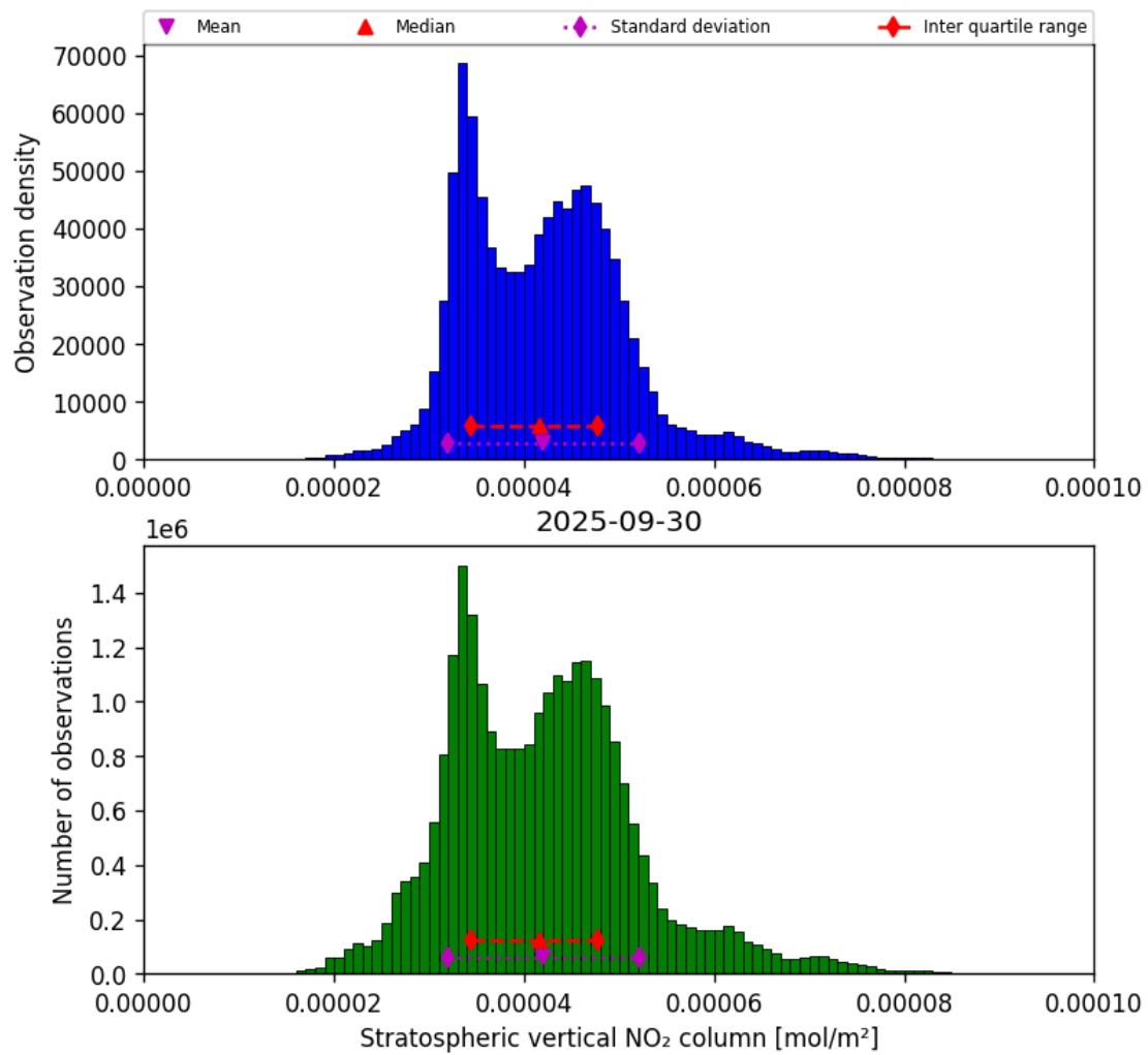
Figure 36: Histogram of “Stratospheric vertical NO 2 column” for 2025-09-29 to 2025-10-01
