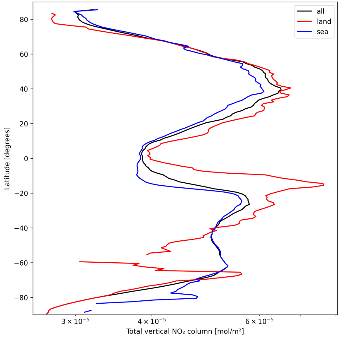
Figure 21: Zonal average of “Total vertical NO 2 column” for 2025-09-29 to 2025-10-01.
