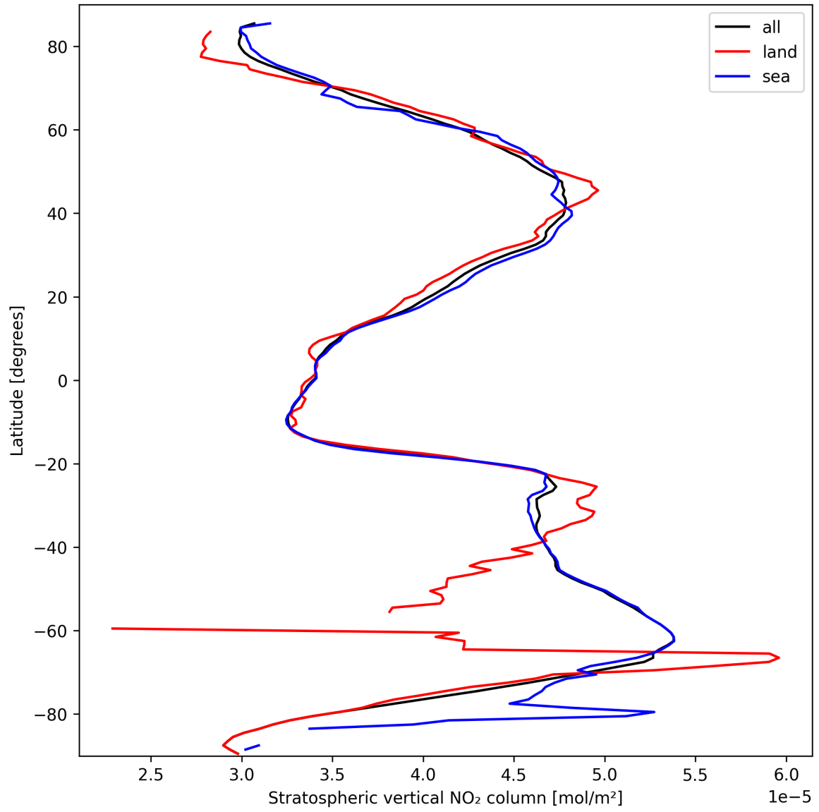
Figure 19: Zonal average of “Stratospheric vertical NO 2 column” for 2025-09-29 to 2025-10-01.
