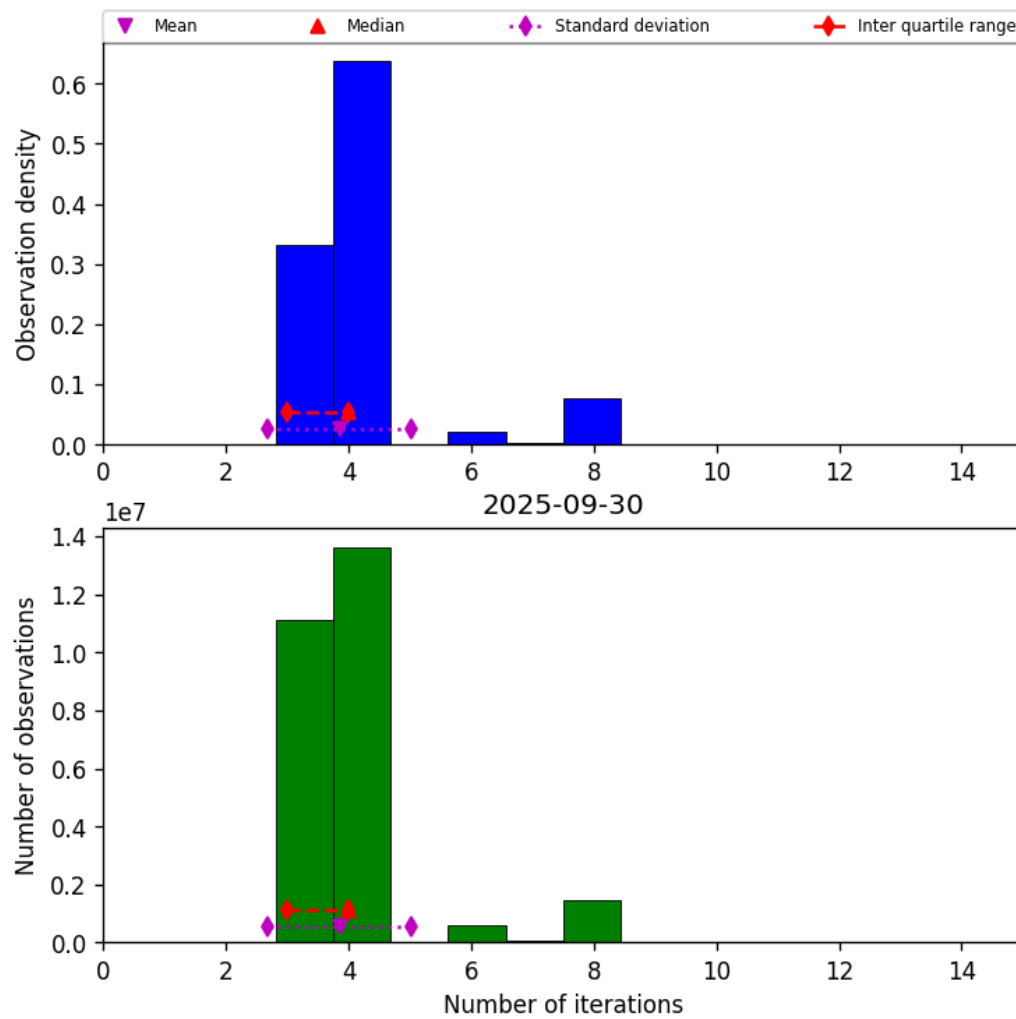
Figure 34: Histogram of “Number of iterations” for 2025-09-29 to 2025-10-01
