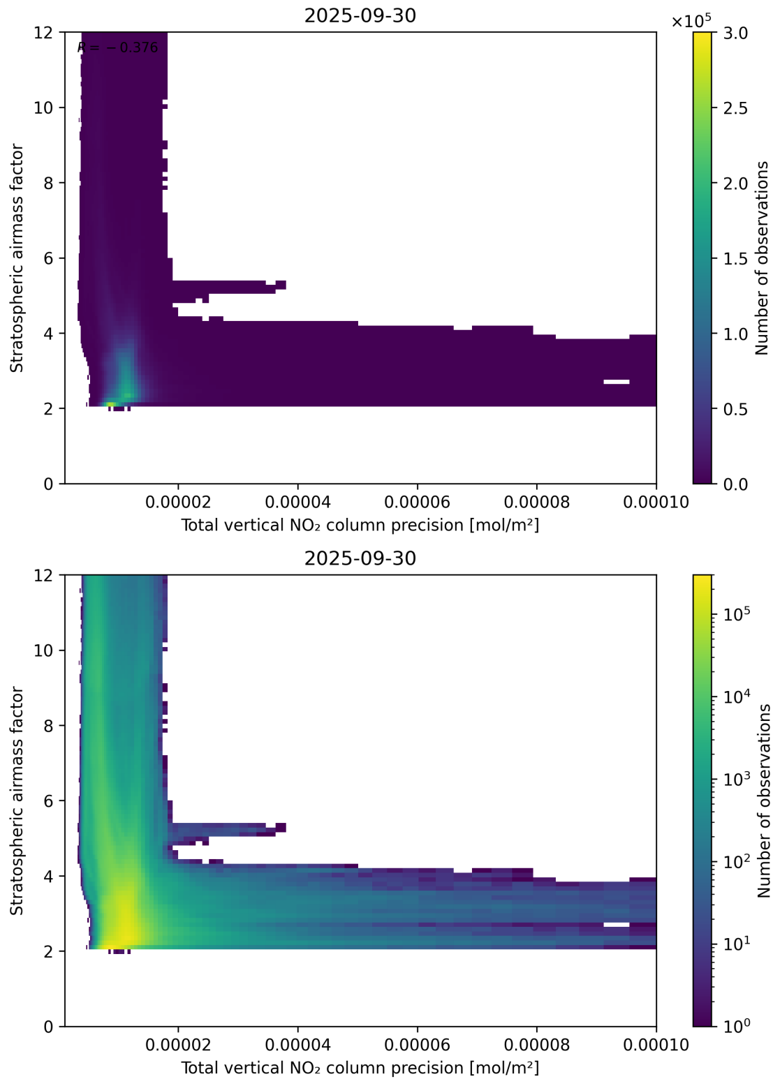
Figure 115: Scatter density plot of “Total vertical NO 2 column precision” against “Stratospheric airmass factor” for 2025-09-29 to 2025-10-01.
