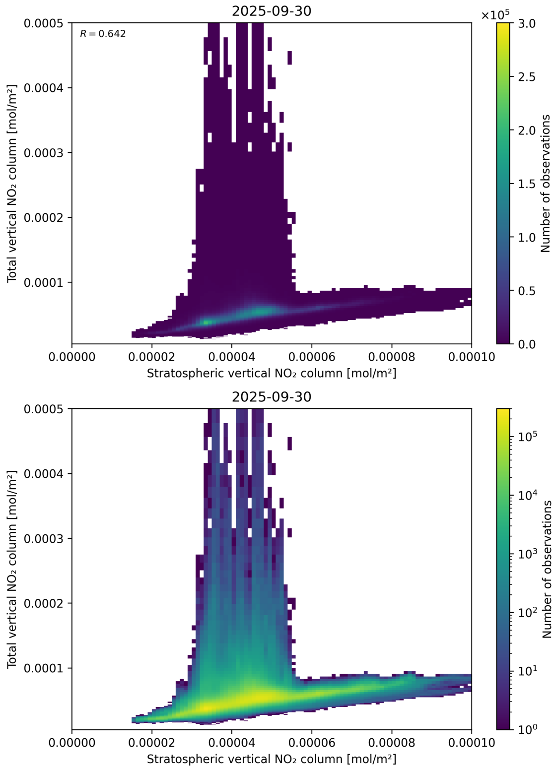
Figure 100: Scatter density plot of “Stratospheric vertical NO 2 column” against “Total vertical NO 2 column” for 2025-09-29 to 2025-10-01.
