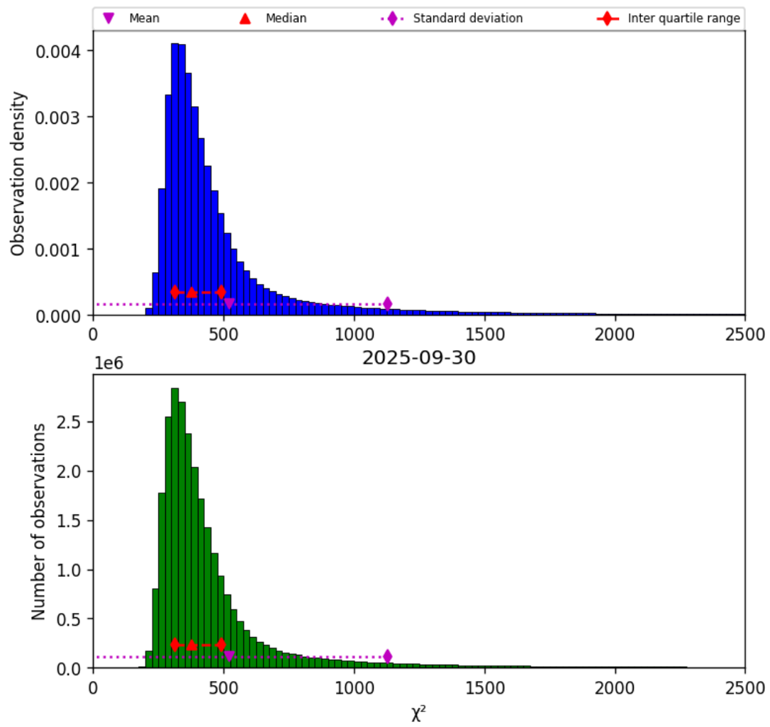
Figure 42: Histogram of “ \chi^2 ” for 2025-09-29 to 2025-10-01
