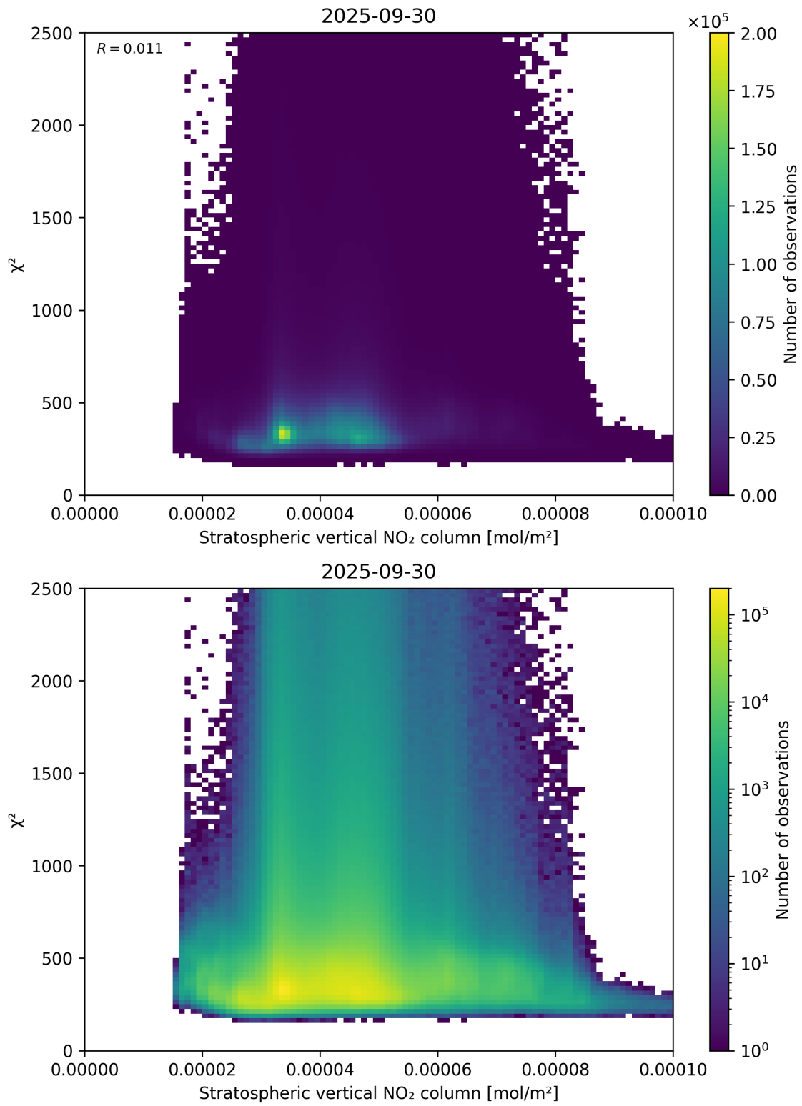
Figure 97: Scatter density plot of “Stratospheric vertical NO 2 column” against “ \chi^2 ” for 2025-09-29 to 2025-10-01.
