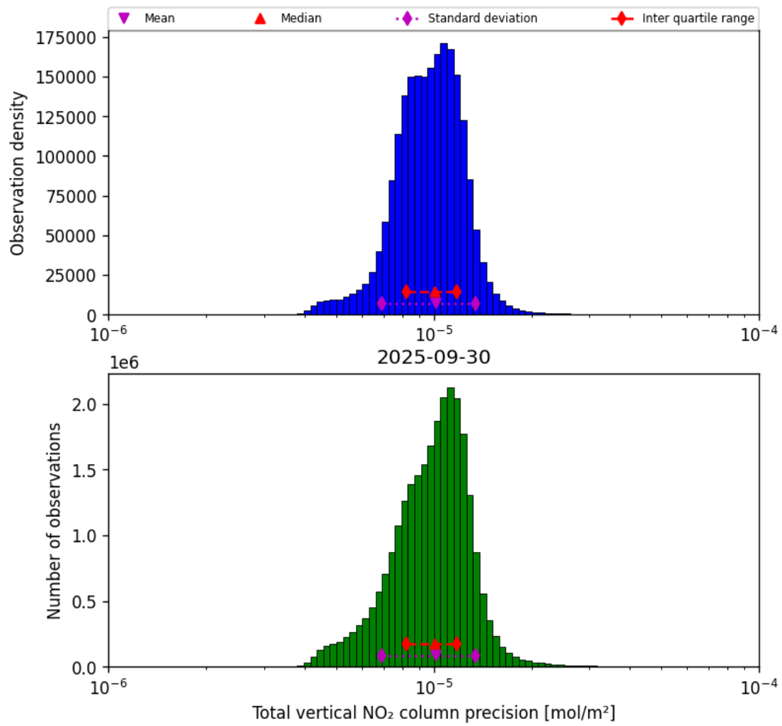
Figure 39: Histogram of “Total vertical NO 2 column precision” for 2025-09-29 to 2025-10-01
