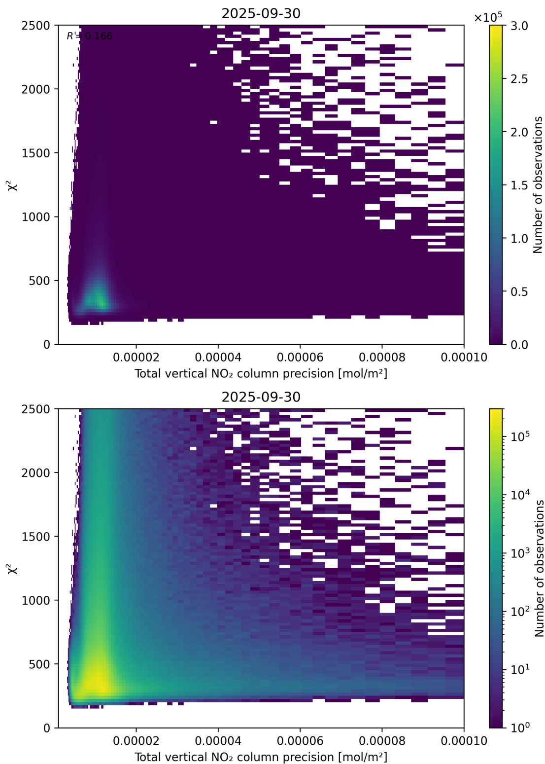
Figure 116: Scatter density plot of "Total vertical NO 2 column precision" against " \chi^2 " for 2025-09-29 to 2025-10-01.
