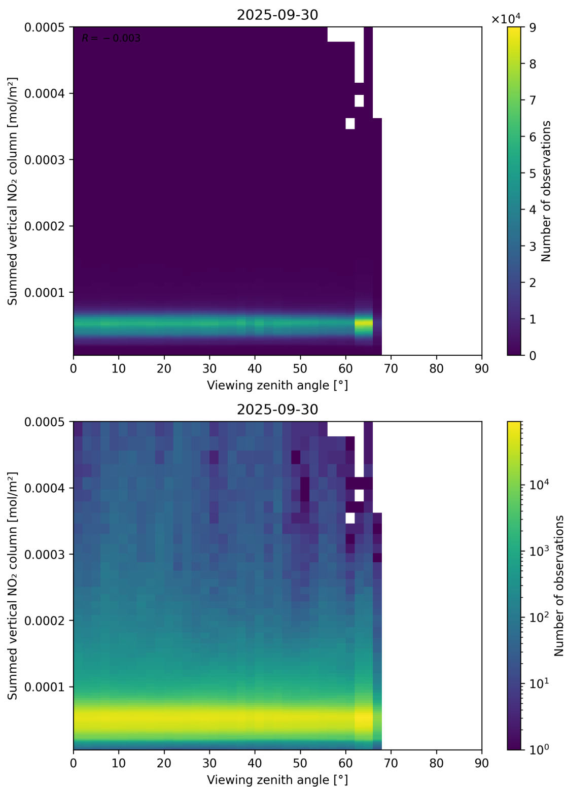
Figure 165: Scatter density plot of “Viewing zenith angle” against “Summed vertical NO 2 column” for 2025-09-29 to 2025-10-01.
