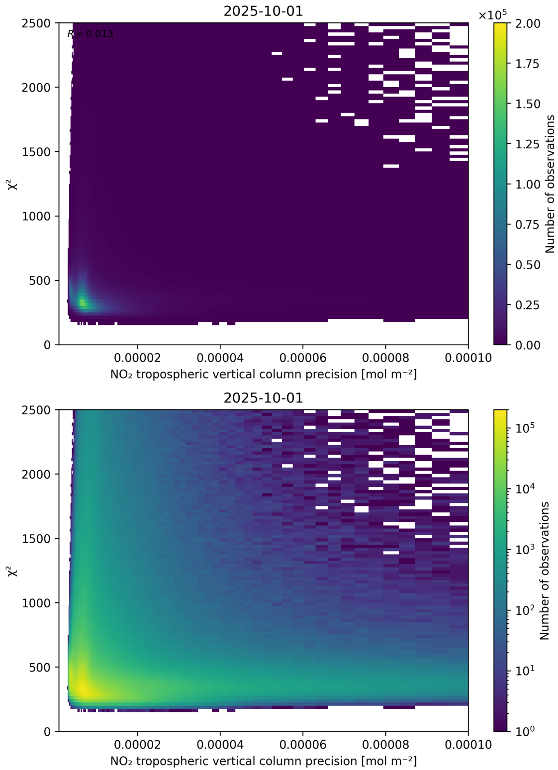
Figure 134: Scatter density plot of “NO 2 tropospheric vertical column precision” against “ \chi^2 ” for 2025-10-01 to 2025-10-02.
