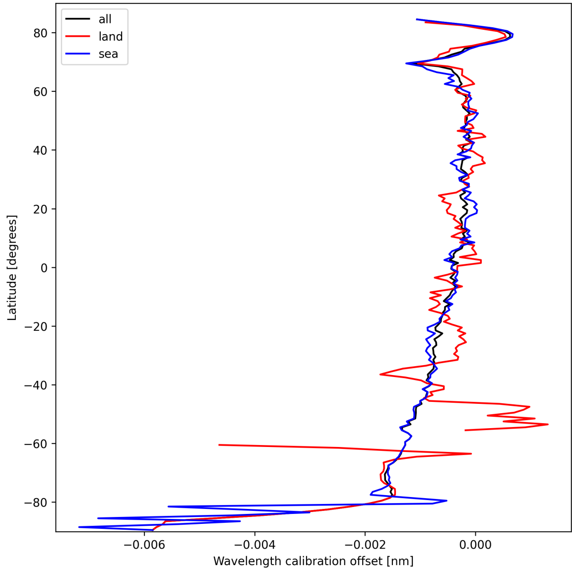
Figure 18: Zonal average of “Wavelength calibration offset” for 2025-10-01 to 2025-10-02.
