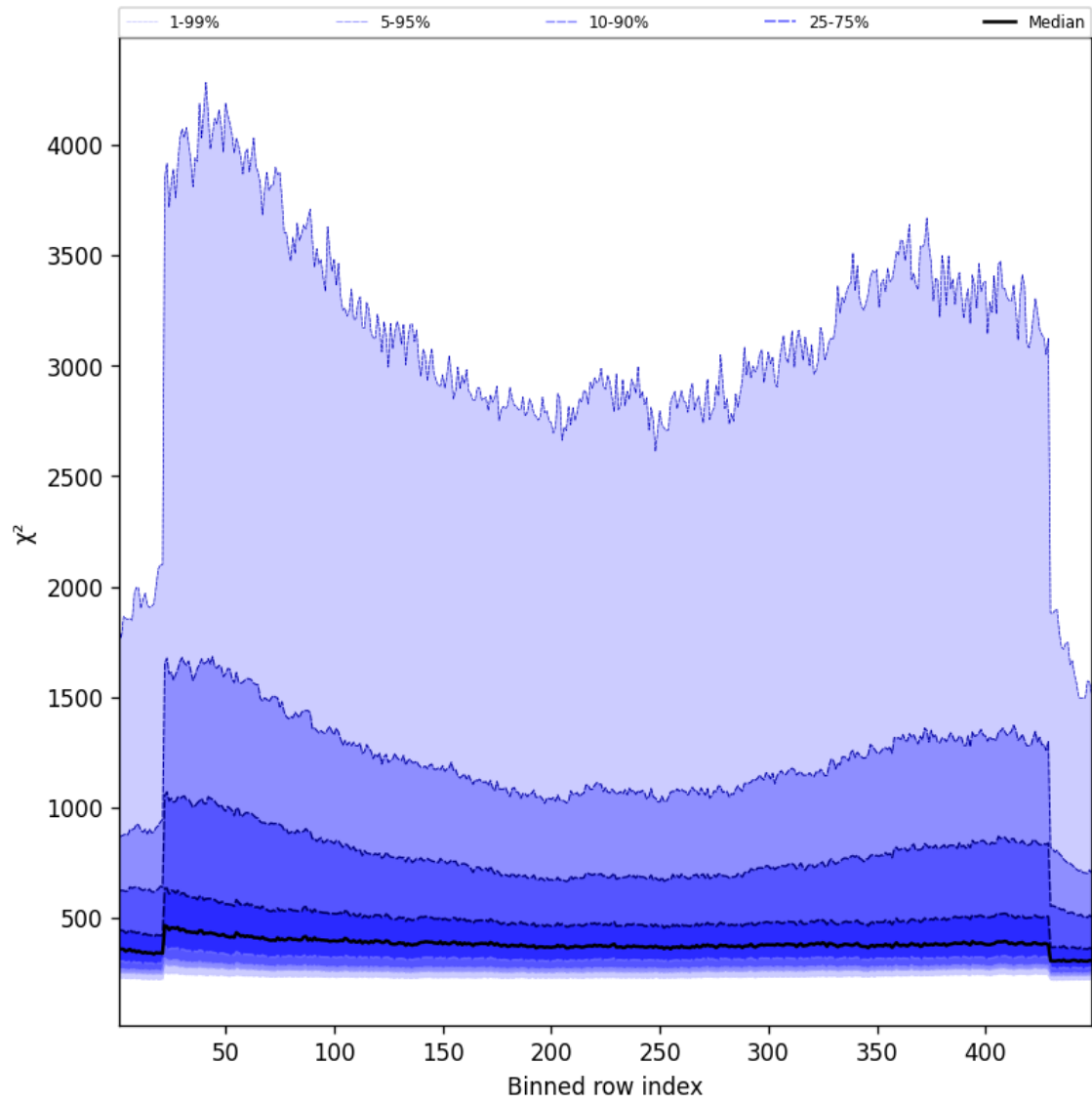
Figure 59: Along track statistics of “ \chi^2 ” for 2025-10-01 to 2025-10-02
