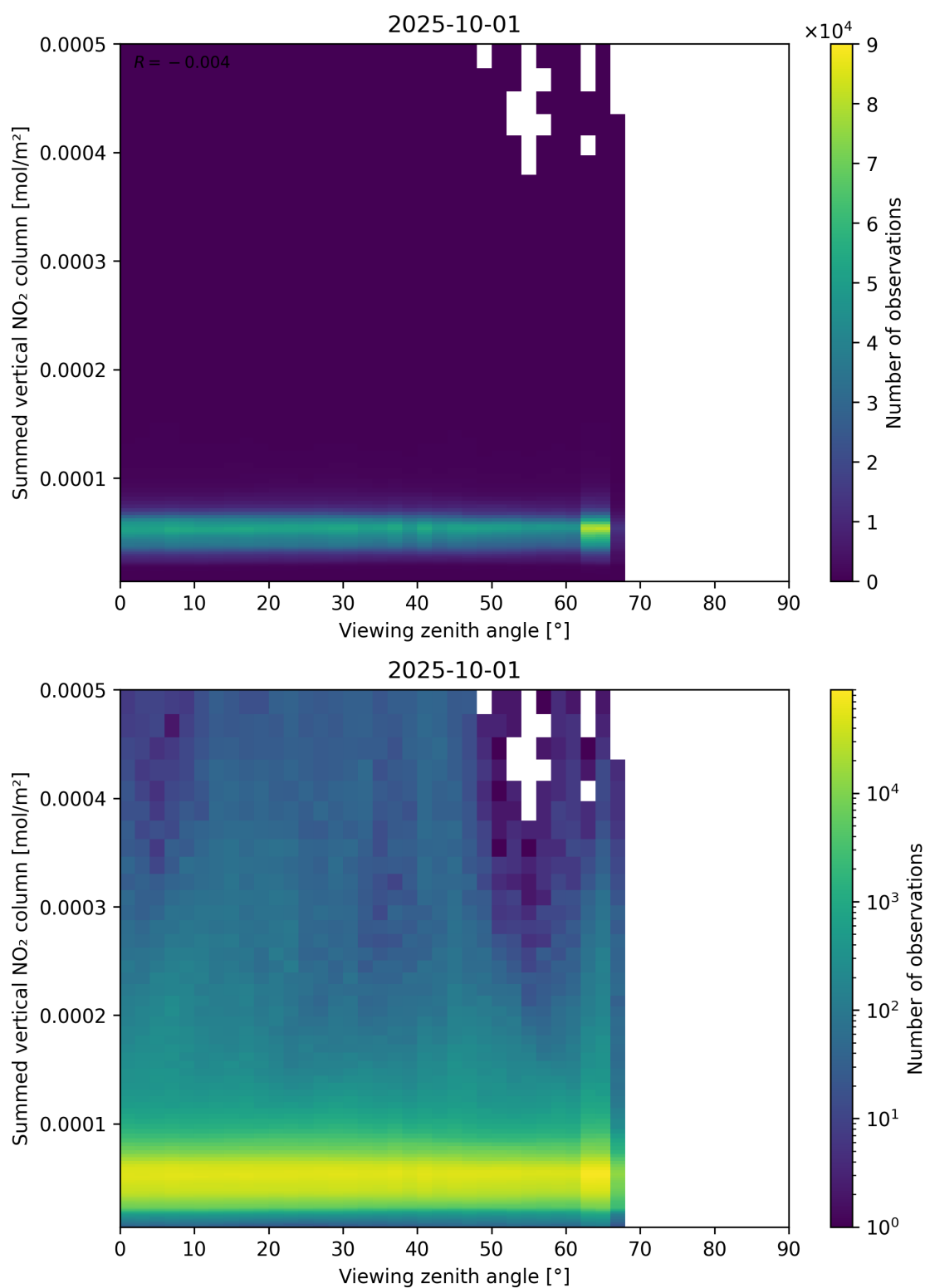
Figure 165: Scatter density plot of “Viewing zenith angle” against “Summed vertical NO 2 column” for 2025-10-01 to 2025-10-02.
