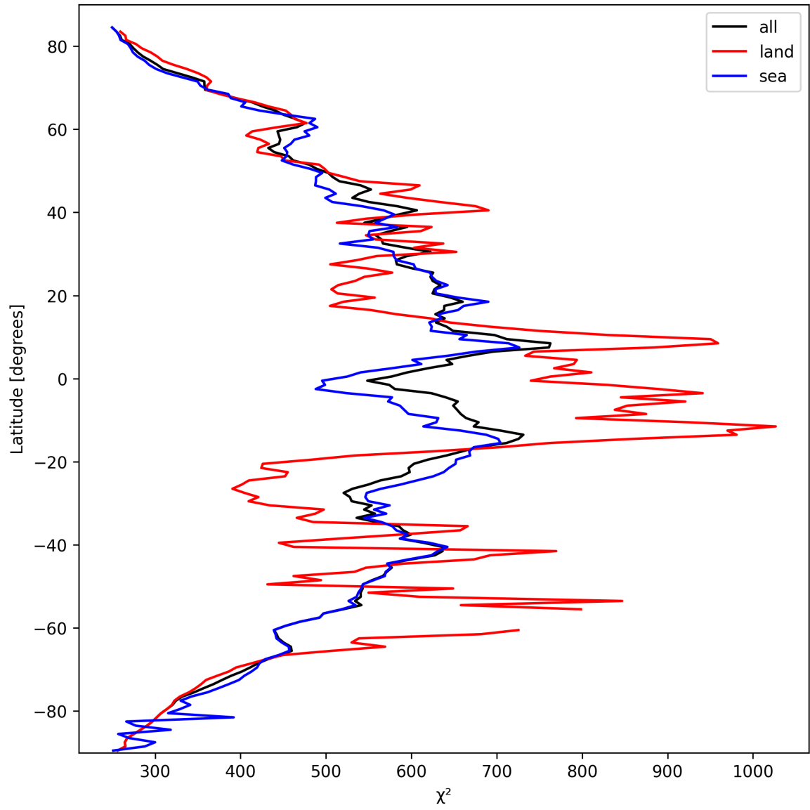
Figure 25: Zonal average of “ \chi^2 ” for 2025-10-01 to 2025-10-02.
