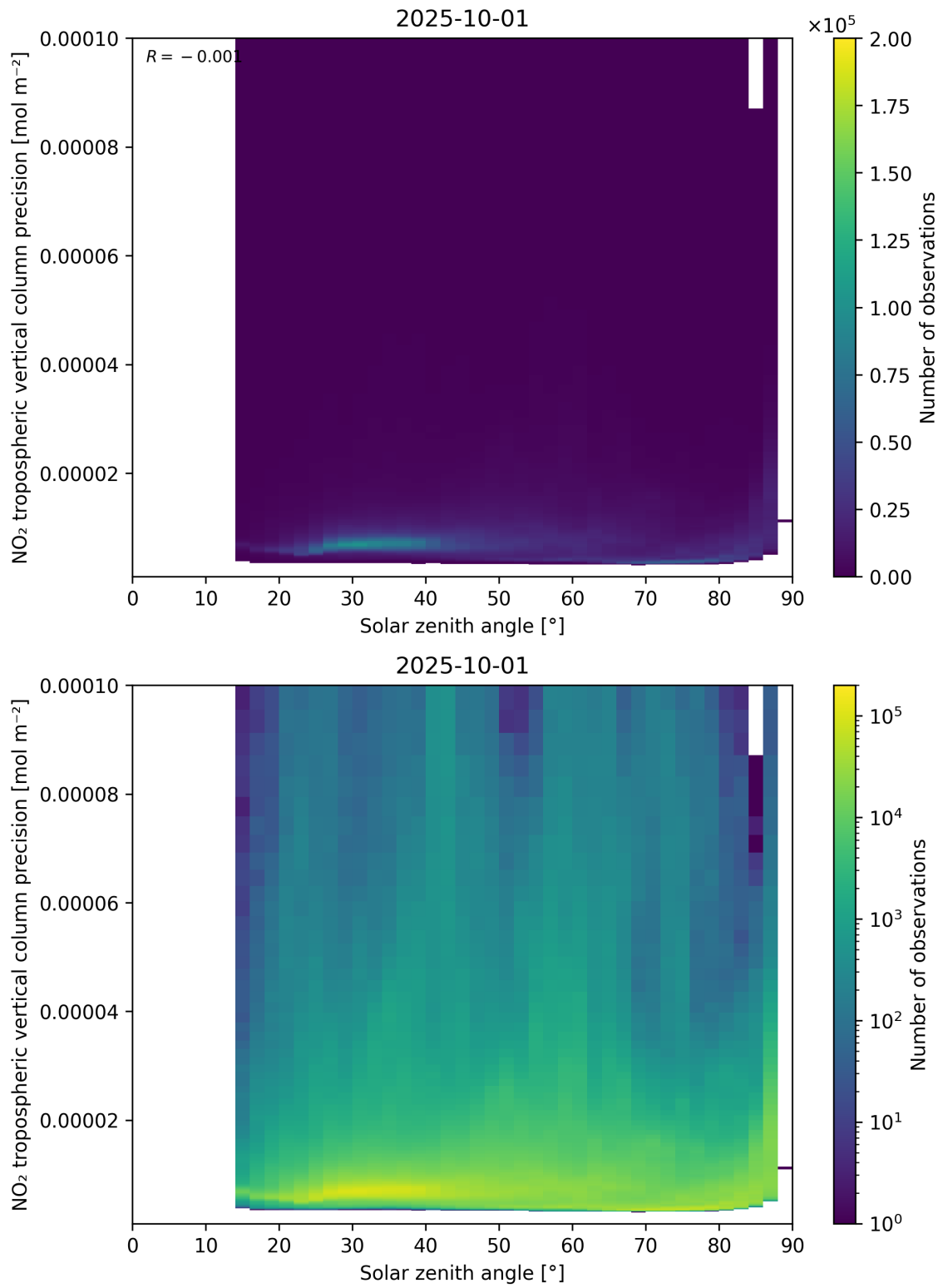
Figure 156: Scatter density plot of “Solar zenith angle” against “NO 2 tropospheric vertical column precision” for 2025-10-01 to 2025-10-02.
