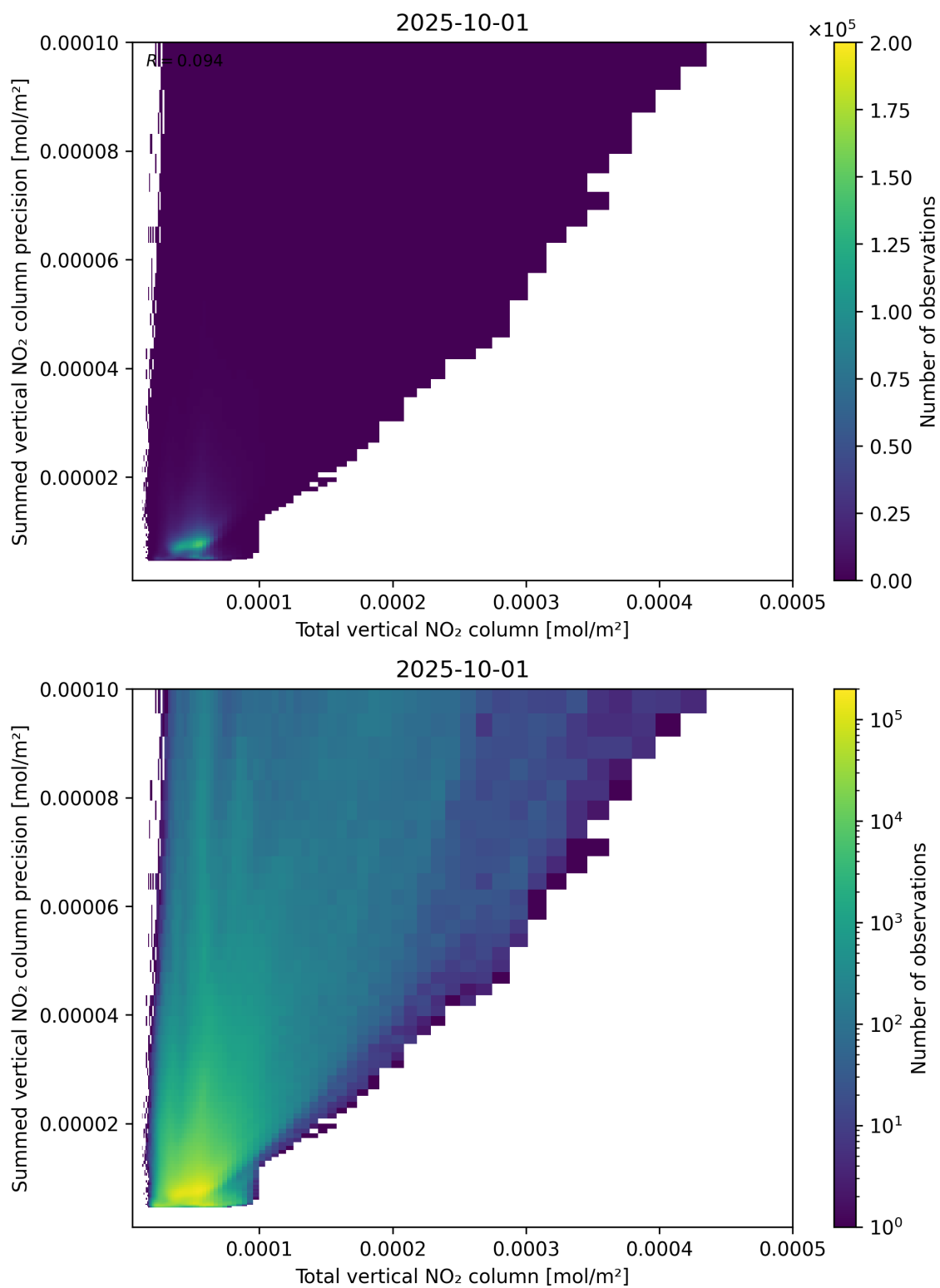
Figure 113: Scatter density plot of “Total vertical NO 2 column” against “Summed vertical NO 2 column precision” for 2025-10-01 to 2025-10-02.
