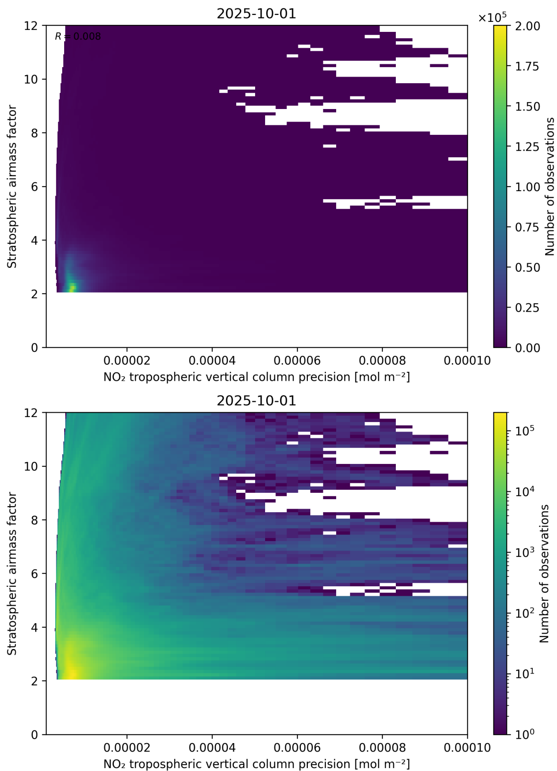
Figure 131: Scatter density plot of “NO 2 tropospheric vertical column precision” against “Stratospheric airmass factor” for 2025-10-01 to 2025-10-02.
