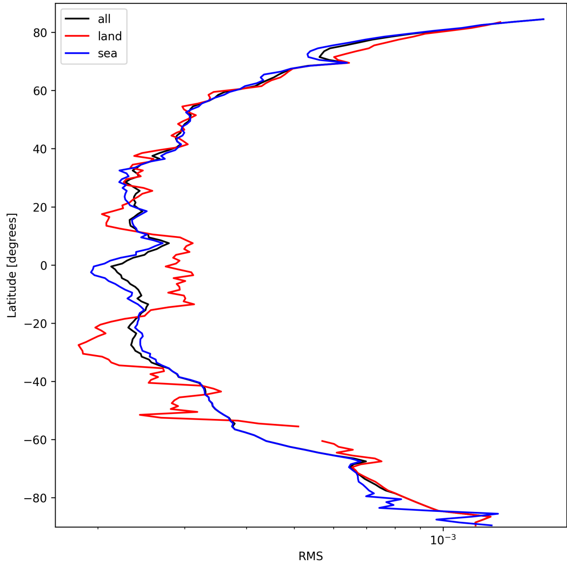
Figure 26: Zonal average of “RMS” for 2025-10-01 to 2025-10-02.
