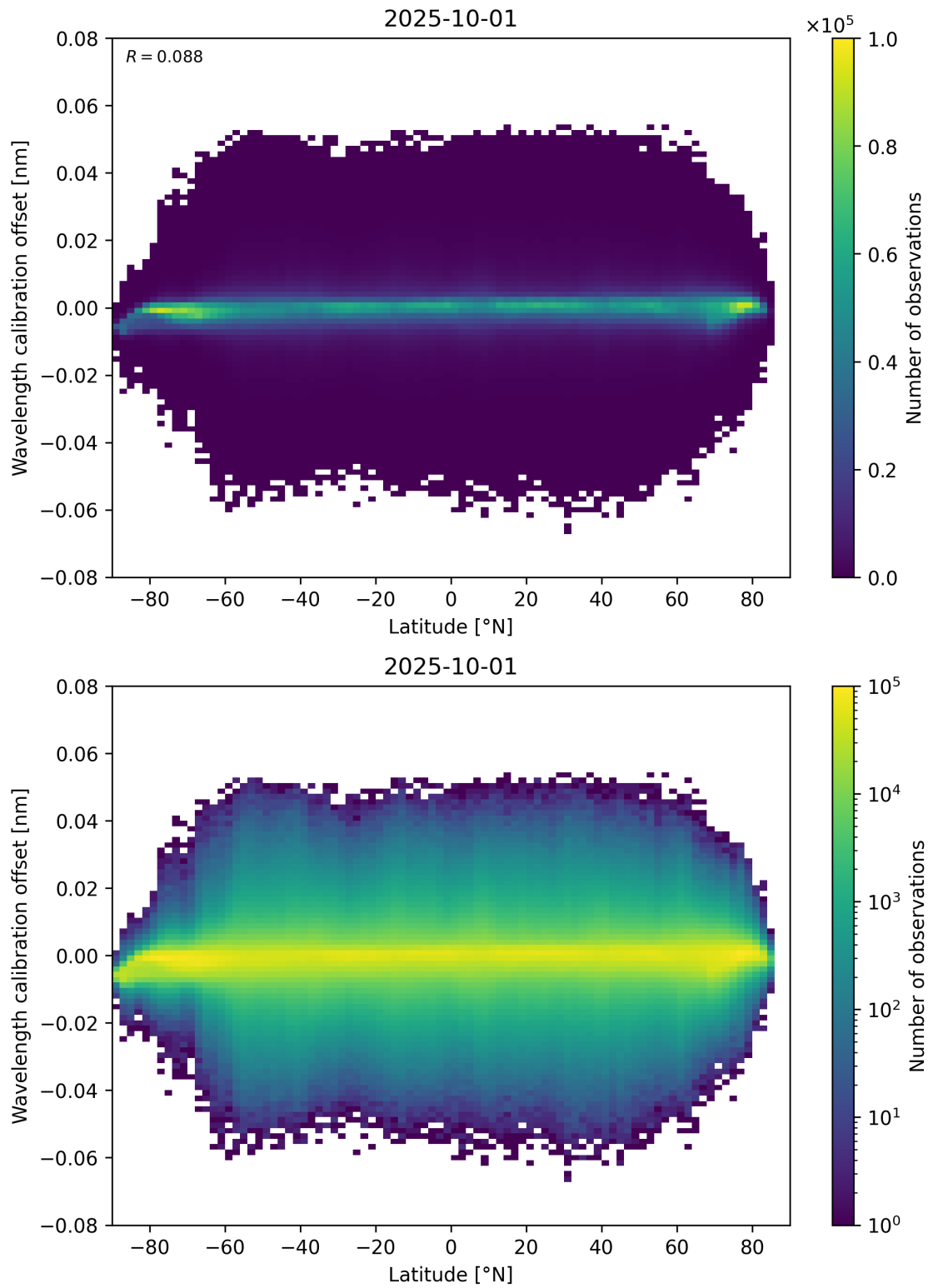
Figure 95: Scatter density plot of “Latitude” against “Wavelength calibration offset” for 2025-10-01 to 2025-10-02.
