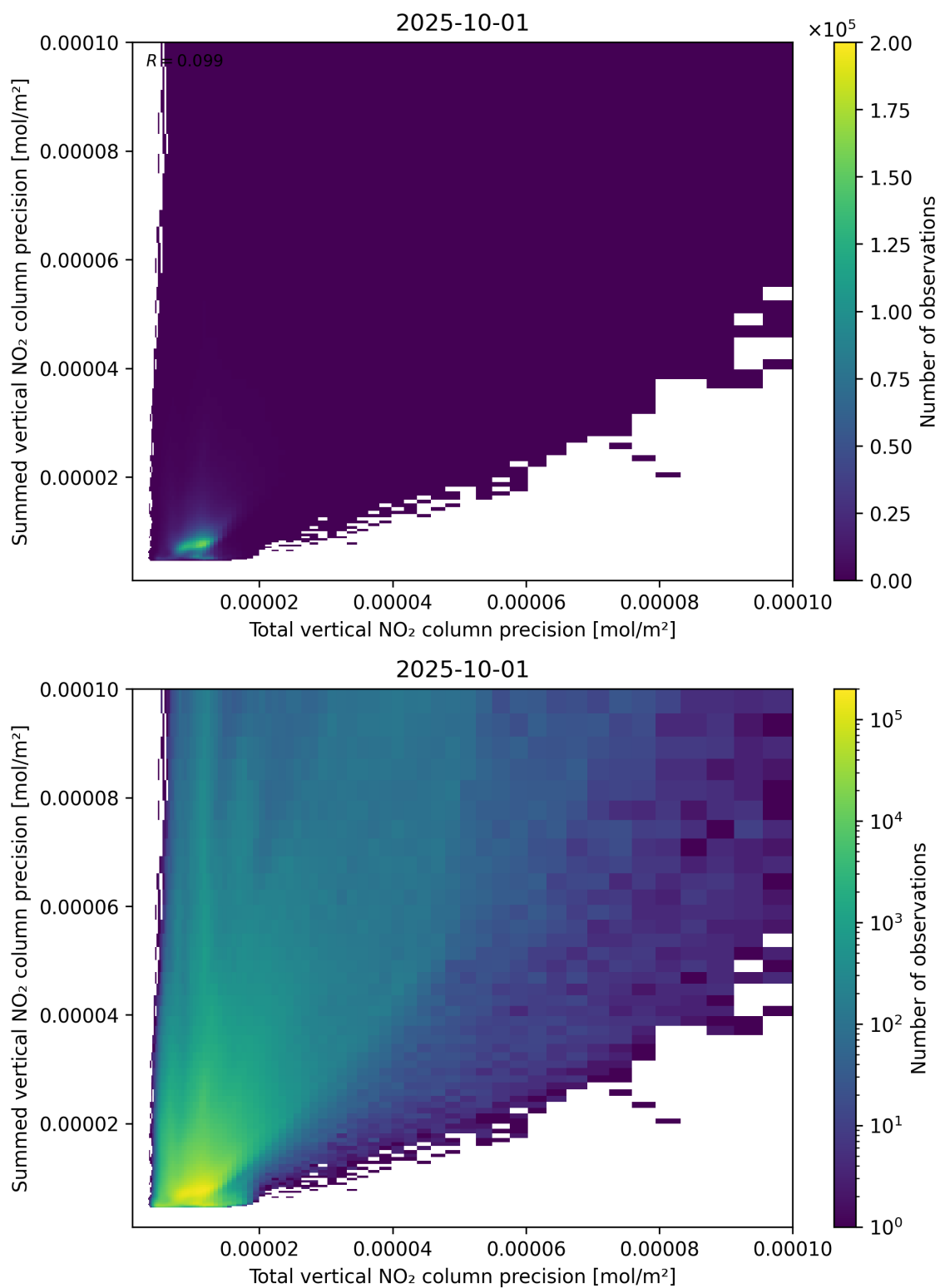
Figure 118: Scatter density plot of “Total vertical NO 2 column precision” against “Summed vertical NO 2 column precision” for 2025-10-01 to 2025-10-02.
