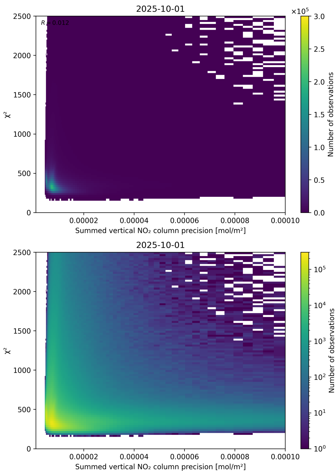
Figure 107: Scatter density plot of “Summed vertical NO 2 column precision” against “ \chi^2 ” for 2025-10-01 to 2025-10-02.
