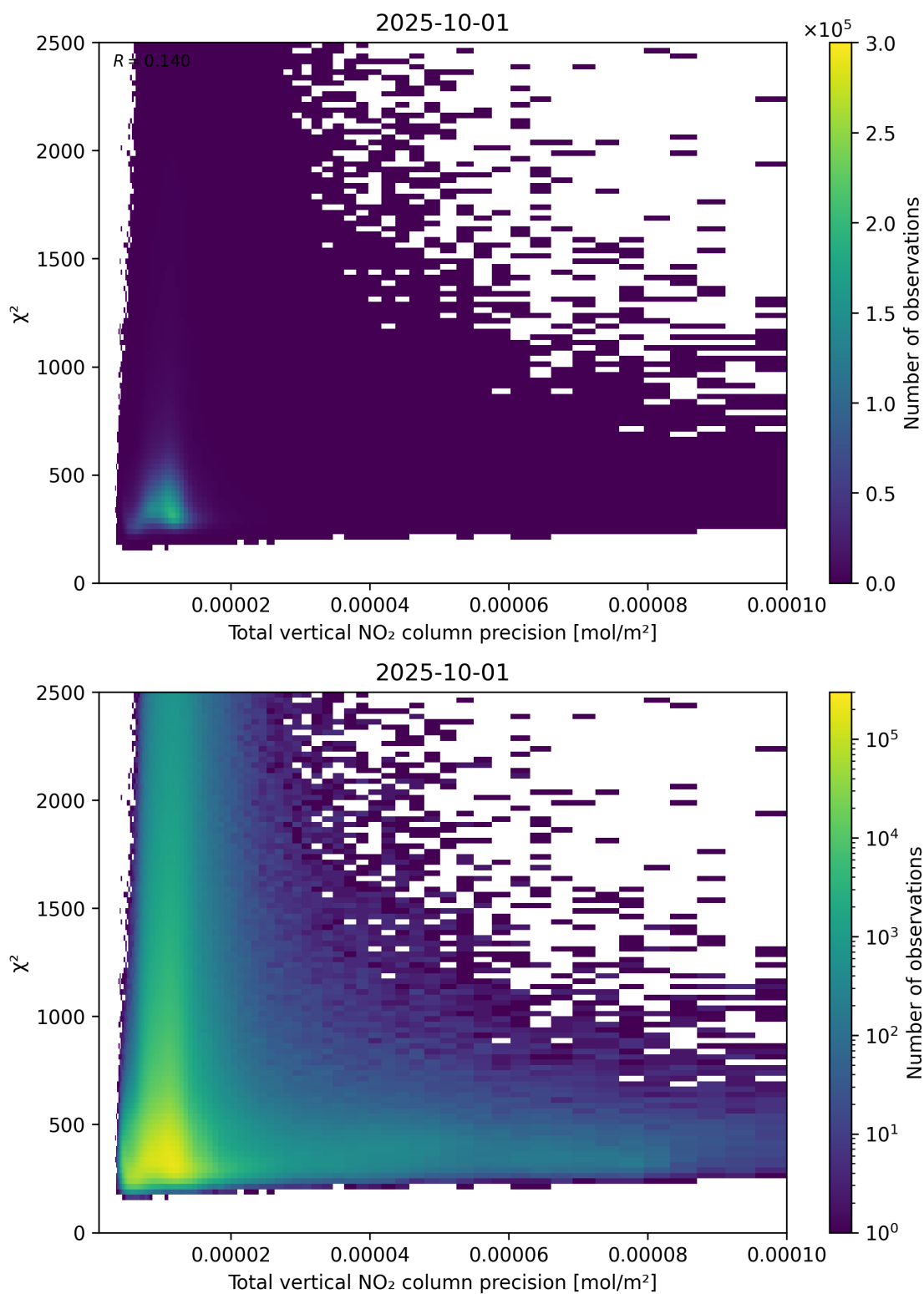
Figure 116: Scatter density plot of “Total vertical NO 2 column precision” against “ \chi^2 ” for 2025-10-01 to 2025-10-02.
