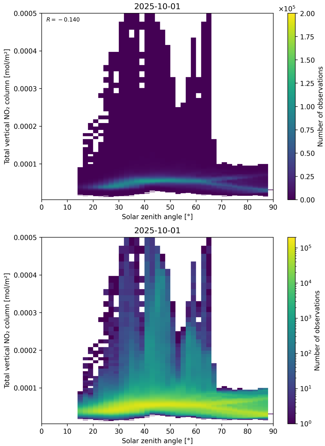
Figure 153: Scatter density plot of “Solar zenith angle” against “Total vertical NO 2 column” for 2025-10-01 to 2025-10-02.
