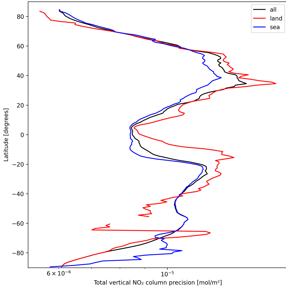
Figure 22: Zonal average of “Total vertical NO 2 column precision” for 2025-10-01 to 2025-10-02.
