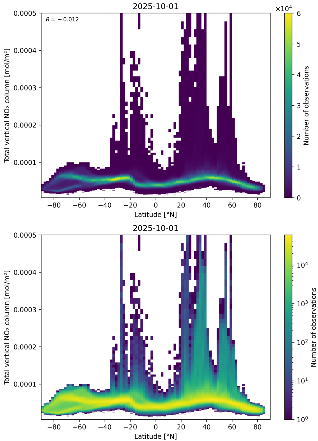
Figure 90: Scatter density plot of “Latitude” against “Total vertical NO 2 column” for 2025-10-01 to 2025-10-02.
