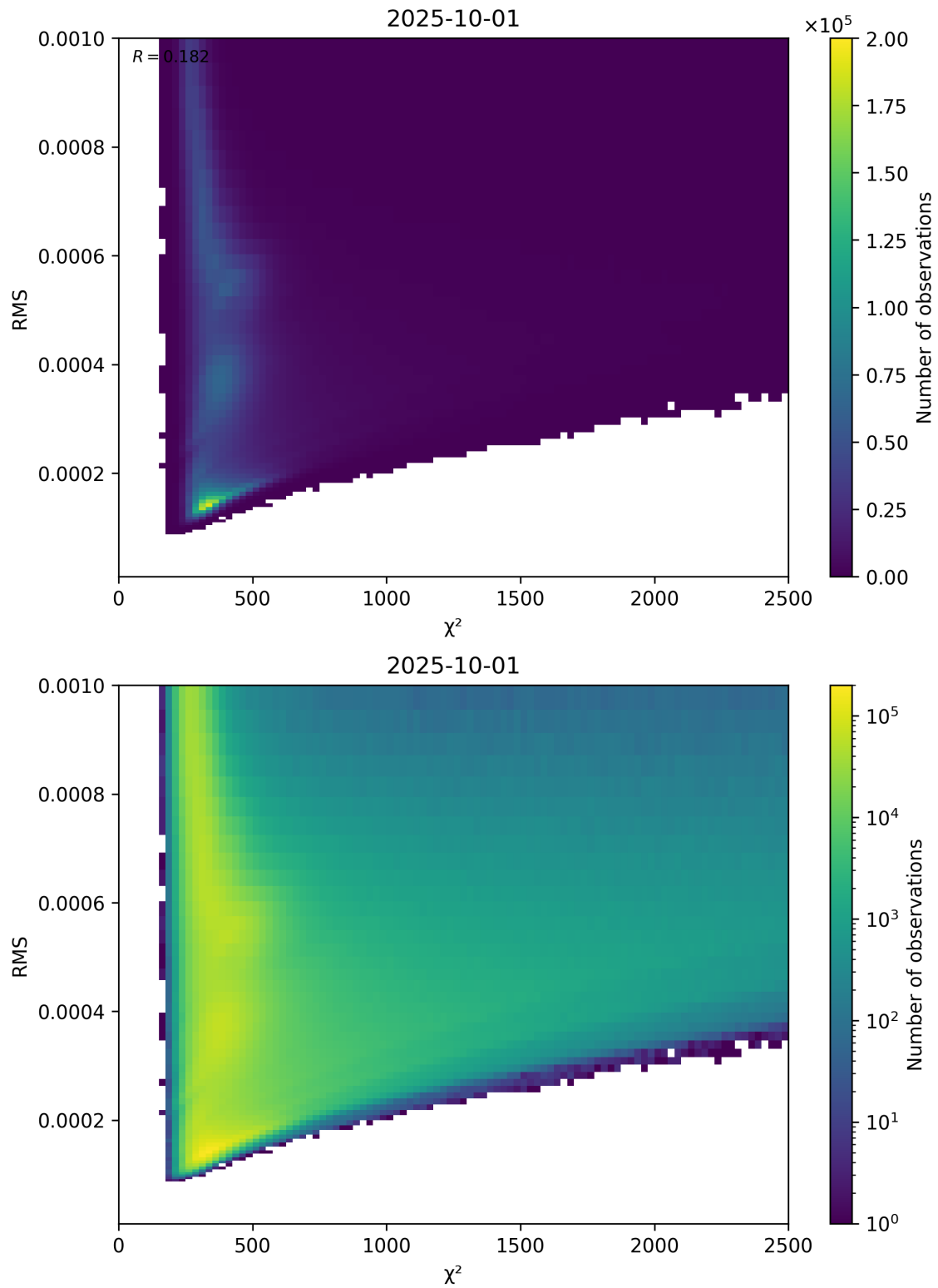
Figure 82: Scatter density plot of “ \chi^2 ” against “RMS” for 2025-10-01 to 2025-10-02.
