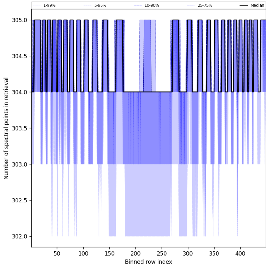
Figure 50: Along track statistics of “Number of spectral points in retrieval” for 2025-10-01 to 2025-10-02
