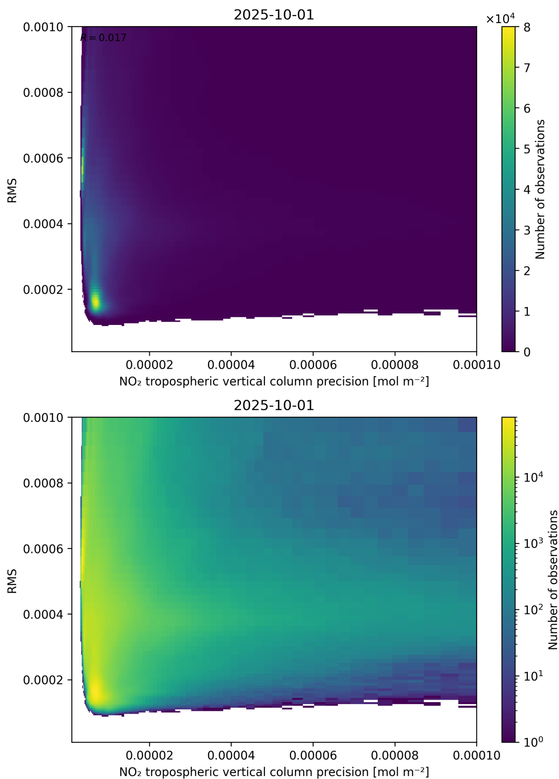
Figure 140: Scatter density plot of “NO 2 tropospheric vertical column precision” against “RMS” for 2025-10-01 to 2025-10-02.
