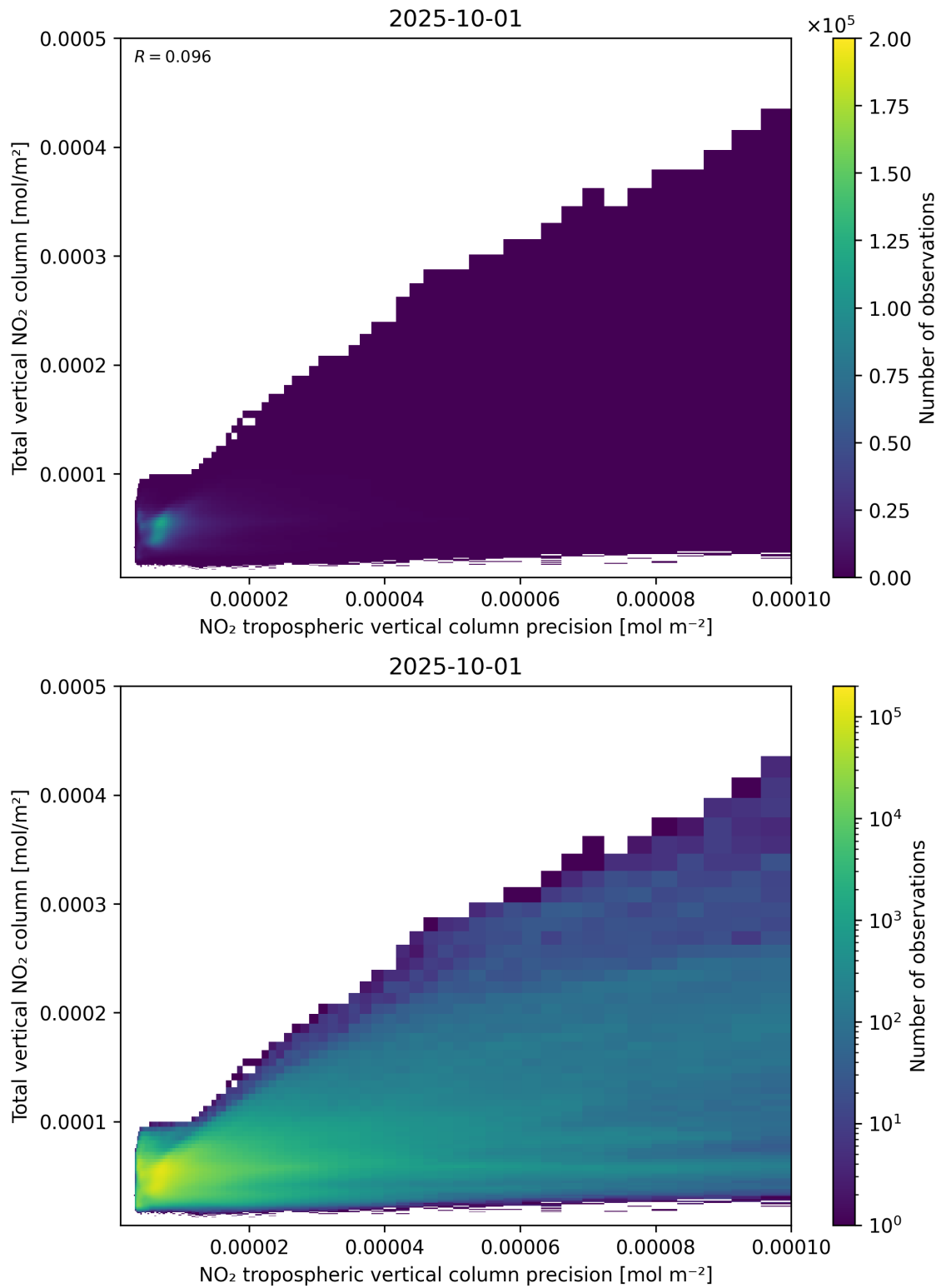
Figure 138: Scatter density plot of “NO 2 tropospheric vertical column precision” against “Total vertical NO 2 column” for 2025-10-01 to 2025-10-02.
