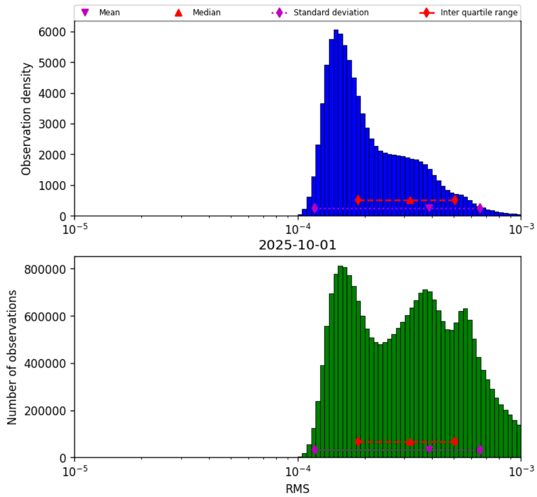
Figure 43: Histogram of “RMS” for 2025-10-01 to 2025-10-02
