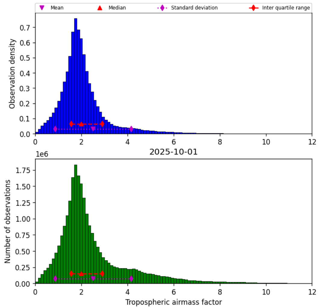
Figure 31: Histogram of “Tropospheric airmass factor” for 2025-10-01 to 2025-10-02
