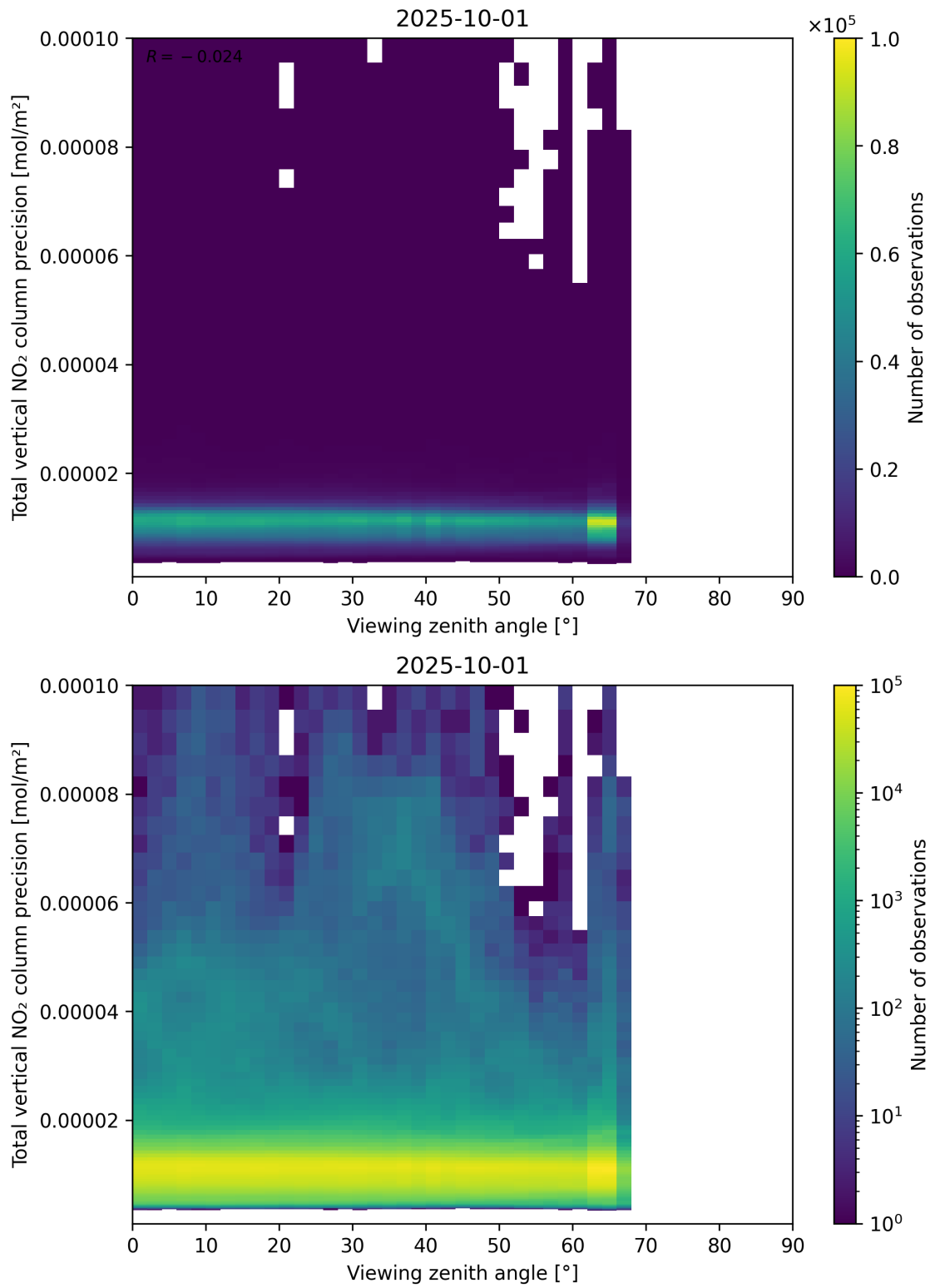
Figure 168: Scatter density plot of “Viewing zenith angle” against “Total vertical NO 2 column precision” for 2025-10-01 to 2025-10-02.
