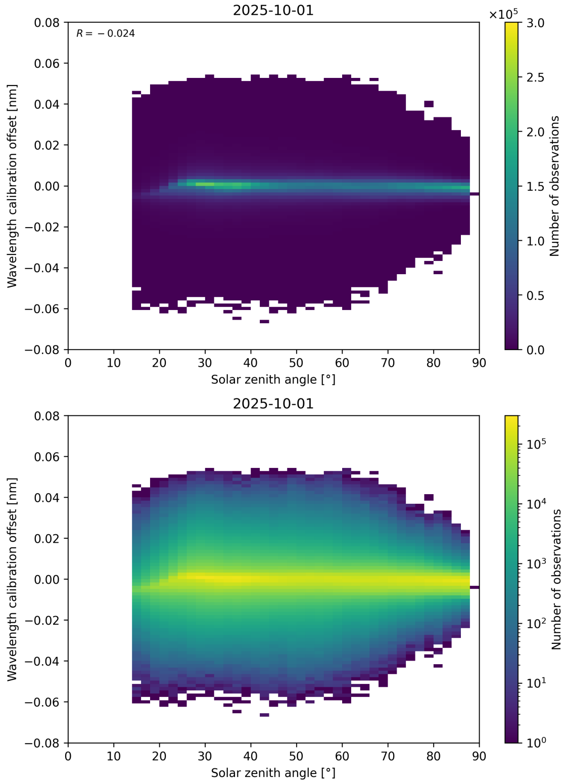
Figure 158: Scatter density plot of “Solar zenith angle” against “Wavelength calibration offset” for 2025-10-01 to 2025-10-02.
