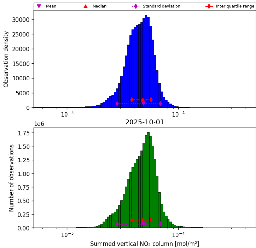
Figure 40: Histogram of “Summed vertical NO 2 column” for 2025-10-01 to 2025-10-02
