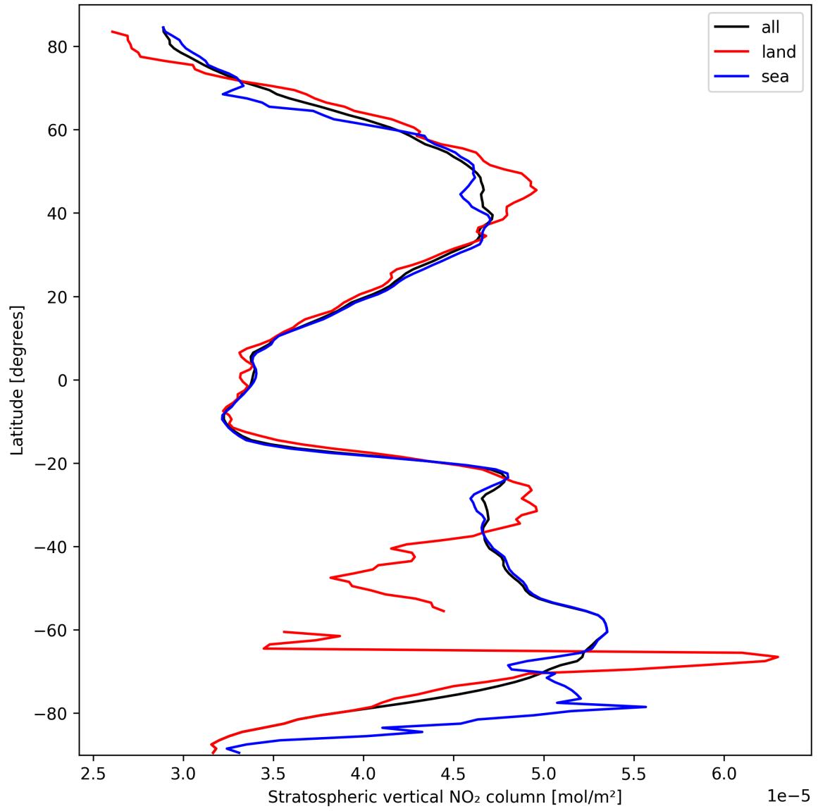
Figure 19: Zonal average of “Stratospheric vertical NO 2 column” for 2025-10-01 to 2025-10-02.
