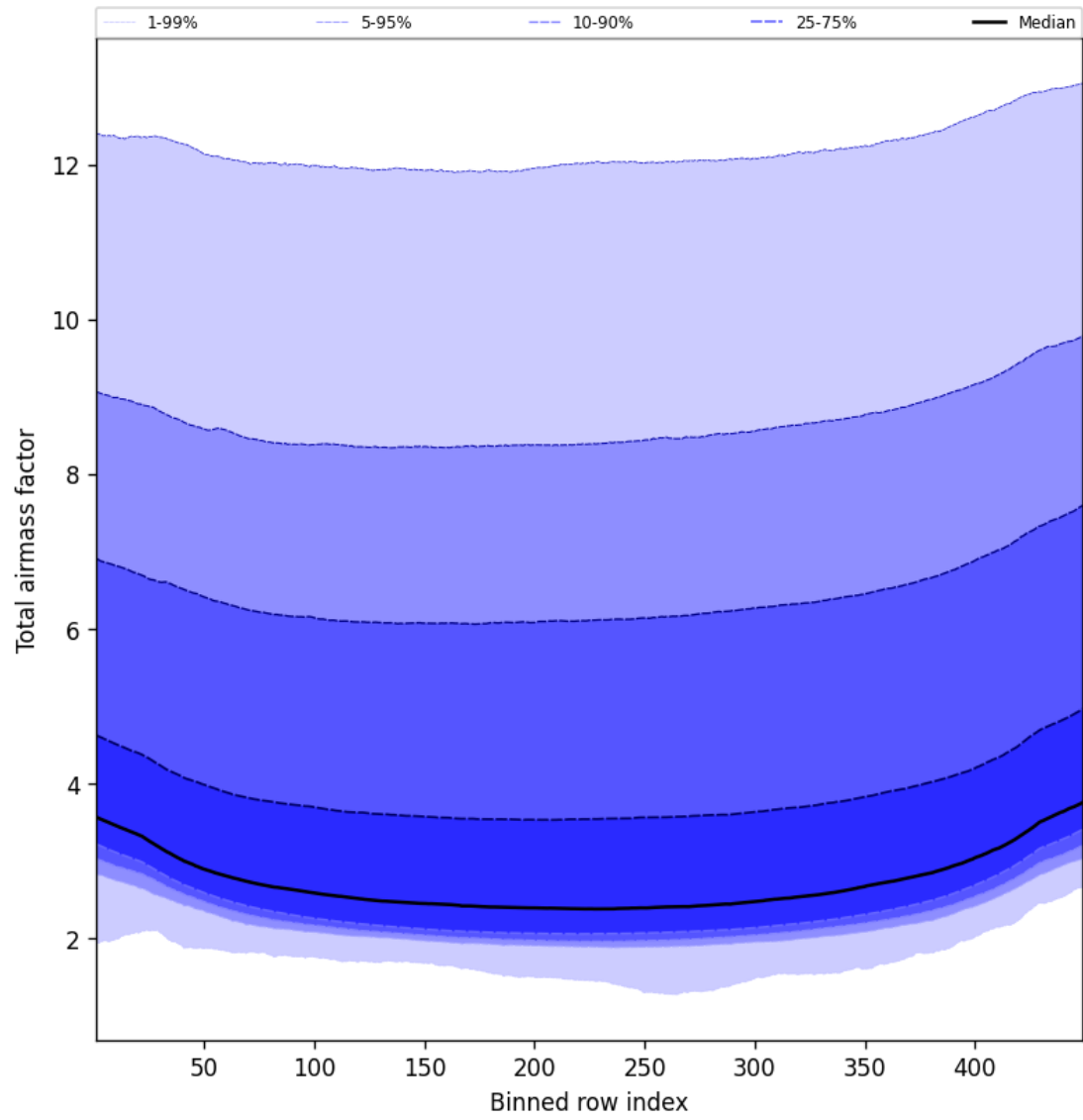
Figure 49: Along track statistics of “Total airmass factor” for 2025-10-01 to 2025-10-02
