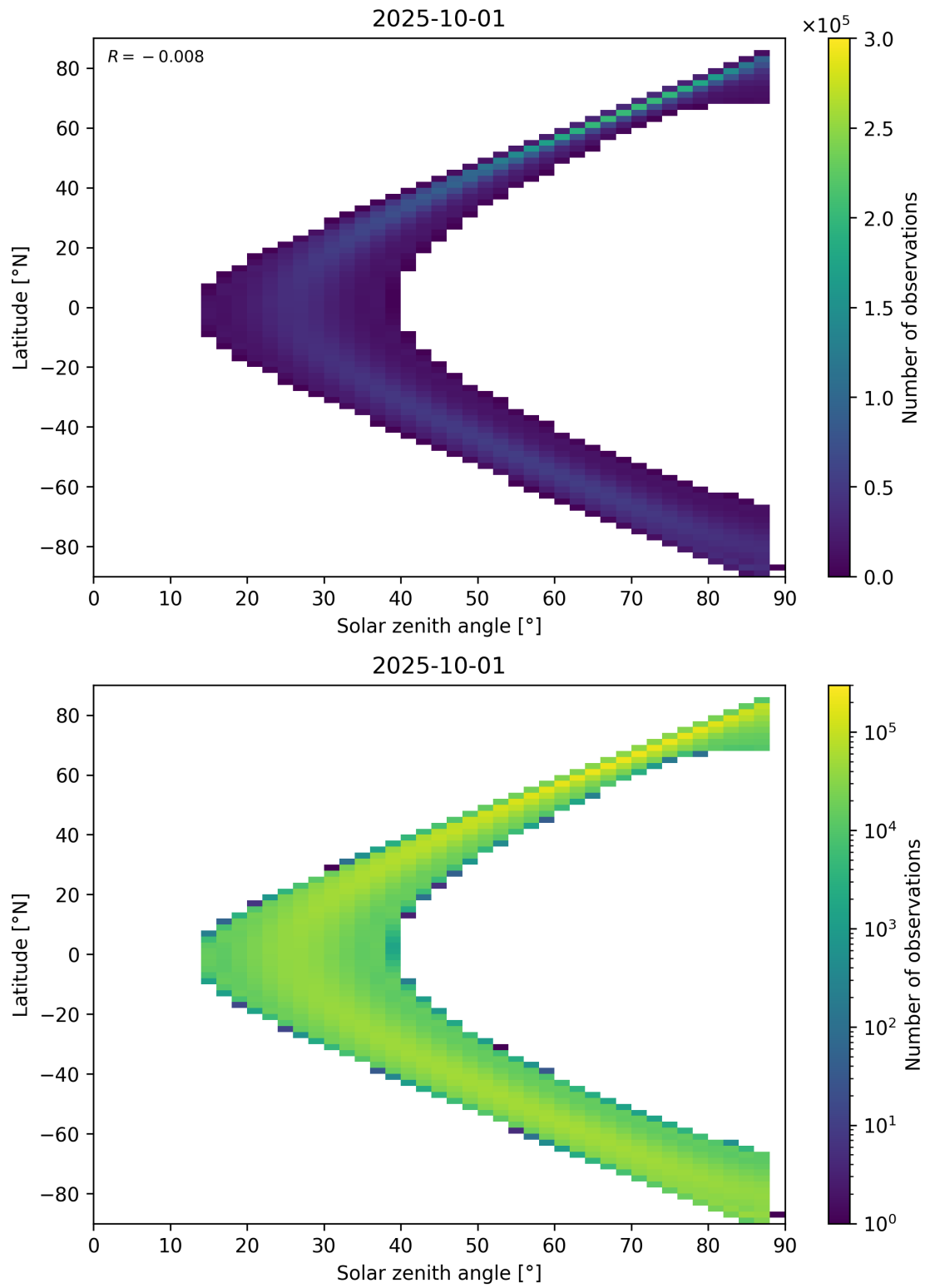
Figure 149: Scatter density plot of “Solar zenith angle” against “Latitude” for 2025-10-01 to 2025-10-02.
