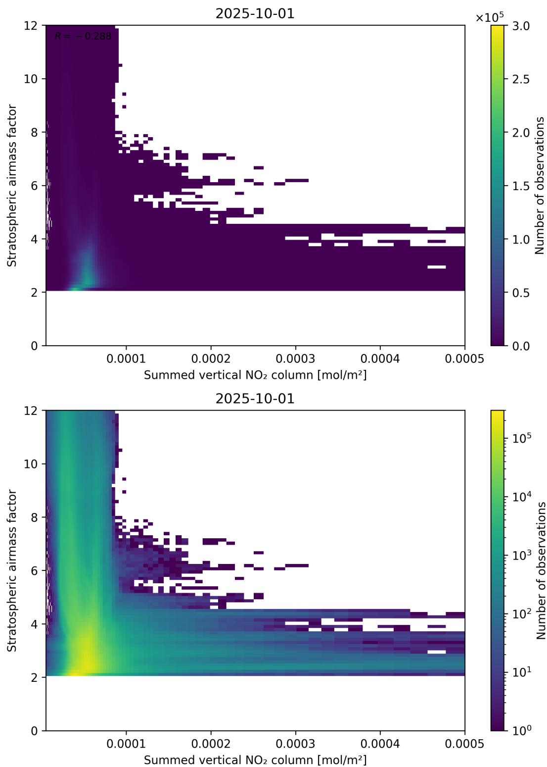
Figure 103: Scatter density plot of “Summed vertical NO 2 column” against “Stratospheric airmass factor” for 2025-10-01 to 2025-10-02.
