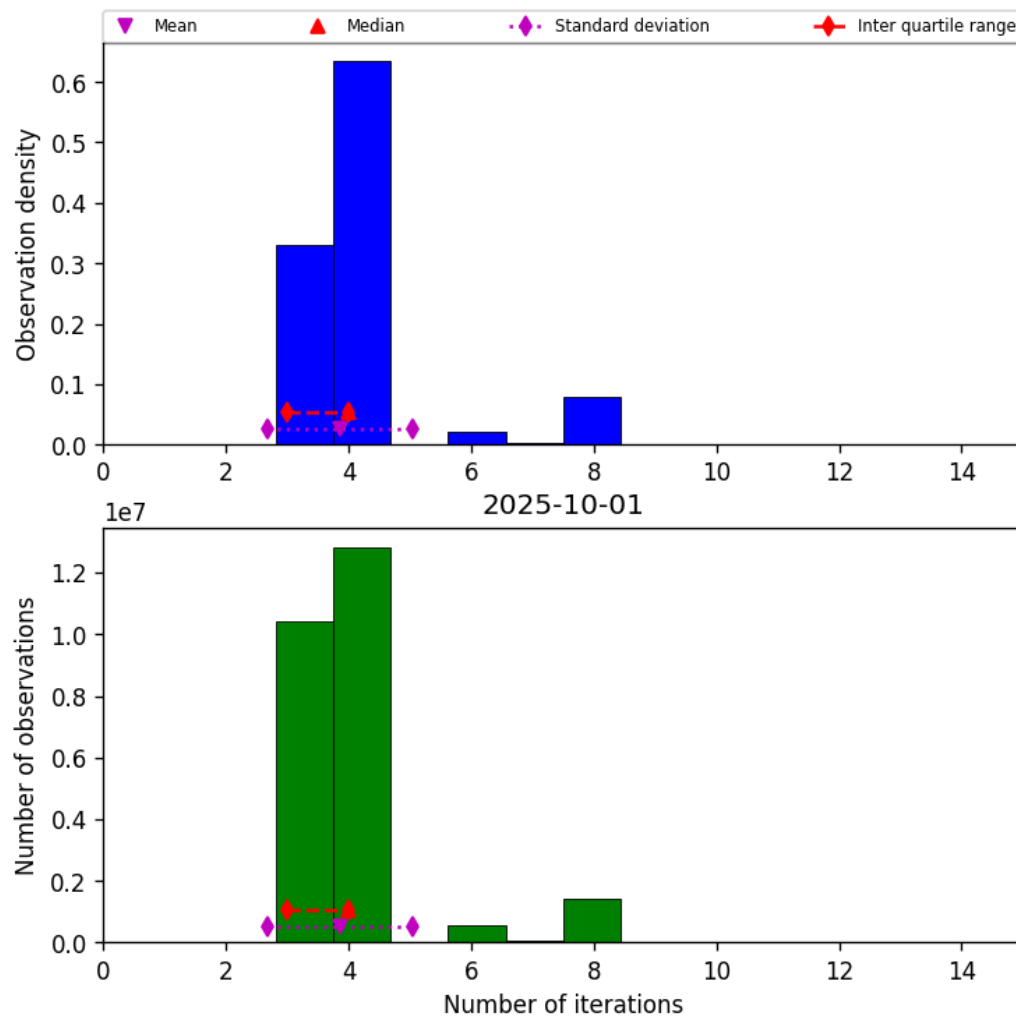
Figure 34: Histogram of “Number of iterations” for 2025-10-01 to 2025-10-02
