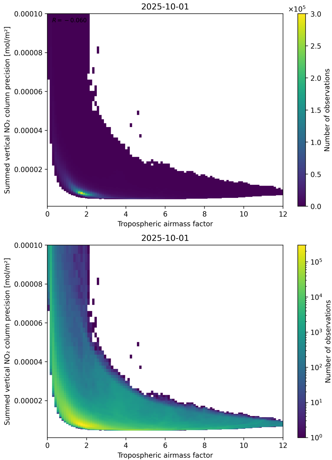
Figure 76: Scatter density plot of “Tropospheric air mass factor” against “Summed vertical NO 2 column precision” for 2025-10-01 to 2025-10-02.
