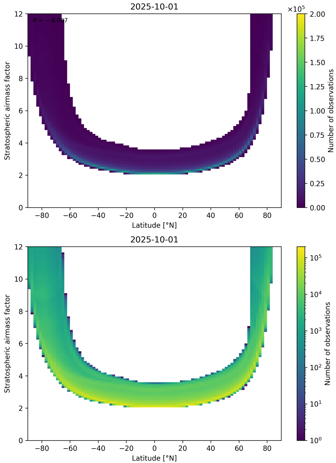
Figure 83: Scatter density plot of “Latitude” against “Stratospheric airmass factor” for 2025-10-01 to 2025-10-02.
