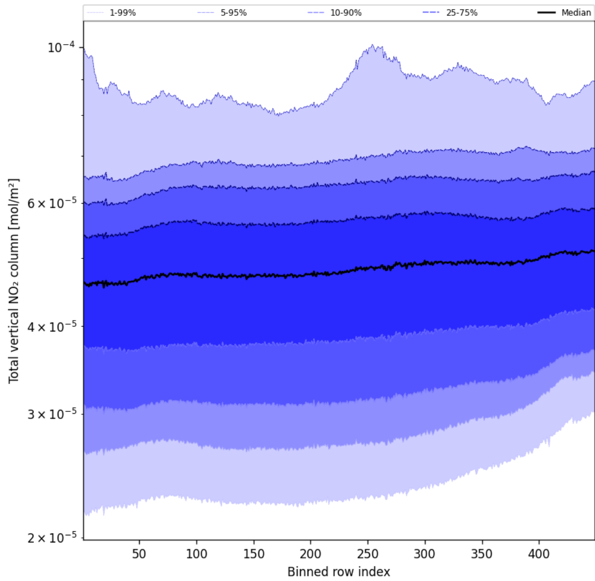
Figure 55: Along track statistics of “Total vertical NO 2 column” for 2025-10-01 to 2025-10-02
