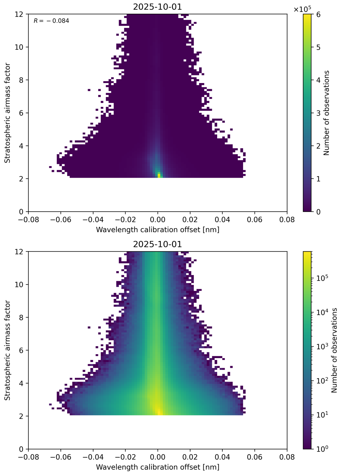
Figure 174: Scatter density plot of “Wavelength calibration offset” against “Stratospheric air mass factor” for 2025-10-01 to 2025-10-02.
