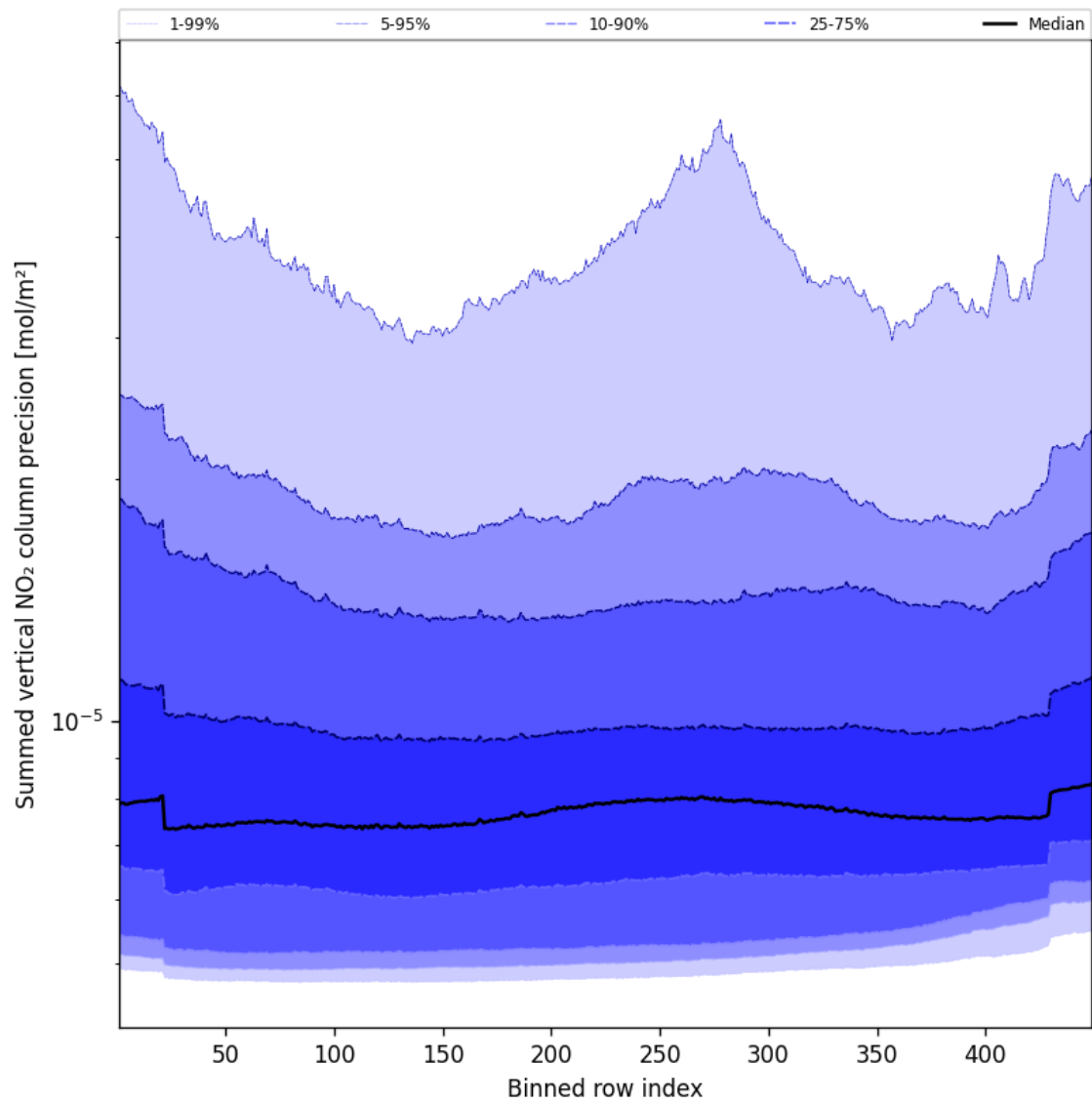
Figure 58: Along track statistics of “Summed vertical NO 2 column precision” for 2025-10-01 to 2025-10-02
