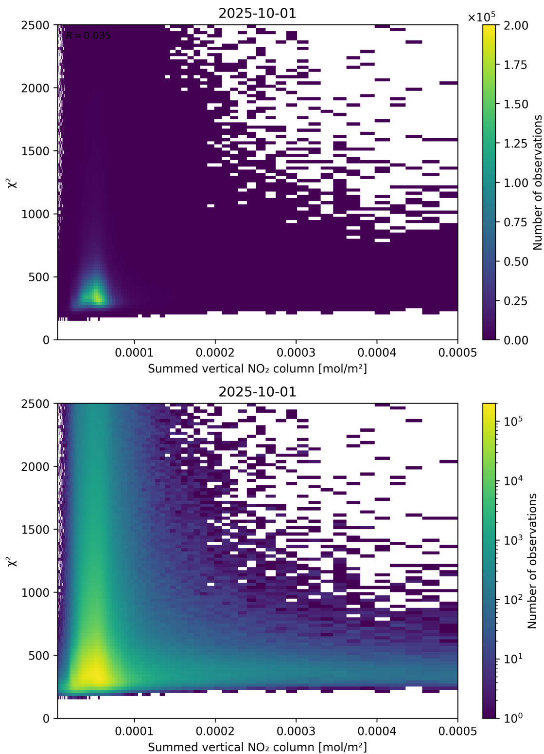
Figure 104: Scatter density plot of “Summed vertical NO 2 column” against “ \chi^2 ” for 2025-10-01 to 2025-10-02.
