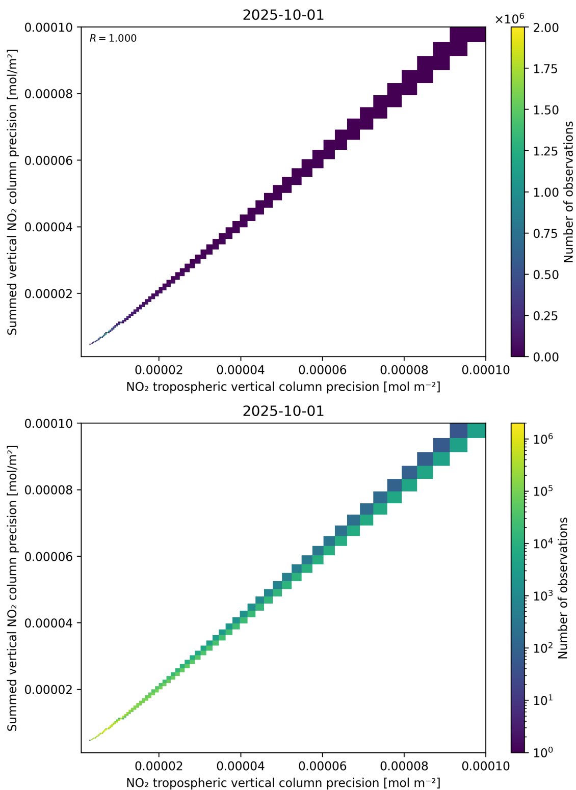
Figure 137: Scatter density plot of “NO 2 tropospheric vertical column precision” against “Summed vertical NO 2 column precision” for 2025-10-01 to 2025-10-02.
