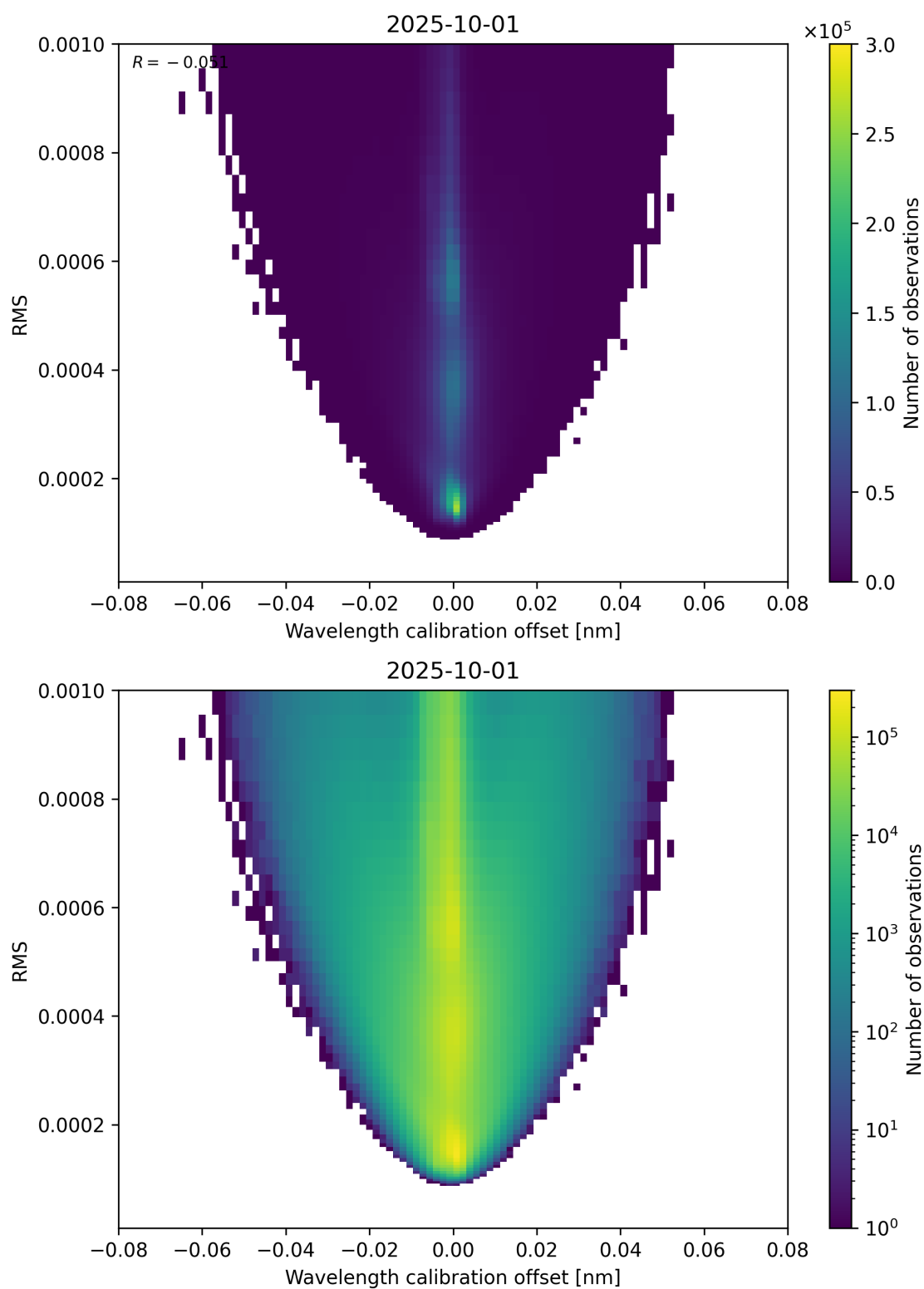
Figure 181: Scatter density plot of “Wavelength calibration offset” against “RMS” for 2025-10-01 to 2025-10-02.
