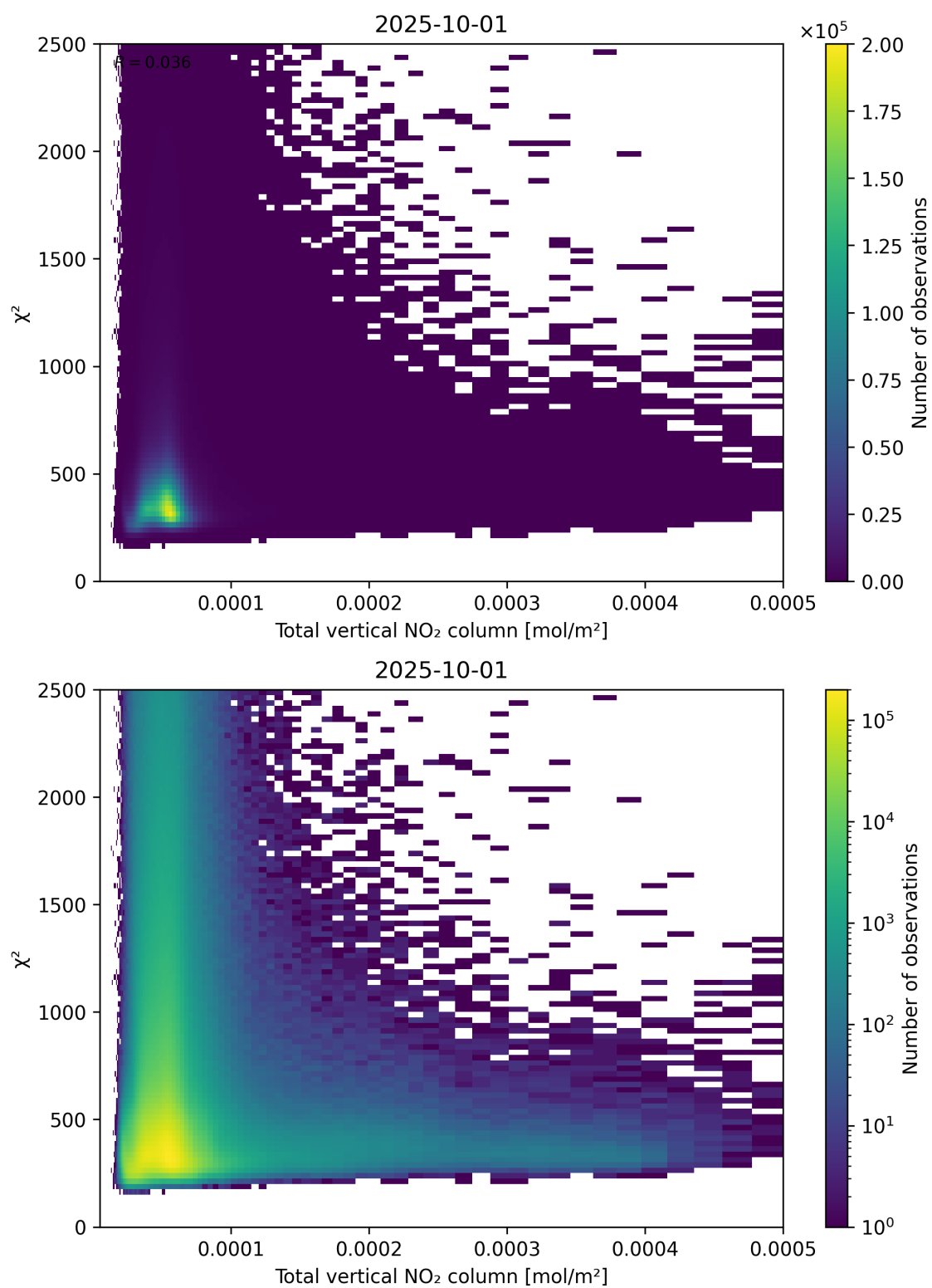
Figure 111: Scatter density plot of “Total vertical NO 2 column” against “ \chi^2 ” for 2025-10-01 to 2025-10-02.
