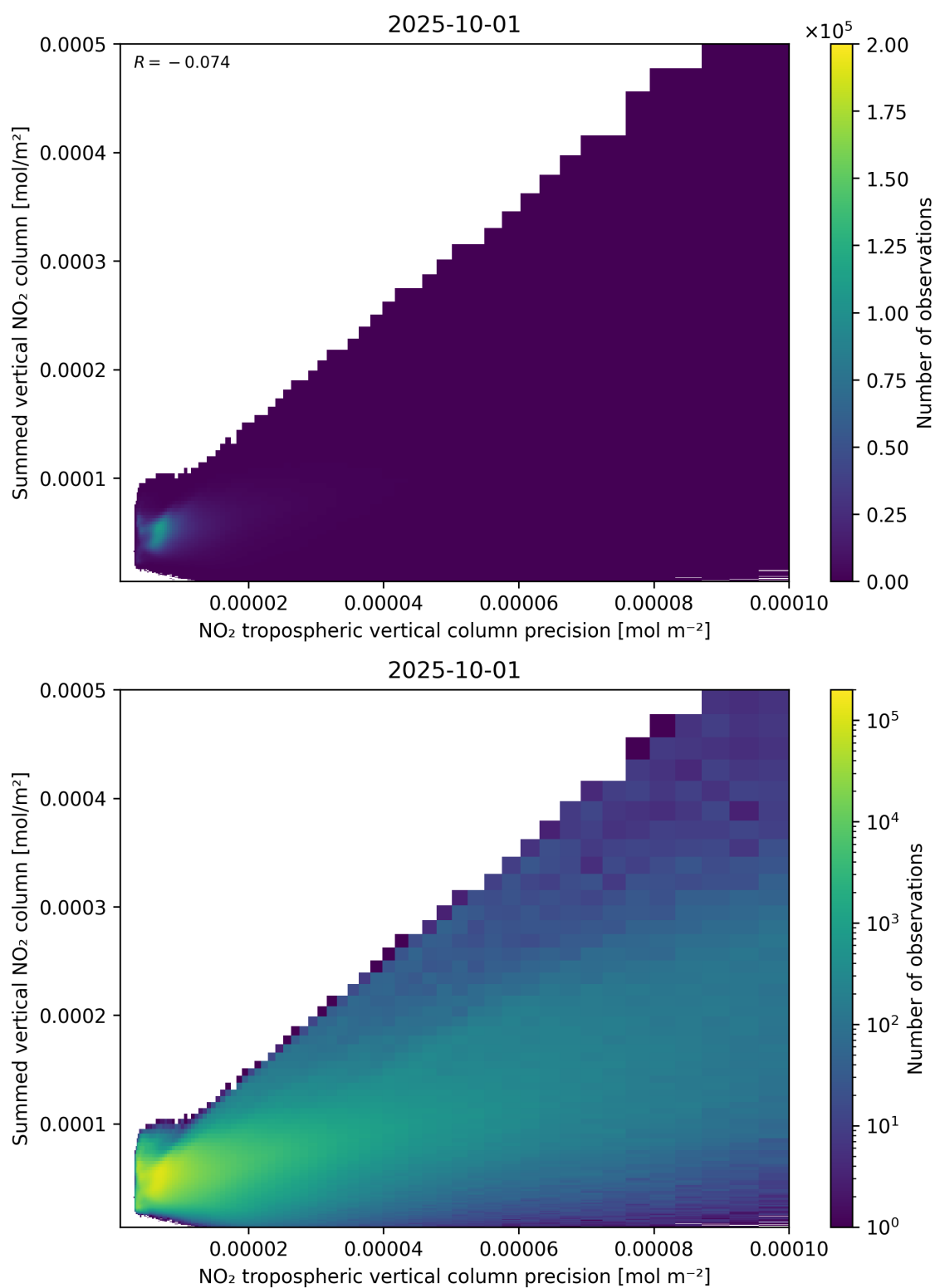
Figure 136: Scatter density plot of “NO 2 tropospheric vertical column precision” against “Summed vertical NO 2 column” for 2025-10-01 to 2025-10-02.
