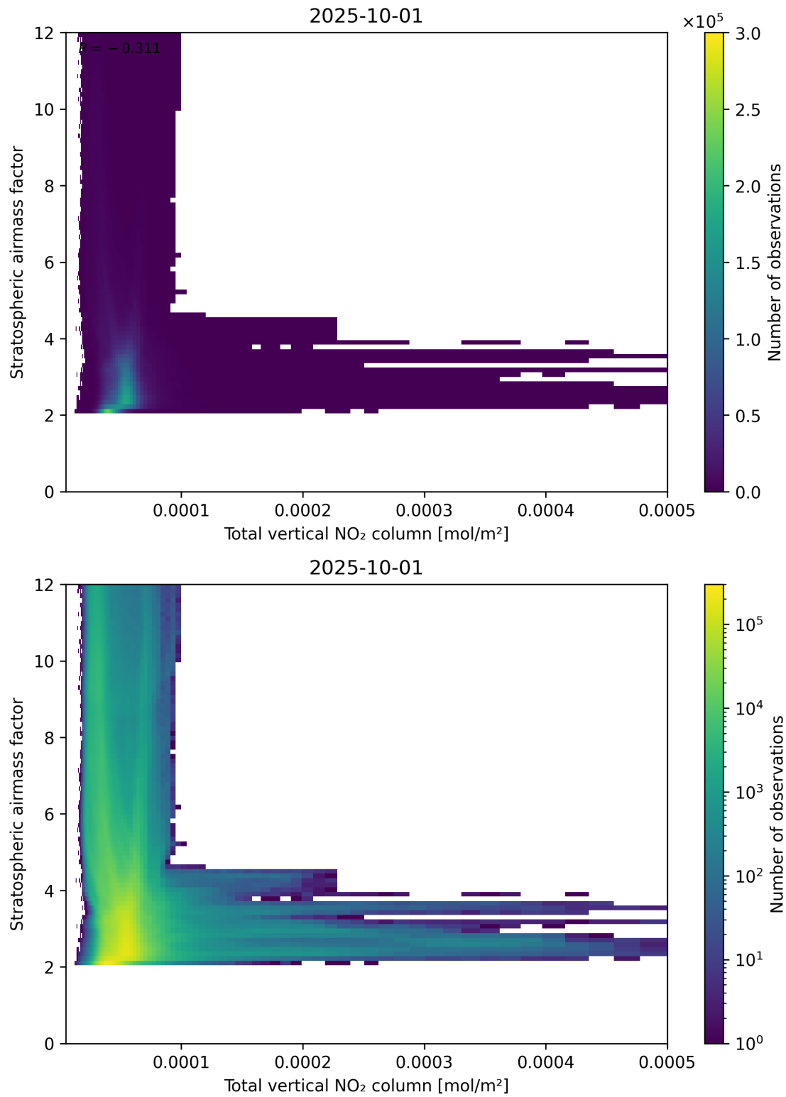
Figure 110: Scatter density plot of “Total vertical NO 2 column” against “Stratospheric airmass factor” for 2025-10-01 to 2025-10-02.
