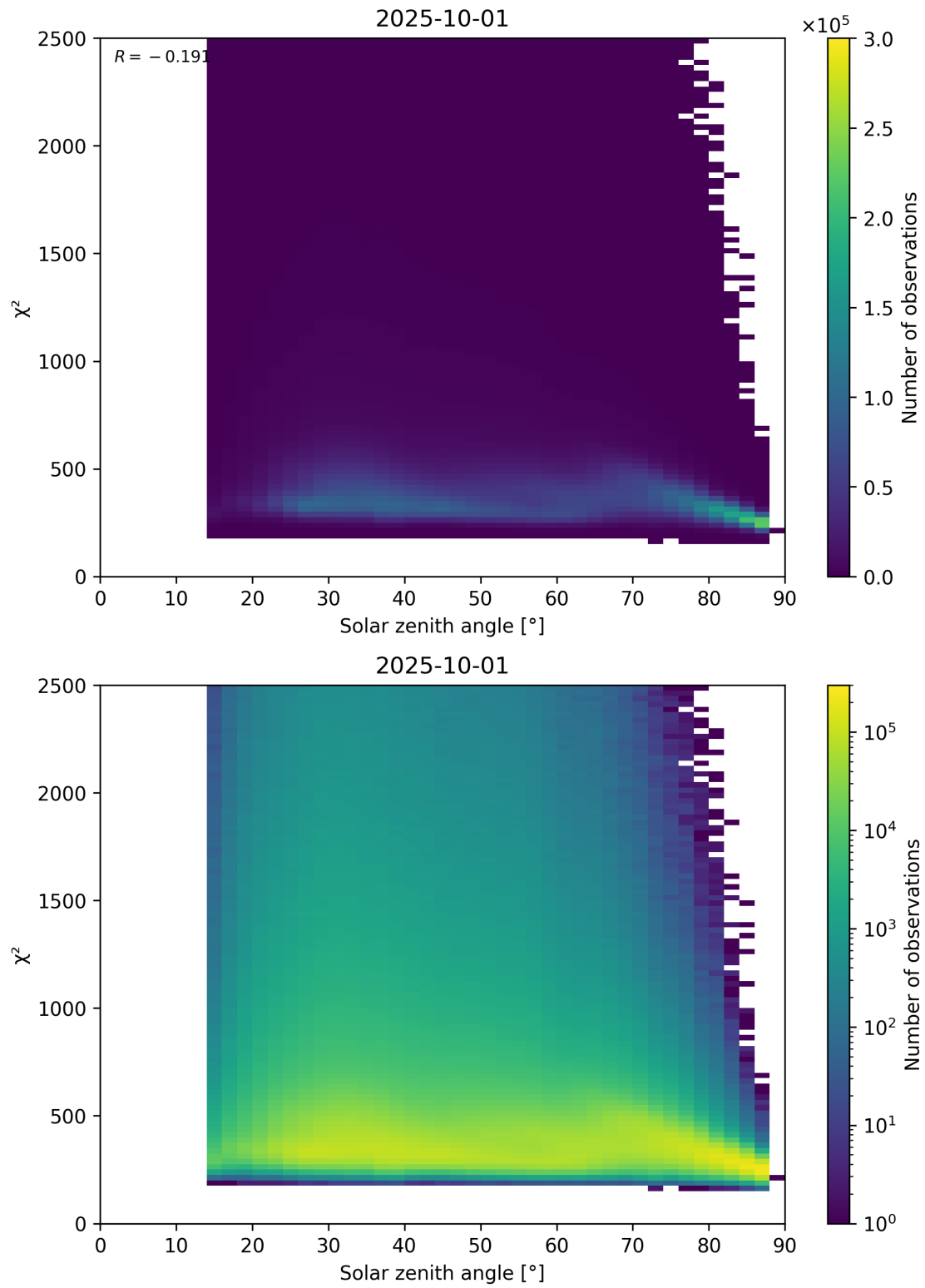
Figure 148: Scatter density plot of “Solar zenith angle” against “ \chi^2 ” for 2025-10-01 to 2025-10-02.
