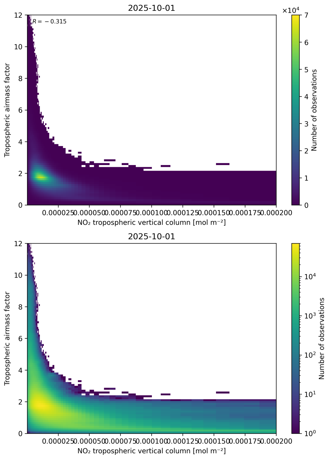
Figure 123: Scatter density plot of “NO 2 tropospheric vertical column” against “Tropospheric air mass factor” for 2025-10-01 to 2025-10-02.
