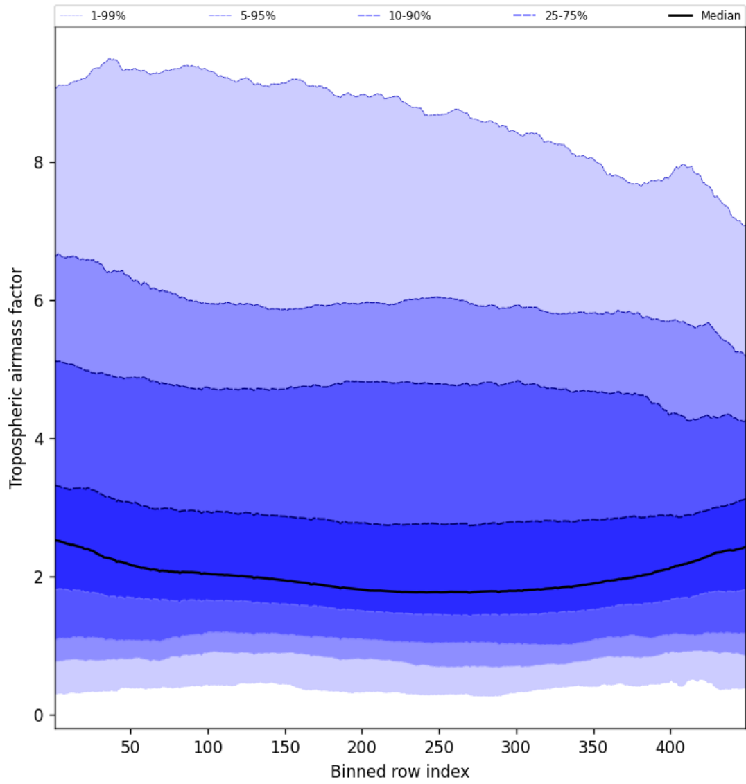
Figure 48: Along track statistics of “Tropospheric air mass factor” for 2025-10-01 to 2025-10-02
