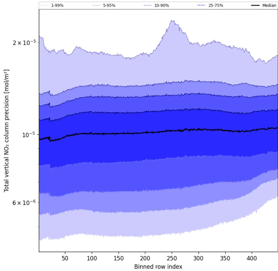
Figure 56: Along track statistics of “Total vertical NO 2 column precision” for 2025-10-01 to 2025-10-02
