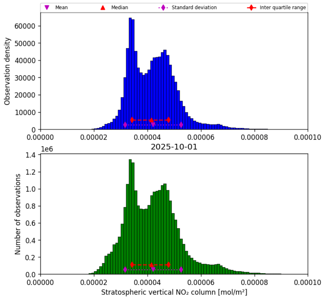
Figure 36: Histogram of “Stratospheric vertical NO 2 column” for 2025-10-01 to 2025-10-02
