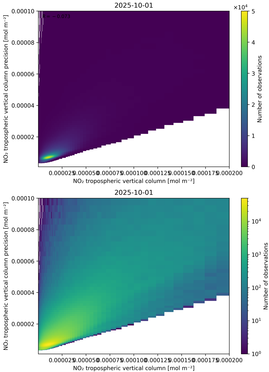
Figure 130: Scatter density plot of “NO 2 tropospheric vertical column” against “NO 2 tropospheric vertical column precision” for 2025-10-01 to 2025-10-02.
