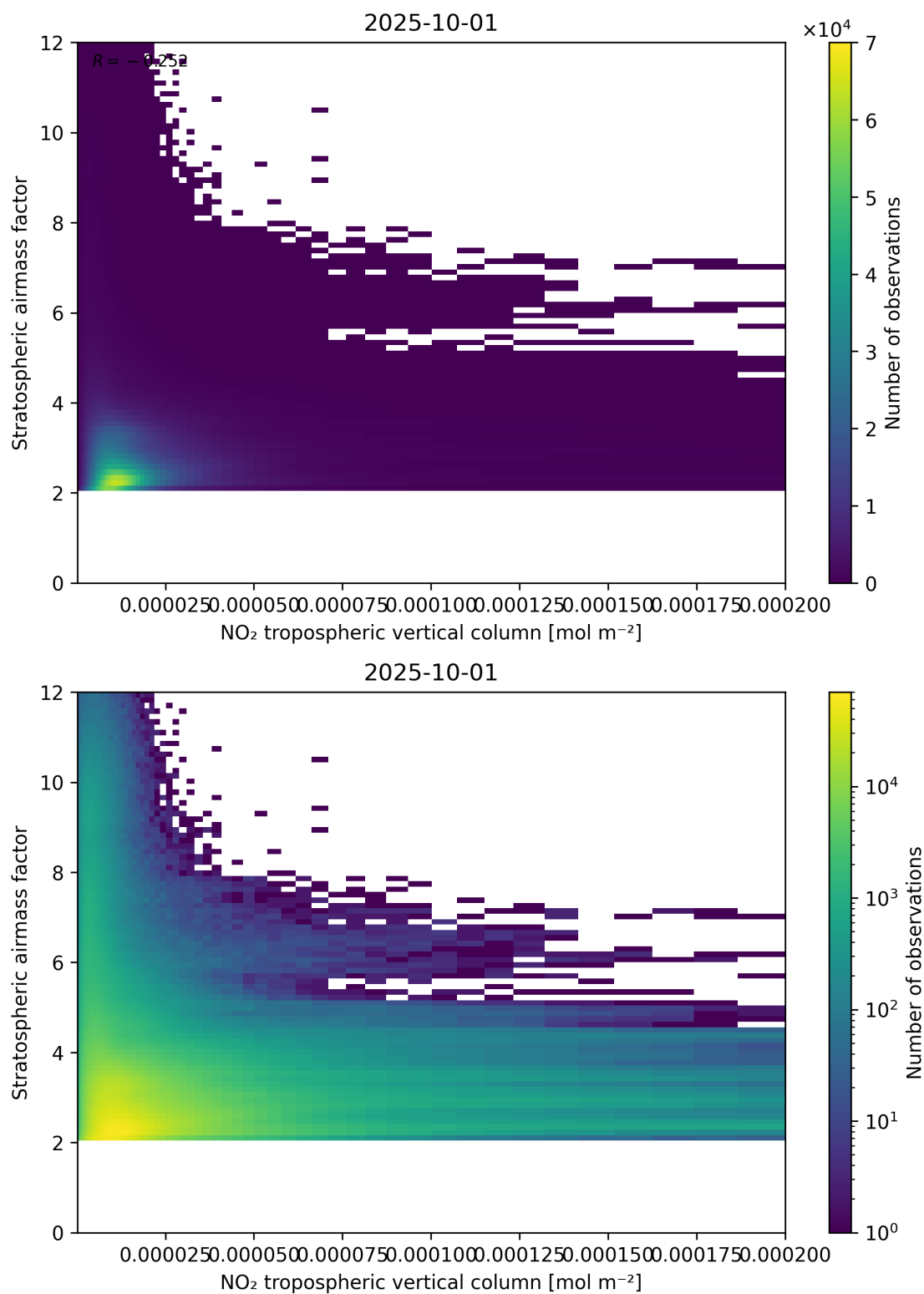
Figure 121: Scatter density plot of “NO 2 tropospheric vertical column” against “Stratospheric air mass factor” for 2025-10-01 to 2025-10-02.
