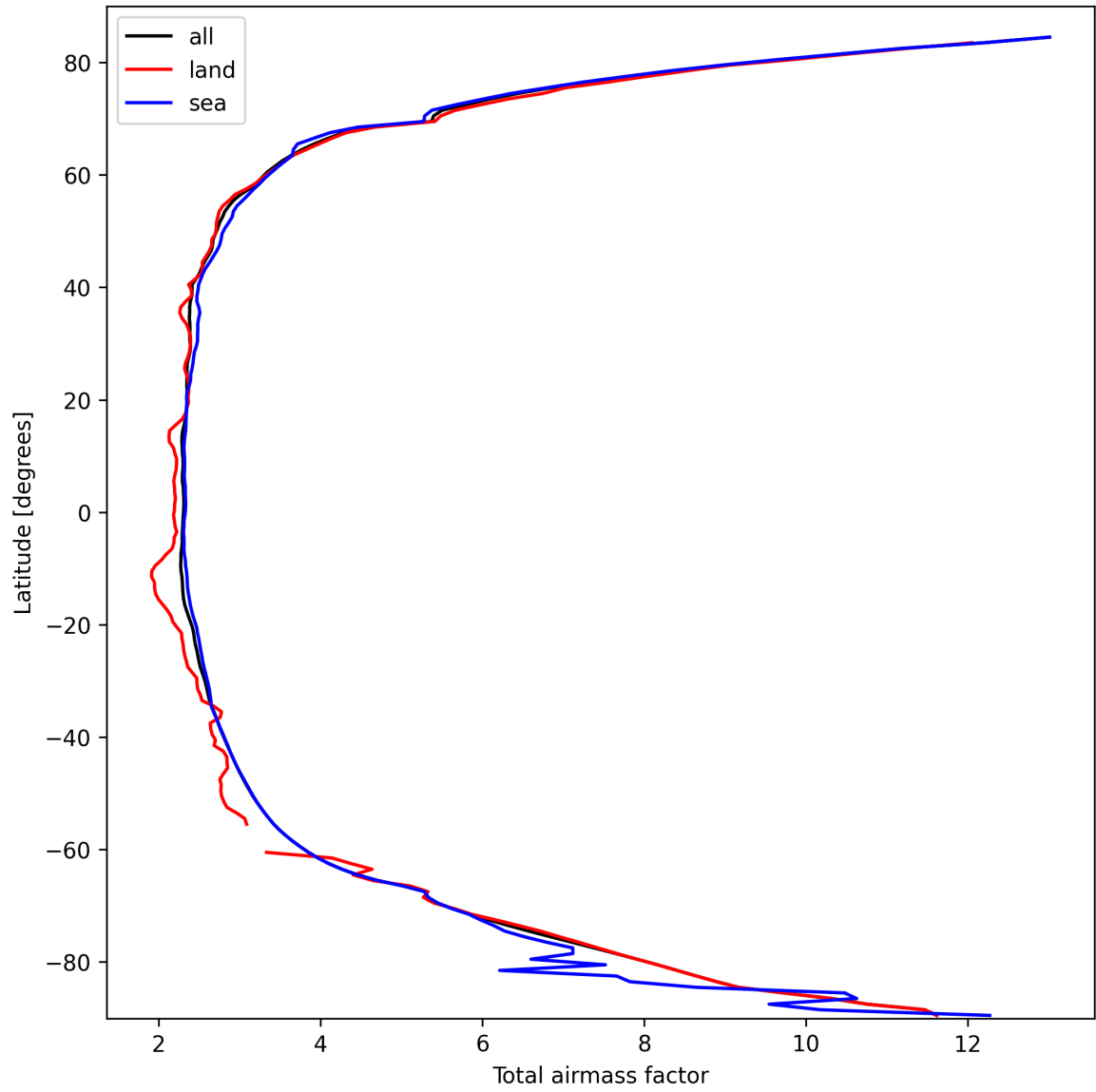
Figure 15: Zonal average of “Total airmass factor” for 2025-10-01 to 2025-10-02.
