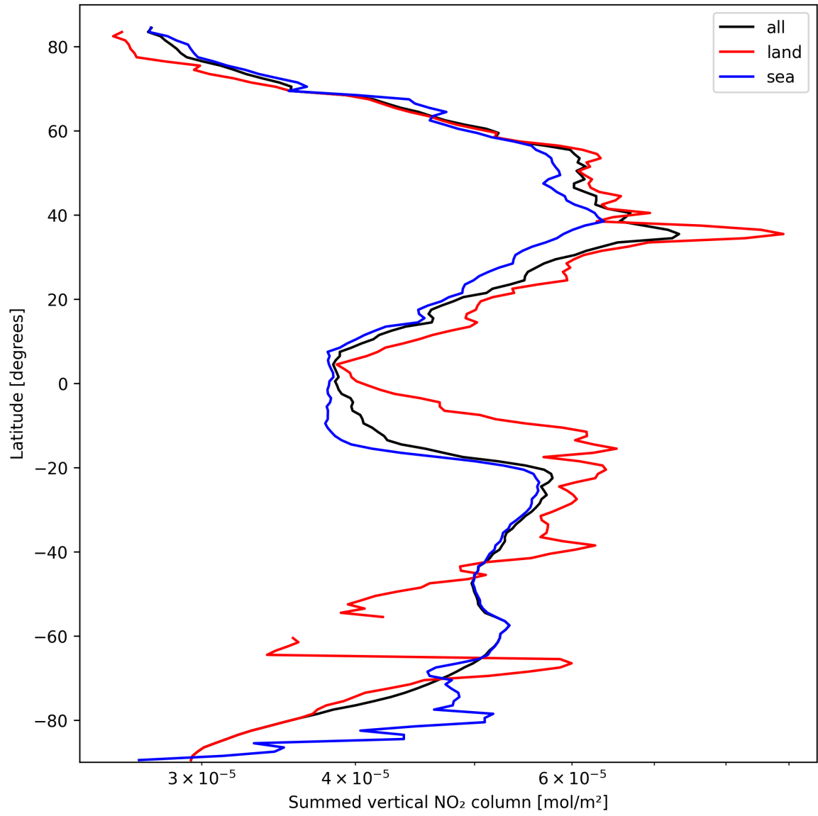
Figure 23: Zonal average of “Summed vertical NO 2 column” for 2025-10-01 to 2025-10-02.
