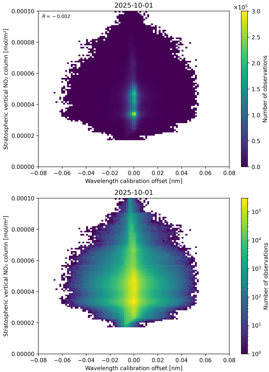
Figure 176: Scatter density plot of “Wavelength calibration offset” against “Stratospheric vertical NO 2 column” for 2025-10-01 to 2025-10-02.
