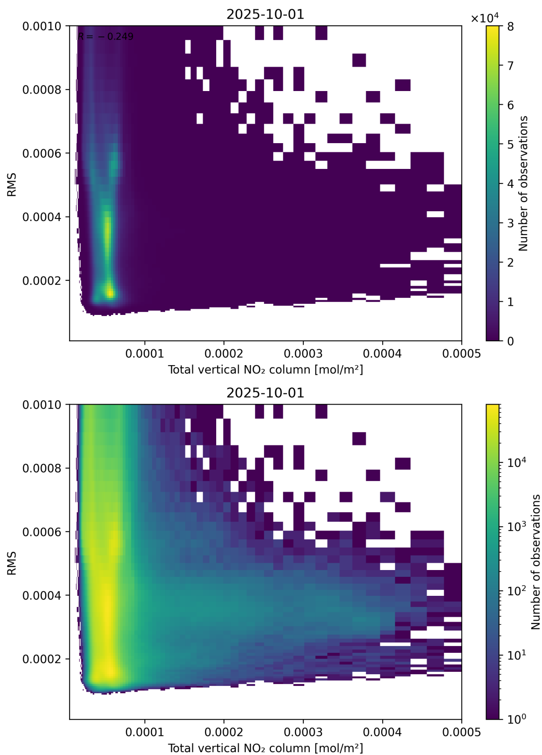
Figure 120: Scatter density plot of “Total vertical NO 2 column” against “RMS” for 2025-10-01 to 2025-10-02.
