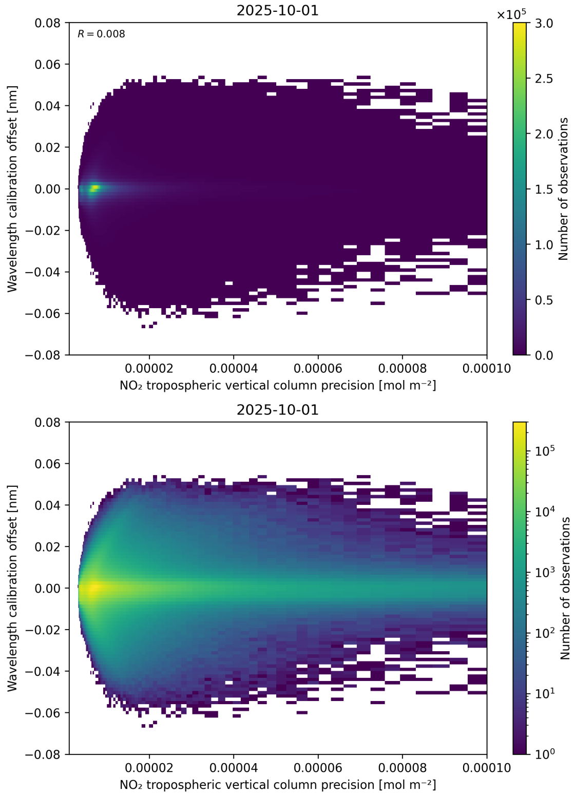
Figure 141: Scatter density plot of “NO 2 tropospheric vertical column precision” against “Wavelength calibration offset” for 2025-10-01 to 2025-10-02.
