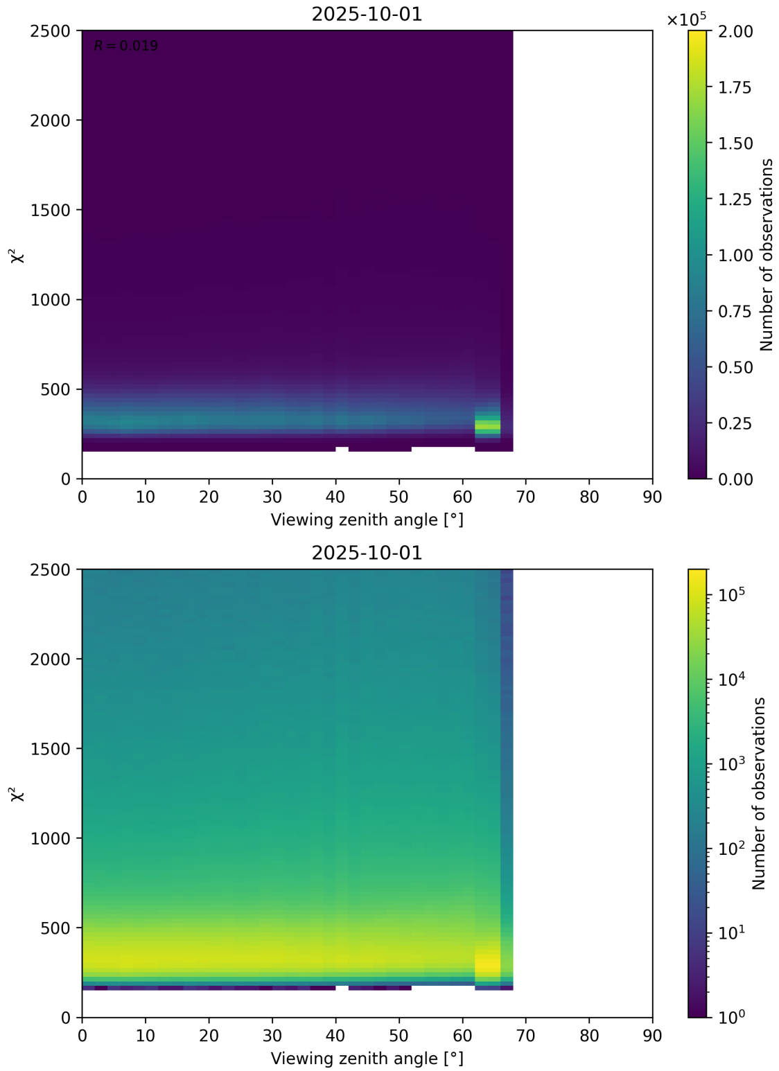
Figure 162: Scatter density plot of “Viewing zenith angle” against “ \chi^2 ” for 2025-10-01 to 2025-10-02.
