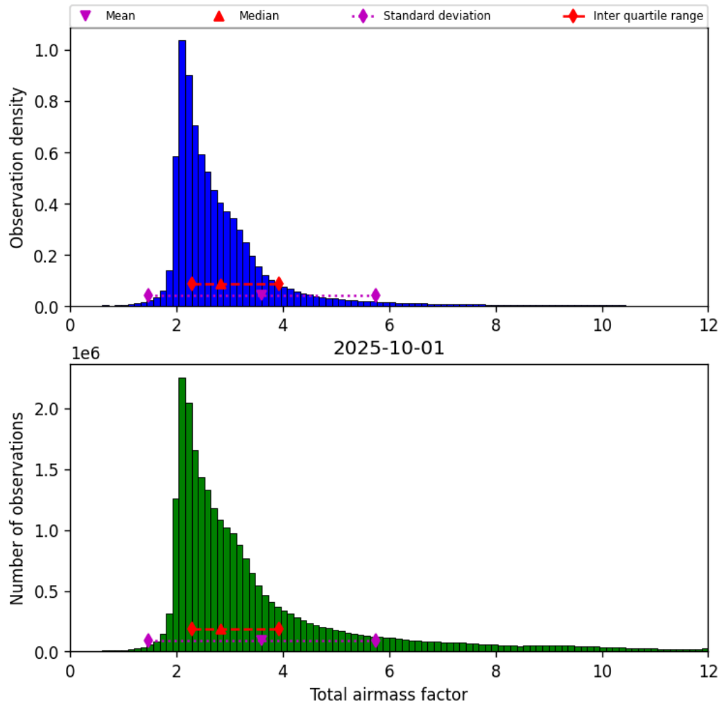
Figure 32: Histogram of “Total airmass factor” for 2025-10-01 to 2025-10-02
