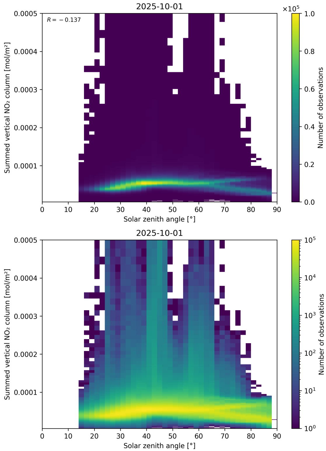
Figure 151: Scatter density plot of “Solar zenith angle” against “Summed vertical NO 2 column” for 2025-10-01 to 2025-10-02.
