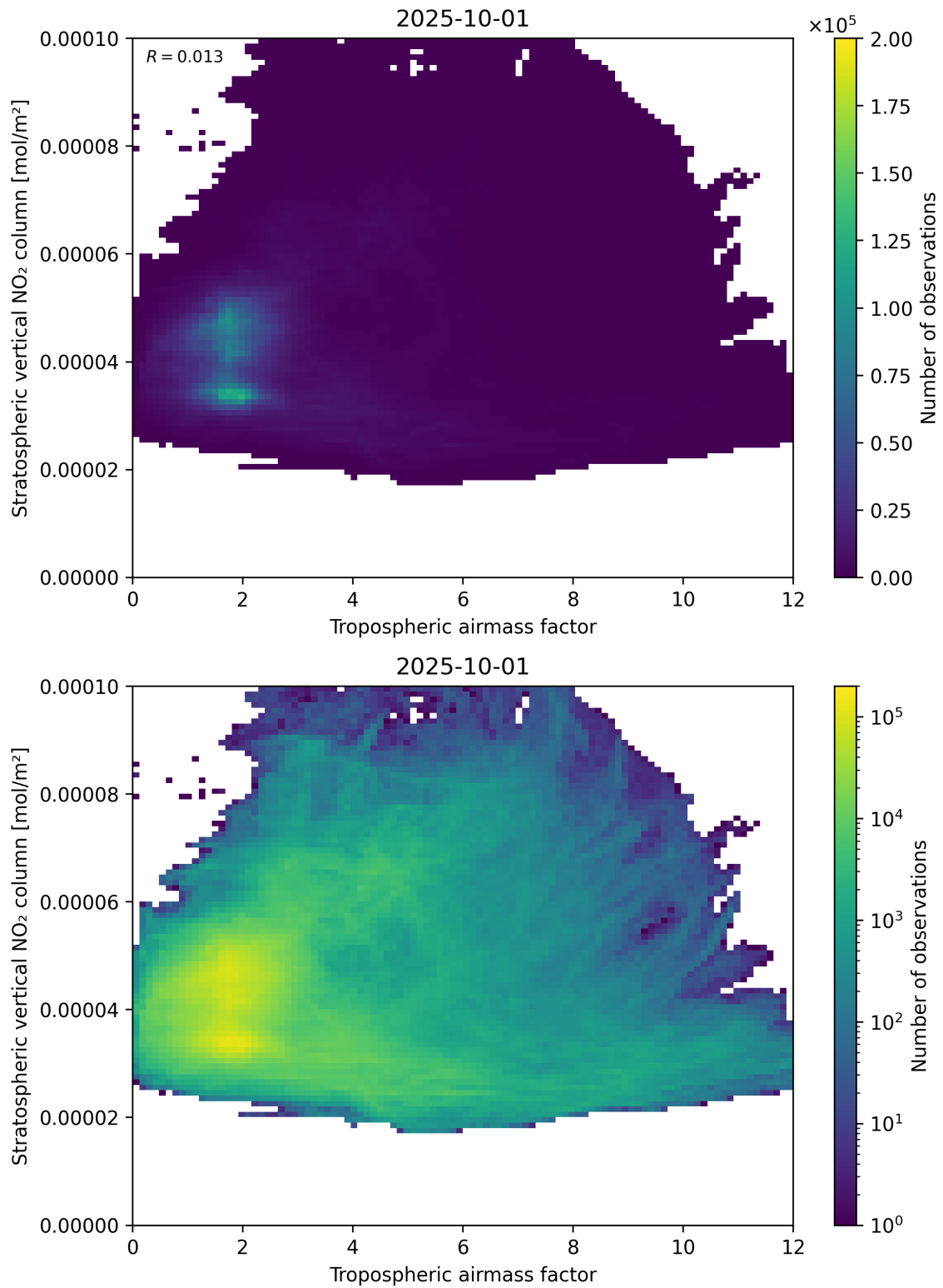
Figure 74: Scatter density plot of “Tropospheric air mass factor” against “Stratospheric vertical NO 2 column” for 2025-10-01 to 2025-10-02.
