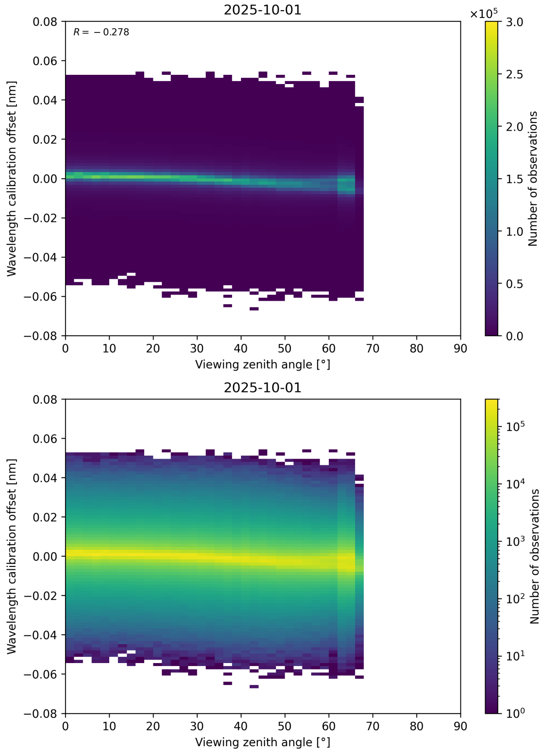
Figure 173: Scatter density plot of “Viewing zenith angle” against “Wavelength calibration offset” for 2025-10-01 to 2025-10-02.
