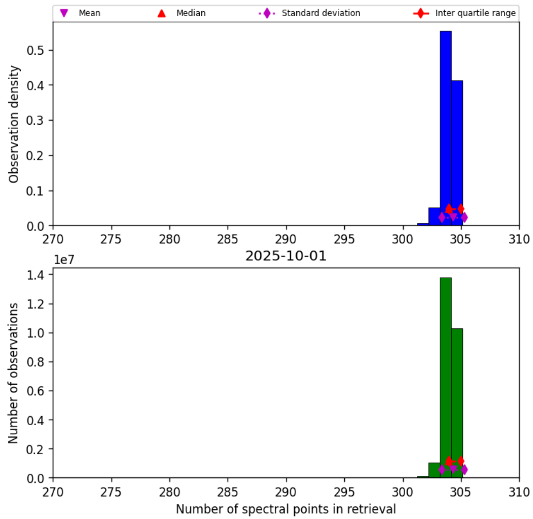
Figure 33: Histogram of “Number of spectral points in retrieval” for 2025-10-01 to 2025-10-02
