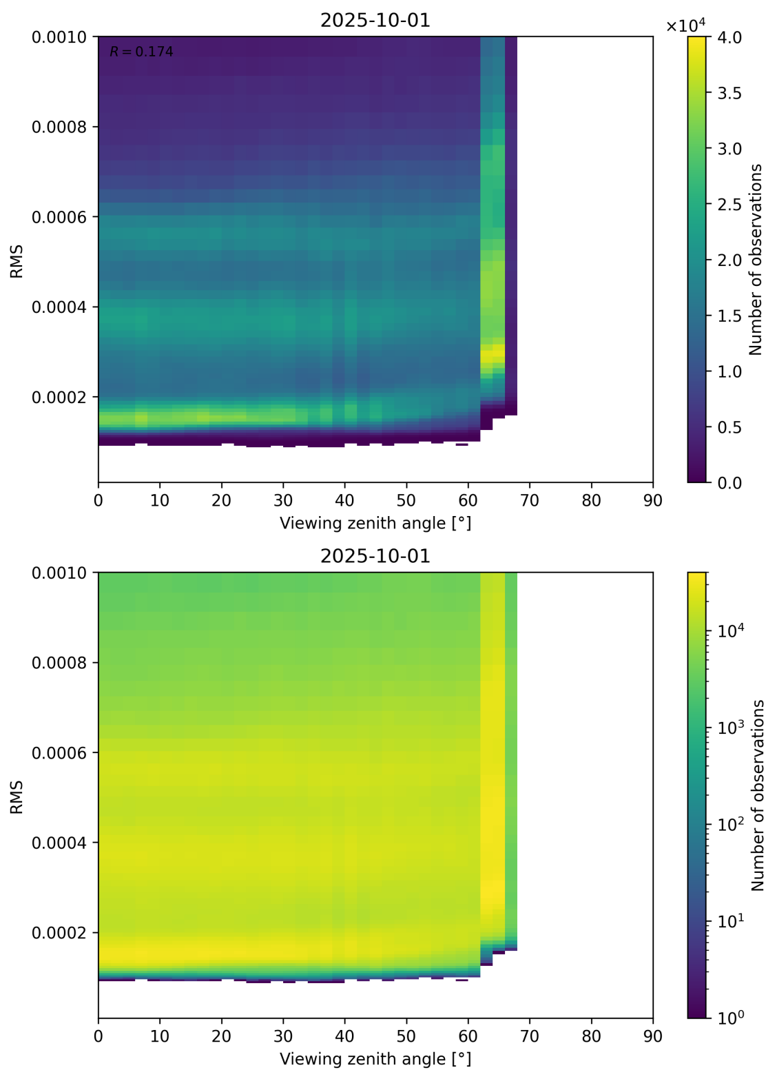
Figure 171: Scatter density plot of “Viewing zenith angle” against “RMS” for 2025-10-01 to 2025-10-02.
