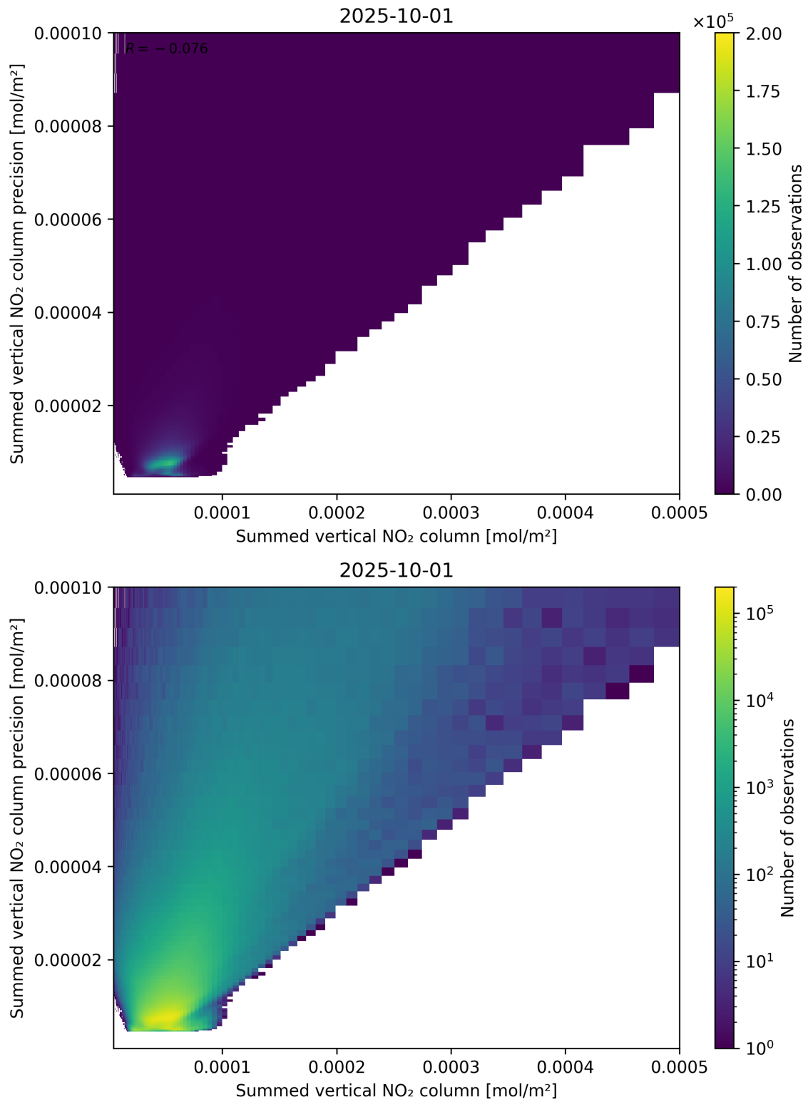
Figure 105: Scatter density plot of “Summed vertical NO 2 column” against “Summed vertical NO 2 column precision” for 2025-10-01 to 2025-10-02.
