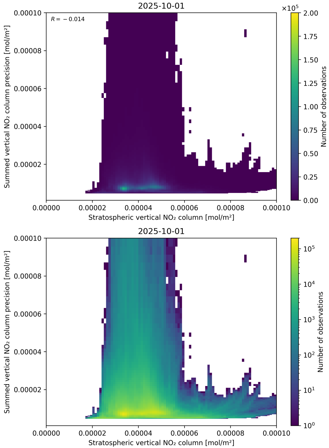
Figure 99: Scatter density plot of “Stratospheric vertical NO 2 column” against “Summed vertical NO 2 column precision” for 2025-10-01 to 2025-10-02.
