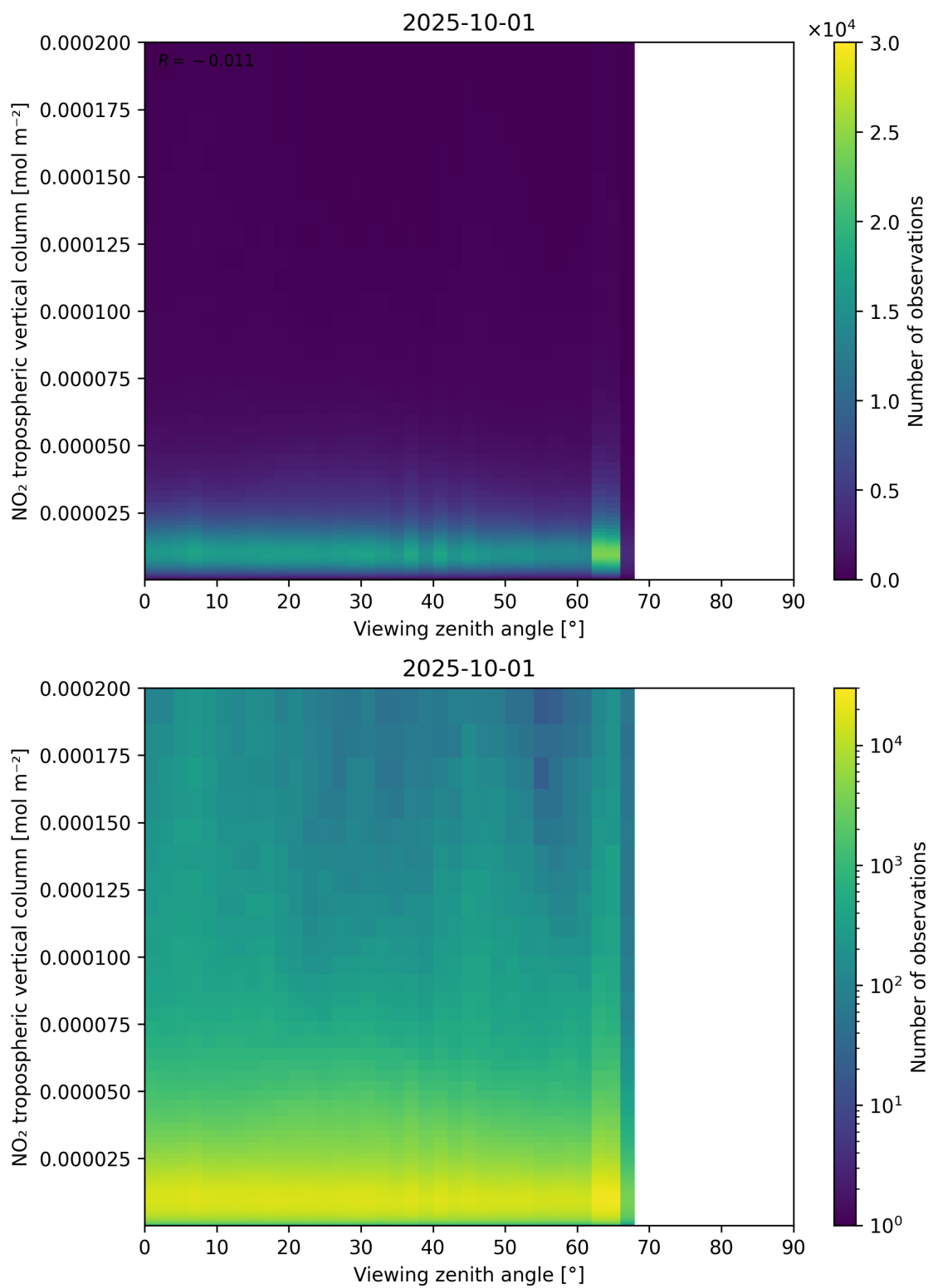
Figure 169: Scatter density plot of “Viewing zenith angle” against “NO 2 tropospheric vertical column” for 2025-10-01 to 2025-10-02.
