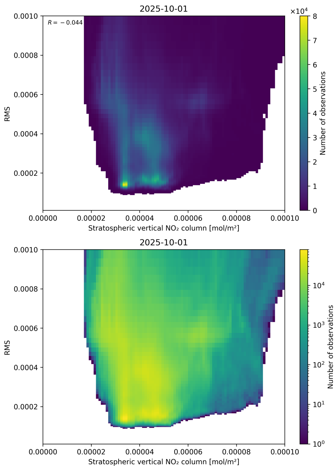
Figure 102: Scatter density plot of “Stratospheric vertical NO 2 column” against “RMS” for 2025-10-01 to 2025-10-02.
