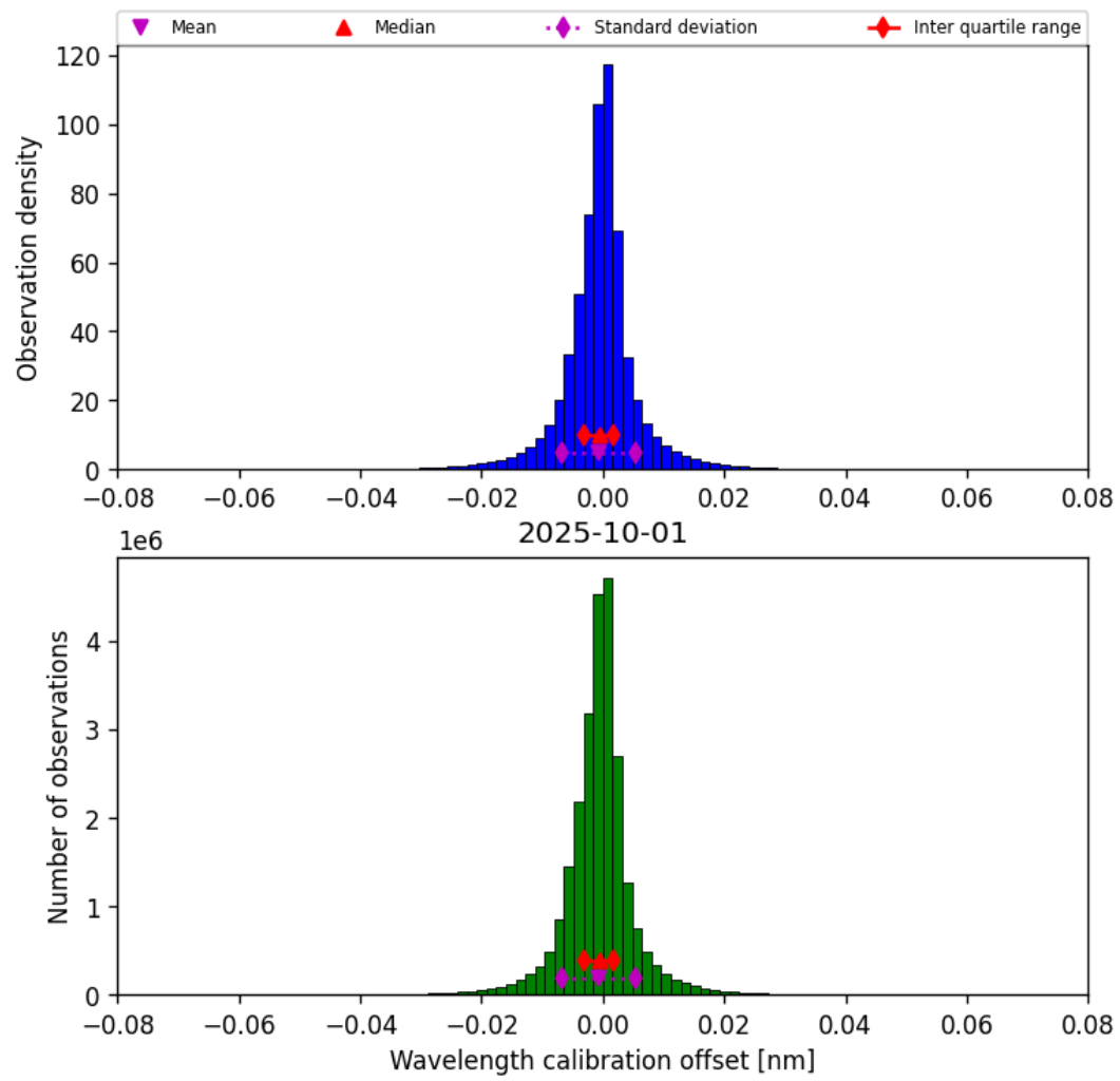
Figure 35: Histogram of “Wavelength calibration offset” for 2025-10-01 to 2025-10-02
