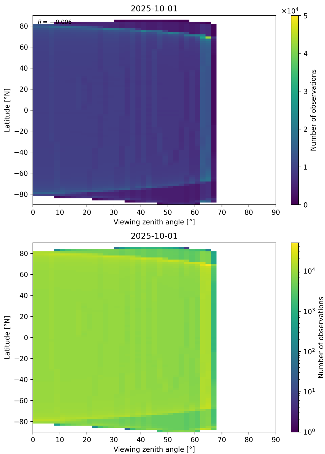
Figure 163: Scatter density plot of “Viewing zenith angle” against “Latitude” for 2025-10-01 to 2025-10-02.
