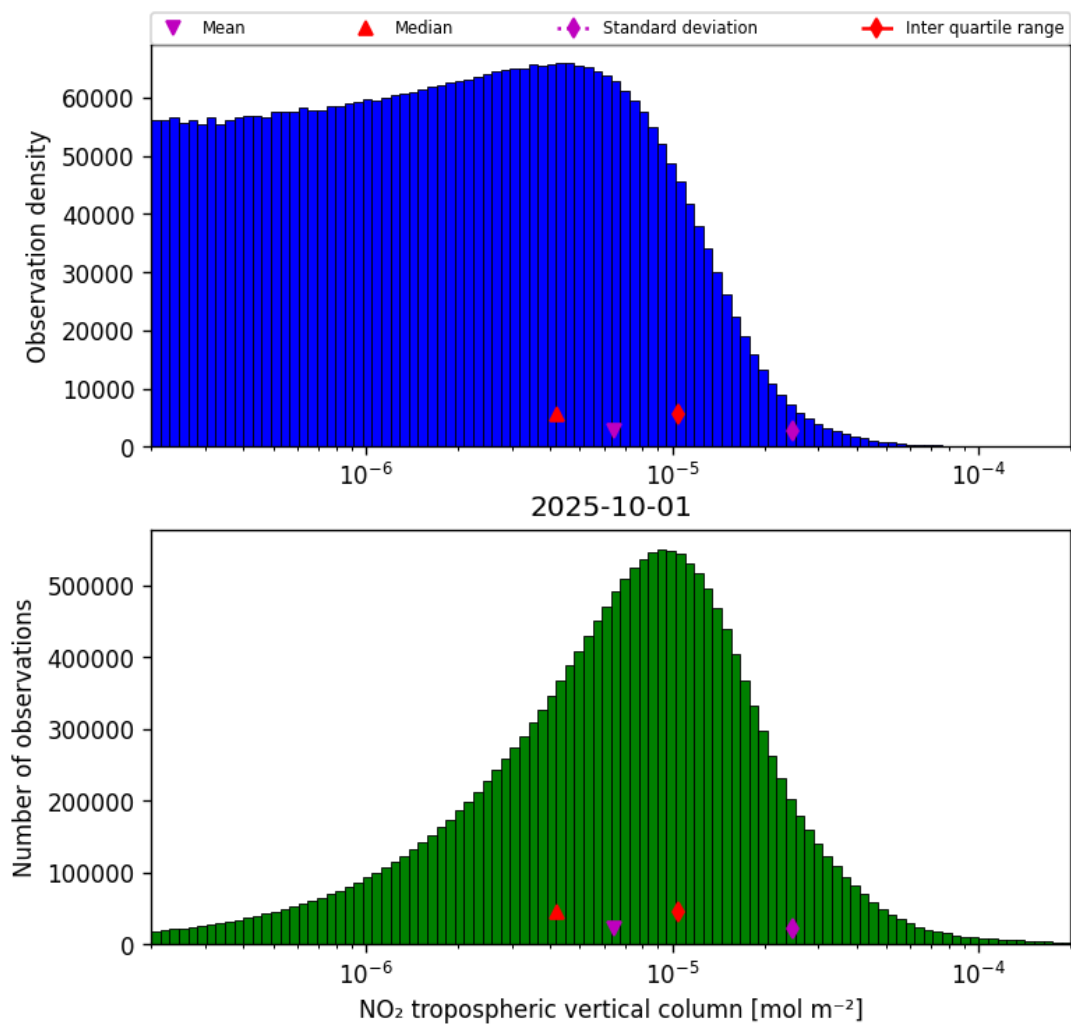
Figure 29: Histogram of “NO 2 tropospheric vertical column” for 2025-10-01 to 2025-10-02
