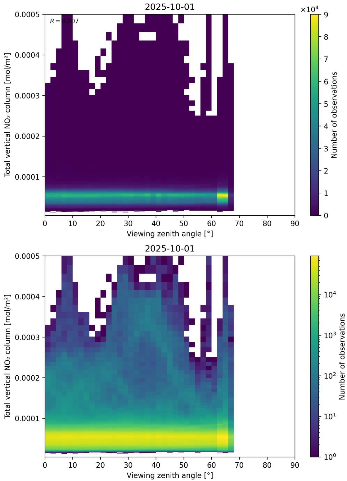
Figure 167: Scatter density plot of “Viewing zenith angle” against “Total vertical NO 2 column” for 2025-10-01 to 2025-10-02.
