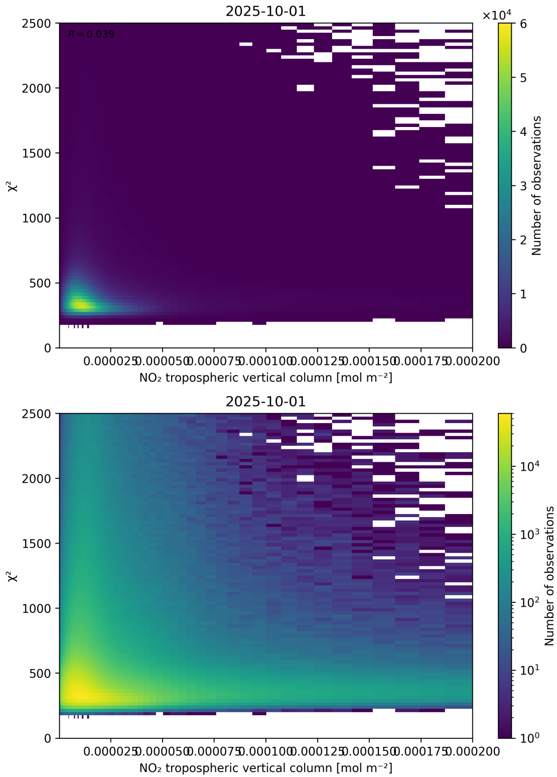
Figure 124: Scatter density plot of “NO 2 tropospheric vertical column” against “ \chi^2 ” for 2025-10-01 to 2025-10-02.
