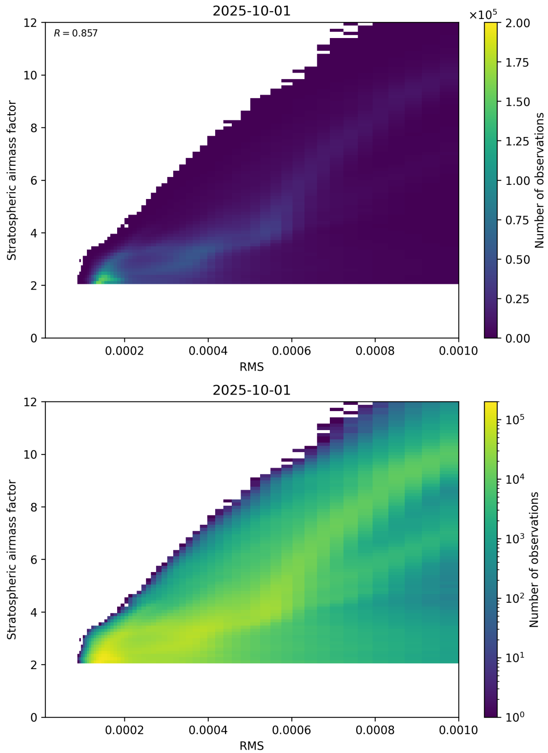
Figure 144: Scatter density plot of “RMS” against “Stratospheric airmass factor” for 2025-10-01 to 2025-10-02.
