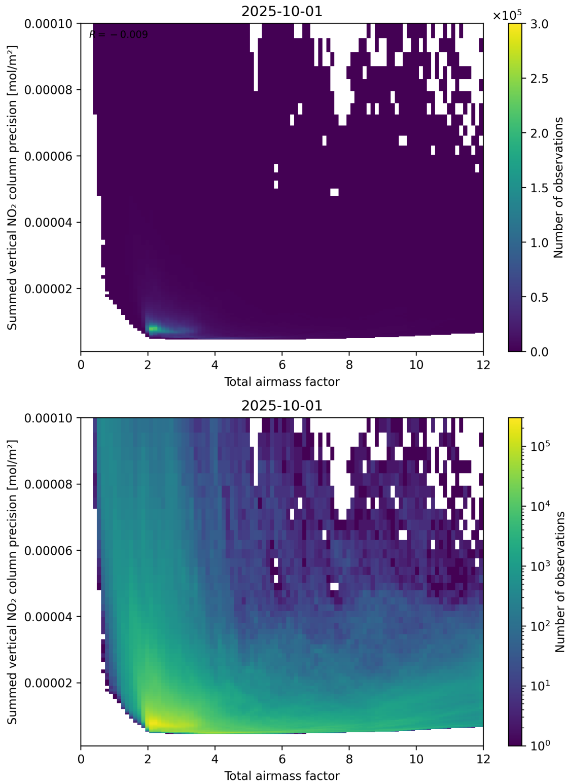
Figure 66: Scatter density plot of “Total airmass factor” against “Summed vertical NO 2 column precision” for 2025-10-01 to 2025-10-02.
