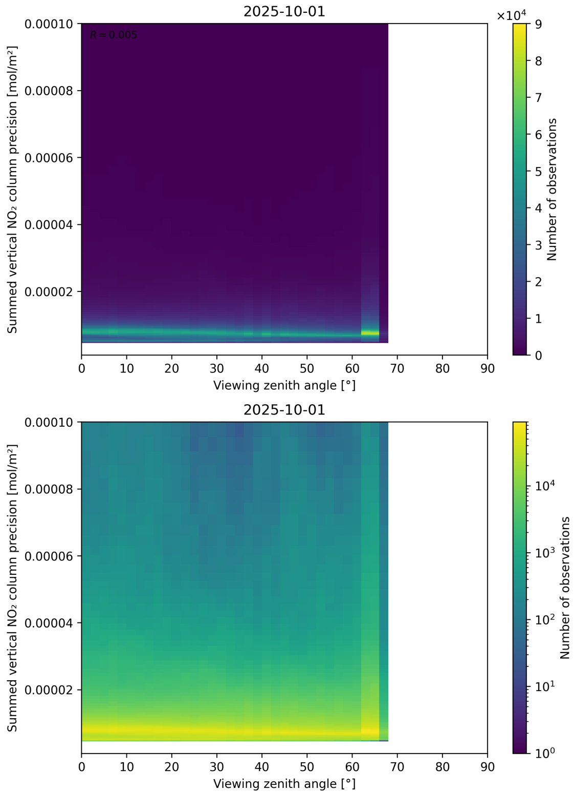
Figure 166: Scatter density plot of “Viewing zenith angle” against “Summed vertical NO 2 column precision” for 2025-10-01 to 2025-10-02.
