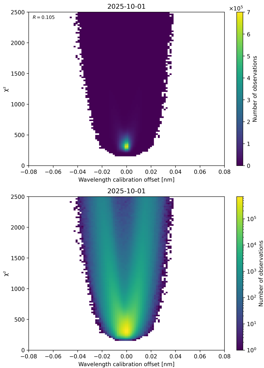
Figure 175: Scatter density plot of “Wavelength calibration offset” against “ \chi^2 ” for 2025-10-01 to 2025-10-02.
