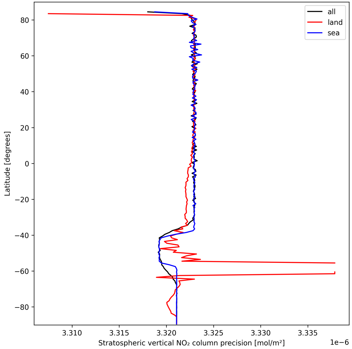
Figure 20: Zonal average of “Stratospheric vertical NO 2 column precision” for 2025-10-01 to 2025-10-02.
