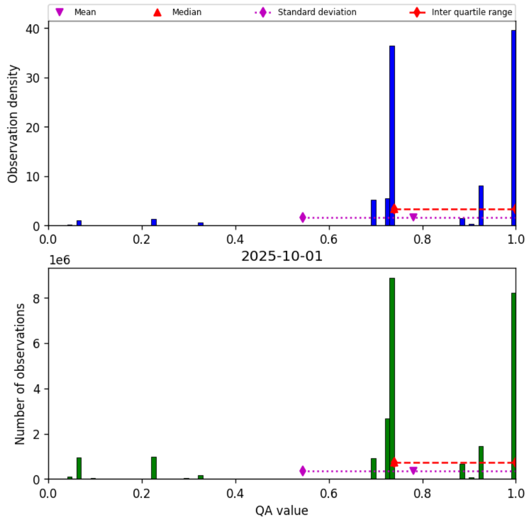
Figure 28: Histogram of “QA value” for 2025-10-01 to 2025-10-02
