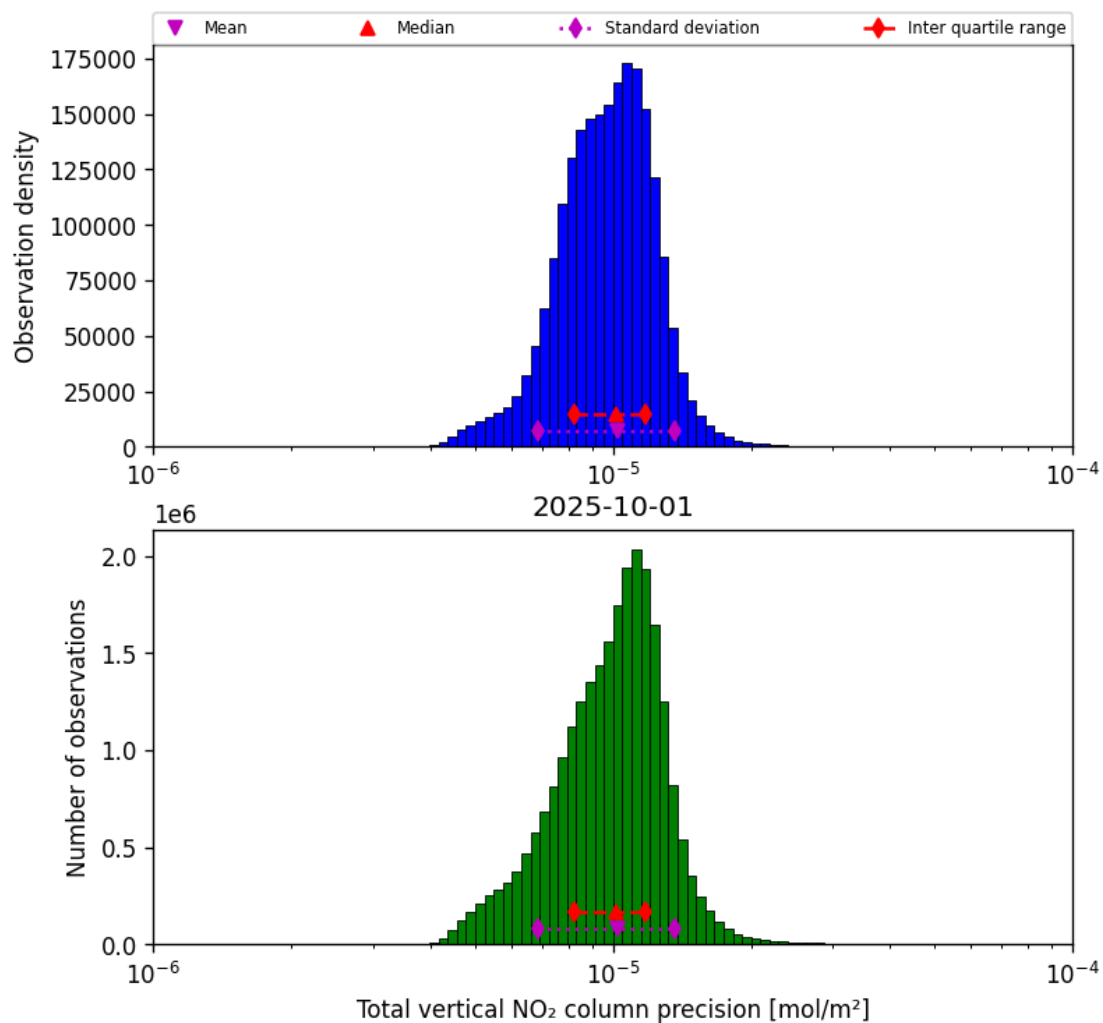
Figure 39: Histogram of “Total vertical NO 2 column precision” for 2025-10-01 to 2025-10-02
