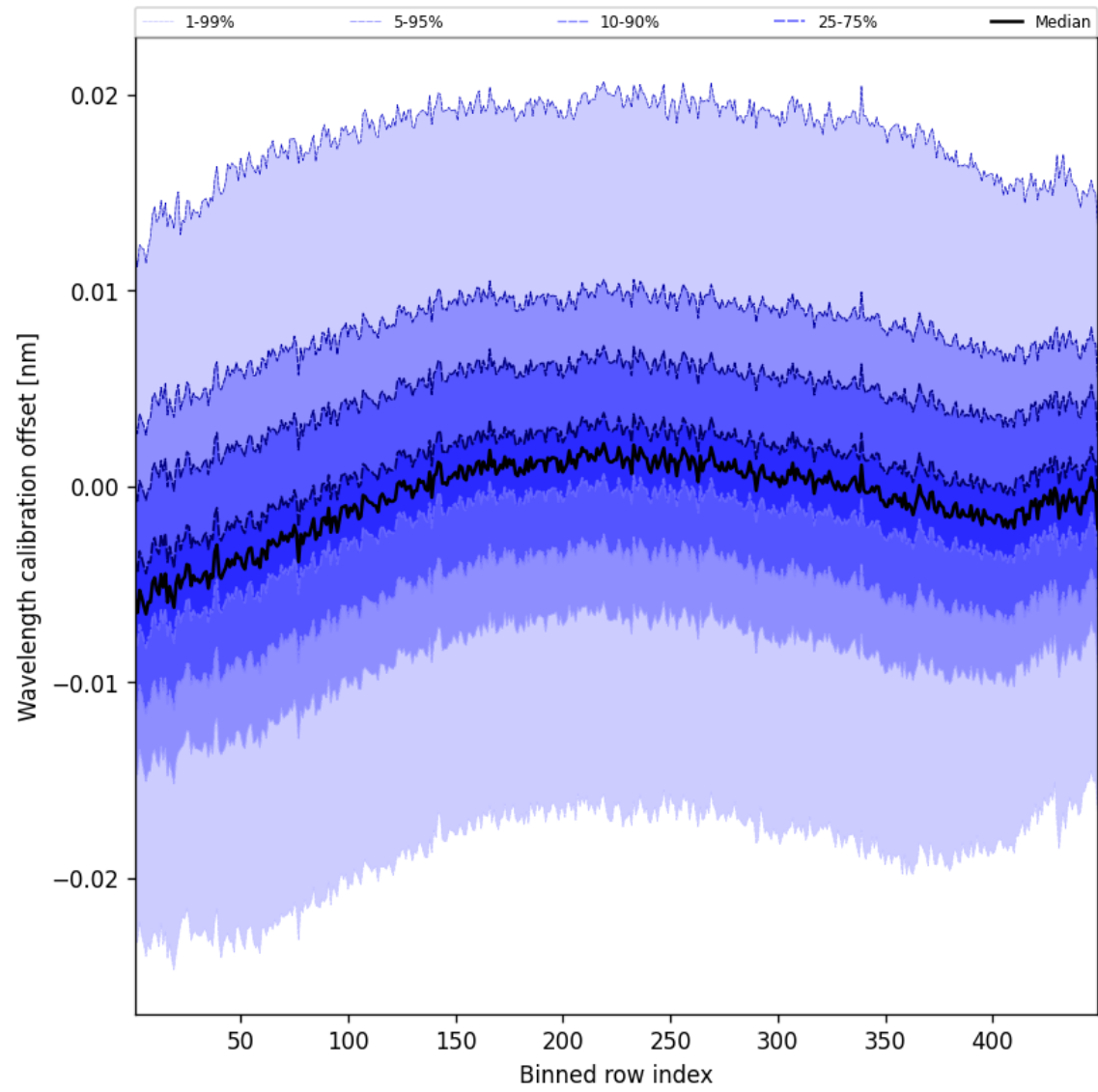
Figure 52: Along track statistics of “Wavelength calibration offset” for 2025-10-01 to 2025-10-02
