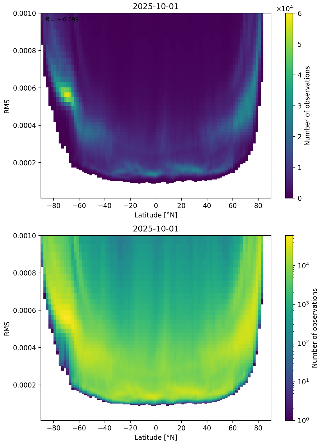
Figure 94: Scatter density plot of “Latitude” against “RMS” for 2025-10-01 to 2025-10-02.
