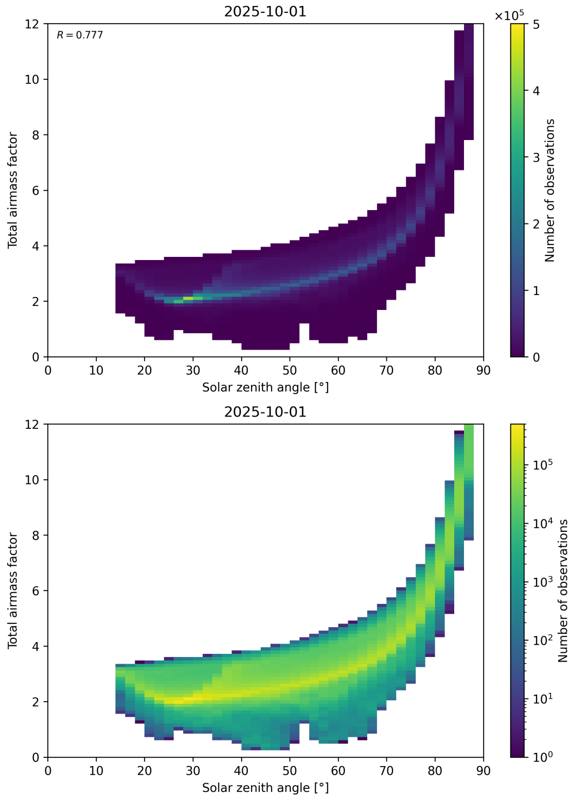
Figure 146: Scatter density plot of “Solar zenith angle” against “Total airmass factor” for 2025-10-01 to 2025-10-02.
