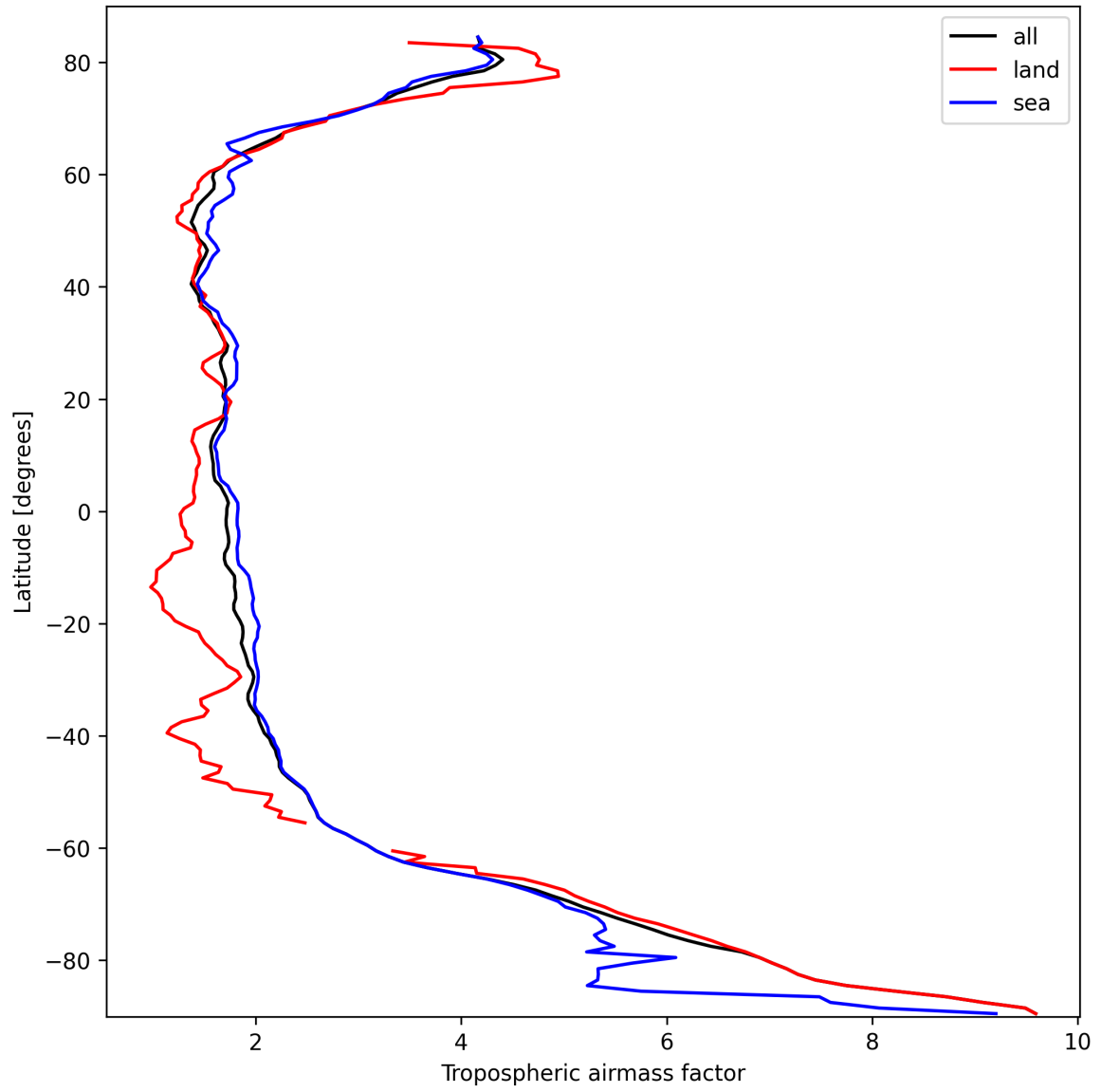
Figure 14: Zonal average of “Tropospheric airmass factor” for 2025-10-01 to 2025-10-02.
