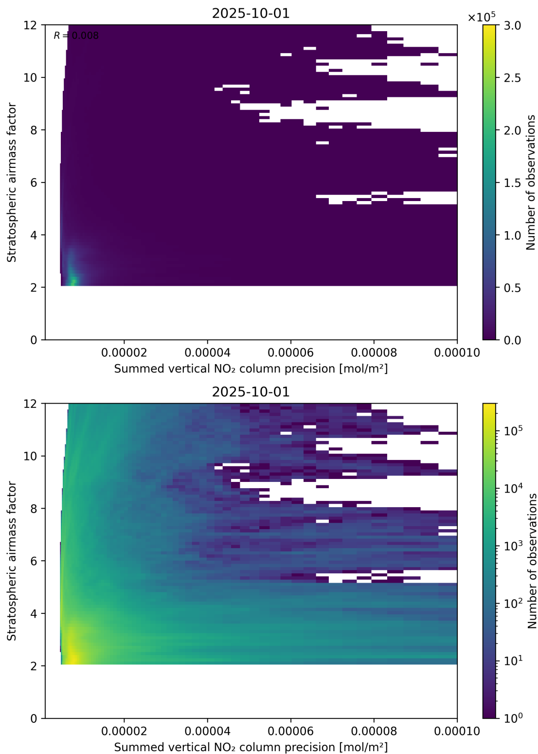
Figure 106: Scatter density plot of “Summed vertical NO 2 column precision” against “Stratospheric airmass factor” for 2025-10-01 to 2025-10-02.
