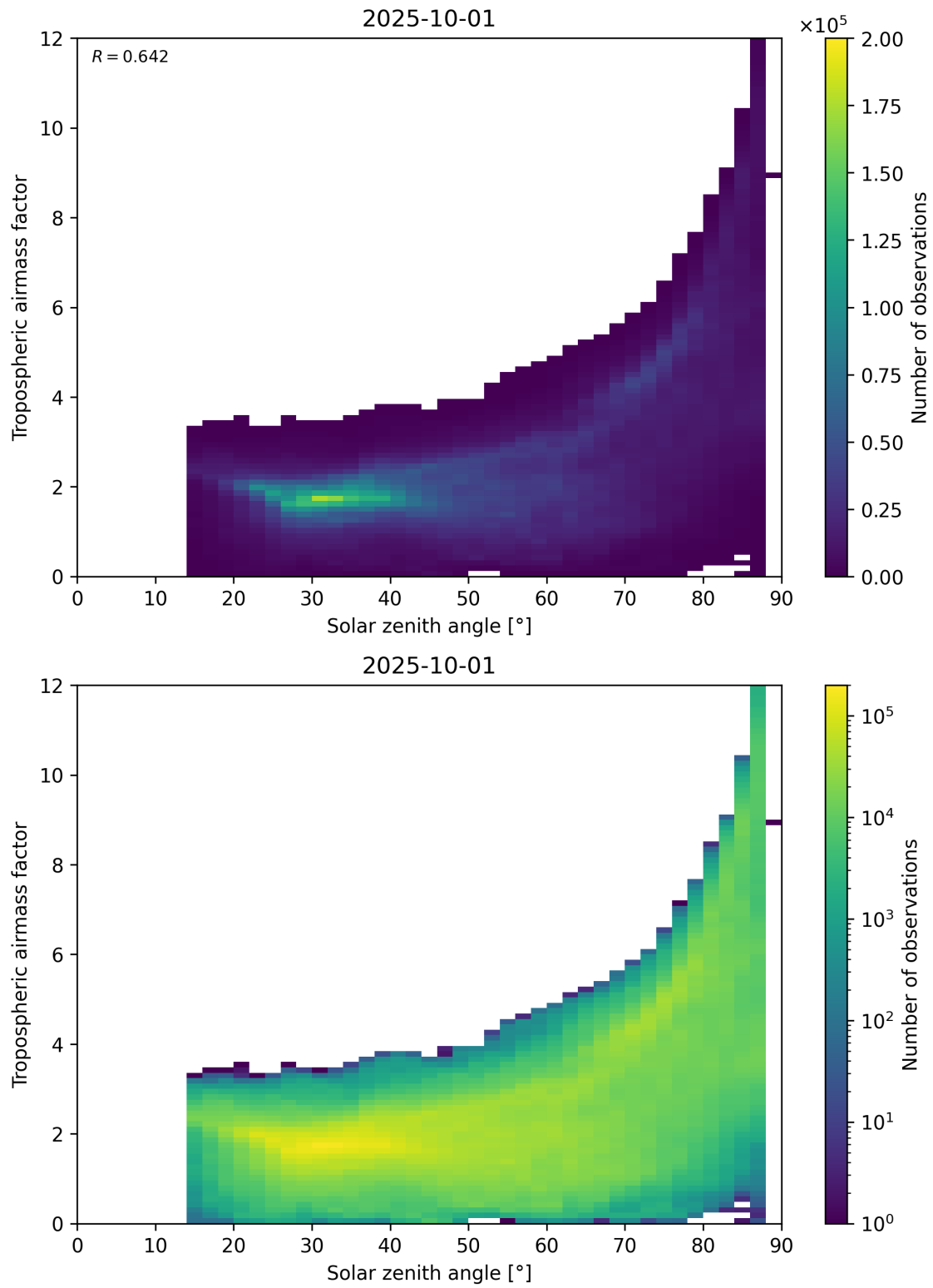
Figure 147: Scatter density plot of “Solar zenith angle” against “Tropospheric airmass factor” for 2025-10-01 to 2025-10-02.
