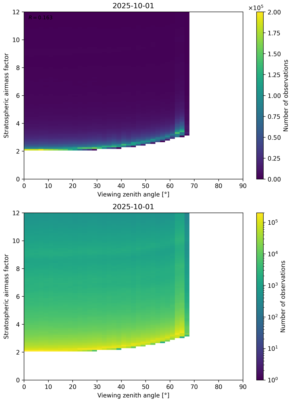
Figure 159: Scatter density plot of “Viewing zenith angle” against “Stratospheric airmass factor” for 2025-10-01 to 2025-10-02.
