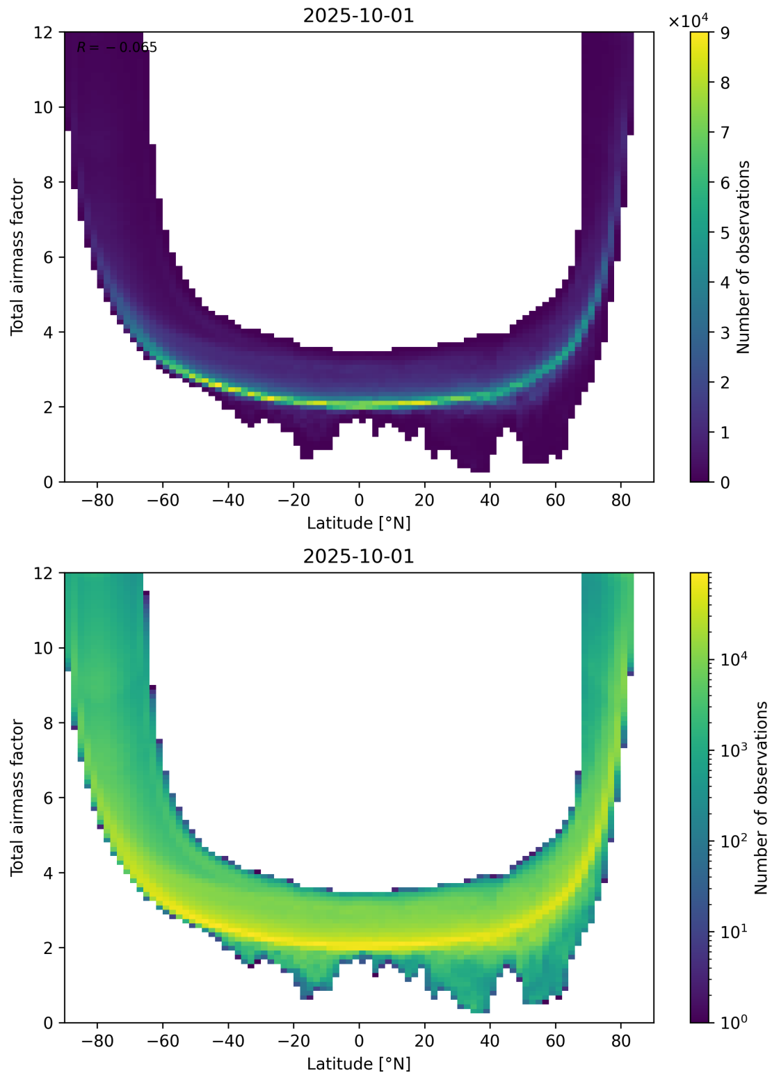
Figure 84: Scatter density plot of “Latitude” against “Total airmass factor” for 2025-10-01 to 2025-10-02.
