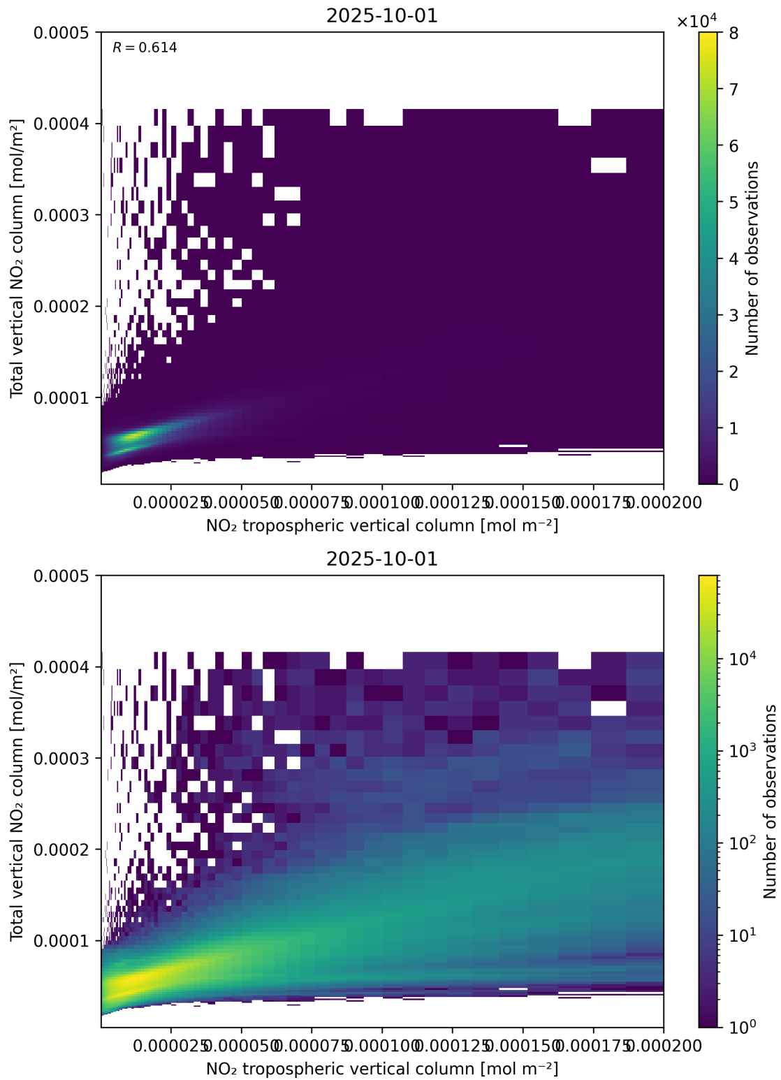
Figure 128: Scatter density plot of “NO 2 tropospheric vertical column” against “Total vertical NO 2 column” for 2025-10-01 to 2025-10-02.
