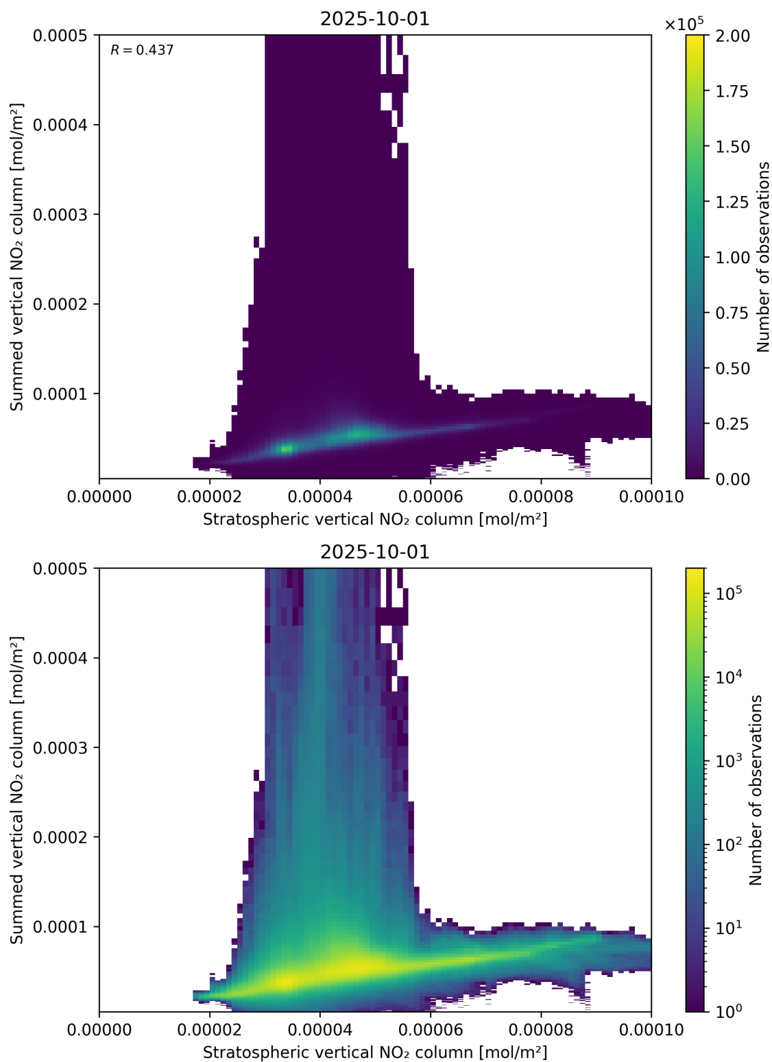
Figure 98: Scatter density plot of “Stratospheric vertical NO 2 column” against “Summed vertical NO 2 column” for 2025-10-01 to 2025-10-02.
