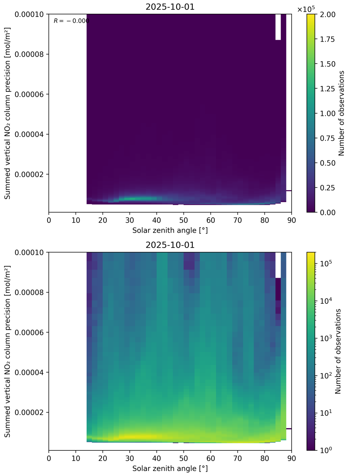
Figure 152: Scatter density plot of “Solar zenith angle” against “Summed vertical NO 2 column precision” for 2025-10-01 to 2025-10-02.
