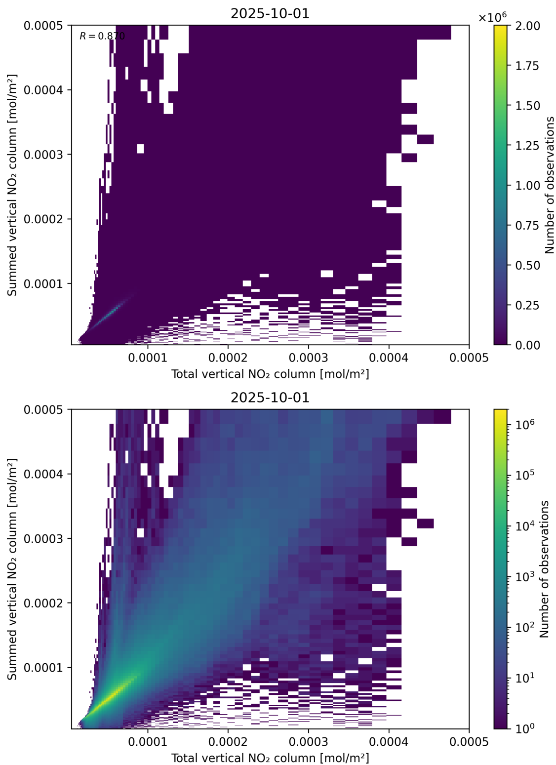
Figure 112: Scatter density plot of “Total vertical NO 2 column” against “Summed vertical NO 2 column” for 2025-10-01 to 2025-10-02.
