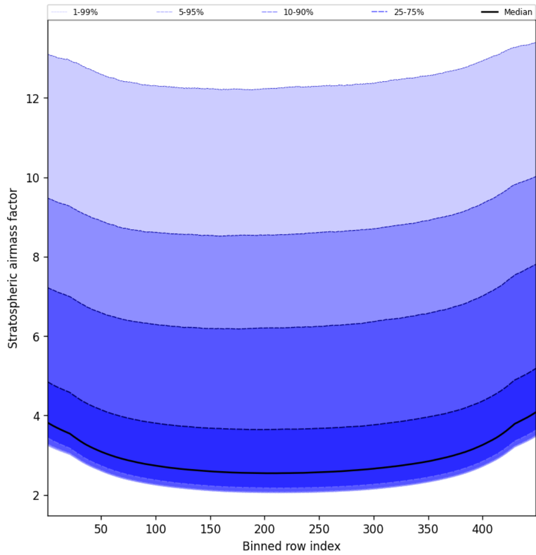
Figure 61: Along track statistics of “Stratospheric air mass factor” for 2025-10-01 to 2025-10-02
