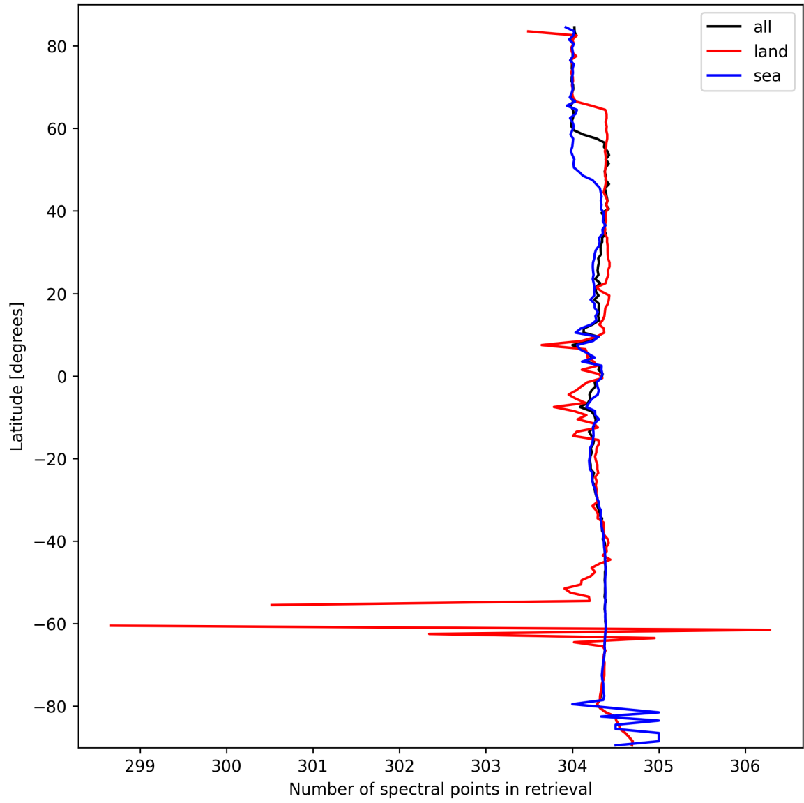
Figure 16: Zonal average of “Number of spectral points in retrieval” for 2025-10-01 to 2025-10-02.
