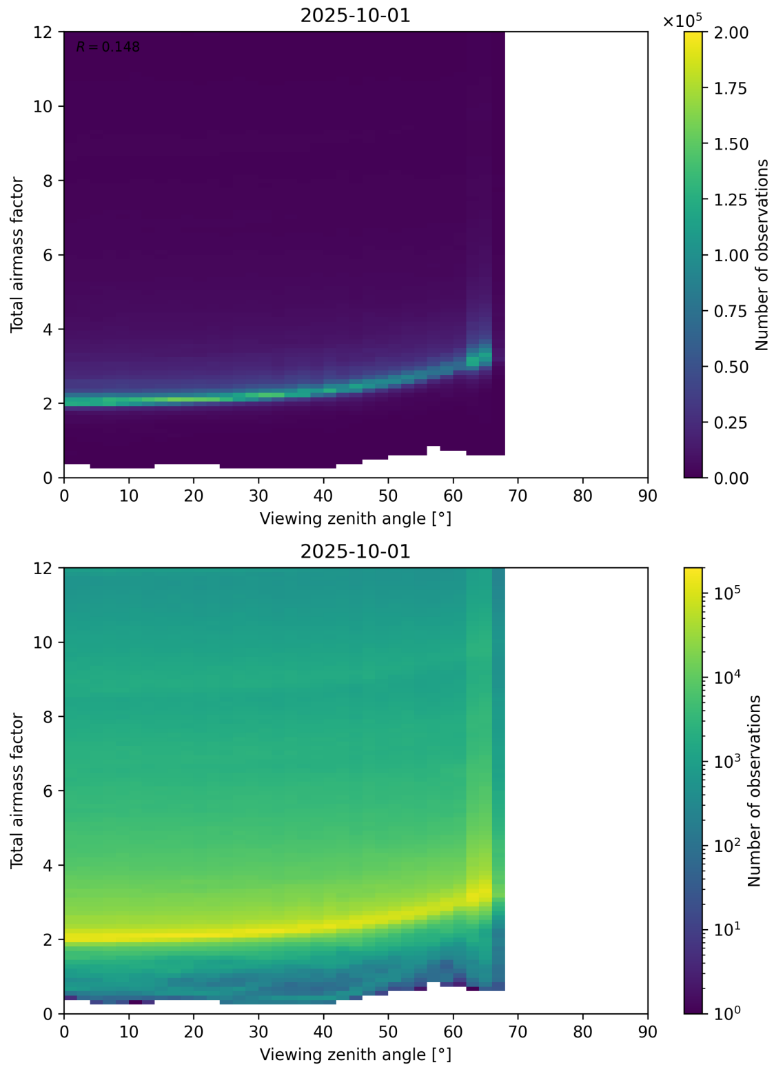
Figure 160: Scatter density plot of “Viewing zenith angle” against “Total airmass factor” for 2025-10-01 to 2025-10-02.
