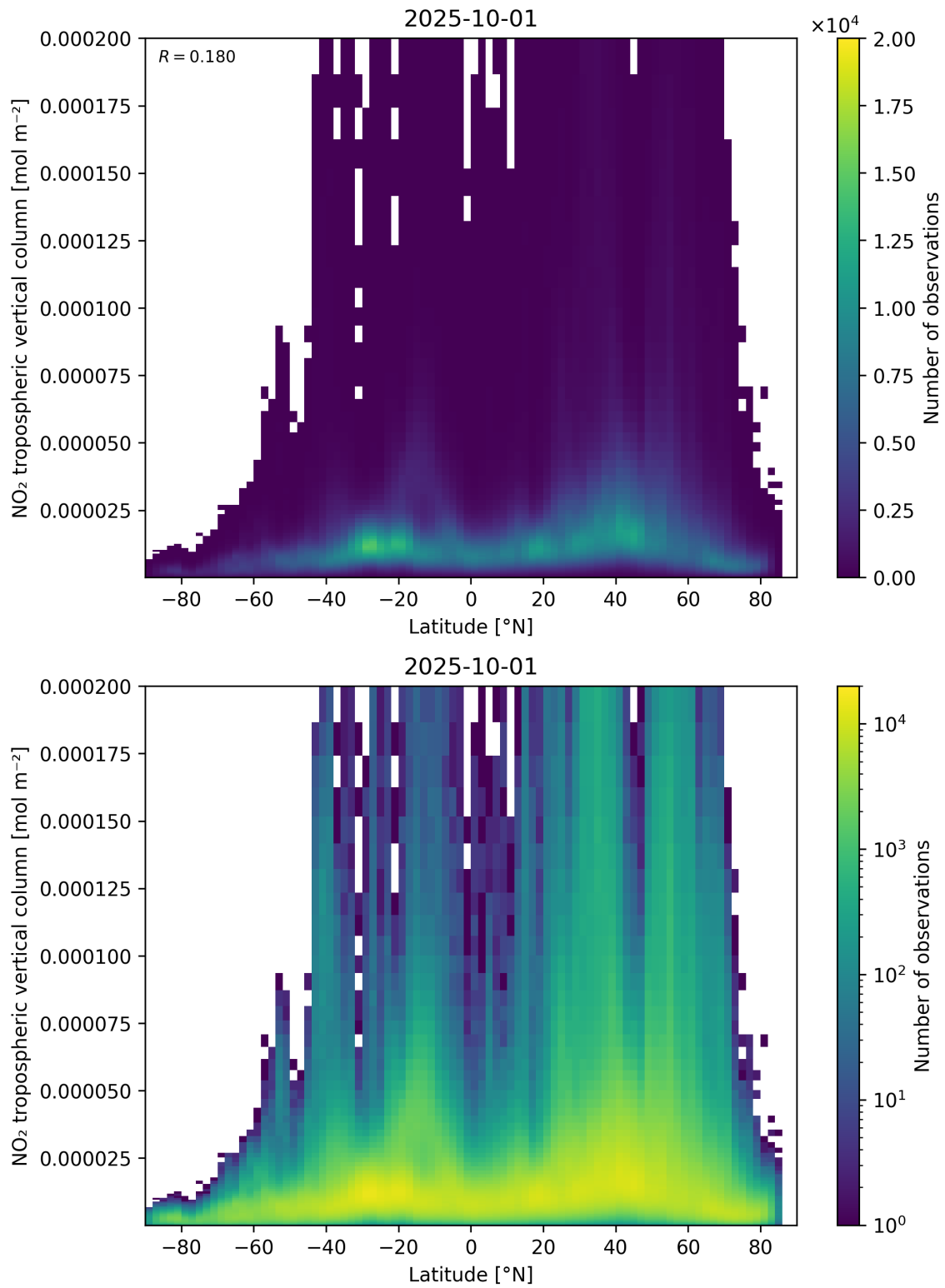
Figure 92: Scatter density plot of “Latitude” against “NO 2 tropospheric vertical column” for 2025-10-01 to 2025-10-02.
