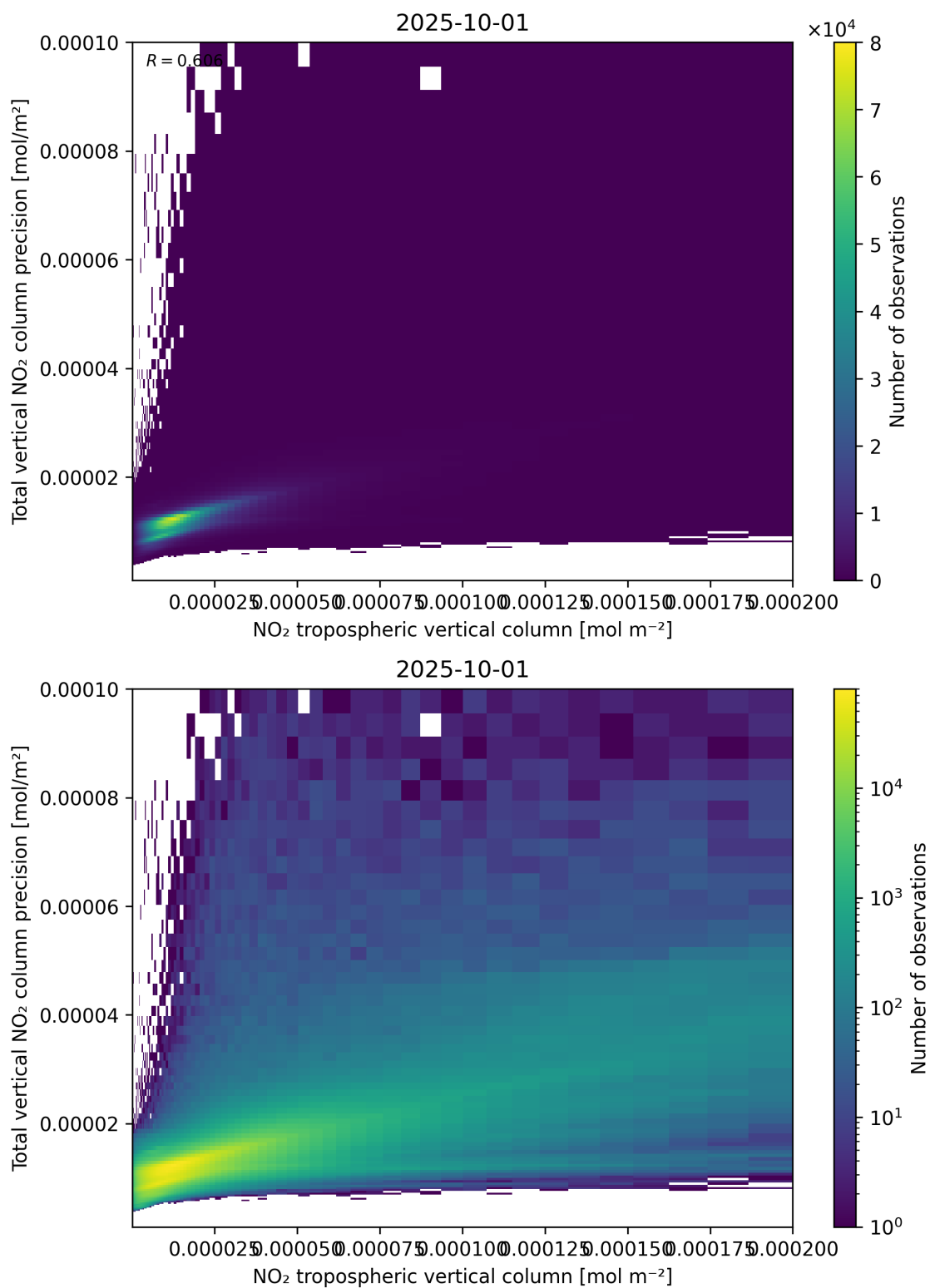
Figure 129: Scatter density plot of “NO 2 tropospheric vertical column” against “Total vertical NO 2 column precision” for 2025-10-01 to 2025-10-02.
