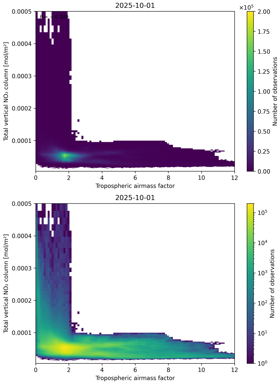
Figure 77: Scatter density plot of “Tropospheric airmass factor” against “Total vertical NO 2 column” for 2025-10-01 to 2025-10-02.
