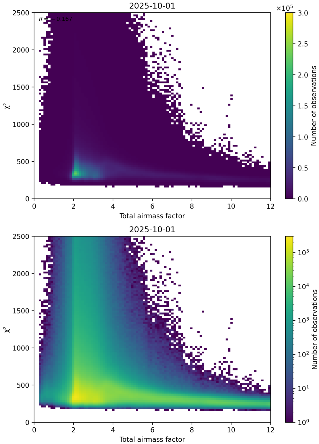
Figure 63: Scatter density plot of “Total airmass factor” against “ \chi^2 ” for 2025-10-01 to 2025-10-02.
