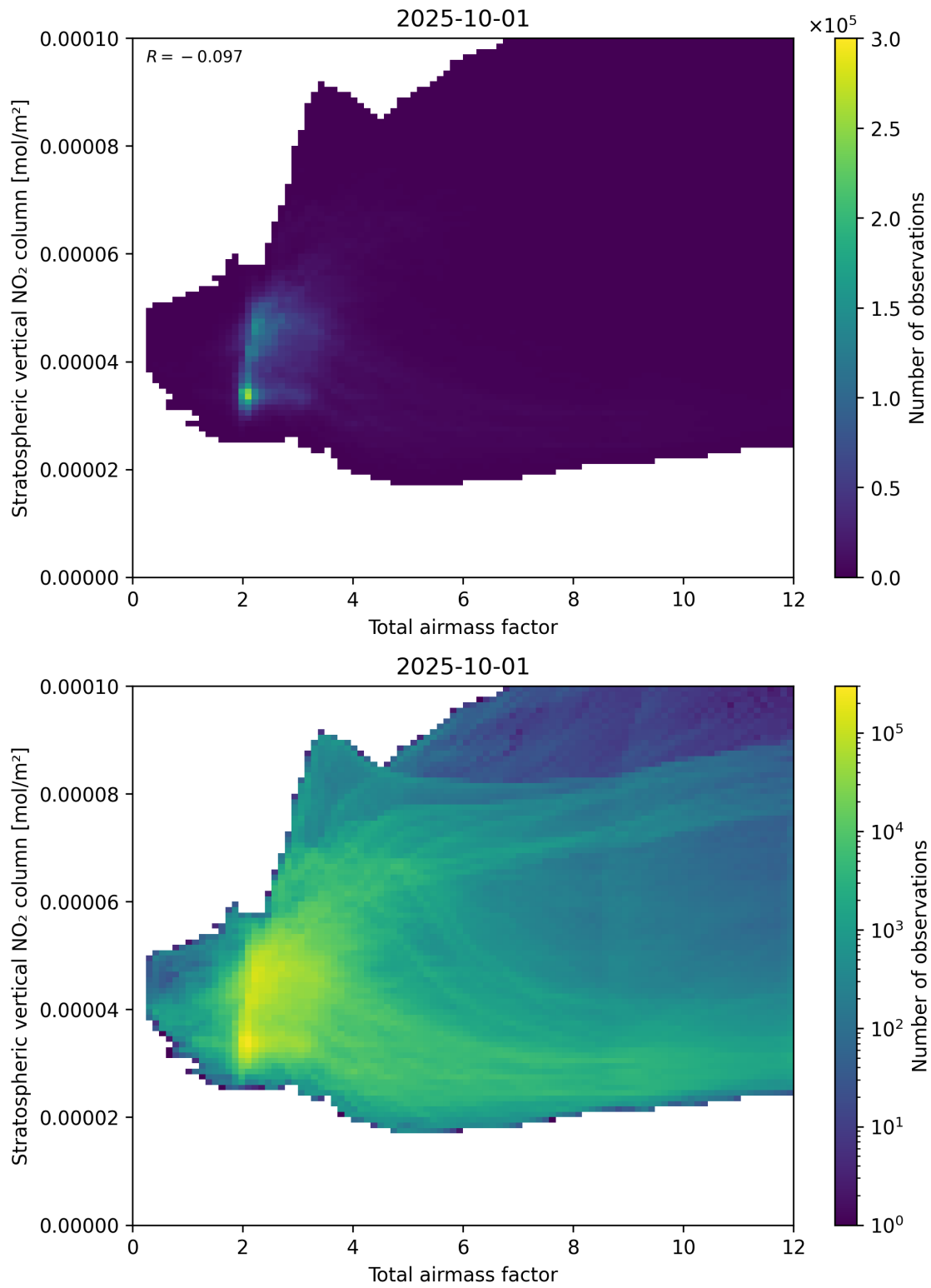
Figure 64: Scatter density plot of “Total airmass factor” against “Stratospheric vertical NO 2 column” for 2025-10-01 to 2025-10-02.
