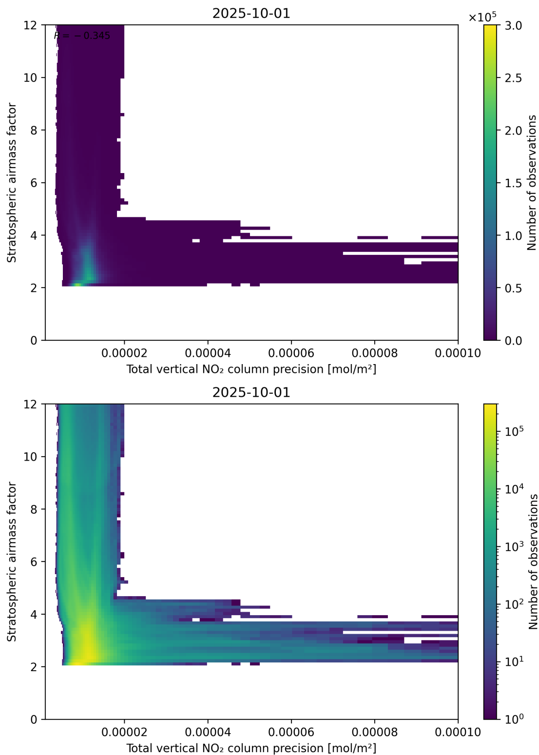
Figure 115: Scatter density plot of “Total vertical NO 2 column precision” against “Stratospheric air mass factor” for 2025-10-01 to 2025-10-02.
