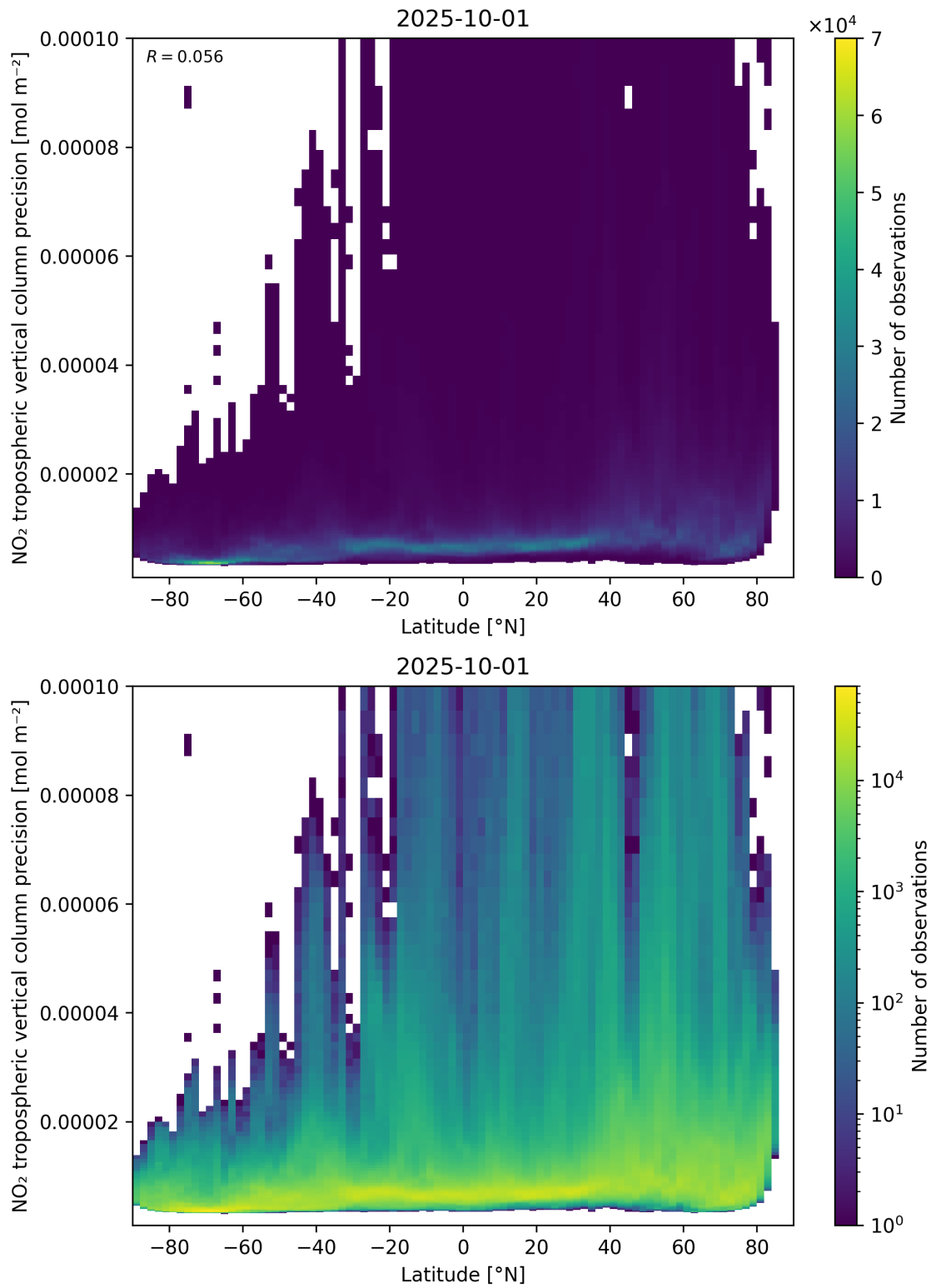
Figure 93: Scatter density plot of “Latitude” against “NO 2 tropospheric vertical column precision” for 2025-10-01 to 2025-10-02.
