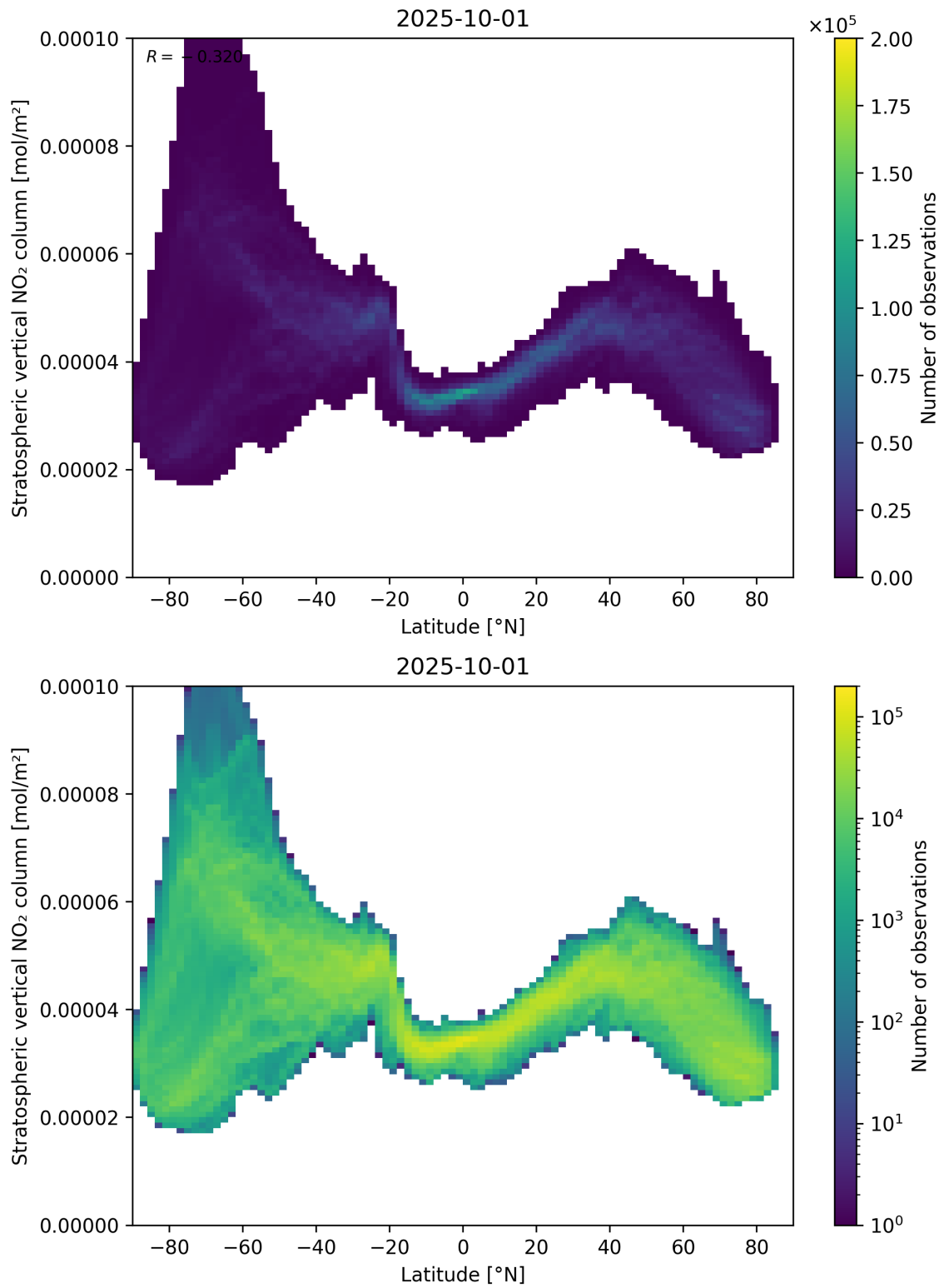
Figure 87: Scatter density plot of “Latitude” against “Stratospheric vertical NO 2 column” for 2025-10-01 to 2025-10-02.
