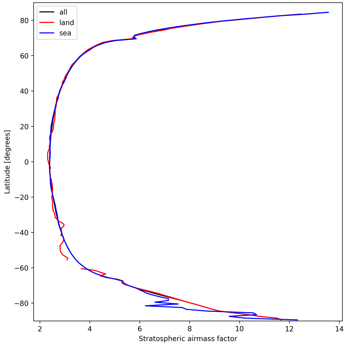
Figure 27: Zonal average of “Stratospheric airmass factor” for 2025-10-01 to 2025-10-02.
