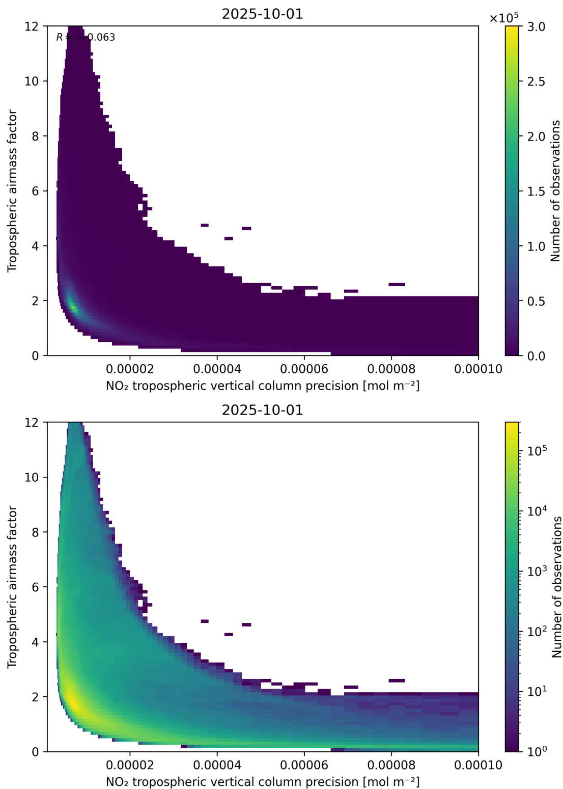
Figure 133: Scatter density plot of “NO 2 tropospheric vertical column precision” against “Tropospheric air mass factor” for 2025-10-01 to 2025-10-02.
