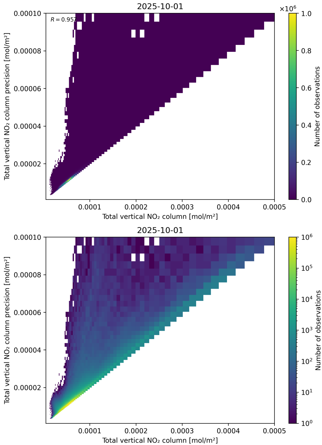
Figure 114: Scatter density plot of “Total vertical NO 2 column” against “Total vertical NO 2 column precision” for 2025-10-01 to 2025-10-02.
