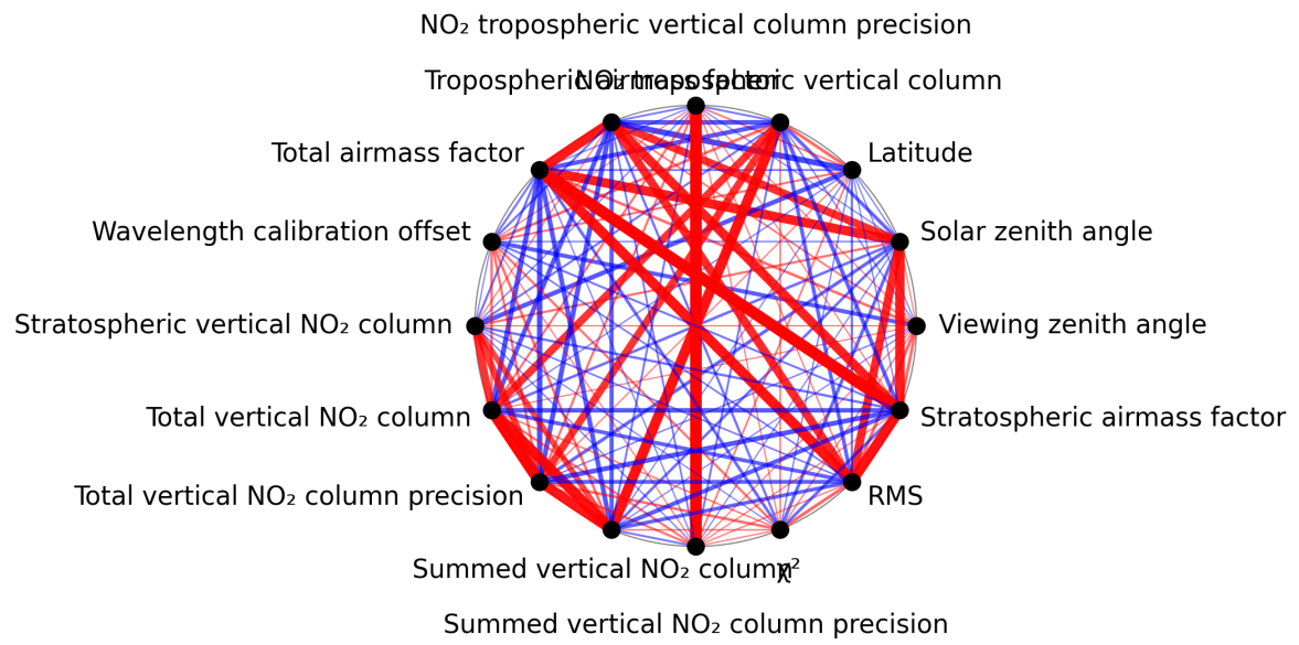
Figure 1: Map of correlation graph for 2025-10-01 to 2025-10-02.
