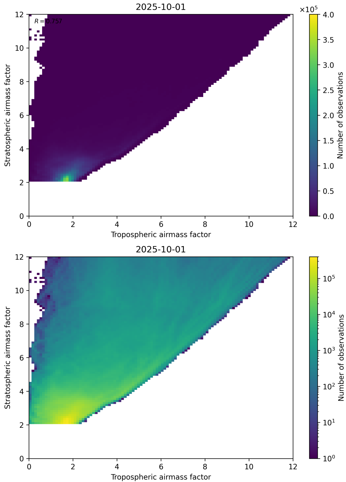
Figure 71: Scatter density plot of “Tropospheric airmass factor” against “Stratospheric airmass factor” for 2025-10-01 to 2025-10-02.
