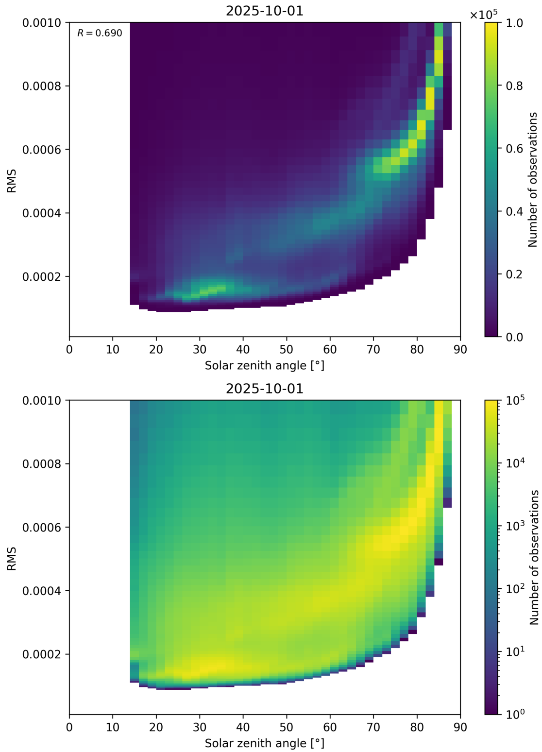
Figure 157: Scatter density plot of “Solar zenith angle” against “RMS” for 2025-10-01 to 2025-10-02.
