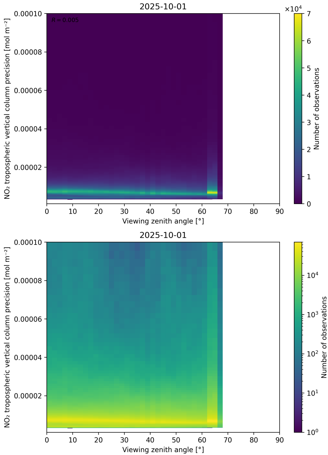
Figure 170: Scatter density plot of “Viewing zenith angle” against “NO 2 tropospheric vertical column precision” for 2025-10-01 to 2025-10-02.
