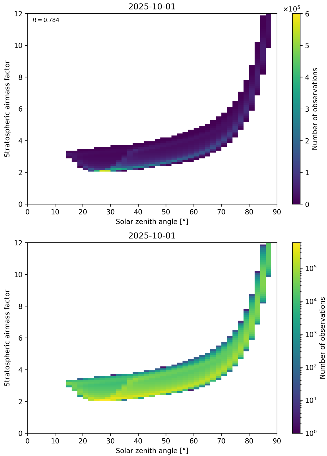
Figure 145: Scatter density plot of “Solar zenith angle” against “Stratospheric airmass factor” for 2025-10-01 to 2025-10-02.
