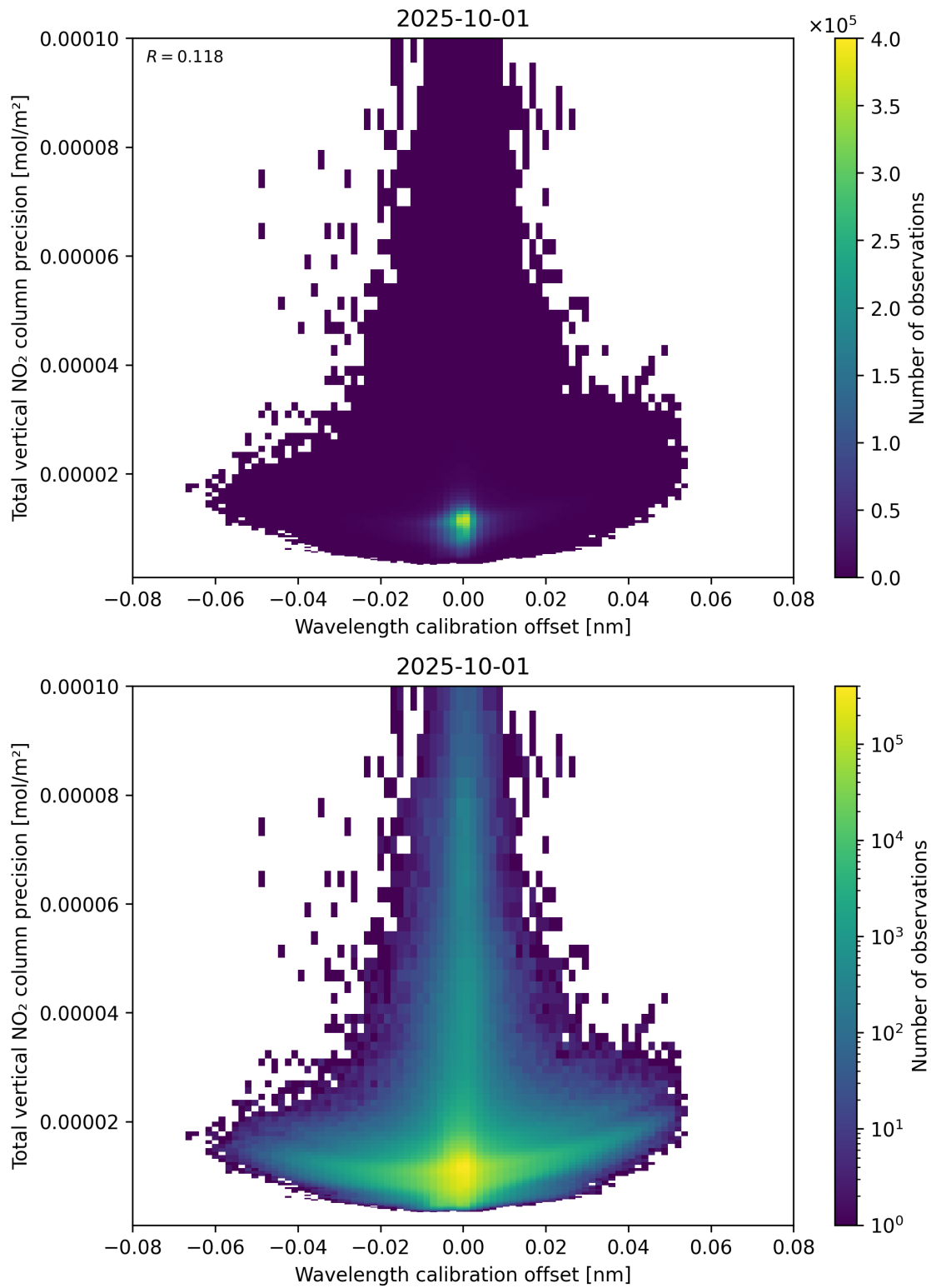
Figure 180: Scatter density plot of “Wavelength calibration offset” against “Total vertical NO 2 column precision” for 2025-10-01 to 2025-10-02.
