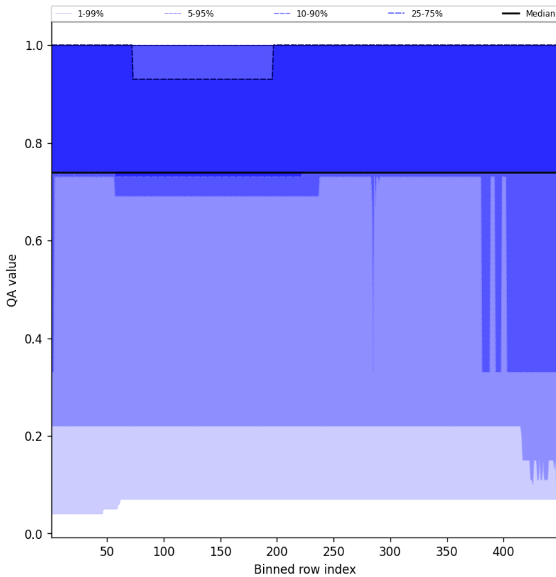
Figure 45: Along track statistics of “QA value” for 2025-10-01 to 2025-10-02
