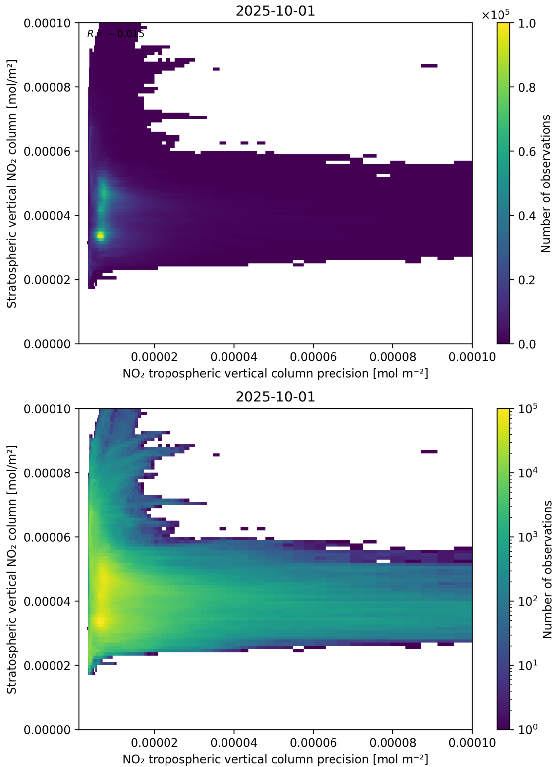
Figure 135: Scatter density plot of “NO 2 tropospheric vertical column precision” against “Stratospheric vertical NO 2 column” for 2025-10-01 to 2025-10-02.
