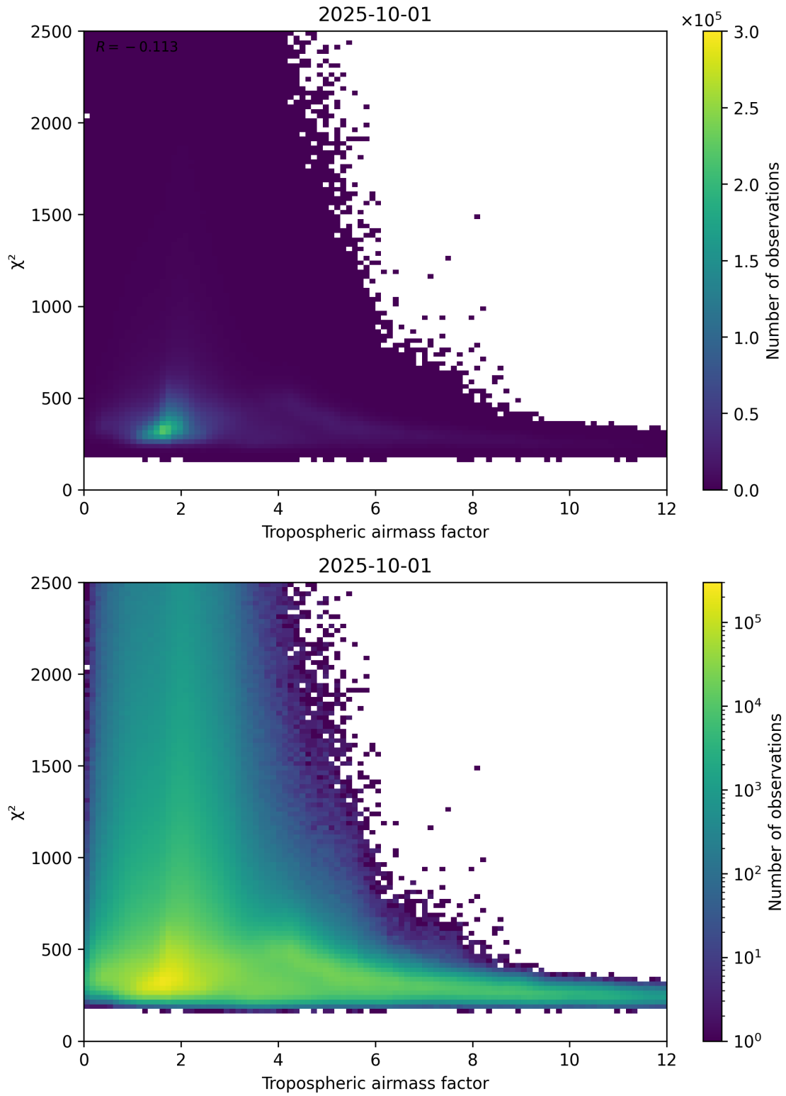
Figure 73: Scatter density plot of “Tropospheric airmass factor” against “ \chi^2 ” for 2025-10-01 to 2025-10-02.
