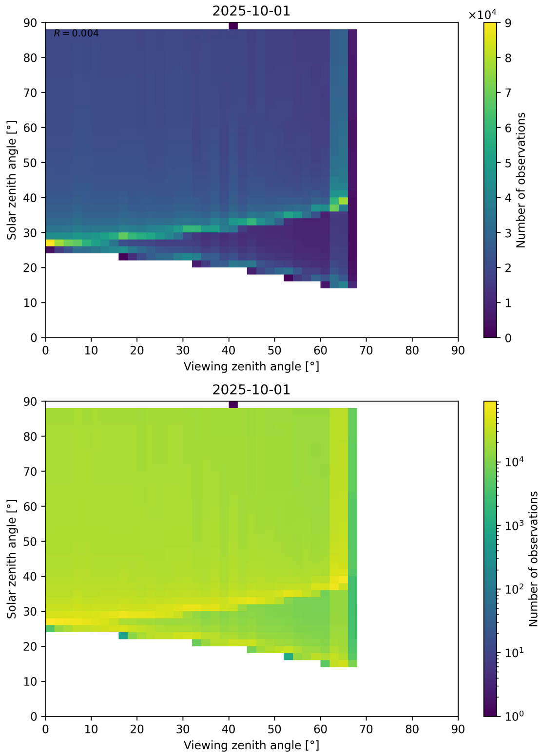
Figure 172: Scatter density plot of “Viewing zenith angle” against “Solar zenith angle” for 2025-10-01 to 2025-10-02.
