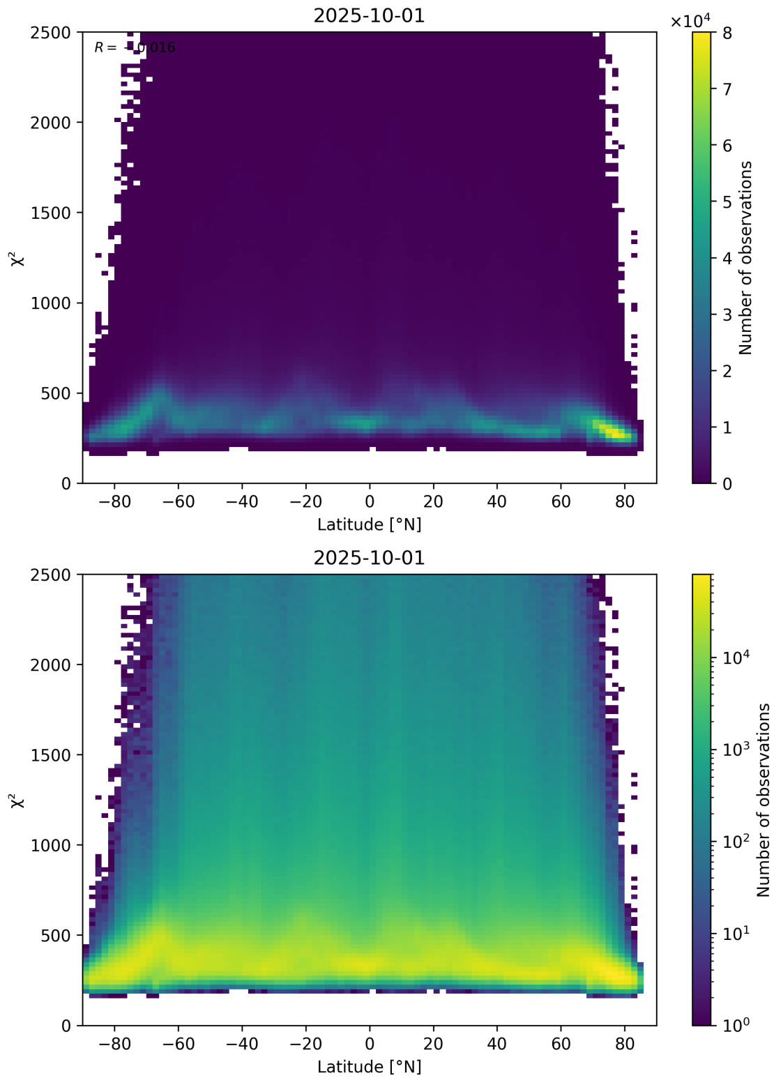
Figure 86: Scatter density plot of “Latitude” against “ \chi^2 ” for 2025-10-01 to 2025-10-02.
