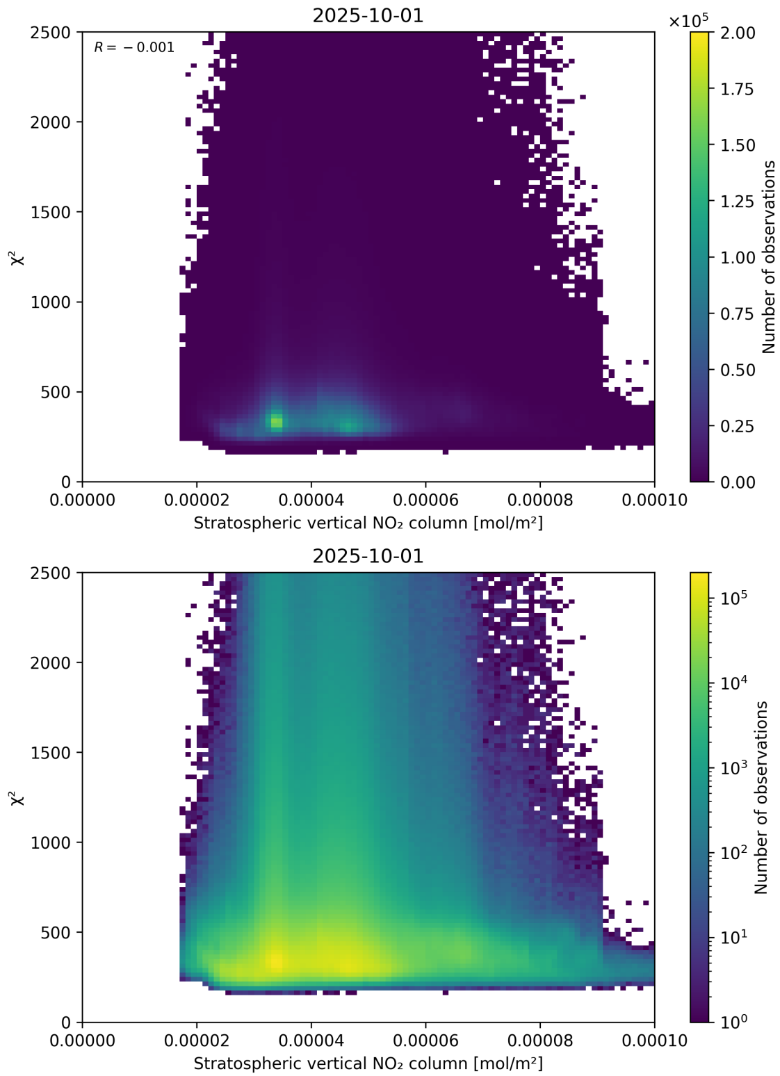
Figure 97: Scatter density plot of “Stratospheric vertical NO 2 column” against “ \chi^2 ” for 2025-10-01 to 2025-10-02.
