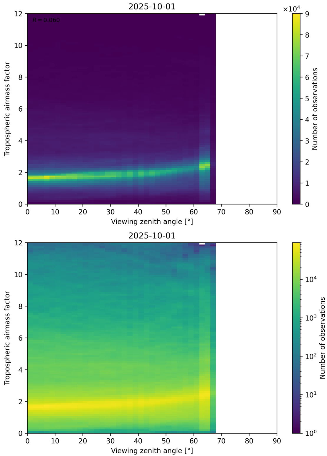
Figure 161: Scatter density plot of “Viewing zenith angle” against “Tropospheric air mass factor” for 2025-10-01 to 2025-10-02.
