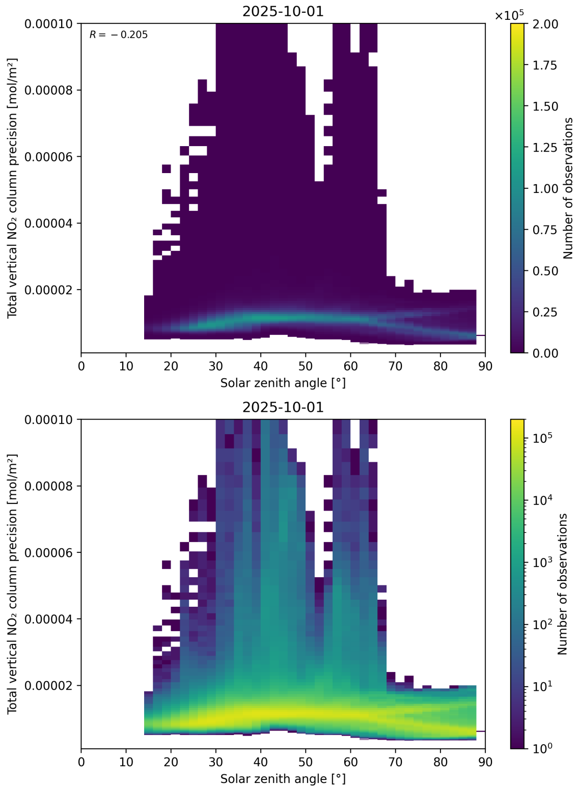
Figure 154: Scatter density plot of “Solar zenith angle” against “Total vertical NO 2 column precision” for 2025-10-01 to 2025-10-02.
