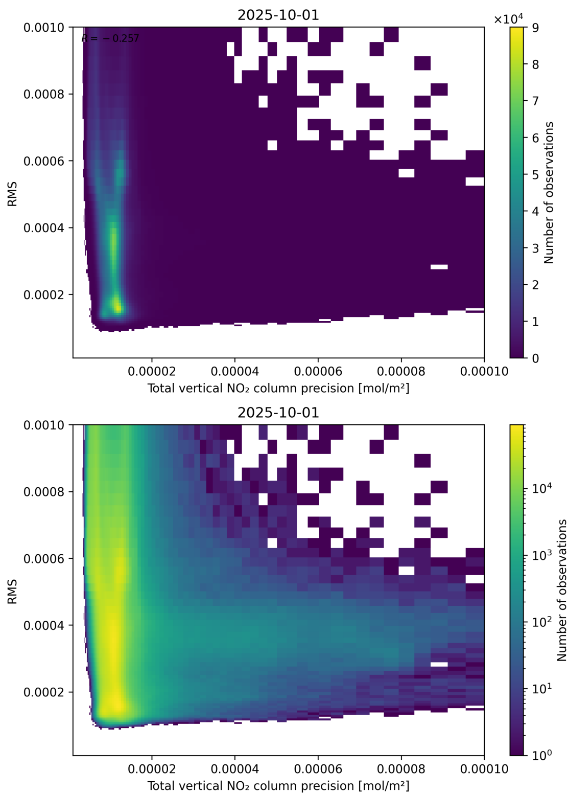
Figure 119: Scatter density plot of “Total vertical NO 2 column precision” against “RMS” for 2025-10-01 to 2025-10-02.
