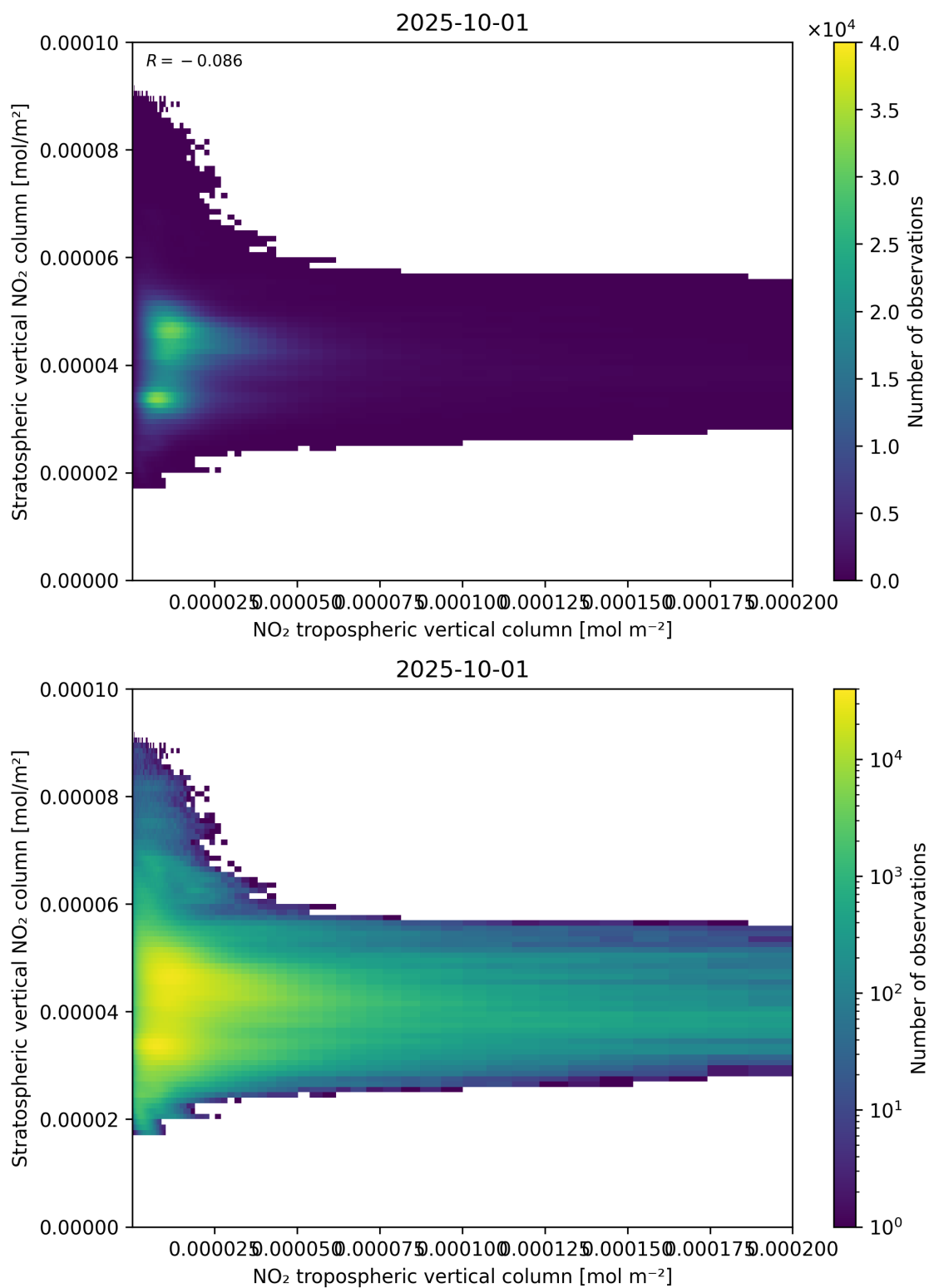
Figure 125: Scatter density plot of “NO 2 tropospheric vertical column” against “Stratospheric vertical NO 2 column” for 2025-10-01 to 2025-10-02.
