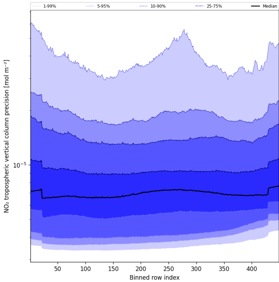
Figure 47: Along track statistics of “NO 2 tropospheric vertical column precision” for 2025-10-01 to 2025-10-02
