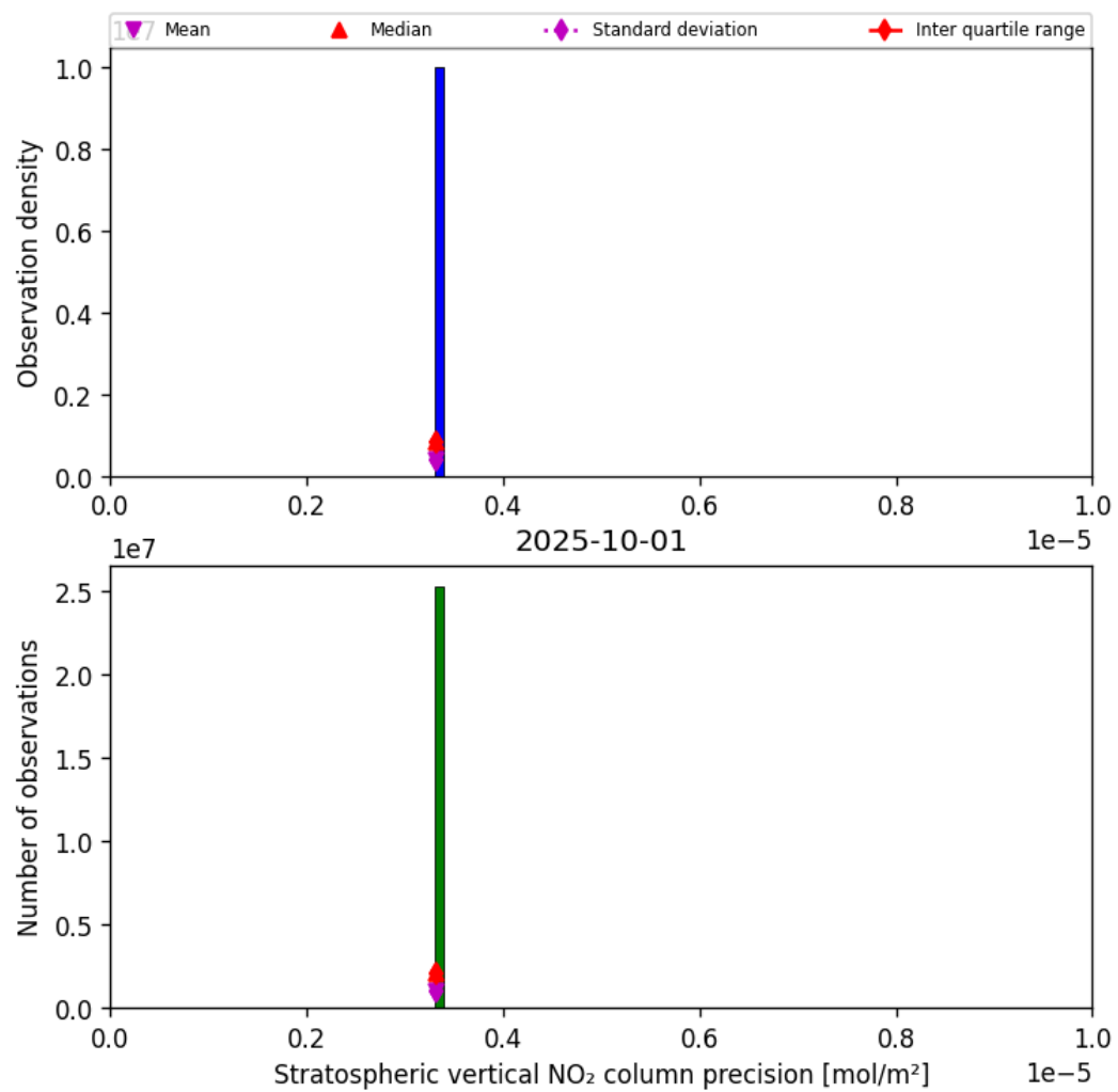
Figure 37: Histogram of “Stratospheric vertical NO 2 column precision” for 2025-10-01 to 2025-10-02
