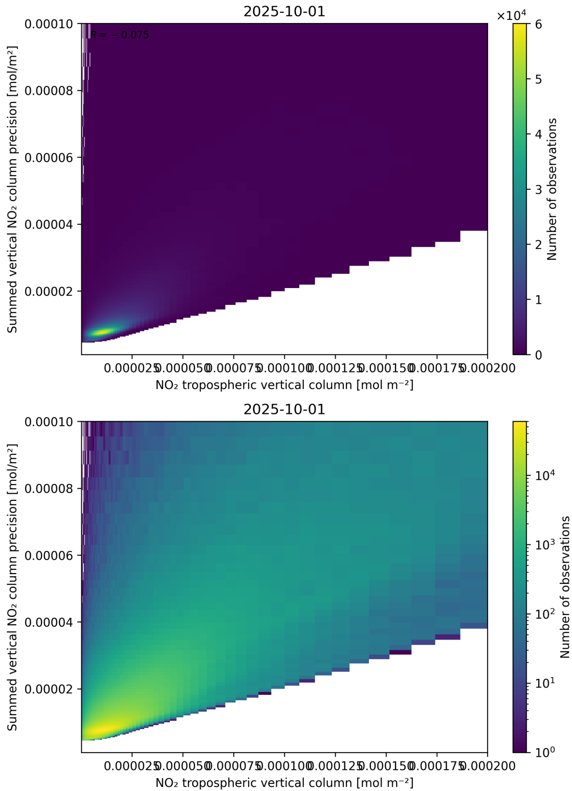
Figure 127: Scatter density plot of “NO 2 tropospheric vertical column” against “Summed vertical NO 2 column precision” for 2025-10-01 to 2025-10-02.
