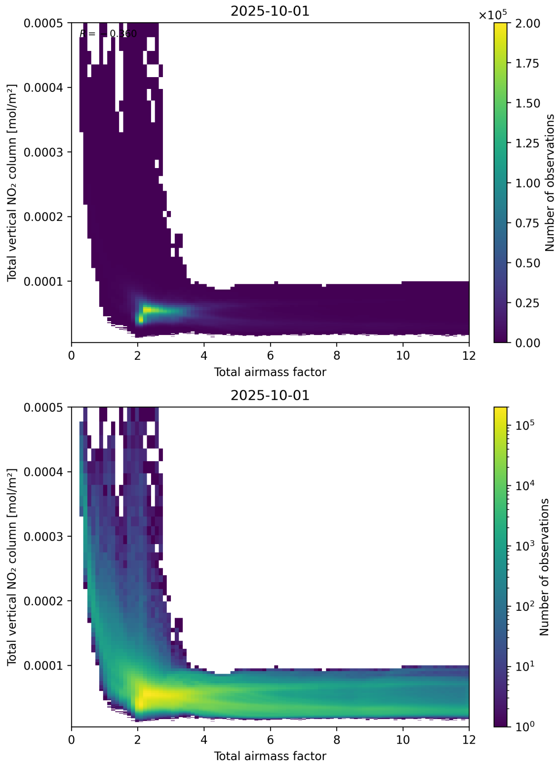
Figure 67: Scatter density plot of “Total airmass factor” against “Total vertical NO 2 column” for 2025-10-01 to 2025-10-02.
