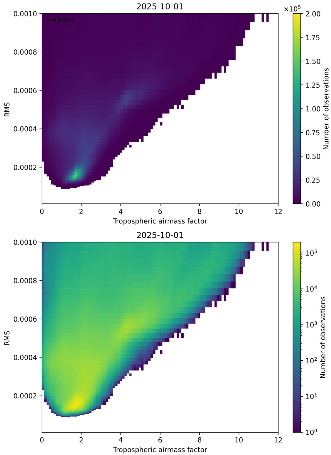
Figure 79: Scatter density plot of “Tropospheric airmass factor” against “RMS” for 2025-10-01 to 2025-10-02.
