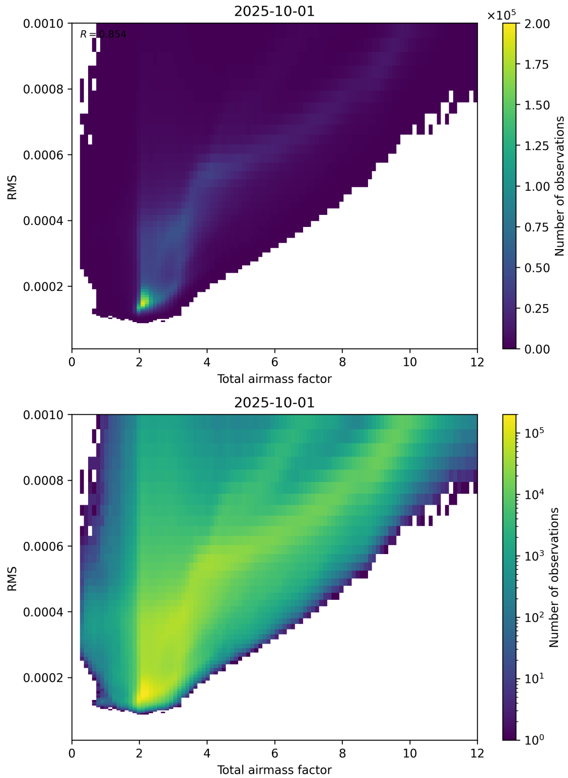
Figure 69: Scatter density plot of “Total airmass factor” against “RMS” for 2025-10-01 to 2025-10-02.
