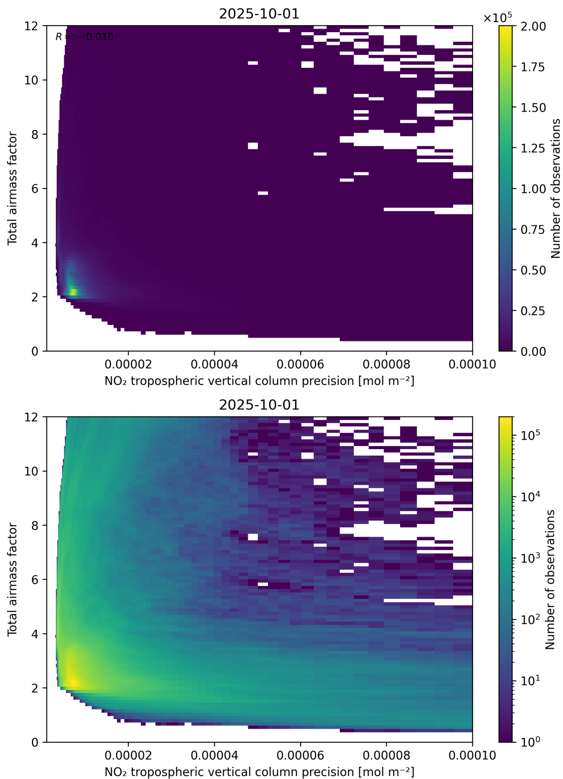
Figure 132: Scatter density plot of “NO 2 tropospheric vertical column precision” against “Total air mass factor” for 2025-10-01 to 2025-10-02.
