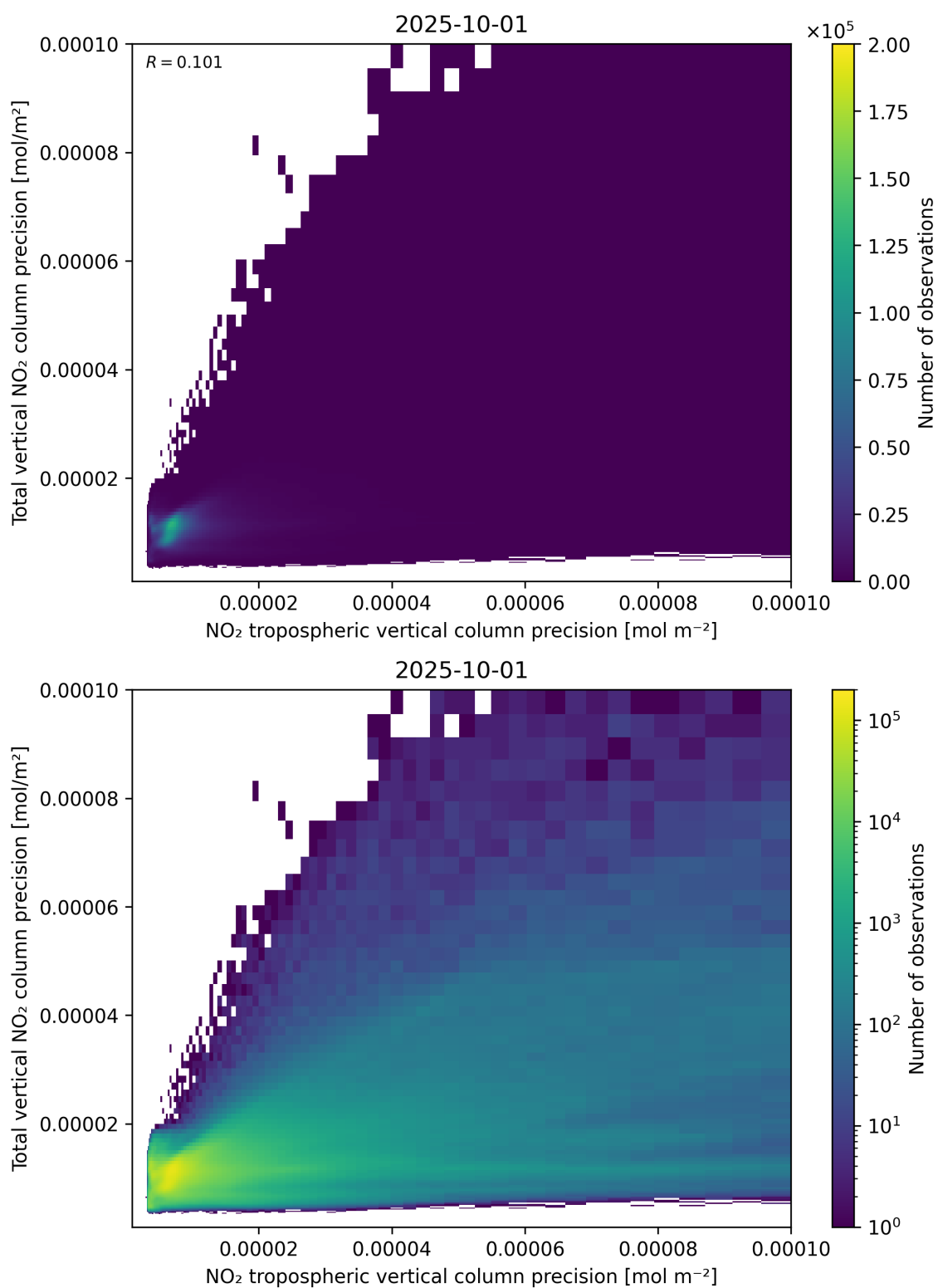
Figure 139: Scatter density plot of “NO 2 tropospheric vertical column precision” against “Total vertical NO 2 column precision” for 2025-10-01 to 2025-10-02.
