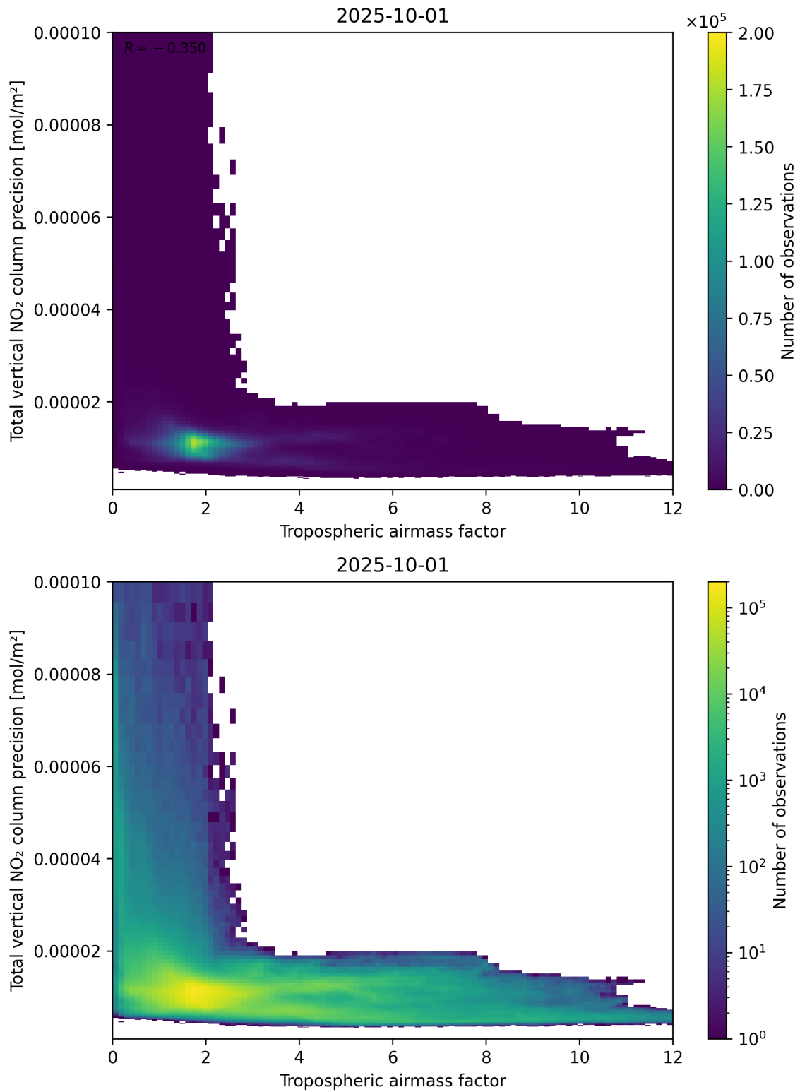
Figure 78: Scatter density plot of “Tropospheric air mass factor” against “Total vertical NO 2 column precision” for 2025-10-01 to 2025-10-02.
