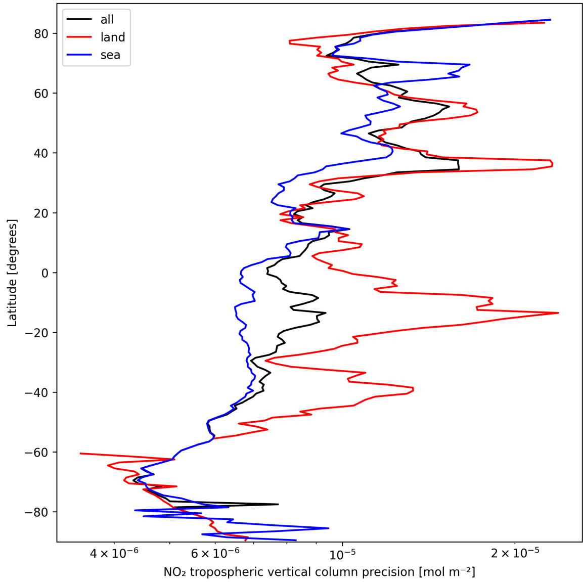
Figure 13: Zonal average of “NO 2 tropospheric vertical column precision” for 2025-10-01 to 2025-10-02.
