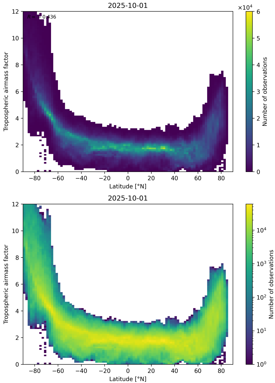
Figure 85: Scatter density plot of “Latitude” against “Tropospheric airmass factor” for 2025-10-01 to 2025-10-02.
