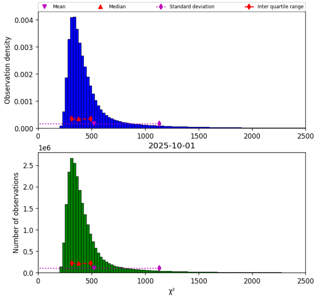
Figure 42: Histogram of “ \chi^2 ” for 2025-10-01 to 2025-10-02
