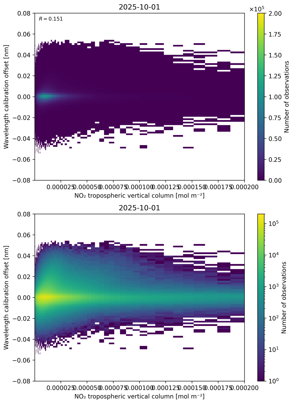
Figure 143: Scatter density plot of “NO 2 tropospheric vertical column” against “Wavelength calibration offset” for 2025-10-01 to 2025-10-02.
