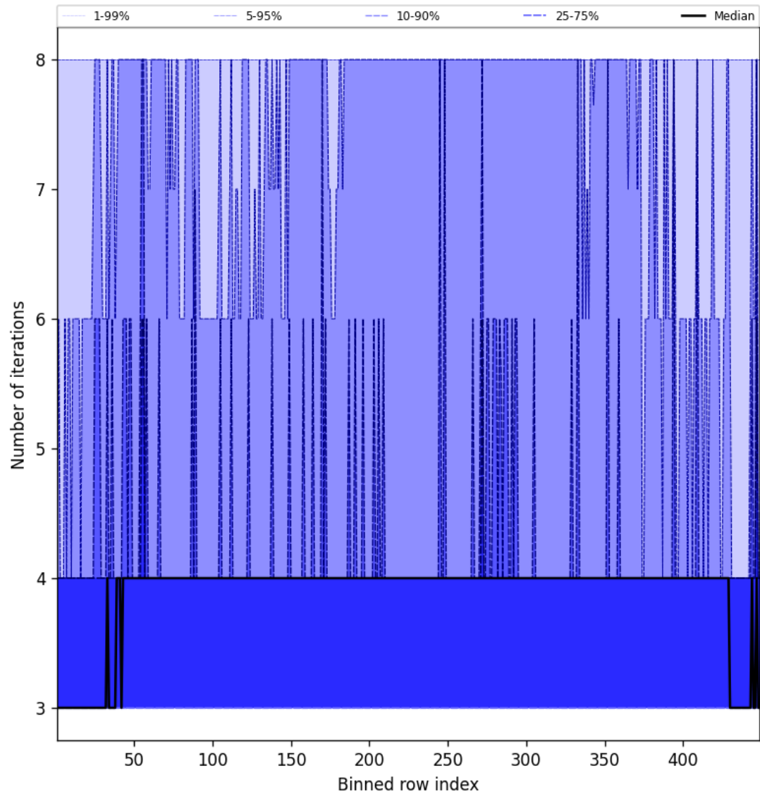
Figure 51: Along track statistics of “Number of iterations” for 2025-10-01 to 2025-10-02
