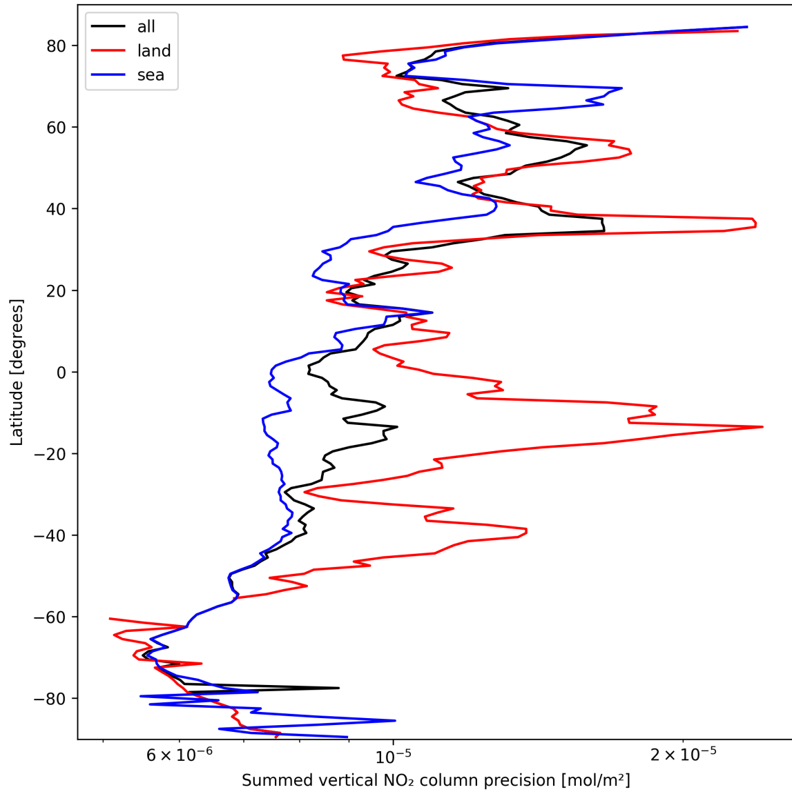
Figure 24: Zonal average of “Summed vertical NO 2 column precision” for 2025-10-01 to 2025-10-02.
