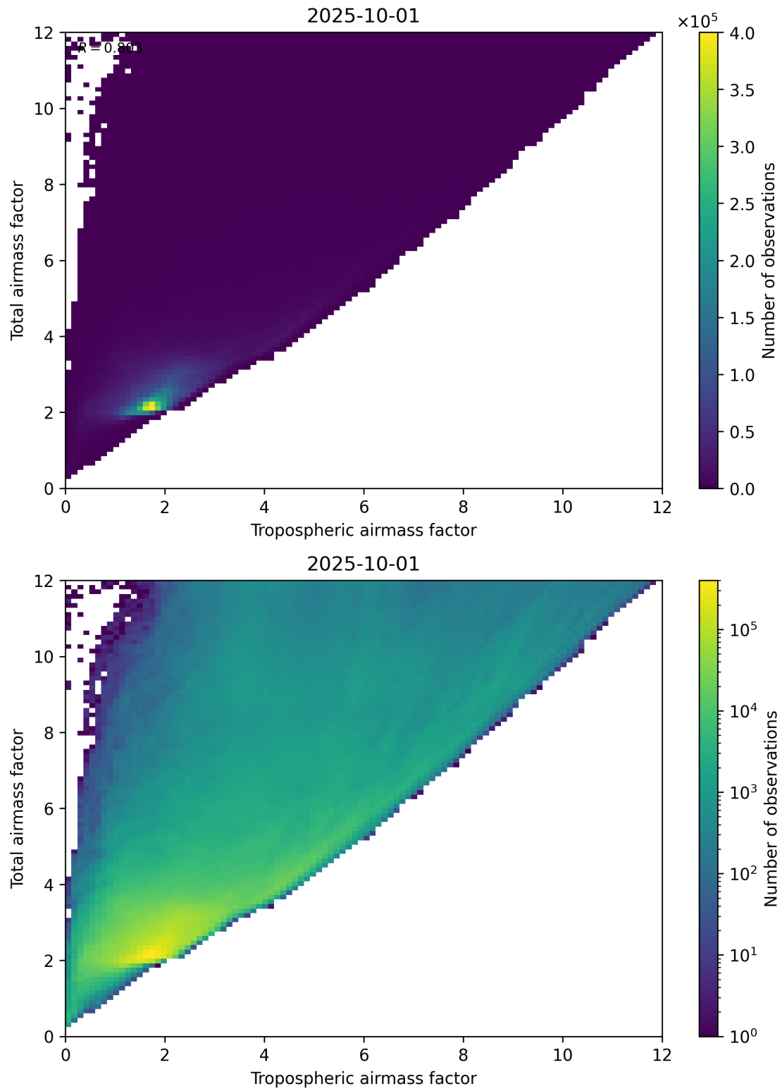
Figure 72: Scatter density plot of “Tropospheric airmass factor” against “Total airmass factor” for 2025-10-01 to 2025-10-02.
