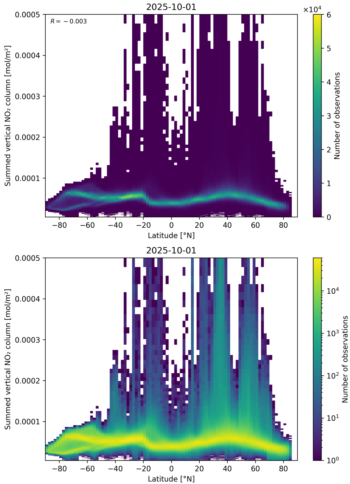
Figure 88: Scatter density plot of “Latitude” against “Summed vertical NO 2 column” for 2025-10-01 to 2025-10-02.
