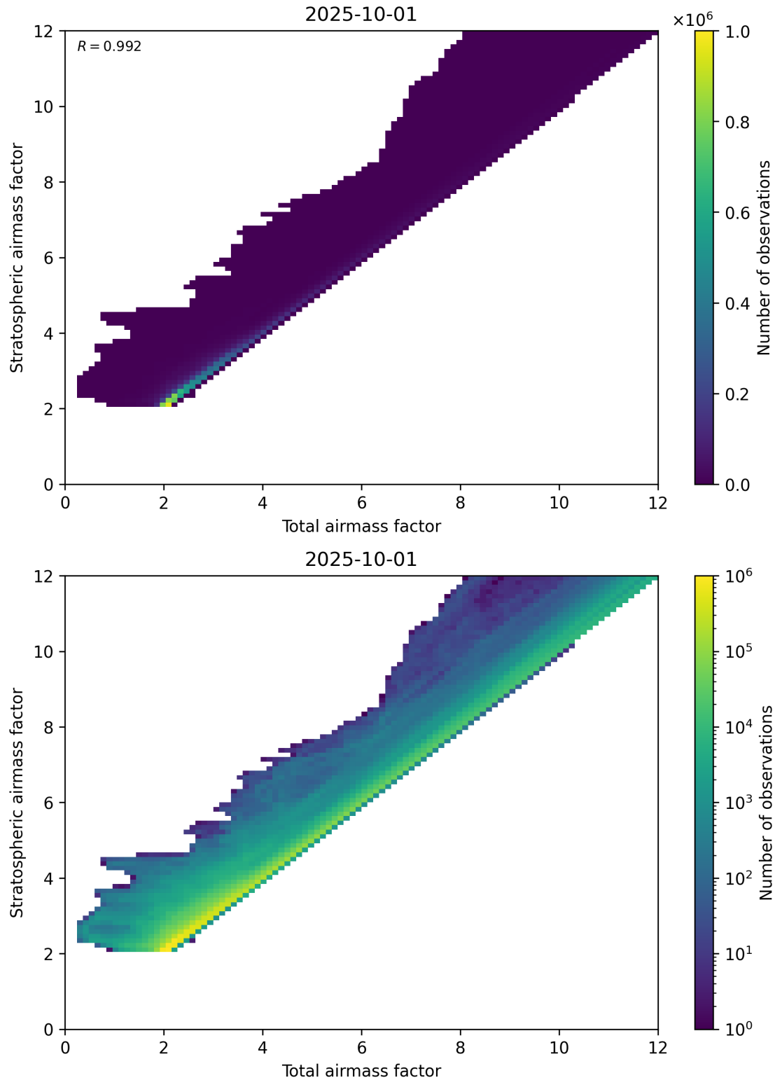
Figure 62: Scatter density plot of “Total airmass factor” against “Stratospheric airmass factor” for 2025-10-01 to 2025-10-02.
