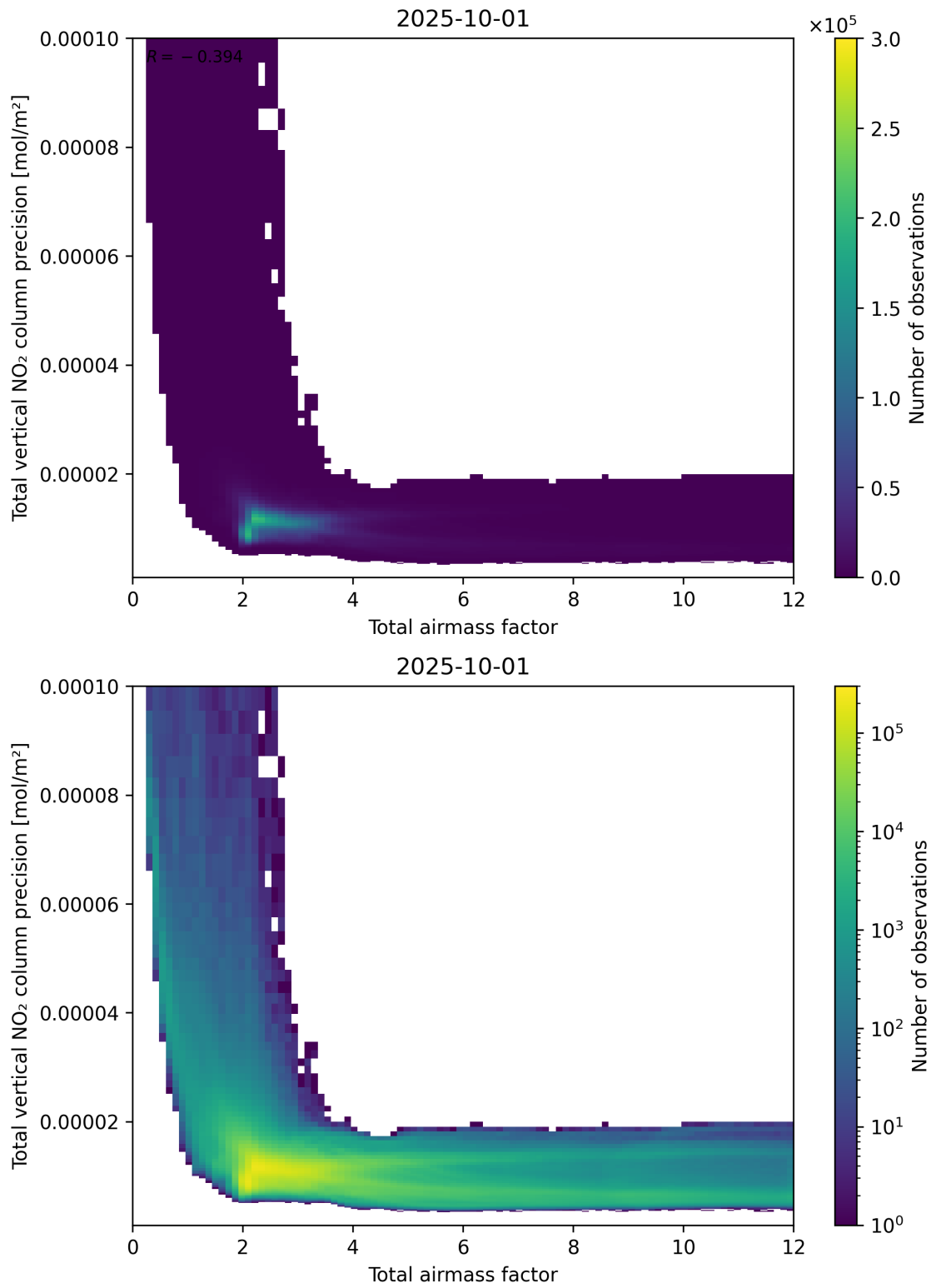
Figure 68: Scatter density plot of “Total airmass factor” against “Total vertical NO 2 column precision” for 2025-10-01 to 2025-10-02.
