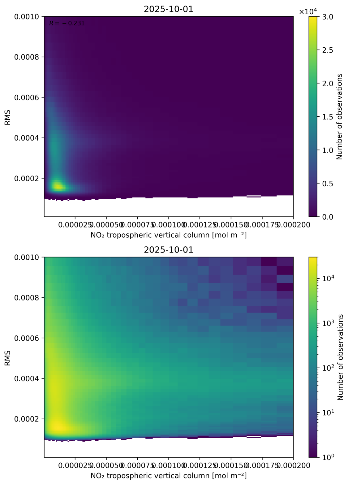
Figure 142: Scatter density plot of “NO 2 tropospheric vertical column” against “RMS” for 2025-10-01 to 2025-10-02.
