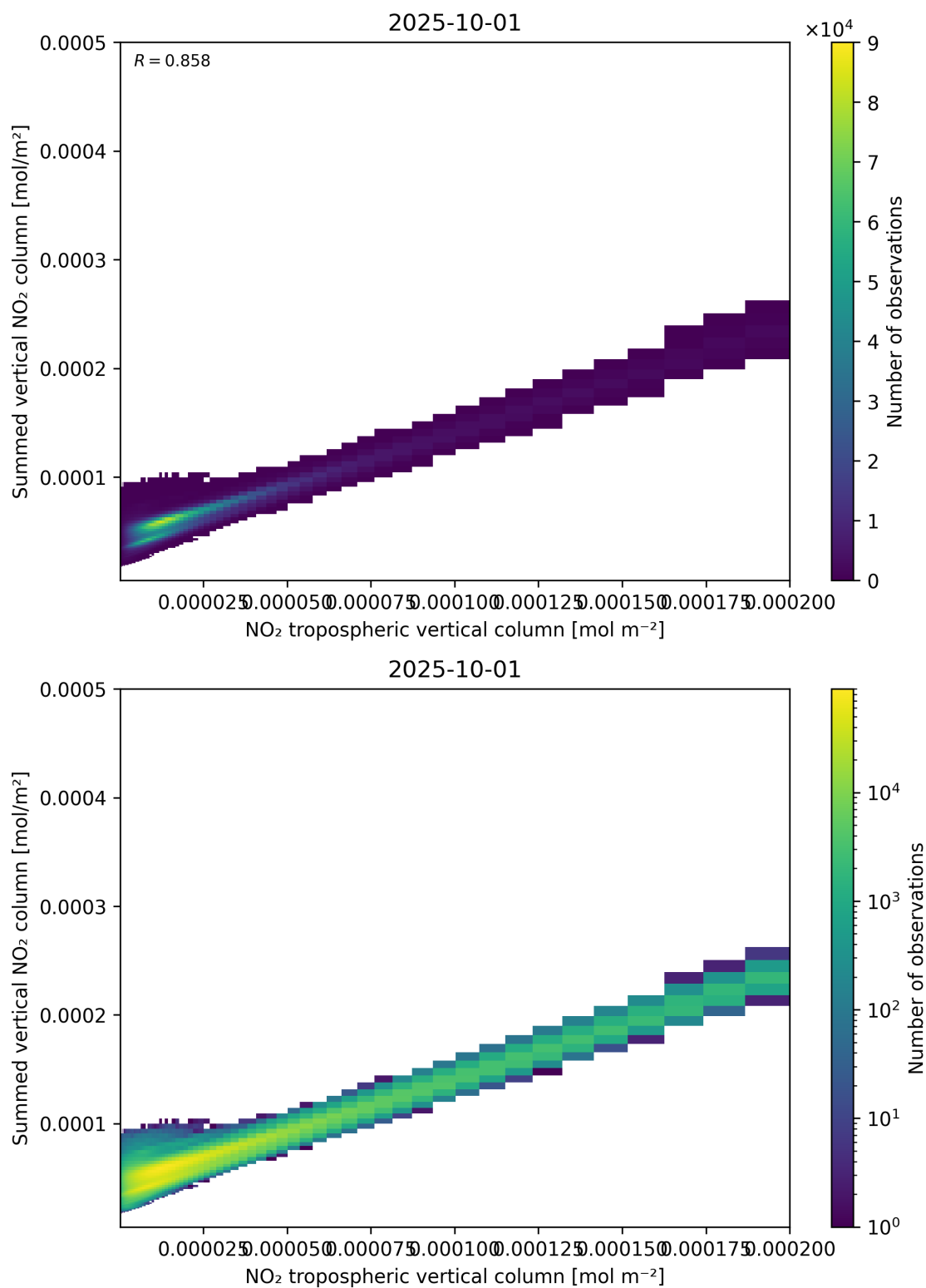
Figure 126: Scatter density plot of “NO 2 tropospheric vertical column” against “Summed vertical NO 2 column” for 2025-10-01 to 2025-10-02.
