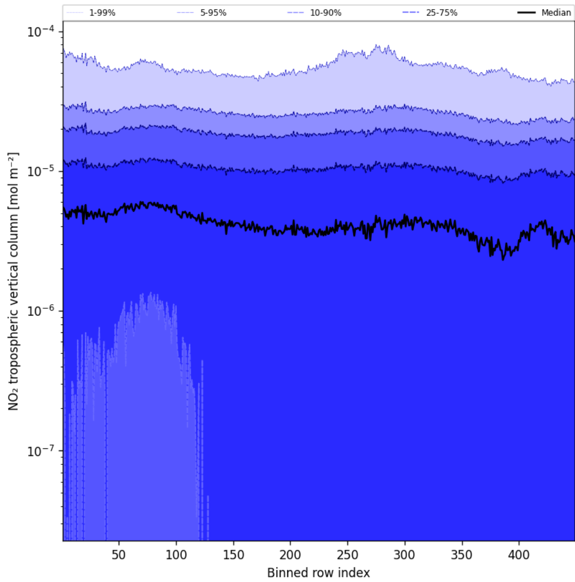
Figure 46: Along track statistics of “NO 2 tropospheric vertical column” for 2025-10-01 to 2025-10-02
