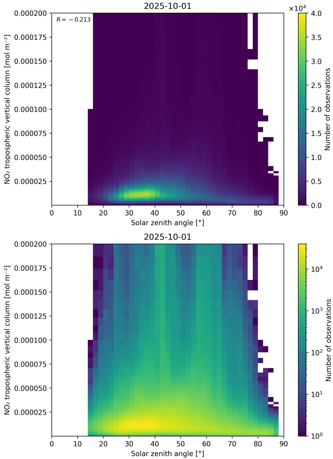
Figure 155: Scatter density plot of “Solar zenith angle” against “NO 2 tropospheric vertical column” for 2025-10-01 to 2025-10-02.
