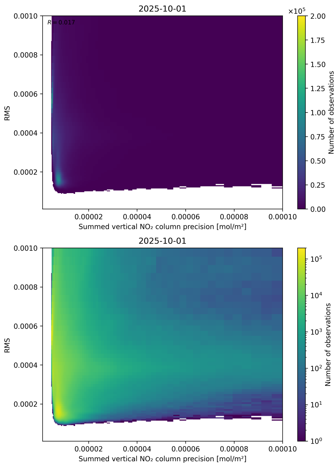
Figure 108: Scatter density plot of “Summed vertical NO 2 column precision” against “RMS” for 2025-10-01 to 2025-10-02.
