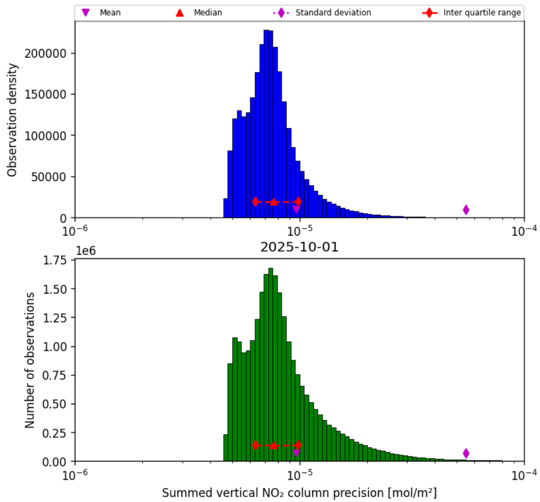
Figure 41: Histogram of “Summed vertical NO 2 column precision” for 2025-10-01 to 2025-10-02
