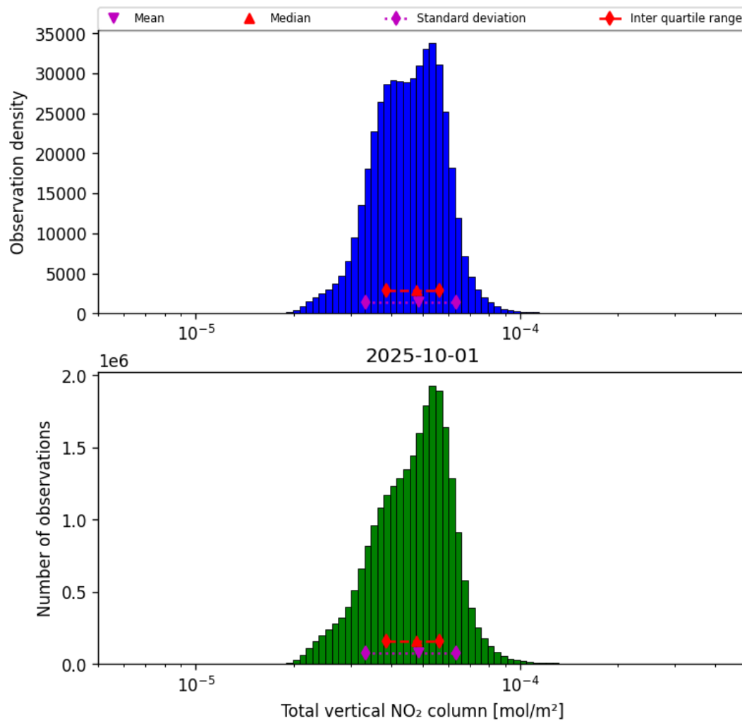
Figure 38: Histogram of “Total vertical NO 2 column” for 2025-10-01 to 2025-10-02
