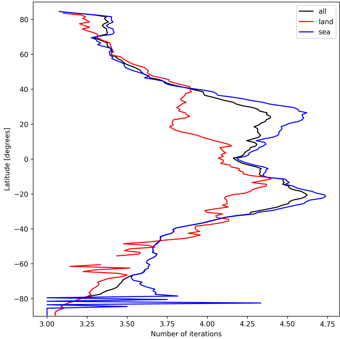
Figure 17: Zonal average of “Number of iterations” for 2025-10-01 to 2025-10-02.
