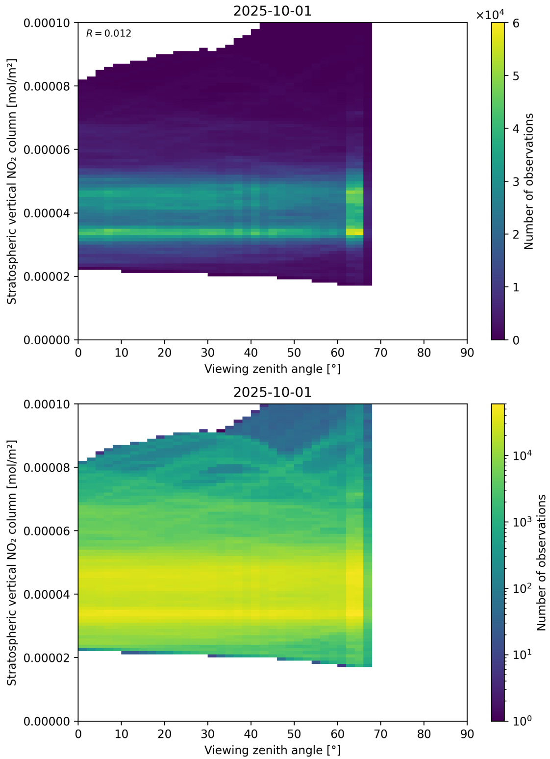
Figure 164: Scatter density plot of “Viewing zenith angle” against “Stratospheric vertical NO 2 column” for 2025-10-01 to 2025-10-02.
