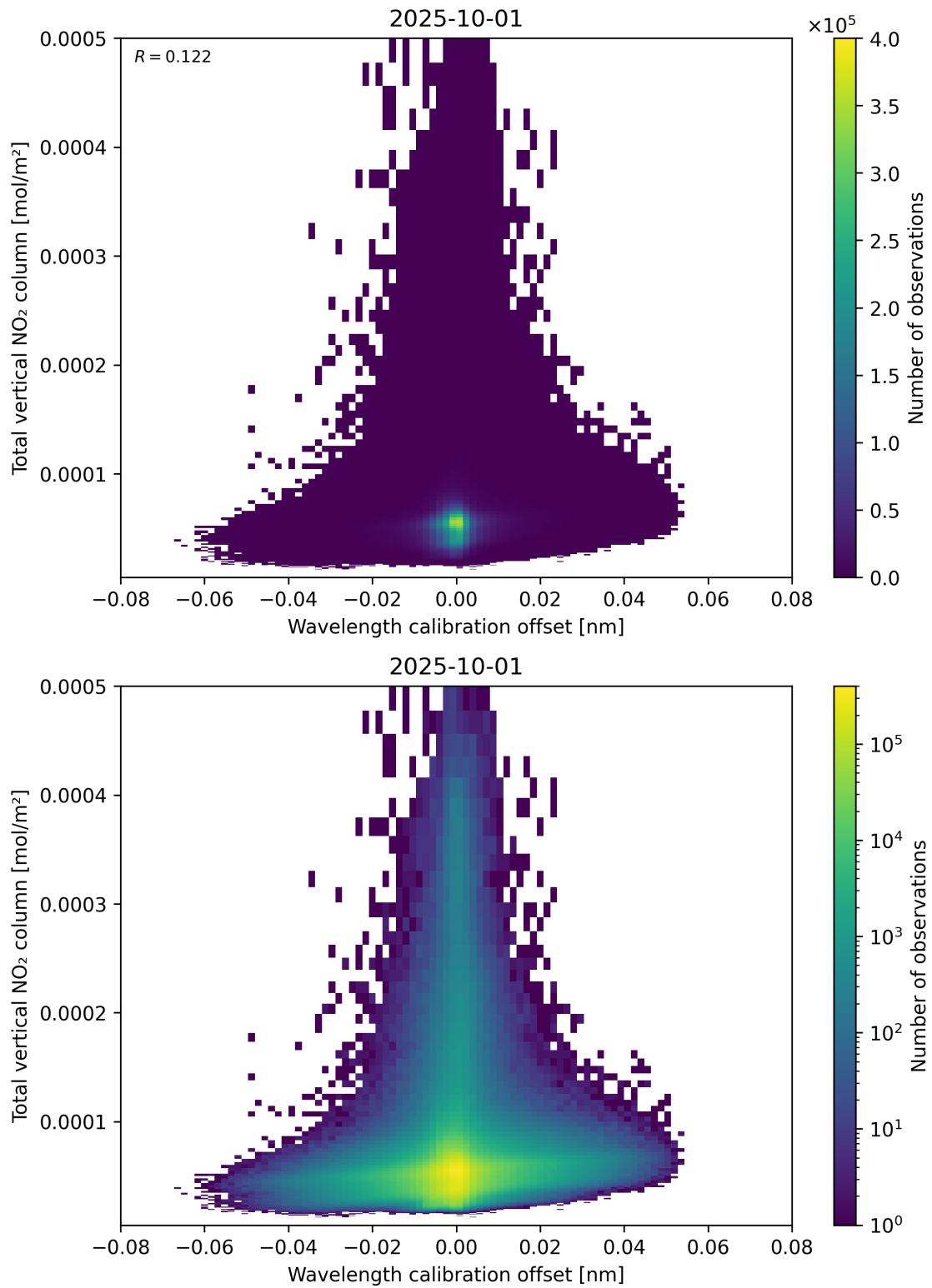
Figure 179: Scatter density plot of “Wavelength calibration offset” against “Total vertical NO 2 column” for 2025-10-01 to 2025-10-02.
