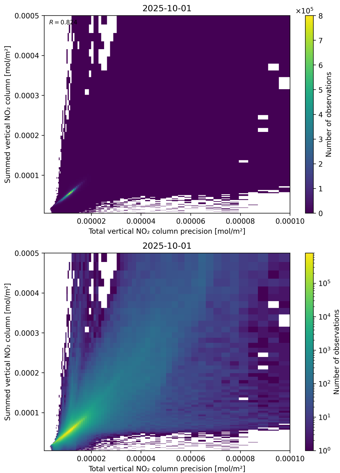
Figure 117: Scatter density plot of “Total vertical NO 2 column precision” against “Summed vertical NO 2 column” for 2025-10-01 to 2025-10-02.
