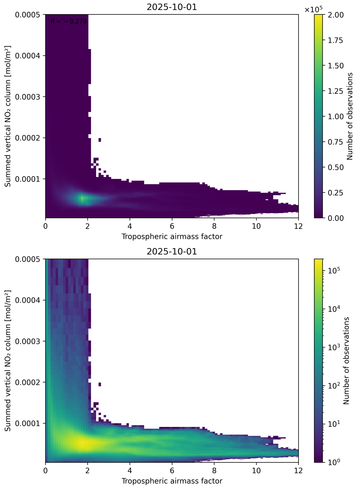
Figure 75: Scatter density plot of “Tropospheric air mass factor” against “Summed vertical NO 2 column” for 2025-10-01 to 2025-10-02.
