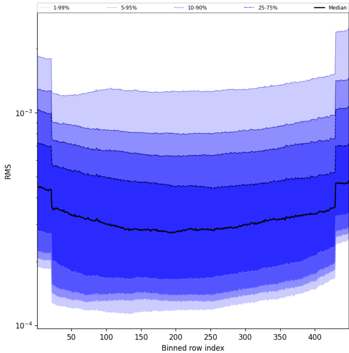
Figure 60: Along track statistics of “RMS” for 2025-10-01 to 2025-10-02
