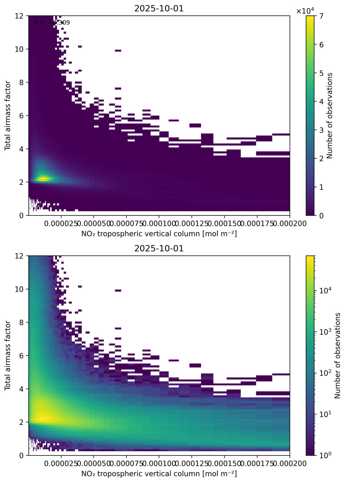
Figure 122: Scatter density plot of “NO 2 tropospheric vertical column” against “Total air mass factor” for 2025-10-01 to 2025-10-02.
