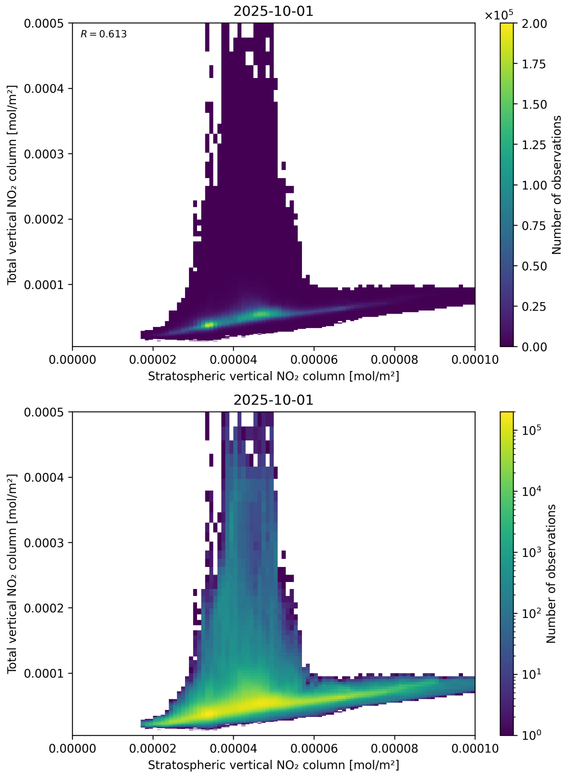
Figure 100: Scatter density plot of “Stratospheric vertical NO 2 column” against “Total vertical NO 2 column” for 2025-10-01 to 2025-10-02.
