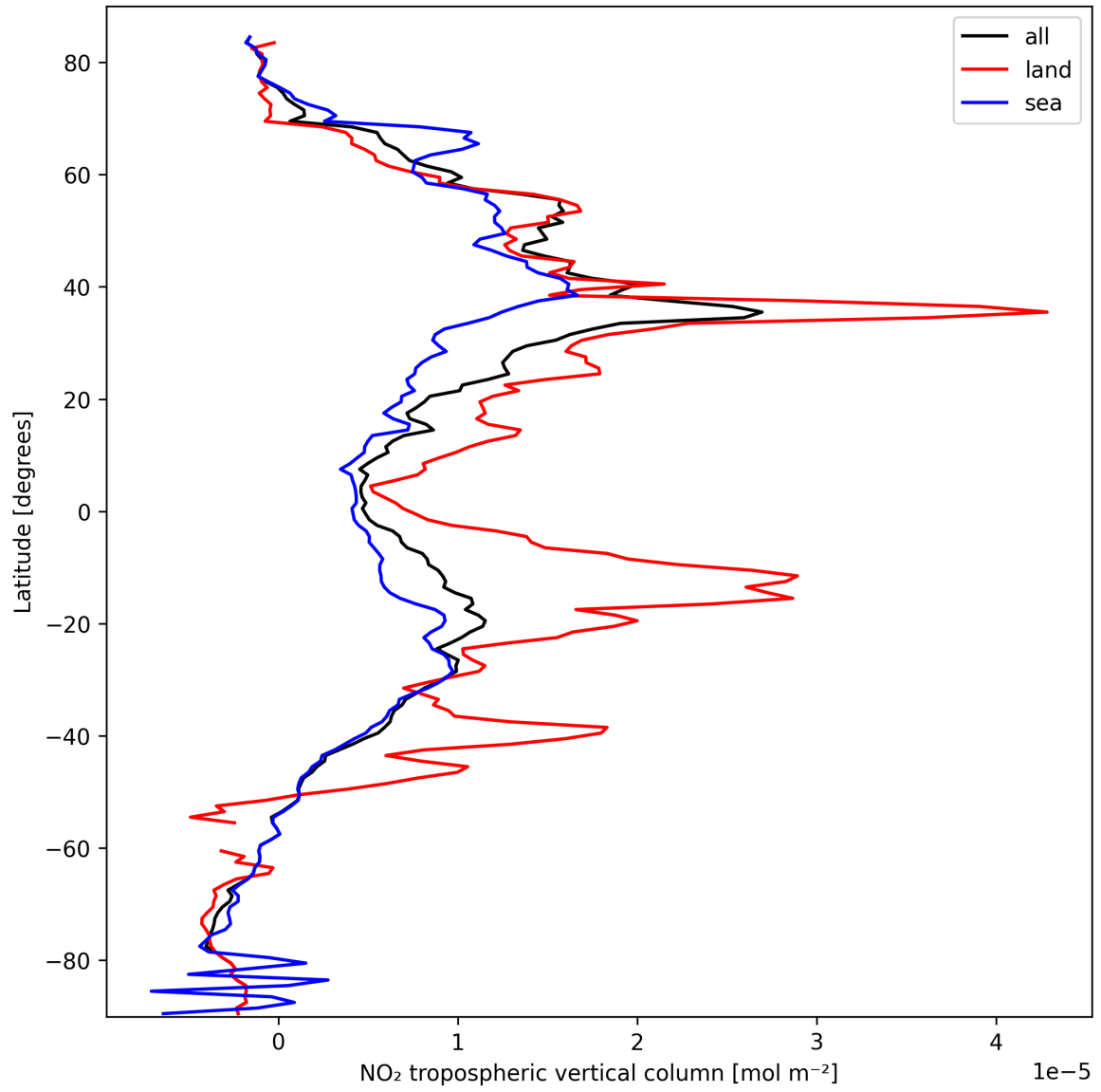
Figure 12: Zonal average of “NO 2 tropospheric vertical column” for 2025-10-01 to 2025-10-02.
