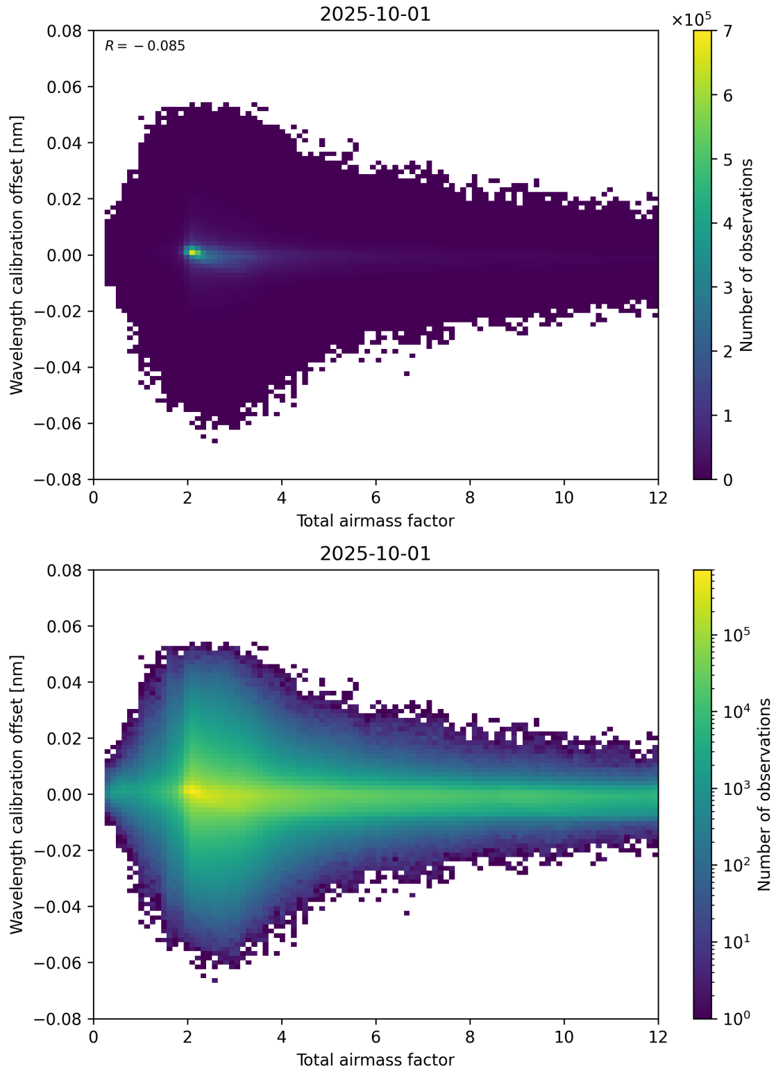
Figure 70: Scatter density plot of “Total airmass factor” against “Wavelength calibration offset” for 2025-10-01 to 2025-10-02.
