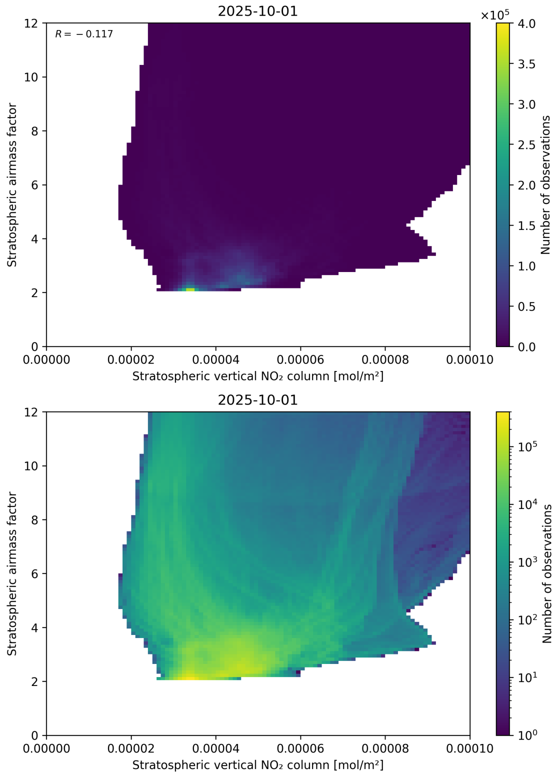
Figure 96: Scatter density plot of “Stratospheric vertical NO 2 column” against “Stratospheric airmass factor” for 2025-10-01 to 2025-10-02.
