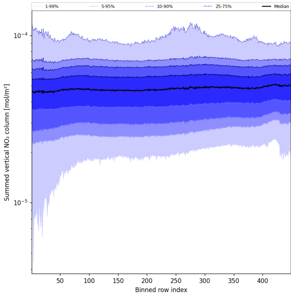
Figure 57: Along track statistics of “Summed vertical NO 2 column” for 2025-10-01 to 2025-10-02
