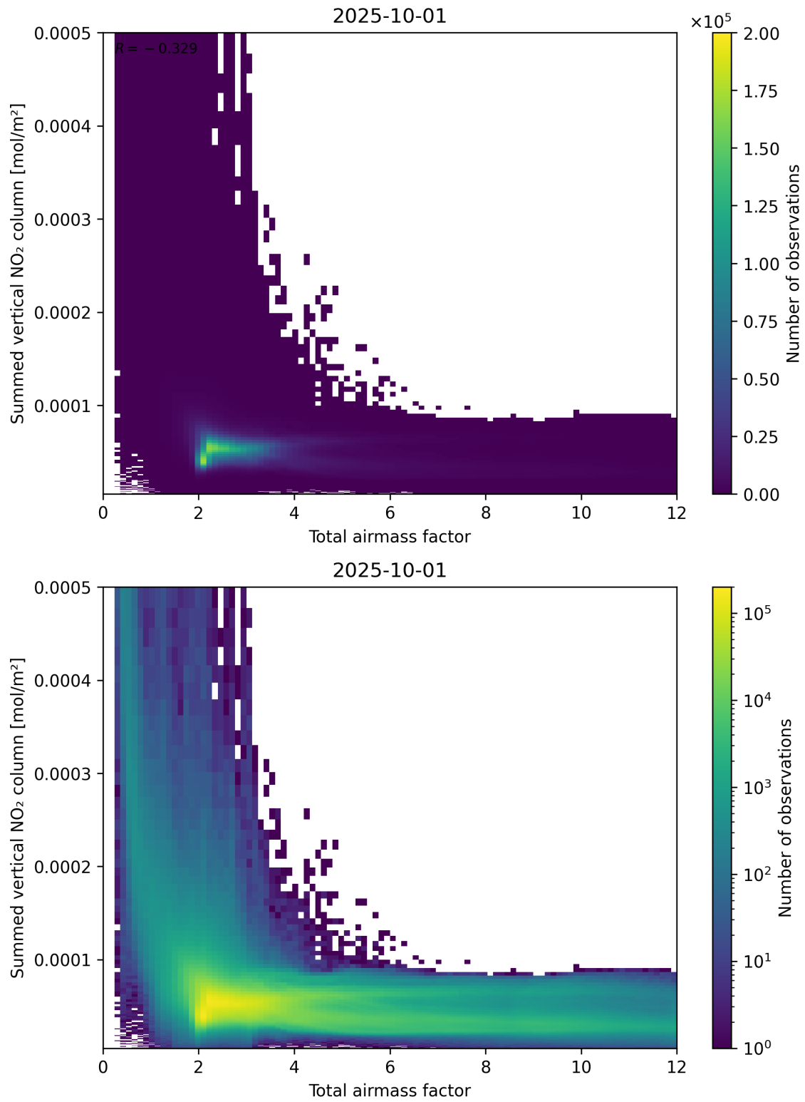
Figure 65: Scatter density plot of “Total airmass factor” against “Summed vertical NO 2 column” for 2025-10-01 to 2025-10-02.
