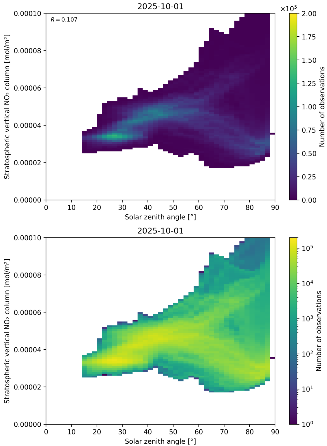
Figure 150: Scatter density plot of “Solar zenith angle” against “Stratospheric vertical NO 2 column” for 2025-10-01 to 2025-10-02.
