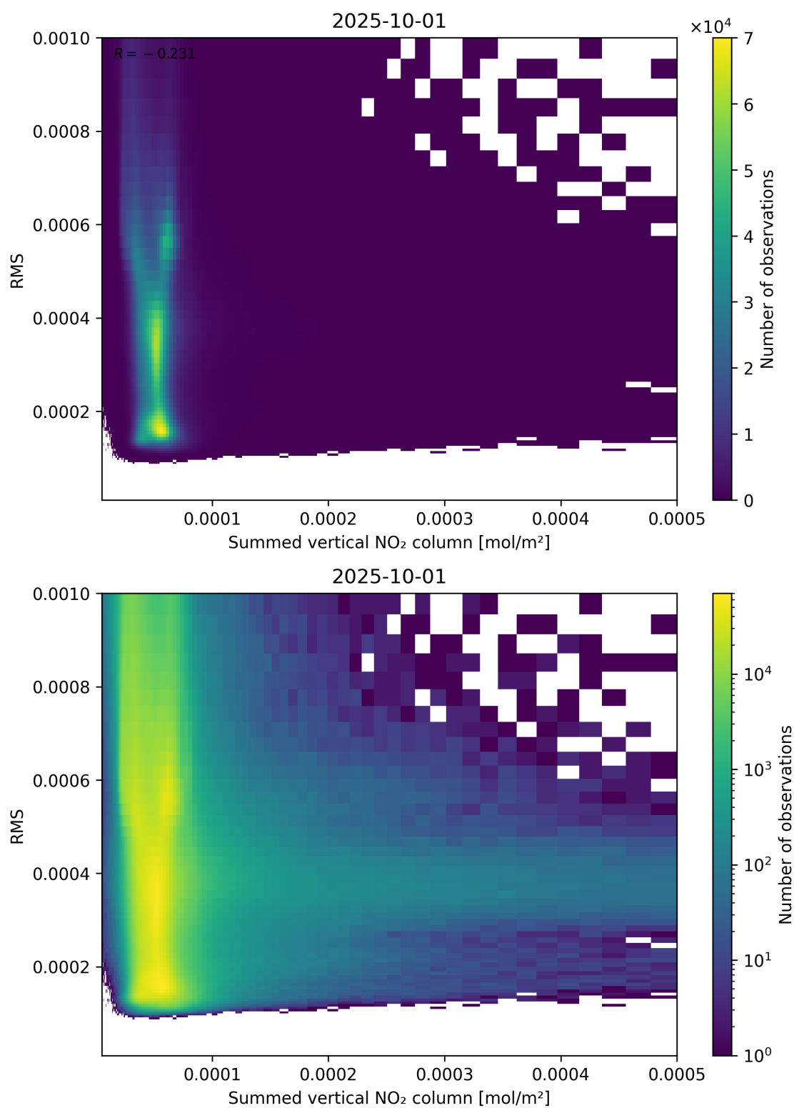
Figure 109: Scatter density plot of “Summed vertical NO 2 column” against “RMS” for 2025-10-01 to 2025-10-02.
