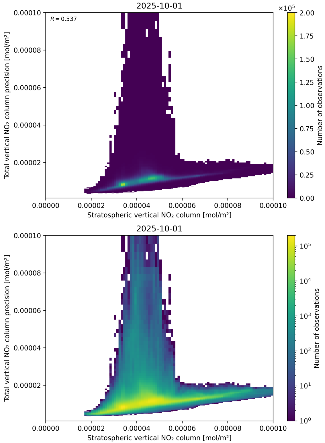
Figure 101: Scatter density plot of “Stratospheric vertical NO 2 column” against “Total vertical NO 2 column precision” for 2025-10-01 to 2025-10-02.
