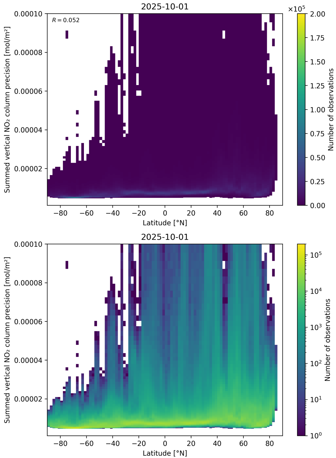
Figure 89: Scatter density plot of “Latitude” against “Summed vertical NO 2 column precision” for 2025-10-01 to 2025-10-02.
