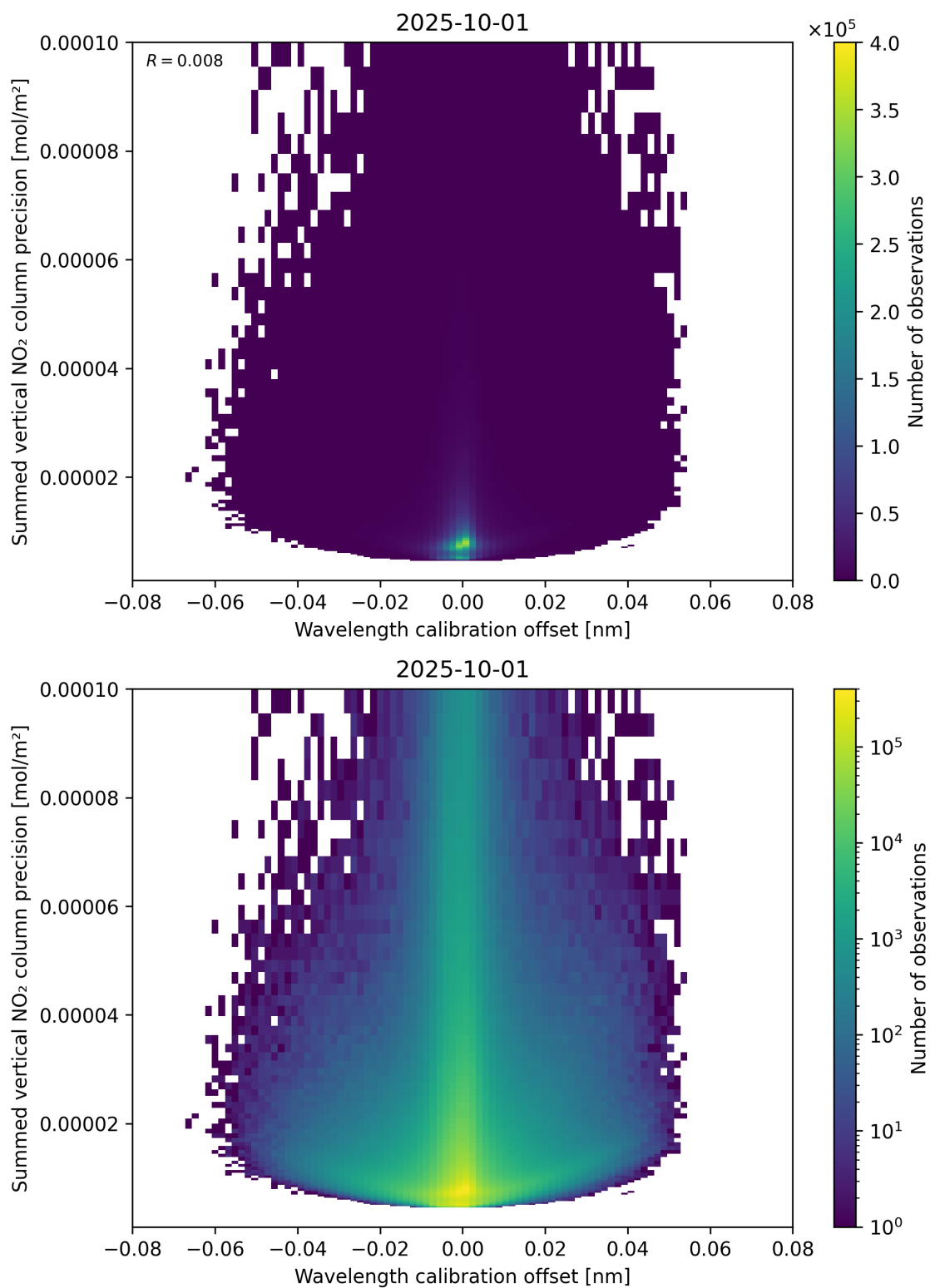
Figure 178: Scatter density plot of “Wavelength calibration offset” against “Summed vertical NO 2 column precision” for 2025-10-01 to 2025-10-02.
