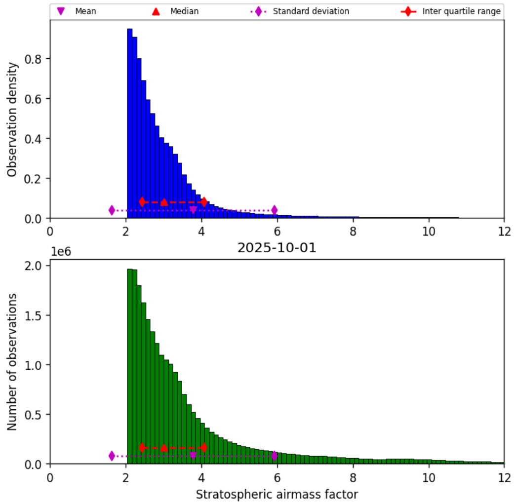
Figure 44: Histogram of “Stratospheric airmass factor” for 2025-10-01 to 2025-10-02
