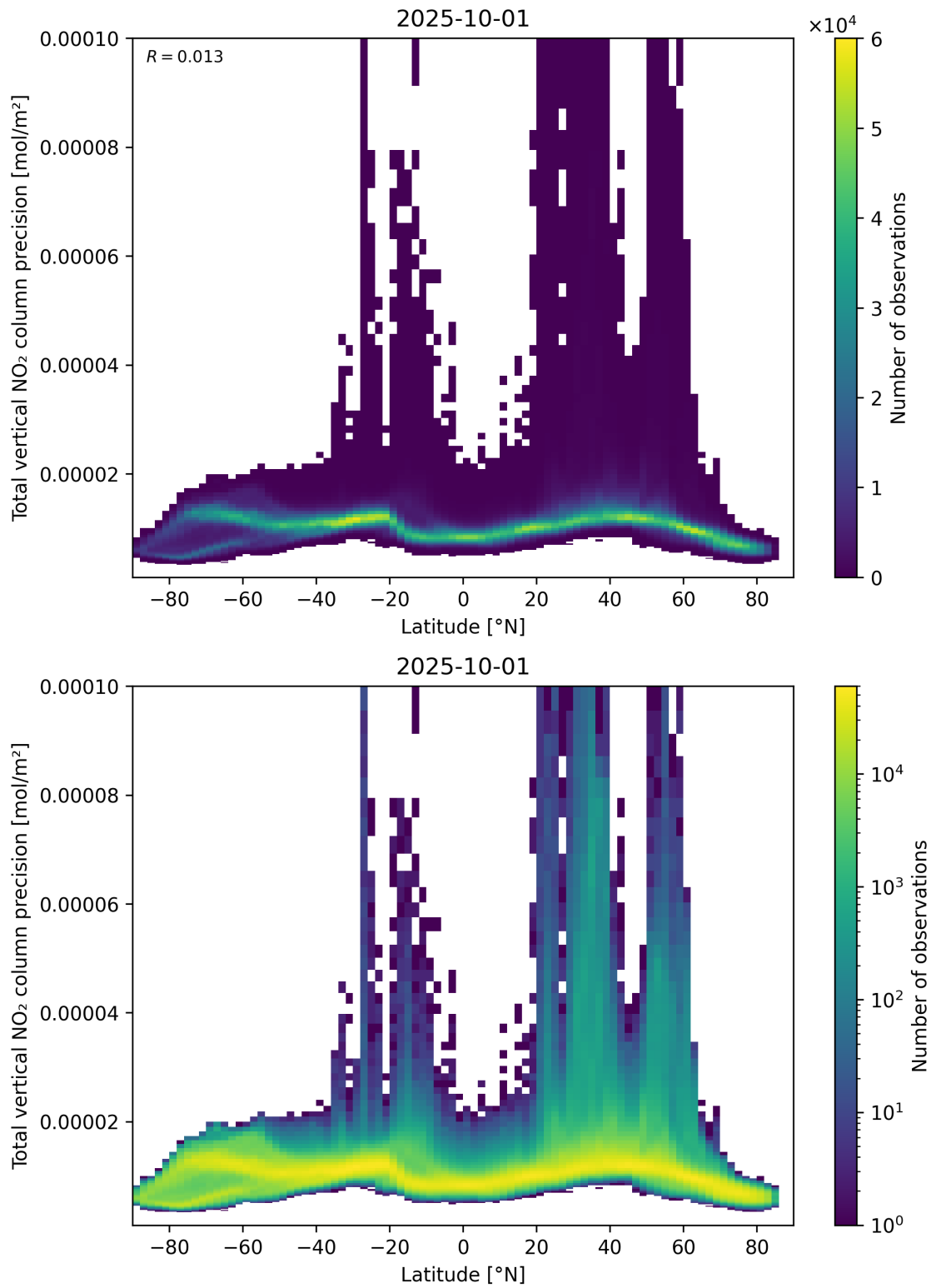
Figure 91: Scatter density plot of “Latitude” against “Total vertical NO 2 column precision” for 2025-10-01 to 2025-10-02.
