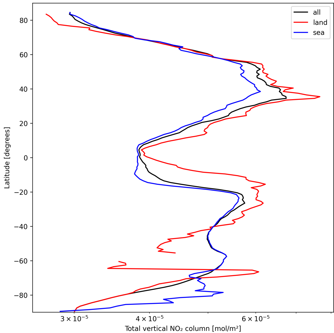
Figure 21: Zonal average of “Total vertical NO 2 column” for 2025-10-01 to 2025-10-02.
