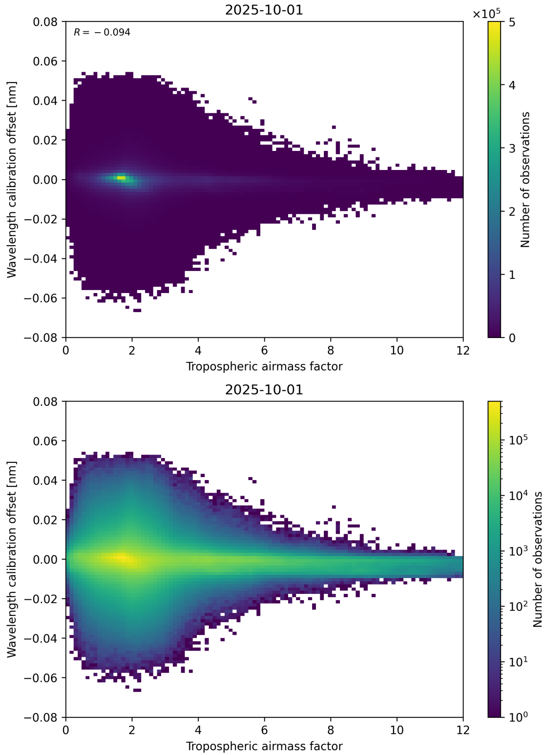
Figure 80: Scatter density plot of “Tropospheric air mass factor” against “Wavelength calibration offset” for 2025-10-01 to 2025-10-02.
