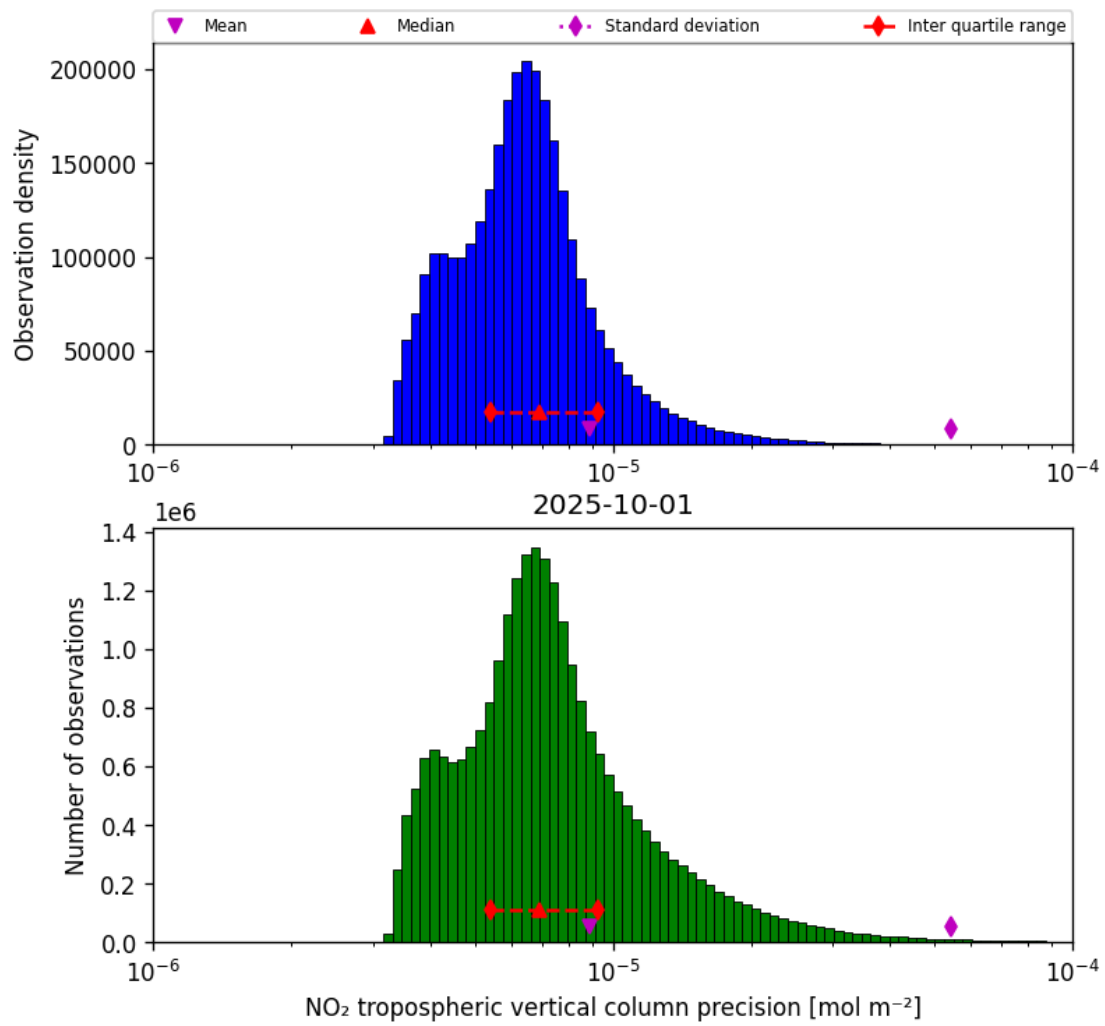
Figure 30: Histogram of “NO 2 tropospheric vertical column precision” for 2025-10-01 to 2025-10-02
