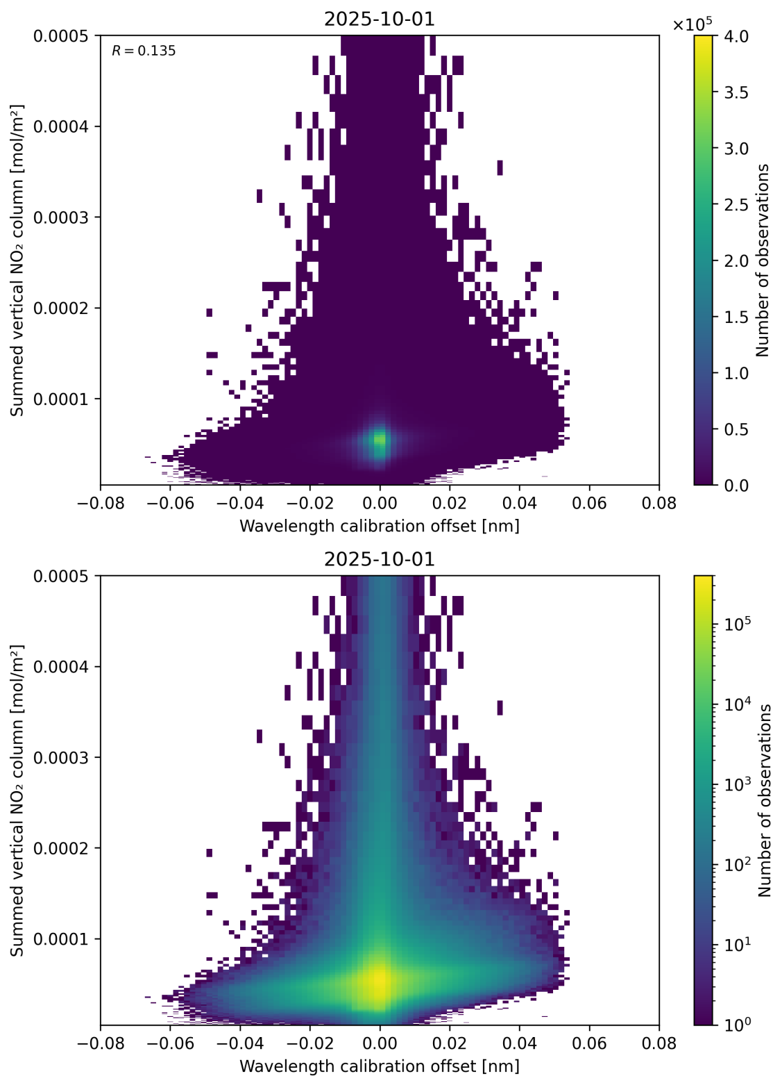
Figure 177: Scatter density plot of “Wavelength calibration offset” against “Summed vertical NO 2 column” for 2025-10-01 to 2025-10-02.
