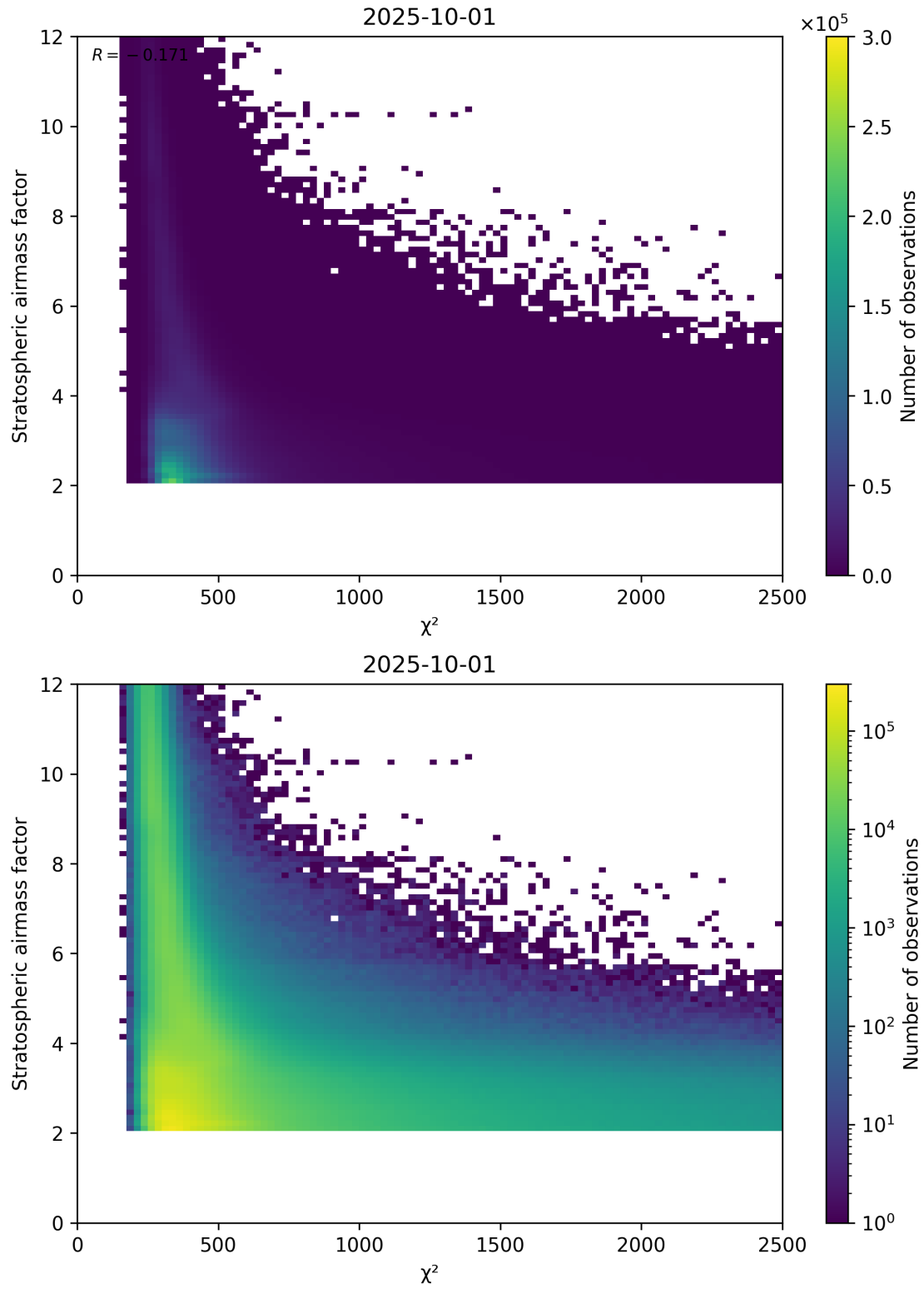
Figure 81: Scatter density plot of “ \chi^2 ” against “Stratospheric airmass factor” for 2025-10-01 to 2025-10-02.
