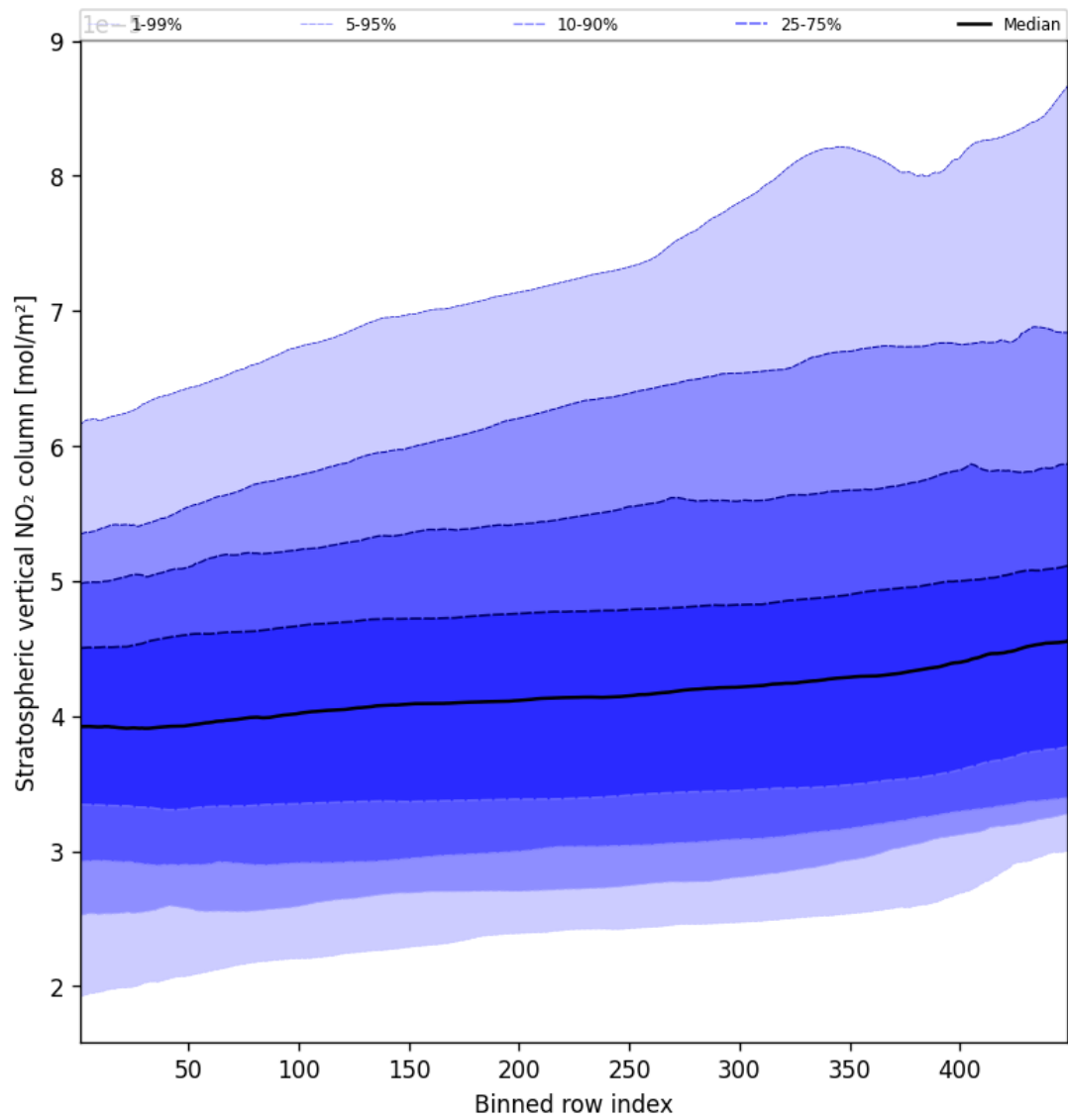
Figure 53: Along track statistics of “Stratospheric vertical NO 2 column” for 2025-10-01 to 2025-10-02
