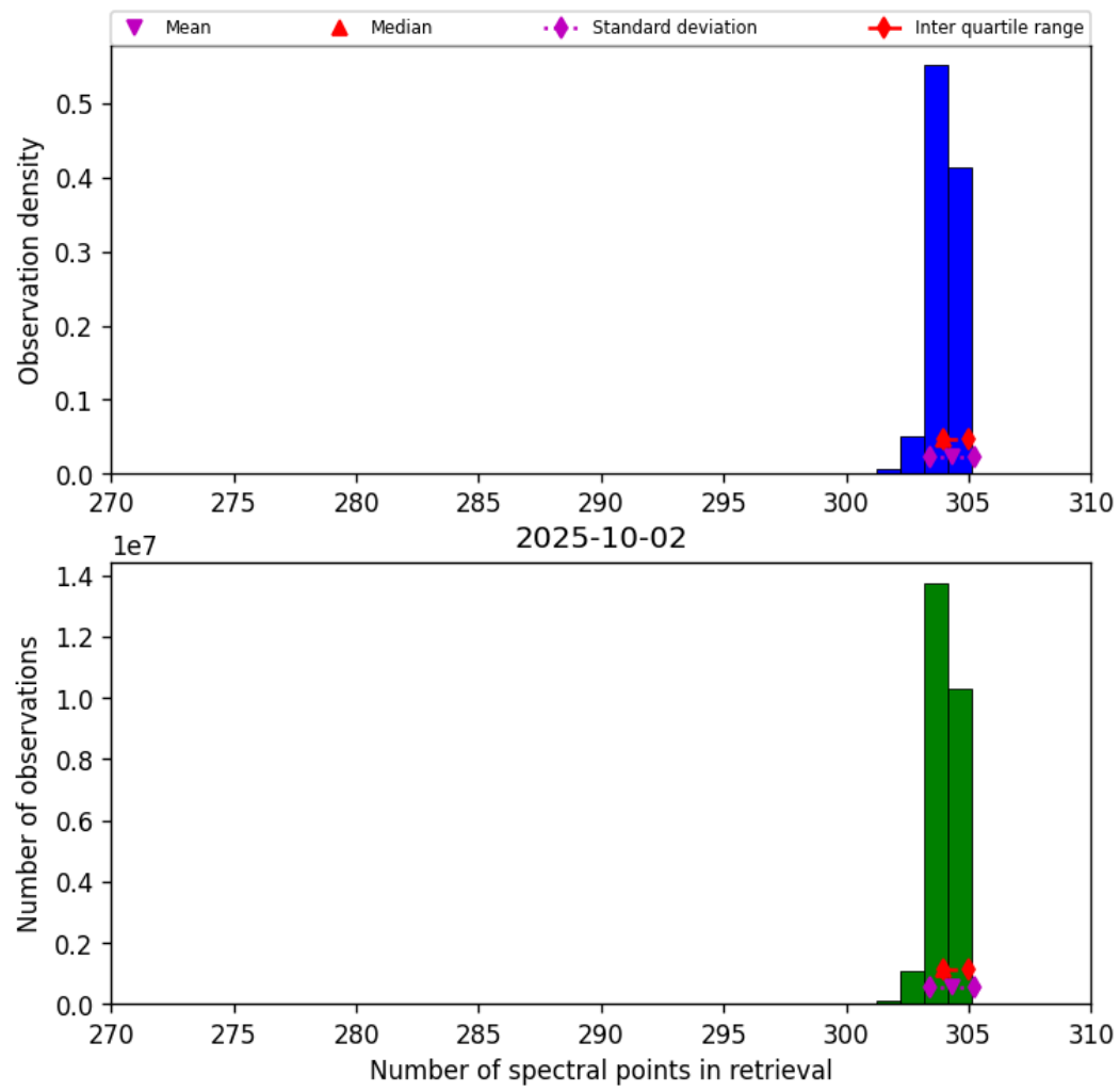
Figure 33: Histogram of “Number of spectral points in retrieval” for 2025-10-01 to 2025-10-03
