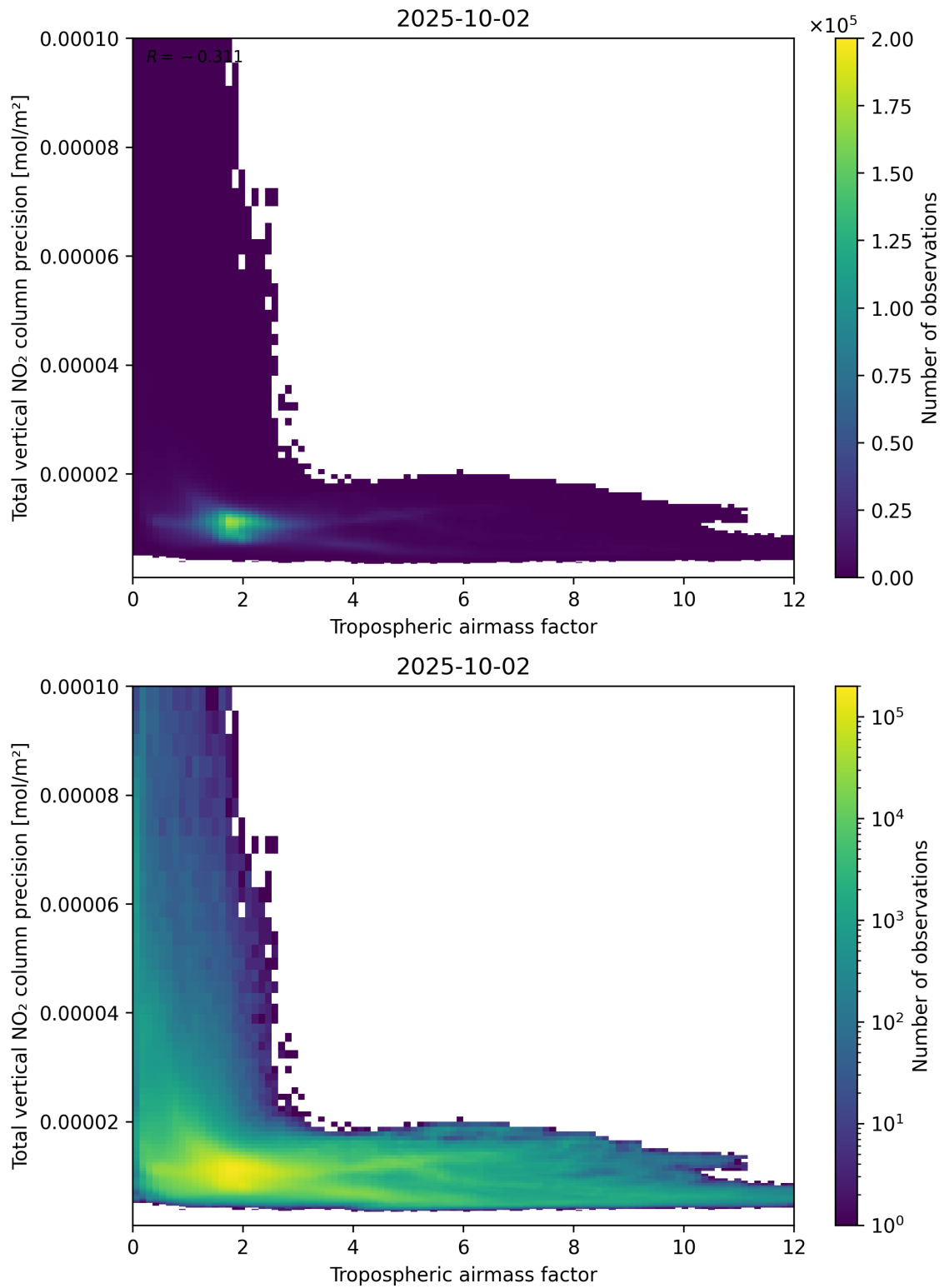
Figure 78: Scatter density plot of “Tropospheric airmass factor” against “Total vertical NO 2 column precision” for 2025-10-01 to 2025-10-03.
