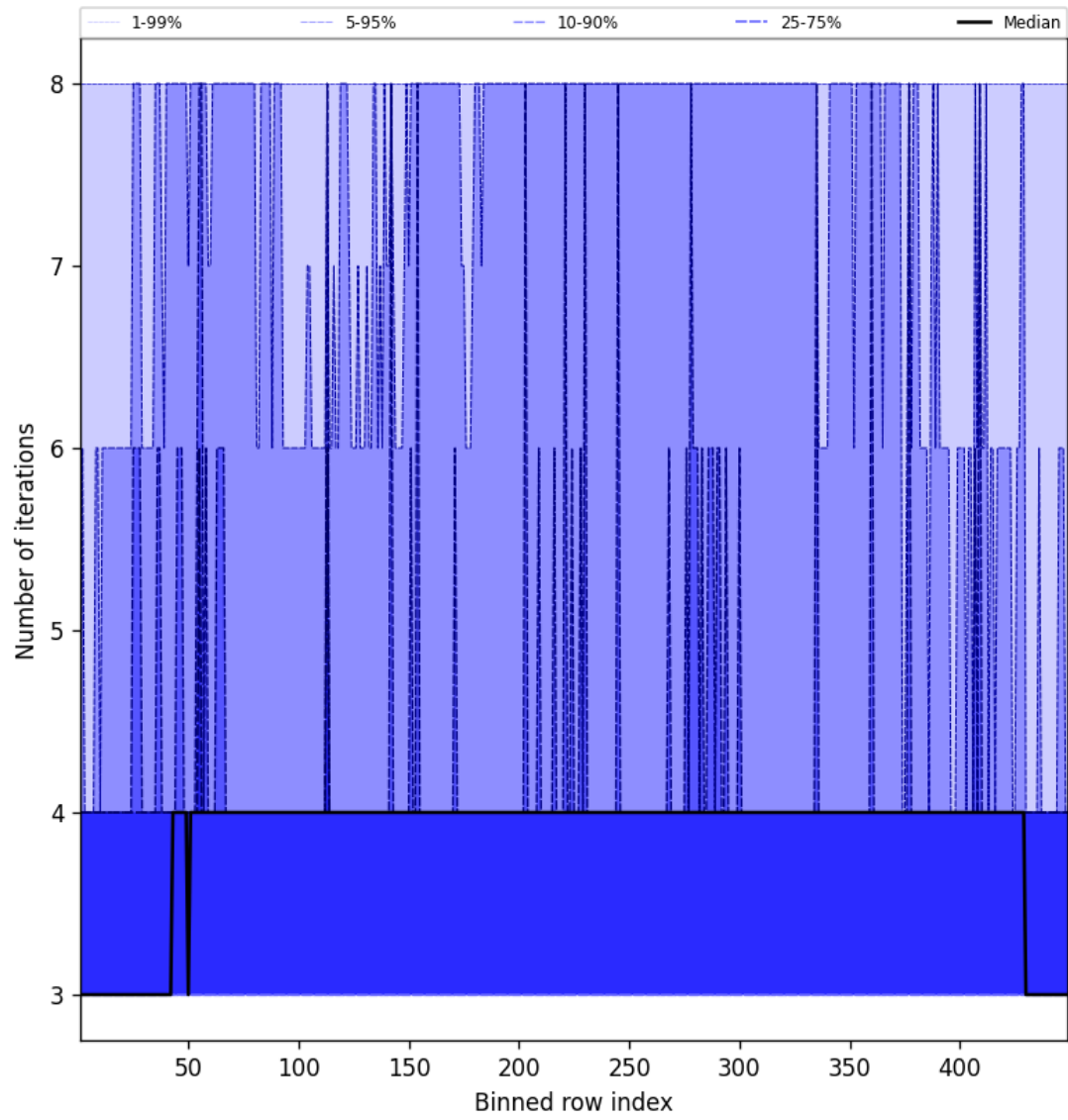
Figure 51: Along track statistics of “Number of iterations” for 2025-10-01 to 2025-10-03
