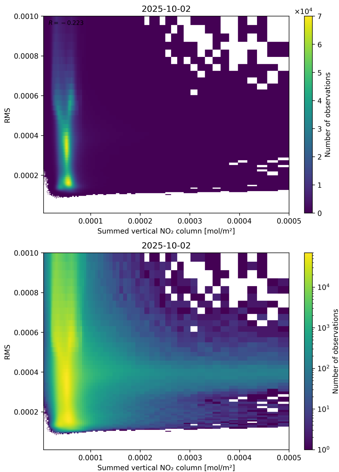
Figure 109: Scatter density plot of “Summed vertical NO 2 column” against “RMS” for 2025-10-01 to 2025-10-03.
