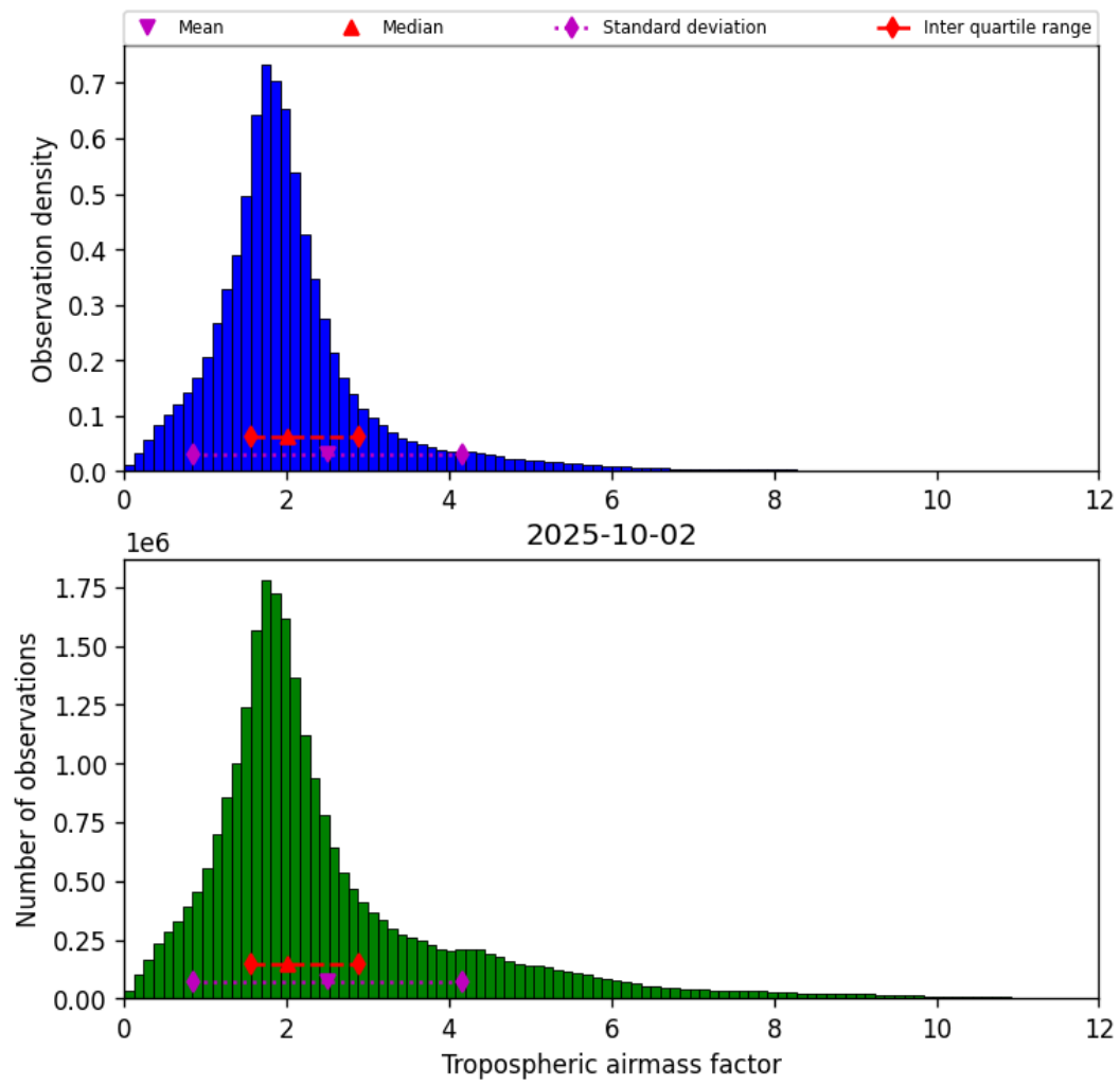
Figure 31: Histogram of “Tropospheric airmass factor” for 2025-10-01 to 2025-10-03
