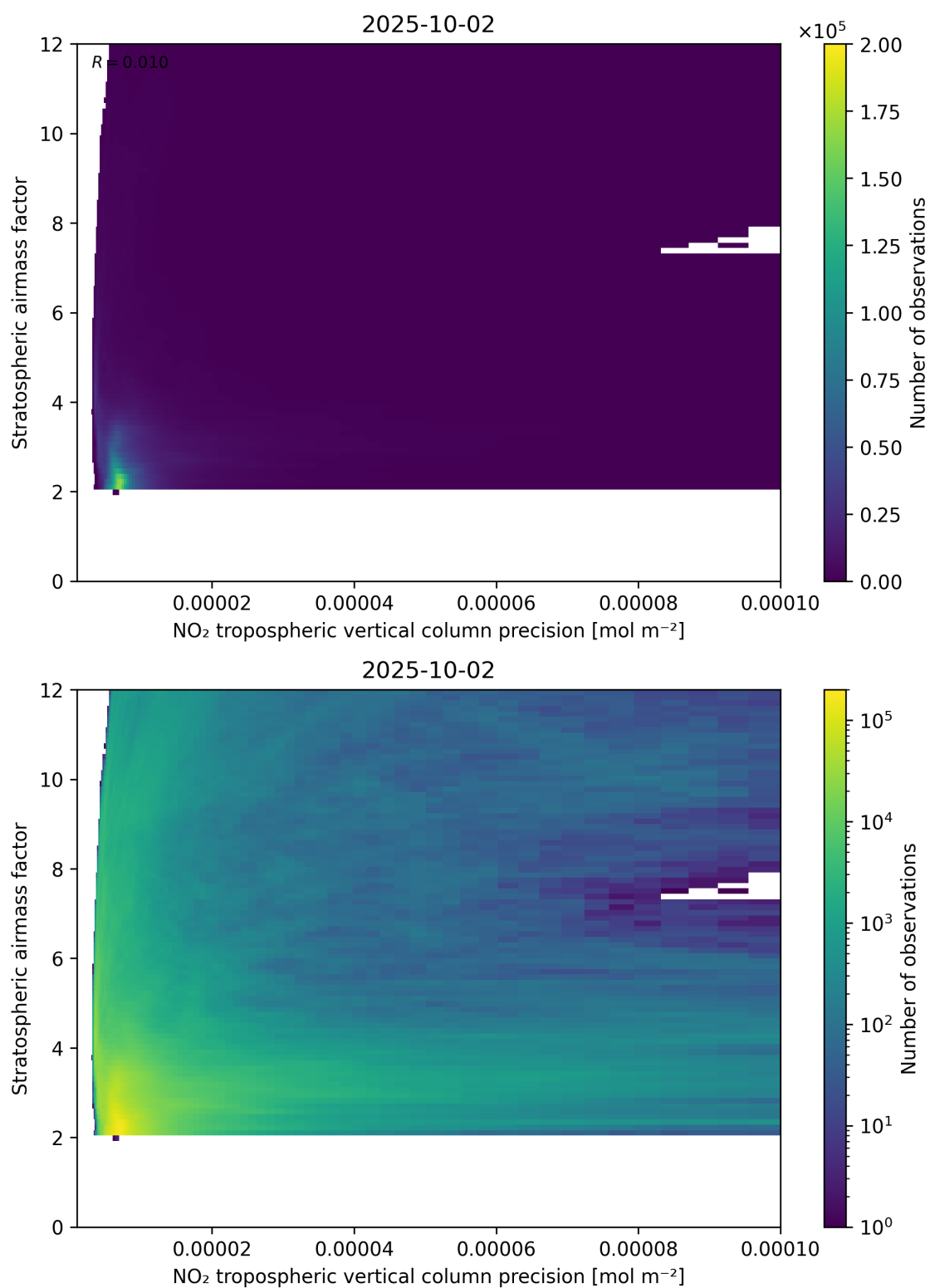
Figure 131: Scatter density plot of “NO 2 tropospheric vertical column precision” against “Stratospheric airmass factor” for 2025-10-01 to 2025-10-03.
