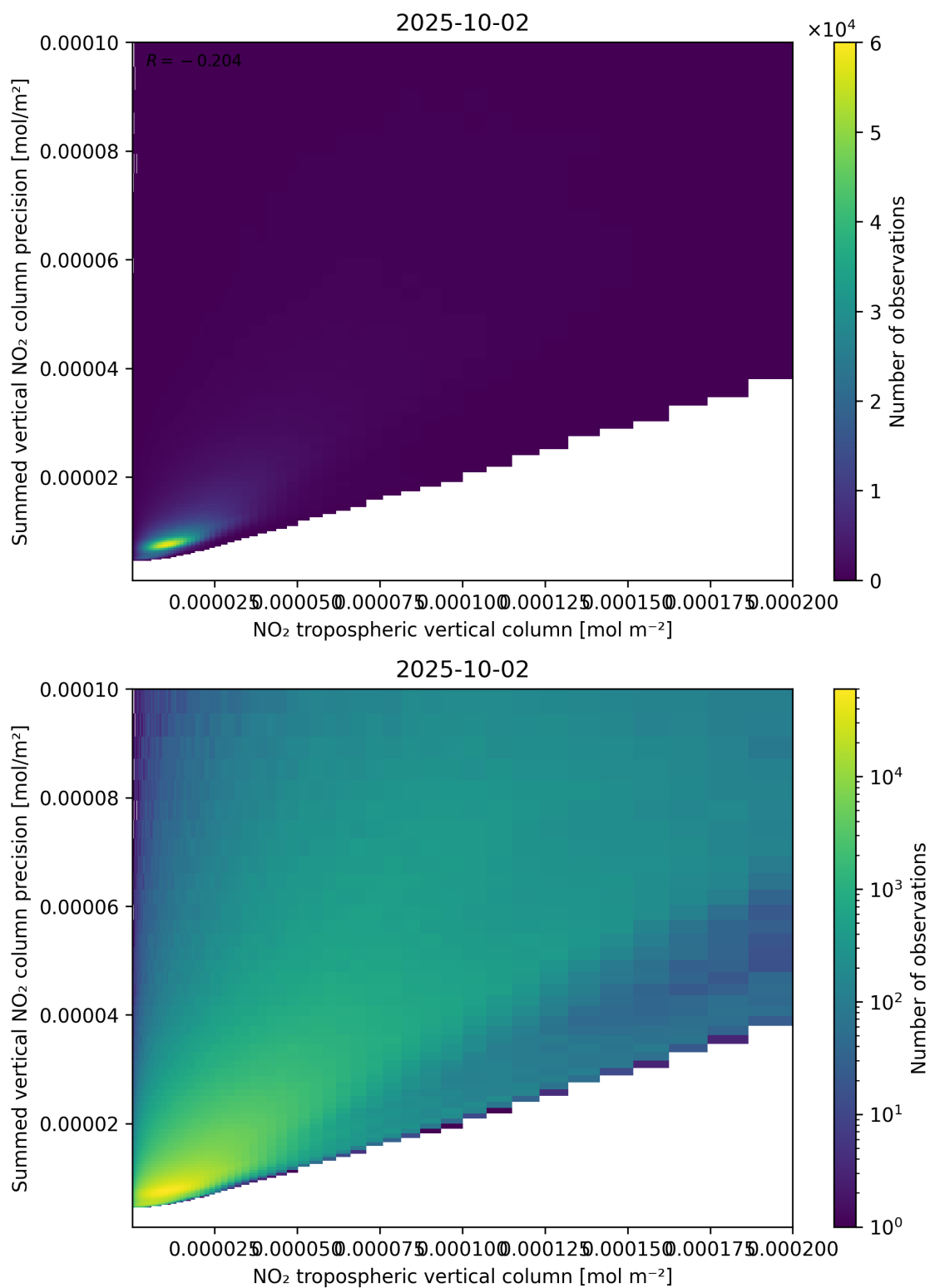
Figure 127: Scatter density plot of “NO 2 tropospheric vertical column” against “Summed vertical NO 2 column precision” for 2025-10-01 to 2025-10-03.
