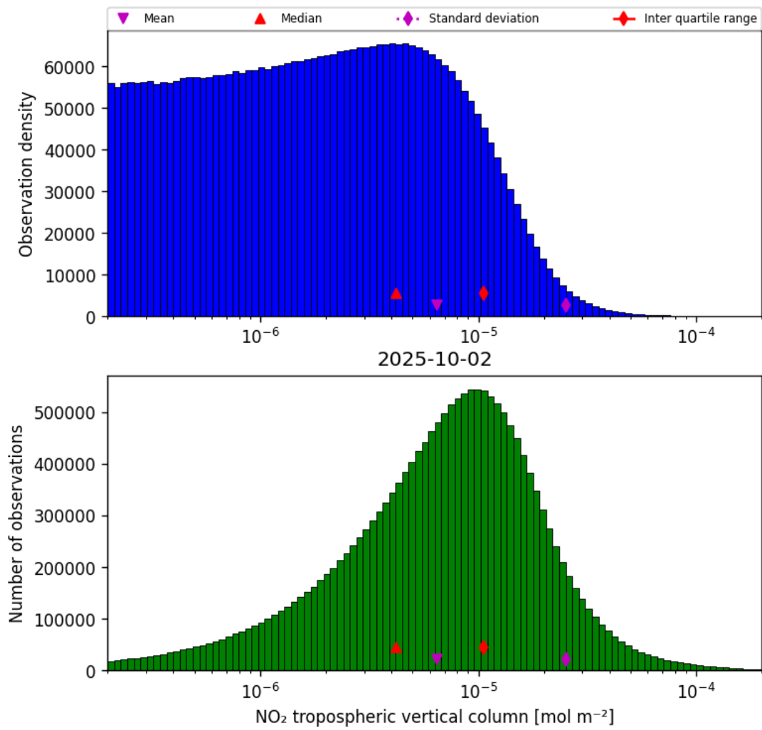
Figure 29: Histogram of “NO 2 tropospheric vertical column” for 2025-10-01 to 2025-10-03
