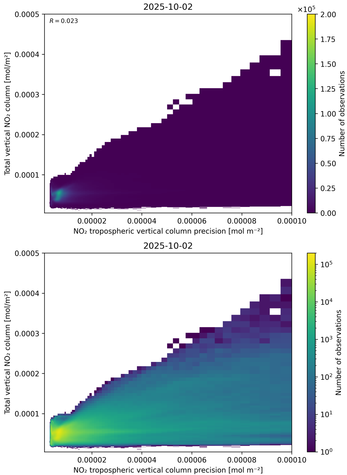
Figure 138: Scatter density plot of “NO 2 tropospheric vertical column precision” against “Total vertical NO 2 column” for 2025-10-01 to 2025-10-03.
