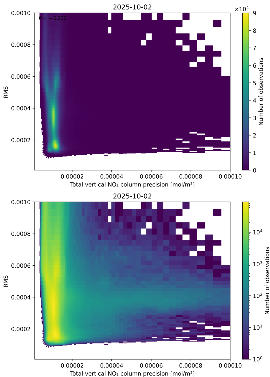
Figure 119: Scatter density plot of “Total vertical NO 2 column precision” against “RMS” for 2025-10-01 to 2025-10-03.
