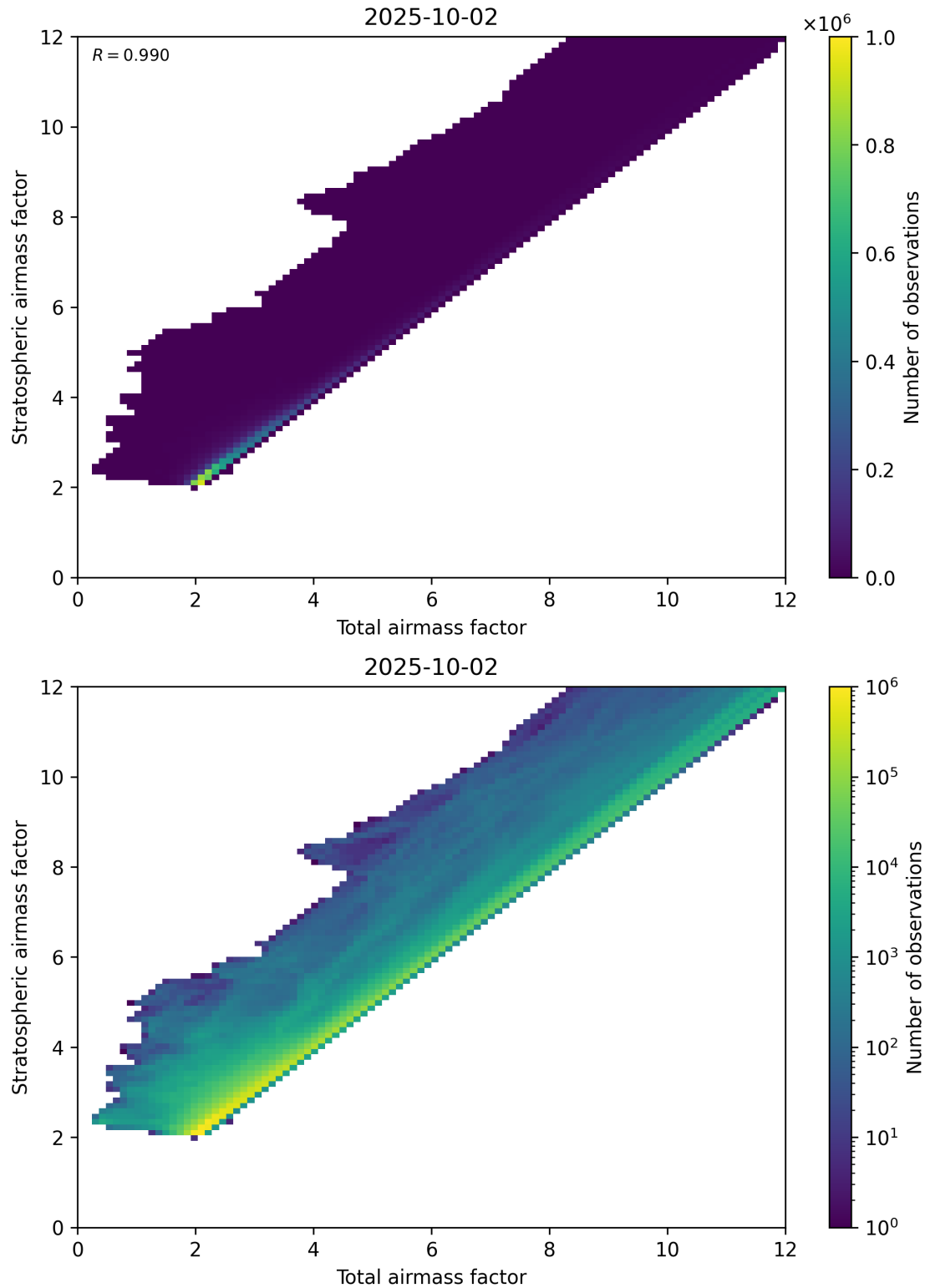
Figure 62: Scatter density plot of “Total airmass factor” against “Stratospheric airmass factor” for 2025-10-01 to 2025-10-03.
