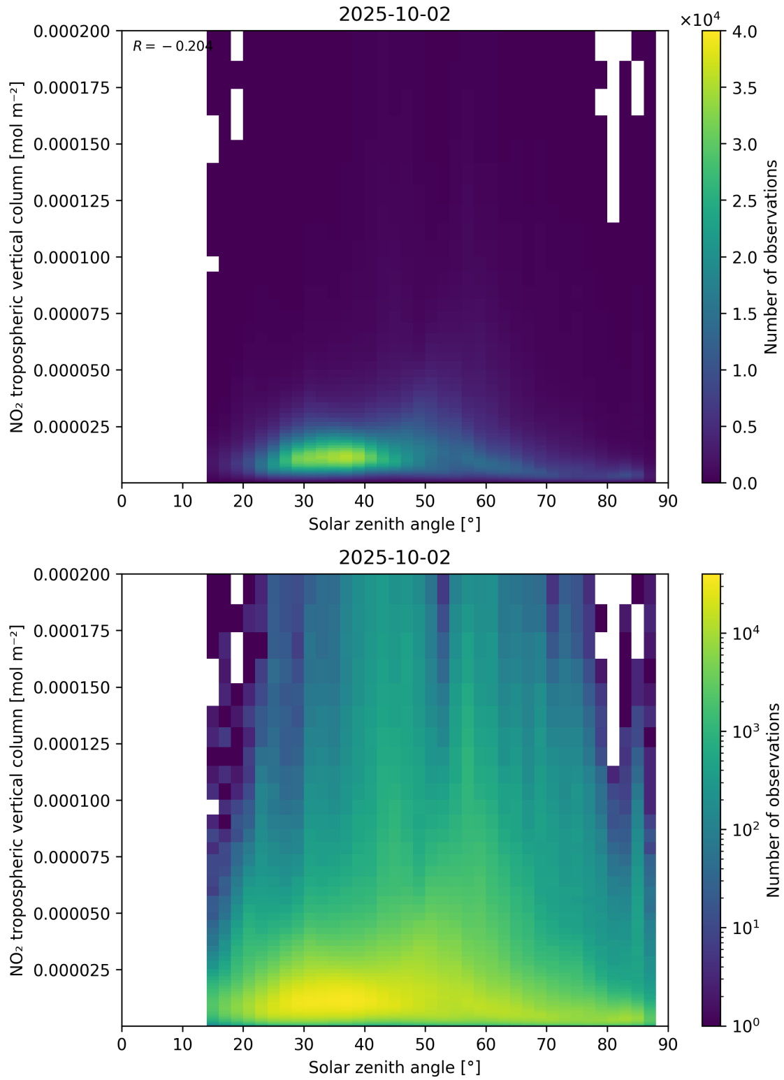
Figure 155: Scatter density plot of “Solar zenith angle” against “NO 2 tropospheric vertical column” for 2025-10-01 to 2025-10-03.
