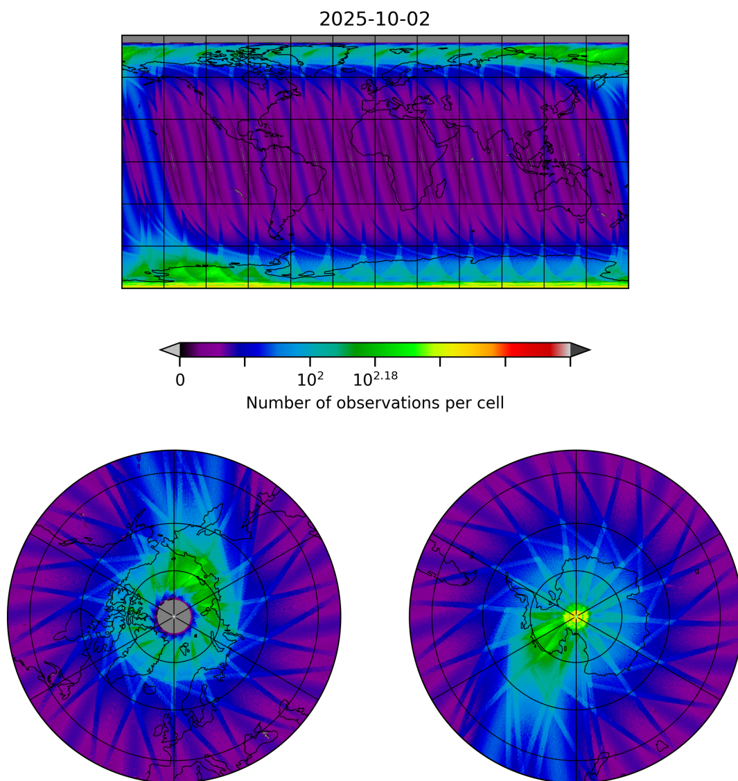
Figure 10: Map of the number of observations for 2025-10-01 to 2025-10-03
