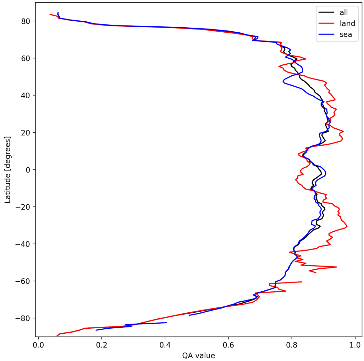
Figure 11: Zonal average of “QA value” for 2025-10-01 to 2025-10-03.
