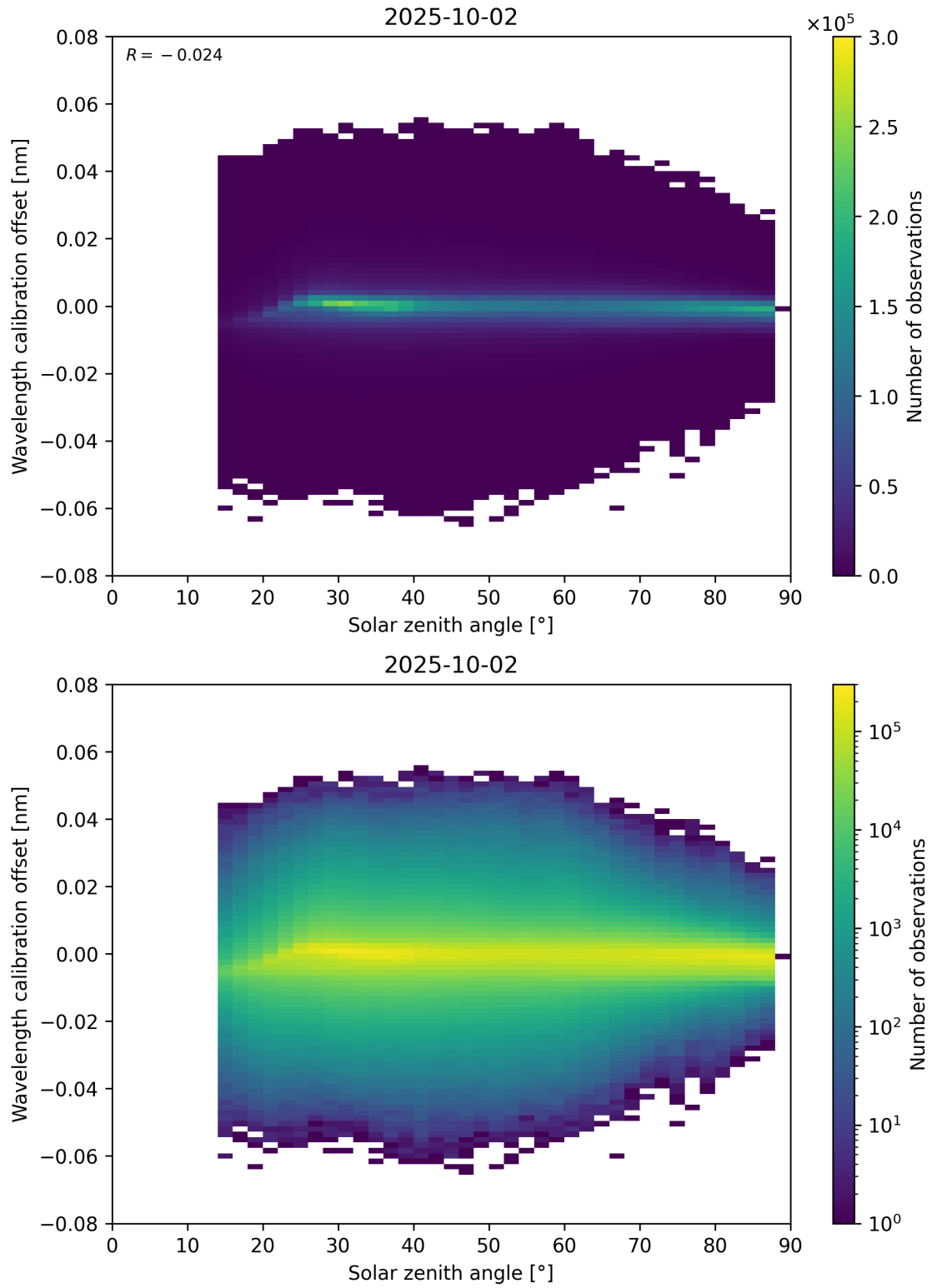
Figure 158: Scatter density plot of “Solar zenith angle” against “Wavelength calibration offset” for 2025-10-01 to 2025-10-03.
