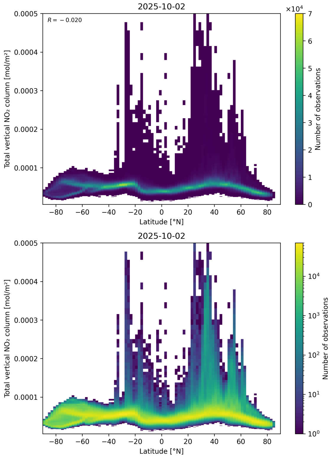
Figure 90: Scatter density plot of “Latitude” against “Total vertical NO 2 column” for 2025-10-01 to 2025-10-03.
