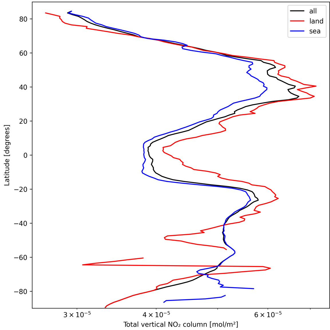
Figure 21: Zonal average of “Total vertical NO 2 column” for 2025-10-01 to 2025-10-03.
