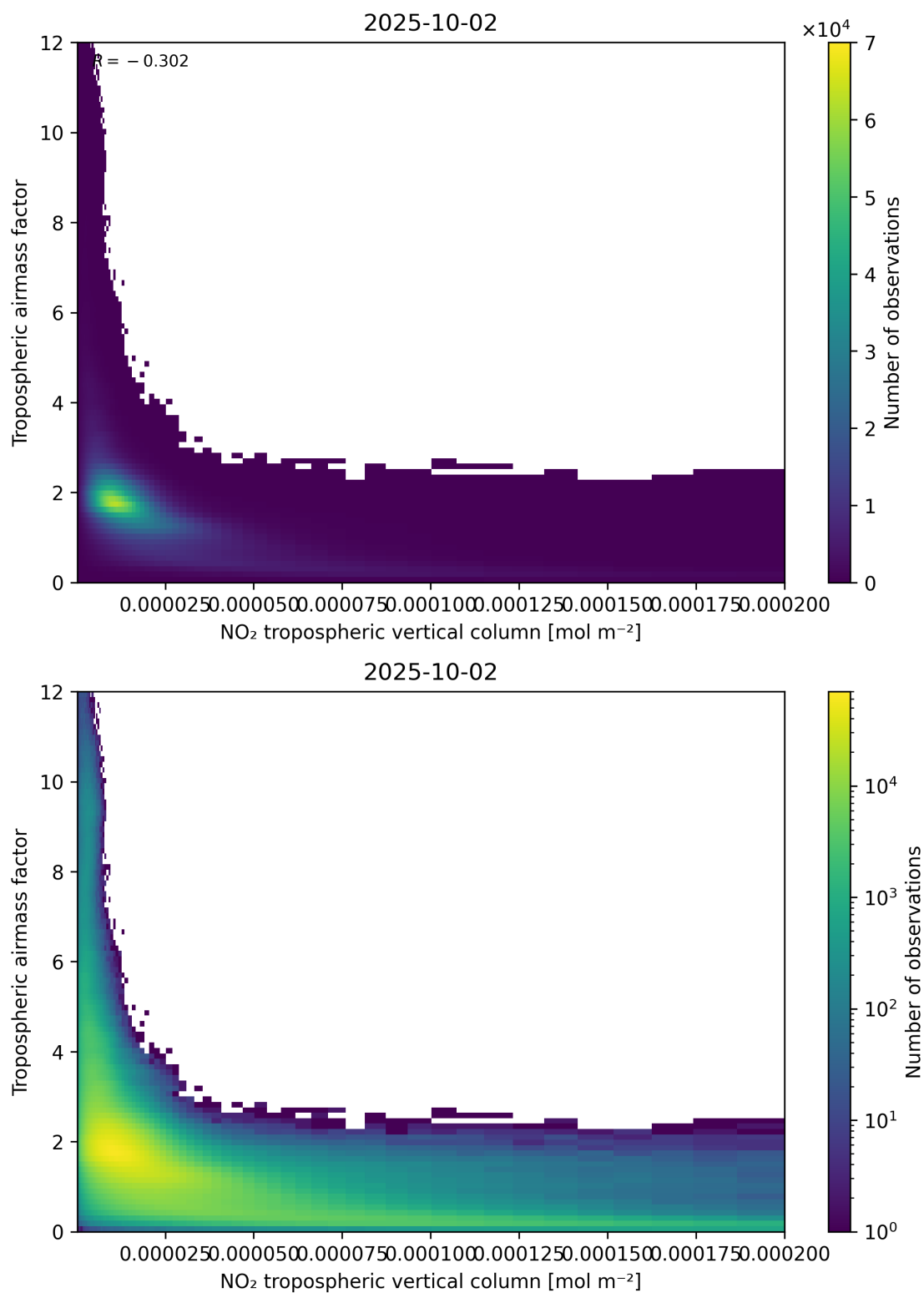
Figure 123: Scatter density plot of “NO 2 tropospheric vertical column” against “Tropospheric air mass factor” for 2025-10-01 to 2025-10-03.
