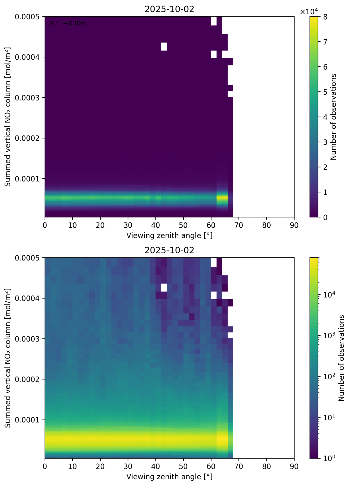
Figure 165: Scatter density plot of “Viewing zenith angle” against “Summed vertical NO 2 column” for 2025-10-01 to 2025-10-03.
