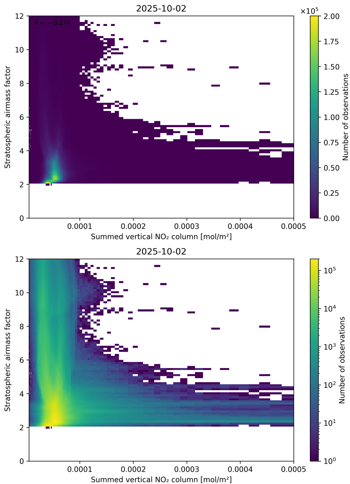
Figure 103: Scatter density plot of “Summed vertical NO 2 column” against “Stratospheric airmass factor” for 2025-10-01 to 2025-10-03.
