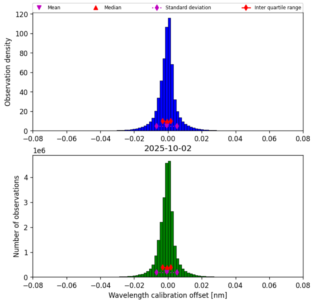
Figure 35: Histogram of “Wavelength calibration offset” for 2025-10-01 to 2025-10-03
