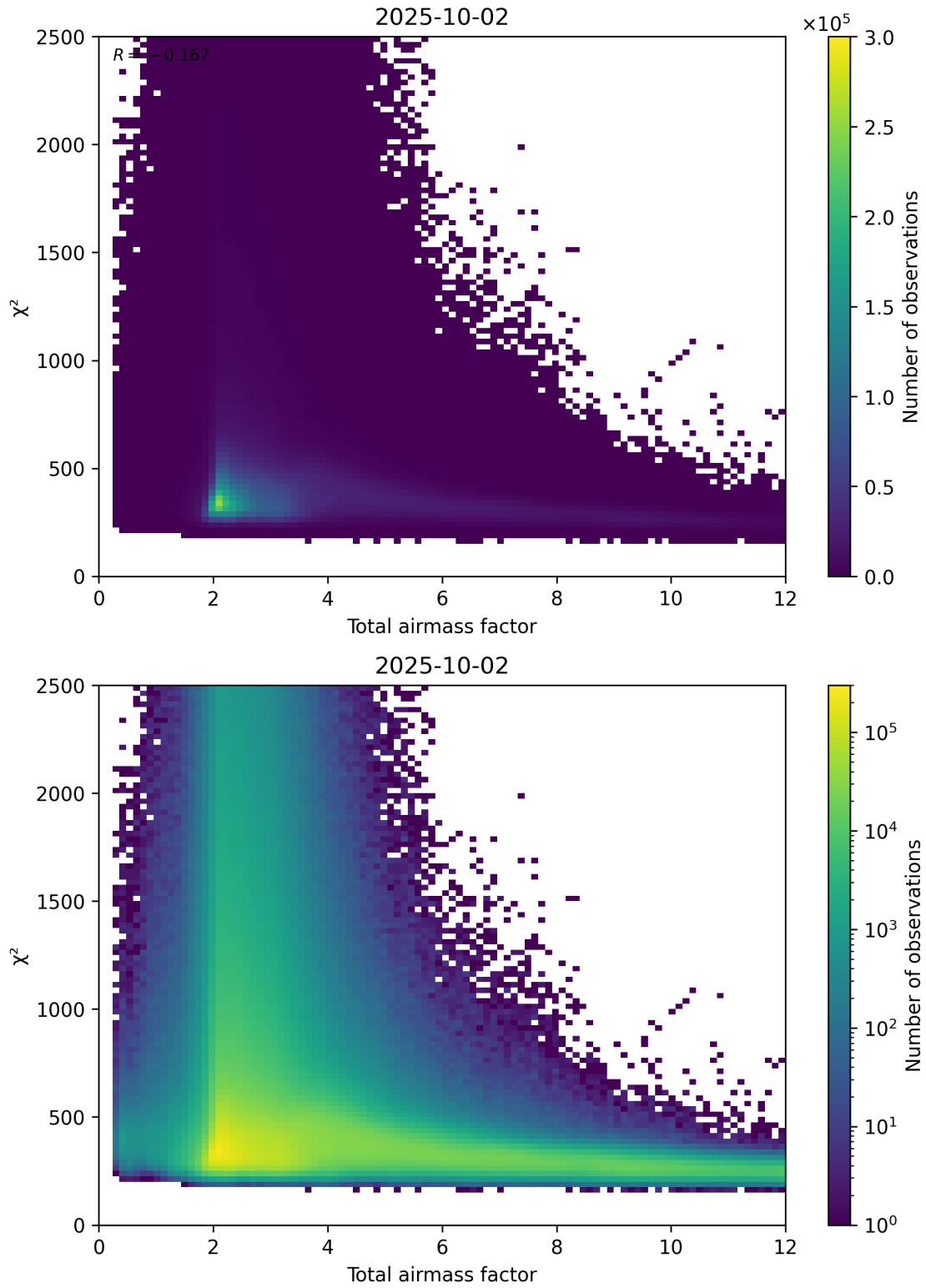
Figure 63: Scatter density plot of “Total airmass factor” against “ \chi^2 ” for 2025-10-01 to 2025-10-03.
