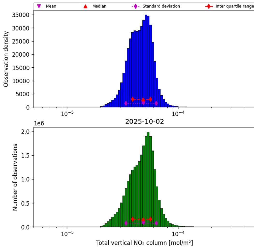
Figure 38: Histogram of “Total vertical NO 2 column” for 2025-10-01 to 2025-10-03
