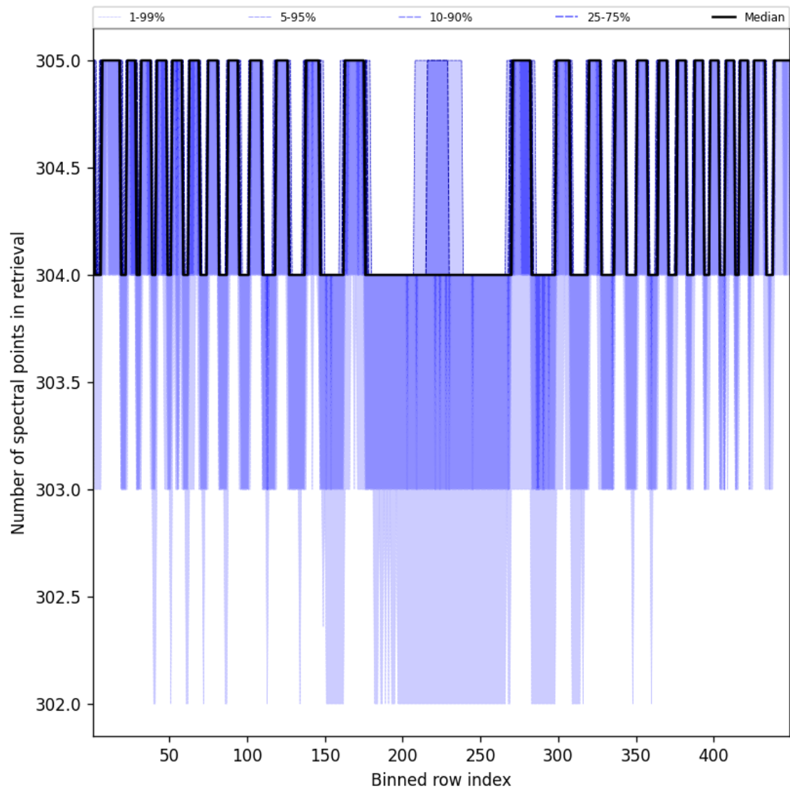
Figure 50: Along track statistics of “Number of spectral points in retrieval” for 2025-10-01 to 2025-10-03
