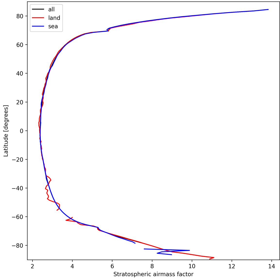
Figure 27: Zonal average of “Stratospheric air mass factor” for 2025-10-01 to 2025-10-03.
