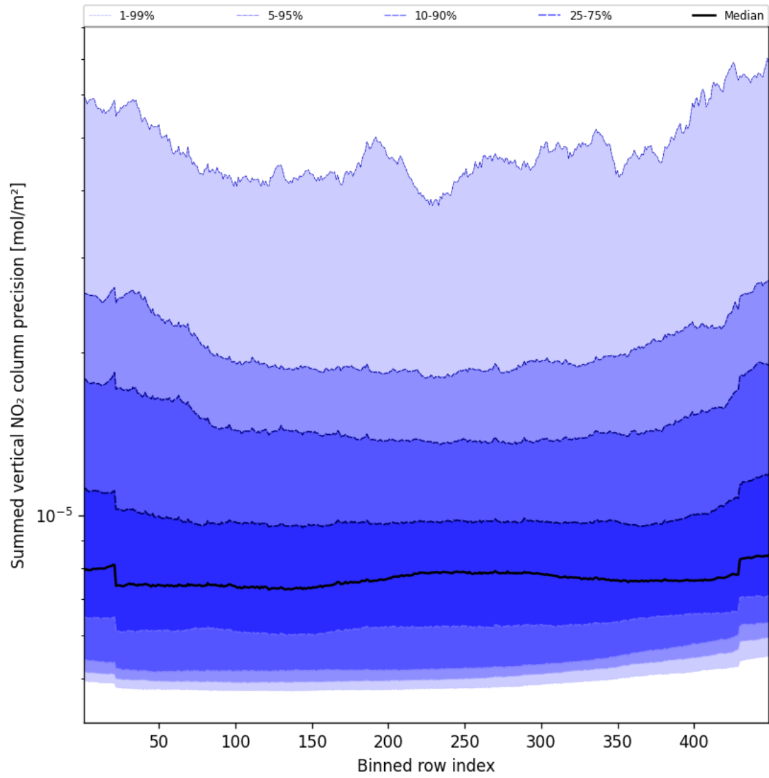
Figure 58: Along track statistics of “Summed vertical NO 2 column precision” for 2025-10-01 to 2025-10-03
