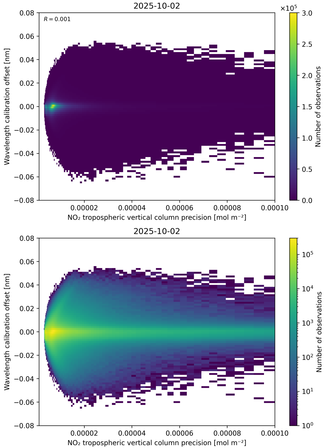
Figure 141: Scatter density plot of “NO 2 tropospheric vertical column precision” against “Wavelength calibration offset” for 2025-10-01 to 2025-10-03.
