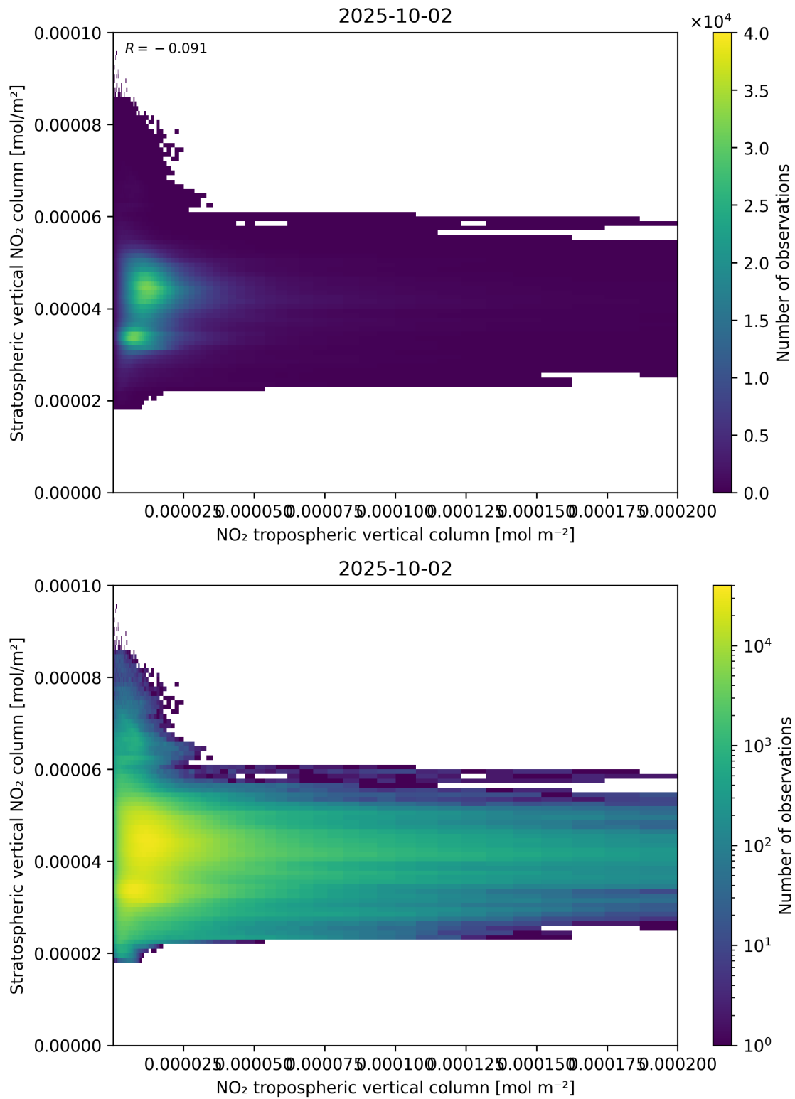
Figure 125: Scatter density plot of “NO 2 tropospheric vertical column” against “Stratospheric vertical NO 2 column” for 2025-10-01 to 2025-10-03.
