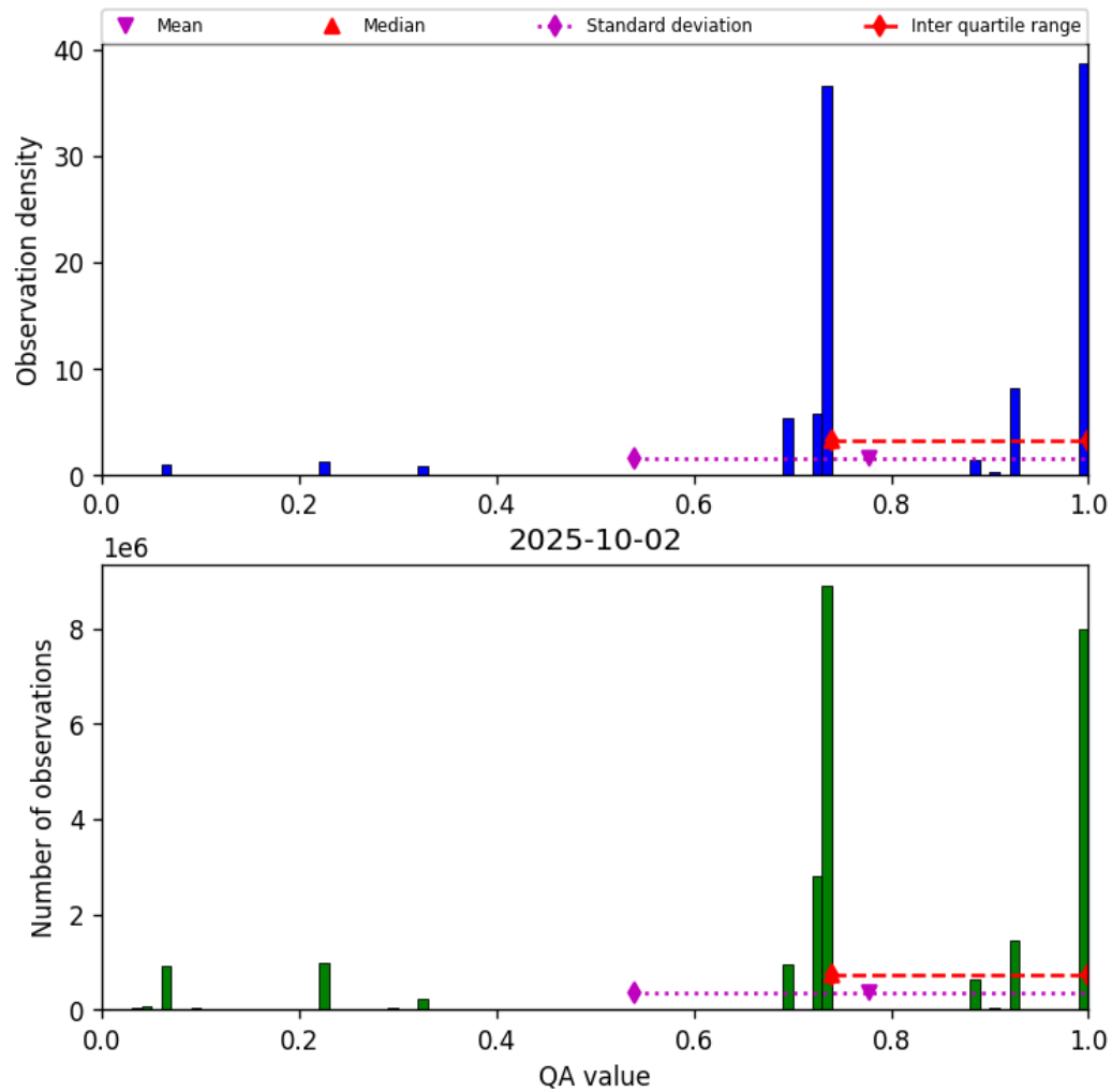
Figure 28: Histogram of “QA value” for 2025-10-01 to 2025-10-03
