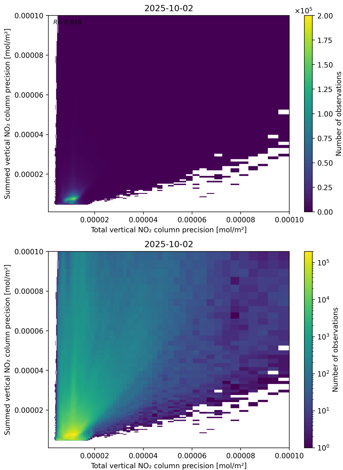
Figure 118: Scatter density plot of “Total vertical NO 2 column precision” against “Summed vertical NO 2 column precision” for 2025-10-01 to 2025-10-03.
