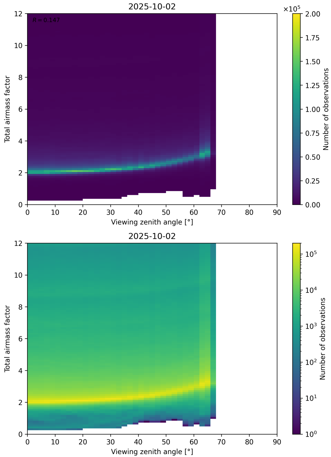
Figure 160: Scatter density plot of “Viewing zenith angle” against “Total airmass factor” for 2025-10-01 to 2025-10-03.
