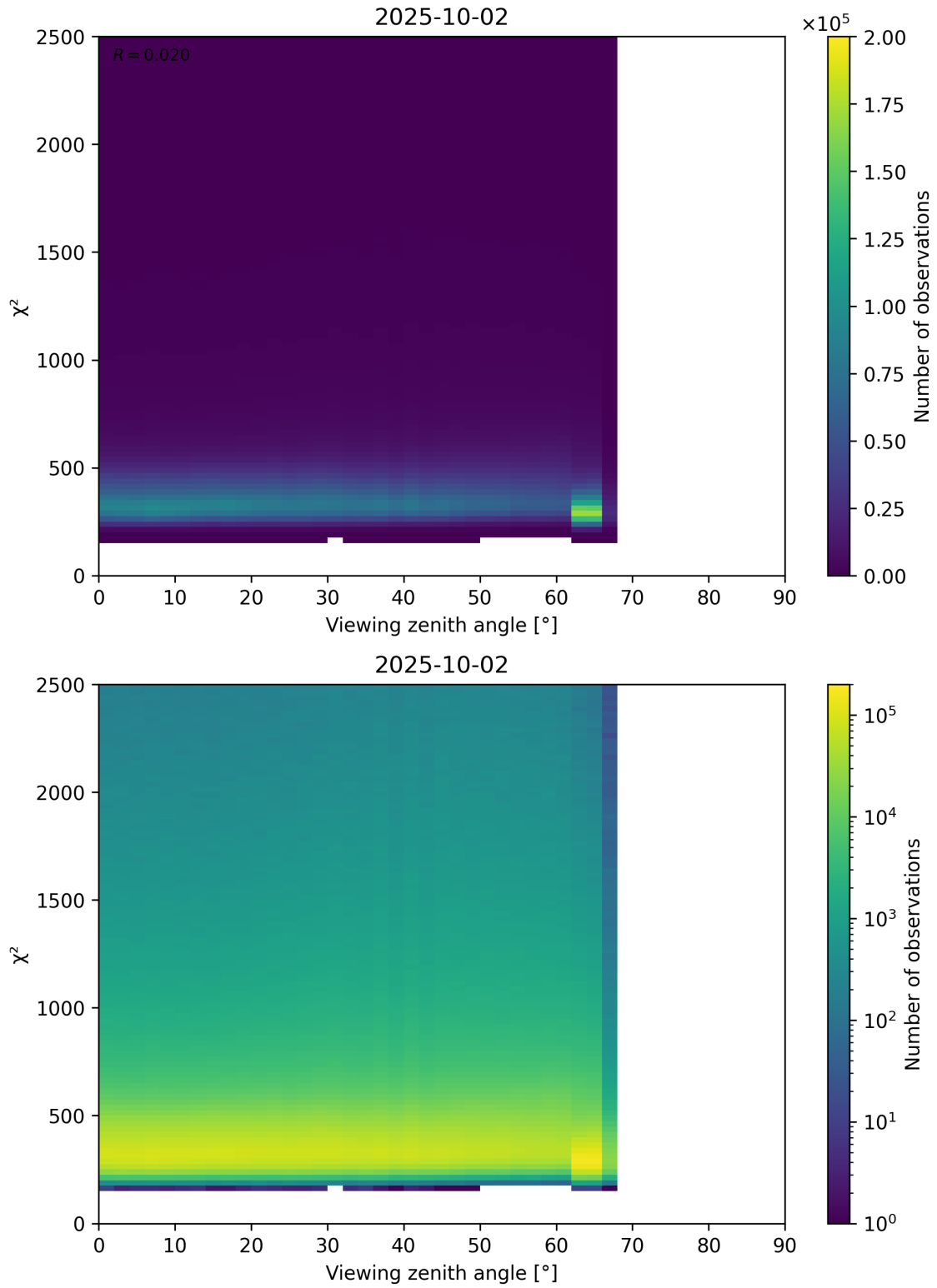
Figure 162: Scatter density plot of “Viewing zenith angle” against “ \chi^2 ” for 2025-10-01 to 2025-10-03.
