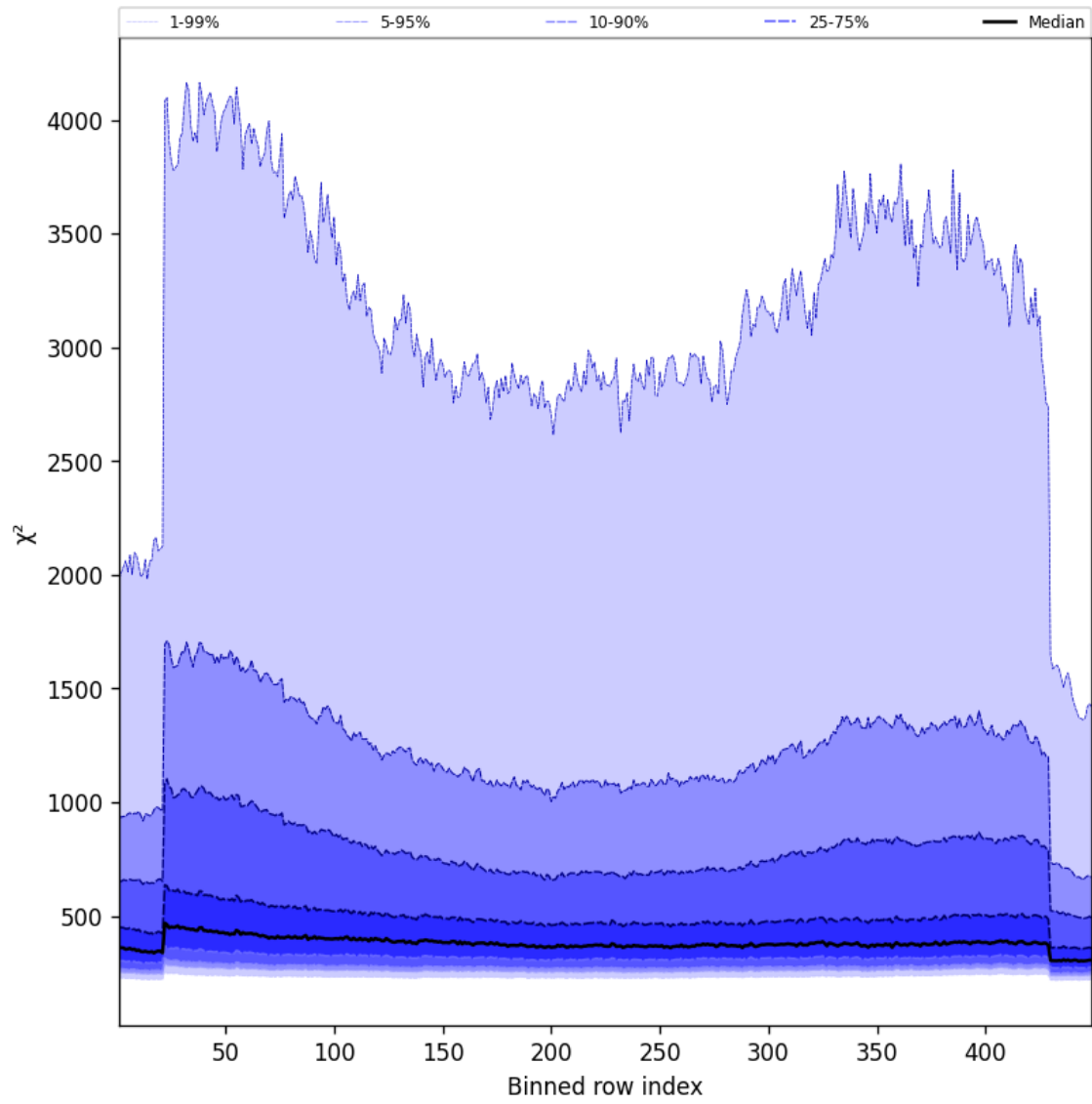
Figure 59: Along track statistics of “ \chi^2 ” for 2025-10-01 to 2025-10-03
