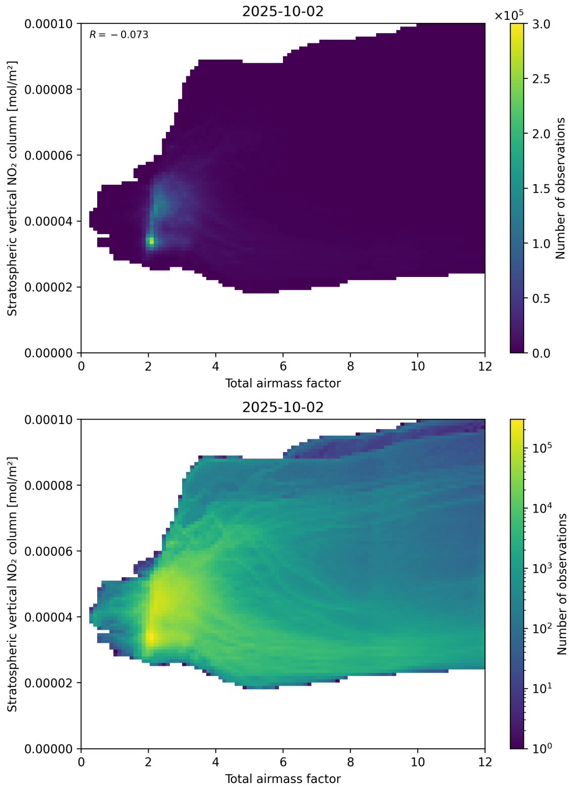
Figure 64: Scatter density plot of “Total airmass factor” against “Stratospheric vertical \text{NO}_2 column” for 2025-10-01 to 2025-10-03.
