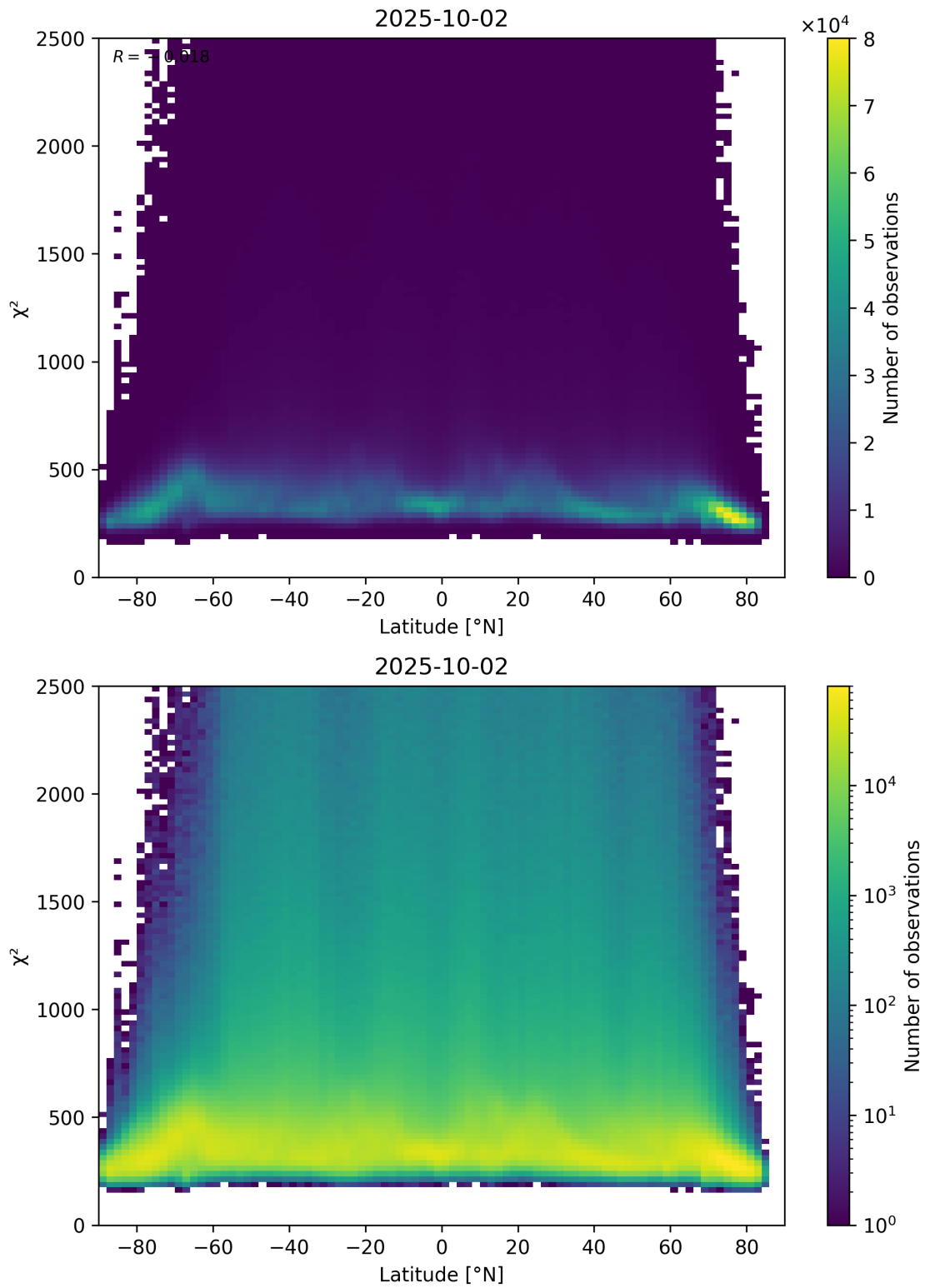
Figure 86: Scatter density plot of “Latitude” against “ \chi^2 ” for 2025-10-01 to 2025-10-03.
