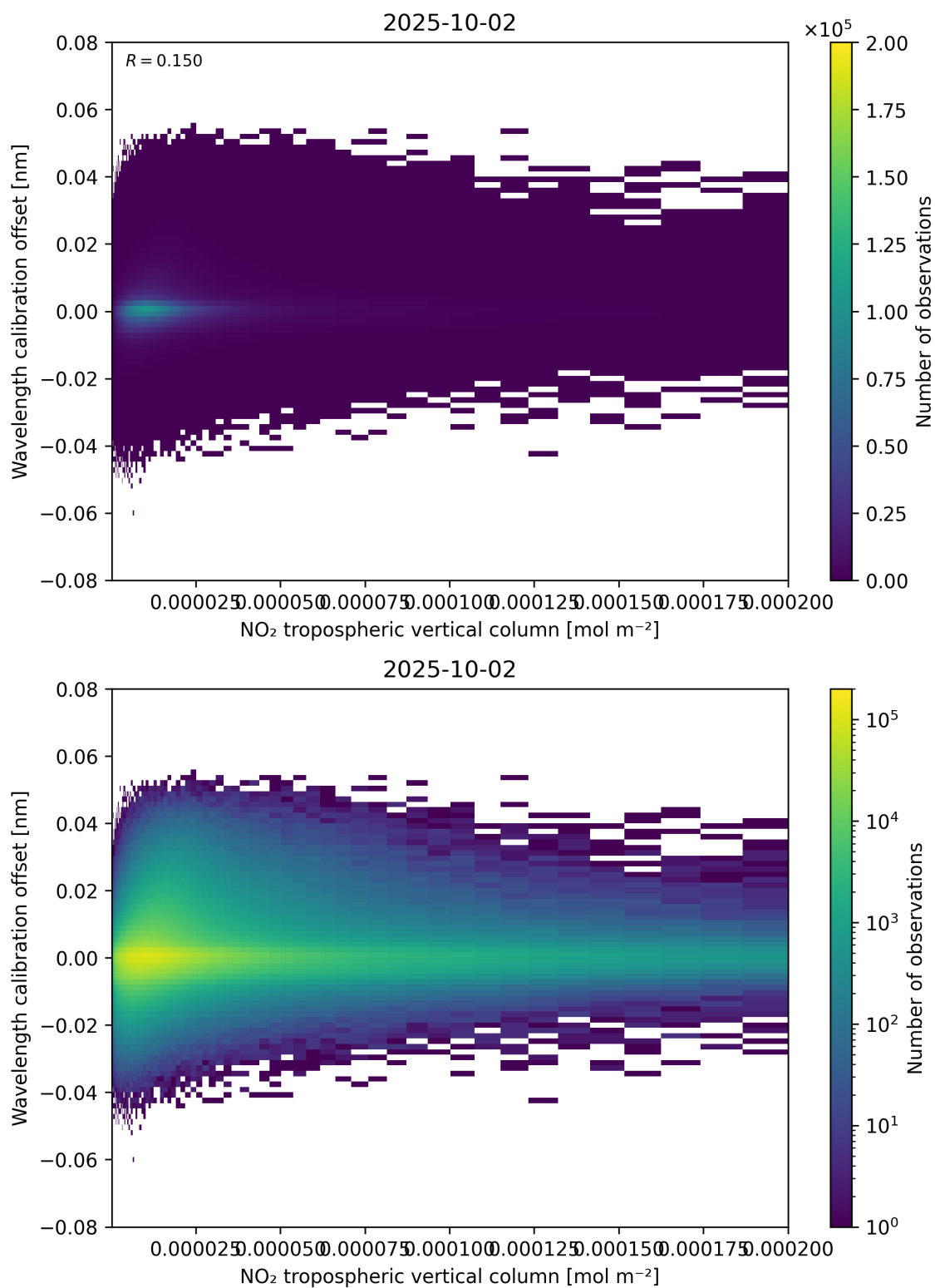
Figure 143: Scatter density plot of “NO 2 tropospheric vertical column” against “Wavelength calibration offset” for 2025-10-01 to 2025-10-03.
