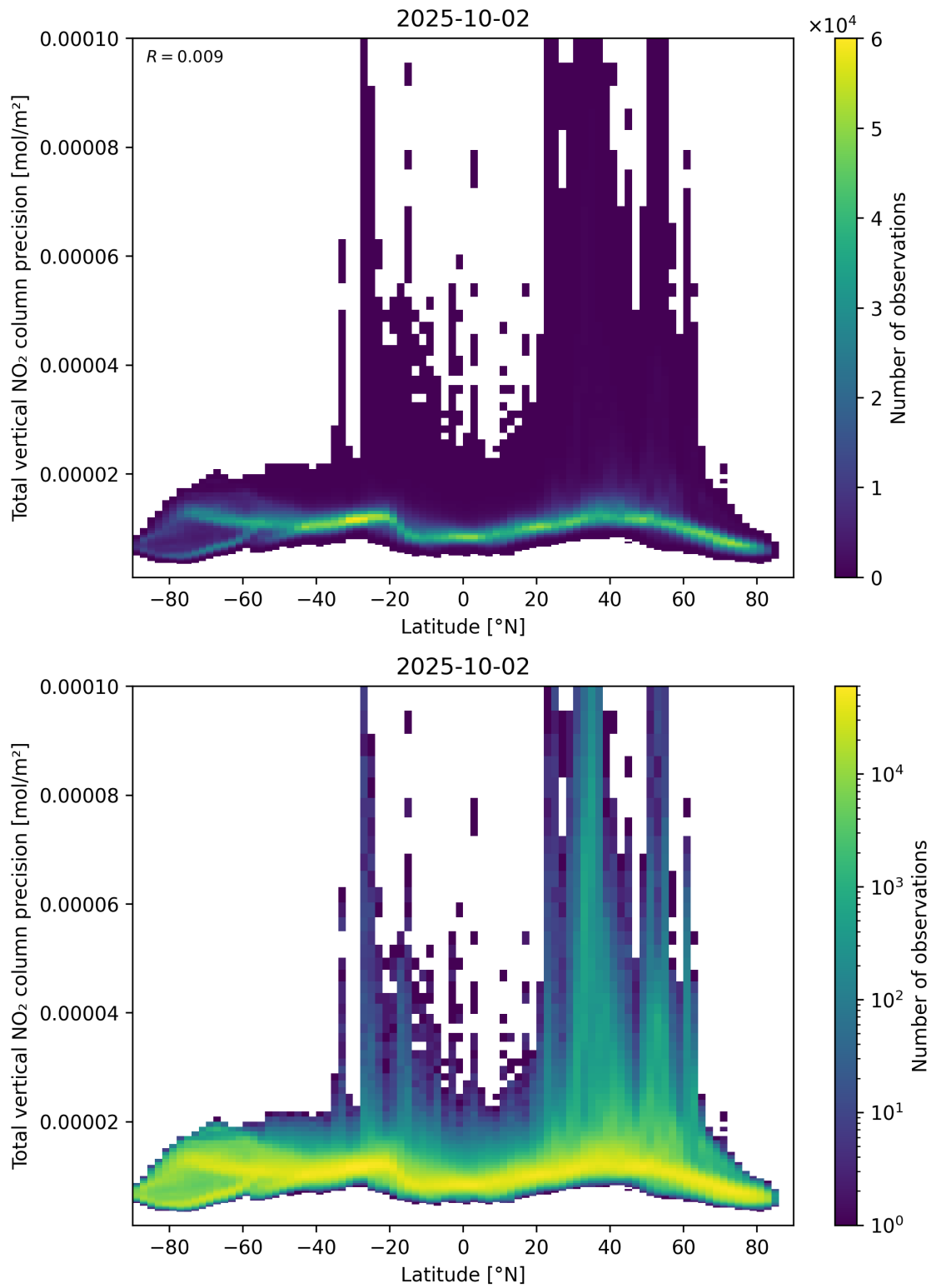
Figure 91: Scatter density plot of “Latitude” against “Total vertical NO 2 column precision” for 2025-10-01 to 2025-10-03.
