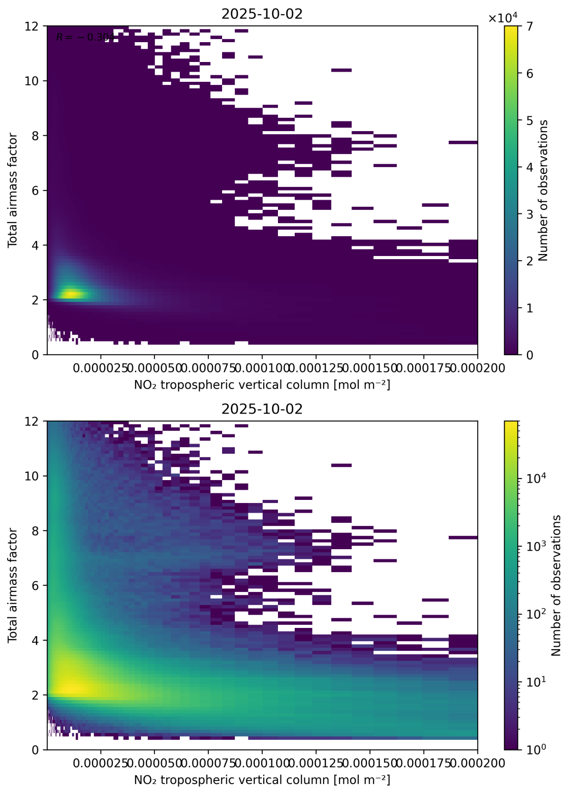
Figure 122: Scatter density plot of “NO 2 tropospheric vertical column” against “Total air mass factor” for 2025-10-01 to 2025-10-03.
