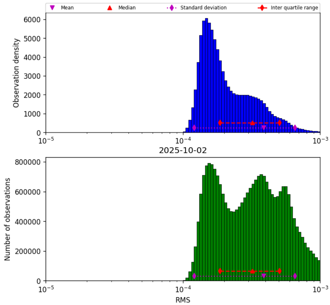
Figure 43: Histogram of “RMS” for 2025-10-01 to 2025-10-03
