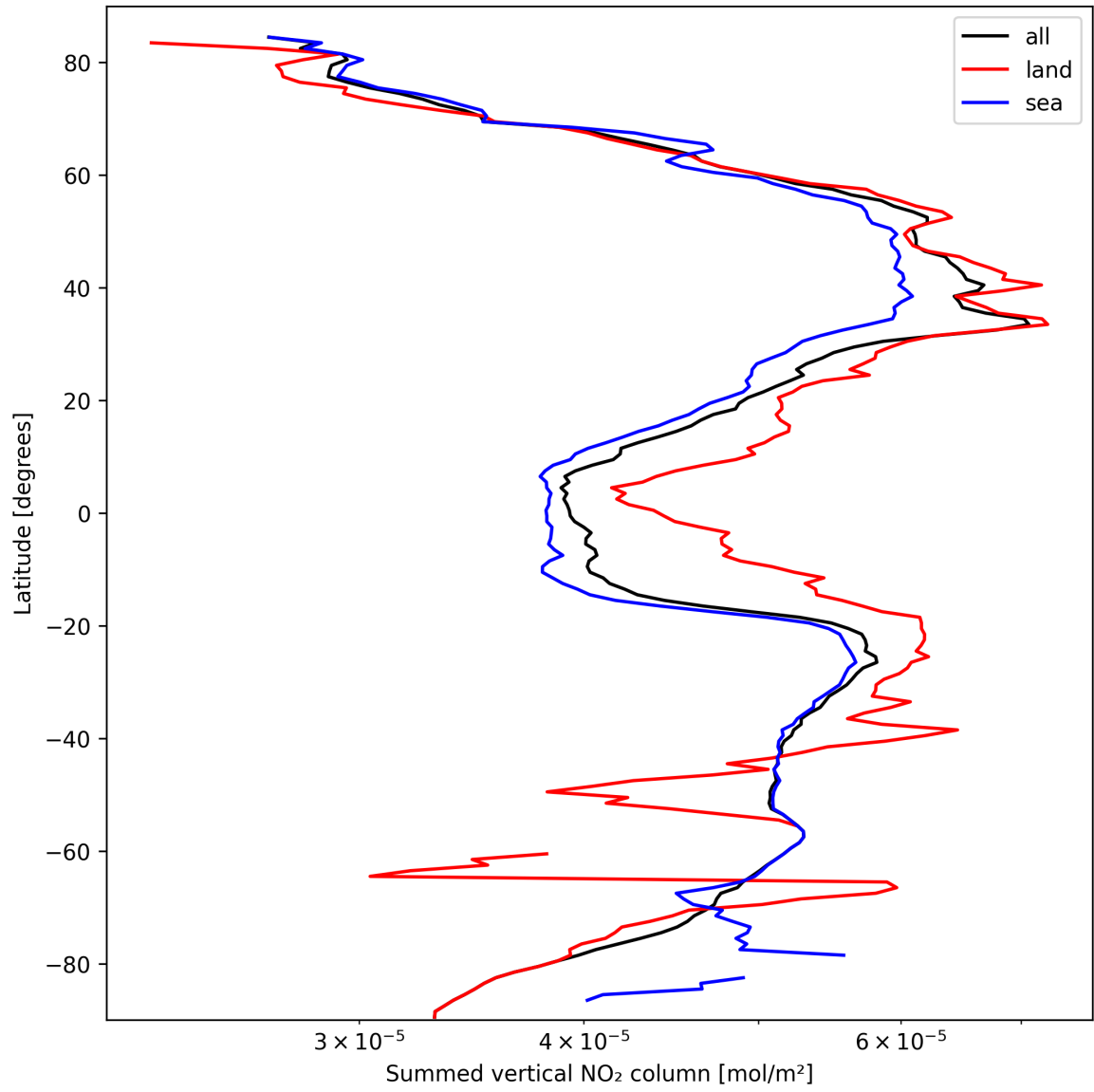
Figure 23: Zonal average of “Summed vertical NO 2 column” for 2025-10-01 to 2025-10-03.
