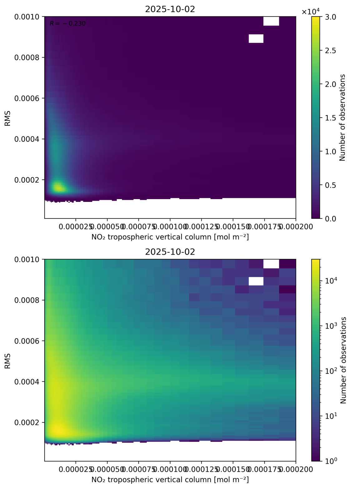
Figure 142: Scatter density plot of “NO 2 tropospheric vertical column” against “RMS” for 2025-10-01 to 2025-10-03.
