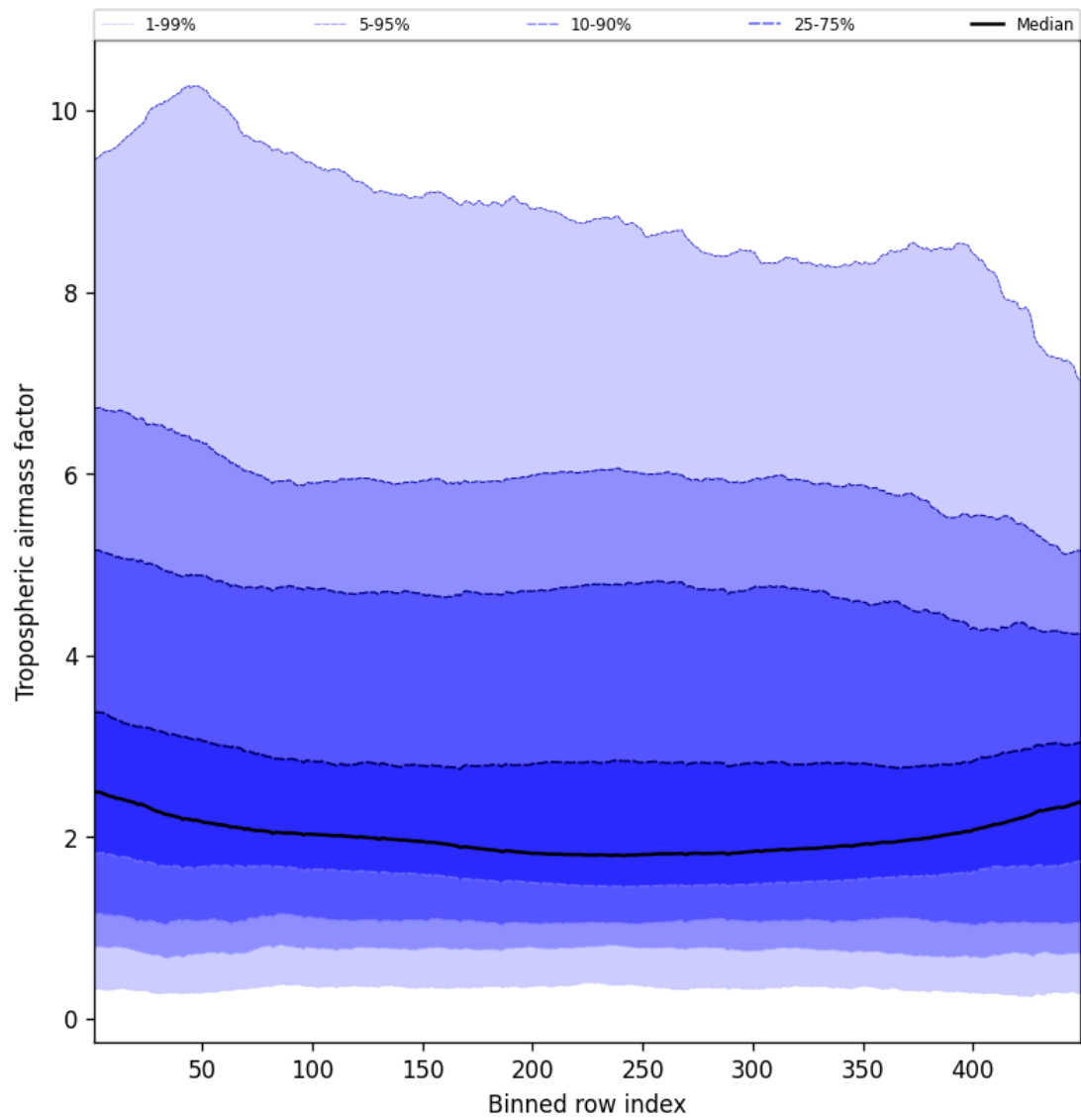
Figure 48: Along track statistics of “Tropospheric air mass factor” for 2025-10-01 to 2025-10-03
