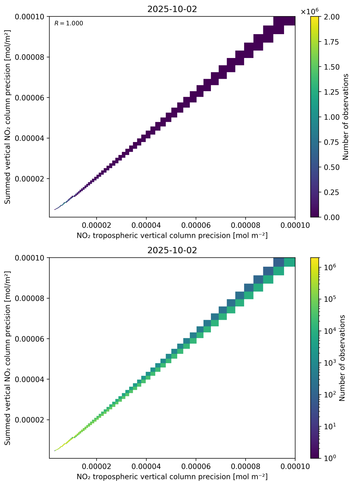
Figure 137: Scatter density plot of “NO 2 tropospheric vertical column precision” against “Summed vertical NO 2 column precision” for 2025-10-01 to 2025-10-03.
