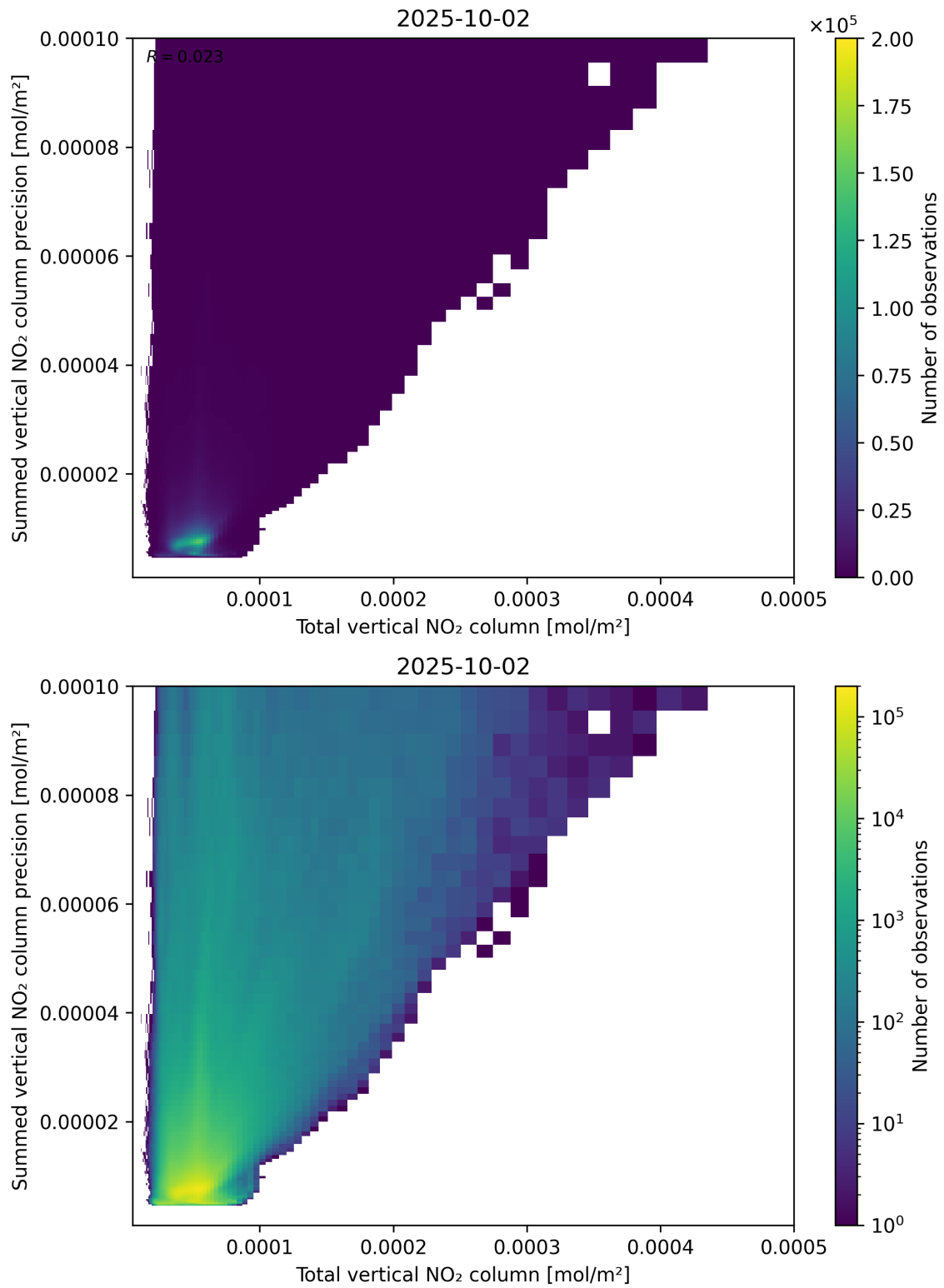
Figure 113: Scatter density plot of “Total vertical NO 2 column” against “Summed vertical NO 2 column precision” for 2025-10-01 to 2025-10-03.
