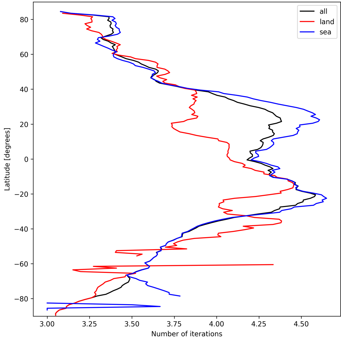
Figure 17: Zonal average of “Number of iterations” for 2025-10-01 to 2025-10-03.
