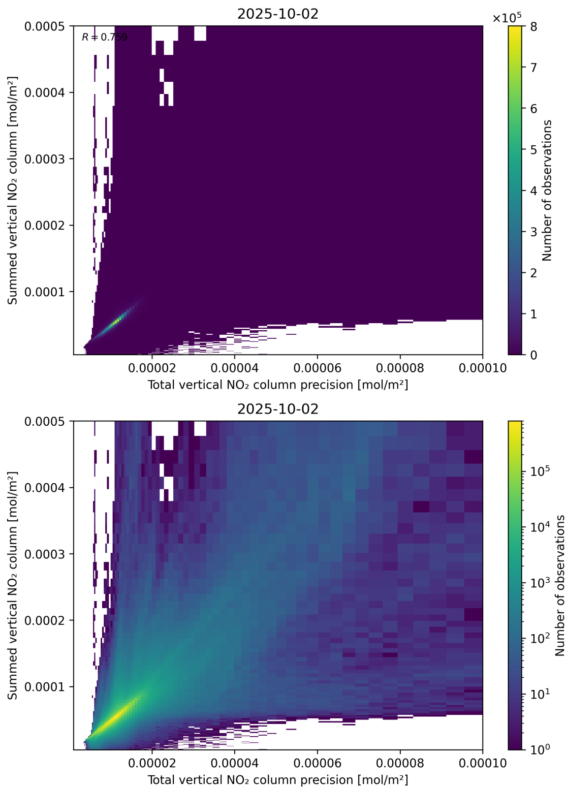
Figure 117: Scatter density plot of “Total vertical NO 2 column precision” against “Summed vertical NO 2 column” for 2025-10-01 to 2025-10-03.
