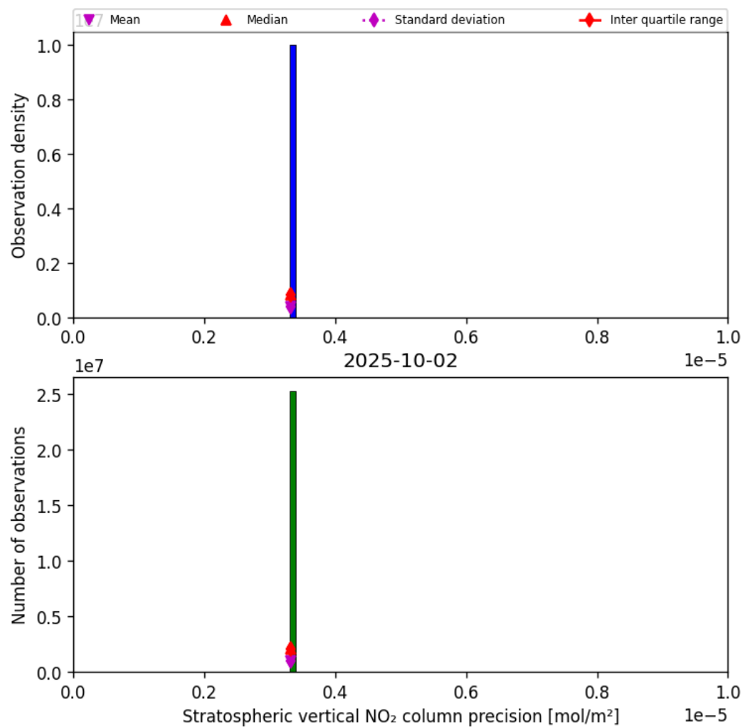
Figure 37: Histogram of “Stratospheric vertical NO 2 column precision” for 2025-10-01 to 2025-10-03
