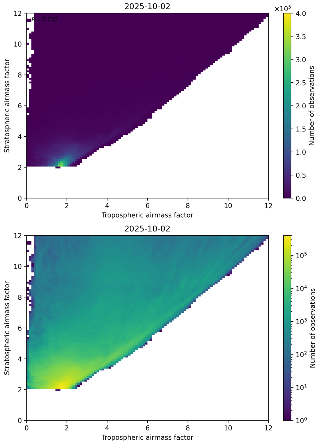
Figure 71: Scatter density plot of “Tropospheric airmass factor” against “Stratospheric airmass factor” for 2025-10-01 to 2025-10-03.
