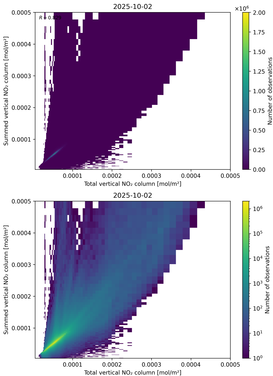
Figure 112: Scatter density plot of “Total vertical NO 2 column” against “Summed vertical NO 2 column” for 2025-10-01 to 2025-10-03.
