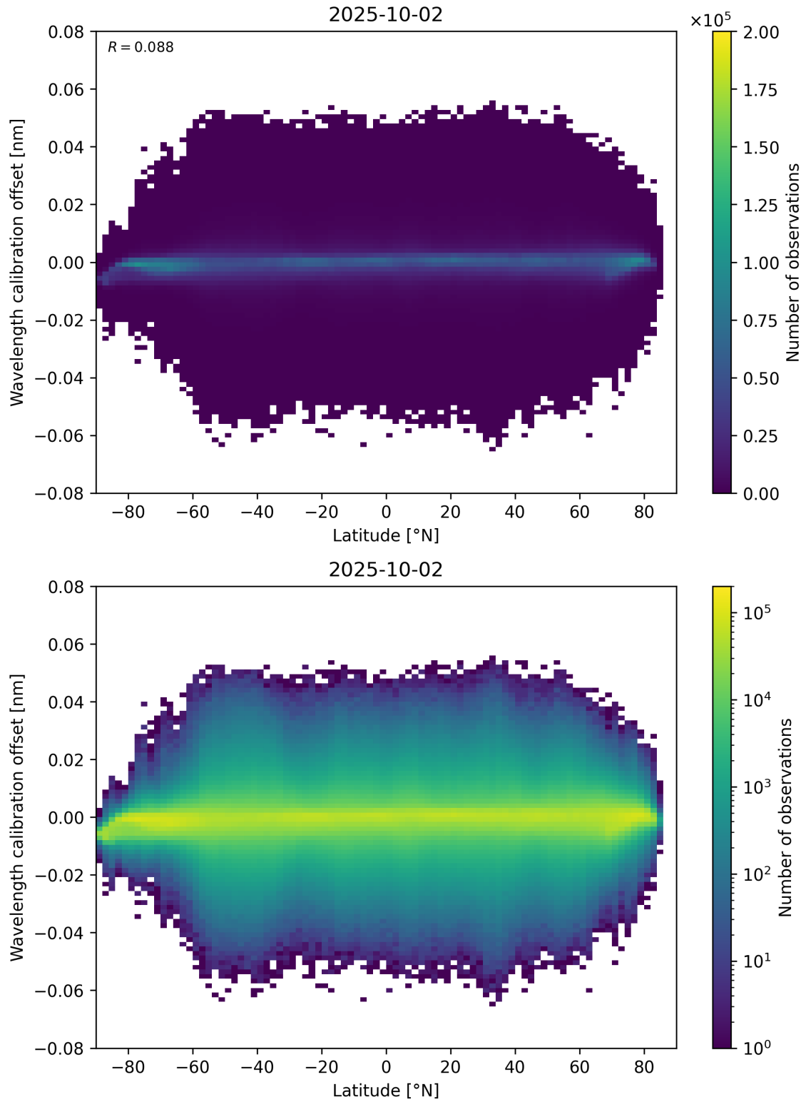
Figure 95: Scatter density plot of “Latitude” against “Wavelength calibration offset” for 2025-10-01 to 2025-10-03.
