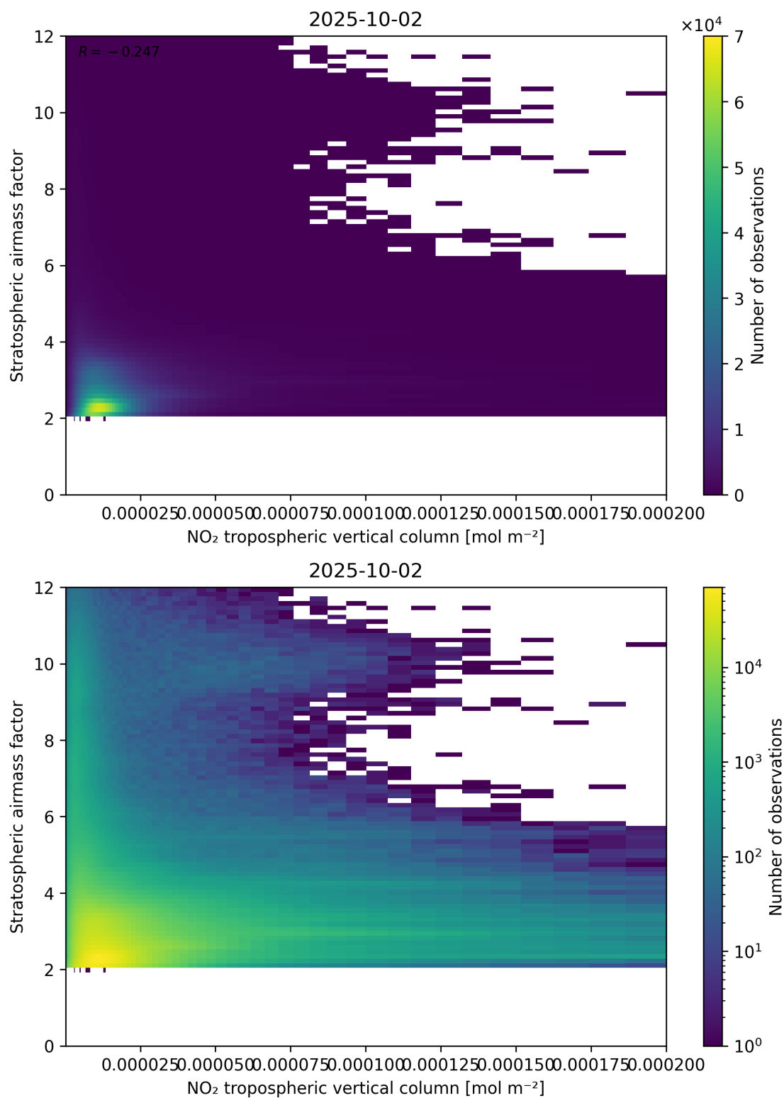
Figure 121: Scatter density plot of “NO 2 tropospheric vertical column” against “Stratospheric air mass factor” for 2025-10-01 to 2025-10-03.
