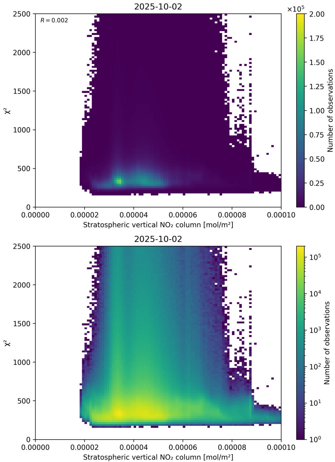
Figure 97: Scatter density plot of “Stratospheric vertical NO 2 column” against “ \chi^2 ” for 2025-10-01 to 2025-10-03.
