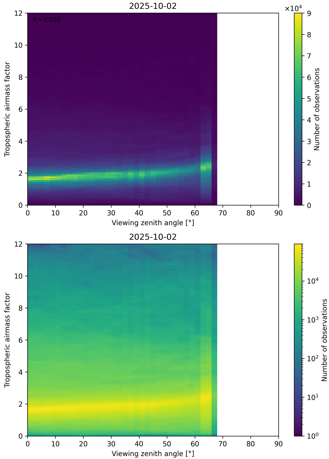
Figure 161: Scatter density plot of “Viewing zenith angle” against “Tropospheric airmass factor” for 2025-10-01 to 2025-10-03.
