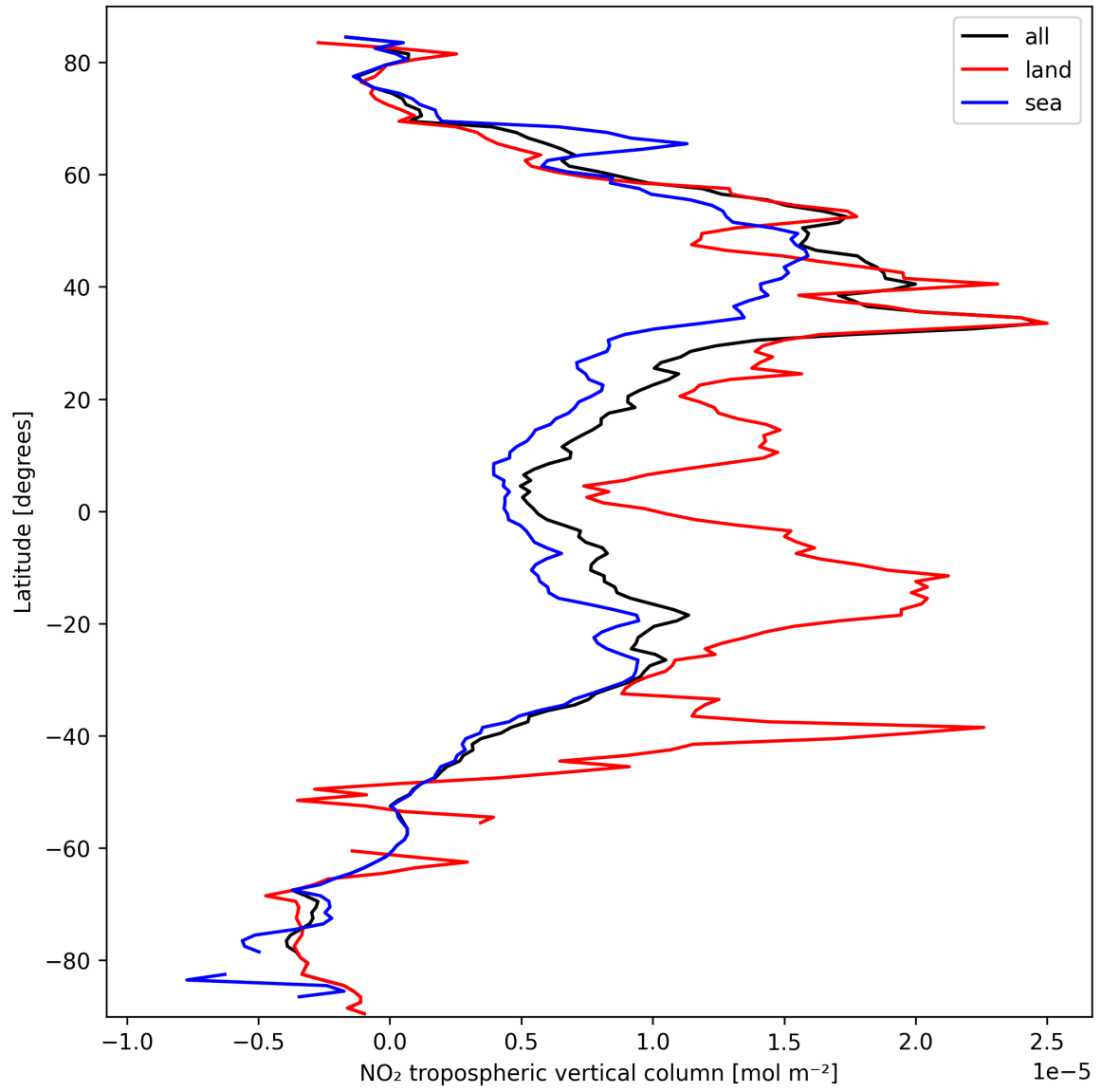
Figure 12: Zonal average of “NO 2 tropospheric vertical column” for 2025-10-01 to 2025-10-03.
