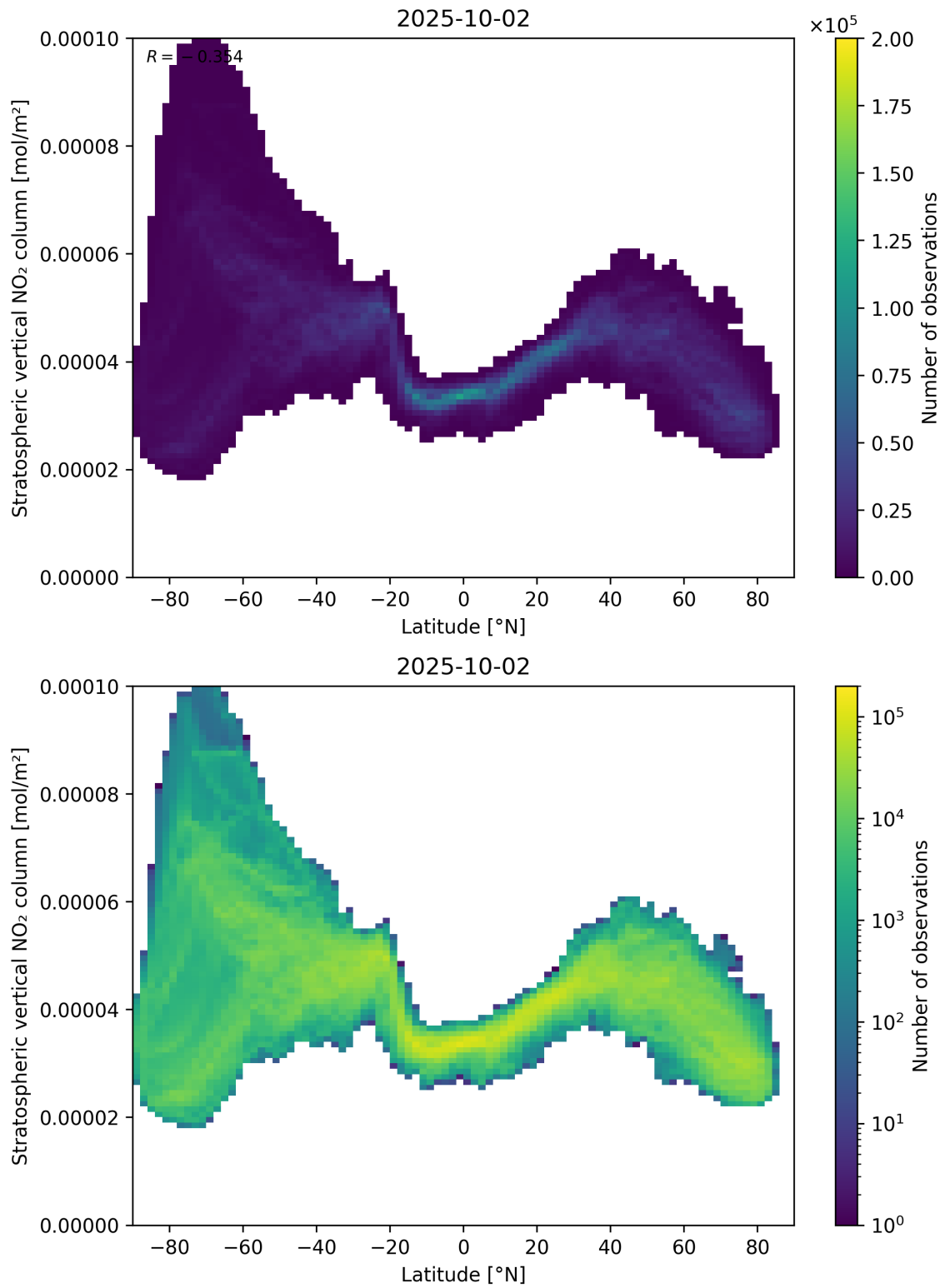
Figure 87: Scatter density plot of “Latitude” against “Stratospheric vertical NO 2 column” for 2025-10-01 to 2025-10-03.
