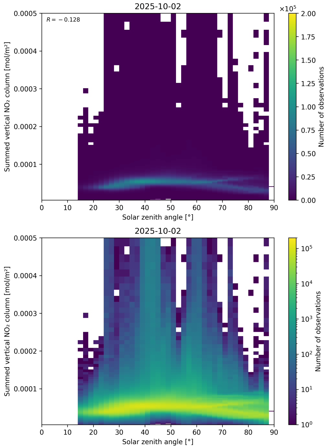
Figure 151: Scatter density plot of “Solar zenith angle” against “Summed vertical NO 2 column” for 2025-10-01 to 2025-10-03.
