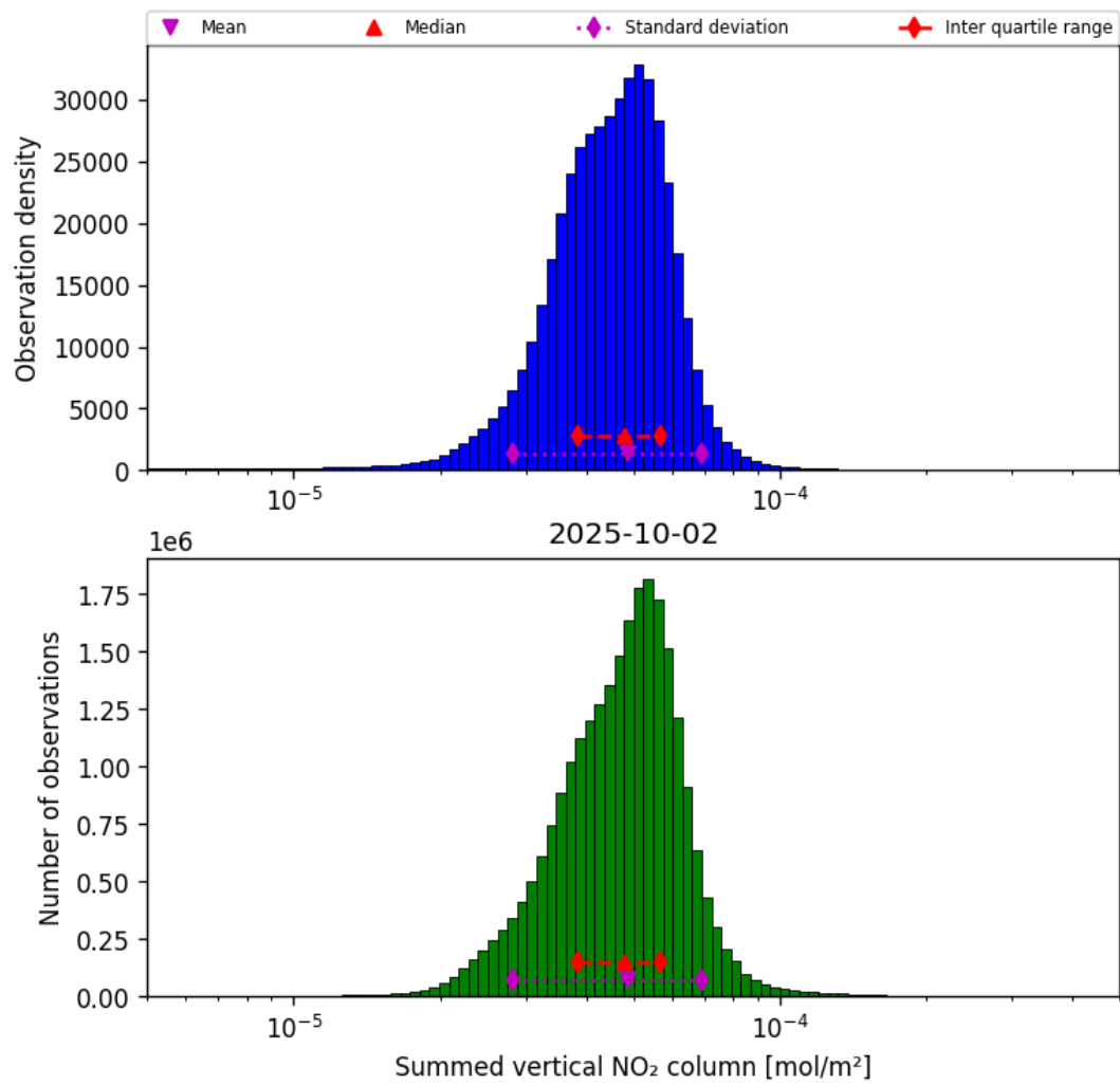
Figure 40: Histogram of “Summed vertical NO 2 column” for 2025-10-01 to 2025-10-03
