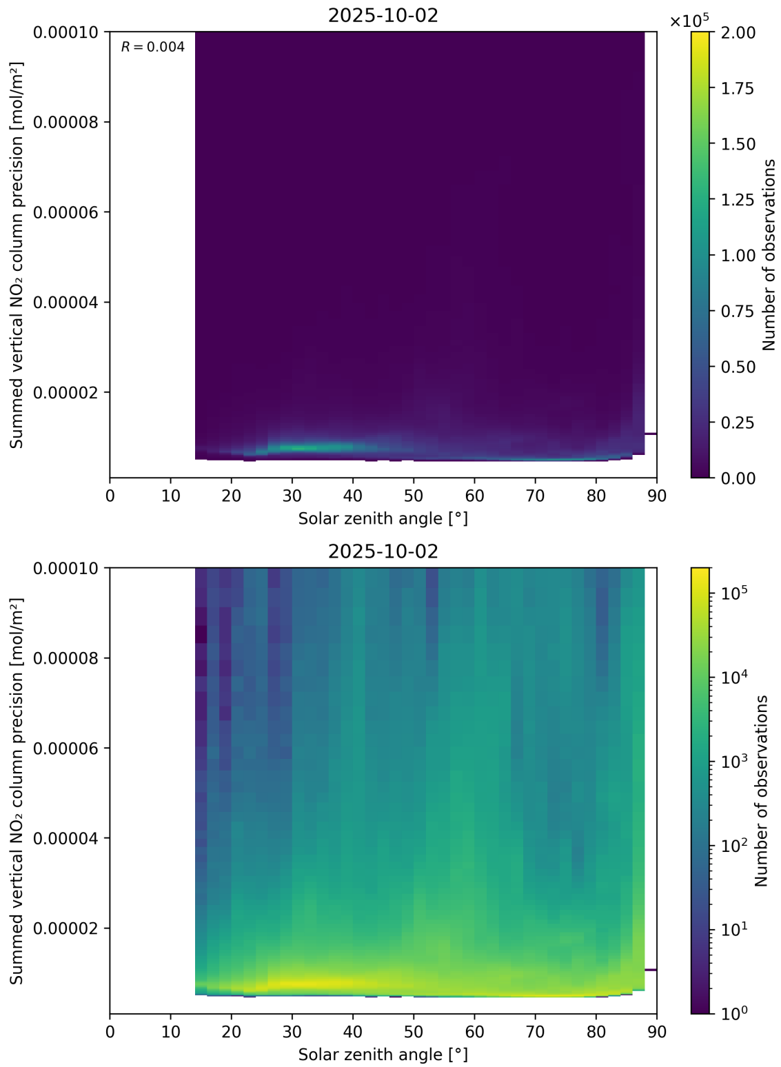
Figure 152: Scatter density plot of “Solar zenith angle” against “Summed vertical NO 2 column precision” for 2025-10-01 to 2025-10-03.
