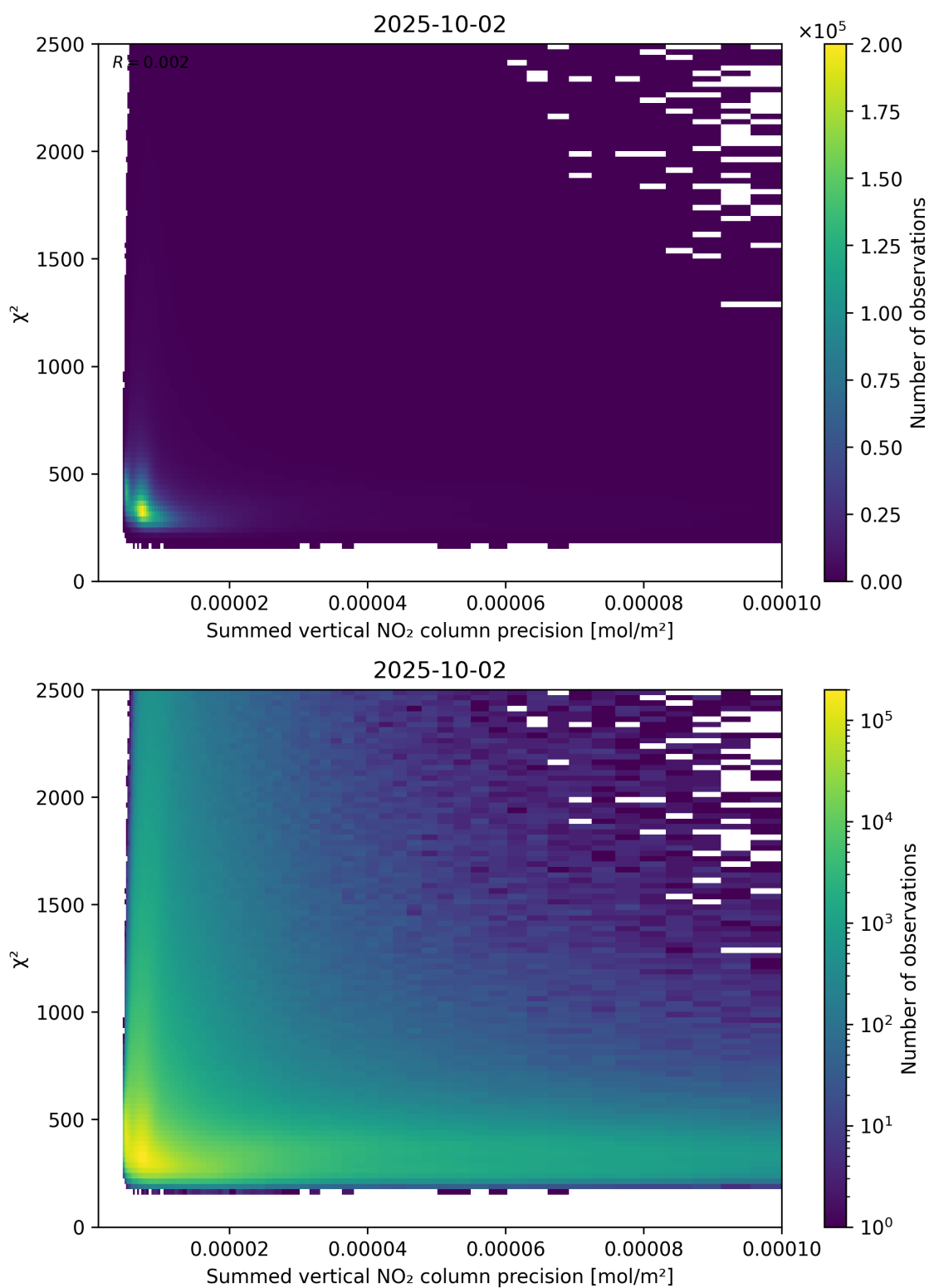
Figure 107: Scatter density plot of “Summed vertical NO 2 column precision” against “ \chi^2 ” for 2025-10-01 to 2025-10-03.
