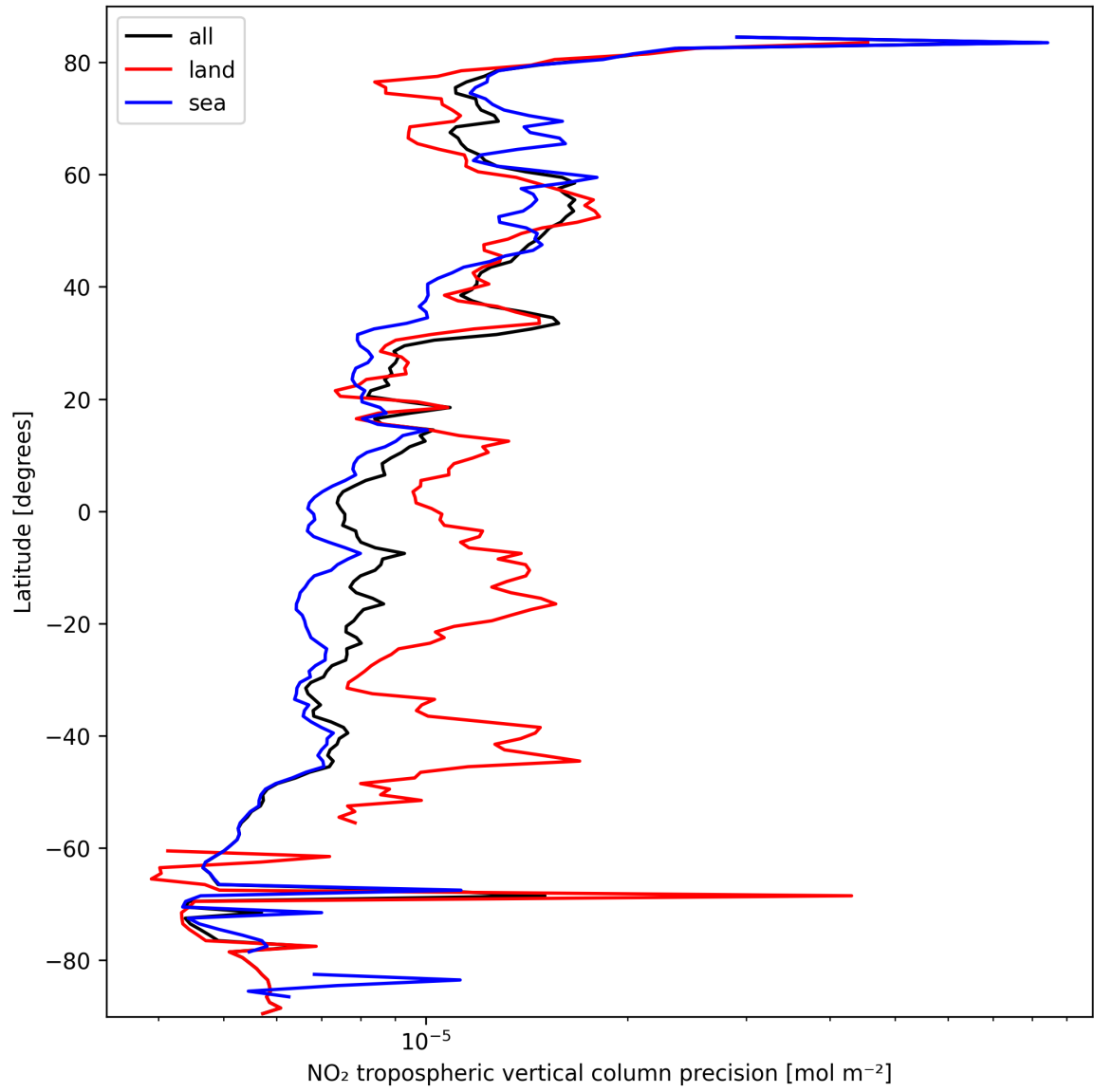
Figure 13: Zonal average of "NO 2 tropospheric vertical column precision" for 2025-10-01 to 2025-10-03.
