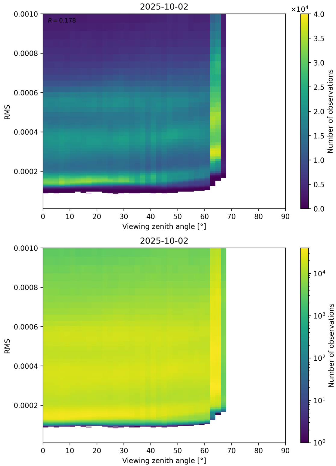
Figure 171: Scatter density plot of “Viewing zenith angle” against “RMS” for 2025-10-01 to 2025-10-03.
