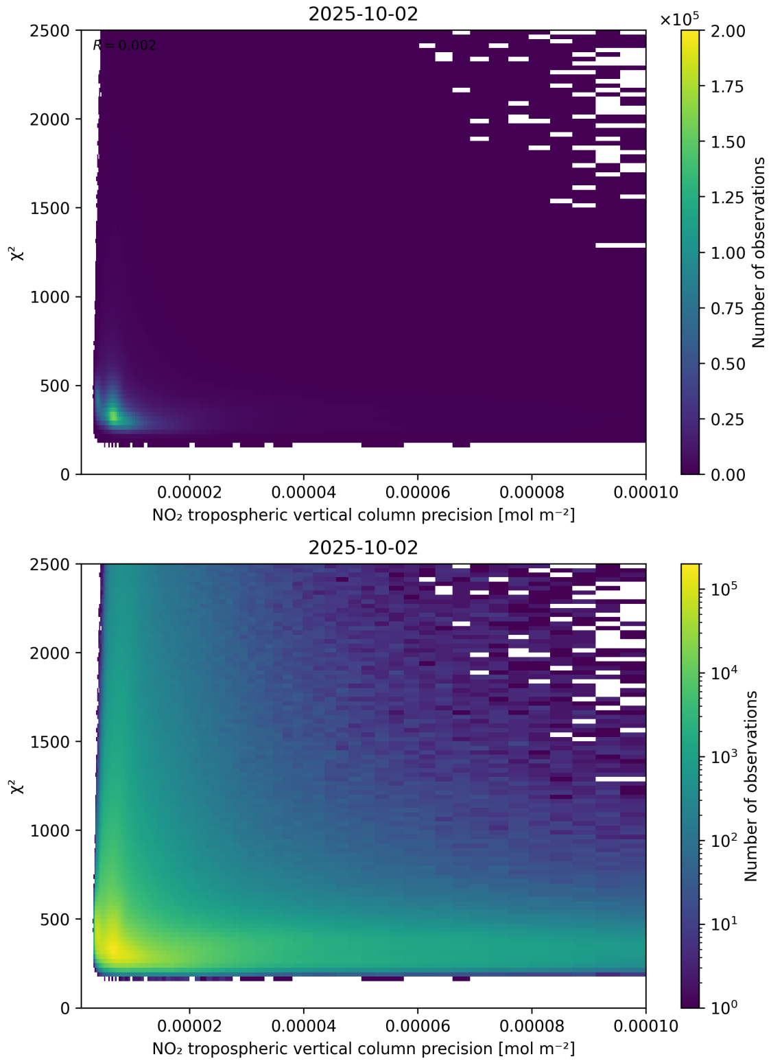
Figure 134: Scatter density plot of “NO 2 tropospheric vertical column precision” against “ \chi^2 ” for 2025-10-01 to 2025-10-03.
