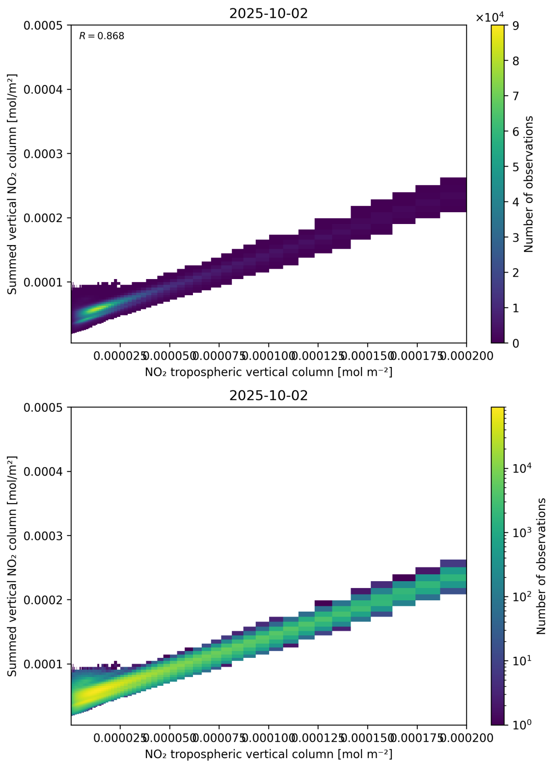
Figure 126: Scatter density plot of “NO 2 tropospheric vertical column” against “Summed vertical NO 2 column” for 2025-10-01 to 2025-10-03.
