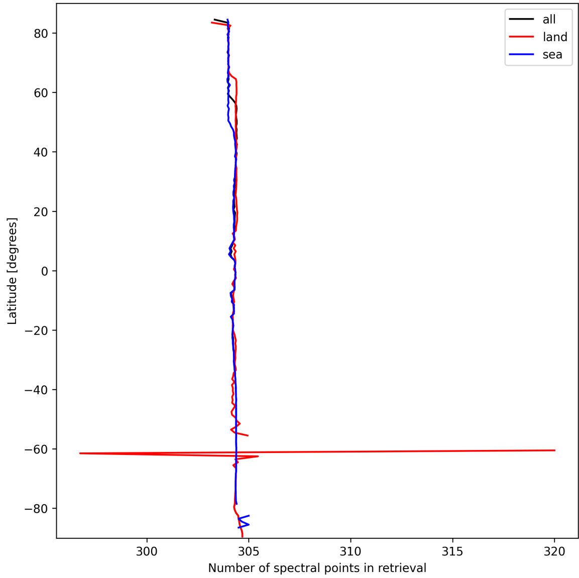
Figure 16: Zonal average of “Number of spectral points in retrieval” for 2025-10-01 to 2025-10-03.
