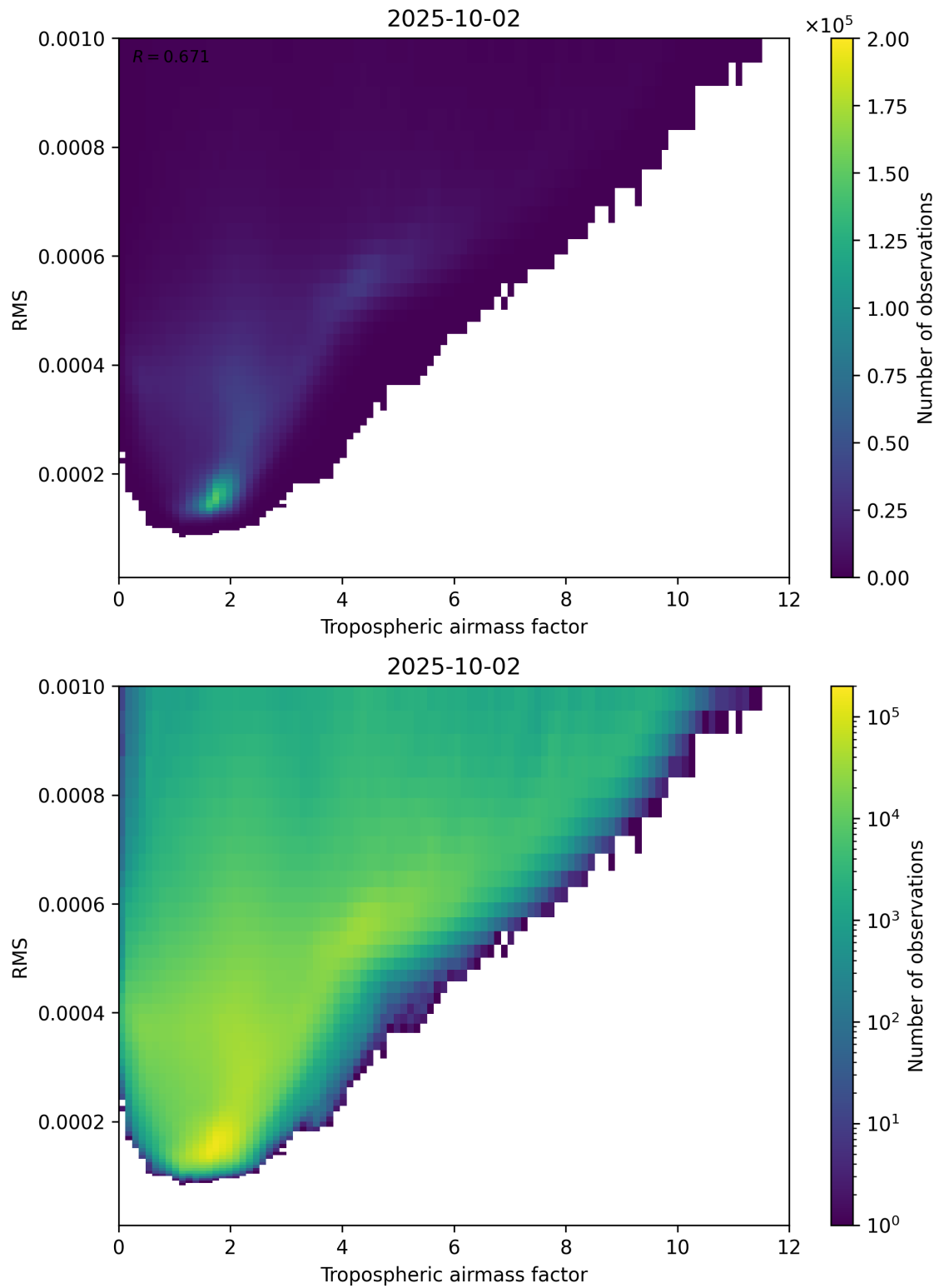
Figure 79: Scatter density plot of “Tropospheric airmass factor” against “RMS” for 2025-10-01 to 2025-10-03.
