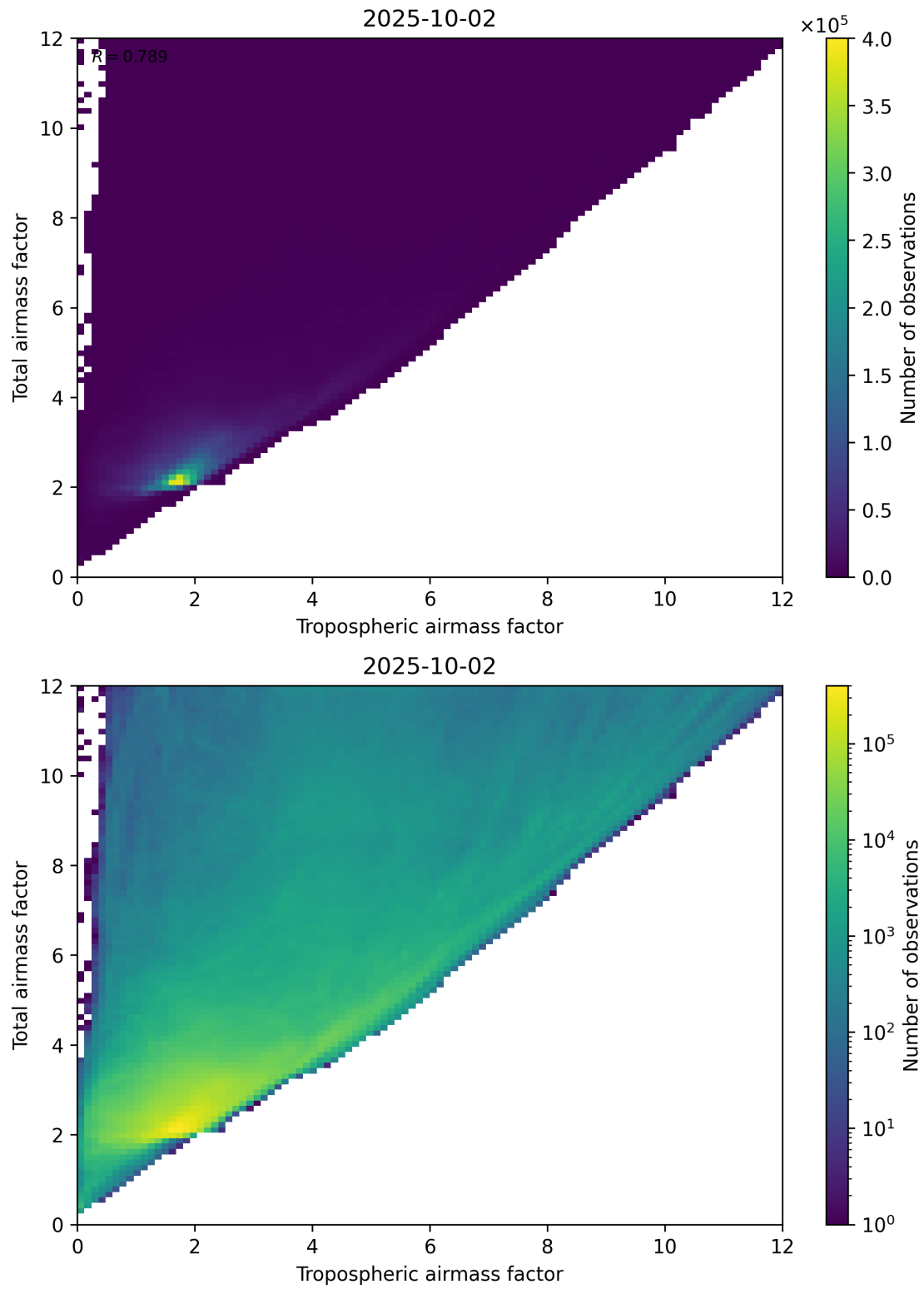
Figure 72: Scatter density plot of “Tropospheric airmass factor” against “Total airmass factor” for 2025-10-01 to 2025-10-03.
