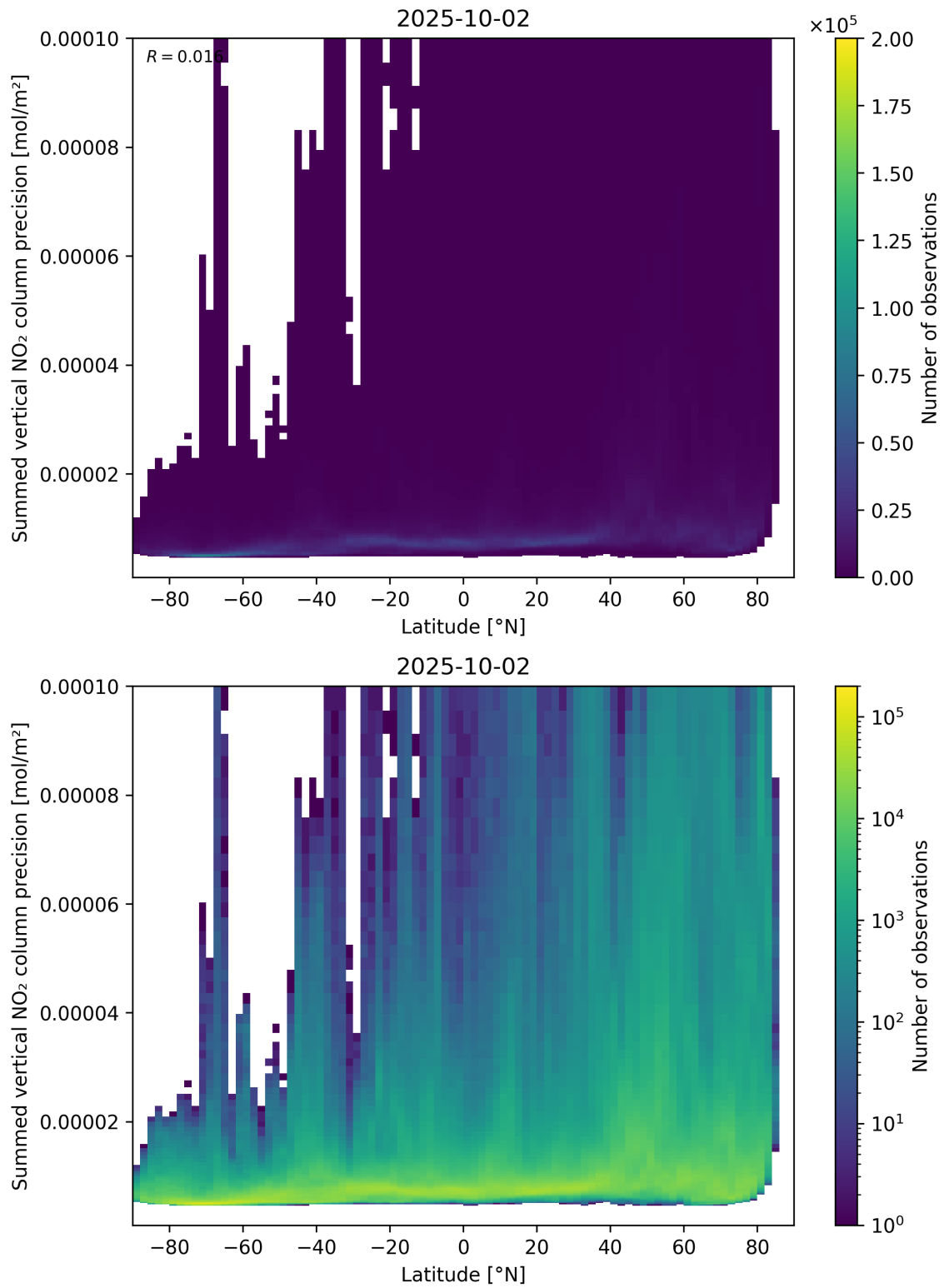
Figure 89: Scatter density plot of “Latitude” against “Summed vertical NO 2 column precision” for 2025-10-01 to 2025-10-03.
