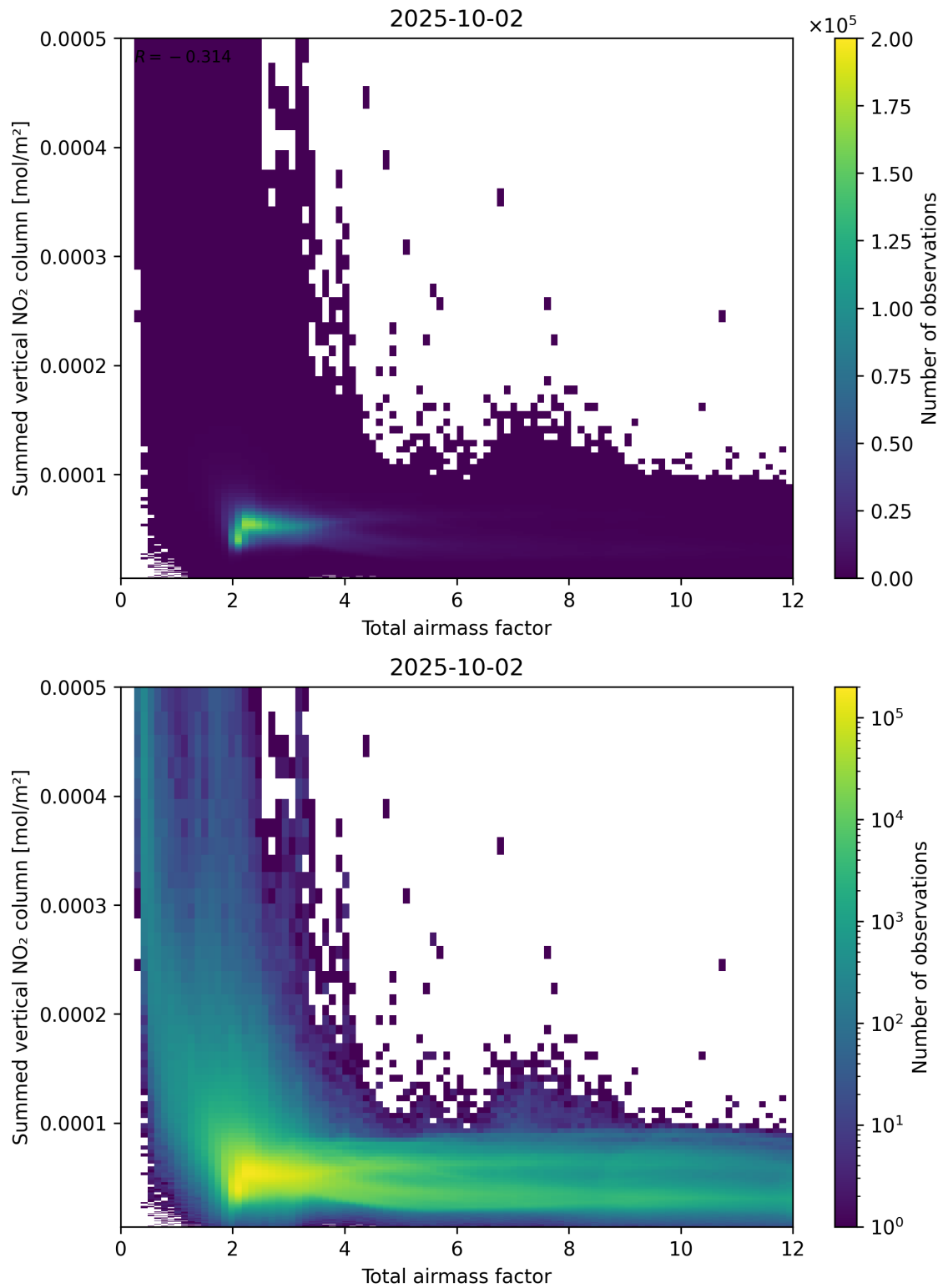
Figure 65: Scatter density plot of “Total airmass factor” against “Summed vertical NO 2 column” for 2025-10-01 to 2025-10-03.
