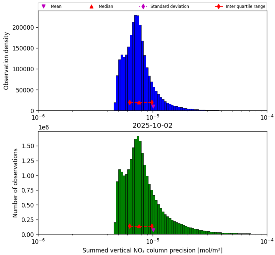
Figure 41: Histogram of "Summed vertical NO 2 column precision" for 2025-10-01 to 2025-10-03
