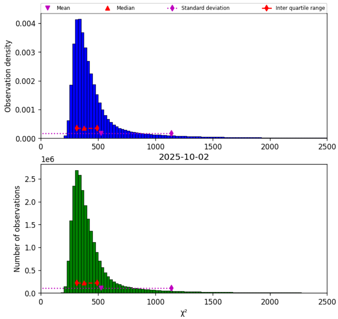
Figure 42: Histogram of “ \chi^2 ” for 2025-10-01 to 2025-10-03
