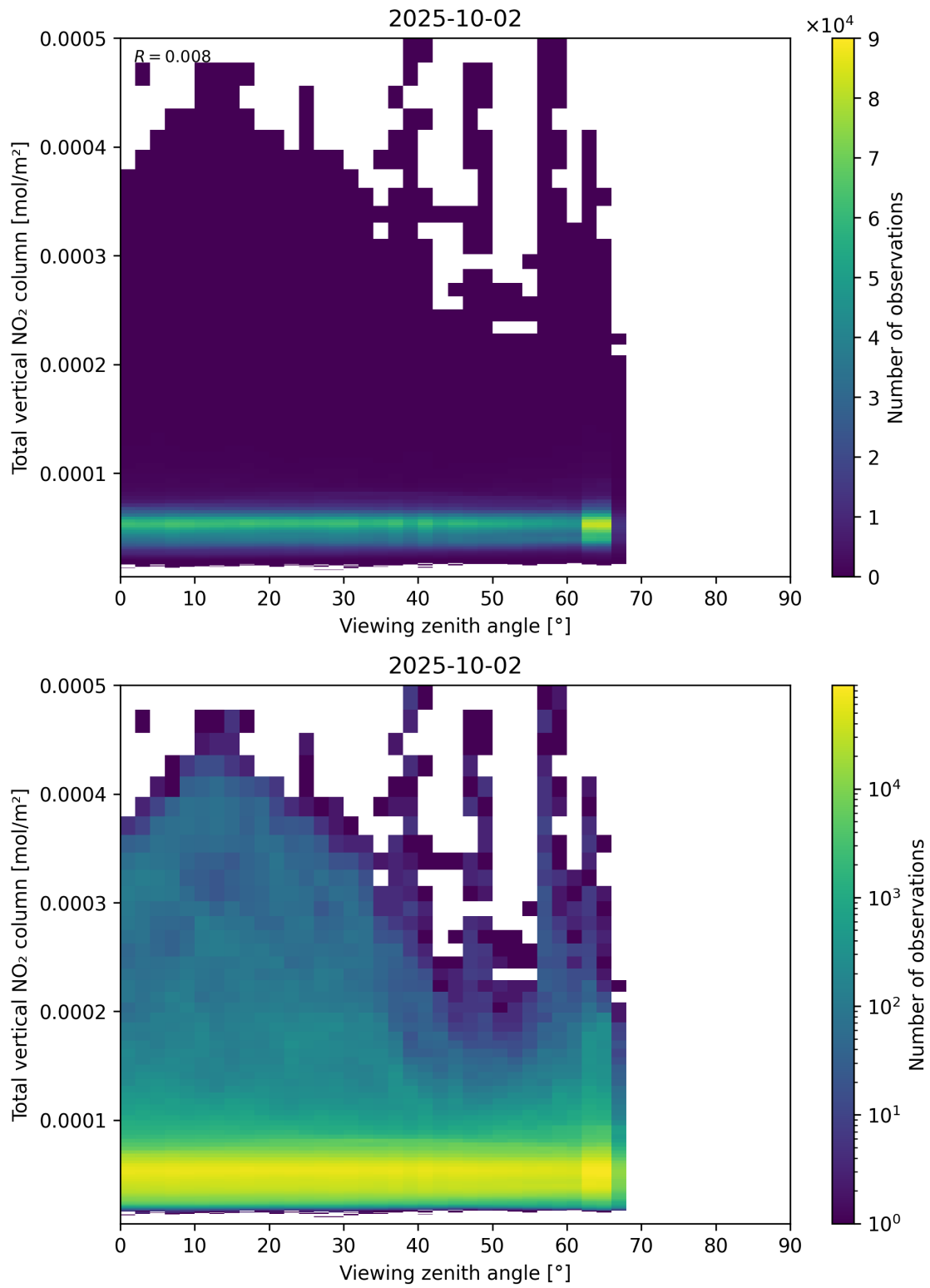
Figure 167: Scatter density plot of “Viewing zenith angle” against “Total vertical NO 2 column” for 2025-10-01 to 2025-10-03.
