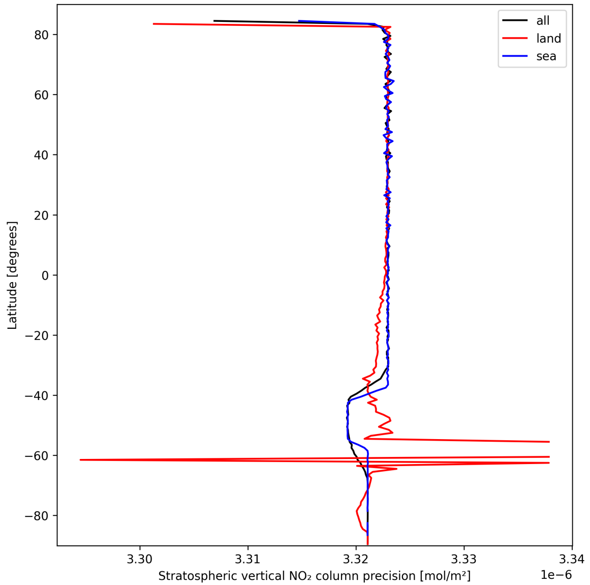
Figure 20: Zonal average of “Stratospheric vertical NO 2 column precision” for 2025-10-01 to 2025-10-03.
