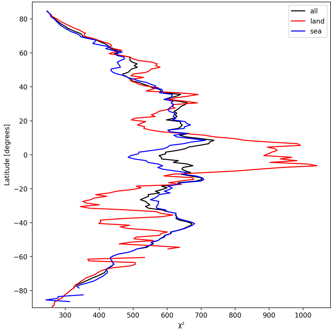
Figure 25: Zonal average of “ \chi^2 ” for 2025-10-01 to 2025-10-03.
