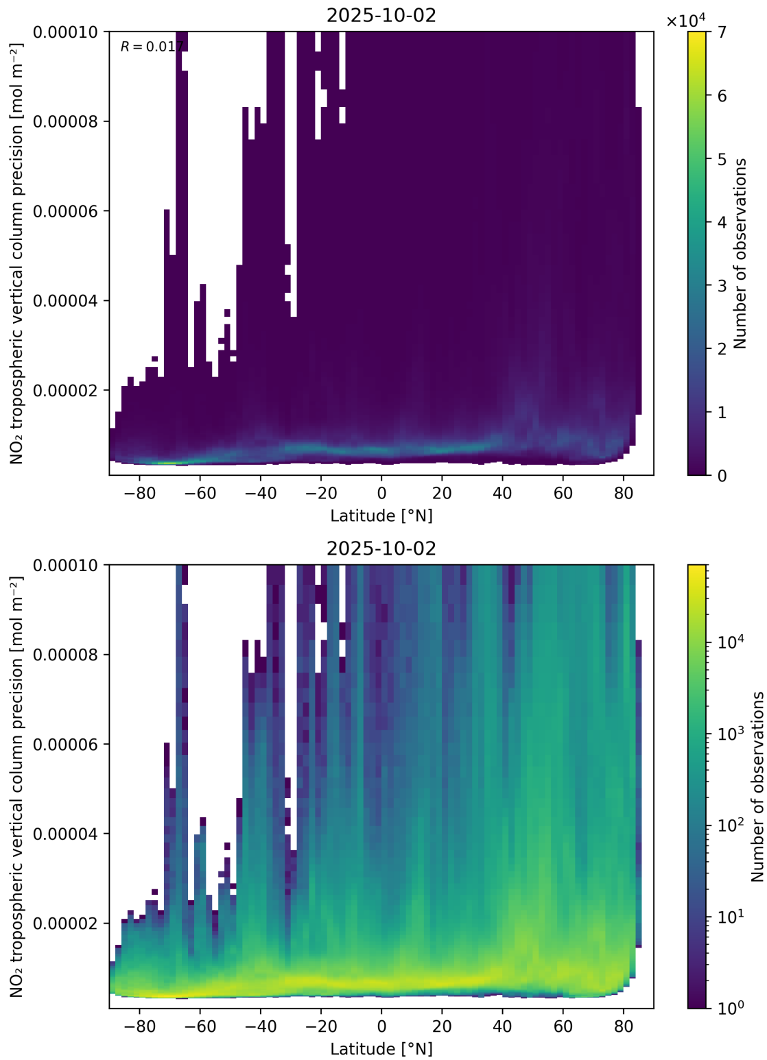
Figure 93: Scatter density plot of “Latitude” against “NO 2 tropospheric vertical column precision” for 2025-10-01 to 2025-10-03.
