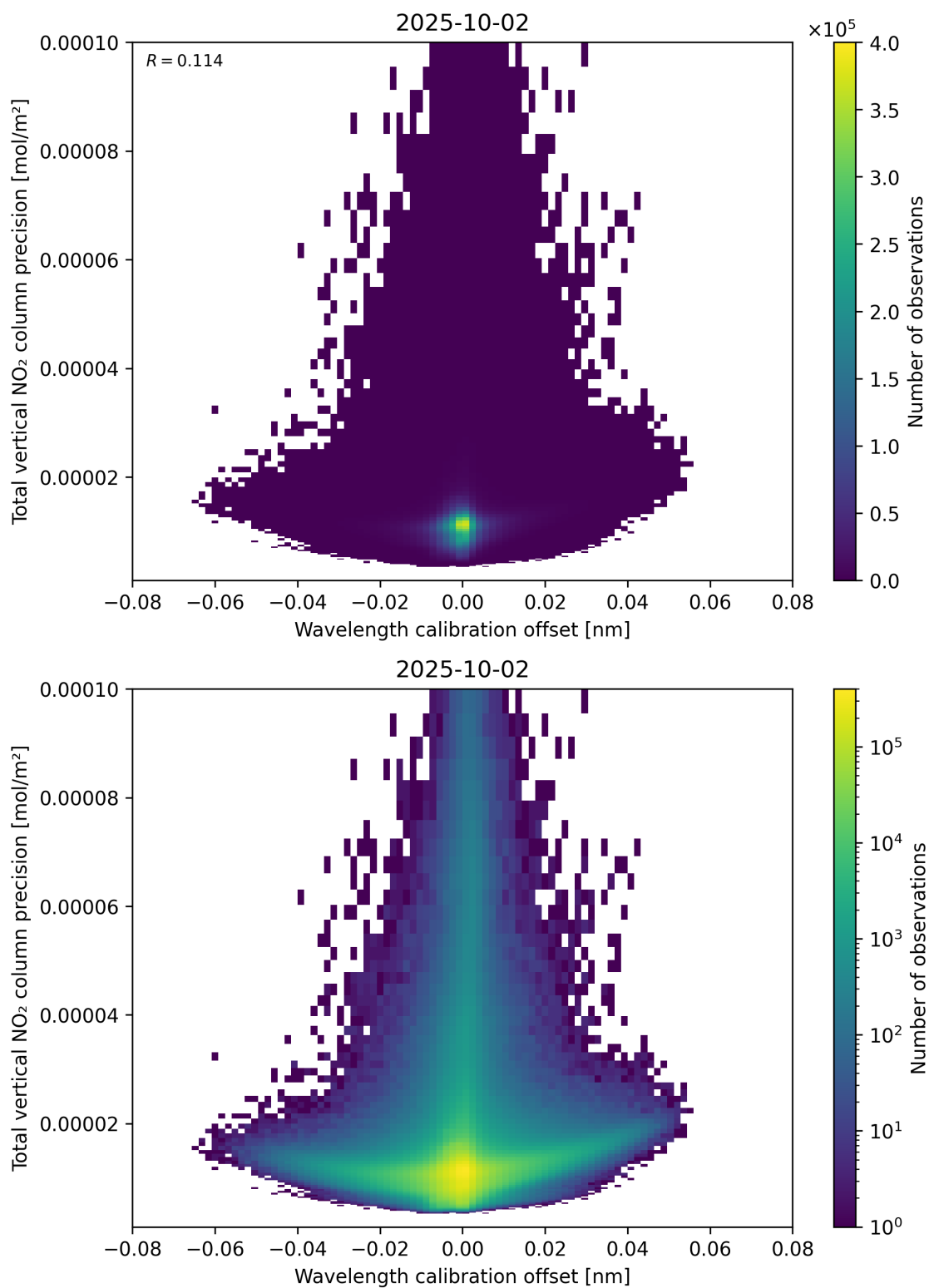
Figure 180: Scatter density plot of “Wavelength calibration offset” against “Total vertical NO 2 column precision” for 2025-10-01 to 2025-10-03.
