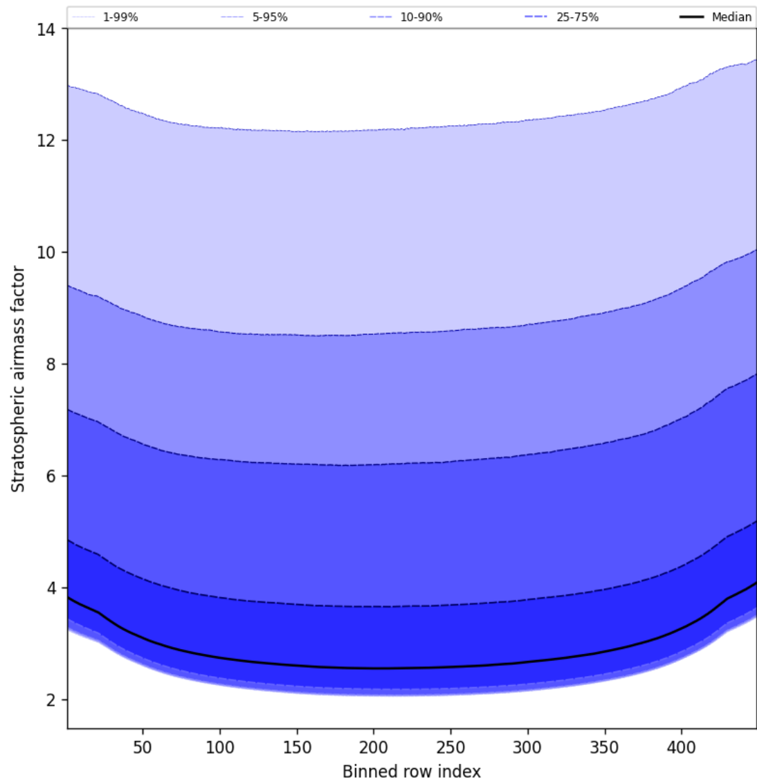
Figure 61: Along track statistics of “Stratospheric air mass factor” for 2025-10-01 to 2025-10-03
