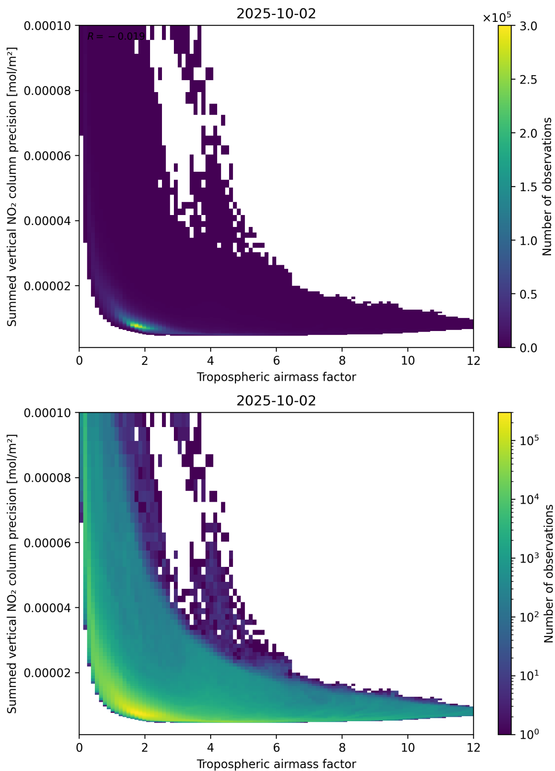
Figure 76: Scatter density plot of “Tropospheric air mass factor” against “Summed vertical NO 2 column precision” for 2025-10-01 to 2025-10-03.
