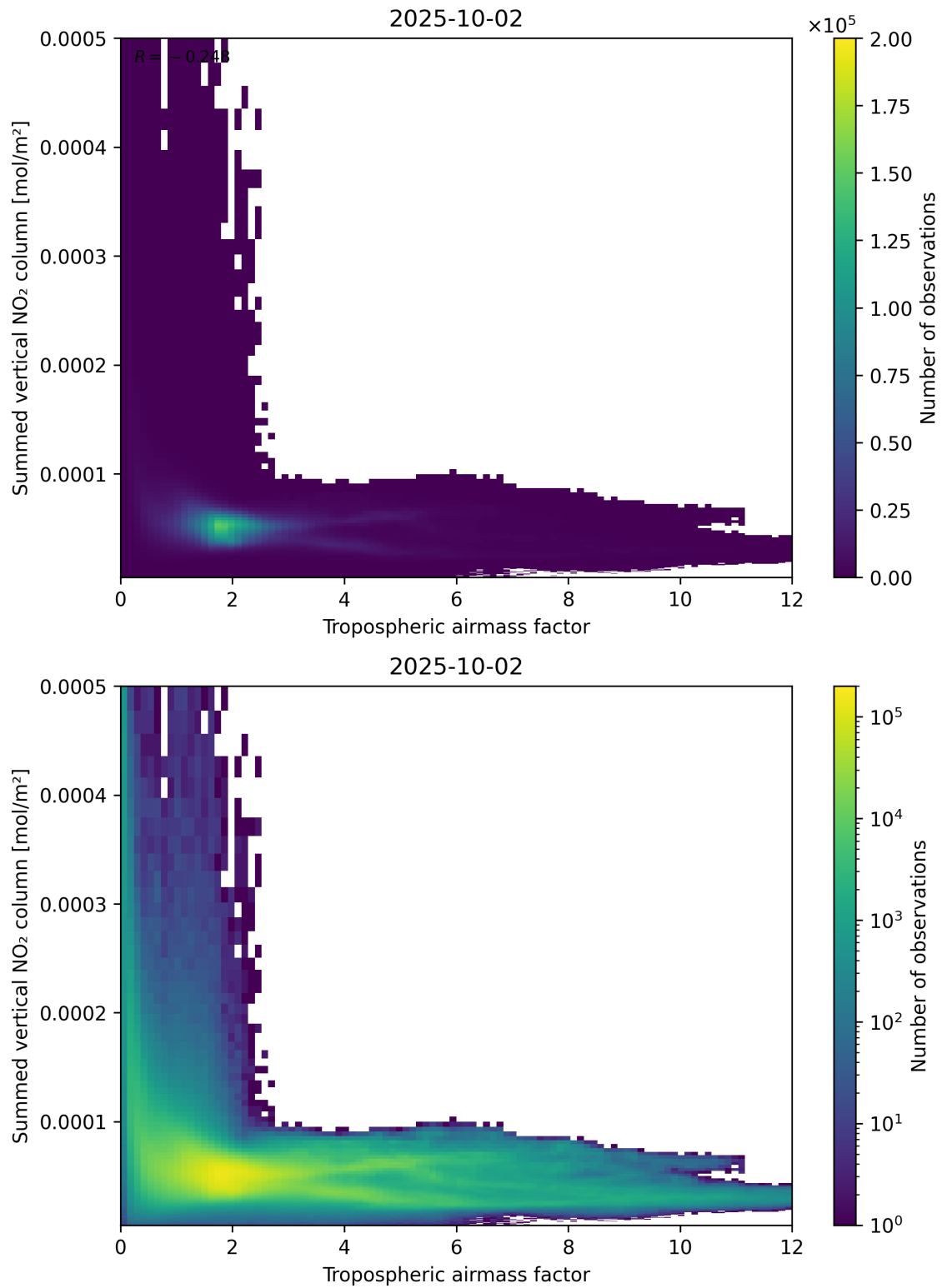
Figure 75: Scatter density plot of “Tropospheric air mass factor” against “Summed vertical NO 2 column” for 2025-10-01 to 2025-10-03.
