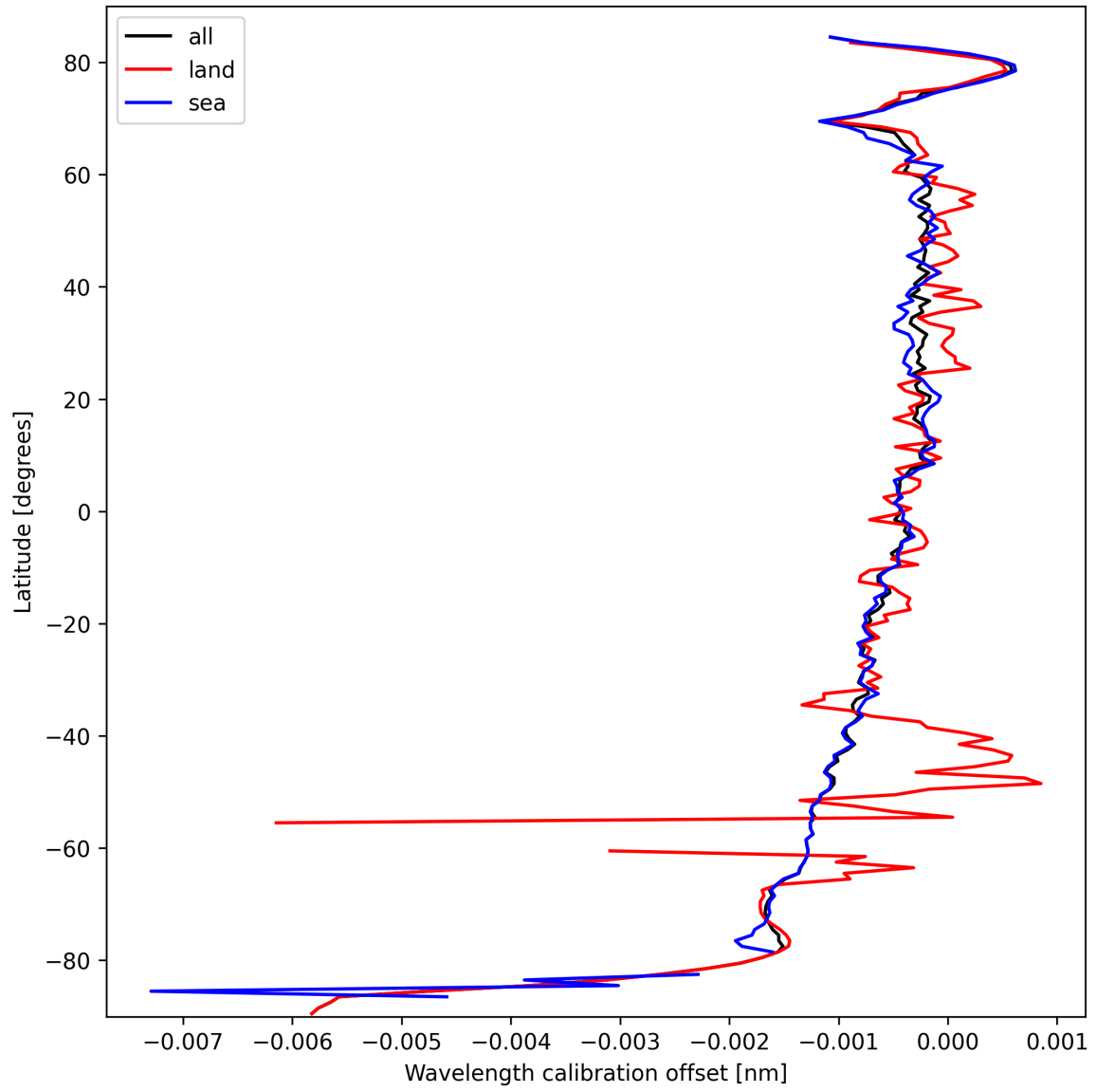
Figure 18: Zonal average of “Wavelength calibration offset” for 2025-10-01 to 2025-10-03.
