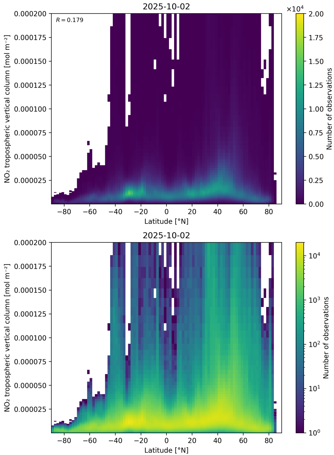
Figure 92: Scatter density plot of “Latitude” against “NO 2 tropospheric vertical column” for 2025-10-01 to 2025-10-03.
