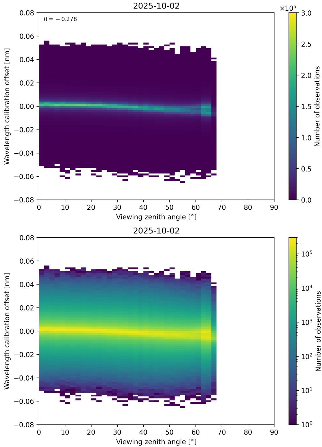
Figure 173: Scatter density plot of “Viewing zenith angle” against “Wavelength calibration offset” for 2025-10-01 to 2025-10-03.
