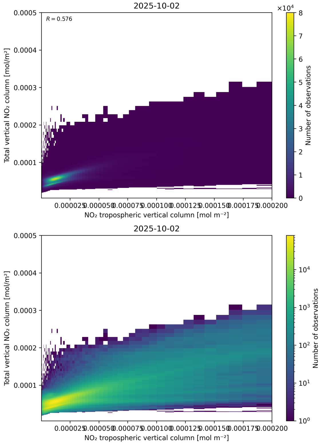
Figure 128: Scatter density plot of “NO 2 tropospheric vertical column” against “Total vertical NO 2 column” for 2025-10-01 to 2025-10-03.
