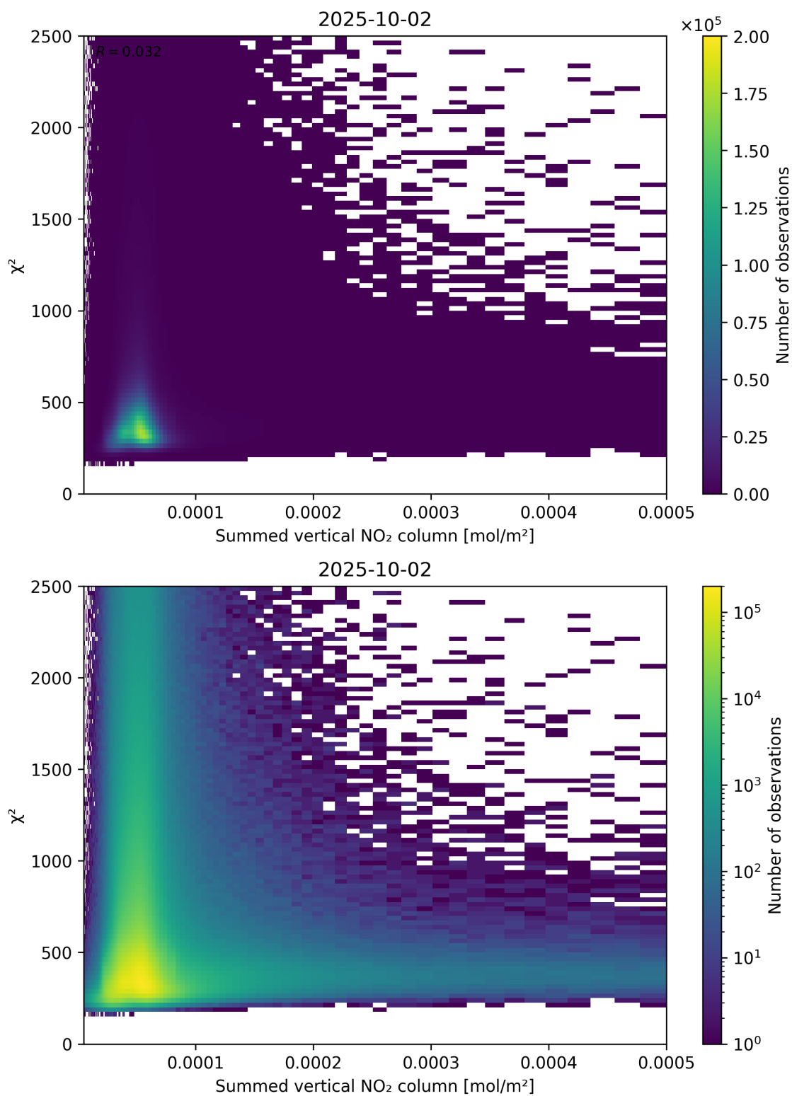
Figure 104: Scatter density plot of “Summed vertical NO 2 column” against “ \chi^2 ” for 2025-10-01 to 2025-10-03.
