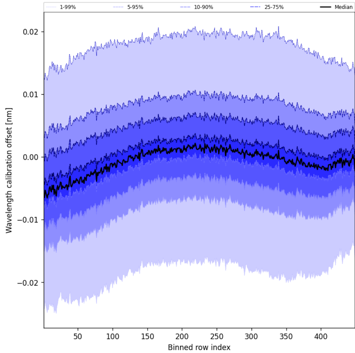
Figure 52: Along track statistics of “Wavelength calibration offset” for 2025-10-01 to 2025-10-03
