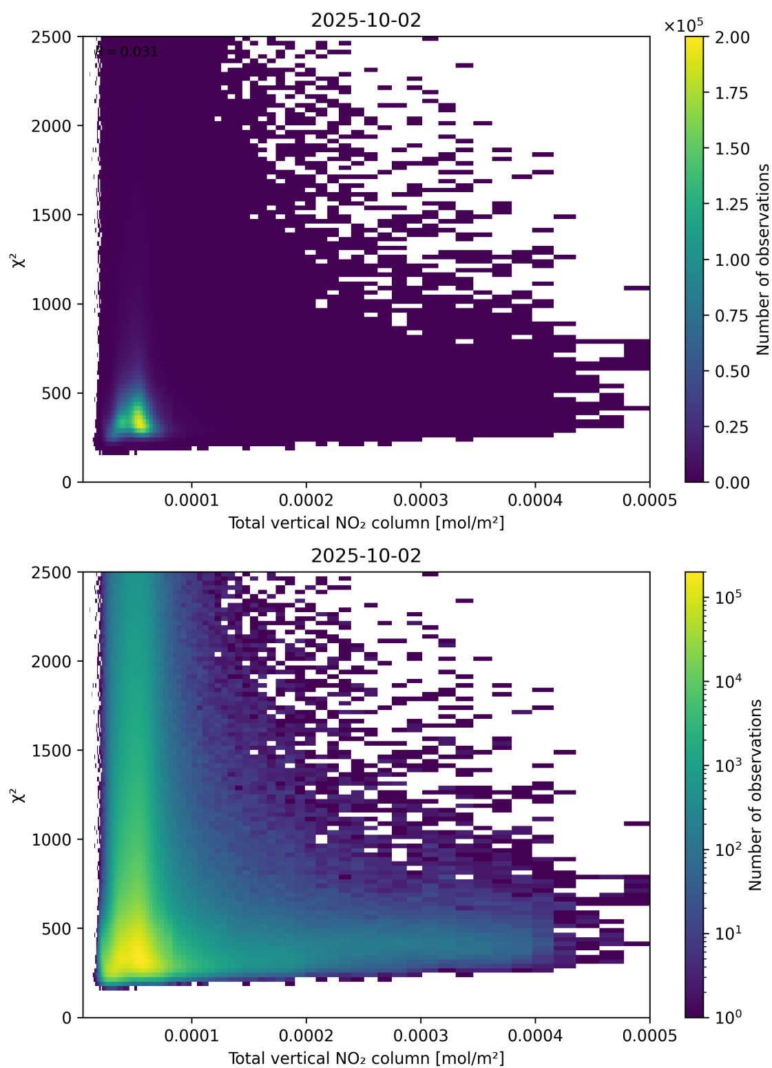
Figure 111: Scatter density plot of “Total vertical NO 2 column” against “ \chi^2 ” for 2025-10-01 to 2025-10-03.
