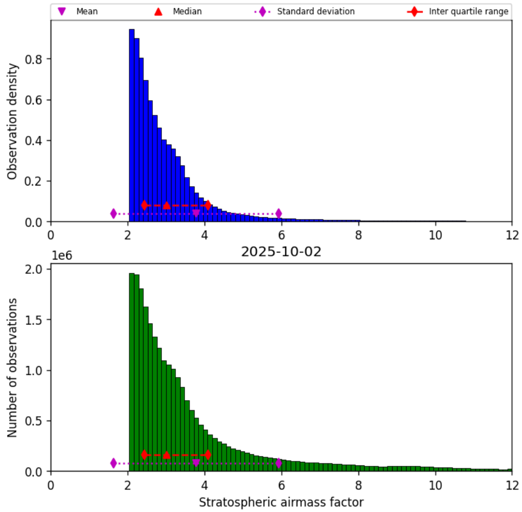
Figure 44: Histogram of “Stratospheric airmass factor” for 2025-10-01 to 2025-10-03
