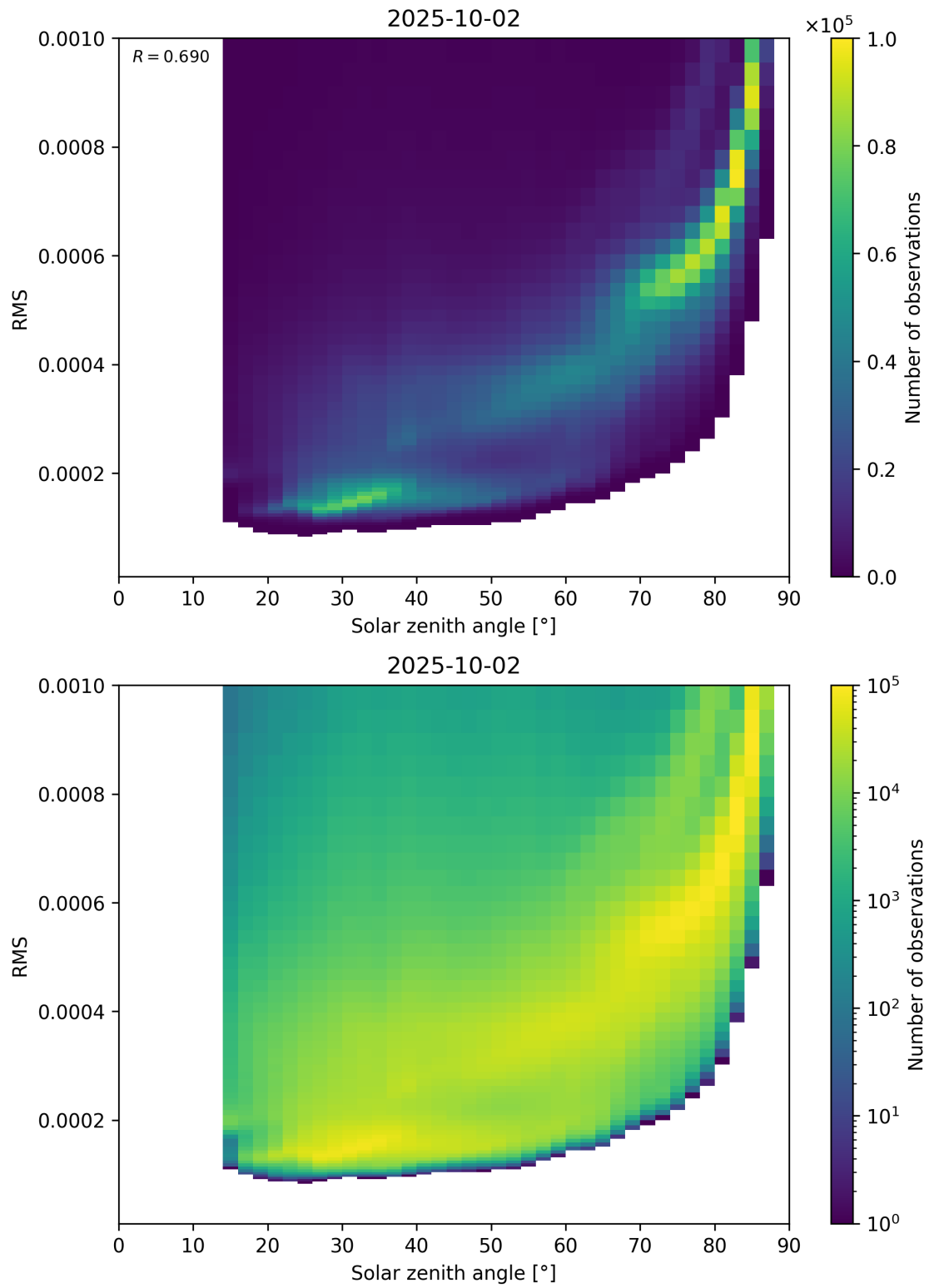
Figure 157: Scatter density plot of “Solar zenith angle” against “RMS” for 2025-10-01 to 2025-10-03.
