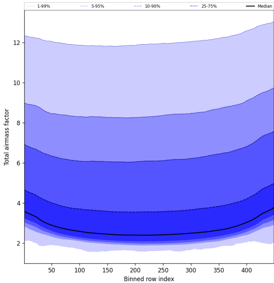
Figure 49: Along track statistics of “Total airmass factor” for 2025-10-01 to 2025-10-03
