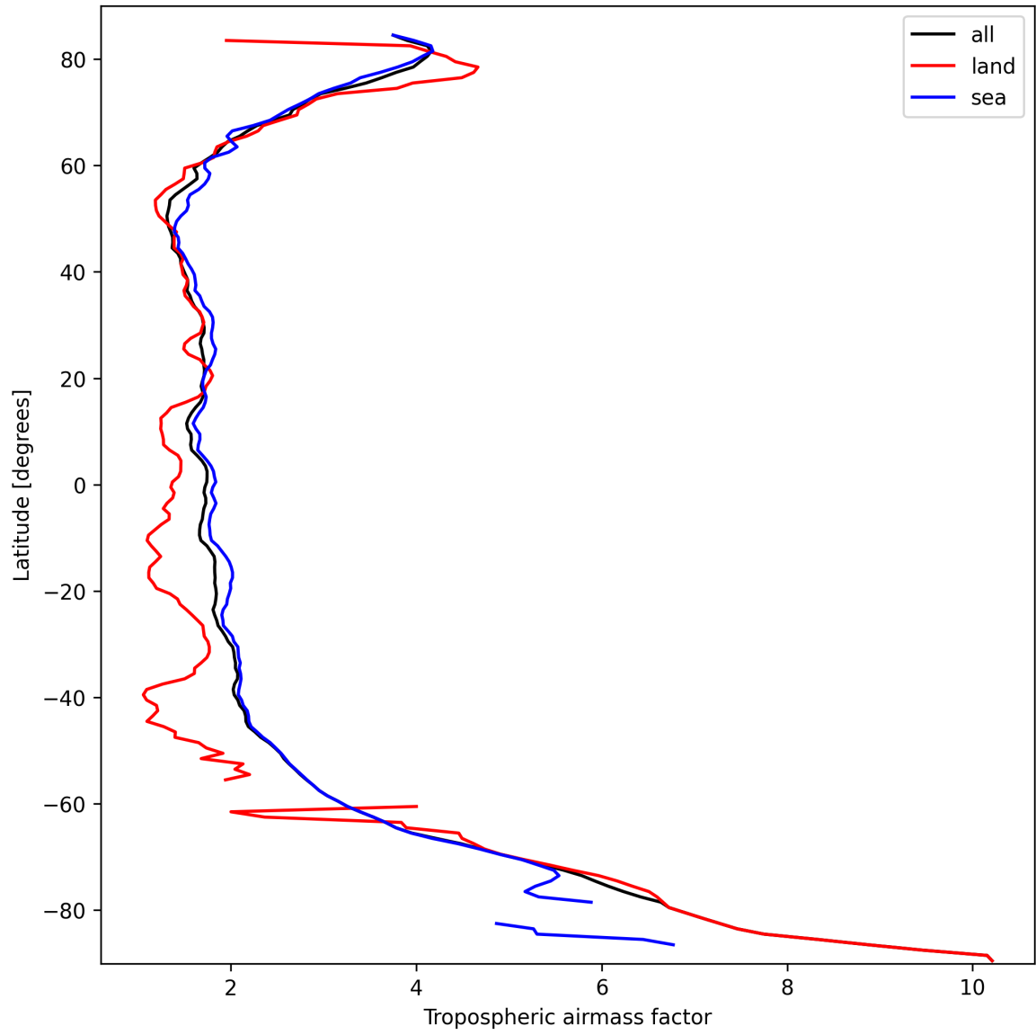
Figure 14: Zonal average of “Tropospheric air mass factor” for 2025-10-01 to 2025-10-03.
