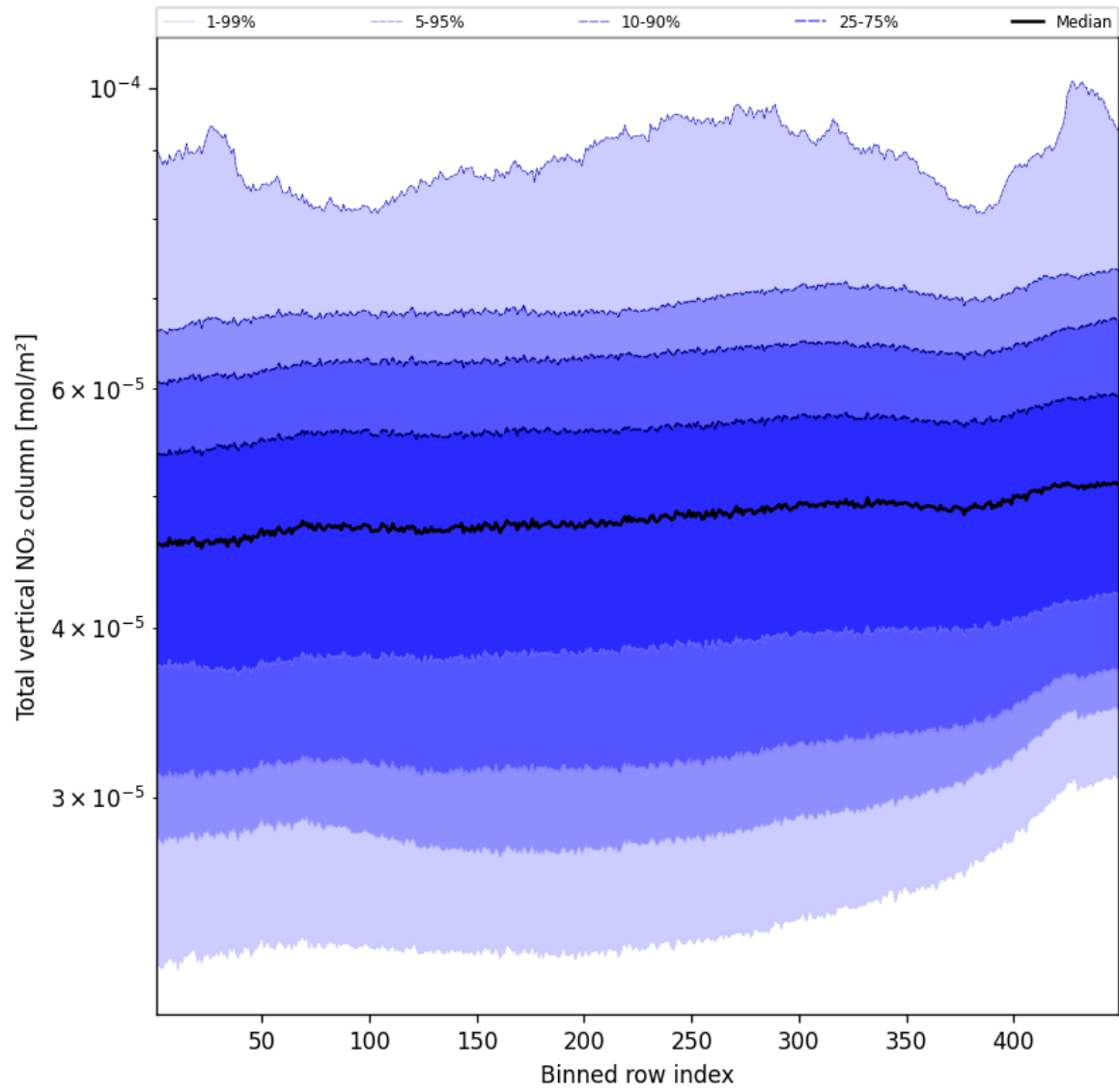
Figure 55: Along track statistics of “Total vertical NO 2 column” for 2025-10-01 to 2025-10-03
