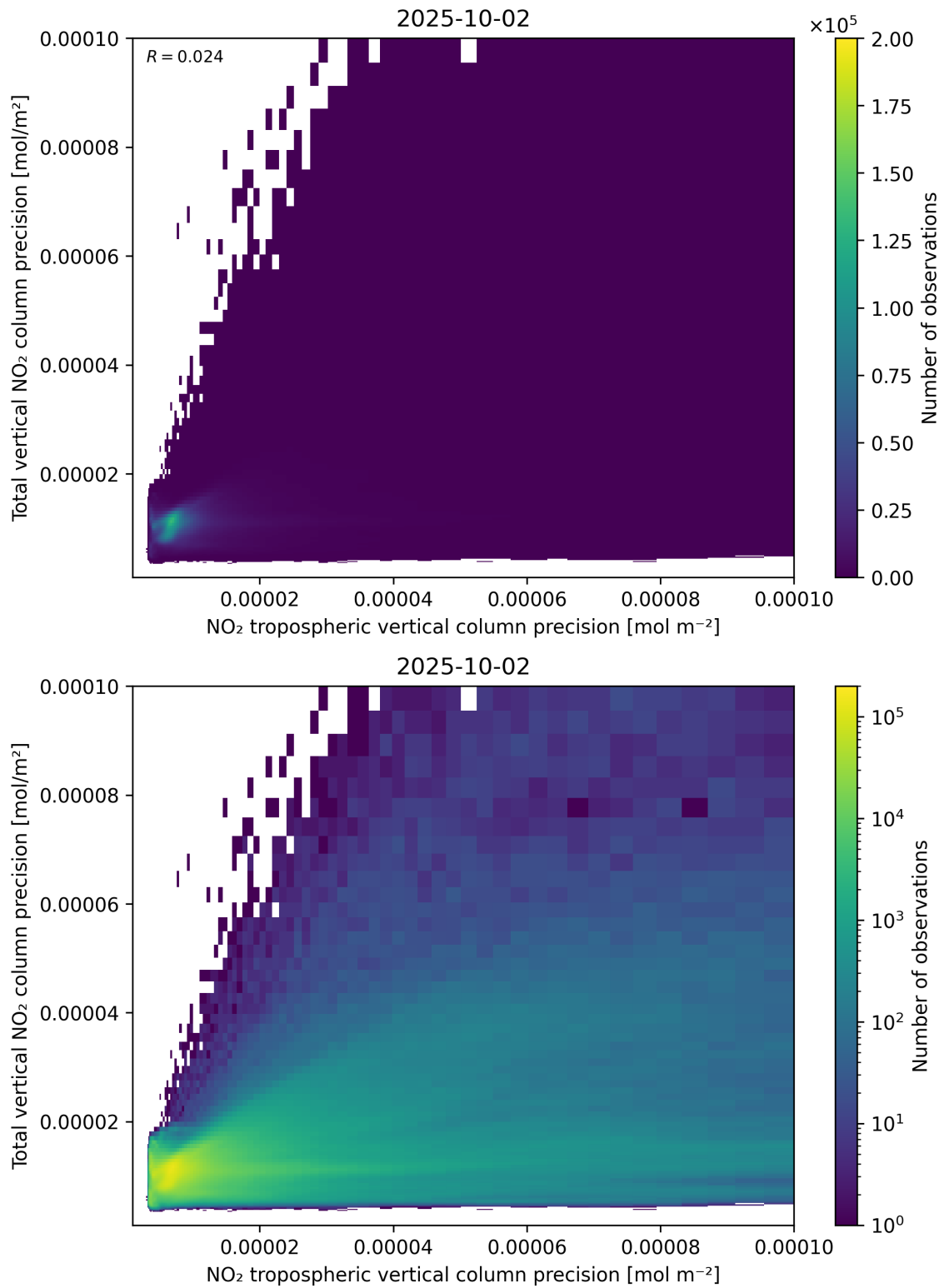
Figure 139: Scatter density plot of “NO 2 tropospheric vertical column precision” against “Total vertical NO 2 column precision” for 2025-10-01 to 2025-10-03.
