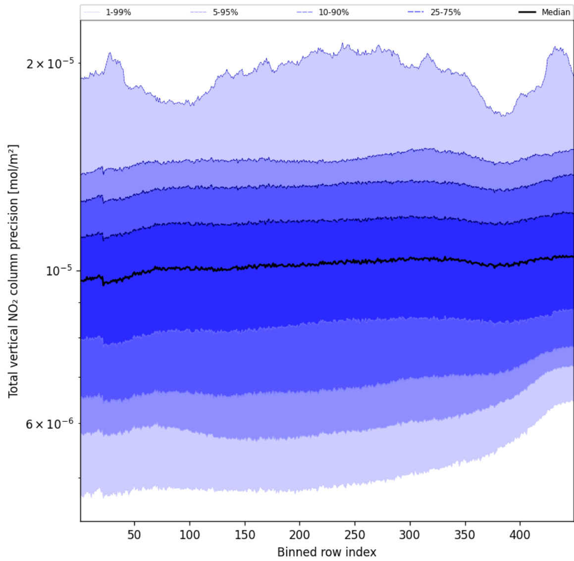
Figure 56: Along track statistics of “Total vertical NO 2 column precision” for 2025-10-01 to 2025-10-03
