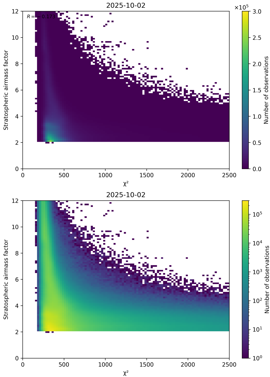
Figure 81: Scatter density plot of “ \chi^2 ” against “Stratospheric airmass factor” for 2025-10-01 to 2025-10-03.
