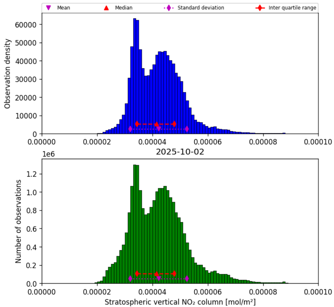
Figure 36: Histogram of “Stratospheric vertical NO 2 column” for 2025-10-01 to 2025-10-03
