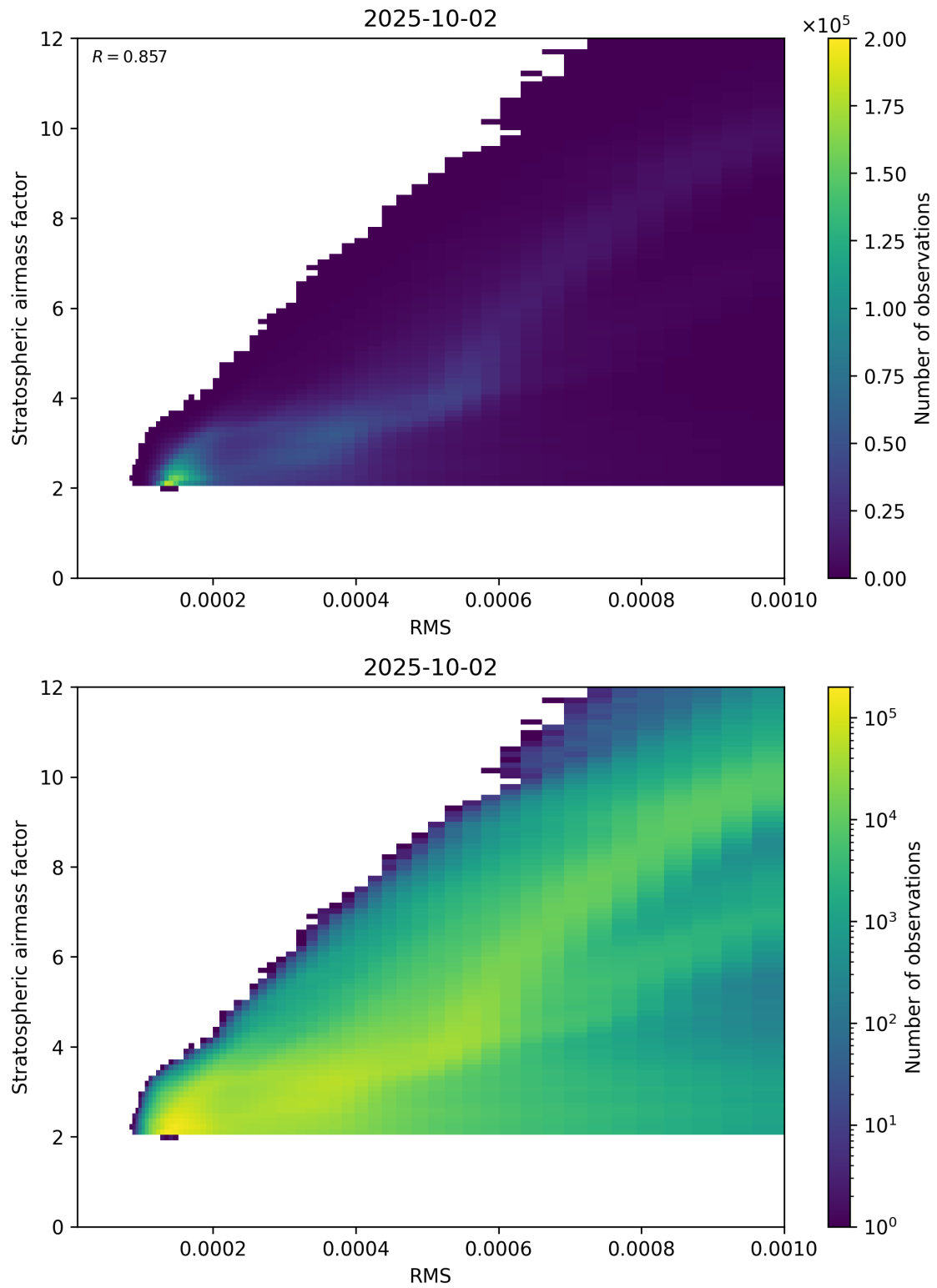
Figure 144: Scatter density plot of “RMS” against “Stratospheric airmass factor” for 2025-10-01 to 2025-10-03.
