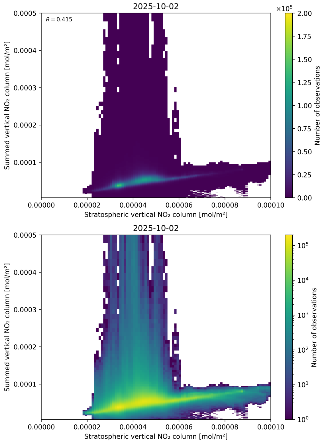
Figure 98: Scatter density plot of “Stratospheric vertical NO 2 column” against “Summed vertical NO 2 column” for 2025-10-01 to 2025-10-03.
