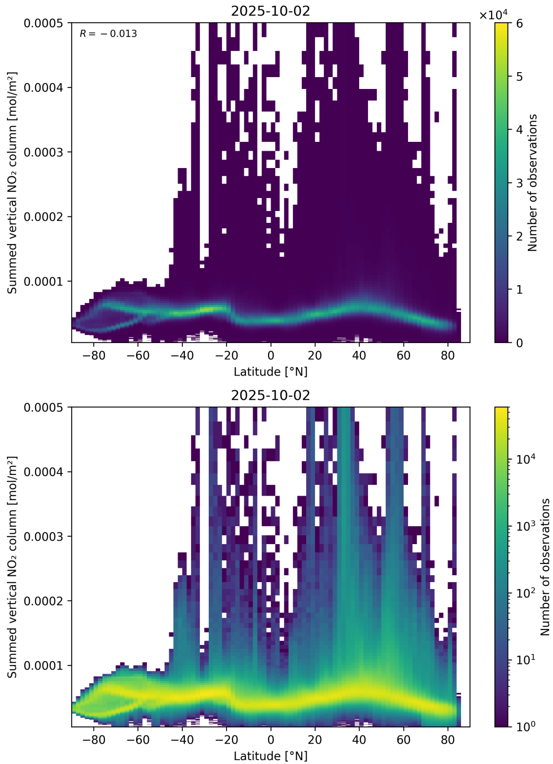
Figure 88: Scatter density plot of “Latitude” against “Summed vertical NO 2 column” for 2025-10-01 to 2025-10-03.
