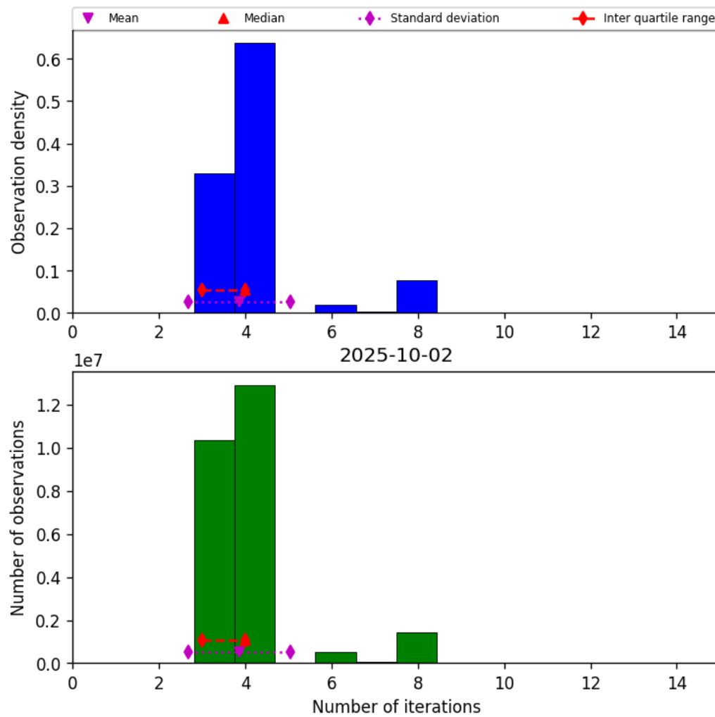
Figure 34: Histogram of “Number of iterations” for 2025-10-01 to 2025-10-03
