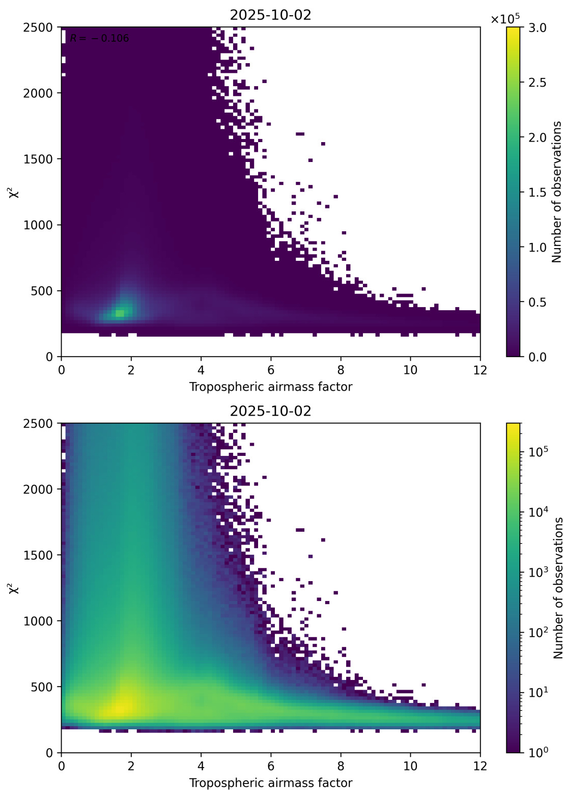
Figure 73: Scatter density plot of “Tropospheric airmass factor” against “ \chi^2 ” for 2025-10-01 to 2025-10-03.
