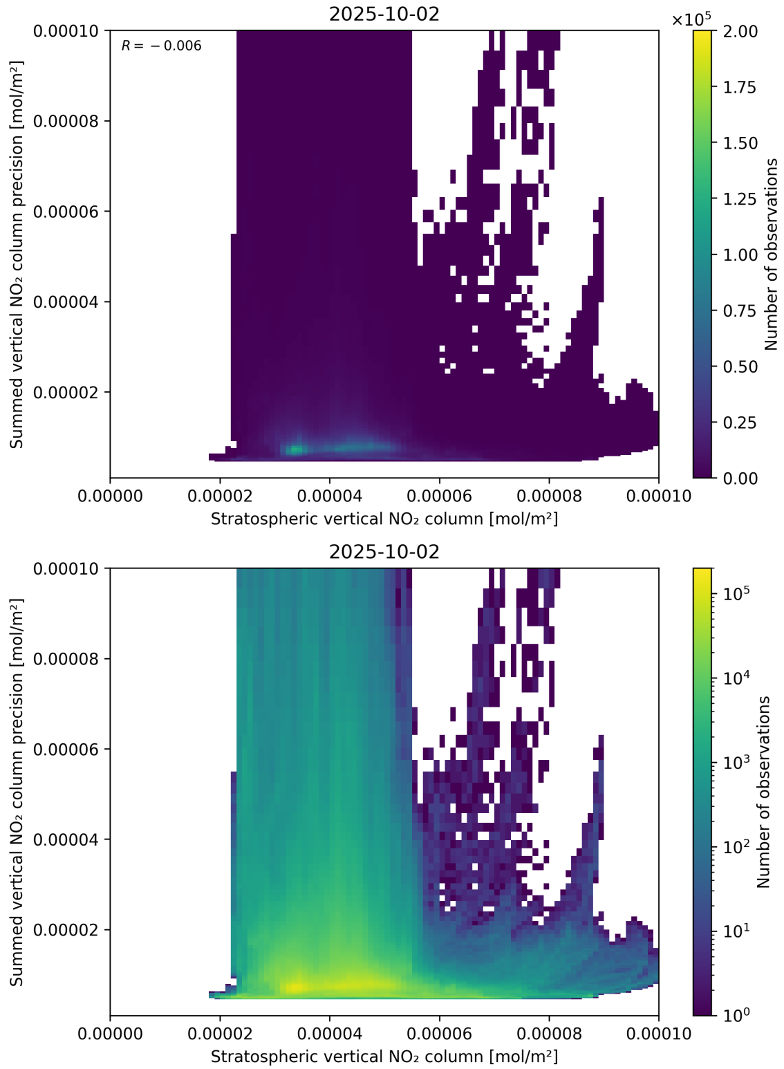
Figure 99: Scatter density plot of “Stratospheric vertical NO 2 column” against “Summed vertical NO 2 column precision” for 2025-10-01 to 2025-10-03.
