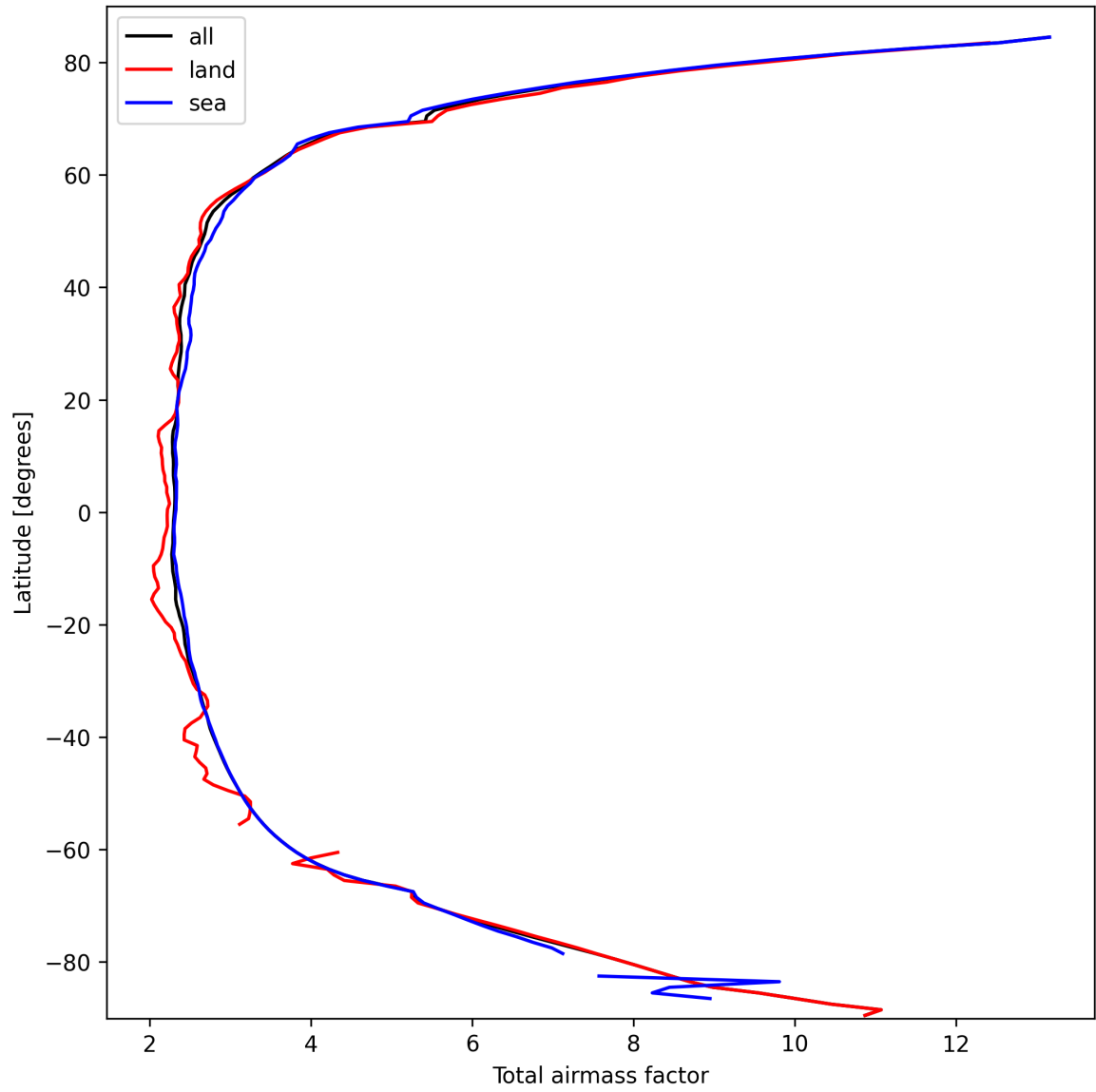
Figure 15: Zonal average of “Total airmass factor” for 2025-10-01 to 2025-10-03.
