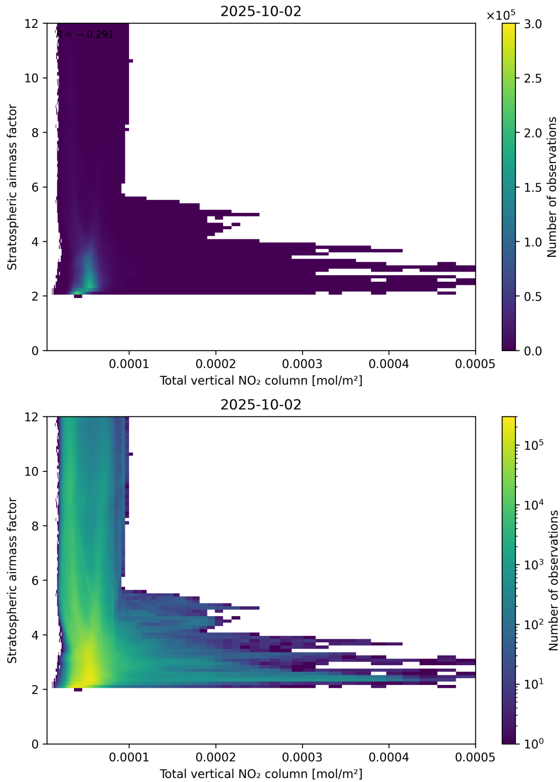
Figure 110: Scatter density plot of “Total vertical NO 2 column” against “Stratospheric airmass factor” for 2025-10-01 to 2025-10-03.
