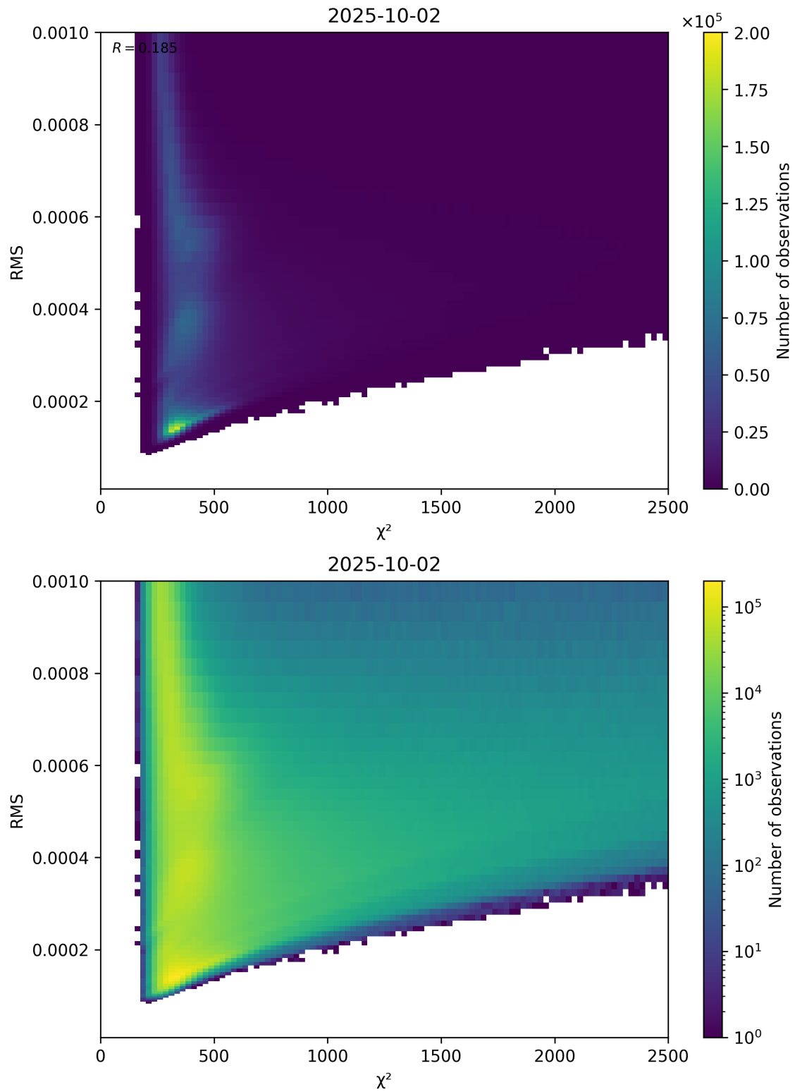
Figure 82: Scatter density plot of “ \chi^2 ” against “RMS” for 2025-10-01 to 2025-10-03.
