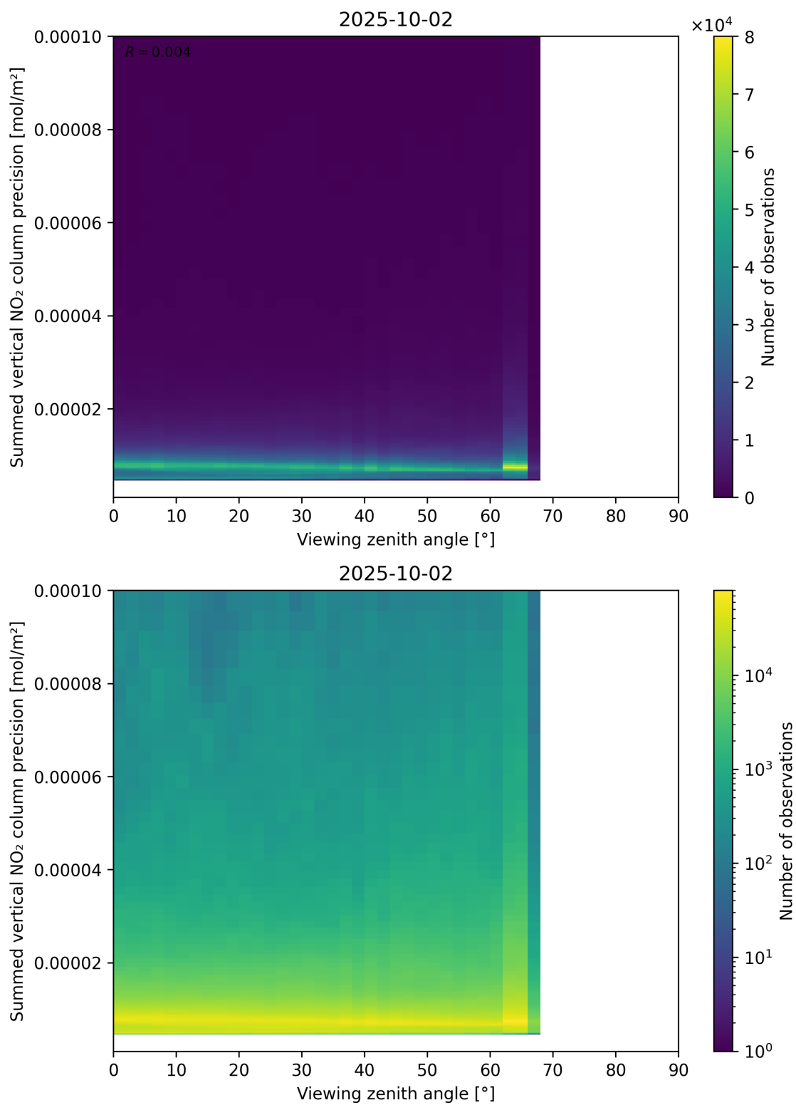
Figure 166: Scatter density plot of “Viewing zenith angle” against “Summed vertical NO 2 column precision” for 2025-10-01 to 2025-10-03.
