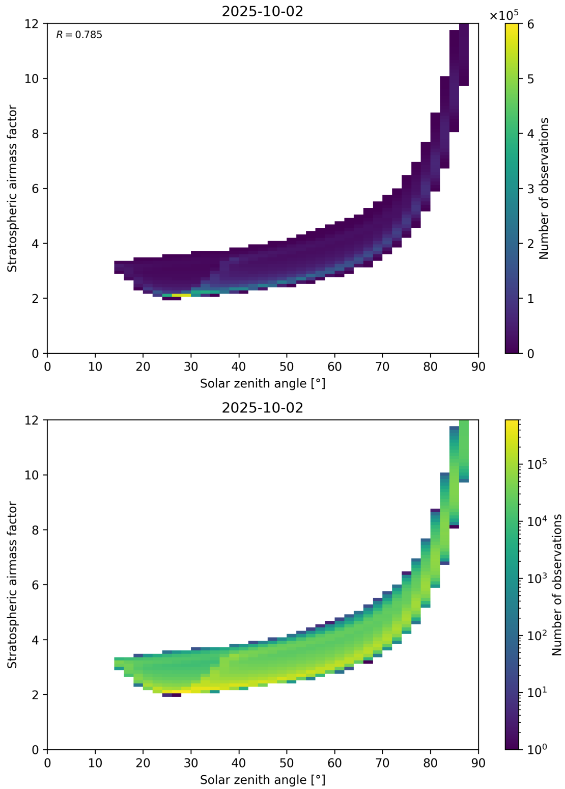
Figure 145: Scatter density plot of “Solar zenith angle” against “Stratospheric airmass factor” for 2025-10-01 to 2025-10-03.
