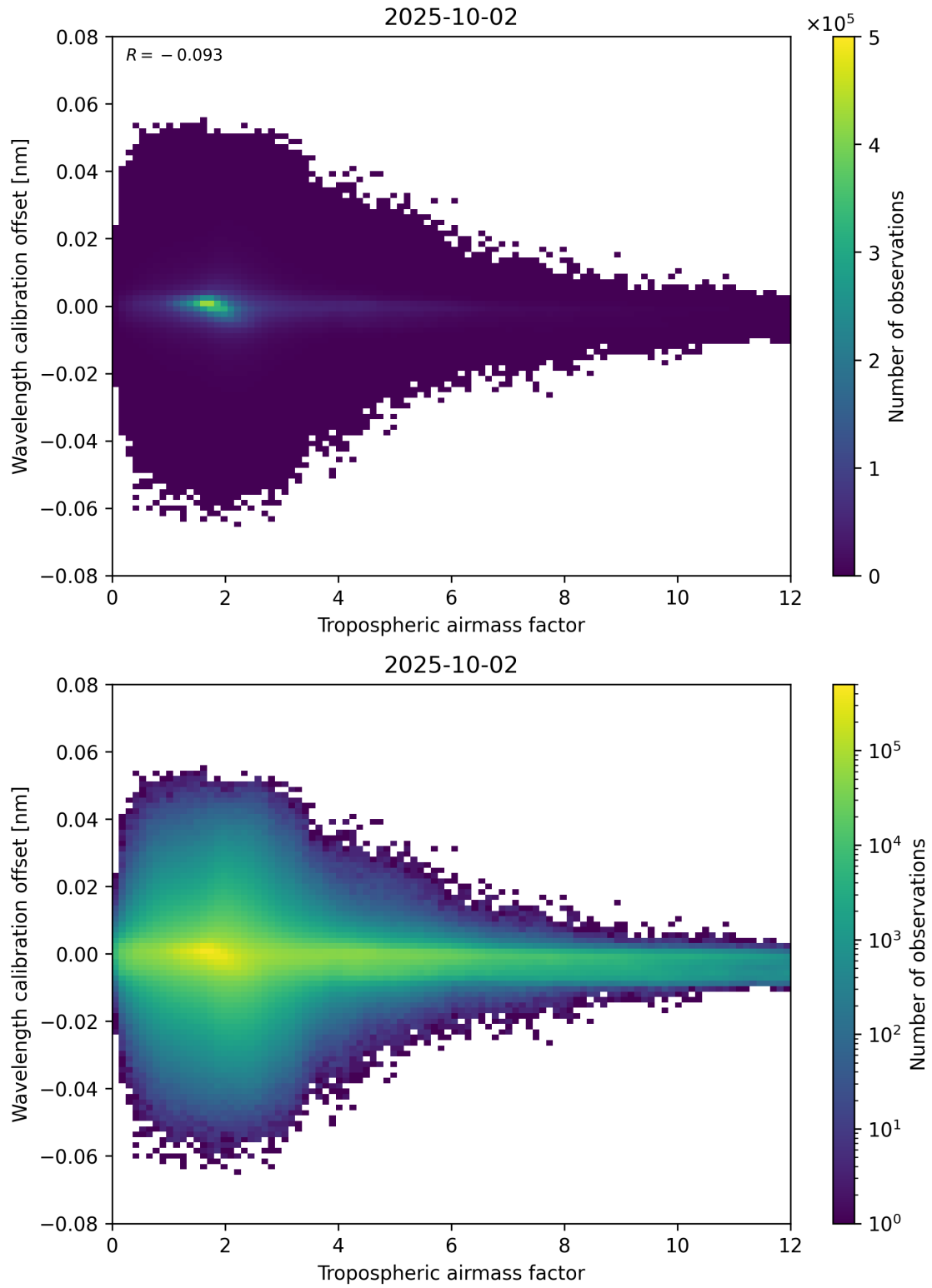
Figure 80: Scatter density plot of “Tropospheric airmass factor” against “Wavelength calibration offset” for 2025-10-01 to 2025-10-03.
