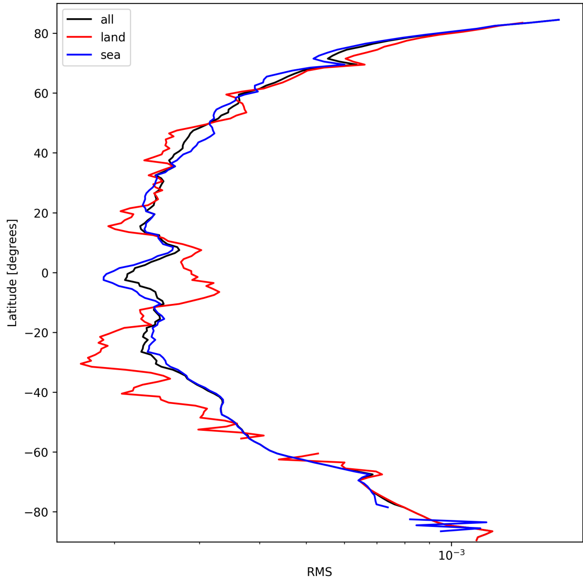
Figure 26: Zonal average of “RMS” for 2025-10-01 to 2025-10-03.
