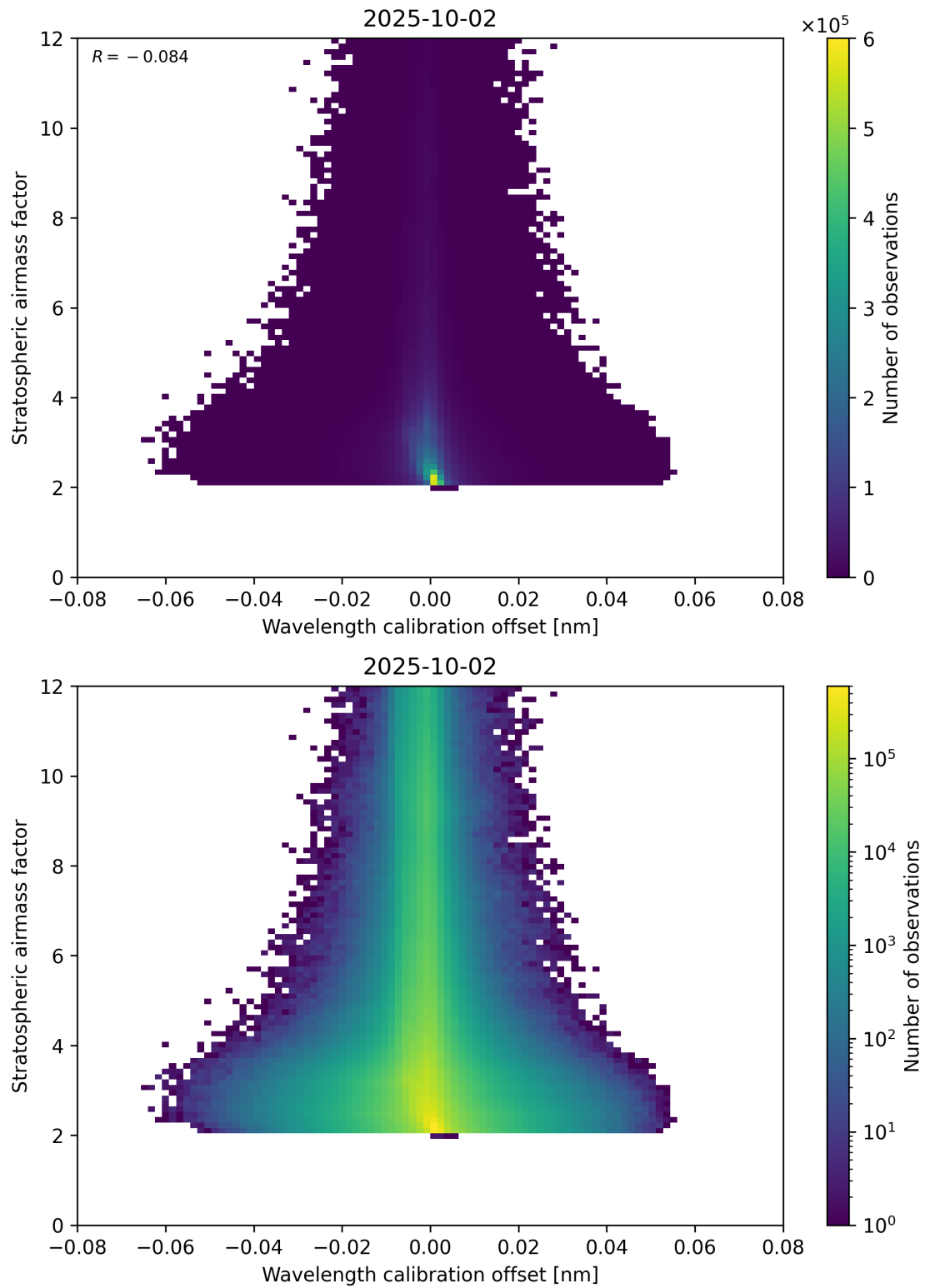
Figure 174: Scatter density plot of “Wavelength calibration offset” against “Stratospheric airmass factor” for 2025-10-01 to 2025-10-03.
