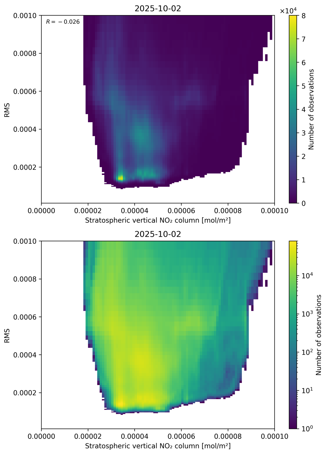
Figure 102: Scatter density plot of “Stratospheric vertical NO 2 column” against “RMS” for 2025-10-01 to 2025-10-03.
