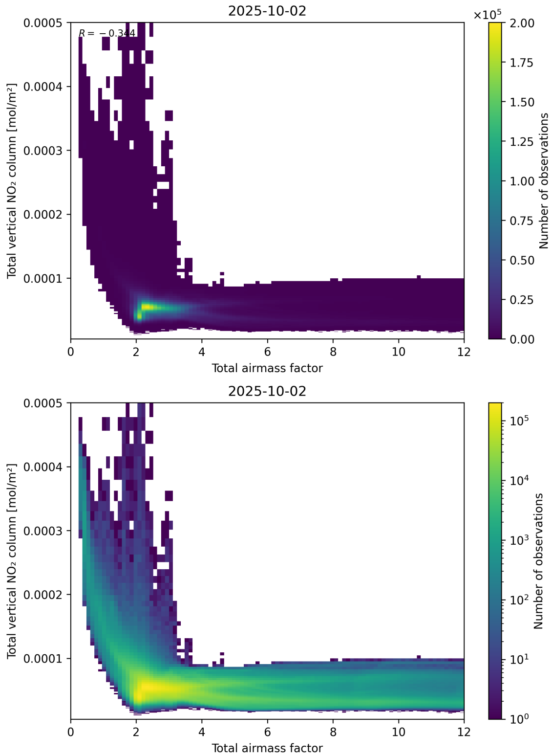
Figure 67: Scatter density plot of “Total airmass factor” against “Total vertical NO 2 column” for 2025-10-01 to 2025-10-03.
