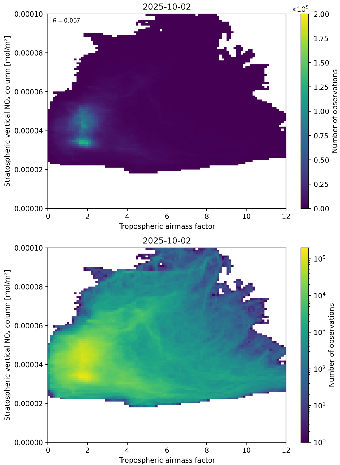
Figure 74: Scatter density plot of “Tropospheric air mass factor” against “Stratospheric vertical NO 2 column” for 2025-10-01 to 2025-10-03.
