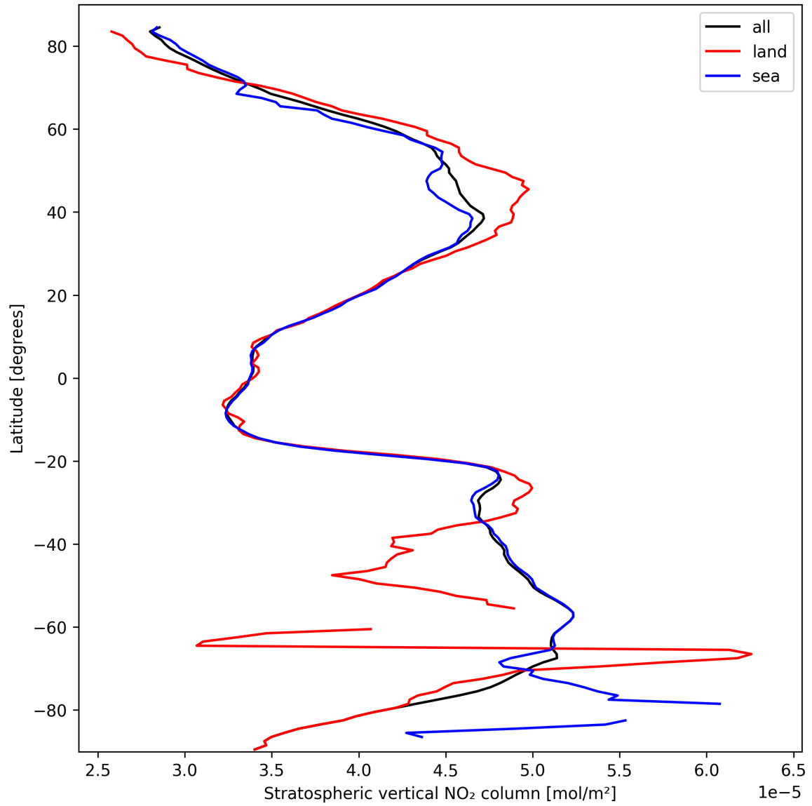
Figure 19: Zonal average of “Stratospheric vertical NO 2 column” for 2025-10-01 to 2025-10-03.
