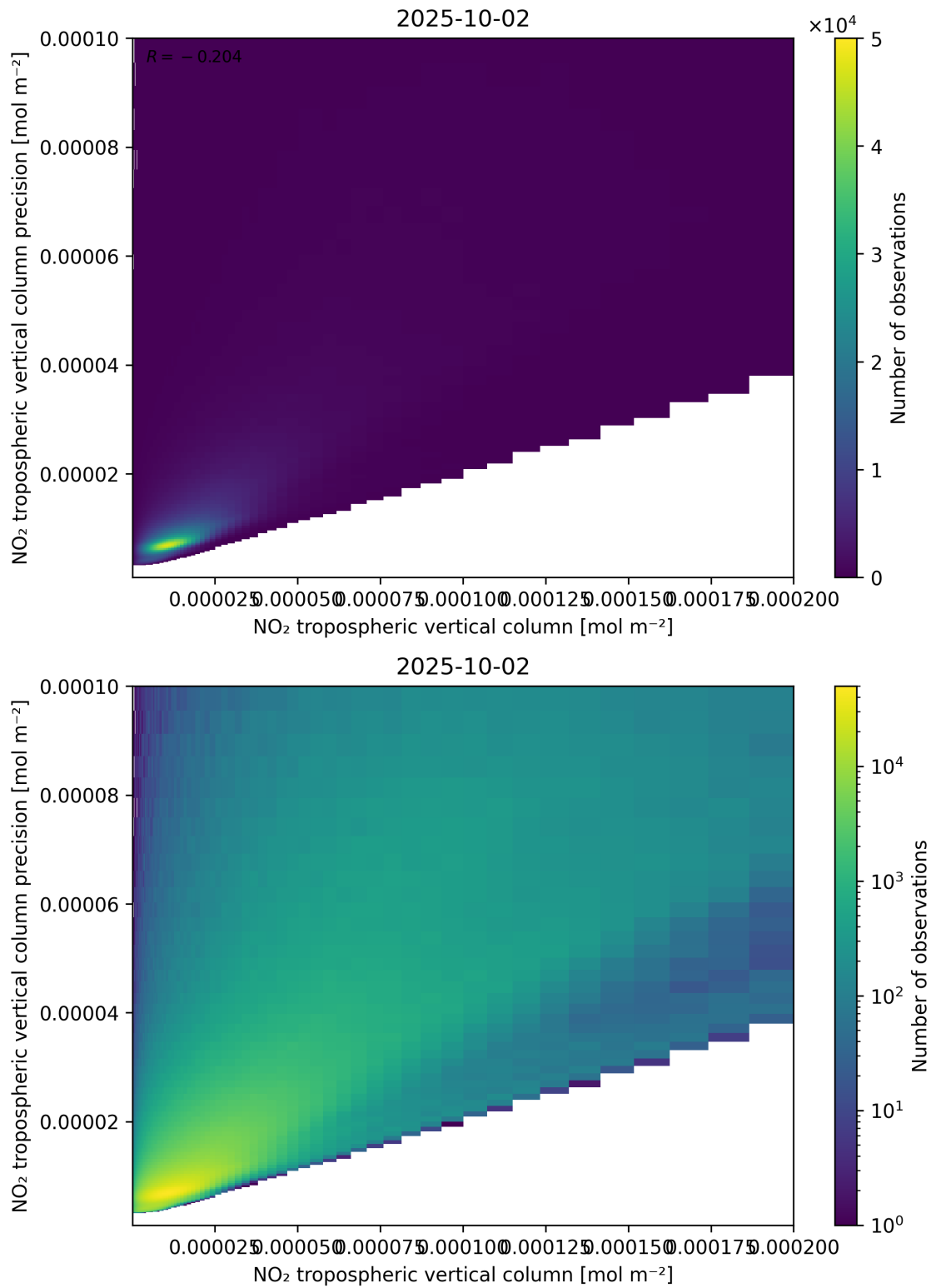
Figure 130: Scatter density plot of “NO 2 tropospheric vertical column” against “NO 2 tropospheric vertical column precision” for 2025-10-01 to 2025-10-03.
