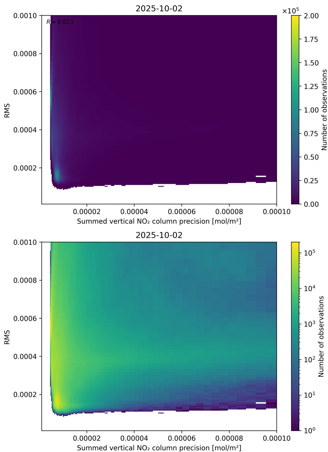
Figure 108: Scatter density plot of “Summed vertical NO 2 column precision” against “RMS” for 2025-10-01 to 2025-10-03.
