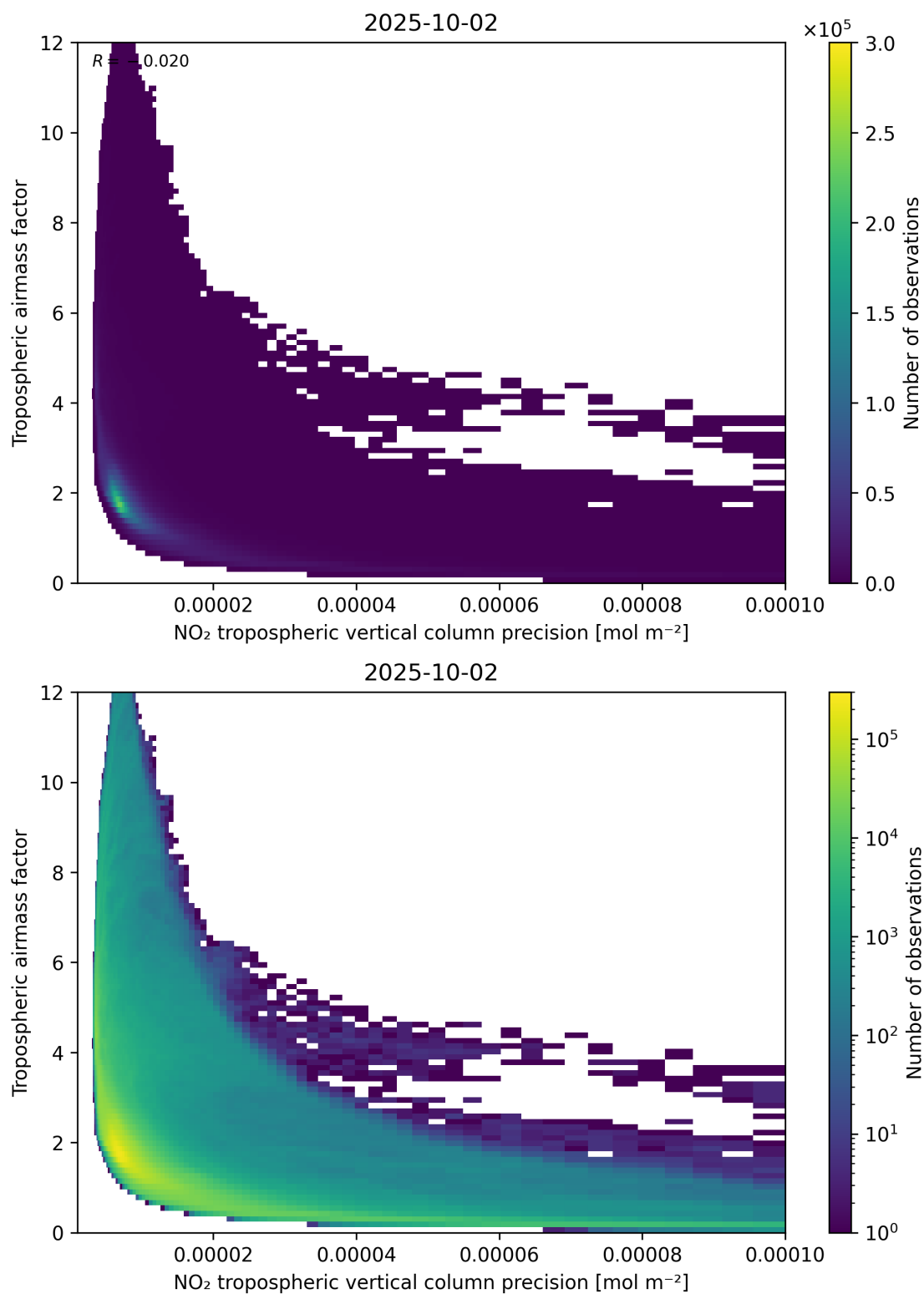
Figure 133: Scatter density plot of “NO 2 tropospheric vertical column precision” against “Tropospheric air mass factor” for 2025-10-01 to 2025-10-03.
