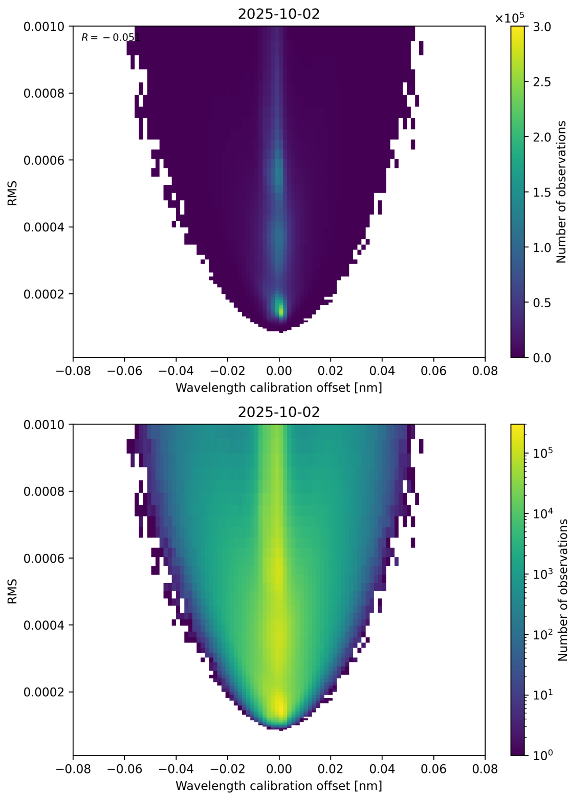
Figure 181: Scatter density plot of “Wavelength calibration offset” against “RMS” for 2025-10-01 to 2025-10-03.
