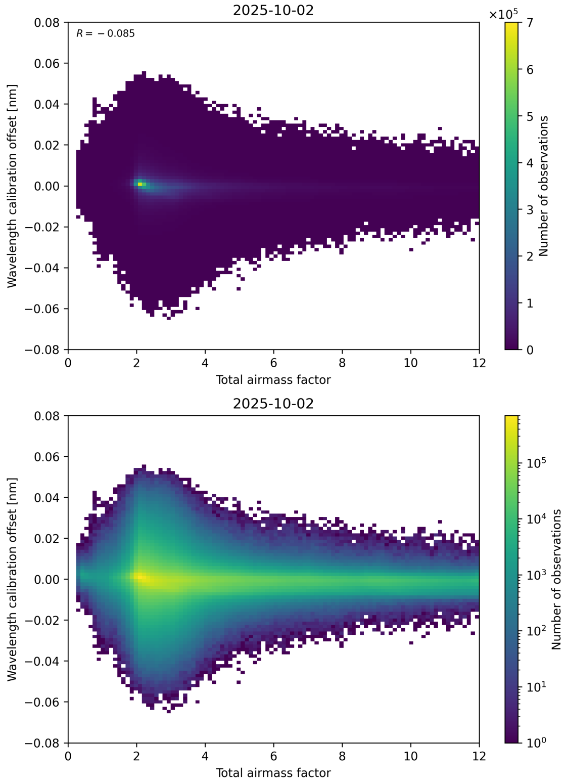
Figure 70: Scatter density plot of “Total airmass factor” against “Wavelength calibration offset” for 2025-10-01 to 2025-10-03.
