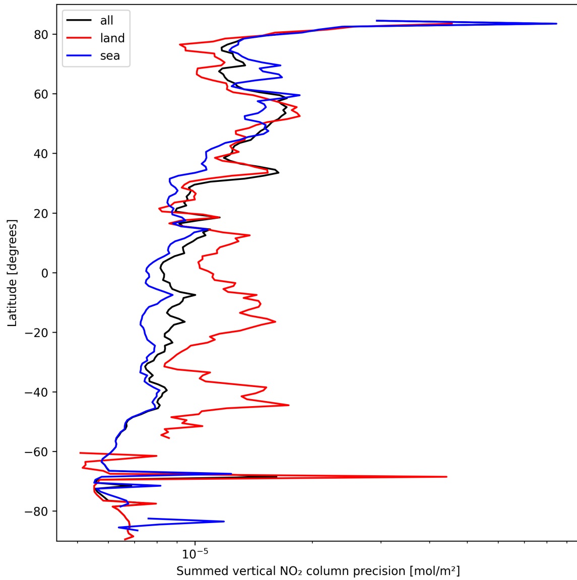
Figure 24: Zonal average of “Summed vertical NO 2 column precision” for 2025-10-01 to 2025-10-03.
