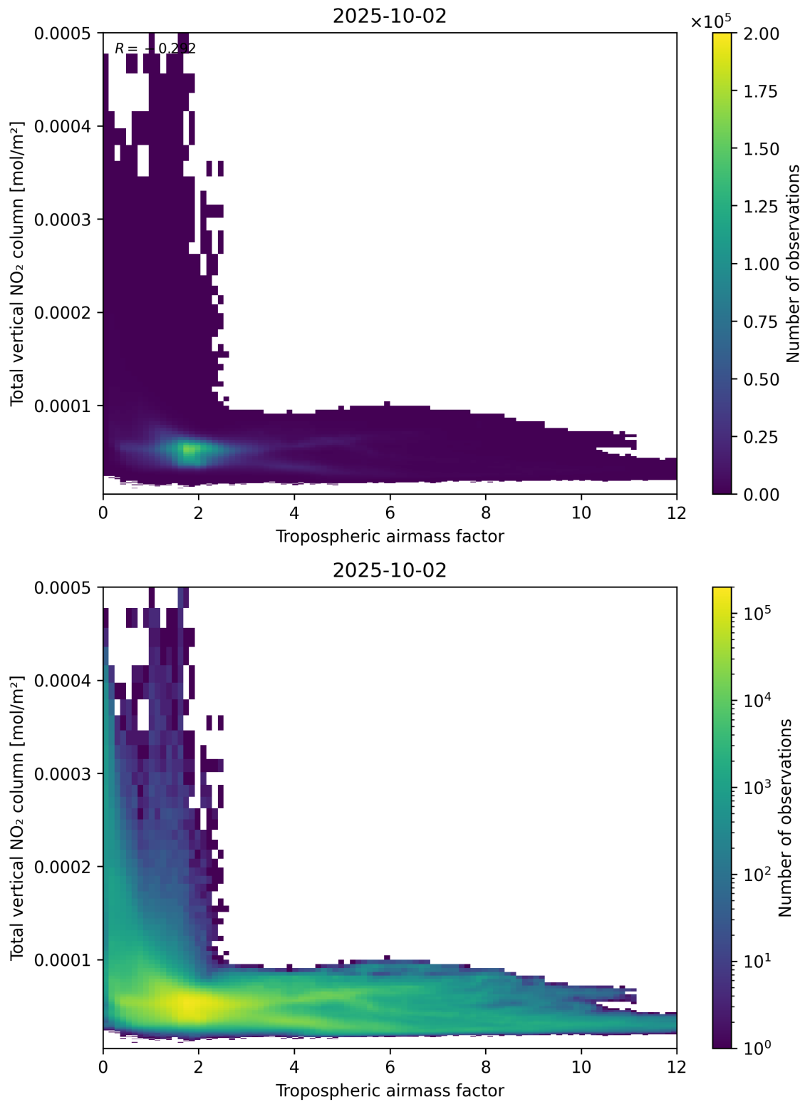
Figure 77: Scatter density plot of “Tropospheric airmass factor” against “Total vertical NO 2 column” for 2025-10-01 to 2025-10-03.
