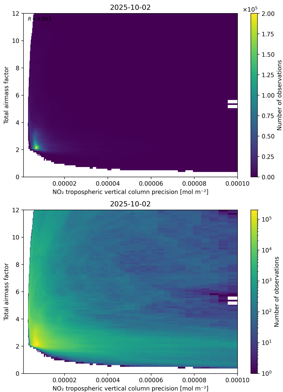
Figure 132: Scatter density plot of “NO 2 tropospheric vertical column precision” against “Total air mass factor” for 2025-10-01 to 2025-10-03.
