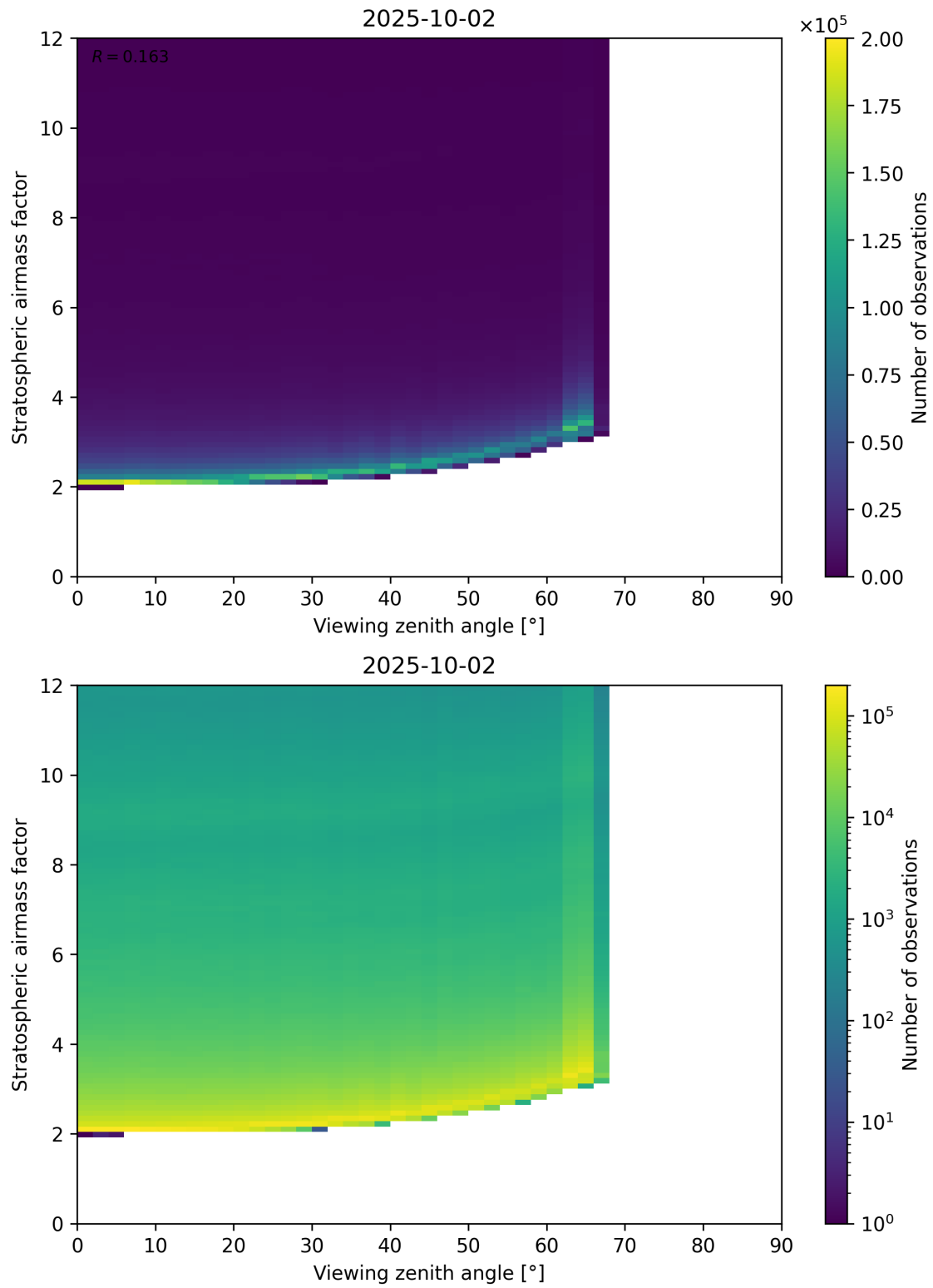
Figure 159: Scatter density plot of “Viewing zenith angle” against “Stratospheric airmass factor” for 2025-10-01 to 2025-10-03.
