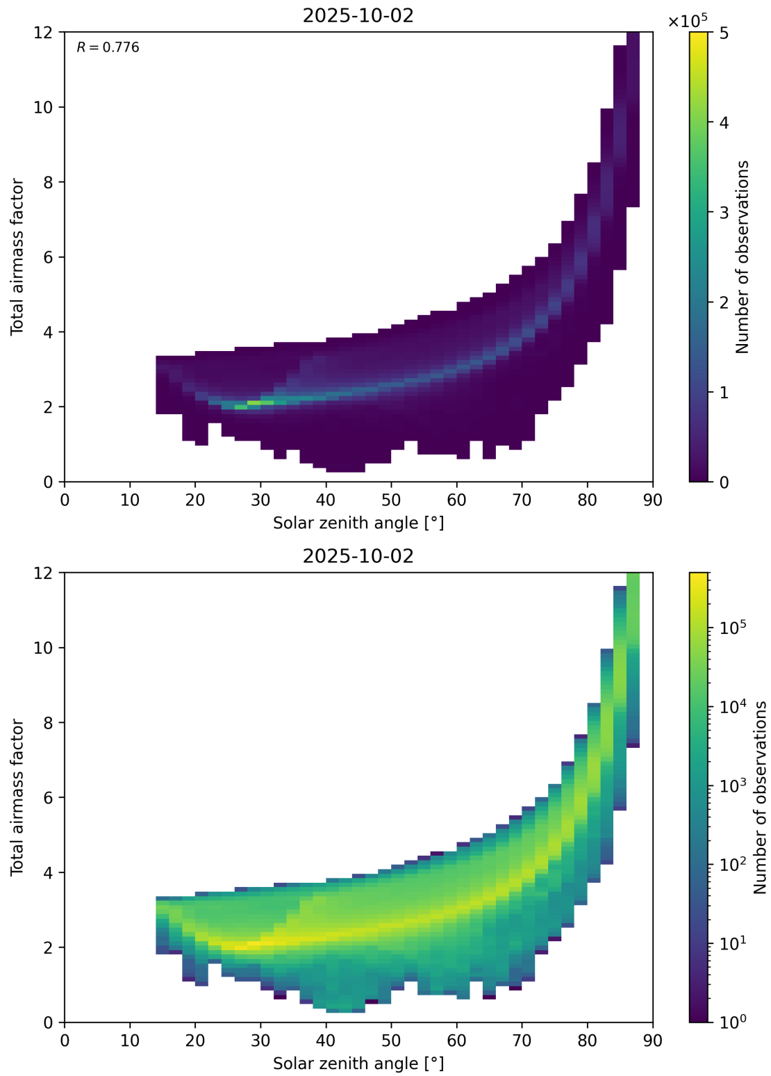
Figure 146: Scatter density plot of “Solar zenith angle” against “Total airmass factor” for 2025-10-01 to 2025-10-03.
