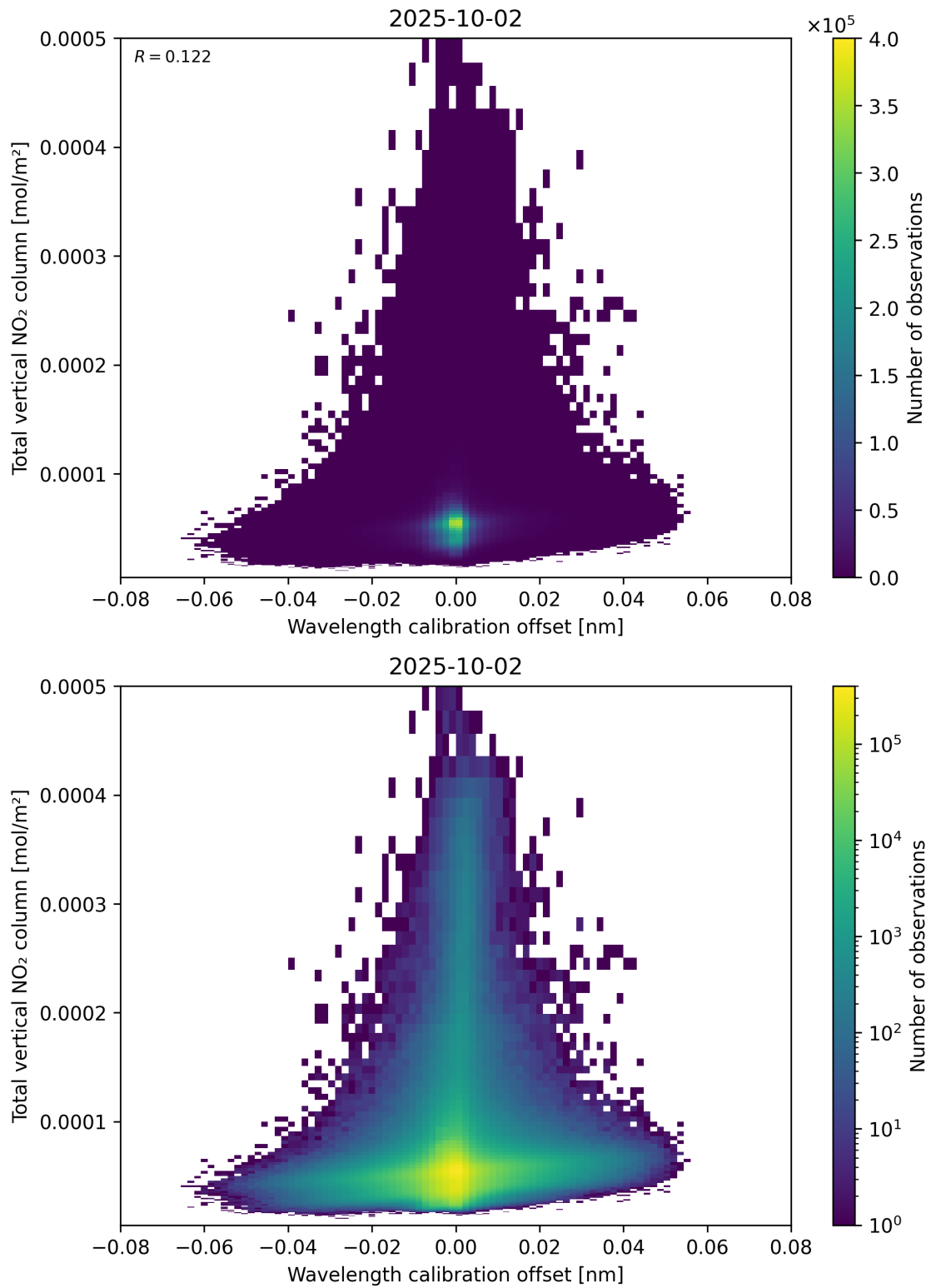
Figure 179: Scatter density plot of “Wavelength calibration offset” against “Total vertical NO 2 column” for 2025-10-01 to 2025-10-03.
