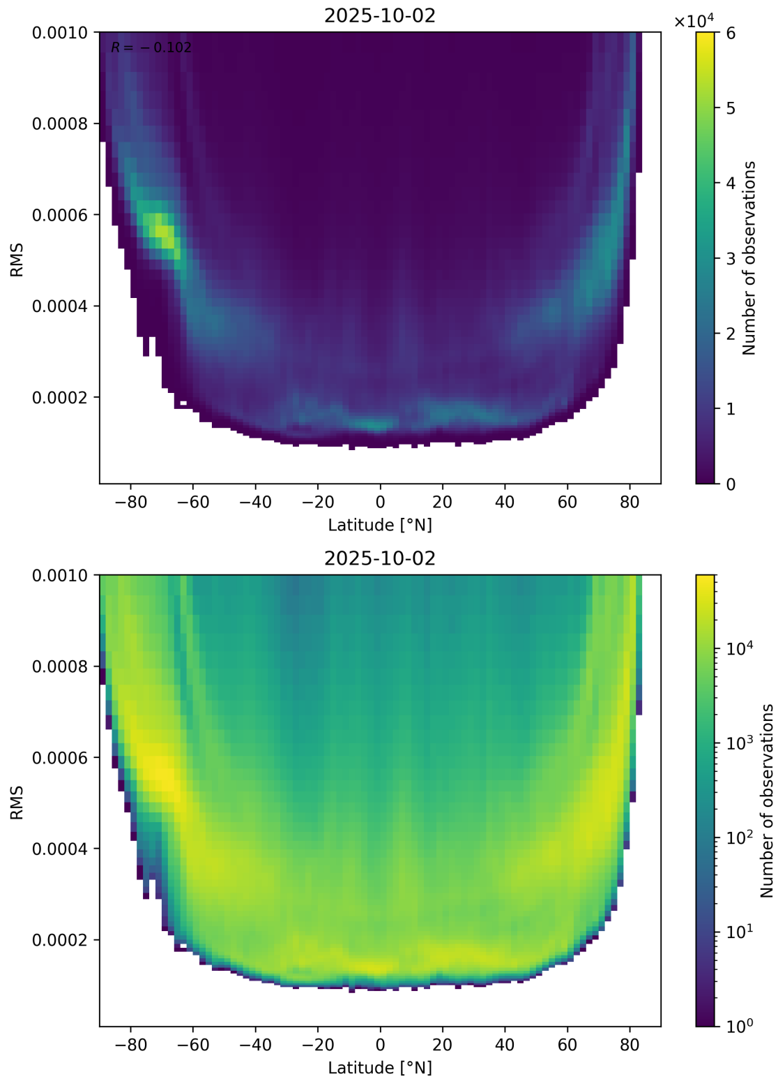
Figure 94: Scatter density plot of “Latitude” against “RMS” for 2025-10-01 to 2025-10-03.
