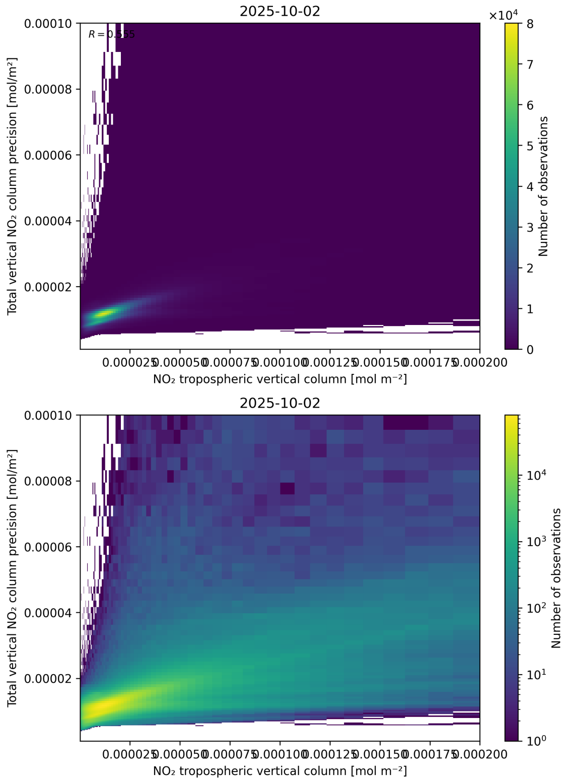
Figure 129: Scatter density plot of “NO 2 tropospheric vertical column” against “Total vertical NO 2 column precision” for 2025-10-01 to 2025-10-03.
