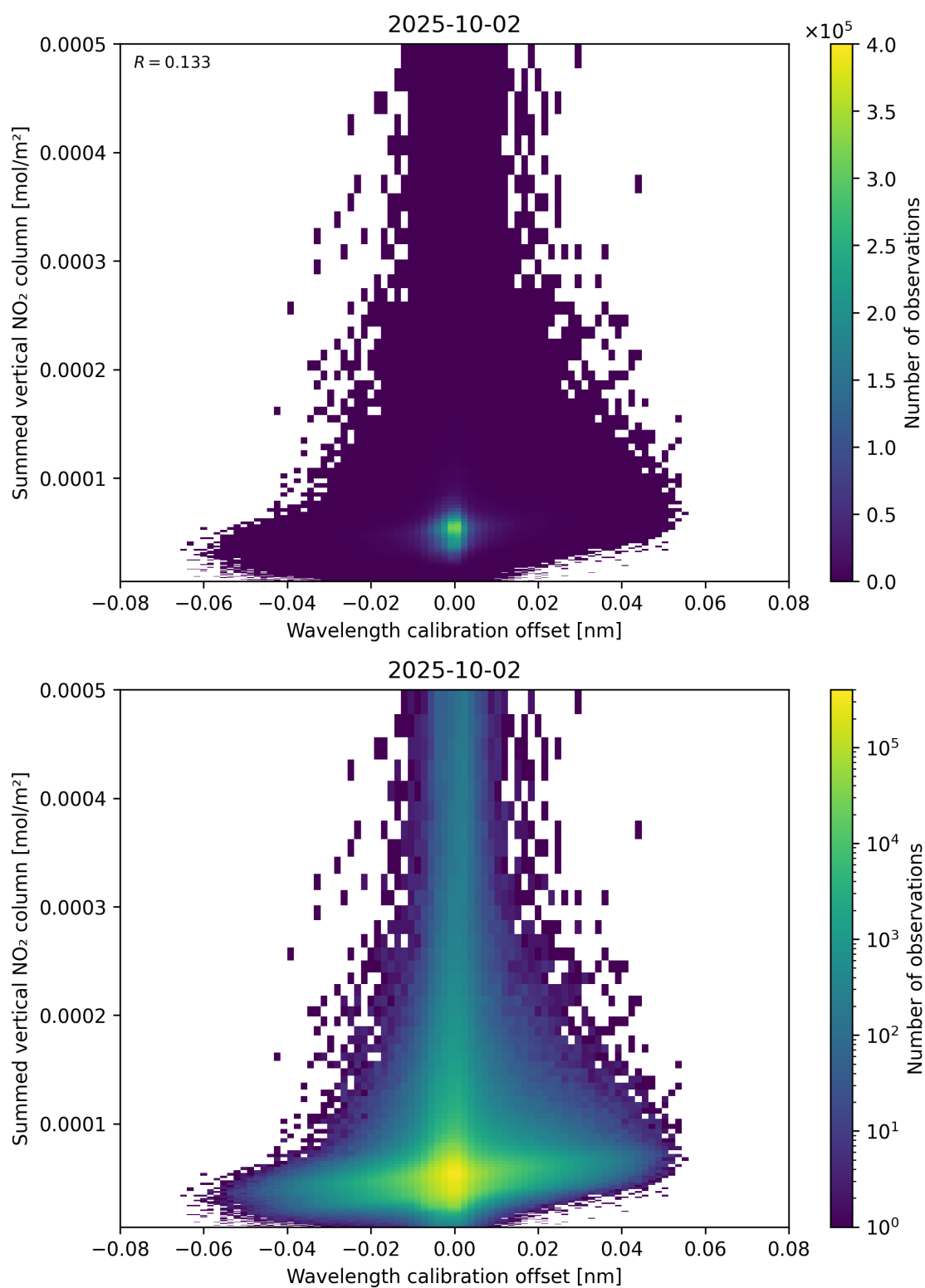
Figure 177: Scatter density plot of “Wavelength calibration offset” against “Summed vertical NO 2 column” for 2025-10-01 to 2025-10-03.
