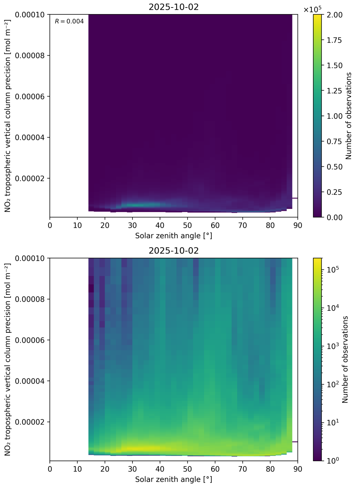
Figure 156: Scatter density plot of “Solar zenith angle” against “NO 2 tropospheric vertical column precision” for 2025-10-01 to 2025-10-03.
