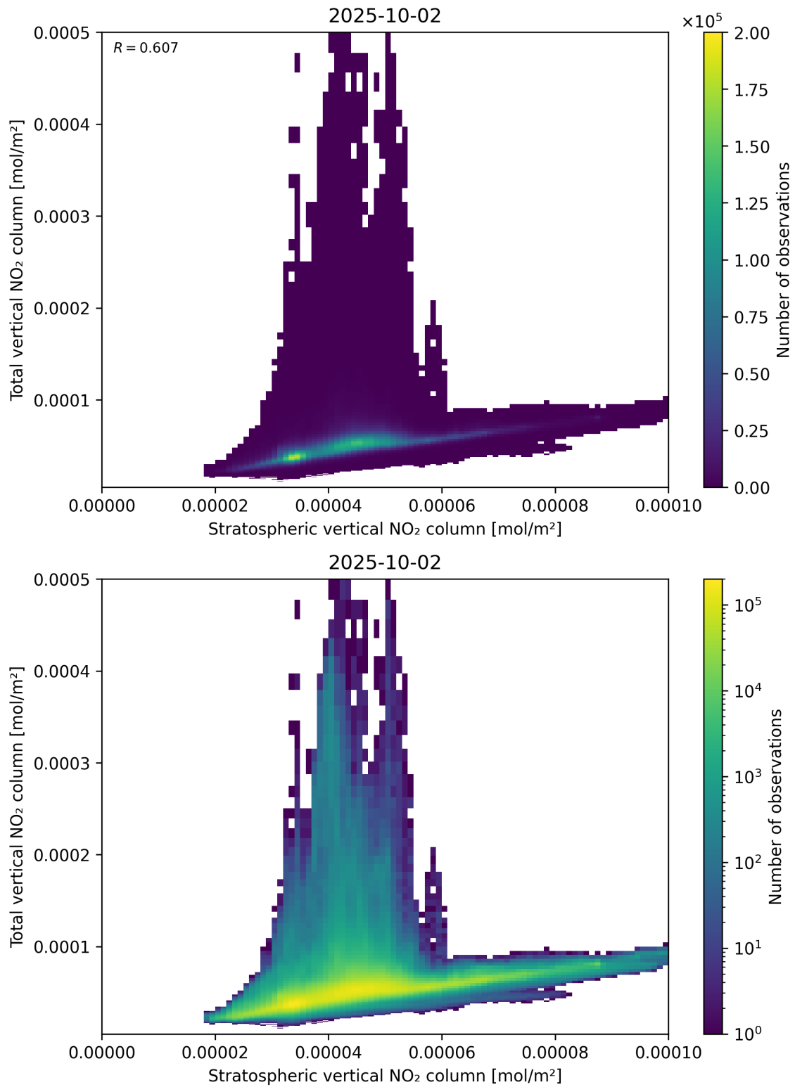
Figure 100: Scatter density plot of “Stratospheric vertical NO 2 column” against “Total vertical NO 2 column” for 2025-10-01 to 2025-10-03.
