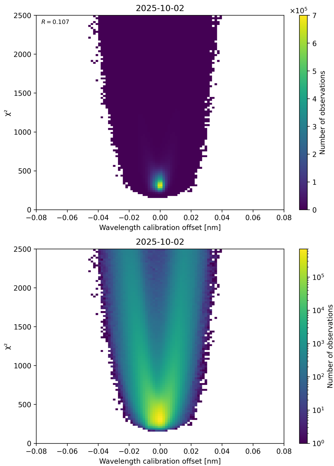
Figure 175: Scatter density plot of “Wavelength calibration offset” against “ \chi^2 ” for 2025-10-01 to 2025-10-03.
