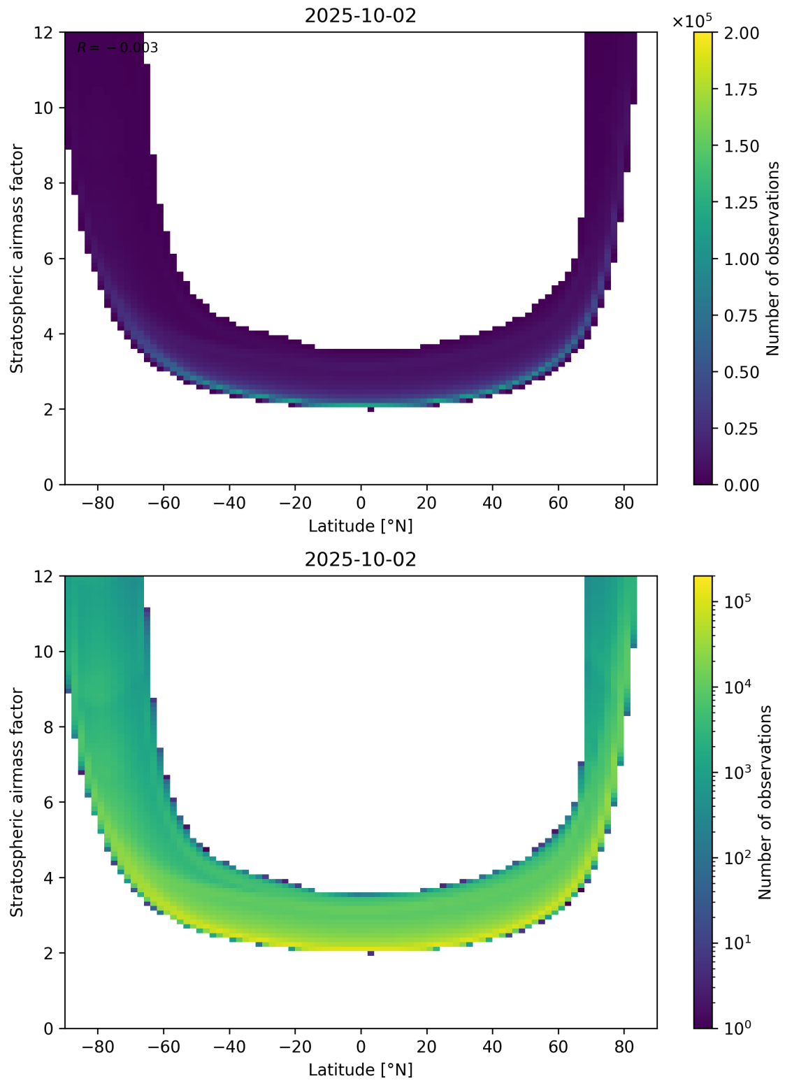
Figure 83: Scatter density plot of “Latitude” against “Stratospheric air mass factor” for 2025-10-01 to 2025-10-03.
