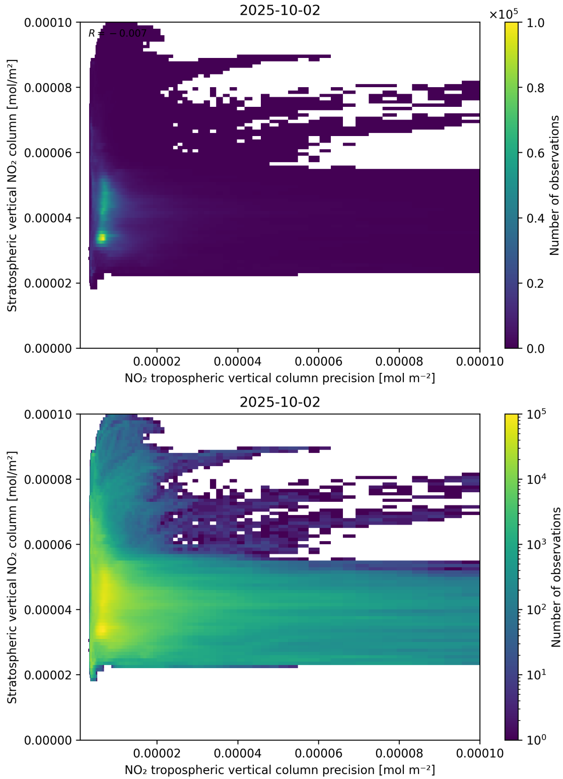
Figure 135: Scatter density plot of “NO 2 tropospheric vertical column precision” against “Stratospheric vertical NO 2 column” for 2025-10-01 to 2025-10-03.
