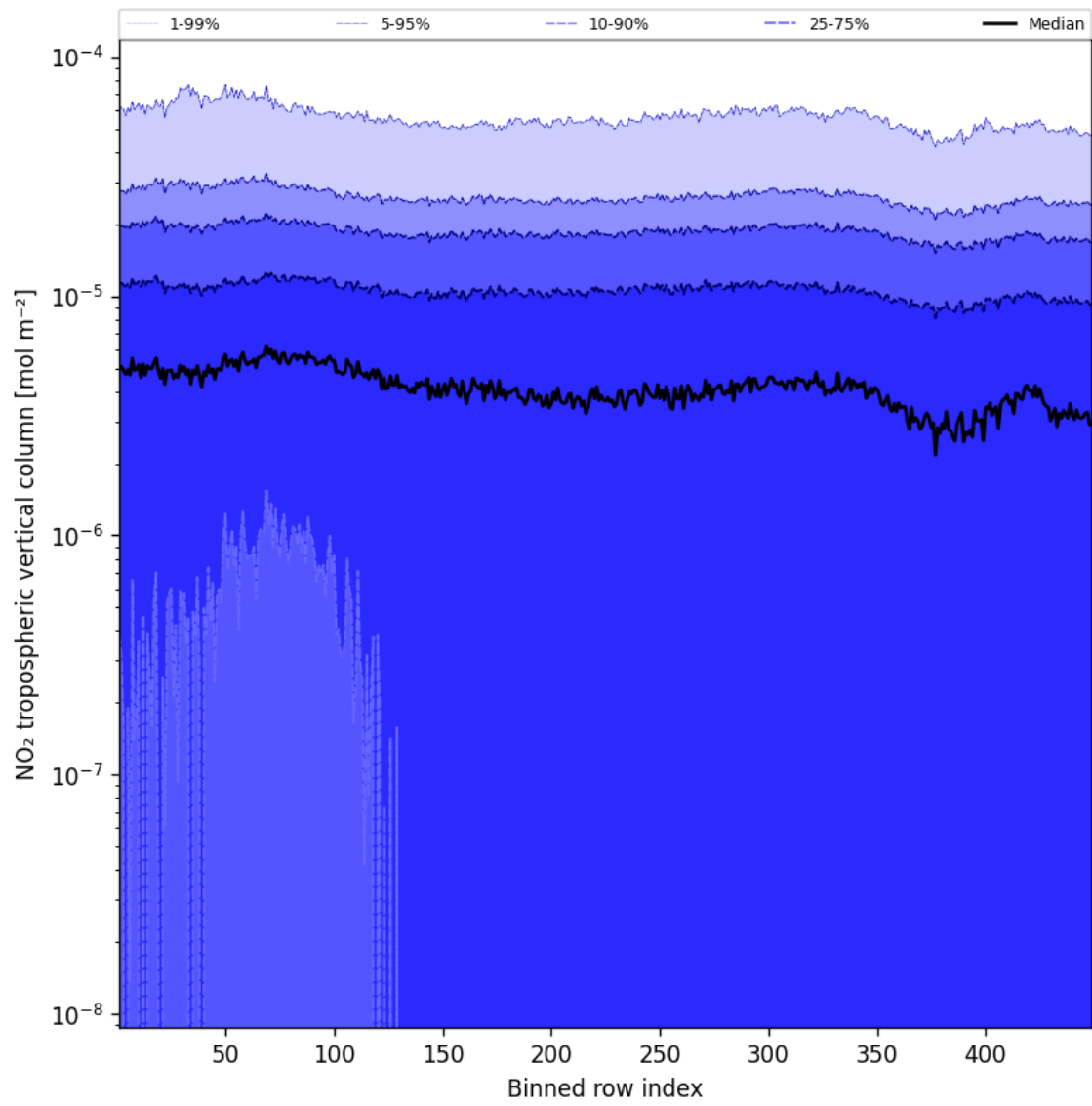
Figure 46: Along track statistics of “NO 2 tropospheric vertical column” for 2025-10-01 to 2025-10-03
