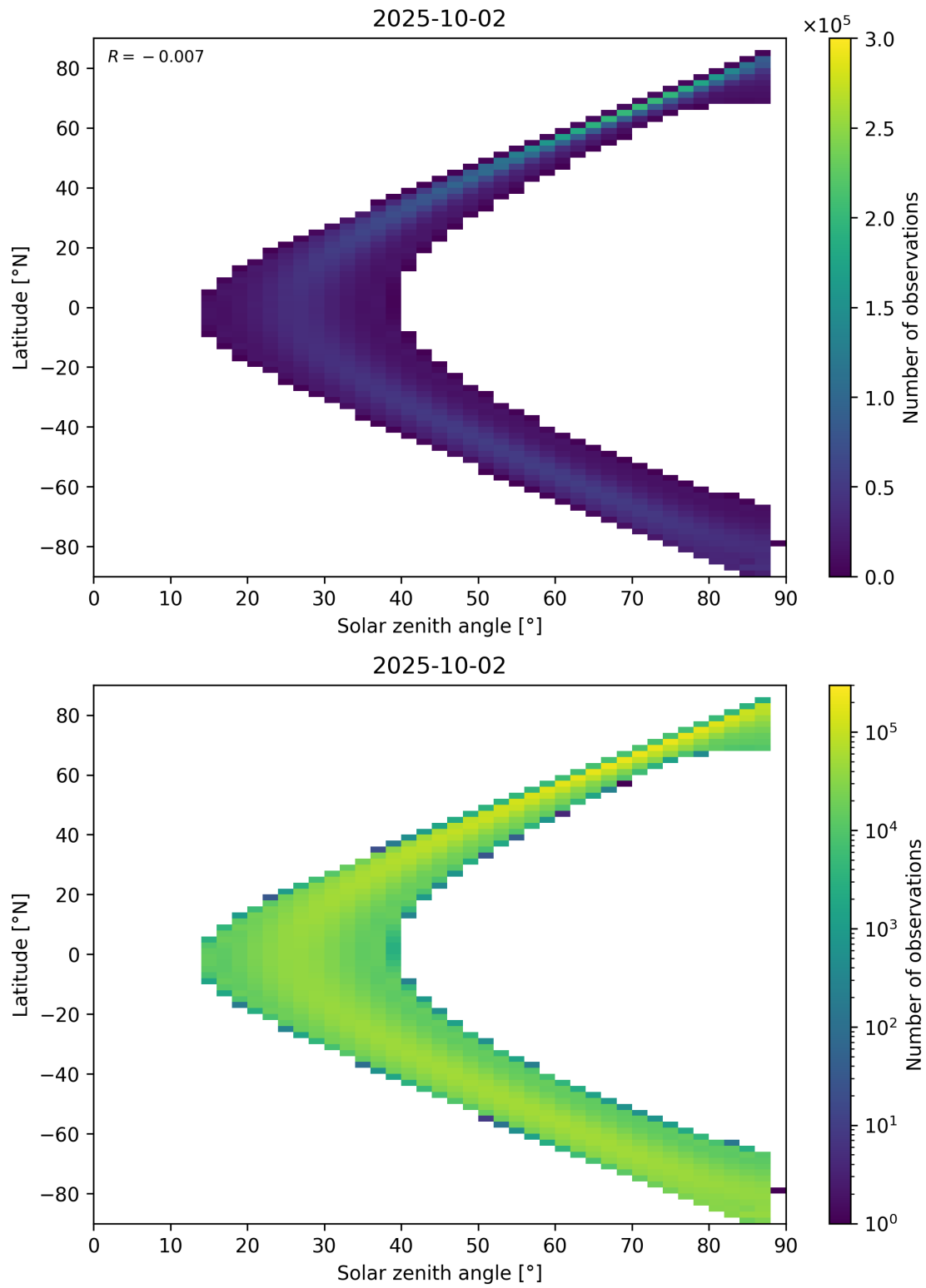
Figure 149: Scatter density plot of “Solar zenith angle” against “Latitude” for 2025-10-01 to 2025-10-03.
