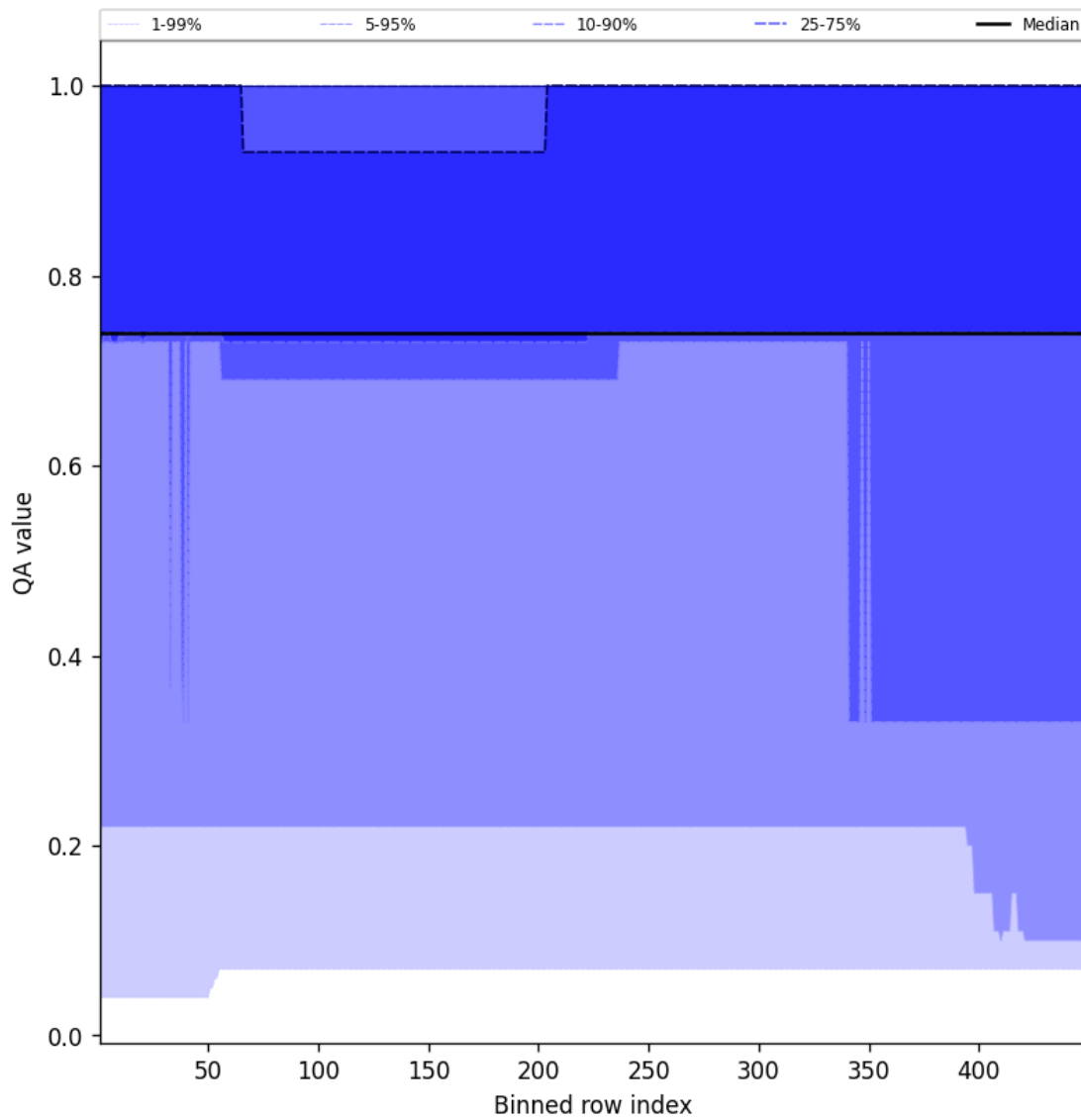
Figure 45: Along track statistics of “QA value” for 2025-10-01 to 2025-10-03
