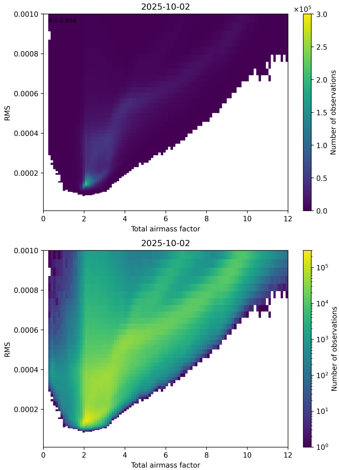
Figure 69: Scatter density plot of “Total airmass factor” against “RMS” for 2025-10-01 to 2025-10-03.
