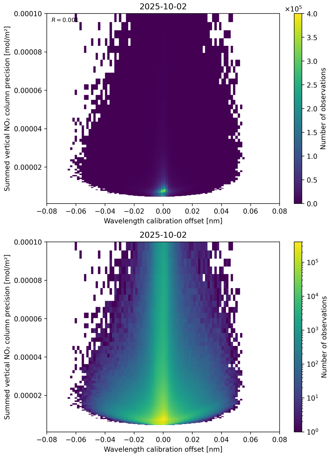
Figure 178: Scatter density plot of “Wavelength calibration offset” against “Summed vertical NO 2 column precision” for 2025-10-01 to 2025-10-03.
