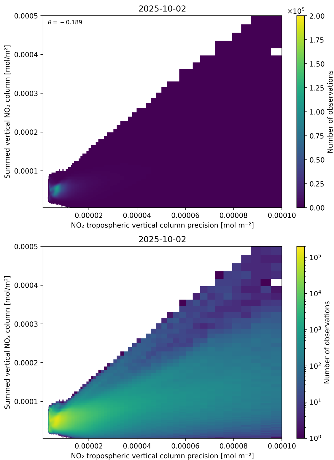
Figure 136: Scatter density plot of “NO 2 tropospheric vertical column precision” against “Summed vertical NO 2 column” for 2025-10-01 to 2025-10-03.
