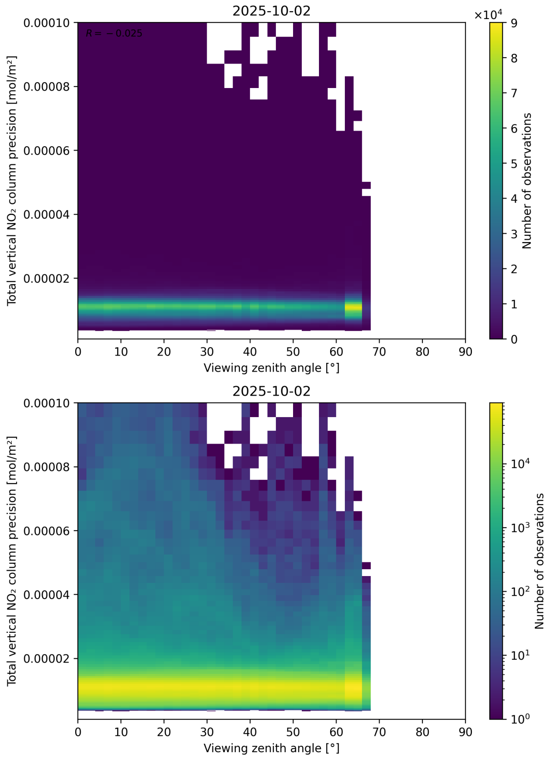
Figure 168: Scatter density plot of “Viewing zenith angle” against “Total vertical NO 2 column precision” for 2025-10-01 to 2025-10-03.
