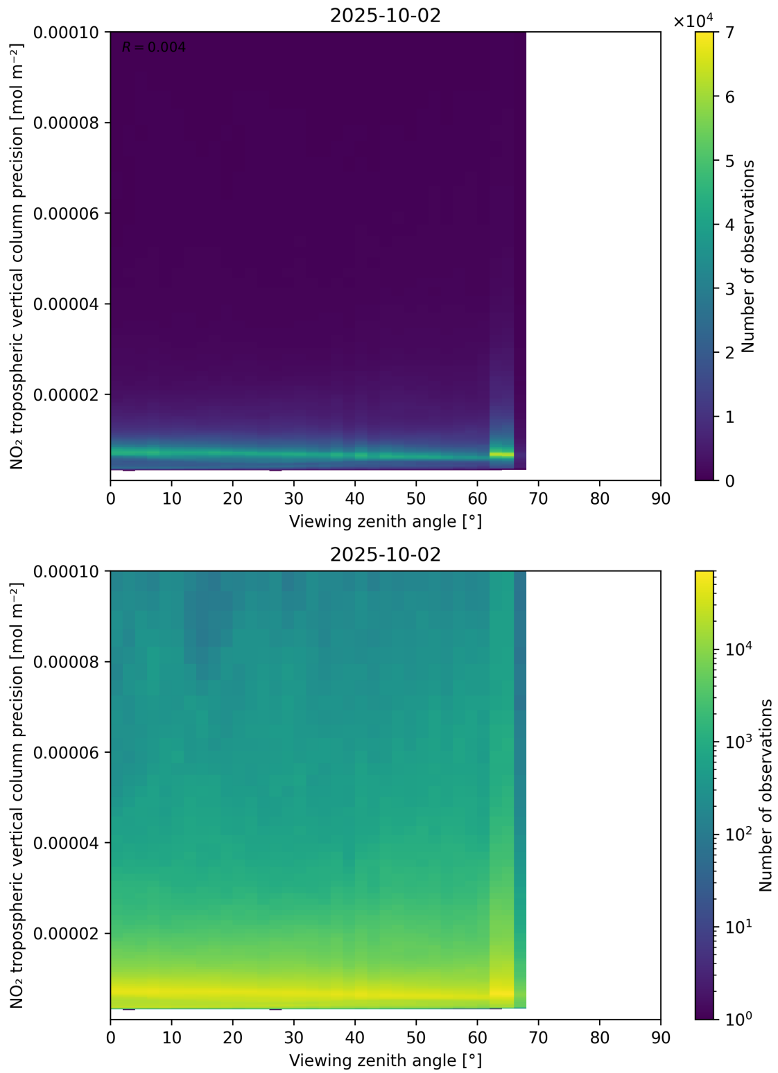
Figure 170: Scatter density plot of “Viewing zenith angle” against “NO 2 tropospheric vertical column precision” for 2025-10-01 to 2025-10-03.
