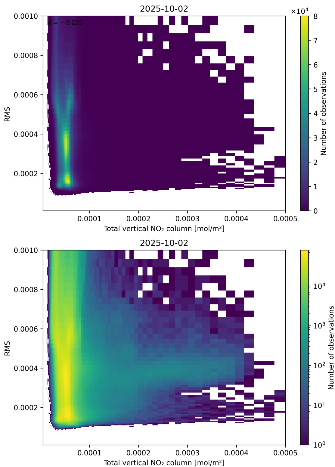
Figure 120: Scatter density plot of “Total vertical NO 2 column” against “RMS” for 2025-10-01 to 2025-10-03.
