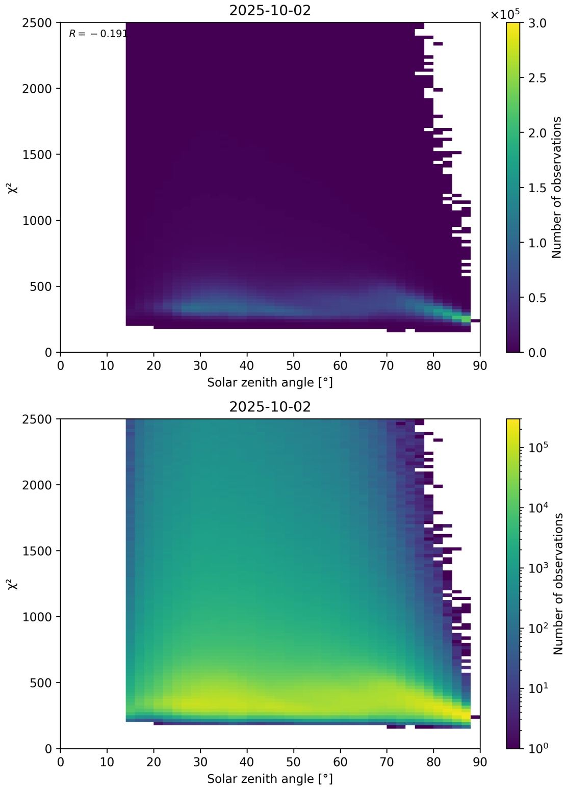
Figure 148: Scatter density plot of “Solar zenith angle” against “ \chi^2 ” for 2025-10-01 to 2025-10-03.
