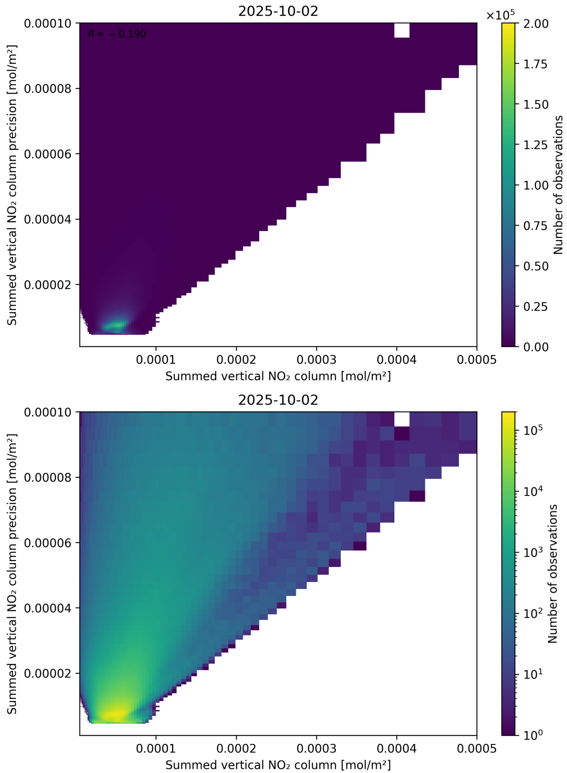
Figure 105: Scatter density plot of “Summed vertical NO 2 column” against “Summed vertical NO 2 column precision” for 2025-10-01 to 2025-10-03.
