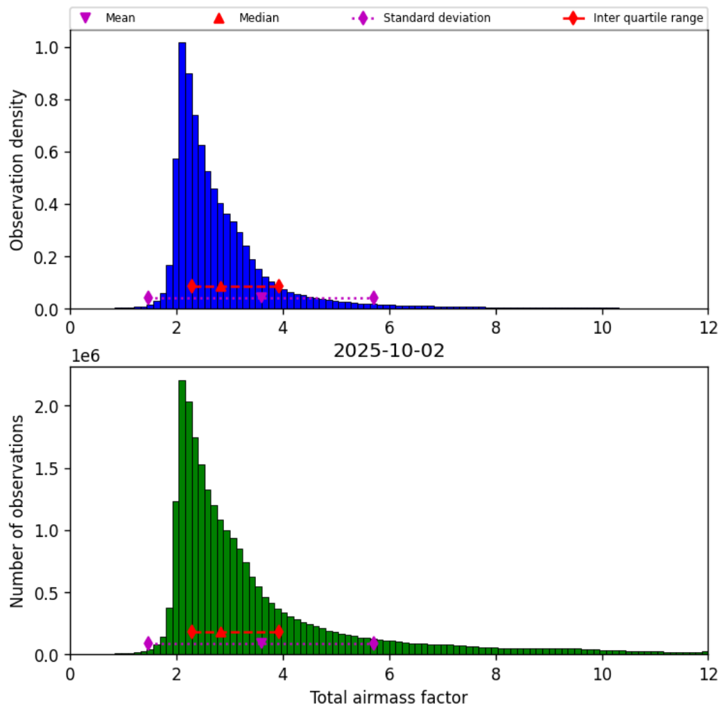
Figure 32: Histogram of “Total airmass factor” for 2025-10-01 to 2025-10-03
