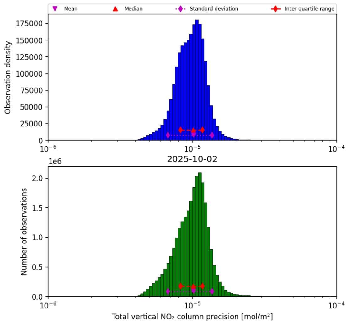
Figure 39: Histogram of "Total vertical NO 2 column precision" for 2025-10-01 to 2025-10-03
