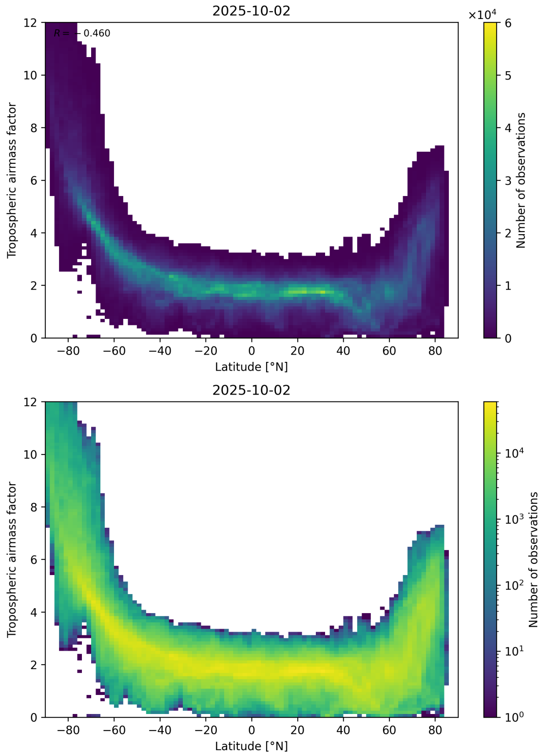
Figure 85: Scatter density plot of “Latitude” against “Tropospheric airmass factor” for 2025-10-01 to 2025-10-03.
