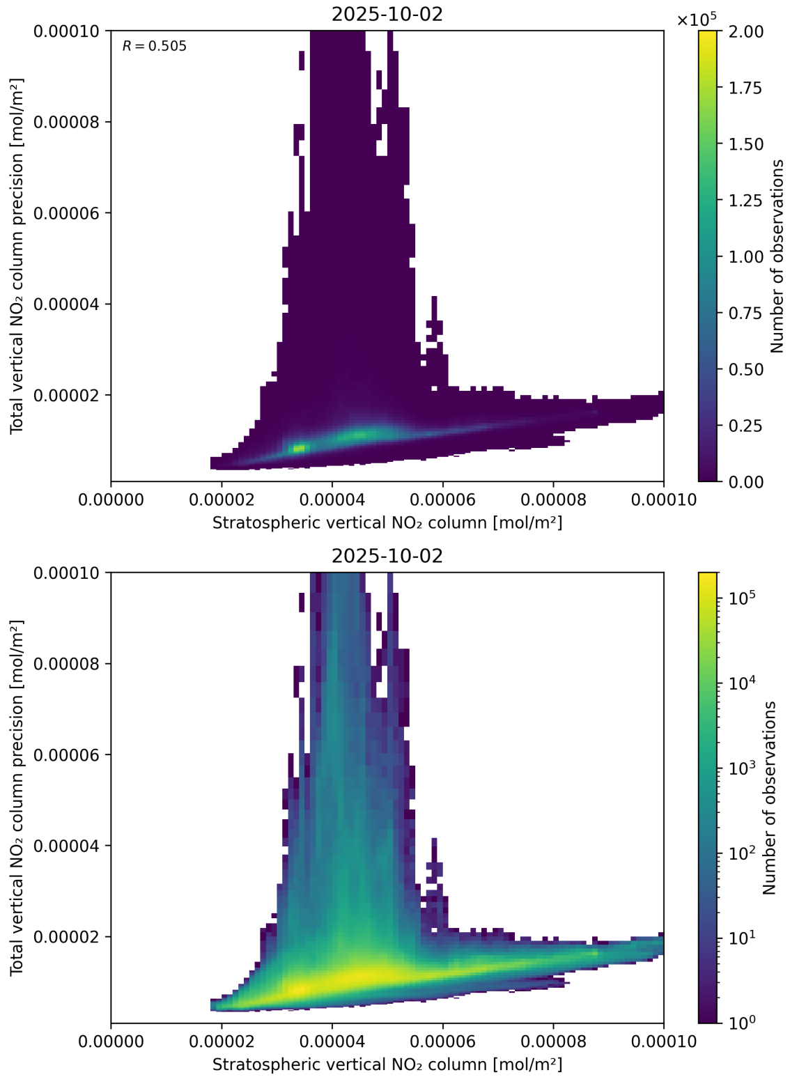
Figure 101: Scatter density plot of “Stratospheric vertical NO 2 column” against “Total vertical NO 2 column precision” for 2025-10-01 to 2025-10-03.
