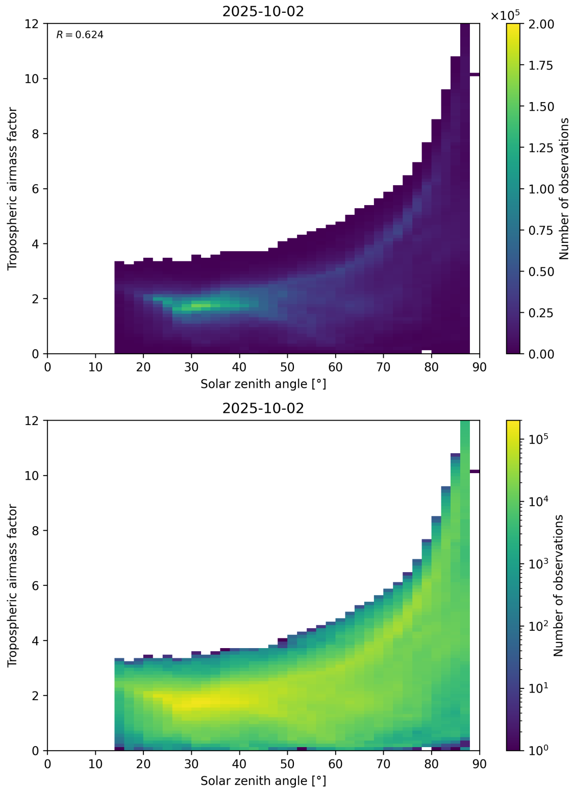
Figure 147: Scatter density plot of “Solar zenith angle” against “Tropospheric airmass factor” for 2025-10-01 to 2025-10-03.
