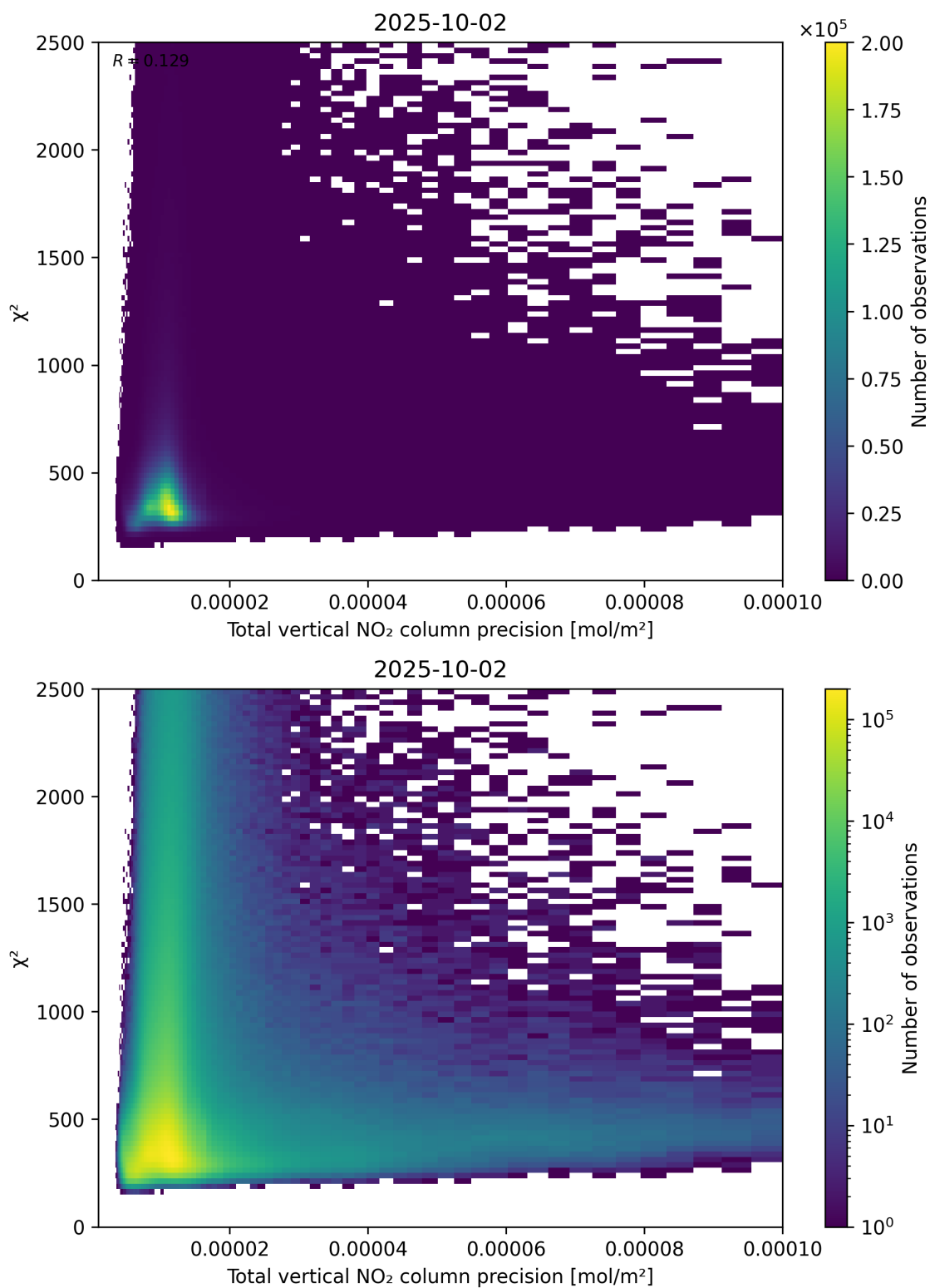
Figure 116: Scatter density plot of “Total vertical NO 2 column precision” against “ \chi^2 ” for 2025-10-01 to 2025-10-03.
