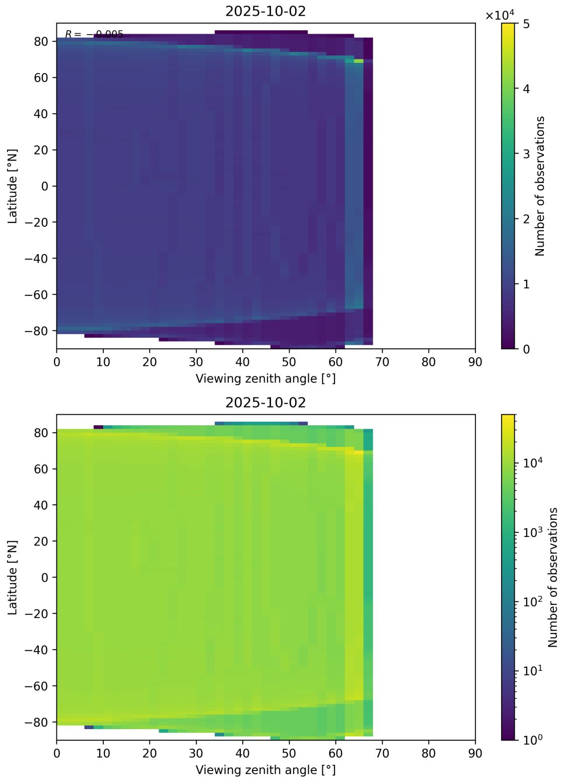
Figure 163: Scatter density plot of “Viewing zenith angle” against “Latitude” for 2025-10-01 to 2025-10-03.
