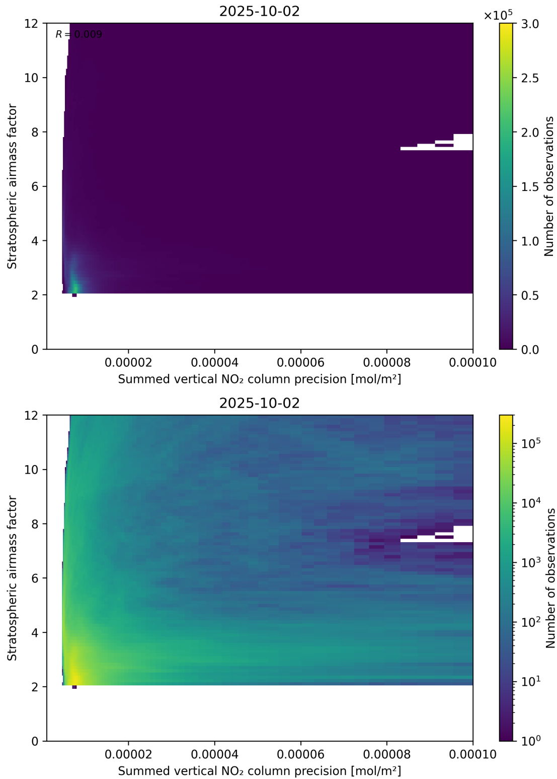
Figure 106: Scatter density plot of “Summed vertical NO 2 column precision” against “Stratospheric airmass factor” for 2025-10-01 to 2025-10-03.
