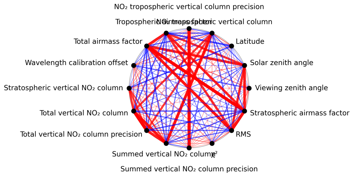
Figure 1: Map of correlation graph for 2025-10-01 to 2025-10-03.
