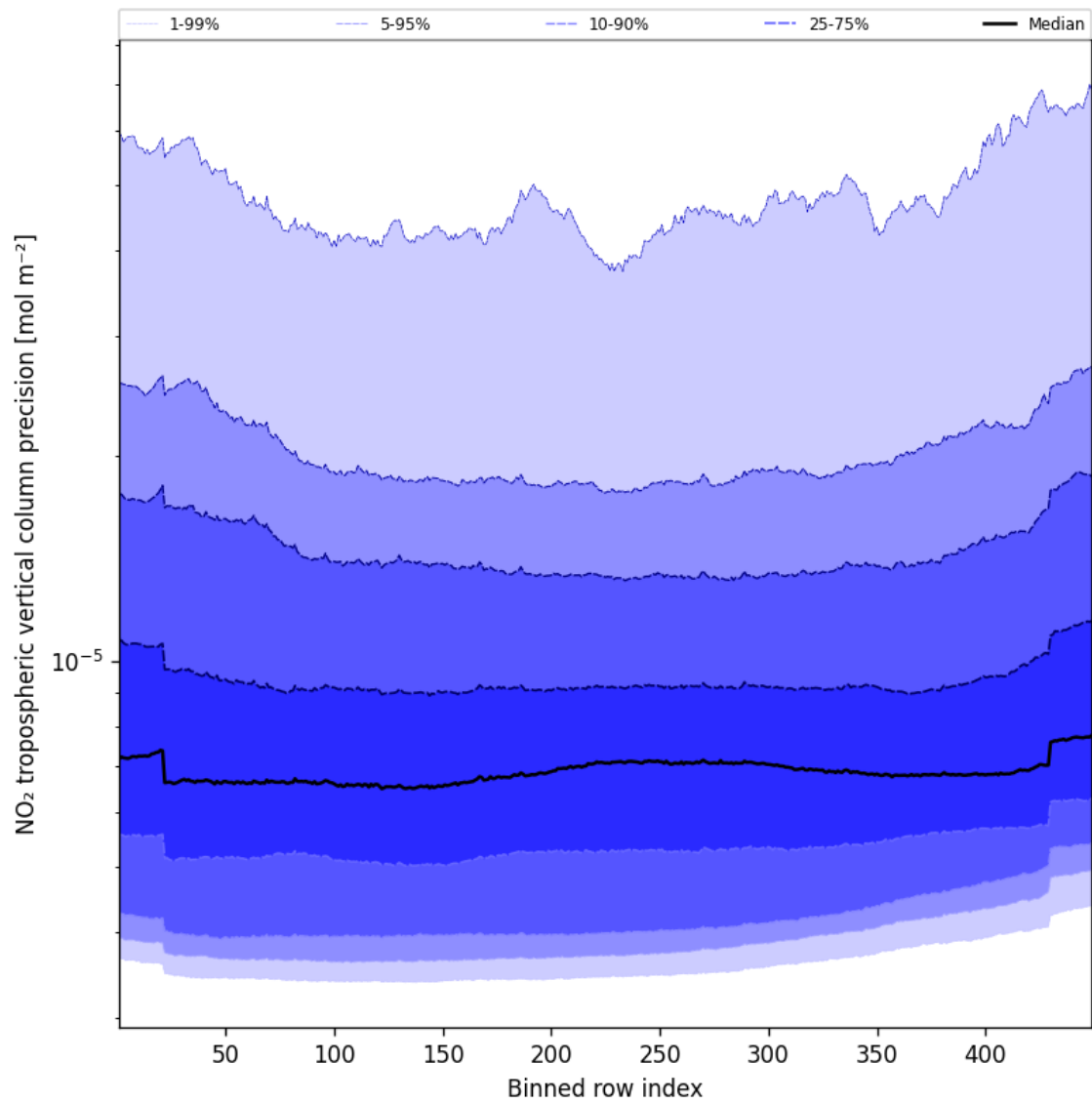
Figure 47: Along track statistics of “NO 2 tropospheric vertical column precision” for 2025-10-01 to 2025-10-03
