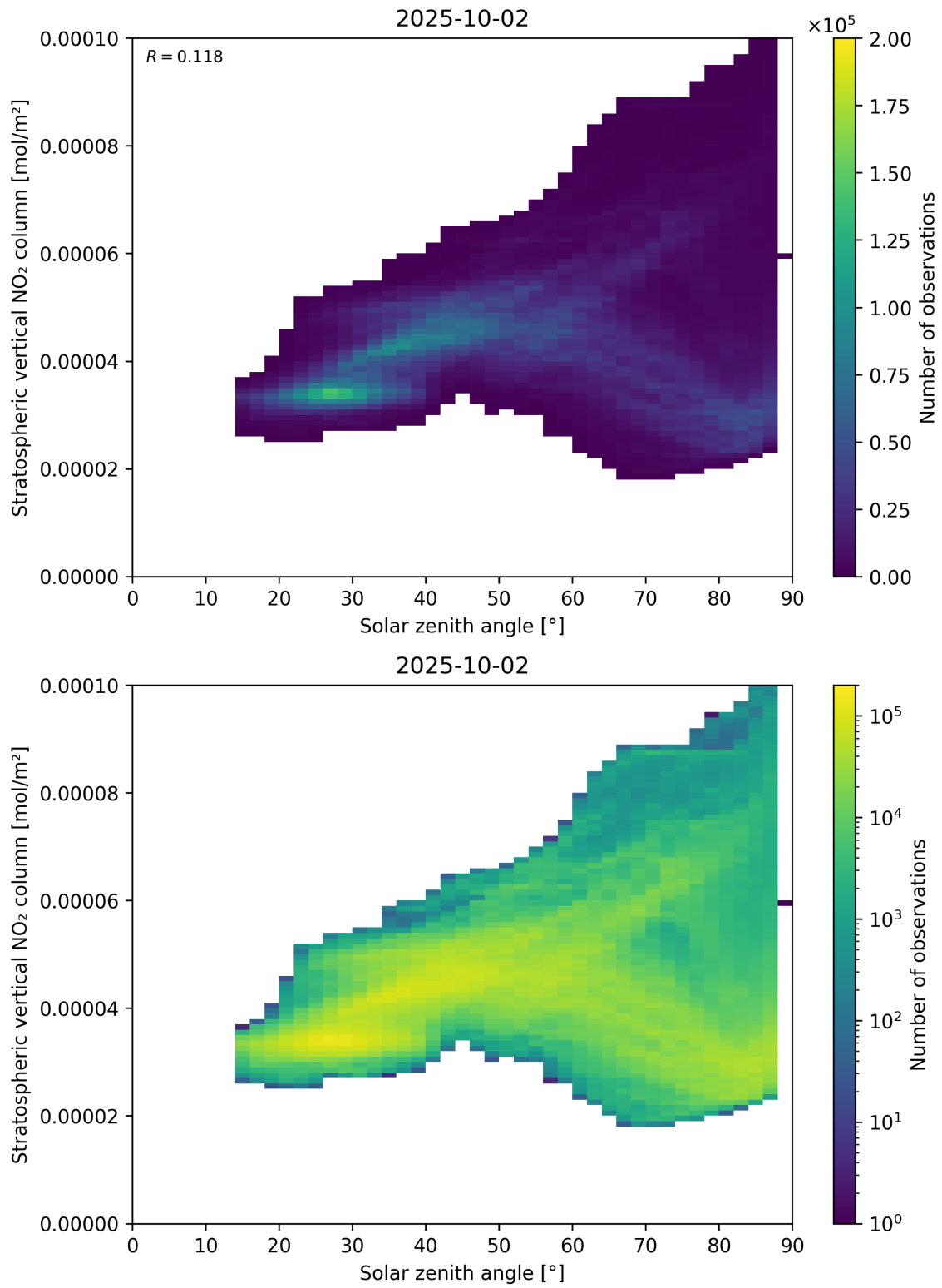
Figure 150: Scatter density plot of “Solar zenith angle” against “Stratospheric vertical NO 2 column” for 2025-10-01 to 2025-10-03.
