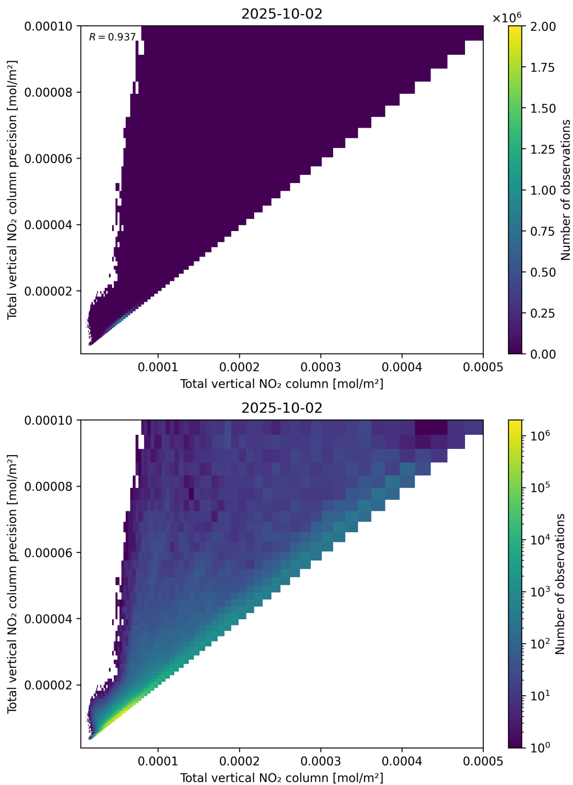
Figure 114: Scatter density plot of “Total vertical NO 2 column” against “Total vertical NO 2 column precision” for 2025-10-01 to 2025-10-03.
