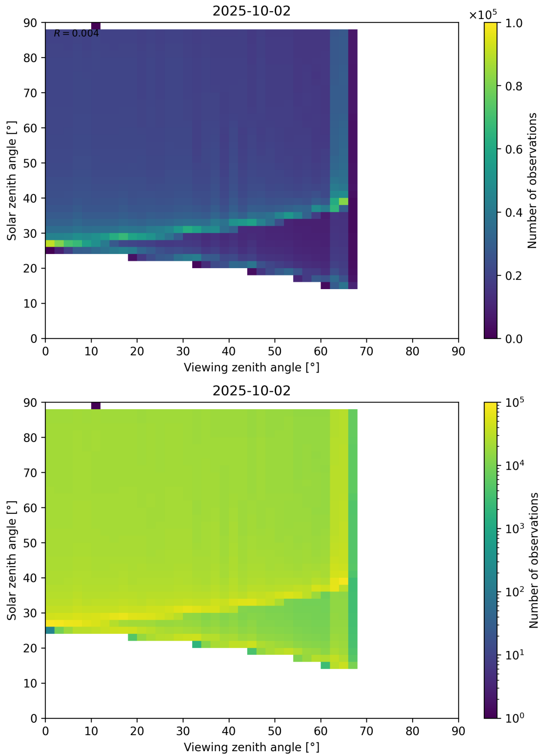
Figure 172: Scatter density plot of “Viewing zenith angle” against “Solar zenith angle” for 2025-10-01 to 2025-10-03.
