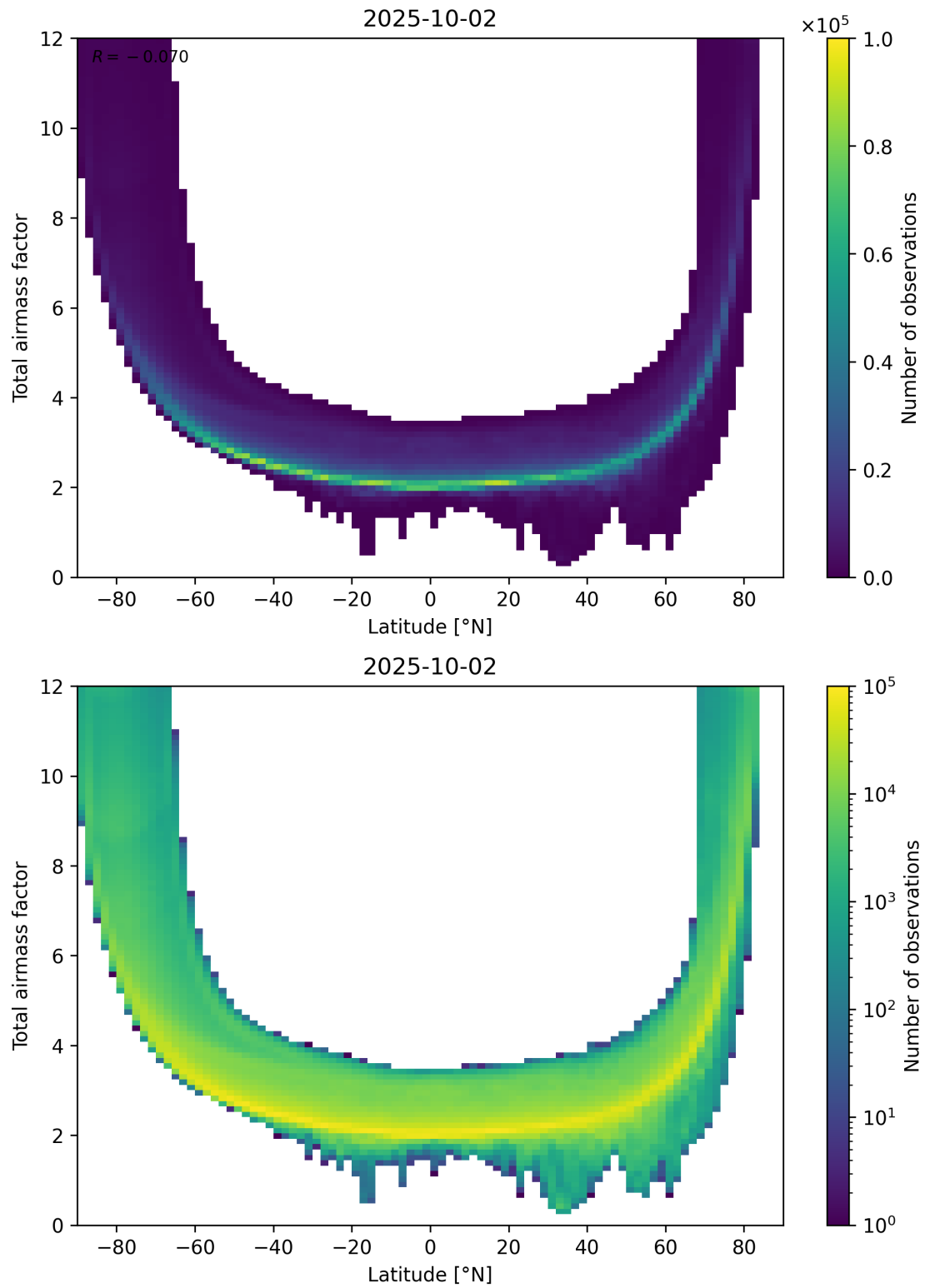
Figure 84: Scatter density plot of “Latitude” against “Total airmass factor” for 2025-10-01 to 2025-10-03.
