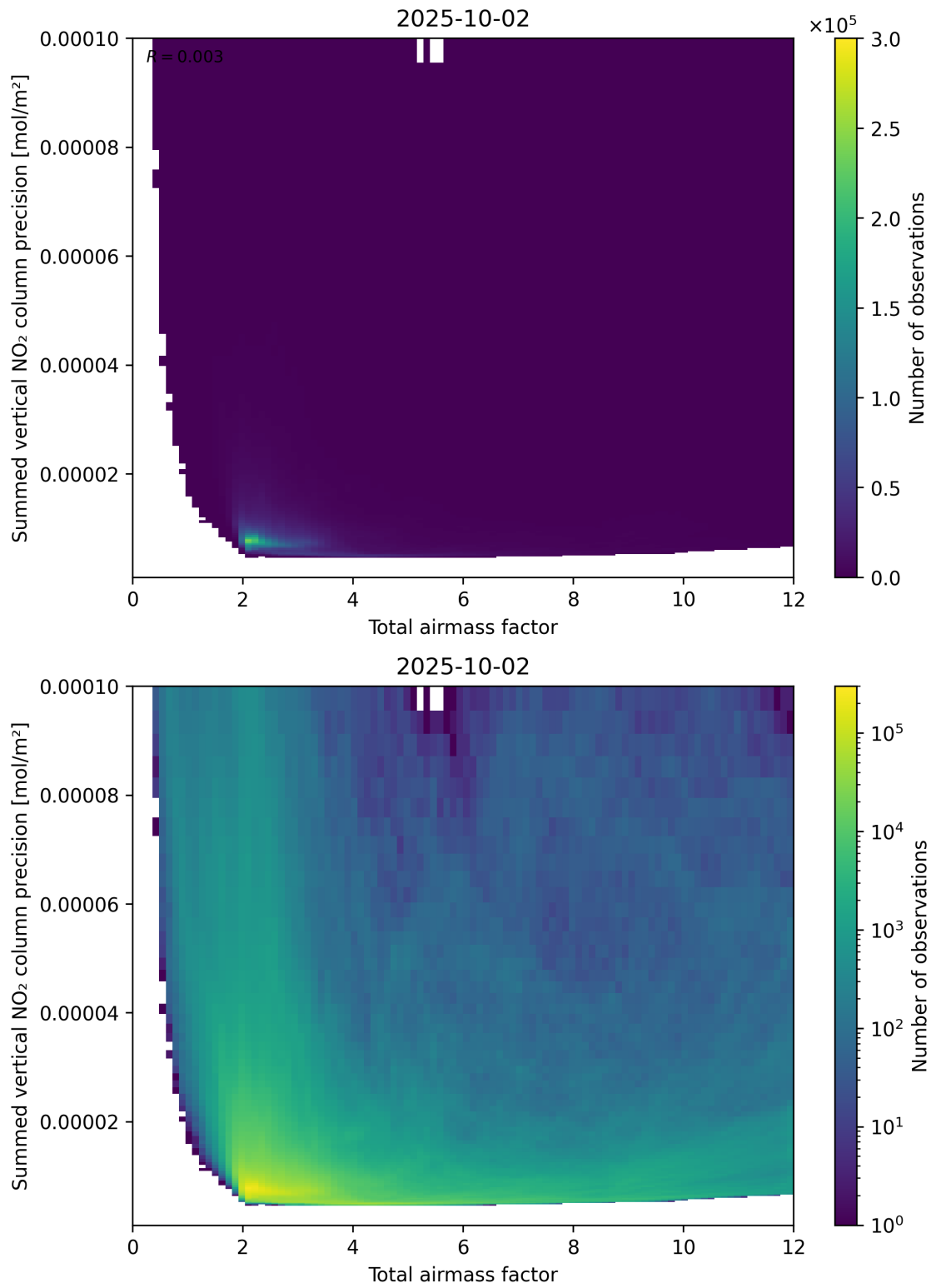
Figure 66: Scatter density plot of “Total airmass factor” against “Summed vertical NO 2 column precision” for 2025-10-01 to 2025-10-03.
