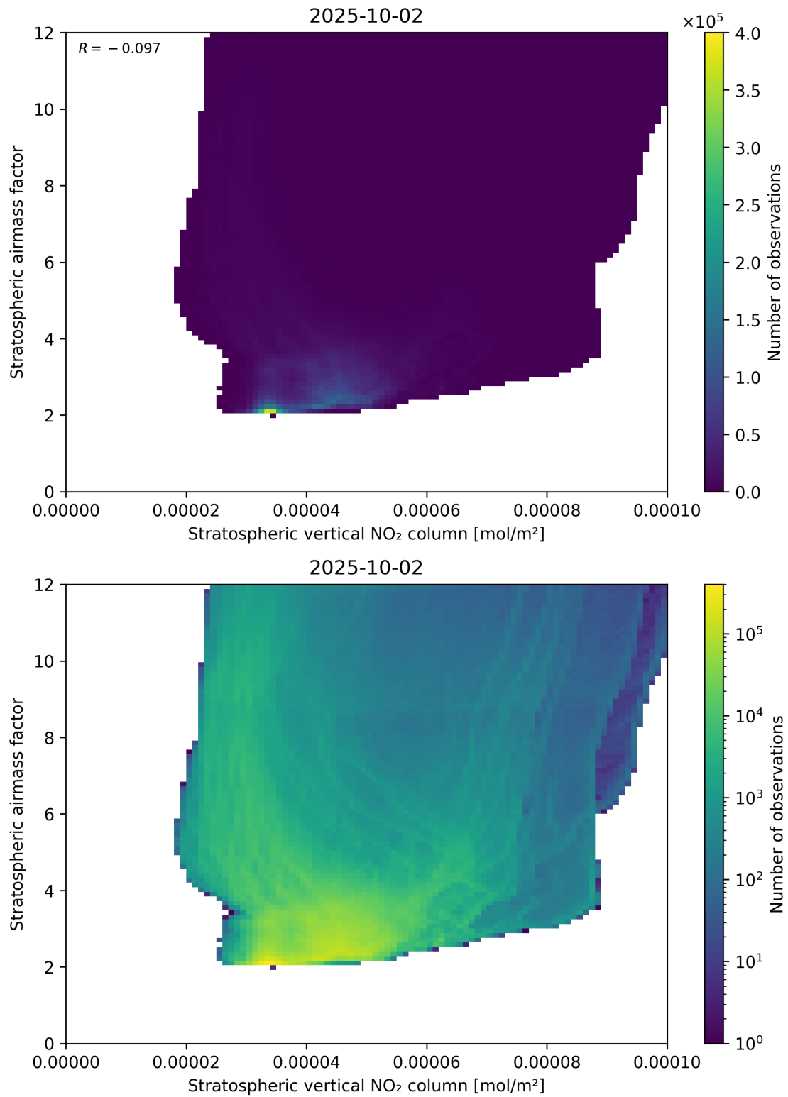
Figure 96: Scatter density plot of “Stratospheric vertical NO 2 column” against “Stratospheric airmass factor” for 2025-10-01 to 2025-10-03.
