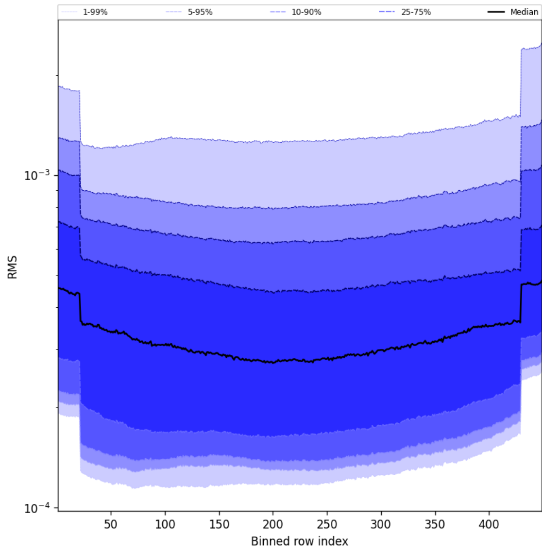
Figure 60: Along track statistics of “RMS” for 2025-10-01 to 2025-10-03
