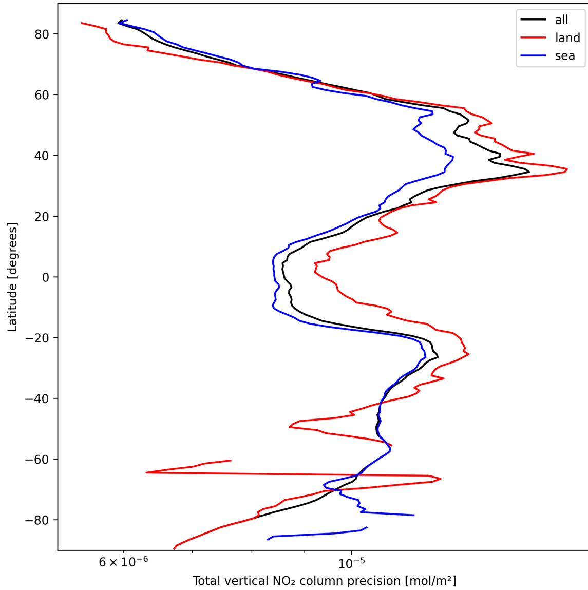
Figure 22: Zonal average of “Total vertical NO 2 column precision” for 2025-10-01 to 2025-10-03.
