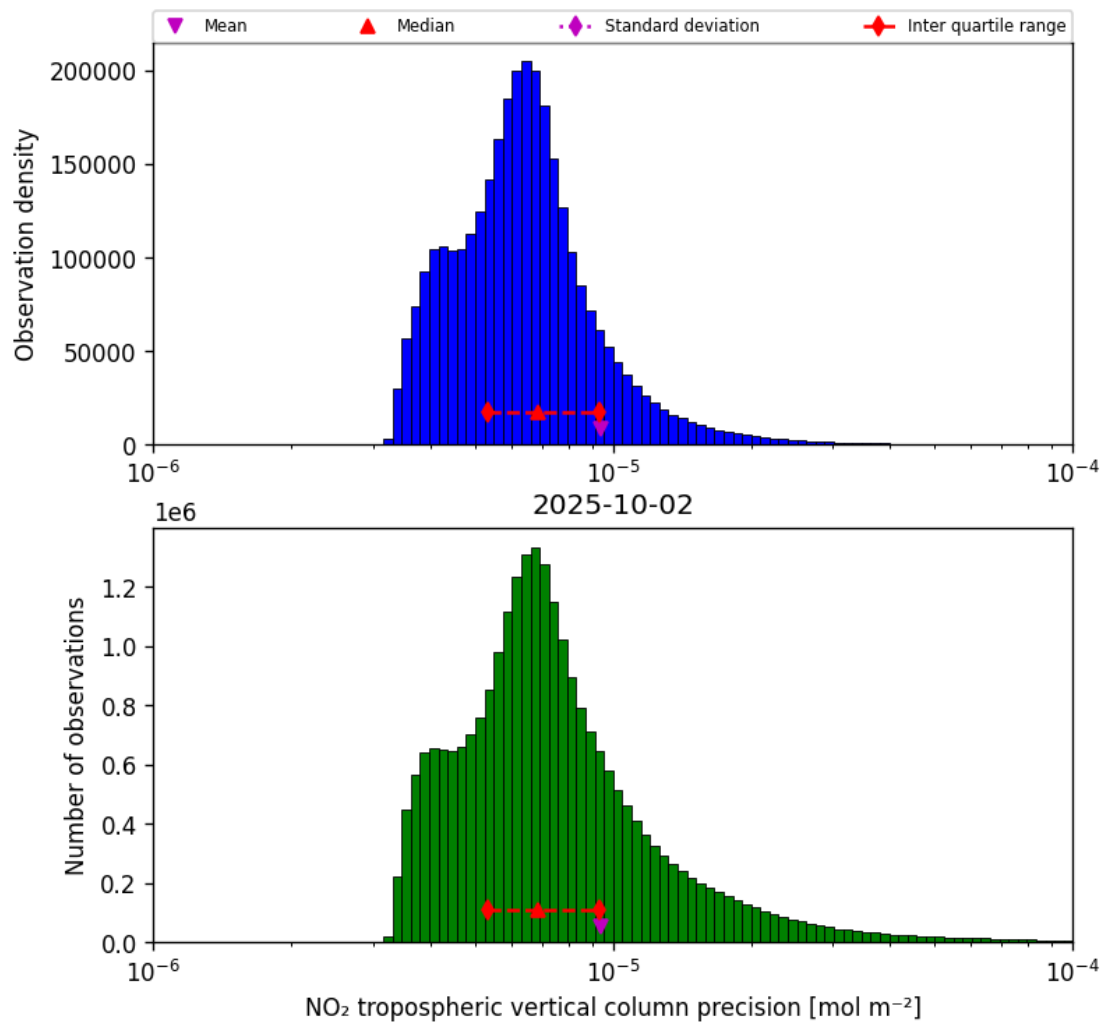
Figure 30: Histogram of “NO 2 tropospheric vertical column precision” for 2025-10-01 to 2025-10-03
