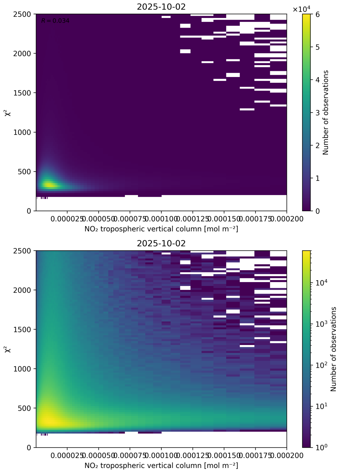
Figure 124: Scatter density plot of “NO 2 tropospheric vertical column” against “ \chi^2 ” for 2025-10-01 to 2025-10-03.
