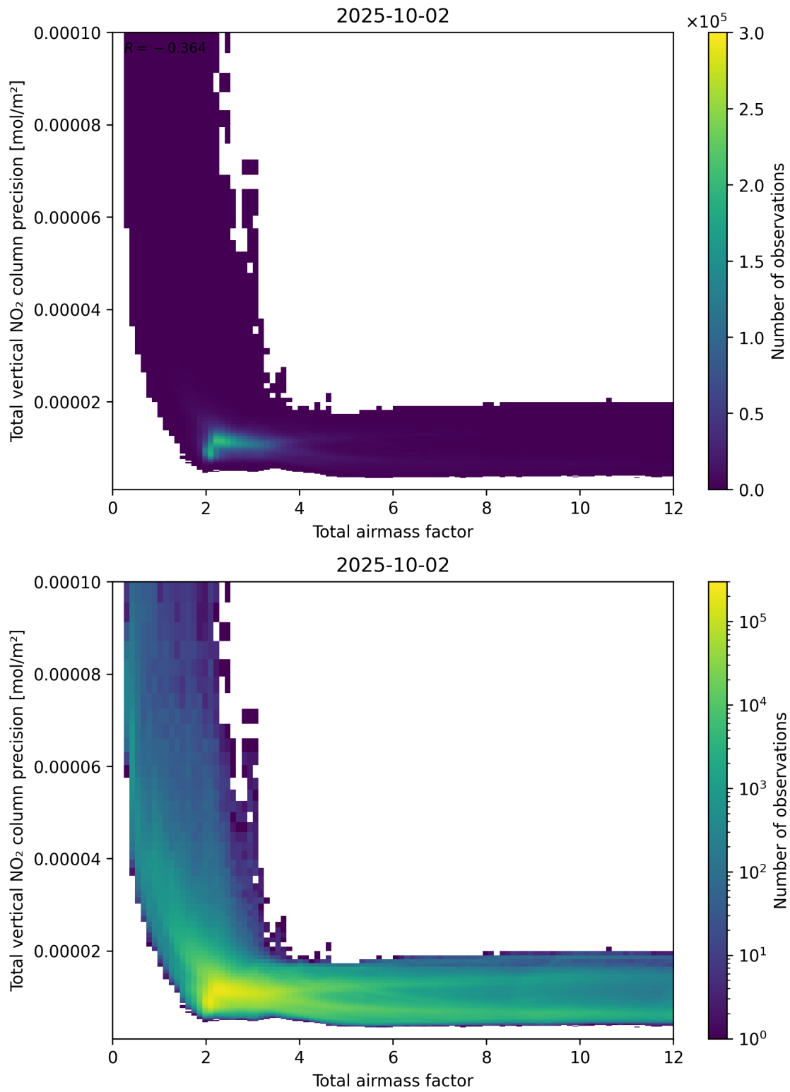
Figure 68: Scatter density plot of “Total airmass factor” against “Total vertical NO 2 column precision” for 2025-10-01 to 2025-10-03.
