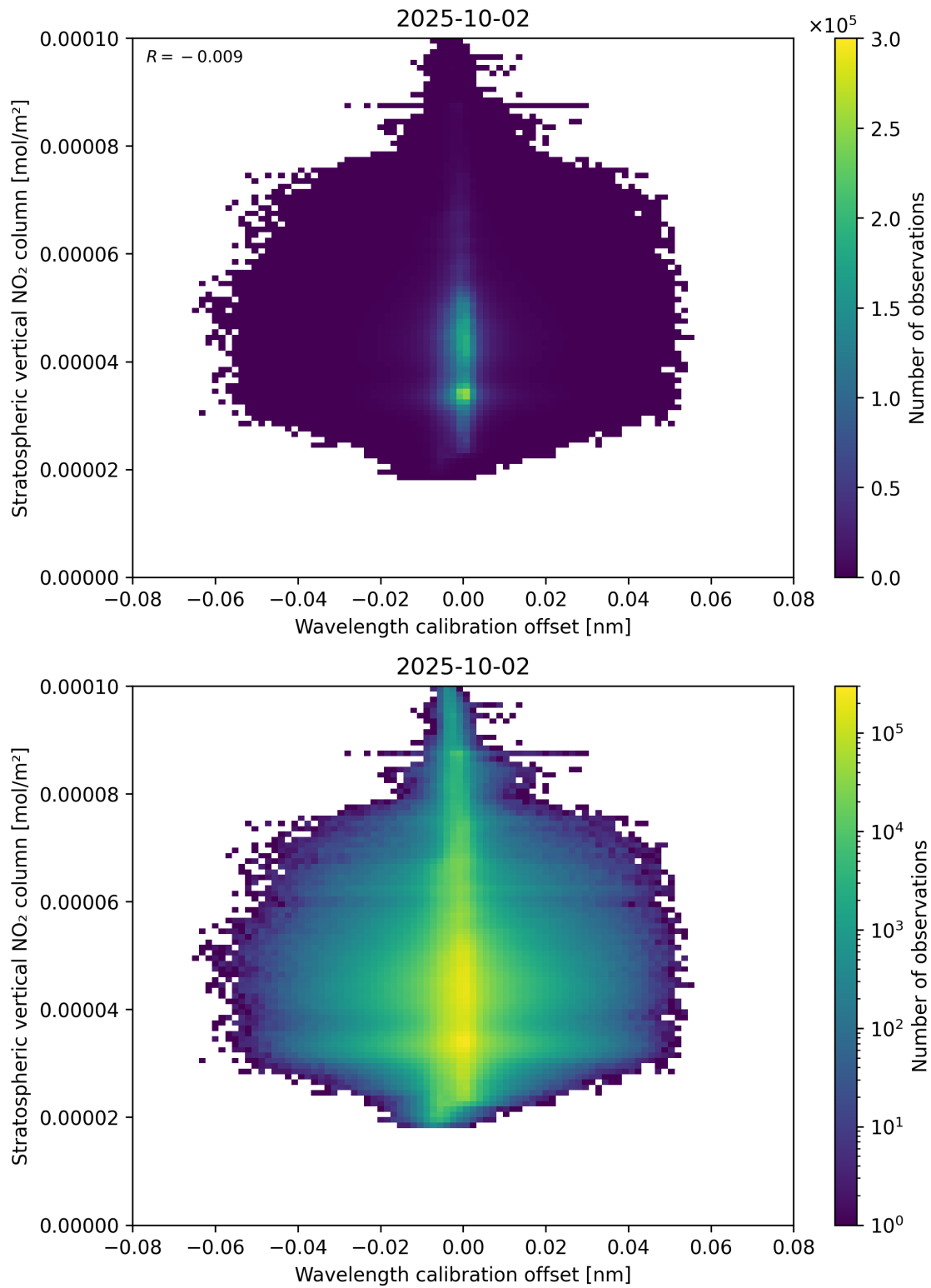
Figure 176: Scatter density plot of “Wavelength calibration offset” against “Stratospheric vertical NO 2 column” for 2025-10-01 to 2025-10-03.
