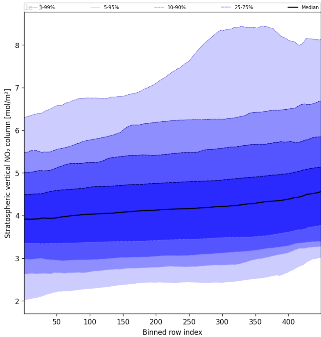
Figure 53: Along track statistics of “Stratospheric vertical NO 2 column” for 2025-10-01 to 2025-10-03
