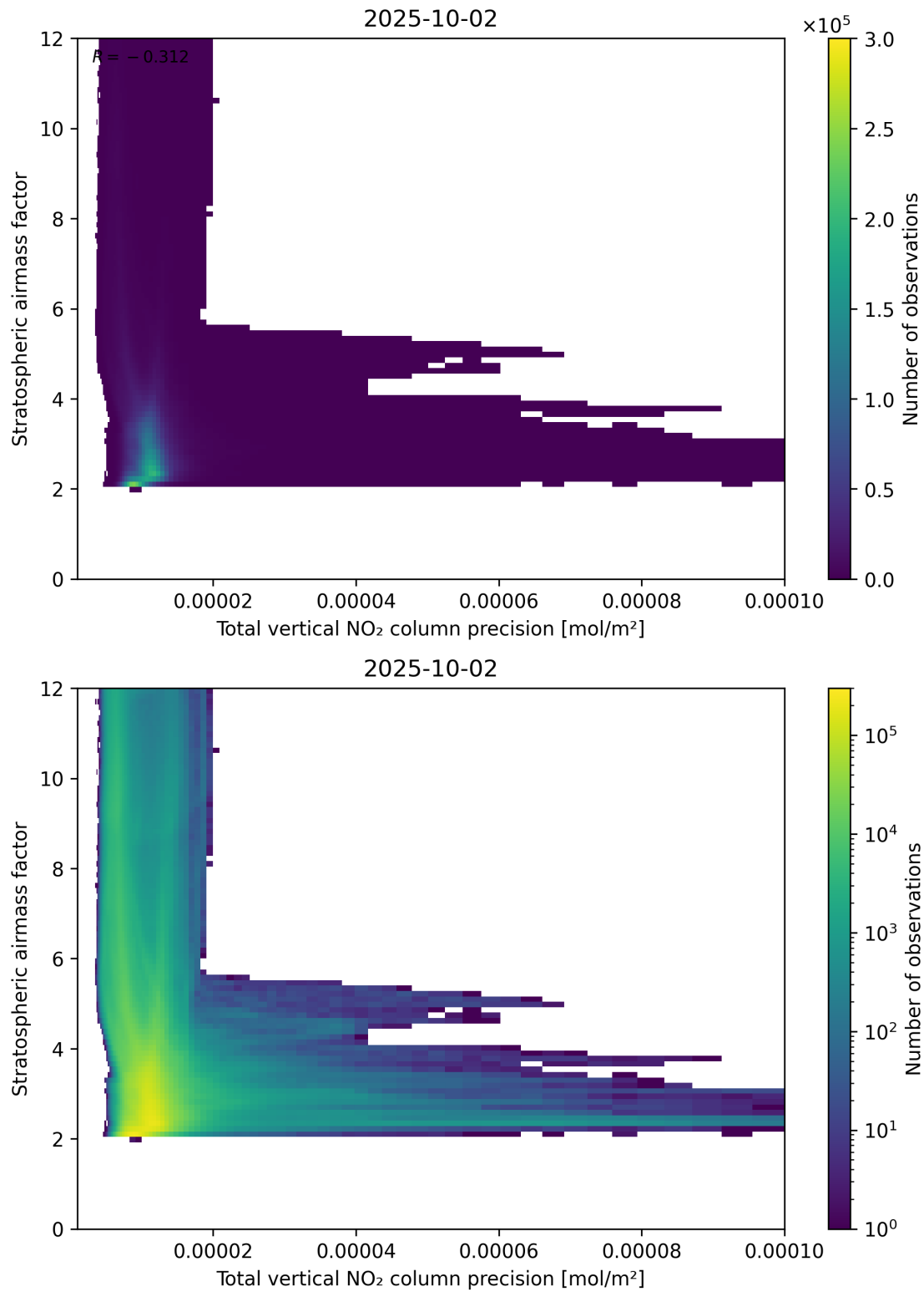
Figure 115: Scatter density plot of “Total vertical NO 2 column precision” against “Stratospheric airmass factor” for 2025-10-01 to 2025-10-03.
