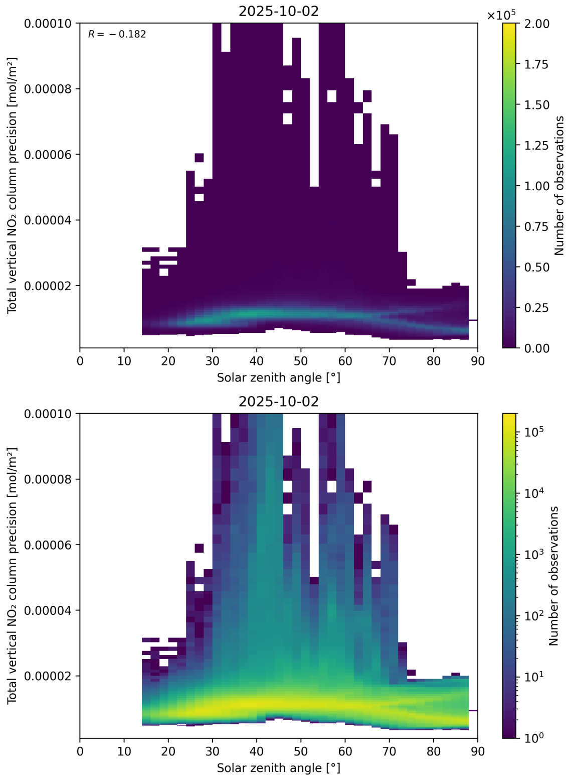
Figure 154: Scatter density plot of “Solar zenith angle” against “Total vertical NO 2 column precision” for 2025-10-01 to 2025-10-03.
