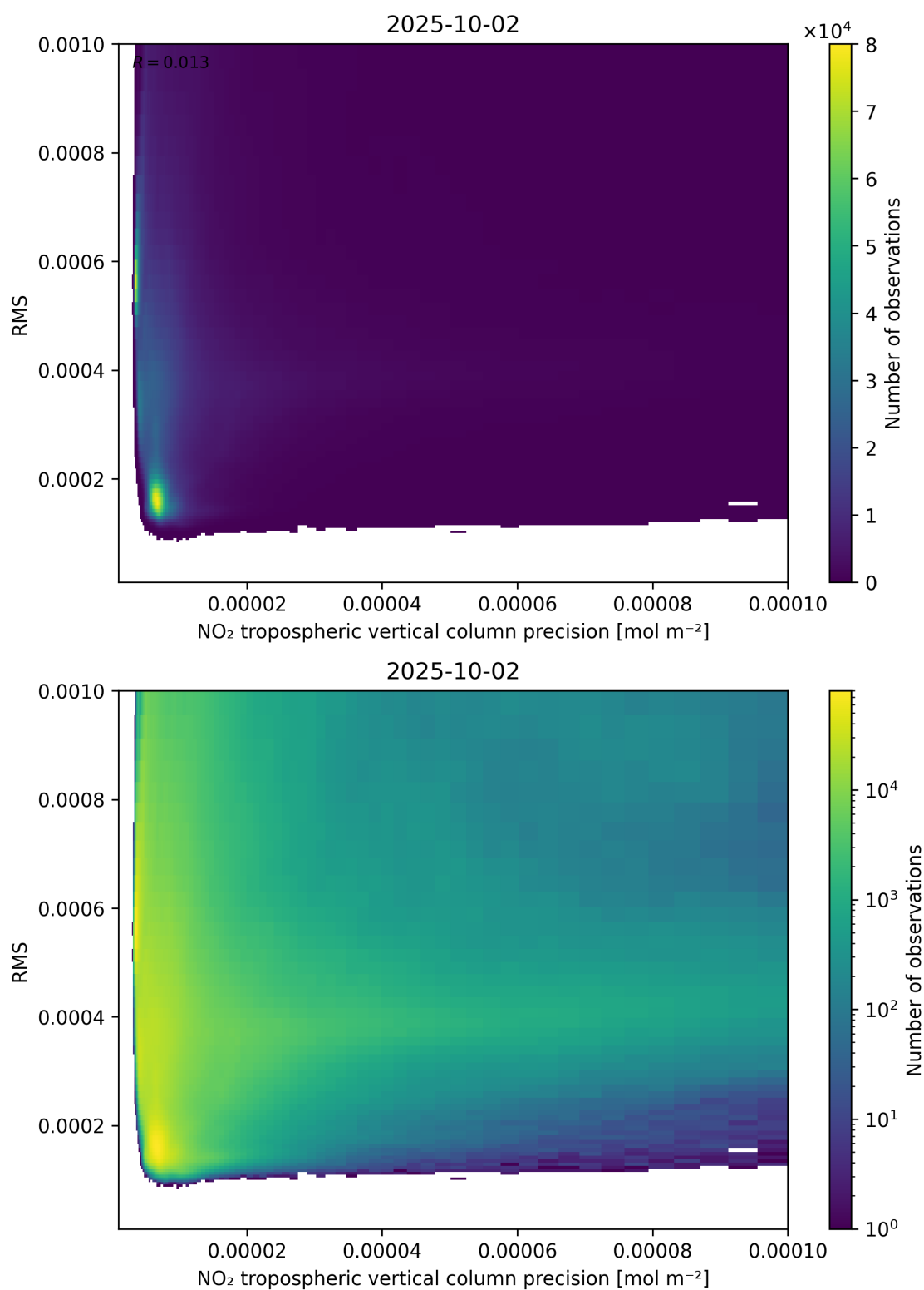
Figure 140: Scatter density plot of “NO 2 tropospheric vertical column precision” against “RMS” for 2025-10-01 to 2025-10-03.
