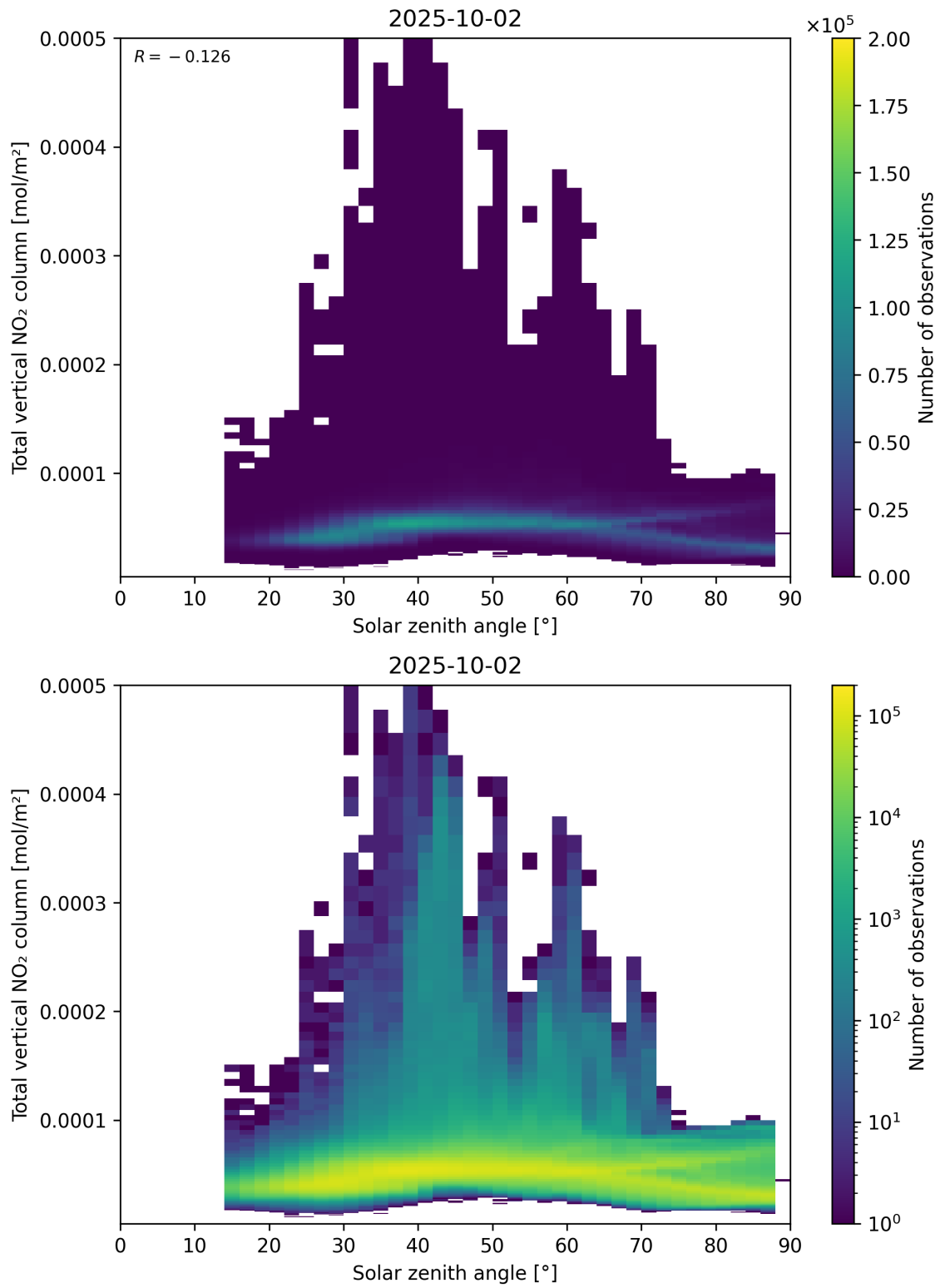
Figure 153: Scatter density plot of “Solar zenith angle” against “Total vertical NO 2 column” for 2025-10-01 to 2025-10-03.
