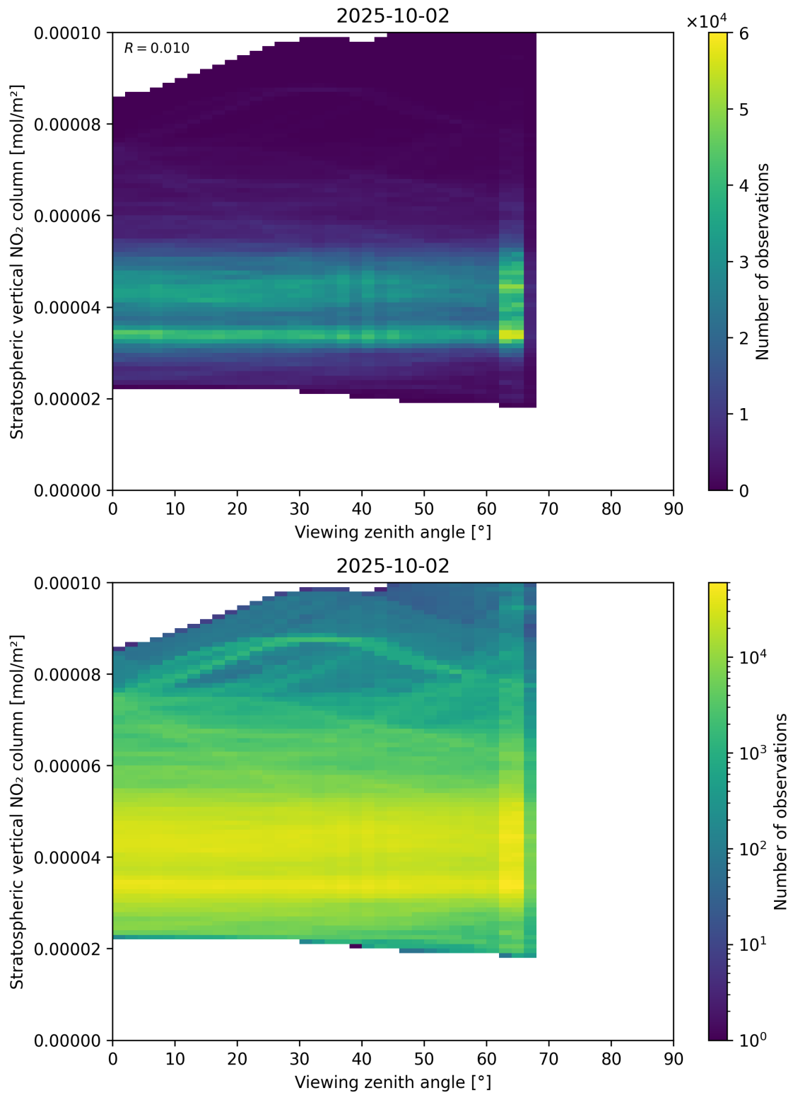
Figure 164: Scatter density plot of “Viewing zenith angle” against “Stratospheric vertical NO 2 column” for 2025-10-01 to 2025-10-03.
