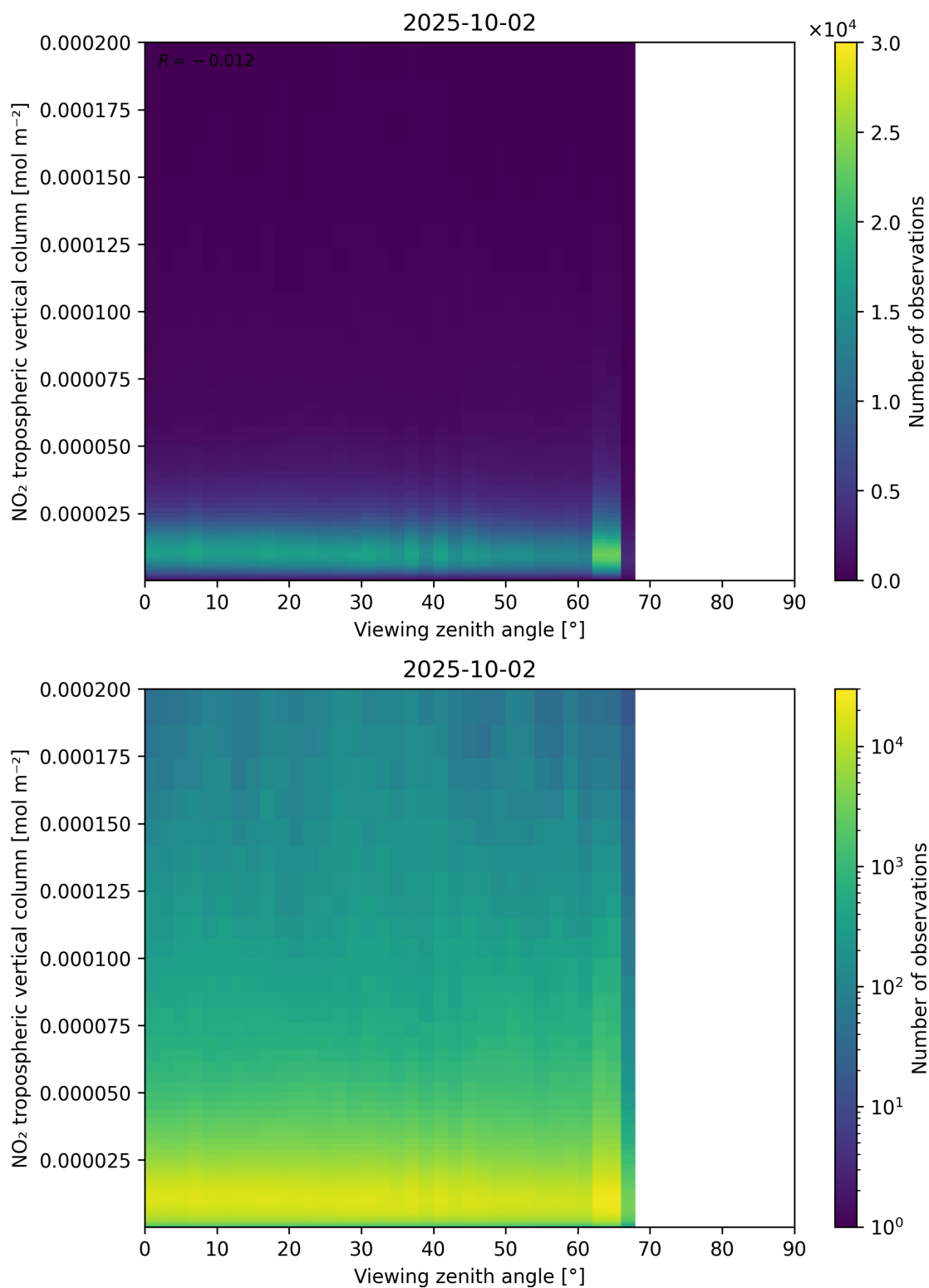
Figure 169: Scatter density plot of “Viewing zenith angle” against “NO 2 tropospheric vertical column” for 2025-10-01 to 2025-10-03.
