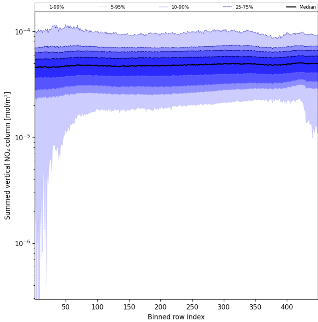
Figure 57: Along track statistics of “Summed vertical NO 2 column” for 2025-10-01 to 2025-10-03
