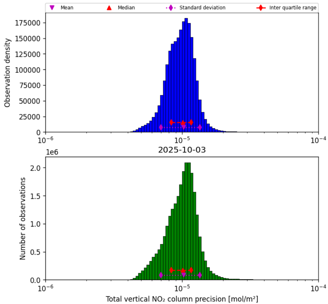
Figure 39: Histogram of "Total vertical NO 2 column precision" for 2025-10-02 to 2025-10-04
