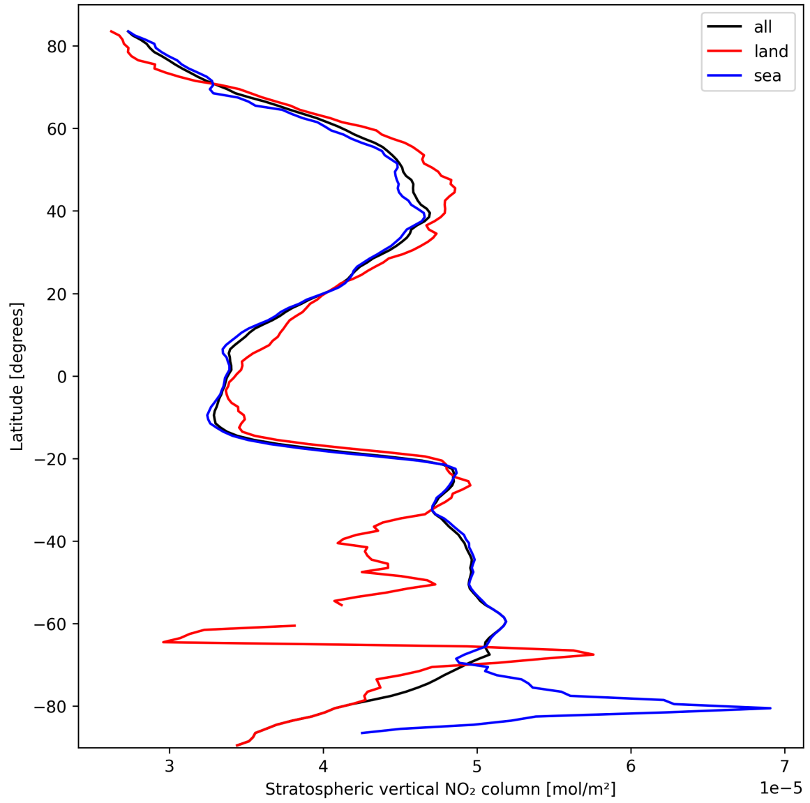
Figure 19: Zonal average of “Stratospheric vertical NO 2 column” for 2025-10-02 to 2025-10-04.
