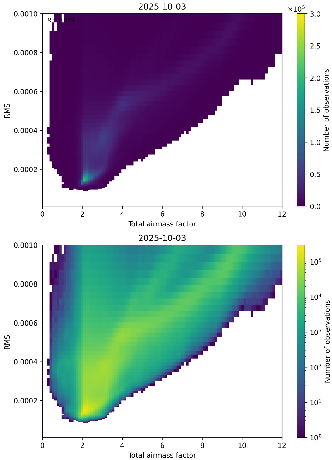
Figure 69: Scatter density plot of “Total airmass factor” against “RMS” for 2025-10-02 to 2025-10-04.
