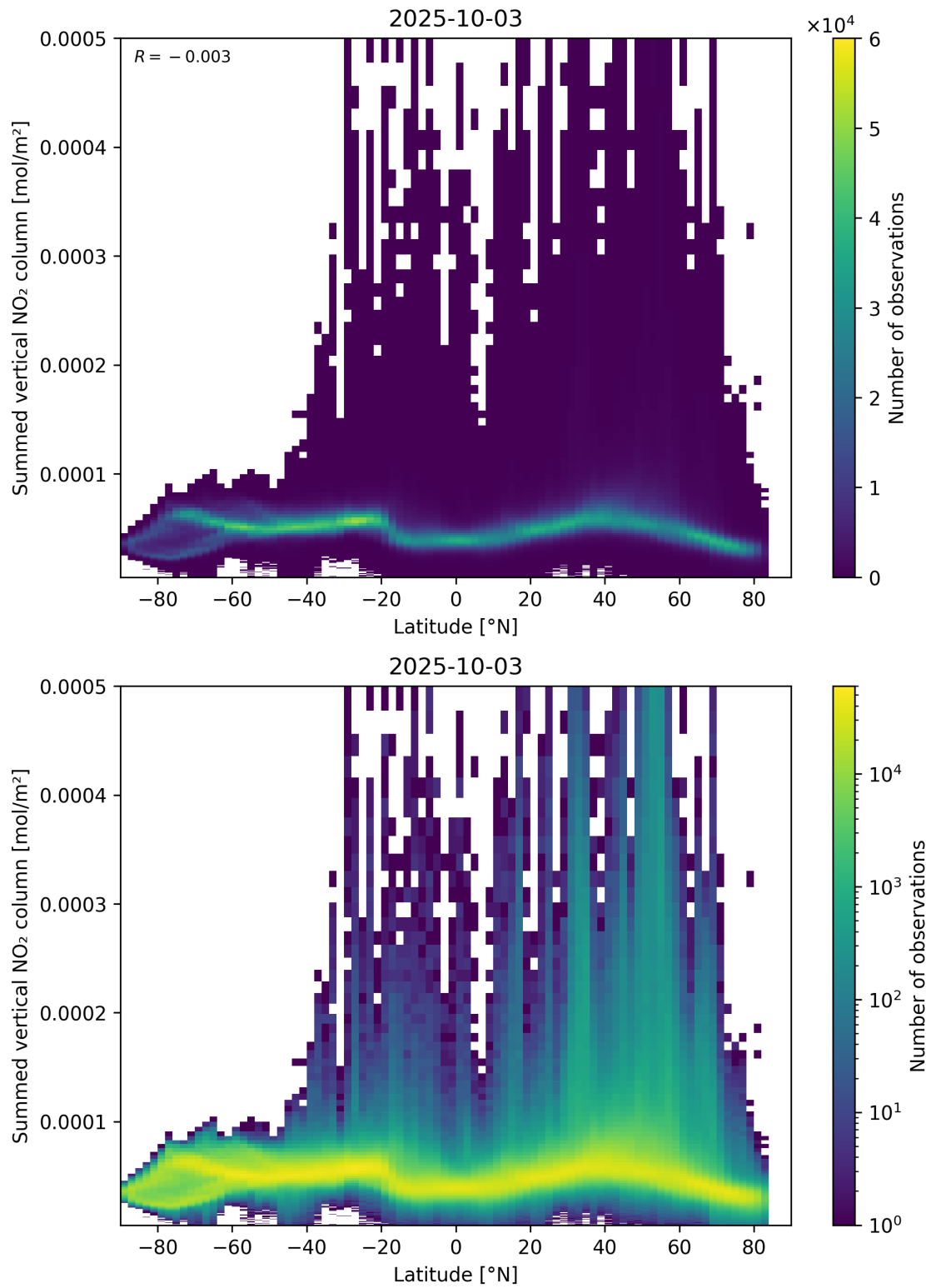
Figure 88: Scatter density plot of “Latitude” against “Summed vertical NO 2 column” for 2025-10-02 to 2025-10-04.
