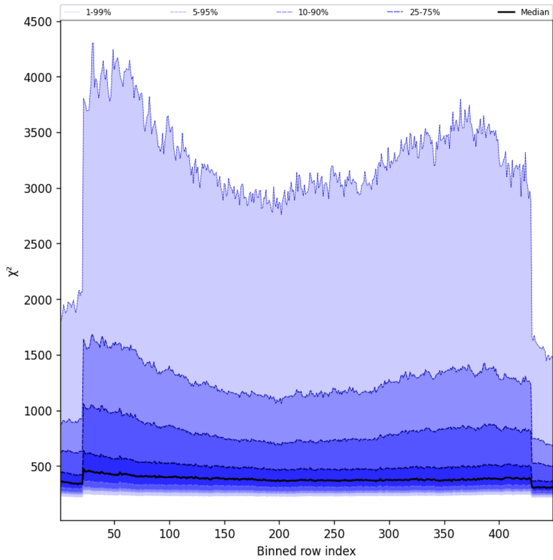
Figure 59: Along track statistics of “ \chi^2 ” for 2025-10-02 to 2025-10-04
