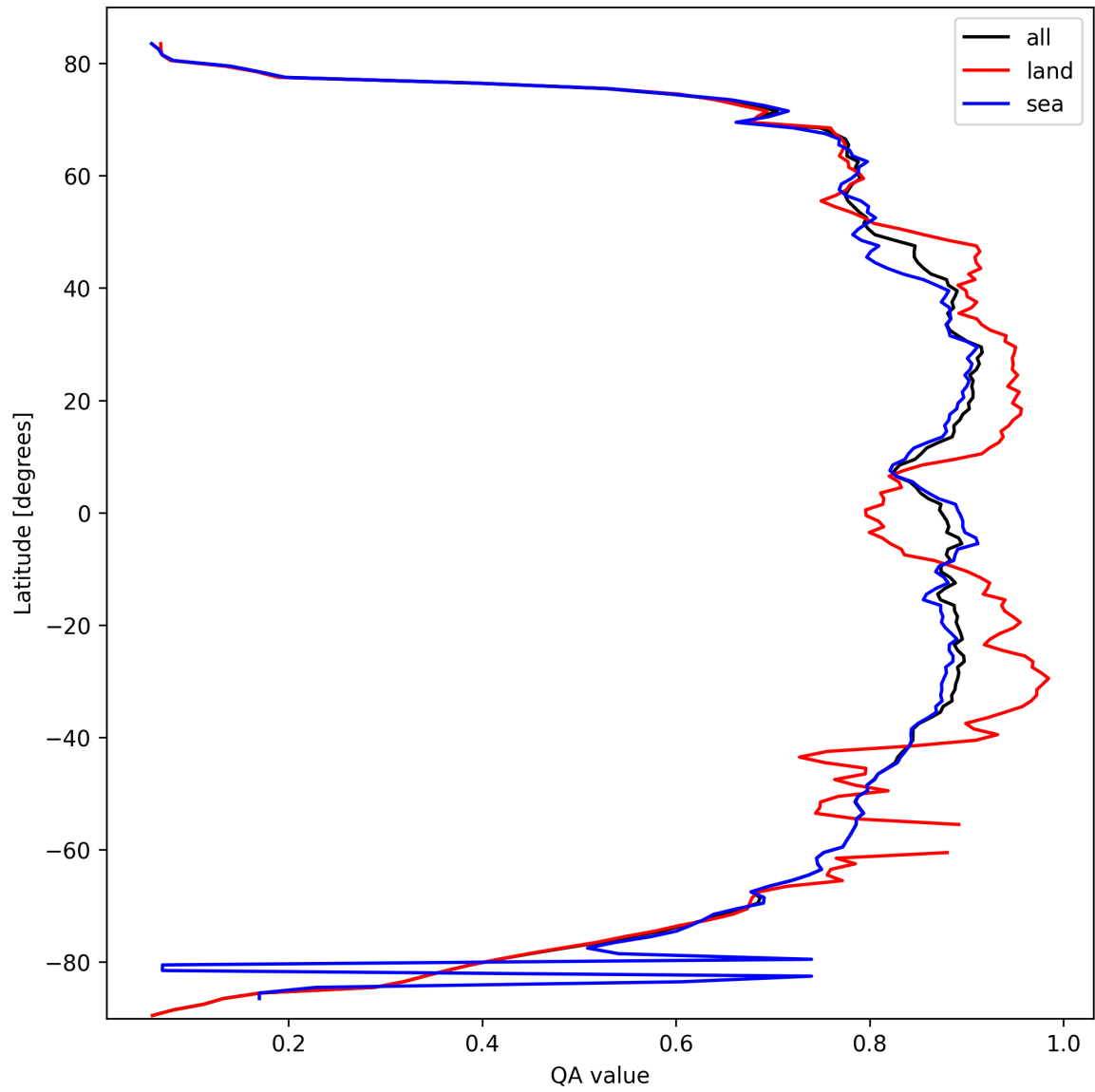
Figure 11: Zonal average of “QA value” for 2025-10-02 to 2025-10-04.
