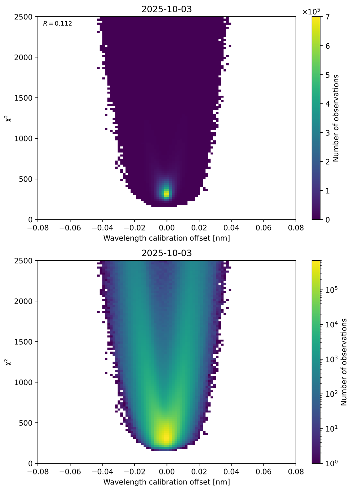
Figure 175: Scatter density plot of “Wavelength calibration offset” against “ \chi^2 ” for 2025-10-02 to 2025-10-04.
