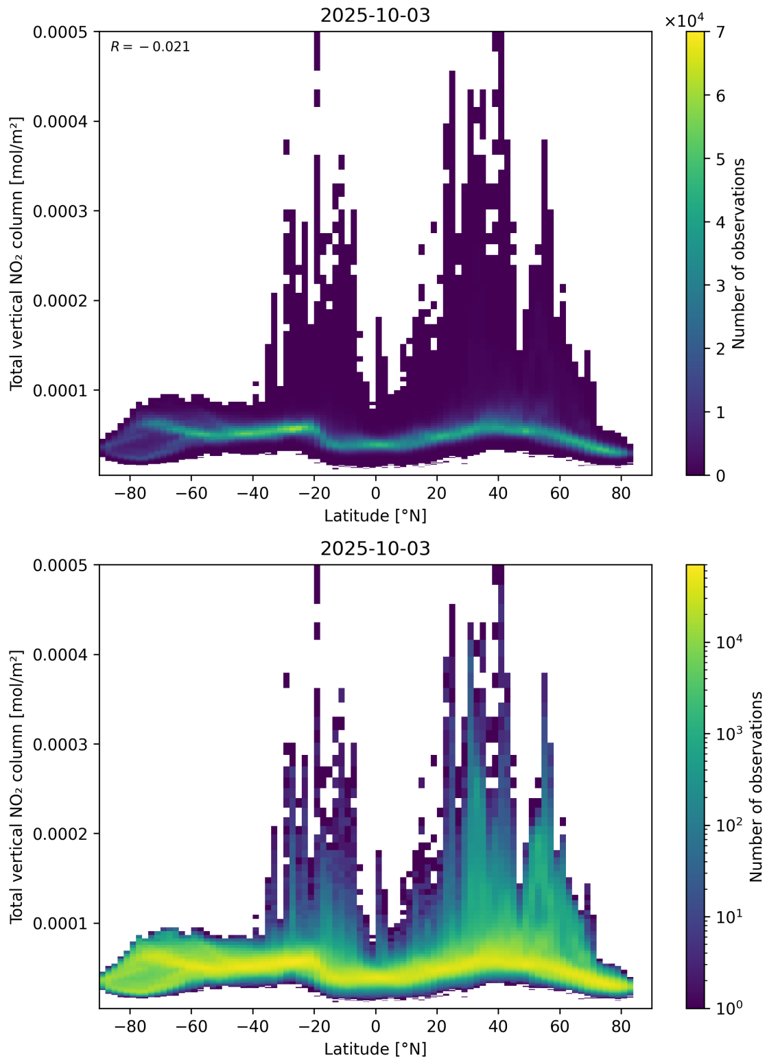
Figure 90: Scatter density plot of “Latitude” against “Total vertical NO 2 column” for 2025-10-02 to 2025-10-04.
