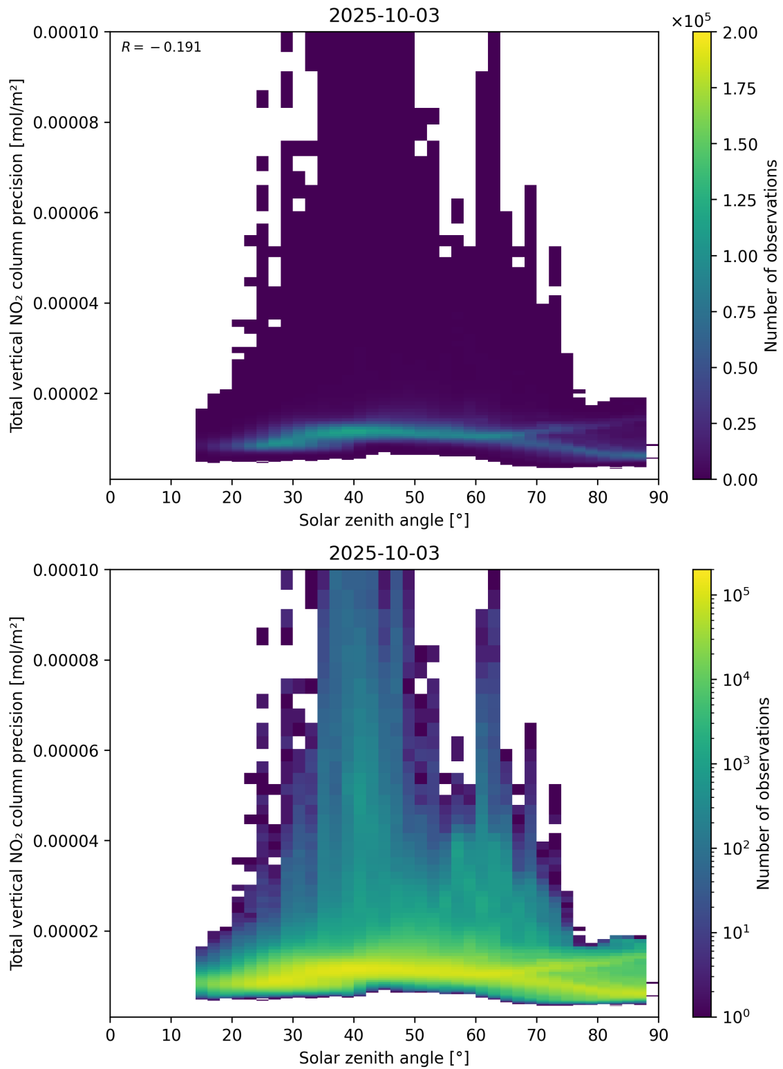
Figure 154: Scatter density plot of “Solar zenith angle” against “Total vertical NO 2 column precision” for 2025-10-02 to 2025-10-04.
