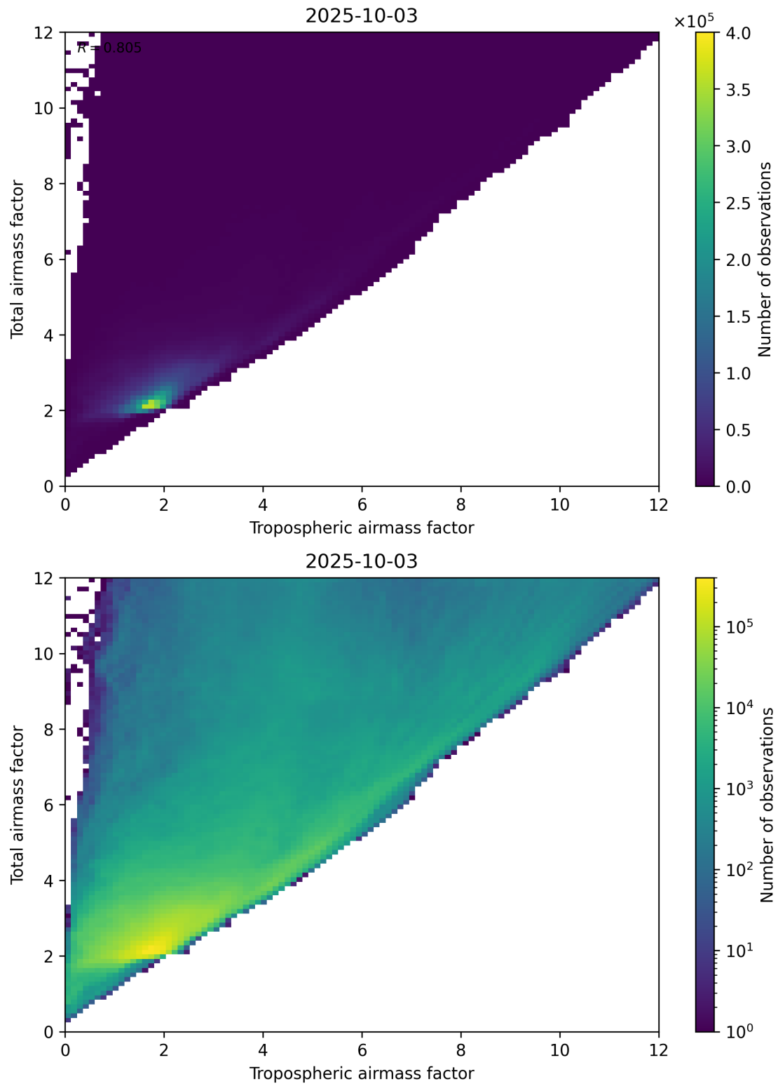
Figure 72: Scatter density plot of “Tropospheric airmass factor” against “Total airmass factor” for 2025-10-02 to 2025-10-04.
