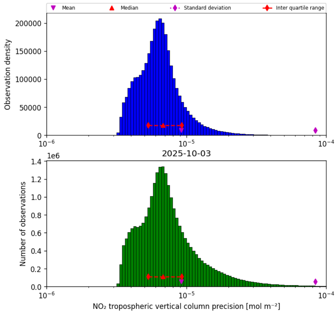
Figure 30: Histogram of “NO 2 tropospheric vertical column precision” for 2025-10-02 to 2025-10-04
