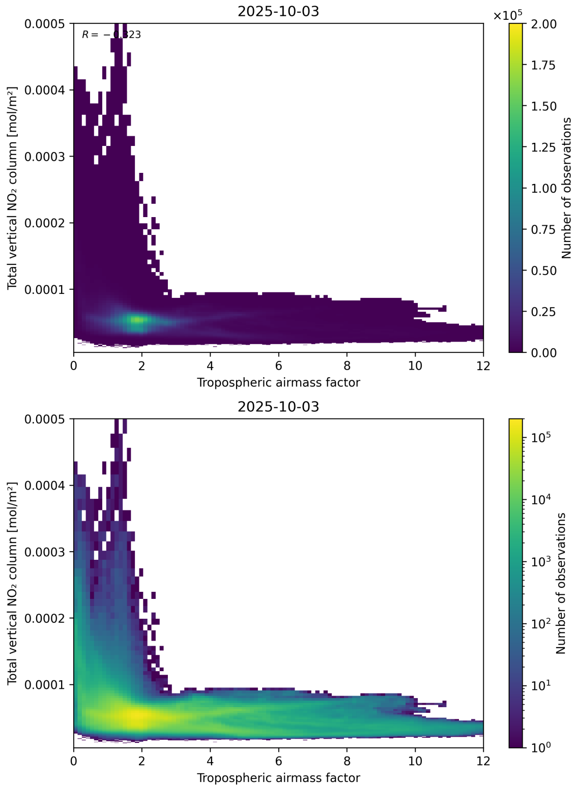
Figure 77: Scatter density plot of “Tropospheric airmass factor” against “Total vertical NO 2 column” for 2025-10-02 to 2025-10-04.
