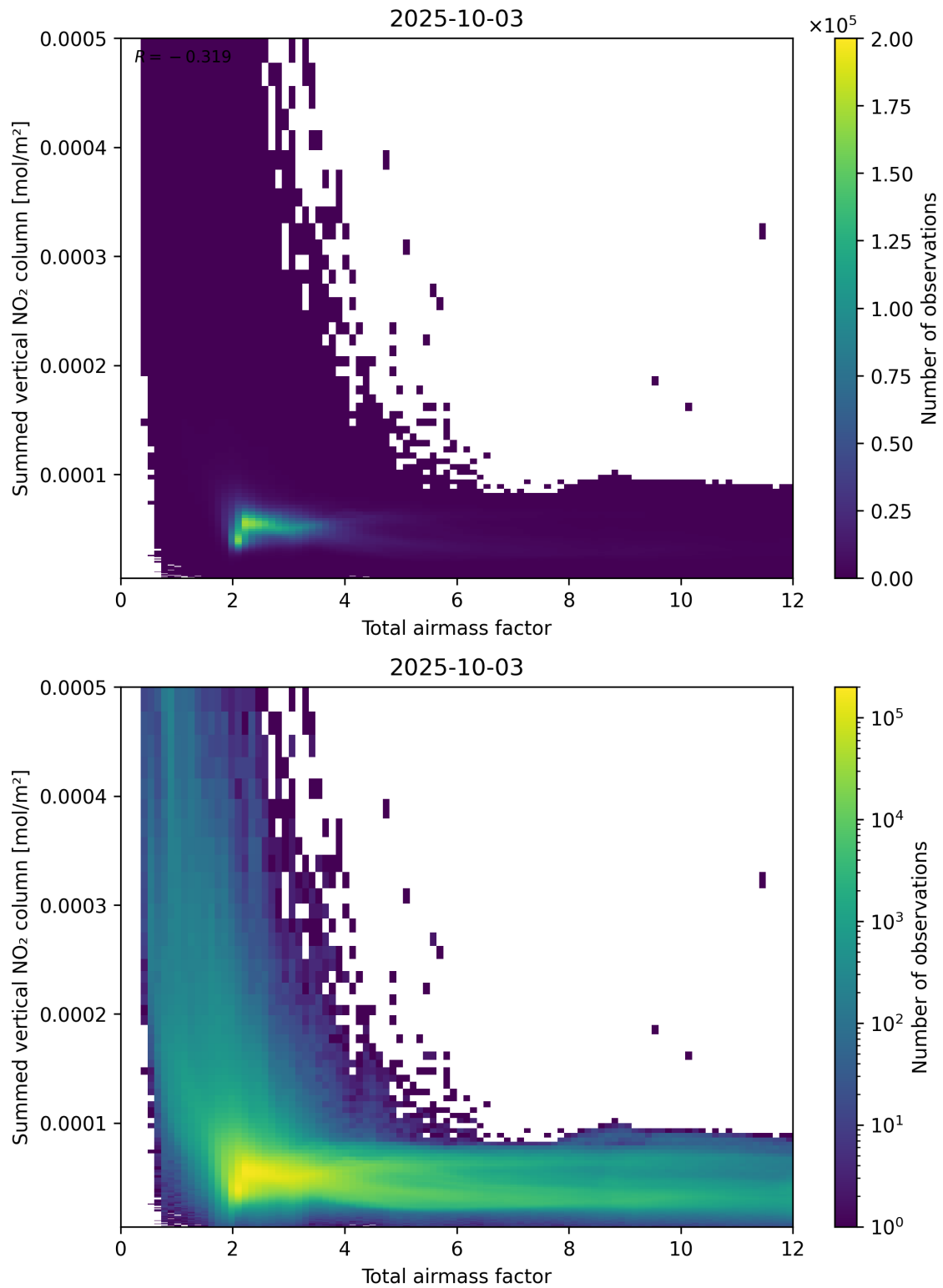
Figure 65: Scatter density plot of “Total airmass factor” against “Summed vertical NO 2 column” for 2025-10-02 to 2025-10-04.
