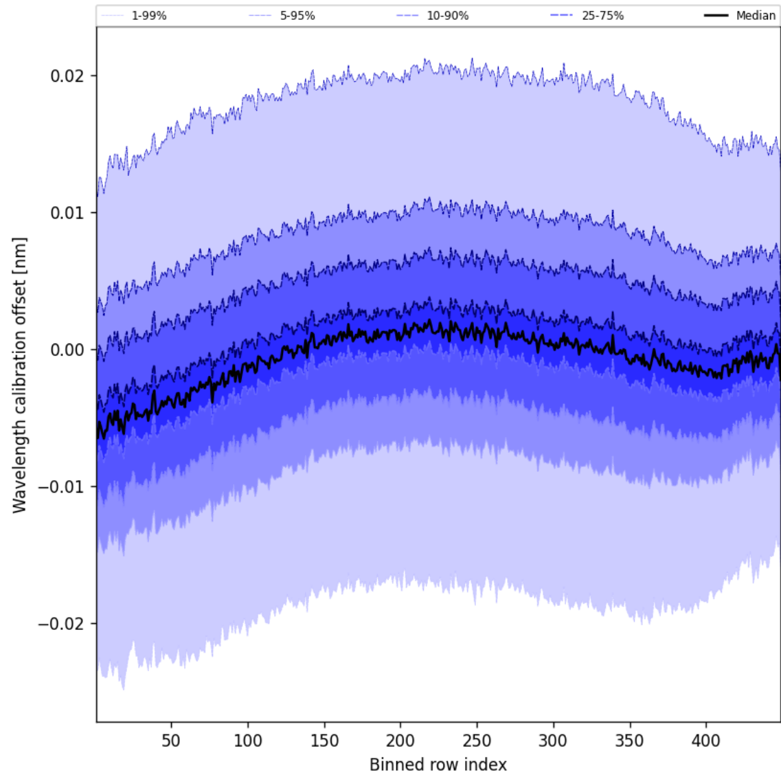
Figure 52: Along track statistics of “Wavelength calibration offset” for 2025-10-02 to 2025-10-04
