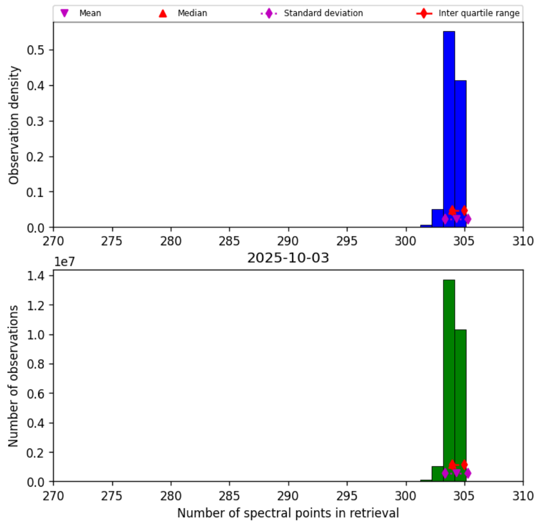
Figure 33: Histogram of “Number of spectral points in retrieval” for 2025-10-02 to 2025-10-04
