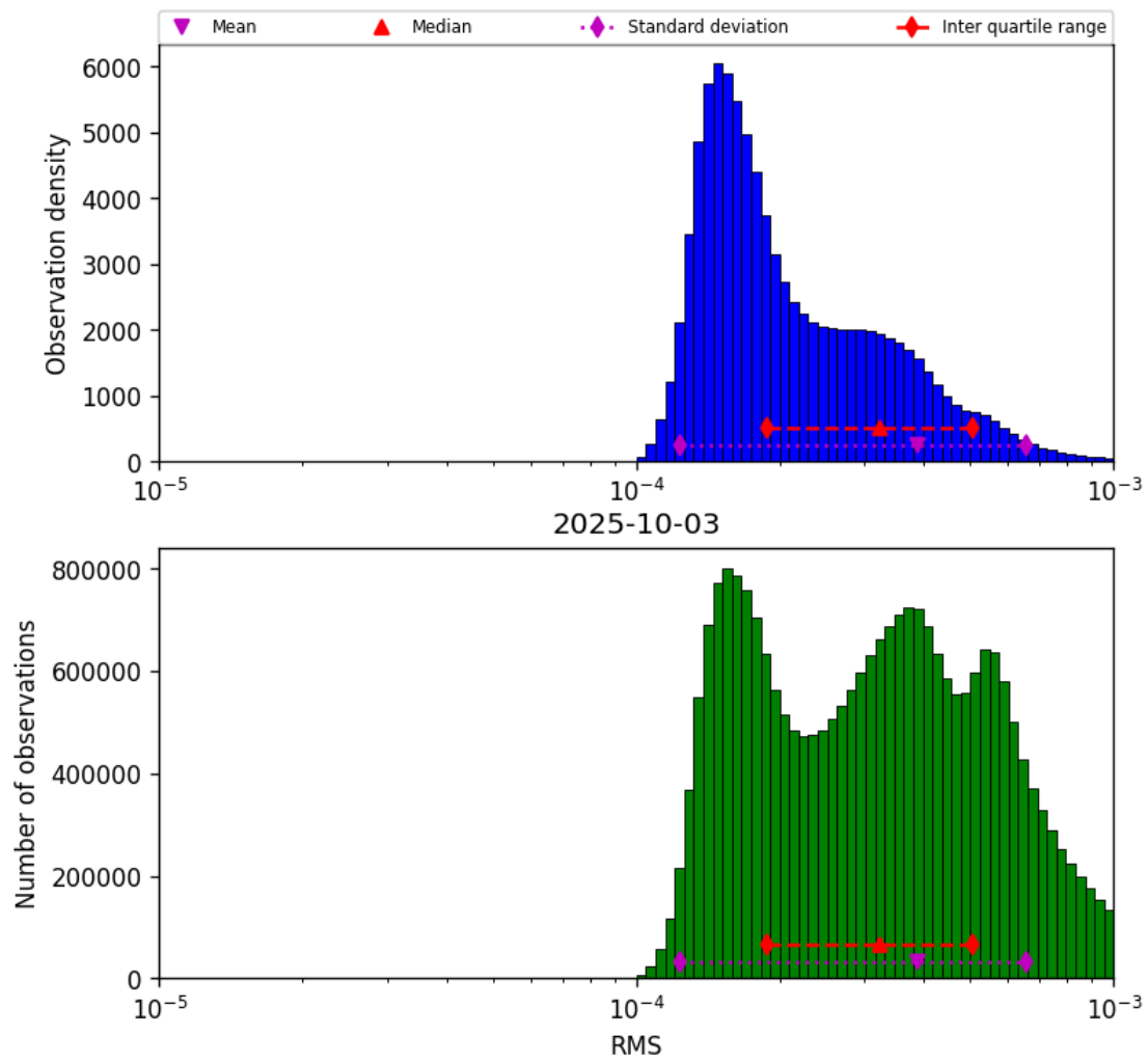
Figure 43: Histogram of “RMS” for 2025-10-02 to 2025-10-04
