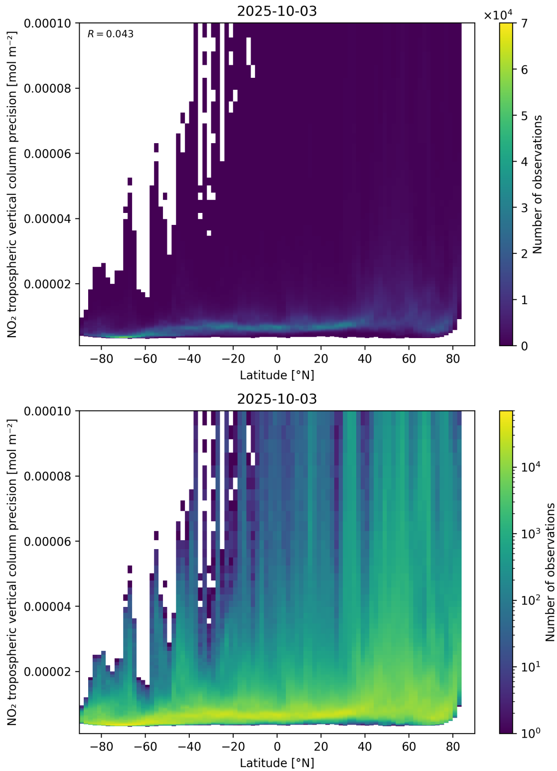
Figure 93: Scatter density plot of “Latitude” against “NO 2 tropospheric vertical column precision” for 2025-10-02 to 2025-10-04.
