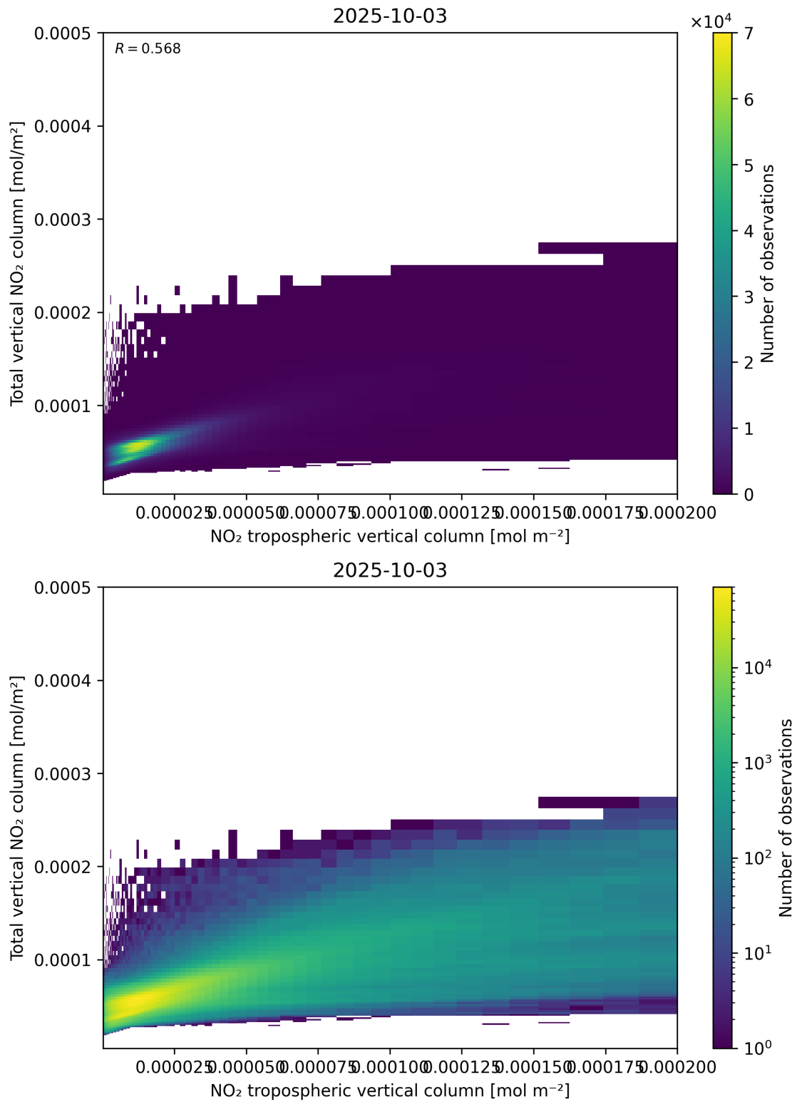
Figure 128: Scatter density plot of “NO 2 tropospheric vertical column” against “Total vertical NO 2 column” for 2025-10-02 to 2025-10-04.
