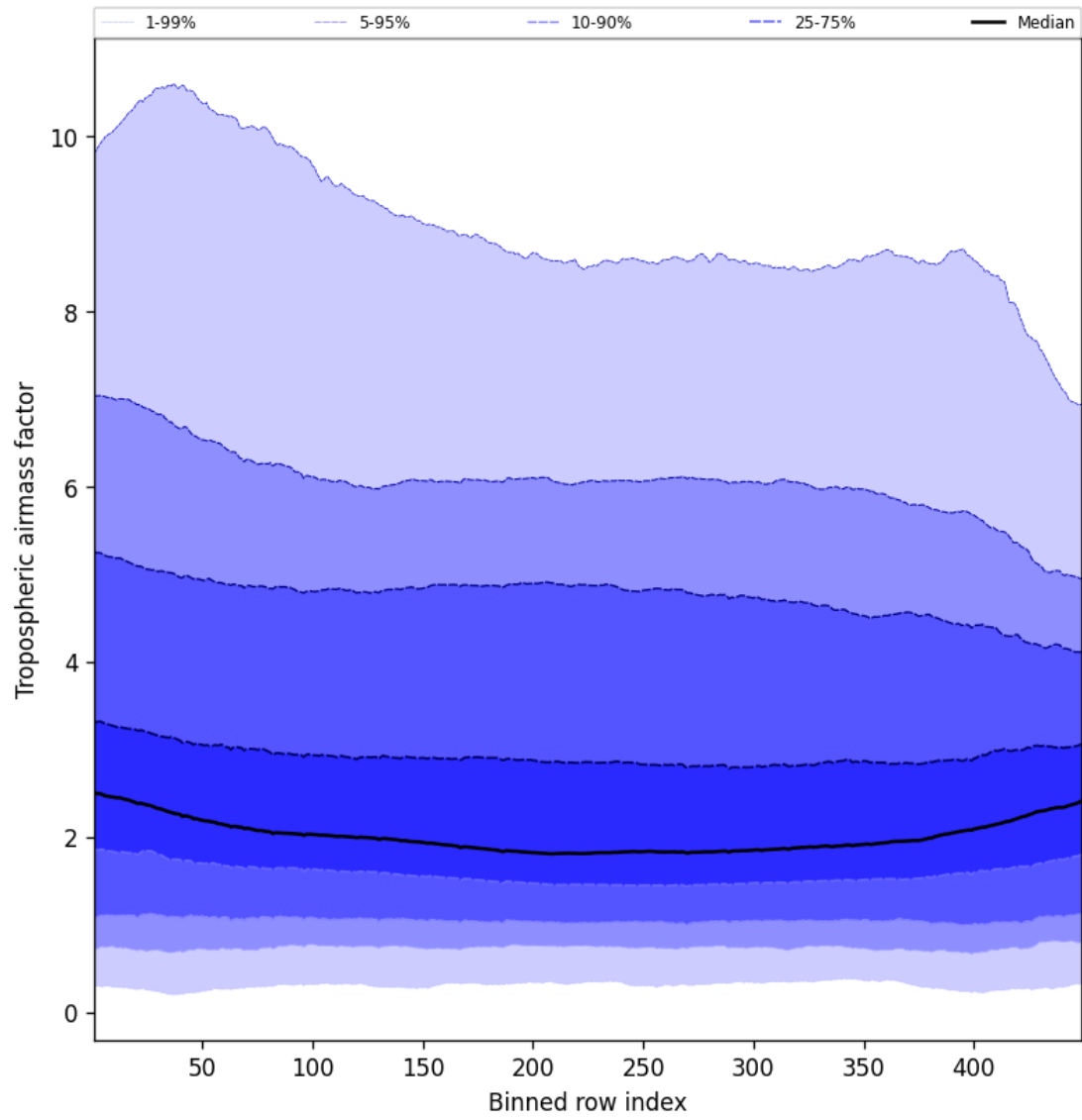
Figure 48: Along track statistics of “Tropospheric air mass factor” for 2025-10-02 to 2025-10-04
