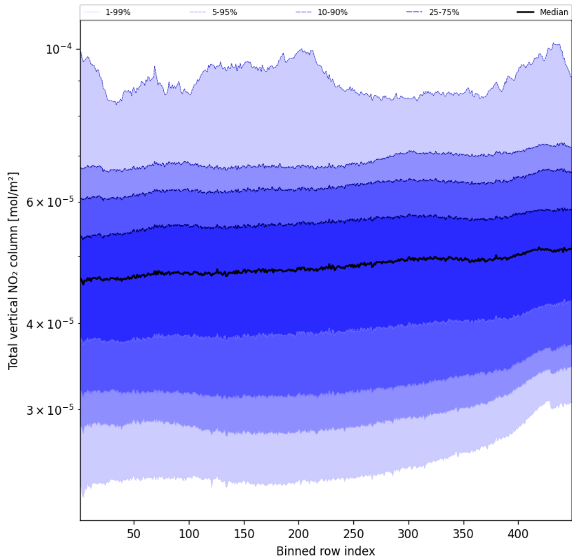
Figure 55: Along track statistics of “Total vertical NO 2 column” for 2025-10-02 to 2025-10-04
