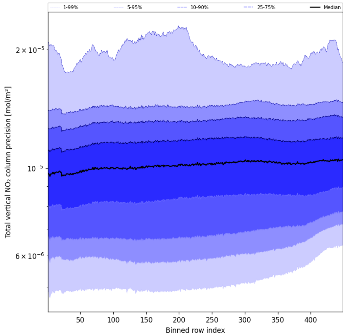
Figure 56: Along track statistics of “Total vertical NO 2 column precision” for 2025-10-02 to 2025-10-04
