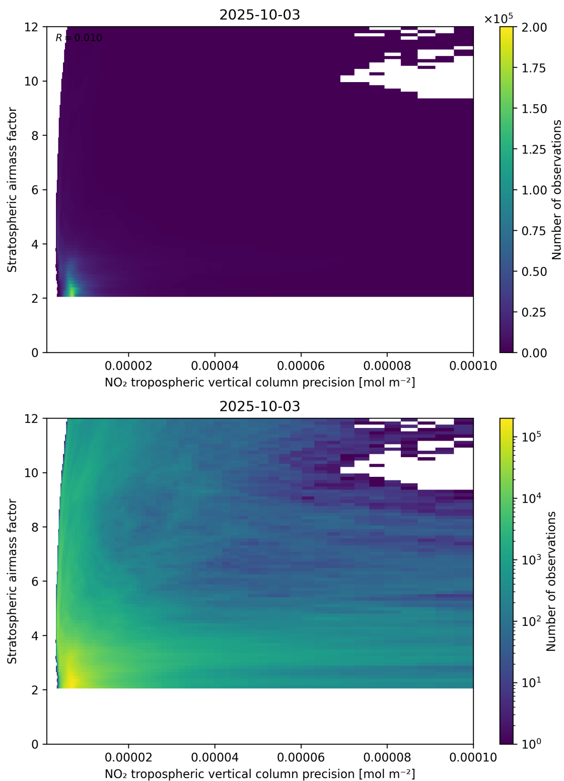
Figure 131: Scatter density plot of “NO 2 tropospheric vertical column precision” against “Stratospheric airmass factor” for 2025-10-02 to 2025-10-04.
