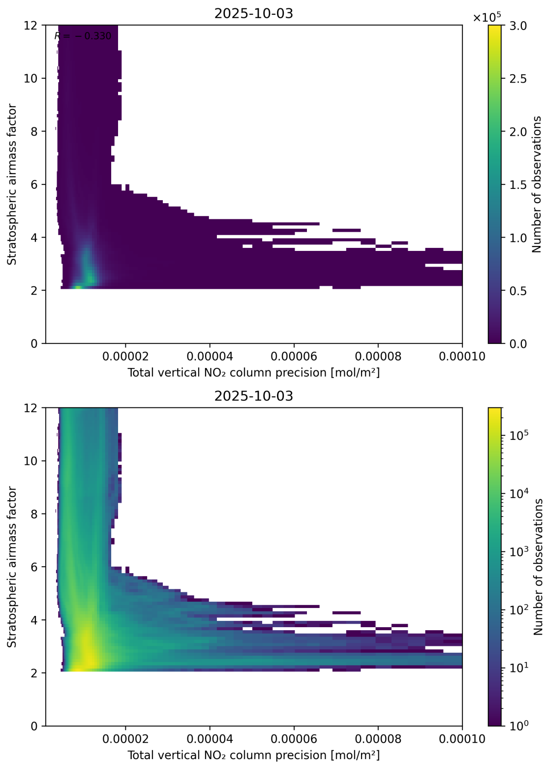
Figure 115: Scatter density plot of “Total vertical NO 2 column precision” against “Stratospheric air mass factor” for 2025-10-02 to 2025-10-04.
