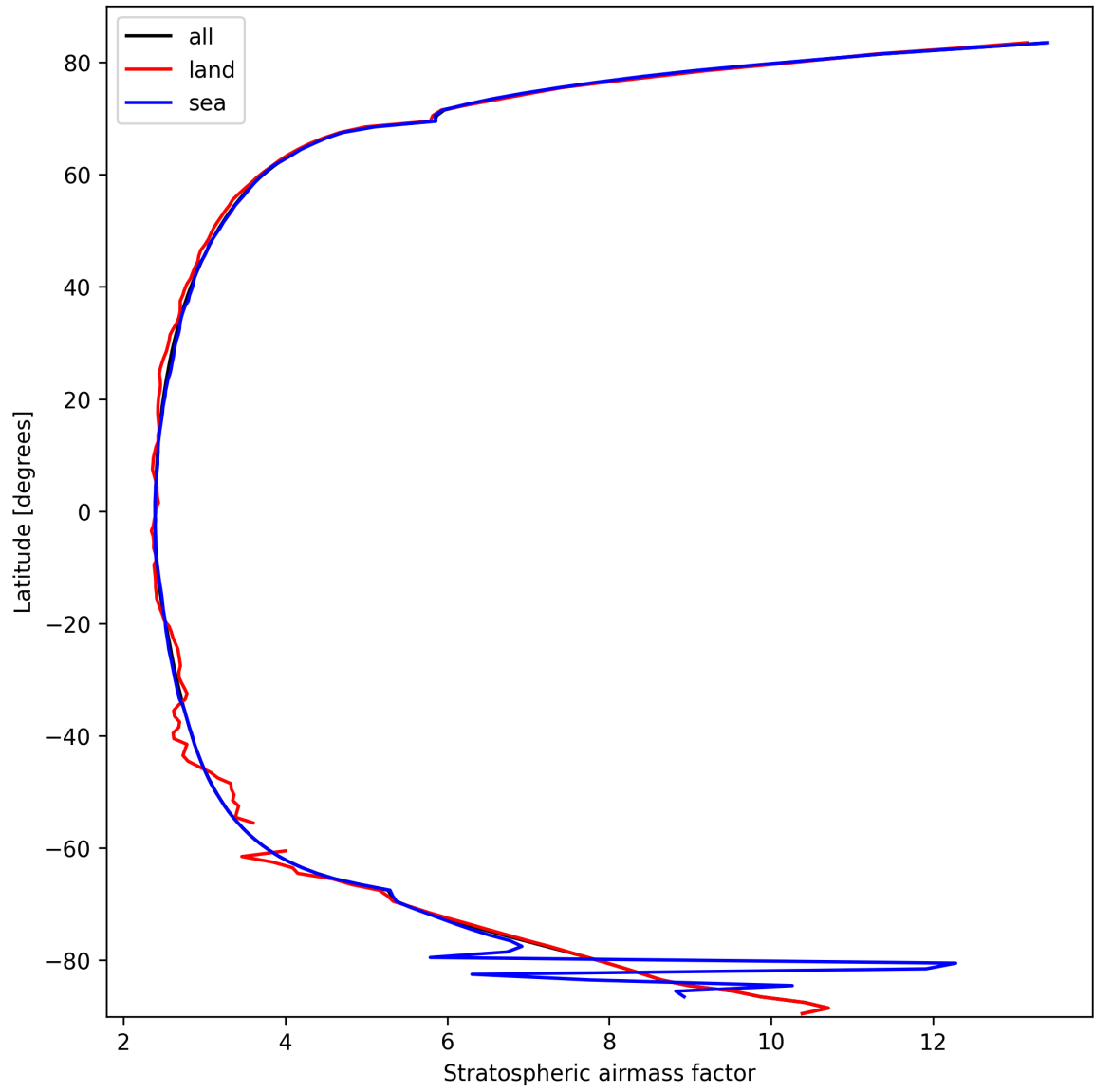
Figure 27: Zonal average of “Stratospheric air mass factor” for 2025-10-02 to 2025-10-04.
