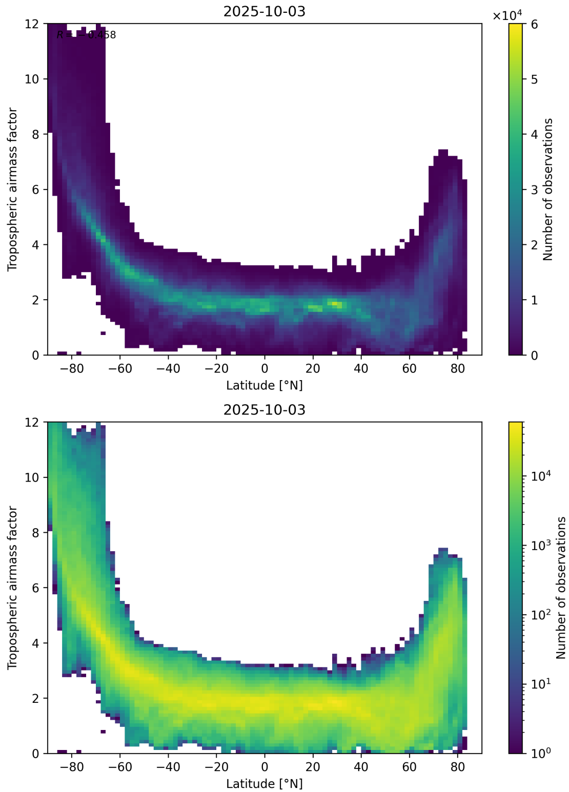
Figure 85: Scatter density plot of “Latitude” against “Tropospheric airmass factor” for 2025-10-02 to 2025-10-04.
