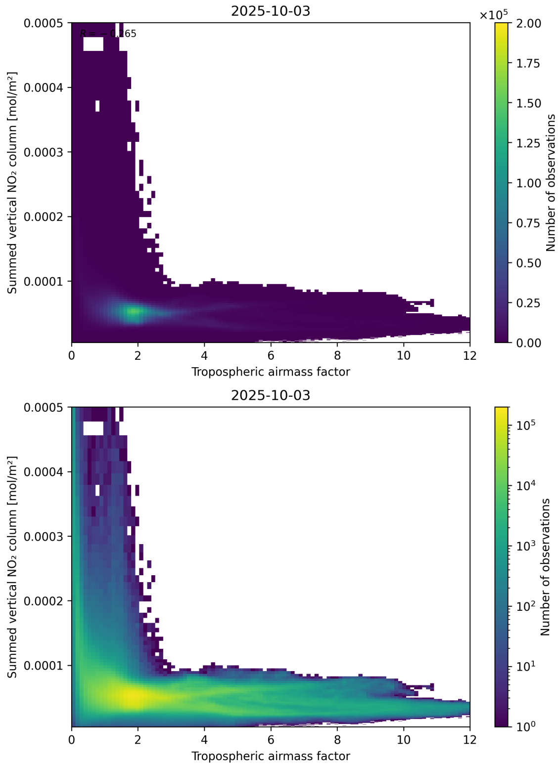
Figure 75: Scatter density plot of “Tropospheric airmass factor” against “Summed vertical NO 2 column” for 2025-10-02 to 2025-10-04.
