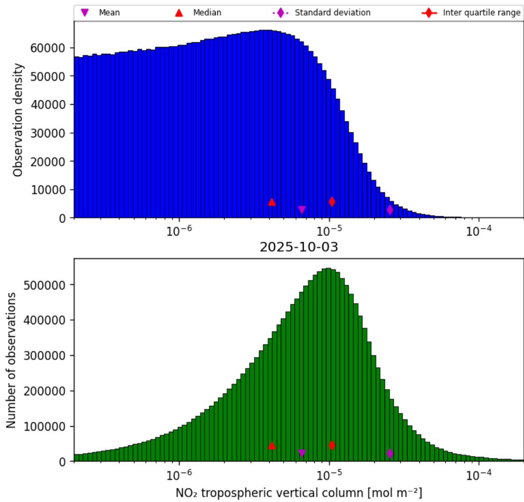
Figure 29: Histogram of “NO 2 tropospheric vertical column” for 2025-10-02 to 2025-10-04
