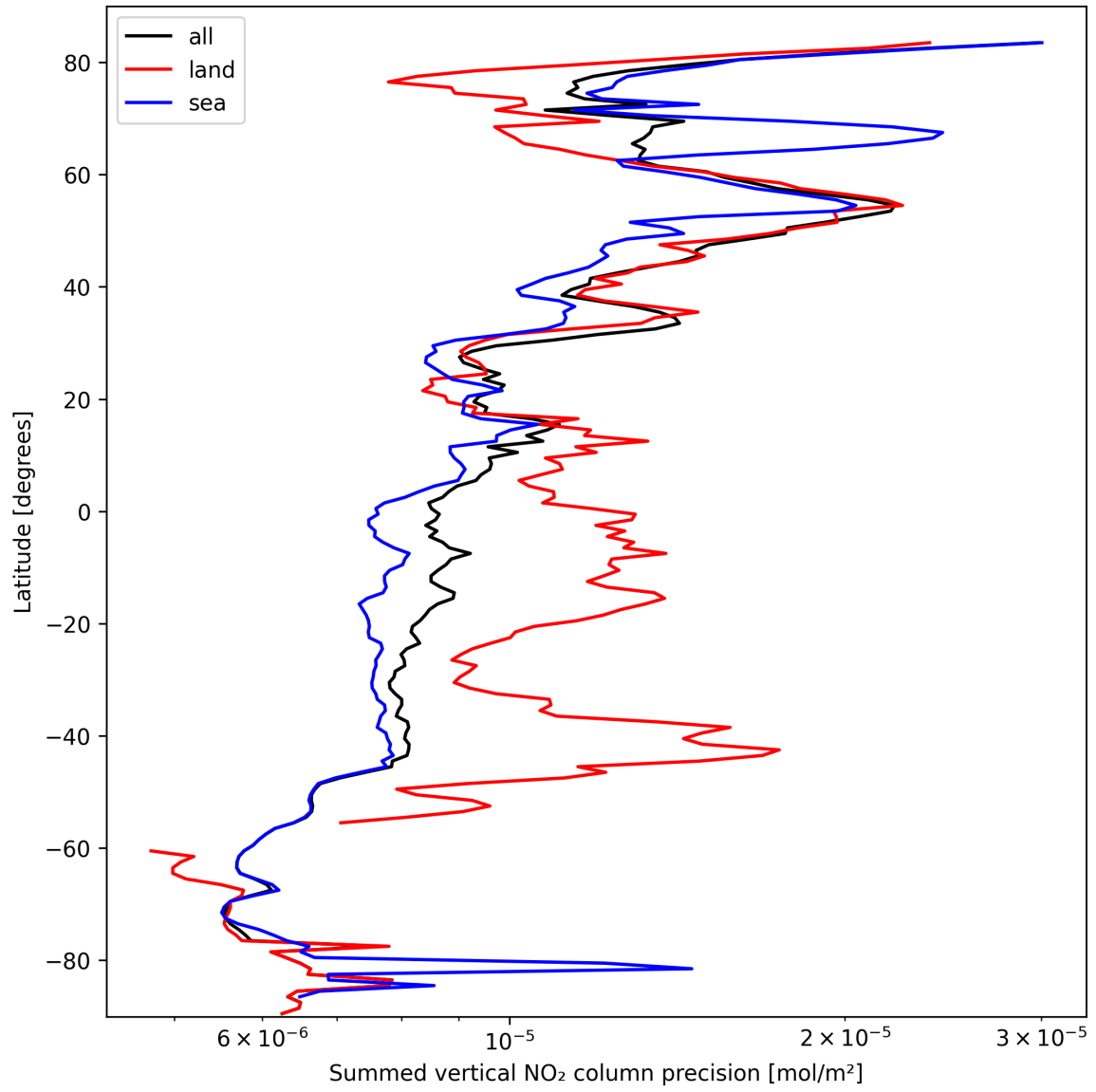
Figure 24: Zonal average of “Summed vertical NO 2 column precision” for 2025-10-02 to 2025-10-04.
