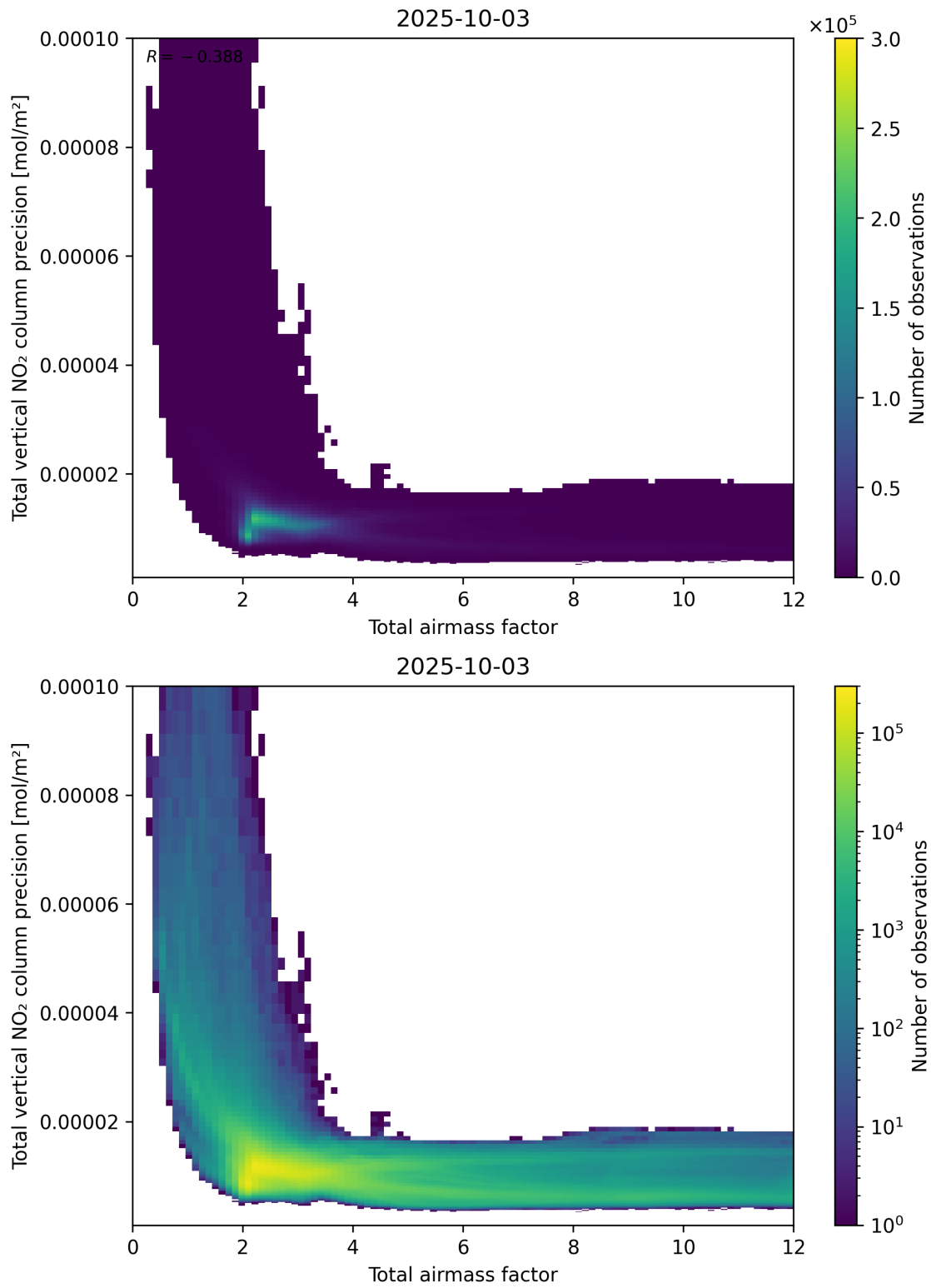
Figure 68: Scatter density plot of “Total airmass factor” against “Total vertical NO 2 column precision” for 2025-10-02 to 2025-10-04.
