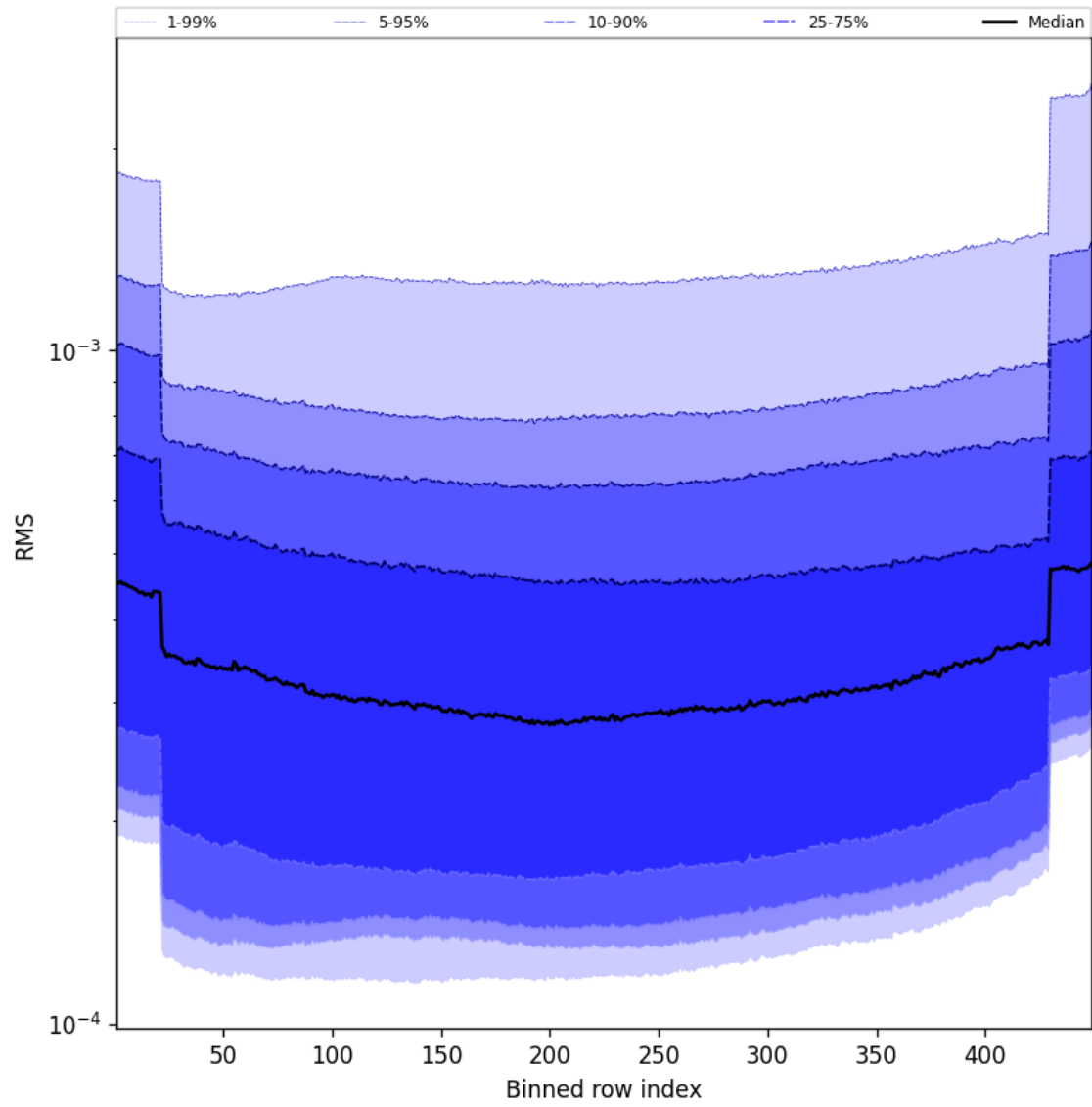
Figure 60: Along track statistics of “RMS” for 2025-10-02 to 2025-10-04
