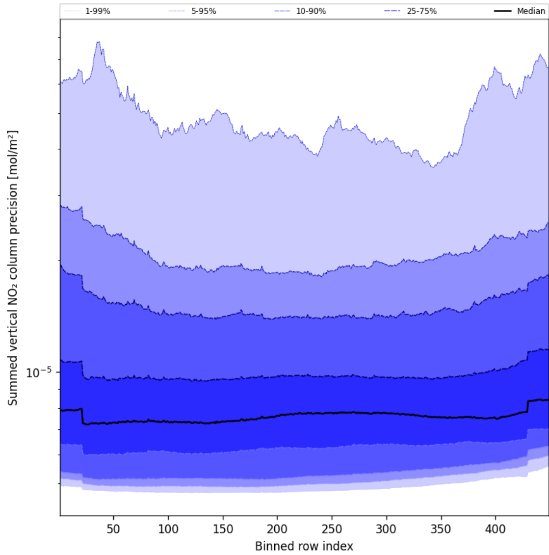
Figure 58: Along track statistics of “Summed vertical NO 2 column precision” for 2025-10-02 to 2025-10-04
