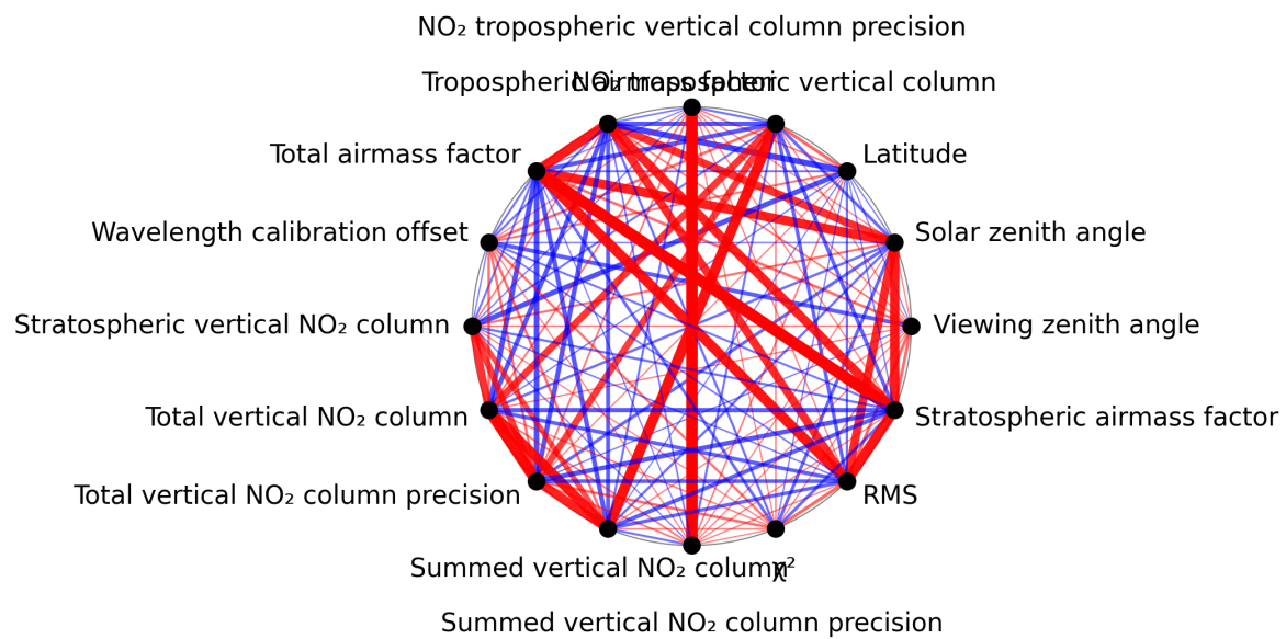
Figure 1: Map of correlation graph for 2025-10-02 to 2025-10-04.
