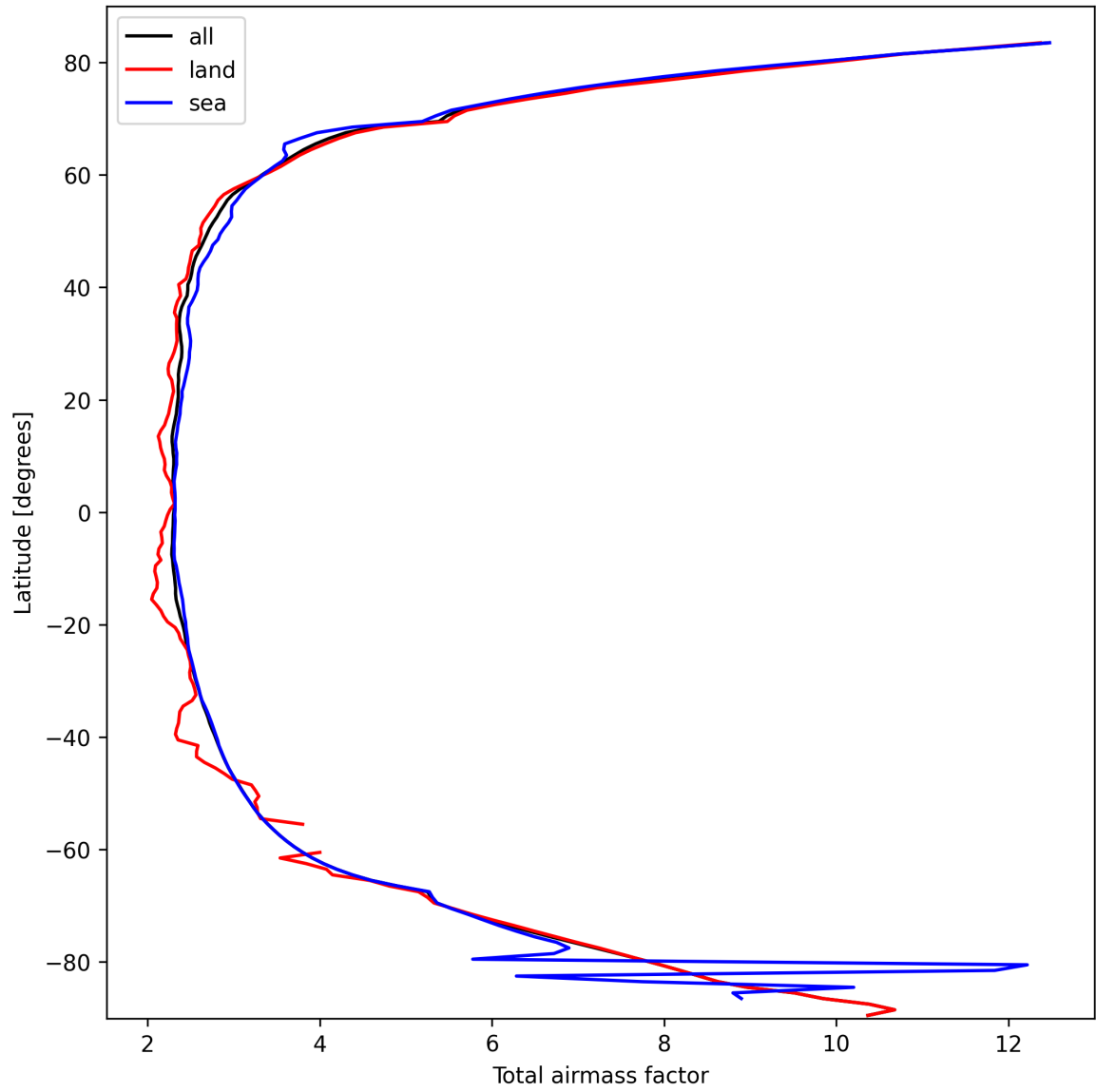
Figure 15: Zonal average of “Total airmass factor” for 2025-10-02 to 2025-10-04.
