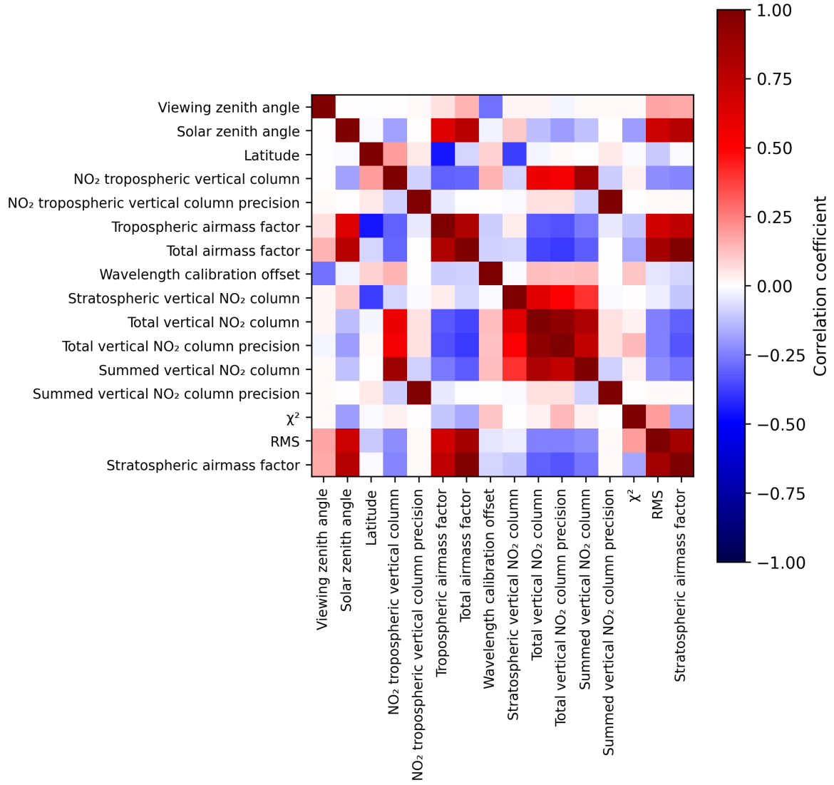
Figure 2: Map of correlation matrix for 2025-10-02 to 2025-10-04.
