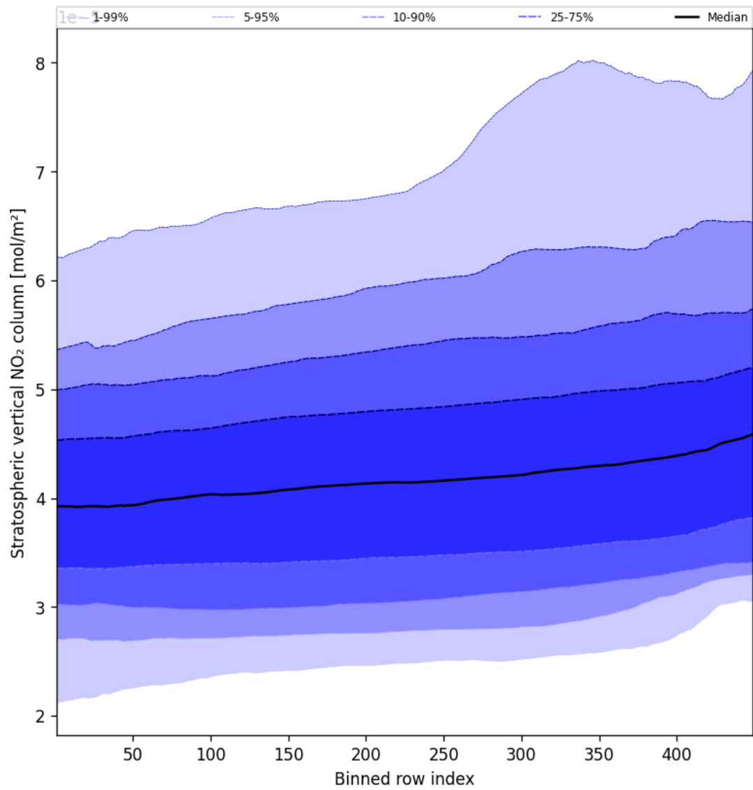
Figure 53: Along track statistics of “Stratospheric vertical NO 2 column” for 2025-10-02 to 2025-10-04
