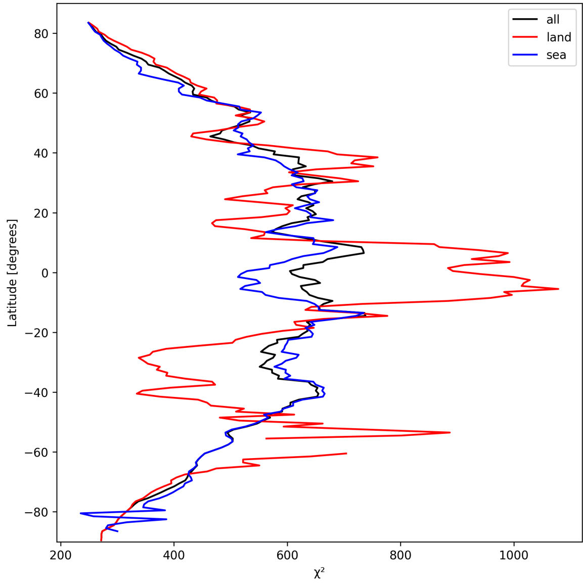
Figure 25: Zonal average of “ \chi^2 ” for 2025-10-02 to 2025-10-04.
