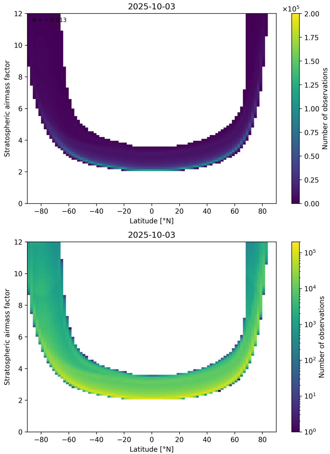
Figure 83: Scatter density plot of “Latitude” against “Stratospheric airmass factor” for 2025-10-02 to 2025-10-04.
