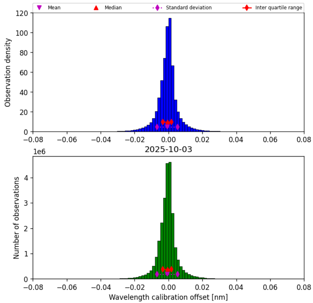
Figure 35: Histogram of “Wavelength calibration offset” for 2025-10-02 to 2025-10-04
