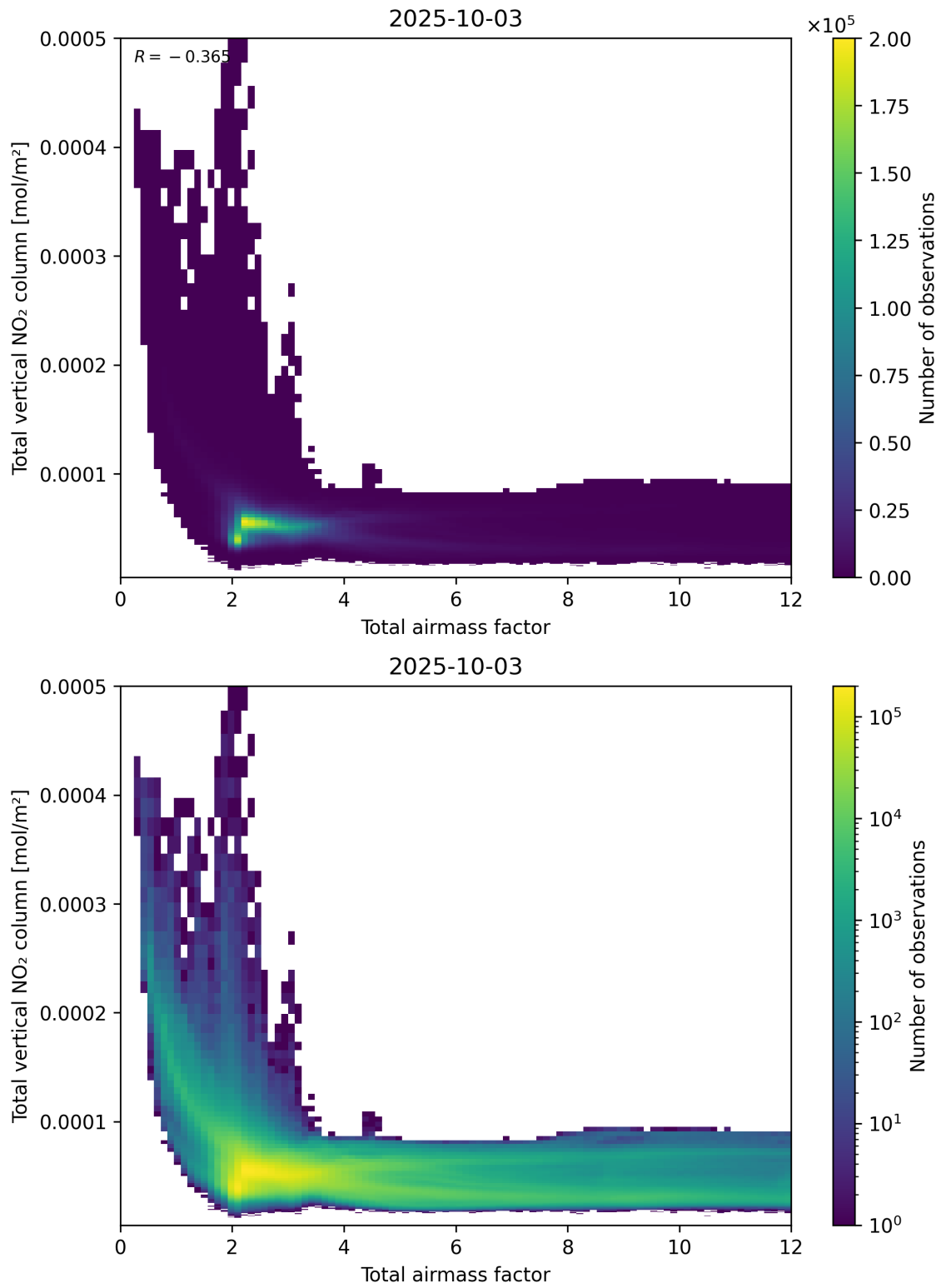
Figure 67: Scatter density plot of “Total airmass factor” against “Total vertical NO 2 column” for 2025-10-02 to 2025-10-04.
