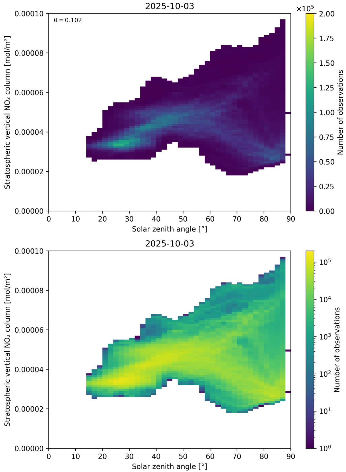
Figure 150: Scatter density plot of “Solar zenith angle” against “Stratospheric vertical NO 2 column” for 2025-10-02 to 2025-10-04.
