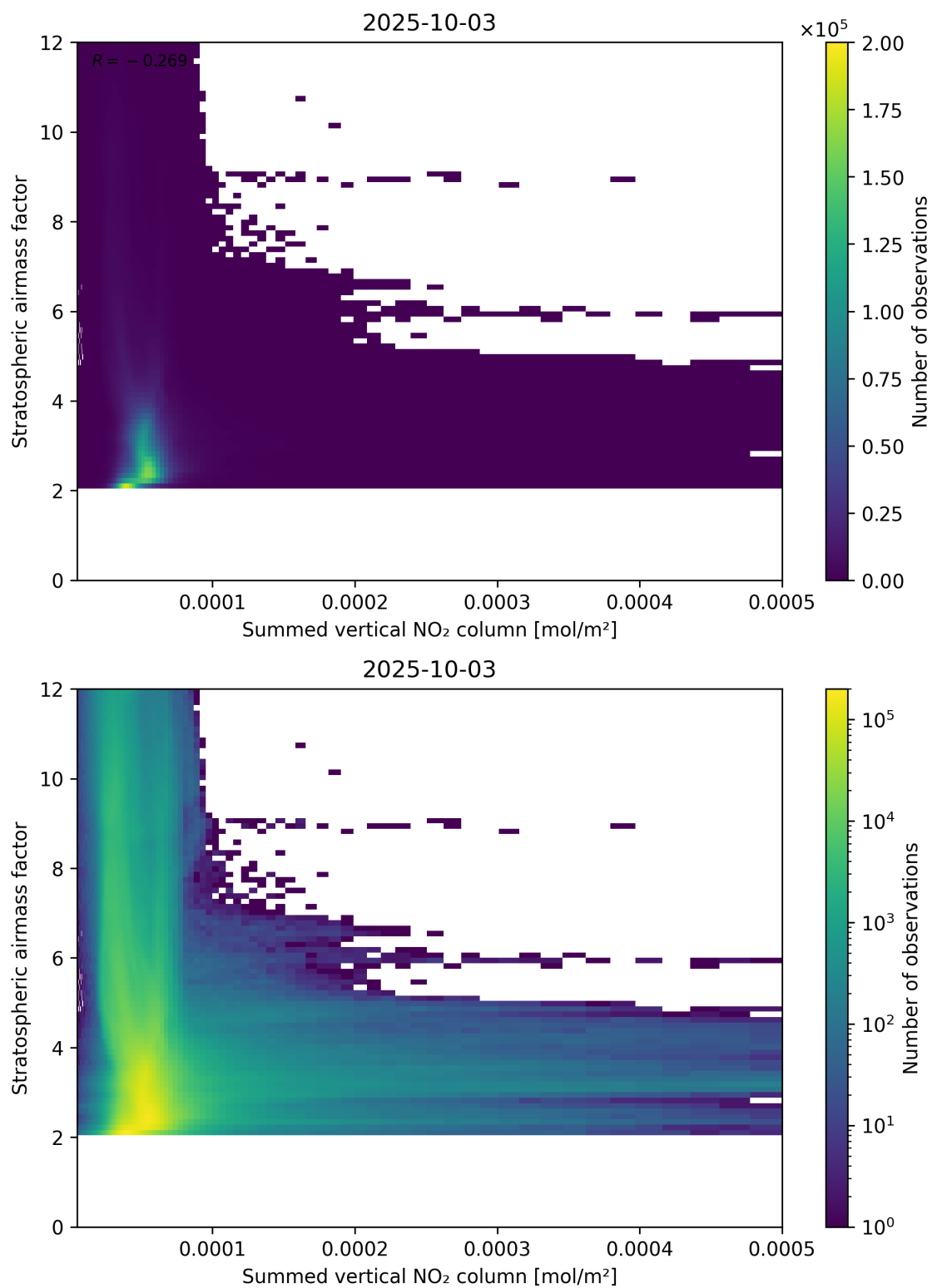
Figure 103: Scatter density plot of “Summed vertical NO 2 column” against “Stratospheric airmass factor” for 2025-10-02 to 2025-10-04.
