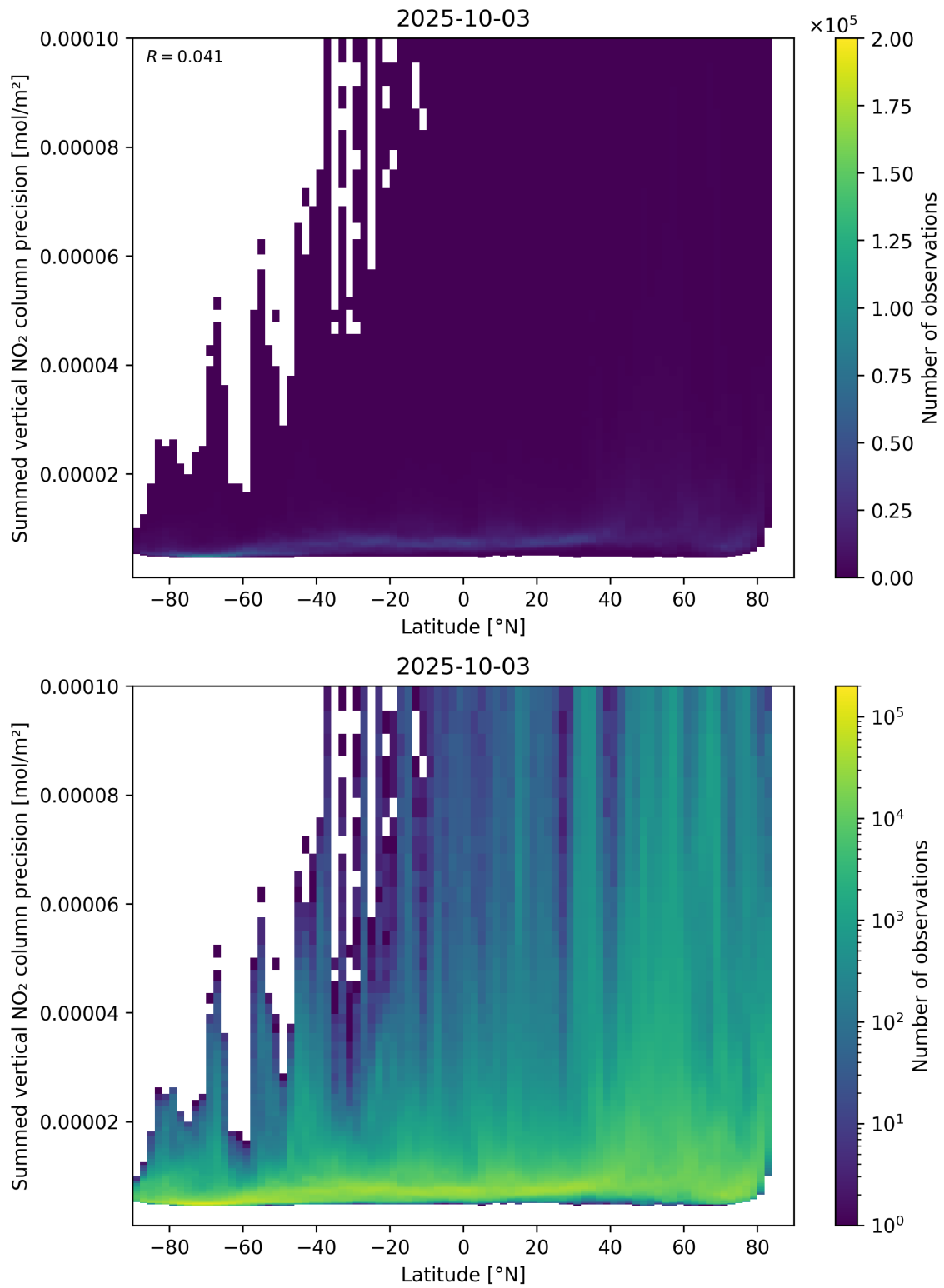
Figure 89: Scatter density plot of “Latitude” against “Summed vertical NO 2 column precision” for 2025-10-02 to 2025-10-04.
