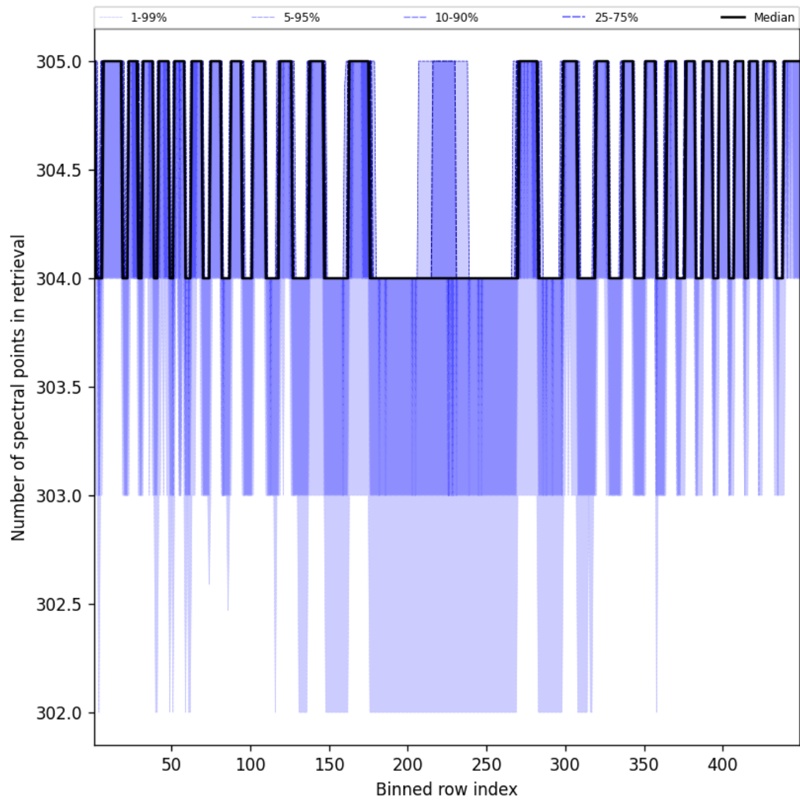
Figure 50: Along track statistics of “Number of spectral points in retrieval” for 2025-10-02 to 2025-10-04
