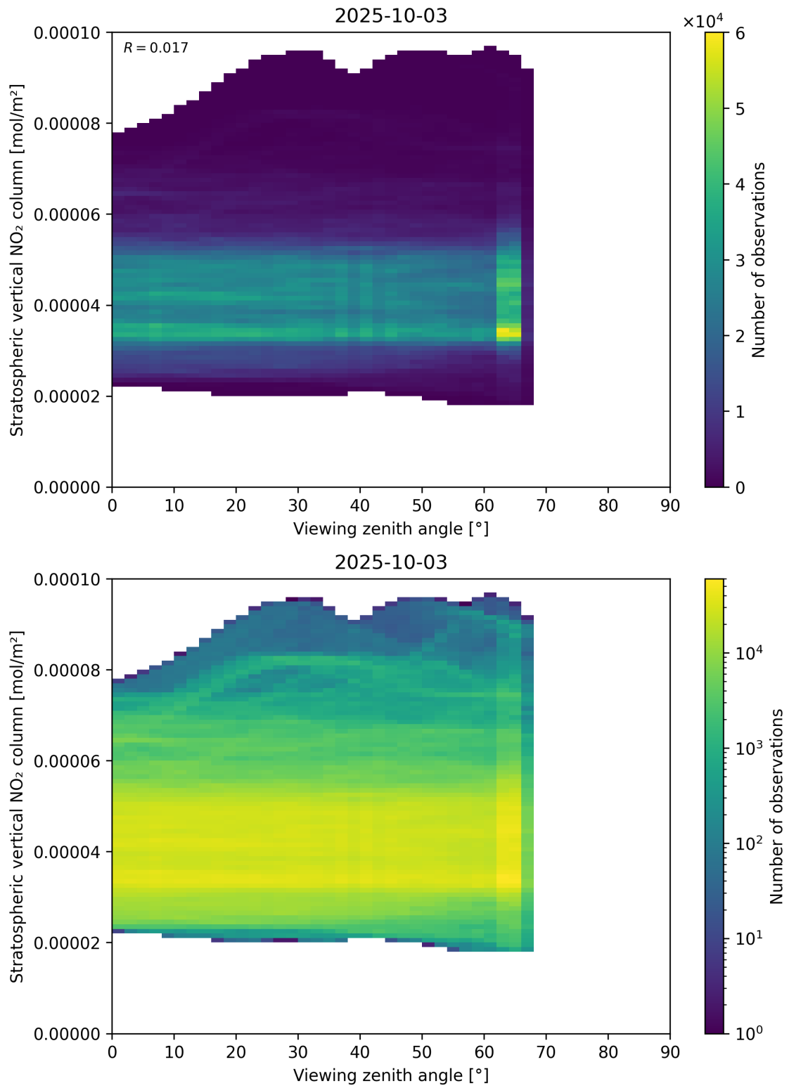
Figure 164: Scatter density plot of “Viewing zenith angle” against “Stratospheric vertical NO 2 column” for 2025-10-02 to 2025-10-04.
