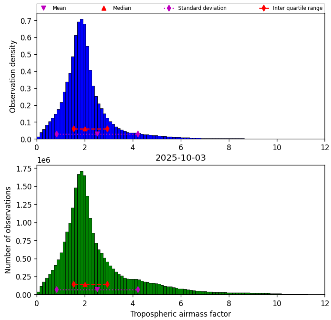
Figure 31: Histogram of “Tropospheric airmass factor” for 2025-10-02 to 2025-10-04
