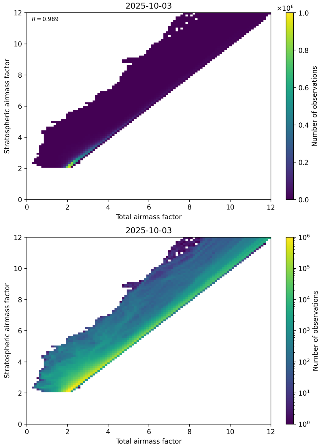
Figure 62: Scatter density plot of “Total airmass factor” against “Stratospheric airmass factor” for 2025-10-02 to 2025-10-04.
