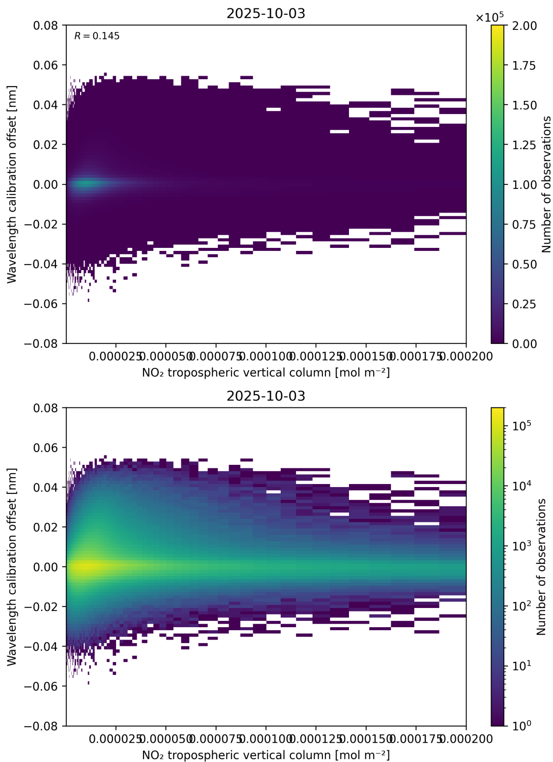
Figure 143: Scatter density plot of “NO 2 tropospheric vertical column” against “Wavelength calibration offset” for 2025-10-02 to 2025-10-04.
