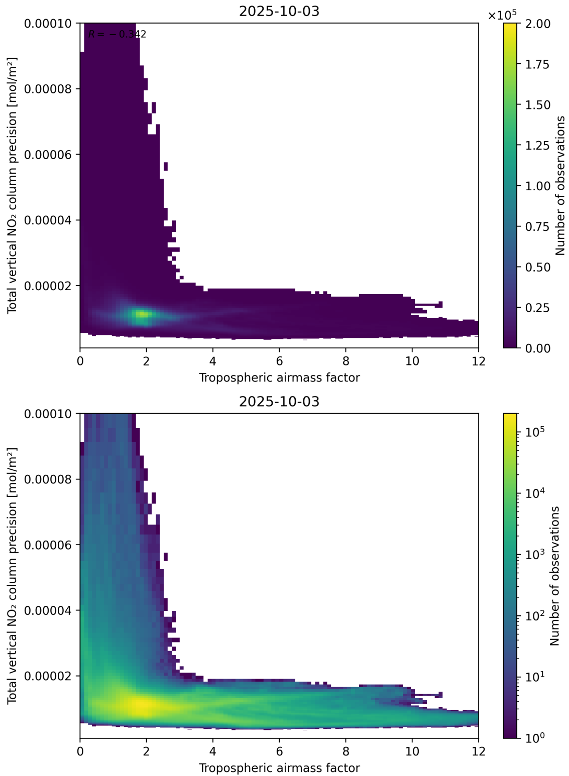
Figure 78: Scatter density plot of “Tropospheric air mass factor” against “Total vertical NO 2 column precision” for 2025-10-02 to 2025-10-04.
