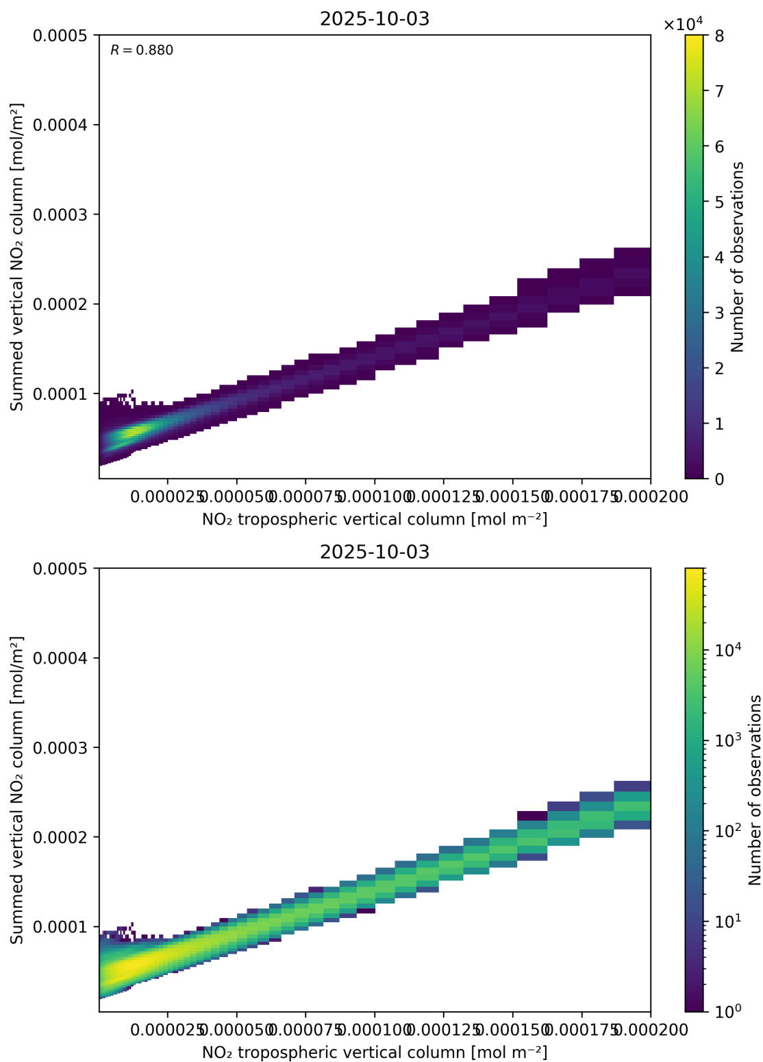
Figure 126: Scatter density plot of “NO 2 tropospheric vertical column” against “Summed vertical NO 2 column” for 2025-10-02 to 2025-10-04.
