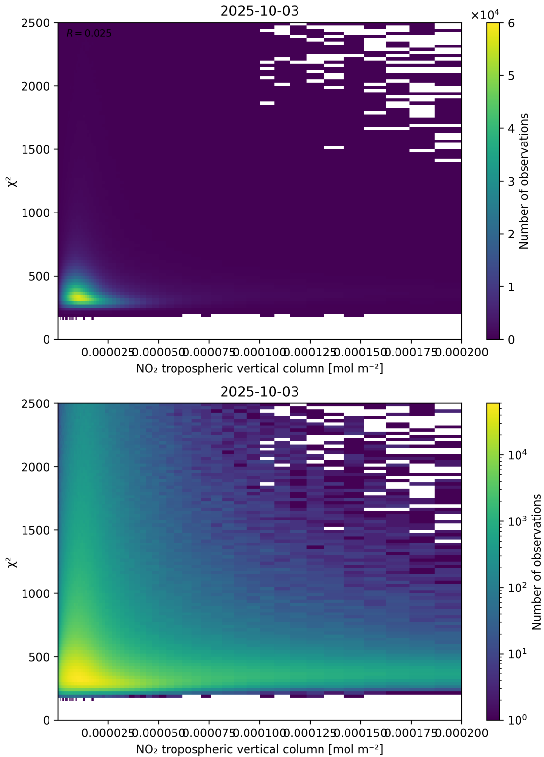
Figure 124: Scatter density plot of “NO 2 tropospheric vertical column” against “ \chi^2 ” for 2025-10-02 to 2025-10-04.
