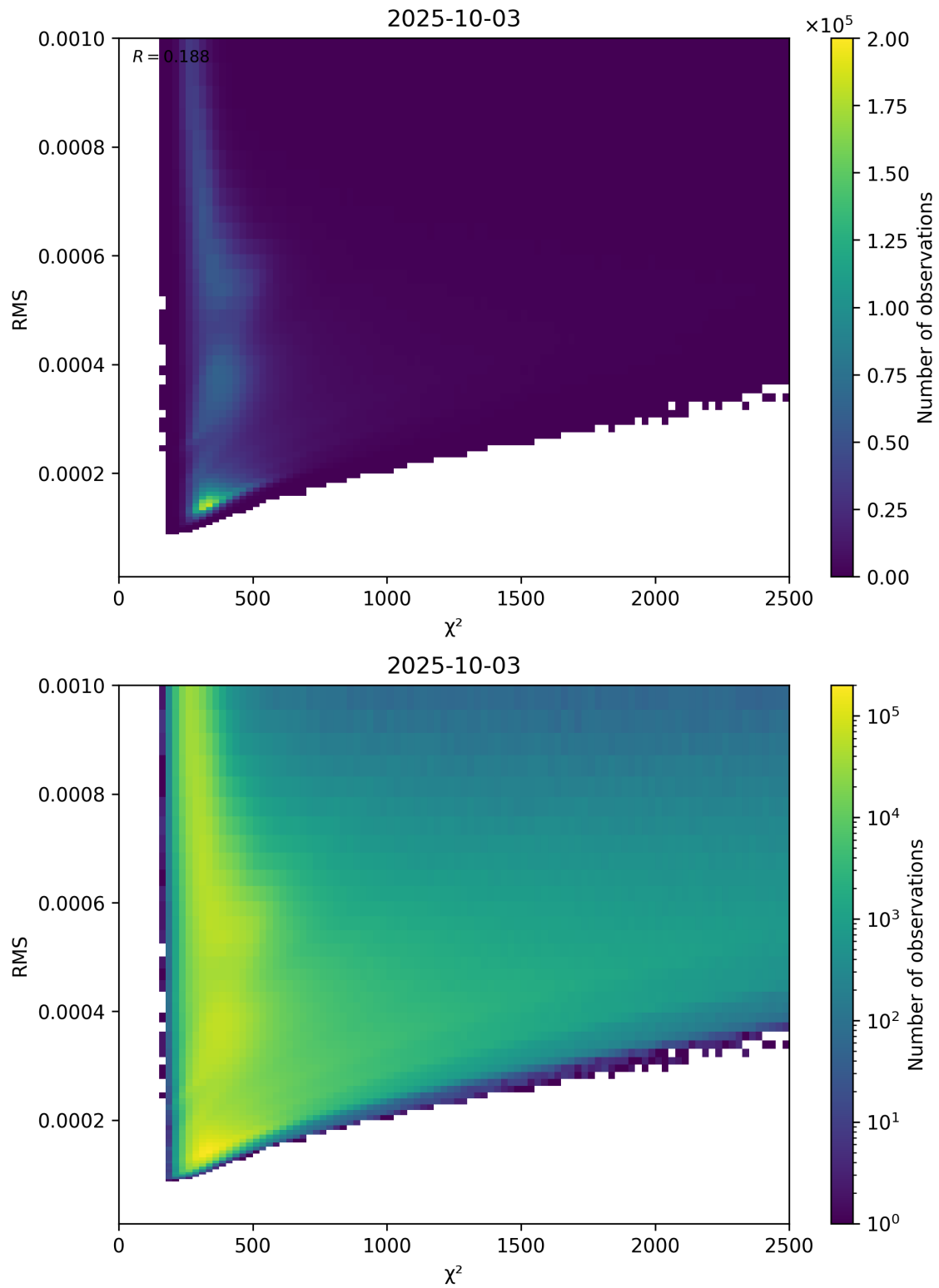
Figure 82: Scatter density plot of “ \chi^2 ” against “RMS” for 2025-10-02 to 2025-10-04.
