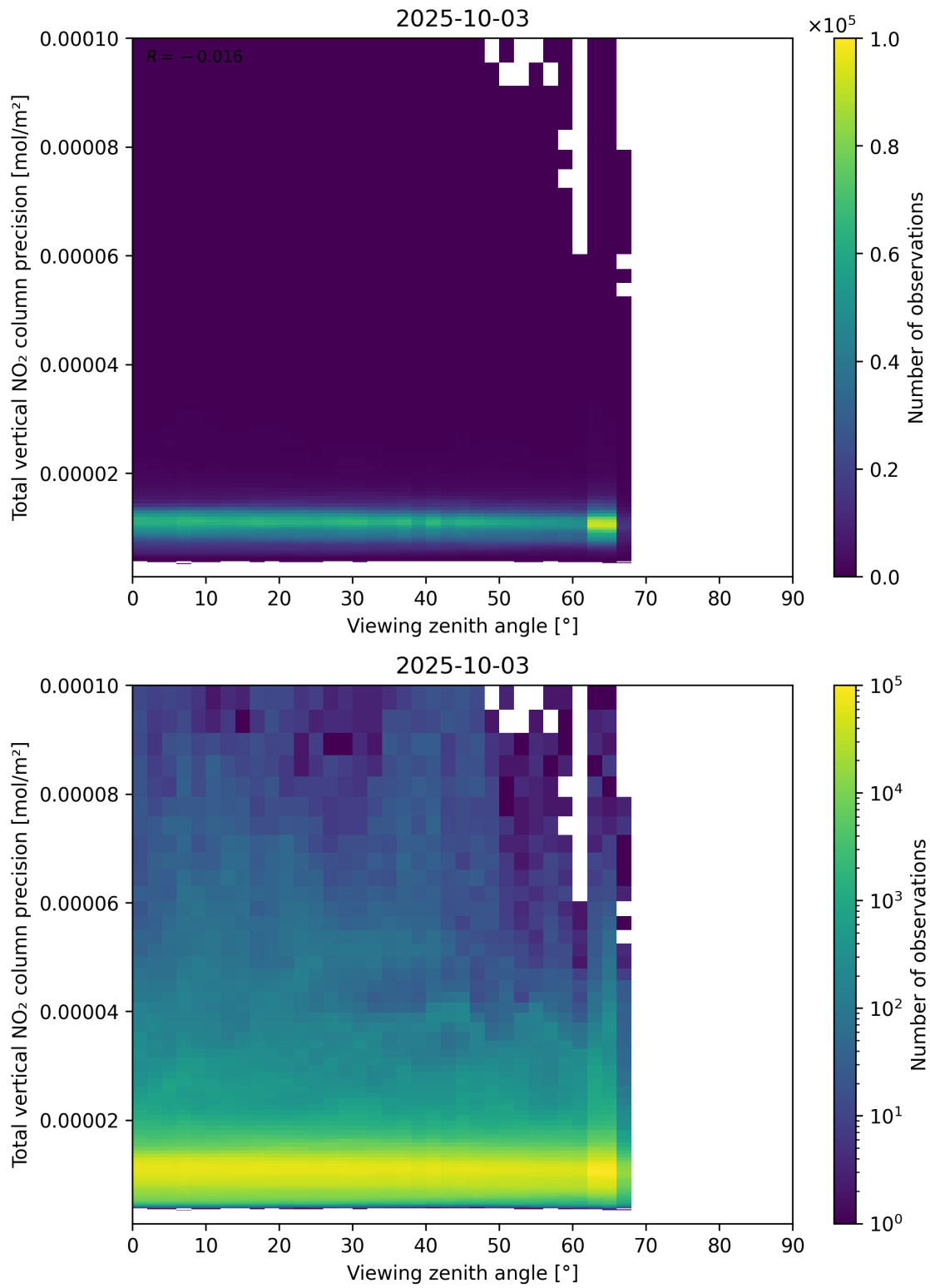
Figure 168: Scatter density plot of “Viewing zenith angle” against “Total vertical NO 2 column precision” for 2025-10-02 to 2025-10-04.
