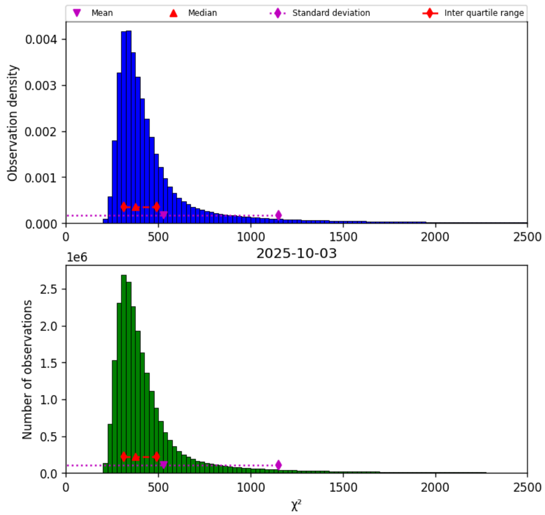
Figure 42: Histogram of “ \chi^2 ” for 2025-10-02 to 2025-10-04
