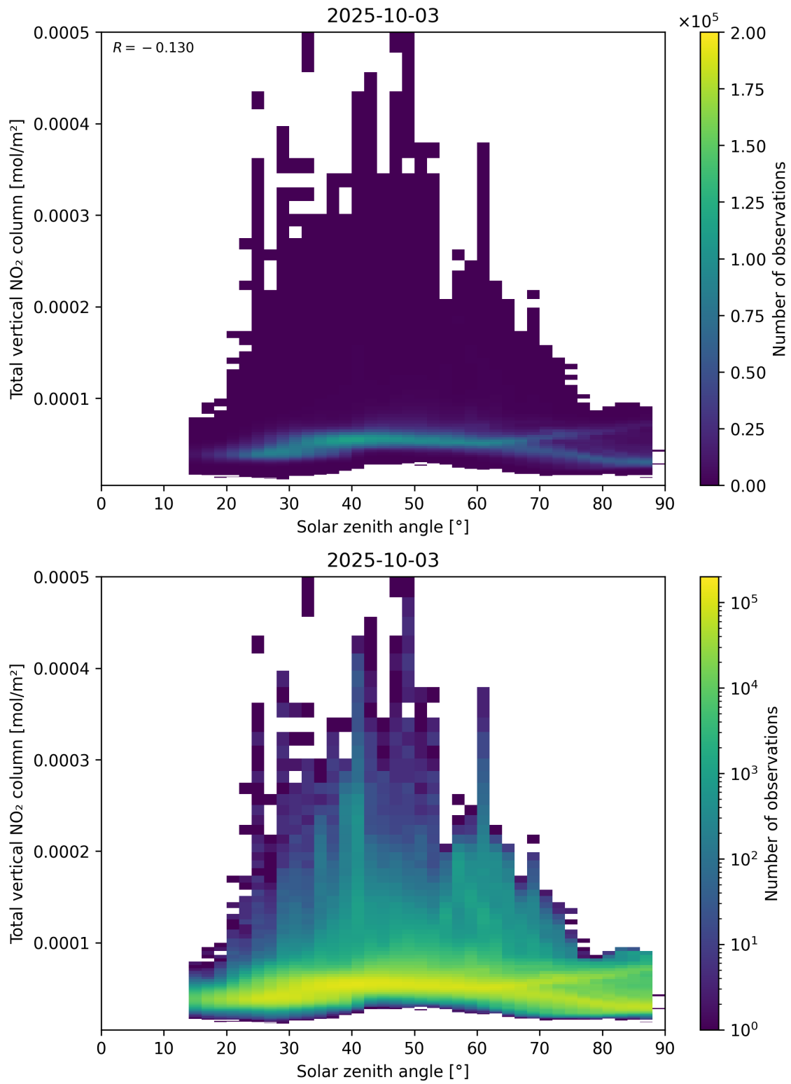
Figure 153: Scatter density plot of “Solar zenith angle” against “Total vertical NO 2 column” for 2025-10-02 to 2025-10-04.
