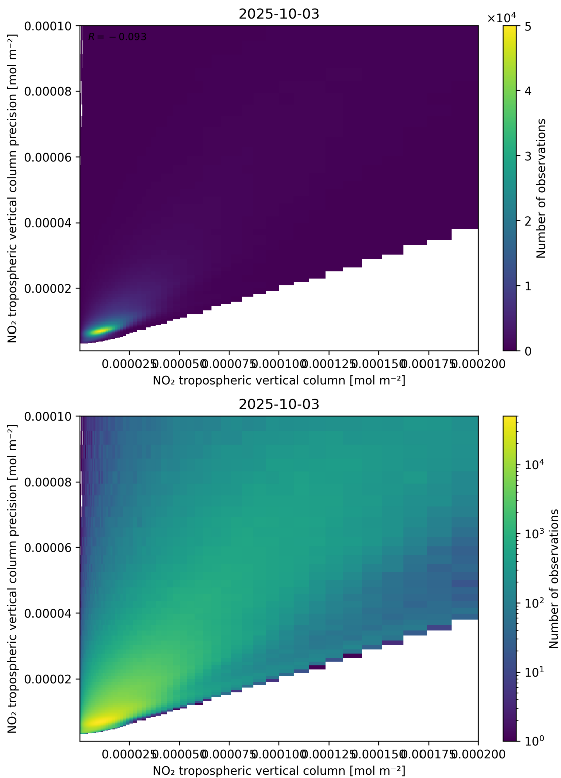
Figure 130: Scatter density plot of “NO 2 tropospheric vertical column” against “NO 2 tropospheric vertical column precision” for 2025-10-02 to 2025-10-04.
