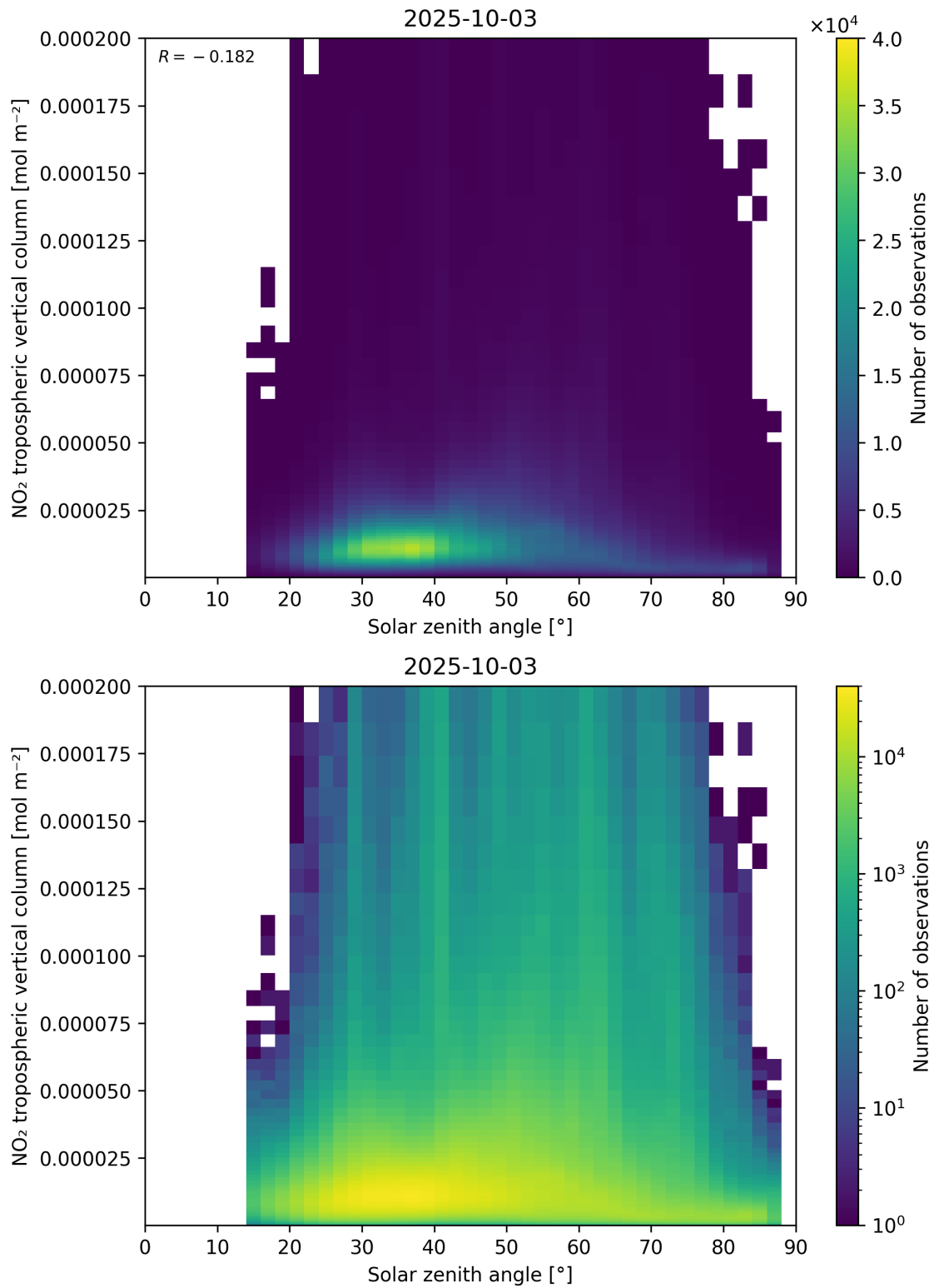
Figure 155: Scatter density plot of “Solar zenith angle” against “NO 2 tropospheric vertical column” for 2025-10-02 to 2025-10-04.
