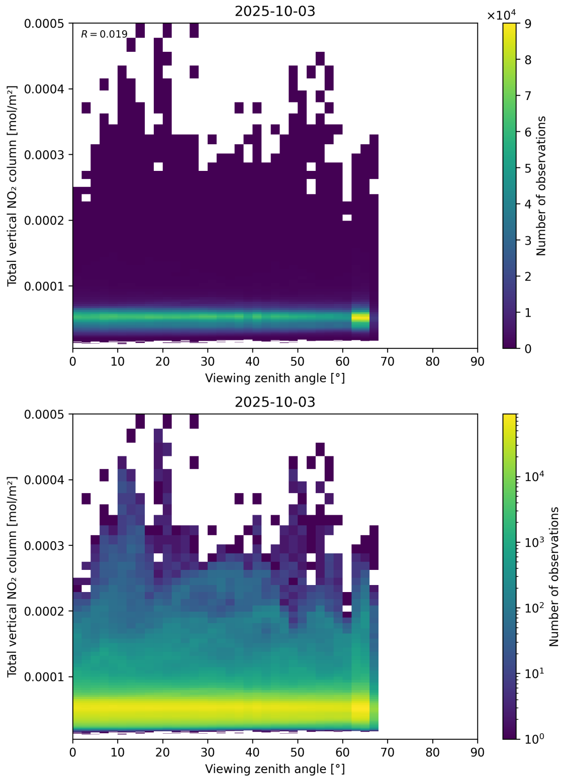
Figure 167: Scatter density plot of “Viewing zenith angle” against “Total vertical NO 2 column” for 2025-10-02 to 2025-10-04.
