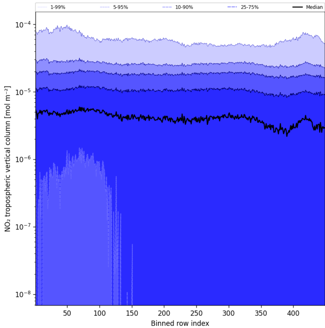
Figure 46: Along track statistics of “NO 2 tropospheric vertical column” for 2025-10-02 to 2025-10-04
