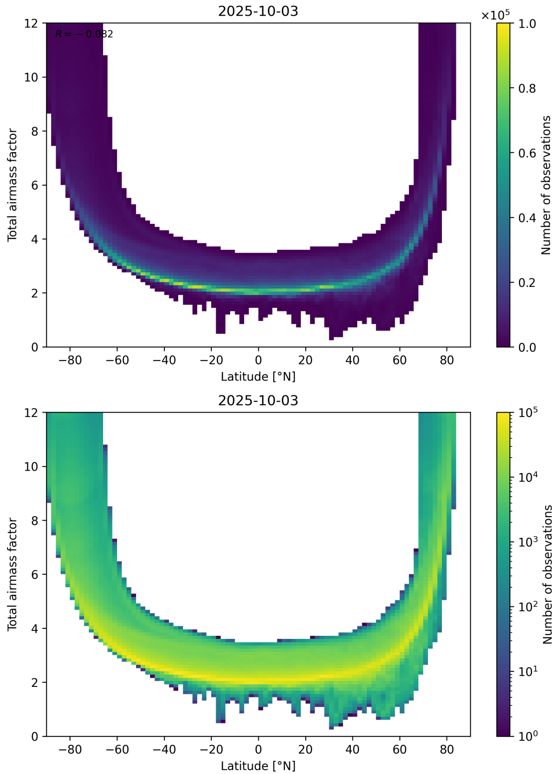
Figure 84: Scatter density plot of “Latitude” against “Total airmass factor” for 2025-10-02 to 2025-10-04.
