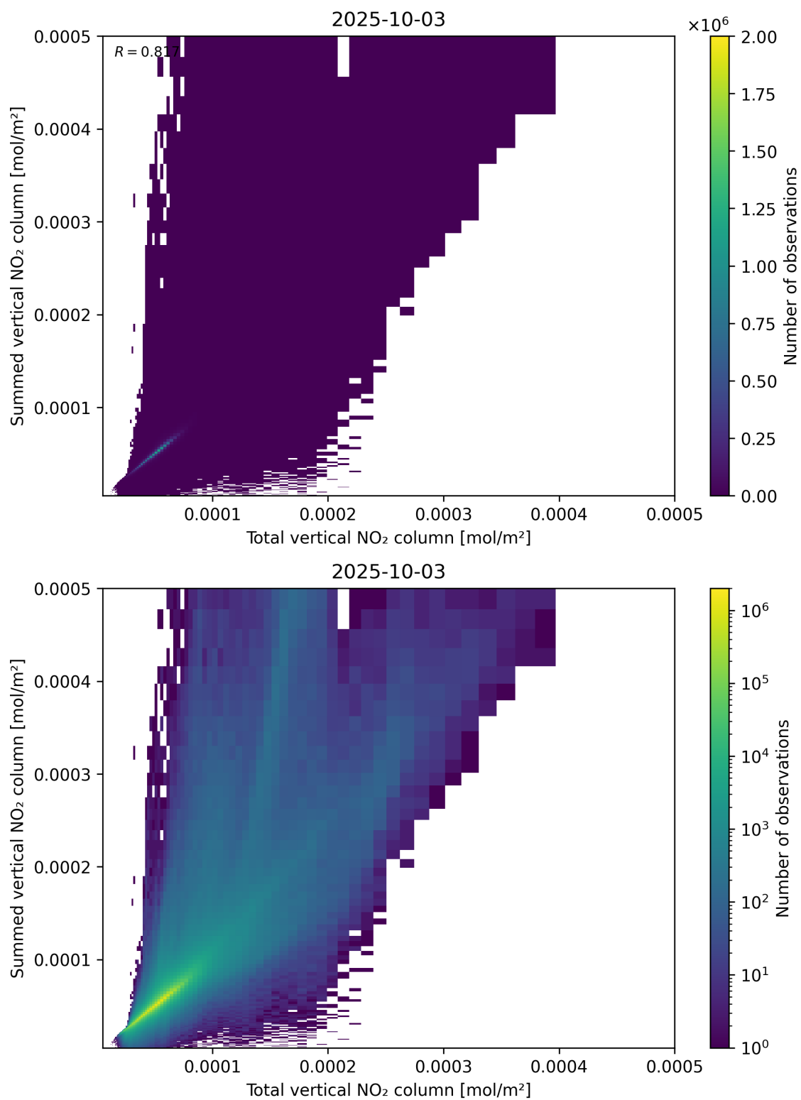
Figure 112: Scatter density plot of “Total vertical NO 2 column” against “Summed vertical NO 2 column” for 2025-10-02 to 2025-10-04.
