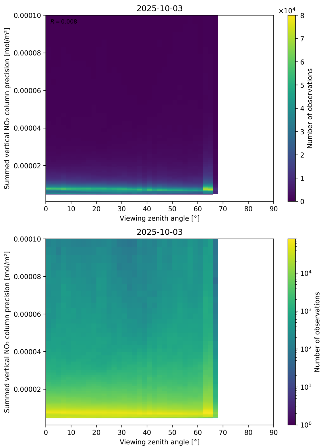
Figure 166: Scatter density plot of “Viewing zenith angle” against “Summed vertical NO 2 column precision” for 2025-10-02 to 2025-10-04.
