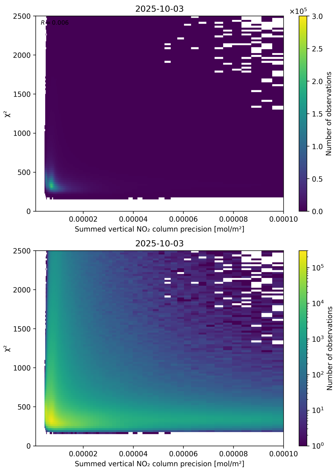
Figure 107: Scatter density plot of “Summed vertical NO 2 column precision” against “ \chi^2 ” for 2025-10-02 to 2025-10-04.
