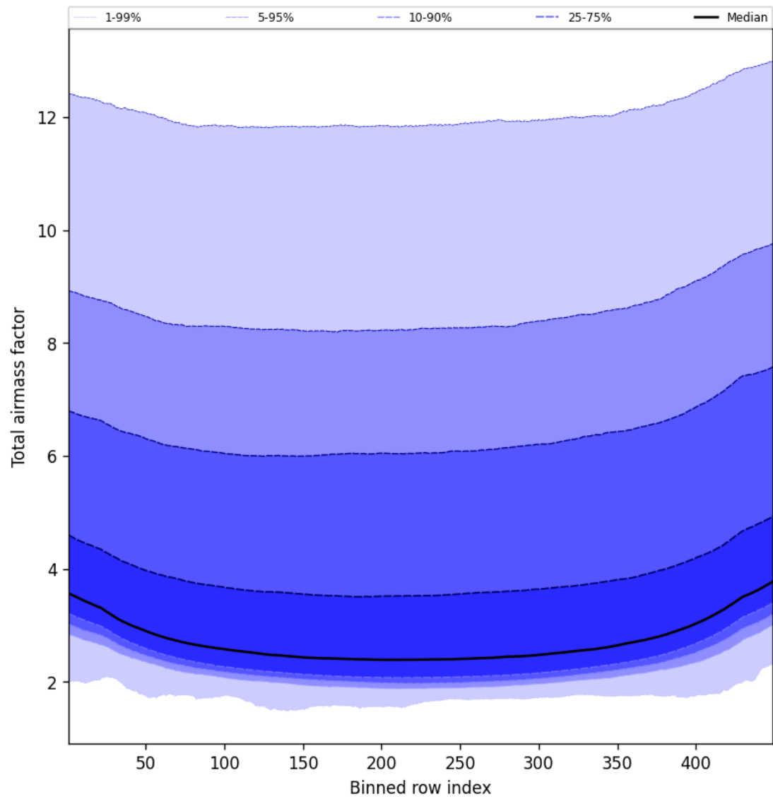
Figure 49: Along track statistics of “Total airmass factor” for 2025-10-02 to 2025-10-04
