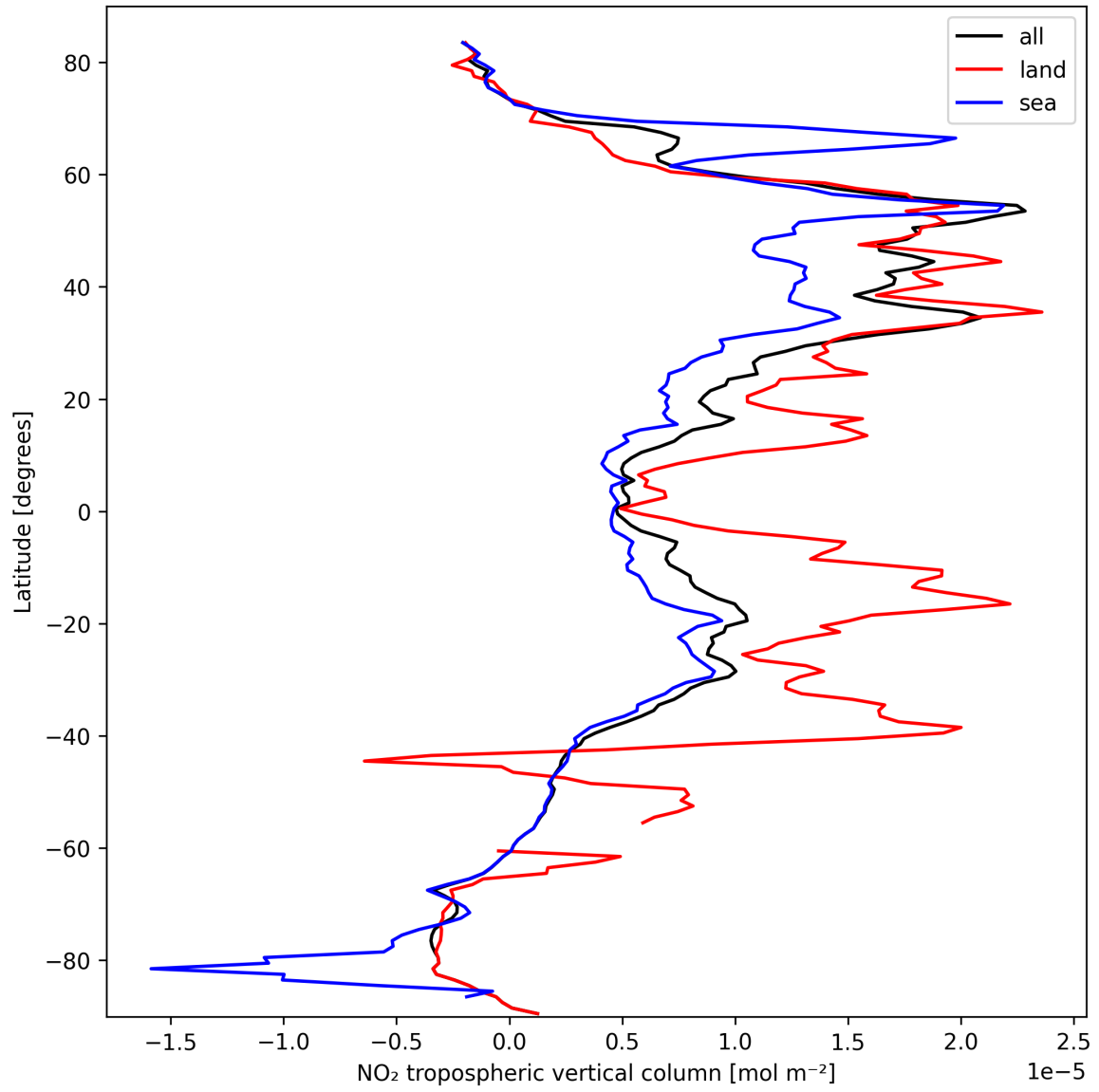
Figure 12: Zonal average of “NO 2 tropospheric vertical column” for 2025-10-02 to 2025-10-04.
