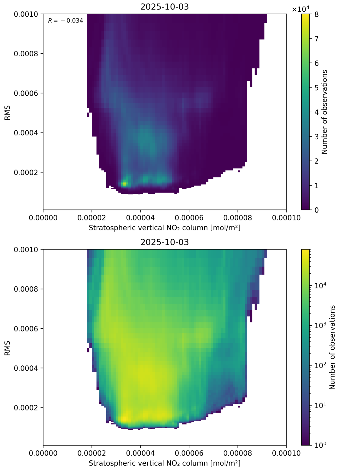
Figure 102: Scatter density plot of “Stratospheric vertical NO 2 column” against “RMS” for 2025-10-02 to 2025-10-04.
