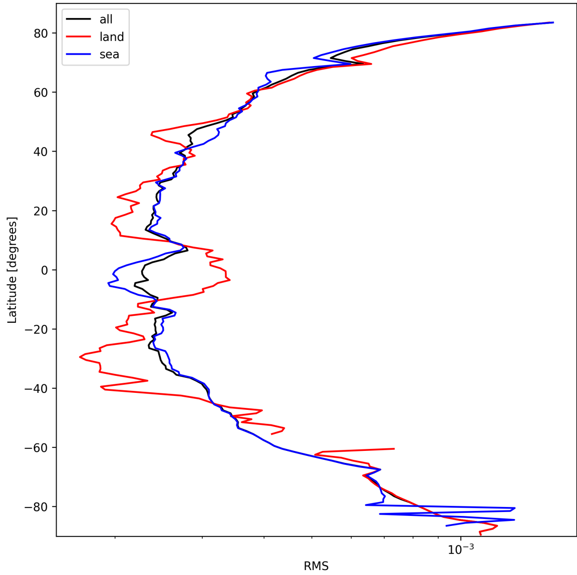
Figure 26: Zonal average of “RMS” for 2025-10-02 to 2025-10-04.
