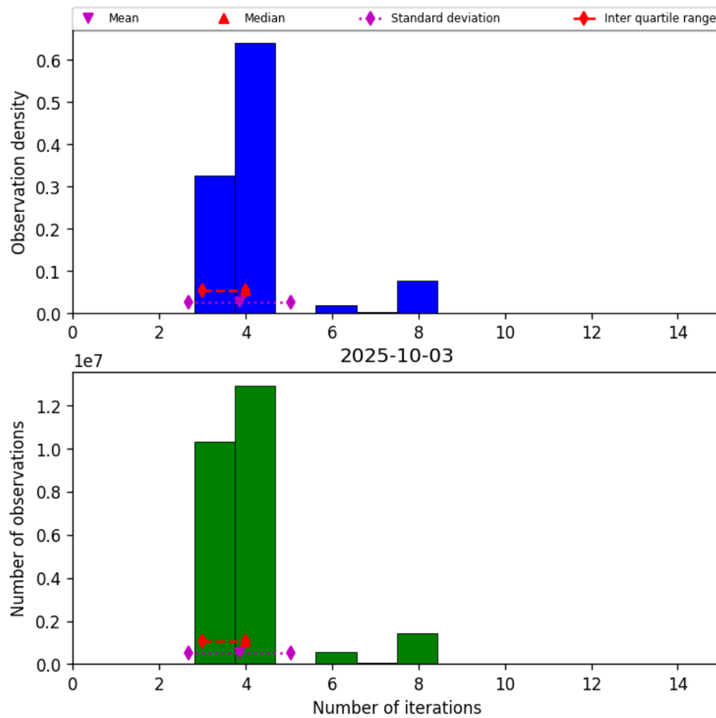
Figure 34: Histogram of “Number of iterations” for 2025-10-02 to 2025-10-04
