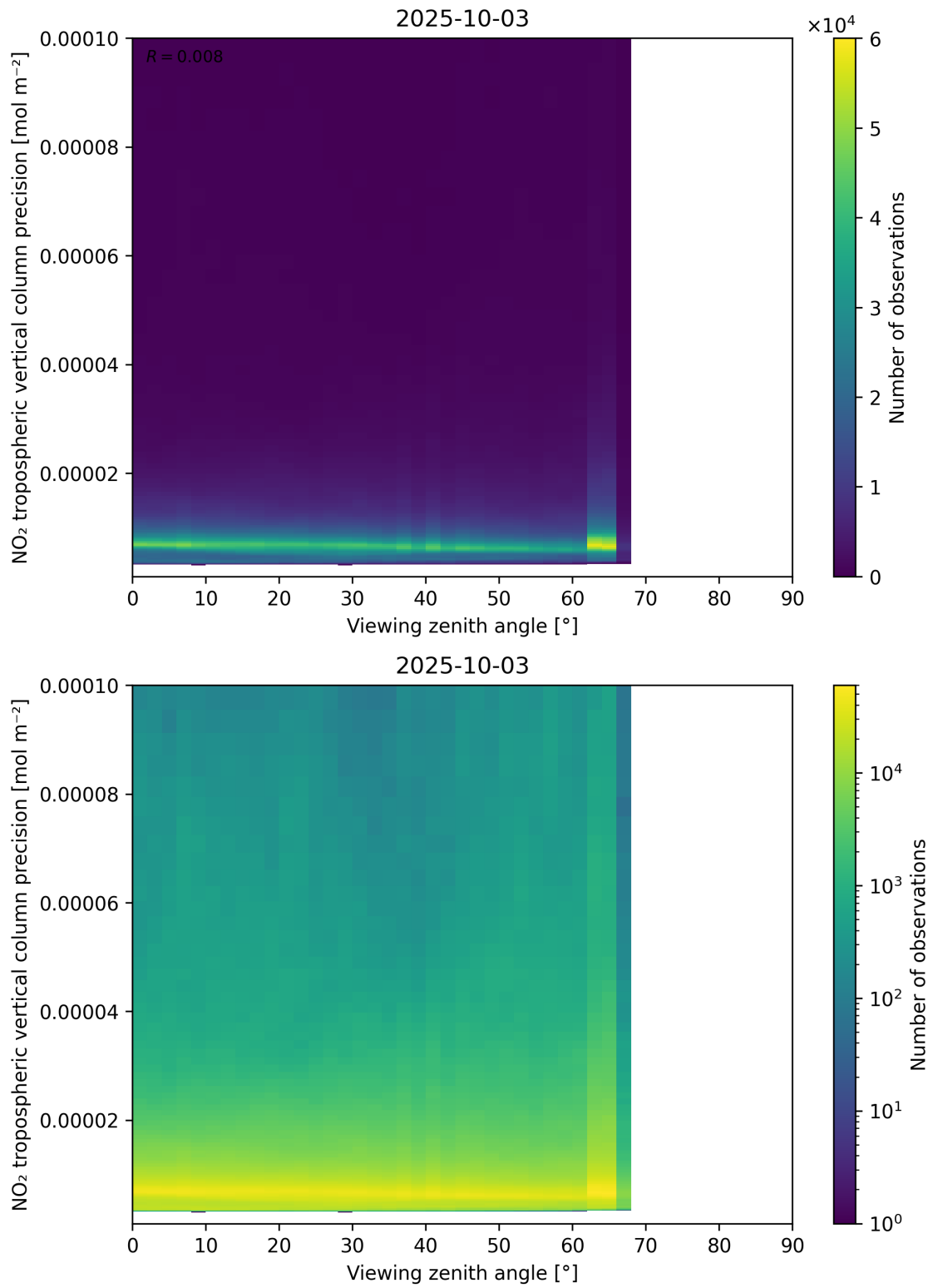
Figure 170: Scatter density plot of “Viewing zenith angle” against “NO 2 tropospheric vertical column precision” for 2025-10-02 to 2025-10-04.
