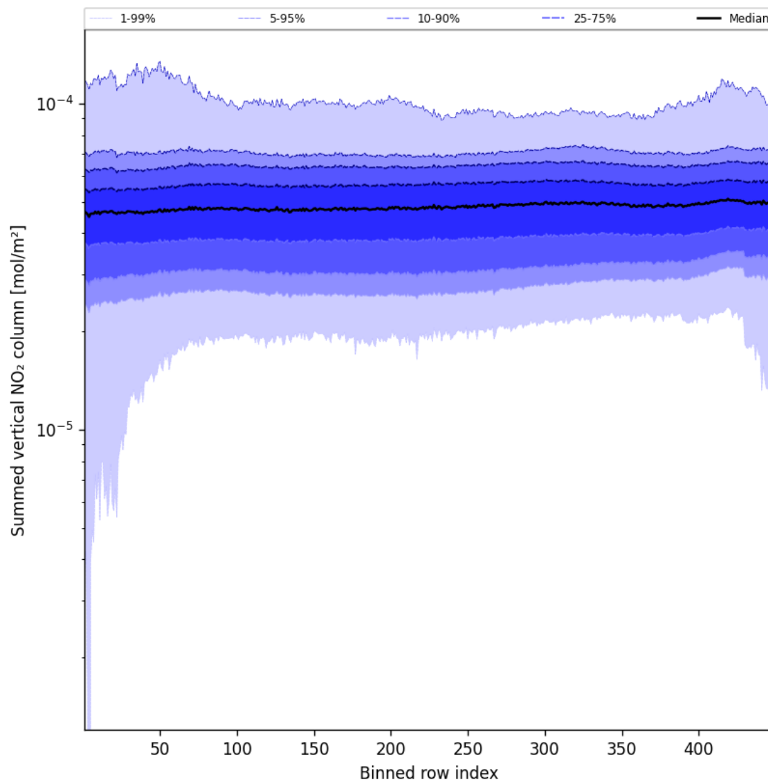
Figure 57: Along track statistics of “Summed vertical NO 2 column” for 2025-10-02 to 2025-10-04
