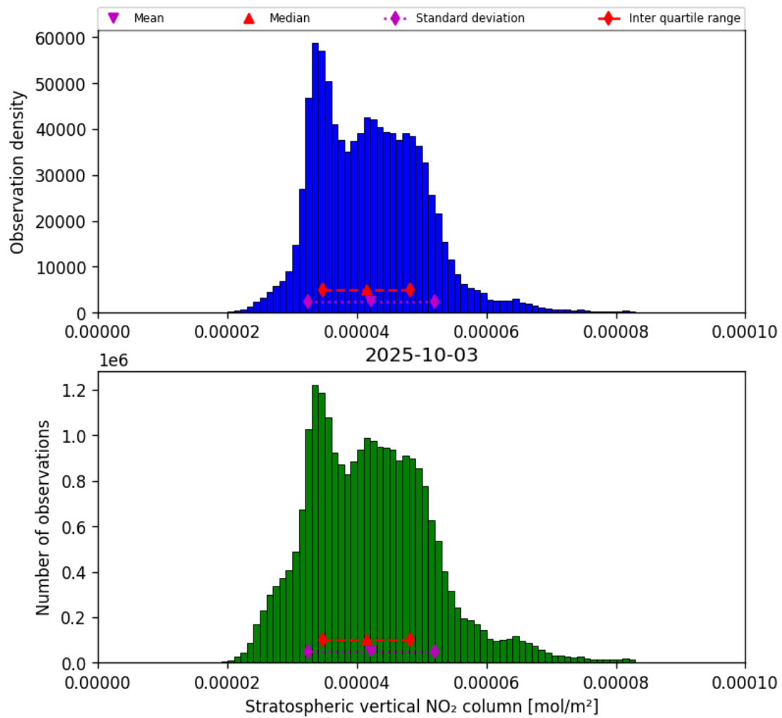
Figure 36: Histogram of “Stratospheric vertical NO 2 column” for 2025-10-02 to 2025-10-04
