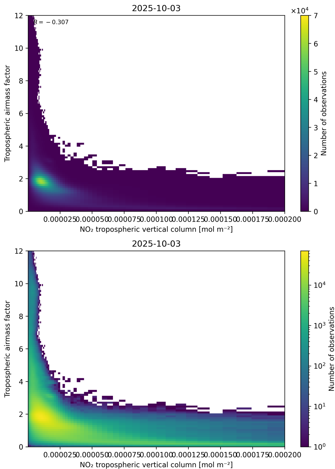
Figure 123: Scatter density plot of “NO 2 tropospheric vertical column” against “Tropospheric air mass factor” for 2025-10-02 to 2025-10-04.
