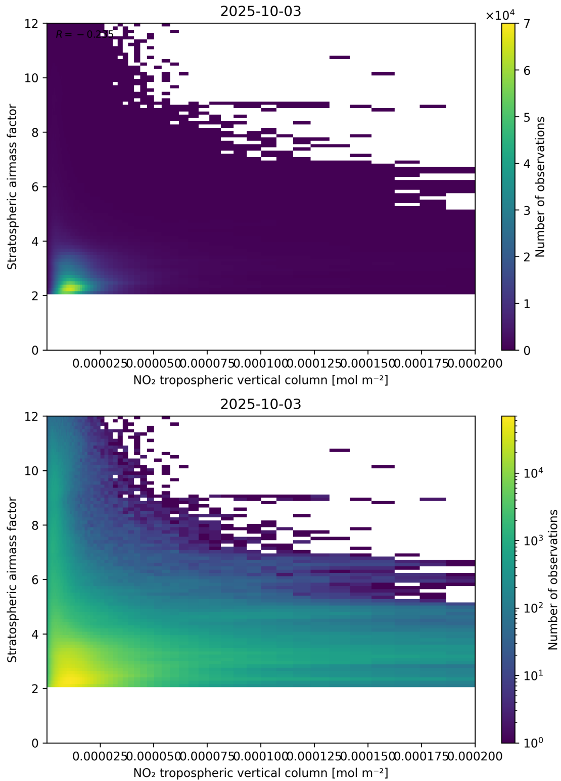
Figure 121: Scatter density plot of “NO 2 tropospheric vertical column” against “Stratospheric air mass factor” for 2025-10-02 to 2025-10-04.
