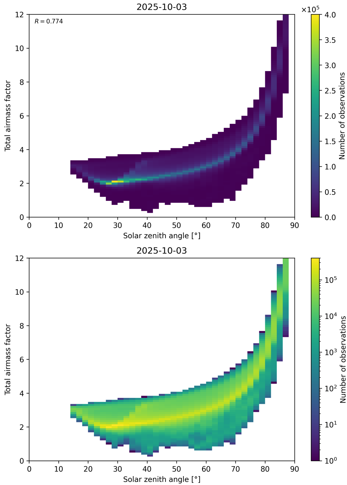
Figure 146: Scatter density plot of “Solar zenith angle” against “Total air mass factor” for 2025-10-02 to 2025-10-04.
