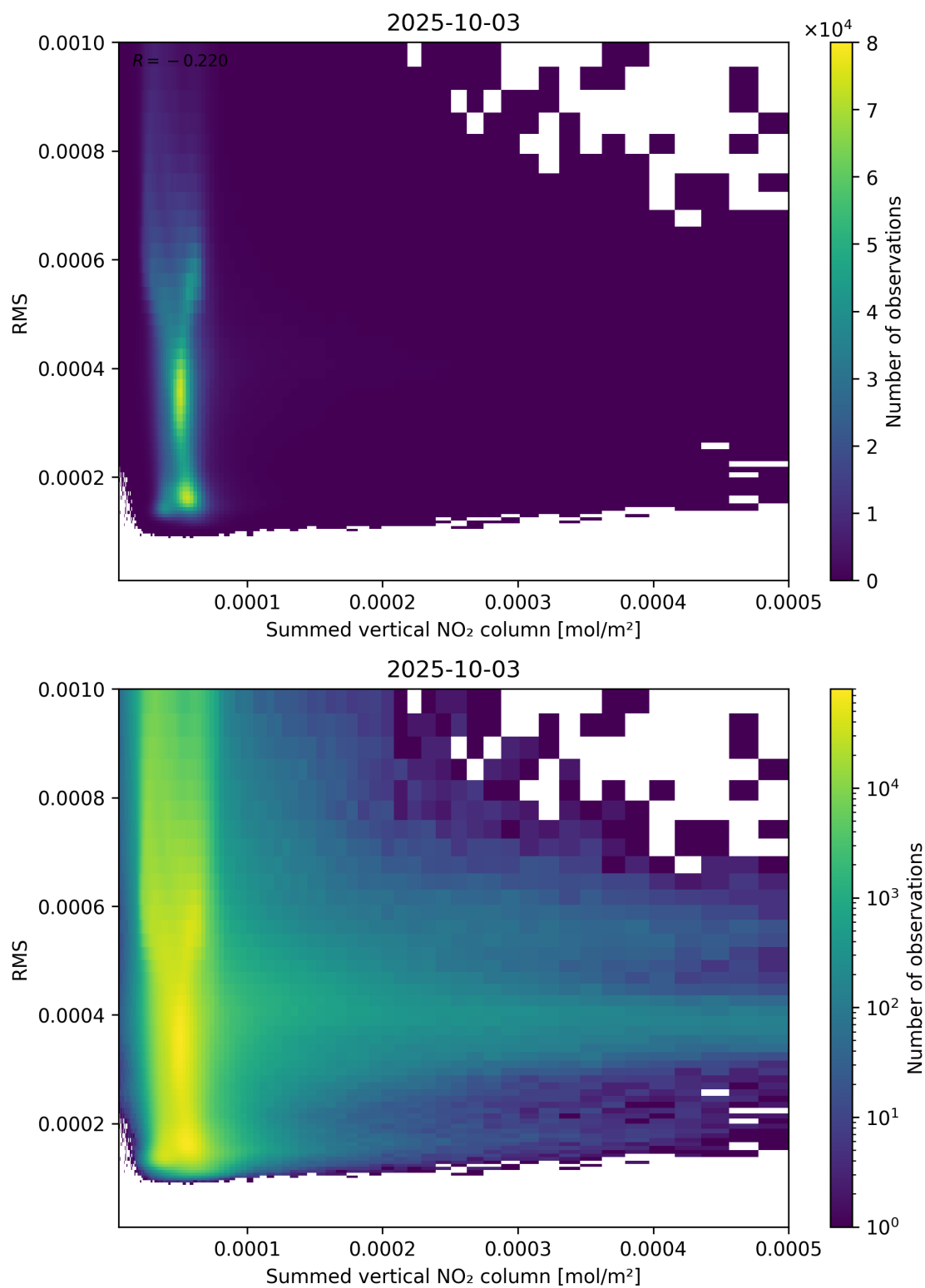
Figure 109: Scatter density plot of “Summed vertical NO 2 column” against “RMS” for 2025-10-02 to 2025-10-04.
