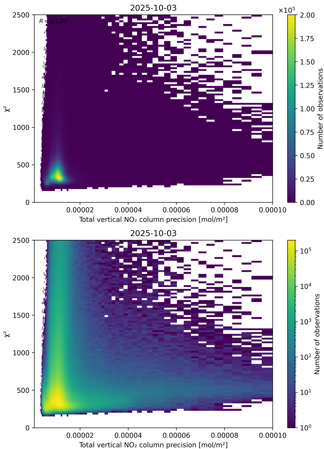
Figure 116: Scatter density plot of “Total vertical NO 2 column precision” against “ \chi^2 ” for 2025-10-02 to 2025-10-04.
