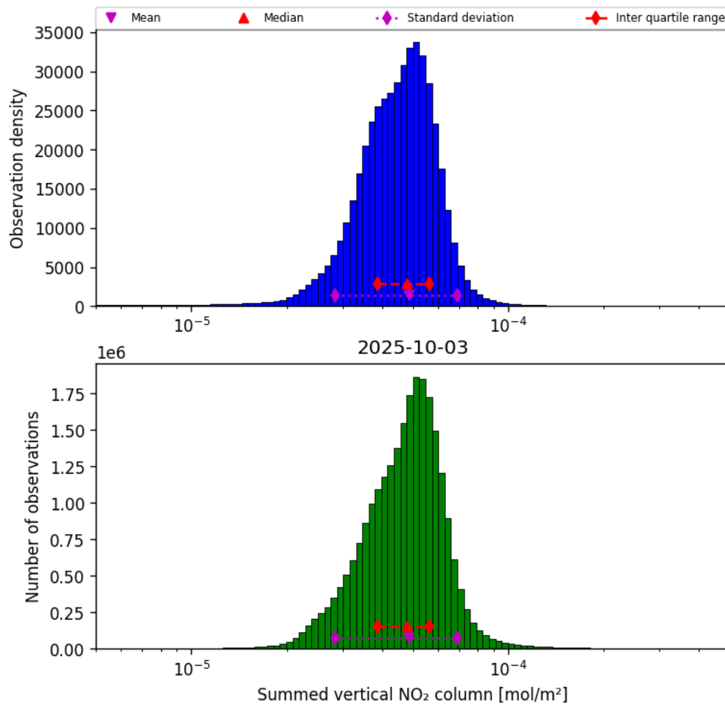
Figure 40: Histogram of “Summed vertical NO 2 column” for 2025-10-02 to 2025-10-04
