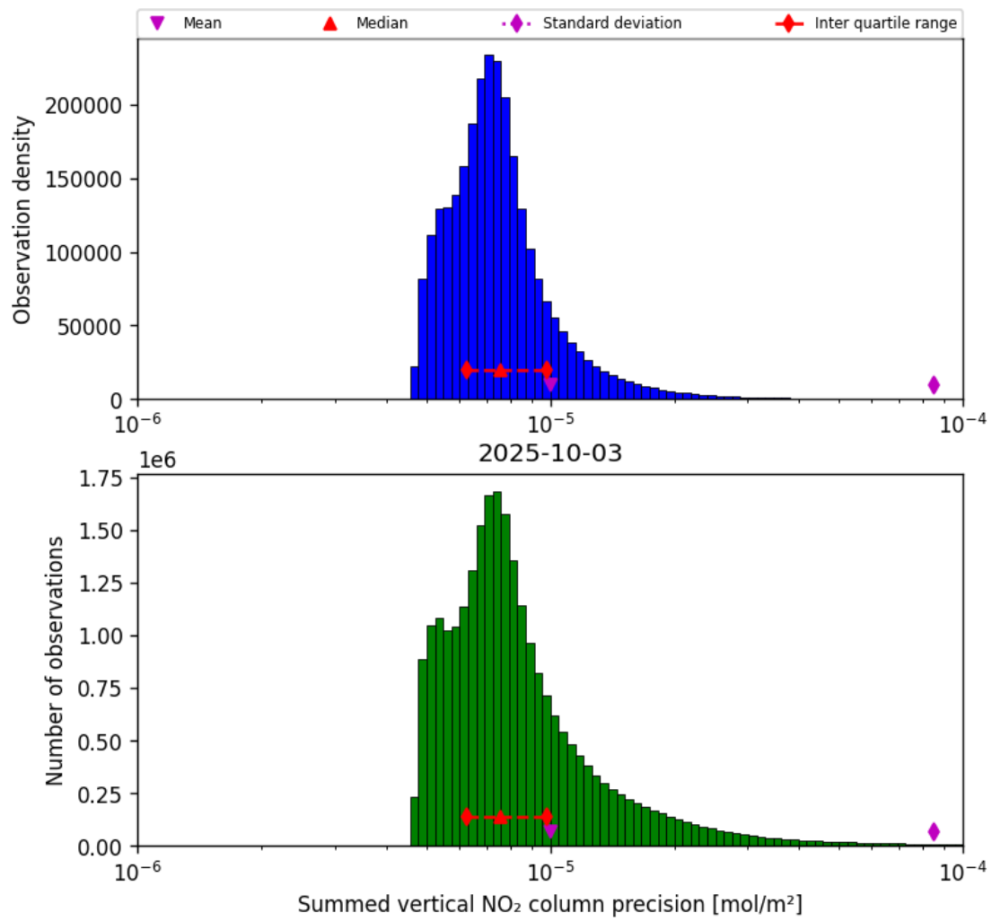
Figure 41: Histogram of “Summed vertical NO 2 column precision” for 2025-10-02 to 2025-10-04
