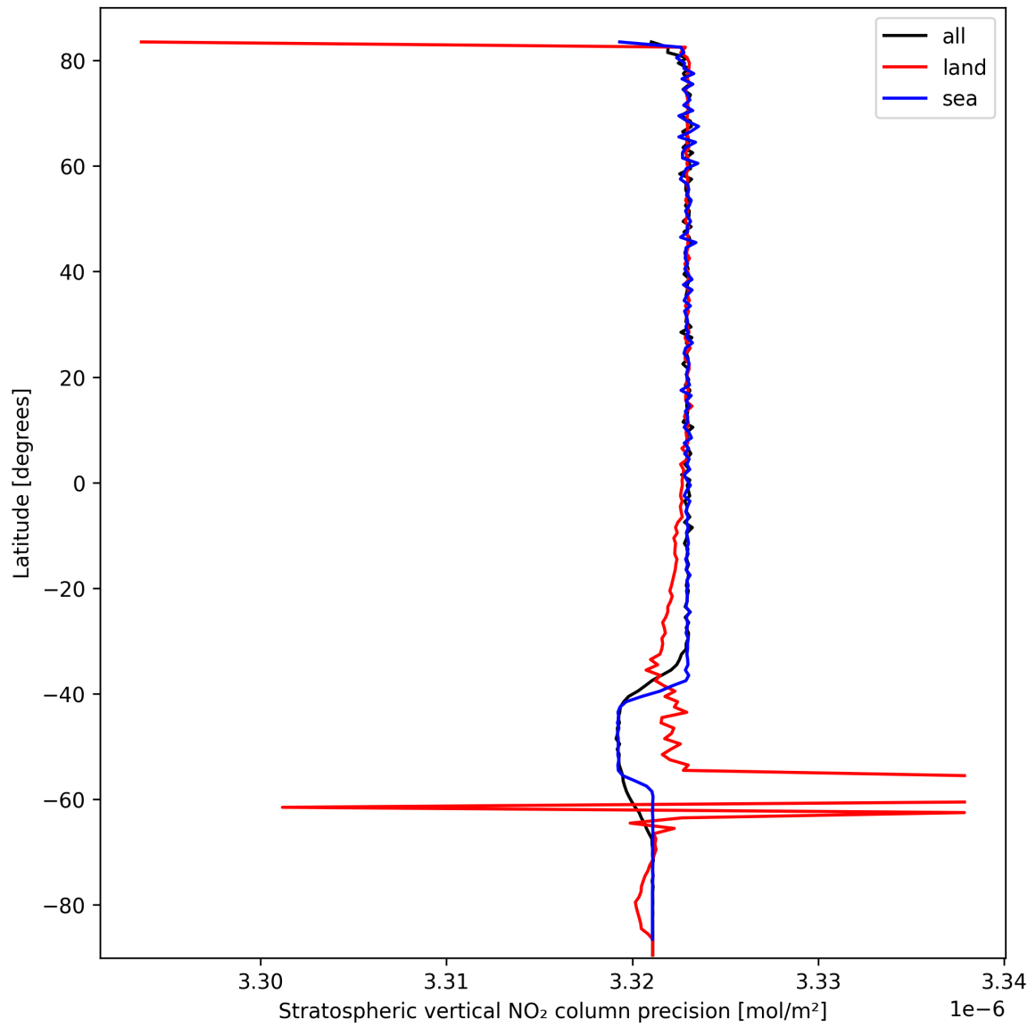
Figure 20: Zonal average of “Stratospheric vertical NO 2 column precision” for 2025-10-02 to 2025-10-04.
