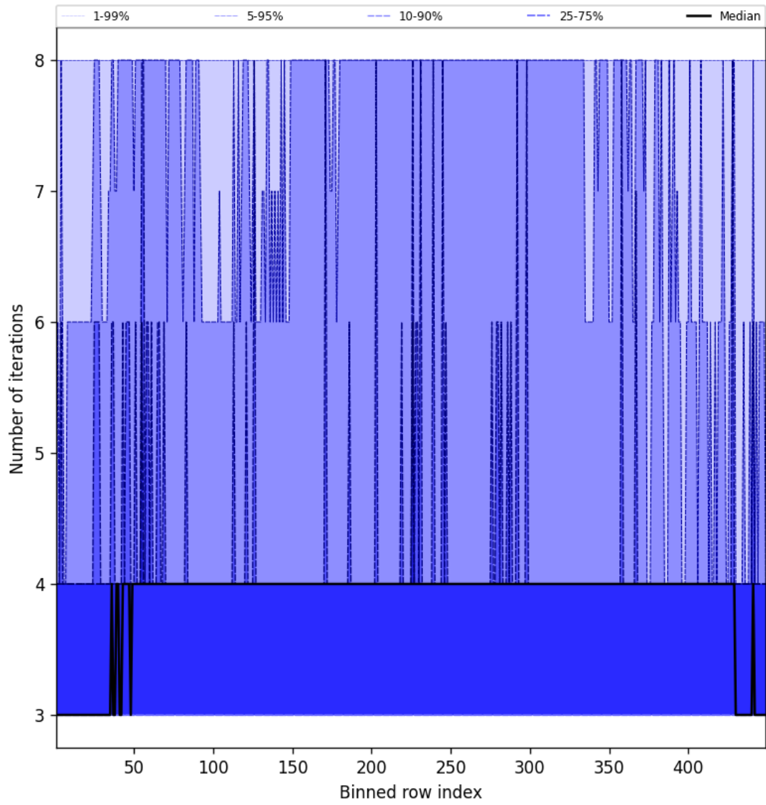
Figure 51: Along track statistics of “Number of iterations” for 2025-10-02 to 2025-10-04
