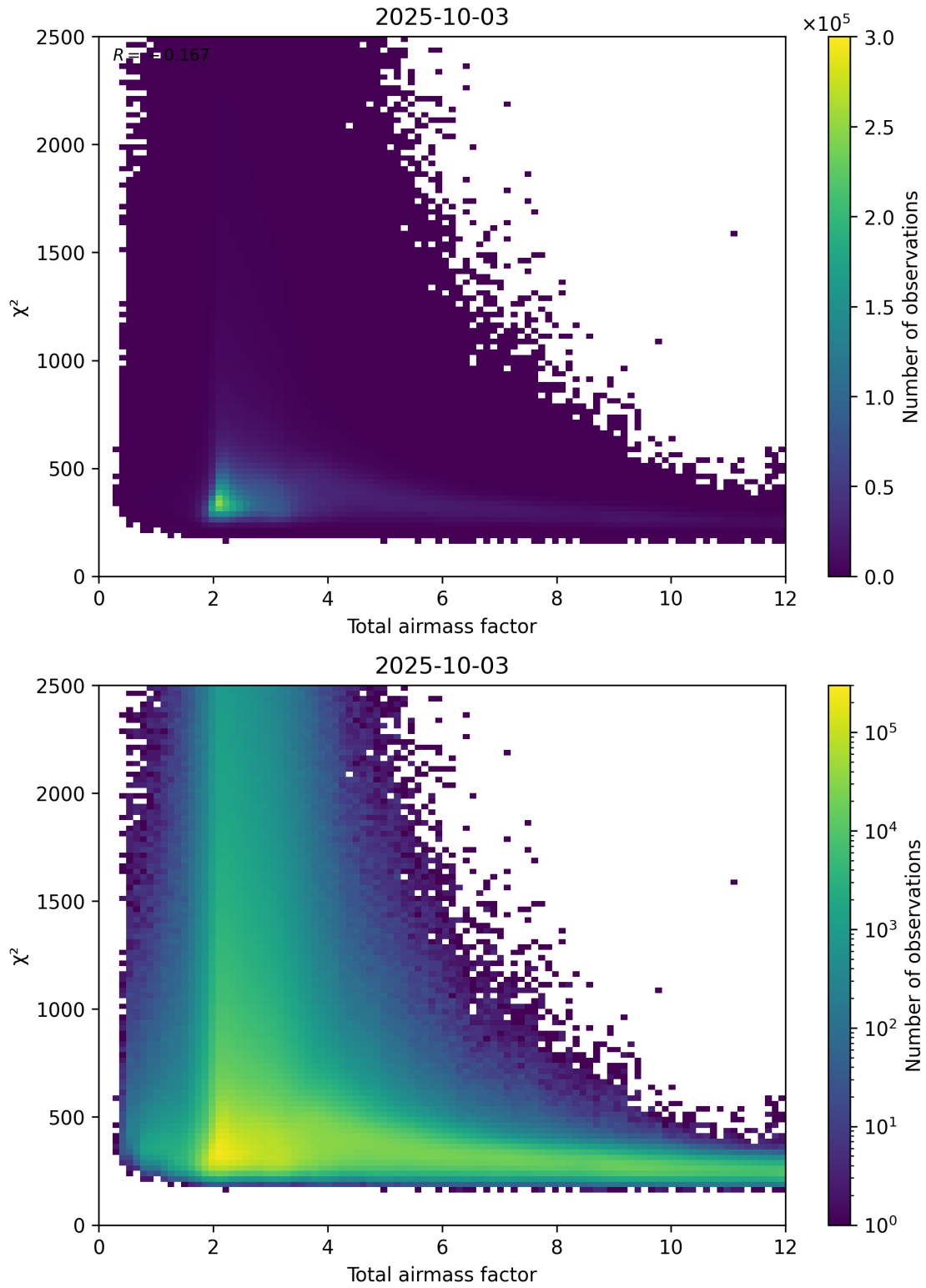
Figure 63: Scatter density plot of “Total airmass factor” against “ \chi^2 ” for 2025-10-02 to 2025-10-04.
