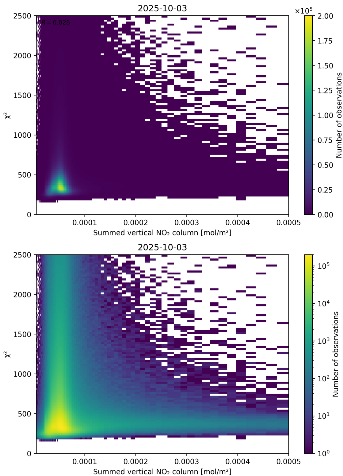
Figure 104: Scatter density plot of “Summed vertical NO 2 column” against “ \chi^2 ” for 2025-10-02 to 2025-10-04.
