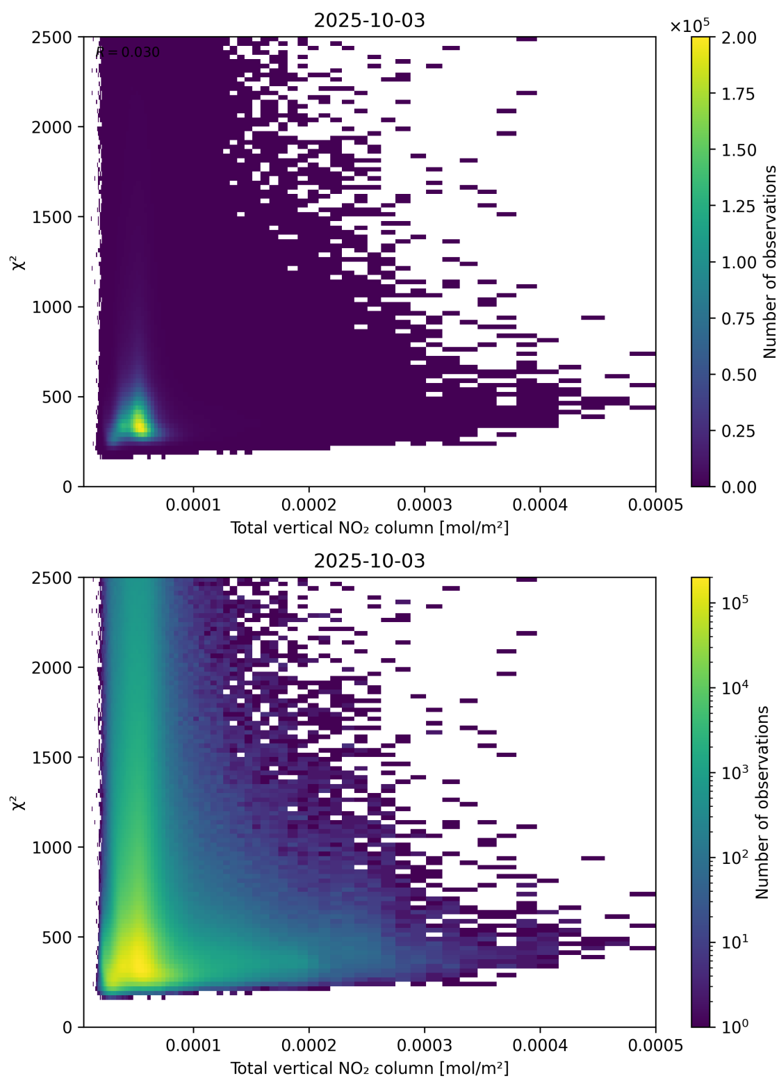
Figure 111: Scatter density plot of “Total vertical NO 2 column” against “ \chi^2 ” for 2025-10-02 to 2025-10-04.
