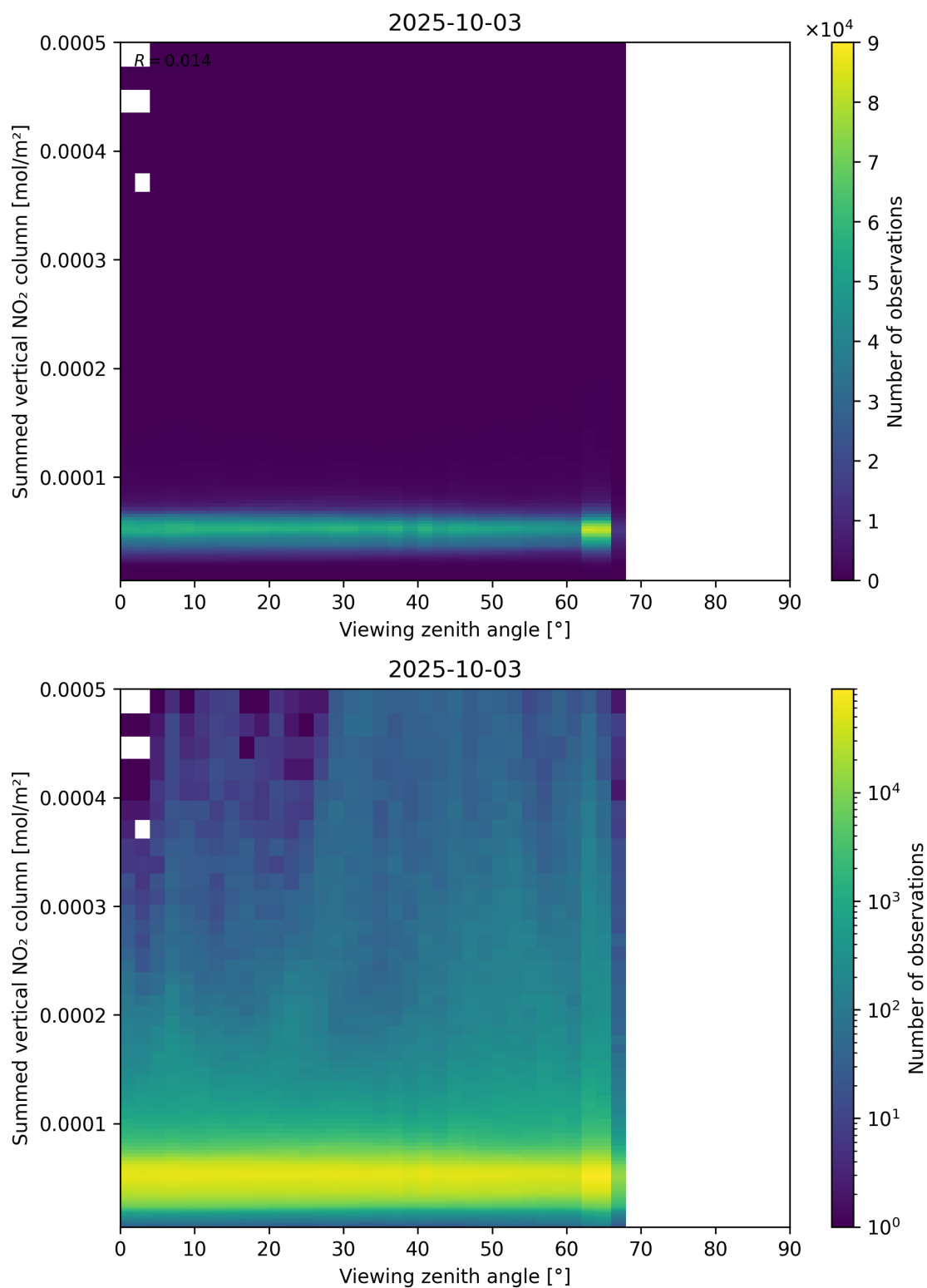
Figure 165: Scatter density plot of “Viewing zenith angle” against “Summed vertical NO 2 column” for 2025-10-02 to 2025-10-04.
