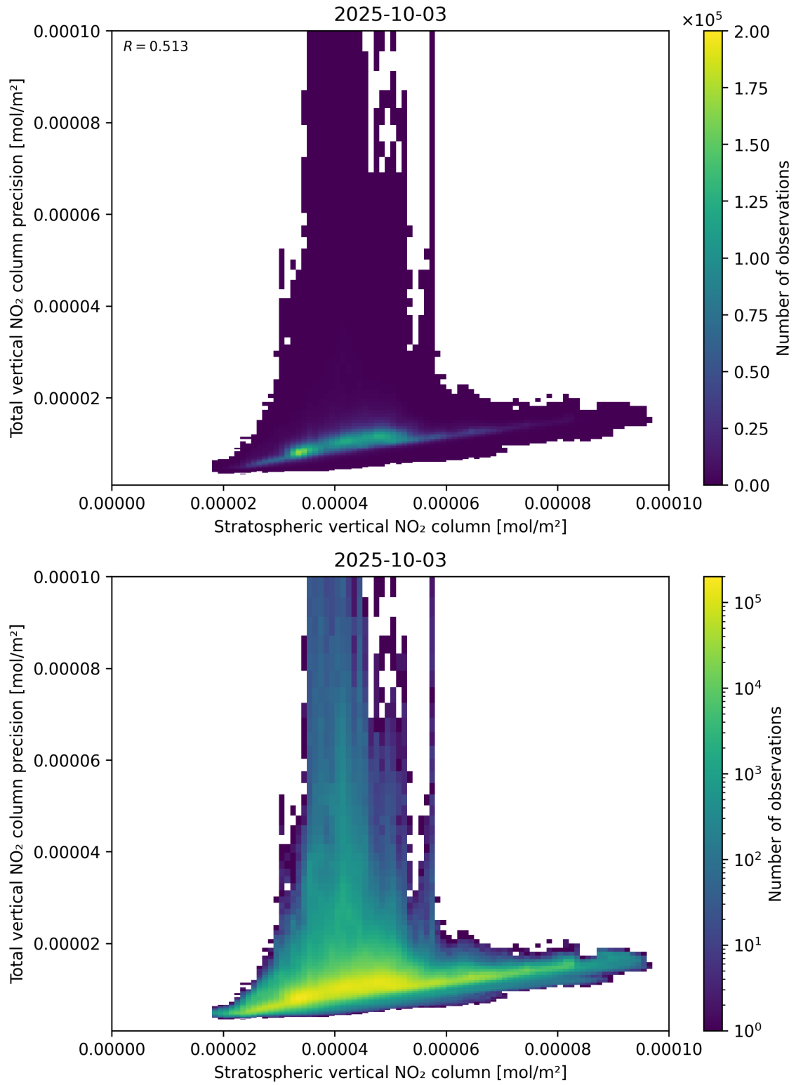
Figure 101: Scatter density plot of “Stratospheric vertical NO 2 column” against “Total vertical NO 2 column precision” for 2025-10-02 to 2025-10-04.
