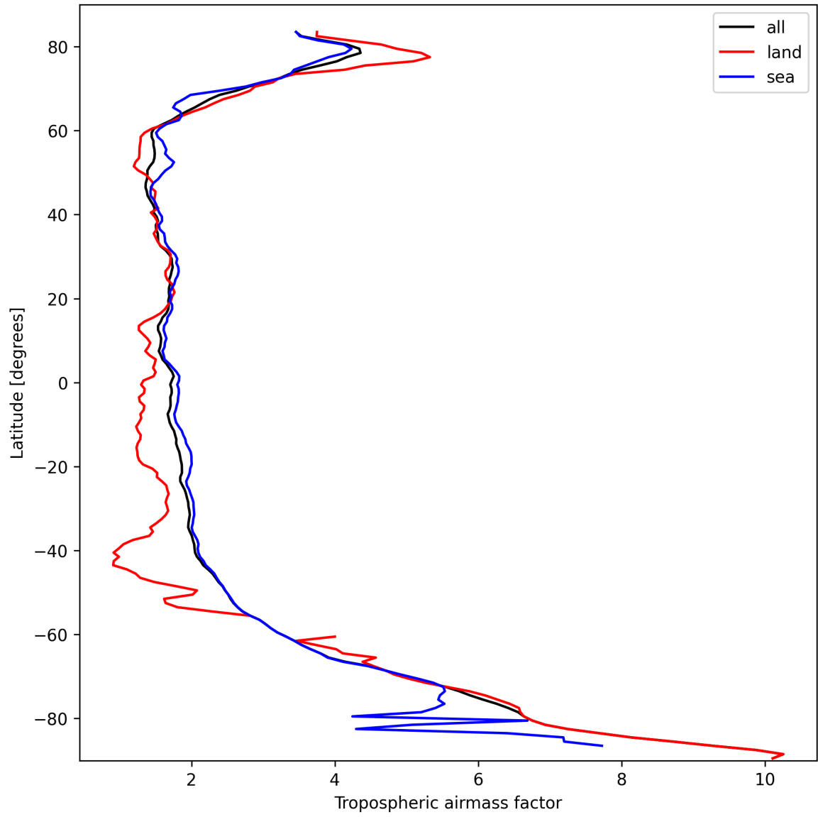
Figure 14: Zonal average of “Tropospheric airmass factor” for 2025-10-02 to 2025-10-04.
