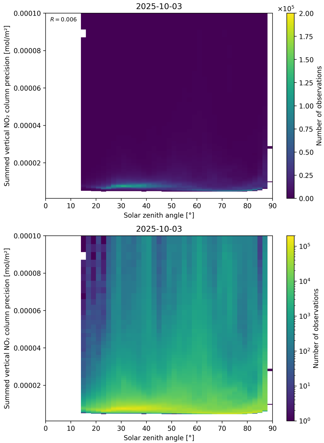
Figure 152: Scatter density plot of “Solar zenith angle” against “Summed vertical NO 2 column precision” for 2025-10-02 to 2025-10-04.
