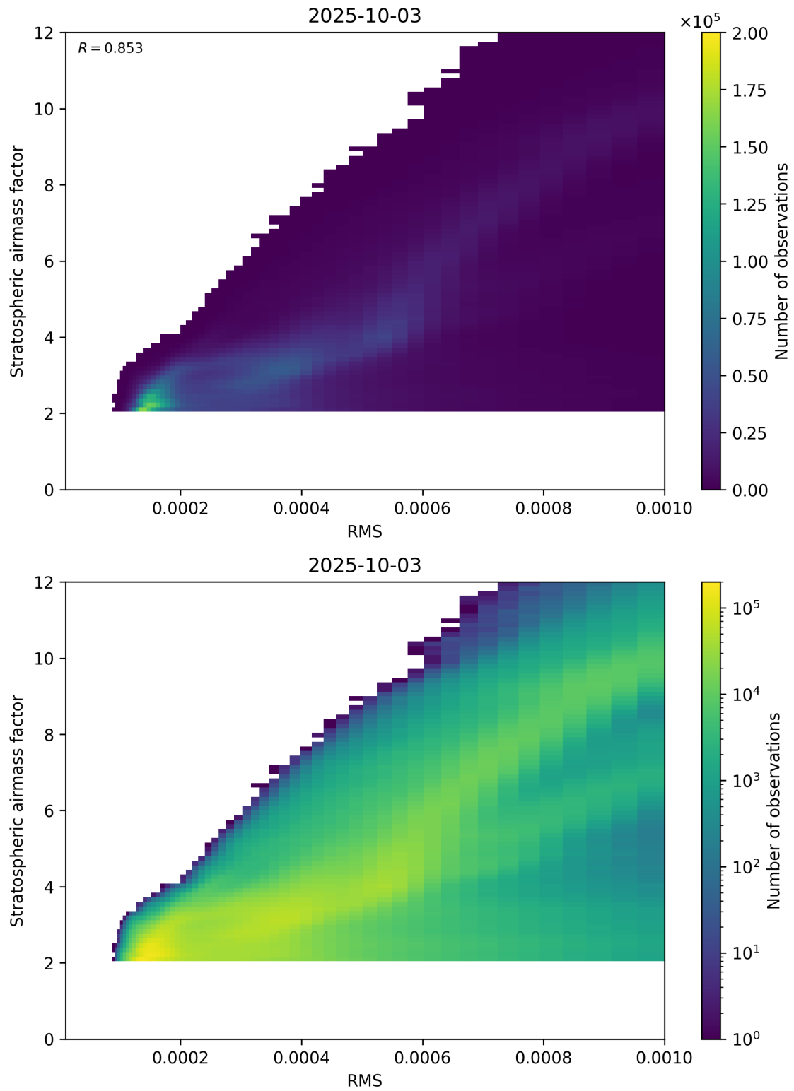
Figure 144: Scatter density plot of “RMS” against “Stratospheric airmass factor” for 2025-10-02 to 2025-10-04.
