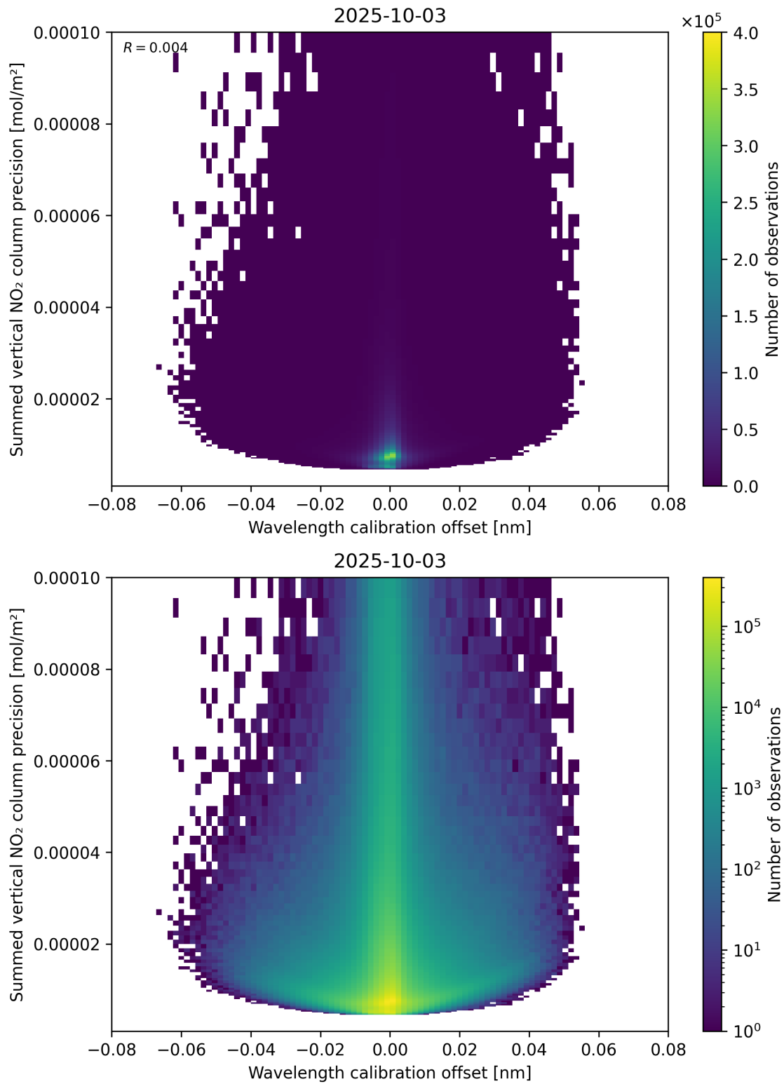
Figure 178: Scatter density plot of “Wavelength calibration offset” against “Summed vertical NO 2 column precision” for 2025-10-02 to 2025-10-04.
