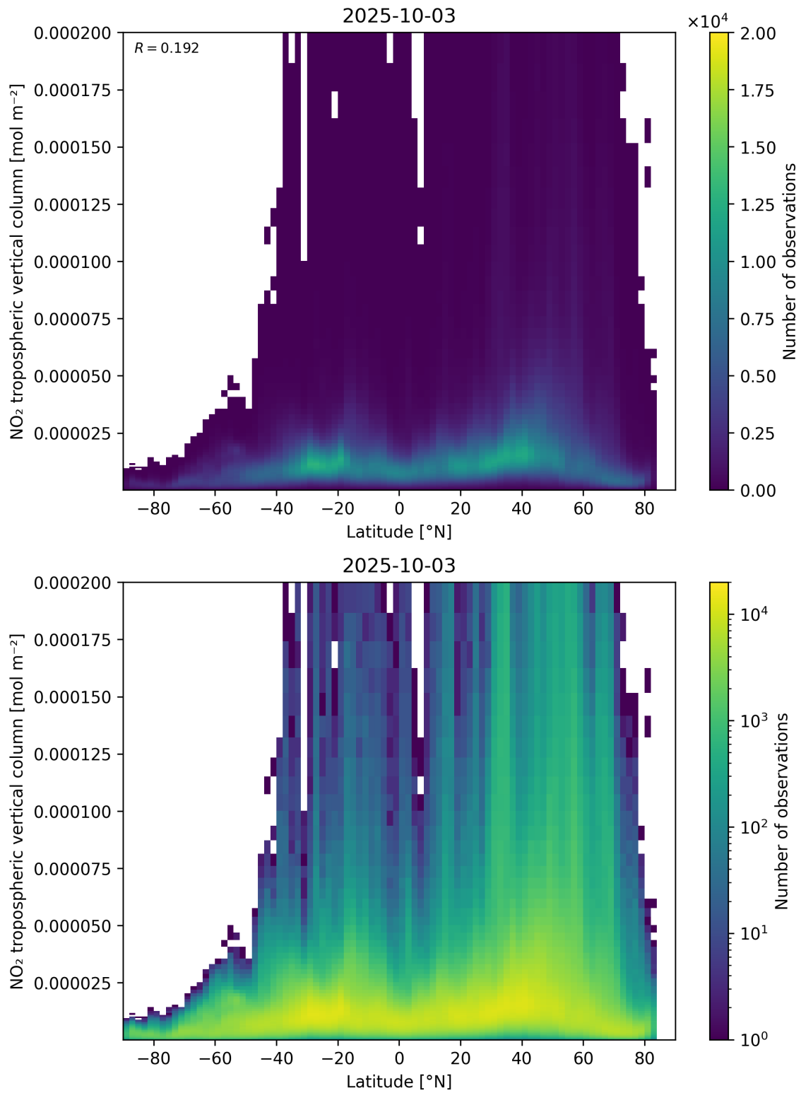
Figure 92: Scatter density plot of “Latitude” against “NO 2 tropospheric vertical column” for 2025-10-02 to 2025-10-04.
