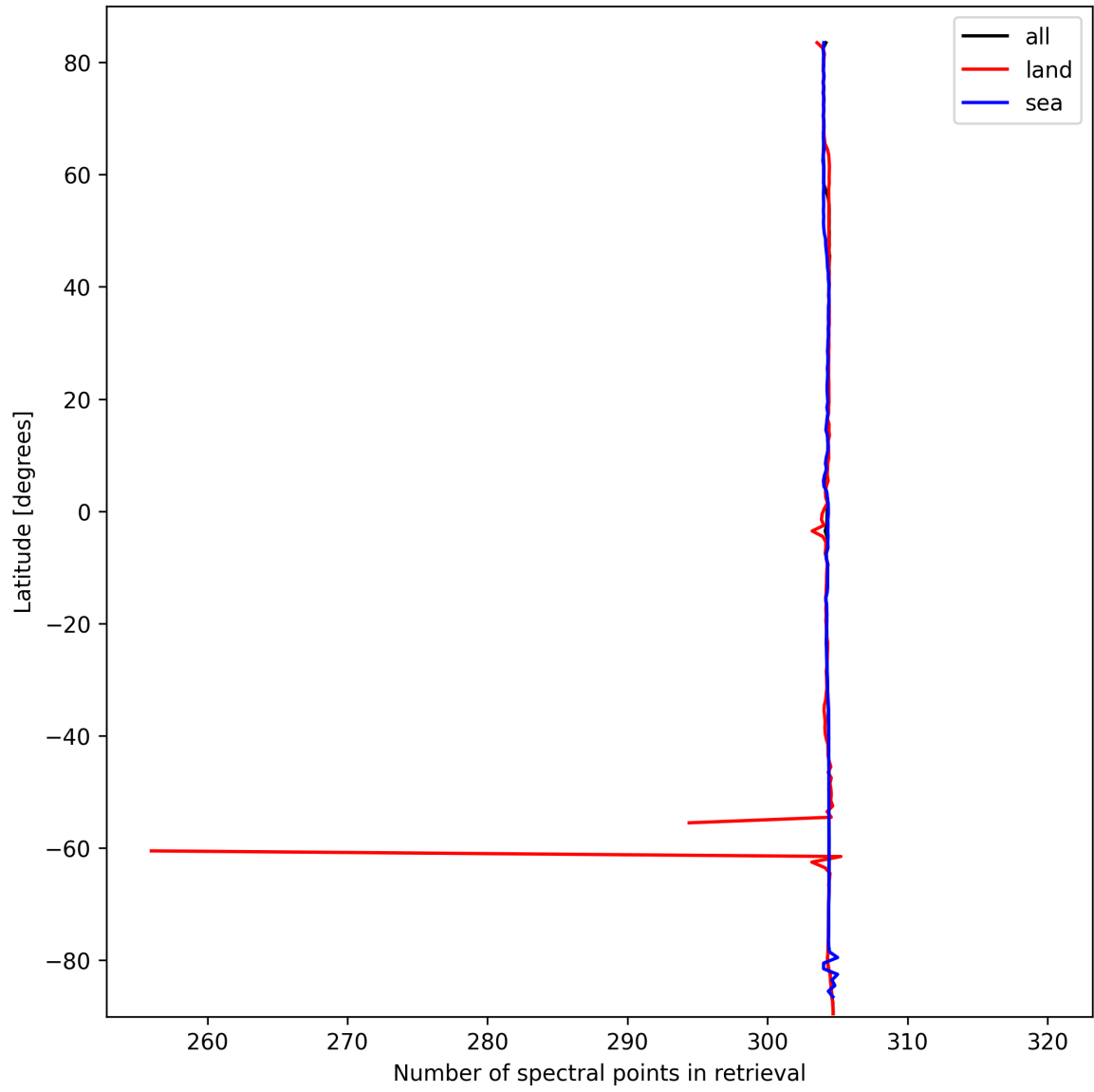
Figure 16: Zonal average of “Number of spectral points in retrieval” for 2025-10-02 to 2025-10-04.
