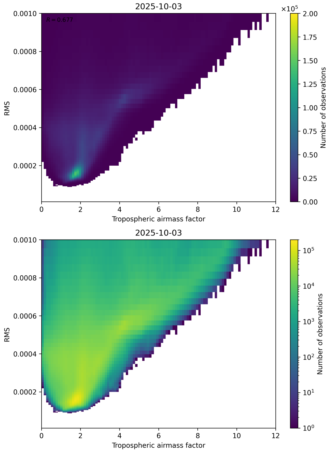
Figure 79: Scatter density plot of “Tropospheric airmass factor” against “RMS” for 2025-10-02 to 2025-10-04.
