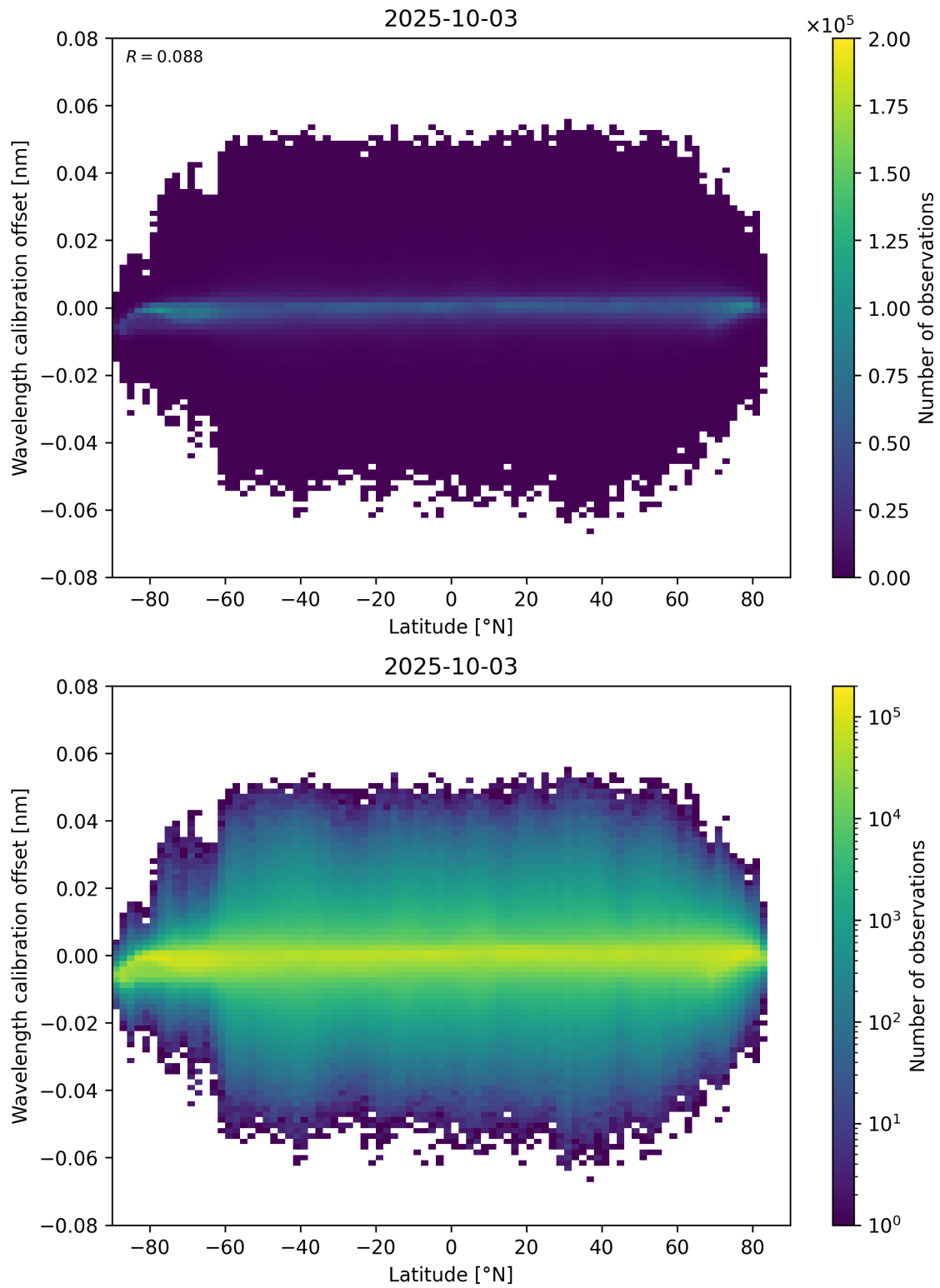
Figure 95: Scatter density plot of “Latitude” against “Wavelength calibration offset” for 2025-10-02 to 2025-10-04.
