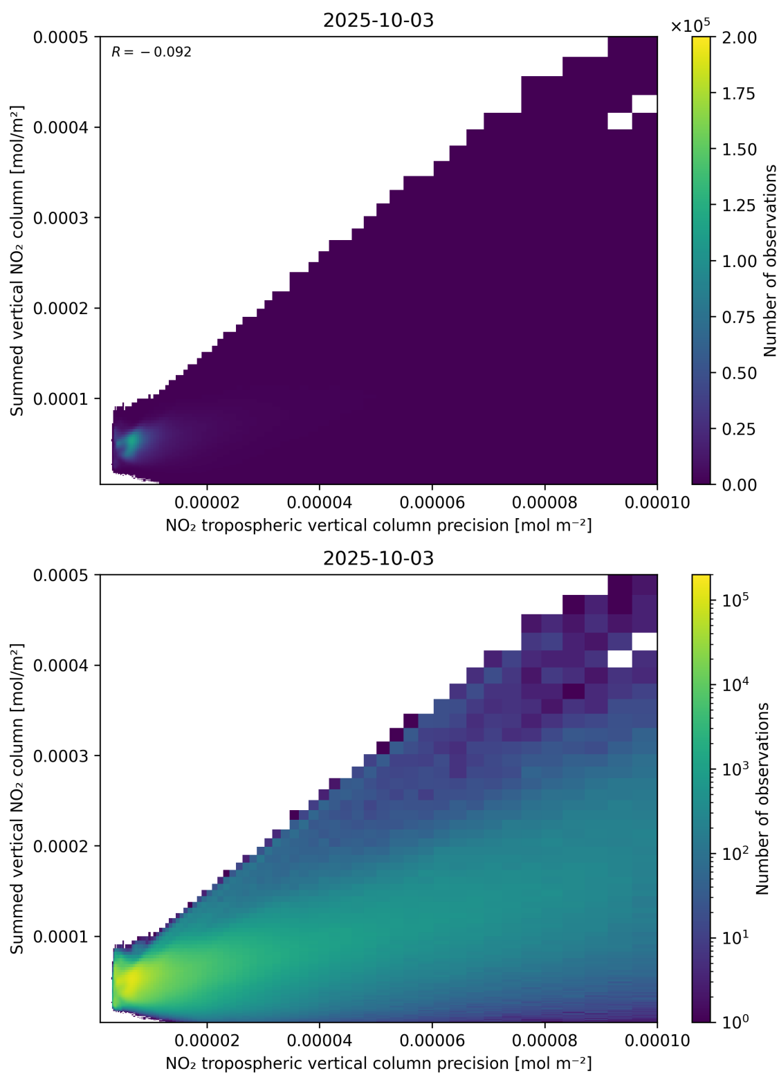
Figure 136: Scatter density plot of “NO 2 tropospheric vertical column precision” against “Summed vertical NO 2 column” for 2025-10-02 to 2025-10-04.
