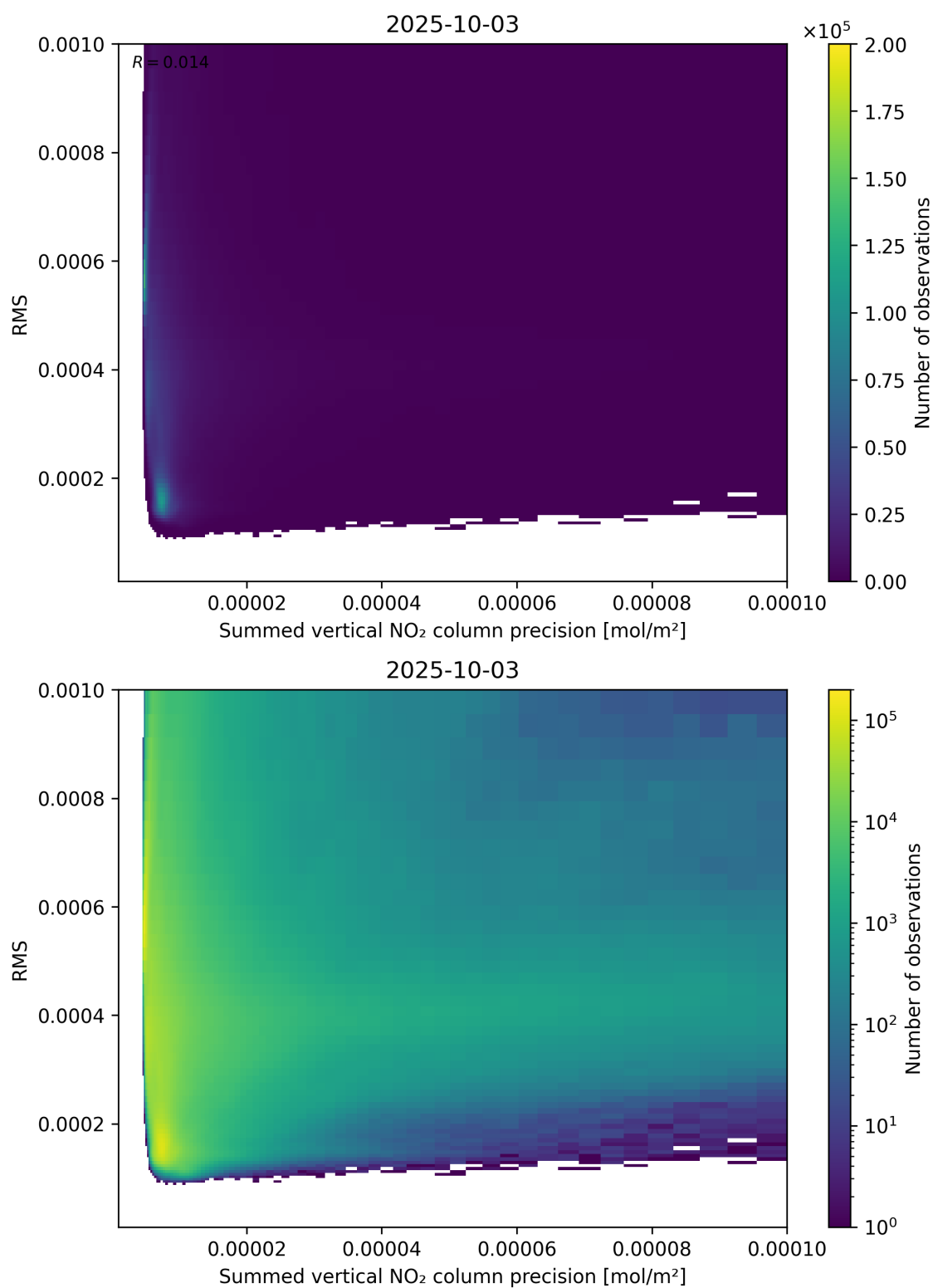
Figure 108: Scatter density plot of “Summed vertical NO 2 column precision” against “RMS” for 2025-10-02 to 2025-10-04.
