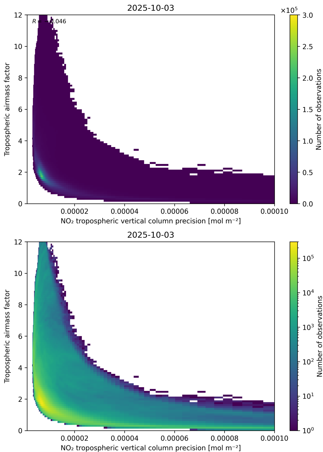
Figure 133: Scatter density plot of “NO 2 tropospheric vertical column precision” against “Tropospheric air mass factor” for 2025-10-02 to 2025-10-04.
