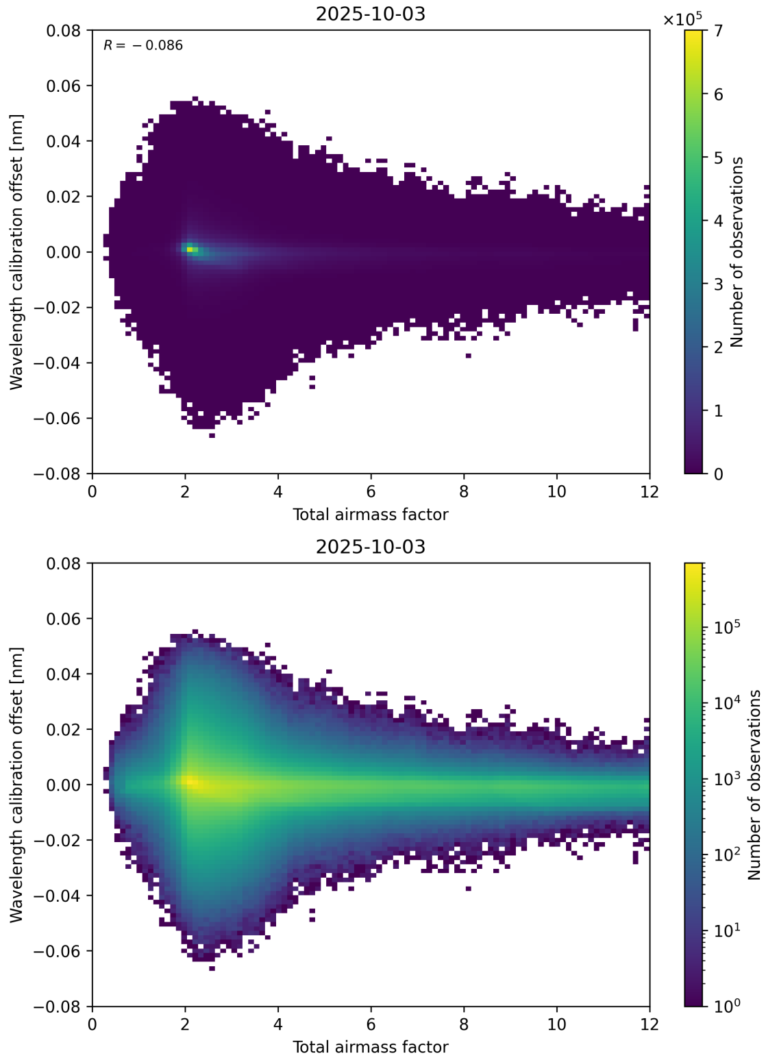
Figure 70: Scatter density plot of “Total airmass factor” against “Wavelength calibration offset” for 2025-10-02 to 2025-10-04.
