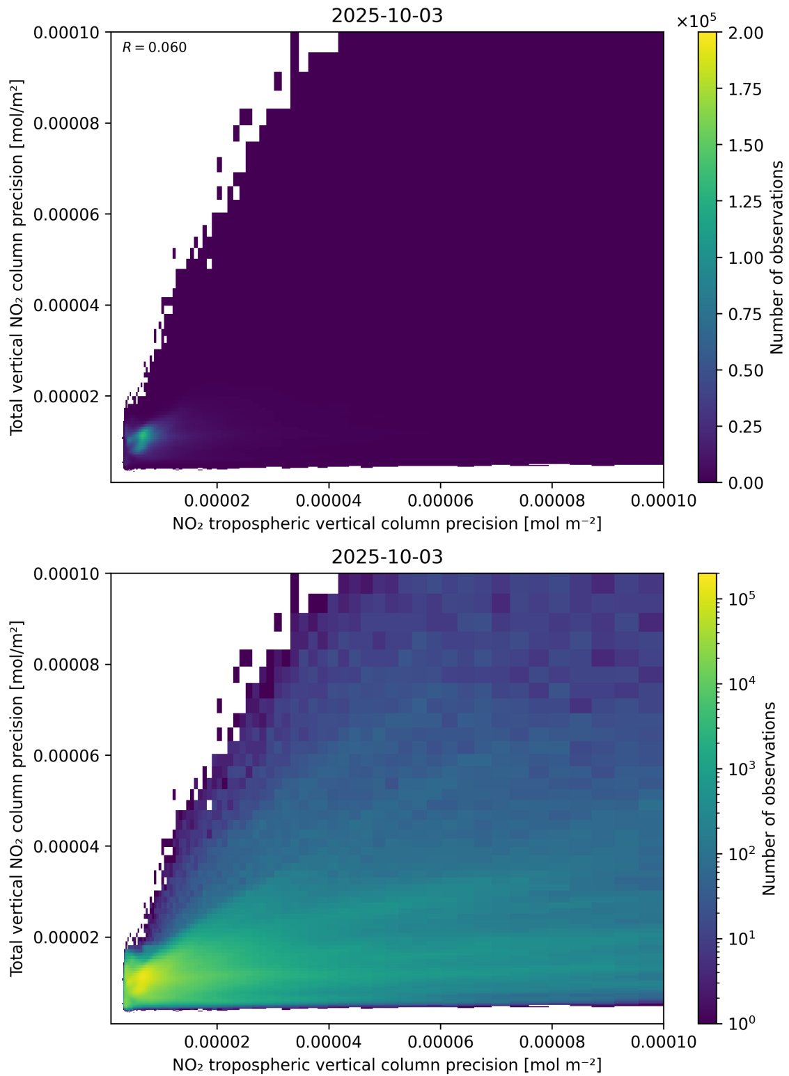
Figure 139: Scatter density plot of “NO 2 tropospheric vertical column precision” against “Total vertical NO 2 column precision” for 2025-10-02 to 2025-10-04.
