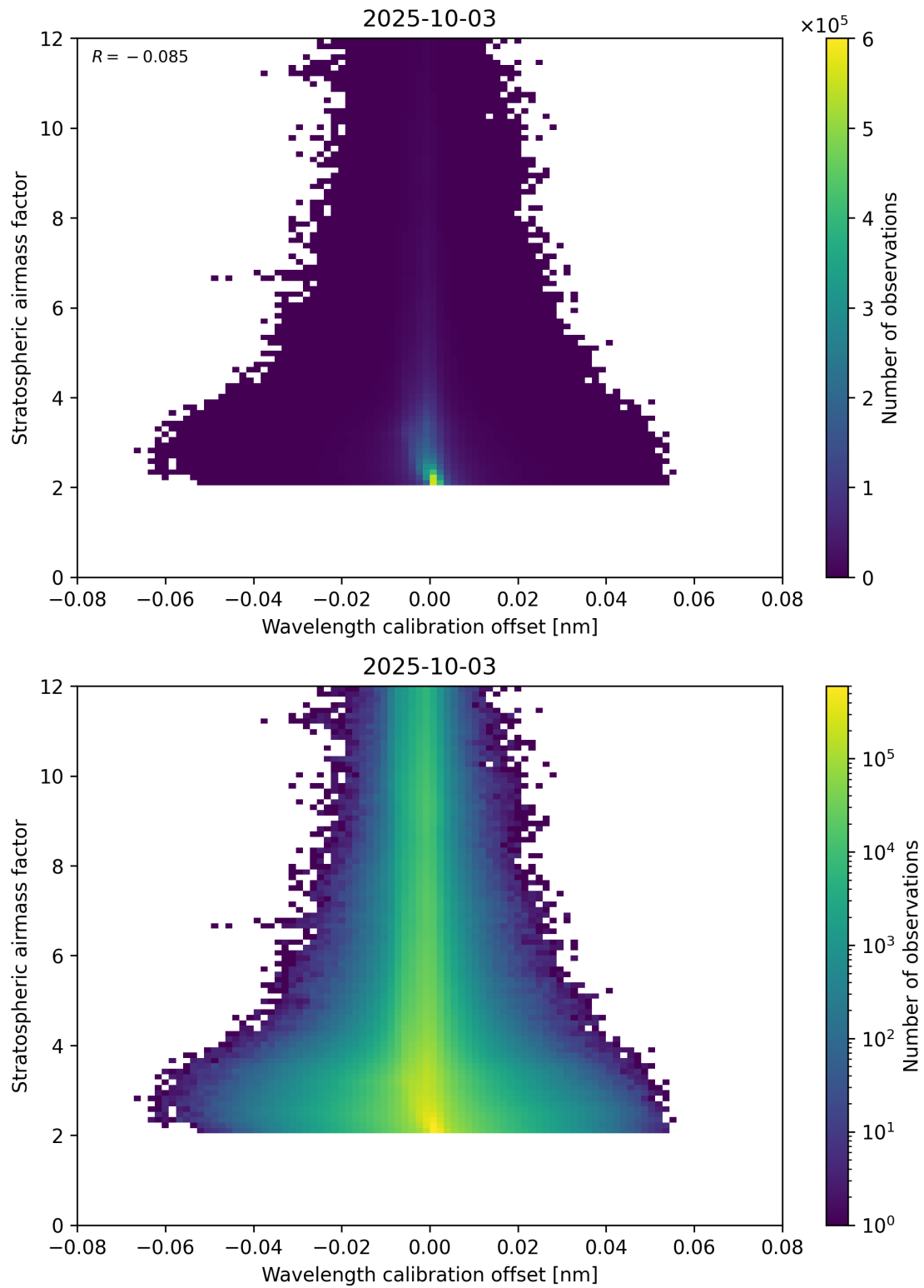
Figure 174: Scatter density plot of “Wavelength calibration offset” against “Stratospheric air mass factor” for 2025-10-02 to 2025-10-04.
