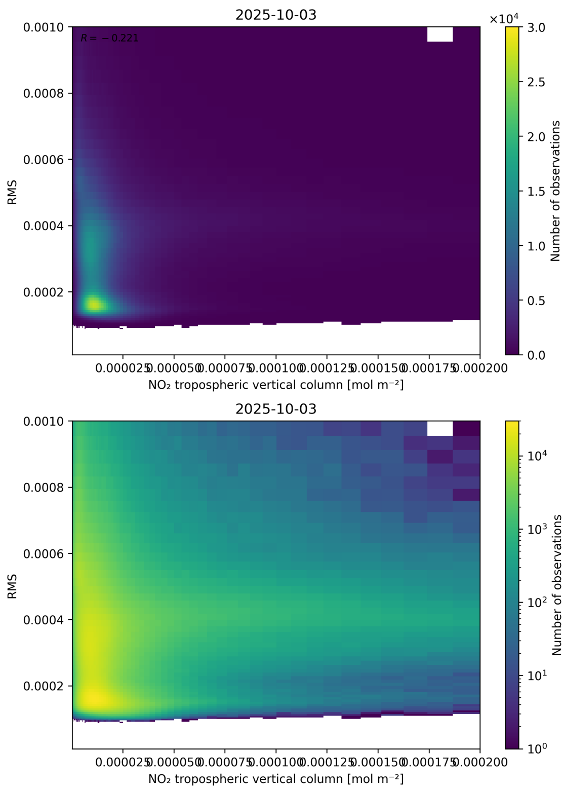
Figure 142: Scatter density plot of “NO 2 tropospheric vertical column” against “RMS” for 2025-10-02 to 2025-10-04.
