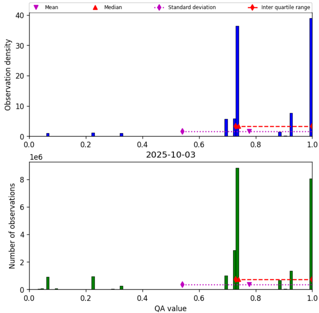
Figure 28: Histogram of “QA value” for 2025-10-02 to 2025-10-04
