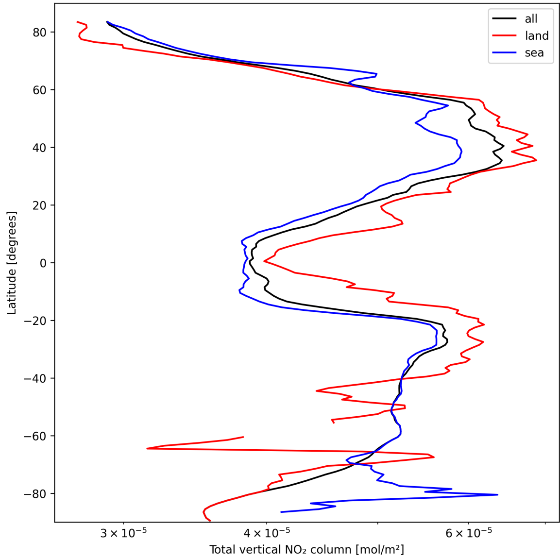
Figure 21: Zonal average of “Total vertical NO 2 column” for 2025-10-02 to 2025-10-04.
