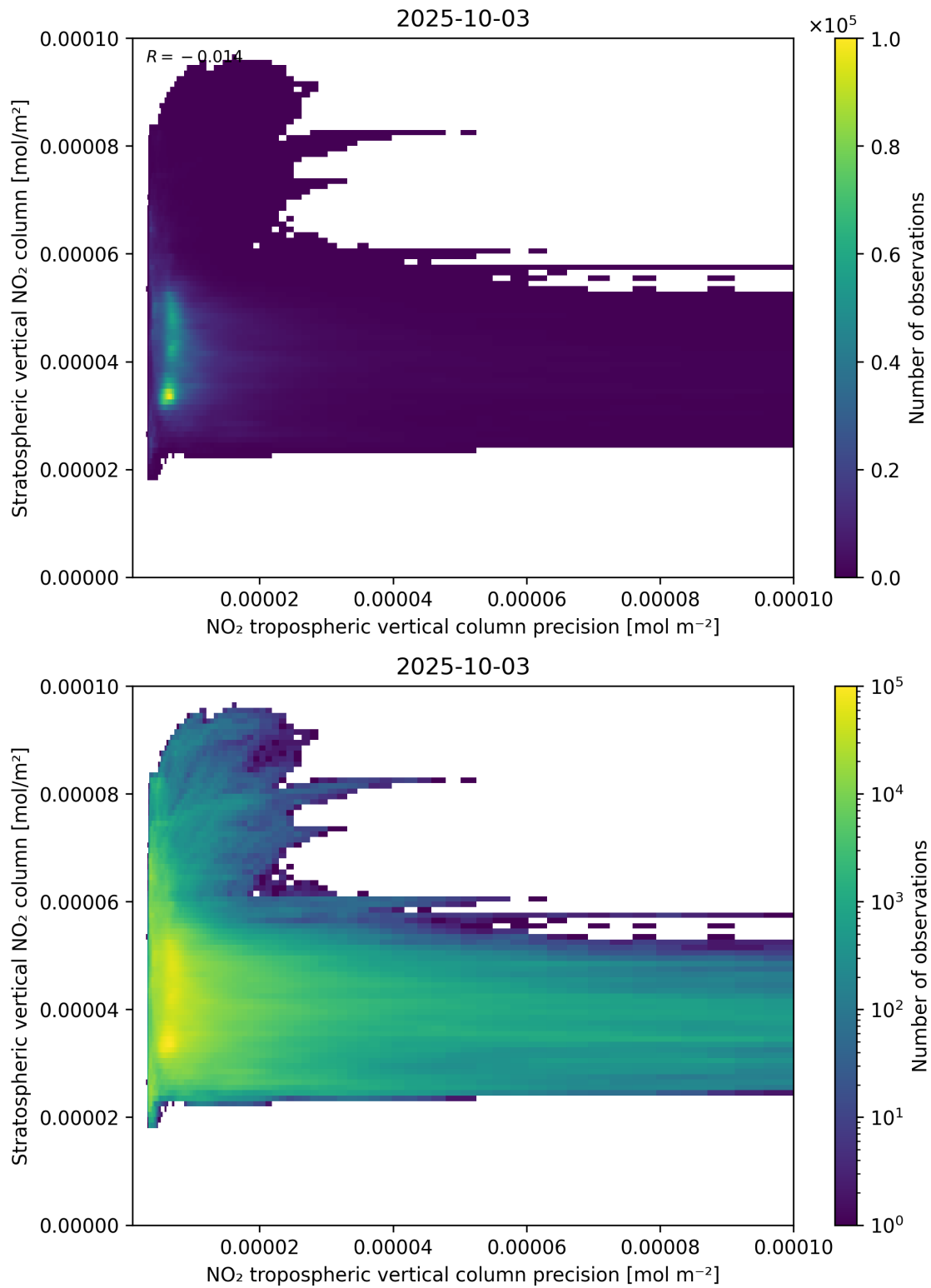
Figure 135: Scatter density plot of “NO 2 tropospheric vertical column precision” against “Stratospheric vertical NO 2 column” for 2025-10-02 to 2025-10-04.
