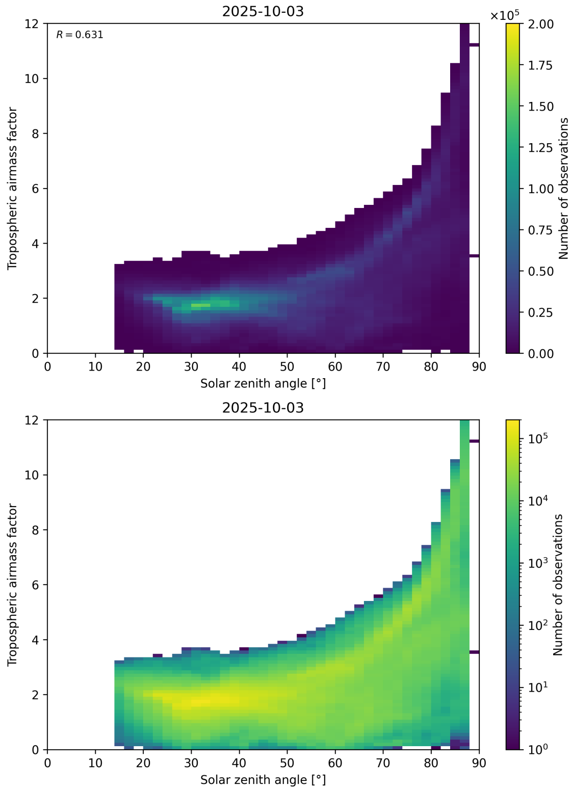
Figure 147: Scatter density plot of “Solar zenith angle” against “Tropospheric airmass factor” for 2025-10-02 to 2025-10-04.
