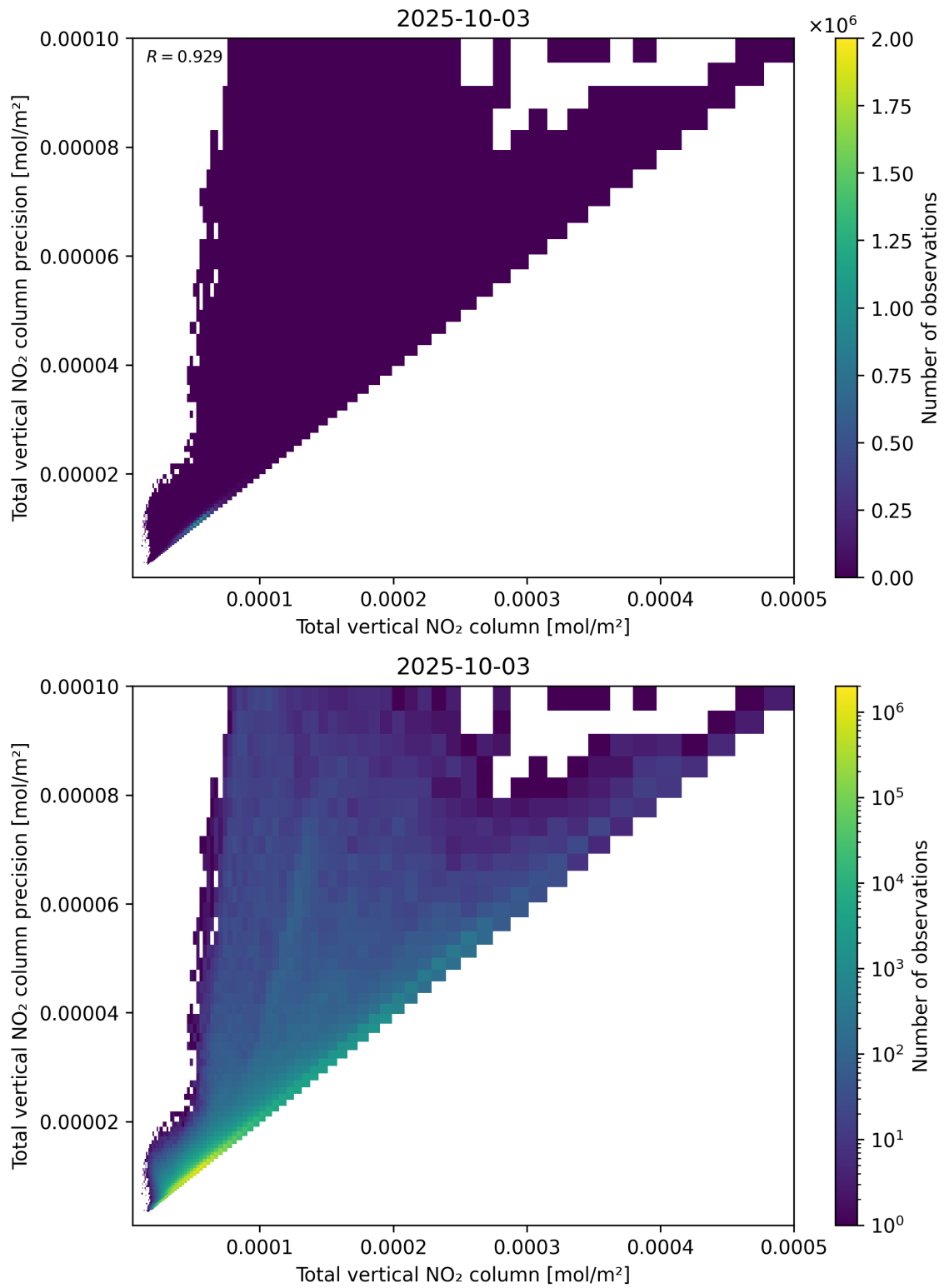
Figure 114: Scatter density plot of “Total vertical NO 2 column” against “Total vertical NO 2 column precision” for 2025-10-02 to 2025-10-04.
