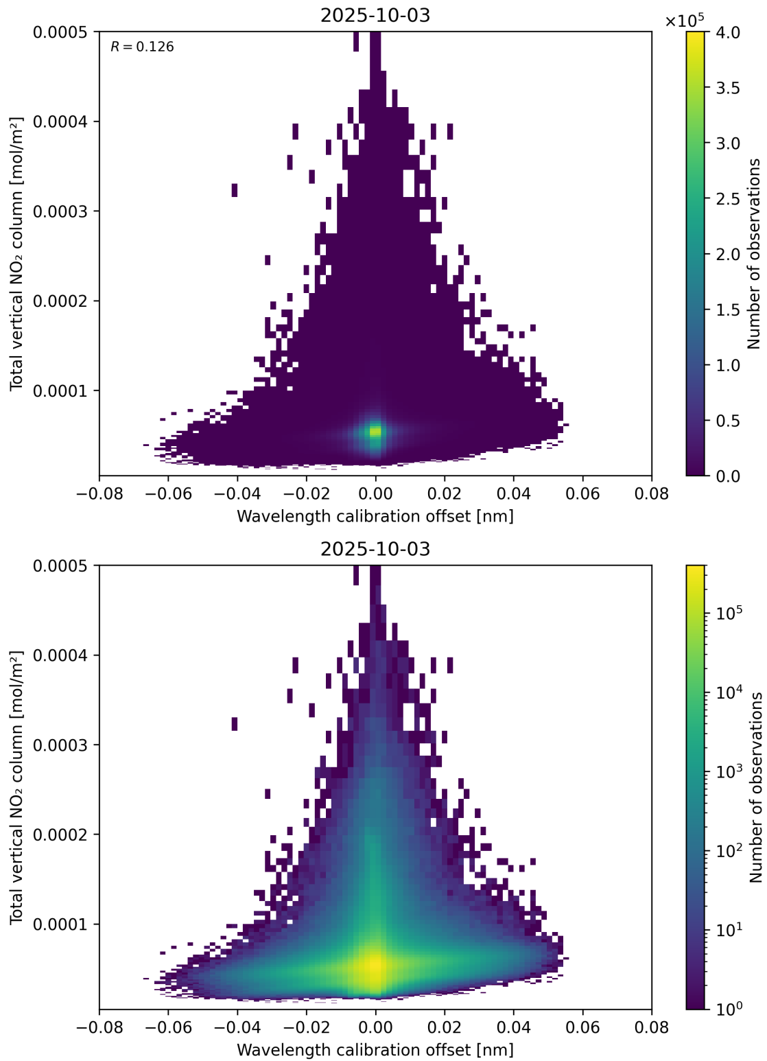
Figure 179: Scatter density plot of “Wavelength calibration offset” against “Total vertical NO 2 column” for 2025-10-02 to 2025-10-04.
