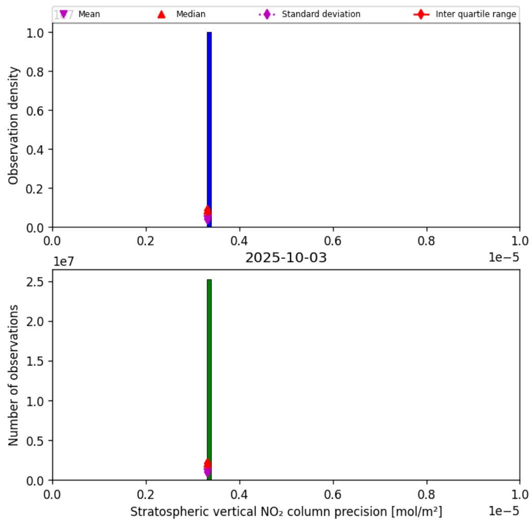
Figure 37: Histogram of “Stratospheric vertical NO 2 column precision” for 2025-10-02 to 2025-10-04
