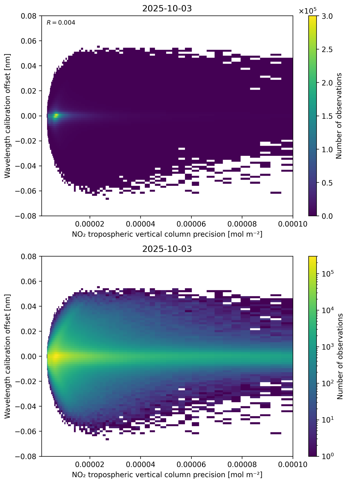
Figure 141: Scatter density plot of “NO 2 tropospheric vertical column precision” against “Wavelength calibration offset” for 2025-10-02 to 2025-10-04.
