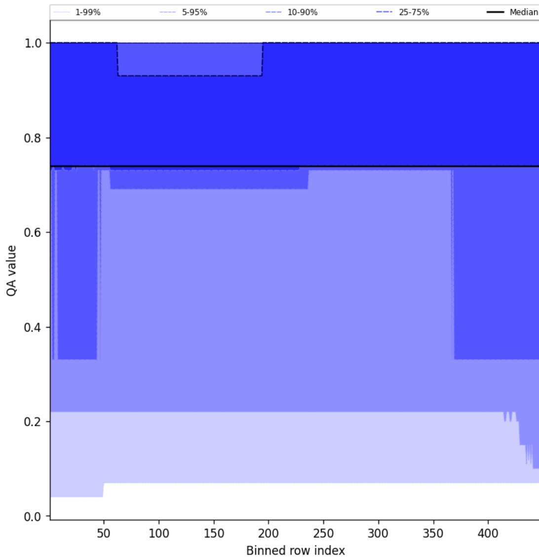
Figure 45: Along track statistics of "QA value" for 2025-10-02 to 2025-10-04
