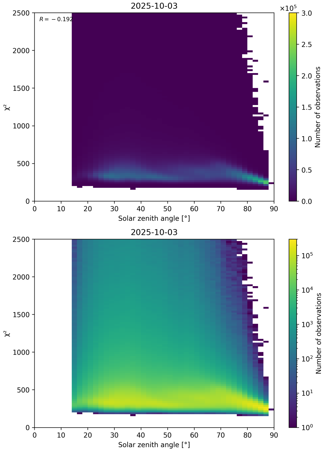
Figure 148: Scatter density plot of “Solar zenith angle” against “ \chi^2 ” for 2025-10-02 to 2025-10-04.
