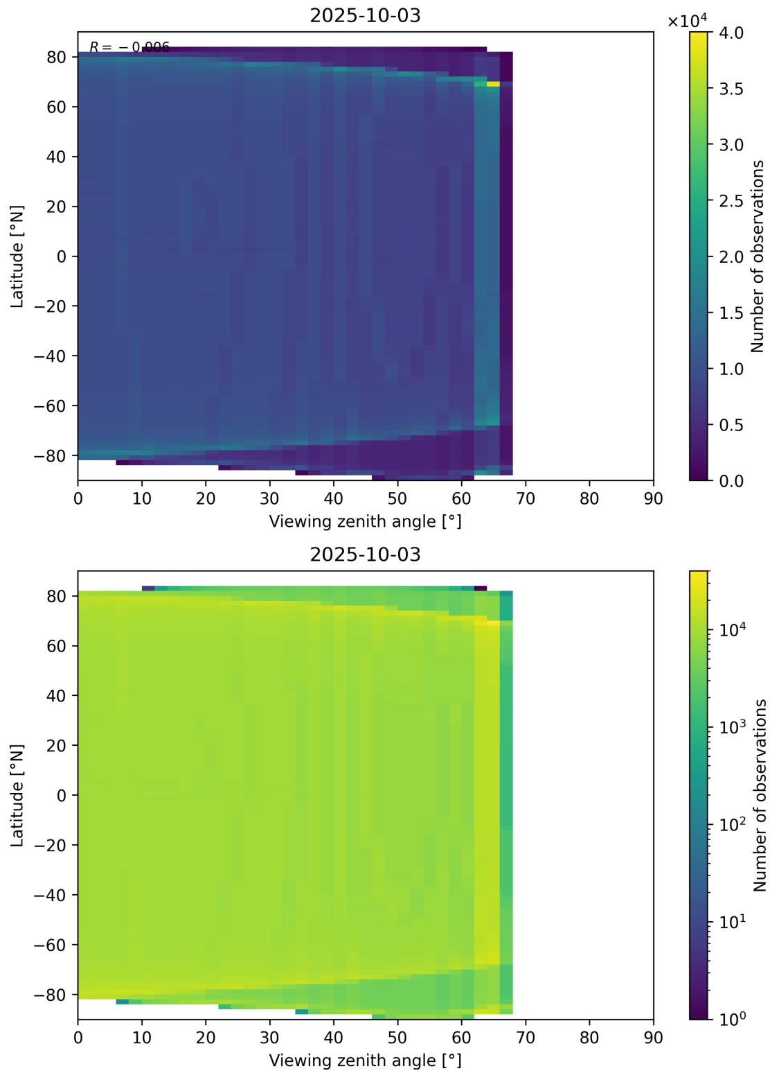
Figure 163: Scatter density plot of “Viewing zenith angle” against “Latitude” for 2025-10-02 to 2025-10-04.
