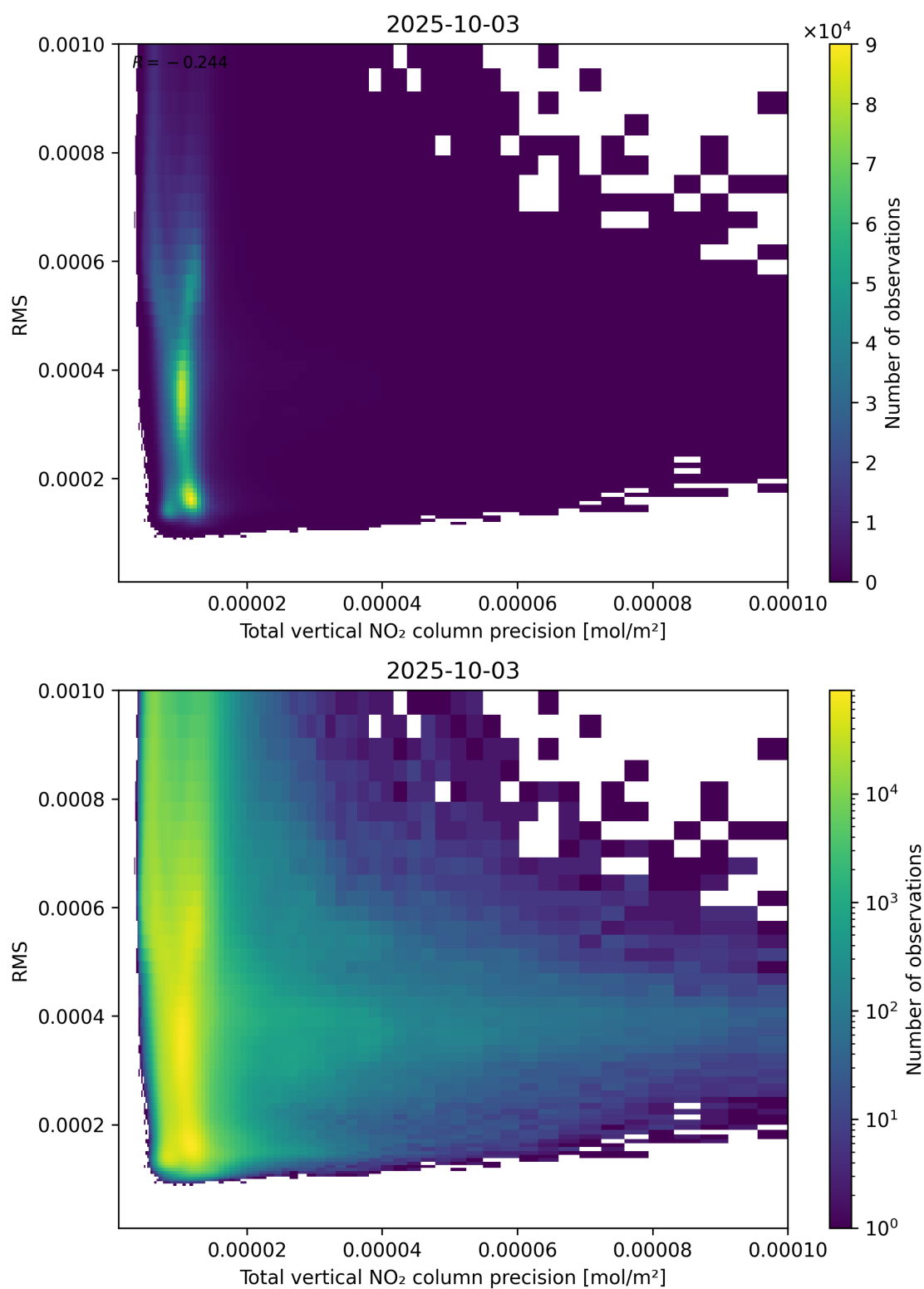
Figure 119: Scatter density plot of “Total vertical NO 2 column precision” against “RMS” for 2025-10-02 to 2025-10-04.
