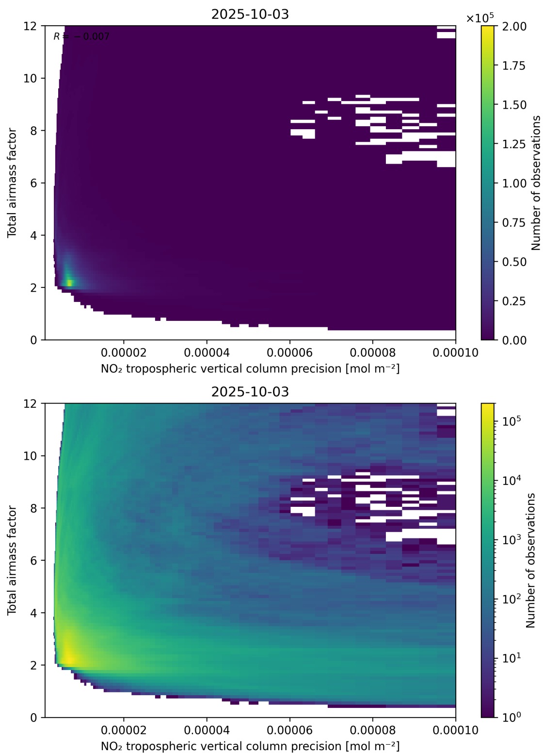
Figure 132: Scatter density plot of “NO 2 tropospheric vertical column precision” against “Total air mass factor” for 2025-10-02 to 2025-10-04.
