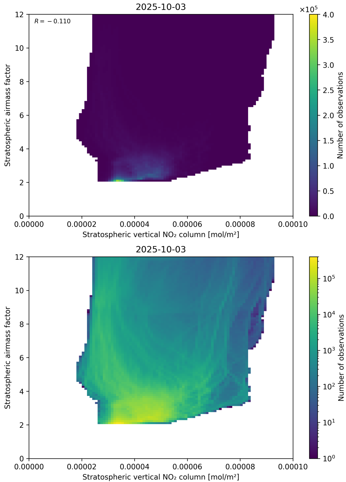
Figure 96: Scatter density plot of “Stratospheric vertical NO 2 column” against “Stratospheric airmass factor” for 2025-10-02 to 2025-10-04.
