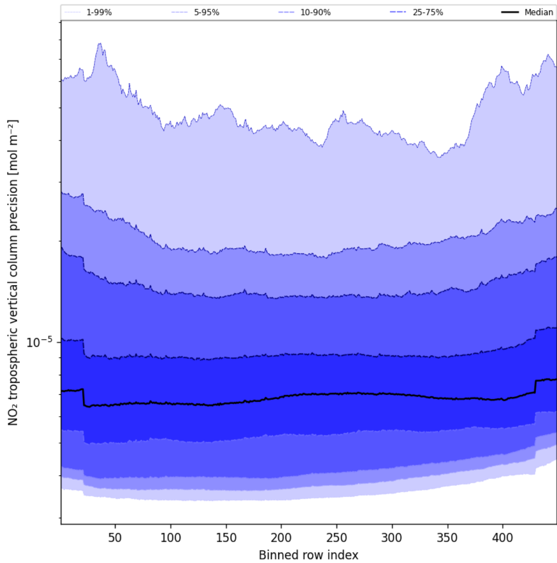
Figure 47: Along track statistics of “NO 2 tropospheric vertical column precision” for 2025-10-02 to 2025-10-04
