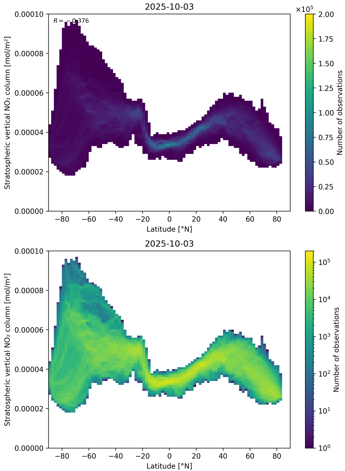
Figure 87: Scatter density plot of “Latitude” against “Stratospheric vertical NO 2 column” for 2025-10-02 to 2025-10-04.
