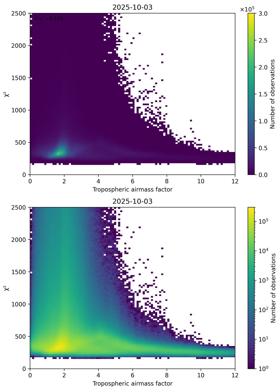
Figure 73: Scatter density plot of “Tropospheric airmass factor” against “ \chi^2 ” for 2025-10-02 to 2025-10-04.
