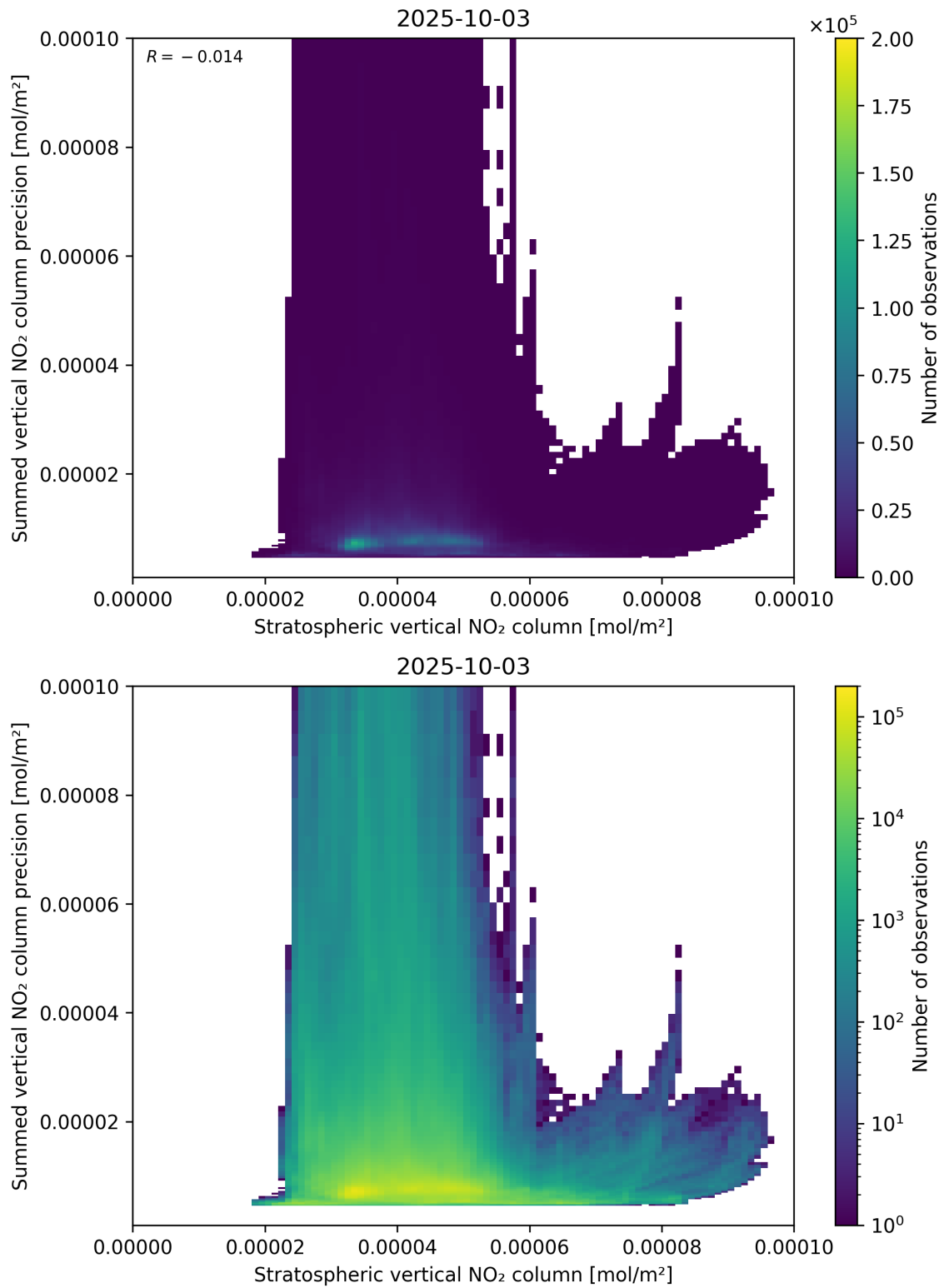
Figure 99: Scatter density plot of “Stratospheric vertical NO 2 column” against “Summed vertical NO 2 column precision” for 2025-10-02 to 2025-10-04.
