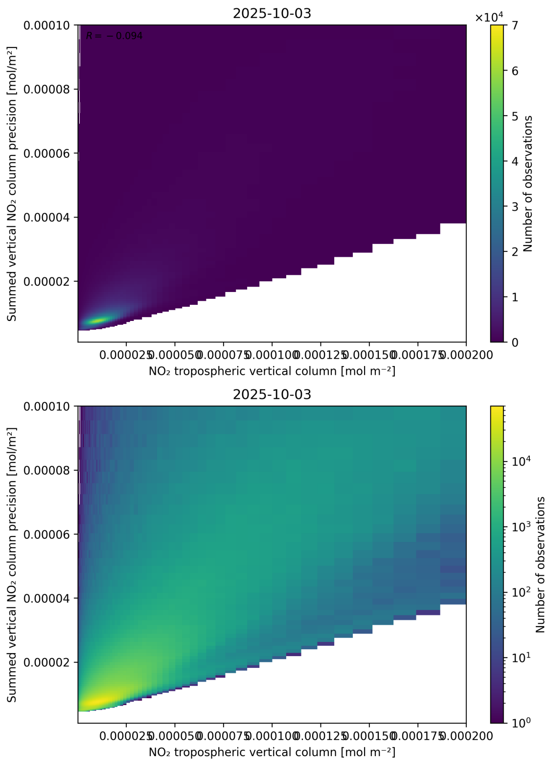
Figure 127: Scatter density plot of “NO 2 tropospheric vertical column” against “Summed vertical NO 2 column precision” for 2025-10-02 to 2025-10-04.
