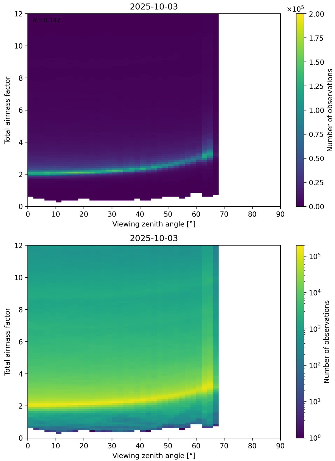
Figure 160: Scatter density plot of “Viewing zenith angle” against “Total airmass factor” for 2025-10-02 to 2025-10-04.
