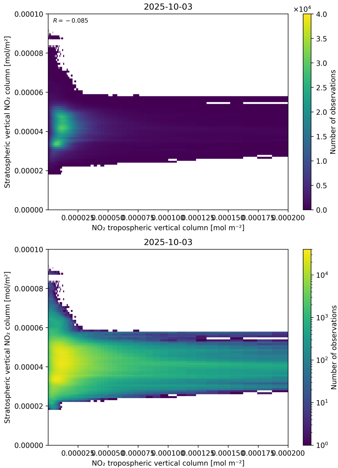
Figure 125: Scatter density plot of “NO 2 tropospheric vertical column” against “Stratospheric vertical NO 2 column” for 2025-10-02 to 2025-10-04.
