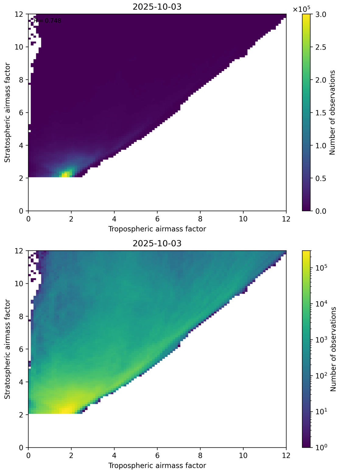
Figure 71: Scatter density plot of “Tropospheric airmass factor” against “Stratospheric airmass factor” for 2025-10-02 to 2025-10-04.
