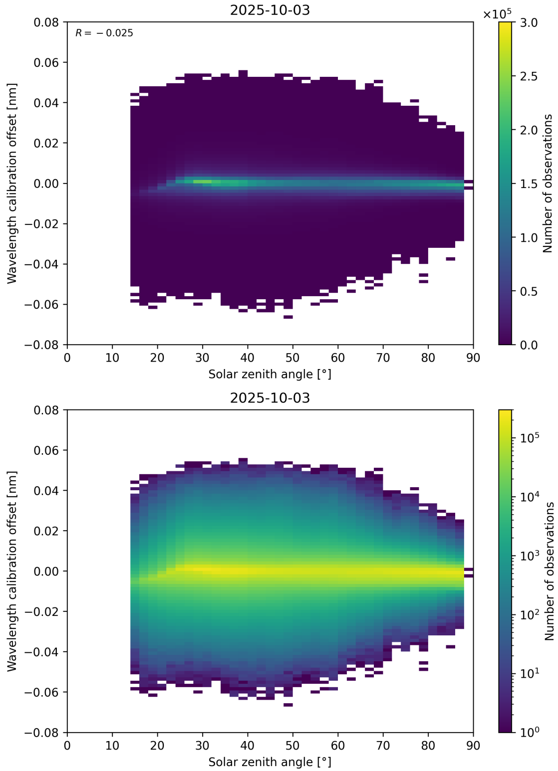
Figure 158: Scatter density plot of “Solar zenith angle” against “Wavelength calibration offset” for 2025-10-02 to 2025-10-04.
