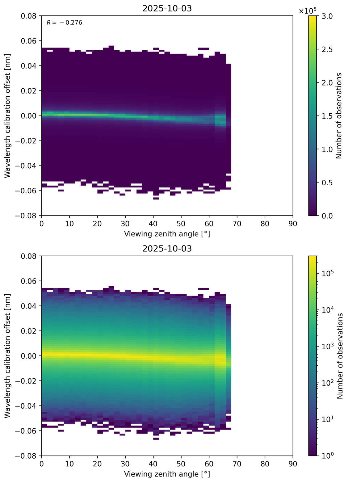
Figure 173: Scatter density plot of “Viewing zenith angle” against “Wavelength calibration offset” for 2025-10-02 to 2025-10-04.
