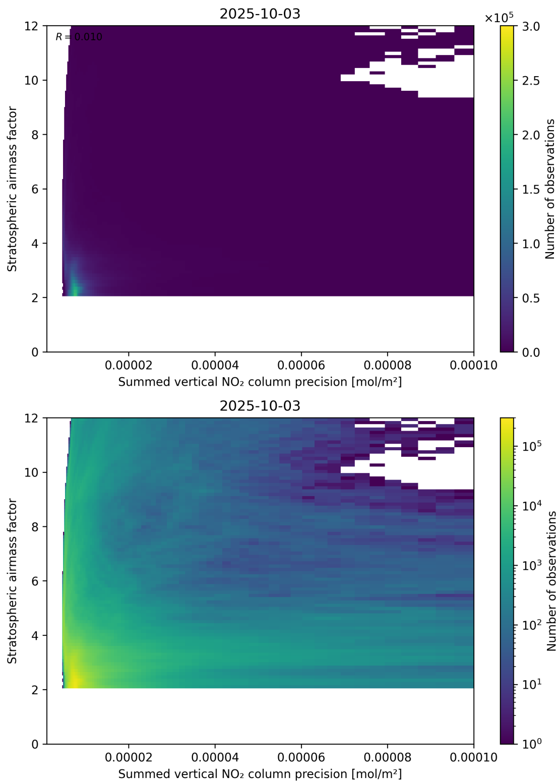
Figure 106: Scatter density plot of “Summed vertical NO 2 column precision” against “Stratospheric airmass factor” for 2025-10-02 to 2025-10-04.
