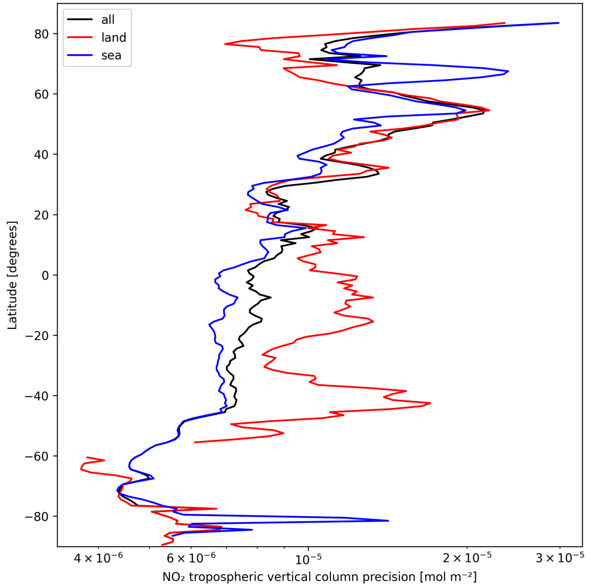
Figure 13: Zonal average of “NO 2 tropospheric vertical column precision” for 2025-10-02 to 2025-10-04.
