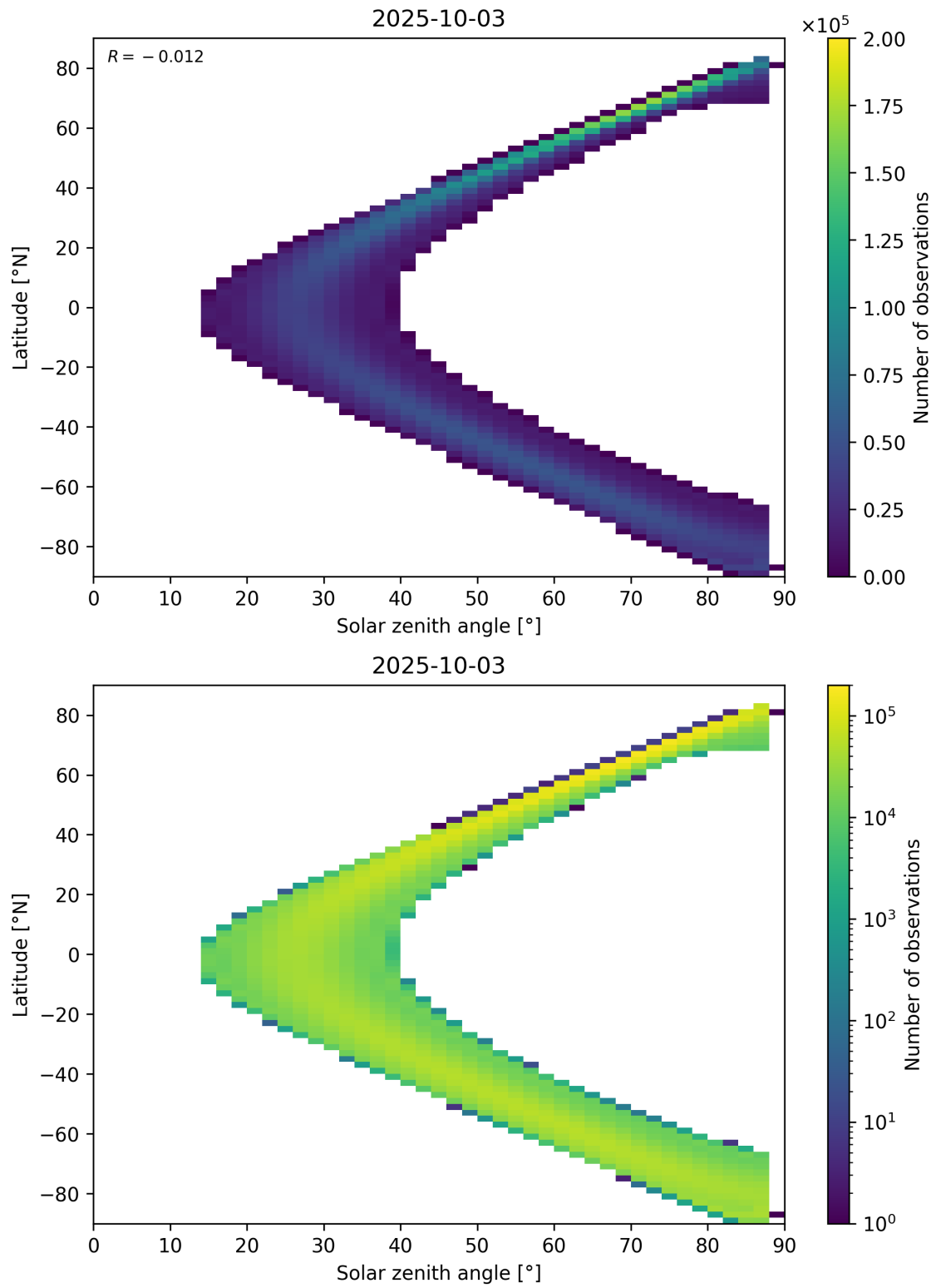
Figure 149: Scatter density plot of “Solar zenith angle” against “Latitude” for 2025-10-02 to 2025-10-04.
