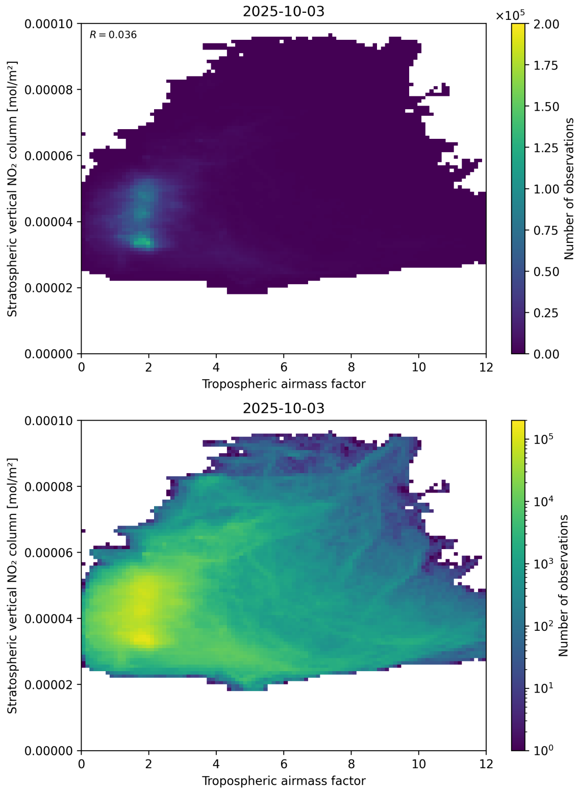
Figure 74: Scatter density plot of “Tropospheric air mass factor” against “Stratospheric vertical NO 2 column” for 2025-10-02 to 2025-10-04.
