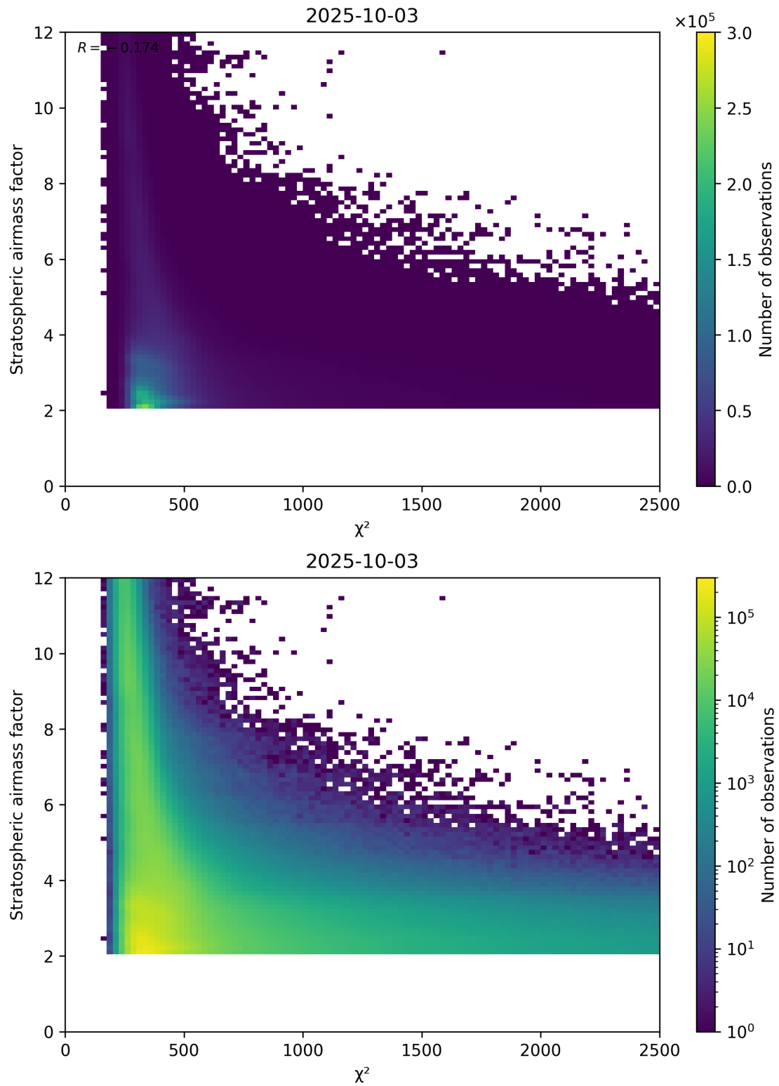
Figure 81: Scatter density plot of “ \chi^2 ” against “Stratospheric air mass factor” for 2025-10-02 to 2025-10-04.
