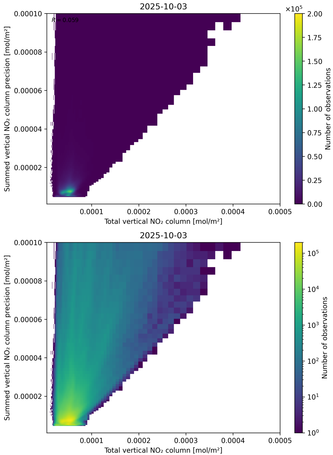
Figure 113: Scatter density plot of “Total vertical NO 2 column” against “Summed vertical NO 2 column precision” for 2025-10-02 to 2025-10-04.
