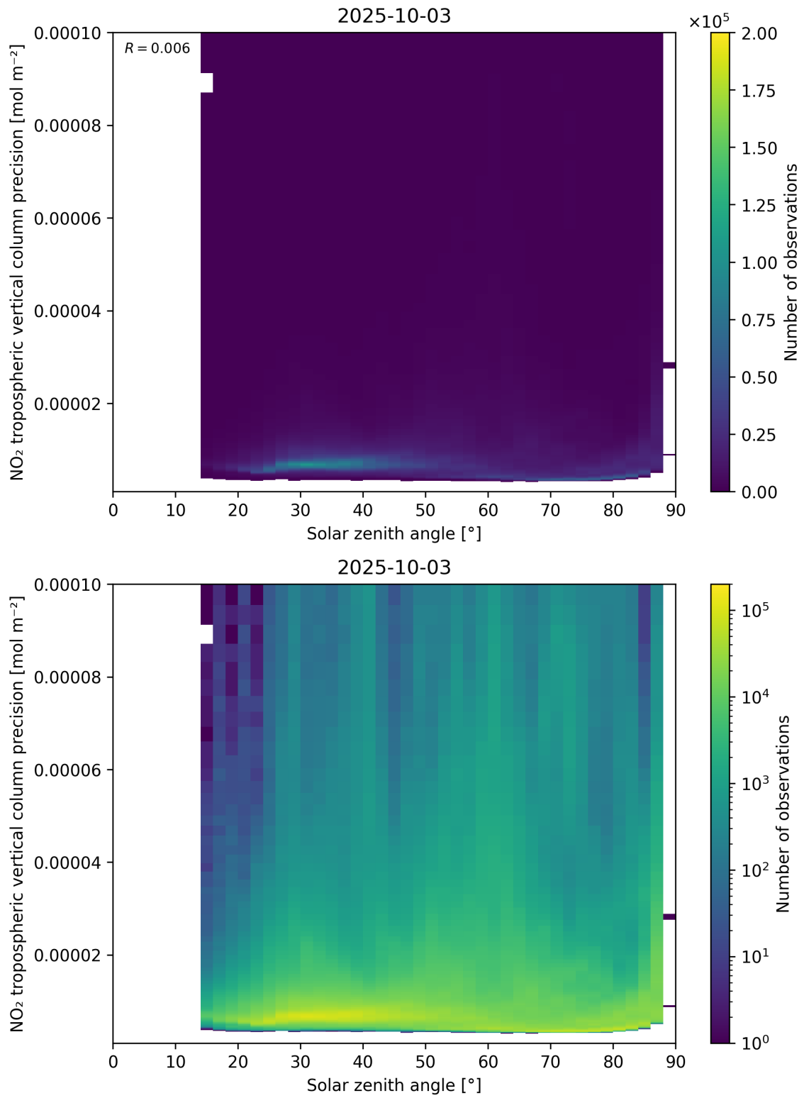
Figure 156: Scatter density plot of “Solar zenith angle” against “NO 2 tropospheric vertical column precision” for 2025-10-02 to 2025-10-04.
