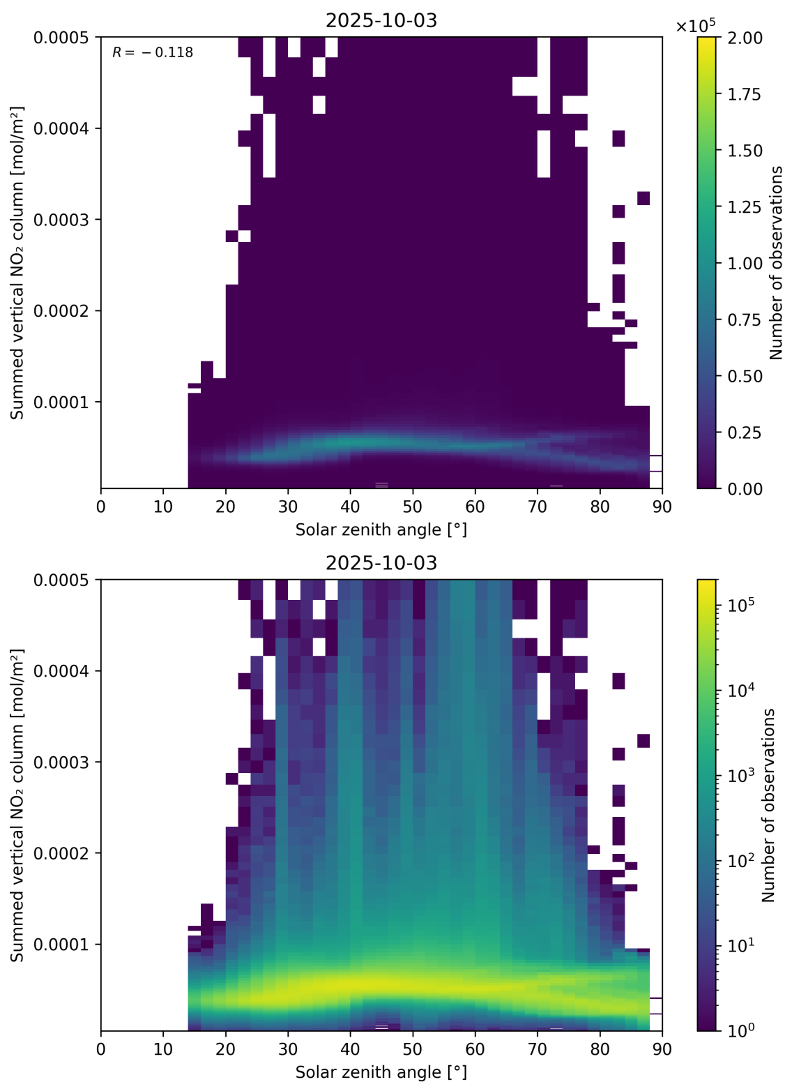
Figure 151: Scatter density plot of “Solar zenith angle” against “Summed vertical NO 2 column” for 2025-10-02 to 2025-10-04.
