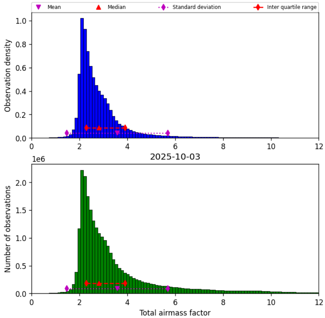
Figure 32: Histogram of “Total airmass factor” for 2025-10-02 to 2025-10-04
