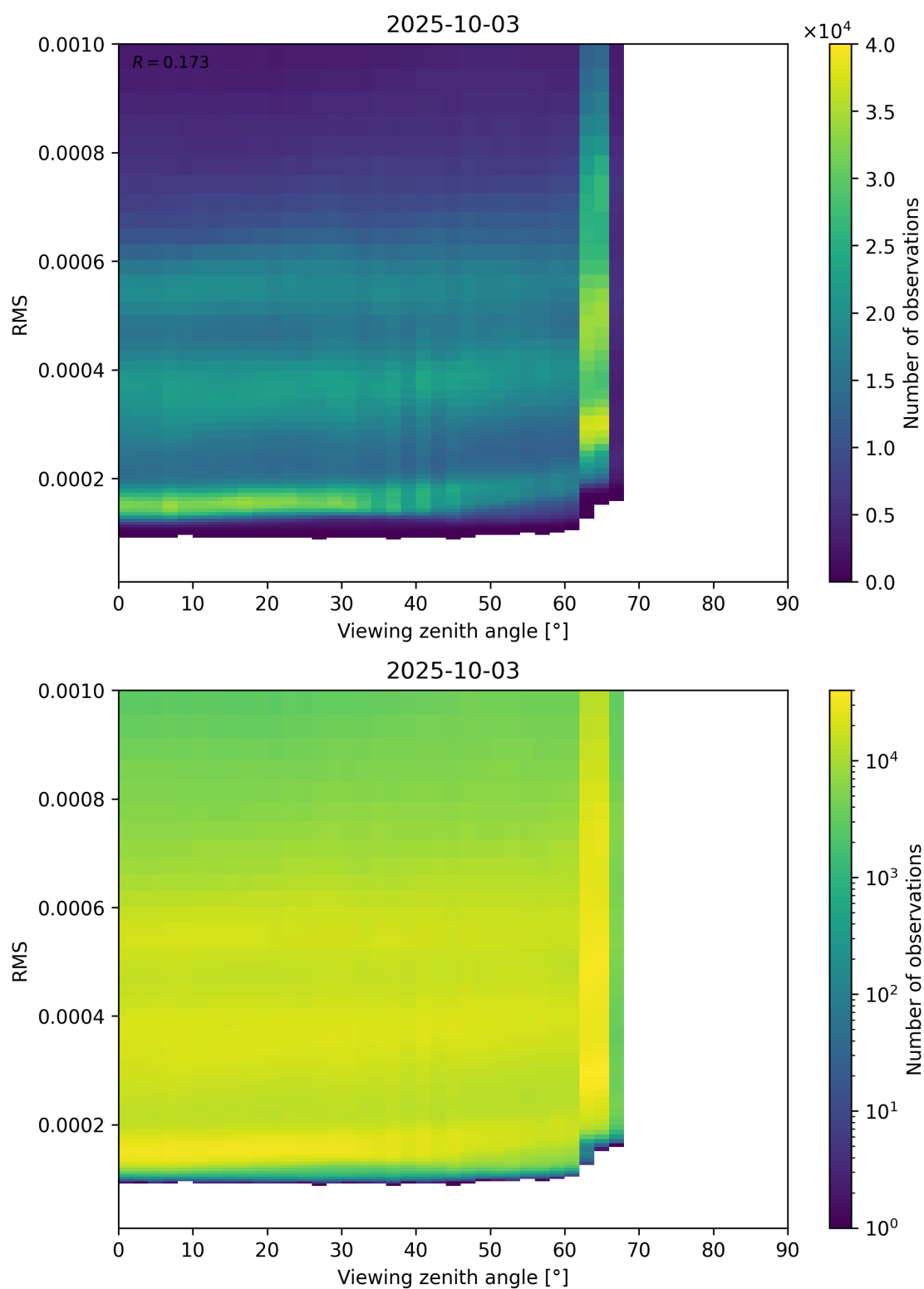
Figure 171: Scatter density plot of “Viewing zenith angle” against “RMS” for 2025-10-02 to 2025-10-04.
