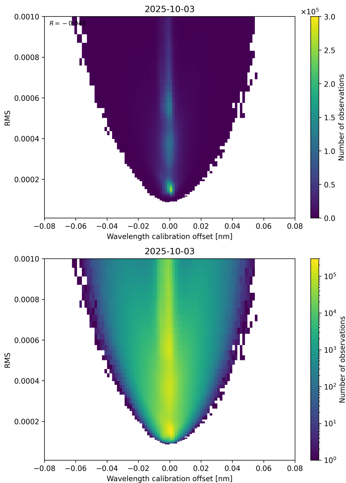
Figure 181: Scatter density plot of “Wavelength calibration offset” against “RMS” for 2025-10-02 to 2025-10-04.
