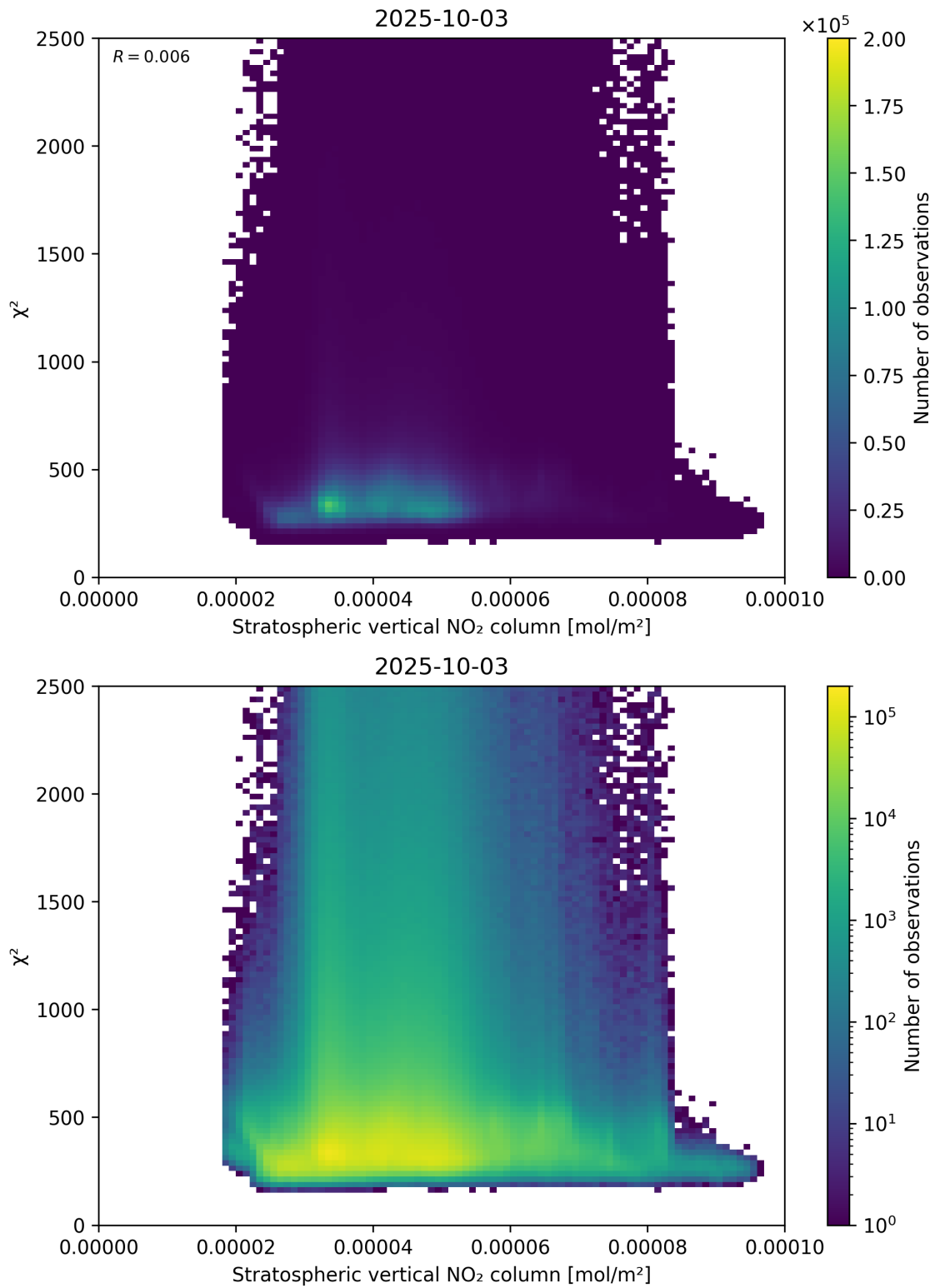
Figure 97: Scatter density plot of “Stratospheric vertical NO 2 column” against “ \chi^2 ” for 2025-10-02 to 2025-10-04.
