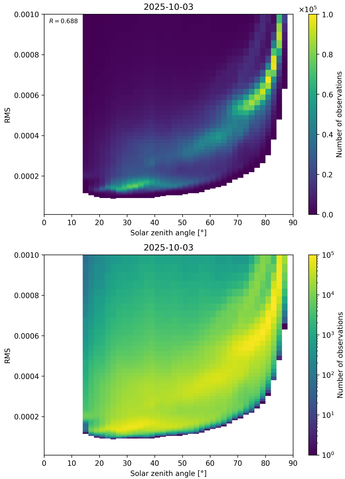
Figure 157: Scatter density plot of “Solar zenith angle” against “RMS” for 2025-10-02 to 2025-10-04.
