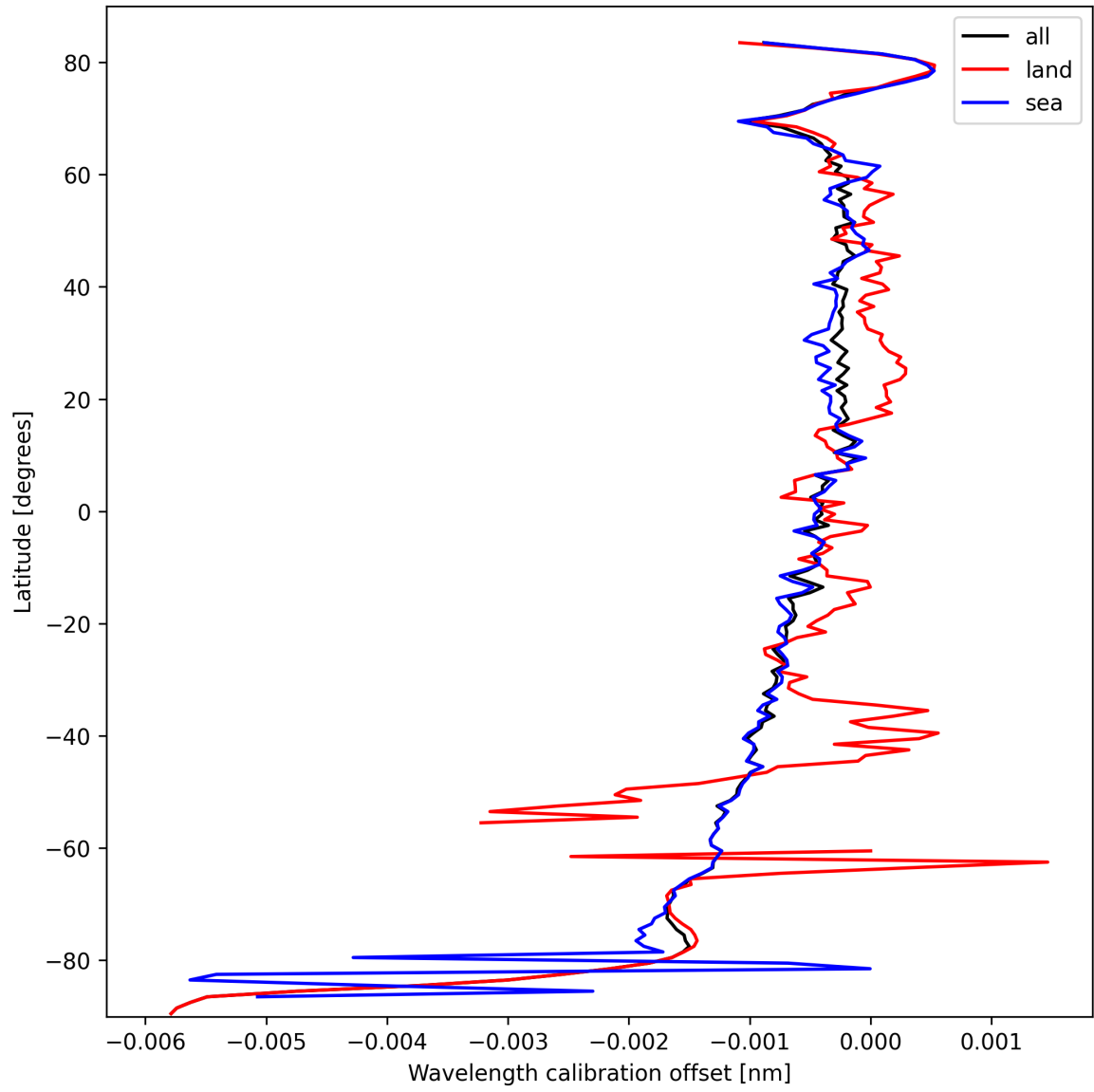
Figure 18: Zonal average of “Wavelength calibration offset” for 2025-10-02 to 2025-10-04.
