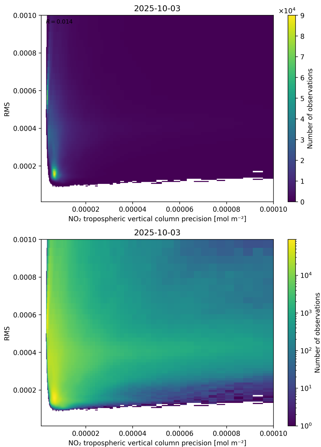
Figure 140: Scatter density plot of “NO 2 tropospheric vertical column precision” against “RMS” for 2025-10-02 to 2025-10-04.
