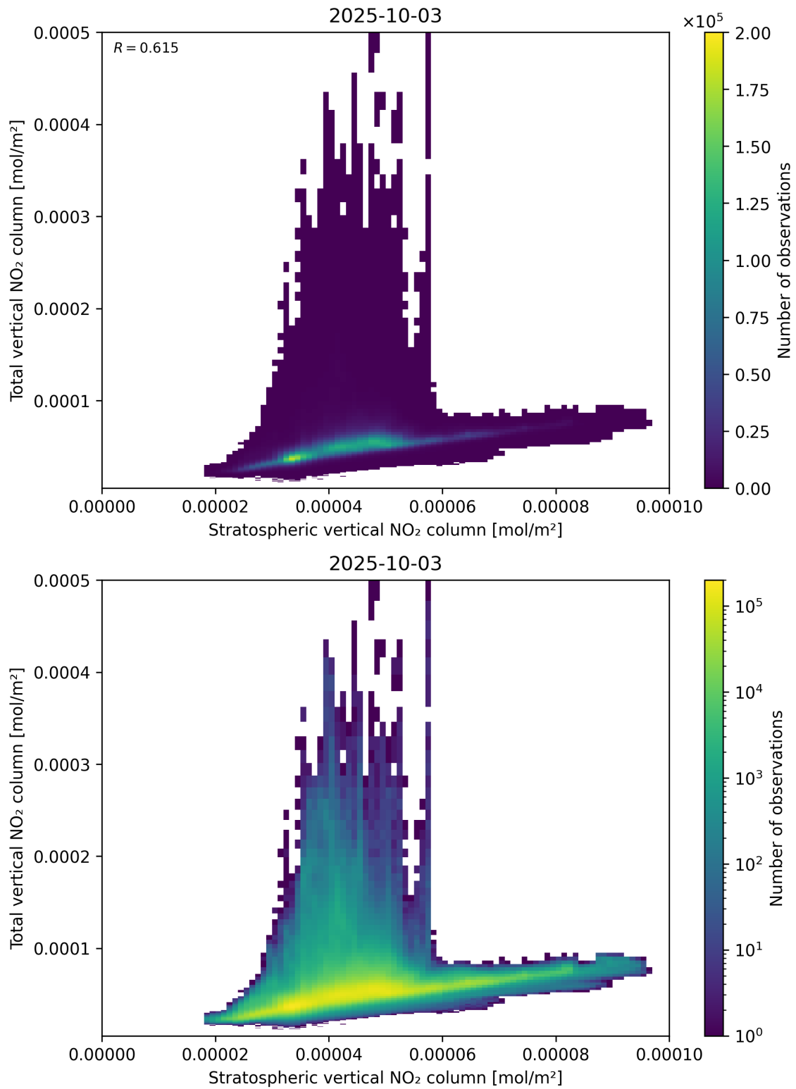
Figure 100: Scatter density plot of “Stratospheric vertical NO 2 column” against “Total vertical NO 2 column” for 2025-10-02 to 2025-10-04.
