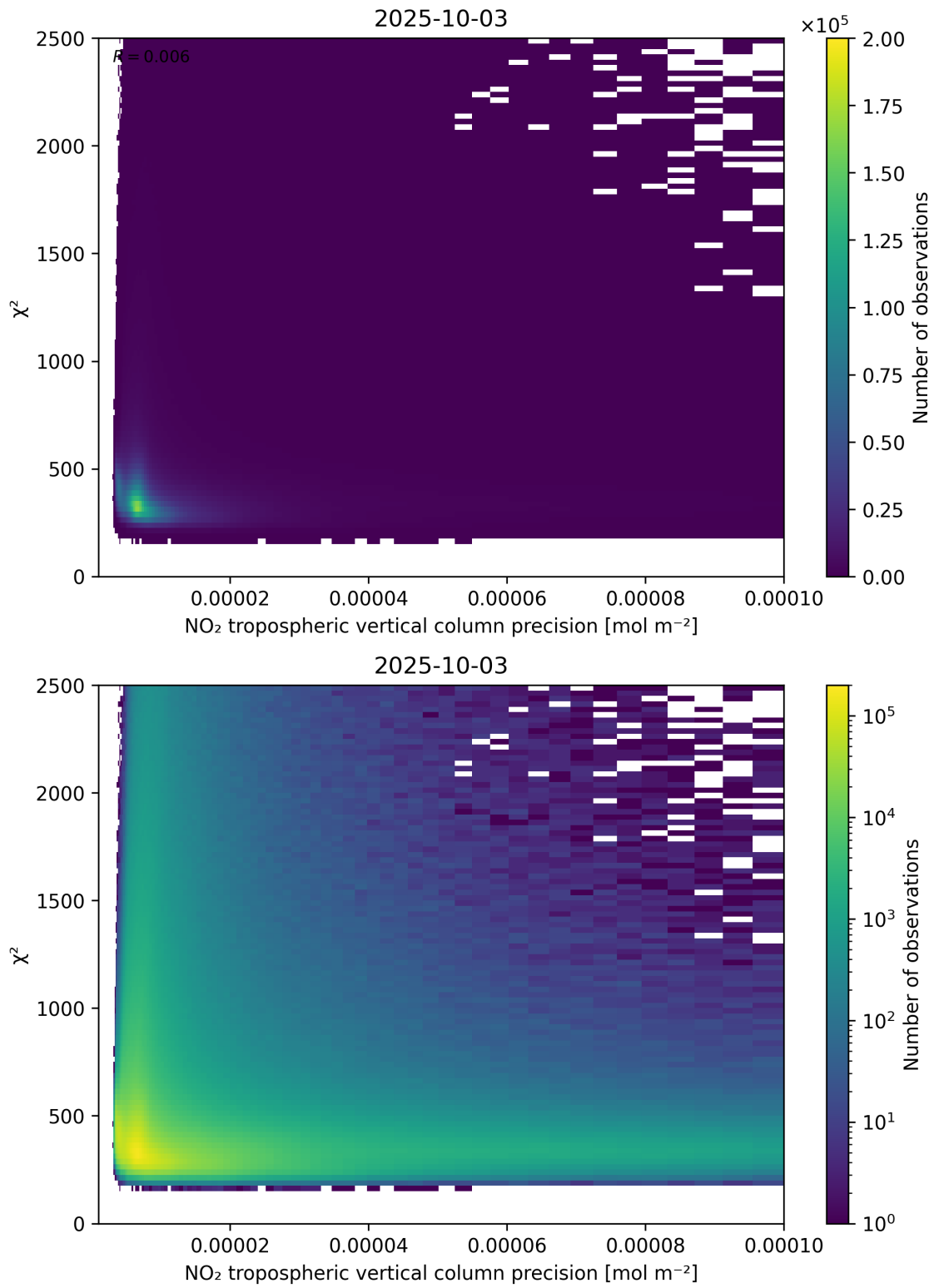
Figure 134: Scatter density plot of “NO 2 tropospheric vertical column precision” against “ \chi^2 ” for 2025-10-02 to 2025-10-04.
