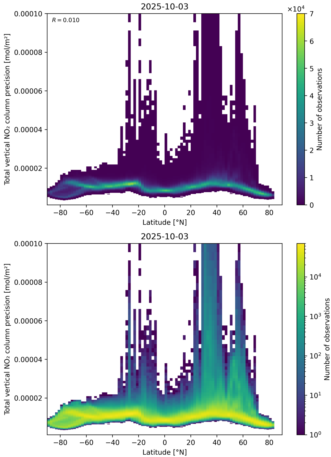
Figure 91: Scatter density plot of “Latitude” against “Total vertical NO 2 column precision” for 2025-10-02 to 2025-10-04.
