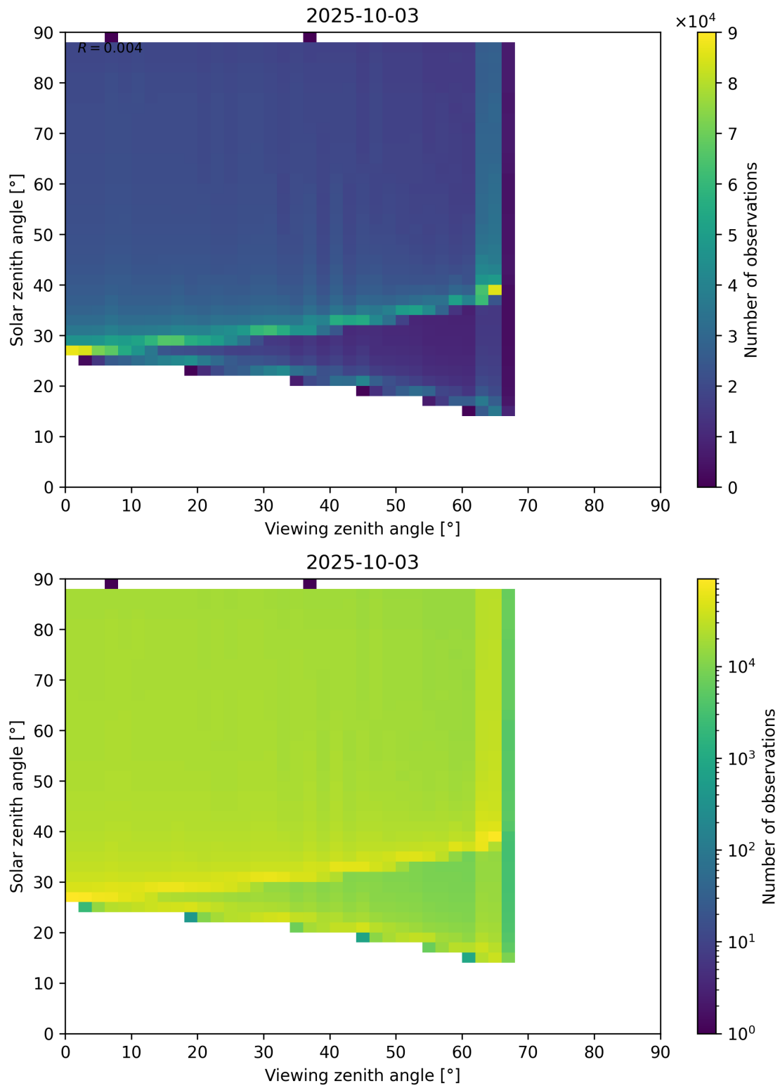
Figure 172: Scatter density plot of “Viewing zenith angle” against “Solar zenith angle” for 2025-10-02 to 2025-10-04.
