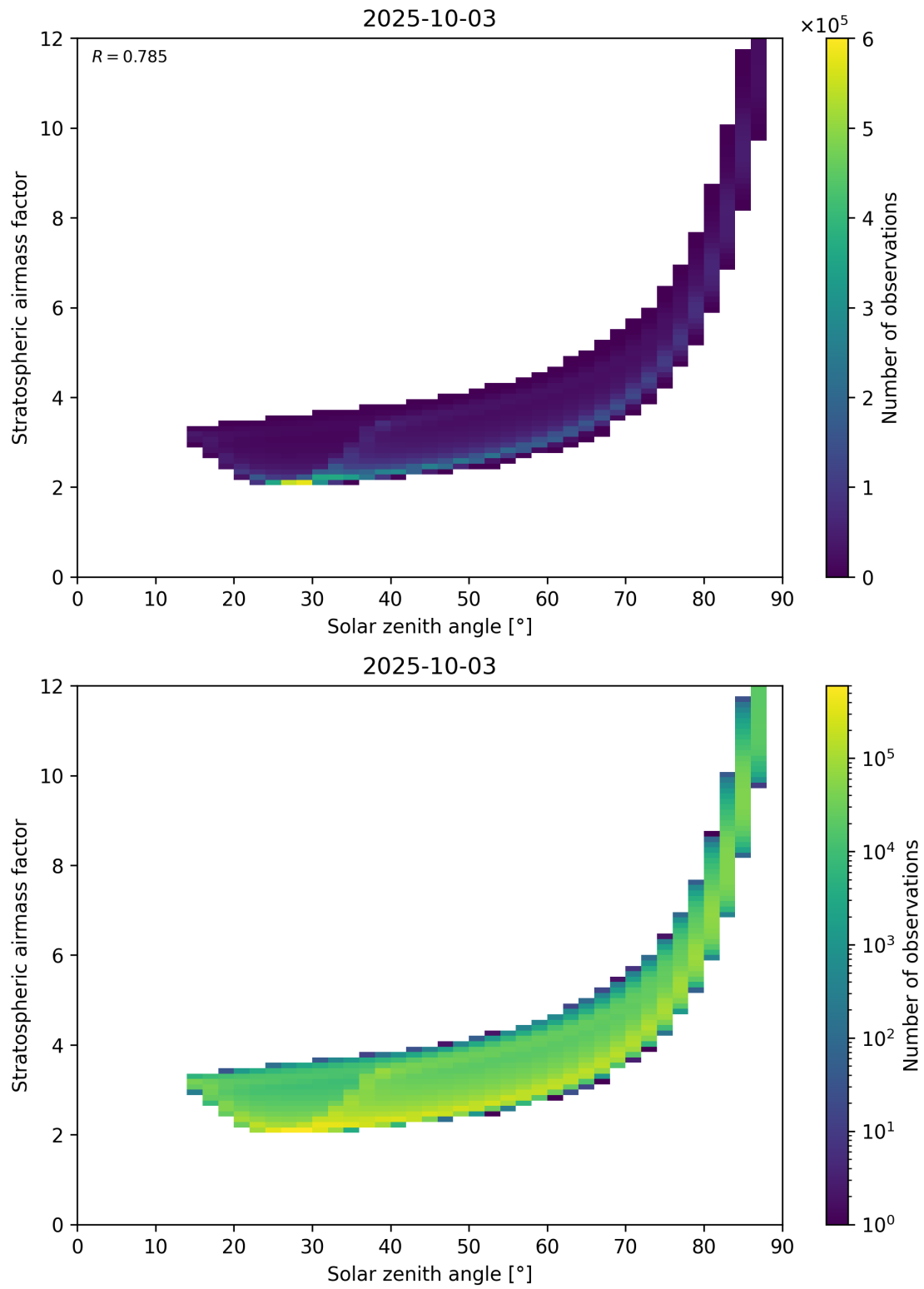
Figure 145: Scatter density plot of “Solar zenith angle” against “Stratospheric airmass factor” for 2025-10-02 to 2025-10-04.
