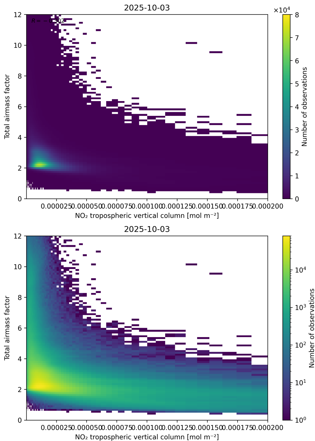
Figure 122: Scatter density plot of “NO 2 tropospheric vertical column” against “Total air mass factor” for 2025-10-02 to 2025-10-04.
