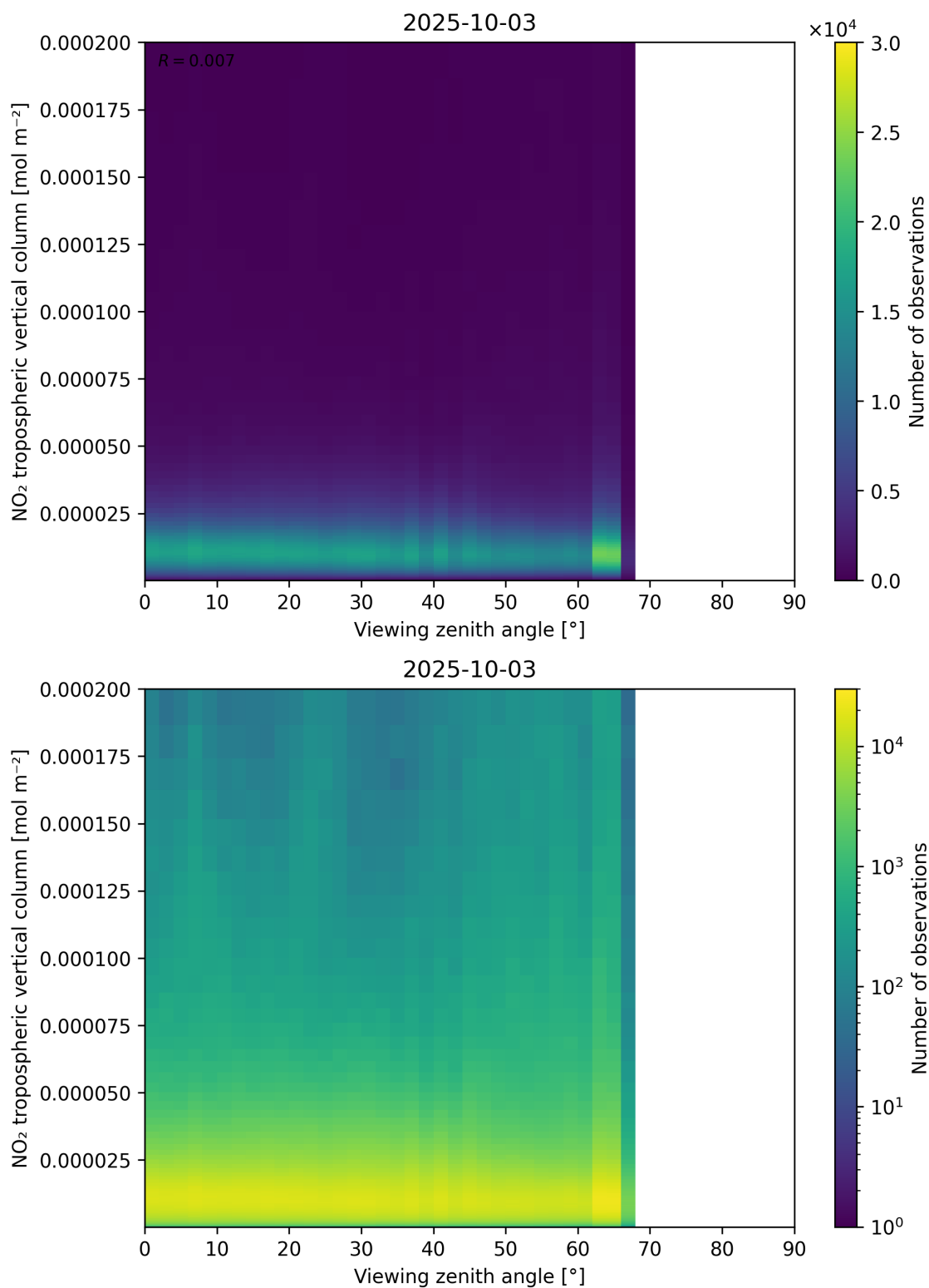
Figure 169: Scatter density plot of “Viewing zenith angle” against “NO 2 tropospheric vertical column” for 2025-10-02 to 2025-10-04.
