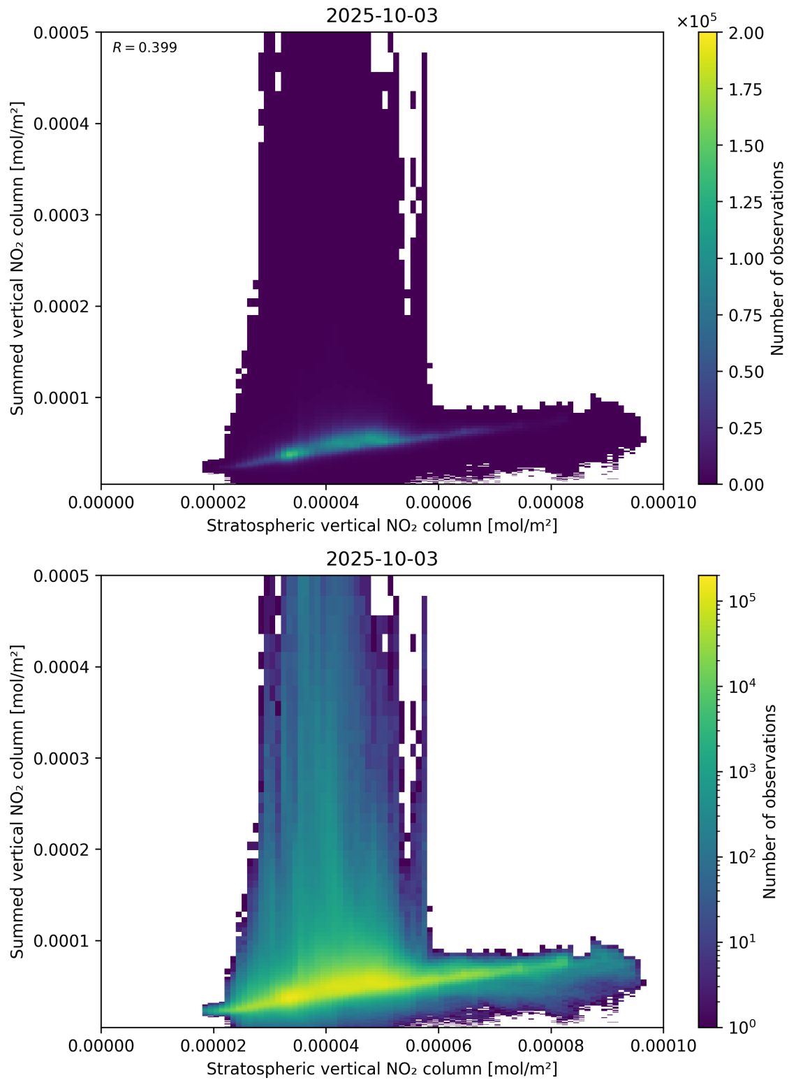
Figure 98: Scatter density plot of “Stratospheric vertical NO 2 column” against “Summed vertical NO 2 column” for 2025-10-02 to 2025-10-04.
