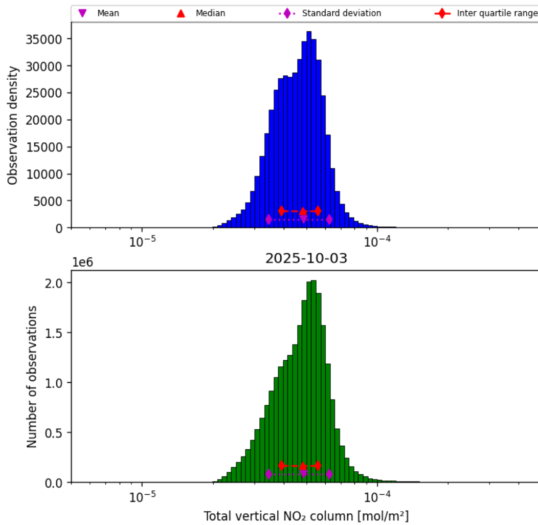
Figure 38: Histogram of “Total vertical NO 2 column” for 2025-10-02 to 2025-10-04
