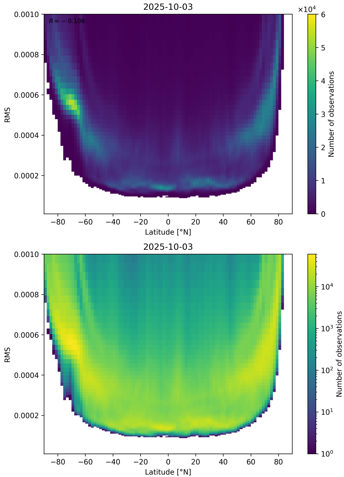
Figure 94: Scatter density plot of “Latitude” against “RMS” for 2025-10-02 to 2025-10-04.
