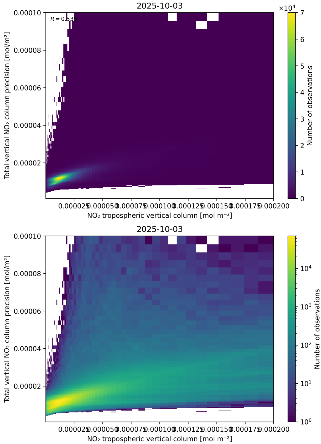
Figure 129: Scatter density plot of “NO 2 tropospheric vertical column” against “Total vertical NO 2 column precision” for 2025-10-02 to 2025-10-04.
