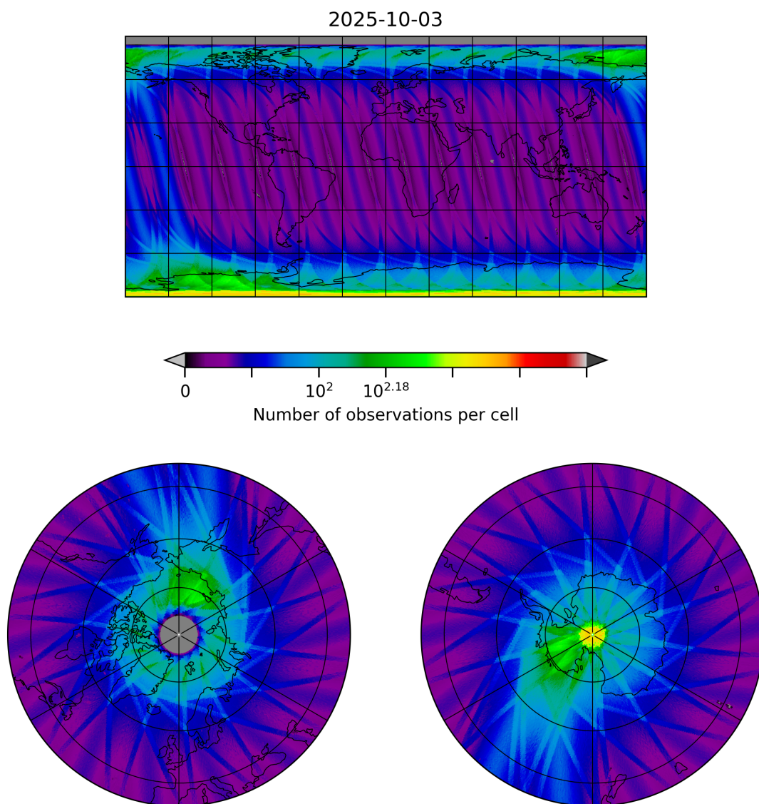
Figure 10: Map of the number of observations for 2025-10-02 to 2025-10-04
