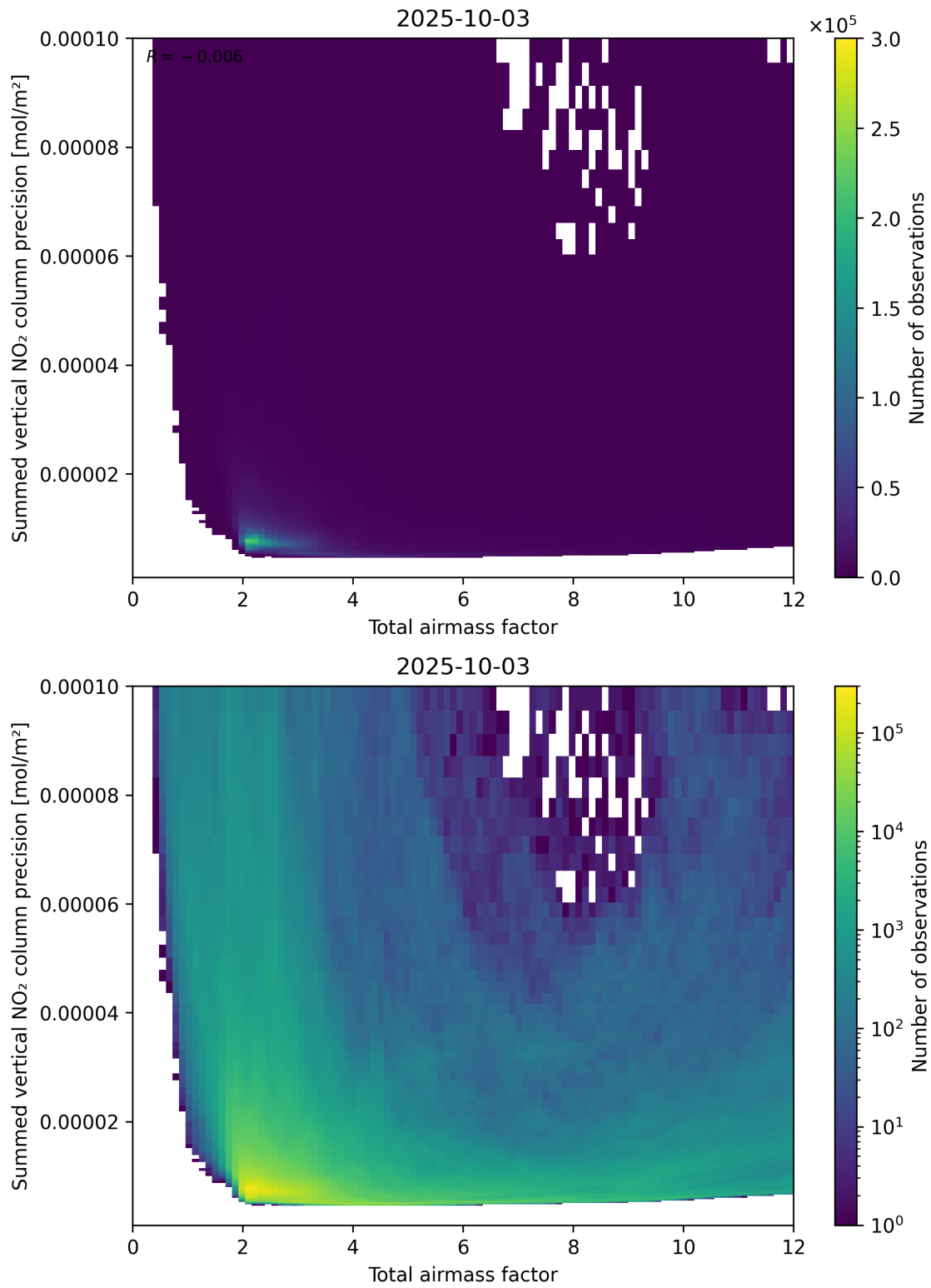
Figure 66: Scatter density plot of “Total airmass factor” against “Summed vertical NO 2 column precision” for 2025-10-02 to 2025-10-04.
