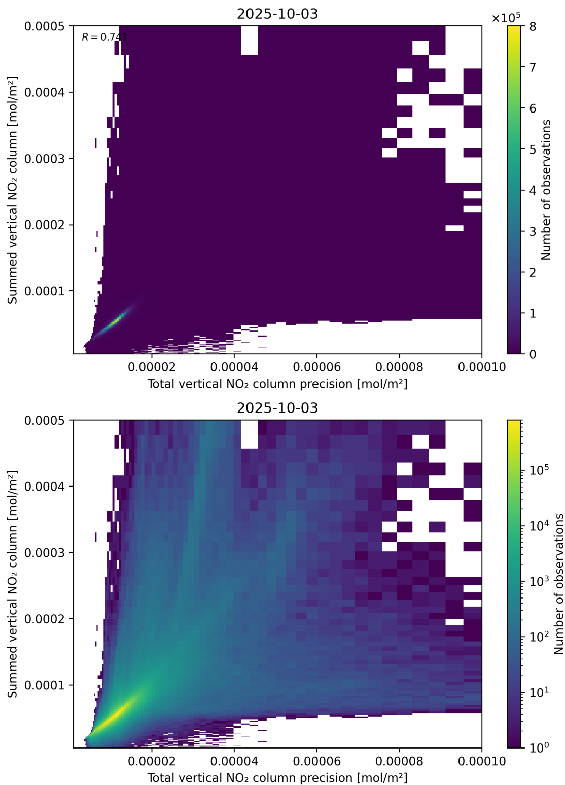
Figure 117: Scatter density plot of “Total vertical NO 2 column precision” against “Summed vertical NO 2 column” for 2025-10-02 to 2025-10-04.
