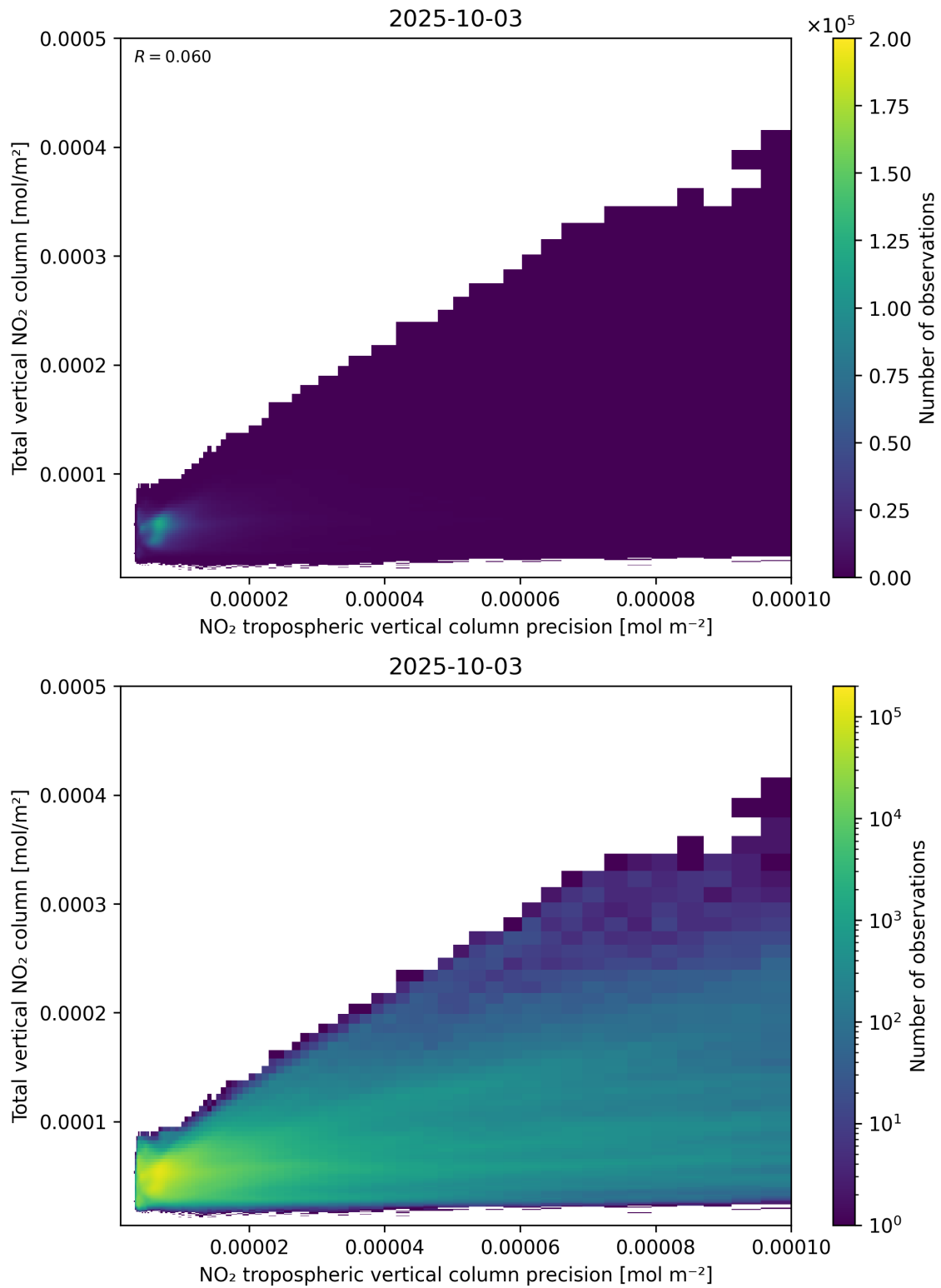
Figure 138: Scatter density plot of “NO 2 tropospheric vertical column precision” against “Total vertical NO 2 column” for 2025-10-02 to 2025-10-04.
