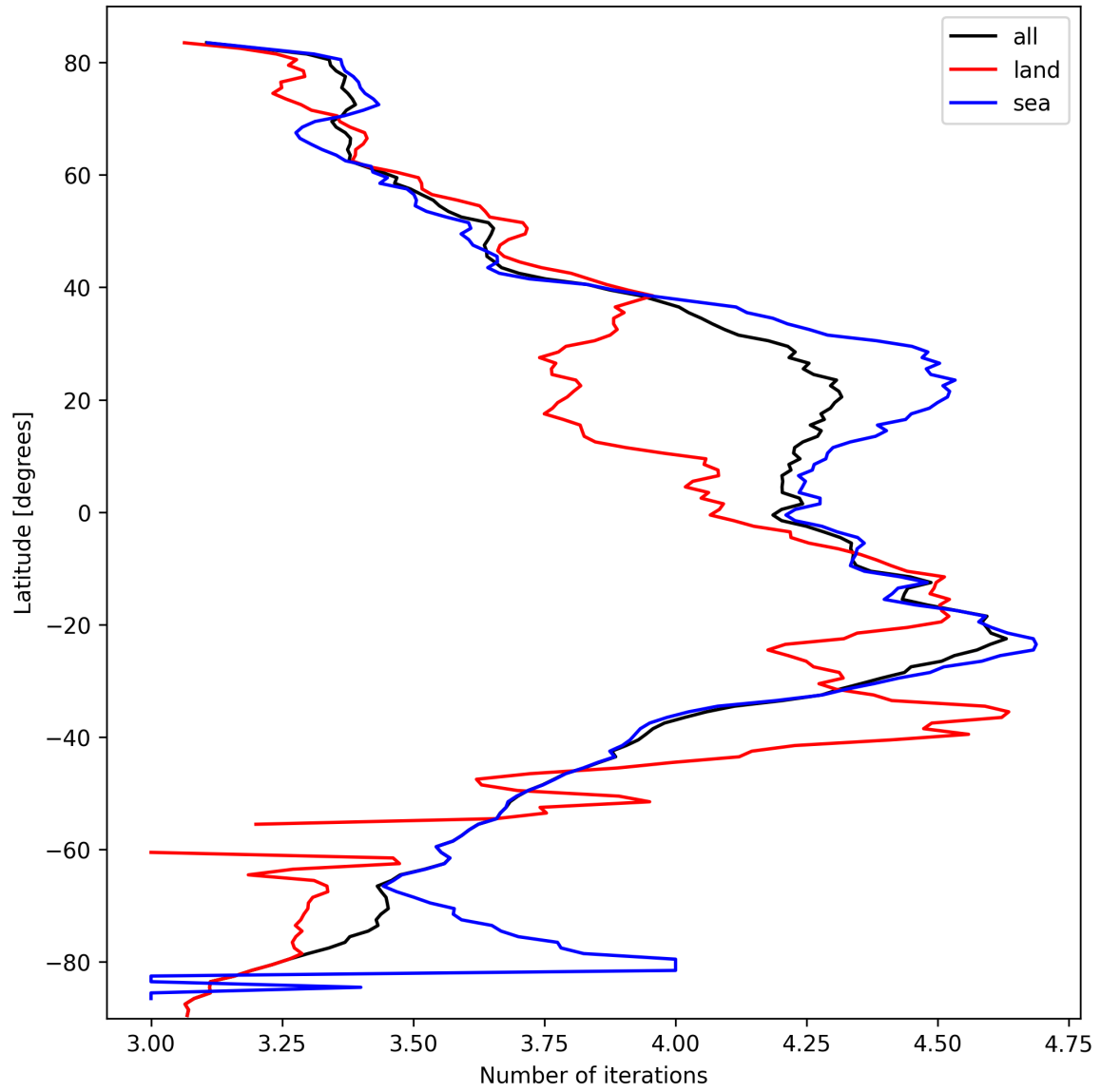
Figure 17: Zonal average of “Number of iterations” for 2025-10-02 to 2025-10-04.
