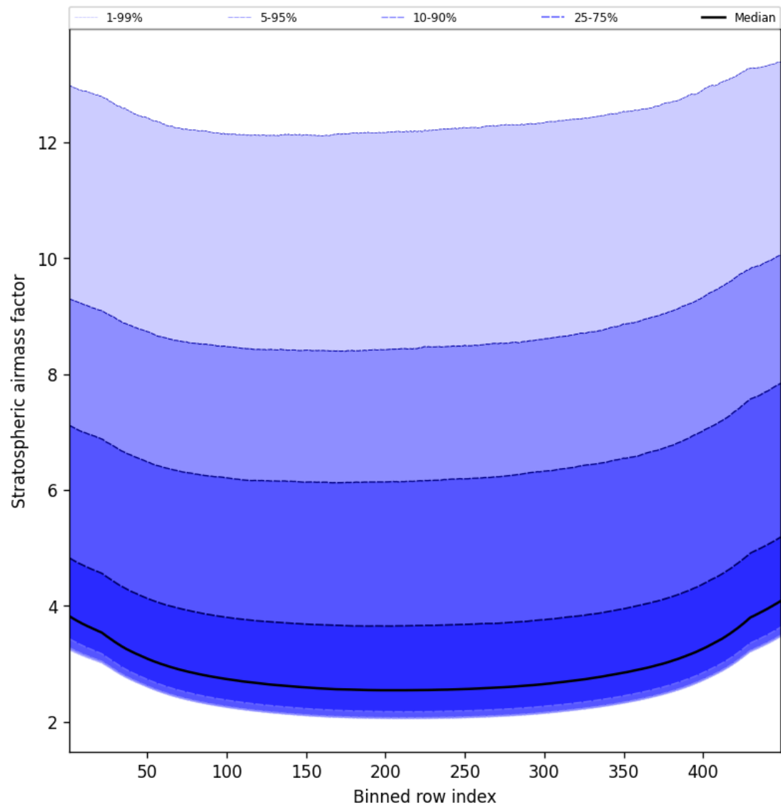
Figure 61: Along track statistics of “Stratospheric air mass factor” for 2025-10-02 to 2025-10-04
