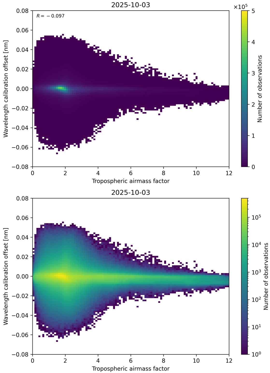
Figure 80: Scatter density plot of “Tropospheric airmass factor” against “Wavelength calibration offset” for 2025-10-02 to 2025-10-04.
