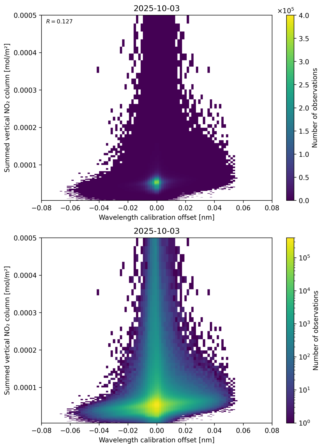
Figure 177: Scatter density plot of “Wavelength calibration offset” against “Summed vertical NO 2 column” for 2025-10-02 to 2025-10-04.
