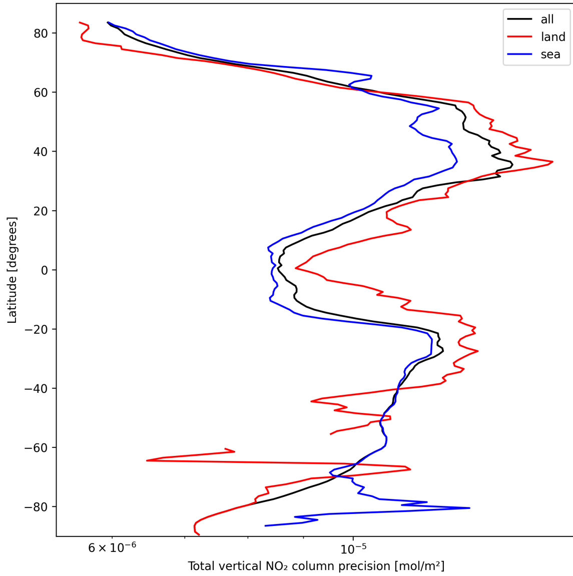
Figure 22: Zonal average of “Total vertical NO 2 column precision” for 2025-10-02 to 2025-10-04.
