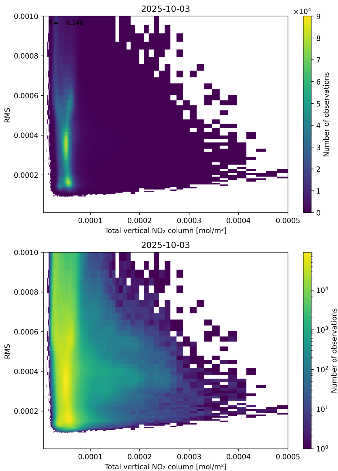
Figure 120: Scatter density plot of “Total vertical NO 2 column” against “RMS” for 2025-10-02 to 2025-10-04.
