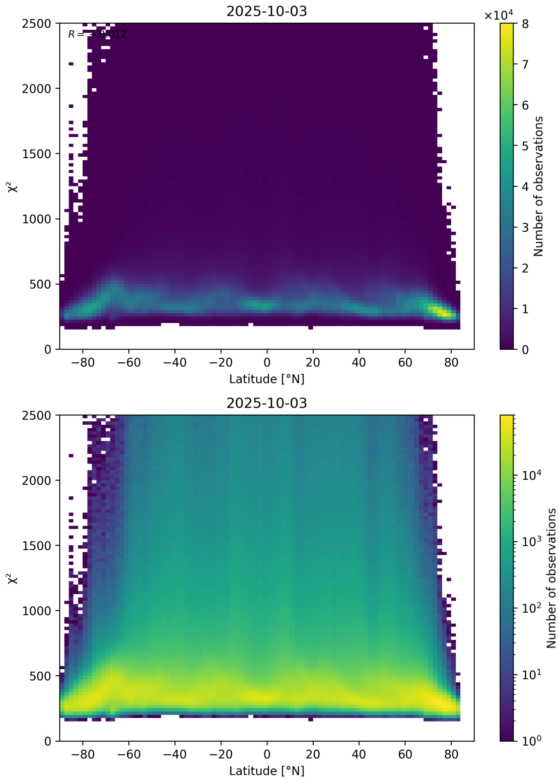
Figure 86: Scatter density plot of “Latitude” against “ \chi^2 ” for 2025-10-02 to 2025-10-04.
