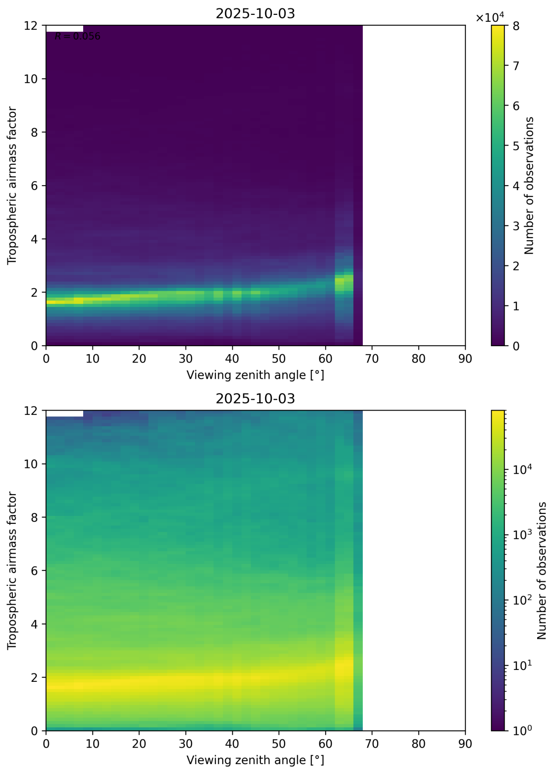
Figure 161: Scatter density plot of “Viewing zenith angle” against “Tropospheric air mass factor” for 2025-10-02 to 2025-10-04.
