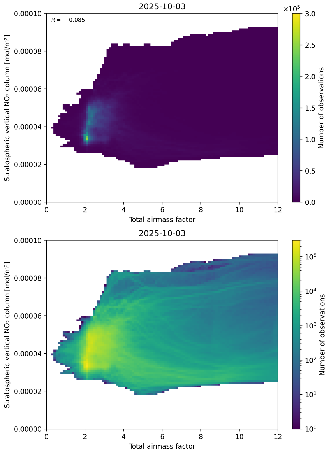
Figure 64: Scatter density plot of “Total airmass factor” against “Stratospheric vertical NO 2 column” for 2025-10-02 to 2025-10-04.
