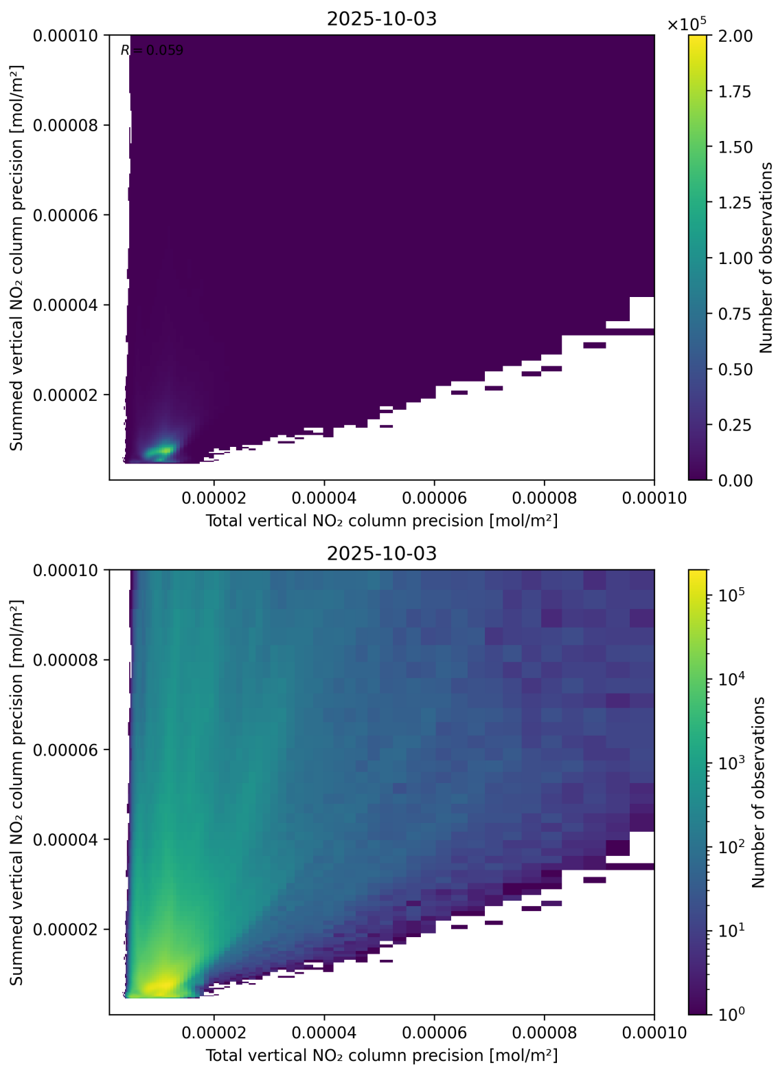
Figure 118: Scatter density plot of “Total vertical NO 2 column precision” against “Summed vertical NO 2 column precision” for 2025-10-02 to 2025-10-04.
