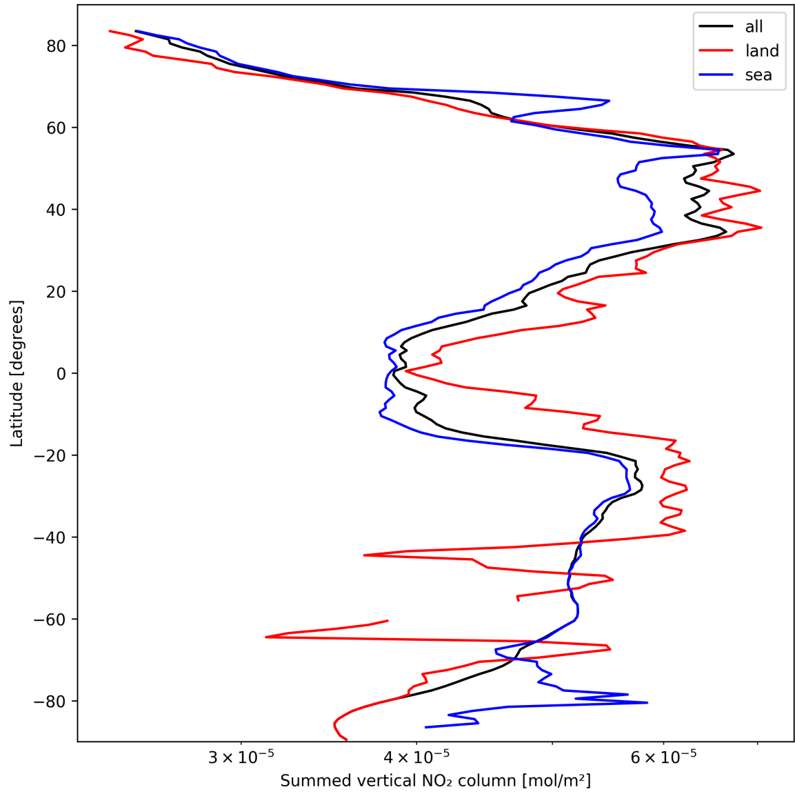
Figure 23: Zonal average of “Summed vertical NO 2 column” for 2025-10-02 to 2025-10-04.
