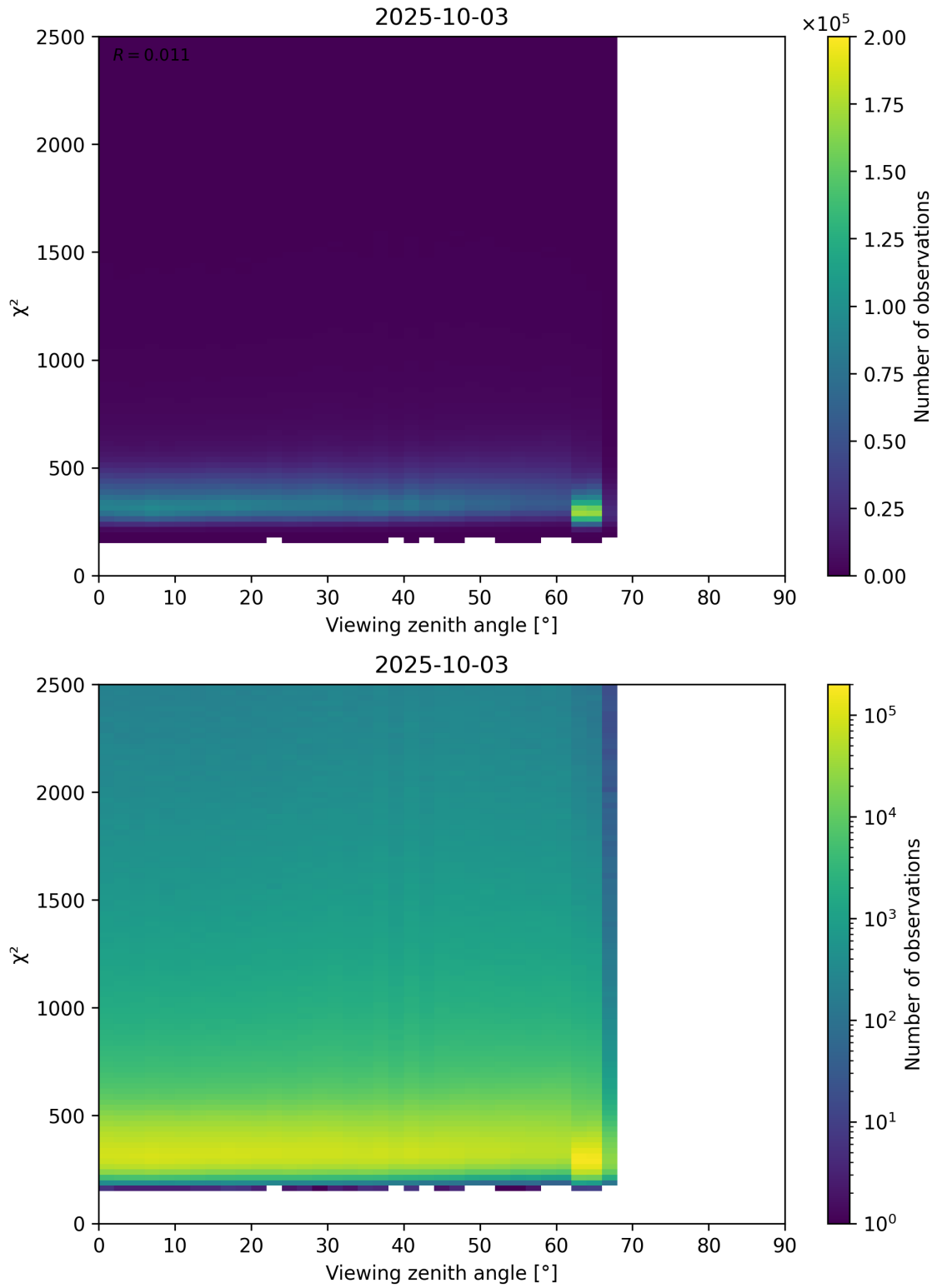
Figure 162: Scatter density plot of “Viewing zenith angle” against “ \chi^2 ” for 2025-10-02 to 2025-10-04.
