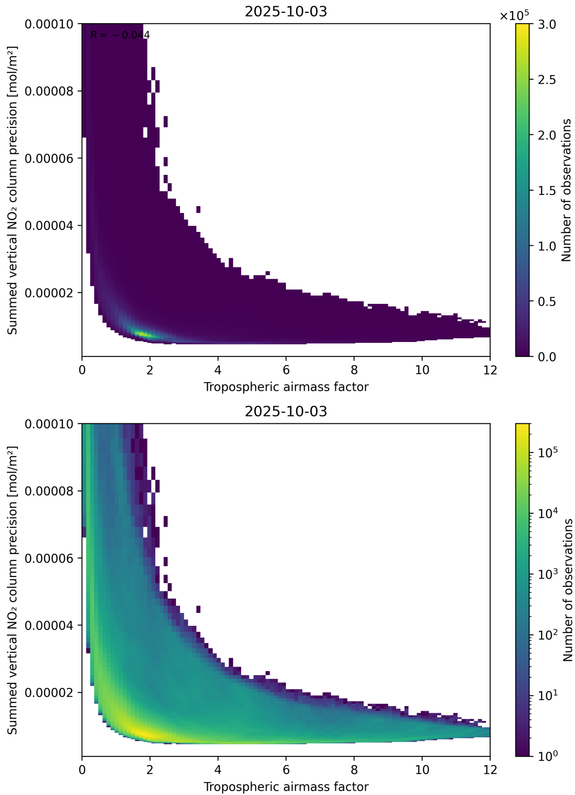
Figure 76: Scatter density plot of “Tropospheric air mass factor” against “Summed vertical NO 2 column precision” for 2025-10-02 to 2025-10-04.
