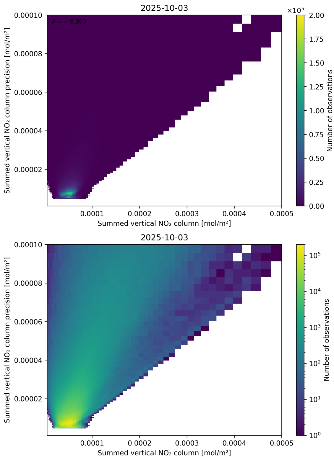
Figure 105: Scatter density plot of “Summed vertical NO 2 column” against “Summed vertical NO 2 column precision” for 2025-10-02 to 2025-10-04.
