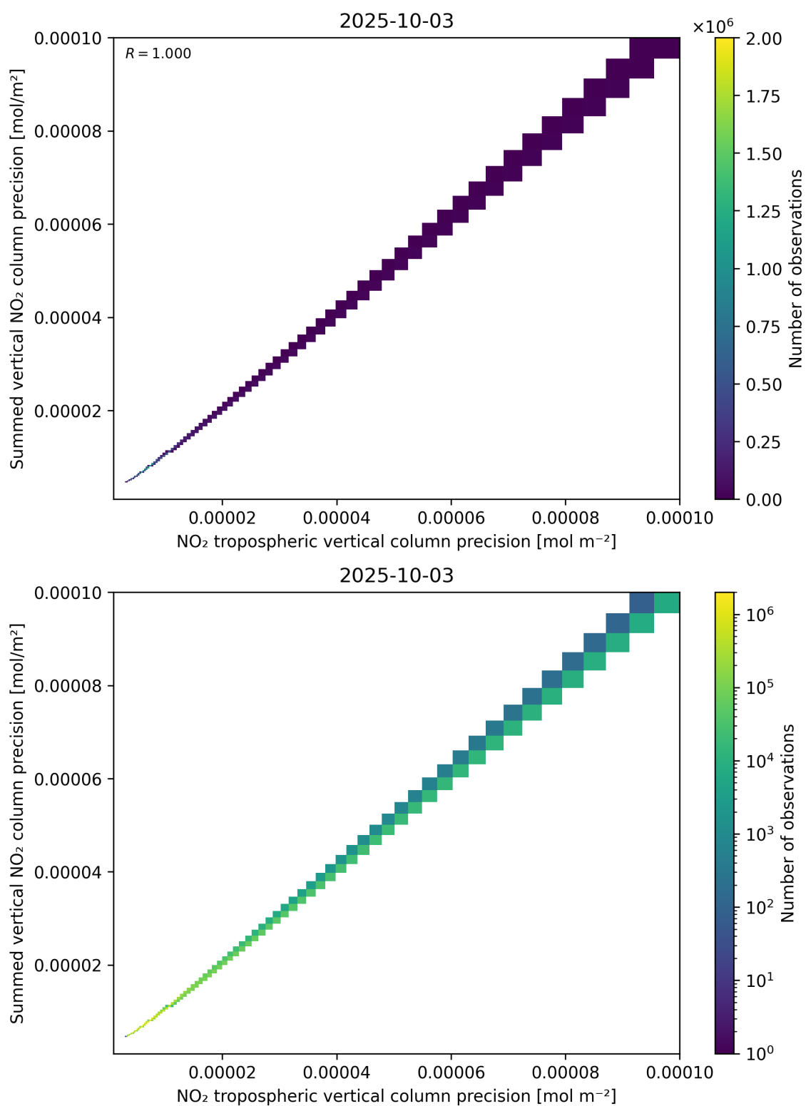
Figure 137: Scatter density plot of “NO 2 tropospheric vertical column precision” against “Summed vertical NO 2 column precision” for 2025-10-02 to 2025-10-04.
