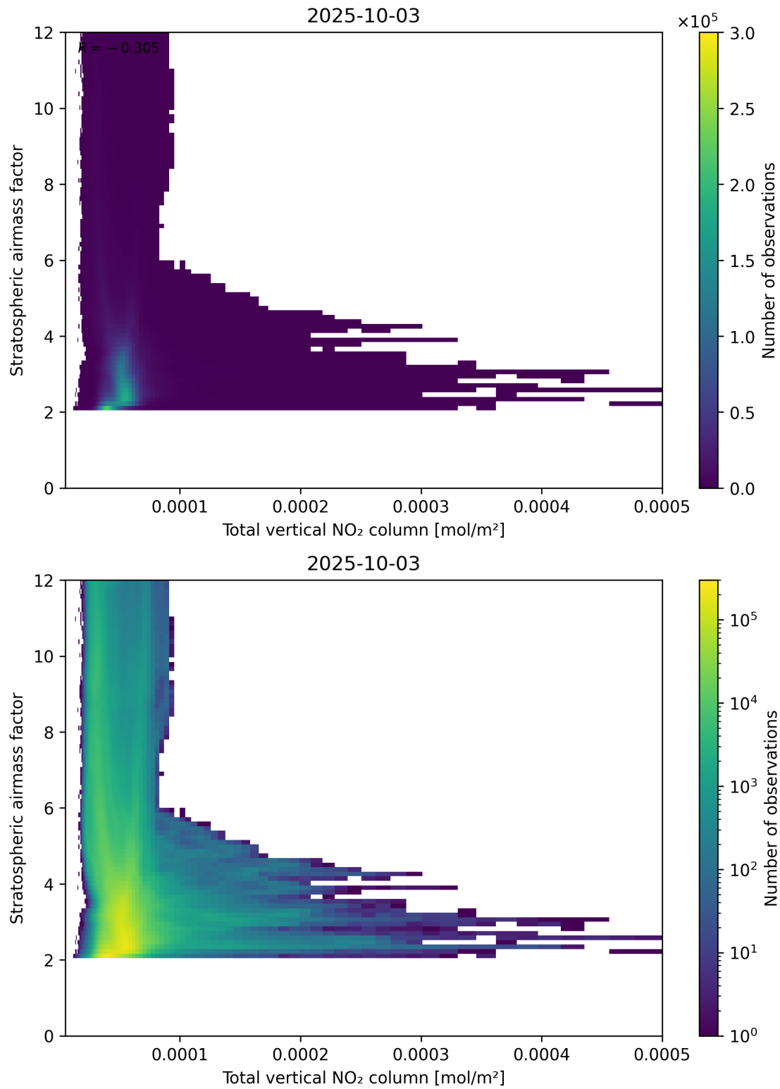
Figure 110: Scatter density plot of “Total vertical NO 2 column” against “Stratospheric airmass factor” for 2025-10-02 to 2025-10-04.
