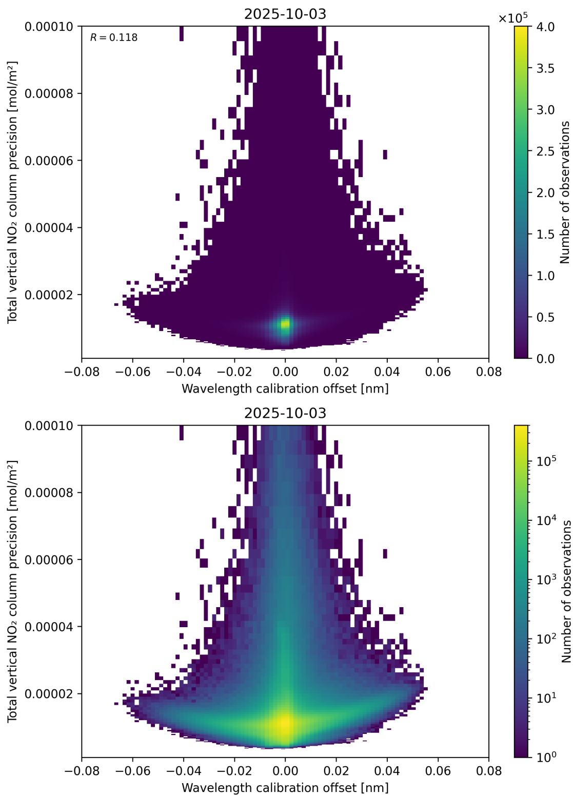
Figure 180: Scatter density plot of “Wavelength calibration offset” against “Total vertical NO 2 column precision” for 2025-10-02 to 2025-10-04.
