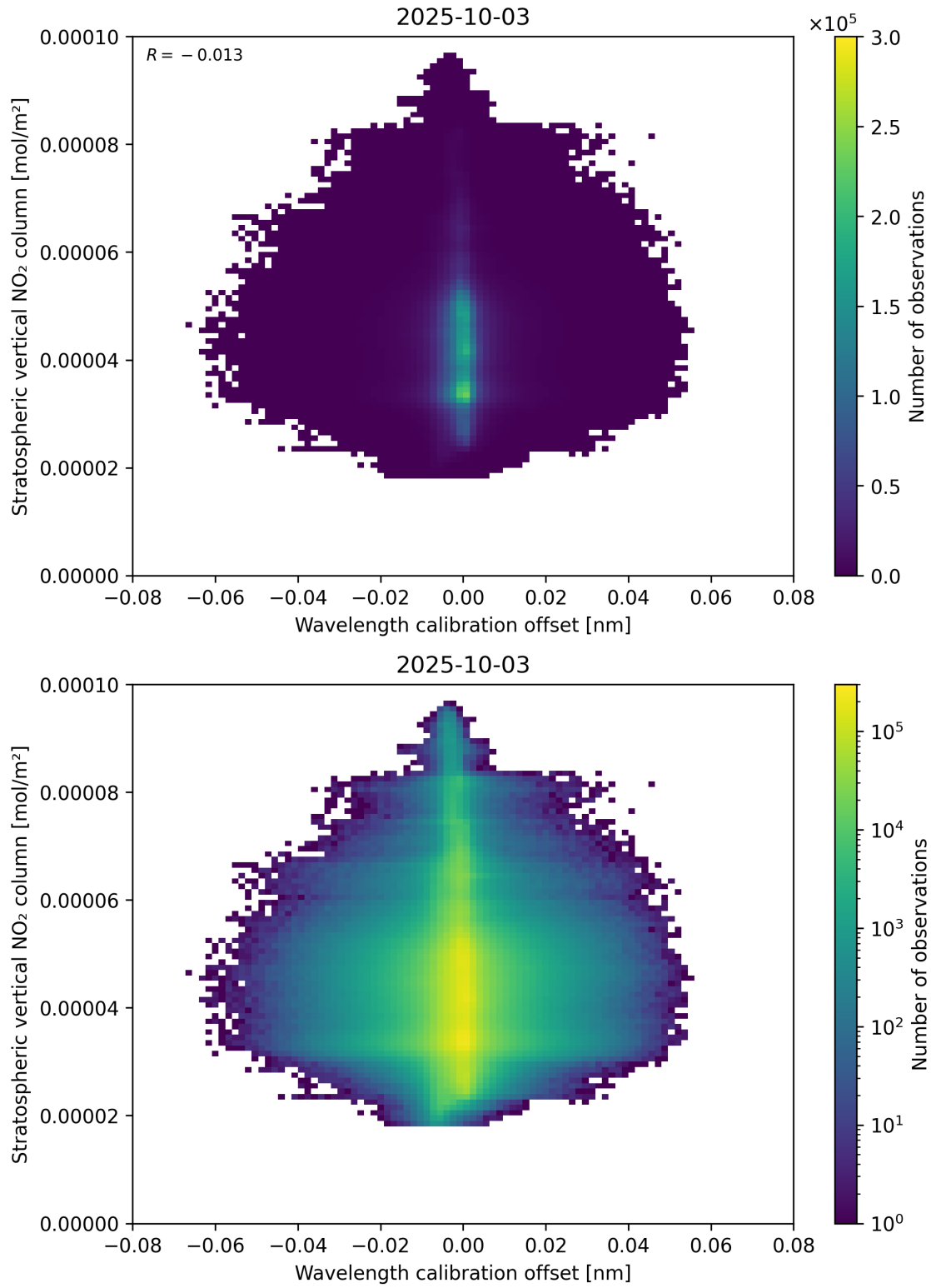
Figure 176: Scatter density plot of “Wavelength calibration offset” against “Stratospheric vertical NO 2 column” for 2025-10-02 to 2025-10-04.
