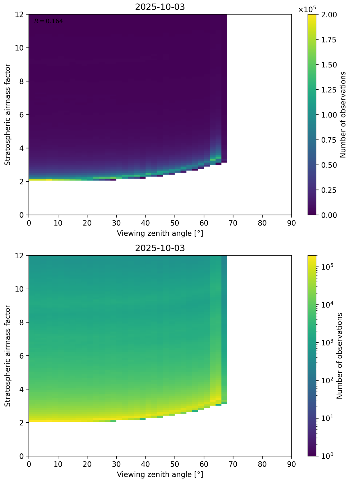
Figure 159: Scatter density plot of “Viewing zenith angle” against “Stratospheric airmass factor” for 2025-10-02 to 2025-10-04.
