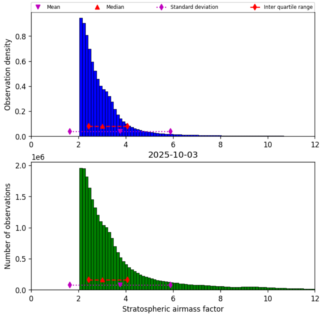
Figure 44: Histogram of “Stratospheric airmass factor” for 2025-10-02 to 2025-10-04
