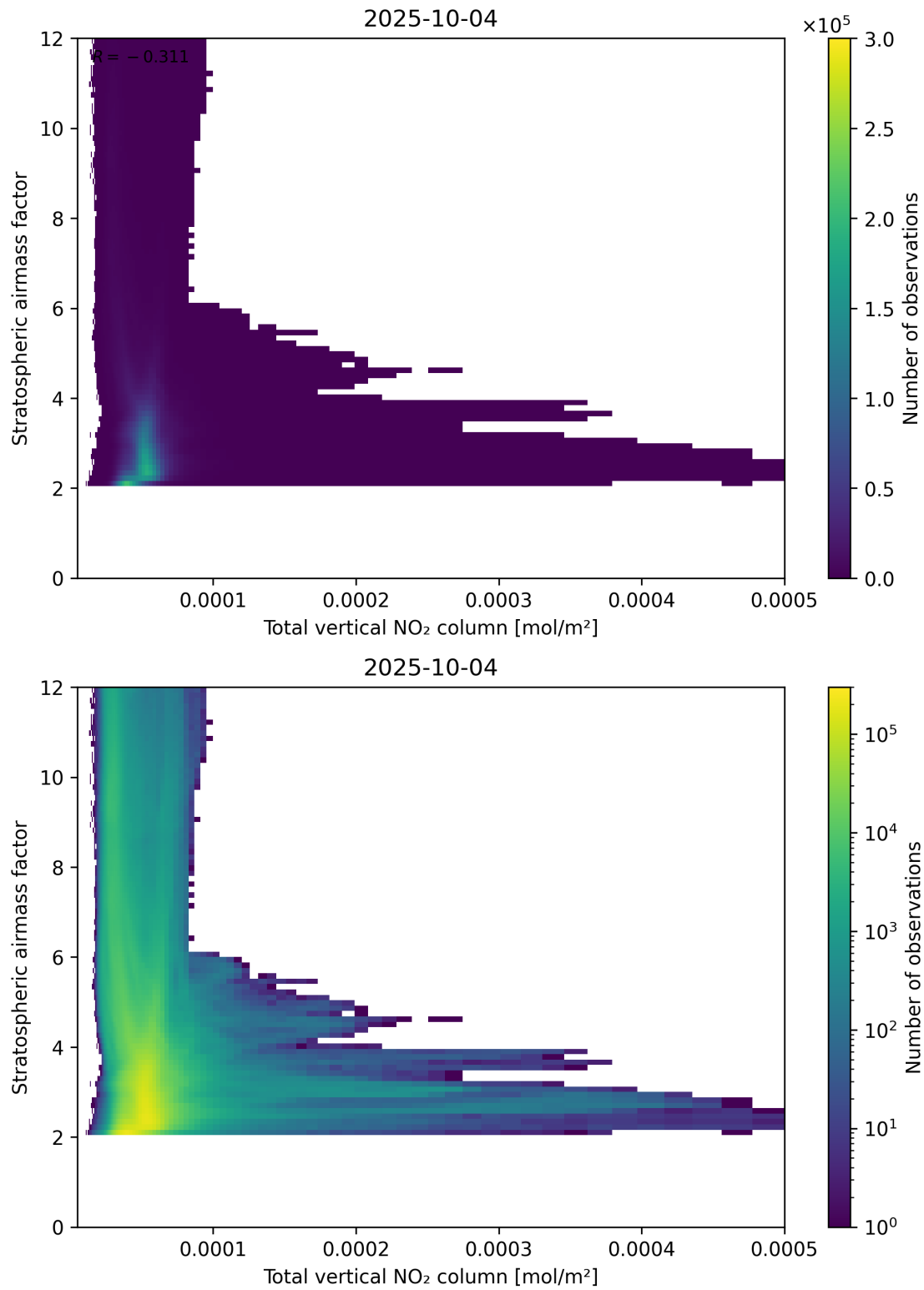
Figure 110: Scatter density plot of “Total vertical NO 2 column” against “Stratospheric airmass factor” for 2025-10-03 to 2025-10-05.
