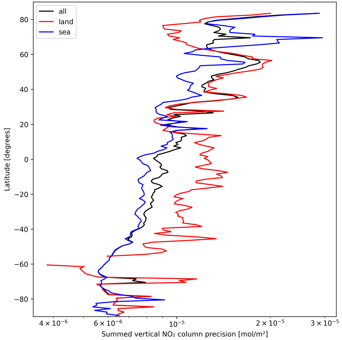
Figure 24: Zonal average of “Summed vertical NO 2 column precision” for 2025-10-03 to 2025-10-05.
