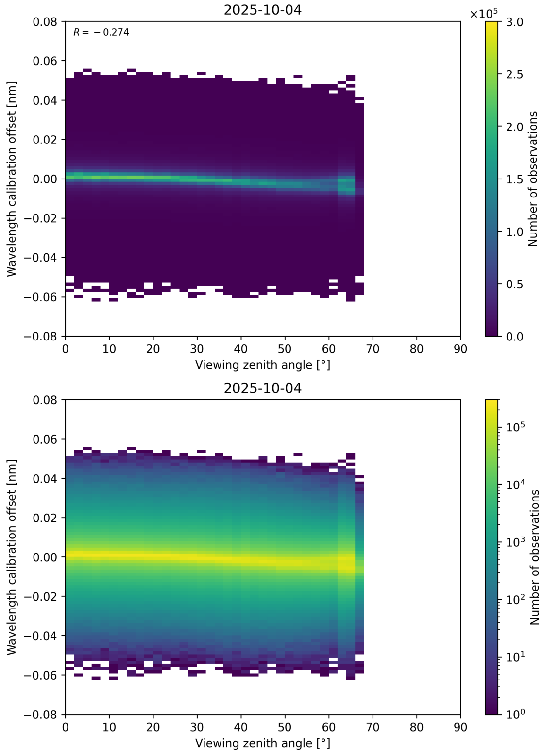
Figure 173: Scatter density plot of “Viewing zenith angle” against “Wavelength calibration offset” for 2025-10-03 to 2025-10-05.
