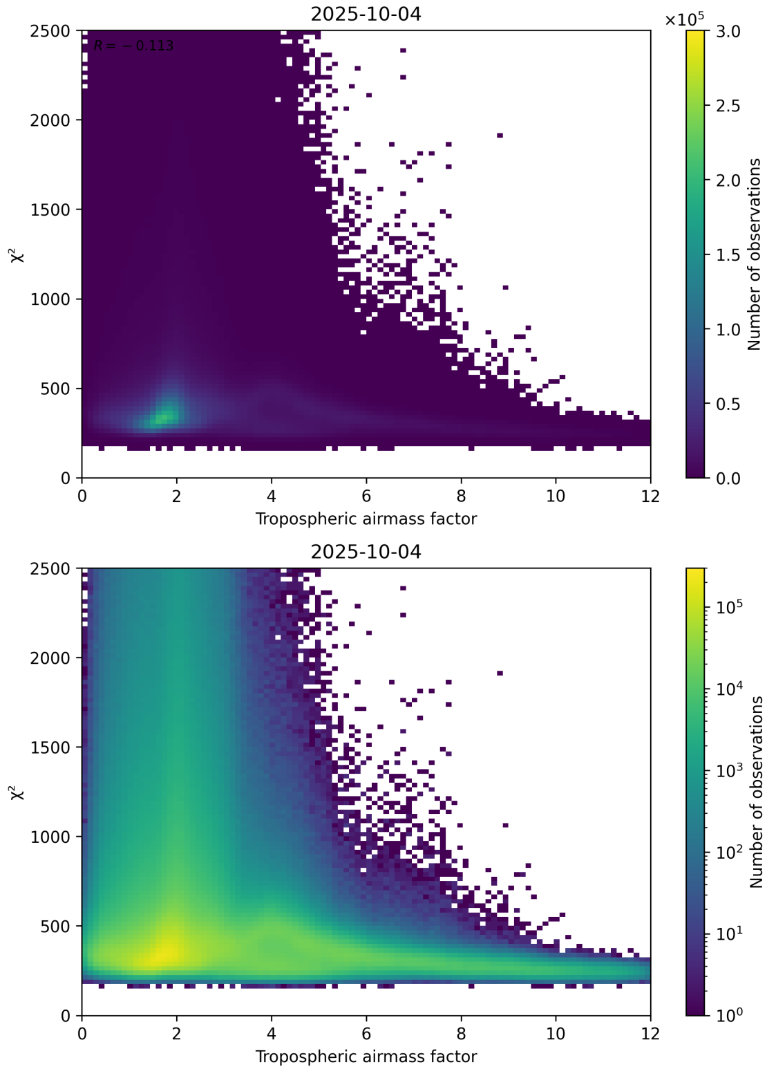
Figure 73: Scatter density plot of “Tropospheric airmass factor” against “ \chi^2 ” for 2025-10-03 to 2025-10-05.
