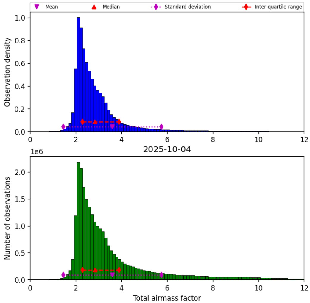
Figure 32: Histogram of “Total airmass factor” for 2025-10-03 to 2025-10-05
