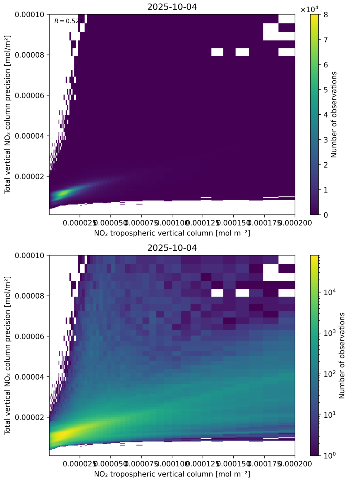
Figure 129: Scatter density plot of “NO 2 tropospheric vertical column” against “Total vertical NO 2 column precision” for 2025-10-03 to 2025-10-05.
