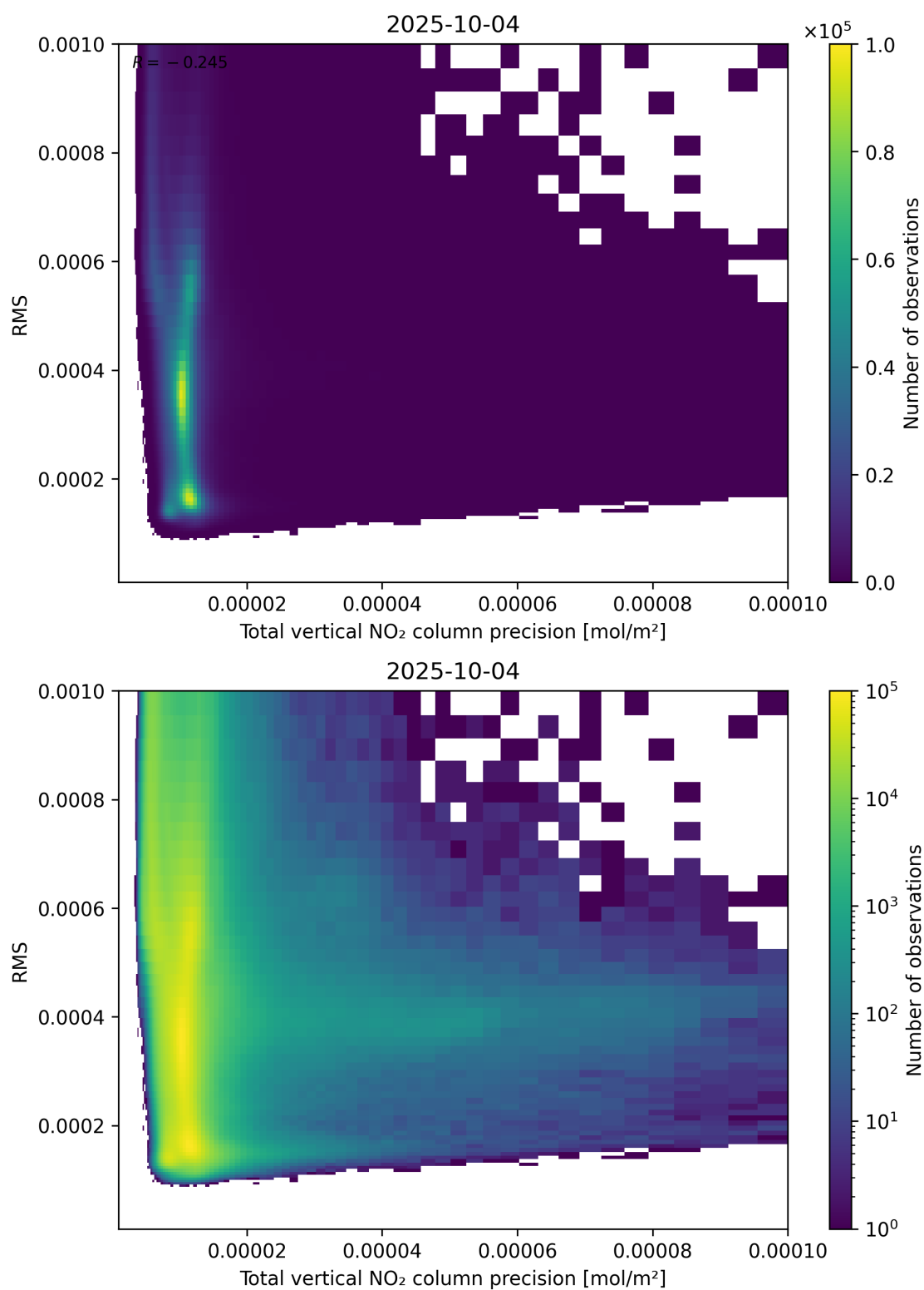
Figure 119: Scatter density plot of “Total vertical NO 2 column precision” against “RMS” for 2025-10-03 to 2025-10-05.
