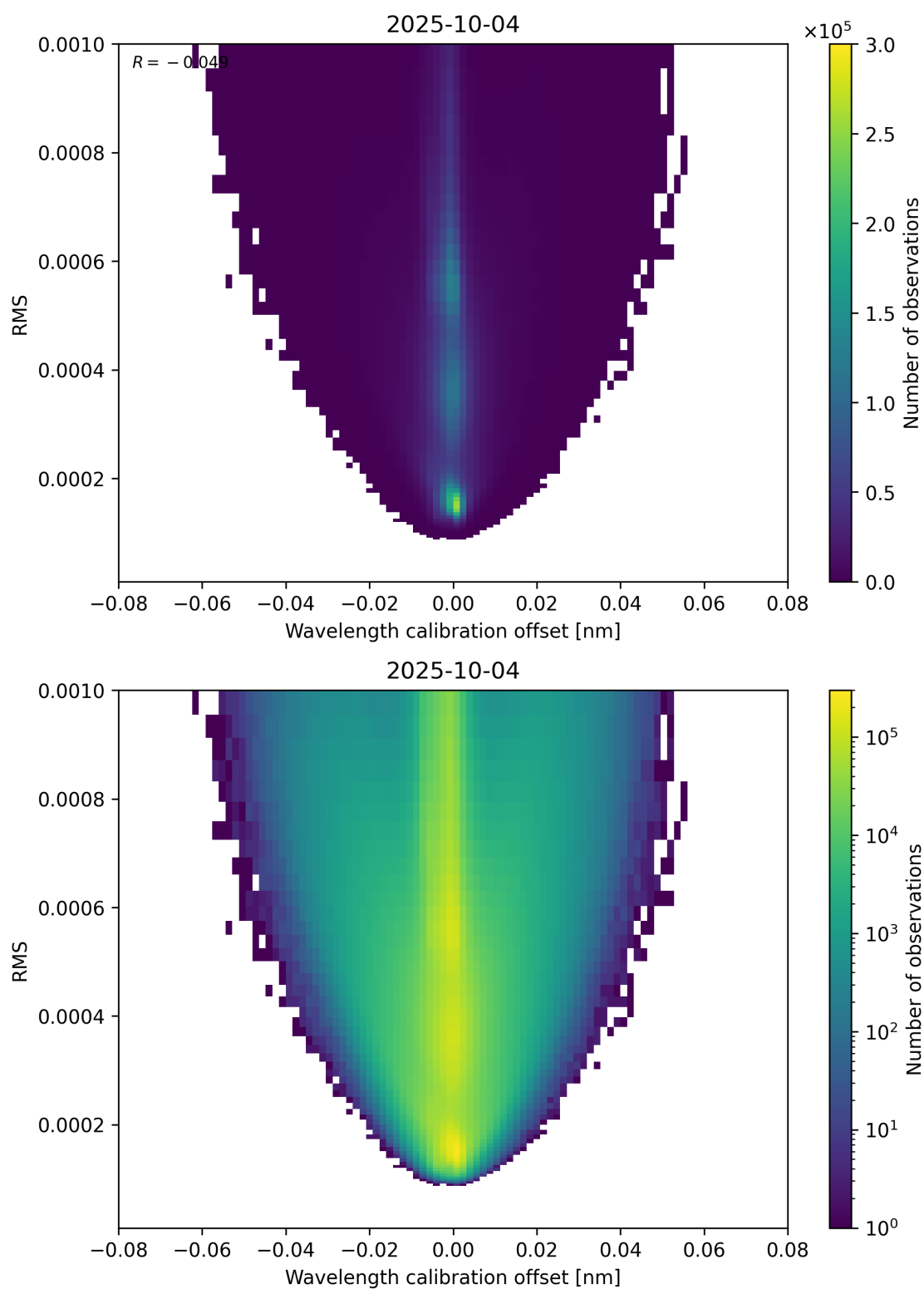
Figure 181: Scatter density plot of “Wavelength calibration offset” against “RMS” for 2025-10-03 to 2025-10-05.
