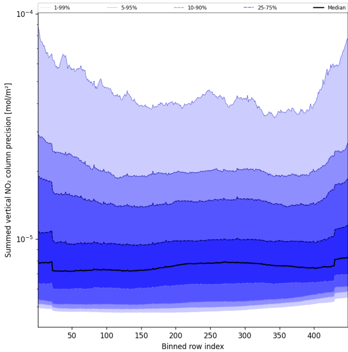
Figure 58: Along track statistics of “Summed vertical NO 2 column precision” for 2025-10-03 to 2025-10-05
