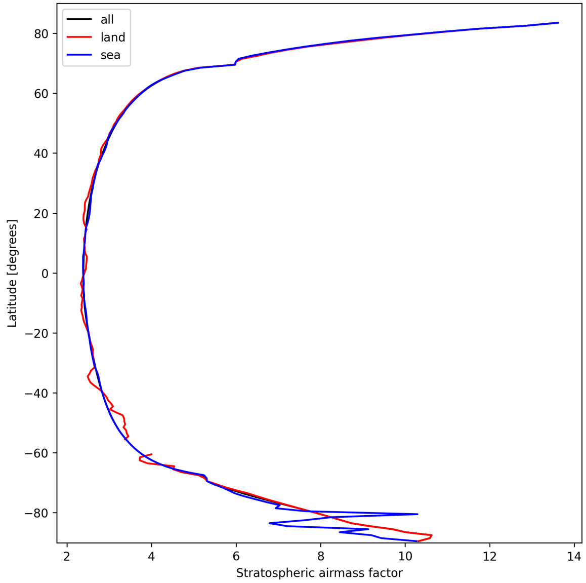
Figure 27: Zonal average of “Stratospheric air mass factor” for 2025-10-03 to 2025-10-05.
