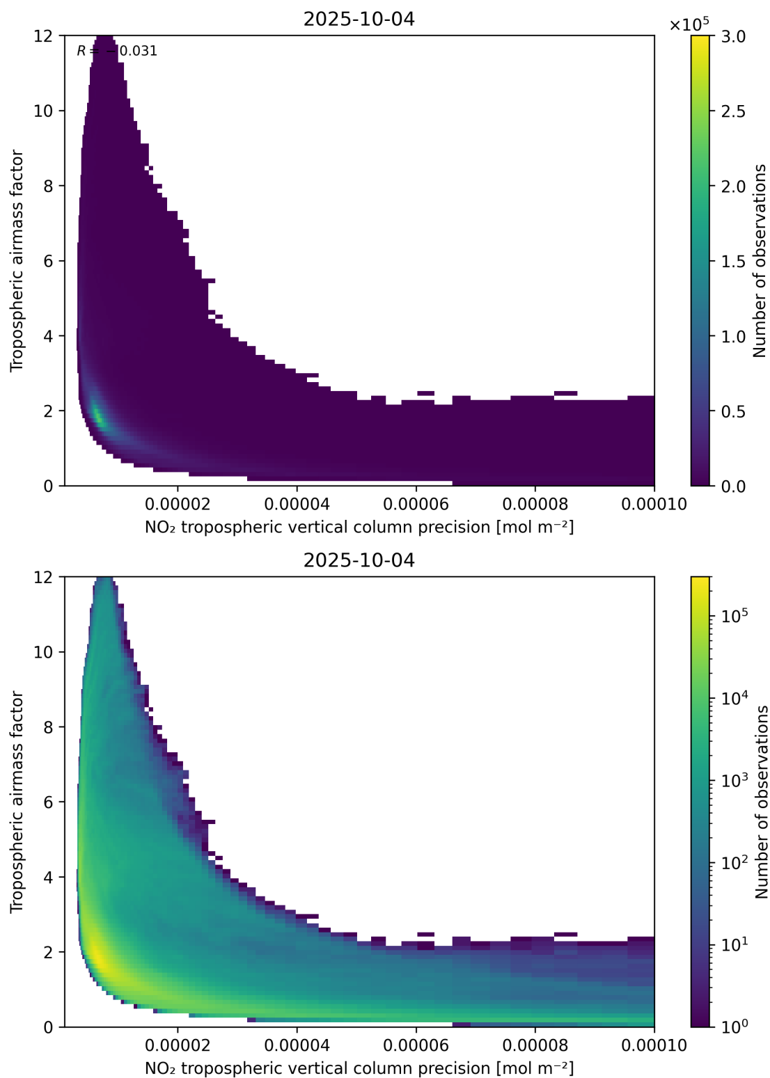
Figure 133: Scatter density plot of “NO 2 tropospheric vertical column precision” against “Tropospheric air mass factor” for 2025-10-03 to 2025-10-05.
