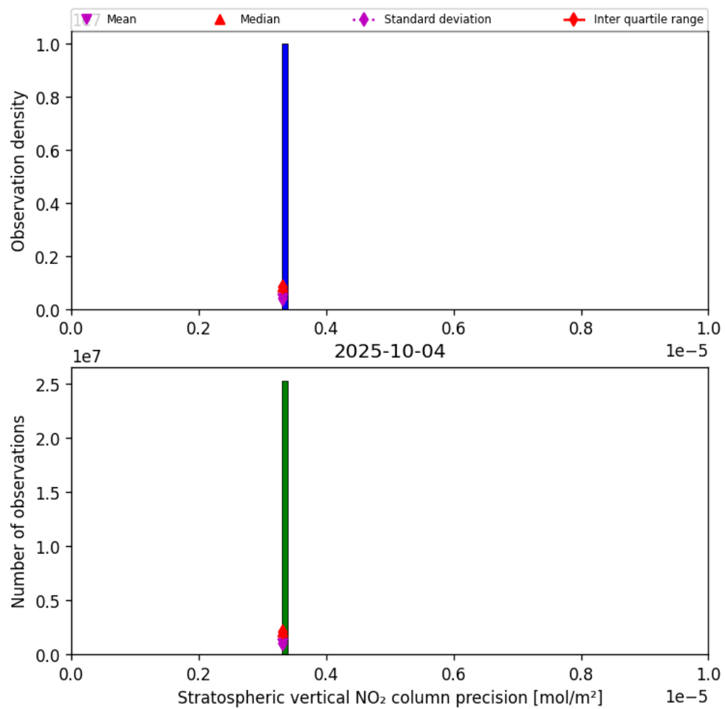
Figure 37: Histogram of “Stratospheric vertical NO 2 column precision” for 2025-10-03 to 2025-10-05
