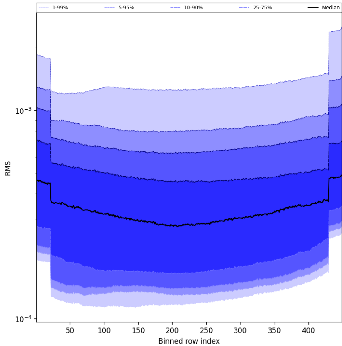
Figure 60: Along track statistics of “RMS” for 2025-10-03 to 2025-10-05
