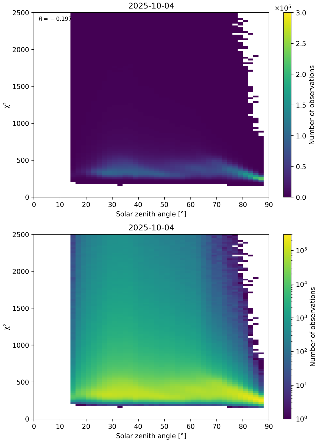
Figure 148: Scatter density plot of “Solar zenith angle” against “ \chi^2 ” for 2025-10-03 to 2025-10-05.
