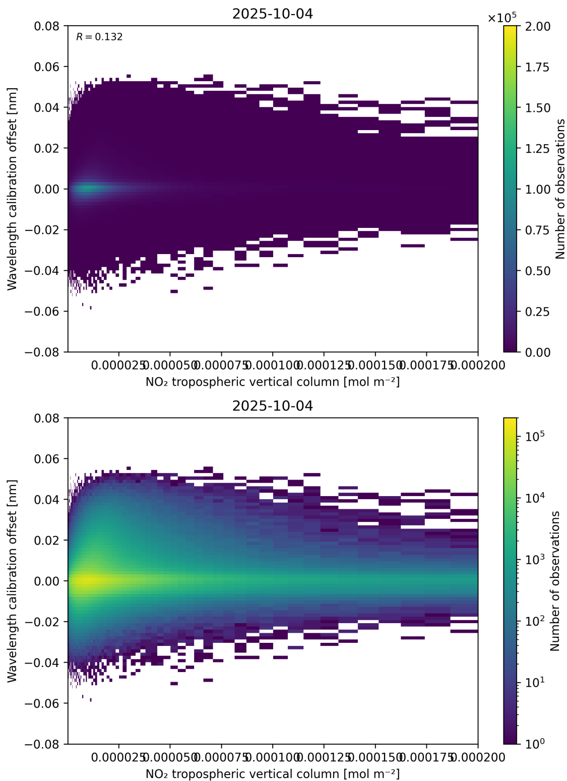
Figure 143: Scatter density plot of “NO 2 tropospheric vertical column” against “Wavelength calibration offset” for 2025-10-03 to 2025-10-05.
