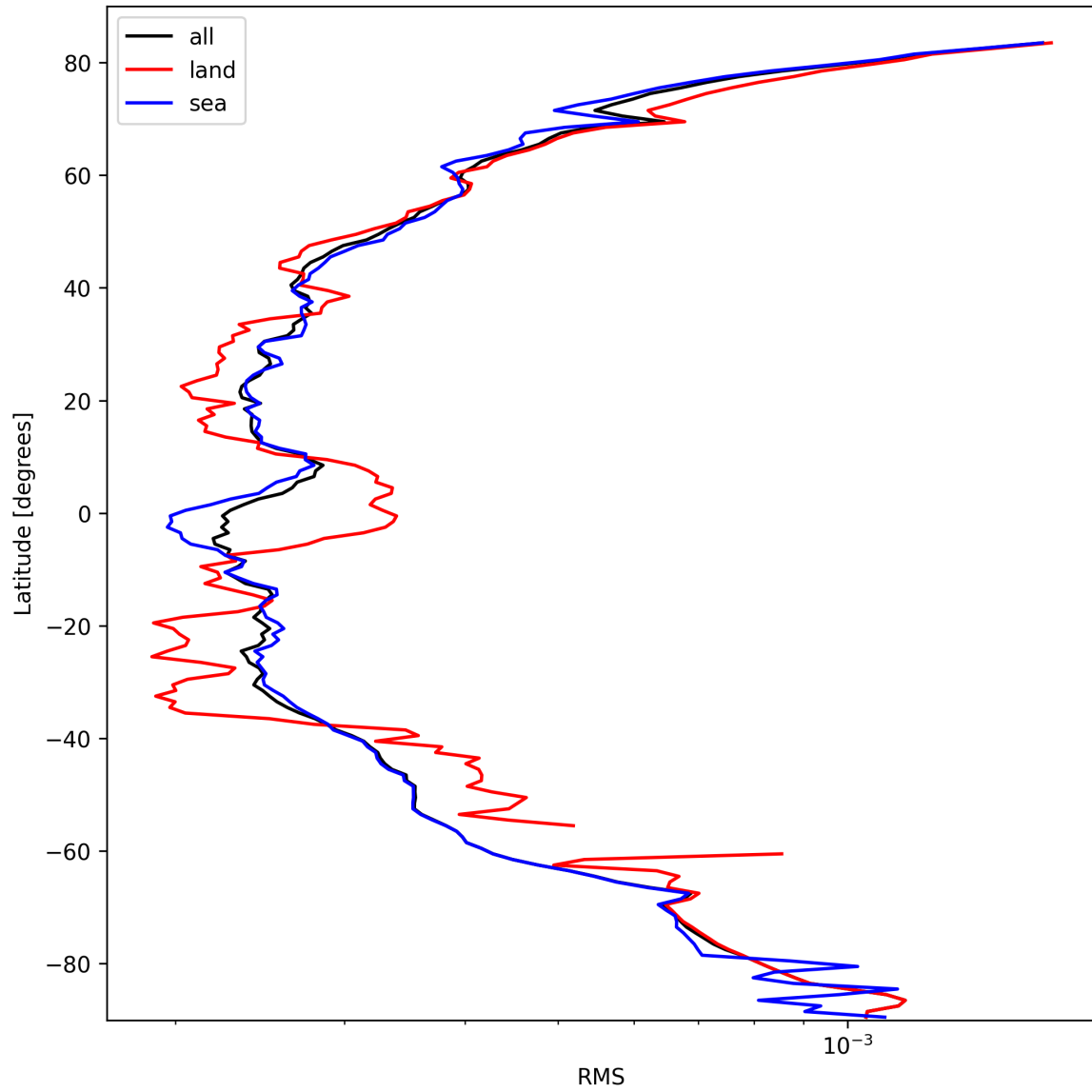
Figure 26: Zonal average of “RMS” for 2025-10-03 to 2025-10-05.
