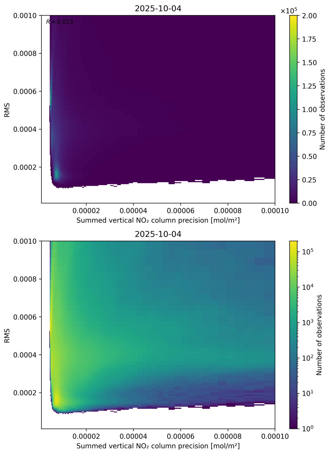
Figure 108: Scatter density plot of “Summed vertical NO 2 column precision” against “RMS” for 2025-10-03 to 2025-10-05.
