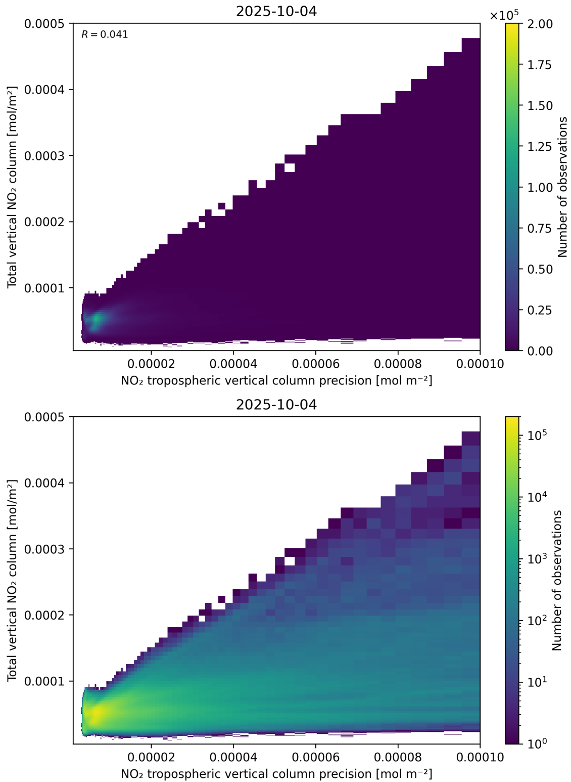
Figure 138: Scatter density plot of “NO 2 tropospheric vertical column precision” against “Total vertical NO 2 column” for 2025-10-03 to 2025-10-05.
