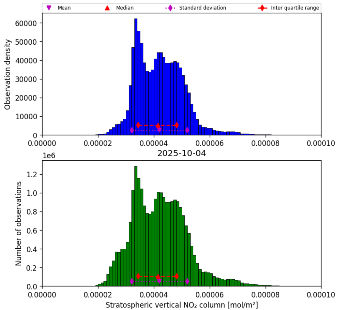
Figure 36: Histogram of “Stratospheric vertical NO 2 column” for 2025-10-03 to 2025-10-05
