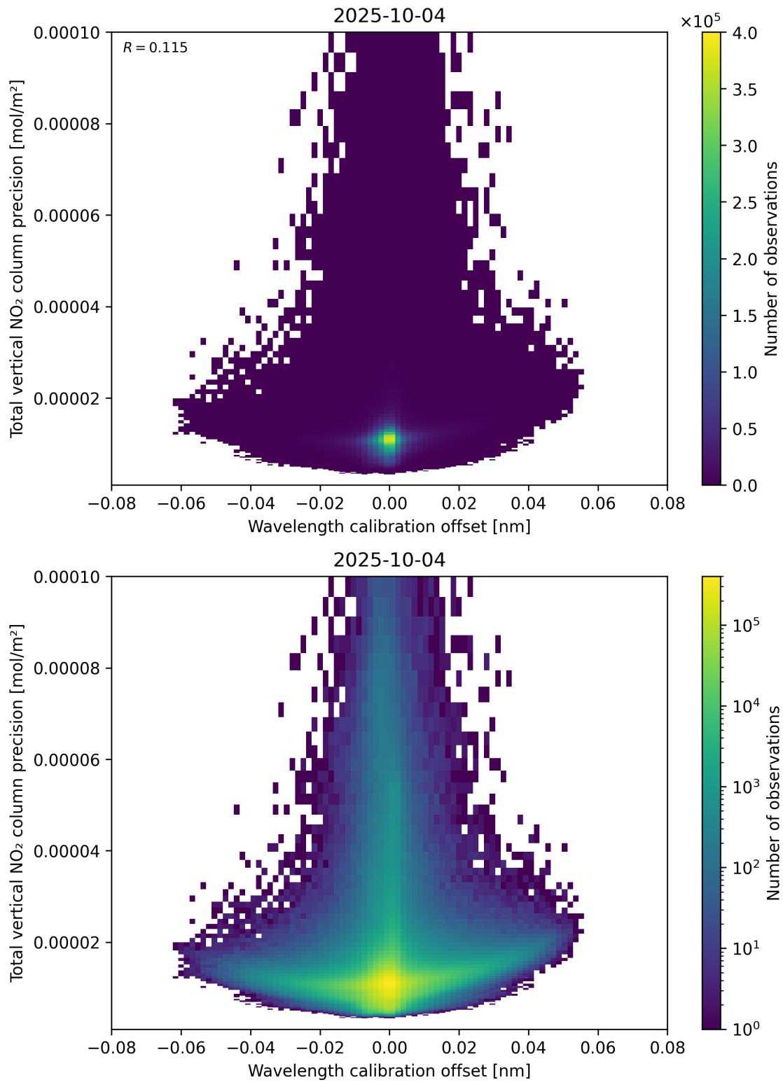
Figure 180: Scatter density plot of “Wavelength calibration offset” against “Total vertical NO 2 column precision” for 2025-10-03 to 2025-10-05.
