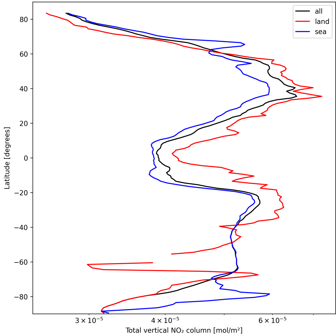
Figure 21: Zonal average of “Total vertical NO 2 column” for 2025-10-03 to 2025-10-05.
