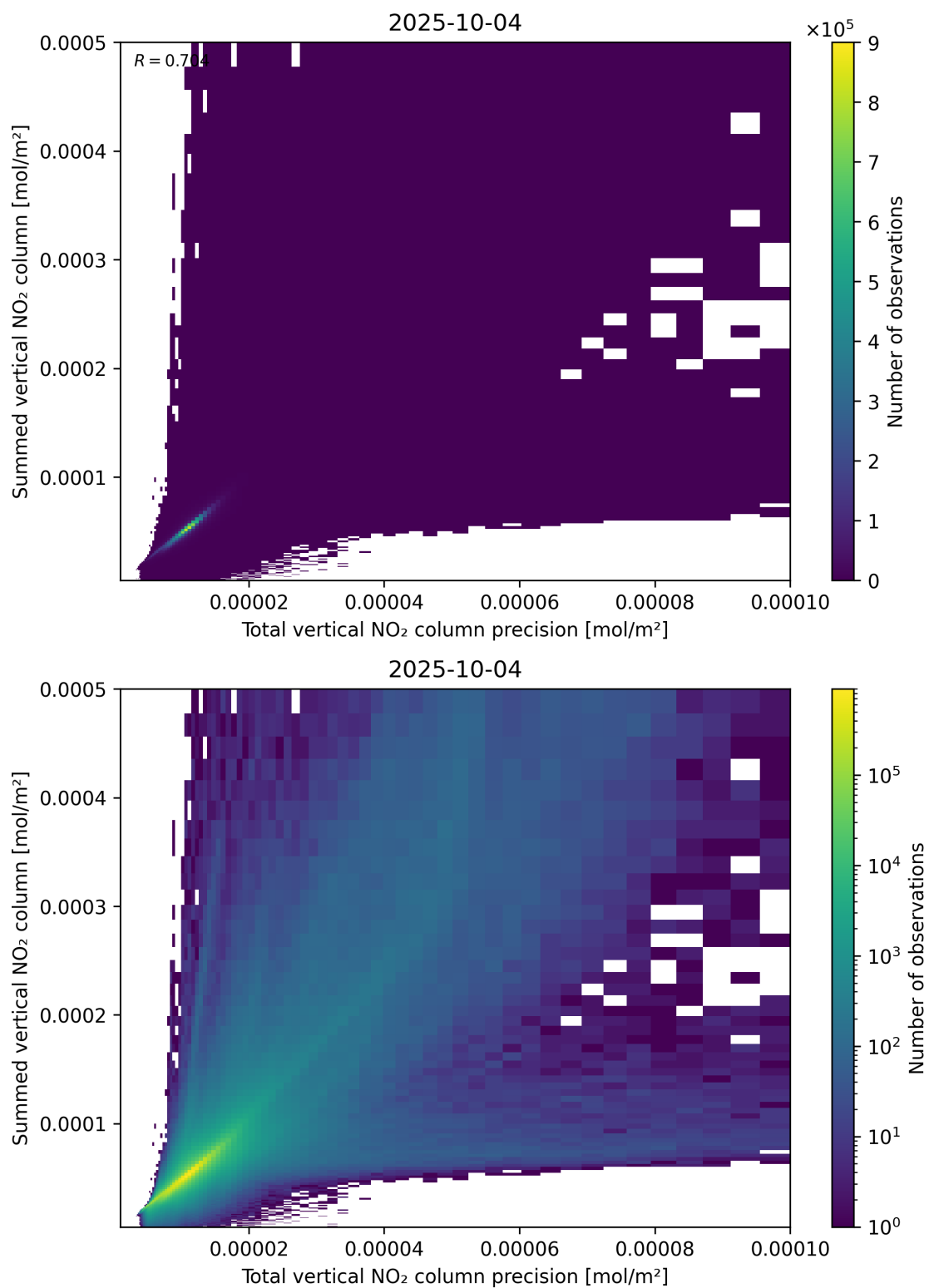
Figure 117: Scatter density plot of “Total vertical NO 2 column precision” against “Summed vertical NO 2 column” for 2025-10-03 to 2025-10-05.
