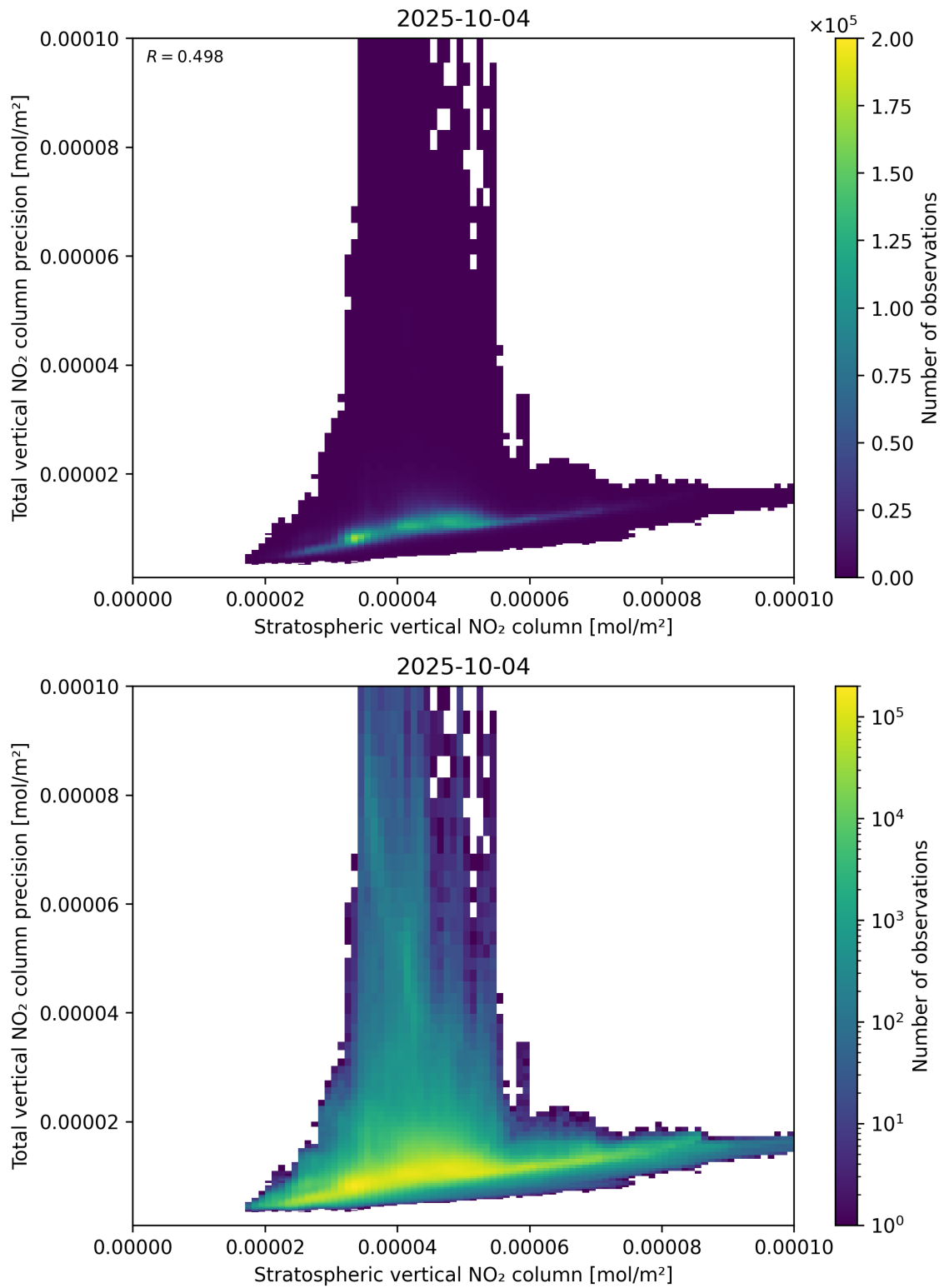
Figure 101: Scatter density plot of “Stratospheric vertical NO 2 column” against “Total vertical NO 2 column precision” for 2025-10-03 to 2025-10-05.
