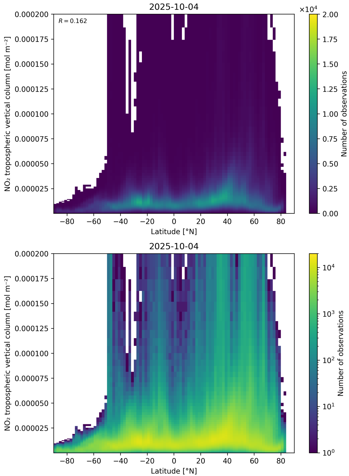
Figure 92: Scatter density plot of “Latitude” against “NO 2 tropospheric vertical column” for 2025-10-03 to 2025-10-05.
