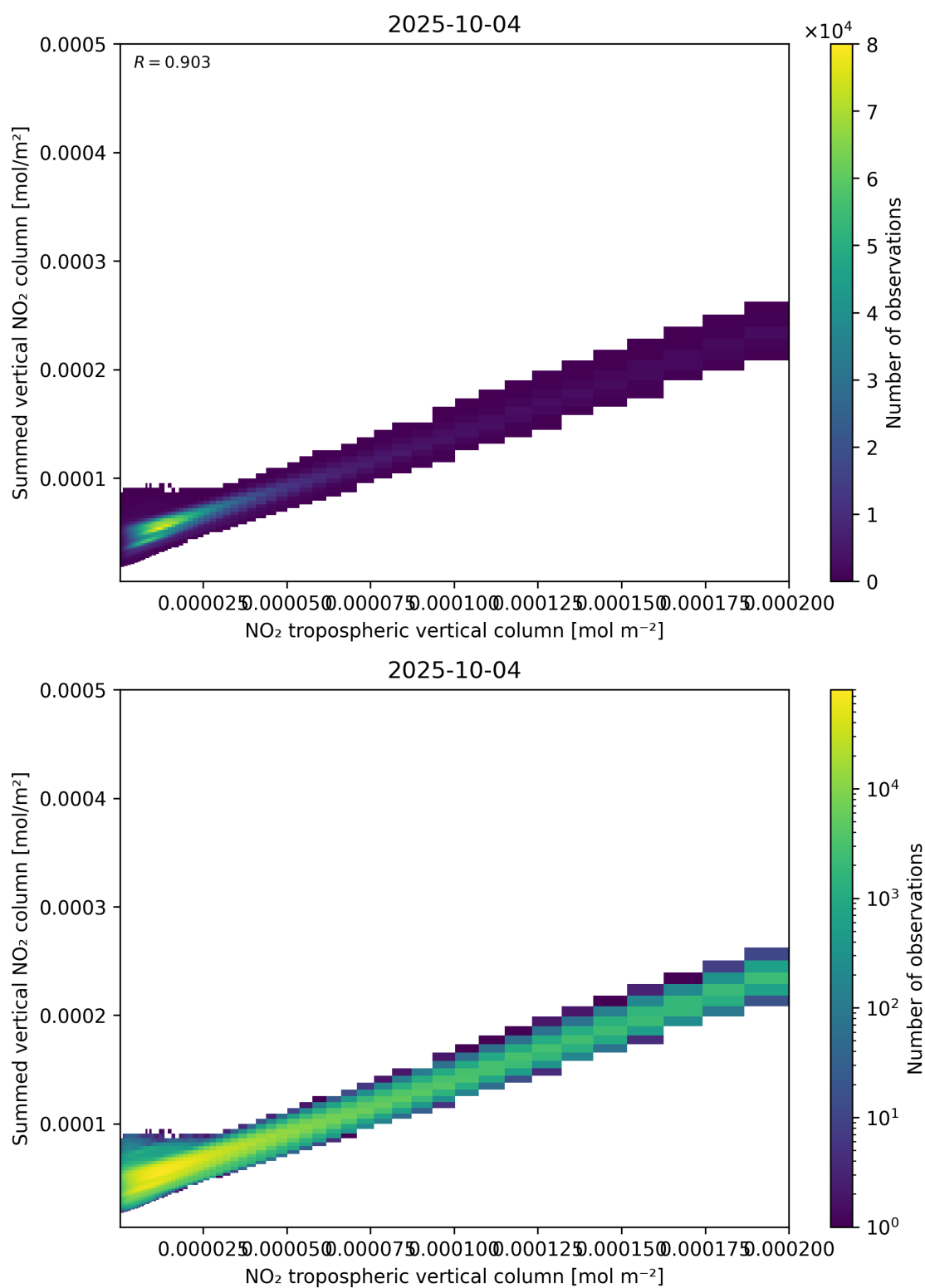
Figure 126: Scatter density plot of “NO 2 tropospheric vertical column” against “Summed vertical NO 2 column” for 2025-10-03 to 2025-10-05.
