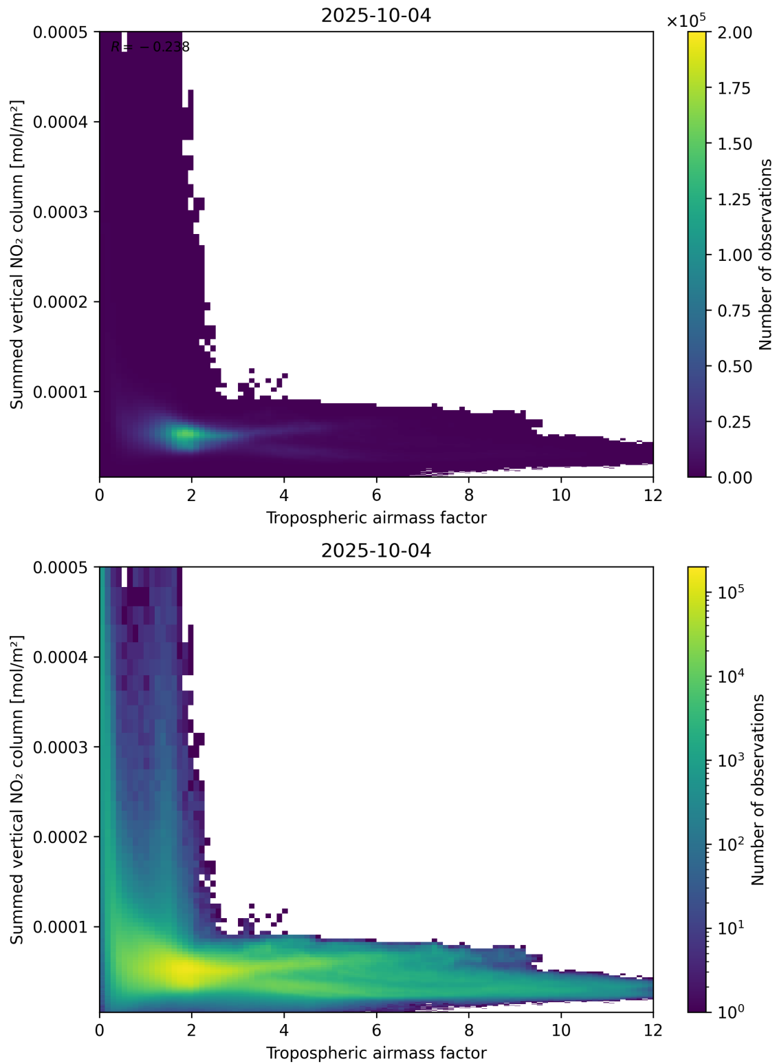
Figure 75: Scatter density plot of “Tropospheric air mass factor” against “Summed vertical NO 2 column” for 2025-10-03 to 2025-10-05.
