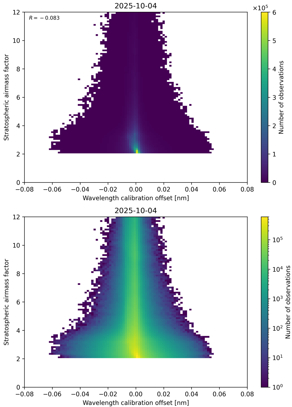
Figure 174: Scatter density plot of “Wavelength calibration offset” against “Stratospheric airmass factor” for 2025-10-03 to 2025-10-05.
