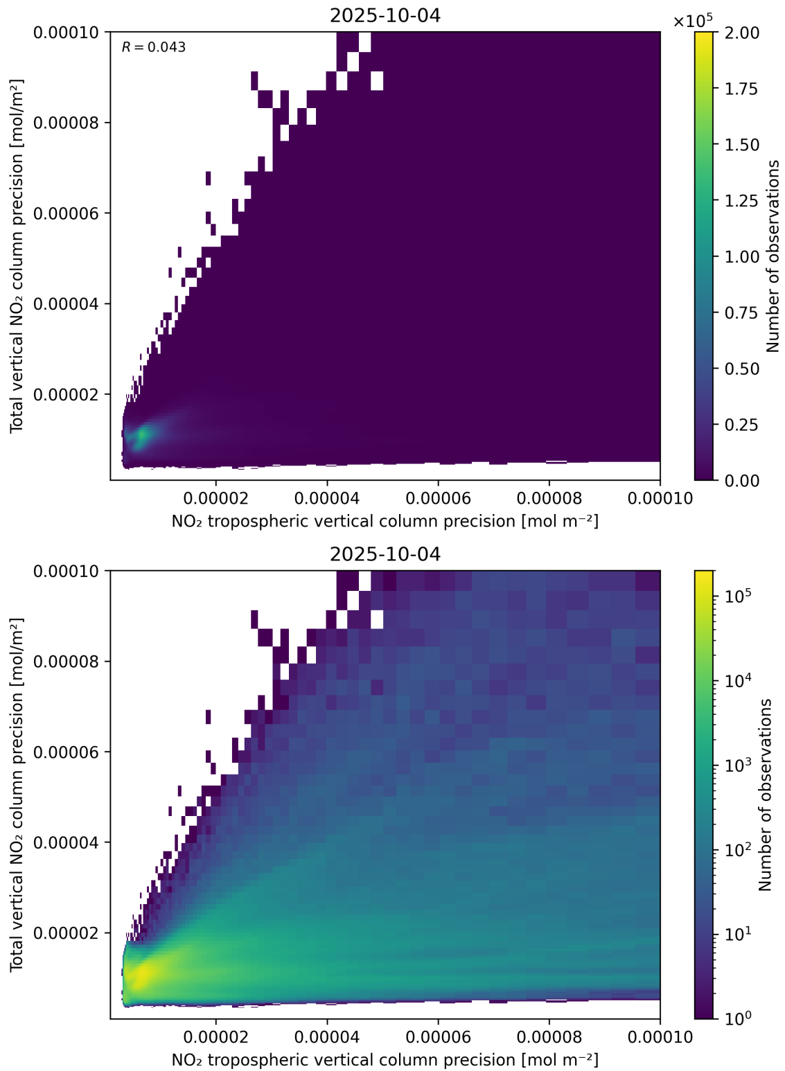
Figure 139: Scatter density plot of “NO 2 tropospheric vertical column precision” against “Total vertical NO 2 column precision” for 2025-10-03 to 2025-10-05.
