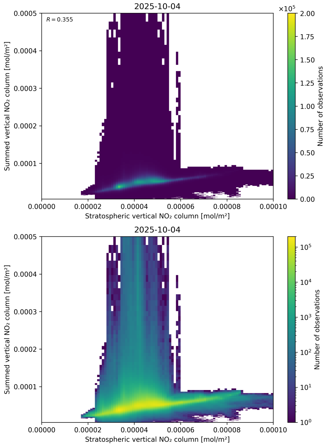
Figure 98: Scatter density plot of “Stratospheric vertical NO 2 column” against “Summed vertical NO 2 column” for 2025-10-03 to 2025-10-05.
