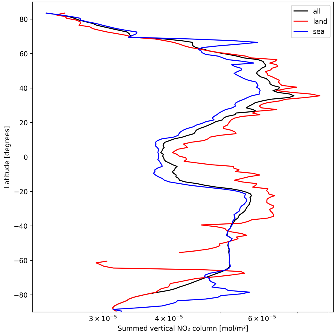
Figure 23: Zonal average of “Summed vertical NO 2 column” for 2025-10-03 to 2025-10-05.
