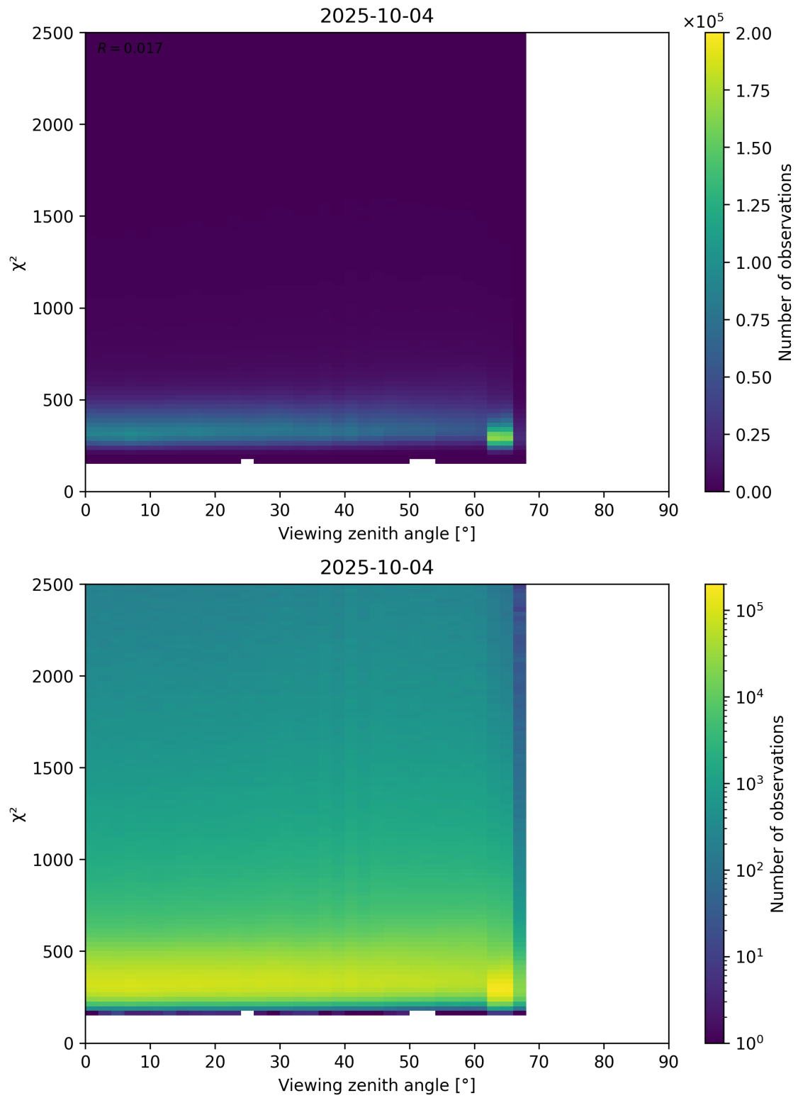
Figure 162: Scatter density plot of “Viewing zenith angle” against “ \chi^2 ” for 2025-10-03 to 2025-10-05.
