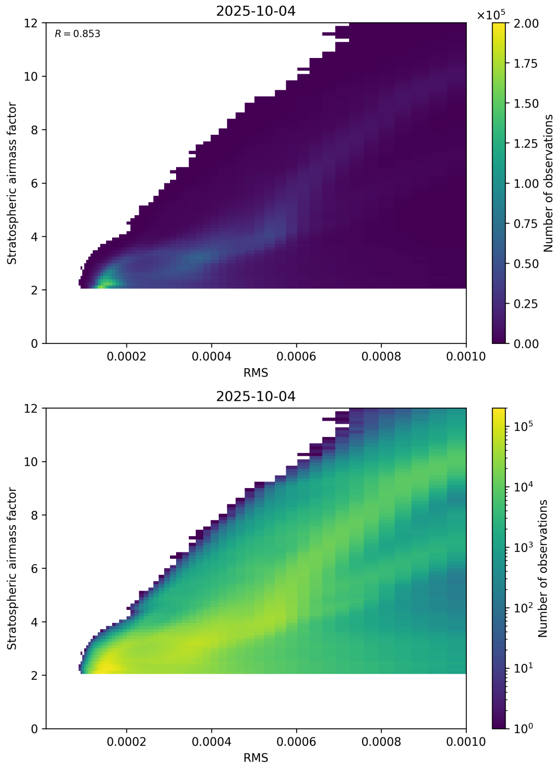
Figure 144: Scatter density plot of “RMS” against “Stratospheric airmass factor” for 2025-10-03 to 2025-10-05.
