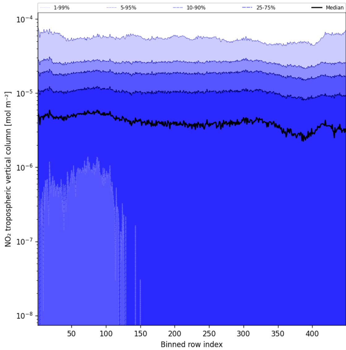
Figure 46: Along track statistics of “NO 2 tropospheric vertical column” for 2025-10-03 to 2025-10-05
