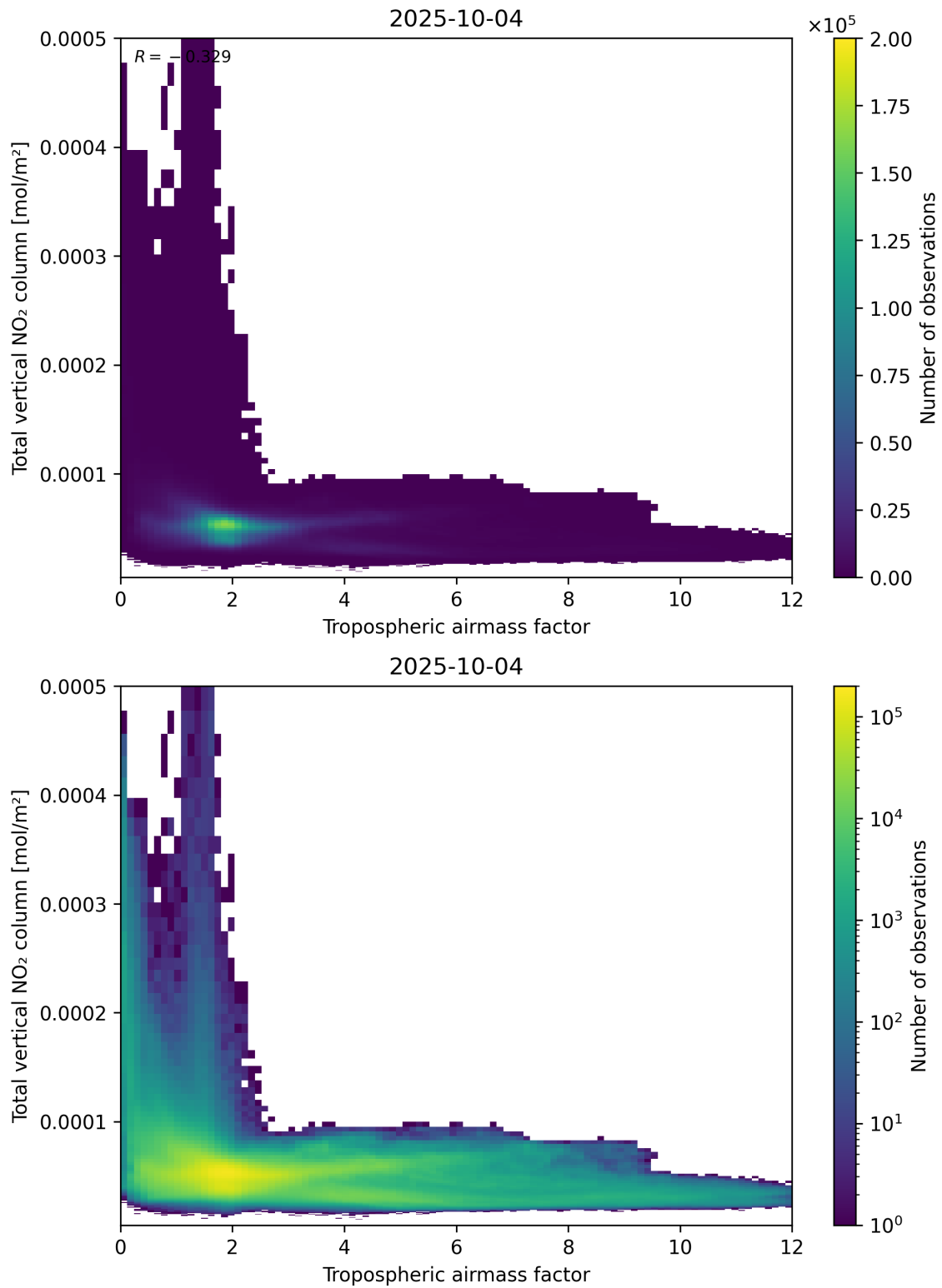
Figure 77: Scatter density plot of “Tropospheric airmass factor” against “Total vertical NO 2 column” for 2025-10-03 to 2025-10-05.
