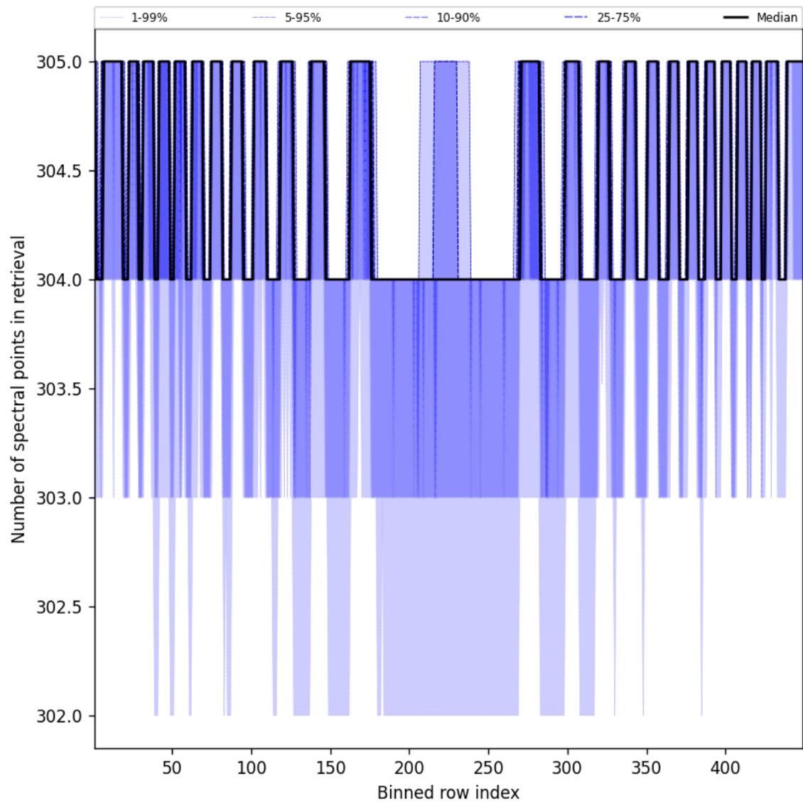
Figure 50: Along track statistics of “Number of spectral points in retrieval” for 2025-10-03 to 2025-10-05
