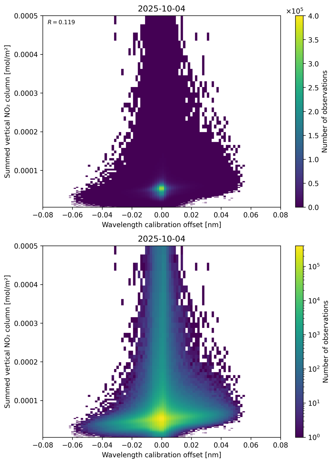
Figure 177: Scatter density plot of “Wavelength calibration offset” against “Summed vertical NO 2 column” for 2025-10-03 to 2025-10-05.
