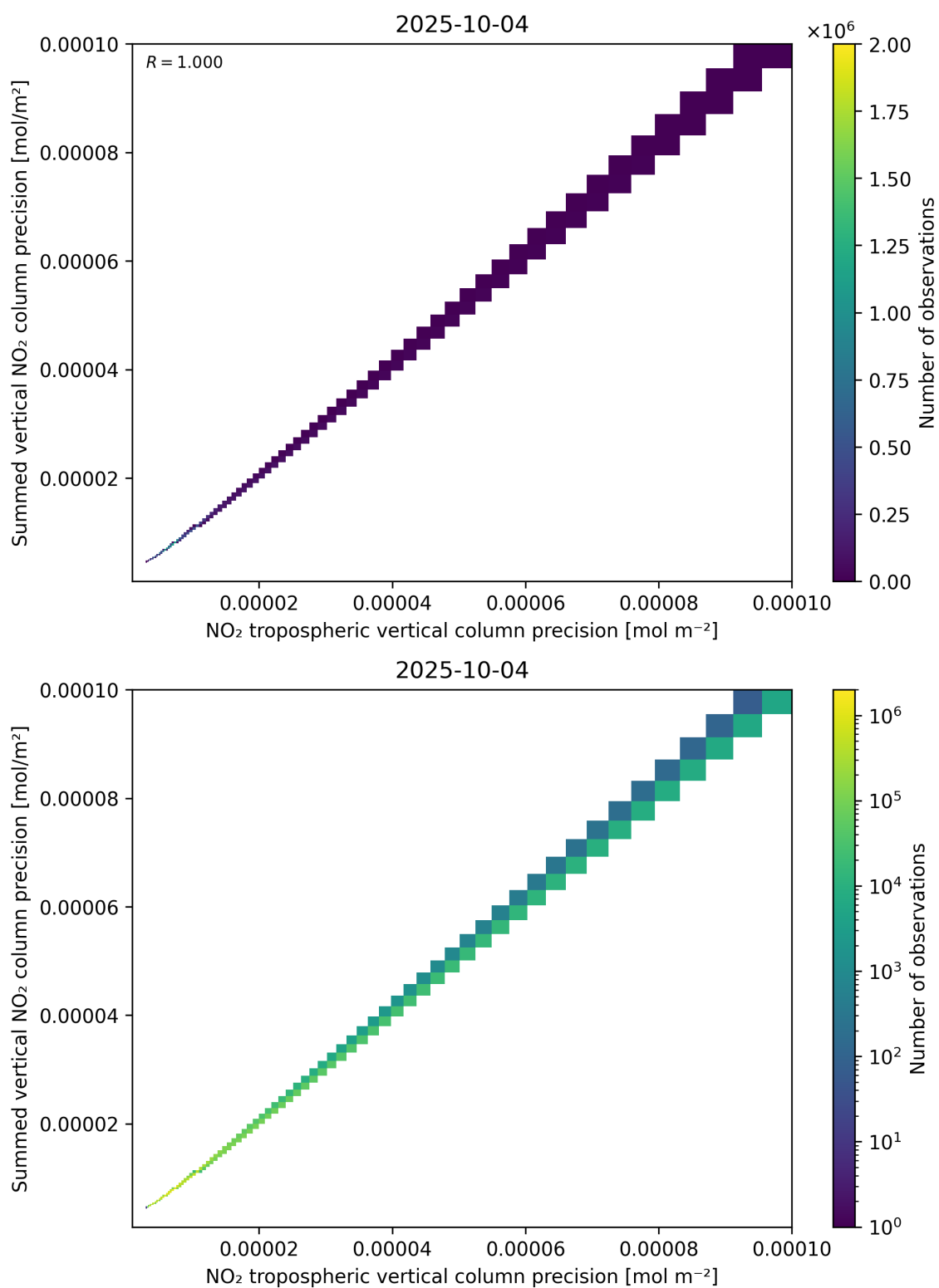
Figure 137: Scatter density plot of “NO 2 tropospheric vertical column precision” against “Summed vertical NO 2 column precision” for 2025-10-03 to 2025-10-05.
