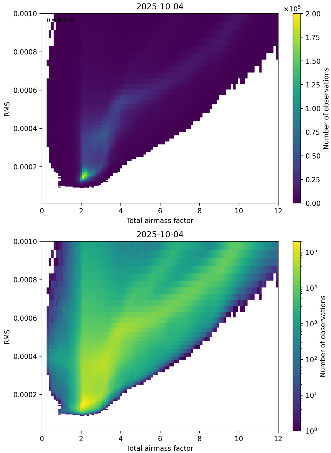
Figure 69: Scatter density plot of “Total airmass factor” against “RMS” for 2025-10-03 to 2025-10-05.
