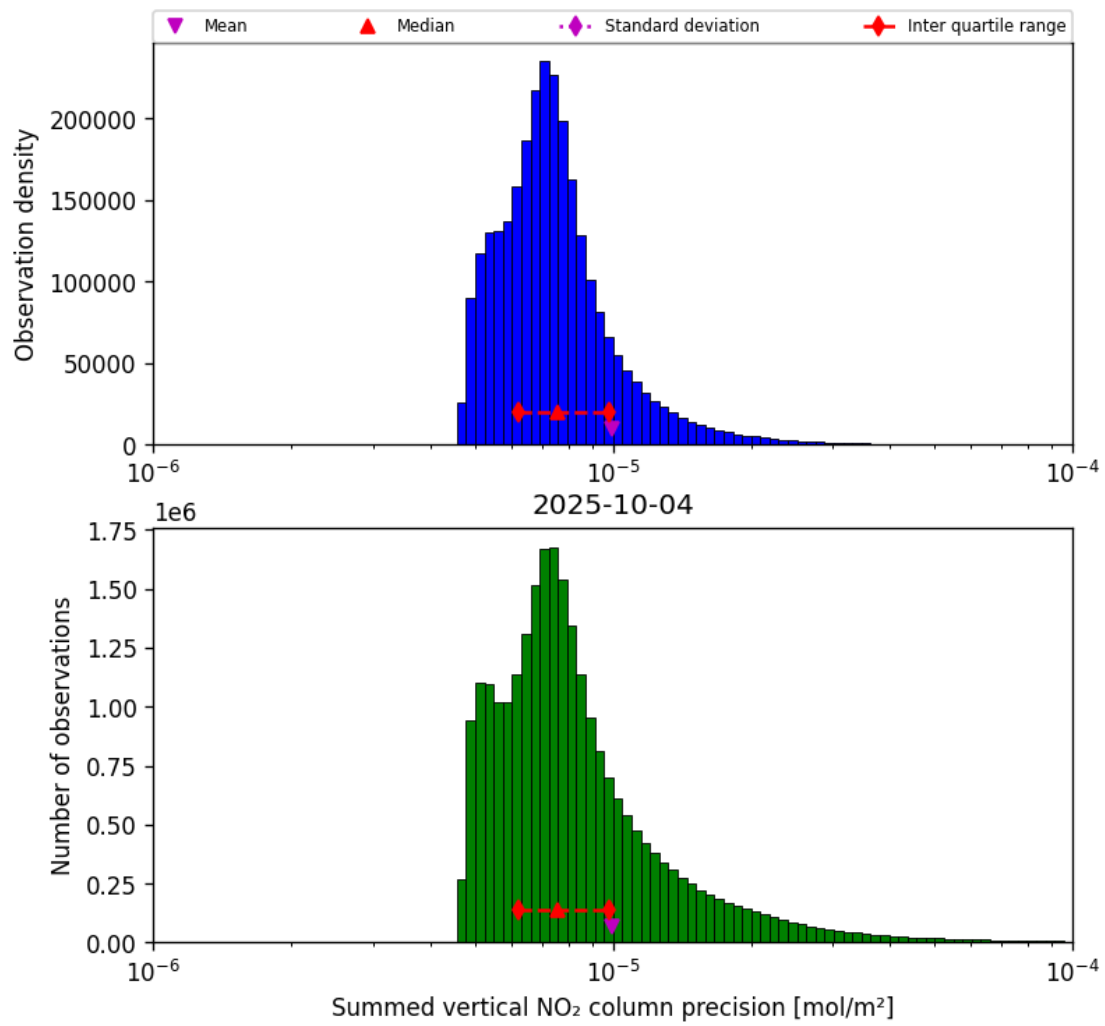
Figure 41: Histogram of "Summed vertical NO 2 column precision" for 2025-10-03 to 2025-10-05
