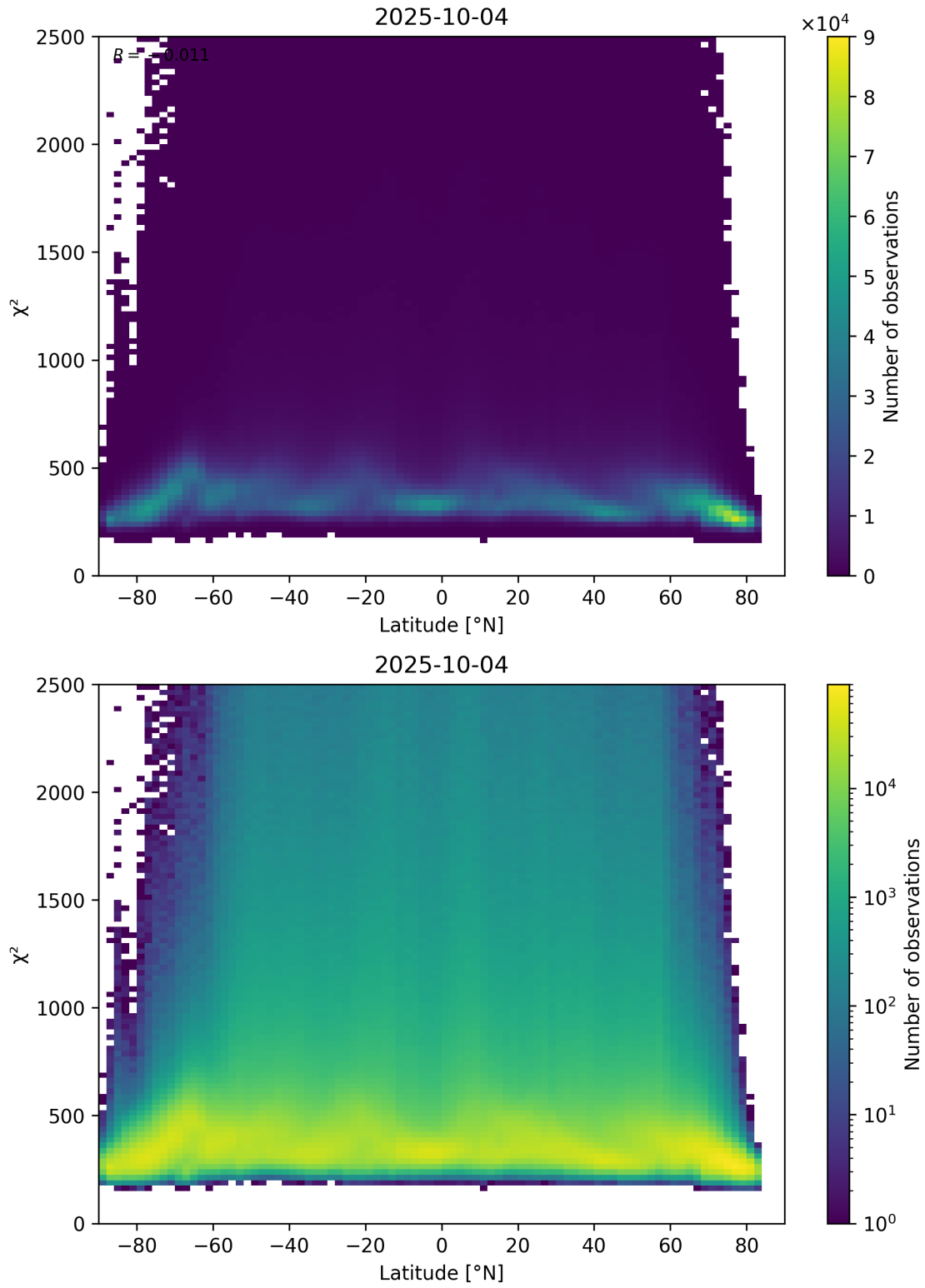
Figure 86: Scatter density plot of “Latitude” against “ \chi^2 ” for 2025-10-03 to 2025-10-05.
