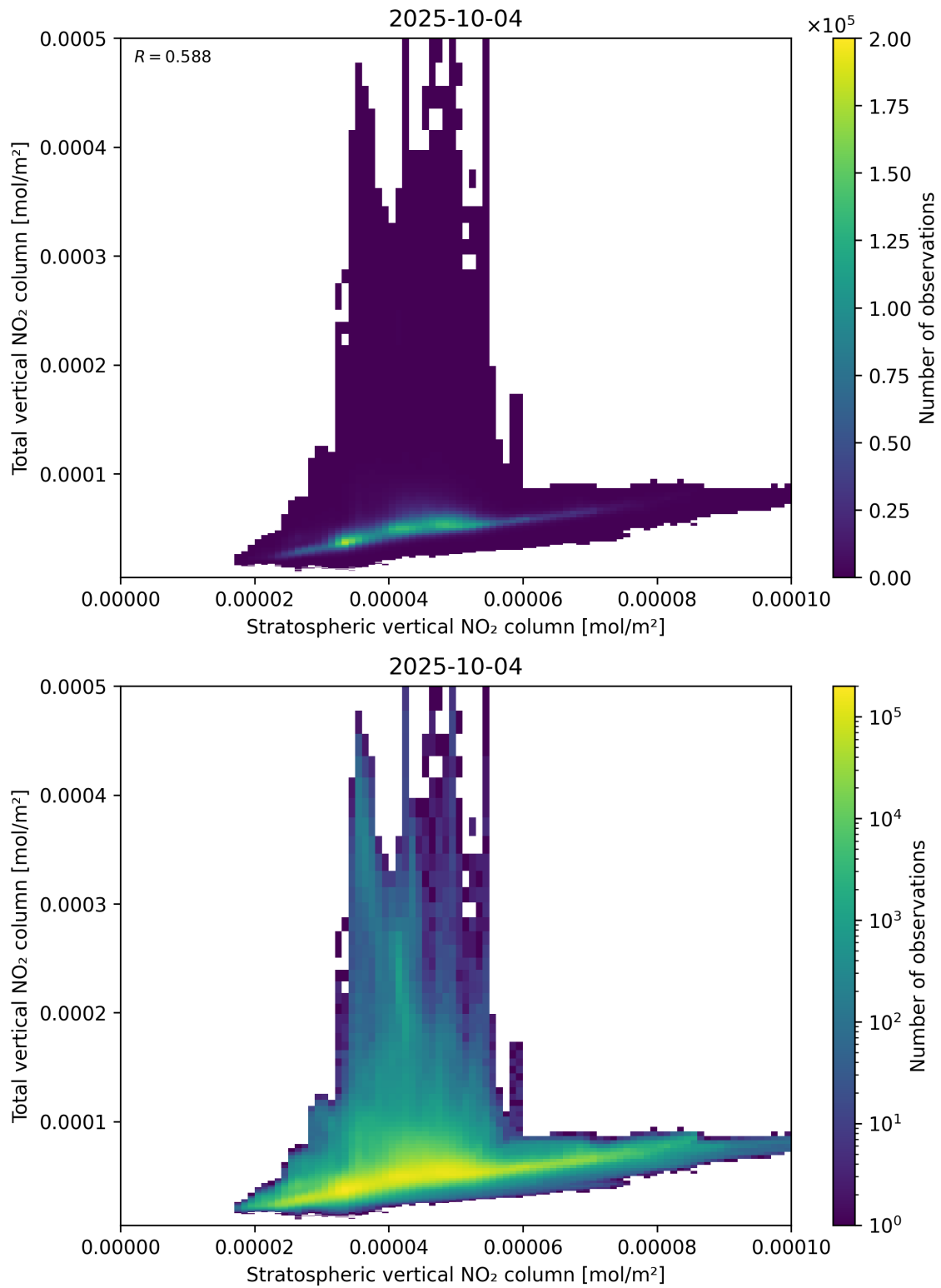
Figure 100: Scatter density plot of “Stratospheric vertical NO 2 column” against “Total vertical NO 2 column” for 2025-10-03 to 2025-10-05.
