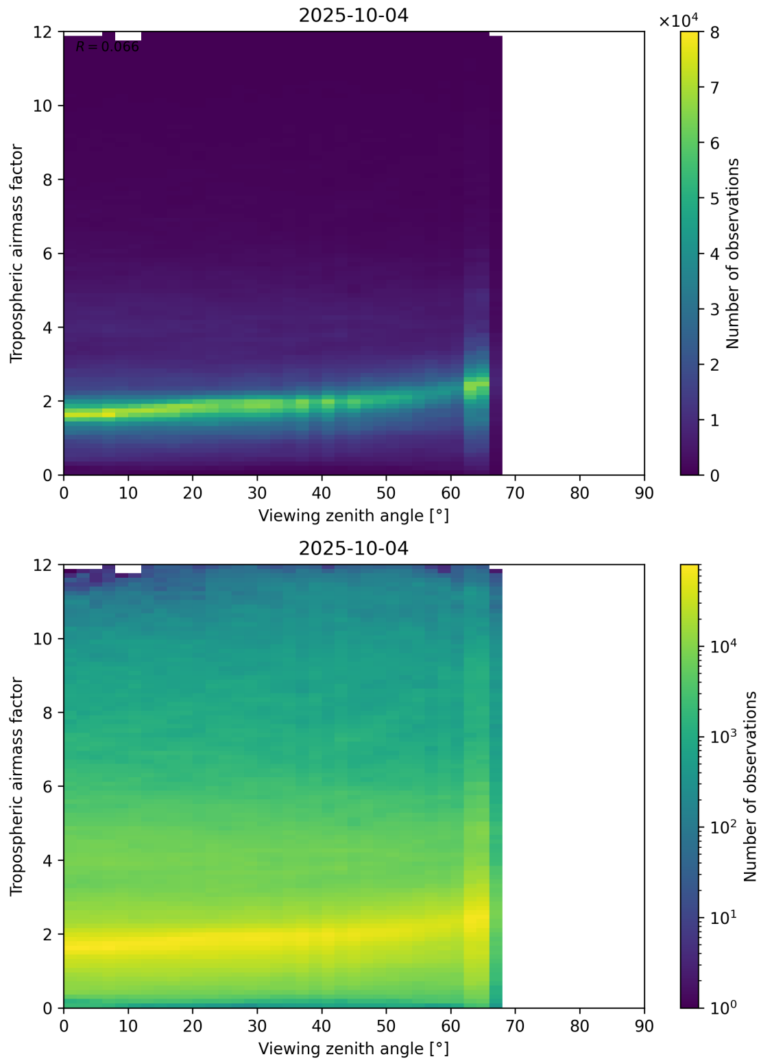
Figure 161: Scatter density plot of “Viewing zenith angle” against “Tropospheric airmass factor” for 2025-10-03 to 2025-10-05.
