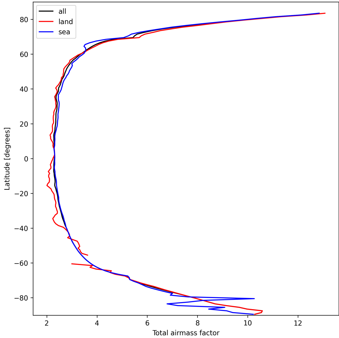
Figure 15: Zonal average of “Total airmass factor” for 2025-10-03 to 2025-10-05.
