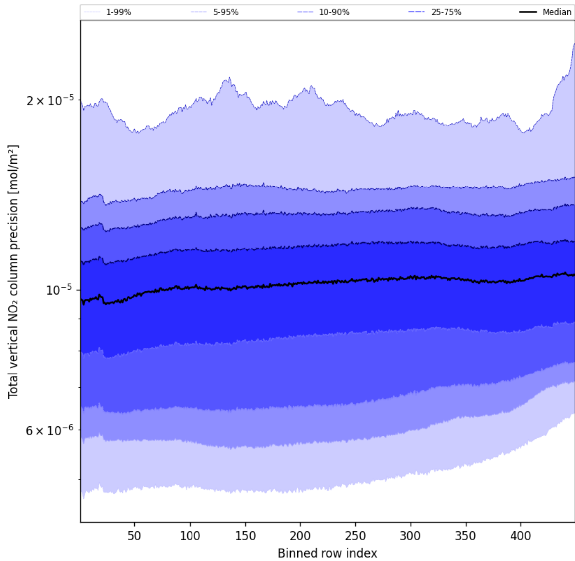
Figure 56: Along track statistics of “Total vertical NO 2 column precision” for 2025-10-03 to 2025-10-05
