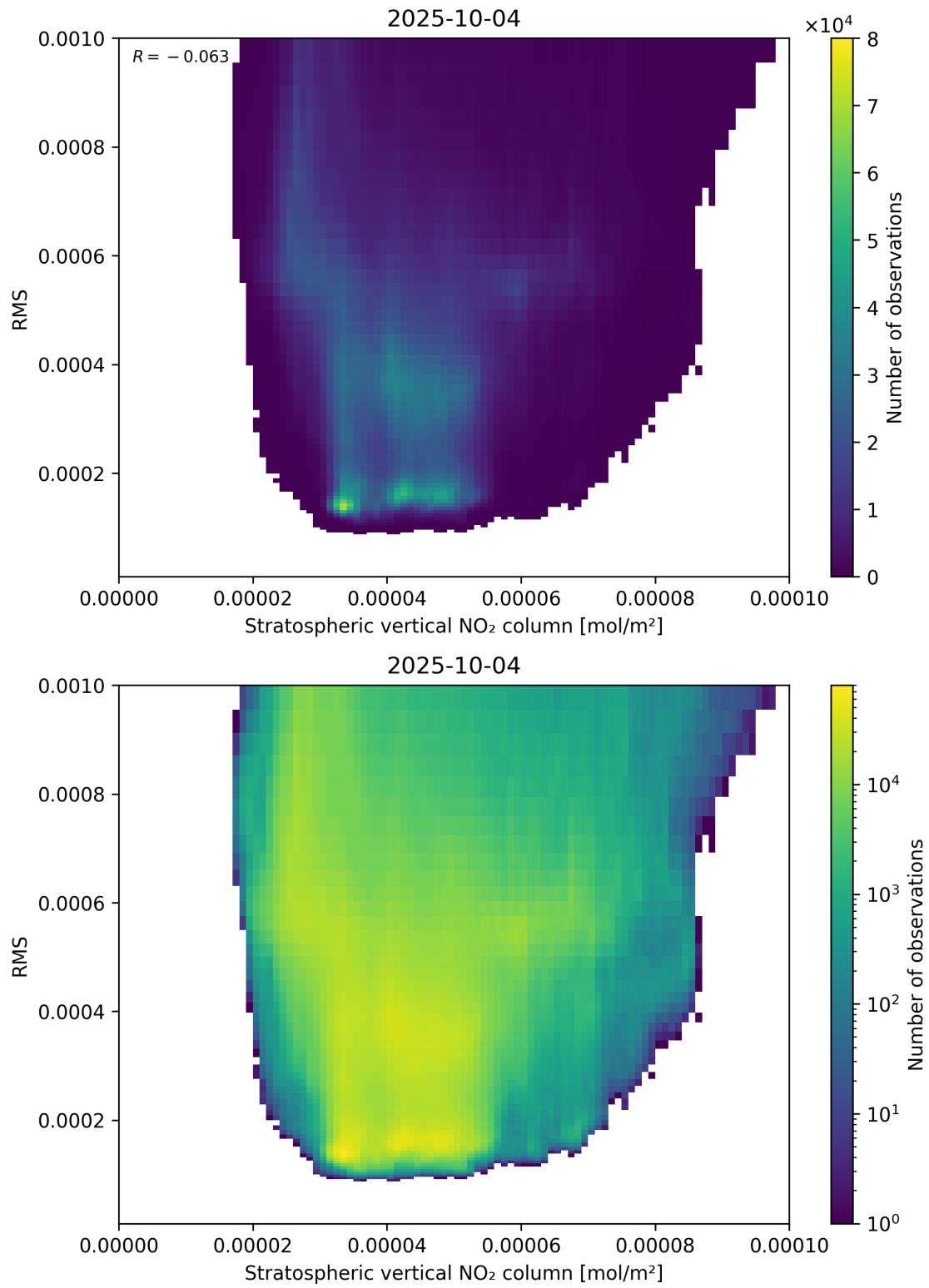
Figure 102: Scatter density plot of “Stratospheric vertical NO 2 column” against “RMS” for 2025-10-03 to 2025-10-05.
