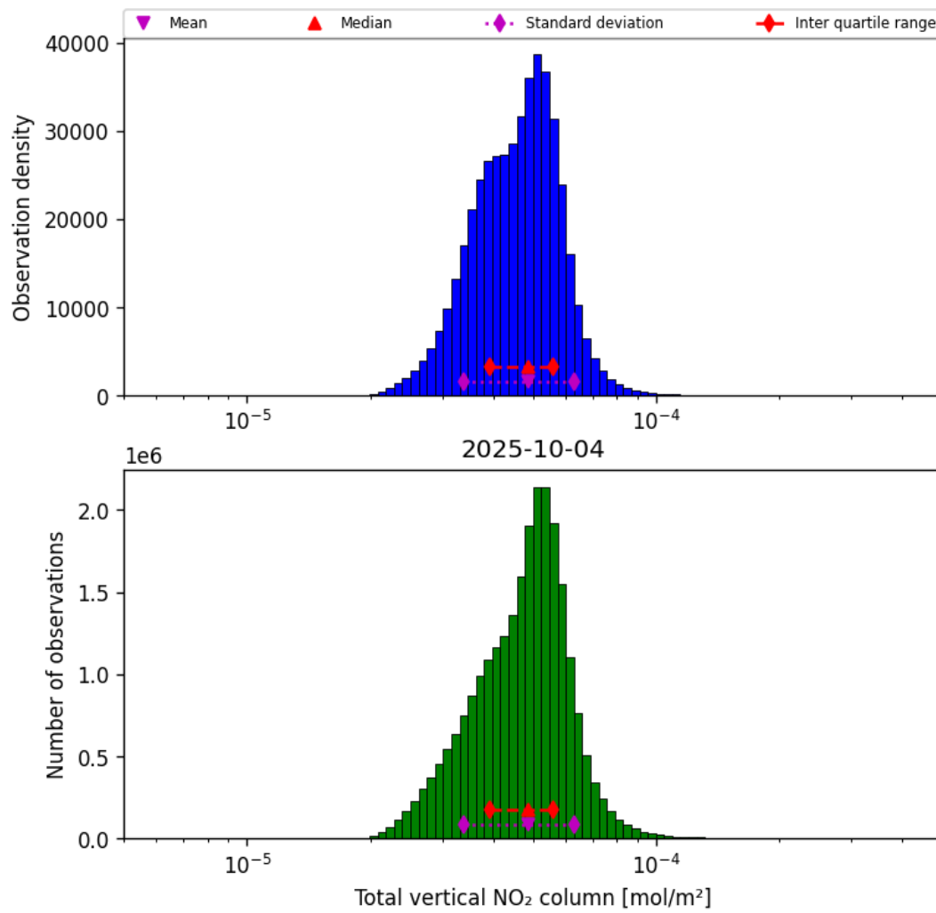
Figure 38: Histogram of “Total vertical NO 2 column” for 2025-10-03 to 2025-10-05
