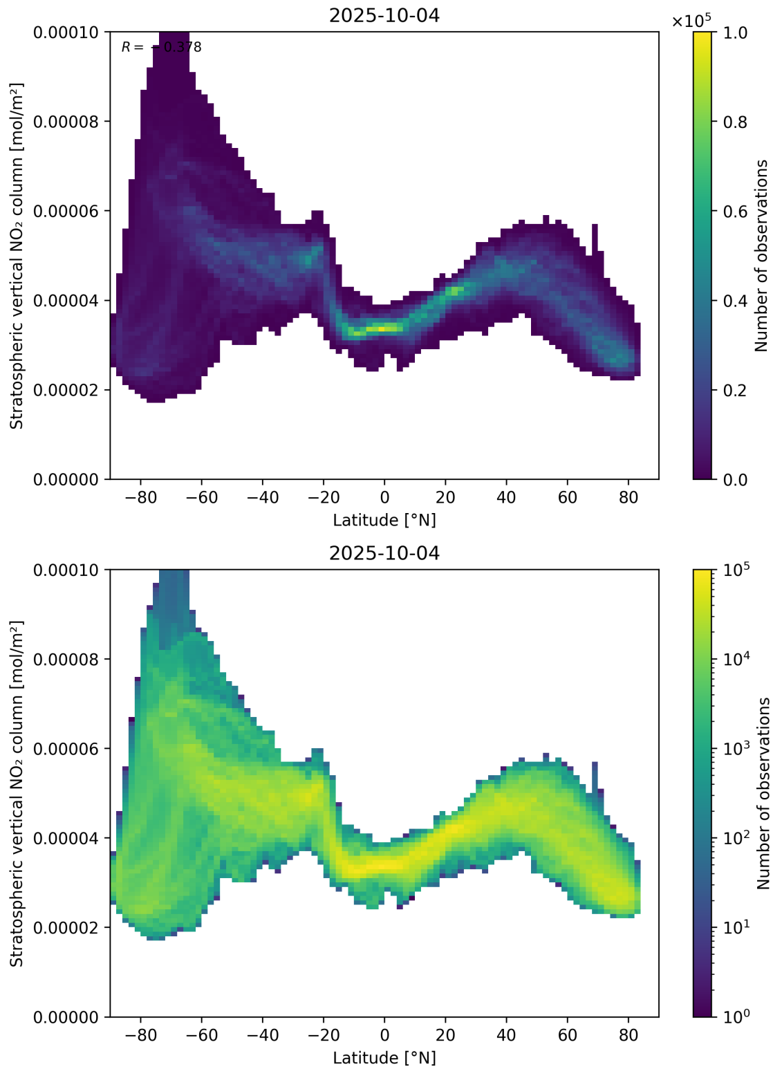
Figure 87: Scatter density plot of “Latitude” against “Stratospheric vertical NO 2 column” for 2025-10-03 to 2025-10-05.
