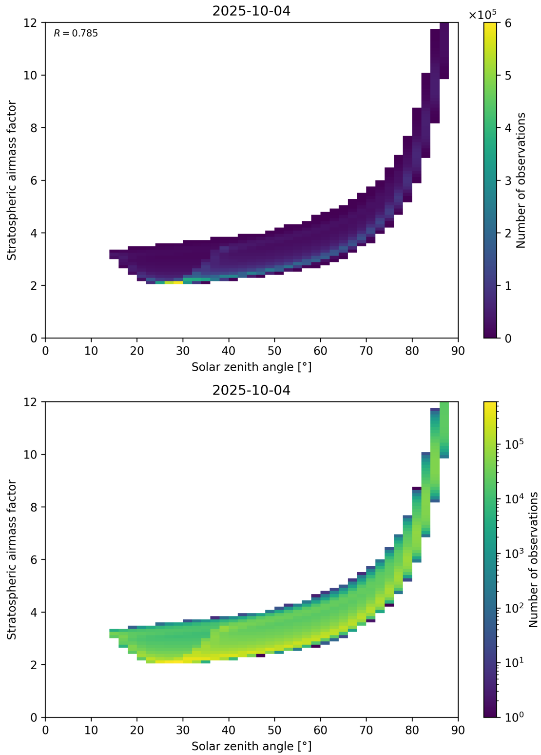
Figure 145: Scatter density plot of “Solar zenith angle” against “Stratospheric airmass factor” for 2025-10-03 to 2025-10-05.
