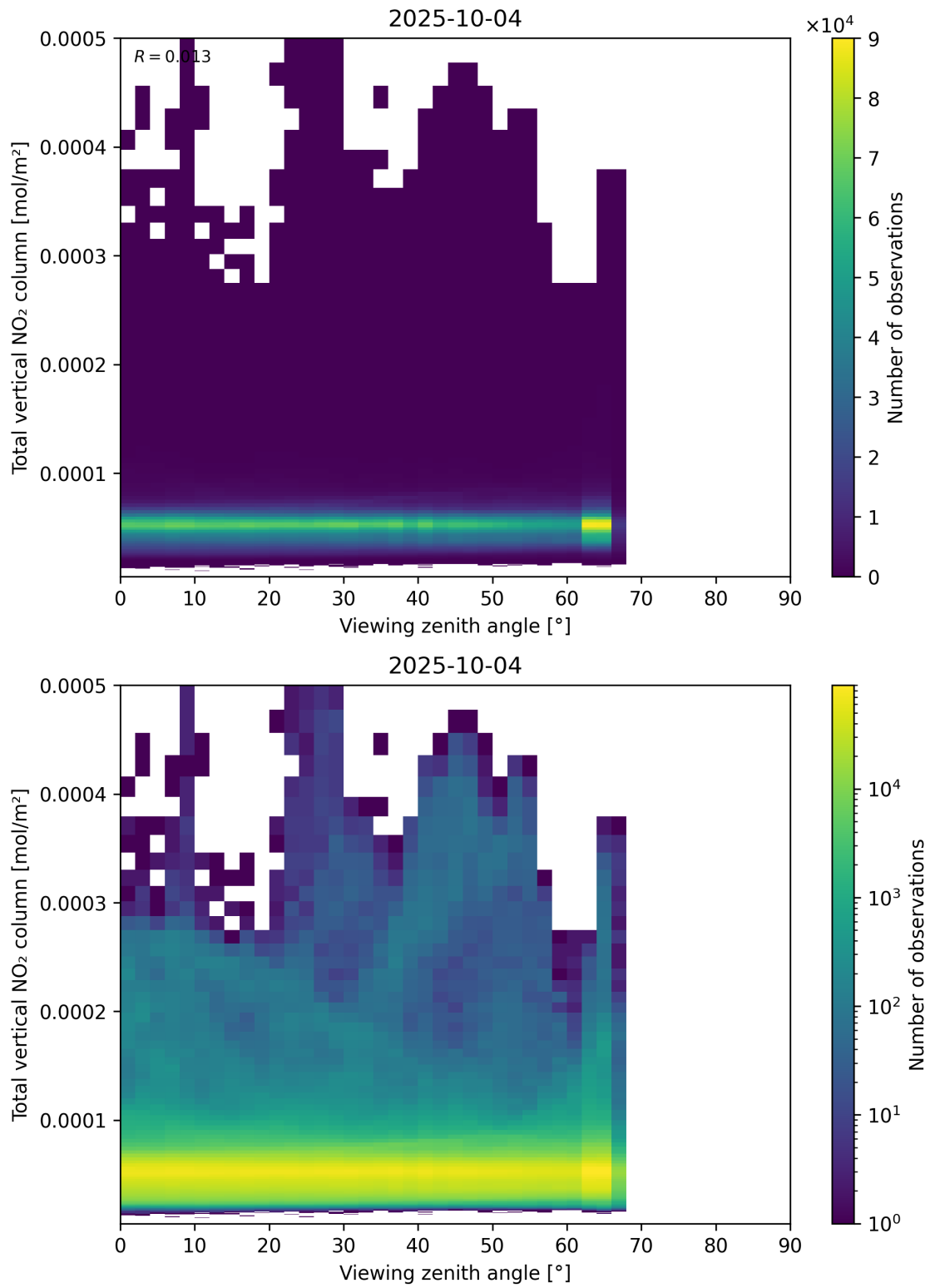
Figure 167: Scatter density plot of “Viewing zenith angle” against “Total vertical NO 2 column” for 2025-10-03 to 2025-10-05.
