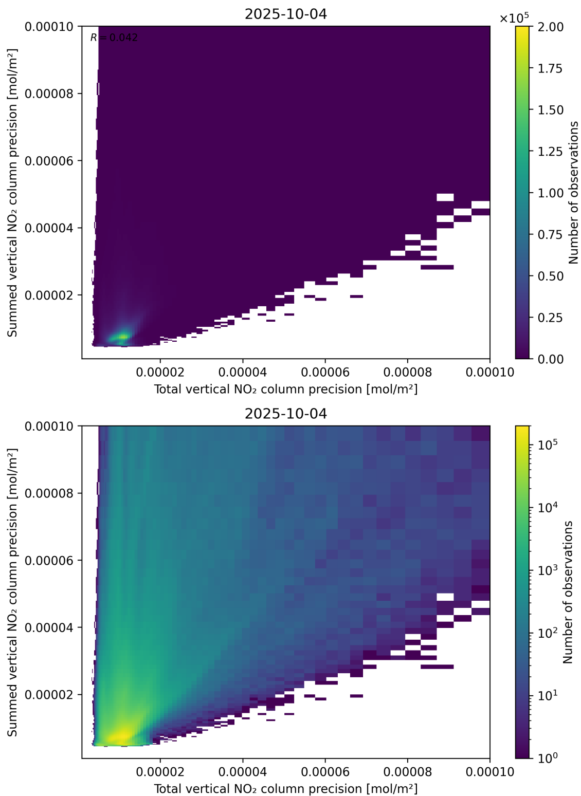
Figure 118: Scatter density plot of “Total vertical NO 2 column precision” against “Summed vertical NO 2 column precision” for 2025-10-03 to 2025-10-05.
