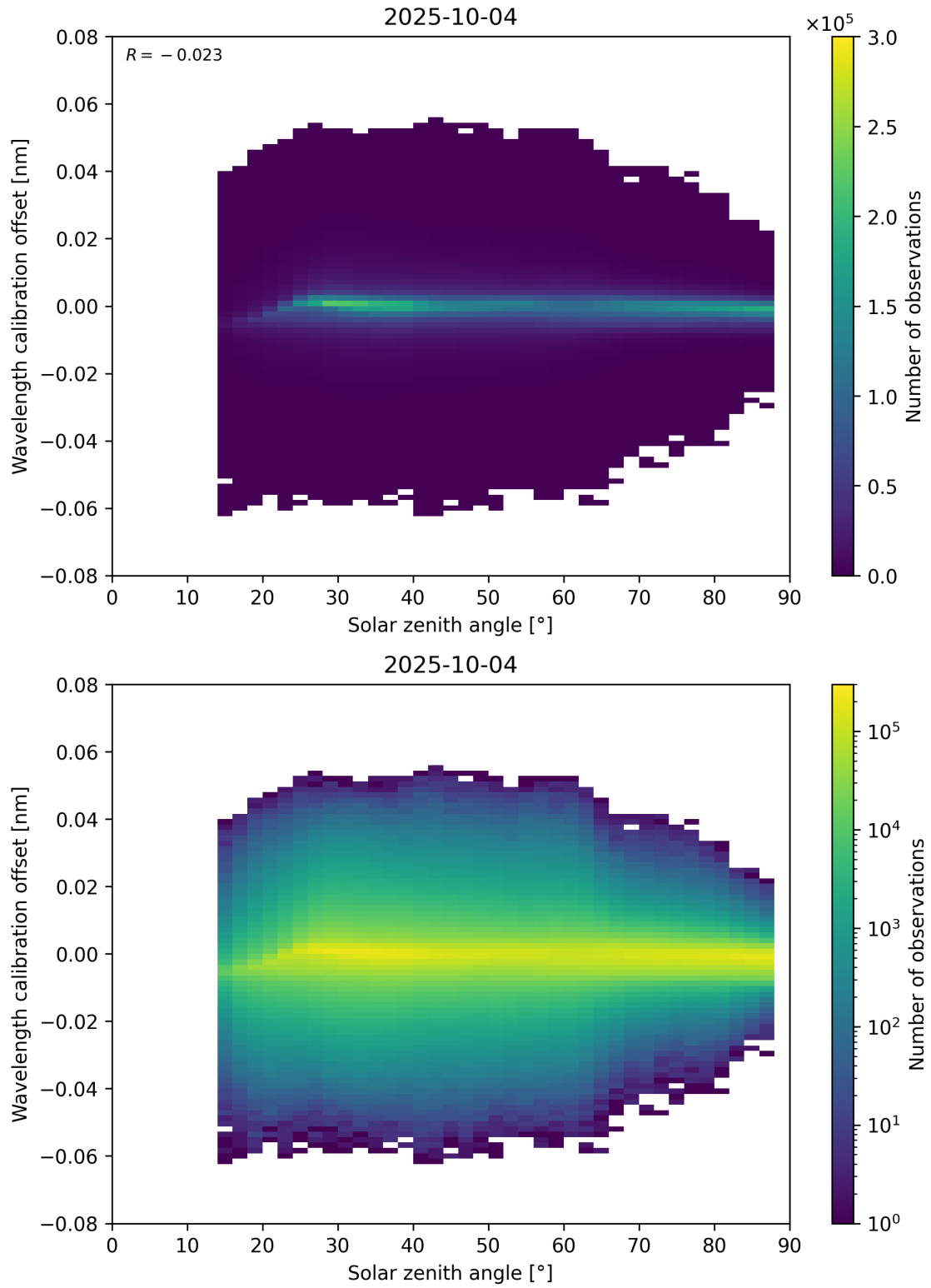
Figure 158: Scatter density plot of “Solar zenith angle” against “Wavelength calibration offset” for 2025-10-03 to 2025-10-05.
