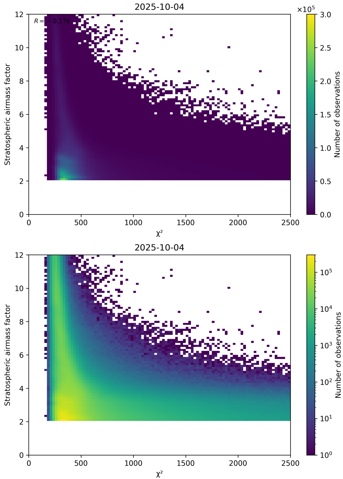
Figure 81: Scatter density plot of “ \chi^2 ” against “Stratospheric airmass factor” for 2025-10-03 to 2025-10-05.
