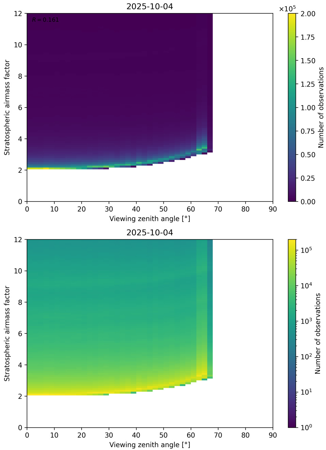
Figure 159: Scatter density plot of “Viewing zenith angle” against “Stratospheric airmass factor” for 2025-10-03 to 2025-10-05.
