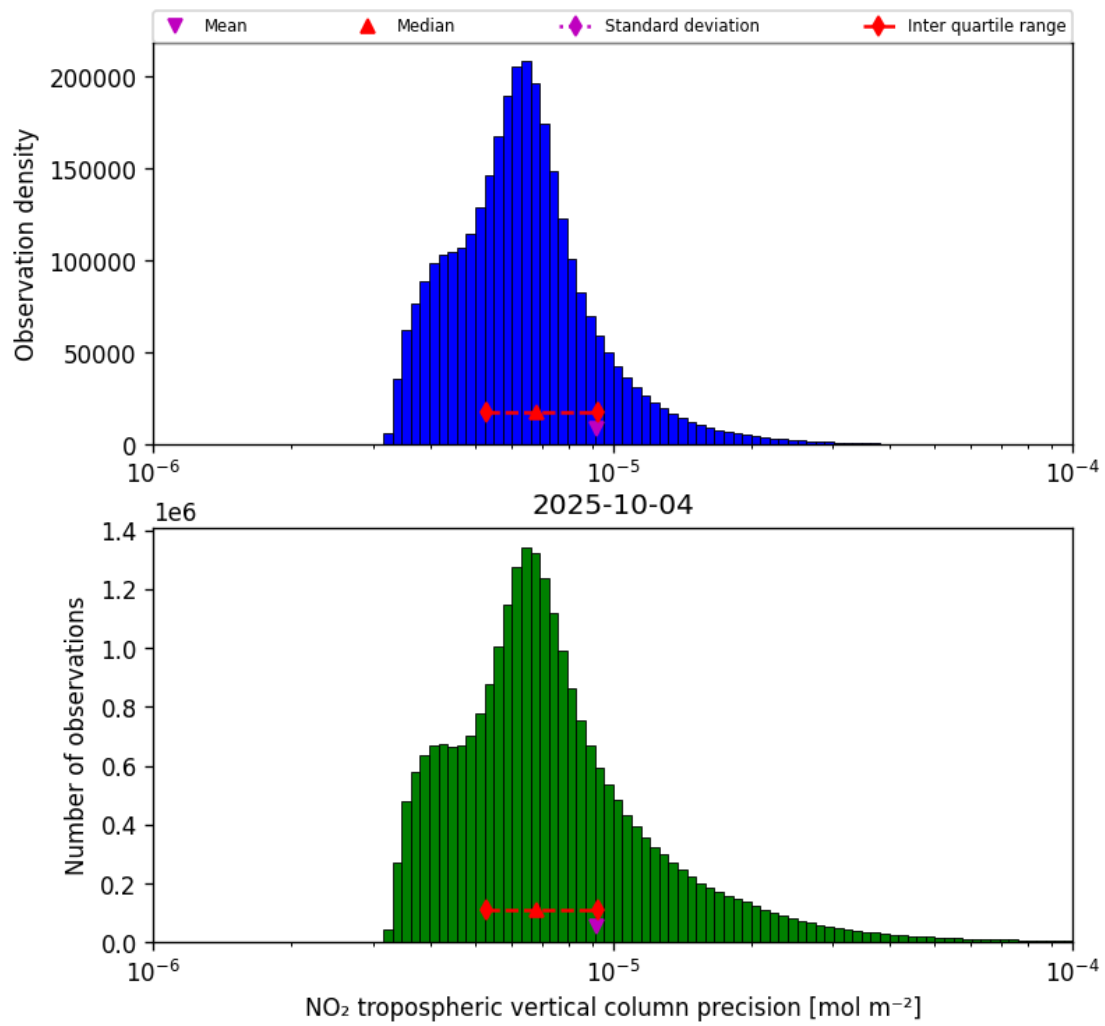
Figure 30: Histogram of “NO 2 tropospheric vertical column precision” for 2025-10-03 to 2025-10-05
