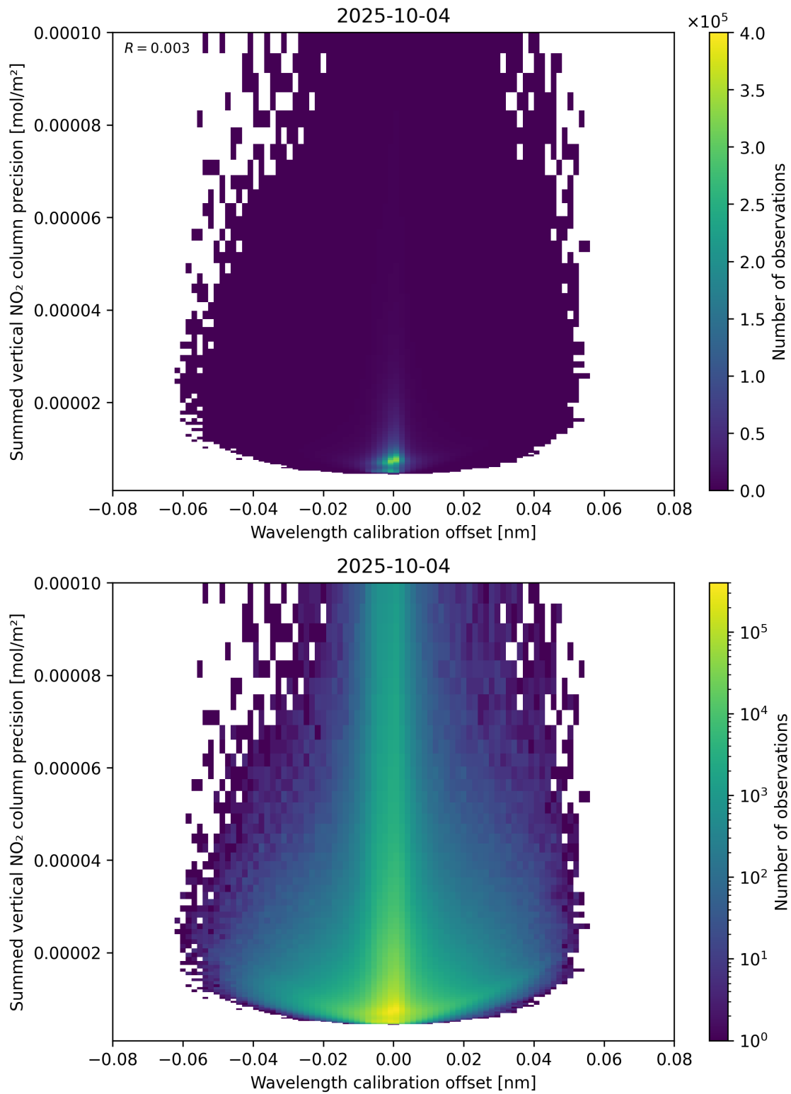
Figure 178: Scatter density plot of “Wavelength calibration offset” against “Summed vertical NO 2 column precision” for 2025-10-03 to 2025-10-05.
