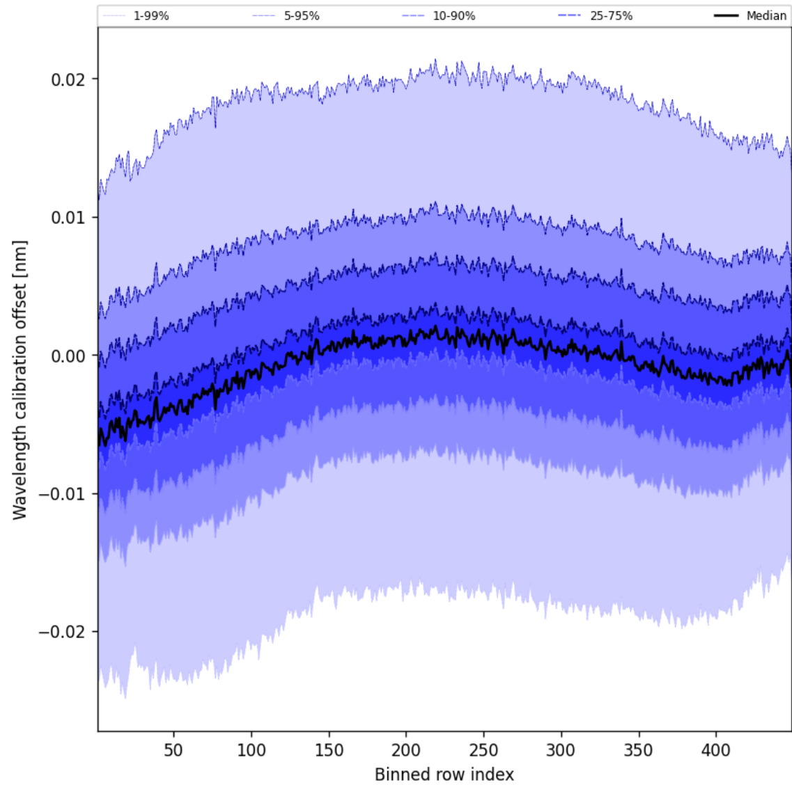
Figure 52: Along track statistics of “Wavelength calibration offset” for 2025-10-03 to 2025-10-05
