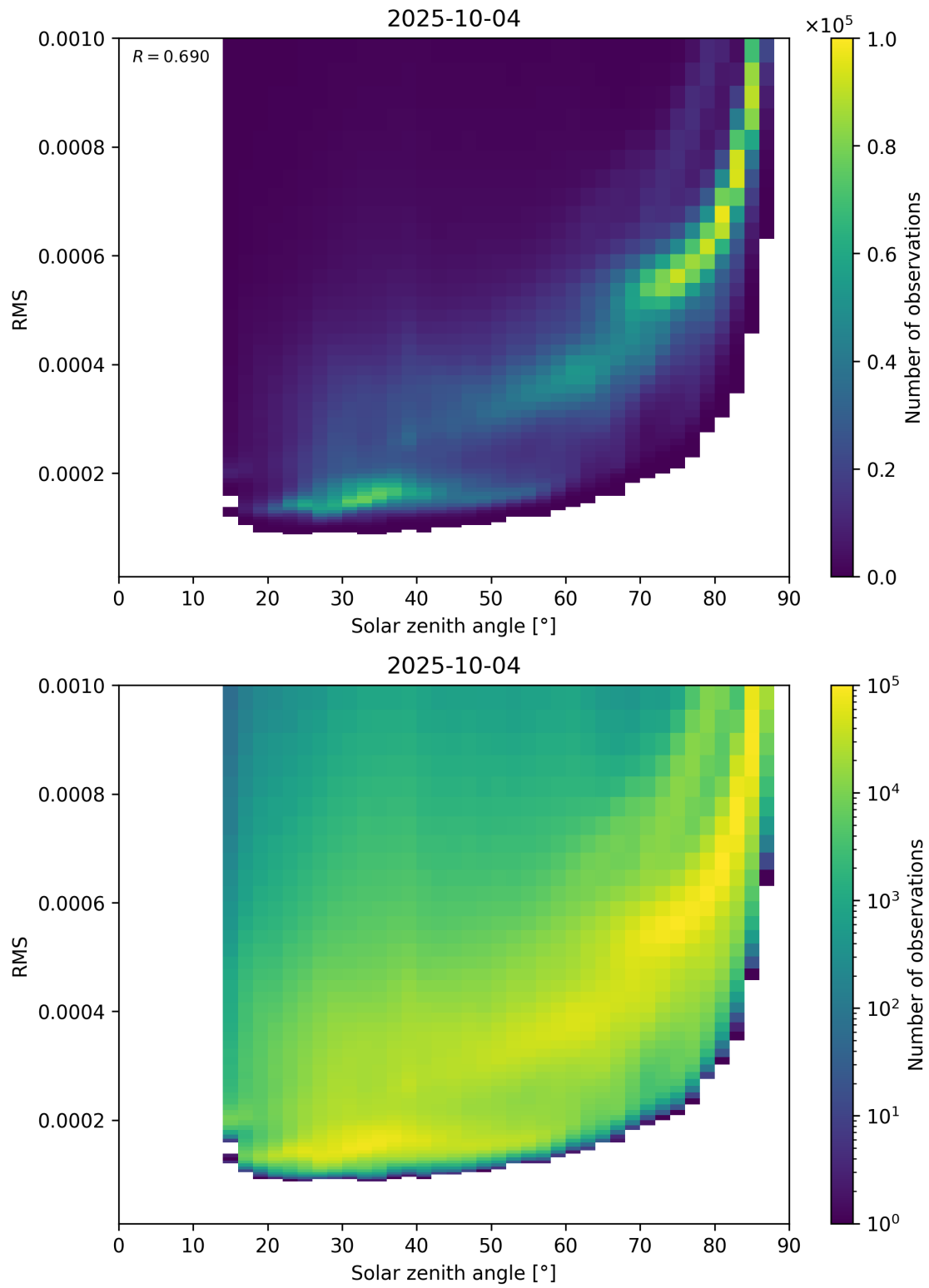
Figure 157: Scatter density plot of “Solar zenith angle” against “RMS” for 2025-10-03 to 2025-10-05.
