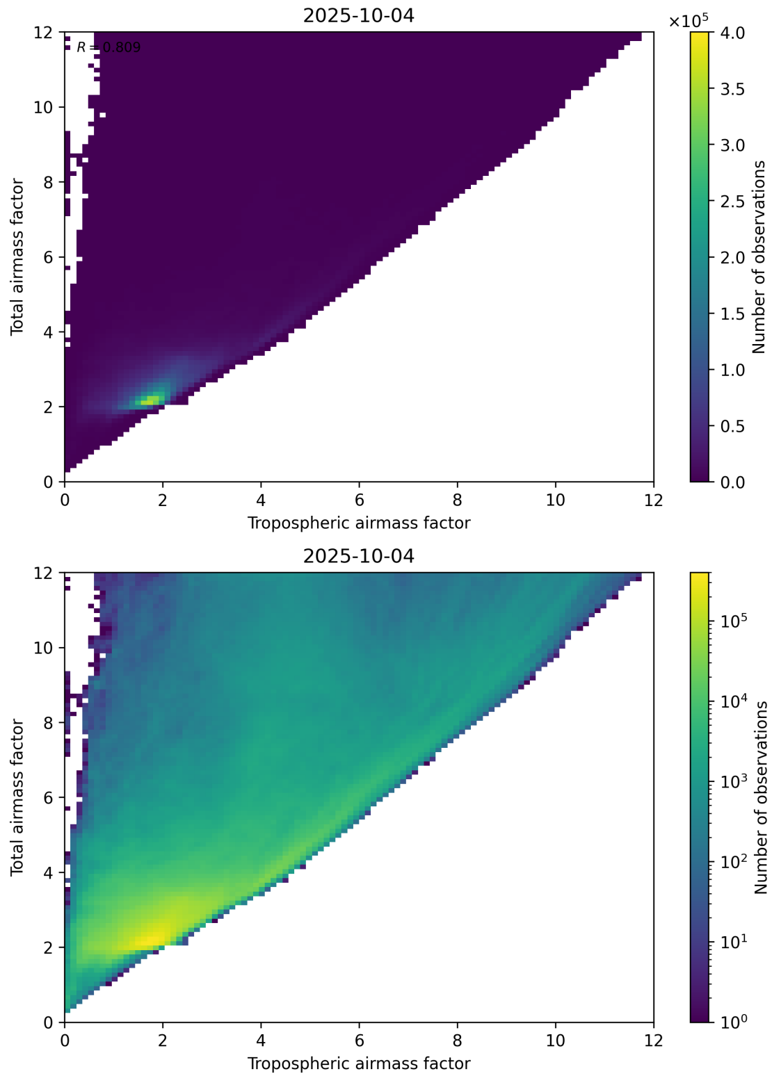
Figure 72: Scatter density plot of “Tropospheric airmass factor” against “Total airmass factor” for 2025-10-03 to 2025-10-05.
