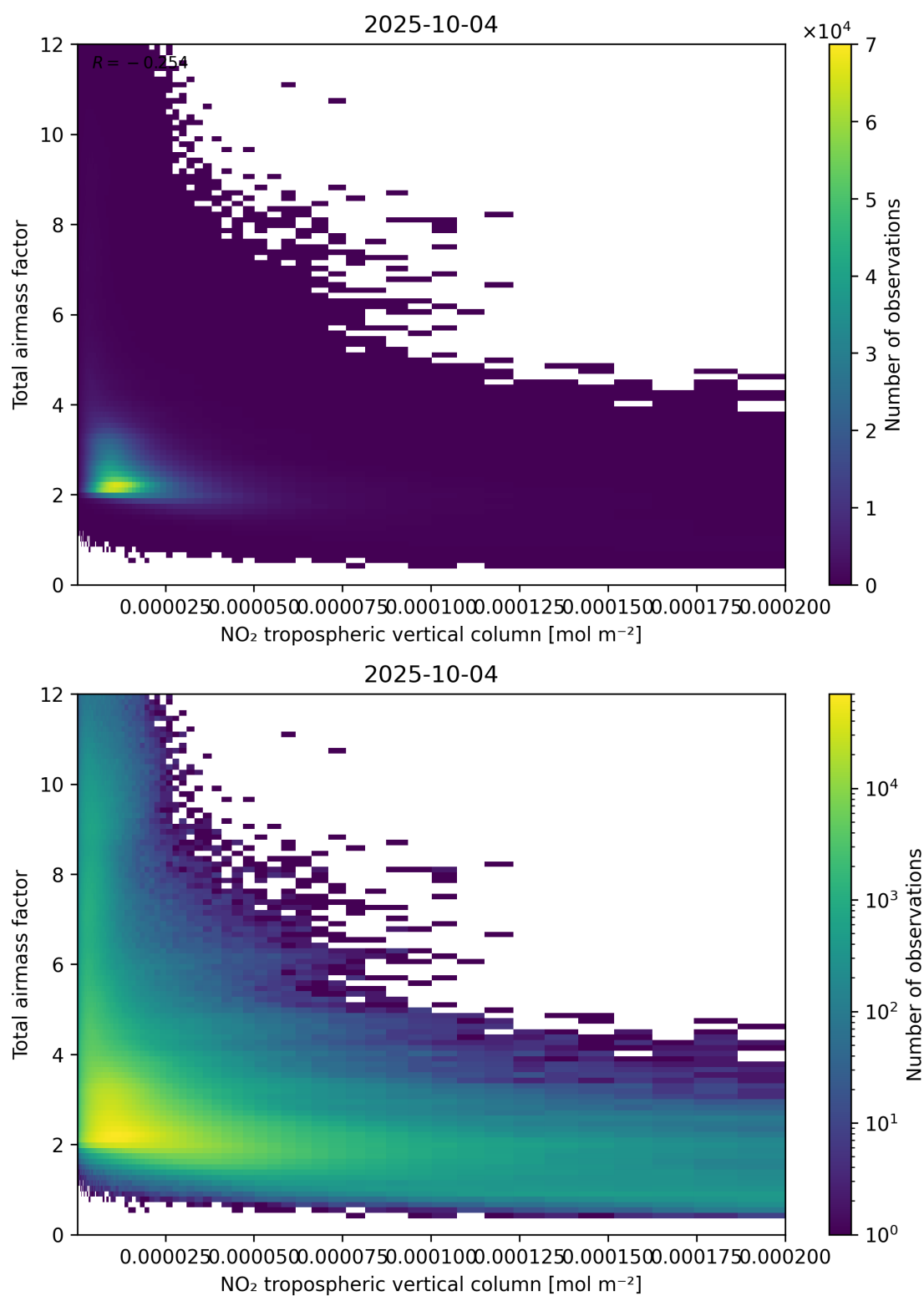
Figure 122: Scatter density plot of “NO 2 tropospheric vertical column” against “Total air mass factor” for 2025-10-03 to 2025-10-05.
