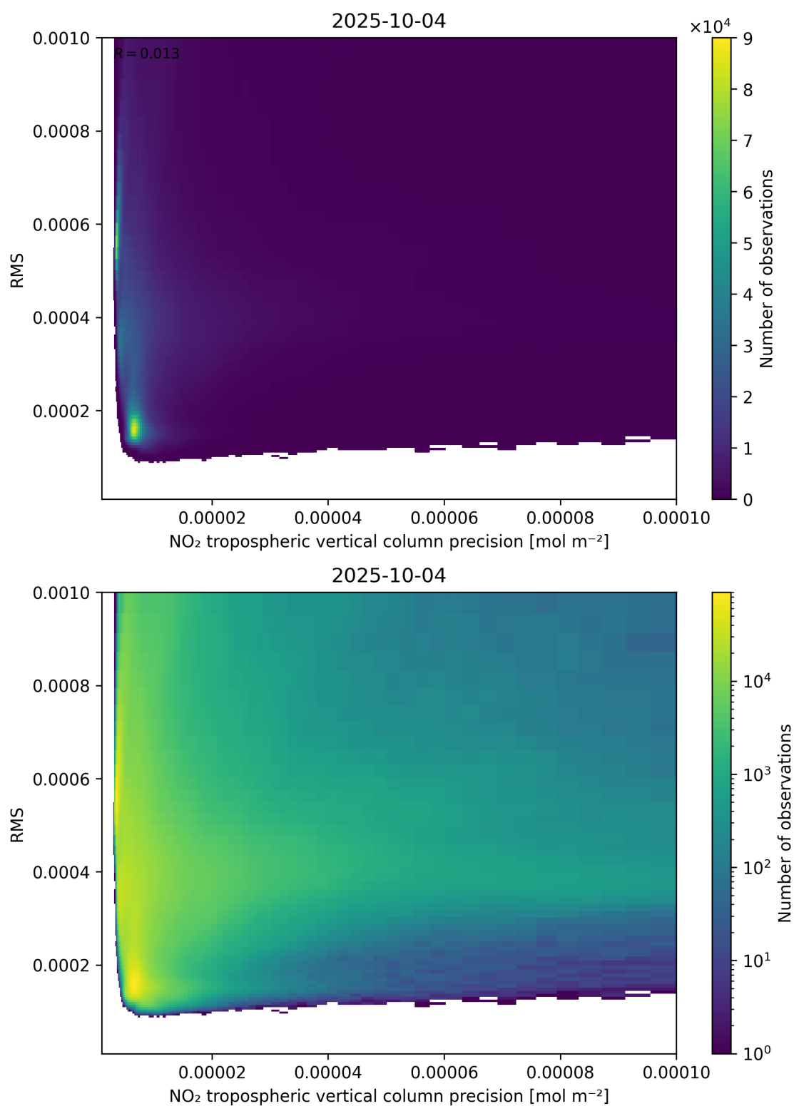
Figure 140: Scatter density plot of “NO 2 tropospheric vertical column precision” against “RMS” for 2025-10-03 to 2025-10-05.
