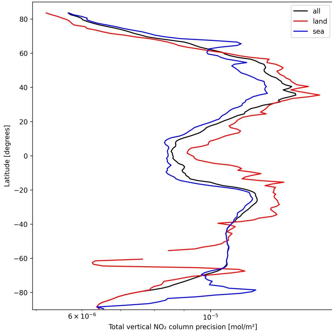
Figure 22: Zonal average of “Total vertical NO 2 column precision” for 2025-10-03 to 2025-10-05.
