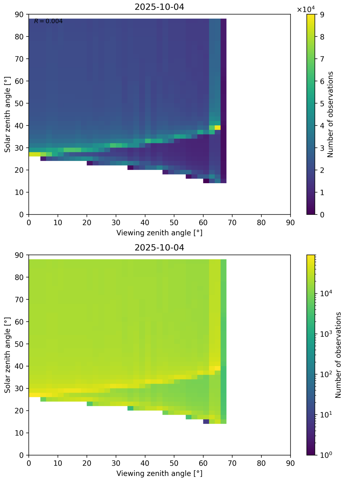
Figure 172: Scatter density plot of “Viewing zenith angle” against “Solar zenith angle” for 2025-10-03 to 2025-10-05.
