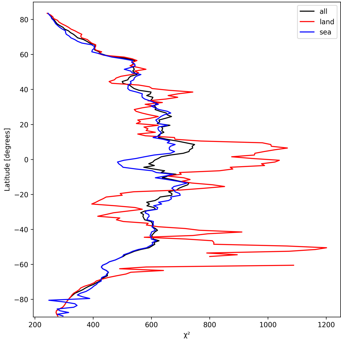
Figure 25: Zonal average of “ \chi^2 ” for 2025-10-03 to 2025-10-05.
