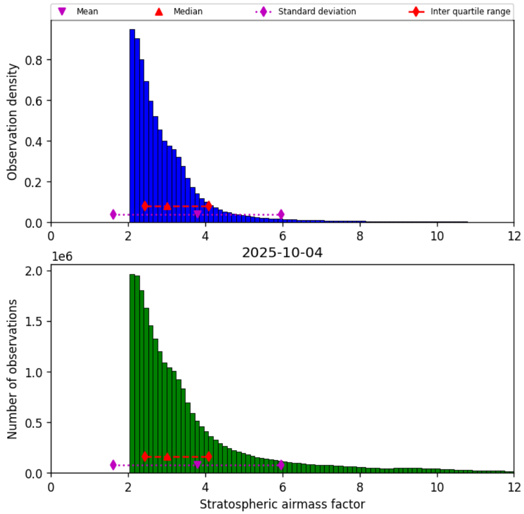
Figure 44: Histogram of “Stratospheric airmass factor” for 2025-10-03 to 2025-10-05
