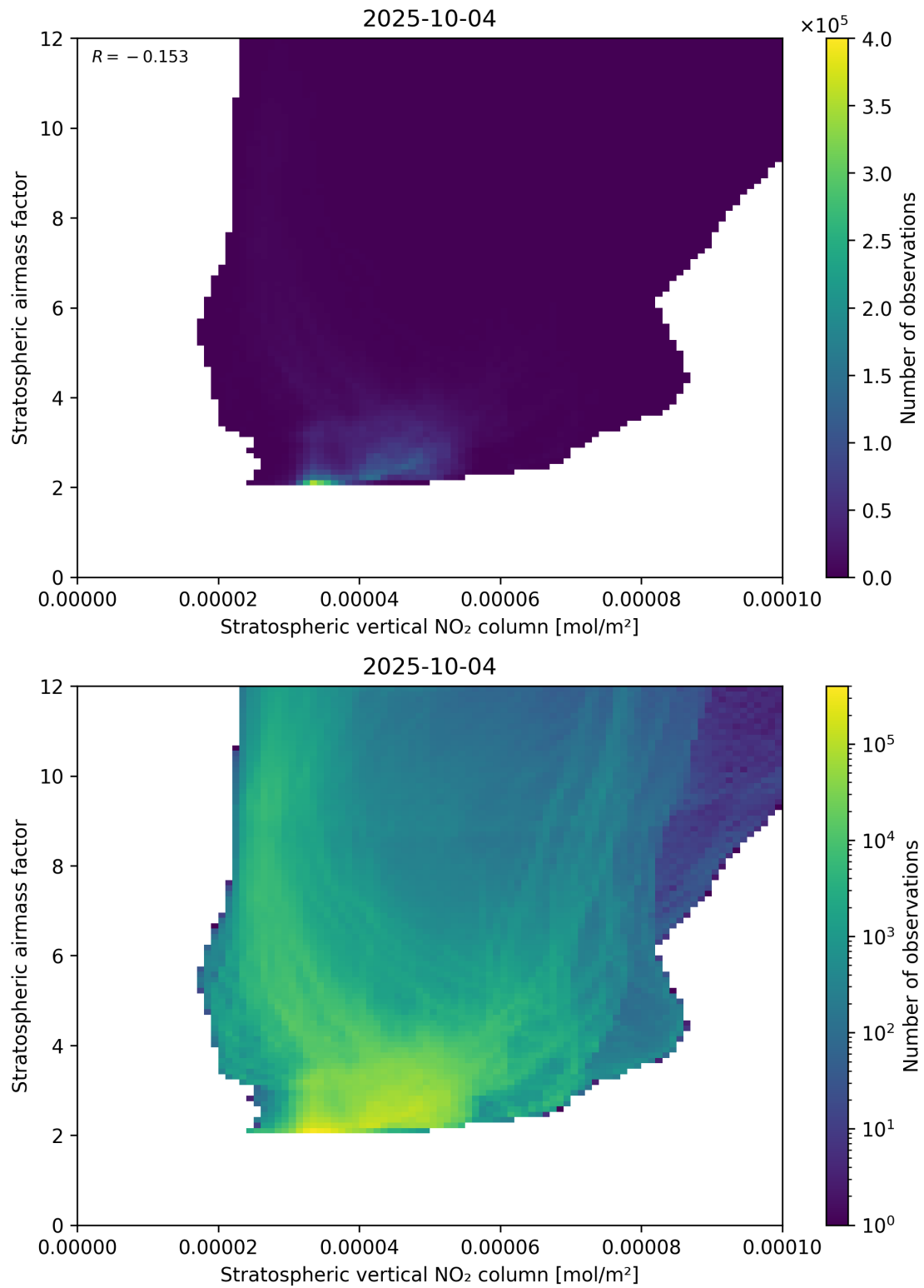
Figure 96: Scatter density plot of “Stratospheric vertical NO 2 column” against “Stratospheric airmass factor” for 2025-10-03 to 2025-10-05.
