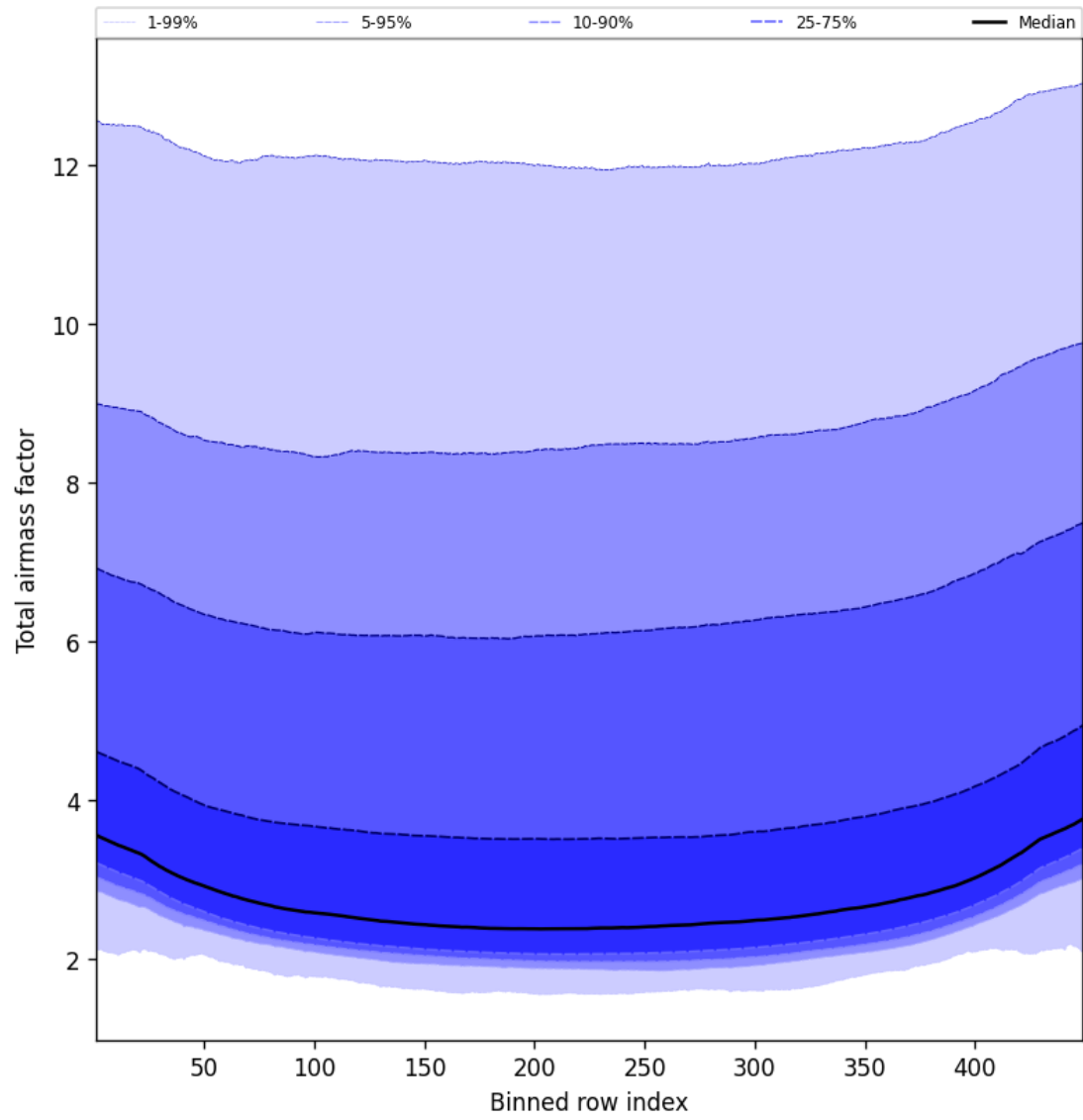
Figure 49: Along track statistics of “Total airmass factor” for 2025-10-03 to 2025-10-05
