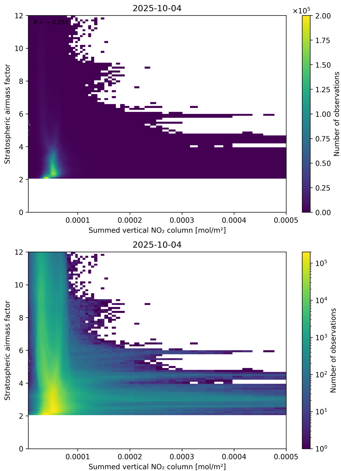
Figure 103: Scatter density plot of “Summed vertical NO 2 column” against “Stratospheric airmass factor” for 2025-10-03 to 2025-10-05.
