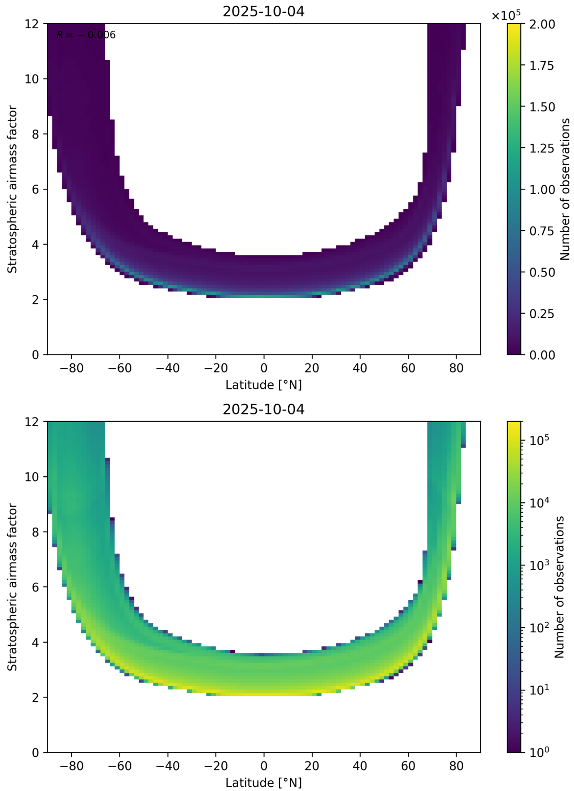
Figure 83: Scatter density plot of “Latitude” against “Stratospheric air mass factor” for 2025-10-03 to 2025-10-05.
