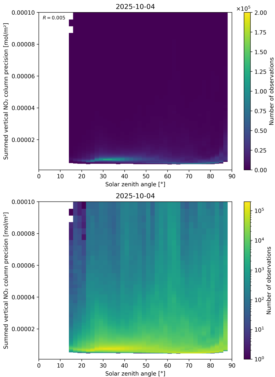
Figure 152: Scatter density plot of “Solar zenith angle” against “Summed vertical NO 2 column precision” for 2025-10-03 to 2025-10-05.
