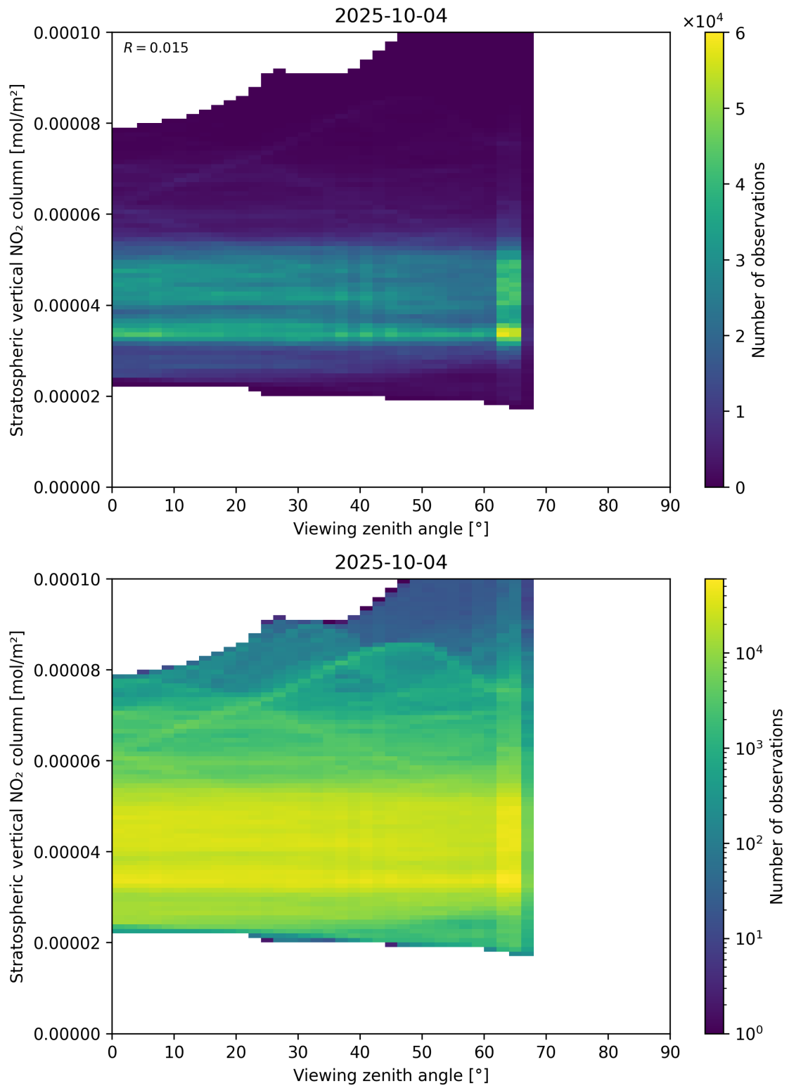
Figure 164: Scatter density plot of “Viewing zenith angle” against “Stratospheric vertical NO 2 column” for 2025-10-03 to 2025-10-05.
