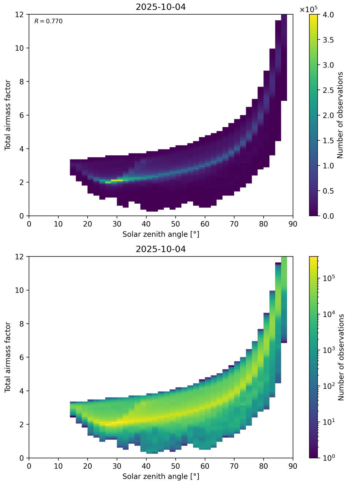
Figure 146: Scatter density plot of “Solar zenith angle” against “Total air mass factor” for 2025-10-03 to 2025-10-05.
