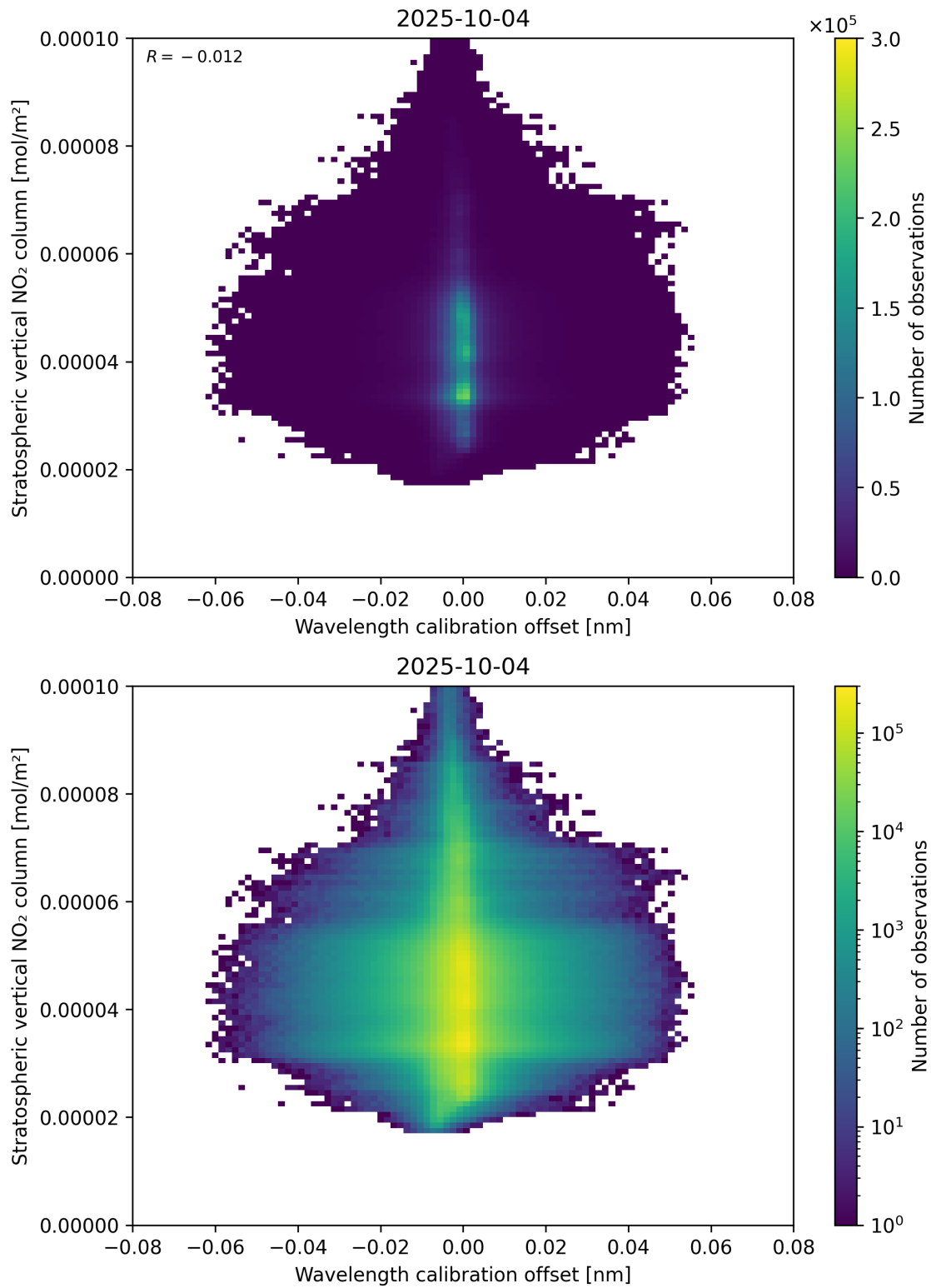
Figure 176: Scatter density plot of “Wavelength calibration offset” against “Stratospheric vertical NO 2 column” for 2025-10-03 to 2025-10-05.
