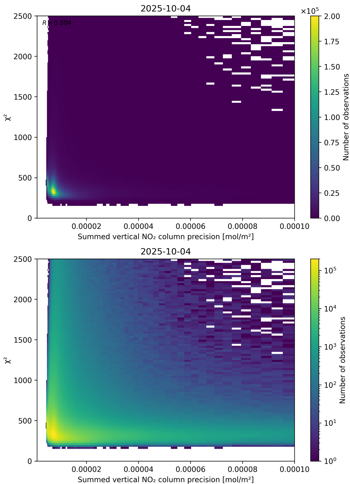
Figure 107: Scatter density plot of “Summed vertical NO 2 column precision” against “ \chi^2 ” for 2025-10-03 to 2025-10-05.
