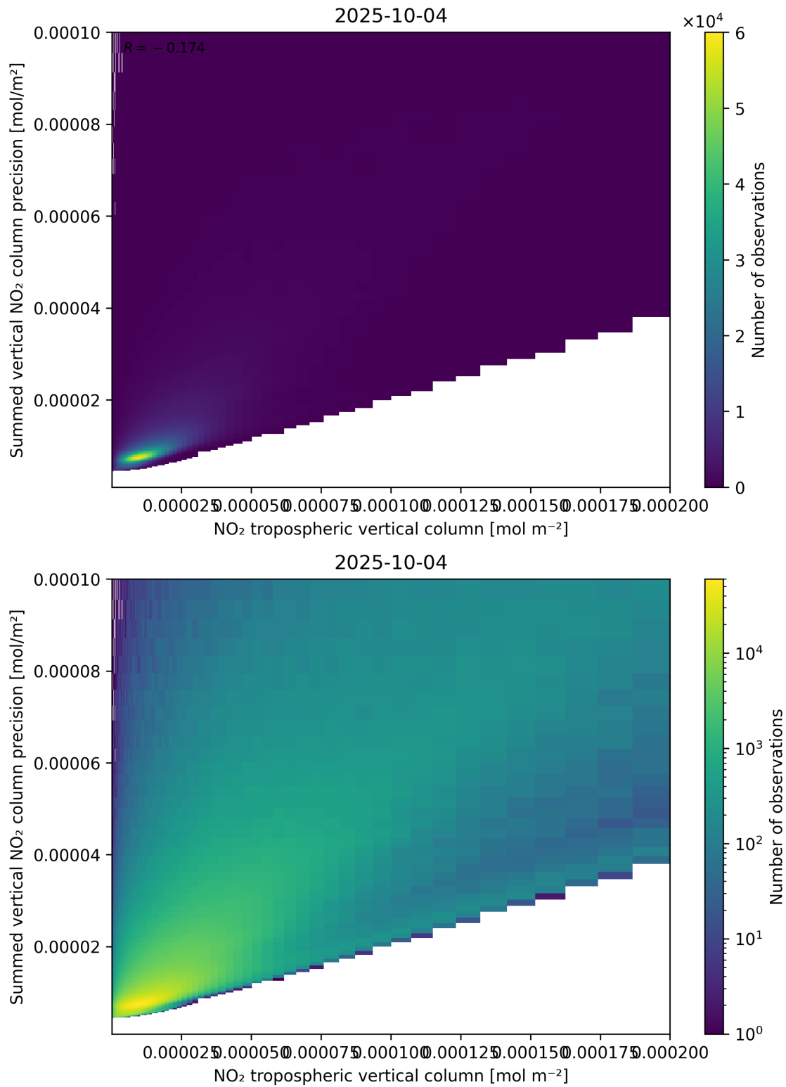
Figure 127: Scatter density plot of “NO 2 tropospheric vertical column” against “Summed vertical NO 2 column precision” for 2025-10-03 to 2025-10-05.
