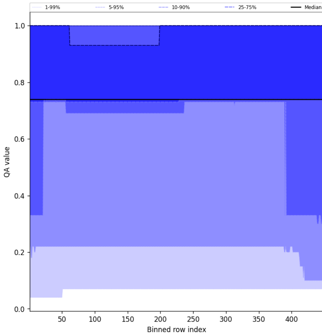
Figure 45: Along track statistics of "QA value" for 2025-10-03 to 2025-10-05
