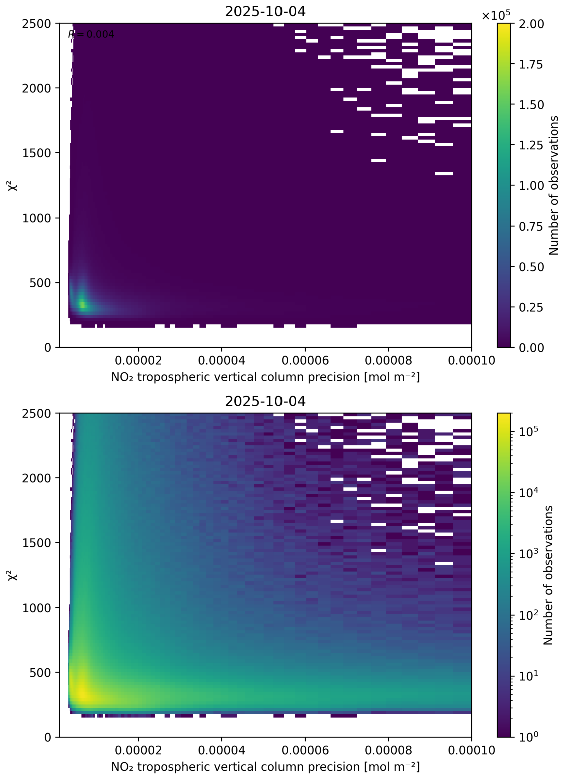
Figure 134: Scatter density plot of “NO 2 tropospheric vertical column precision” against “ \chi^2 ” for 2025-10-03 to 2025-10-05.
