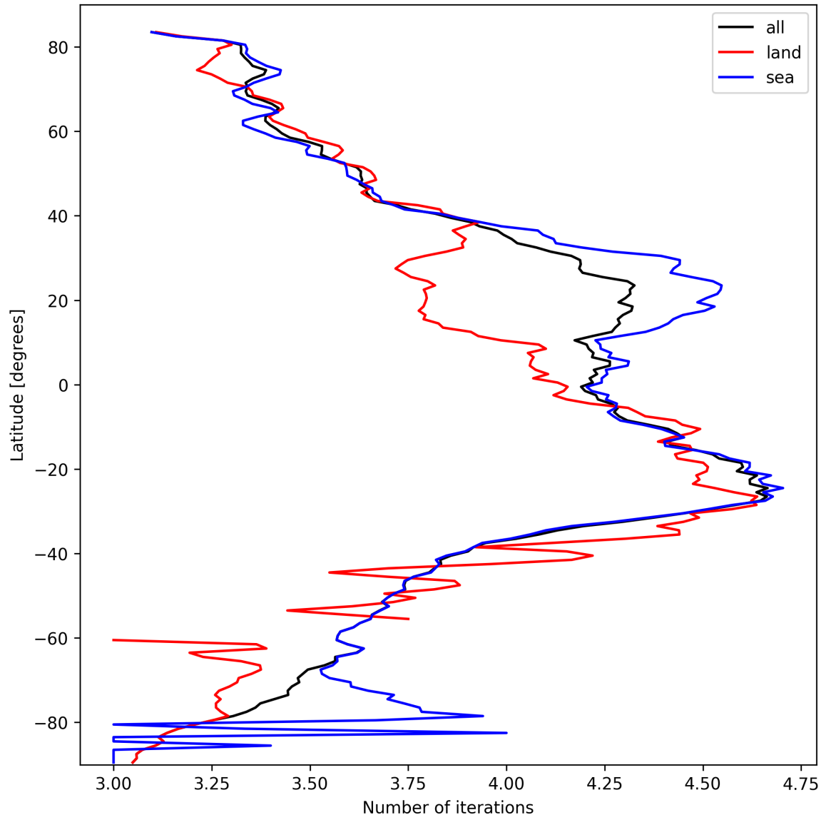
Figure 17: Zonal average of “Number of iterations” for 2025-10-03 to 2025-10-05.
