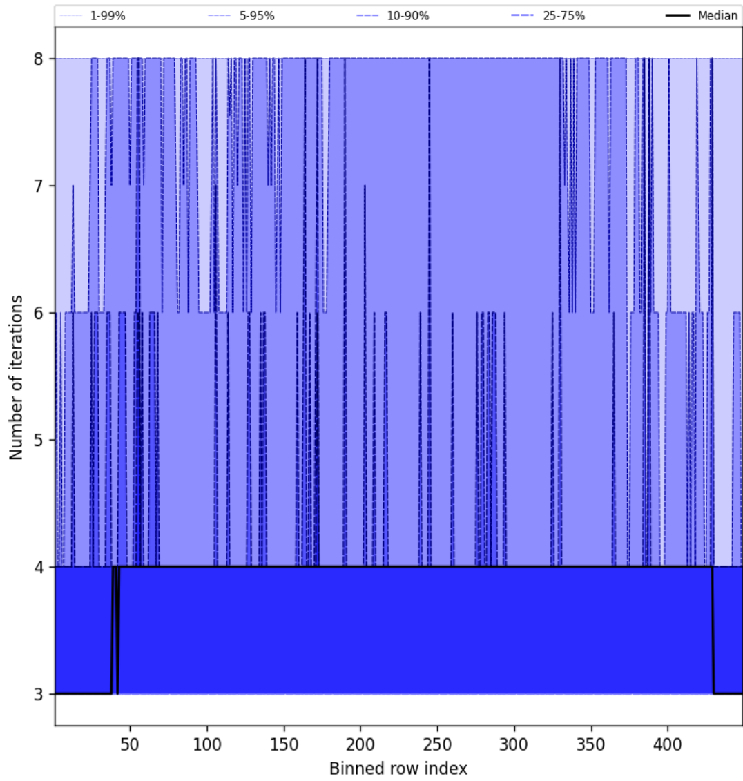
Figure 51: Along track statistics of “Number of iterations” for 2025-10-03 to 2025-10-05
