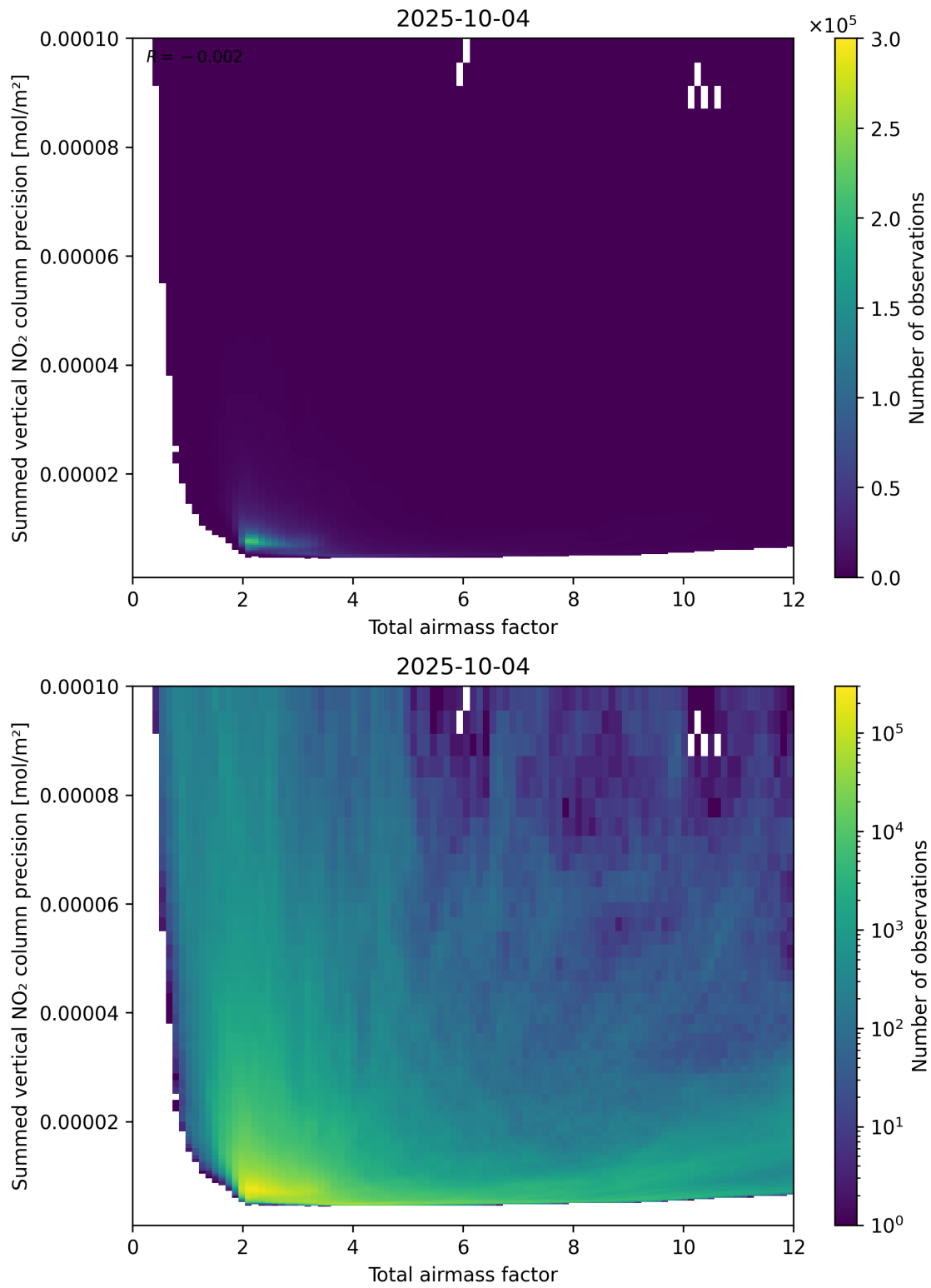
Figure 66: Scatter density plot of “Total airmass factor” against “Summed vertical NO 2 column precision” for 2025-10-03 to 2025-10-05.
