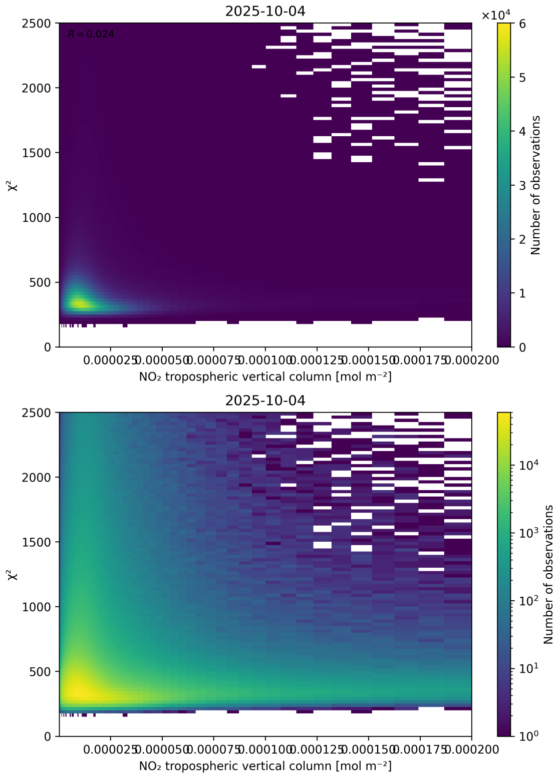
Figure 124: Scatter density plot of “NO 2 tropospheric vertical column” against “ \chi^2 ” for 2025-10-03 to 2025-10-05.
