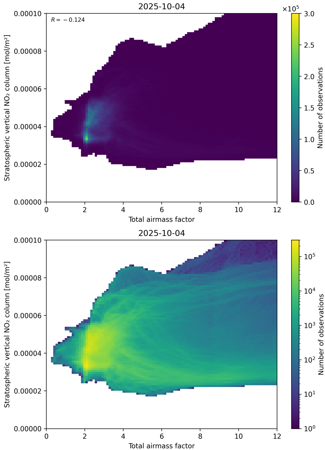
Figure 64: Scatter density plot of “Total airmass factor” against “Stratospheric vertical \text{NO}_2 column” for 2025-10-03 to 2025-10-05.
