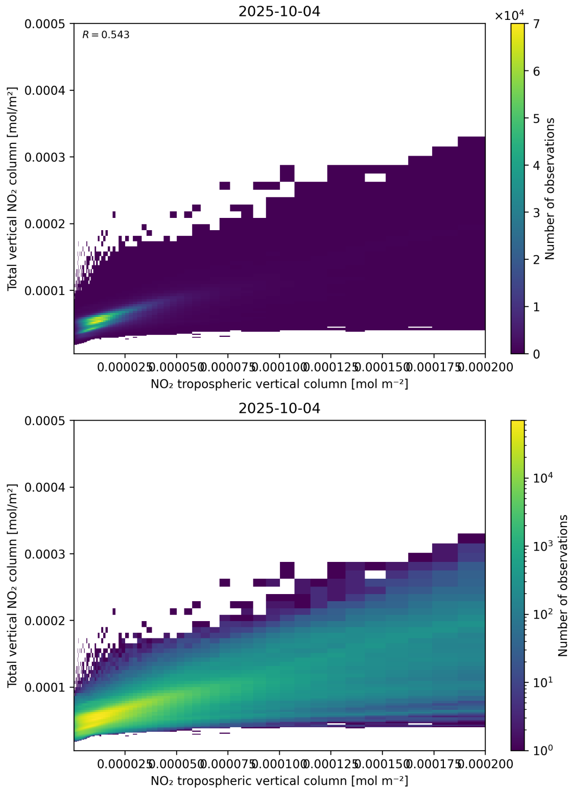
Figure 128: Scatter density plot of “NO 2 tropospheric vertical column” against “Total vertical NO 2 column” for 2025-10-03 to 2025-10-05.
