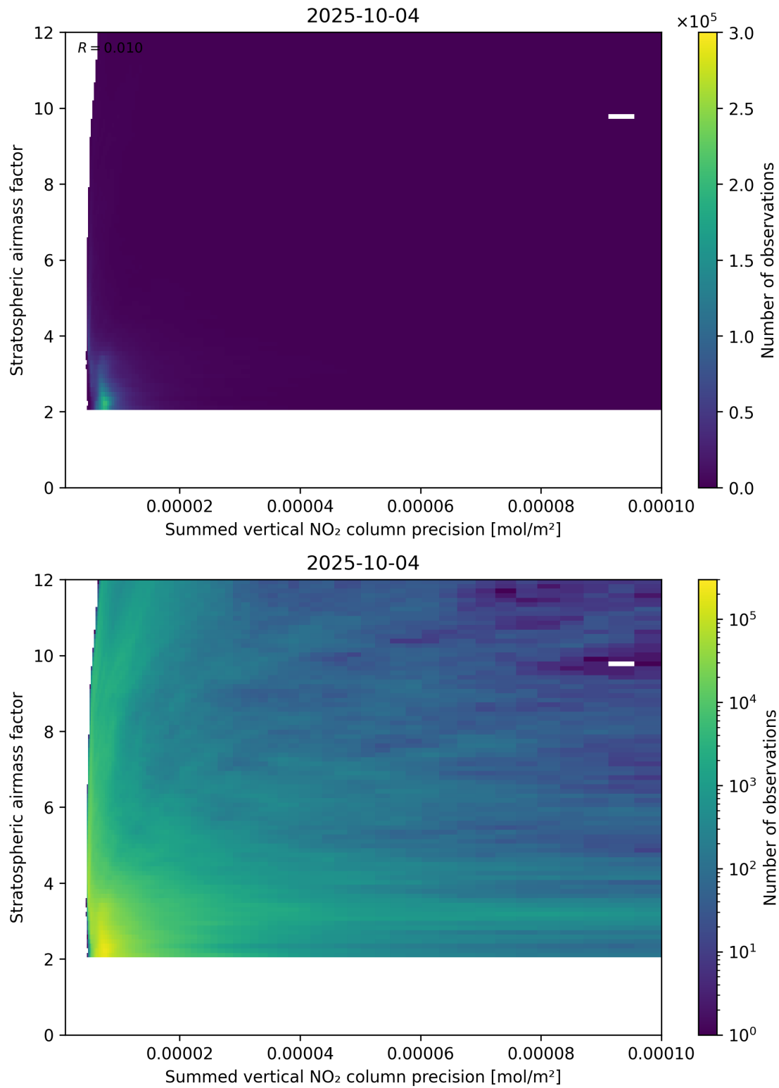
Figure 106: Scatter density plot of “Summed vertical NO 2 column precision” against “Stratospheric airmass factor” for 2025-10-03 to 2025-10-05.
