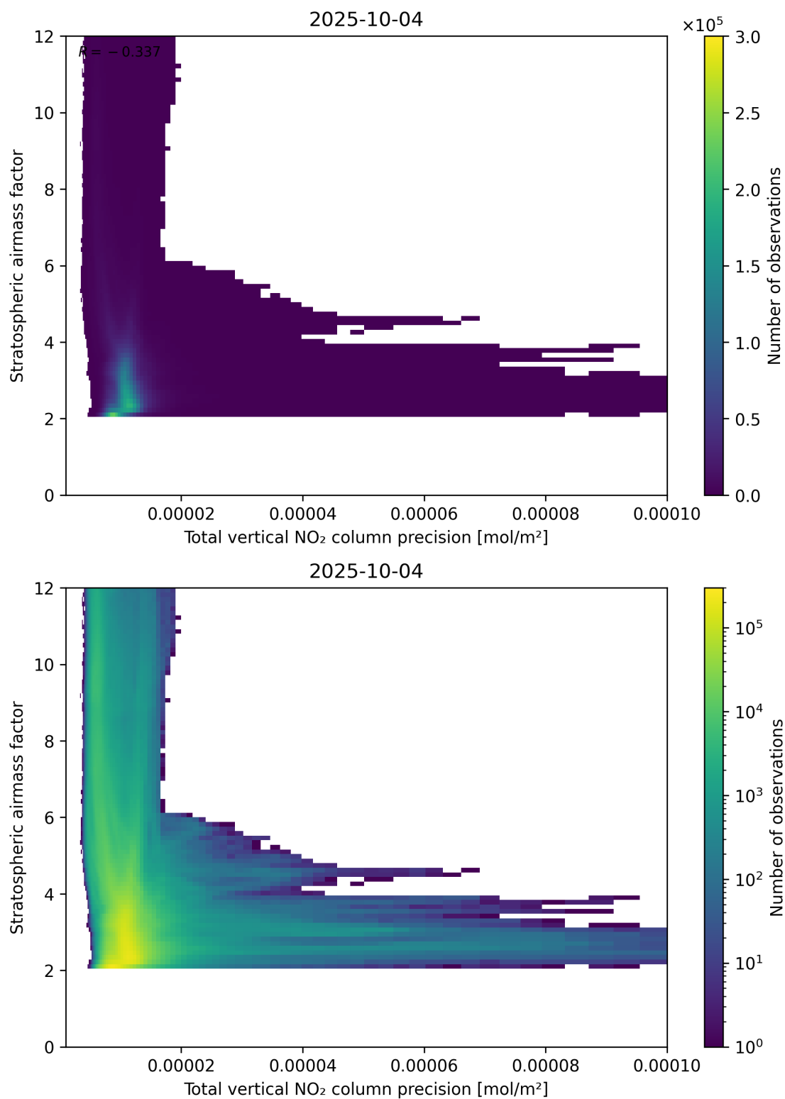
Figure 115: Scatter density plot of “Total vertical NO 2 column precision” against “Stratospheric airmass factor” for 2025-10-03 to 2025-10-05.
