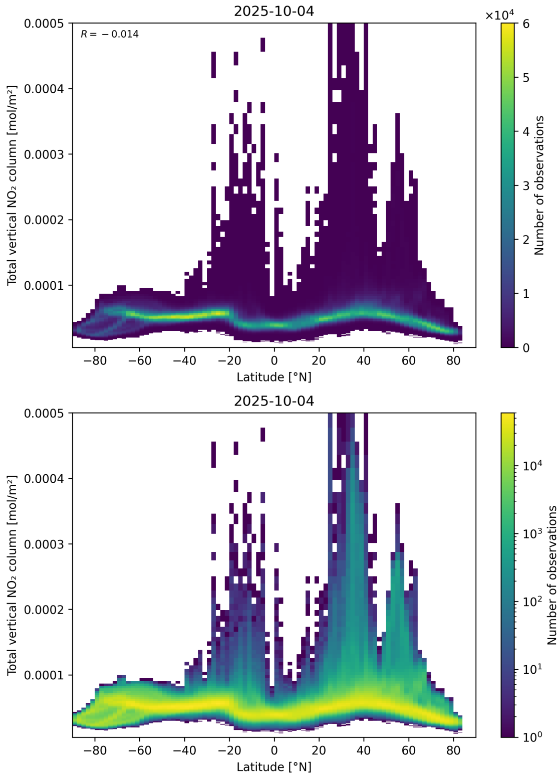
Figure 90: Scatter density plot of “Latitude” against “Total vertical NO 2 column” for 2025-10-03 to 2025-10-05.
