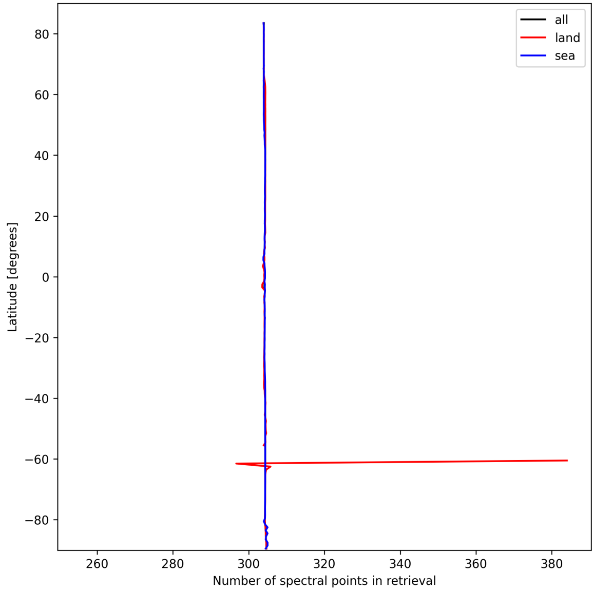
Figure 16: Zonal average of “Number of spectral points in retrieval” for 2025-10-03 to 2025-10-05.
