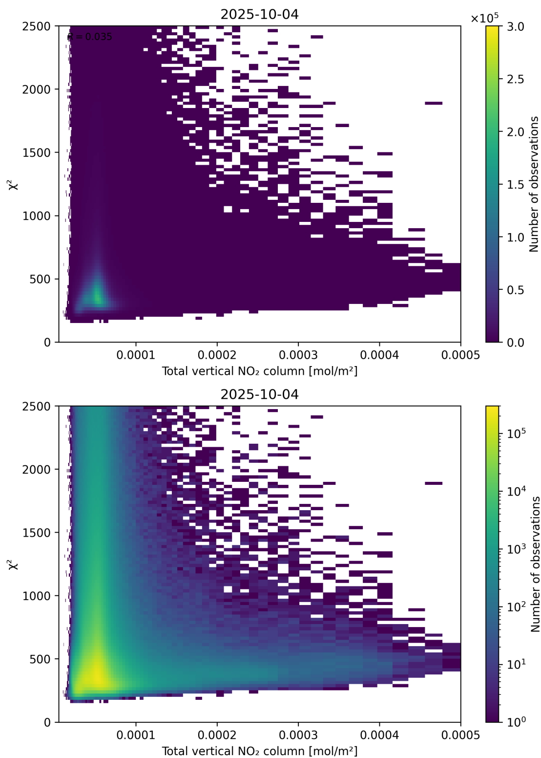
Figure 111: Scatter density plot of “Total vertical NO 2 column” against “ \chi^2 ” for 2025-10-03 to 2025-10-05.
