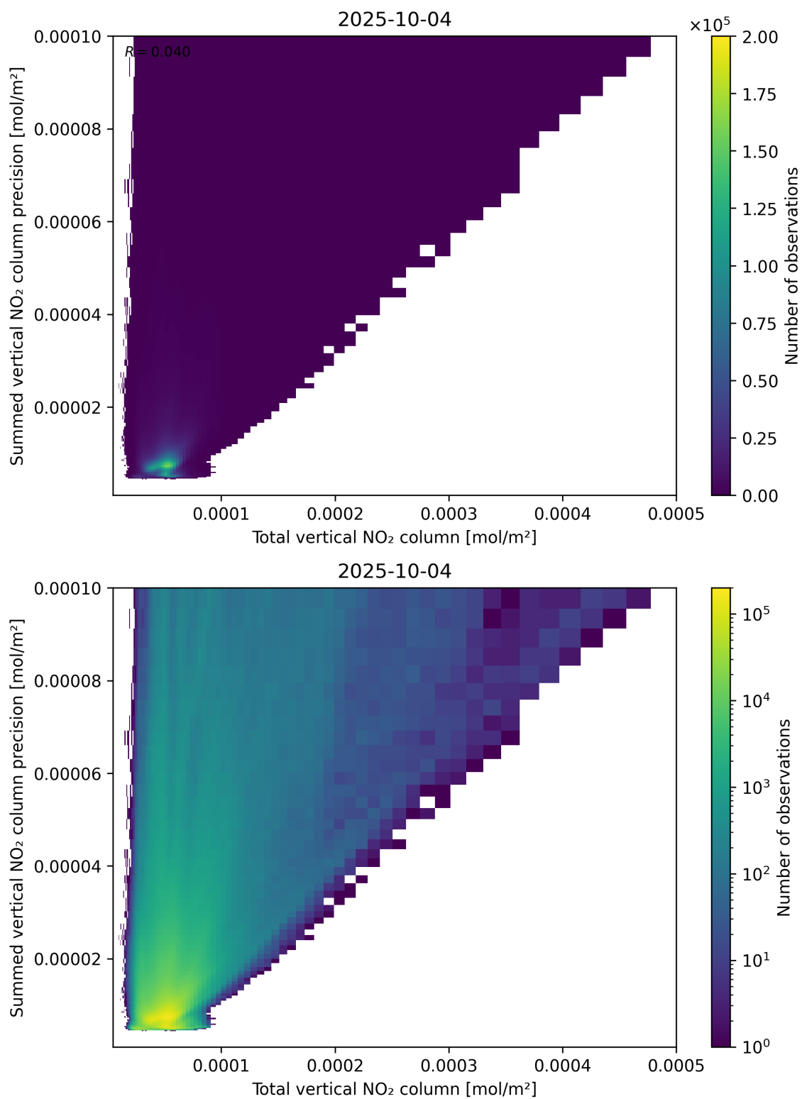
Figure 113: Scatter density plot of “Total vertical NO 2 column” against “Summed vertical NO 2 column precision” for 2025-10-03 to 2025-10-05.
