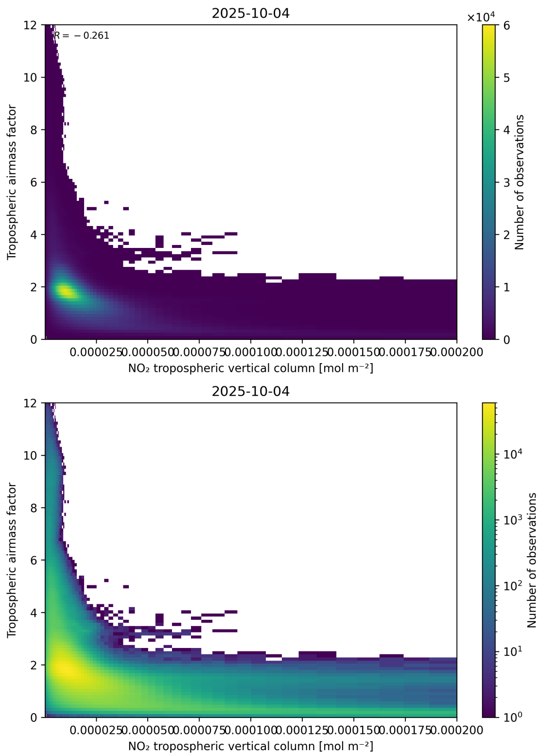
Figure 123: Scatter density plot of “NO 2 tropospheric vertical column” against “Tropospheric air mass factor” for 2025-10-03 to 2025-10-05.
