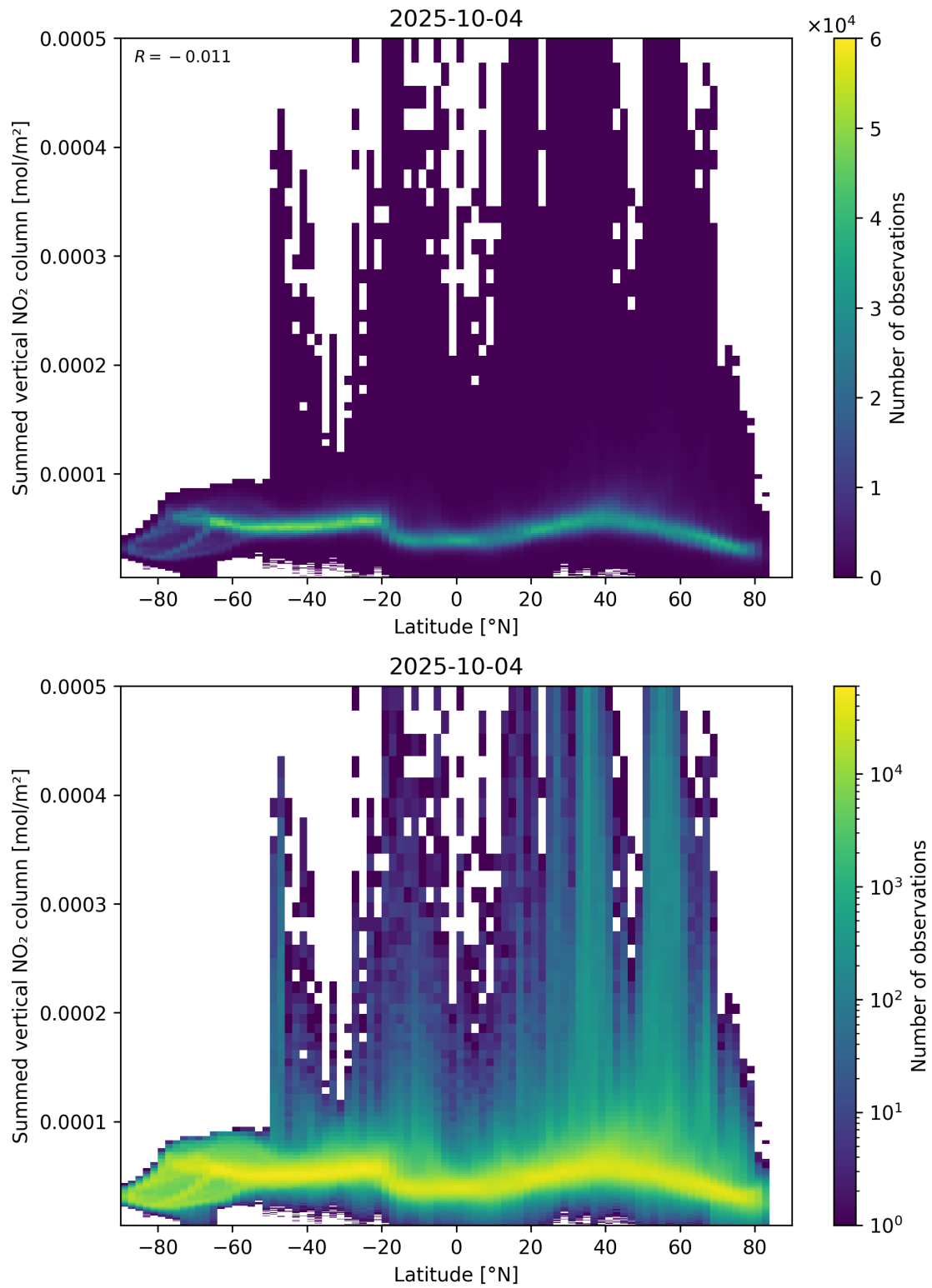
Figure 88: Scatter density plot of “Latitude” against “Summed vertical NO 2 column” for 2025-10-03 to 2025-10-05.
