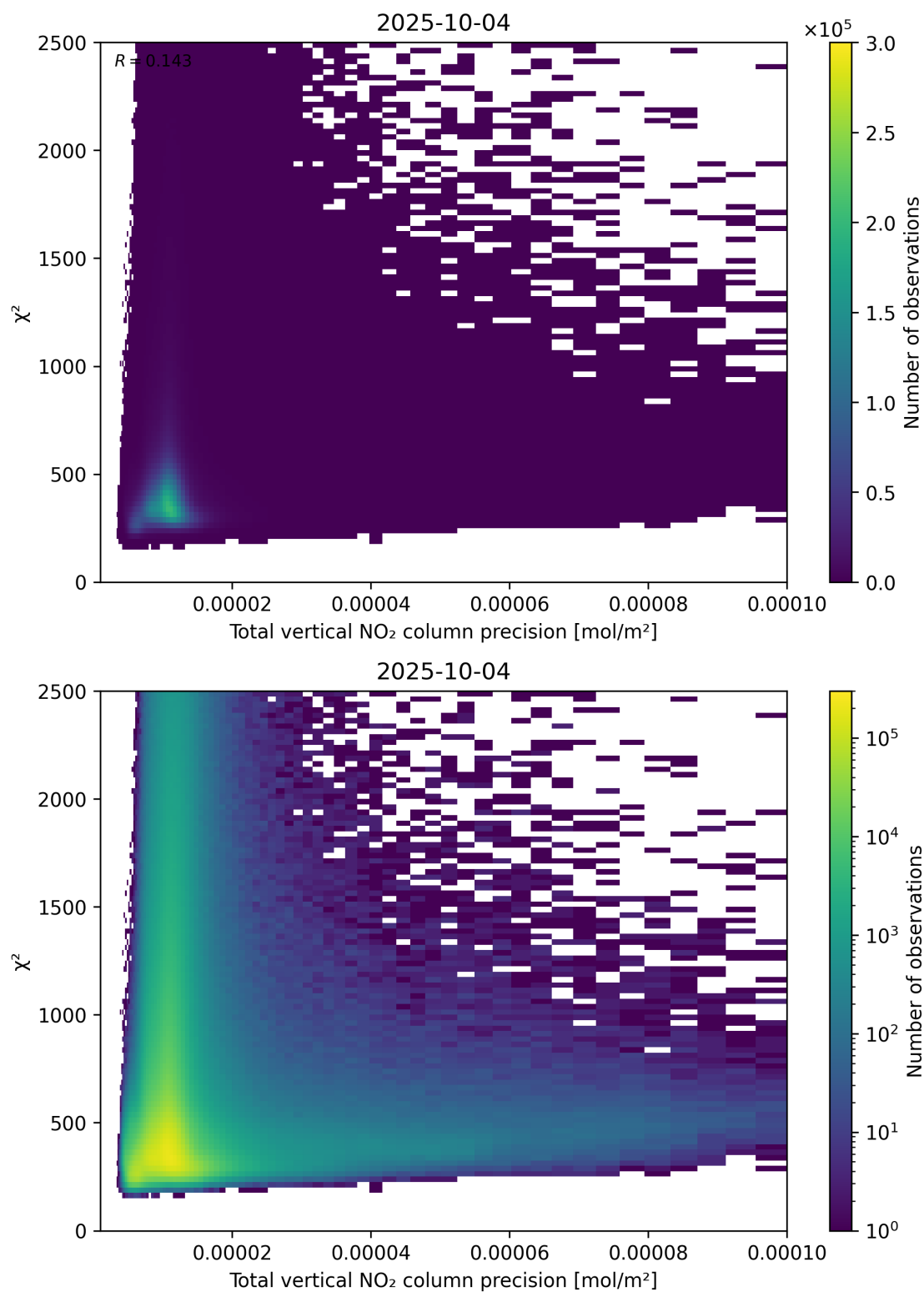
Figure 116: Scatter density plot of “Total vertical NO 2 column precision” against “ \chi^2 ” for 2025-10-03 to 2025-10-05.
