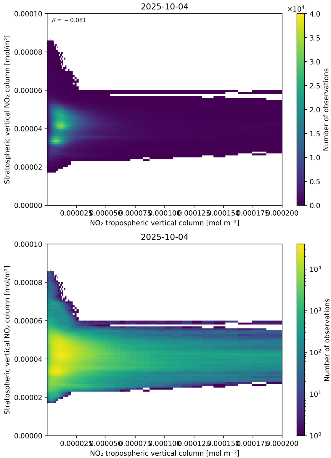
Figure 125: Scatter density plot of “NO 2 tropospheric vertical column” against “Stratospheric vertical NO 2 column” for 2025-10-03 to 2025-10-05.
