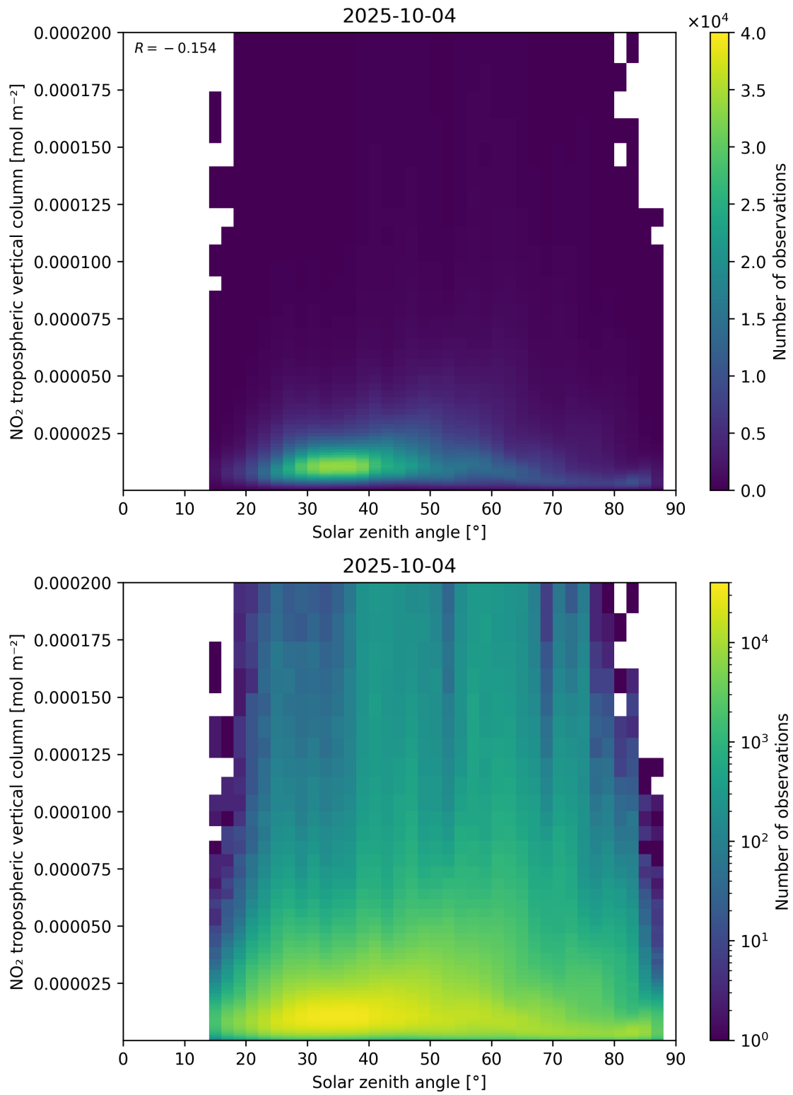
Figure 155: Scatter density plot of “Solar zenith angle” against “NO 2 tropospheric vertical column” for 2025-10-03 to 2025-10-05.
