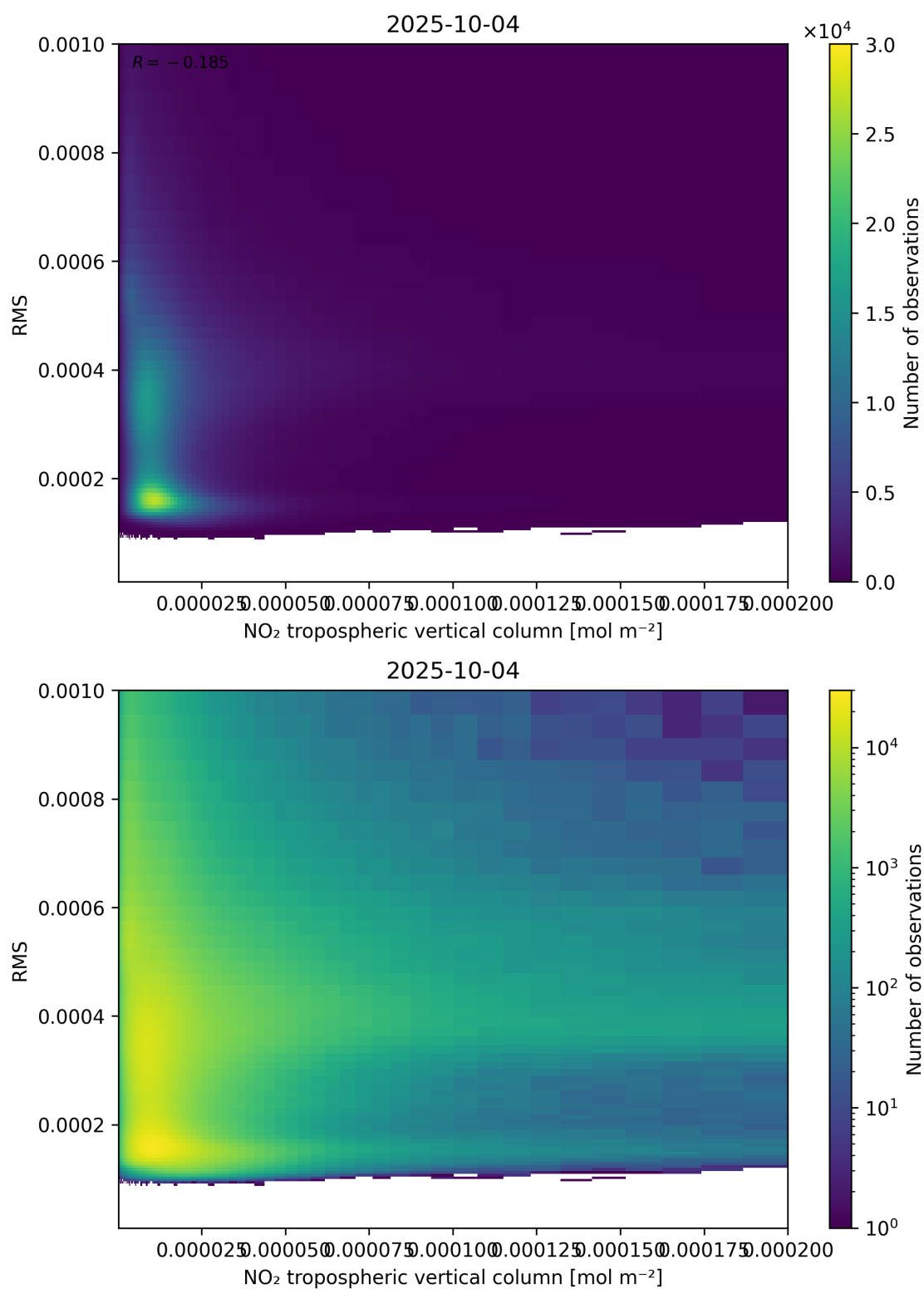
Figure 142: Scatter density plot of “NO 2 tropospheric vertical column” against “RMS” for 2025-10-03 to 2025-10-05.
