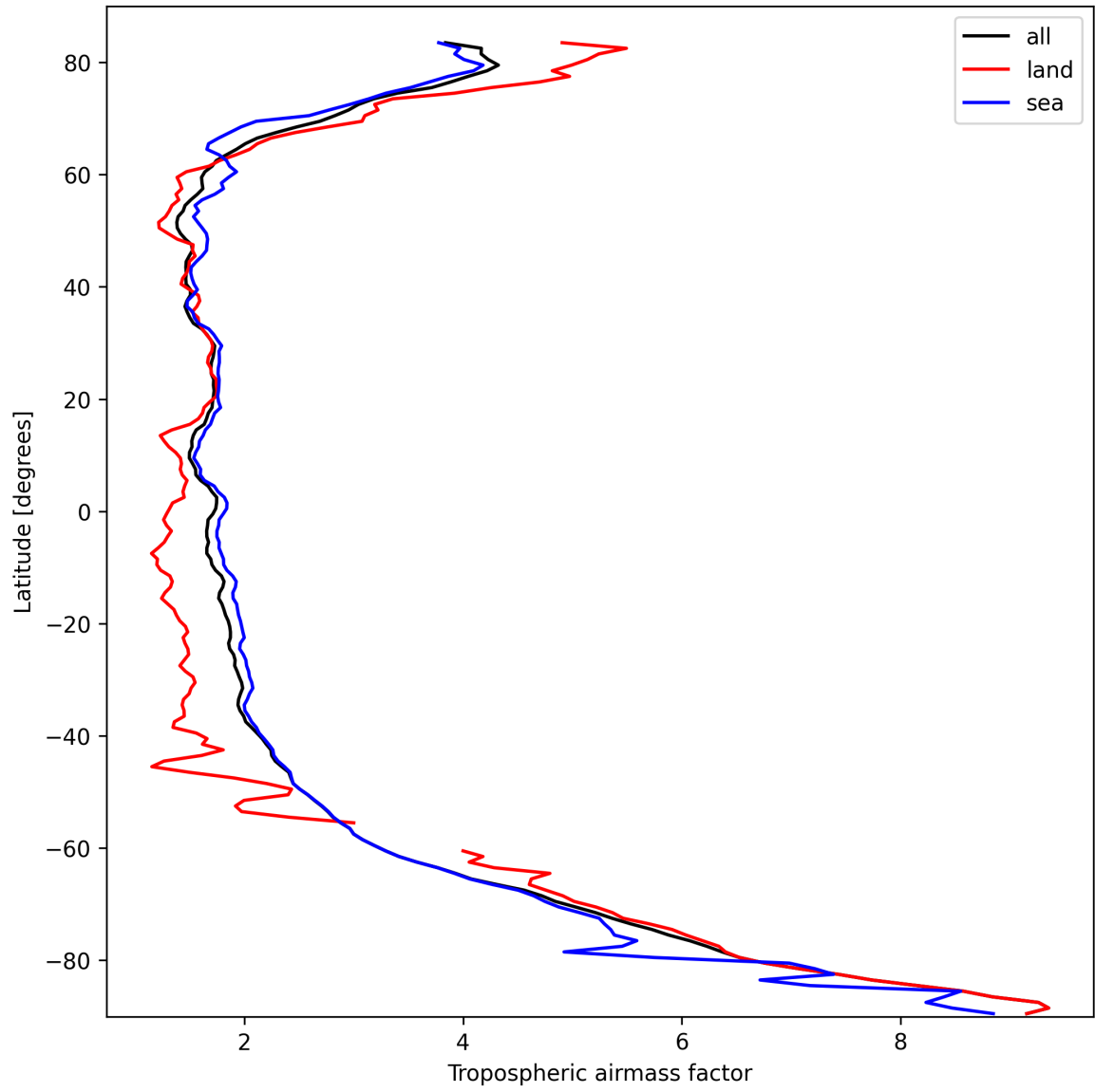
Figure 14: Zonal average of “Tropospheric air mass factor” for 2025-10-03 to 2025-10-05.
