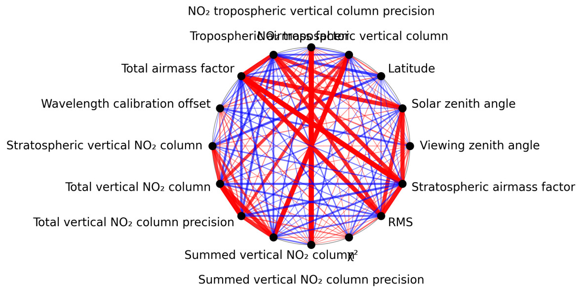
Figure 1: Map of correlation graph for 2025-10-03 to 2025-10-05.
