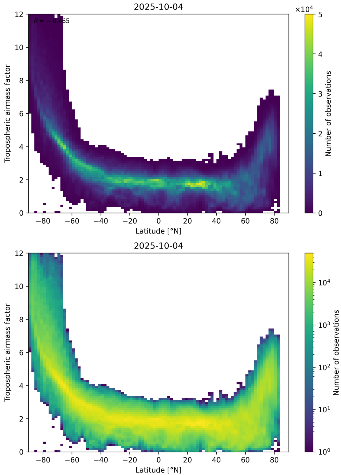
Figure 85: Scatter density plot of “Latitude” against “Tropospheric airmass factor” for 2025-10-03 to 2025-10-05.
