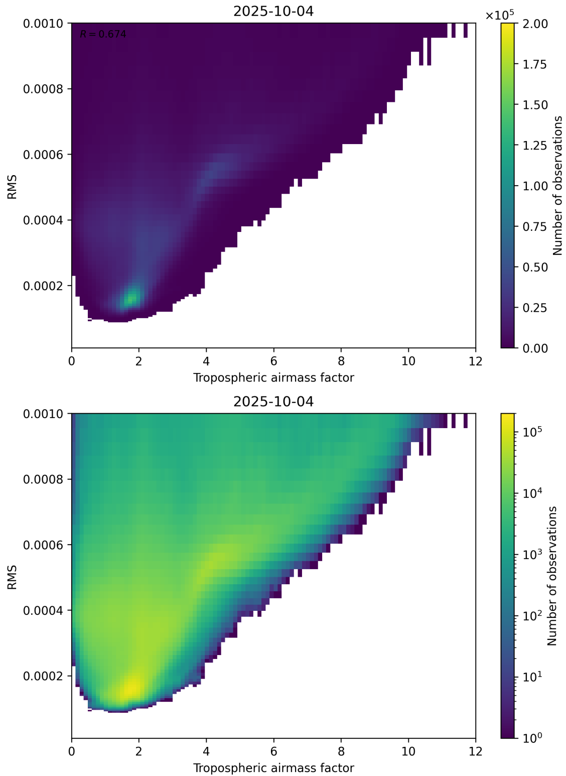
Figure 79: Scatter density plot of “Tropospheric airmass factor” against “RMS” for 2025-10-03 to 2025-10-05.
