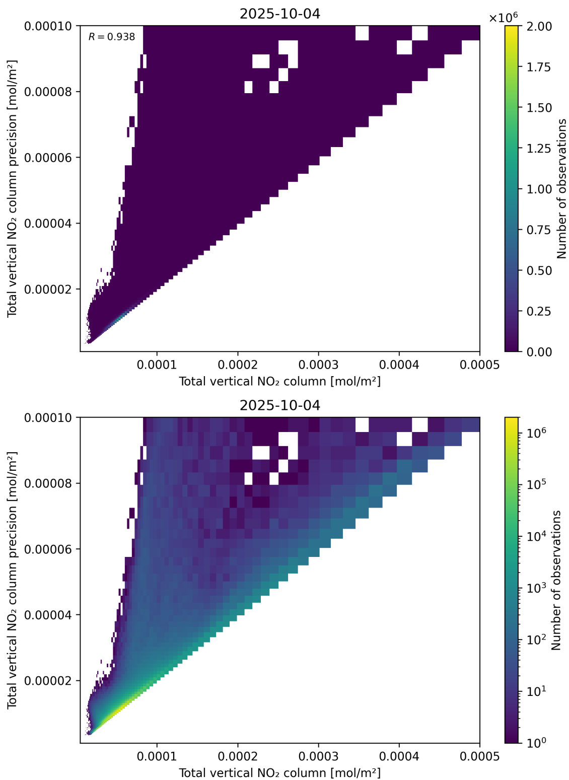
Figure 114: Scatter density plot of “Total vertical NO 2 column” against “Total vertical NO 2 column precision” for 2025-10-03 to 2025-10-05.
