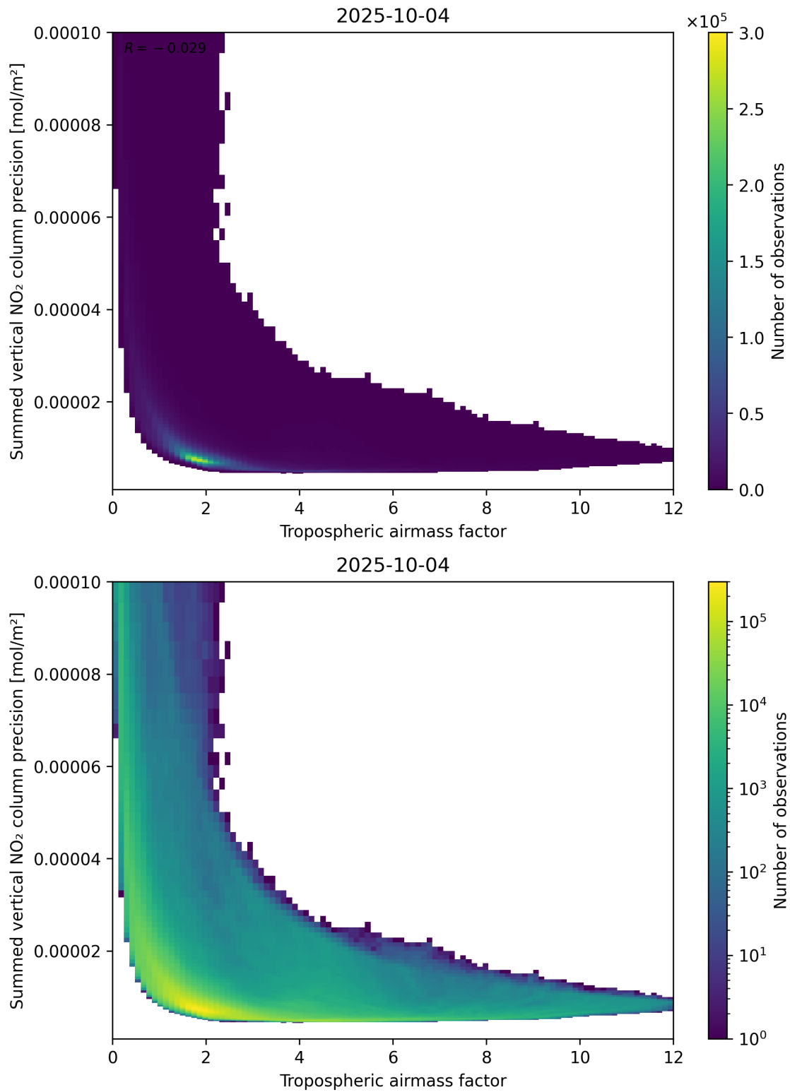
Figure 76: Scatter density plot of “Tropospheric air mass factor” against “Summed vertical NO 2 column precision” for 2025-10-03 to 2025-10-05.
