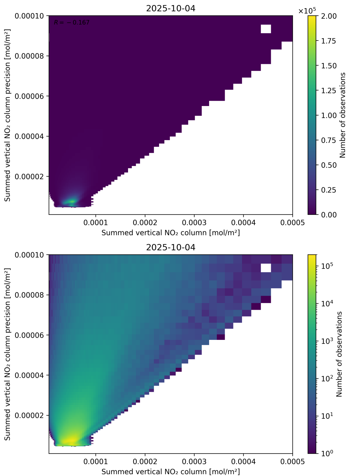
Figure 105: Scatter density plot of “Summed vertical NO 2 column” against “Summed vertical NO 2 column precision” for 2025-10-03 to 2025-10-05.
