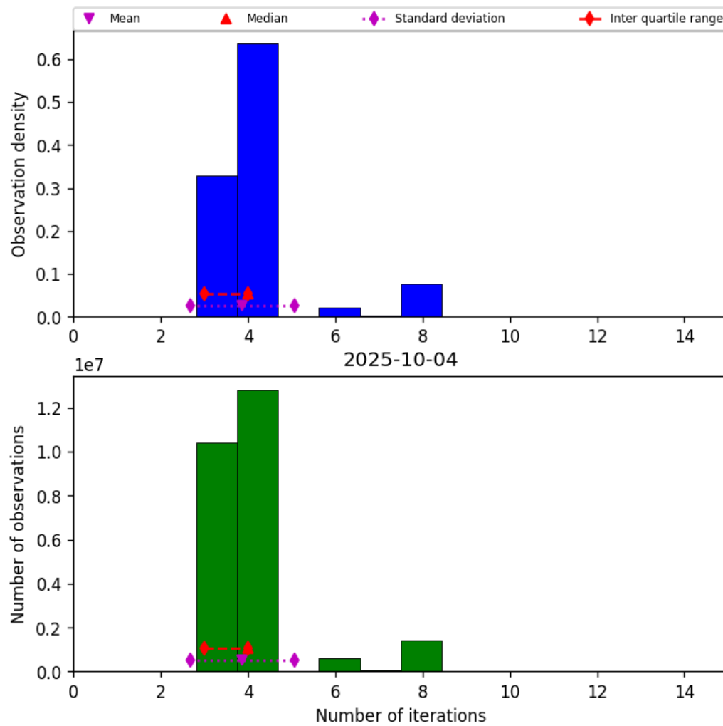
Figure 34: Histogram of “Number of iterations” for 2025-10-03 to 2025-10-05
