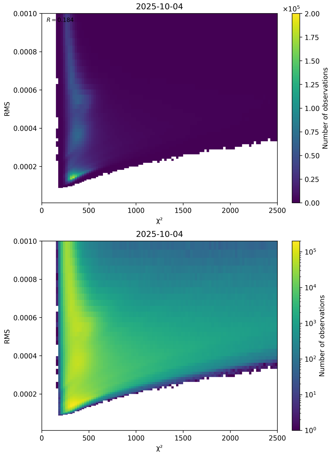
Figure 82: Scatter density plot of “ \chi^2 ” against “RMS” for 2025-10-03 to 2025-10-05.
