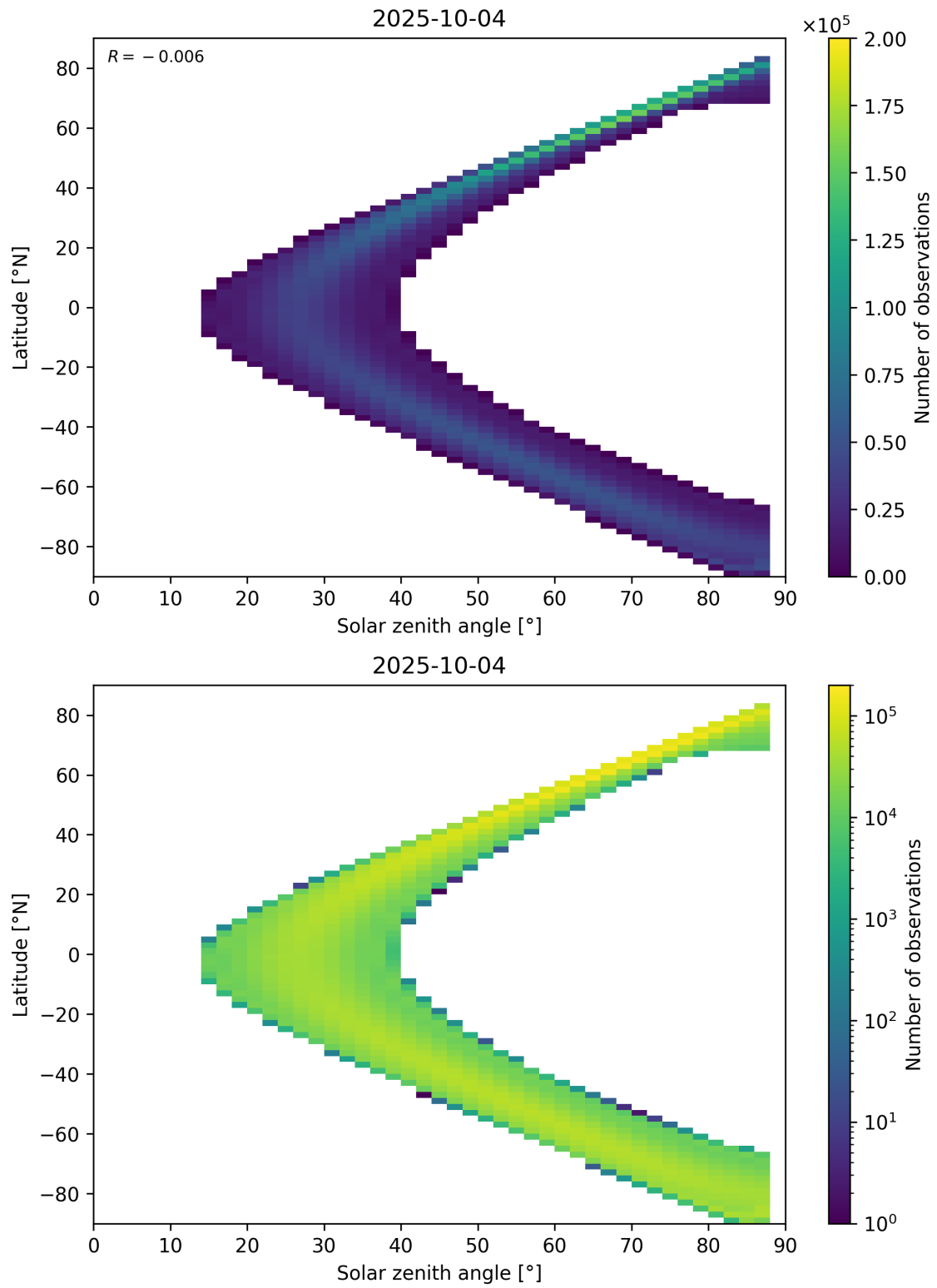
Figure 149: Scatter density plot of “Solar zenith angle” against “Latitude” for 2025-10-03 to 2025-10-05.
