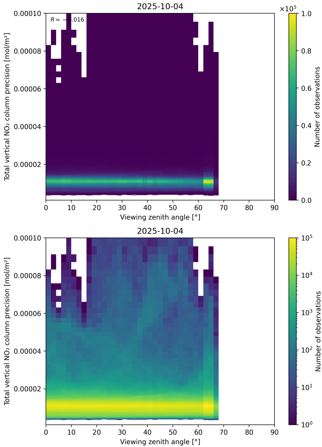
Figure 168: Scatter density plot of “Viewing zenith angle” against “Total vertical NO 2 column precision” for 2025-10-03 to 2025-10-05.
