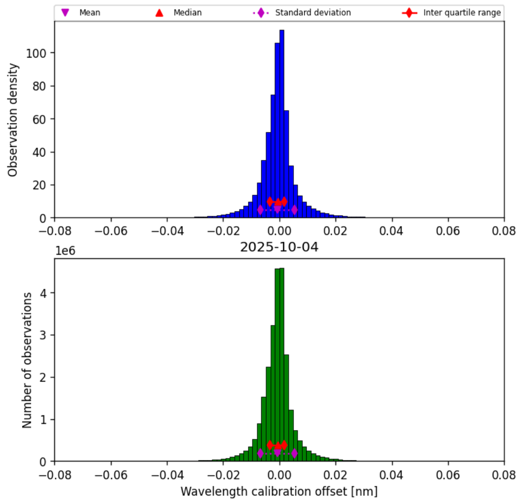
Figure 35: Histogram of “Wavelength calibration offset” for 2025-10-03 to 2025-10-05
