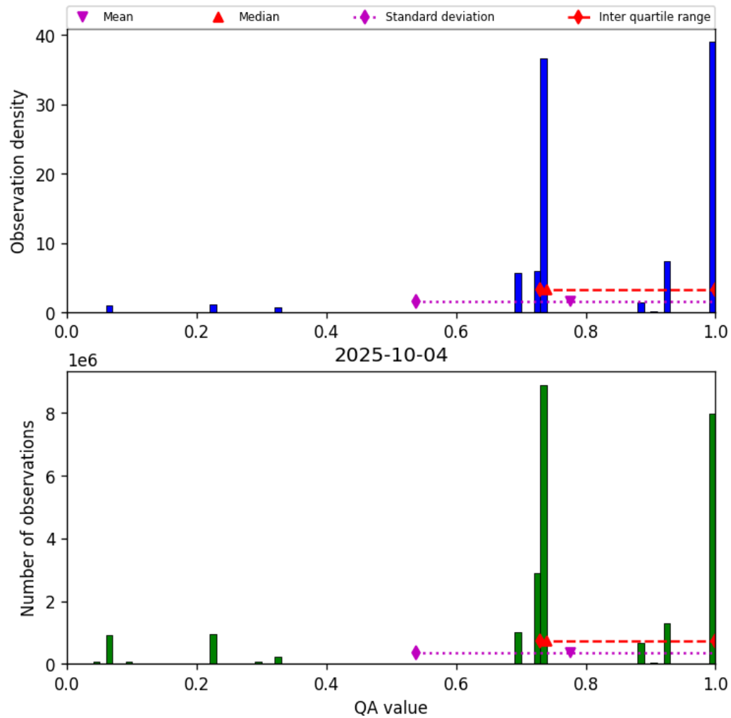
Figure 28: Histogram of “QA value” for 2025-10-03 to 2025-10-05
