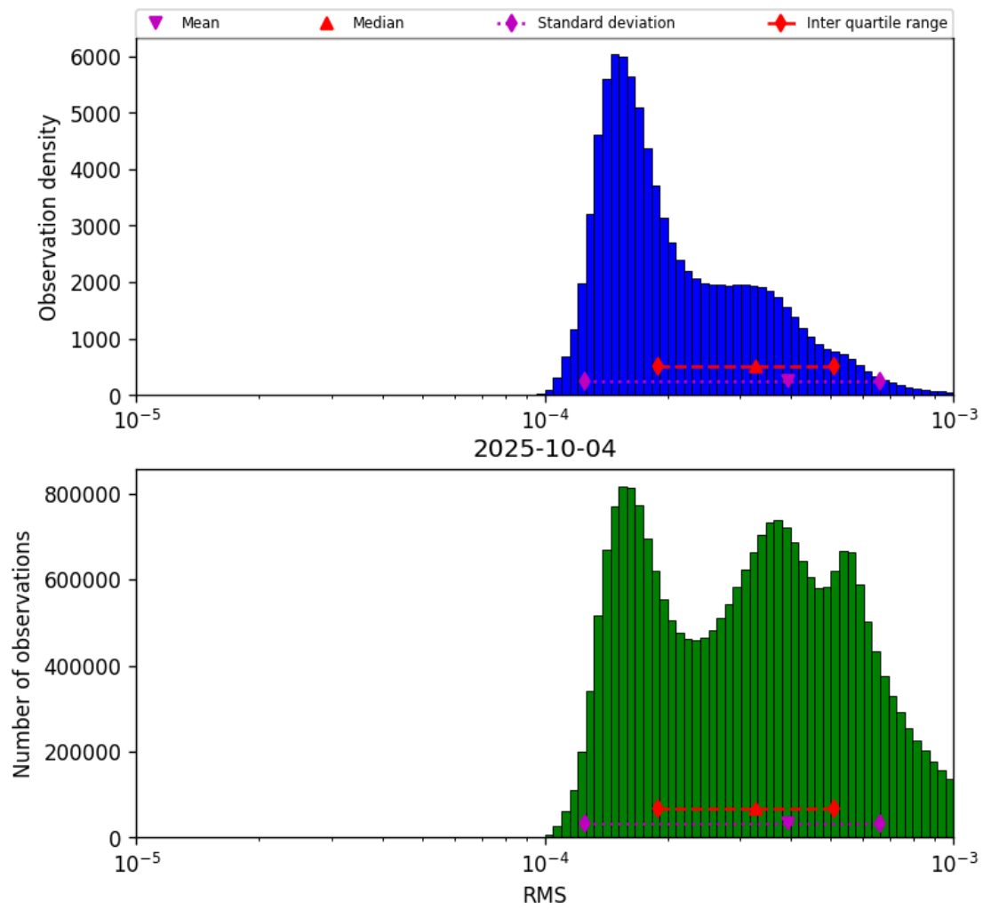
Figure 43: Histogram of “RMS” for 2025-10-03 to 2025-10-05
