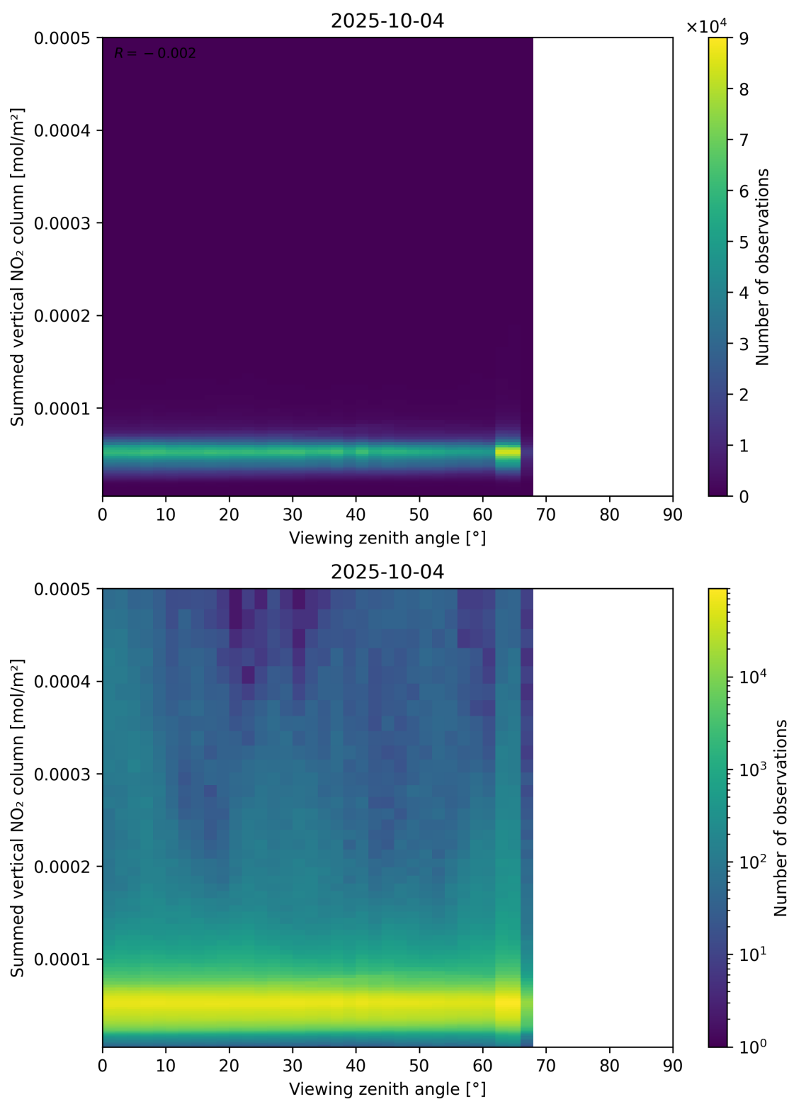
Figure 165: Scatter density plot of “Viewing zenith angle” against “Summed vertical NO 2 column” for 2025-10-03 to 2025-10-05.
