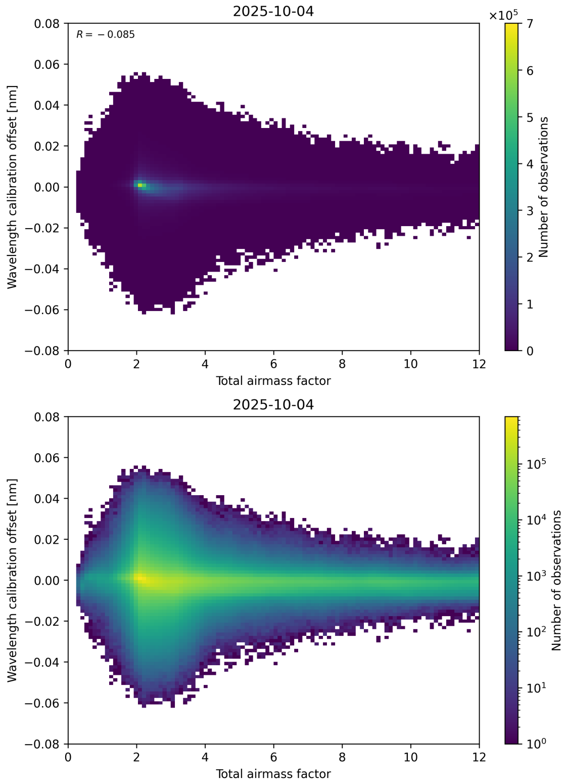
Figure 70: Scatter density plot of “Total airmass factor” against “Wavelength calibration offset” for 2025-10-03 to 2025-10-05.
