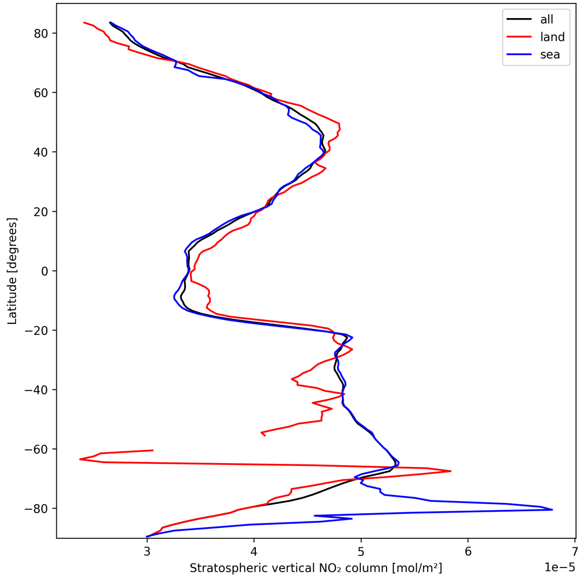
Figure 19: Zonal average of “Stratospheric vertical NO 2 column” for 2025-10-03 to 2025-10-05.
