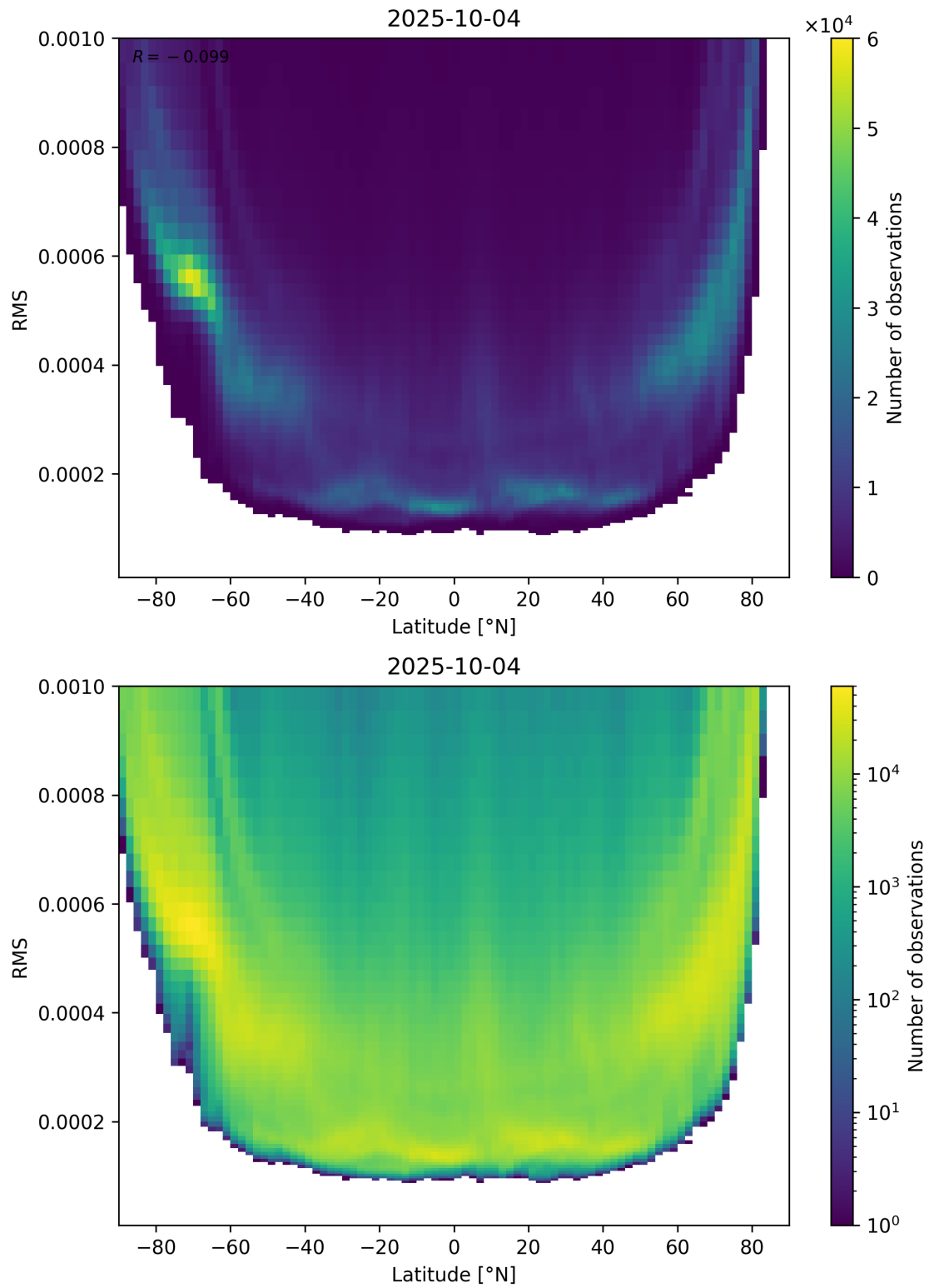
Figure 94: Scatter density plot of “Latitude” against “RMS” for 2025-10-03 to 2025-10-05.
