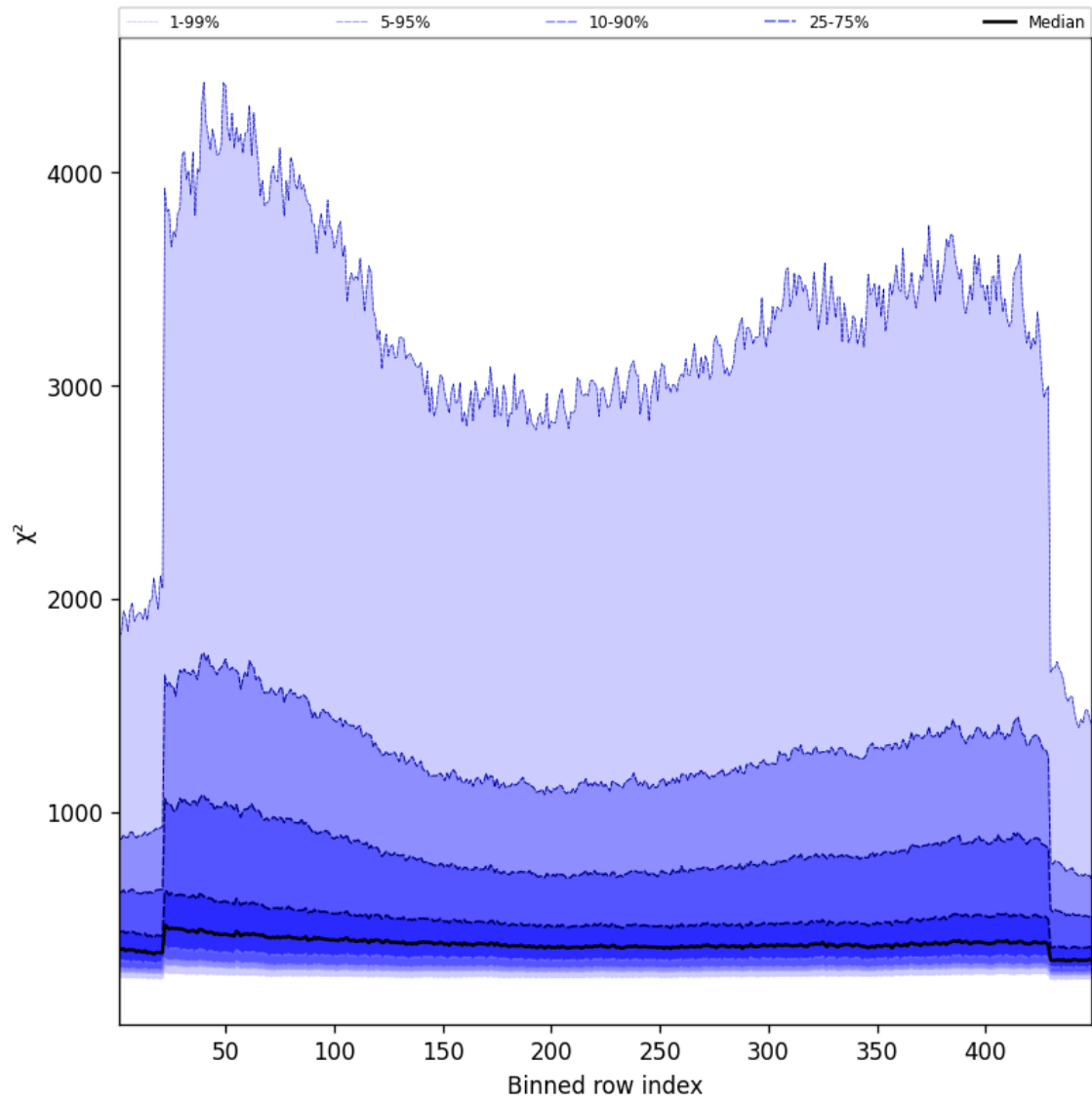
Figure 59: Along track statistics of “ \chi^2 ” for 2025-10-03 to 2025-10-05
