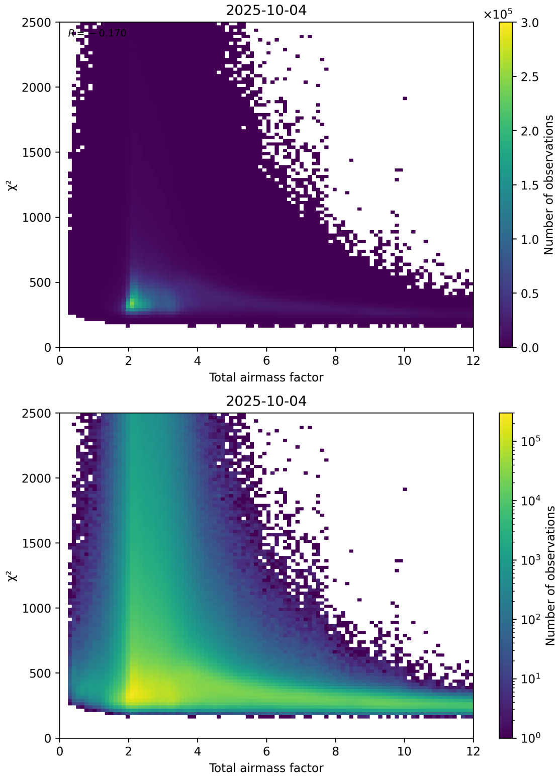
Figure 63: Scatter density plot of “Total airmass factor” against “ \chi^2 ” for 2025-10-03 to 2025-10-05.
