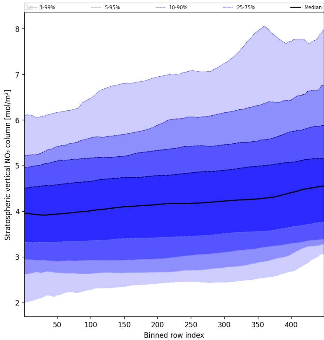
Figure 53: Along track statistics of “Stratospheric vertical NO 2 column” for 2025-10-03 to 2025-10-05
