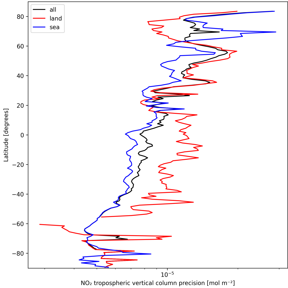
Figure 13: Zonal average of “NO 2 tropospheric vertical column precision” for 2025-10-03 to 2025-10-05.
