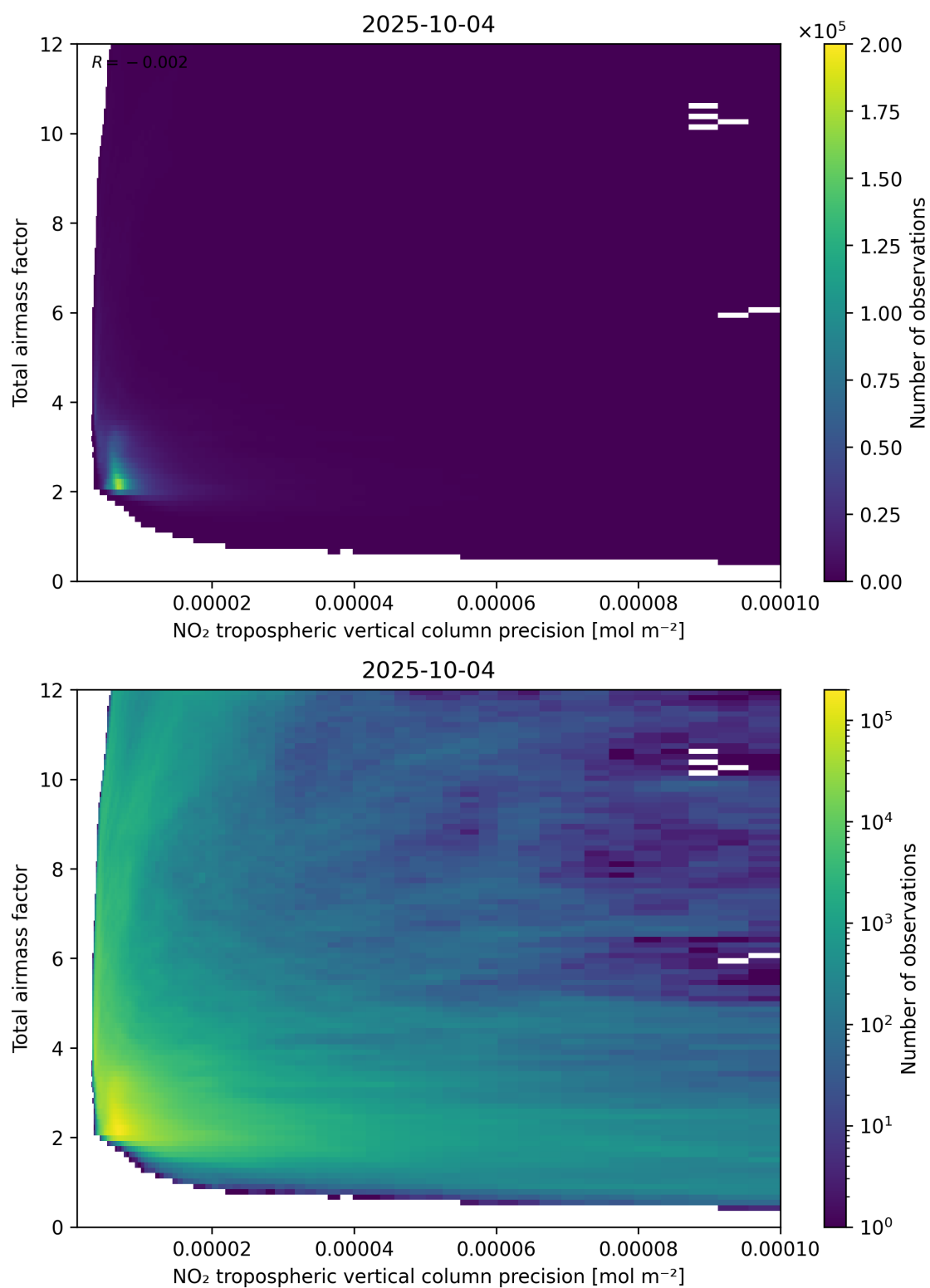
Figure 132: Scatter density plot of “NO 2 tropospheric vertical column precision” against “Total air mass factor” for 2025-10-03 to 2025-10-05.
