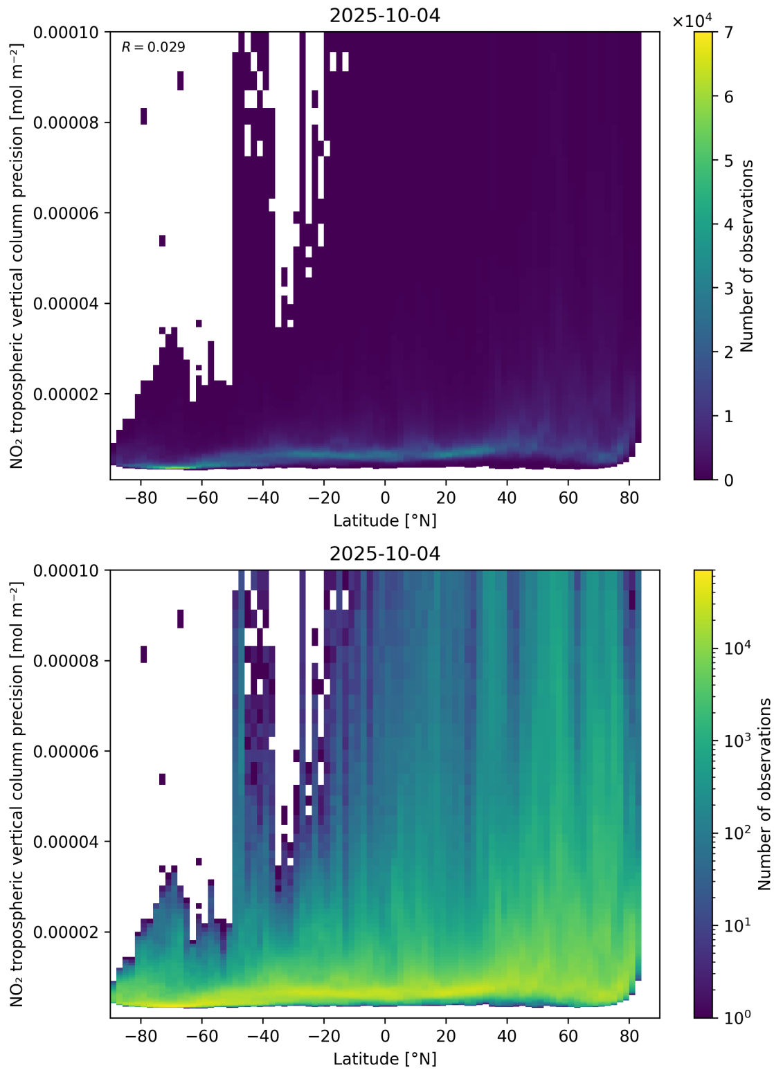
Figure 93: Scatter density plot of “Latitude” against “NO 2 tropospheric vertical column precision” for 2025-10-03 to 2025-10-05.
