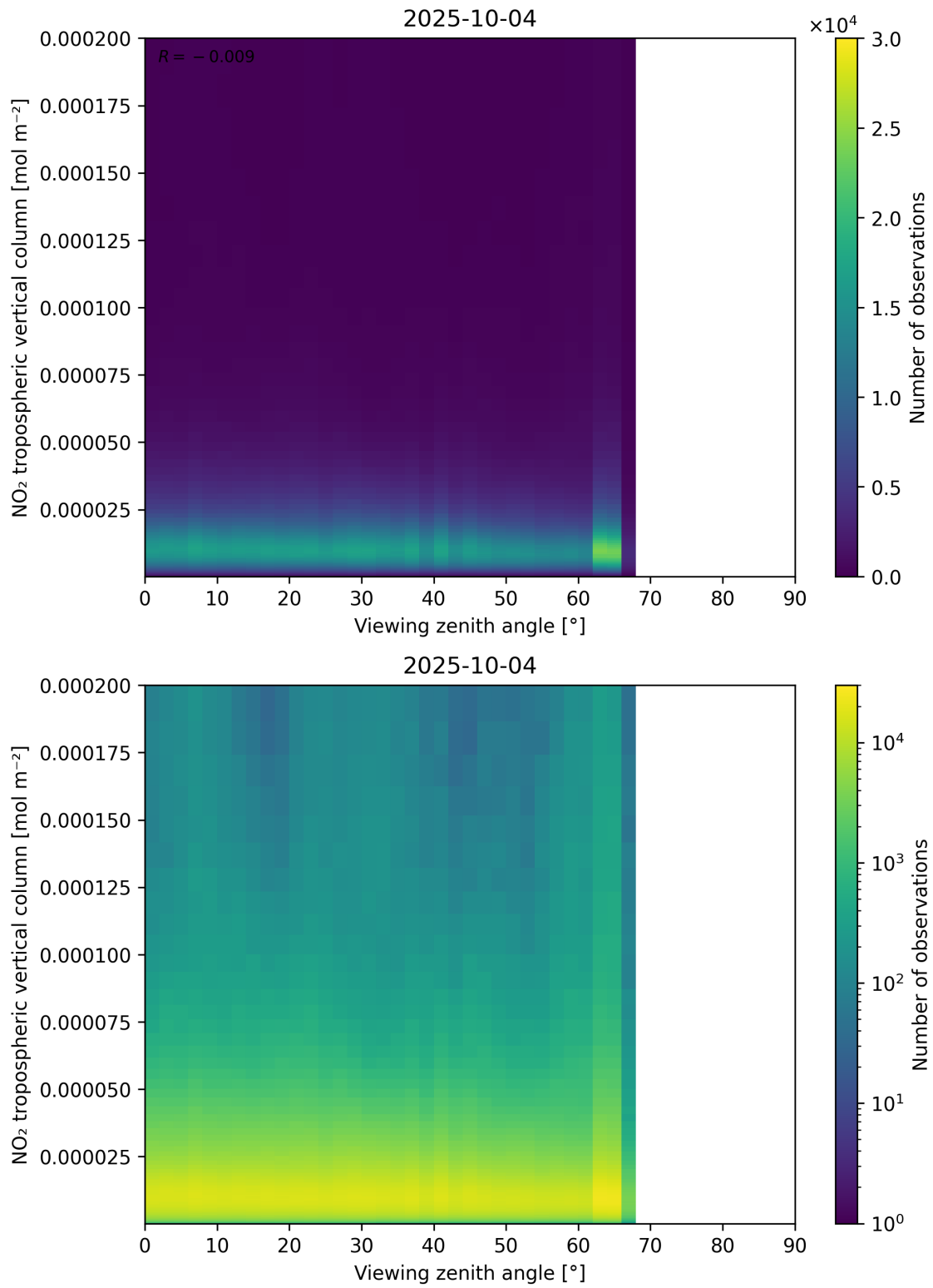
Figure 169: Scatter density plot of “Viewing zenith angle” against “NO 2 tropospheric vertical column” for 2025-10-03 to 2025-10-05.
