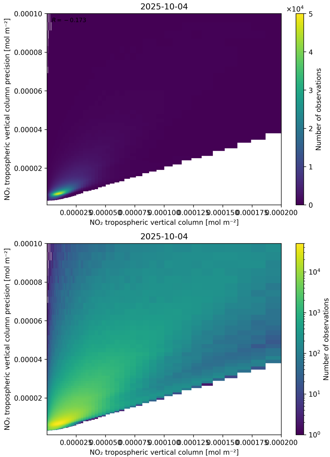
Figure 130: Scatter density plot of “NO 2 tropospheric vertical column” against “NO 2 tropospheric vertical column precision” for 2025-10-03 to 2025-10-05.
