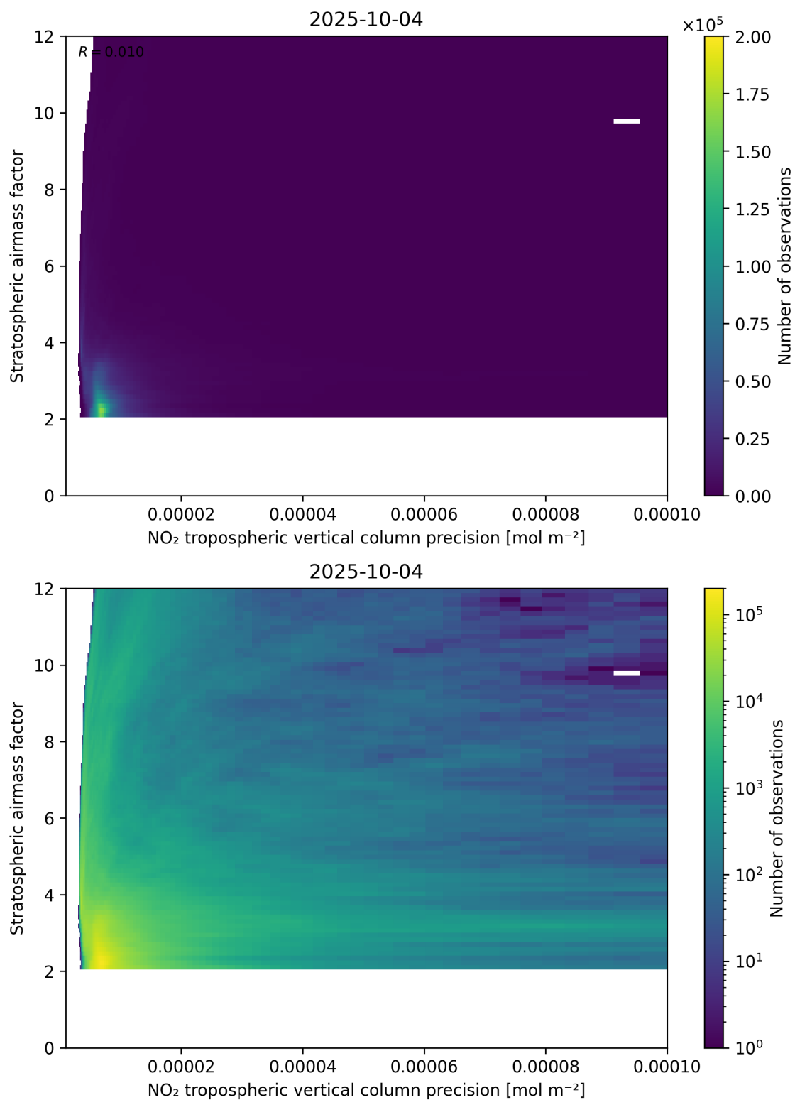
Figure 131: Scatter density plot of “NO 2 tropospheric vertical column precision” against “Stratospheric airmass factor” for 2025-10-03 to 2025-10-05.
