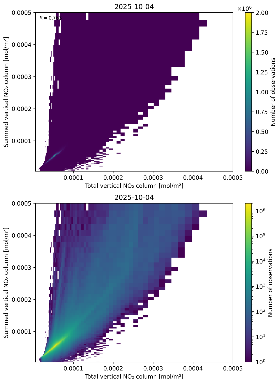
Figure 112: Scatter density plot of “Total vertical NO 2 column” against “Summed vertical NO 2 column” for 2025-10-03 to 2025-10-05.
