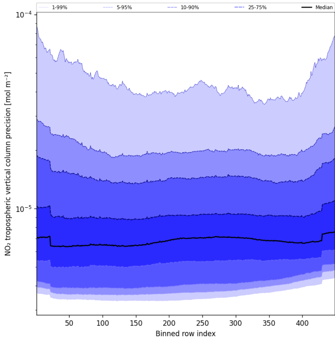
Figure 47: Along track statistics of “NO 2 tropospheric vertical column precision” for 2025-10-03 to 2025-10-05
