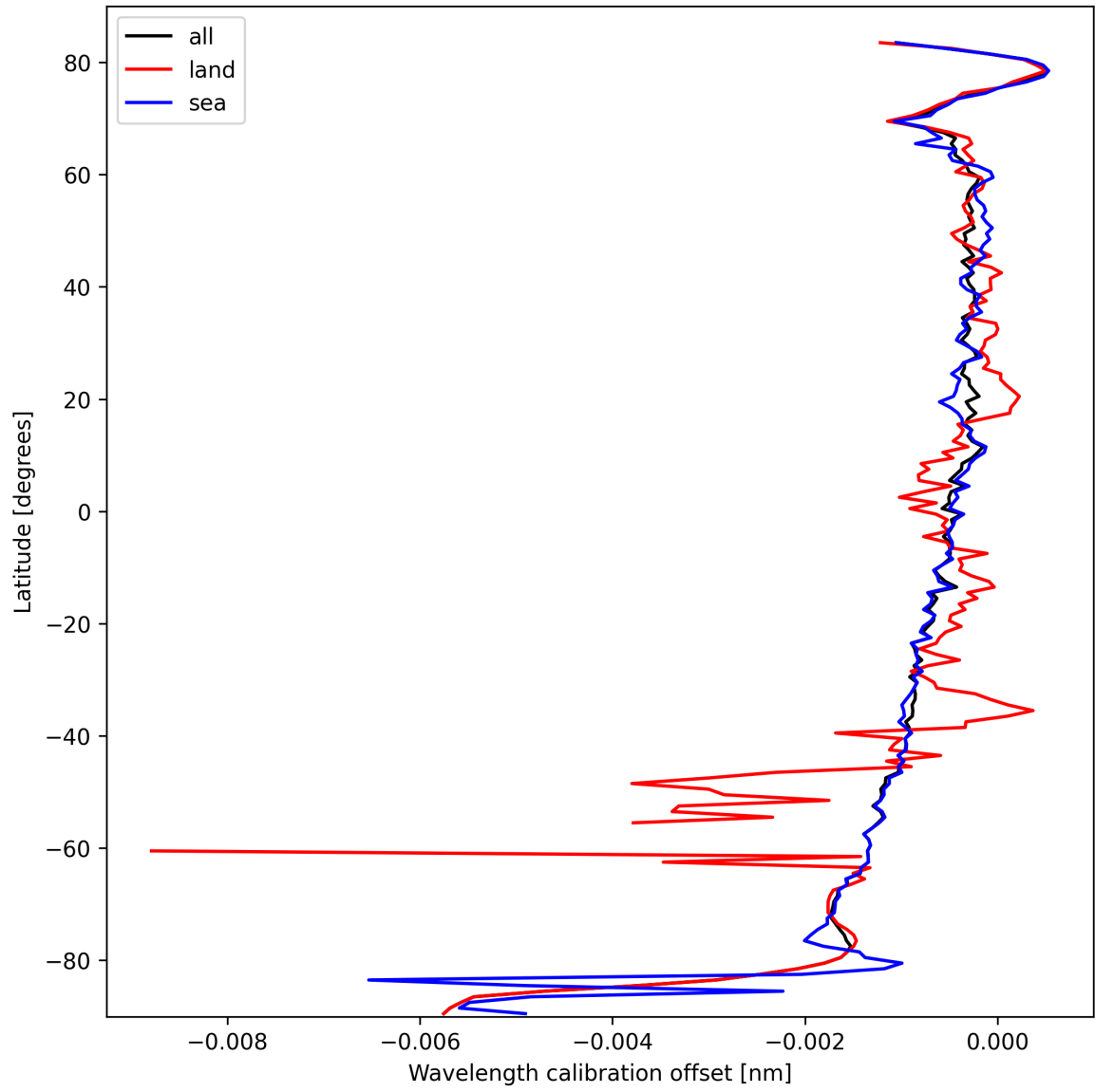
Figure 18: Zonal average of “Wavelength calibration offset” for 2025-10-03 to 2025-10-05.
