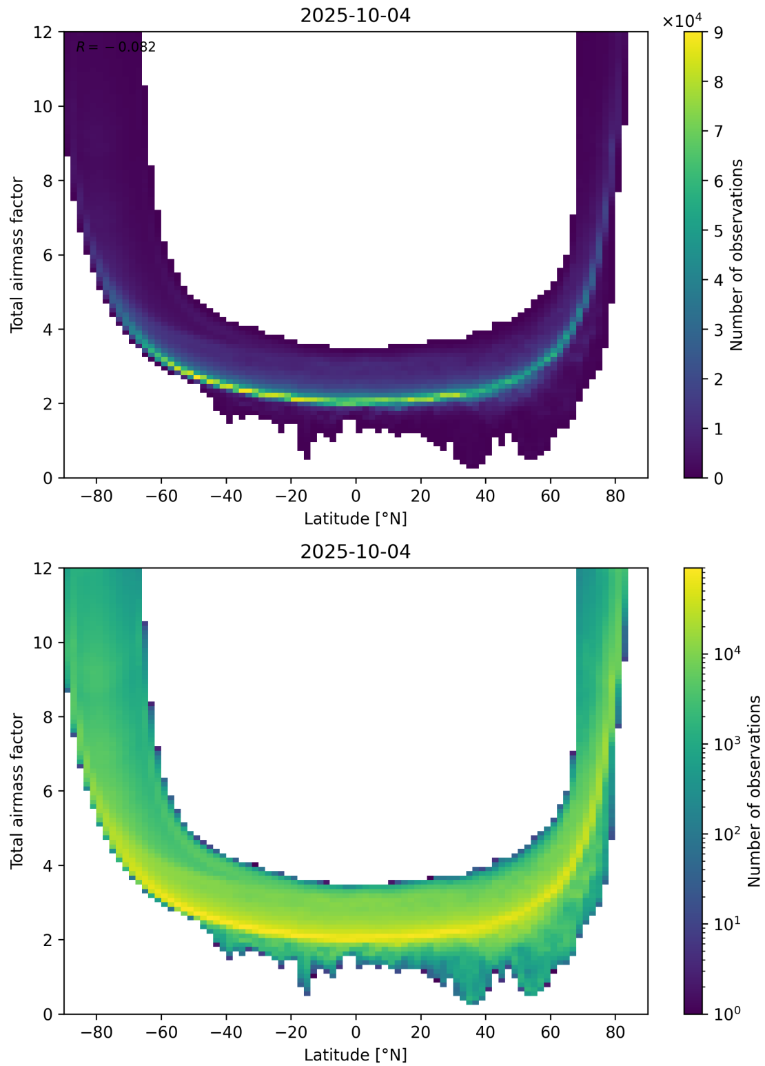
Figure 84: Scatter density plot of “Latitude” against “Total airmass factor” for 2025-10-03 to 2025-10-05.
