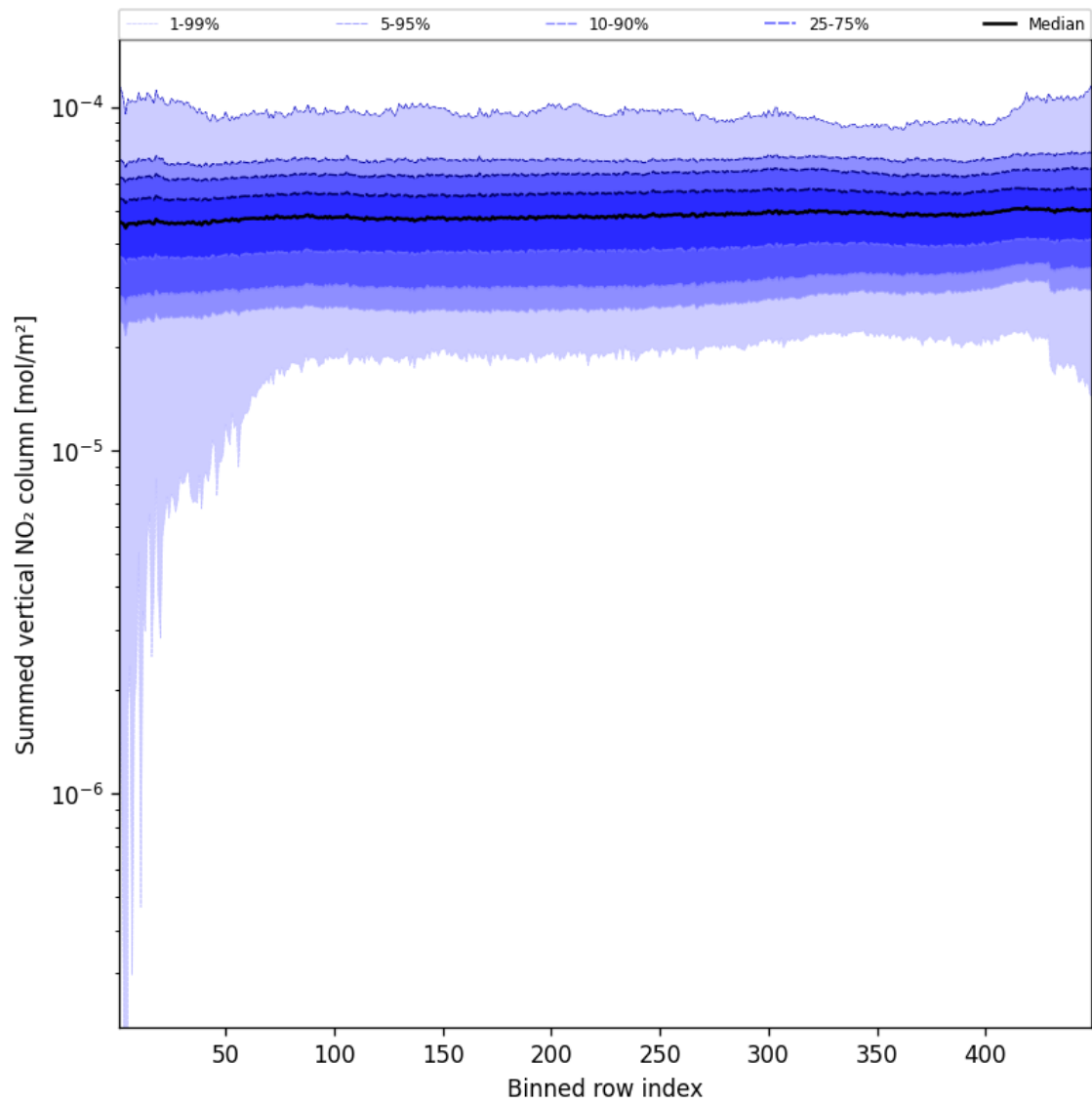
Figure 57: Along track statistics of “Summed vertical NO 2 column” for 2025-10-03 to 2025-10-05
