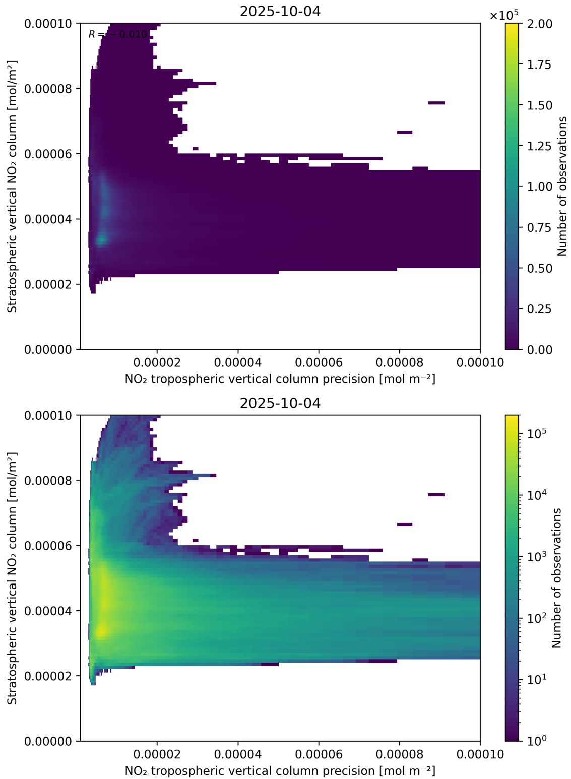
Figure 135: Scatter density plot of “NO 2 tropospheric vertical column precision” against “Stratospheric vertical NO 2 column” for 2025-10-03 to 2025-10-05.
