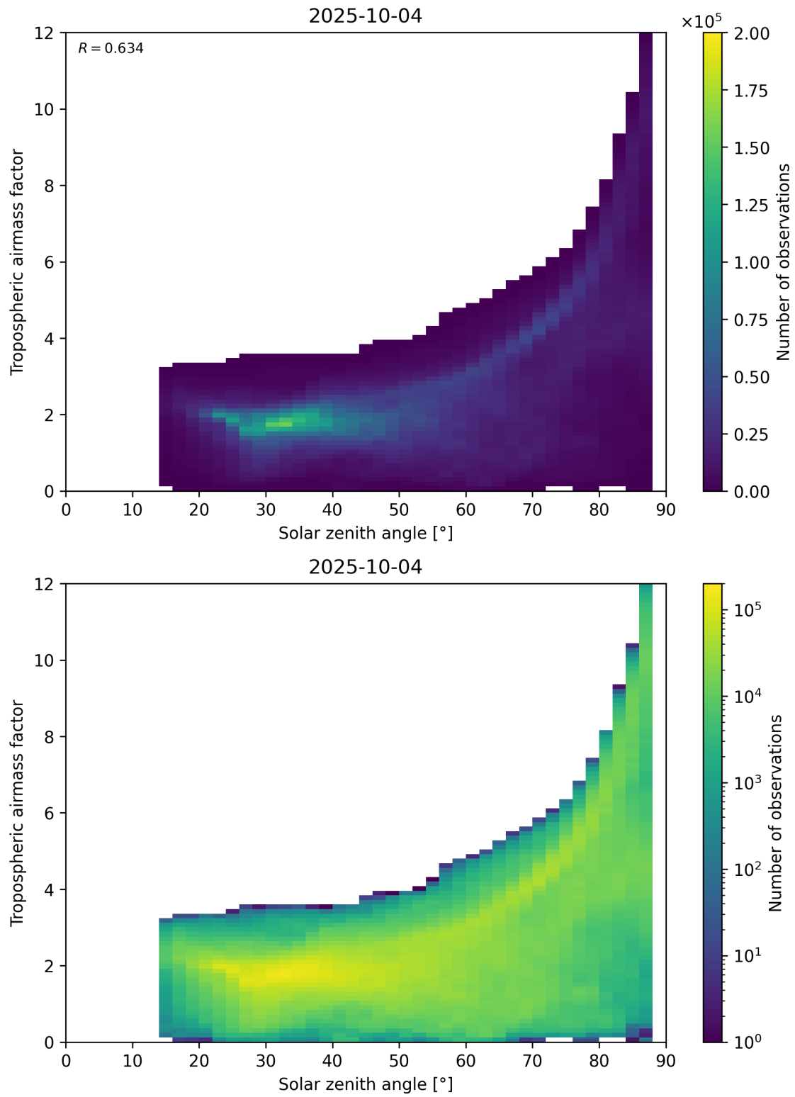
Figure 147: Scatter density plot of “Solar zenith angle” against “Tropospheric airmass factor” for 2025-10-03 to 2025-10-05.
