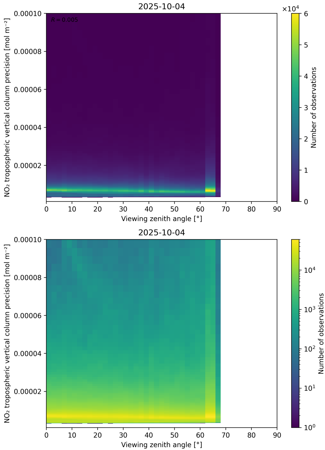
Figure 170: Scatter density plot of “Viewing zenith angle” against “NO 2 tropospheric vertical column precision” for 2025-10-03 to 2025-10-05.
