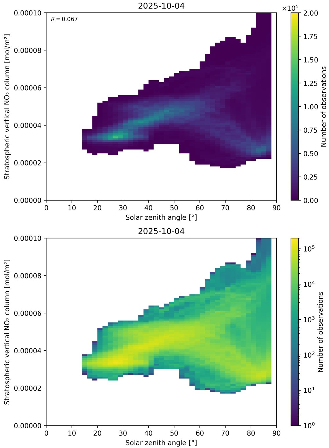
Figure 150: Scatter density plot of “Solar zenith angle” against “Stratospheric vertical NO 2 column” for 2025-10-03 to 2025-10-05.
