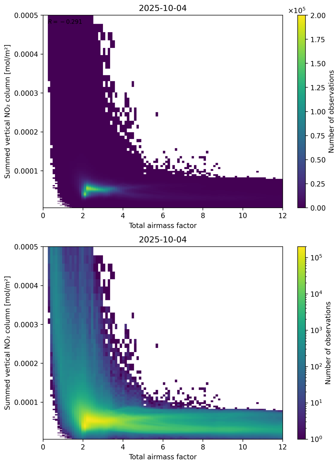
Figure 65: Scatter density plot of “Total airmass factor” against “Summed vertical NO 2 column” for 2025-10-03 to 2025-10-05.
