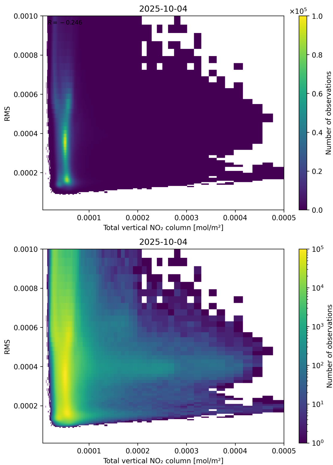
Figure 120: Scatter density plot of “Total vertical NO 2 column” against “RMS” for 2025-10-03 to 2025-10-05.
