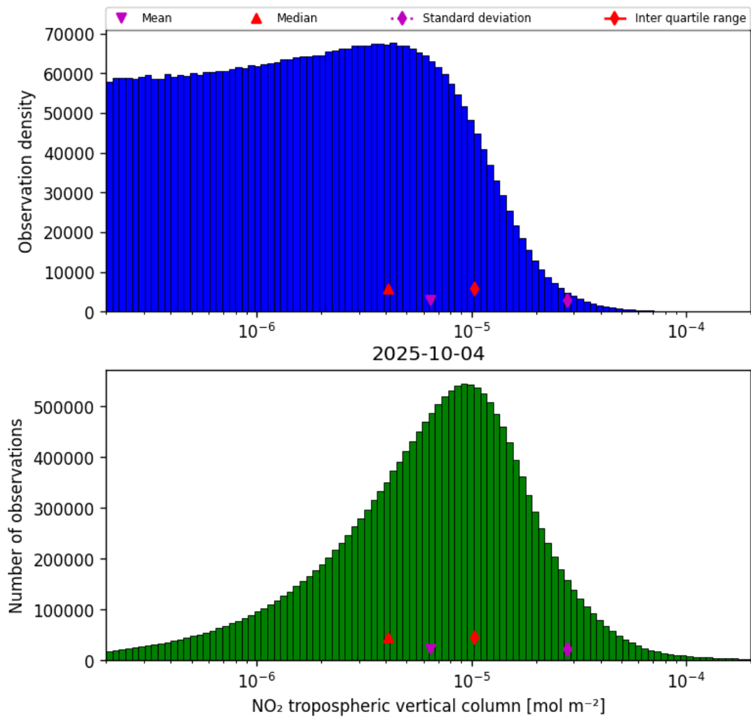
Figure 29: Histogram of “NO 2 tropospheric vertical column” for 2025-10-03 to 2025-10-05
