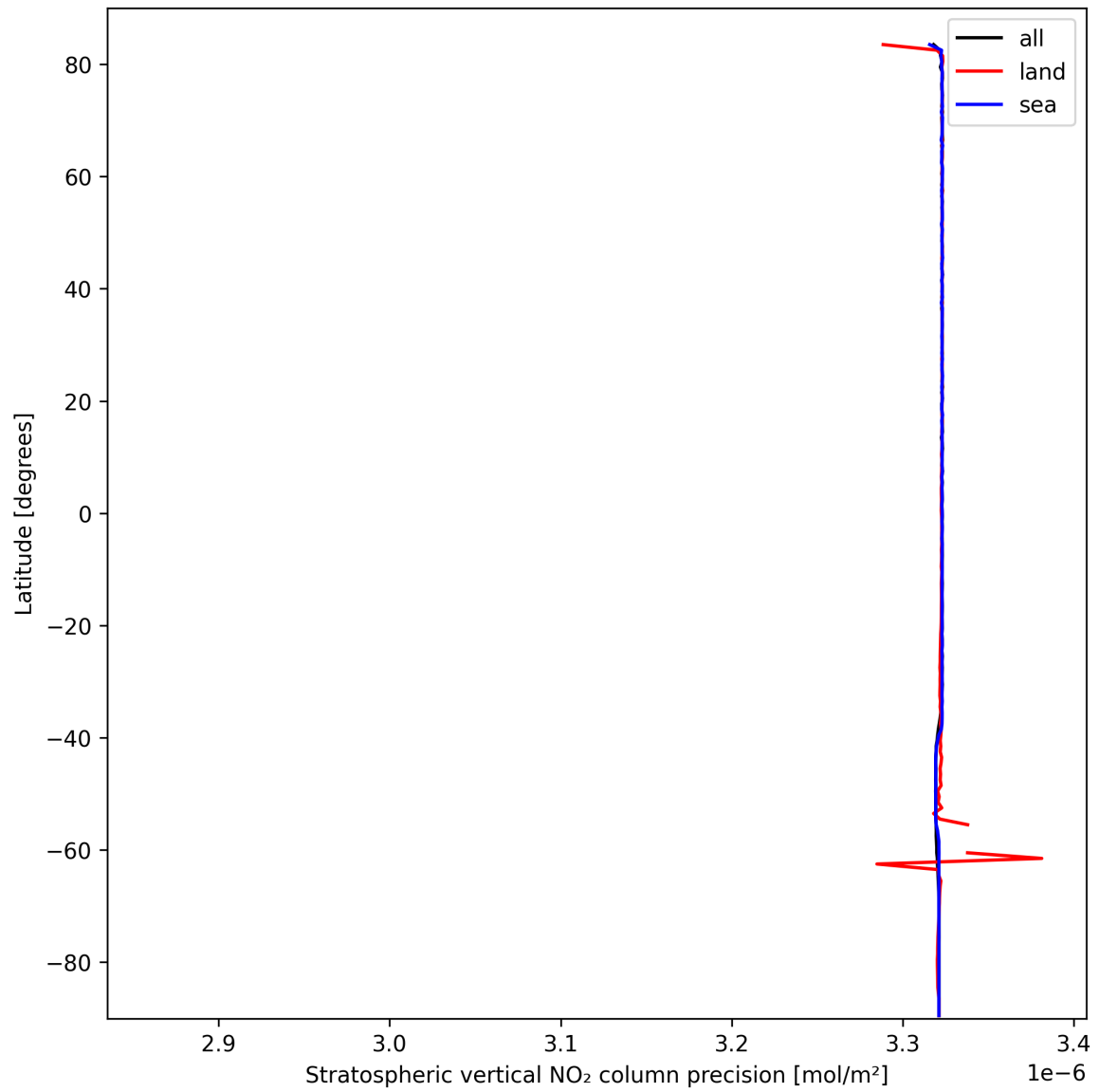
Figure 20: Zonal average of "Stratospheric vertical NO 2 column precision" for 2025-10-03 to 2025-10-05.
