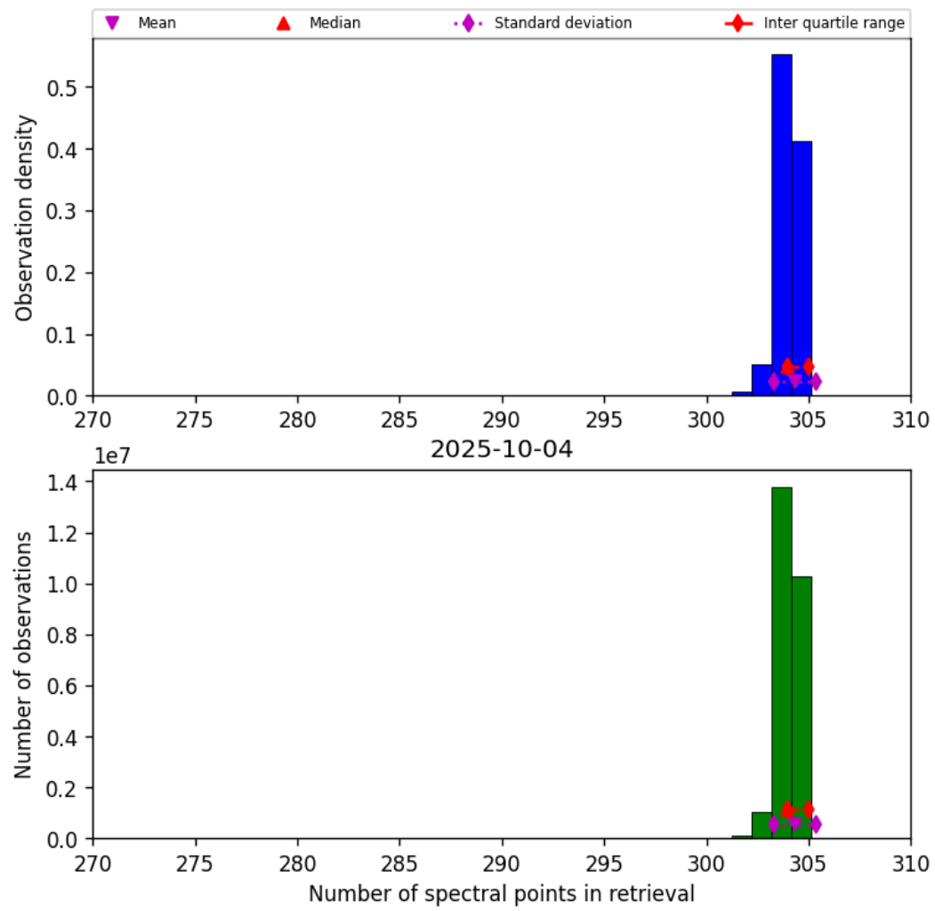
Figure 33: Histogram of “Number of spectral points in retrieval” for 2025-10-03 to 2025-10-05
