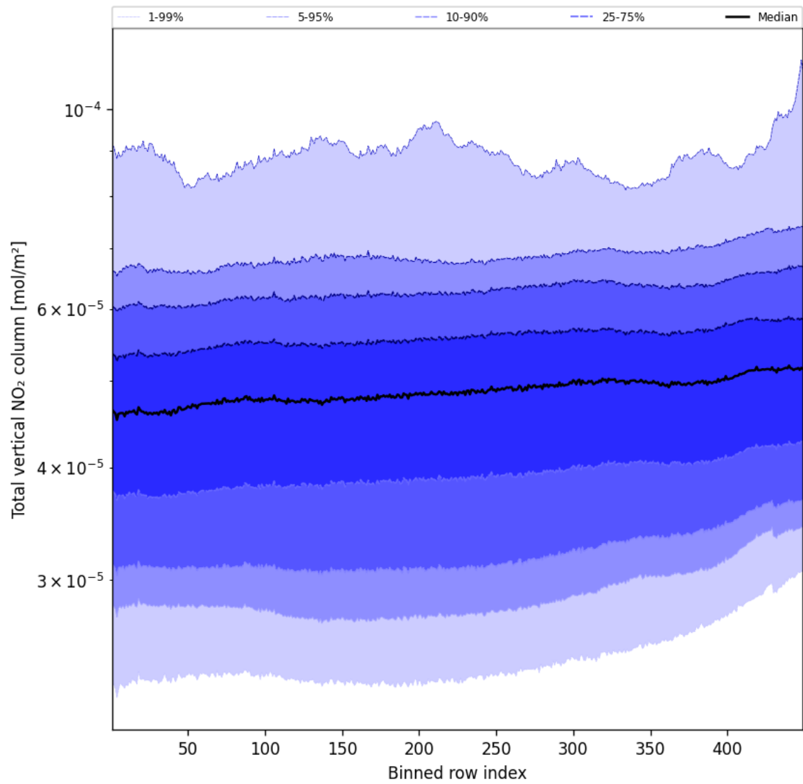
Figure 55: Along track statistics of “Total vertical NO 2 column” for 2025-10-03 to 2025-10-05
