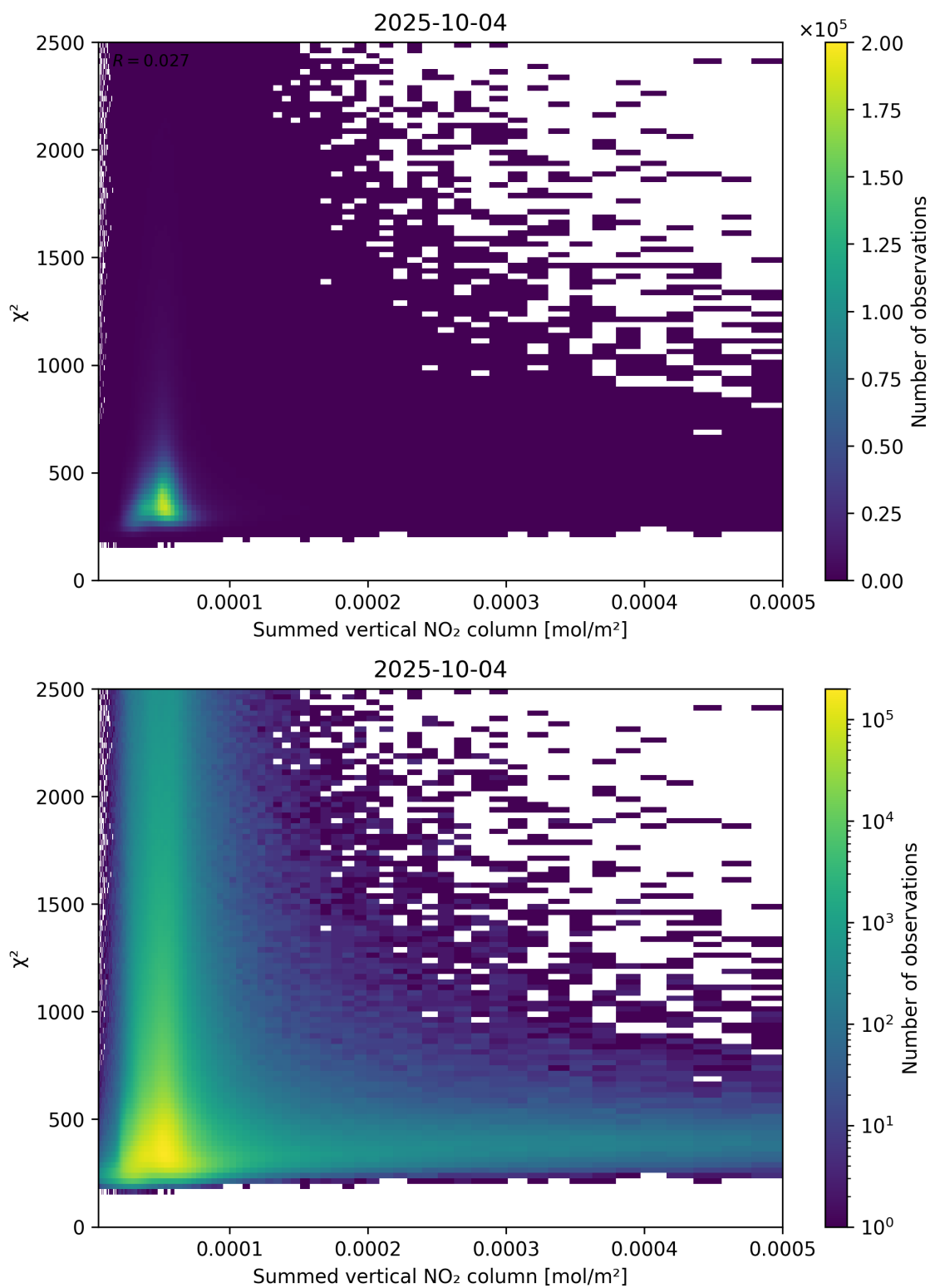
Figure 104: Scatter density plot of “Summed vertical NO 2 column” against “ \chi^2 ” for 2025-10-03 to 2025-10-05.
