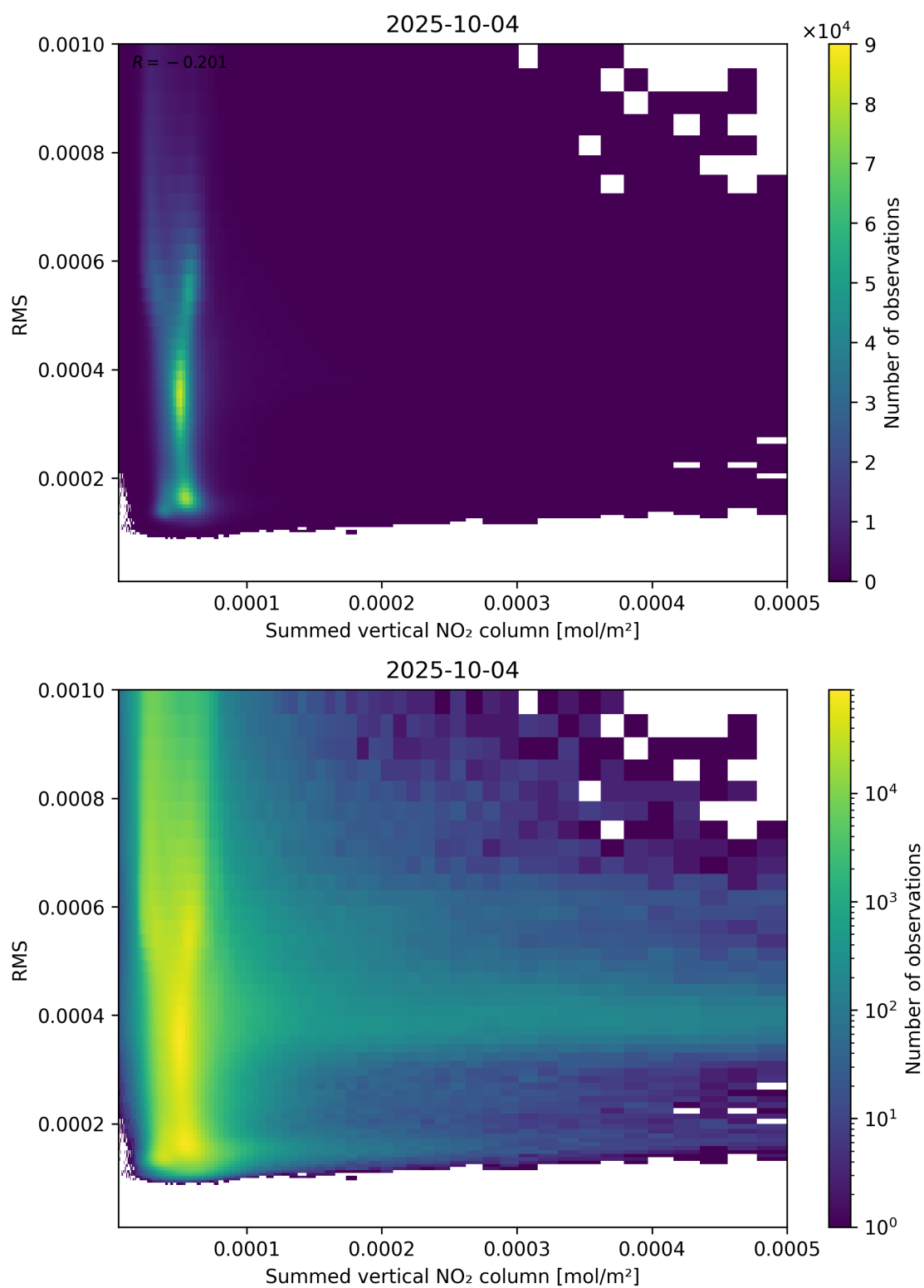
Figure 109: Scatter density plot of “Summed vertical NO 2 column” against “RMS” for 2025-10-03 to 2025-10-05.
