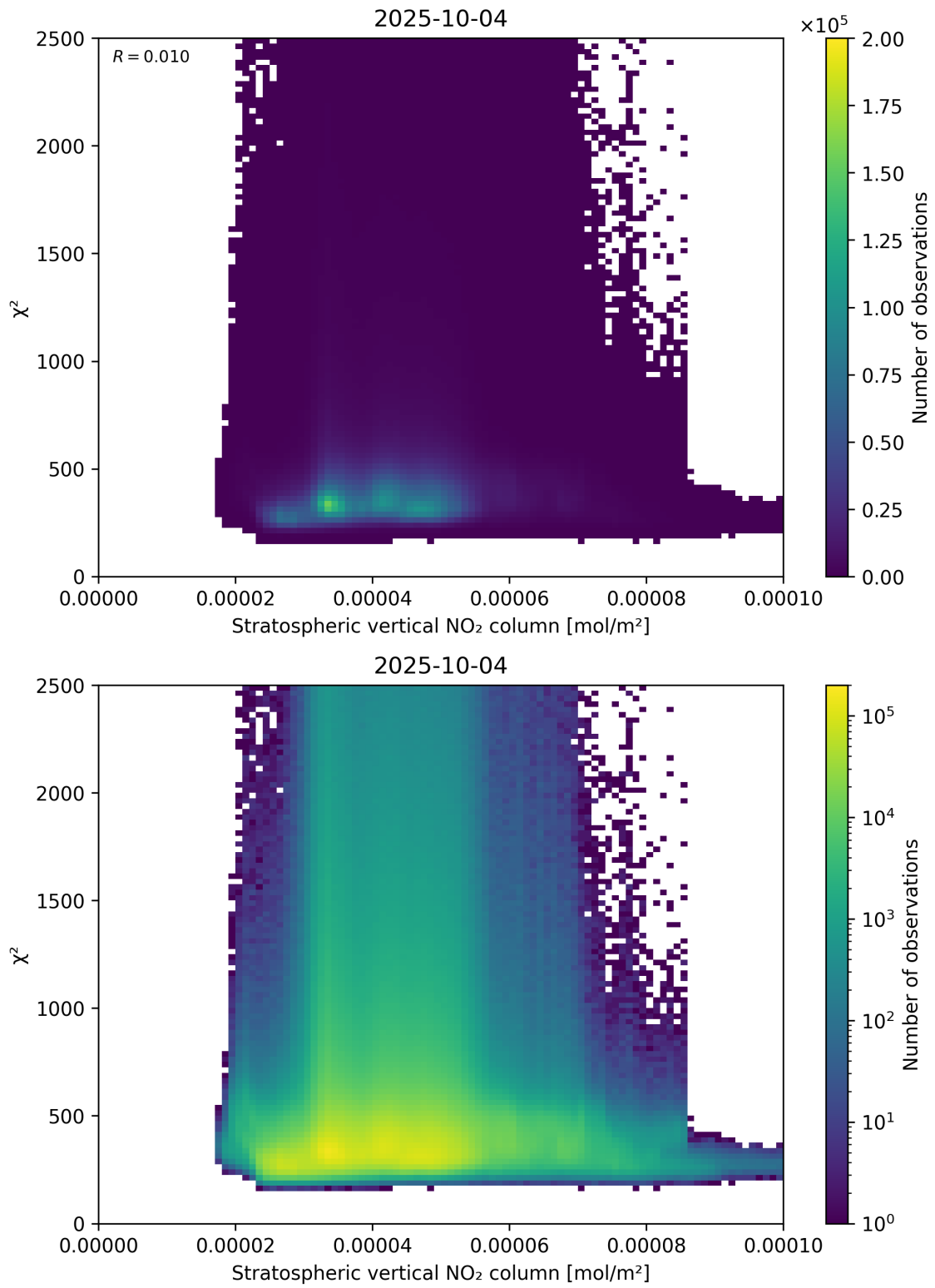
Figure 97: Scatter density plot of “Stratospheric vertical NO 2 column” against “ \chi^2 ” for 2025-10-03 to 2025-10-05.
