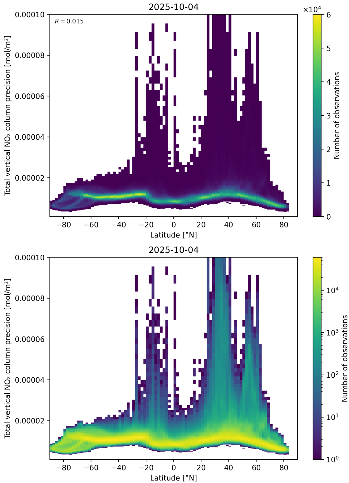
Figure 91: Scatter density plot of “Latitude” against “Total vertical NO 2 column precision” for 2025-10-03 to 2025-10-05.
