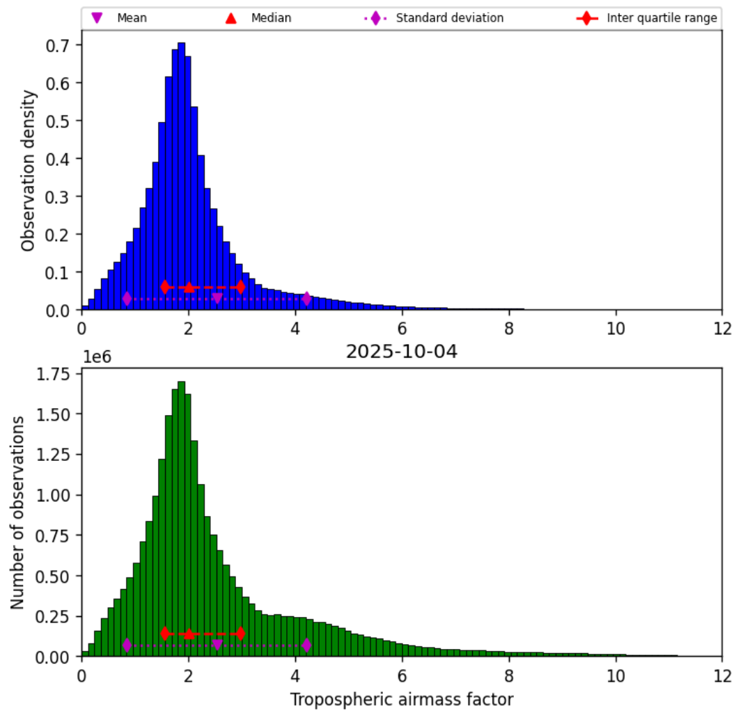
Figure 31: Histogram of “Tropospheric airmass factor” for 2025-10-03 to 2025-10-05
