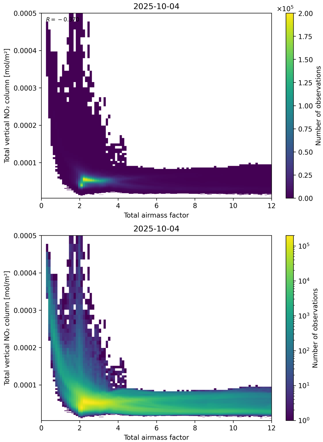
Figure 67: Scatter density plot of “Total airmass factor” against “Total vertical NO 2 column” for 2025-10-03 to 2025-10-05.
