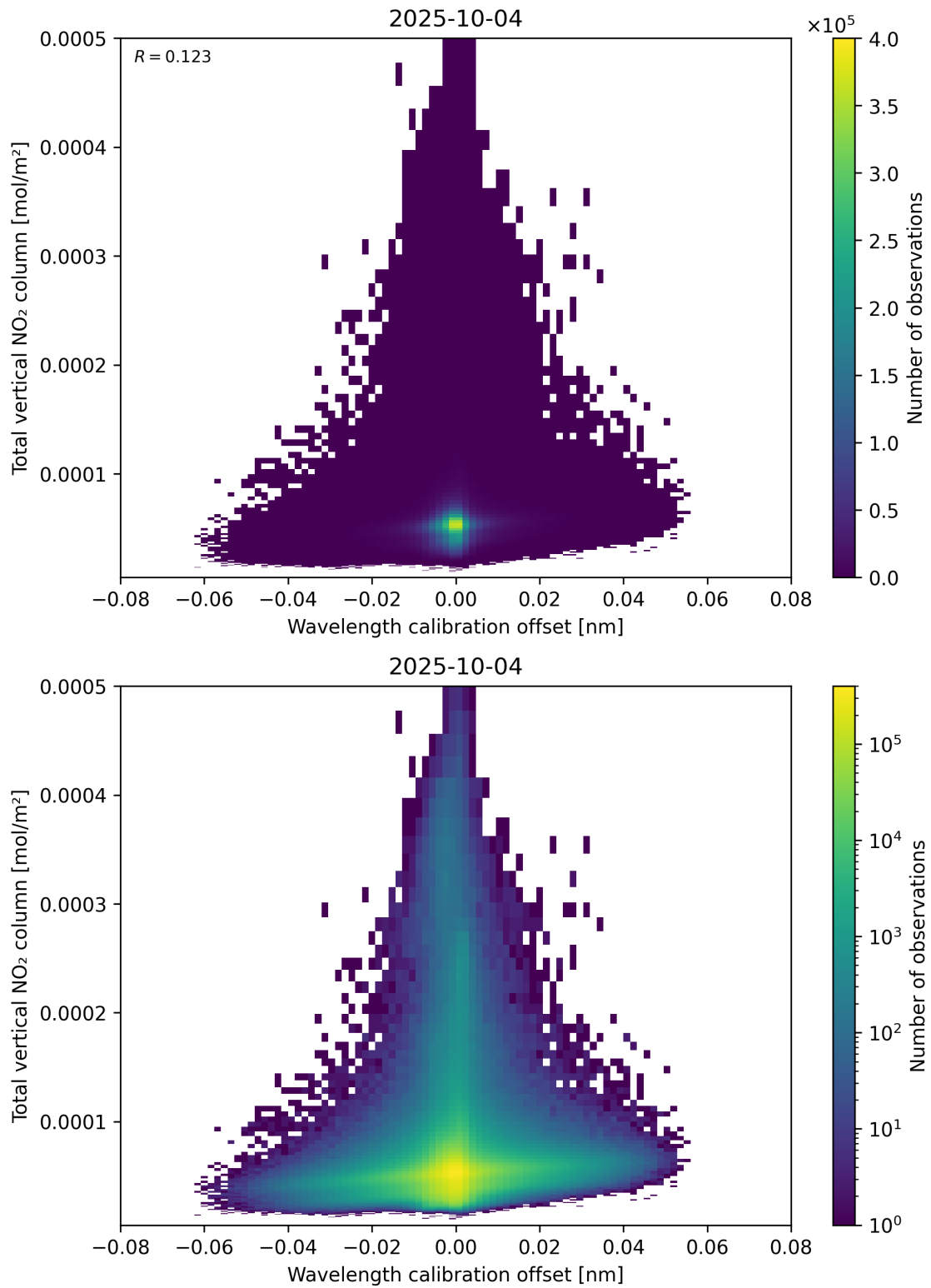
Figure 179: Scatter density plot of “Wavelength calibration offset” against “Total vertical NO 2 column” for 2025-10-03 to 2025-10-05.
