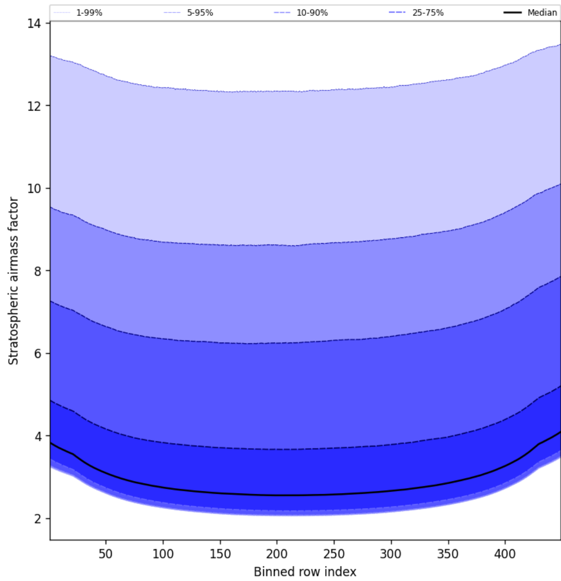
Figure 61: Along track statistics of “Stratospheric airmass factor” for 2025-10-03 to 2025-10-05
