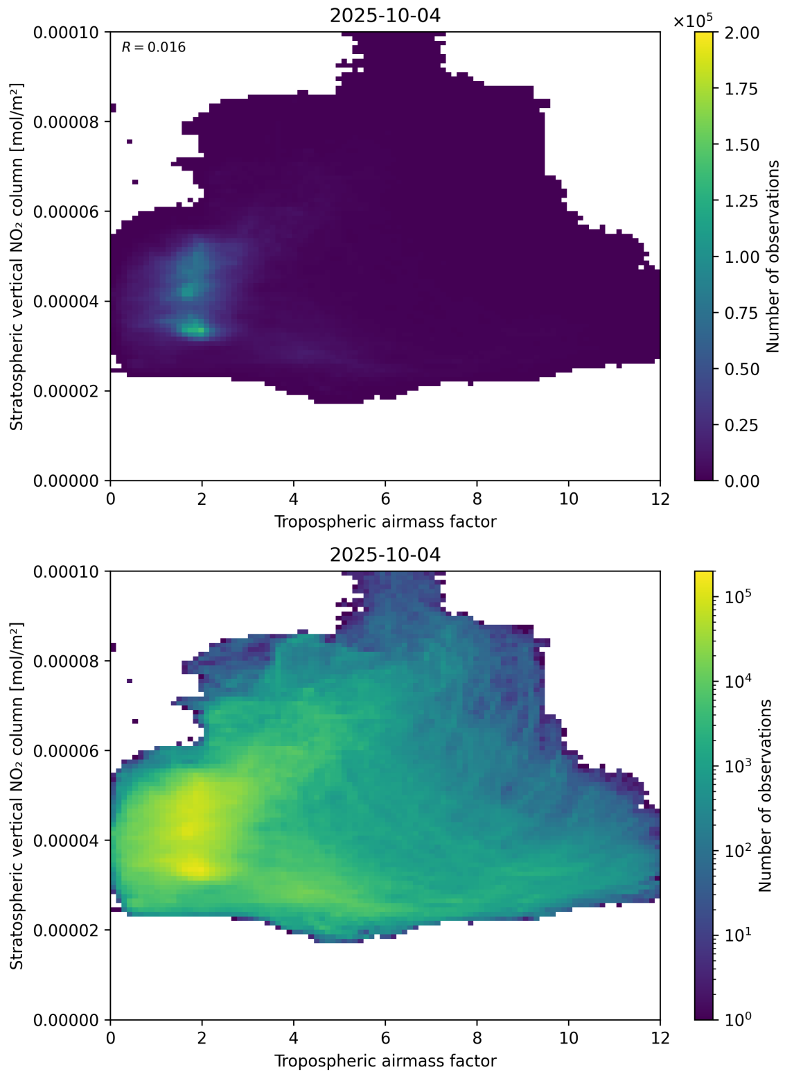
Figure 74: Scatter density plot of “Tropospheric air mass factor” against “Stratospheric vertical NO 2 column” for 2025-10-03 to 2025-10-05.
