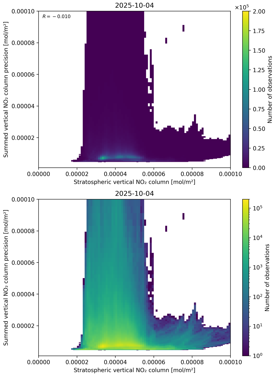
Figure 99: Scatter density plot of “Stratospheric vertical NO 2 column” against “Summed vertical NO 2 column precision” for 2025-10-03 to 2025-10-05.
