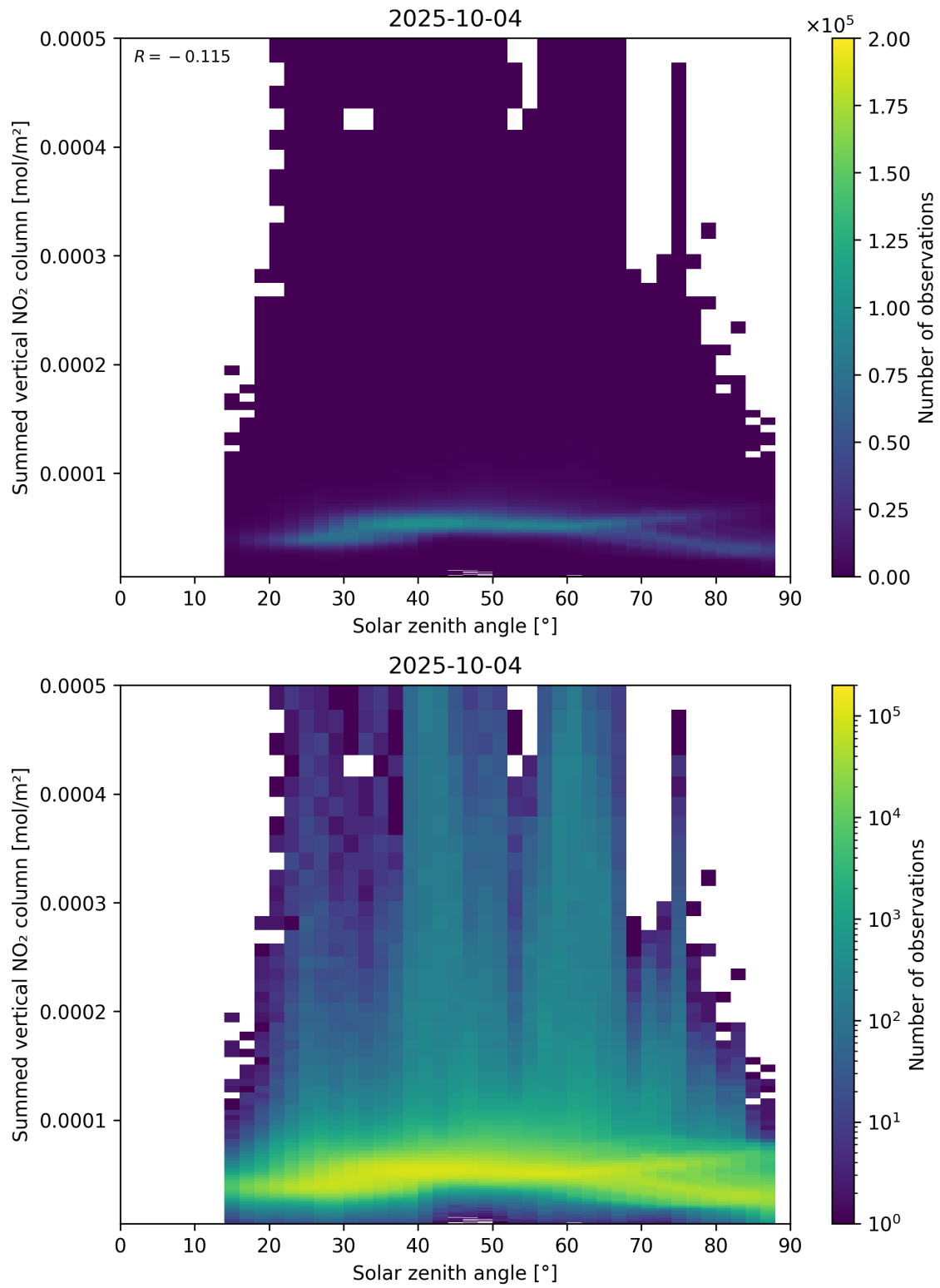
Figure 151: Scatter density plot of “Solar zenith angle” against “Summed vertical NO 2 column” for 2025-10-03 to 2025-10-05.
