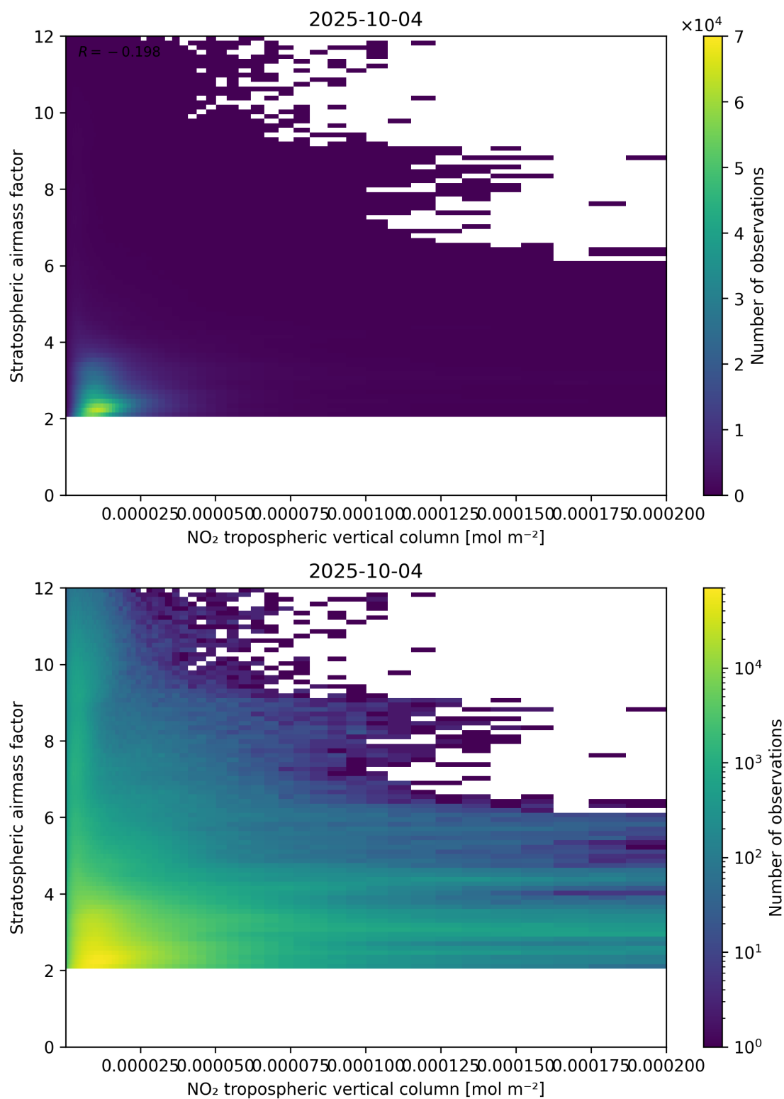
Figure 121: Scatter density plot of “NO 2 tropospheric vertical column” against “Stratospheric air mass factor” for 2025-10-03 to 2025-10-05.
