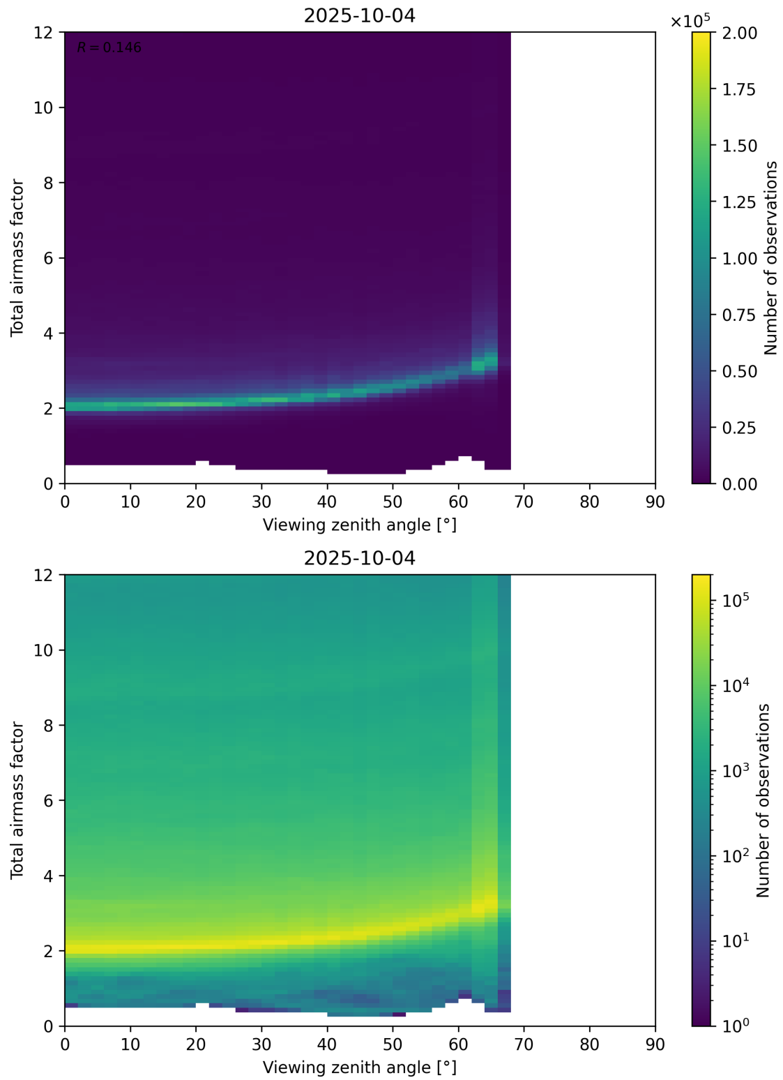
Figure 160: Scatter density plot of “Viewing zenith angle” against “Total airmass factor” for 2025-10-03 to 2025-10-05.
