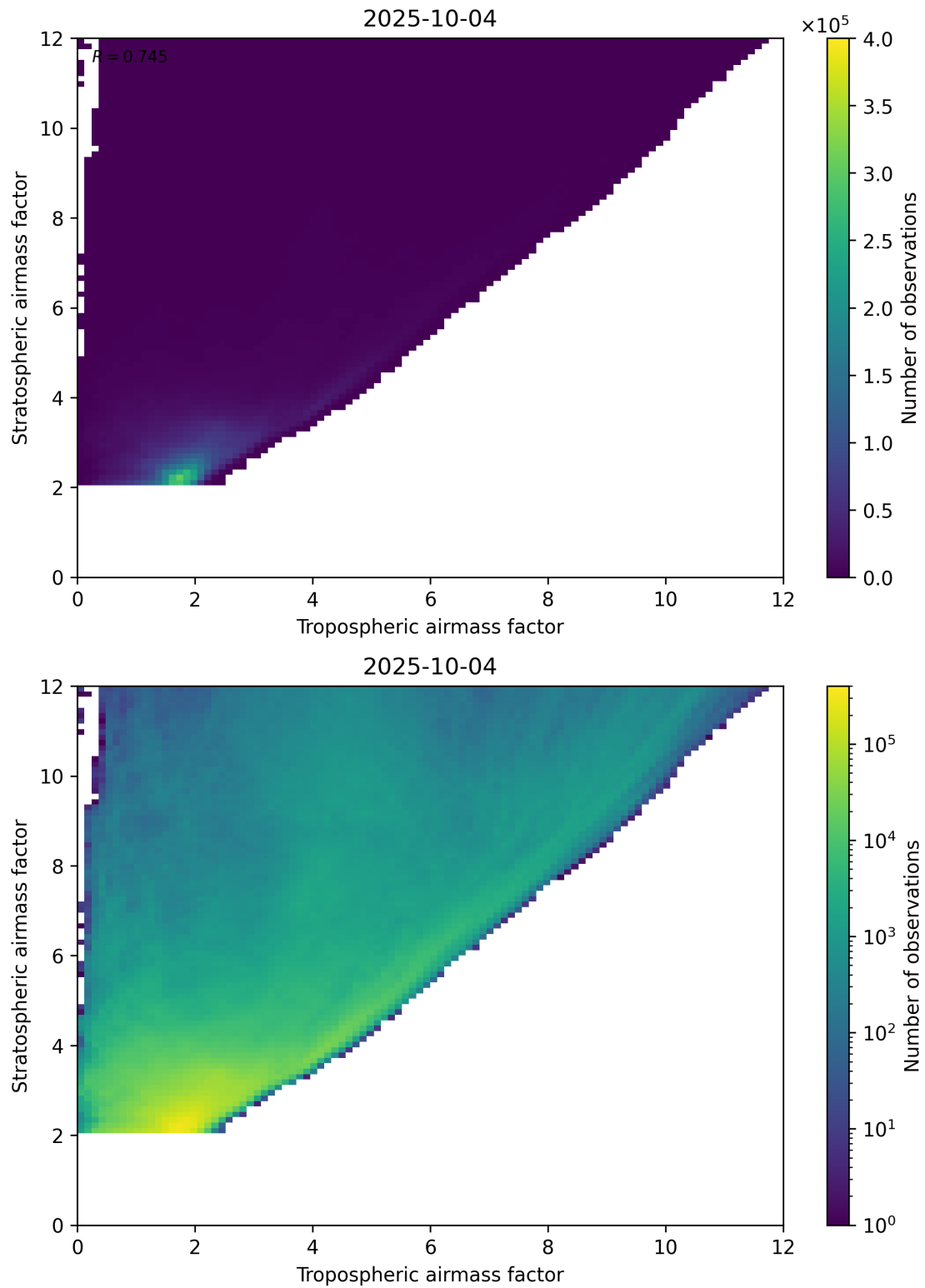
Figure 71: Scatter density plot of “Tropospheric airmass factor” against “Stratospheric airmass factor” for 2025-10-03 to 2025-10-05.
