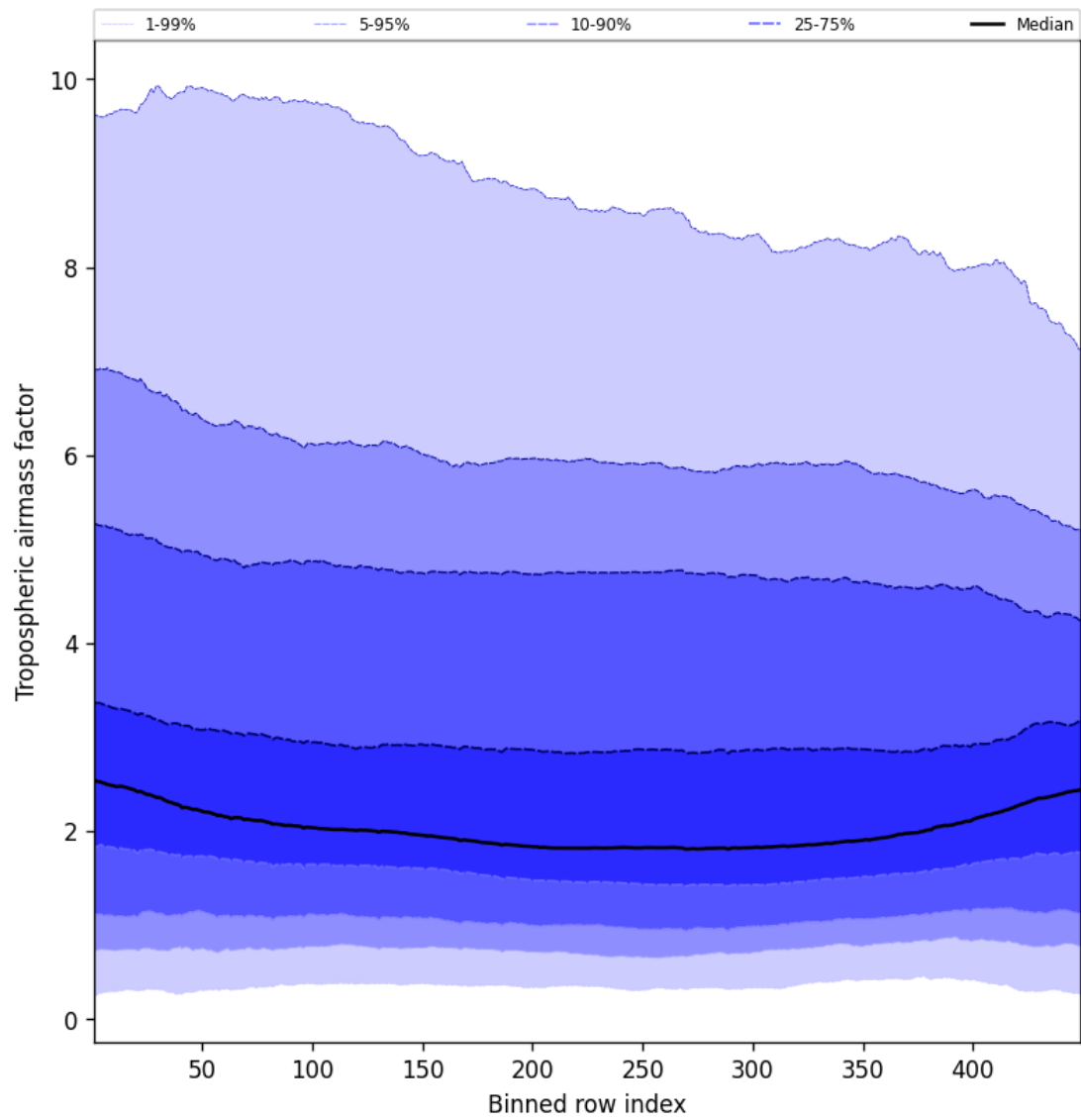
Figure 48: Along track statistics of “Tropospheric airmass factor” for 2025-10-03 to 2025-10-05
