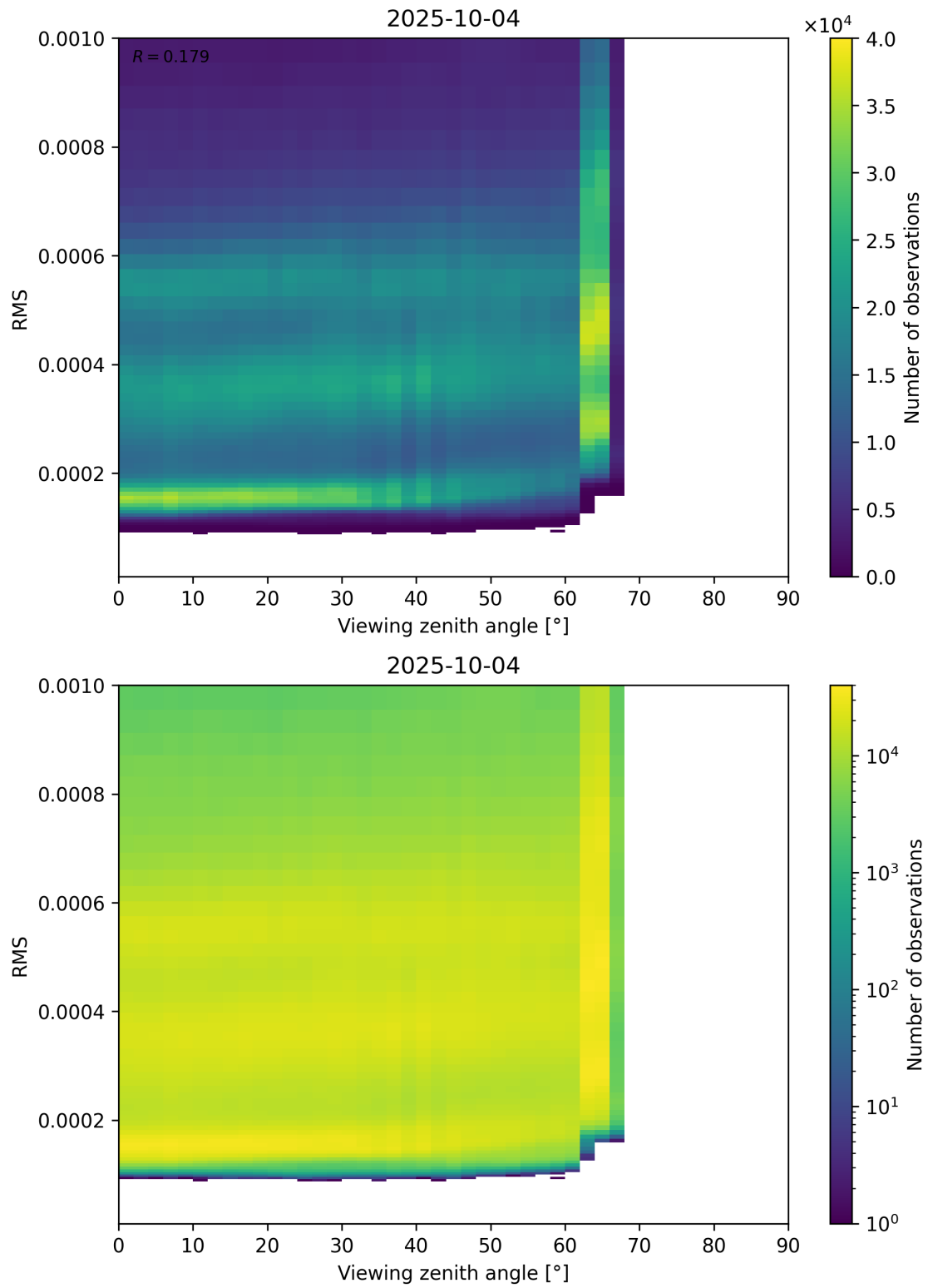
Figure 171: Scatter density plot of “Viewing zenith angle” against “RMS” for 2025-10-03 to 2025-10-05.
