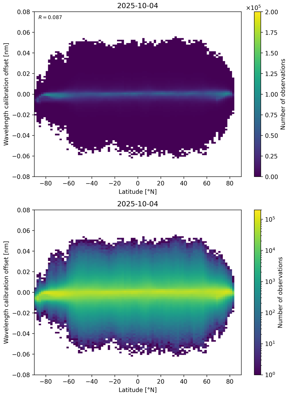
Figure 95: Scatter density plot of “Latitude” against “Wavelength calibration offset” for 2025-10-03 to 2025-10-05.
