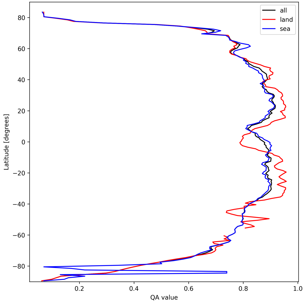
Figure 11: Zonal average of “QA value” for 2025-10-03 to 2025-10-05.
