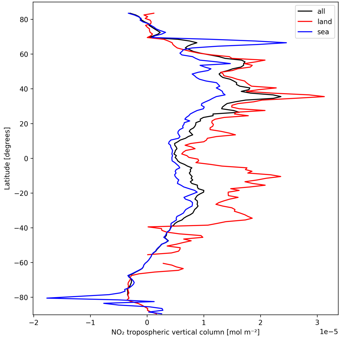
Figure 12: Zonal average of “NO 2 tropospheric vertical column” for 2025-10-03 to 2025-10-05.
