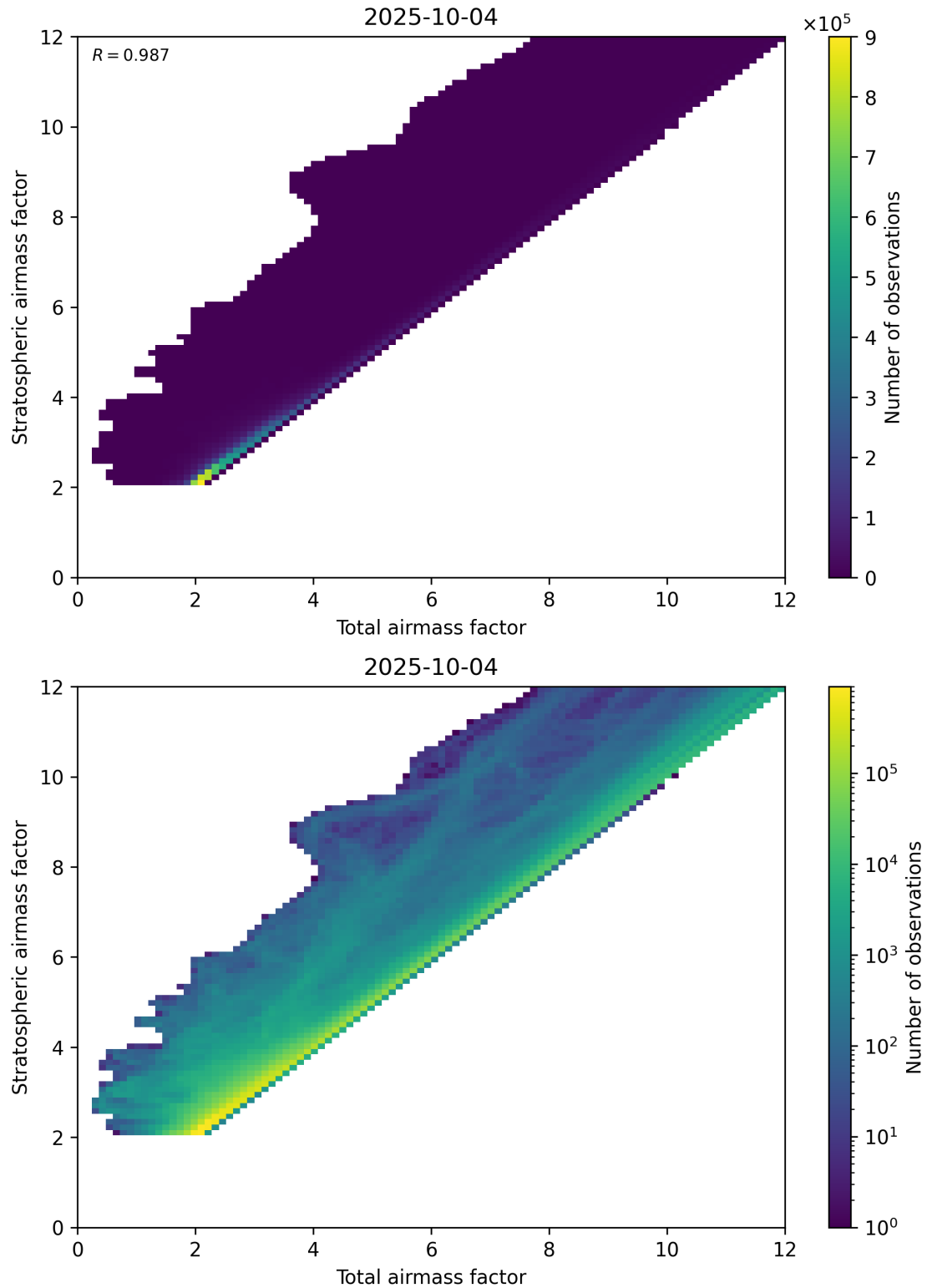
Figure 62: Scatter density plot of “Total airmass factor” against “Stratospheric airmass factor” for 2025-10-03 to 2025-10-05.
