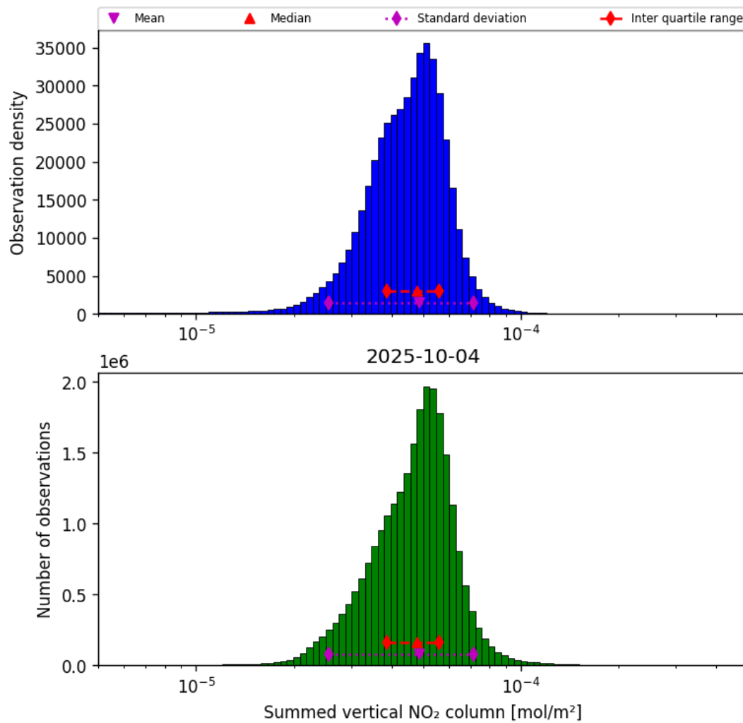
Figure 40: Histogram of “Summed vertical NO 2 column” for 2025-10-03 to 2025-10-05
