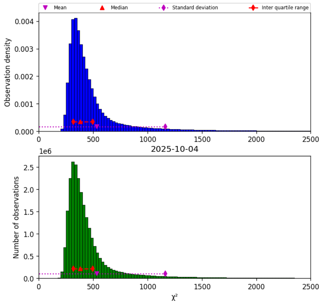
Figure 42: Histogram of " \chi^2 " for 2025-10-03 to 2025-10-05
