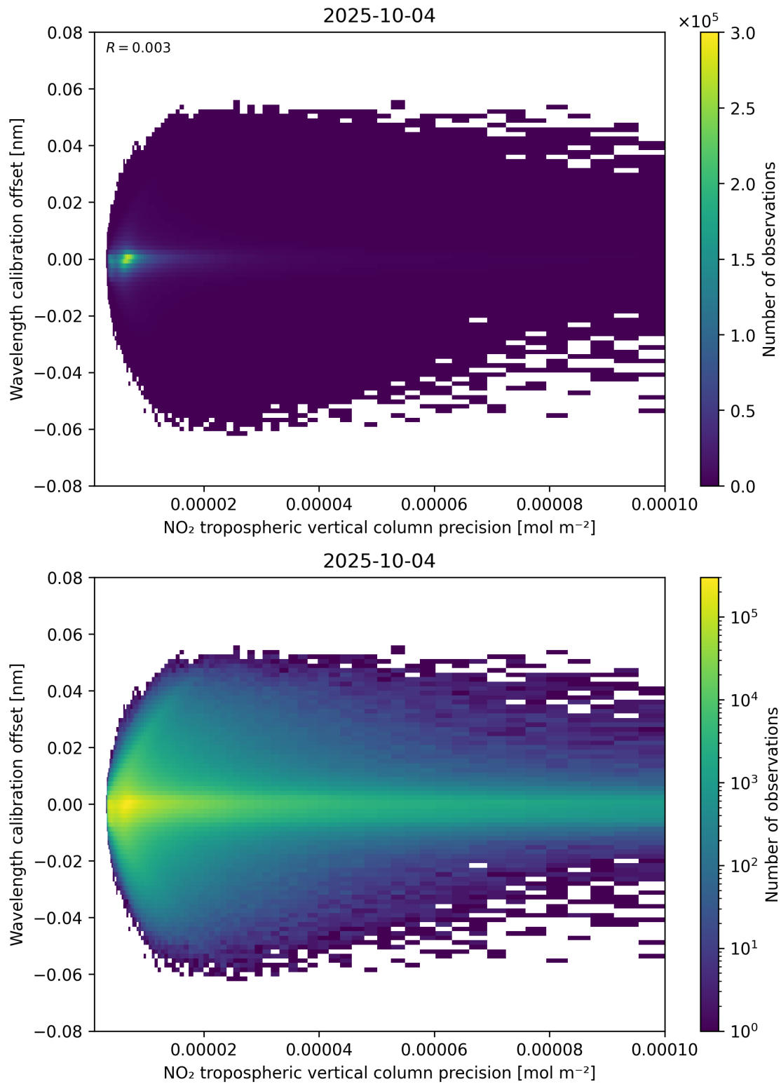
Figure 141: Scatter density plot of “NO 2 tropospheric vertical column precision” against “Wavelength calibration offset” for 2025-10-03 to 2025-10-05.
