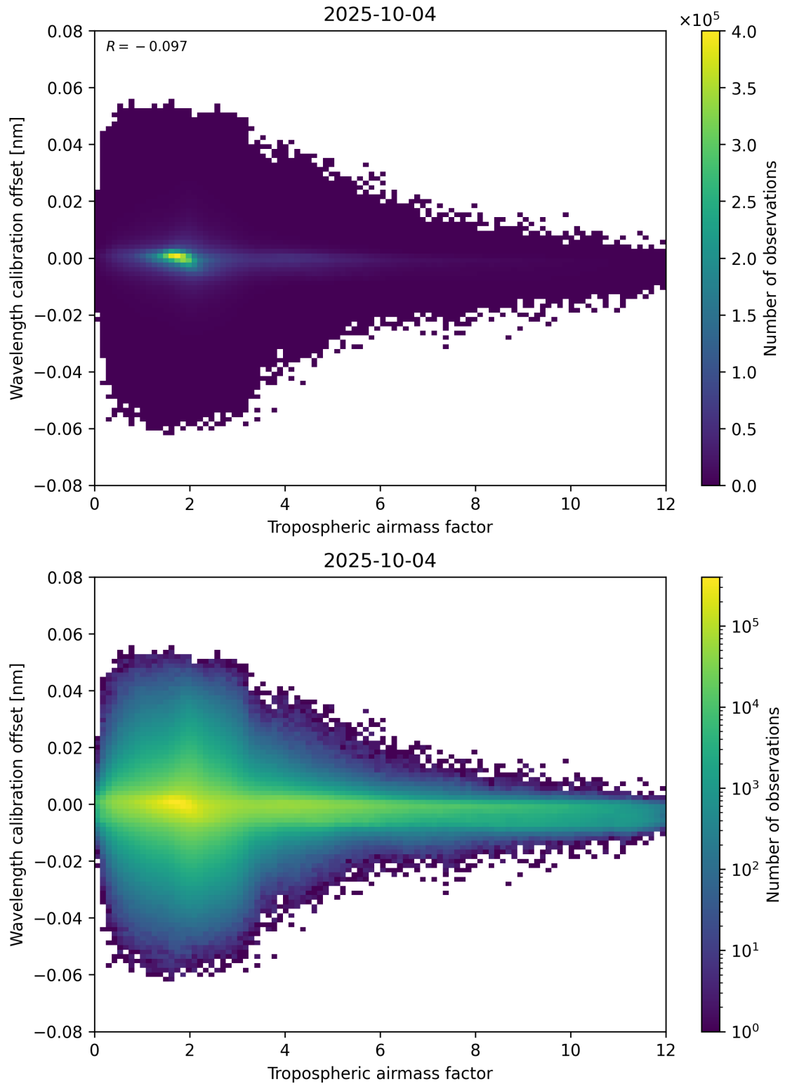
Figure 80: Scatter density plot of “Tropospheric airmass factor” against “Wavelength calibration offset” for 2025-10-03 to 2025-10-05.
