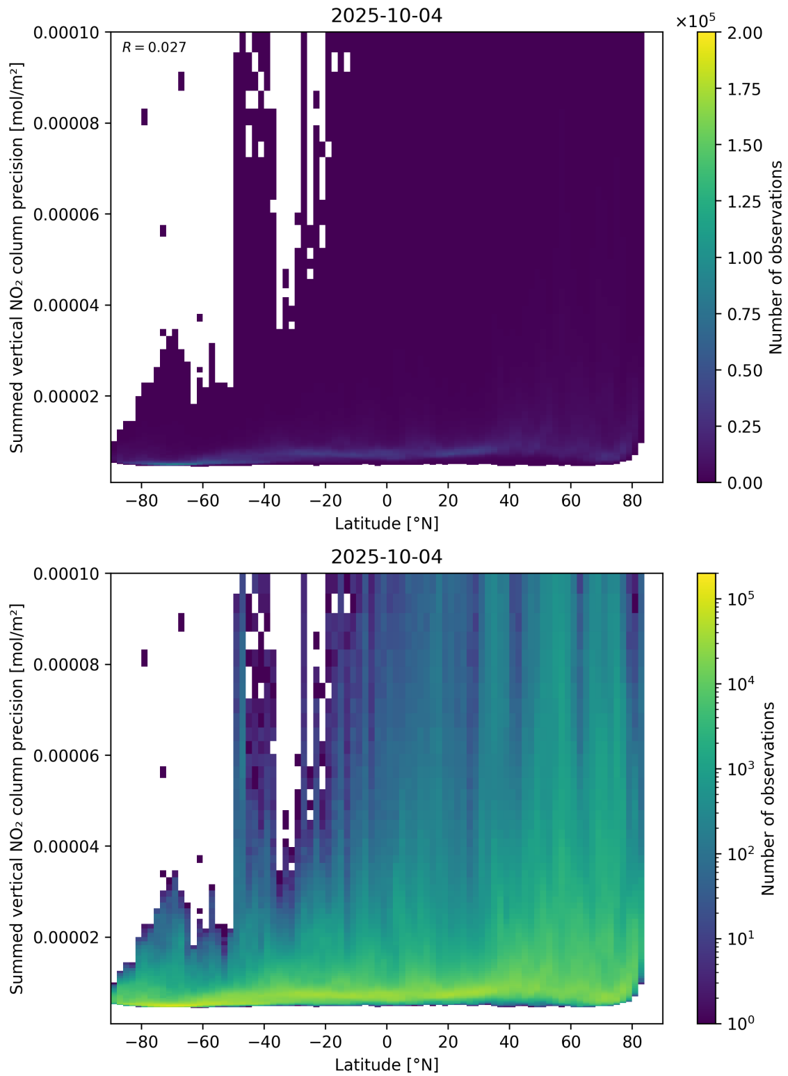
Figure 89: Scatter density plot of “Latitude” against “Summed vertical NO 2 column precision” for 2025-10-03 to 2025-10-05.
