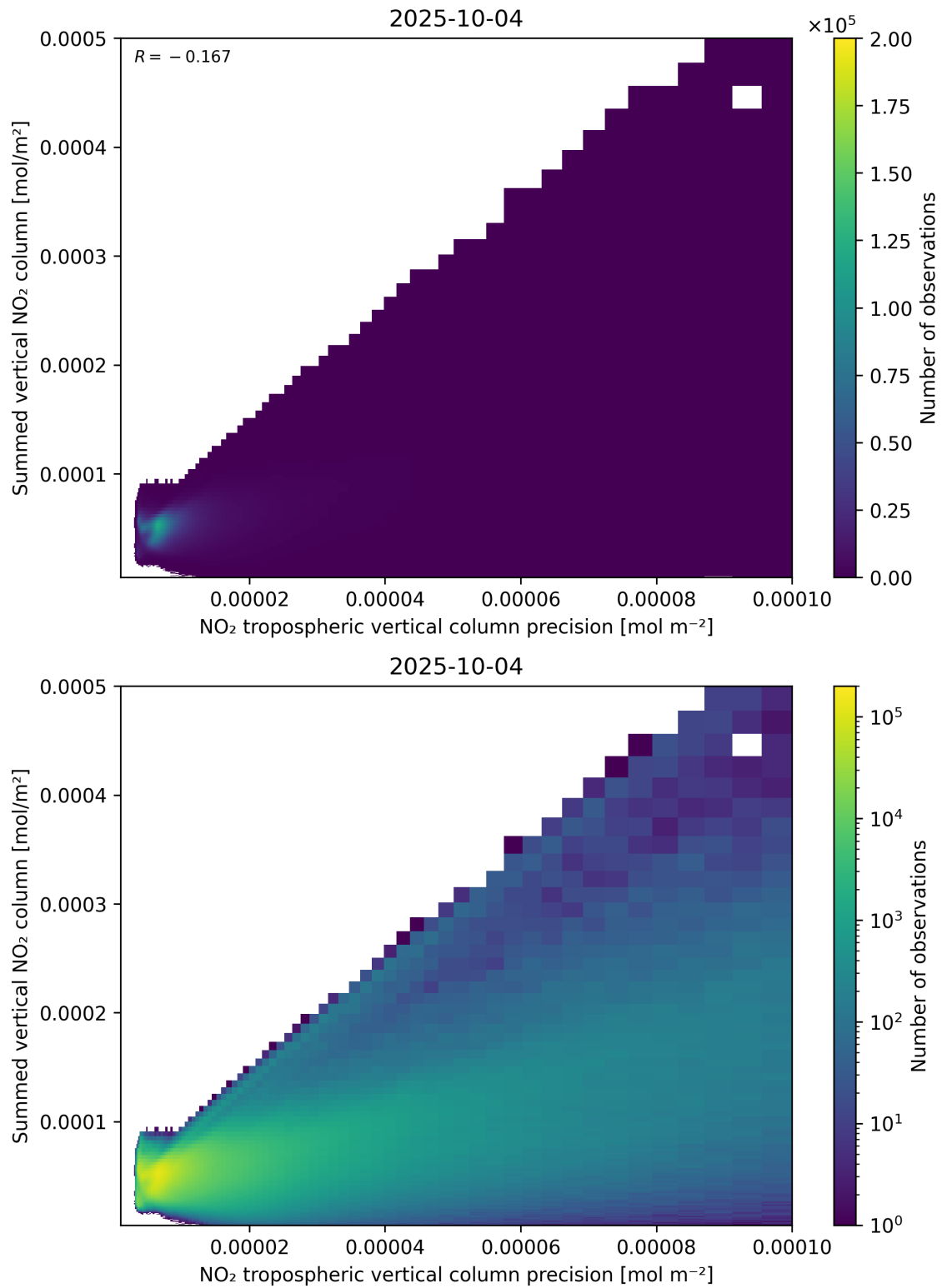
Figure 136: Scatter density plot of “NO 2 tropospheric vertical column precision” against “Summed vertical NO 2 column” for 2025-10-03 to 2025-10-05.
