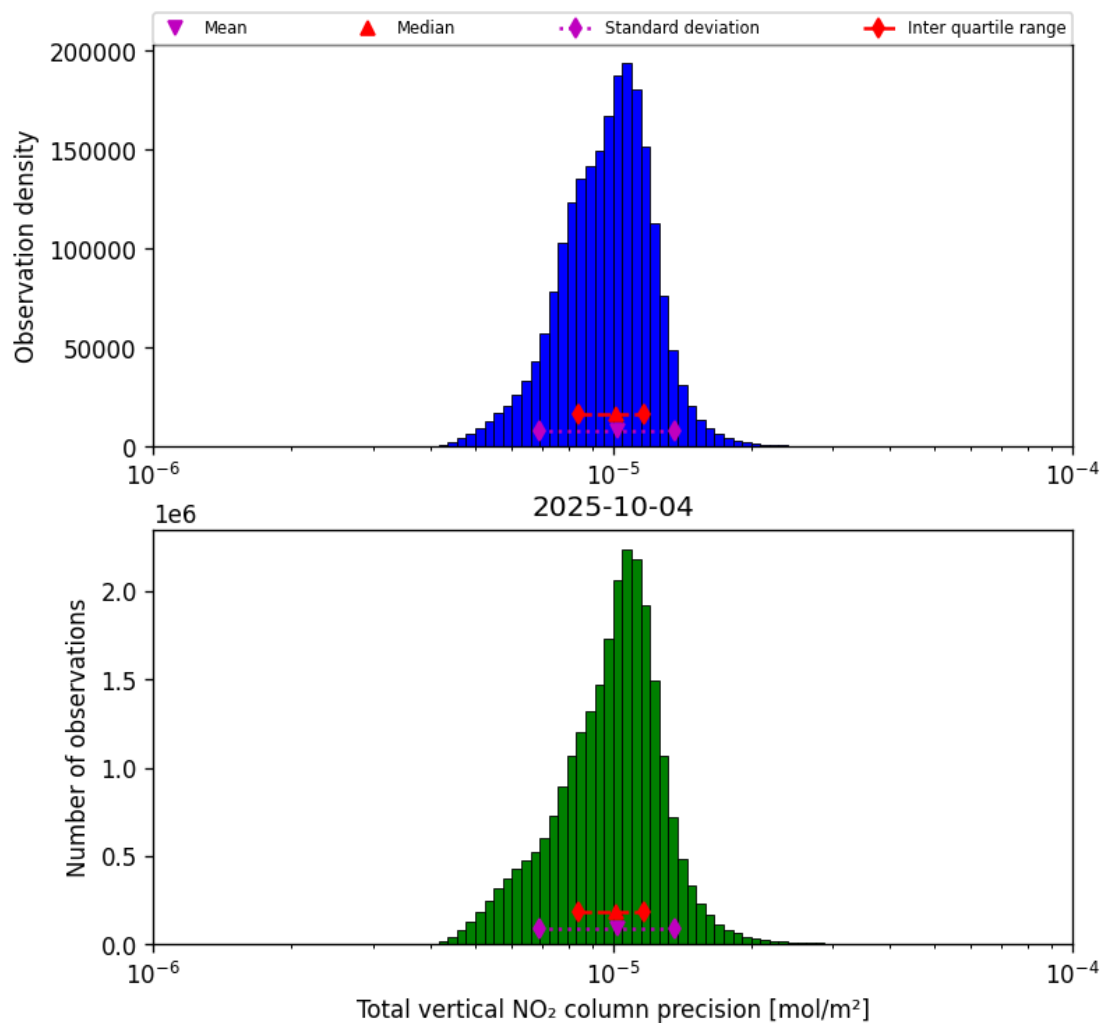
Figure 39: Histogram of “Total vertical NO 2 column precision” for 2025-10-03 to 2025-10-05
