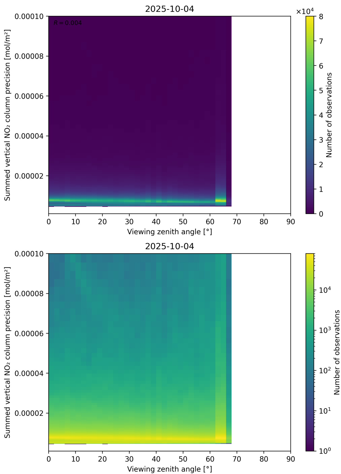
Figure 166: Scatter density plot of “Viewing zenith angle” against “Summed vertical NO 2 column precision” for 2025-10-03 to 2025-10-05.
