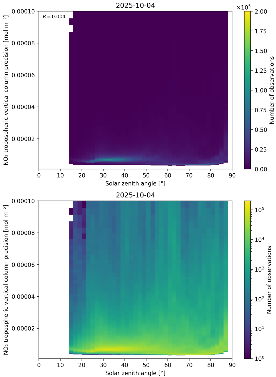
Figure 156: Scatter density plot of “Solar zenith angle” against “NO 2 tropospheric vertical column precision” for 2025-10-03 to 2025-10-05.
