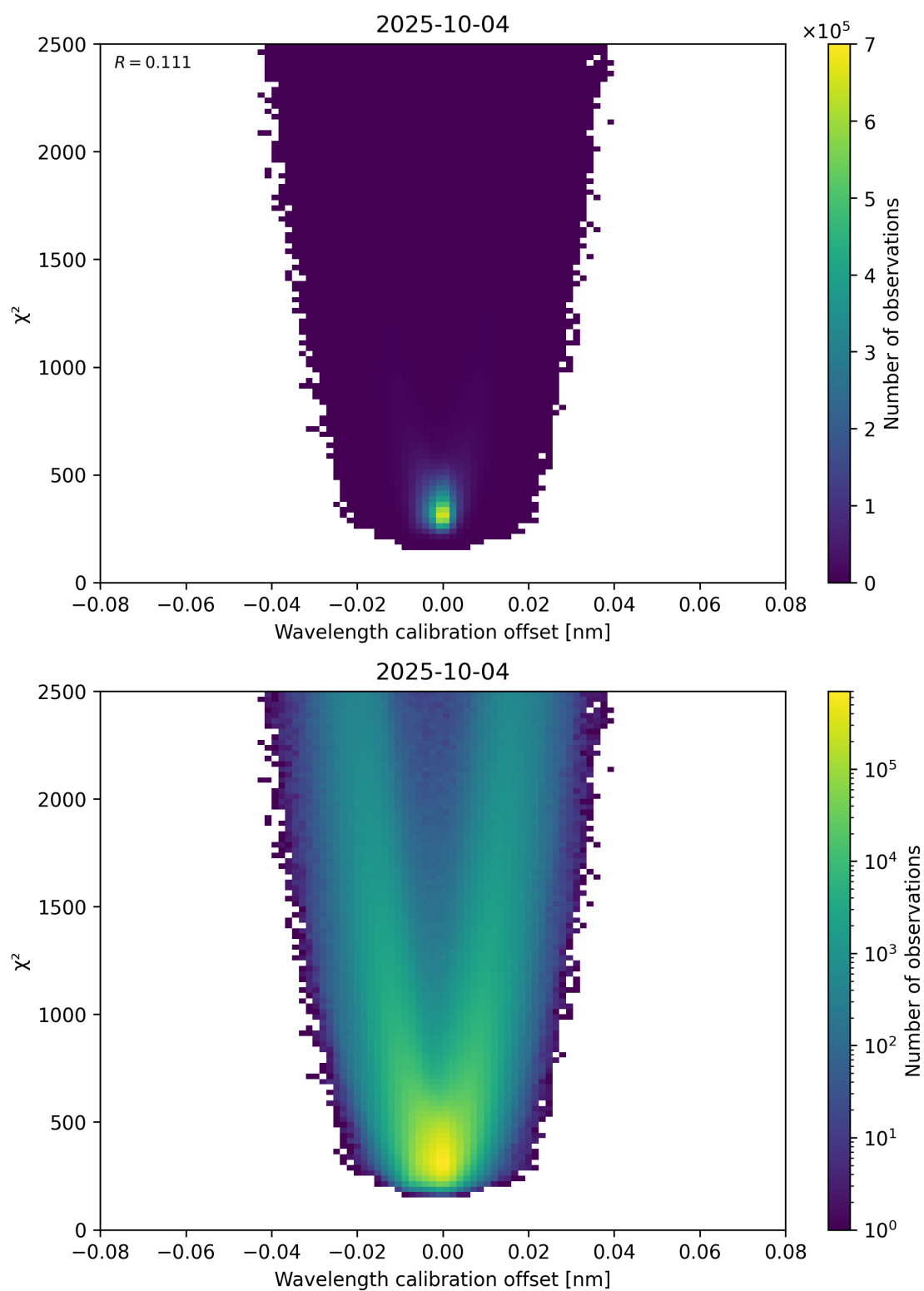
Figure 175: Scatter density plot of “Wavelength calibration offset” against “ \chi^2 ” for 2025-10-03 to 2025-10-05.
