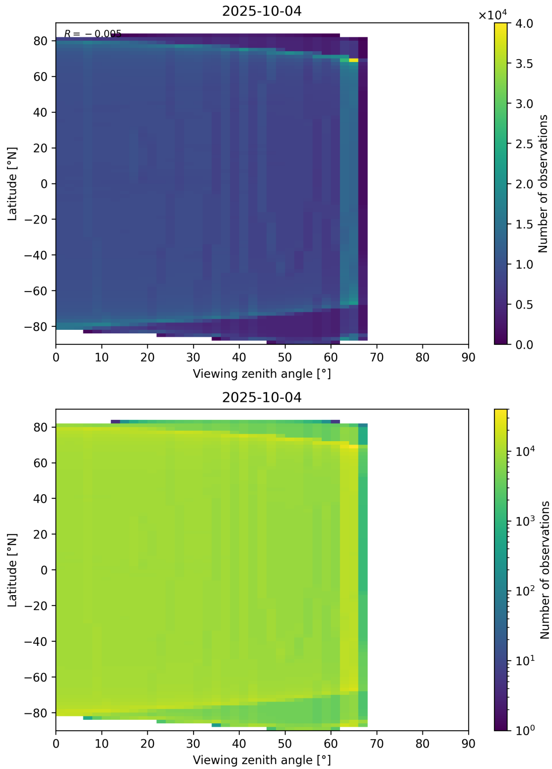
Figure 163: Scatter density plot of “Viewing zenith angle” against “Latitude” for 2025-10-03 to 2025-10-05.
