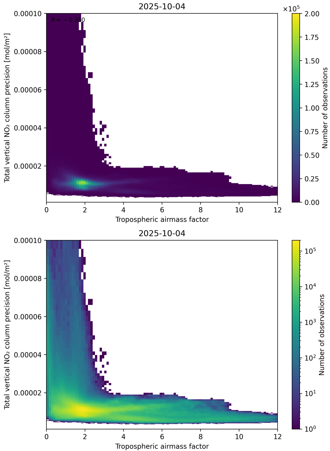
Figure 78: Scatter density plot of “Tropospheric air mass factor” against “Total vertical NO 2 column precision” for 2025-10-03 to 2025-10-05.
