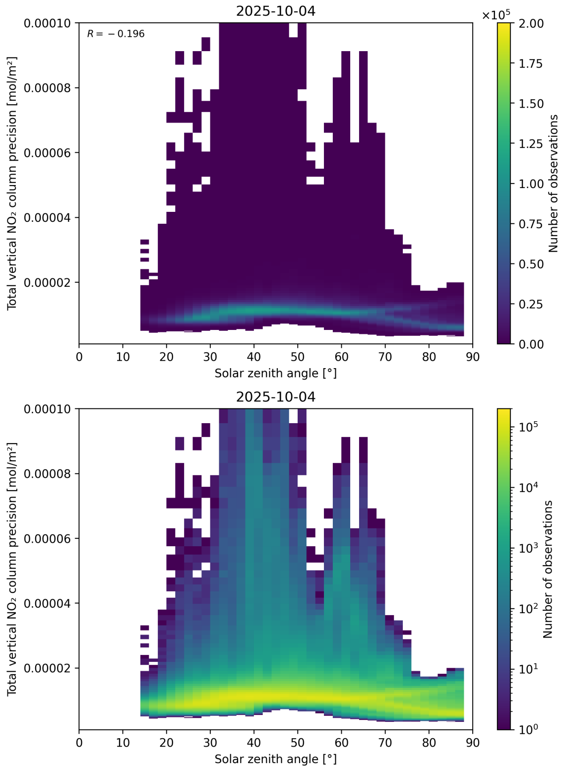
Figure 154: Scatter density plot of “Solar zenith angle” against “Total vertical NO 2 column precision” for 2025-10-03 to 2025-10-05.
