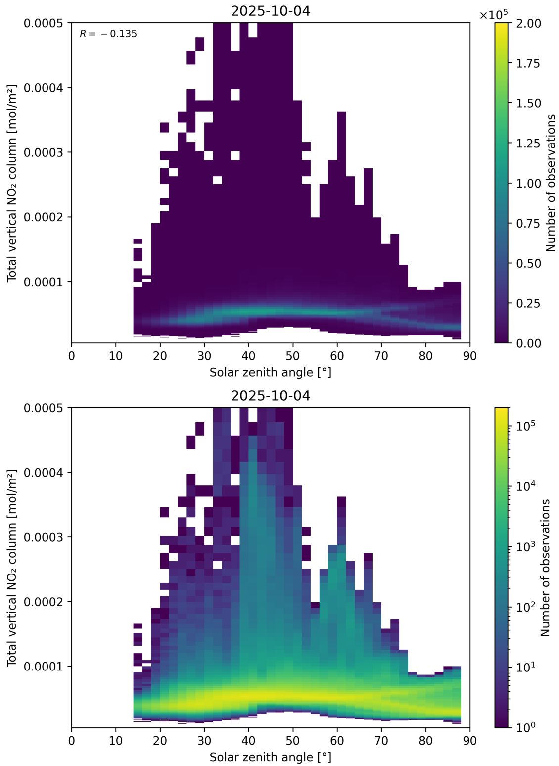
Figure 153: Scatter density plot of “Solar zenith angle” against “Total vertical NO 2 column” for 2025-10-03 to 2025-10-05.
