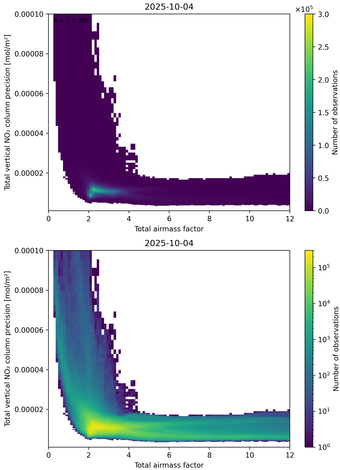
Figure 68: Scatter density plot of “Total airmass factor” against “Total vertical NO 2 column precision” for 2025-10-03 to 2025-10-05.
