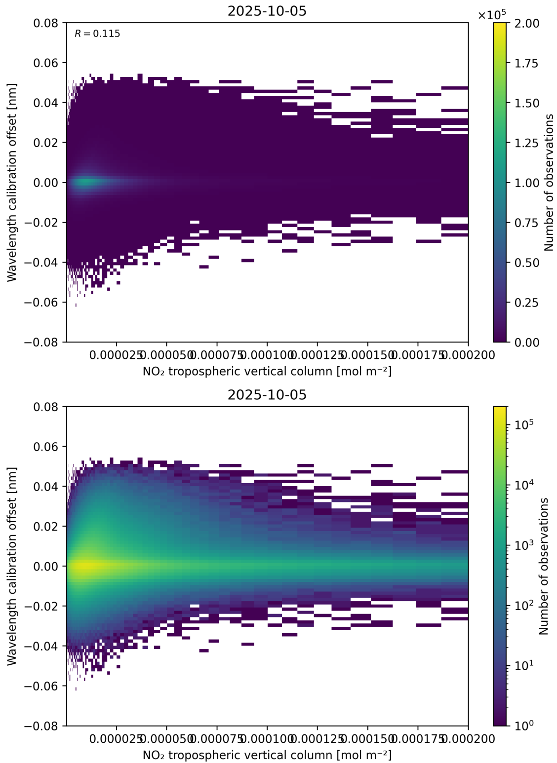
Figure 143: Scatter density plot of “NO 2 tropospheric vertical column” against “Wavelength calibration offset” for 2025-10-04 to 2025-10-06.
