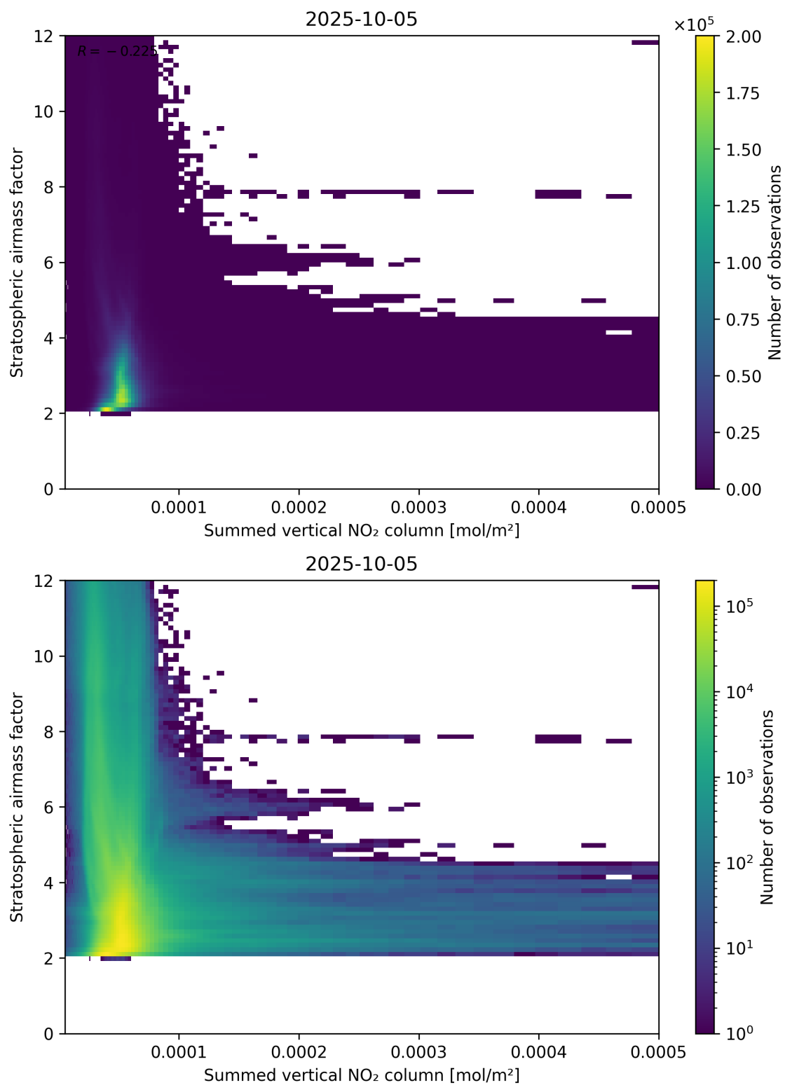
Figure 103: Scatter density plot of “Summed vertical NO 2 column” against “Stratospheric air mass factor” for 2025-10-04 to 2025-10-06.
