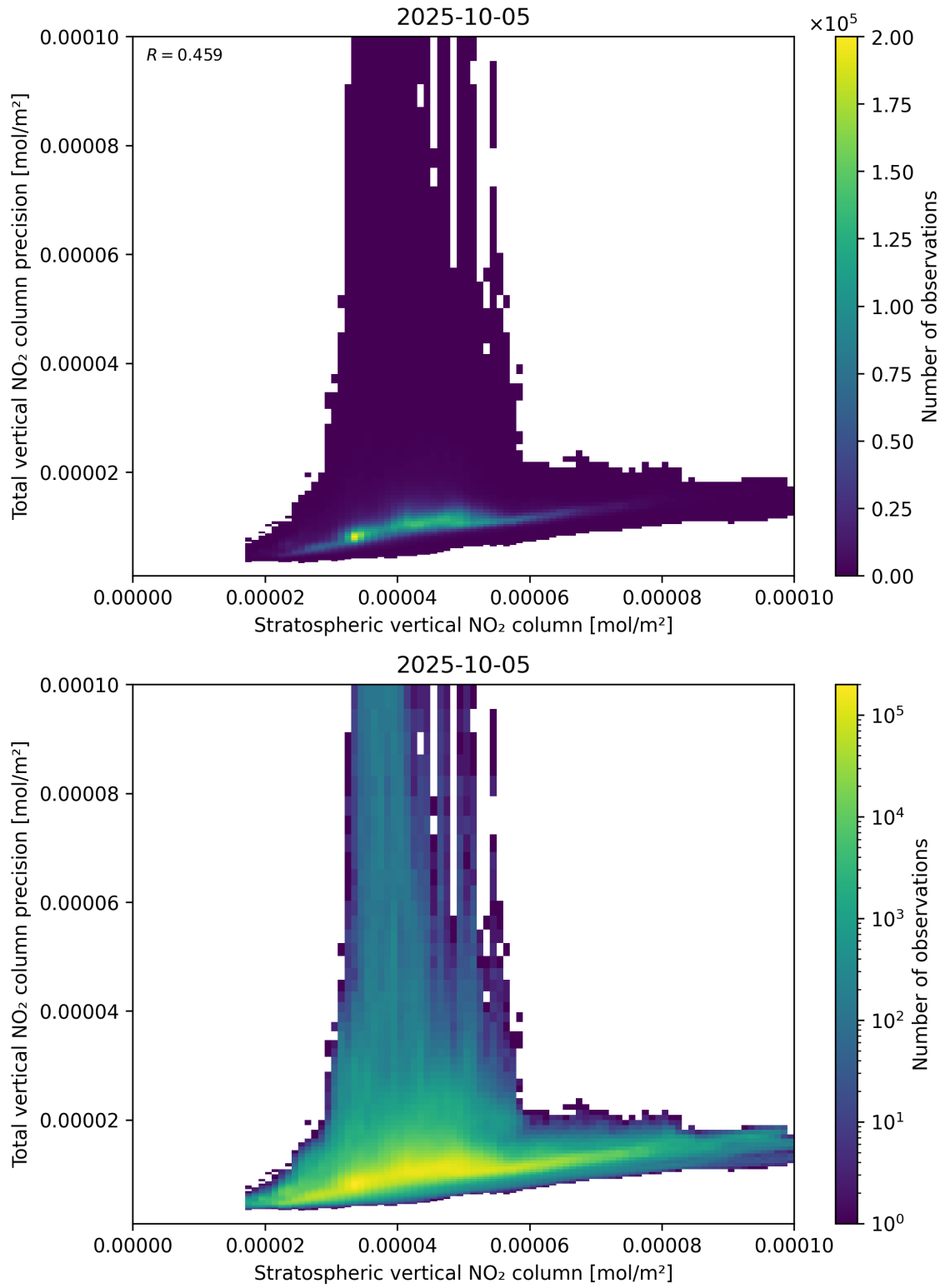
Figure 101: Scatter density plot of “Stratospheric vertical NO 2 column” against “Total vertical NO 2 column precision” for 2025-10-04 to 2025-10-06.
