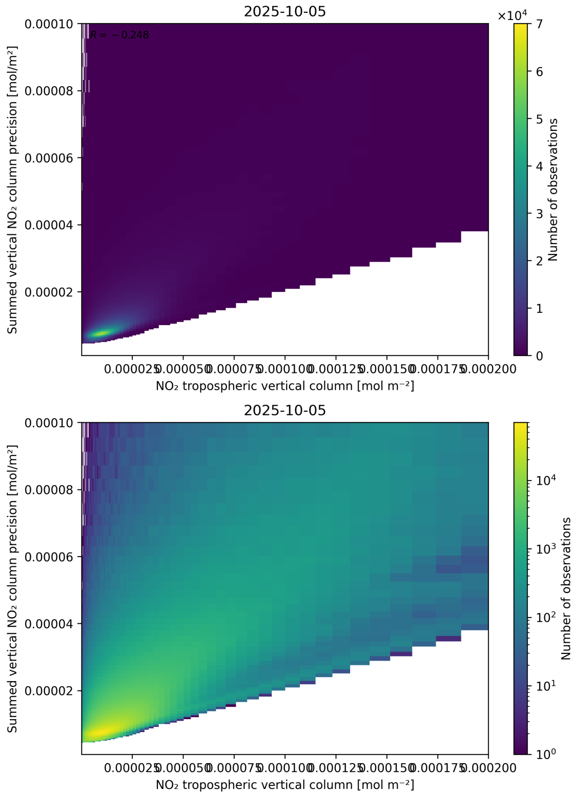
Figure 127: Scatter density plot of “NO 2 tropospheric vertical column” against “Summed vertical NO 2 column precision” for 2025-10-04 to 2025-10-06.
