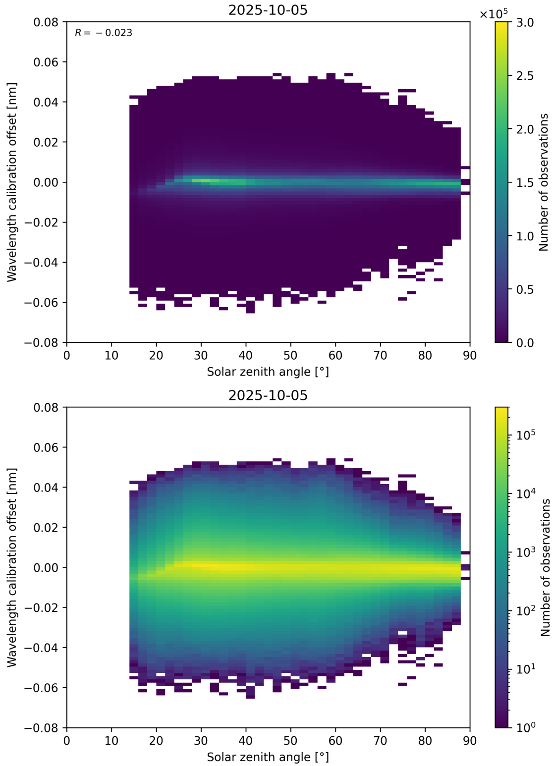
Figure 158: Scatter density plot of “Solar zenith angle” against “Wavelength calibration offset” for 2025-10-04 to 2025-10-06.
