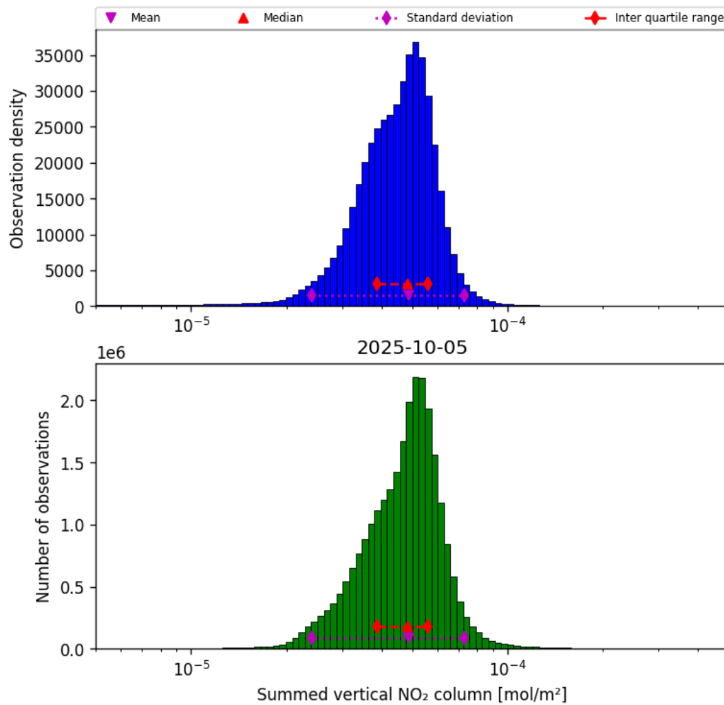
Figure 40: Histogram of “Summed vertical NO 2 column” for 2025-10-04 to 2025-10-06
