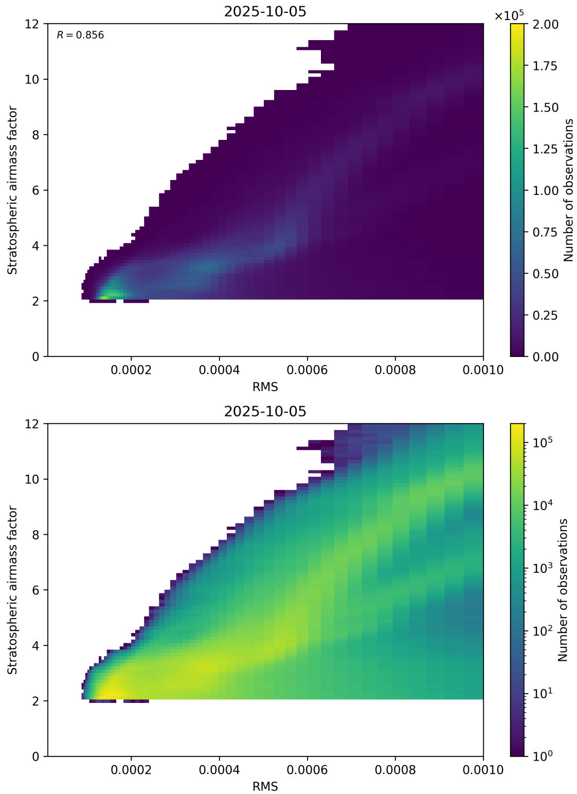
Figure 144: Scatter density plot of “RMS” against “Stratospheric airmass factor” for 2025-10-04 to 2025-10-06.
