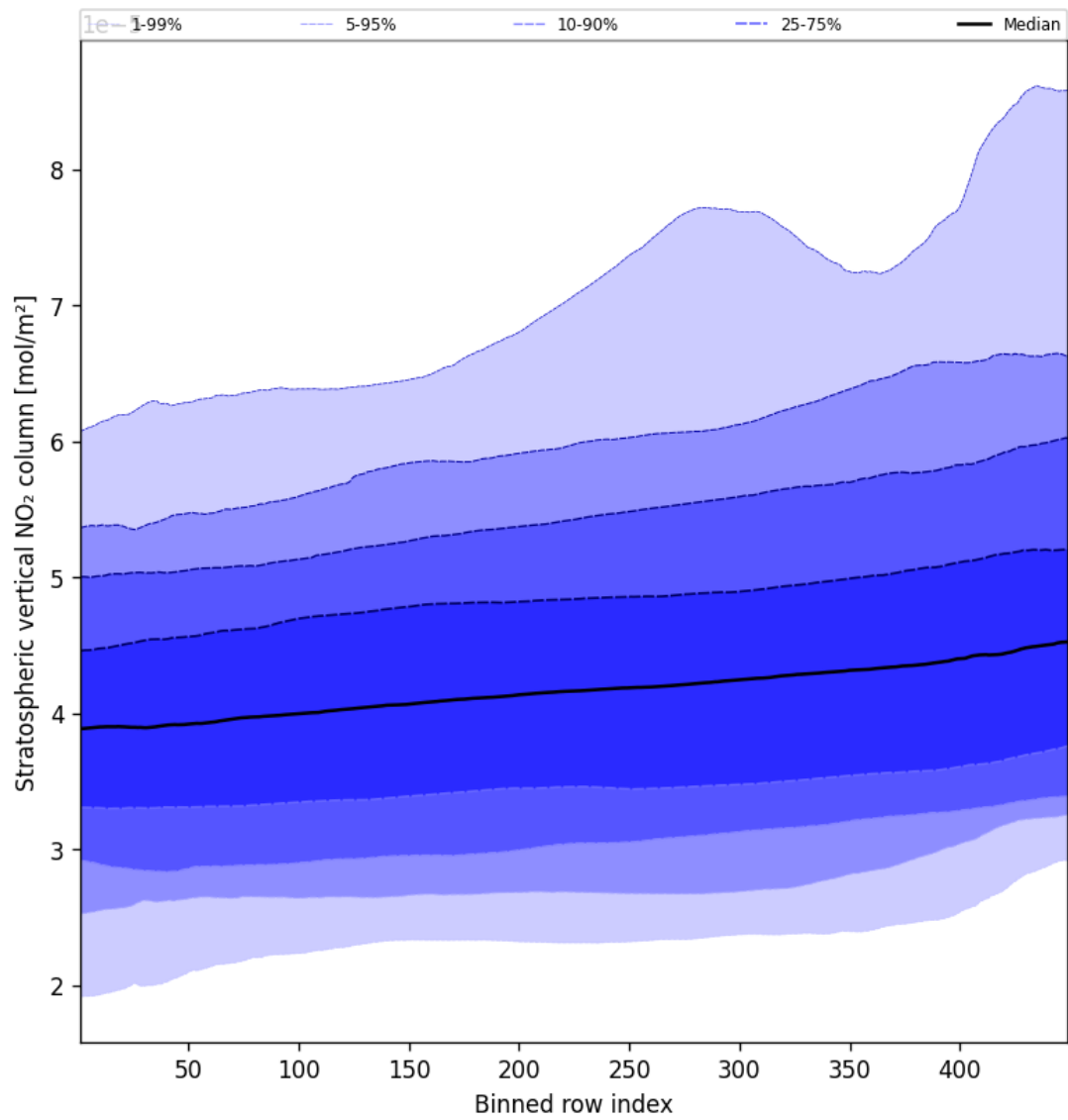
Figure 53: Along track statistics of “Stratospheric vertical NO 2 column” for 2025-10-04 to 2025-10-06
