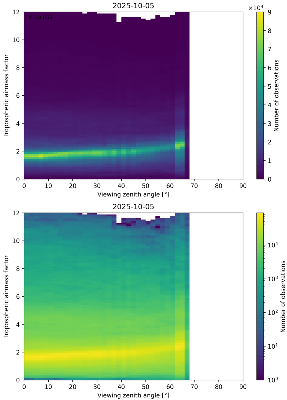
Figure 161: Scatter density plot of “Viewing zenith angle” against “Tropospheric airmass factor” for 2025-10-04 to 2025-10-06.
