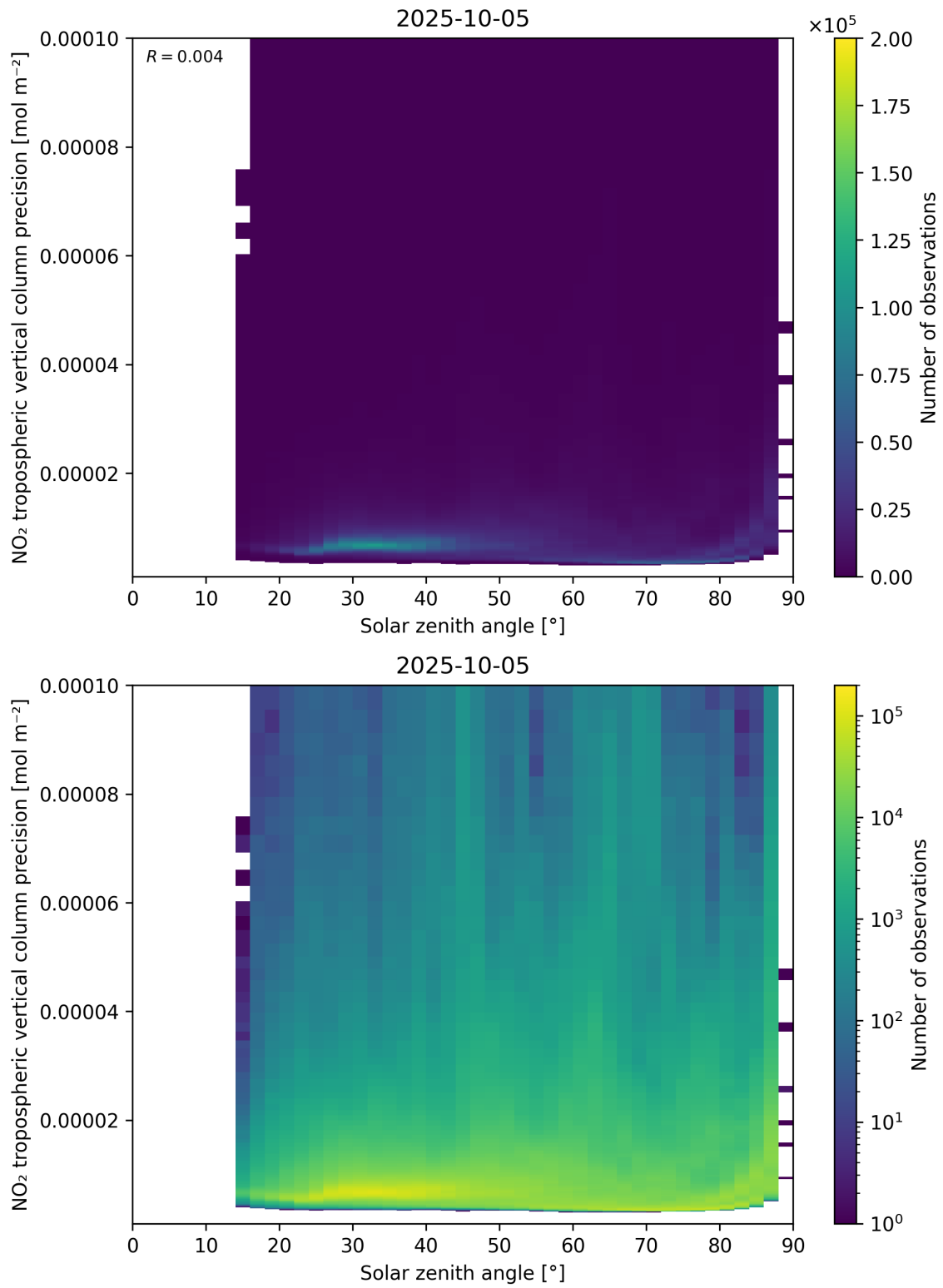
Figure 156: Scatter density plot of “Solar zenith angle” against “NO 2 tropospheric vertical column precision” for 2025-10-04 to 2025-10-06.
