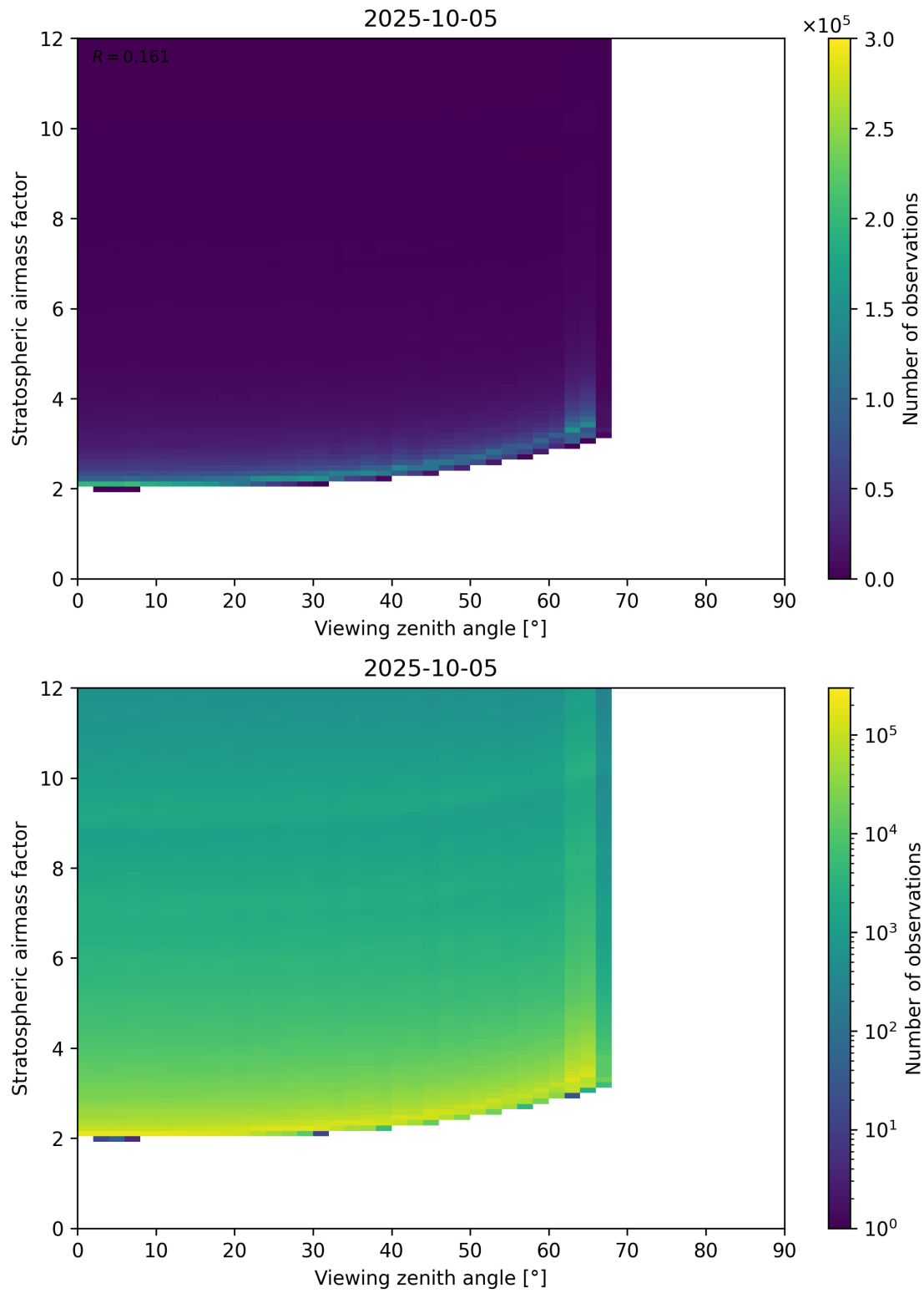
Figure 159: Scatter density plot of “Viewing zenith angle” against “Stratospheric airmass factor” for 2025-10-04 to 2025-10-06.
