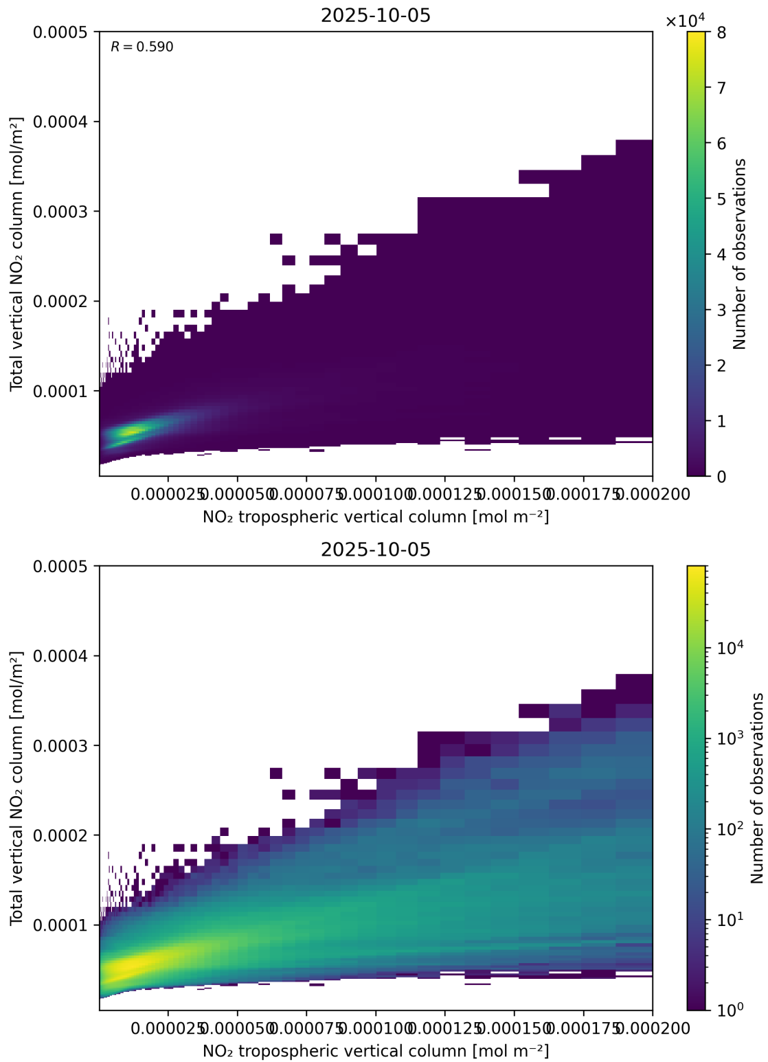
Figure 128: Scatter density plot of “NO 2 tropospheric vertical column” against “Total vertical NO 2 column” for 2025-10-04 to 2025-10-06.
