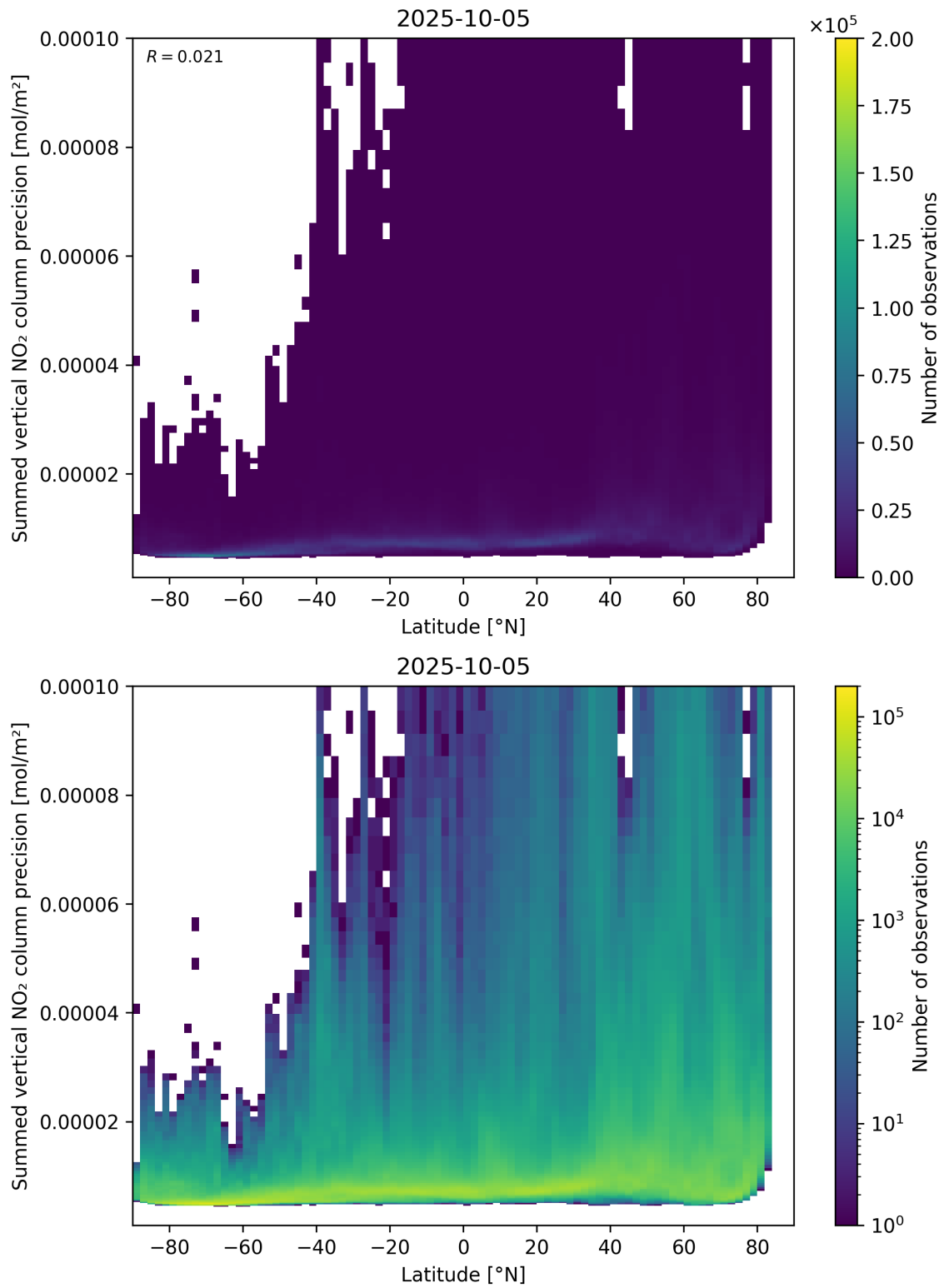
Figure 89: Scatter density plot of “Latitude” against “Summed vertical NO 2 column precision” for 2025-10-04 to 2025-10-06.
