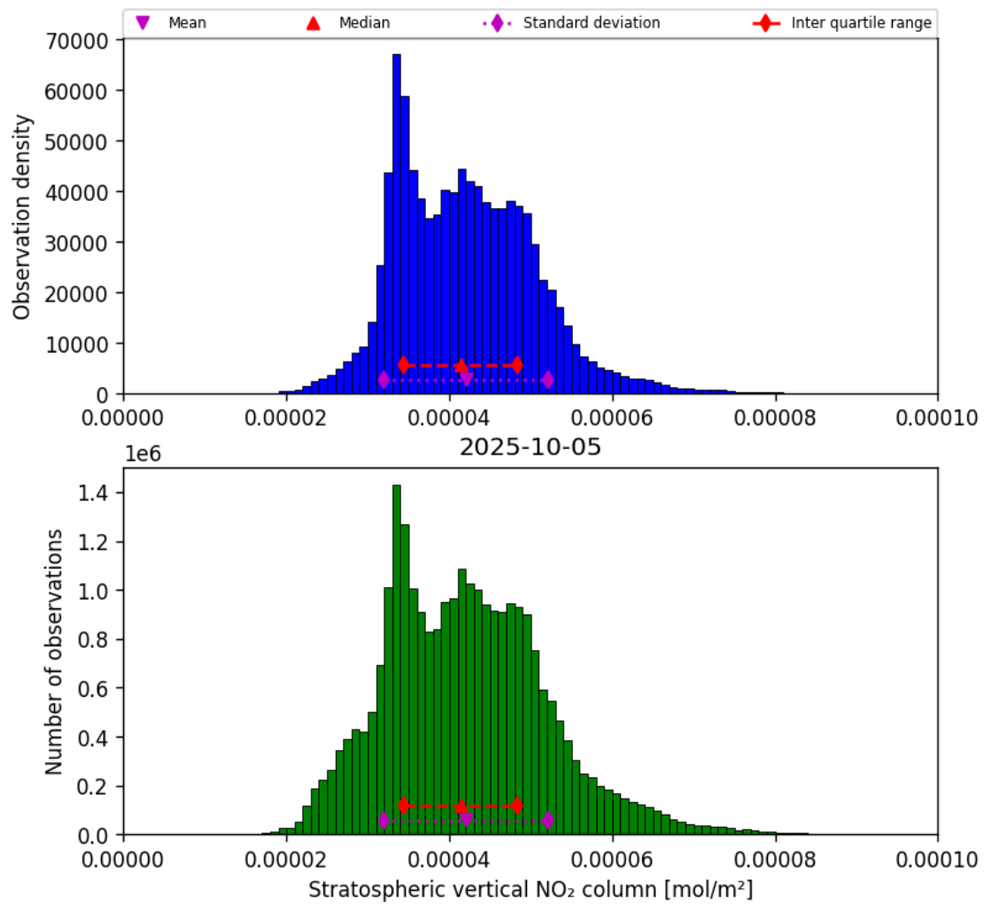
Figure 36: Histogram of “Stratospheric vertical NO 2 column” for 2025-10-04 to 2025-10-06
