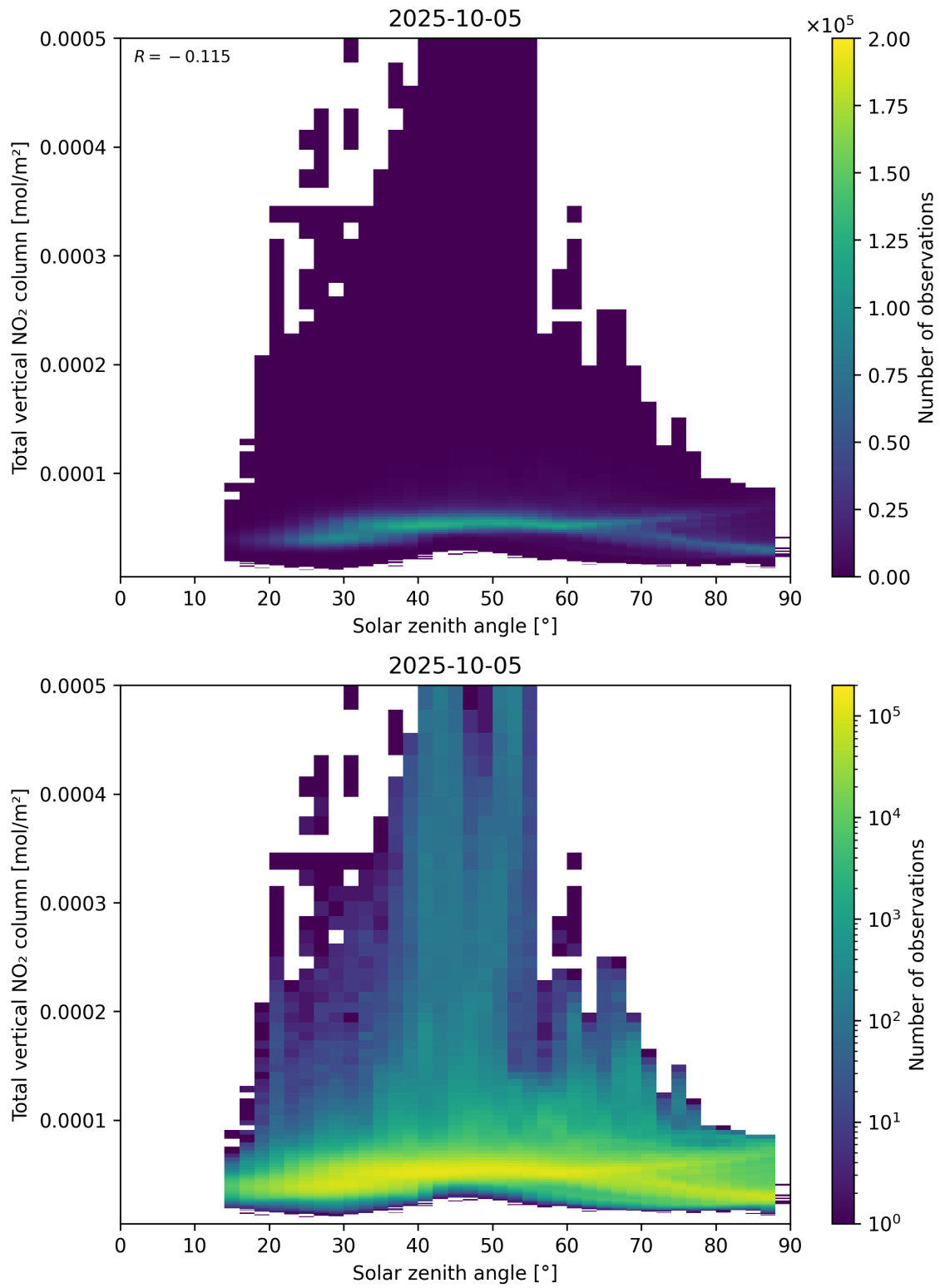
Figure 153: Scatter density plot of “Solar zenith angle” against “Total vertical NO 2 column” for 2025-10-04 to 2025-10-06.
