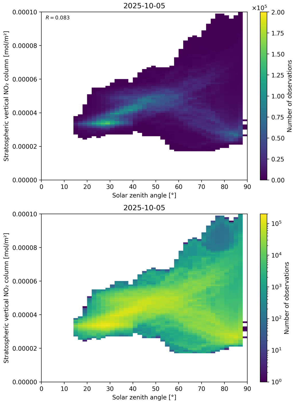
Figure 150: Scatter density plot of “Solar zenith angle” against “Stratospheric vertical NO 2 column” for 2025-10-04 to 2025-10-06.
