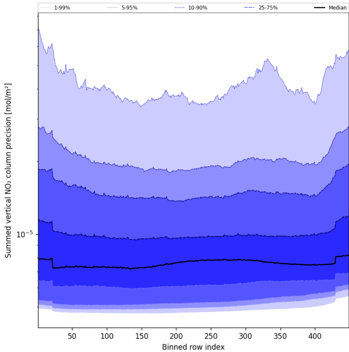
Figure 58: Along track statistics of “Summed vertical NO 2 column precision” for 2025-10-04 to 2025-10-06
