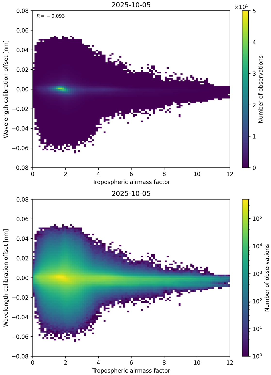
Figure 80: Scatter density plot of “Tropospheric airmass factor” against “Wavelength calibration offset” for 2025-10-04 to 2025-10-06.
