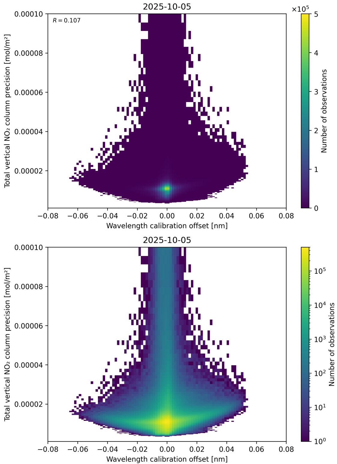
Figure 180: Scatter density plot of “Wavelength calibration offset” against “Total vertical NO 2 column precision” for 2025-10-04 to 2025-10-06.
