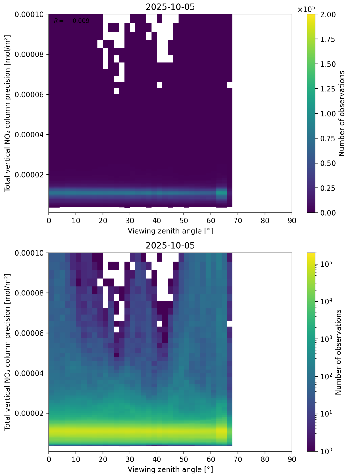
Figure 168: Scatter density plot of “Viewing zenith angle” against “Total vertical NO 2 column precision” for 2025-10-04 to 2025-10-06.
