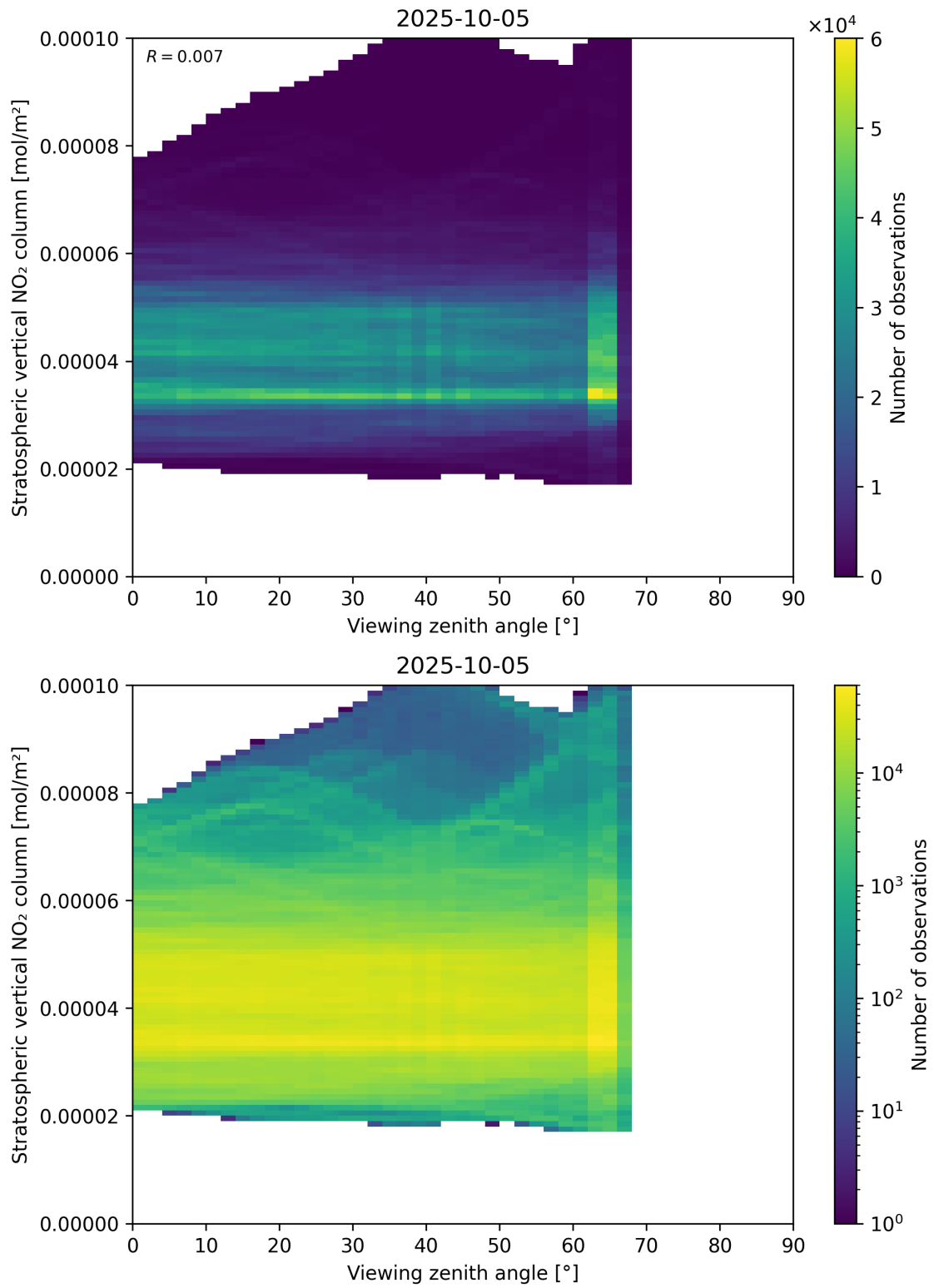
Figure 164: Scatter density plot of “Viewing zenith angle” against “Stratospheric vertical NO 2 column” for 2025-10-04 to 2025-10-06.
