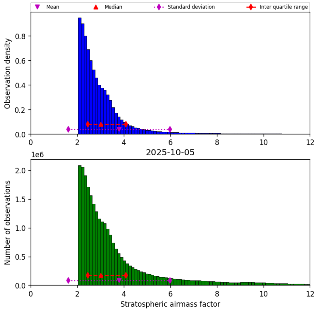
Figure 44: Histogram of “Stratospheric airmass factor” for 2025-10-04 to 2025-10-06
