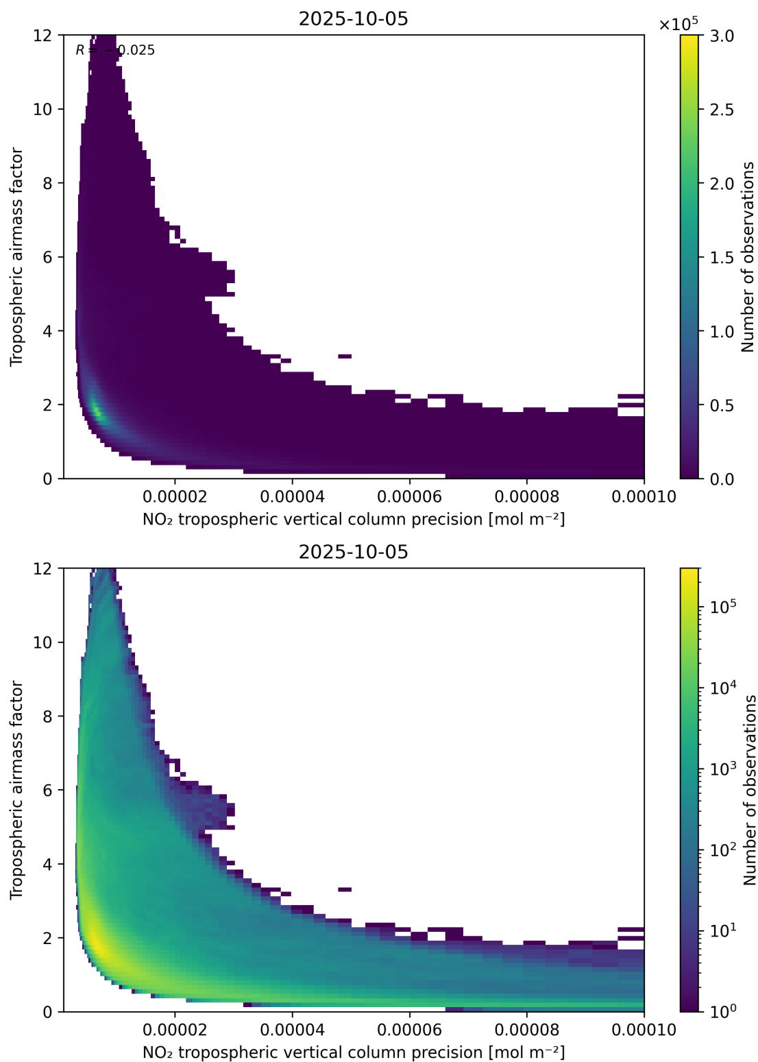
Figure 133: Scatter density plot of “NO 2 tropospheric vertical column precision” against “Tropospheric airmass factor” for 2025-10-04 to 2025-10-06.
