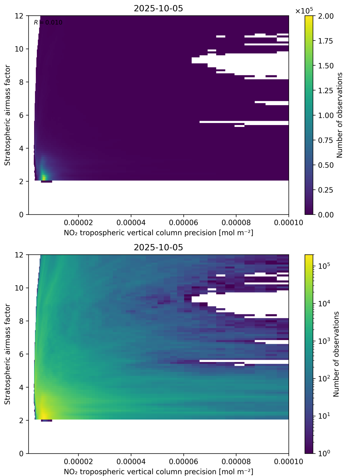
Figure 131: Scatter density plot of “NO 2 tropospheric vertical column precision” against “Stratospheric airmass factor” for 2025-10-04 to 2025-10-06.
