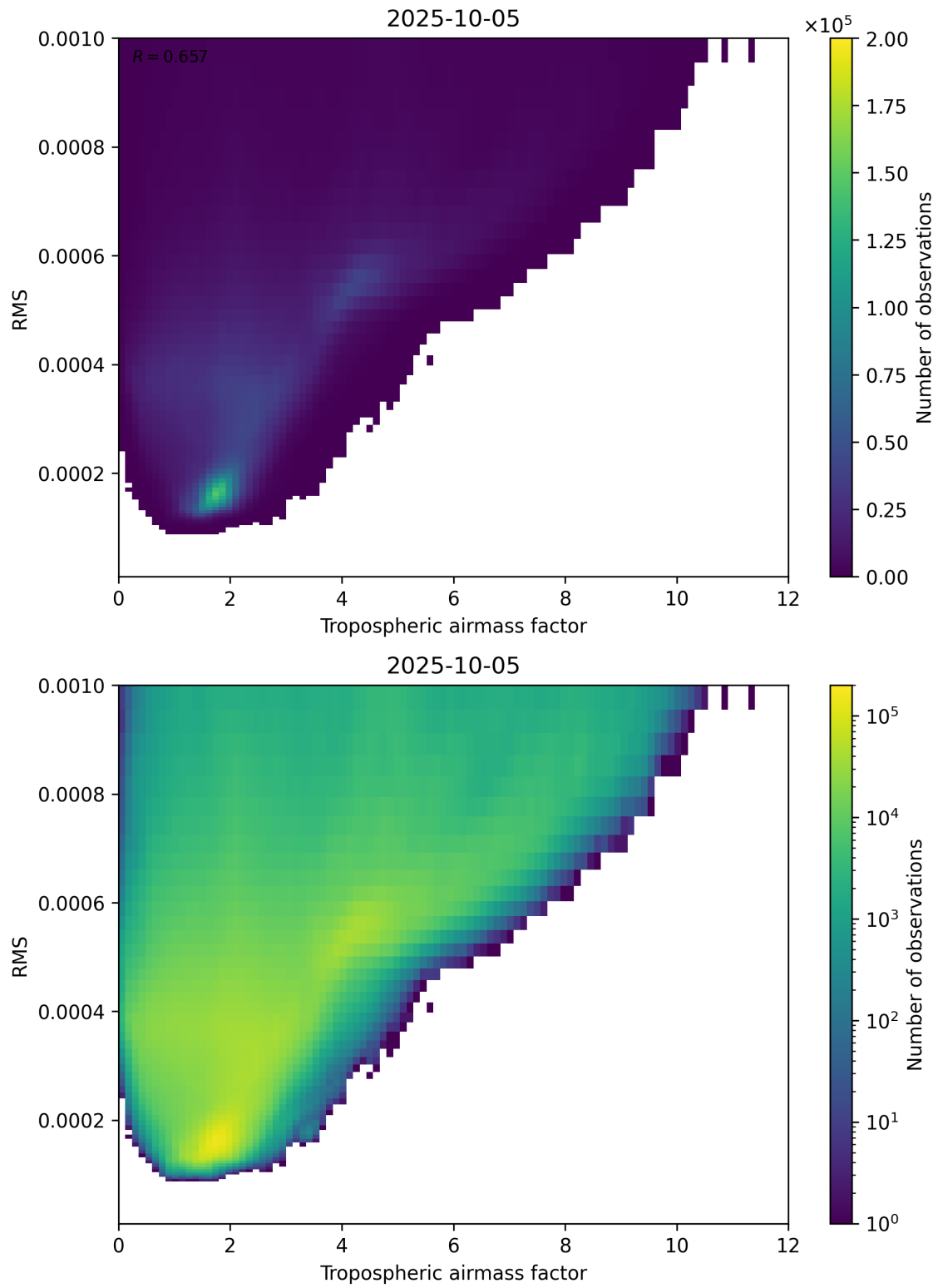
Figure 79: Scatter density plot of “Tropospheric airmass factor” against “RMS” for 2025-10-04 to 2025-10-06.
