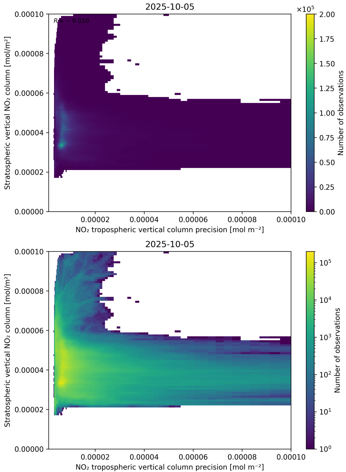
Figure 135: Scatter density plot of “NO 2 tropospheric vertical column precision” against “Stratospheric vertical NO 2 column” for 2025-10-04 to 2025-10-06.
