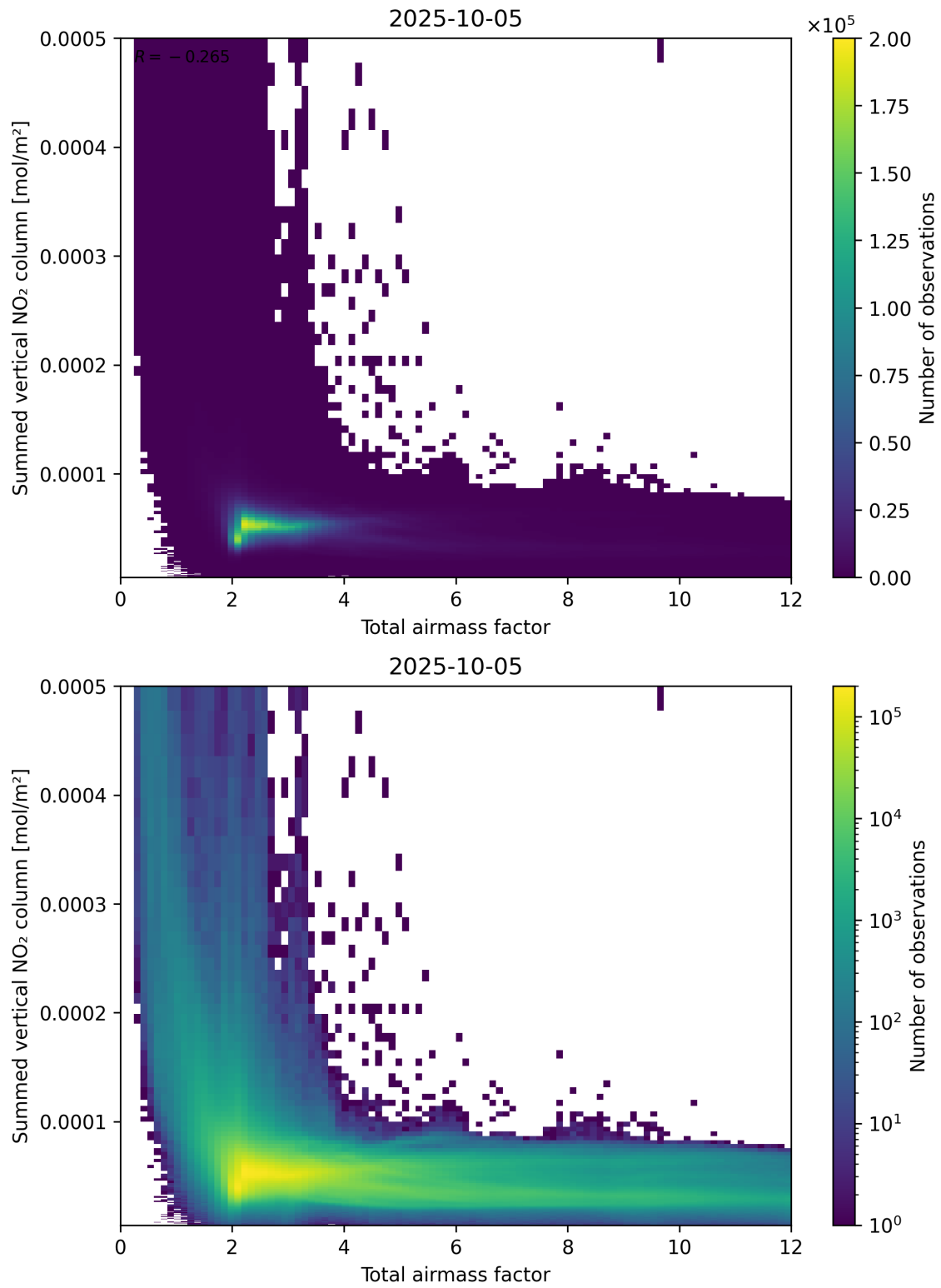
Figure 65: Scatter density plot of “Total airmass factor” against “Summed vertical NO 2 column” for 2025-10-04 to 2025-10-06.
