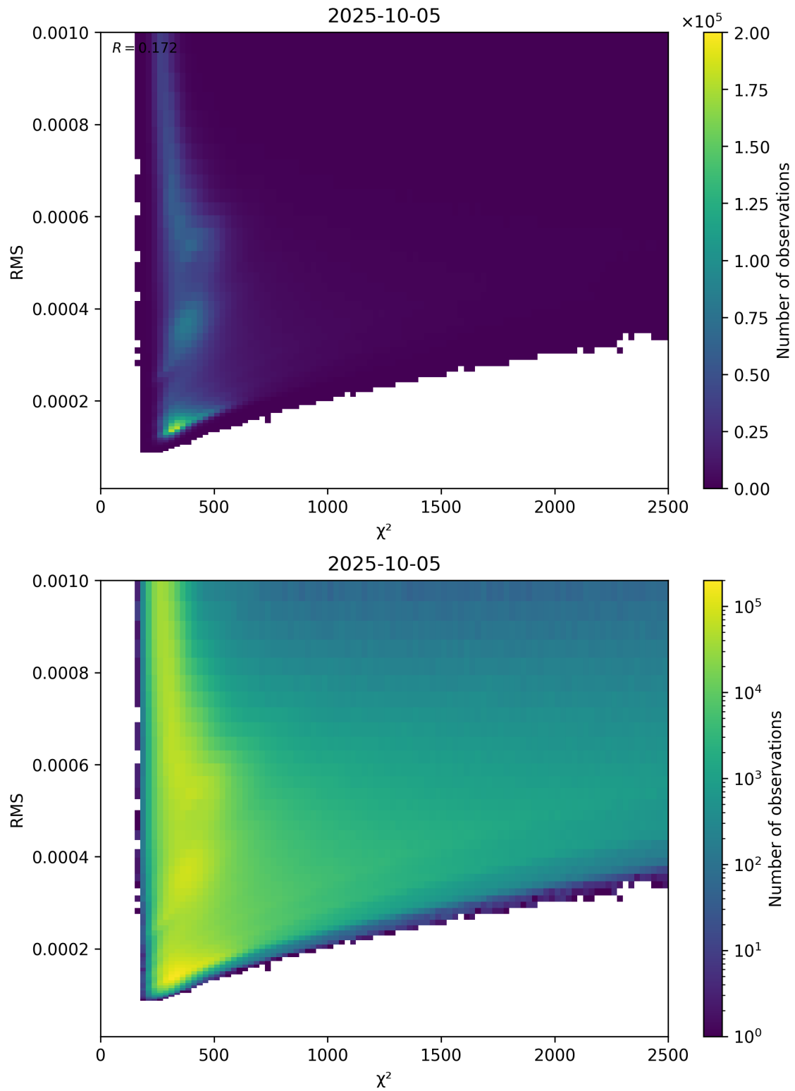
Figure 82: Scatter density plot of “ \chi^2 ” against “RMS” for 2025-10-04 to 2025-10-06.
