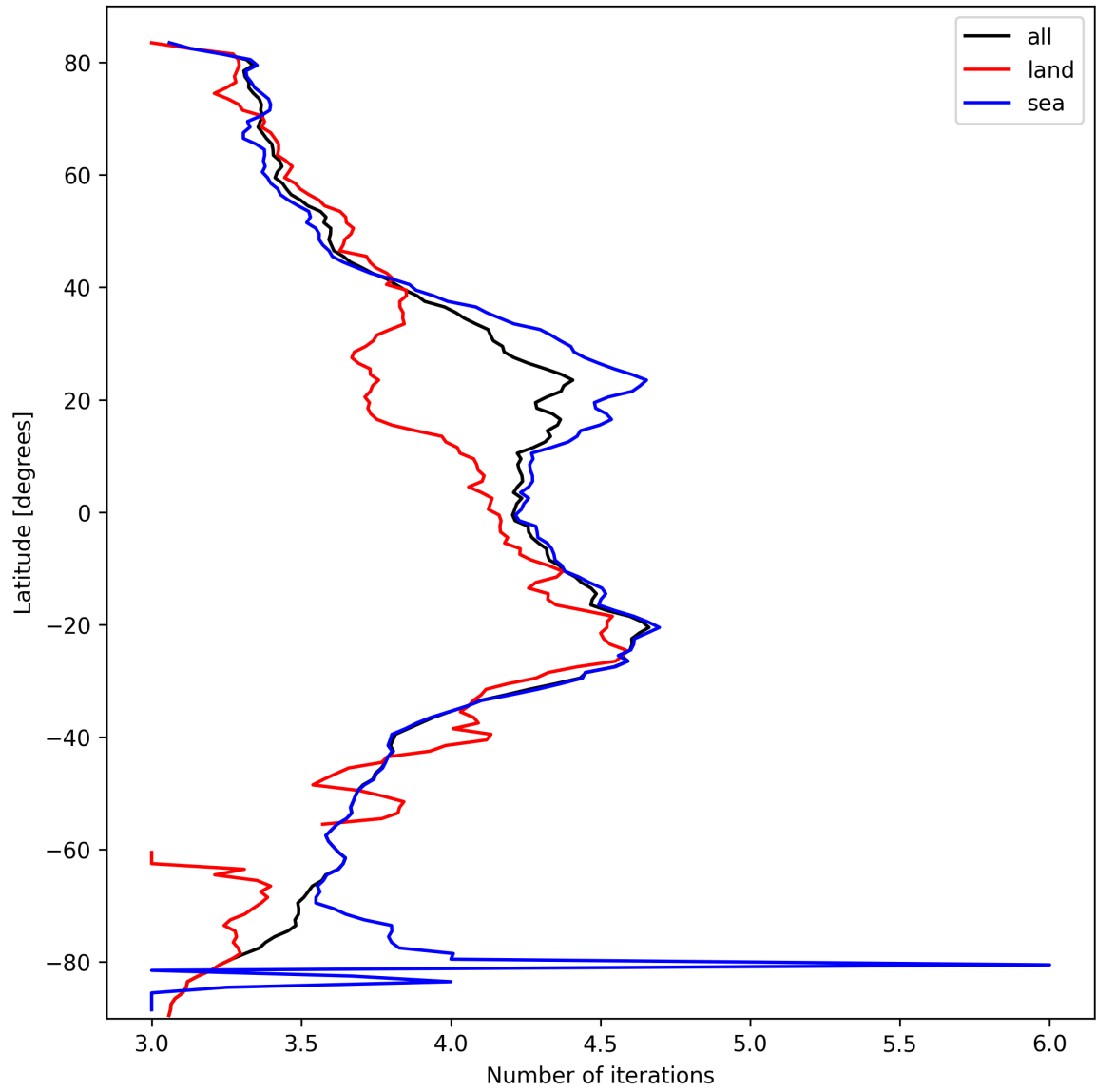
Figure 17: Zonal average of “Number of iterations” for 2025-10-04 to 2025-10-06.
