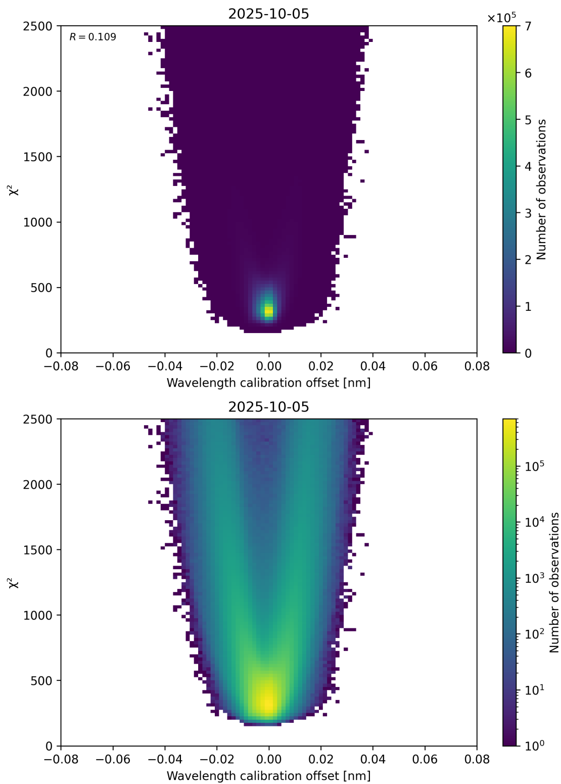
Figure 175: Scatter density plot of “Wavelength calibration offset” against “ \chi^2 ” for 2025-10-04 to 2025-10-06.
