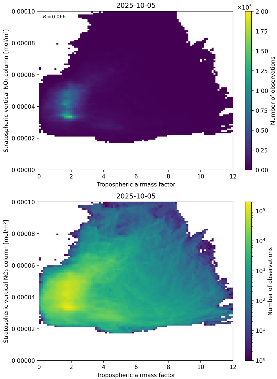
Figure 74: Scatter density plot of “Tropospheric air mass factor” against “Stratospheric vertical \text{NO}_2 column” for 2025-10-04 to 2025-10-06.
