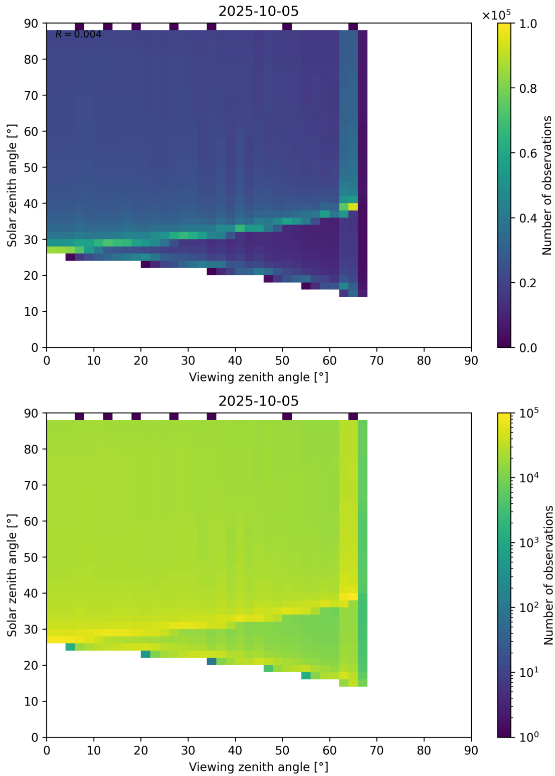
Figure 172: Scatter density plot of “Viewing zenith angle” against “Solar zenith angle” for 2025-10-04 to 2025-10-06.
