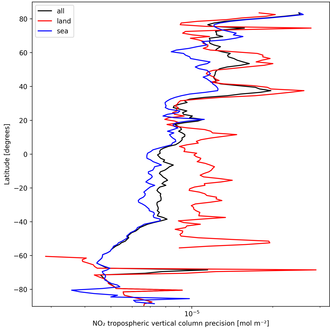
Figure 13: Zonal average of “NO 2 tropospheric vertical column precision” for 2025-10-04 to 2025-10-06.
