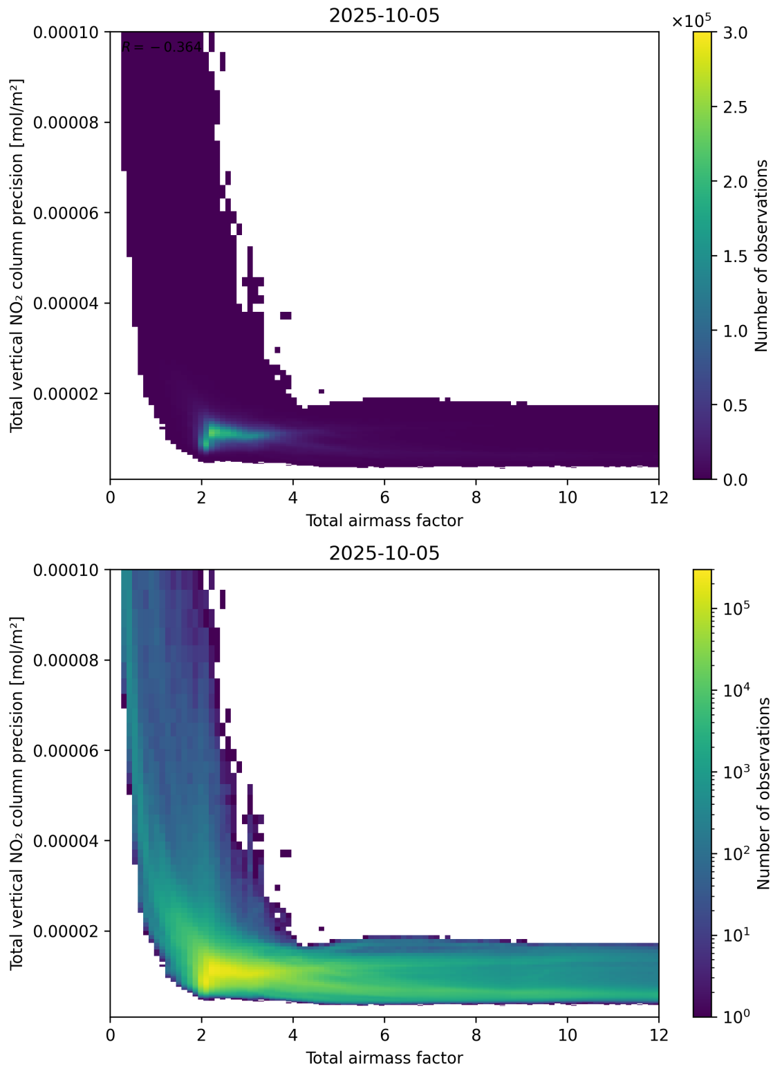
Figure 68: Scatter density plot of “Total airmass factor” against “Total vertical NO 2 column precision” for 2025-10-04 to 2025-10-06.
