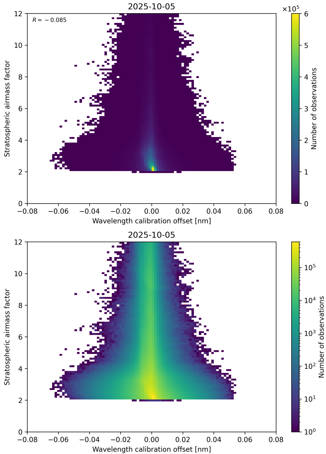
Figure 174: Scatter density plot of “Wavelength calibration offset” against “Stratospheric airmass factor” for 2025-10-04 to 2025-10-06.
