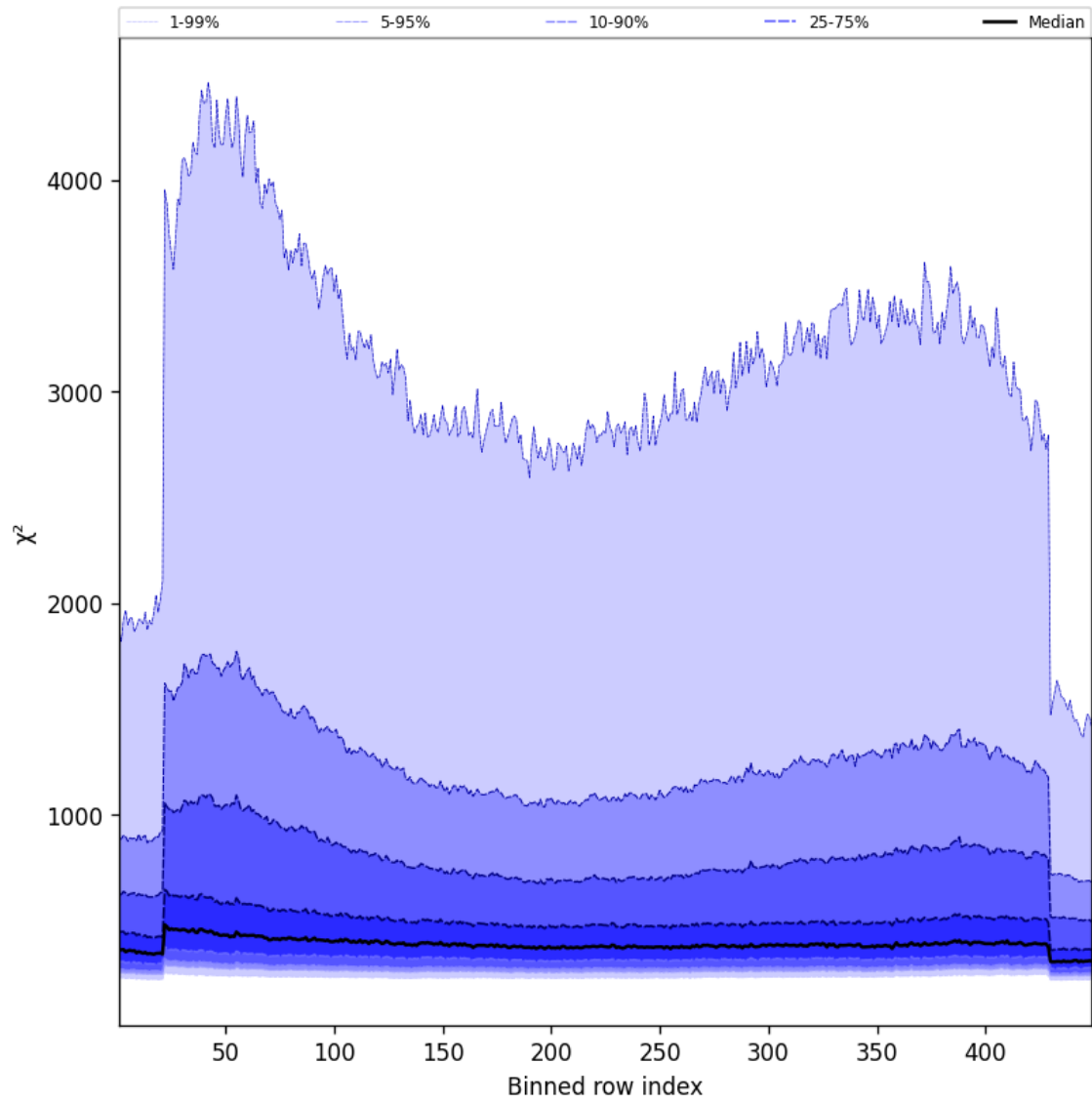
Figure 59: Along track statistics of “ \chi^2 ” for 2025-10-04 to 2025-10-06
