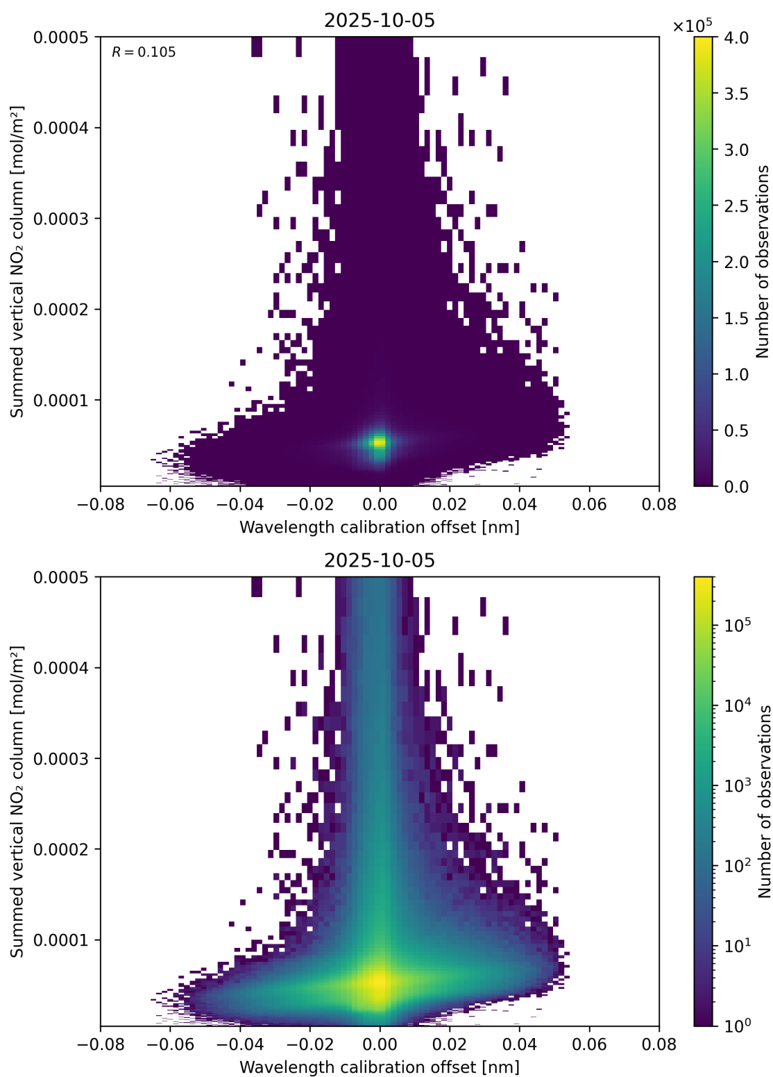
Figure 177: Scatter density plot of “Wavelength calibration offset” against “Summed vertical NO 2 column” for 2025-10-04 to 2025-10-06.
