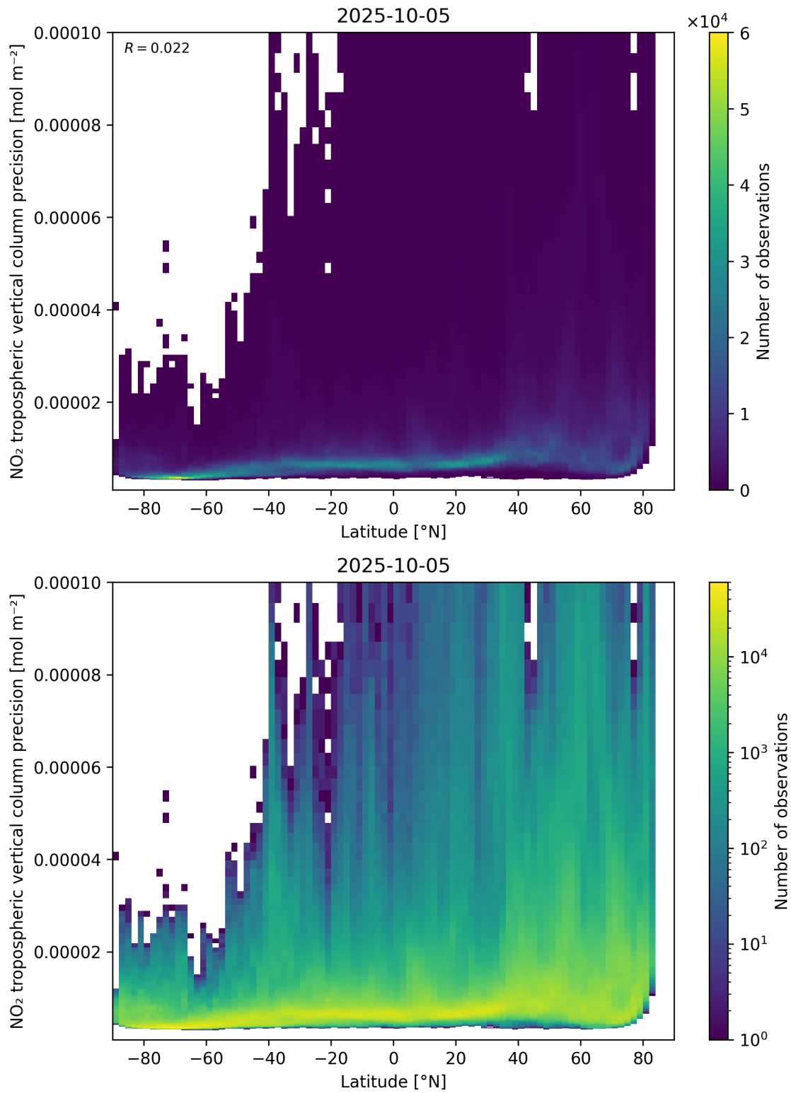
Figure 93: Scatter density plot of “Latitude” against “NO 2 tropospheric vertical column precision” for 2025-10-04 to 2025-10-06.
