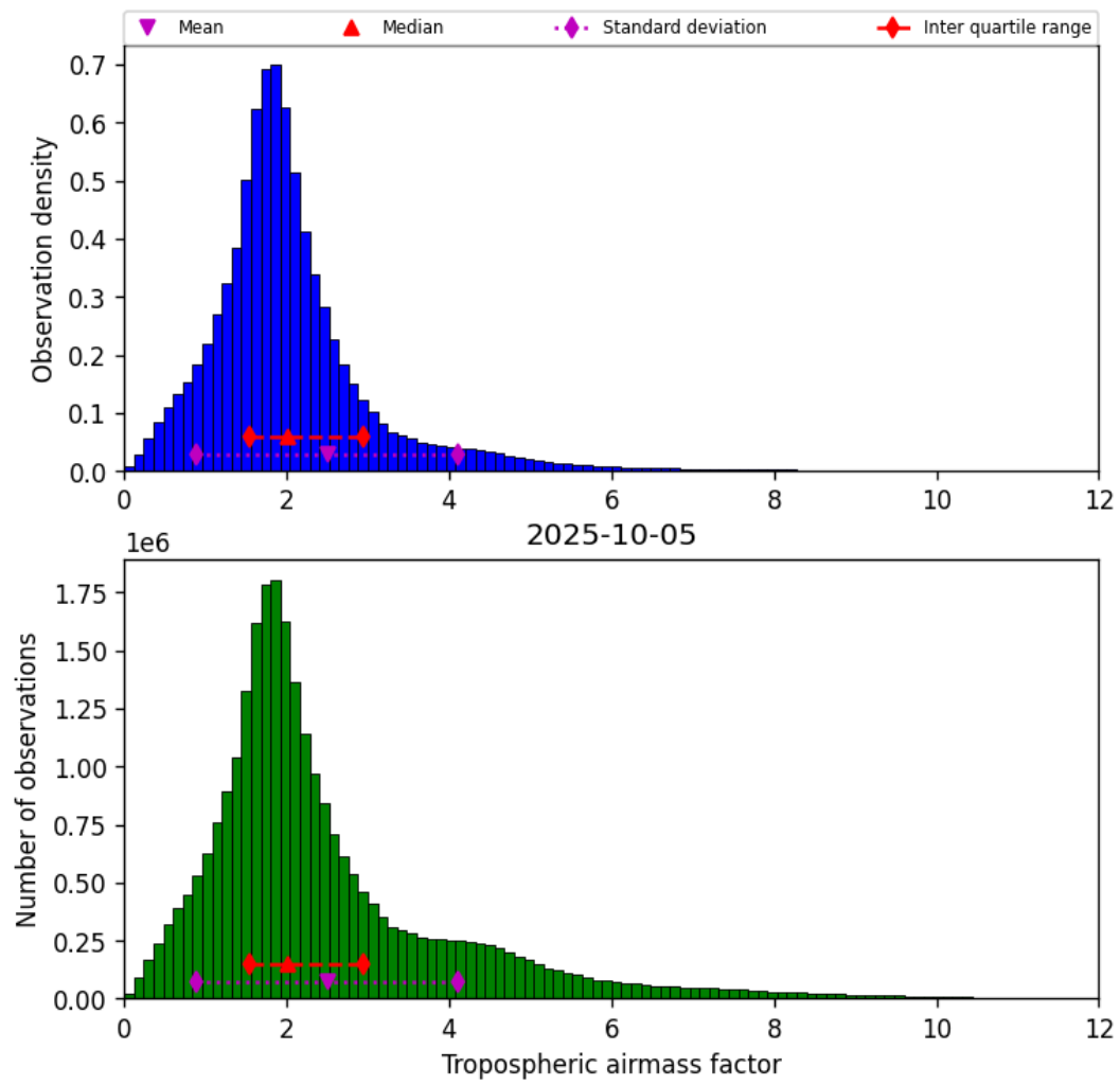
Figure 31: Histogram of “Tropospheric airmass factor” for 2025-10-04 to 2025-10-06
