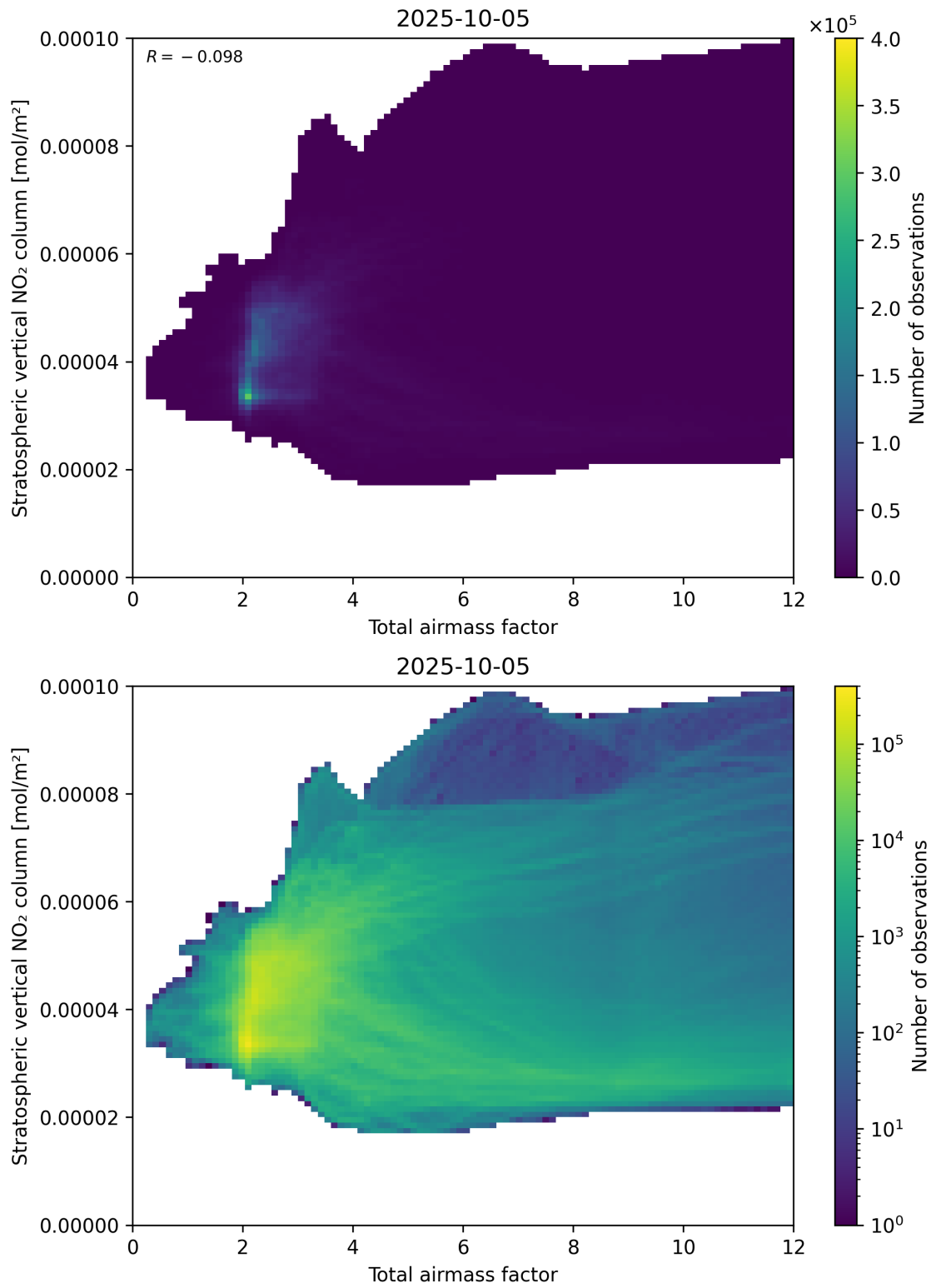
Figure 64: Scatter density plot of “Total airmass factor” against “Stratospheric vertical \text{NO}_2 column” for 2025-10-04 to 2025-10-06.
