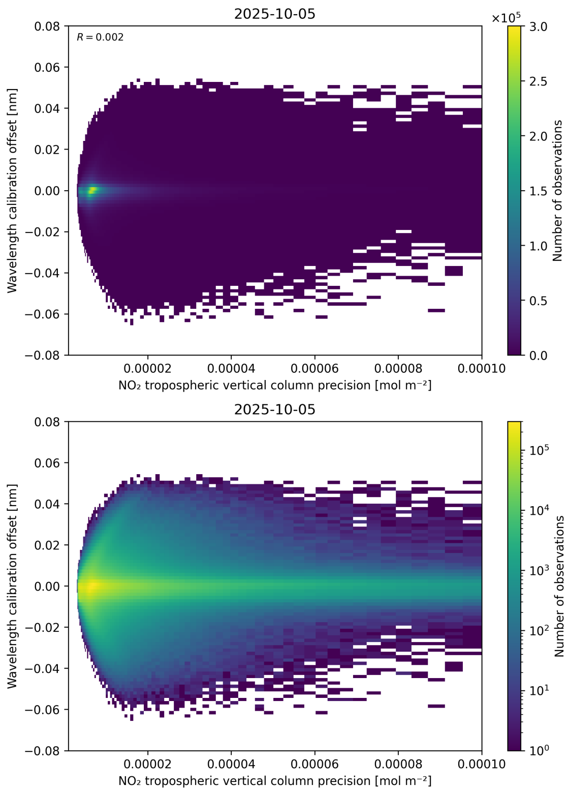
Figure 141: Scatter density plot of “NO 2 tropospheric vertical column precision” against “Wavelength calibration offset” for 2025-10-04 to 2025-10-06.
