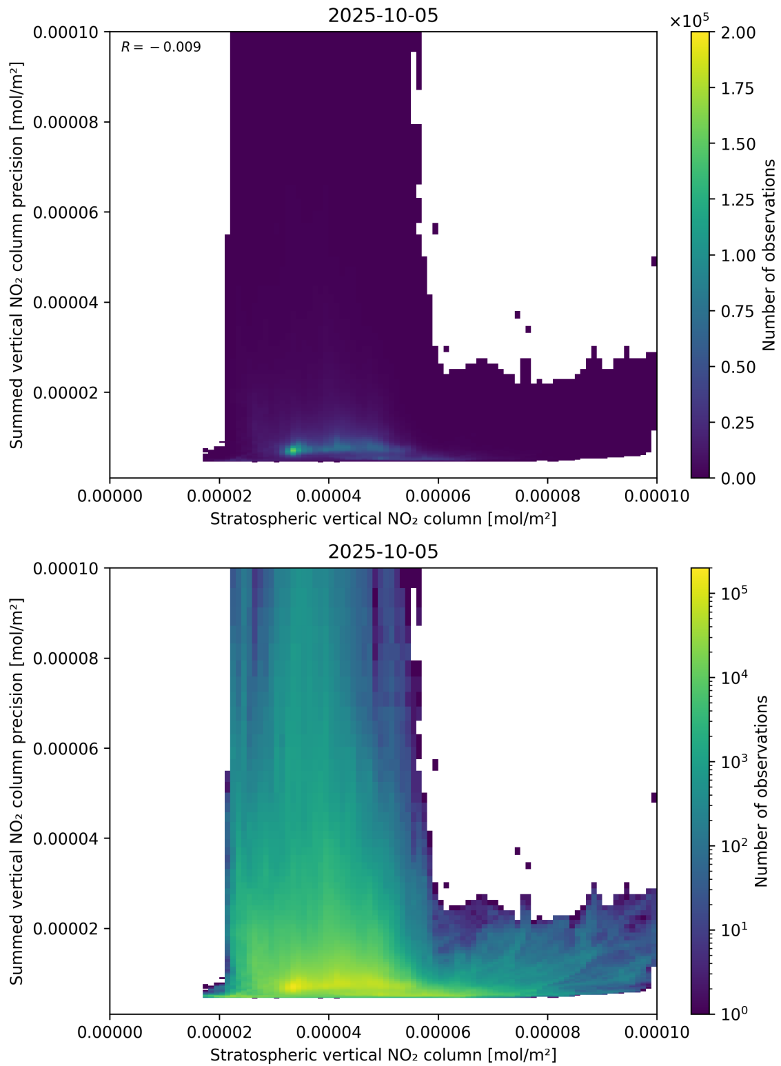
Figure 99: Scatter density plot of “Stratospheric vertical NO 2 column” against “Summed vertical NO 2 column precision” for 2025-10-04 to 2025-10-06.
