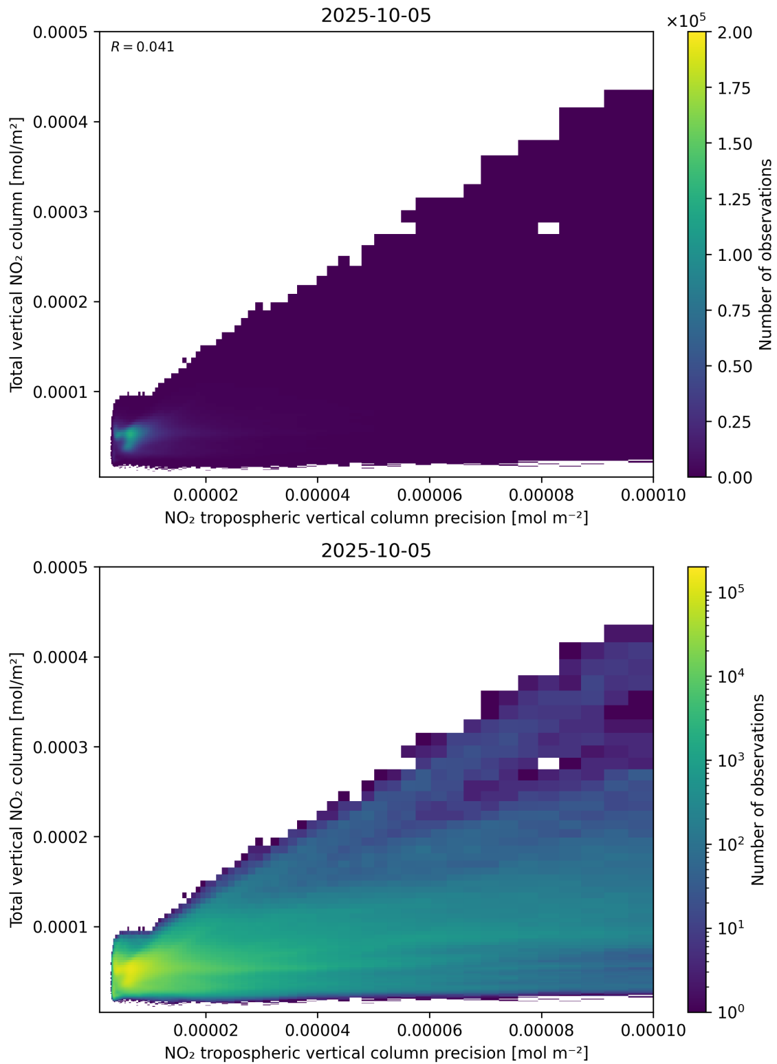
Figure 138: Scatter density plot of “NO 2 tropospheric vertical column precision” against “Total vertical NO 2 column” for 2025-10-04 to 2025-10-06.
