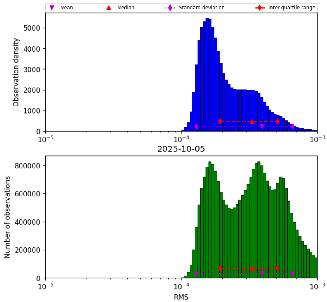
Figure 43: Histogram of “RMS” for 2025-10-04 to 2025-10-06
