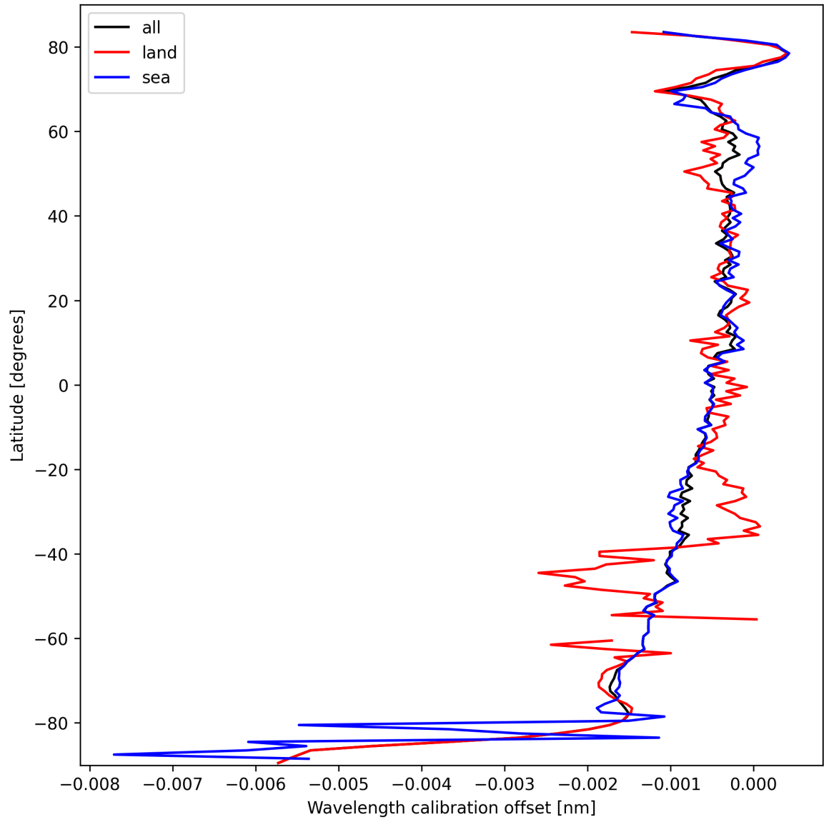
Figure 18: Zonal average of “Wavelength calibration offset” for 2025-10-04 to 2025-10-06.
