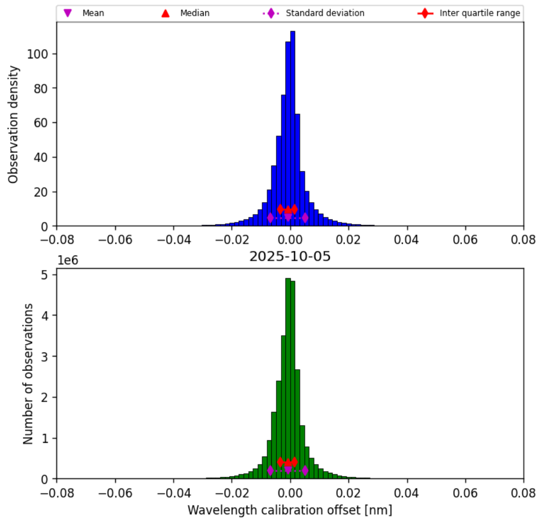
Figure 35: Histogram of “Wavelength calibration offset” for 2025-10-04 to 2025-10-06
