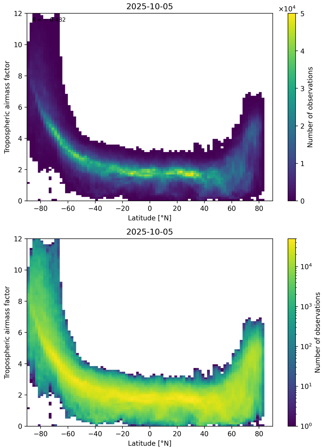
Figure 85: Scatter density plot of “Latitude” against “Tropospheric airmass factor” for 2025-10-04 to 2025-10-06.
