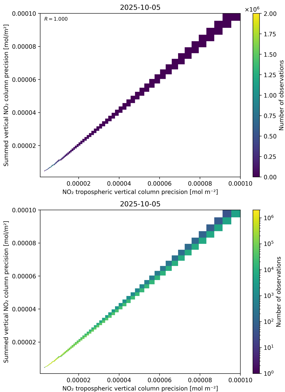
Figure 137: Scatter density plot of “NO 2 tropospheric vertical column precision” against “Summed vertical NO 2 column precision” for 2025-10-04 to 2025-10-06.
