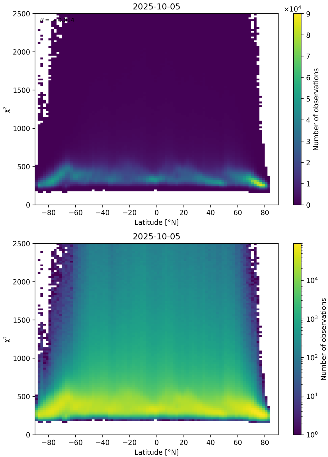
Figure 86: Scatter density plot of “Latitude” against “ \chi^2 ” for 2025-10-04 to 2025-10-06.
