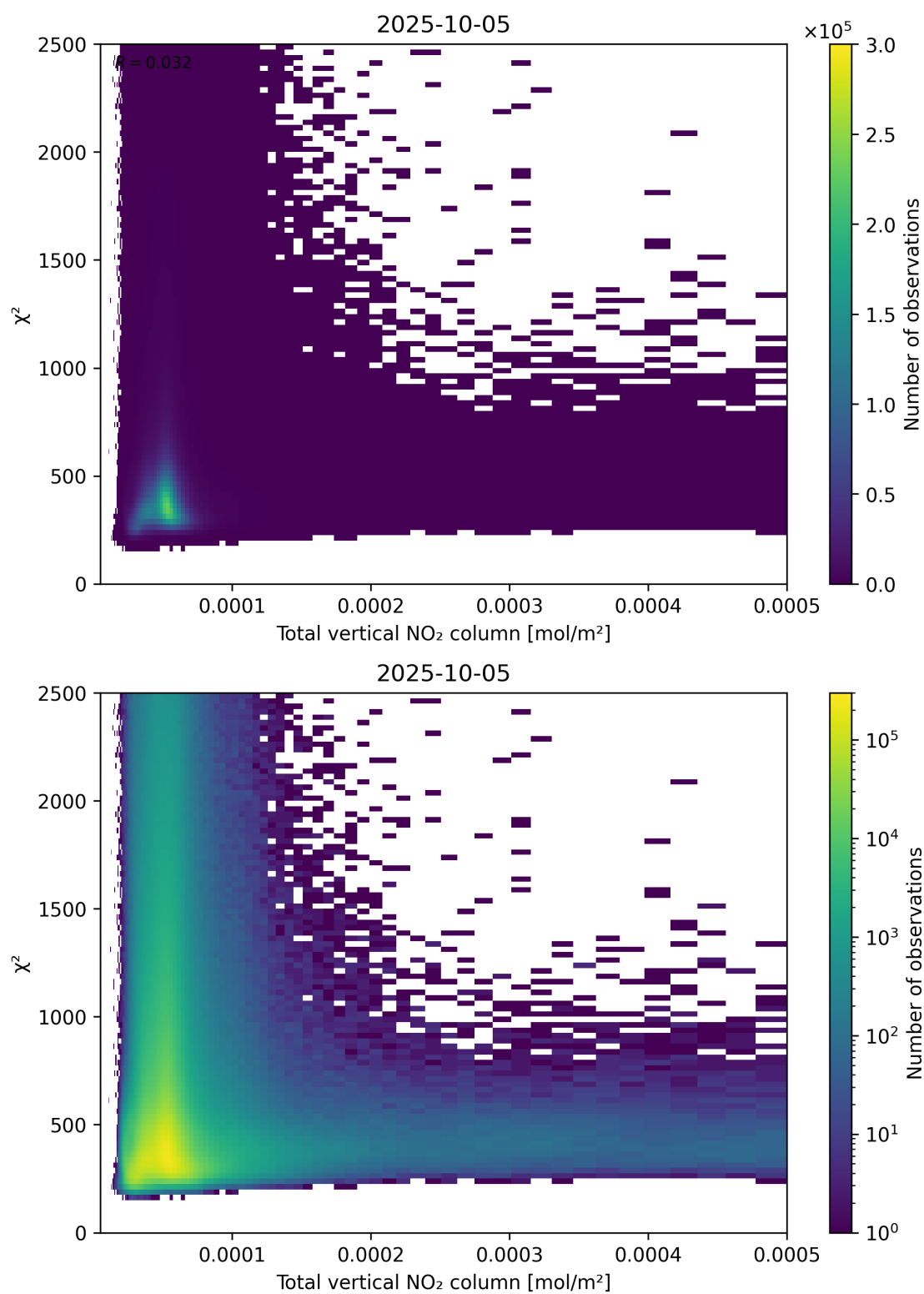
Figure 111: Scatter density plot of “Total vertical NO 2 column” against “ \chi^2 ” for 2025-10-04 to 2025-10-06.
