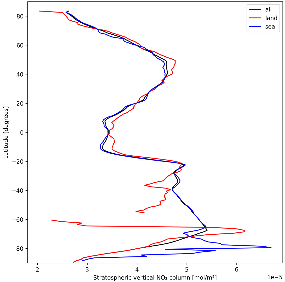
Figure 19: Zonal average of “Stratospheric vertical NO 2 column” for 2025-10-04 to 2025-10-06.
