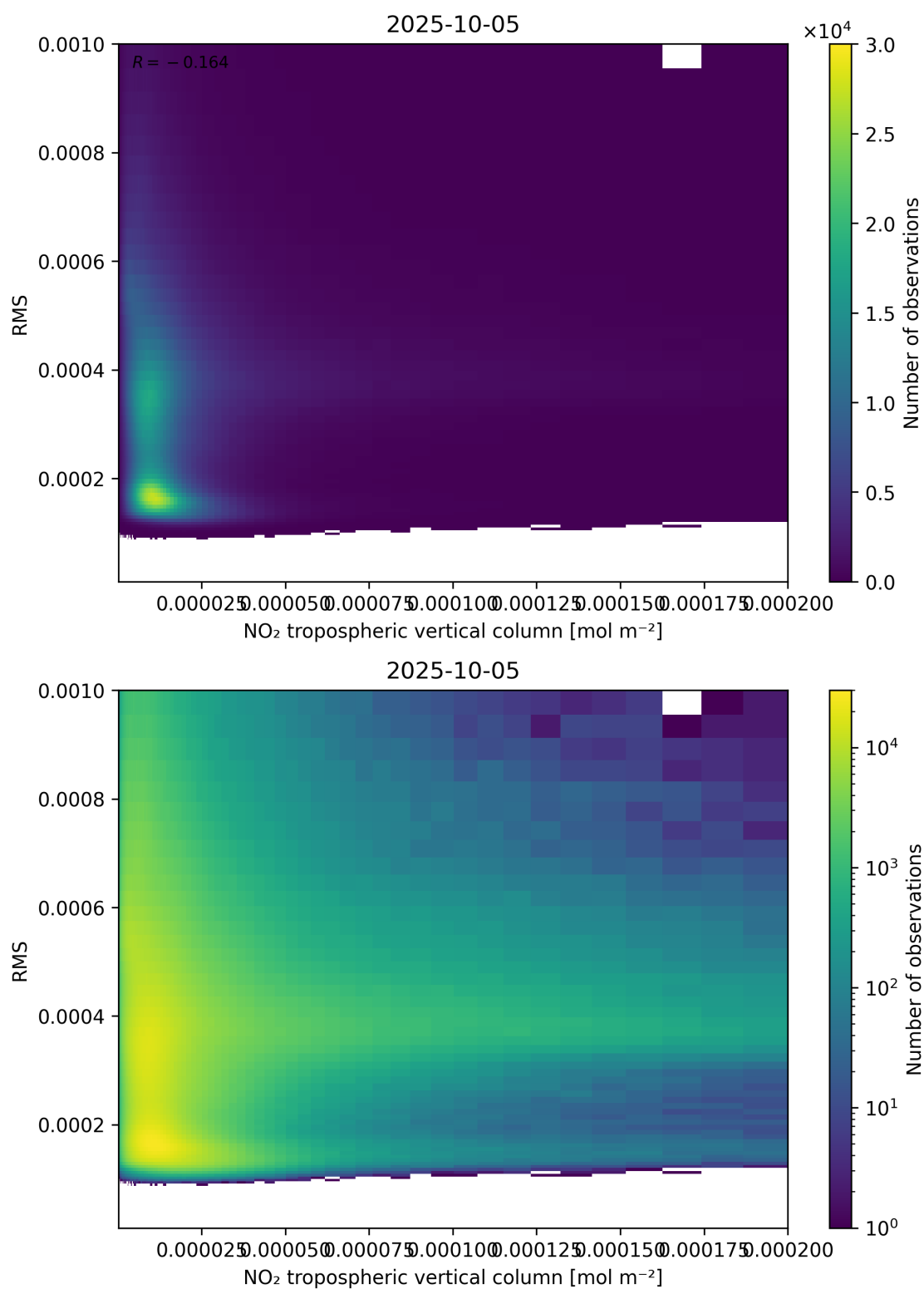
Figure 142: Scatter density plot of “NO 2 tropospheric vertical column” against “RMS” for 2025-10-04 to 2025-10-06.
