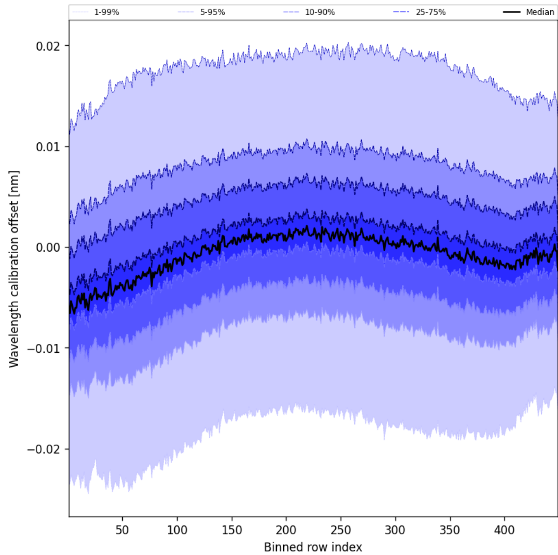
Figure 52: Along track statistics of “Wavelength calibration offset” for 2025-10-04 to 2025-10-06
