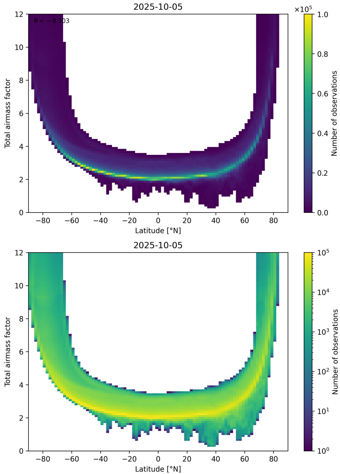
Figure 84: Scatter density plot of “Latitude” against “Total airmass factor” for 2025-10-04 to 2025-10-06.
