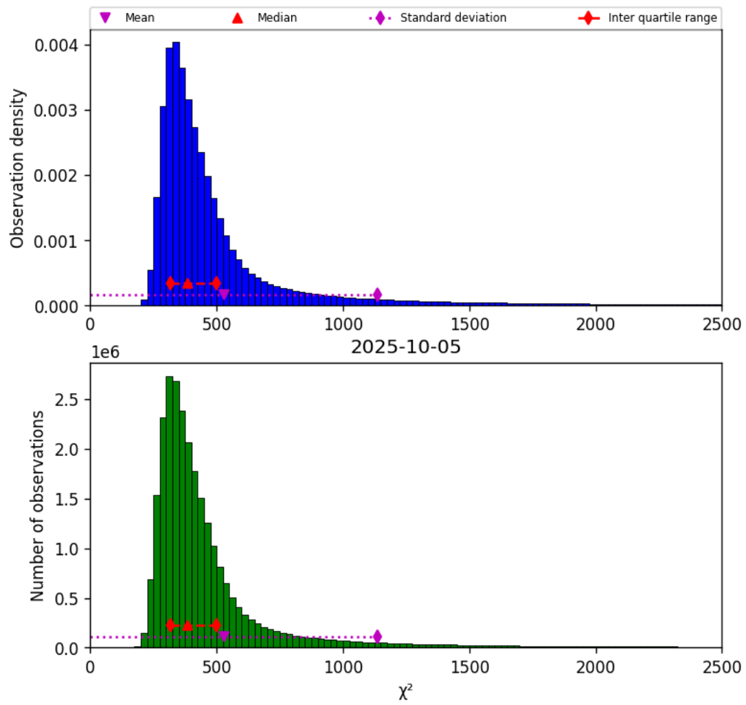
Figure 42: Histogram of " \chi^2 " for 2025-10-04 to 2025-10-06
