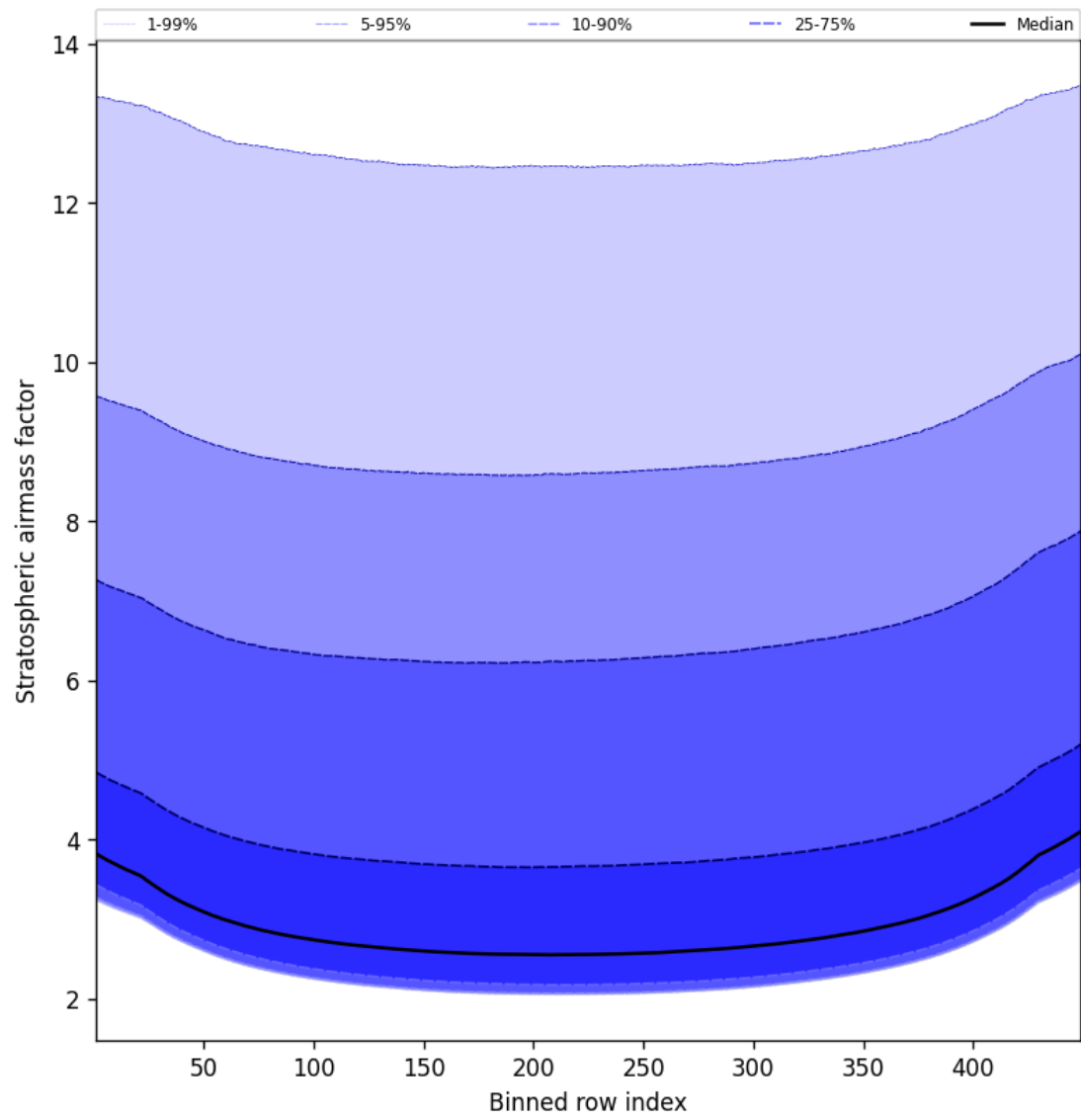
Figure 61: Along track statistics of “Stratospheric airmass factor” for 2025-10-04 to 2025-10-06
