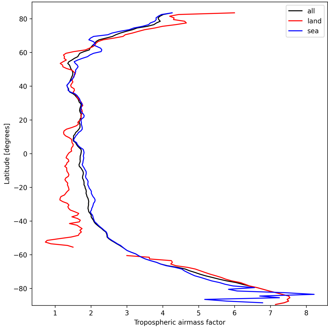
Figure 14: Zonal average of “Tropospheric air mass factor” for 2025-10-04 to 2025-10-06.
