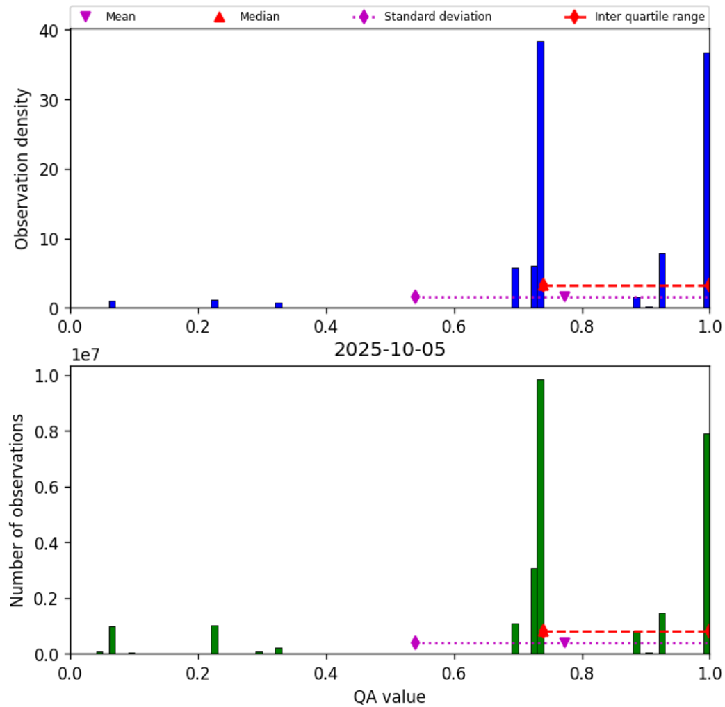
Figure 28: Histogram of “QA value” for 2025-10-04 to 2025-10-06
