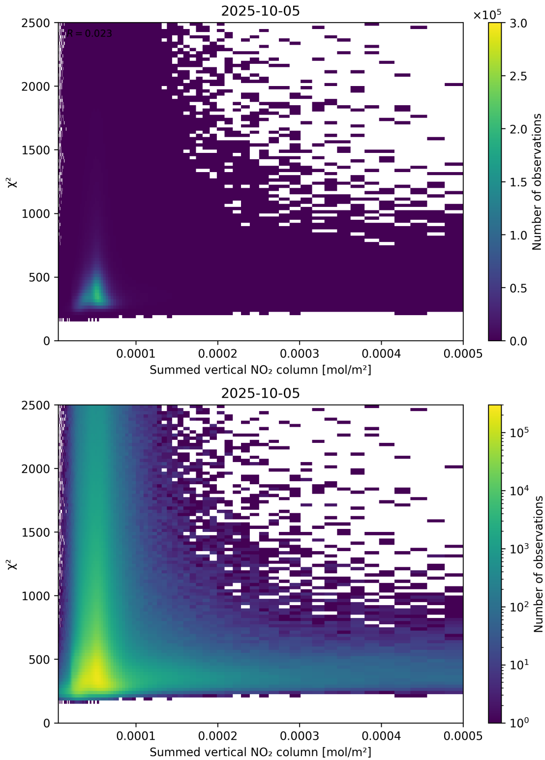
Figure 104: Scatter density plot of “Summed vertical NO 2 column” against “ \chi^2 ” for 2025-10-04 to 2025-10-06.
