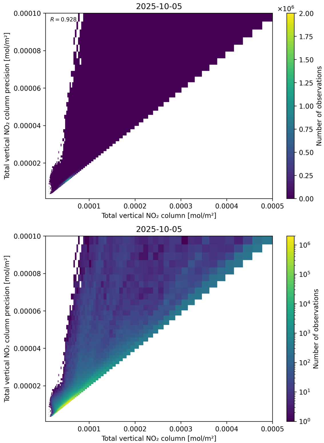
Figure 114: Scatter density plot of “Total vertical NO 2 column” against “Total vertical NO 2 column precision” for 2025-10-04 to 2025-10-06.
