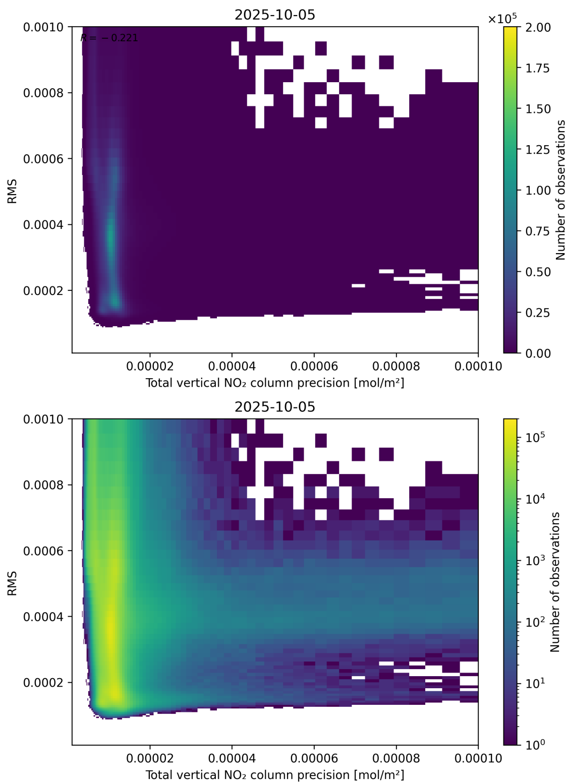
Figure 119: Scatter density plot of “Total vertical NO 2 column precision” against “RMS” for 2025-10-04 to 2025-10-06.
