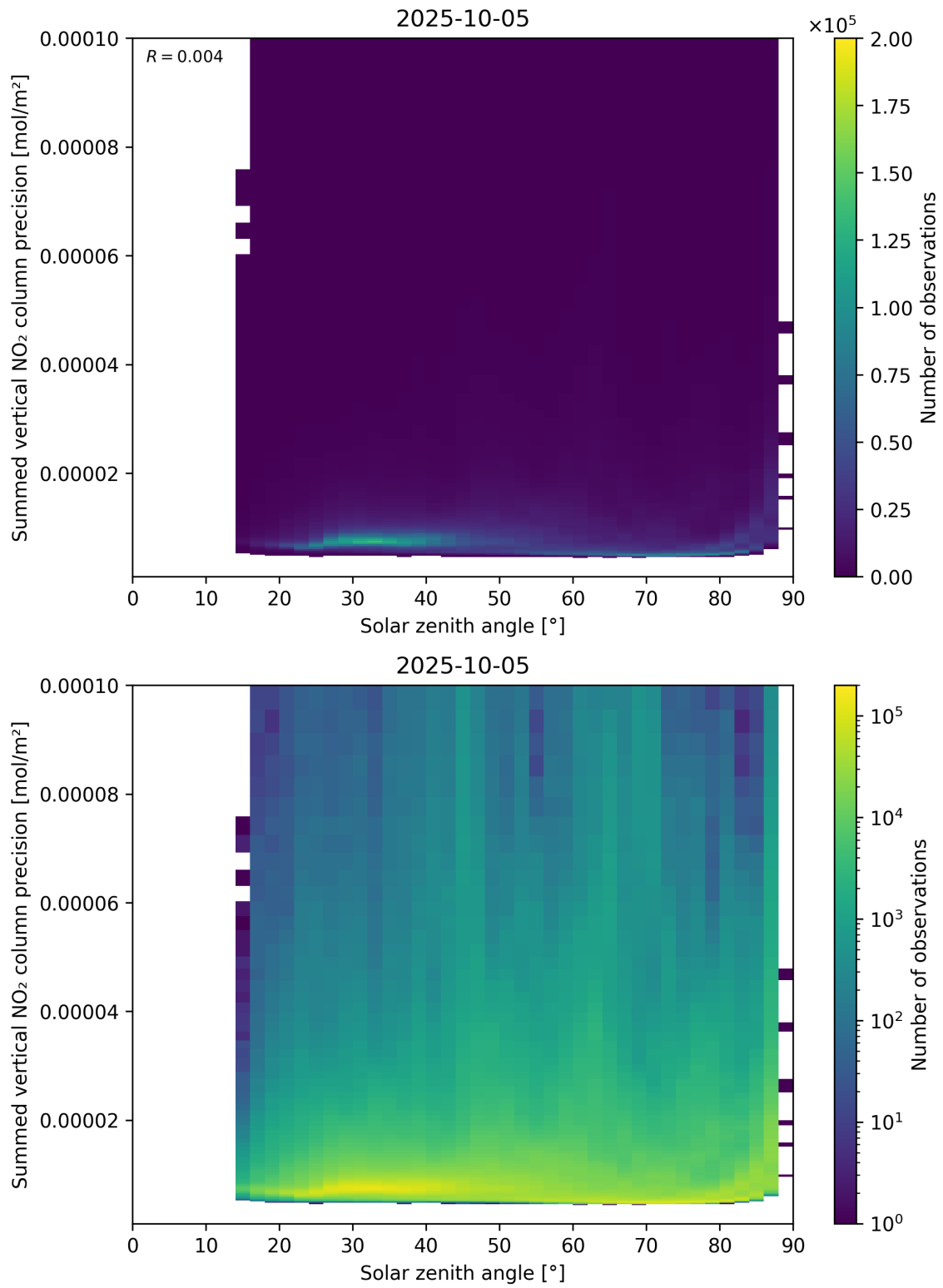
Figure 152: Scatter density plot of “Solar zenith angle” against “Summed vertical NO 2 column precision” for 2025-10-04 to 2025-10-06.
