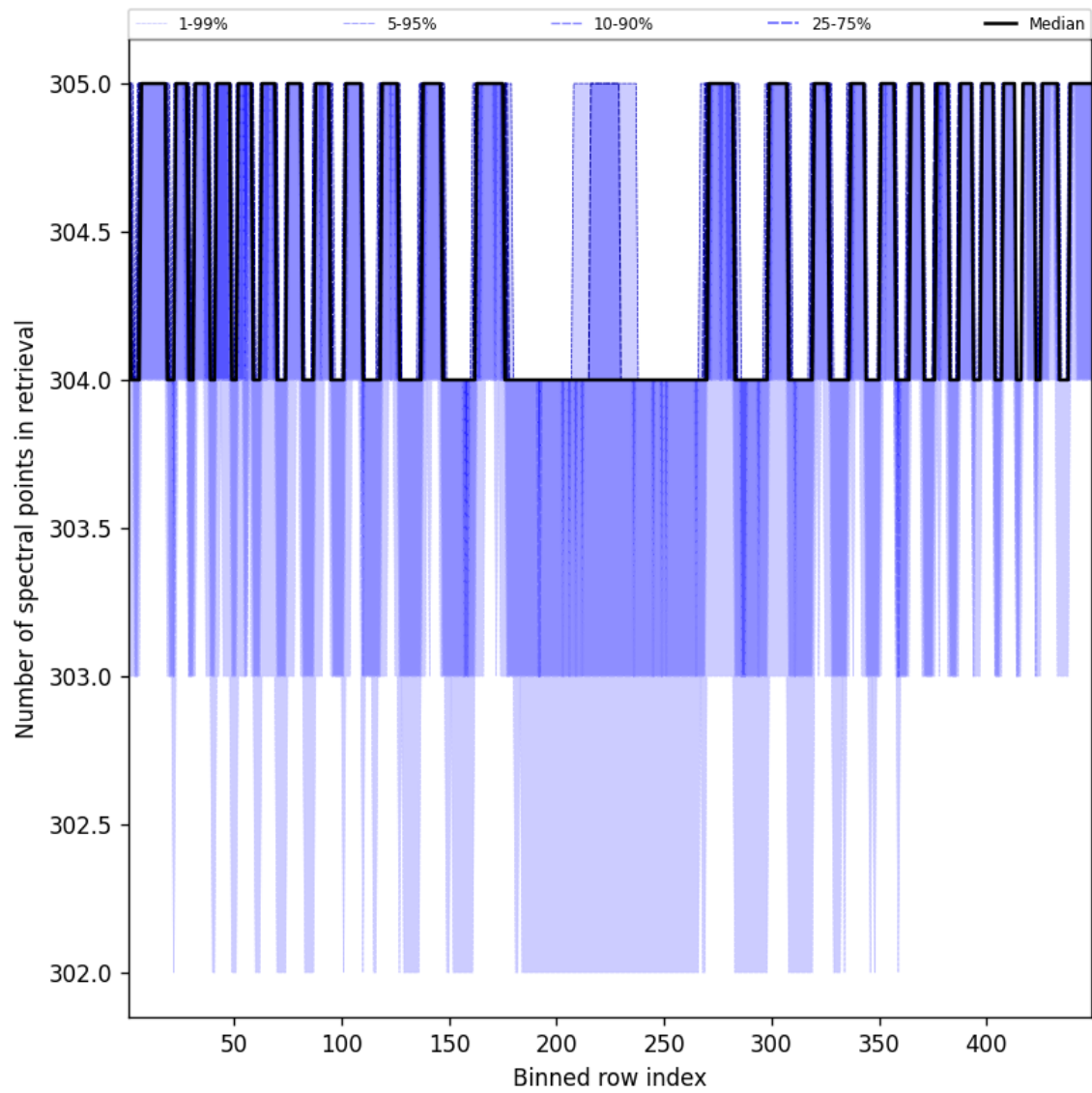
Figure 50: Along track statistics of “Number of spectral points in retrieval” for 2025-10-04 to 2025-10-06
