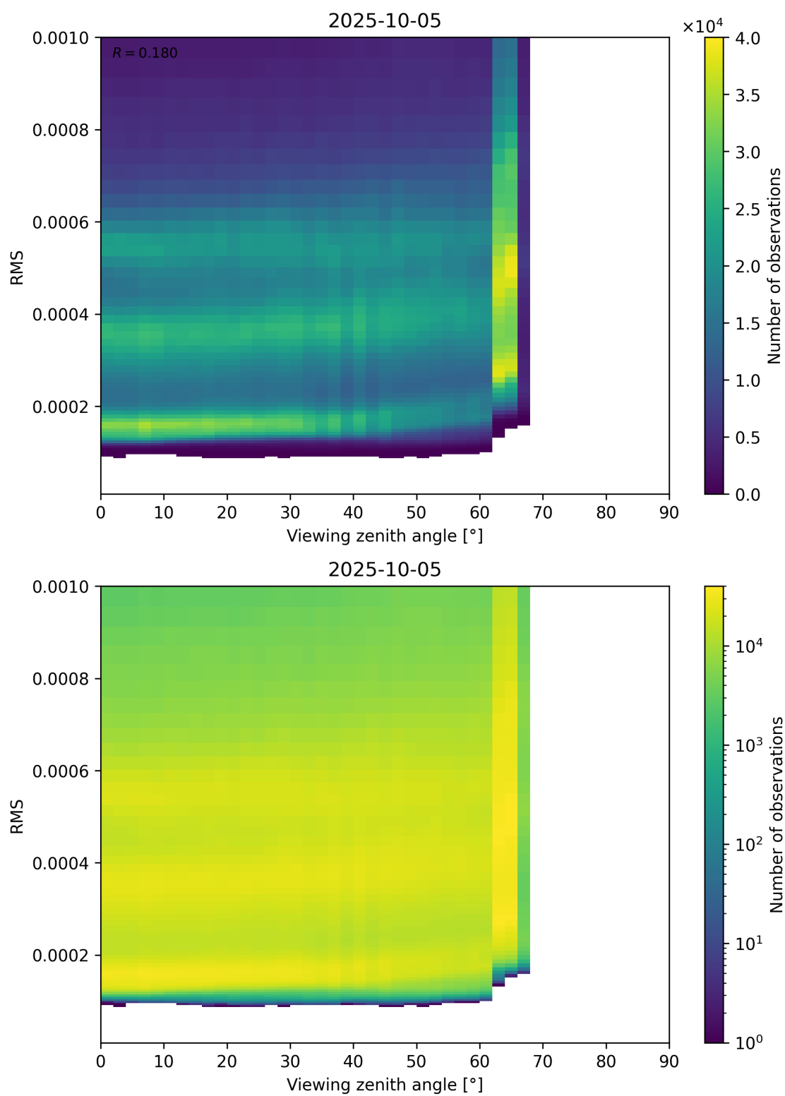
Figure 171: Scatter density plot of “Viewing zenith angle” against “RMS” for 2025-10-04 to 2025-10-06.
