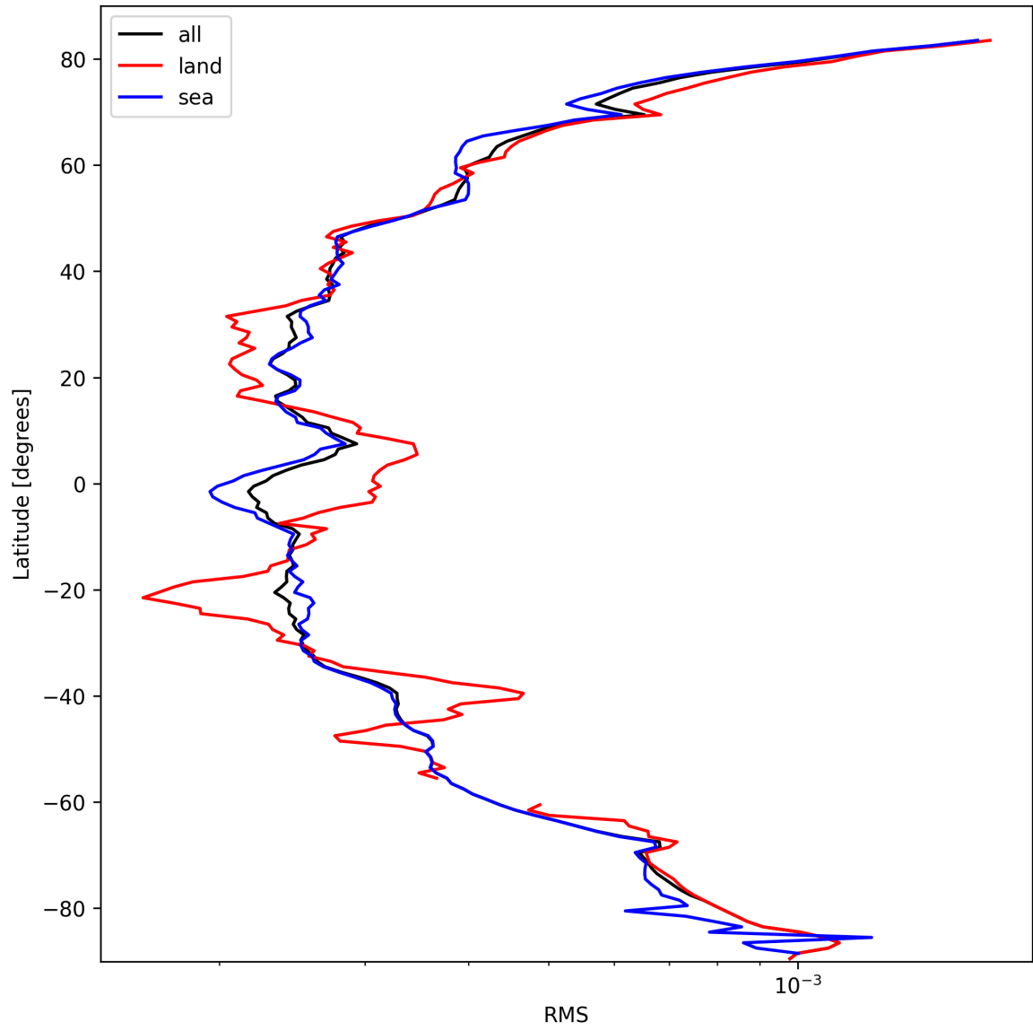
Figure 26: Zonal average of “RMS” for 2025-10-04 to 2025-10-06.
