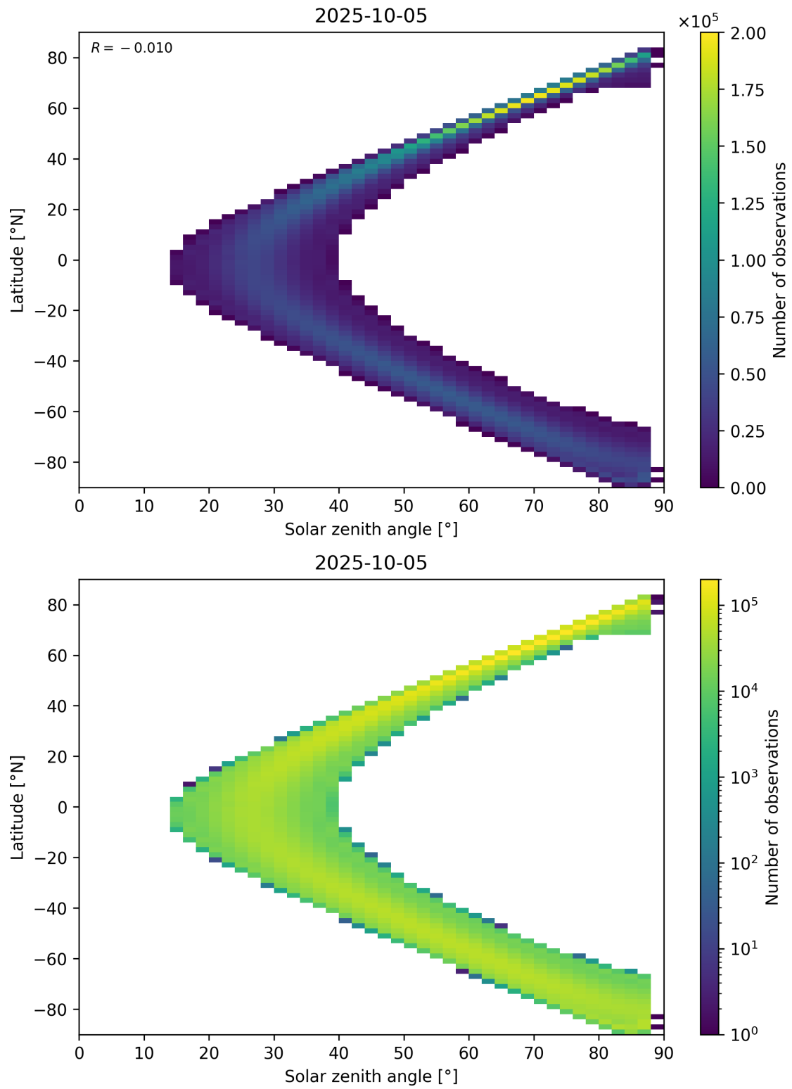
Figure 149: Scatter density plot of “Solar zenith angle” against “Latitude” for 2025-10-04 to 2025-10-06.
