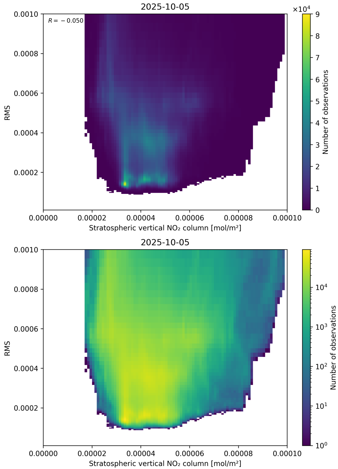
Figure 102: Scatter density plot of “Stratospheric vertical NO 2 column” against “RMS” for 2025-10-04 to 2025-10-06.
