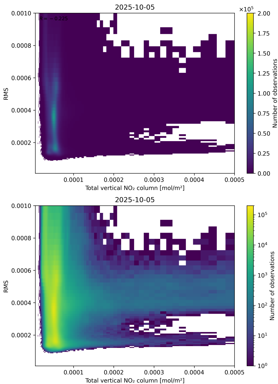
Figure 120: Scatter density plot of “Total vertical NO 2 column” against “RMS” for 2025-10-04 to 2025-10-06.
