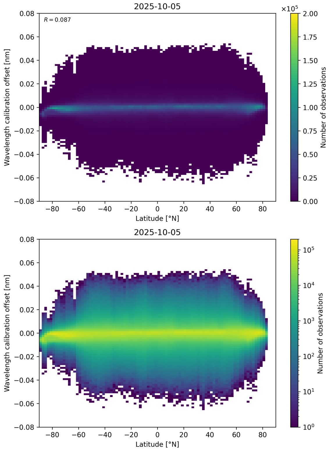
Figure 95: Scatter density plot of “Latitude” against “Wavelength calibration offset” for 2025-10-04 to 2025-10-06.
