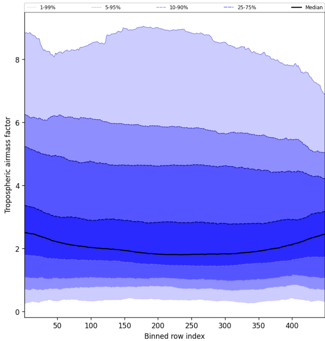
Figure 48: Along track statistics of “Tropospheric air mass factor” for 2025-10-04 to 2025-10-06
