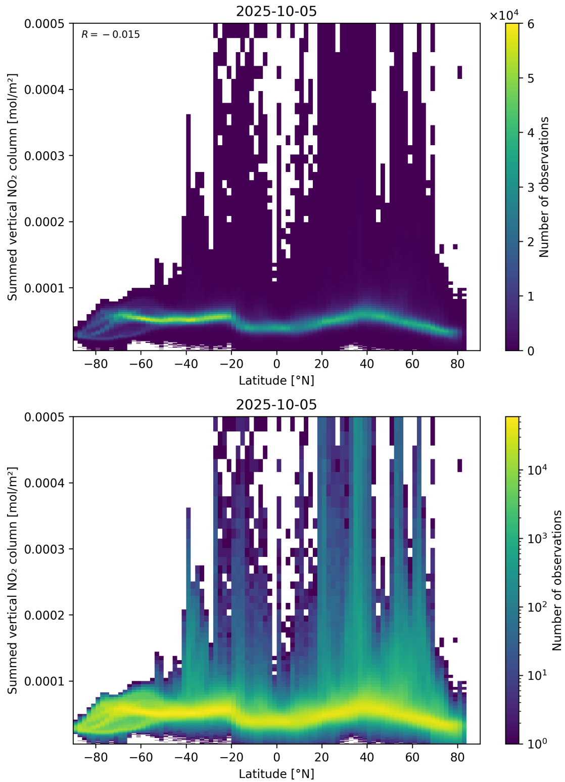
Figure 88: Scatter density plot of “Latitude” against “Summed vertical NO 2 column” for 2025-10-04 to 2025-10-06.
