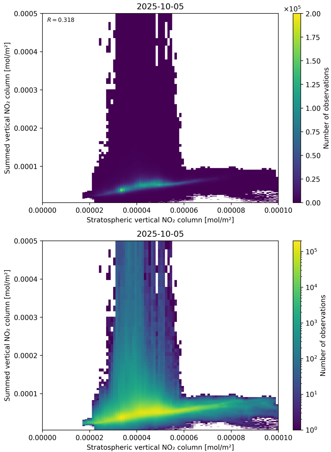
Figure 98: Scatter density plot of “Stratospheric vertical NO 2 column” against “Summed vertical NO 2 column” for 2025-10-04 to 2025-10-06.
