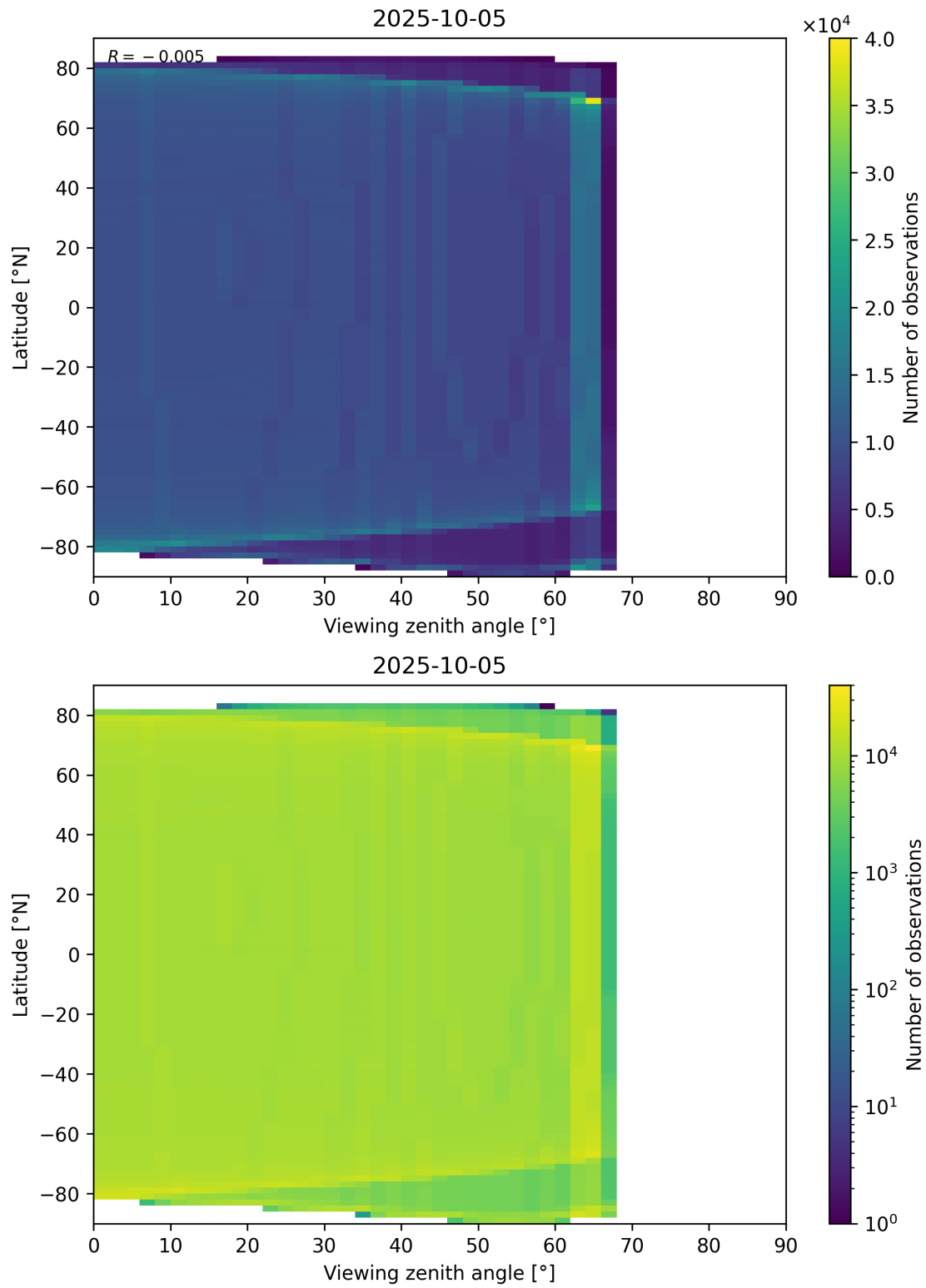
Figure 163: Scatter density plot of “Viewing zenith angle” against “Latitude” for 2025-10-04 to 2025-10-06.
