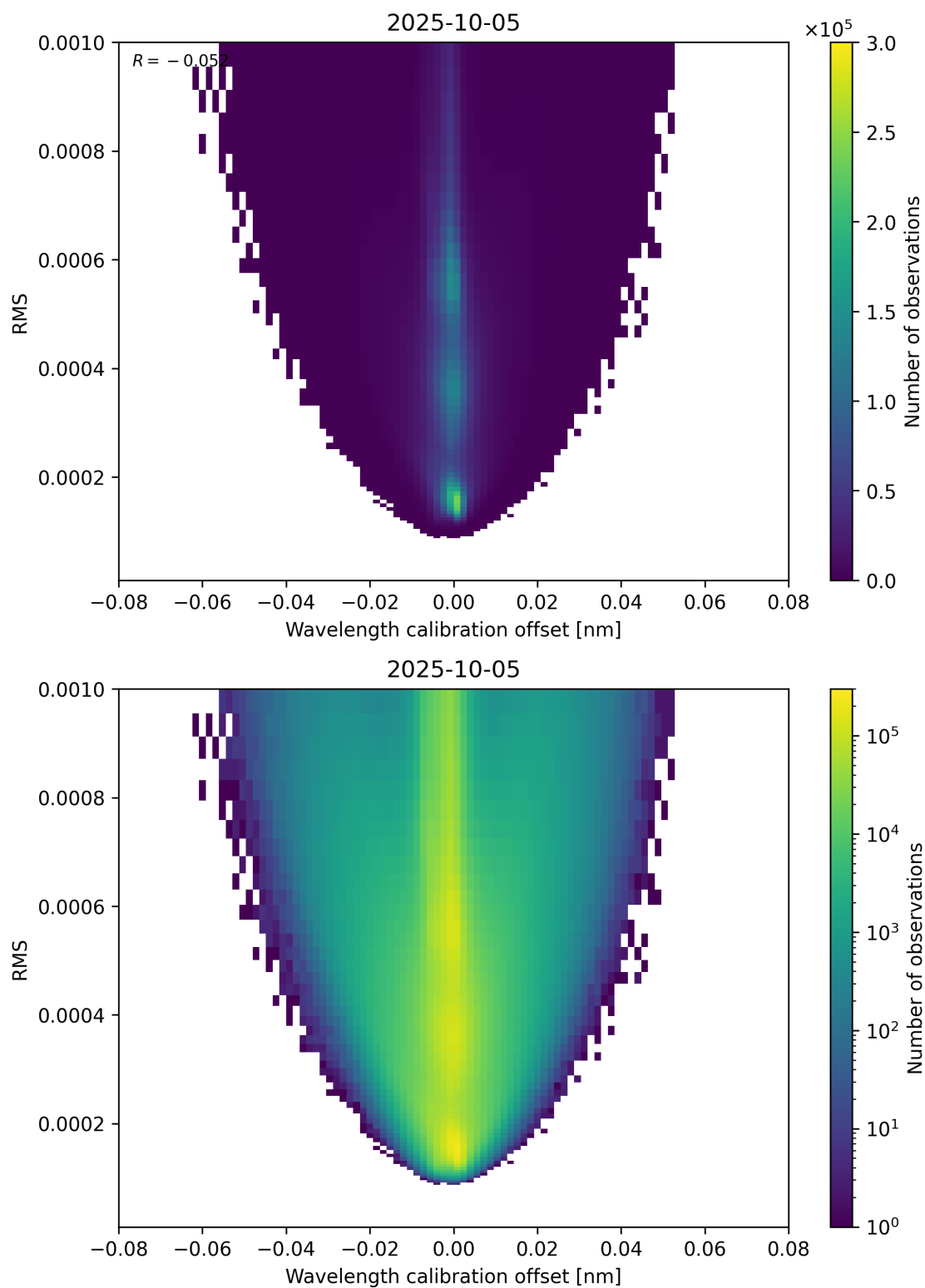
Figure 181: Scatter density plot of “Wavelength calibration offset” against “RMS” for 2025-10-04 to 2025-10-06.
