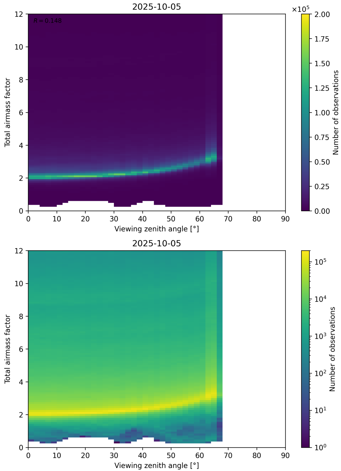
Figure 160: Scatter density plot of “Viewing zenith angle” against “Total airmass factor” for 2025-10-04 to 2025-10-06.
