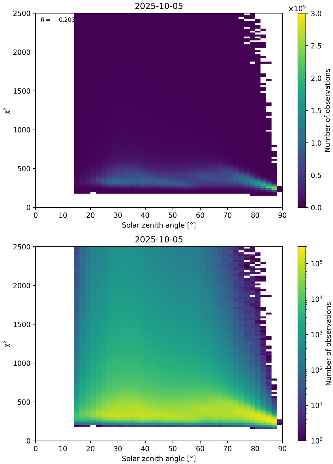
Figure 148: Scatter density plot of “Solar zenith angle” against “ \chi^2 ” for 2025-10-04 to 2025-10-06.
