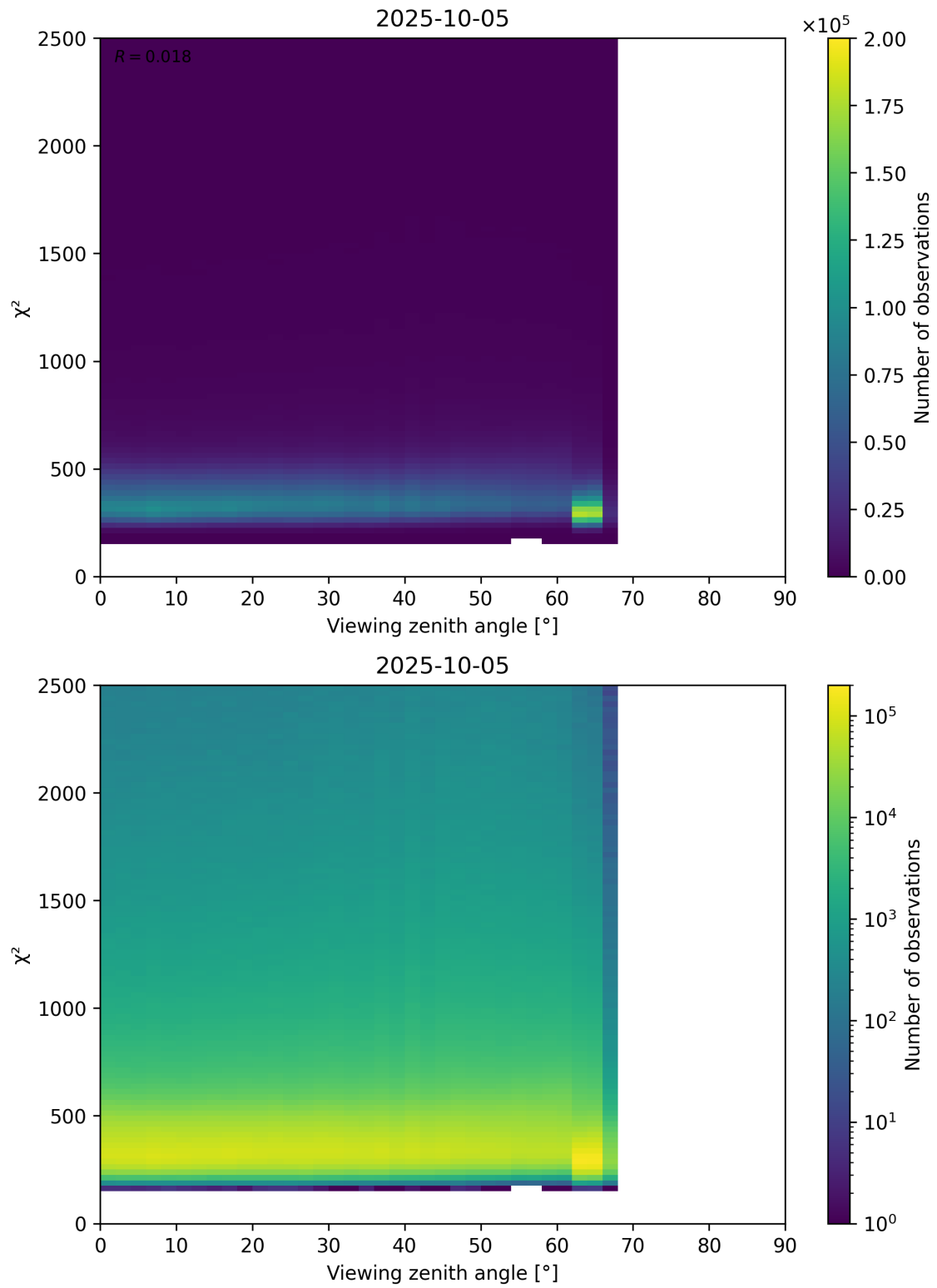
Figure 162: Scatter density plot of “Viewing zenith angle” against “ \chi^2 ” for 2025-10-04 to 2025-10-06.
