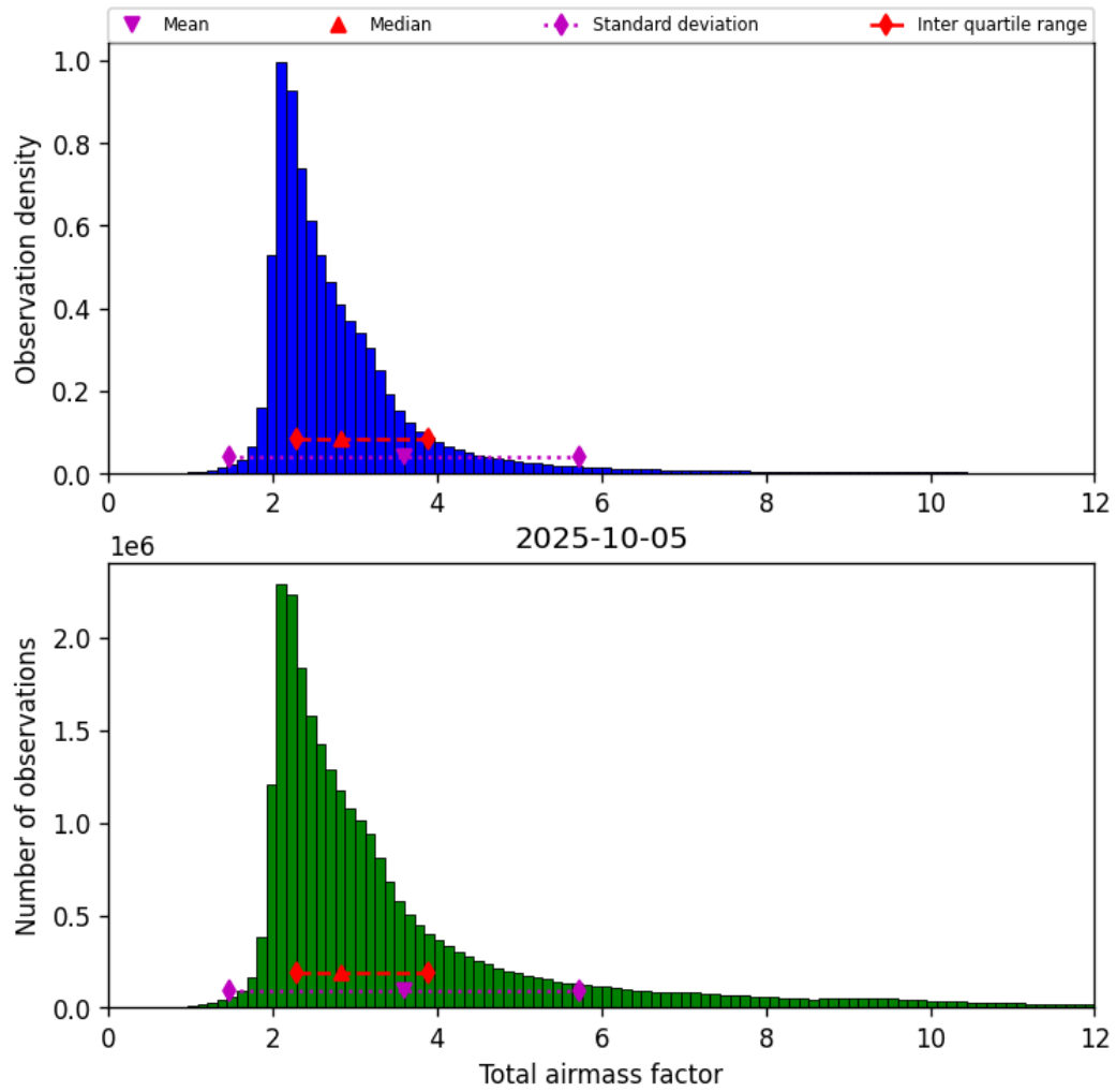
Figure 32: Histogram of “Total airmass factor” for 2025-10-04 to 2025-10-06
