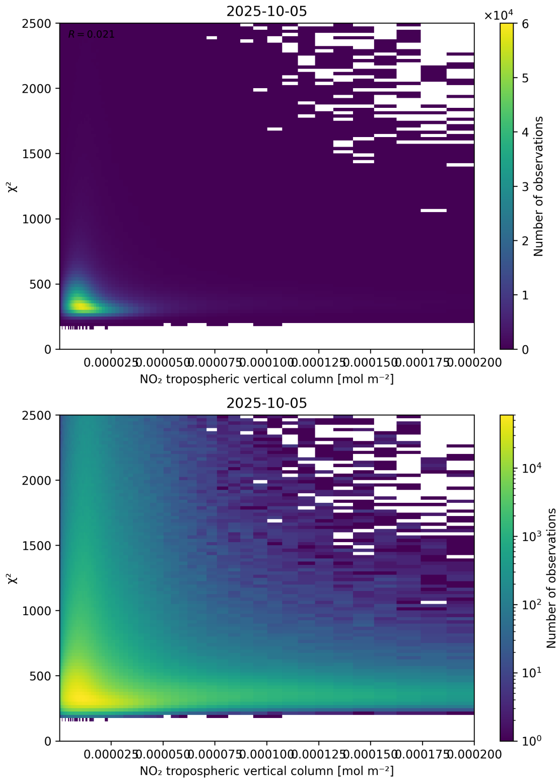
Figure 124: Scatter density plot of “NO 2 tropospheric vertical column” against “ \chi^2 ” for 2025-10-04 to 2025-10-06.
