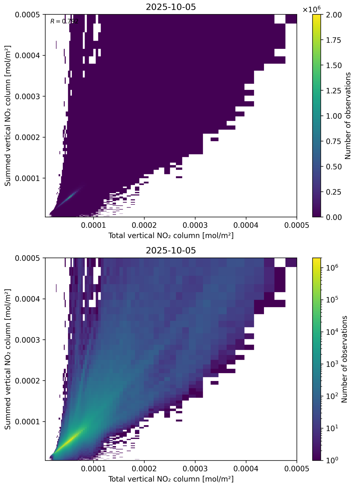
Figure 112: Scatter density plot of “Total vertical NO 2 column” against “Summed vertical NO 2 column” for 2025-10-04 to 2025-10-06.
