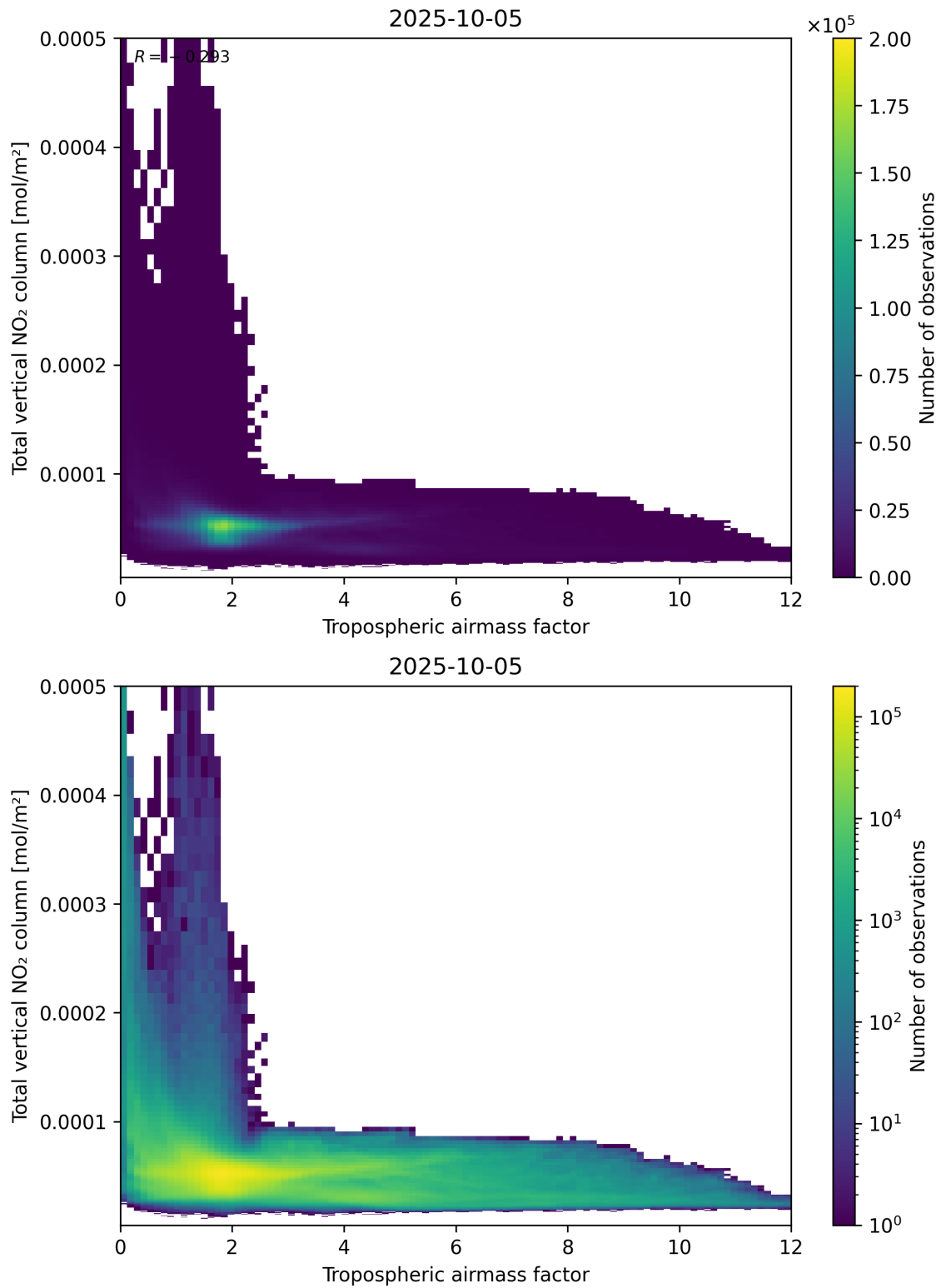
Figure 77: Scatter density plot of “Tropospheric airmass factor” against “Total vertical NO 2 column” for 2025-10-04 to 2025-10-06.
