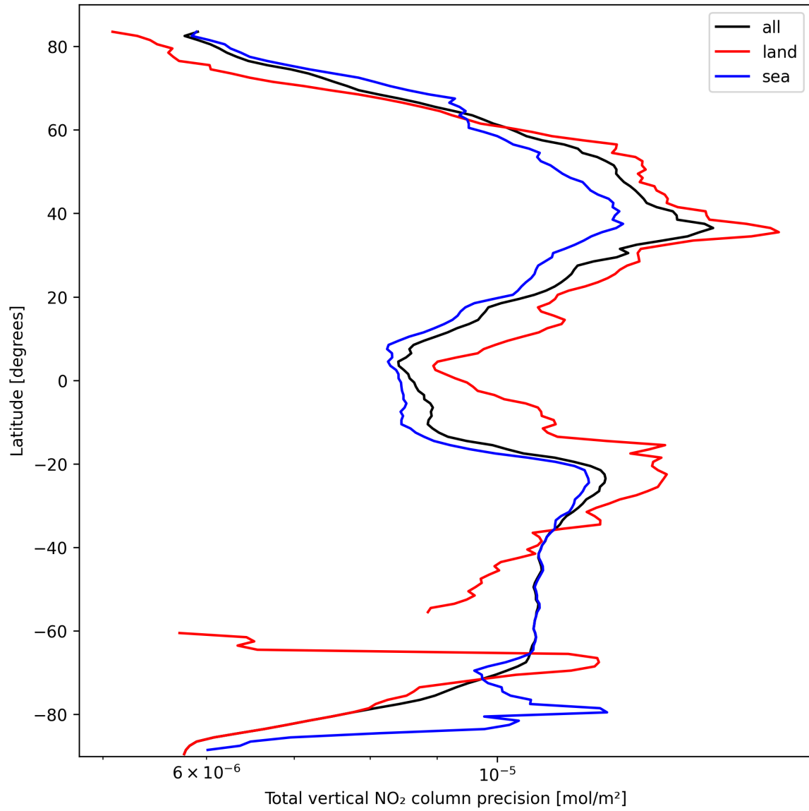
Figure 22: Zonal average of “Total vertical NO 2 column precision” for 2025-10-04 to 2025-10-06.
