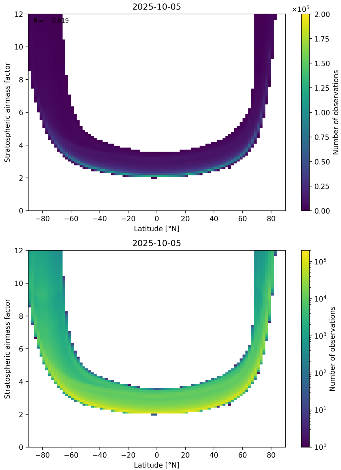
Figure 83: Scatter density plot of “Latitude” against “Stratospheric air mass factor” for 2025-10-04 to 2025-10-06.
