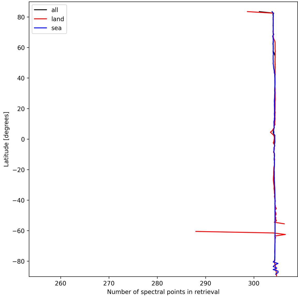
Figure 16: Zonal average of “Number of spectral points in retrieval” for 2025-10-04 to 2025-10-06.
