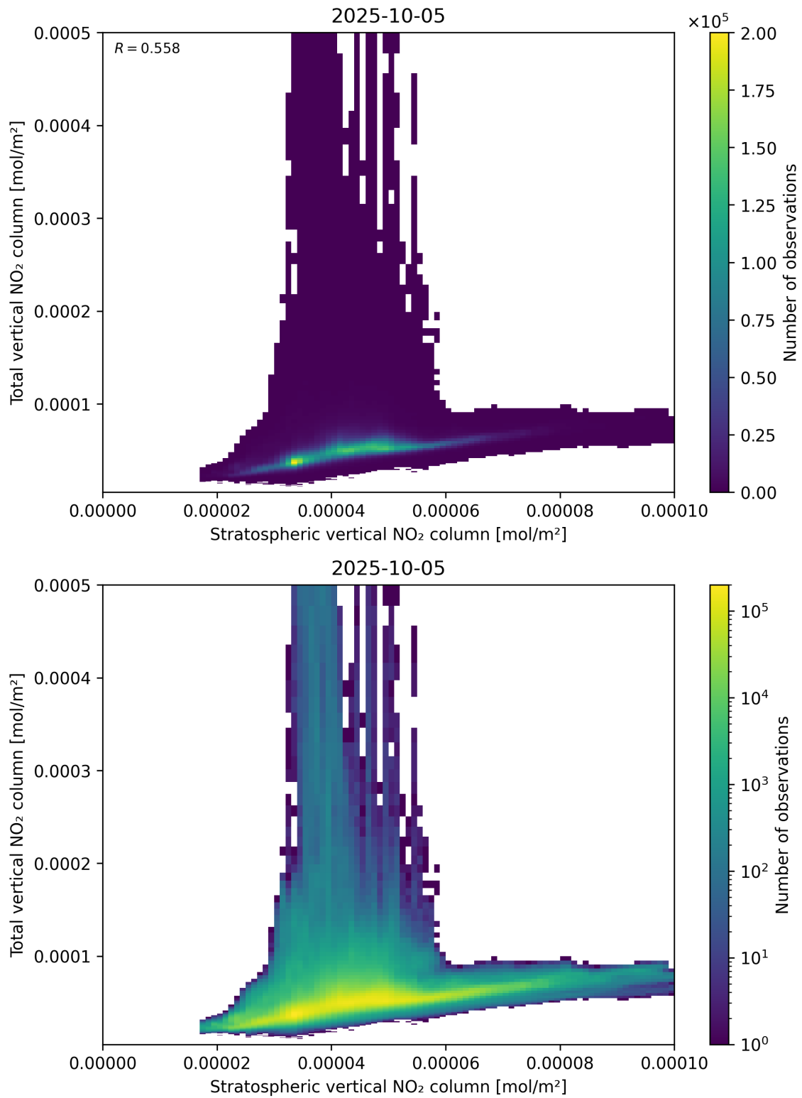
Figure 100: Scatter density plot of “Stratospheric vertical NO 2 column” against “Total vertical NO 2 column” for 2025-10-04 to 2025-10-06.
