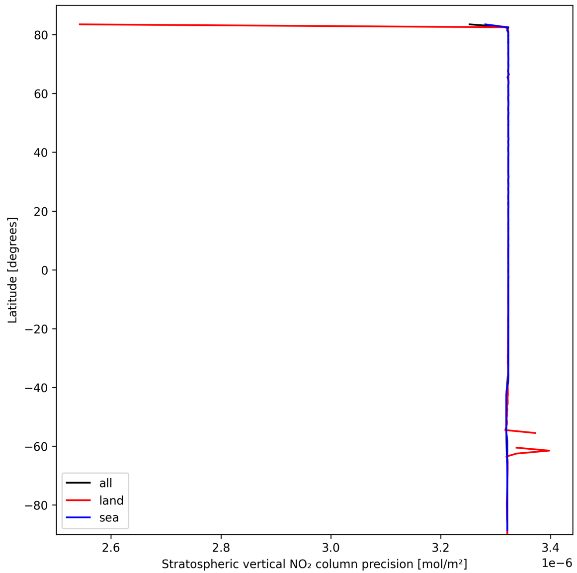
Figure 20: Zonal average of “Stratospheric vertical NO 2 column precision” for 2025-10-04 to 2025-10-06.
