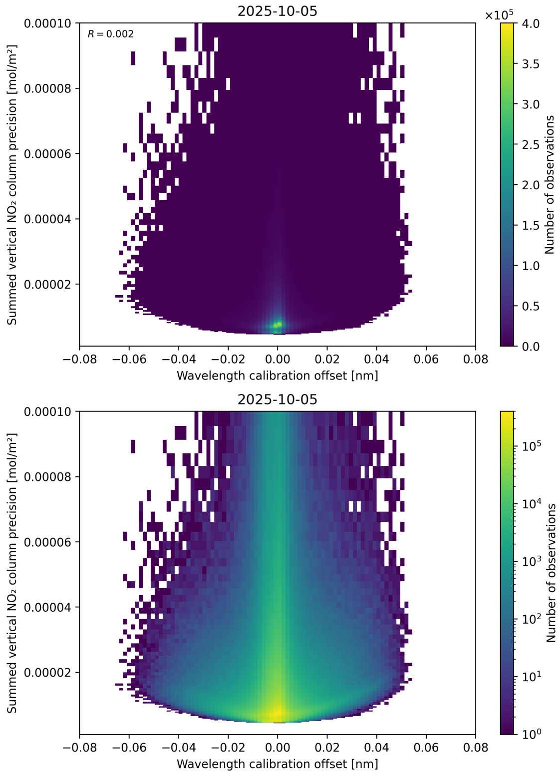
Figure 178: Scatter density plot of “Wavelength calibration offset” against “Summed vertical NO 2 column precision” for 2025-10-04 to 2025-10-06.
