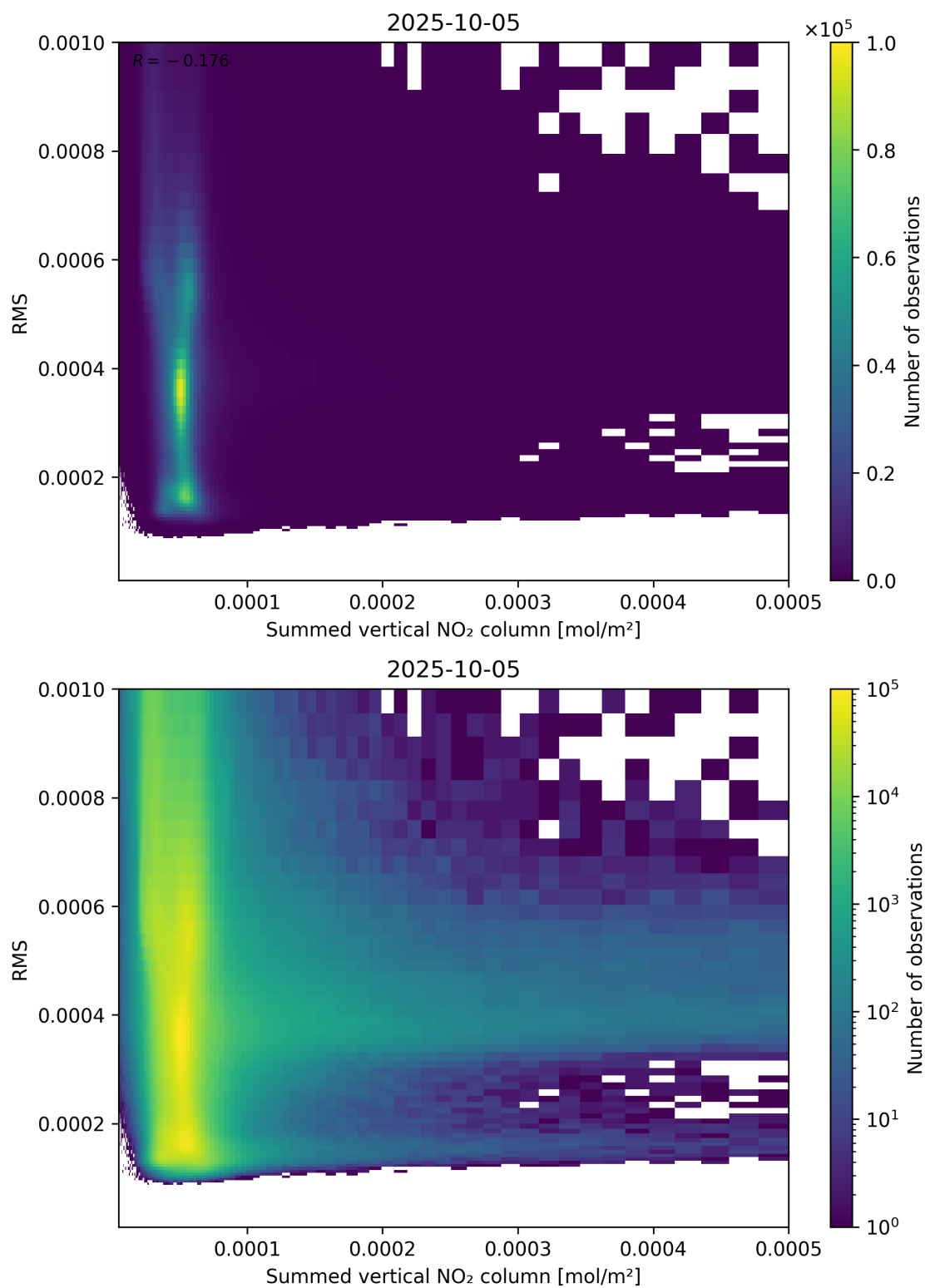
Figure 109: Scatter density plot of “Summed vertical NO 2 column” against “RMS” for 2025-10-04 to 2025-10-06.
