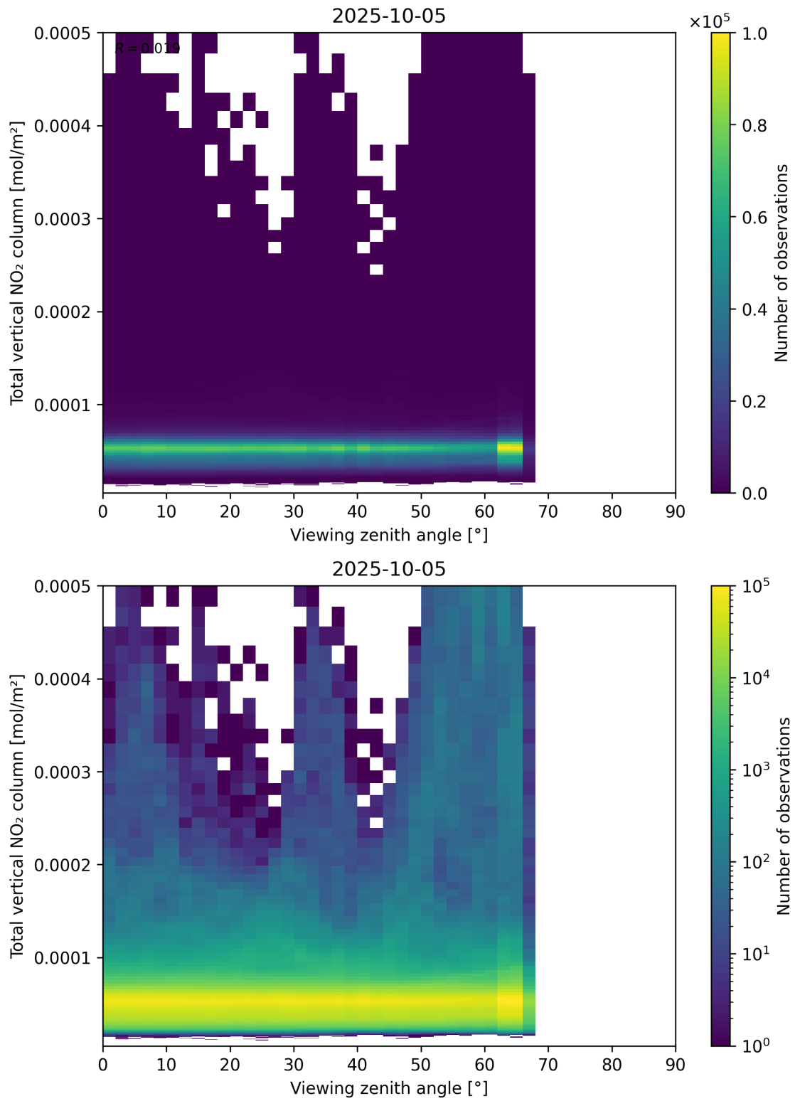
Figure 167: Scatter density plot of “Viewing zenith angle” against “Total vertical NO 2 column” for 2025-10-04 to 2025-10-06.
