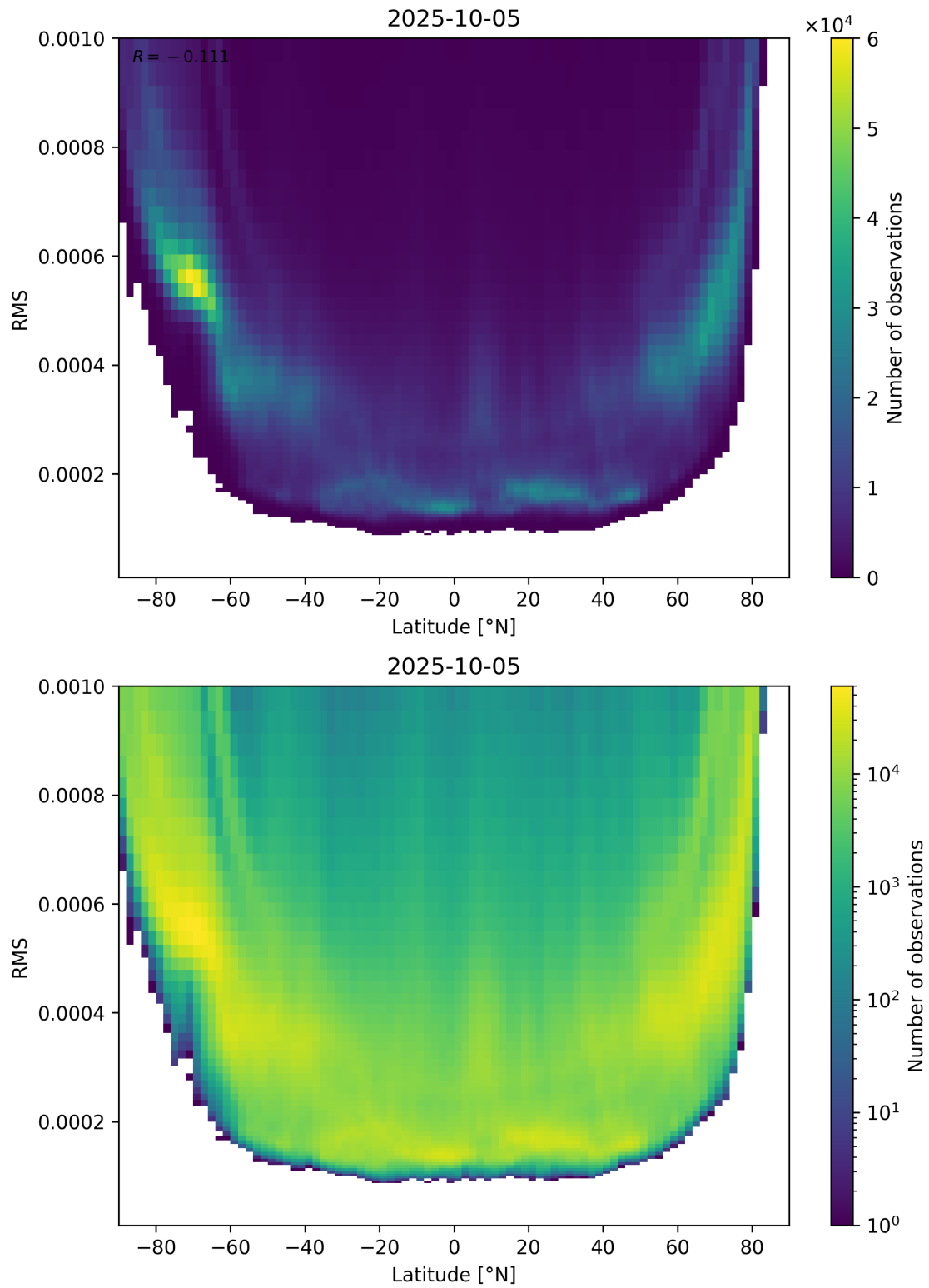
Figure 94: Scatter density plot of “Latitude” against “RMS” for 2025-10-04 to 2025-10-06.
