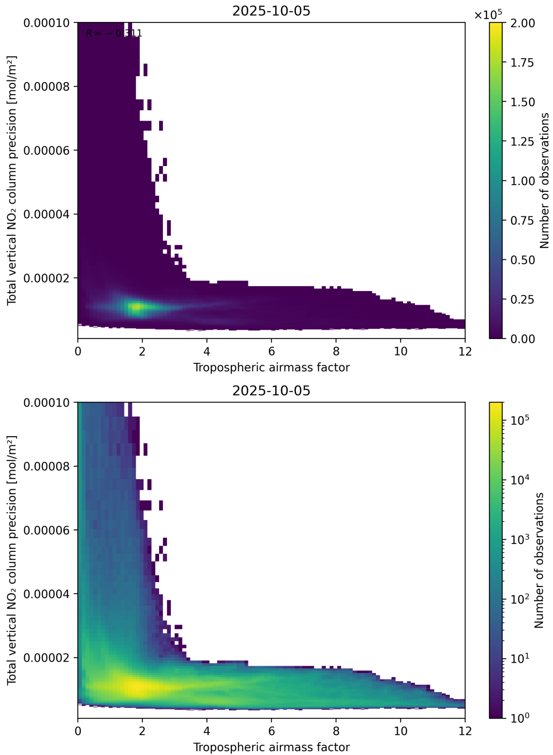
Figure 78: Scatter density plot of “Tropospheric air mass factor” against “Total vertical NO 2 column precision” for 2025-10-04 to 2025-10-06.
