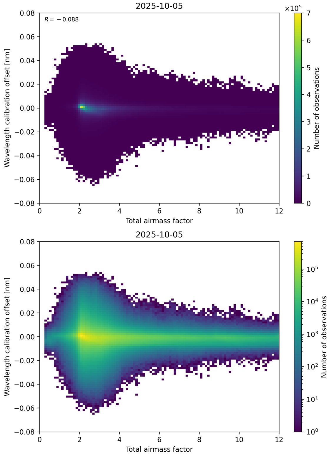
Figure 70: Scatter density plot of “Total airmass factor” against “Wavelength calibration offset” for 2025-10-04 to 2025-10-06.
