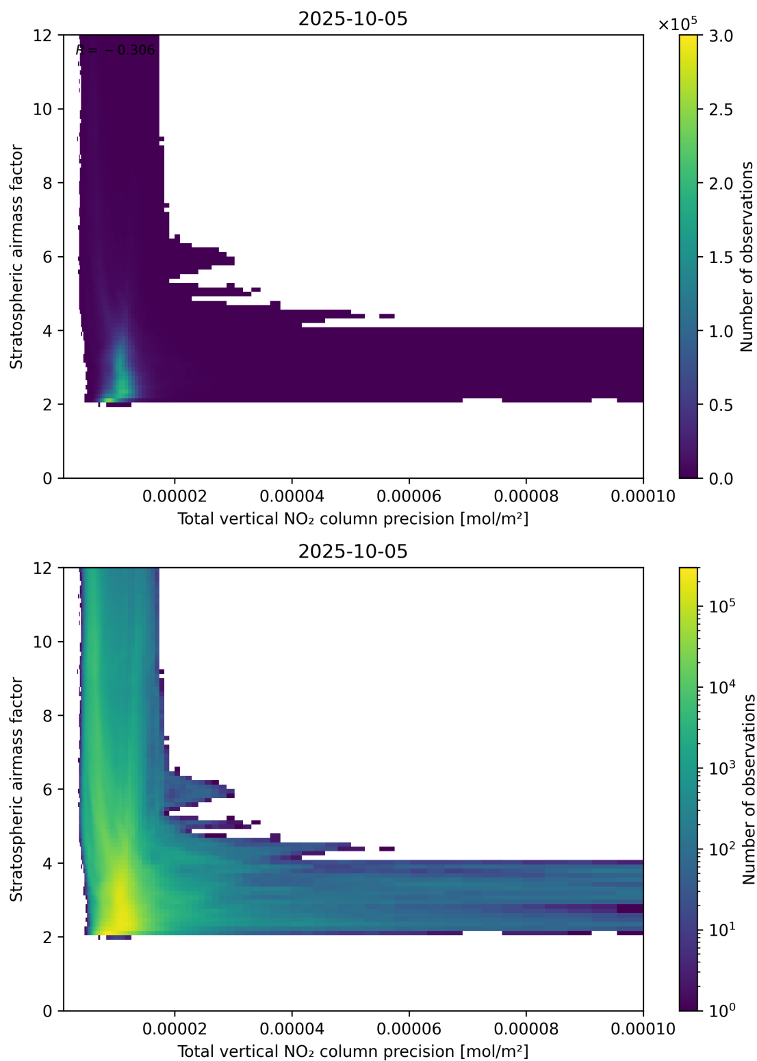
Figure 115: Scatter density plot of “Total vertical NO 2 column precision” against “Stratospheric airmass factor” for 2025-10-04 to 2025-10-06.
