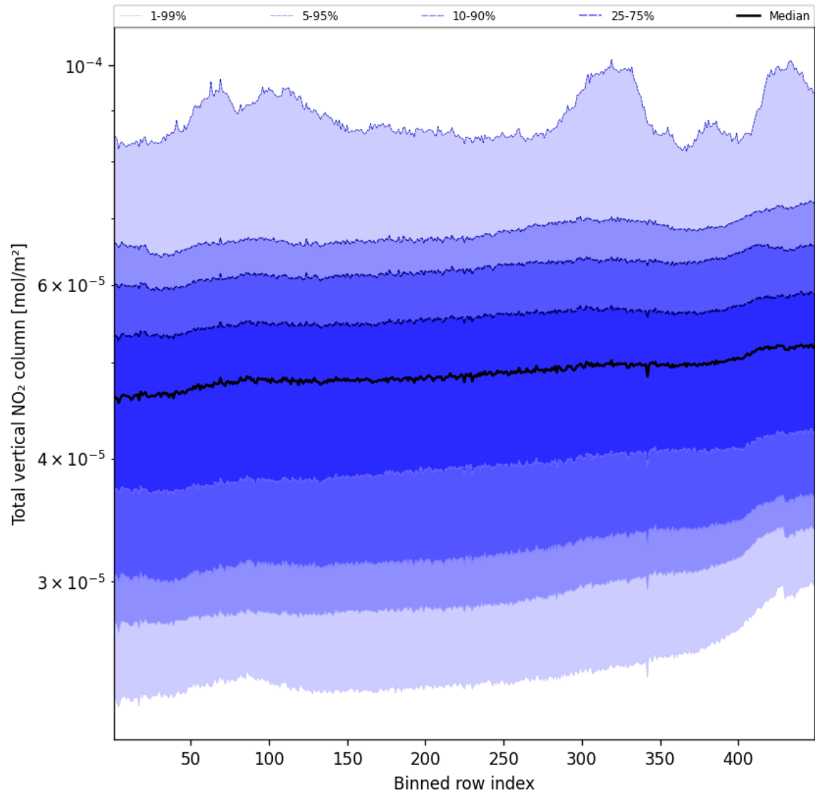
Figure 55: Along track statistics of “Total vertical NO 2 column” for 2025-10-04 to 2025-10-06
