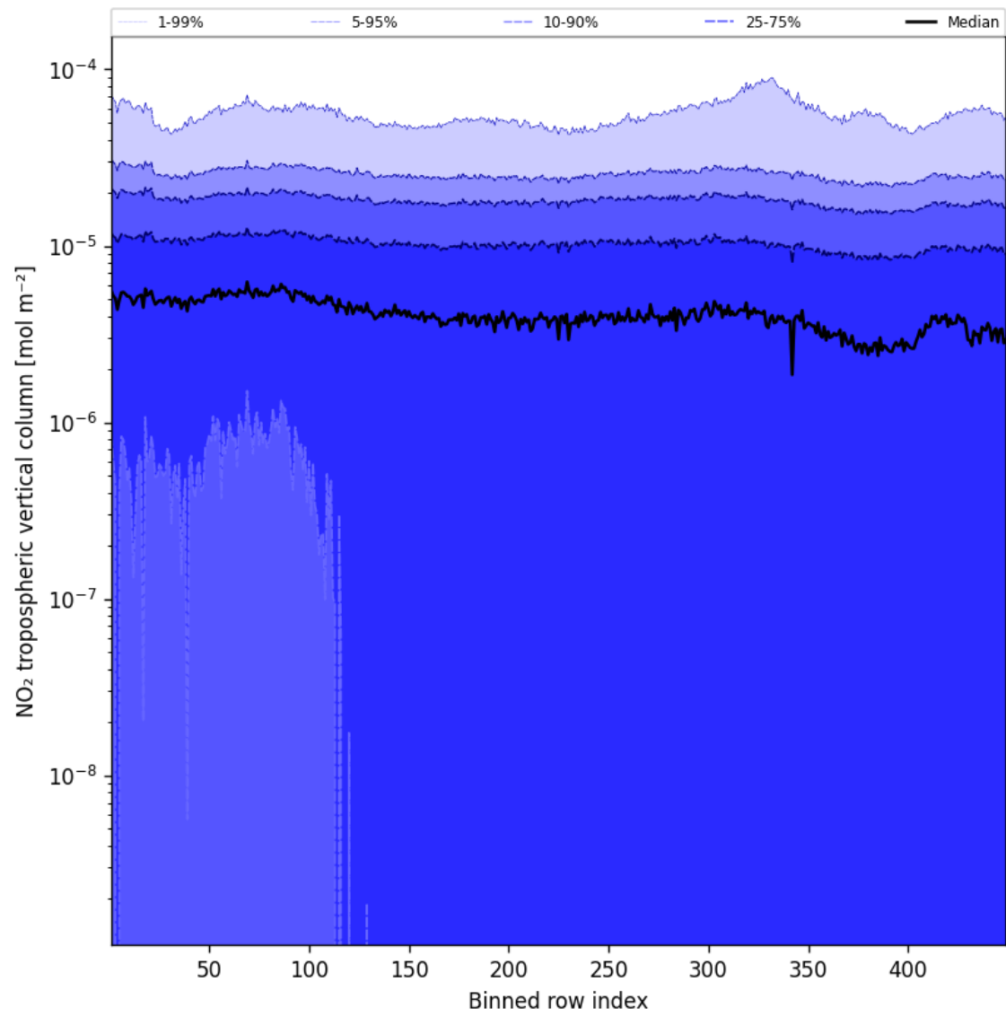
Figure 46: Along track statistics of “NO 2 tropospheric vertical column” for 2025-10-04 to 2025-10-06
