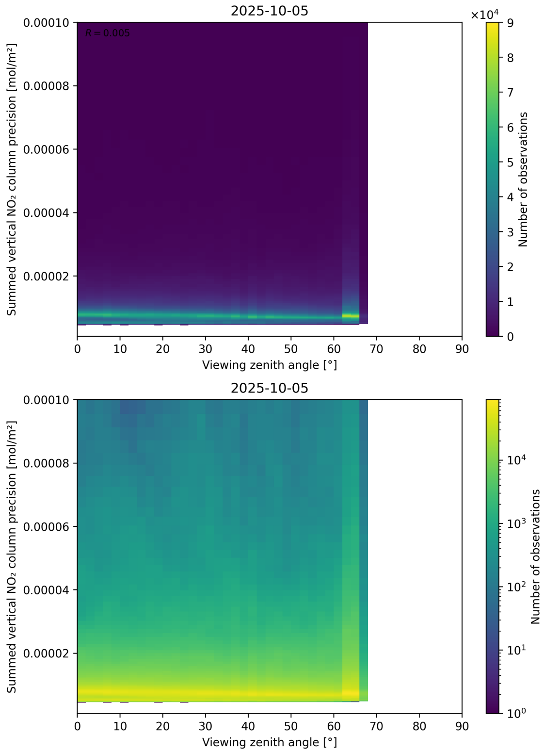
Figure 166: Scatter density plot of “Viewing zenith angle” against “Summed vertical NO 2 column precision” for 2025-10-04 to 2025-10-06.
