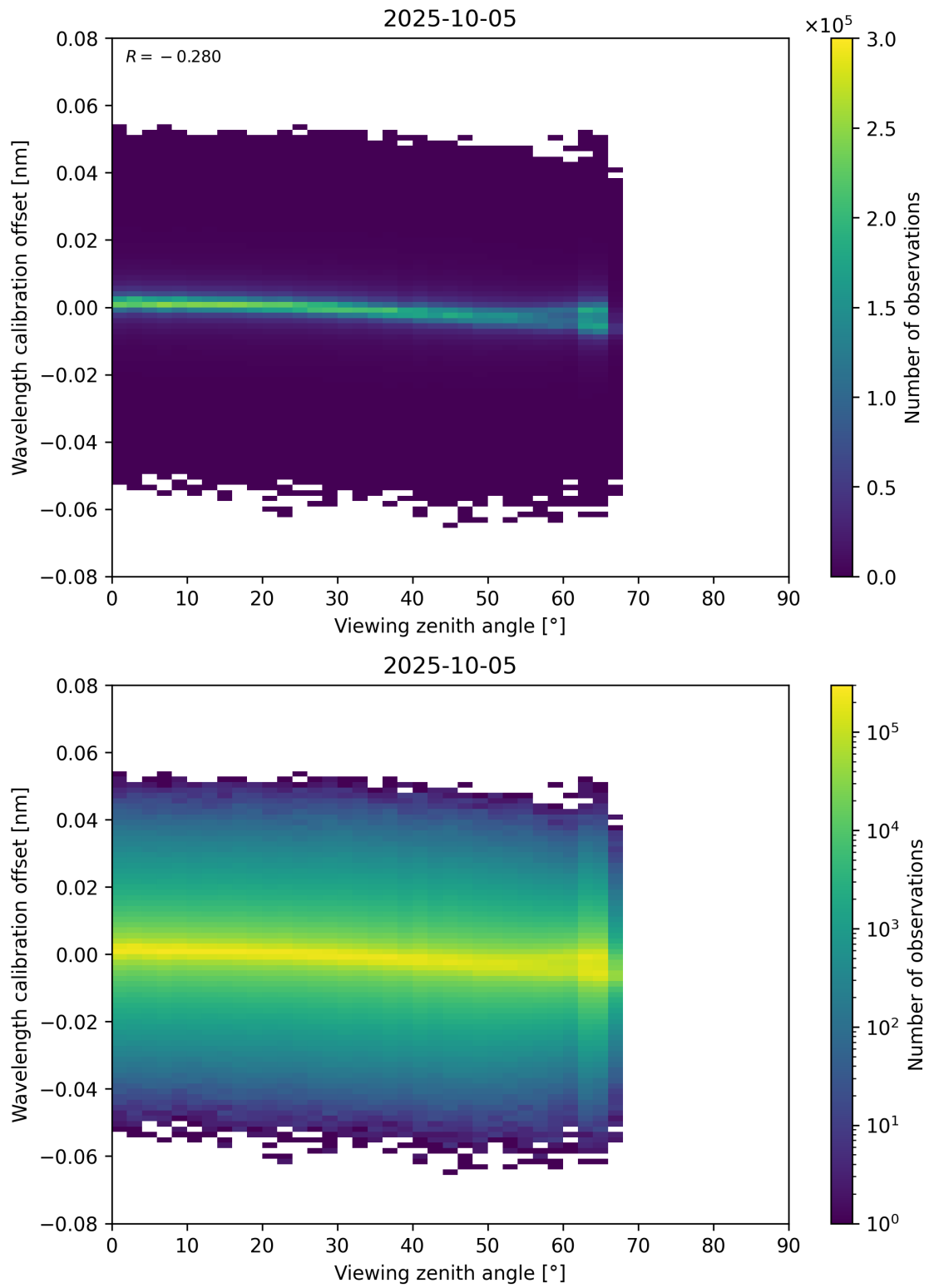
Figure 173: Scatter density plot of “Viewing zenith angle” against “Wavelength calibration offset” for 2025-10-04 to 2025-10-06.
