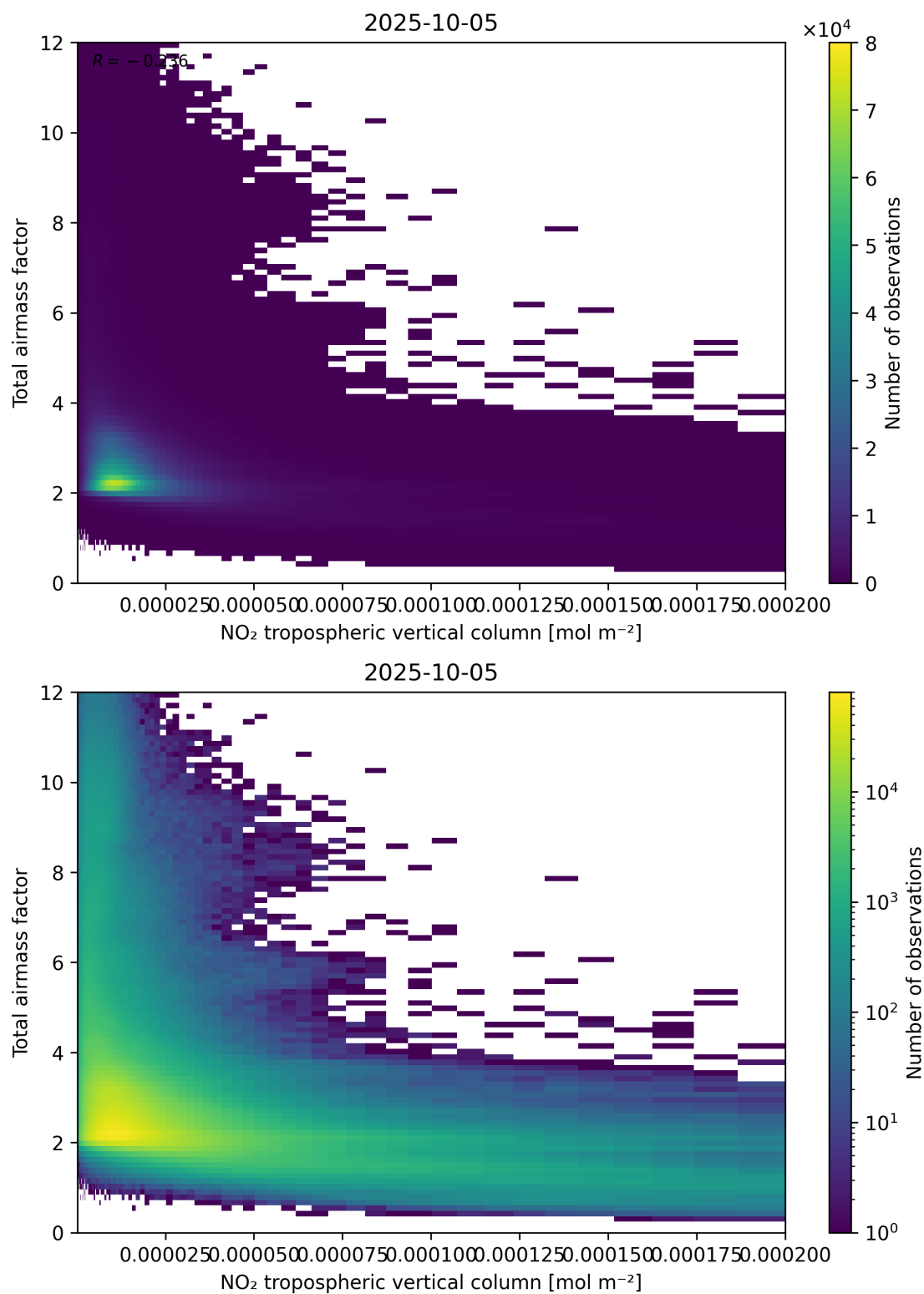
Figure 122: Scatter density plot of “NO 2 tropospheric vertical column” against “Total air mass factor” for 2025-10-04 to 2025-10-06.
