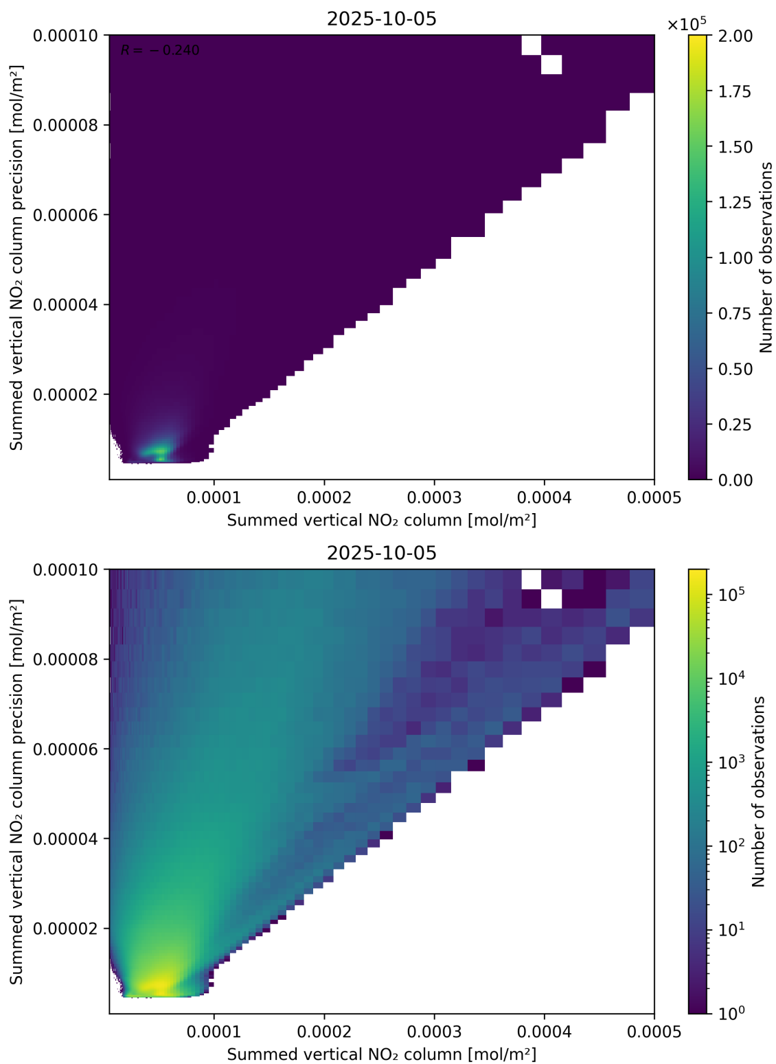
Figure 105: Scatter density plot of “Summed vertical NO 2 column” against “Summed vertical NO 2 column precision” for 2025-10-04 to 2025-10-06.
