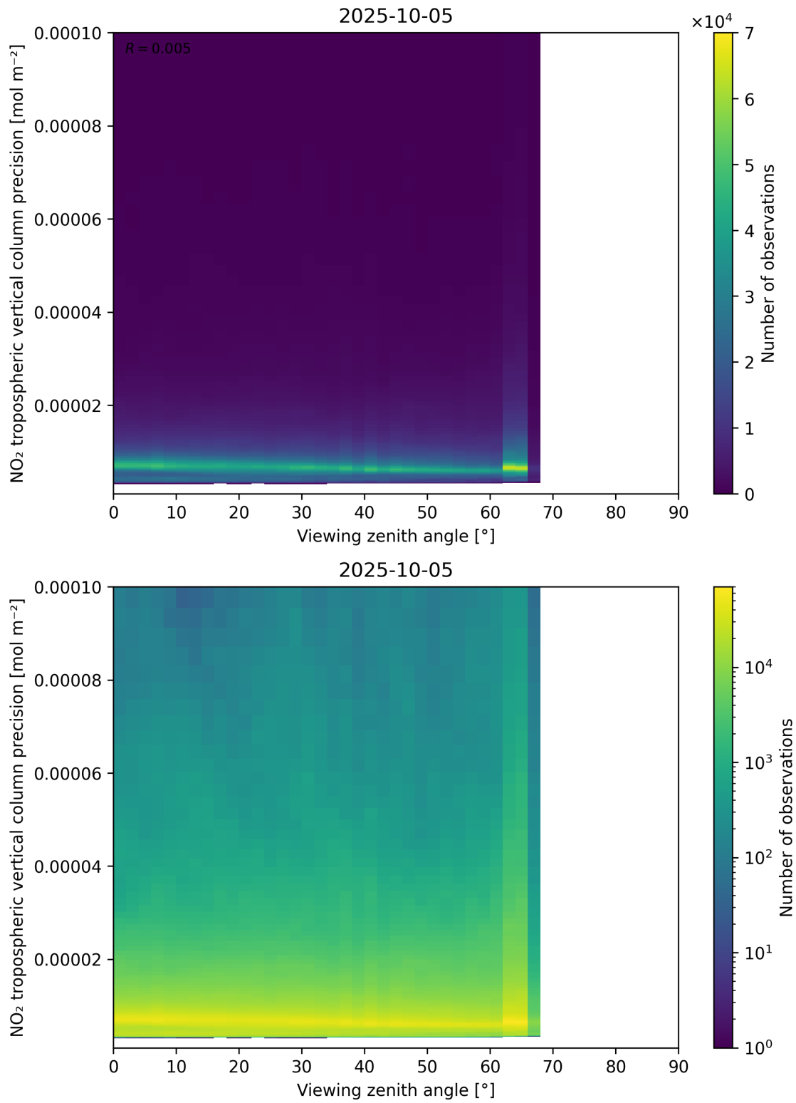
Figure 170: Scatter density plot of “Viewing zenith angle” against “NO 2 tropospheric vertical column precision” for 2025-10-04 to 2025-10-06.
