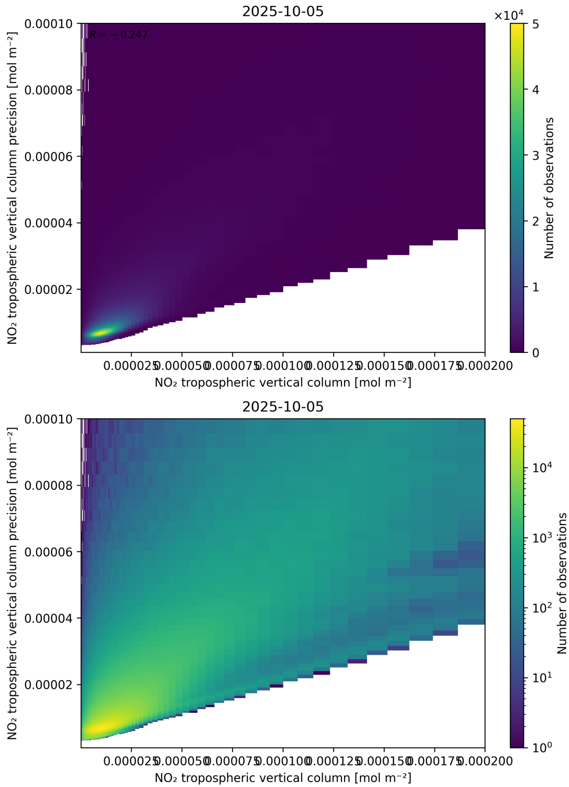
Figure 130: Scatter density plot of “NO 2 tropospheric vertical column” against “NO 2 tropospheric vertical column precision” for 2025-10-04 to 2025-10-06.
