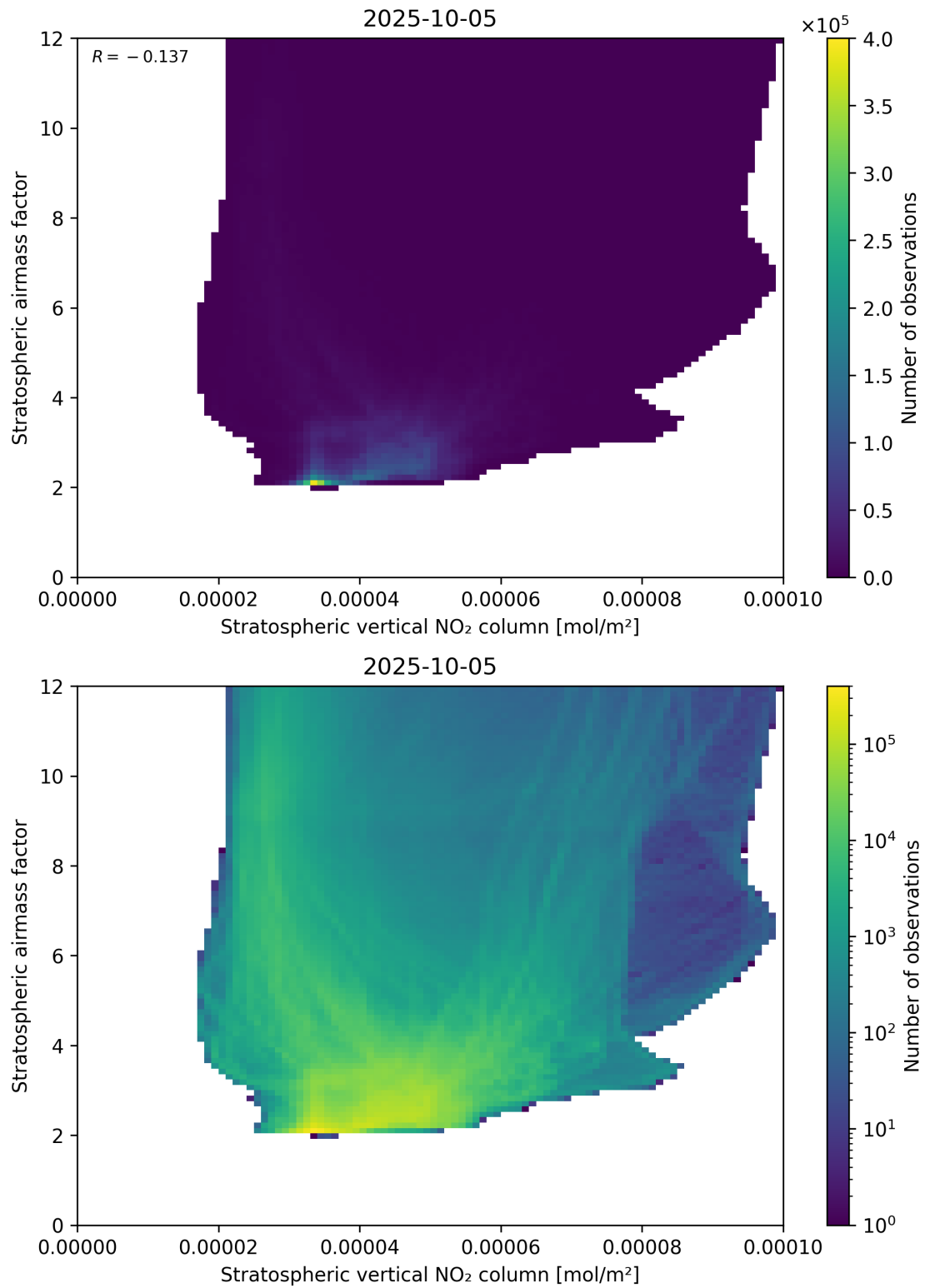
Figure 96: Scatter density plot of “Stratospheric vertical NO 2 column” against “Stratospheric airmass factor” for 2025-10-04 to 2025-10-06.
