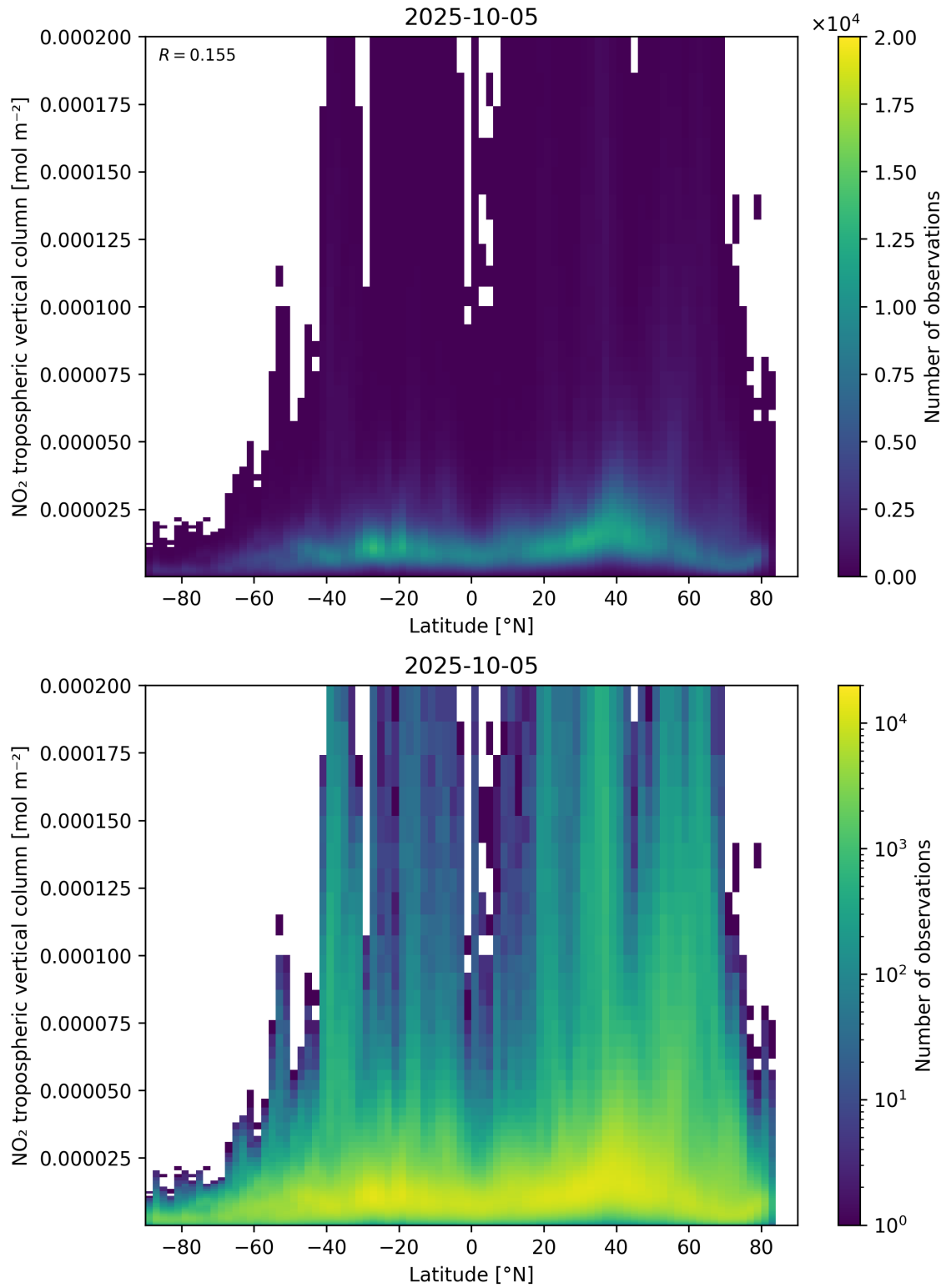
Figure 92: Scatter density plot of “Latitude” against “NO 2 tropospheric vertical column” for 2025-10-04 to 2025-10-06.
