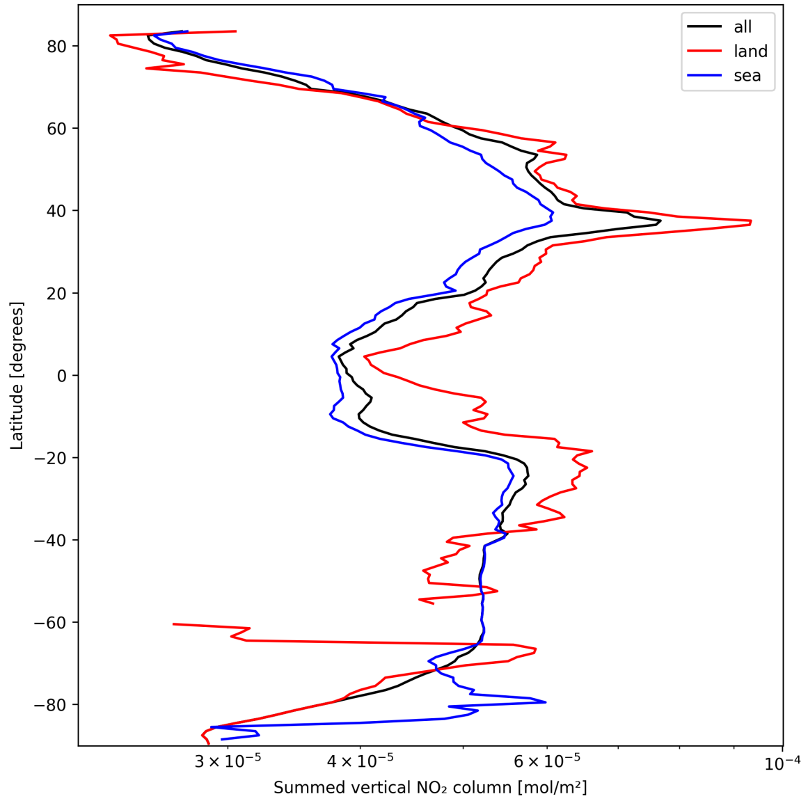
Figure 23: Zonal average of “Summed vertical NO 2 column” for 2025-10-04 to 2025-10-06.
