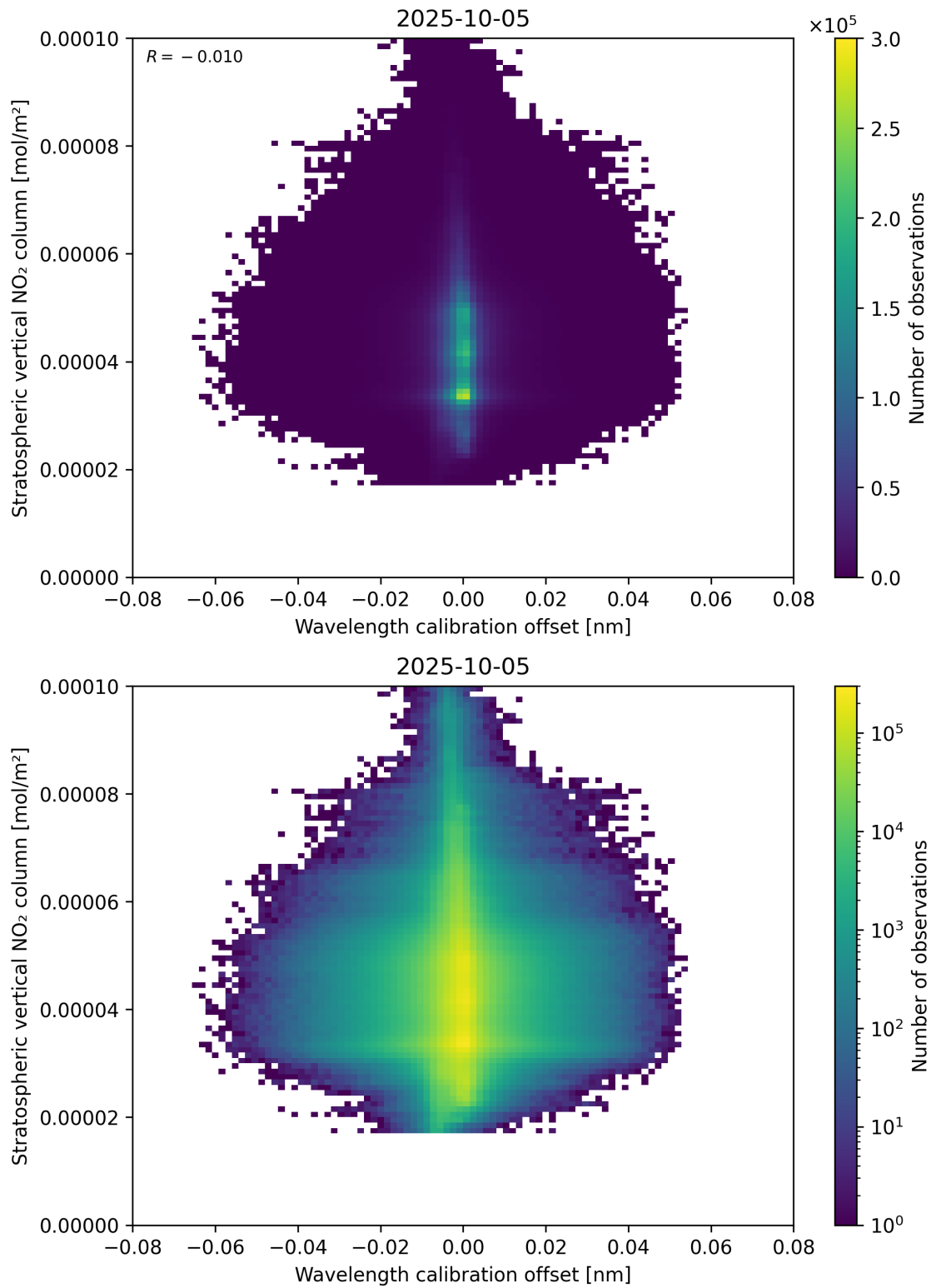
Figure 176: Scatter density plot of “Wavelength calibration offset” against “Stratospheric vertical NO 2 column” for 2025-10-04 to 2025-10-06.
