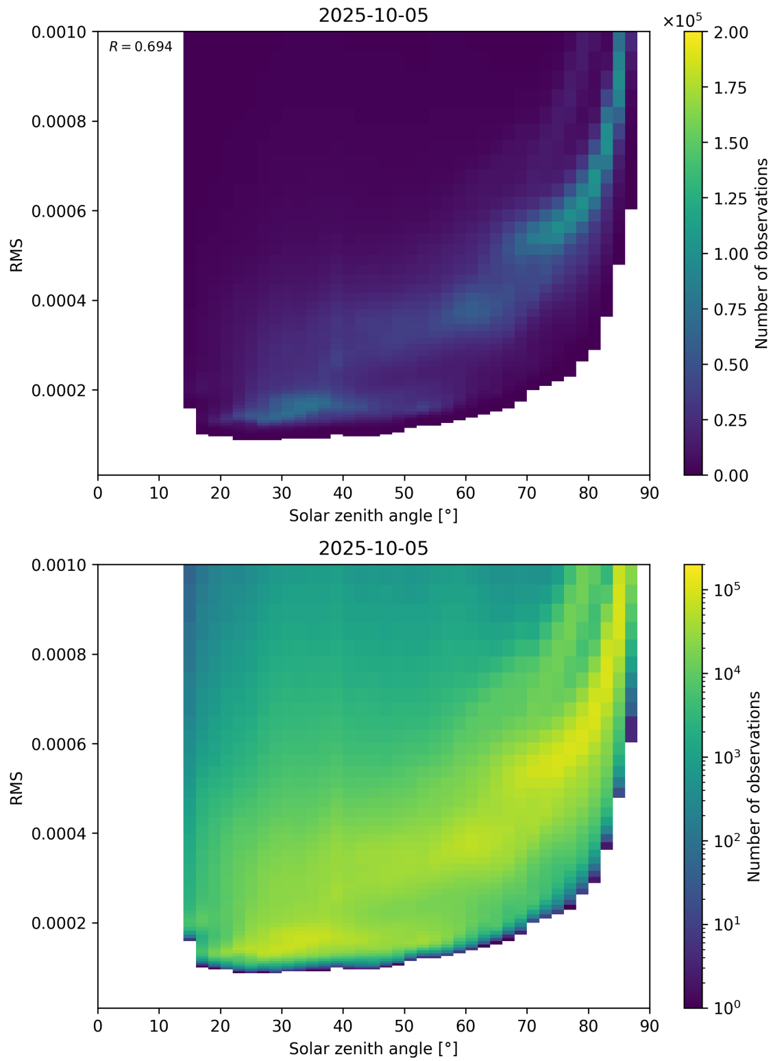
Figure 157: Scatter density plot of “Solar zenith angle” against “RMS” for 2025-10-04 to 2025-10-06.
