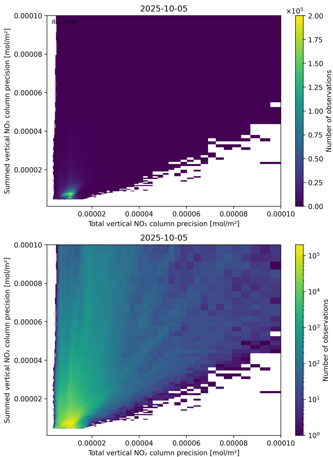
Figure 118: Scatter density plot of “Total vertical NO 2 column precision” against “Summed vertical NO 2 column precision” for 2025-10-04 to 2025-10-06.
