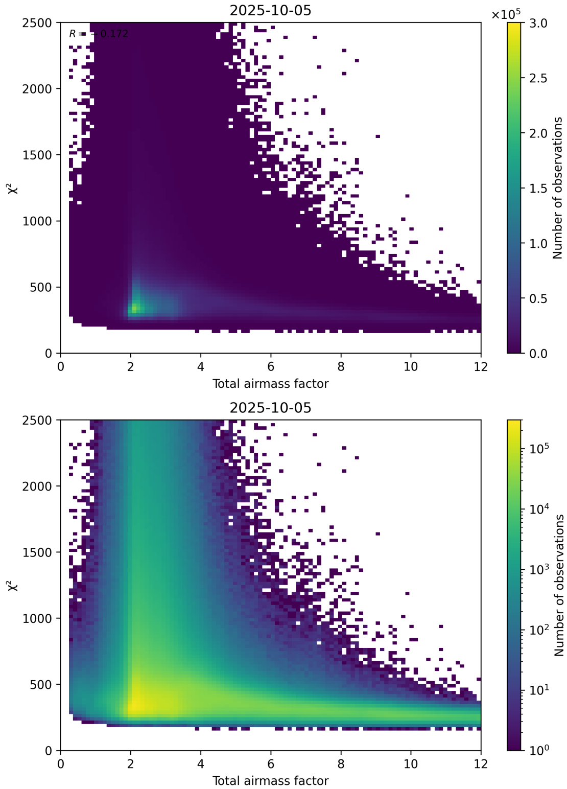
Figure 63: Scatter density plot of “Total airmass factor” against “ \chi^2 ” for 2025-10-04 to 2025-10-06.
