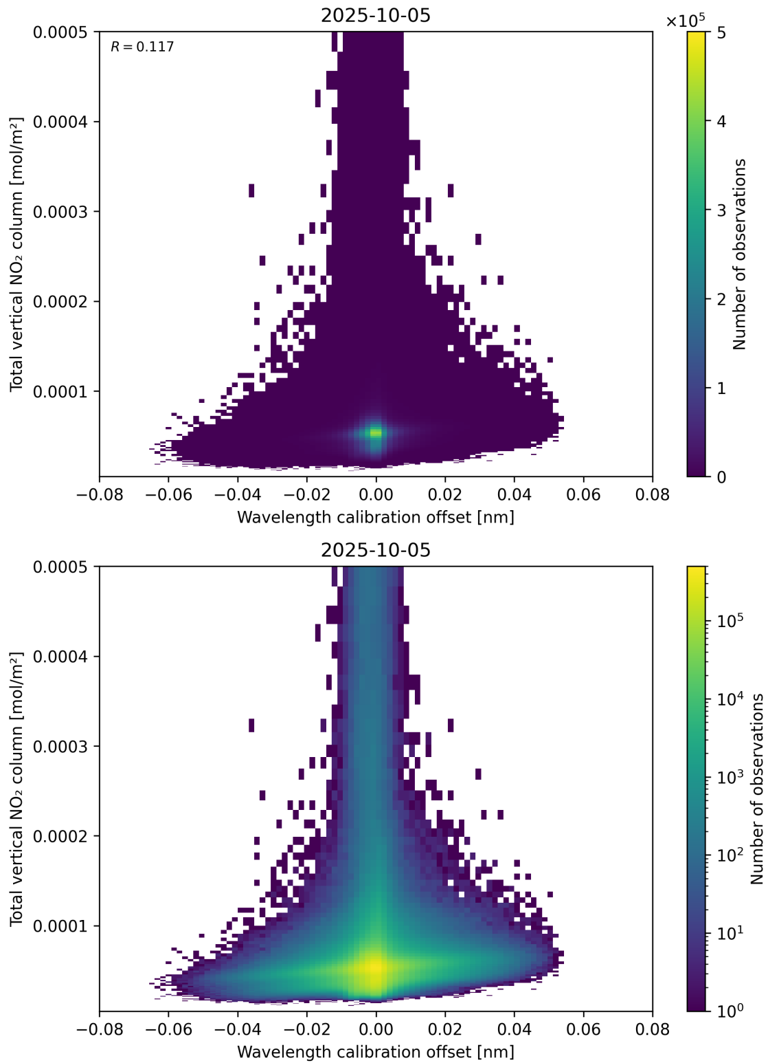
Figure 179: Scatter density plot of “Wavelength calibration offset” against “Total vertical NO 2 column” for 2025-10-04 to 2025-10-06.
