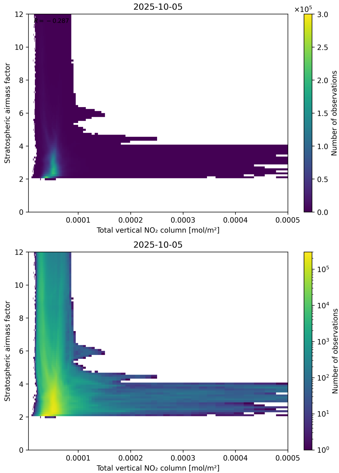
Figure 110: Scatter density plot of “Total vertical NO 2 column” against “Stratospheric airmass factor” for 2025-10-04 to 2025-10-06.
