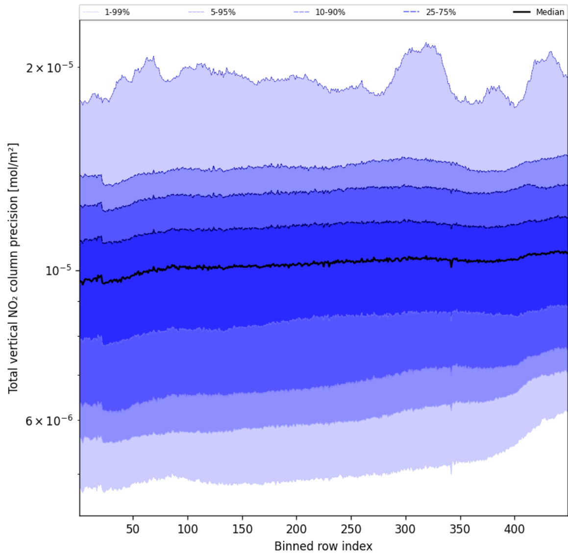
Figure 56: Along track statistics of “Total vertical NO 2 column precision” for 2025-10-04 to 2025-10-06
