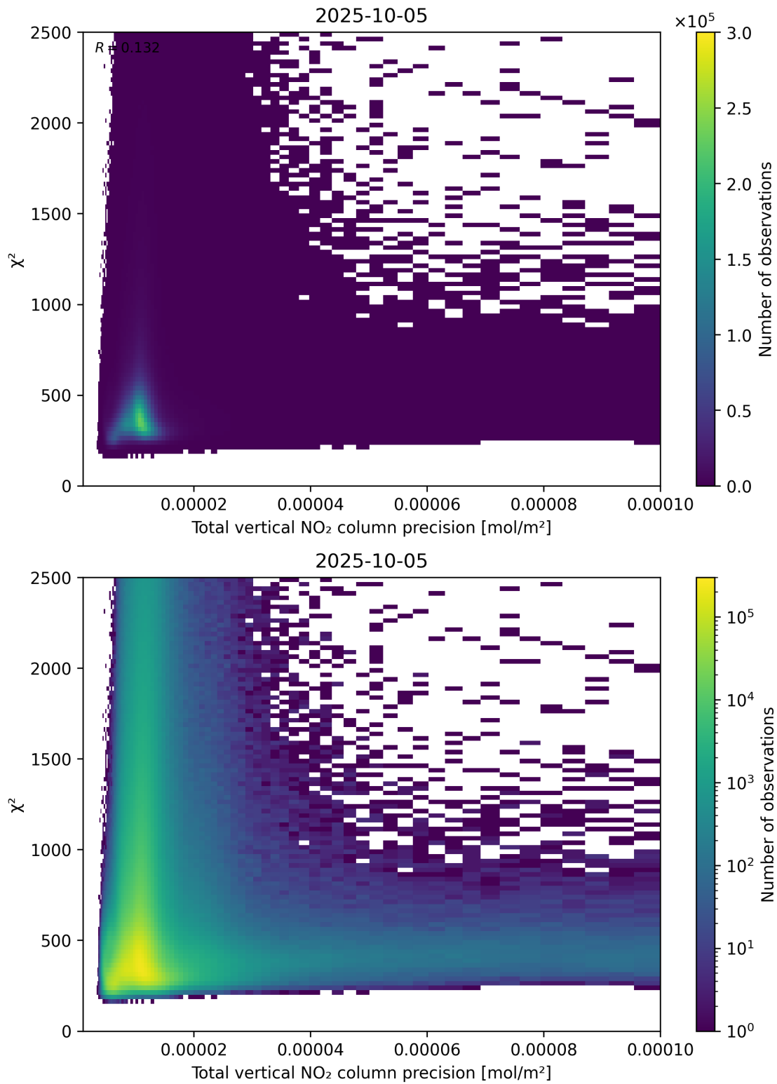
Figure 116: Scatter density plot of “Total vertical NO 2 column precision” against “ \chi^2 ” for 2025-10-04 to 2025-10-06.
