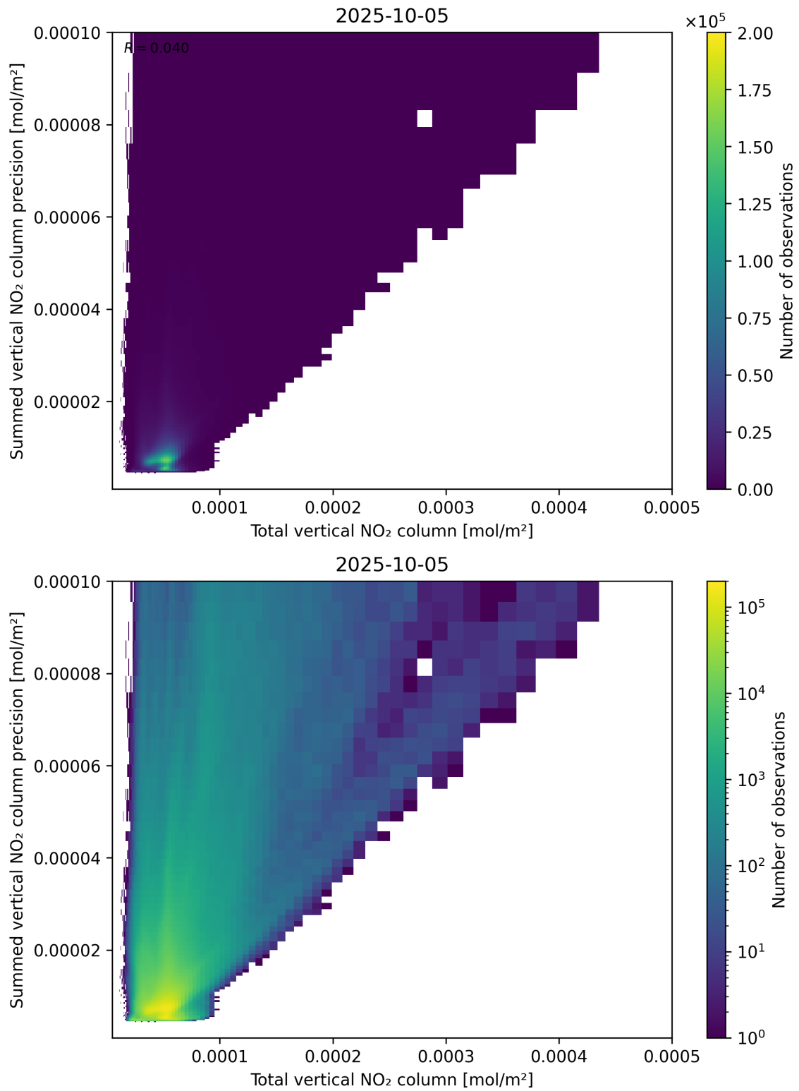
Figure 113: Scatter density plot of “Total vertical NO 2 column” against “Summed vertical NO 2 column precision” for 2025-10-04 to 2025-10-06.
