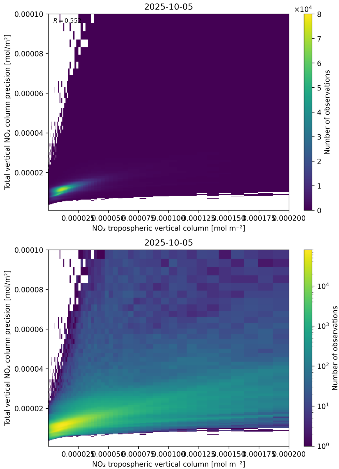
Figure 129: Scatter density plot of “NO 2 tropospheric vertical column” against “Total vertical NO 2 column precision” for 2025-10-04 to 2025-10-06.
