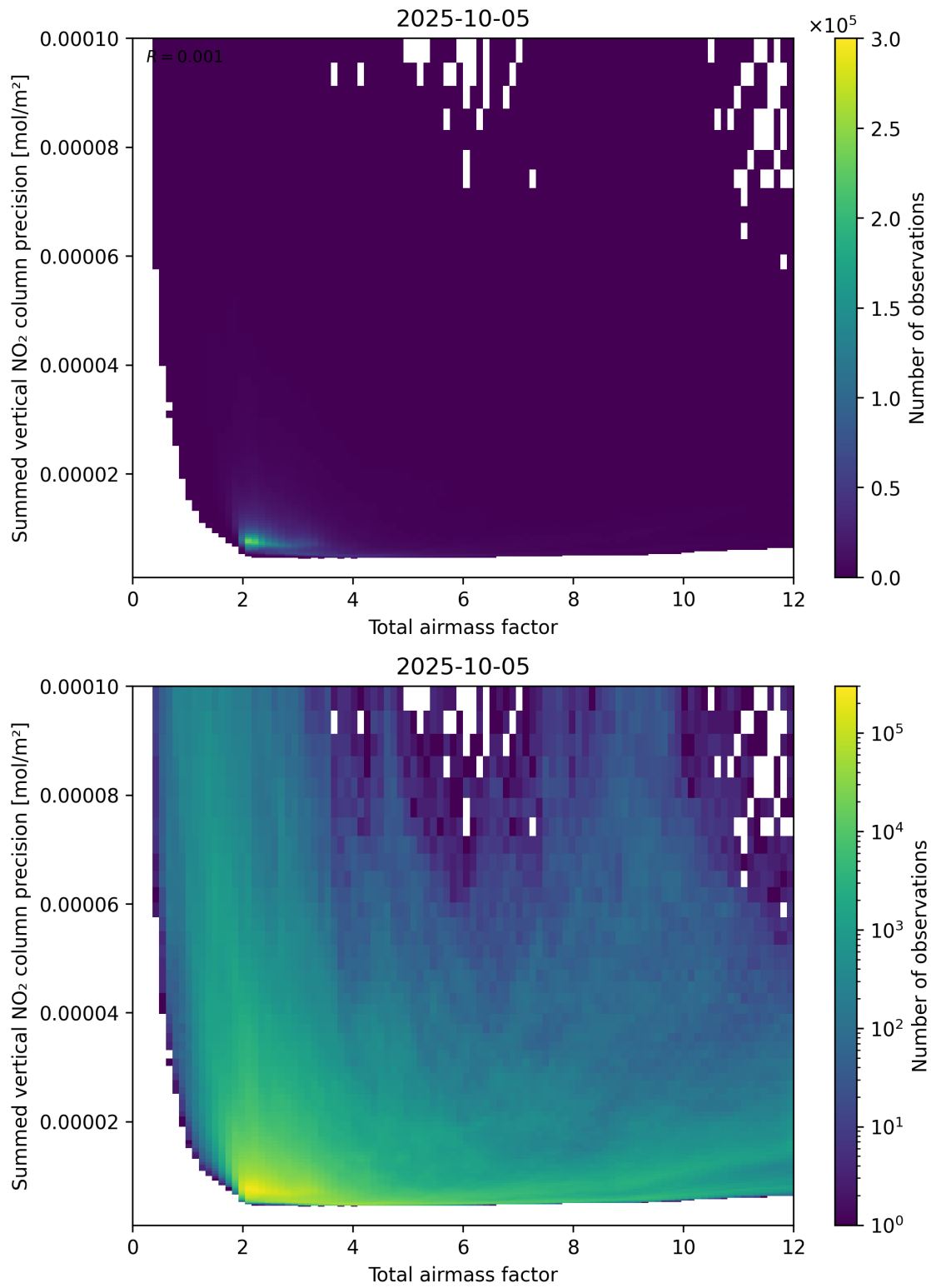
Figure 66: Scatter density plot of “Total airmass factor” against “Summed vertical NO 2 column precision” for 2025-10-04 to 2025-10-06.
