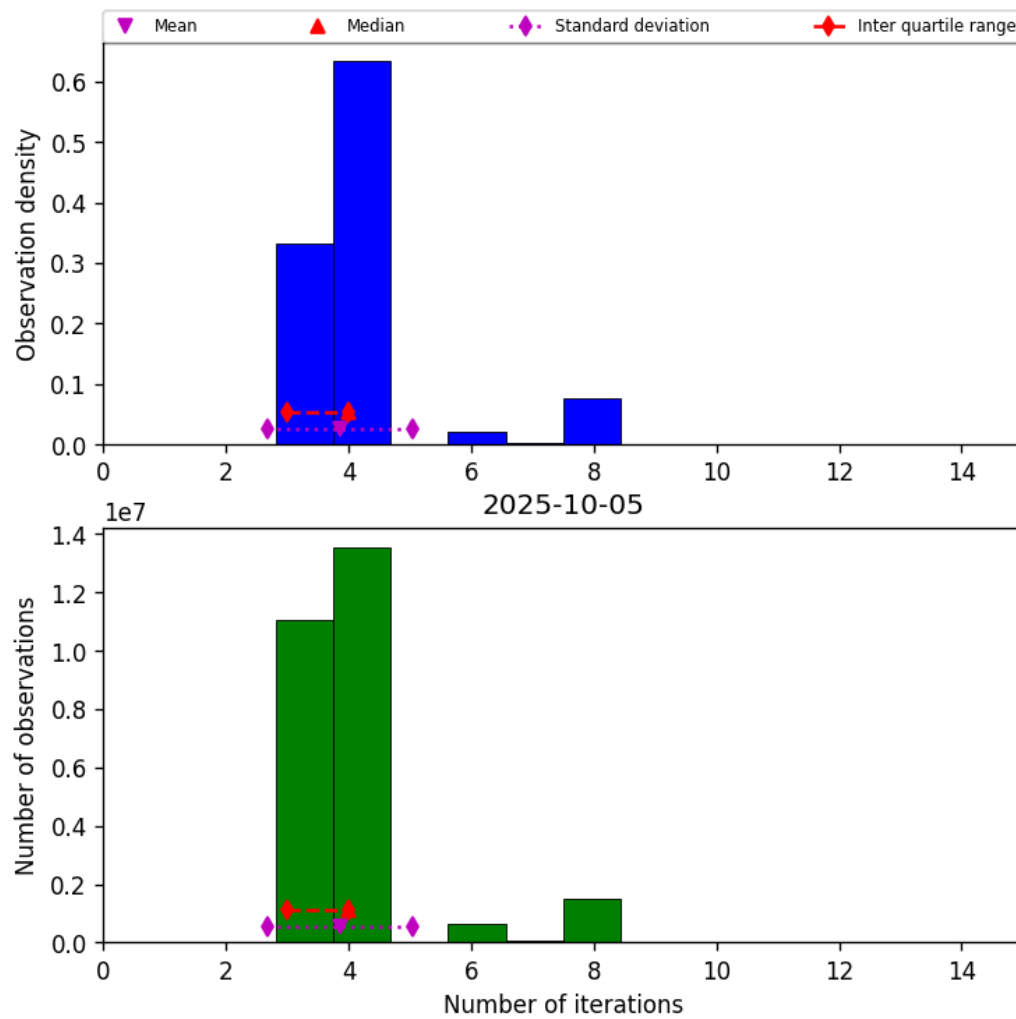
Figure 34: Histogram of “Number of iterations” for 2025-10-04 to 2025-10-06
