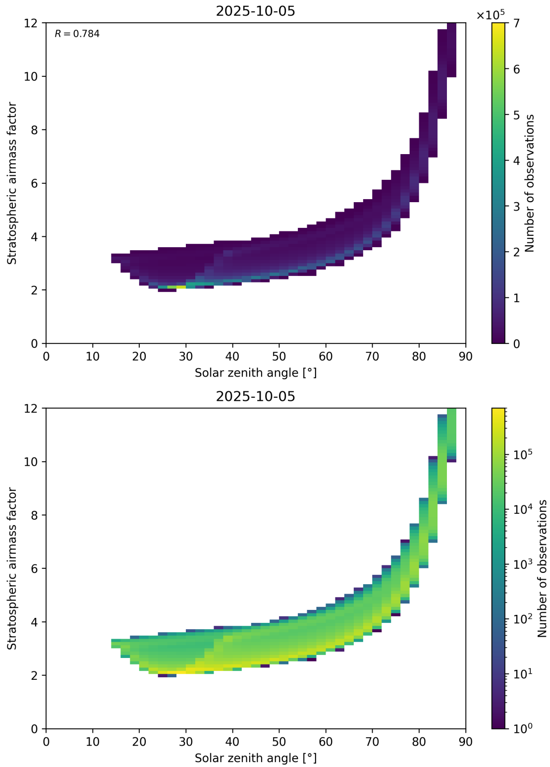
Figure 145: Scatter density plot of “Solar zenith angle” against “Stratospheric airmass factor” for 2025-10-04 to 2025-10-06.
