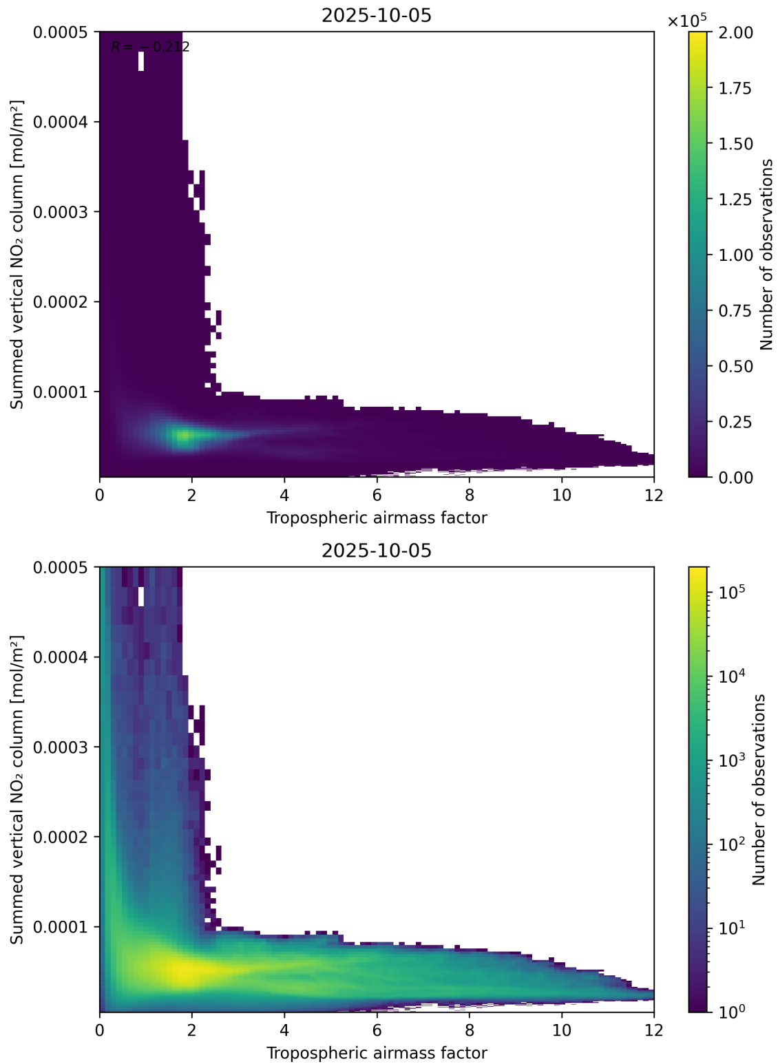
Figure 75: Scatter density plot of “Tropospheric air mass factor” against “Summed vertical NO 2 column” for 2025-10-04 to 2025-10-06.
