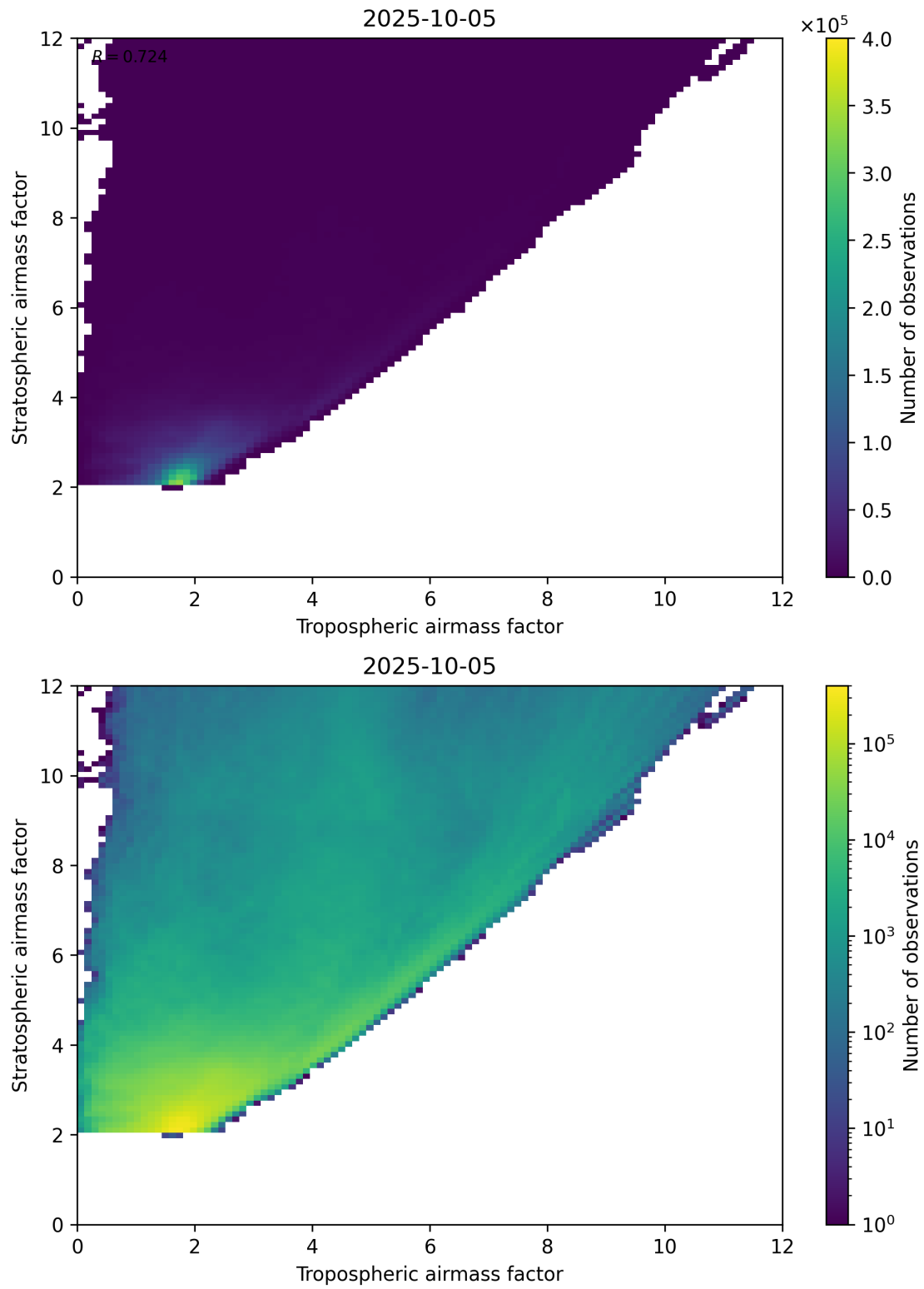
Figure 71: Scatter density plot of “Tropospheric airmass factor” against “Stratospheric airmass factor” for 2025-10-04 to 2025-10-06.
