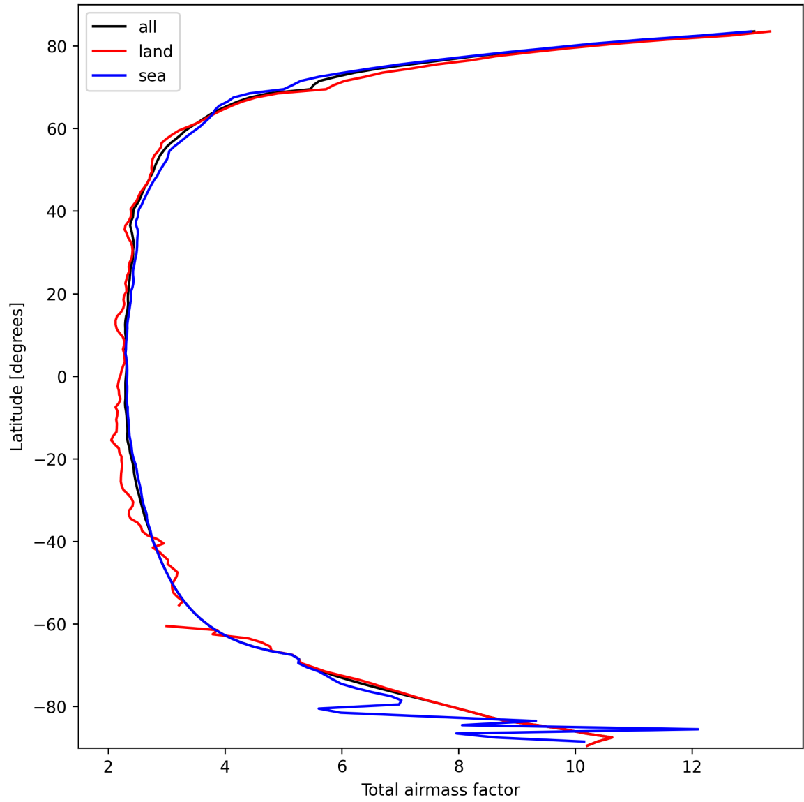
Figure 15: Zonal average of “Total airmass factor” for 2025-10-04 to 2025-10-06.
