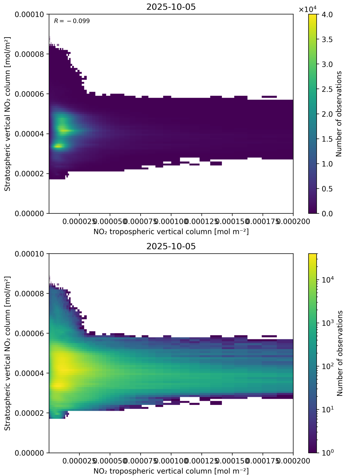
Figure 125: Scatter density plot of “NO 2 tropospheric vertical column” against “Stratospheric vertical NO 2 column” for 2025-10-04 to 2025-10-06.
