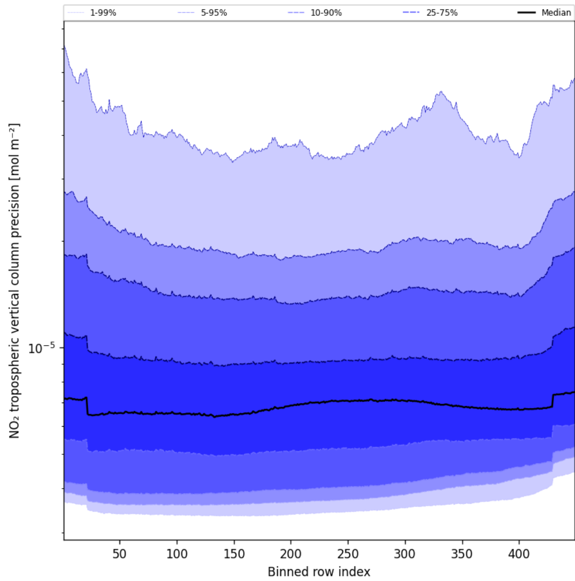
Figure 47: Along track statistics of “NO 2 tropospheric vertical column precision” for 2025-10-04 to 2025-10-06
