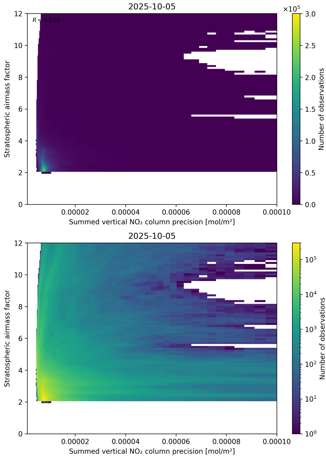
Figure 106: Scatter density plot of “Summed vertical NO 2 column precision” against “Stratospheric airmass factor” for 2025-10-04 to 2025-10-06.
