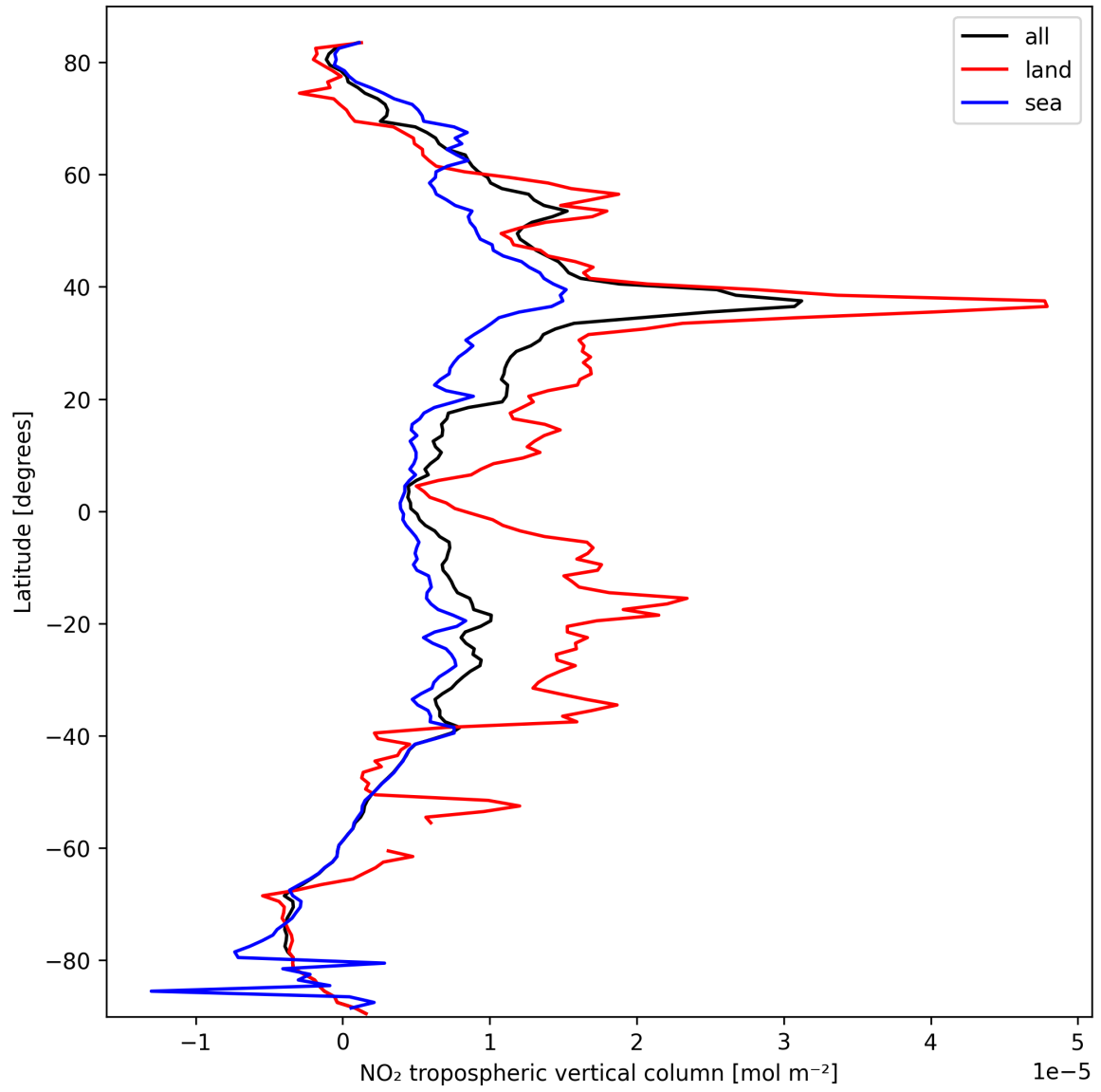
Figure 12: Zonal average of “NO 2 tropospheric vertical column” for 2025-10-04 to 2025-10-06.
