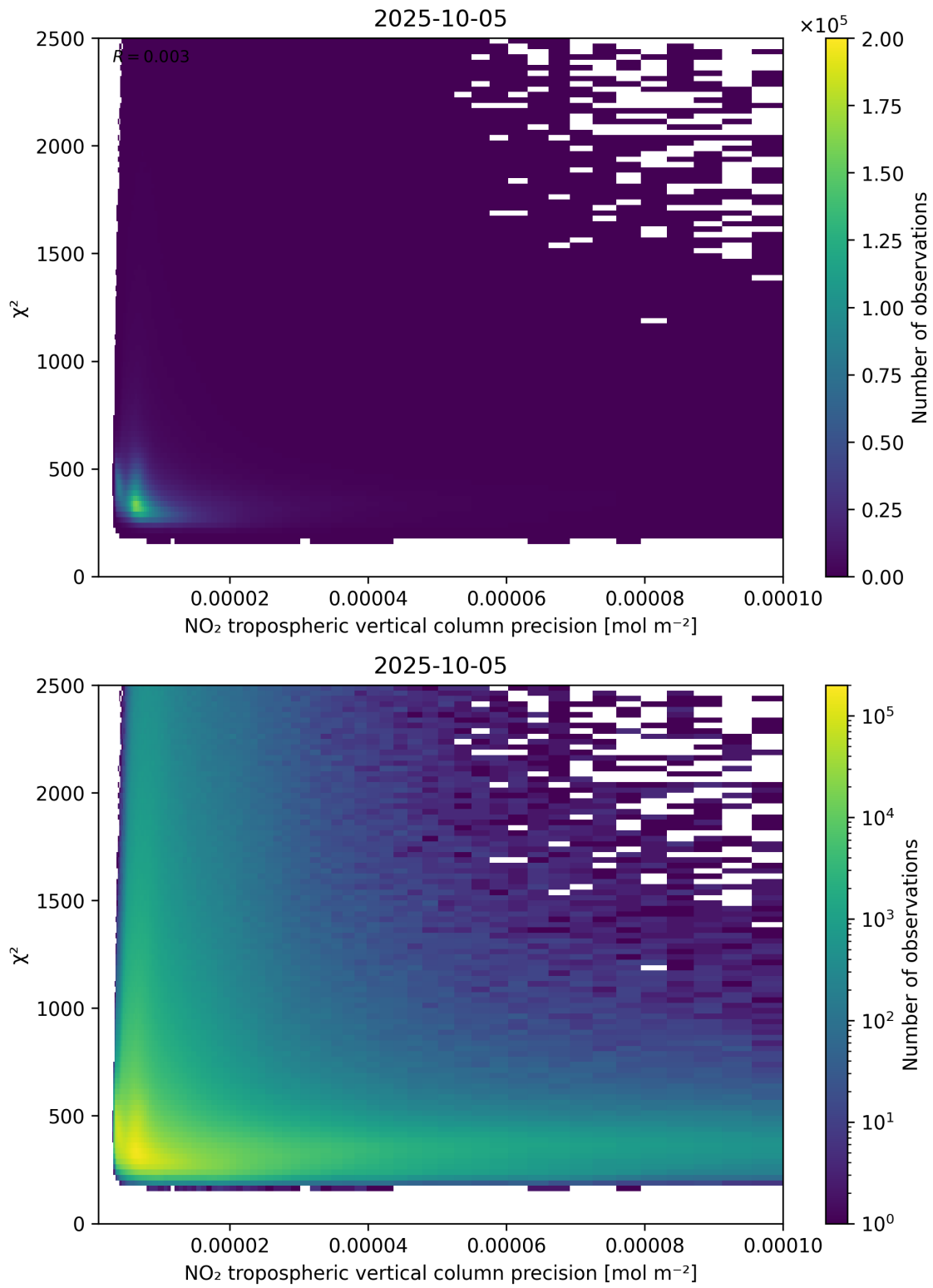
Figure 134: Scatter density plot of “NO 2 tropospheric vertical column precision” against “ \chi^2 ” for 2025-10-04 to 2025-10-06.
