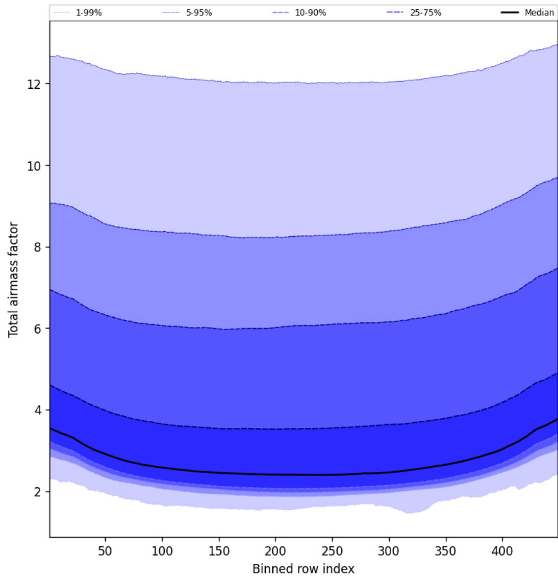
Figure 49: Along track statistics of “Total airmass factor” for 2025-10-04 to 2025-10-06
