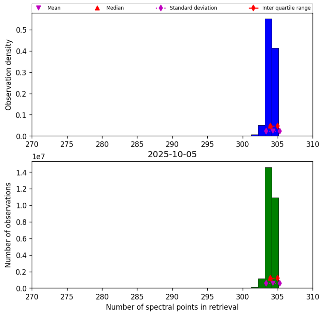
Figure 33: Histogram of “Number of spectral points in retrieval” for 2025-10-04 to 2025-10-06
