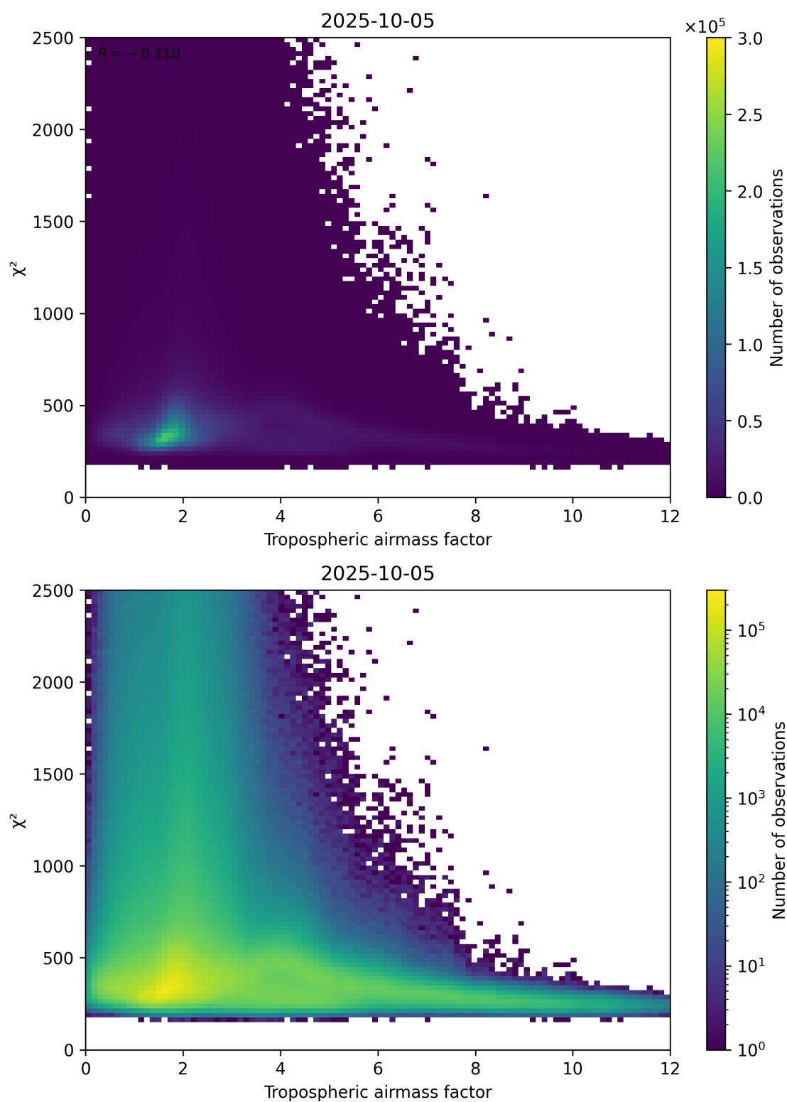
Figure 73: Scatter density plot of “Tropospheric airmass factor” against “ \chi^2 ” for 2025-10-04 to 2025-10-06.
