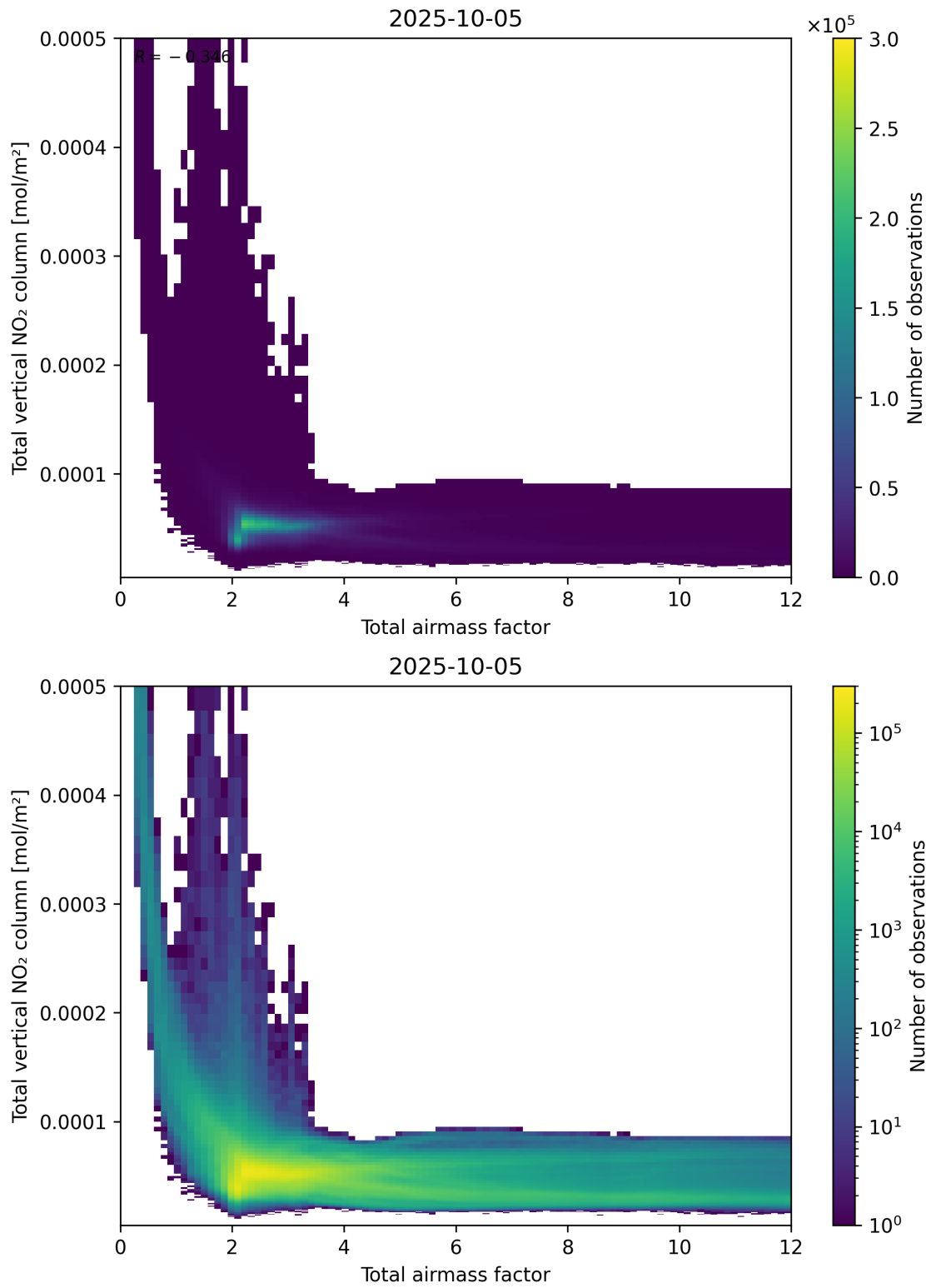
Figure 67: Scatter density plot of “Total airmass factor” against “Total vertical NO 2 column” for 2025-10-04 to 2025-10-06.
