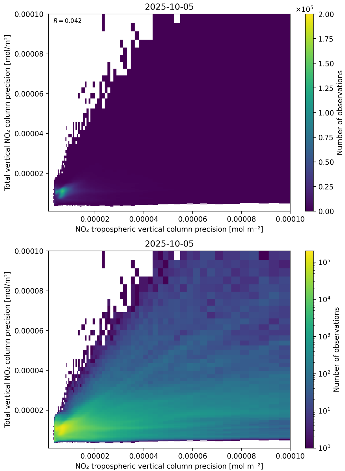
Figure 139: Scatter density plot of “NO 2 tropospheric vertical column precision” against “Total vertical NO 2 column precision” for 2025-10-04 to 2025-10-06.
