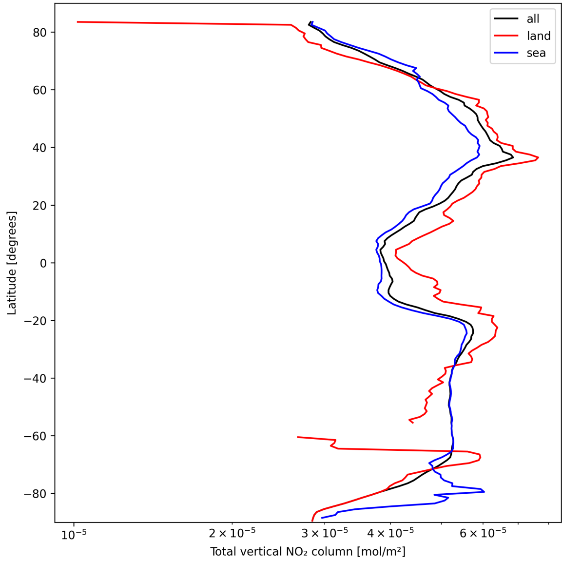
Figure 21: Zonal average of “Total vertical NO 2 column” for 2025-10-04 to 2025-10-06.
