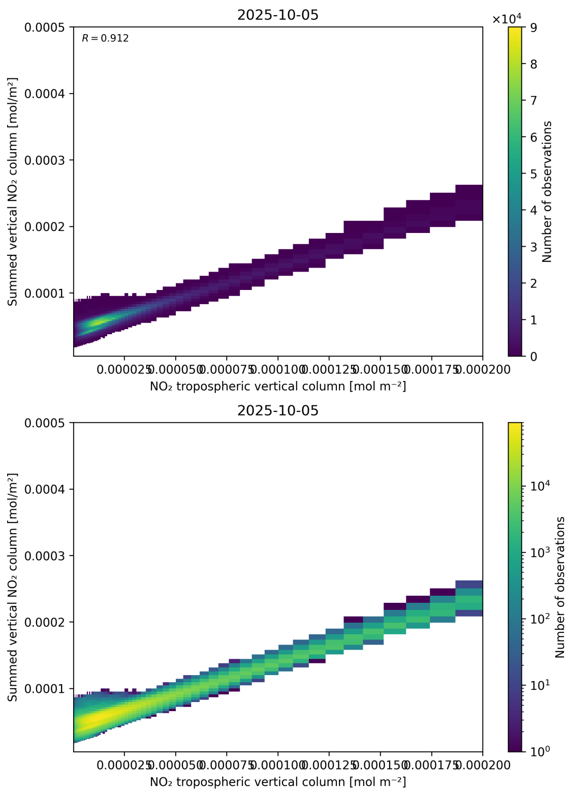
Figure 126: Scatter density plot of “NO 2 tropospheric vertical column” against “Summed vertical NO 2 column” for 2025-10-04 to 2025-10-06.
