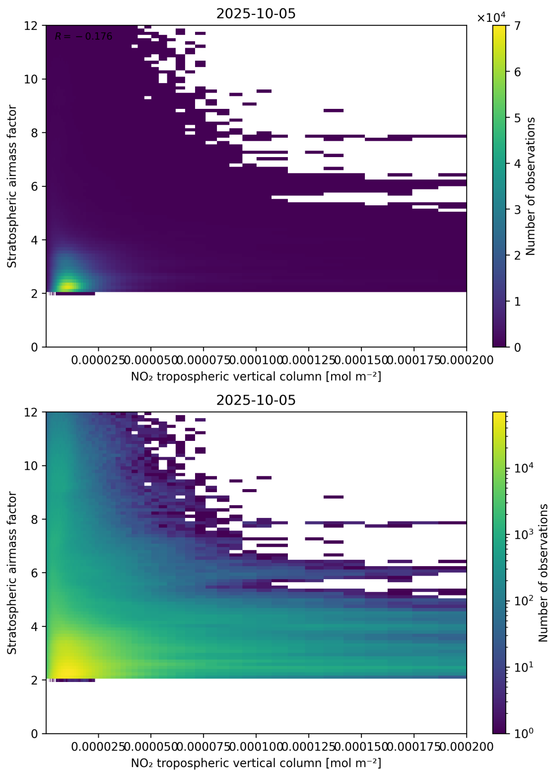
Figure 121: Scatter density plot of “NO 2 tropospheric vertical column” against “Stratospheric air mass factor” for 2025-10-04 to 2025-10-06.
