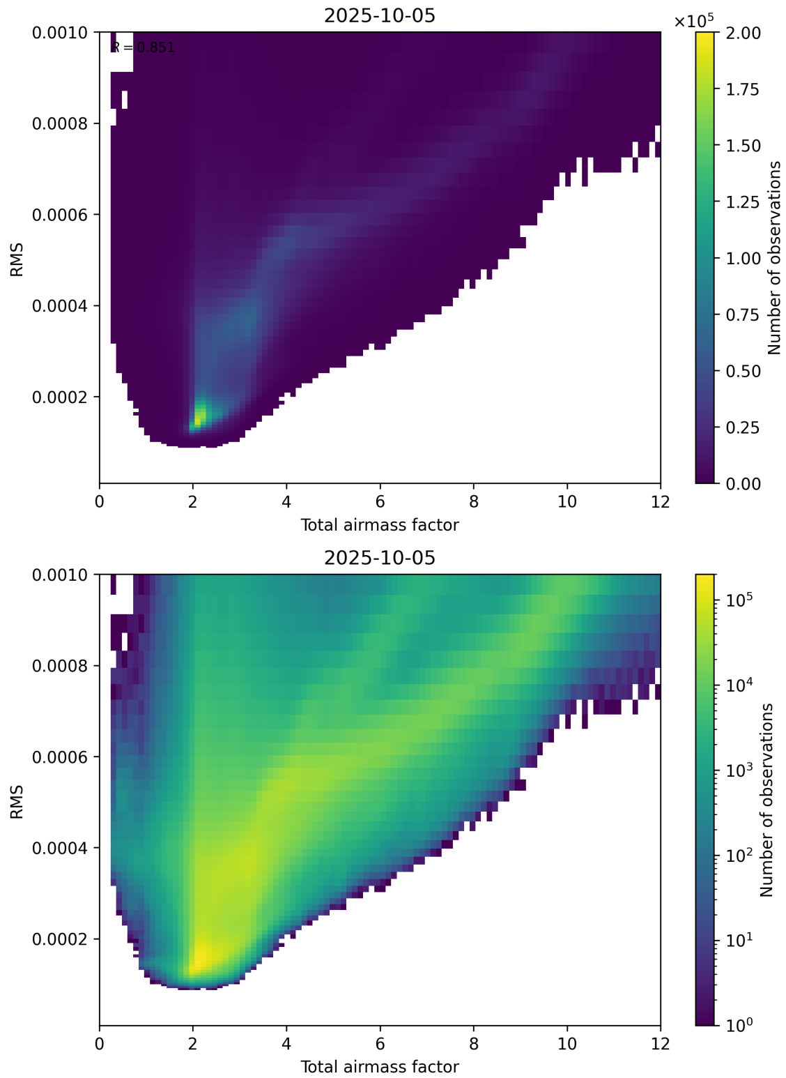
Figure 69: Scatter density plot of “Total airmass factor” against “RMS” for 2025-10-04 to 2025-10-06.
