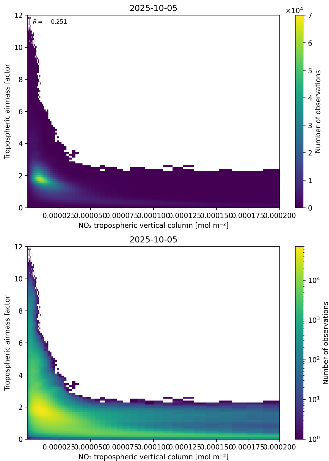
Figure 123: Scatter density plot of “NO 2 tropospheric vertical column” against “Tropospheric air mass factor” for 2025-10-04 to 2025-10-06.
