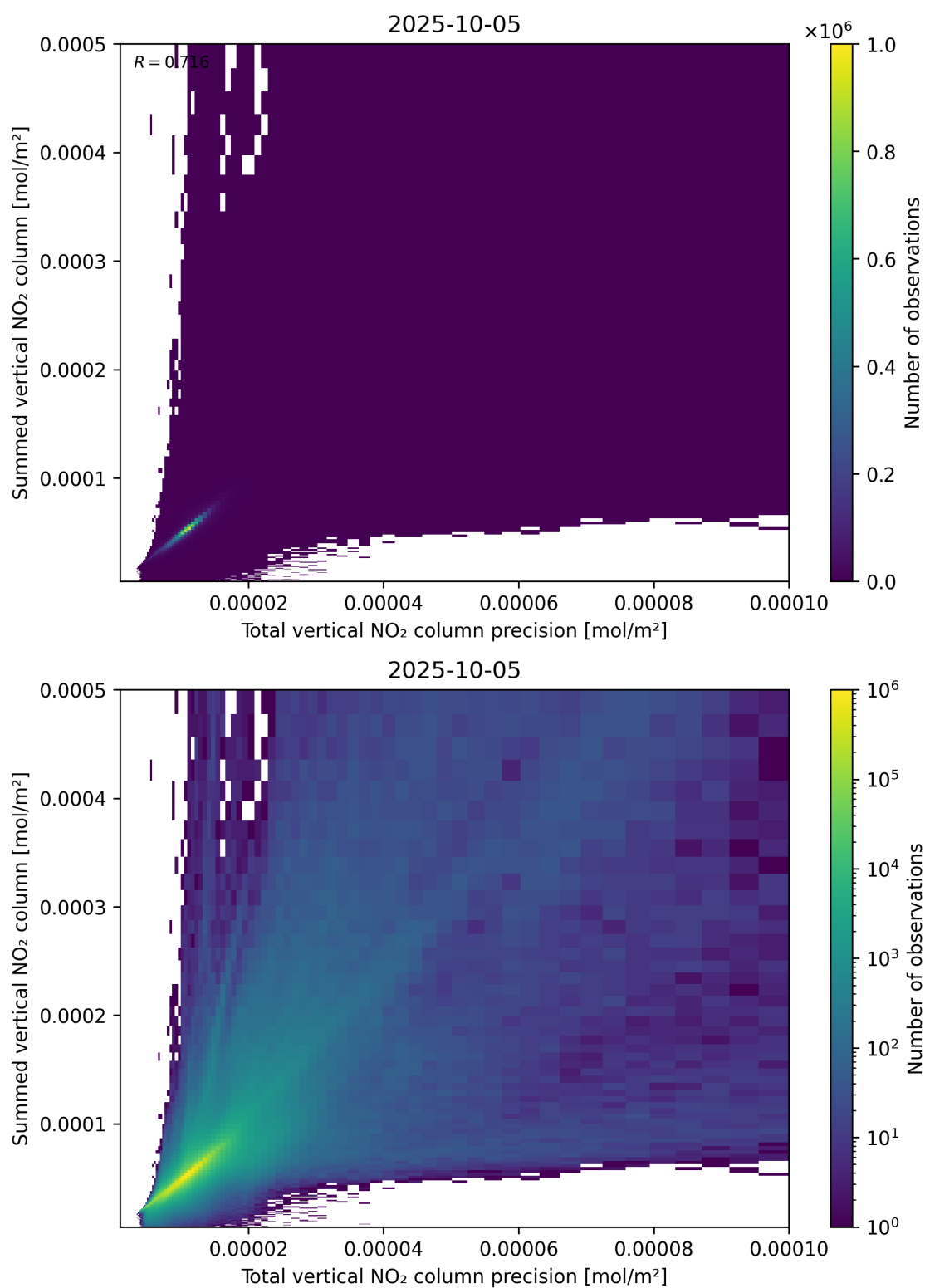
Figure 117: Scatter density plot of “Total vertical NO 2 column precision” against “Summed vertical NO 2 column” for 2025-10-04 to 2025-10-06.
