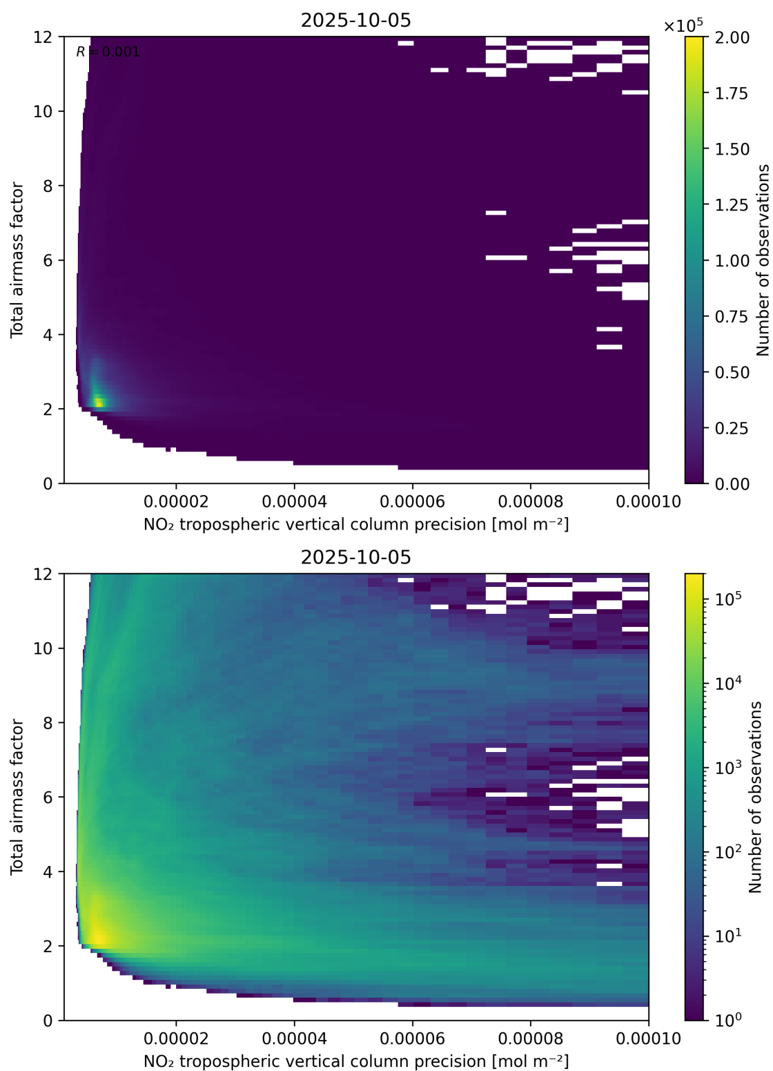
Figure 132: Scatter density plot of “NO 2 tropospheric vertical column precision” against “Total air mass factor” for 2025-10-04 to 2025-10-06.
