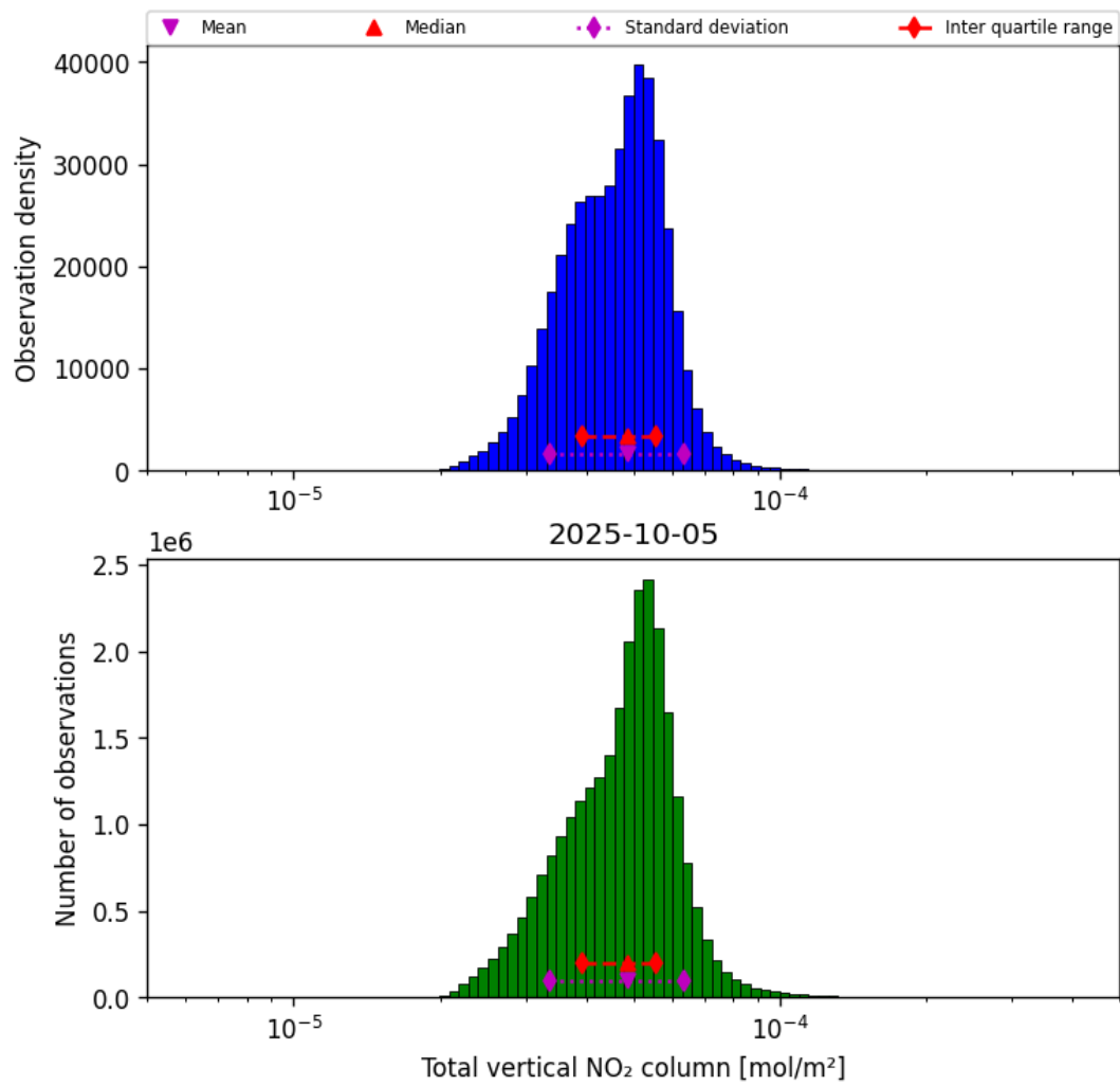
Figure 38: Histogram of “Total vertical NO 2 column” for 2025-10-04 to 2025-10-06
