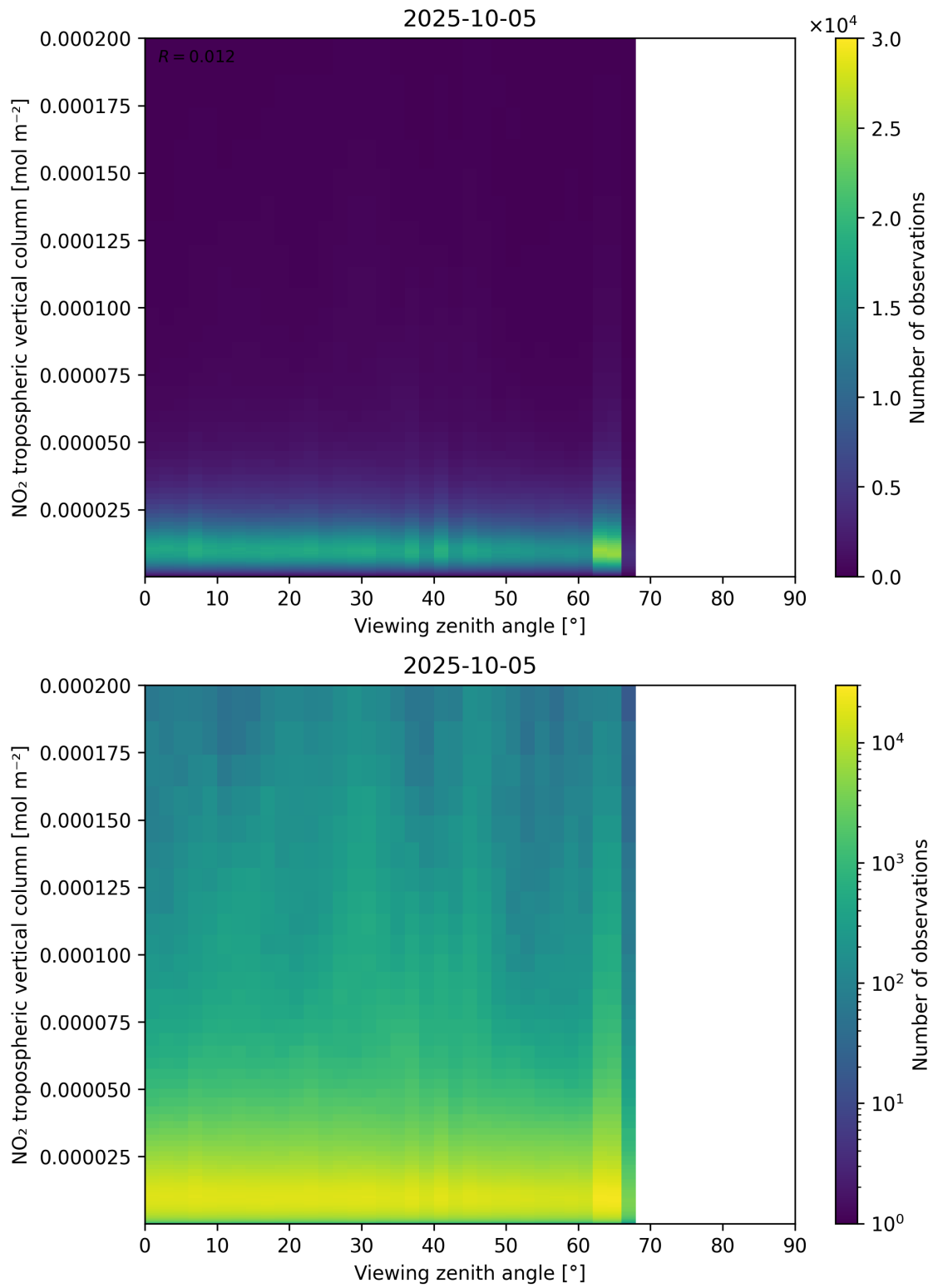
Figure 169: Scatter density plot of “Viewing zenith angle” against “NO 2 tropospheric vertical column” for 2025-10-04 to 2025-10-06.
