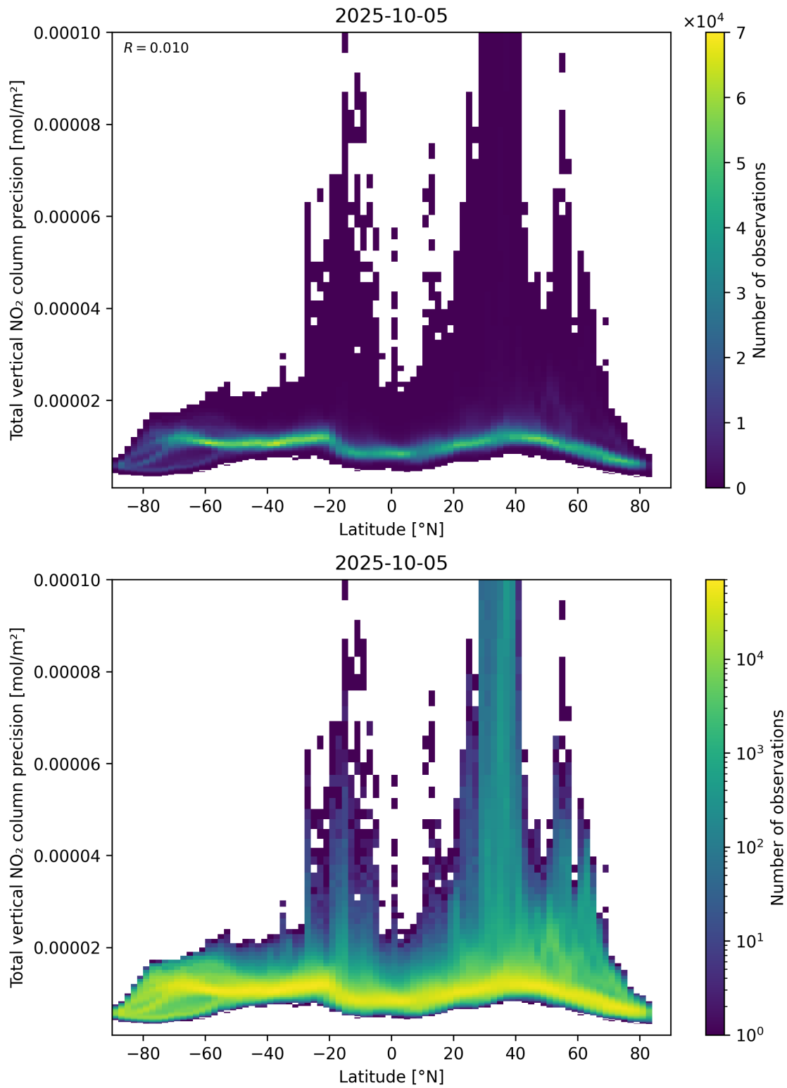
Figure 91: Scatter density plot of “Latitude” against “Total vertical NO 2 column precision” for 2025-10-04 to 2025-10-06.
