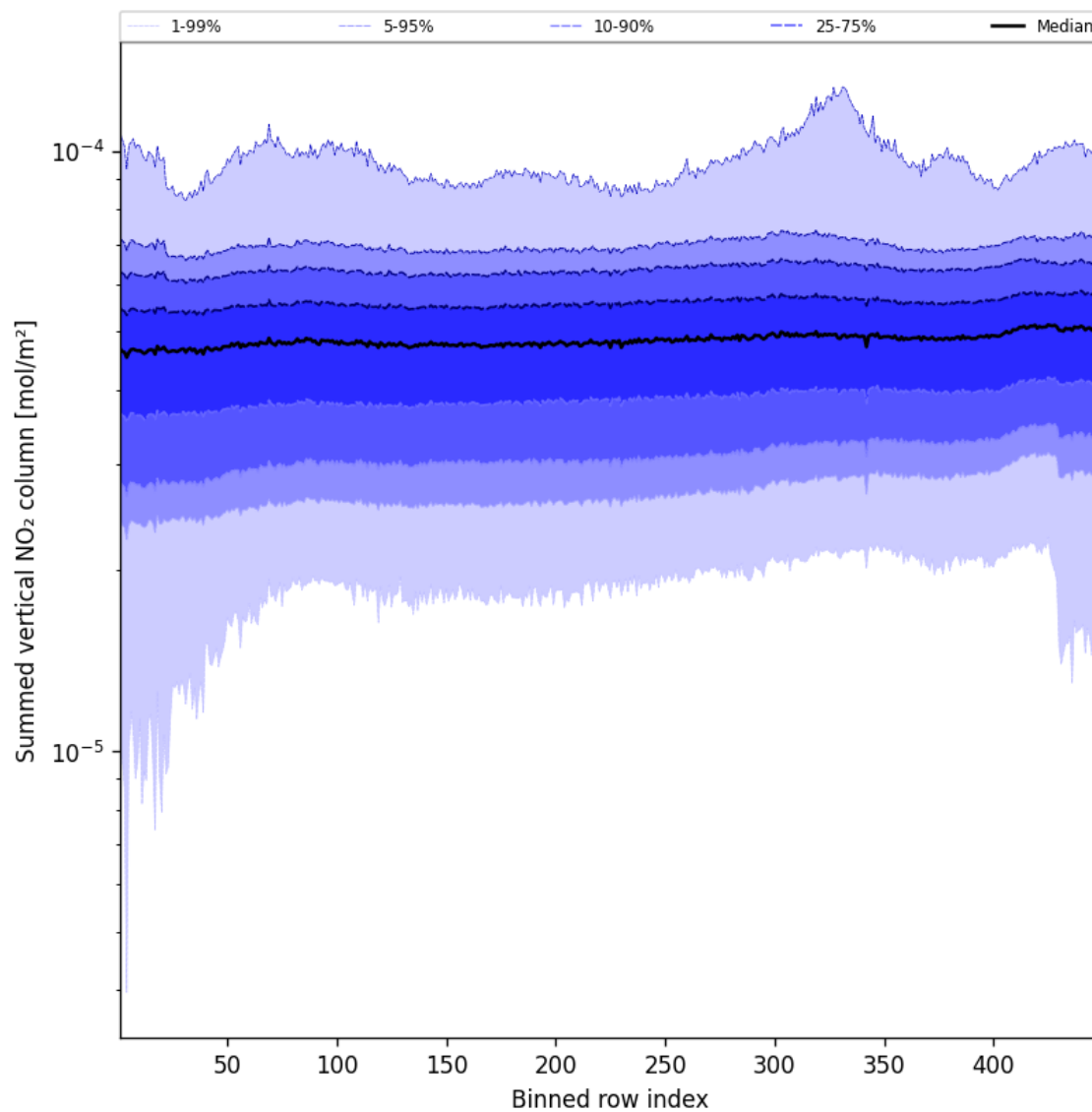
Figure 57: Along track statistics of “Summed vertical NO 2 column” for 2025-10-04 to 2025-10-06
