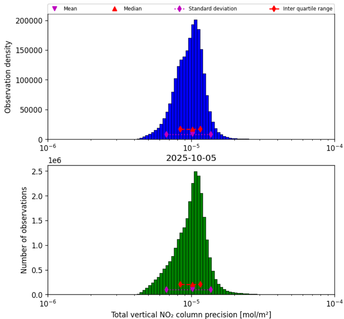
Figure 39: Histogram of "Total vertical NO 2 column precision" for 2025-10-04 to 2025-10-06
