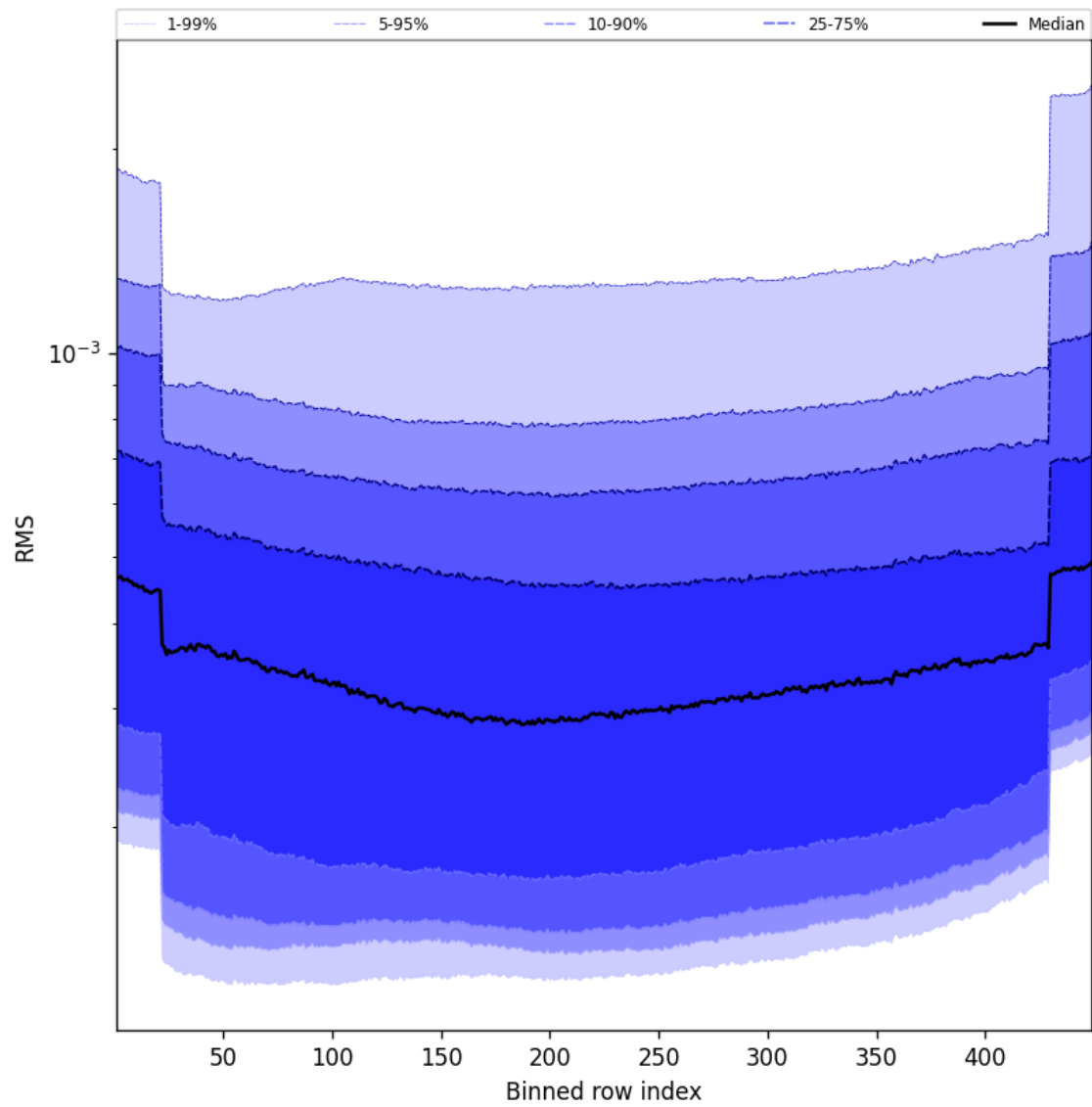
Figure 60: Along track statistics of “RMS” for 2025-10-04 to 2025-10-06
