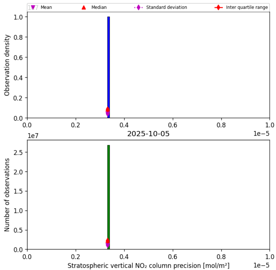
Figure 37: Histogram of “Stratospheric vertical NO 2 column precision” for 2025-10-04 to 2025-10-06
