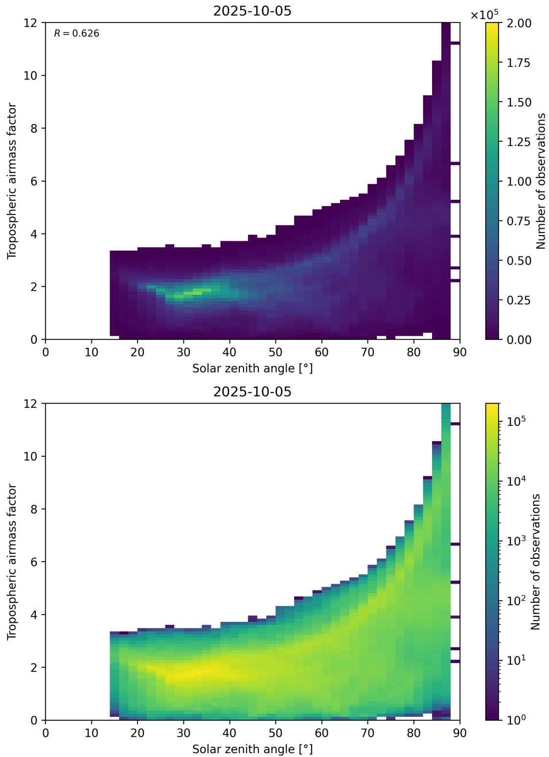
Figure 147: Scatter density plot of “Solar zenith angle” against “Tropospheric airmass factor” for 2025-10-04 to 2025-10-06.
