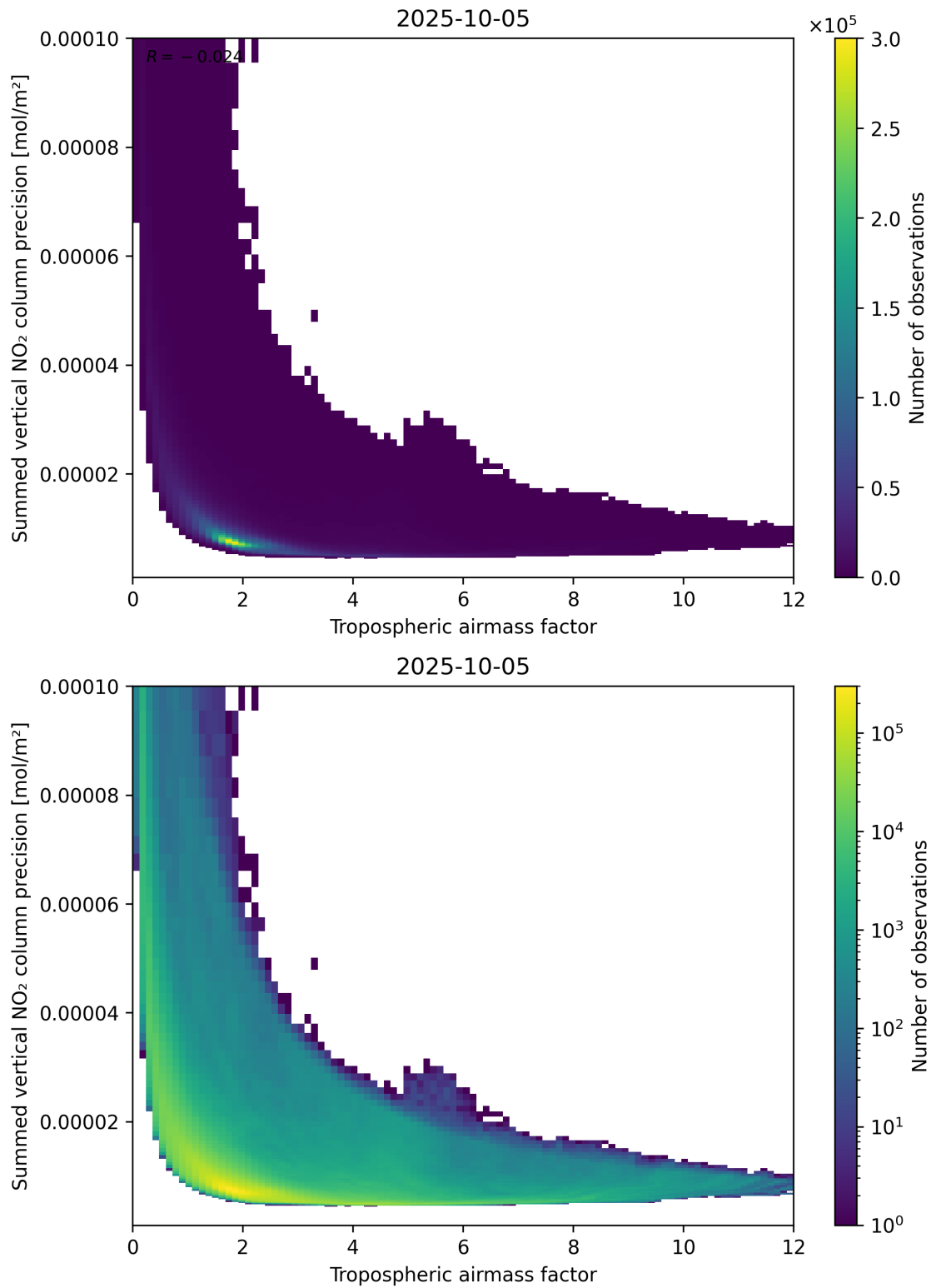
Figure 76: Scatter density plot of “Tropospheric air mass factor” against “Summed vertical NO 2 column precision” for 2025-10-04 to 2025-10-06.
