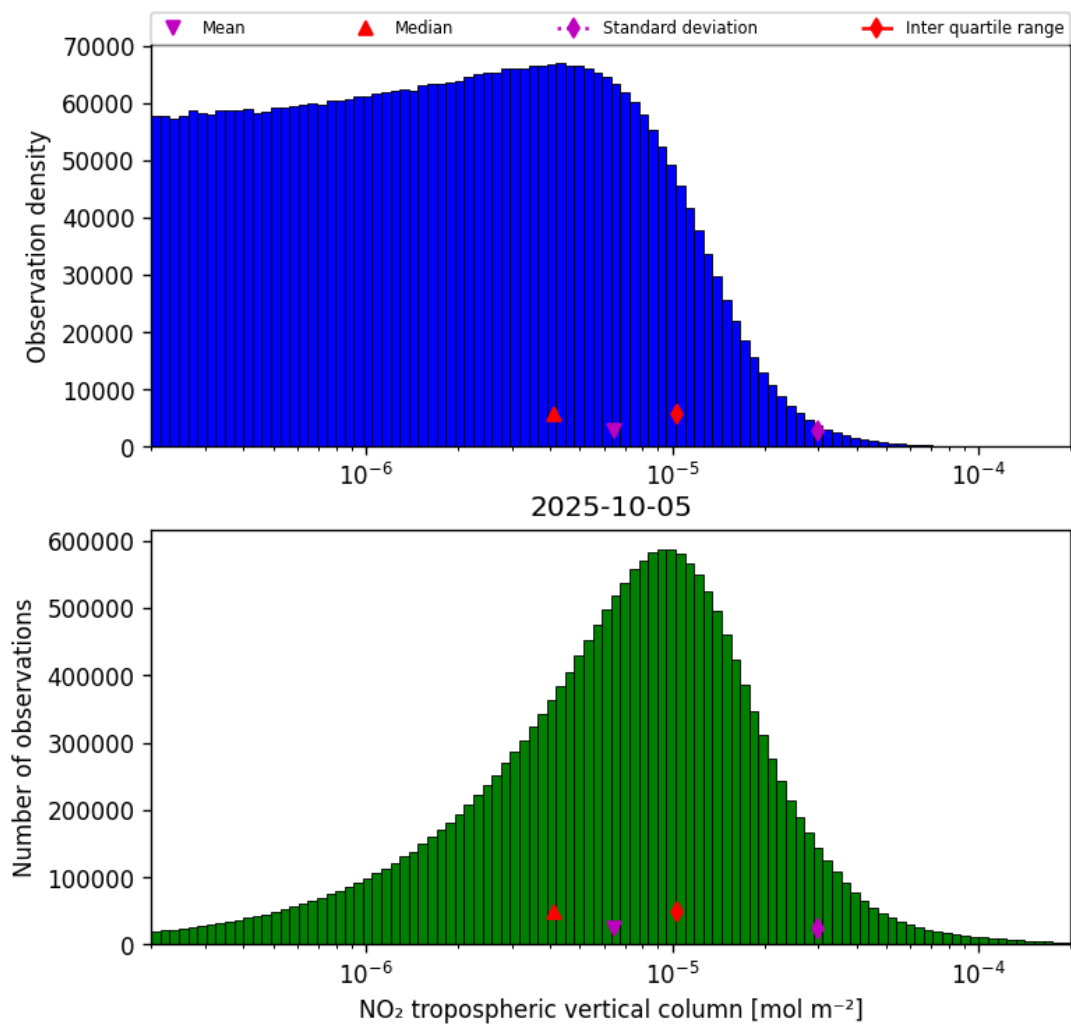
Figure 29: Histogram of “ \text{NO}_2 tropospheric vertical column” for 2025-10-04 to 2025-10-06
