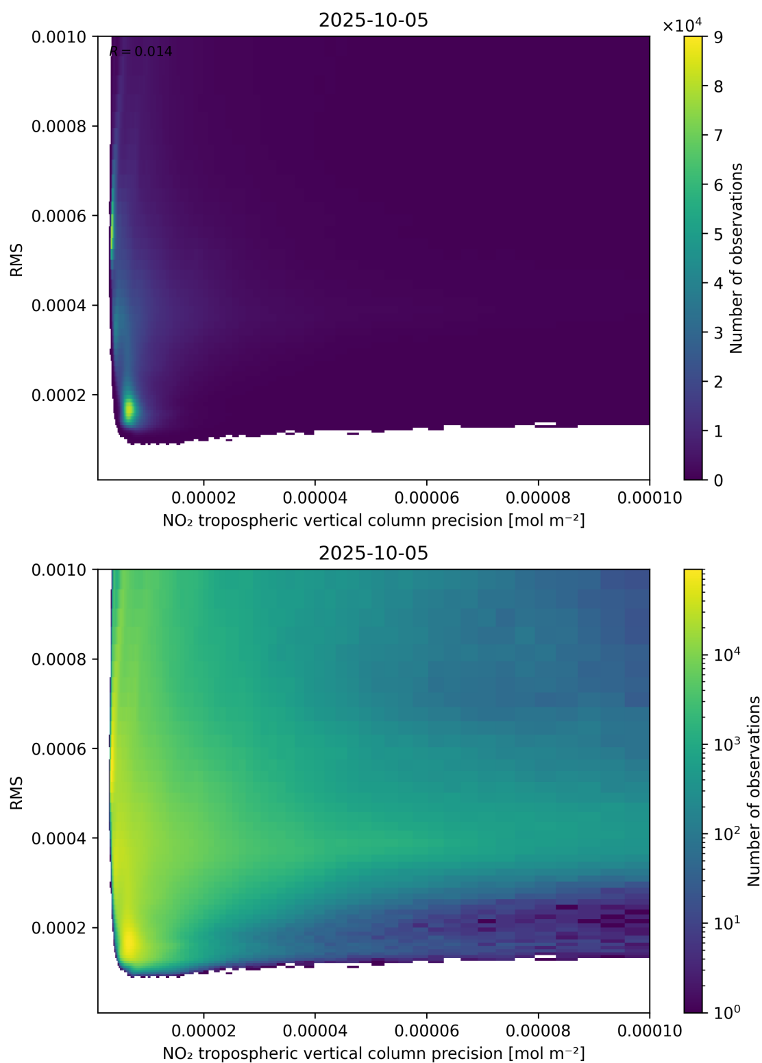
Figure 140: Scatter density plot of “NO 2 tropospheric vertical column precision” against “RMS” for 2025-10-04 to 2025-10-06.
