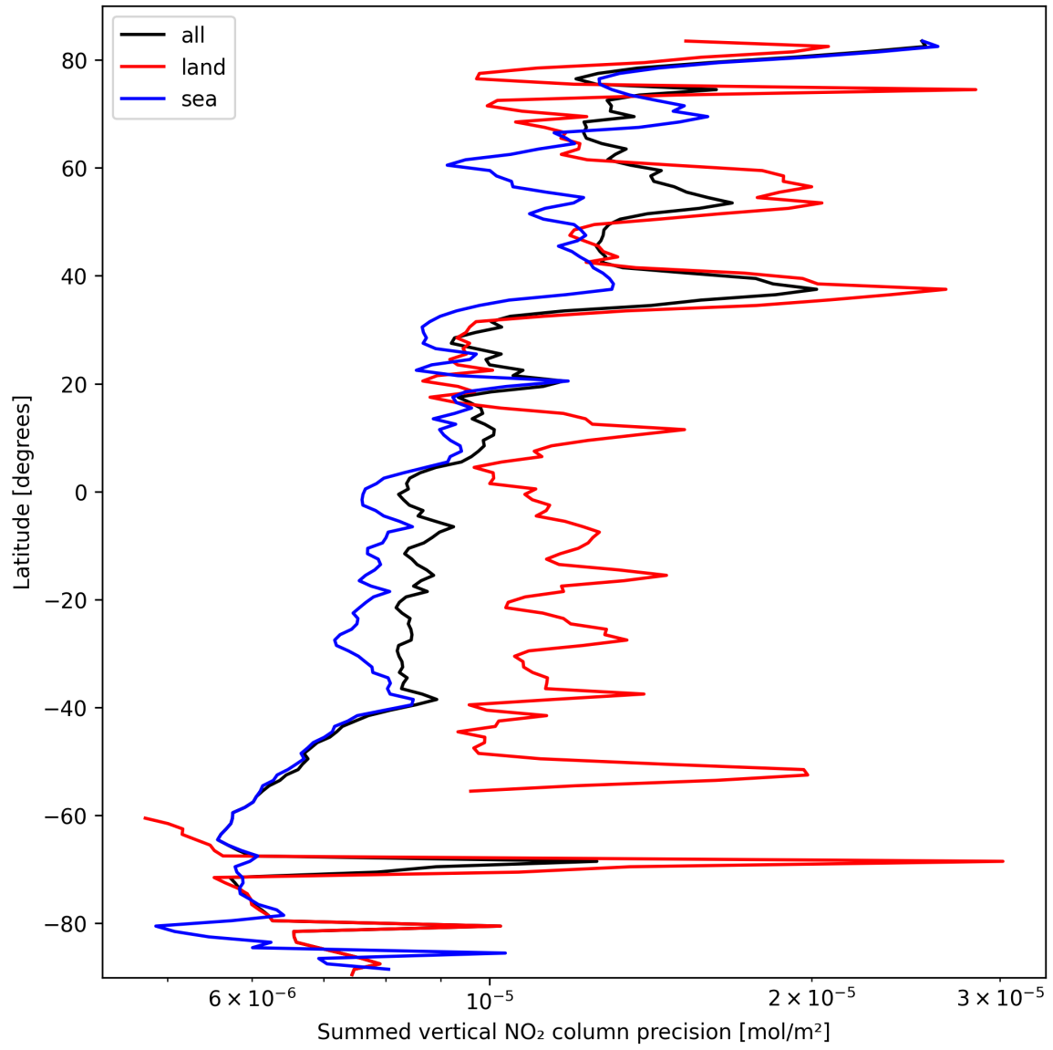
Figure 24: Zonal average of “Summed vertical NO 2 column precision” for 2025-10-04 to 2025-10-06.
