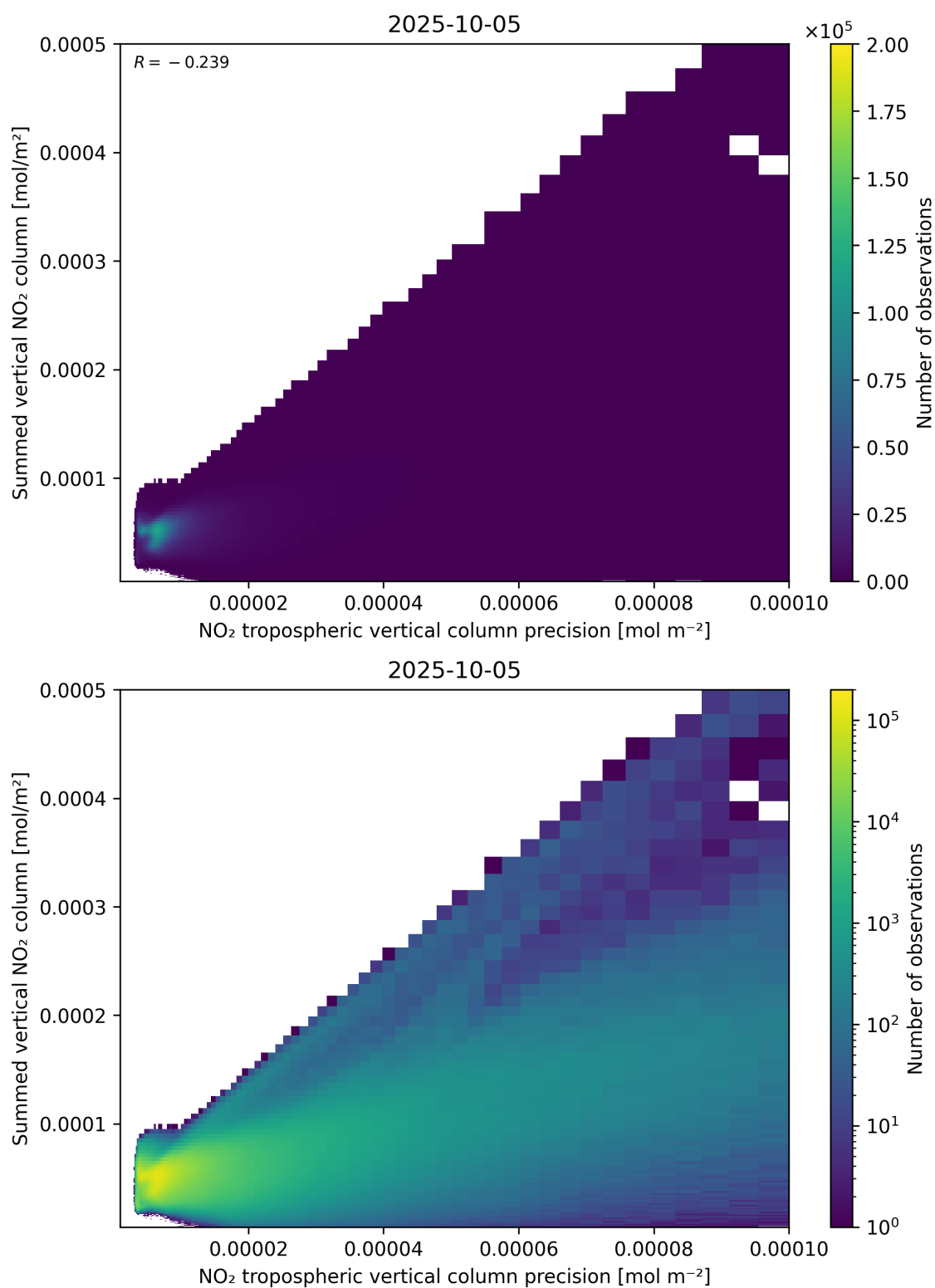
Figure 136: Scatter density plot of “NO 2 tropospheric vertical column precision” against “Summed vertical NO 2 column” for 2025-10-04 to 2025-10-06.
