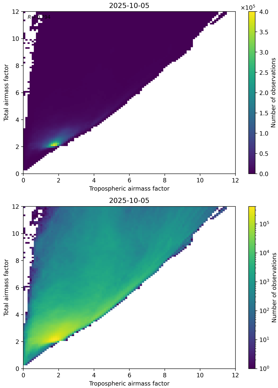
Figure 72: Scatter density plot of “Tropospheric airmass factor” against “Total airmass factor” for 2025-10-04 to 2025-10-06.
