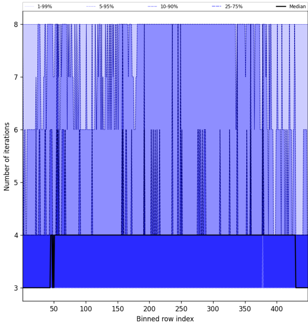
Figure 51: Along track statistics of “Number of iterations” for 2025-10-04 to 2025-10-06
