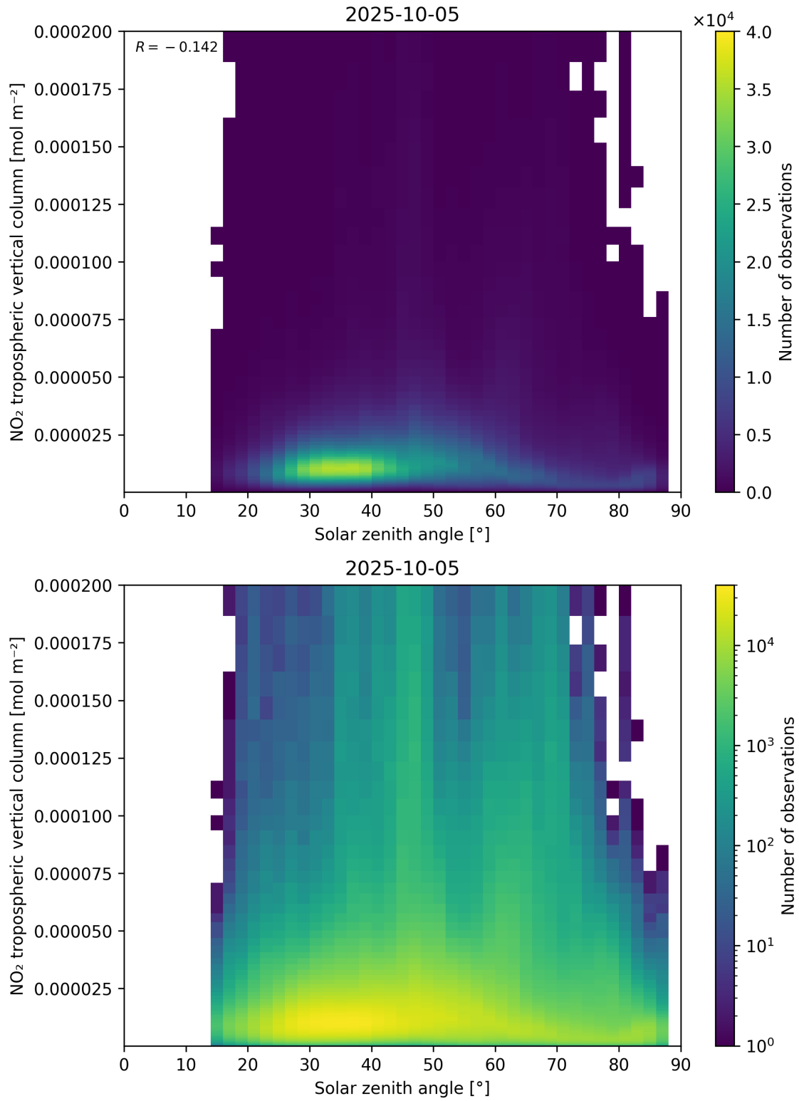
Figure 155: Scatter density plot of “Solar zenith angle” against “NO 2 tropospheric vertical column” for 2025-10-04 to 2025-10-06.
