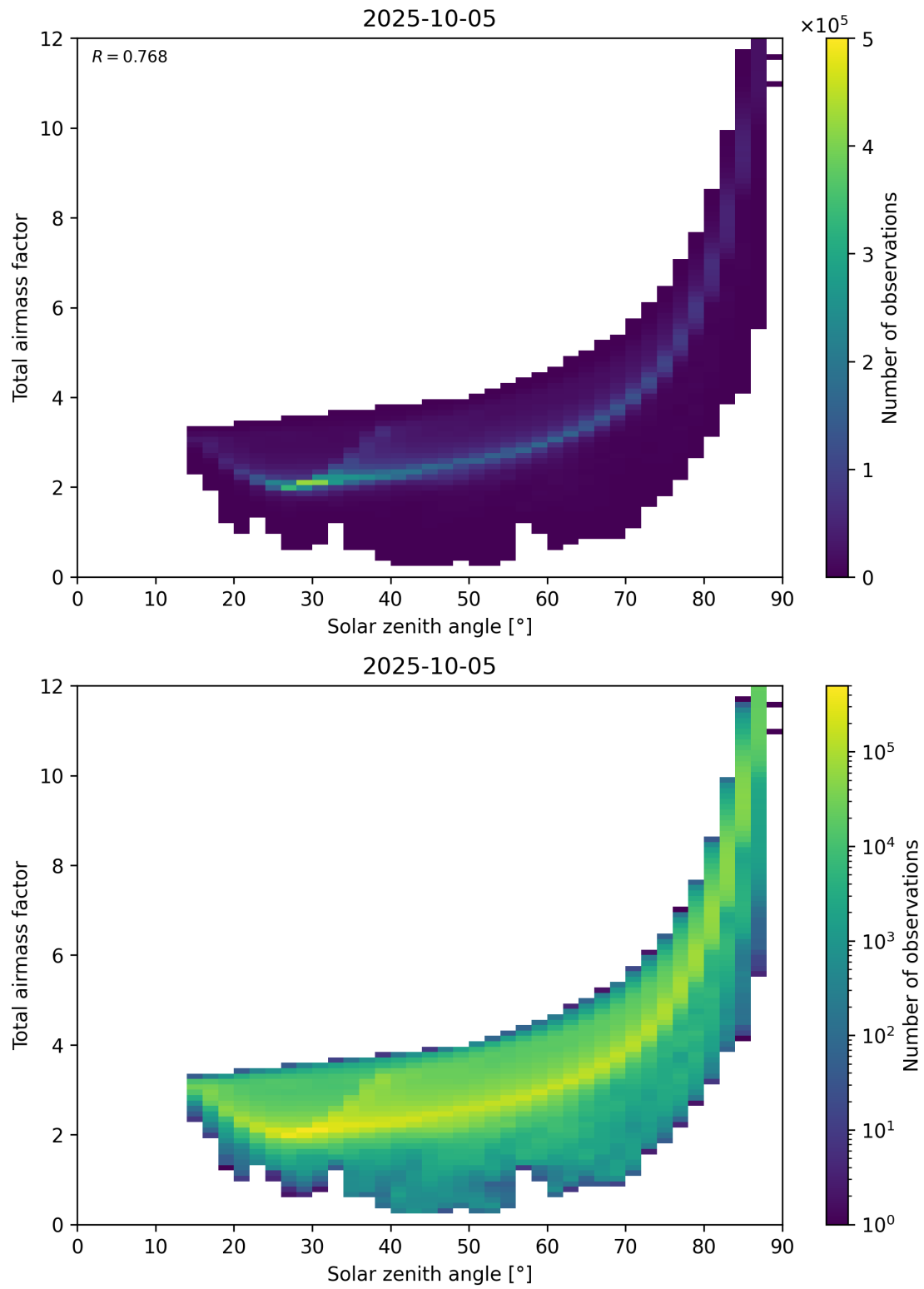
Figure 146: Scatter density plot of “Solar zenith angle” against “Total airmass factor” for 2025-10-04 to 2025-10-06.
