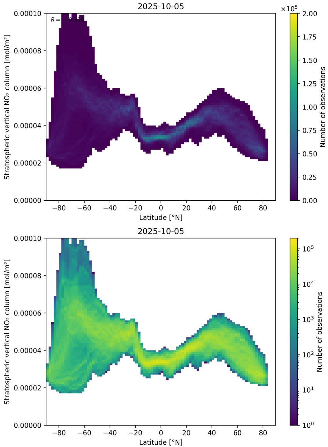
Figure 87: Scatter density plot of “Latitude” against “Stratospheric vertical NO 2 column” for 2025-10-04 to 2025-10-06.
