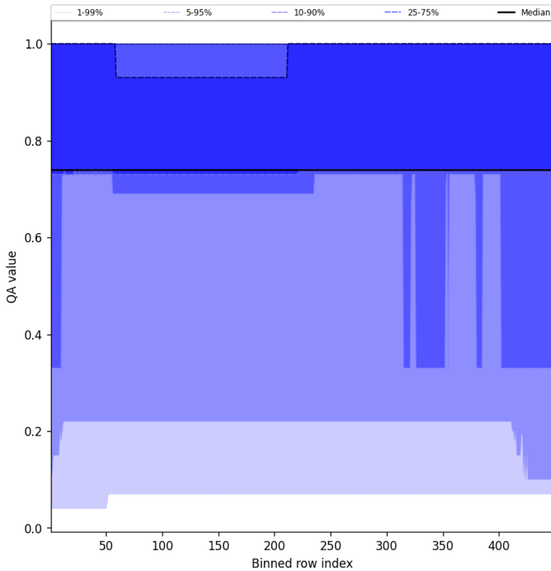
Figure 45: Along track statistics of “QA value” for 2025-10-04 to 2025-10-06
