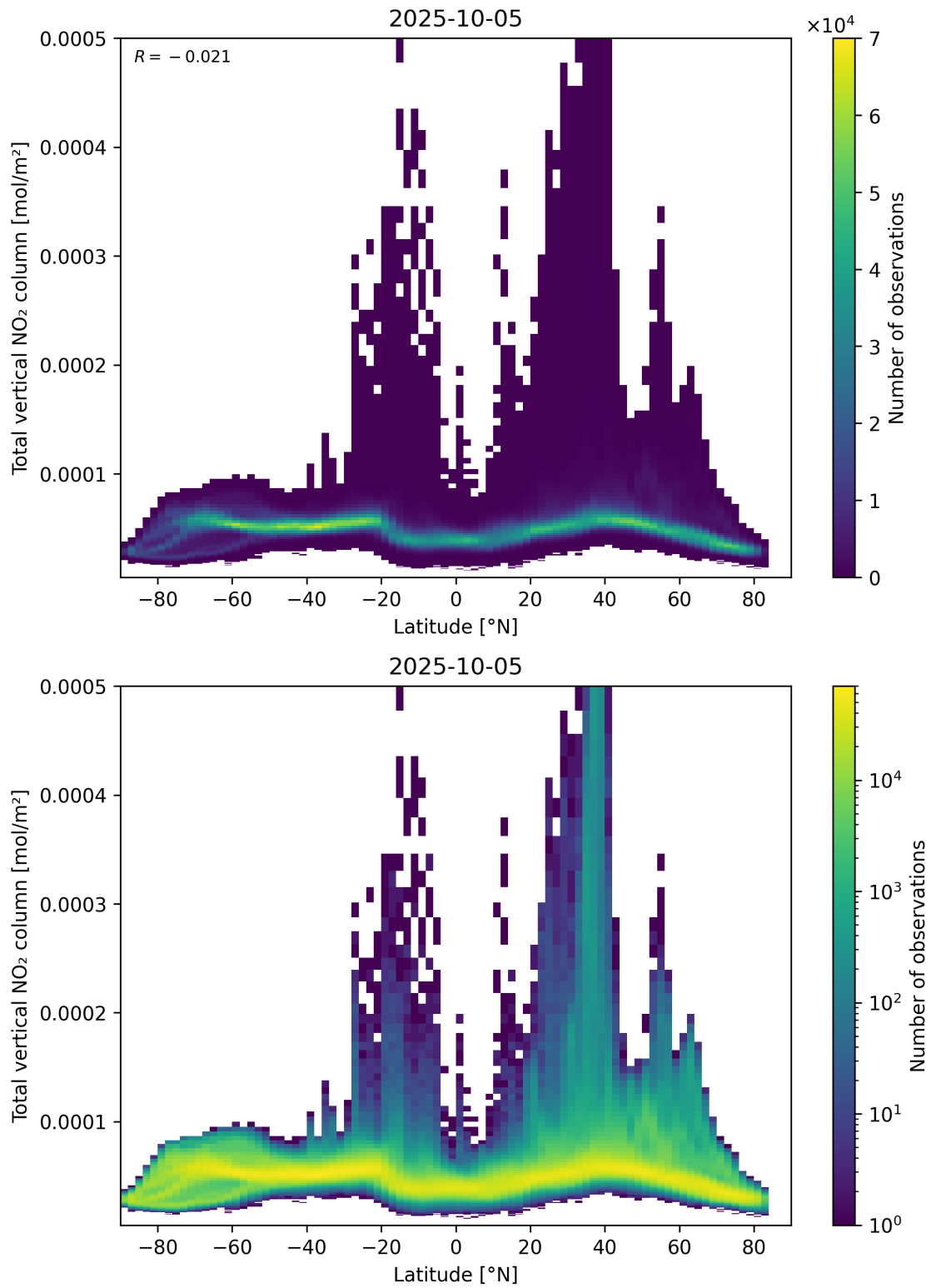
Figure 90: Scatter density plot of “Latitude” against “Total vertical NO 2 column” for 2025-10-04 to 2025-10-06.
