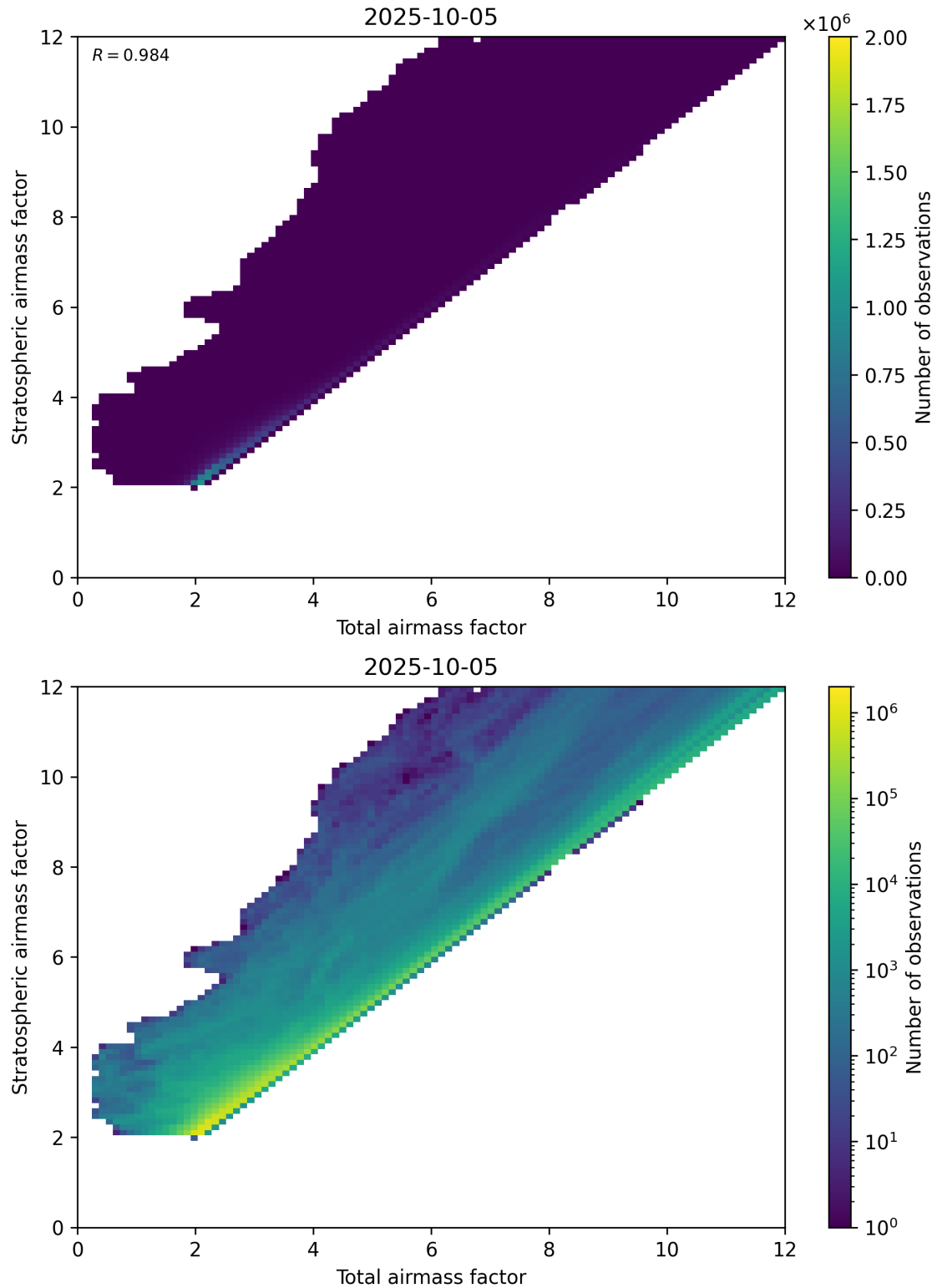
Figure 62: Scatter density plot of “Total airmass factor” against “Stratospheric airmass factor” for 2025-10-04 to 2025-10-06.
