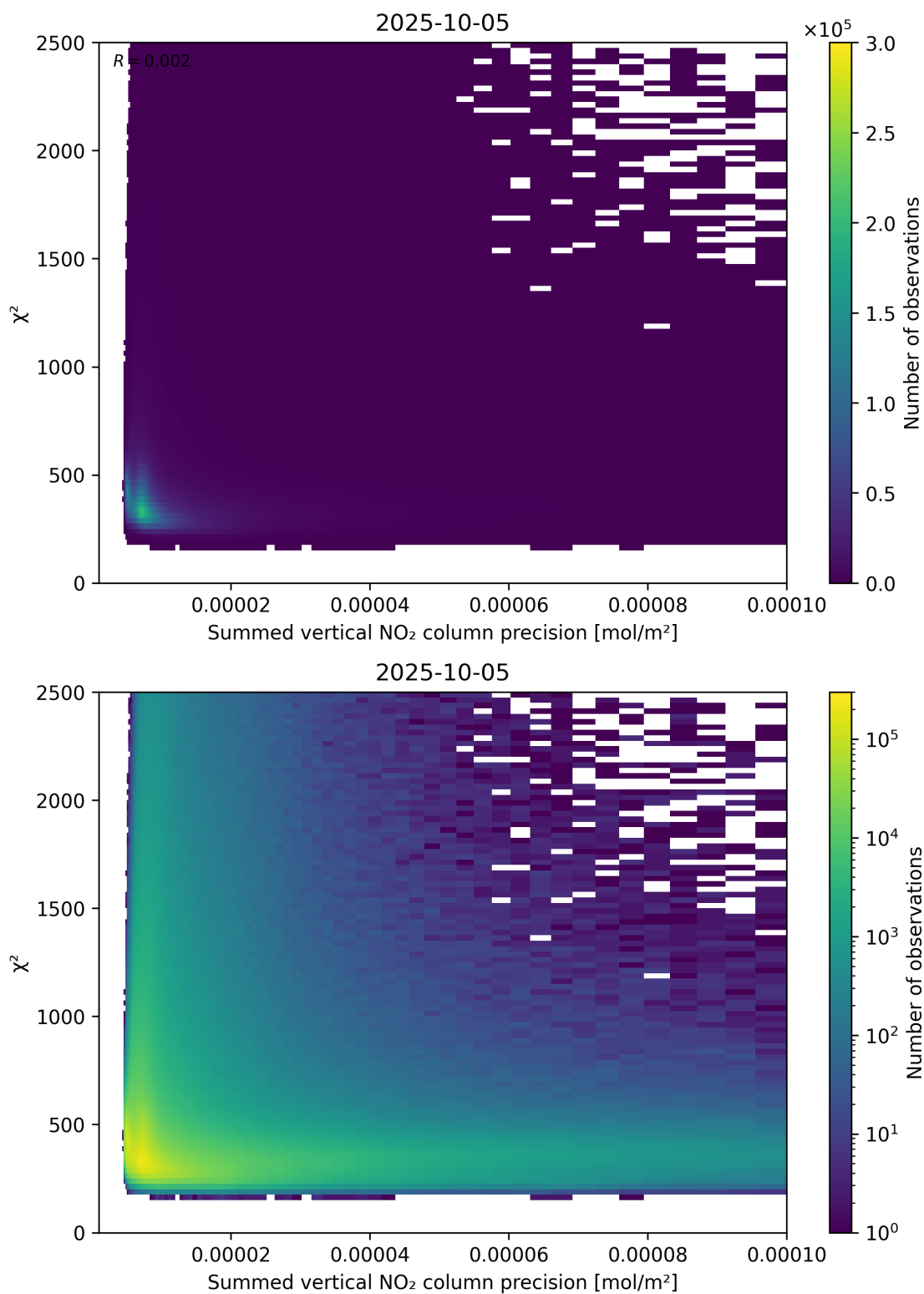
Figure 107: Scatter density plot of “Summed vertical NO 2 column precision” against “ \chi^2 ” for 2025-10-04 to 2025-10-06.
