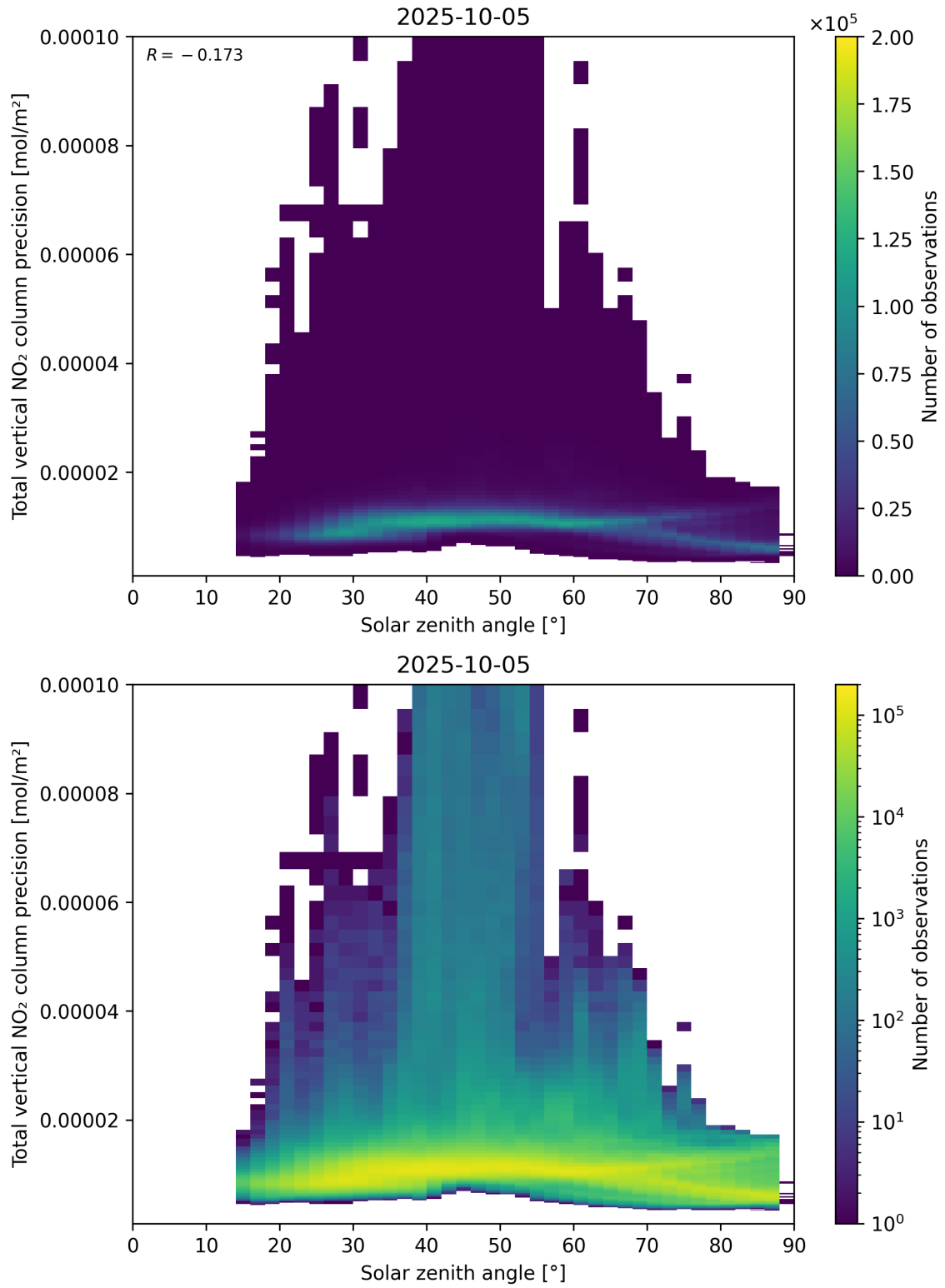
Figure 154: Scatter density plot of “Solar zenith angle” against “Total vertical NO 2 column precision” for 2025-10-04 to 2025-10-06.
