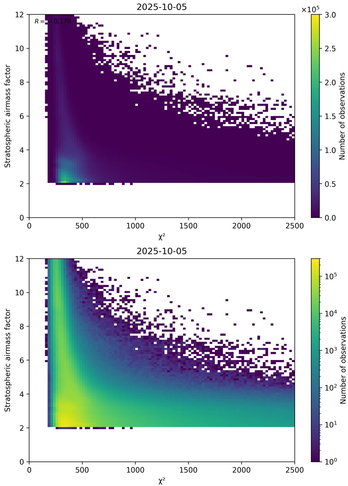
Figure 81: Scatter density plot of “ \chi^2 ” against “Stratospheric airmass factor” for 2025-10-04 to 2025-10-06.
