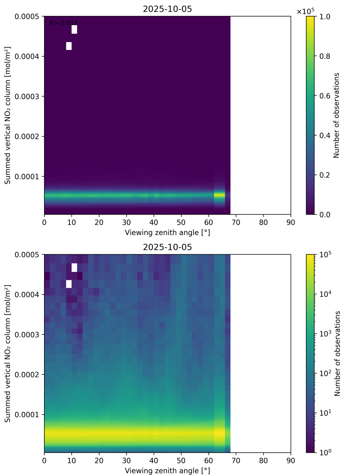
Figure 165: Scatter density plot of “Viewing zenith angle” against “Summed vertical NO 2 column” for 2025-10-04 to 2025-10-06.
