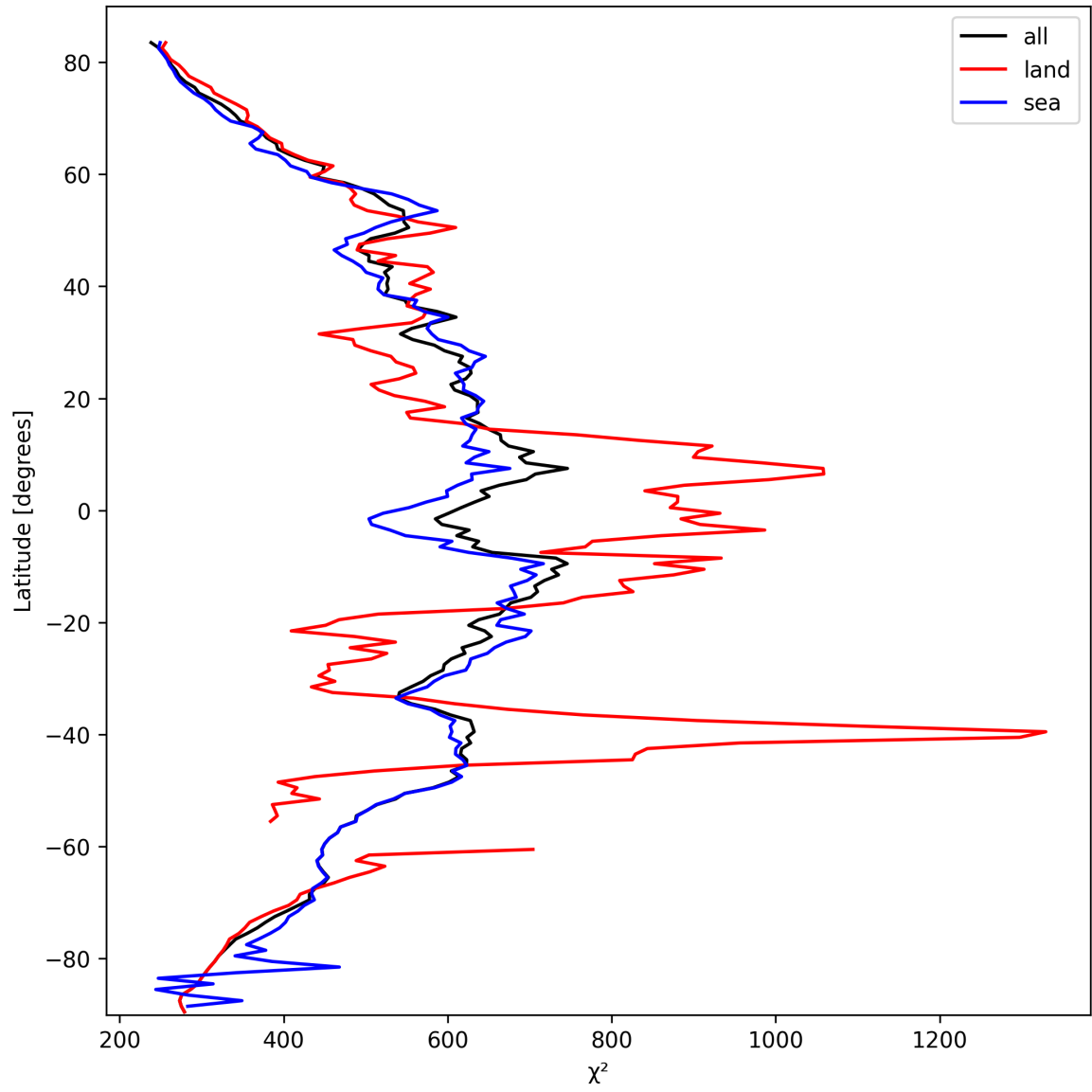
Figure 25: Zonal average of “ \chi^2 ” for 2025-10-04 to 2025-10-06.
