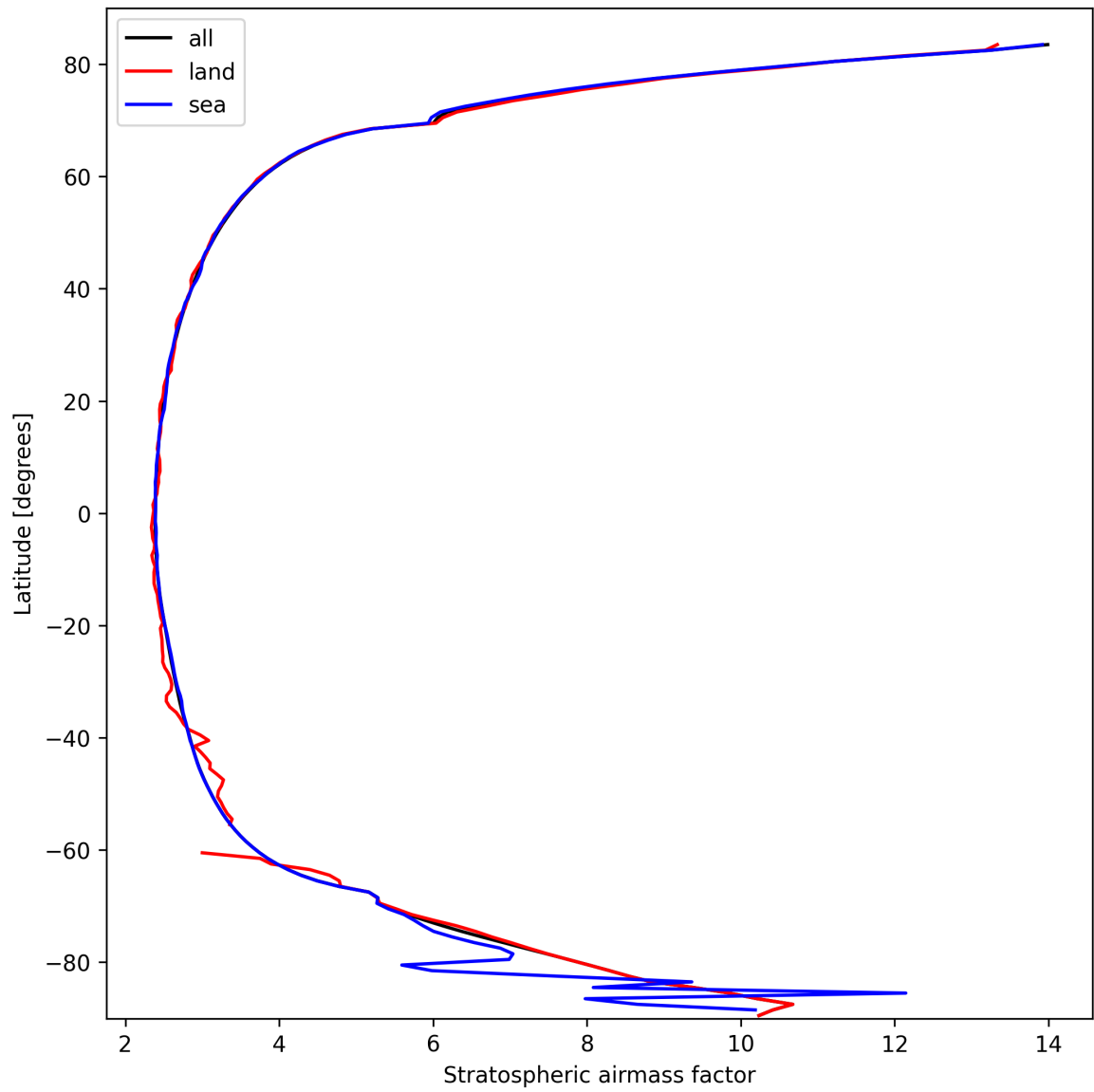
Figure 27: Zonal average of “Stratospheric air mass factor” for 2025-10-04 to 2025-10-06.
