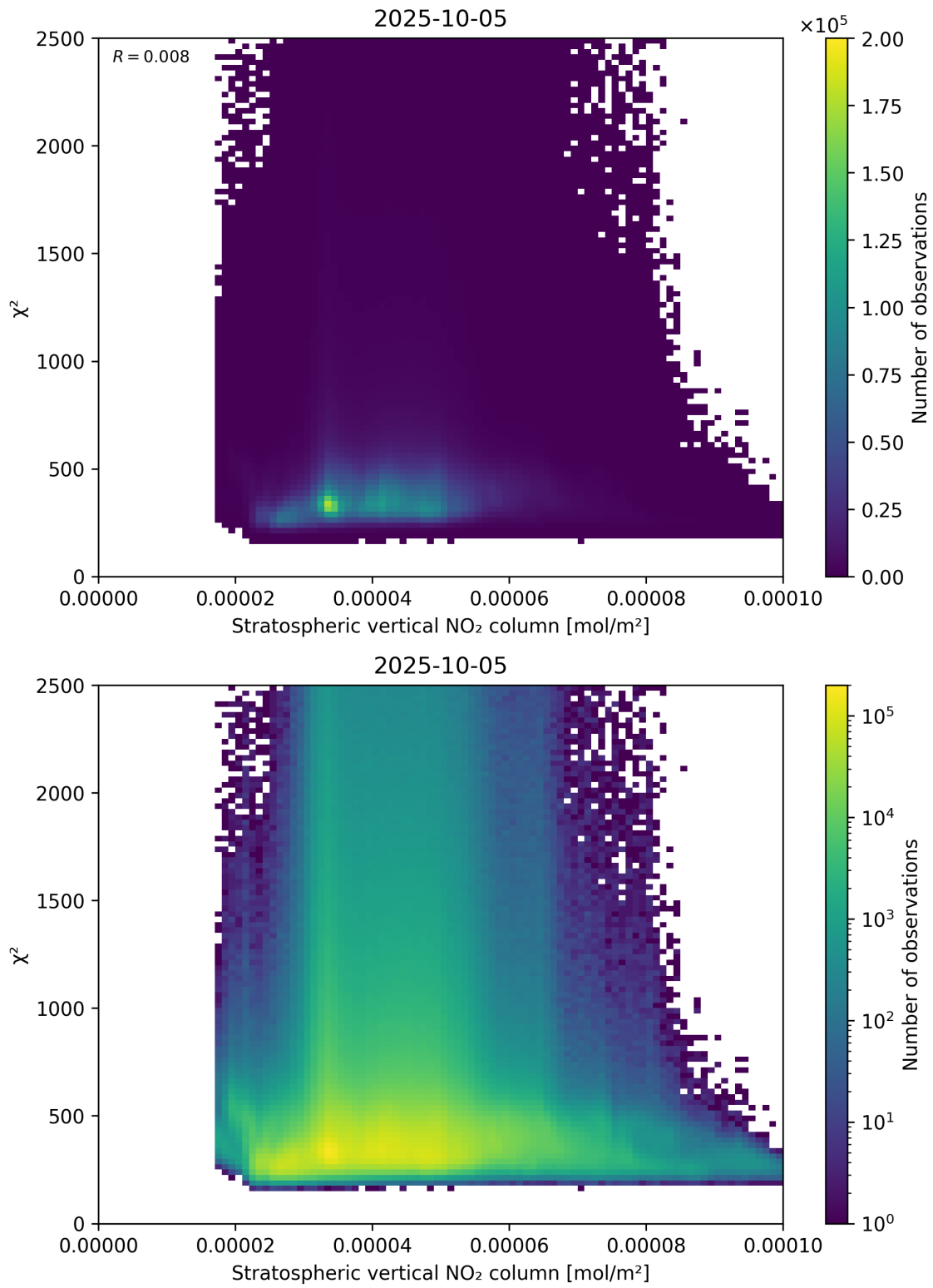
Figure 97: Scatter density plot of “Stratospheric vertical NO 2 column” against “ \chi^2 ” for 2025-10-04 to 2025-10-06.
