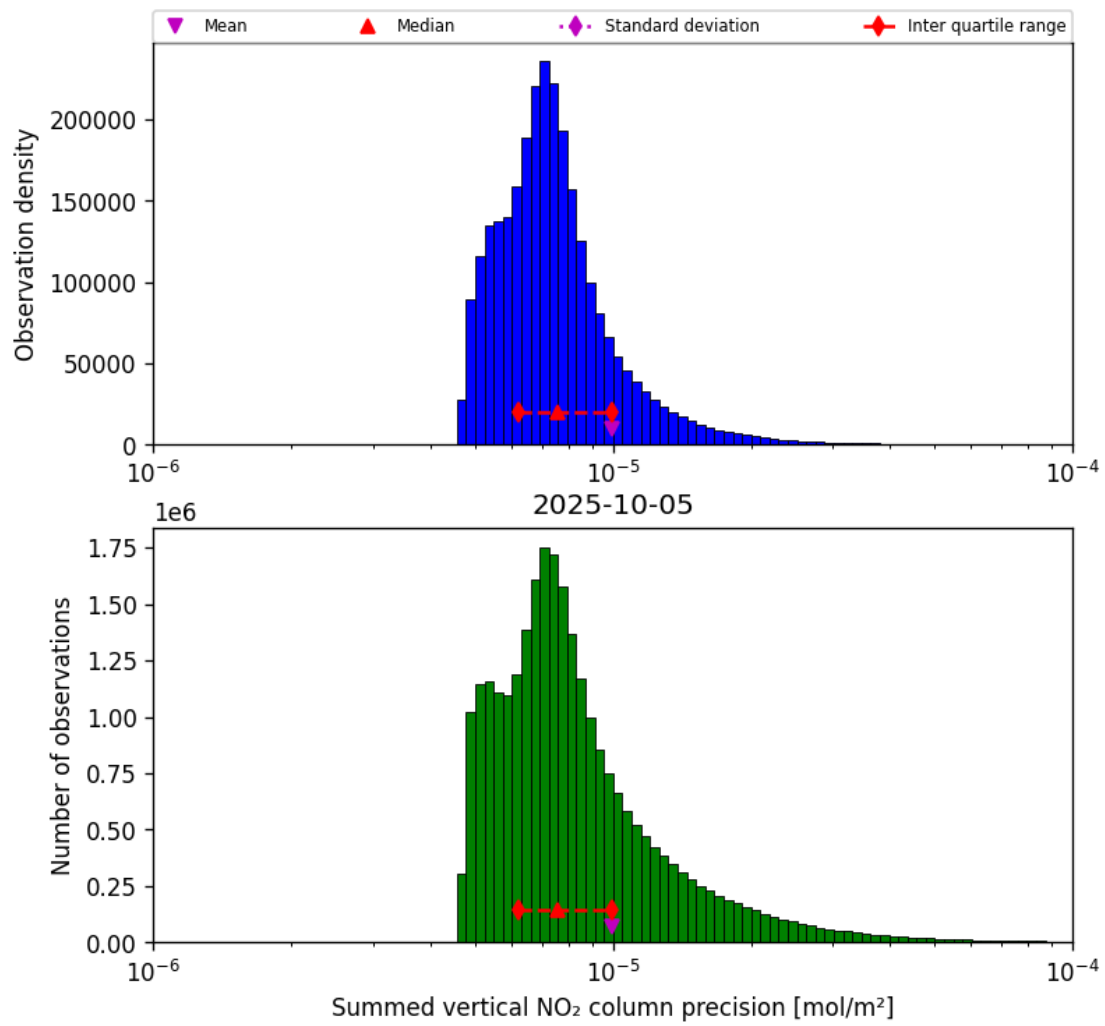
Figure 41: Histogram of "Summed vertical NO 2 column precision" for 2025-10-04 to 2025-10-06
