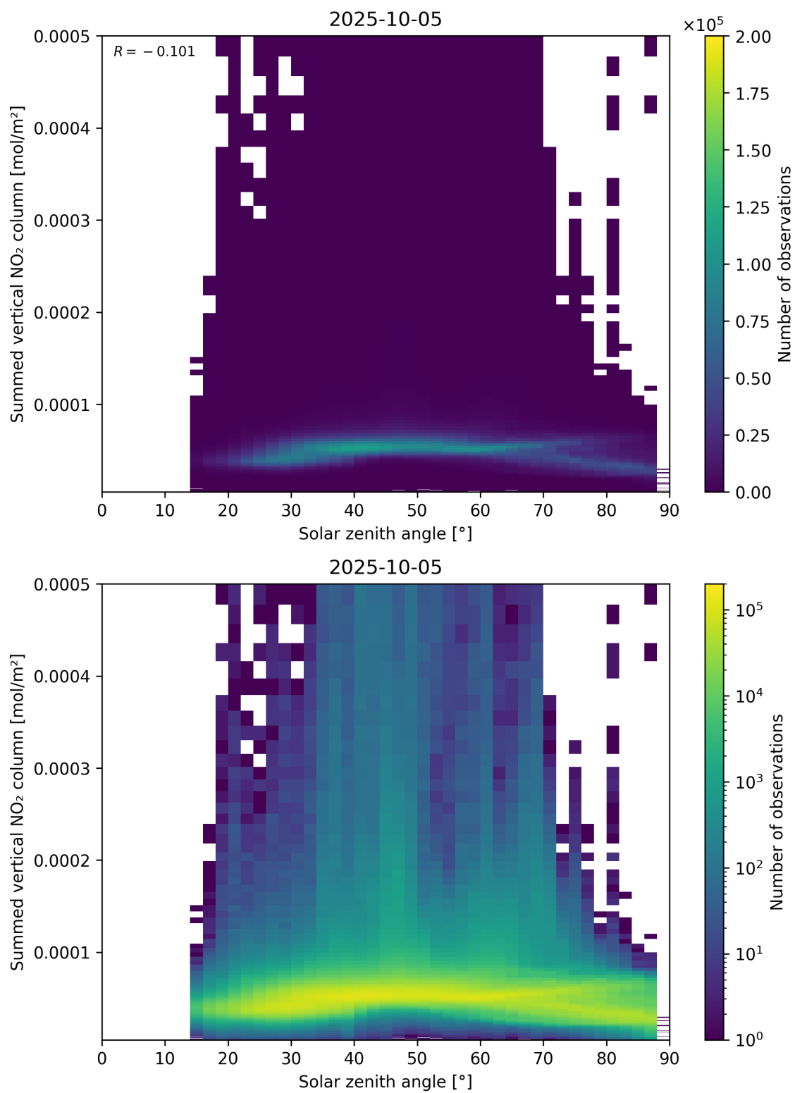
Figure 151: Scatter density plot of “Solar zenith angle” against “Summed vertical NO 2 column” for 2025-10-04 to 2025-10-06.
