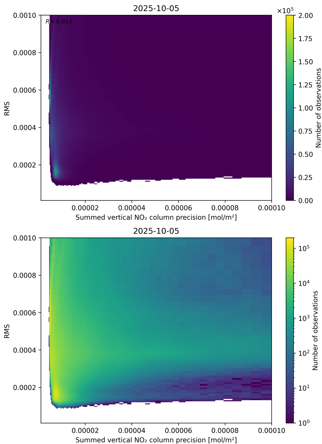
Figure 108: Scatter density plot of “Summed vertical NO 2 column precision” against “RMS” for 2025-10-04 to 2025-10-06.
