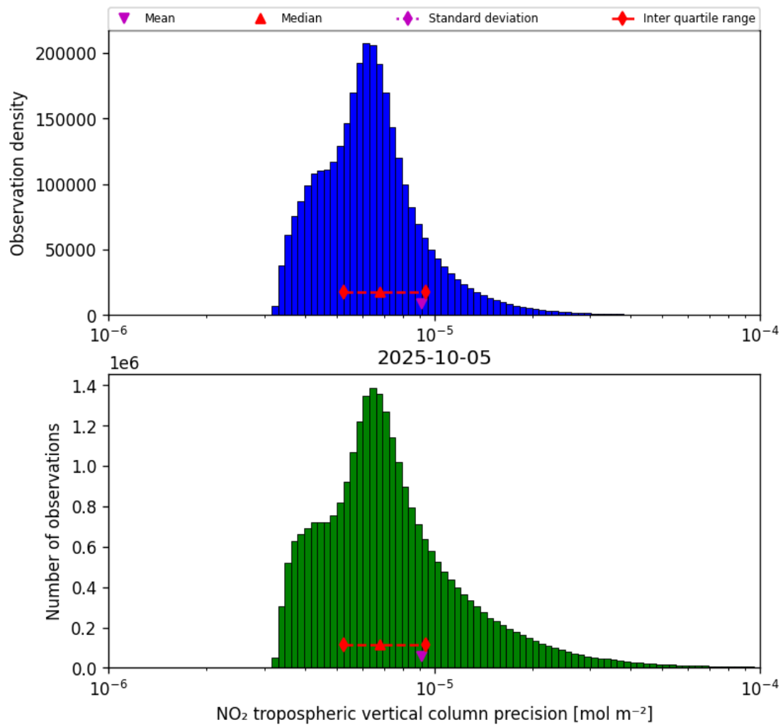
Figure 30: Histogram of “NO 2 tropospheric vertical column precision” for 2025-10-04 to 2025-10-06
