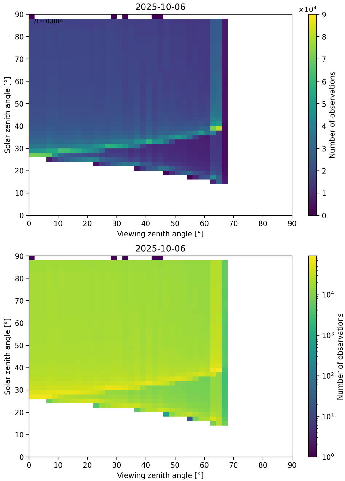
Figure 172: Scatter density plot of “Viewing zenith angle” against “Solar zenith angle” for 2025-10-06 to 2025-10-07.
