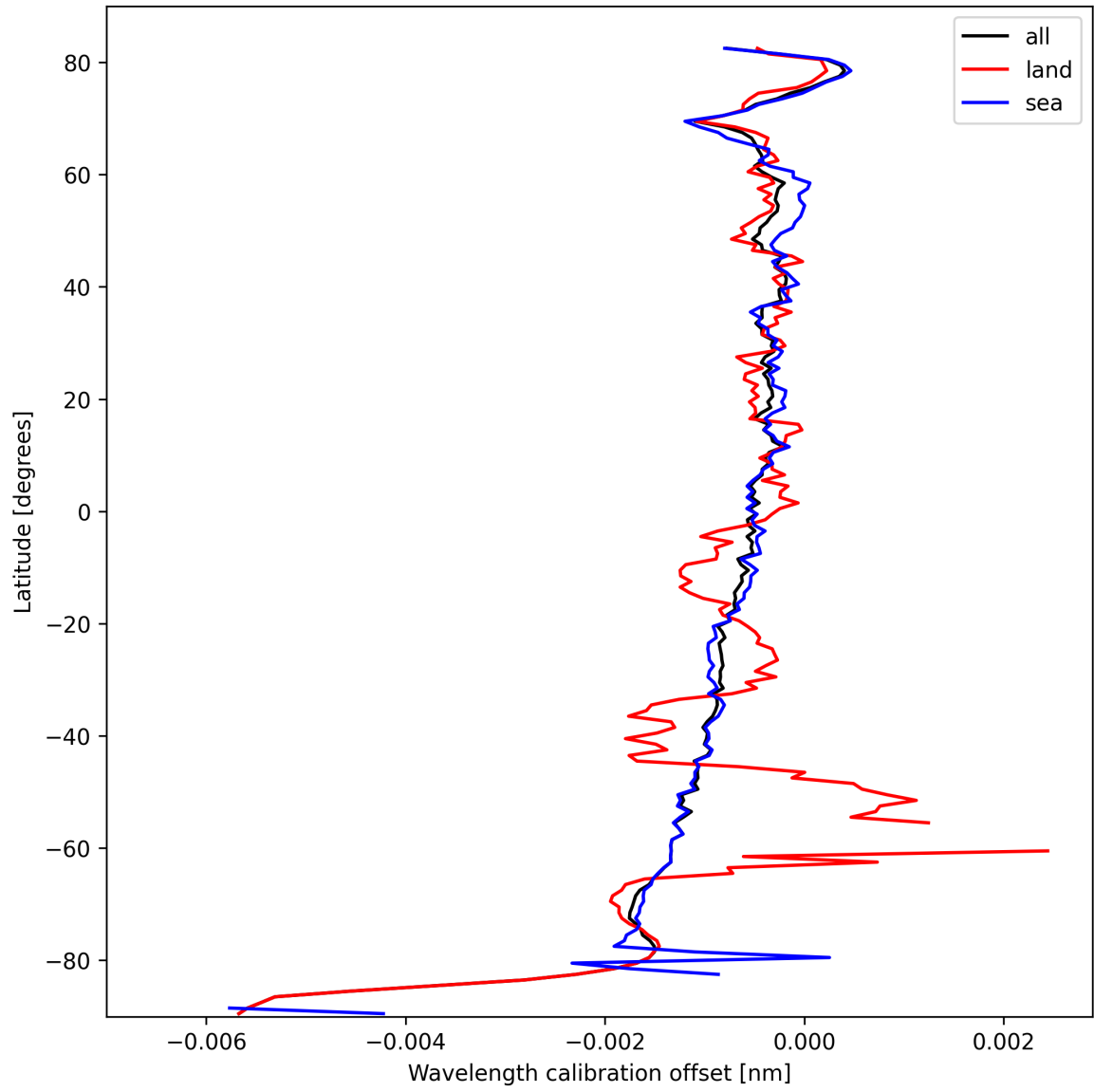
Figure 18: Zonal average of “Wavelength calibration offset” for 2025-10-06 to 2025-10-07.
