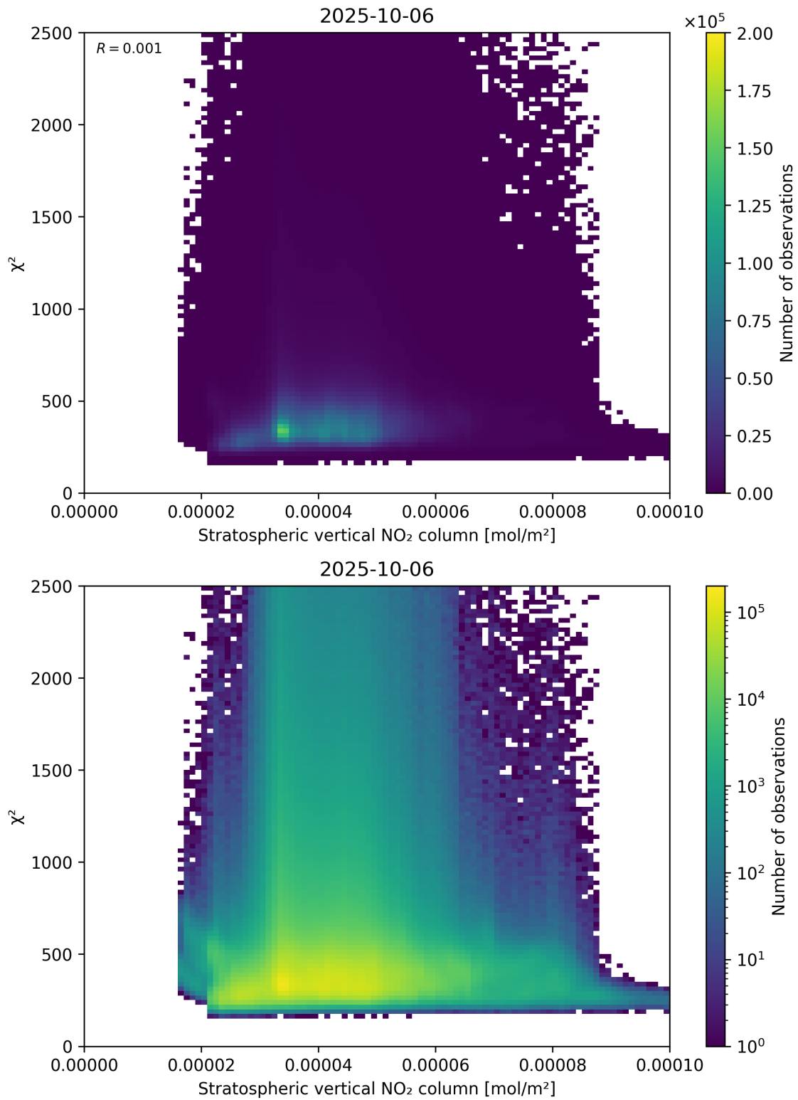
Figure 97: Scatter density plot of “Stratospheric vertical NO 2 column” against “ \chi^2 ” for 2025-10-06 to 2025-10-07.
