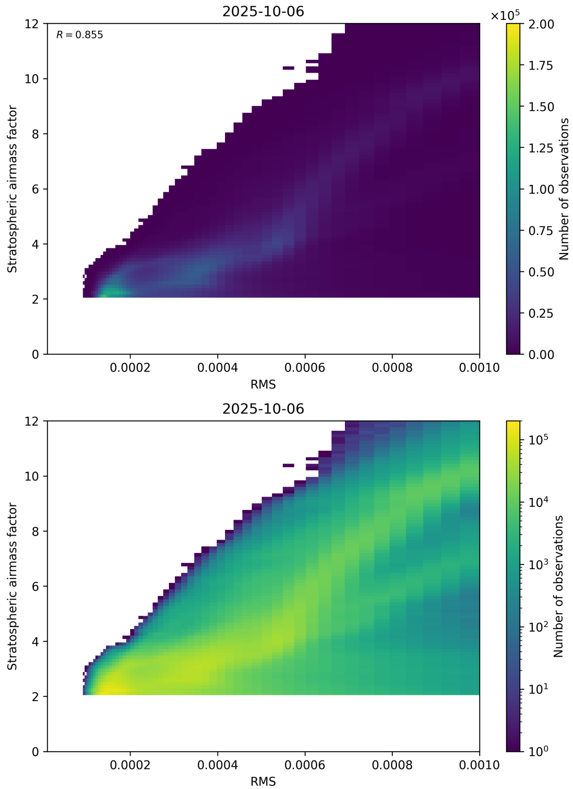
Figure 144: Scatter density plot of “RMS” against “Stratospheric airmass factor” for 2025-10-06 to 2025-10-07.
