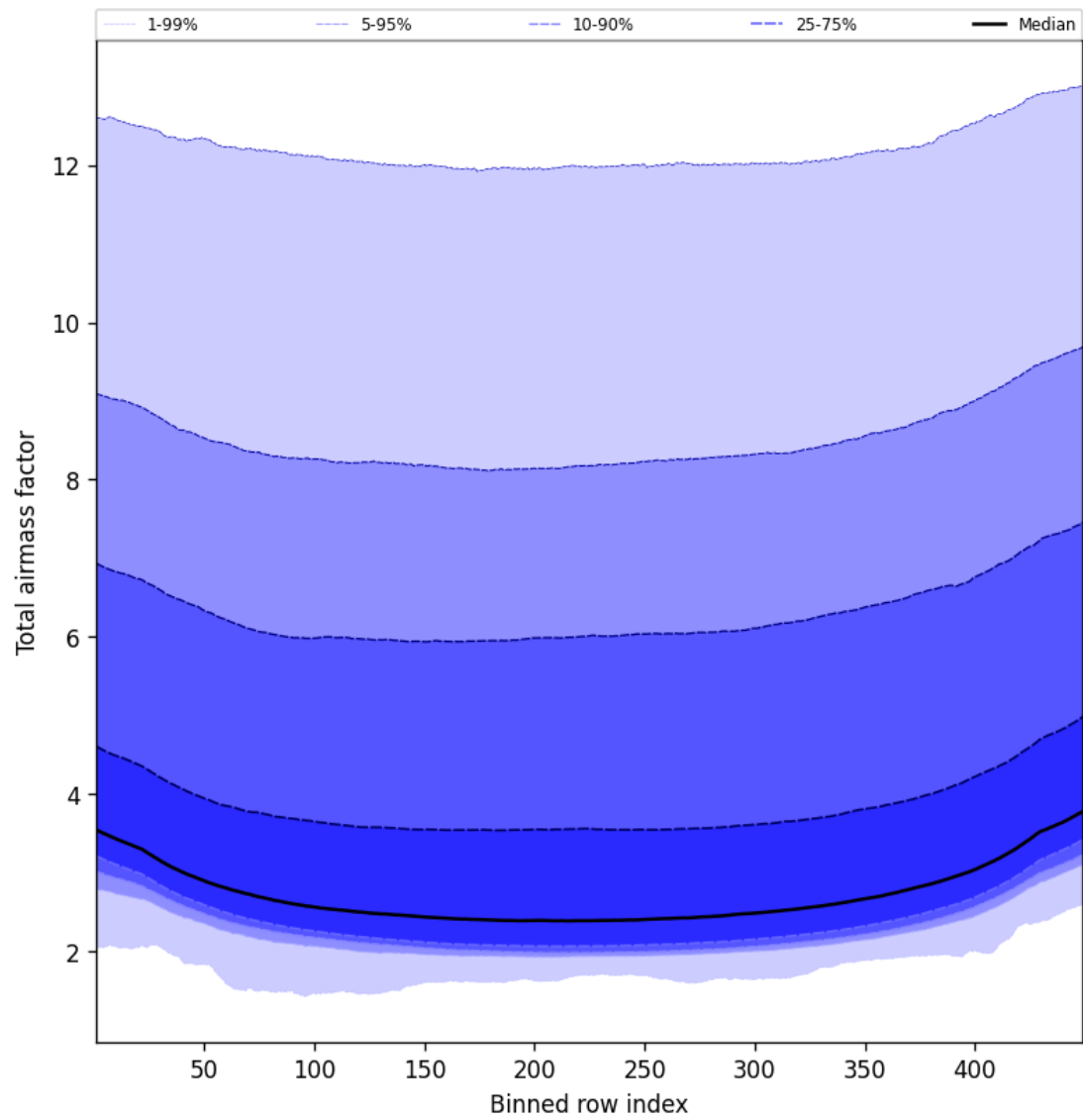
Figure 49: Along track statistics of “Total airmass factor” for 2025-10-06 to 2025-10-07
