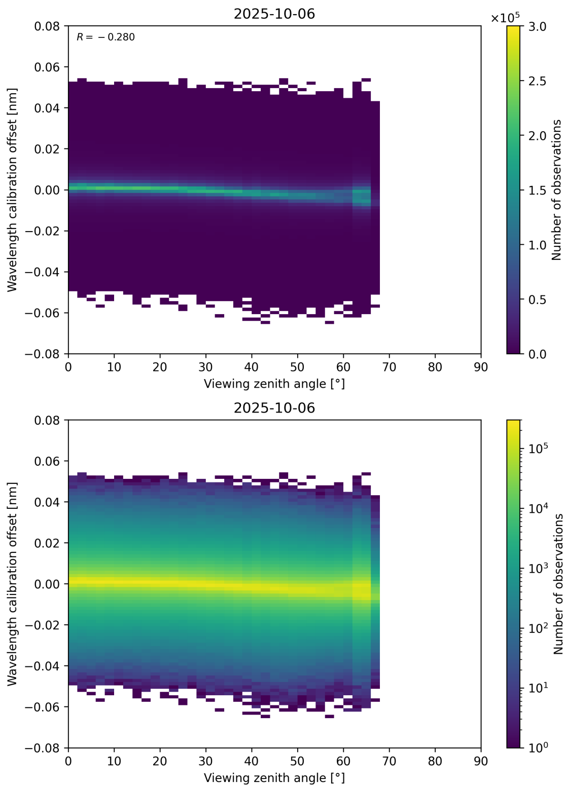
Figure 173: Scatter density plot of “Viewing zenith angle” against “Wavelength calibration offset” for 2025-10-06 to 2025-10-07.
