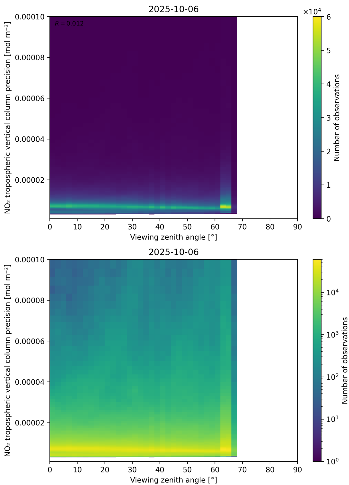
Figure 170: Scatter density plot of “Viewing zenith angle” against “NO 2 tropospheric vertical column precision” for 2025-10-06 to 2025-10-07.
