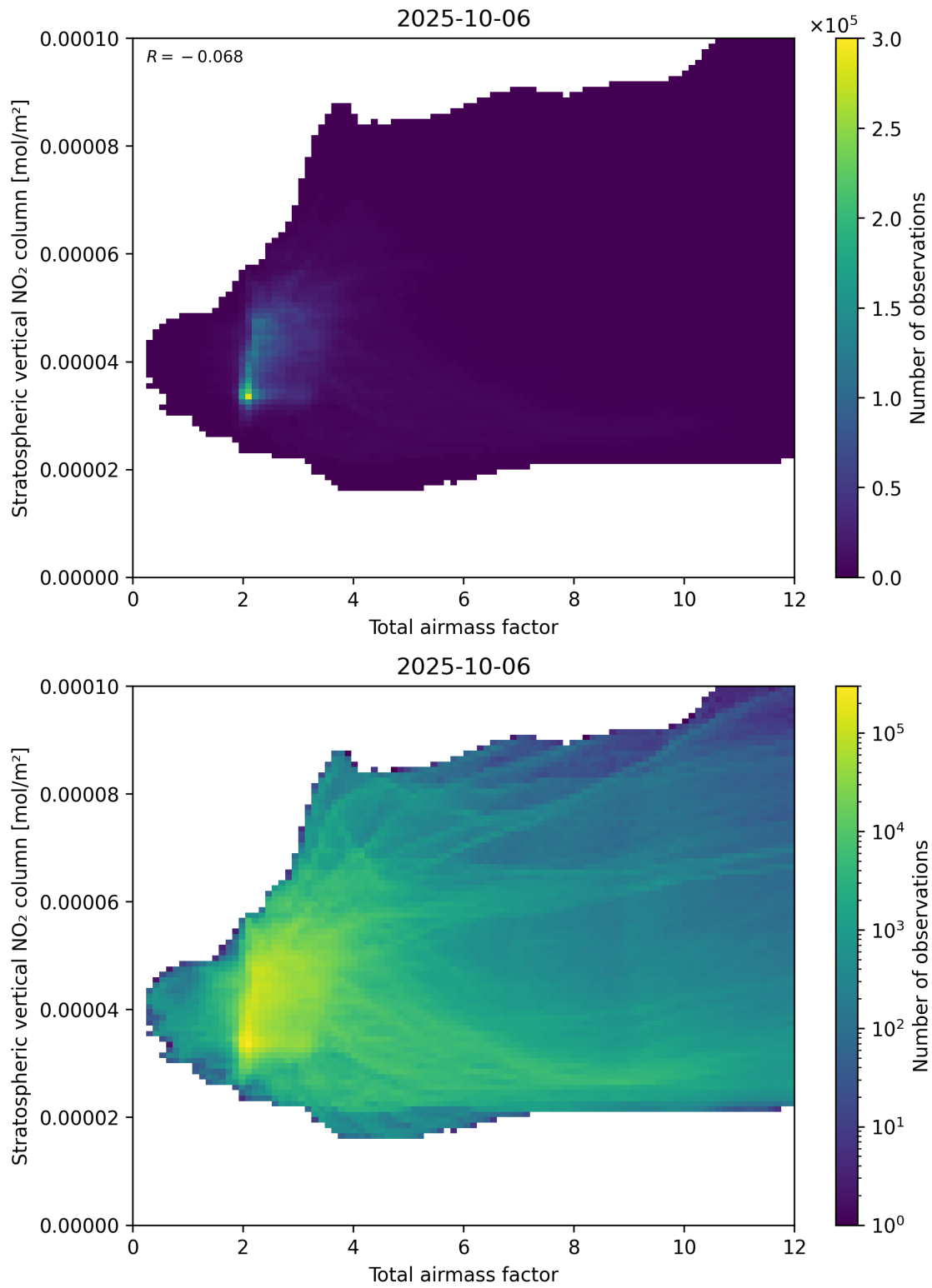
Figure 64: Scatter density plot of “Total airmass factor” against “Stratospheric vertical \text{NO}_2 column” for 2025-10-06 to 2025-10-07.
