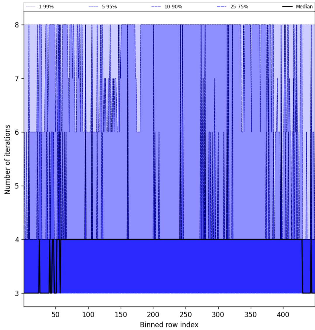
Figure 51: Along track statistics of “Number of iterations” for 2025-10-06 to 2025-10-07
