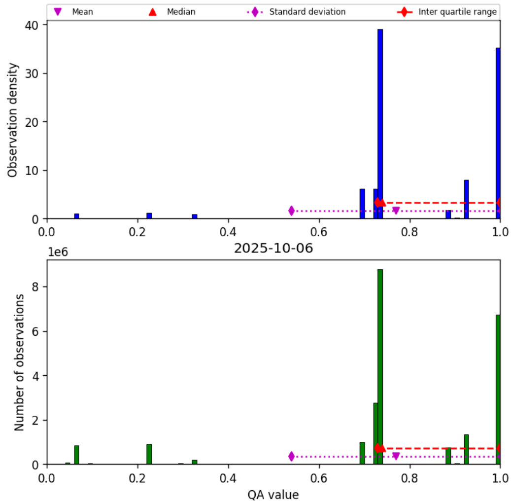
Figure 28: Histogram of “QA value” for 2025-10-06 to 2025-10-07
