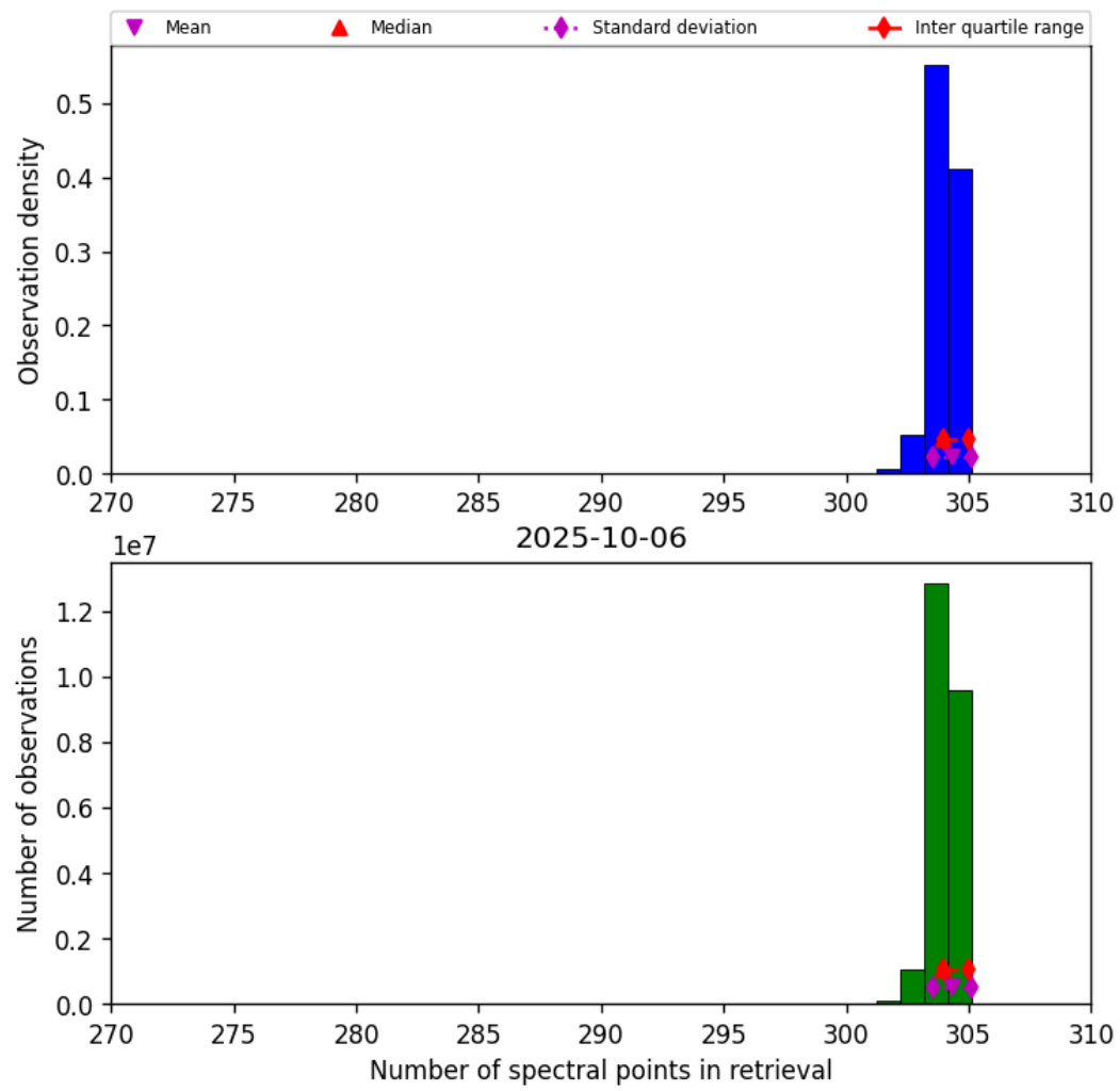
Figure 33: Histogram of “Number of spectral points in retrieval” for 2025-10-06 to 2025-10-07
