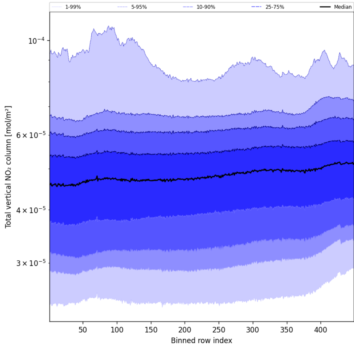
Figure 55: Along track statistics of “Total vertical NO 2 column” for 2025-10-06 to 2025-10-07
