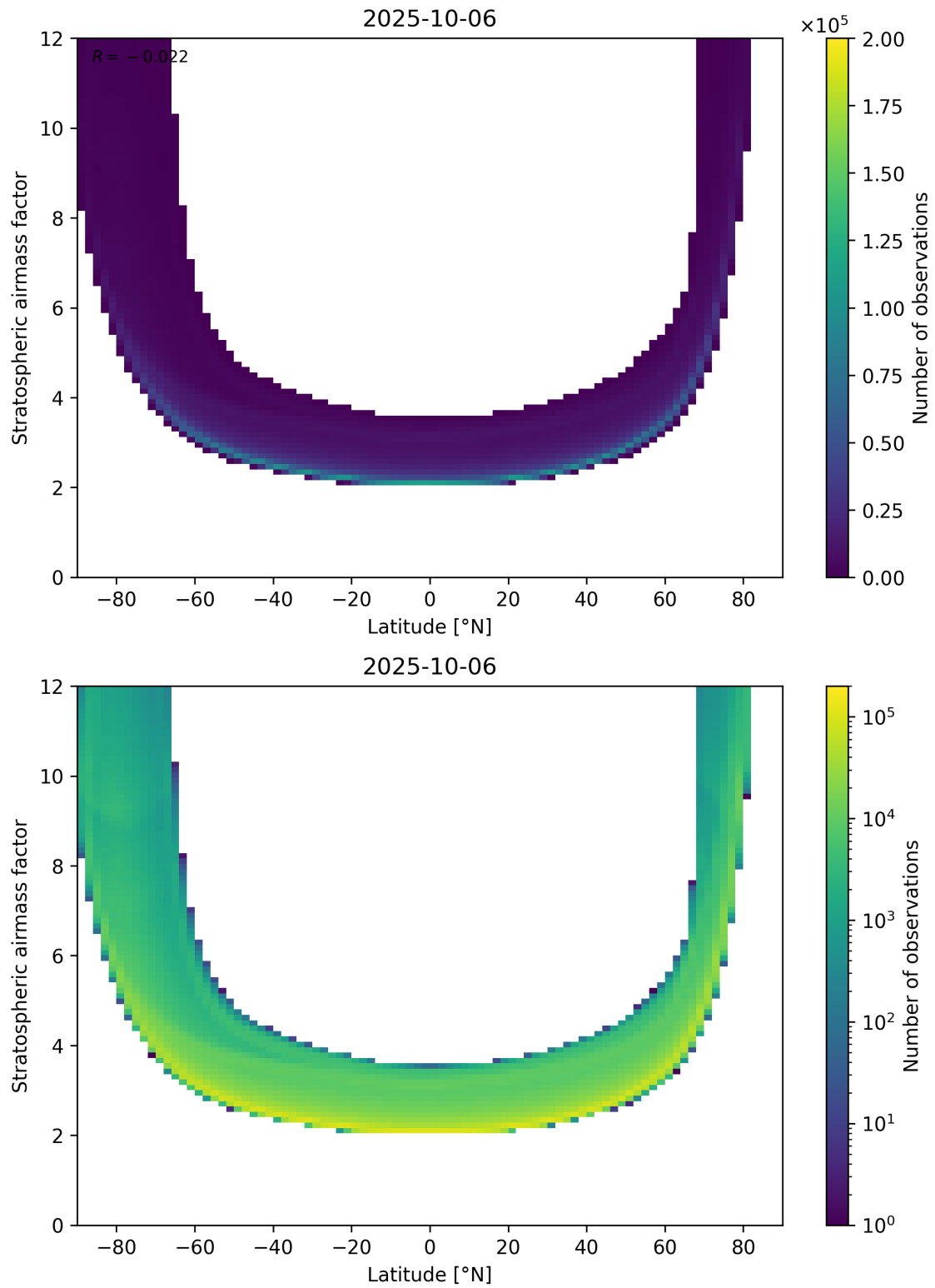
Figure 83: Scatter density plot of “Latitude” against “Stratospheric airmass factor” for 2025-10-06 to 2025-10-07.
