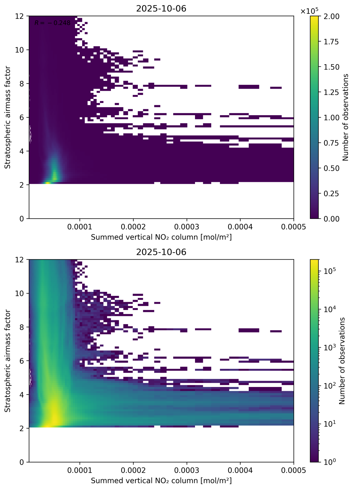
Figure 103: Scatter density plot of “Summed vertical NO 2 column” against “Stratospheric air mass factor” for 2025-10-06 to 2025-10-07.
