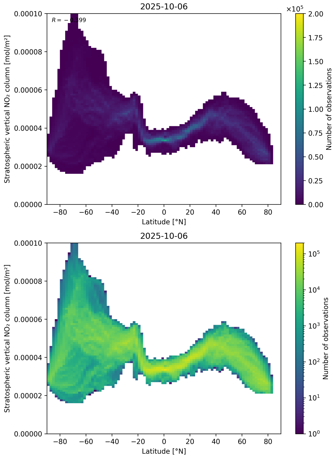
Figure 87: Scatter density plot of “Latitude” against “Stratospheric vertical NO 2 column” for 2025-10-06 to 2025-10-07.
