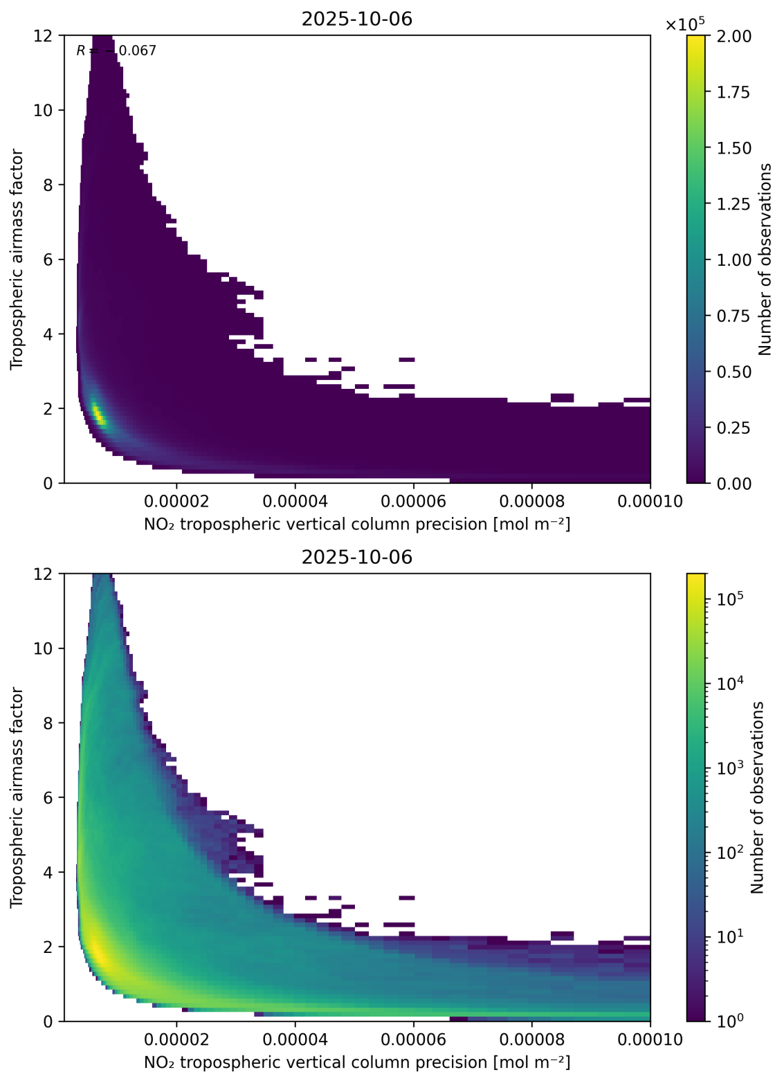
Figure 133: Scatter density plot of “NO 2 tropospheric vertical column precision” against “Tropospheric air mass factor” for 2025-10-06 to 2025-10-07.
