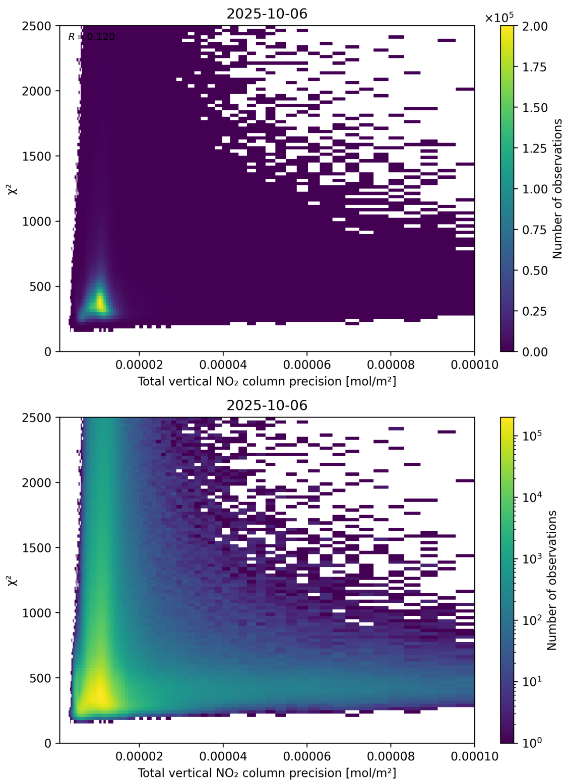
Figure 116: Scatter density plot of “Total vertical NO 2 column precision” against “ \chi^2 ” for 2025-10-06 to 2025-10-07.
