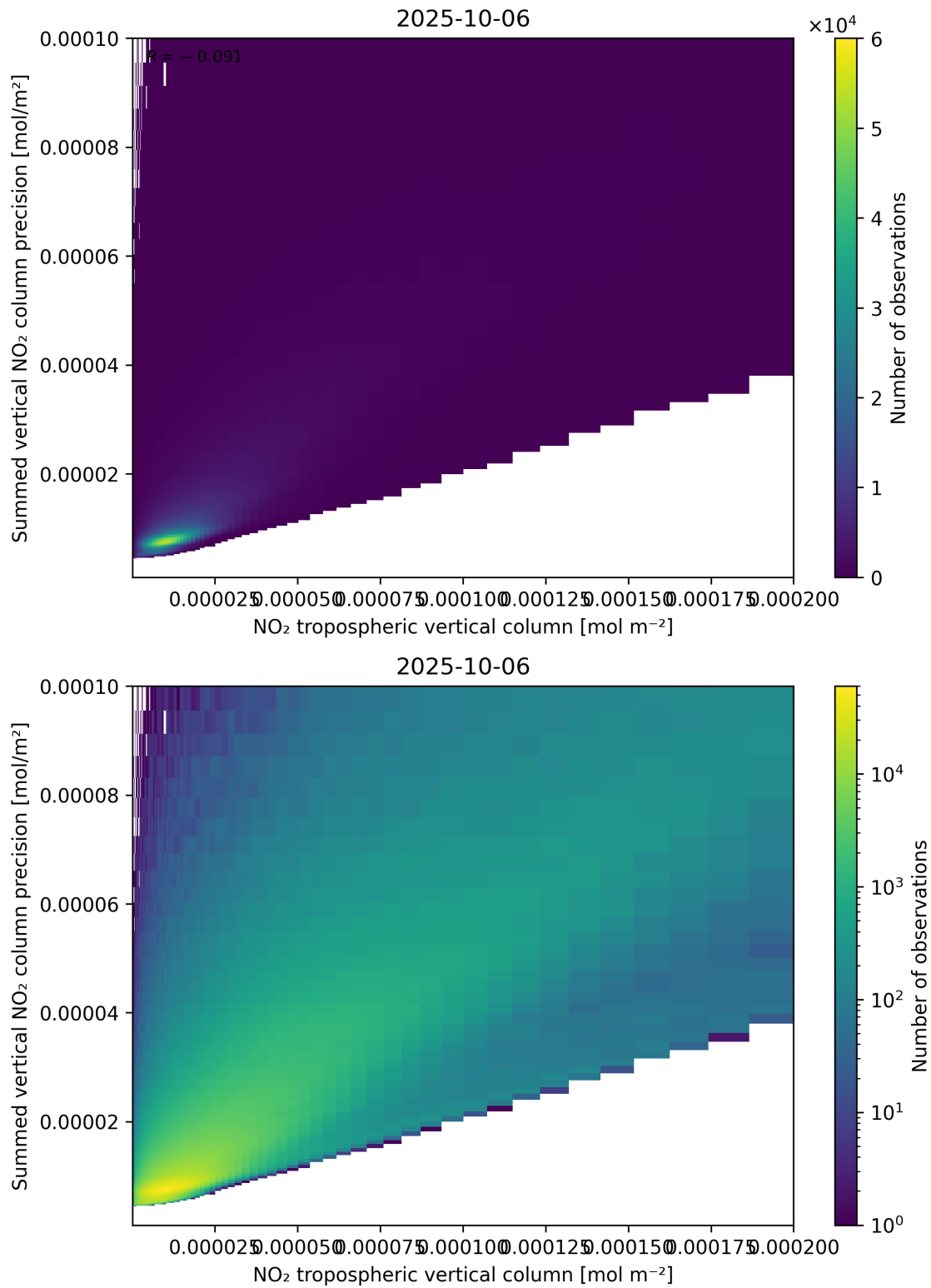
Figure 127: Scatter density plot of “NO 2 tropospheric vertical column” against “Summed vertical NO 2 column precision” for 2025-10-06 to 2025-10-07.
