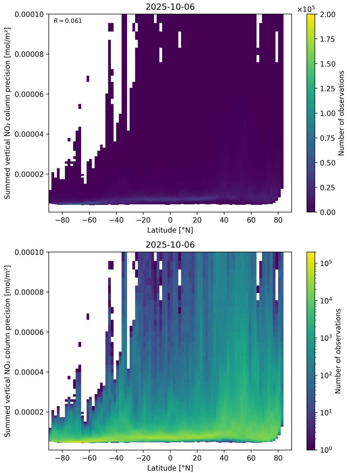
Figure 89: Scatter density plot of “Latitude” against “Summed vertical NO 2 column precision” for 2025-10-06 to 2025-10-07.
