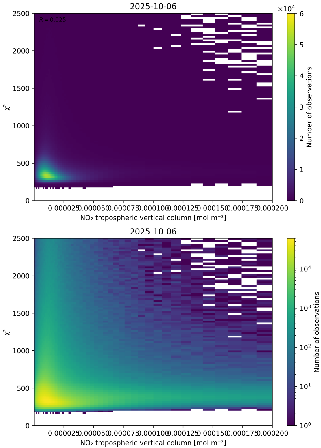
Figure 124: Scatter density plot of “NO 2 tropospheric vertical column” against “ \chi^2 ” for 2025-10-06 to 2025-10-07.
