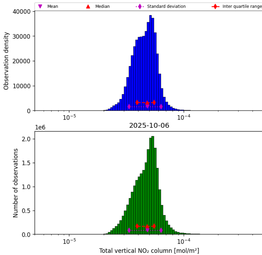
Figure 38: Histogram of “Total vertical NO 2 column” for 2025-10-06 to 2025-10-07
