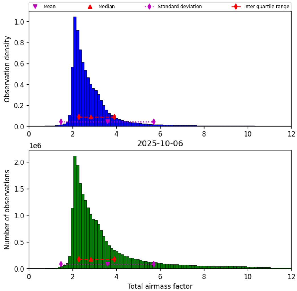
Figure 32: Histogram of “Total airmass factor” for 2025-10-06 to 2025-10-07
