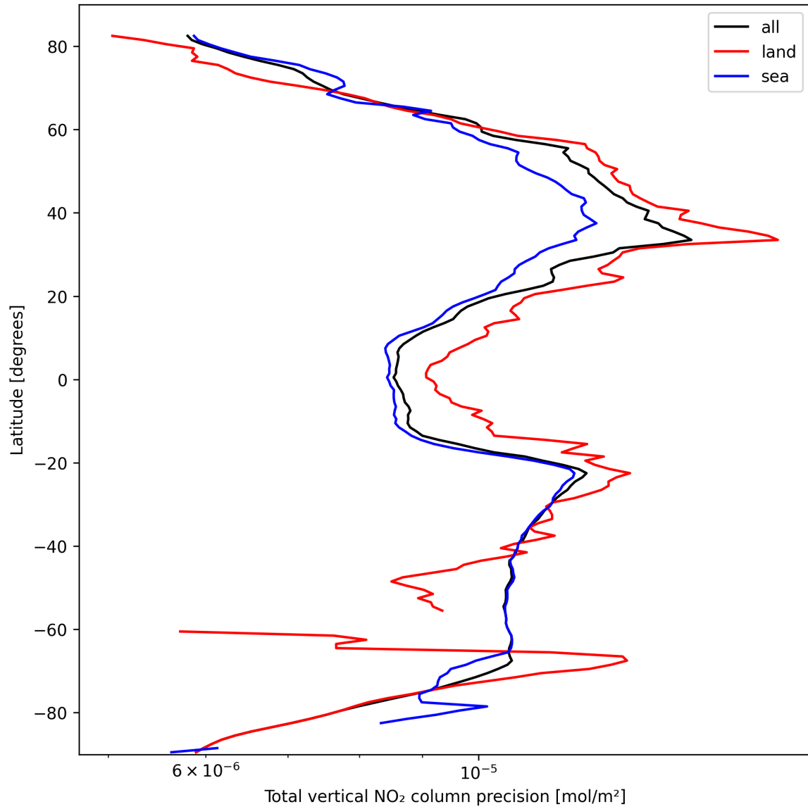
Figure 22: Zonal average of “Total vertical NO 2 column precision” for 2025-10-06 to 2025-10-07.
