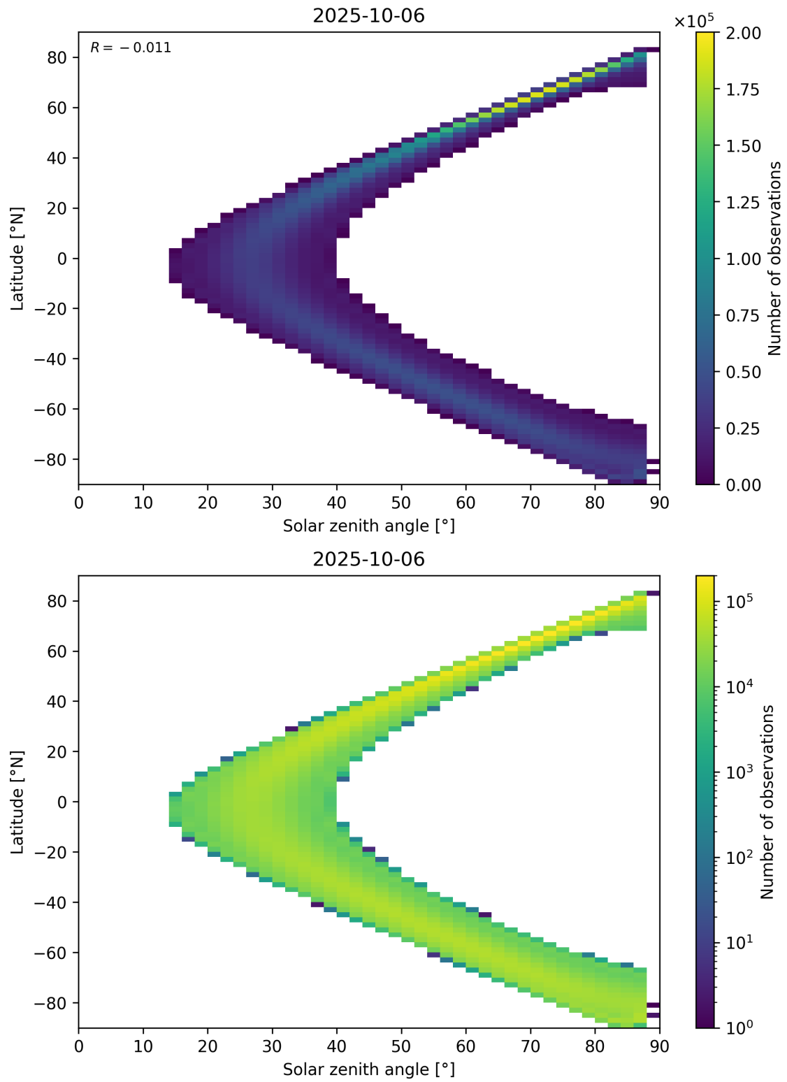
Figure 149: Scatter density plot of “Solar zenith angle” against “Latitude” for 2025-10-06 to 2025-10-07.
