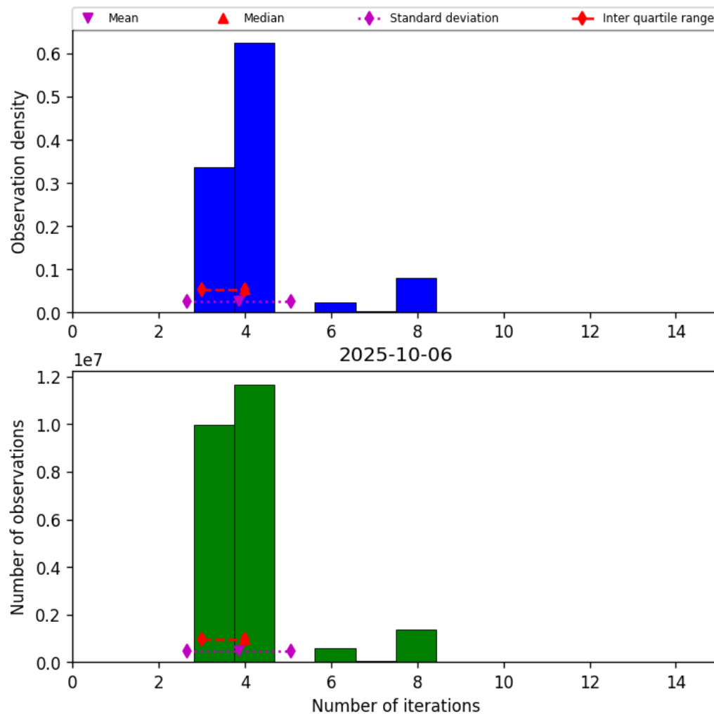
Figure 34: Histogram of “Number of iterations” for 2025-10-06 to 2025-10-07
