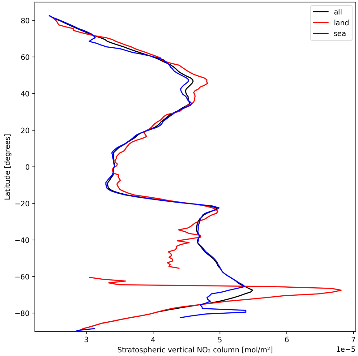
Figure 19: Zonal average of “Stratospheric vertical NO 2 column” for 2025-10-06 to 2025-10-07.
