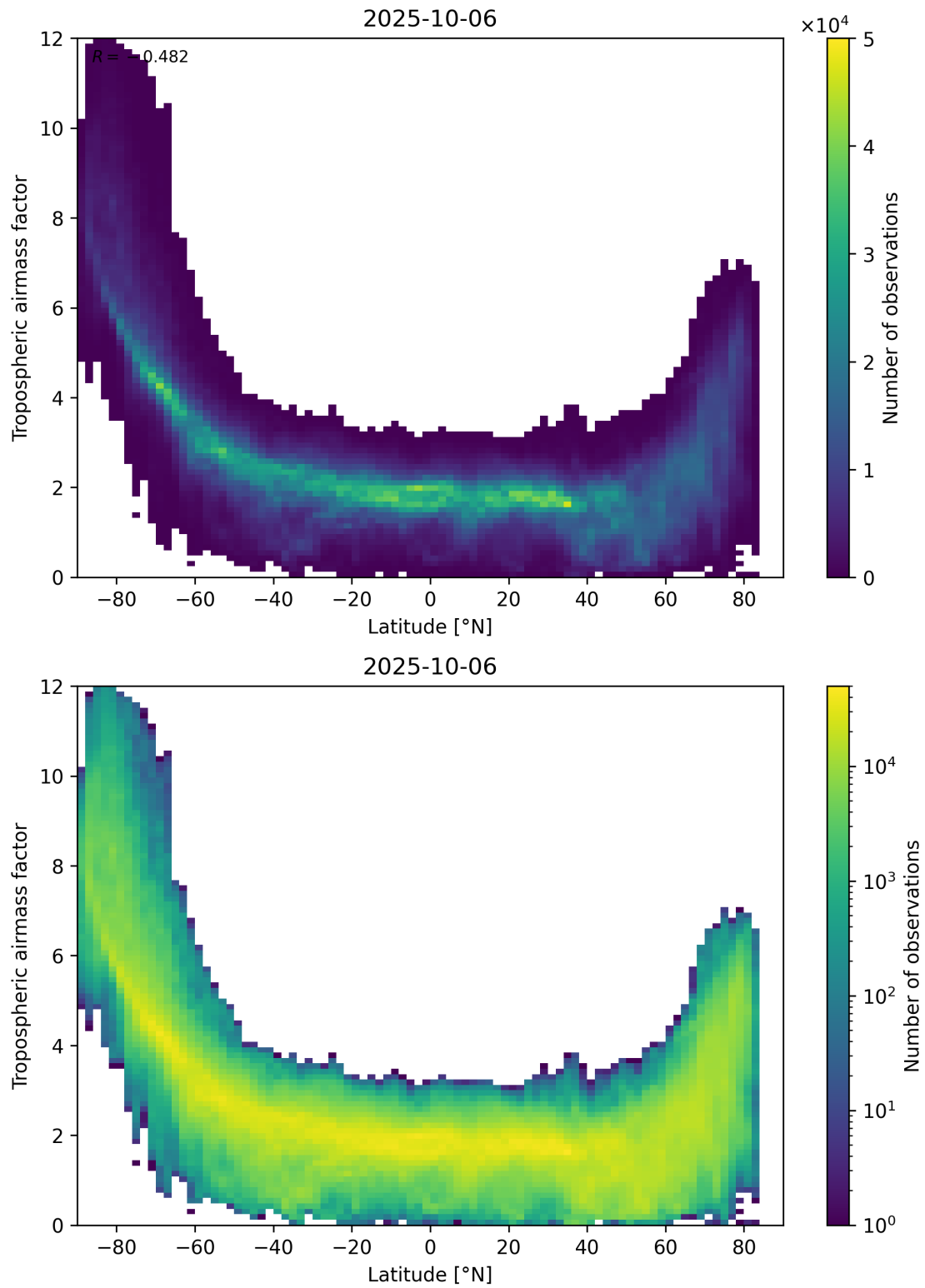
Figure 85: Scatter density plot of “Latitude” against “Tropospheric airmass factor” for 2025-10-06 to 2025-10-07.
