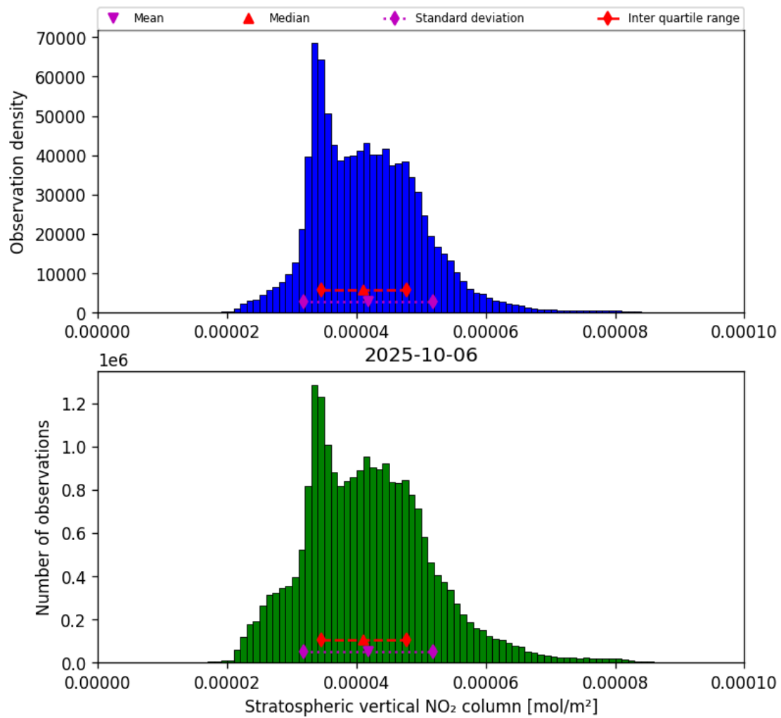
Figure 36: Histogram of “Stratospheric vertical NO 2 column” for 2025-10-06 to 2025-10-07
