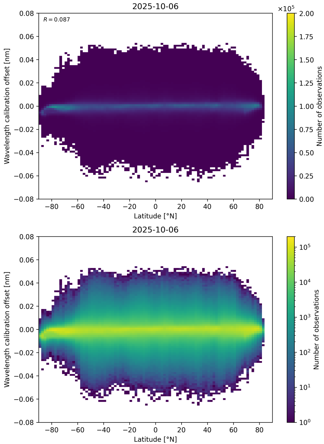
Figure 95: Scatter density plot of “Latitude” against “Wavelength calibration offset” for 2025-10-06 to 2025-10-07.
