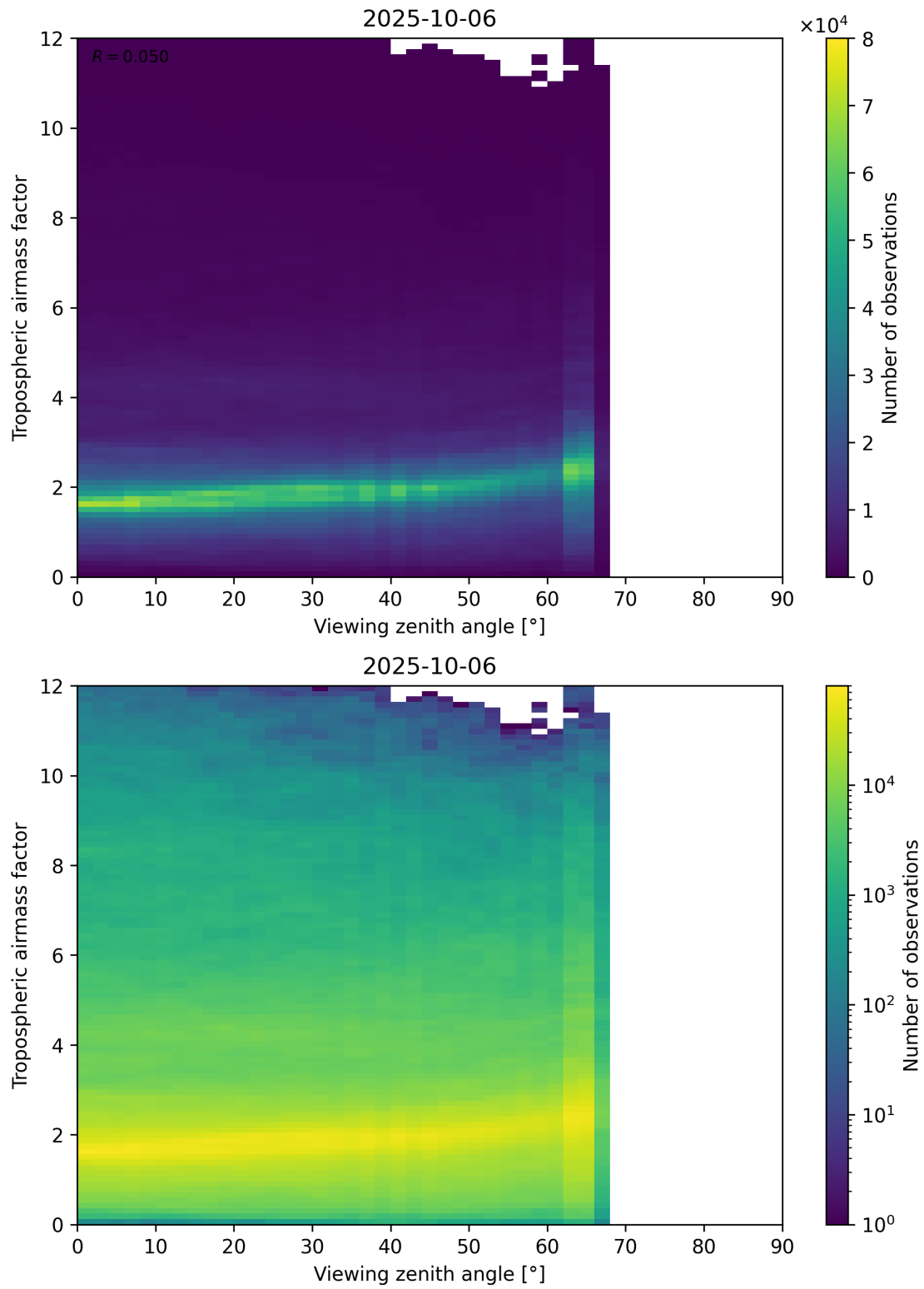
Figure 161: Scatter density plot of “Viewing zenith angle” against “Tropospheric airmass factor” for 2025-10-06 to 2025-10-07.
