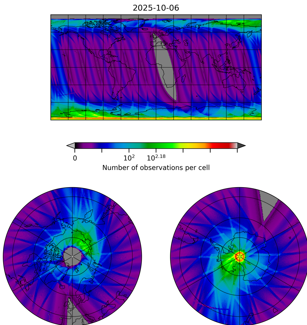
Figure 10: Map of the number of observations for 2025-10-06 to 2025-10-07
