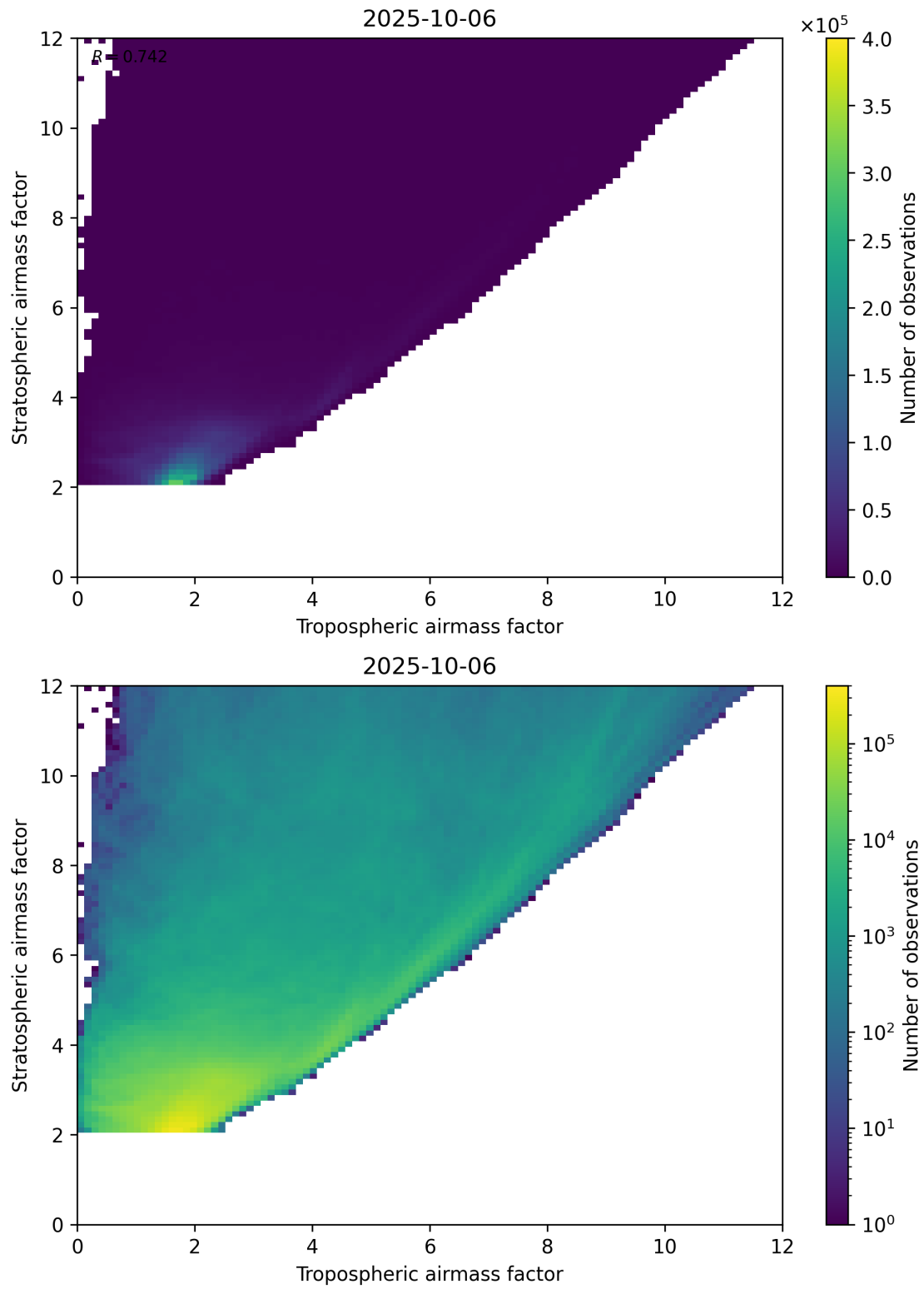
Figure 71: Scatter density plot of “Tropospheric airmass factor” against “Stratospheric airmass factor” for 2025-10-06 to 2025-10-07.
