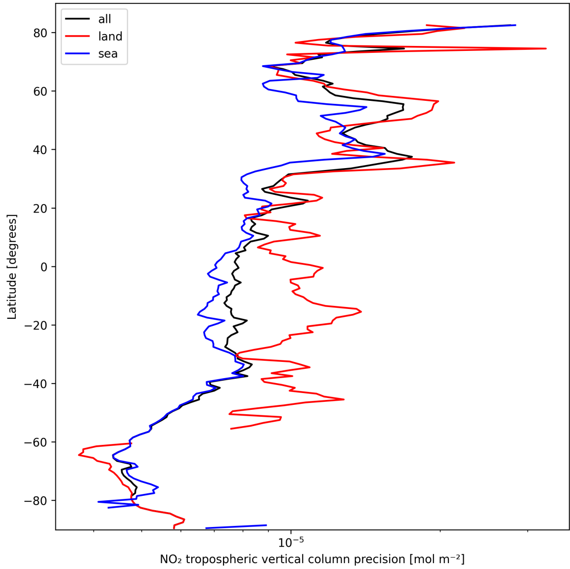
Figure 13: Zonal average of “NO 2 tropospheric vertical column precision” for 2025-10-06 to 2025-10-07.
