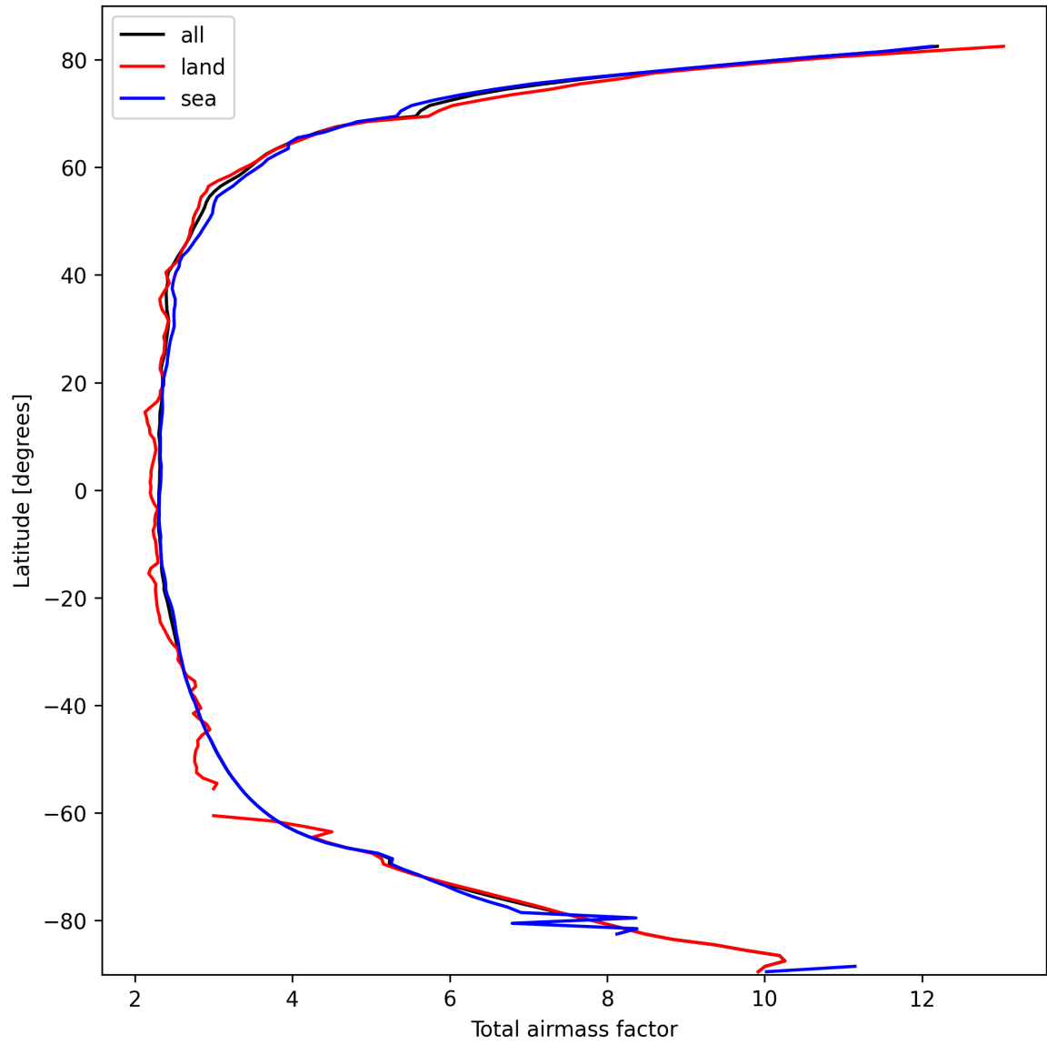
Figure 15: Zonal average of “Total airmass factor” for 2025-10-06 to 2025-10-07.
