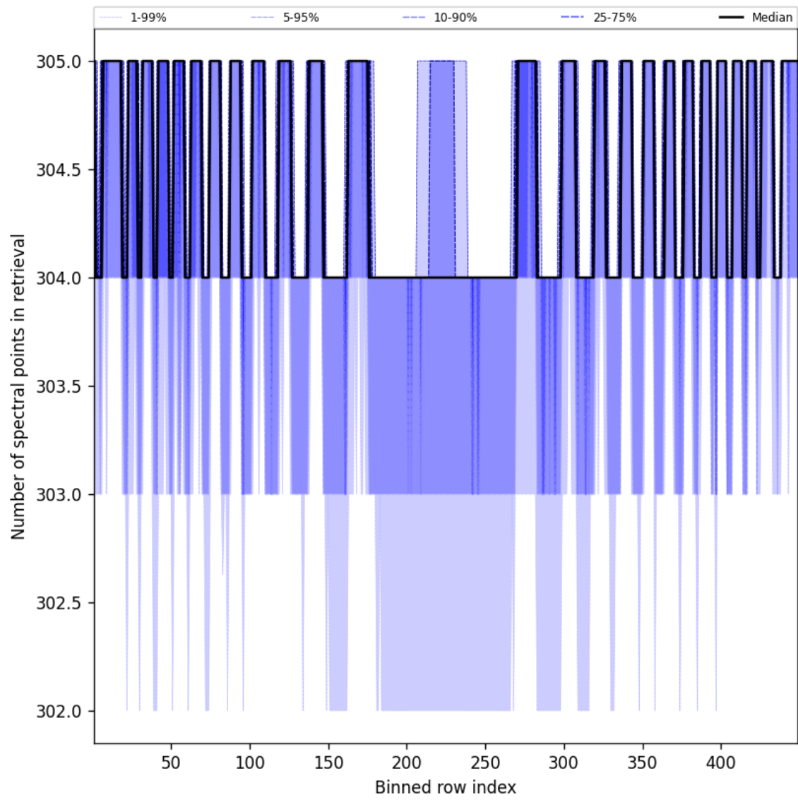
Figure 50: Along track statistics of “Number of spectral points in retrieval” for 2025-10-06 to 2025-10-07
