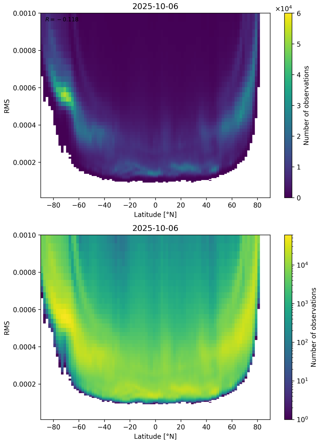
Figure 94: Scatter density plot of “Latitude” against “RMS” for 2025-10-06 to 2025-10-07.
