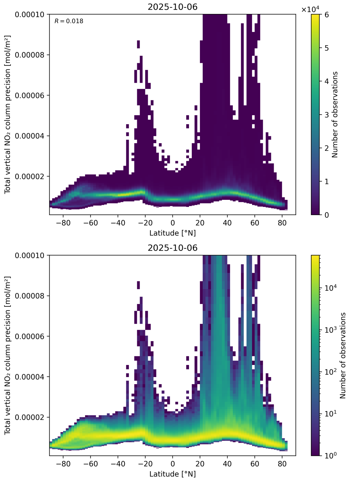
Figure 91: Scatter density plot of “Latitude” against “Total vertical NO 2 column precision” for 2025-10-06 to 2025-10-07.
