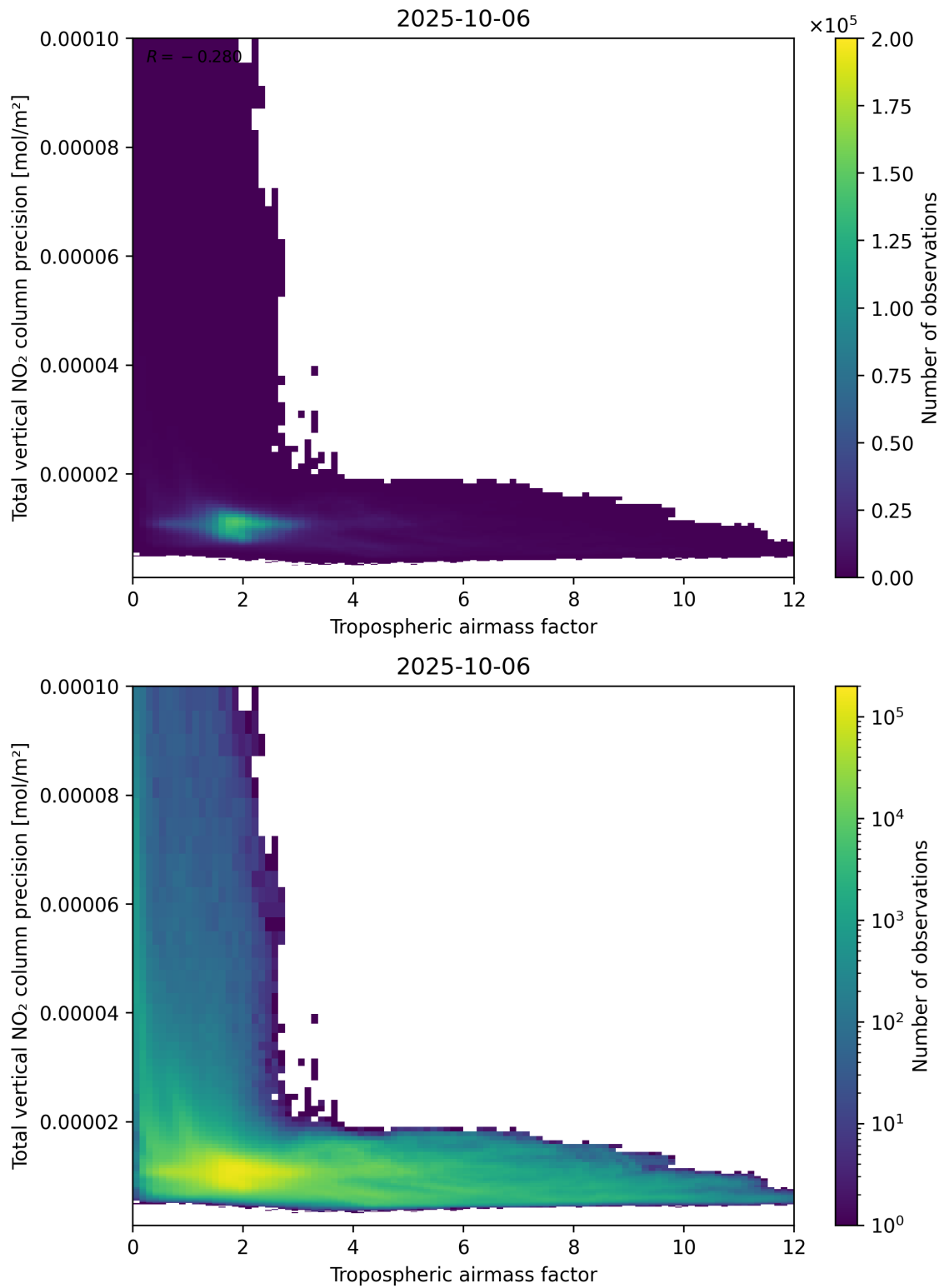
Figure 78: Scatter density plot of “Tropospheric air mass factor” against “Total vertical NO 2 column precision” for 2025-10-06 to 2025-10-07.
