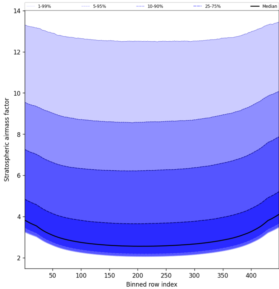
Figure 61: Along track statistics of “Stratospheric air mass factor” for 2025-10-06 to 2025-10-07
