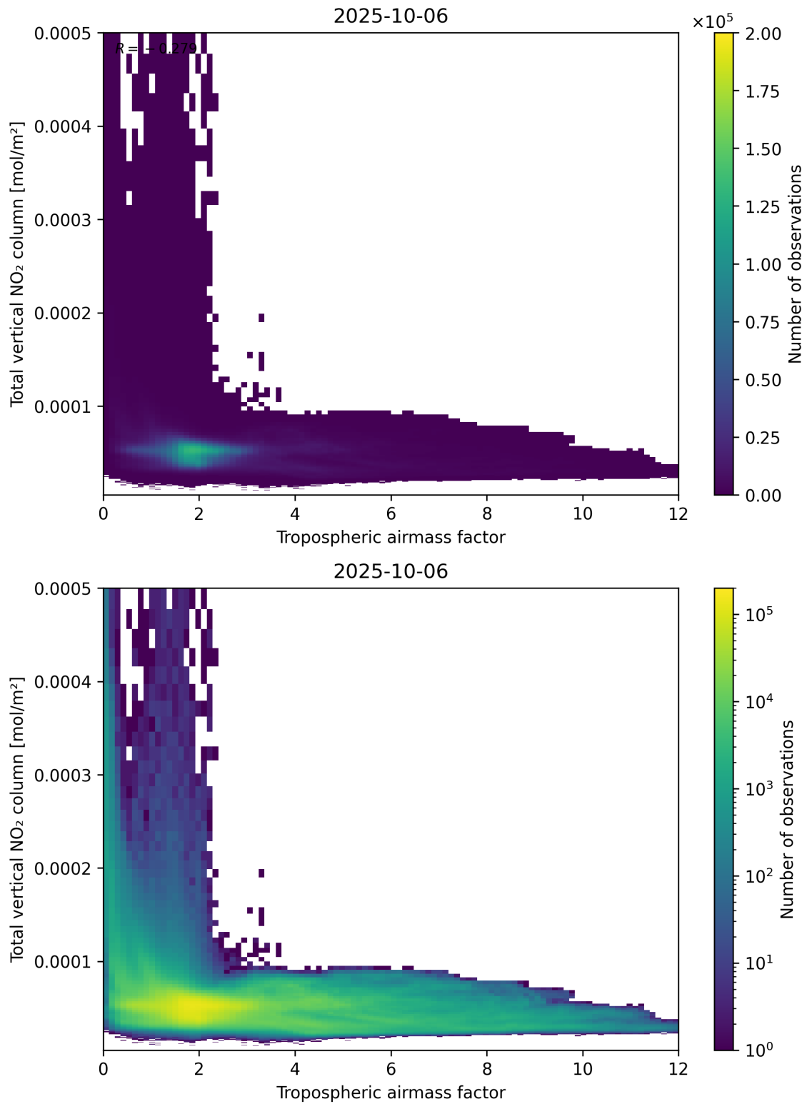
Figure 77: Scatter density plot of “Tropospheric airmass factor” against “Total vertical \text{NO}_2 column” for 2025-10-06 to 2025-10-07.
