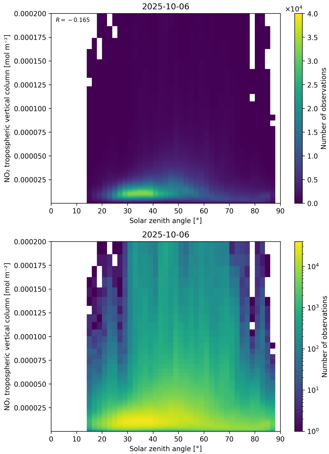
Figure 155: Scatter density plot of “Solar zenith angle” against “NO 2 tropospheric vertical column” for 2025-10-06 to 2025-10-07.
