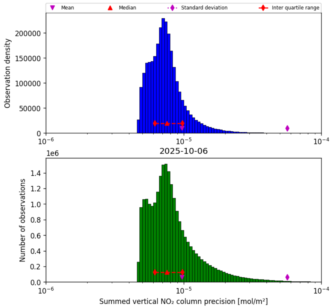
Figure 41: Histogram of “Summed vertical NO 2 column precision” for 2025-10-06 to 2025-10-07
