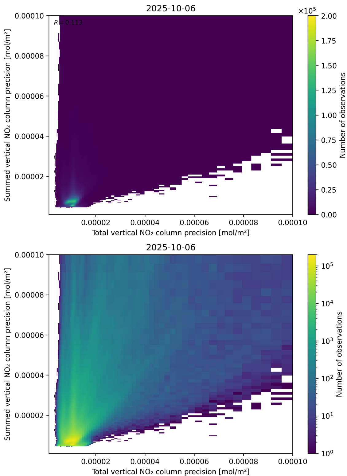
Figure 118: Scatter density plot of “Total vertical NO 2 column precision” against “Summed vertical NO 2 column precision” for 2025-10-06 to 2025-10-07.
