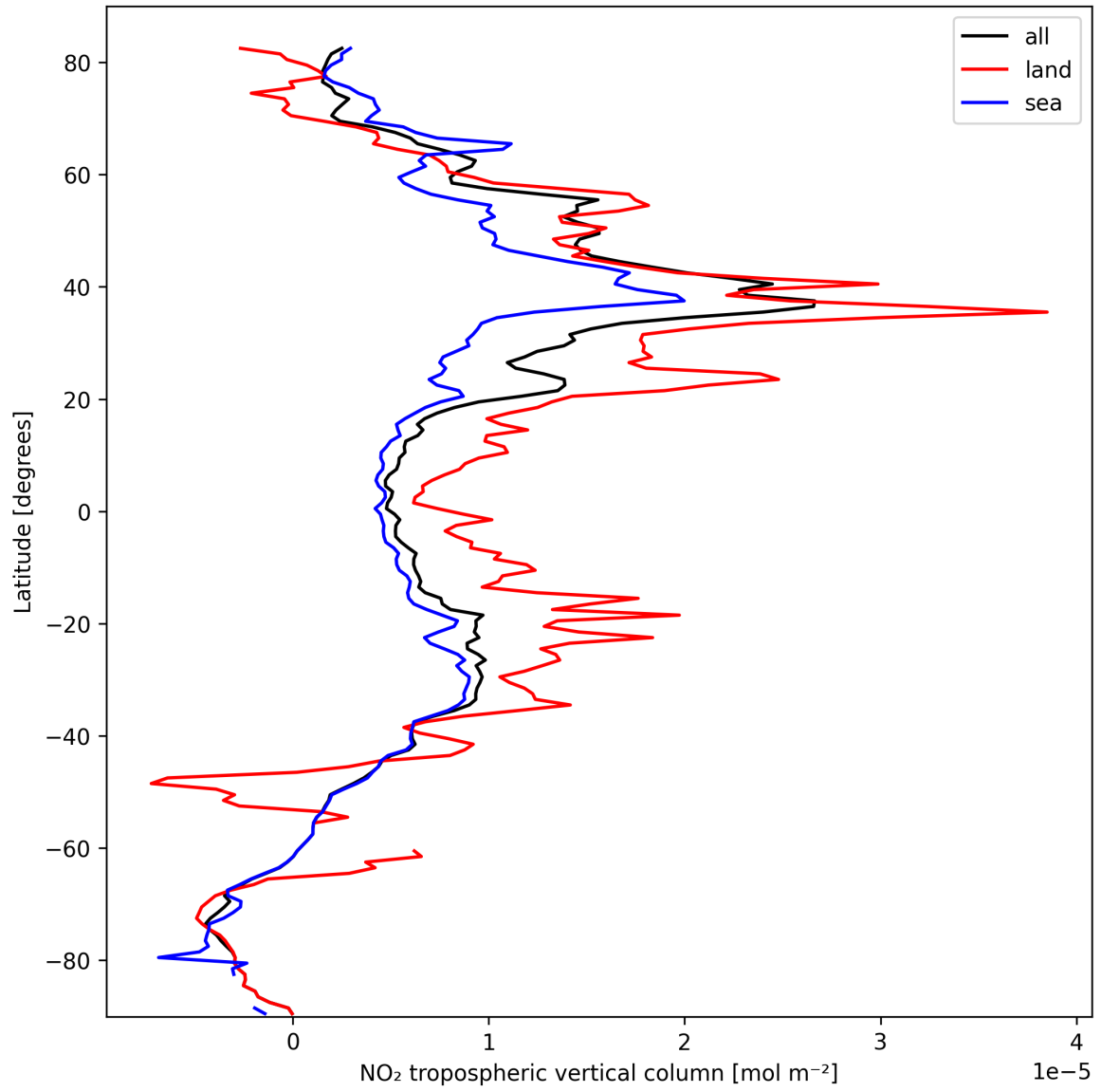
Figure 12: Zonal average of “NO 2 tropospheric vertical column” for 2025-10-06 to 2025-10-07.
