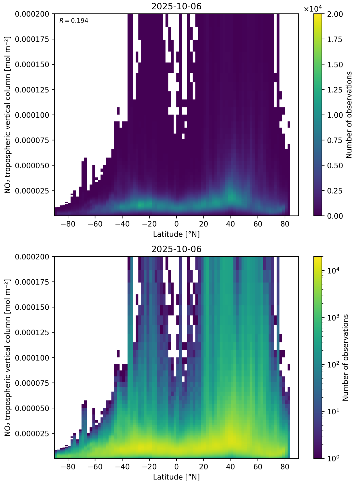
Figure 92: Scatter density plot of “Latitude” against “NO 2 tropospheric vertical column” for 2025-10-06 to 2025-10-07.
