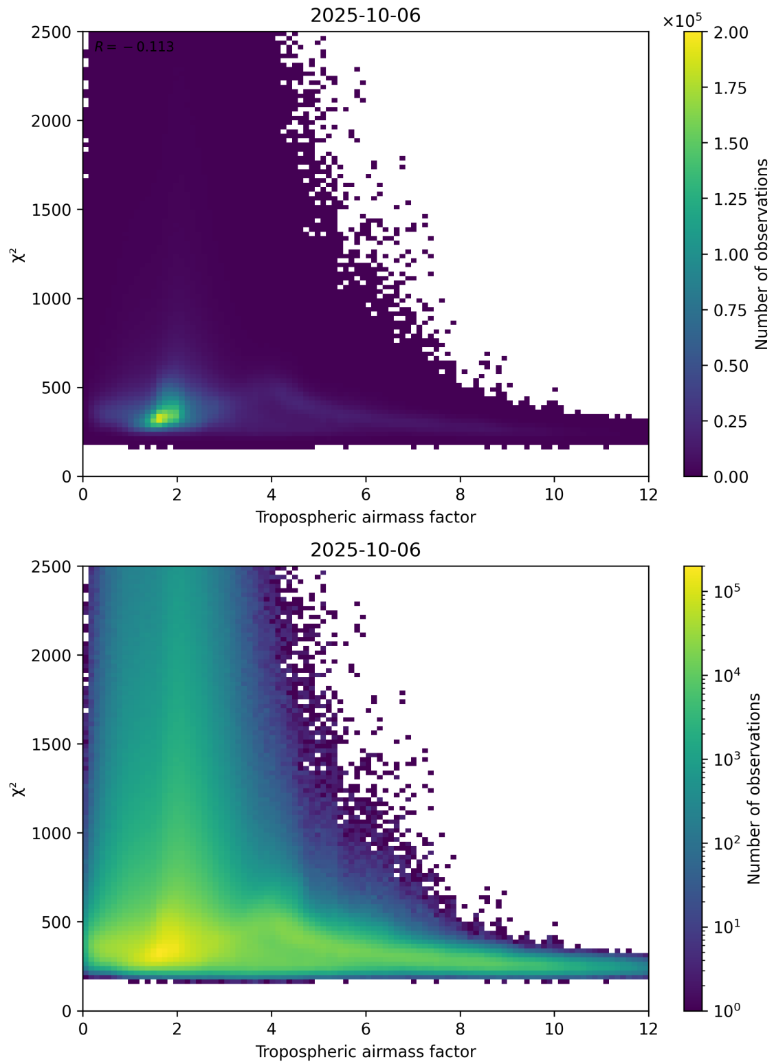
Figure 73: Scatter density plot of “Tropospheric airmass factor” against “ \chi^2 ” for 2025-10-06 to 2025-10-07.
