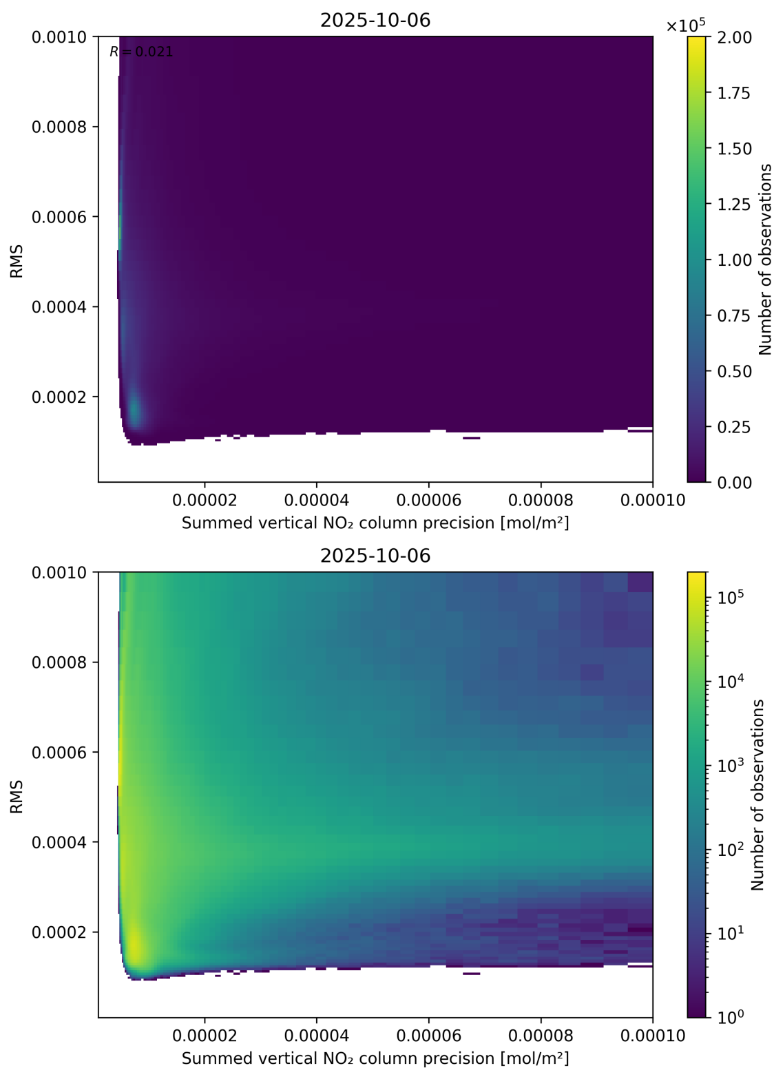
Figure 108: Scatter density plot of “Summed vertical NO 2 column precision” against “RMS” for 2025-10-06 to 2025-10-07.
