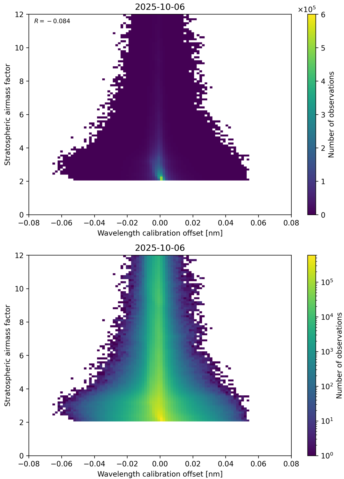
Figure 174: Scatter density plot of “Wavelength calibration offset” against “Stratospheric air mass factor” for 2025-10-06 to 2025-10-07.
