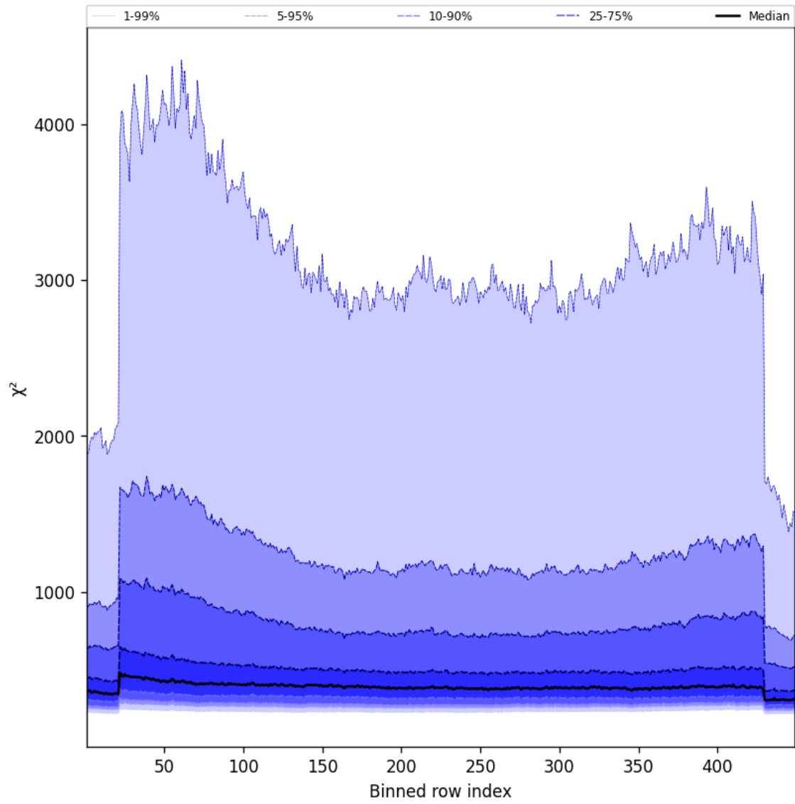
Figure 59: Along track statistics of “ \chi^2 ” for 2025-10-06 to 2025-10-07
