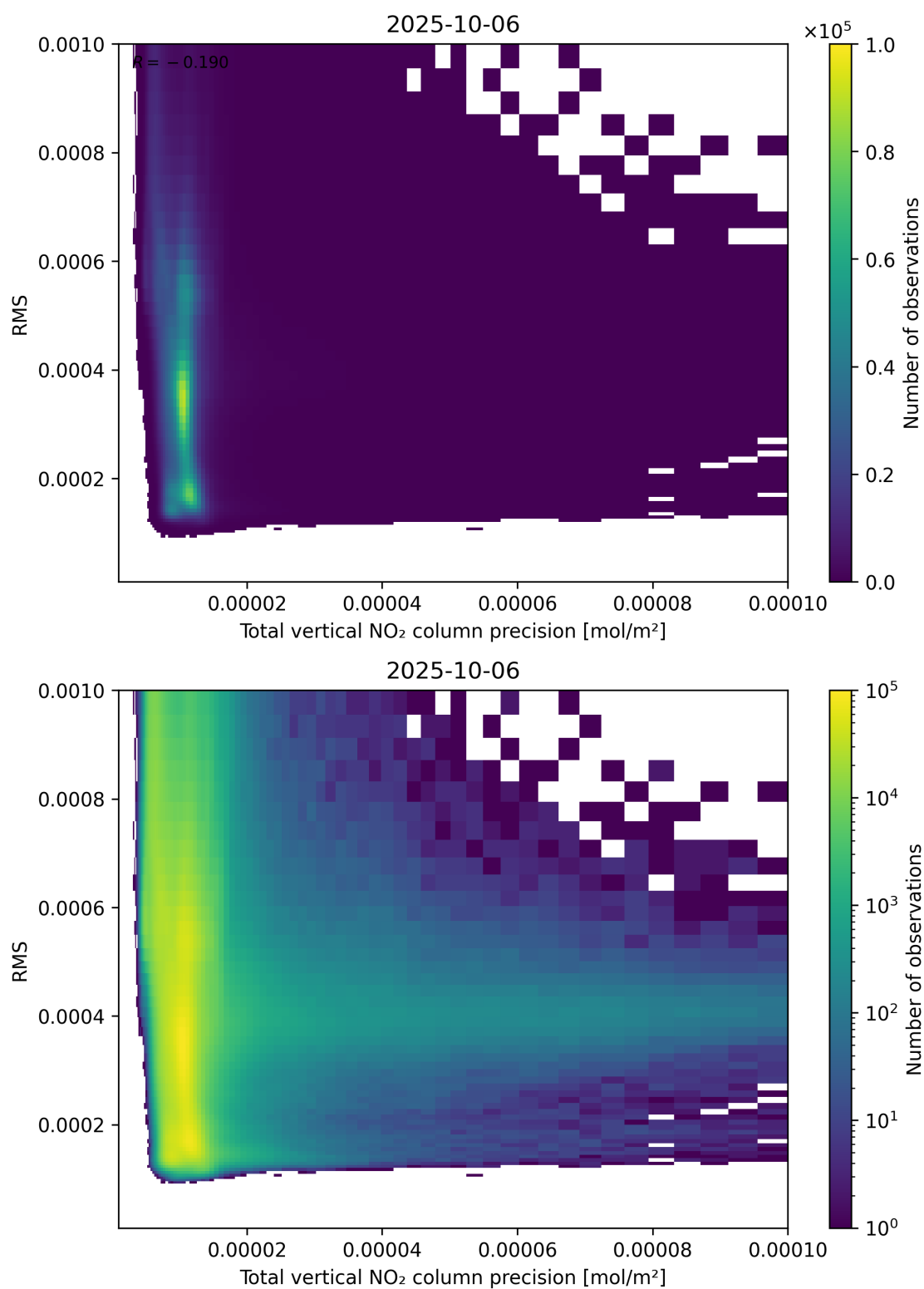
Figure 119: Scatter density plot of “Total vertical NO 2 column precision” against “RMS” for 2025-10-06 to 2025-10-07.
