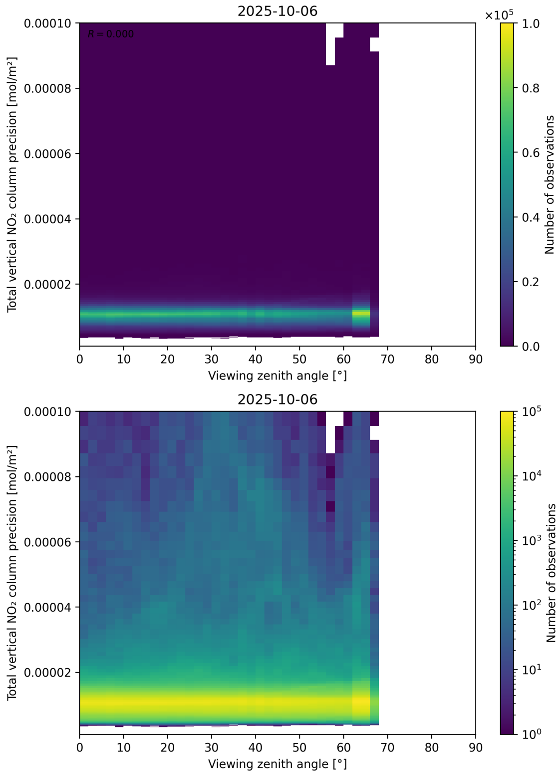
Figure 168: Scatter density plot of “Viewing zenith angle” against “Total vertical NO 2 column precision” for 2025-10-06 to 2025-10-07.
