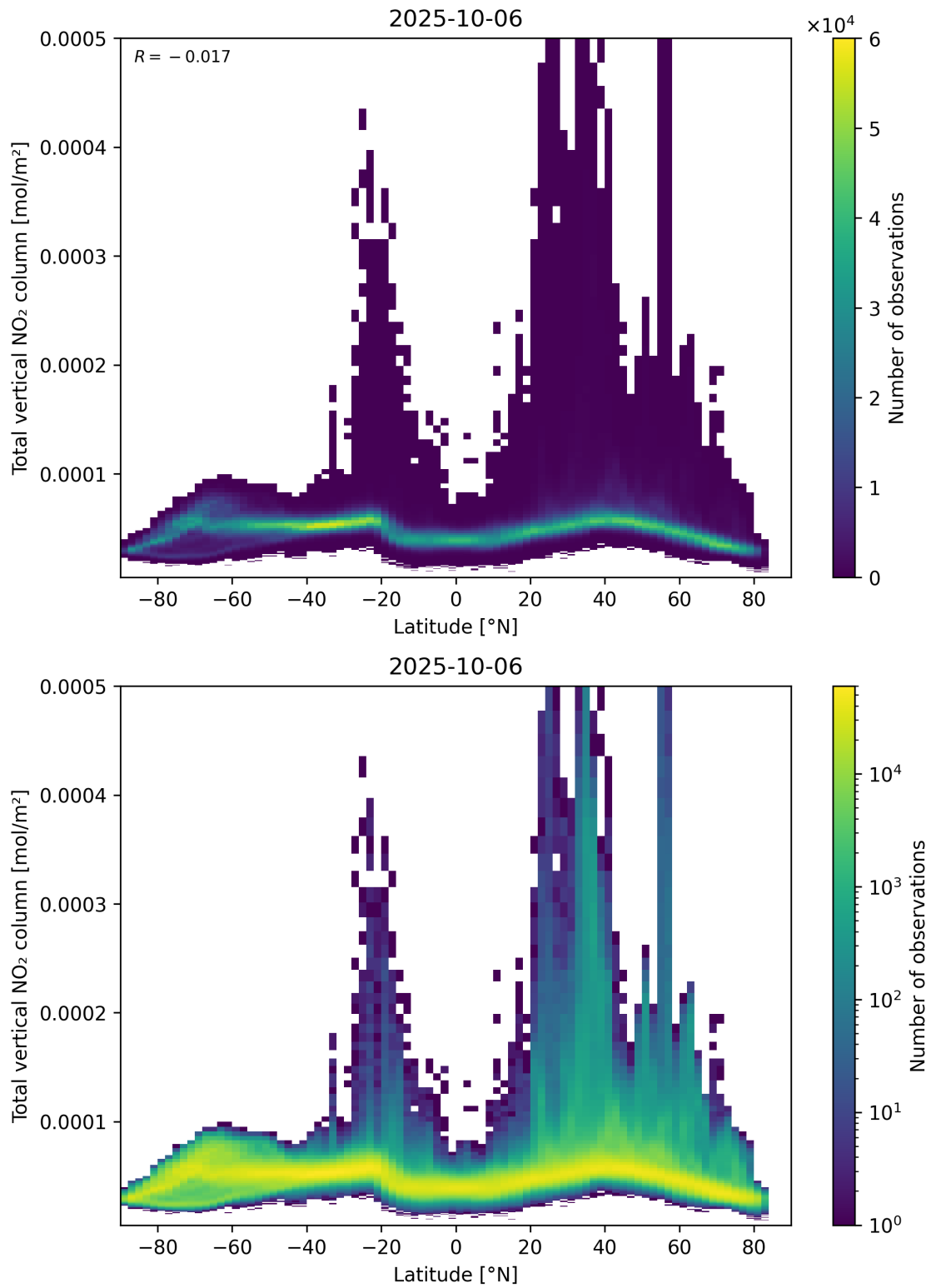
Figure 90: Scatter density plot of “Latitude” against “Total vertical NO 2 column” for 2025-10-06 to 2025-10-07.
