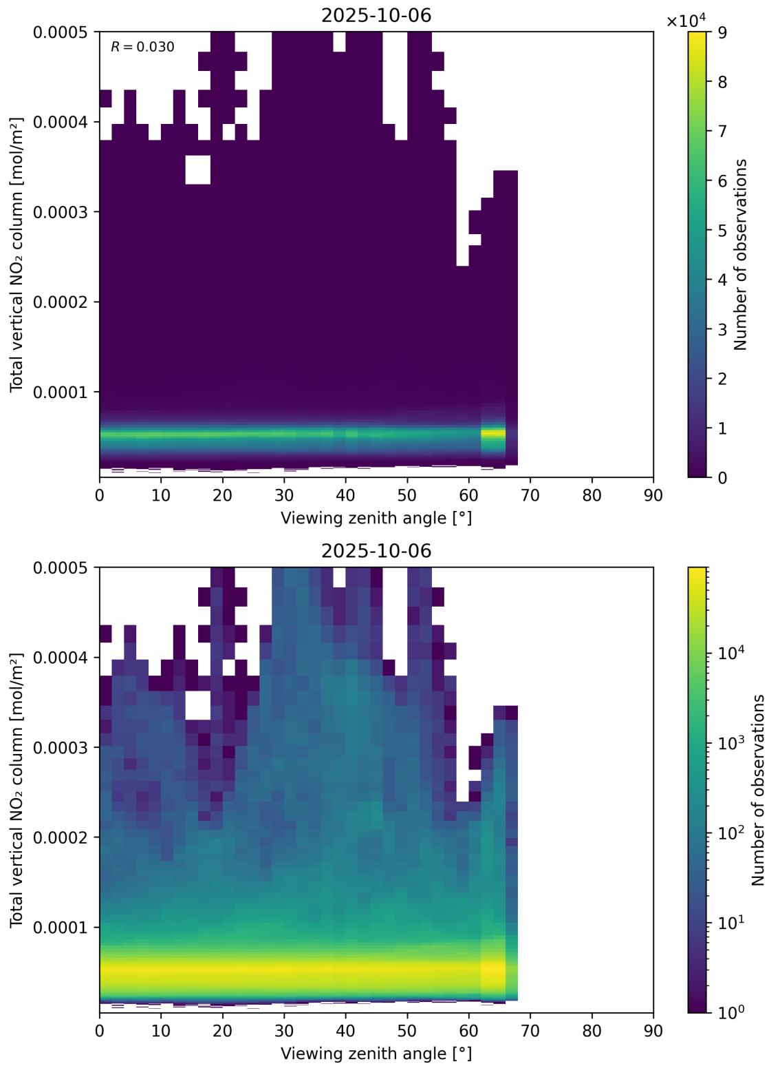
Figure 167: Scatter density plot of “Viewing zenith angle” against “Total vertical NO 2 column” for 2025-10-06 to 2025-10-07.
