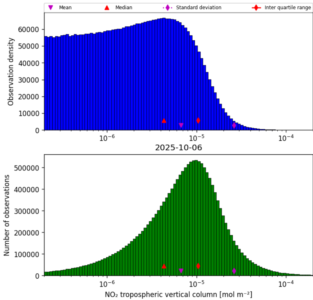
Figure 29: Histogram of “NO 2 tropospheric vertical column” for 2025-10-06 to 2025-10-07
