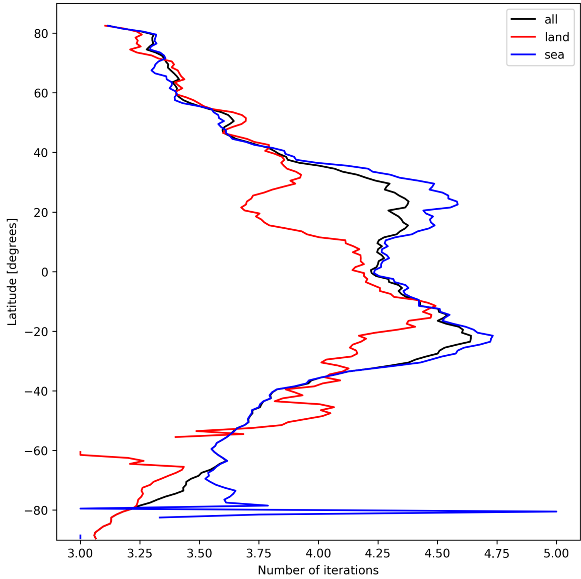
Figure 17: Zonal average of “Number of iterations” for 2025-10-06 to 2025-10-07.
