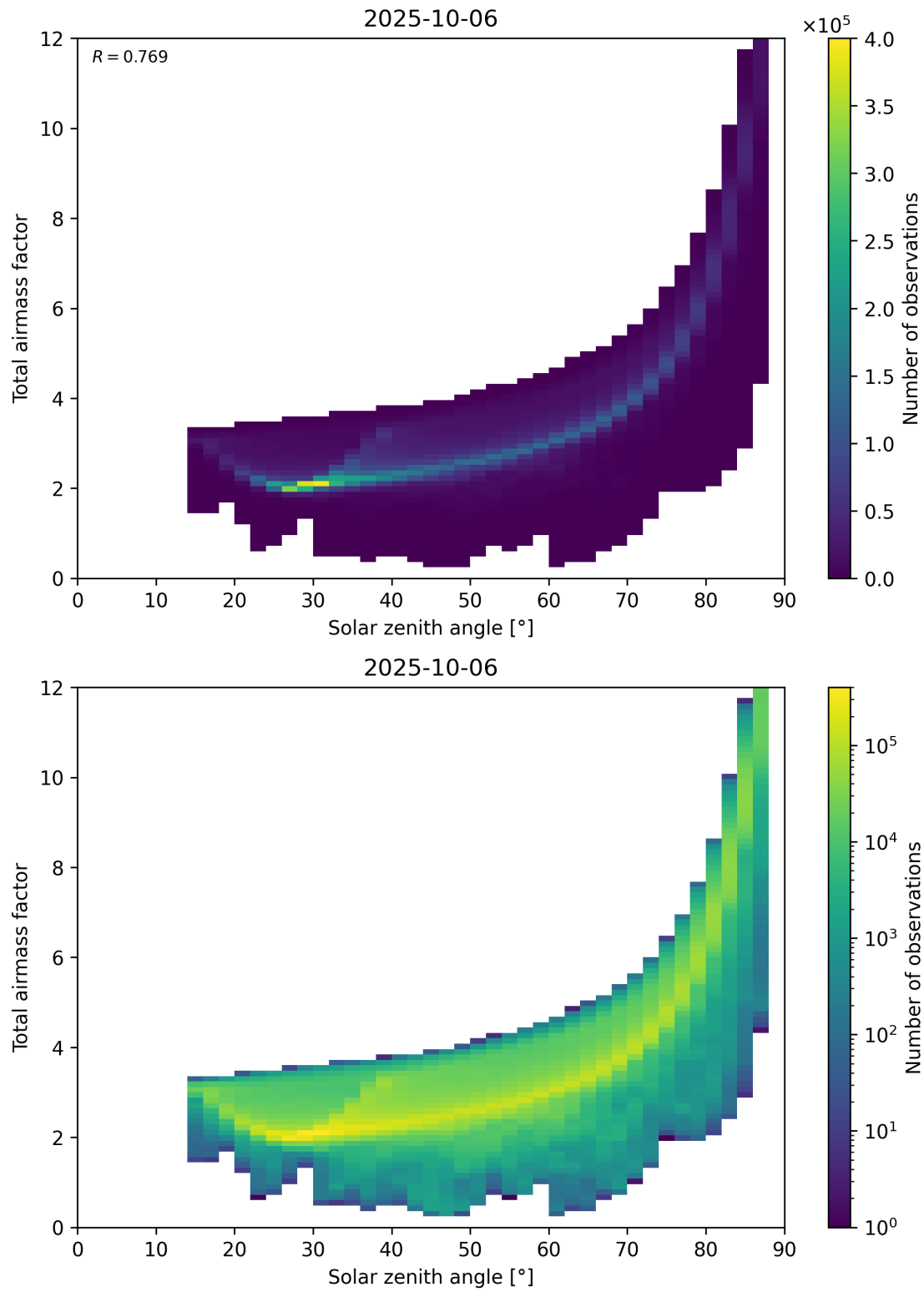
Figure 146: Scatter density plot of “Solar zenith angle” against “Total air mass factor” for 2025-10-06 to 2025-10-07.
