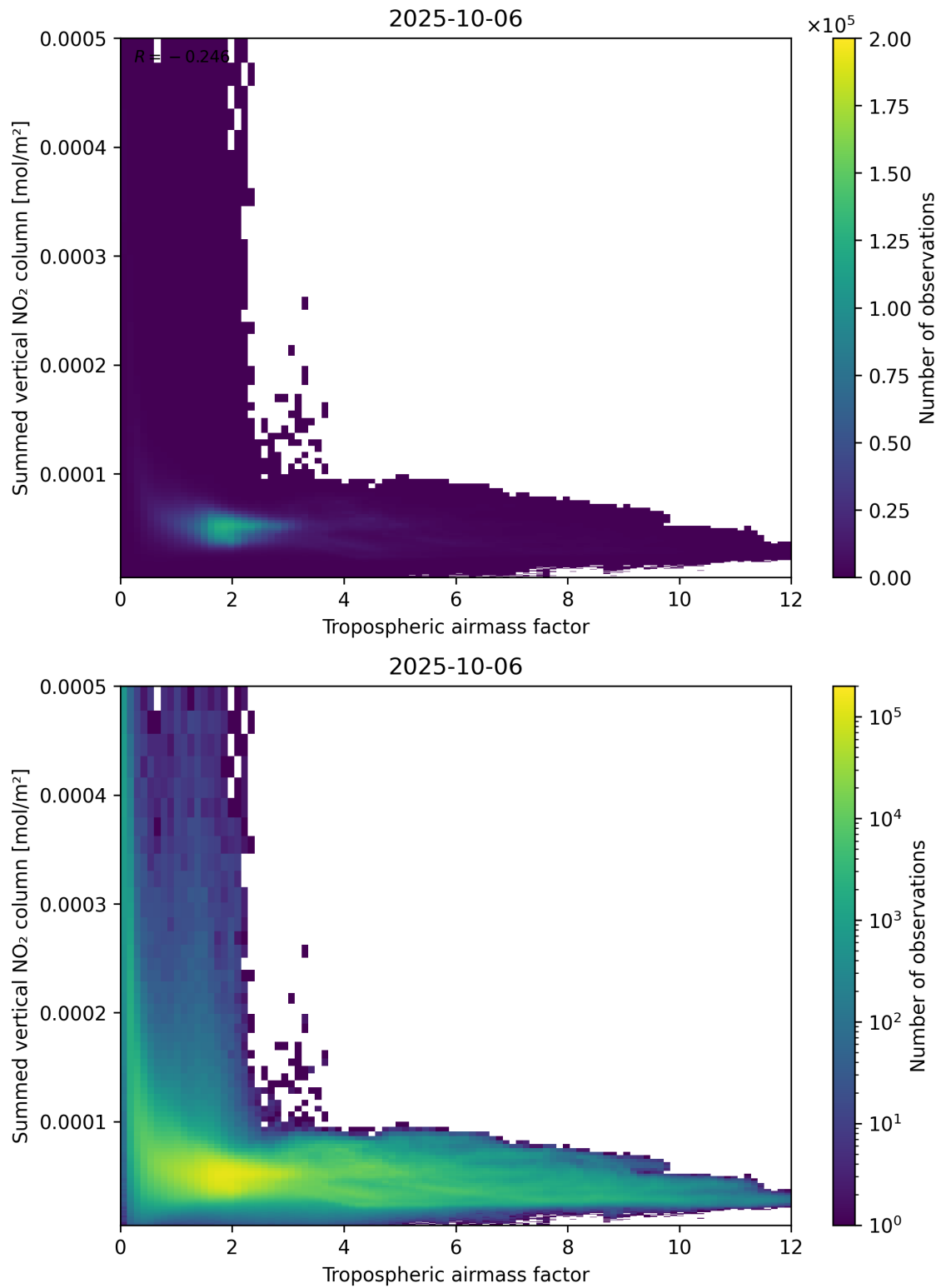
Figure 75: Scatter density plot of “Tropospheric airmass factor” against “Summed vertical NO 2 column” for 2025-10-06 to 2025-10-07.
