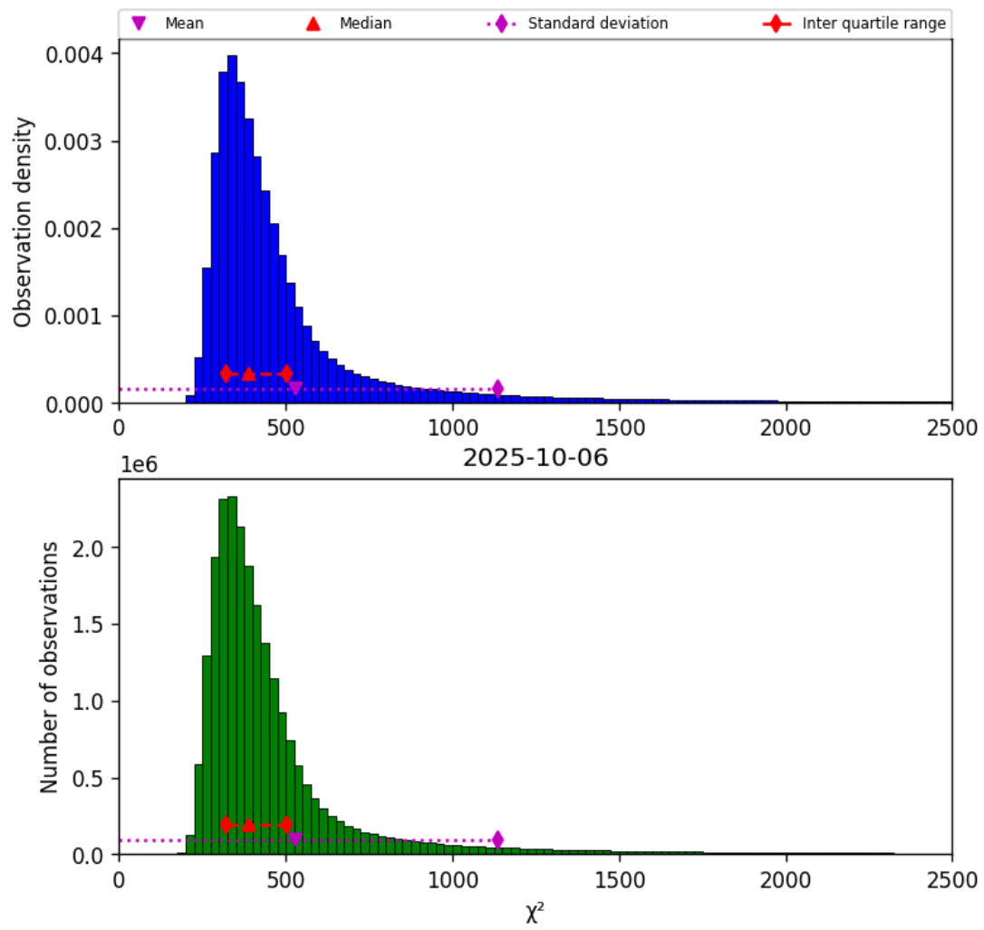
Figure 42: Histogram of “ \chi^2 ” for 2025-10-06 to 2025-10-07
