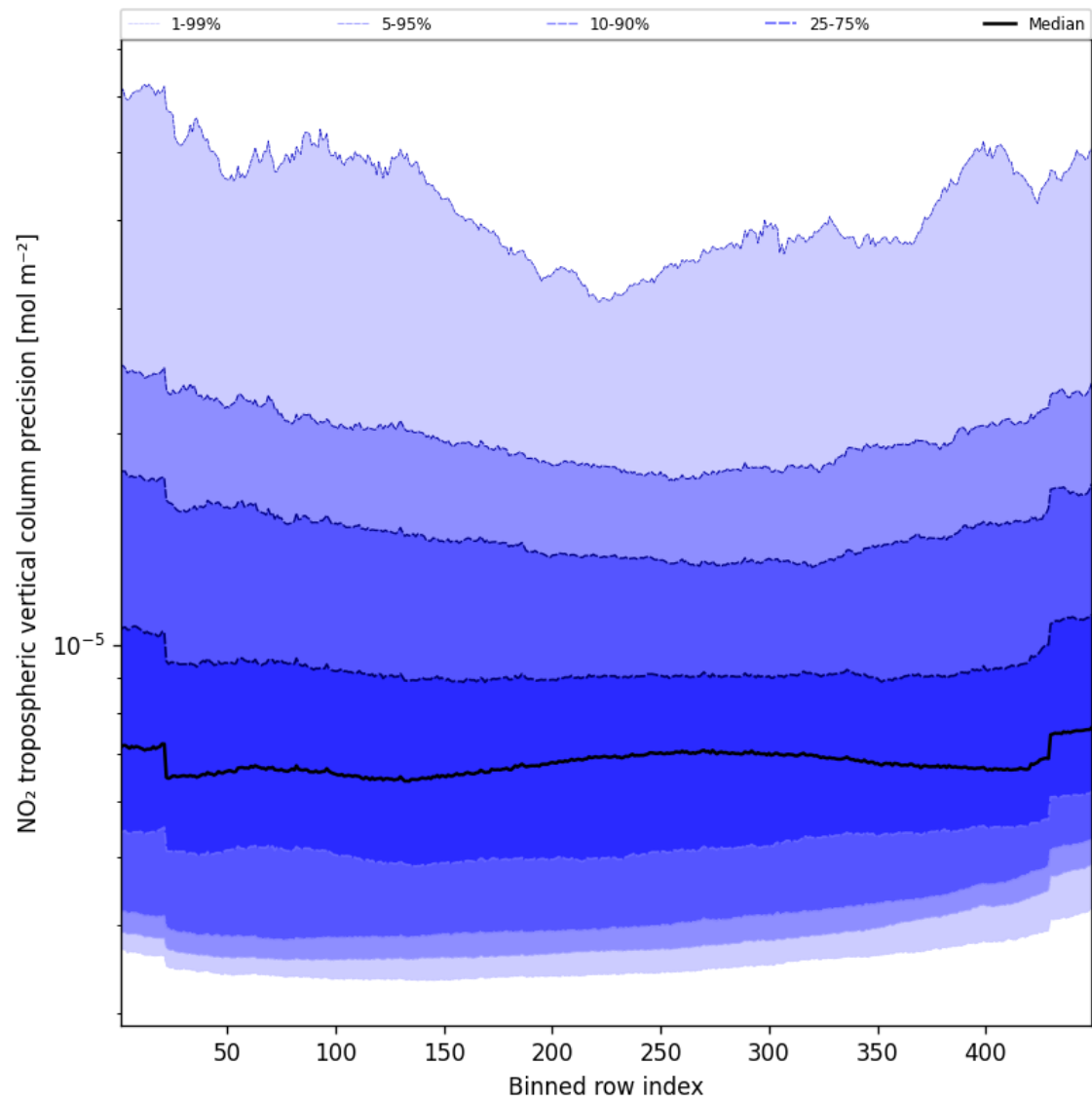
Figure 47: Along track statistics of “NO 2 tropospheric vertical column precision” for 2025-10-06 to 2025-10-07
