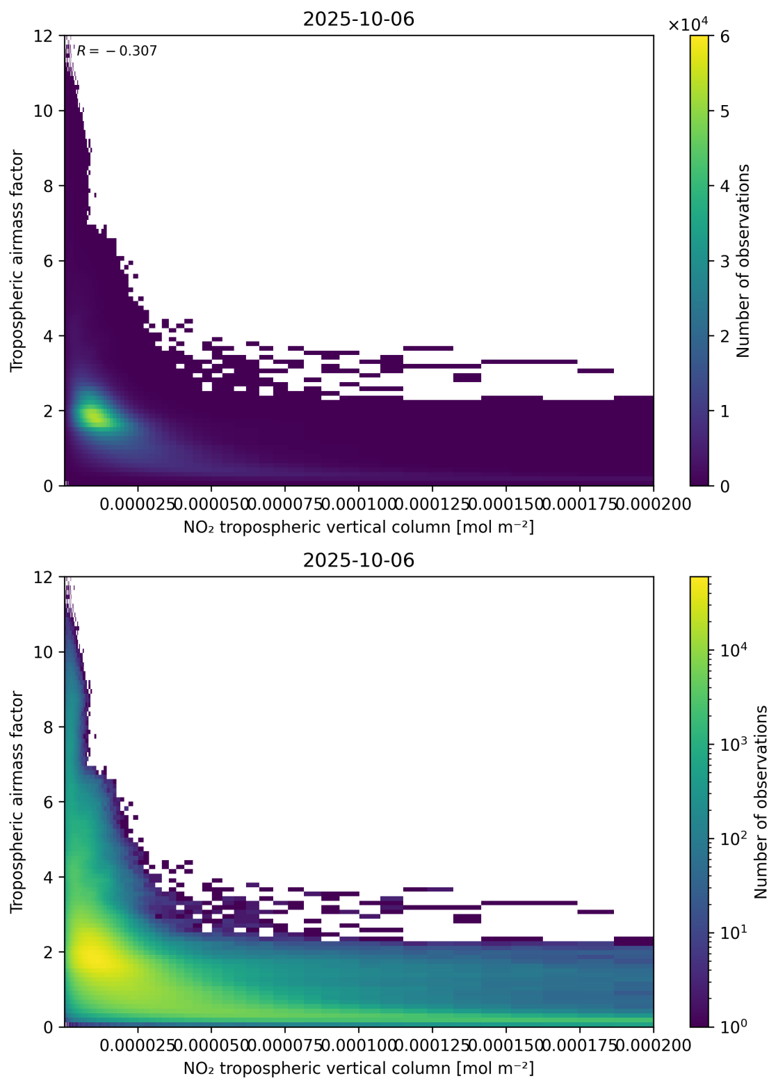
Figure 123: Scatter density plot of “NO 2 tropospheric vertical column” against “Tropospheric air mass factor” for 2025-10-06 to 2025-10-07.
