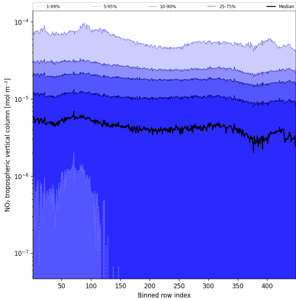
Figure 46: Along track statistics of “NO 2 tropospheric vertical column” for 2025-10-06 to 2025-10-07
