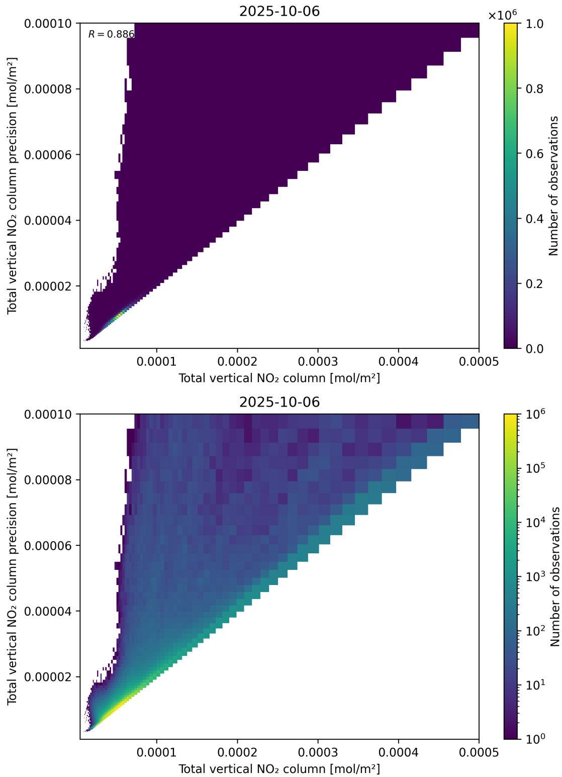
Figure 114: Scatter density plot of “Total vertical NO 2 column” against “Total vertical NO 2 column precision” for 2025-10-06 to 2025-10-07.
