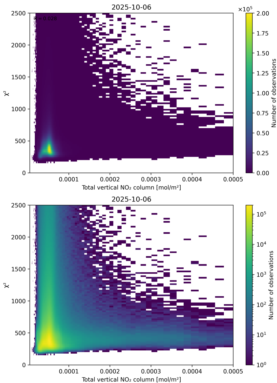
Figure 111: Scatter density plot of “Total vertical NO 2 column” against “ \chi^2 ” for 2025-10-06 to 2025-10-07.
