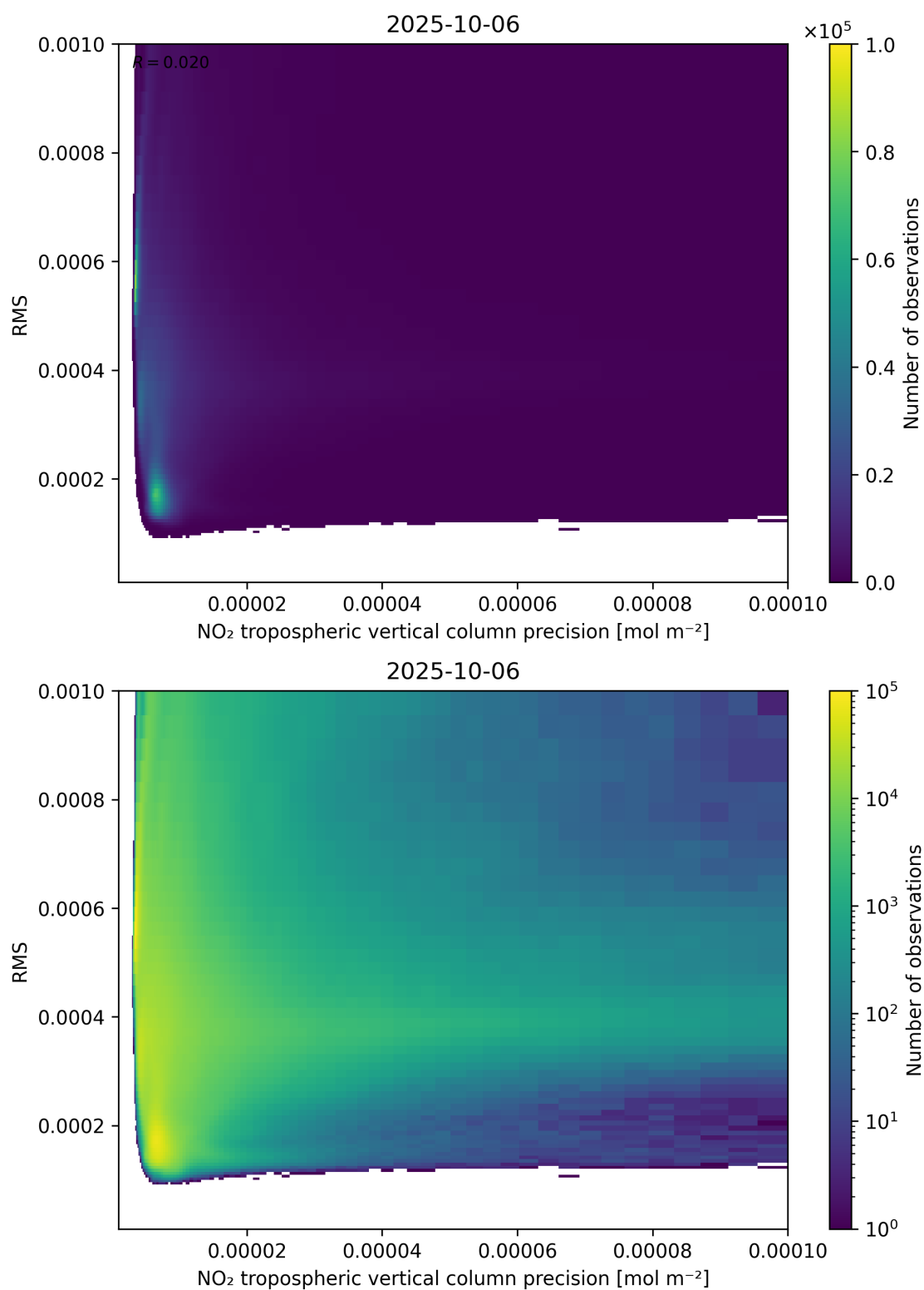
Figure 140: Scatter density plot of “NO 2 tropospheric vertical column precision” against “RMS” for 2025-10-06 to 2025-10-07.
