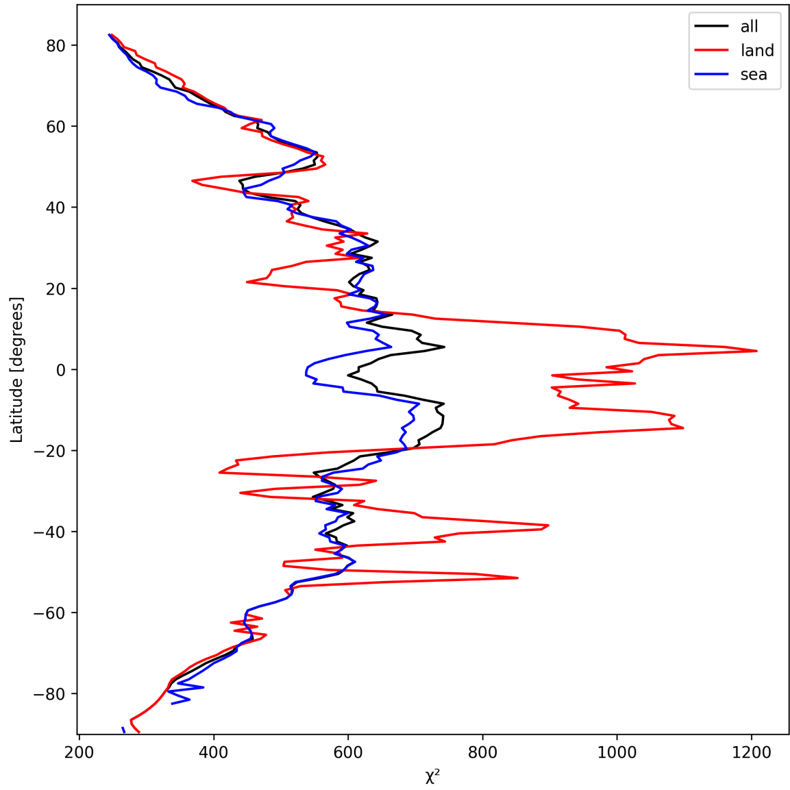
Figure 25: Zonal average of “ \chi^2 ” for 2025-10-06 to 2025-10-07.
