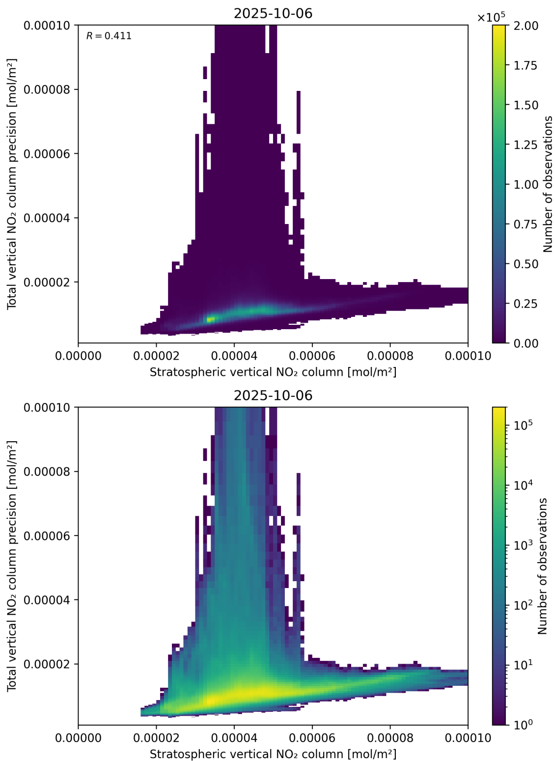
Figure 101: Scatter density plot of “Stratospheric vertical NO 2 column” against “Total vertical NO 2 column precision” for 2025-10-06 to 2025-10-07.
