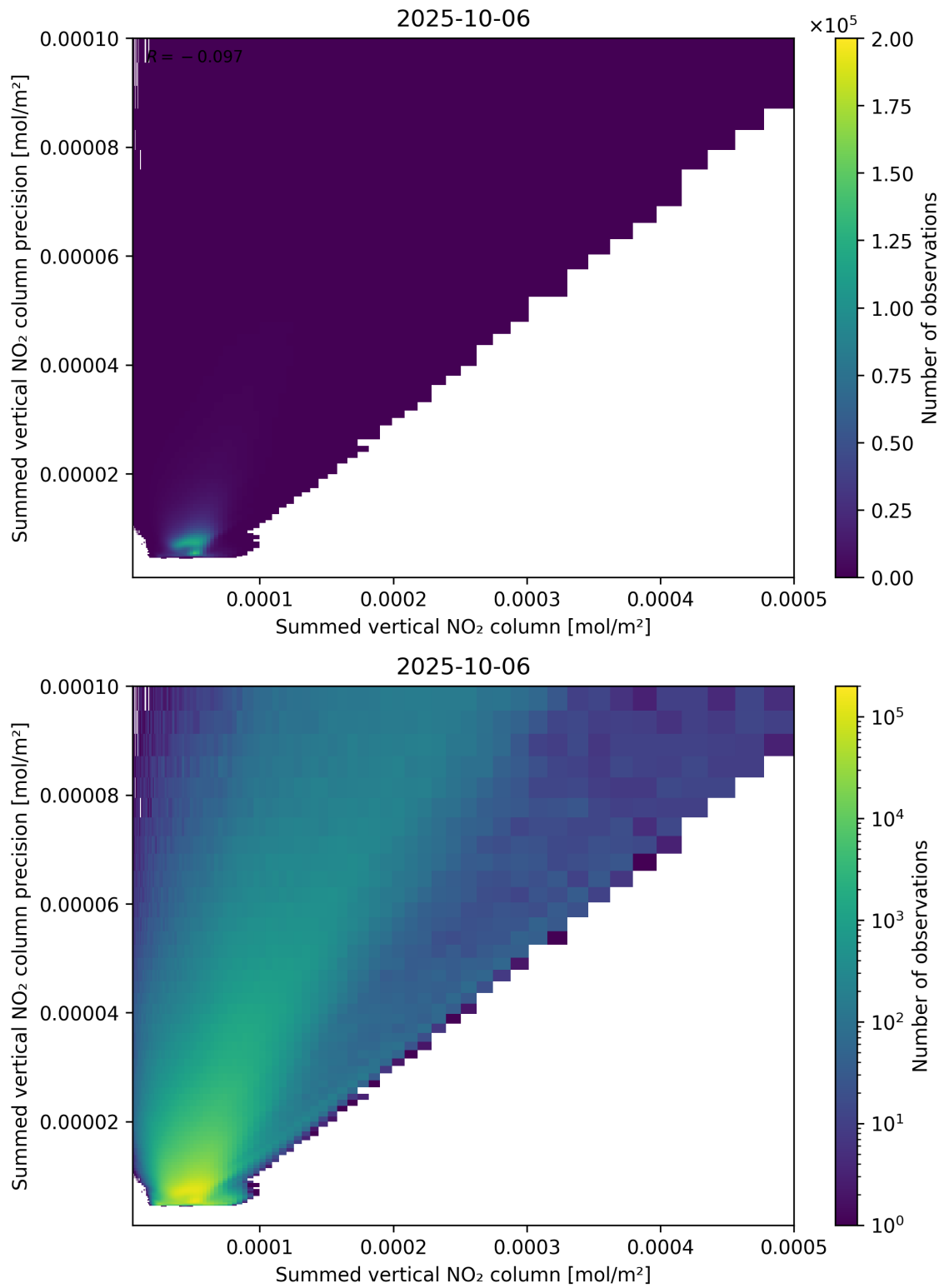
Figure 105: Scatter density plot of “Summed vertical NO 2 column” against “Summed vertical NO 2 column precision” for 2025-10-06 to 2025-10-07.
