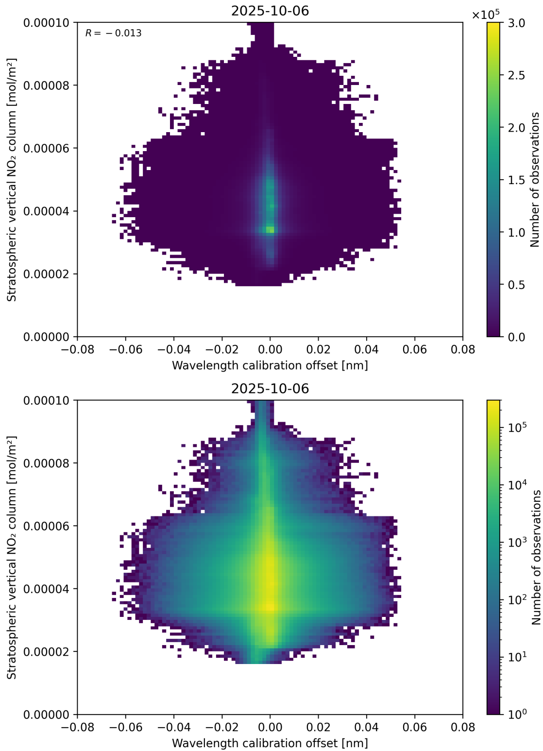
Figure 176: Scatter density plot of “Wavelength calibration offset” against “Stratospheric vertical NO 2 column” for 2025-10-06 to 2025-10-07.
