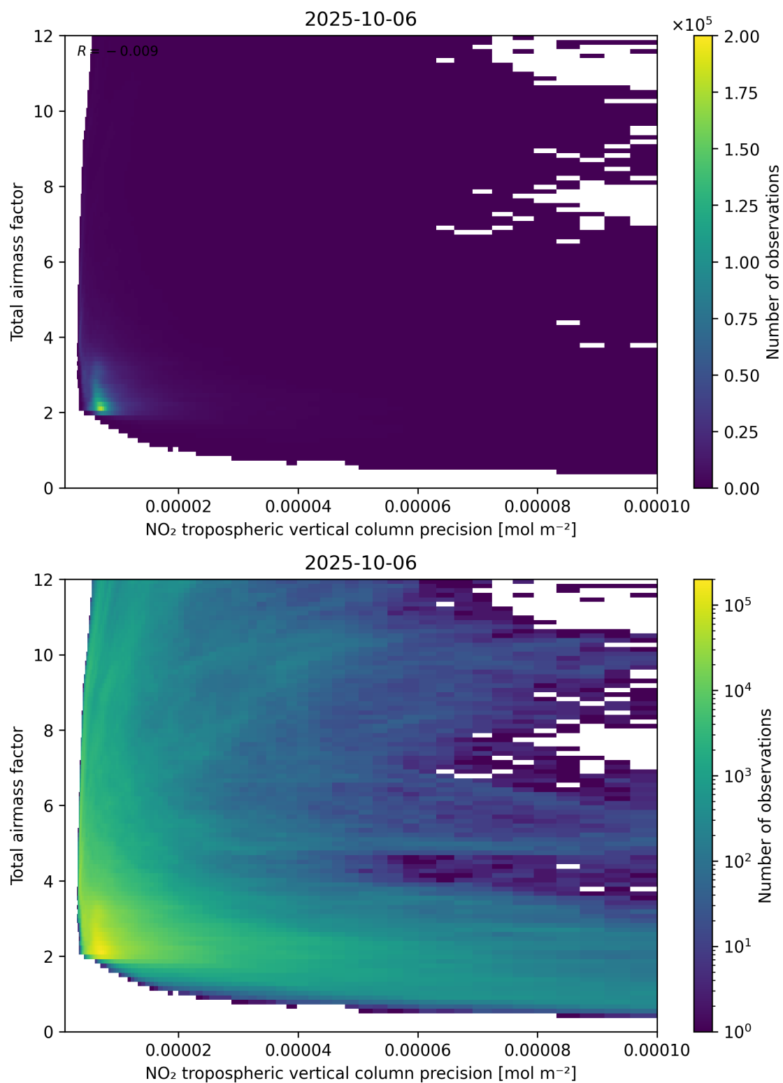
Figure 132: Scatter density plot of “NO 2 tropospheric vertical column precision” against “Total air mass factor” for 2025-10-06 to 2025-10-07.
