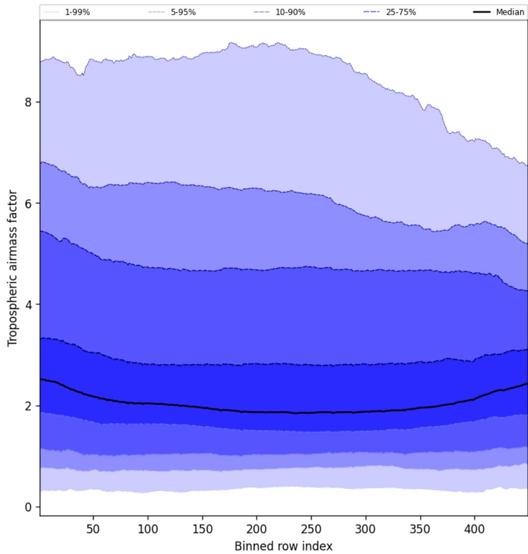
Figure 48: Along track statistics of “Tropospheric air mass factor” for 2025-10-06 to 2025-10-07
