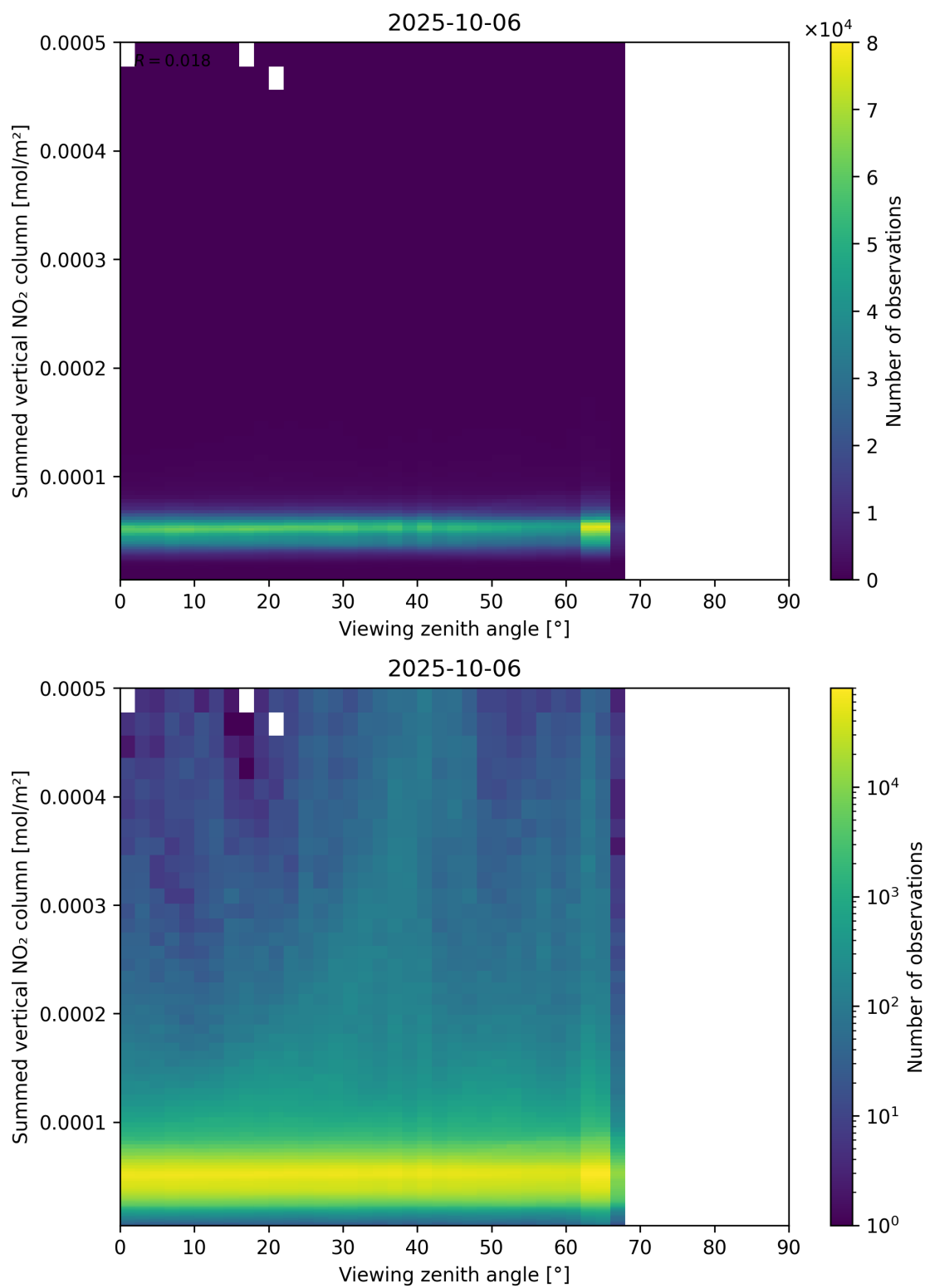
Figure 165: Scatter density plot of “Viewing zenith angle” against “Summed vertical NO 2 column” for 2025-10-06 to 2025-10-07.
