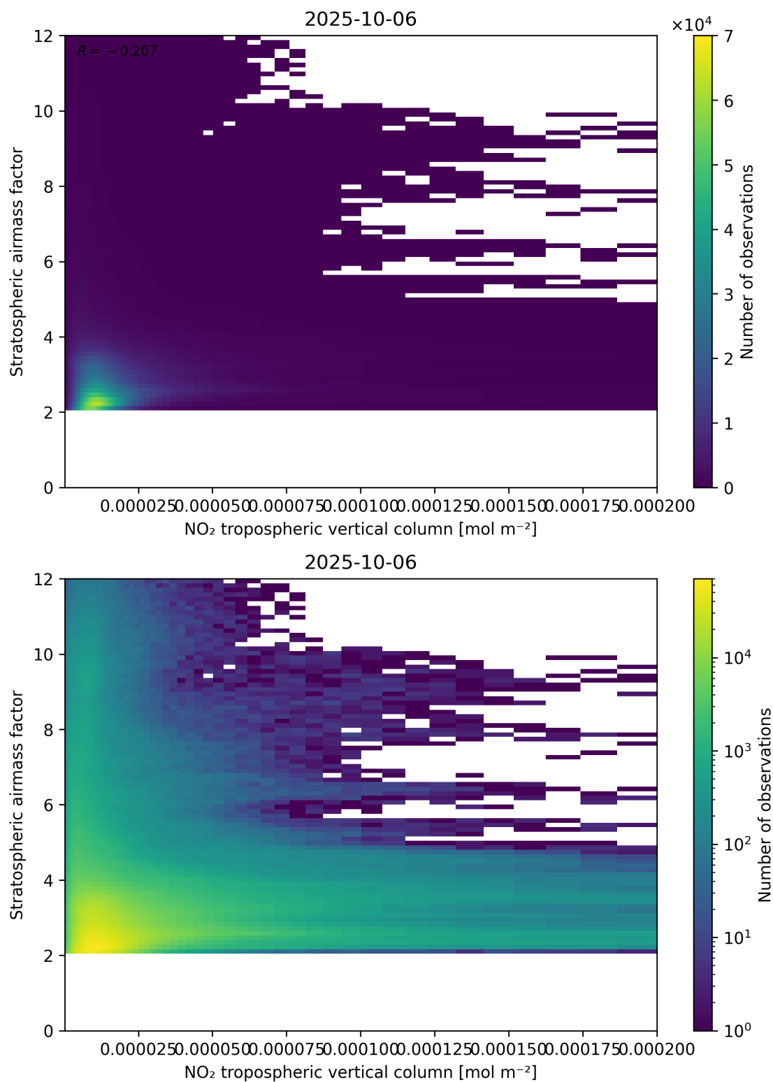
Figure 121: Scatter density plot of “NO 2 tropospheric vertical column” against “Stratospheric air mass factor” for 2025-10-06 to 2025-10-07.
