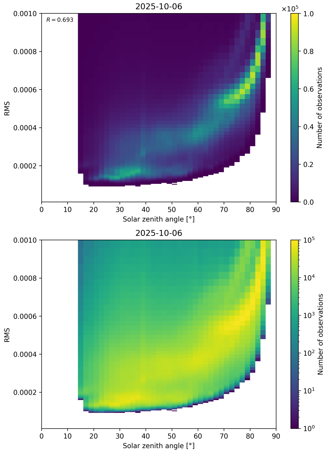
Figure 157: Scatter density plot of “Solar zenith angle” against “RMS” for 2025-10-06 to 2025-10-07.
