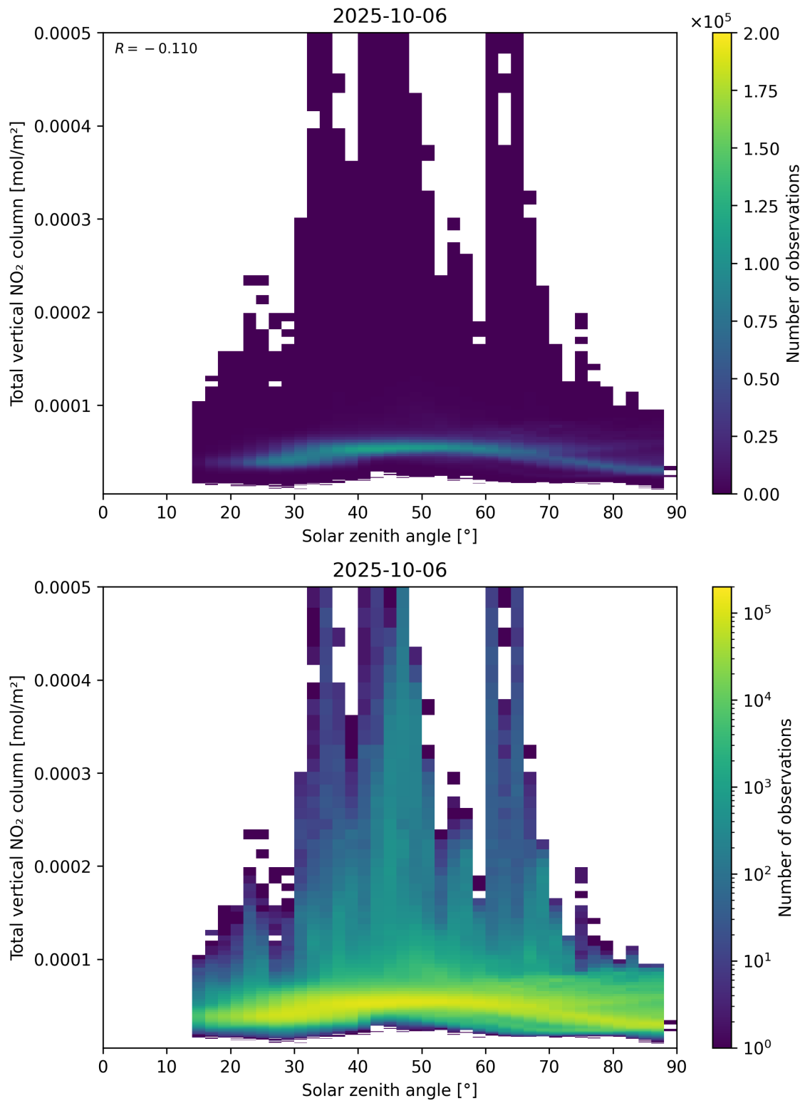
Figure 153: Scatter density plot of “Solar zenith angle” against “Total vertical NO 2 column” for 2025-10-06 to 2025-10-07.
