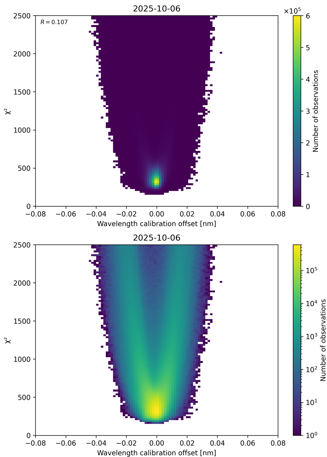
Figure 175: Scatter density plot of “Wavelength calibration offset” against “ \chi^2 ” for 2025-10-06 to 2025-10-07.
