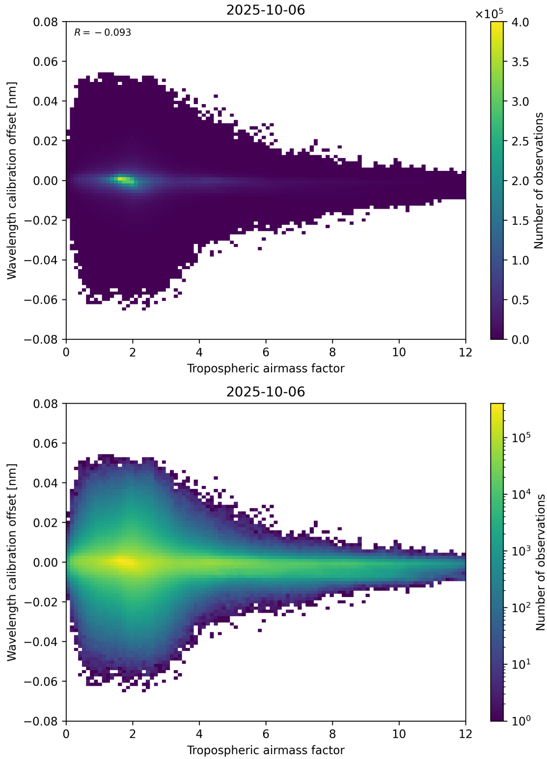
Figure 80: Scatter density plot of “Tropospheric airmass factor” against “Wavelength calibration offset” for 2025-10-06 to 2025-10-07.
