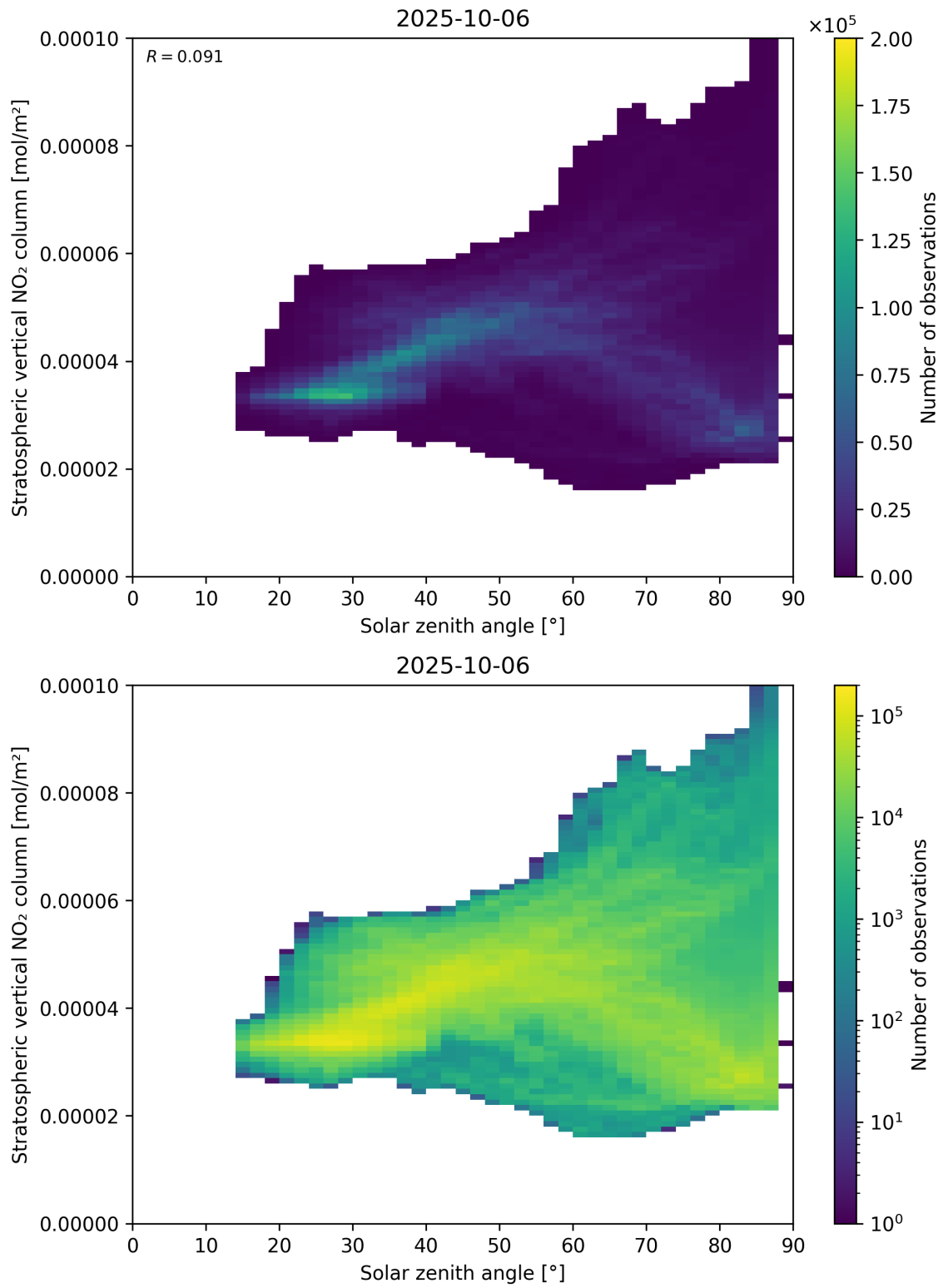
Figure 150: Scatter density plot of “Solar zenith angle” against “Stratospheric vertical NO 2 column” for 2025-10-06 to 2025-10-07.
