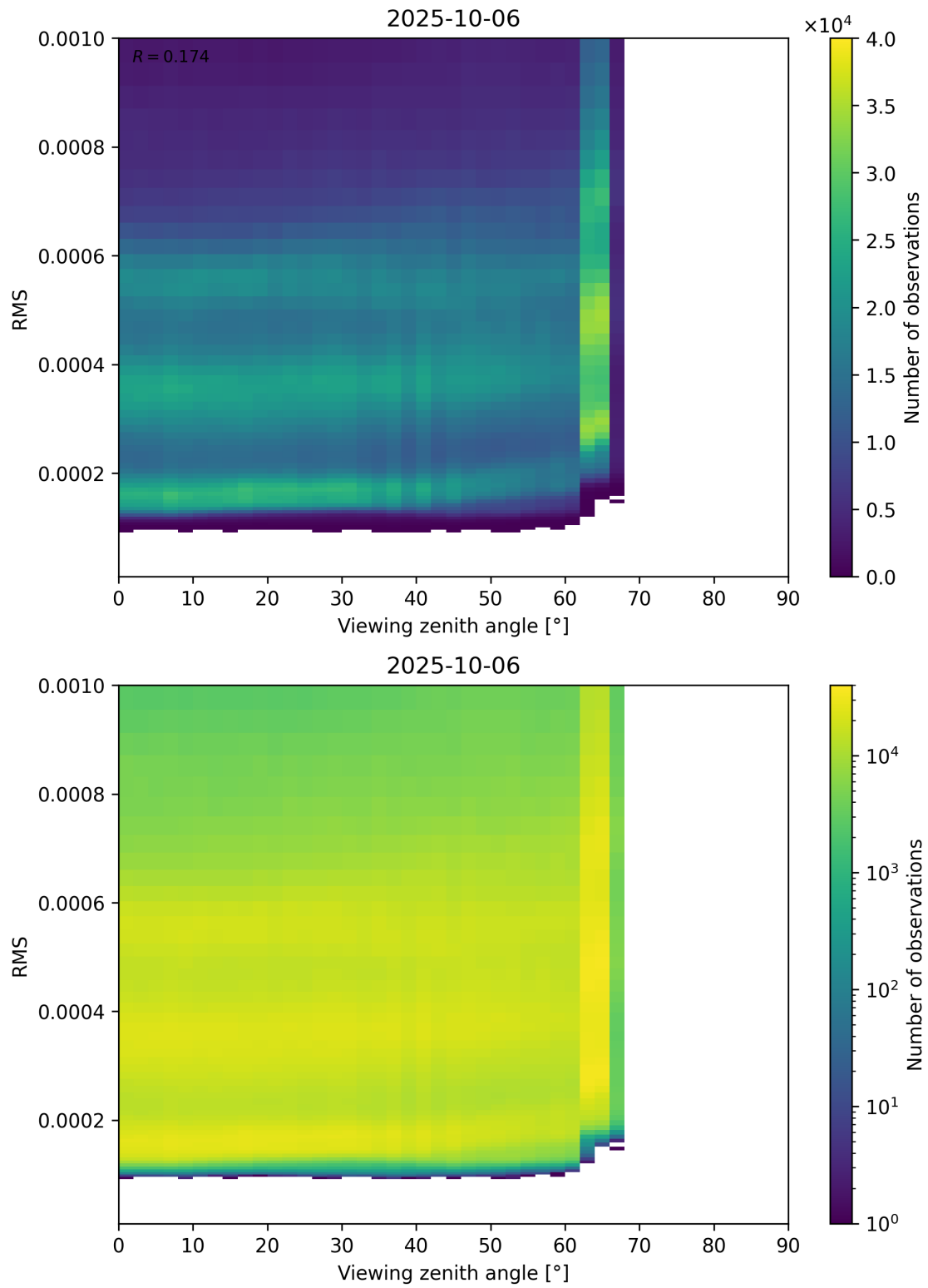
Figure 171: Scatter density plot of “Viewing zenith angle” against “RMS” for 2025-10-06 to 2025-10-07.
