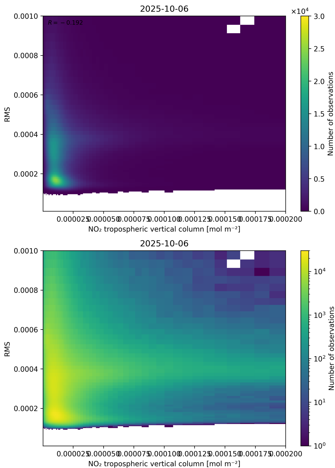
Figure 142: Scatter density plot of “NO 2 tropospheric vertical column” against “RMS” for 2025-10-06 to 2025-10-07.
