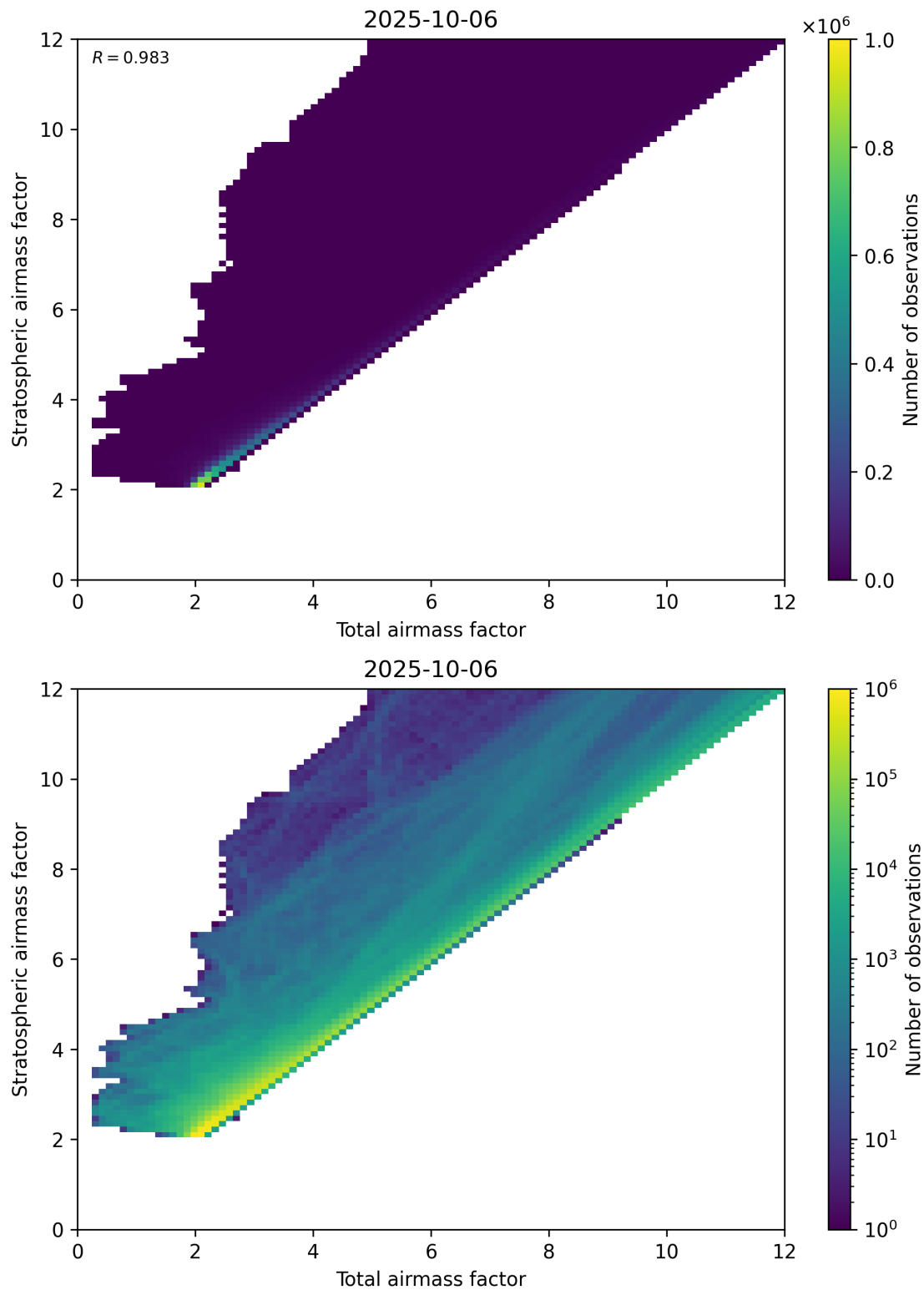
Figure 62: Scatter density plot of “Total airmass factor” against “Stratospheric airmass factor” for 2025-10-06 to 2025-10-07.
