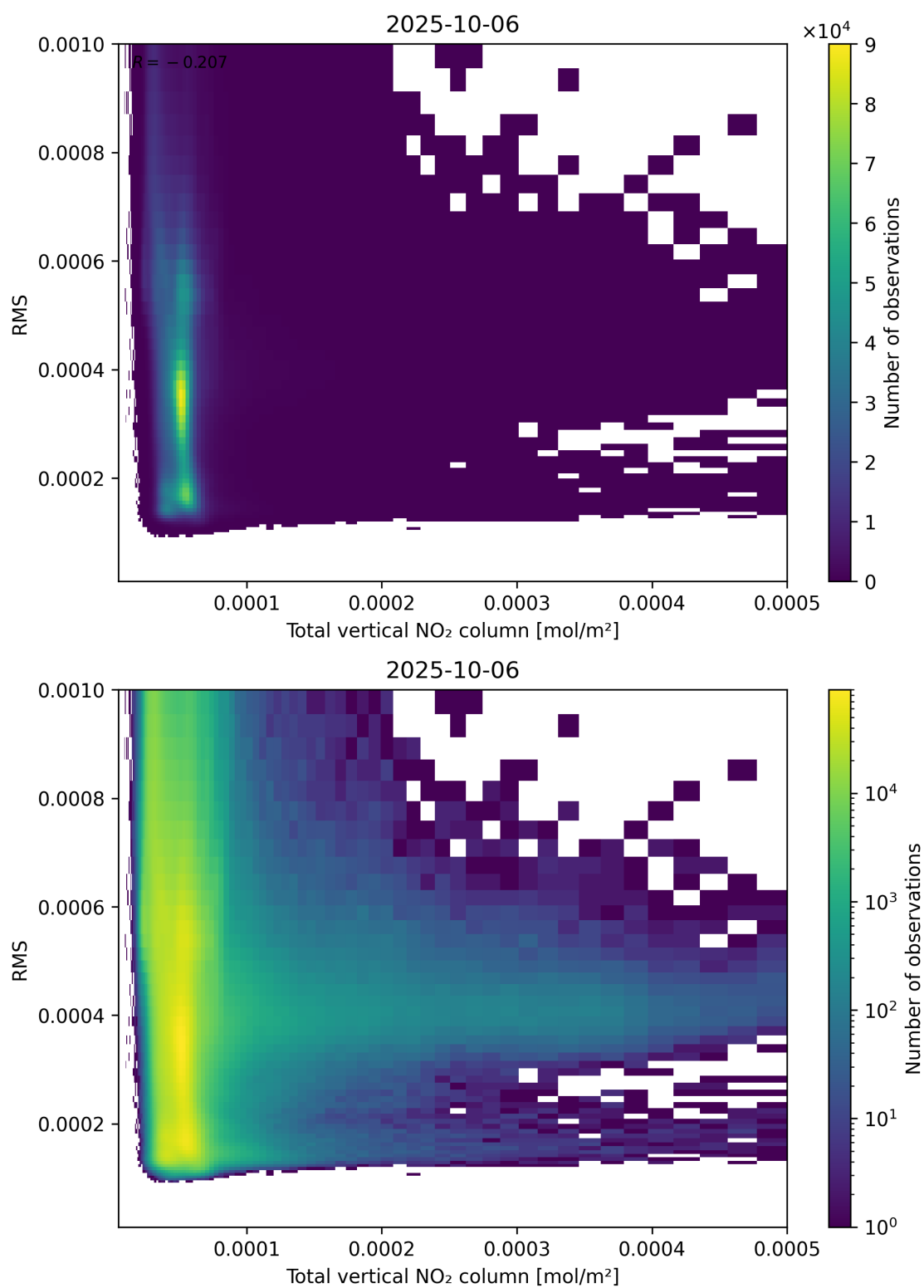
Figure 120: Scatter density plot of “Total vertical NO 2 column” against “RMS” for 2025-10-06 to 2025-10-07.
