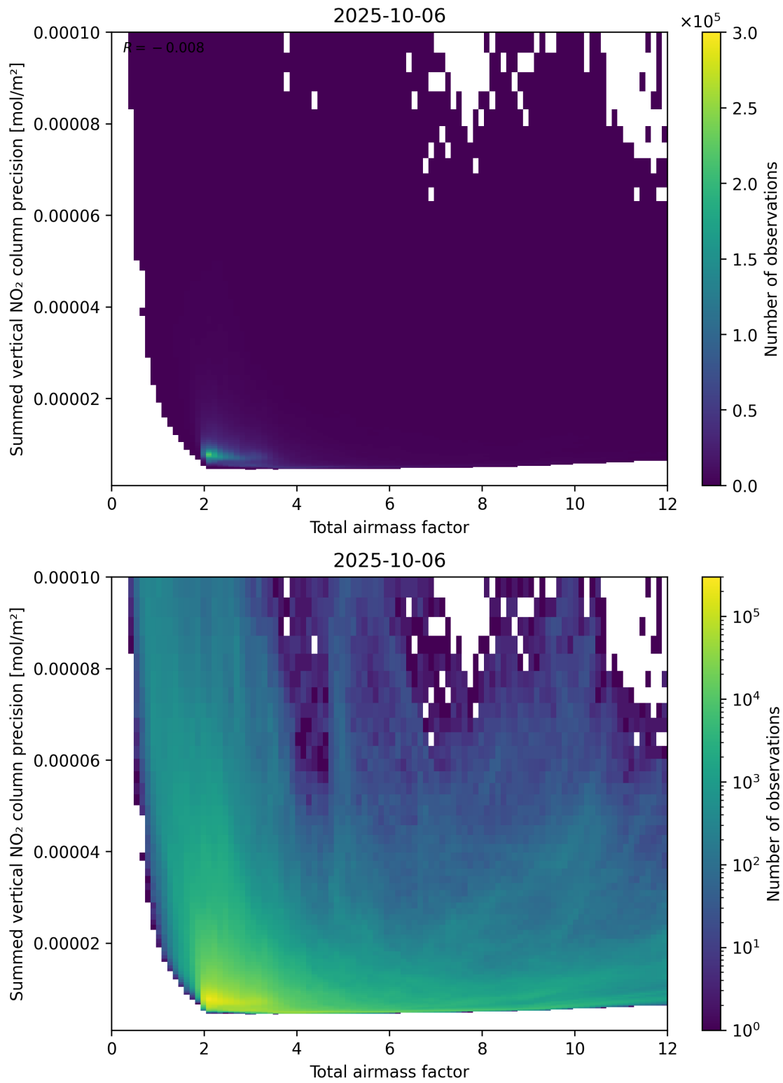
Figure 66: Scatter density plot of “Total airmass factor” against “Summed vertical NO 2 column precision” for 2025-10-06 to 2025-10-07.
