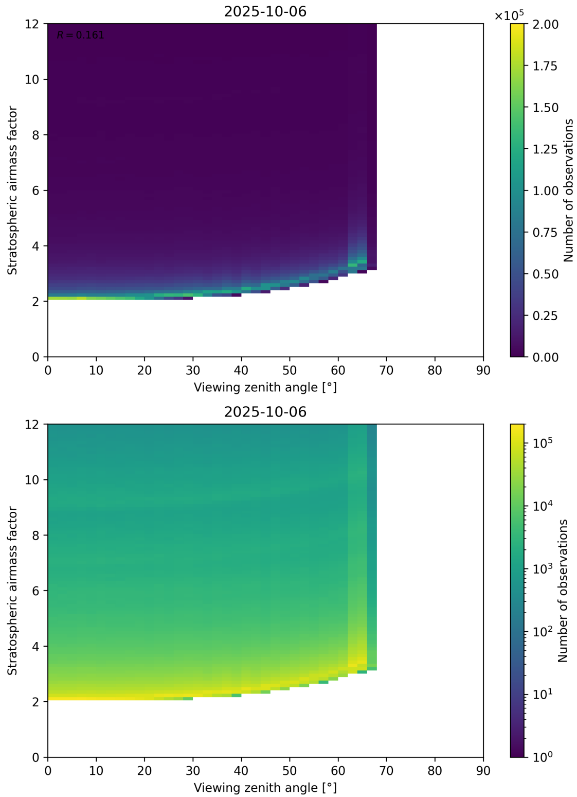
Figure 159: Scatter density plot of “Viewing zenith angle” against “Stratospheric airmass factor” for 2025-10-06 to 2025-10-07.
