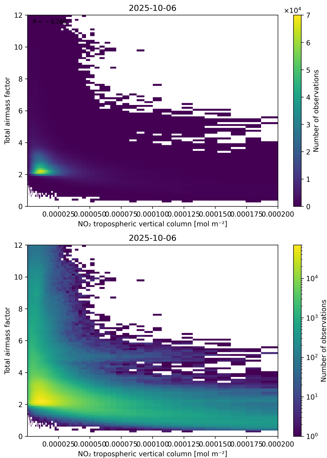
Figure 122: Scatter density plot of “NO 2 tropospheric vertical column” against “Total air mass factor” for 2025-10-06 to 2025-10-07.
