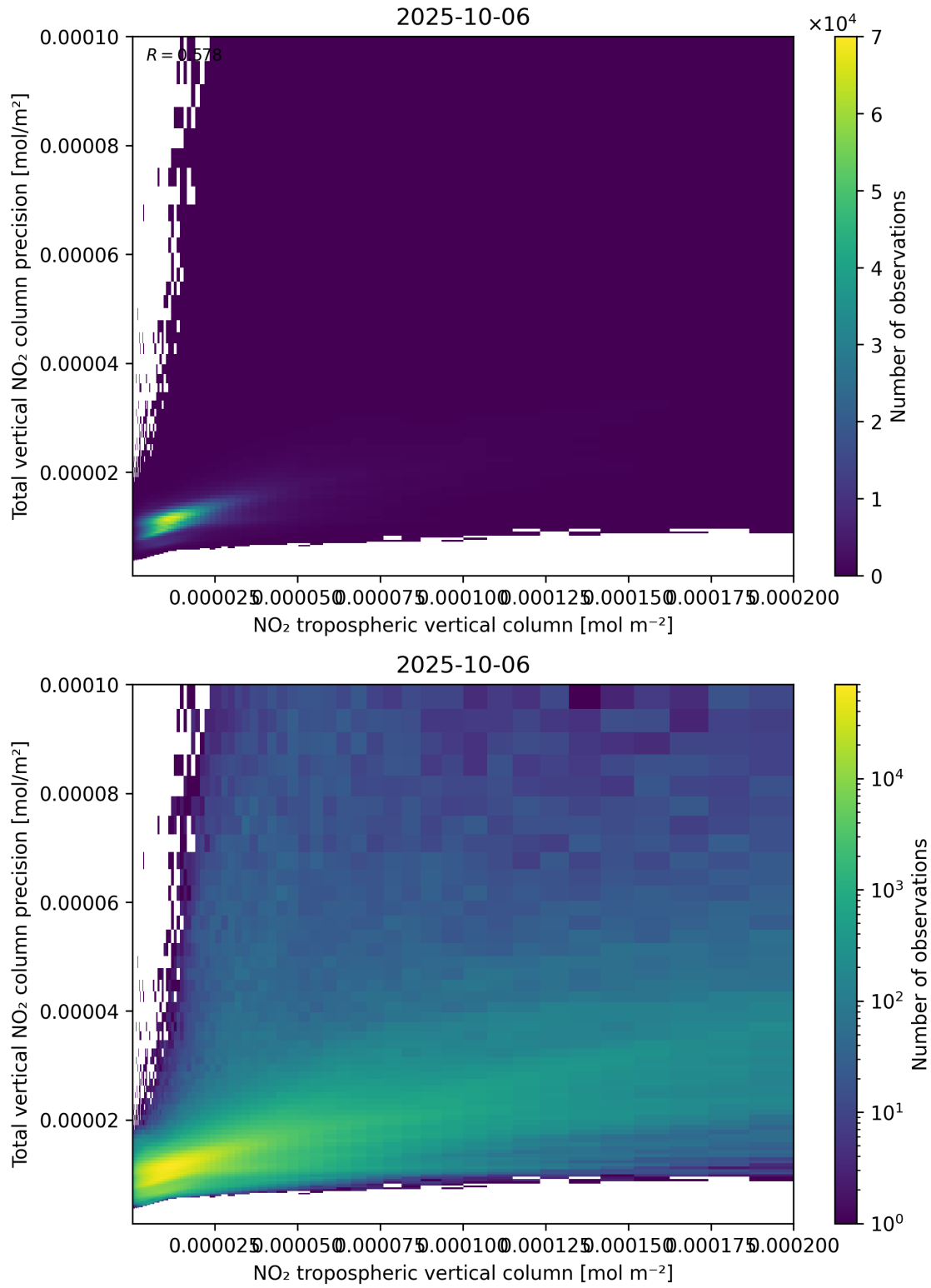
Figure 129: Scatter density plot of “NO 2 tropospheric vertical column” against “Total vertical NO 2 column precision” for 2025-10-06 to 2025-10-07.
