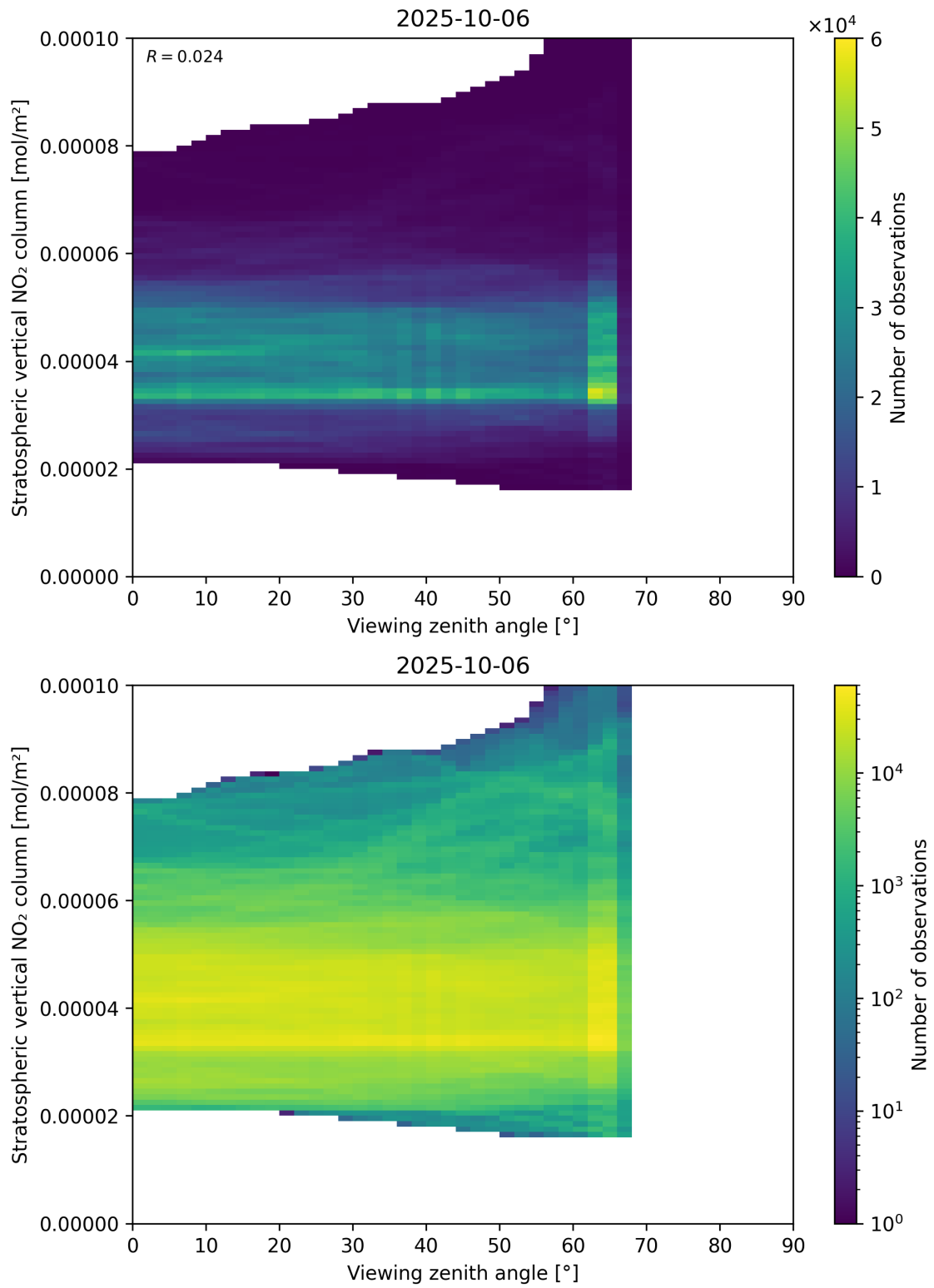
Figure 164: Scatter density plot of “Viewing zenith angle” against “Stratospheric vertical NO 2 column” for 2025-10-06 to 2025-10-07.
