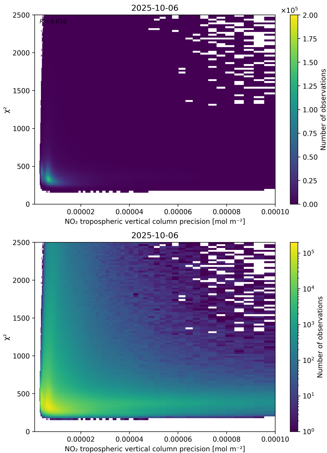
Figure 134: Scatter density plot of “NO 2 tropospheric vertical column precision” against “ \chi^2 ” for 2025-10-06 to 2025-10-07.
