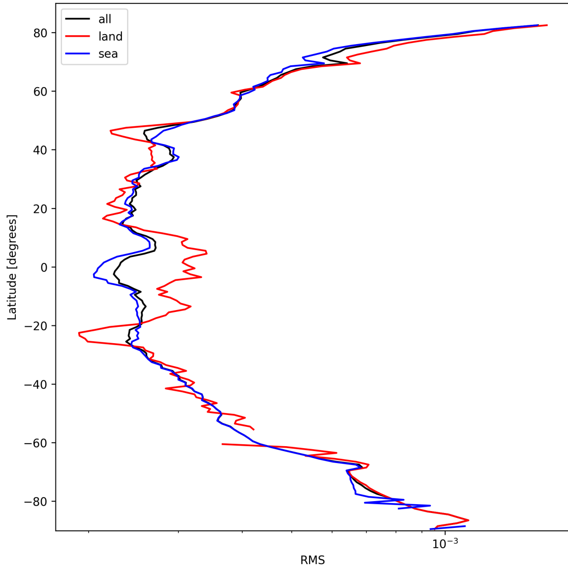
Figure 26: Zonal average of “RMS” for 2025-10-06 to 2025-10-07.
