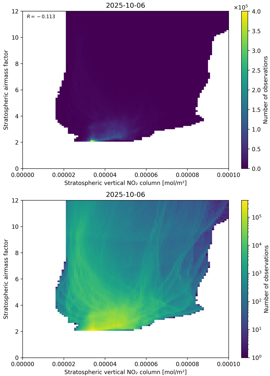
Figure 96: Scatter density plot of “Stratospheric vertical NO 2 column” against “Stratospheric airmass factor” for 2025-10-06 to 2025-10-07.
