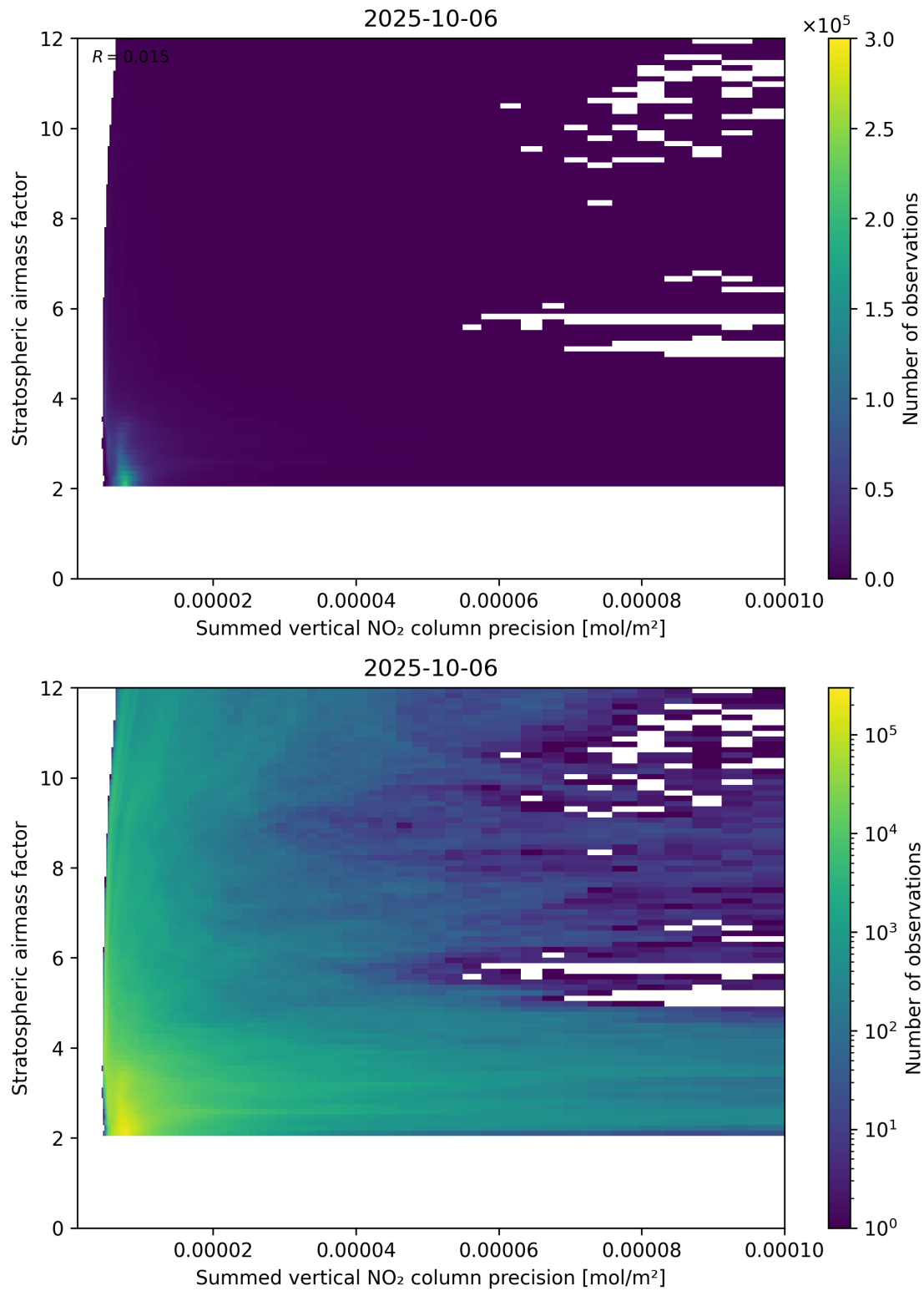
Figure 106: Scatter density plot of “Summed vertical NO 2 column precision” against “Stratospheric airmass factor” for 2025-10-06 to 2025-10-07.
