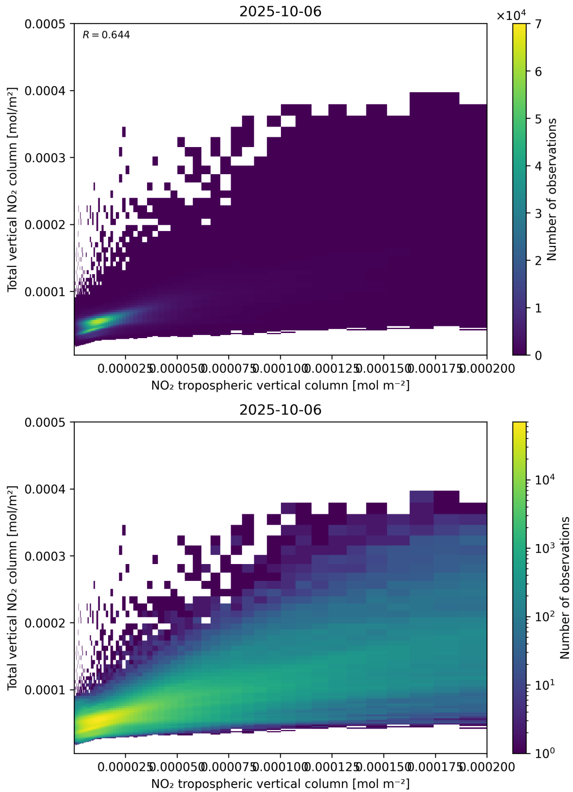
Figure 128: Scatter density plot of “NO 2 tropospheric vertical column” against “Total vertical NO 2 column” for 2025-10-06 to 2025-10-07.
