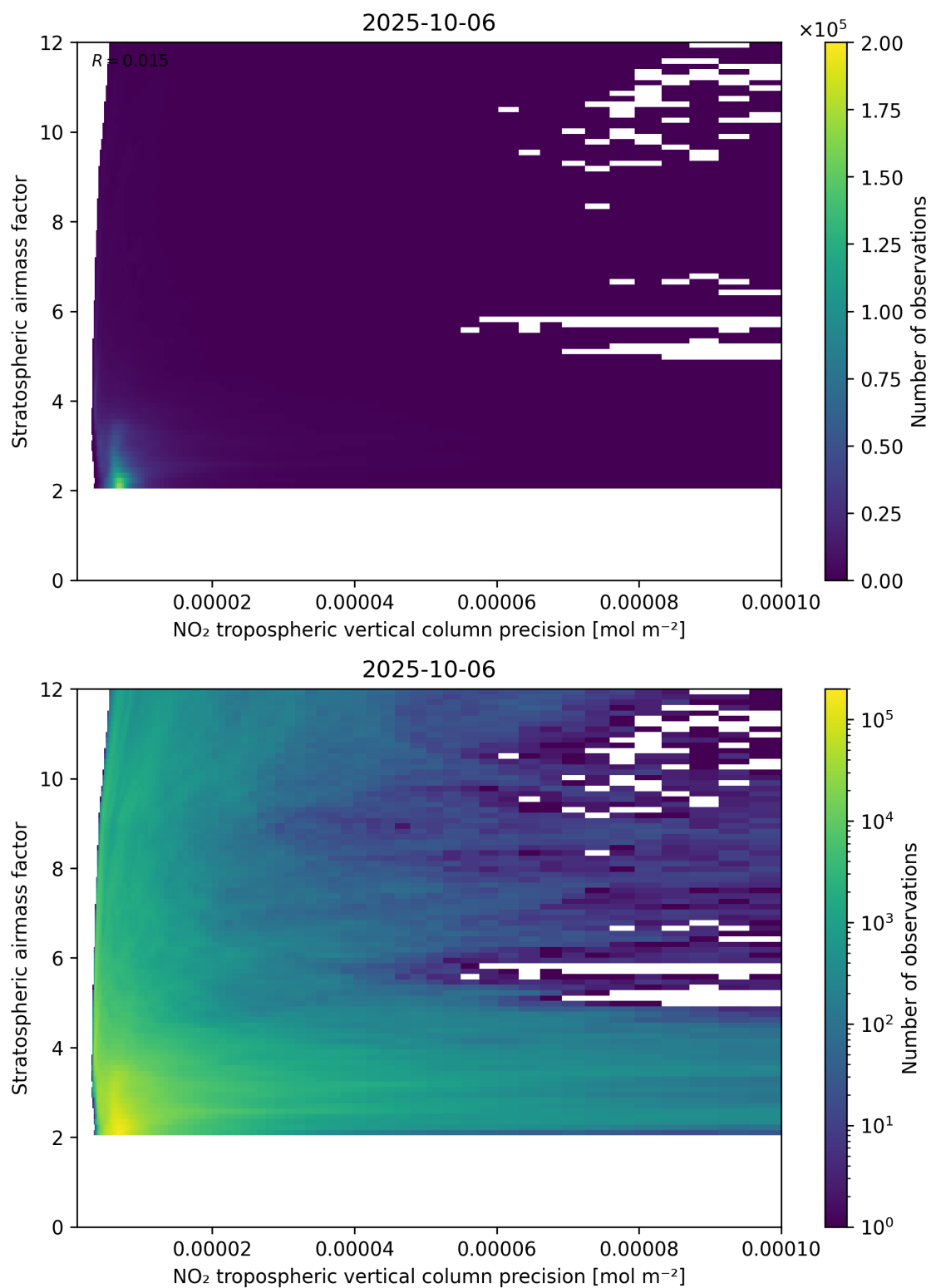
Figure 131: Scatter density plot of “NO 2 tropospheric vertical column precision” against “Stratospheric airmass factor” for 2025-10-06 to 2025-10-07.
