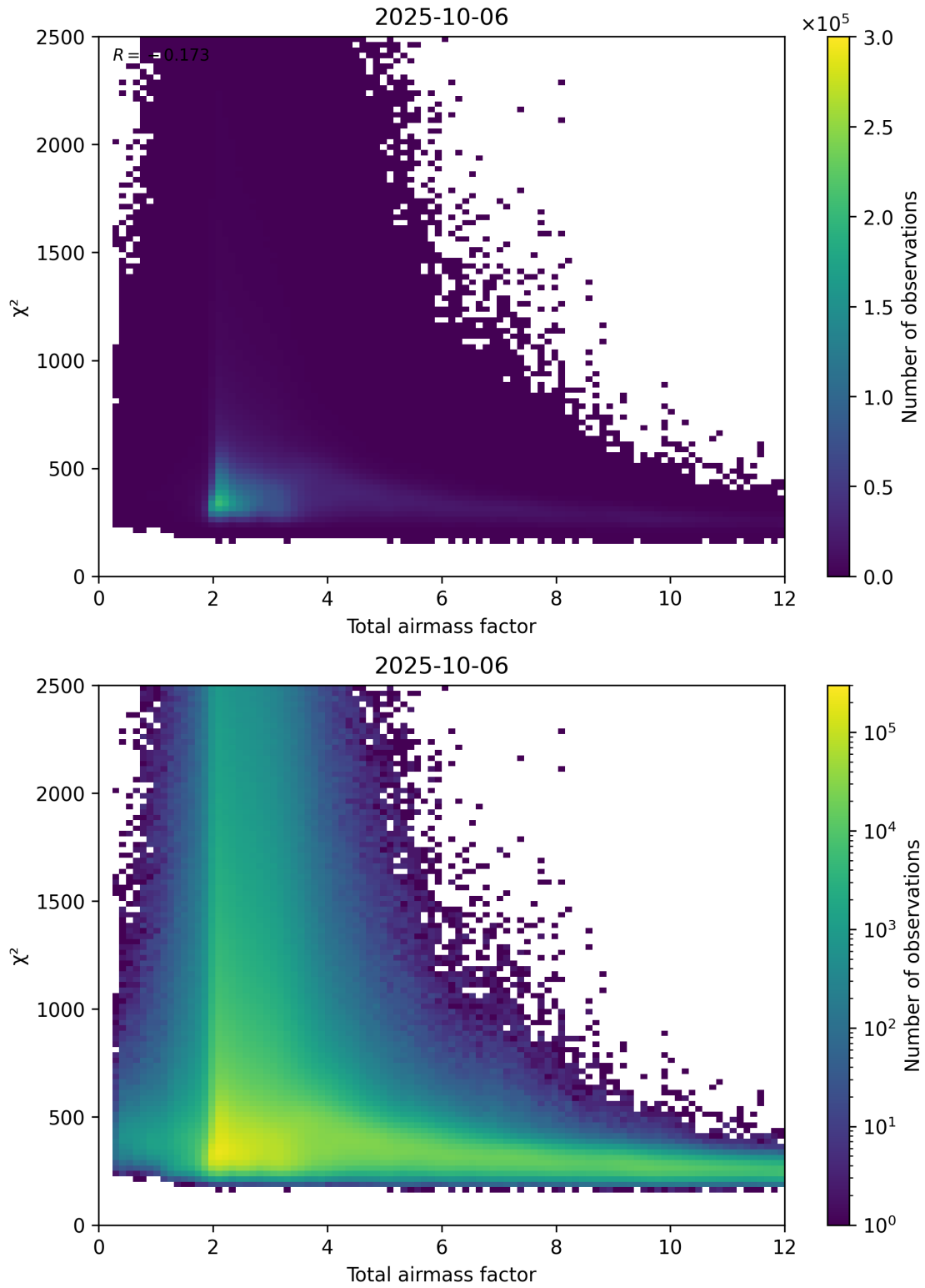
Figure 63: Scatter density plot of “Total airmass factor” against “ \chi^2 ” for 2025-10-06 to 2025-10-07.
