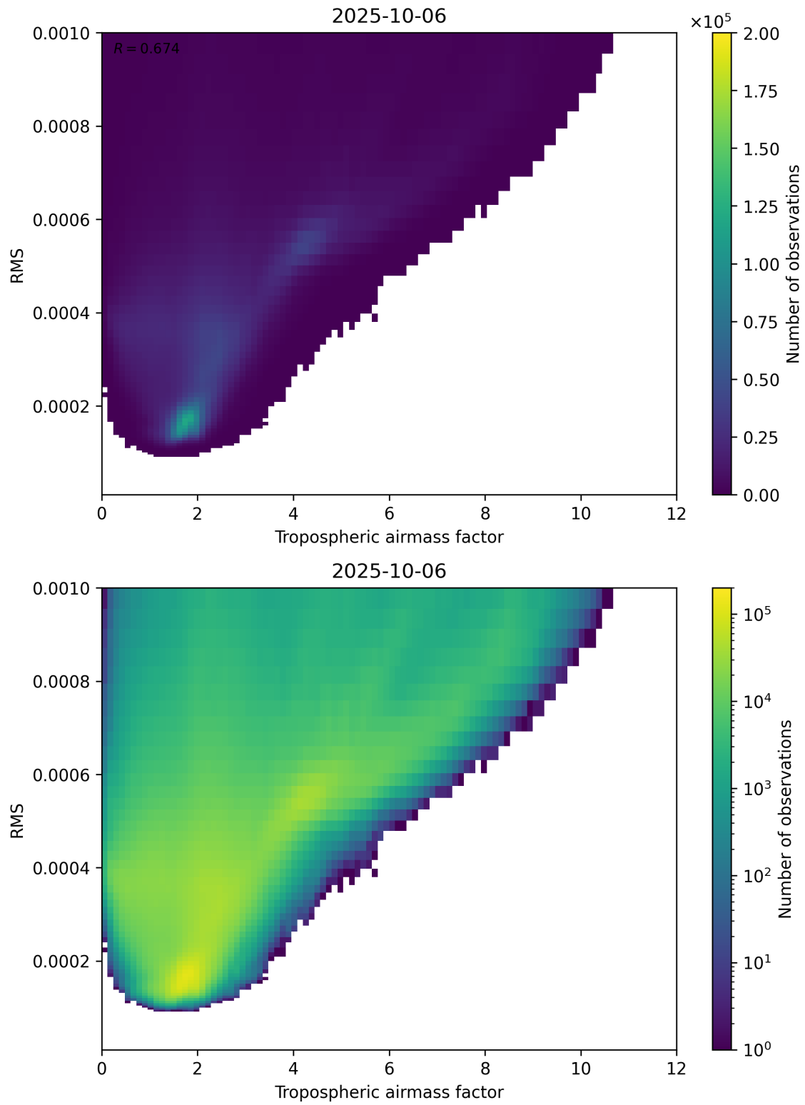
Figure 79: Scatter density plot of “Tropospheric airmass factor” against “RMS” for 2025-10-06 to 2025-10-07.
