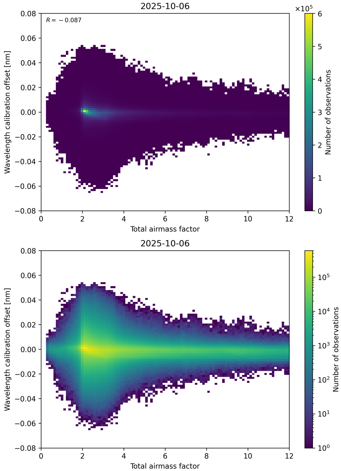
Figure 70: Scatter density plot of “Total airmass factor” against “Wavelength calibration offset” for 2025-10-06 to 2025-10-07.
