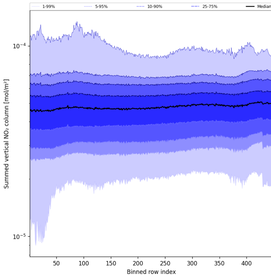
Figure 57: Along track statistics of “Summed vertical NO 2 column” for 2025-10-06 to 2025-10-07
