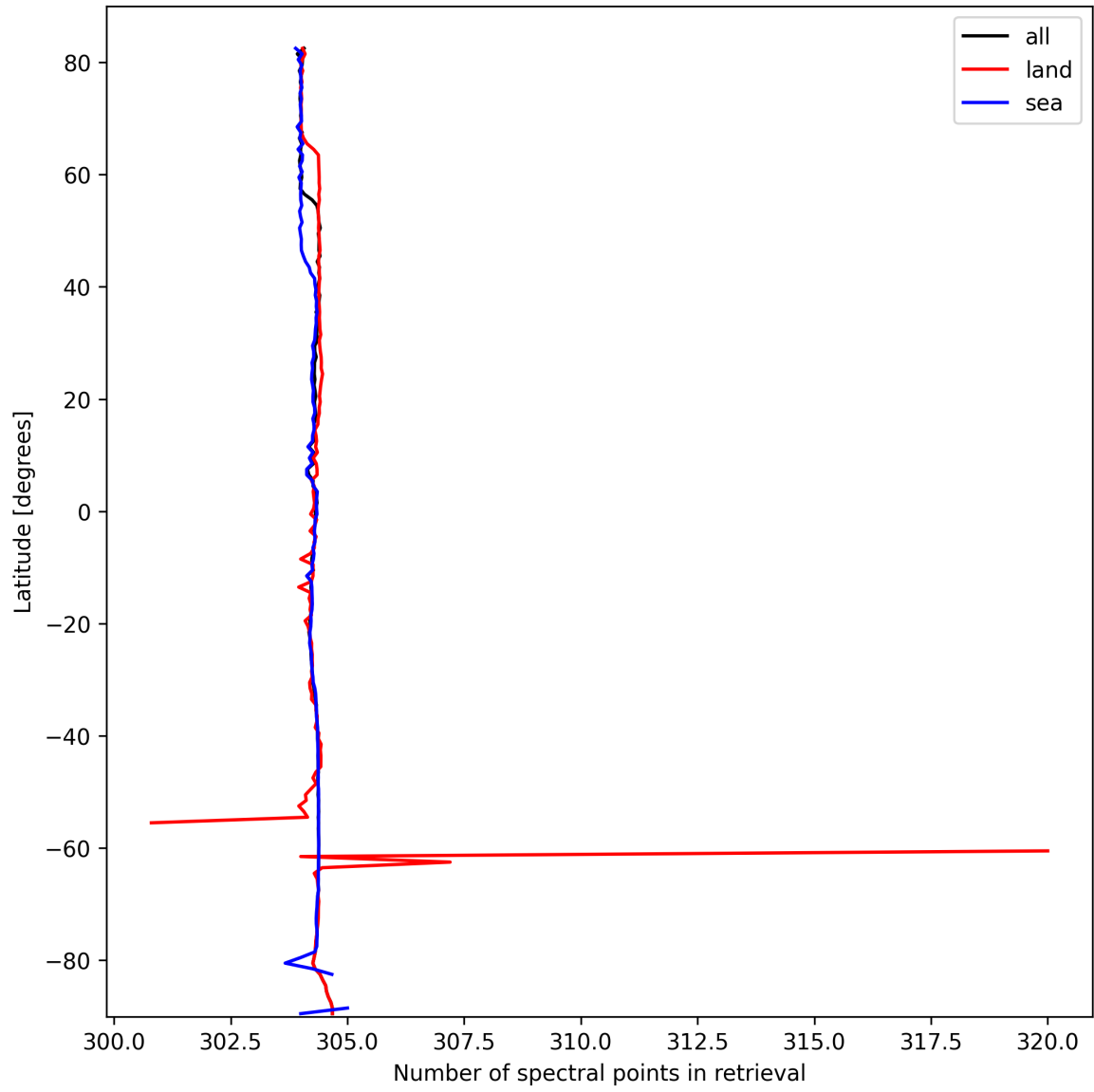
Figure 16: Zonal average of “Number of spectral points in retrieval” for 2025-10-06 to 2025-10-07.
