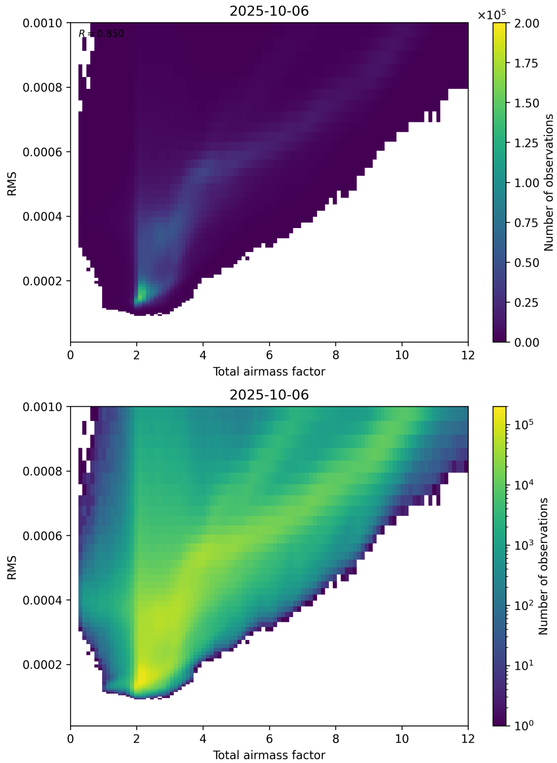
Figure 69: Scatter density plot of “Total airmass factor” against “RMS” for 2025-10-06 to 2025-10-07.
