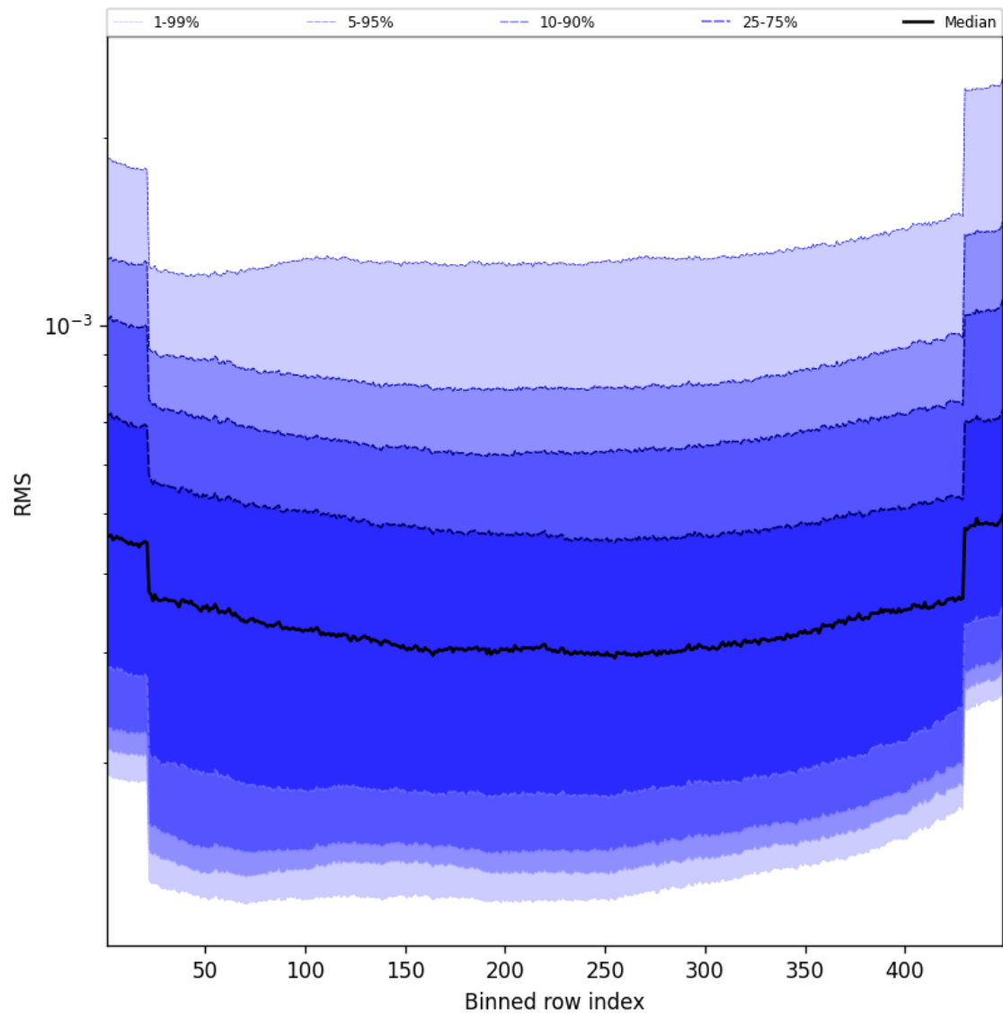
Figure 60: Along track statistics of “RMS” for 2025-10-06 to 2025-10-07
