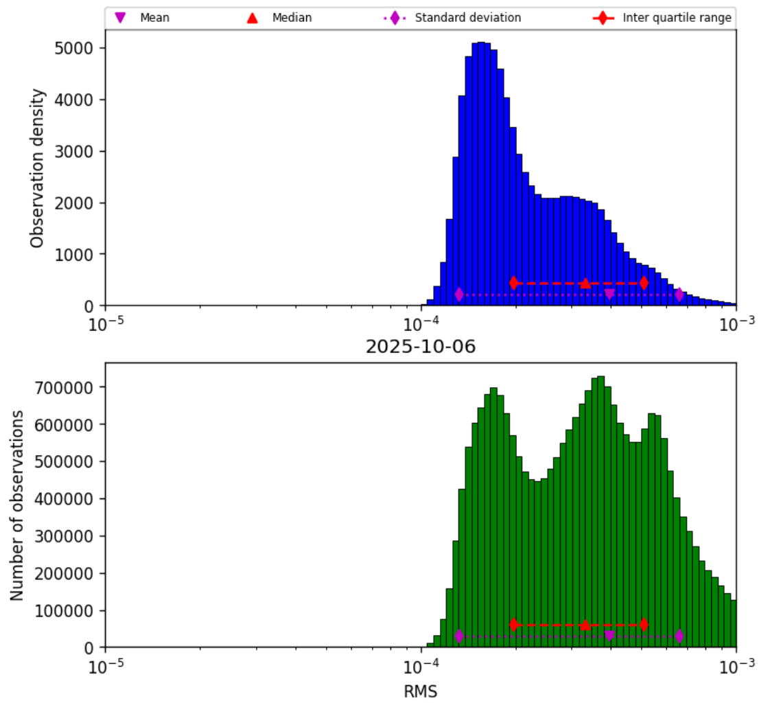
Figure 43: Histogram of “RMS” for 2025-10-06 to 2025-10-07
