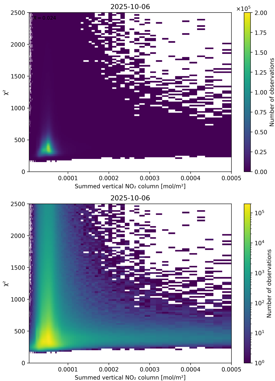
Figure 104: Scatter density plot of “Summed vertical NO 2 column” against “ \chi^2 ” for 2025-10-06 to 2025-10-07.
