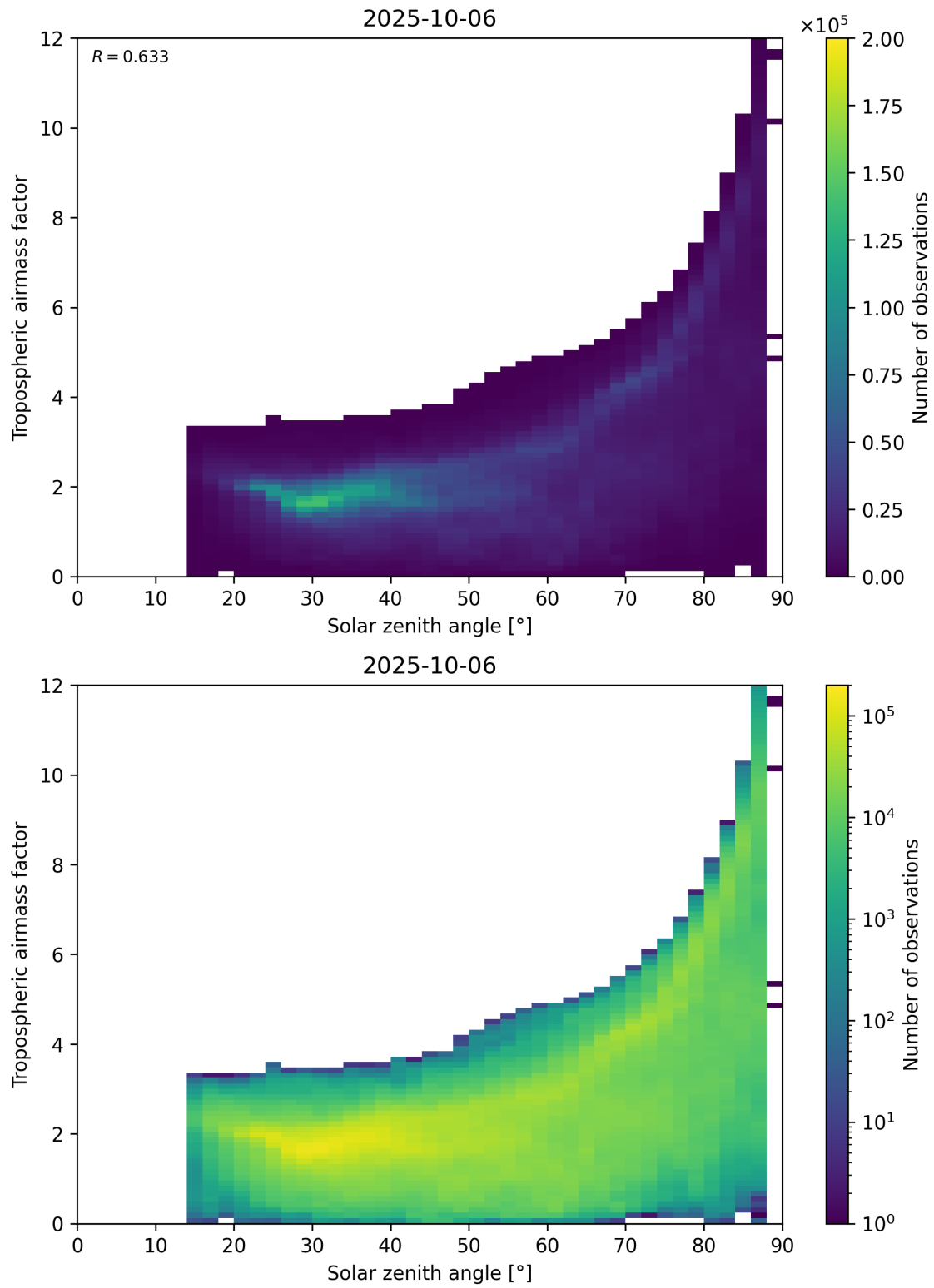
Figure 147: Scatter density plot of “Solar zenith angle” against “Tropospheric airmass factor” for 2025-10-06 to 2025-10-07.
