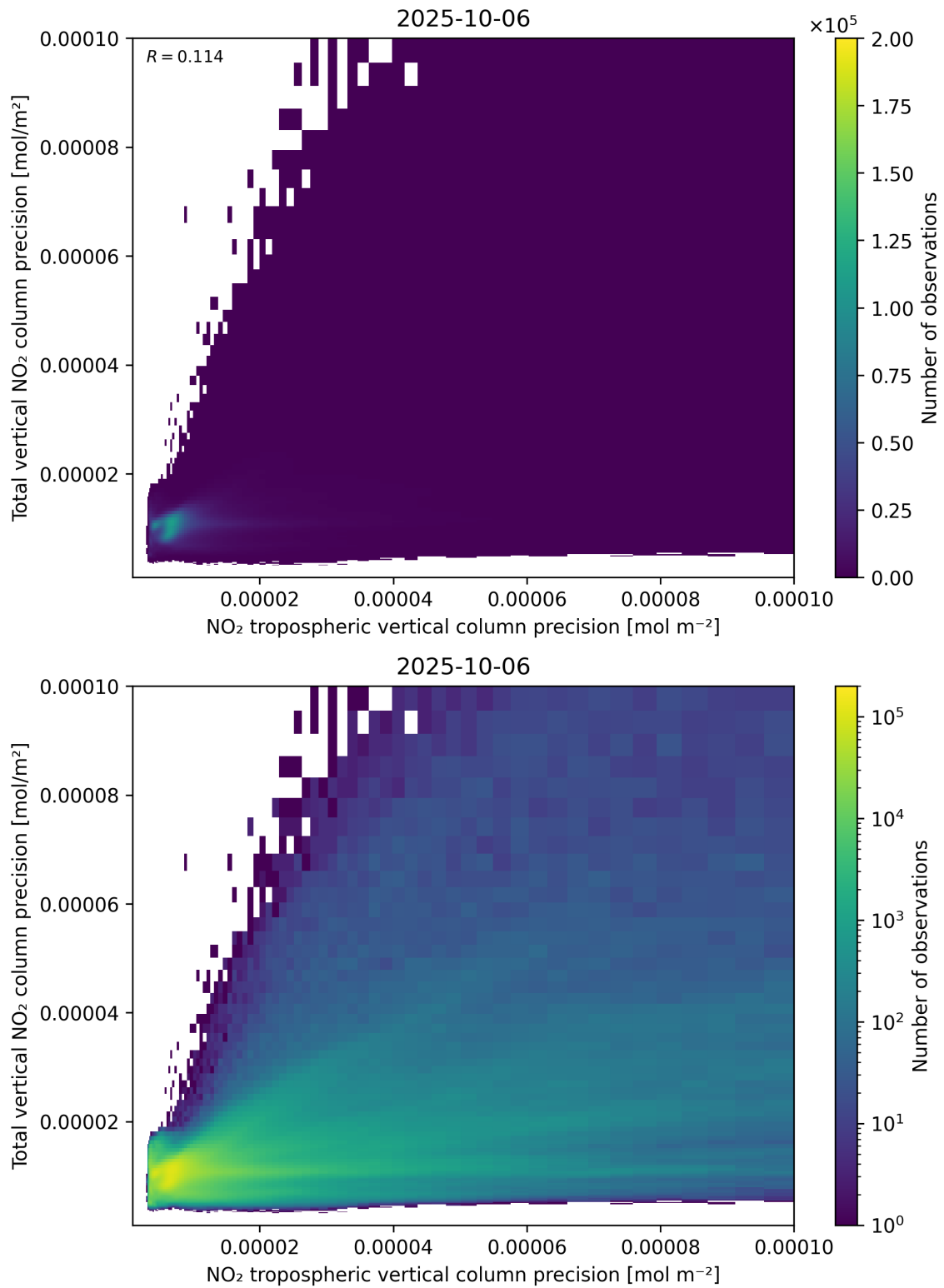
Figure 139: Scatter density plot of “NO 2 tropospheric vertical column precision” against “Total vertical NO 2 column precision” for 2025-10-06 to 2025-10-07.
