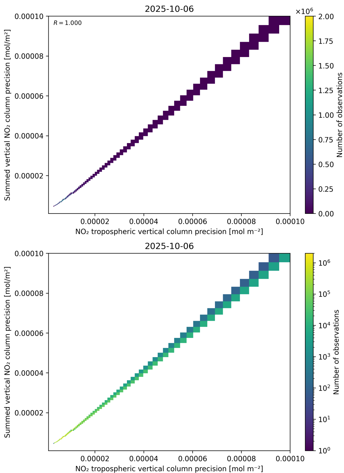
Figure 137: Scatter density plot of “NO 2 tropospheric vertical column precision” against “Summed vertical NO 2 column precision” for 2025-10-06 to 2025-10-07.
