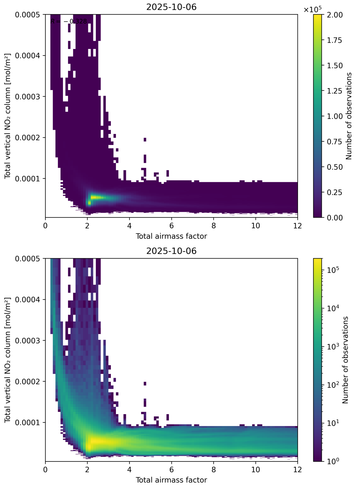
Figure 67: Scatter density plot of “Total airmass factor” against “Total vertical NO 2 column” for 2025-10-06 to 2025-10-07.
