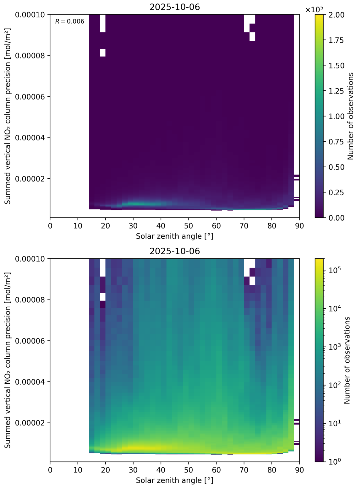
Figure 152: Scatter density plot of “Solar zenith angle” against “Summed vertical NO 2 column precision” for 2025-10-06 to 2025-10-07.
