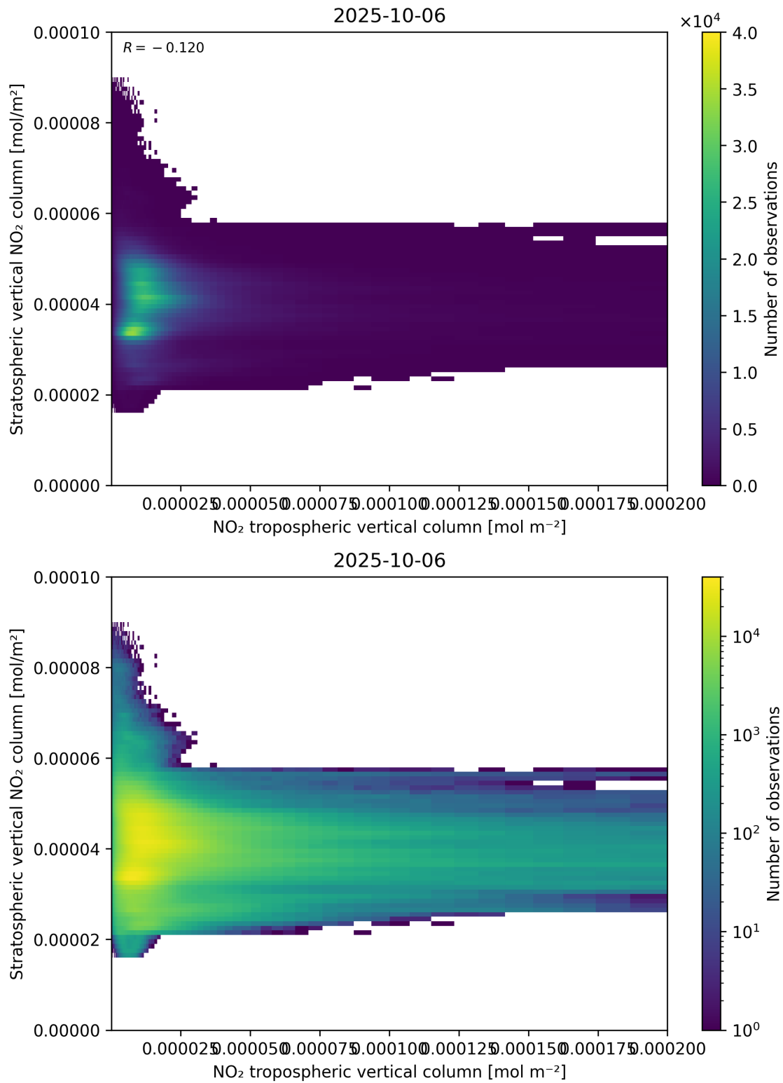
Figure 125: Scatter density plot of “NO 2 tropospheric vertical column” against “Stratospheric vertical NO 2 column” for 2025-10-06 to 2025-10-07.
