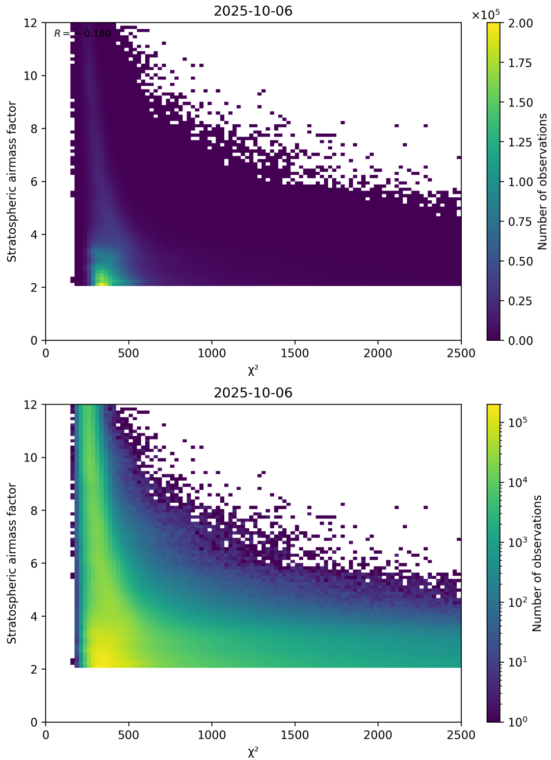
Figure 81: Scatter density plot of “ \chi^2 ” against “Stratospheric airmass factor” for 2025-10-06 to 2025-10-07.
