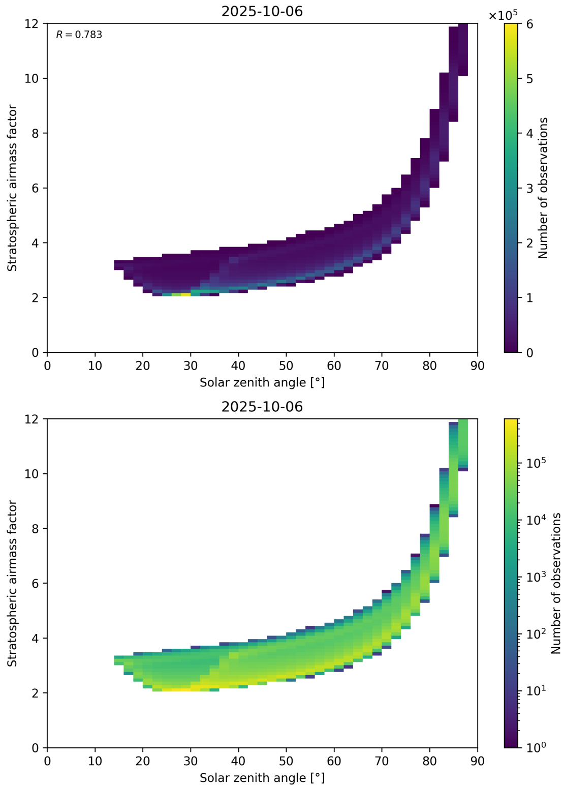
Figure 145: Scatter density plot of “Solar zenith angle” against “Stratospheric airmass factor” for 2025-10-06 to 2025-10-07.
