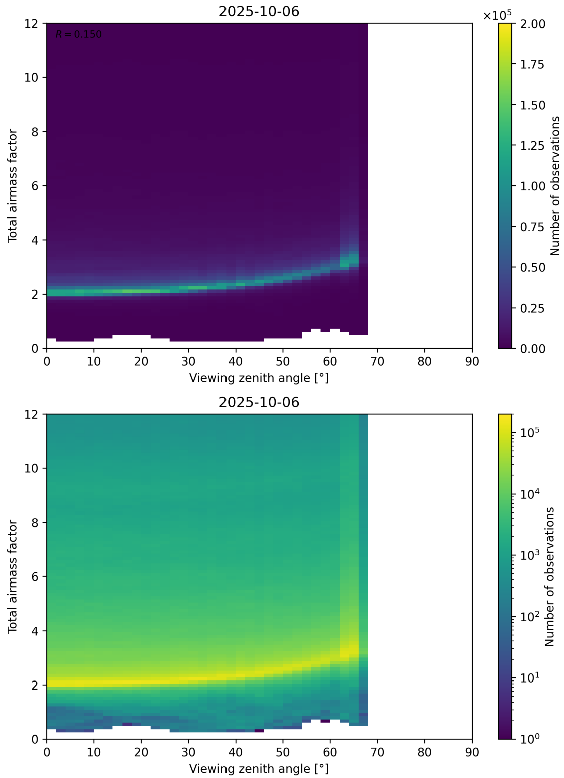
Figure 160: Scatter density plot of “Viewing zenith angle” against “Total airmass factor” for 2025-10-06 to 2025-10-07.
