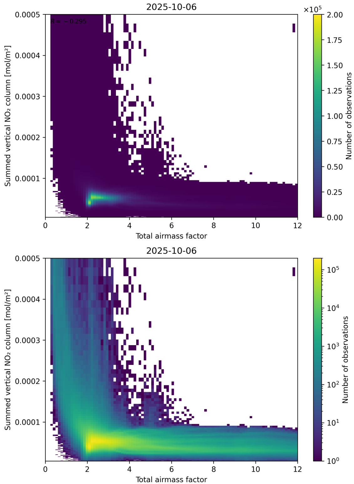
Figure 65: Scatter density plot of “Total airmass factor” against “Summed vertical NO 2 column” for 2025-10-06 to 2025-10-07.
