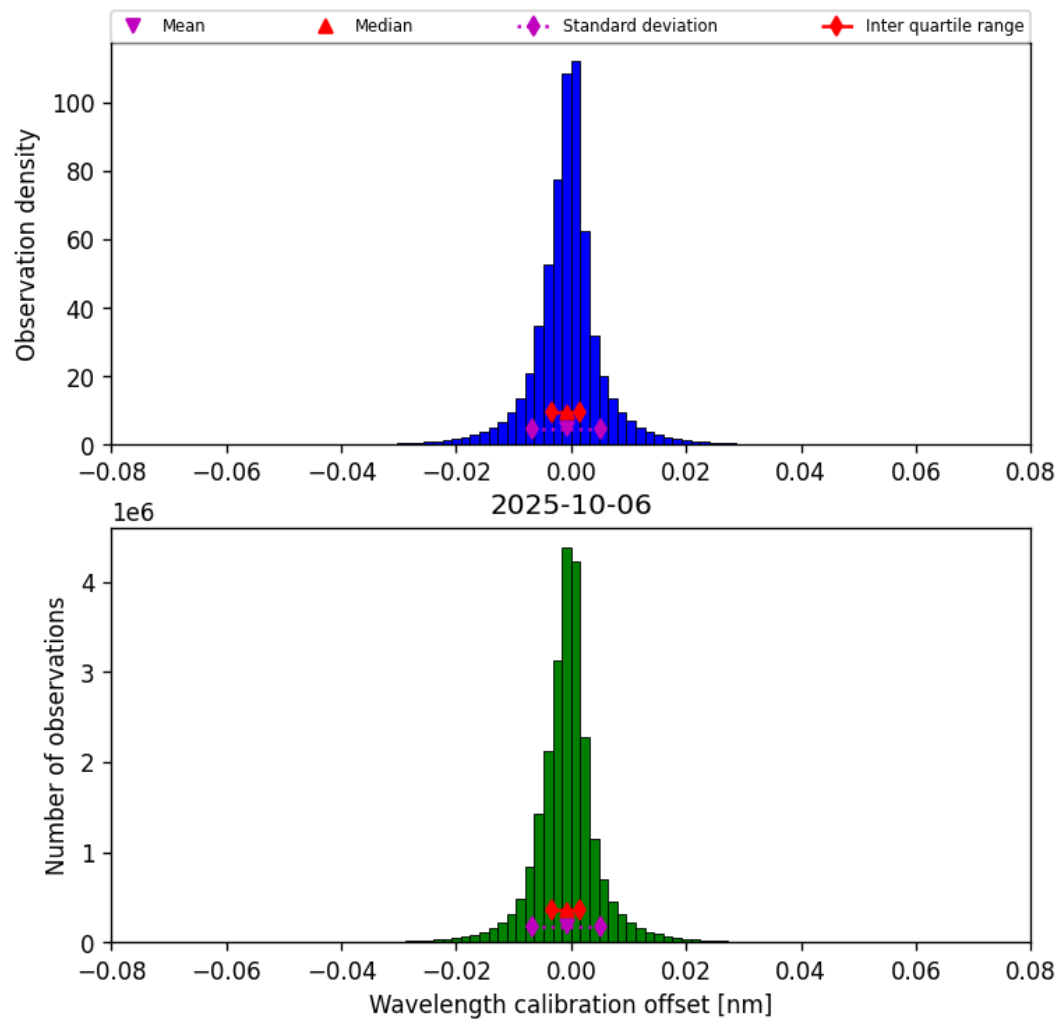
Figure 35: Histogram of “Wavelength calibration offset” for 2025-10-06 to 2025-10-07
