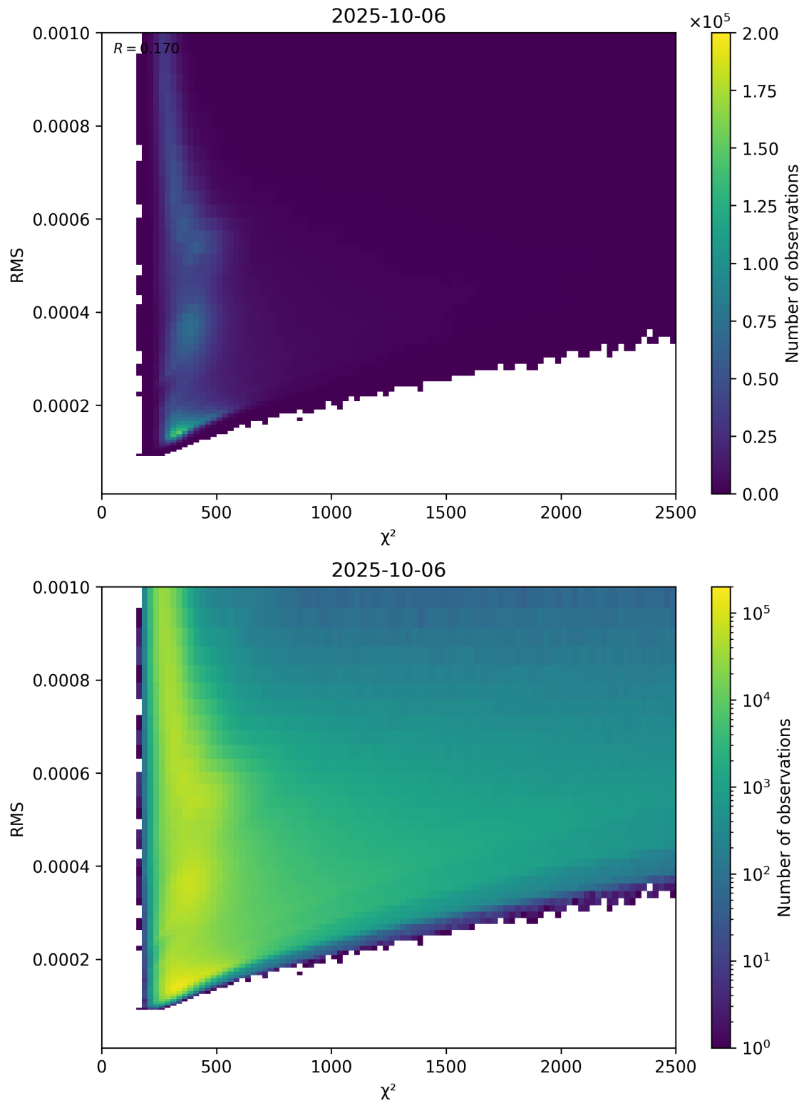
Figure 82: Scatter density plot of “ \chi^2 ” against “RMS” for 2025-10-06 to 2025-10-07.
