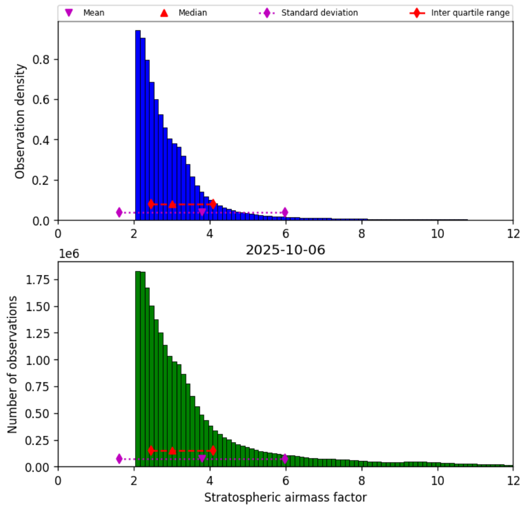
Figure 44: Histogram of “Stratospheric airmass factor” for 2025-10-06 to 2025-10-07
