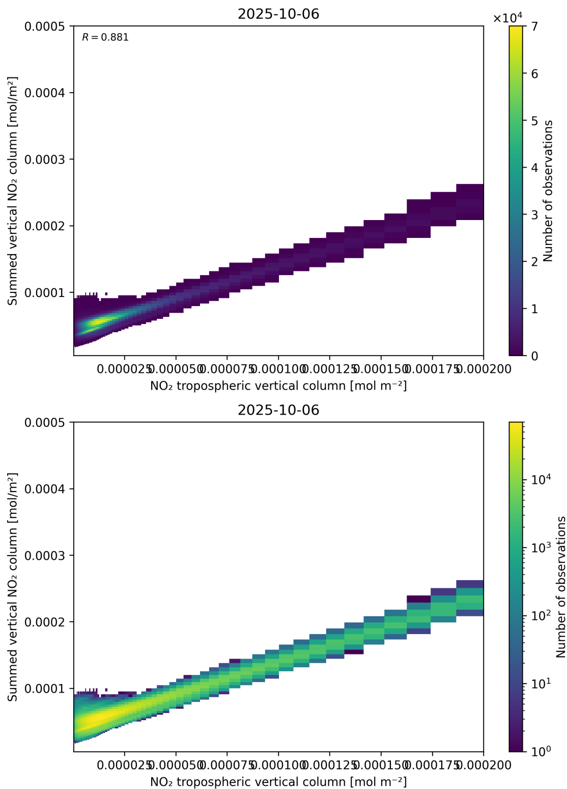
Figure 126: Scatter density plot of “NO 2 tropospheric vertical column” against “Summed vertical NO 2 column” for 2025-10-06 to 2025-10-07.
