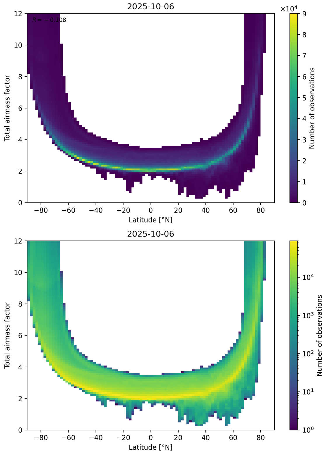
Figure 84: Scatter density plot of “Latitude” against “Total airmass factor” for 2025-10-06 to 2025-10-07.
