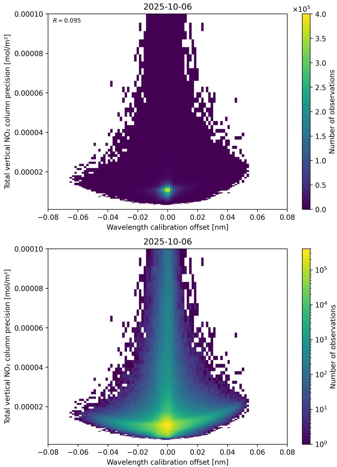
Figure 180: Scatter density plot of “Wavelength calibration offset” against “Total vertical NO 2 column precision” for 2025-10-06 to 2025-10-07.
