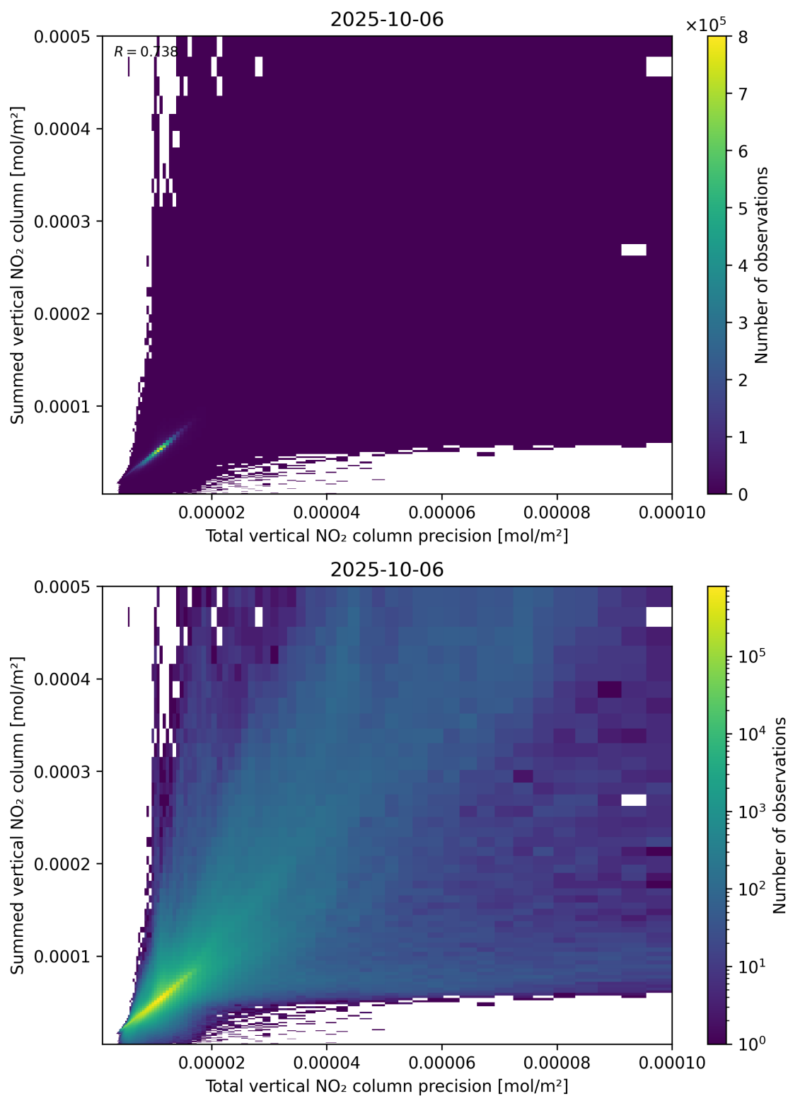
Figure 117: Scatter density plot of “Total vertical NO 2 column precision” against “Summed vertical NO 2 column” for 2025-10-06 to 2025-10-07.
