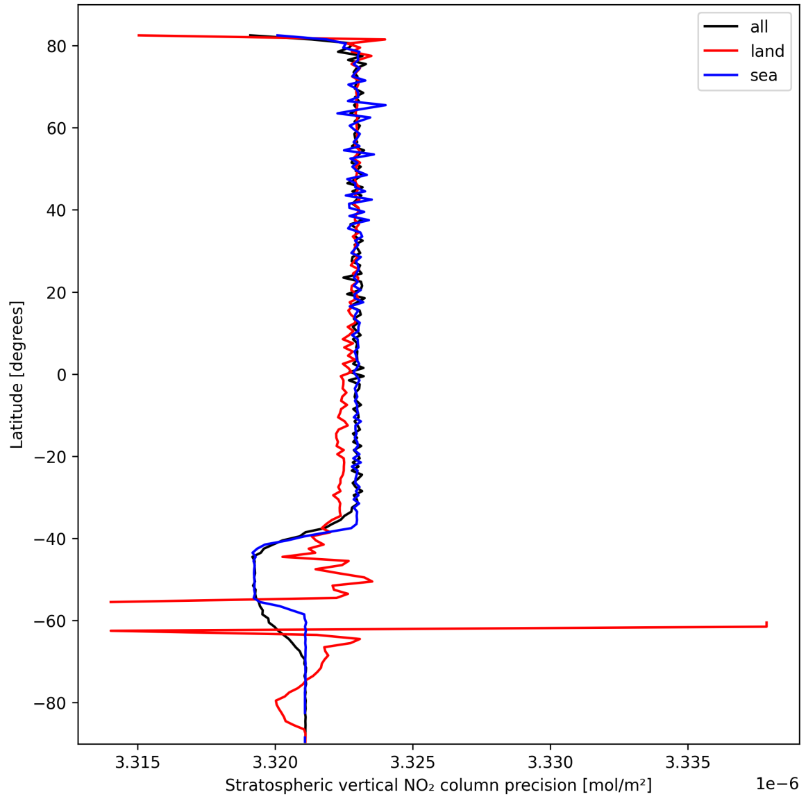
Figure 20: Zonal average of “Stratospheric vertical NO 2 column precision” for 2025-10-06 to 2025-10-07.
