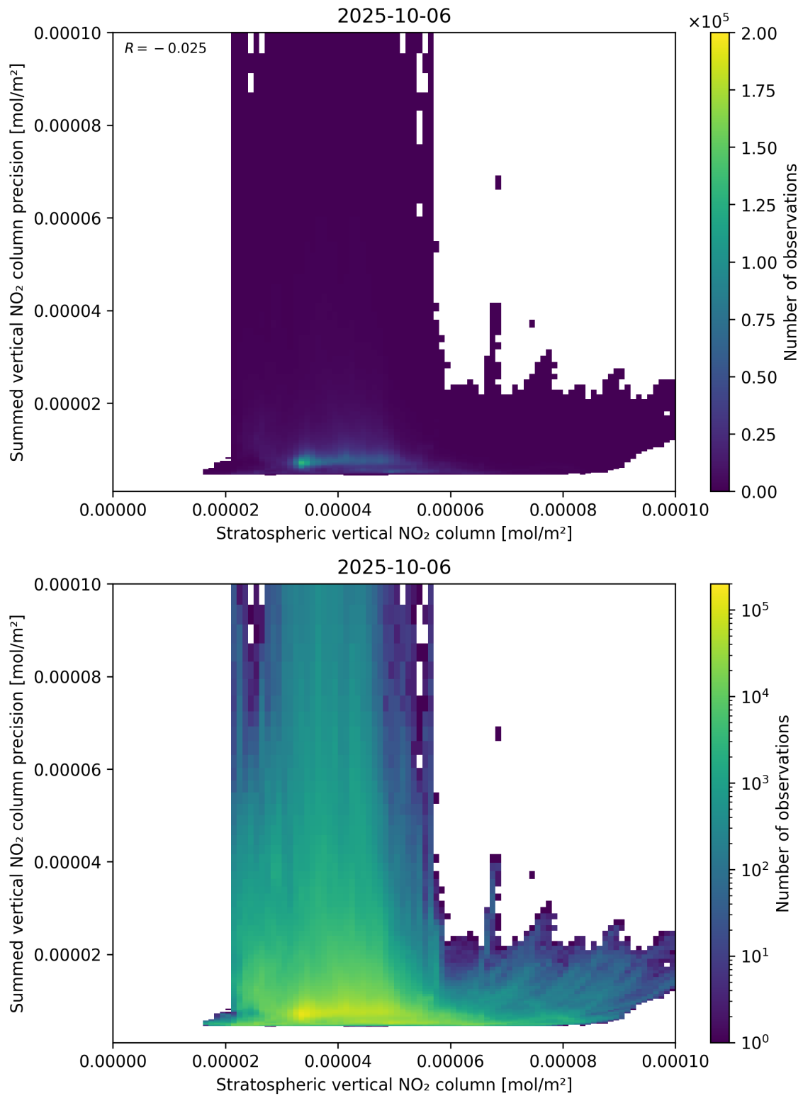
Figure 99: Scatter density plot of “Stratospheric vertical NO 2 column” against “Summed vertical NO 2 column precision” for 2025-10-06 to 2025-10-07.
