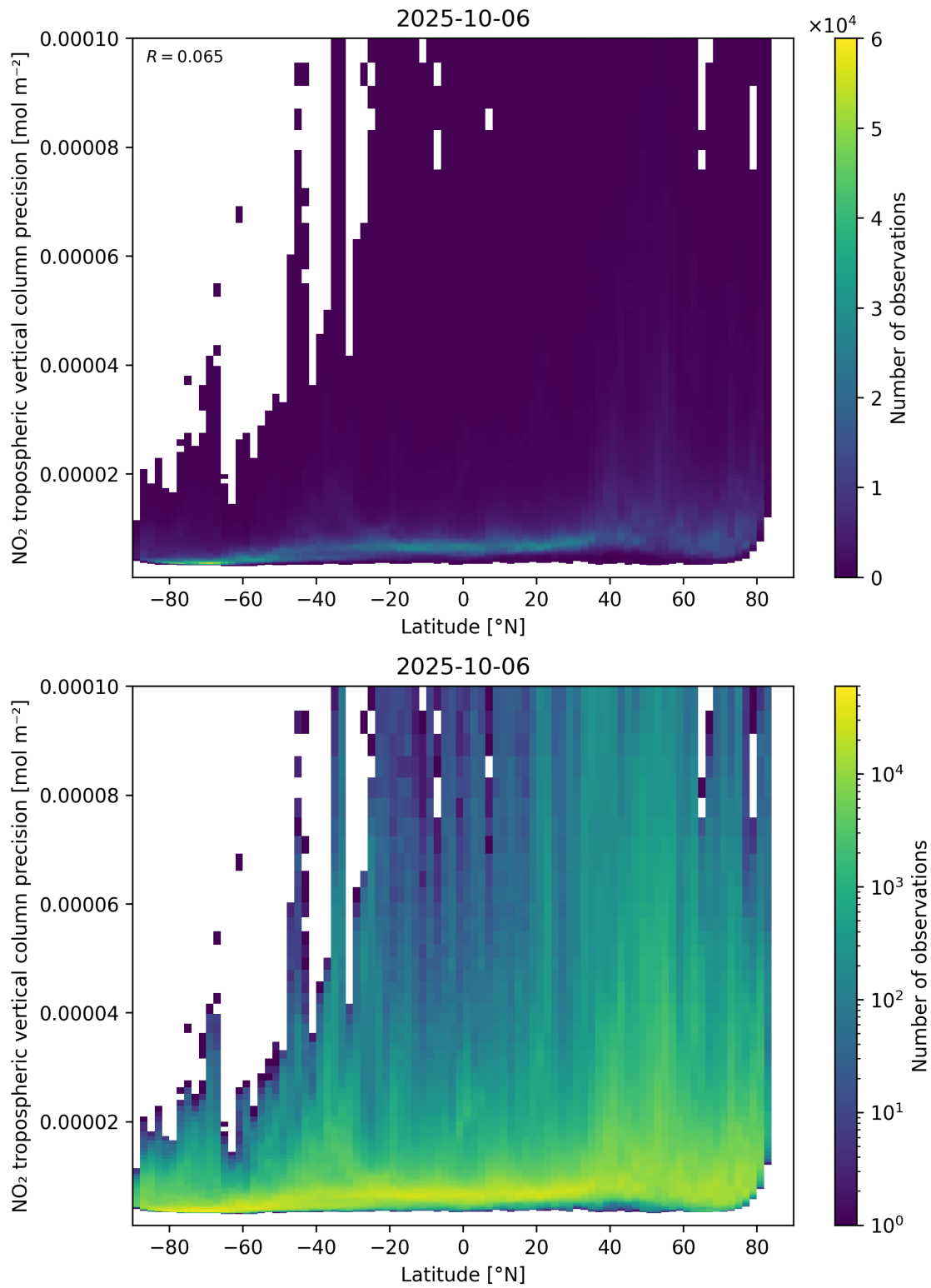
Figure 93: Scatter density plot of “Latitude” against “NO 2 tropospheric vertical column precision” for 2025-10-06 to 2025-10-07.
