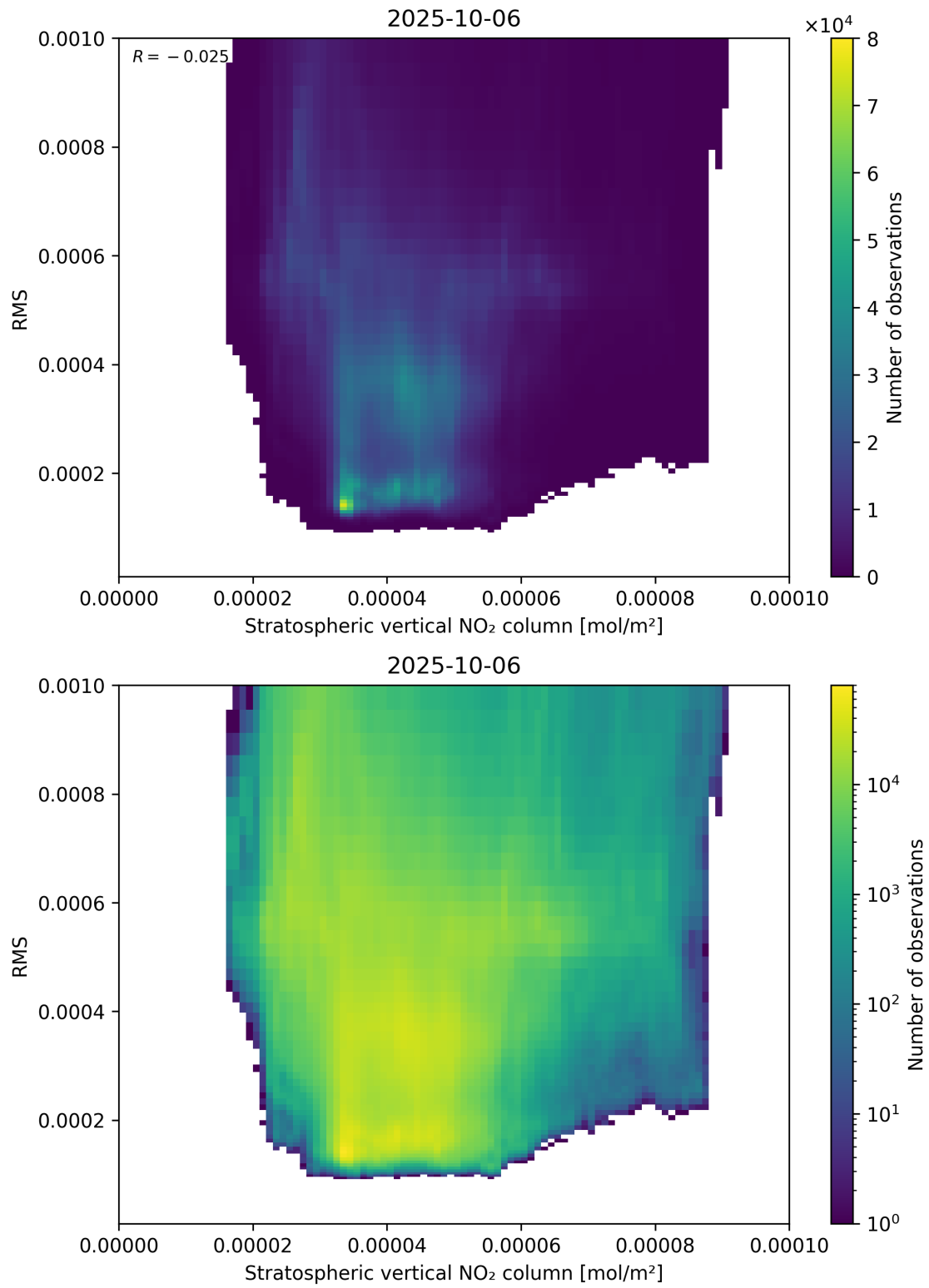
Figure 102: Scatter density plot of “Stratospheric vertical NO 2 column” against “RMS” for 2025-10-06 to 2025-10-07.
