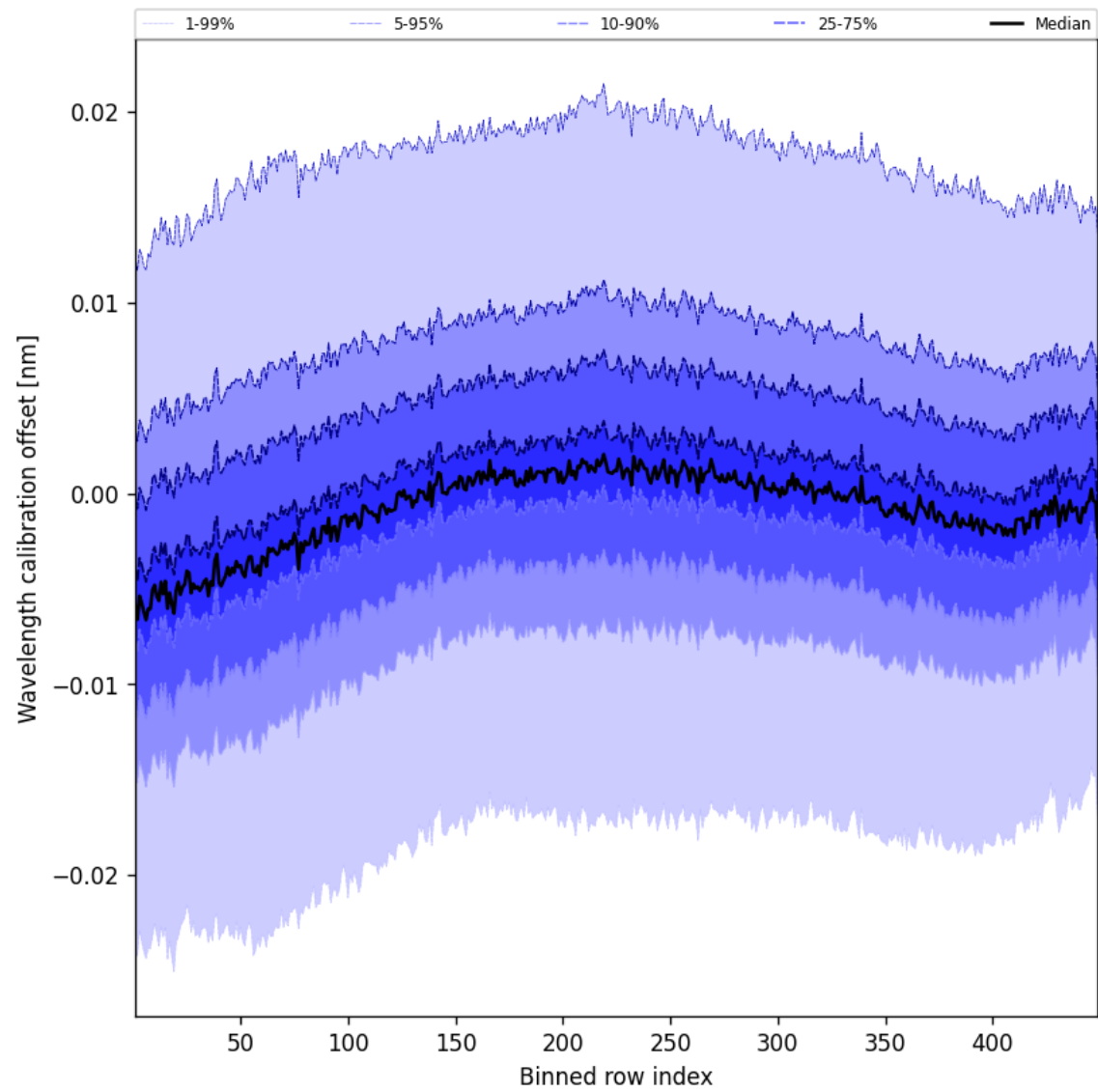
Figure 52: Along track statistics of “Wavelength calibration offset” for 2025-10-06 to 2025-10-07
