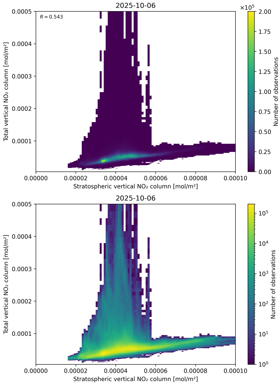
Figure 100: Scatter density plot of “Stratospheric vertical NO 2 column” against “Total vertical NO 2 column” for 2025-10-06 to 2025-10-07.
