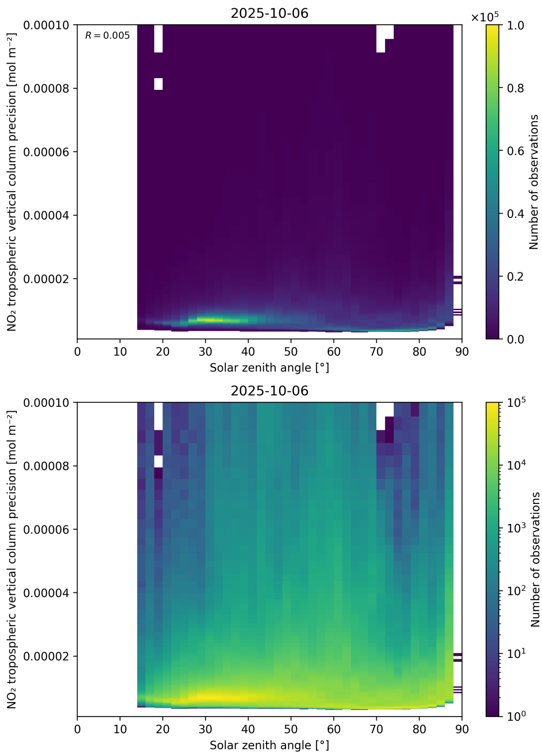
Figure 156: Scatter density plot of “Solar zenith angle” against “NO 2 tropospheric vertical column precision” for 2025-10-06 to 2025-10-07.
