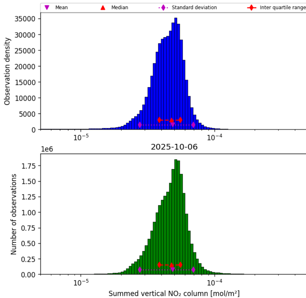
Figure 40: Histogram of “Summed vertical NO 2 column” for 2025-10-06 to 2025-10-07
