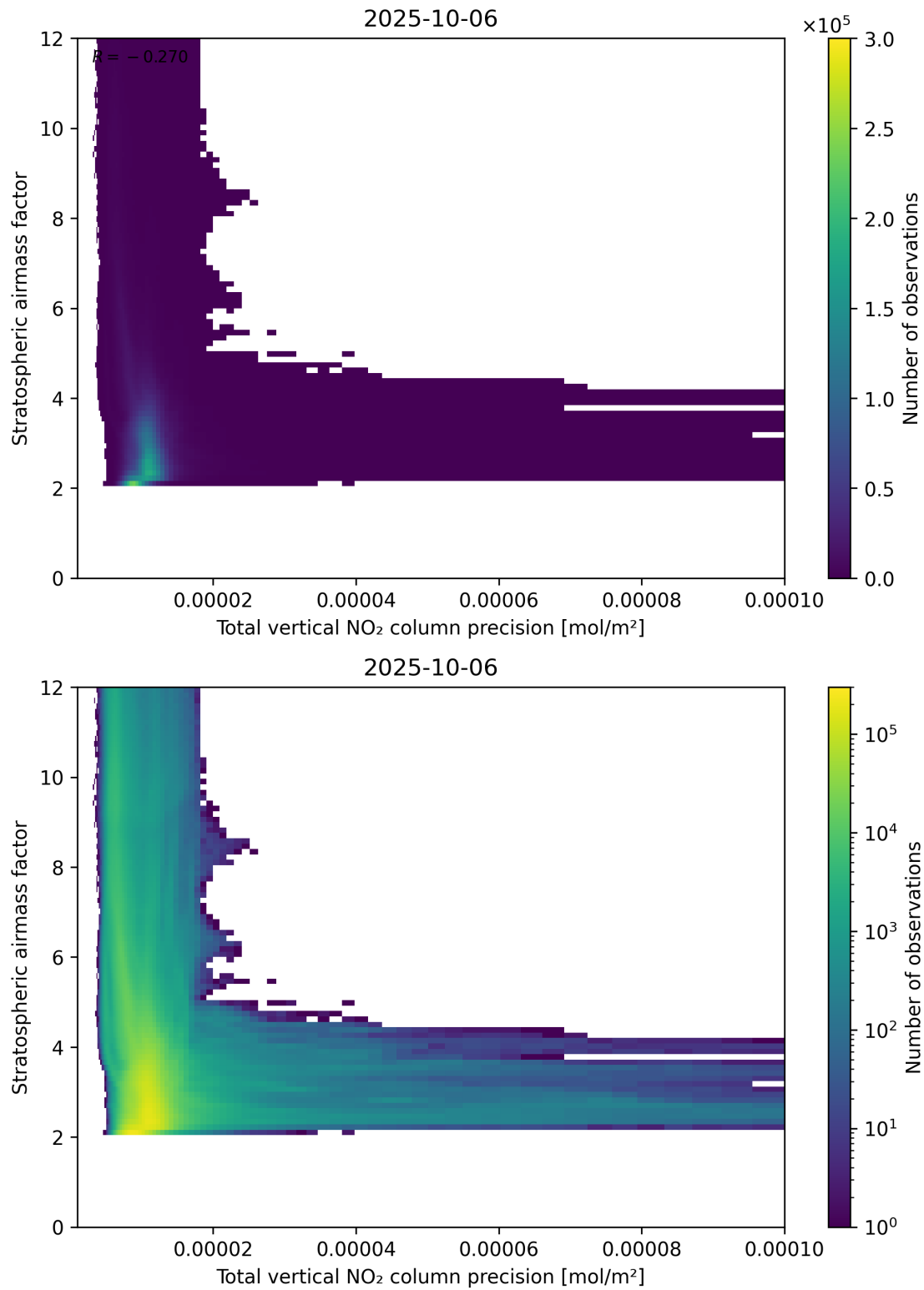
Figure 115: Scatter density plot of “Total vertical NO 2 column precision” against “Stratospheric air mass factor” for 2025-10-06 to 2025-10-07.
