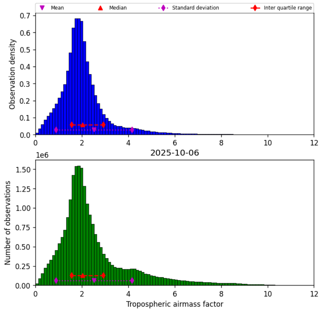
Figure 31: Histogram of “Tropospheric airmass factor” for 2025-10-06 to 2025-10-07
