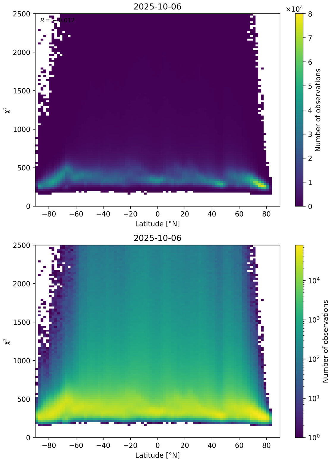
Figure 86: Scatter density plot of “Latitude” against “ \chi^2 ” for 2025-10-06 to 2025-10-07.
