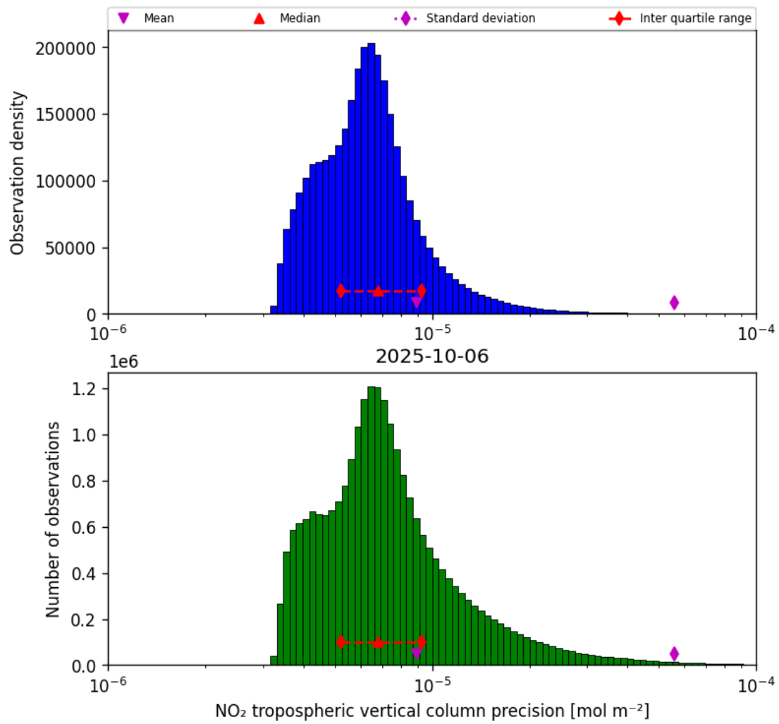
Figure 30: Histogram of “NO 2 tropospheric vertical column precision” for 2025-10-06 to 2025-10-07
