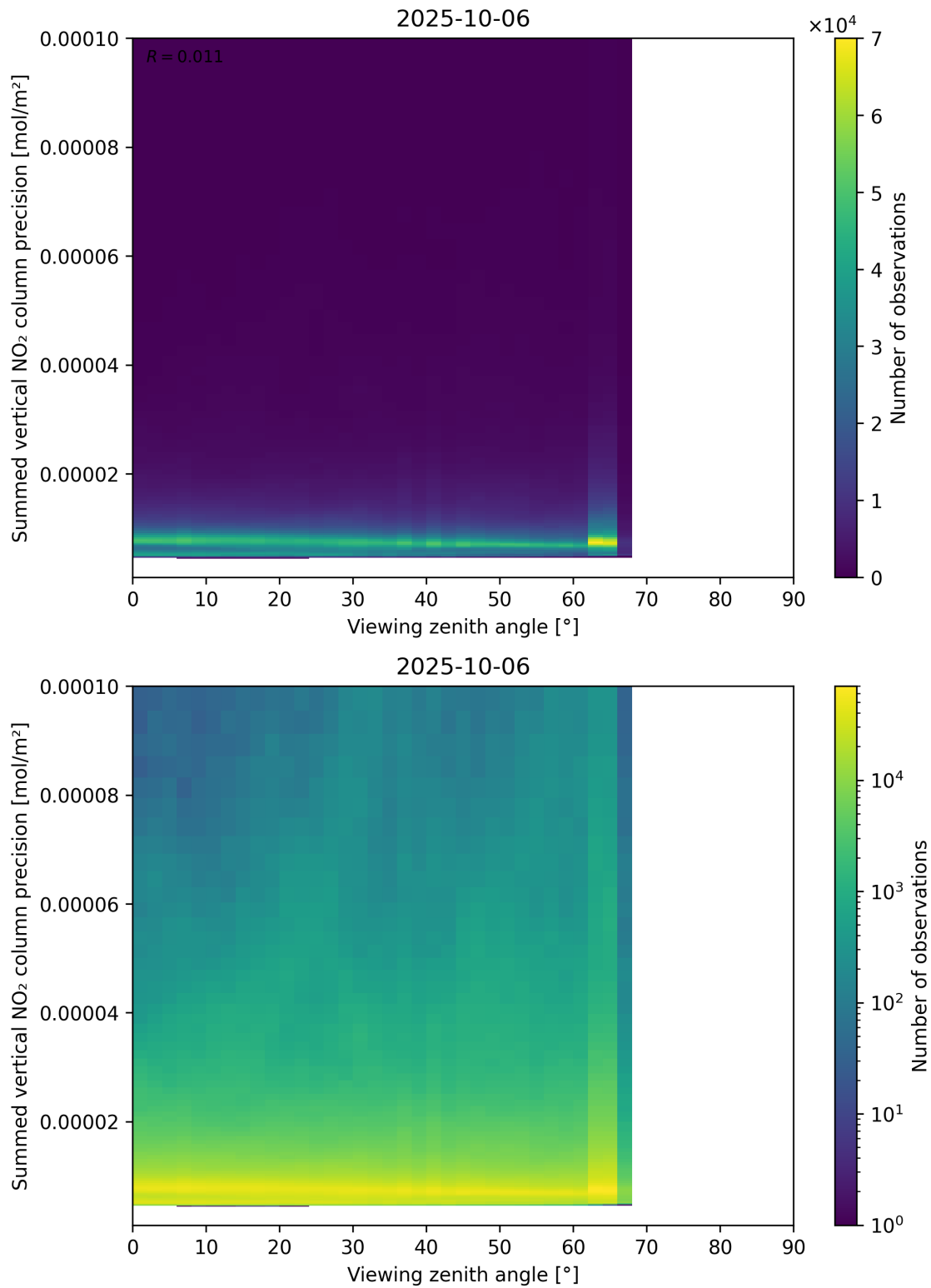
Figure 166: Scatter density plot of “Viewing zenith angle” against “Summed vertical NO 2 column precision” for 2025-10-06 to 2025-10-07.
