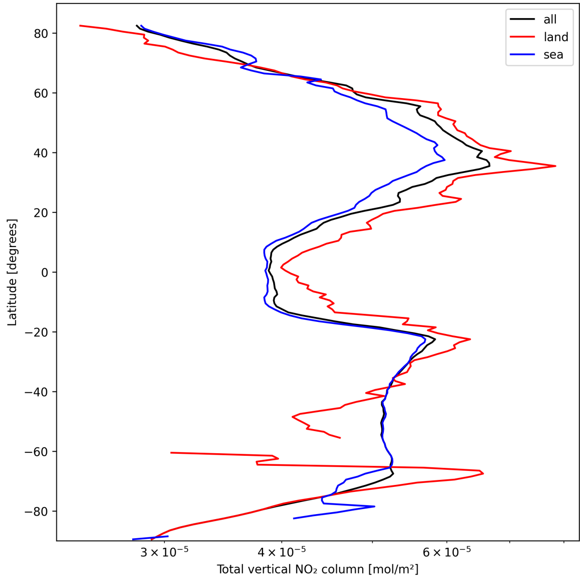
Figure 21: Zonal average of “Total vertical NO 2 column” for 2025-10-06 to 2025-10-07.
