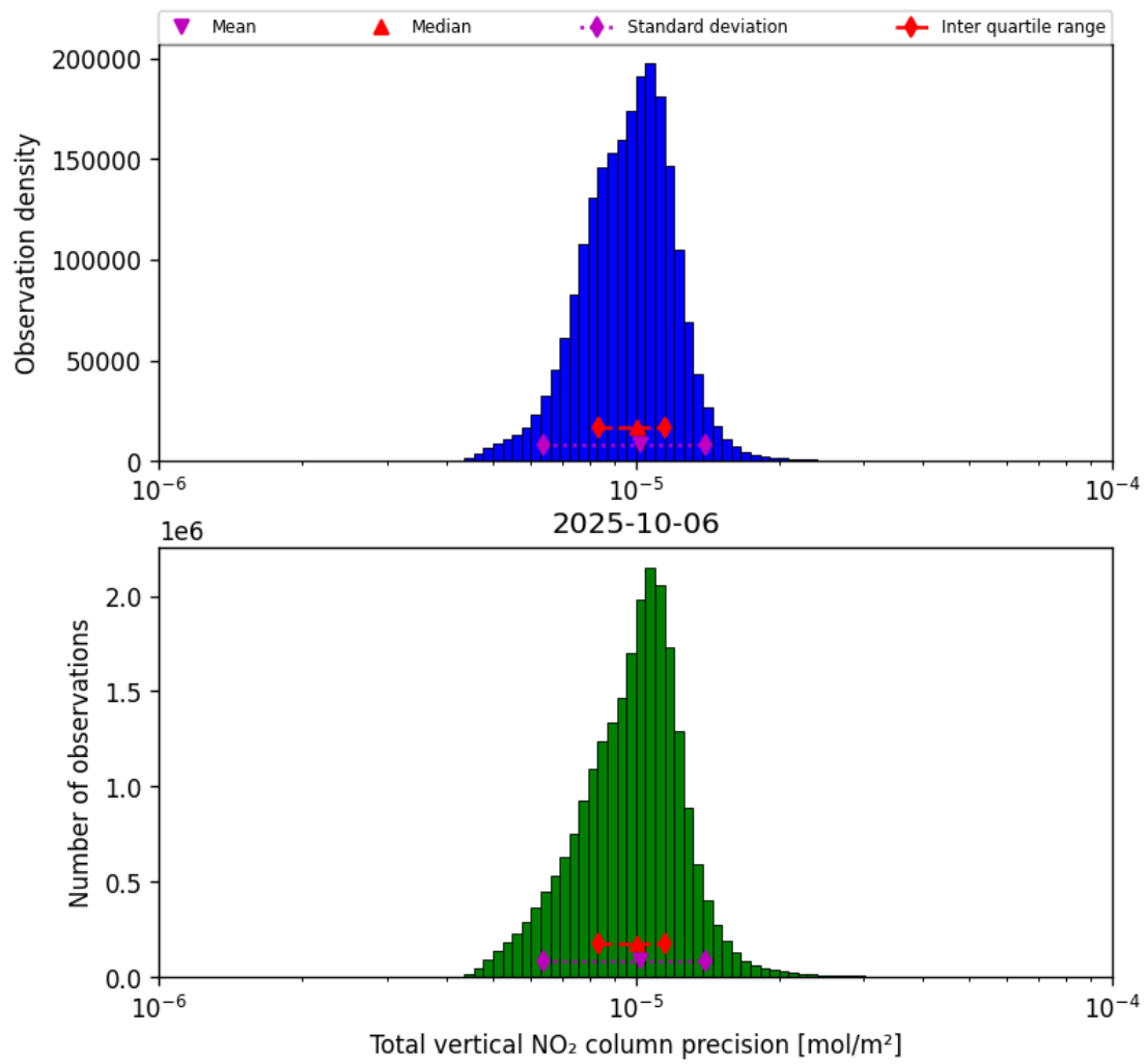
Figure 39: Histogram of "Total vertical NO 2 column precision" for 2025-10-06 to 2025-10-07
