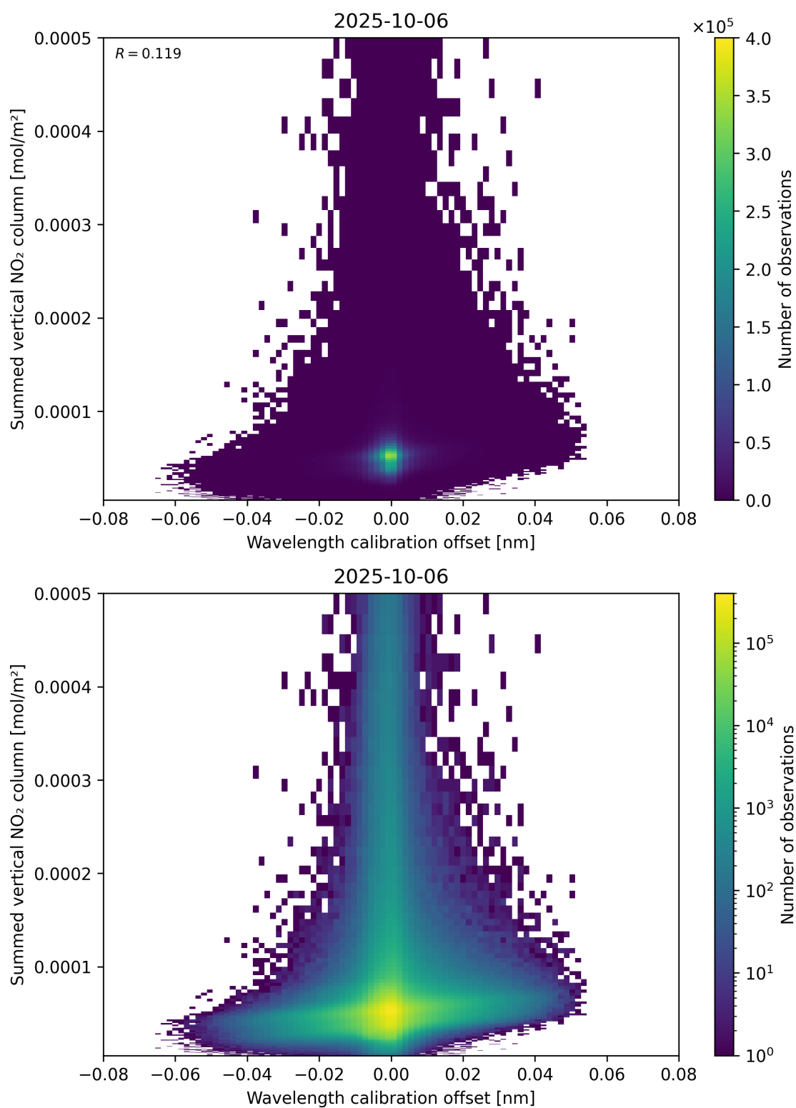
Figure 177: Scatter density plot of “Wavelength calibration offset” against “Summed vertical NO 2 column” for 2025-10-06 to 2025-10-07.
