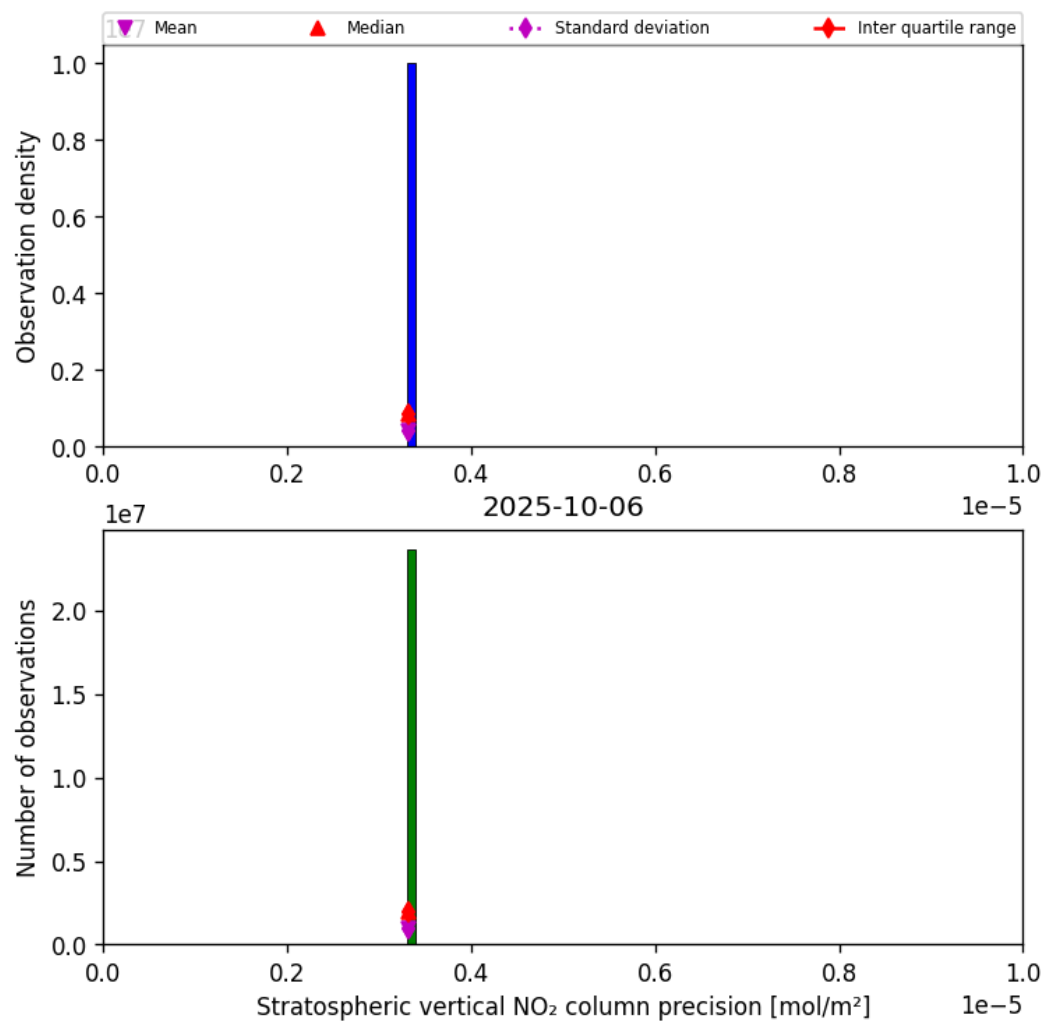
Figure 37: Histogram of “Stratospheric vertical NO 2 column precision” for 2025-10-06 to 2025-10-07
