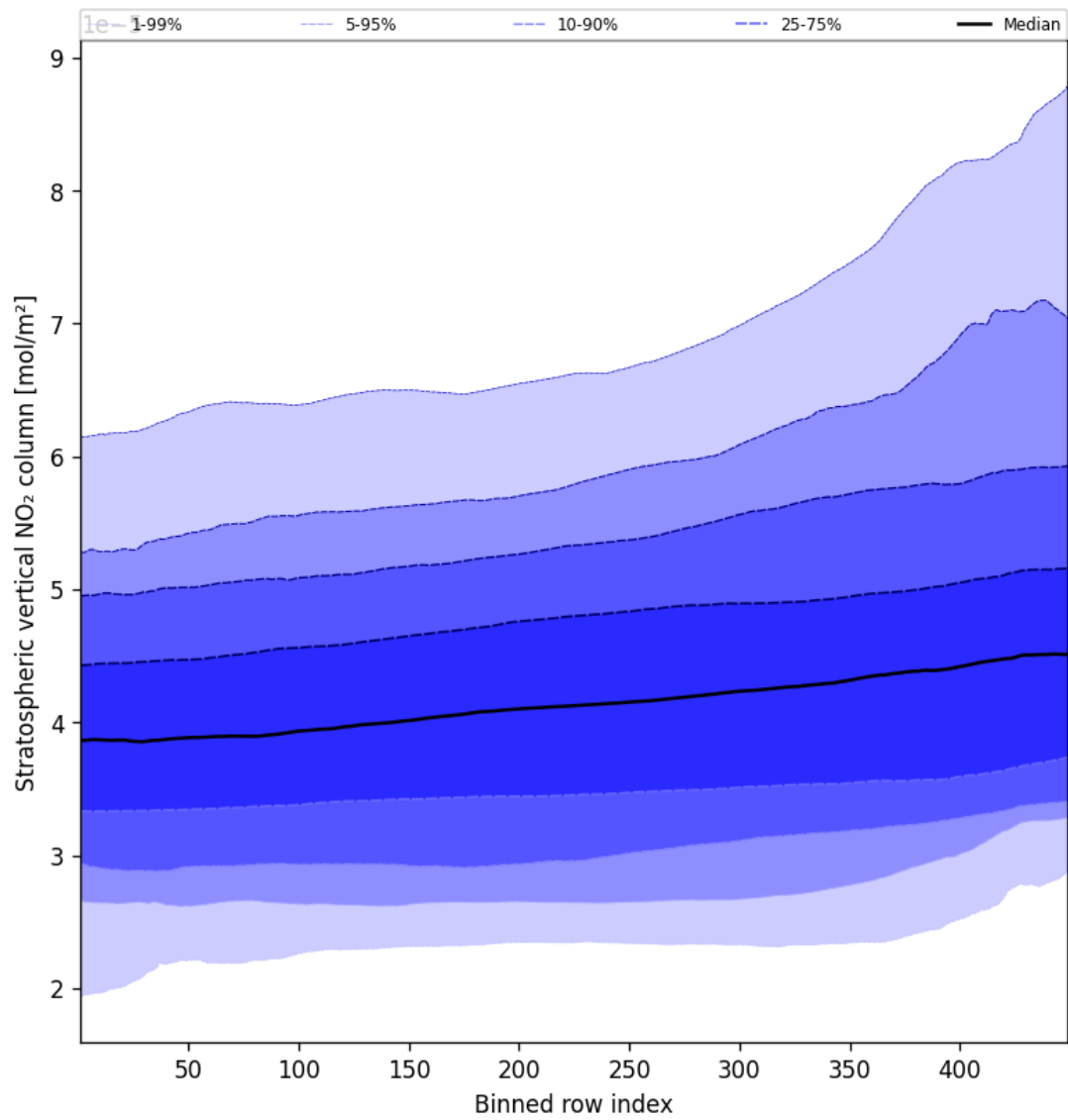
Figure 53: Along track statistics of “Stratospheric vertical NO 2 column” for 2025-10-06 to 2025-10-07
