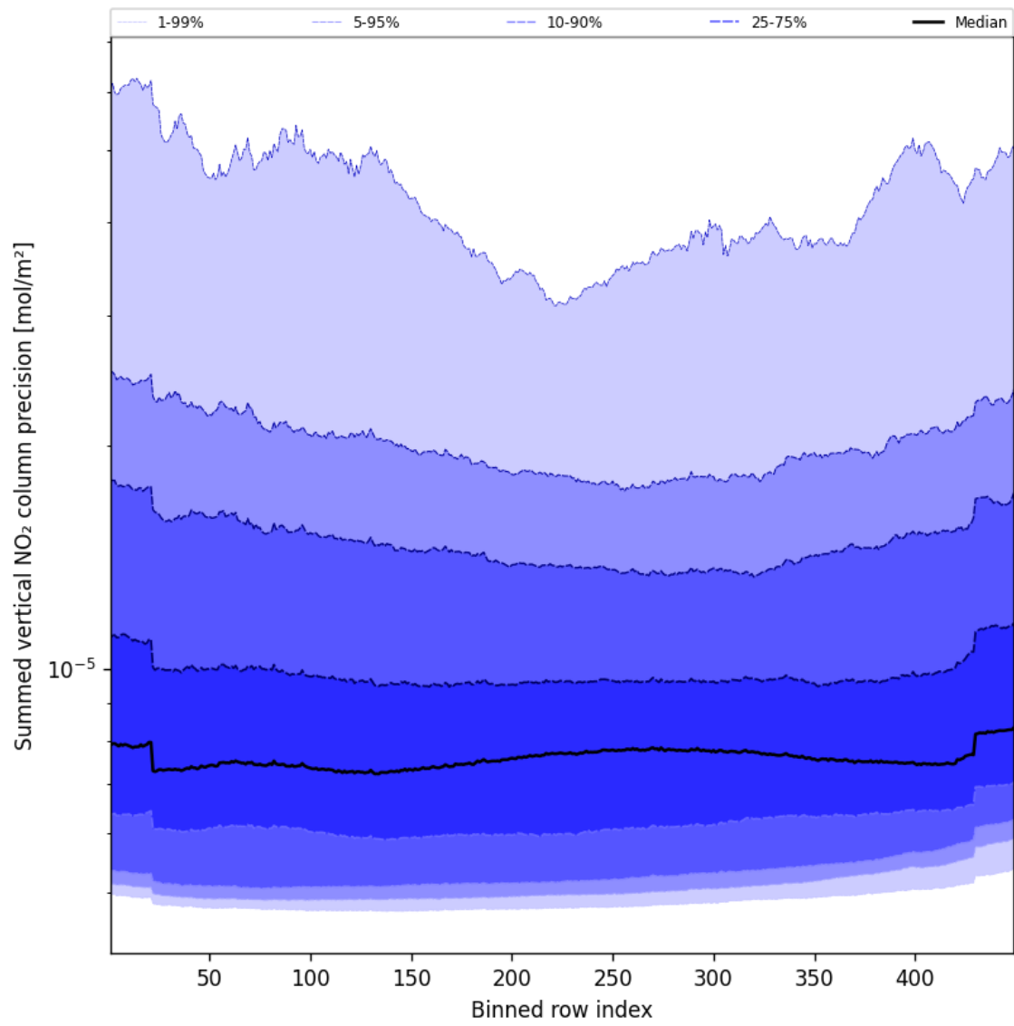
Figure 58: Along track statistics of “Summed vertical NO 2 column precision” for 2025-10-06 to 2025-10-07
