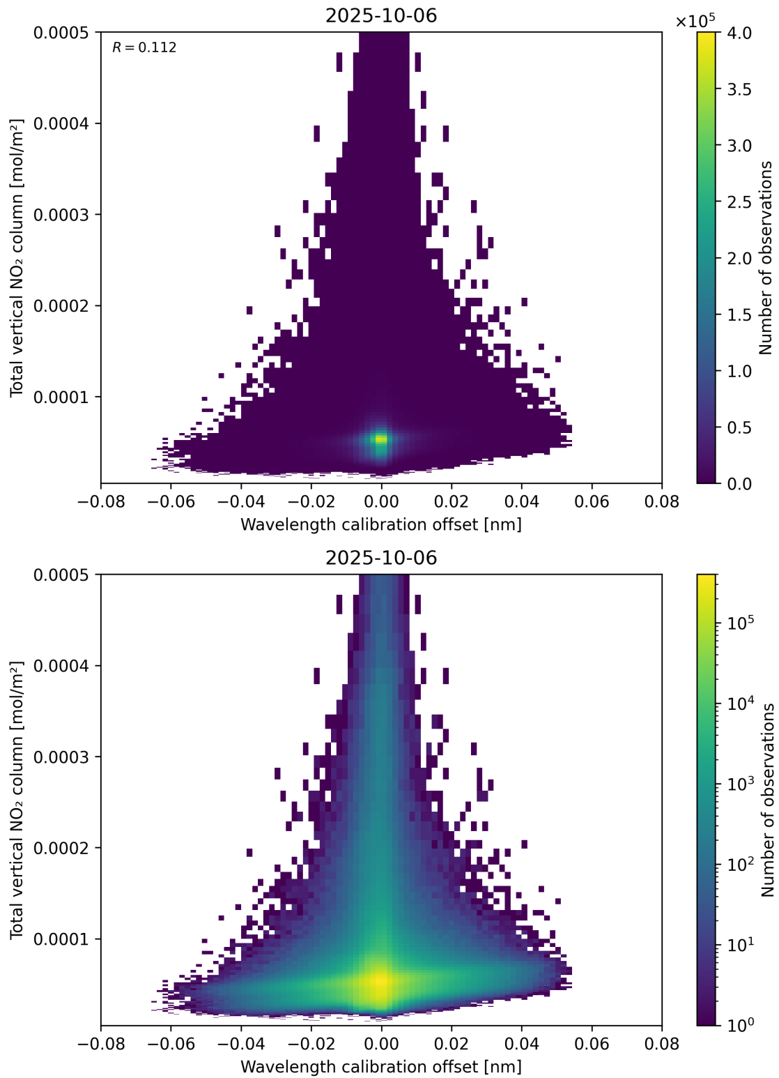
Figure 179: Scatter density plot of “Wavelength calibration offset” against “Total vertical NO 2 column” for 2025-10-06 to 2025-10-07.
