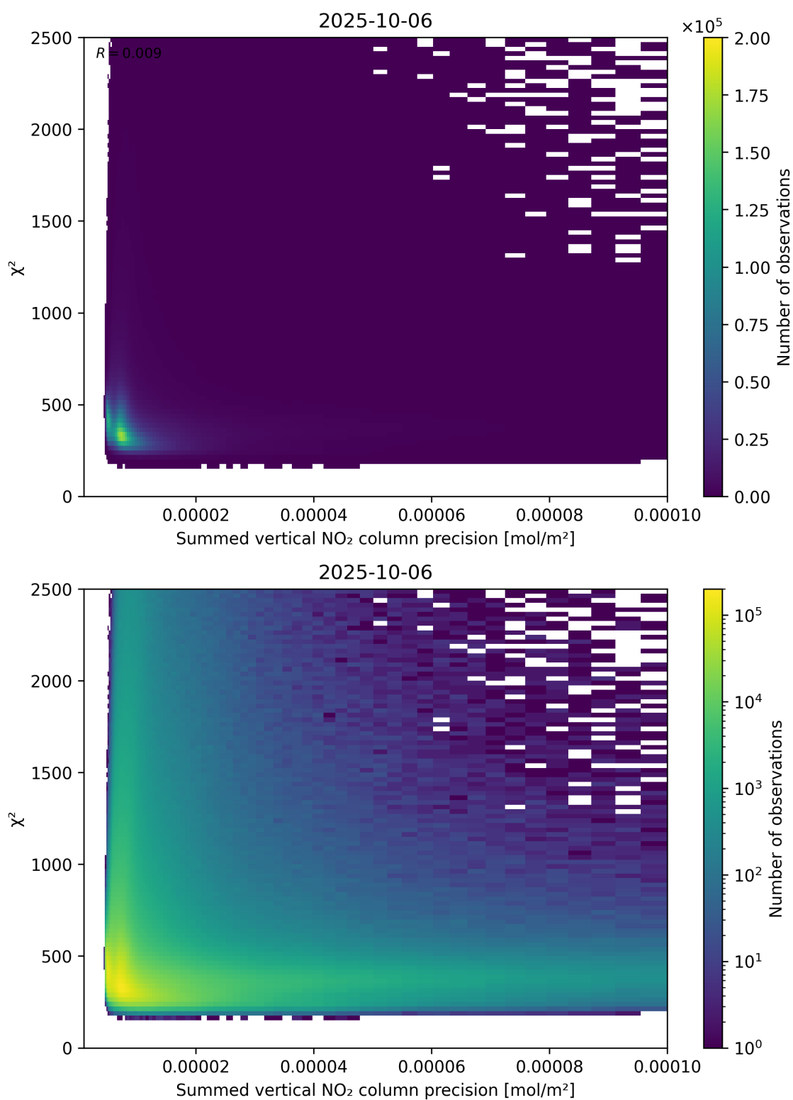
Figure 107: Scatter density plot of “Summed vertical NO 2 column precision” against “ \chi^2 ” for 2025-10-06 to 2025-10-07.
