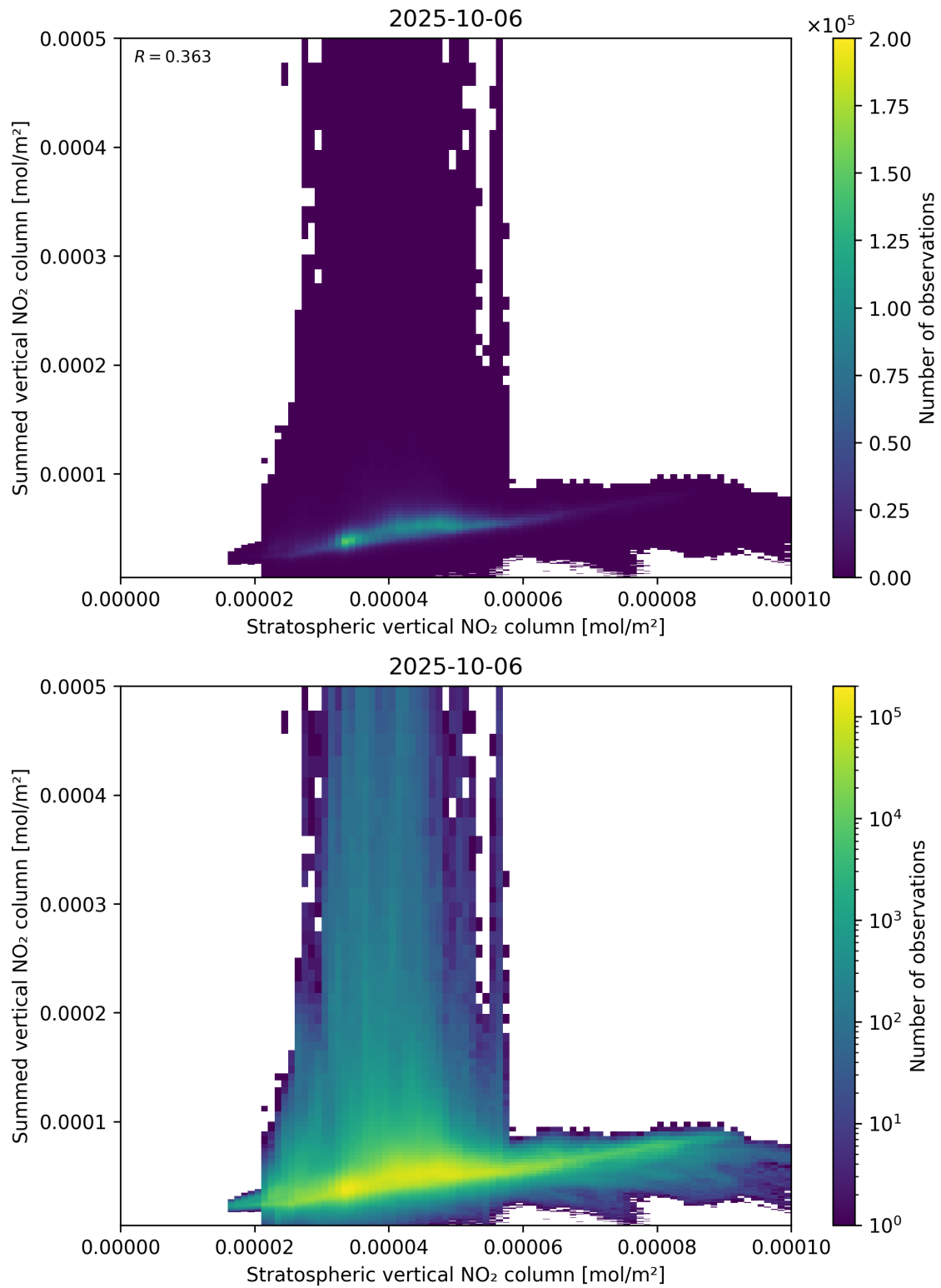
Figure 98: Scatter density plot of “Stratospheric vertical NO 2 column” against “Summed vertical NO 2 column” for 2025-10-06 to 2025-10-07.
