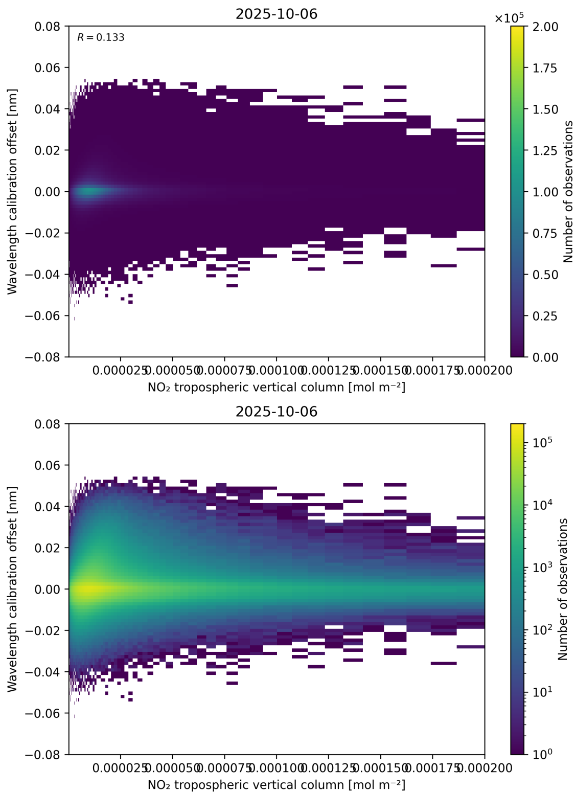
Figure 143: Scatter density plot of “NO 2 tropospheric vertical column” against “Wavelength calibration offset” for 2025-10-06 to 2025-10-07.
