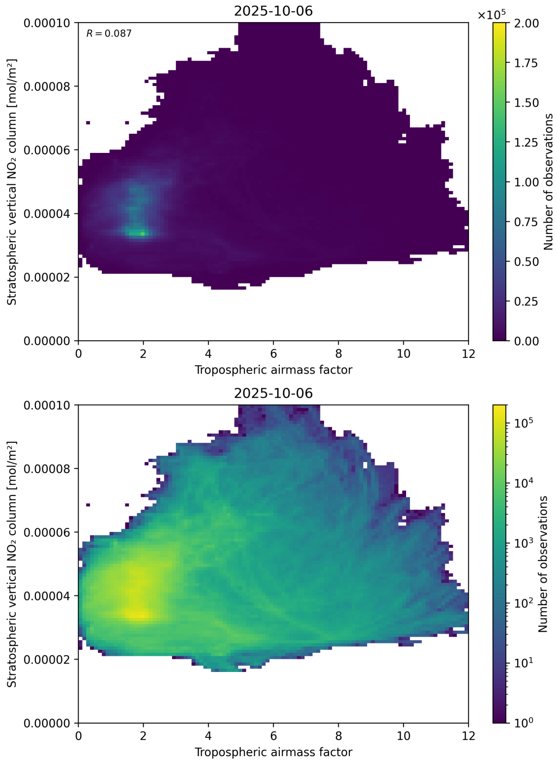
Figure 74: Scatter density plot of “Tropospheric air mass factor” against “Stratospheric vertical NO 2 column” for 2025-10-06 to 2025-10-07.
