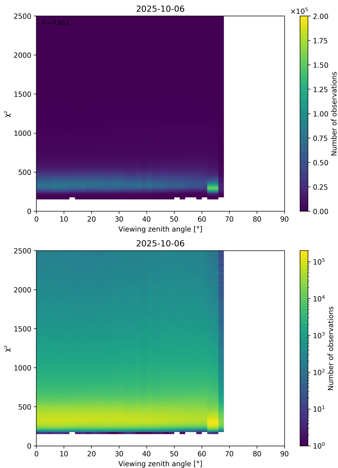
Figure 162: Scatter density plot of “Viewing zenith angle” against “ \chi^2 ” for 2025-10-06 to 2025-10-07.
