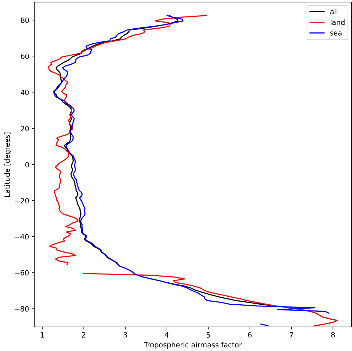
Figure 14: Zonal average of “Tropospheric airmass factor” for 2025-10-06 to 2025-10-07.
