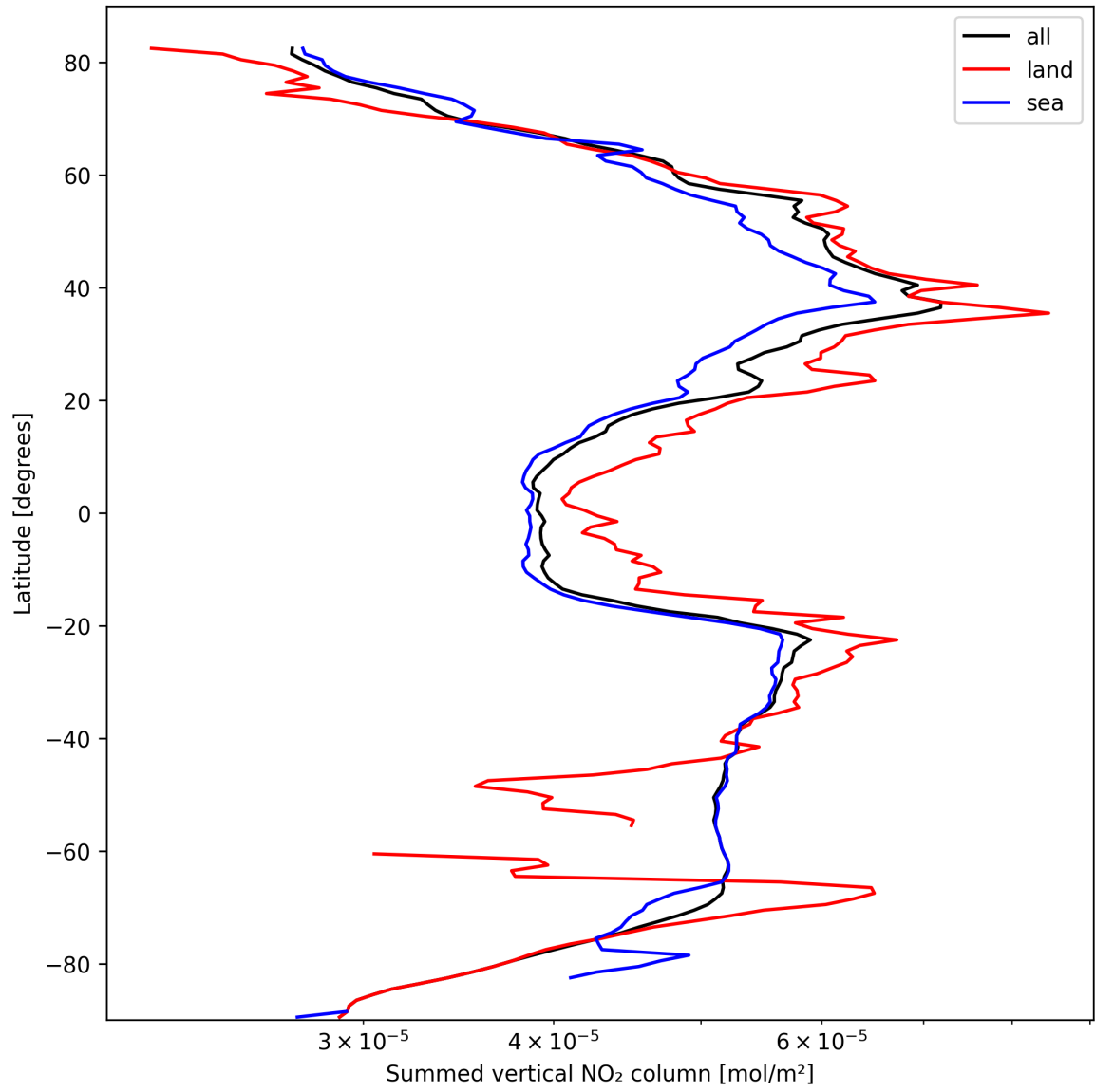
Figure 23: Zonal average of “Summed vertical NO 2 column” for 2025-10-06 to 2025-10-07.
