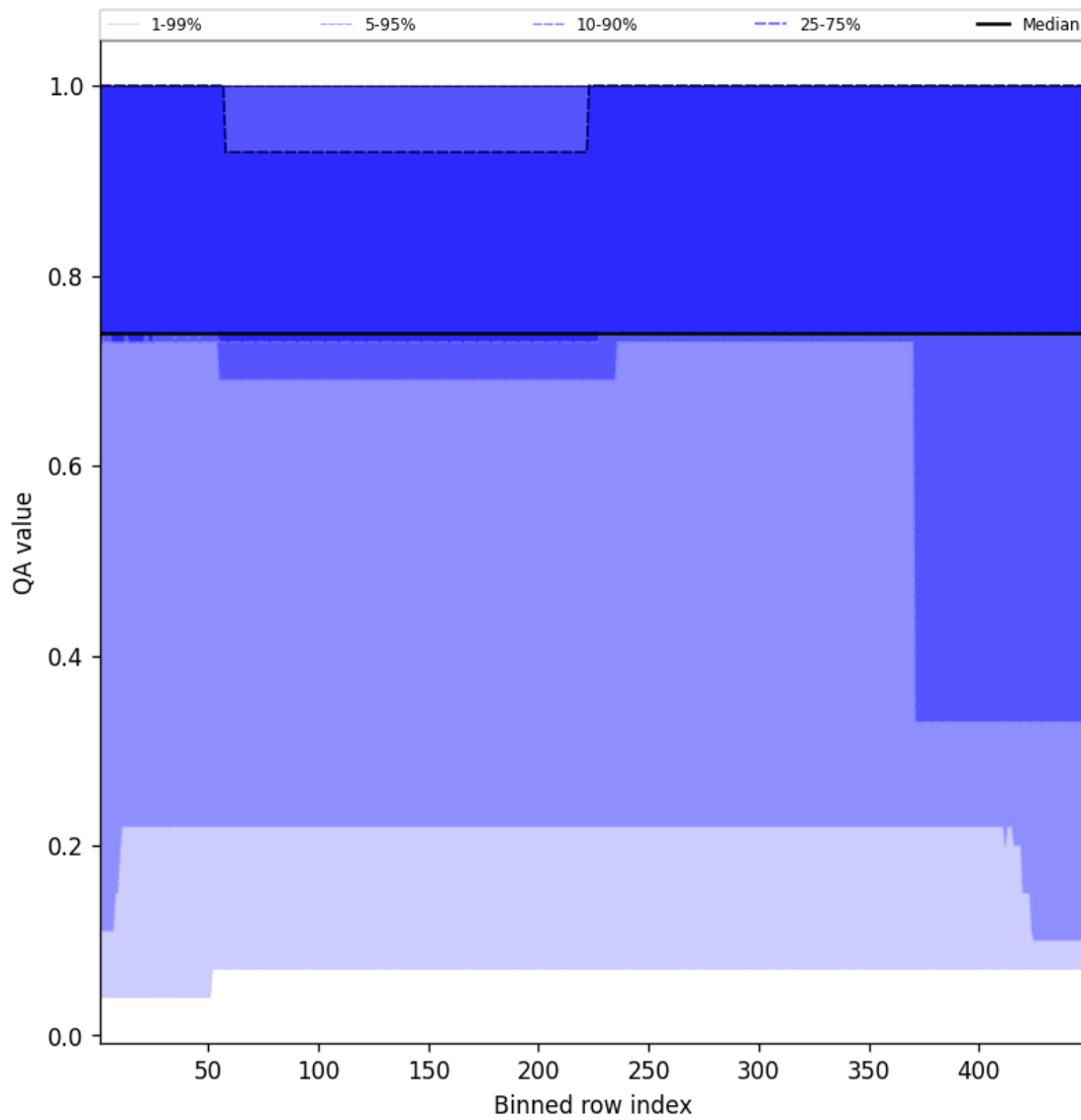
Figure 45: Along track statistics of “QA value” for 2025-10-06 to 2025-10-07
