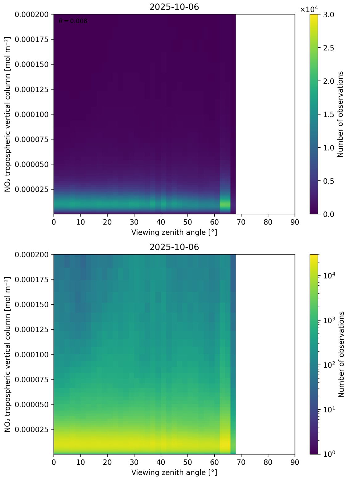
Figure 169: Scatter density plot of “Viewing zenith angle” against “NO 2 tropospheric vertical column” for 2025-10-06 to 2025-10-07.
