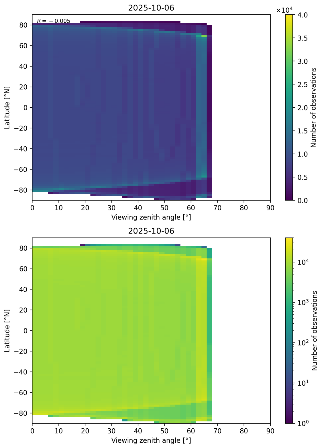
Figure 163: Scatter density plot of “Viewing zenith angle” against “Latitude” for 2025-10-06 to 2025-10-07.
