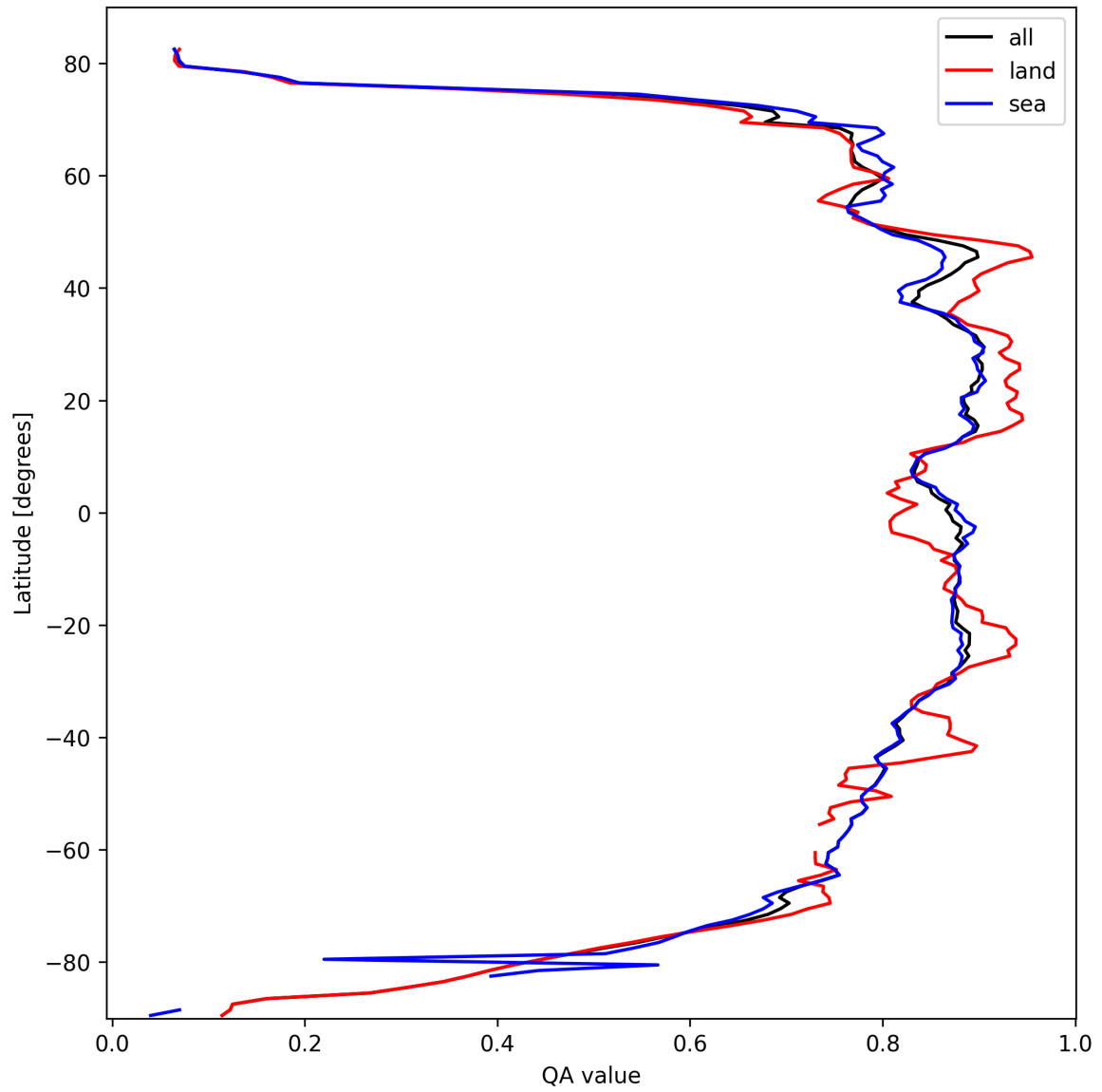
Figure 11: Zonal average of “QA value” for 2025-10-06 to 2025-10-07.
