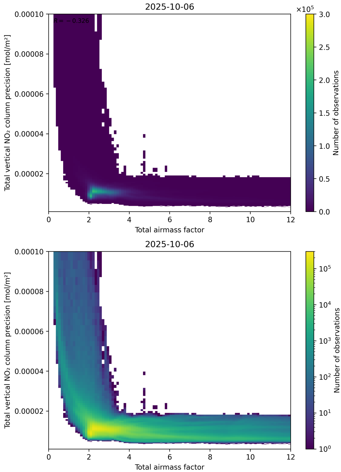
Figure 68: Scatter density plot of “Total airmass factor” against “Total vertical NO 2 column precision” for 2025-10-06 to 2025-10-07.
