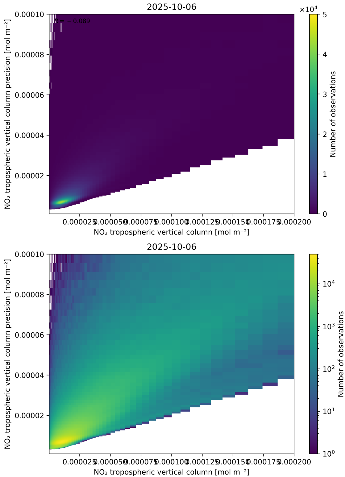
Figure 130: Scatter density plot of “NO 2 tropospheric vertical column” against “NO 2 tropospheric vertical column precision” for 2025-10-06 to 2025-10-07.
