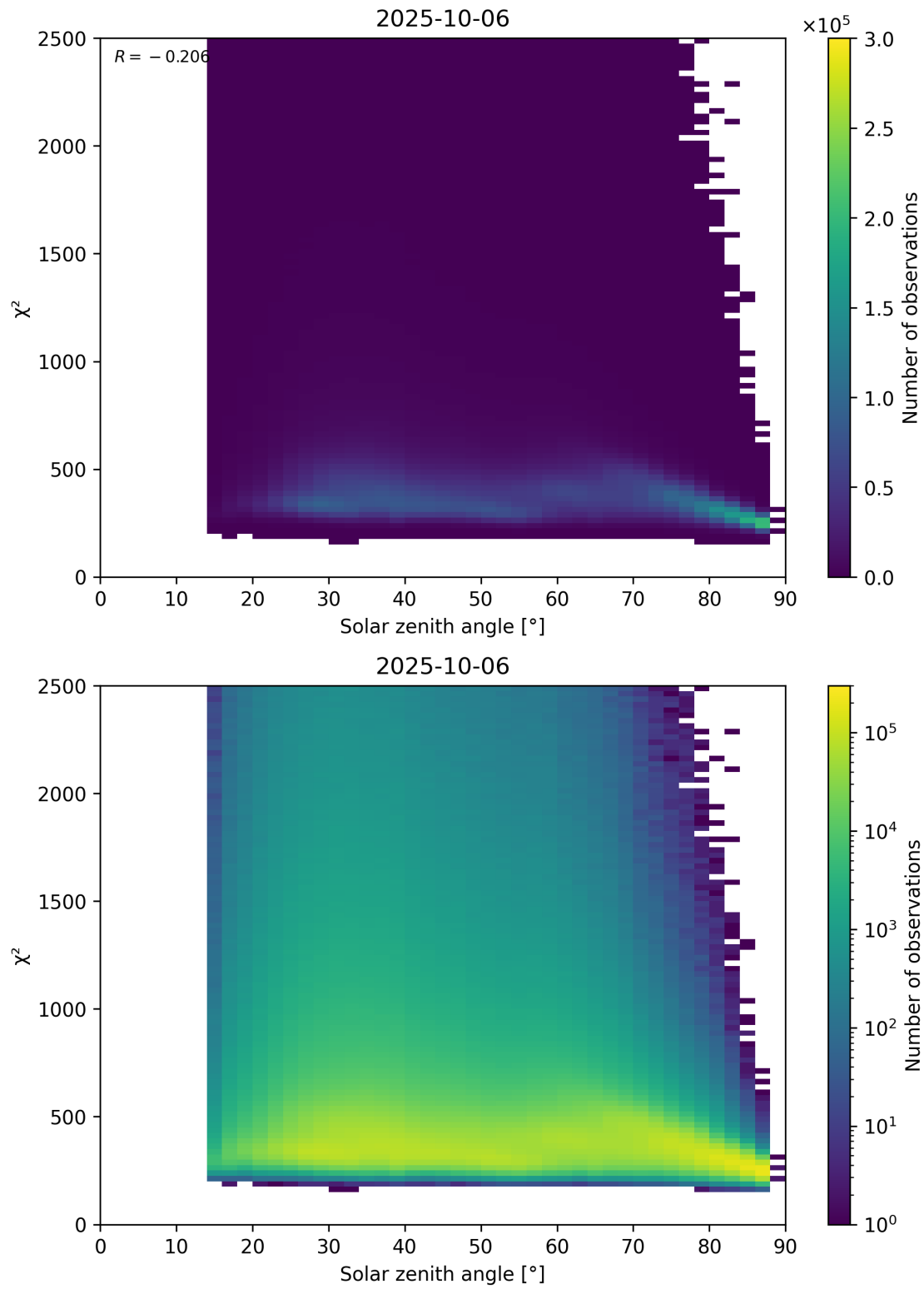
Figure 148: Scatter density plot of “Solar zenith angle” against “ \chi^2 ” for 2025-10-06 to 2025-10-07.
