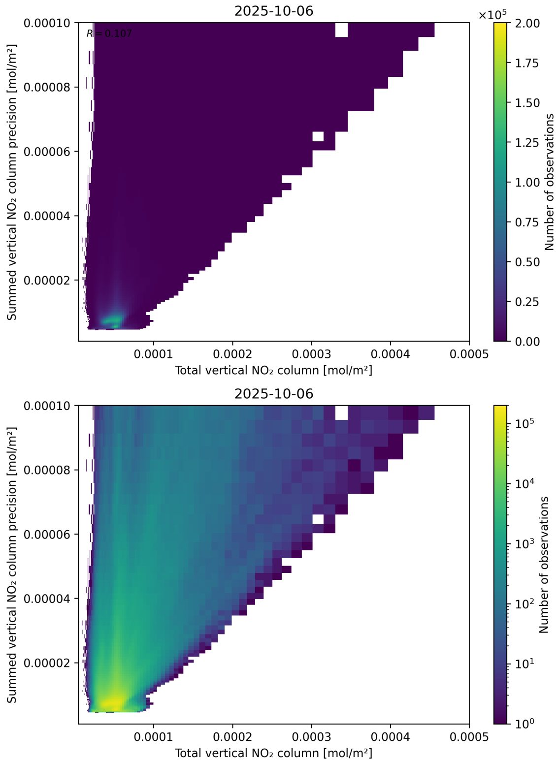
Figure 113: Scatter density plot of “Total vertical NO 2 column” against “Summed vertical NO 2 column precision” for 2025-10-06 to 2025-10-07.
