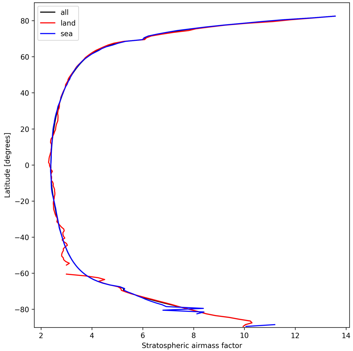
Figure 27: Zonal average of “Stratospheric airmass factor” for 2025-10-06 to 2025-10-07.
