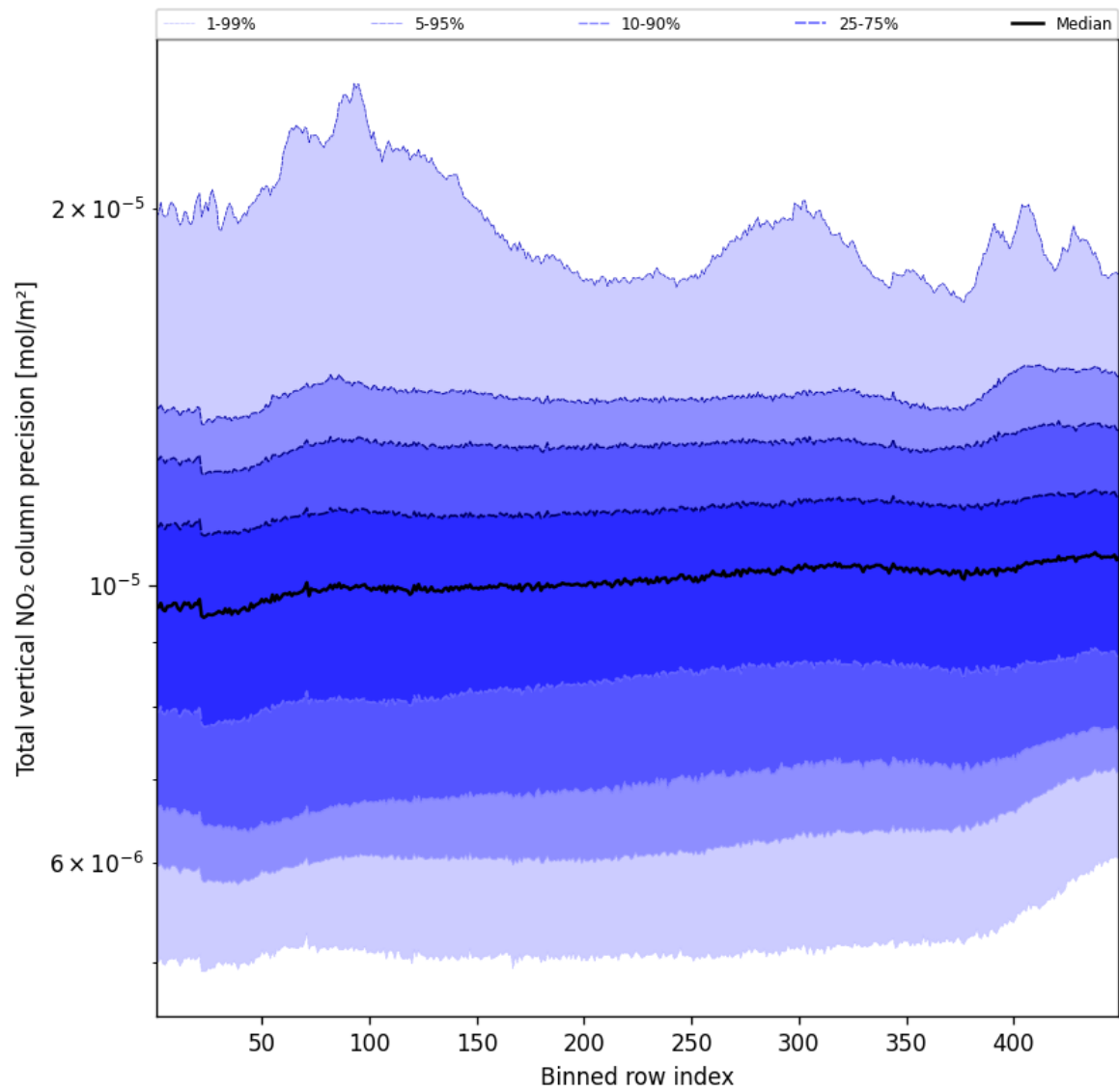
Figure 56: Along track statistics of “Total vertical NO 2 column precision” for 2025-10-06 to 2025-10-07
