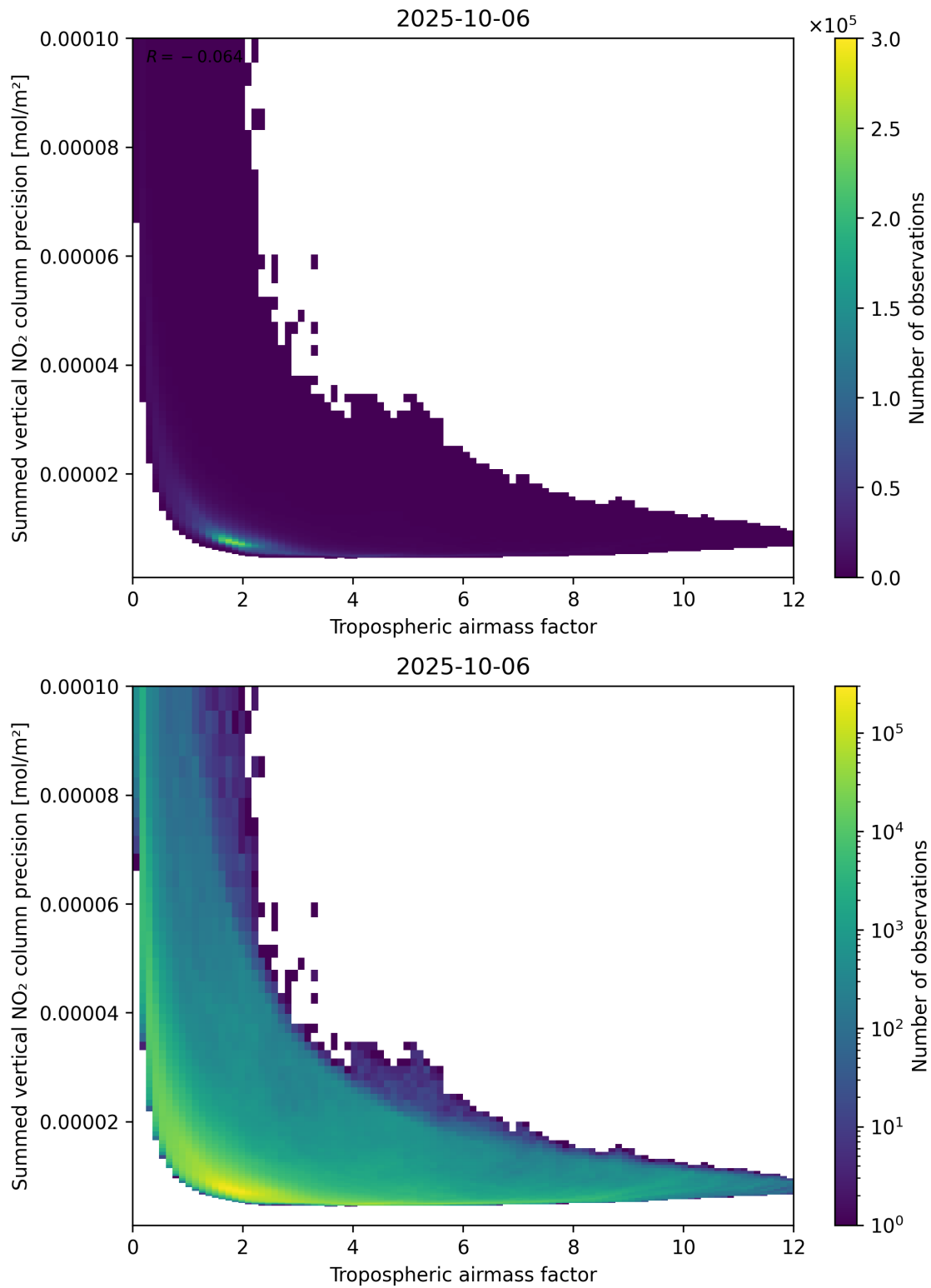
Figure 76: Scatter density plot of “Tropospheric air mass factor” against “Summed vertical NO 2 column precision” for 2025-10-06 to 2025-10-07.
