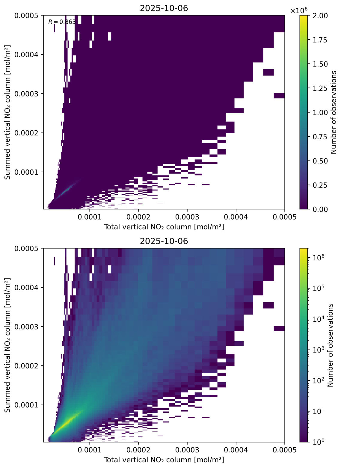
Figure 112: Scatter density plot of “Total vertical NO 2 column” against “Summed vertical NO 2 column” for 2025-10-06 to 2025-10-07.
