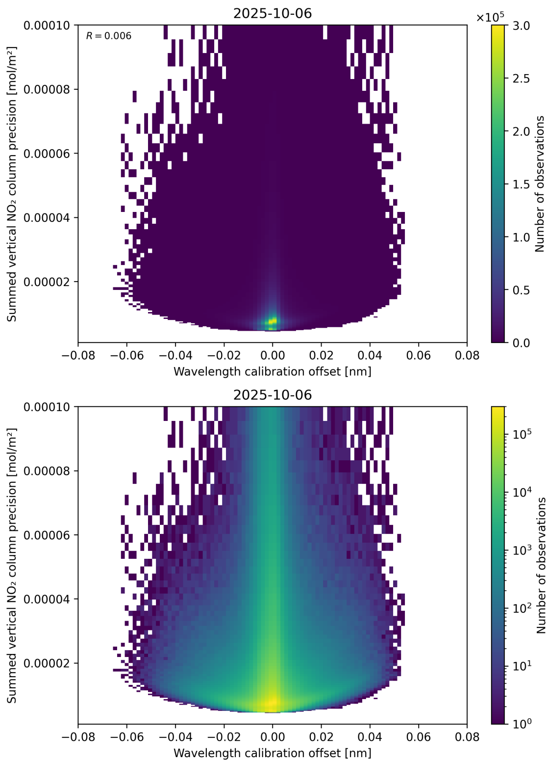
Figure 178: Scatter density plot of “Wavelength calibration offset” against “Summed vertical NO 2 column precision” for 2025-10-06 to 2025-10-07.
