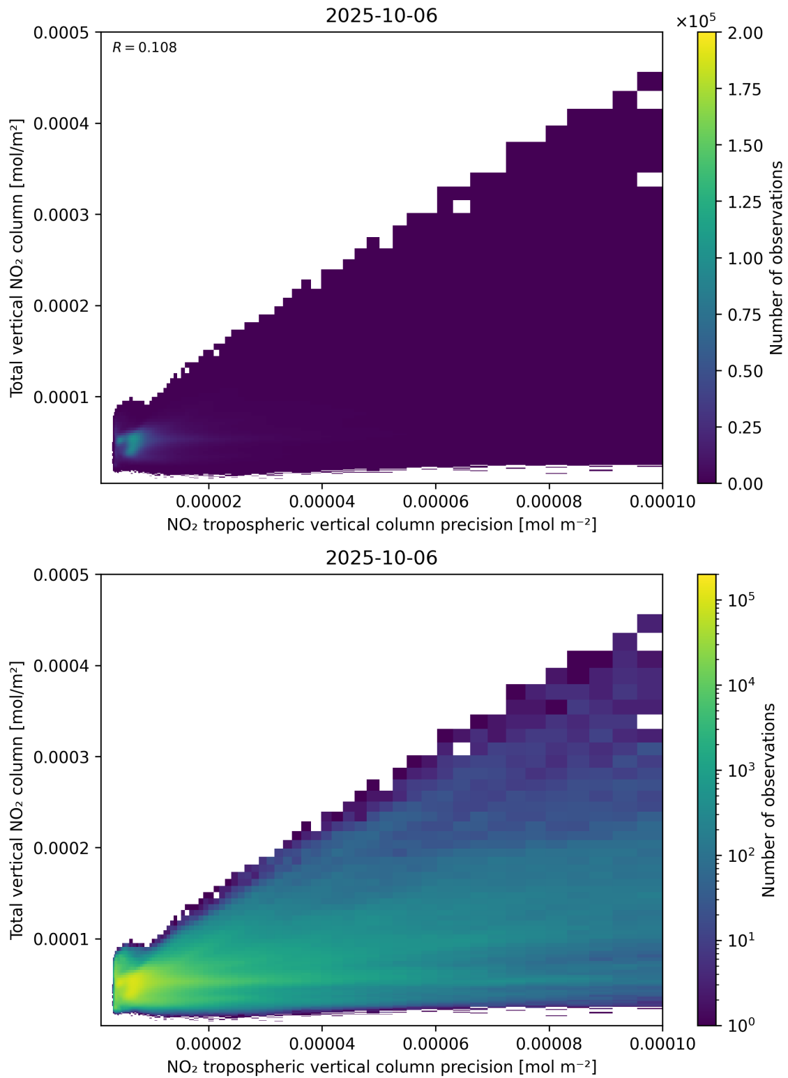
Figure 138: Scatter density plot of “NO 2 tropospheric vertical column precision” against “Total vertical NO 2 column” for 2025-10-06 to 2025-10-07.
