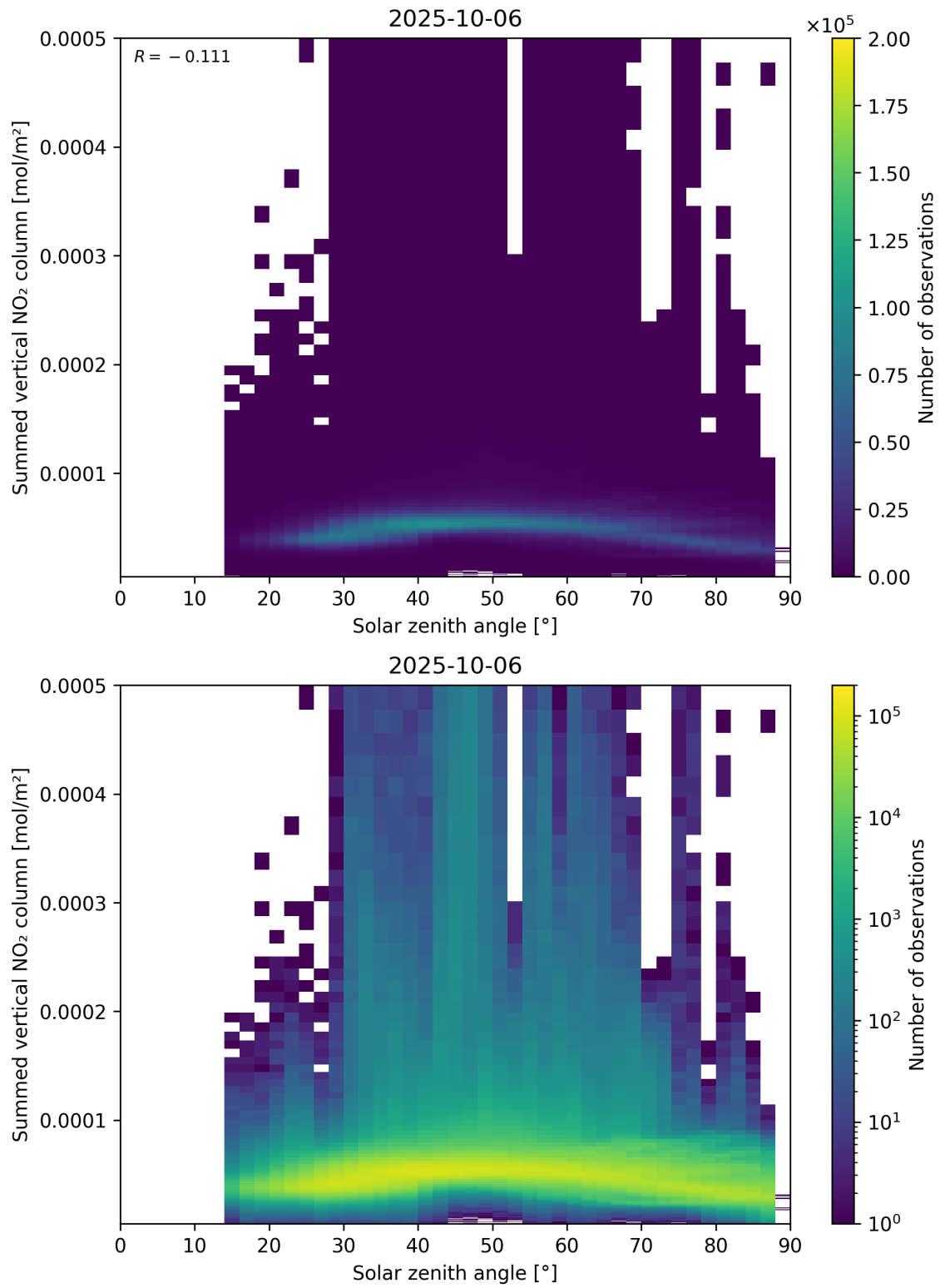
Figure 151: Scatter density plot of “Solar zenith angle” against “Summed vertical NO 2 column” for 2025-10-06 to 2025-10-07.
