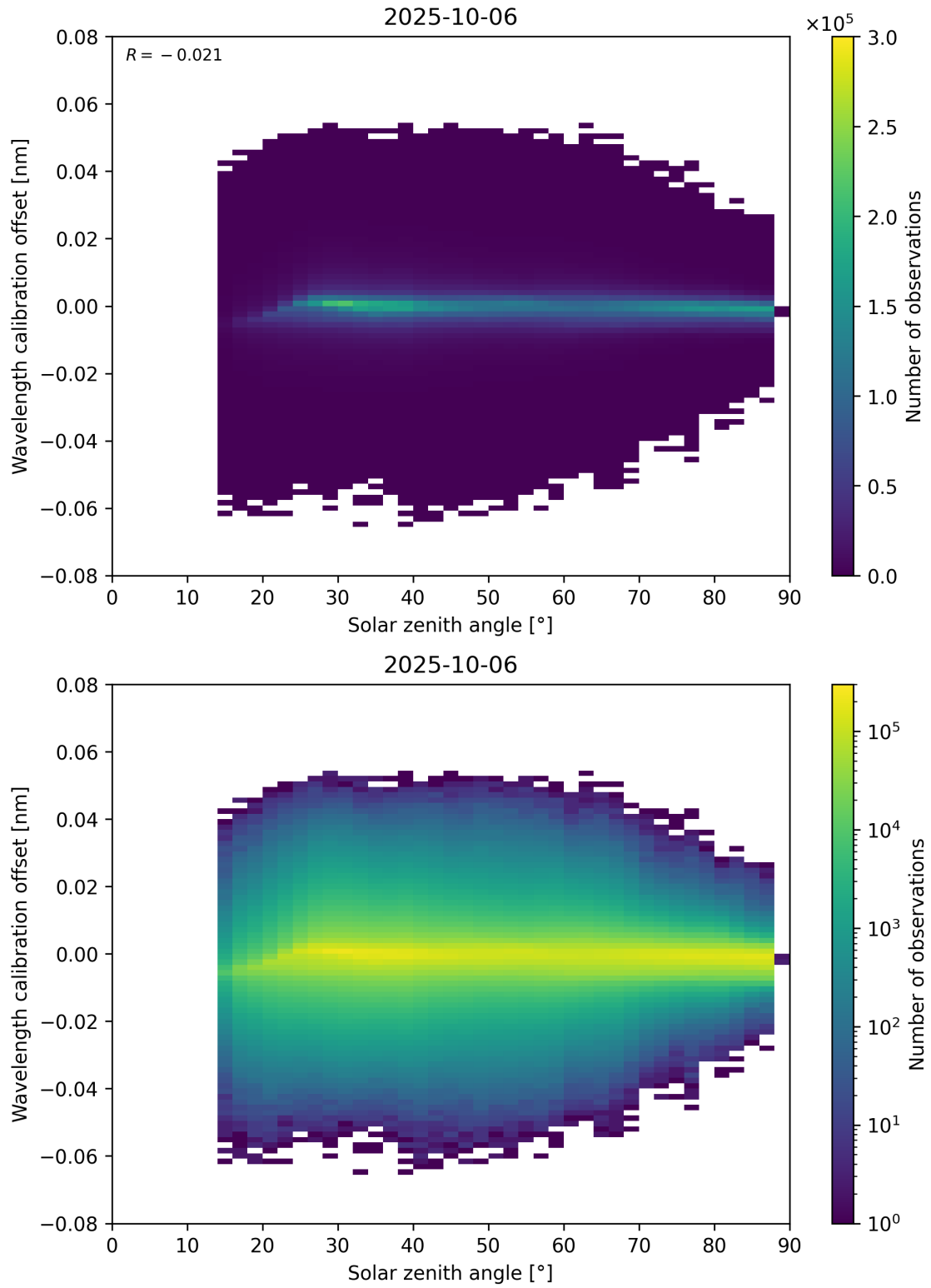
Figure 158: Scatter density plot of “Solar zenith angle” against “Wavelength calibration offset” for 2025-10-06 to 2025-10-07.
