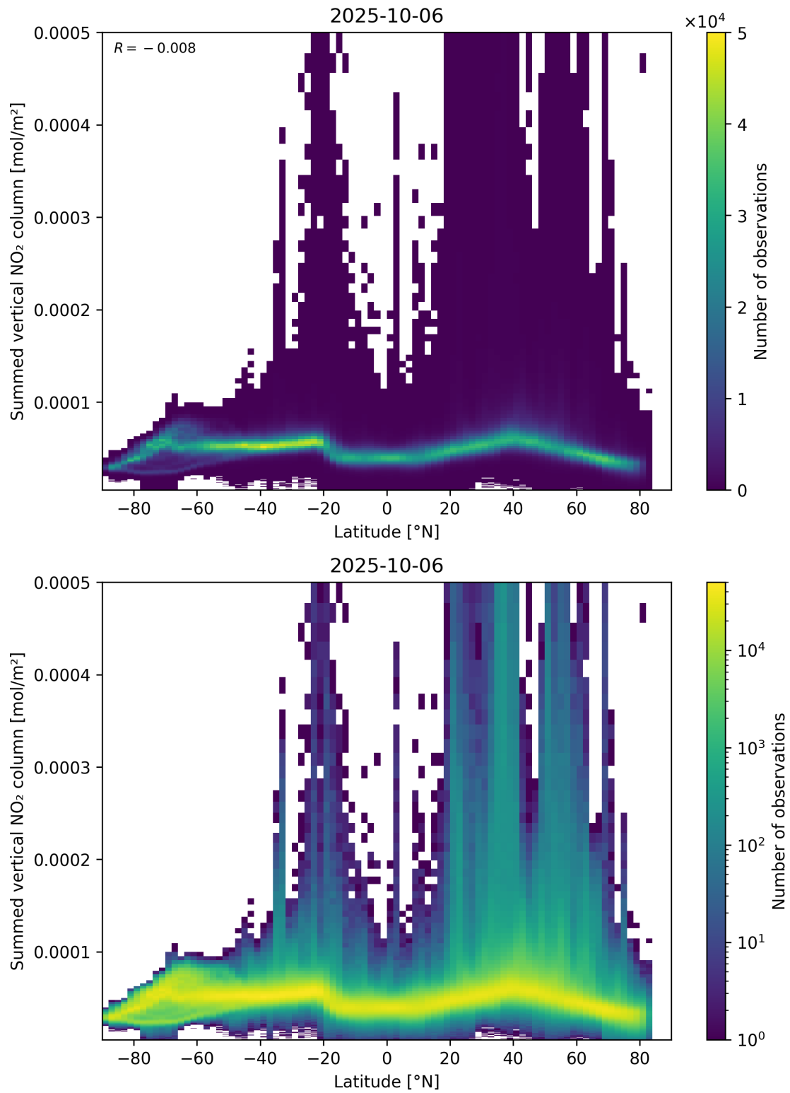
Figure 88: Scatter density plot of “Latitude” against “Summed vertical NO 2 column” for 2025-10-06 to 2025-10-07.
