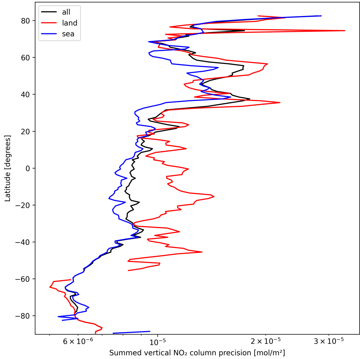
Figure 24: Zonal average of “Summed vertical NO 2 column precision” for 2025-10-06 to 2025-10-07.
