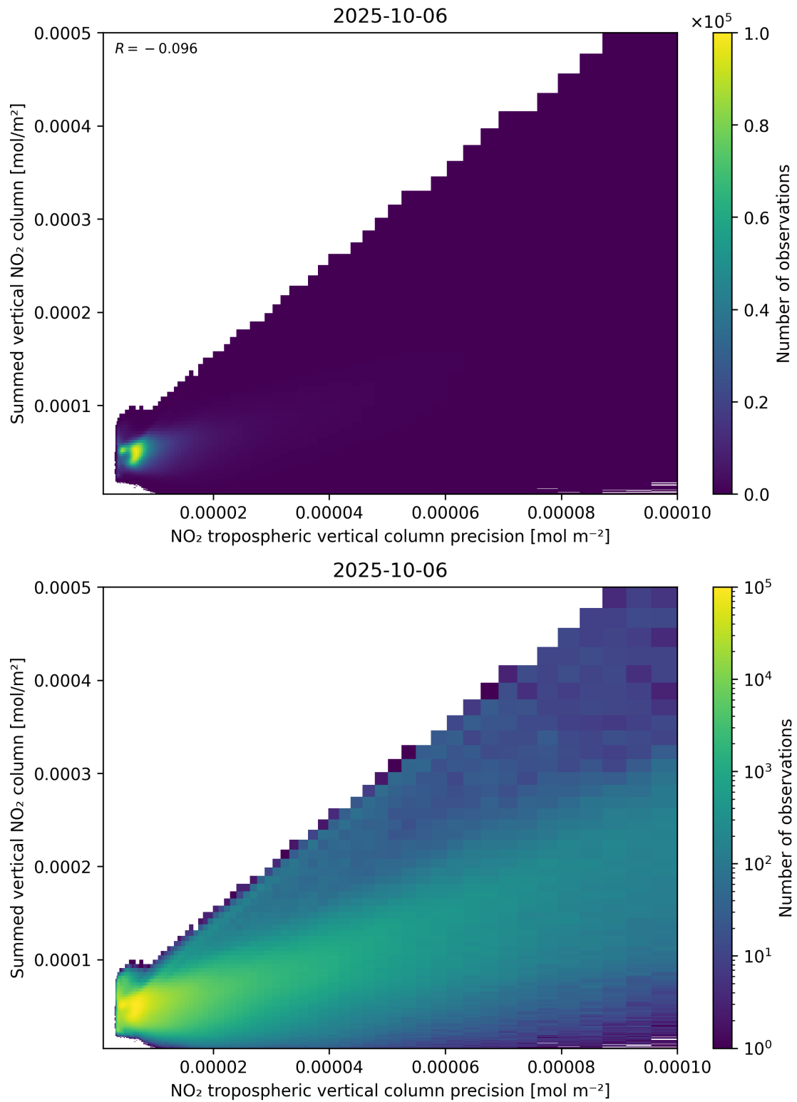
Figure 136: Scatter density plot of “NO 2 tropospheric vertical column precision” against “Summed vertical NO 2 column” for 2025-10-06 to 2025-10-07.
