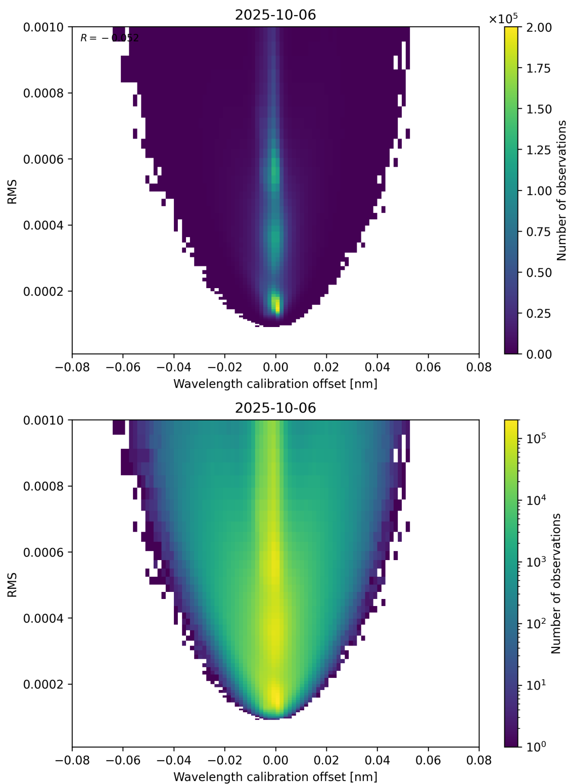
Figure 181: Scatter density plot of “Wavelength calibration offset” against “RMS” for 2025-10-06 to 2025-10-07.
