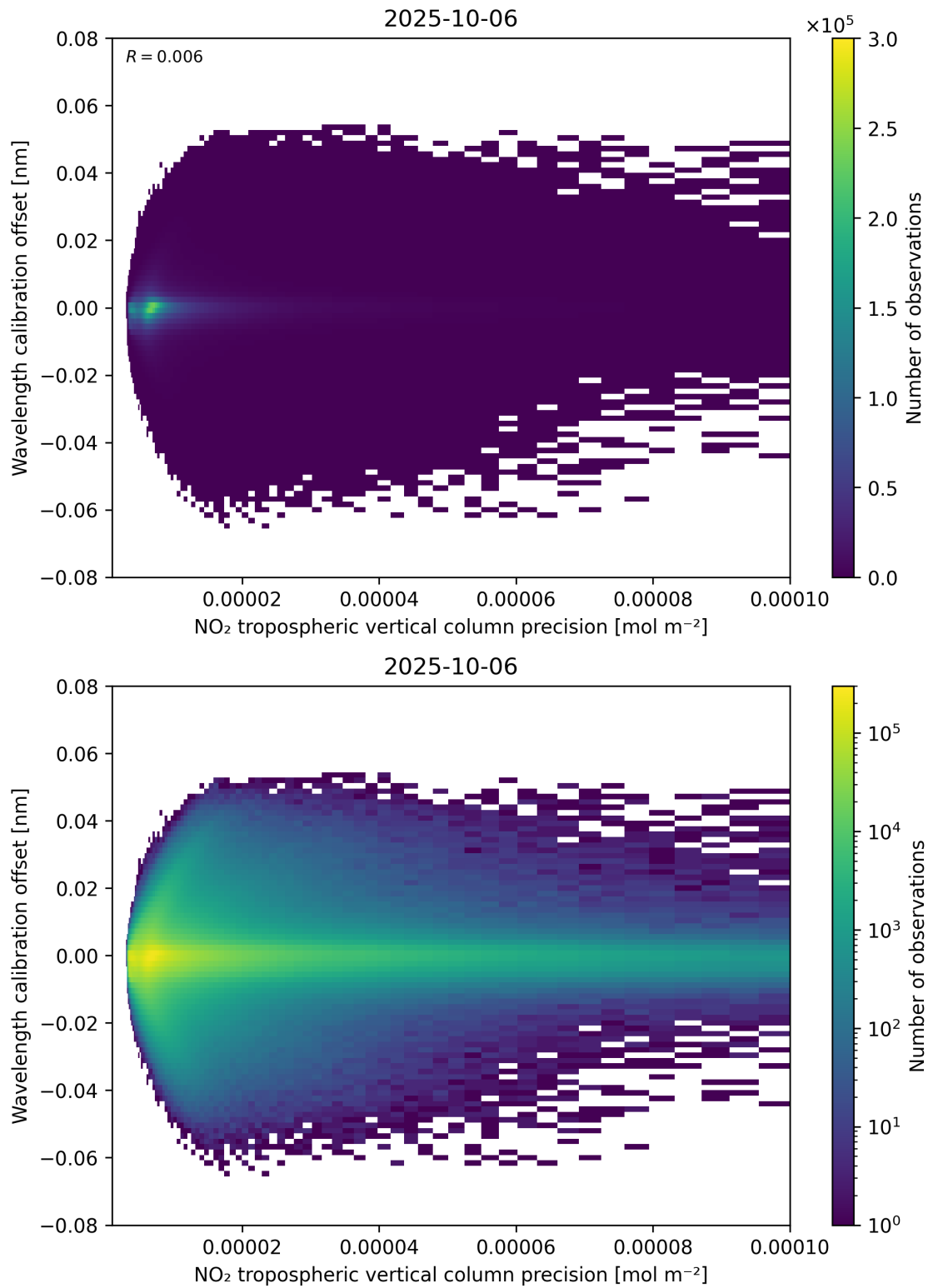
Figure 141: Scatter density plot of “NO 2 tropospheric vertical column precision” against “Wavelength calibration offset” for 2025-10-06 to 2025-10-07.
