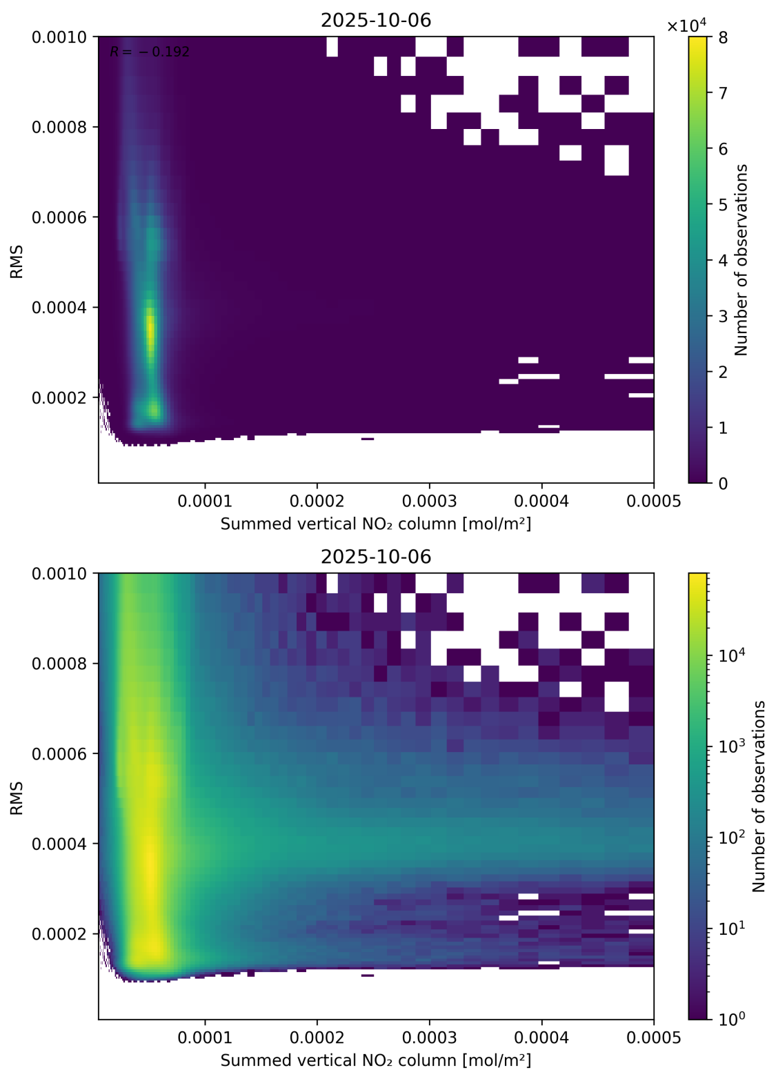
Figure 109: Scatter density plot of “Summed vertical NO 2 column” against “RMS” for 2025-10-06 to 2025-10-07.
