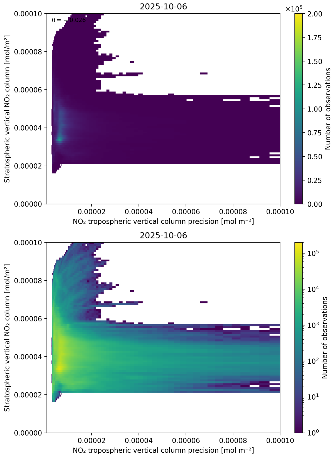
Figure 135: Scatter density plot of “NO 2 tropospheric vertical column precision” against “Stratospheric vertical NO 2 column” for 2025-10-06 to 2025-10-07.
