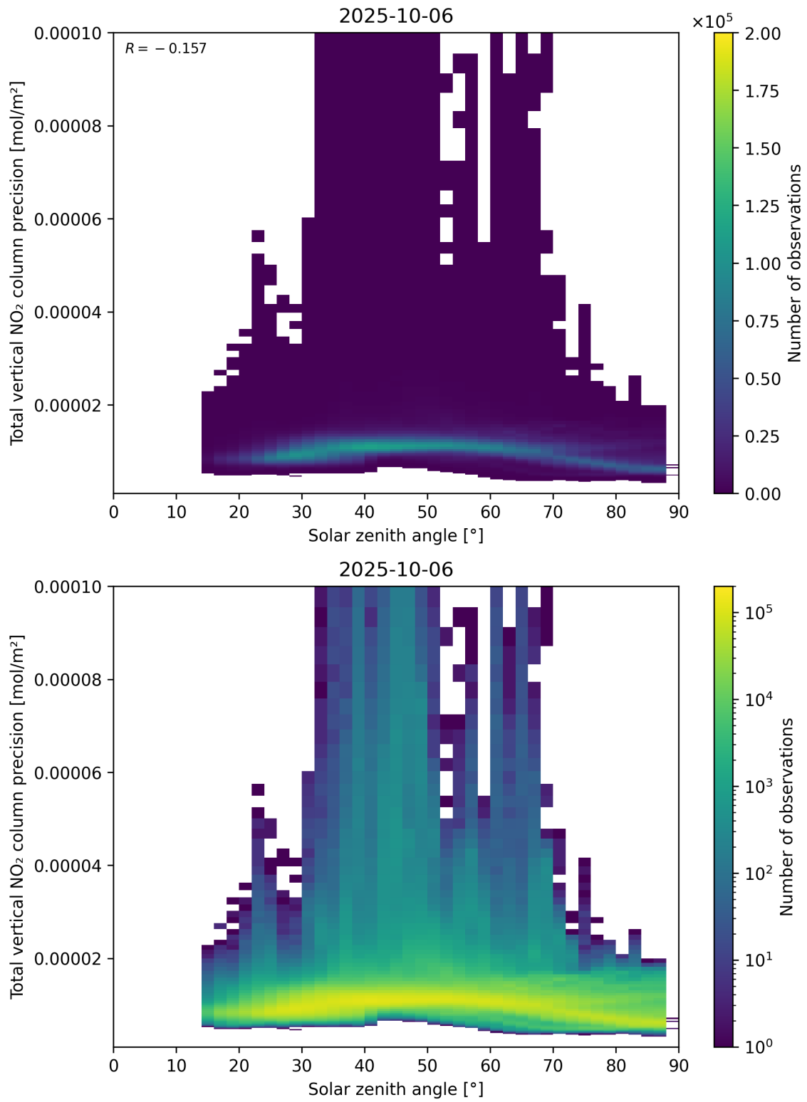
Figure 154: Scatter density plot of “Solar zenith angle” against “Total vertical NO 2 column precision” for 2025-10-06 to 2025-10-07.
