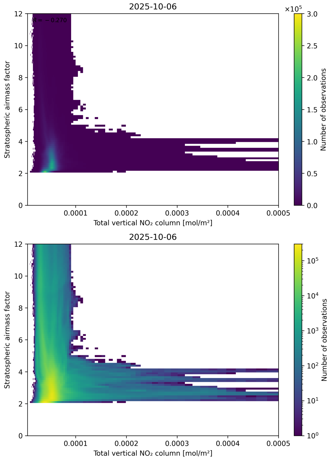
Figure 110: Scatter density plot of “Total vertical NO 2 column” against “Stratospheric airmass factor” for 2025-10-06 to 2025-10-07.
