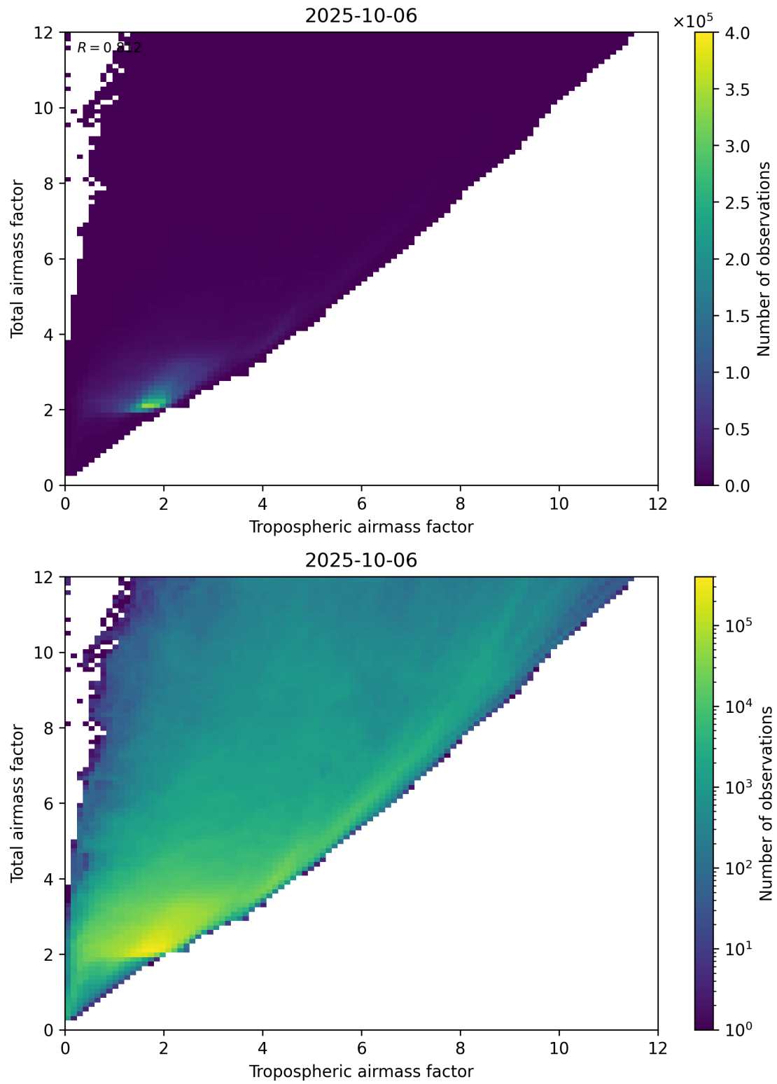
Figure 72: Scatter density plot of “Tropospheric airmass factor” against “Total airmass factor” for 2025-10-06 to 2025-10-07.
