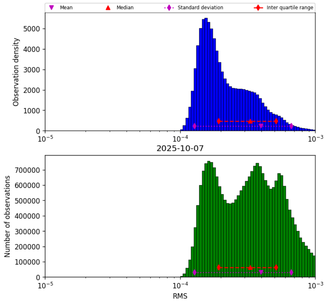
Figure 43: Histogram of “RMS” for 2025-10-06 to 2025-10-08
