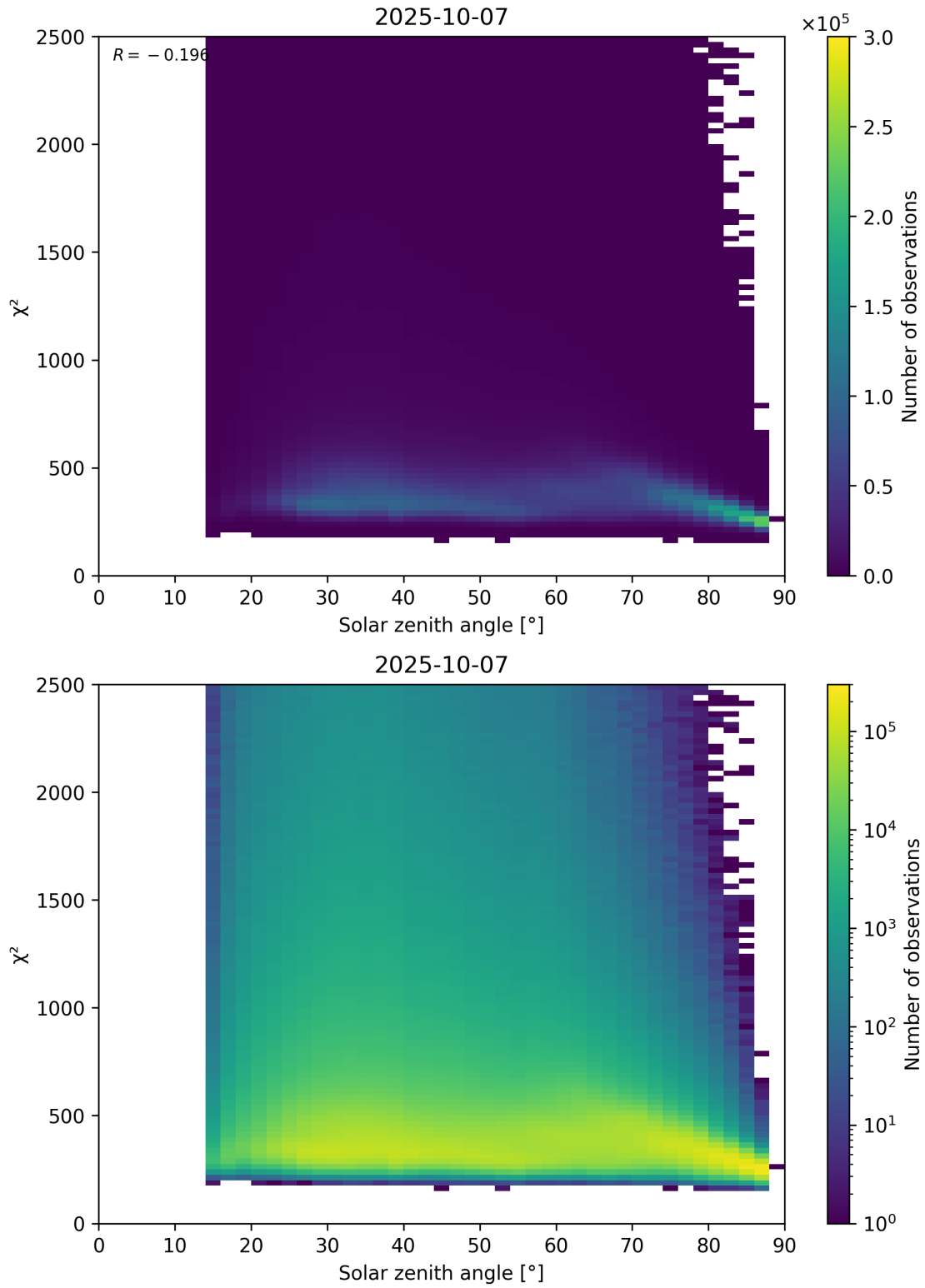
Figure 148: Scatter density plot of “Solar zenith angle” against “ \chi^2 ” for 2025-10-06 to 2025-10-08.
