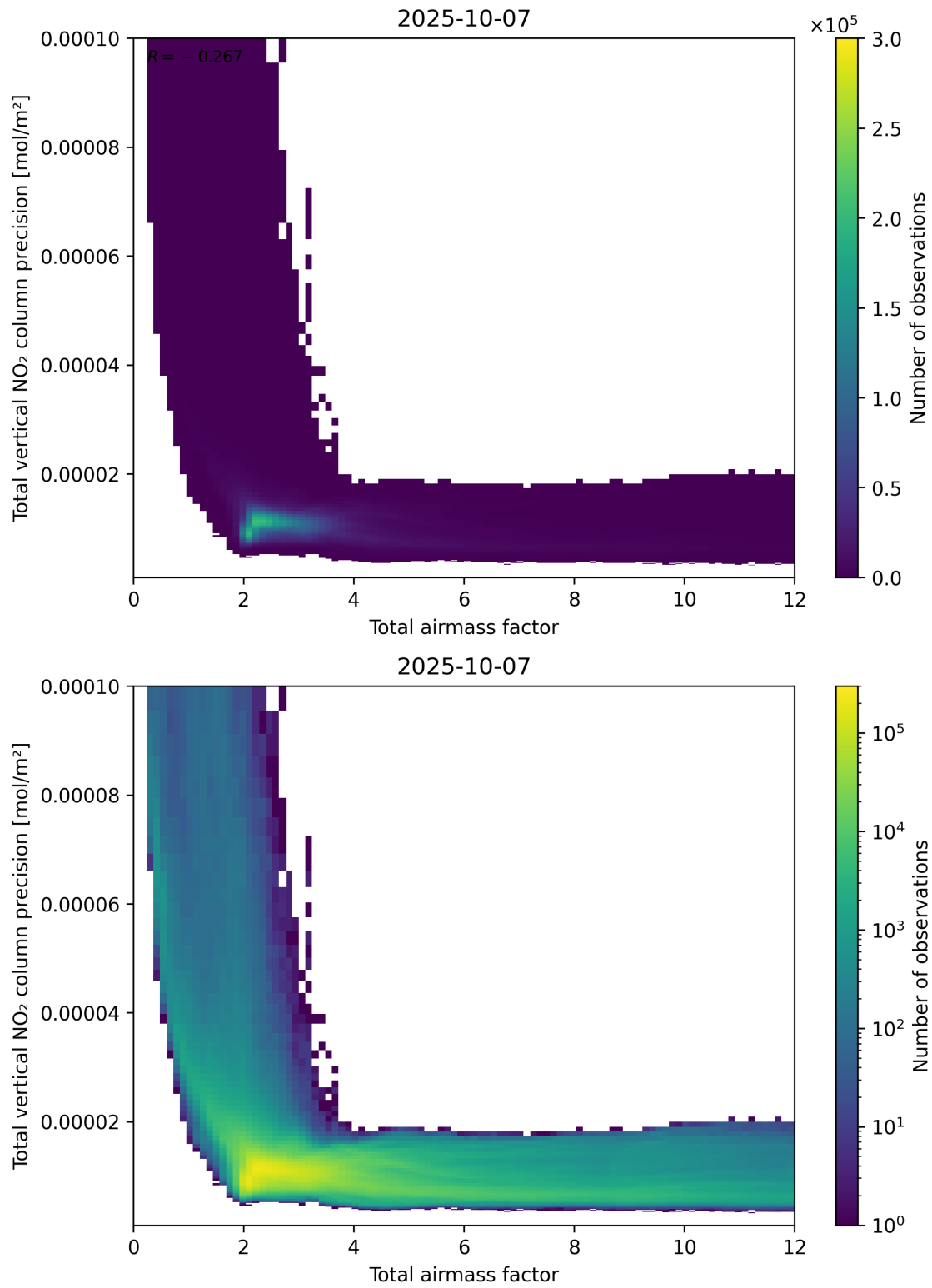
Figure 68: Scatter density plot of “Total airmass factor” against “Total vertical NO 2 column precision” for 2025-10-06 to 2025-10-08.
