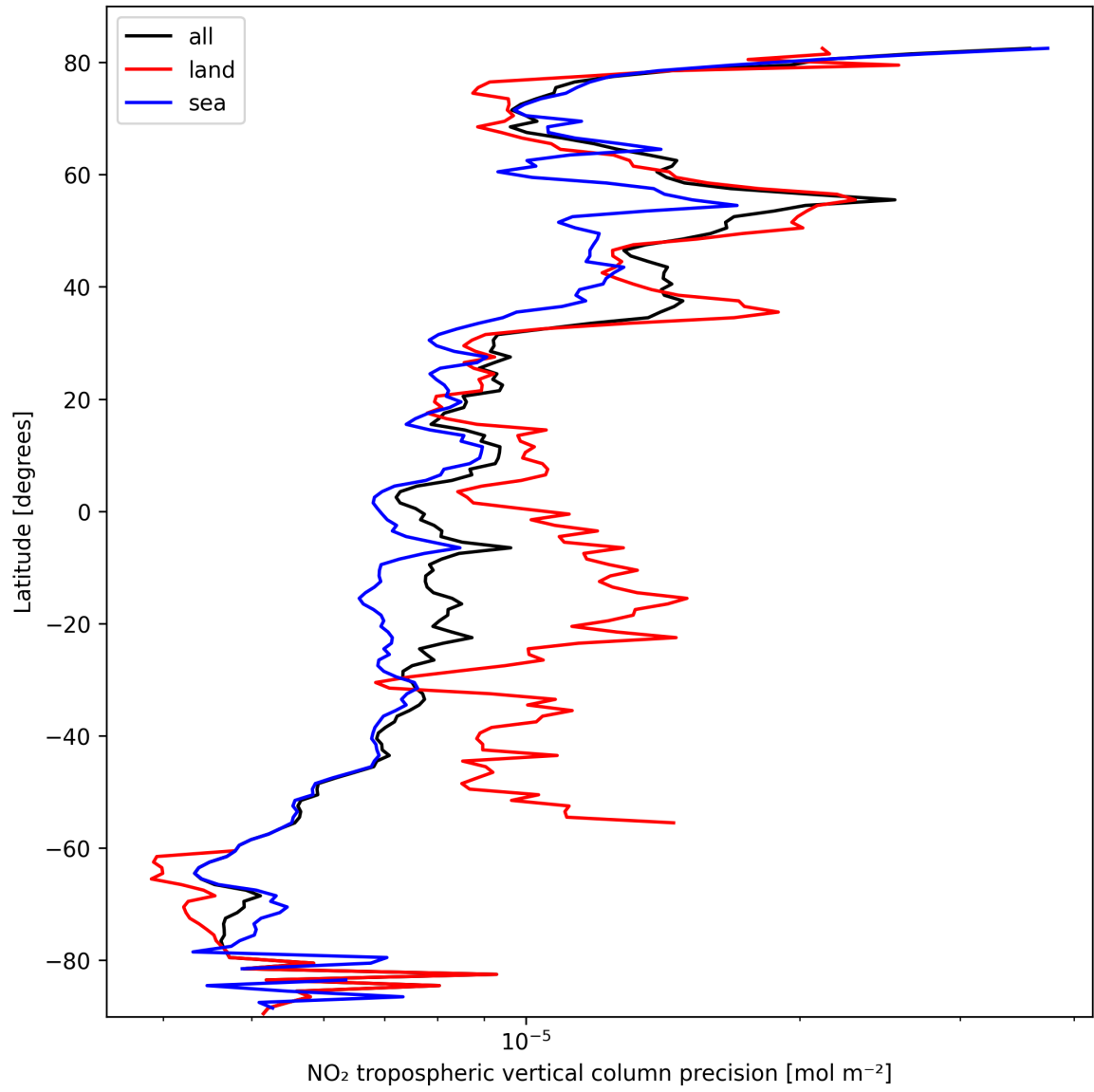
Figure 13: Zonal average of “NO 2 tropospheric vertical column precision” for 2025-10-06 to 2025-10-08.
