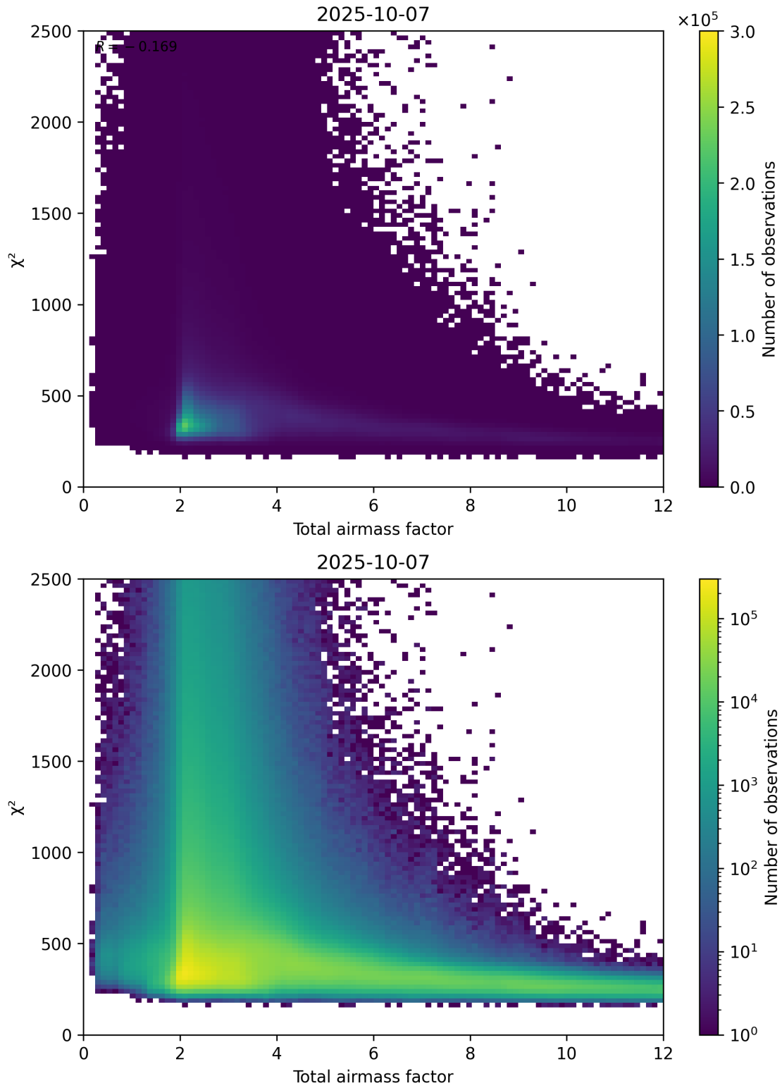
Figure 63: Scatter density plot of “Total airmass factor” against “ \chi^2 ” for 2025-10-06 to 2025-10-08.
