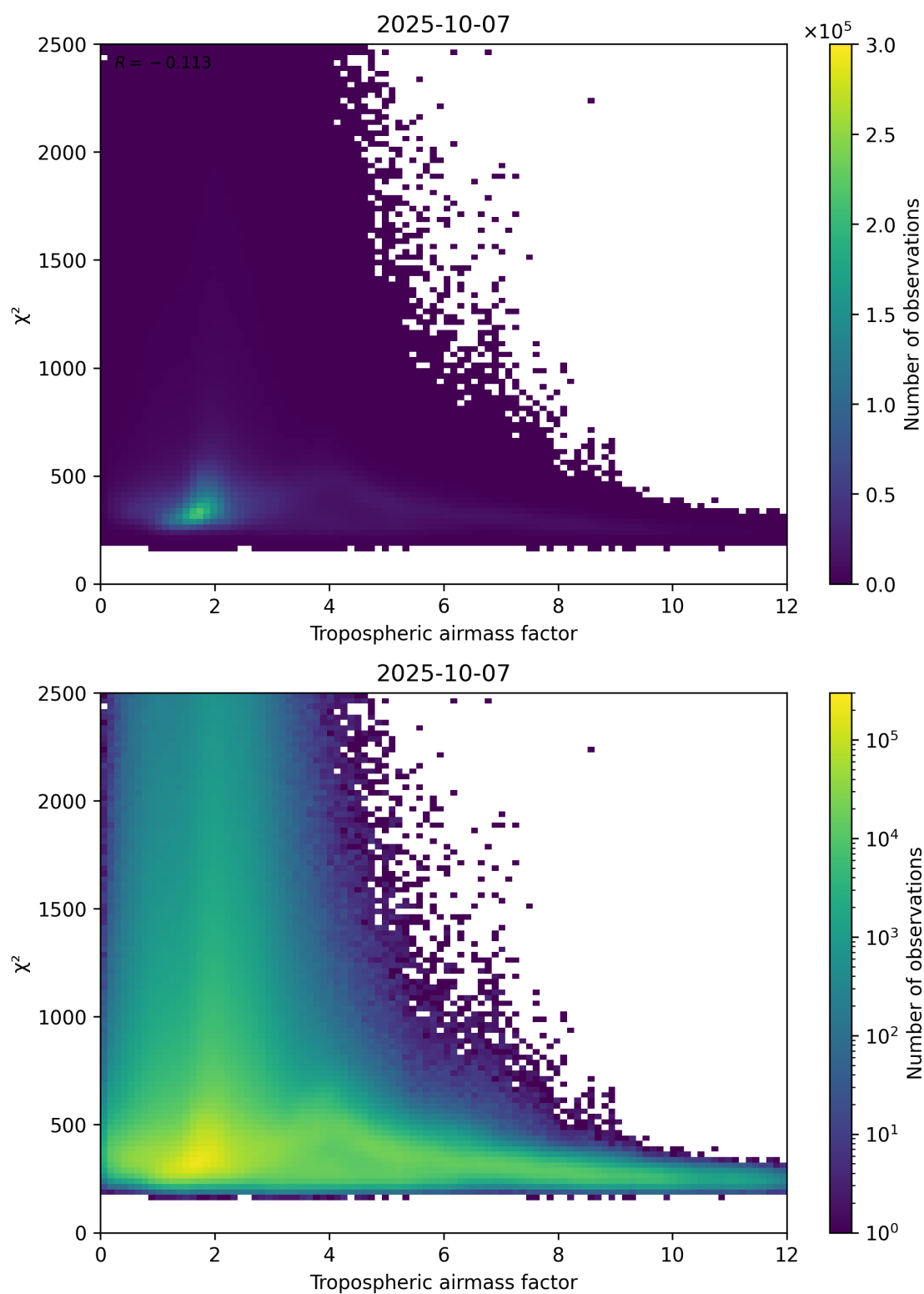
Figure 73: Scatter density plot of “Tropospheric airmass factor” against “ \chi^2 ” for 2025-10-06 to 2025-10-08.
