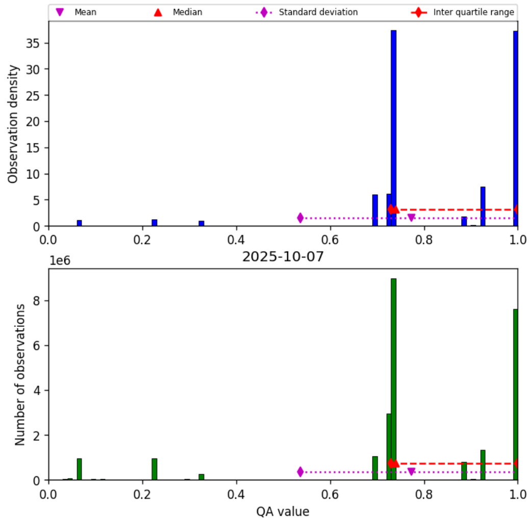
Figure 28: Histogram of “QA value” for 2025-10-06 to 2025-10-08
