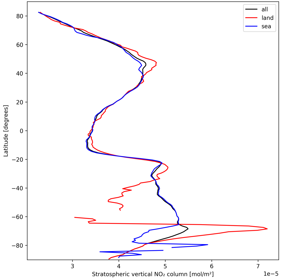
Figure 19: Zonal average of “Stratospheric vertical NO 2 column” for 2025-10-06 to 2025-10-08.
