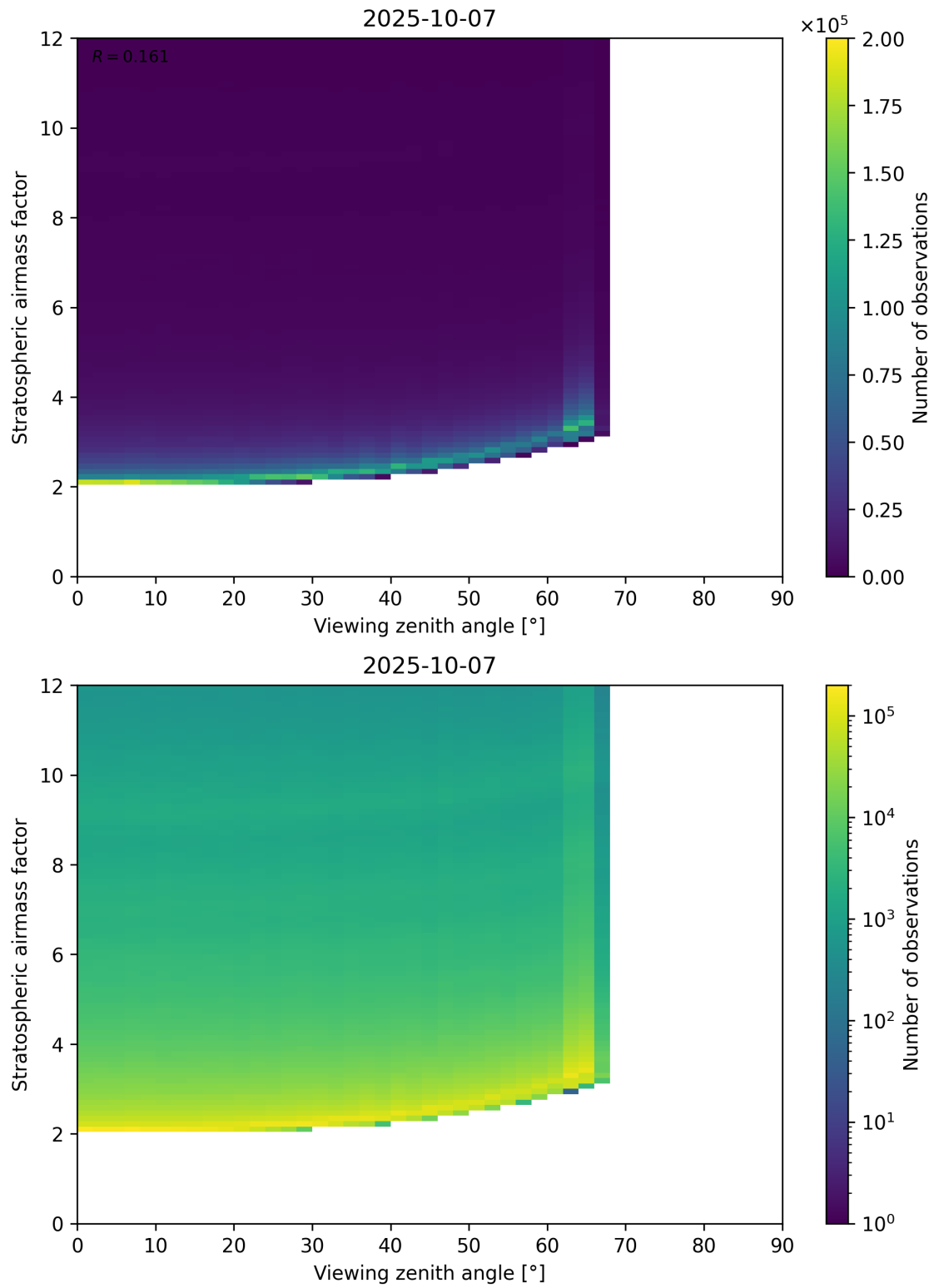
Figure 159: Scatter density plot of “Viewing zenith angle” against “Stratospheric airmass factor” for 2025-10-06 to 2025-10-08.
