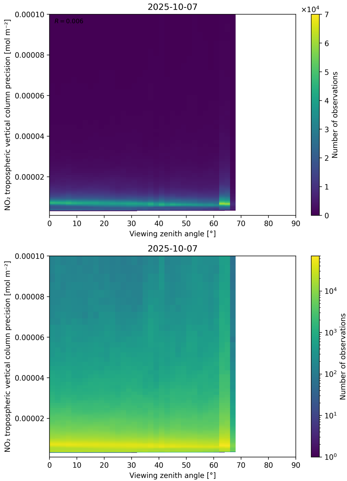
Figure 170: Scatter density plot of “Viewing zenith angle” against “NO 2 tropospheric vertical column precision” for 2025-10-06 to 2025-10-08.
