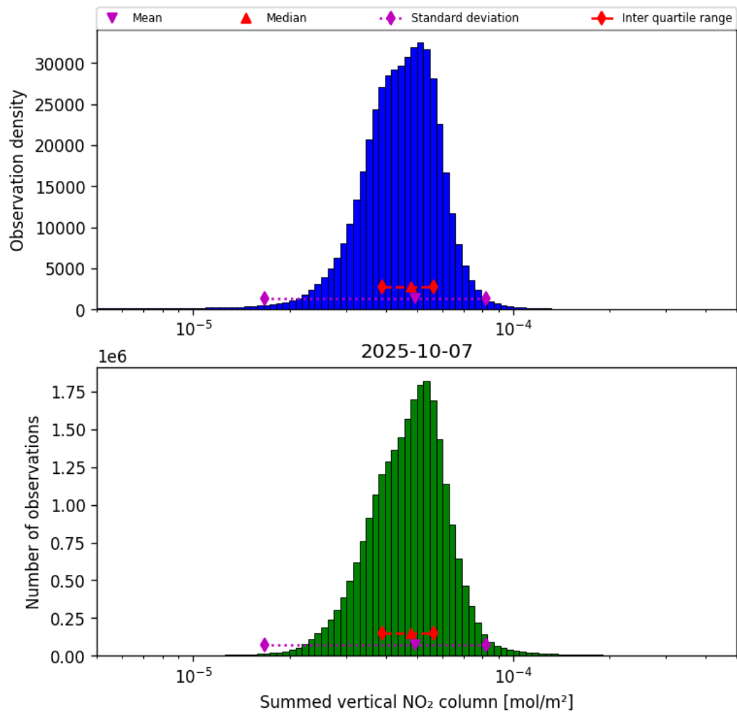
Figure 40: Histogram of “Summed vertical NO 2 column” for 2025-10-06 to 2025-10-08
