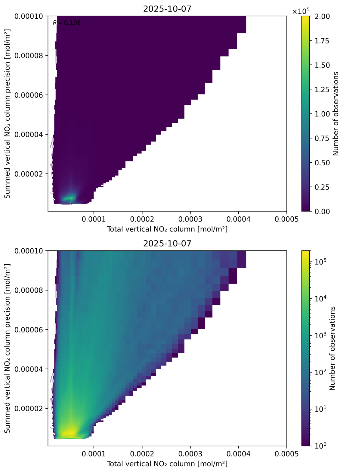
Figure 113: Scatter density plot of “Total vertical NO 2 column” against “Summed vertical NO 2 column precision” for 2025-10-06 to 2025-10-08.
