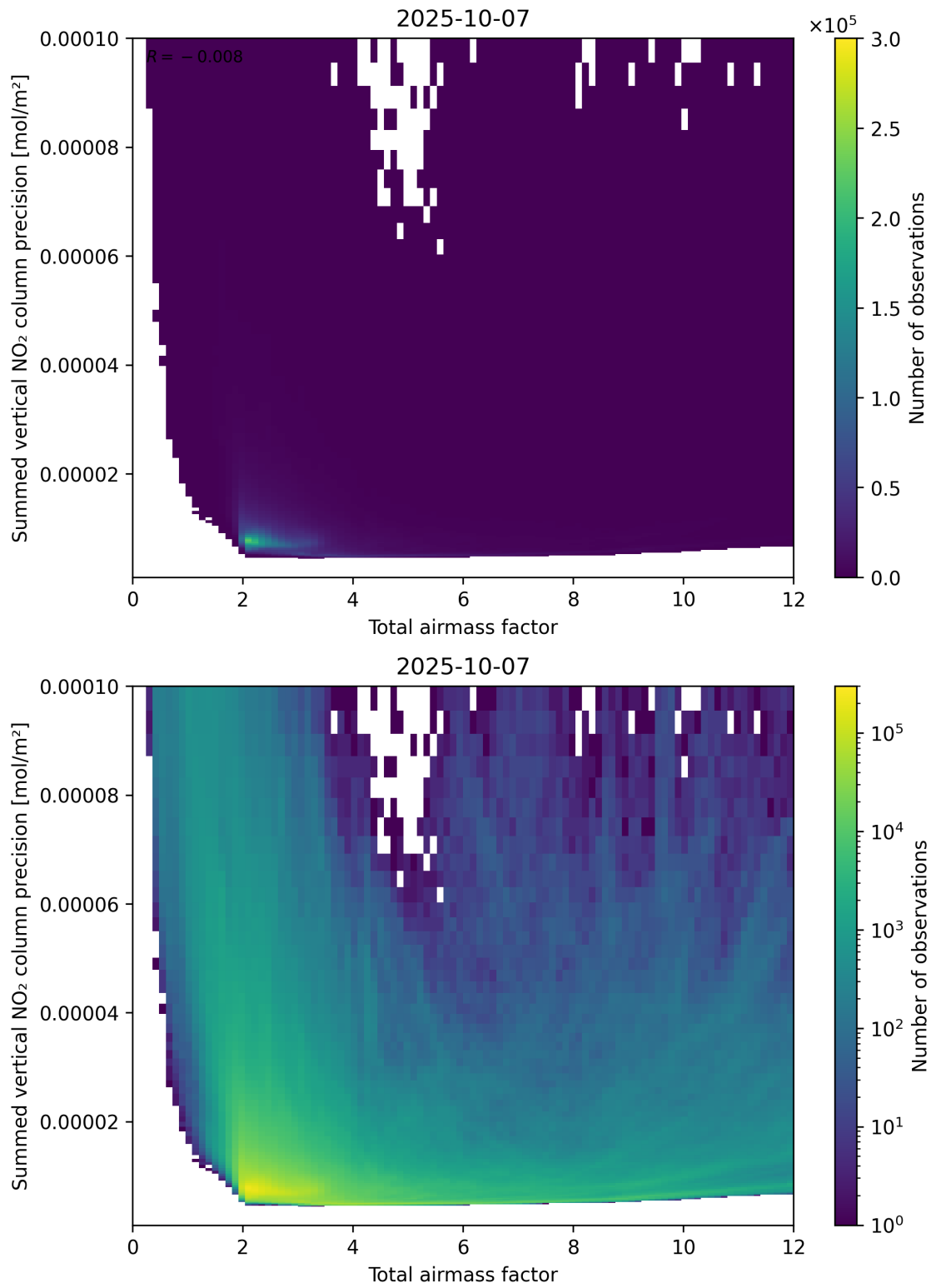
Figure 66: Scatter density plot of “Total airmass factor” against “Summed vertical NO 2 column precision” for 2025-10-06 to 2025-10-08.
