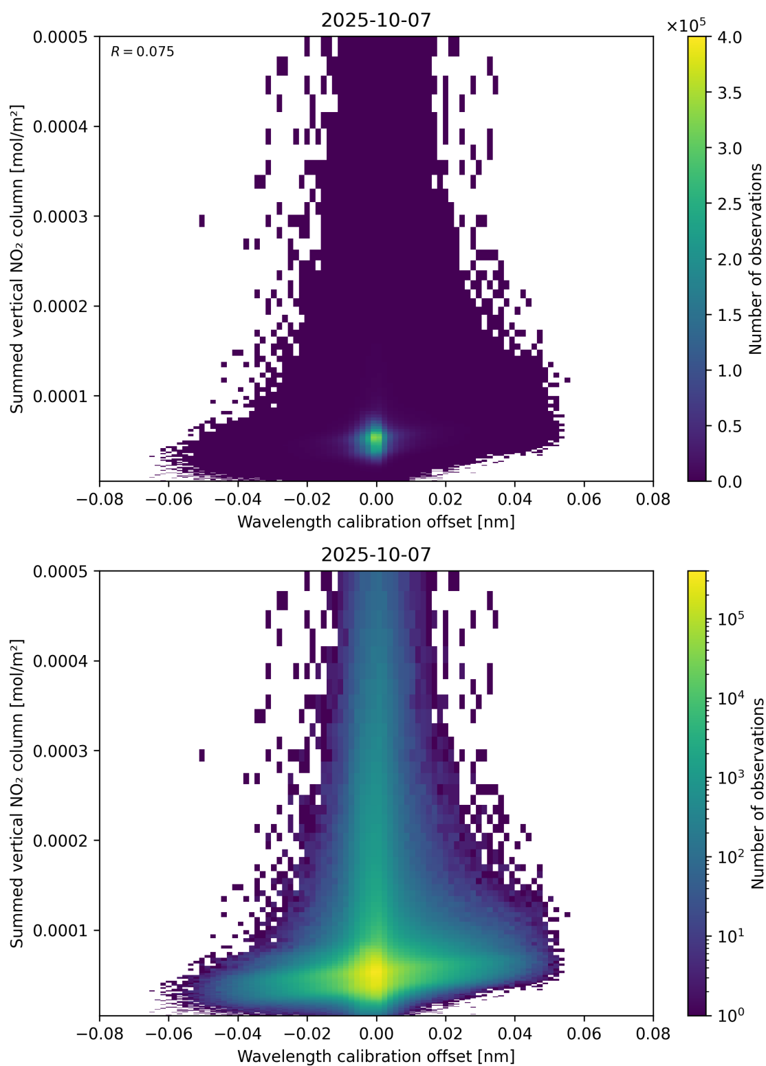
Figure 177: Scatter density plot of “Wavelength calibration offset” against “Summed vertical NO 2 column” for 2025-10-06 to 2025-10-08.
