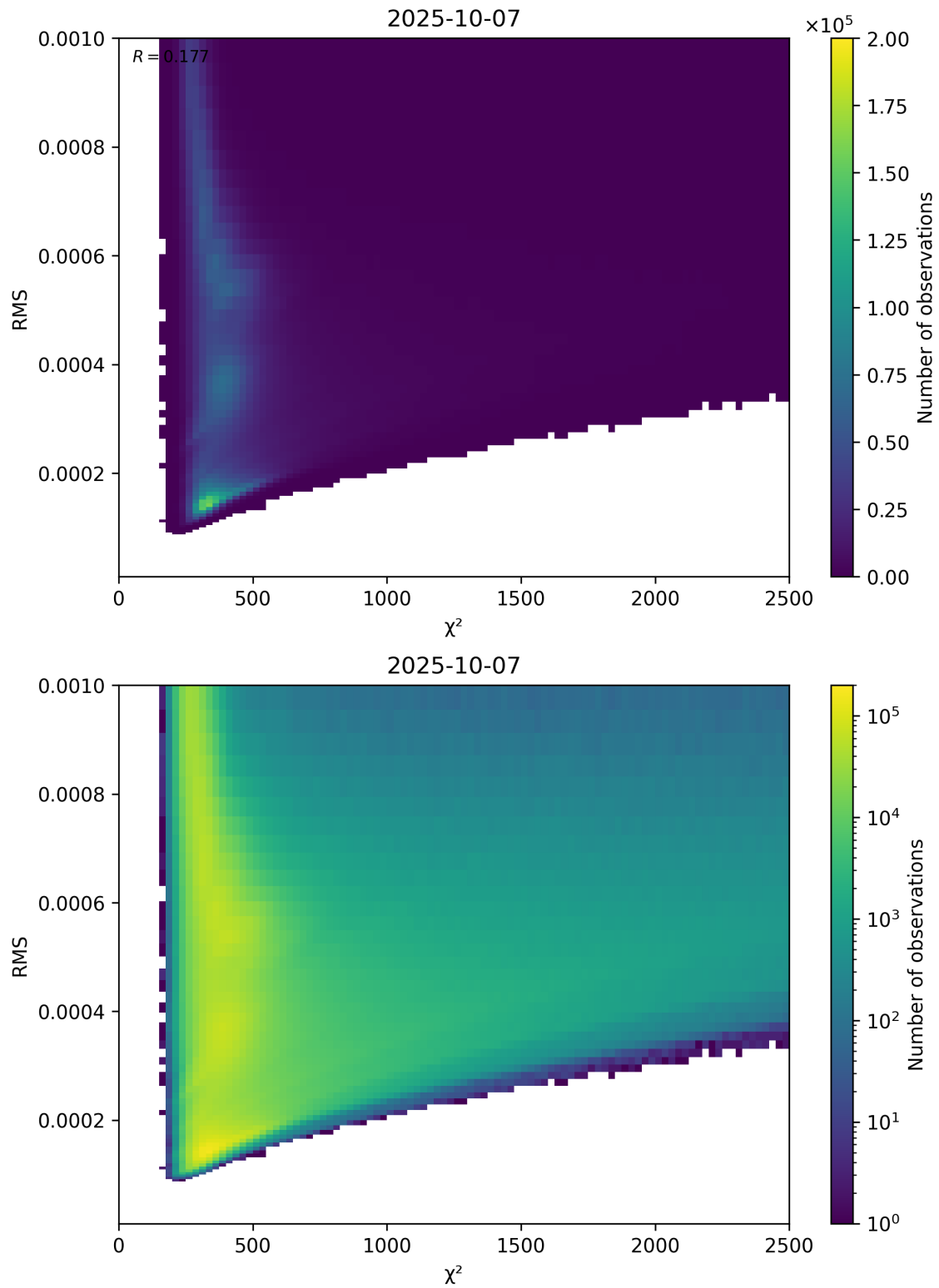
Figure 82: Scatter density plot of “ \chi^2 ” against “RMS” for 2025-10-06 to 2025-10-08.
