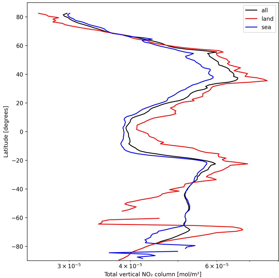
Figure 21: Zonal average of “Total vertical NO 2 column” for 2025-10-06 to 2025-10-08.
