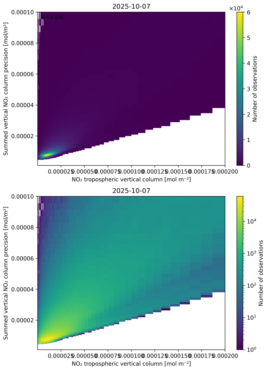
Figure 127: Scatter density plot of “NO 2 tropospheric vertical column” against “Summed vertical NO 2 column precision” for 2025-10-06 to 2025-10-08.
