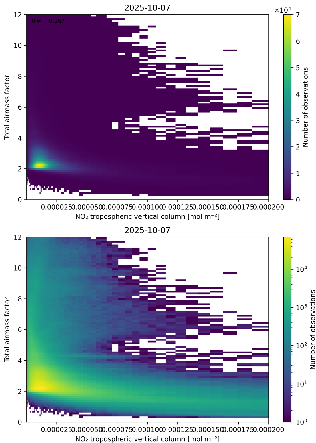
Figure 122: Scatter density plot of “NO 2 tropospheric vertical column” against “Total air mass factor” for 2025-10-06 to 2025-10-08.
