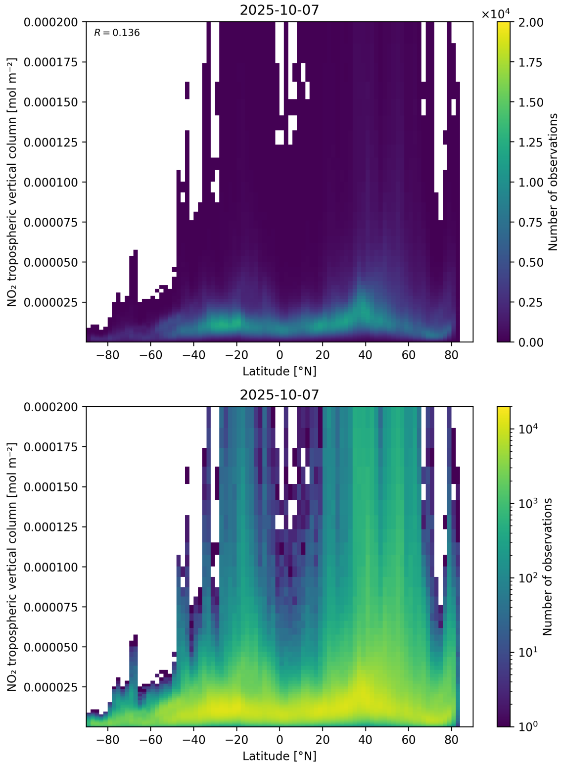
Figure 92: Scatter density plot of “Latitude” against “NO 2 tropospheric vertical column” for 2025-10-06 to 2025-10-08.
