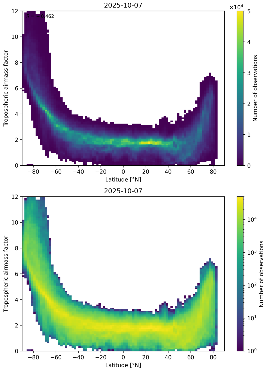
Figure 85: Scatter density plot of “Latitude” against “Tropospheric airmass factor” for 2025-10-06 to 2025-10-08.
