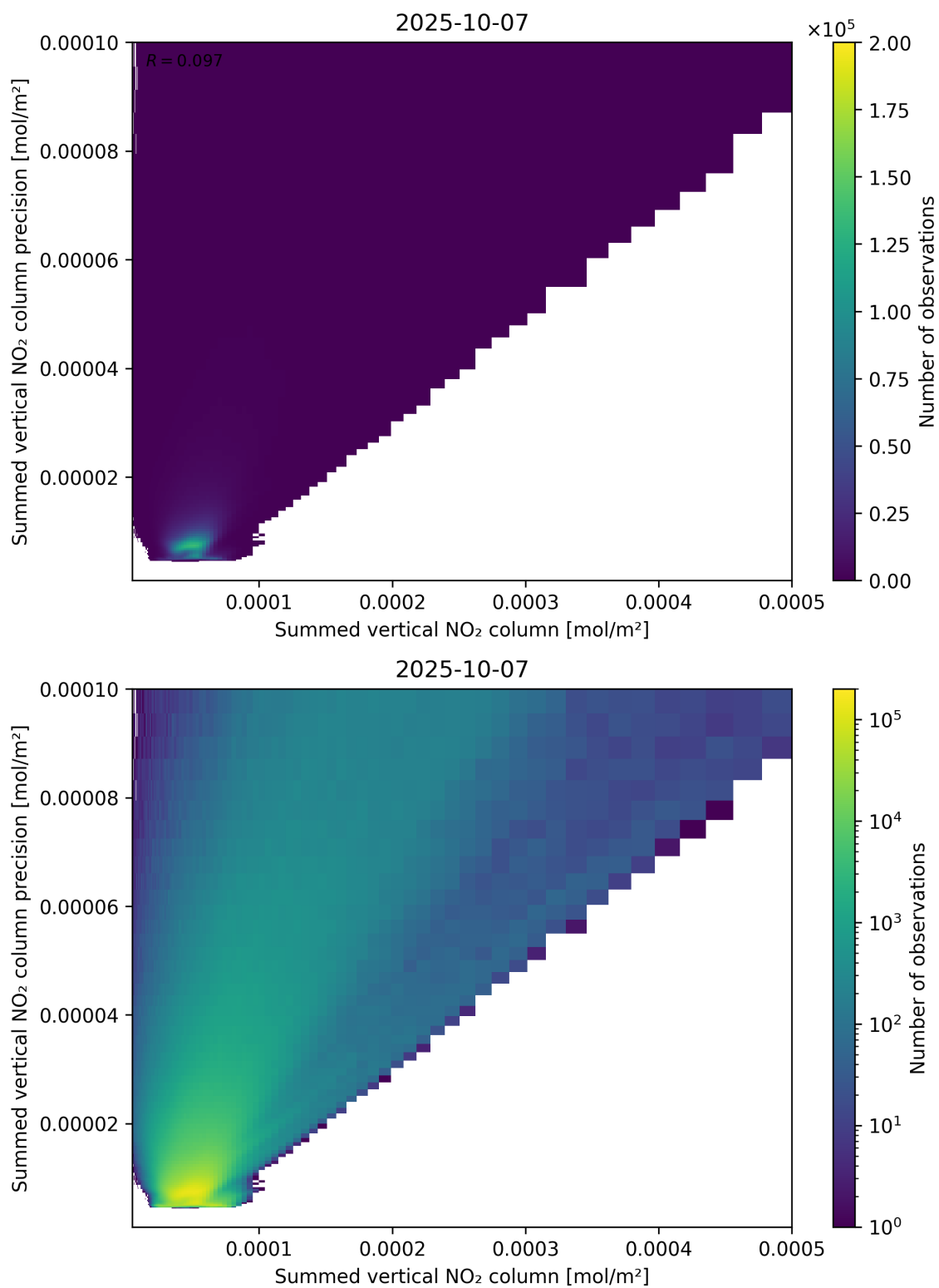
Figure 105: Scatter density plot of “Summed vertical NO 2 column” against “Summed vertical NO 2 column precision” for 2025-10-06 to 2025-10-08.
