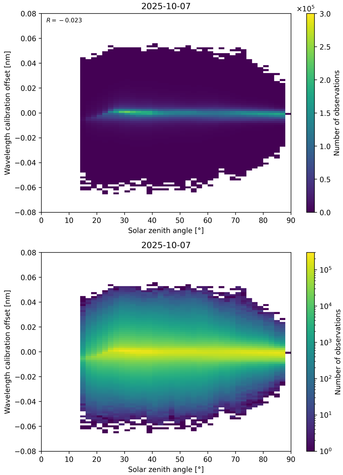
Figure 158: Scatter density plot of “Solar zenith angle” against “Wavelength calibration offset” for 2025-10-06 to 2025-10-08.
