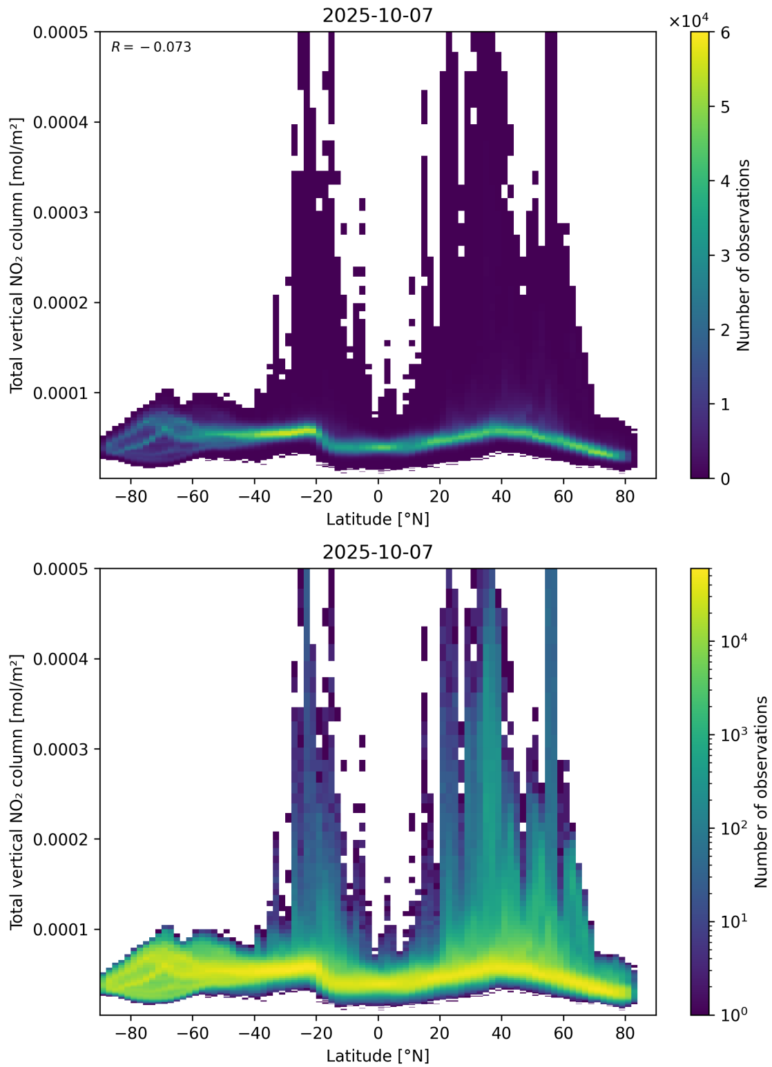
Figure 90: Scatter density plot of “Latitude” against “Total vertical NO 2 column” for 2025-10-06 to 2025-10-08.
