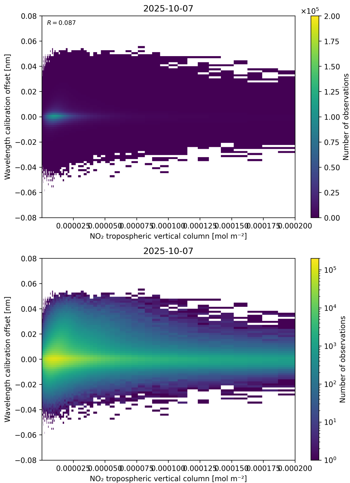
Figure 143: Scatter density plot of “NO 2 tropospheric vertical column” against “Wavelength calibration offset” for 2025-10-06 to 2025-10-08.
