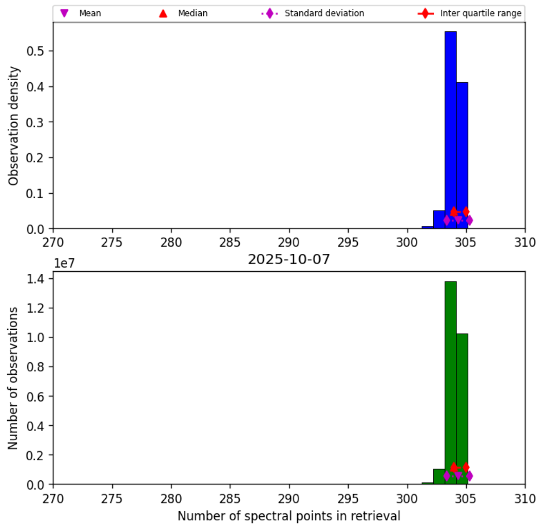
Figure 33: Histogram of “Number of spectral points in retrieval” for 2025-10-06 to 2025-10-08
