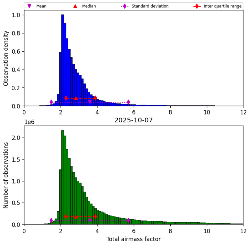
Figure 32: Histogram of “Total airmass factor” for 2025-10-06 to 2025-10-08
