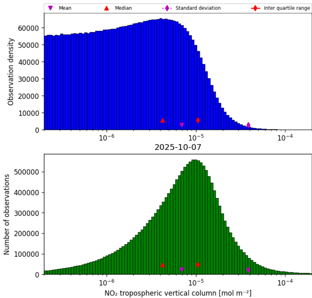
Figure 29: Histogram of “NO 2 tropospheric vertical column” for 2025-10-06 to 2025-10-08
