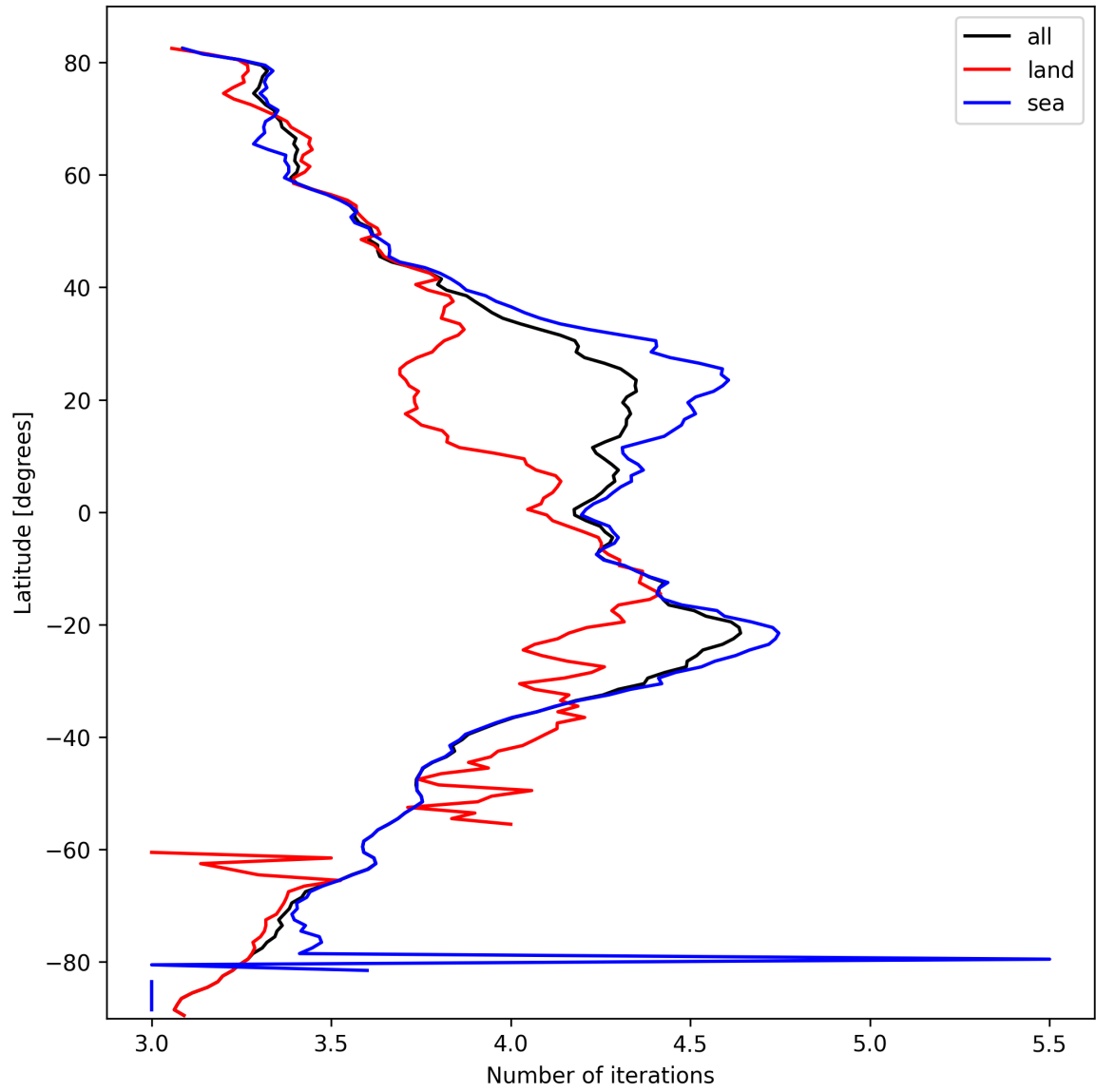
Figure 17: Zonal average of “Number of iterations” for 2025-10-06 to 2025-10-08.
