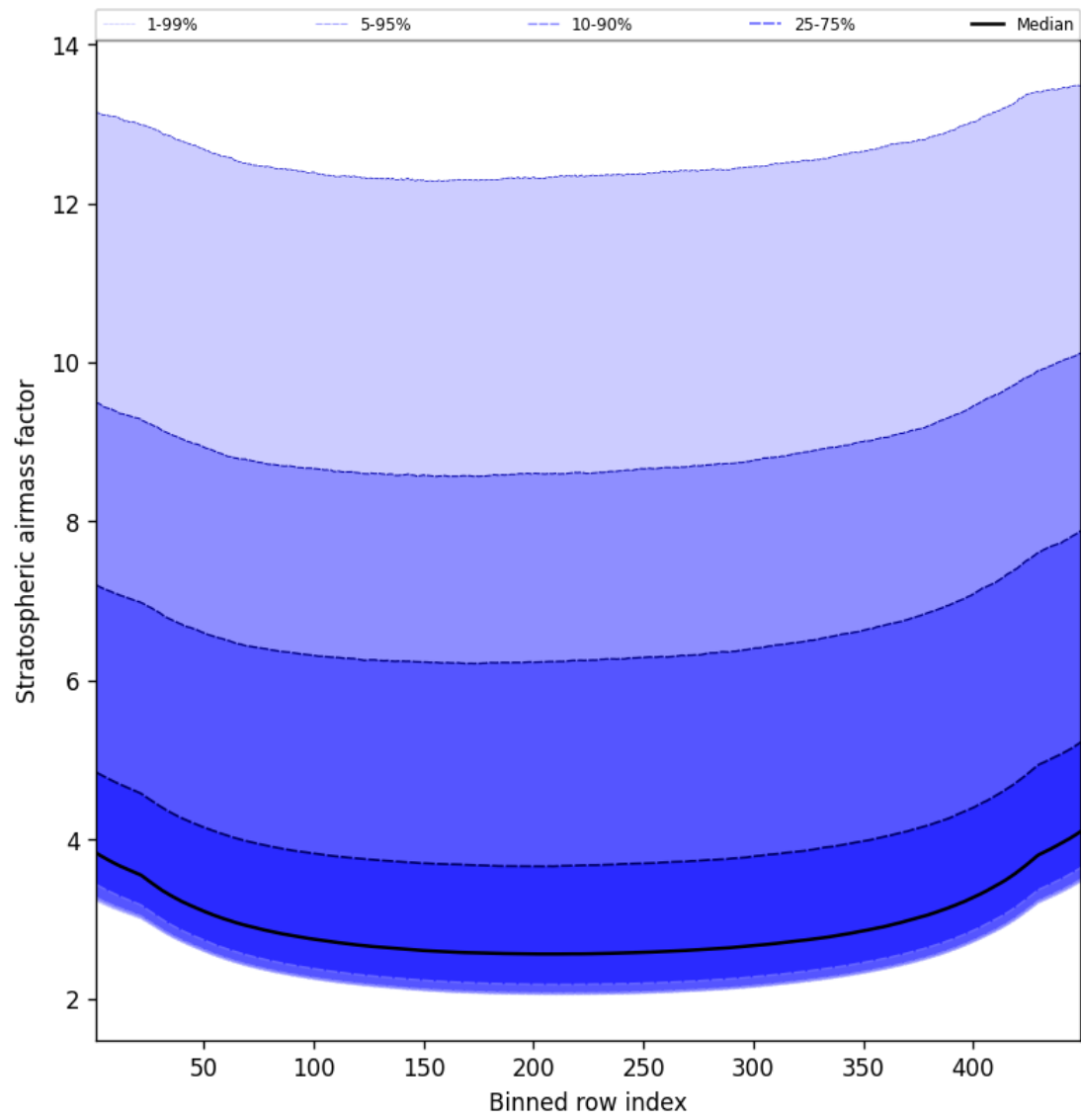
Figure 61: Along track statistics of “Stratospheric air mass factor” for 2025-10-06 to 2025-10-08
