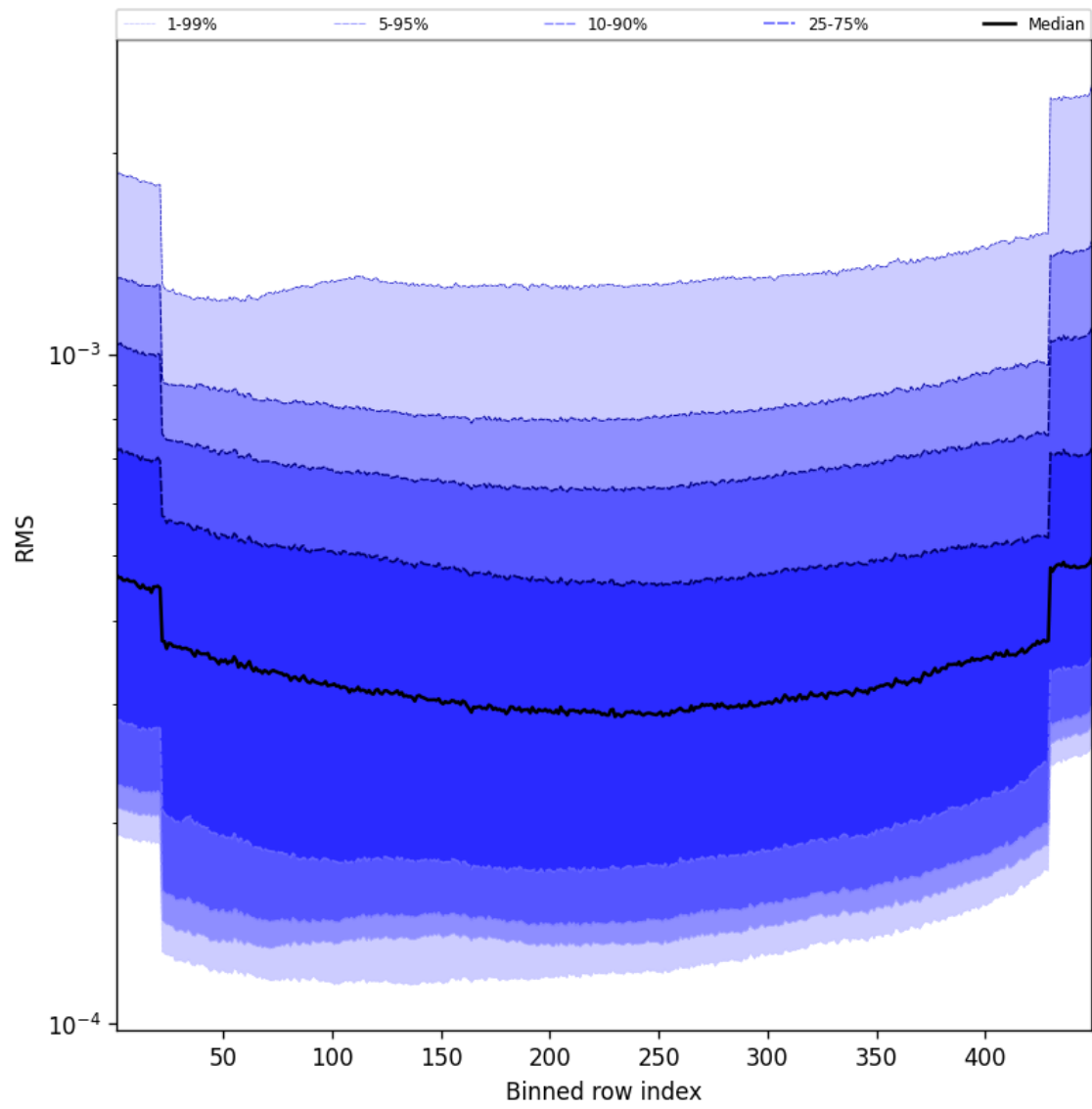
Figure 60: Along track statistics of “RMS” for 2025-10-06 to 2025-10-08
