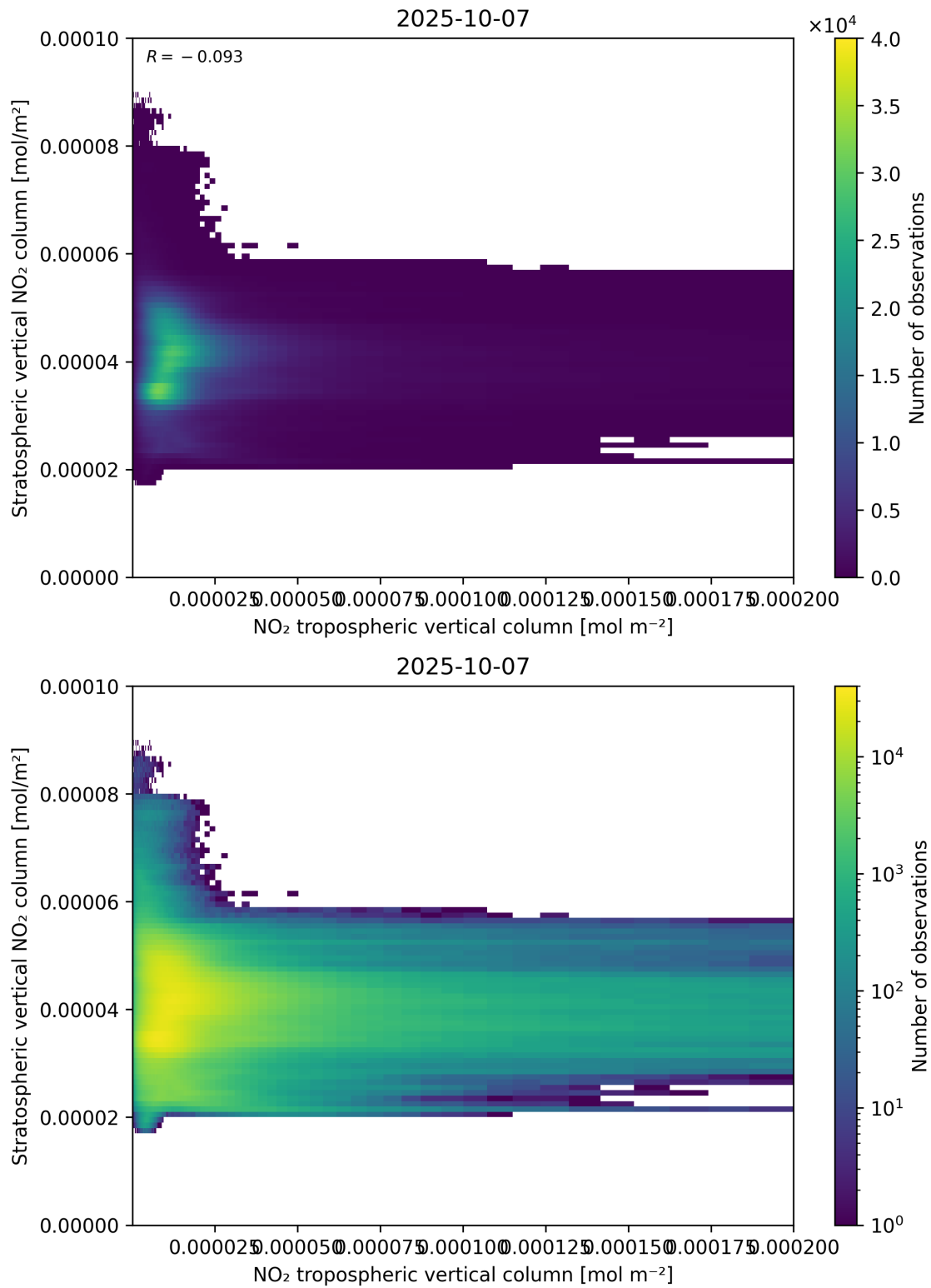
Figure 125: Scatter density plot of “NO 2 tropospheric vertical column” against “Stratospheric vertical NO 2 column” for 2025-10-06 to 2025-10-08.
