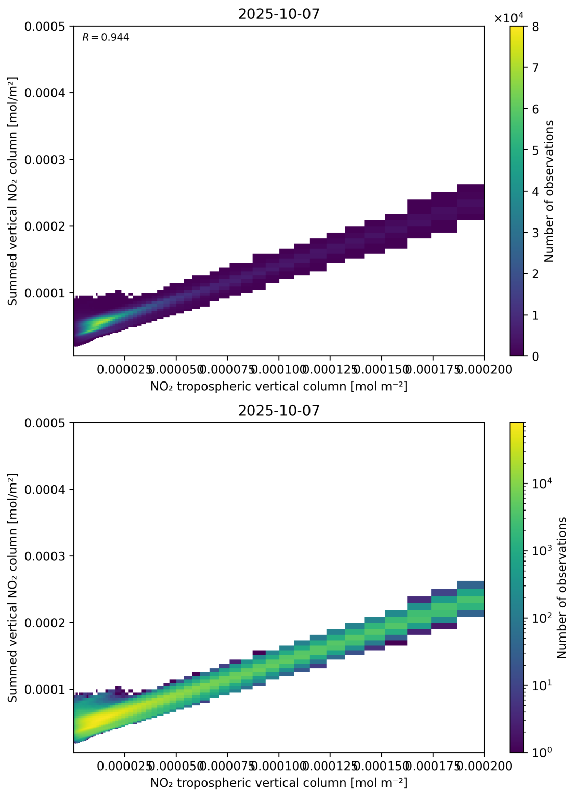
Figure 126: Scatter density plot of “NO 2 tropospheric vertical column” against “Summed vertical NO 2 column” for 2025-10-06 to 2025-10-08.
