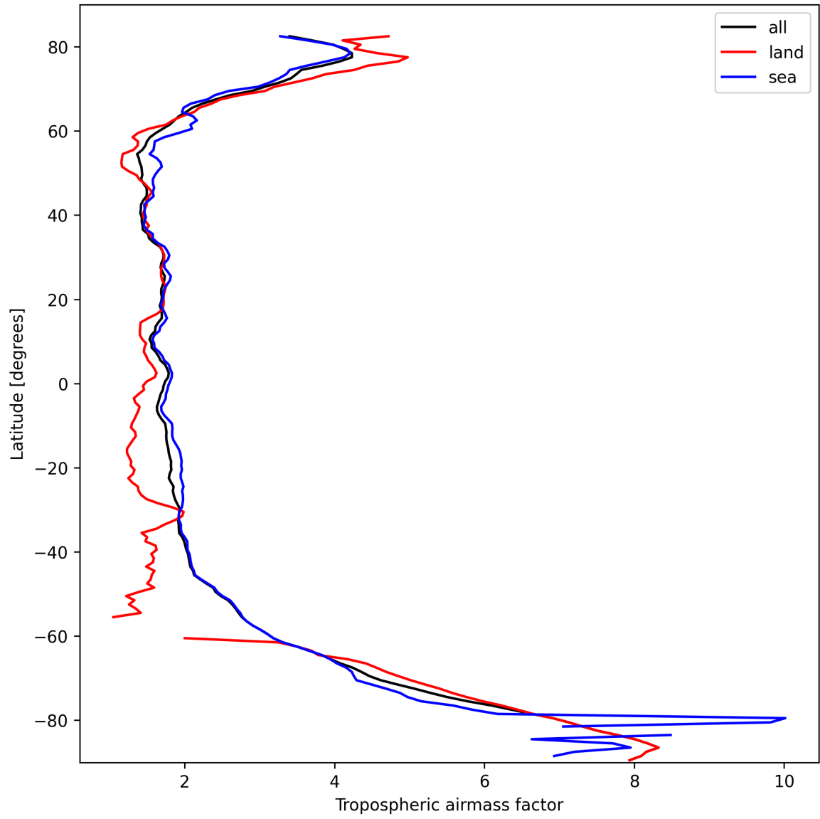
Figure 14: Zonal average of “Tropospheric airmass factor” for 2025-10-06 to 2025-10-08.
