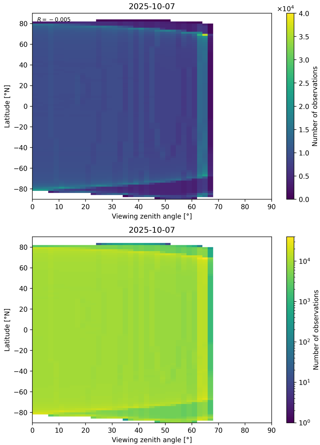
Figure 163: Scatter density plot of “Viewing zenith angle” against “Latitude” for 2025-10-06 to 2025-10-08.
