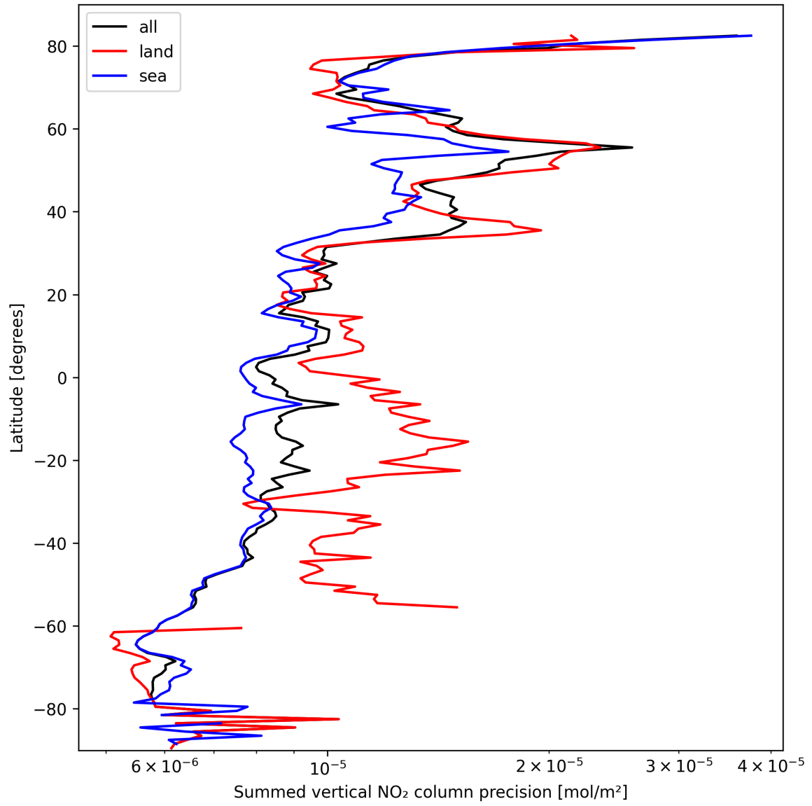
Figure 24: Zonal average of “Summed vertical NO 2 column precision” for 2025-10-06 to 2025-10-08.
