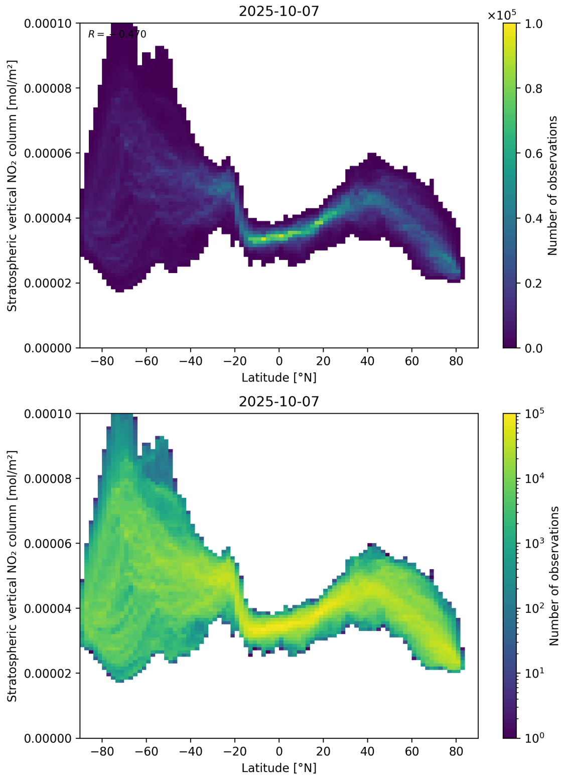
Figure 87: Scatter density plot of “Latitude” against “Stratospheric vertical NO 2 column” for 2025-10-06 to 2025-10-08.
