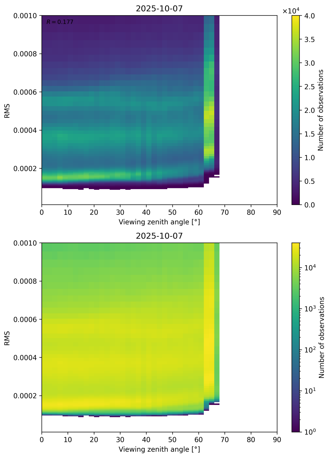
Figure 171: Scatter density plot of “Viewing zenith angle” against “RMS” for 2025-10-06 to 2025-10-08.
