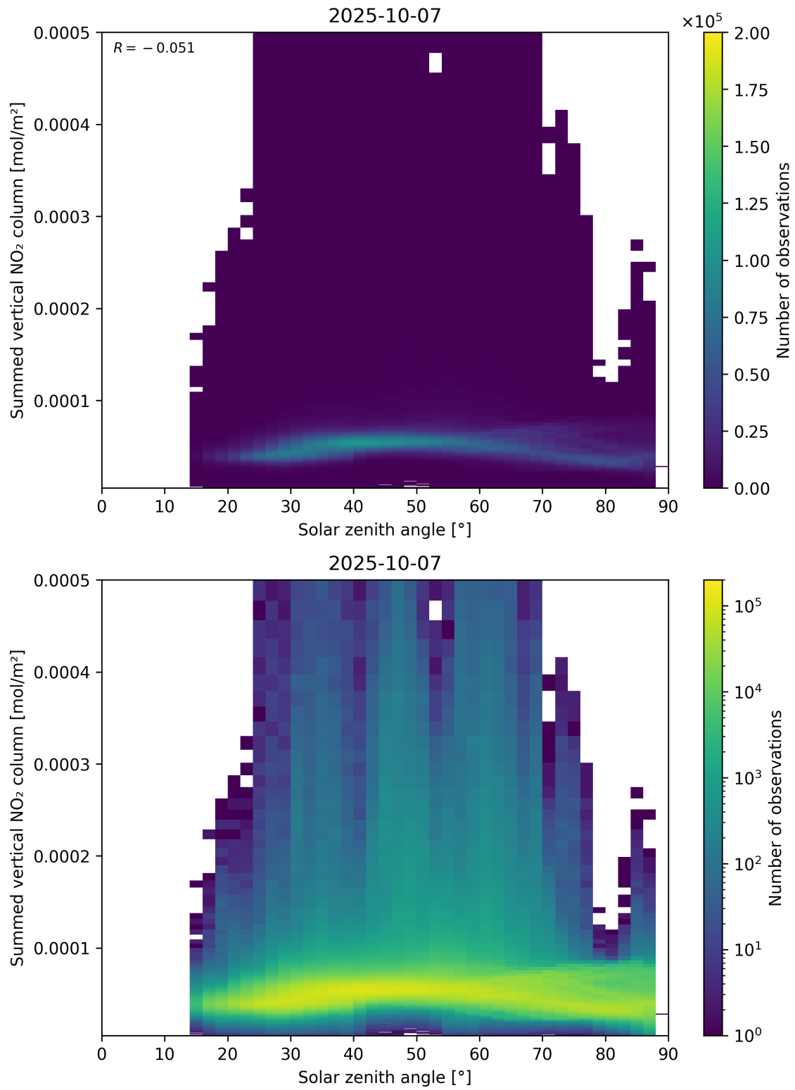
Figure 151: Scatter density plot of “Solar zenith angle” against “Summed vertical NO 2 column” for 2025-10-06 to 2025-10-08.
