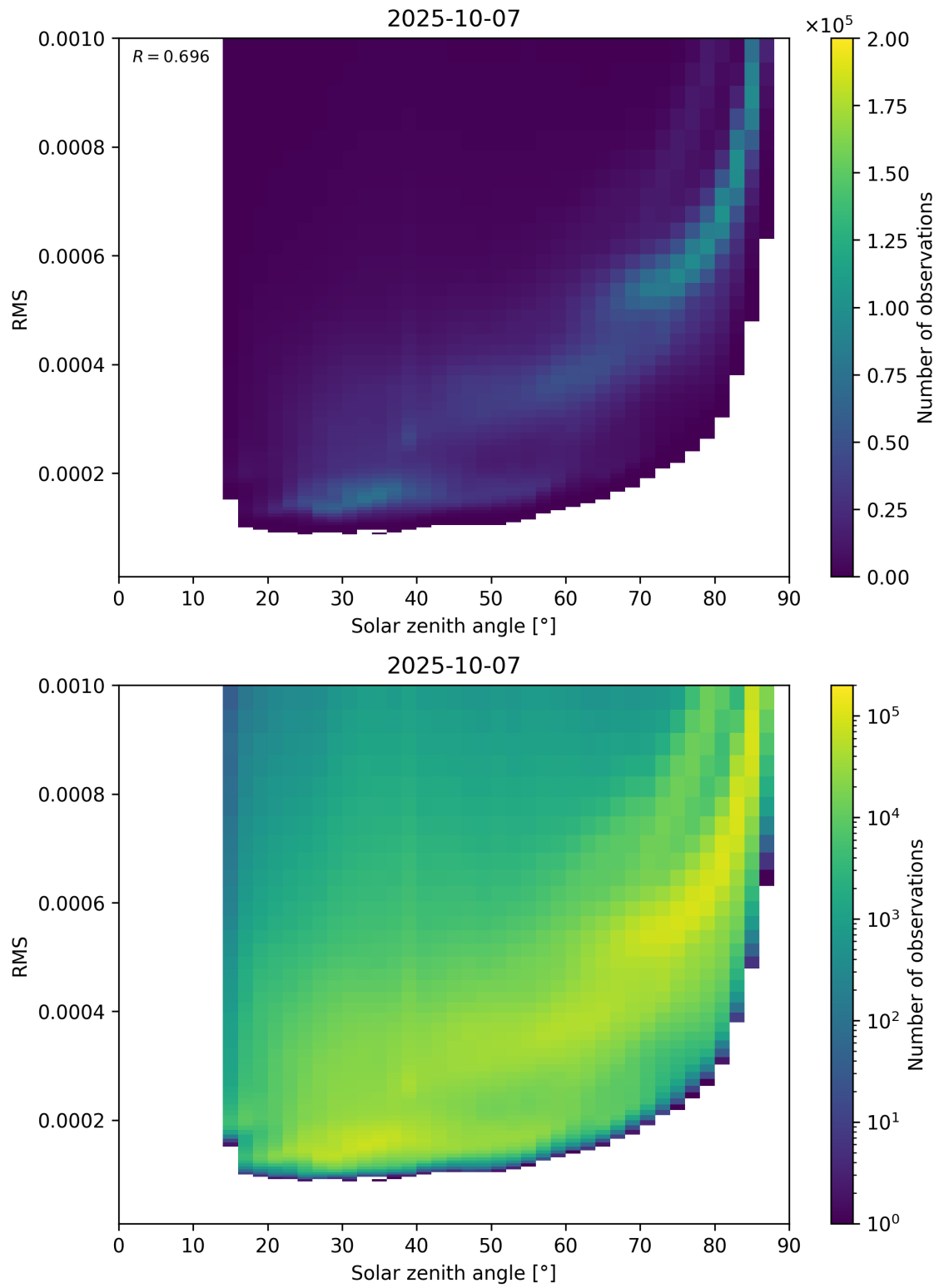
Figure 157: Scatter density plot of “Solar zenith angle” against “RMS” for 2025-10-06 to 2025-10-08.
