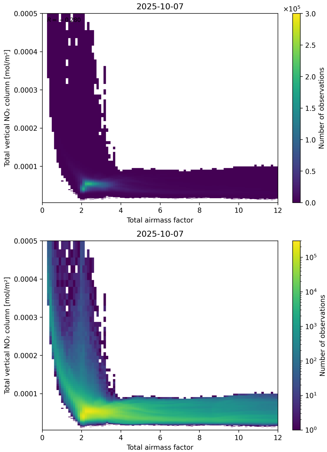
Figure 67: Scatter density plot of “Total airmass factor” against “Total vertical NO 2 column” for 2025-10-06 to 2025-10-08.
