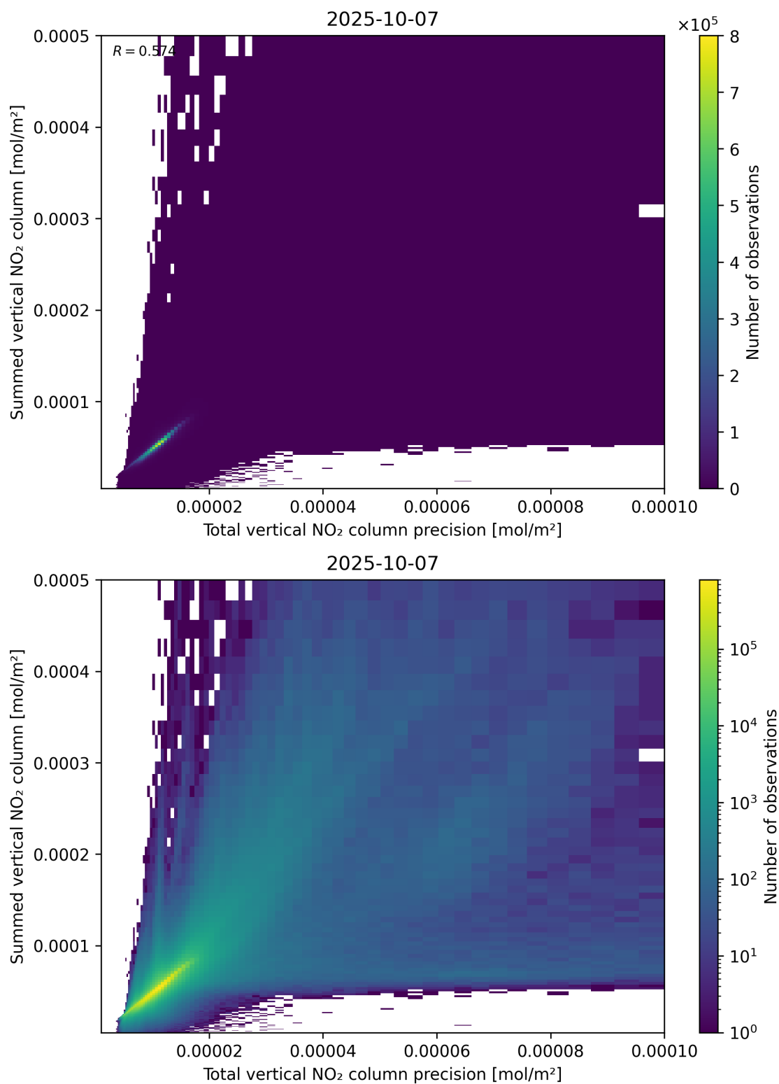
Figure 117: Scatter density plot of “Total vertical NO 2 column precision” against “Summed vertical NO 2 column” for 2025-10-06 to 2025-10-08.
