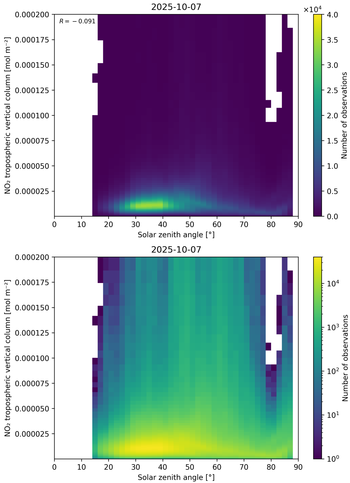
Figure 155: Scatter density plot of “Solar zenith angle” against “NO 2 tropospheric vertical column” for 2025-10-06 to 2025-10-08.
