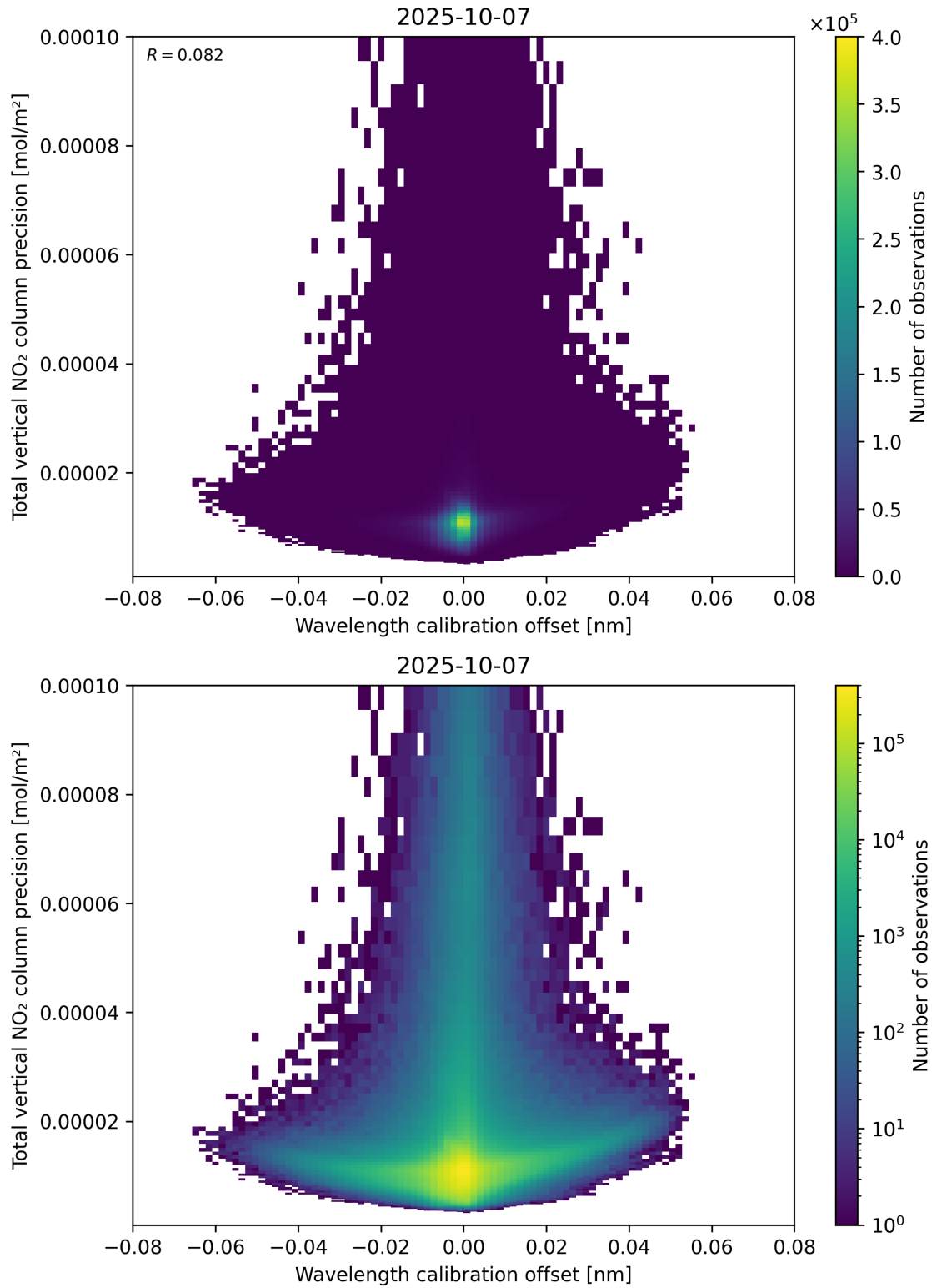
Figure 180: Scatter density plot of “Wavelength calibration offset” against “Total vertical NO 2 column precision” for 2025-10-06 to 2025-10-08.
