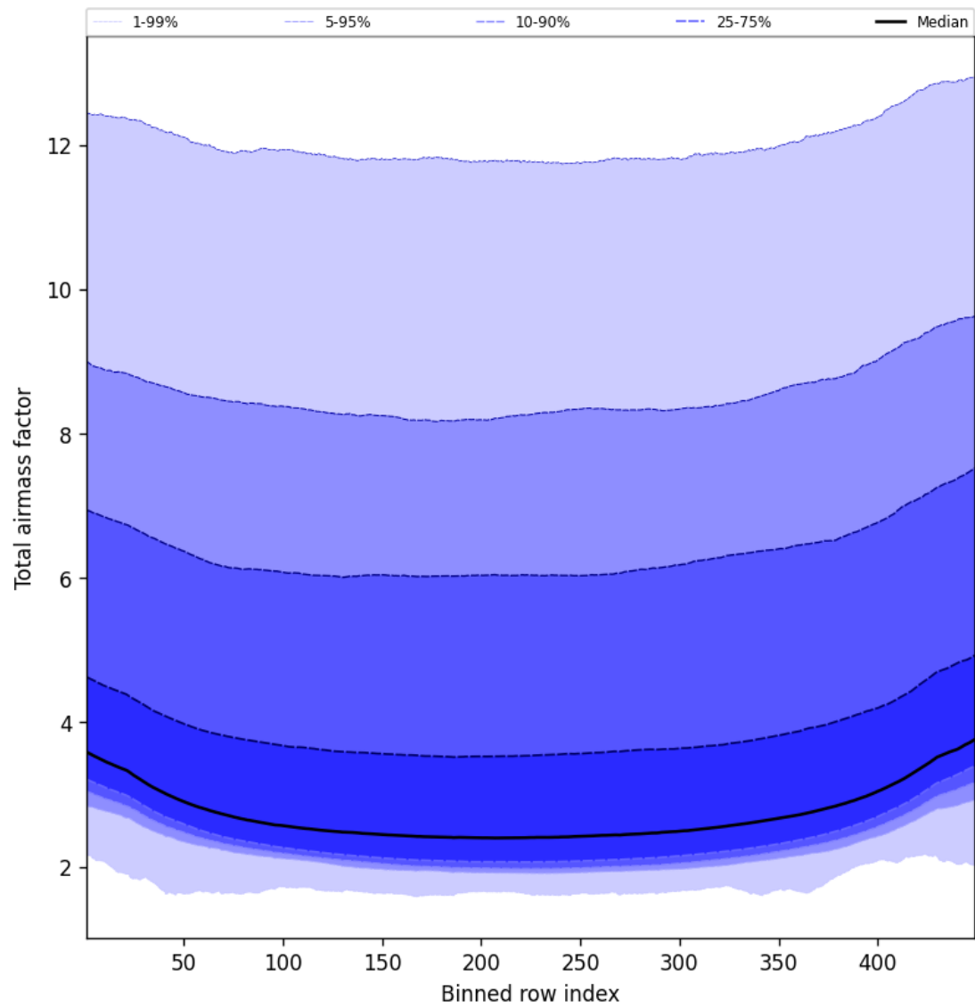
Figure 49: Along track statistics of “Total airmass factor” for 2025-10-06 to 2025-10-08
