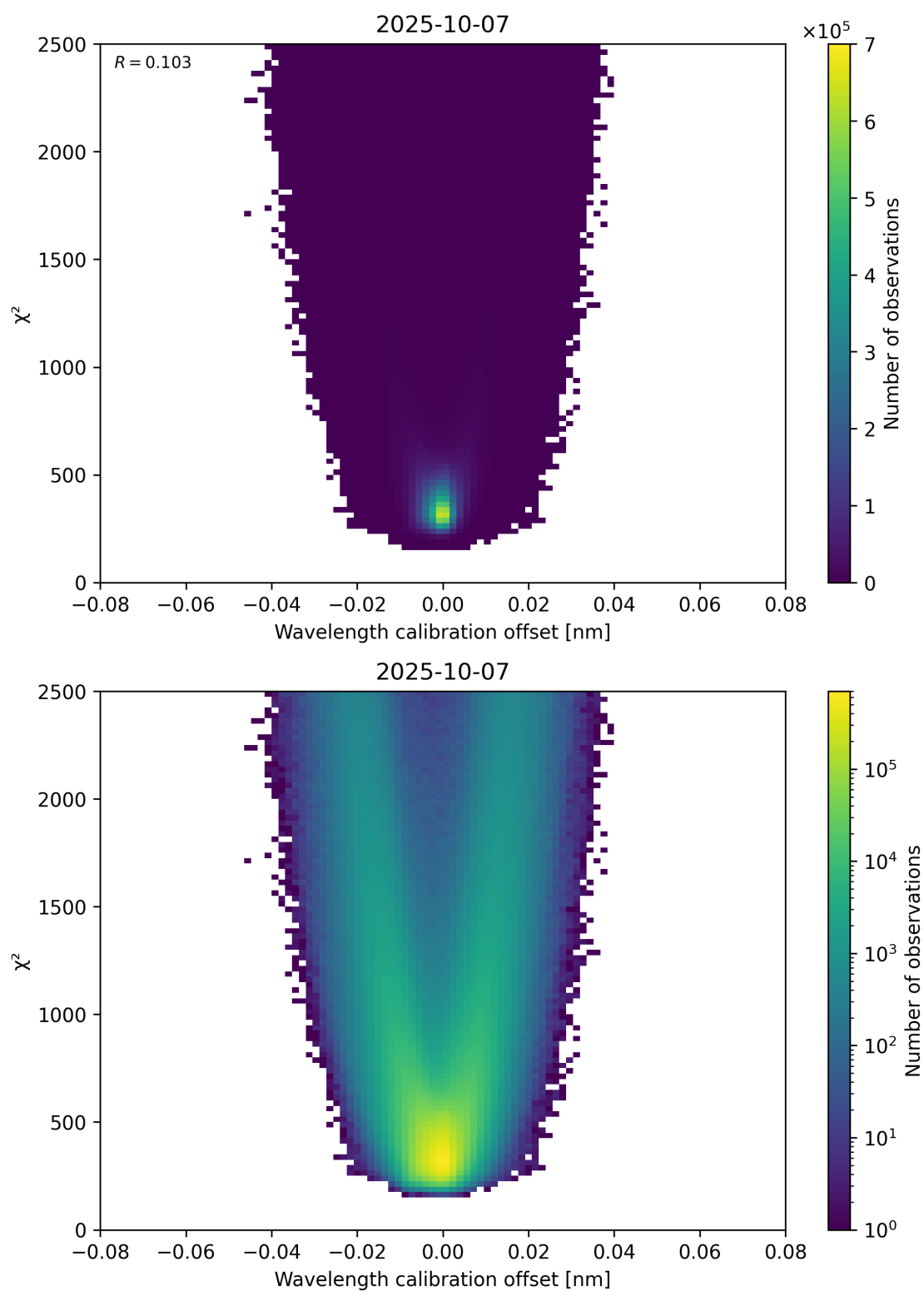
Figure 175: Scatter density plot of “Wavelength calibration offset” against “ \chi^2 ” for 2025-10-06 to 2025-10-08.
