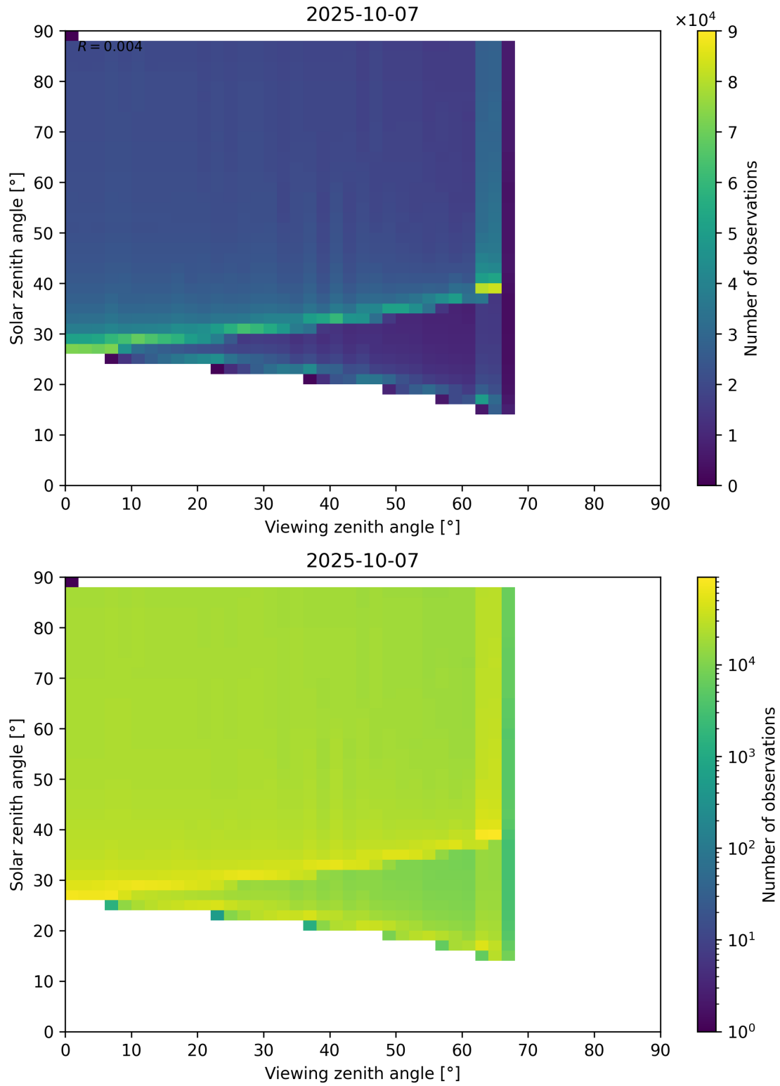
Figure 172: Scatter density plot of “Viewing zenith angle” against “Solar zenith angle” for 2025-10-06 to 2025-10-08.
