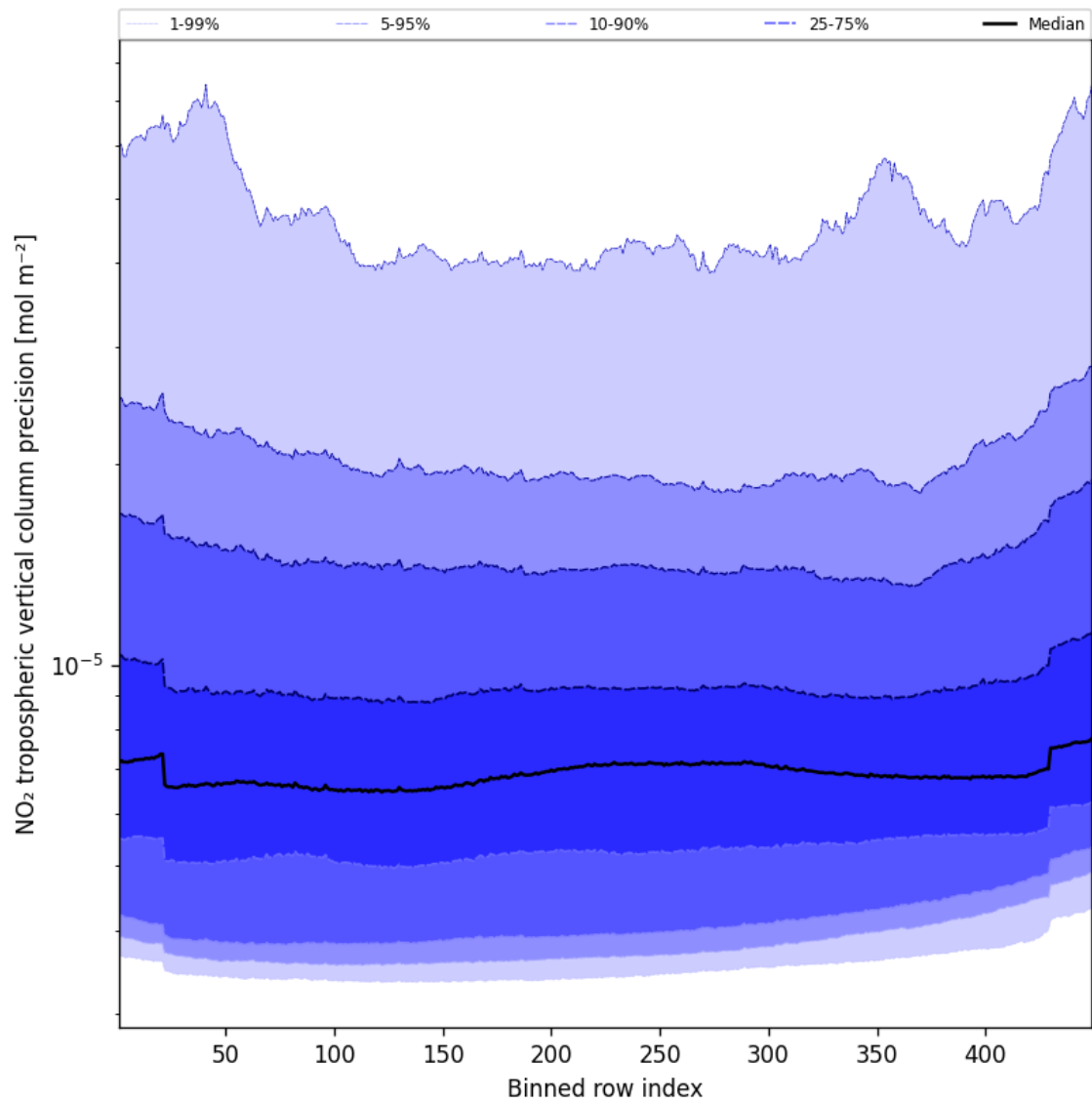
Figure 47: Along track statistics of “NO 2 tropospheric vertical column precision” for 2025-10-06 to 2025-10-08
