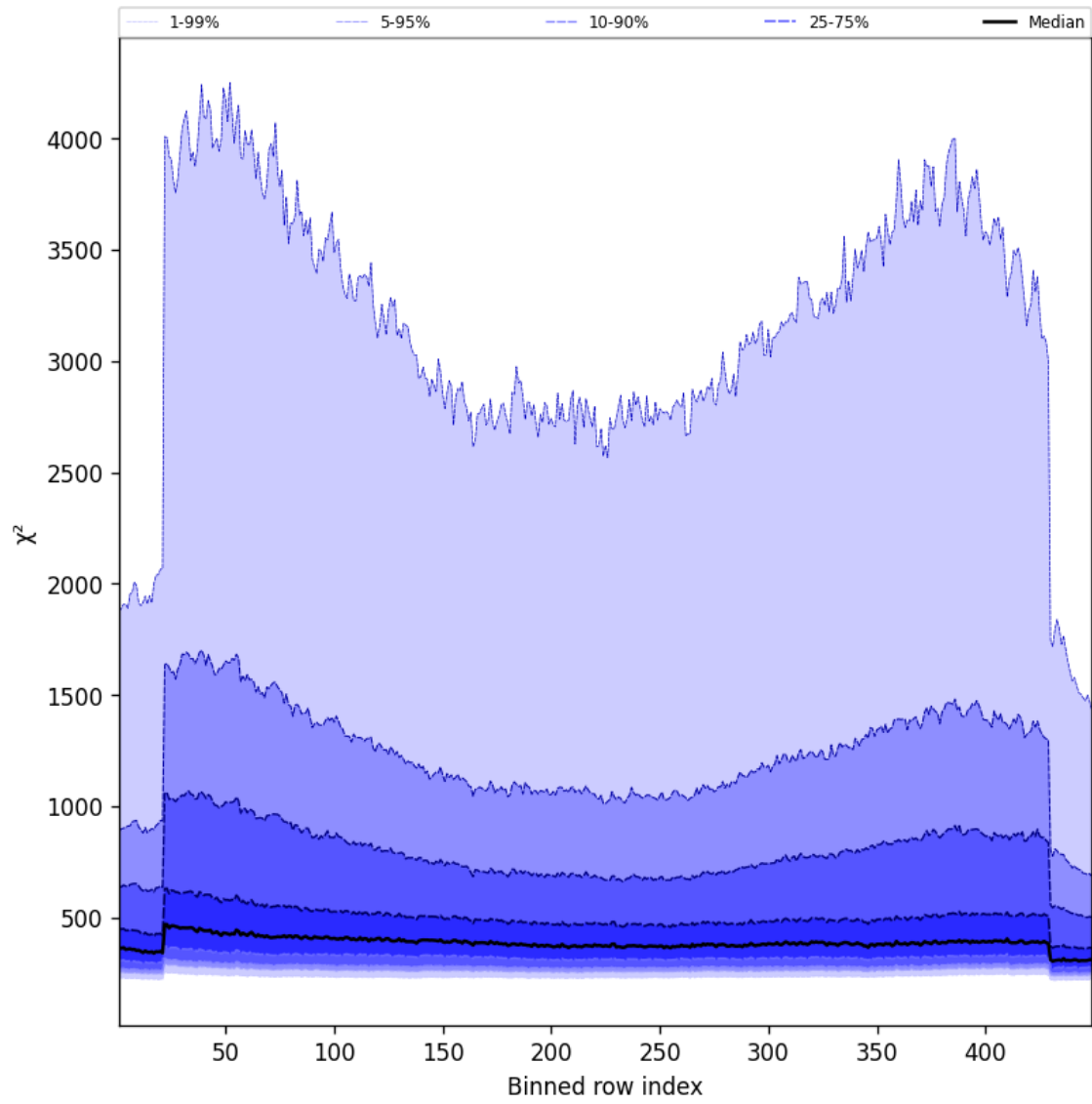
Figure 59: Along track statistics of “ \chi^2 ” for 2025-10-06 to 2025-10-08
