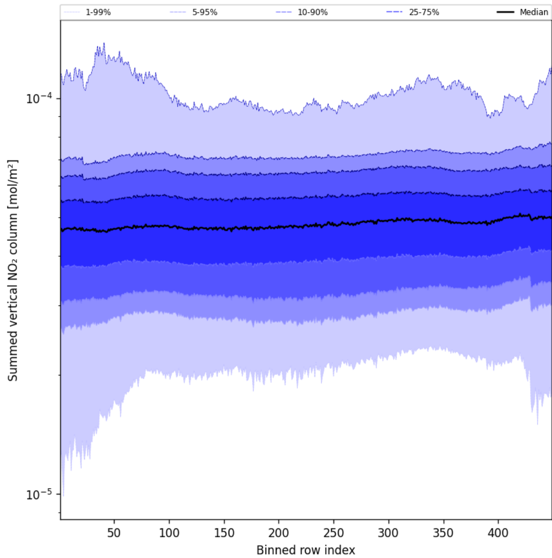
Figure 57: Along track statistics of “Summed vertical NO 2 column” for 2025-10-06 to 2025-10-08
