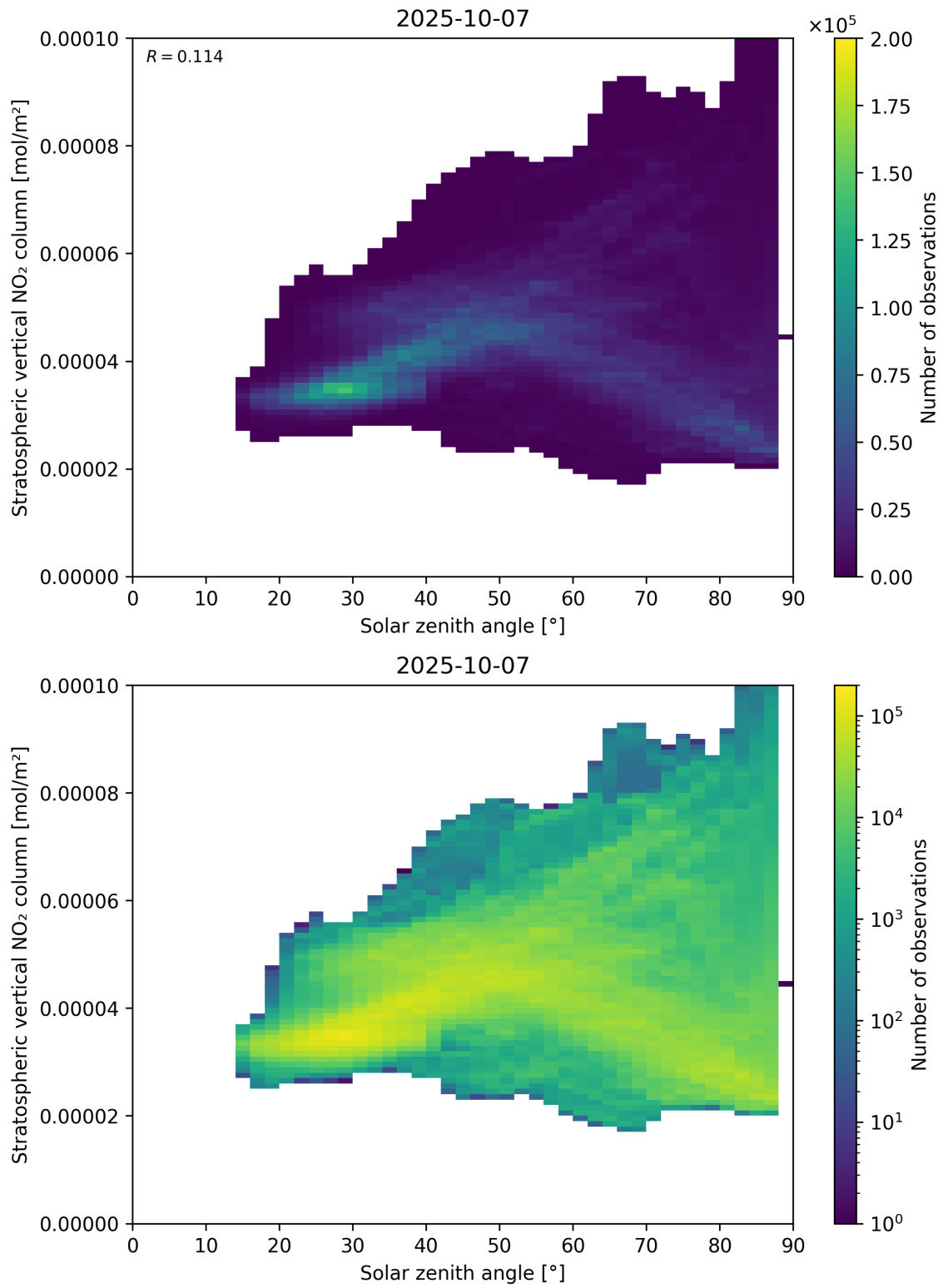
Figure 150: Scatter density plot of “Solar zenith angle” against “Stratospheric vertical NO 2 column” for 2025-10-06 to 2025-10-08.
