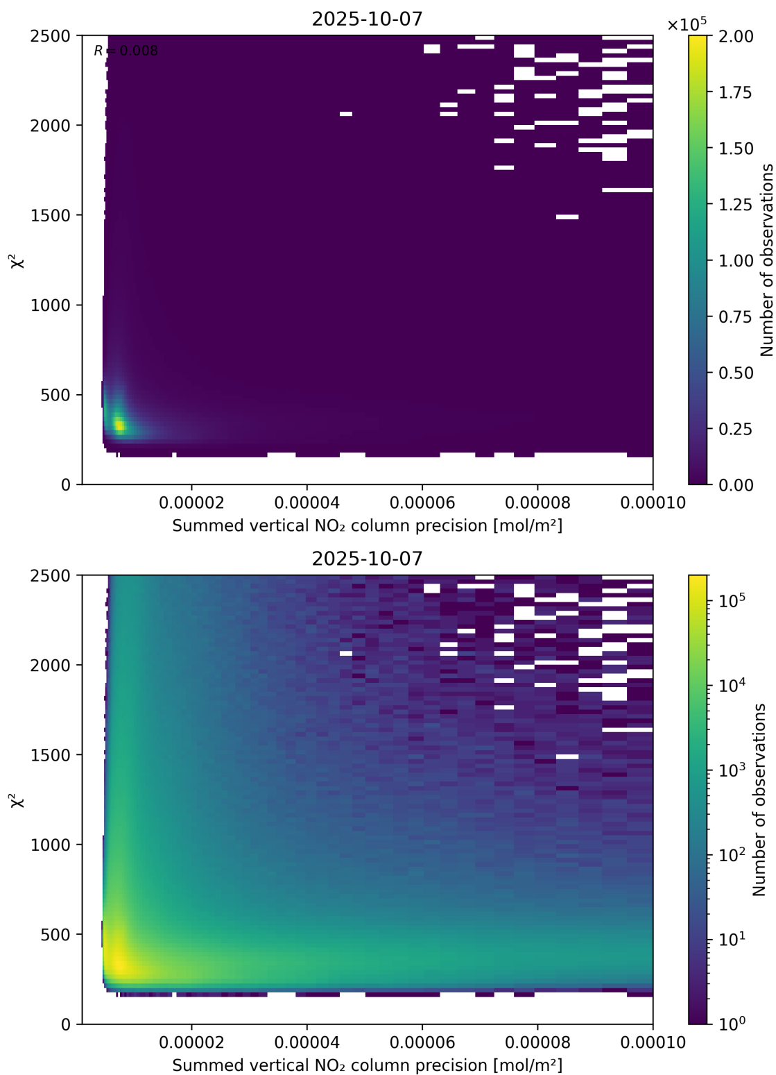
Figure 107: Scatter density plot of “Summed vertical NO 2 column precision” against “ \chi^2 ” for 2025-10-06 to 2025-10-08.
