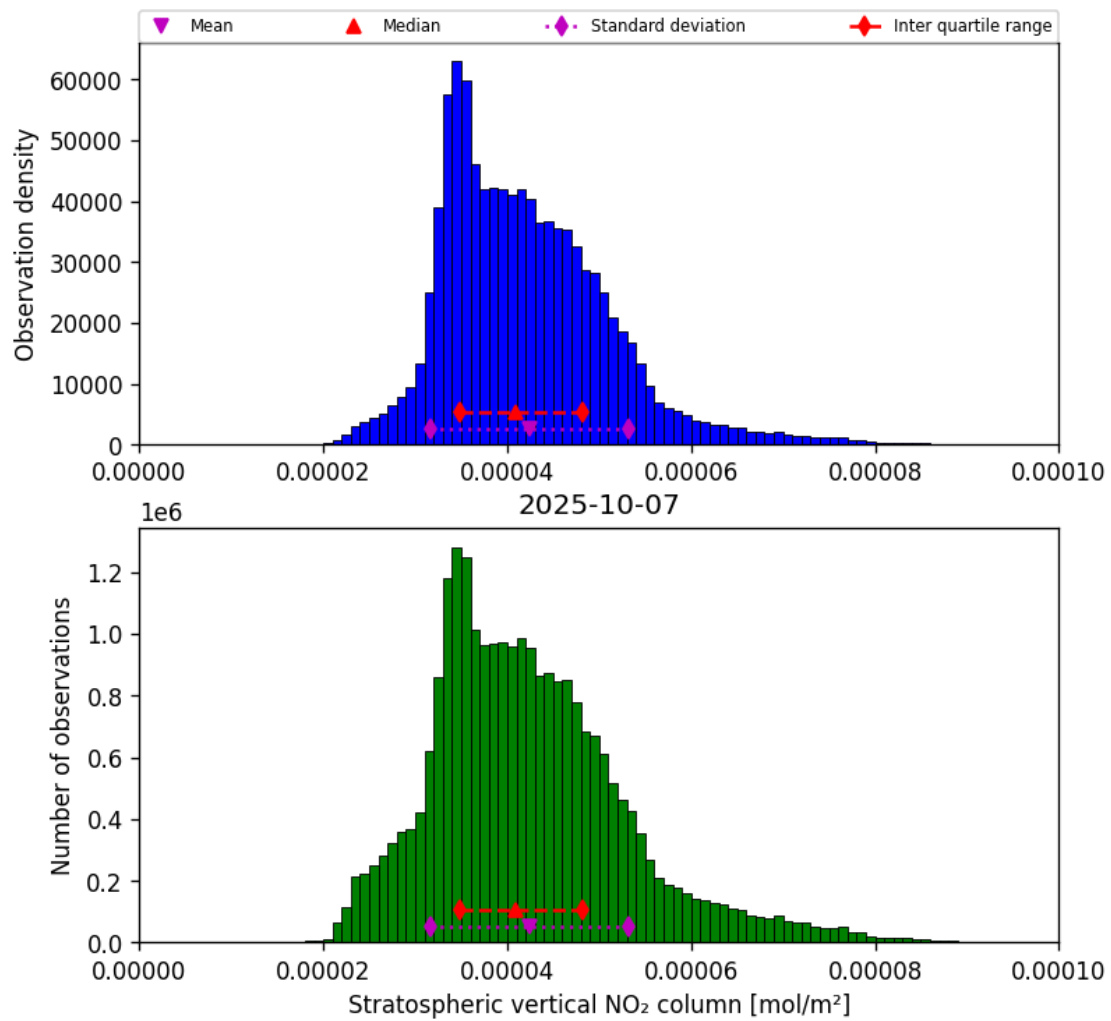
Figure 36: Histogram of “Stratospheric vertical NO 2 column” for 2025-10-06 to 2025-10-08
