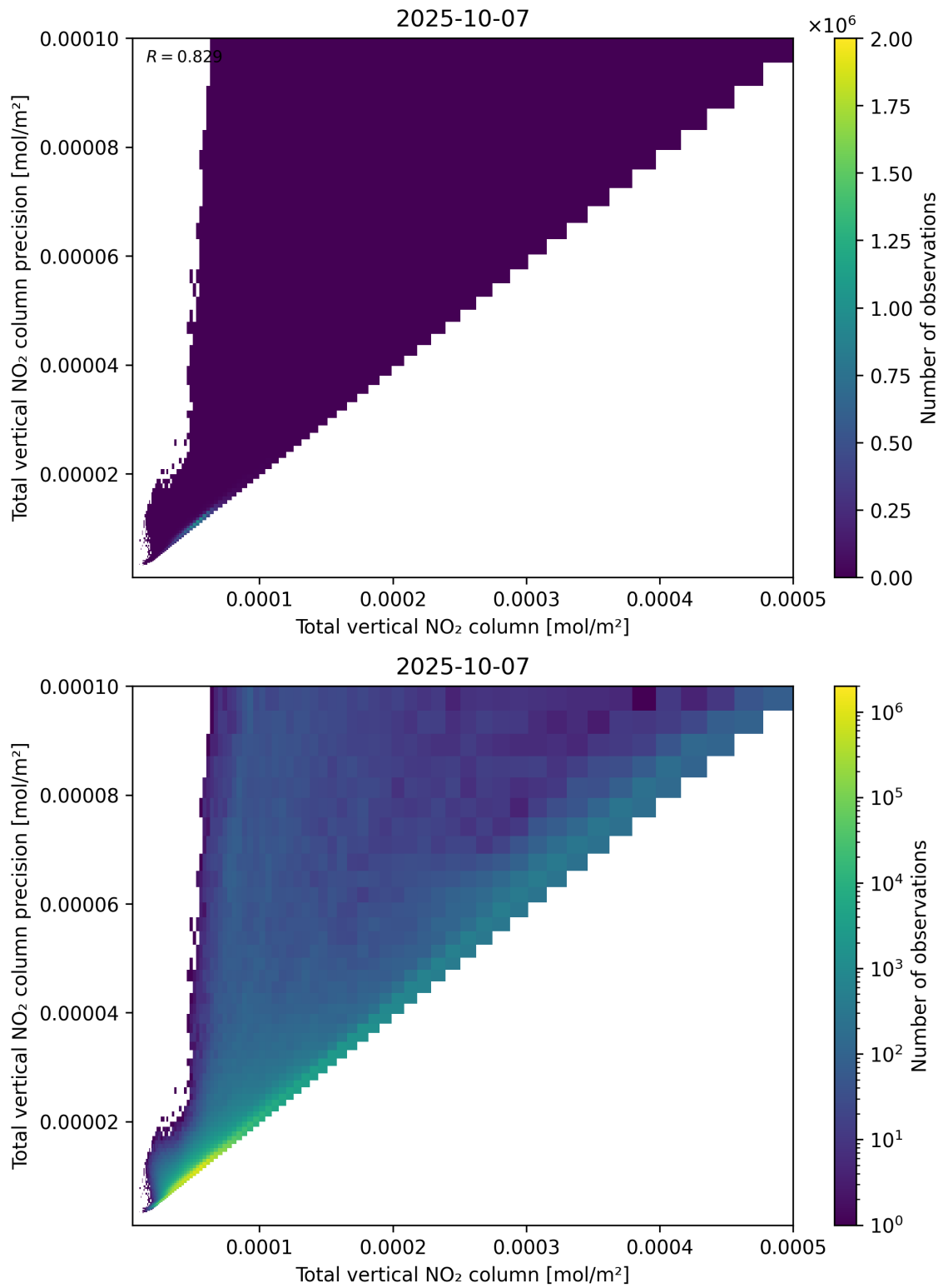
Figure 114: Scatter density plot of “Total vertical NO 2 column” against “Total vertical NO 2 column precision” for 2025-10-06 to 2025-10-08.
