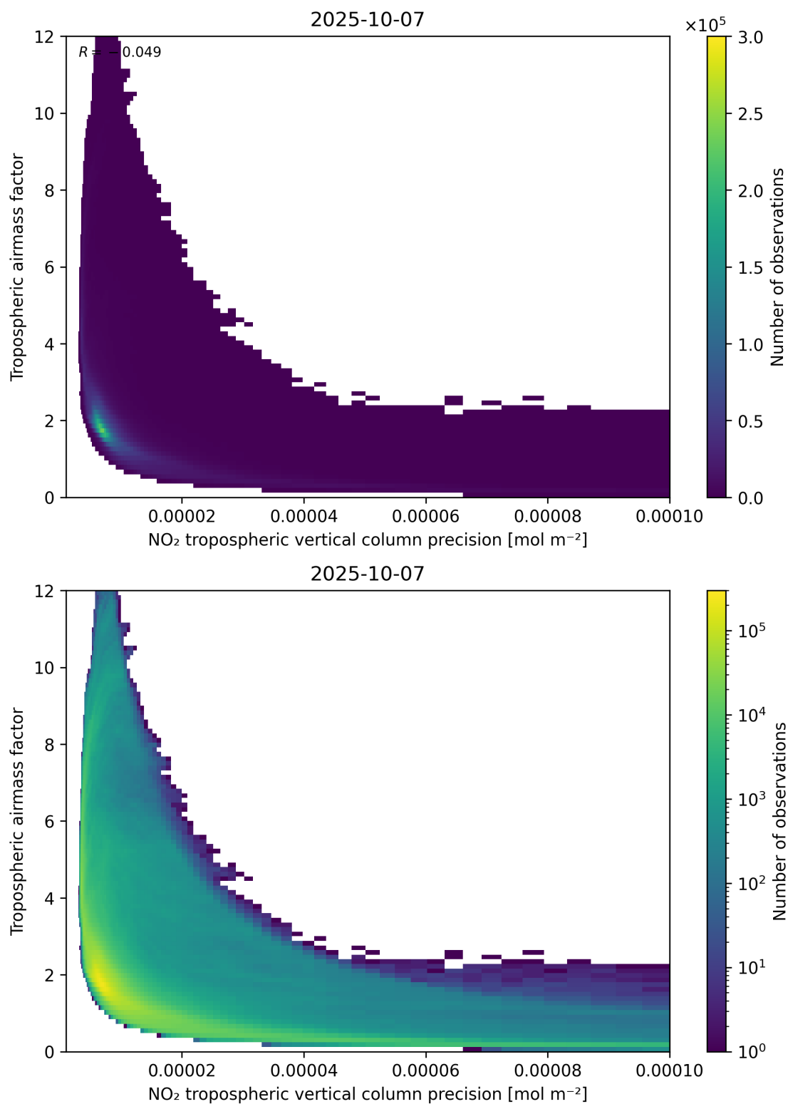
Figure 133: Scatter density plot of “NO 2 tropospheric vertical column precision” against “Tropospheric airmass factor” for 2025-10-06 to 2025-10-08.
