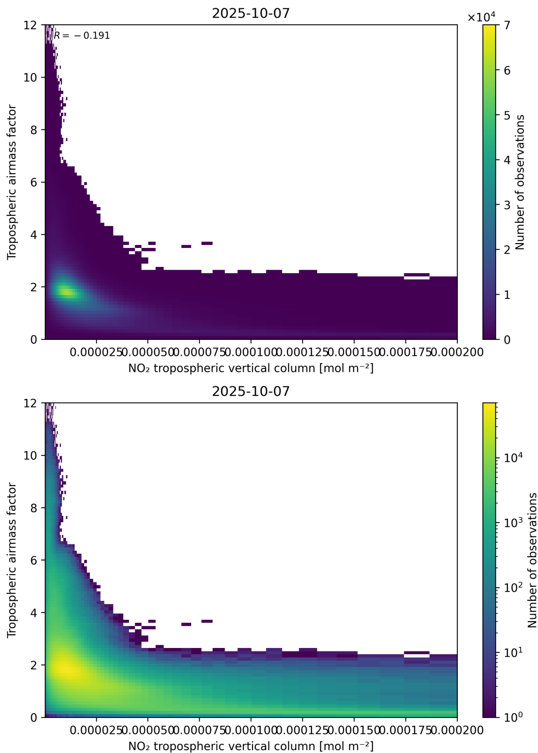
Figure 123: Scatter density plot of “NO 2 tropospheric vertical column” against “Tropospheric air mass factor” for 2025-10-06 to 2025-10-08.
