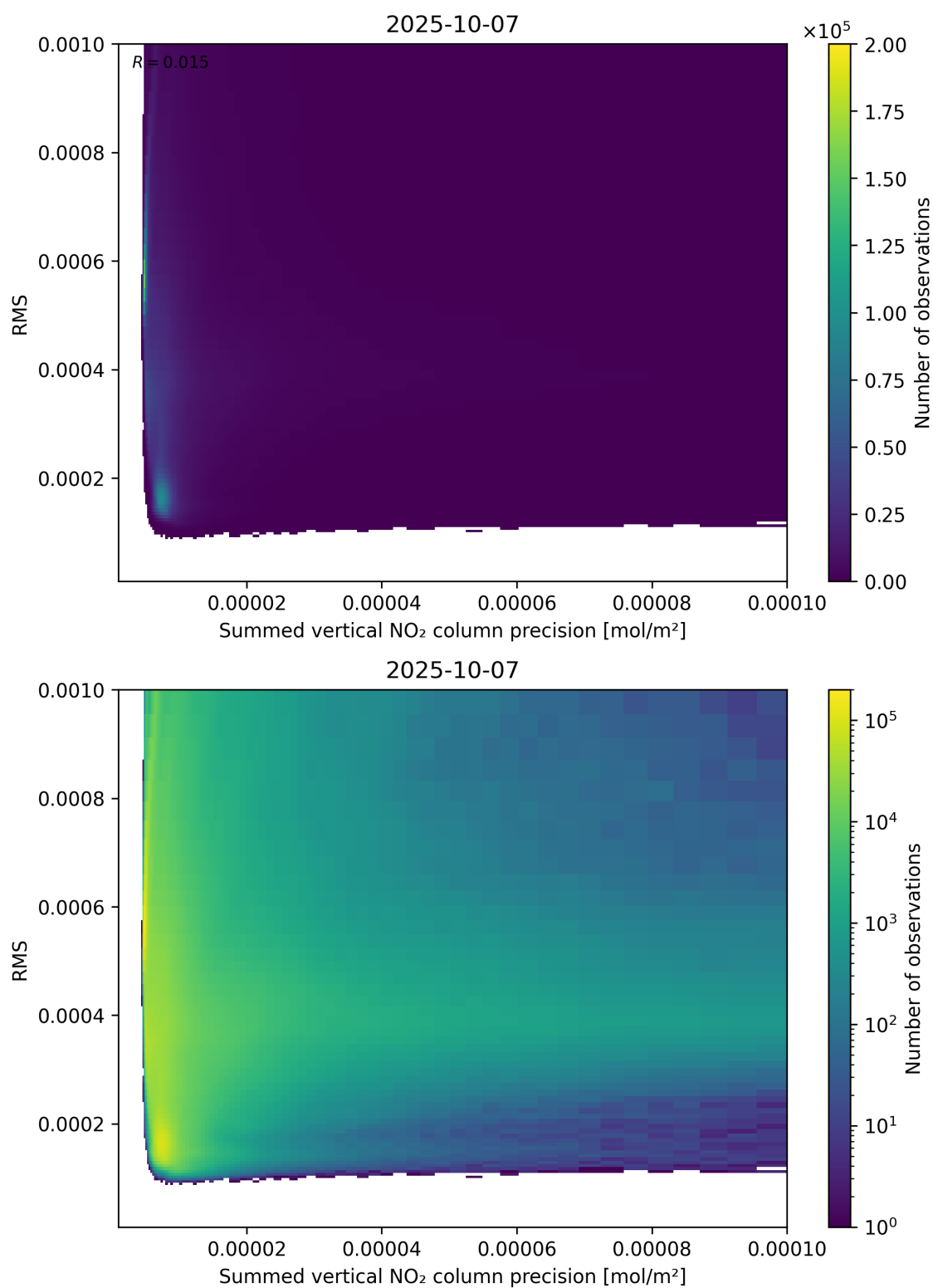
Figure 108: Scatter density plot of “Summed vertical NO 2 column precision” against “RMS” for 2025-10-06 to 2025-10-08.
