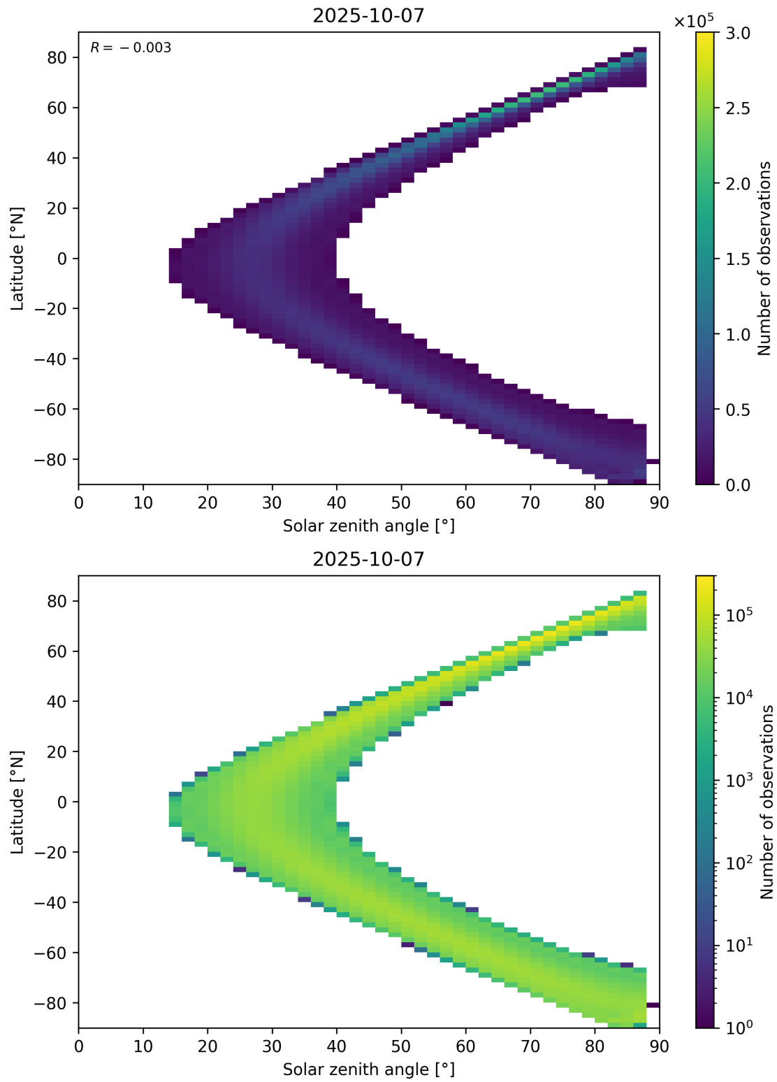
Figure 149: Scatter density plot of “Solar zenith angle” against “Latitude” for 2025-10-06 to 2025-10-08.
