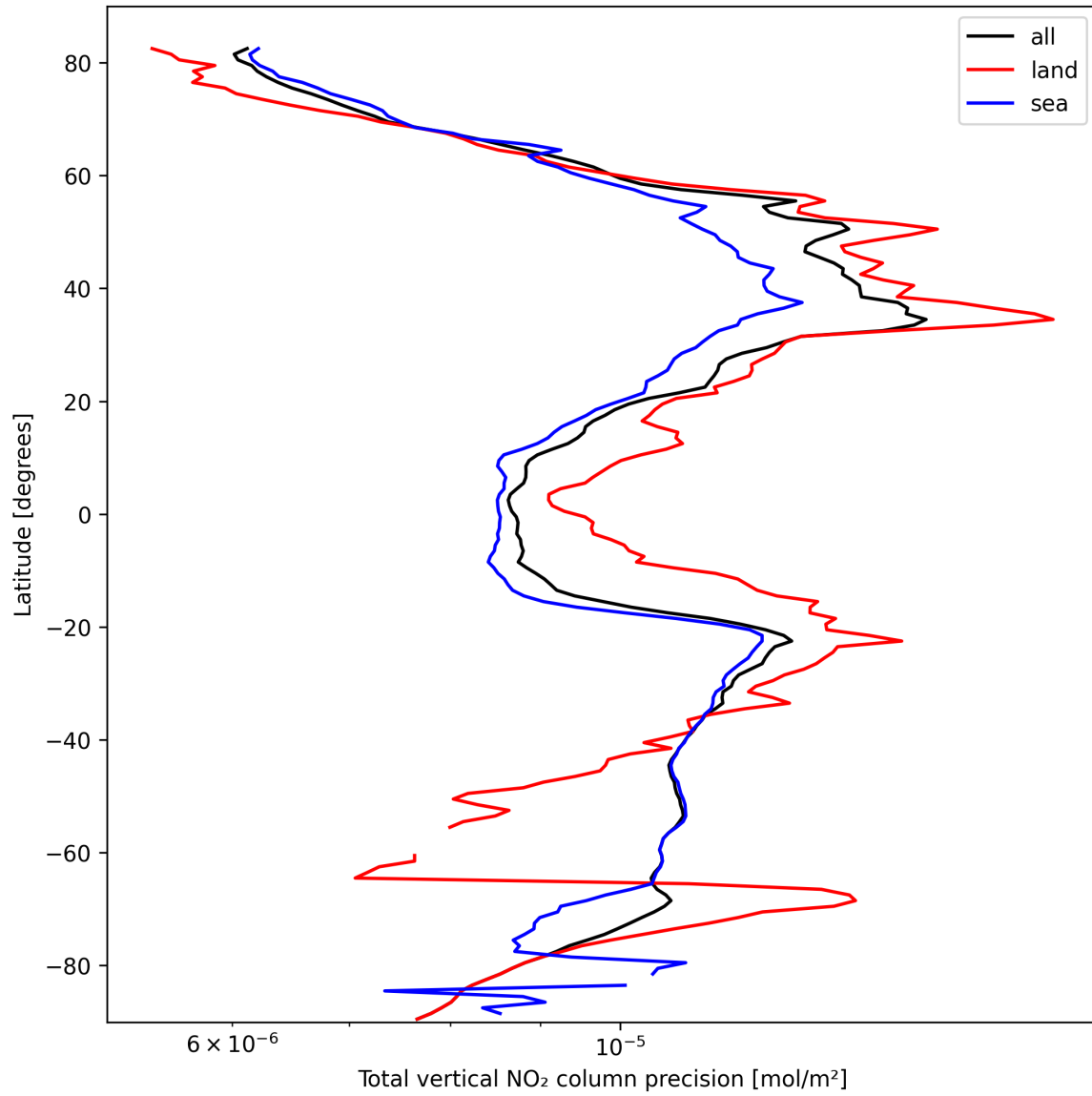
Figure 22: Zonal average of “Total vertical NO 2 column precision” for 2025-10-06 to 2025-10-08.
