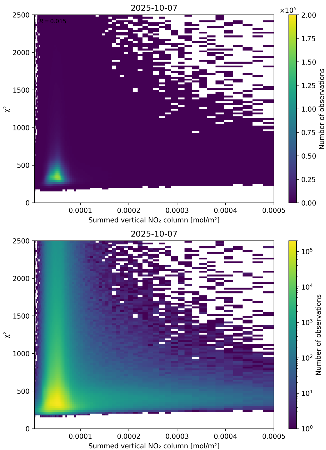
Figure 104: Scatter density plot of “Summed vertical NO 2 column” against “ \chi^2 ” for 2025-10-06 to 2025-10-08.
