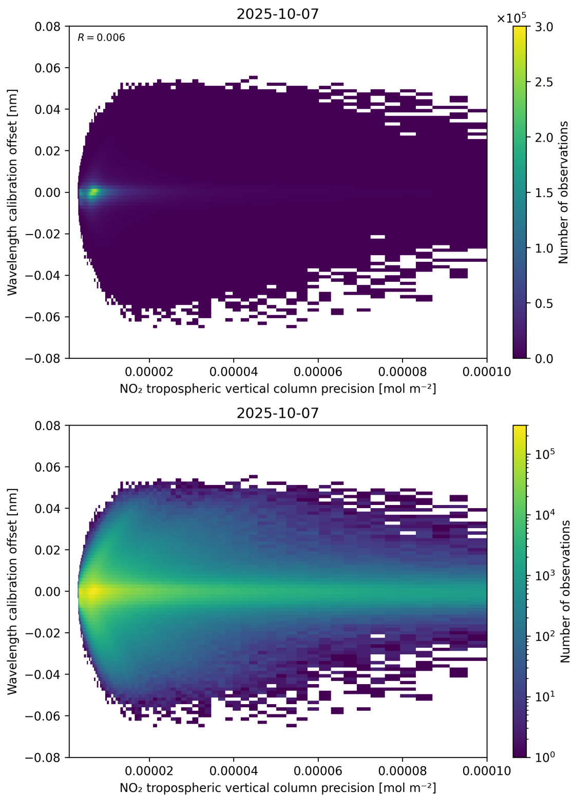
Figure 141: Scatter density plot of “NO 2 tropospheric vertical column precision” against “Wavelength calibration offset” for 2025-10-06 to 2025-10-08.
