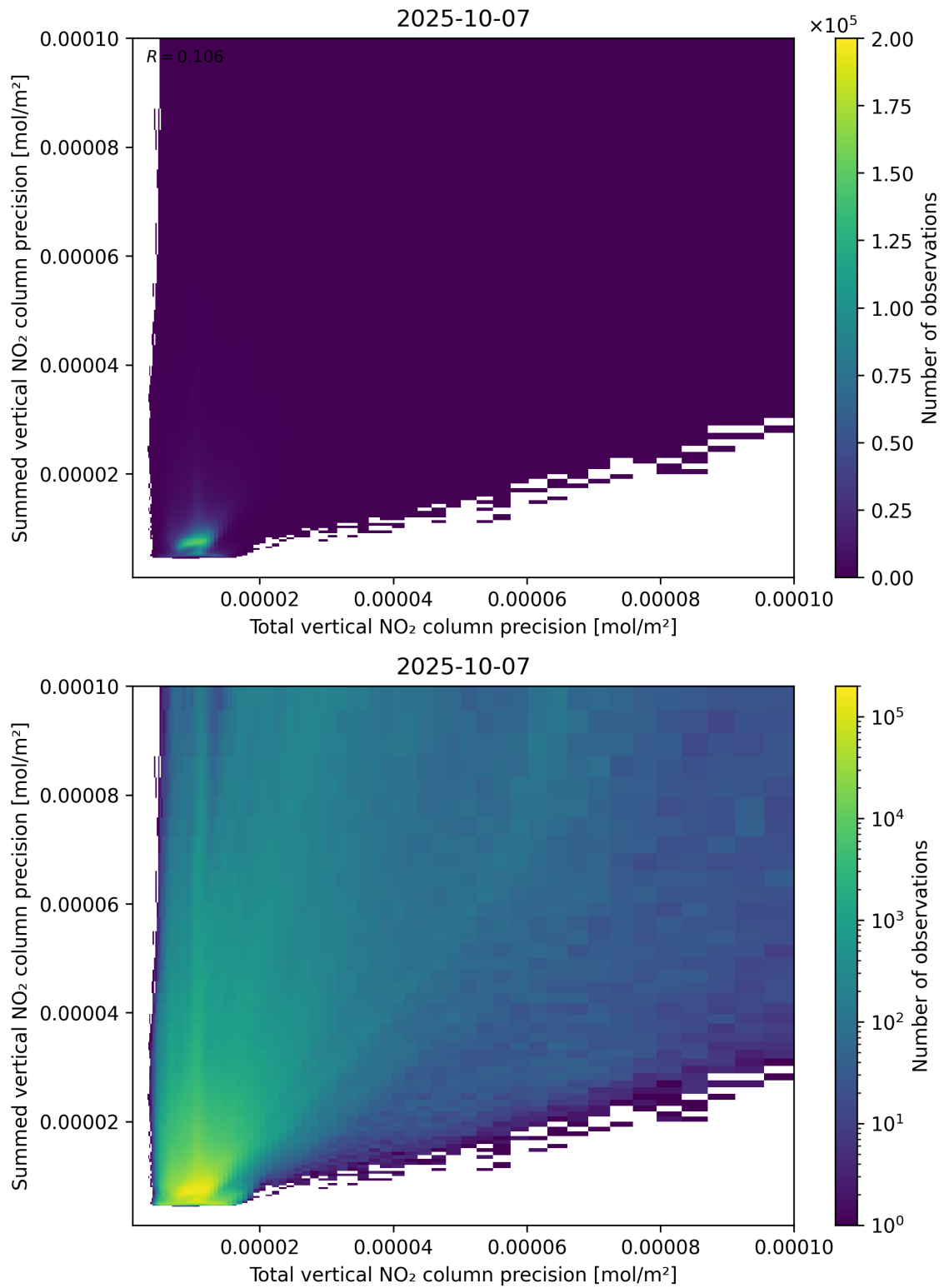
Figure 118: Scatter density plot of “Total vertical NO 2 column precision” against “Summed vertical NO 2 column precision” for 2025-10-06 to 2025-10-08.
