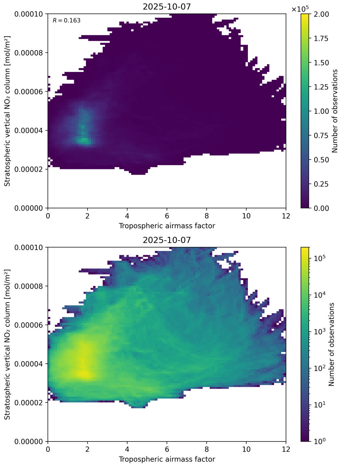
Figure 74: Scatter density plot of “Tropospheric air mass factor” against “Stratospheric vertical \text{NO}_2 column” for 2025-10-06 to 2025-10-08.
