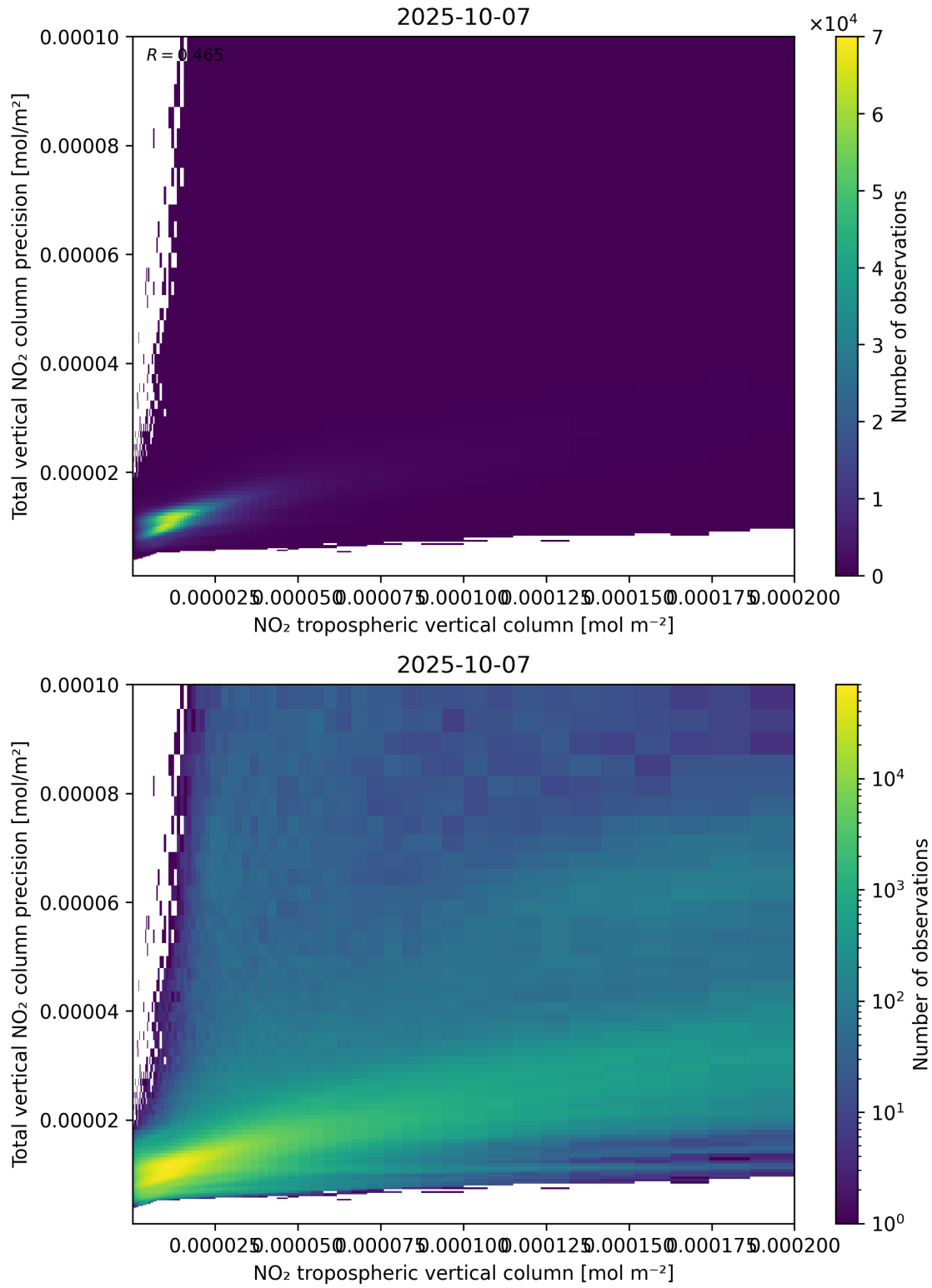
Figure 129: Scatter density plot of “NO 2 tropospheric vertical column” against “Total vertical NO 2 column precision” for 2025-10-06 to 2025-10-08.
