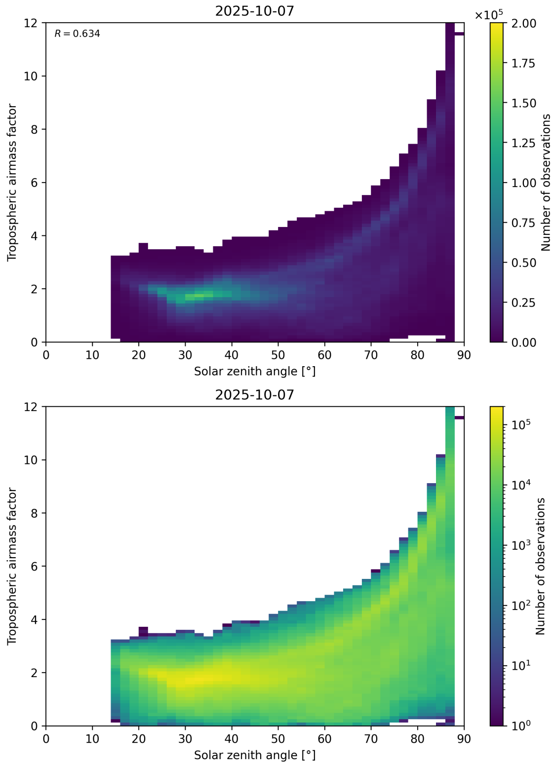
Figure 147: Scatter density plot of “Solar zenith angle” against “Tropospheric airmass factor” for 2025-10-06 to 2025-10-08.
