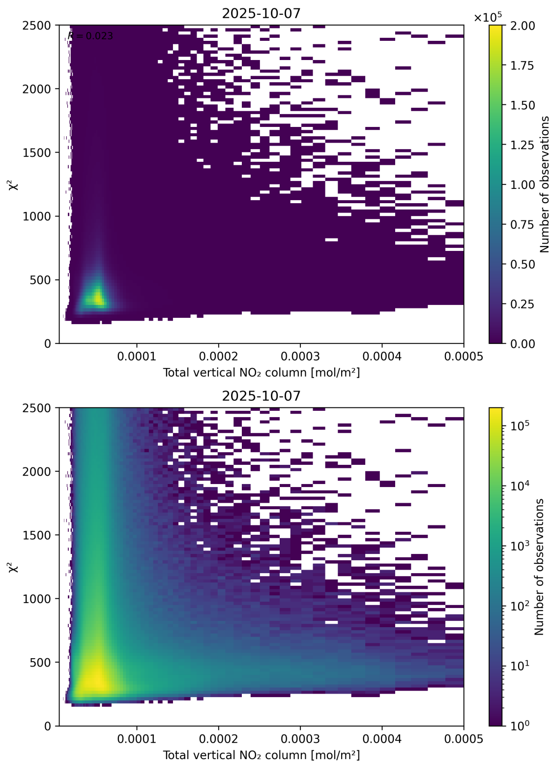
Figure 111: Scatter density plot of “Total vertical NO 2 column” against “ \chi^2 ” for 2025-10-06 to 2025-10-08.
