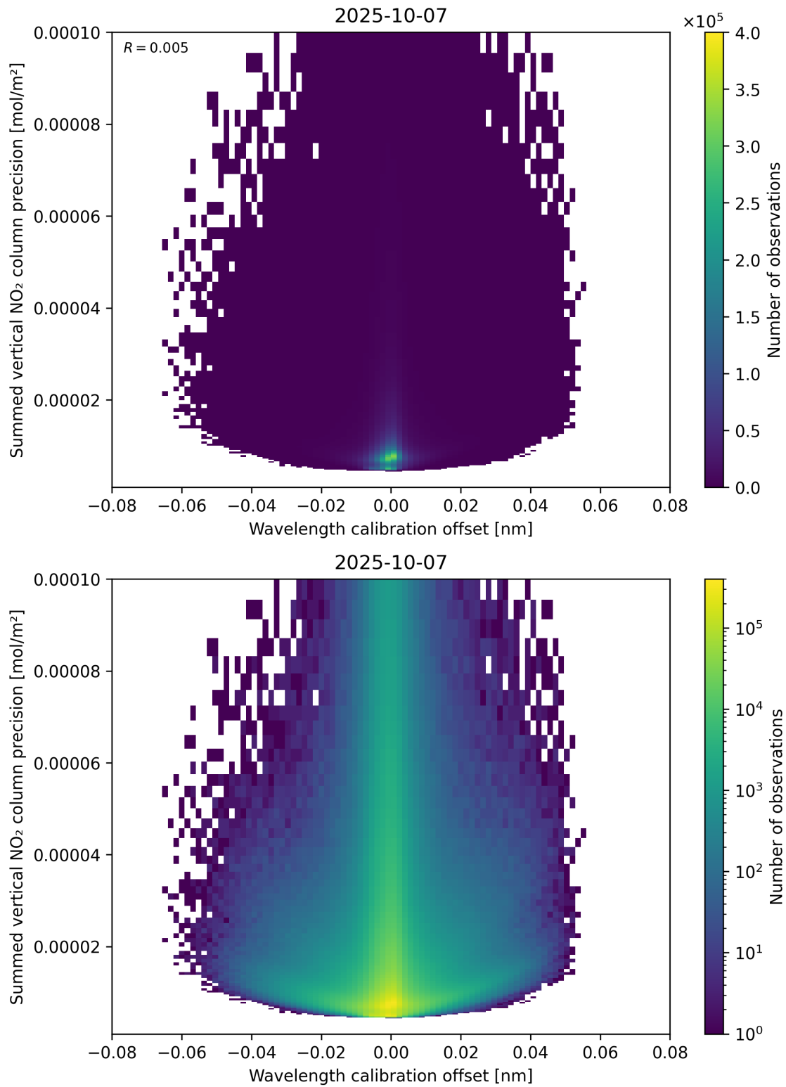
Figure 178: Scatter density plot of “Wavelength calibration offset” against “Summed vertical NO 2 column precision” for 2025-10-06 to 2025-10-08.
