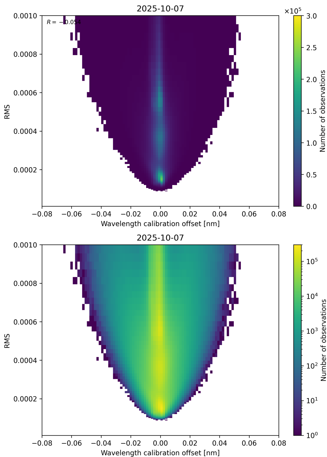
Figure 181: Scatter density plot of “Wavelength calibration offset” against “RMS” for 2025-10-06 to 2025-10-08.
