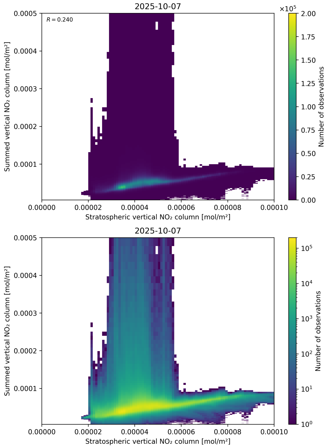
Figure 98: Scatter density plot of “Stratospheric vertical NO 2 column” against “Summed vertical NO 2 column” for 2025-10-06 to 2025-10-08.
