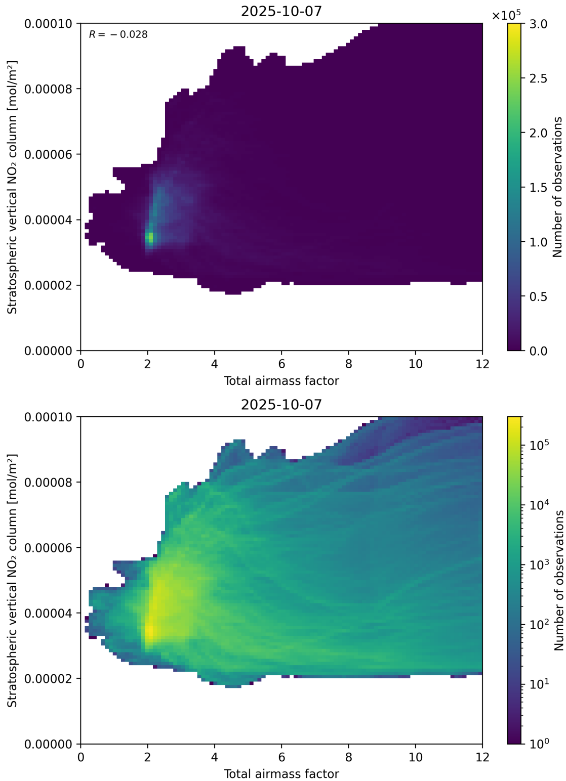
Figure 64: Scatter density plot of “Total airmass factor” against “Stratospheric vertical NO 2 column” for 2025-10-06 to 2025-10-08.
