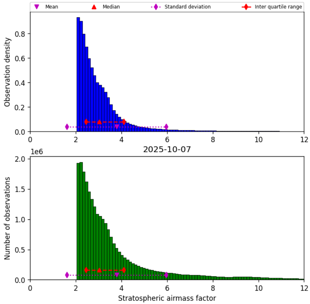
Figure 44: Histogram of “Stratospheric airmass factor” for 2025-10-06 to 2025-10-08
