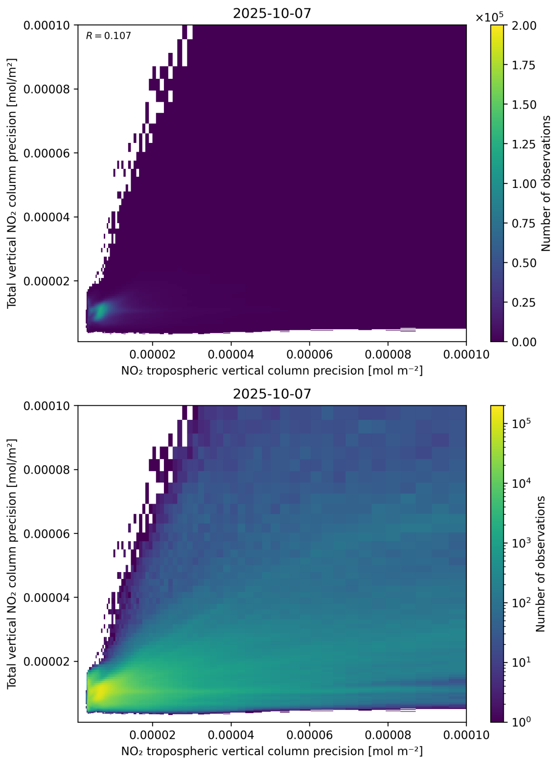
Figure 139: Scatter density plot of “NO 2 tropospheric vertical column precision” against “Total vertical NO 2 column precision” for 2025-10-06 to 2025-10-08.
