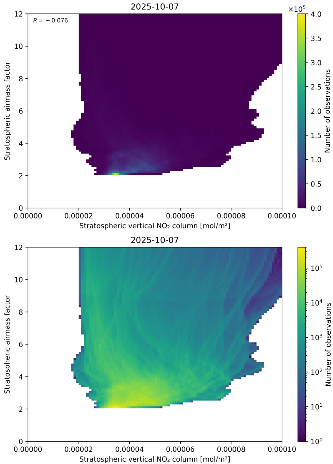
Figure 96: Scatter density plot of “Stratospheric vertical NO 2 column” against “Stratospheric airmass factor” for 2025-10-06 to 2025-10-08.
