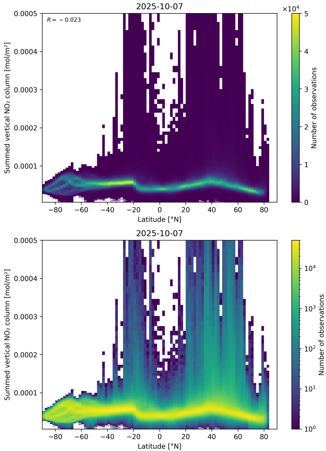
Figure 88: Scatter density plot of “Latitude” against “Summed vertical NO 2 column” for 2025-10-06 to 2025-10-08.
