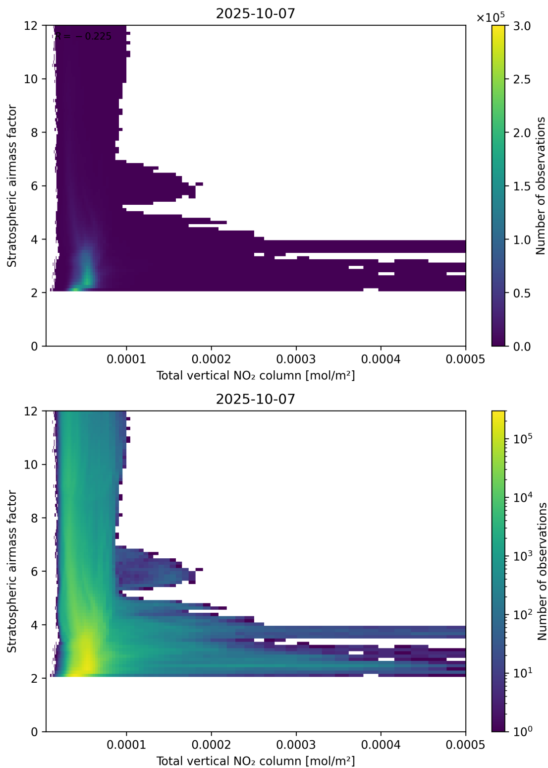
Figure 110: Scatter density plot of “Total vertical NO 2 column” against “Stratospheric airmass factor” for 2025-10-06 to 2025-10-08.
