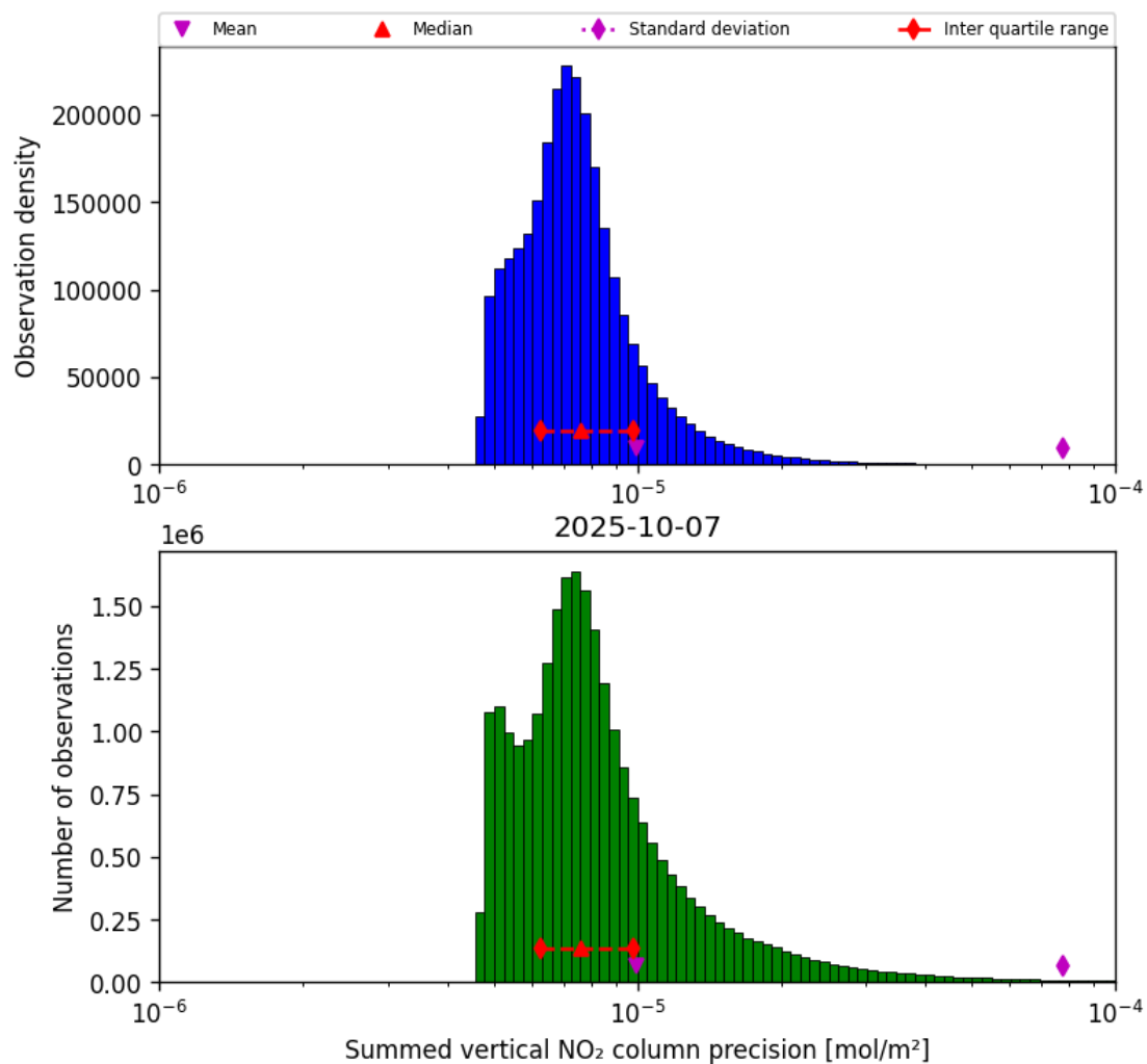
Figure 41: Histogram of “Summed vertical NO 2 column precision” for 2025-10-06 to 2025-10-08
