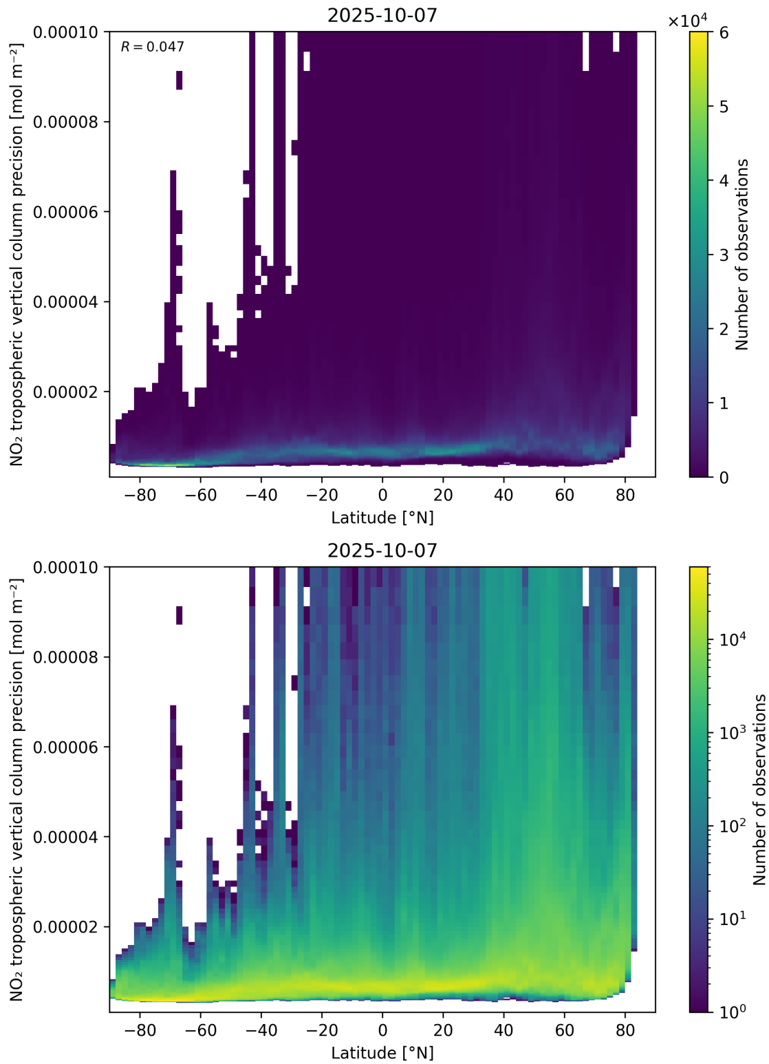
Figure 93: Scatter density plot of “Latitude” against “NO 2 tropospheric vertical column precision” for 2025-10-06 to 2025-10-08.
