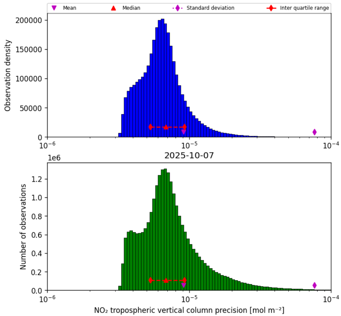
Figure 30: Histogram of “NO 2 tropospheric vertical column precision” for 2025-10-06 to 2025-10-08
