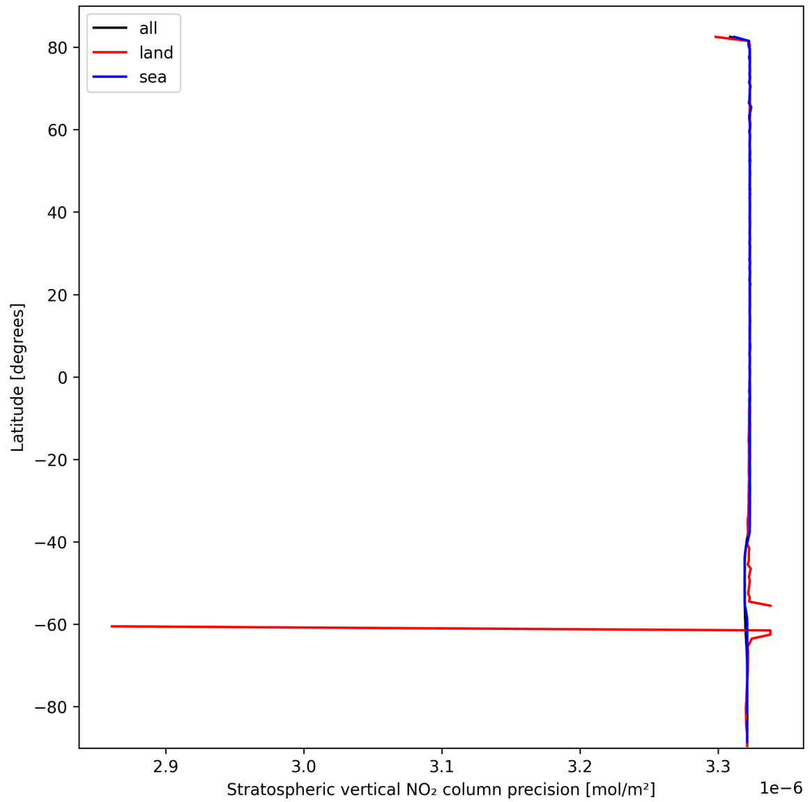
Figure 20: Zonal average of “Stratospheric vertical NO 2 column precision” for 2025-10-06 to 2025-10-08.
