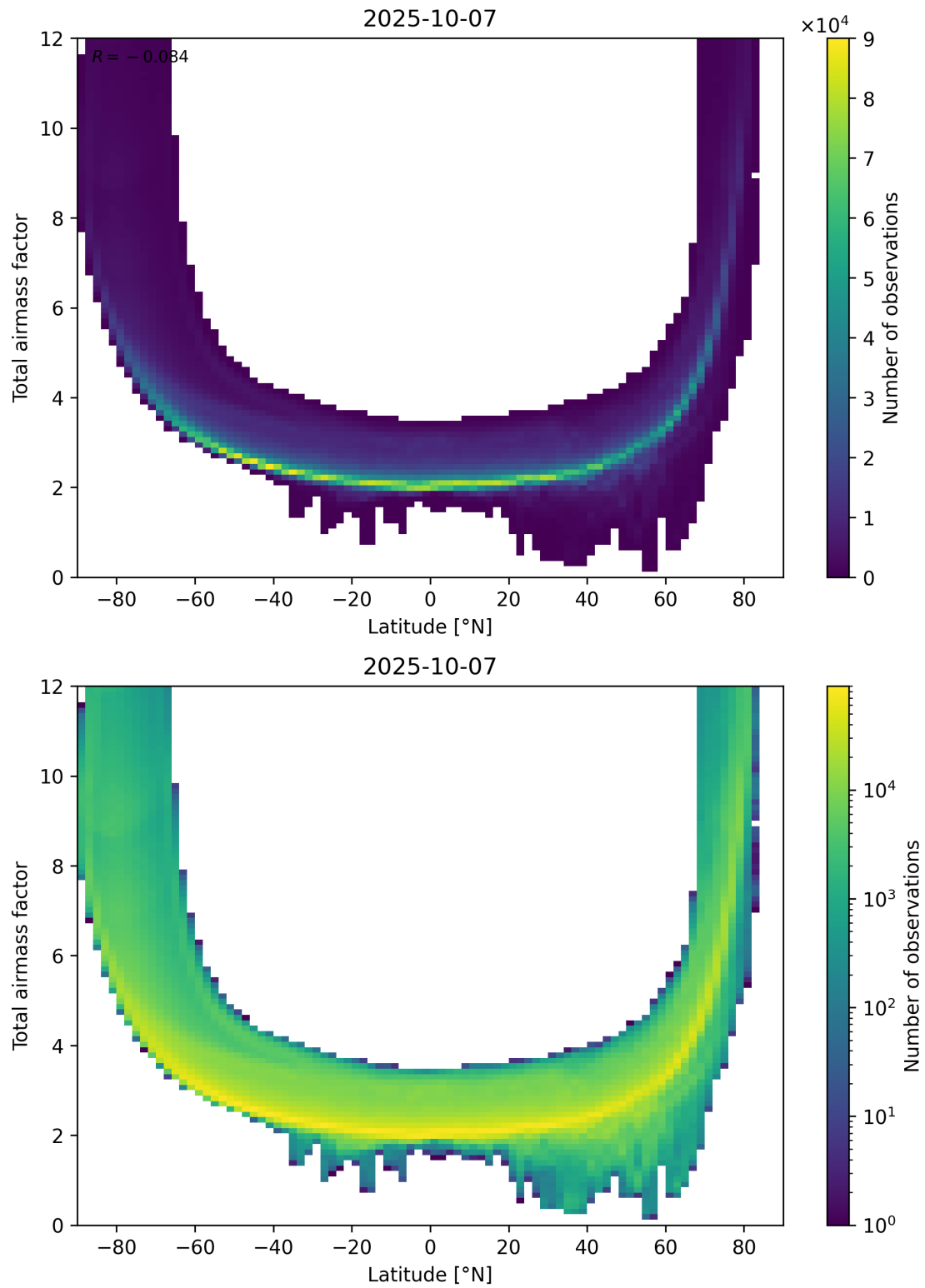
Figure 84: Scatter density plot of “Latitude” against “Total airmass factor” for 2025-10-06 to 2025-10-08.
