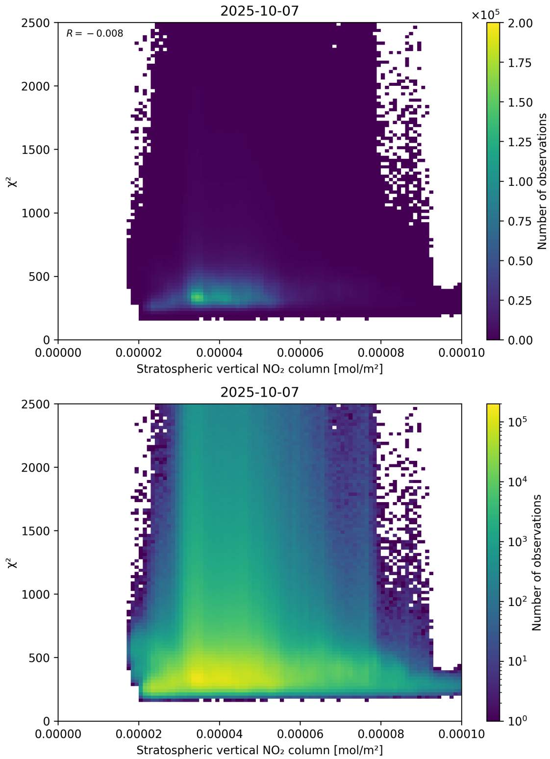
Figure 97: Scatter density plot of “Stratospheric vertical NO 2 column” against “ \chi^2 ” for 2025-10-06 to 2025-10-08.
