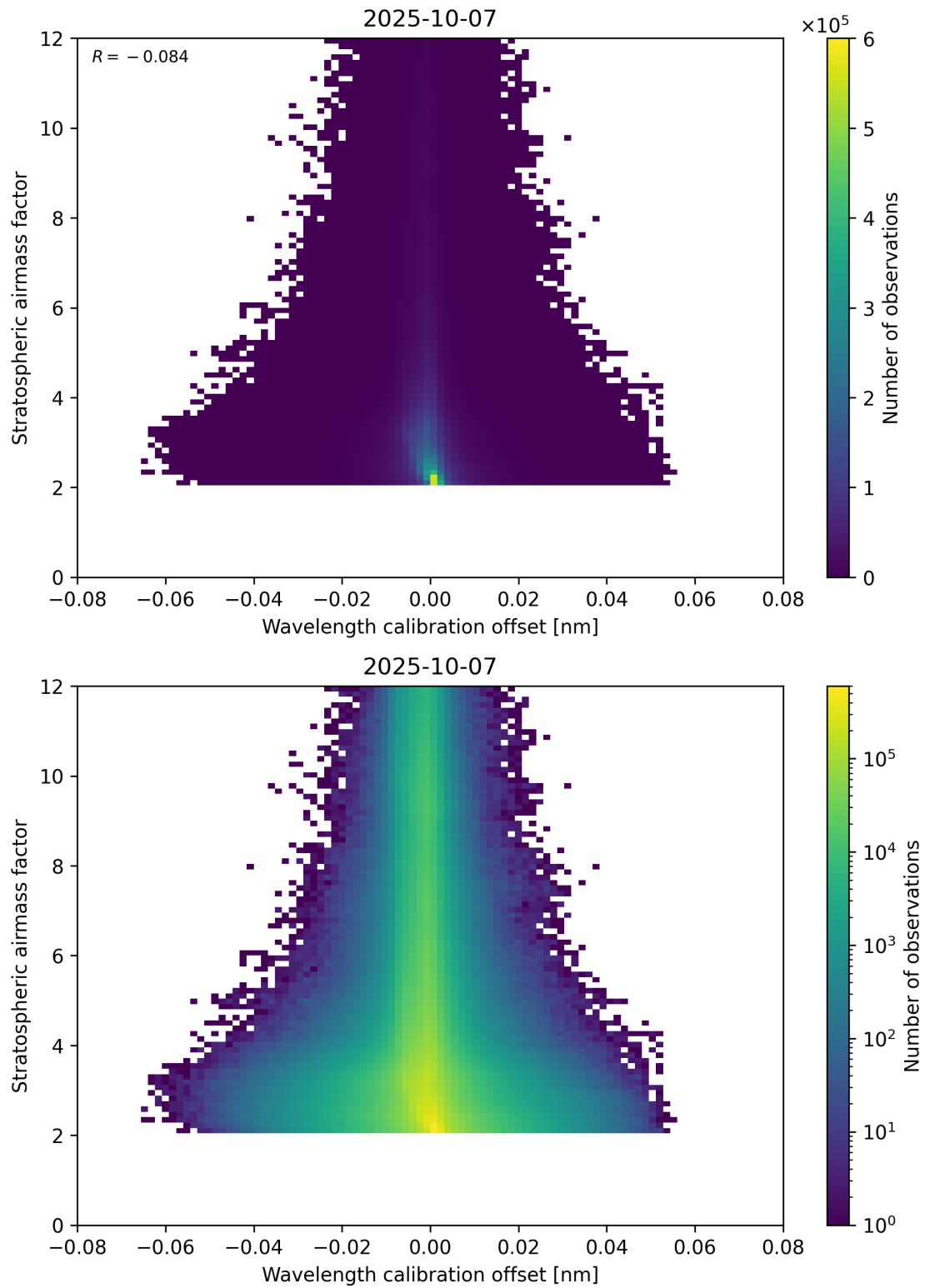
Figure 174: Scatter density plot of “Wavelength calibration offset” against “Stratospheric airmass factor” for 2025-10-06 to 2025-10-08.
