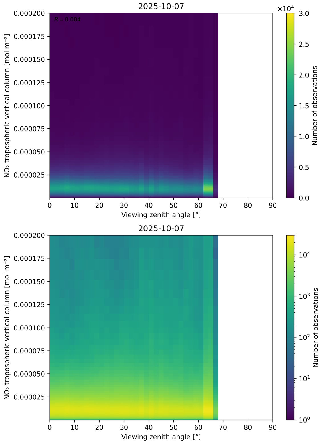
Figure 169: Scatter density plot of “Viewing zenith angle” against “NO 2 tropospheric vertical column” for 2025-10-06 to 2025-10-08.
