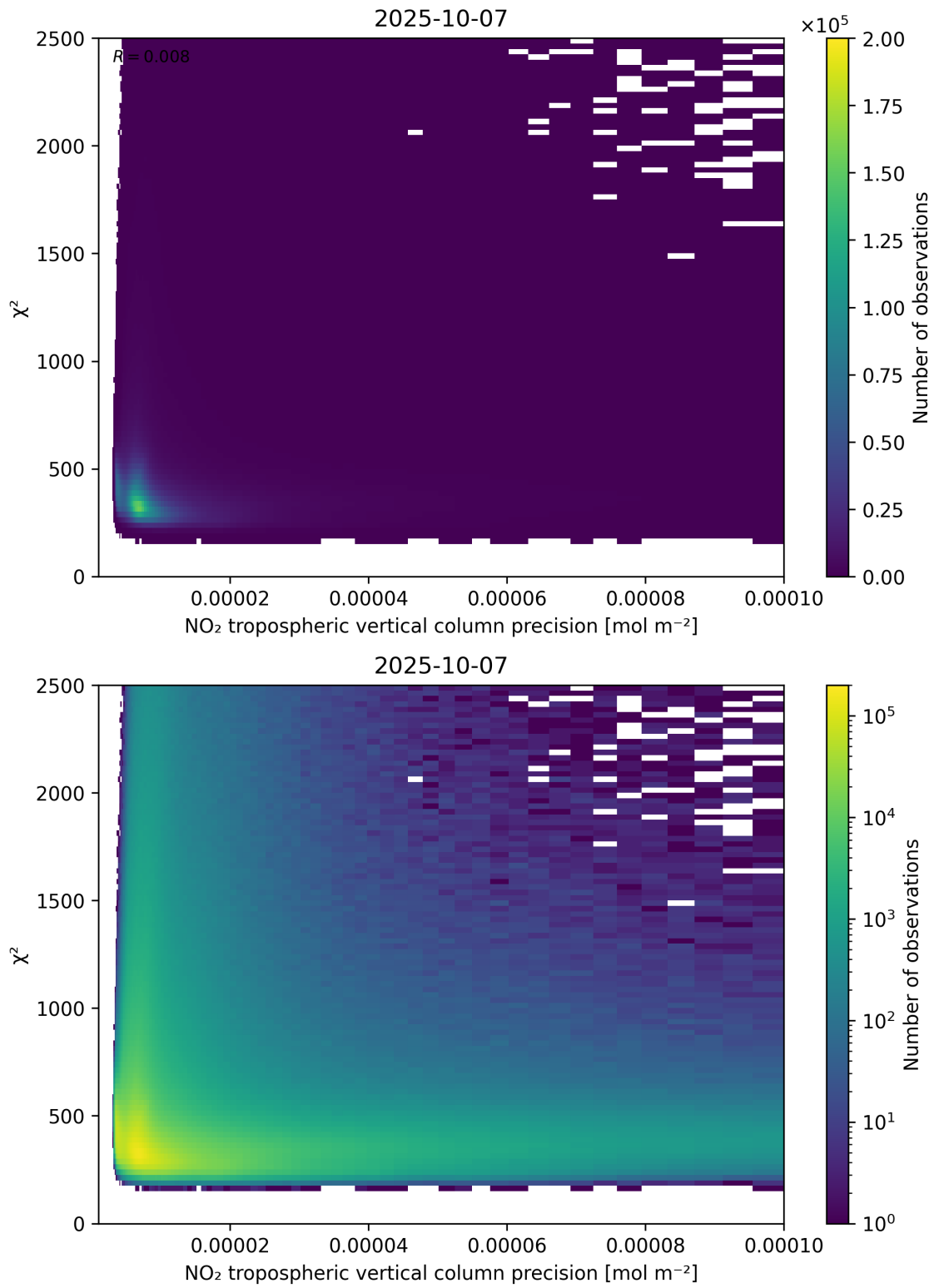
Figure 134: Scatter density plot of “NO 2 tropospheric vertical column precision” against “ \chi^2 ” for 2025-10-06 to 2025-10-08.
