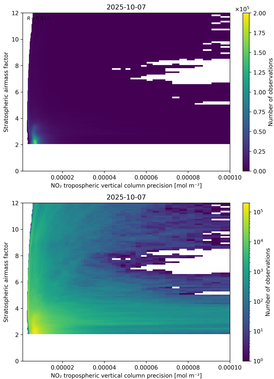
Figure 131: Scatter density plot of “NO 2 tropospheric vertical column precision” against “Stratospheric airmass factor” for 2025-10-06 to 2025-10-08.
