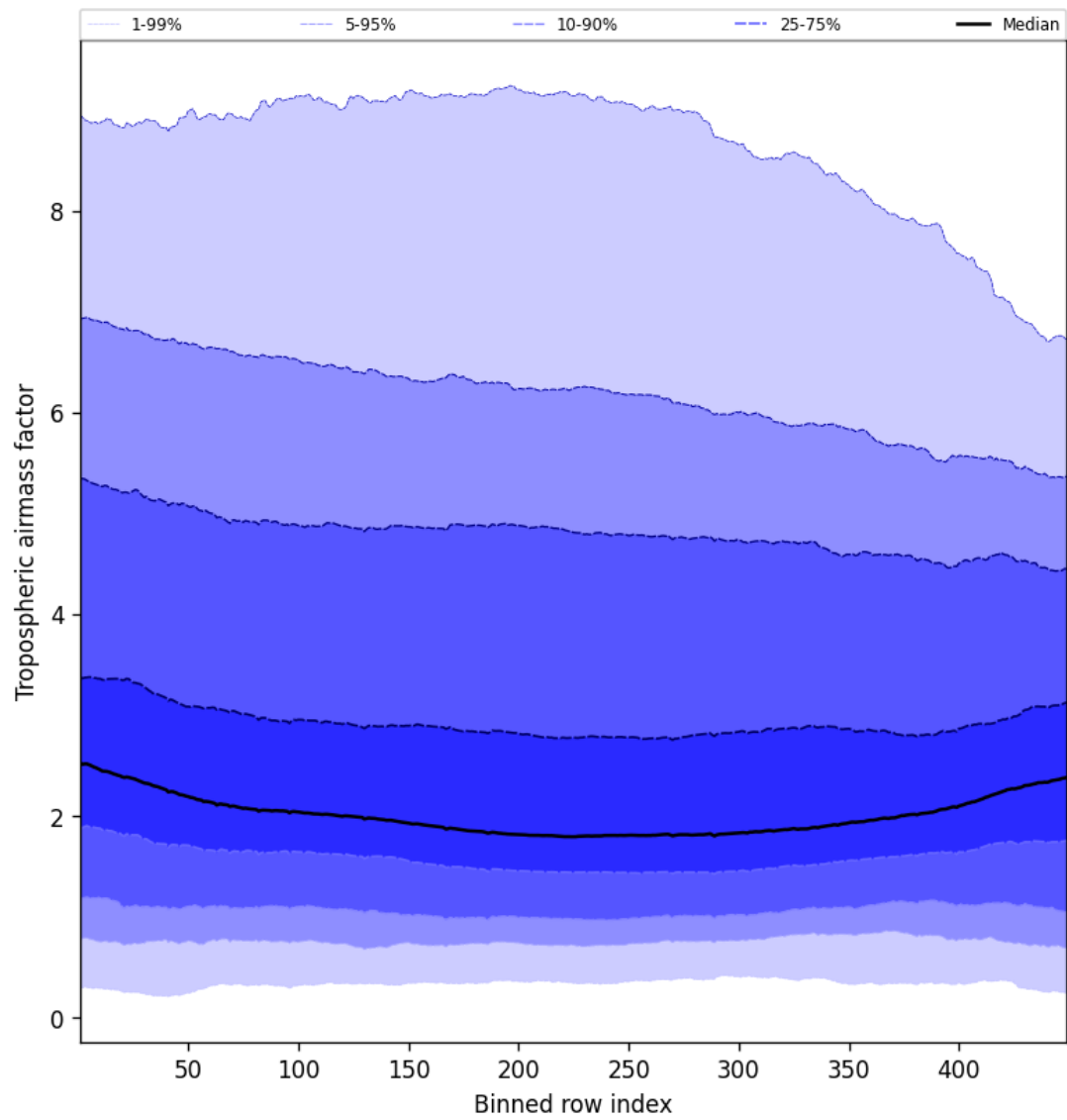
Figure 48: Along track statistics of “Tropospheric air mass factor” for 2025-10-06 to 2025-10-08
