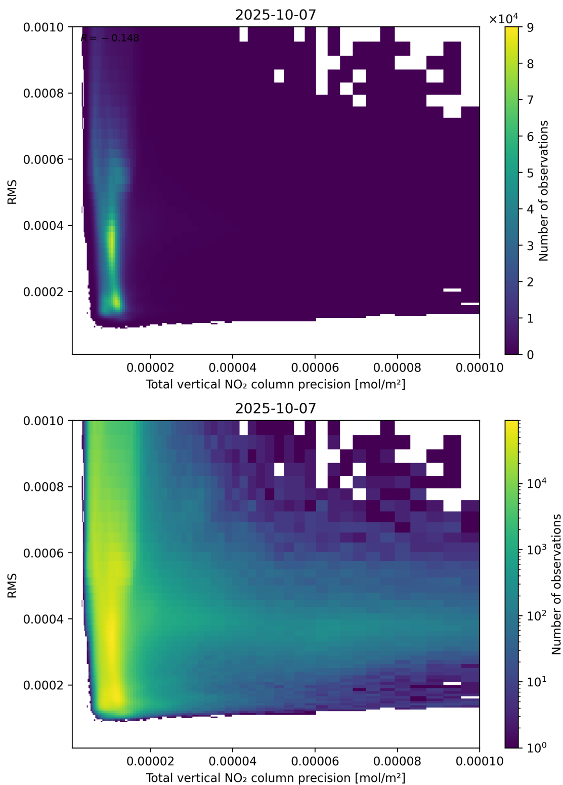
Figure 119: Scatter density plot of “Total vertical NO 2 column precision” against “RMS” for 2025-10-06 to 2025-10-08.
