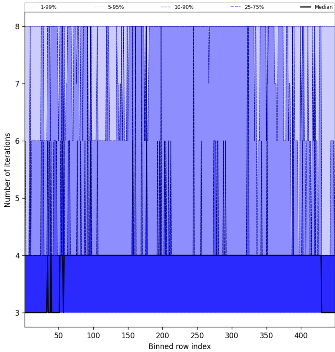
Figure 51: Along track statistics of “Number of iterations” for 2025-10-06 to 2025-10-08
