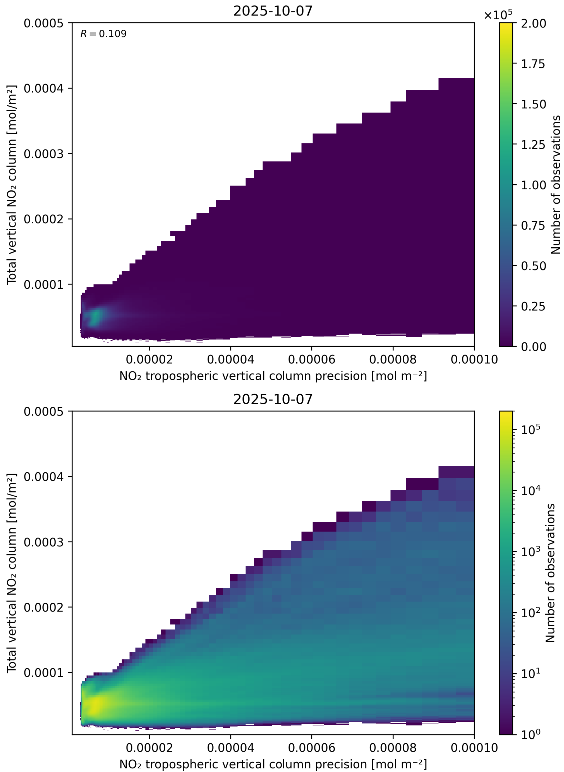
Figure 138: Scatter density plot of “NO 2 tropospheric vertical column precision” against “Total vertical NO 2 column” for 2025-10-06 to 2025-10-08.
