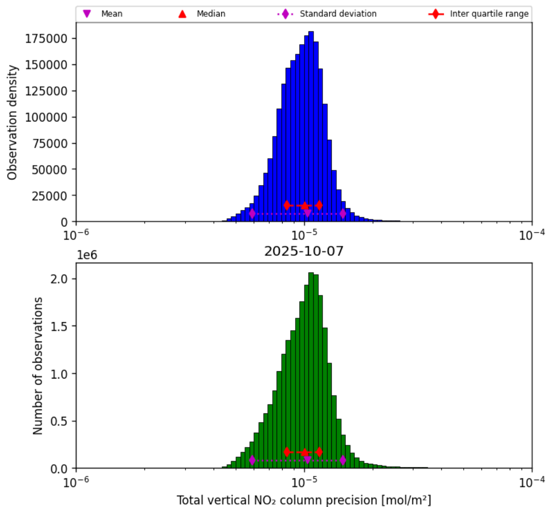
Figure 39: Histogram of “Total vertical NO 2 column precision” for 2025-10-06 to 2025-10-08
