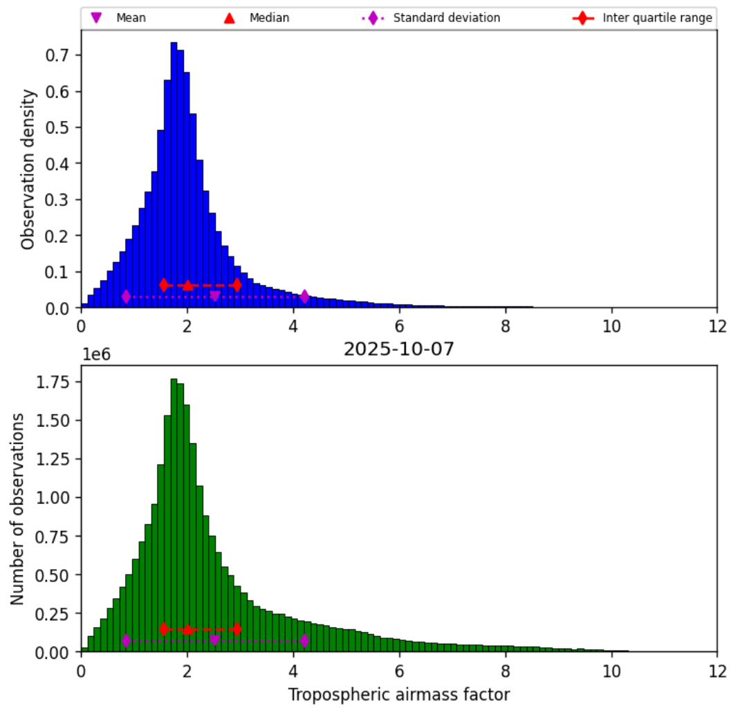
Figure 31: Histogram of “Tropospheric airmass factor” for 2025-10-06 to 2025-10-08
