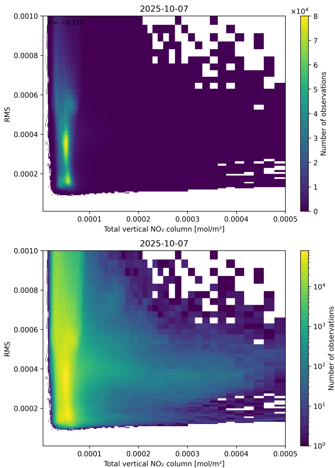
Figure 120: Scatter density plot of “Total vertical NO 2 column” against “RMS” for 2025-10-06 to 2025-10-08.
