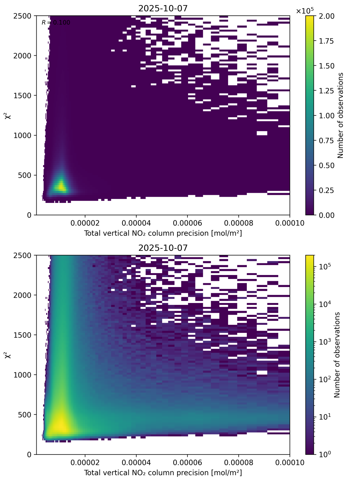
Figure 116: Scatter density plot of “Total vertical NO 2 column precision” against “ \chi^2 ” for 2025-10-06 to 2025-10-08.
