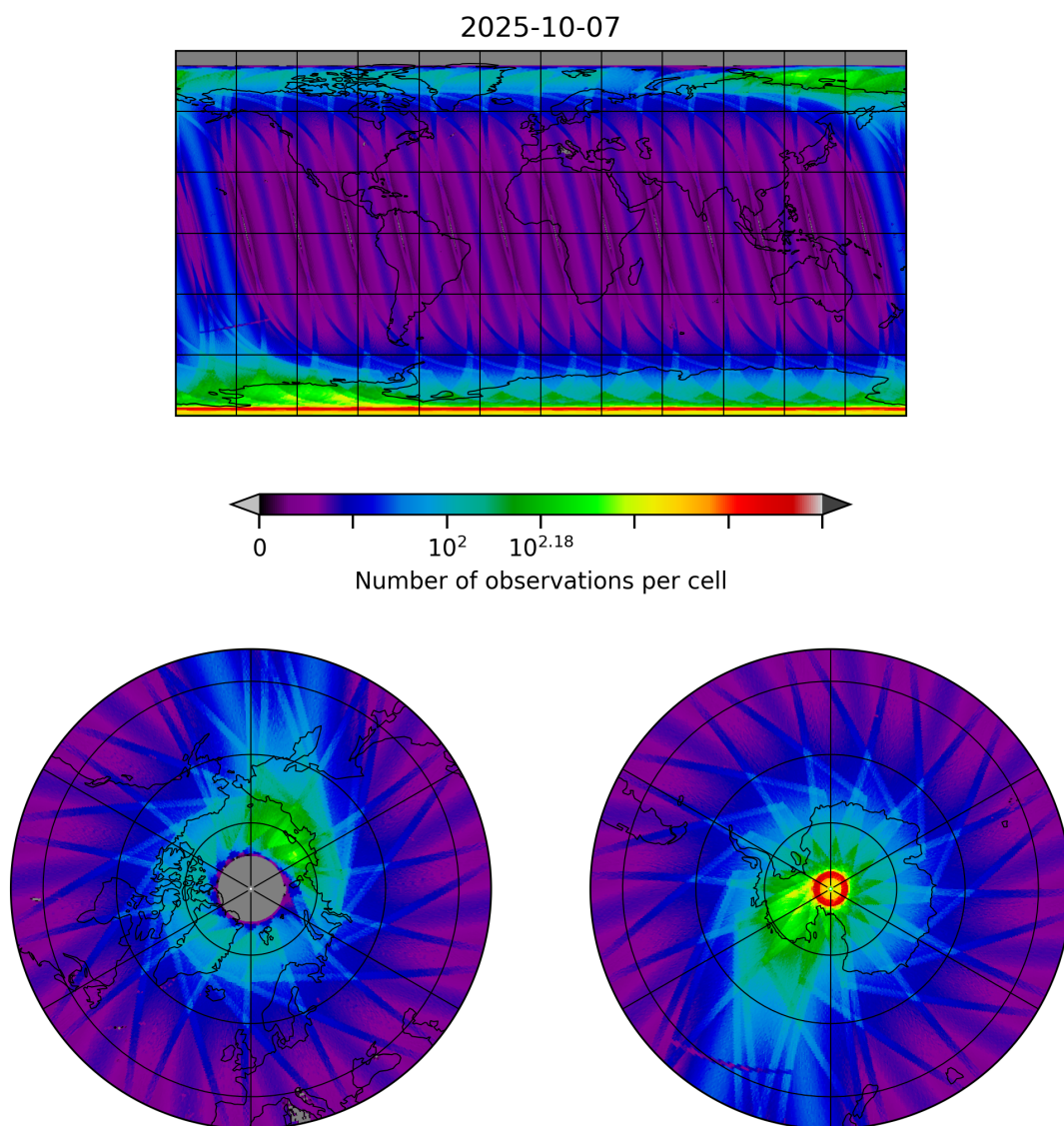
Figure 10: Map of the number of observations for 2025-10-06 to 2025-10-08
