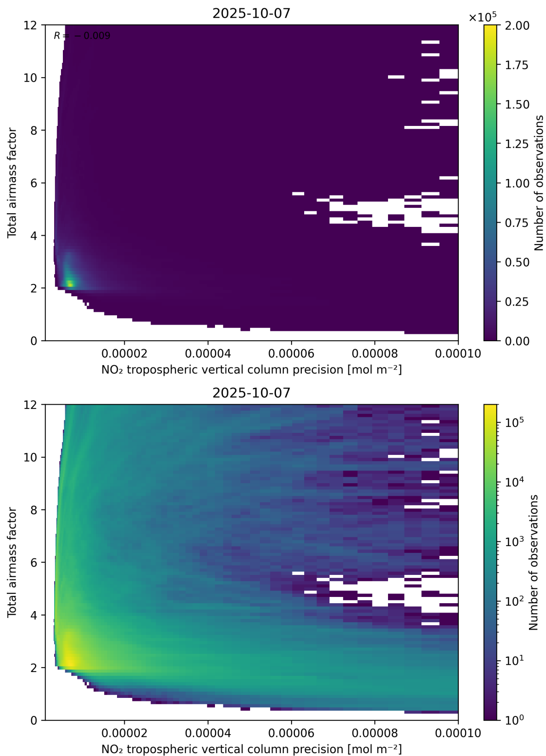
Figure 132: Scatter density plot of “NO 2 tropospheric vertical column precision” against “Total air mass factor” for 2025-10-06 to 2025-10-08.
