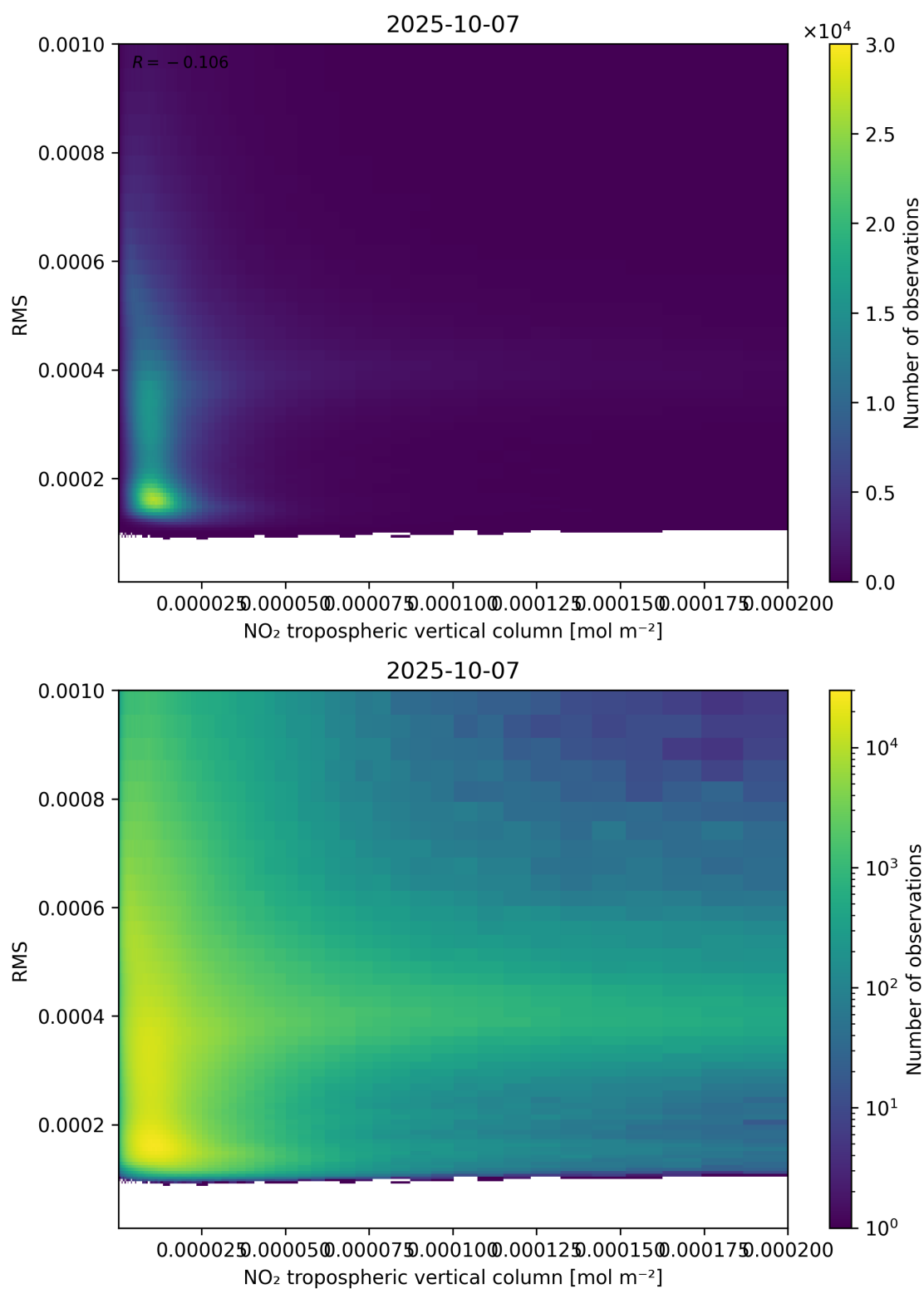
Figure 142: Scatter density plot of “NO 2 tropospheric vertical column” against “RMS” for 2025-10-06 to 2025-10-08.
