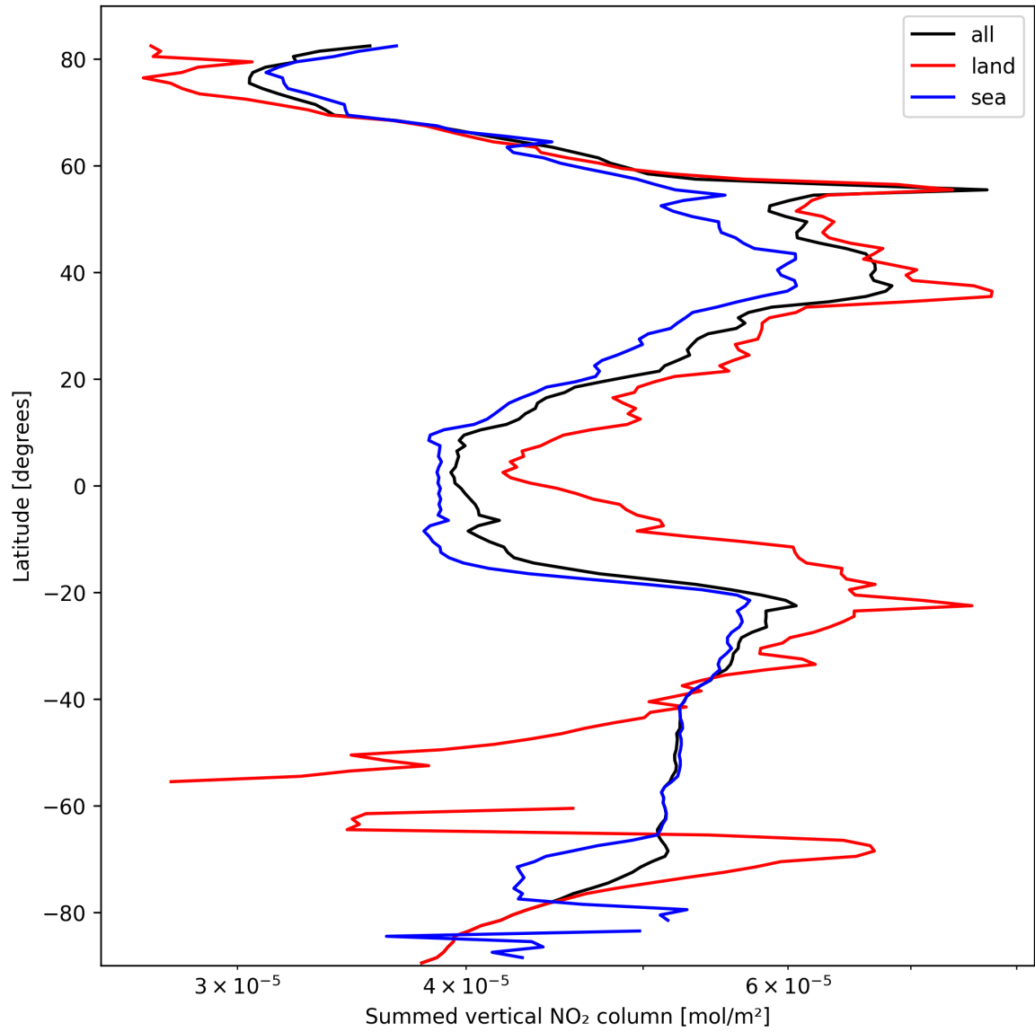
Figure 23: Zonal average of “Summed vertical NO 2 column” for 2025-10-06 to 2025-10-08.
