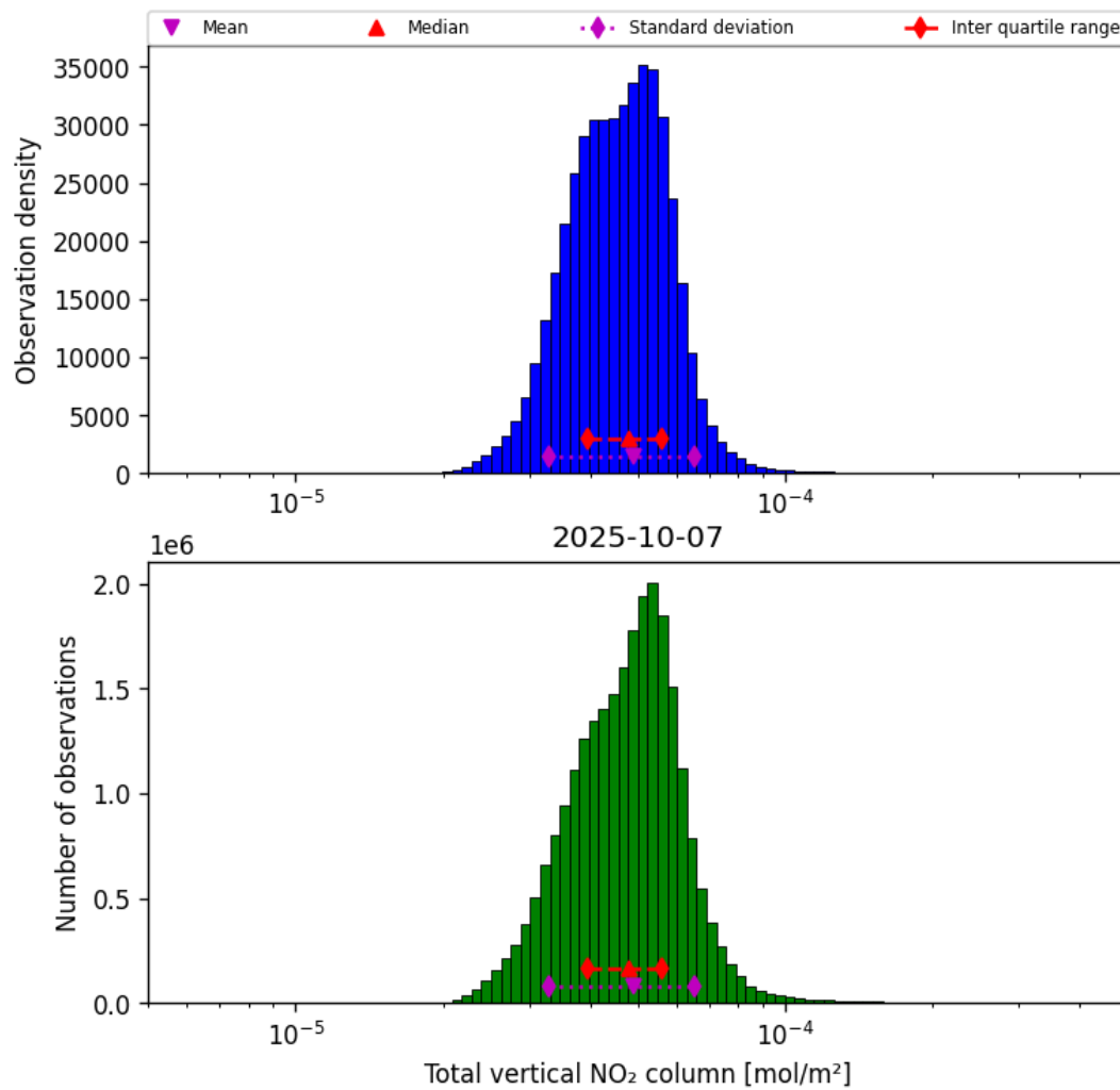
Figure 38: Histogram of “Total vertical NO 2 column” for 2025-10-06 to 2025-10-08
