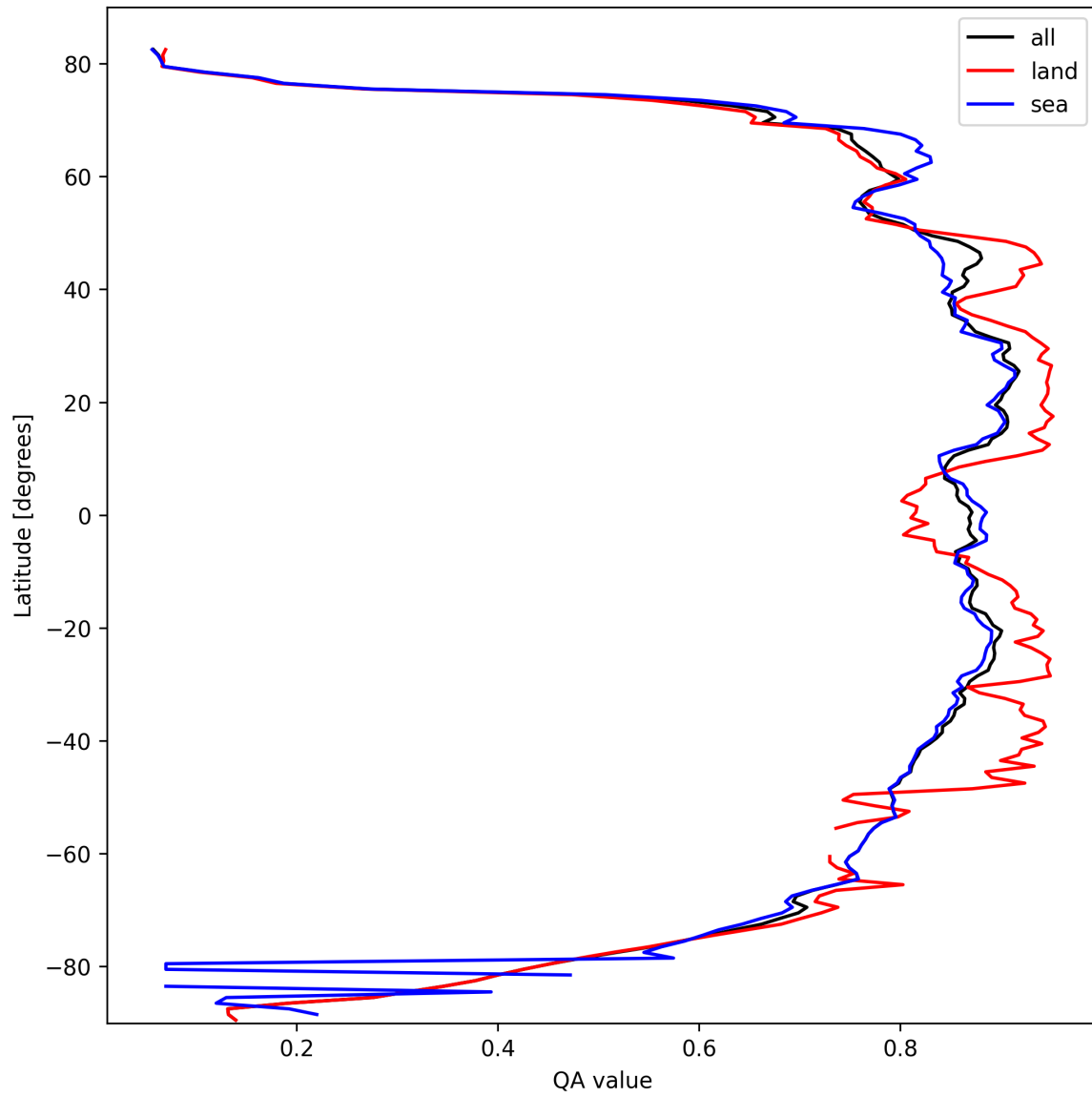
Figure 11: Zonal average of “QA value” for 2025-10-06 to 2025-10-08.
