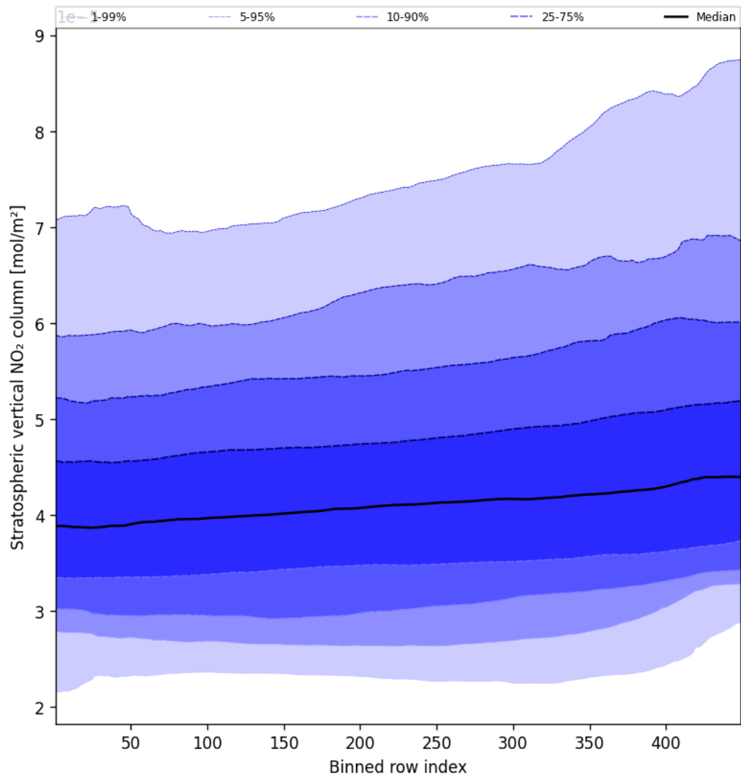
Figure 53: Along track statistics of “Stratospheric vertical NO 2 column” for 2025-10-06 to 2025-10-08
