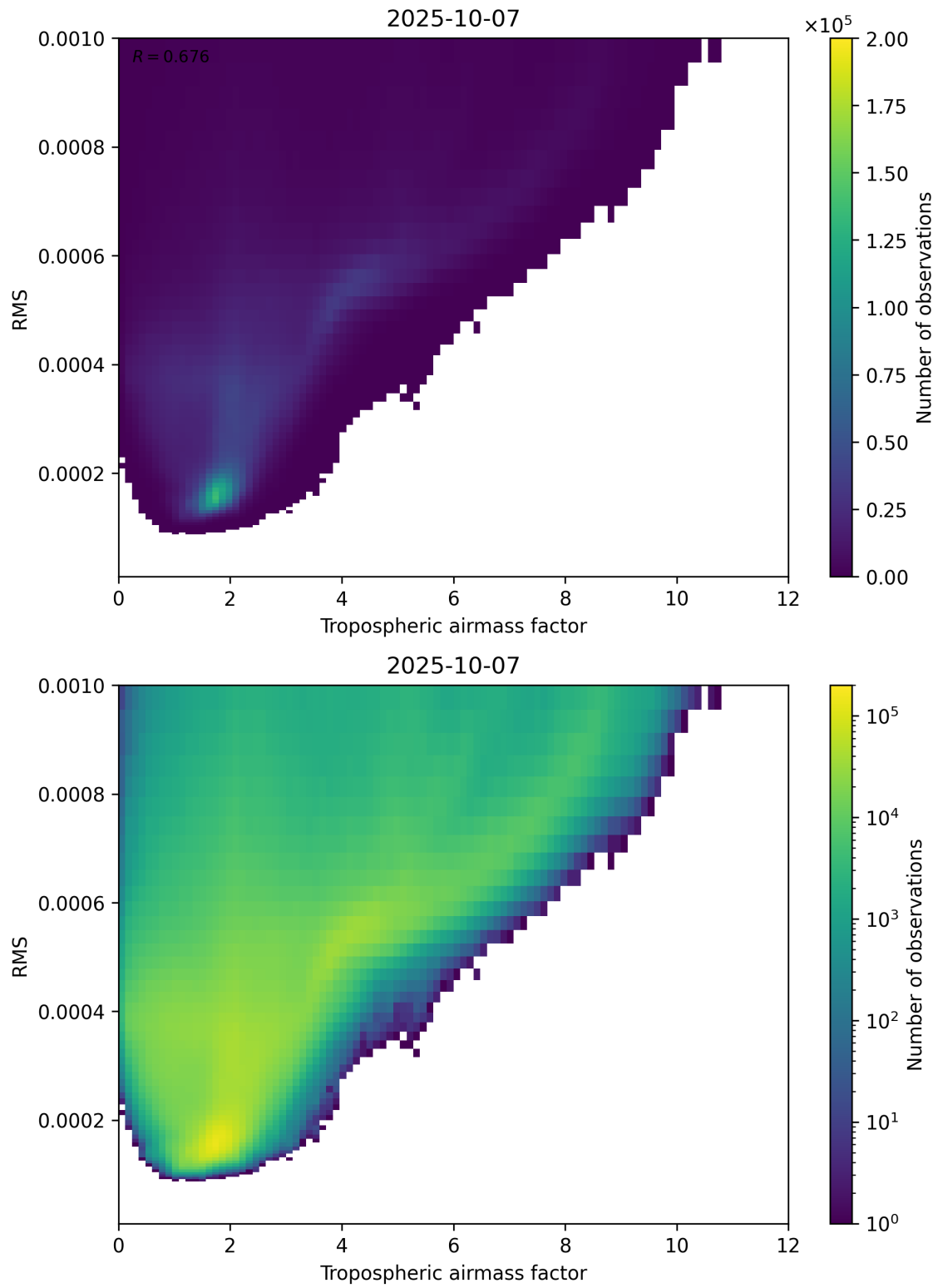
Figure 79: Scatter density plot of “Tropospheric airmass factor” against “RMS” for 2025-10-06 to 2025-10-08.
