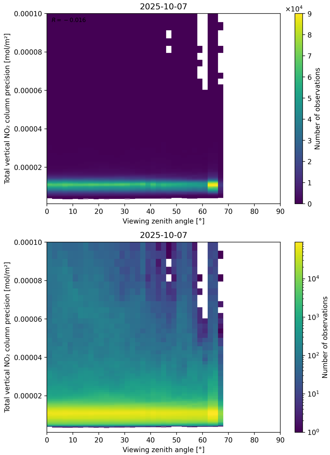
Figure 168: Scatter density plot of “Viewing zenith angle” against “Total vertical NO 2 column precision” for 2025-10-06 to 2025-10-08.
