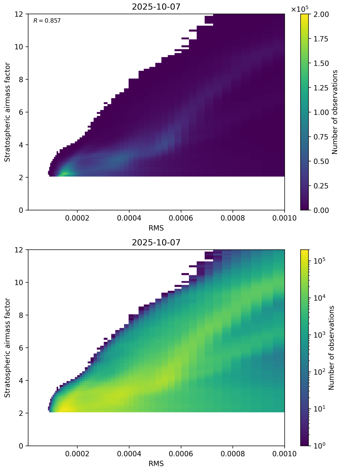
Figure 144: Scatter density plot of “RMS” against “Stratospheric airmass factor” for 2025-10-06 to 2025-10-08.
