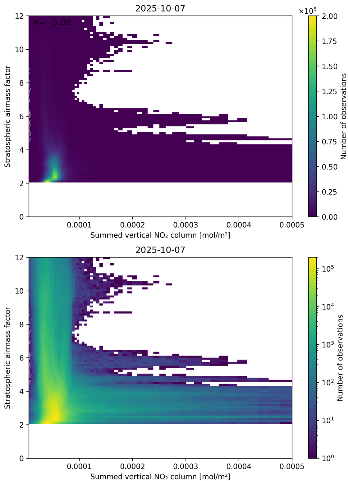
Figure 103: Scatter density plot of “Summed vertical NO 2 column” against “Stratospheric airmass factor” for 2025-10-06 to 2025-10-08.
