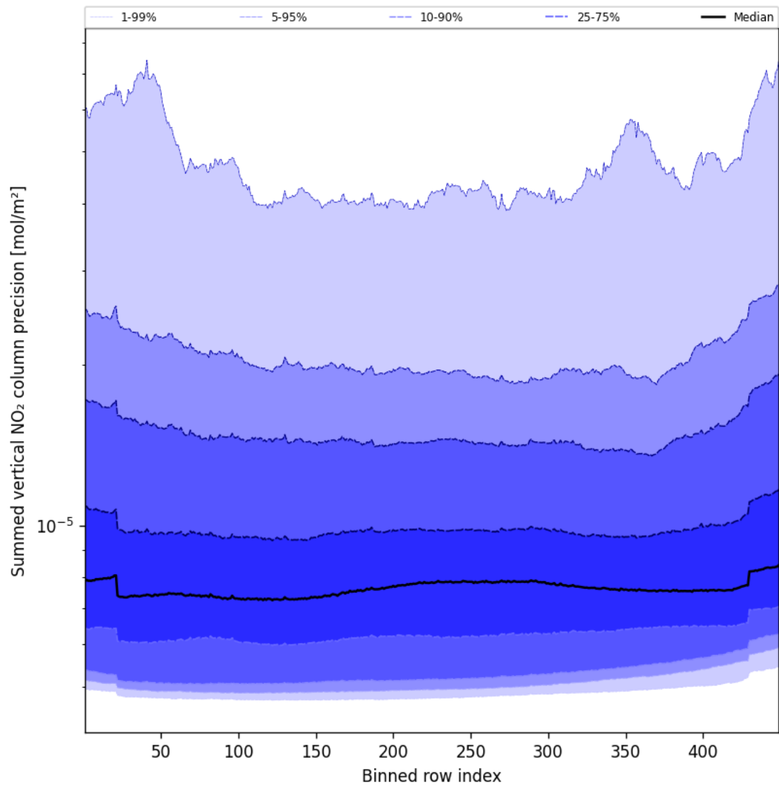
Figure 58: Along track statistics of “Summed vertical NO 2 column precision” for 2025-10-06 to 2025-10-08
