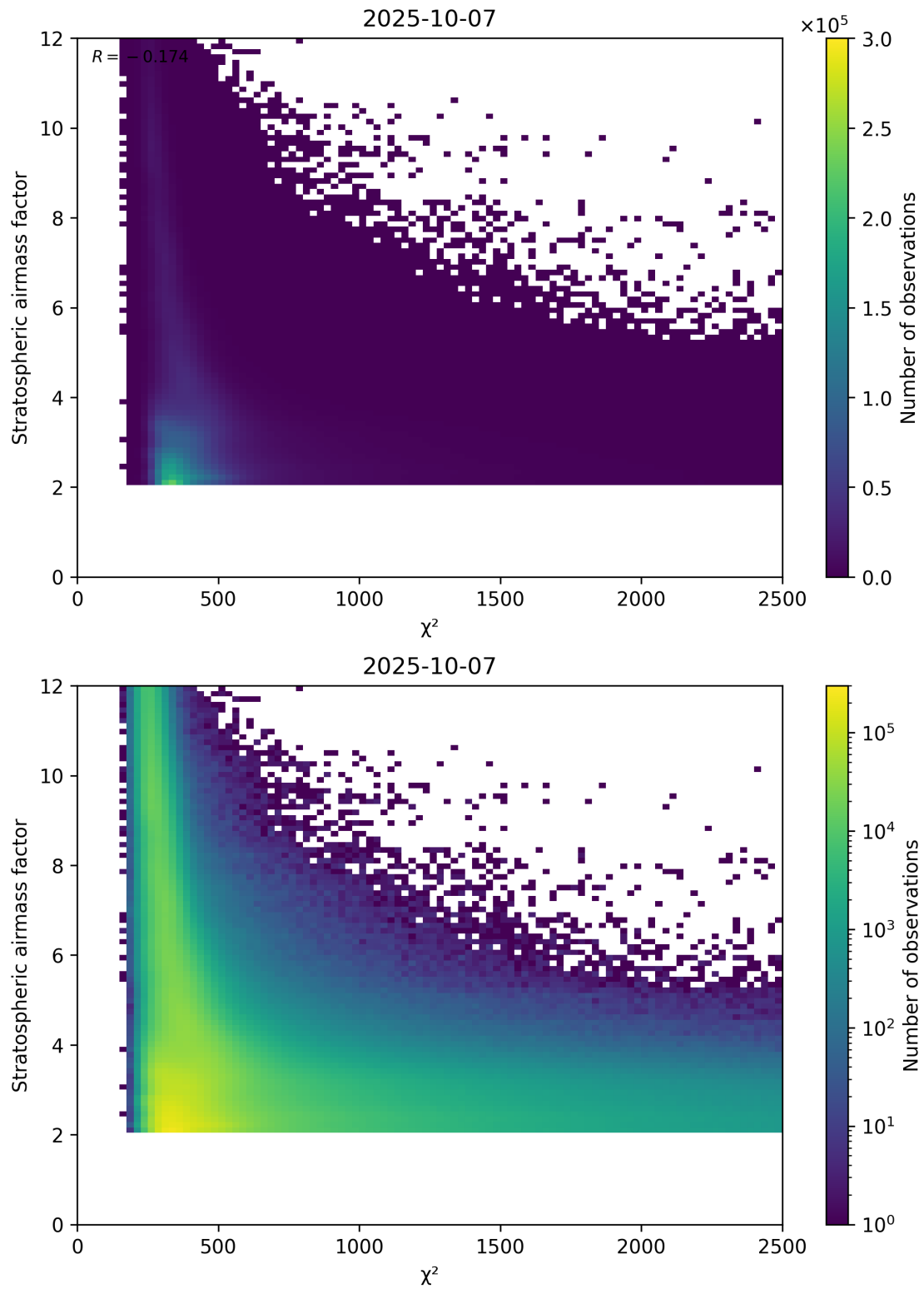
Figure 81: Scatter density plot of “ \chi^2 ” against “Stratospheric airmass factor” for 2025-10-06 to 2025-10-08.
