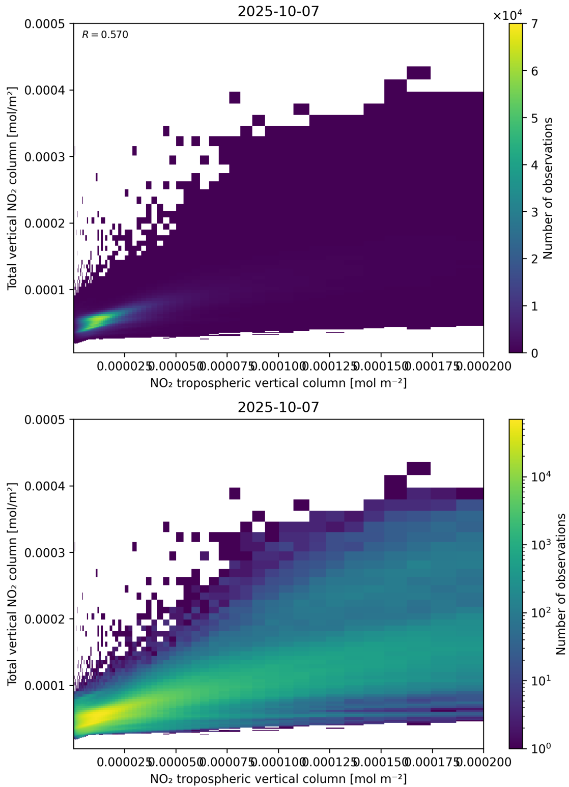
Figure 128: Scatter density plot of “NO 2 tropospheric vertical column” against “Total vertical NO 2 column” for 2025-10-06 to 2025-10-08.
