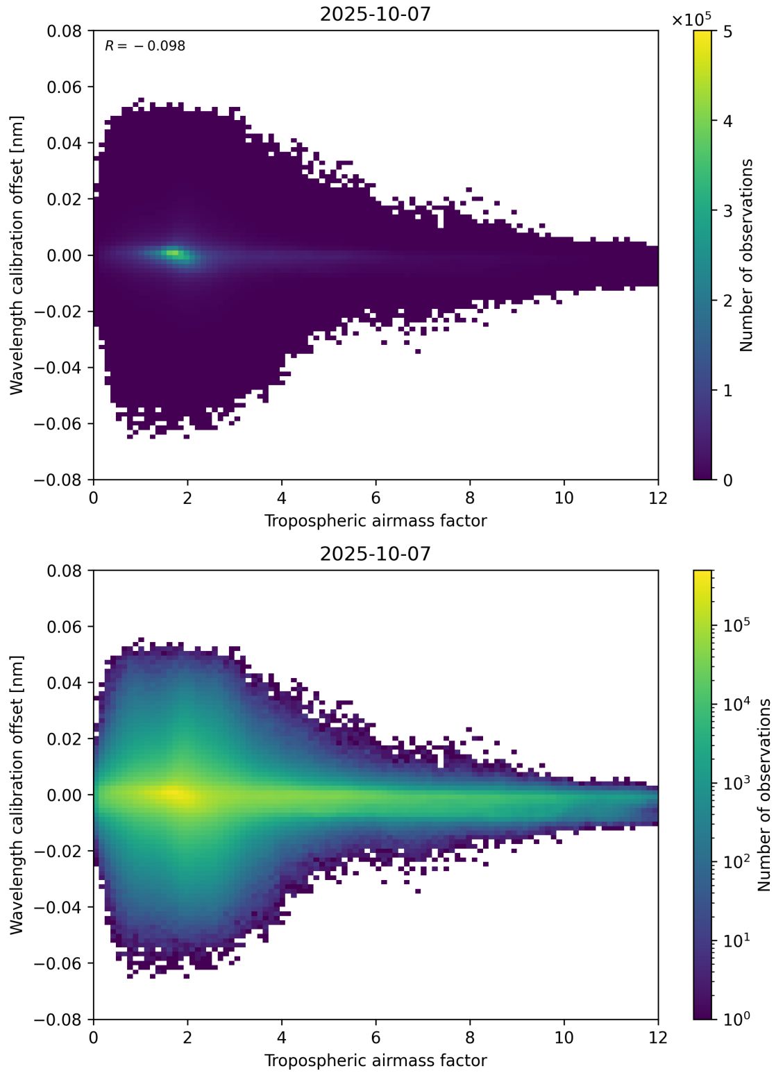
Figure 80: Scatter density plot of “Tropospheric air mass factor” against “Wavelength calibration offset” for 2025-10-06 to 2025-10-08.
