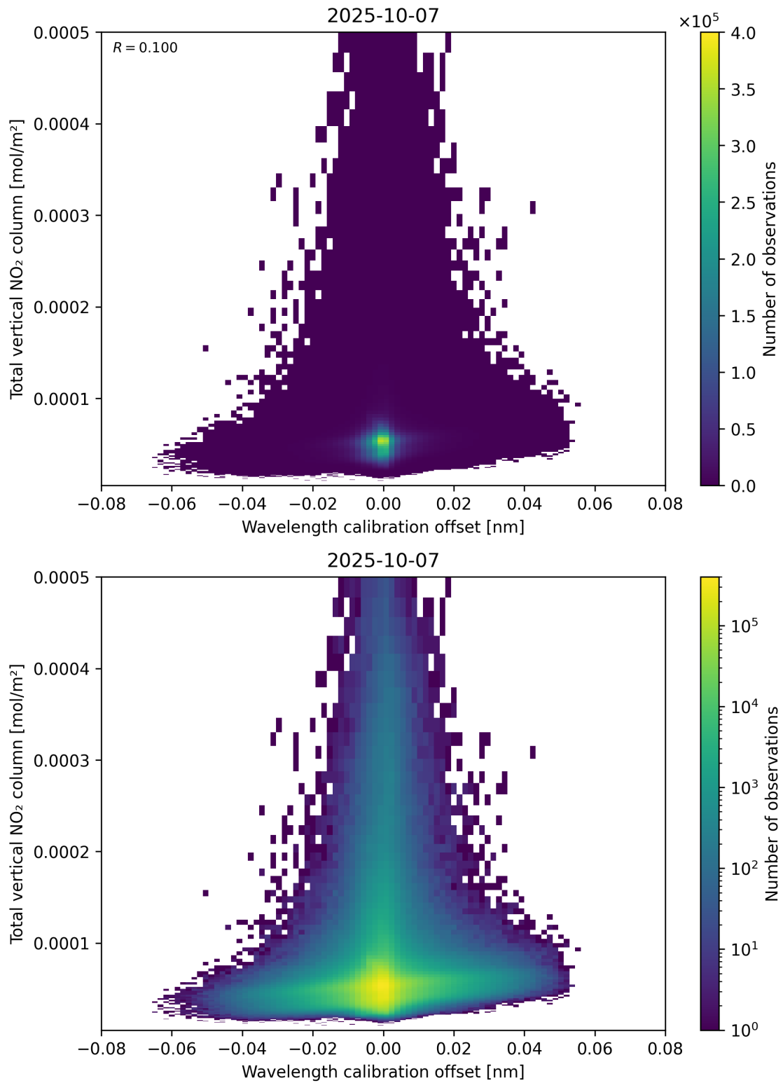
Figure 179: Scatter density plot of “Wavelength calibration offset” against “Total vertical NO 2 column” for 2025-10-06 to 2025-10-08.
