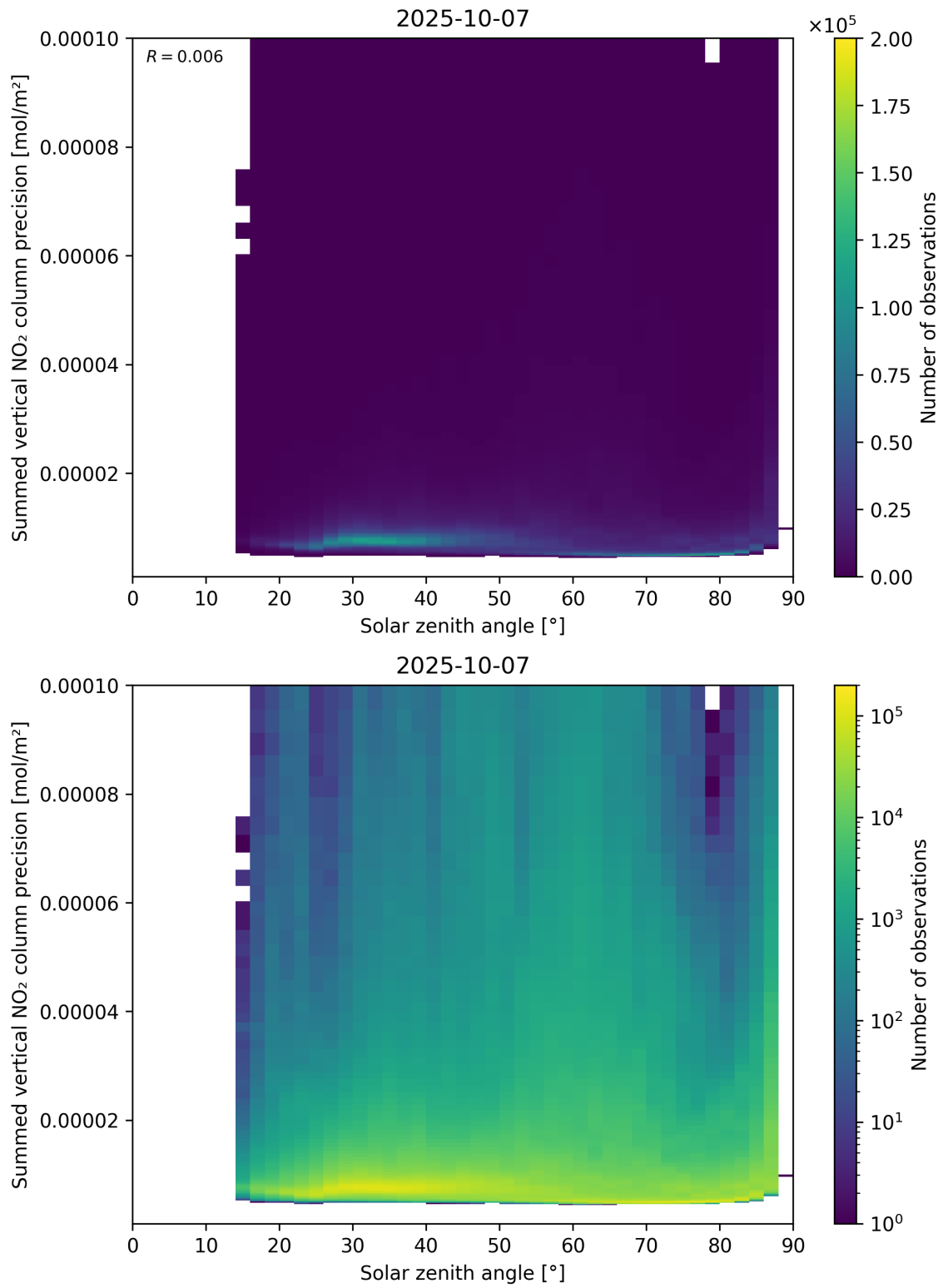
Figure 152: Scatter density plot of “Solar zenith angle” against “Summed vertical NO 2 column precision” for 2025-10-06 to 2025-10-08.
