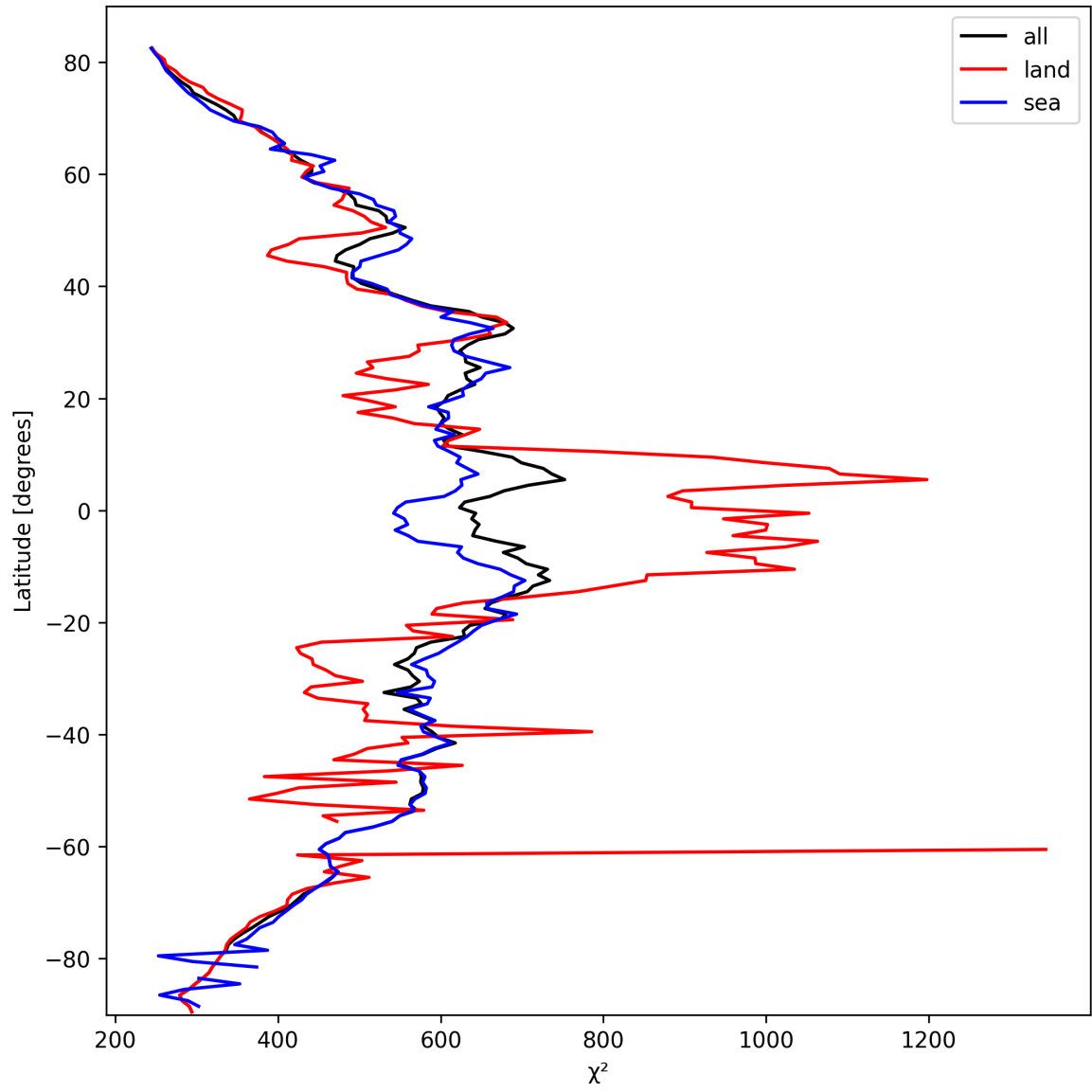
Figure 25: Zonal average of “ \chi^2 ” for 2025-10-06 to 2025-10-08.
