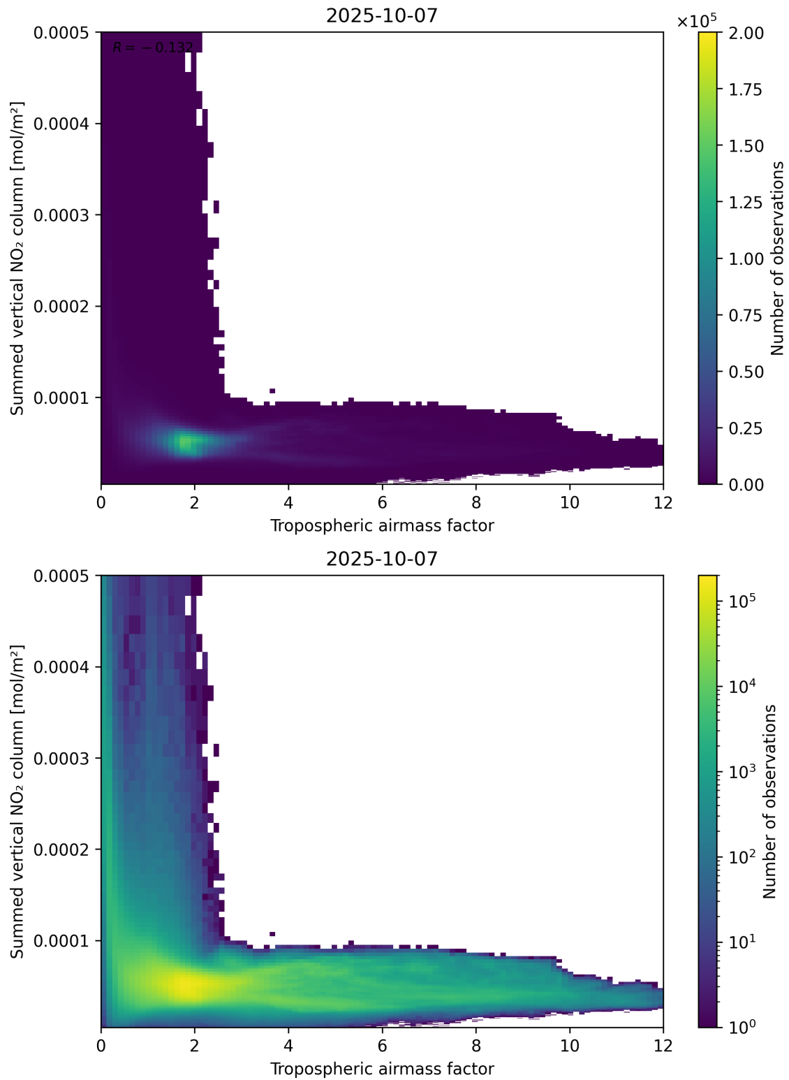
Figure 75: Scatter density plot of “Tropospheric airmass factor” against “Summed vertical NO 2 column” for 2025-10-06 to 2025-10-08.
