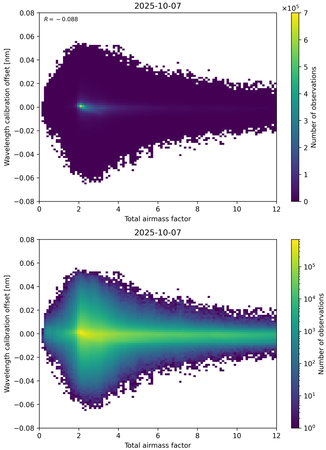
Figure 70: Scatter density plot of “Total airmass factor” against “Wavelength calibration offset” for 2025-10-06 to 2025-10-08.
