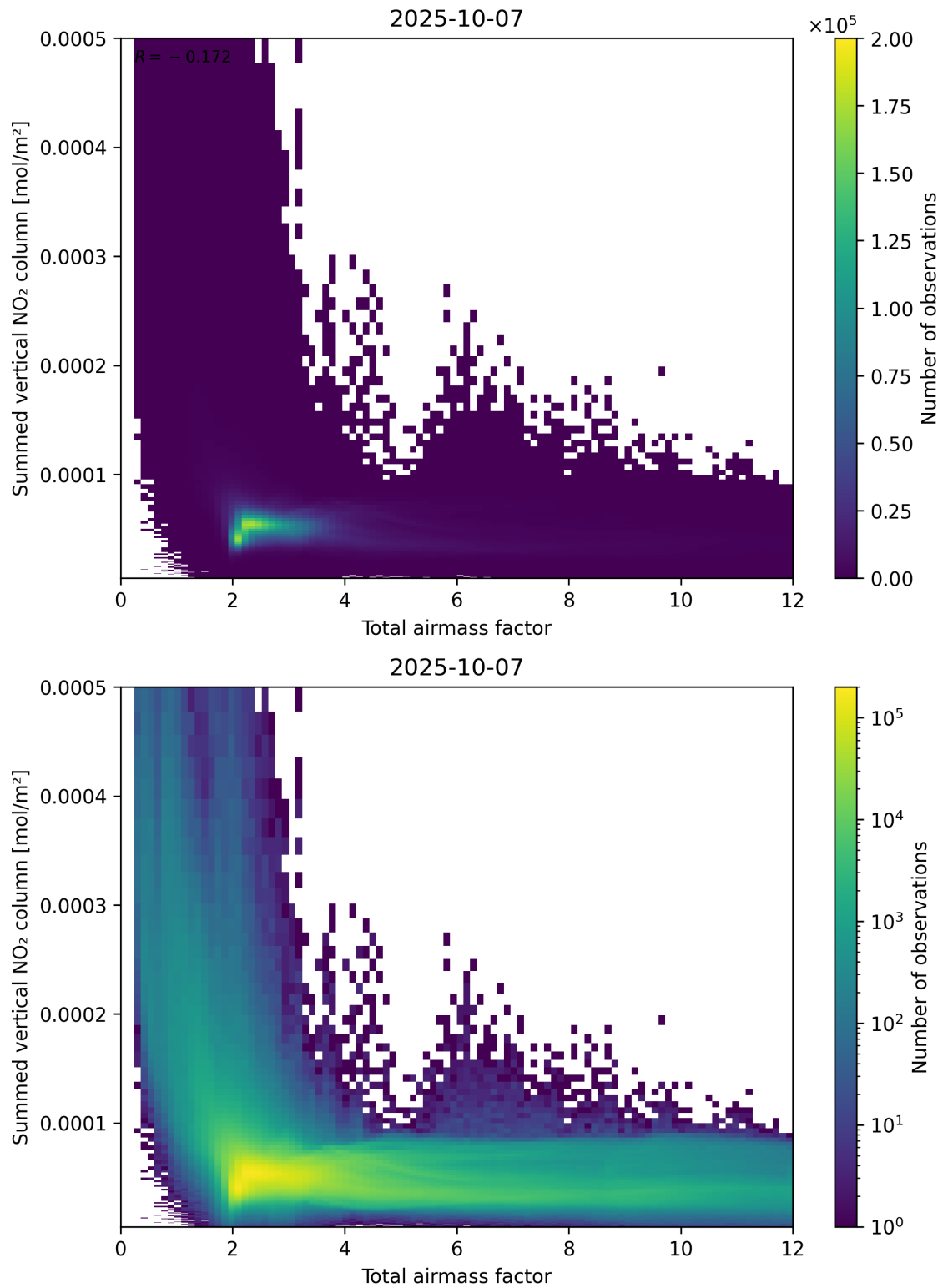
Figure 65: Scatter density plot of “Total airmass factor” against “Summed vertical NO 2 column” for 2025-10-06 to 2025-10-08.
