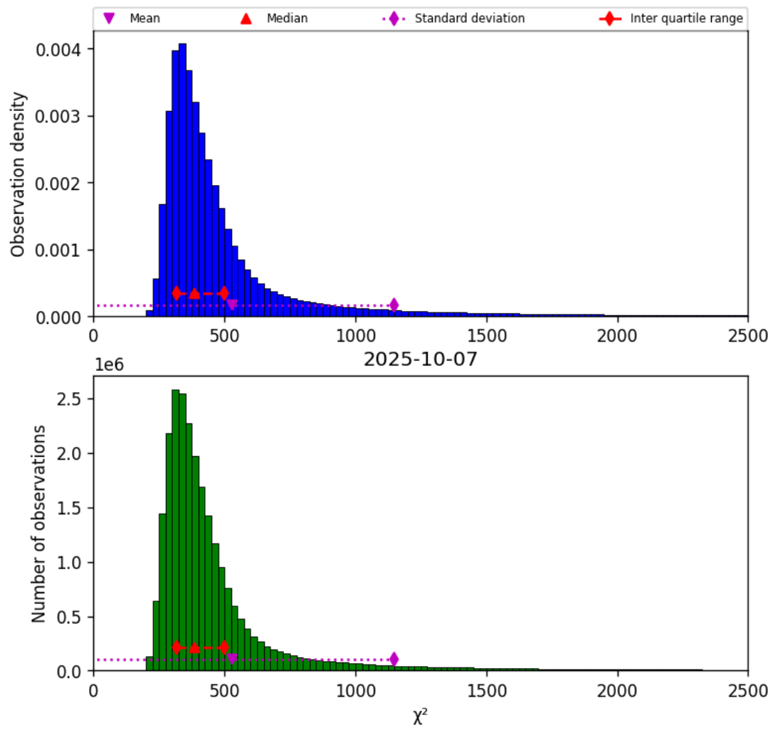
Figure 42: Histogram of “ \chi^2 ” for 2025-10-06 to 2025-10-08
