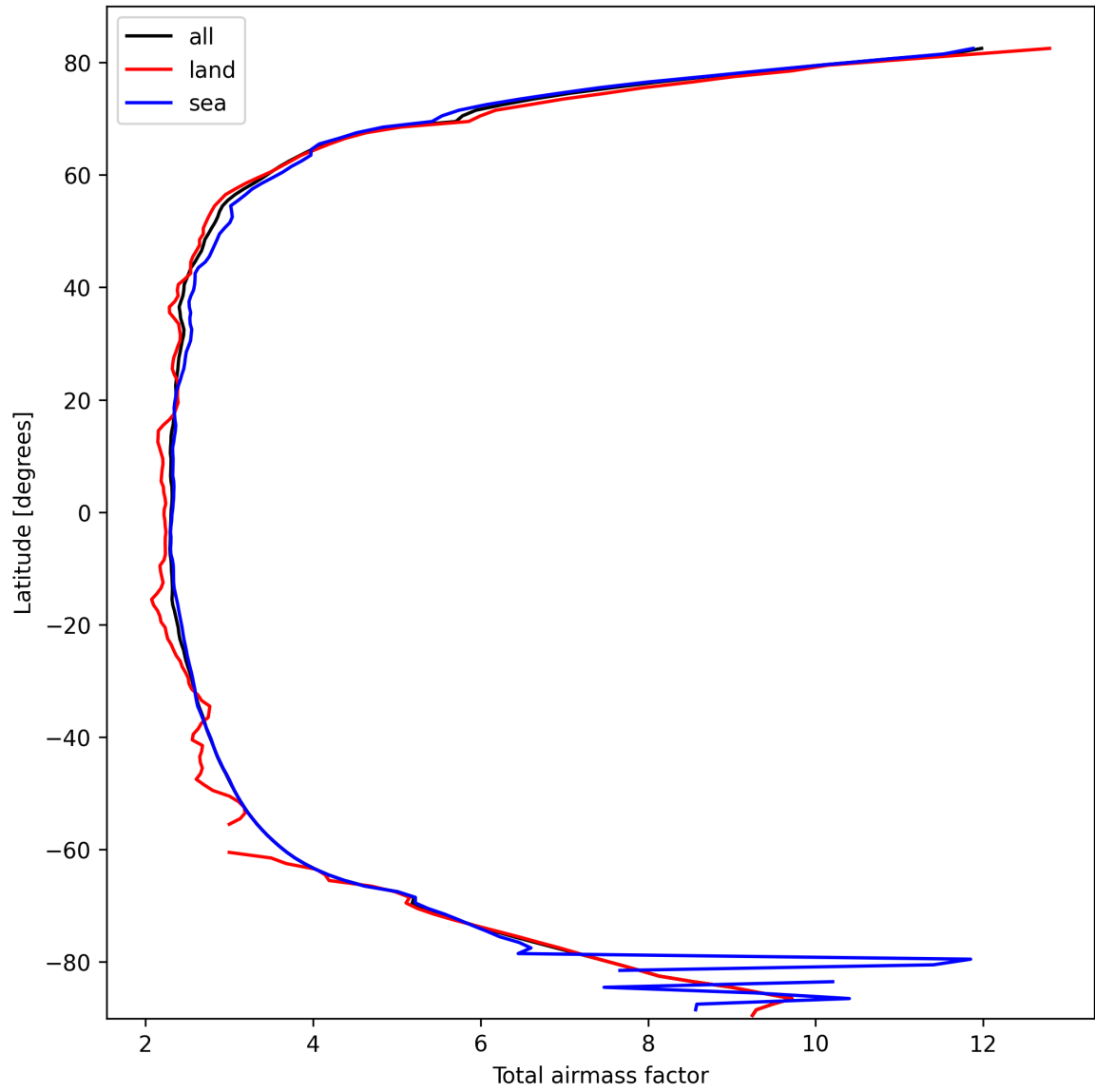
Figure 15: Zonal average of “Total airmass factor” for 2025-10-06 to 2025-10-08.
