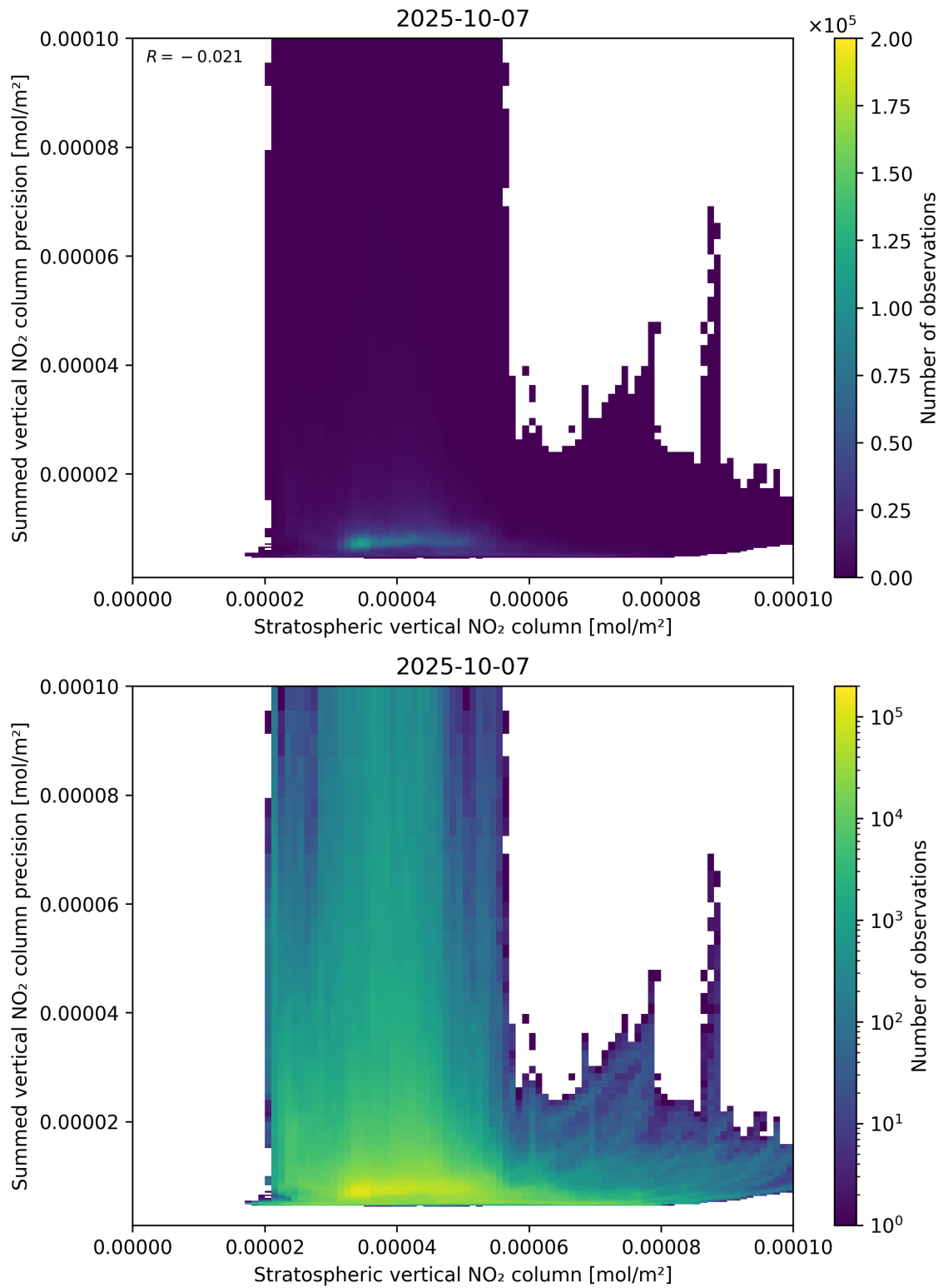
Figure 99: Scatter density plot of “Stratospheric vertical NO 2 column” against “Summed vertical NO 2 column precision” for 2025-10-06 to 2025-10-08.
