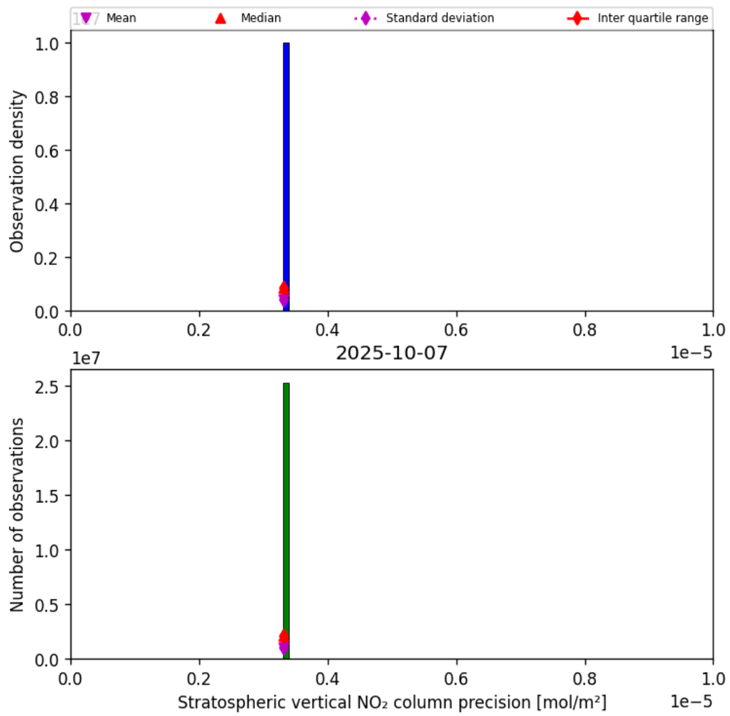
Figure 37: Histogram of “Stratospheric vertical NO 2 column precision” for 2025-10-06 to 2025-10-08
