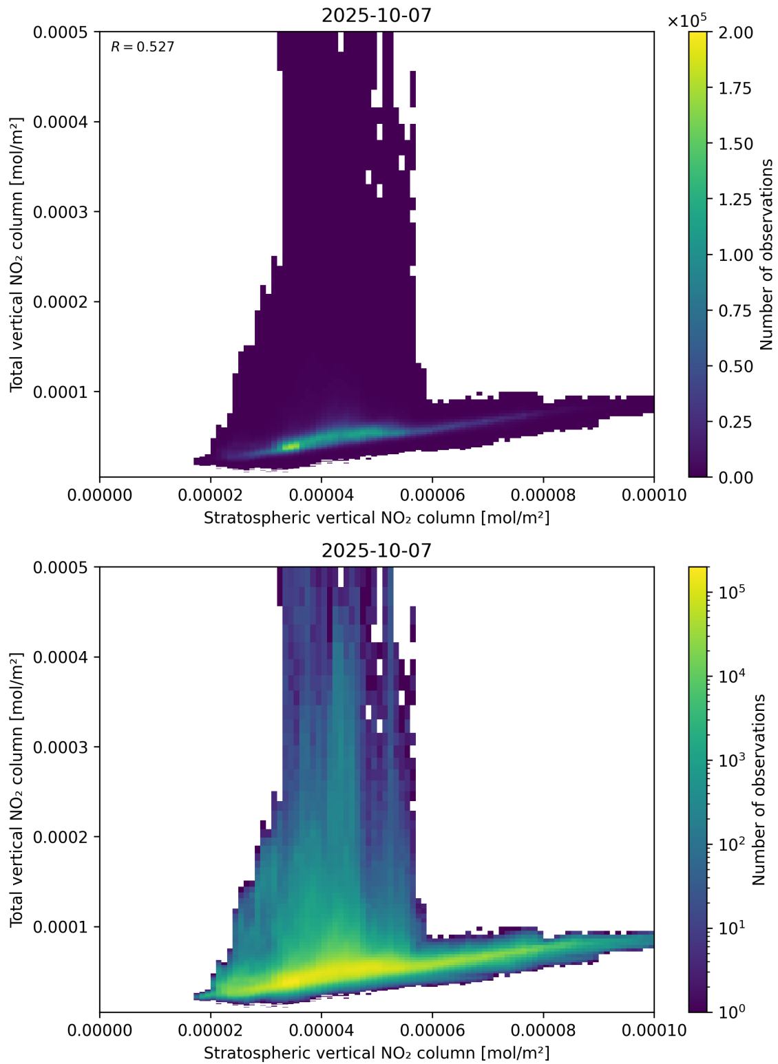
Figure 100: Scatter density plot of “Stratospheric vertical NO 2 column” against “Total vertical NO 2 column” for 2025-10-06 to 2025-10-08.
