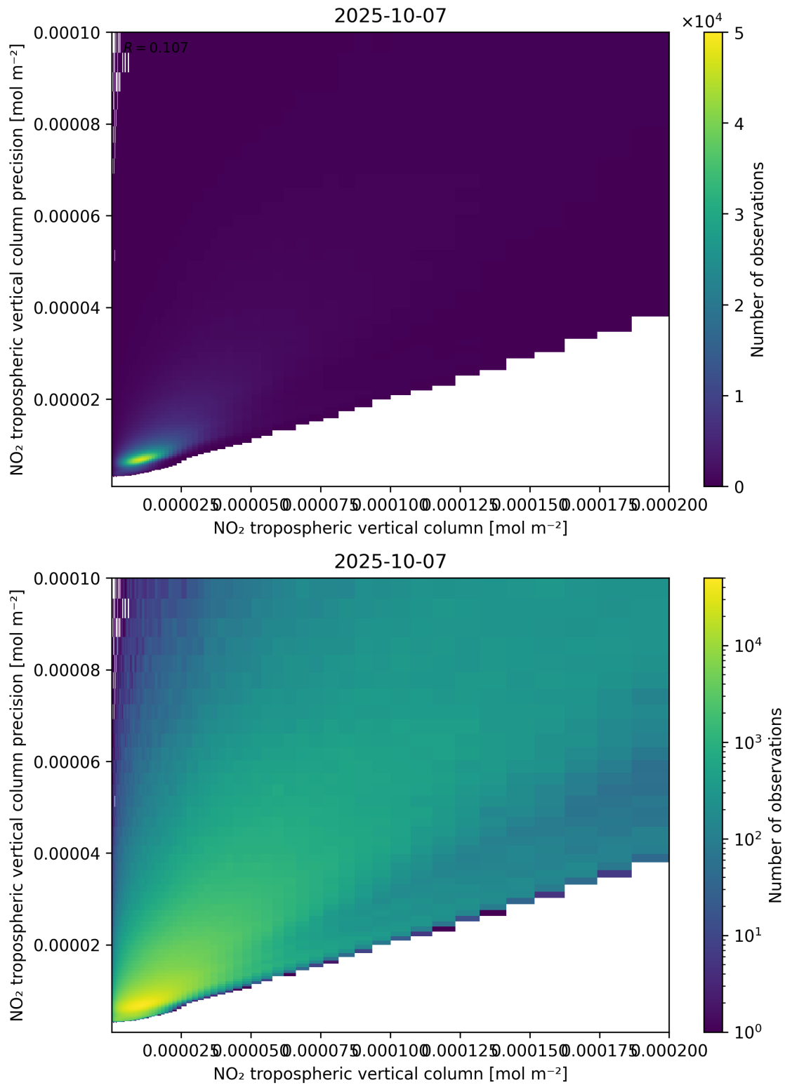
Figure 130: Scatter density plot of “NO 2 tropospheric vertical column” against “NO 2 tropospheric vertical column precision” for 2025-10-06 to 2025-10-08.
