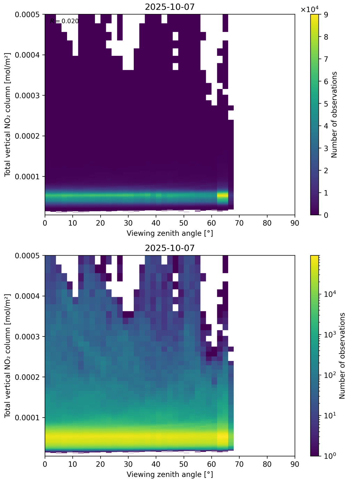
Figure 167: Scatter density plot of “Viewing zenith angle” against “Total vertical NO 2 column” for 2025-10-06 to 2025-10-08.
