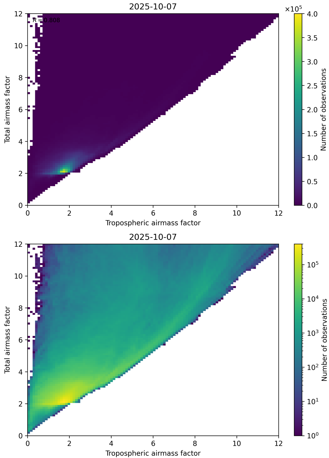
Figure 72: Scatter density plot of “Tropospheric airmass factor” against “Total airmass factor” for 2025-10-06 to 2025-10-08.
