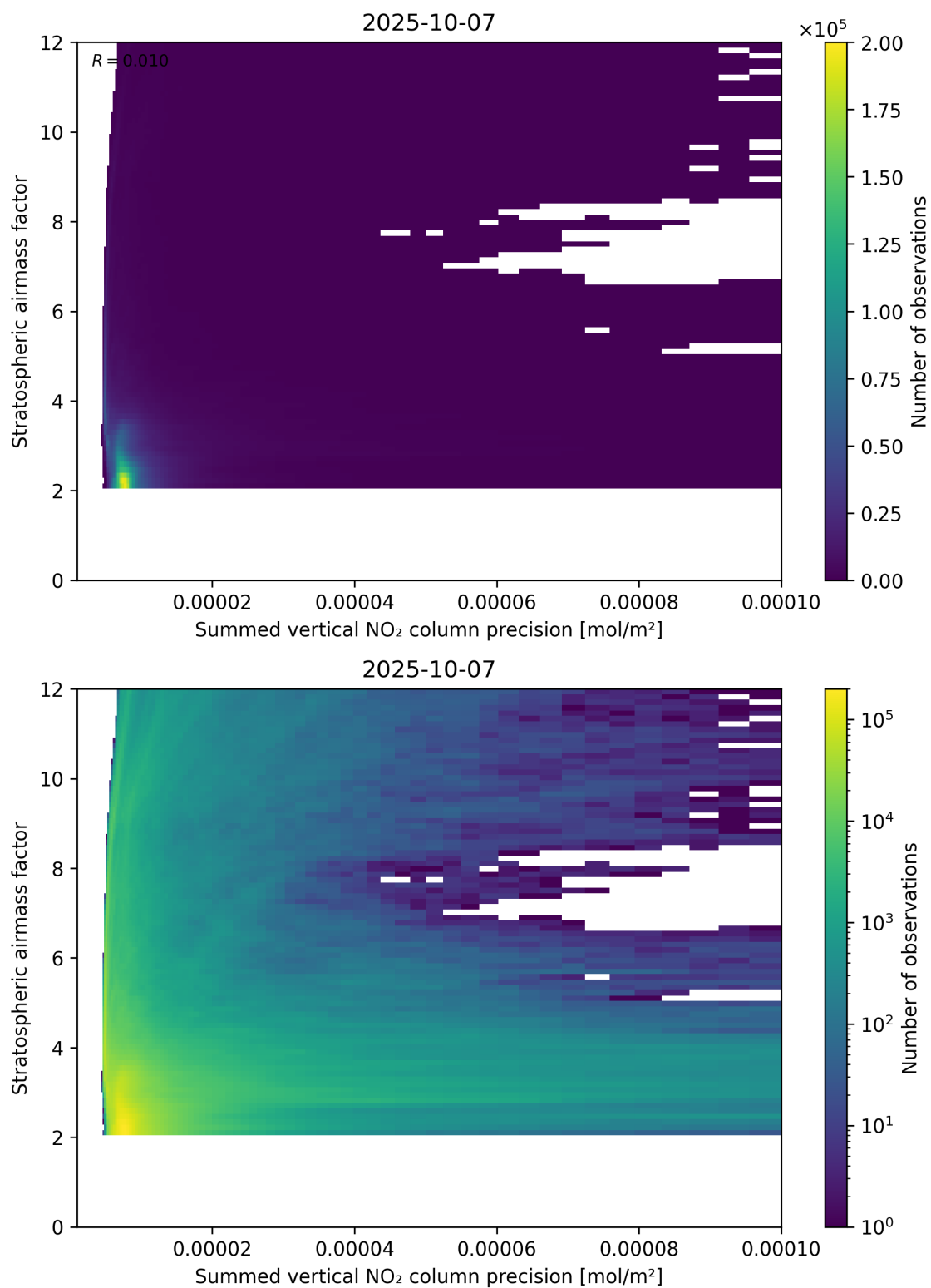
Figure 106: Scatter density plot of “Summed vertical NO 2 column precision” against “Stratospheric airmass factor” for 2025-10-06 to 2025-10-08.
