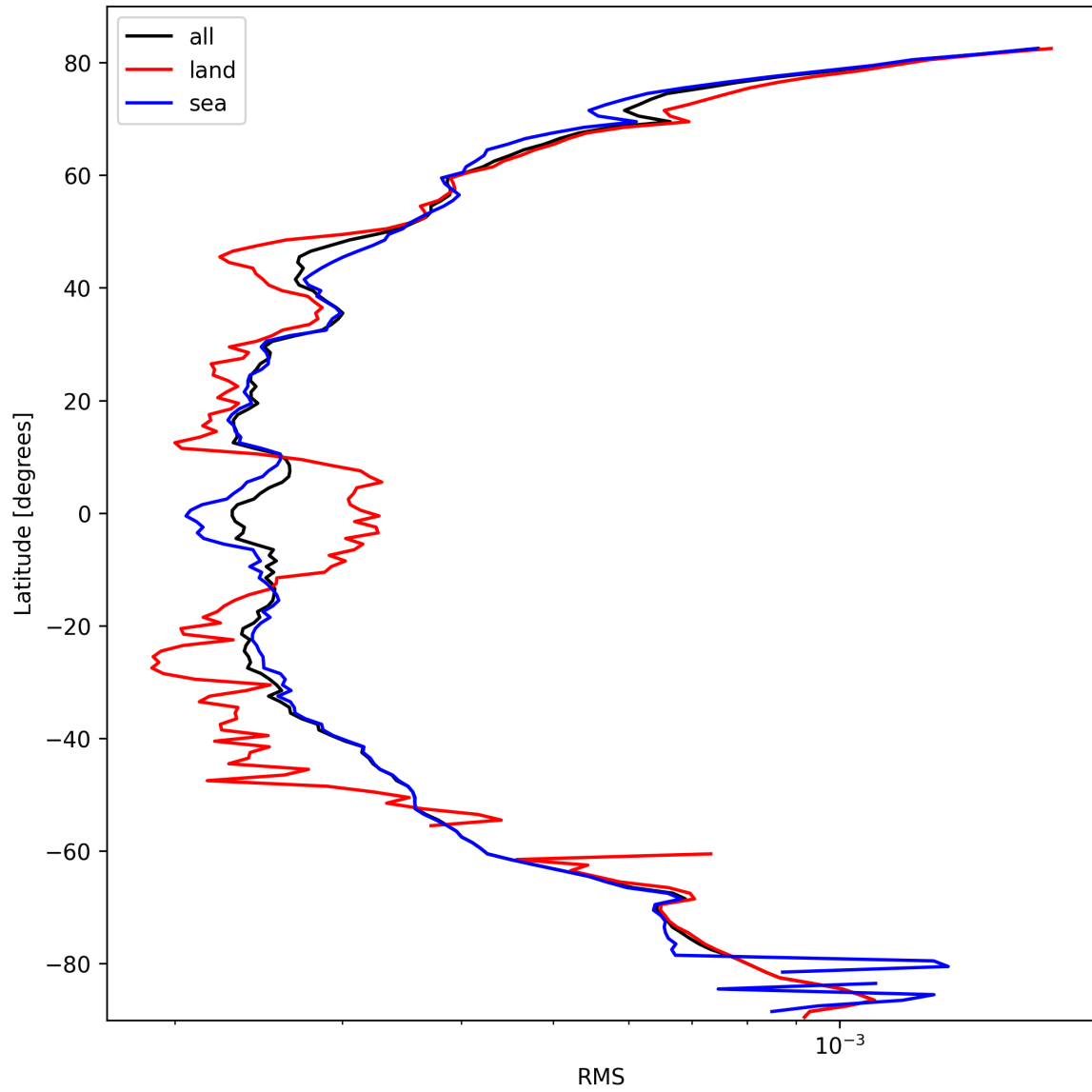
Figure 26: Zonal average of “RMS” for 2025-10-06 to 2025-10-08.
