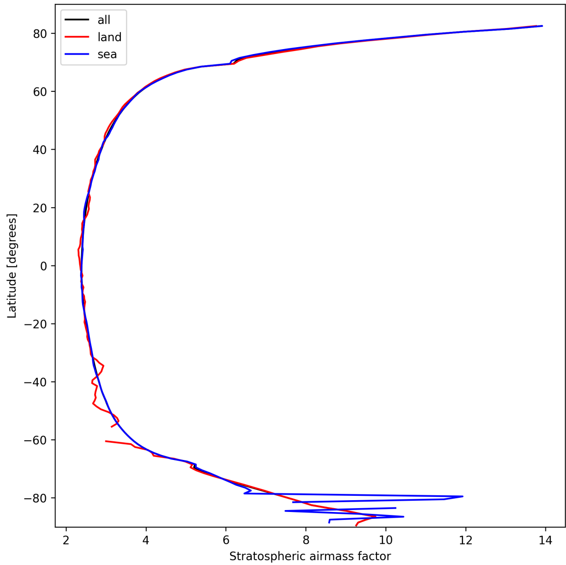
Figure 27: Zonal average of “Stratospheric air mass factor” for 2025-10-06 to 2025-10-08.
