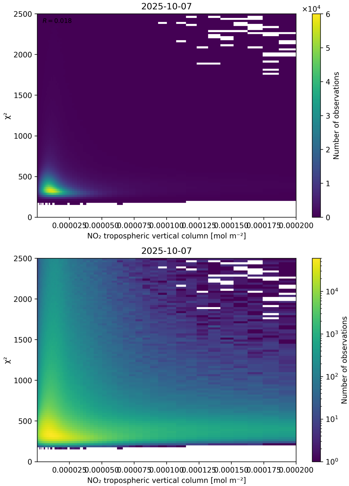
Figure 124: Scatter density plot of “NO 2 tropospheric vertical column” against “ \chi^2 ” for 2025-10-06 to 2025-10-08.
