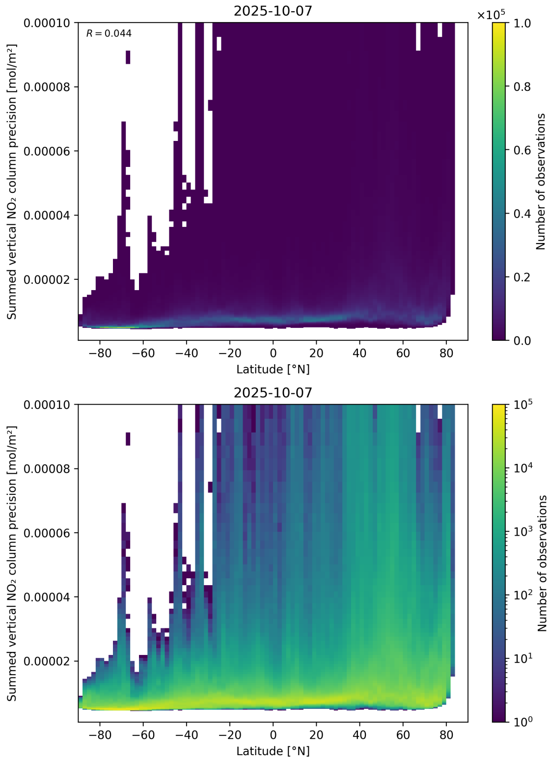
Figure 89: Scatter density plot of “Latitude” against “Summed vertical NO 2 column precision” for 2025-10-06 to 2025-10-08.
