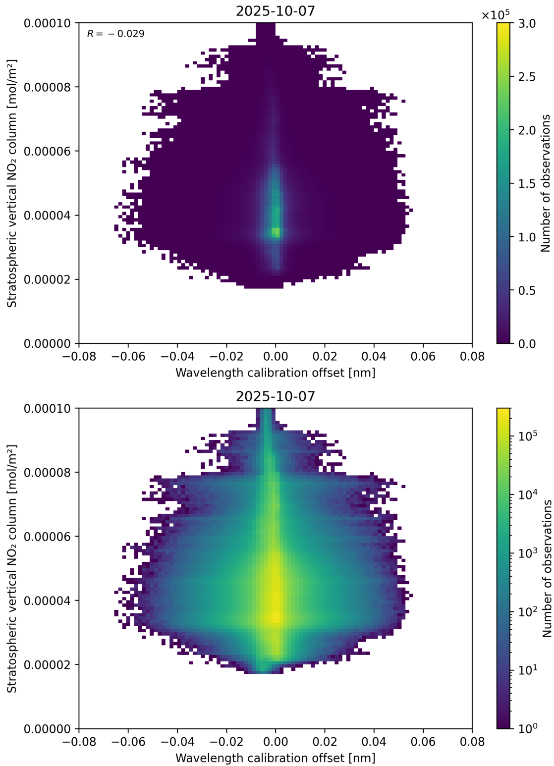
Figure 176: Scatter density plot of “Wavelength calibration offset” against “Stratospheric vertical NO 2 column” for 2025-10-06 to 2025-10-08.
