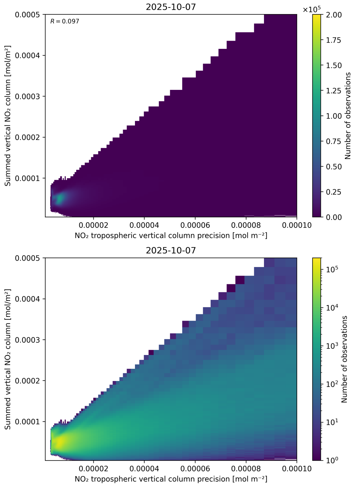
Figure 136: Scatter density plot of “NO 2 tropospheric vertical column precision” against “Summed vertical NO 2 column” for 2025-10-06 to 2025-10-08.
