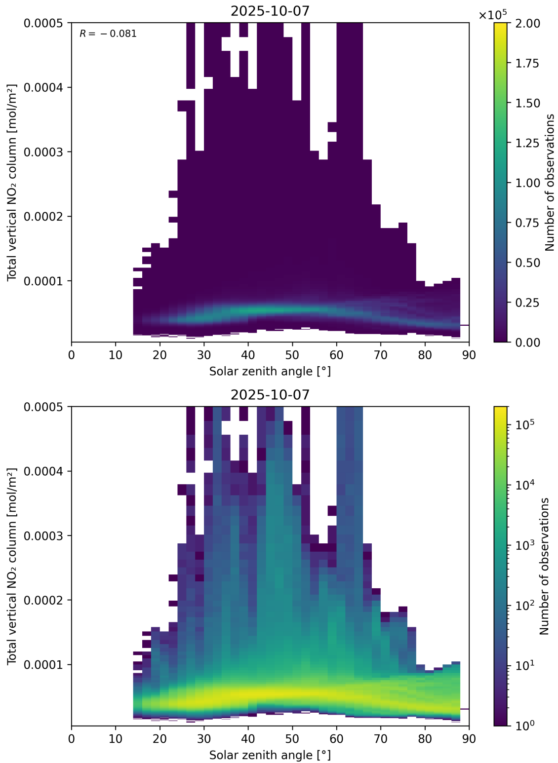
Figure 153: Scatter density plot of “Solar zenith angle” against “Total vertical NO 2 column” for 2025-10-06 to 2025-10-08.
