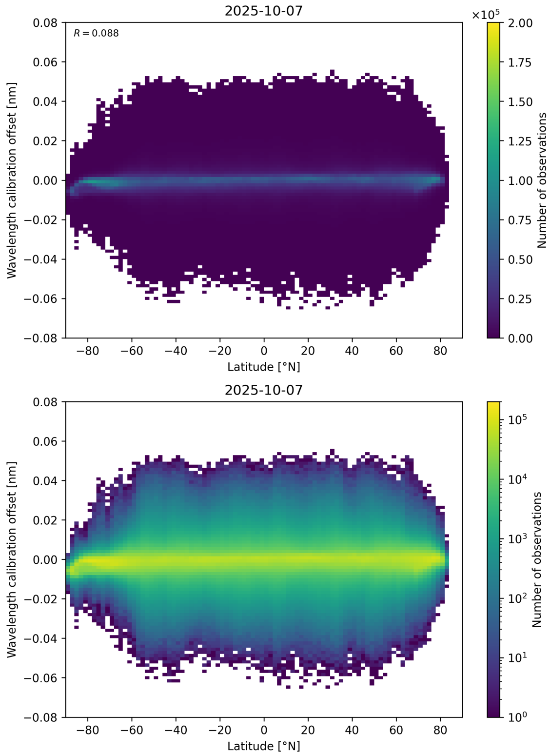
Figure 95: Scatter density plot of “Latitude” against “Wavelength calibration offset” for 2025-10-06 to 2025-10-08.
