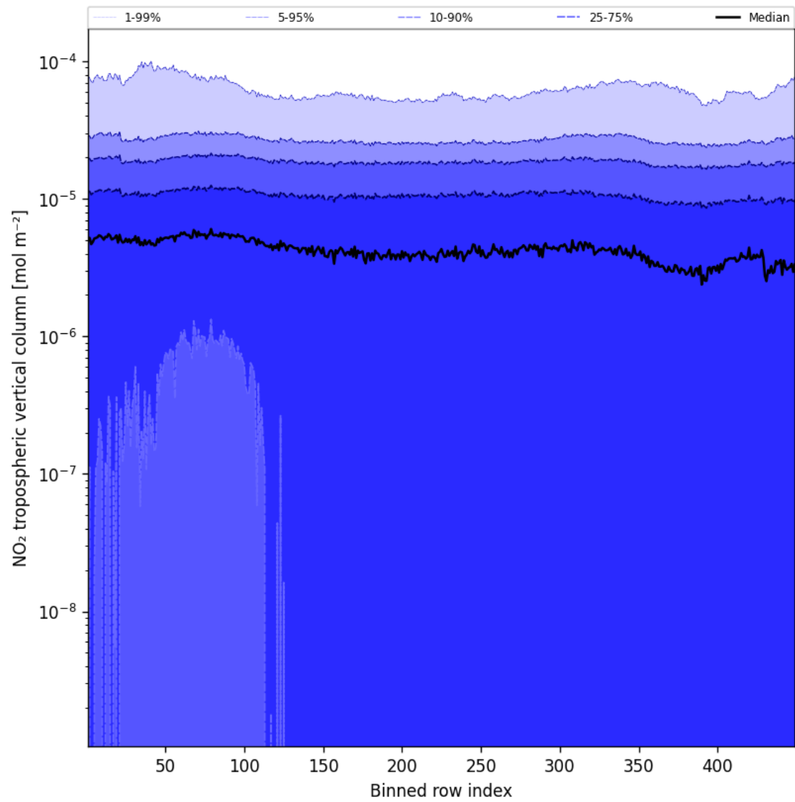
Figure 46: Along track statistics of “NO 2 tropospheric vertical column” for 2025-10-06 to 2025-10-08
