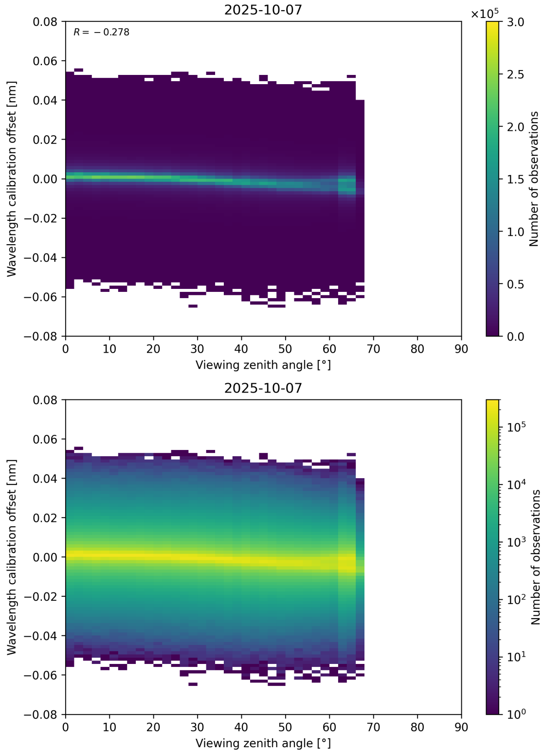
Figure 173: Scatter density plot of “Viewing zenith angle” against “Wavelength calibration offset” for 2025-10-06 to 2025-10-08.
