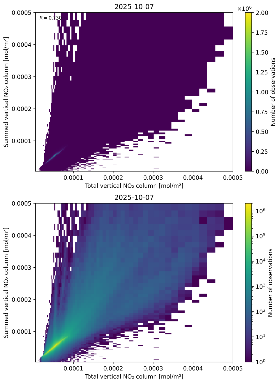
Figure 112: Scatter density plot of “Total vertical NO 2 column” against “Summed vertical NO 2 column” for 2025-10-06 to 2025-10-08.
