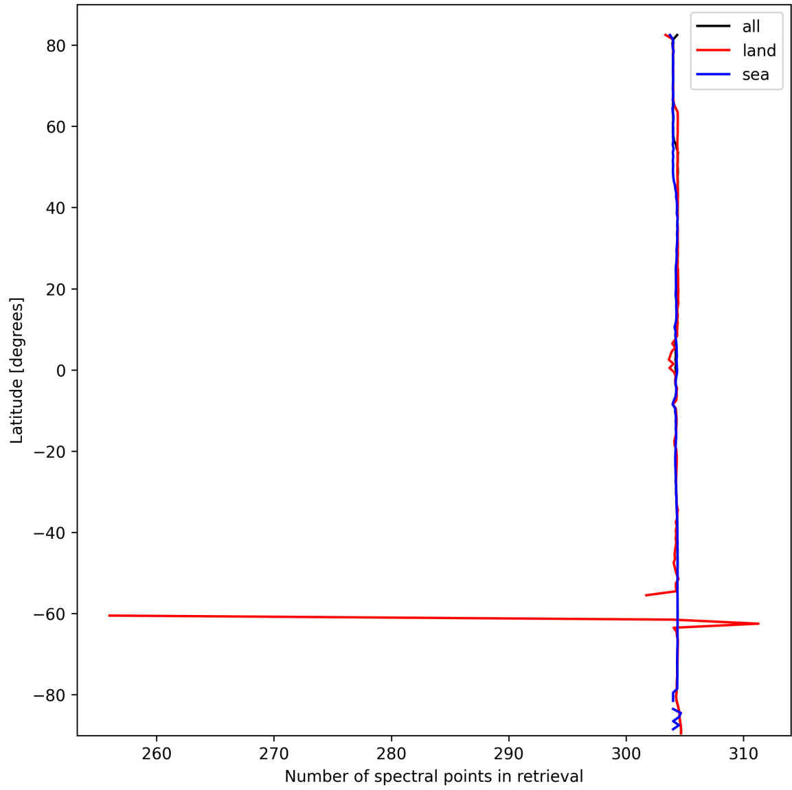
Figure 16: Zonal average of “Number of spectral points in retrieval” for 2025-10-06 to 2025-10-08.
