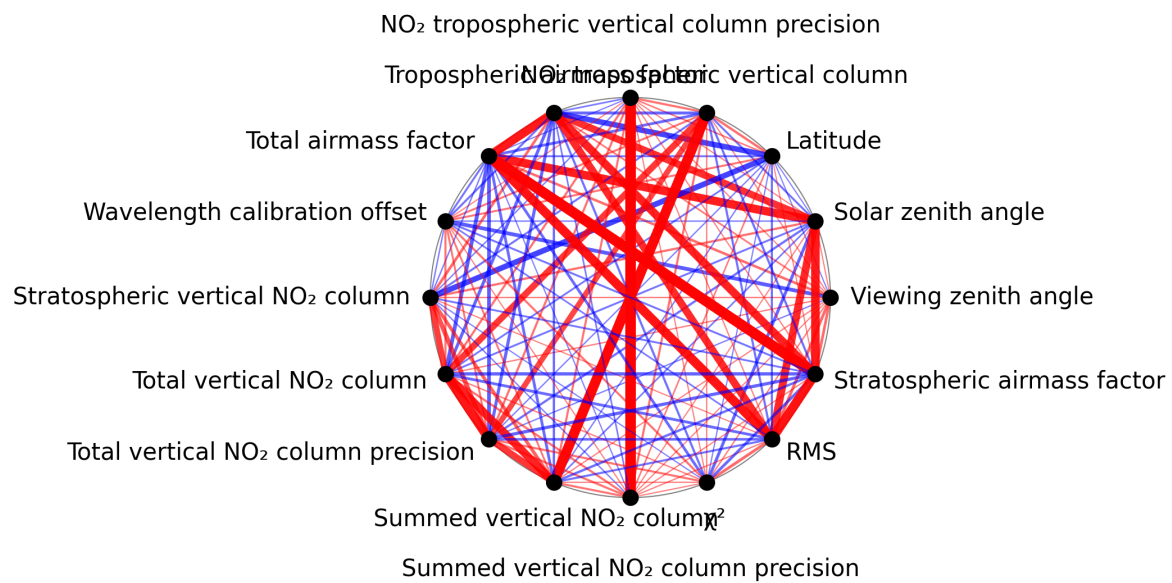
Figure 1: Map of correlation graph for 2025-10-06 to 2025-10-08.
