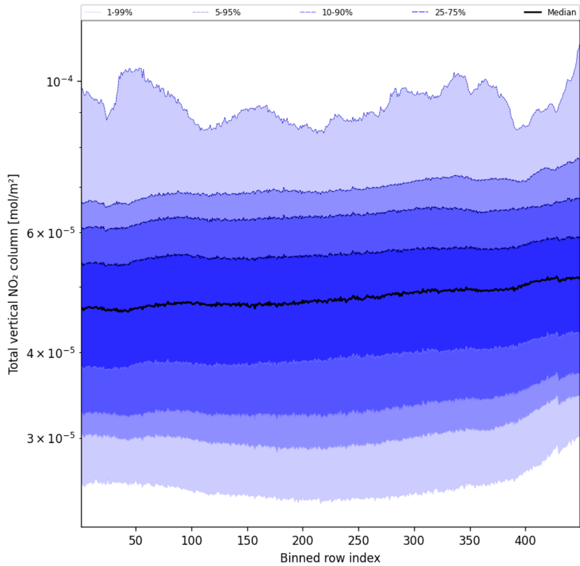
Figure 55: Along track statistics of “Total vertical NO 2 column” for 2025-10-06 to 2025-10-08
