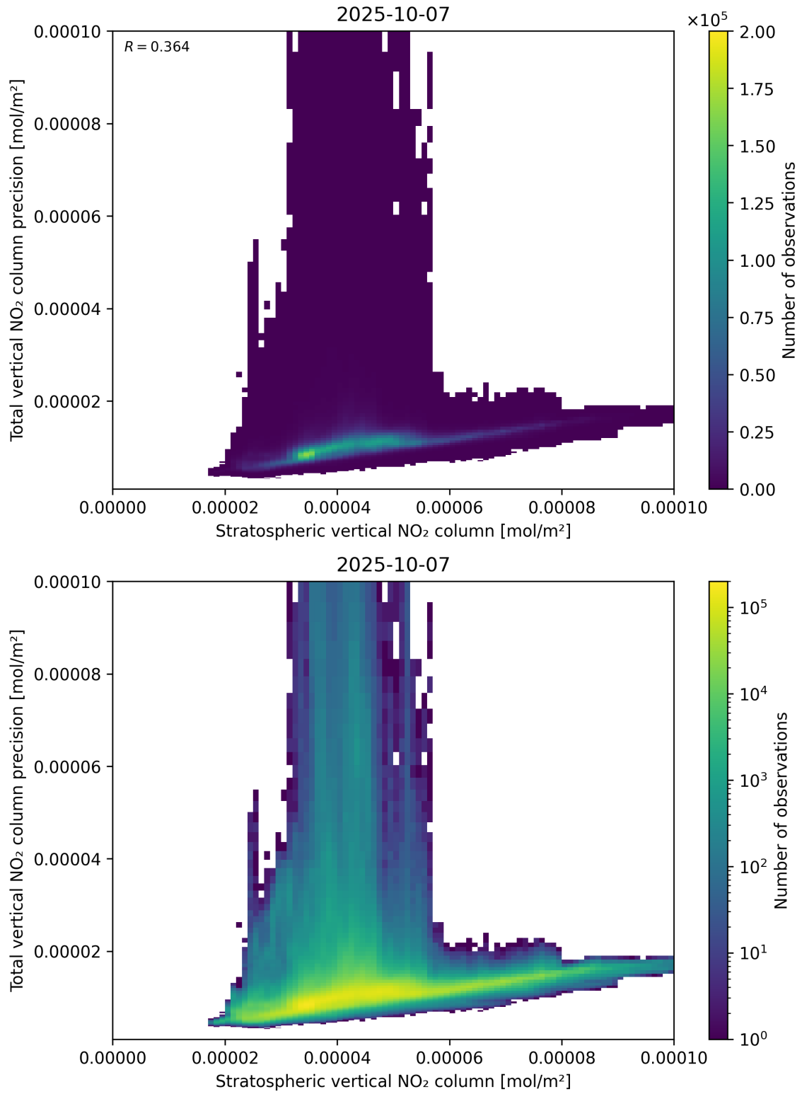
Figure 101: Scatter density plot of “Stratospheric vertical NO 2 column” against “Total vertical NO 2 column precision” for 2025-10-06 to 2025-10-08.
