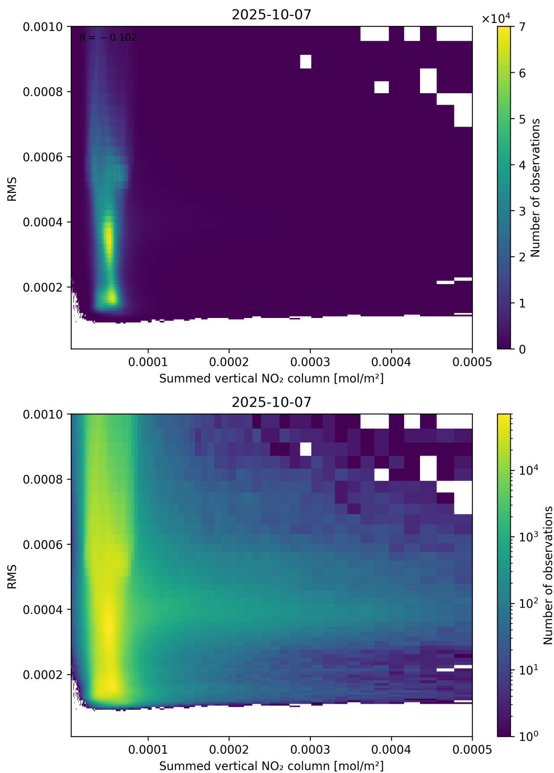
Figure 109: Scatter density plot of “Summed vertical NO 2 column” against “RMS” for 2025-10-06 to 2025-10-08.
