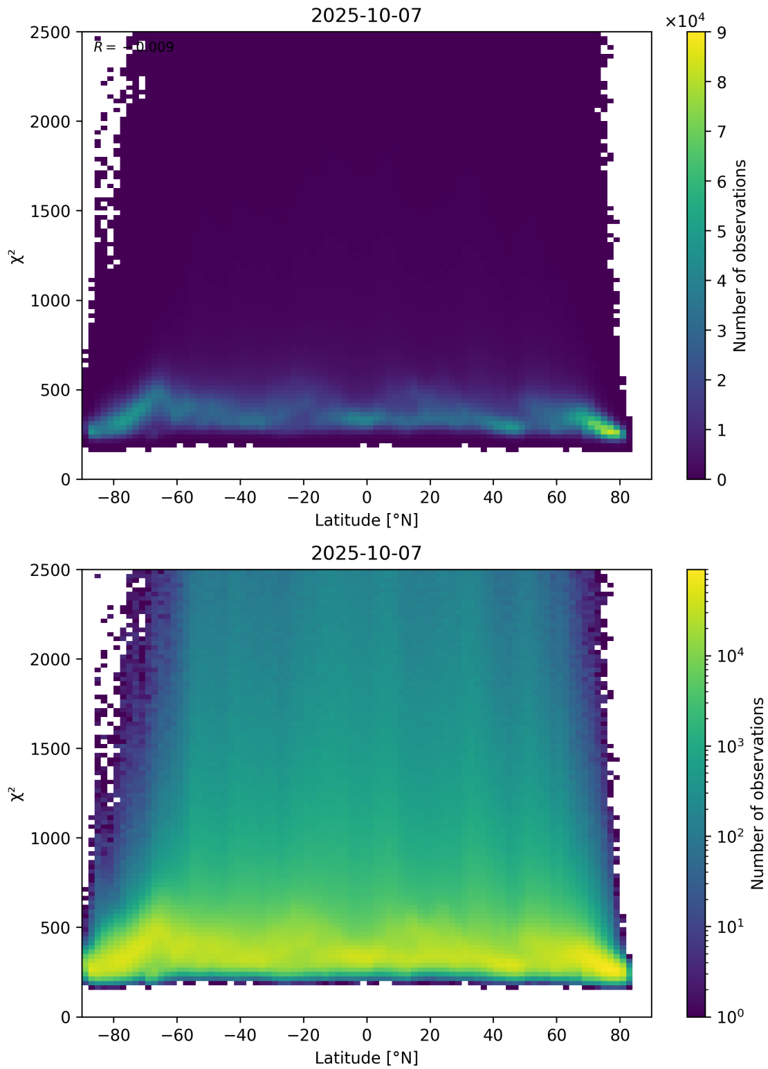
Figure 86: Scatter density plot of “Latitude” against “ \chi^2 ” for 2025-10-06 to 2025-10-08.
