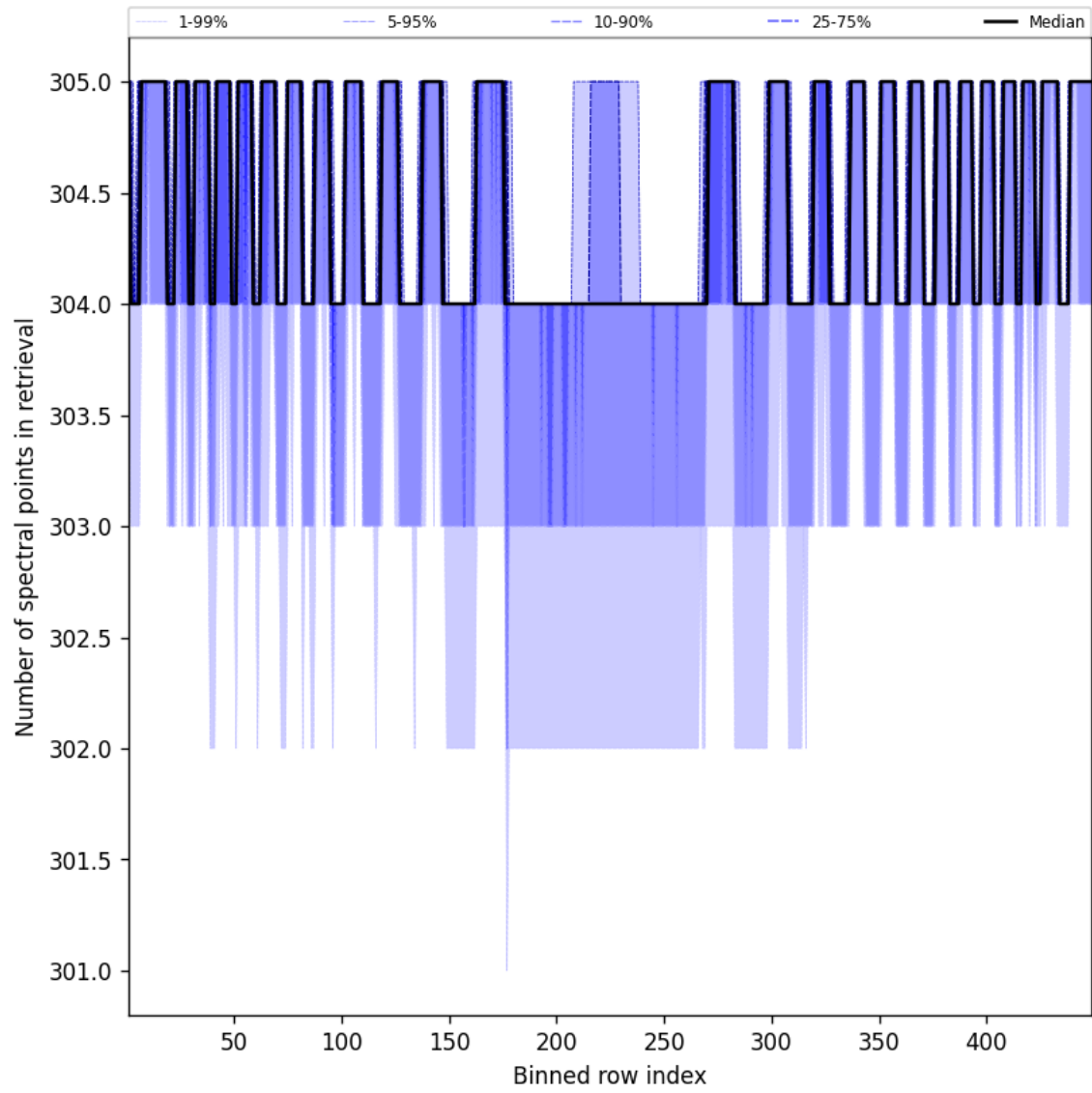
Figure 50: Along track statistics of “Number of spectral points in retrieval” for 2025-10-06 to 2025-10-08
