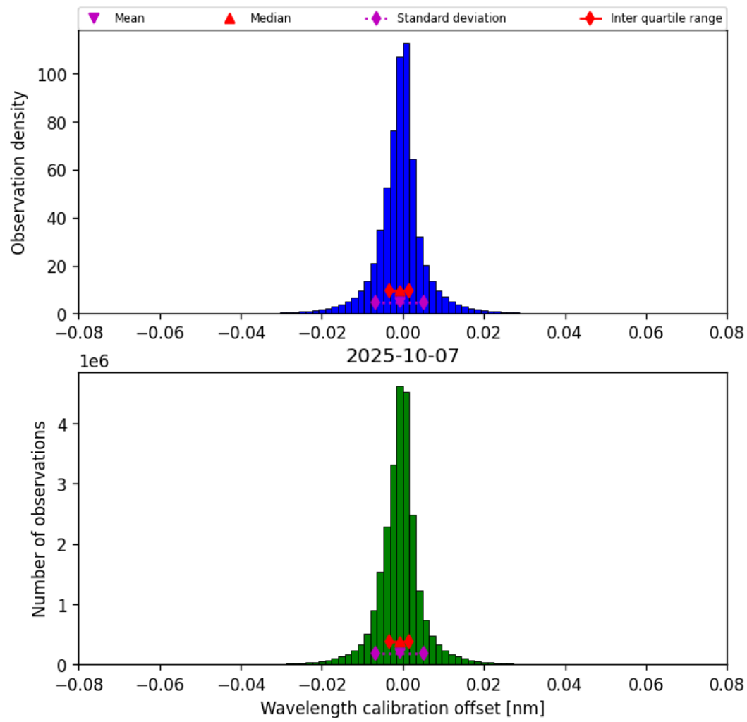
Figure 35: Histogram of “Wavelength calibration offset” for 2025-10-06 to 2025-10-08
