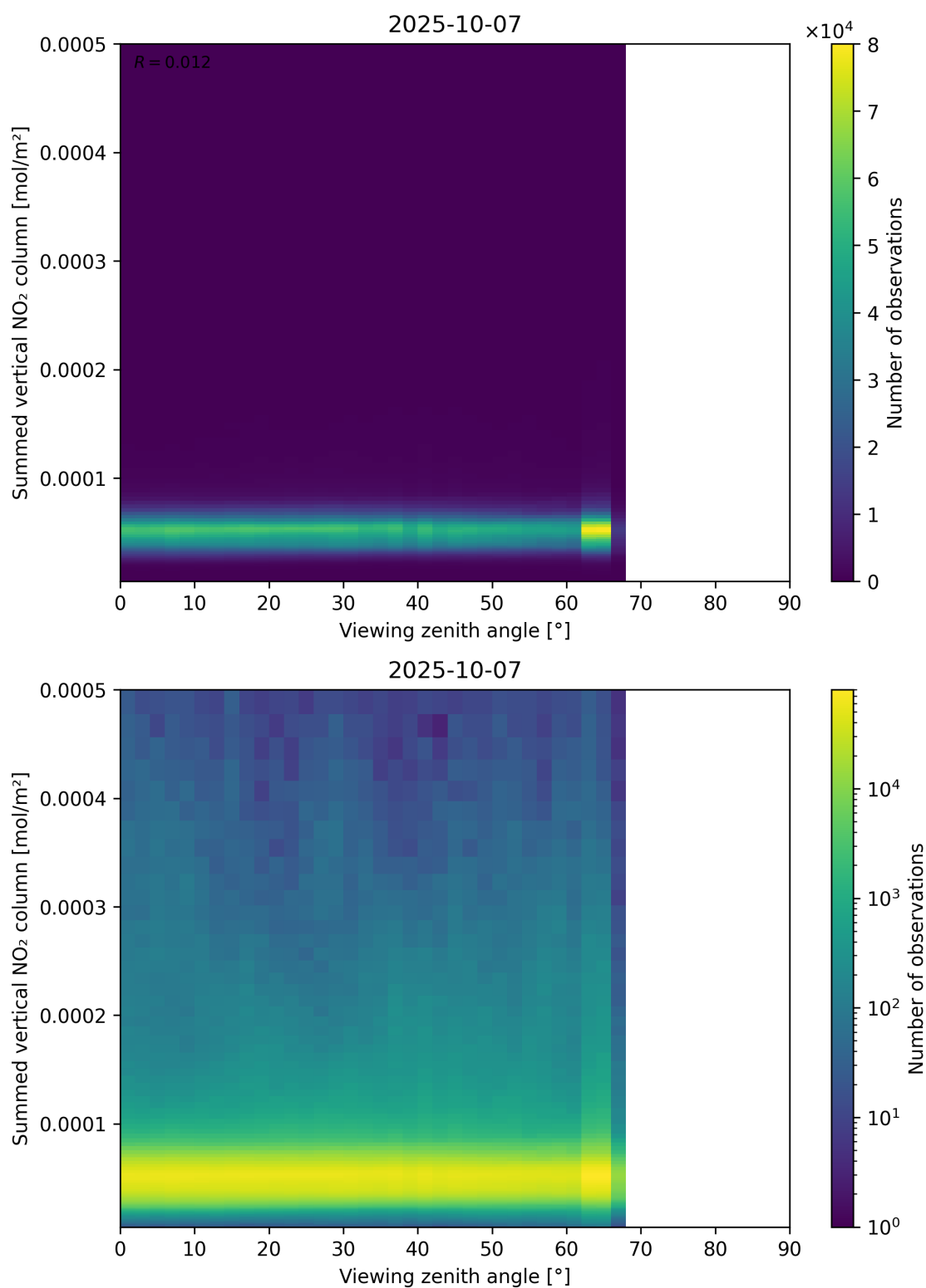
Figure 165: Scatter density plot of “Viewing zenith angle” against “Summed vertical NO 2 column” for 2025-10-06 to 2025-10-08.
