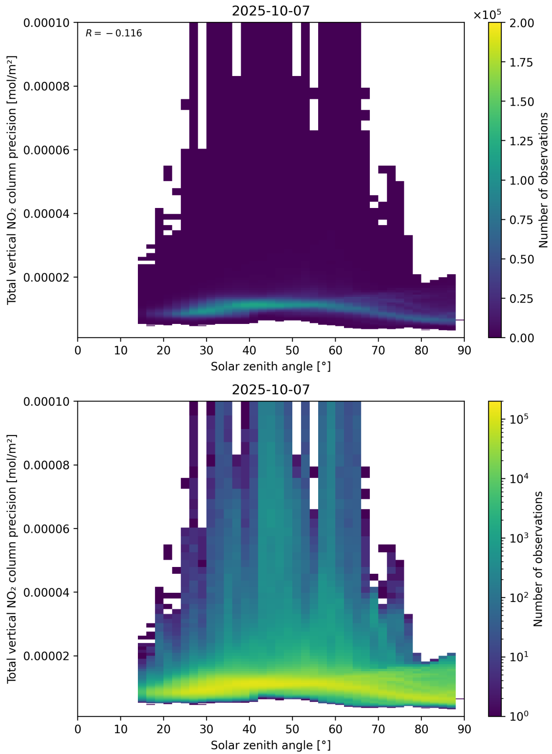
Figure 154: Scatter density plot of “Solar zenith angle” against “Total vertical NO 2 column precision” for 2025-10-06 to 2025-10-08.
