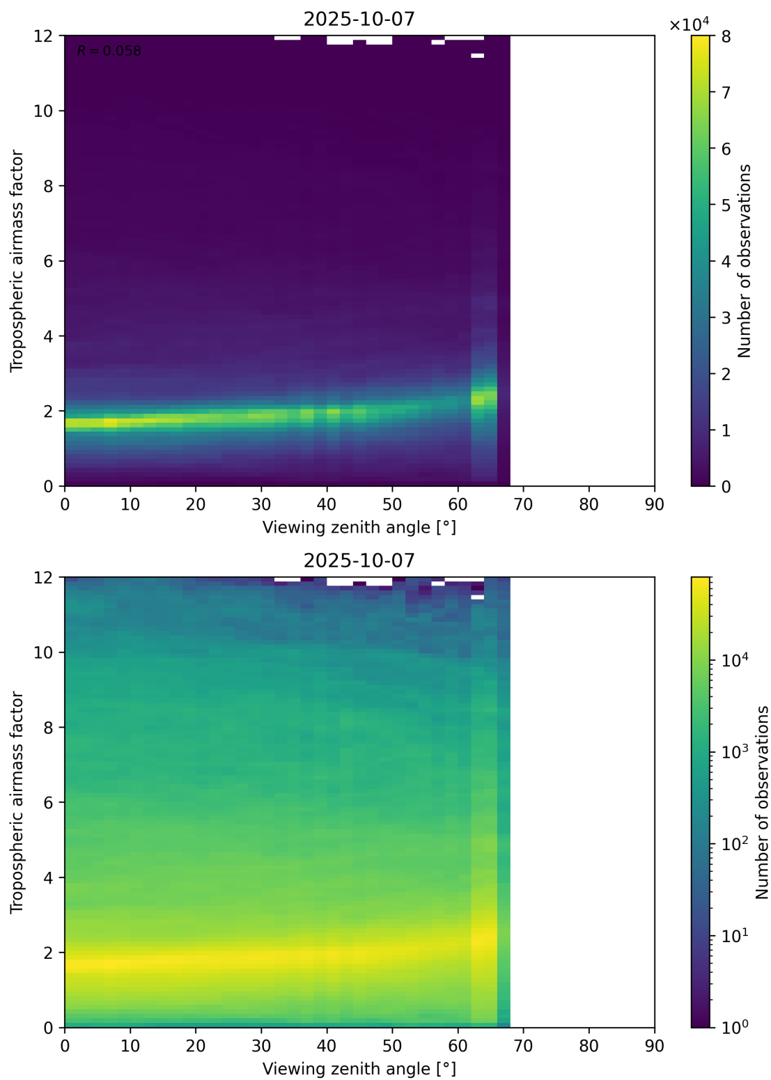
Figure 161: Scatter density plot of “Viewing zenith angle” against “Tropospheric airmass factor” for 2025-10-06 to 2025-10-08.
