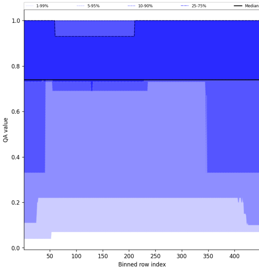
Figure 45: Along track statistics of "QA value" for 2025-10-06 to 2025-10-08
