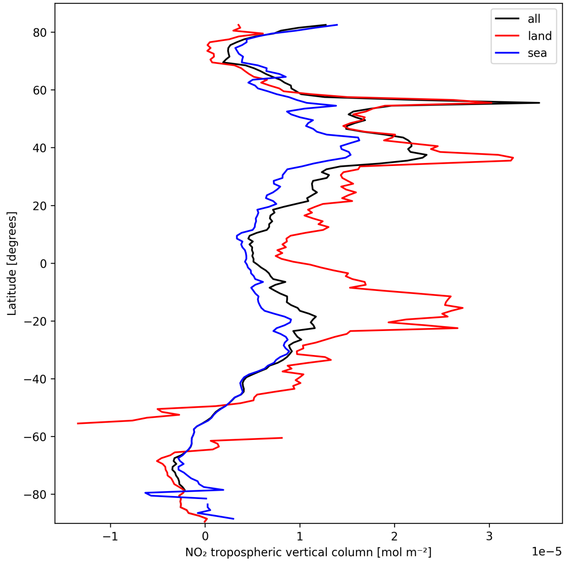
Figure 12: Zonal average of “NO 2 tropospheric vertical column” for 2025-10-06 to 2025-10-08.
