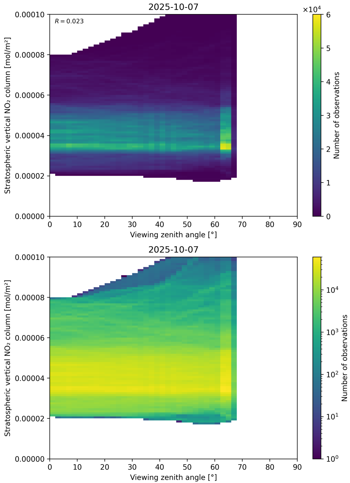
Figure 164: Scatter density plot of “Viewing zenith angle” against “Stratospheric vertical NO 2 column” for 2025-10-06 to 2025-10-08.
