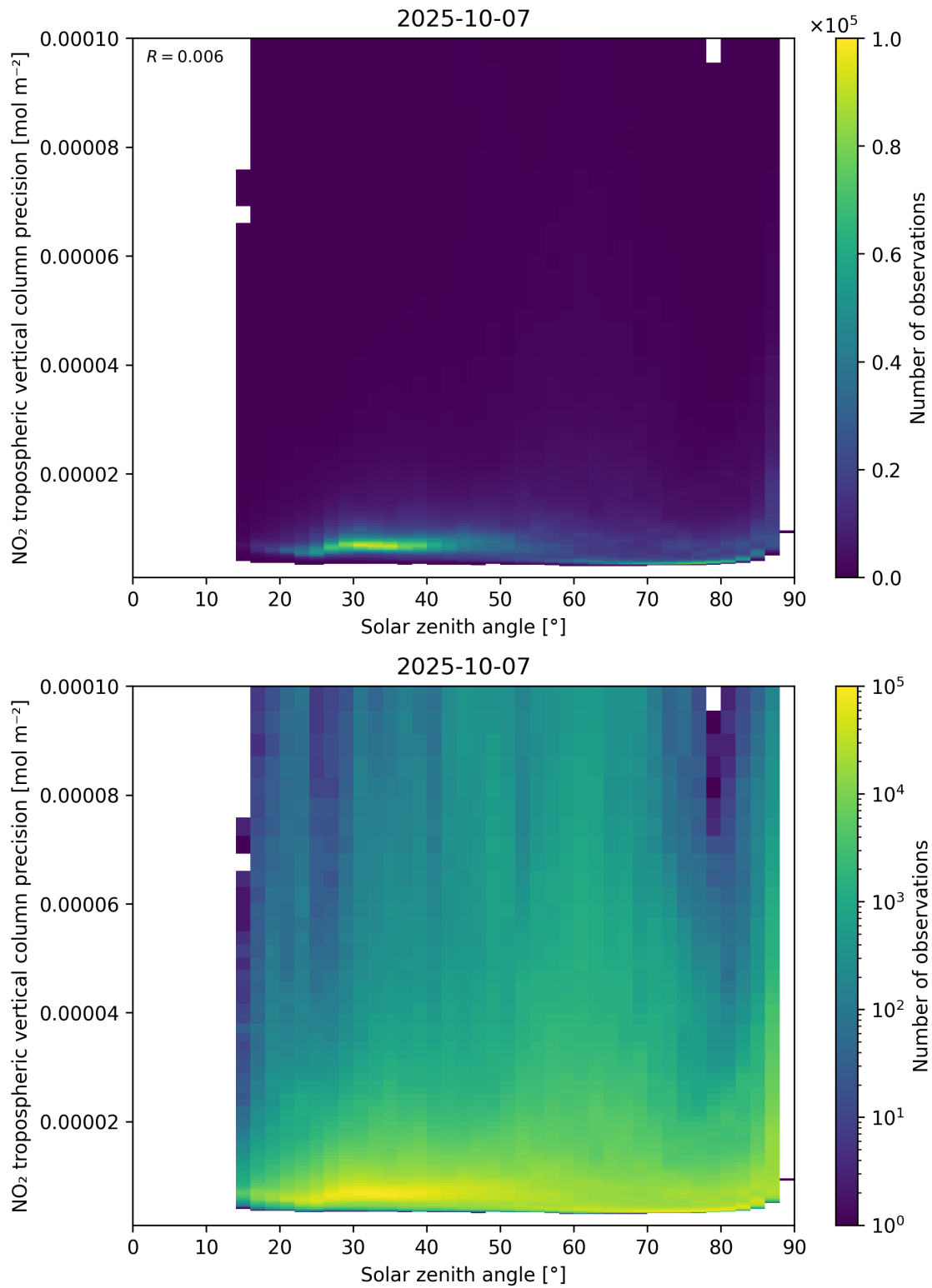
Figure 156: Scatter density plot of “Solar zenith angle” against “NO 2 tropospheric vertical column precision” for 2025-10-06 to 2025-10-08.
