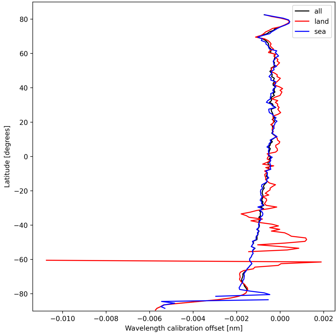
Figure 18: Zonal average of “Wavelength calibration offset” for 2025-10-06 to 2025-10-08.
