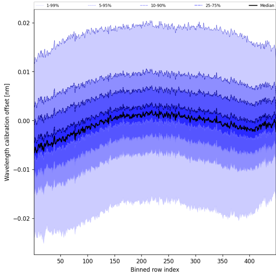
Figure 52: Along track statistics of “Wavelength calibration offset” for 2025-10-06 to 2025-10-08
