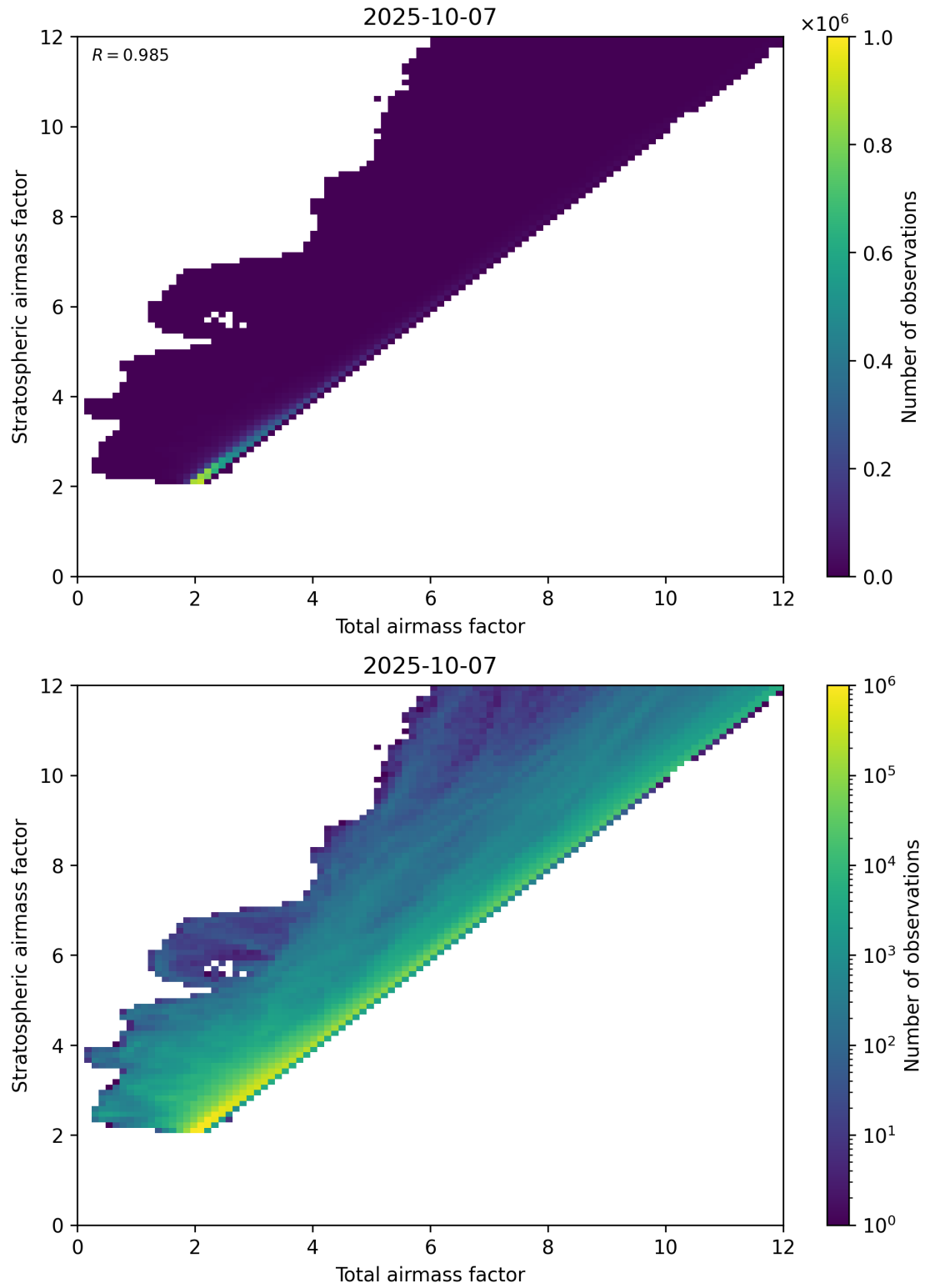
Figure 62: Scatter density plot of “Total airmass factor” against “Stratospheric airmass factor” for 2025-10-06 to 2025-10-08.
