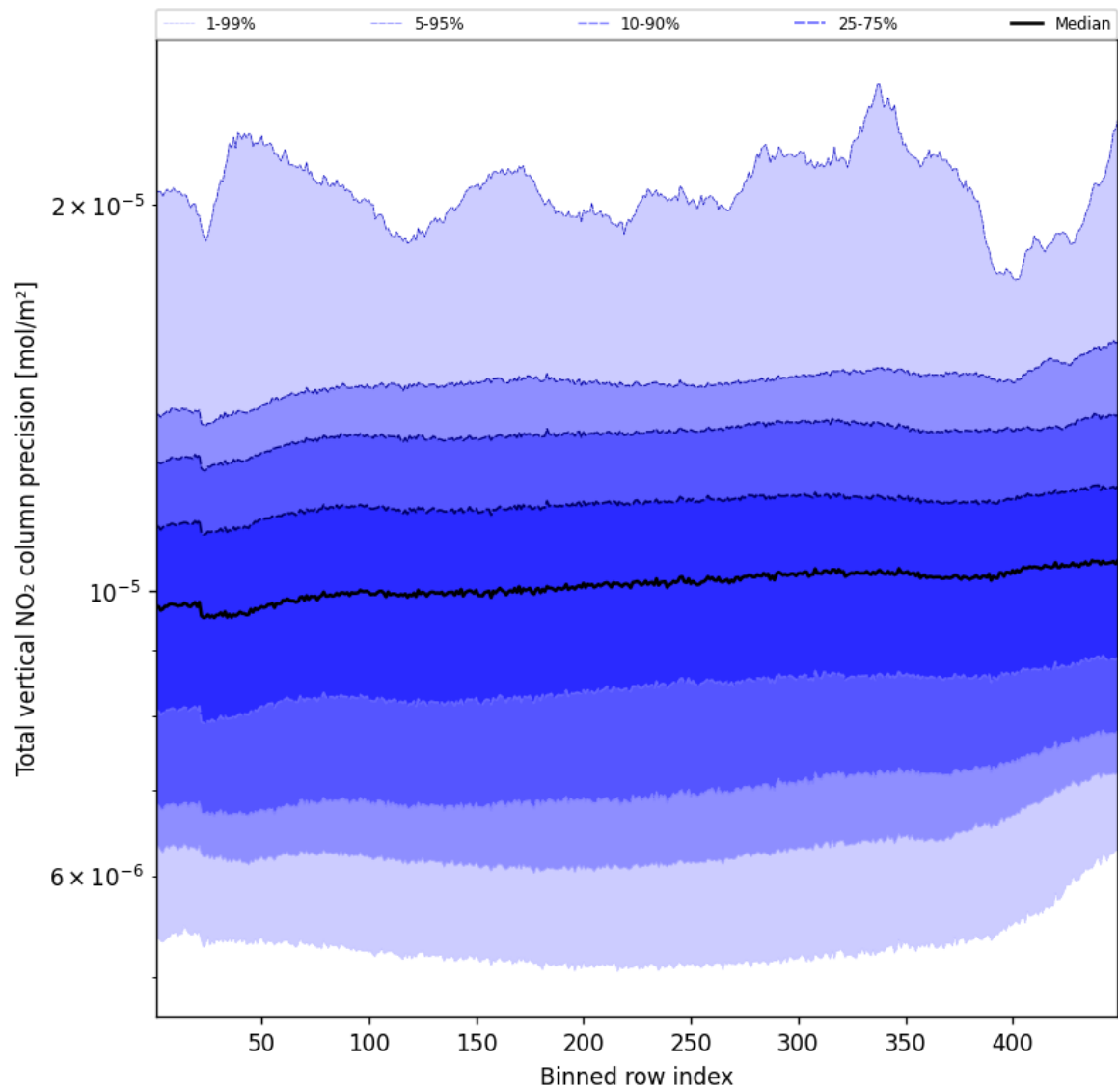
Figure 56: Along track statistics of “Total vertical NO 2 column precision” for 2025-10-06 to 2025-10-08
