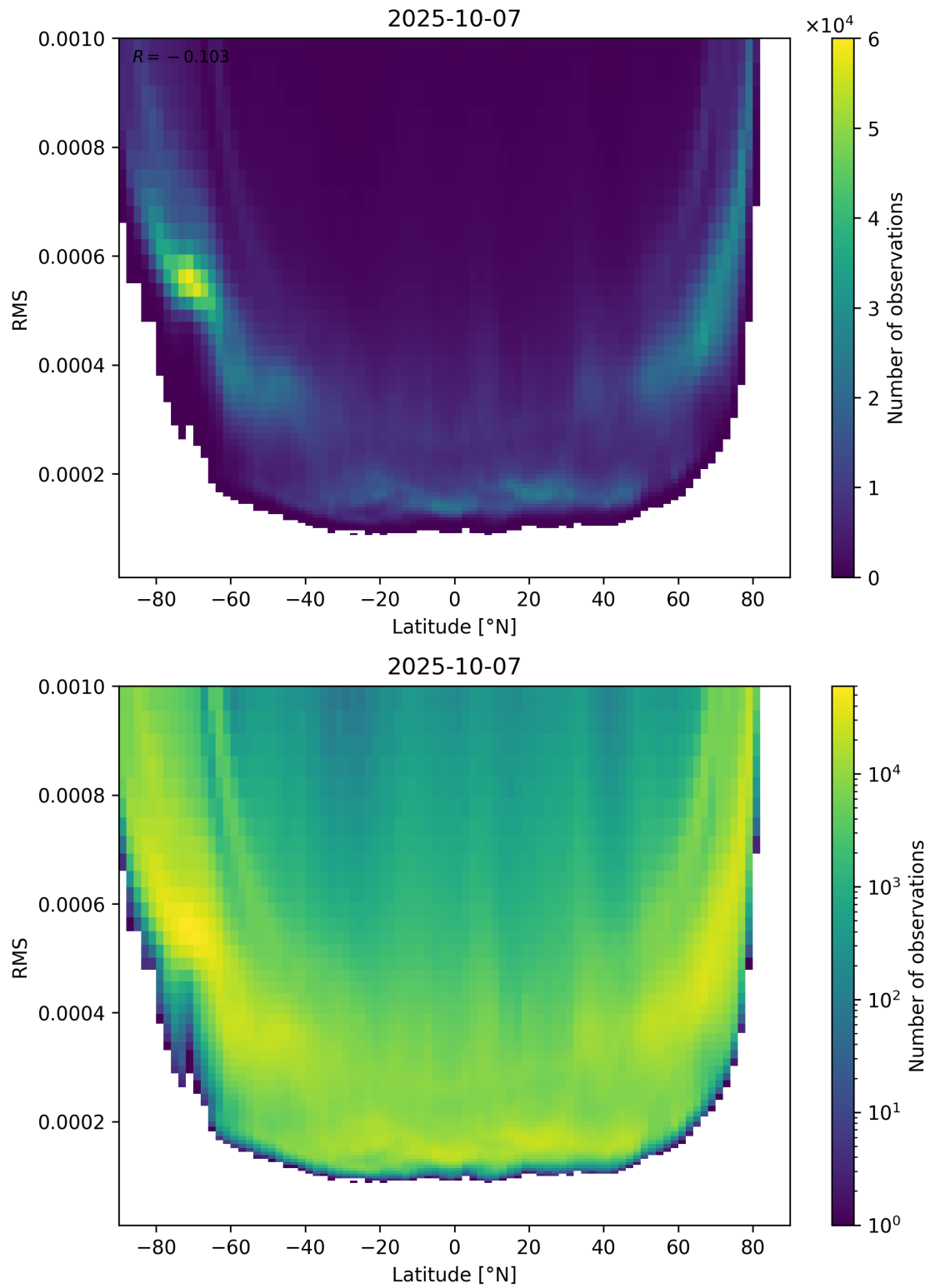
Figure 94: Scatter density plot of “Latitude” against “RMS” for 2025-10-06 to 2025-10-08.
