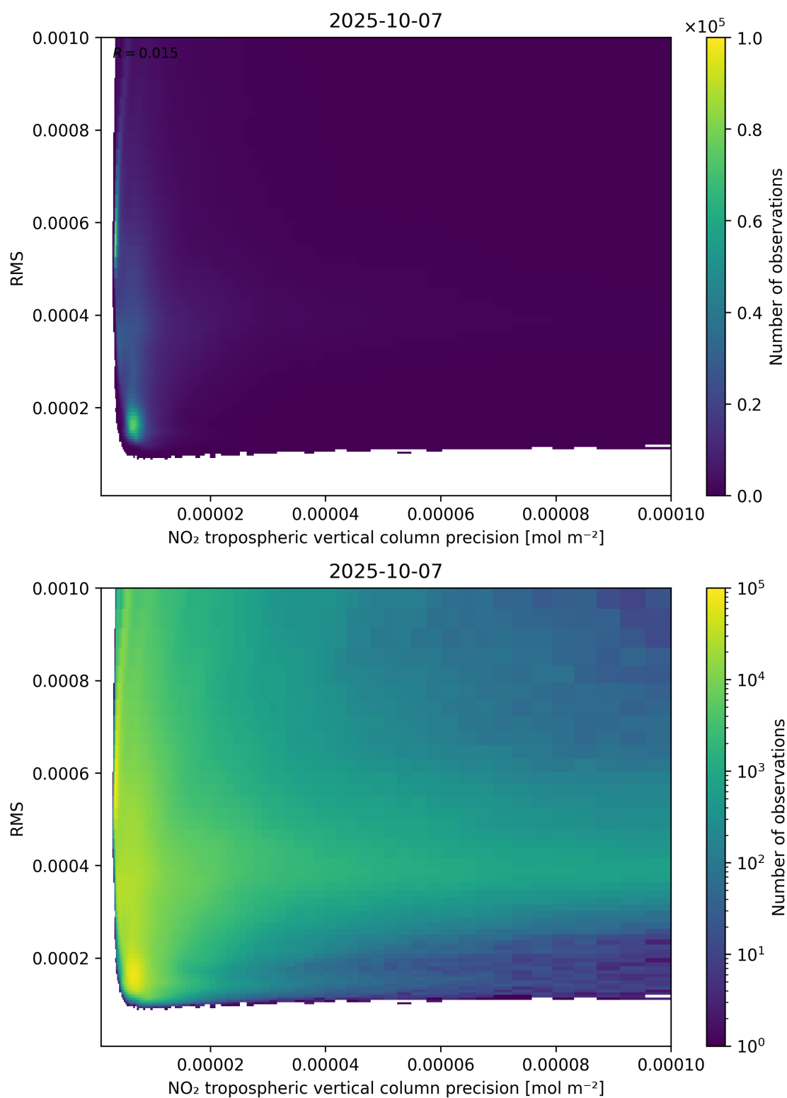
Figure 140: Scatter density plot of “NO 2 tropospheric vertical column precision” against “RMS” for 2025-10-06 to 2025-10-08.
