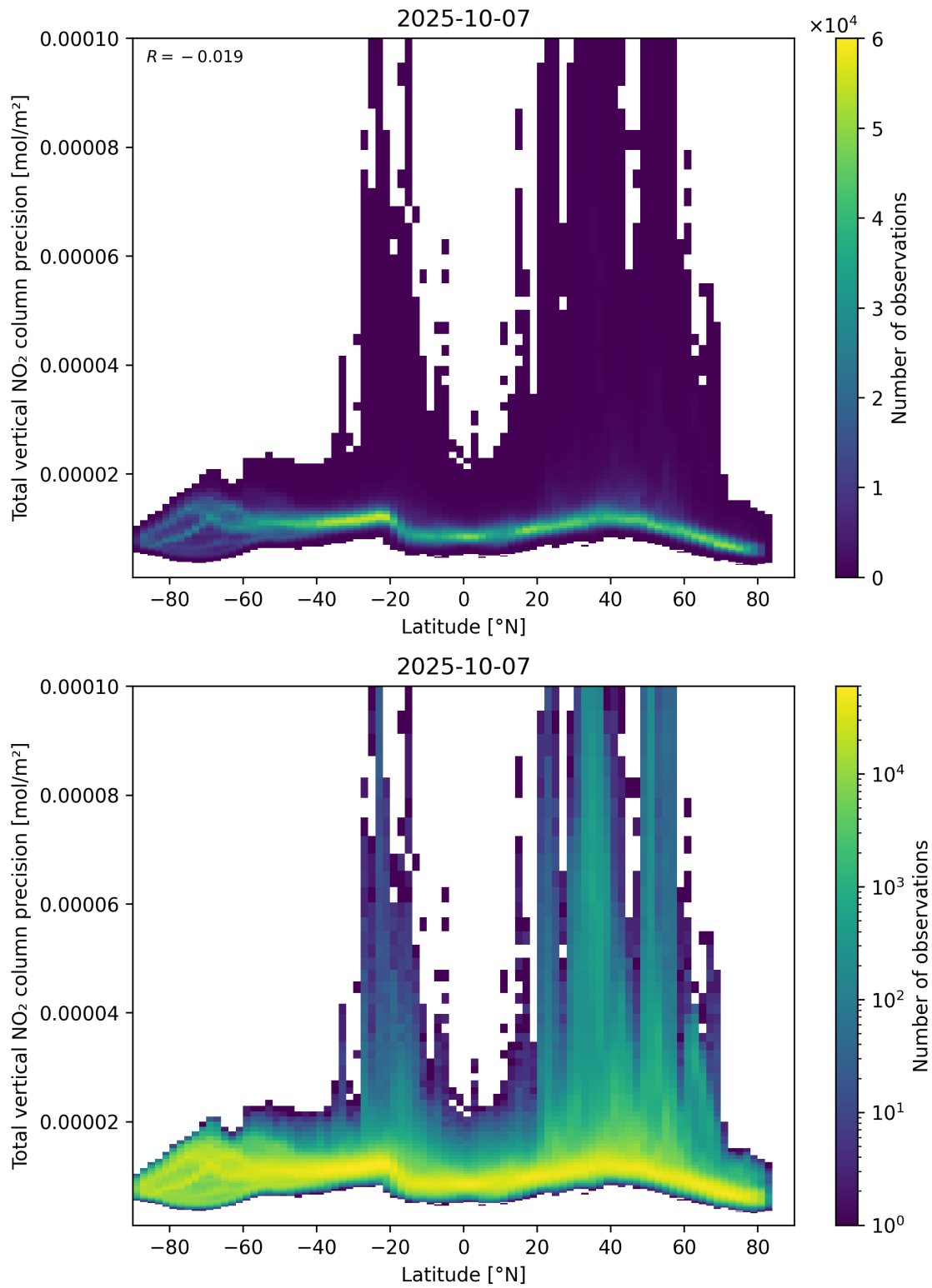
Figure 91: Scatter density plot of “Latitude” against “Total vertical NO 2 column precision” for 2025-10-06 to 2025-10-08.
