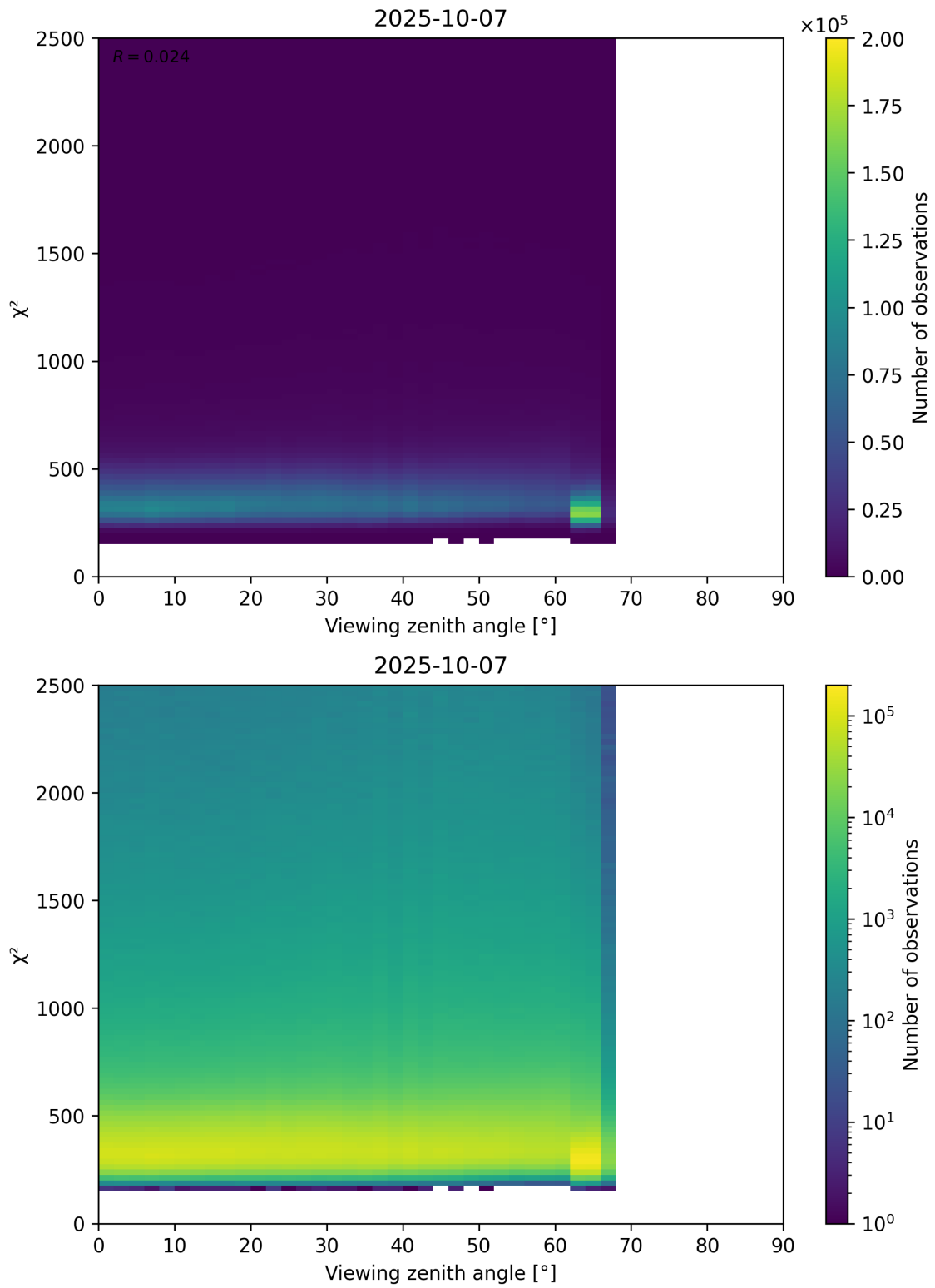
Figure 162: Scatter density plot of “Viewing zenith angle” against “ \chi^2 ” for 2025-10-06 to 2025-10-08.
