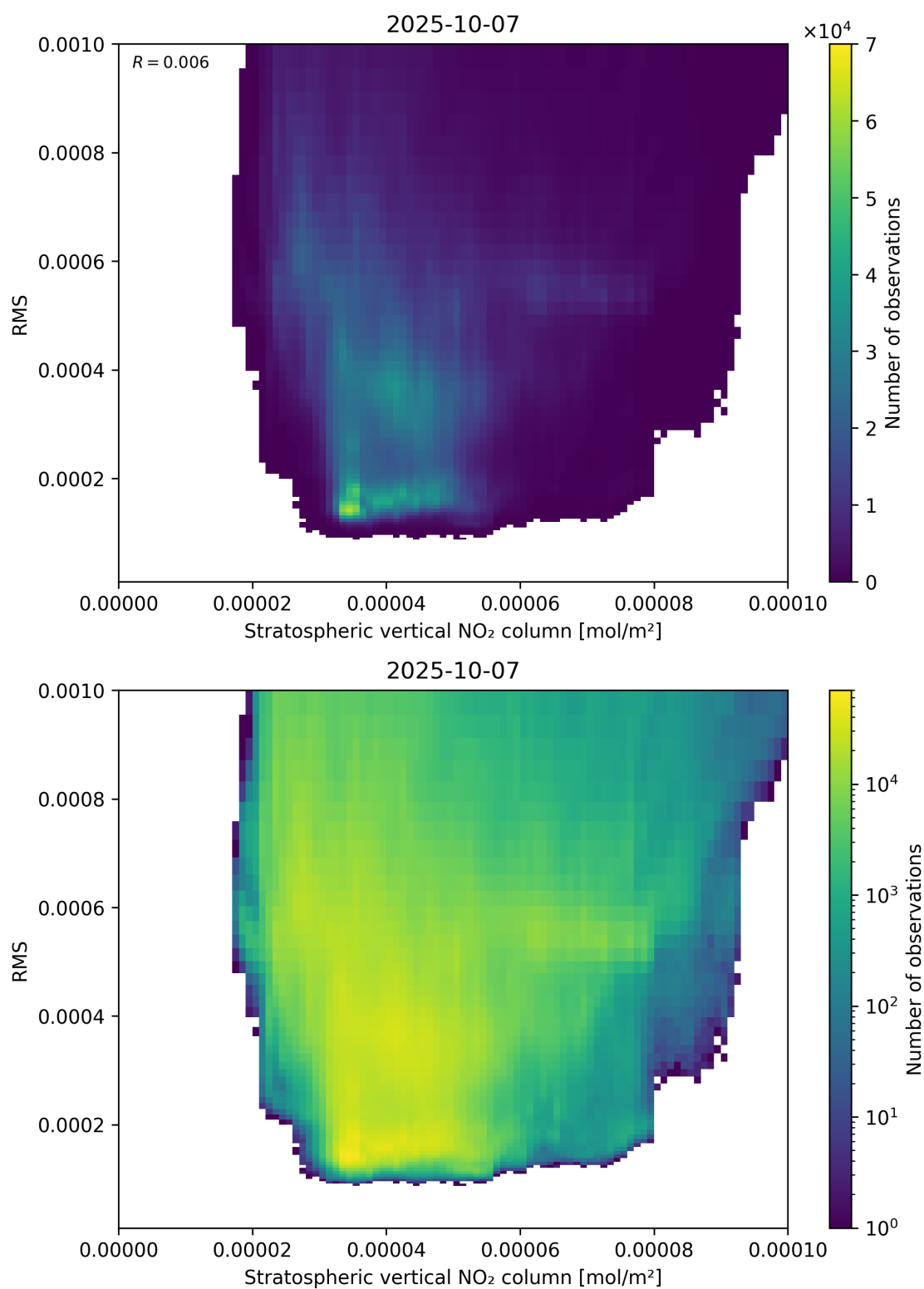
Figure 102: Scatter density plot of “Stratospheric vertical NO 2 column” against “RMS” for 2025-10-06 to 2025-10-08.
