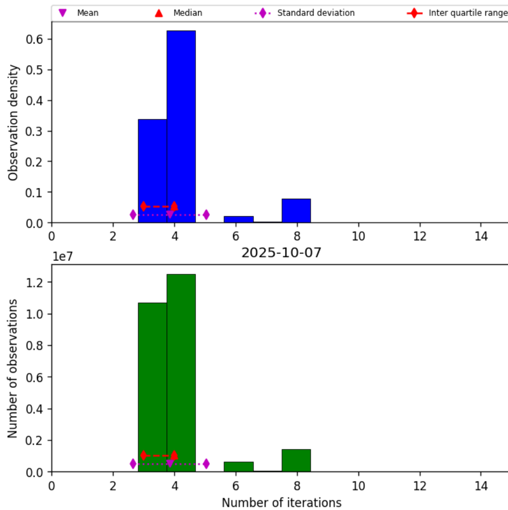
Figure 34: Histogram of “Number of iterations” for 2025-10-06 to 2025-10-08
