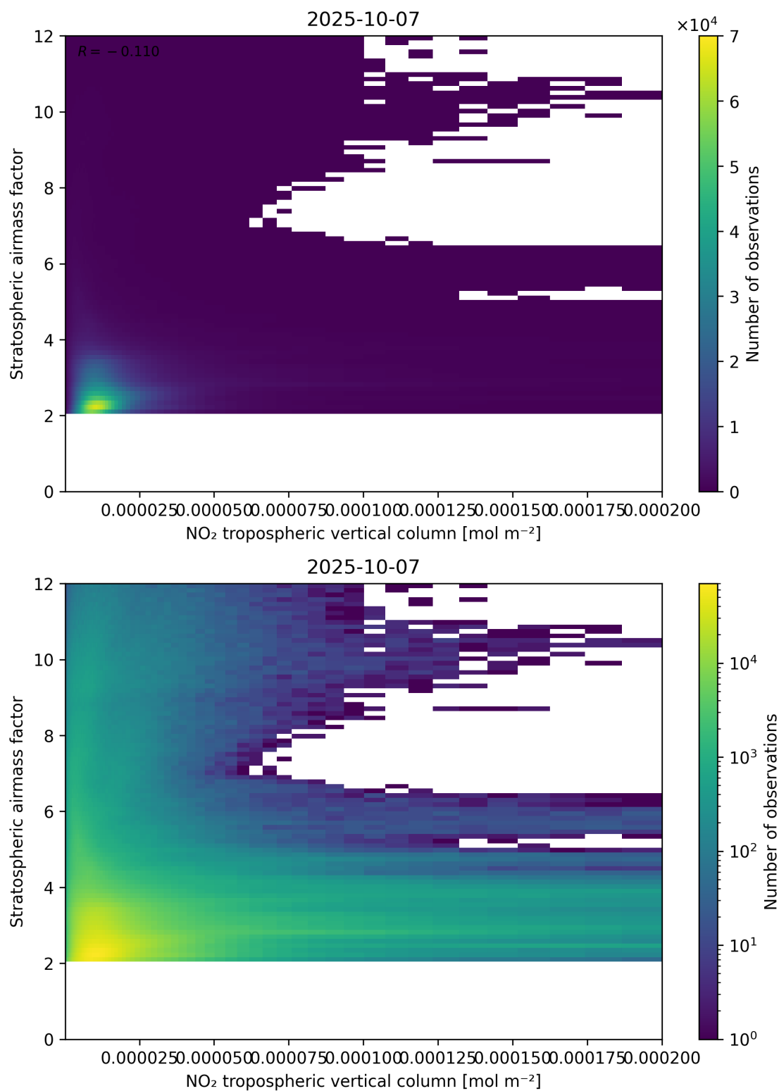
Figure 121: Scatter density plot of “NO 2 tropospheric vertical column” against “Stratospheric air mass factor” for 2025-10-06 to 2025-10-08.
