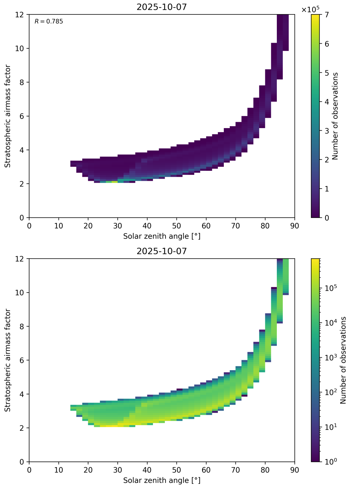
Figure 145: Scatter density plot of “Solar zenith angle” against “Stratospheric airmass factor” for 2025-10-06 to 2025-10-08.
