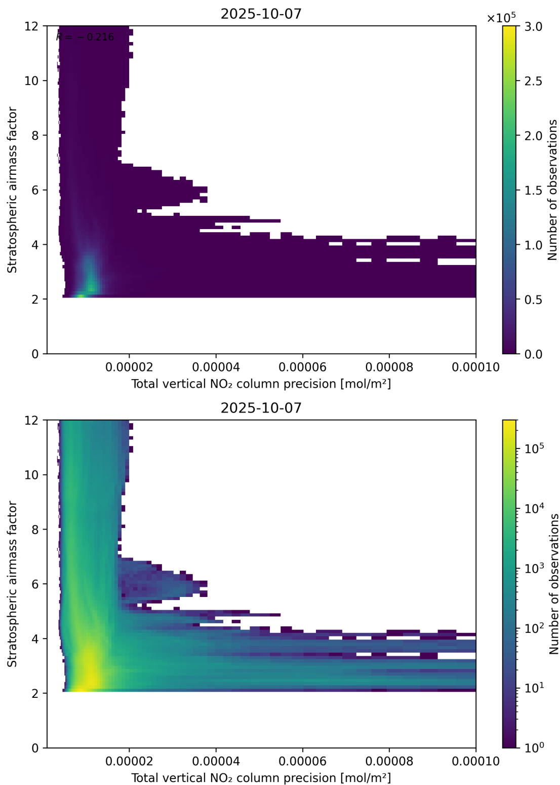
Figure 115: Scatter density plot of “Total vertical NO 2 column precision” against “Stratospheric air mass factor” for 2025-10-06 to 2025-10-08.
