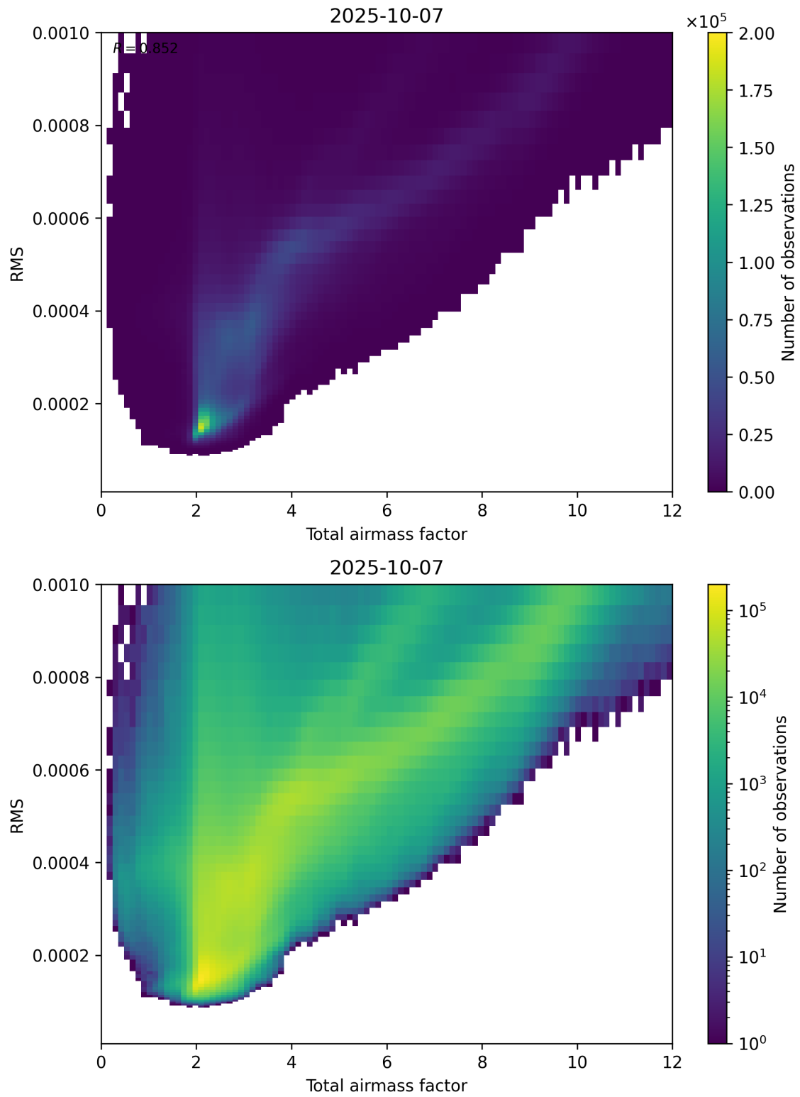
Figure 69: Scatter density plot of “Total airmass factor” against “RMS” for 2025-10-06 to 2025-10-08.
