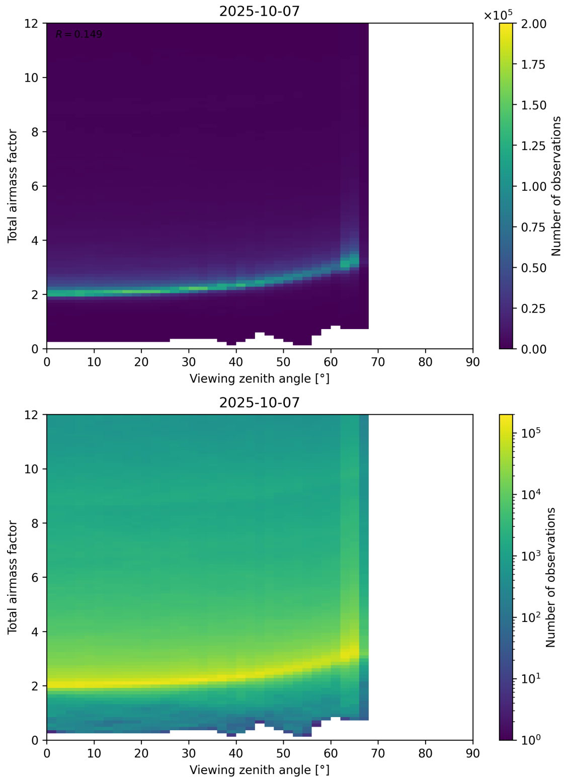
Figure 160: Scatter density plot of “Viewing zenith angle” against “Total airmass factor” for 2025-10-06 to 2025-10-08.
