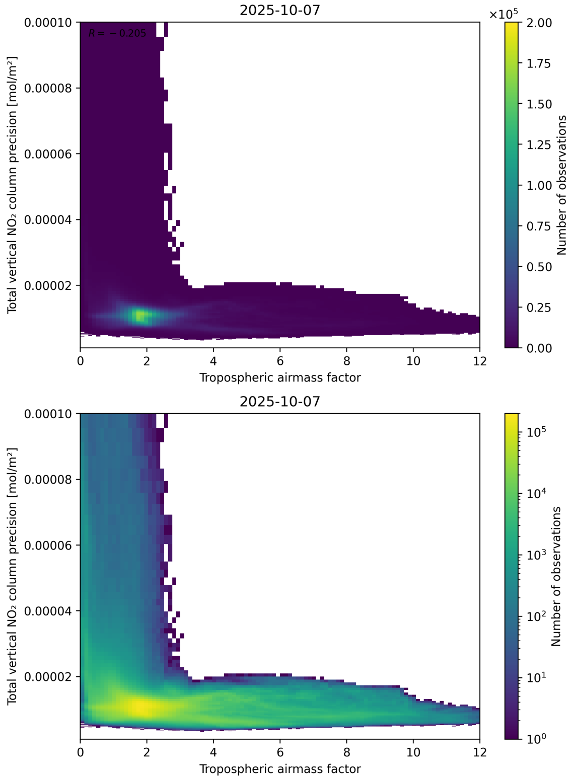
Figure 78: Scatter density plot of “Tropospheric air mass factor” against “Total vertical NO 2 column precision” for 2025-10-06 to 2025-10-08.
