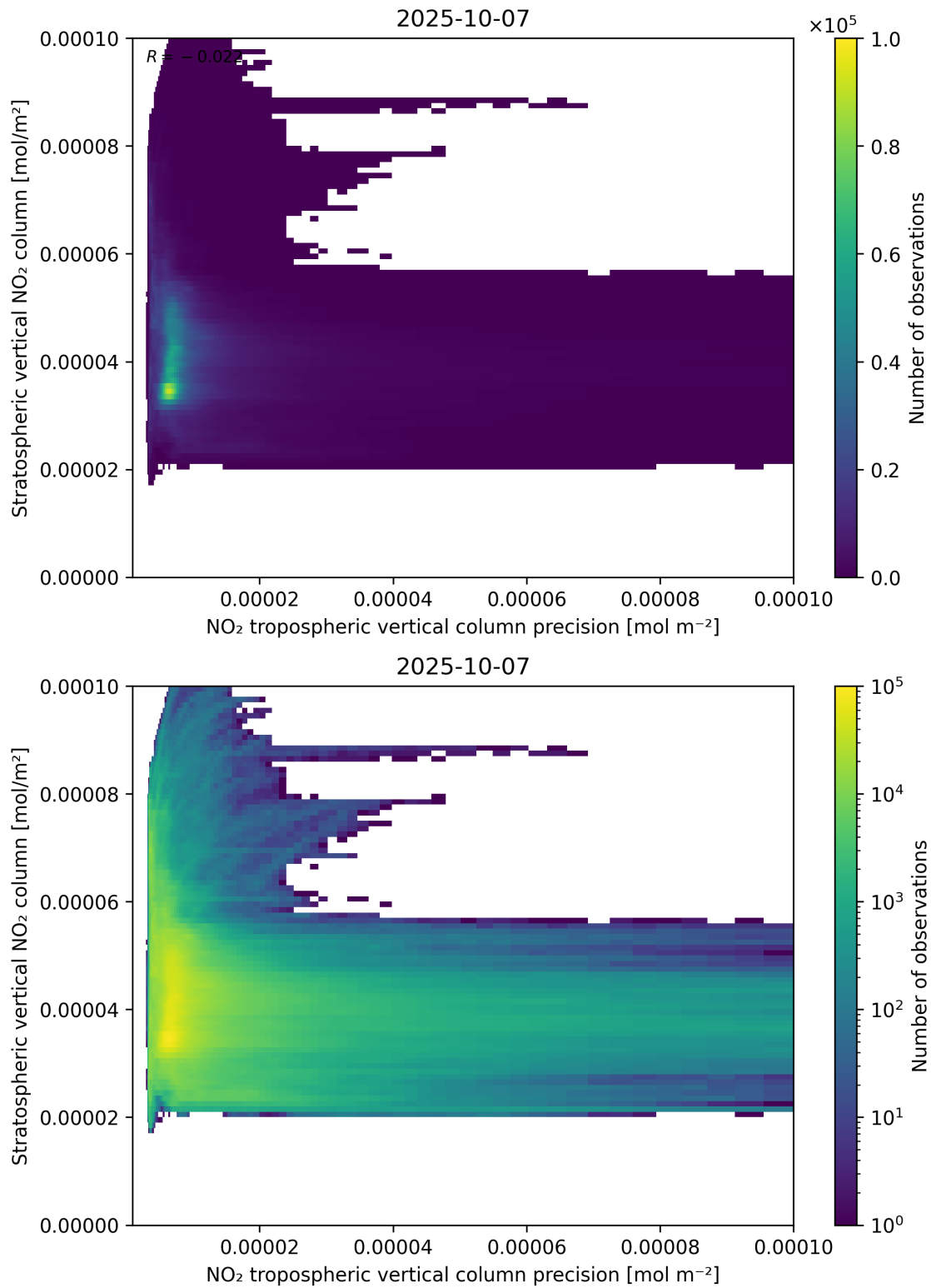
Figure 135: Scatter density plot of “NO 2 tropospheric vertical column precision” against “Stratospheric vertical NO 2 column” for 2025-10-06 to 2025-10-08.
