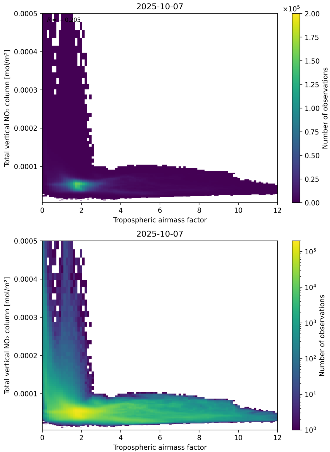
Figure 77: Scatter density plot of “Tropospheric airmass factor” against “Total vertical NO 2 column” for 2025-10-06 to 2025-10-08.
