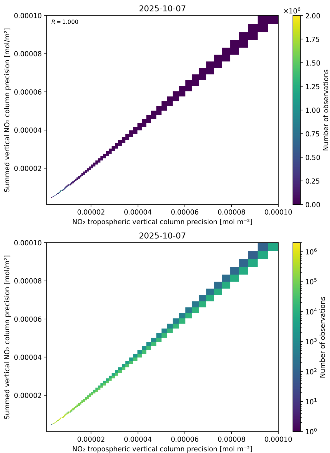
Figure 137: Scatter density plot of “NO 2 tropospheric vertical column precision” against “Summed vertical NO 2 column precision” for 2025-10-06 to 2025-10-08.
