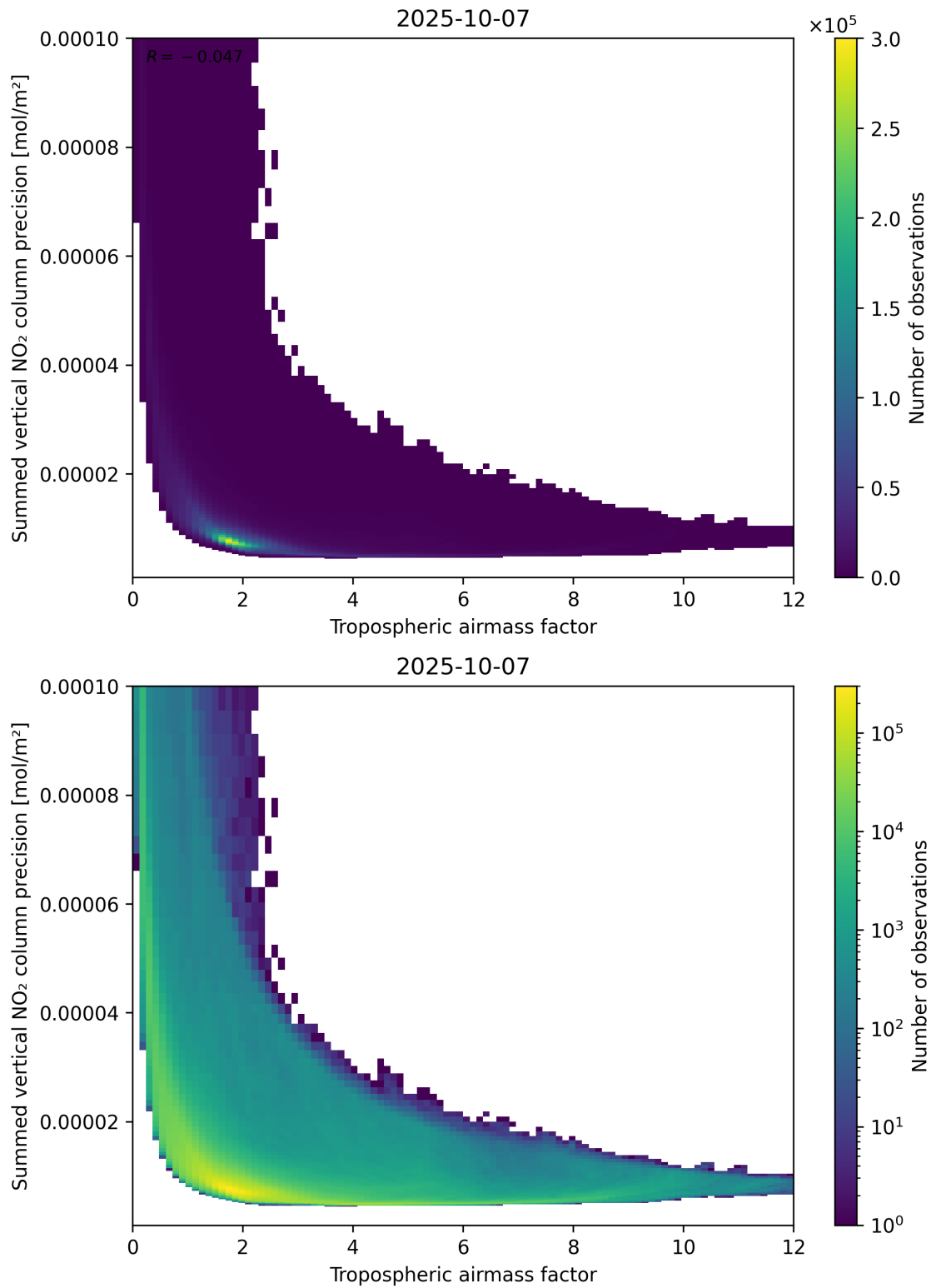
Figure 76: Scatter density plot of “Tropospheric air mass factor” against “Summed vertical NO 2 column precision” for 2025-10-06 to 2025-10-08.
