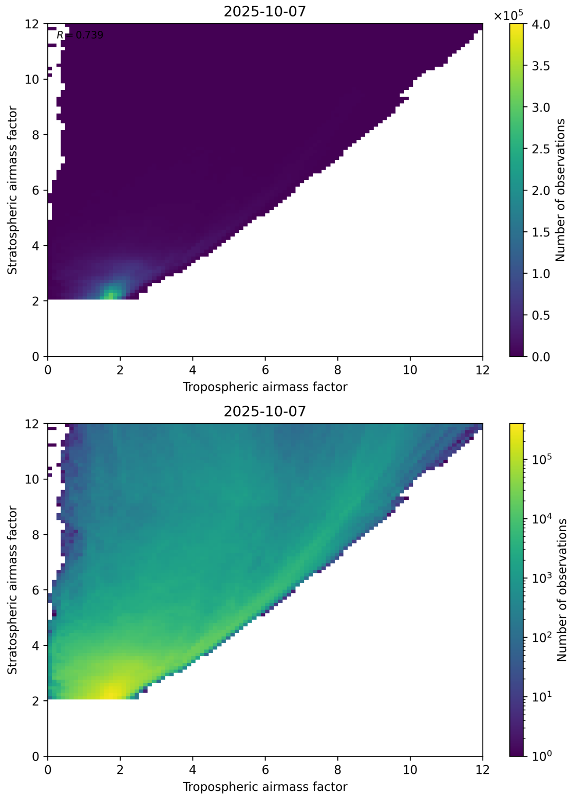
Figure 71: Scatter density plot of “Tropospheric airmass factor” against “Stratospheric airmass factor” for 2025-10-06 to 2025-10-08.
