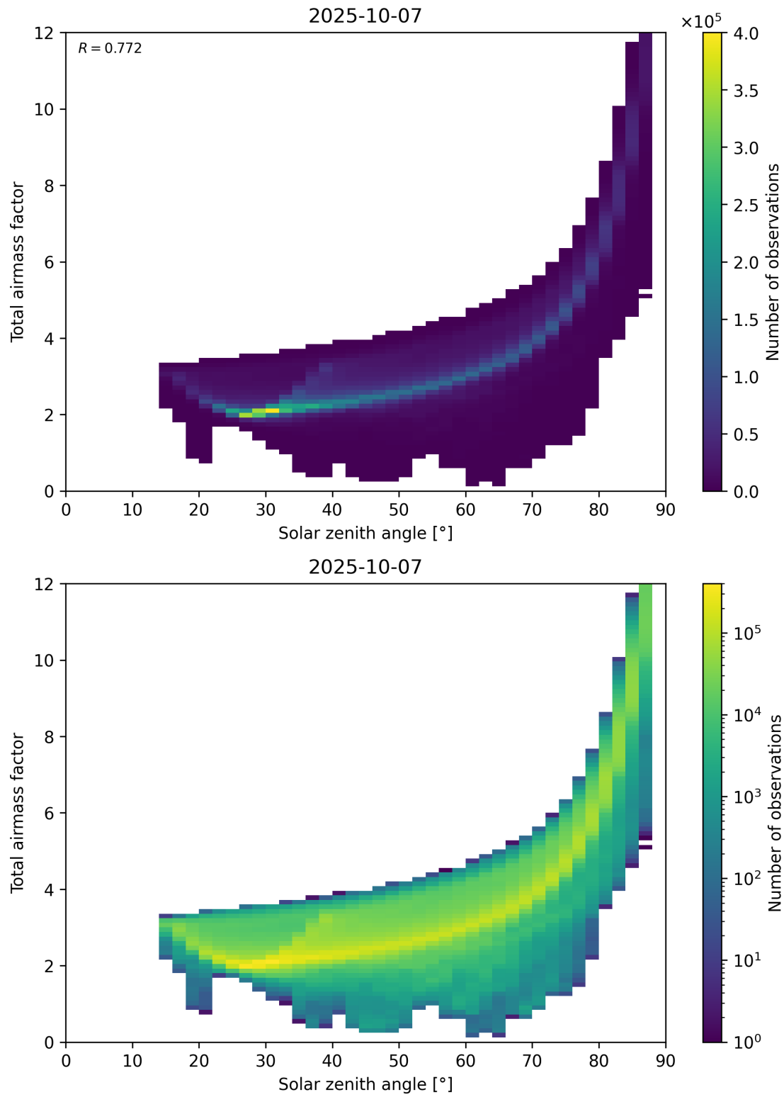
Figure 146: Scatter density plot of “Solar zenith angle” against “Total airmass factor” for 2025-10-06 to 2025-10-08.
