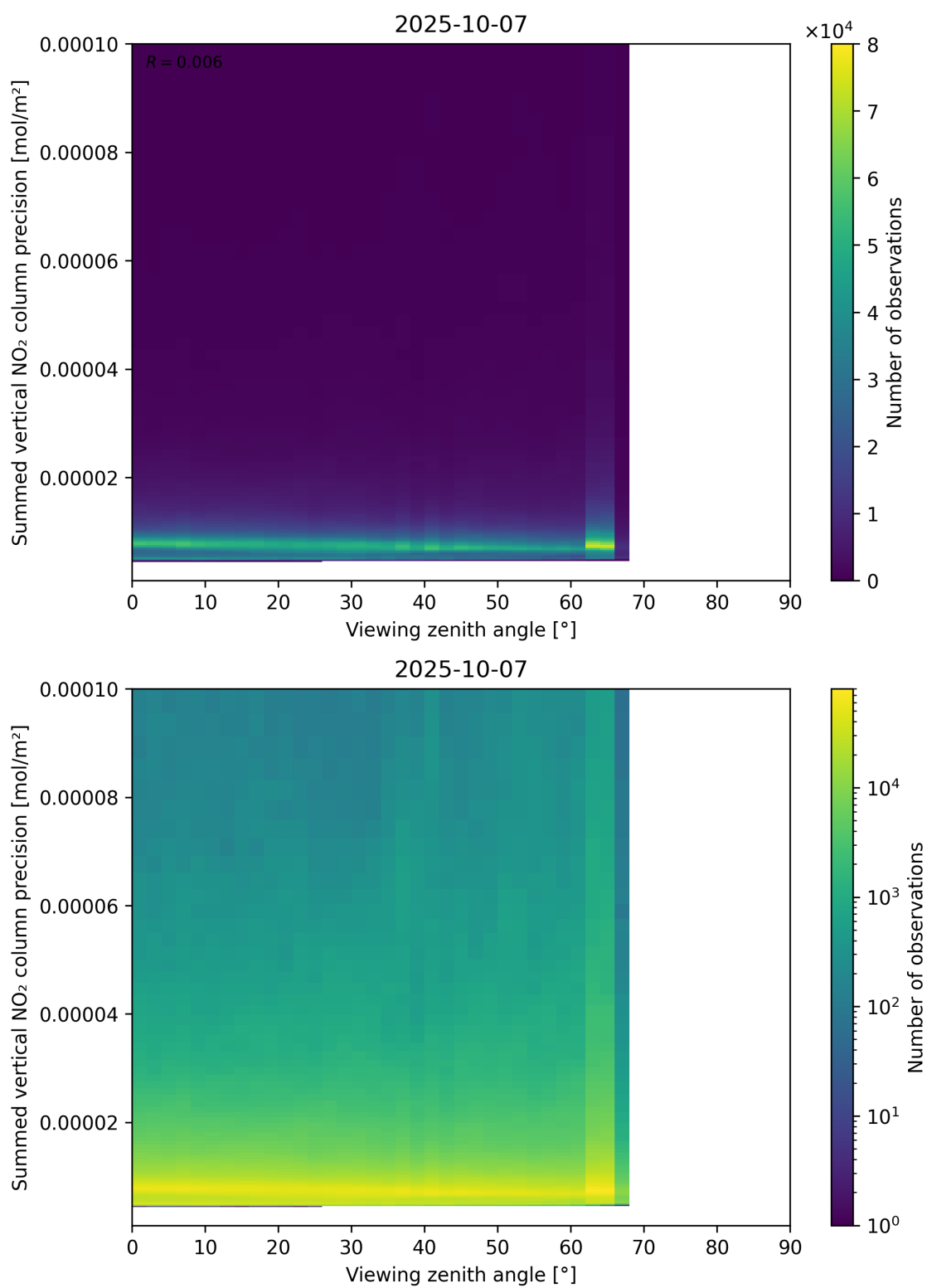
Figure 166: Scatter density plot of “Viewing zenith angle” against “Summed vertical NO 2 column precision” for 2025-10-06 to 2025-10-08.
