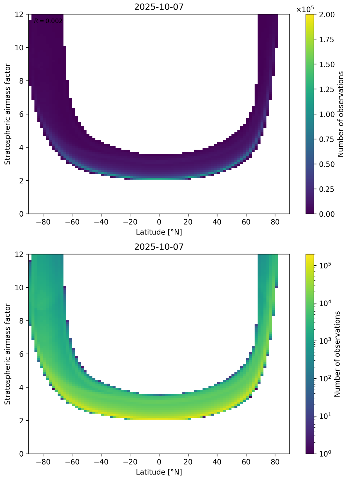
Figure 83: Scatter density plot of “Latitude” against “Stratospheric airmass factor” for 2025-10-06 to 2025-10-08.
