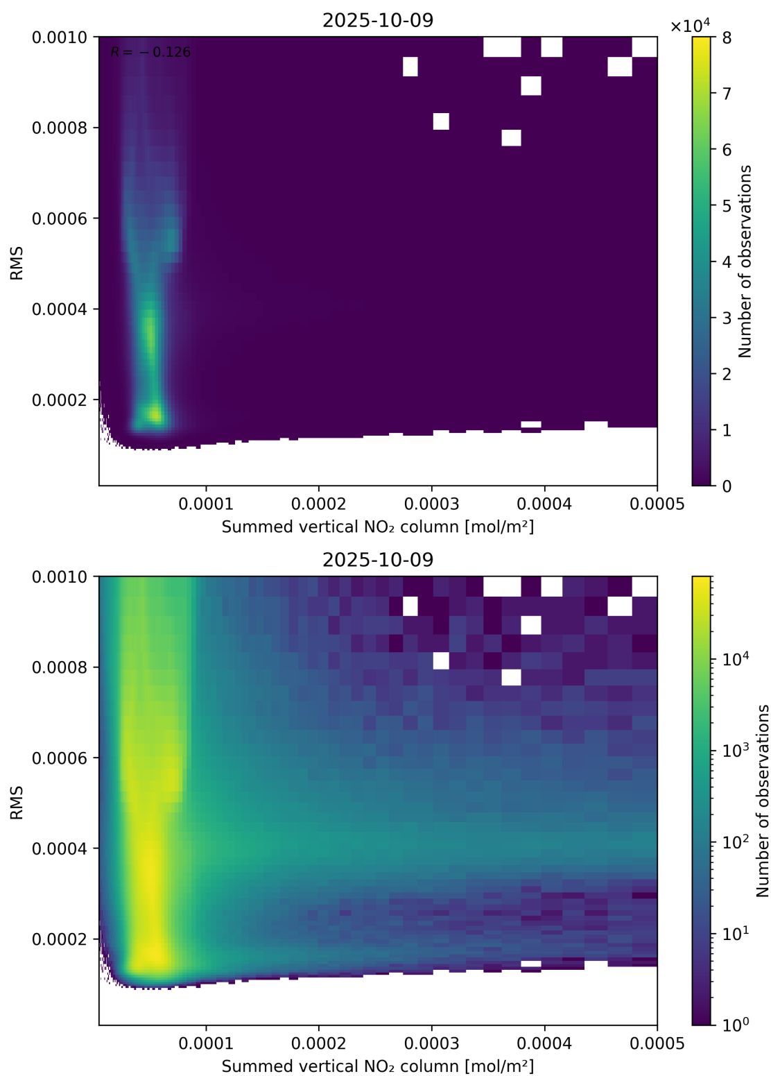
Figure 109: Scatter density plot of “Summed vertical NO 2 column” against “RMS” for 2025-10-08 to 2025-10-10.
