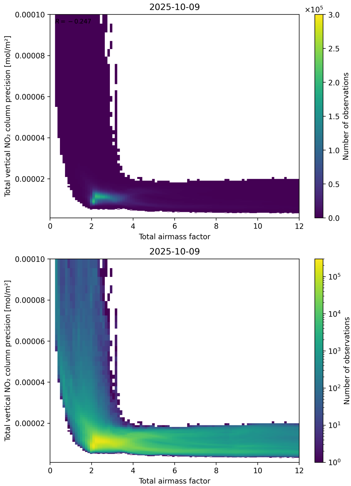
Figure 68: Scatter density plot of “Total airmass factor” against “Total vertical NO 2 column precision” for 2025-10-08 to 2025-10-10.
