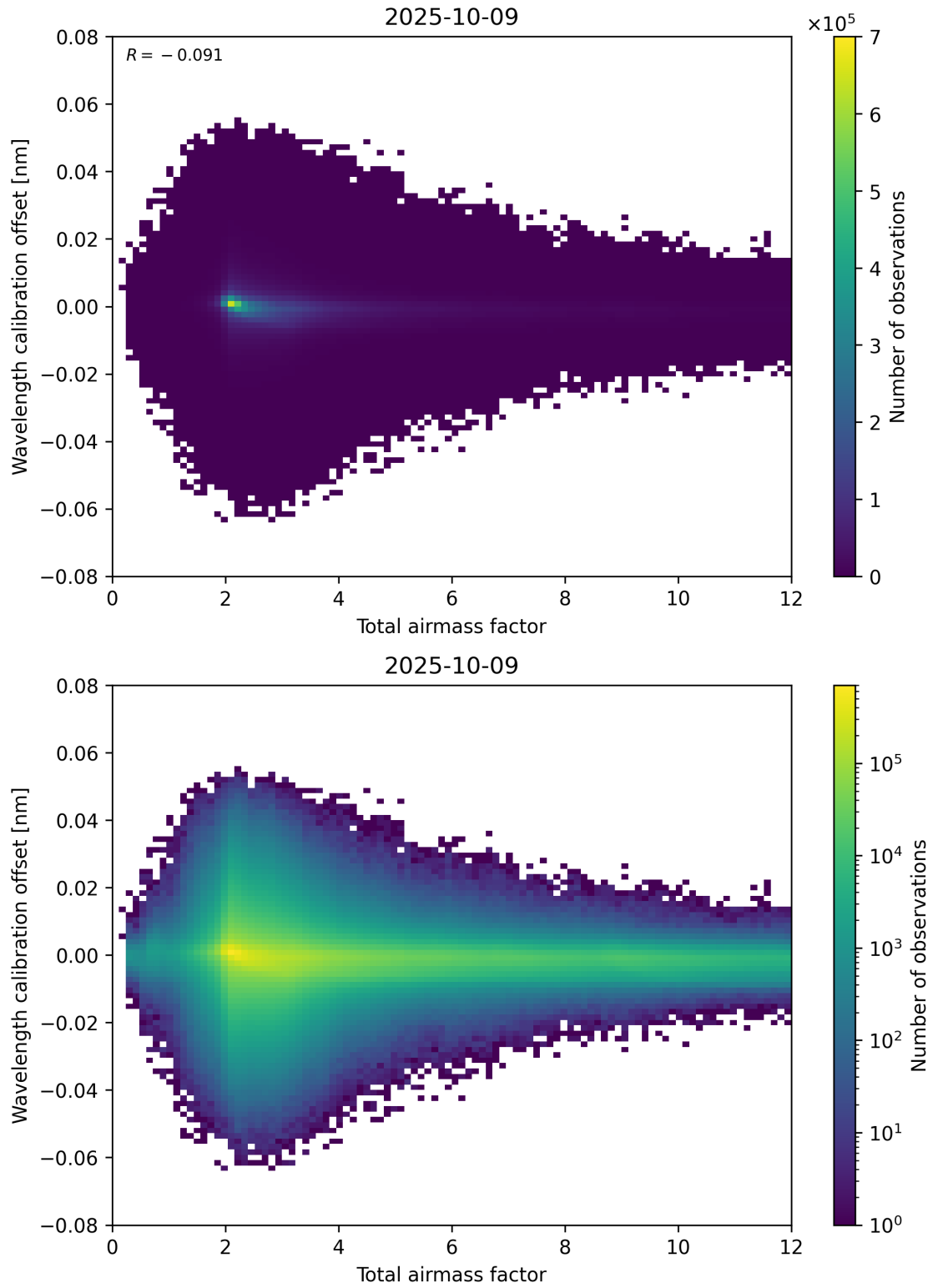
Figure 70: Scatter density plot of “Total airmass factor” against “Wavelength calibration offset” for 2025-10-08 to 2025-10-10.
