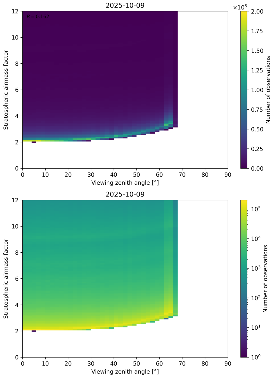
Figure 159: Scatter density plot of “Viewing zenith angle” against “Stratospheric airmass factor” for 2025-10-08 to 2025-10-10.
