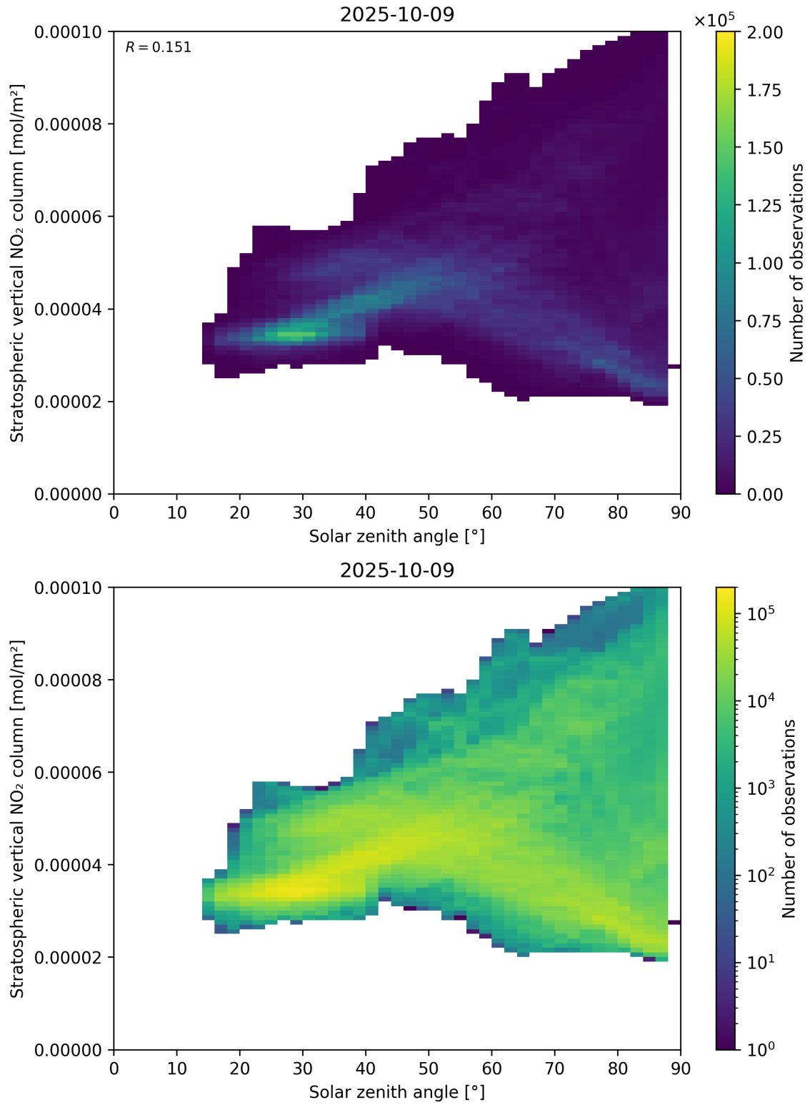
Figure 150: Scatter density plot of “Solar zenith angle” against “Stratospheric vertical NO 2 column” for 2025-10-08 to 2025-10-10.
