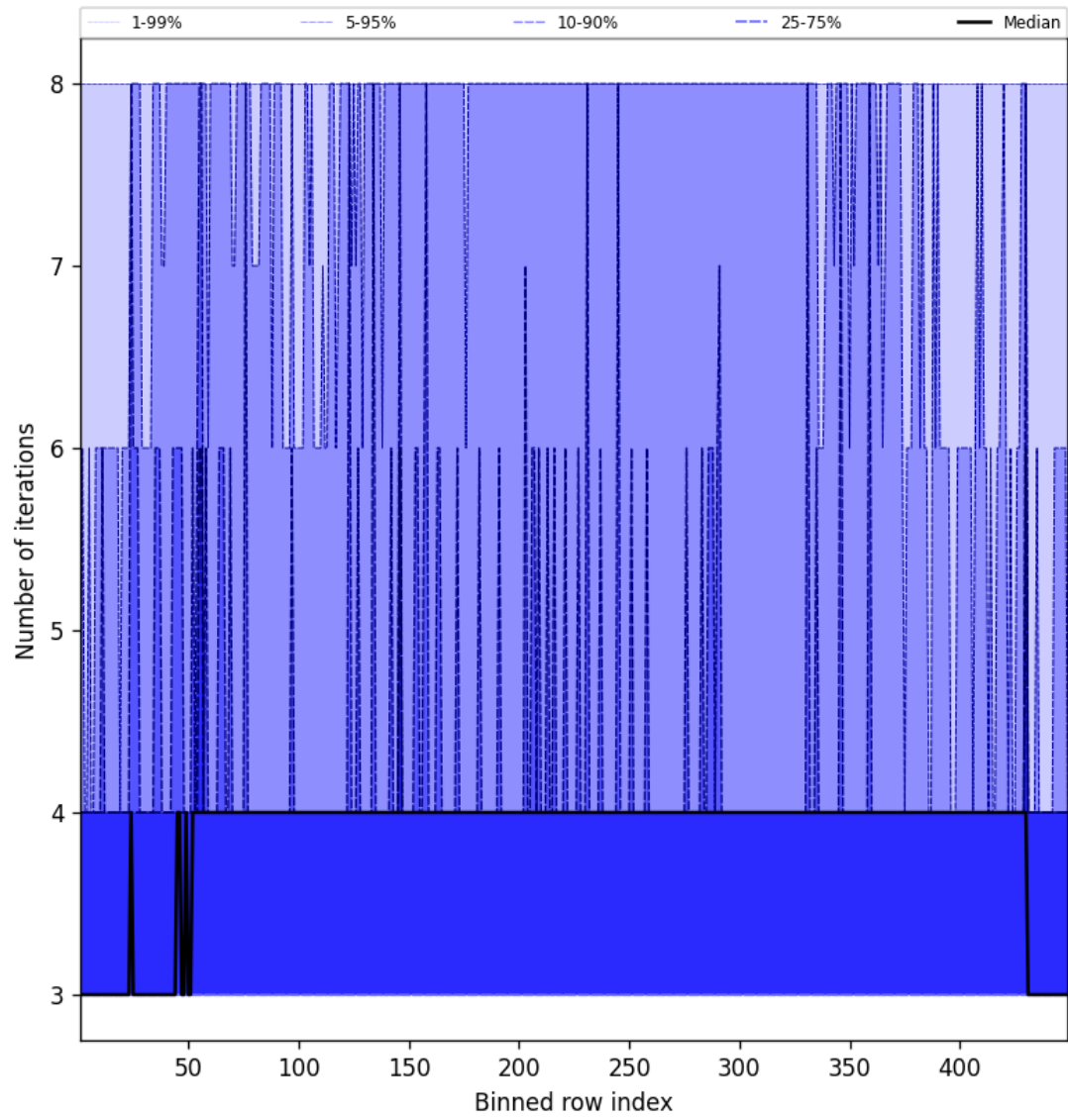
Figure 51: Along track statistics of “Number of iterations” for 2025-10-08 to 2025-10-10
