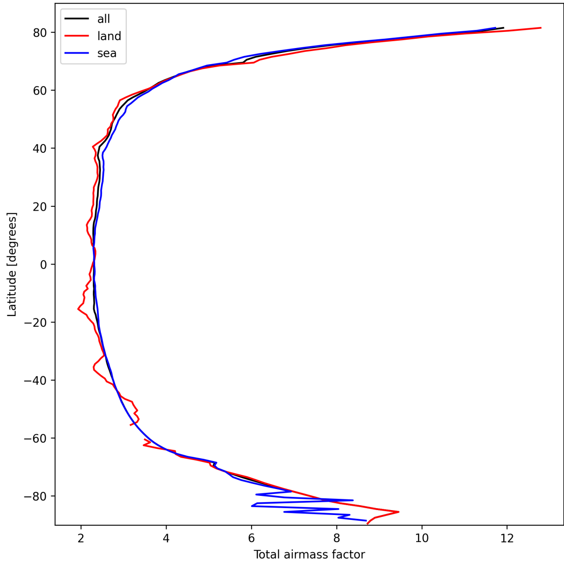
Figure 15: Zonal average of “Total airmass factor” for 2025-10-08 to 2025-10-10.
