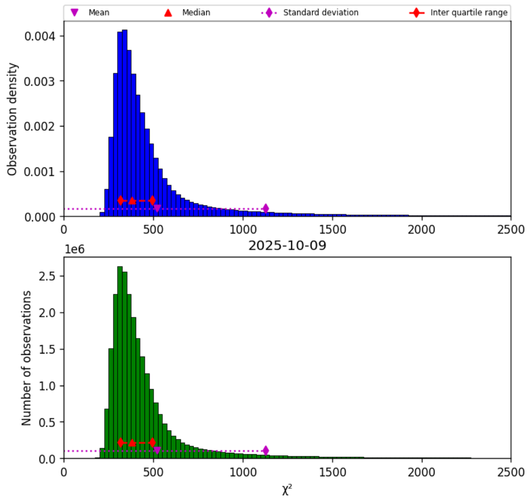
Figure 42: Histogram of “ \chi^2 ” for 2025-10-08 to 2025-10-10
