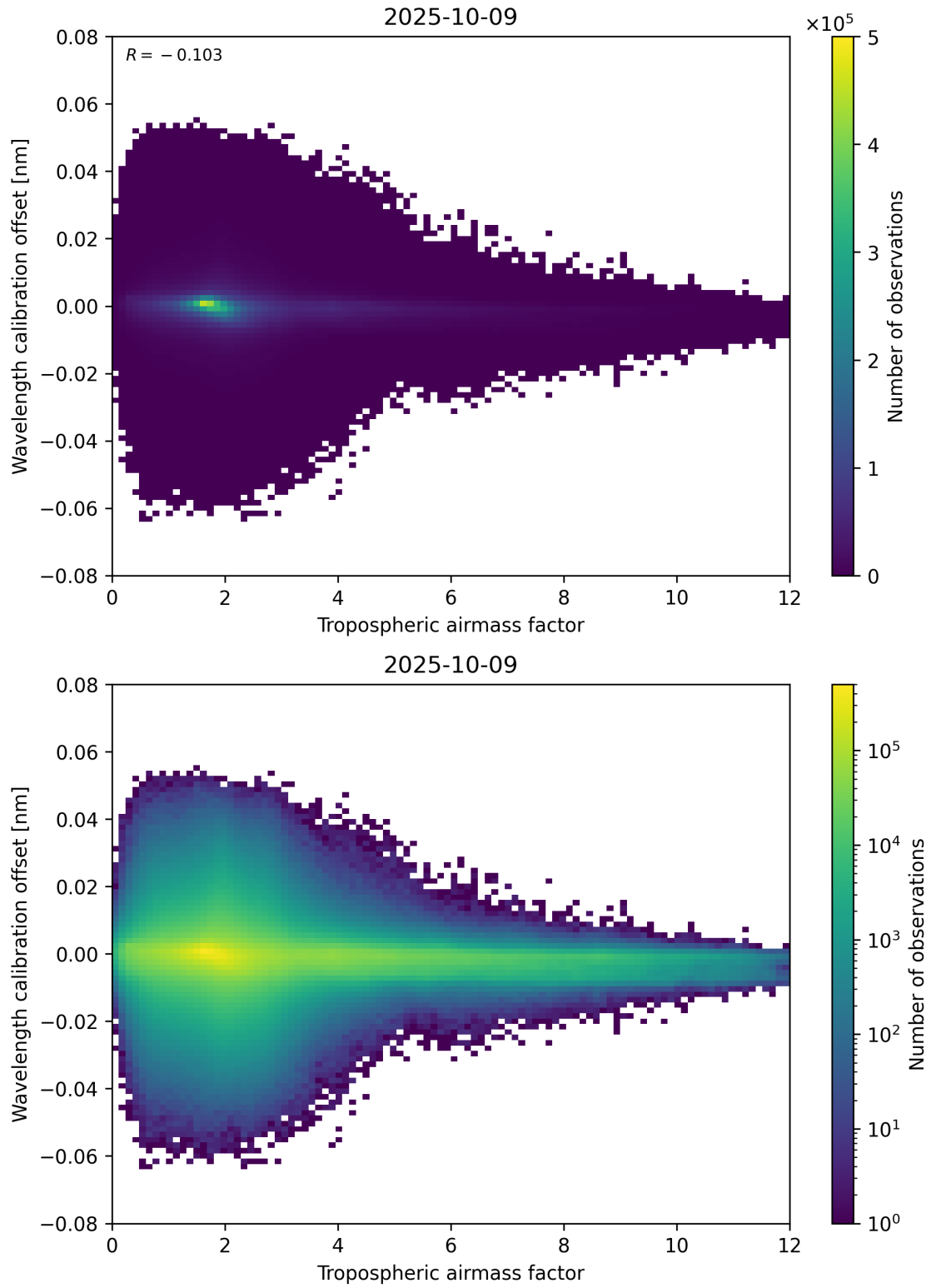
Figure 80: Scatter density plot of “Tropospheric airmass factor” against “Wavelength calibration offset” for 2025-10-08 to 2025-10-10.
