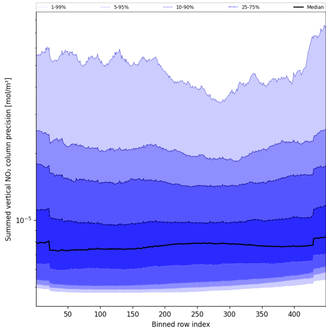
Figure 58: Along track statistics of “Summed vertical NO 2 column precision” for 2025-10-08 to 2025-10-10
