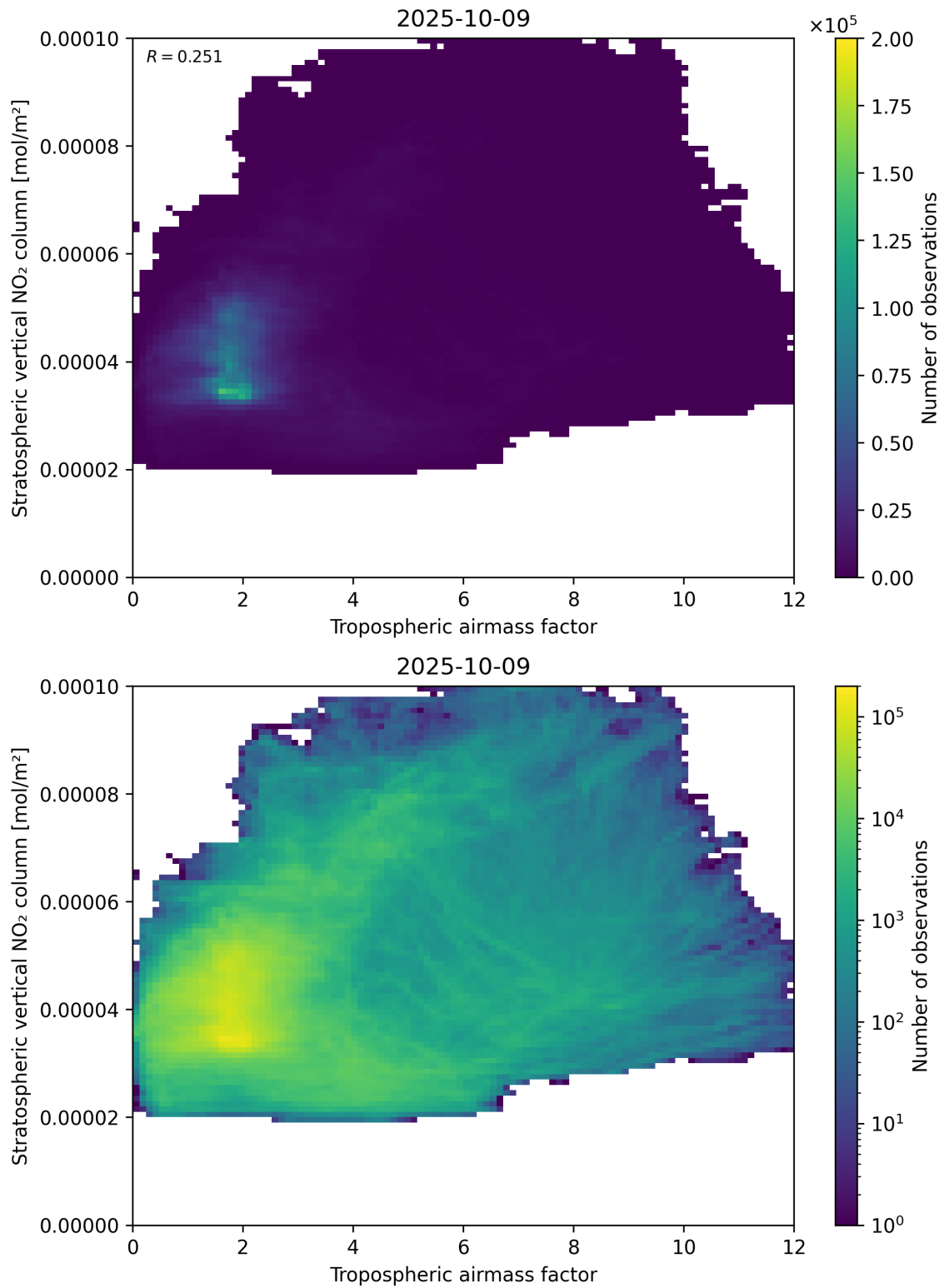
Figure 74: Scatter density plot of “Tropospheric air mass factor” against “Stratospheric vertical NO 2 column” for 2025-10-08 to 2025-10-10.
