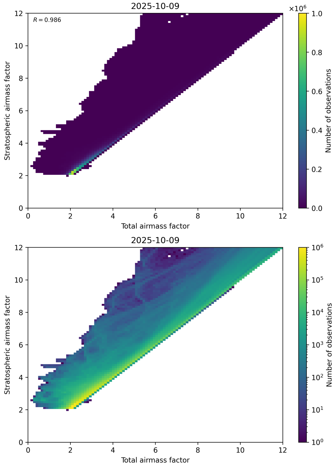
Figure 62: Scatter density plot of “Total airmass factor” against “Stratospheric airmass factor” for 2025-10-08 to 2025-10-10.
