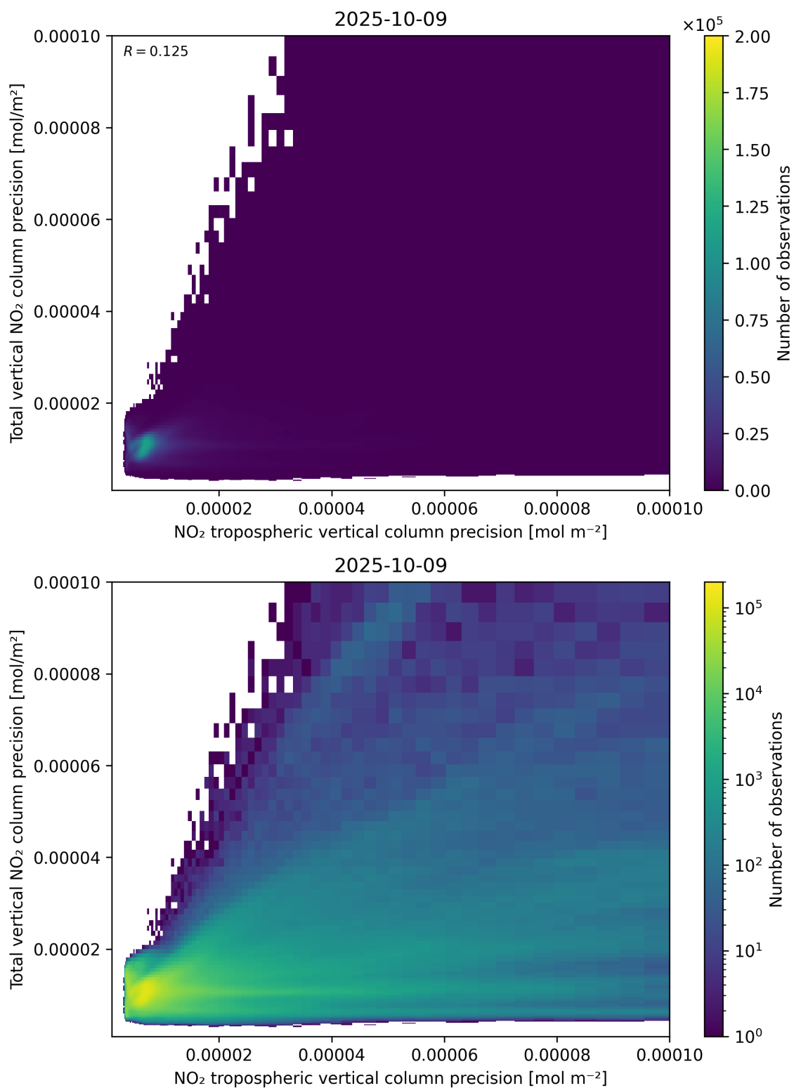
Figure 139: Scatter density plot of “NO 2 tropospheric vertical column precision” against “Total vertical NO 2 column precision” for 2025-10-08 to 2025-10-10.
