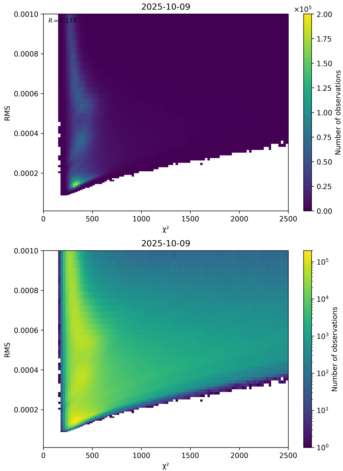
Figure 82: Scatter density plot of “ \chi^2 ” against “RMS” for 2025-10-08 to 2025-10-10.
