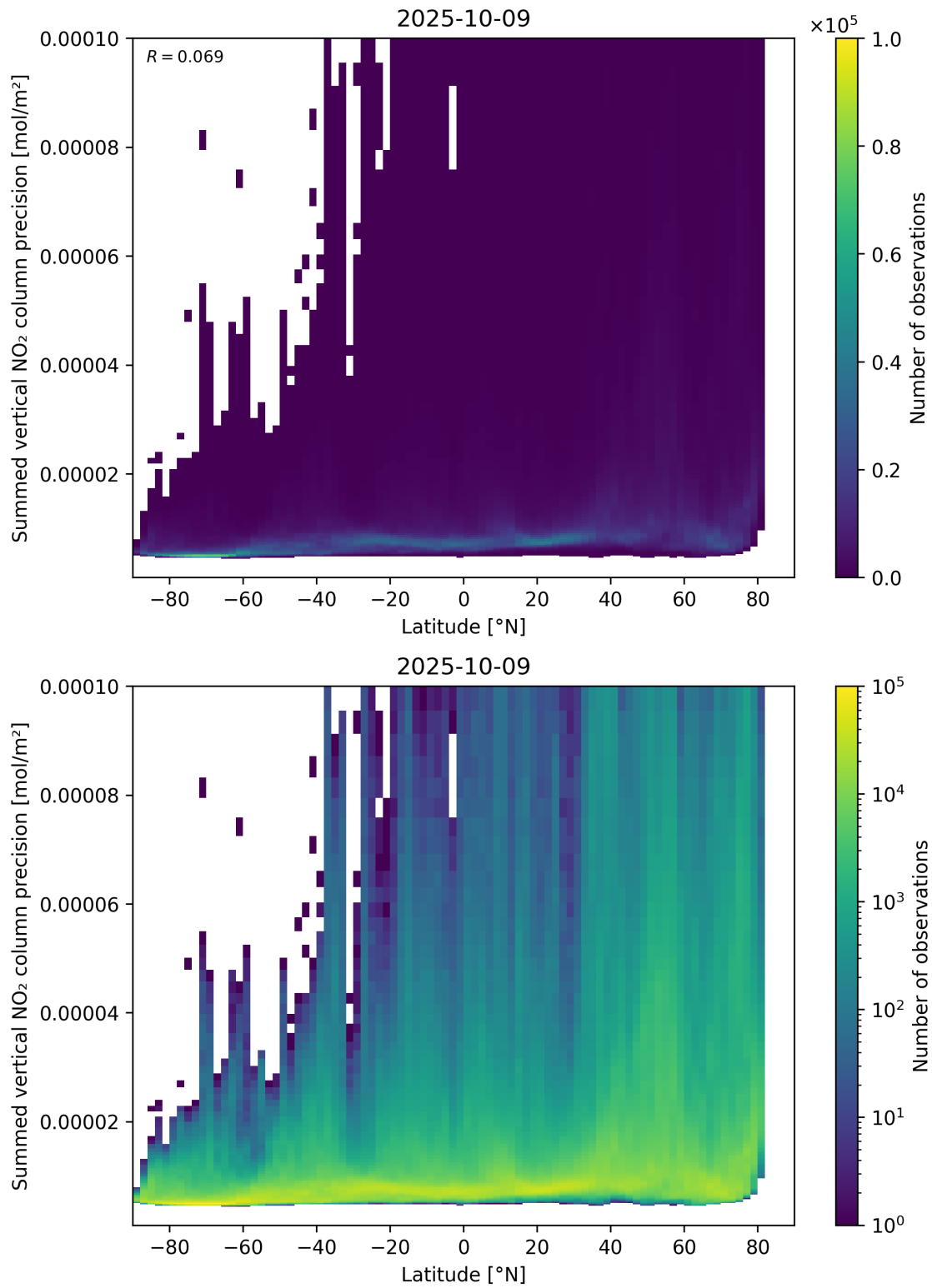
Figure 89: Scatter density plot of “Latitude” against “Summed vertical NO 2 column precision” for 2025-10-08 to 2025-10-10.
