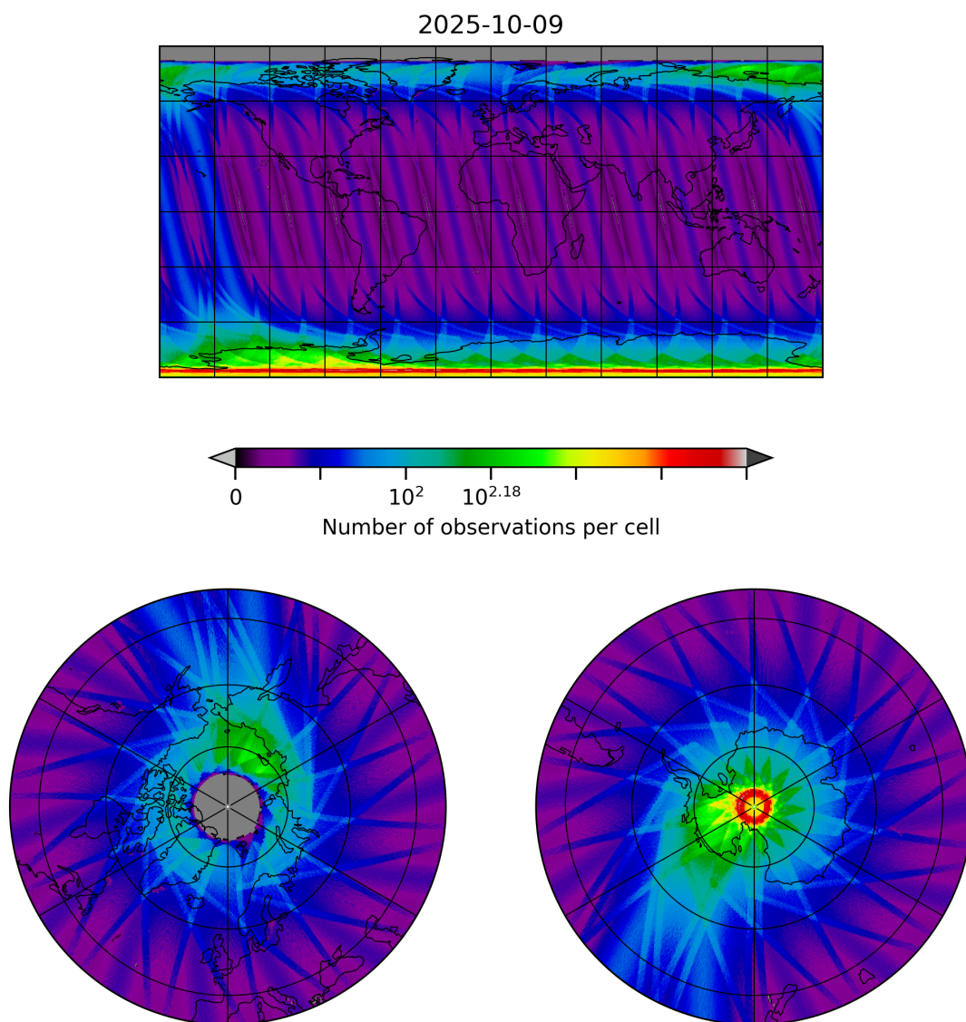
Figure 10: Map of the number of observations for 2025-10-08 to 2025-10-10
