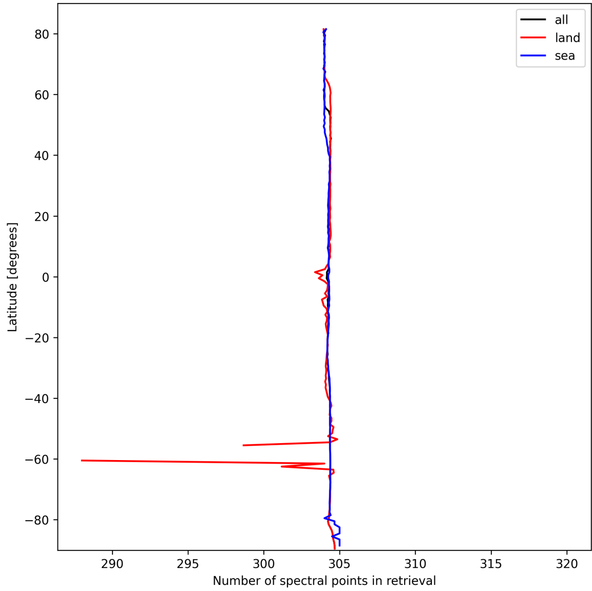
Figure 16: Zonal average of “Number of spectral points in retrieval” for 2025-10-08 to 2025-10-10.
