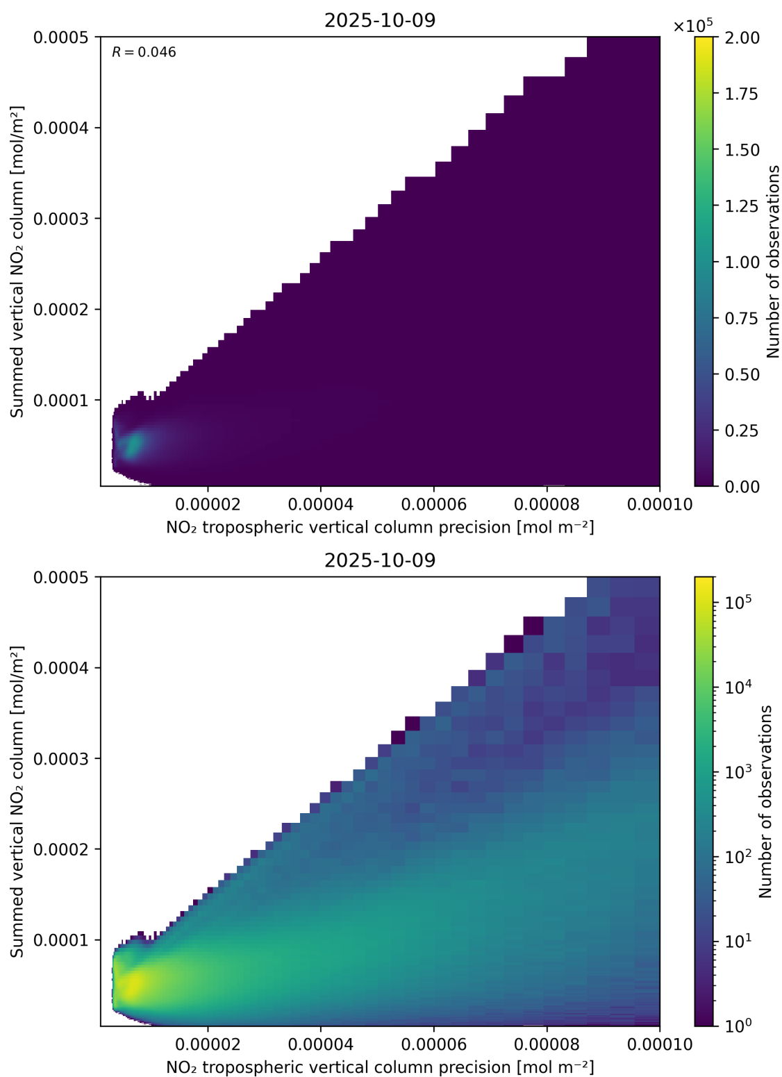
Figure 136: Scatter density plot of “NO 2 tropospheric vertical column precision” against “Summed vertical NO 2 column” for 2025-10-08 to 2025-10-10.
