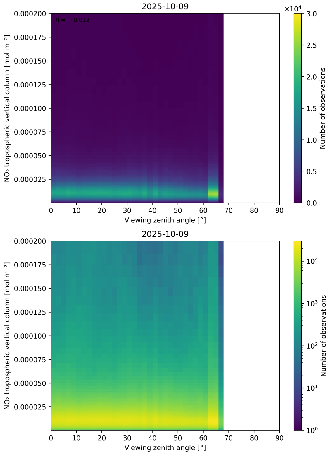
Figure 169: Scatter density plot of “Viewing zenith angle” against “NO 2 tropospheric vertical column” for 2025-10-08 to 2025-10-10.
