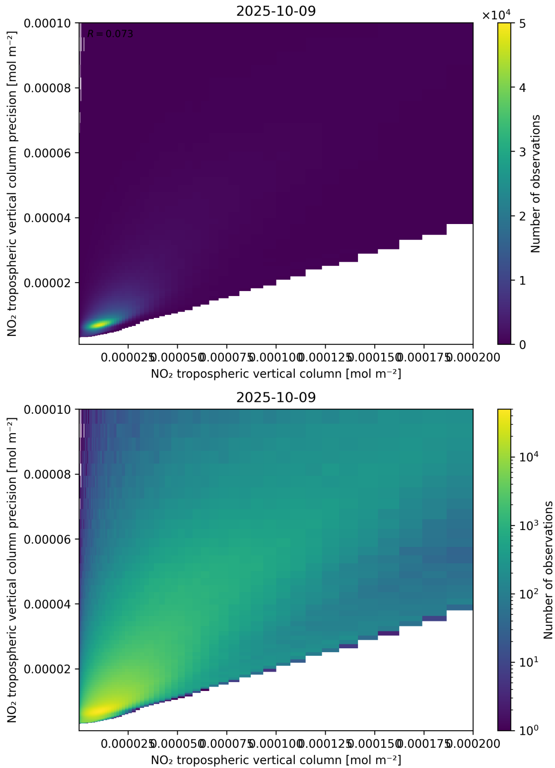
Figure 130: Scatter density plot of “NO 2 tropospheric vertical column” against “NO 2 tropospheric vertical column precision” for 2025-10-08 to 2025-10-10.
