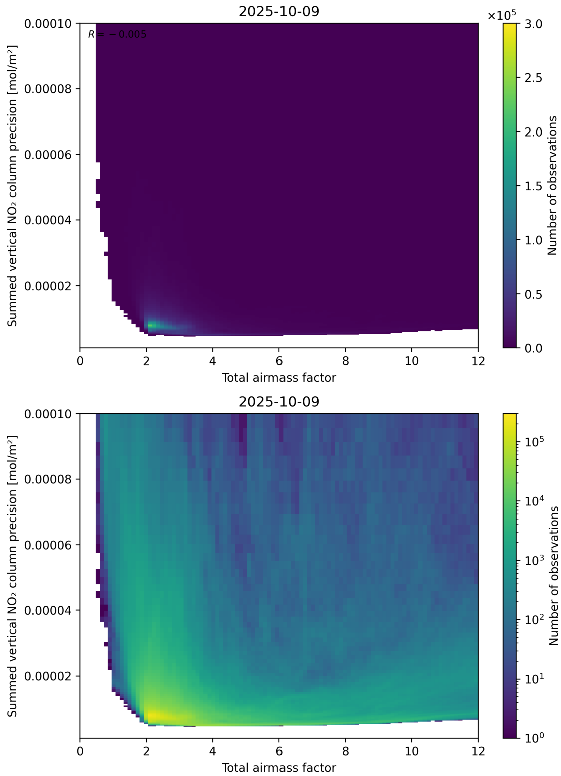
Figure 66: Scatter density plot of “Total airmass factor” against “Summed vertical NO 2 column precision” for 2025-10-08 to 2025-10-10.
