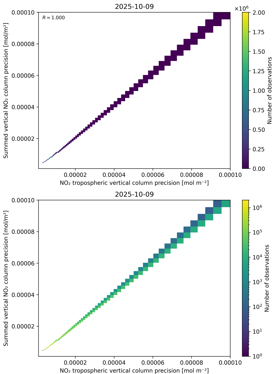
Figure 137: Scatter density plot of “NO 2 tropospheric vertical column precision” against “Summed vertical NO 2 column precision” for 2025-10-08 to 2025-10-10.
