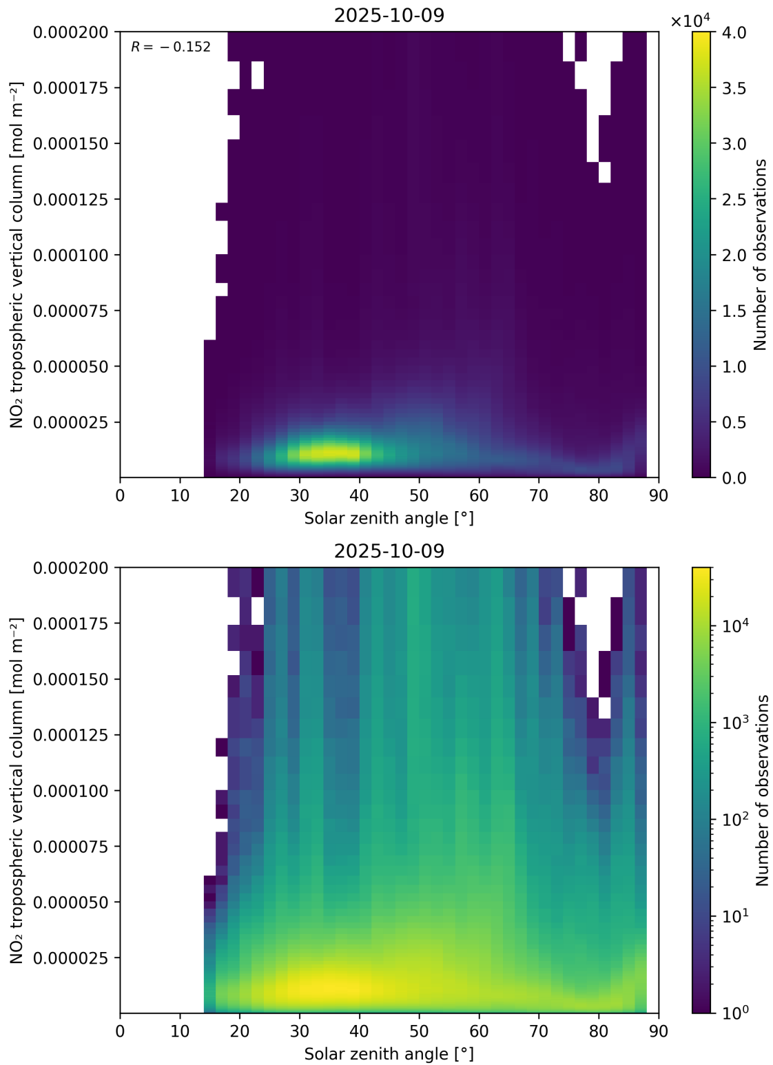
Figure 155: Scatter density plot of “Solar zenith angle” against “NO 2 tropospheric vertical column” for 2025-10-08 to 2025-10-10.
