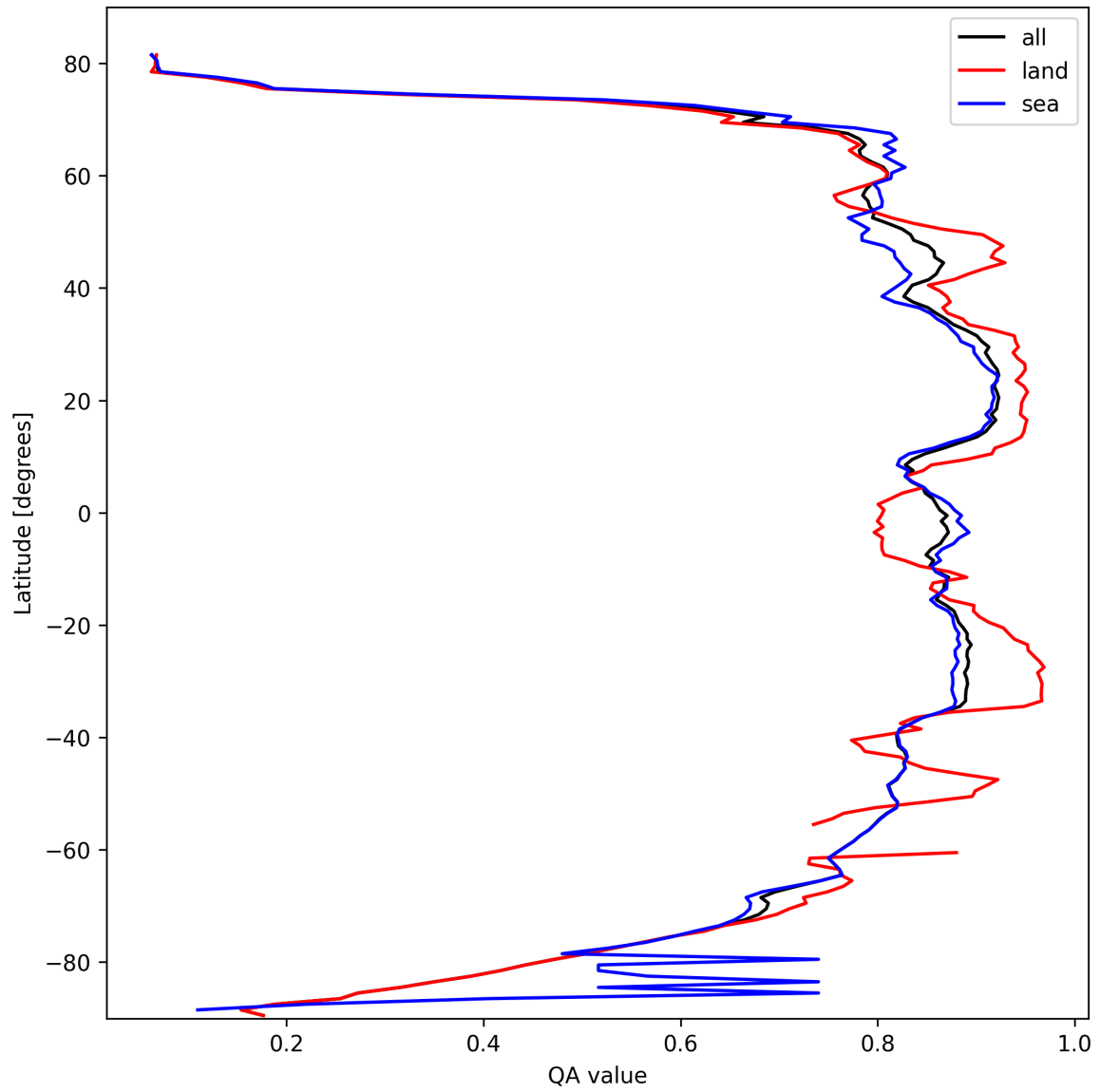
Figure 11: Zonal average of “QA value” for 2025-10-08 to 2025-10-10.
