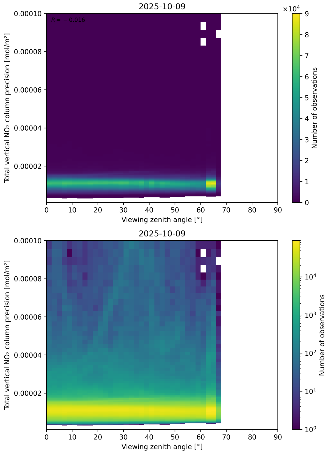
Figure 168: Scatter density plot of “Viewing zenith angle” against “Total vertical NO 2 column precision” for 2025-10-08 to 2025-10-10.
