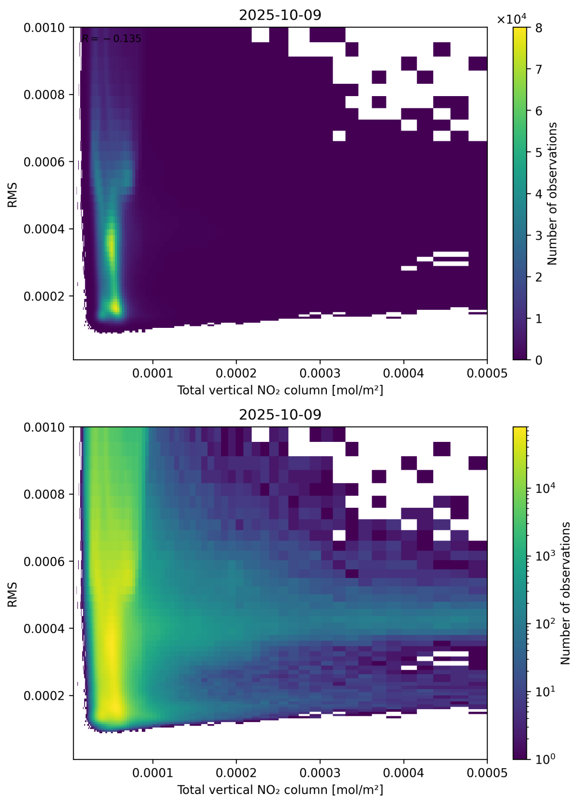
Figure 120: Scatter density plot of “Total vertical NO 2 column” against “RMS” for 2025-10-08 to 2025-10-10.
