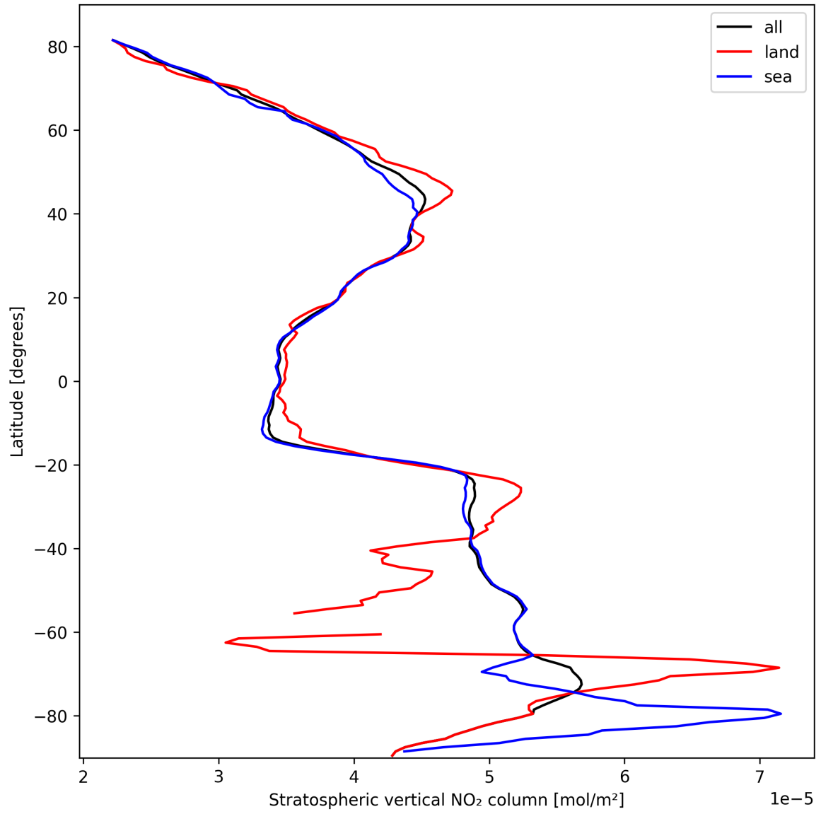
Figure 19: Zonal average of “Stratospheric vertical NO 2 column” for 2025-10-08 to 2025-10-10.
