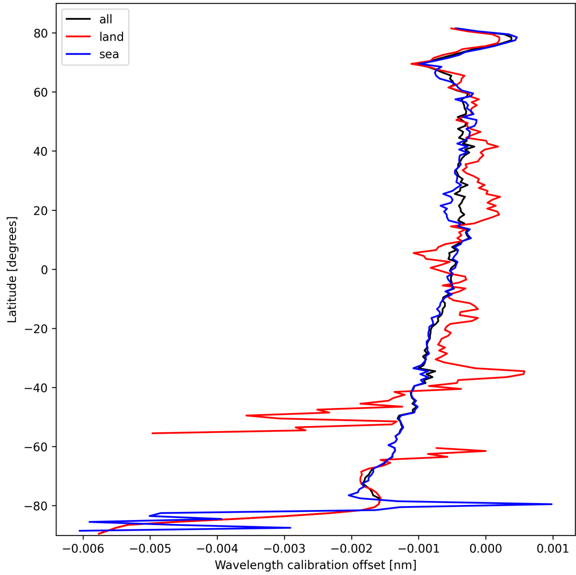
Figure 18: Zonal average of “Wavelength calibration offset” for 2025-10-08 to 2025-10-10.
