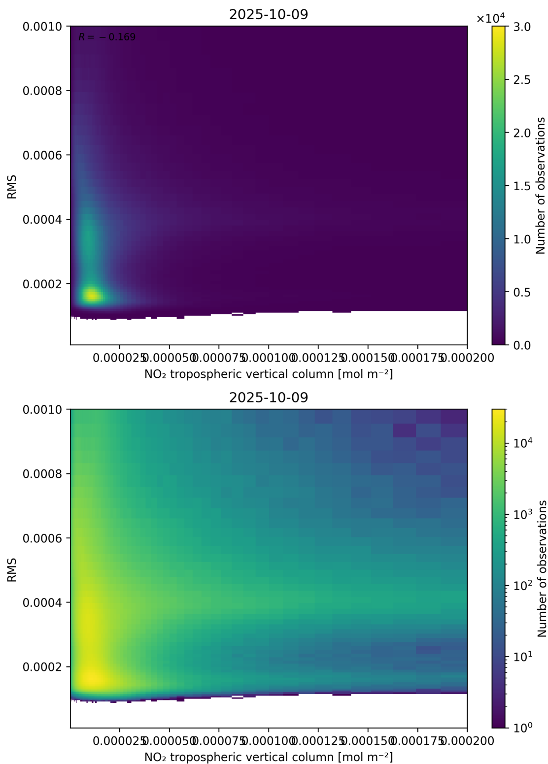
Figure 142: Scatter density plot of “NO 2 tropospheric vertical column” against “RMS” for 2025-10-08 to 2025-10-10.
