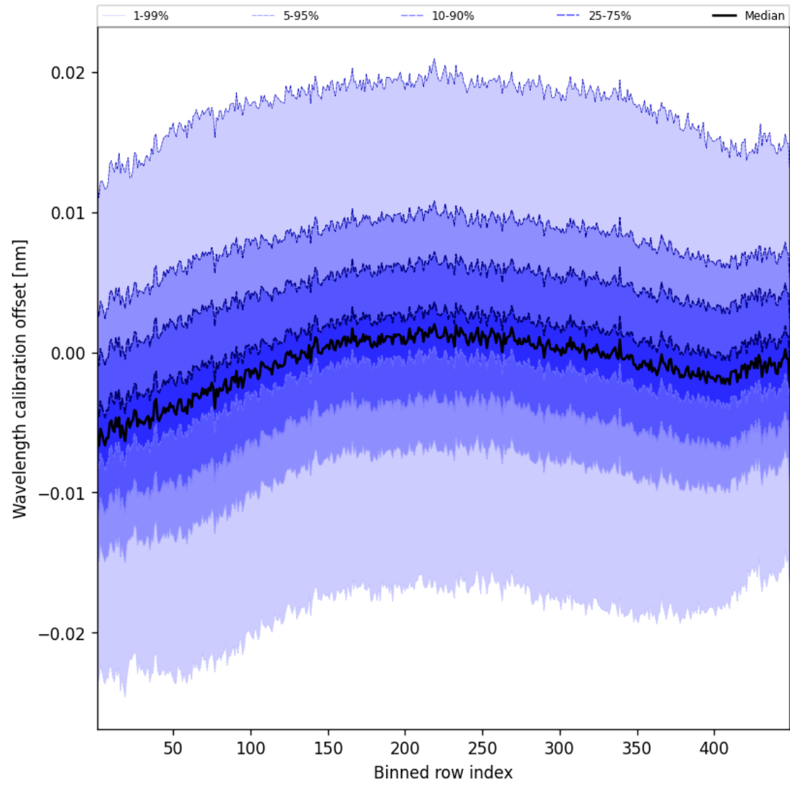
Figure 52: Along track statistics of “Wavelength calibration offset” for 2025-10-08 to 2025-10-10
