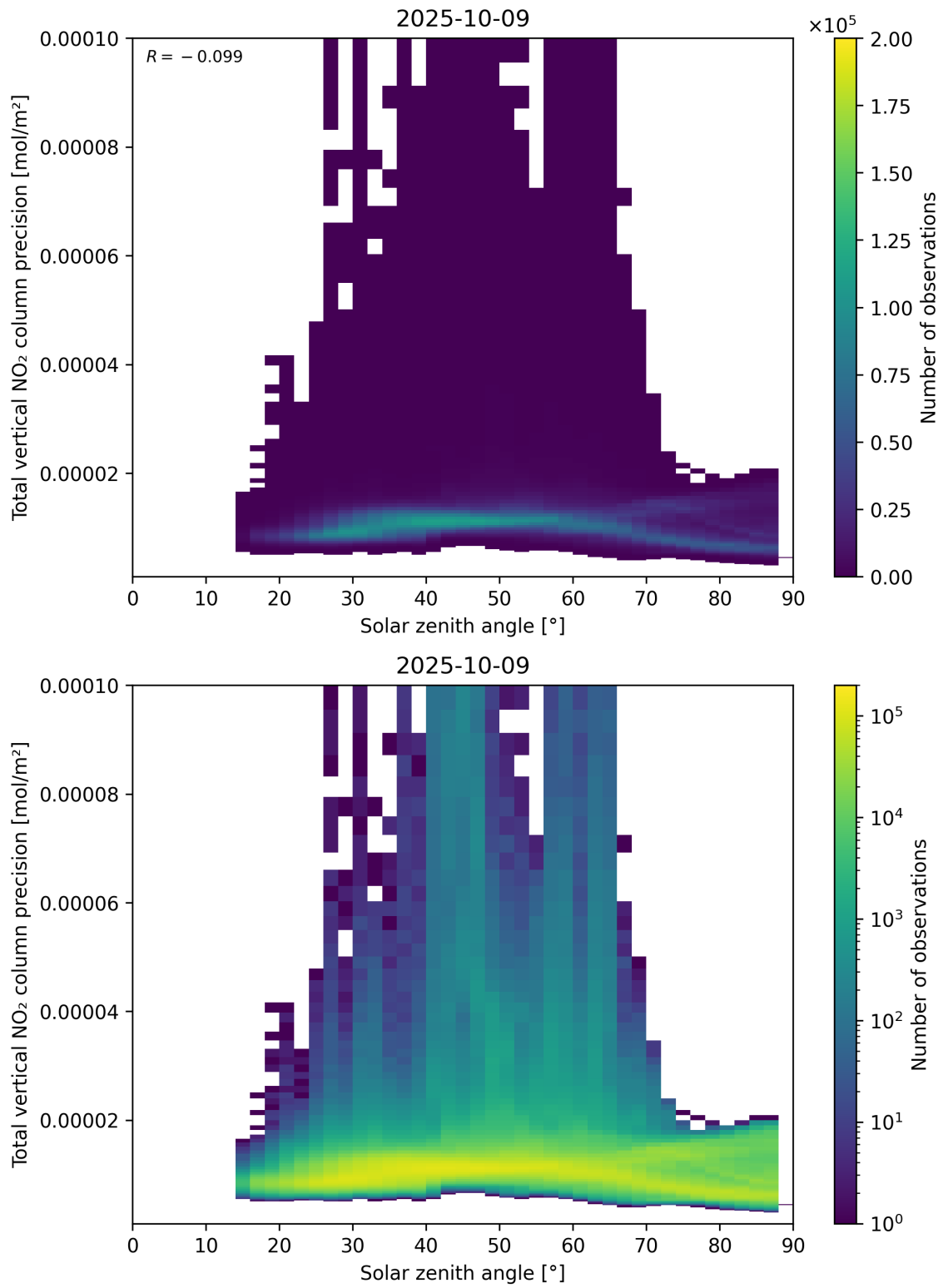
Figure 154: Scatter density plot of “Solar zenith angle” against “Total vertical NO 2 column precision” for 2025-10-08 to 2025-10-10.
