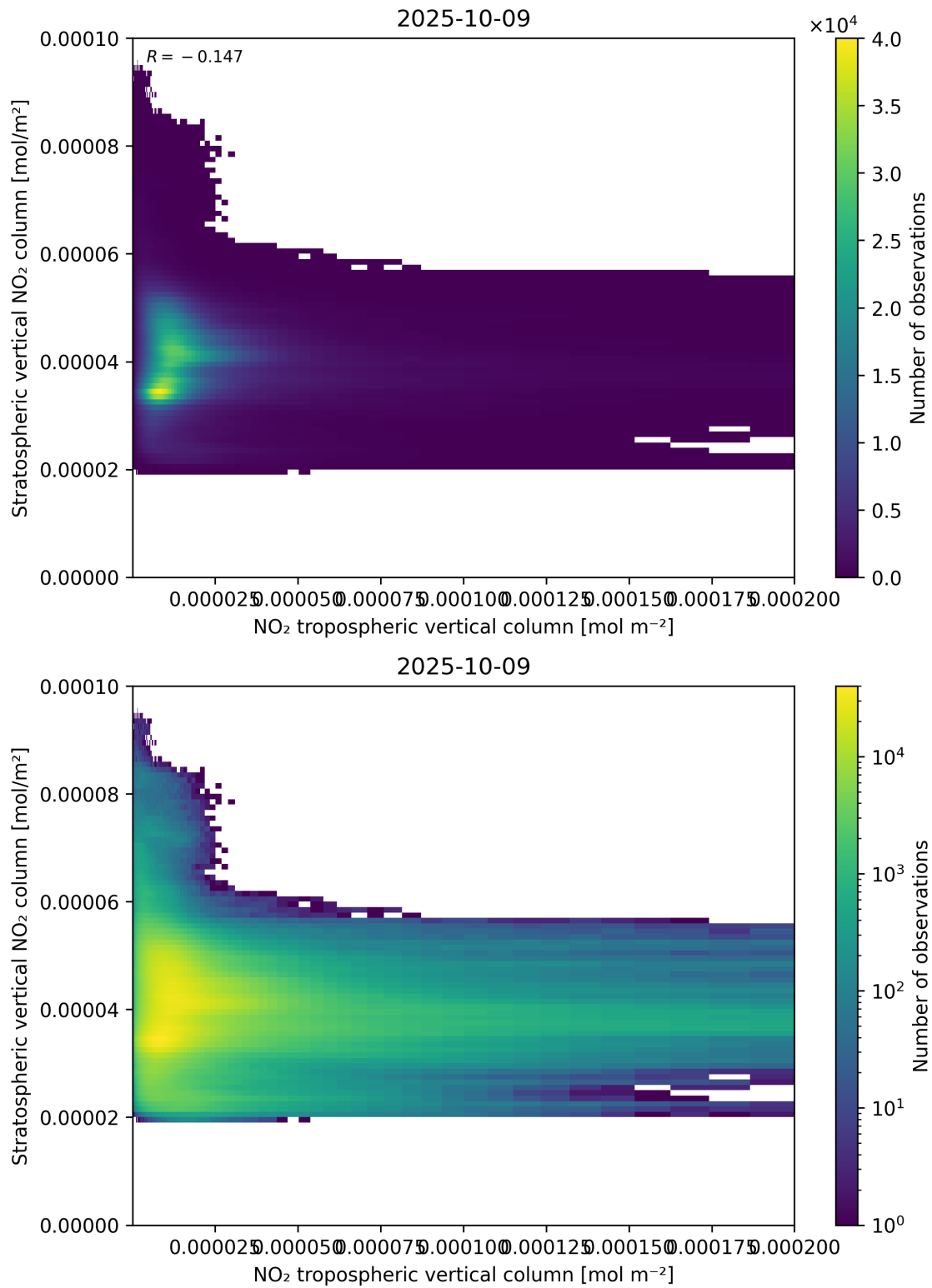
Figure 125: Scatter density plot of “NO 2 tropospheric vertical column” against “Stratospheric vertical NO 2 column” for 2025-10-08 to 2025-10-10.
