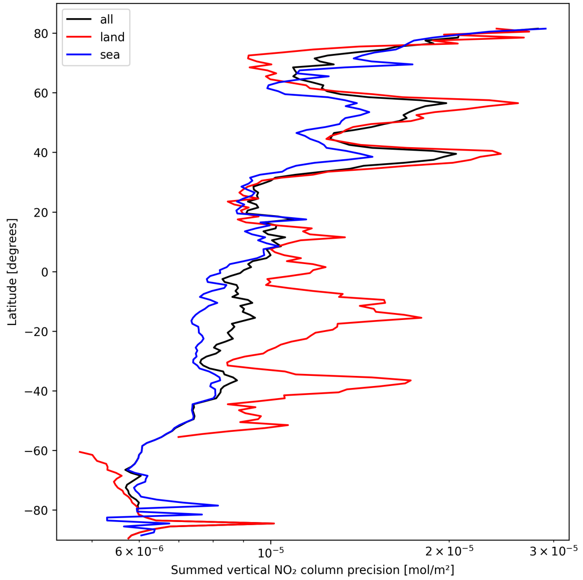
Figure 24: Zonal average of “Summed vertical NO 2 column precision” for 2025-10-08 to 2025-10-10.
