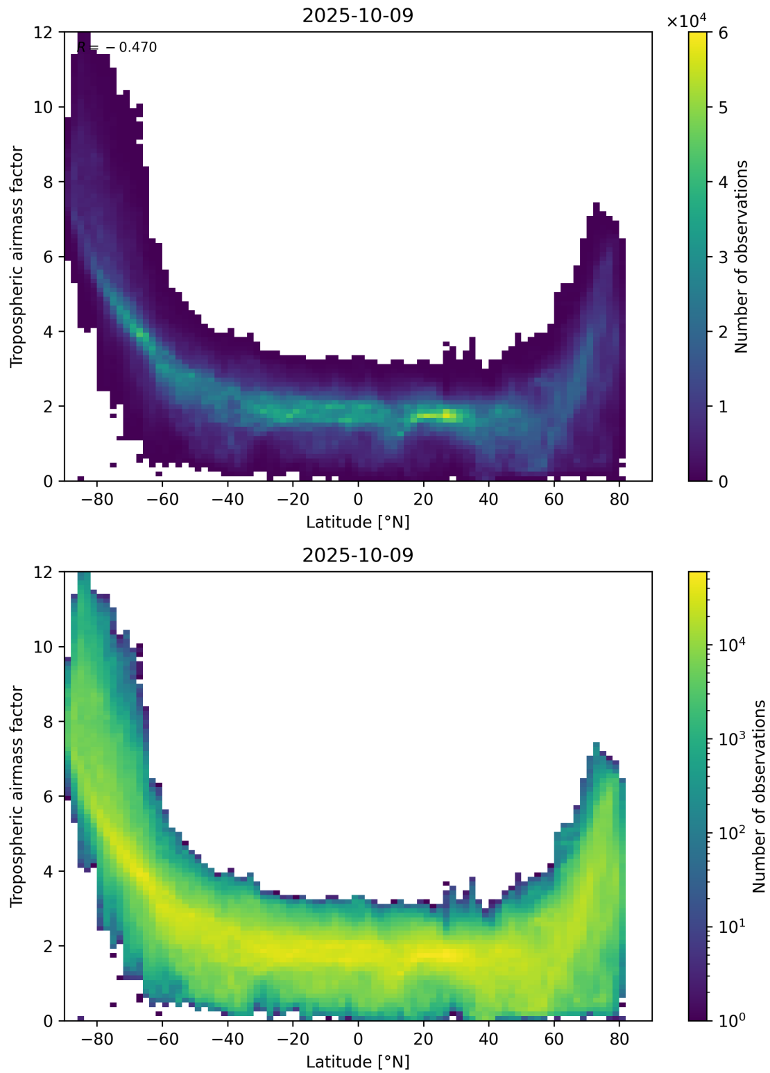
Figure 85: Scatter density plot of “Latitude” against “Tropospheric airmass factor” for 2025-10-08 to 2025-10-10.
