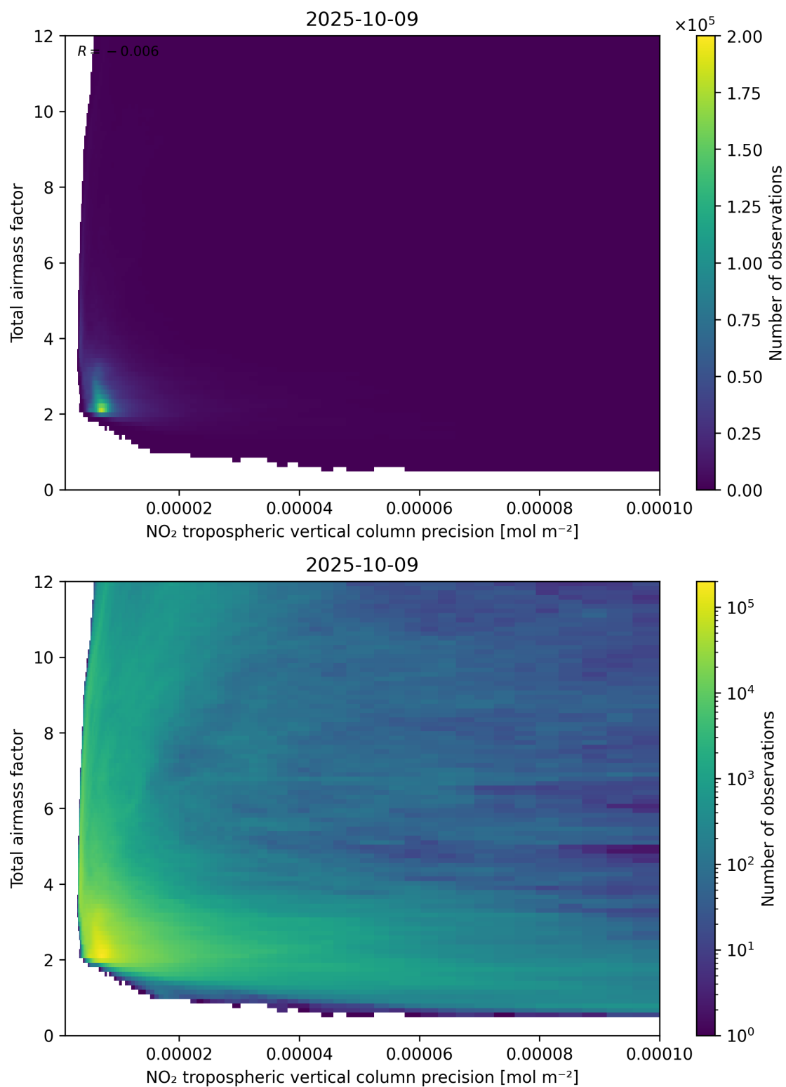
Figure 132: Scatter density plot of “NO 2 tropospheric vertical column precision” against “Total air mass factor” for 2025-10-08 to 2025-10-10.
