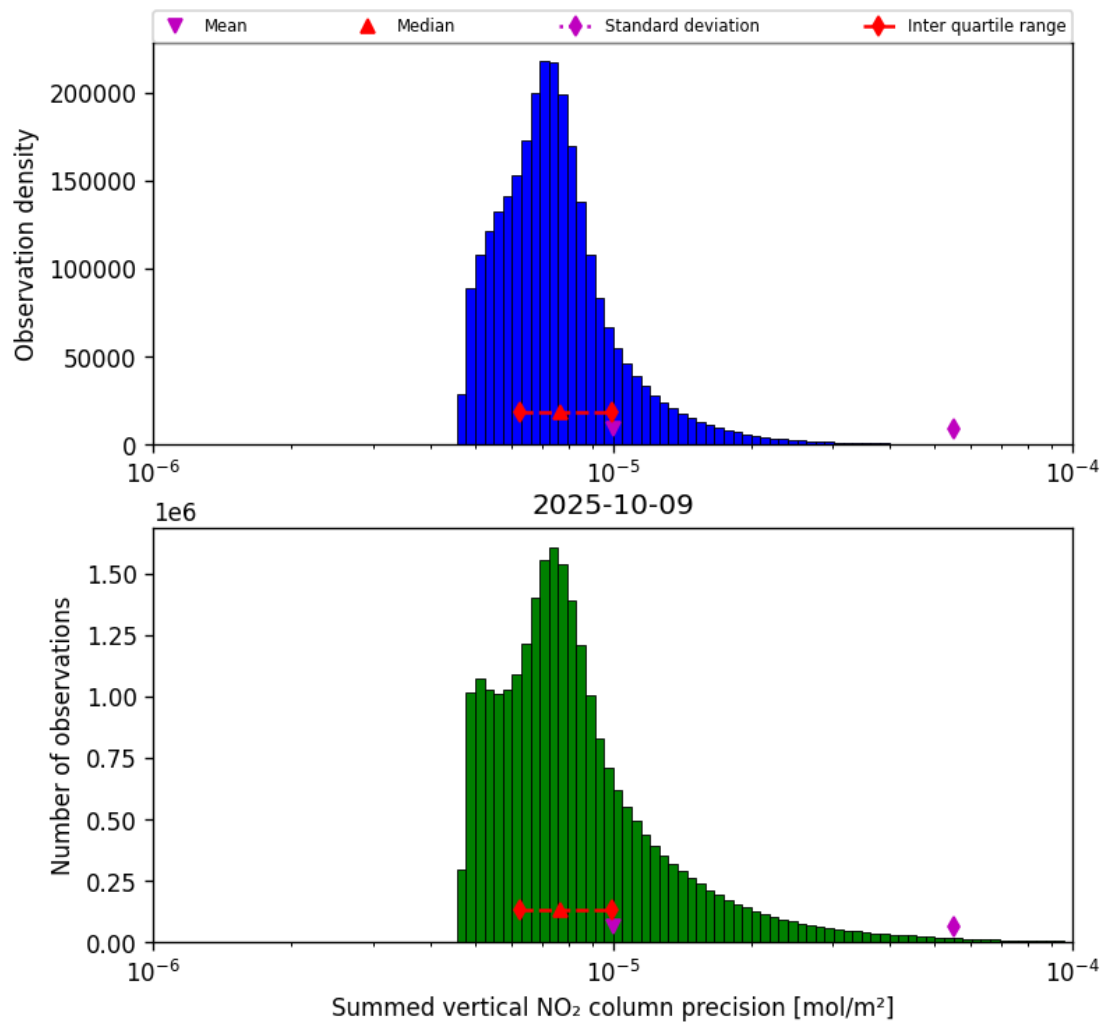
Figure 41: Histogram of "Summed vertical NO 2 column precision" for 2025-10-08 to 2025-10-10
