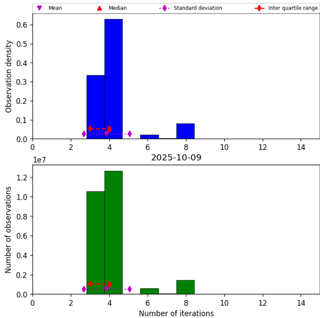
Figure 34: Histogram of “Number of iterations” for 2025-10-08 to 2025-10-10
