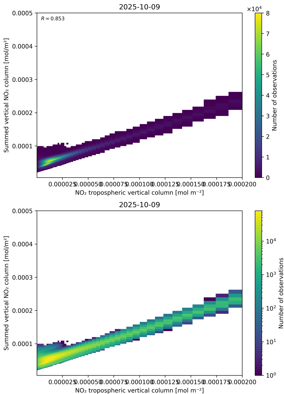
Figure 126: Scatter density plot of “NO 2 tropospheric vertical column” against “Summed vertical NO 2 column” for 2025-10-08 to 2025-10-10.
