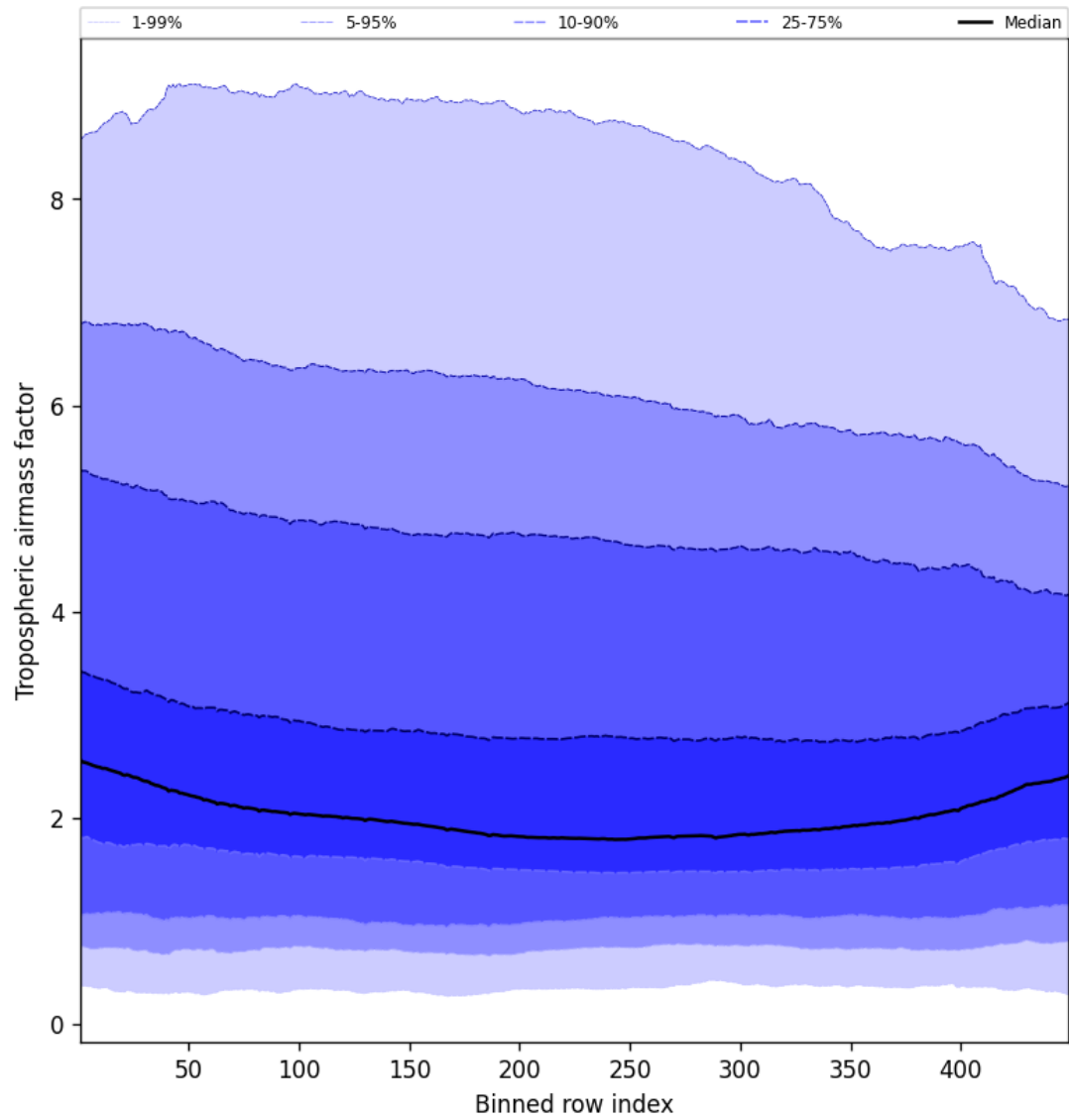
Figure 48: Along track statistics of “Tropospheric air mass factor” for 2025-10-08 to 2025-10-10
