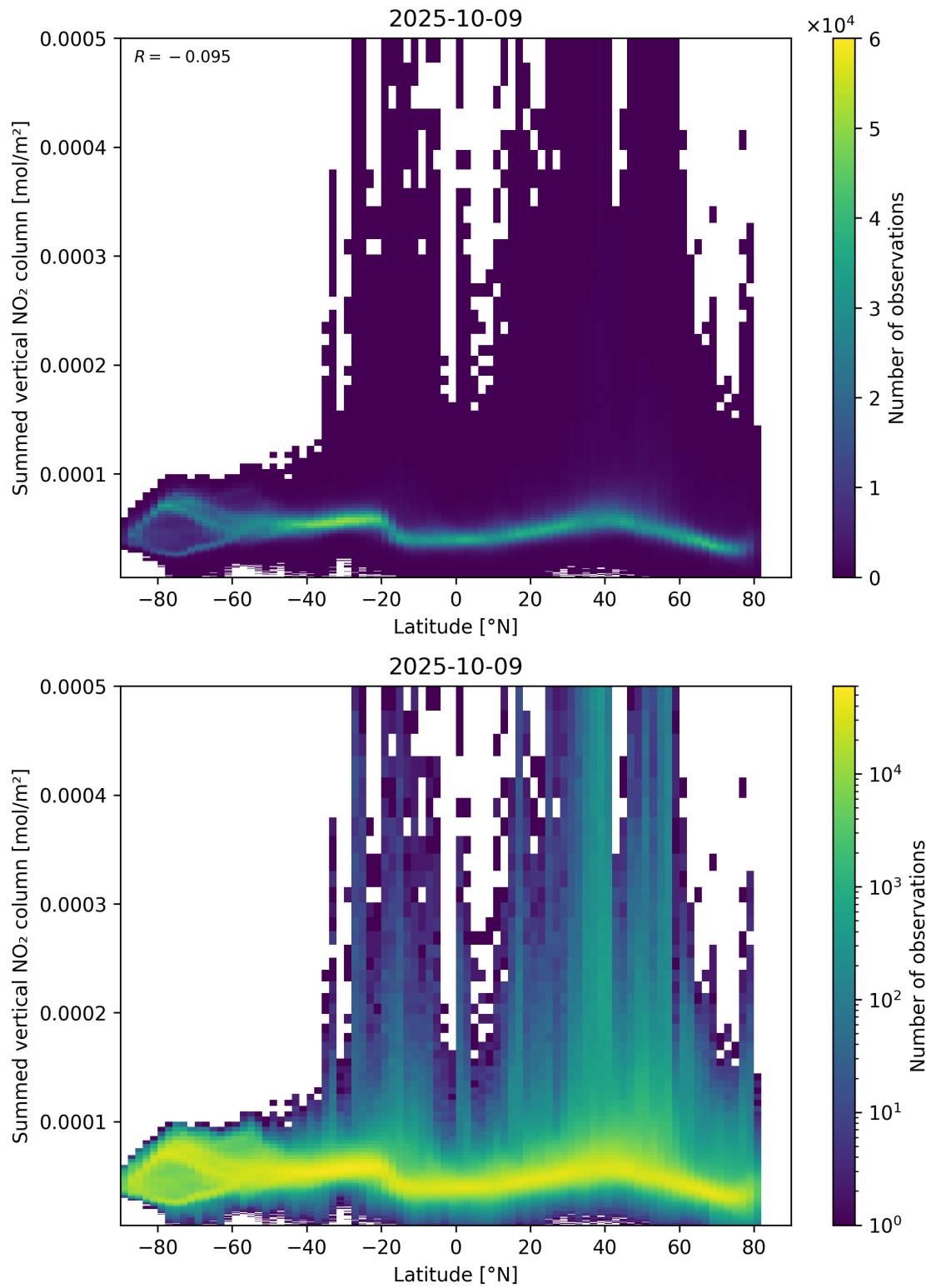
Figure 88: Scatter density plot of “Latitude” against “Summed vertical NO 2 column” for 2025-10-08 to 2025-10-10.
