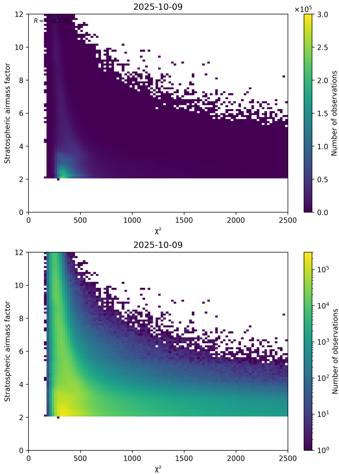
Figure 81: Scatter density plot of “ \chi^2 ” against “Stratospheric airmass factor” for 2025-10-08 to 2025-10-10.
