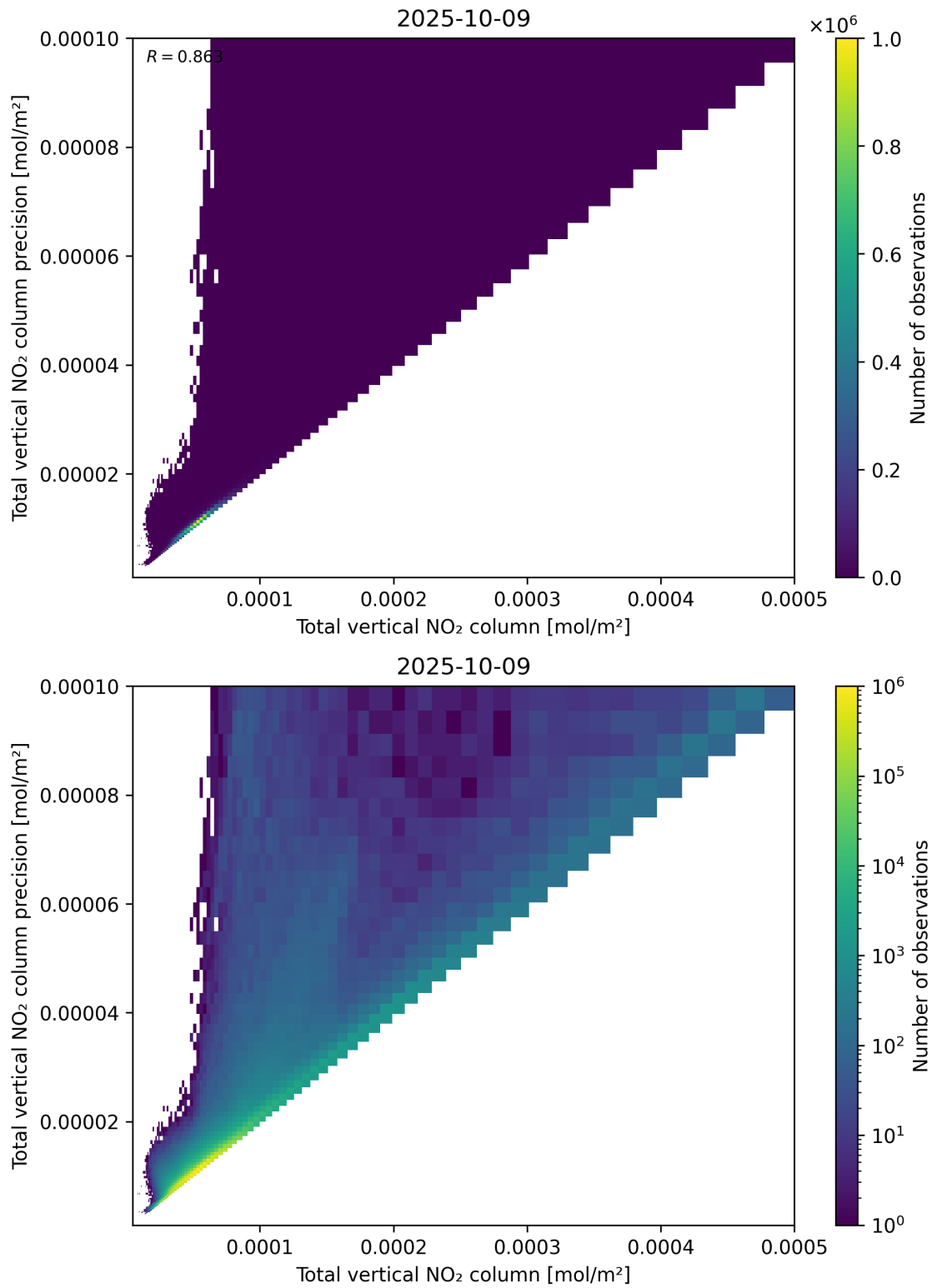
Figure 114: Scatter density plot of “Total vertical NO 2 column” against “Total vertical NO 2 column precision” for 2025-10-08 to 2025-10-10.
