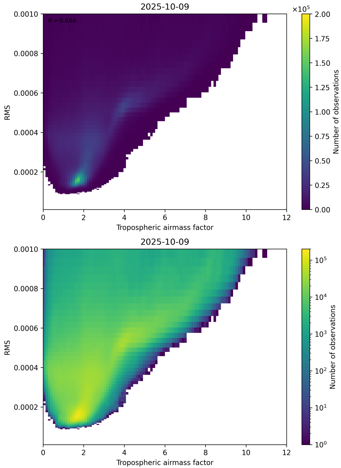
Figure 79: Scatter density plot of “Tropospheric airmass factor” against “RMS” for 2025-10-08 to 2025-10-10.
