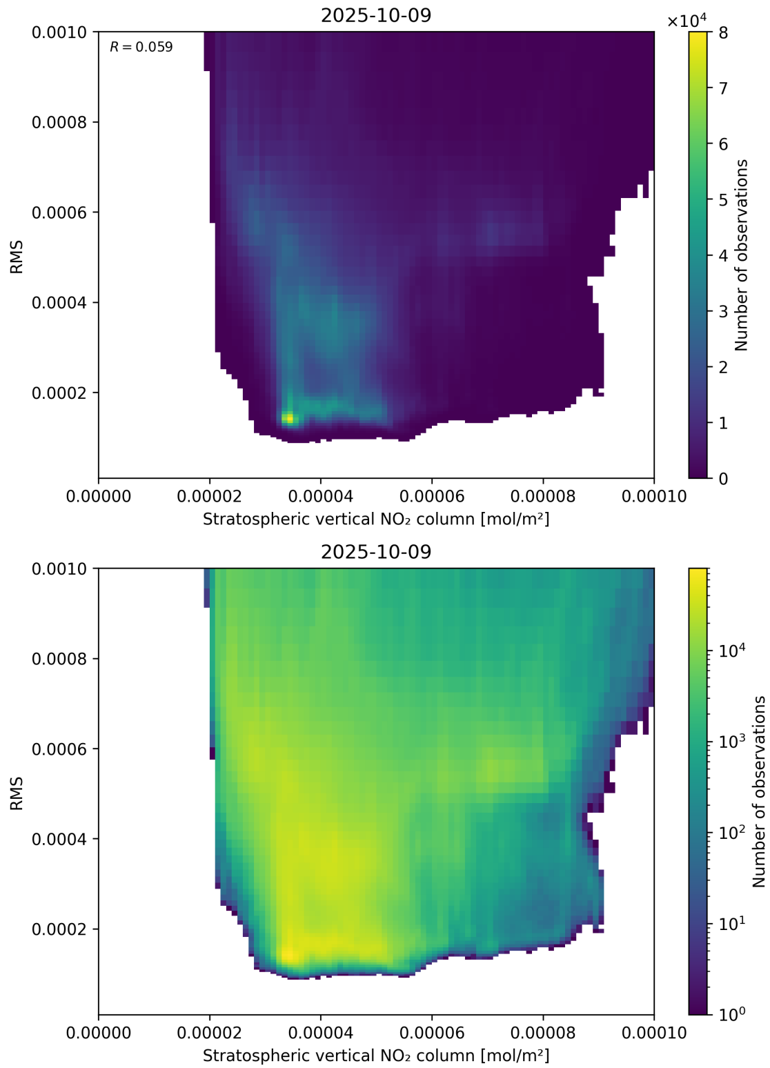
Figure 102: Scatter density plot of “Stratospheric vertical NO 2 column” against “RMS” for 2025-10-08 to 2025-10-10.
