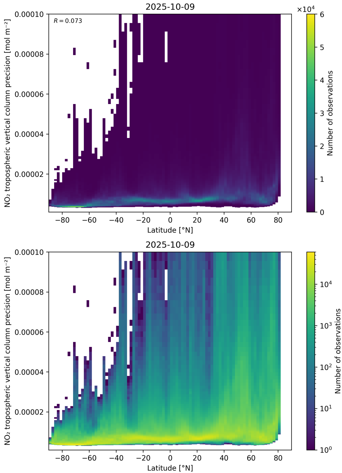
Figure 93: Scatter density plot of “Latitude” against “NO 2 tropospheric vertical column precision” for 2025-10-08 to 2025-10-10.
