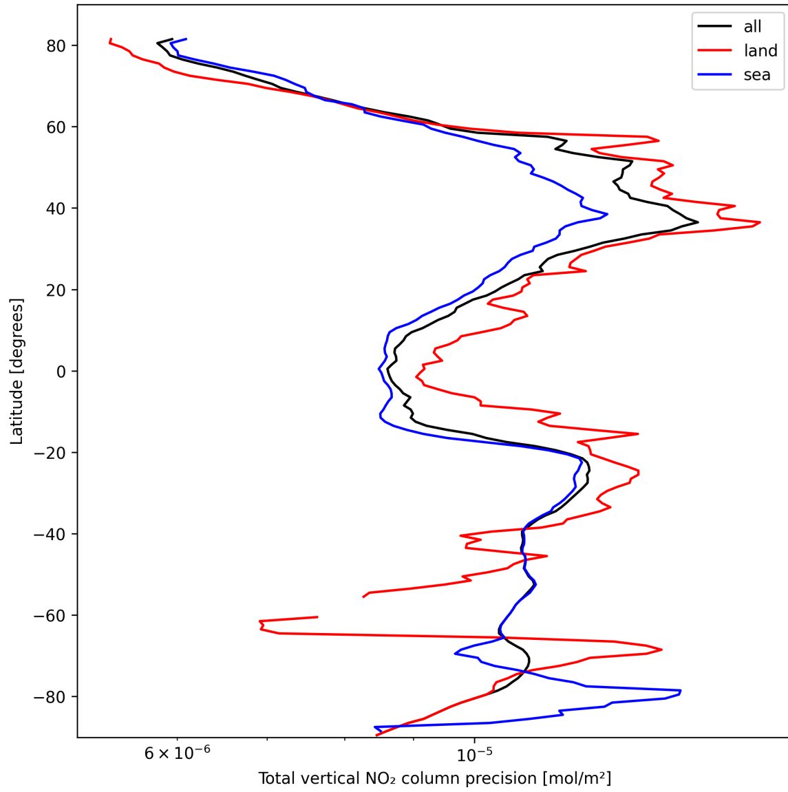
Figure 22: Zonal average of “Total vertical NO 2 column precision” for 2025-10-08 to 2025-10-10.
