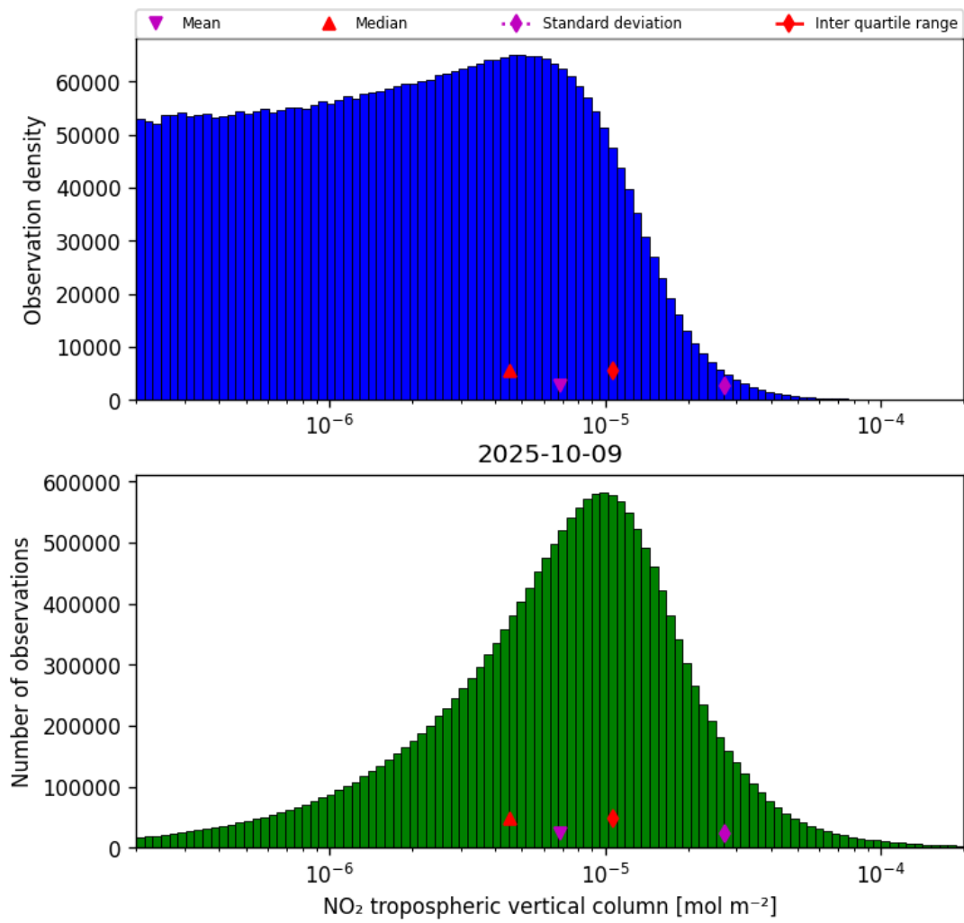
Figure 29: Histogram of “NO 2 tropospheric vertical column” for 2025-10-08 to 2025-10-10
