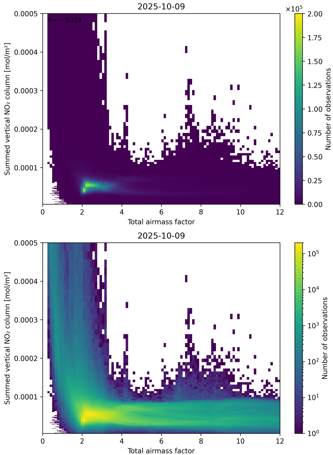
Figure 65: Scatter density plot of “Total air mass factor” against “Summed vertical NO 2 column” for 2025-10-08 to 2025-10-10.
