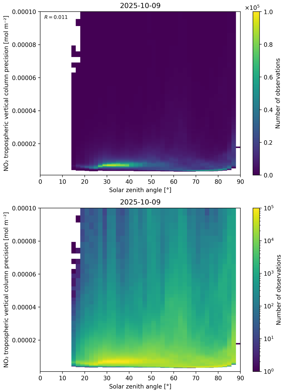
Figure 156: Scatter density plot of “Solar zenith angle” against “NO 2 tropospheric vertical column precision” for 2025-10-08 to 2025-10-10.
