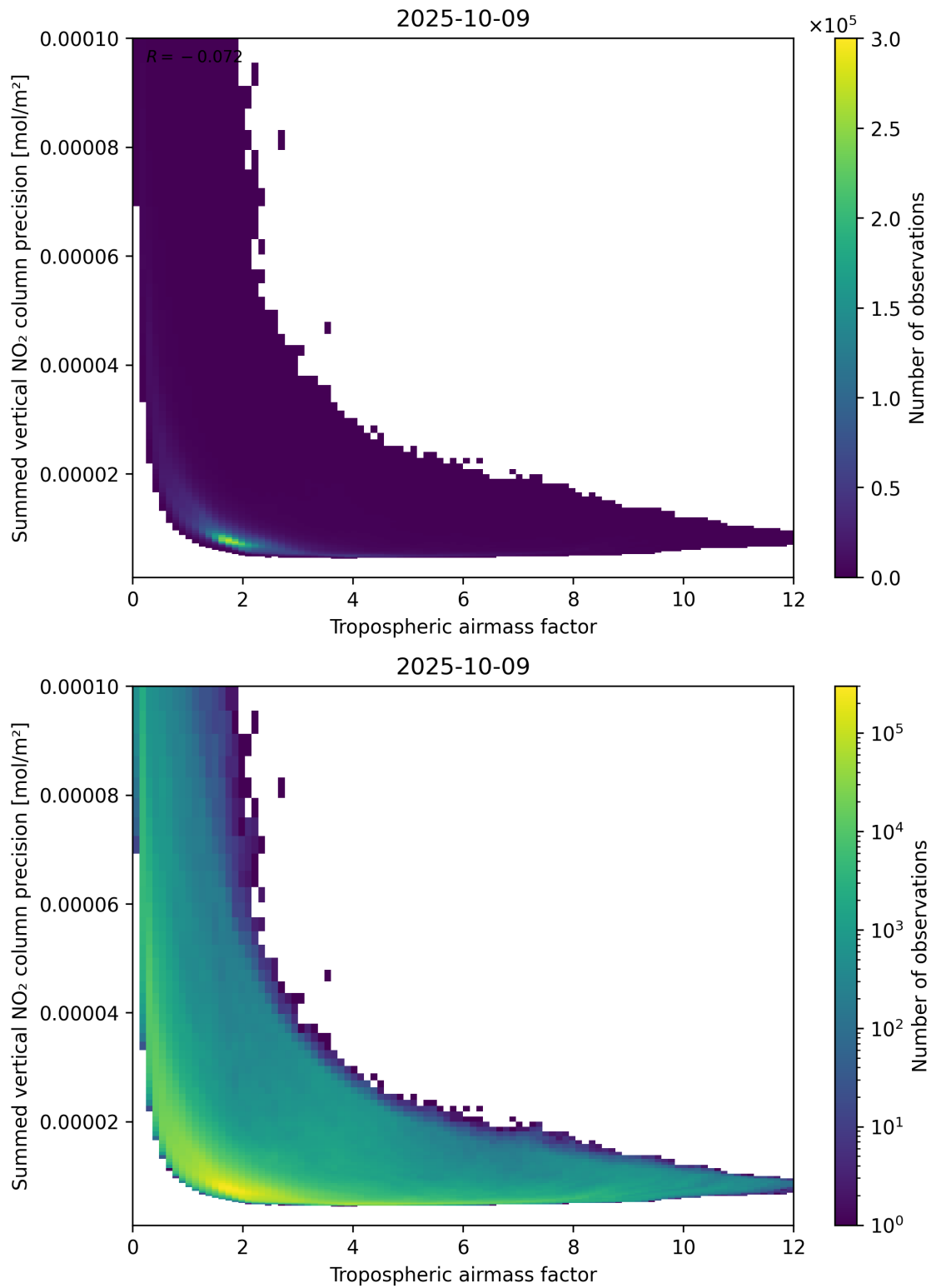
Figure 76: Scatter density plot of “Tropospheric air mass factor” against “Summed vertical NO 2 column precision” for 2025-10-08 to 2025-10-10.
