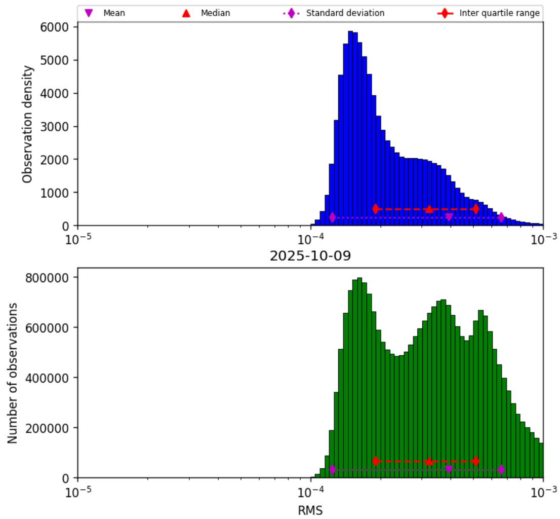
Figure 43: Histogram of “RMS” for 2025-10-08 to 2025-10-10
