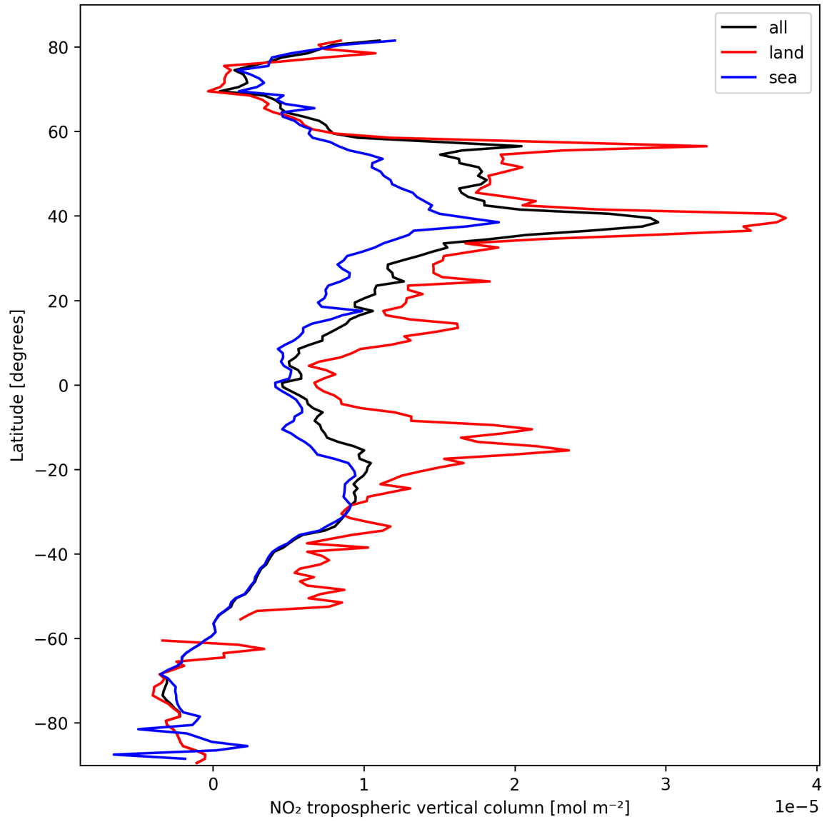
Figure 12: Zonal average of “NO 2 tropospheric vertical column” for 2025-10-08 to 2025-10-10.
