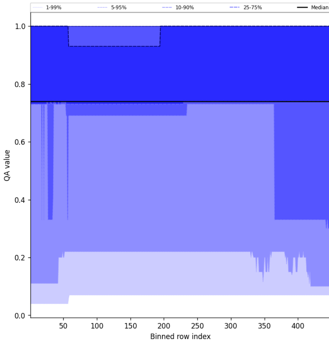
Figure 45: Along track statistics of "QA value" for 2025-10-08 to 2025-10-10
