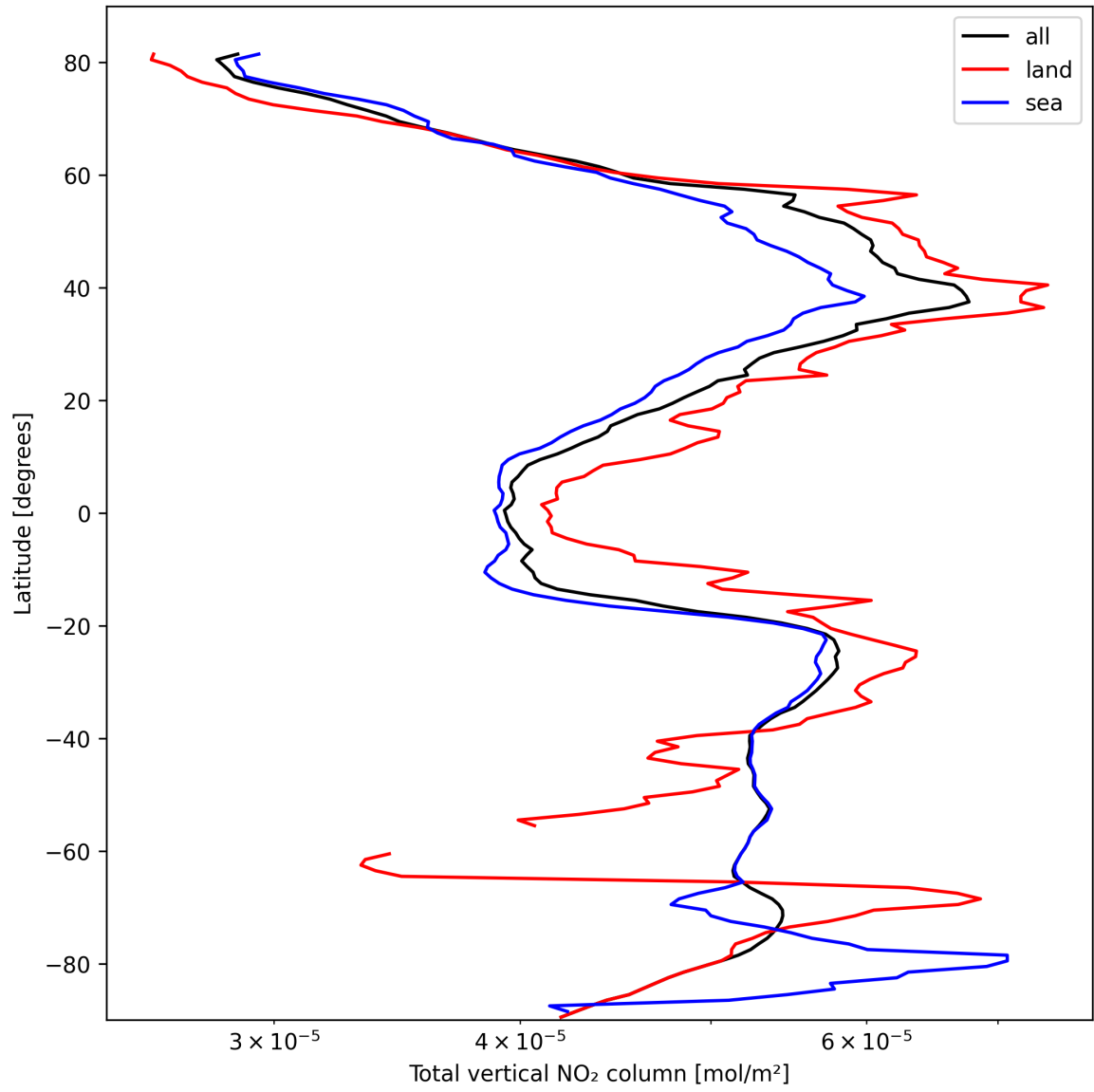
Figure 21: Zonal average of “Total vertical NO 2 column” for 2025-10-08 to 2025-10-10.
