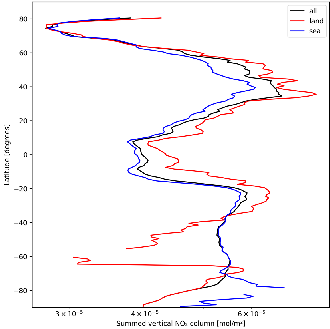
Figure 23: Zonal average of “Summed vertical NO 2 column” for 2025-10-11 to 2025-10-12.
