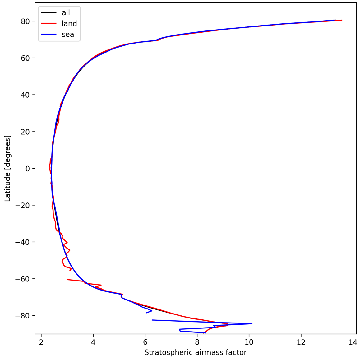
Figure 27: Zonal average of “Stratospheric airmass factor” for 2025-10-11 to 2025-10-12.
