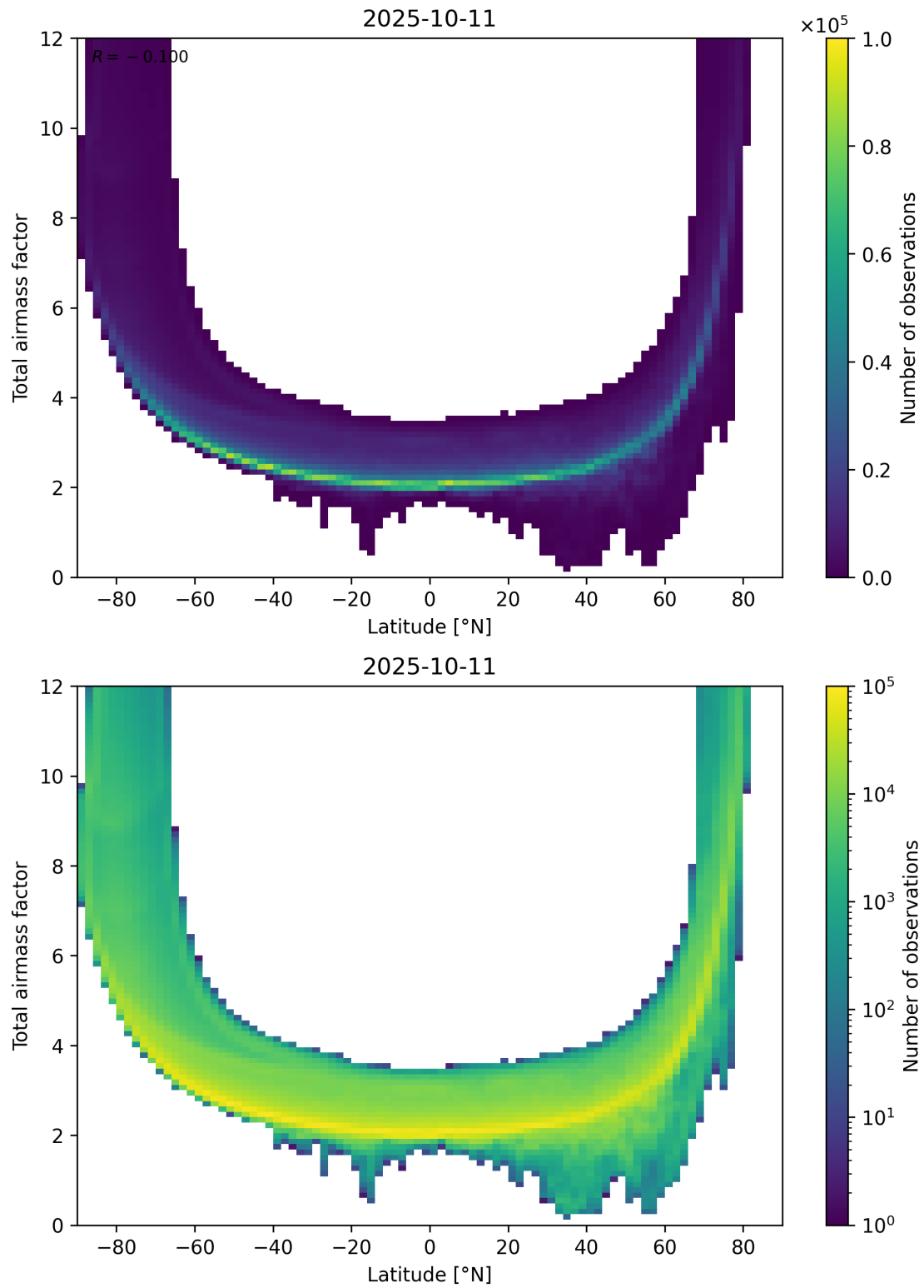
Figure 84: Scatter density plot of “Latitude” against “Total airmass factor” for 2025-10-11 to 2025-10-12.
