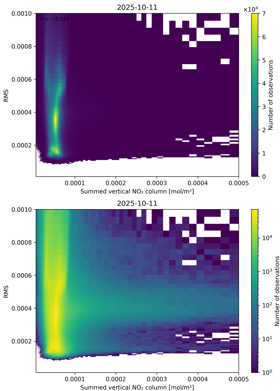
Figure 109: Scatter density plot of “Summed vertical NO 2 column” against “RMS” for 2025-10-11 to 2025-10-12.
