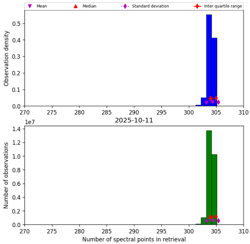
Figure 33: Histogram of “Number of spectral points in retrieval” for 2025-10-11 to 2025-10-12
