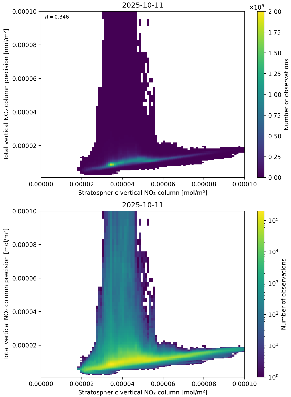
Figure 101: Scatter density plot of “Stratospheric vertical NO 2 column” against “Total vertical NO 2 column precision” for 2025-10-11 to 2025-10-12.
