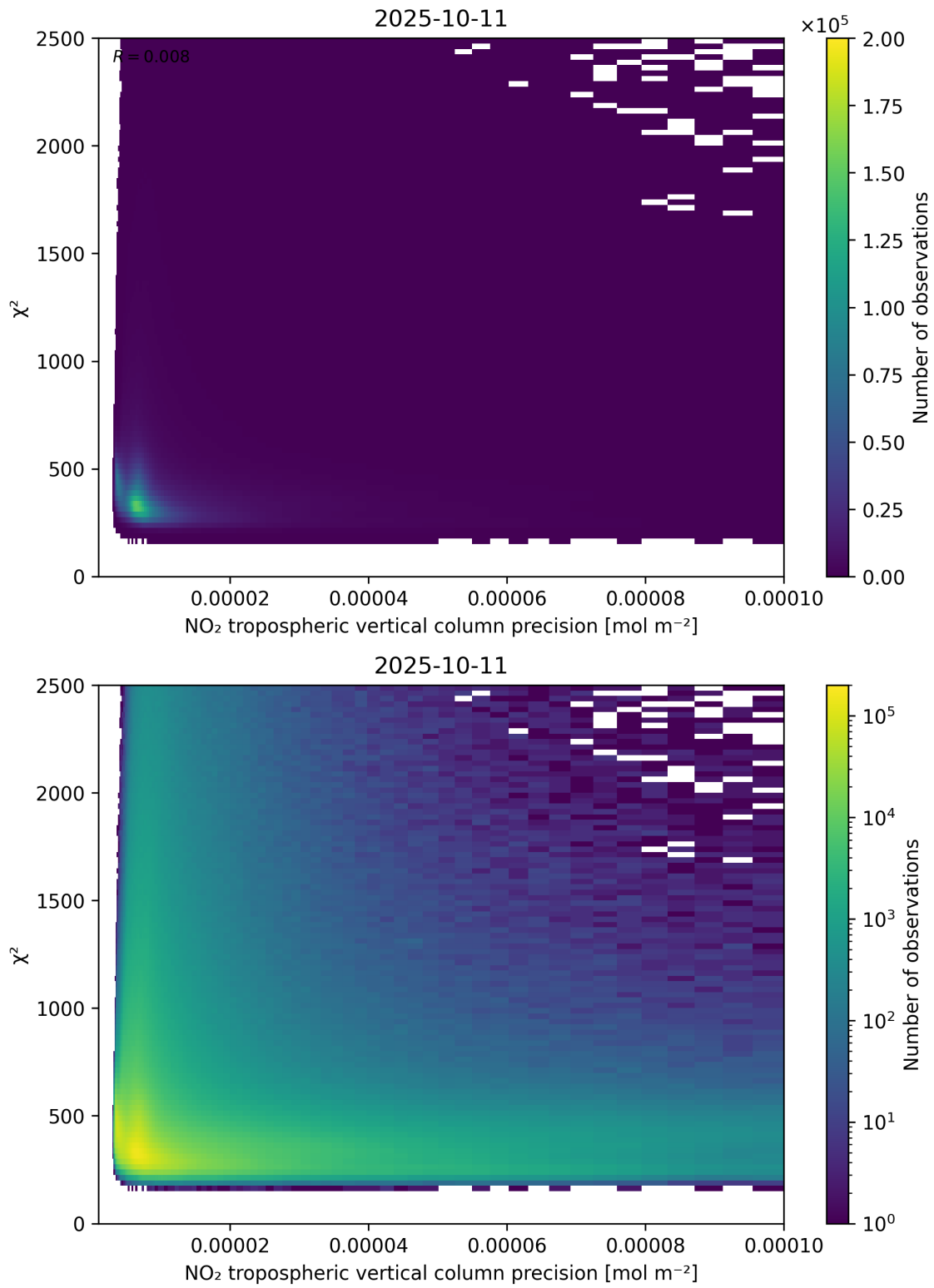
Figure 134: Scatter density plot of “NO 2 tropospheric vertical column precision” against “ \chi^2 ” for 2025-10-11 to 2025-10-12.
