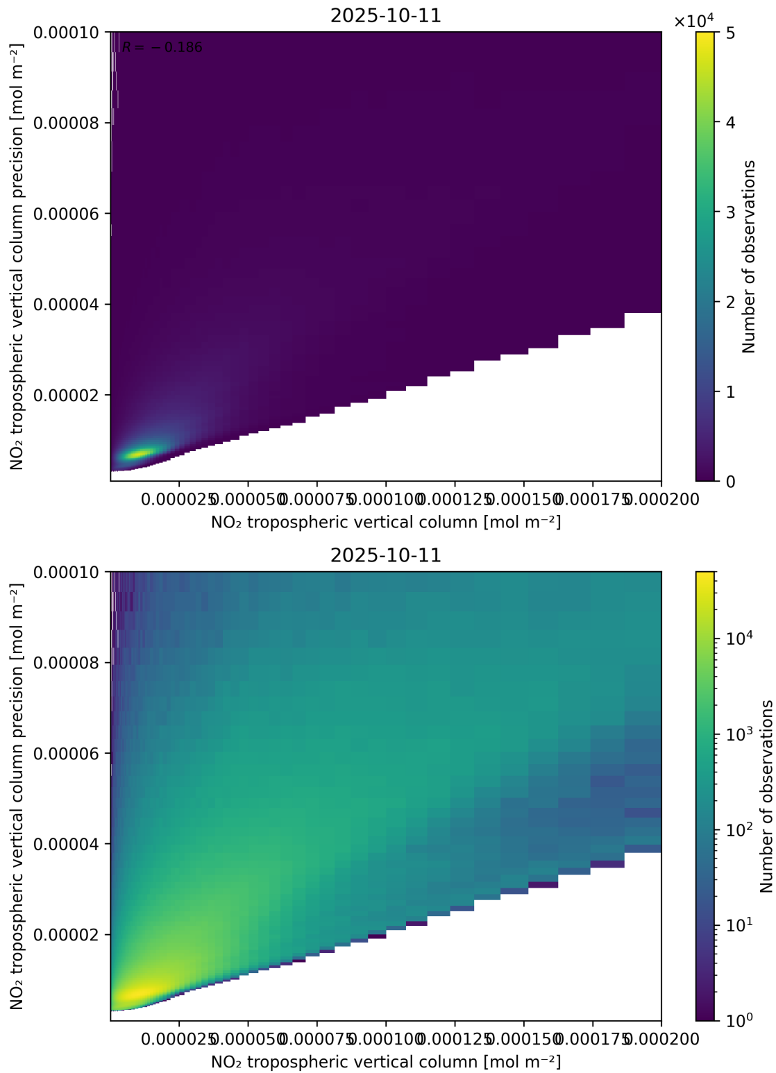
Figure 130: Scatter density plot of “NO 2 tropospheric vertical column” against “NO 2 tropospheric vertical column precision” for 2025-10-11 to 2025-10-12.
