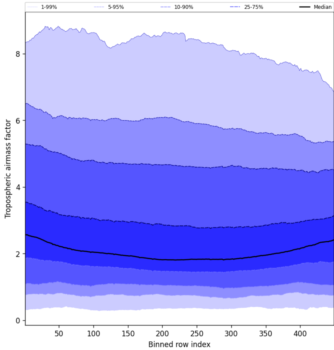
Figure 48: Along track statistics of “Tropospheric airmass factor” for 2025-10-11 to 2025-10-12
