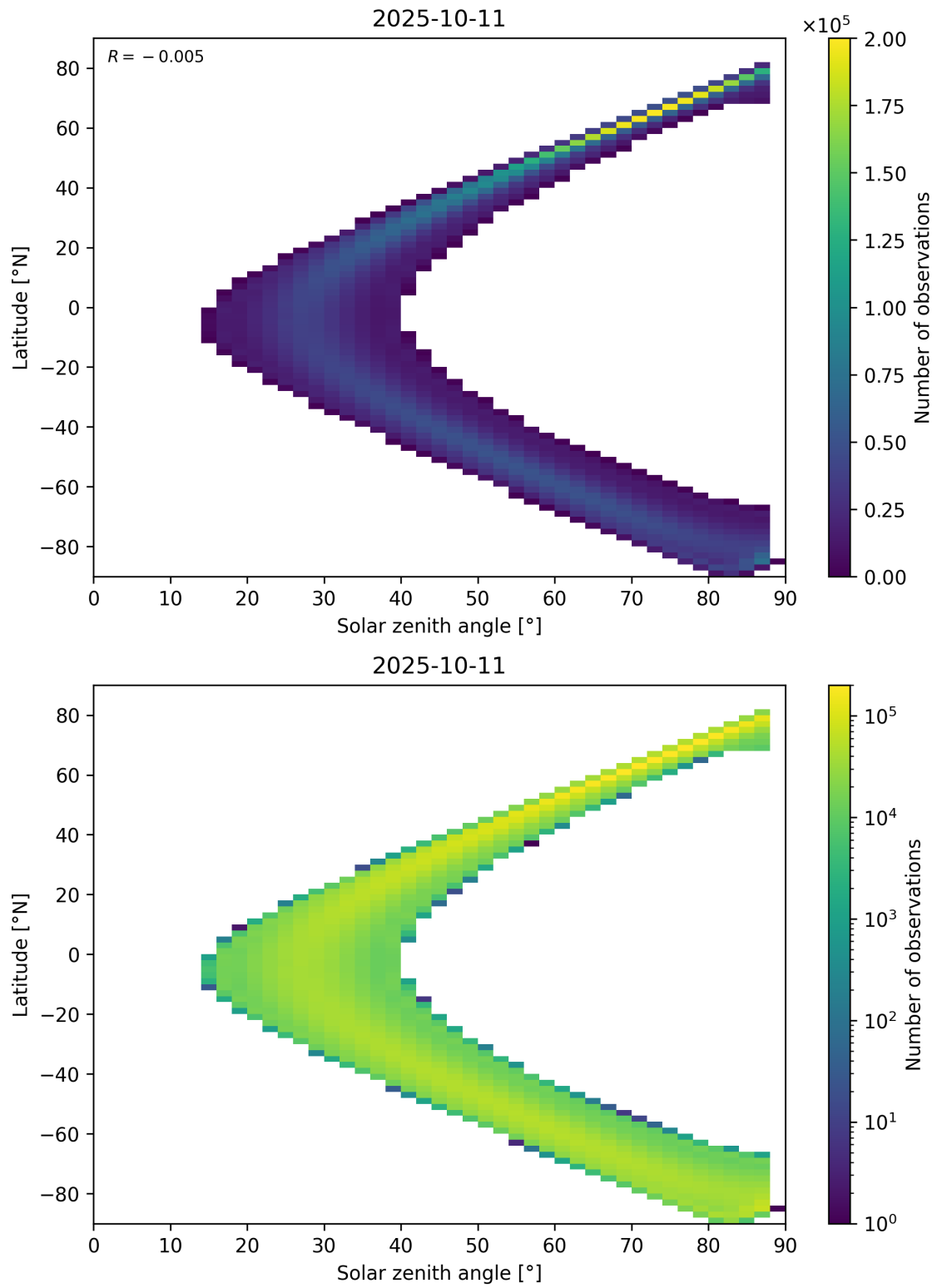
Figure 149: Scatter density plot of “Solar zenith angle” against “Latitude” for 2025-10-11 to 2025-10-12.
