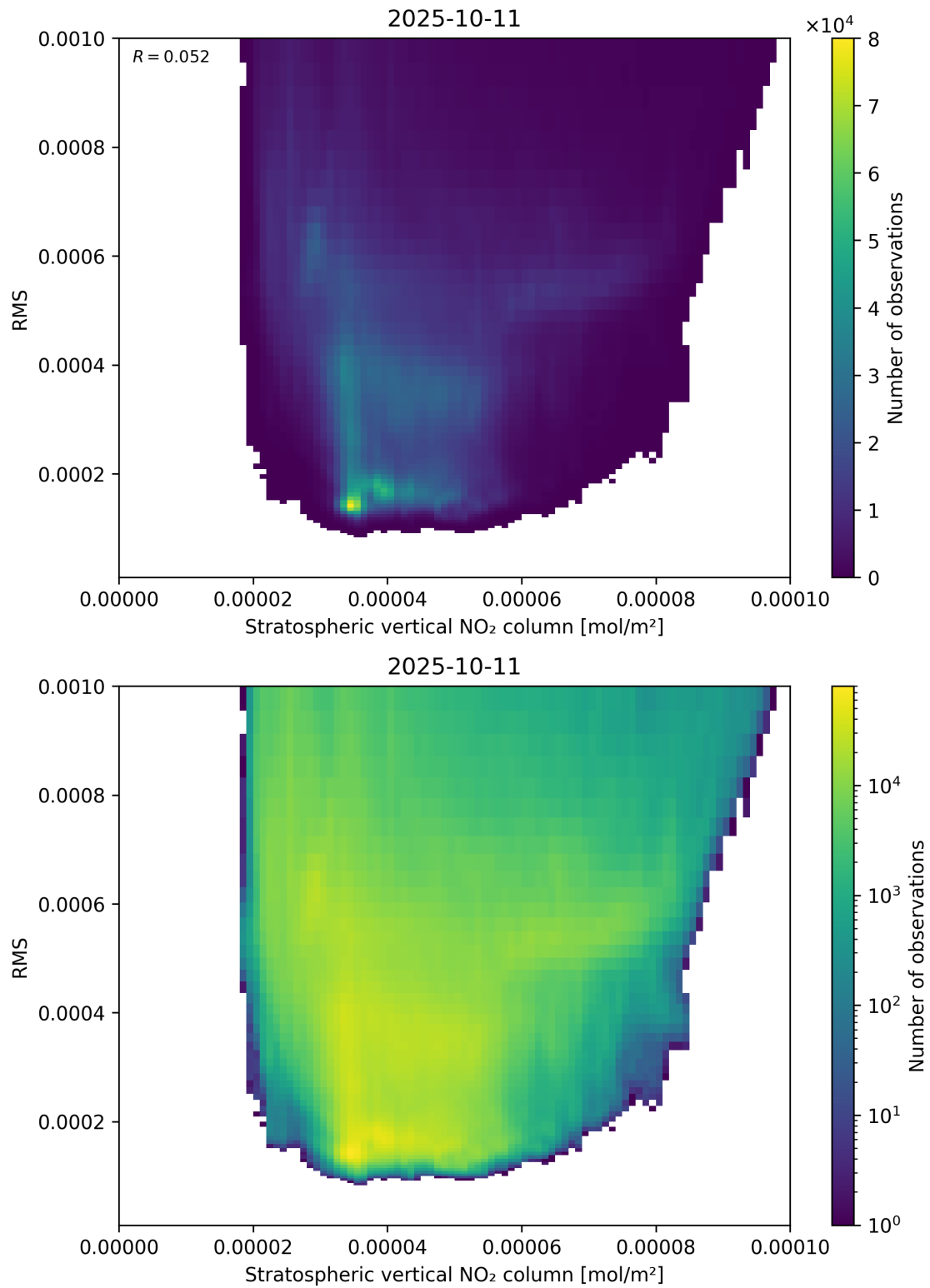
Figure 102: Scatter density plot of “Stratospheric vertical NO 2 column” against “RMS” for 2025-10-11 to 2025-10-12.
