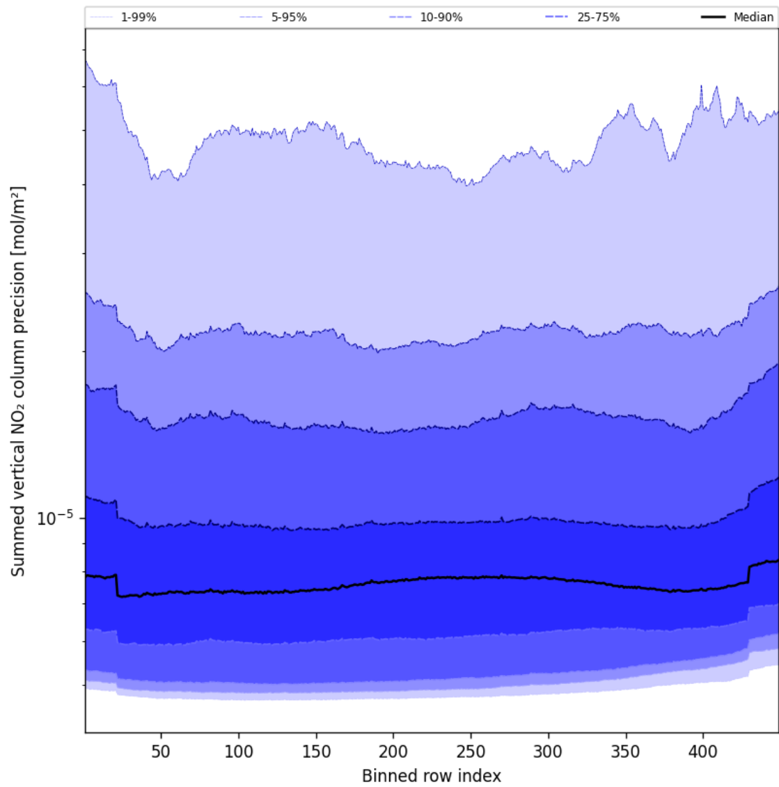
Figure 58: Along track statistics of “Summed vertical NO 2 column precision” for 2025-10-11 to 2025-10-12
