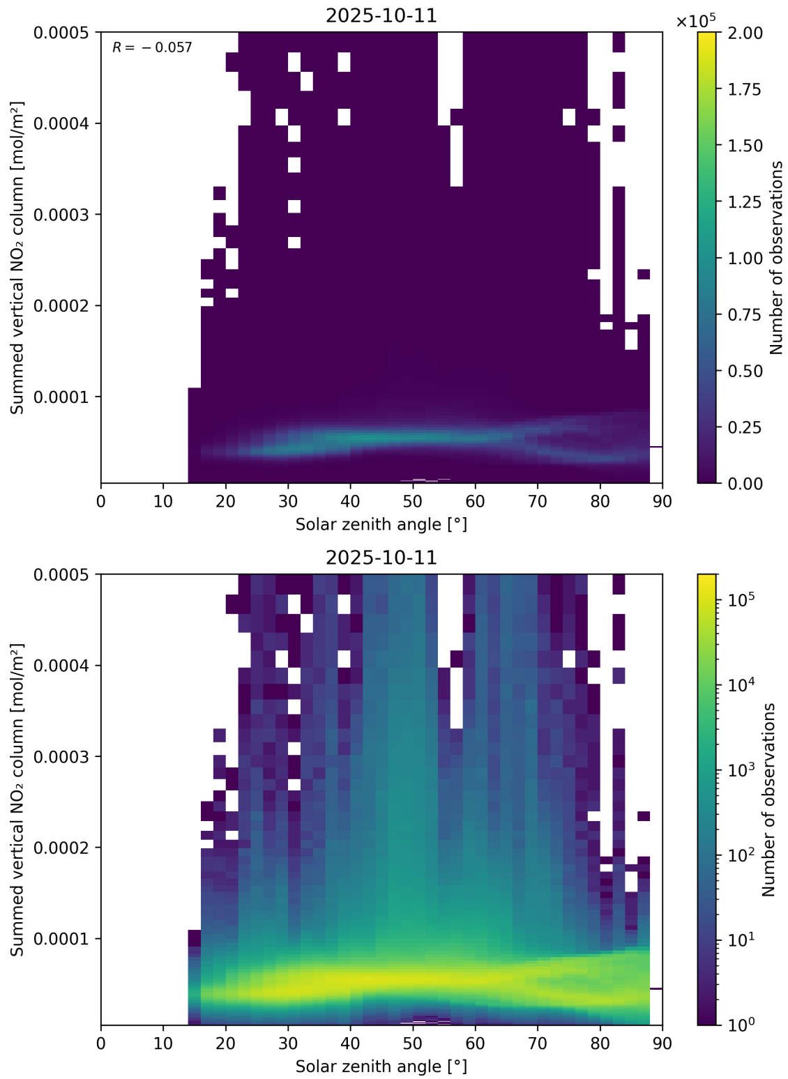
Figure 151: Scatter density plot of “Solar zenith angle” against “Summed vertical NO 2 column” for 2025-10-11 to 2025-10-12.
