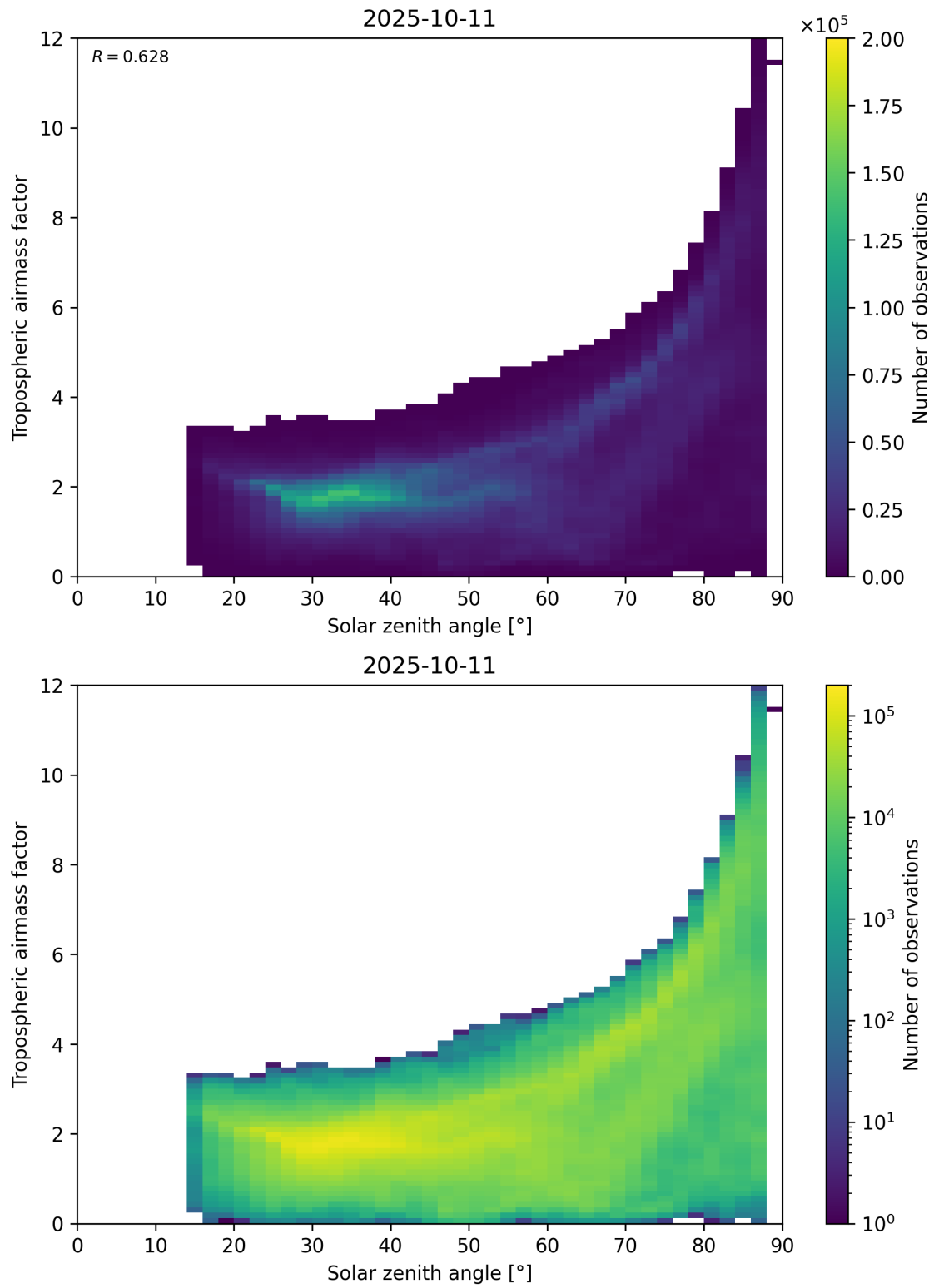
Figure 147: Scatter density plot of “Solar zenith angle” against “Tropospheric airmass factor” for 2025-10-11 to 2025-10-12.
