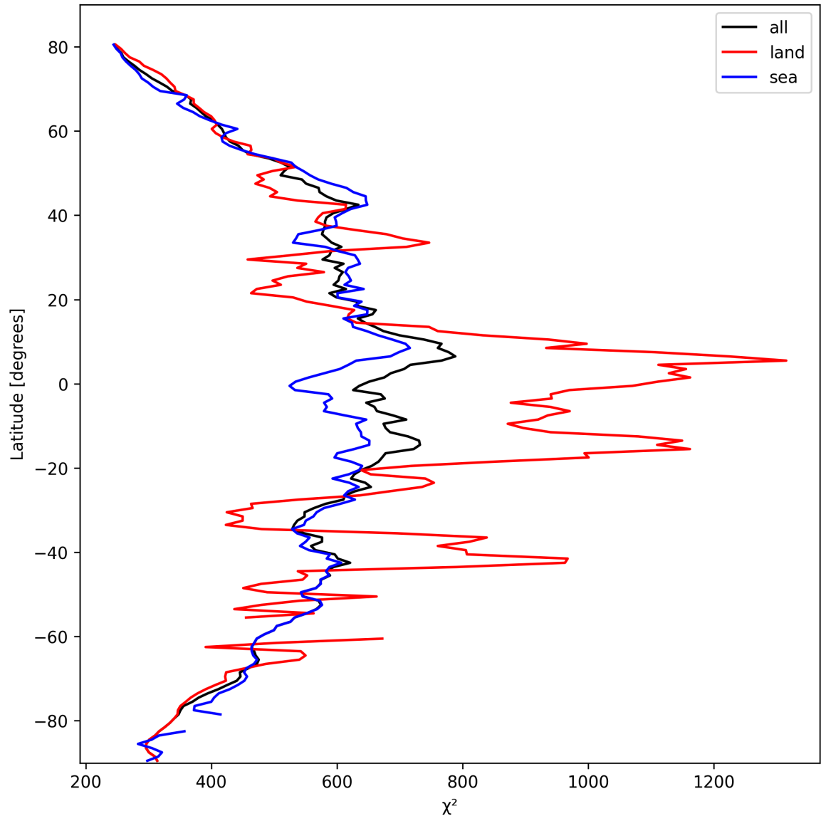
Figure 25: Zonal average of “ \chi^2 ” for 2025-10-11 to 2025-10-12.
