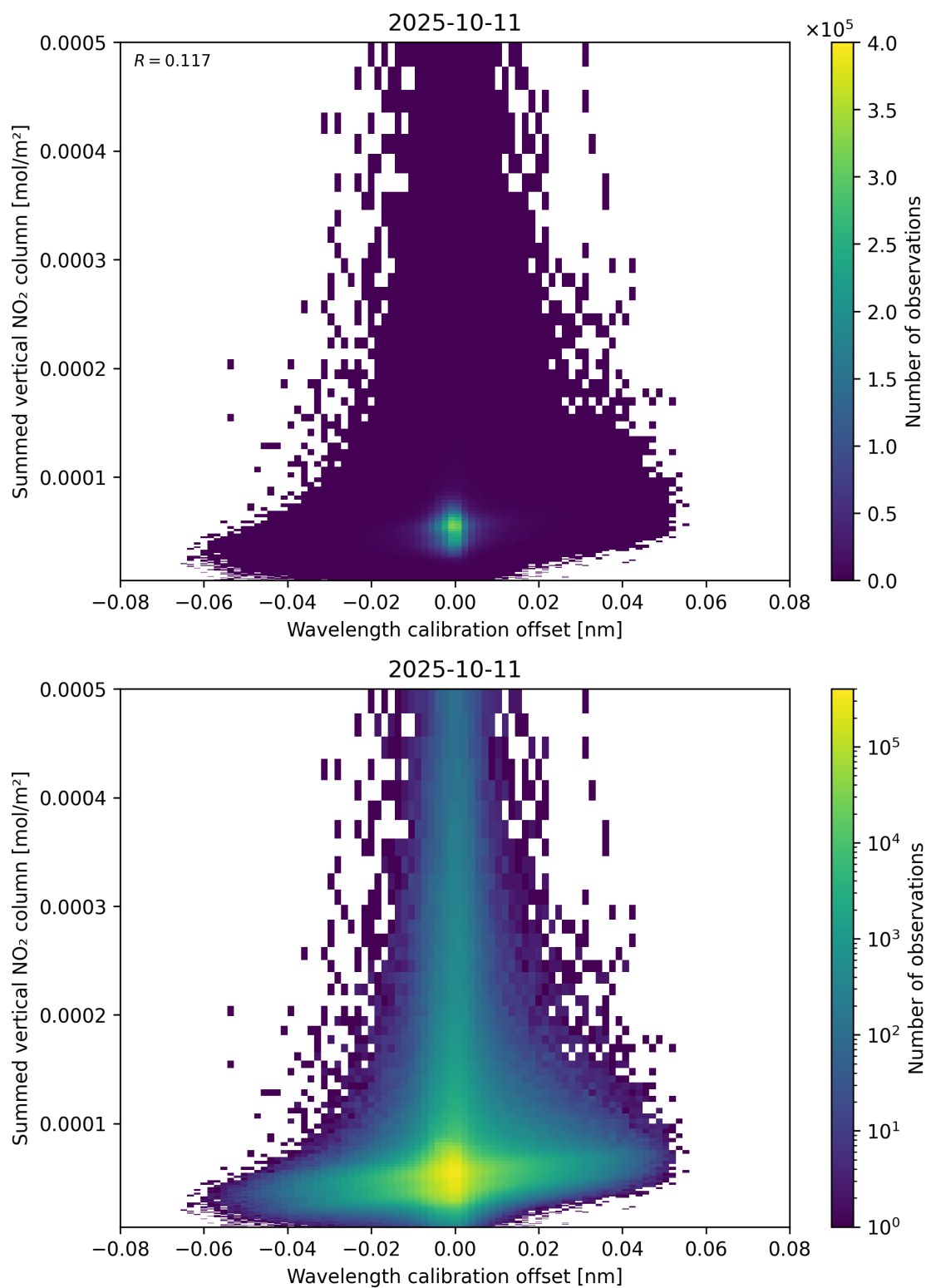
Figure 177: Scatter density plot of “Wavelength calibration offset” against “Summed vertical NO 2 column” for 2025-10-11 to 2025-10-12.
