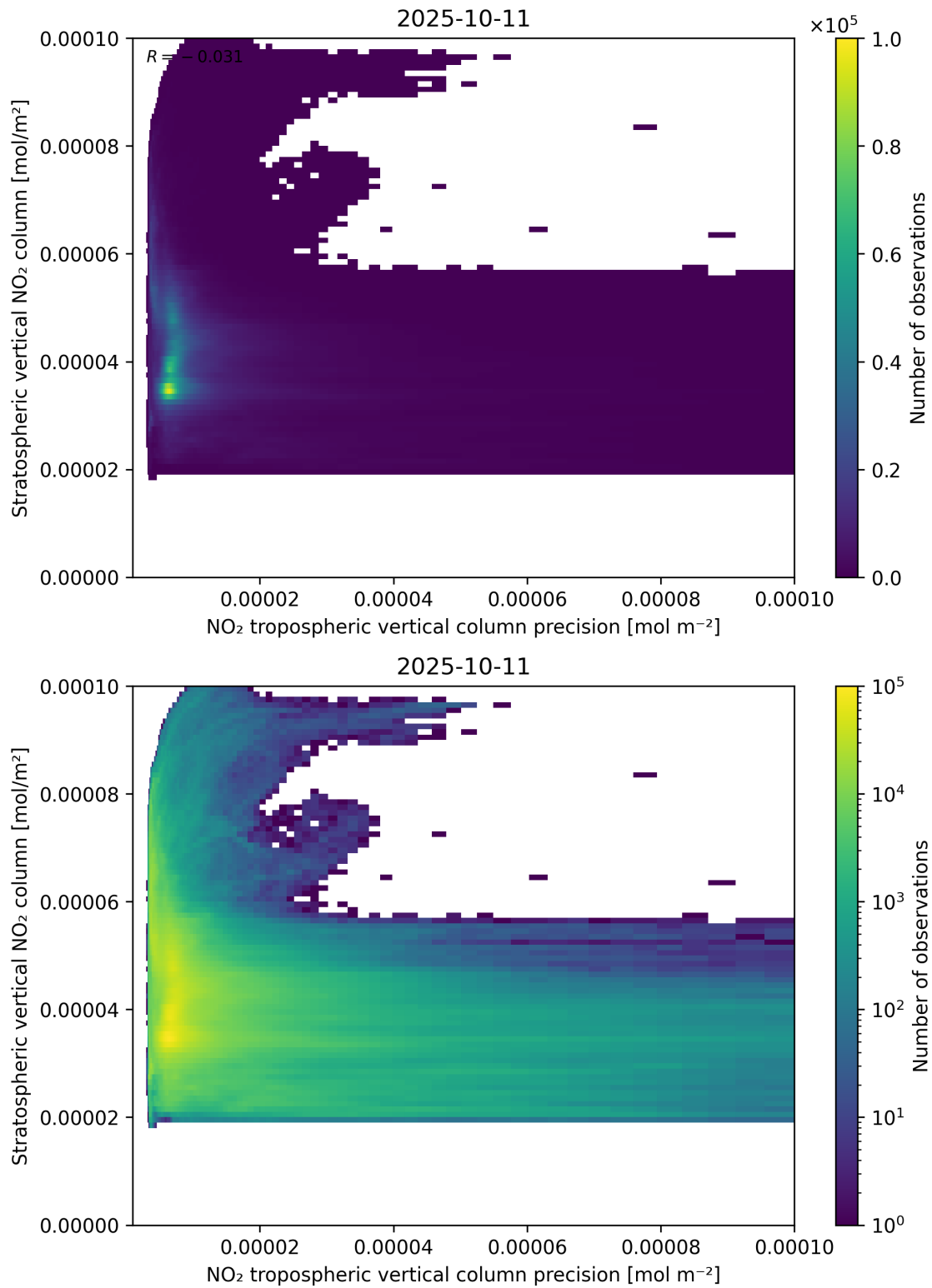
Figure 135: Scatter density plot of “NO 2 tropospheric vertical column precision” against “Stratospheric vertical NO 2 column” for 2025-10-11 to 2025-10-12.
