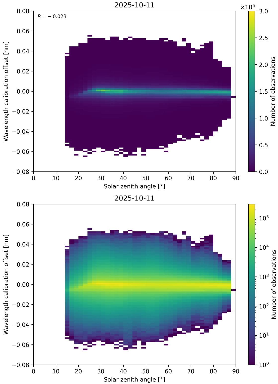
Figure 158: Scatter density plot of “Solar zenith angle” against “Wavelength calibration offset” for 2025-10-11 to 2025-10-12.
