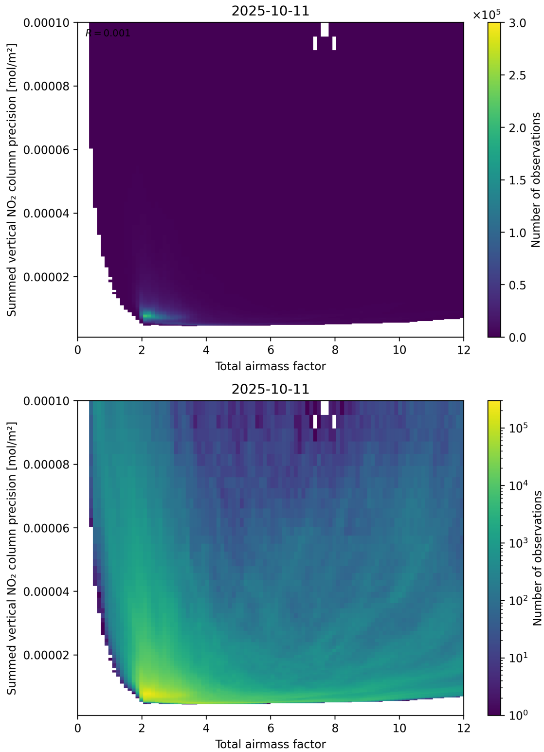
Figure 66: Scatter density plot of “Total airmass factor” against “Summed vertical NO 2 column precision” for 2025-10-11 to 2025-10-12.
