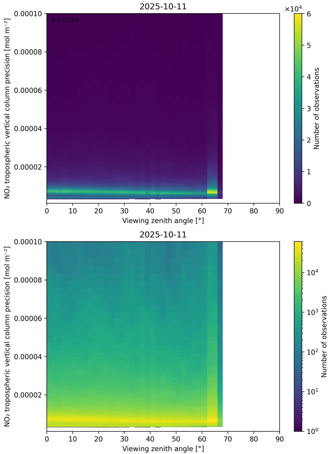
Figure 170: Scatter density plot of “Viewing zenith angle” against “NO 2 tropospheric vertical column precision” for 2025-10-11 to 2025-10-12.
