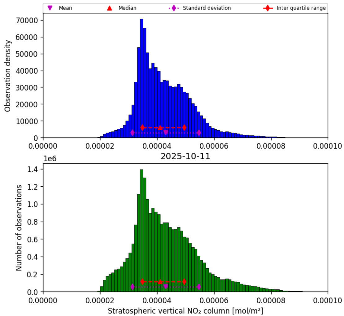
Figure 36: Histogram of “Stratospheric vertical NO 2 column” for 2025-10-11 to 2025-10-12
