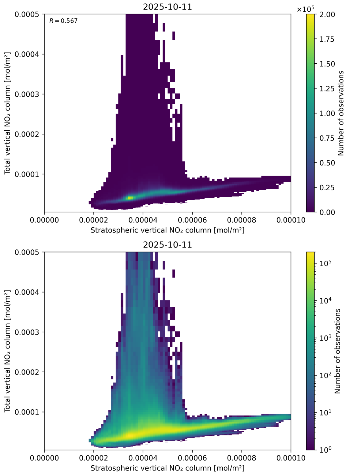
Figure 100: Scatter density plot of “Stratospheric vertical NO 2 column” against “Total vertical NO 2 column” for 2025-10-11 to 2025-10-12.
