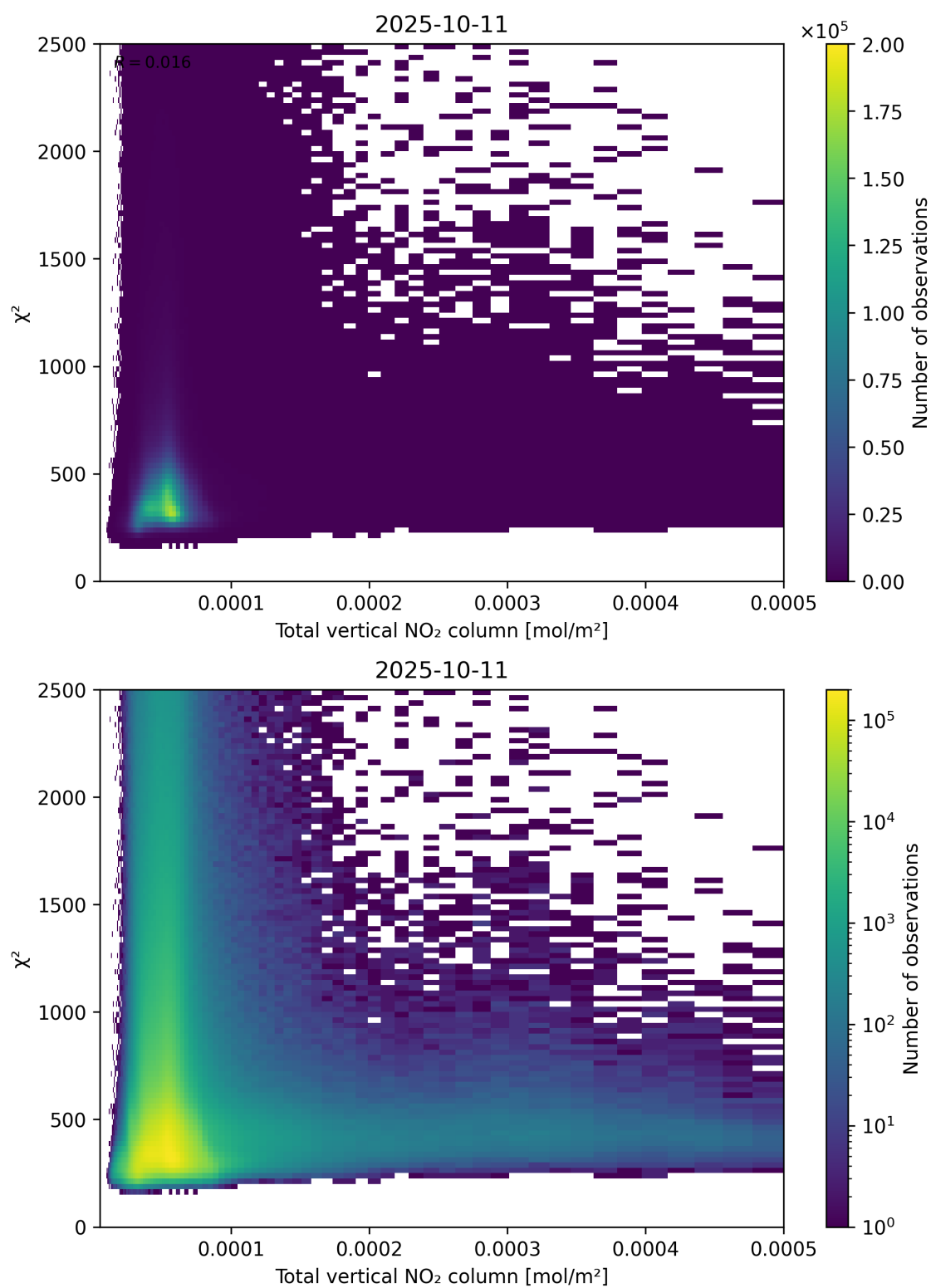
Figure 111: Scatter density plot of “Total vertical NO 2 column” against “ \chi^2 ” for 2025-10-11 to 2025-10-12.
