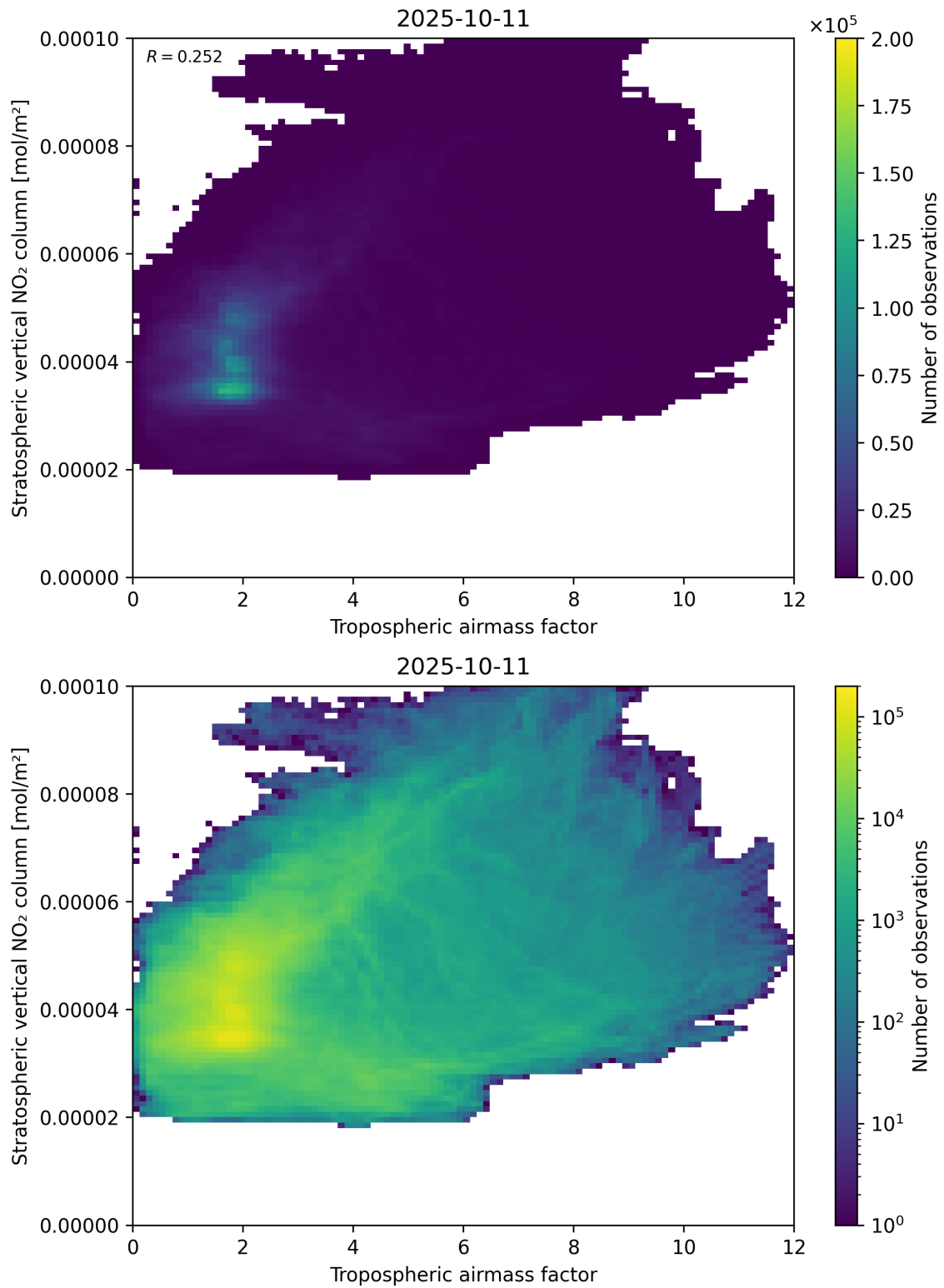
Figure 74: Scatter density plot of “Tropospheric air mass factor” against “Stratospheric vertical NO 2 column” for 2025-10-11 to 2025-10-12.
