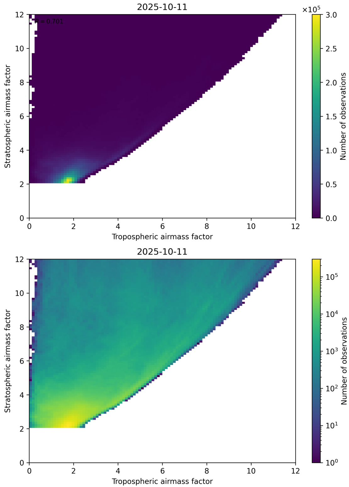
Figure 71: Scatter density plot of “Tropospheric airmass factor” against “Stratospheric airmass factor” for 2025-10-11 to 2025-10-12.
