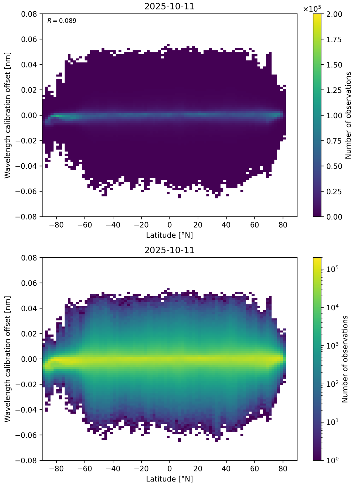
Figure 95: Scatter density plot of “Latitude” against “Wavelength calibration offset” for 2025-10-11 to 2025-10-12.
