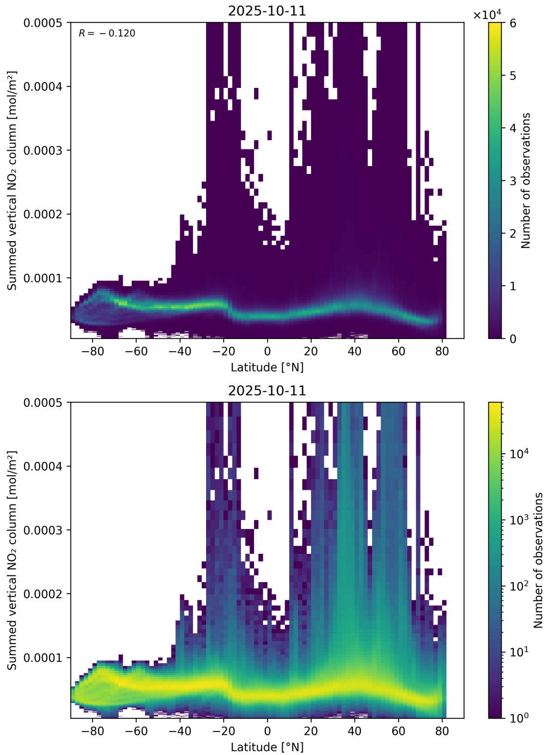
Figure 88: Scatter density plot of “Latitude” against “Summed vertical NO 2 column” for 2025-10-11 to 2025-10-12.
