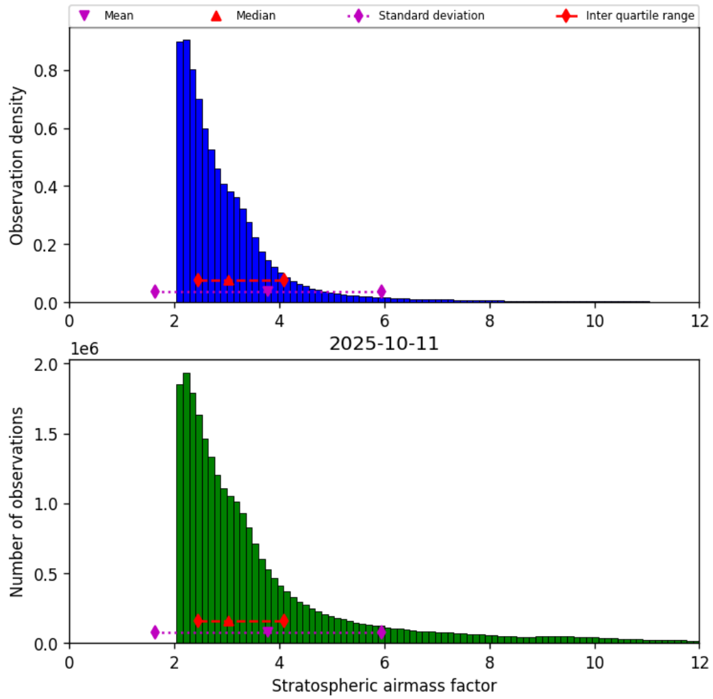
Figure 44: Histogram of “Stratospheric airmass factor” for 2025-10-11 to 2025-10-12
