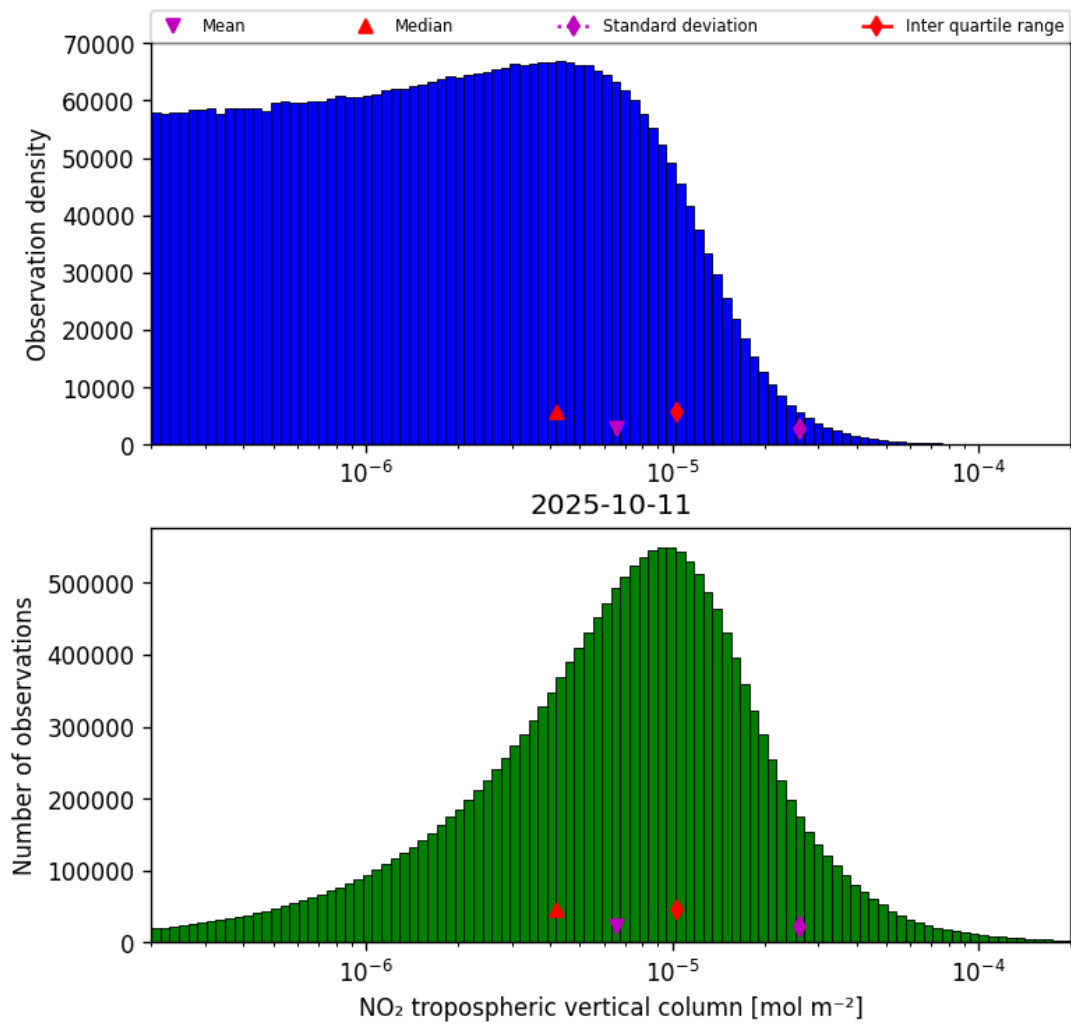
Figure 29: Histogram of “NO 2 tropospheric vertical column” for 2025-10-11 to 2025-10-12
