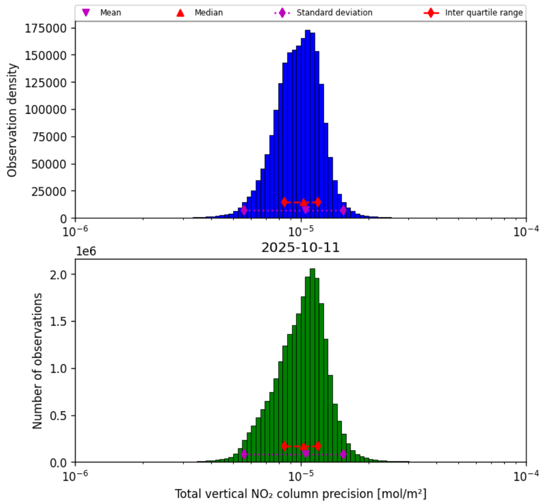
Figure 39: Histogram of “Total vertical NO 2 column precision” for 2025-10-11 to 2025-10-12
