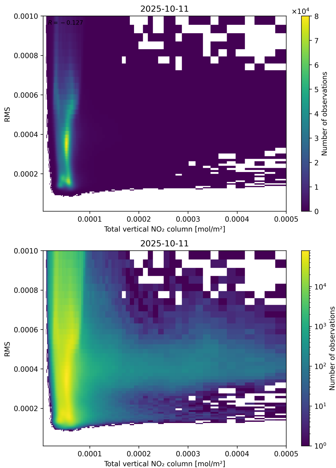
Figure 120: Scatter density plot of “Total vertical NO 2 column” against “RMS” for 2025-10-11 to 2025-10-12.
