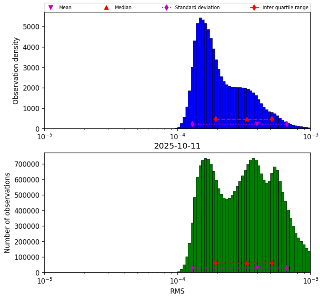
Figure 43: Histogram of “RMS” for 2025-10-11 to 2025-10-12
