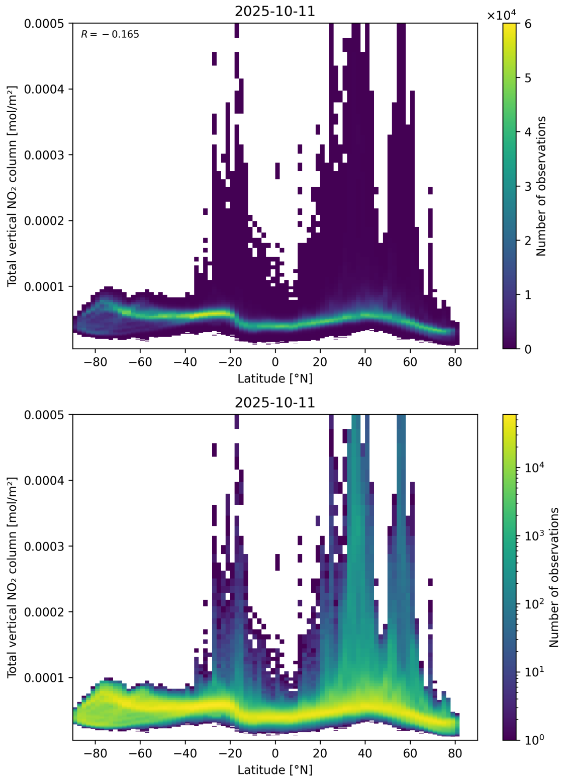
Figure 90: Scatter density plot of “Latitude” against “Total vertical NO 2 column” for 2025-10-11 to 2025-10-12.
