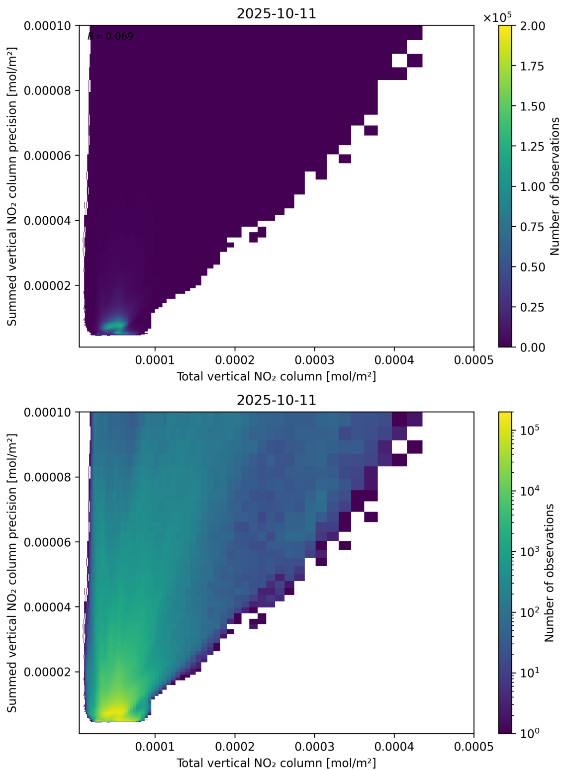
Figure 113: Scatter density plot of “Total vertical NO 2 column” against “Summed vertical NO 2 column precision” for 2025-10-11 to 2025-10-12.
