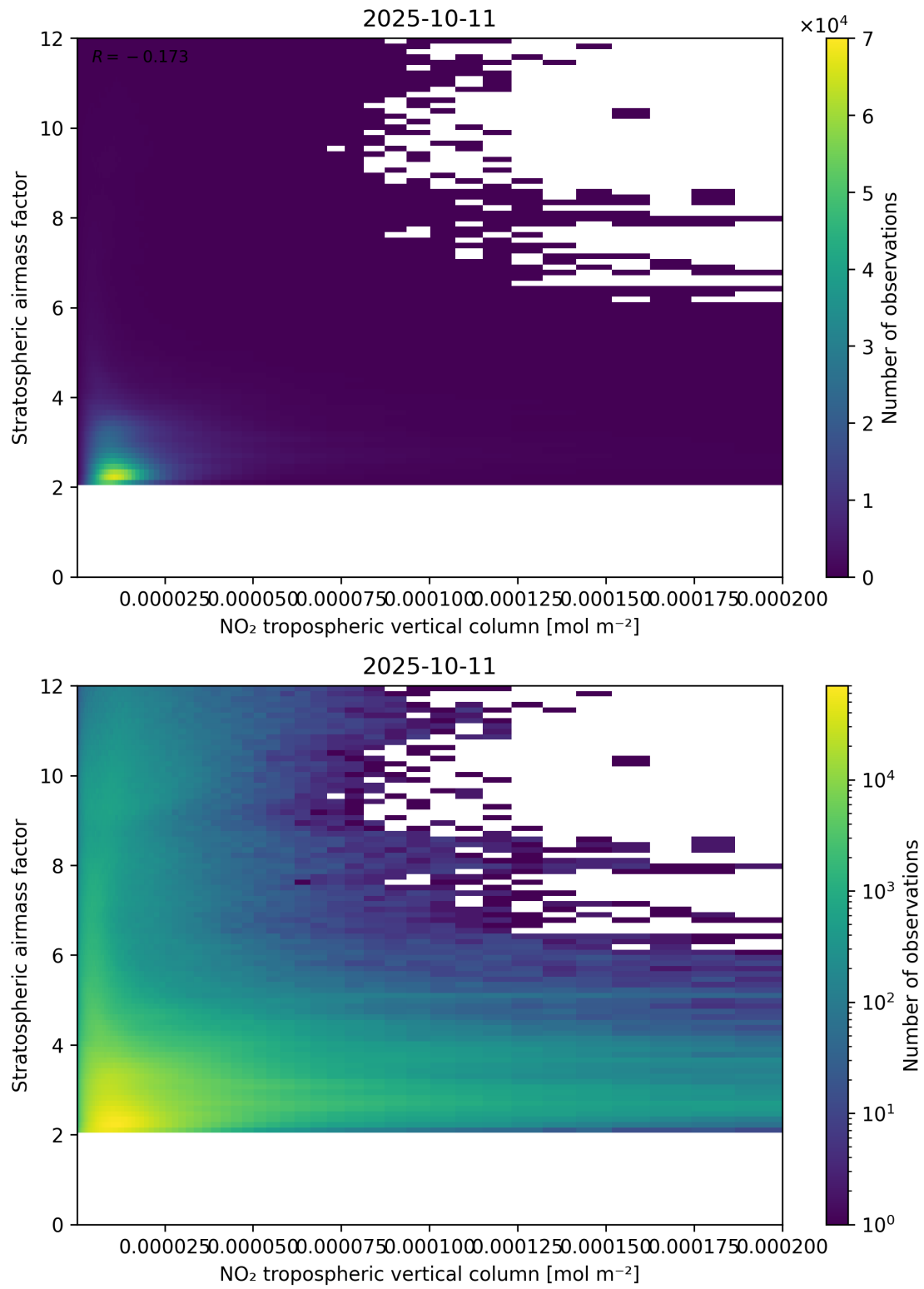
Figure 121: Scatter density plot of “NO 2 tropospheric vertical column” against “Stratospheric air mass factor” for 2025-10-11 to 2025-10-12.
