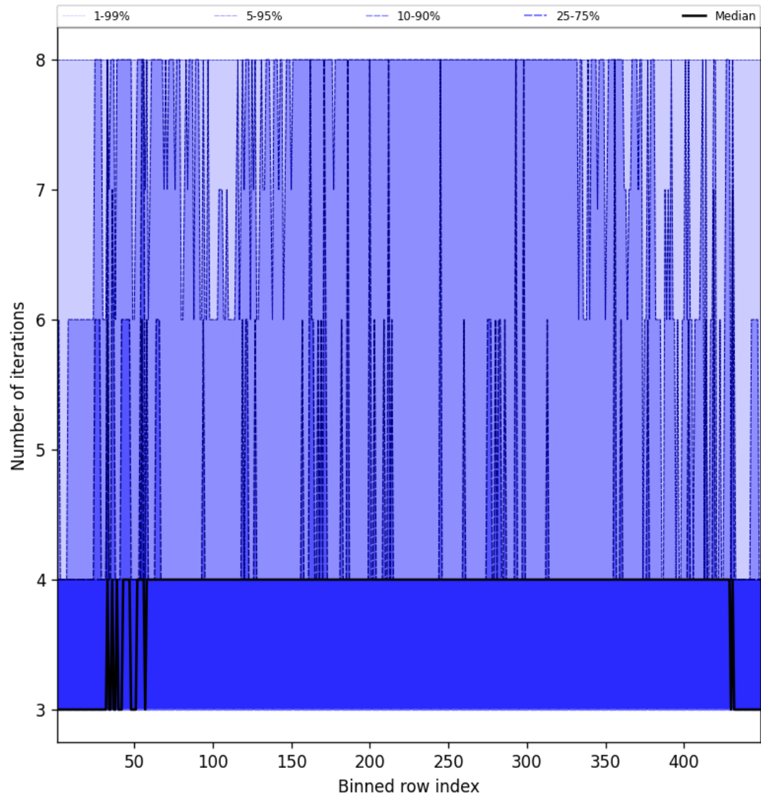
Figure 51: Along track statistics of “Number of iterations” for 2025-10-11 to 2025-10-12
