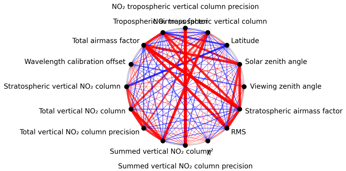
Figure 1: Map of correlation graph for 2025-10-11 to 2025-10-12.
