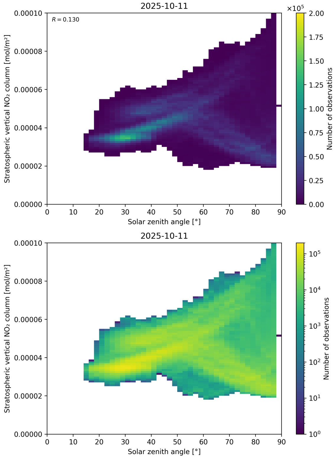
Figure 150: Scatter density plot of “Solar zenith angle” against “Stratospheric vertical \text{NO}_2 column” for 2025-10-11 to 2025-10-12.
