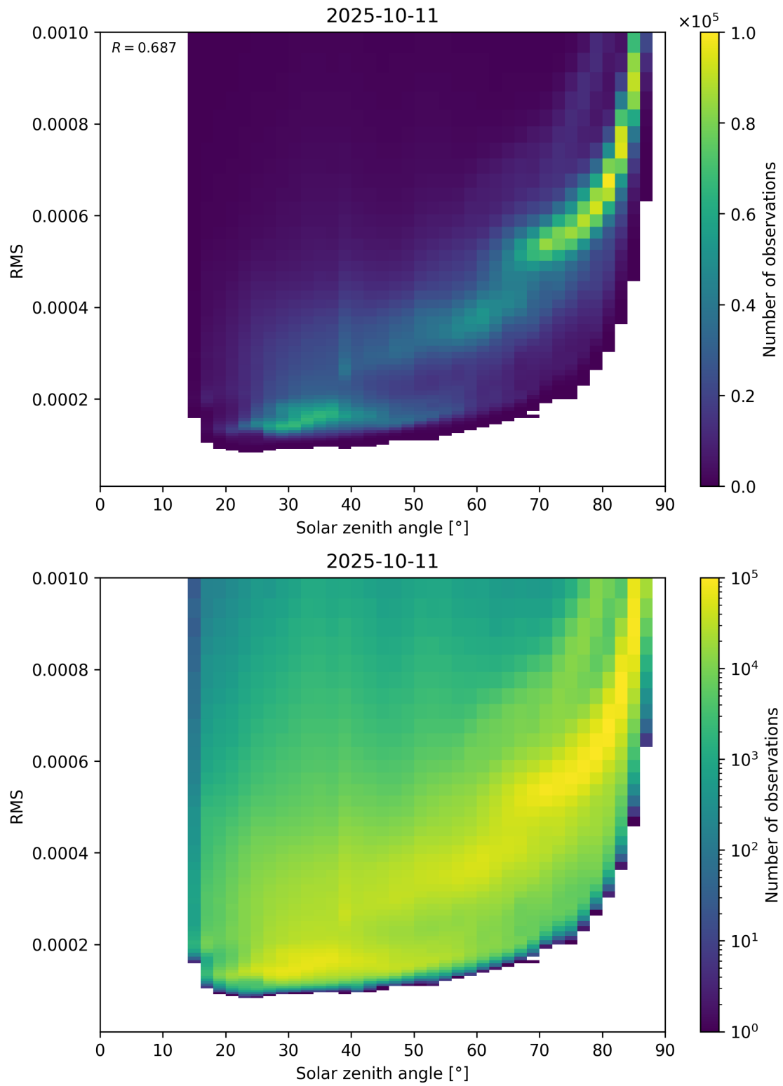
Figure 157: Scatter density plot of “Solar zenith angle” against “RMS” for 2025-10-11 to 2025-10-12.
