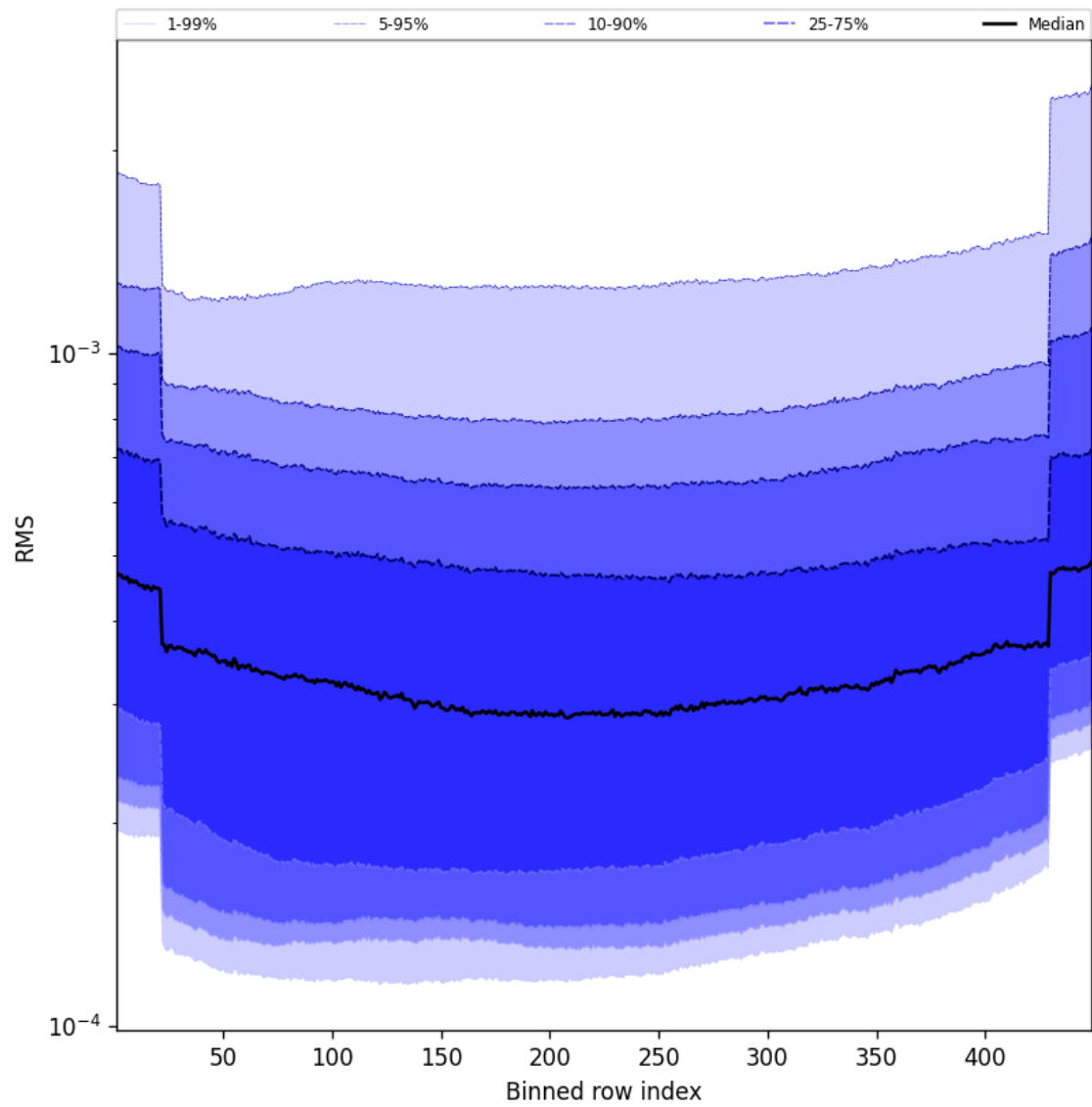
Figure 60: Along track statistics of “RMS” for 2025-10-11 to 2025-10-12
