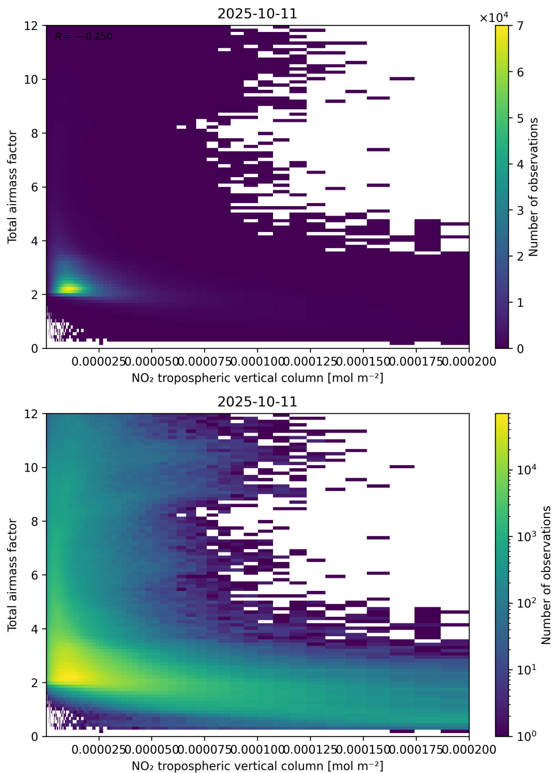
Figure 122: Scatter density plot of “NO 2 tropospheric vertical column” against “Total airmass factor” for 2025-10-11 to 2025-10-12.
