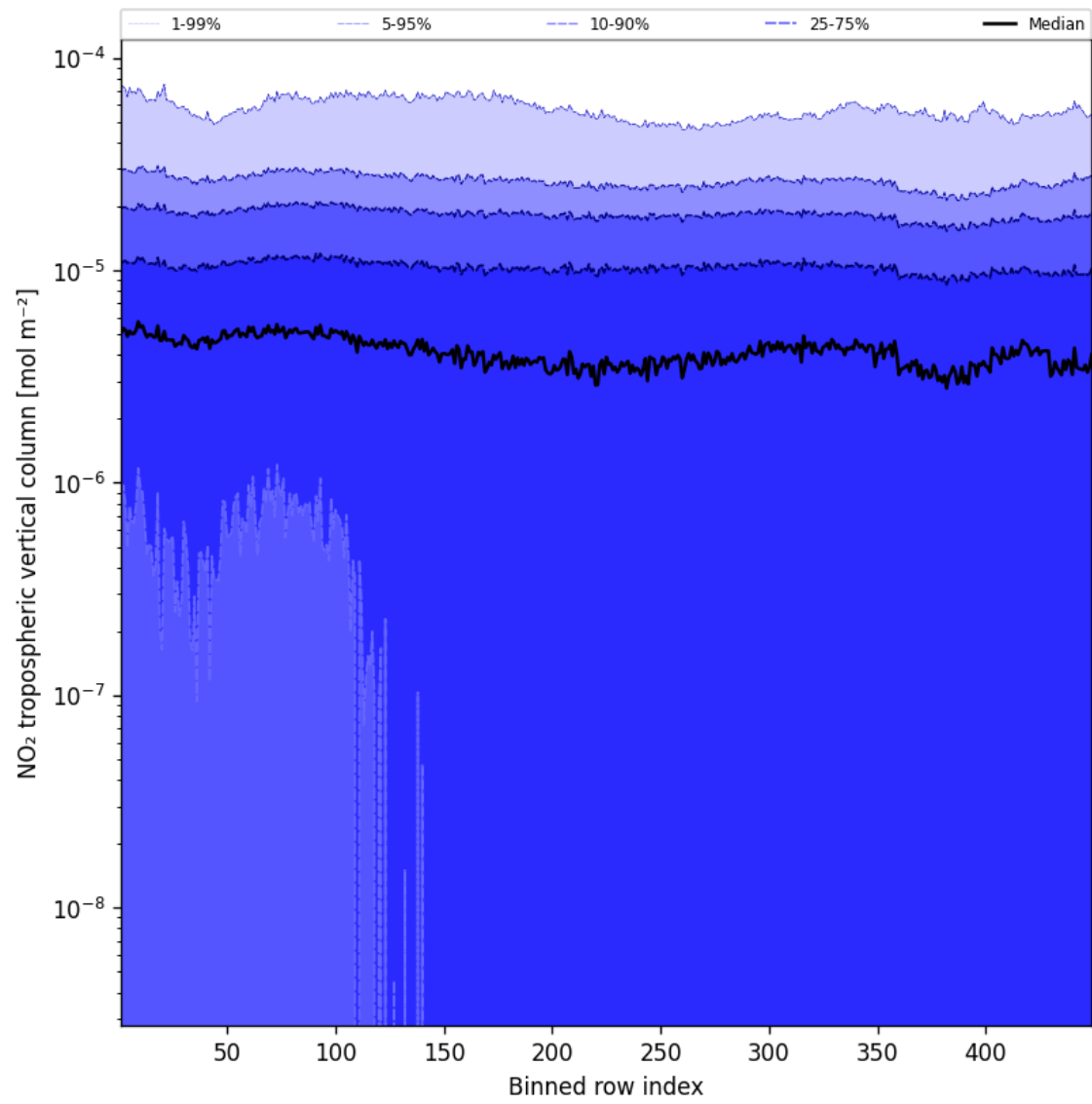
Figure 46: Along track statistics of “NO 2 tropospheric vertical column” for 2025-10-11 to 2025-10-12
