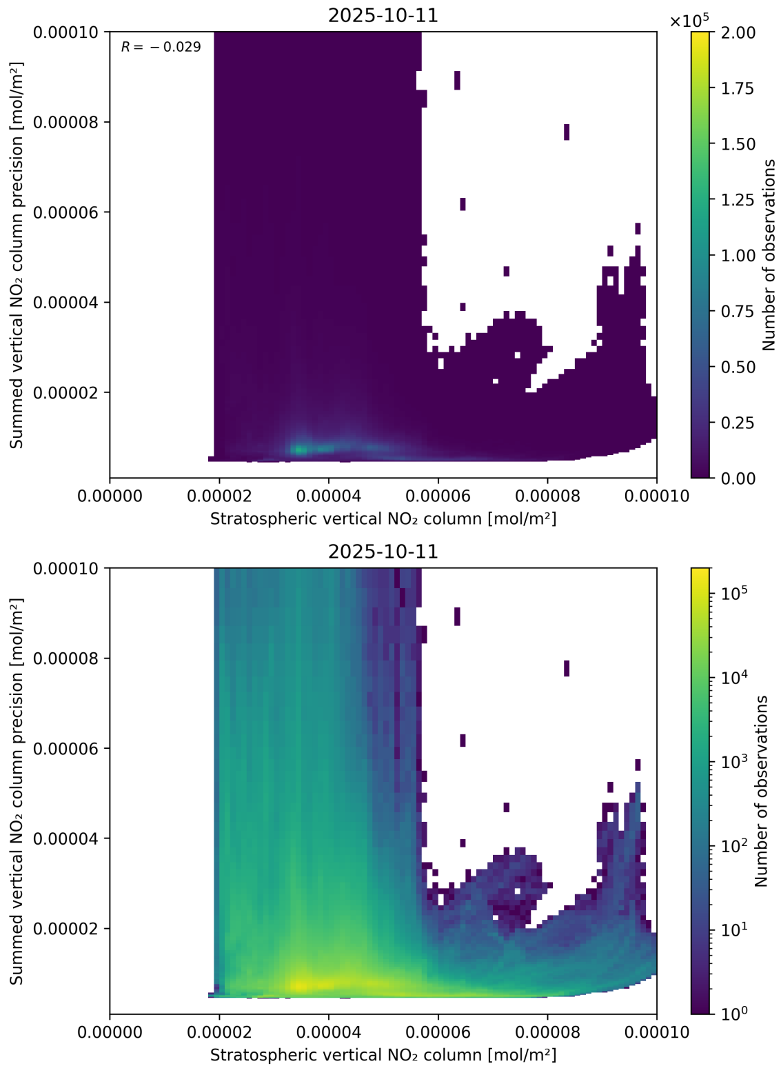
Figure 99: Scatter density plot of “Stratospheric vertical NO 2 column” against “Summed vertical NO 2 column precision” for 2025-10-11 to 2025-10-12.
