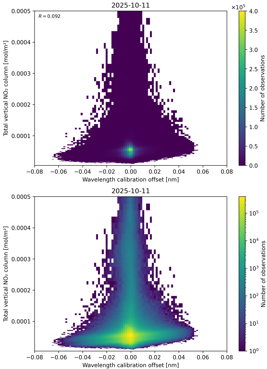
Figure 179: Scatter density plot of “Wavelength calibration offset” against “Total vertical NO 2 column” for 2025-10-11 to 2025-10-12.
