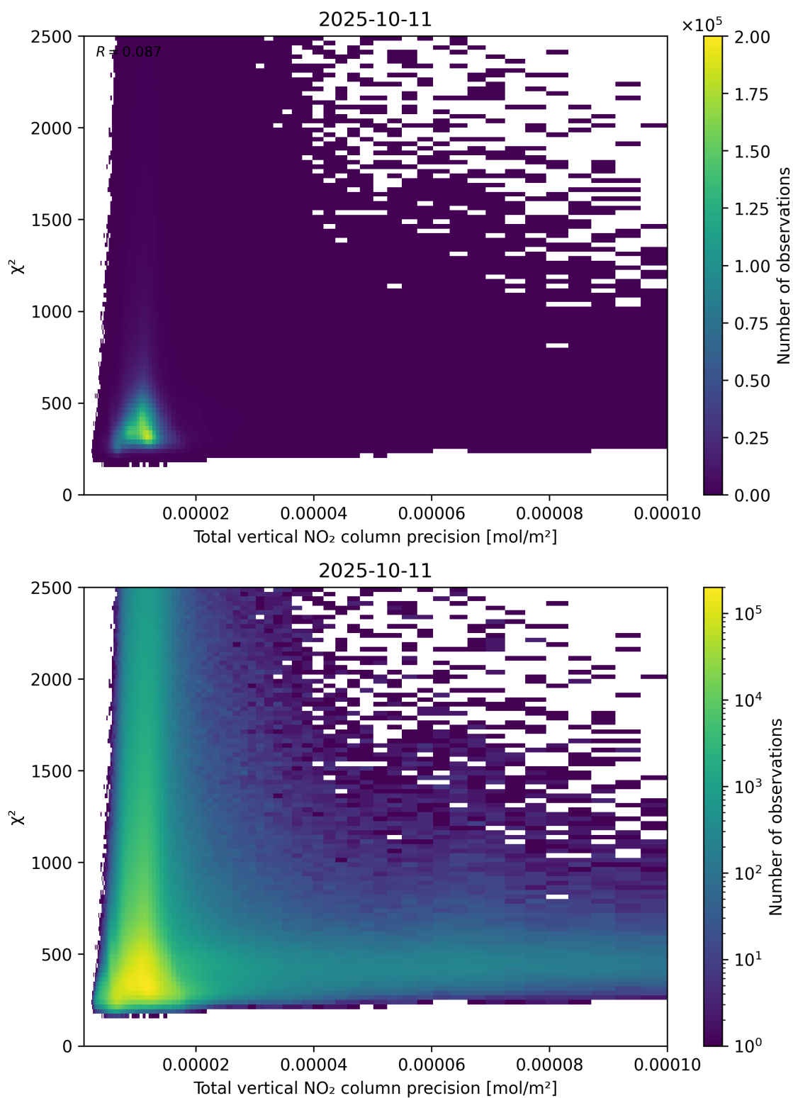
Figure 116: Scatter density plot of “Total vertical NO 2 column precision” against “ \chi^2 ” for 2025-10-11 to 2025-10-12.
