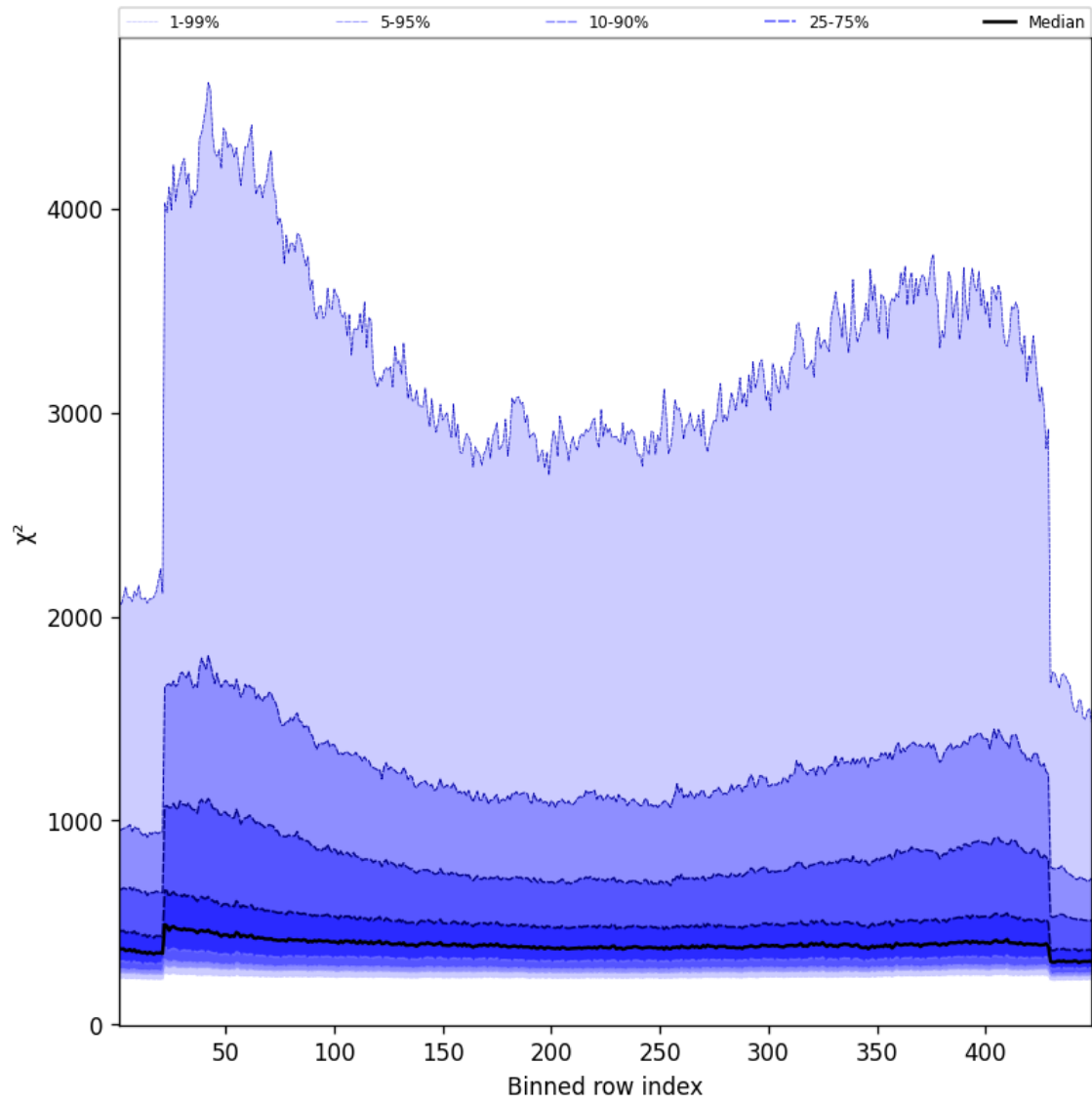
Figure 59: Along track statistics of “ \chi^2 ” for 2025-10-11 to 2025-10-12
