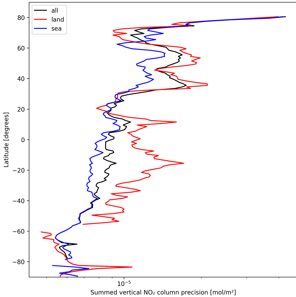
Figure 24: Zonal average of “Summed vertical NO 2 column precision” for 2025-10-11 to 2025-10-12.
