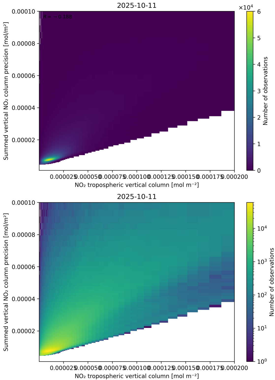
Figure 127: Scatter density plot of “NO 2 tropospheric vertical column” against “Summed vertical NO 2 column precision” for 2025-10-11 to 2025-10-12.
