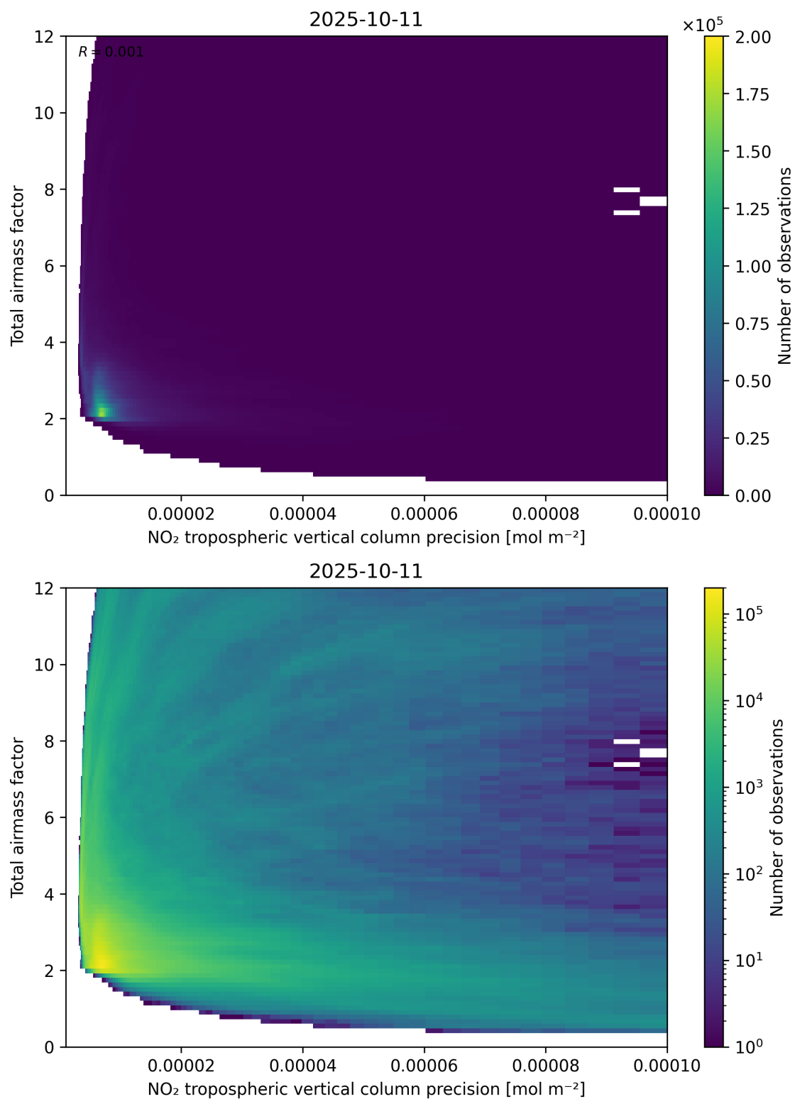
Figure 132: Scatter density plot of “NO 2 tropospheric vertical column precision” against “Total air mass factor” for 2025-10-11 to 2025-10-12.
