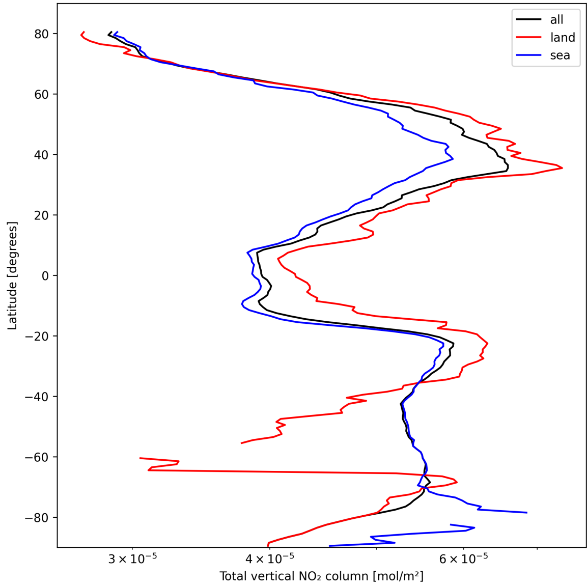
Figure 21: Zonal average of “Total vertical NO 2 column” for 2025-10-11 to 2025-10-12.
