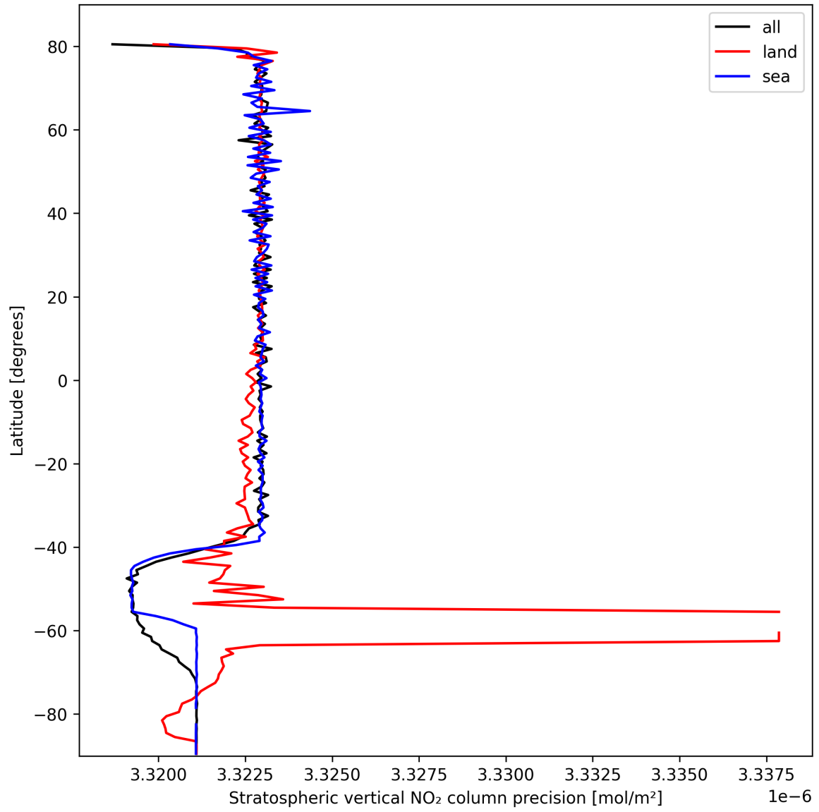
Figure 20: Zonal average of “Stratospheric vertical NO 2 column precision” for 2025-10-11 to 2025-10-12.
