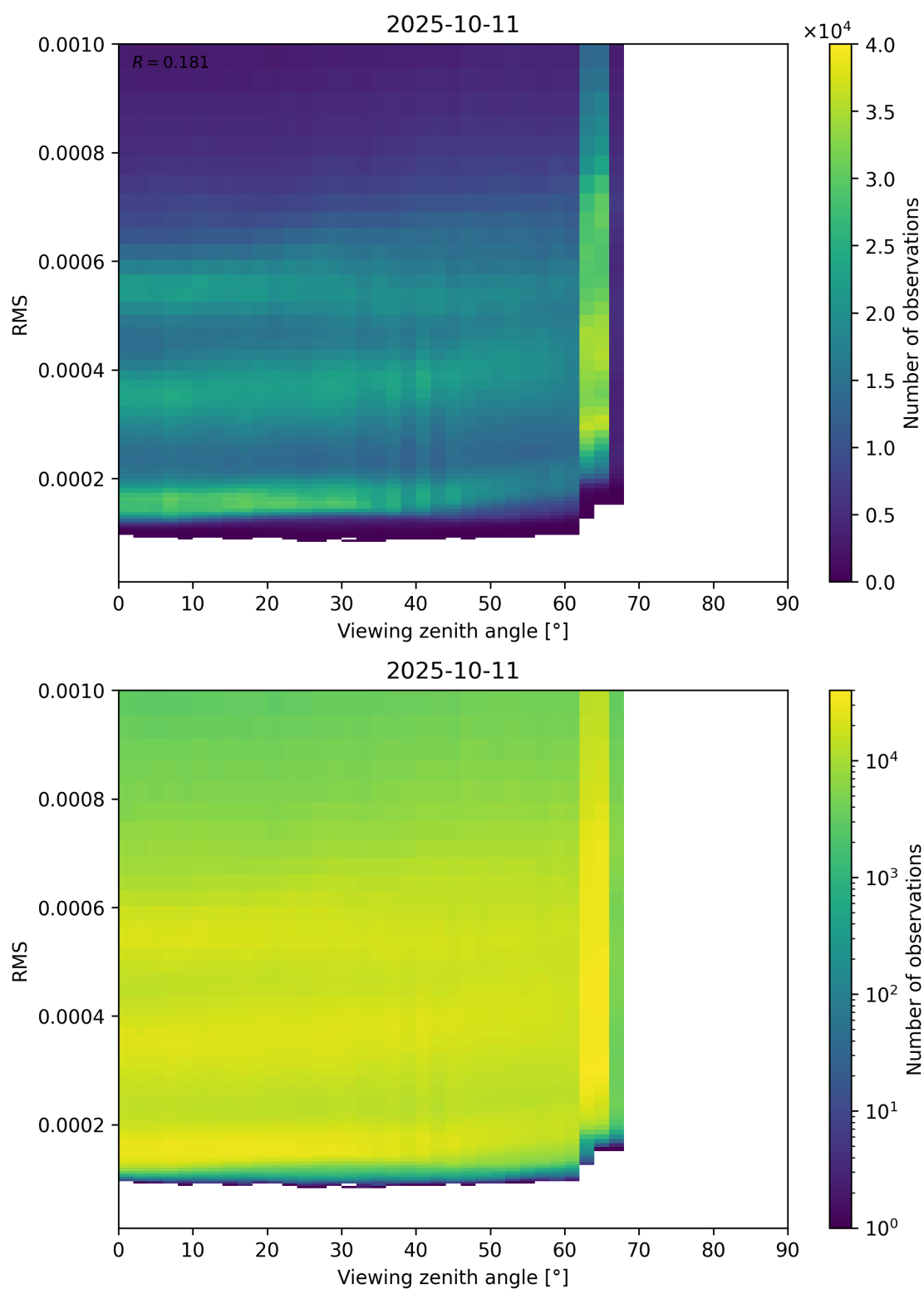
Figure 171: Scatter density plot of “Viewing zenith angle” against “RMS” for 2025-10-11 to 2025-10-12.
