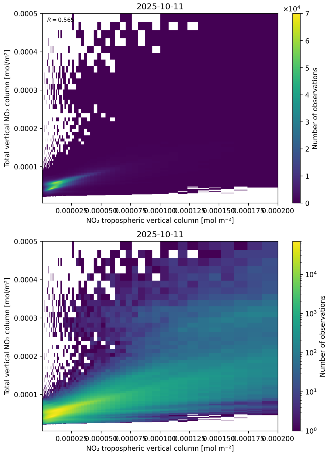
Figure 128: Scatter density plot of “NO 2 tropospheric vertical column” against “Total vertical NO 2 column” for 2025-10-11 to 2025-10-12.
