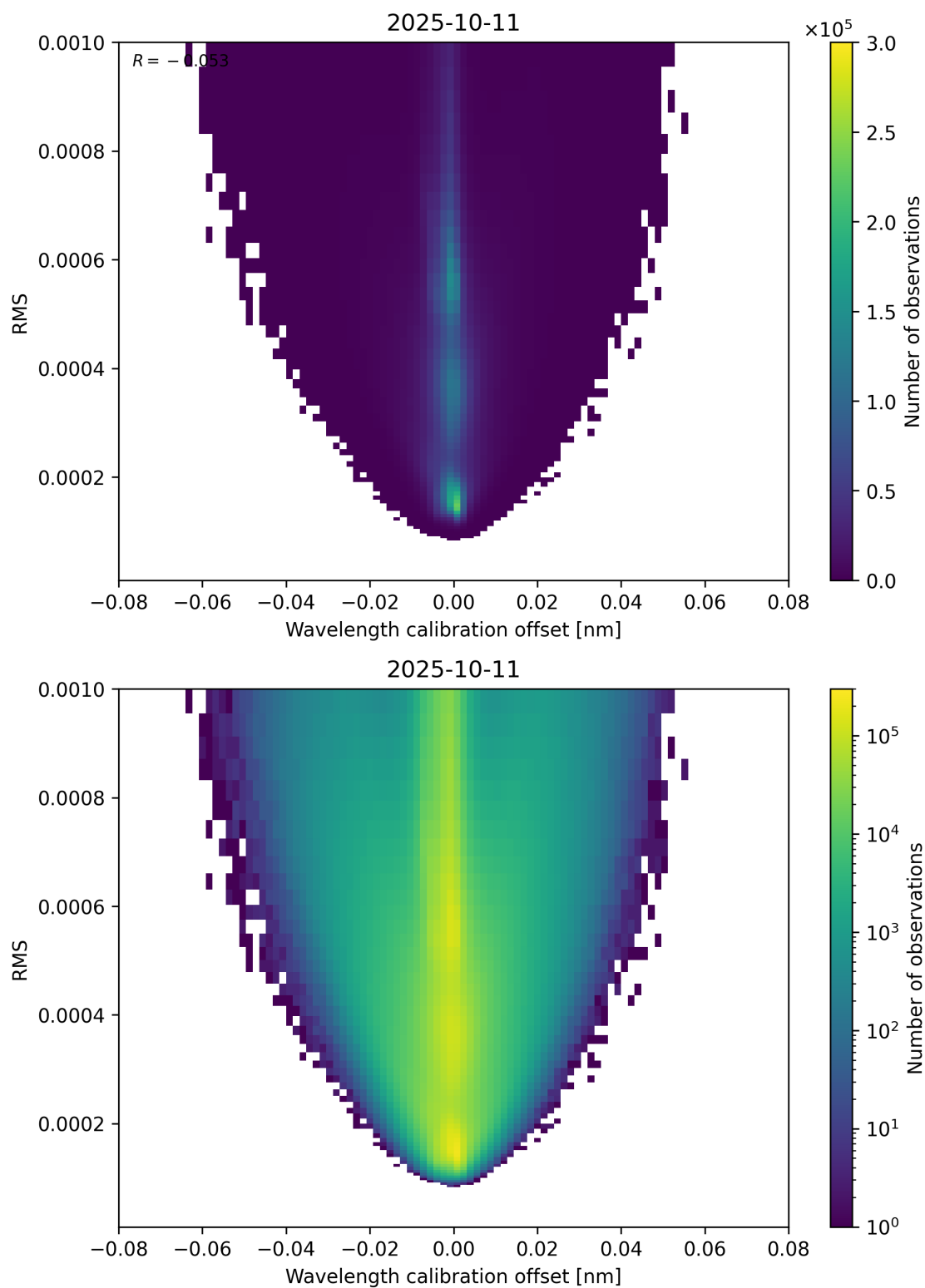
Figure 181: Scatter density plot of “Wavelength calibration offset” against “RMS” for 2025-10-11 to 2025-10-12.
