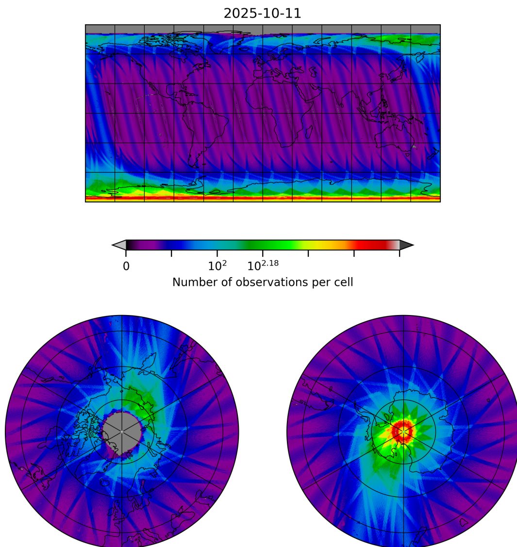
Figure 10: Map of the number of observations for 2025-10-11 to 2025-10-12
