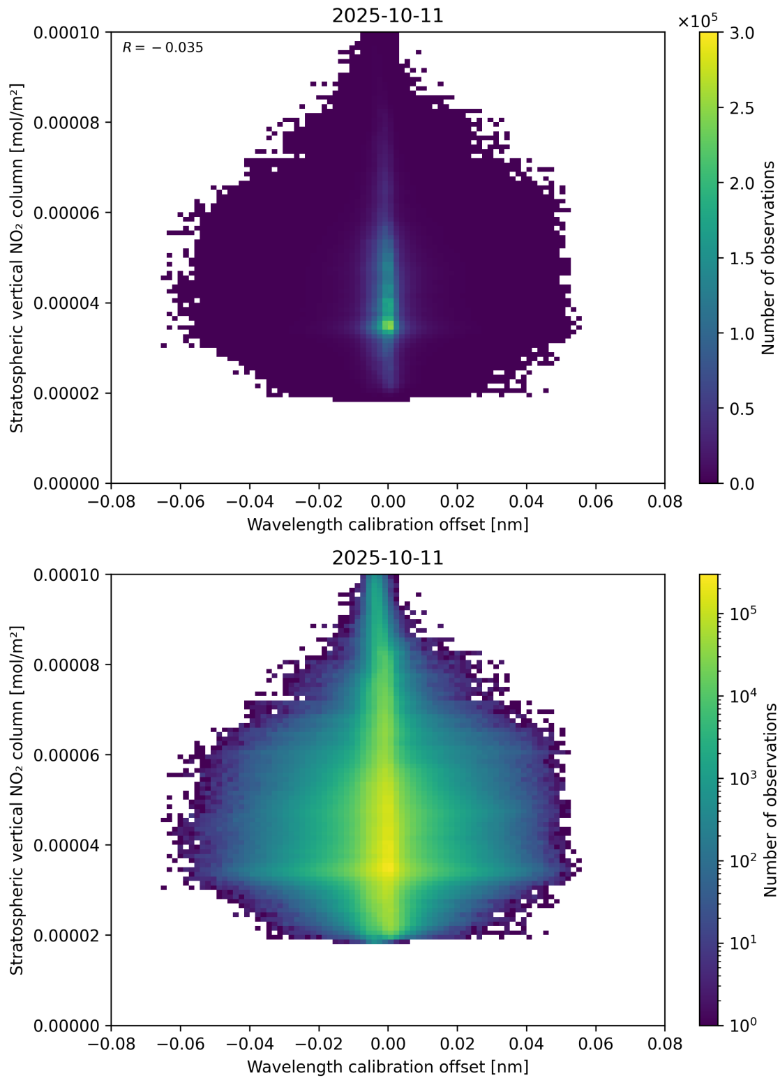
Figure 176: Scatter density plot of “Wavelength calibration offset” against “Stratospheric vertical NO 2 column” for 2025-10-11 to 2025-10-12.
