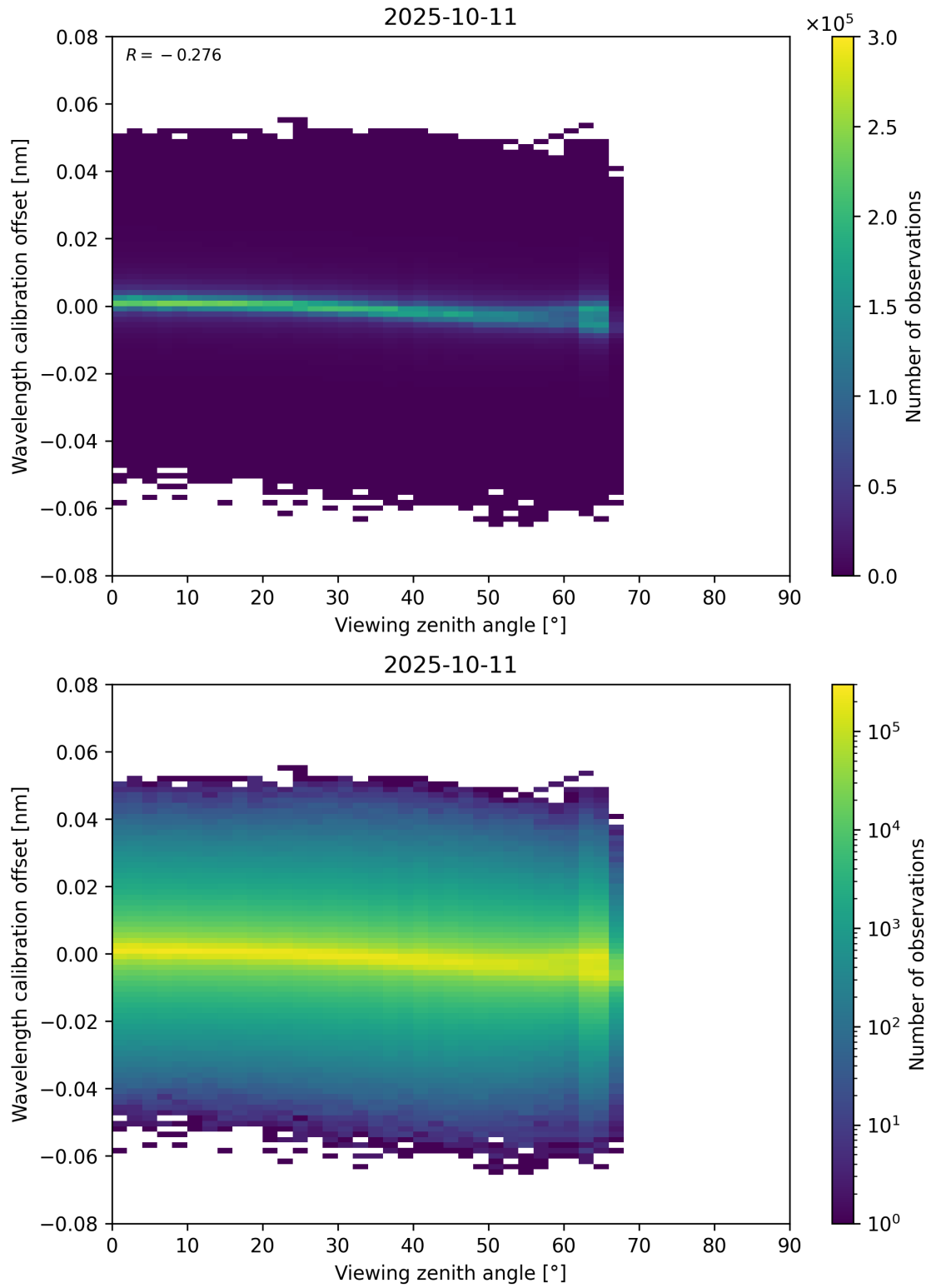
Figure 173: Scatter density plot of “Viewing zenith angle” against “Wavelength calibration offset” for 2025-10-11 to 2025-10-12.
