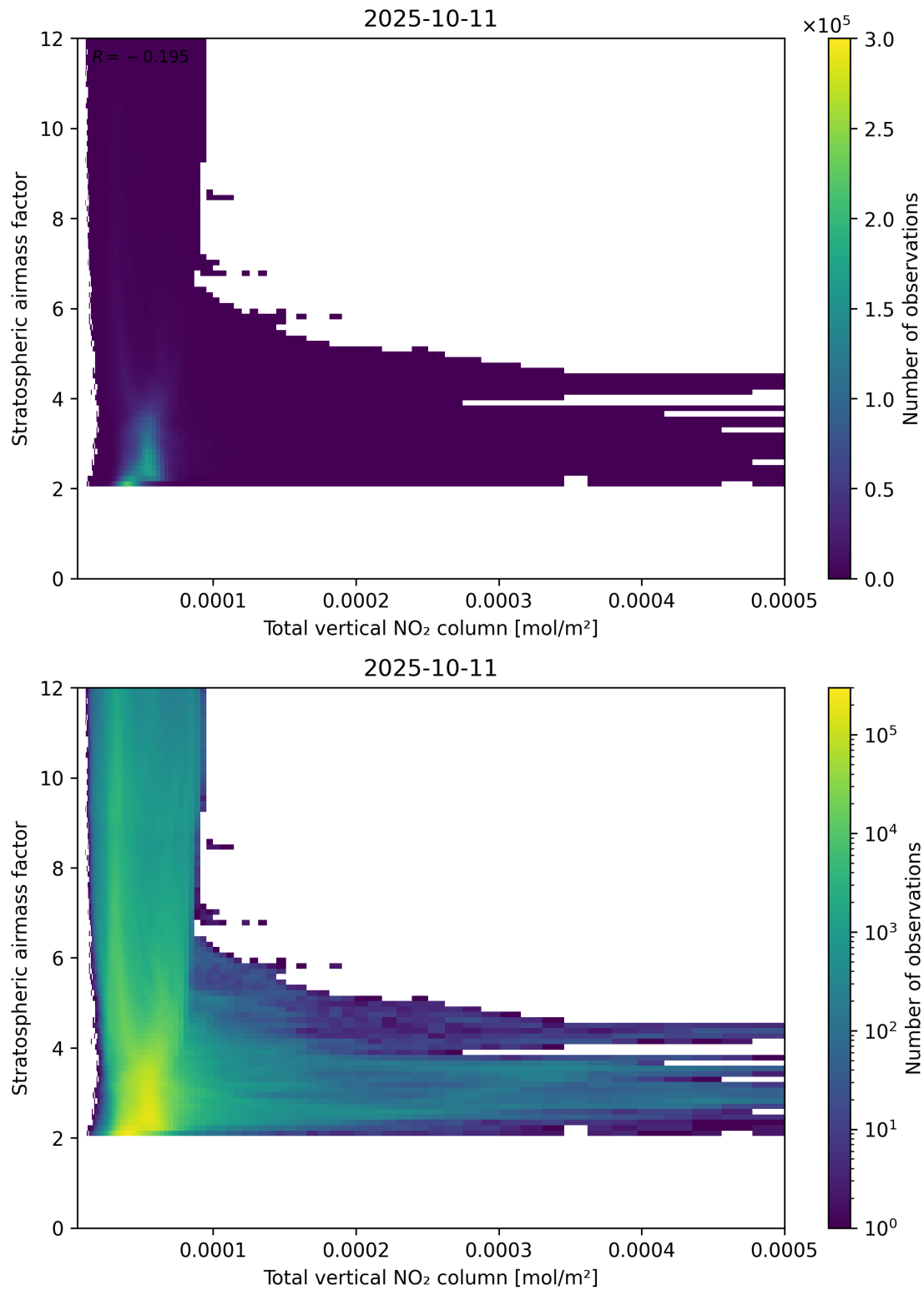
Figure 110: Scatter density plot of “Total vertical NO 2 column” against “Stratospheric airmass factor” for 2025-10-11 to 2025-10-12.
