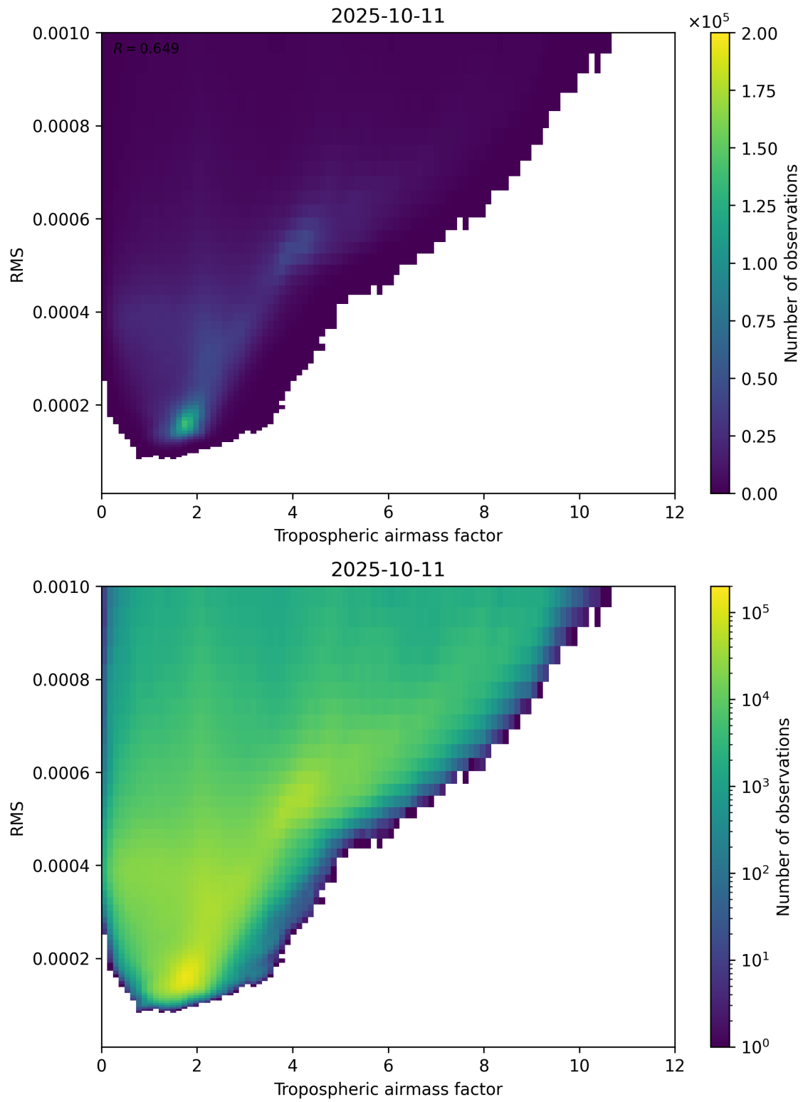
Figure 79: Scatter density plot of “Tropospheric airmass factor” against “RMS” for 2025-10-11 to 2025-10-12.
