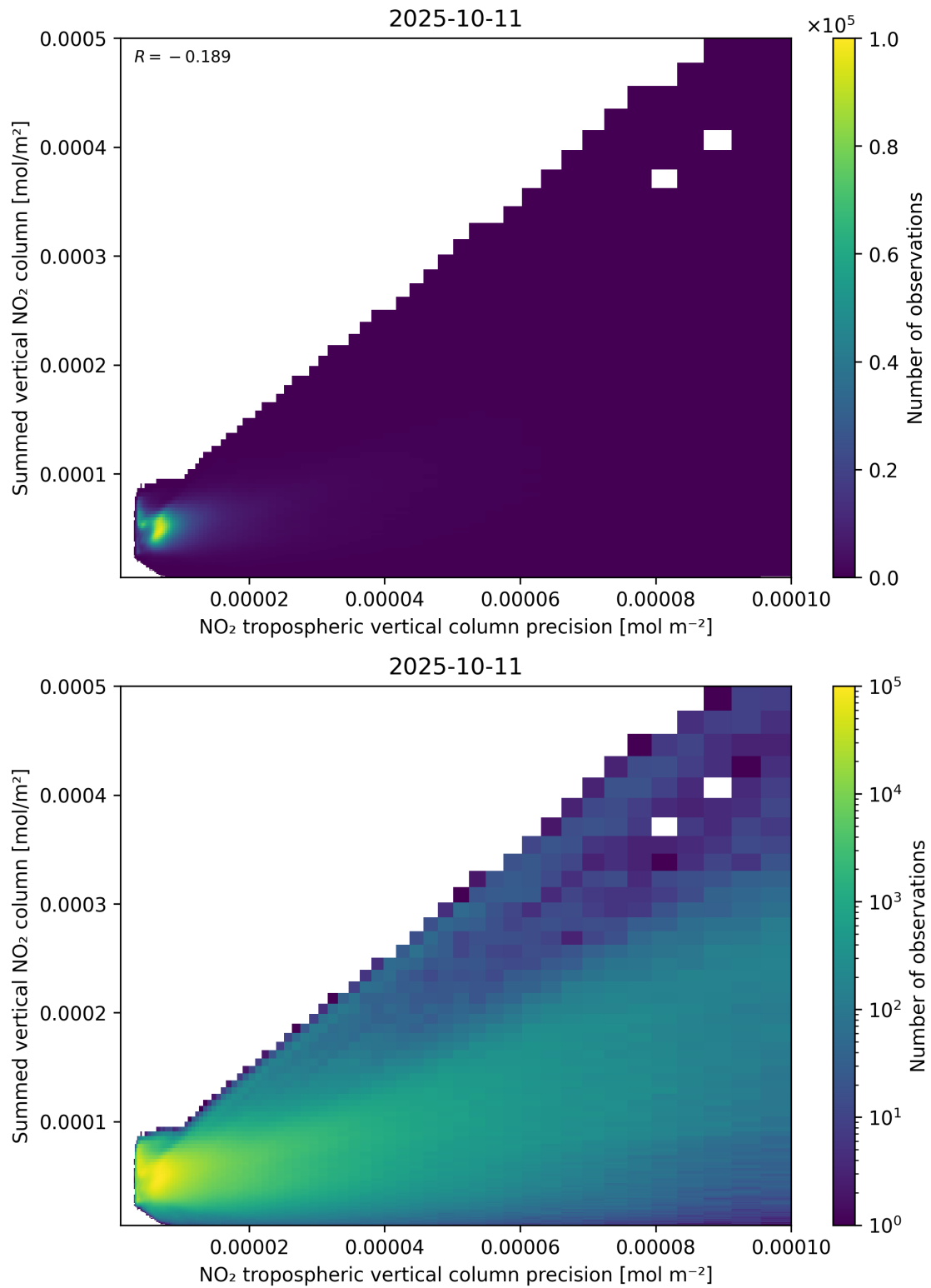
Figure 136: Scatter density plot of “NO 2 tropospheric vertical column precision” against “Summed vertical NO 2 column” for 2025-10-11 to 2025-10-12.
