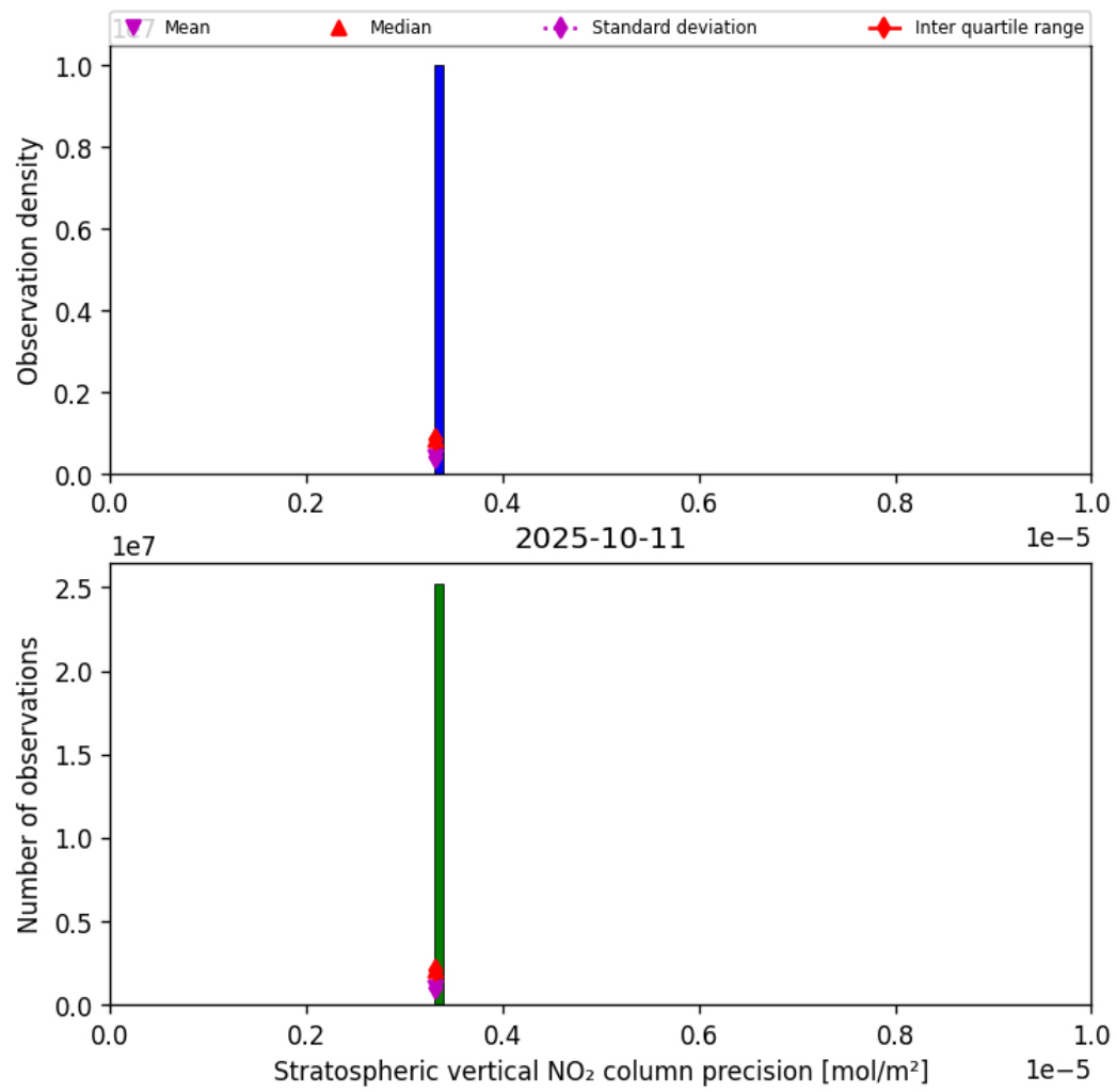
Figure 37: Histogram of “Stratospheric vertical NO 2 column precision” for 2025-10-11 to 2025-10-12
