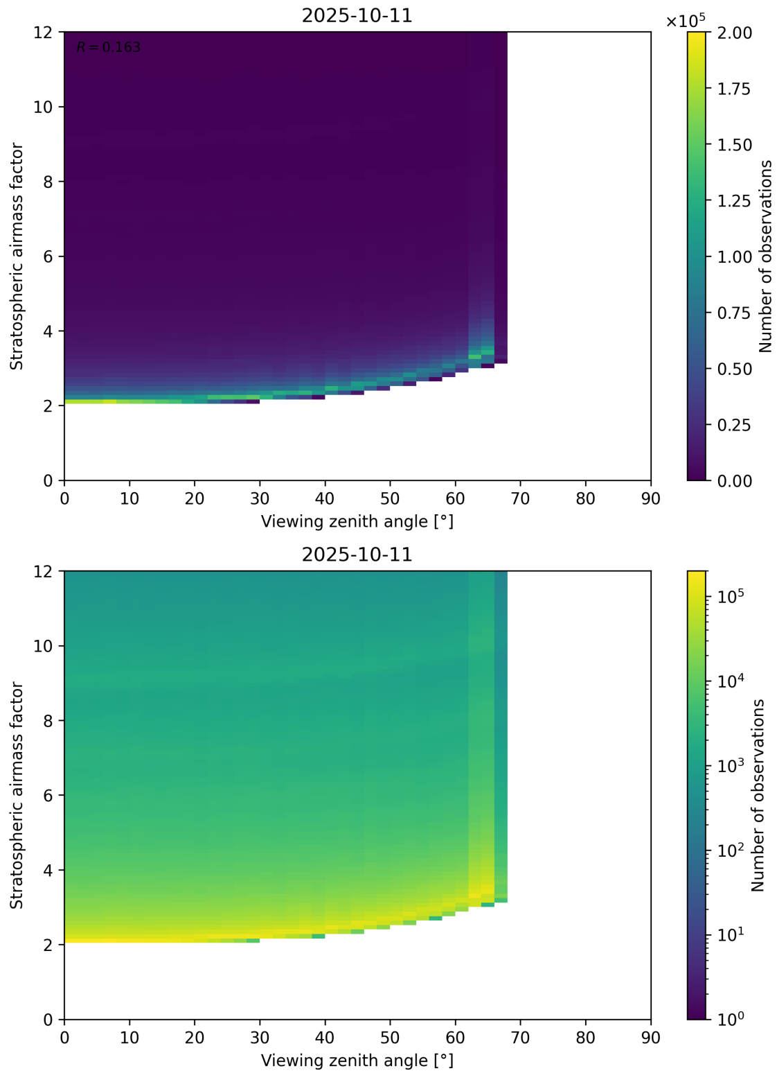
Figure 159: Scatter density plot of “Viewing zenith angle” against “Stratospheric airmass factor” for 2025-10-11 to 2025-10-12.
