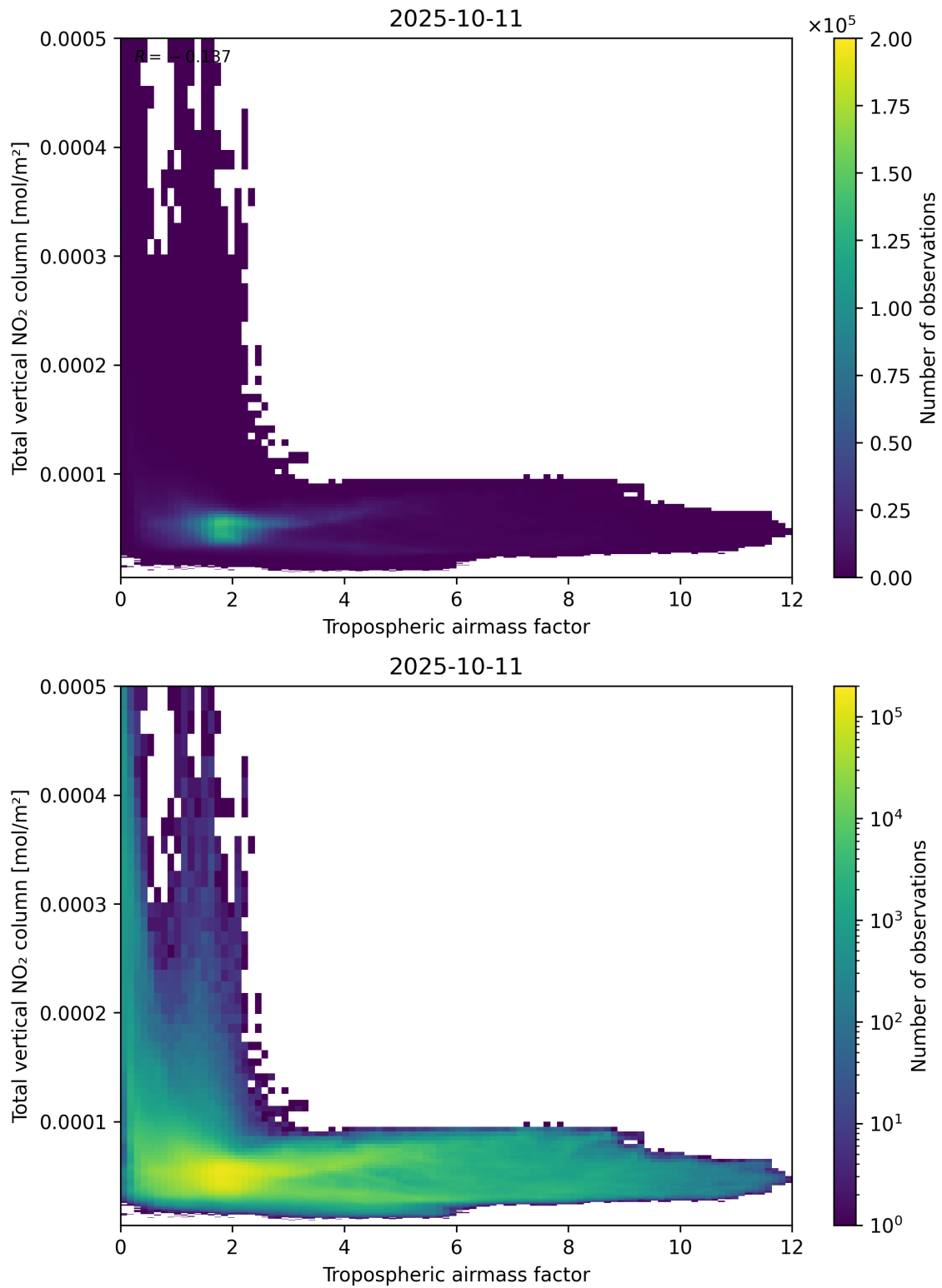
Figure 77: Scatter density plot of “Tropospheric airmass factor” against “Total vertical NO 2 column” for 2025-10-11 to 2025-10-12.
