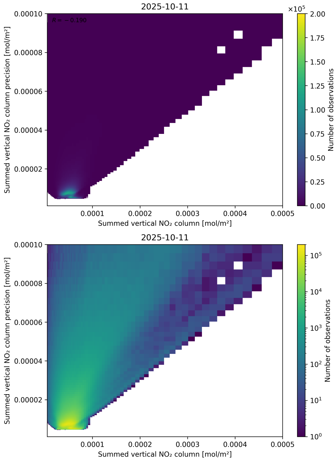
Figure 105: Scatter density plot of “Summed vertical NO 2 column” against “Summed vertical NO 2 column precision” for 2025-10-11 to 2025-10-12.
