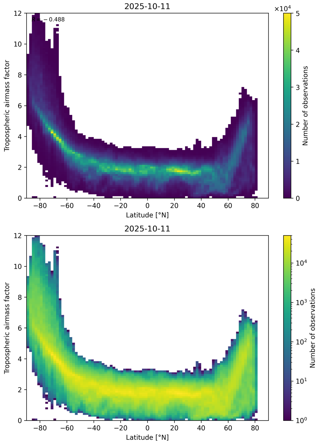
Figure 85: Scatter density plot of “Latitude” against “Tropospheric air mass factor” for 2025-10-11 to 2025-10-12.
