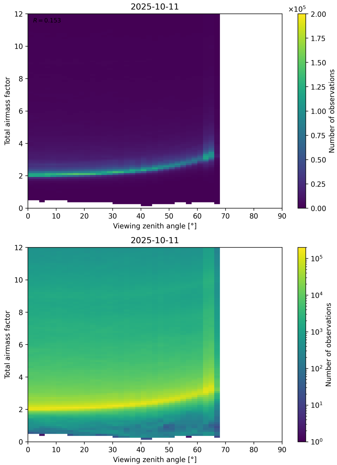
Figure 160: Scatter density plot of “Viewing zenith angle” against “Total airmass factor” for 2025-10-11 to 2025-10-12.
