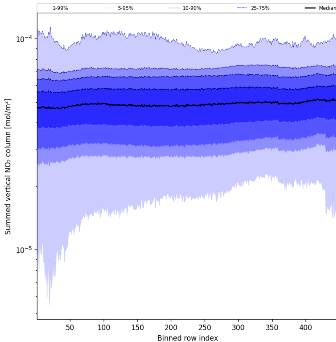
Figure 57: Along track statistics of “Summed vertical NO 2 column” for 2025-10-11 to 2025-10-12
