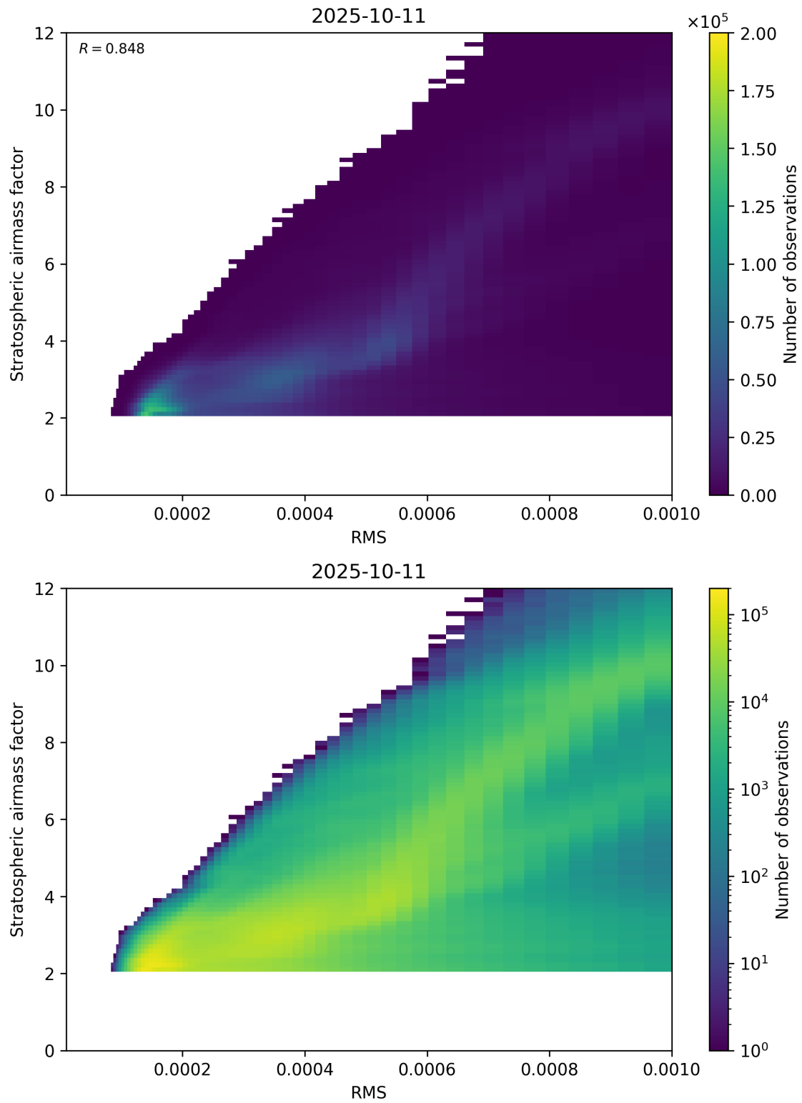
Figure 144: Scatter density plot of “RMS” against “Stratospheric airmass factor” for 2025-10-11 to 2025-10-12.
