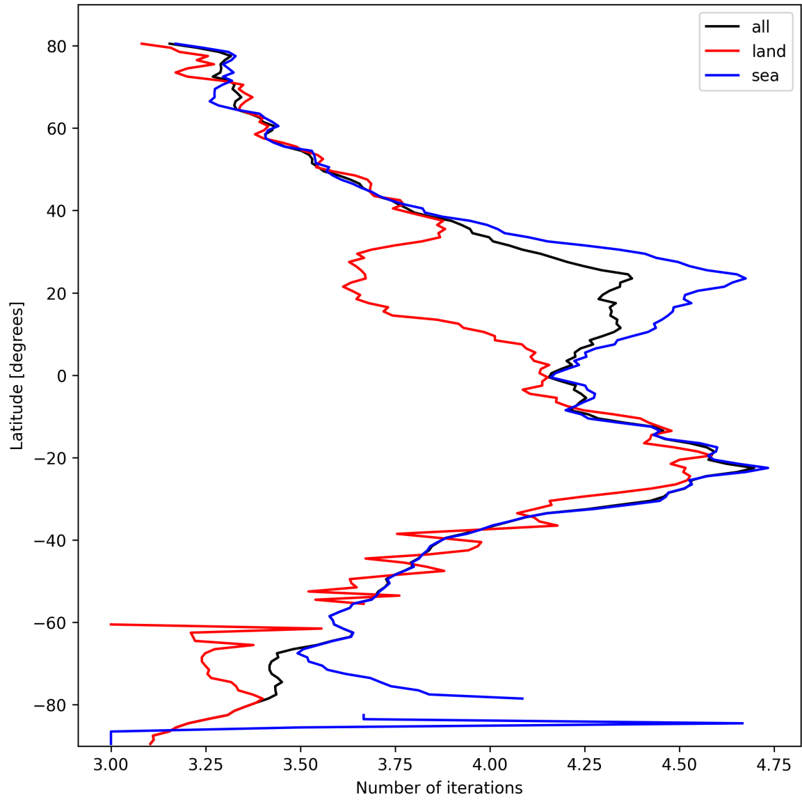
Figure 17: Zonal average of “Number of iterations” for 2025-10-11 to 2025-10-12.
