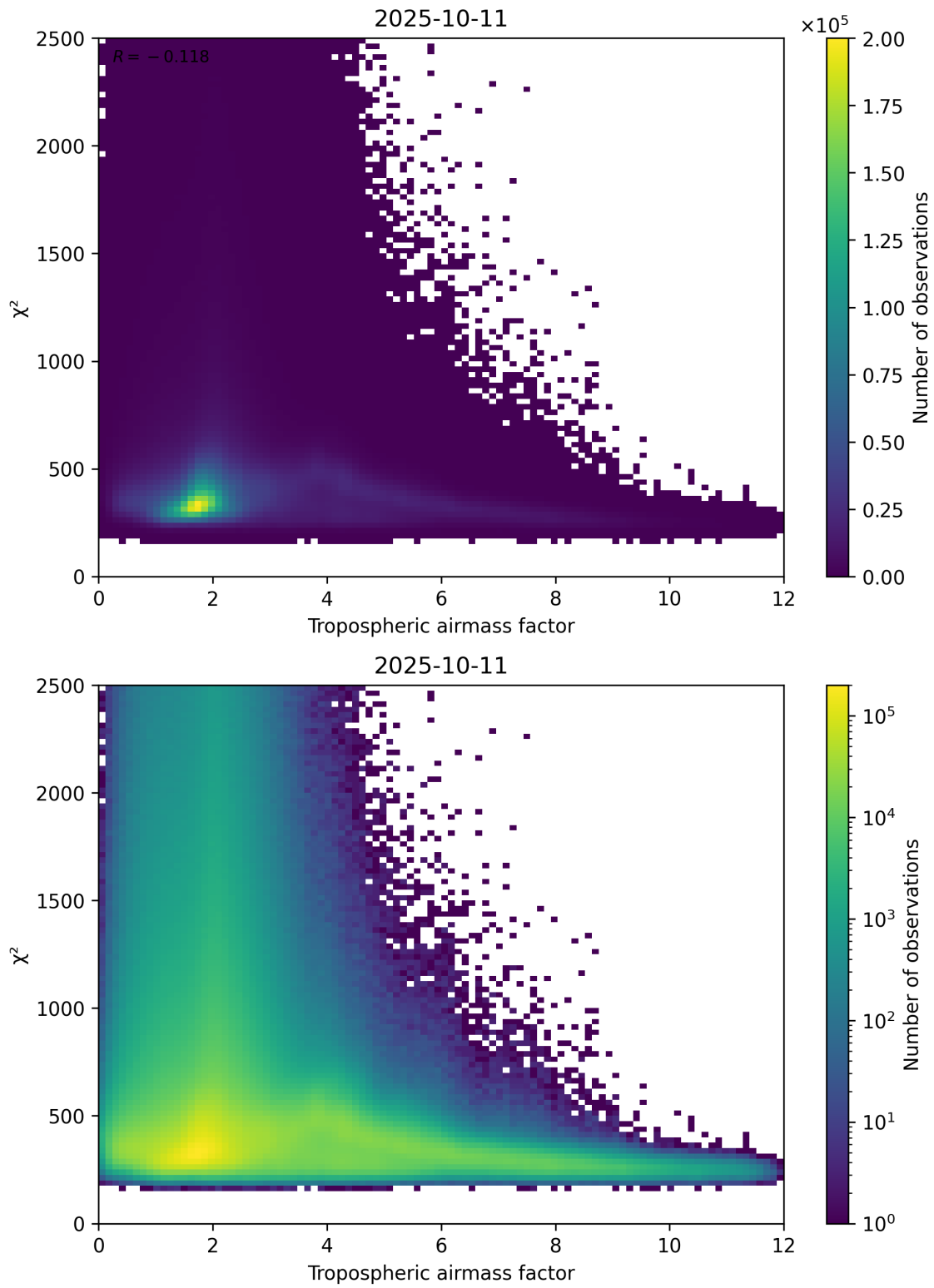
Figure 73: Scatter density plot of “Tropospheric airmass factor” against “ \chi^2 ” for 2025-10-11 to 2025-10-12.
