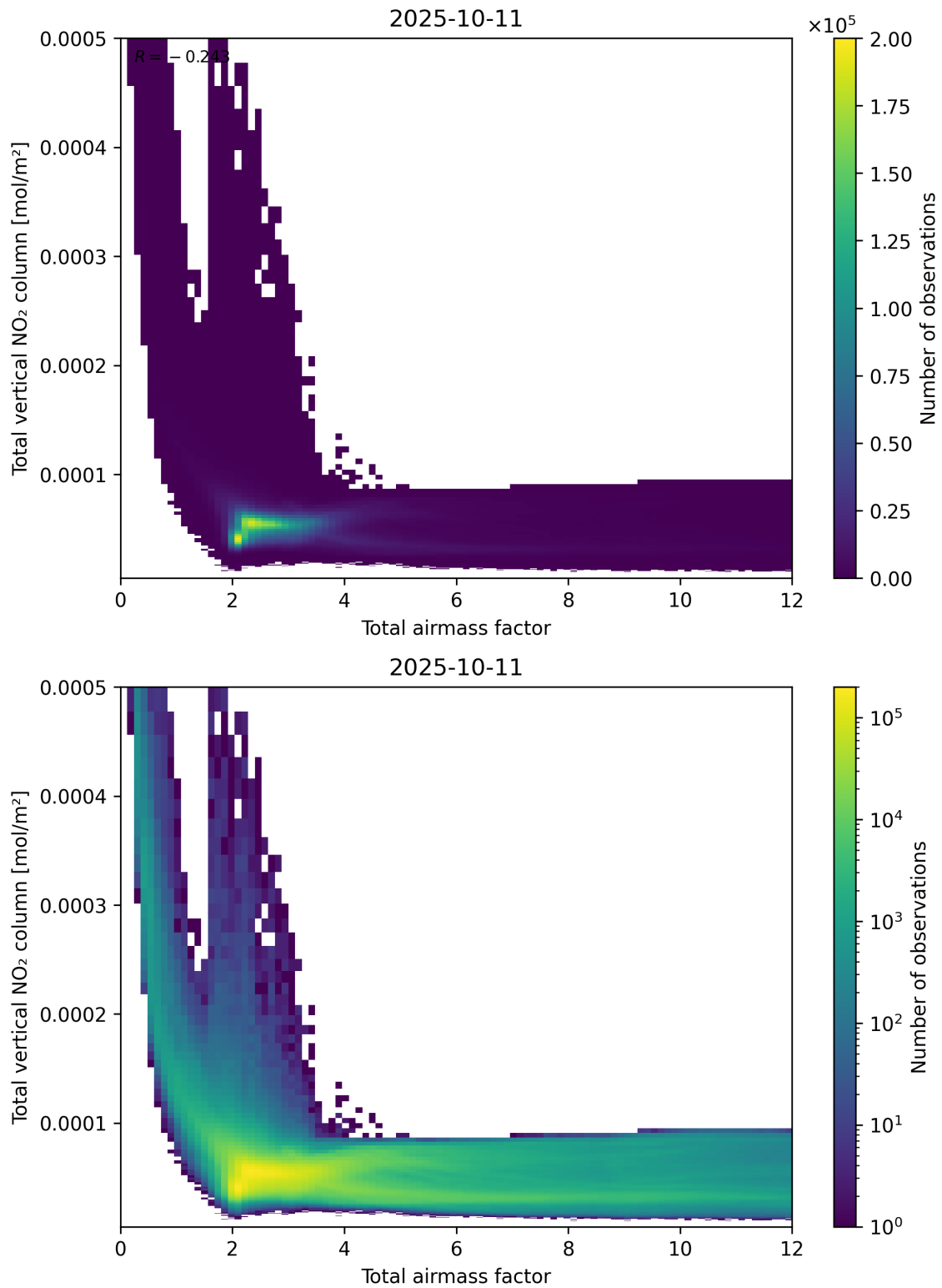
Figure 67: Scatter density plot of “Total airmass factor” against “Total vertical NO 2 column” for 2025-10-11 to 2025-10-12.
