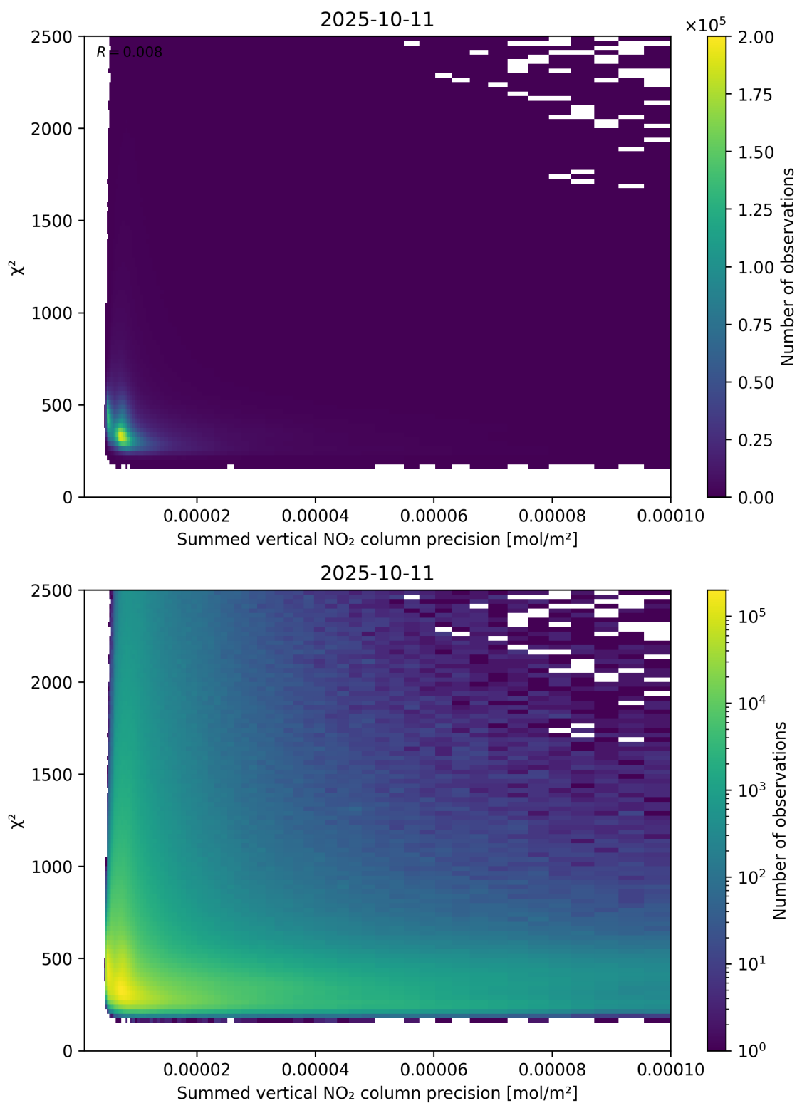
Figure 107: Scatter density plot of “Summed vertical NO 2 column precision” against “ \chi^2 ” for 2025-10-11 to 2025-10-12.
