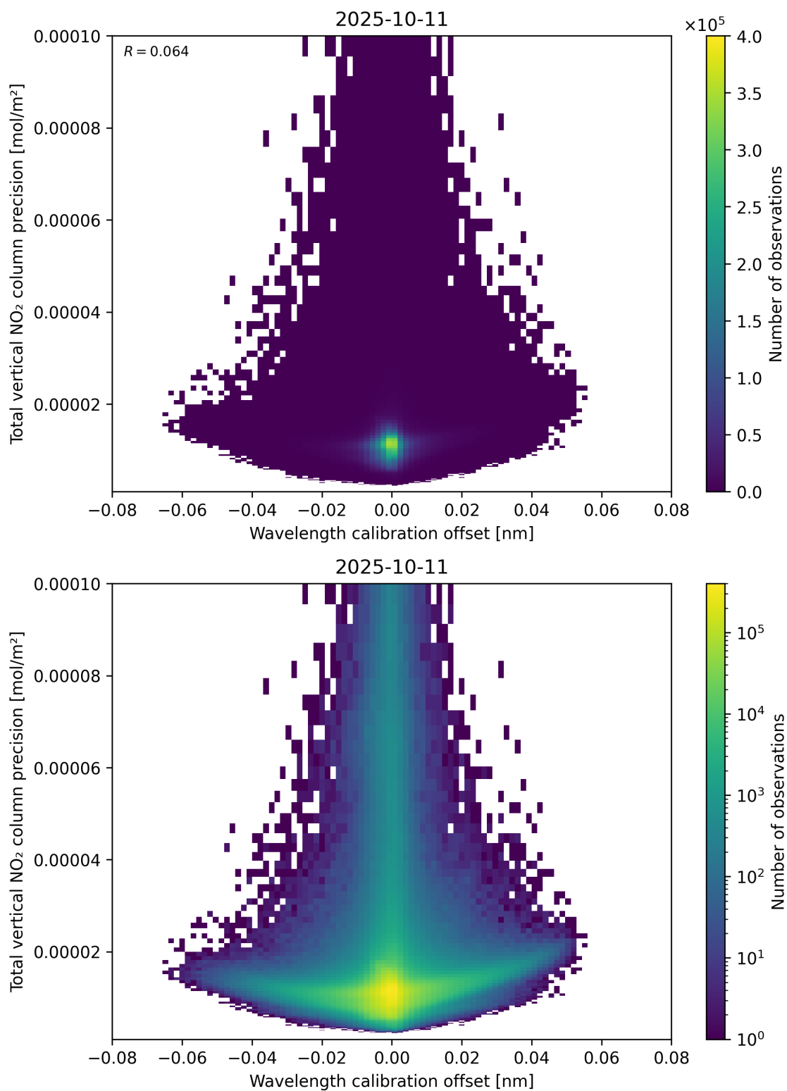
Figure 180: Scatter density plot of “Wavelength calibration offset” against “Total vertical NO 2 column precision” for 2025-10-11 to 2025-10-12.
