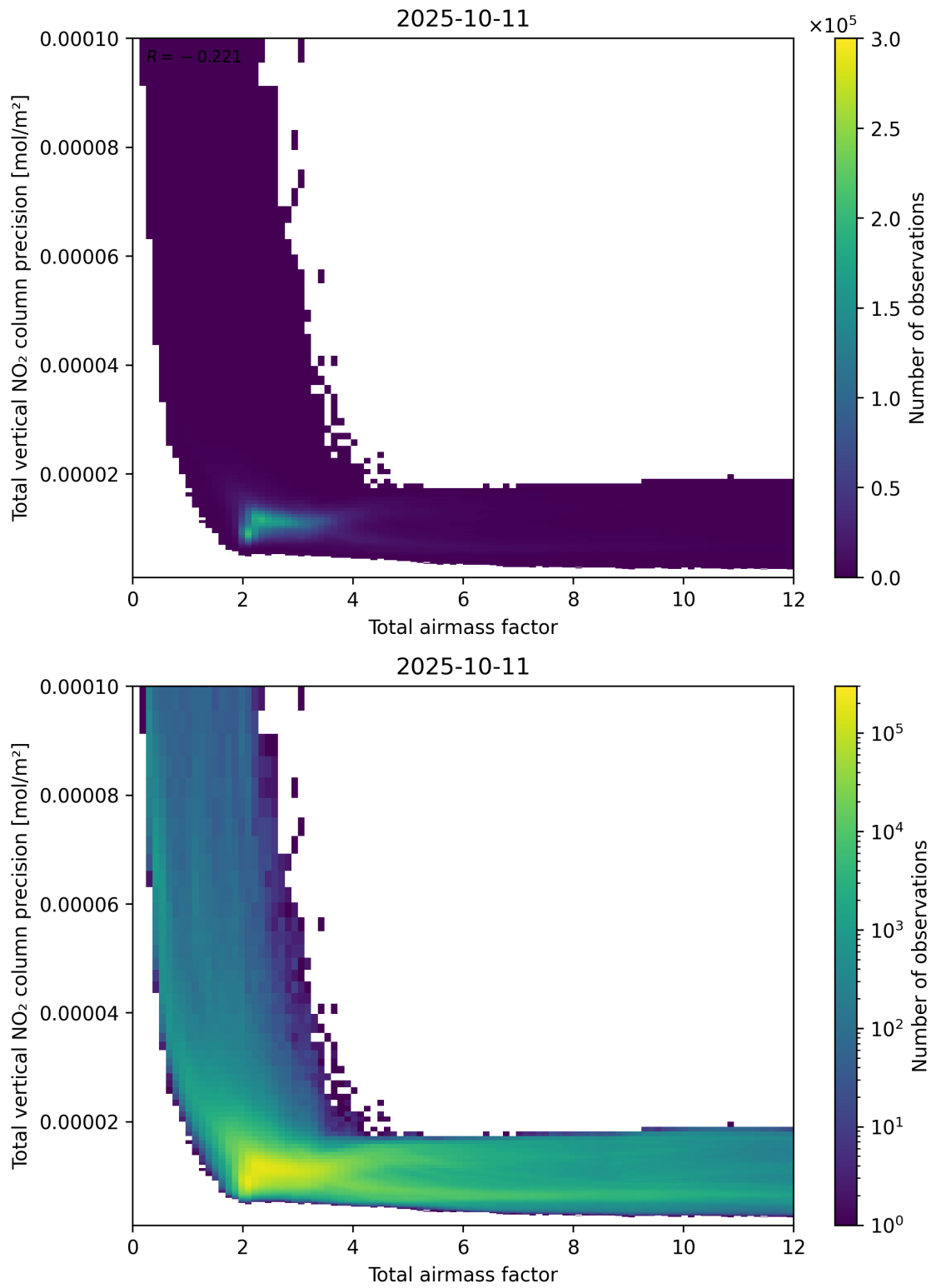
Figure 68: Scatter density plot of “Total airmass factor” against “Total vertical NO 2 column precision” for 2025-10-11 to 2025-10-12.
