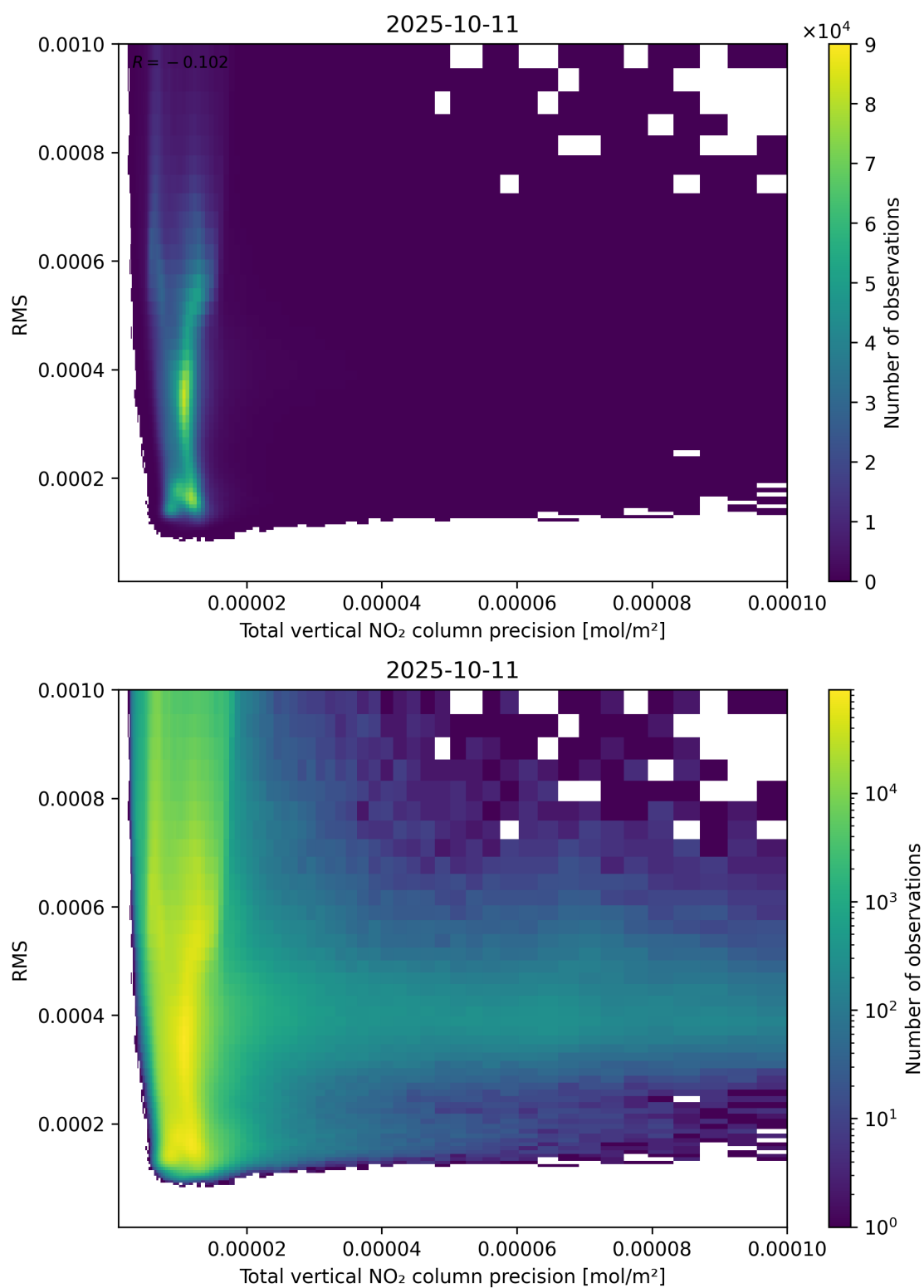
Figure 119: Scatter density plot of “Total vertical NO 2 column precision” against “RMS” for 2025-10-11 to 2025-10-12.
