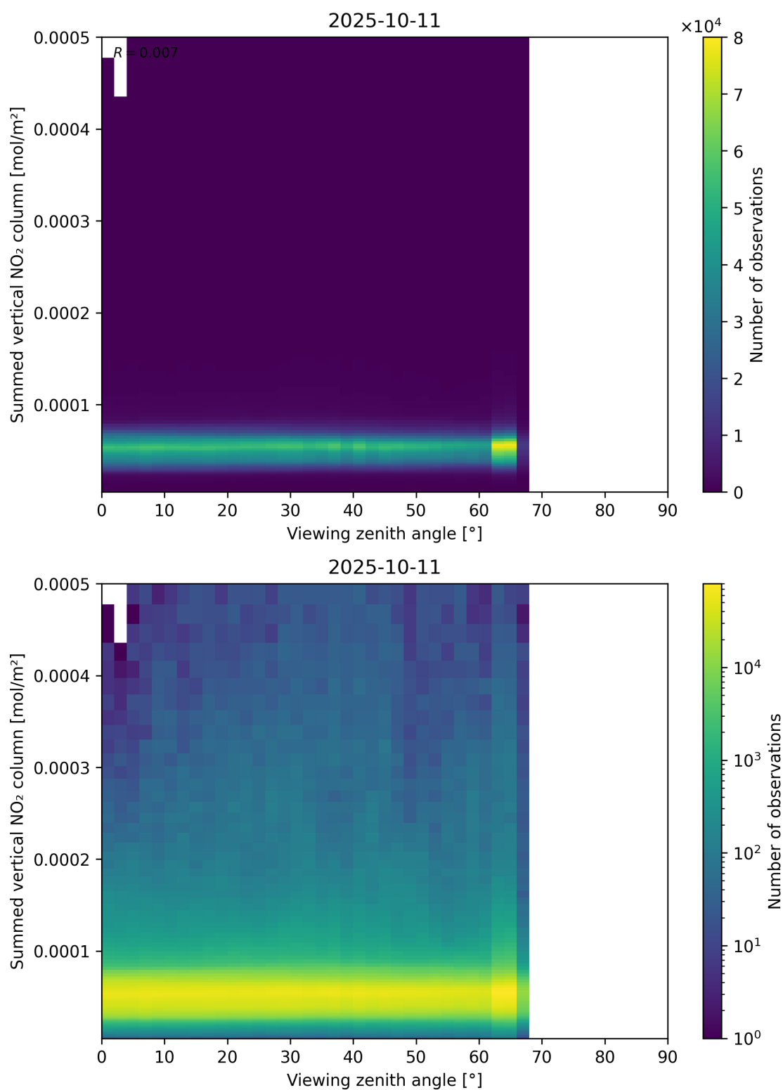
Figure 165: Scatter density plot of “Viewing zenith angle” against “Summed vertical NO 2 column” for 2025-10-11 to 2025-10-12.
