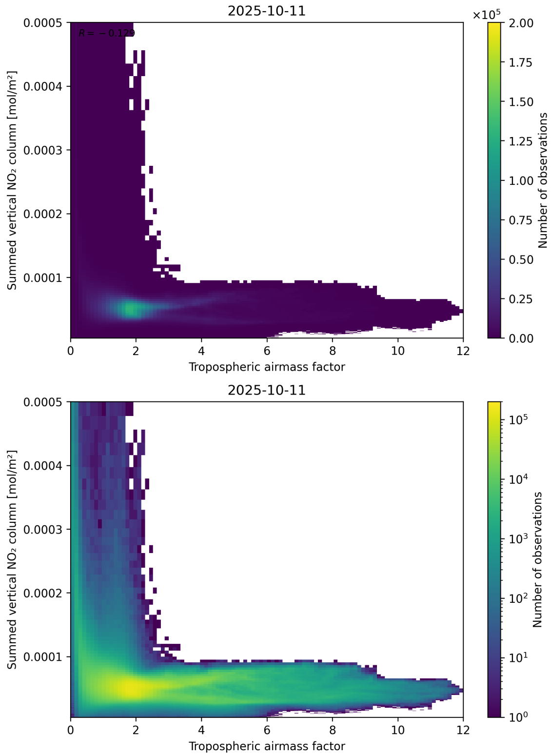
Figure 75: Scatter density plot of “Tropospheric airmass factor” against “Summed vertical NO 2 column” for 2025-10-11 to 2025-10-12.
