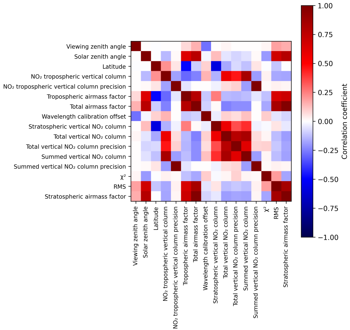
Figure 2: Map of correlation matrix for 2025-10-11 to 2025-10-12.
