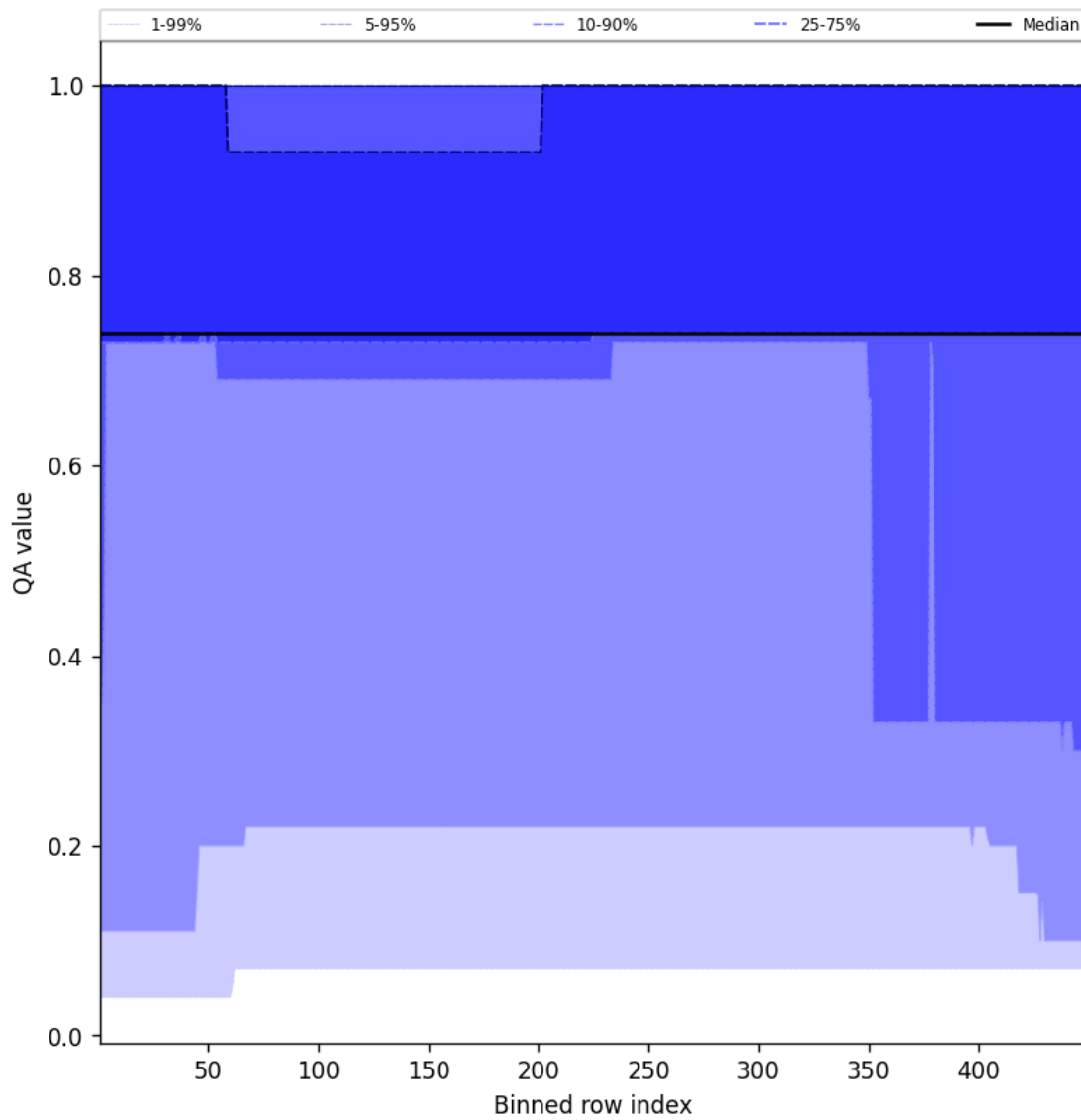
Figure 45: Along track statistics of “QA value” for 2025-10-11 to 2025-10-12
