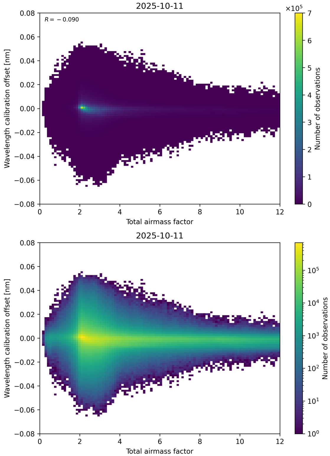
Figure 70: Scatter density plot of “Total airmass factor” against “Wavelength calibration offset” for 2025-10-11 to 2025-10-12.
