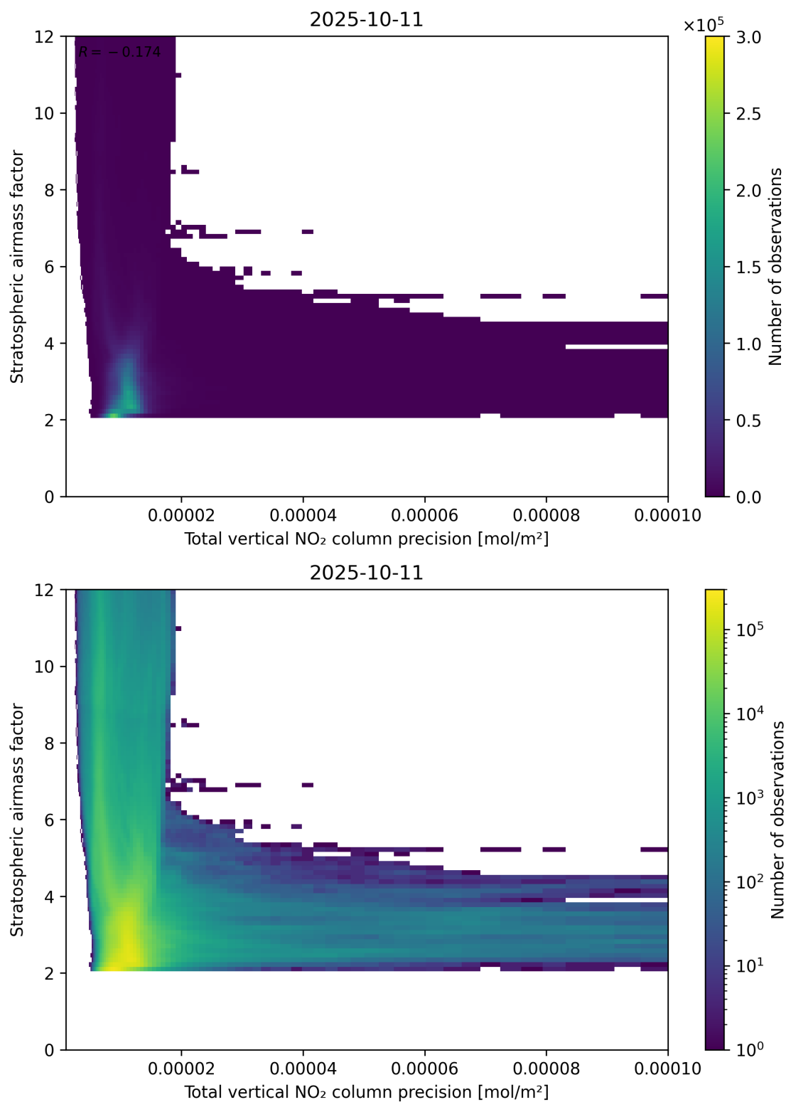
Figure 115: Scatter density plot of “Total vertical NO 2 column precision” against “Stratospheric airmass factor” for 2025-10-11 to 2025-10-12.
