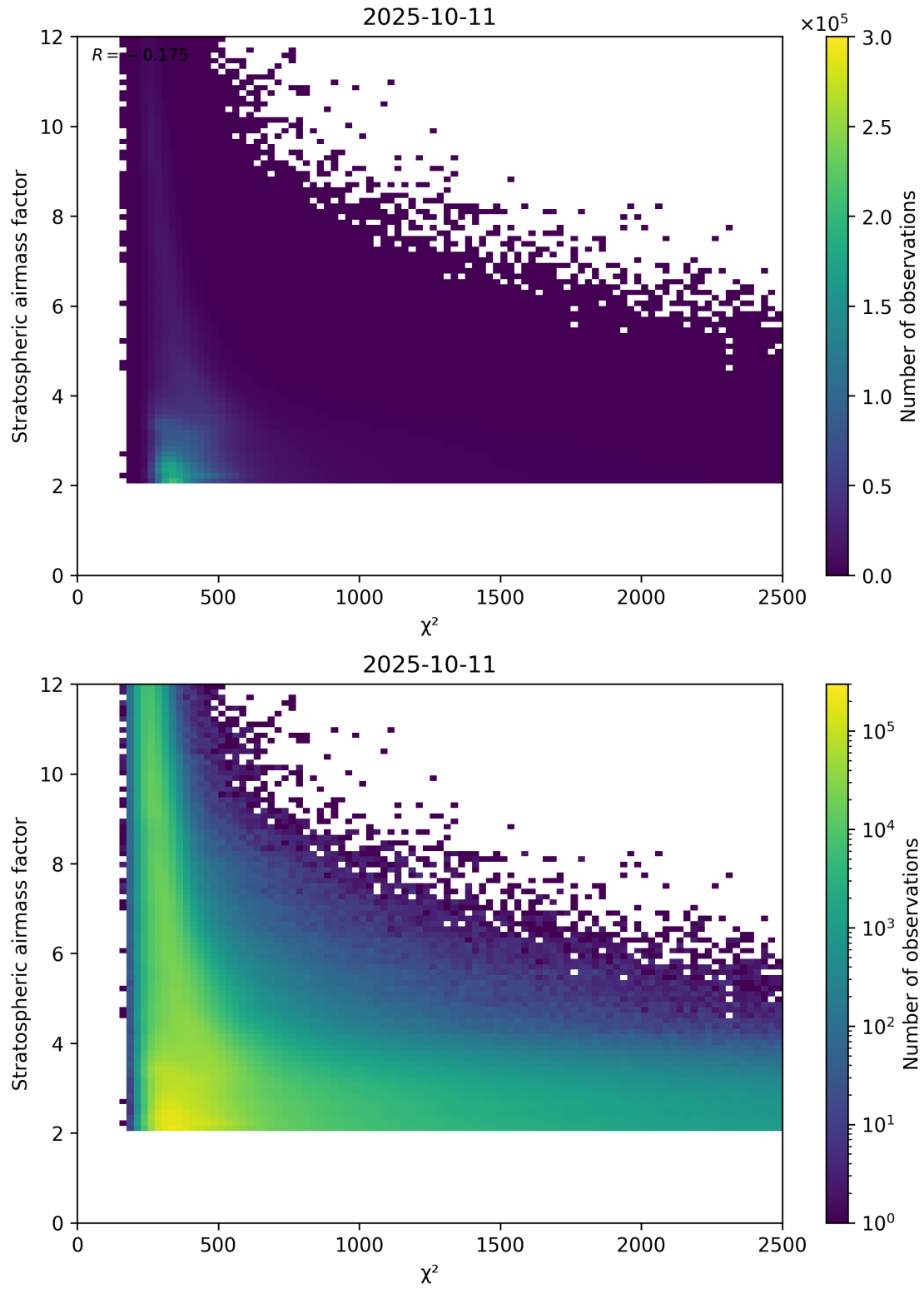
Figure 81: Scatter density plot of " \chi^2 " against "Stratospheric airmass factor" for 2025-10-11 to 2025-10-12.
