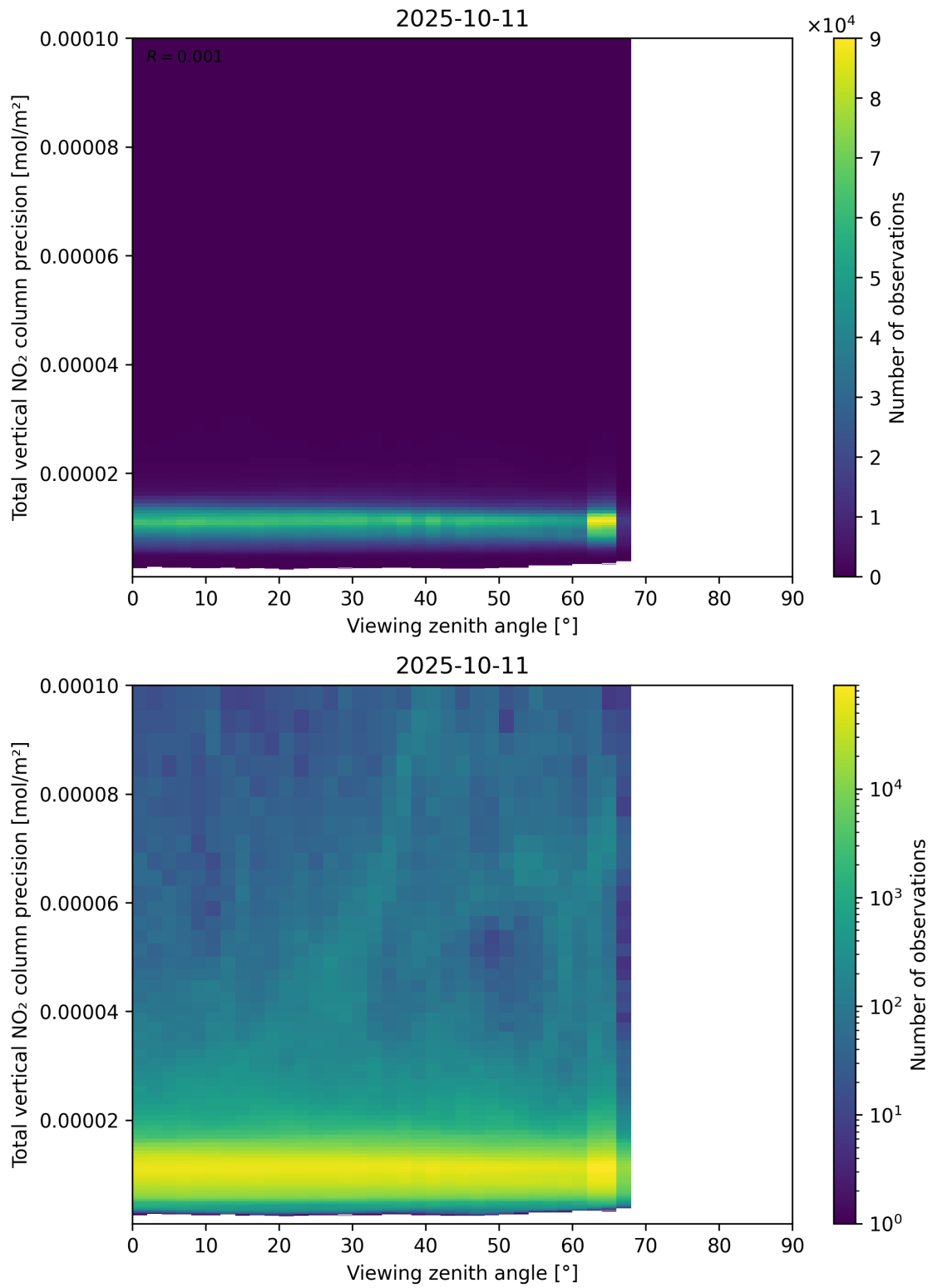
Figure 168: Scatter density plot of “Viewing zenith angle” against “Total vertical NO 2 column precision” for 2025-10-11 to 2025-10-12.
