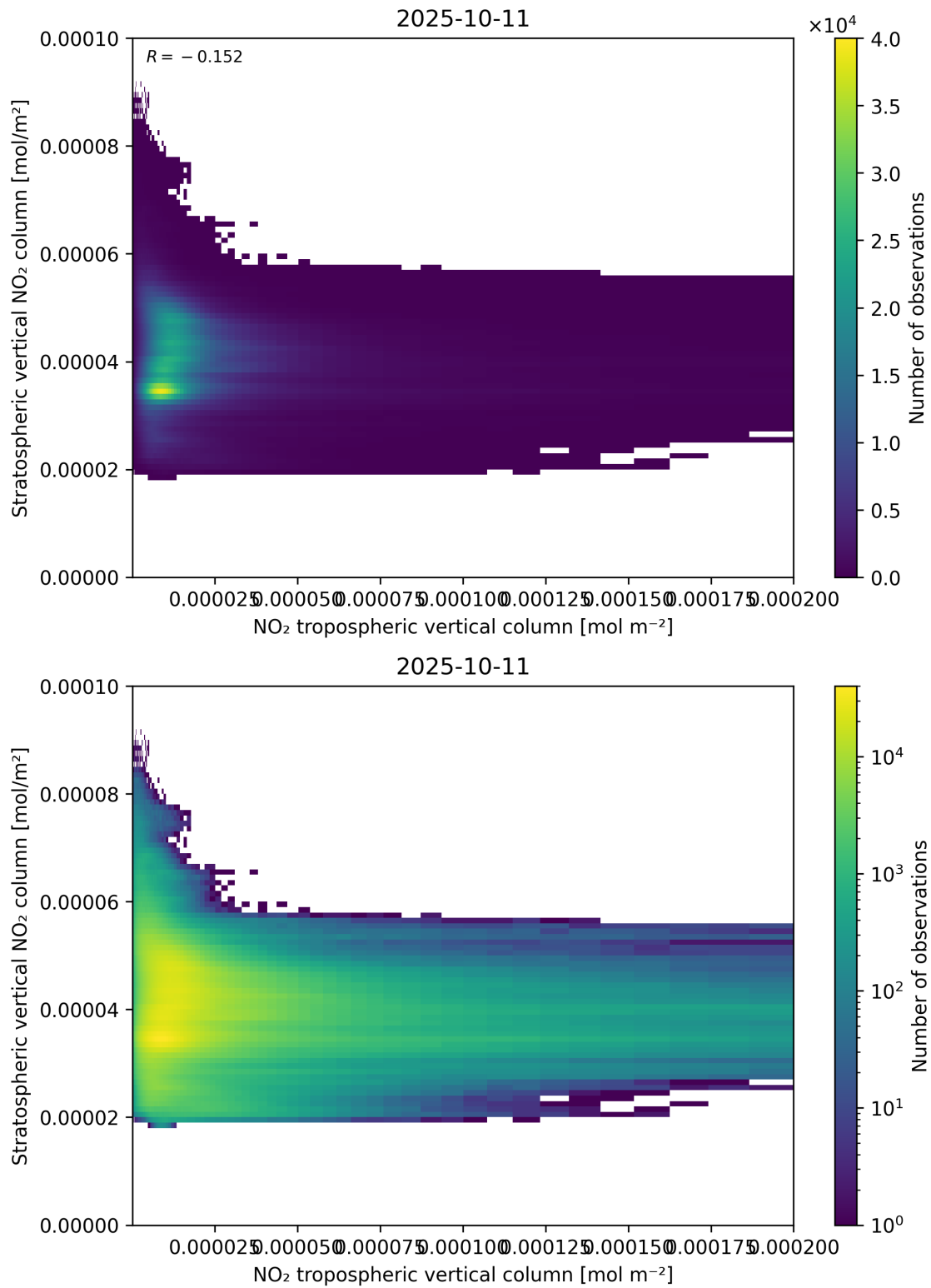
Figure 125: Scatter density plot of “NO 2 tropospheric vertical column” against “Stratospheric vertical NO 2 column” for 2025-10-11 to 2025-10-12.
