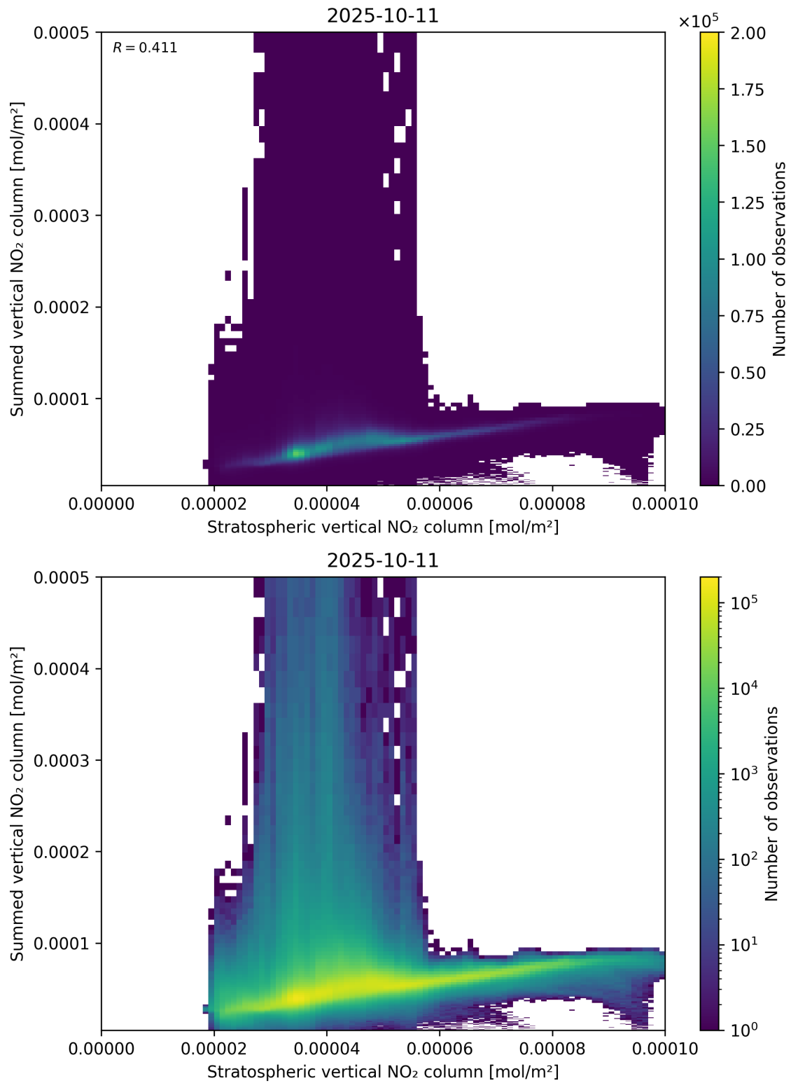
Figure 98: Scatter density plot of “Stratospheric vertical NO 2 column” against “Summed vertical NO 2 column” for 2025-10-11 to 2025-10-12.
