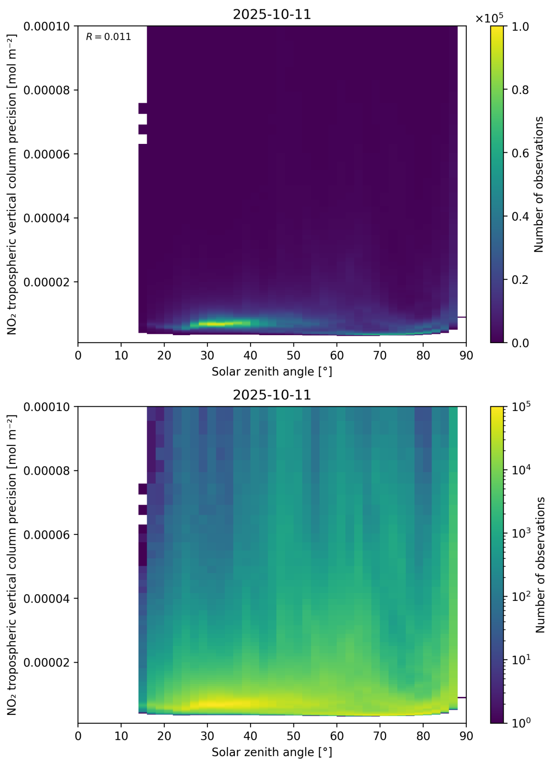
Figure 156: Scatter density plot of “Solar zenith angle” against “NO 2 tropospheric vertical column precision” for 2025-10-11 to 2025-10-12.
