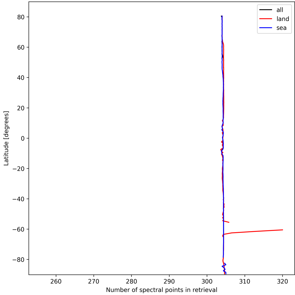
Figure 16: Zonal average of “Number of spectral points in retrieval” for 2025-10-11 to 2025-10-12.
