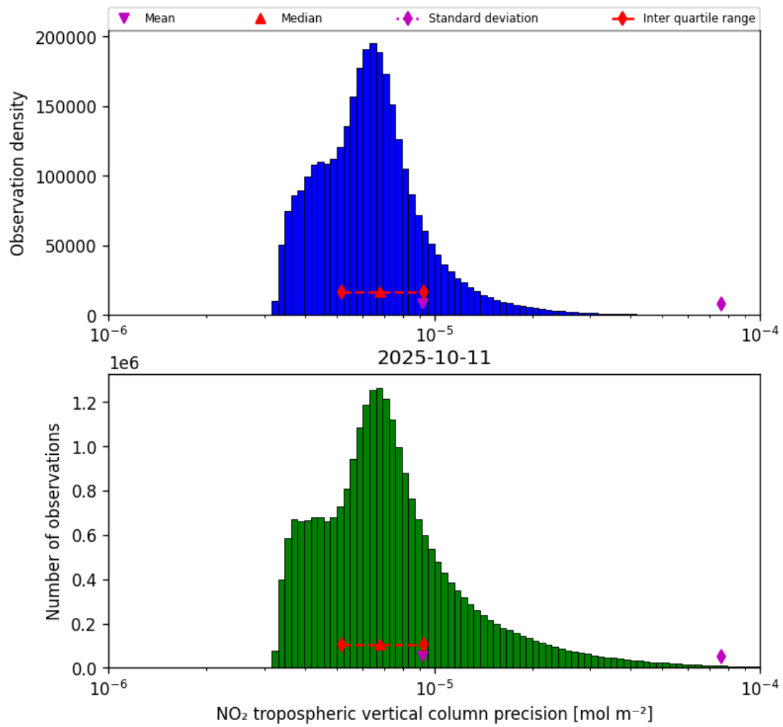
Figure 30: Histogram of “NO 2 tropospheric vertical column precision” for 2025-10-11 to 2025-10-12
