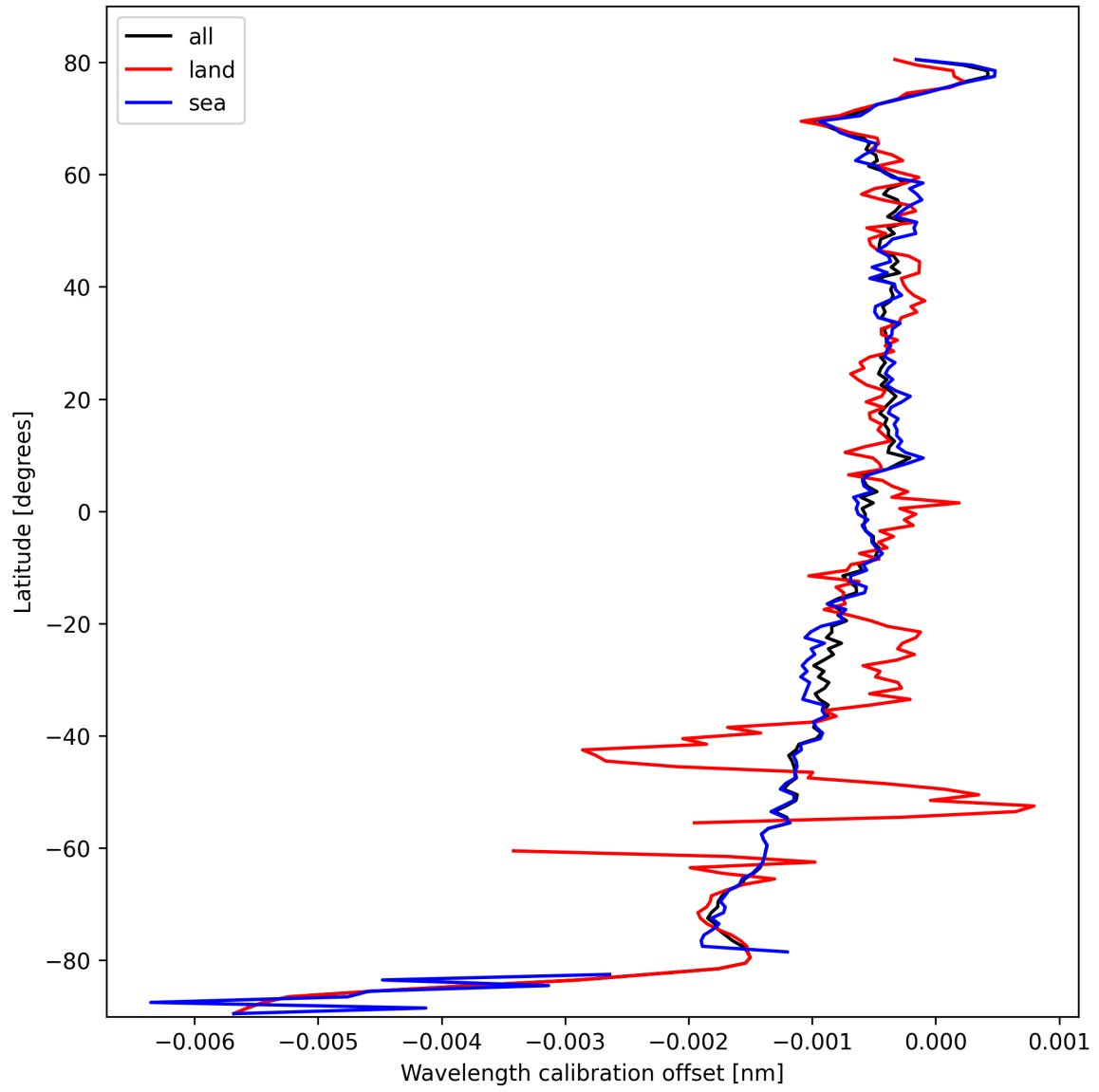
Figure 18: Zonal average of “Wavelength calibration offset” for 2025-10-11 to 2025-10-12.
