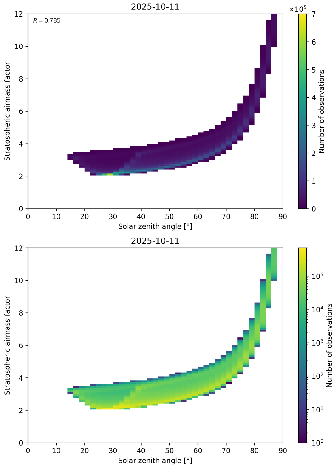
Figure 145: Scatter density plot of “Solar zenith angle” against “Stratospheric airmass factor” for 2025-10-11 to 2025-10-12.
