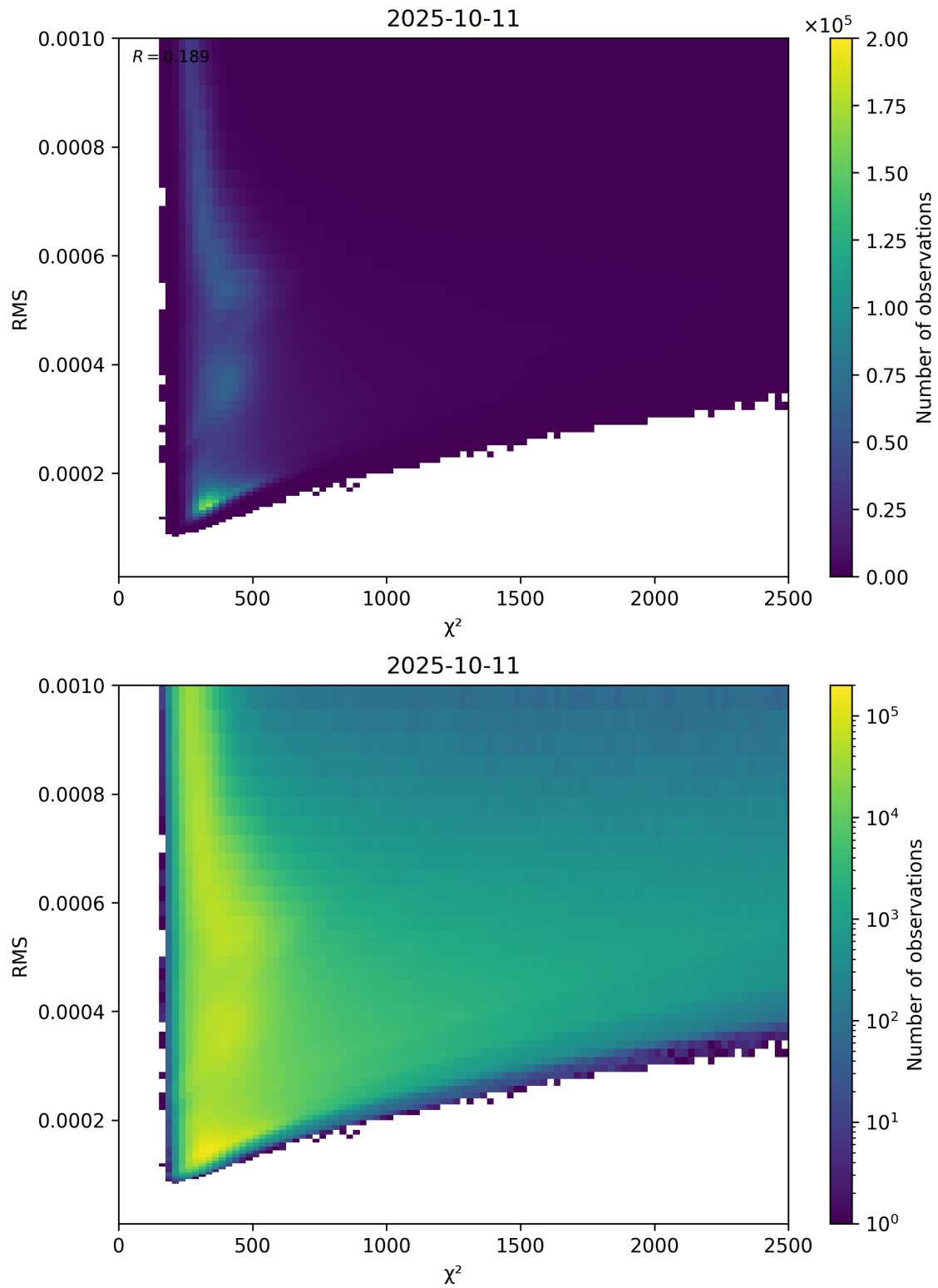
Figure 82: Scatter density plot of “ \chi^2 ” against “RMS” for 2025-10-11 to 2025-10-12.
