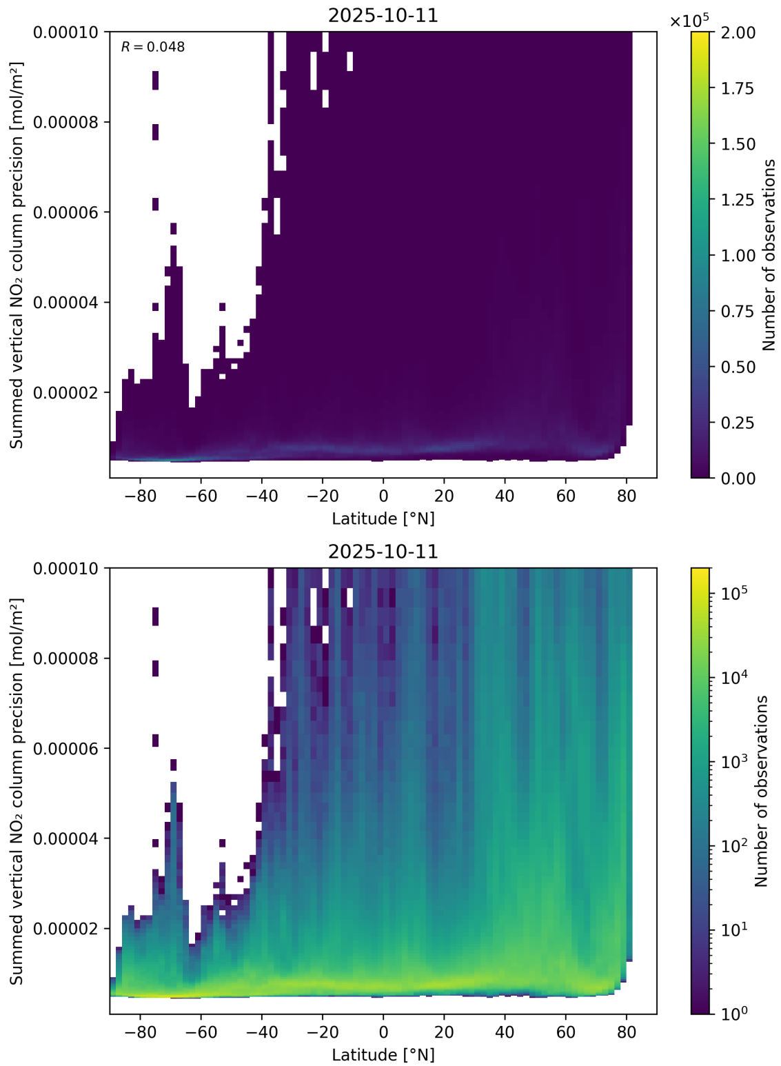
Figure 89: Scatter density plot of “Latitude” against “Summed vertical NO 2 column precision” for 2025-10-11 to 2025-10-12.
