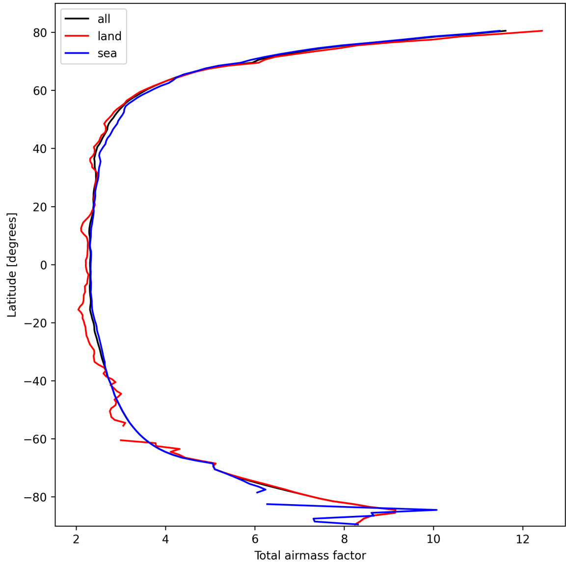
Figure 15: Zonal average of “Total airmass factor” for 2025-10-11 to 2025-10-12.
