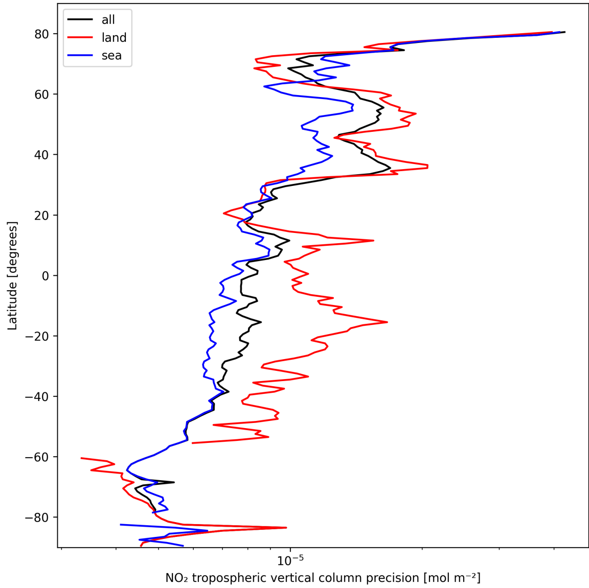
Figure 13: Zonal average of “NO 2 tropospheric vertical column precision” for 2025-10-11 to 2025-10-12.
