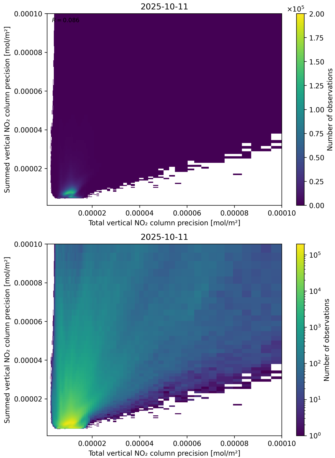
Figure 118: Scatter density plot of “Total vertical NO 2 column precision” against “Summed vertical NO 2 column precision” for 2025-10-11 to 2025-10-12.
