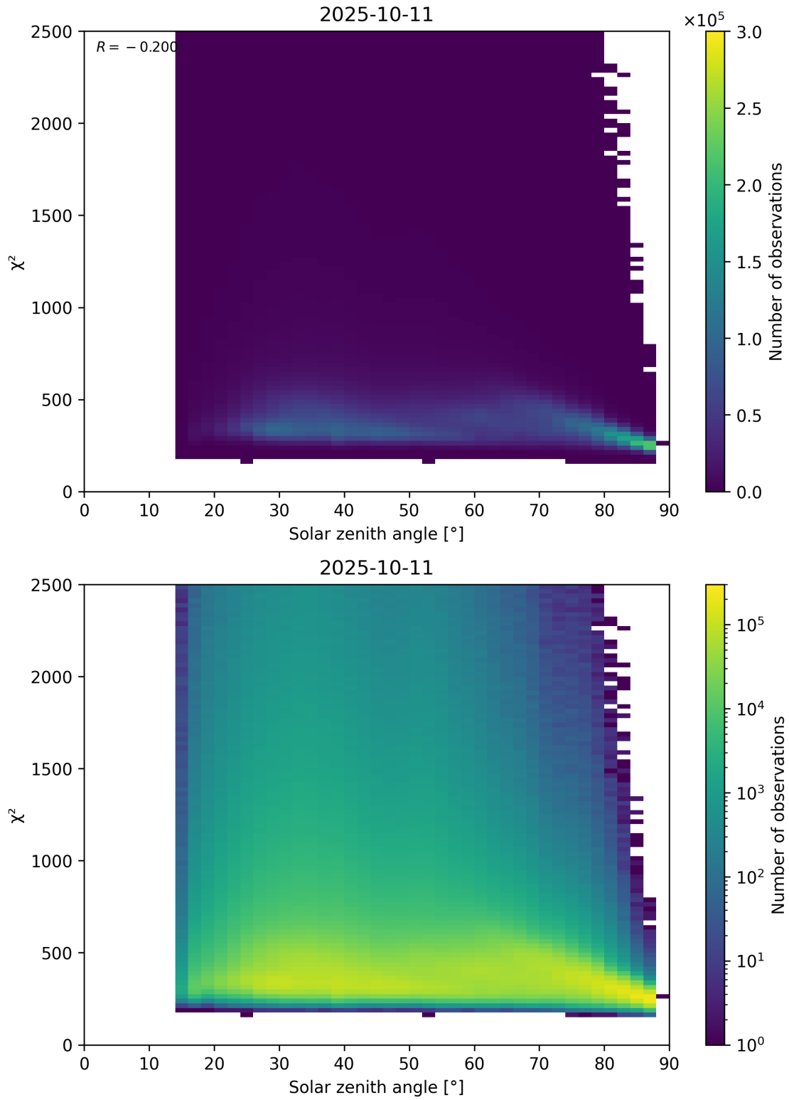
Figure 148: Scatter density plot of “Solar zenith angle” against “ \chi^2 ” for 2025-10-11 to 2025-10-12.
