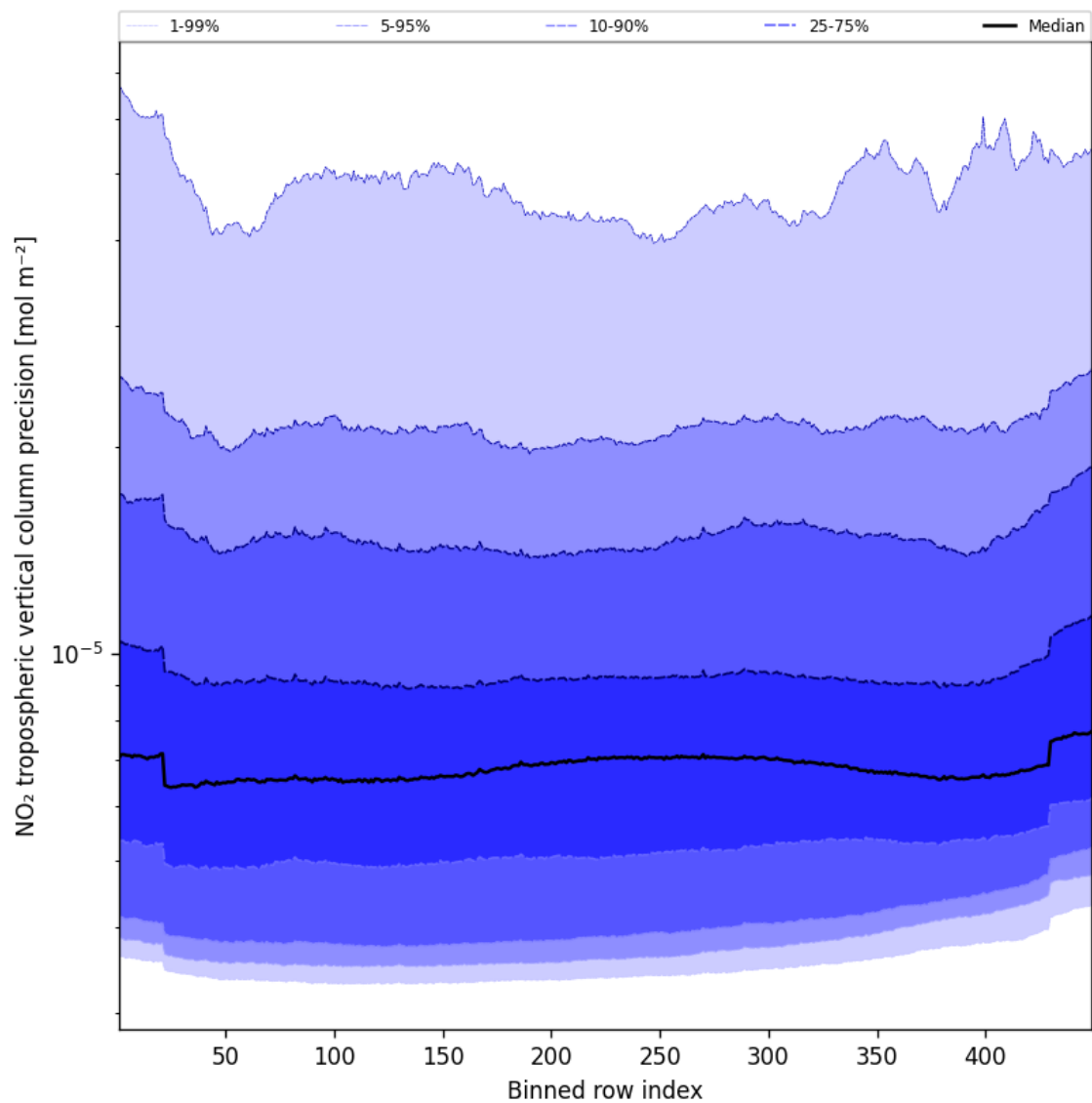
Figure 47: Along track statistics of “NO 2 tropospheric vertical column precision” for 2025-10-11 to 2025-10-12
