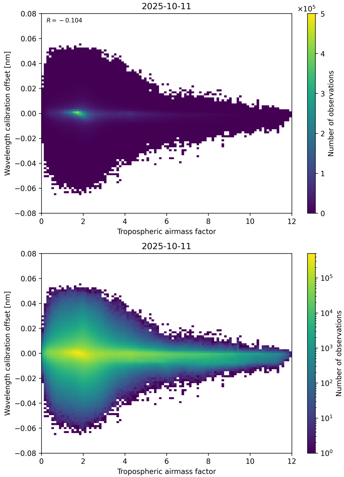
Figure 80: Scatter density plot of “Tropospheric airmass factor” against “Wavelength calibration offset” for 2025-10-11 to 2025-10-12.
