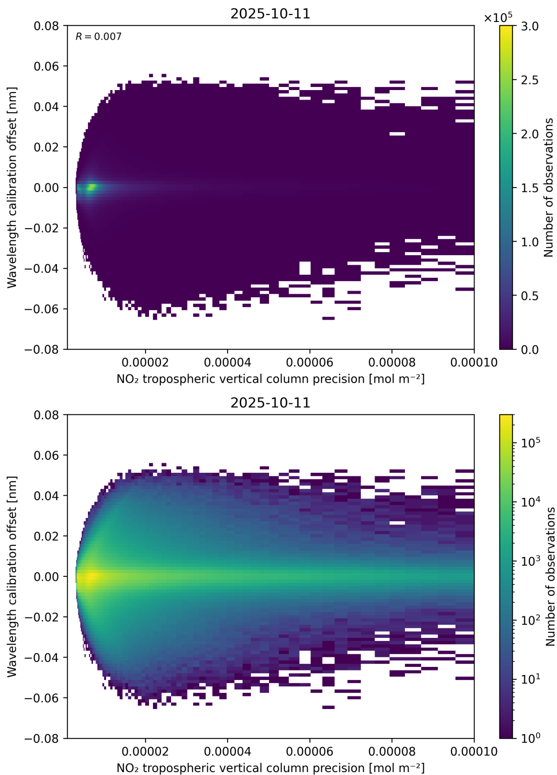
Figure 141: Scatter density plot of “NO 2 tropospheric vertical column precision” against “Wavelength calibration offset” for 2025-10-11 to 2025-10-12.
