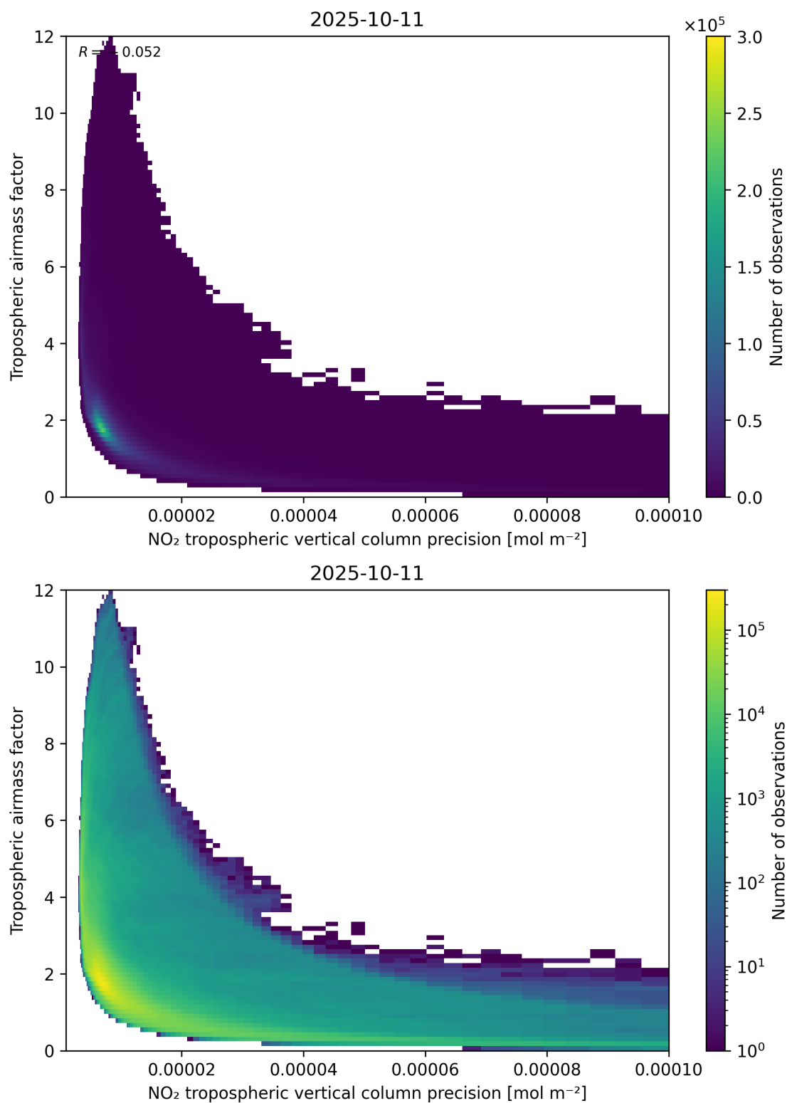
Figure 133: Scatter density plot of “NO 2 tropospheric vertical column precision” against “Tropospheric airmass factor” for 2025-10-11 to 2025-10-12.
