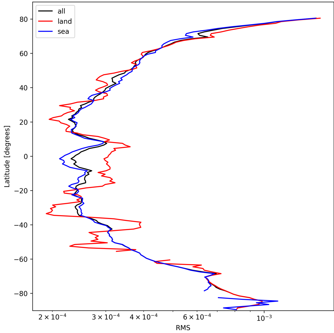
Figure 26: Zonal average of “RMS” for 2025-10-11 to 2025-10-12.
