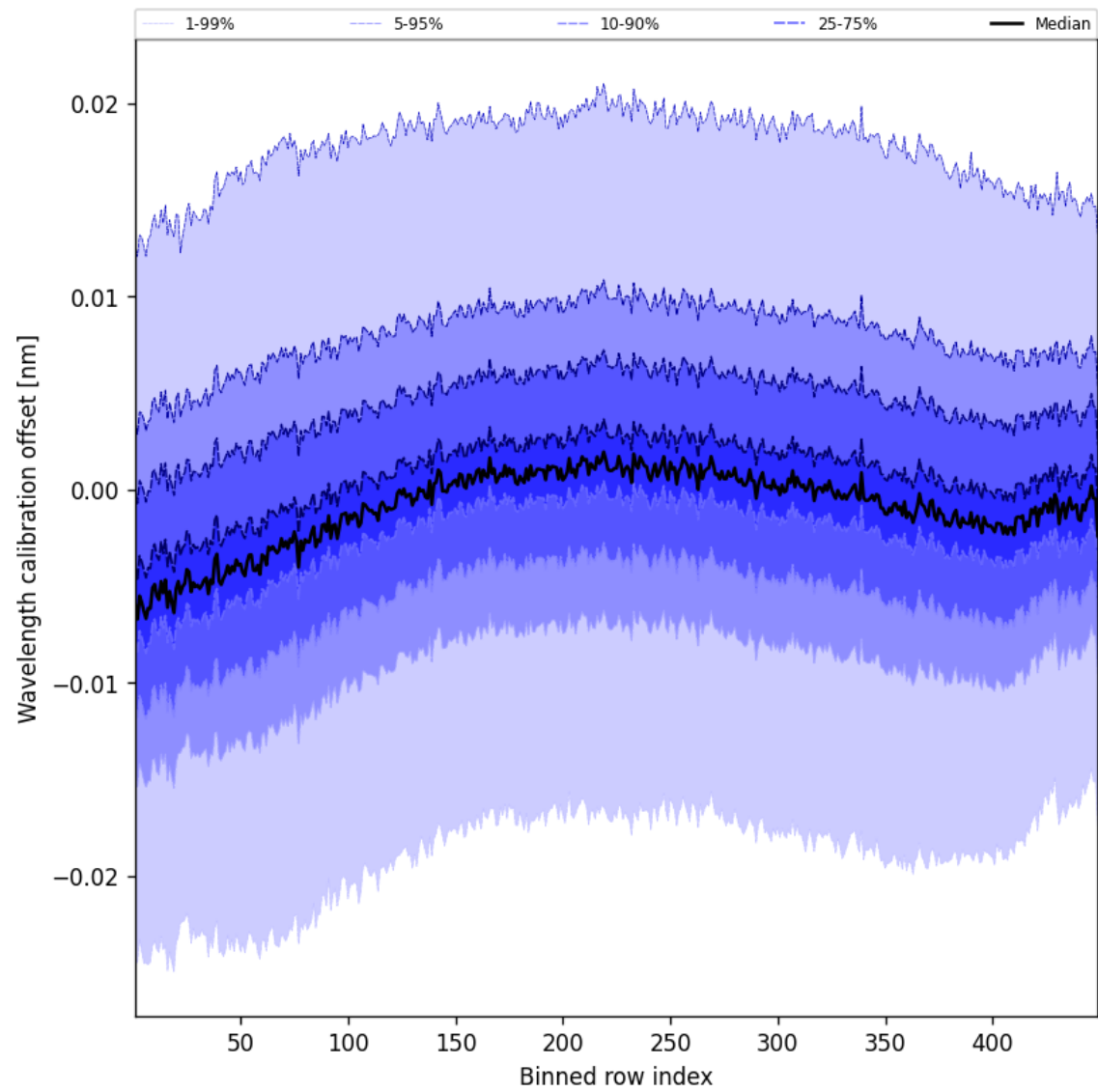
Figure 52: Along track statistics of “Wavelength calibration offset” for 2025-10-11 to 2025-10-12
