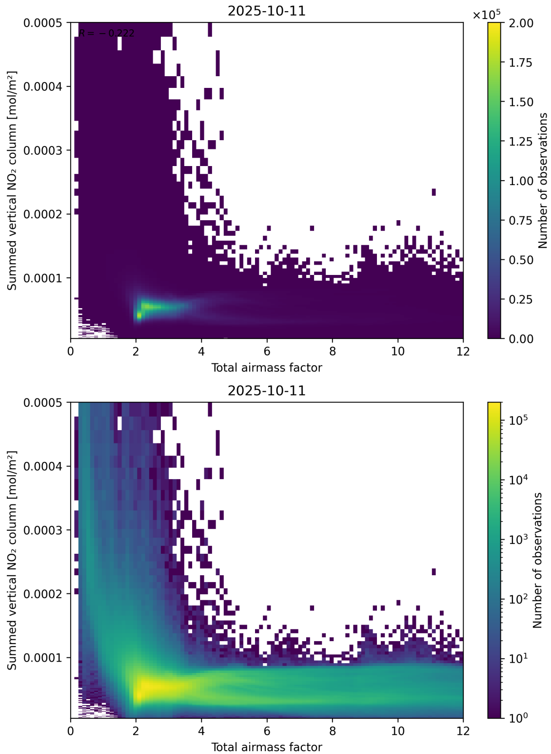
Figure 65: Scatter density plot of “Total airmass factor” against “Summed vertical NO 2 column” for 2025-10-11 to 2025-10-12.
