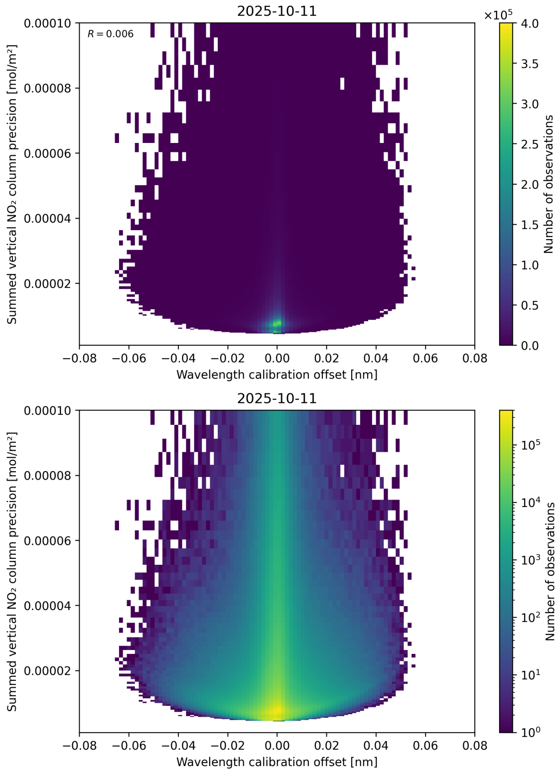
Figure 178: Scatter density plot of “Wavelength calibration offset” against “Summed vertical NO 2 column precision” for 2025-10-11 to 2025-10-12.
