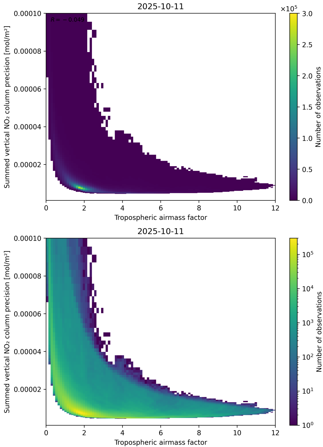
Figure 76: Scatter density plot of “Tropospheric airmass factor” against “Summed vertical NO 2 column precision” for 2025-10-11 to 2025-10-12.
