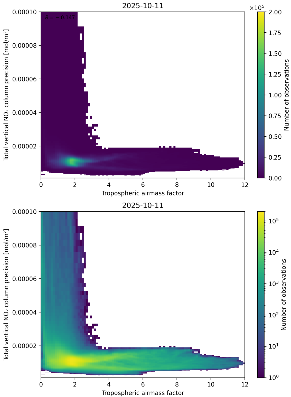
Figure 78: Scatter density plot of “Tropospheric air mass factor” against “Total vertical NO 2 column precision” for 2025-10-11 to 2025-10-12.
