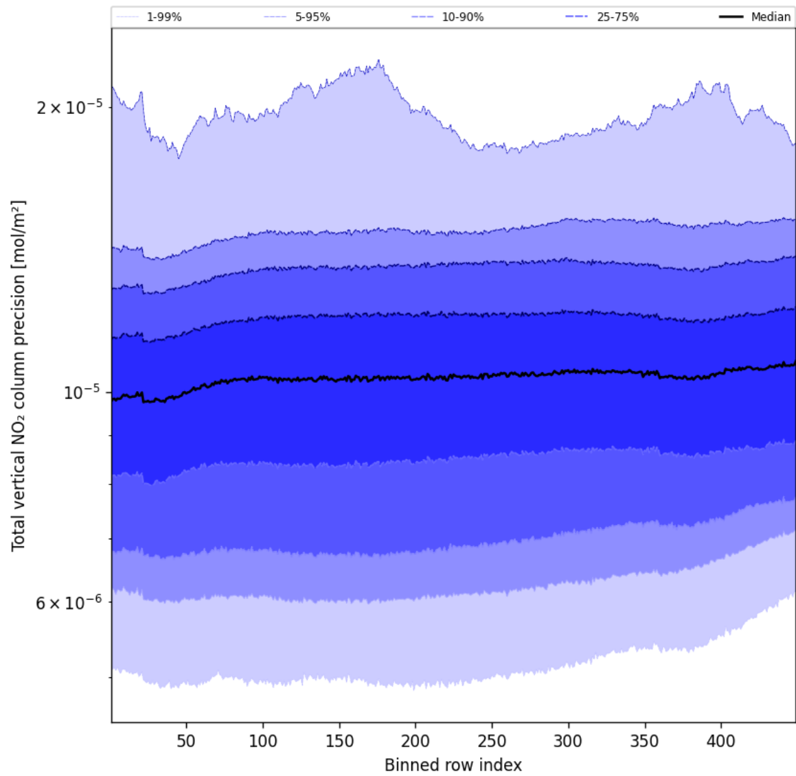
Figure 56: Along track statistics of “Total vertical NO 2 column precision” for 2025-10-11 to 2025-10-12
