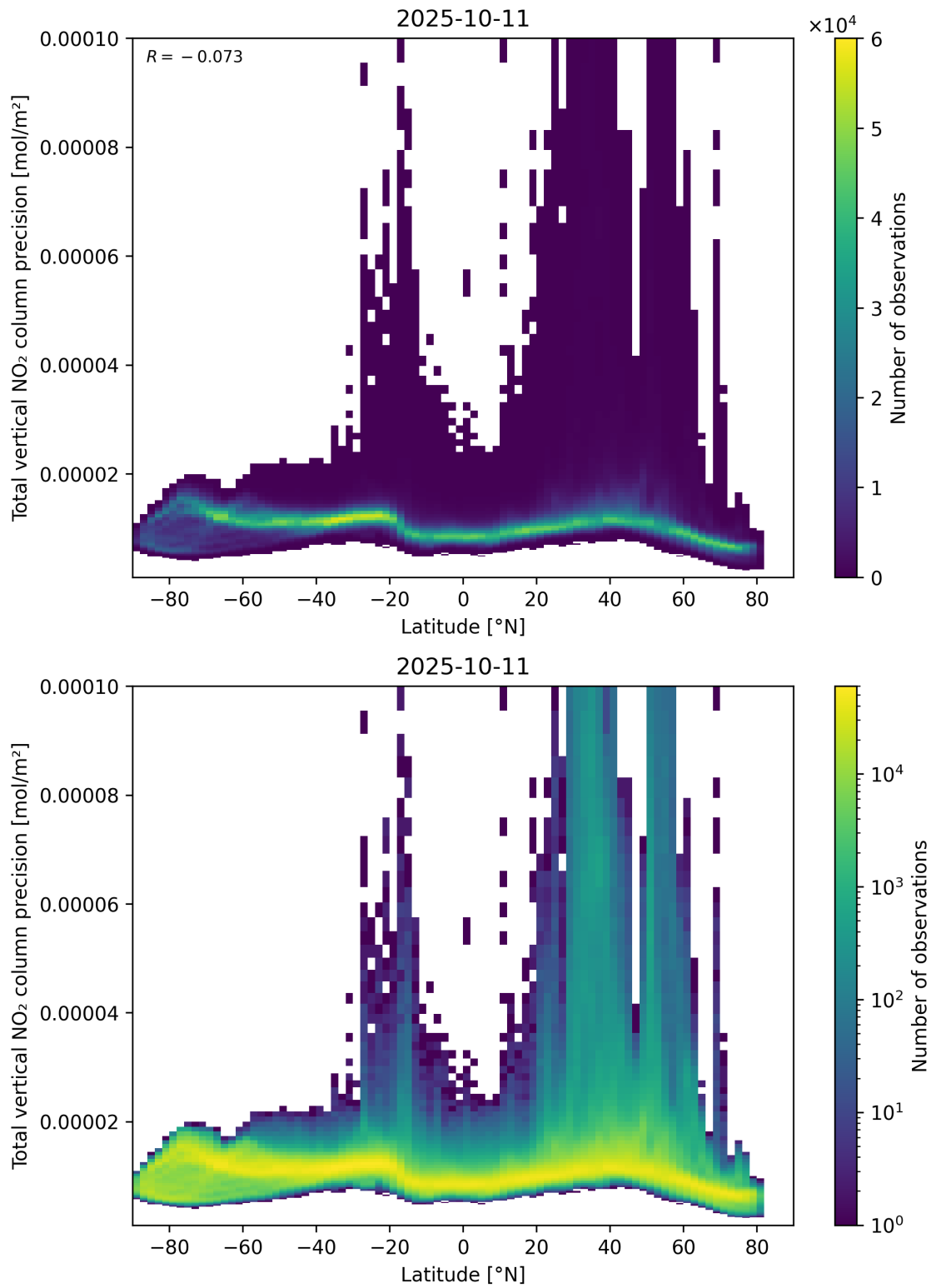
Figure 91: Scatter density plot of “Latitude” against “Total vertical NO 2 column precision” for 2025-10-11 to 2025-10-12.
