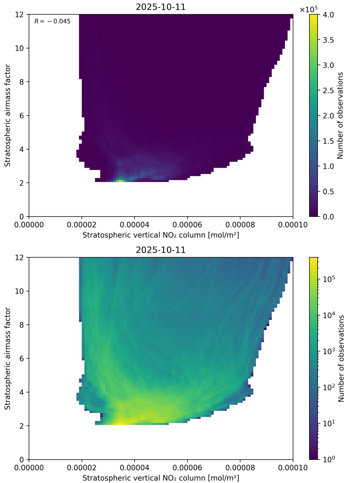
Figure 96: Scatter density plot of “Stratospheric vertical NO 2 column” against “Stratospheric airmass factor” for 2025-10-11 to 2025-10-12.
