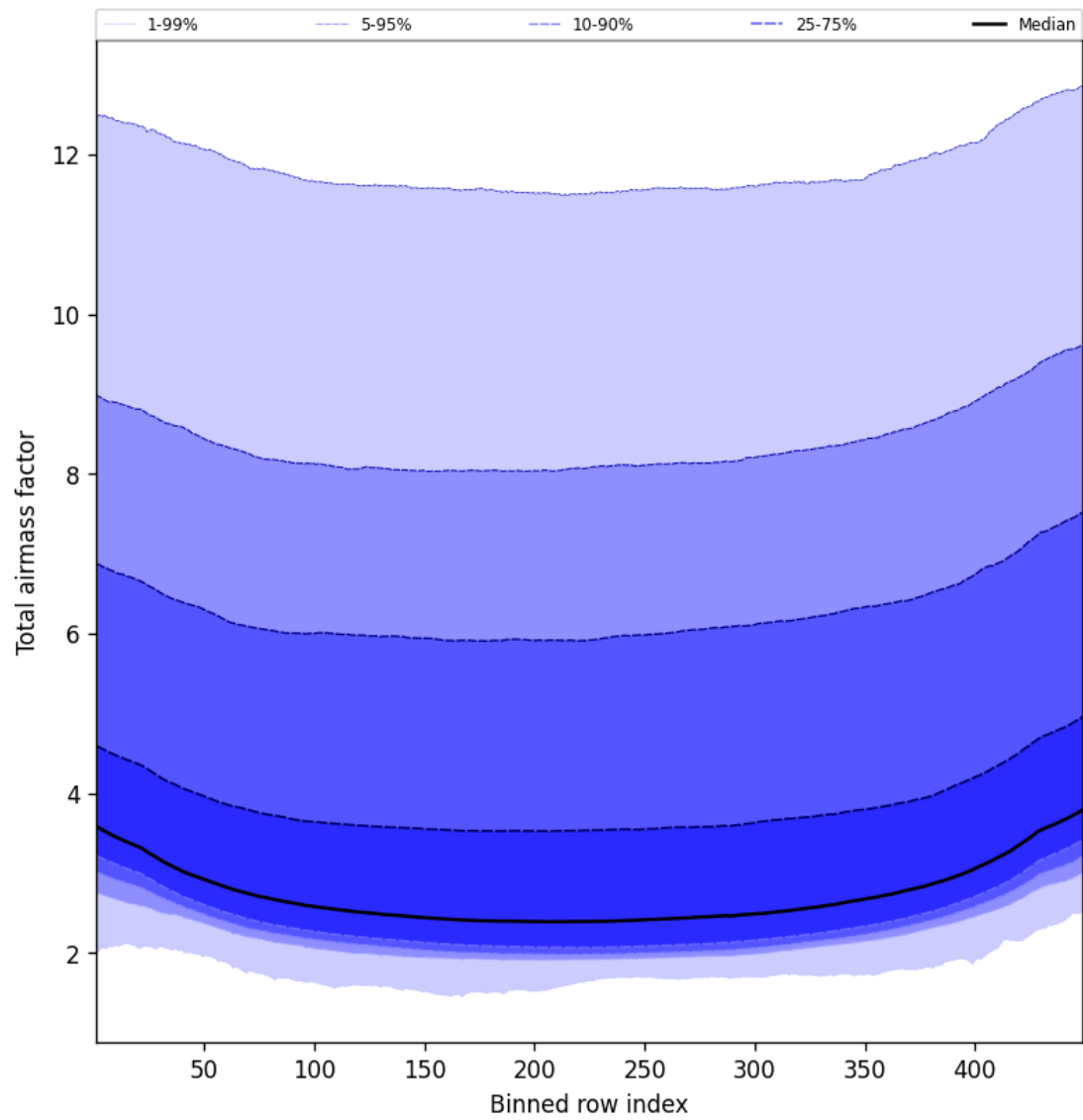
Figure 49: Along track statistics of “Total airmass factor” for 2025-10-11 to 2025-10-12
