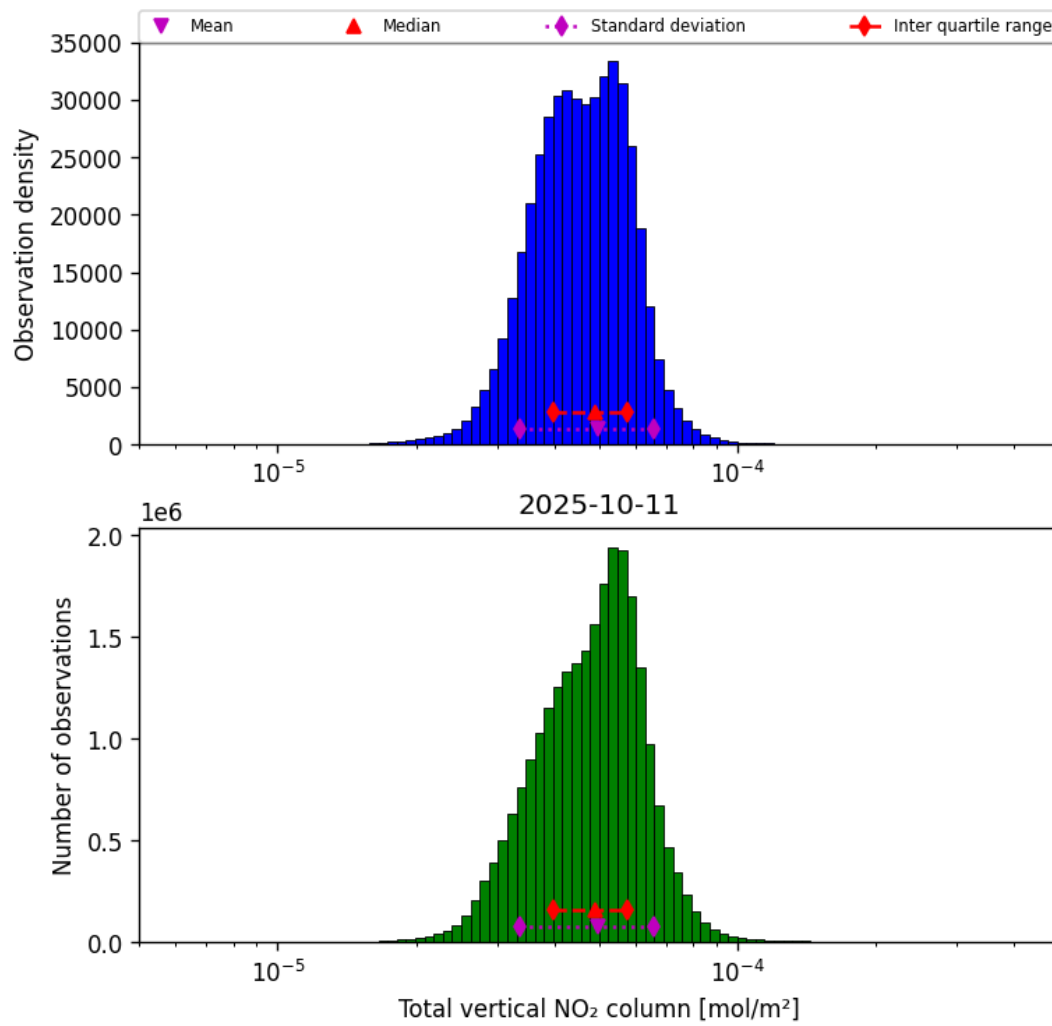
Figure 38: Histogram of “Total vertical NO 2 column” for 2025-10-11 to 2025-10-12
