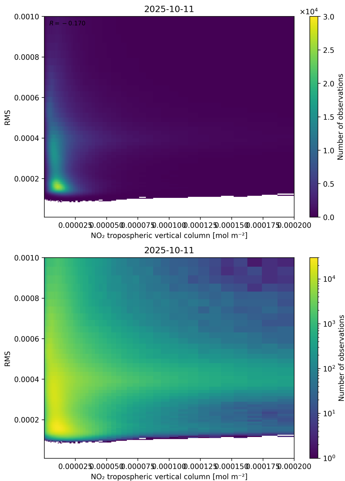
Figure 142: Scatter density plot of “NO 2 tropospheric vertical column” against “RMS” for 2025-10-11 to 2025-10-12.
