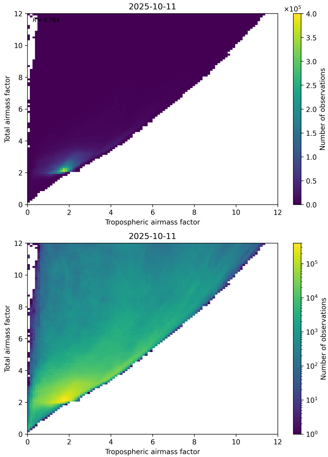
Figure 72: Scatter density plot of “Tropospheric airmass factor” against “Total airmass factor” for 2025-10-11 to 2025-10-12.
