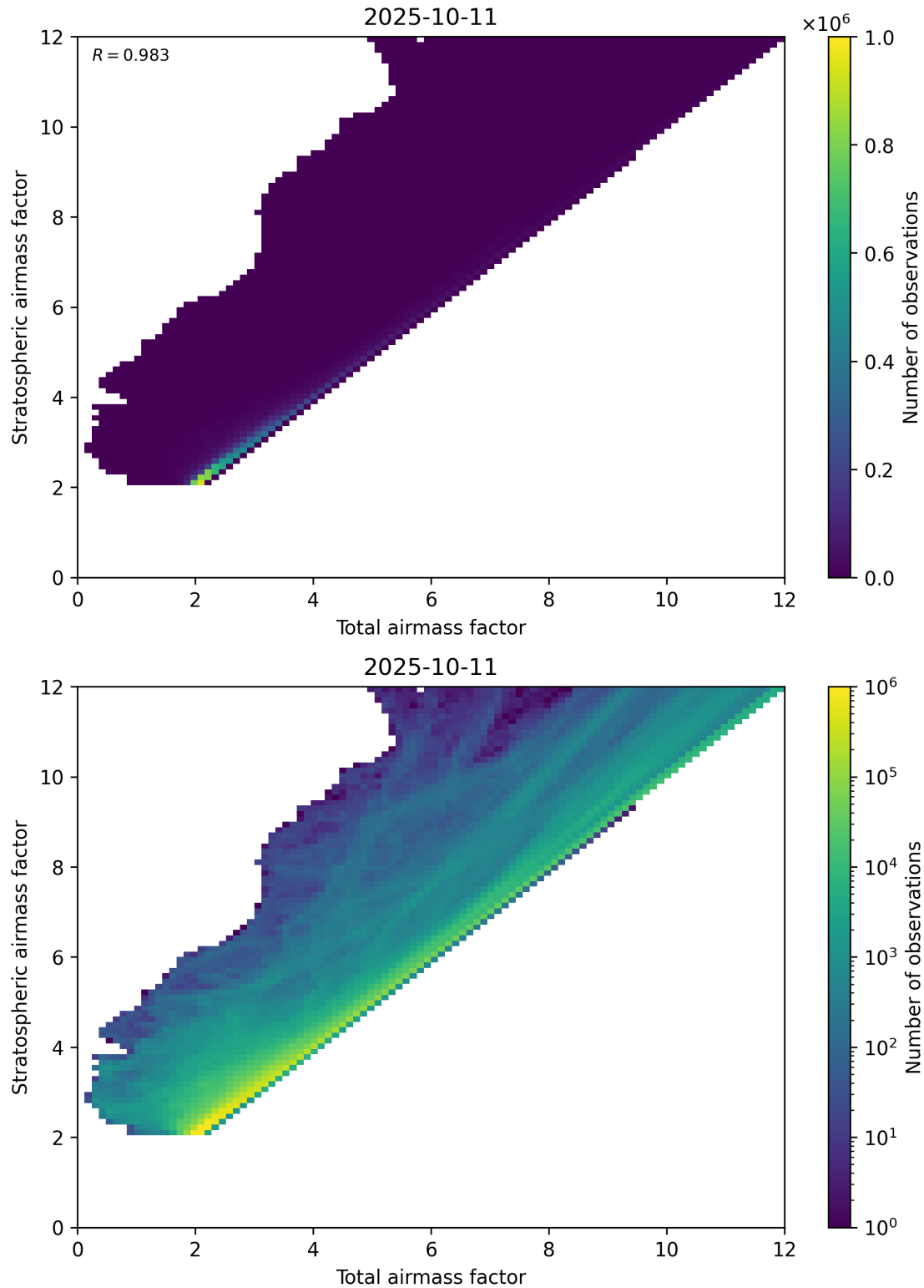
Figure 62: Scatter density plot of “Total airmass factor” against “Stratospheric airmass factor” for 2025-10-11 to 2025-10-12.
