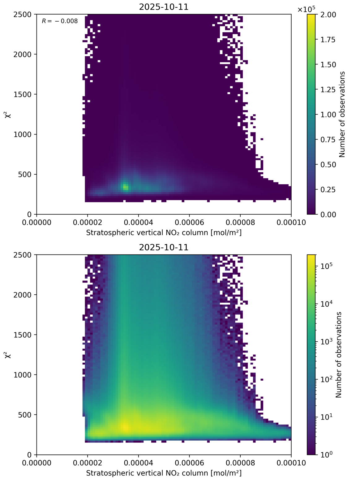
Figure 97: Scatter density plot of “Stratospheric vertical NO 2 column” against “ \chi^2 ” for 2025-10-11 to 2025-10-12.
