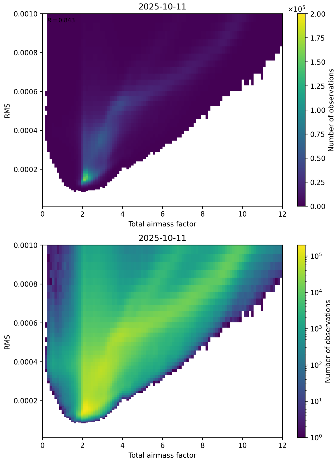
Figure 69: Scatter density plot of “Total airmass factor” against “RMS” for 2025-10-11 to 2025-10-12.
