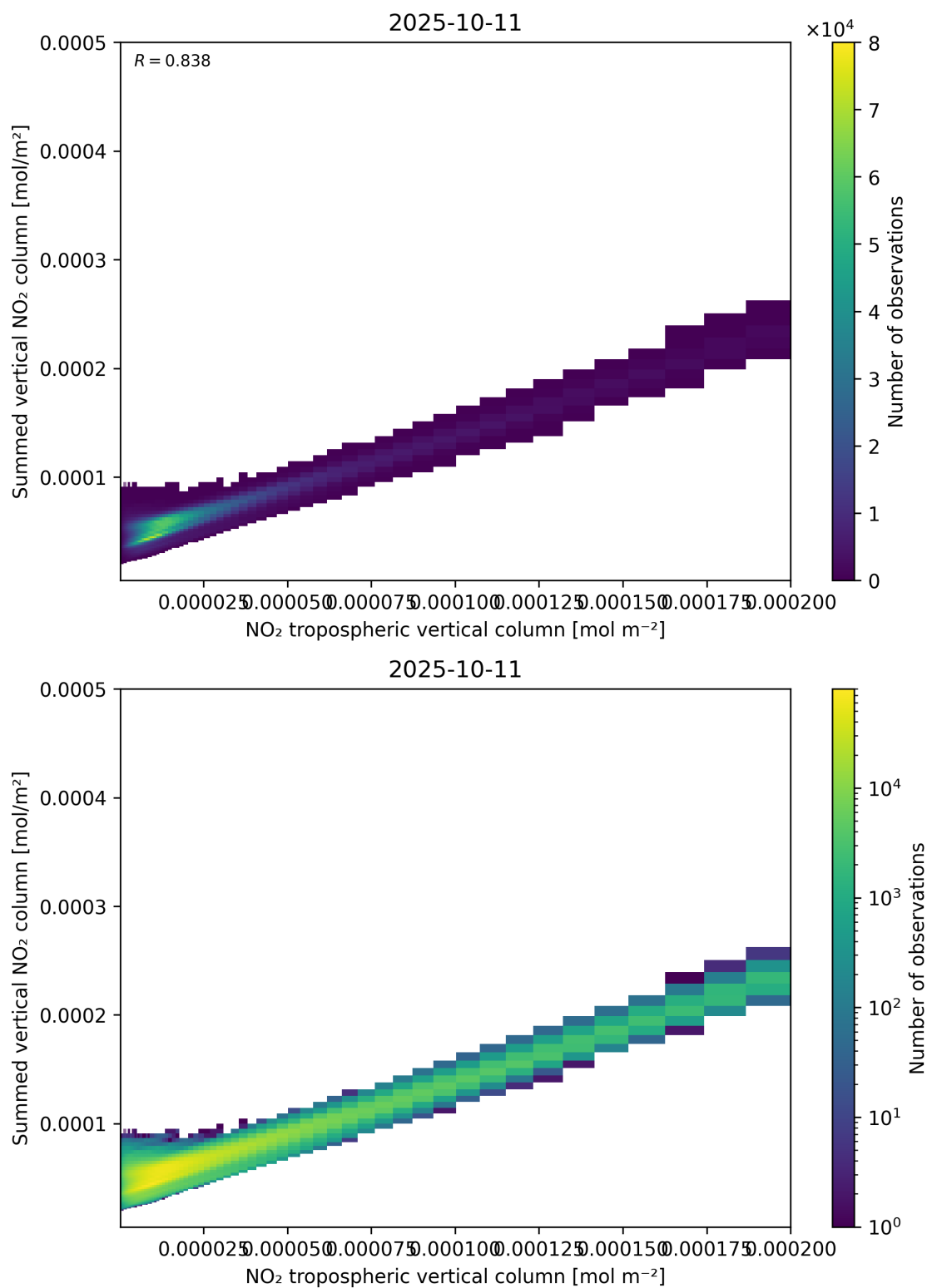
Figure 126: Scatter density plot of “NO 2 tropospheric vertical column” against “Summed vertical NO 2 column” for 2025-10-11 to 2025-10-12.
