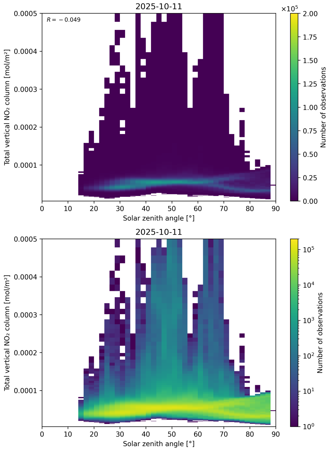
Figure 153: Scatter density plot of “Solar zenith angle” against “Total vertical NO 2 column” for 2025-10-11 to 2025-10-12.
