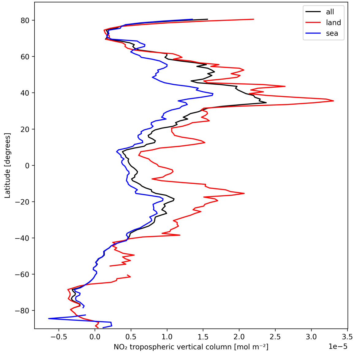
Figure 12: Zonal average of “NO 2 tropospheric vertical column” for 2025-10-11 to 2025-10-12.
