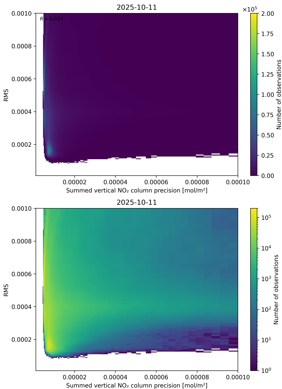
Figure 108: Scatter density plot of “Summed vertical NO 2 column precision” against “RMS” for 2025-10-11 to 2025-10-12.
