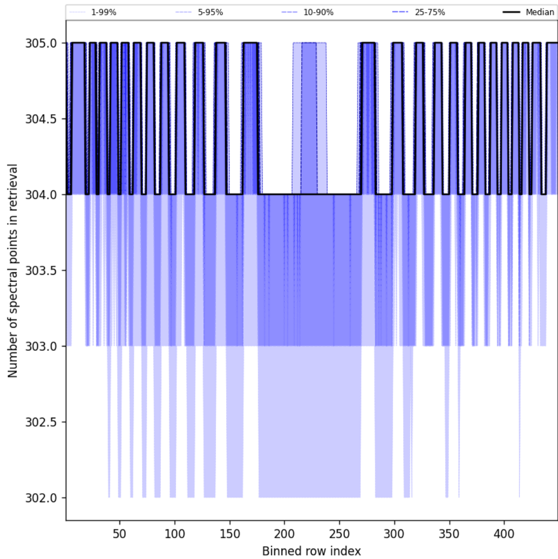
Figure 50: Along track statistics of “Number of spectral points in retrieval” for 2025-10-11 to 2025-10-12
