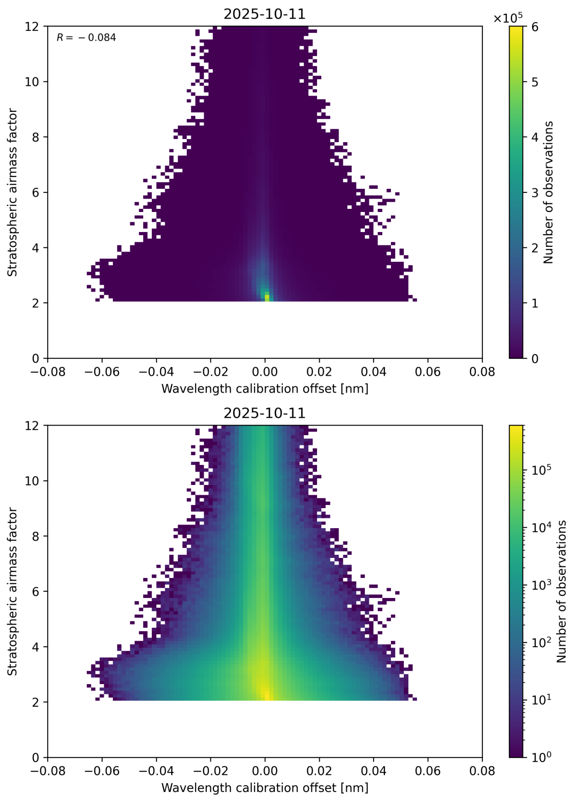
Figure 174: Scatter density plot of “Wavelength calibration offset” against “Stratospheric airmass factor” for 2025-10-11 to 2025-10-12.
