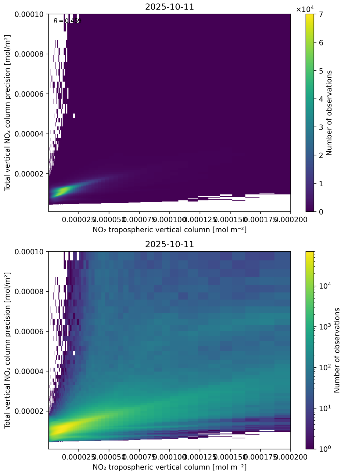
Figure 129: Scatter density plot of “NO 2 tropospheric vertical column” against “Total vertical NO 2 column precision” for 2025-10-11 to 2025-10-12.
