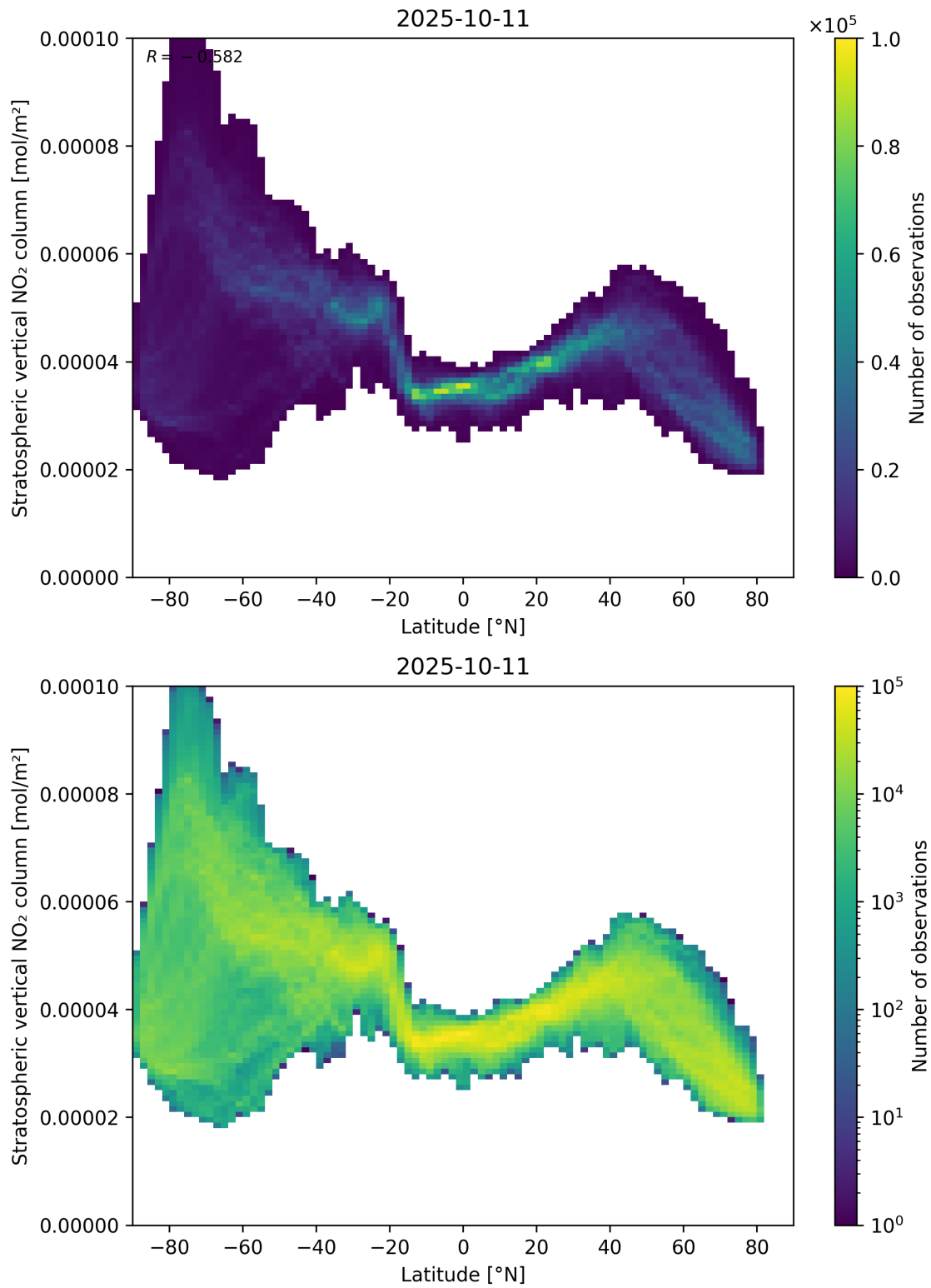
Figure 87: Scatter density plot of “Latitude” against “Stratospheric vertical NO 2 column” for 2025-10-11 to 2025-10-12.
