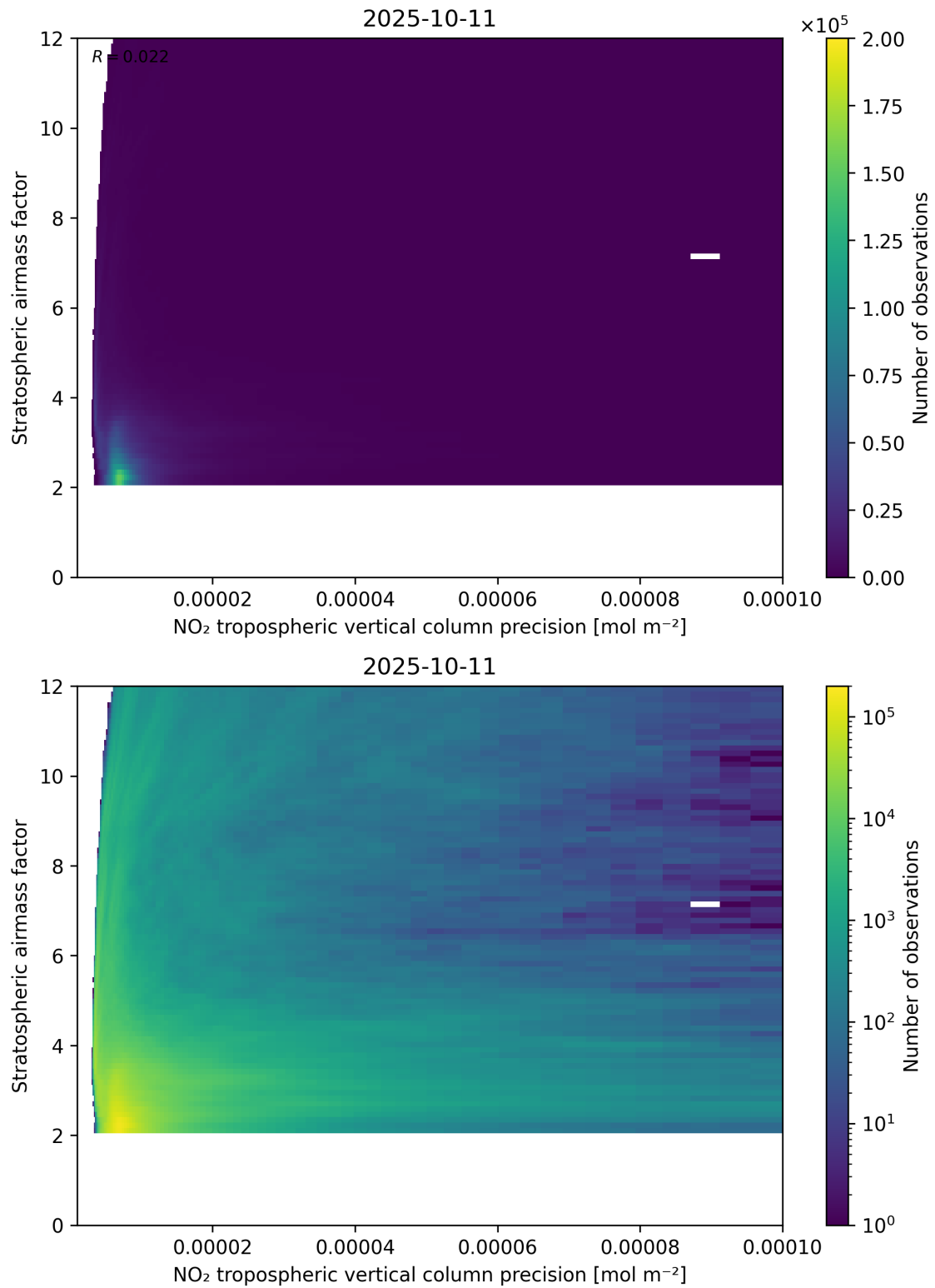
Figure 131: Scatter density plot of “NO 2 tropospheric vertical column precision” against “Stratospheric airmass factor” for 2025-10-11 to 2025-10-12.
