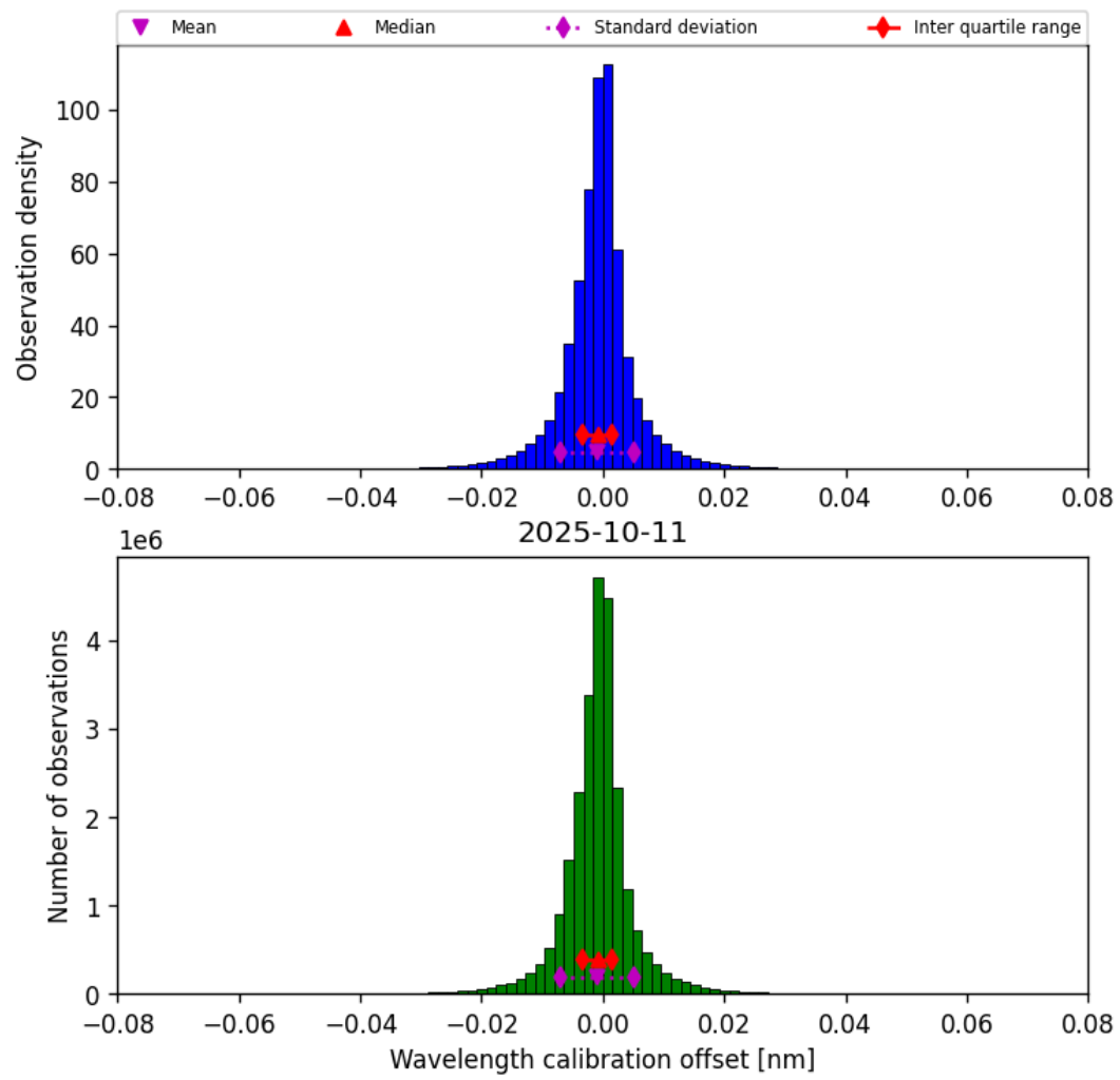
Figure 35: Histogram of “Wavelength calibration offset” for 2025-10-11 to 2025-10-12
