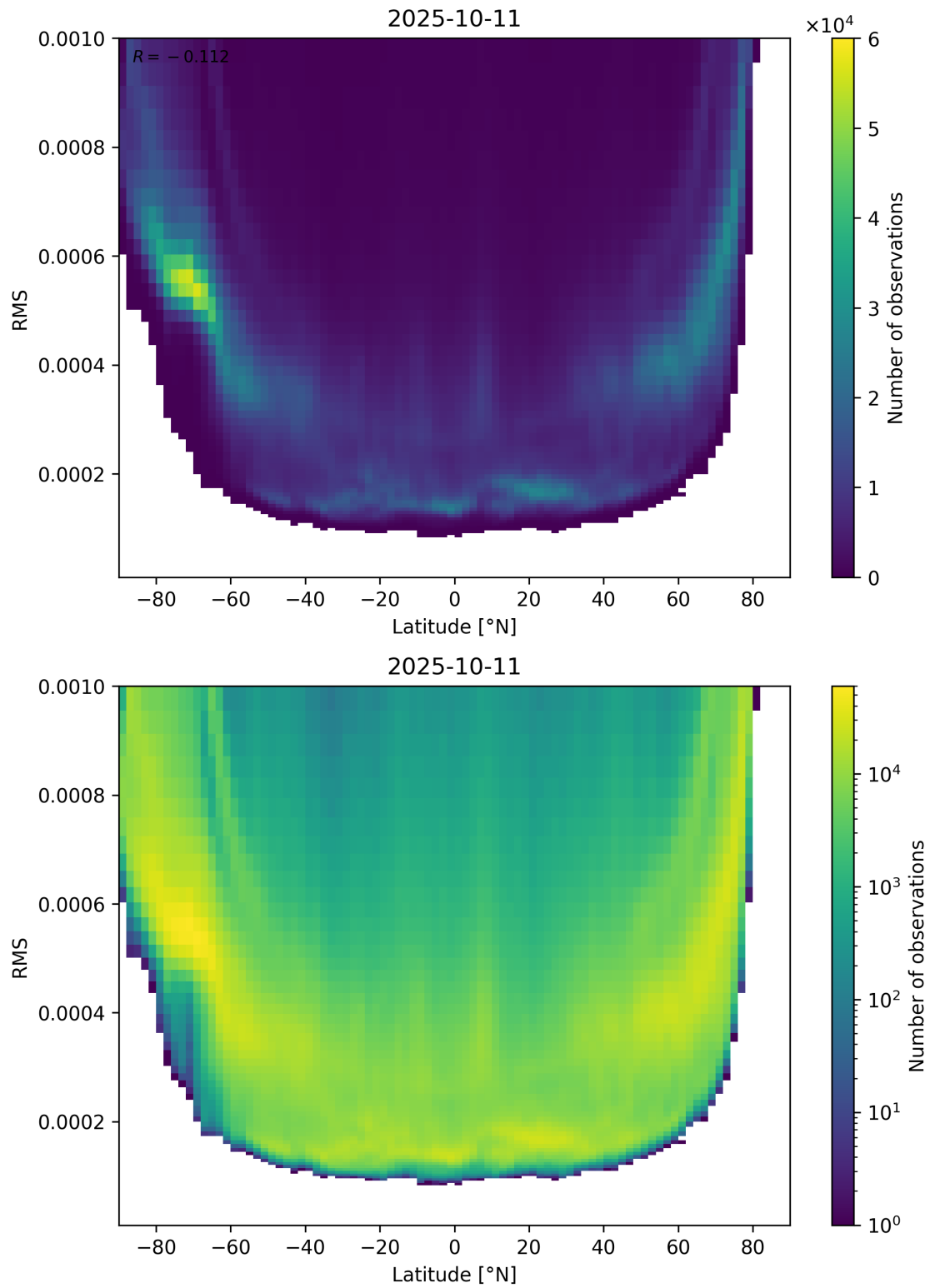
Figure 94: Scatter density plot of “Latitude” against “RMS” for 2025-10-11 to 2025-10-12.
