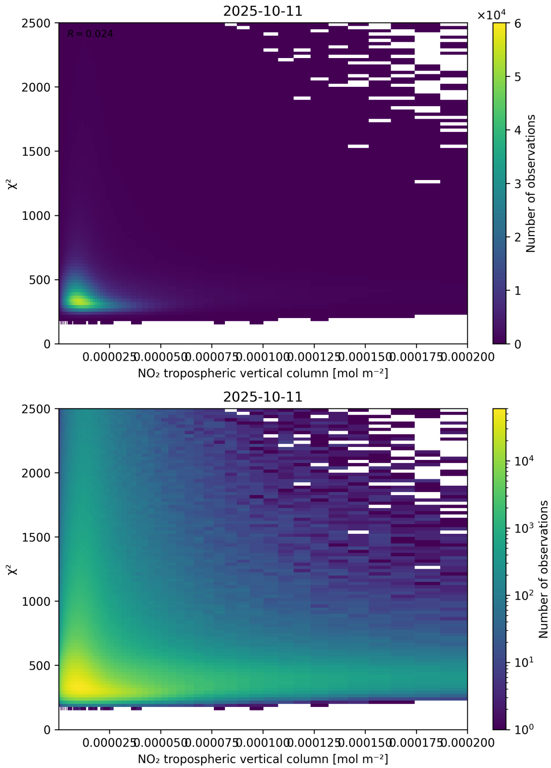
Figure 124: Scatter density plot of “NO 2 tropospheric vertical column” against “ \chi^2 ” for 2025-10-11 to 2025-10-12.
