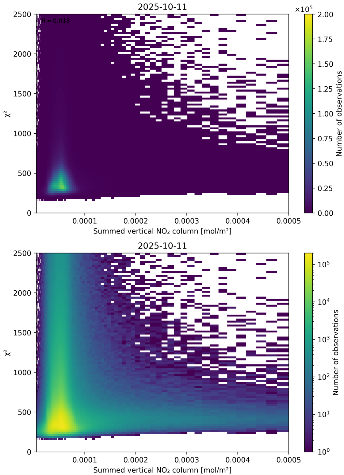
Figure 104: Scatter density plot of “Summed vertical NO 2 column” against “ \chi^2 ” for 2025-10-11 to 2025-10-12.
