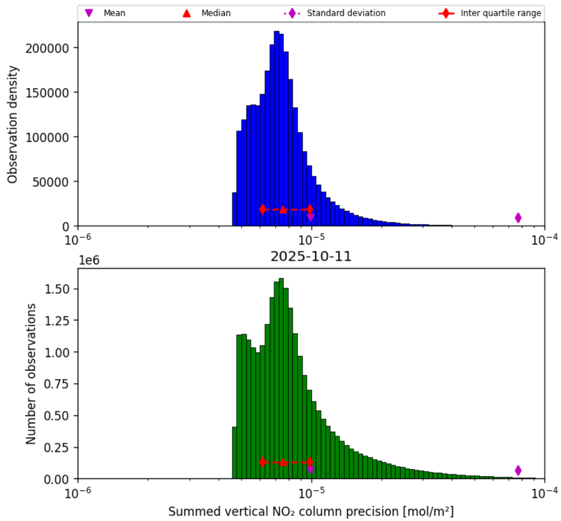
Figure 41: Histogram of “Summed vertical NO 2 column precision” for 2025-10-11 to 2025-10-12
