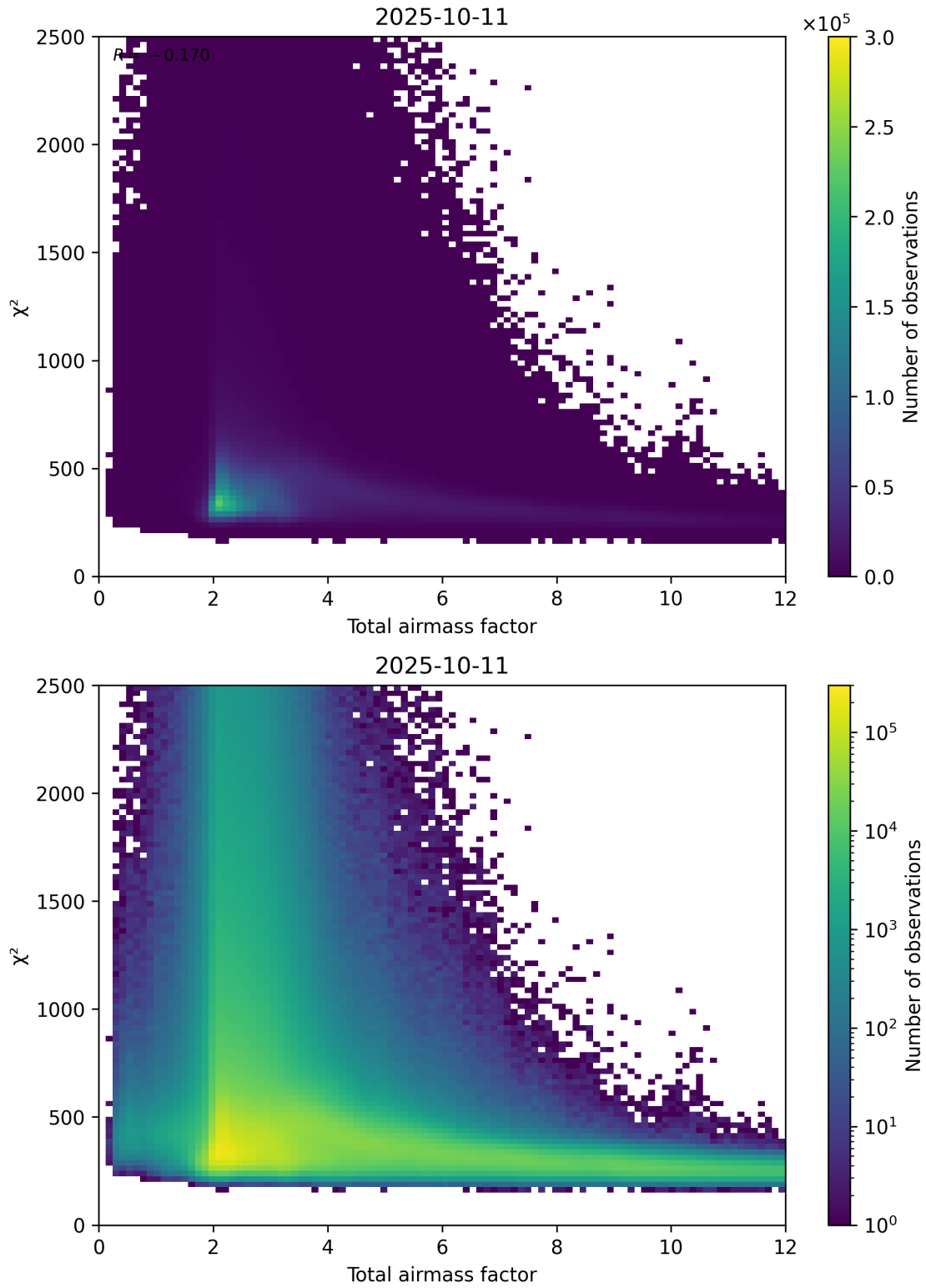
Figure 63: Scatter density plot of “Total airmass factor” against “ \chi^2 ” for 2025-10-11 to 2025-10-12.
