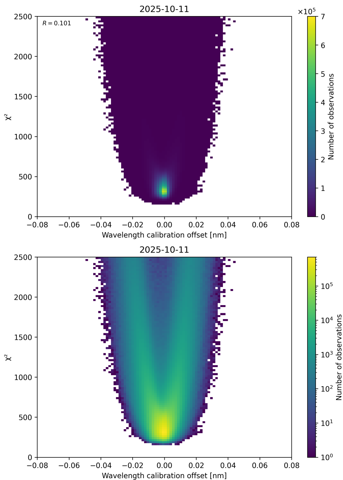
Figure 175: Scatter density plot of “Wavelength calibration offset” against “ \chi^2 ” for 2025-10-11 to 2025-10-12.
