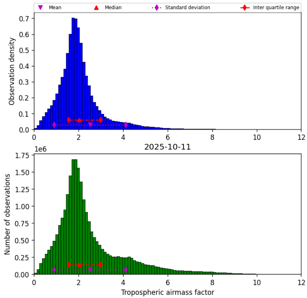
Figure 31: Histogram of “Tropospheric airmass factor” for 2025-10-11 to 2025-10-12
