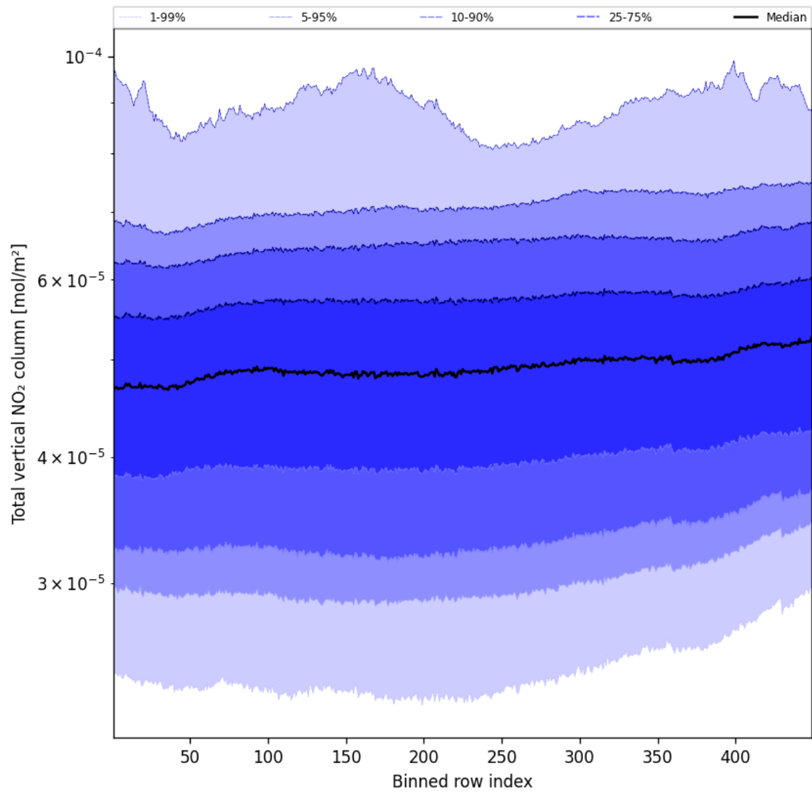
Figure 55: Along track statistics of “Total vertical NO 2 column” for 2025-10-11 to 2025-10-12
