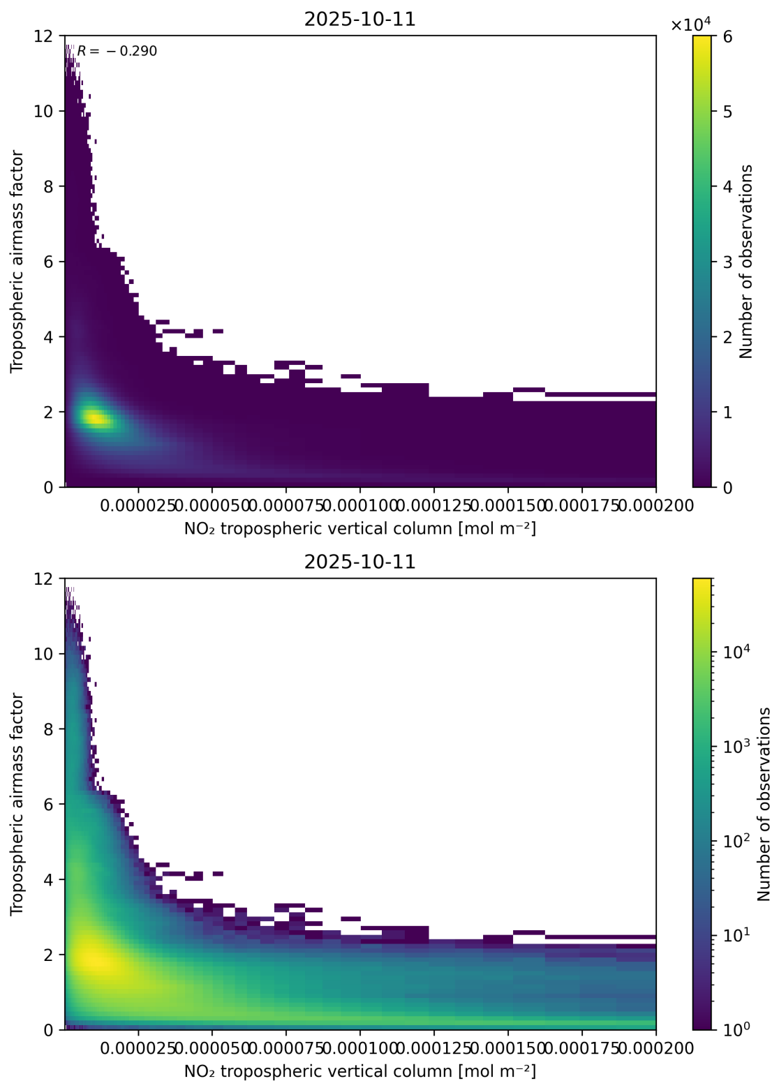
Figure 123: Scatter density plot of “NO 2 tropospheric vertical column” against “Tropospheric air mass factor” for 2025-10-11 to 2025-10-12.
