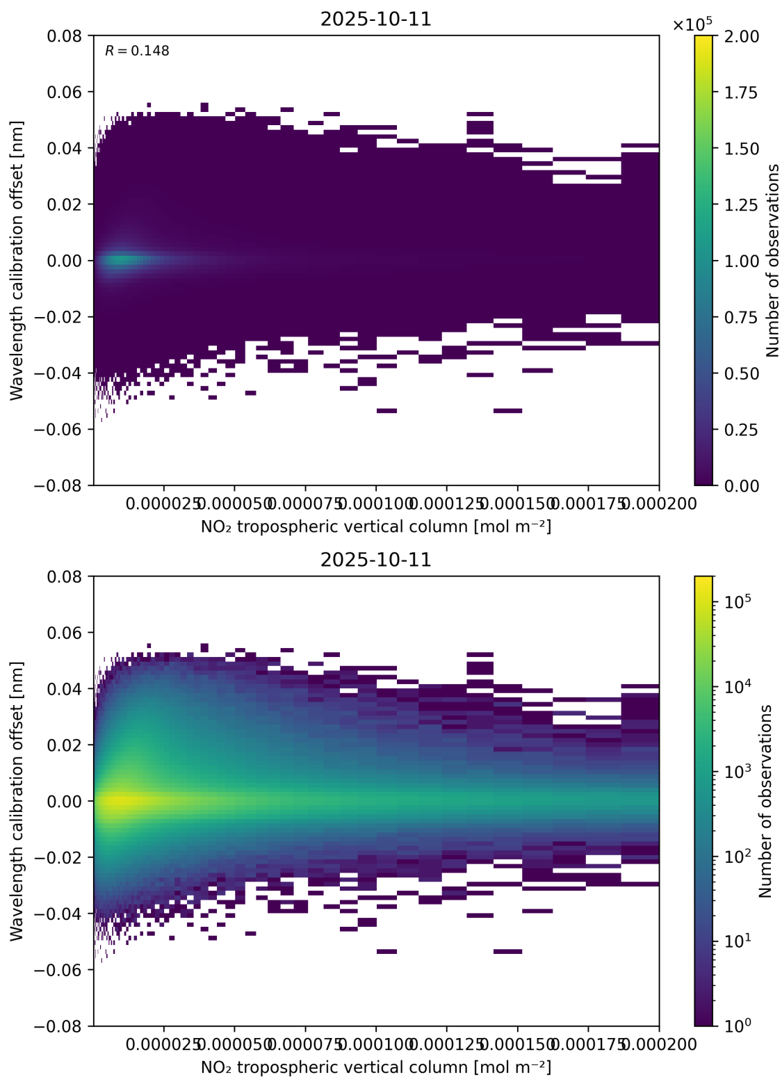
Figure 143: Scatter density plot of “NO 2 tropospheric vertical column” against “Wavelength calibration offset” for 2025-10-11 to 2025-10-12.
