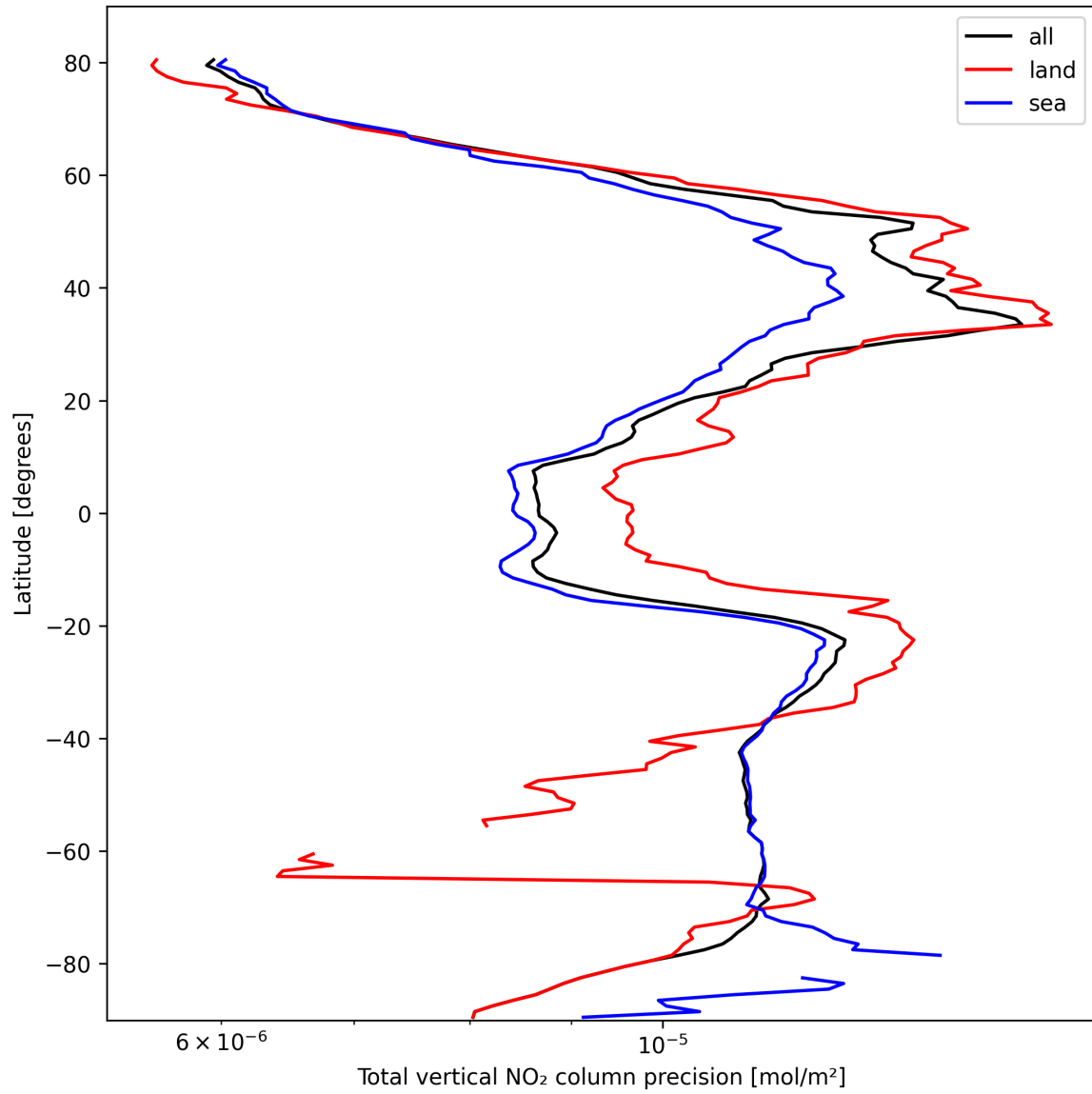
Figure 22: Zonal average of “Total vertical NO 2 column precision” for 2025-10-11 to 2025-10-12.
