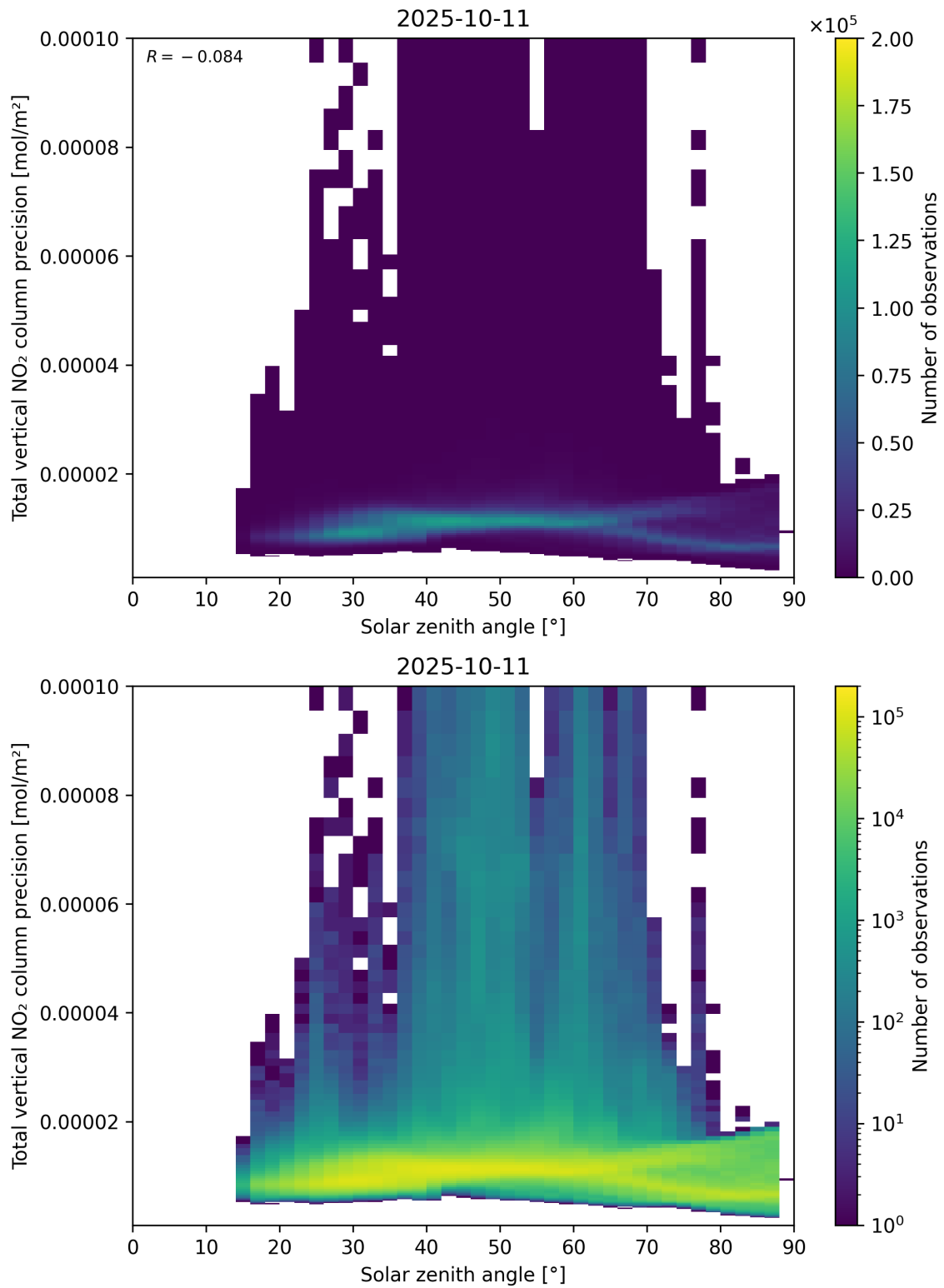
Figure 154: Scatter density plot of “Solar zenith angle” against “Total vertical NO 2 column precision” for 2025-10-11 to 2025-10-12.
