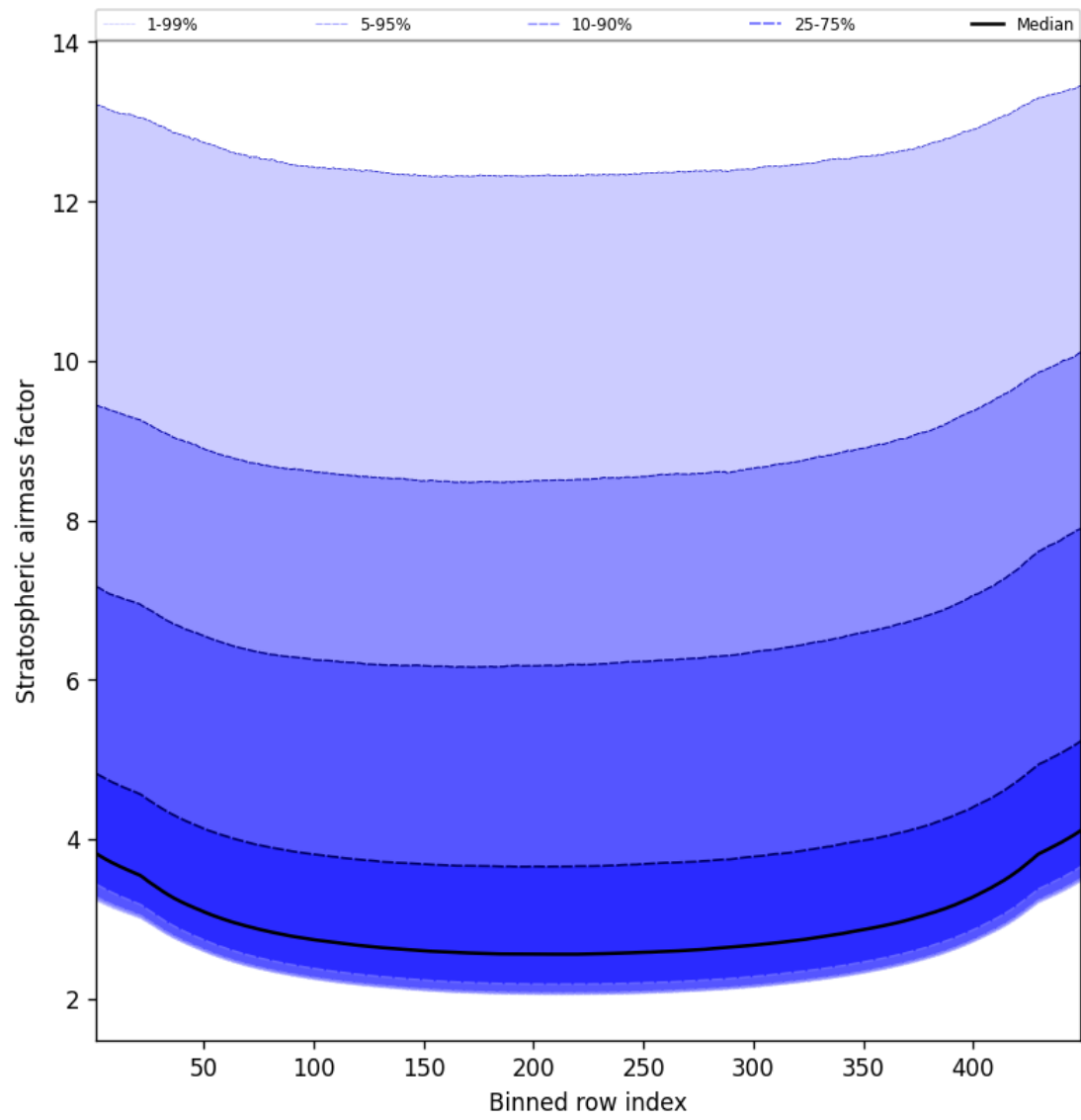
Figure 61: Along track statistics of “Stratospheric air mass factor” for 2025-10-11 to 2025-10-12
