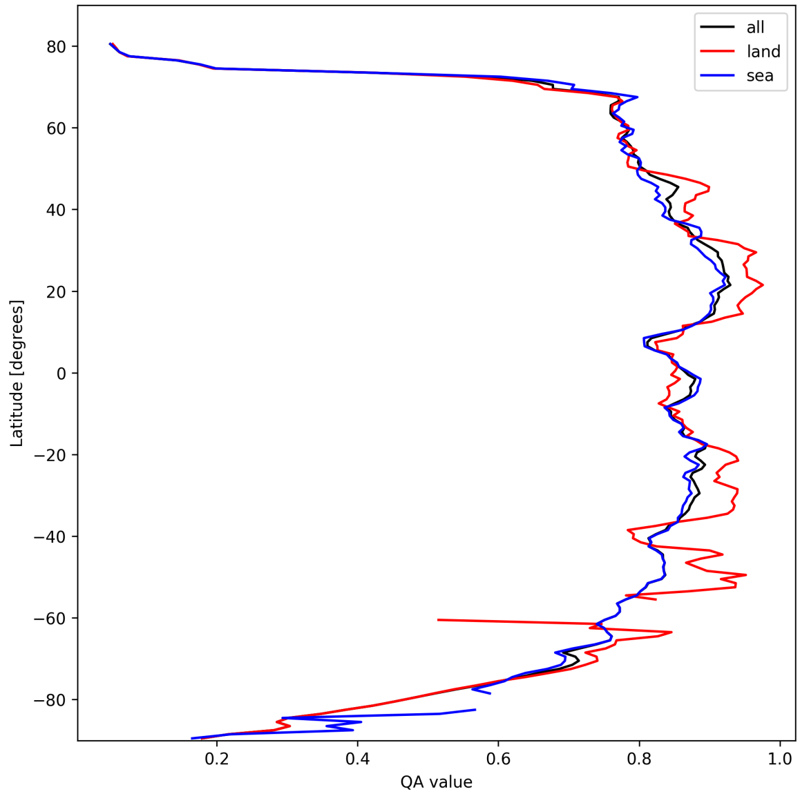
Figure 11: Zonal average of “QA value” for 2025-10-11 to 2025-10-12.
