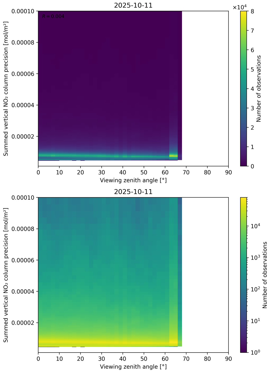
Figure 166: Scatter density plot of “Viewing zenith angle” against “Summed vertical NO 2 column precision” for 2025-10-11 to 2025-10-12.
