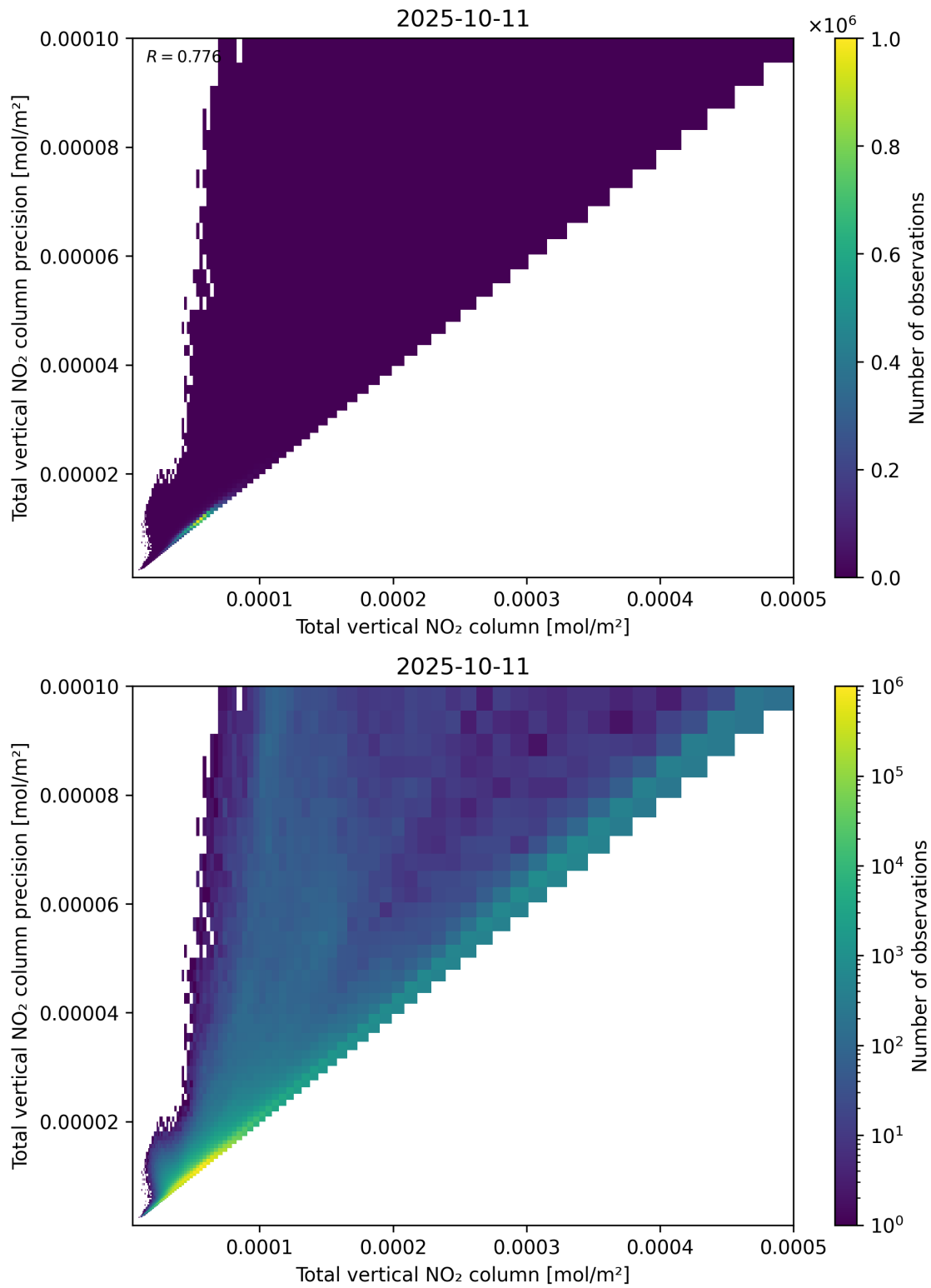
Figure 114: Scatter density plot of “Total vertical NO 2 column” against “Total vertical NO 2 column precision” for 2025-10-11 to 2025-10-12.
