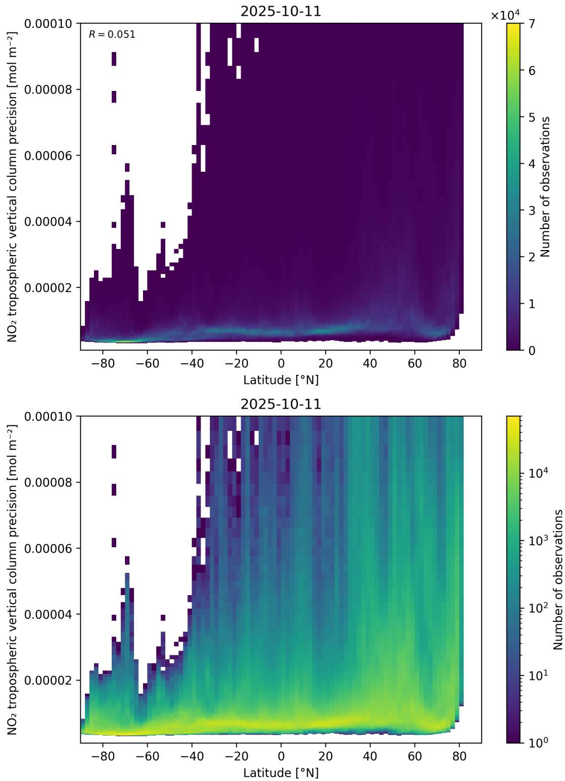
Figure 93: Scatter density plot of “Latitude” against “NO 2 tropospheric vertical column precision” for 2025-10-11 to 2025-10-12.
