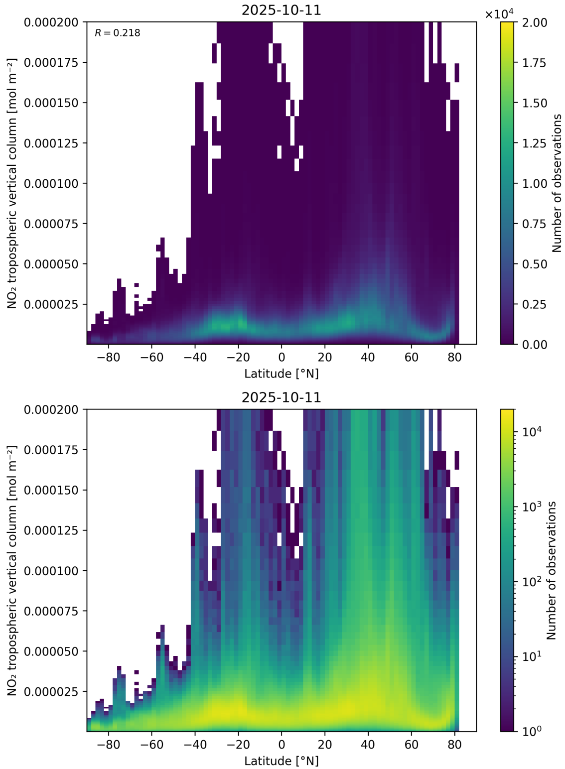
Figure 92: Scatter density plot of “Latitude” against “NO 2 tropospheric vertical column” for 2025-10-11 to 2025-10-12.
