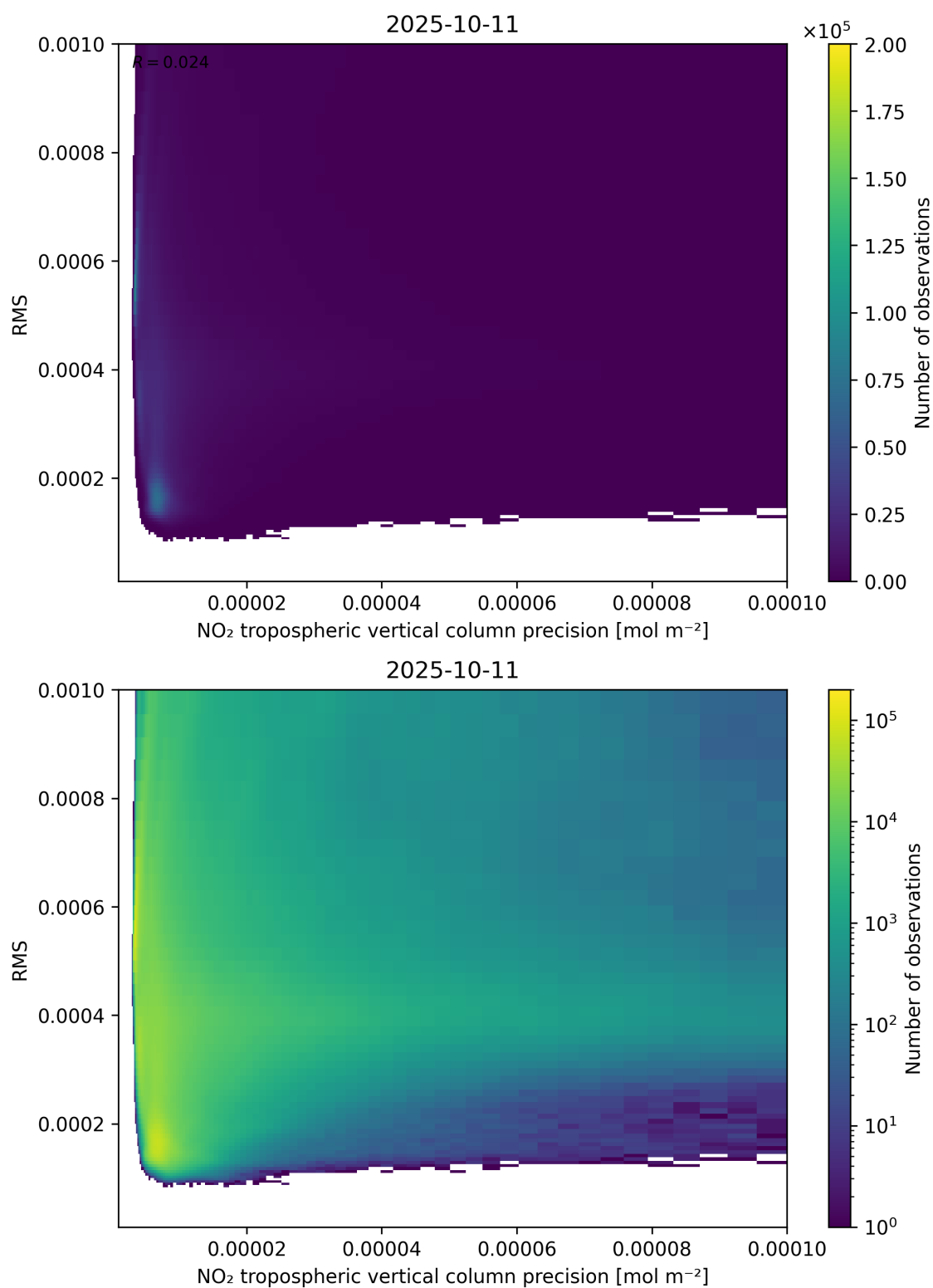
Figure 140: Scatter density plot of “NO 2 tropospheric vertical column precision” against “RMS” for 2025-10-11 to 2025-10-12.
