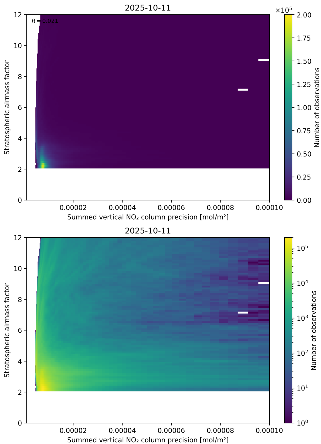
Figure 106: Scatter density plot of “Summed vertical NO 2 column precision” against “Stratospheric airmass factor” for 2025-10-11 to 2025-10-12.
