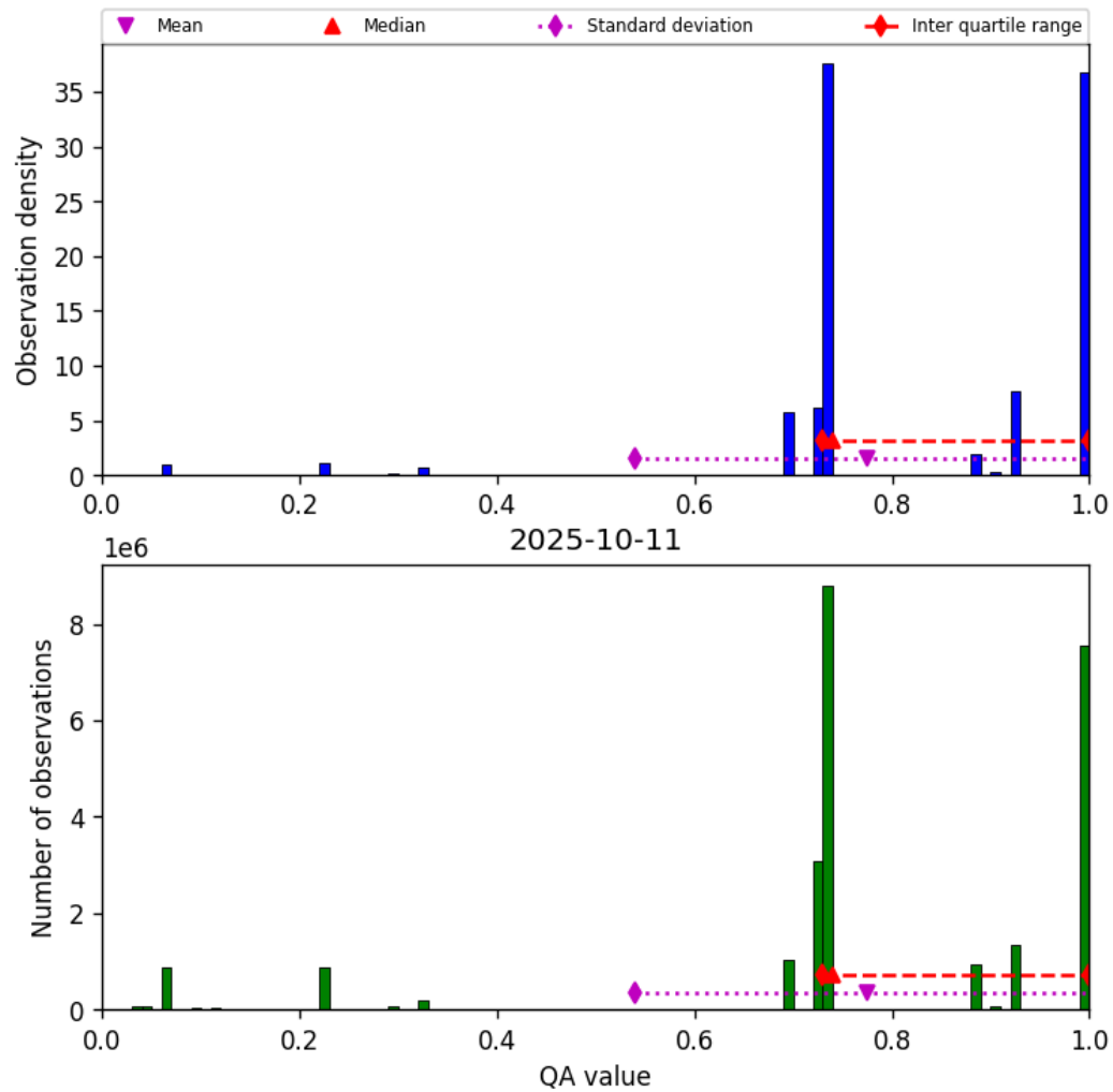
Figure 28: Histogram of “QA value” for 2025-10-11 to 2025-10-12
