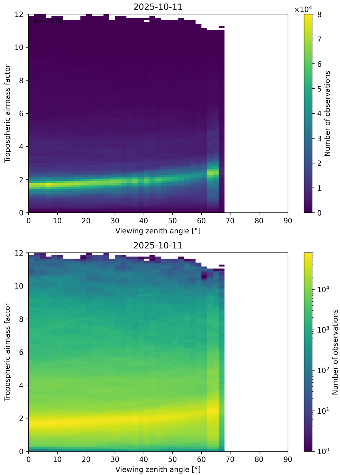
Figure 161: Scatter density plot of “Viewing zenith angle” against “Tropospheric airmass factor” for 2025-10-11 to 2025-10-12.
