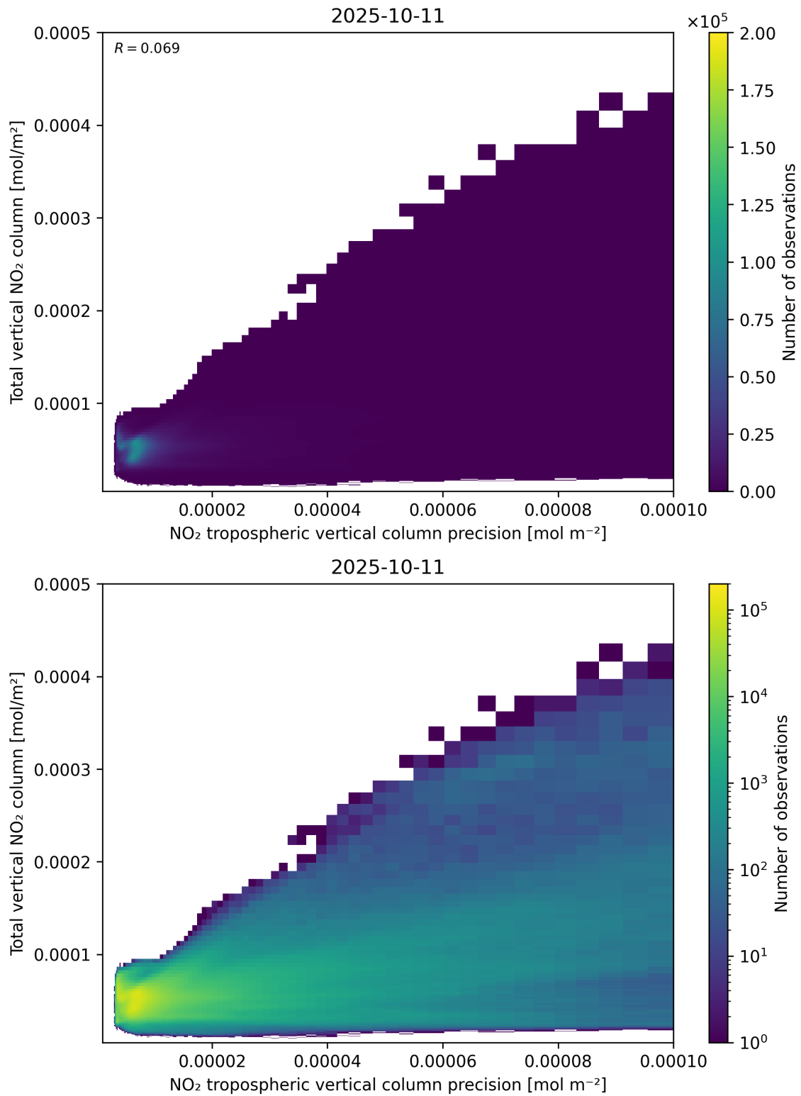
Figure 138: Scatter density plot of “NO 2 tropospheric vertical column precision” against “Total vertical NO 2 column” for 2025-10-11 to 2025-10-12.
