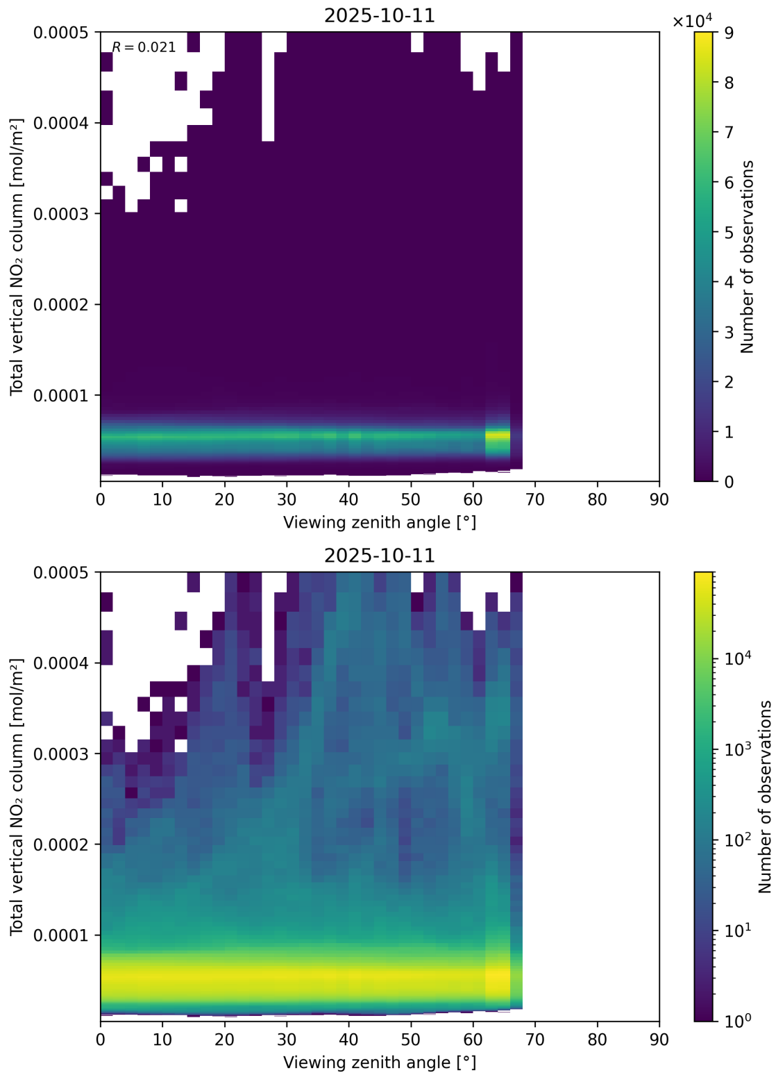
Figure 167: Scatter density plot of “Viewing zenith angle” against “Total vertical NO 2 column” for 2025-10-11 to 2025-10-12.
