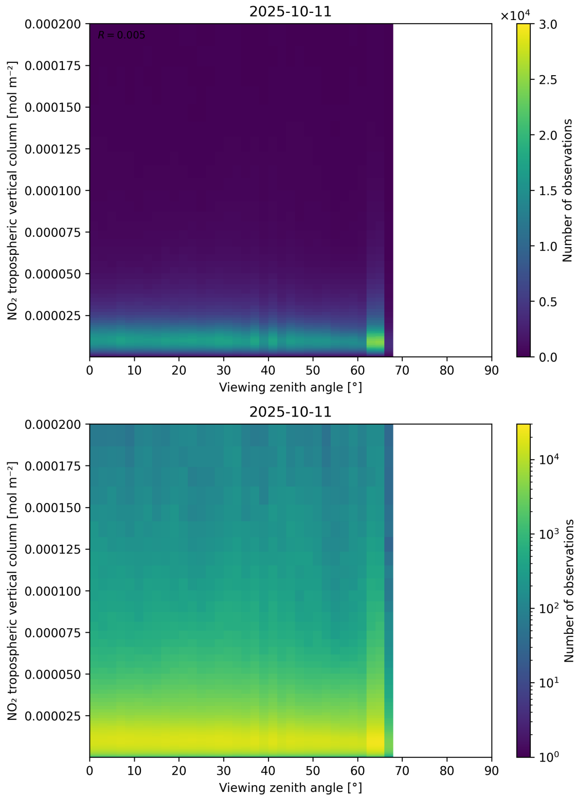
Figure 169: Scatter density plot of “Viewing zenith angle” against “NO 2 tropospheric vertical column” for 2025-10-11 to 2025-10-12.
