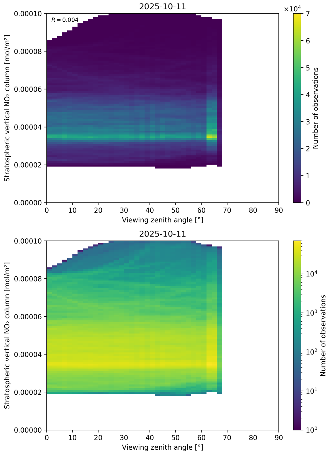
Figure 164: Scatter density plot of “Viewing zenith angle” against “Stratospheric vertical NO 2 column” for 2025-10-11 to 2025-10-12.
