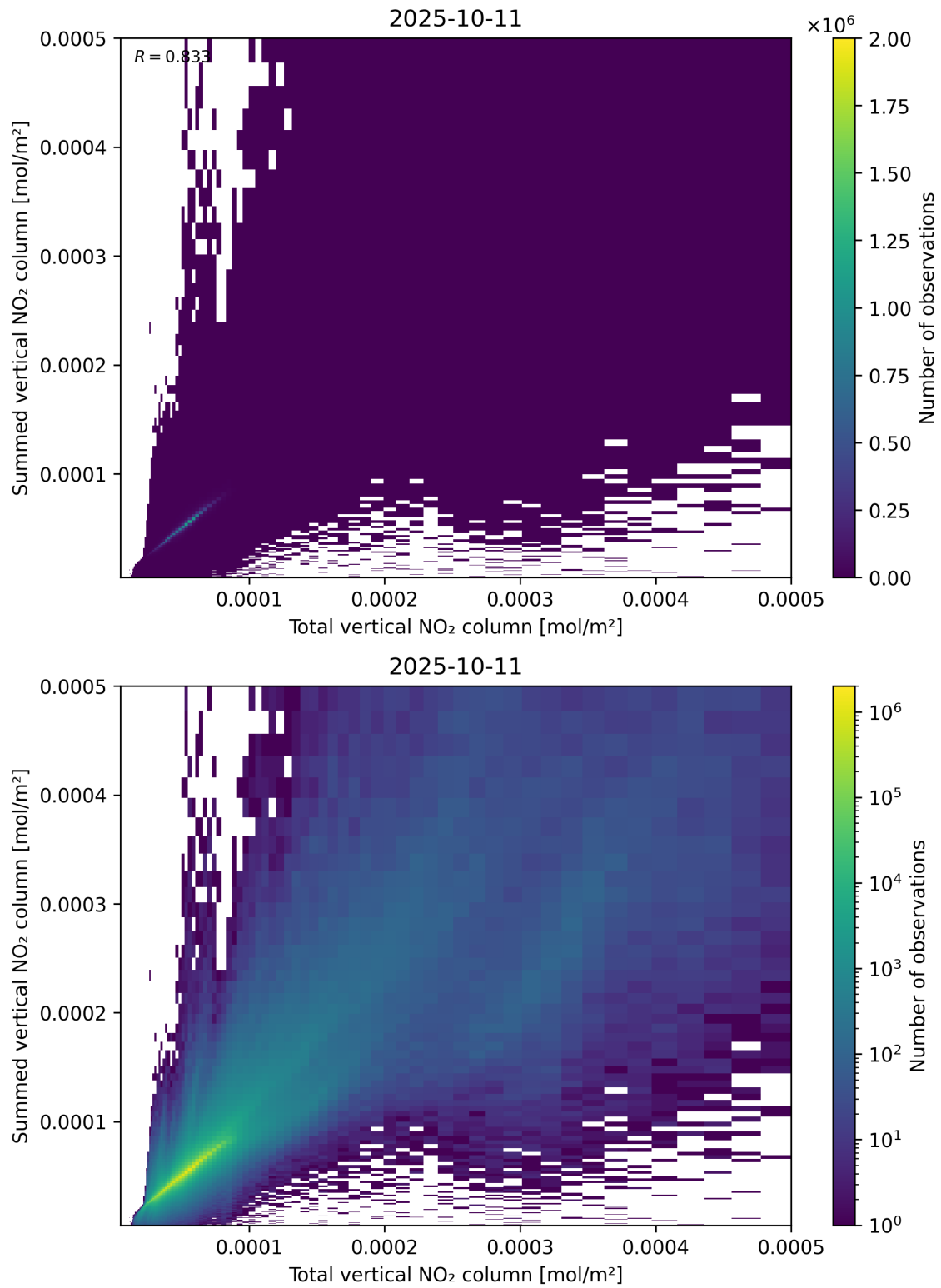
Figure 112: Scatter density plot of “Total vertical NO 2 column” against “Summed vertical NO 2 column” for 2025-10-11 to 2025-10-12.
