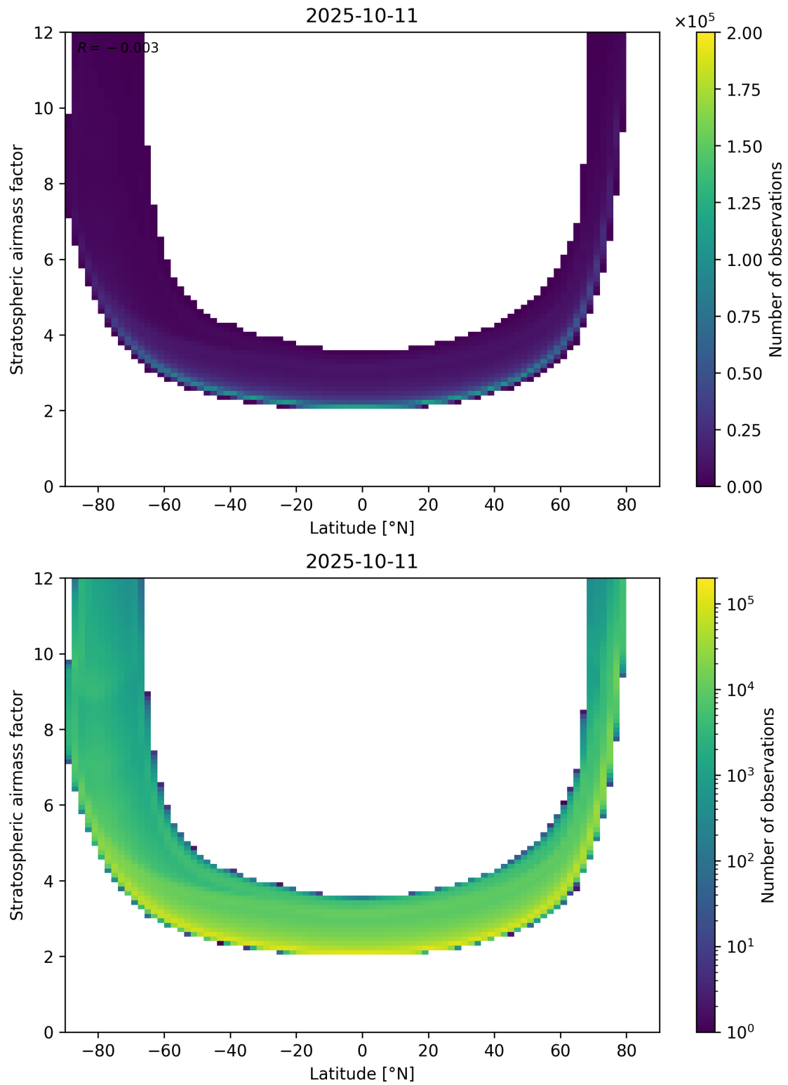
Figure 83: Scatter density plot of “Latitude” against “Stratospheric air mass factor” for 2025-10-11 to 2025-10-12.
