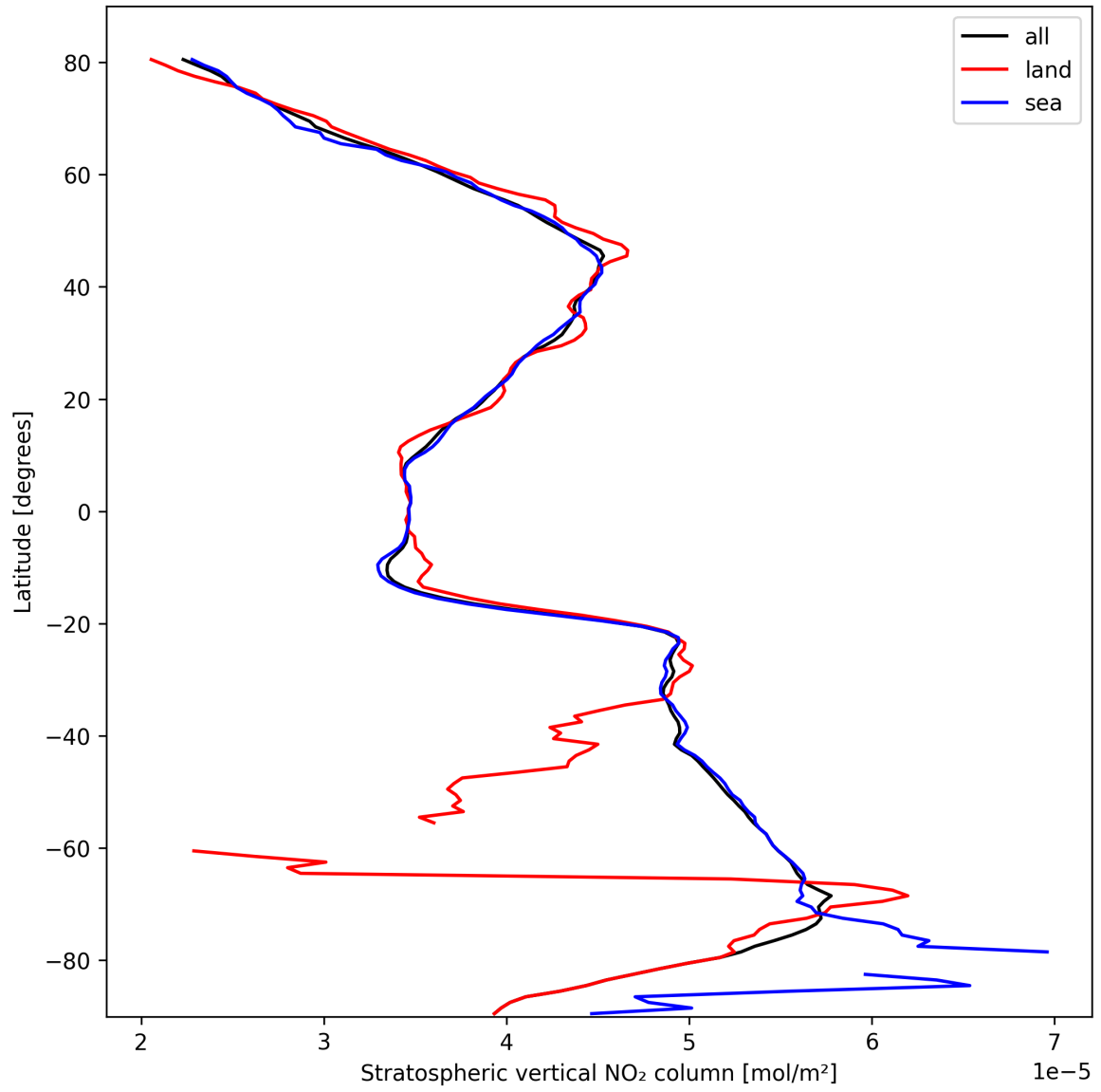
Figure 19: Zonal average of “Stratospheric vertical NO 2 column” for 2025-10-11 to 2025-10-12.
