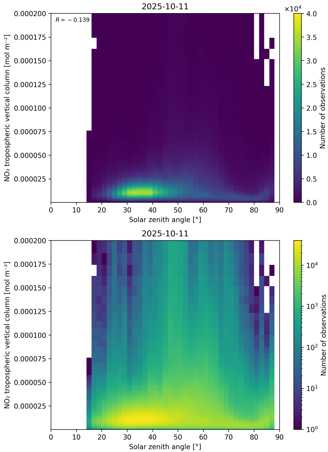
Figure 155: Scatter density plot of “Solar zenith angle” against “NO 2 tropospheric vertical column” for 2025-10-11 to 2025-10-12.
