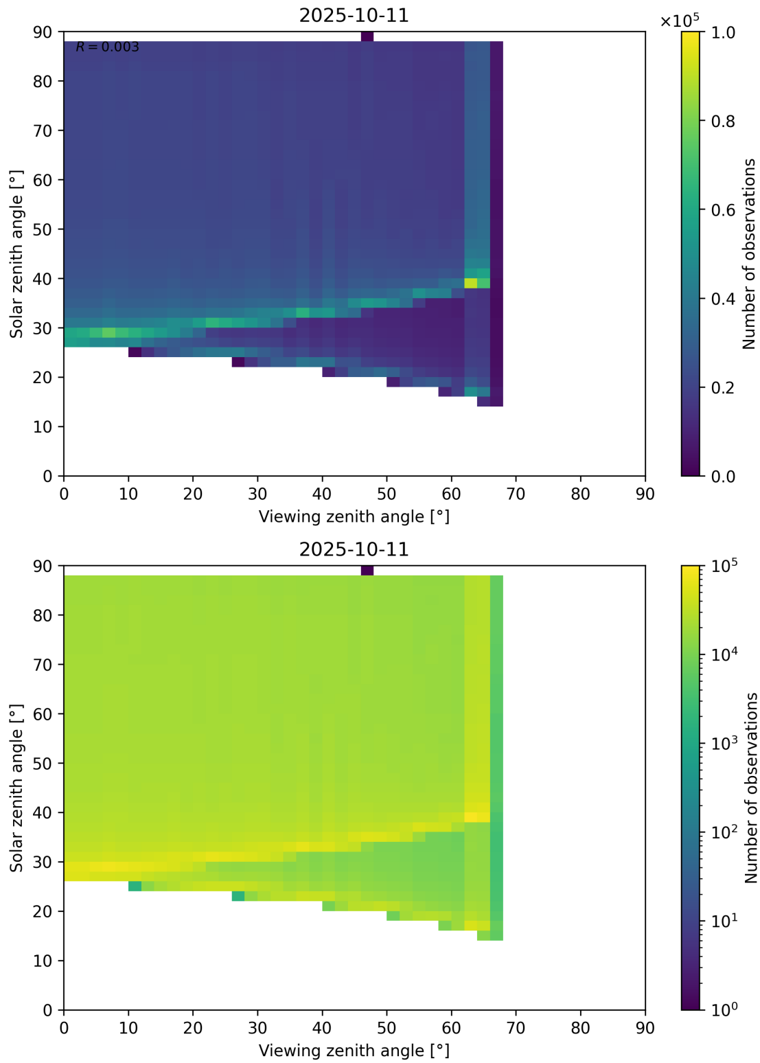
Figure 172: Scatter density plot of “Viewing zenith angle” against “Solar zenith angle” for 2025-10-11 to 2025-10-12.
