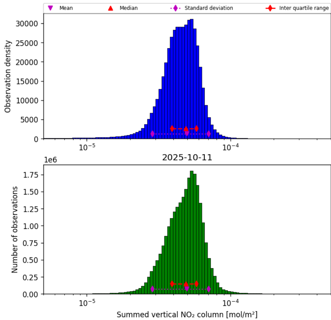
Figure 40: Histogram of “Summed vertical NO 2 column” for 2025-10-11 to 2025-10-12
