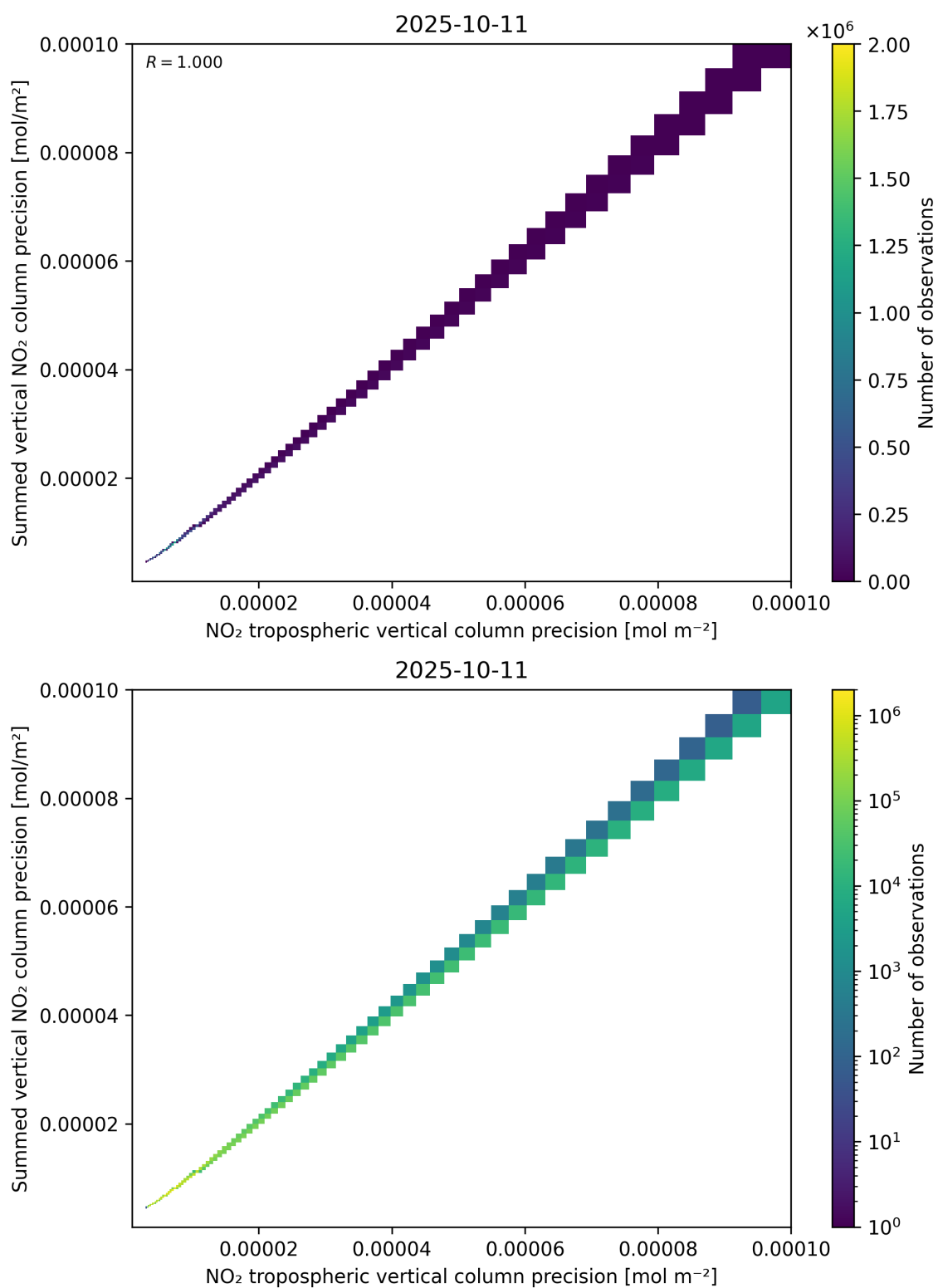
Figure 137: Scatter density plot of “NO 2 tropospheric vertical column precision” against “Summed vertical NO 2 column precision” for 2025-10-11 to 2025-10-12.
