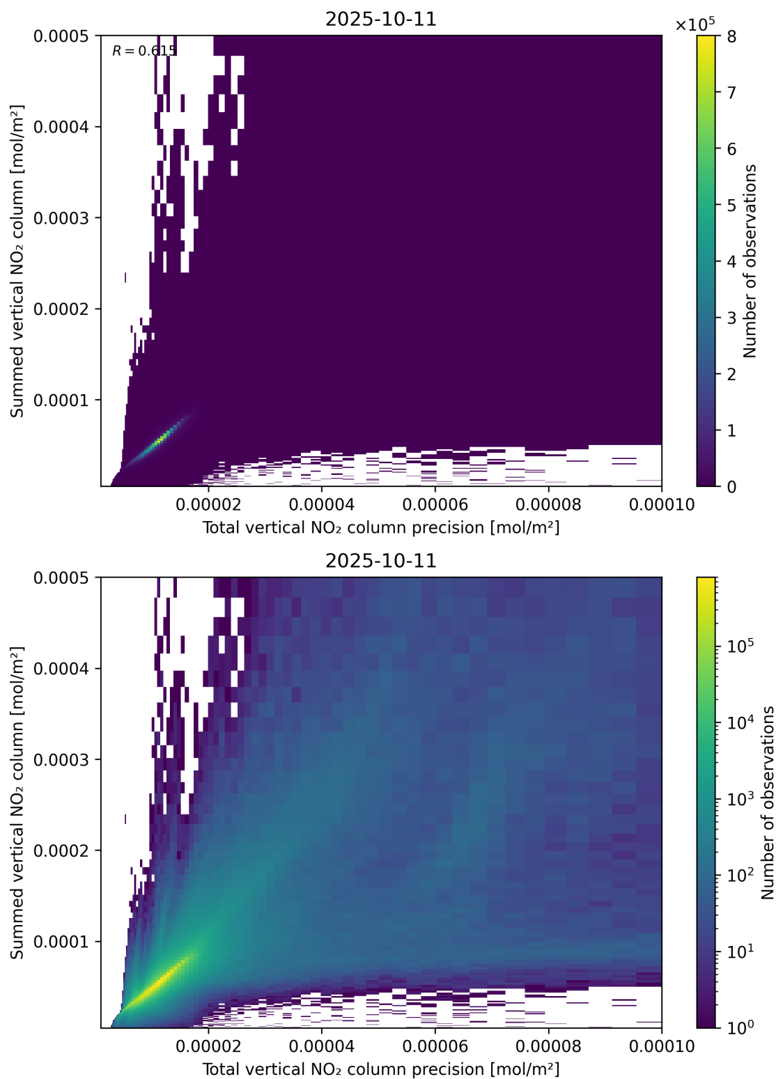
Figure 117: Scatter density plot of “Total vertical NO 2 column precision” against “Summed vertical NO 2 column” for 2025-10-11 to 2025-10-12.
