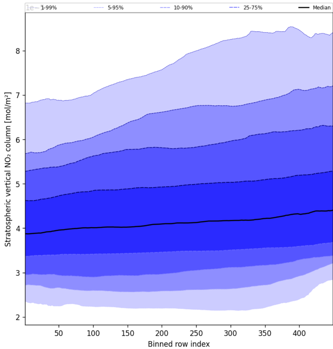
Figure 53: Along track statistics of “Stratospheric vertical NO 2 column” for 2025-10-11 to 2025-10-12
