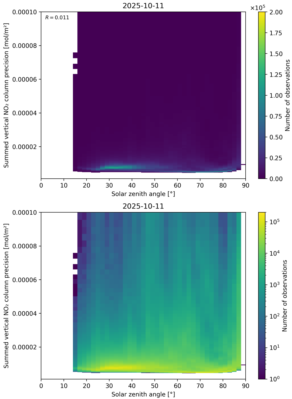
Figure 152: Scatter density plot of “Solar zenith angle” against “Summed vertical NO 2 column precision” for 2025-10-11 to 2025-10-12.
