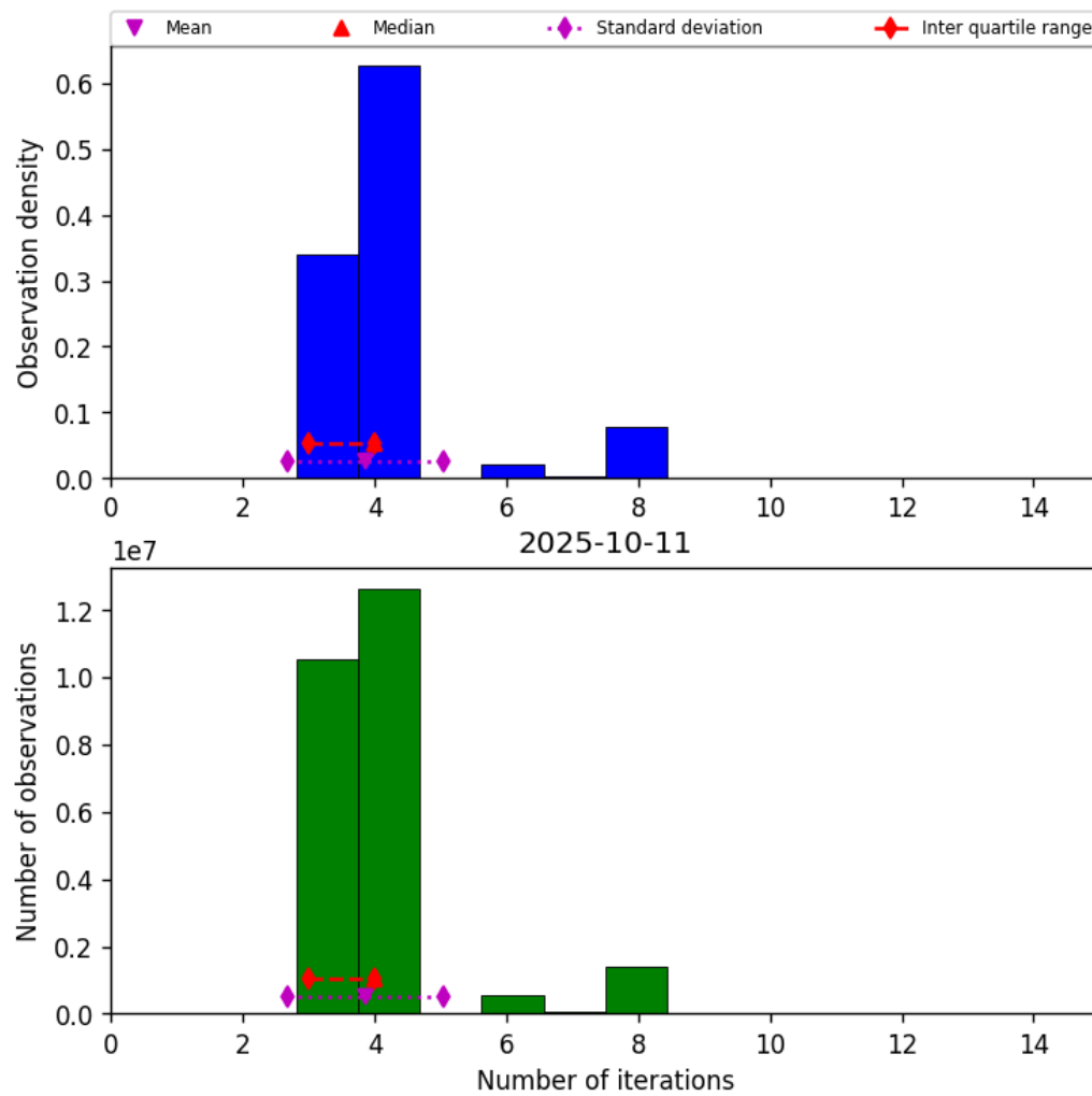
Figure 34: Histogram of “Number of iterations” for 2025-10-11 to 2025-10-12
