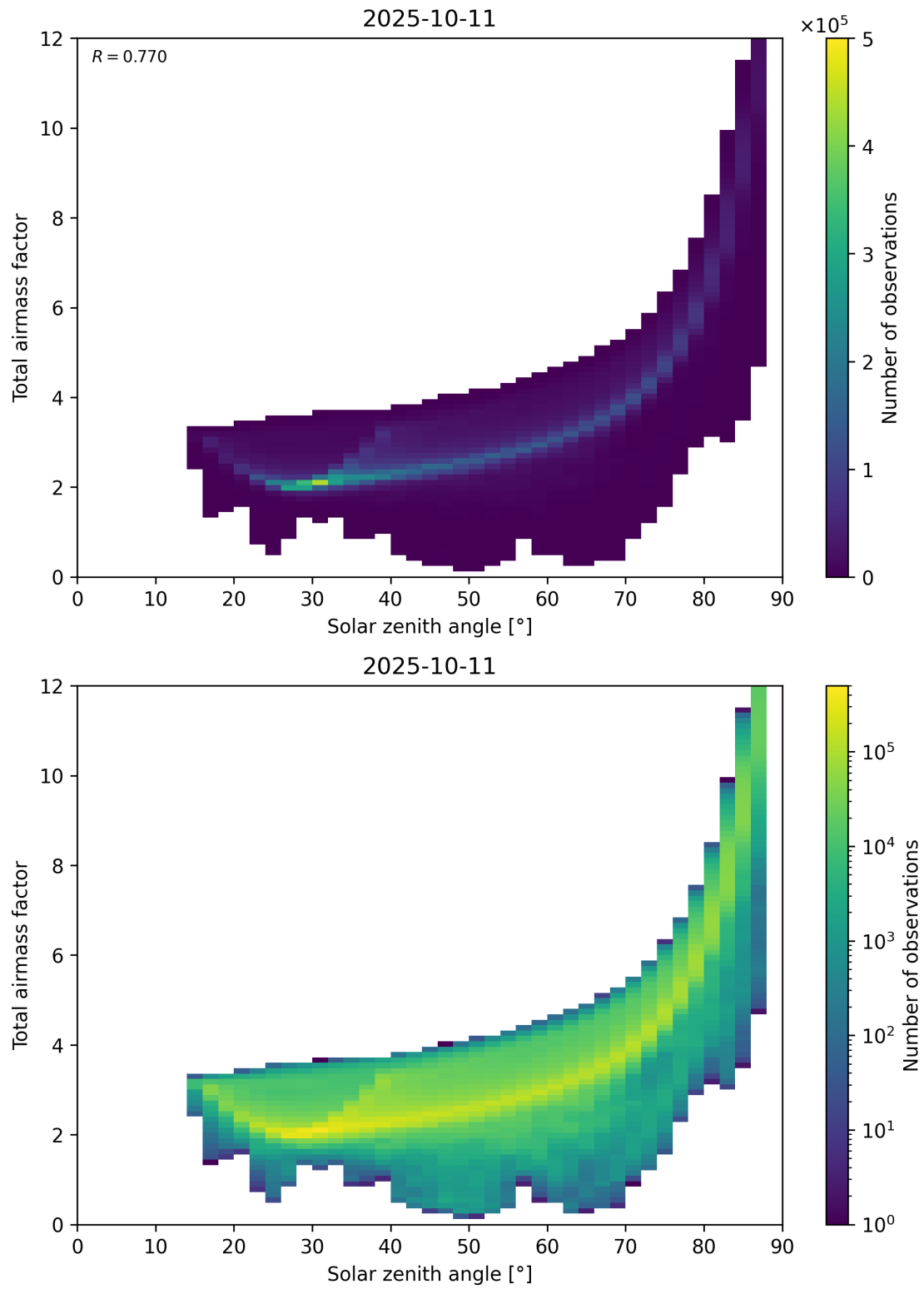
Figure 146: Scatter density plot of “Solar zenith angle” against “Total airmass factor” for 2025-10-11 to 2025-10-12.
