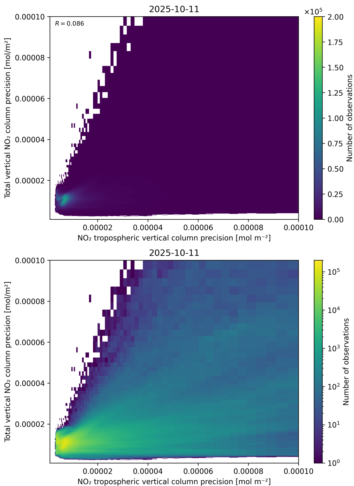
Figure 139: Scatter density plot of “NO 2 tropospheric vertical column precision” against “Total vertical NO 2 column precision” for 2025-10-11 to 2025-10-12.
