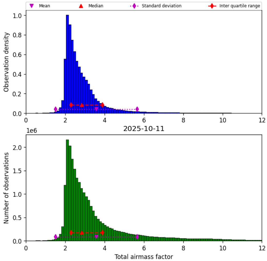
Figure 32: Histogram of “Total airmass factor” for 2025-10-11 to 2025-10-12
