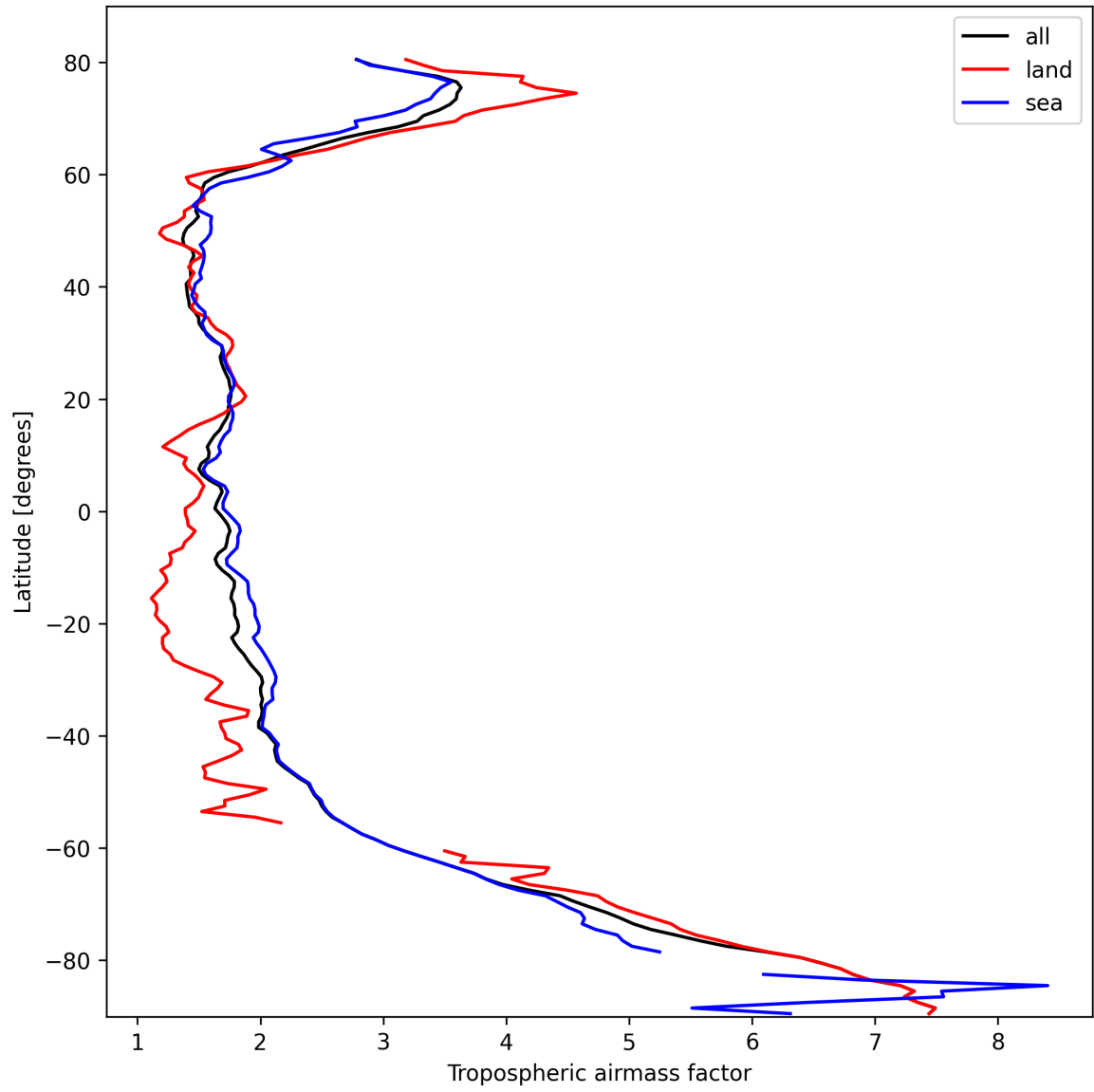
Figure 14: Zonal average of “Tropospheric air mass factor” for 2025-10-11 to 2025-10-12.
