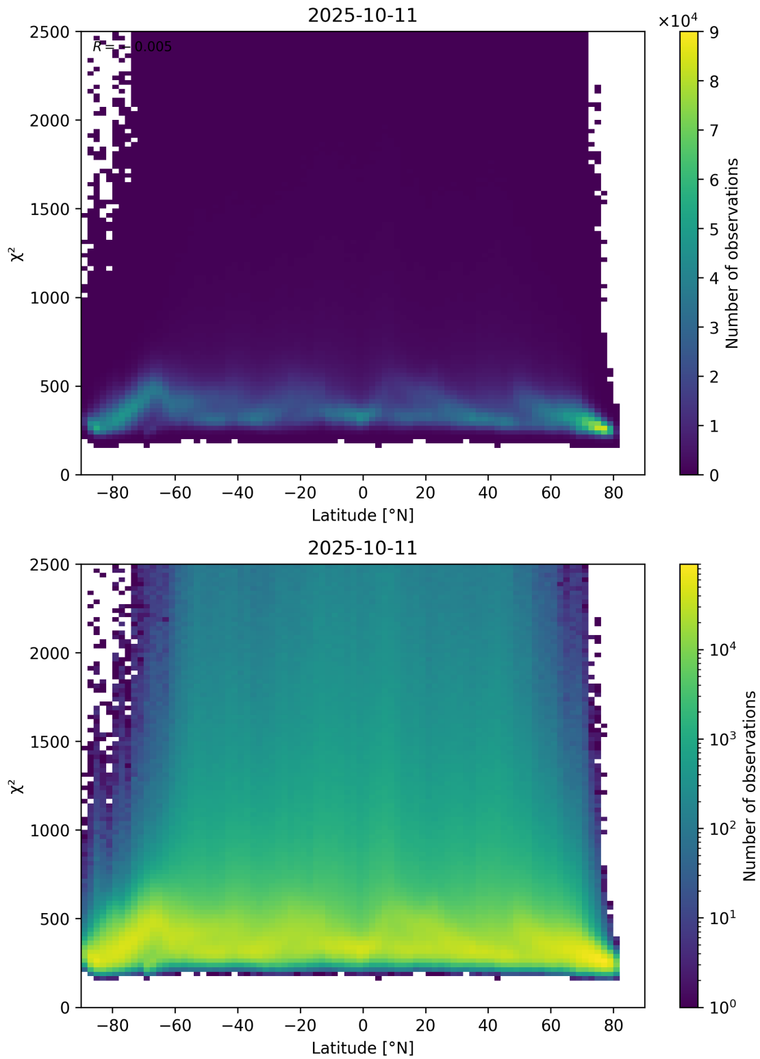
Figure 86: Scatter density plot of “Latitude” against “ \chi^2 ” for 2025-10-11 to 2025-10-12.
