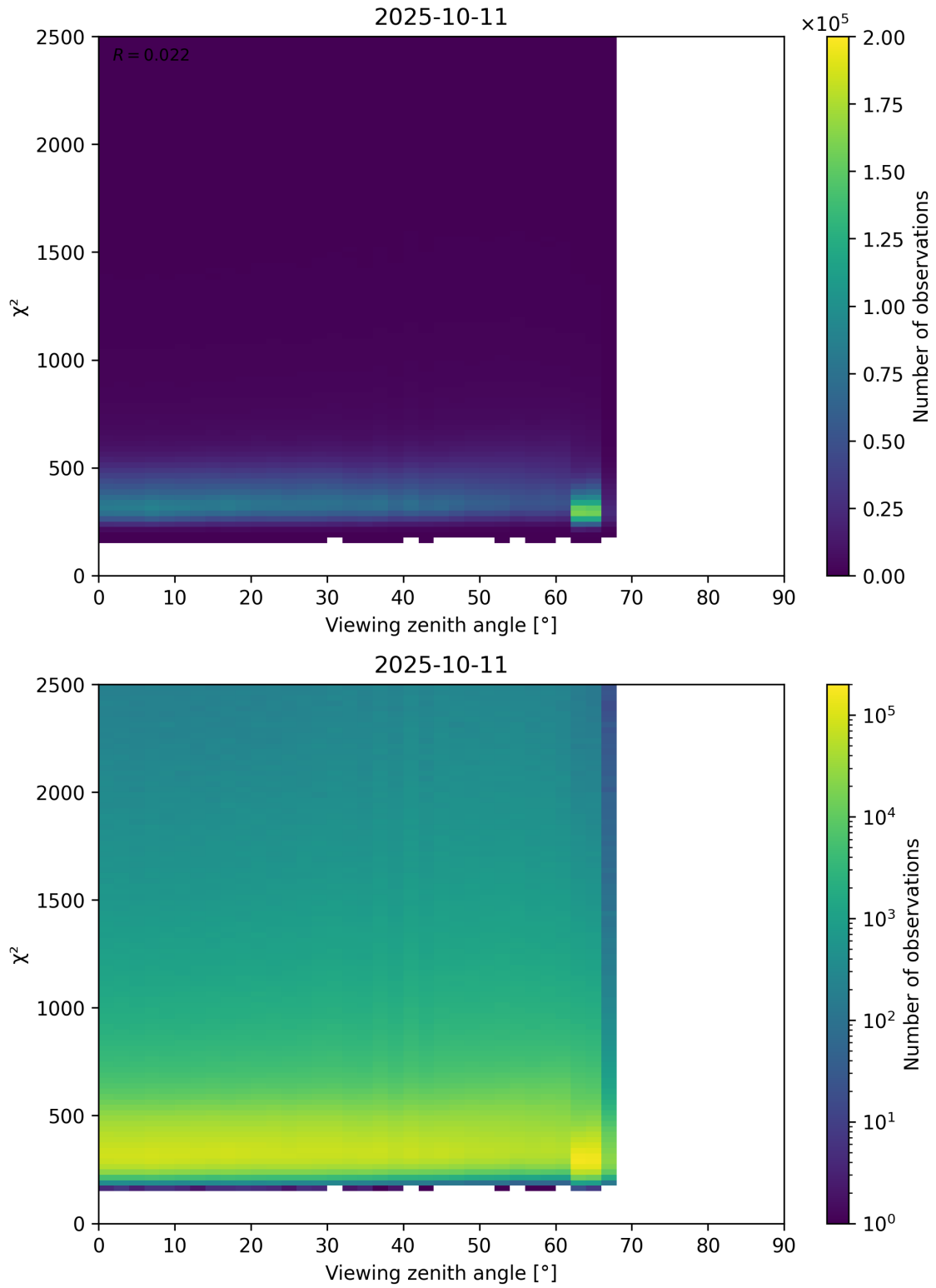
Figure 162: Scatter density plot of “Viewing zenith angle” against “ \chi^2 ” for 2025-10-11 to 2025-10-12.
