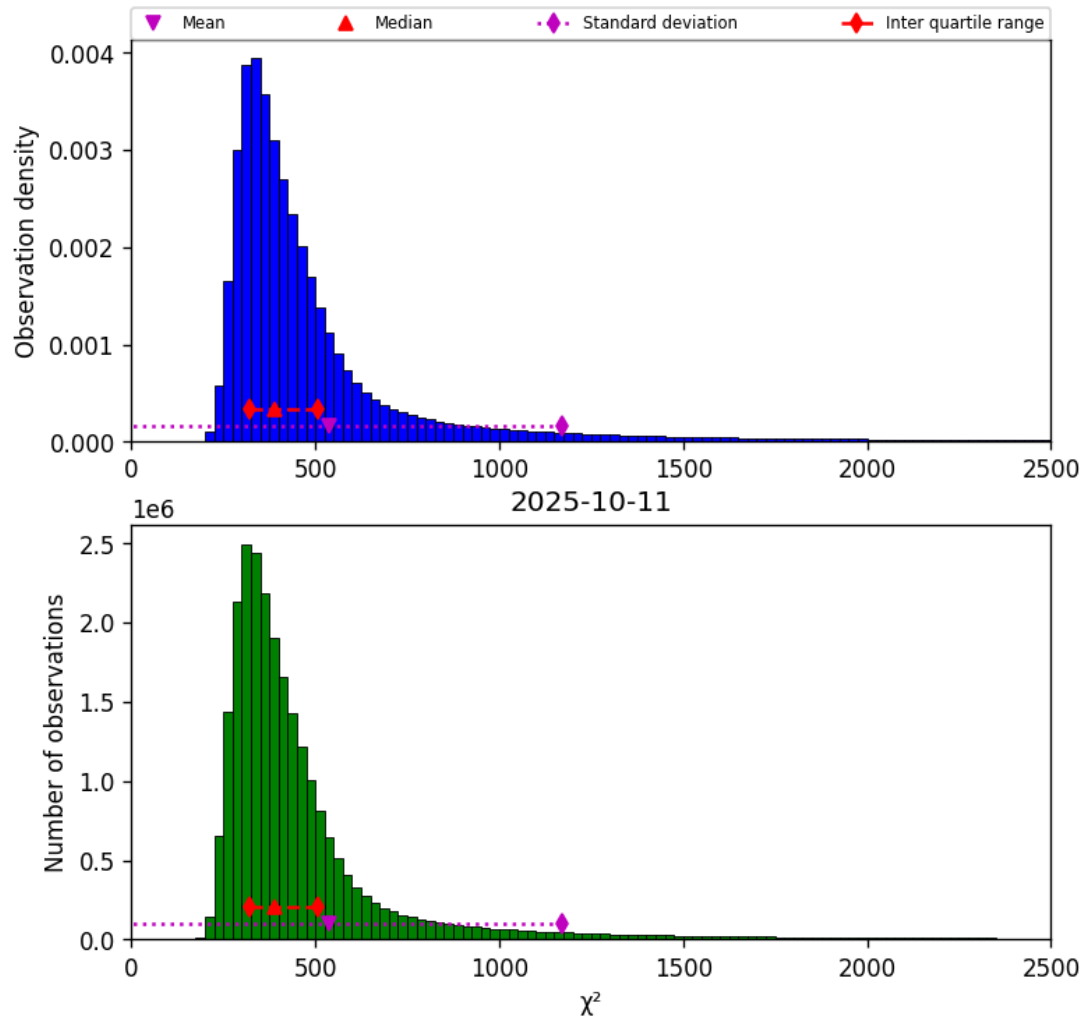
Figure 42: Histogram of “ \chi^2 ” for 2025-10-11 to 2025-10-12
