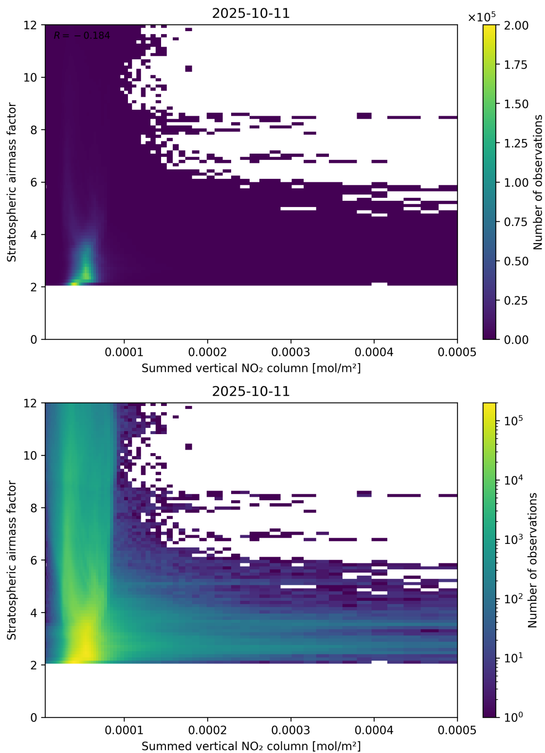
Figure 103: Scatter density plot of “Summed vertical NO 2 column” against “Stratospheric airmass factor” for 2025-10-11 to 2025-10-12.
