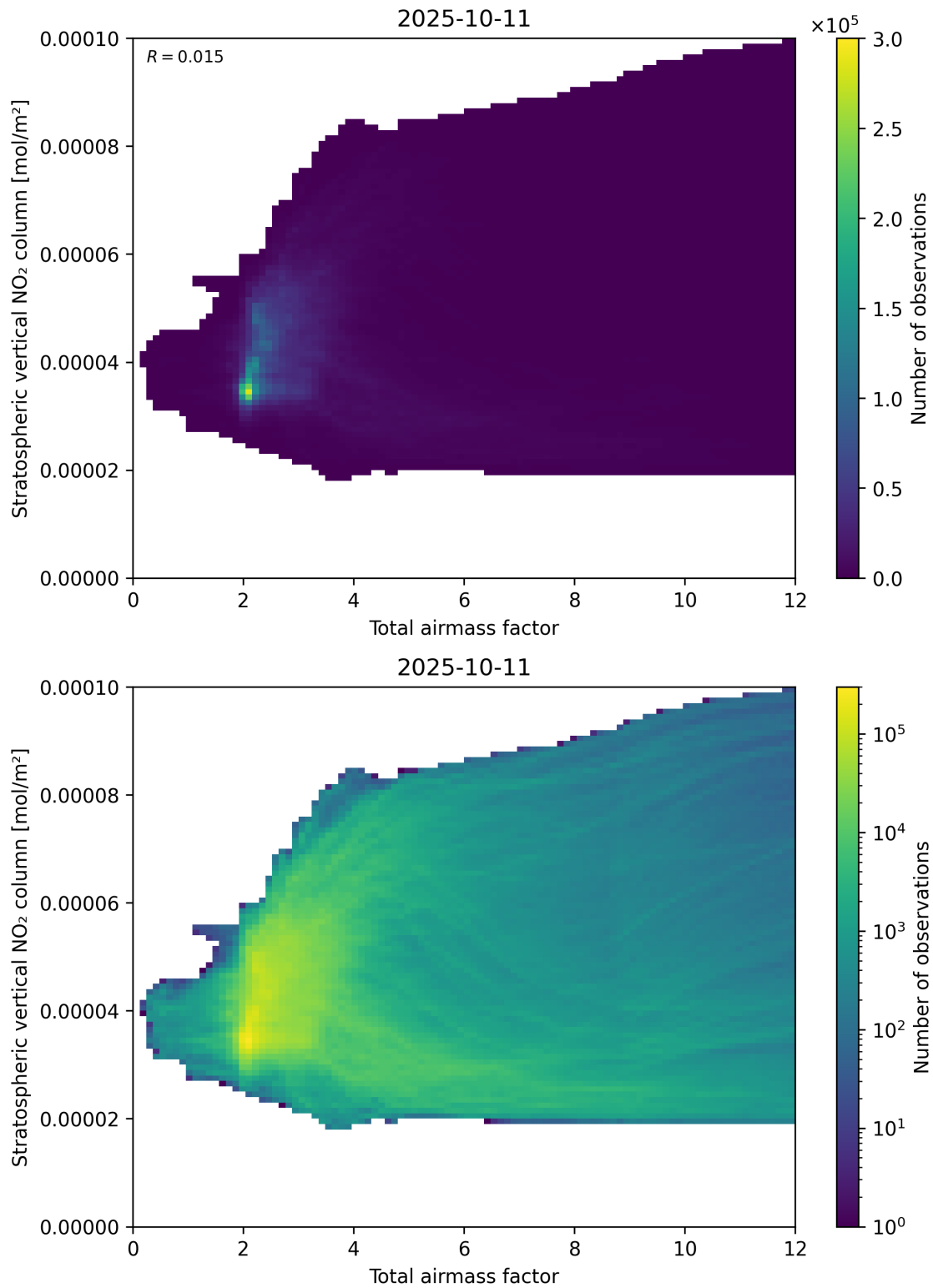
Figure 64: Scatter density plot of “Total airmass factor” against “Stratospheric vertical NO 2 column” for 2025-10-11 to 2025-10-12.
