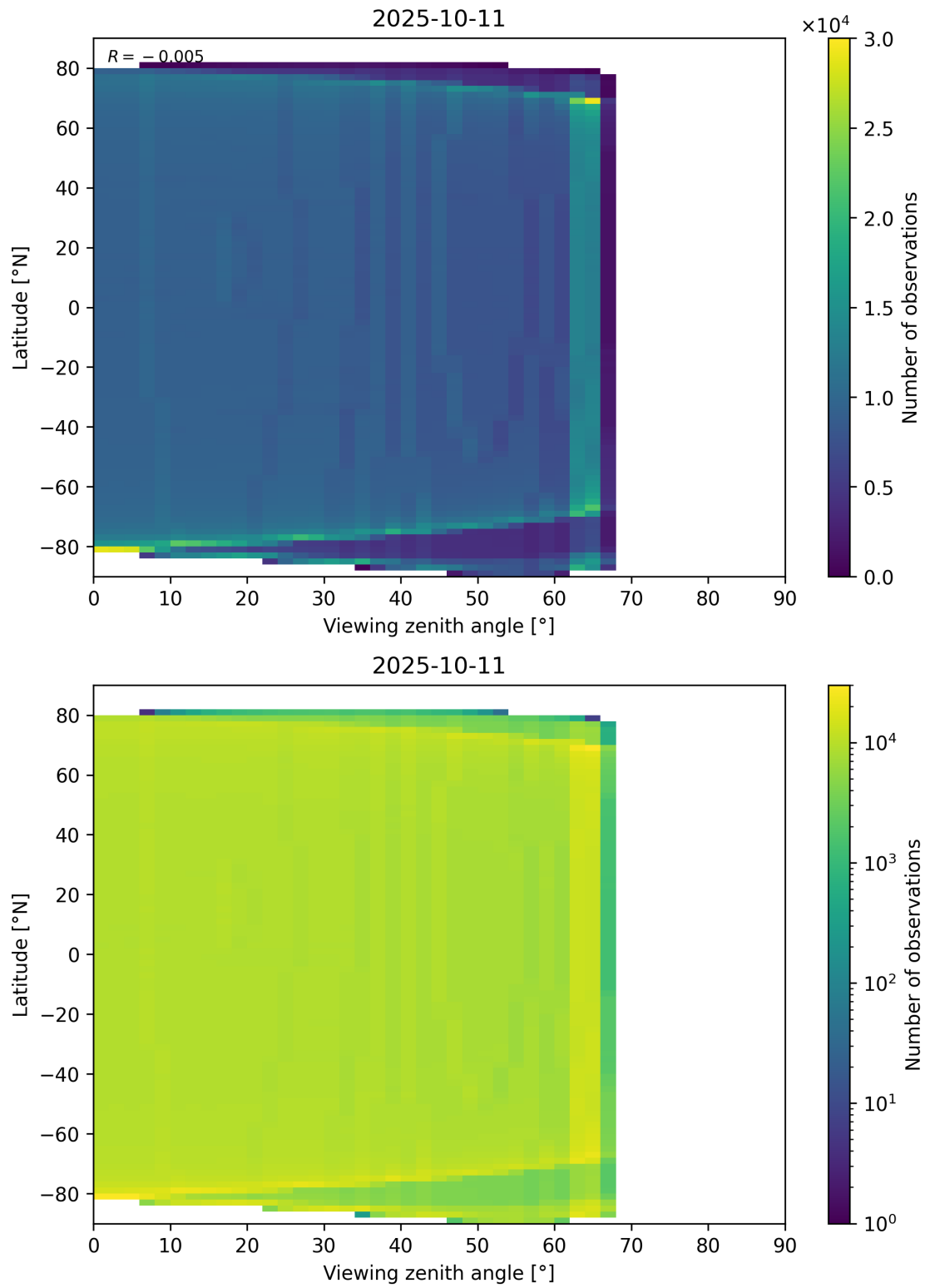
Figure 163: Scatter density plot of “Viewing zenith angle” against “Latitude” for 2025-10-11 to 2025-10-12.
