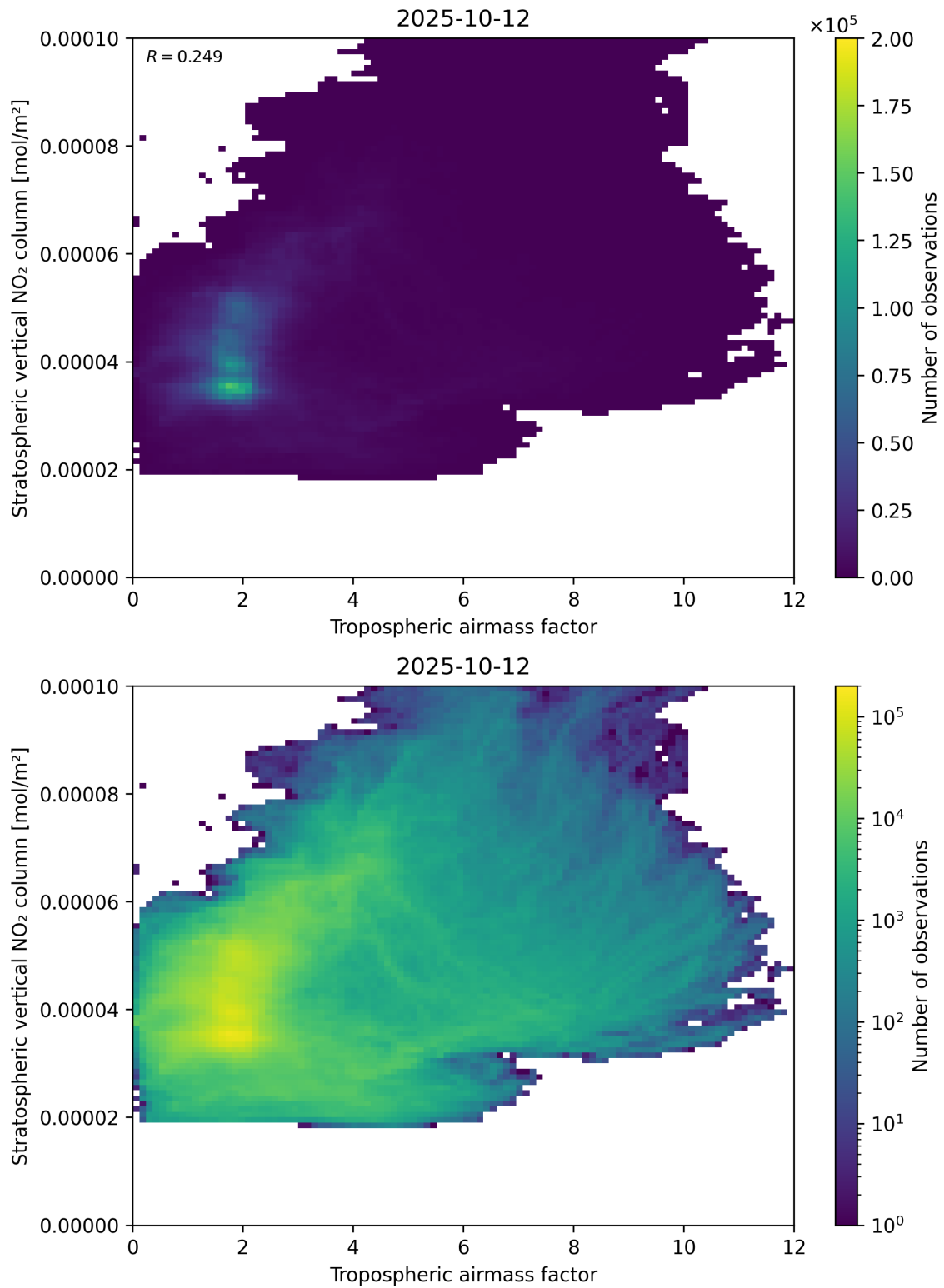
Figure 74: Scatter density plot of “Tropospheric air mass factor” against “Stratospheric vertical NO 2 column” for 2025-10-11 to 2025-10-13.
