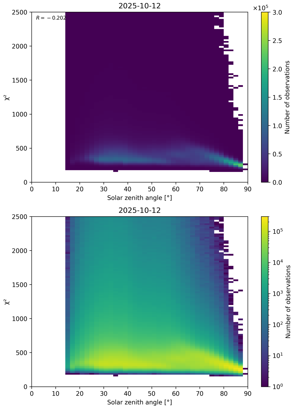
Figure 148: Scatter density plot of “Solar zenith angle” against “ \chi^2 ” for 2025-10-11 to 2025-10-13.
