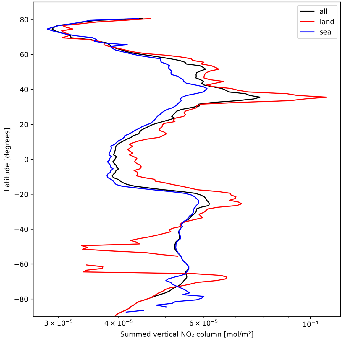
Figure 23: Zonal average of “Summed vertical NO 2 column” for 2025-10-11 to 2025-10-13.
