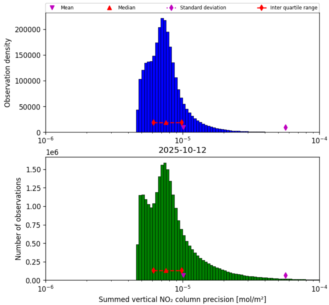
Figure 41: Histogram of "Summed vertical NO 2 column precision" for 2025-10-11 to 2025-10-13
