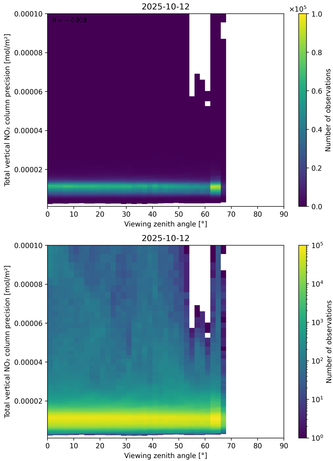
Figure 168: Scatter density plot of “Viewing zenith angle” against “Total vertical NO 2 column precision” for 2025-10-11 to 2025-10-13.
