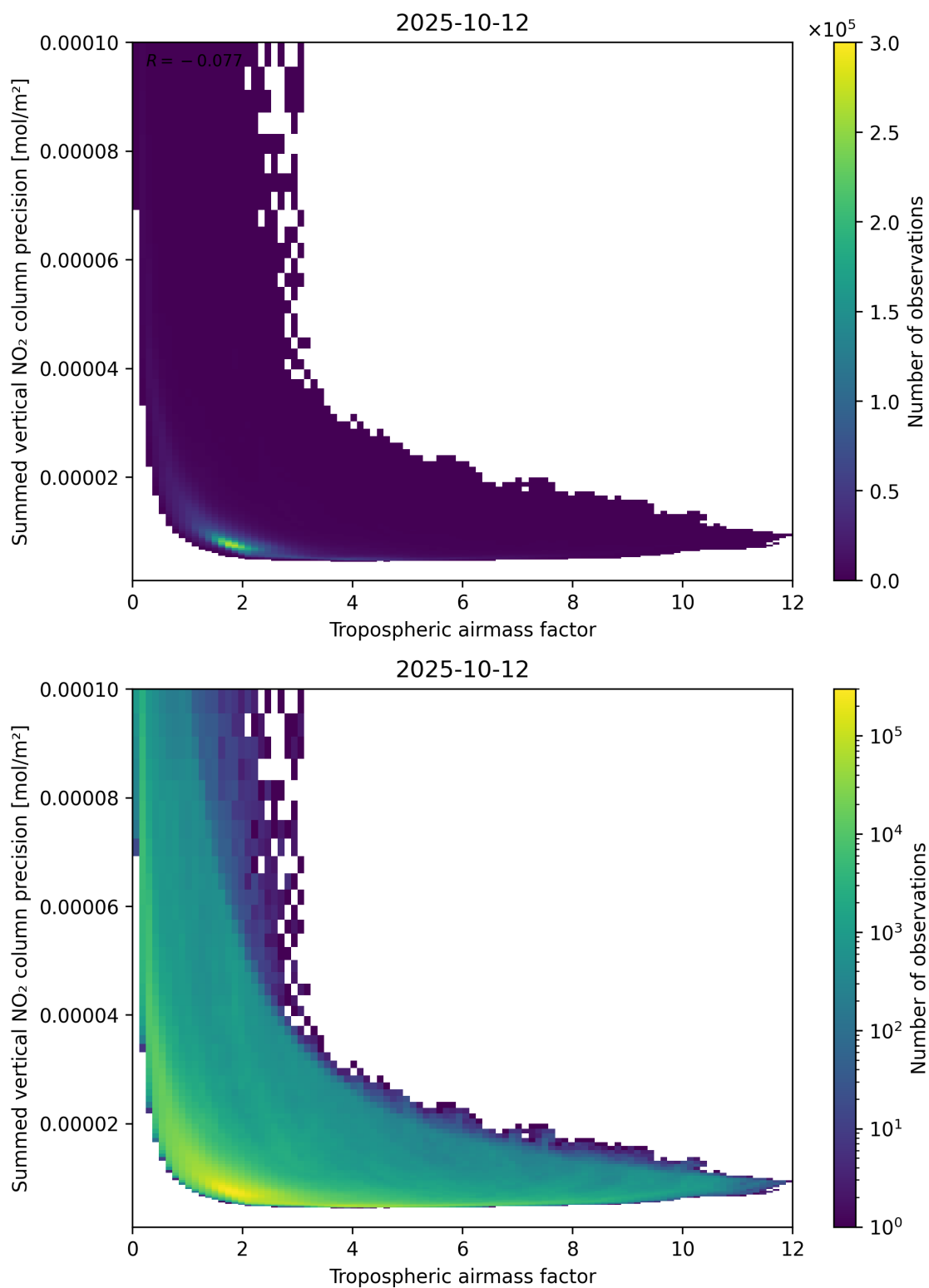
Figure 76: Scatter density plot of “Tropospheric airmass factor” against “Summed vertical NO 2 column precision” for 2025-10-11 to 2025-10-13.
