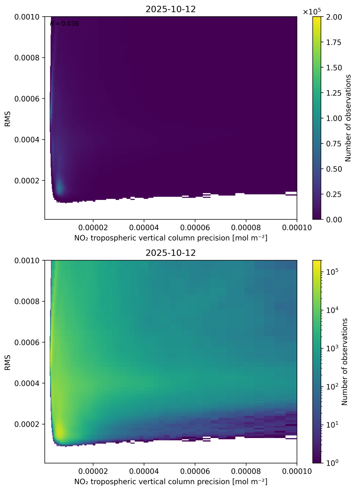
Figure 140: Scatter density plot of “NO 2 tropospheric vertical column precision” against “RMS” for 2025-10-11 to 2025-10-13.
