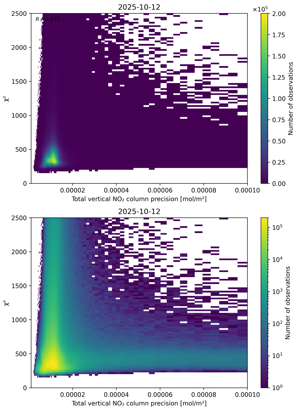
Figure 116: Scatter density plot of “Total vertical NO 2 column precision” against “ \chi^2 ” for 2025-10-11 to 2025-10-13.
