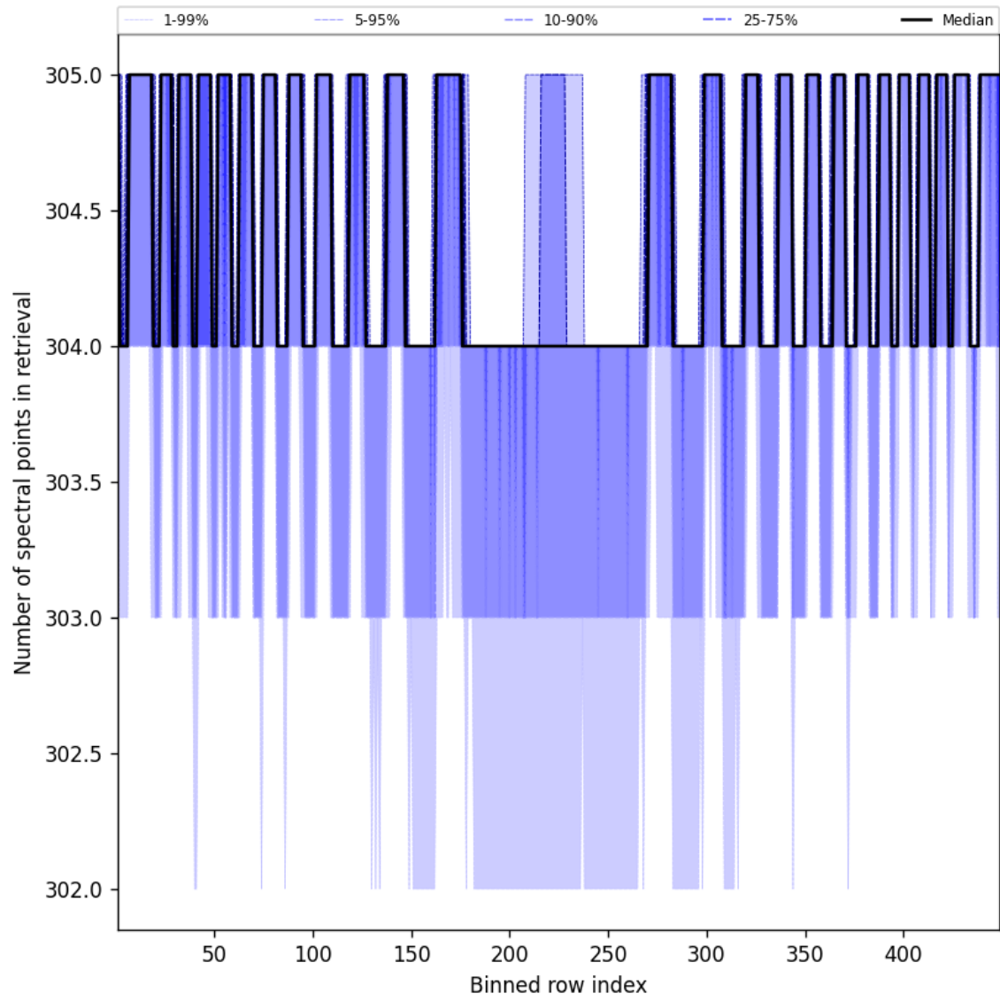
Figure 50: Along track statistics of “Number of spectral points in retrieval” for 2025-10-11 to 2025-10-13
