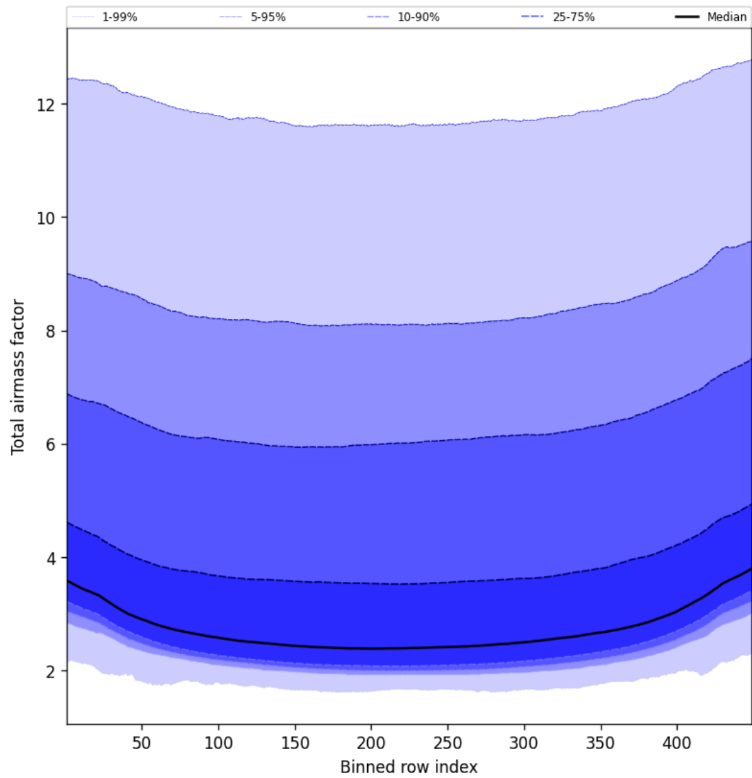
Figure 49: Along track statistics of “Total airmass factor” for 2025-10-11 to 2025-10-13
