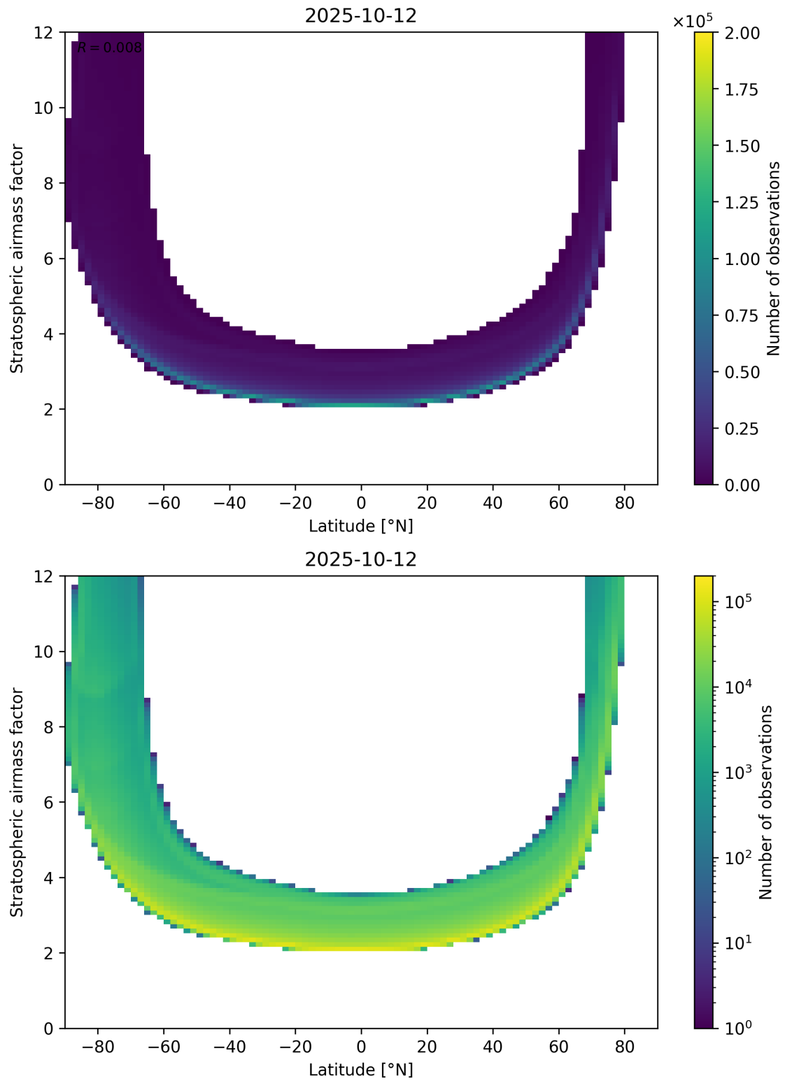
Figure 83: Scatter density plot of “Latitude” against “Stratospheric airmass factor” for 2025-10-11 to 2025-10-13.
