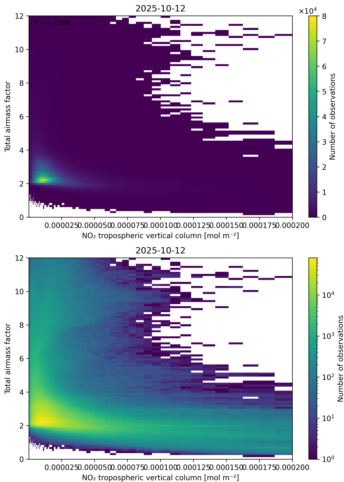
Figure 122: Scatter density plot of “NO 2 tropospheric vertical column” against “Total air mass factor” for 2025-10-11 to 2025-10-13.
