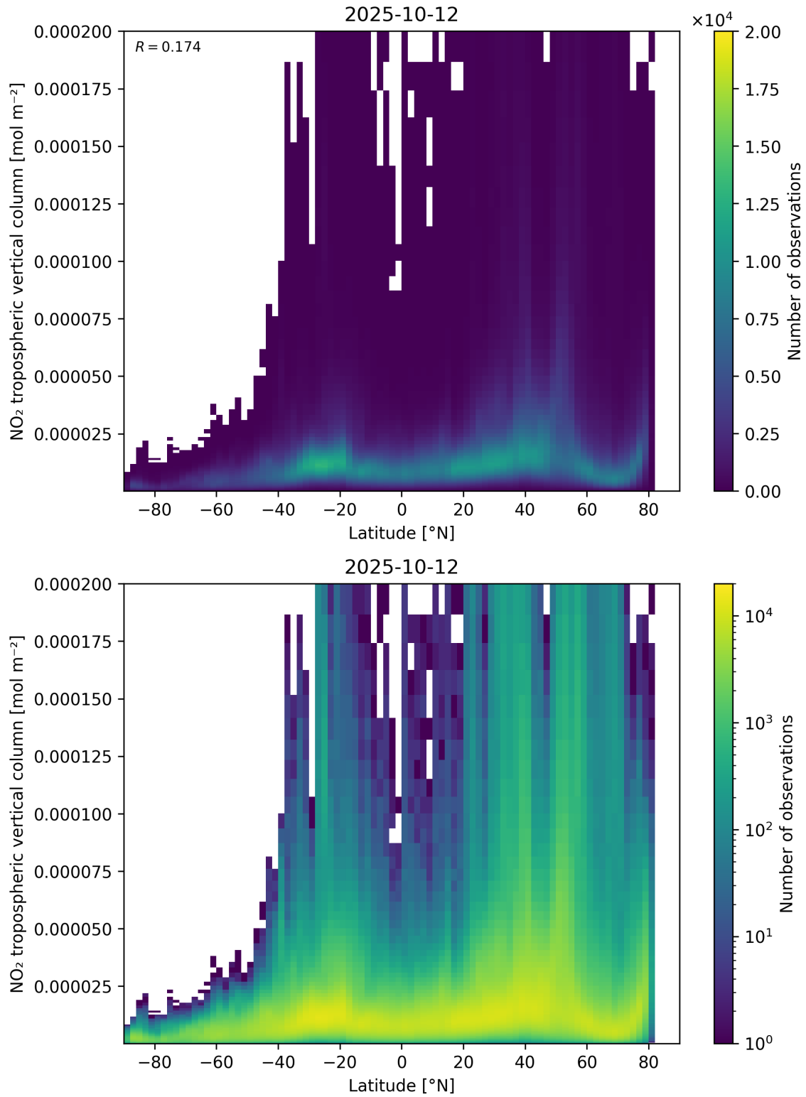
Figure 92: Scatter density plot of “Latitude” against “NO 2 tropospheric vertical column” for 2025-10-11 to 2025-10-13.
