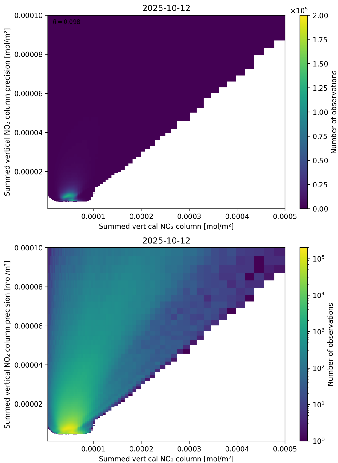
Figure 105: Scatter density plot of “Summed vertical NO 2 column” against “Summed vertical NO 2 column precision” for 2025-10-11 to 2025-10-13.
