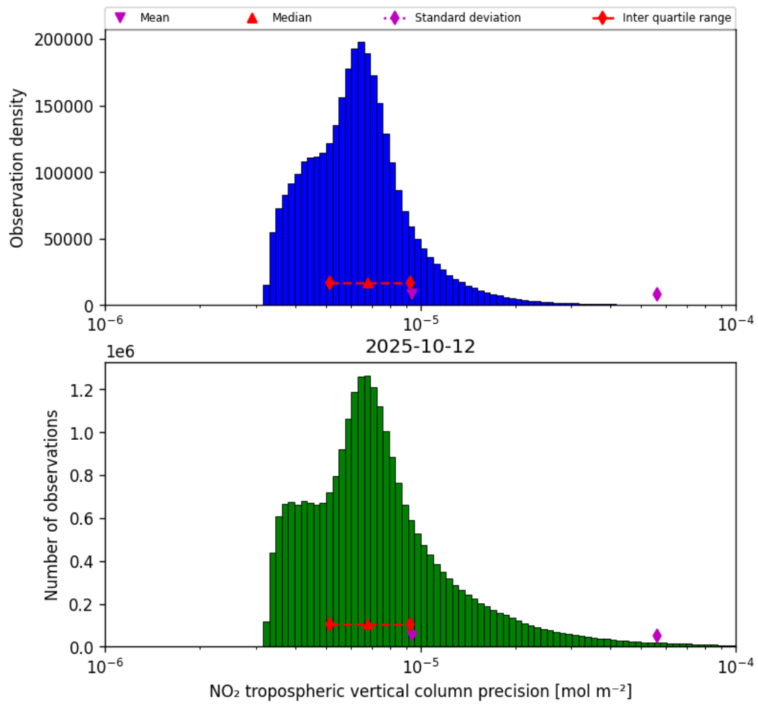
Figure 30: Histogram of “NO 2 tropospheric vertical column precision” for 2025-10-11 to 2025-10-13
