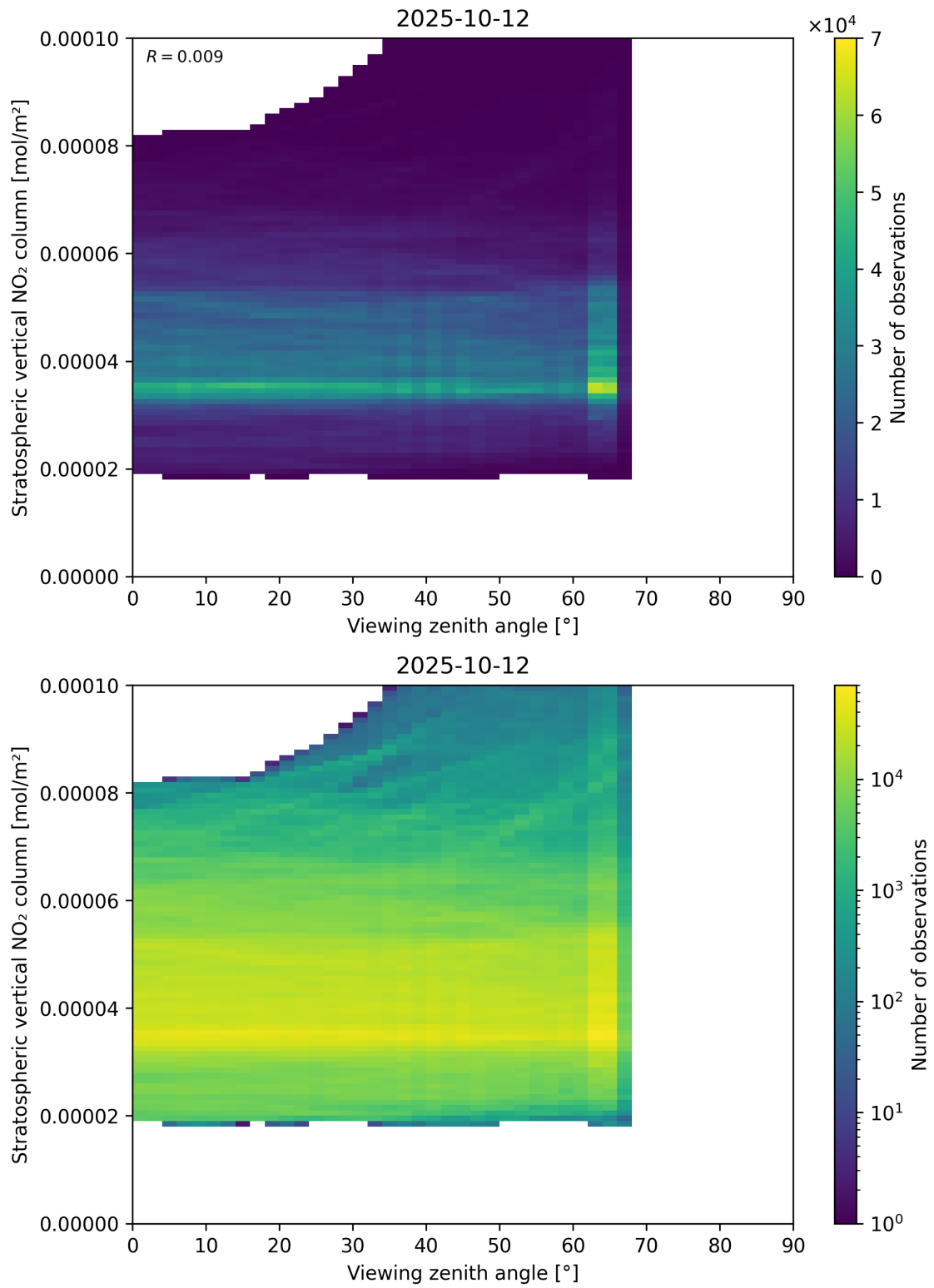
Figure 164: Scatter density plot of “Viewing zenith angle” against “Stratospheric vertical NO 2 column” for 2025-10-11 to 2025-10-13.
