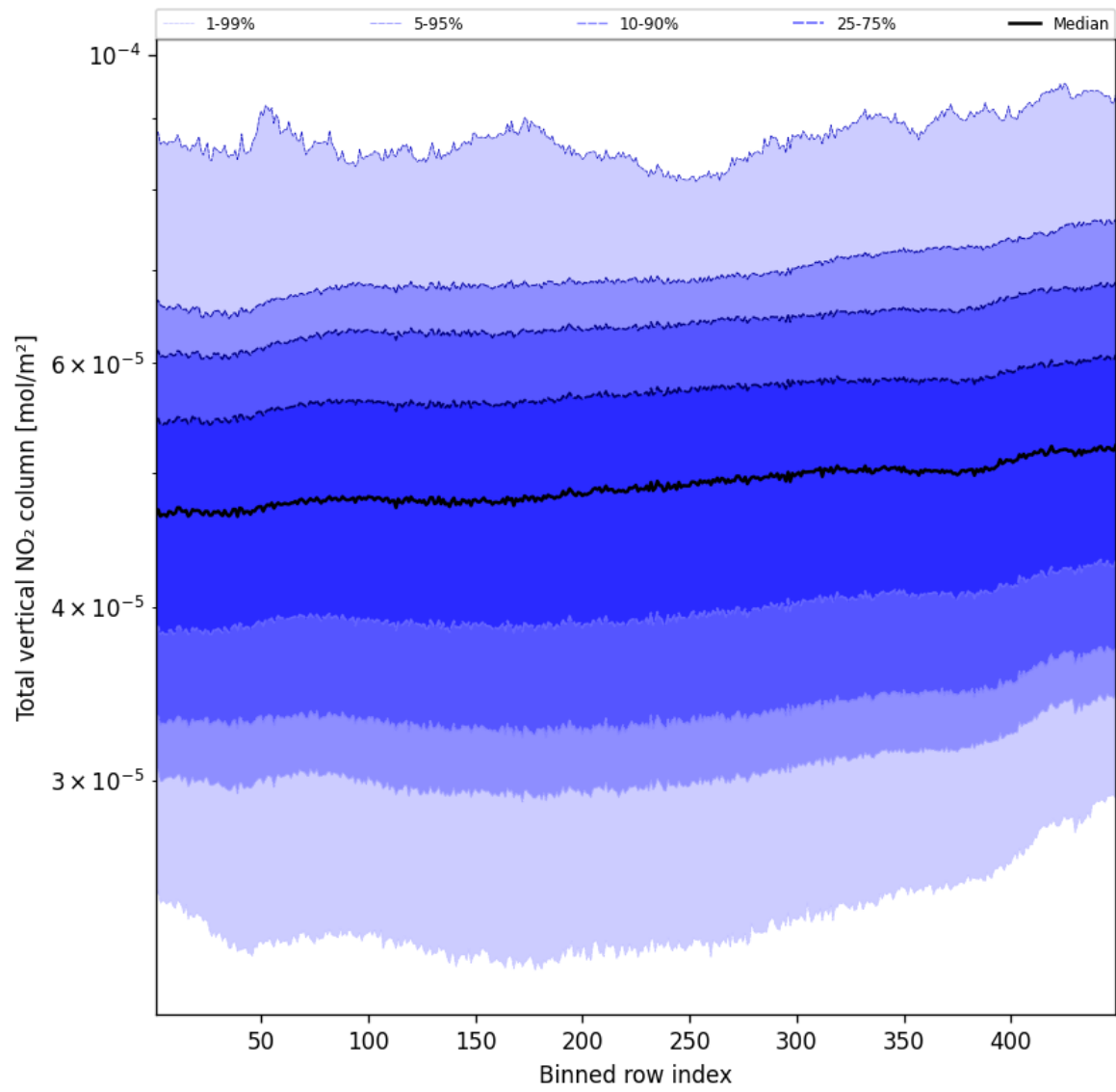
Figure 55: Along track statistics of “Total vertical NO 2 column” for 2025-10-11 to 2025-10-13
