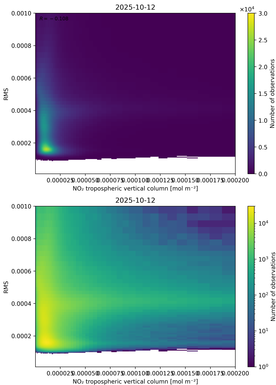
Figure 142: Scatter density plot of “NO 2 tropospheric vertical column” against “RMS” for 2025-10-11 to 2025-10-13.
