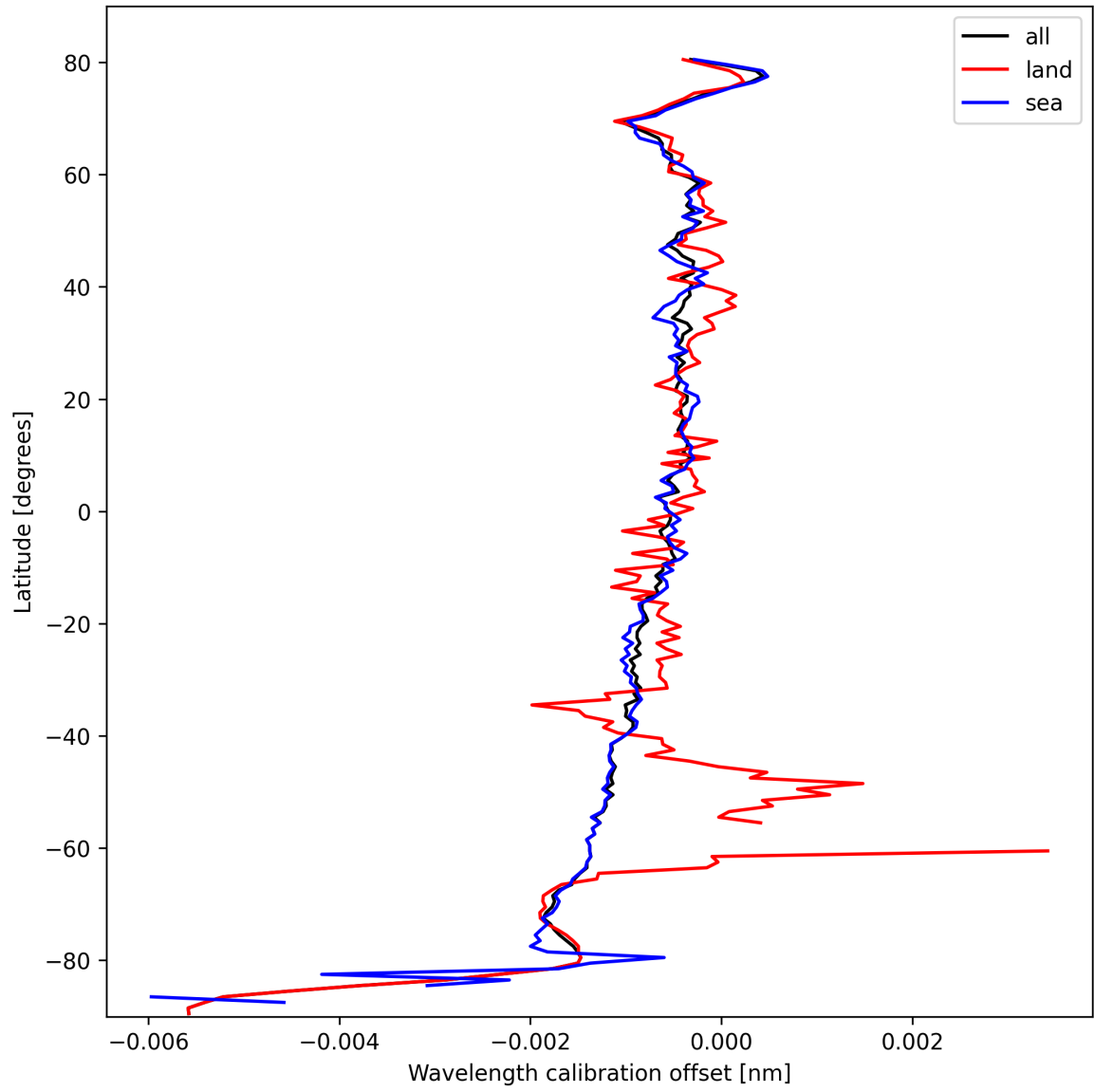
Figure 18: Zonal average of “Wavelength calibration offset” for 2025-10-11 to 2025-10-13.
