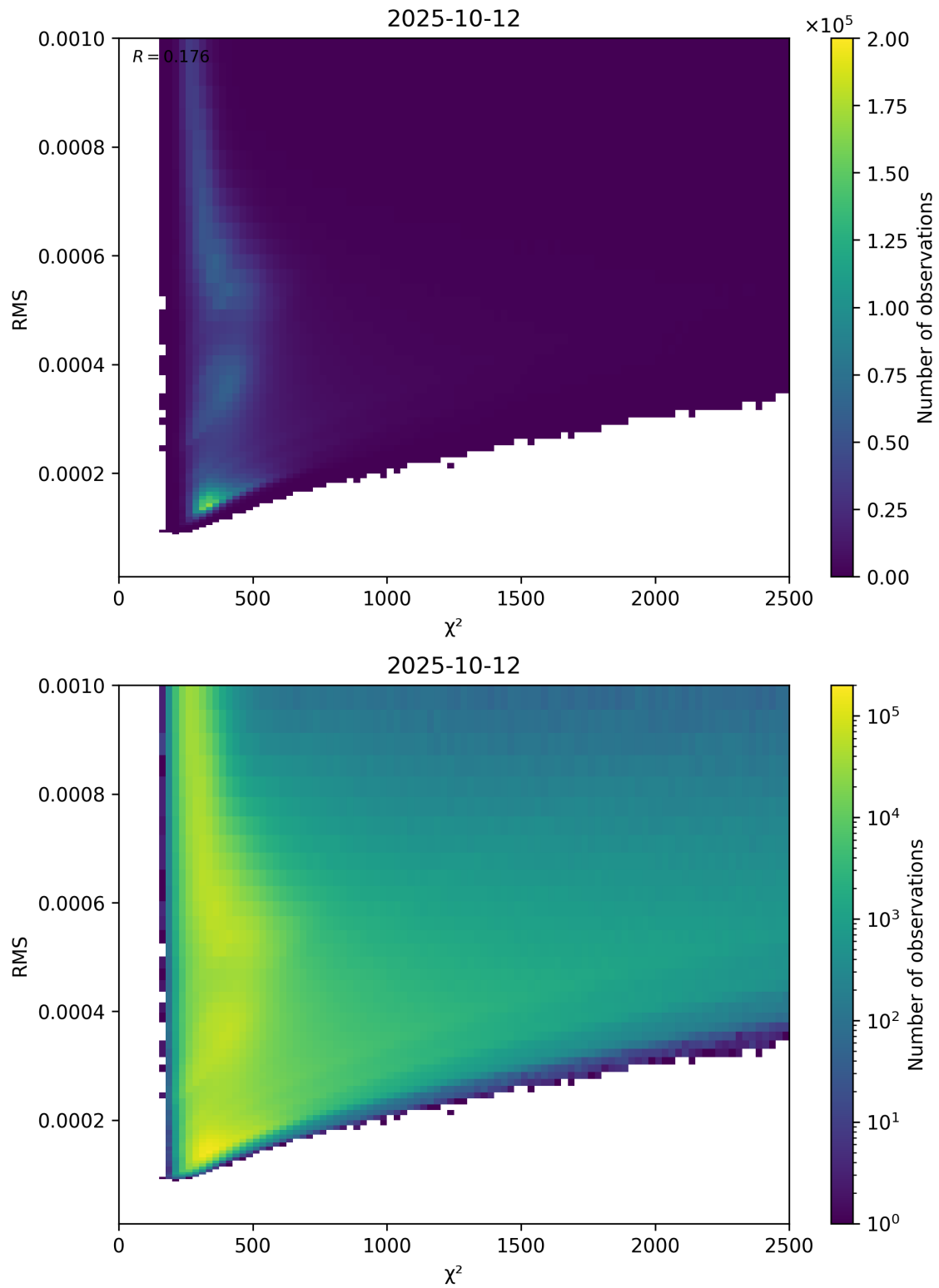
Figure 82: Scatter density plot of “ \chi^2 ” against “RMS” for 2025-10-11 to 2025-10-13.
