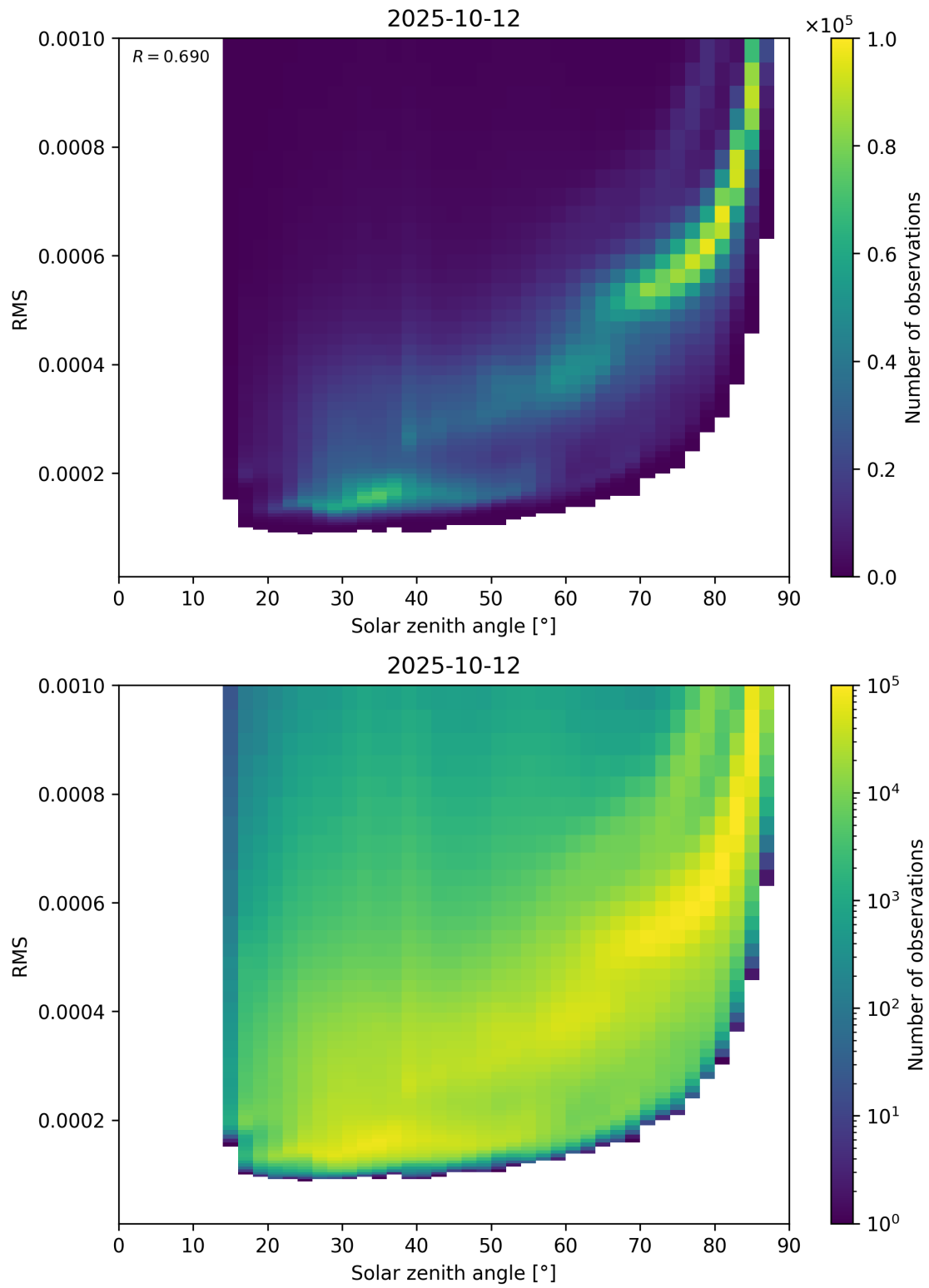
Figure 157: Scatter density plot of “Solar zenith angle” against “RMS” for 2025-10-11 to 2025-10-13.
