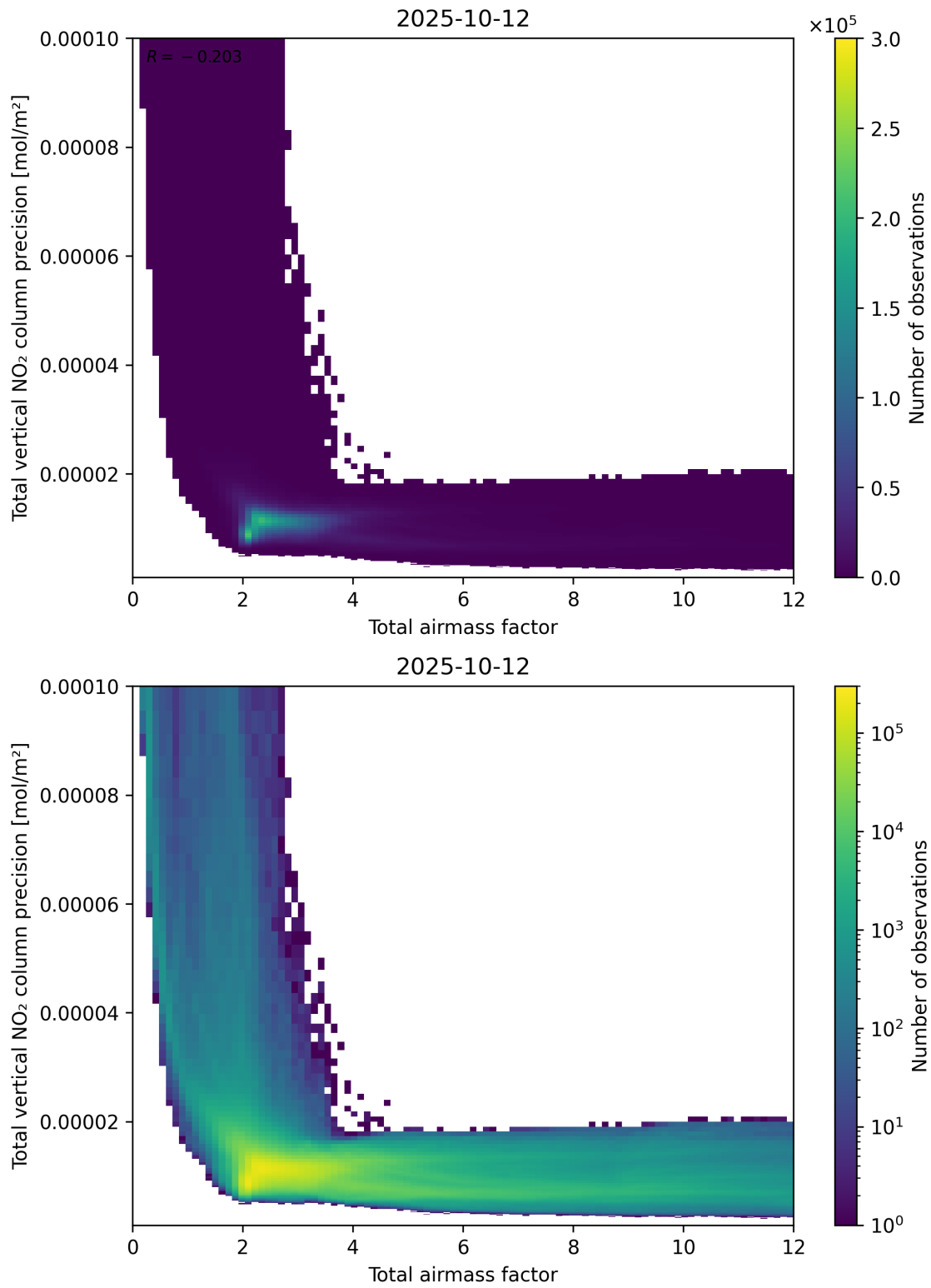
Figure 68: Scatter density plot of “Total airmass factor” against “Total vertical NO 2 column precision” for 2025-10-11 to 2025-10-13.
