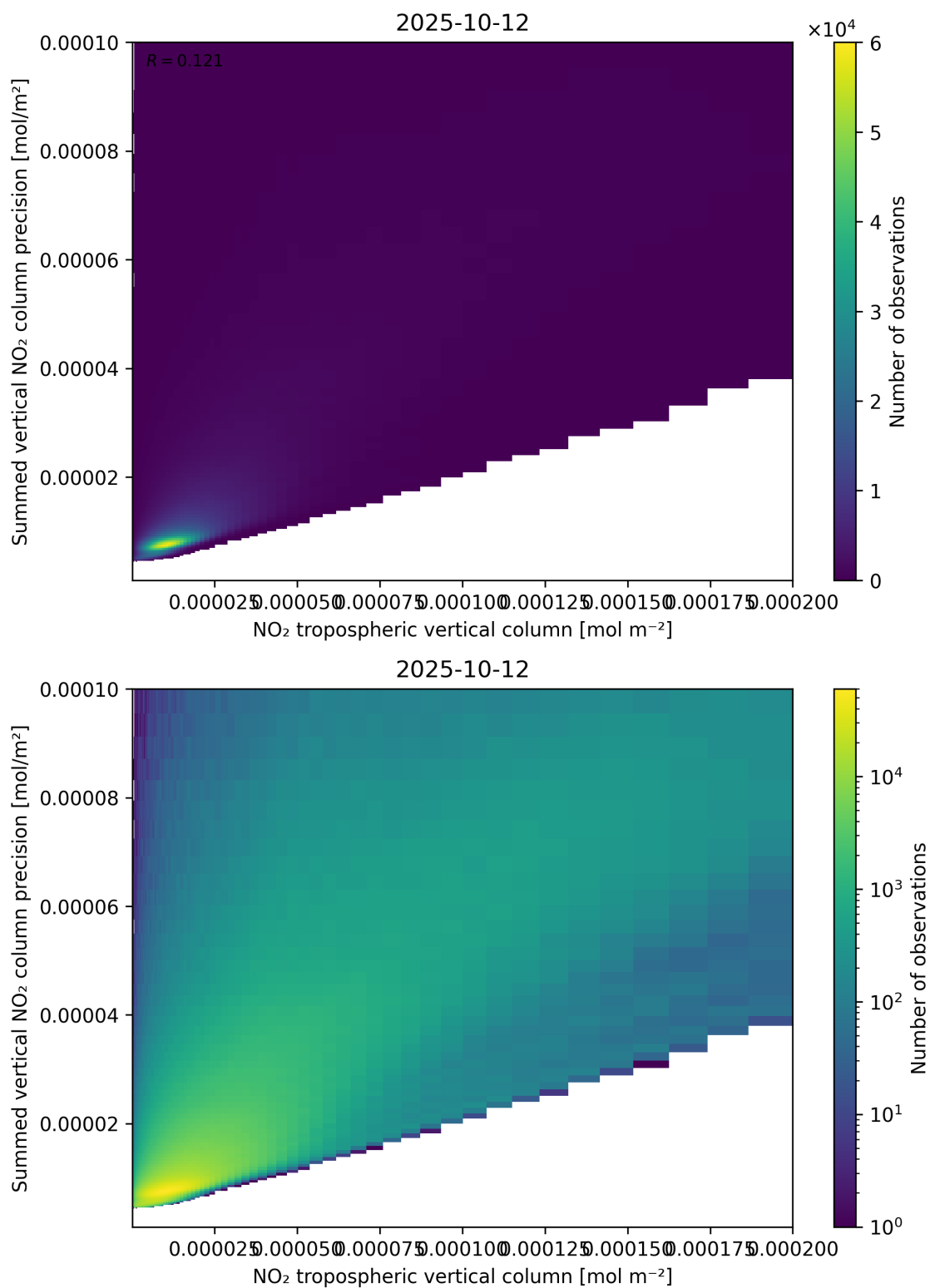
Figure 127: Scatter density plot of “NO 2 tropospheric vertical column” against “Summed vertical NO 2 column precision” for 2025-10-11 to 2025-10-13.
