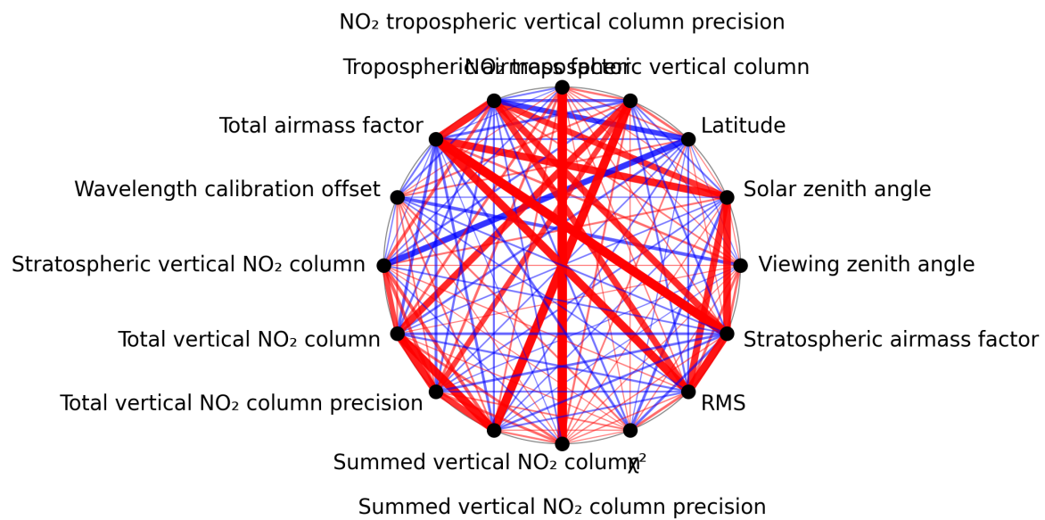
Figure 1: Map of correlation graph for 2025-10-11 to 2025-10-13.
