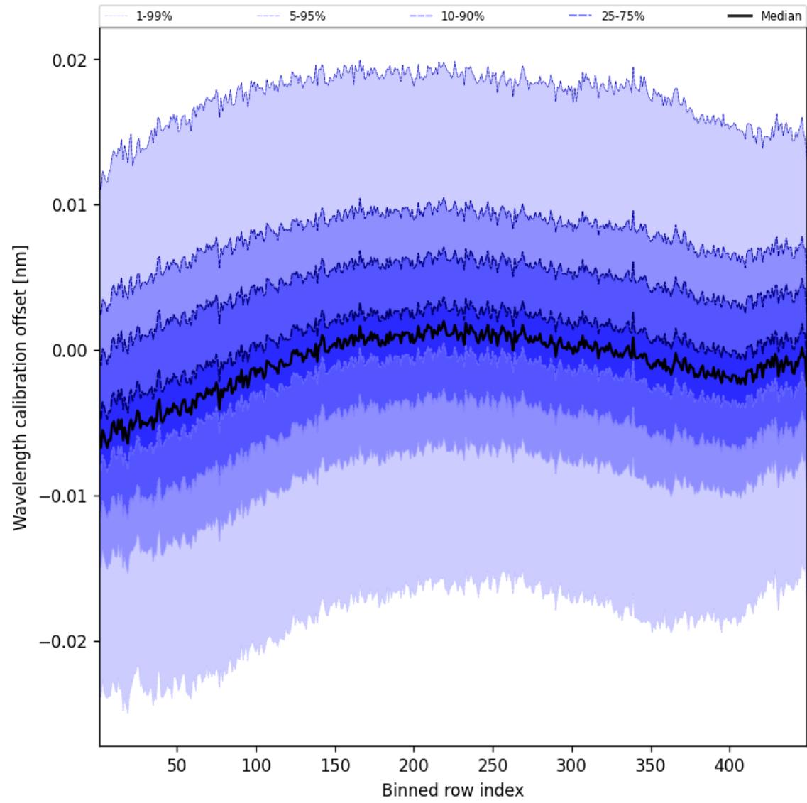
Figure 52: Along track statistics of “Wavelength calibration offset” for 2025-10-11 to 2025-10-13
