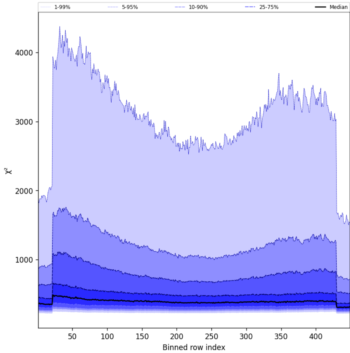
Figure 59: Along track statistics of “ \chi^2 ” for 2025-10-11 to 2025-10-13
