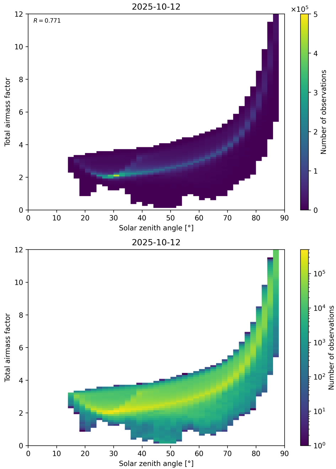
Figure 146: Scatter density plot of “Solar zenith angle” against “Total airmass factor” for 2025-10-11 to 2025-10-13.
