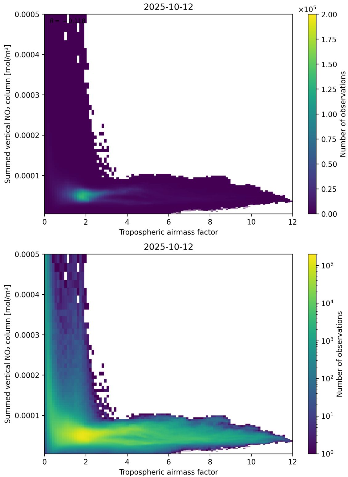
Figure 75: Scatter density plot of “Tropospheric airmass factor” against “Summed vertical NO 2 column” for 2025-10-11 to 2025-10-13.
