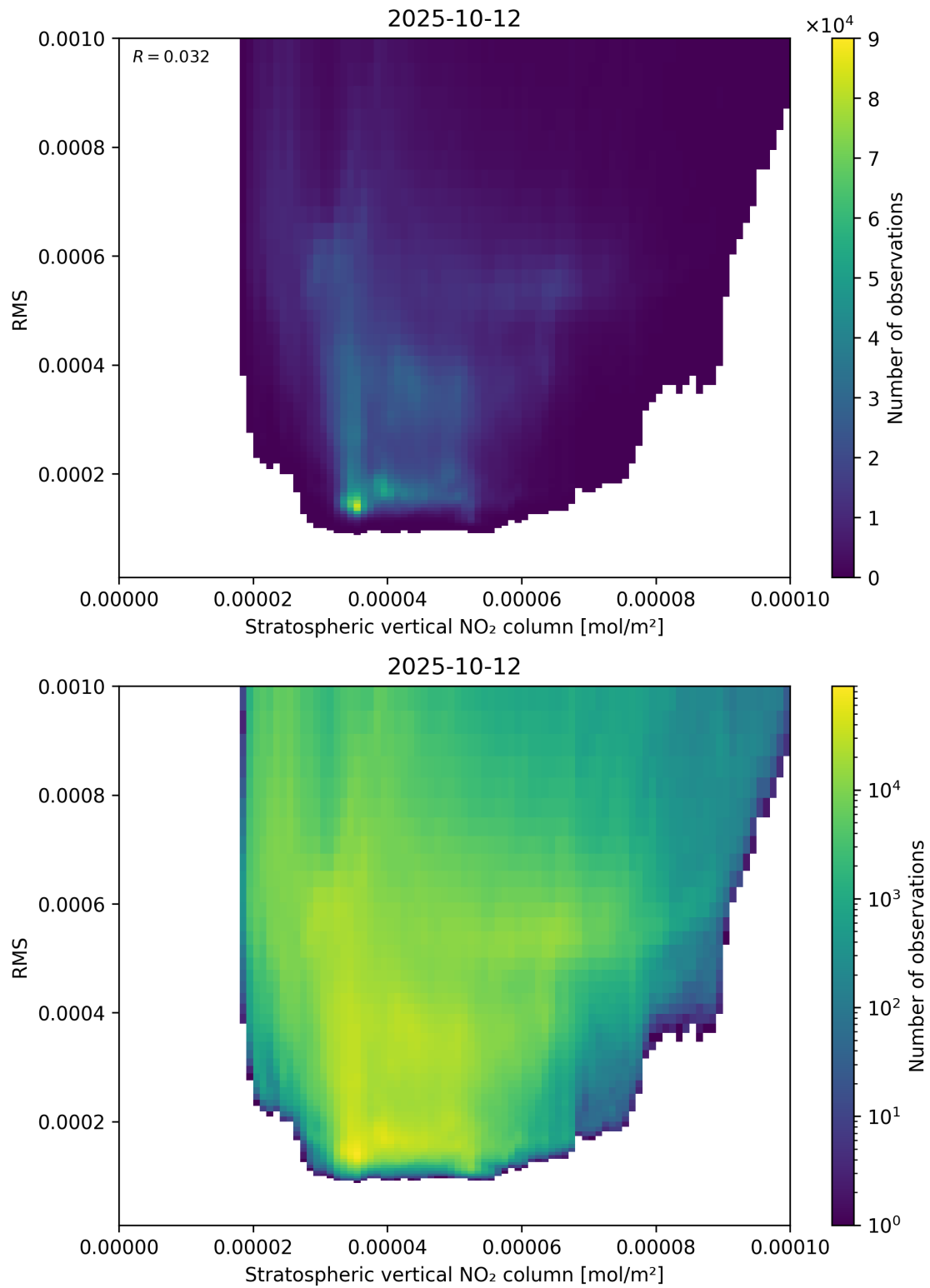
Figure 102: Scatter density plot of “Stratospheric vertical NO 2 column” against “RMS” for 2025-10-11 to 2025-10-13.
