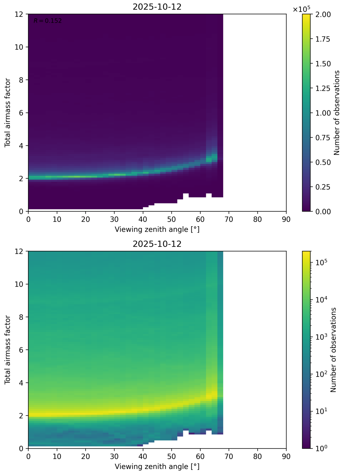
Figure 160: Scatter density plot of “Viewing zenith angle” against “Total airmass factor” for 2025-10-11 to 2025-10-13.
