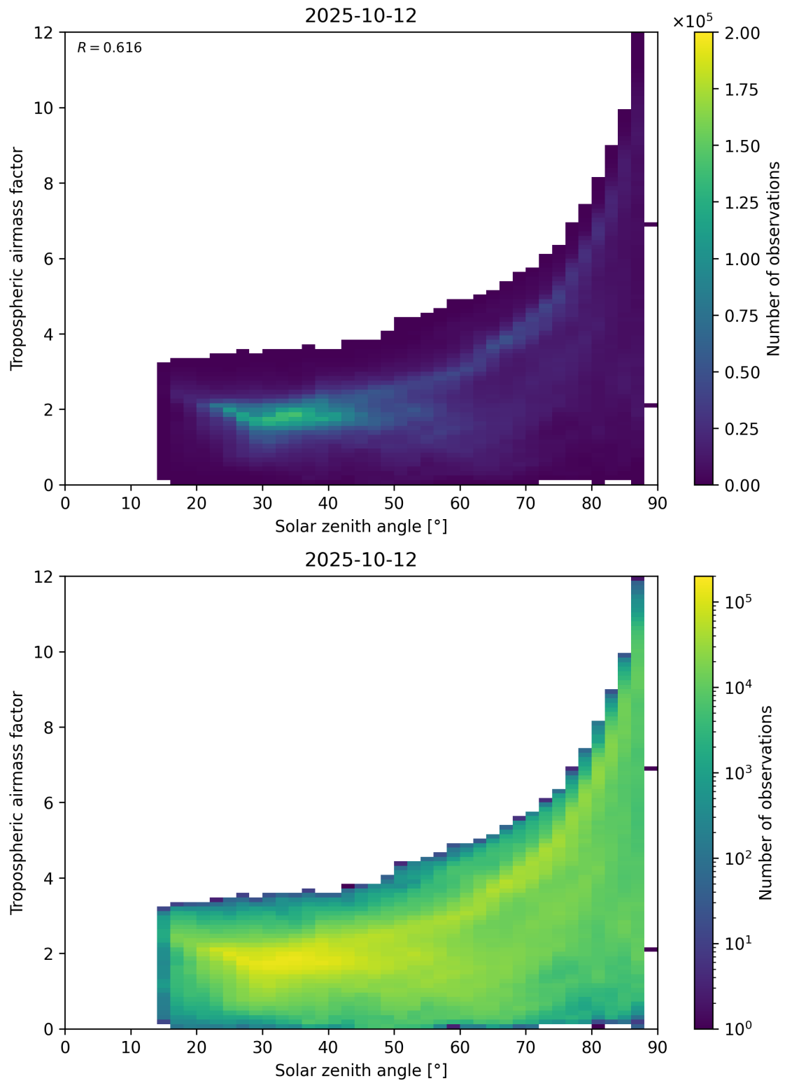
Figure 147: Scatter density plot of “Solar zenith angle” against “Tropospheric airmass factor” for 2025-10-11 to 2025-10-13.
