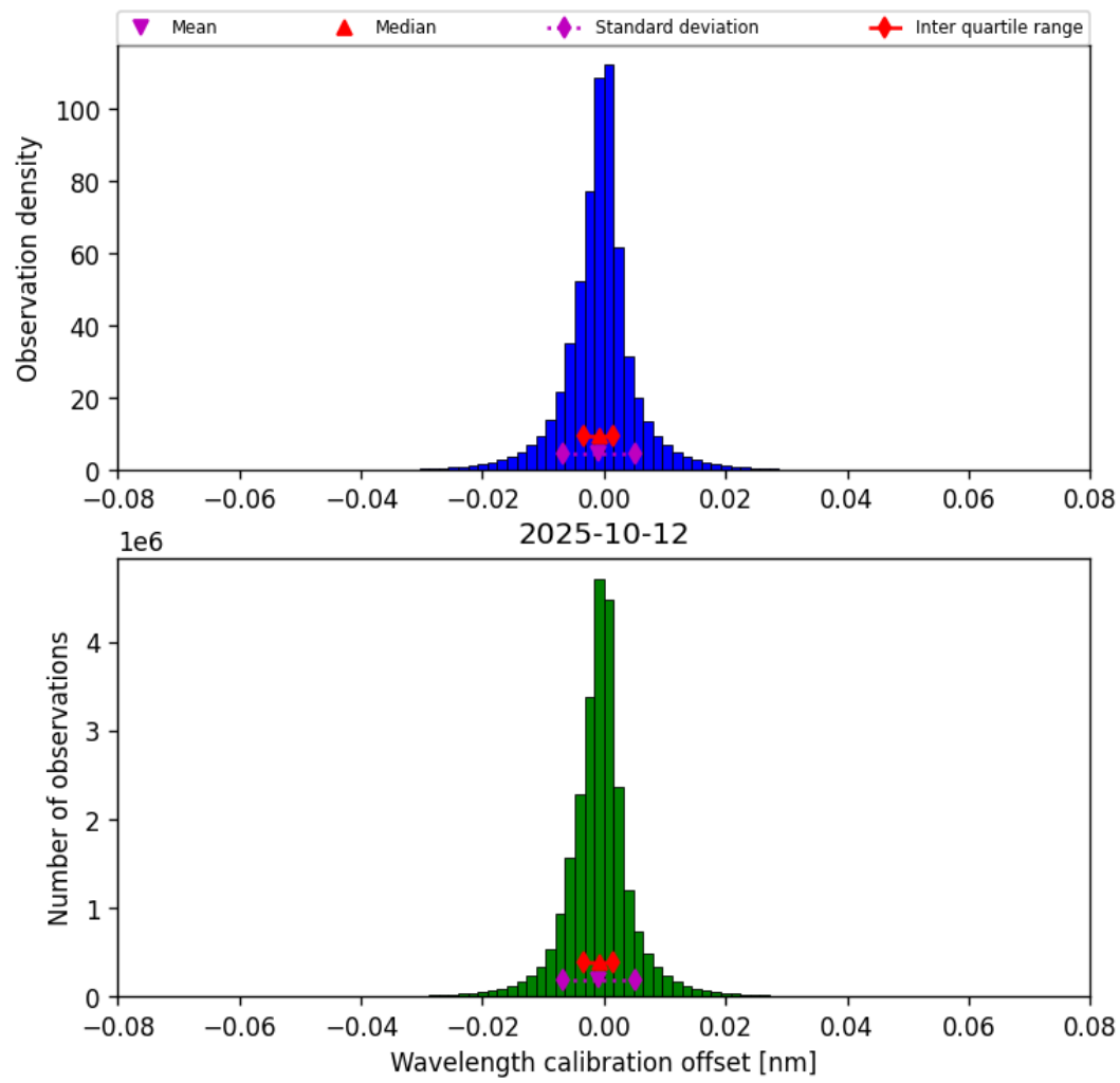
Figure 35: Histogram of “Wavelength calibration offset” for 2025-10-11 to 2025-10-13
