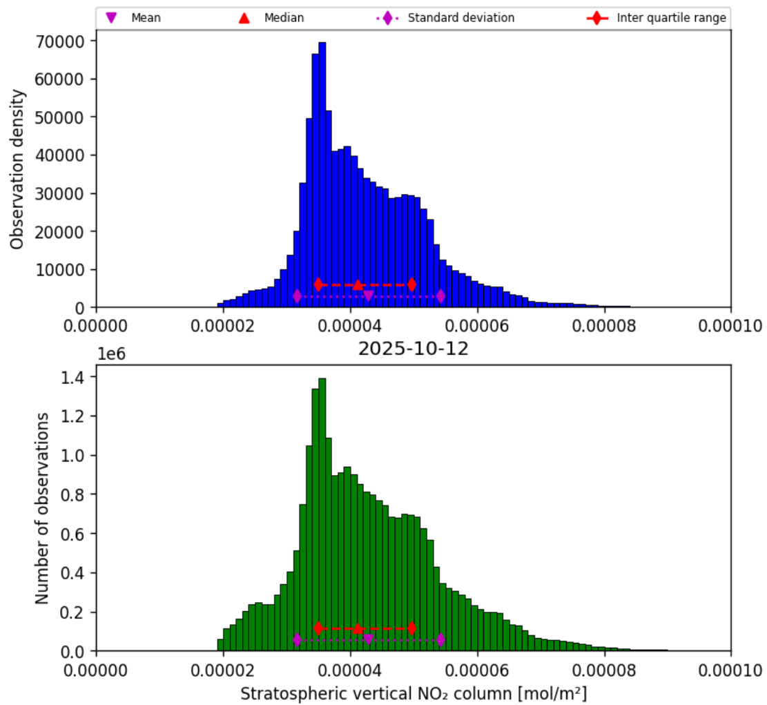
Figure 36: Histogram of “Stratospheric vertical NO 2 column” for 2025-10-11 to 2025-10-13
