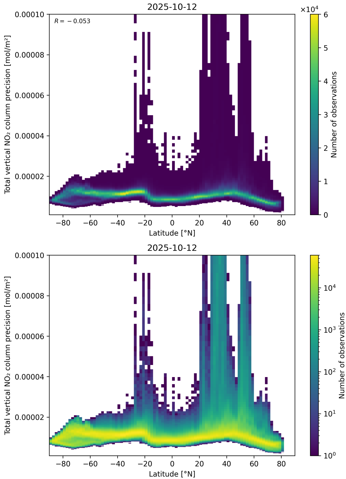
Figure 91: Scatter density plot of “Latitude” against “Total vertical NO 2 column precision” for 2025-10-11 to 2025-10-13.
