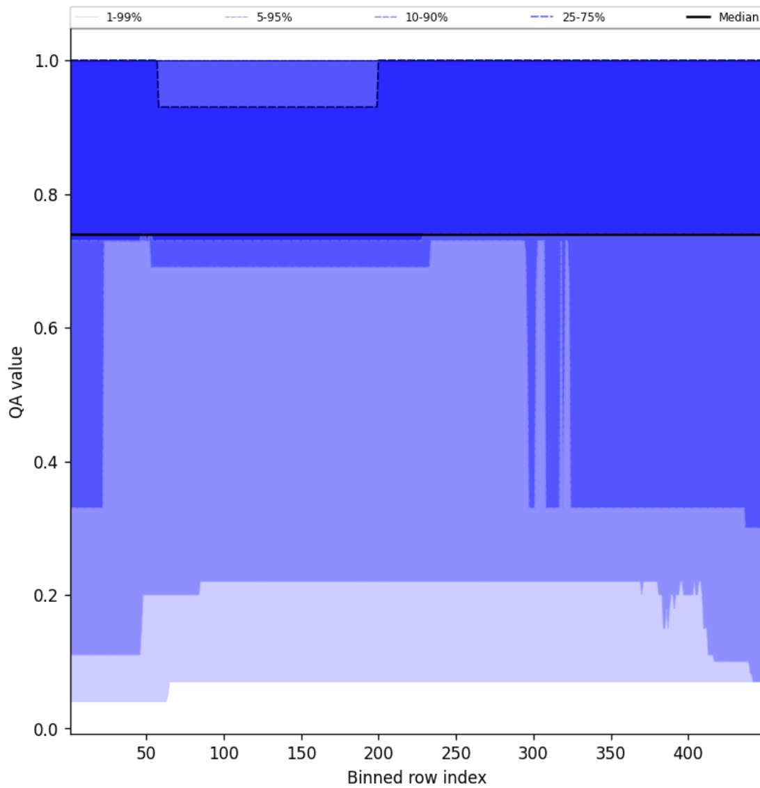
Figure 45: Along track statistics of “QA value” for 2025-10-11 to 2025-10-13
