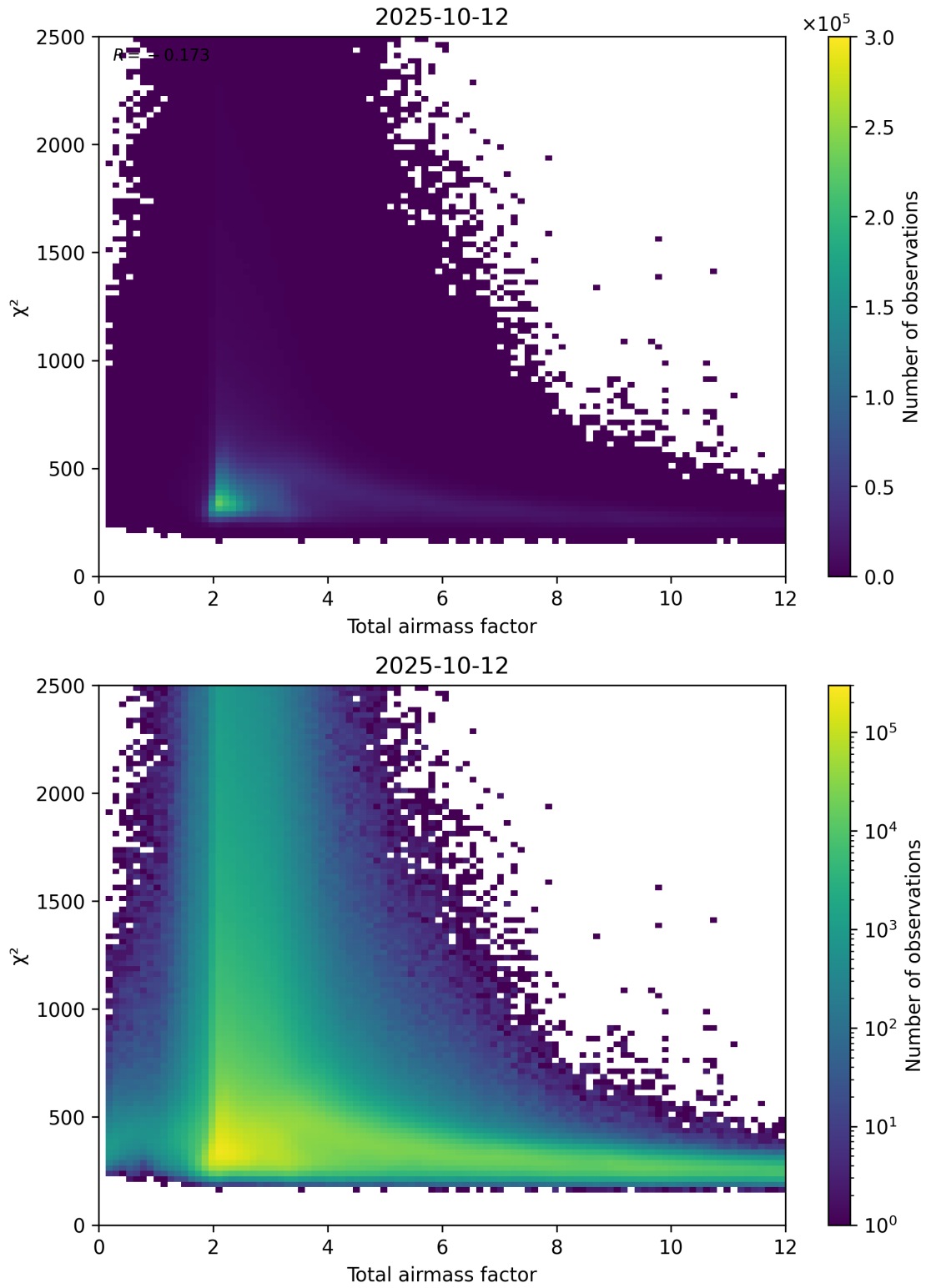
Figure 63: Scatter density plot of “Total airmass factor” against “ \chi^2 ” for 2025-10-11 to 2025-10-13.
