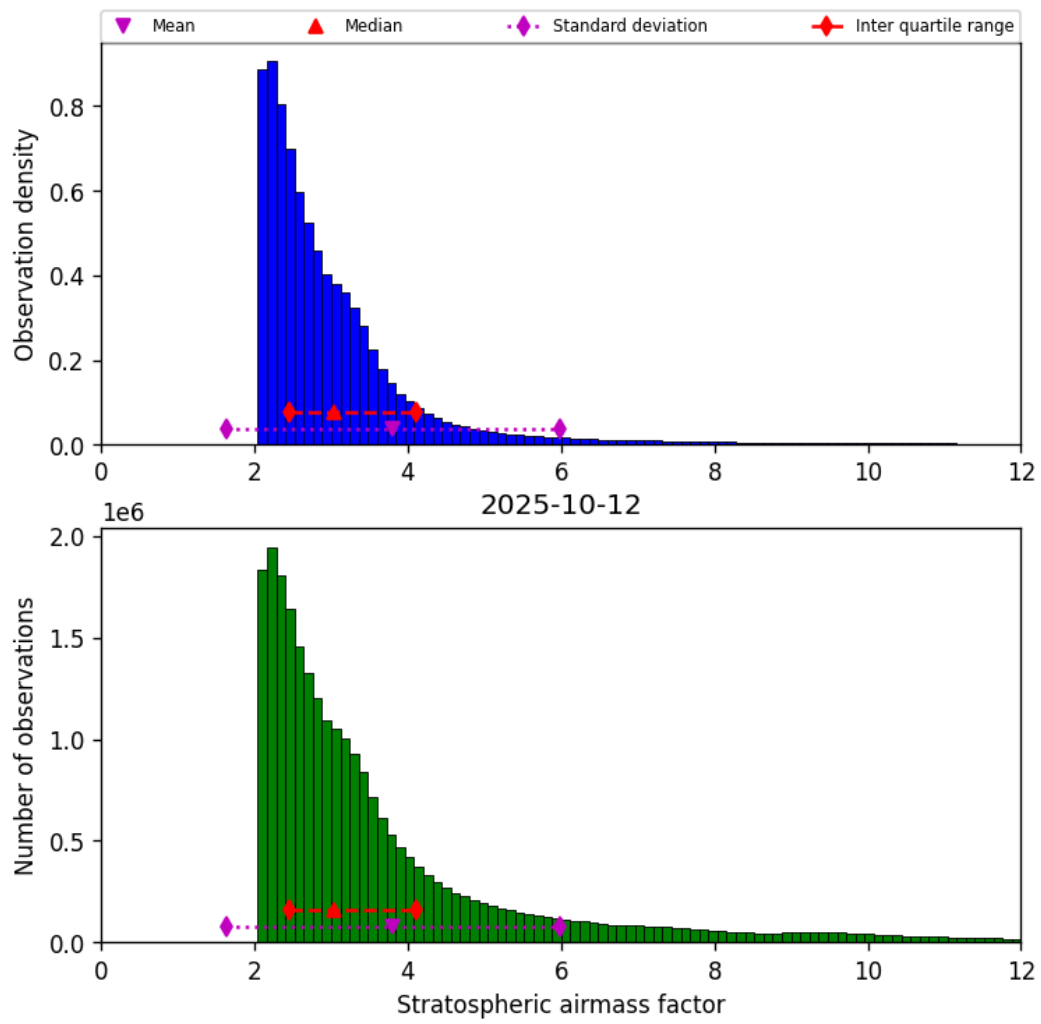
Figure 44: Histogram of “Stratospheric airmass factor” for 2025-10-11 to 2025-10-13
