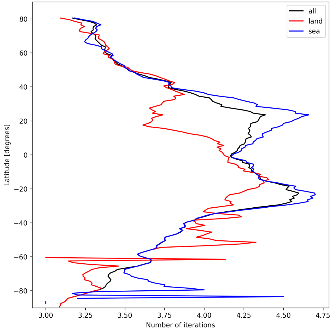
Figure 17: Zonal average of “Number of iterations” for 2025-10-11 to 2025-10-13.
