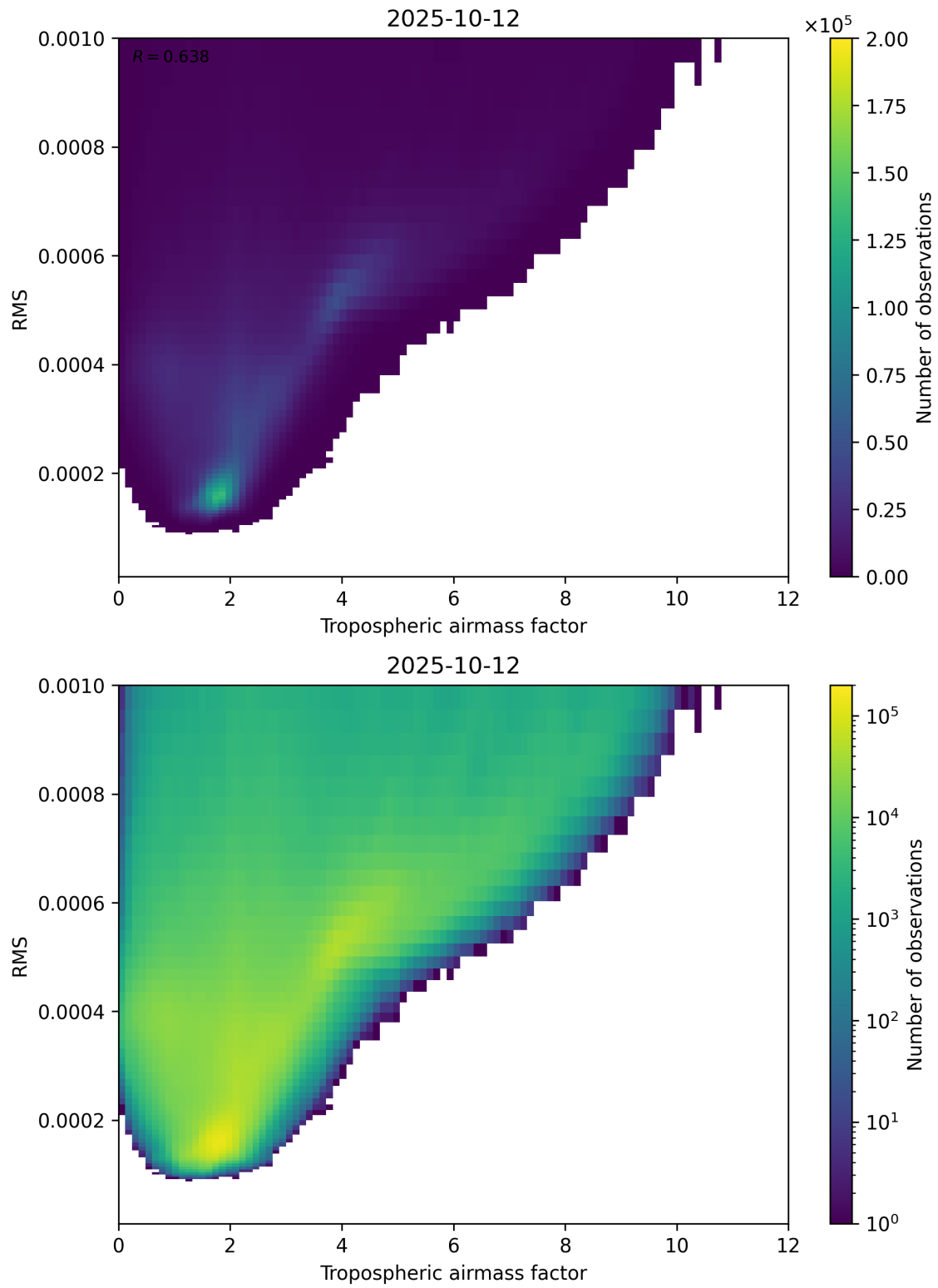
Figure 79: Scatter density plot of “Tropospheric airmass factor” against “RMS” for 2025-10-11 to 2025-10-13.
