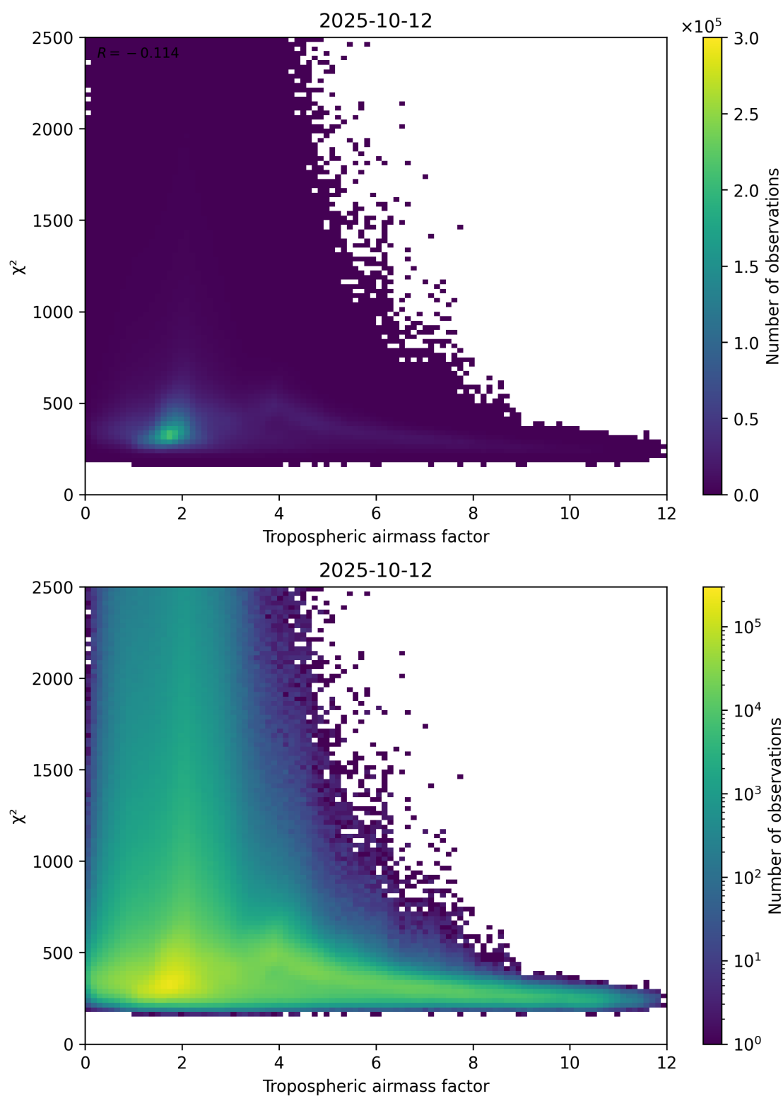
Figure 73: Scatter density plot of “Tropospheric airmass factor” against “ \chi^2 ” for 2025-10-11 to 2025-10-13.
