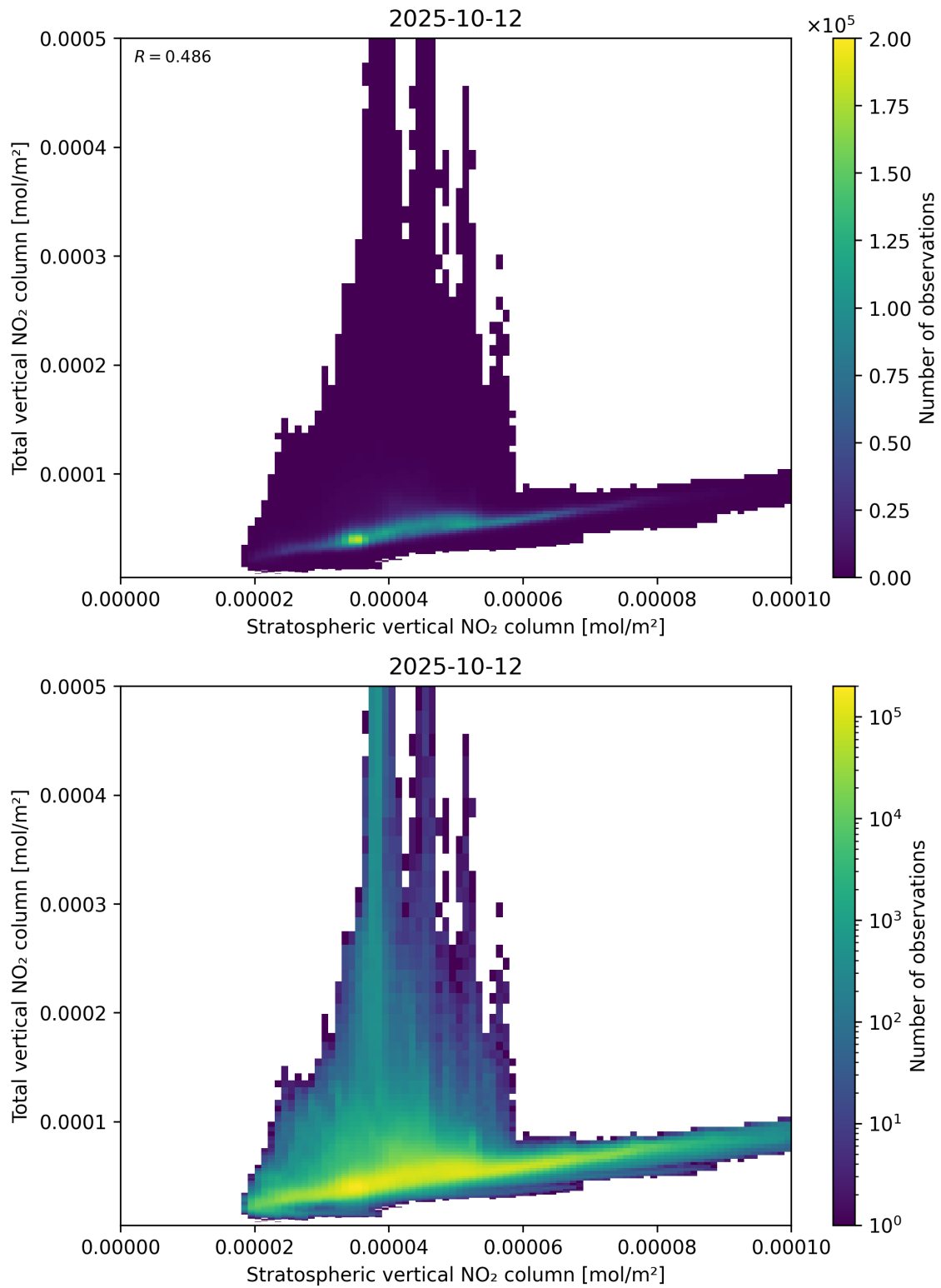
Figure 100: Scatter density plot of “Stratospheric vertical NO 2 column” against “Total vertical NO 2 column” for 2025-10-11 to 2025-10-13.
