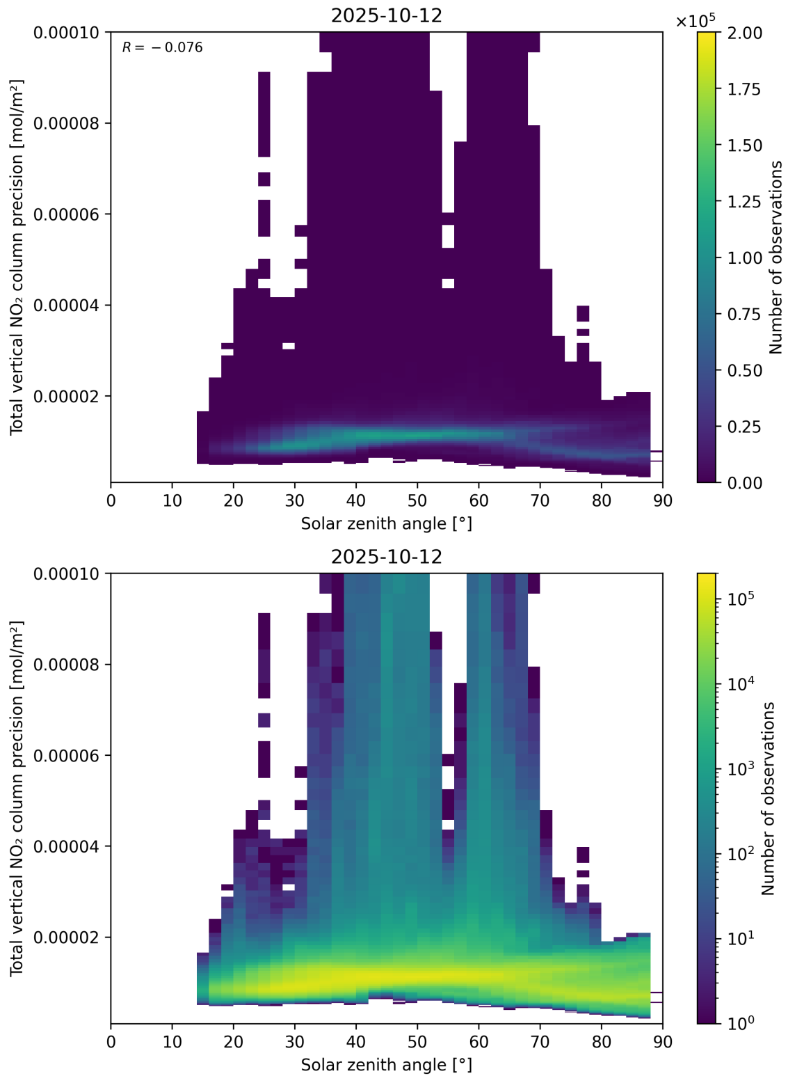
Figure 154: Scatter density plot of “Solar zenith angle” against “Total vertical NO 2 column precision” for 2025-10-11 to 2025-10-13.
