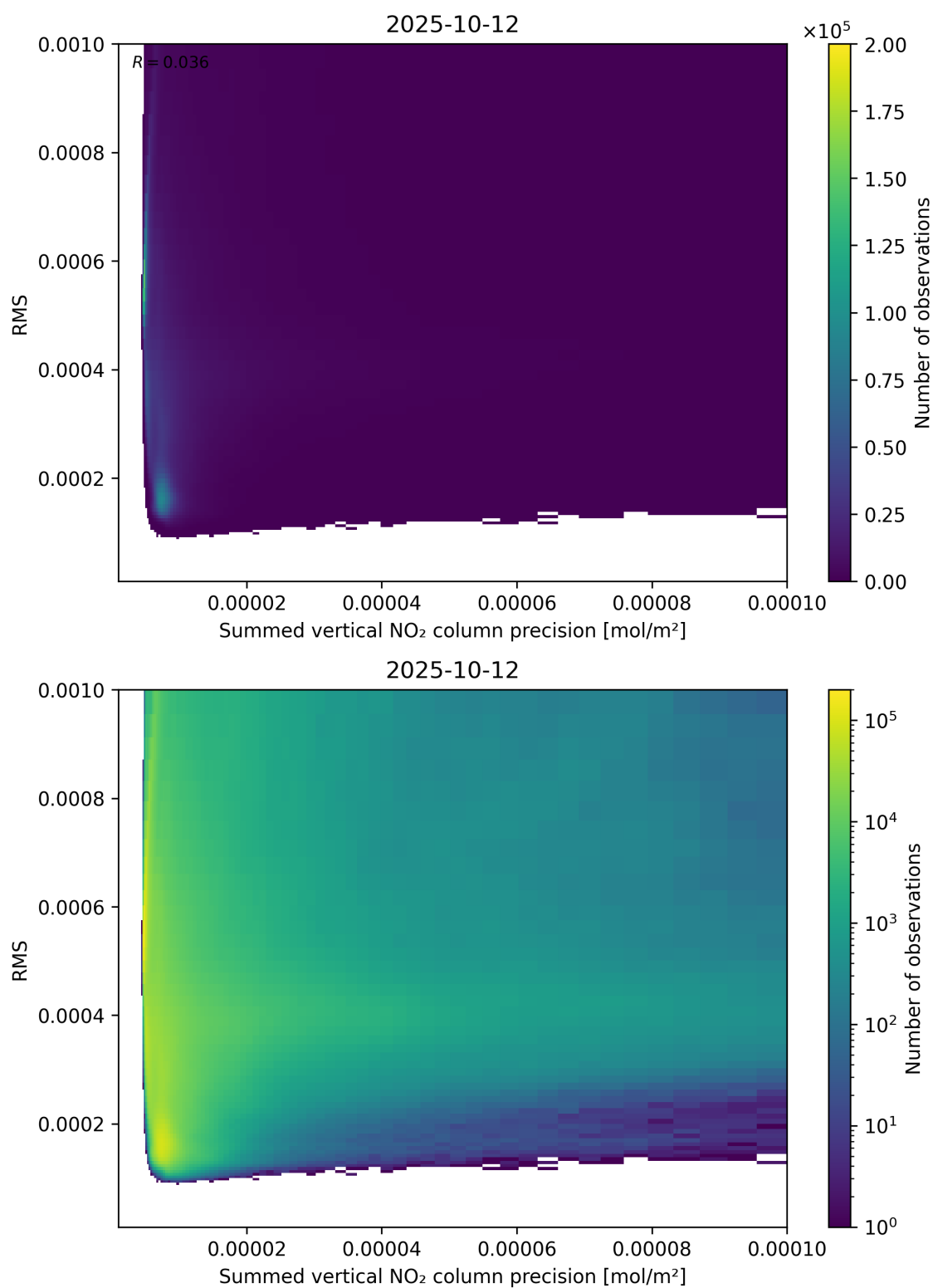
Figure 108: Scatter density plot of “Summed vertical NO 2 column precision” against “RMS” for 2025-10-11 to 2025-10-13.
