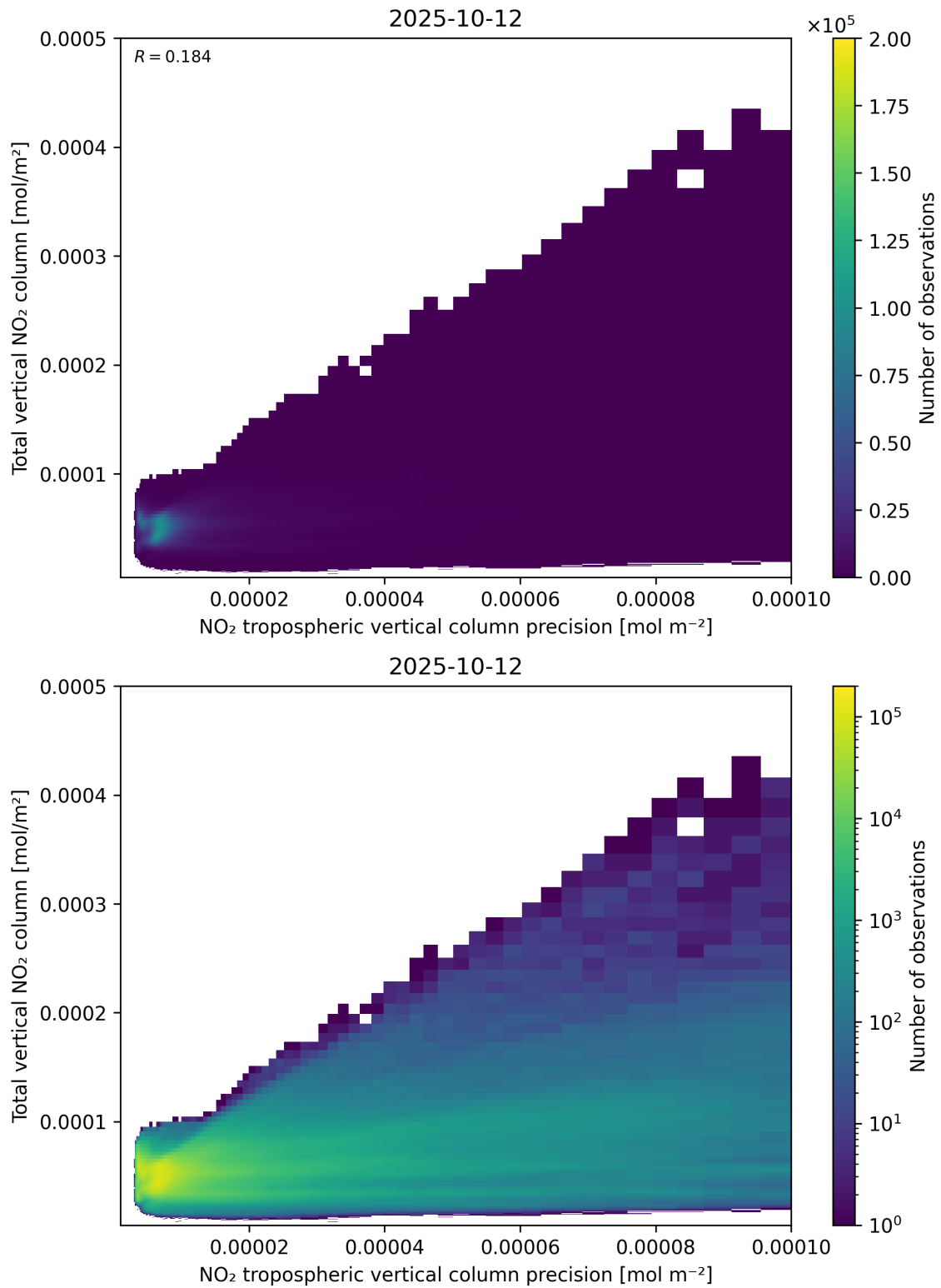
Figure 138: Scatter density plot of “NO 2 tropospheric vertical column precision” against “Total vertical NO 2 column” for 2025-10-11 to 2025-10-13.
