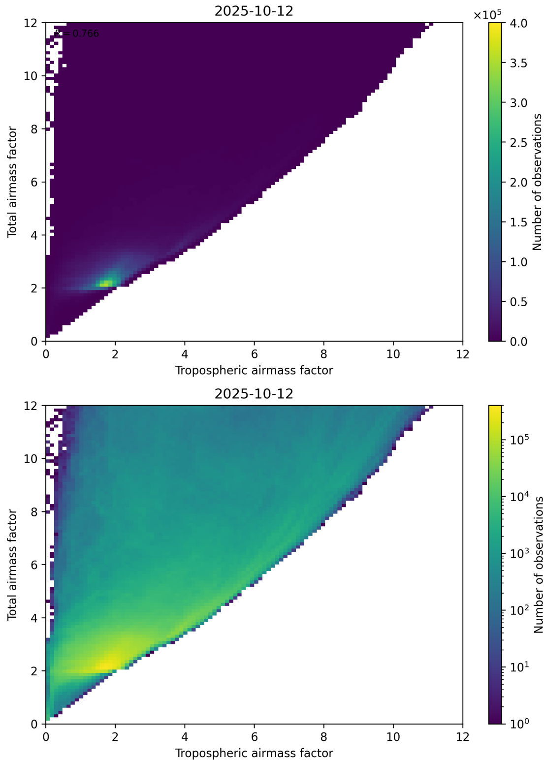
Figure 72: Scatter density plot of “Tropospheric airmass factor” against “Total airmass factor” for 2025-10-11 to 2025-10-13.
