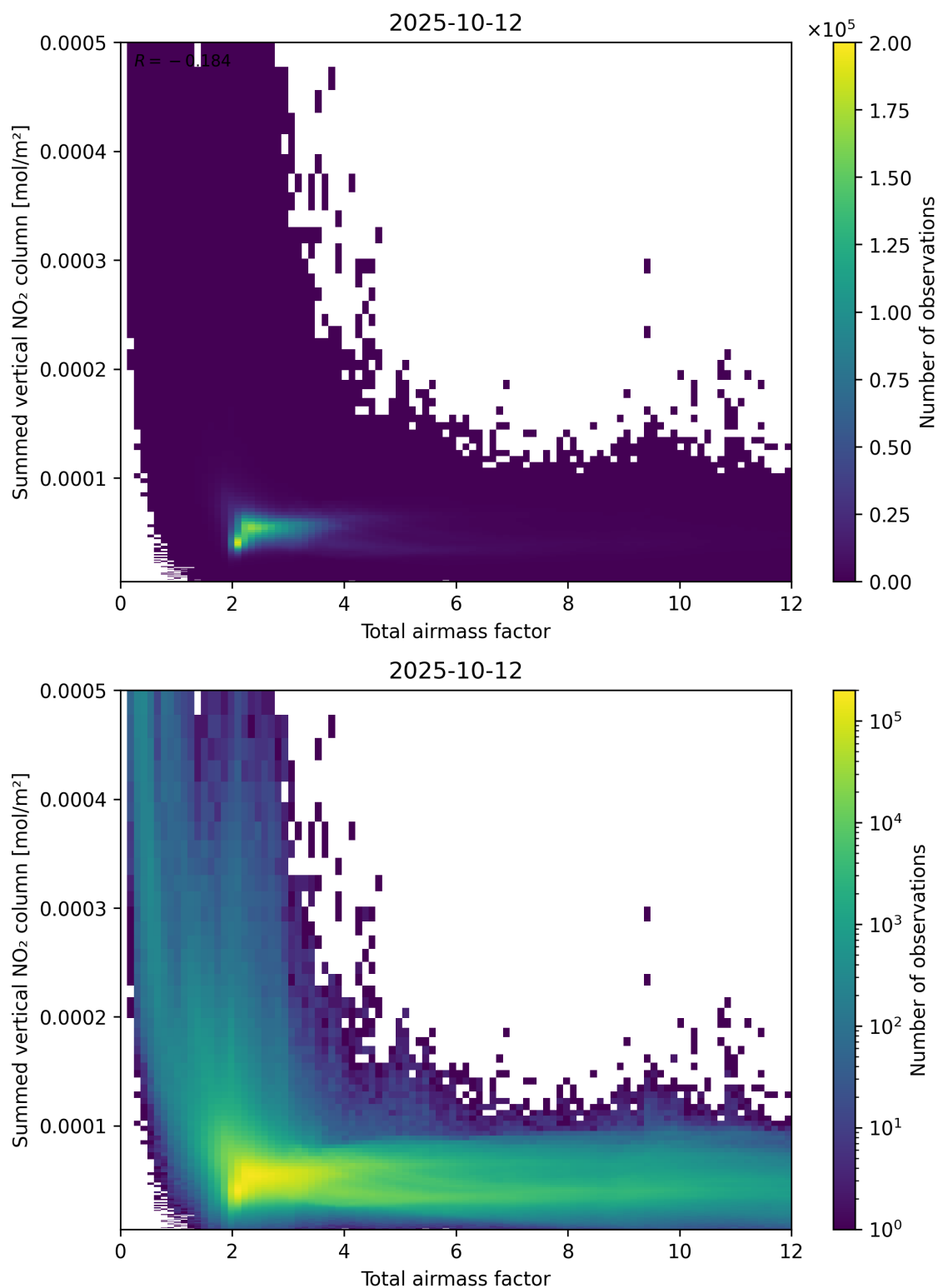
Figure 65: Scatter density plot of “Total airmass factor” against “Summed vertical NO 2 column” for 2025-10-11 to 2025-10-13.
