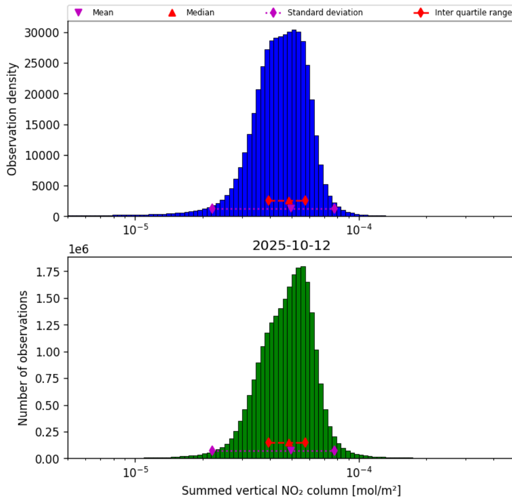
Figure 40: Histogram of “Summed vertical NO 2 column” for 2025-10-11 to 2025-10-13
