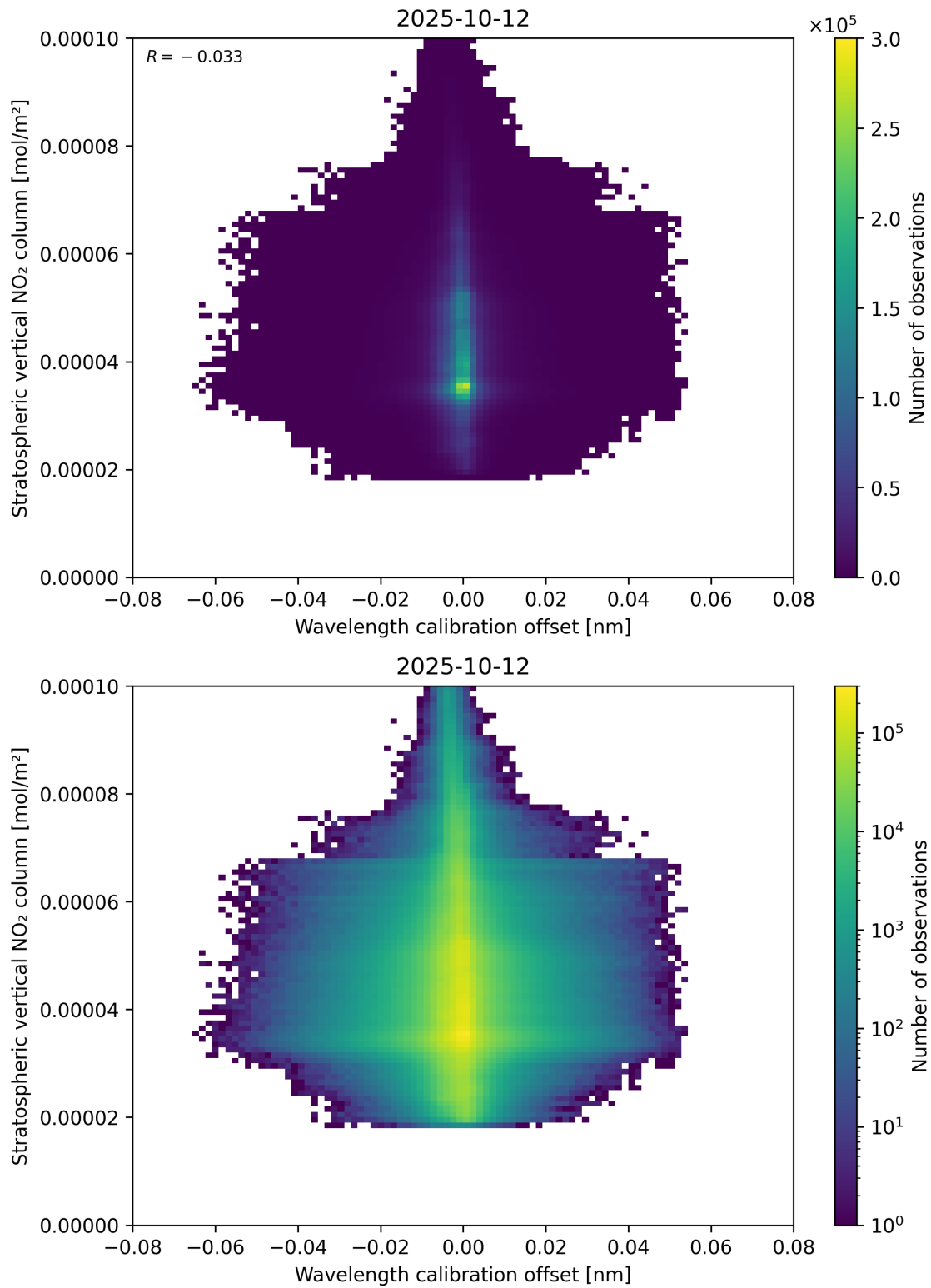
Figure 176: Scatter density plot of “Wavelength calibration offset” against “Stratospheric vertical NO 2 column” for 2025-10-11 to 2025-10-13.
