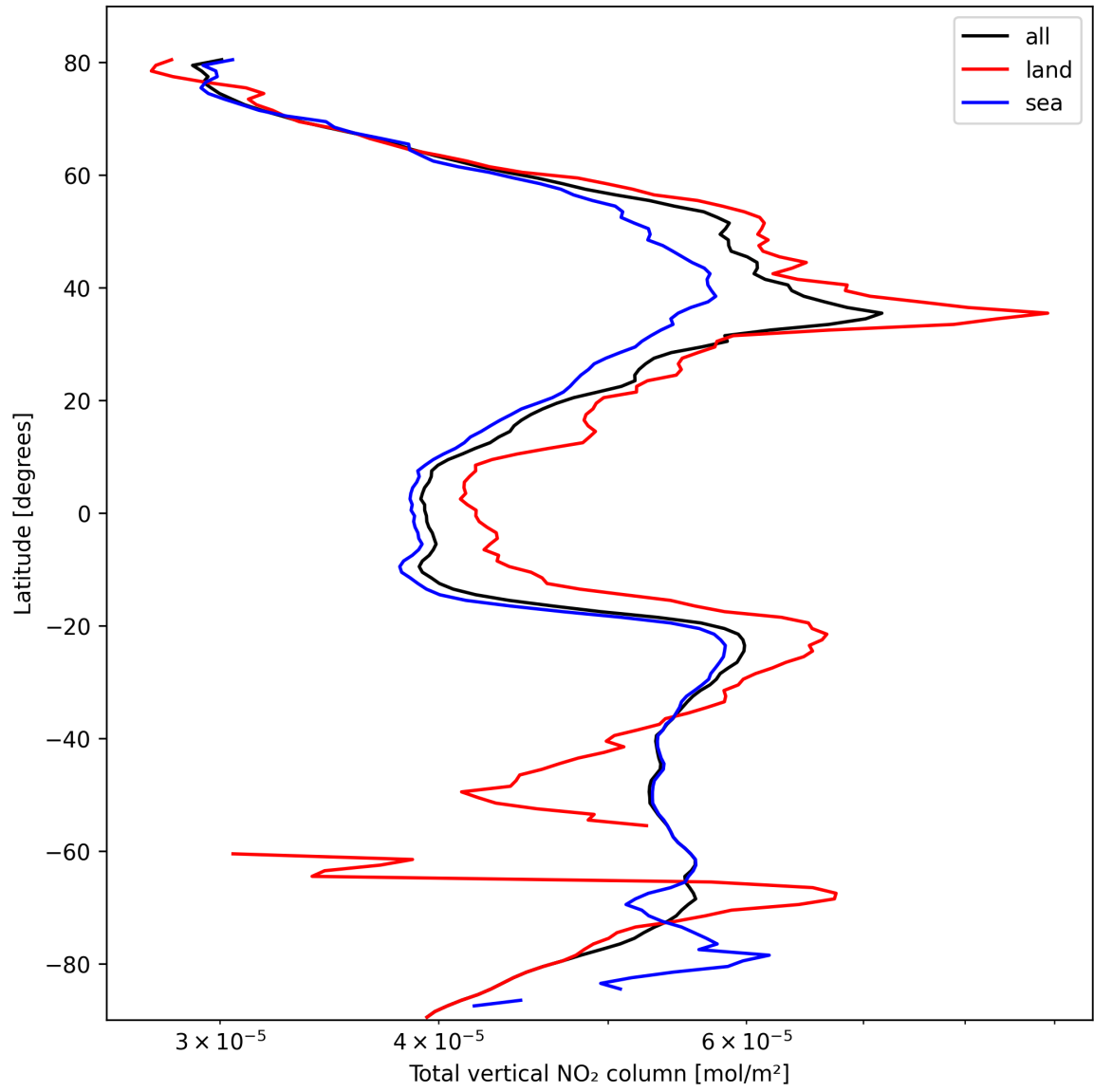
Figure 21: Zonal average of “Total vertical NO 2 column” for 2025-10-11 to 2025-10-13.
