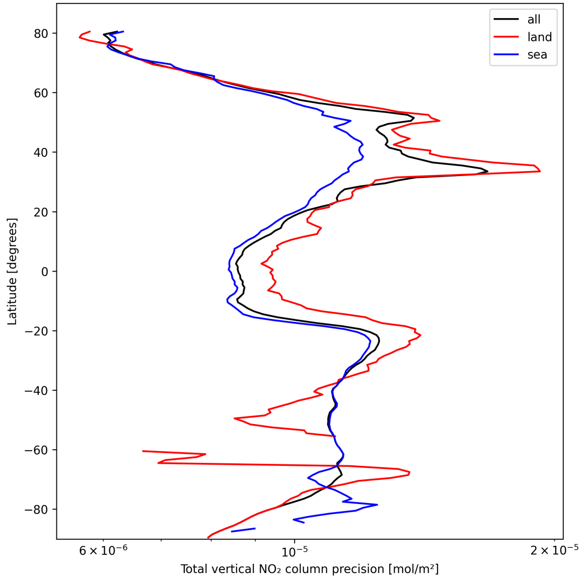
Figure 22: Zonal average of “Total vertical NO 2 column precision” for 2025-10-11 to 2025-10-13.
