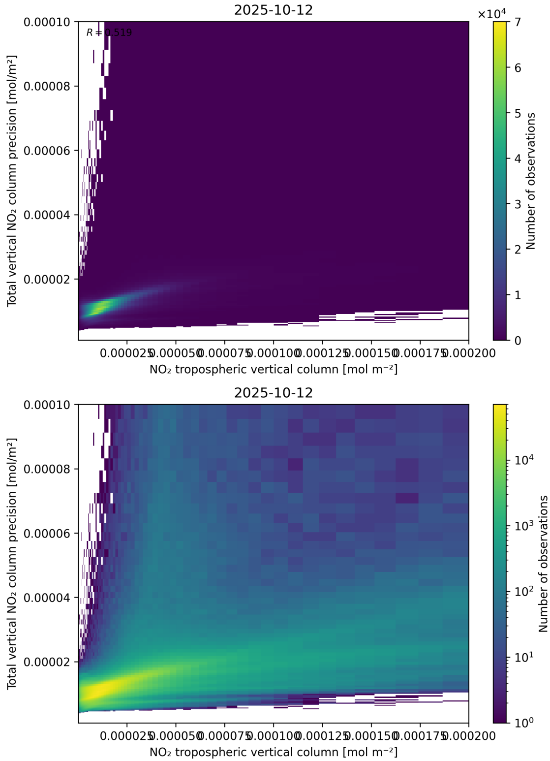
Figure 129: Scatter density plot of “NO 2 tropospheric vertical column” against “Total vertical NO 2 column precision” for 2025-10-11 to 2025-10-13.
