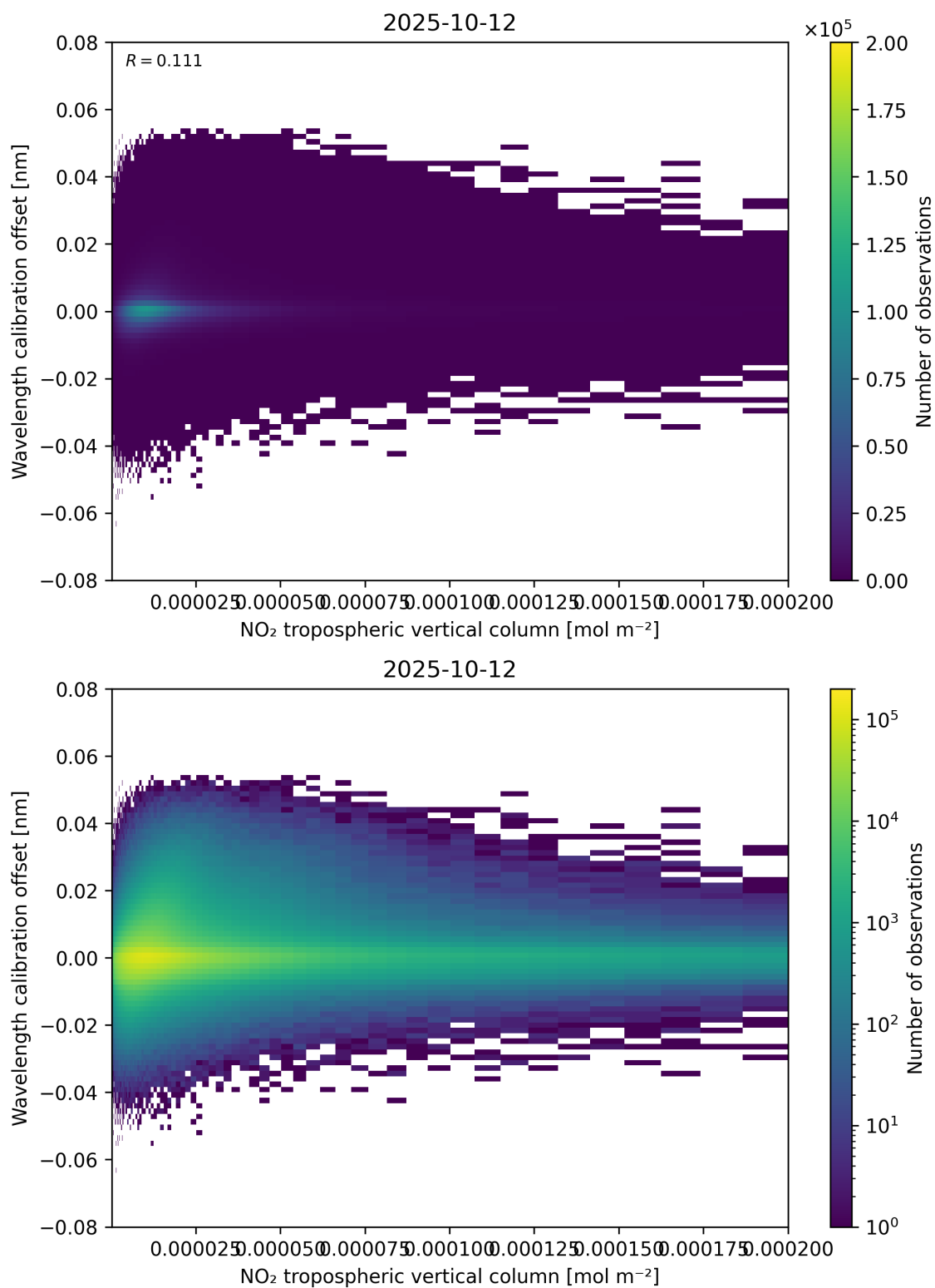
Figure 143: Scatter density plot of “NO 2 tropospheric vertical column” against “Wavelength calibration offset” for 2025-10-11 to 2025-10-13.
