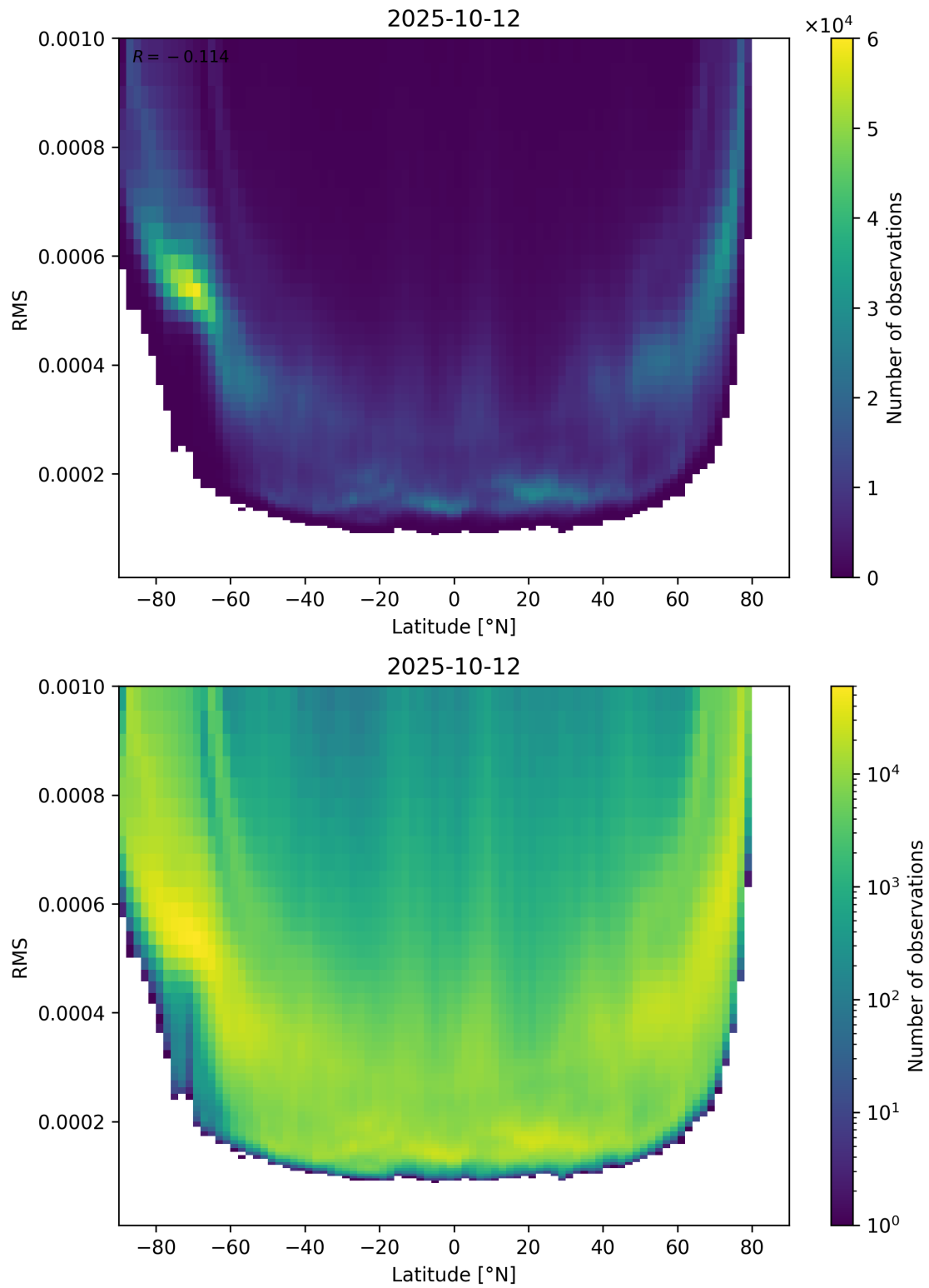
Figure 94: Scatter density plot of “Latitude” against “RMS” for 2025-10-11 to 2025-10-13.
