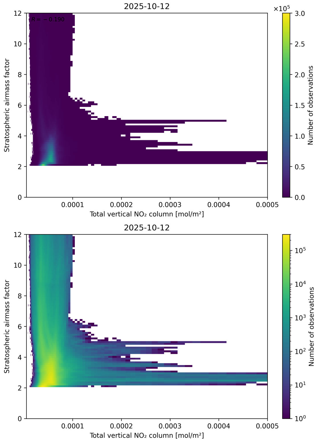
Figure 110: Scatter density plot of “Total vertical NO 2 column” against “Stratospheric airmass factor” for 2025-10-11 to 2025-10-13.
