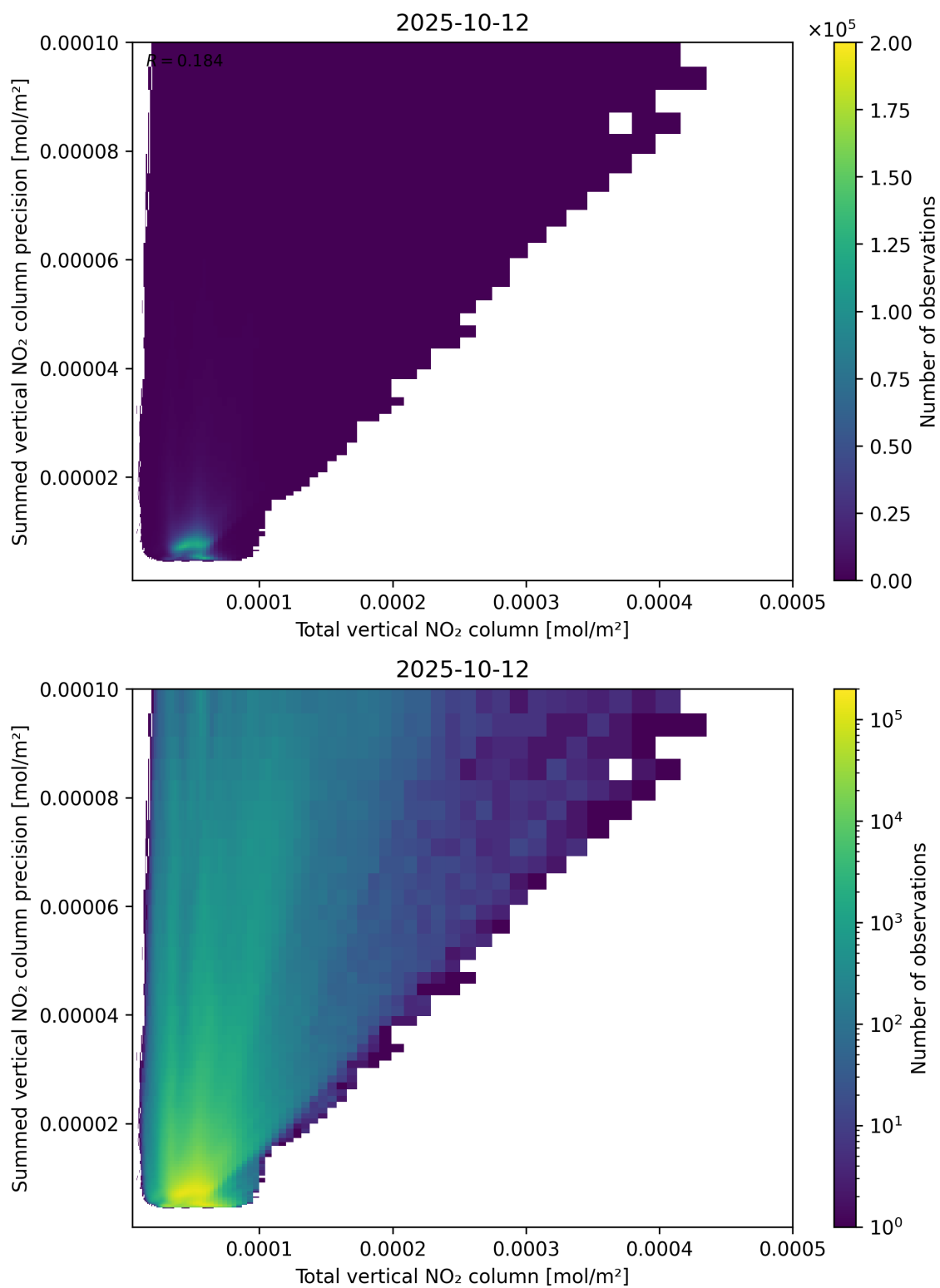
Figure 113: Scatter density plot of “Total vertical NO 2 column” against “Summed vertical NO 2 column precision” for 2025-10-11 to 2025-10-13.
