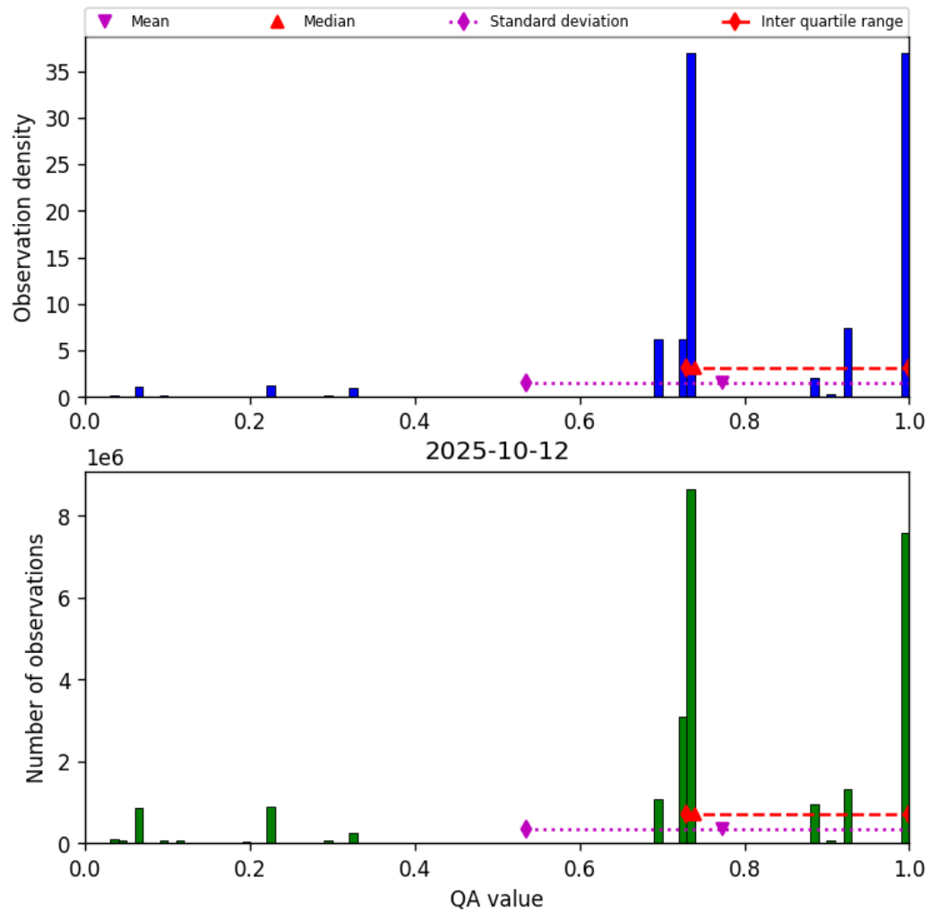
Figure 28: Histogram of “QA value” for 2025-10-11 to 2025-10-13
