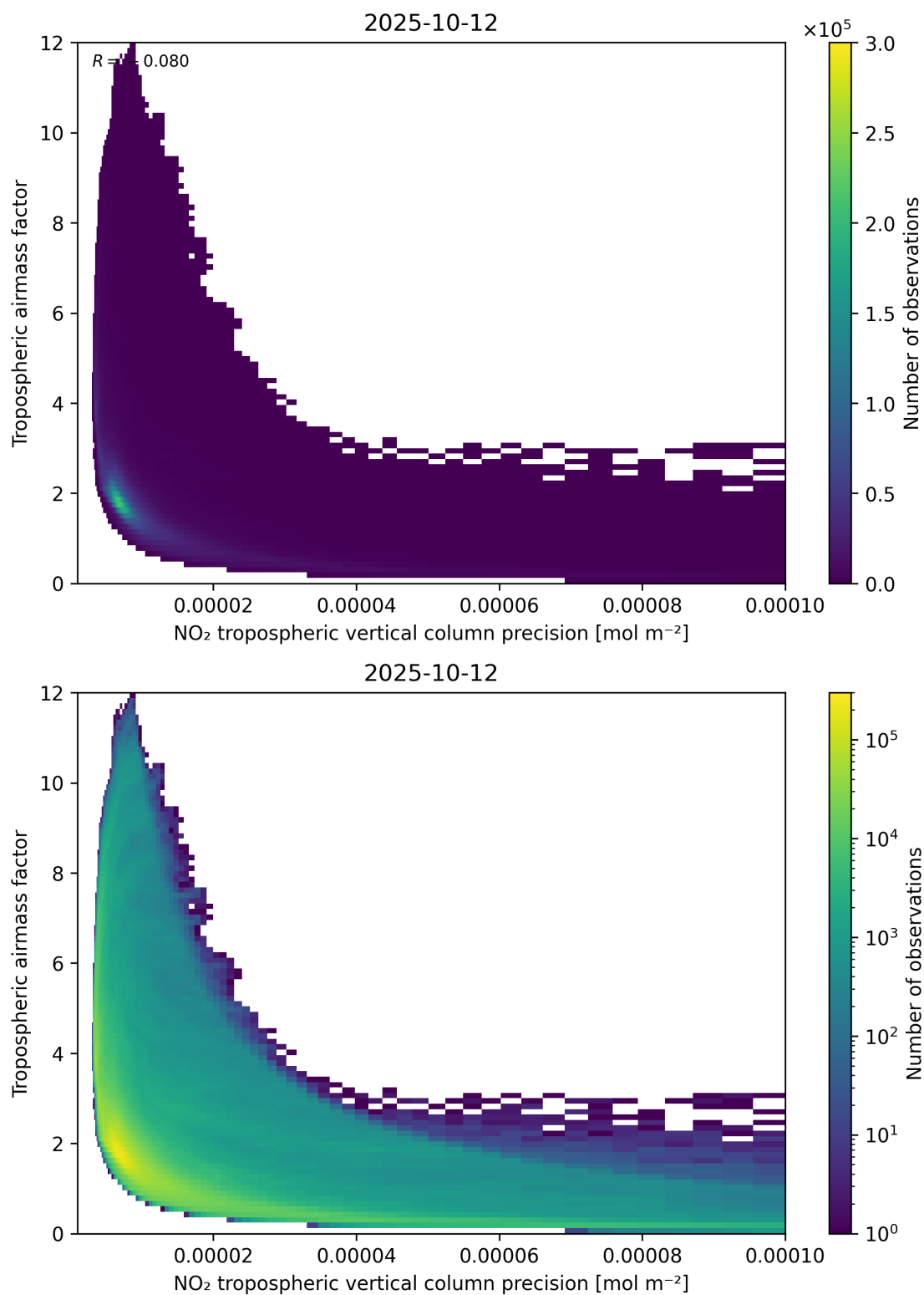
Figure 133: Scatter density plot of “NO 2 tropospheric vertical column precision” against “Tropospheric air mass factor” for 2025-10-11 to 2025-10-13.
