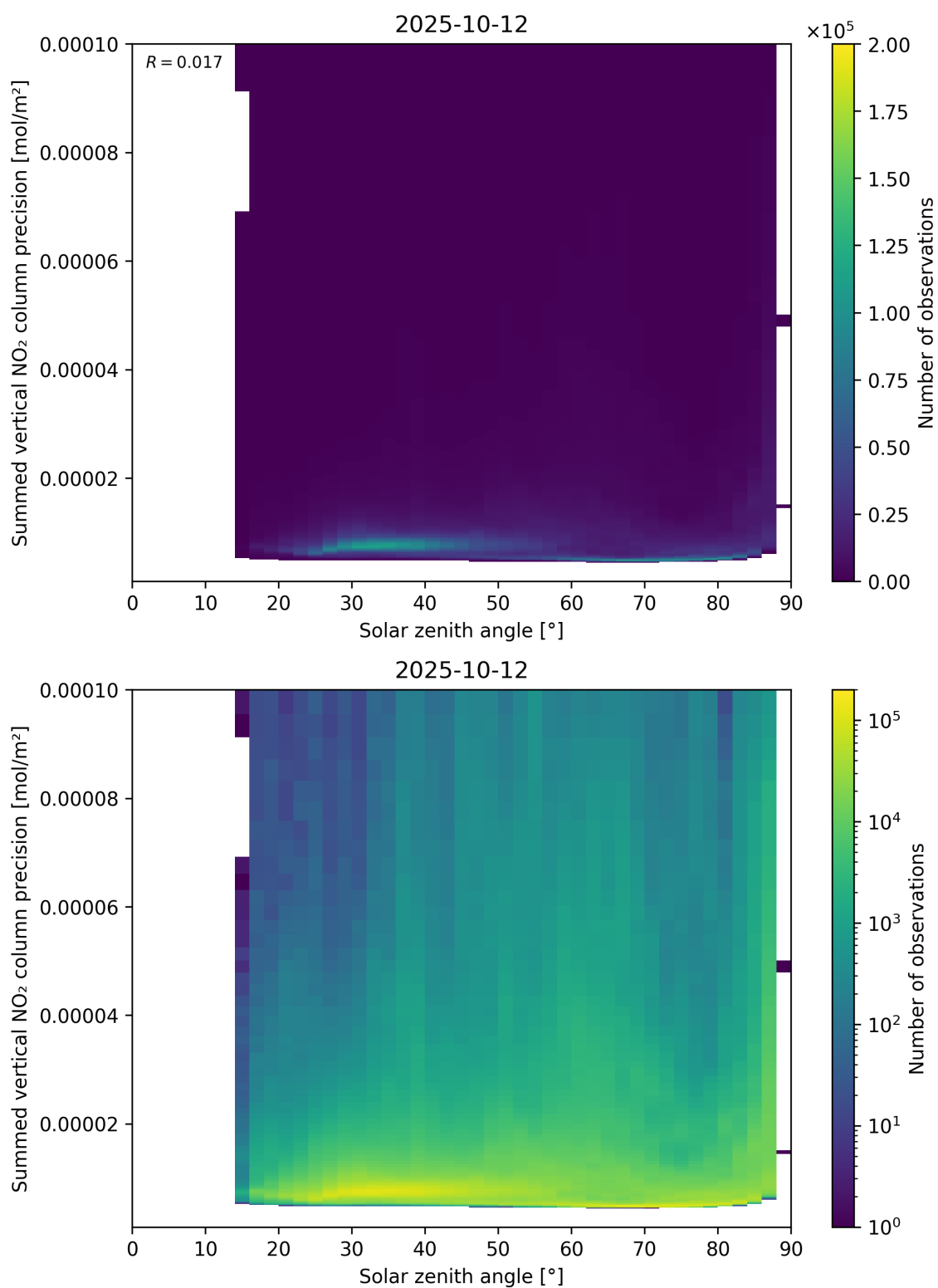
Figure 152: Scatter density plot of “Solar zenith angle” against “Summed vertical NO 2 column precision” for 2025-10-11 to 2025-10-13.
