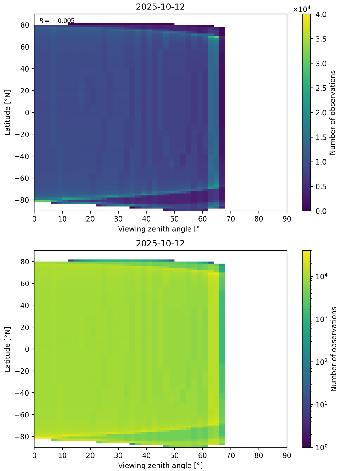
Figure 163: Scatter density plot of “Viewing zenith angle” against “Latitude” for 2025-10-11 to 2025-10-13.
