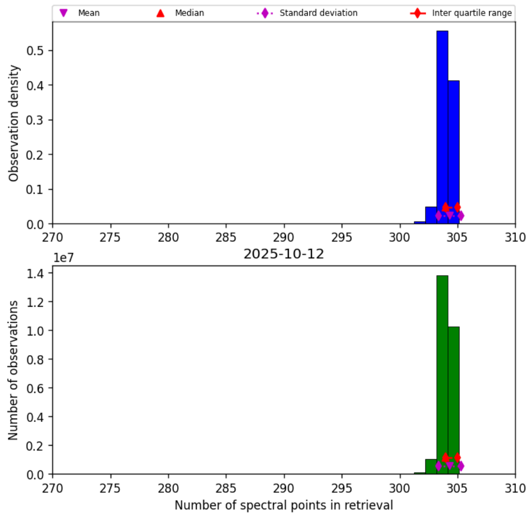
Figure 33: Histogram of “Number of spectral points in retrieval” for 2025-10-11 to 2025-10-13
