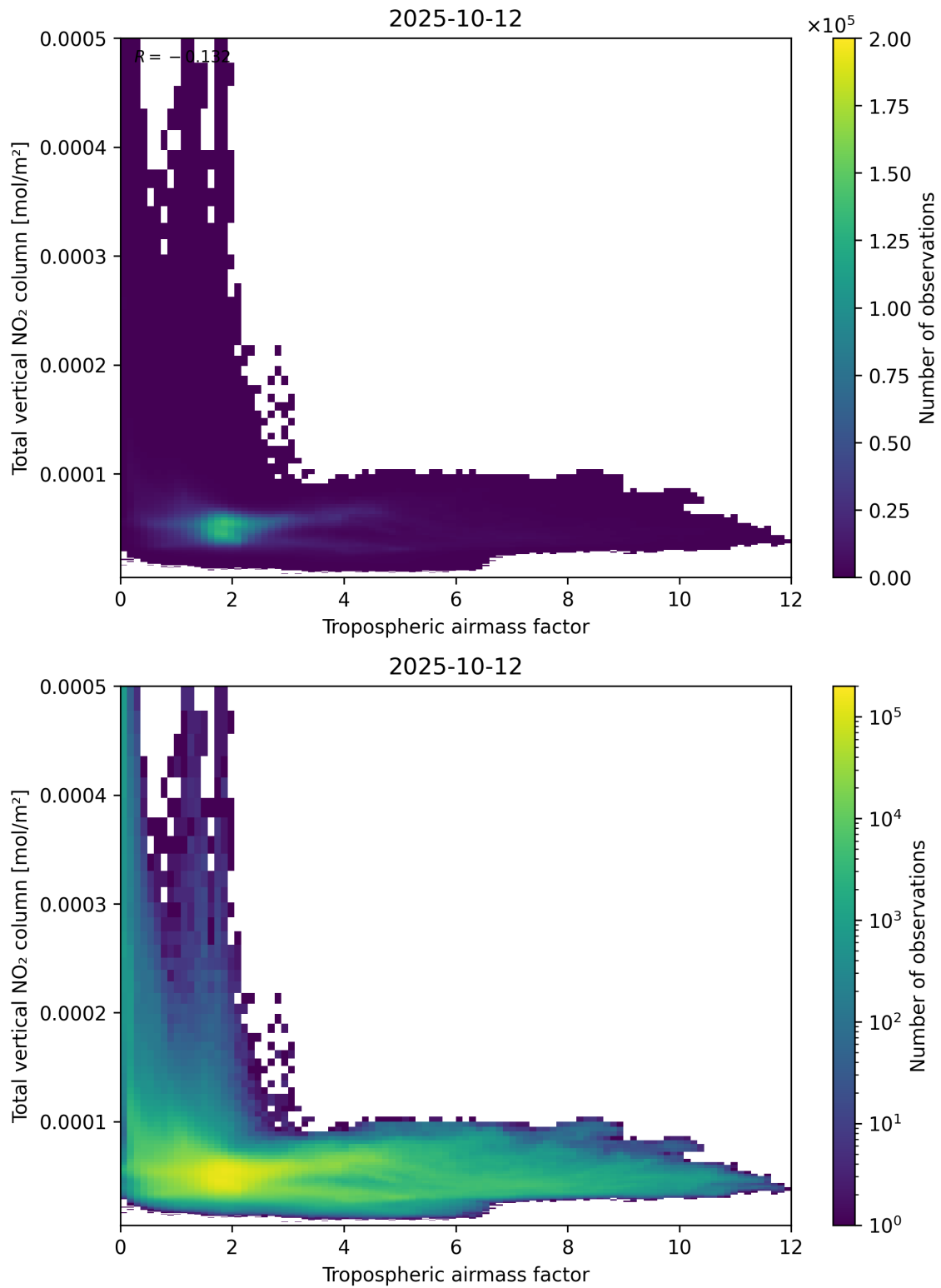
Figure 77: Scatter density plot of “Tropospheric airmass factor” against “Total vertical NO 2 column” for 2025-10-11 to 2025-10-13.
