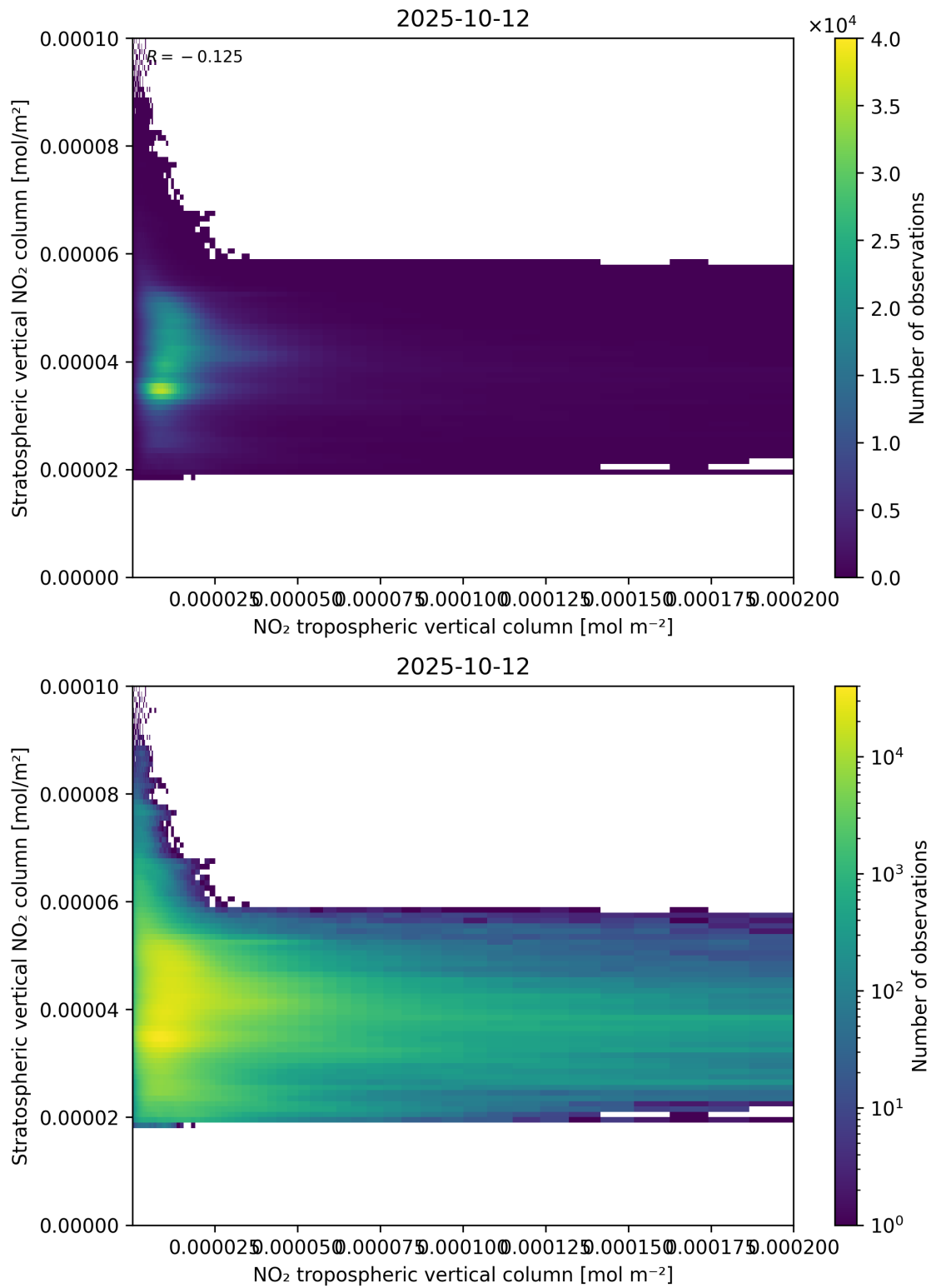
Figure 125: Scatter density plot of “NO 2 tropospheric vertical column” against “Stratospheric vertical NO 2 column” for 2025-10-11 to 2025-10-13.
