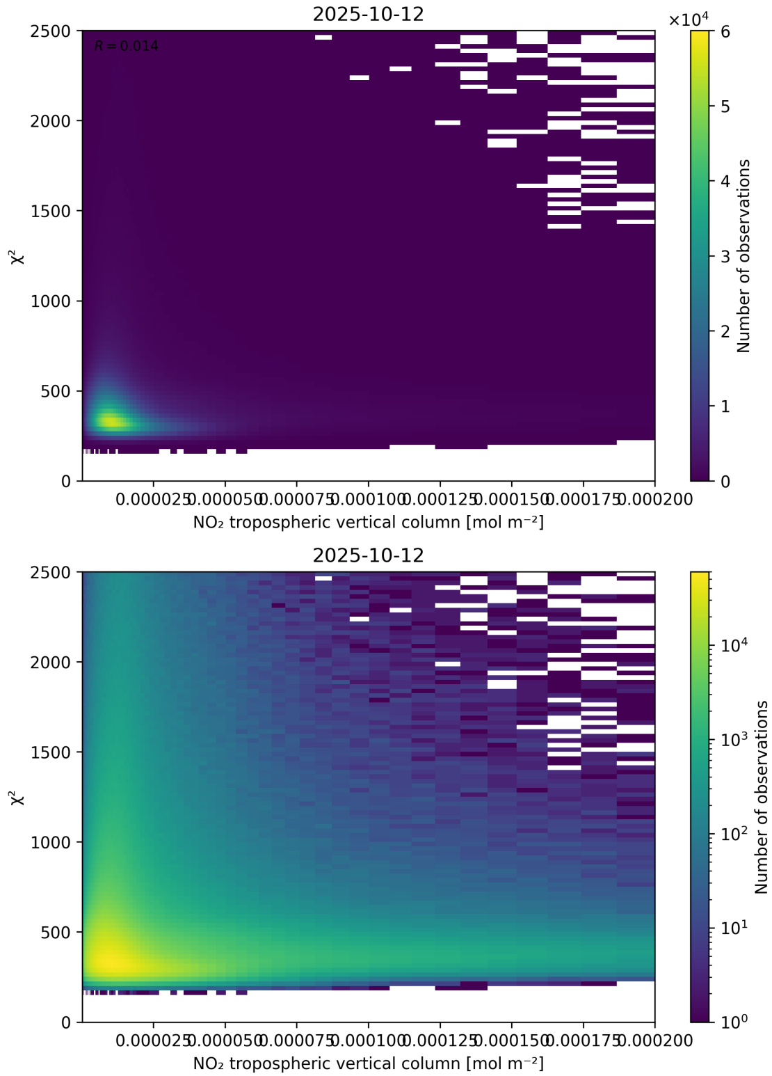
Figure 124: Scatter density plot of “NO 2 tropospheric vertical column” against “ \chi^2 ” for 2025-10-11 to 2025-10-13.
