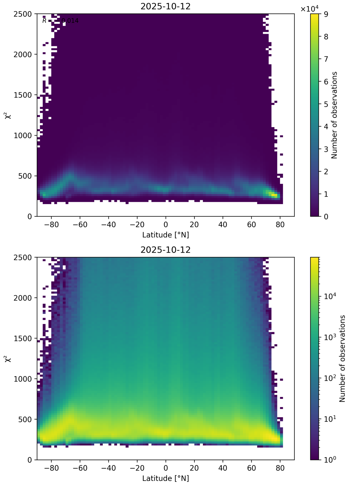
Figure 86: Scatter density plot of “Latitude” against “ \chi^2 ” for 2025-10-11 to 2025-10-13.
