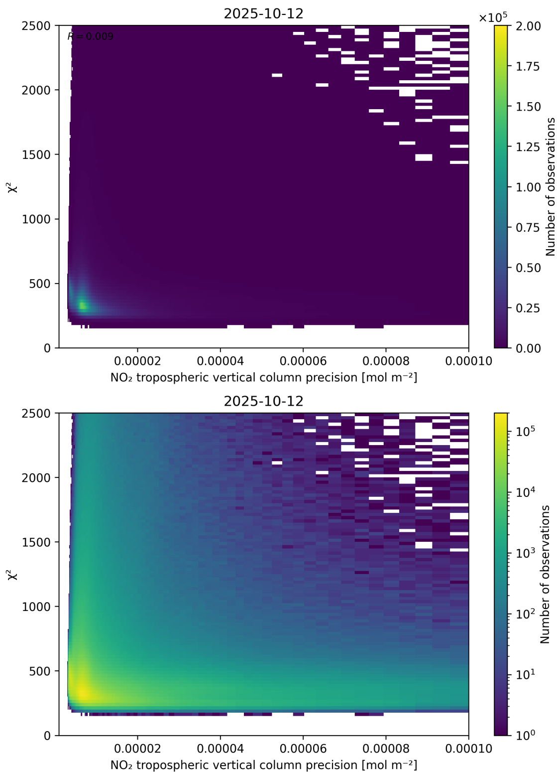
Figure 134: Scatter density plot of “NO 2 tropospheric vertical column precision” against “ \chi^2 ” for 2025-10-11 to 2025-10-13.
