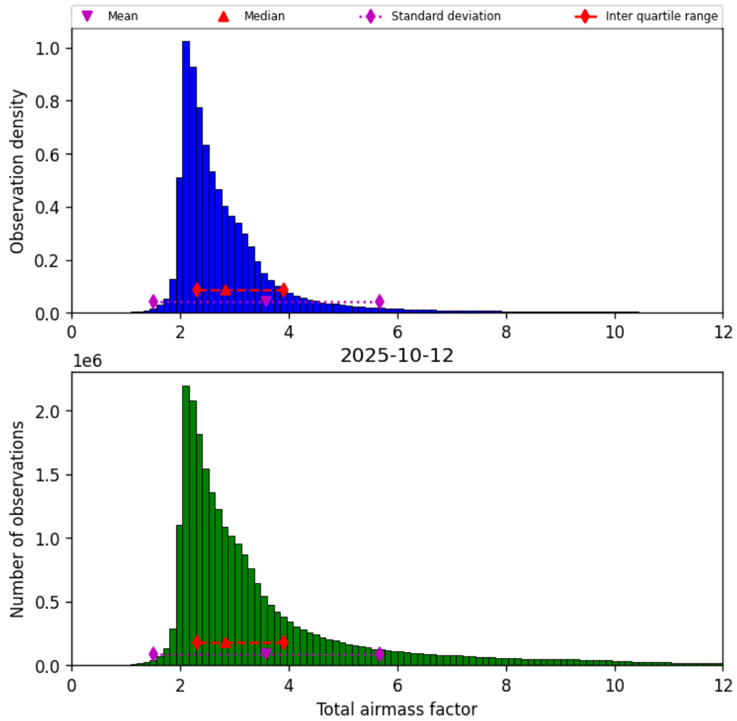
Figure 32: Histogram of “Total airmass factor” for 2025-10-11 to 2025-10-13
