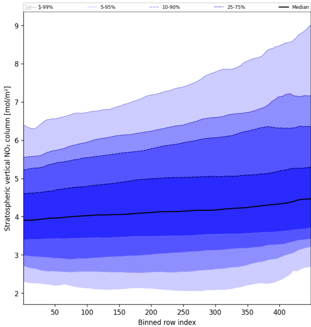
Figure 53: Along track statistics of “Stratospheric vertical NO 2 column” for 2025-10-11 to 2025-10-13
