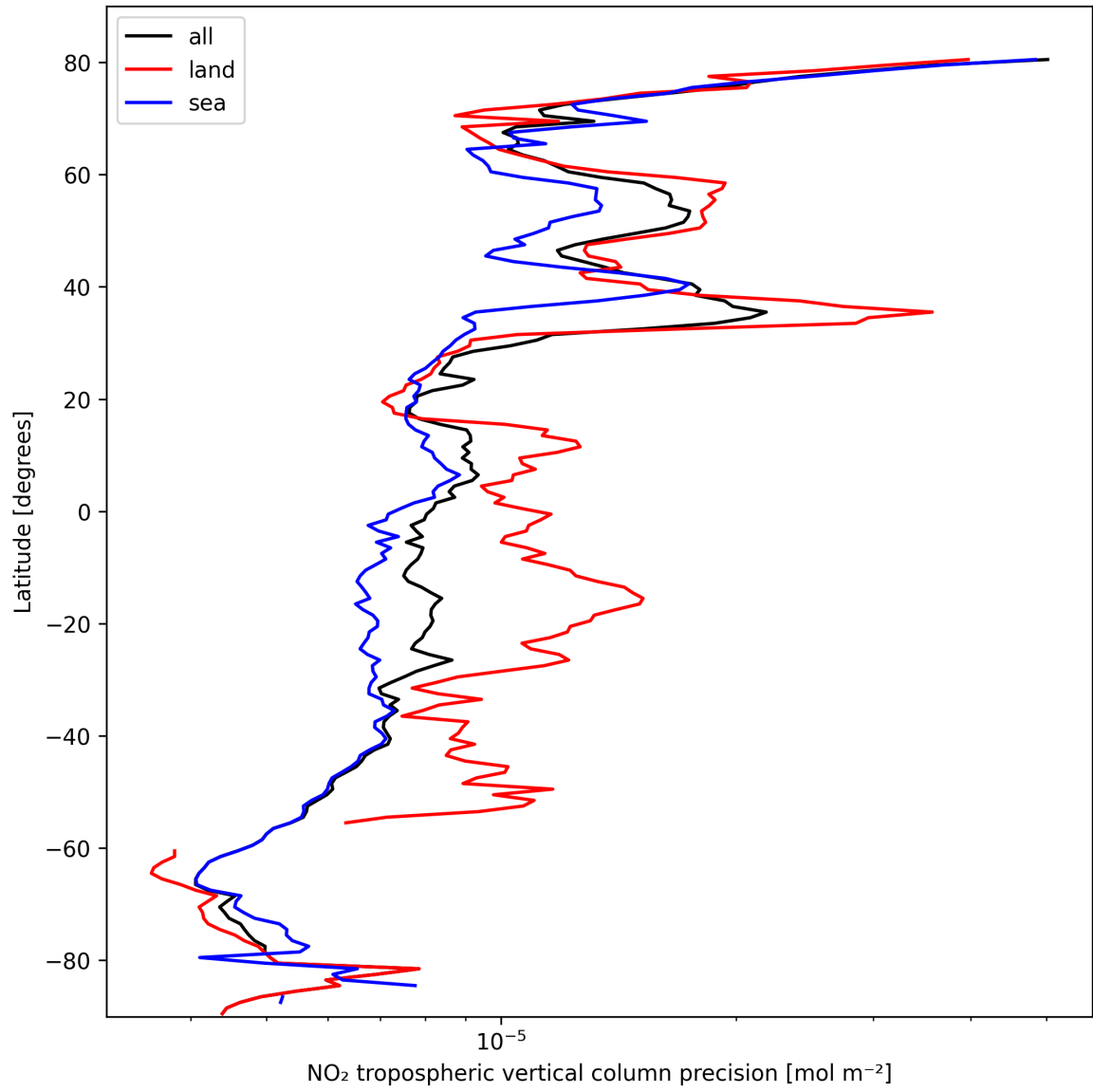
Figure 13: Zonal average of “NO 2 tropospheric vertical column precision” for 2025-10-11 to 2025-10-13.
