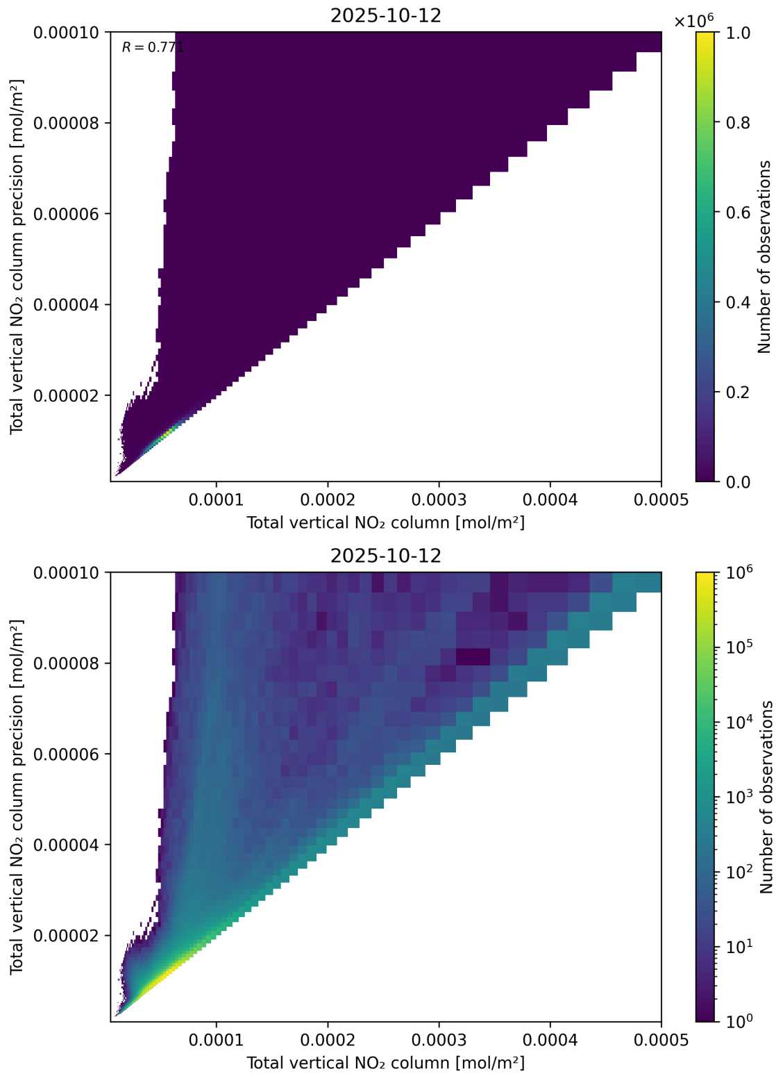
Figure 114: Scatter density plot of “Total vertical NO 2 column” against “Total vertical NO 2 column precision” for 2025-10-11 to 2025-10-13.
