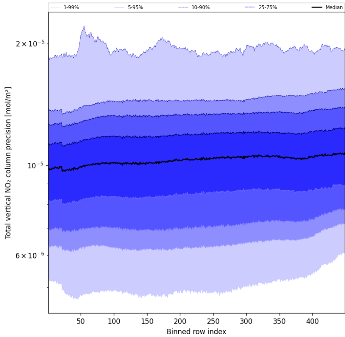
Figure 56: Along track statistics of “Total vertical NO 2 column precision” for 2025-10-11 to 2025-10-13
