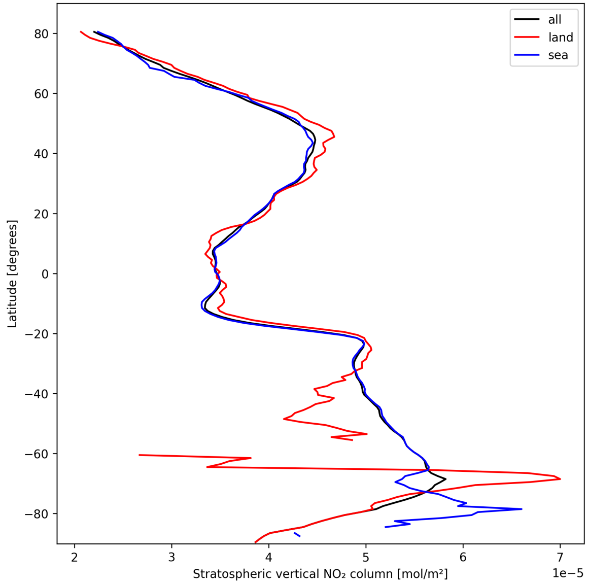
Figure 19: Zonal average of “Stratospheric vertical NO 2 column” for 2025-10-11 to 2025-10-13.
