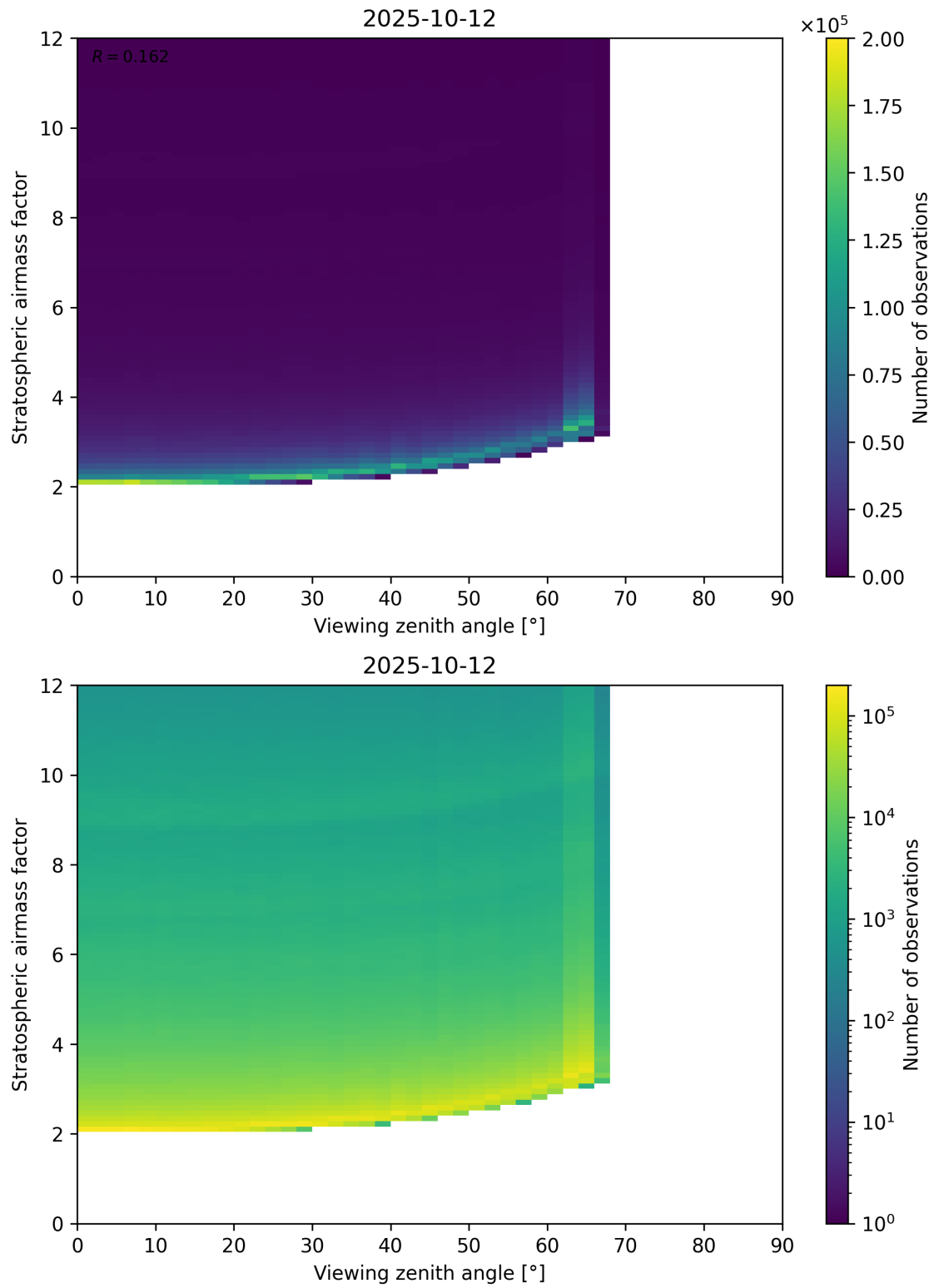
Figure 159: Scatter density plot of “Viewing zenith angle” against “Stratospheric airmass factor” for 2025-10-11 to 2025-10-13.
