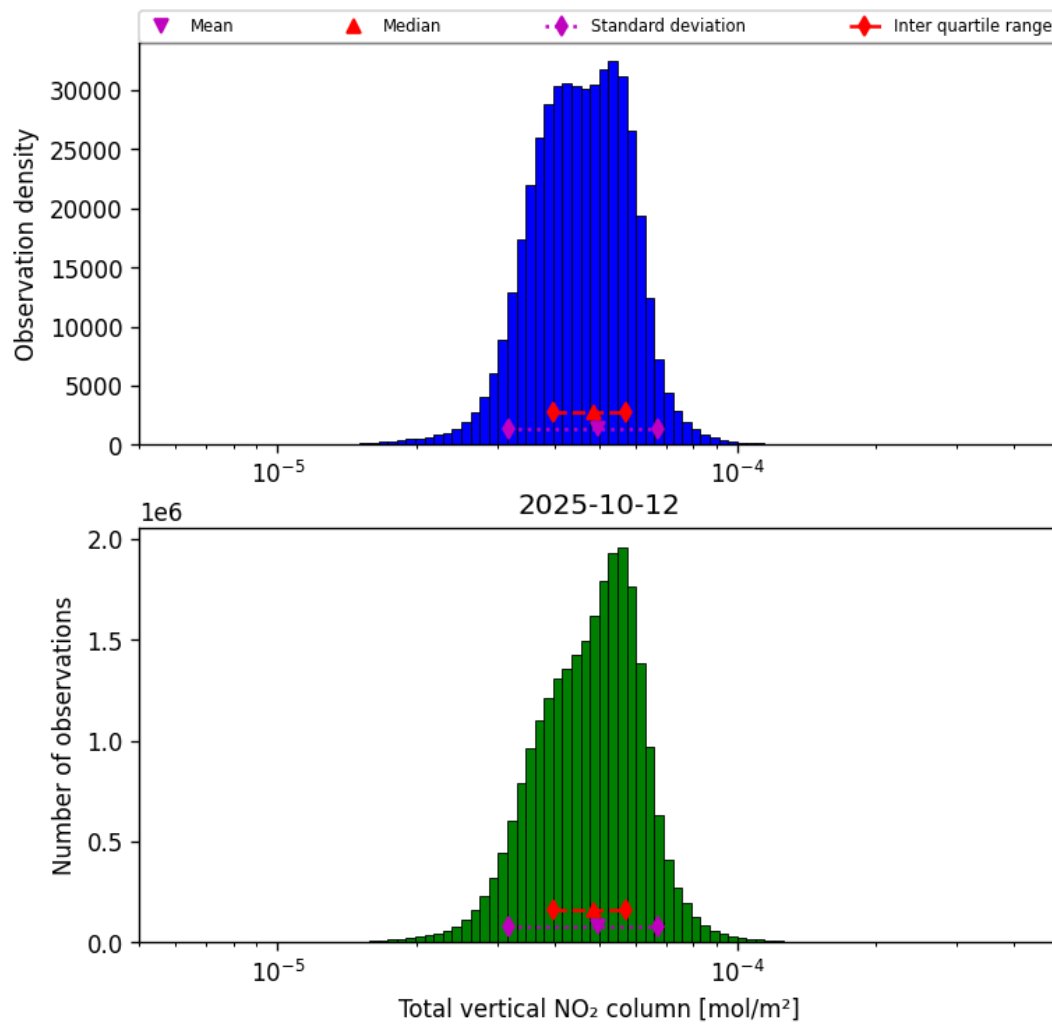
Figure 38: Histogram of "Total vertical NO 2 column" for 2025-10-11 to 2025-10-13
