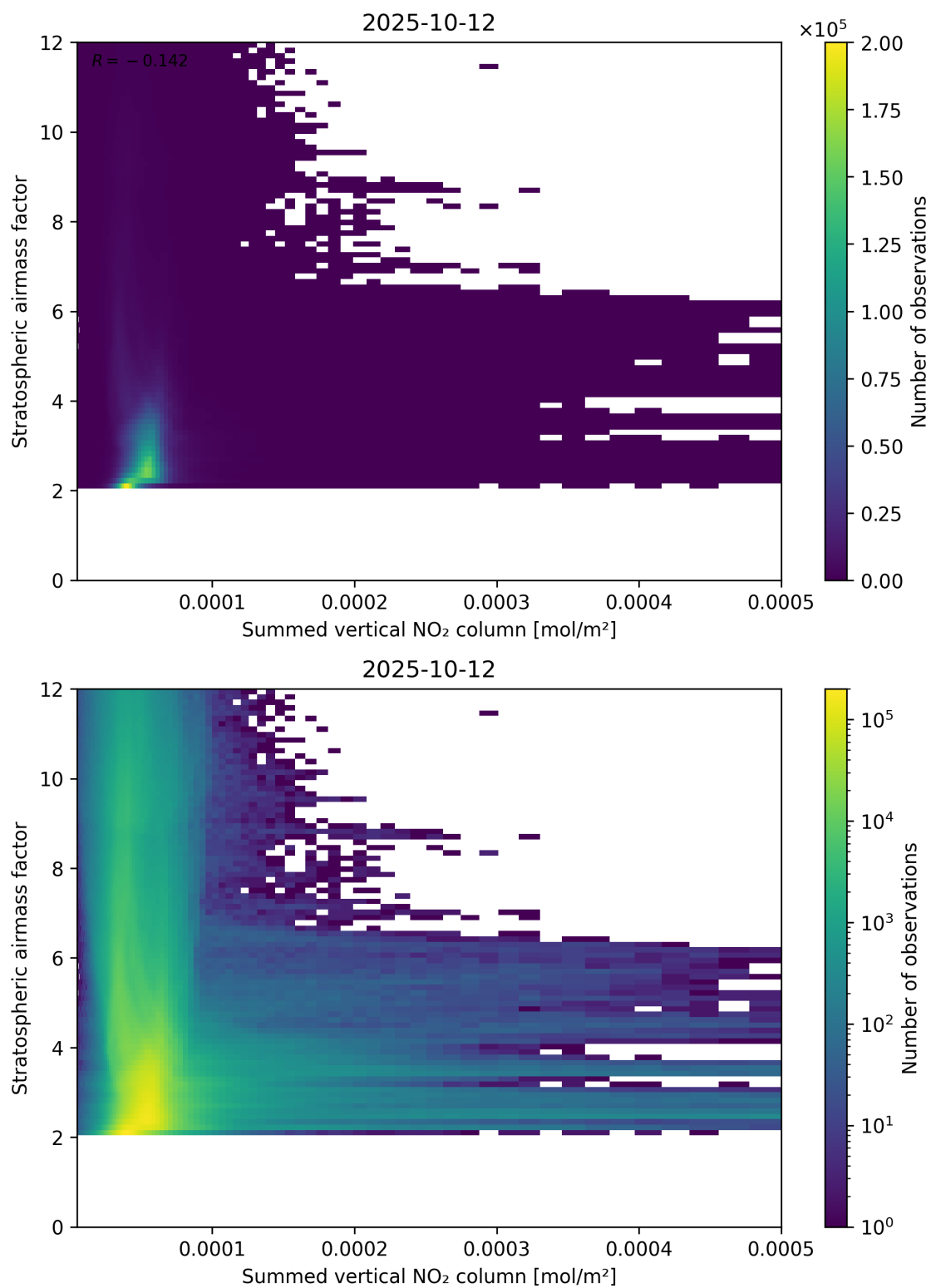
Figure 103: Scatter density plot of “Summed vertical NO 2 column” against “Stratospheric airmass factor” for 2025-10-11 to 2025-10-13.
