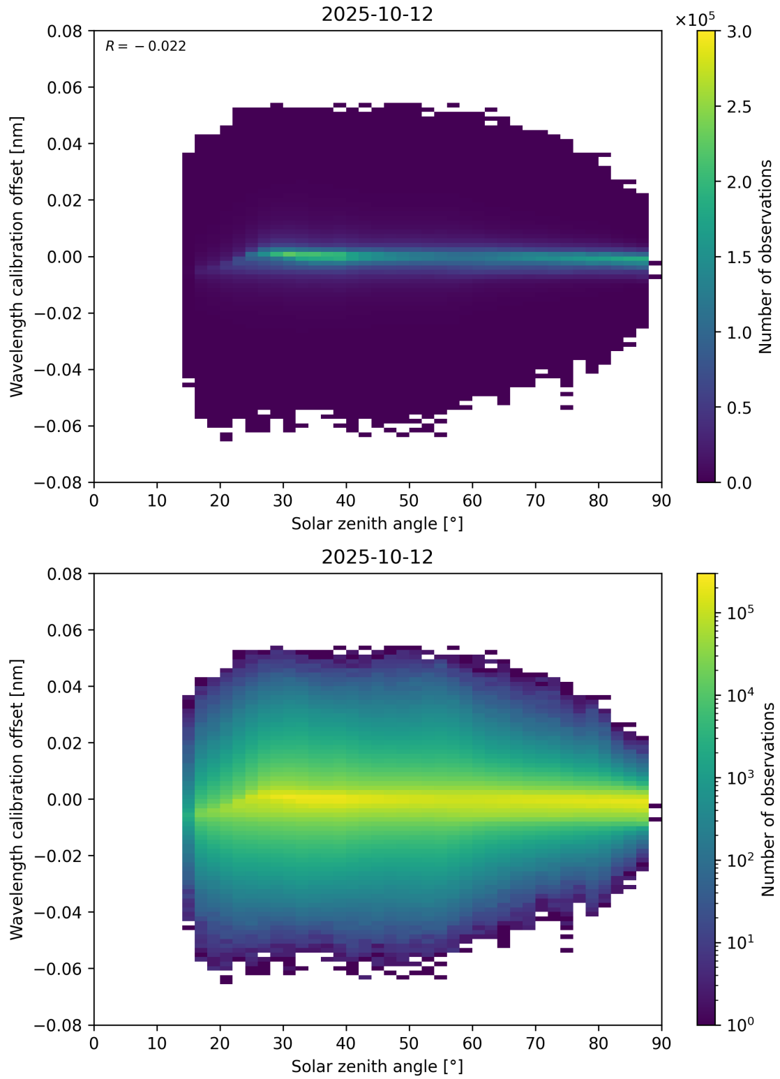
Figure 158: Scatter density plot of “Solar zenith angle” against “Wavelength calibration offset” for 2025-10-11 to 2025-10-13.
