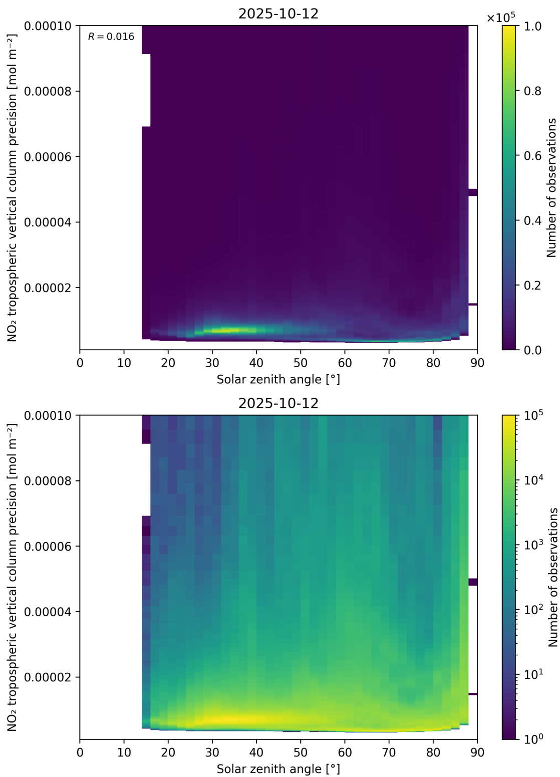
Figure 156: Scatter density plot of “Solar zenith angle” against “NO 2 tropospheric vertical column precision” for 2025-10-11 to 2025-10-13.
