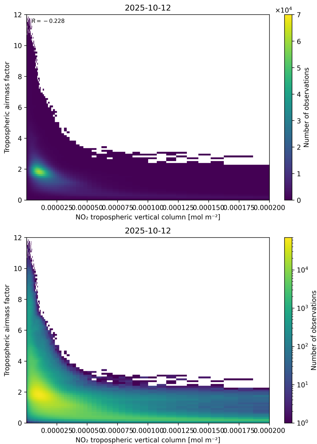
Figure 123: Scatter density plot of “NO 2 tropospheric vertical column” against “Tropospheric air mass factor” for 2025-10-11 to 2025-10-13.
