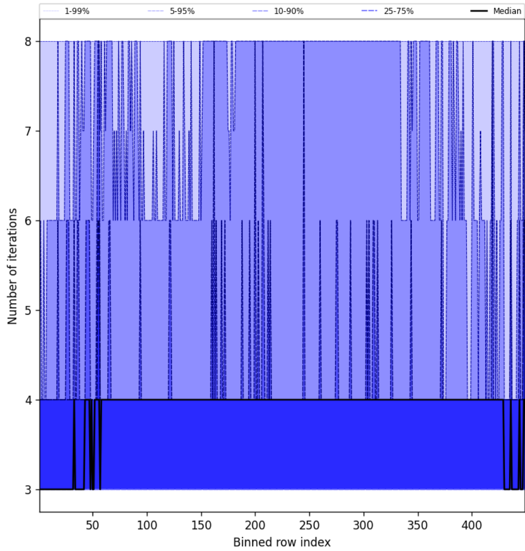
Figure 51: Along track statistics of “Number of iterations” for 2025-10-11 to 2025-10-13
