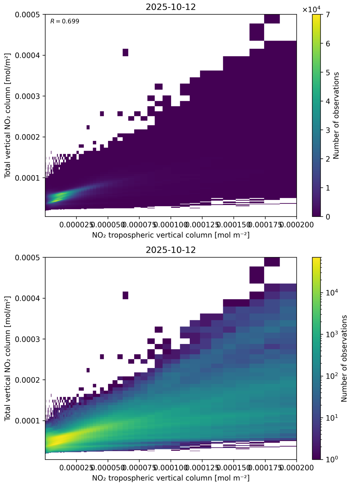
Figure 128: Scatter density plot of “NO 2 tropospheric vertical column” against “Total vertical NO 2 column” for 2025-10-11 to 2025-10-13.
