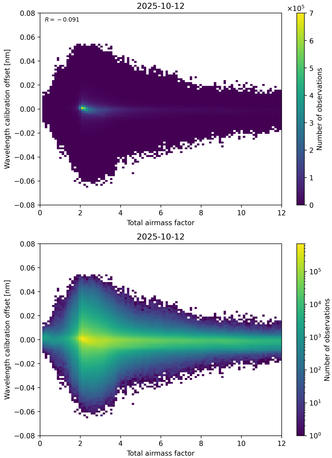
Figure 70: Scatter density plot of “Total airmass factor” against “Wavelength calibration offset” for 2025-10-11 to 2025-10-13.
