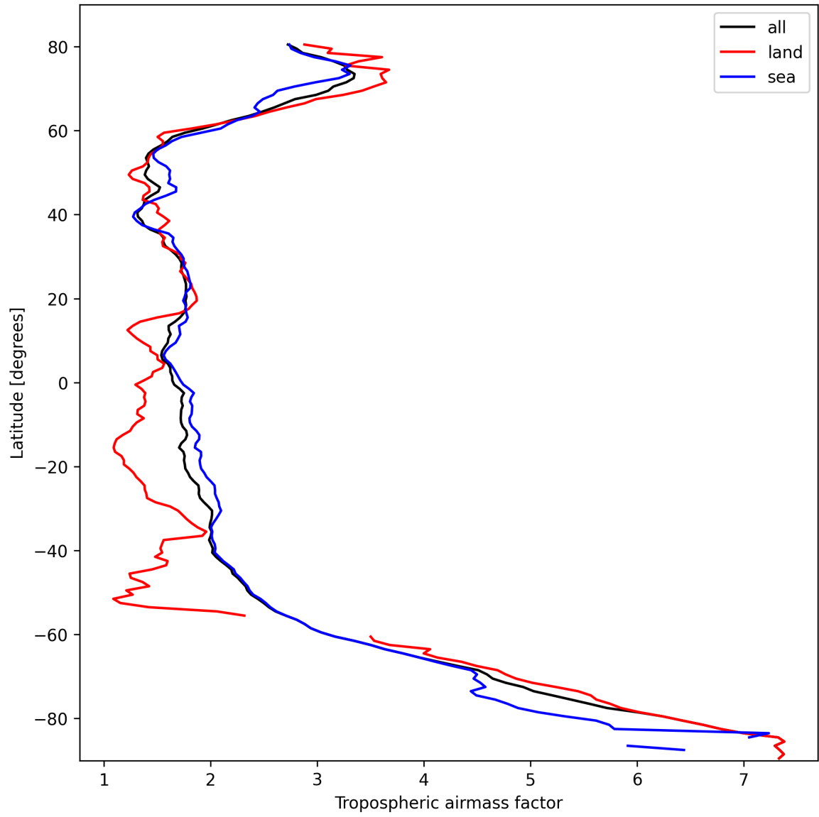
Figure 14: Zonal average of “Tropospheric airmass factor” for 2025-10-11 to 2025-10-13.
