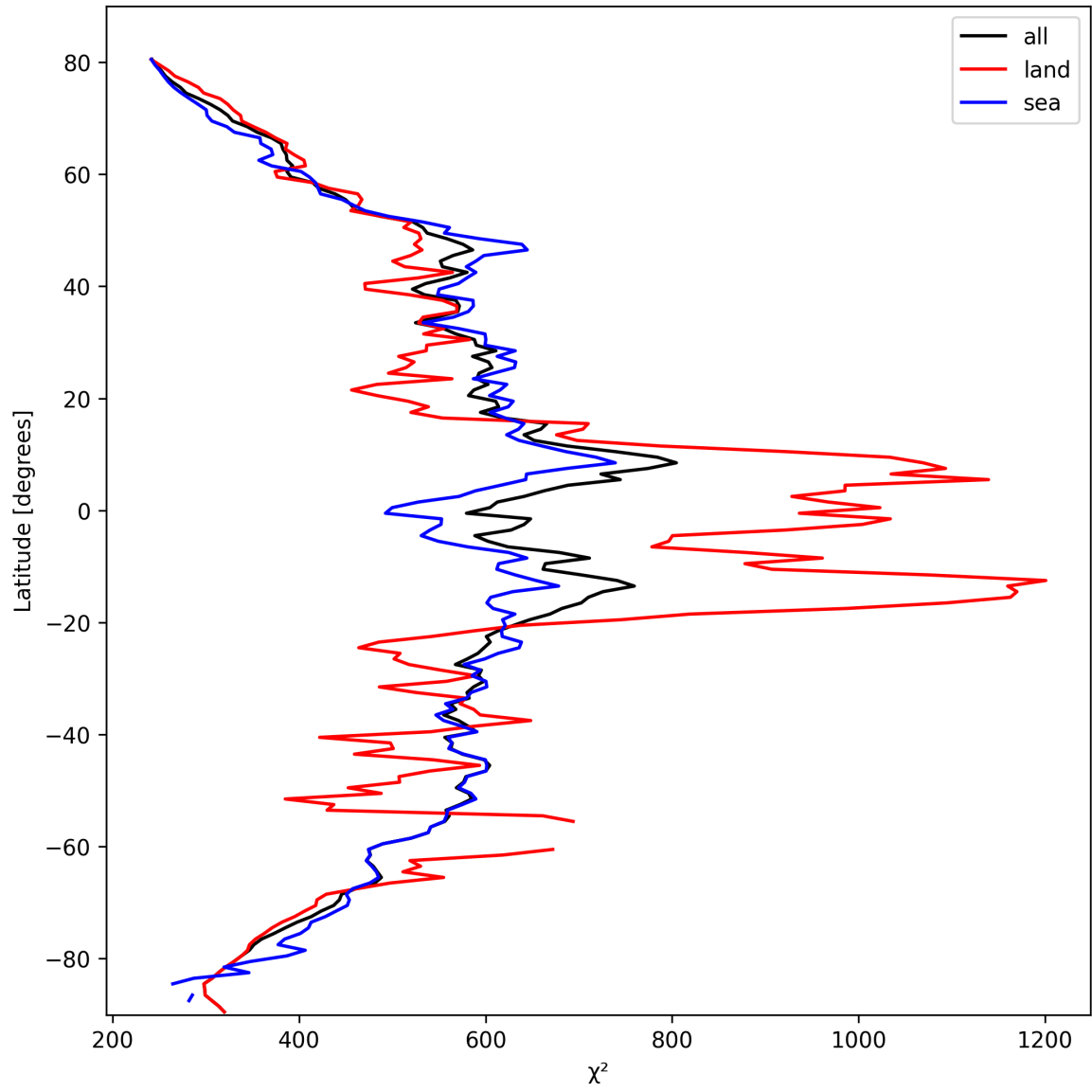
Figure 25: Zonal average of “ \chi^2 ” for 2025-10-11 to 2025-10-13.
