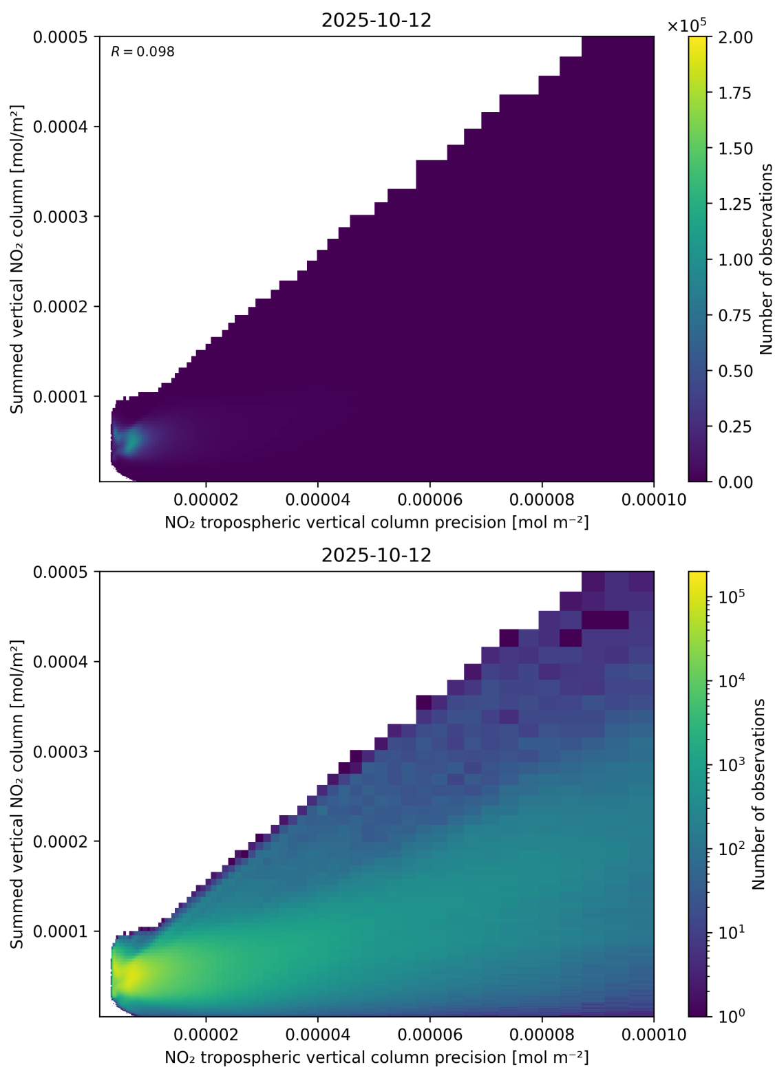
Figure 136: Scatter density plot of “NO 2 tropospheric vertical column precision” against “Summed vertical NO 2 column” for 2025-10-11 to 2025-10-13.
