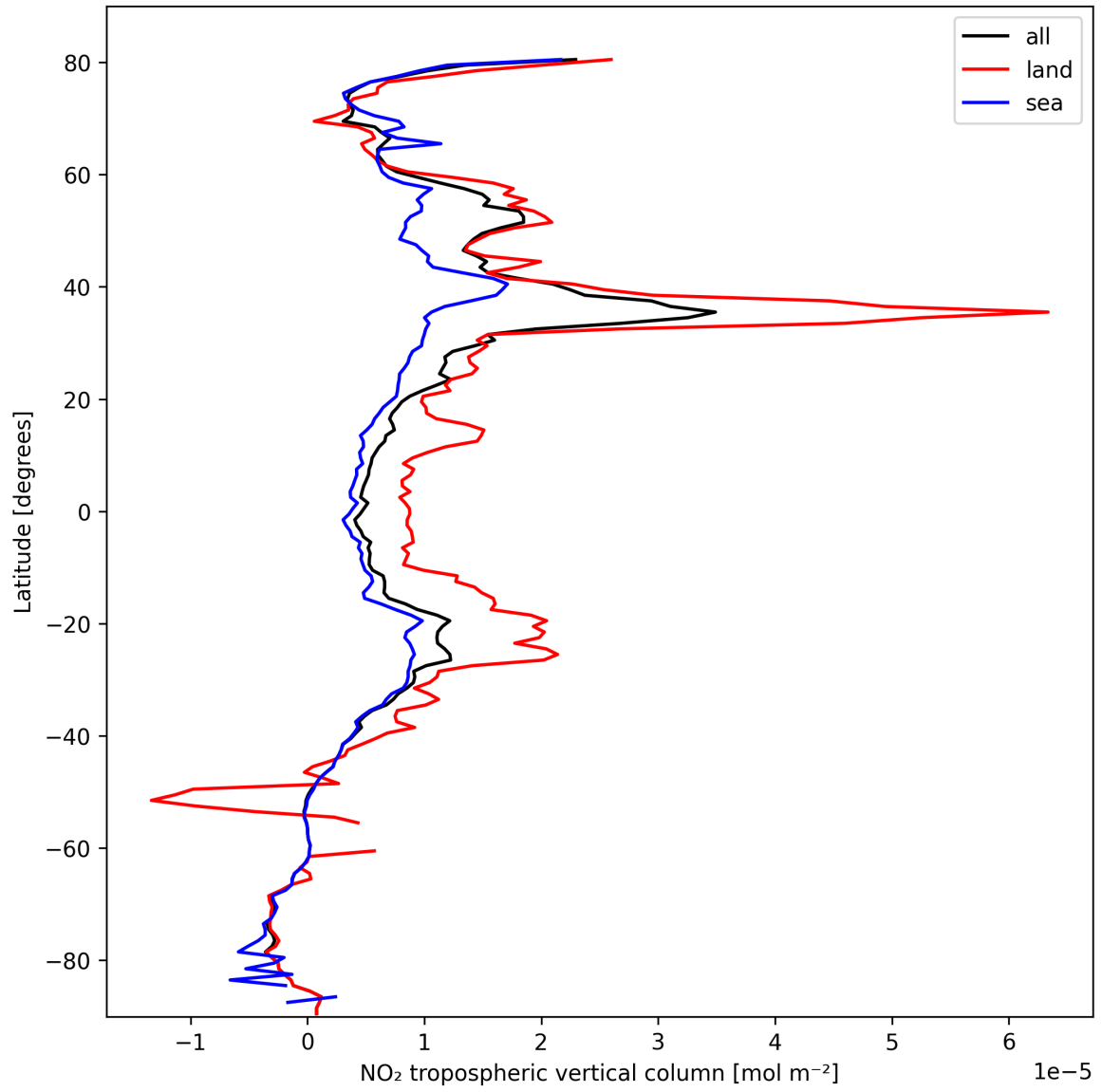
Figure 12: Zonal average of “NO 2 tropospheric vertical column” for 2025-10-11 to 2025-10-13.
