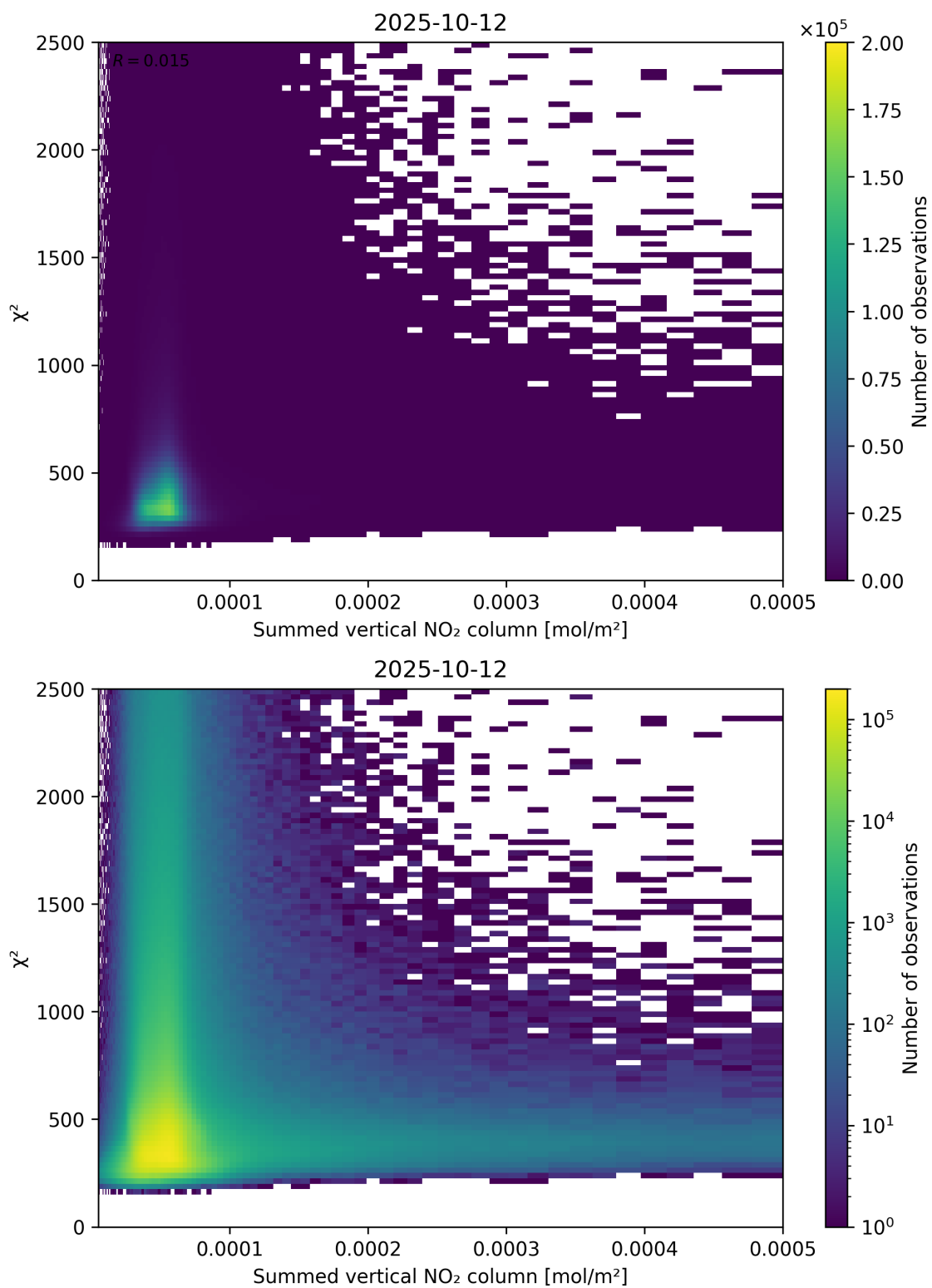
Figure 104: Scatter density plot of “Summed vertical NO 2 column” against “ \chi^2 ” for 2025-10-11 to 2025-10-13.
