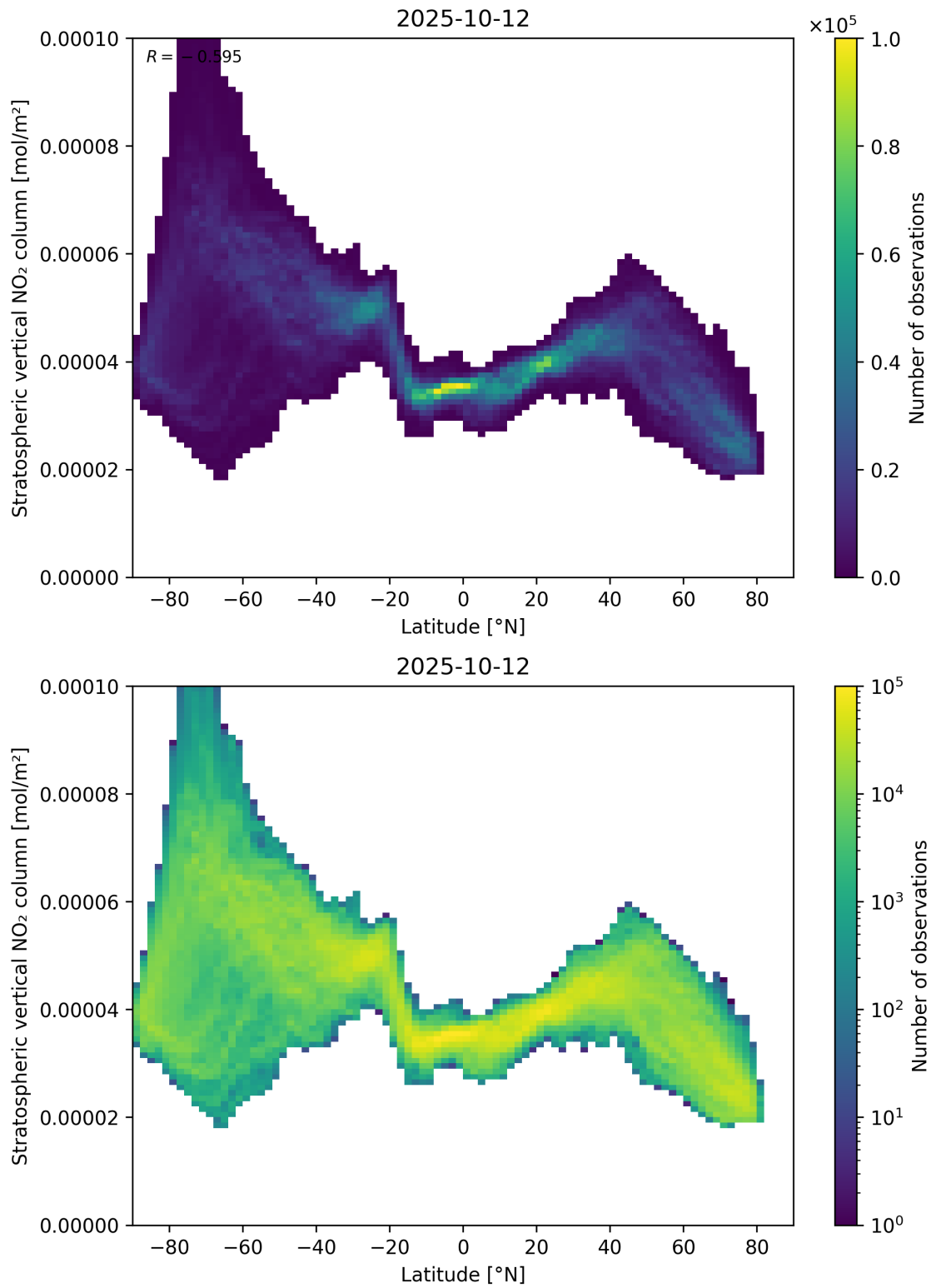
Figure 87: Scatter density plot of “Latitude” against “Stratospheric vertical \text{NO}_2 column” for 2025-10-11 to 2025-10-13.
