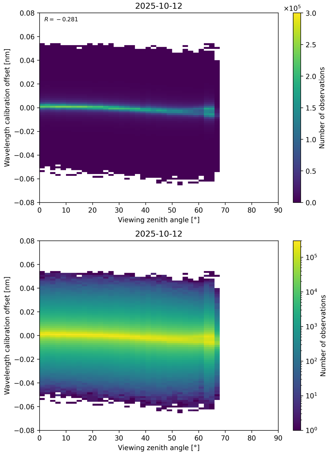
Figure 173: Scatter density plot of “Viewing zenith angle” against “Wavelength calibration offset” for 2025-10-11 to 2025-10-13.
