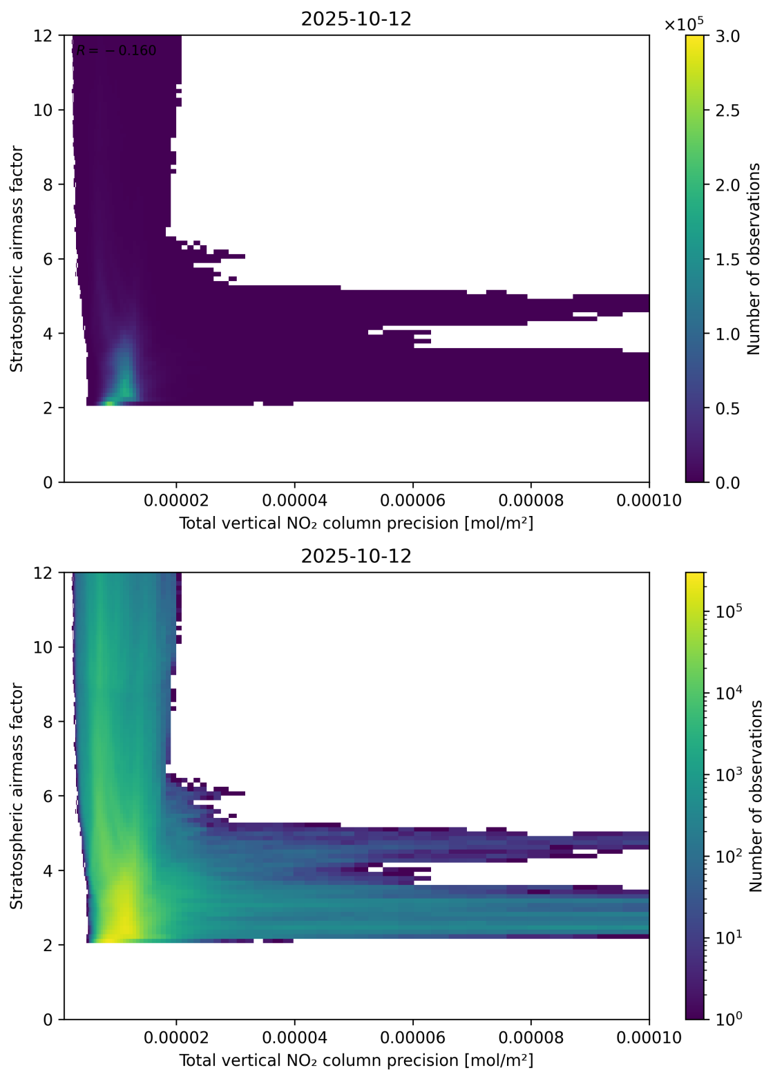
Figure 115: Scatter density plot of “Total vertical NO 2 column precision” against “Stratospheric air mass factor” for 2025-10-11 to 2025-10-13.
