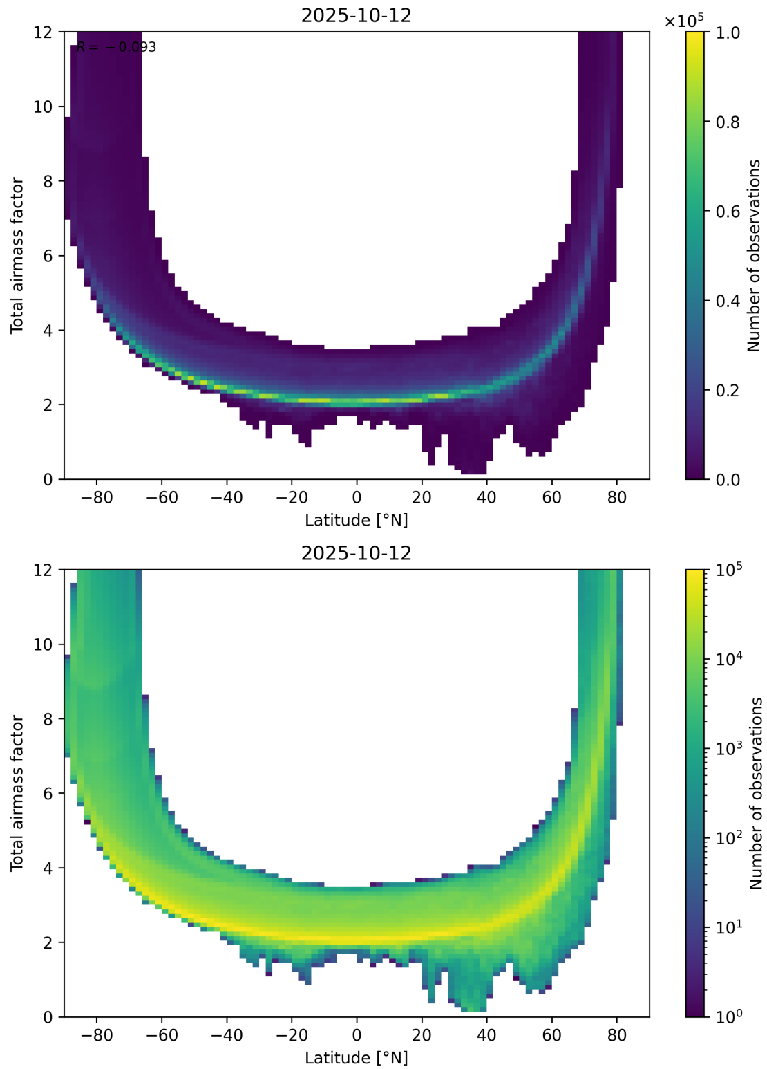
Figure 84: Scatter density plot of “Latitude” against “Total airmass factor” for 2025-10-11 to 2025-10-13.
