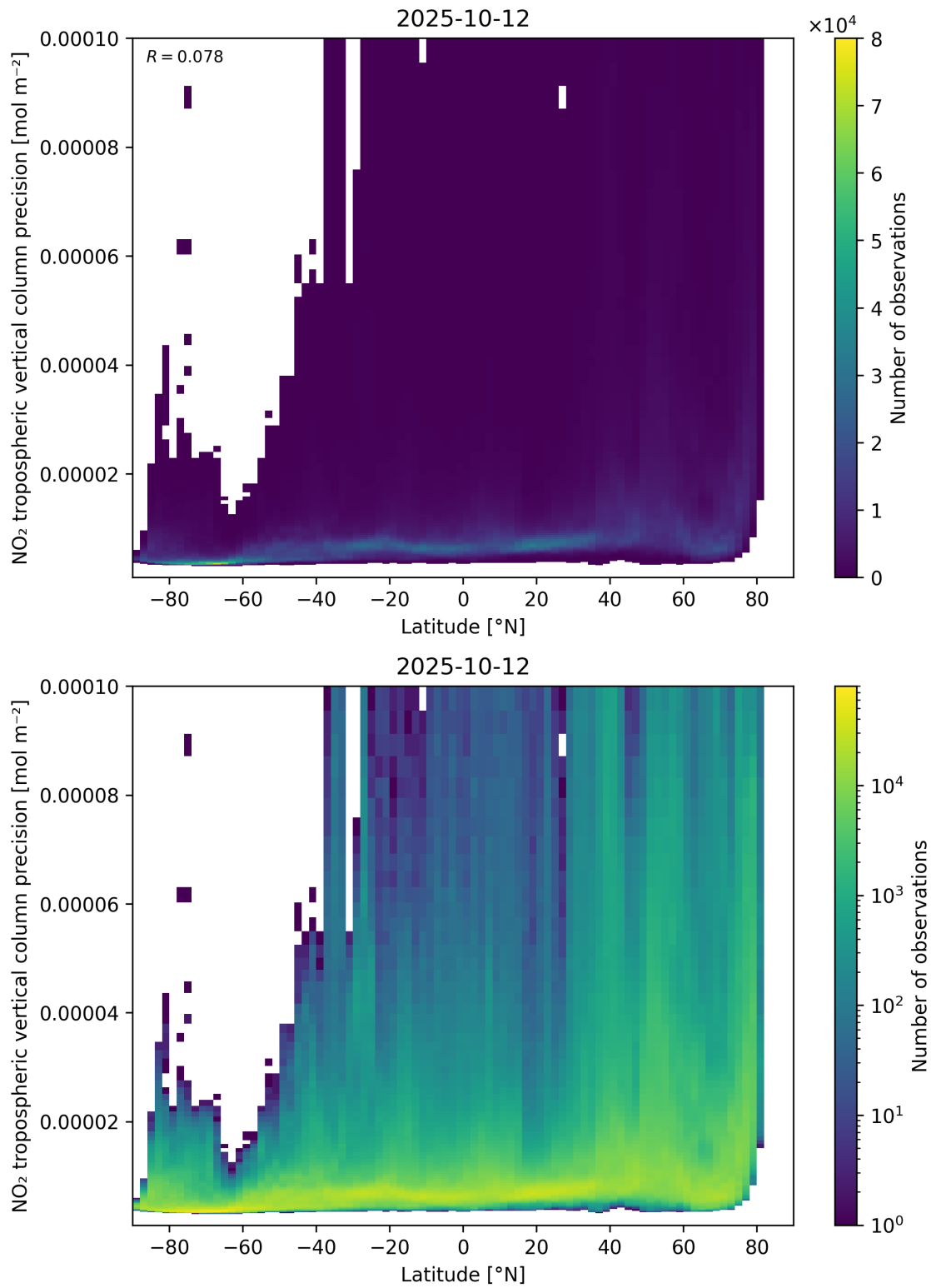
Figure 93: Scatter density plot of “Latitude” against “NO 2 tropospheric vertical column precision” for 2025-10-11 to 2025-10-13.
