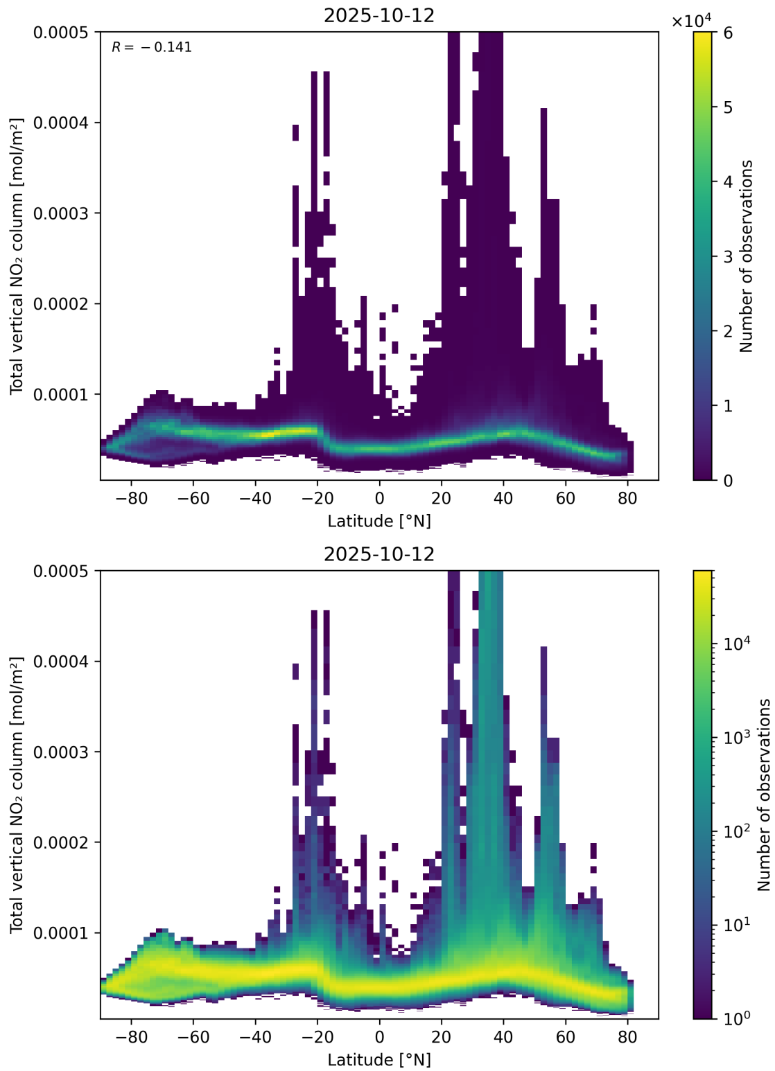
Figure 90: Scatter density plot of “Latitude” against “Total vertical NO 2 column” for 2025-10-11 to 2025-10-13.
