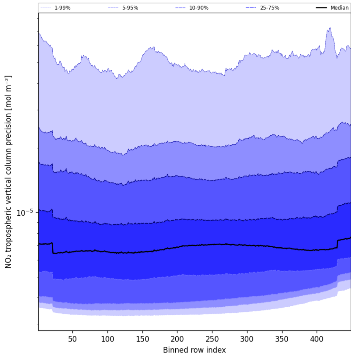
Figure 47: Along track statistics of “NO 2 tropospheric vertical column precision” for 2025-10-11 to 2025-10-13
