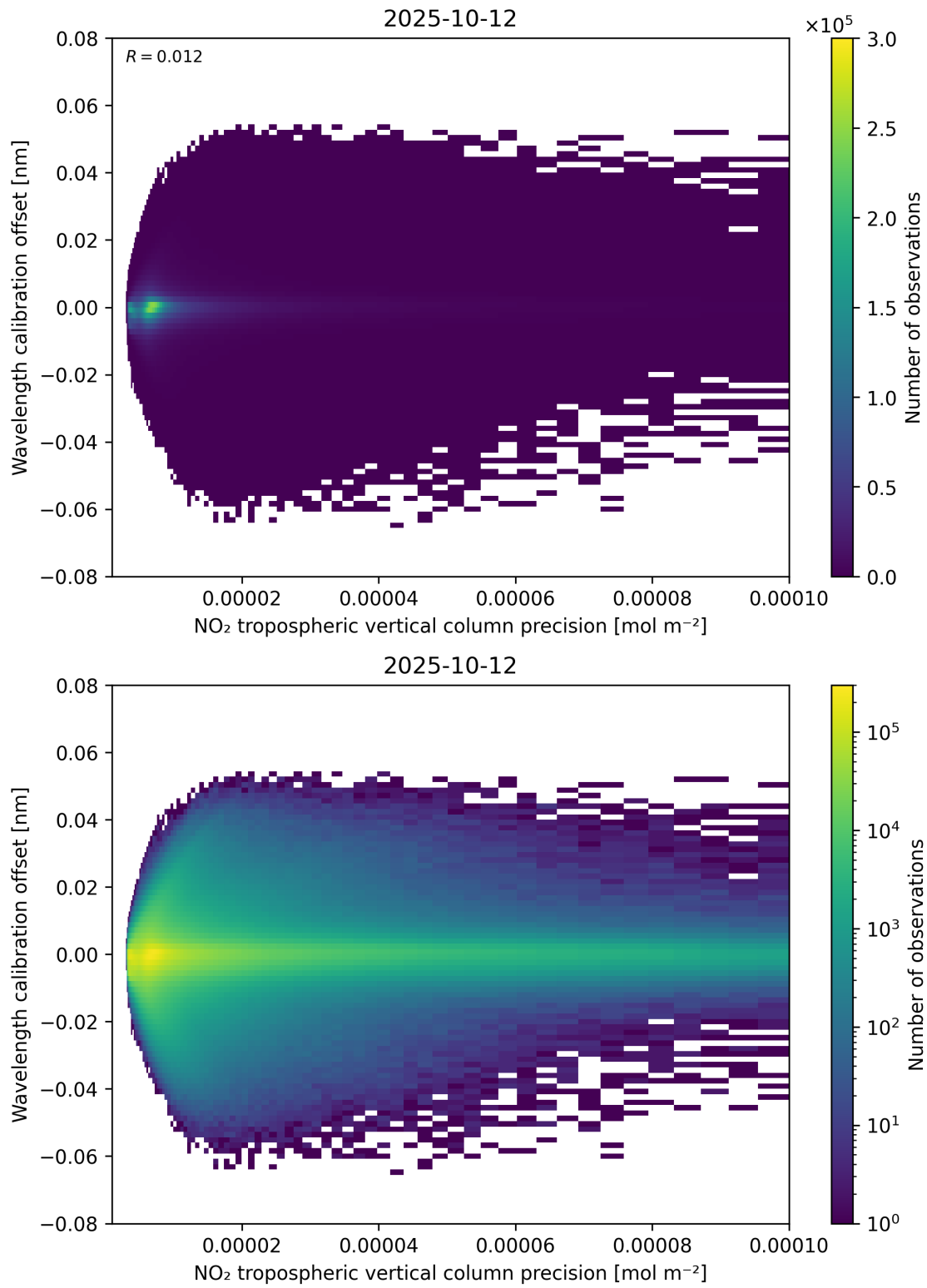
Figure 141: Scatter density plot of “NO 2 tropospheric vertical column precision” against “Wavelength calibration offset” for 2025-10-11 to 2025-10-13.
