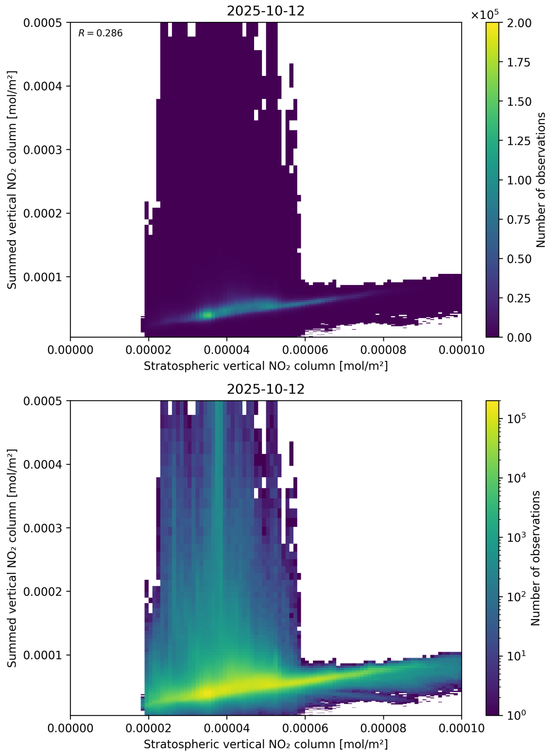
Figure 98: Scatter density plot of “Stratospheric vertical NO 2 column” against “Summed vertical NO 2 column” for 2025-10-11 to 2025-10-13.
