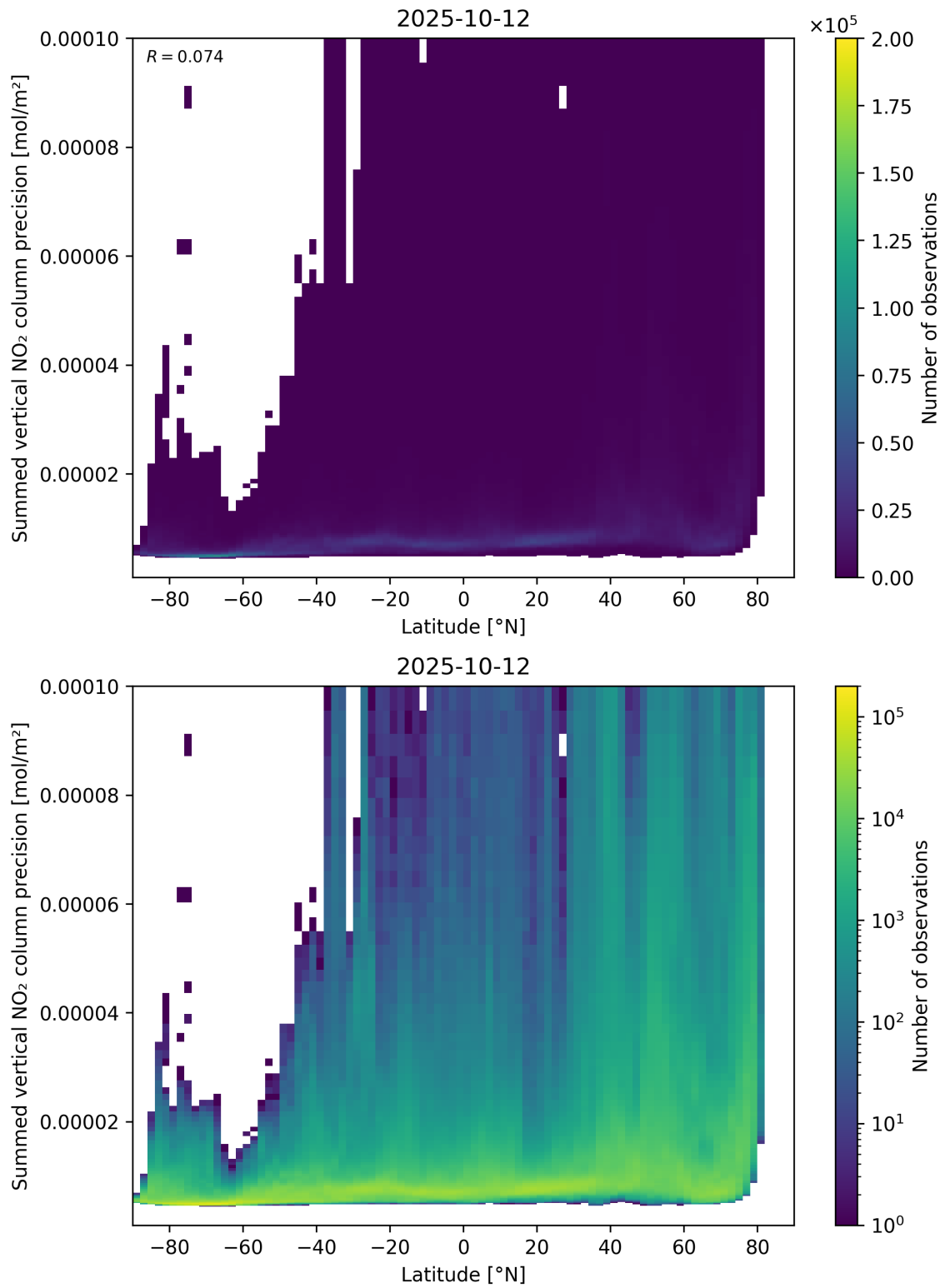
Figure 89: Scatter density plot of “Latitude” against “Summed vertical NO 2 column precision” for 2025-10-11 to 2025-10-13.
