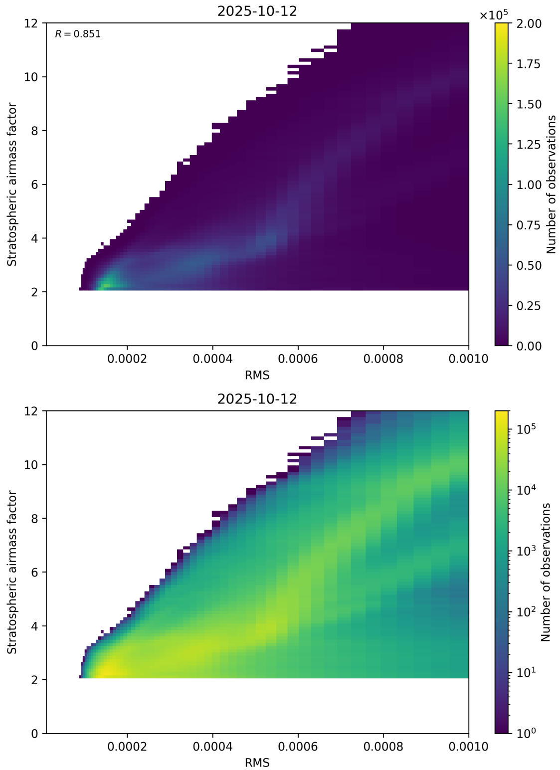
Figure 144: Scatter density plot of “RMS” against “Stratospheric airmass factor” for 2025-10-11 to 2025-10-13.
