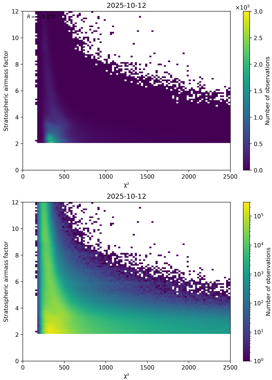
Figure 81: Scatter density plot of “ \chi^2 ” against “Stratospheric airmass factor” for 2025-10-11 to 2025-10-13.
