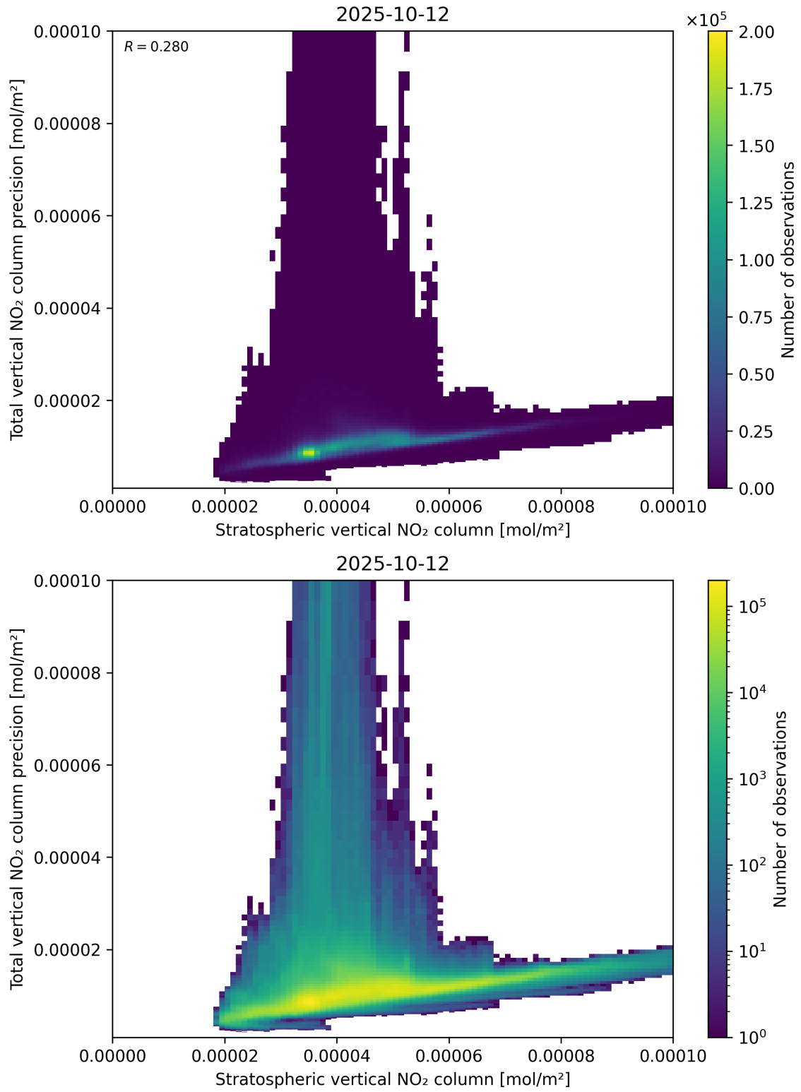
Figure 101: Scatter density plot of “Stratospheric vertical NO 2 column” against “Total vertical NO 2 column precision” for 2025-10-11 to 2025-10-13.
