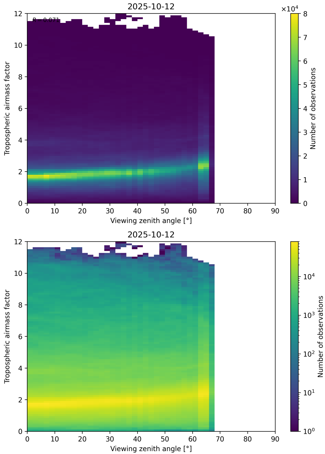
Figure 161: Scatter density plot of “Viewing zenith angle” against “Tropospheric airmass factor” for 2025-10-11 to 2025-10-13.
