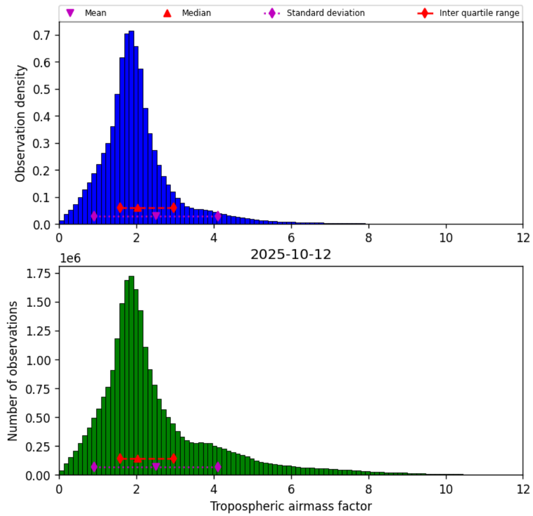
Figure 31: Histogram of “Tropospheric airmass factor” for 2025-10-11 to 2025-10-13
