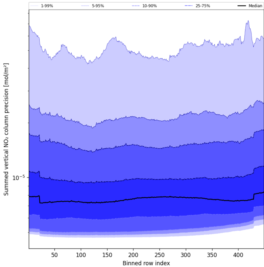
Figure 58: Along track statistics of “Summed vertical NO 2 column precision” for 2025-10-11 to 2025-10-13
