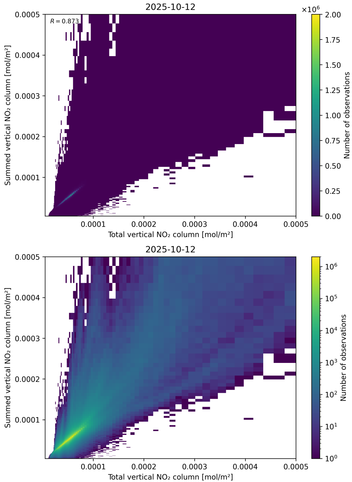
Figure 112: Scatter density plot of “Total vertical NO 2 column” against “Summed vertical NO 2 column” for 2025-10-11 to 2025-10-13.
