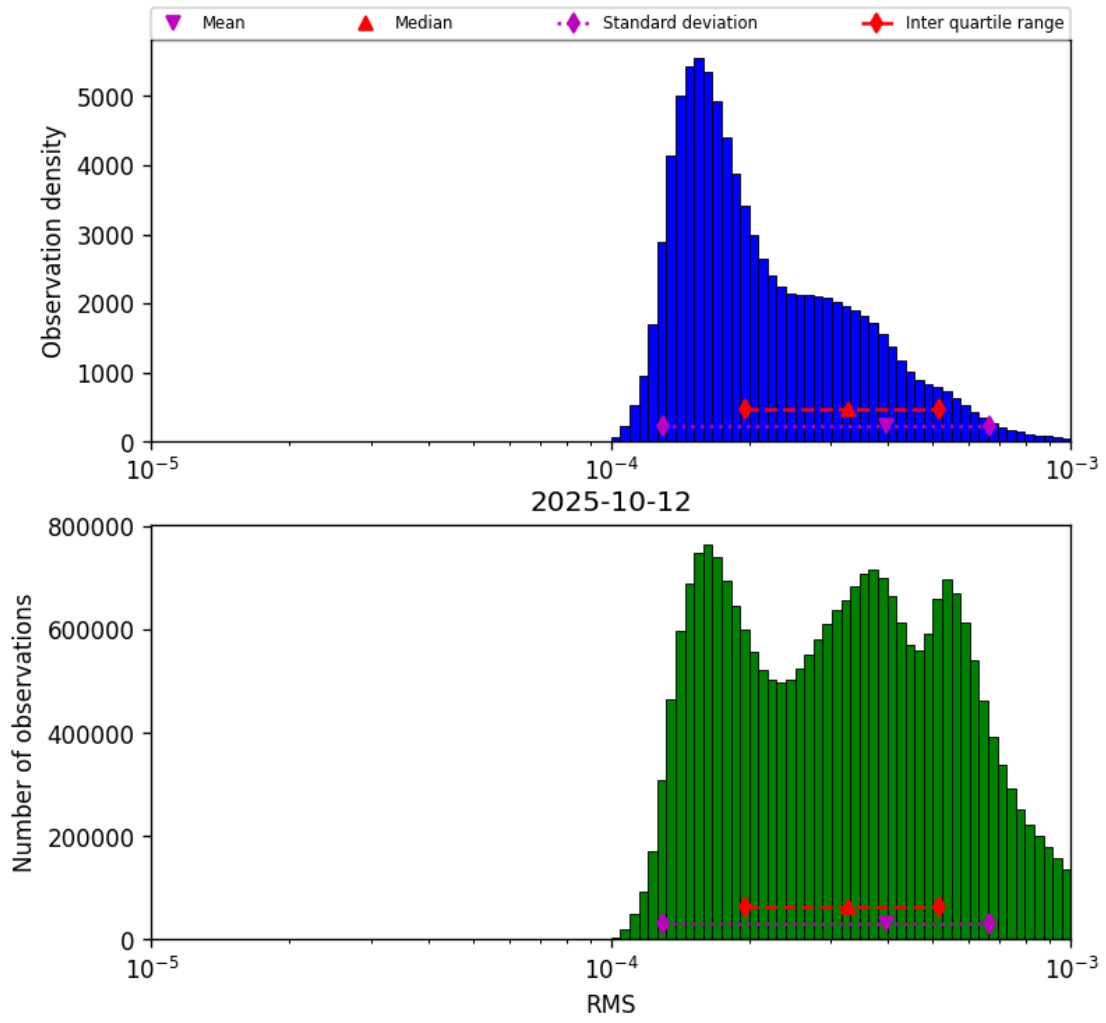
Figure 43: Histogram of “RMS” for 2025-10-11 to 2025-10-13
