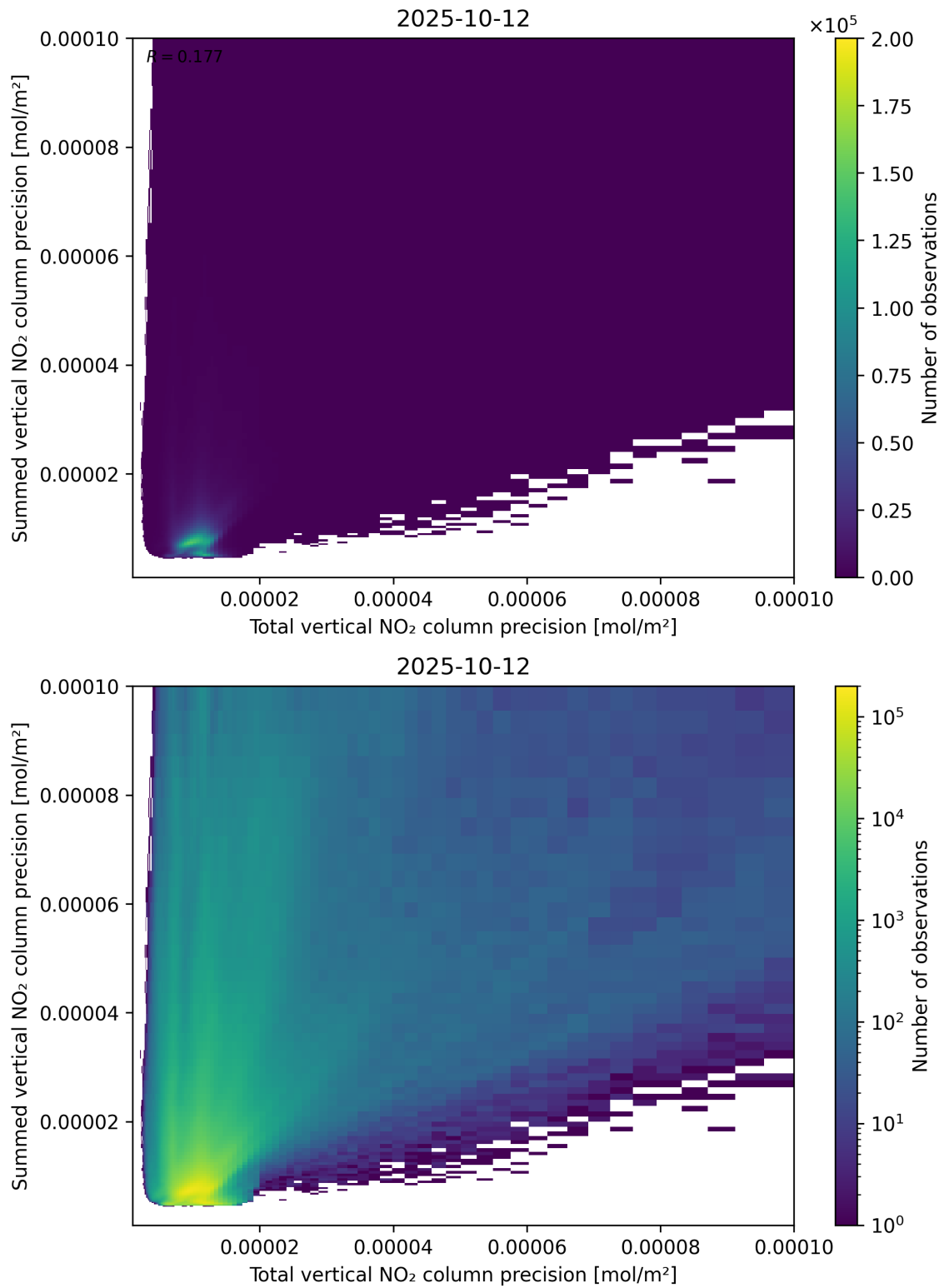
Figure 118: Scatter density plot of “Total vertical NO 2 column precision” against “Summed vertical NO 2 column precision” for 2025-10-11 to 2025-10-13.
