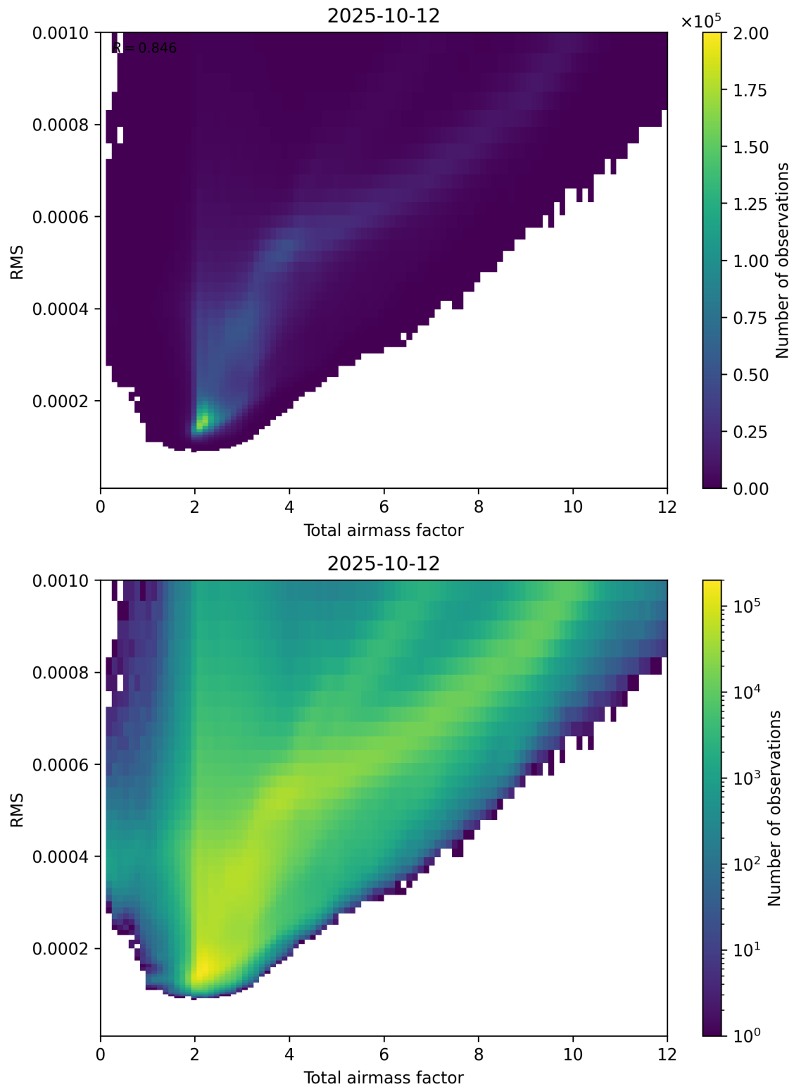
Figure 69: Scatter density plot of “Total airmass factor” against “RMS” for 2025-10-11 to 2025-10-13.
