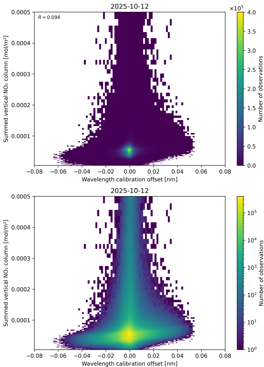
Figure 177: Scatter density plot of “Wavelength calibration offset” against “Summed vertical NO 2 column” for 2025-10-11 to 2025-10-13.
