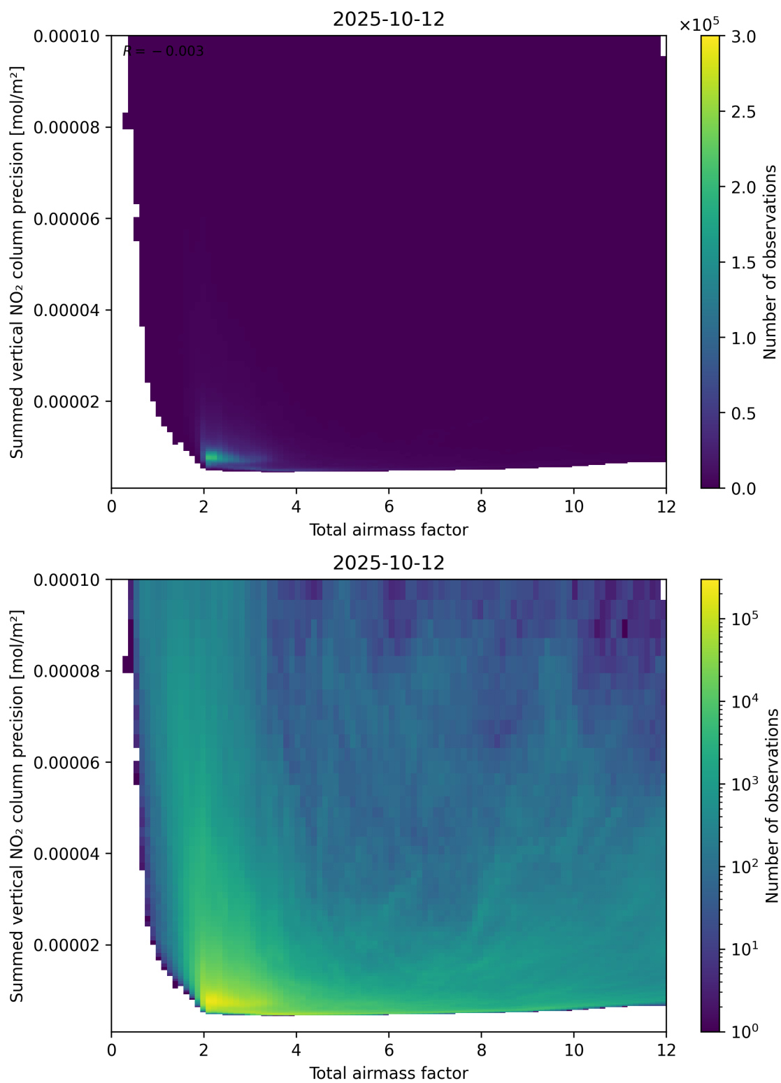
Figure 66: Scatter density plot of “Total airmass factor” against “Summed vertical NO 2 column precision” for 2025-10-11 to 2025-10-13.
