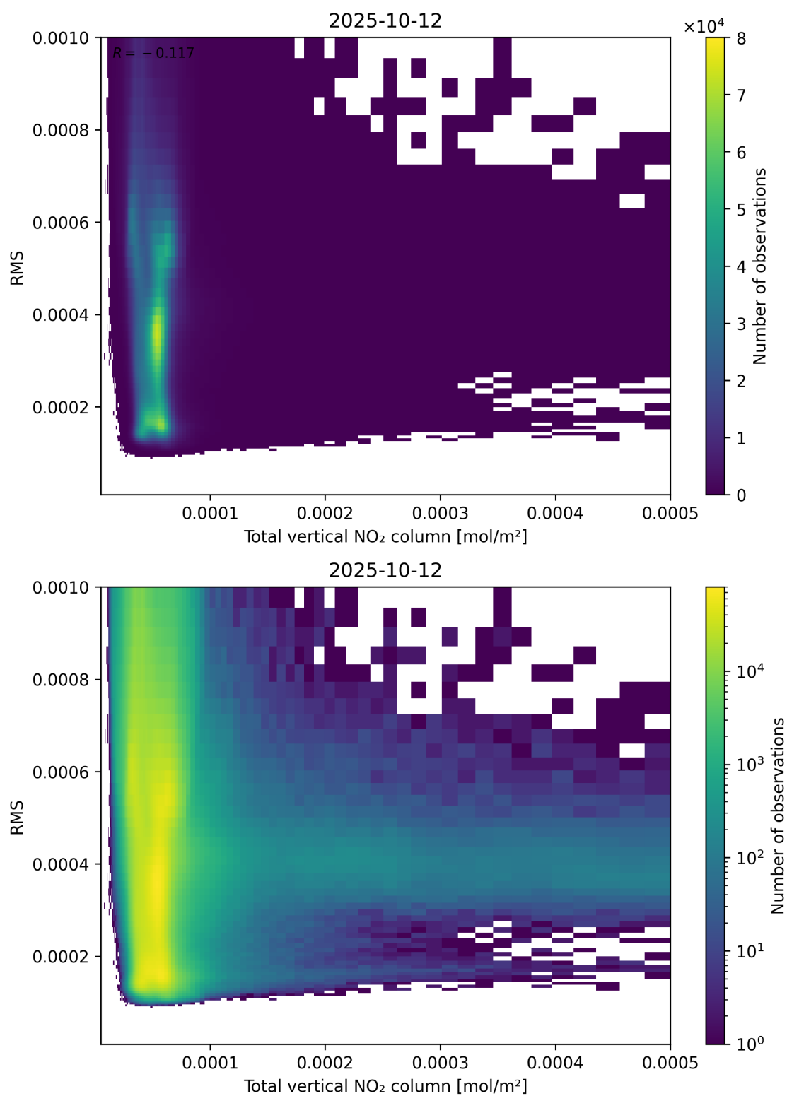
Figure 120: Scatter density plot of “Total vertical NO 2 column” against “RMS” for 2025-10-11 to 2025-10-13.
