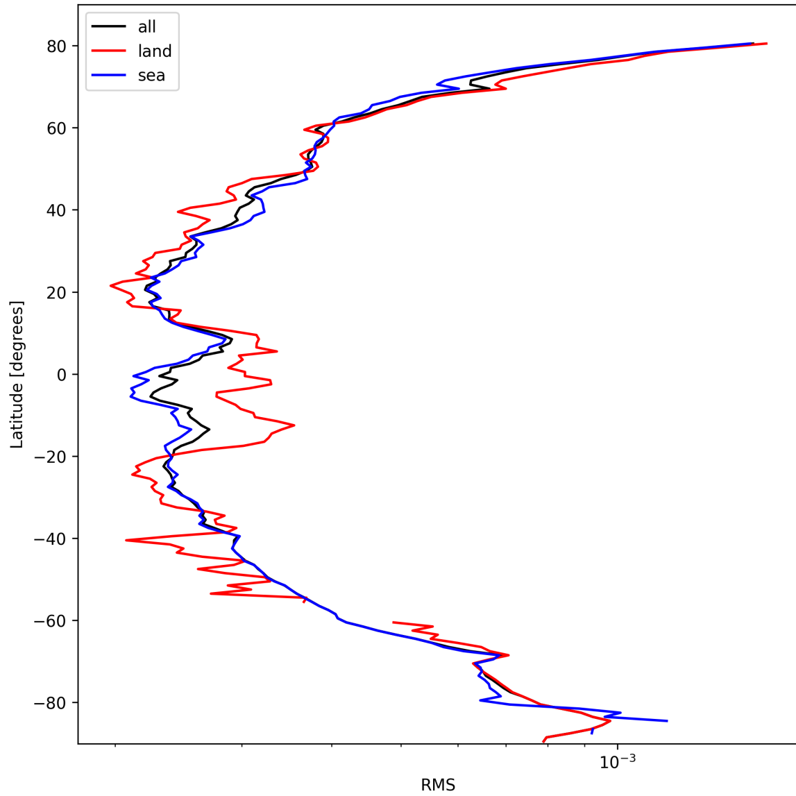
Figure 26: Zonal average of “RMS” for 2025-10-11 to 2025-10-13.
