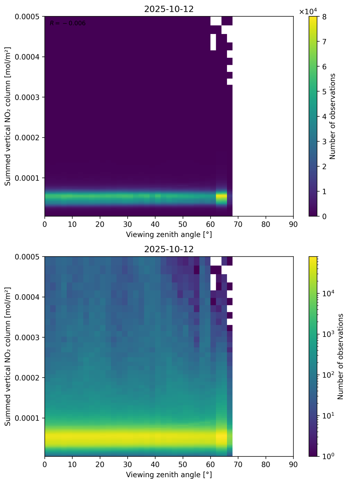
Figure 165: Scatter density plot of “Viewing zenith angle” against “Summed vertical NO 2 column” for 2025-10-11 to 2025-10-13.
