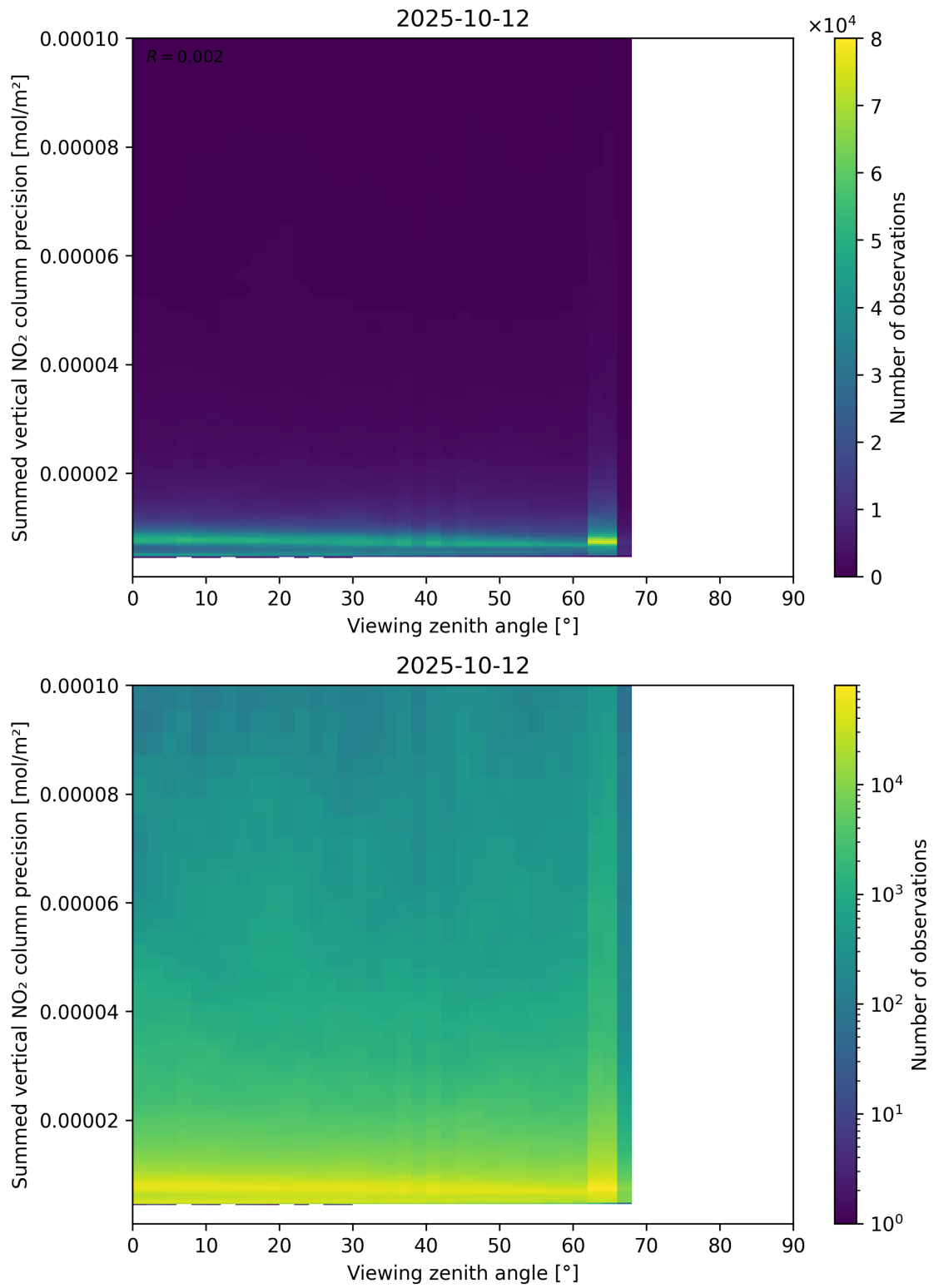
Figure 166: Scatter density plot of “Viewing zenith angle” against “Summed vertical NO 2 column precision” for 2025-10-11 to 2025-10-13.
