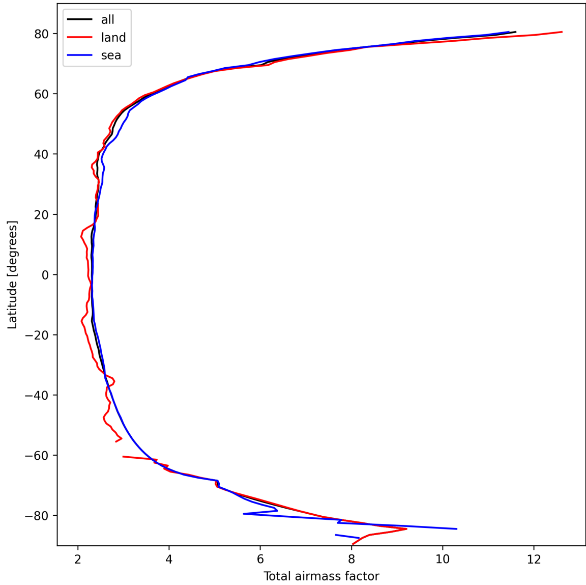
Figure 15: Zonal average of “Total airmass factor” for 2025-10-11 to 2025-10-13.
