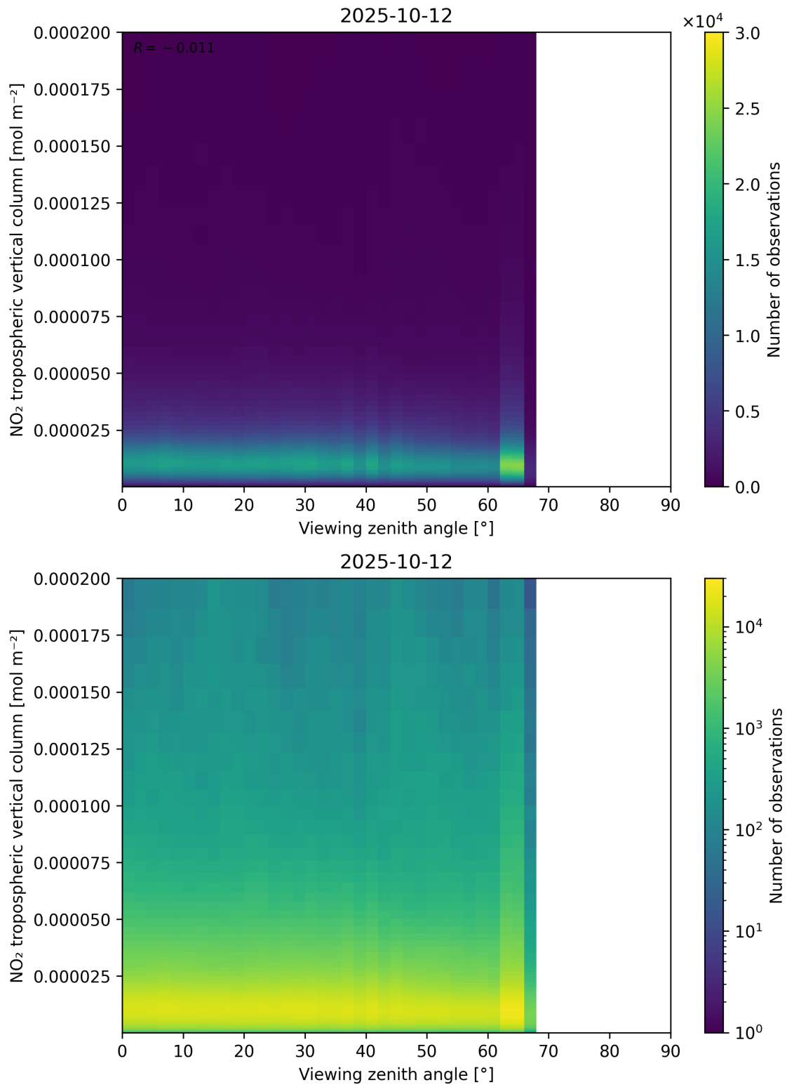
Figure 169: Scatter density plot of “Viewing zenith angle” against “NO 2 tropospheric vertical column” for 2025-10-11 to 2025-10-13.
