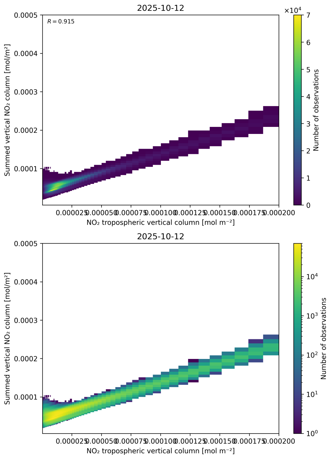
Figure 126: Scatter density plot of “NO 2 tropospheric vertical column” against “Summed vertical NO 2 column” for 2025-10-11 to 2025-10-13.
