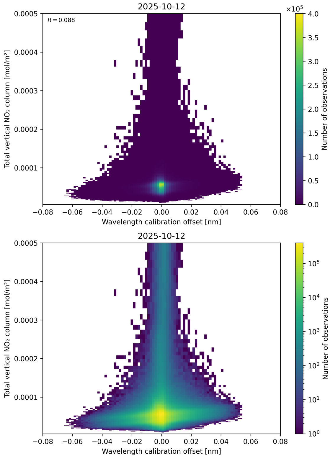
Figure 179: Scatter density plot of “Wavelength calibration offset” against “Total vertical NO 2 column” for 2025-10-11 to 2025-10-13.
