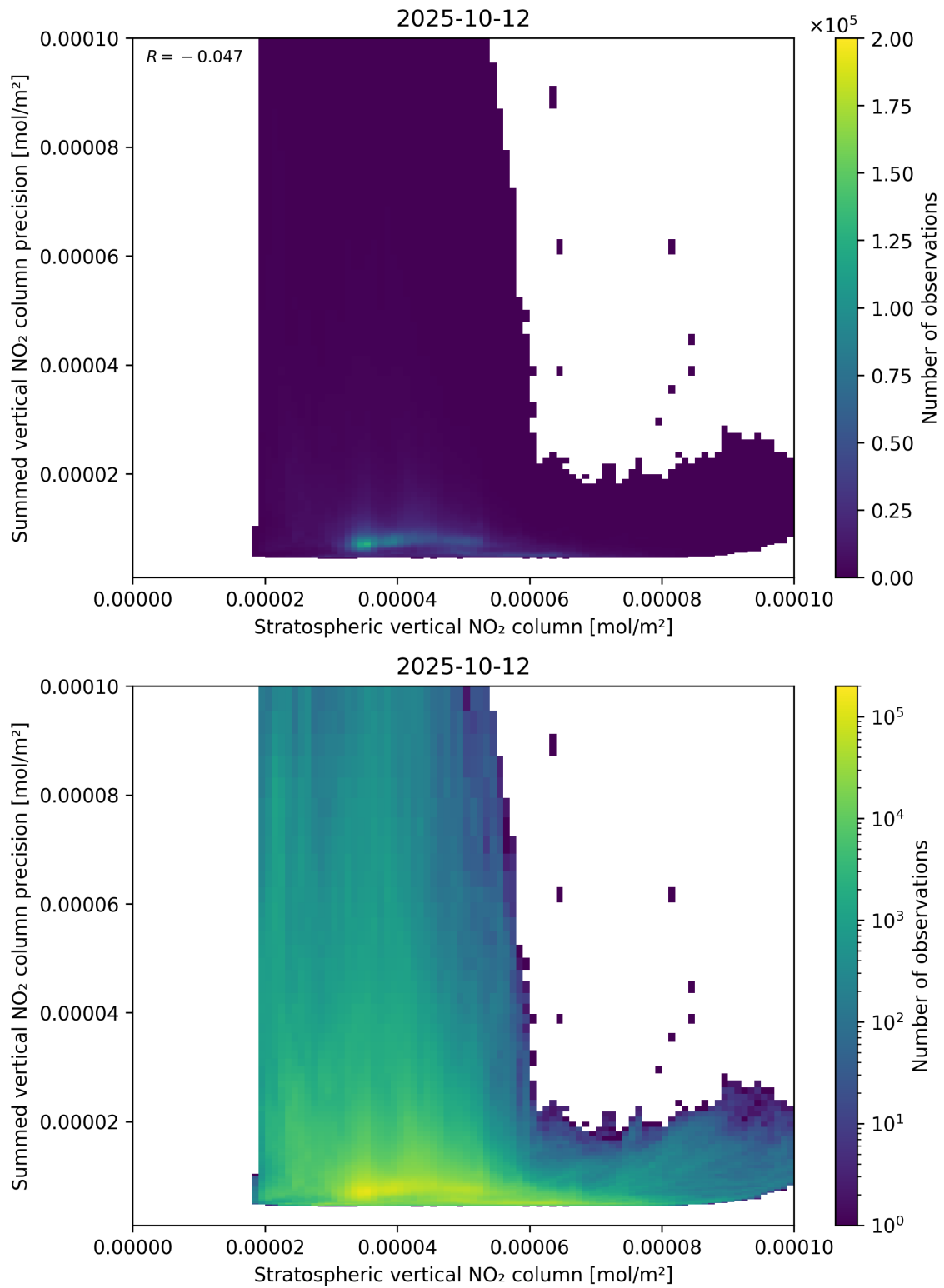
Figure 99: Scatter density plot of “Stratospheric vertical NO 2 column” against “Summed vertical NO 2 column precision” for 2025-10-11 to 2025-10-13.
