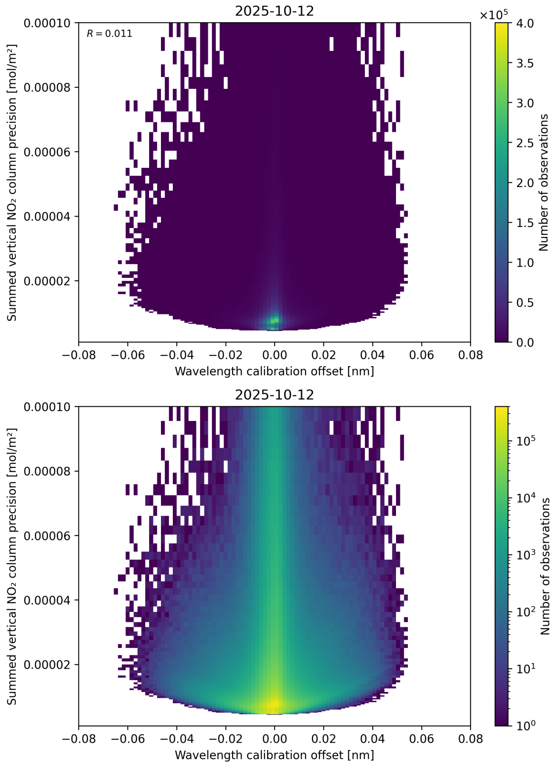
Figure 178: Scatter density plot of “Wavelength calibration offset” against “Summed vertical NO 2 column precision” for 2025-10-11 to 2025-10-13.
