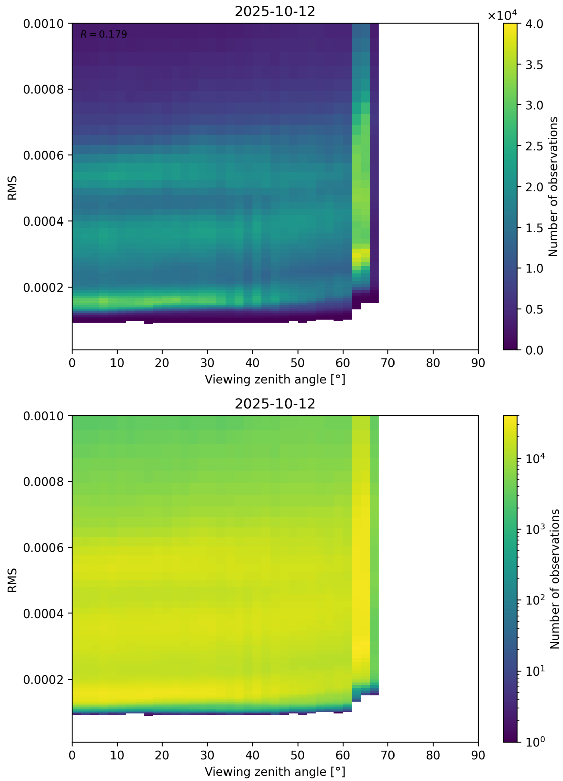
Figure 171: Scatter density plot of “Viewing zenith angle” against “RMS” for 2025-10-11 to 2025-10-13.
