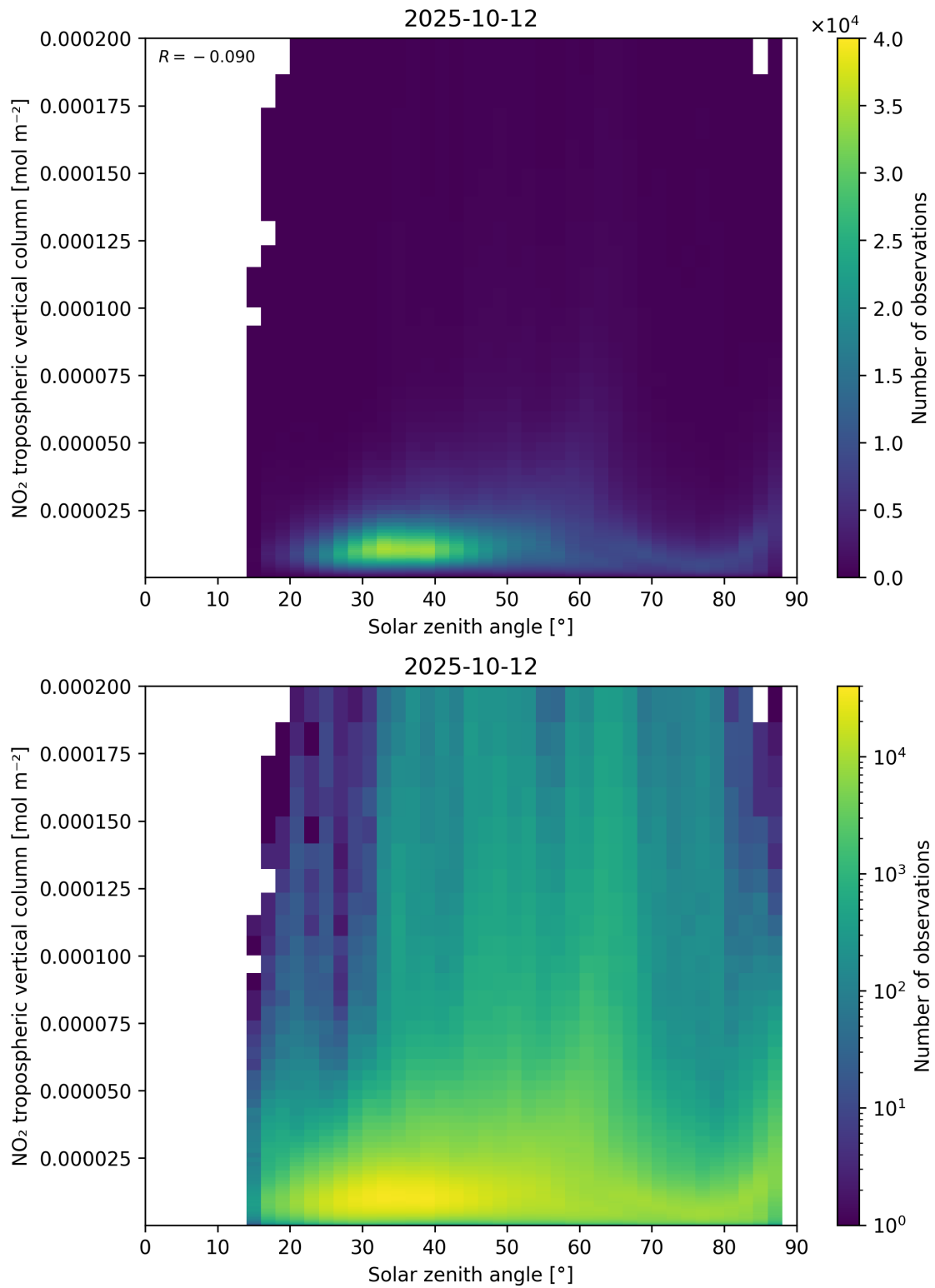
Figure 155: Scatter density plot of “Solar zenith angle” against “NO 2 tropospheric vertical column” for 2025-10-11 to 2025-10-13.
