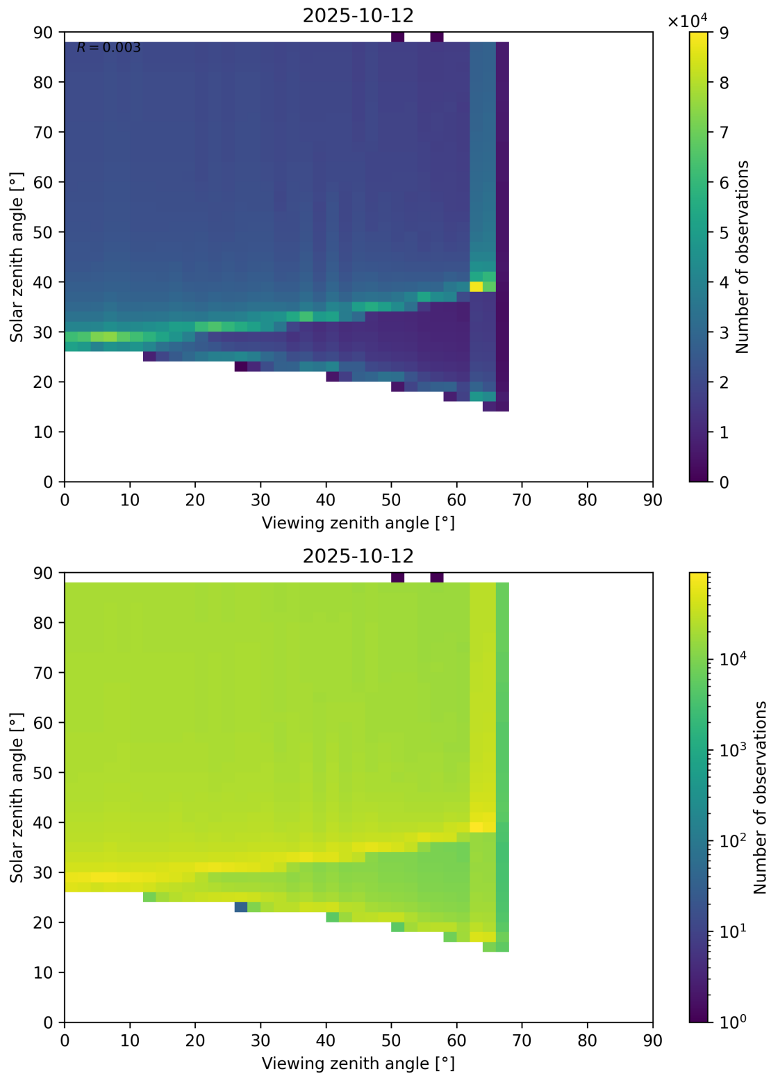
Figure 172: Scatter density plot of “Viewing zenith angle” against “Solar zenith angle” for 2025-10-11 to 2025-10-13.
