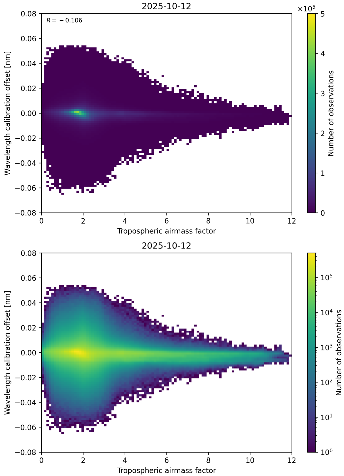
Figure 80: Scatter density plot of “Tropospheric airmass factor” against “Wavelength calibration offset” for 2025-10-11 to 2025-10-13.
