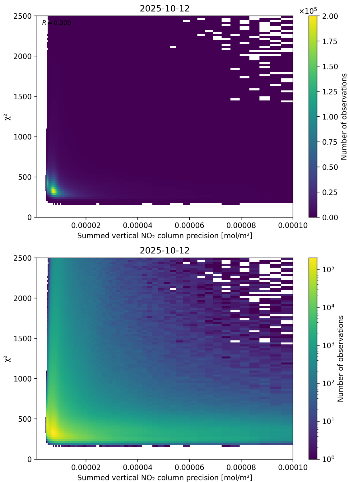
Figure 107: Scatter density plot of “Summed vertical NO 2 column precision” against “ \chi^2 ” for 2025-10-11 to 2025-10-13.
