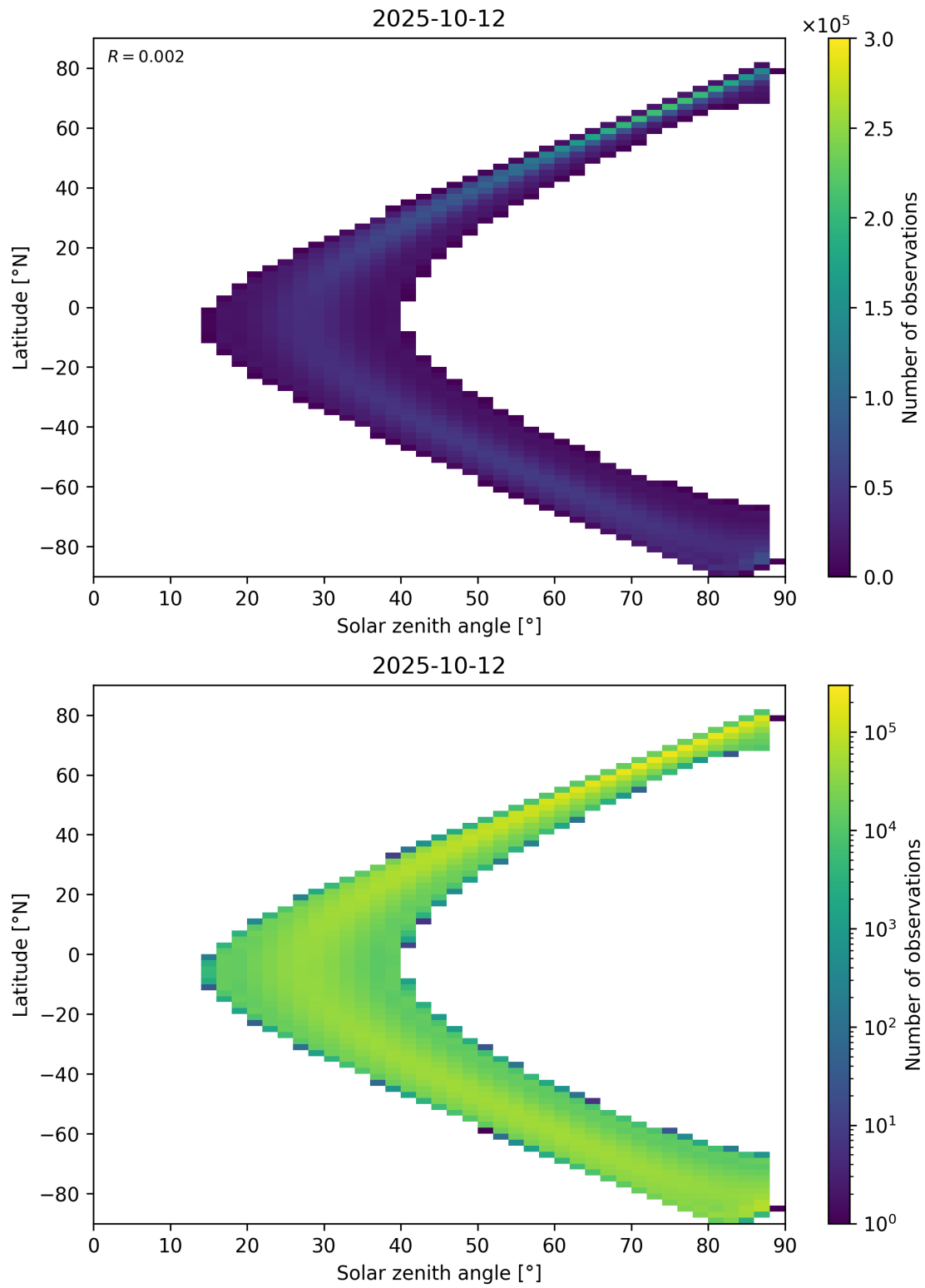
Figure 149: Scatter density plot of “Solar zenith angle” against “Latitude” for 2025-10-11 to 2025-10-13.
