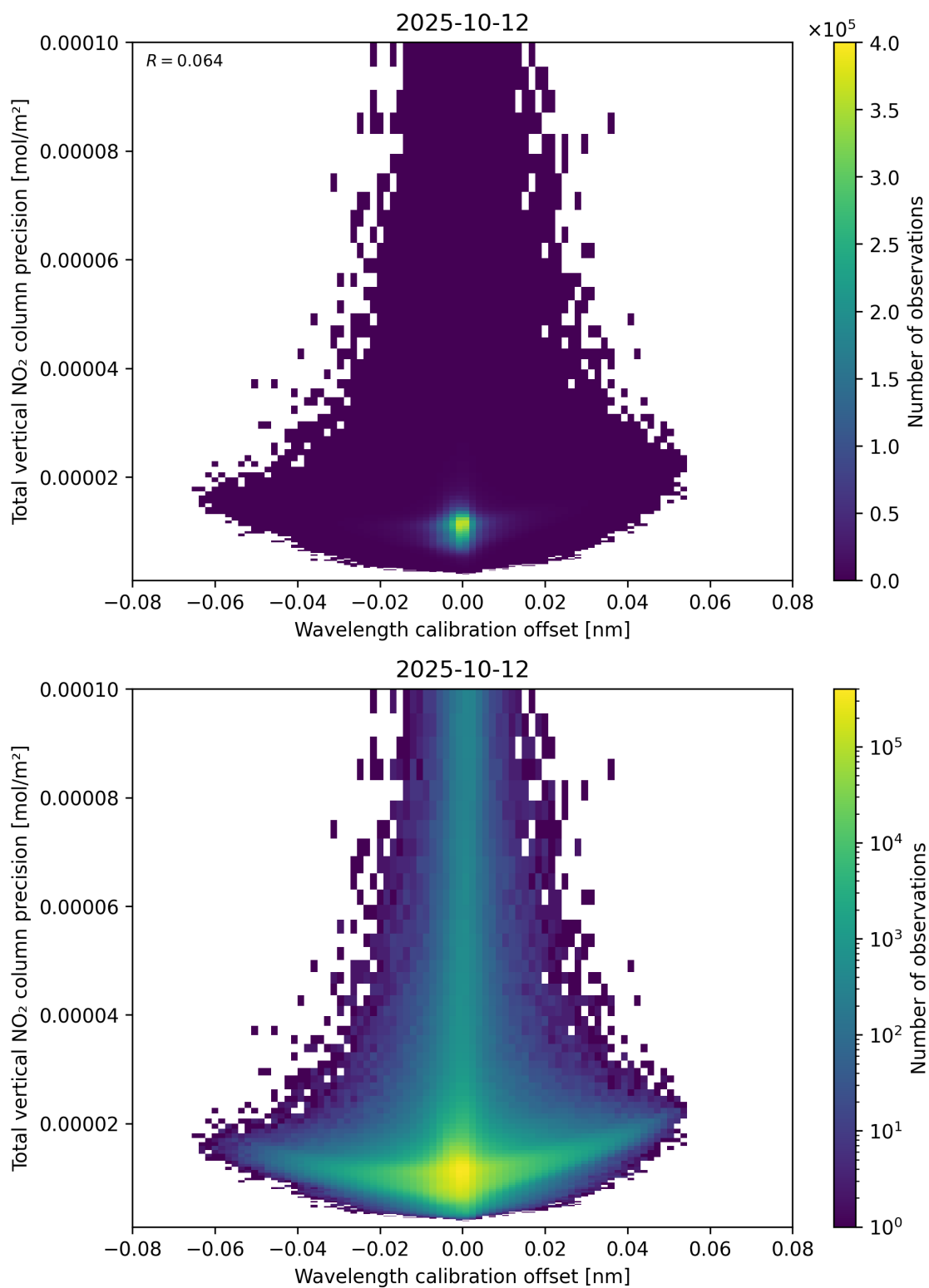
Figure 180: Scatter density plot of “Wavelength calibration offset” against “Total vertical NO 2 column precision” for 2025-10-11 to 2025-10-13.
