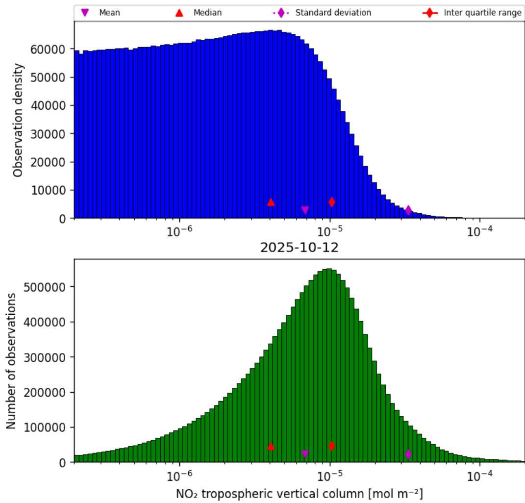
Figure 29: Histogram of “NO 2 tropospheric vertical column” for 2025-10-11 to 2025-10-13
