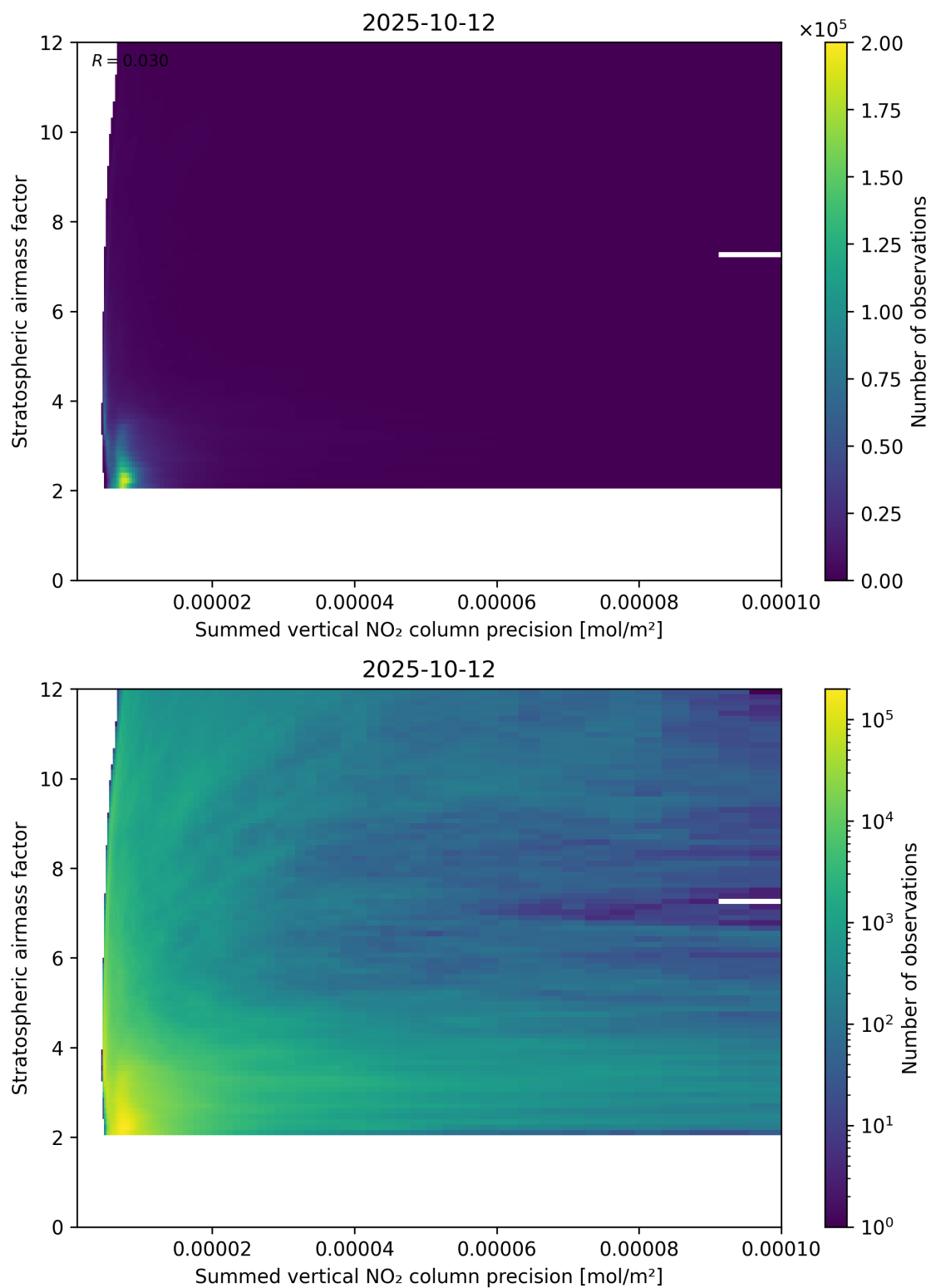
Figure 106: Scatter density plot of “Summed vertical NO 2 column precision” against “Stratospheric airmass factor” for 2025-10-11 to 2025-10-13.
