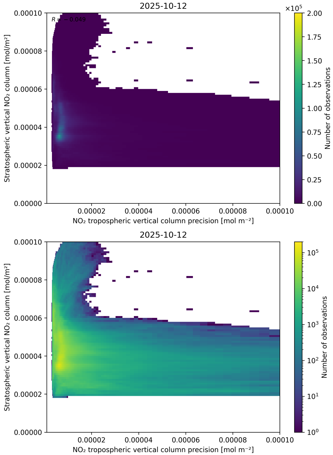
Figure 135: Scatter density plot of “NO 2 tropospheric vertical column precision” against “Stratospheric vertical NO 2 column” for 2025-10-11 to 2025-10-13.
