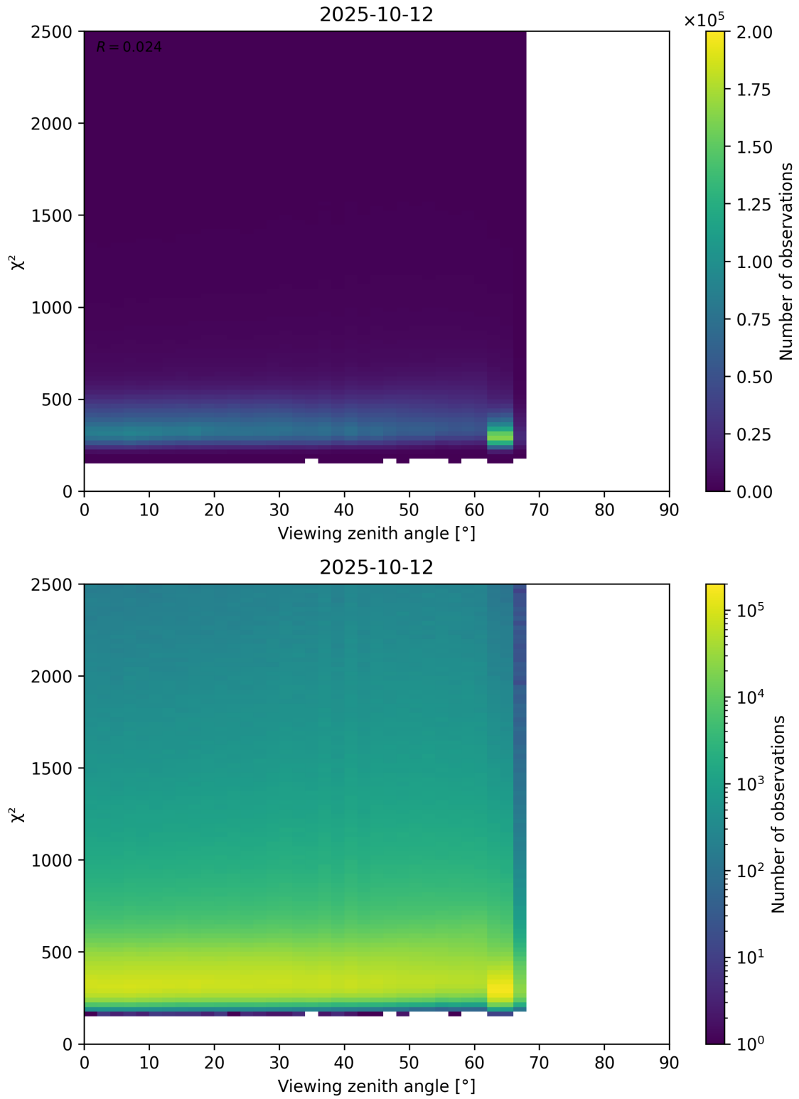
Figure 162: Scatter density plot of “Viewing zenith angle” against “ \chi^2 ” for 2025-10-11 to 2025-10-13.
