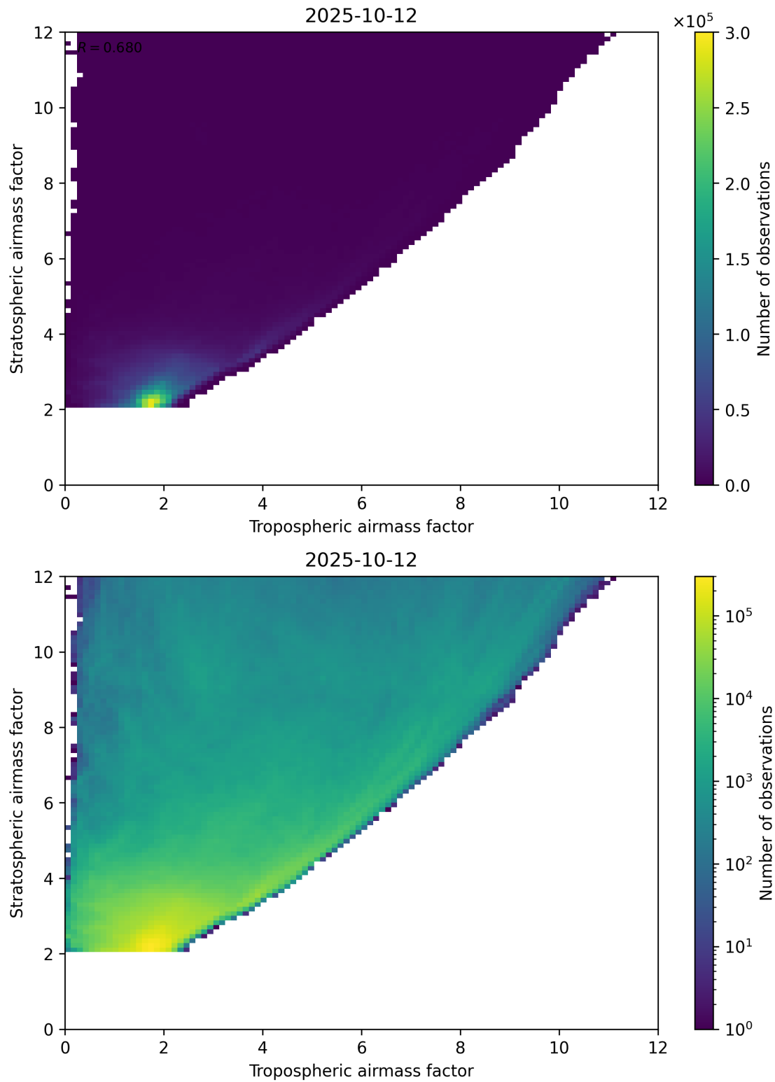
Figure 71: Scatter density plot of “Tropospheric airmass factor” against “Stratospheric airmass factor” for 2025-10-11 to 2025-10-13.
