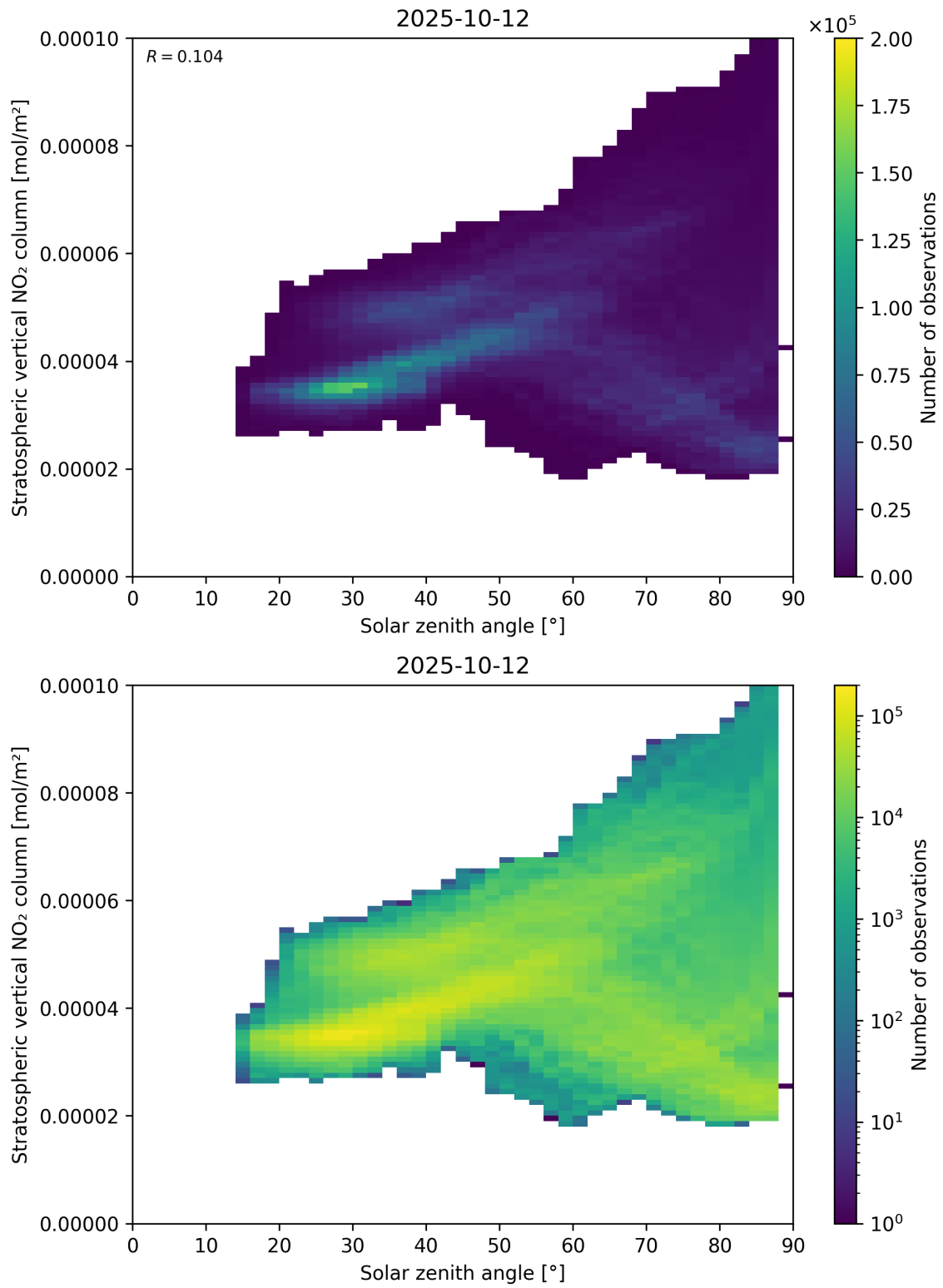
Figure 150: Scatter density plot of “Solar zenith angle” against “Stratospheric vertical NO 2 column” for 2025-10-11 to 2025-10-13.
