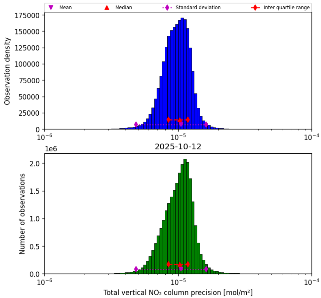
Figure 39: Histogram of "Total vertical NO 2 column precision" for 2025-10-11 to 2025-10-13
