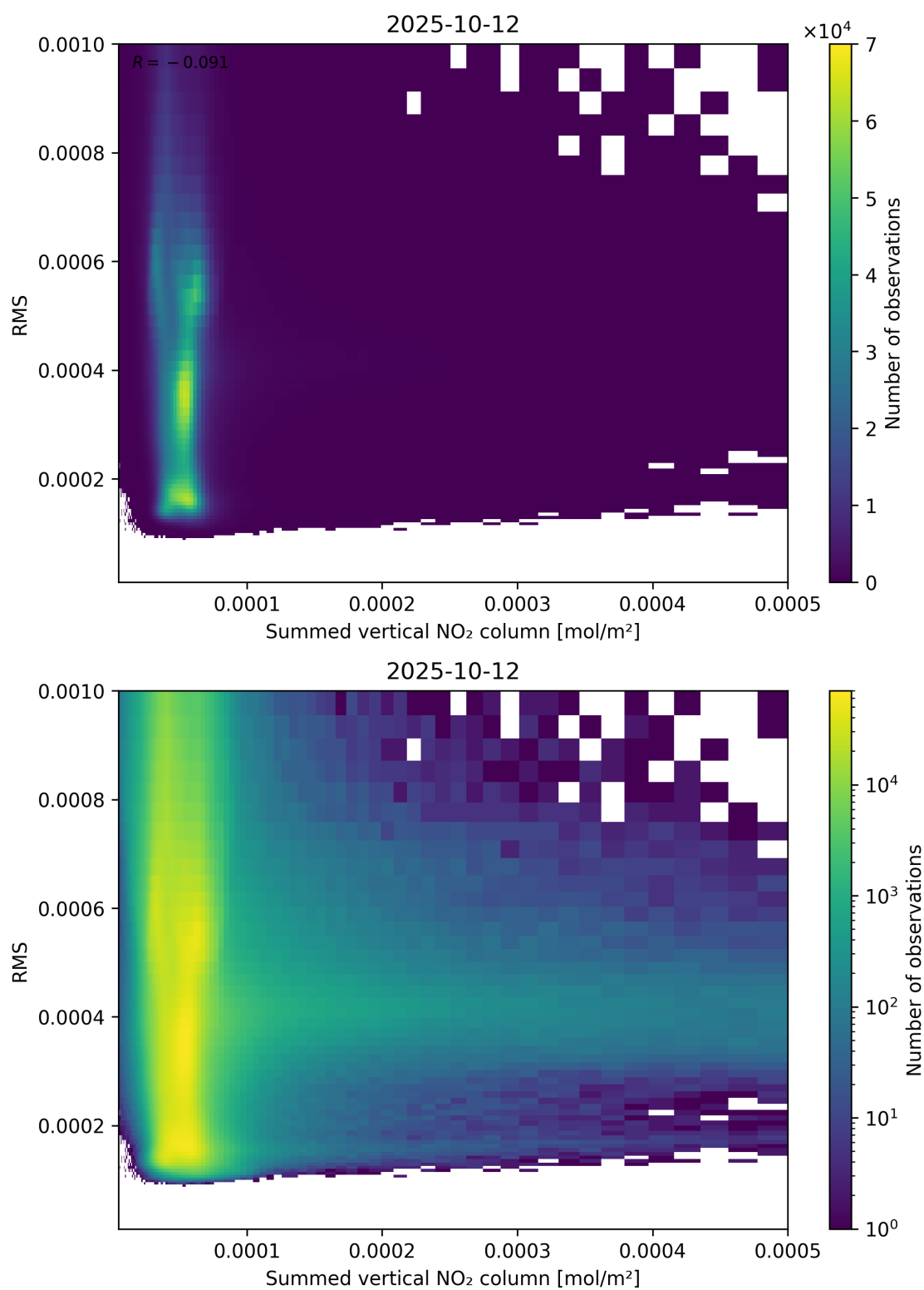
Figure 109: Scatter density plot of “Summed vertical NO 2 column” against “RMS” for 2025-10-11 to 2025-10-13.
