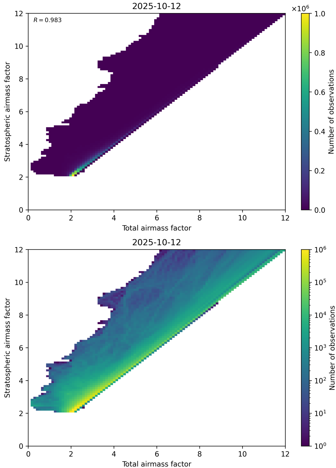
Figure 62: Scatter density plot of “Total airmass factor” against “Stratospheric airmass factor” for 2025-10-11 to 2025-10-13.
