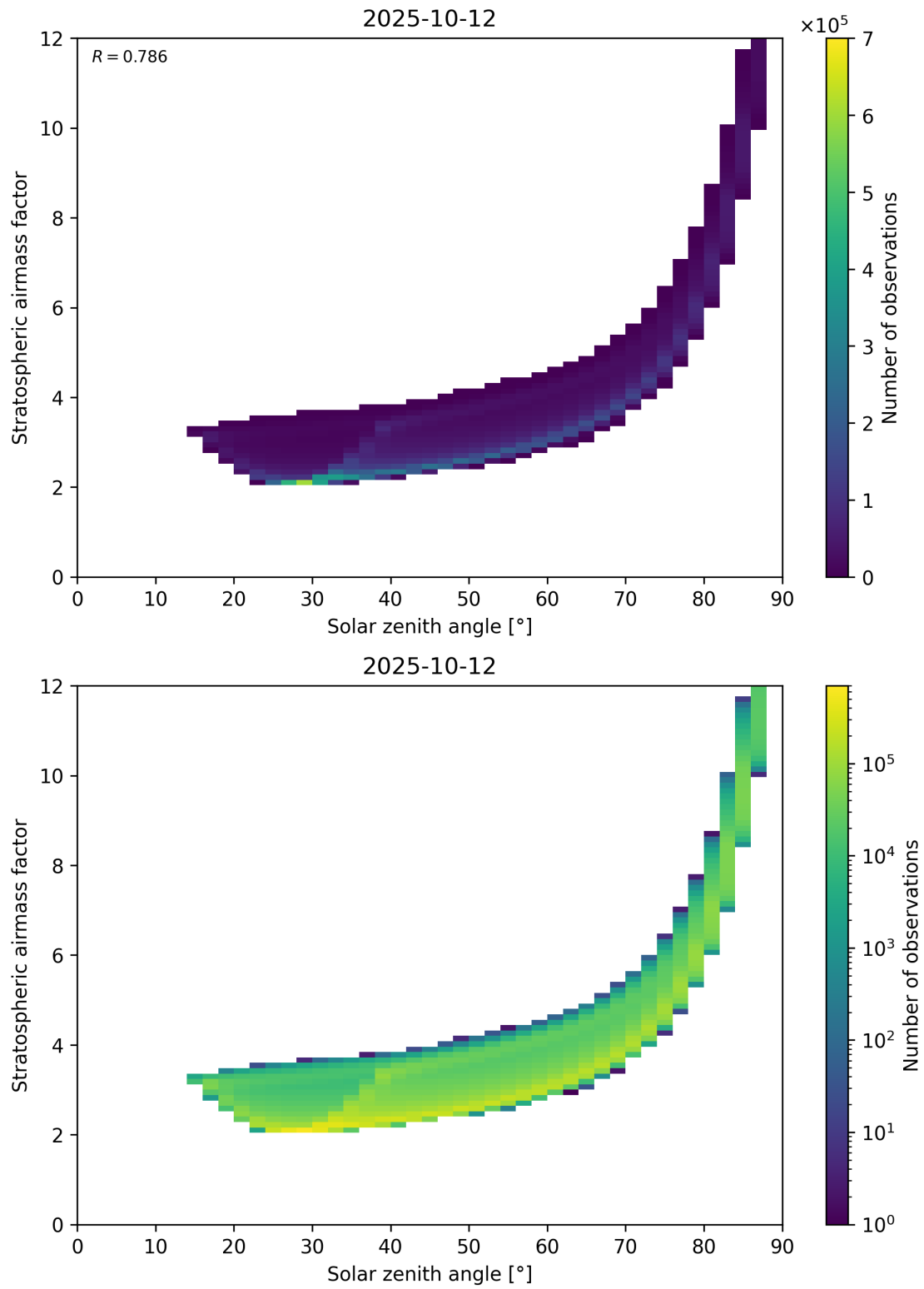
Figure 145: Scatter density plot of “Solar zenith angle” against “Stratospheric airmass factor” for 2025-10-11 to 2025-10-13.
