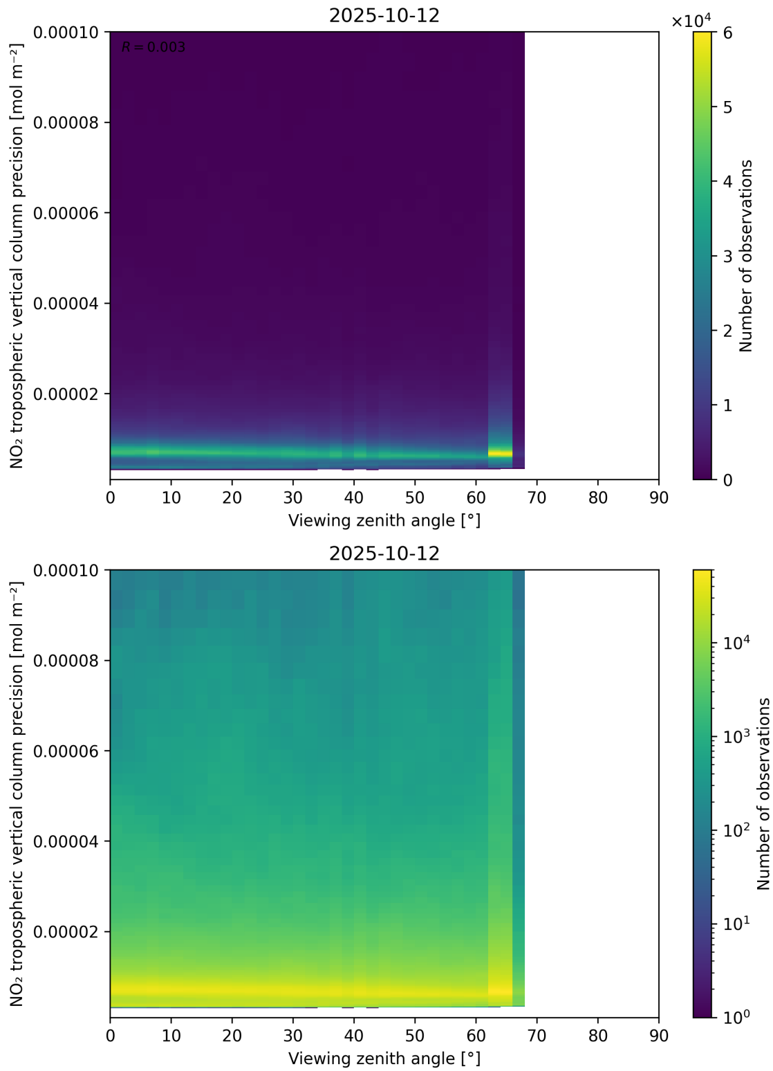
Figure 170: Scatter density plot of “Viewing zenith angle” against “NO 2 tropospheric vertical column precision” for 2025-10-11 to 2025-10-13.
