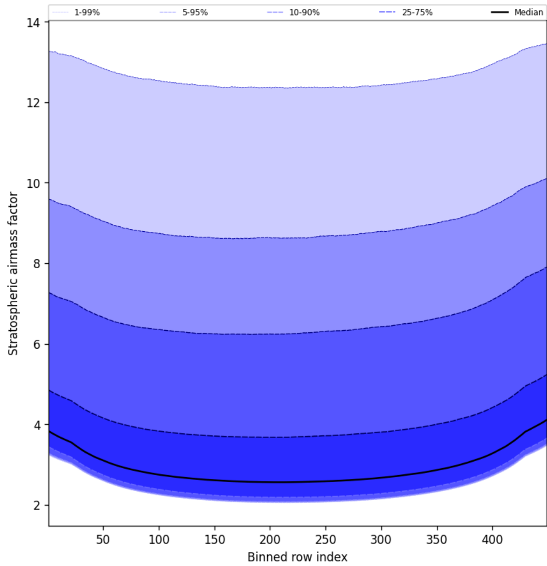
Figure 61: Along track statistics of “Stratospheric airmass factor” for 2025-10-11 to 2025-10-13
