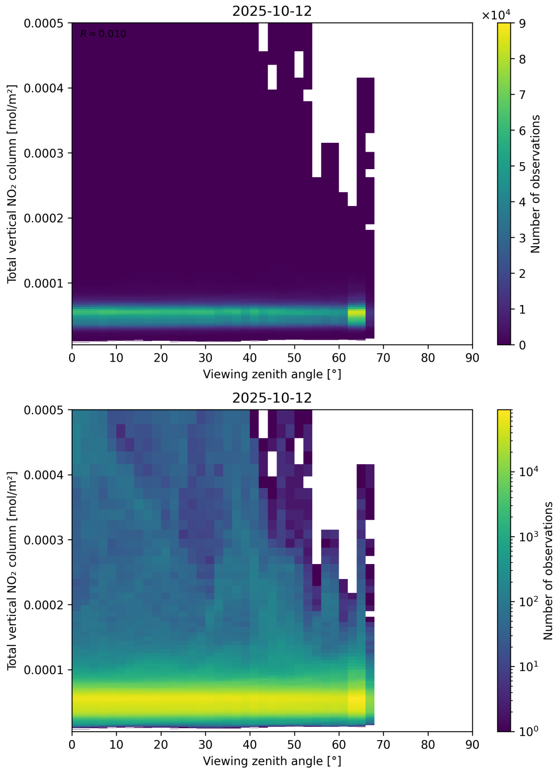
Figure 167: Scatter density plot of “Viewing zenith angle” against “Total vertical NO 2 column” for 2025-10-11 to 2025-10-13.
