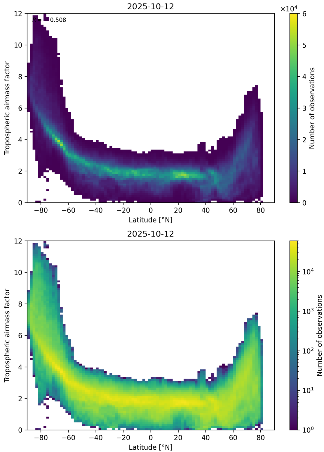
Figure 85: Scatter density plot of “Latitude” against “Tropospheric airmass factor” for 2025-10-11 to 2025-10-13.
