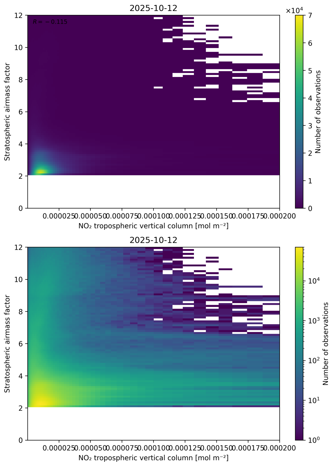
Figure 121: Scatter density plot of “NO 2 tropospheric vertical column” against “Stratospheric air mass factor” for 2025-10-11 to 2025-10-13.
