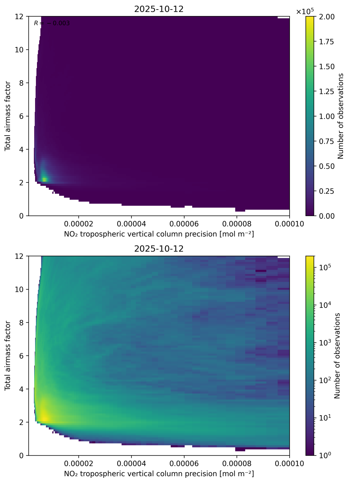
Figure 132: Scatter density plot of “NO 2 tropospheric vertical column precision” against “Total air mass factor” for 2025-10-11 to 2025-10-13.
