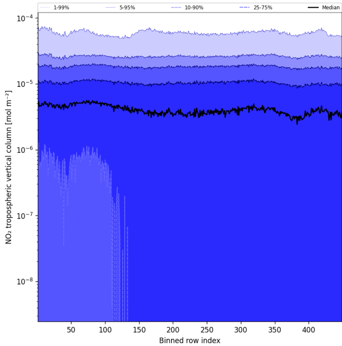
Figure 46: Along track statistics of “NO 2 tropospheric vertical column” for 2025-10-11 to 2025-10-13
