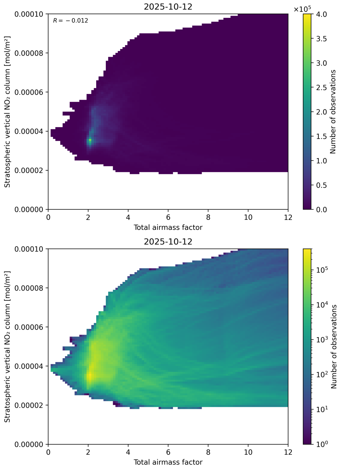
Figure 64: Scatter density plot of “Total airmass factor” against “Stratospheric vertical NO 2 column” for 2025-10-11 to 2025-10-13.
