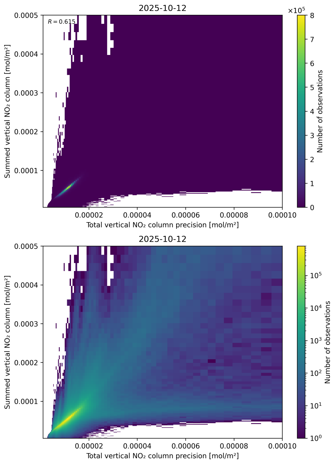
Figure 117: Scatter density plot of “Total vertical NO 2 column precision” against “Summed vertical NO 2 column” for 2025-10-11 to 2025-10-13.
