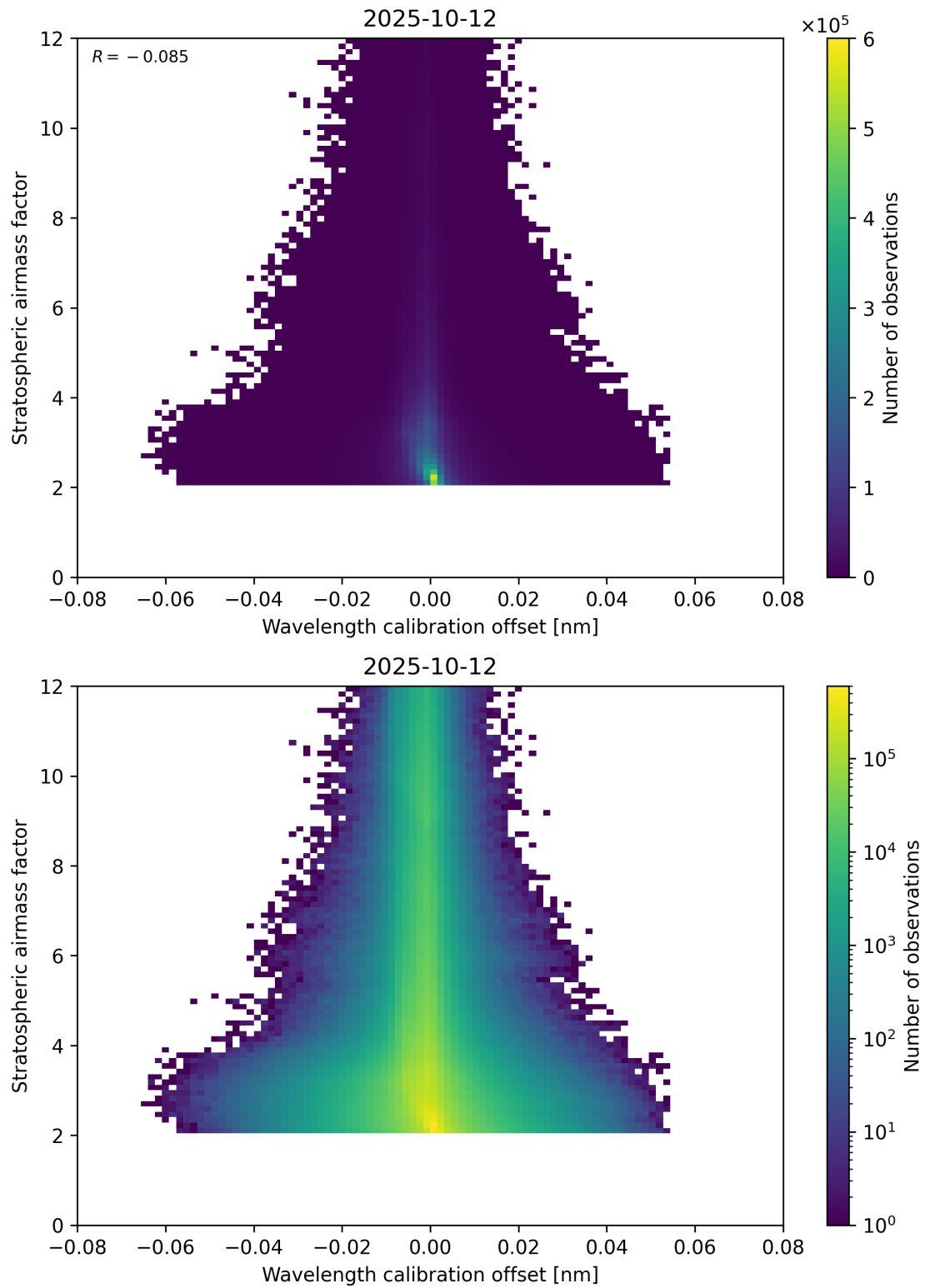
Figure 174: Scatter density plot of “Wavelength calibration offset” against “Stratospheric airmass factor” for 2025-10-11 to 2025-10-13.
