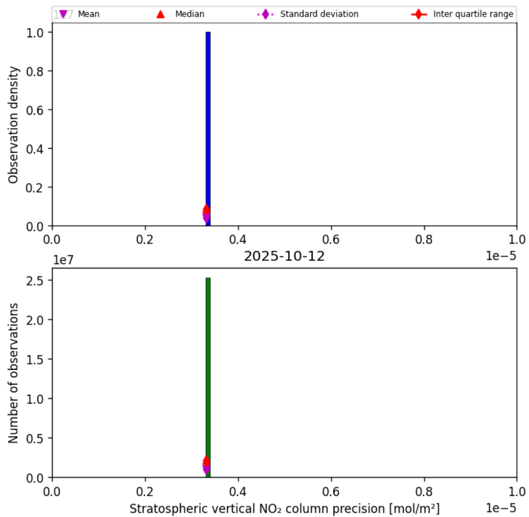
Figure 37: Histogram of “Stratospheric vertical NO 2 column precision” for 2025-10-11 to 2025-10-13
