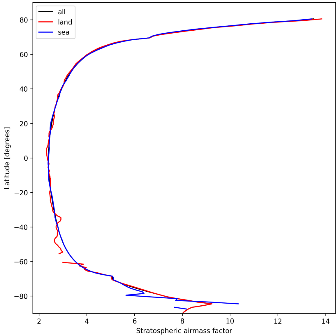
Figure 27: Zonal average of “Stratospheric air mass factor” for 2025-10-11 to 2025-10-13.
