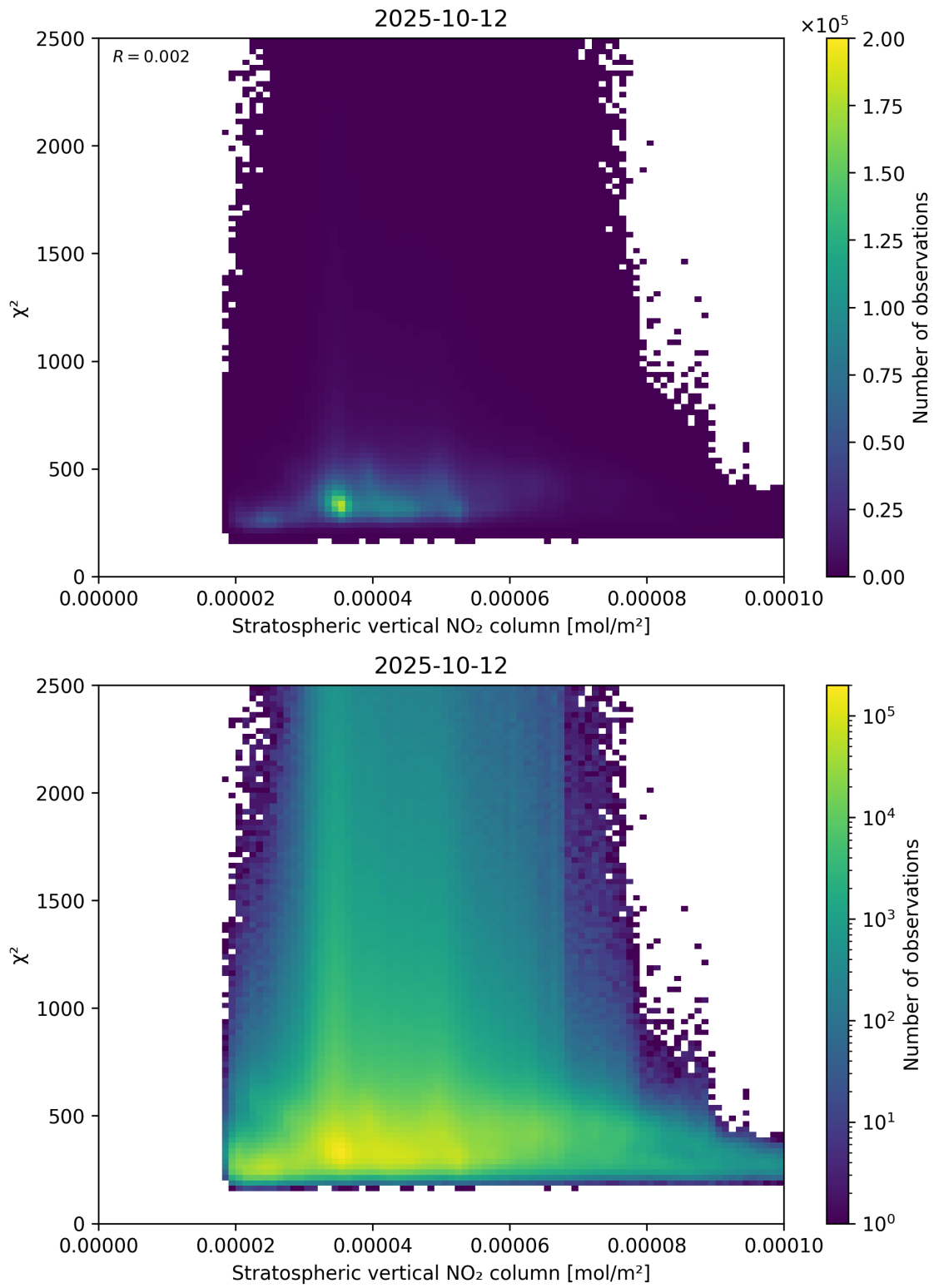
Figure 97: Scatter density plot of “Stratospheric vertical NO 2 column” against “ \chi^2 ” for 2025-10-11 to 2025-10-13.
