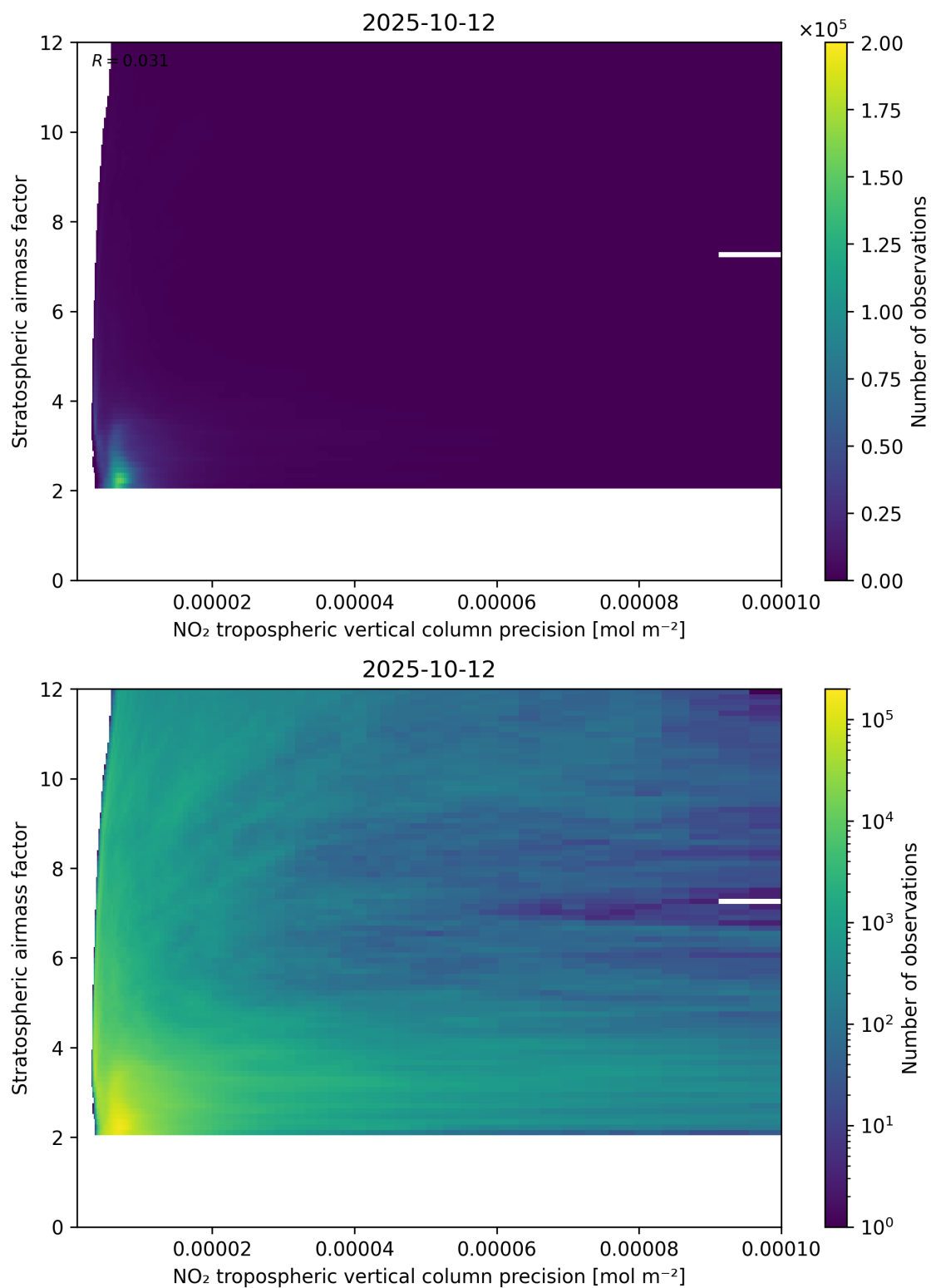
Figure 131: Scatter density plot of “NO 2 tropospheric vertical column precision” against “Stratospheric airmass factor” for 2025-10-11 to 2025-10-13.
