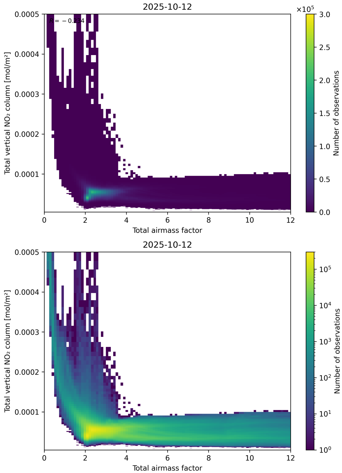
Figure 67: Scatter density plot of “Total airmass factor” against “Total vertical NO 2 column” for 2025-10-11 to 2025-10-13.
