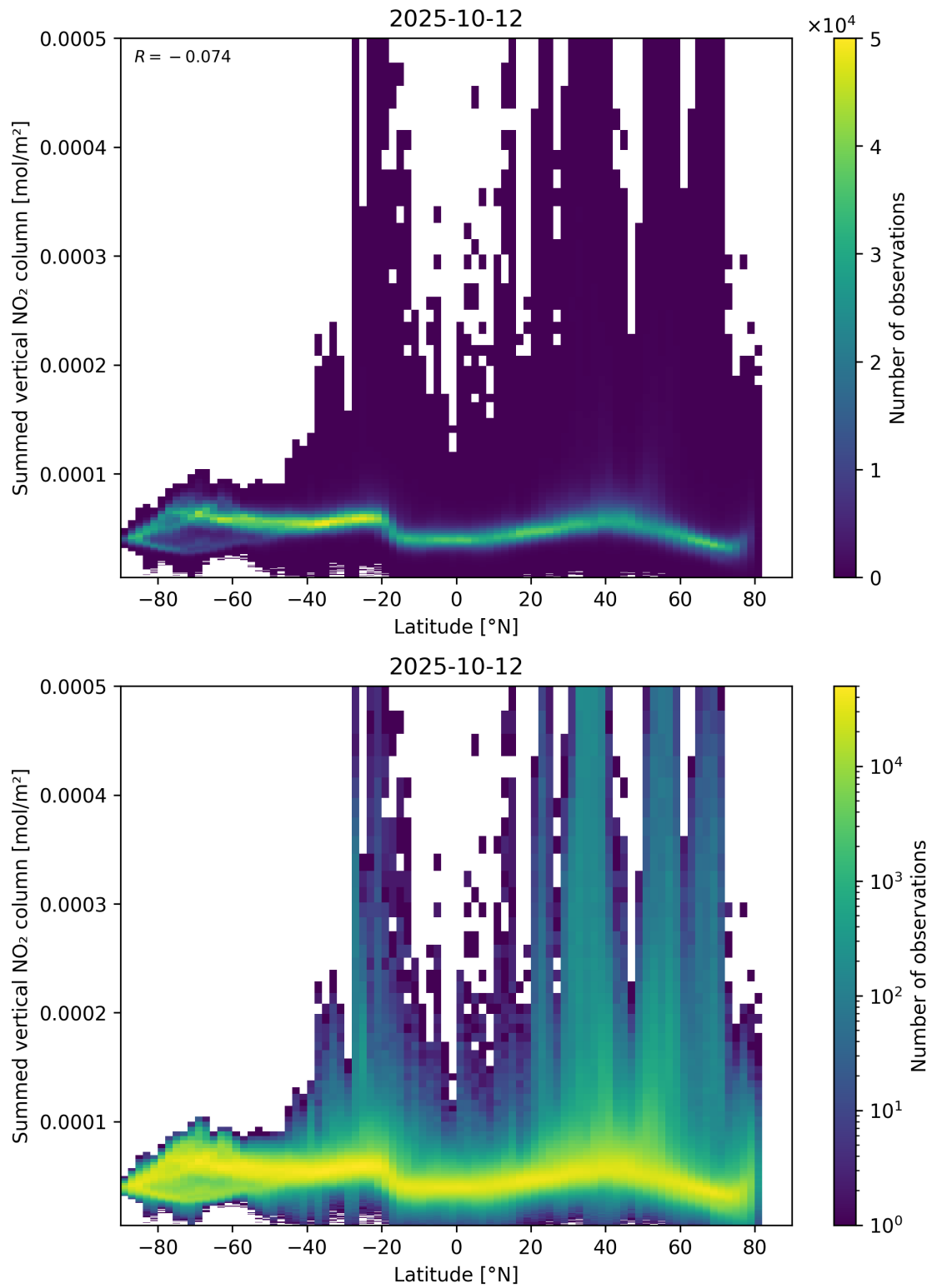
Figure 88: Scatter density plot of “Latitude” against “Summed vertical NO 2 column” for 2025-10-11 to 2025-10-13.
