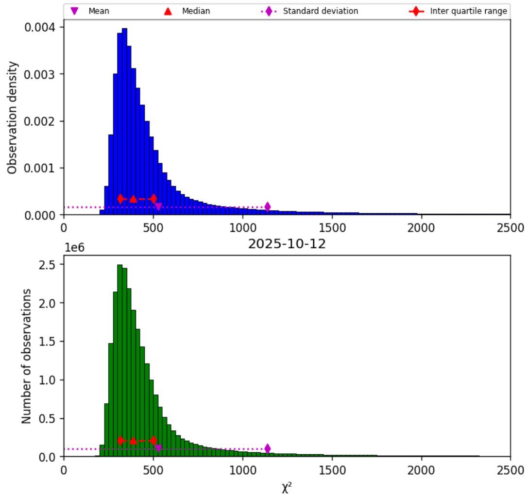
Figure 42: Histogram of “ \chi^2 ” for 2025-10-11 to 2025-10-13
