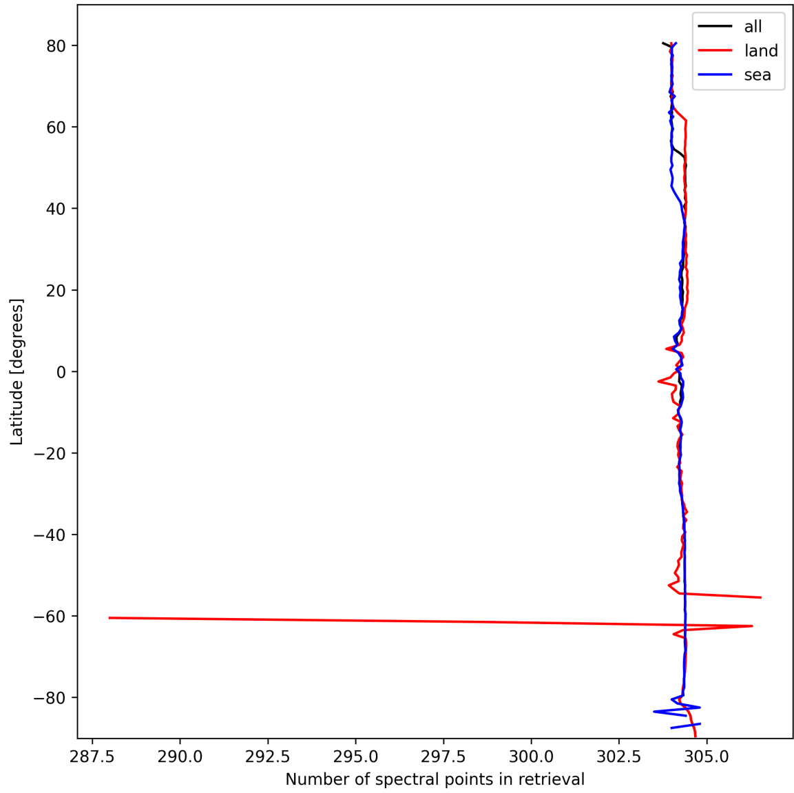
Figure 16: Zonal average of “Number of spectral points in retrieval” for 2025-10-11 to 2025-10-13.
