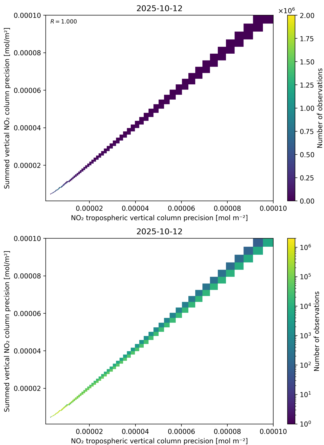
Figure 137: Scatter density plot of “NO 2 tropospheric vertical column precision” against “Summed vertical NO 2 column precision” for 2025-10-11 to 2025-10-13.
