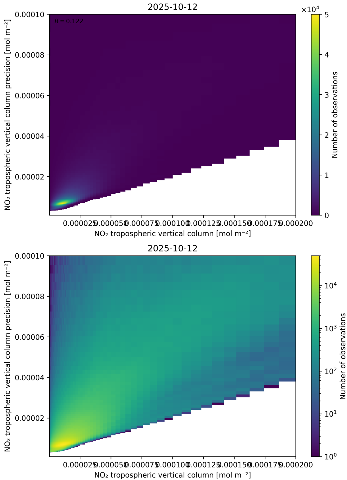
Figure 130: Scatter density plot of “NO 2 tropospheric vertical column” against “NO 2 tropospheric vertical column precision” for 2025-10-11 to 2025-10-13.
