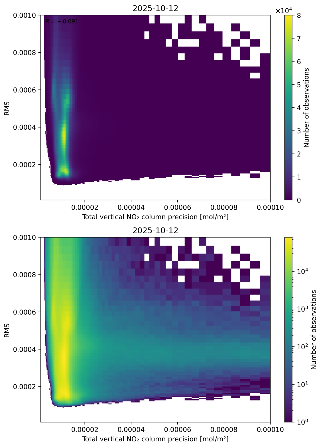
Figure 119: Scatter density plot of “Total vertical NO 2 column precision” against “RMS” for 2025-10-11 to 2025-10-13.
