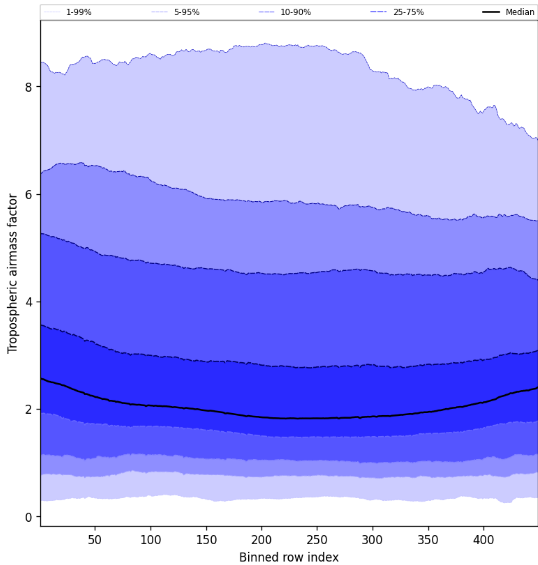
Figure 48: Along track statistics of “Tropospheric airmass factor” for 2025-10-11 to 2025-10-13
