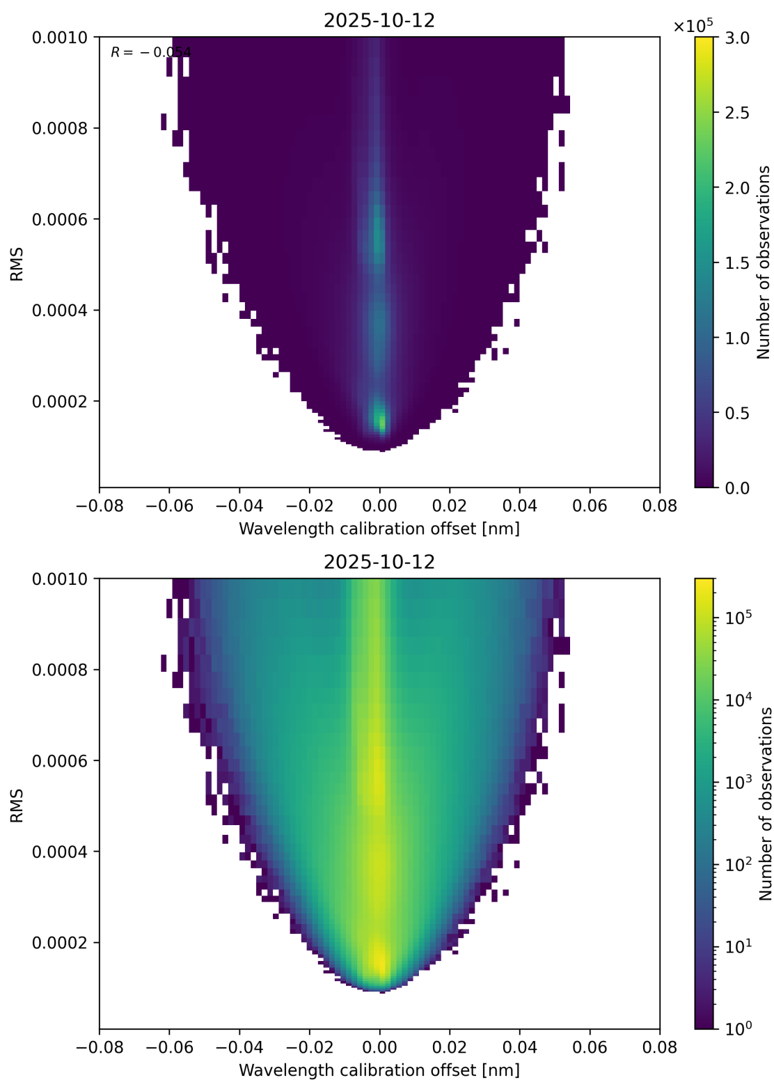
Figure 181: Scatter density plot of “Wavelength calibration offset” against “RMS” for 2025-10-11 to 2025-10-13.
