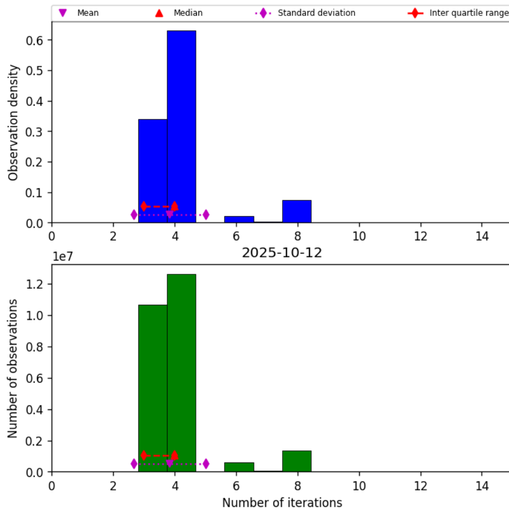
Figure 34: Histogram of “Number of iterations” for 2025-10-11 to 2025-10-13
