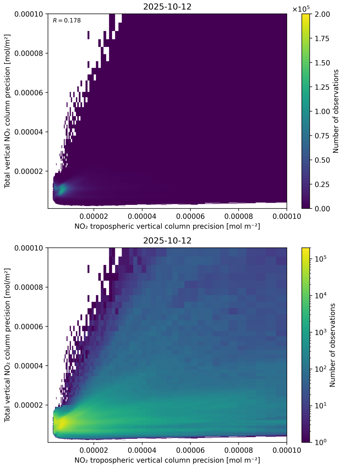
Figure 139: Scatter density plot of “NO 2 tropospheric vertical column precision” against “Total vertical NO 2 column precision” for 2025-10-11 to 2025-10-13.
