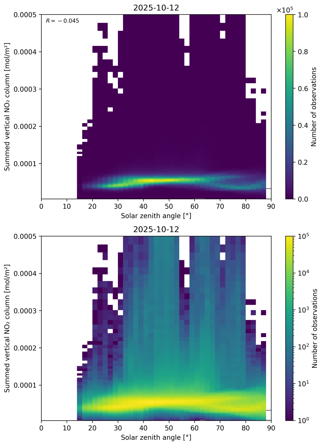
Figure 151: Scatter density plot of “Solar zenith angle” against “Summed vertical NO 2 column” for 2025-10-11 to 2025-10-13.
