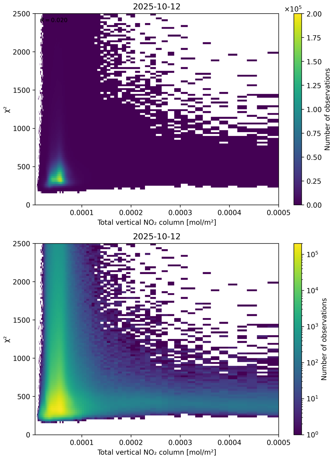
Figure 111: Scatter density plot of “Total vertical NO 2 column” against “ \chi^2 ” for 2025-10-11 to 2025-10-13.
