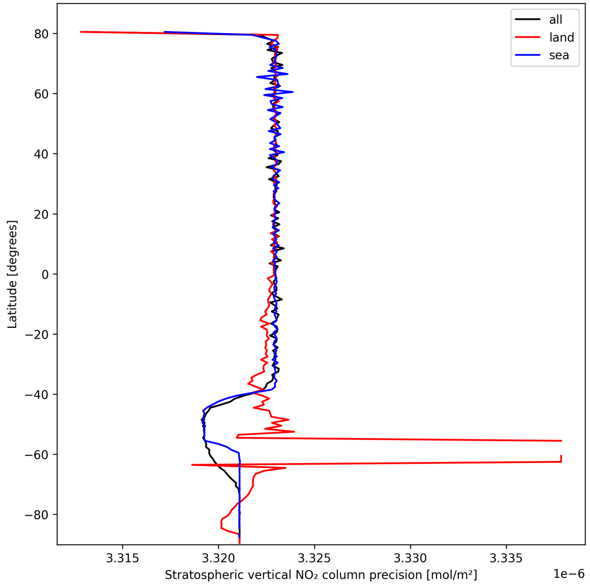
Figure 20: Zonal average of “Stratospheric vertical NO 2 column precision” for 2025-10-11 to 2025-10-13.
