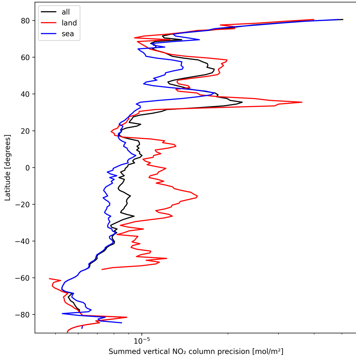
Figure 24: Zonal average of “Summed vertical NO 2 column precision” for 2025-10-11 to 2025-10-13.
