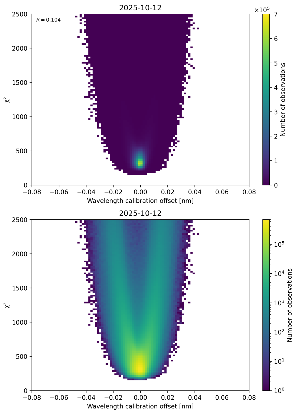
Figure 175: Scatter density plot of “Wavelength calibration offset” against “ \chi^2 ” for 2025-10-11 to 2025-10-13.
