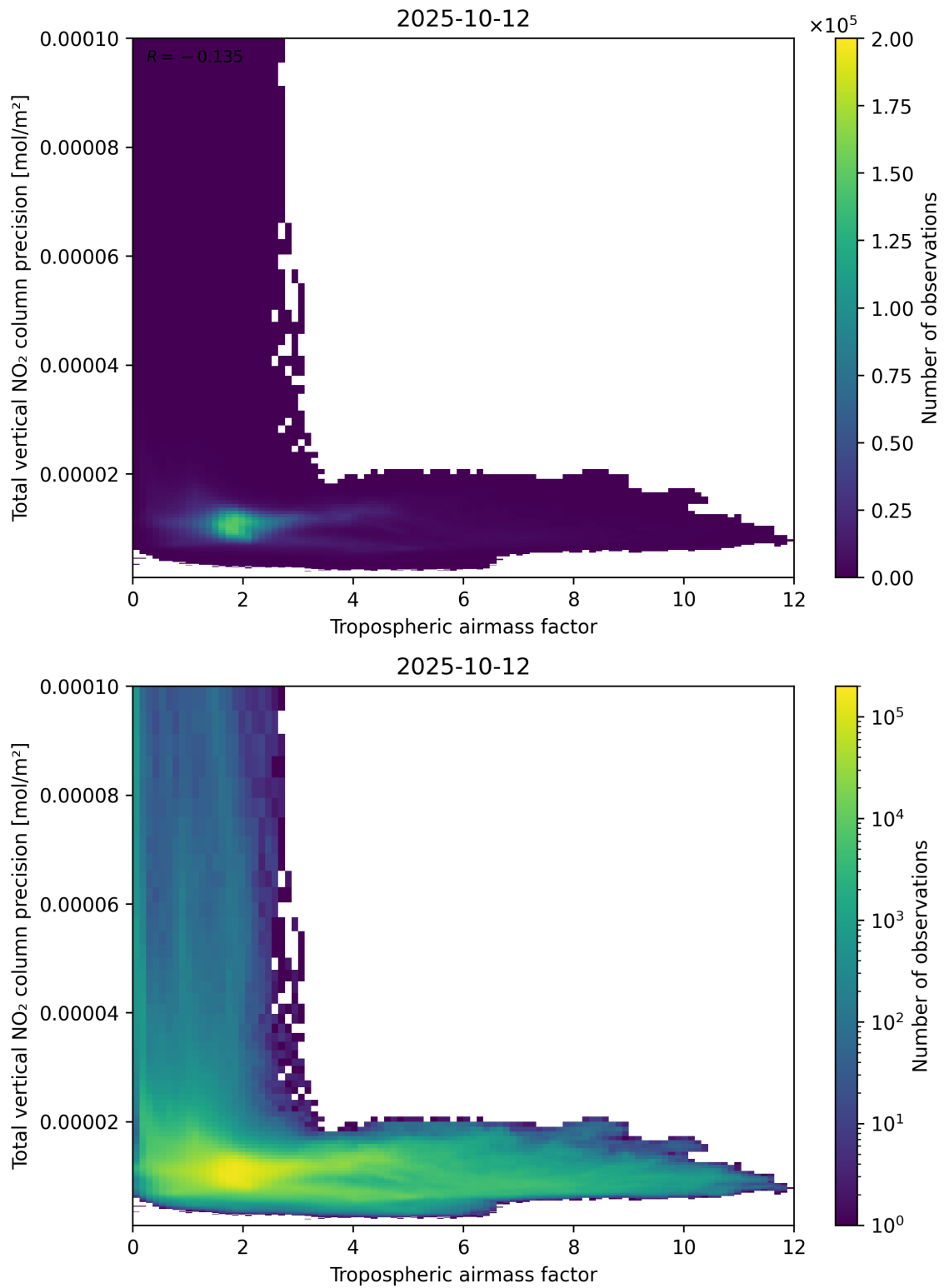
Figure 78: Scatter density plot of “Tropospheric airmass factor” against “Total vertical NO 2 column precision” for 2025-10-11 to 2025-10-13.
