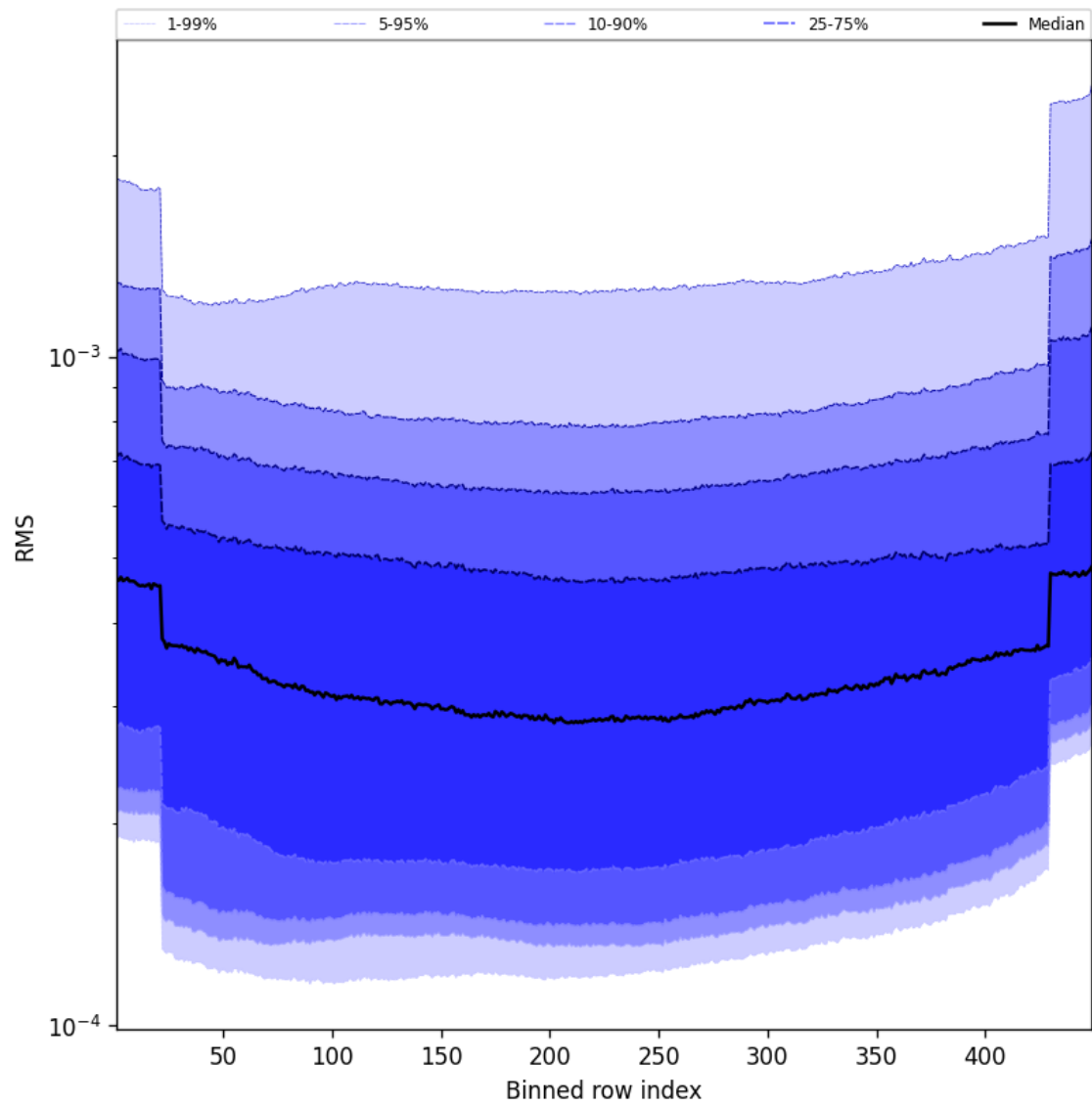
Figure 60: Along track statistics of “RMS” for 2025-10-11 to 2025-10-13
