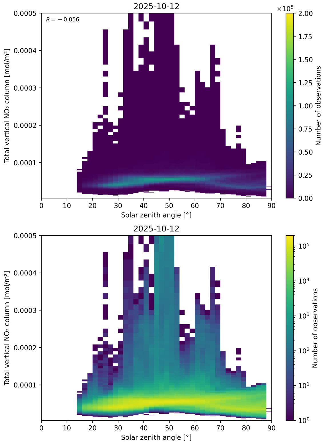
Figure 153: Scatter density plot of “Solar zenith angle” against “Total vertical NO 2 column” for 2025-10-11 to 2025-10-13.
