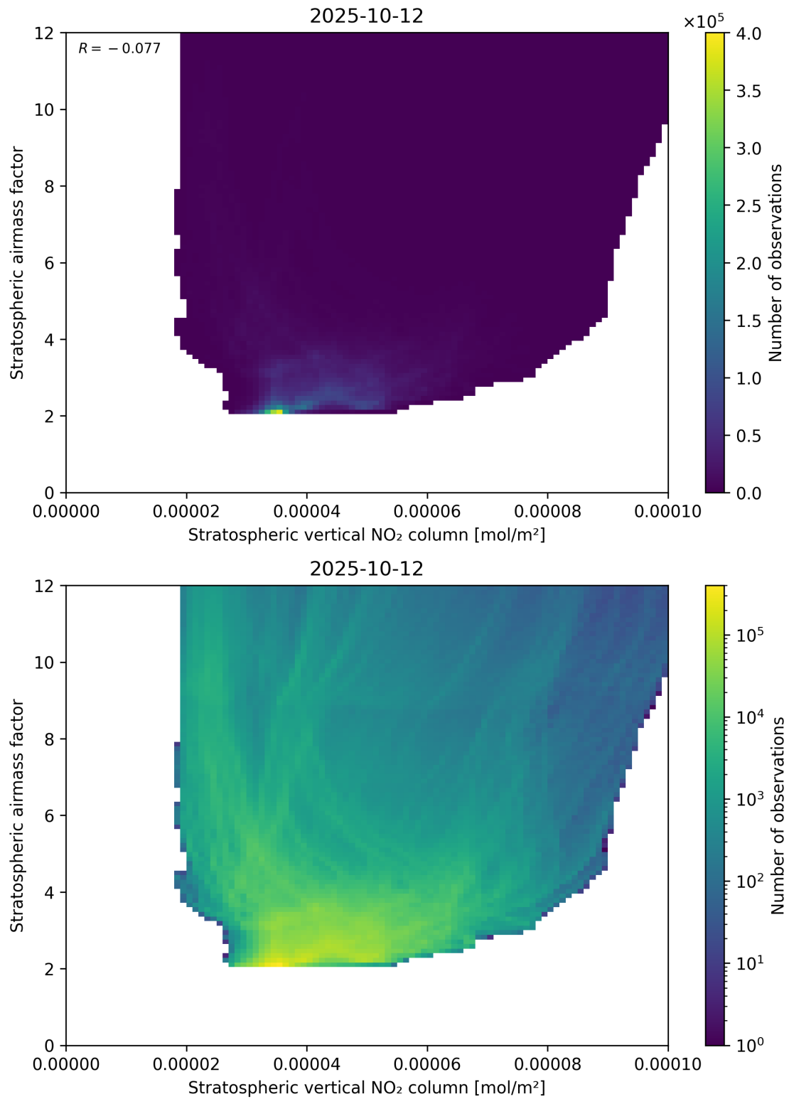
Figure 96: Scatter density plot of “Stratospheric vertical NO 2 column” against “Stratospheric airmass factor” for 2025-10-11 to 2025-10-13.
