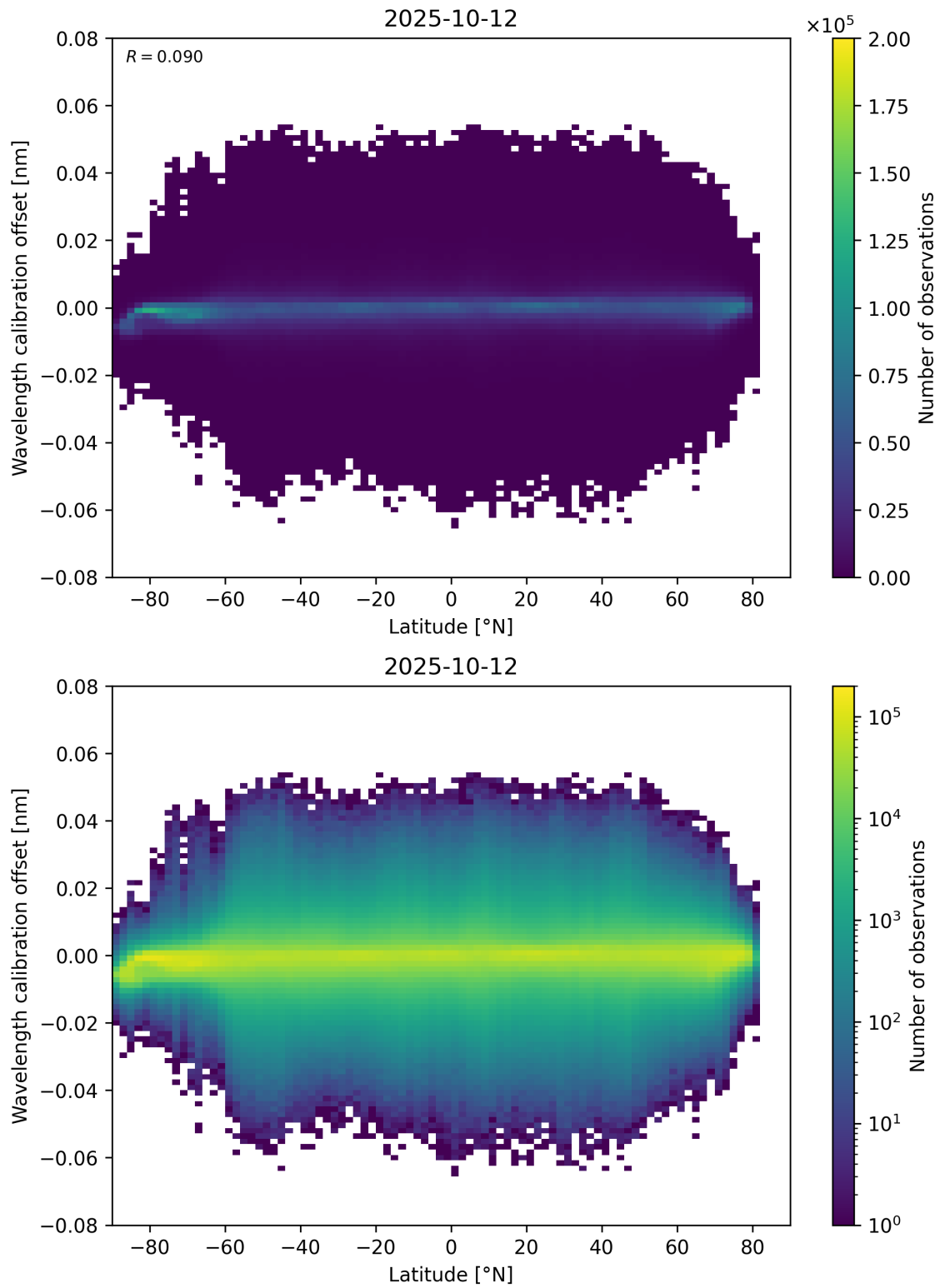
Figure 95: Scatter density plot of “Latitude” against “Wavelength calibration offset” for 2025-10-11 to 2025-10-13.
