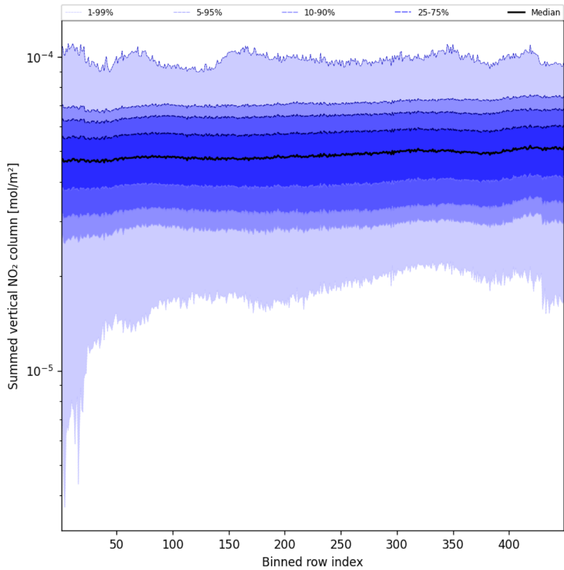
Figure 57: Along track statistics of “Summed vertical NO 2 column” for 2025-10-11 to 2025-10-13
