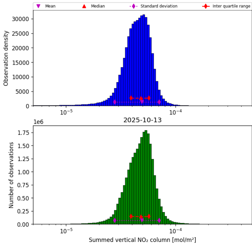
Figure 40: Histogram of “Summed vertical NO 2 column” for 2025-10-12 to 2025-10-14
