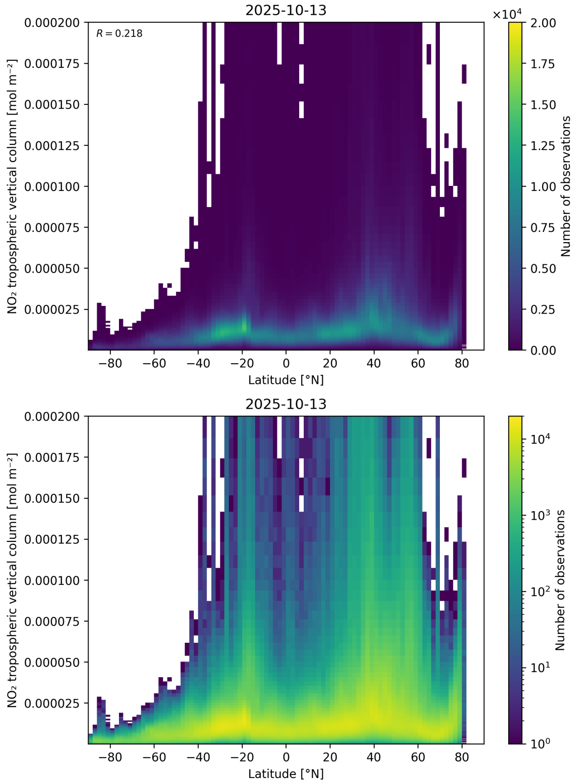
Figure 92: Scatter density plot of “Latitude” against “NO 2 tropospheric vertical column” for 2025-10-12 to 2025-10-14.
