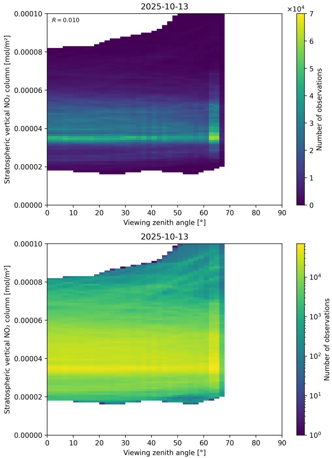
Figure 164: Scatter density plot of “Viewing zenith angle” against “Stratospheric vertical NO 2 column” for 2025-10-12 to 2025-10-14.
