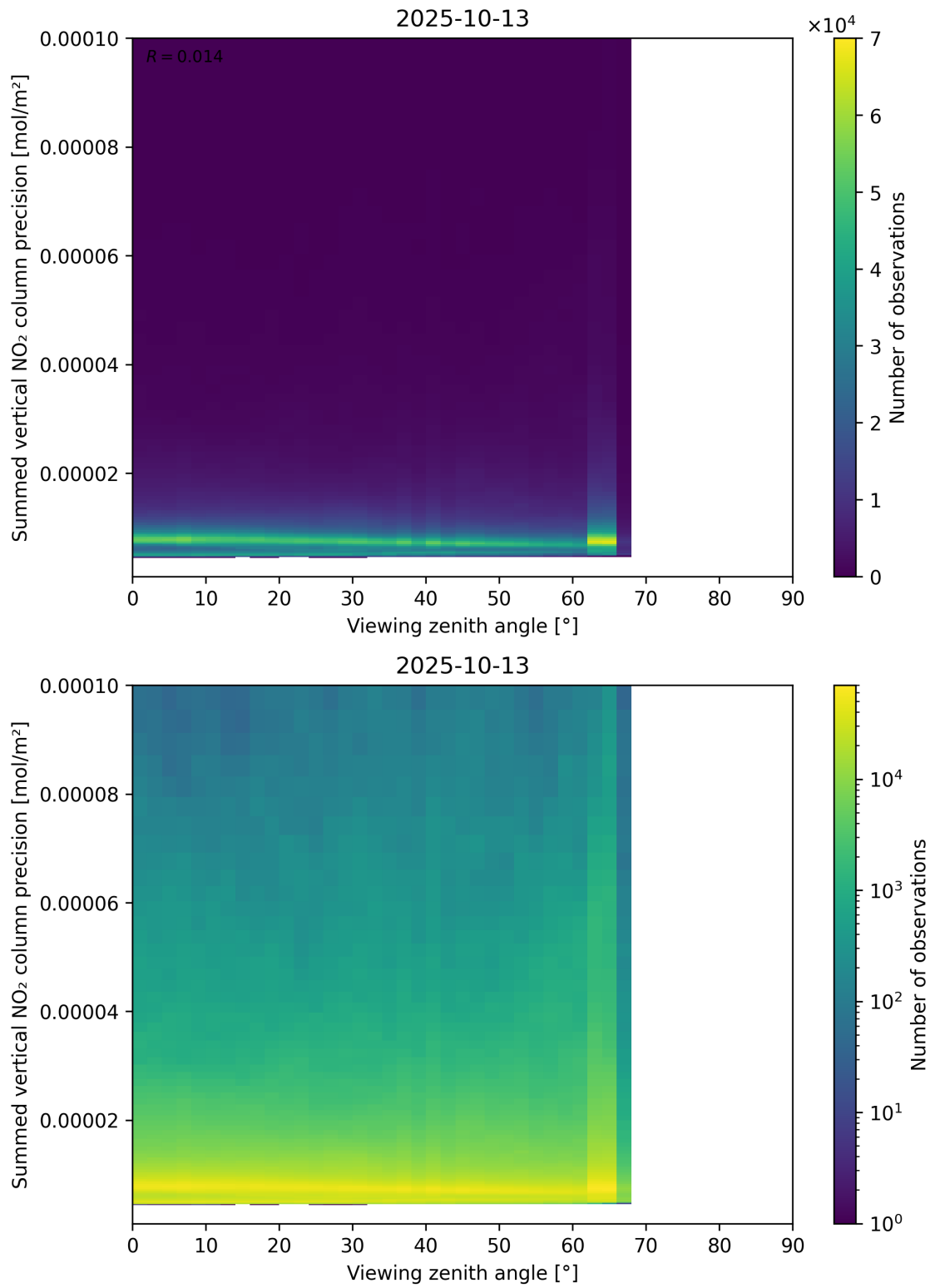
Figure 166: Scatter density plot of “Viewing zenith angle” against “Summed vertical NO 2 column precision” for 2025-10-12 to 2025-10-14.
