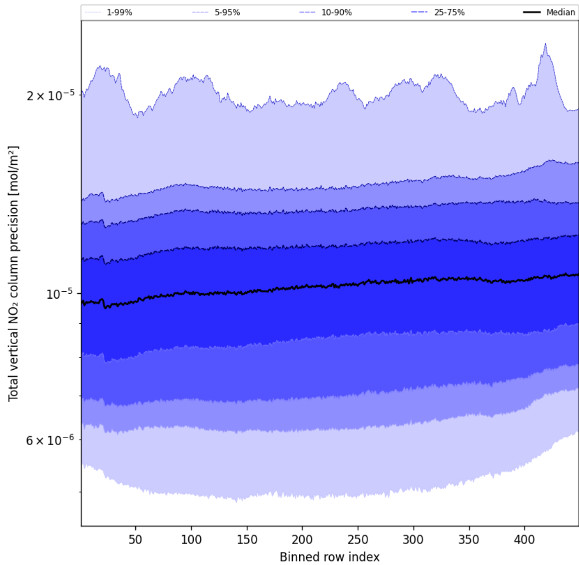
Figure 56: Along track statistics of "Total vertical NO 2 column precision" for 2025-10-12 to 2025-10-14
