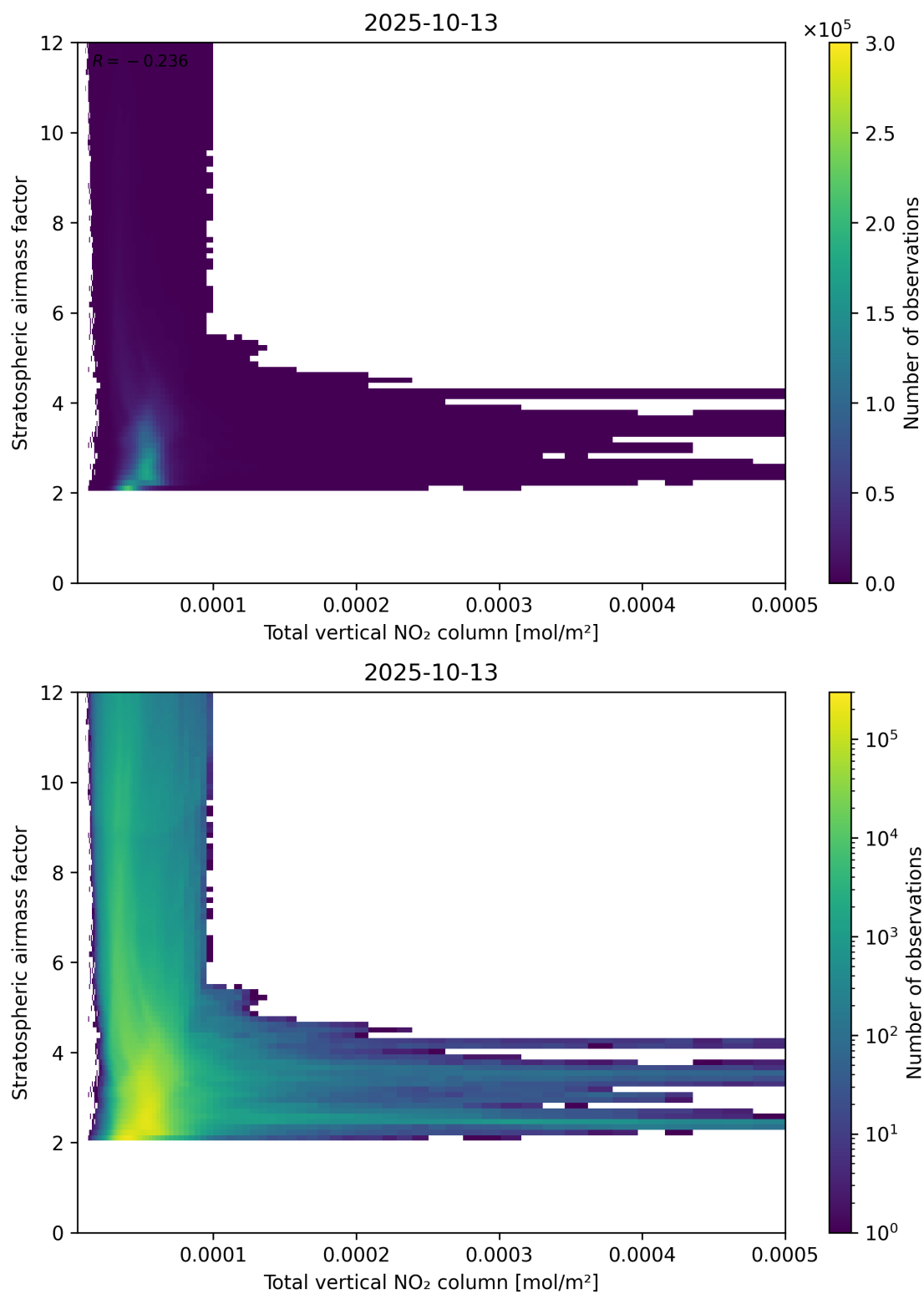
Figure 110: Scatter density plot of “Total vertical NO 2 column” against “Stratospheric airmass factor” for 2025-10-12 to 2025-10-14.
