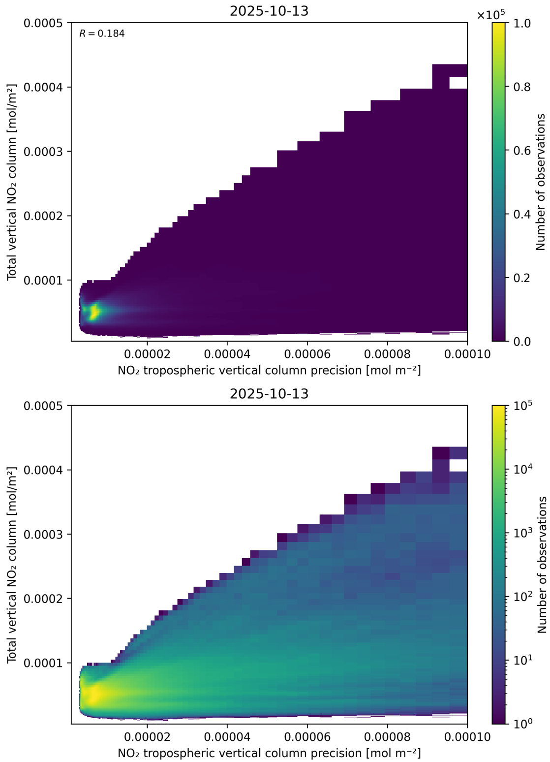
Figure 138: Scatter density plot of “NO 2 tropospheric vertical column precision” against “Total vertical NO 2 column” for 2025-10-12 to 2025-10-14.
