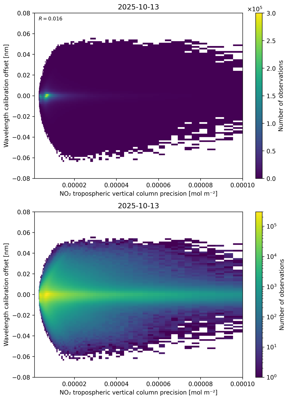
Figure 141: Scatter density plot of “NO 2 tropospheric vertical column precision” against “Wavelength calibration offset” for 2025-10-12 to 2025-10-14.
