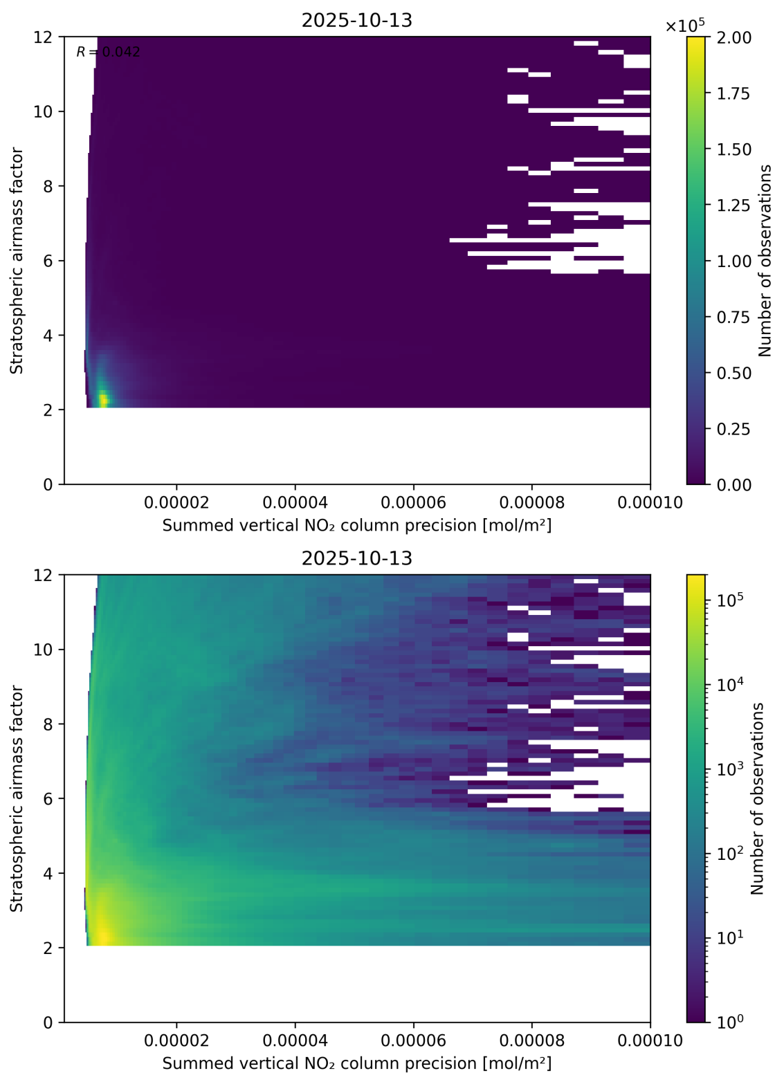
Figure 106: Scatter density plot of “Summed vertical NO 2 column precision” against “Stratospheric airmass factor” for 2025-10-12 to 2025-10-14.
