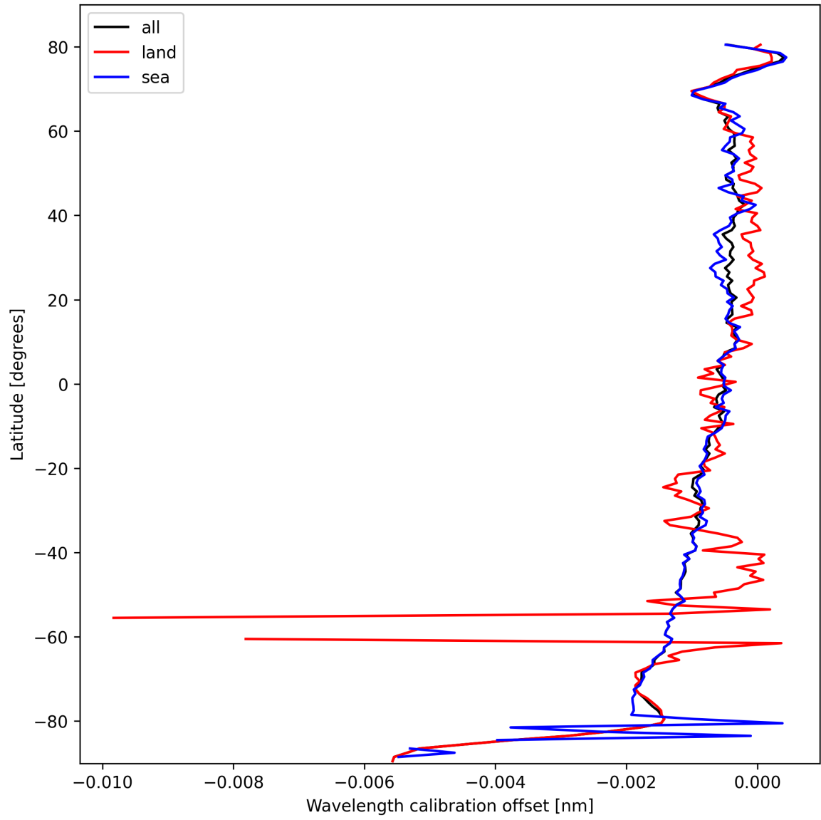
Figure 18: Zonal average of “Wavelength calibration offset” for 2025-10-12 to 2025-10-14.
