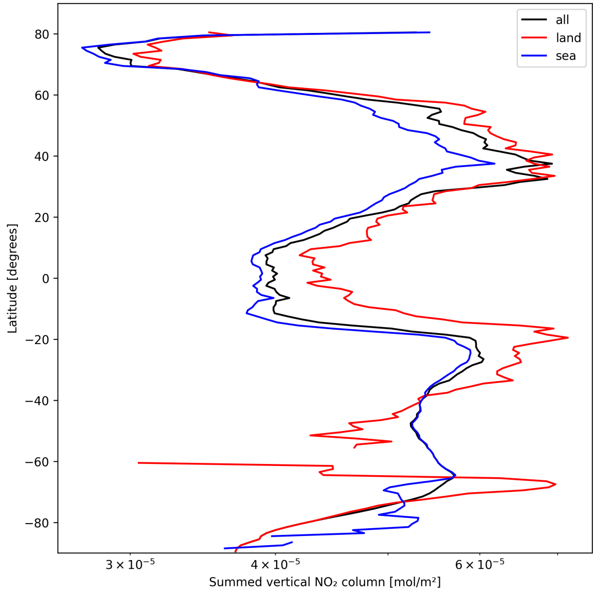
Figure 23: Zonal average of “Summed vertical NO 2 column” for 2025-10-12 to 2025-10-14.
