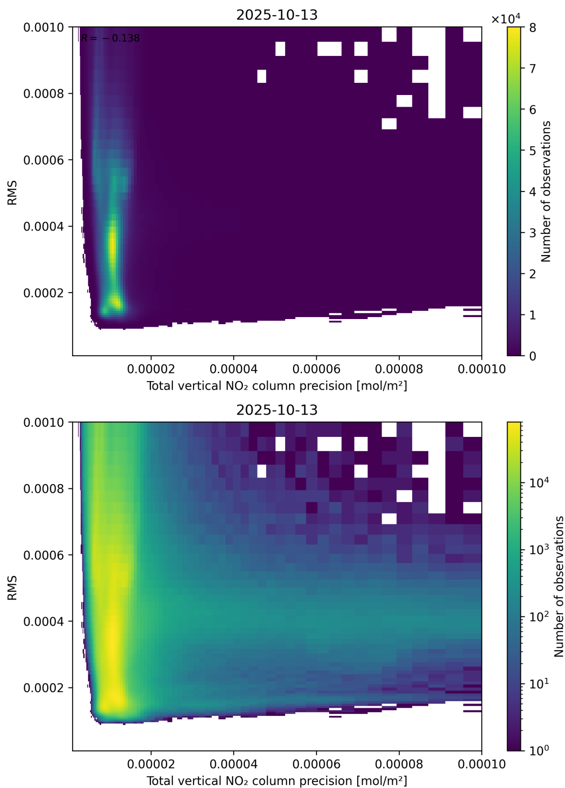
Figure 119: Scatter density plot of “Total vertical NO 2 column precision” against “RMS” for 2025-10-12 to 2025-10-14.
