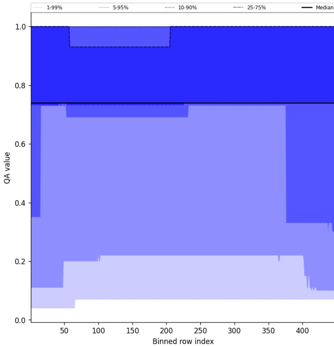
Figure 45: Along track statistics of “QA value” for 2025-10-12 to 2025-10-14
