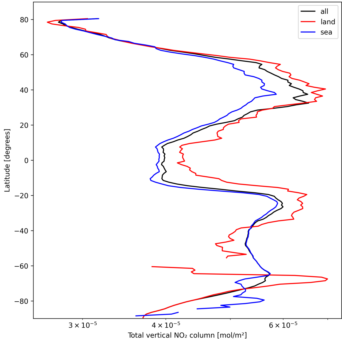
Figure 21: Zonal average of “Total vertical NO 2 column” for 2025-10-12 to 2025-10-14.
