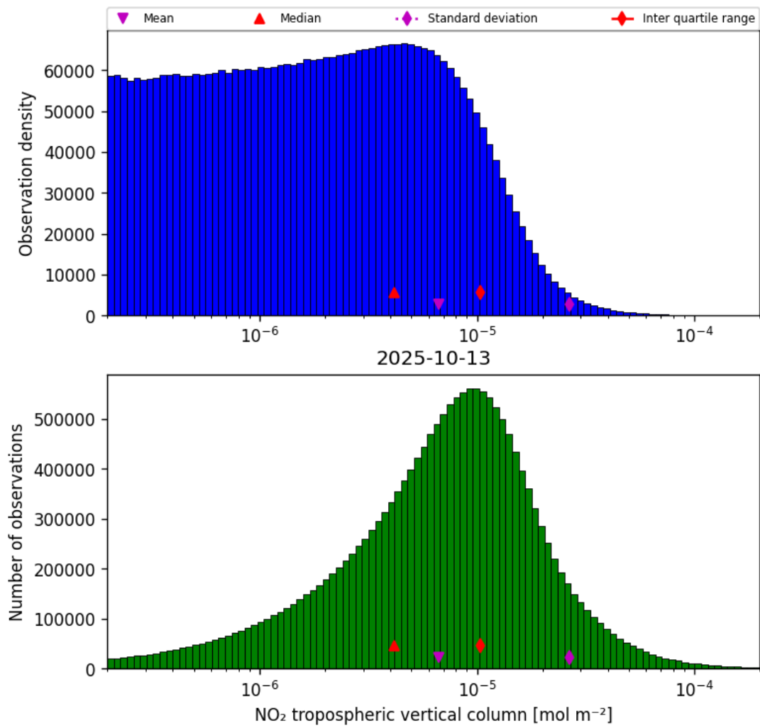
Figure 29: Histogram of “NO 2 tropospheric vertical column” for 2025-10-12 to 2025-10-14
