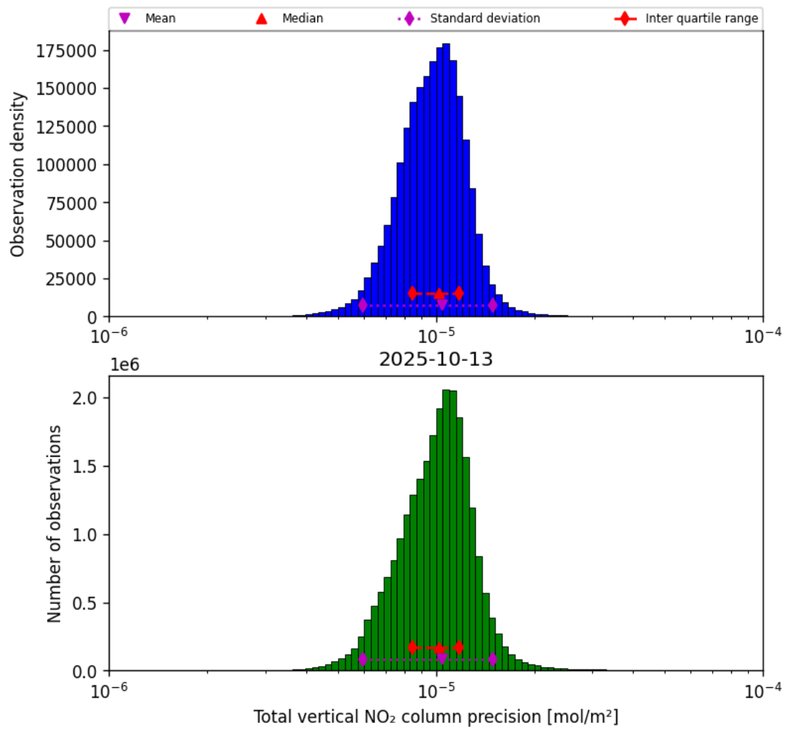
Figure 39: Histogram of “Total vertical NO 2 column precision” for 2025-10-12 to 2025-10-14
