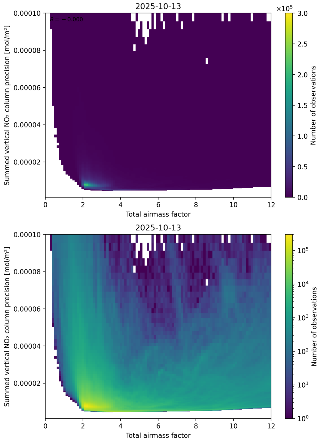
Figure 66: Scatter density plot of “Total airmass factor” against “Summed vertical NO 2 column precision” for 2025-10-12 to 2025-10-14.
