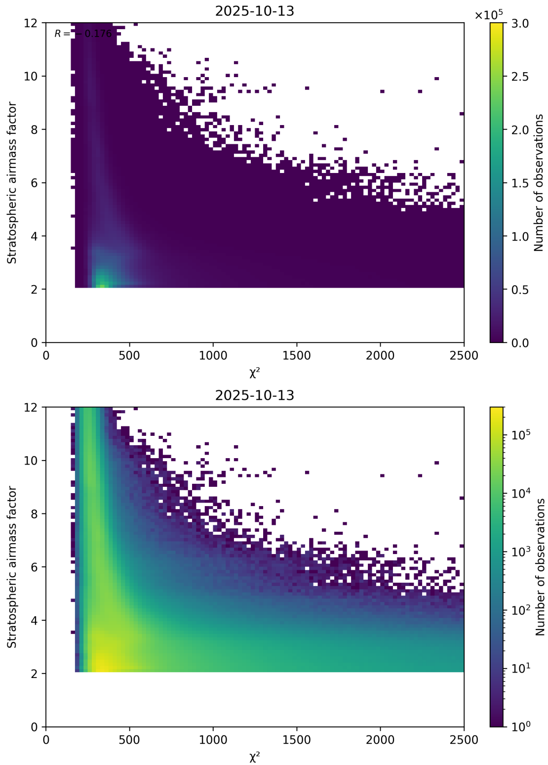
Figure 81: Scatter density plot of “ \chi^2 ” against “Stratospheric airmass factor” for 2025-10-12 to 2025-10-14.
