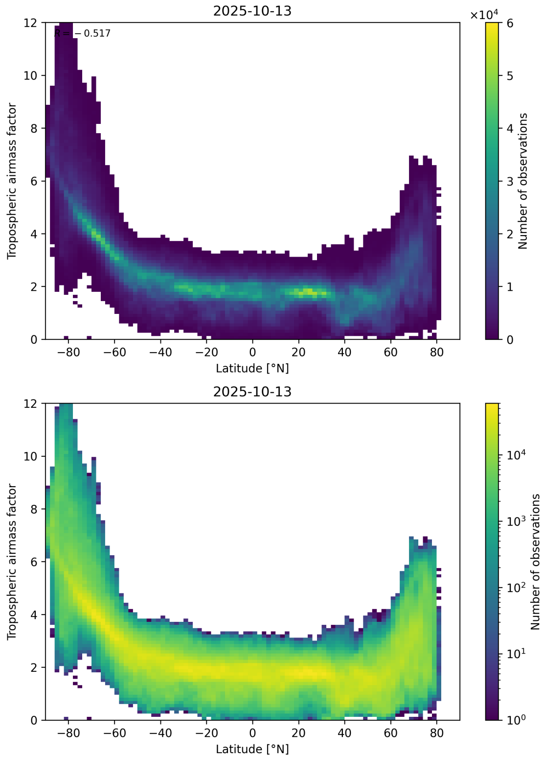
Figure 85: Scatter density plot of “Latitude” against “Tropospheric airmass factor” for 2025-10-12 to 2025-10-14.
