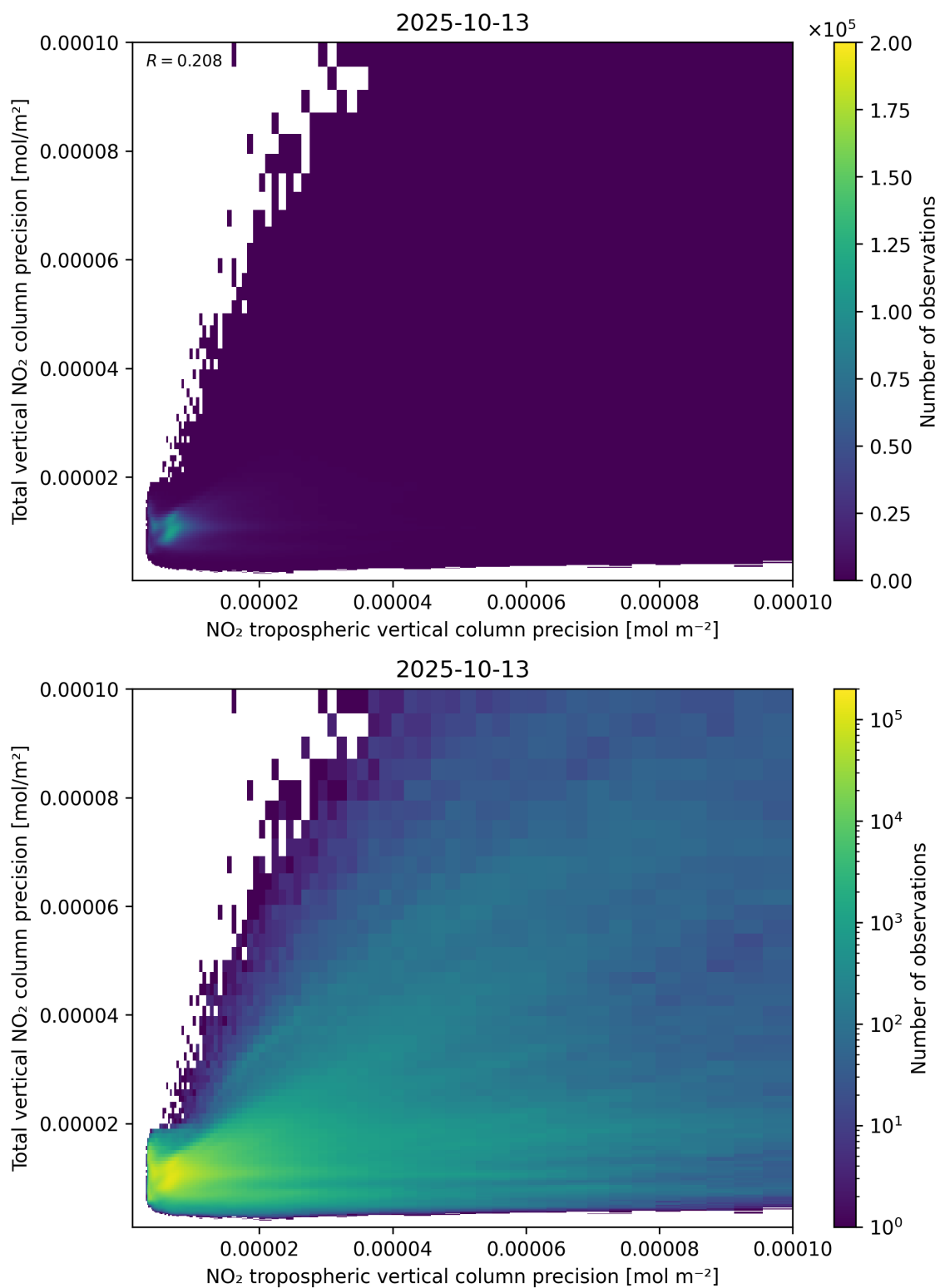
Figure 139: Scatter density plot of “NO 2 tropospheric vertical column precision” against “Total vertical NO 2 column precision” for 2025-10-12 to 2025-10-14.
