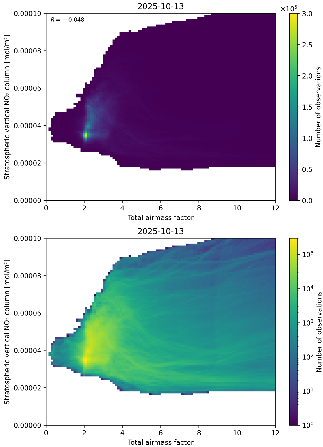
Figure 64: Scatter density plot of “Total airmass factor” against “Stratospheric vertical NO 2 column” for 2025-10-12 to 2025-10-14.
