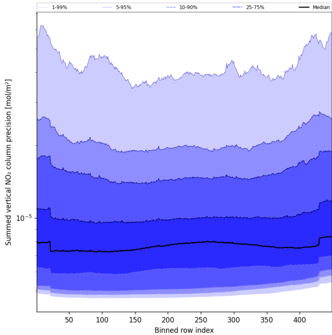
Figure 58: Along track statistics of “Summed vertical NO 2 column precision” for 2025-10-12 to 2025-10-14
