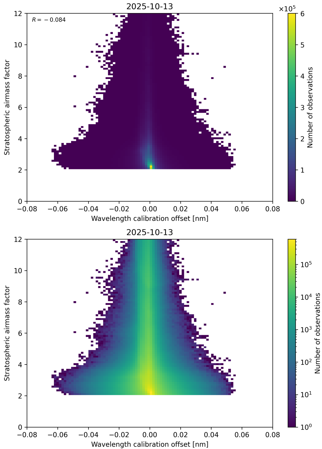
Figure 174: Scatter density plot of “Wavelength calibration offset” against “Stratospheric airmass factor” for 2025-10-12 to 2025-10-14.
