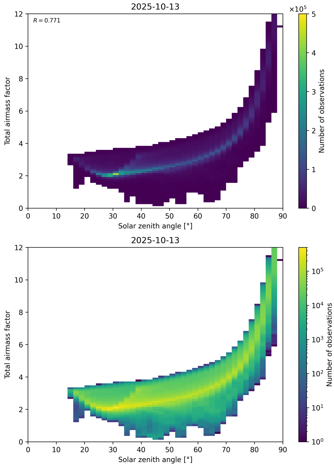
Figure 146: Scatter density plot of “Solar zenith angle” against “Total airmass factor” for 2025-10-12 to 2025-10-14.
