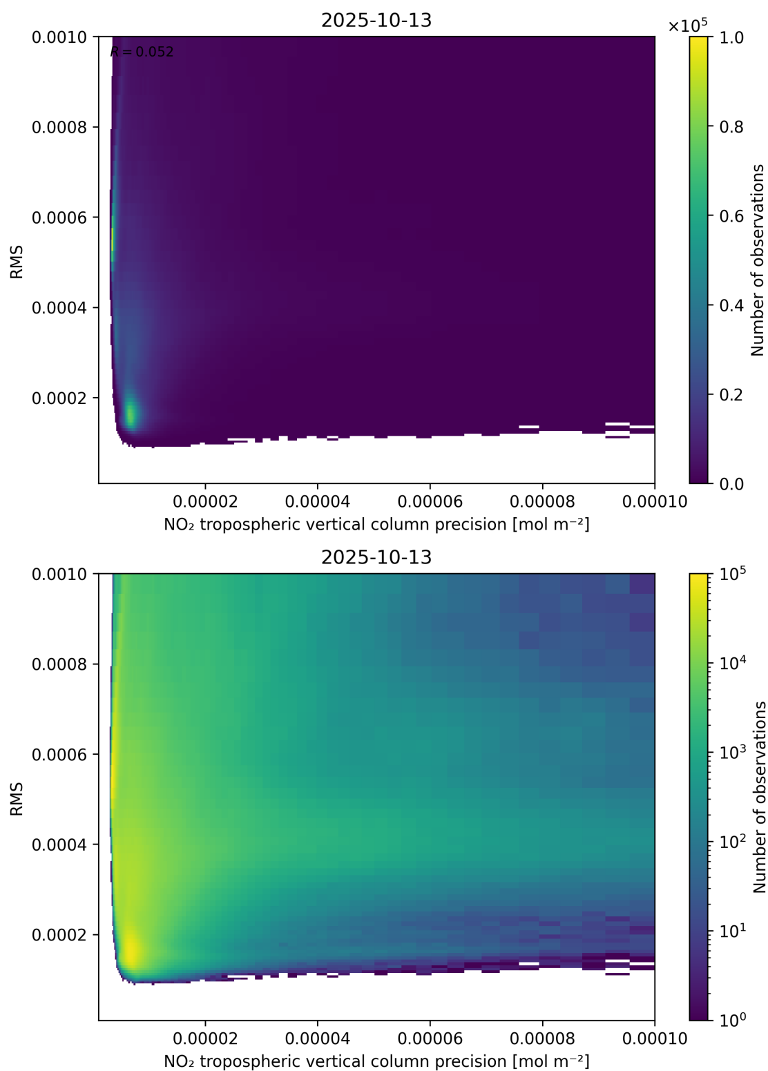
Figure 140: Scatter density plot of “NO 2 tropospheric vertical column precision” against “RMS” for 2025-10-12 to 2025-10-14.
