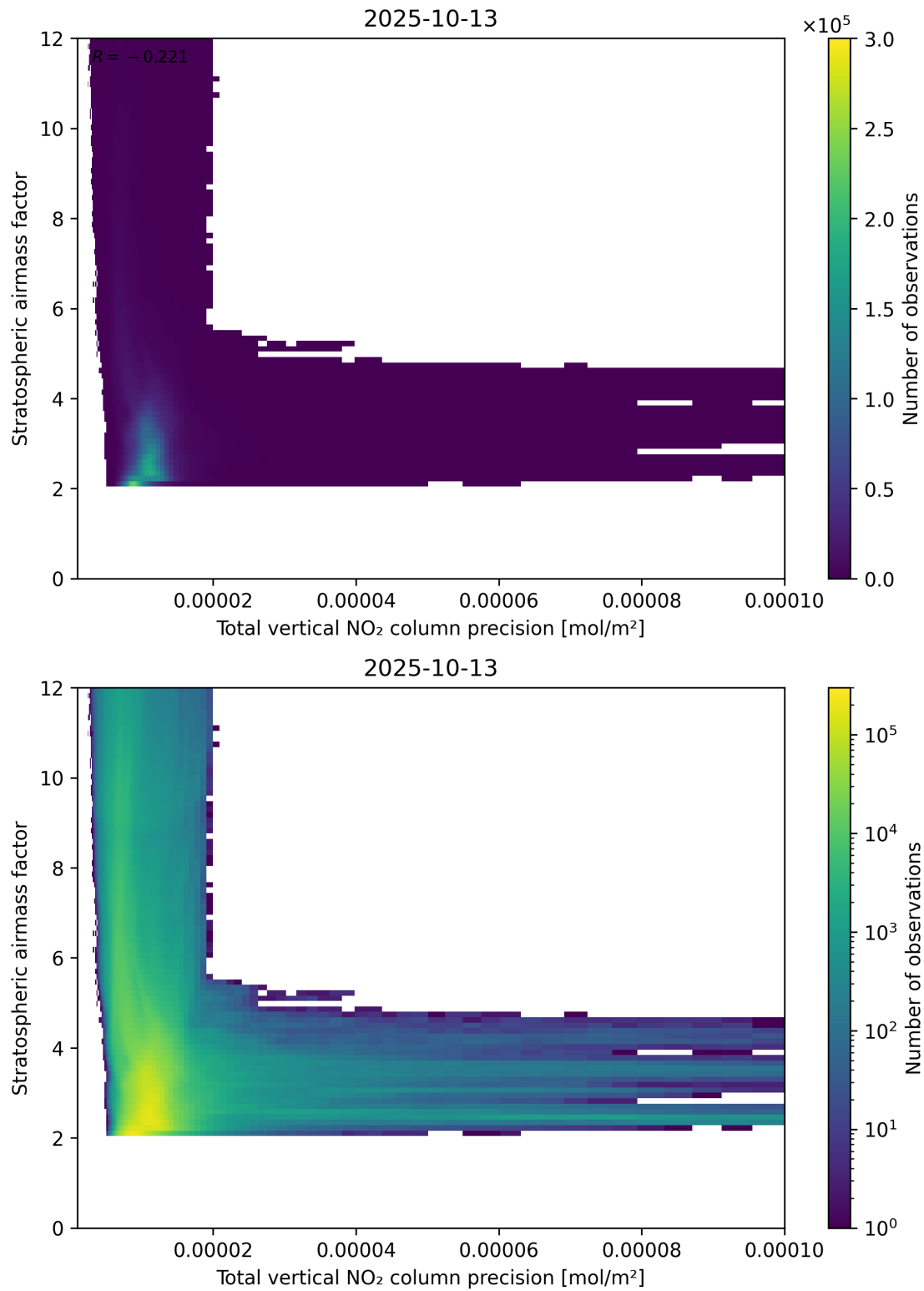
Figure 115: Scatter density plot of “Total vertical NO 2 column precision” against “Stratospheric airmass factor” for 2025-10-12 to 2025-10-14.
