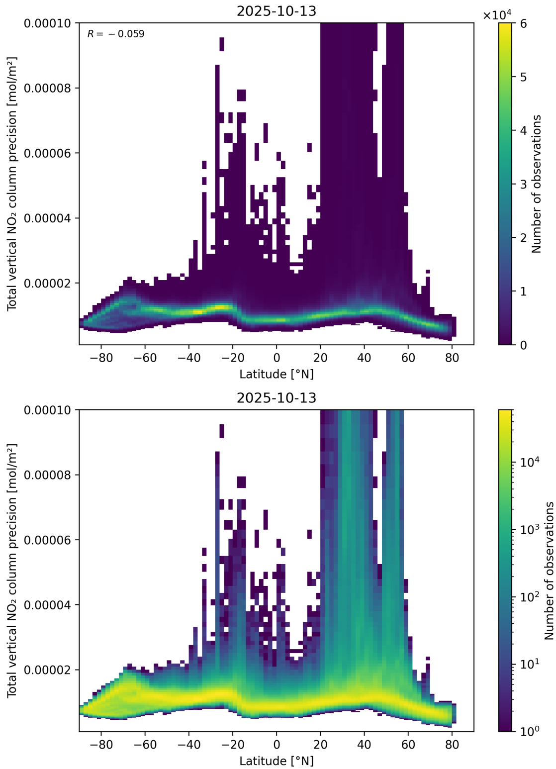
Figure 91: Scatter density plot of “Latitude” against “Total vertical NO 2 column precision” for 2025-10-12 to 2025-10-14.
