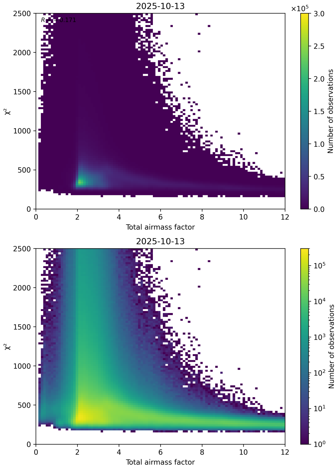
Figure 63: Scatter density plot of “Total airmass factor” against “ \chi^2 ” for 2025-10-12 to 2025-10-14.
