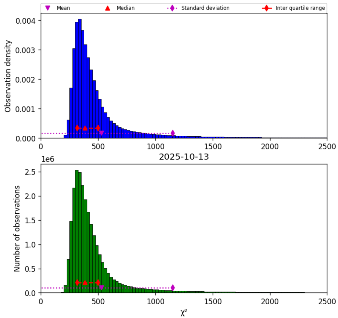
Figure 42: Histogram of “ \chi^2 ” for 2025-10-12 to 2025-10-14
