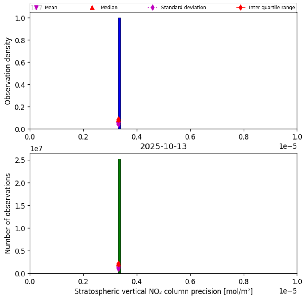
Figure 37: Histogram of “Stratospheric vertical NO 2 column precision” for 2025-10-12 to 2025-10-14
