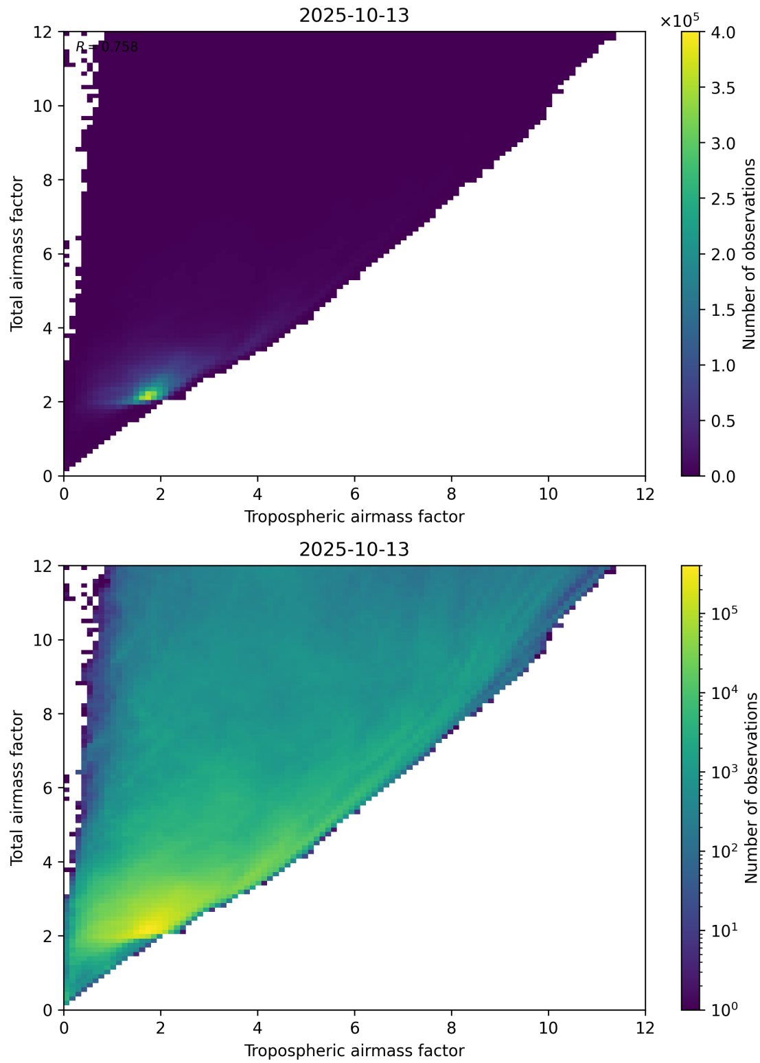
Figure 72: Scatter density plot of “Tropospheric airmass factor” against “Total airmass factor” for 2025-10-12 to 2025-10-14.
