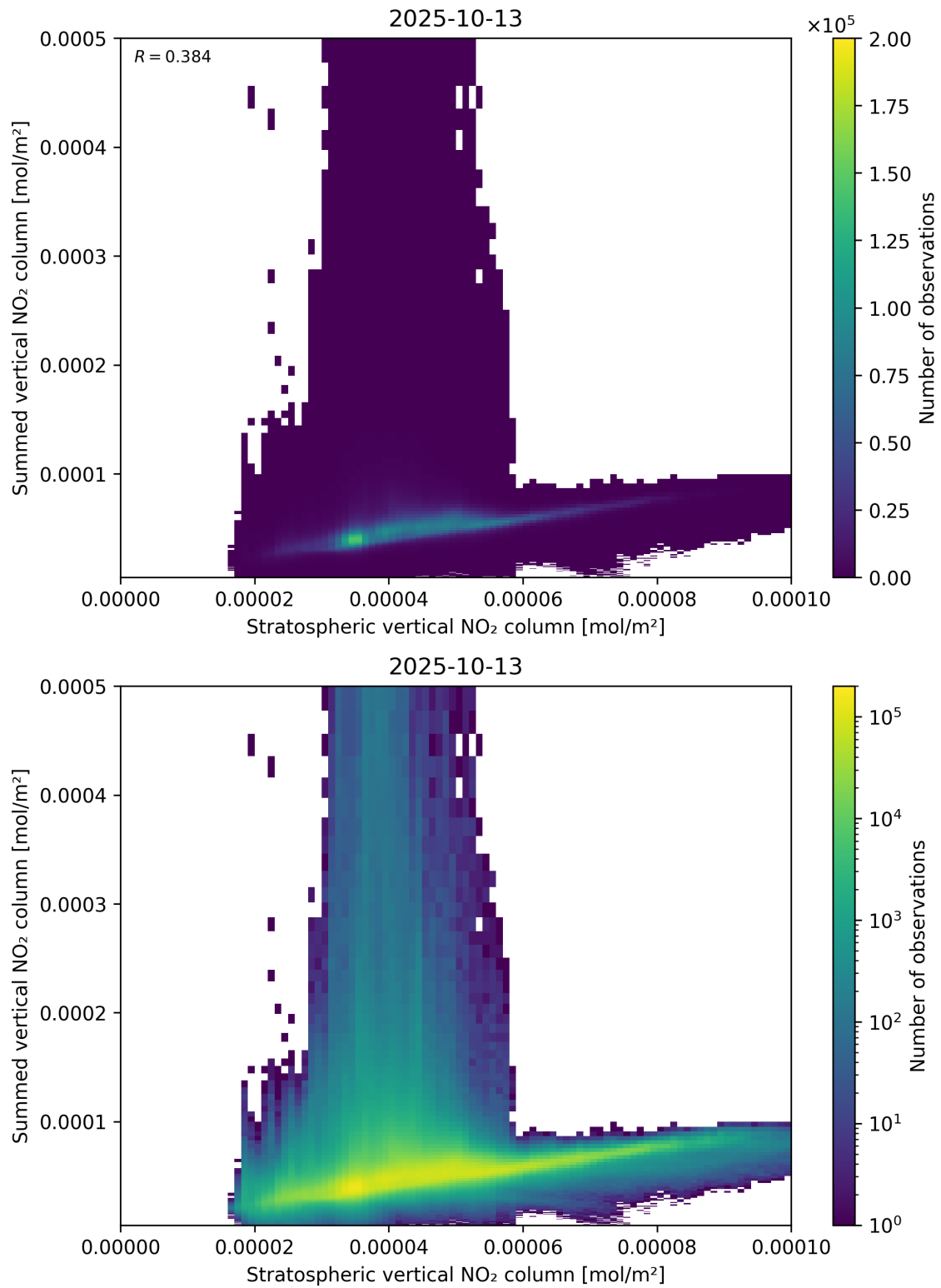
Figure 98: Scatter density plot of “Stratospheric vertical NO 2 column” against “Summed vertical NO 2 column” for 2025-10-12 to 2025-10-14.
