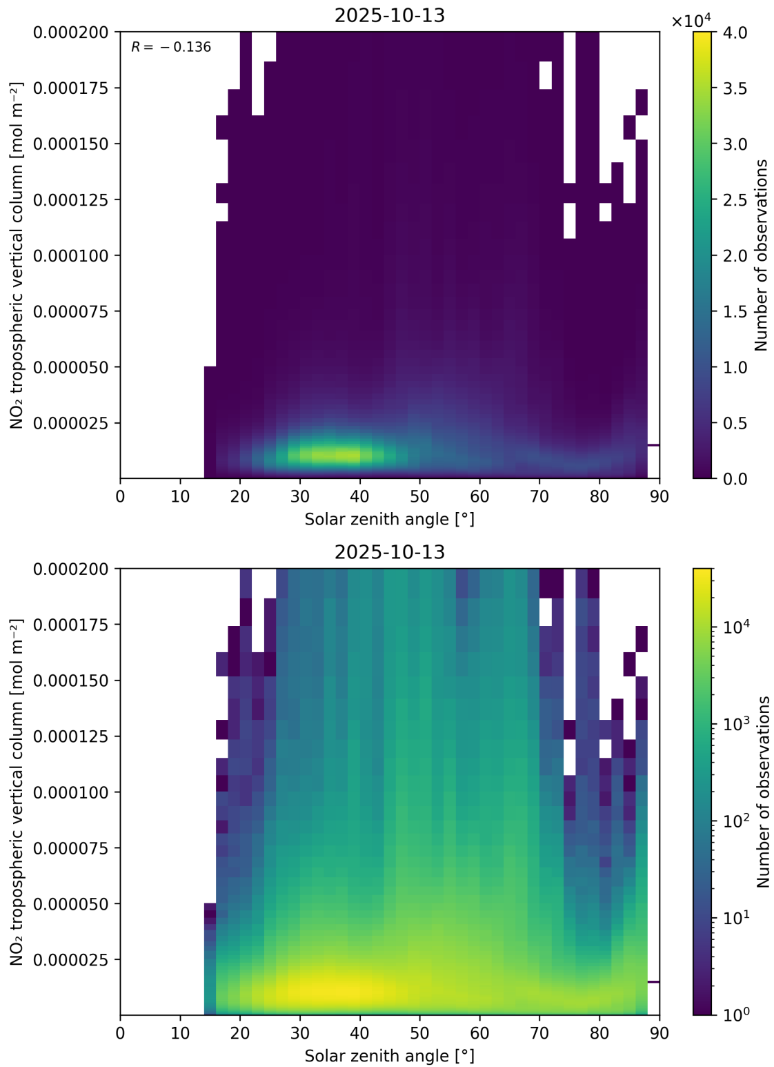
Figure 155: Scatter density plot of “Solar zenith angle” against “NO 2 tropospheric vertical column” for 2025-10-12 to 2025-10-14.
