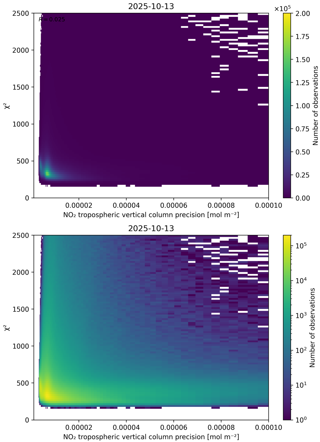
Figure 134: Scatter density plot of “NO 2 tropospheric vertical column precision” against “ \chi^2 ” for 2025-10-12 to 2025-10-14.
