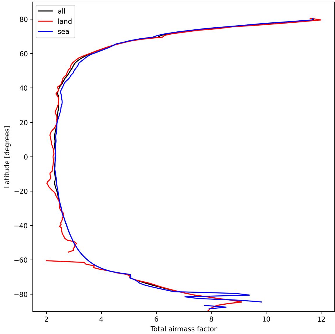
Figure 15: Zonal average of “Total airmass factor” for 2025-10-12 to 2025-10-14.
