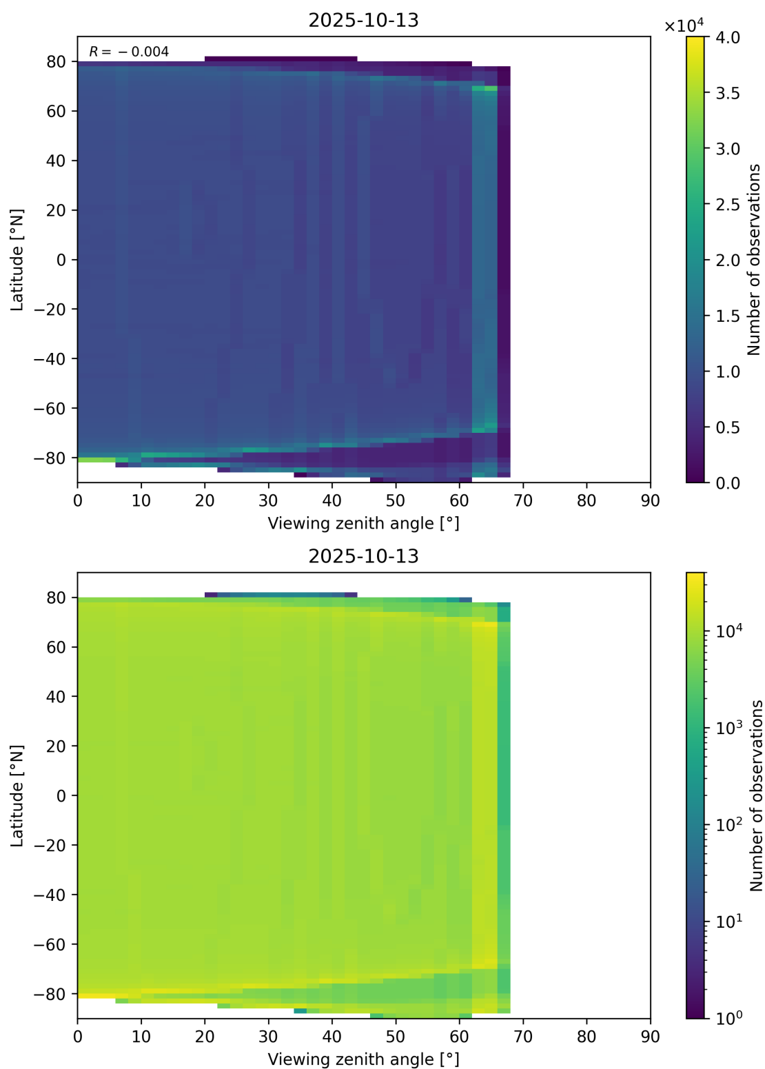
Figure 163: Scatter density plot of “Viewing zenith angle” against “Latitude” for 2025-10-12 to 2025-10-14.
