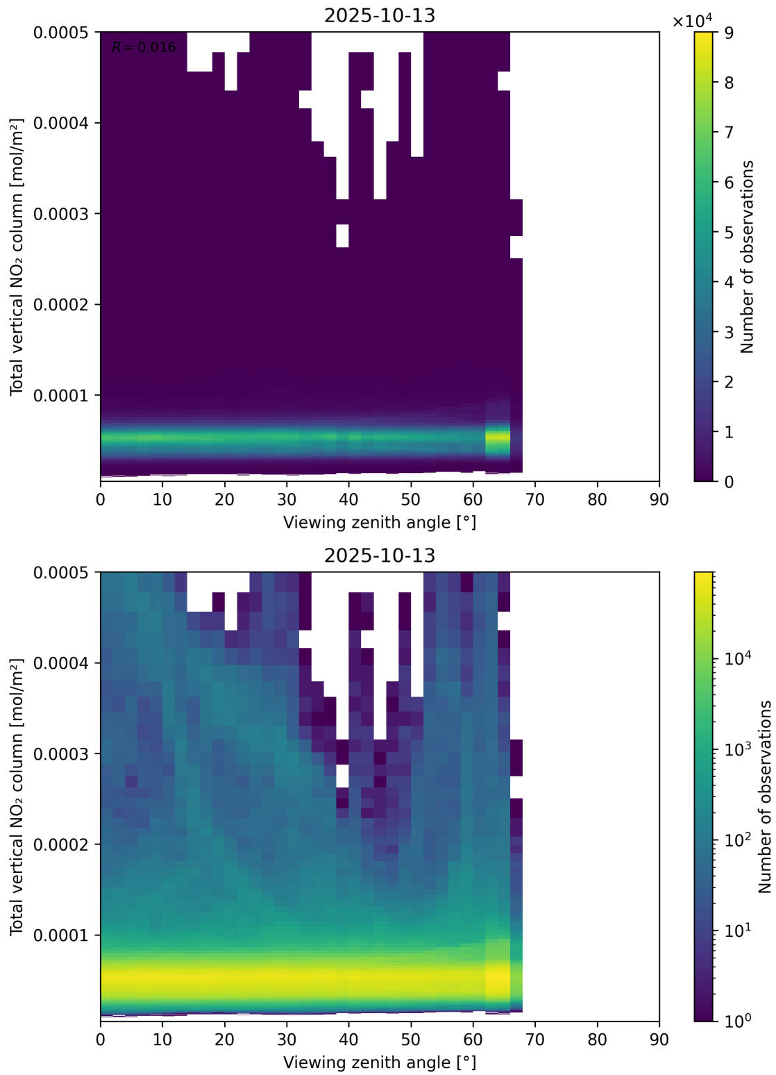
Figure 167: Scatter density plot of “Viewing zenith angle” against “Total vertical NO 2 column” for 2025-10-12 to 2025-10-14.
