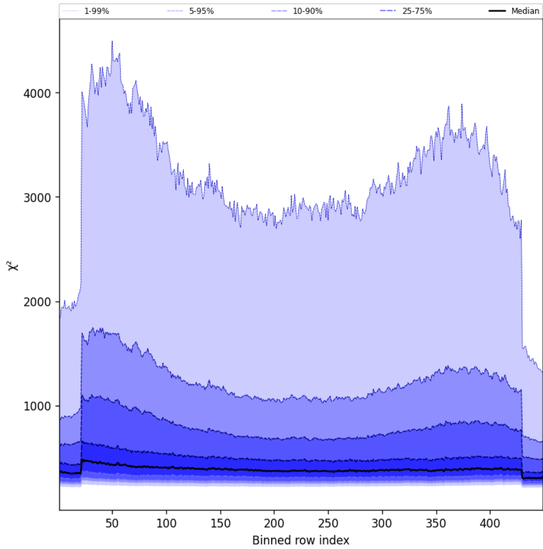
Figure 59: Along track statistics of “ \chi^2 ” for 2025-10-12 to 2025-10-14
