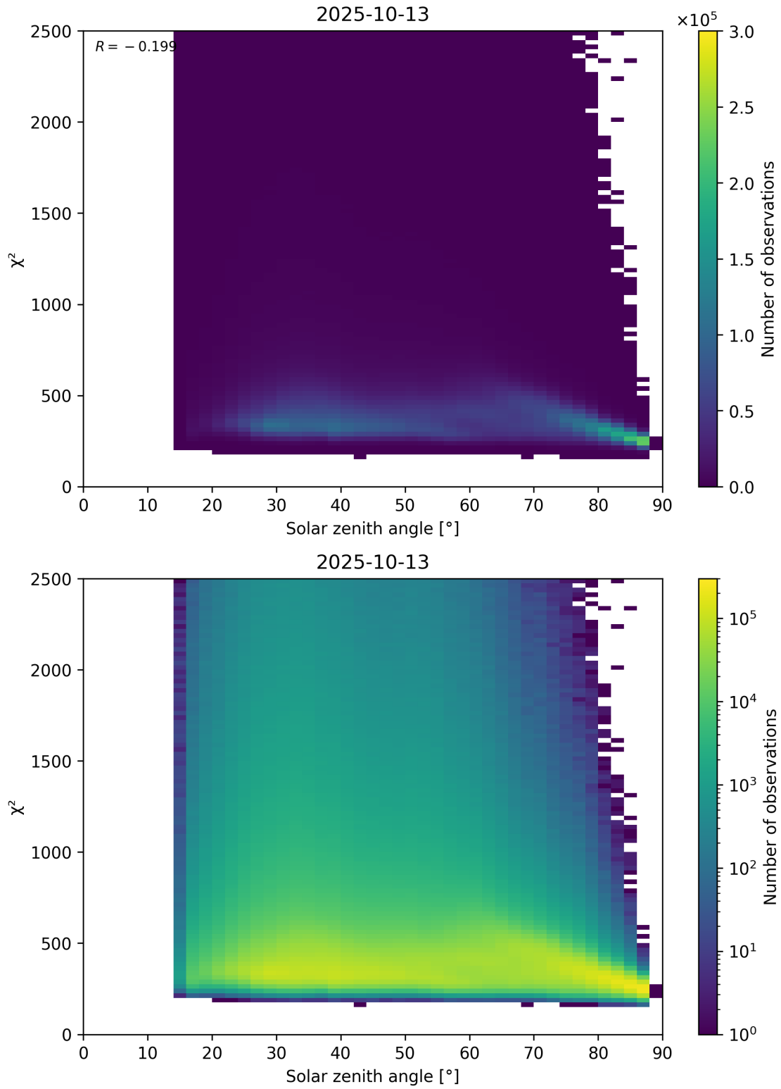
Figure 148: Scatter density plot of “Solar zenith angle” against “ \chi^2 ” for 2025-10-12 to 2025-10-14.
