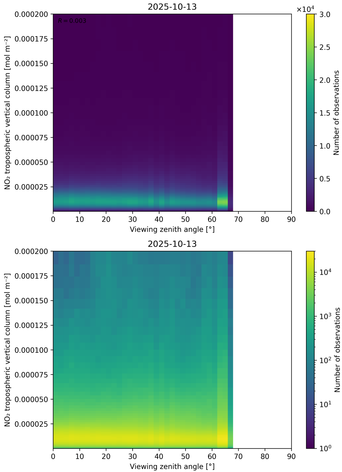
Figure 169: Scatter density plot of “Viewing zenith angle” against “NO 2 tropospheric vertical column” for 2025-10-12 to 2025-10-14.
