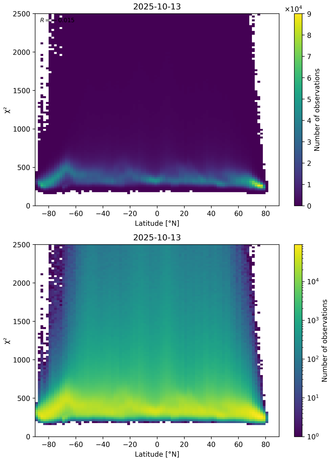
Figure 86: Scatter density plot of “Latitude” against “ \chi^2 ” for 2025-10-12 to 2025-10-14.
