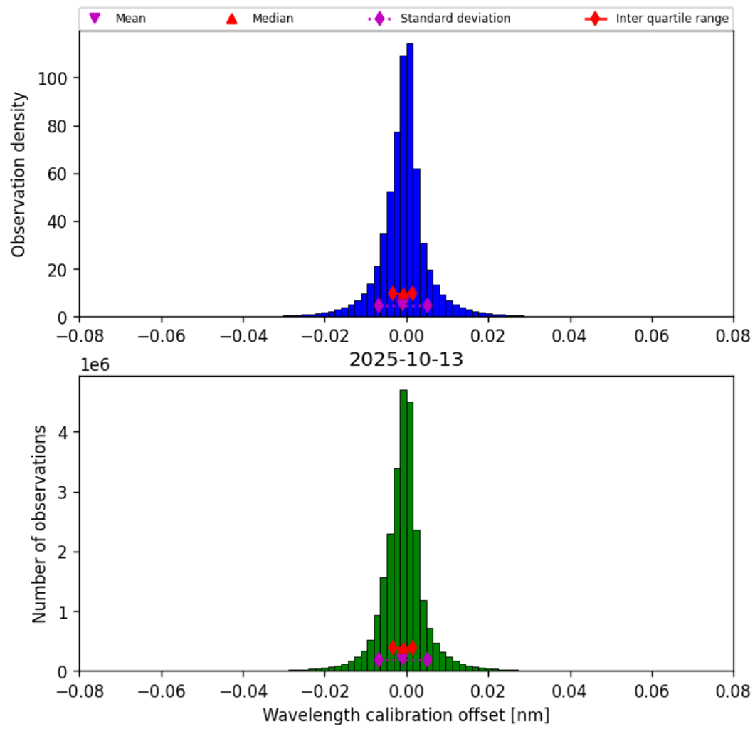
Figure 35: Histogram of “Wavelength calibration offset” for 2025-10-12 to 2025-10-14
