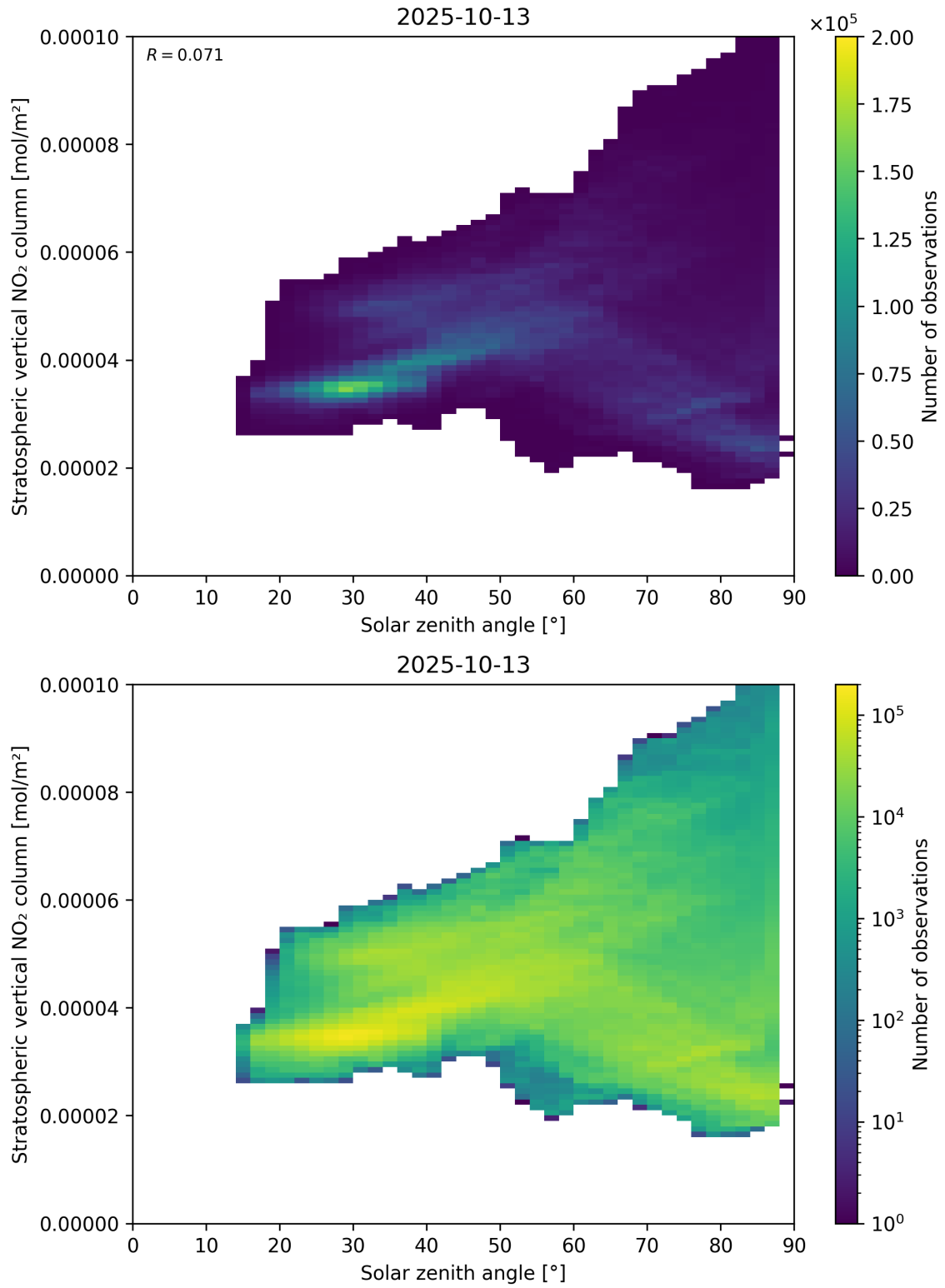
Figure 150: Scatter density plot of “Solar zenith angle” against “Stratospheric vertical NO 2 column” for 2025-10-12 to 2025-10-14.
