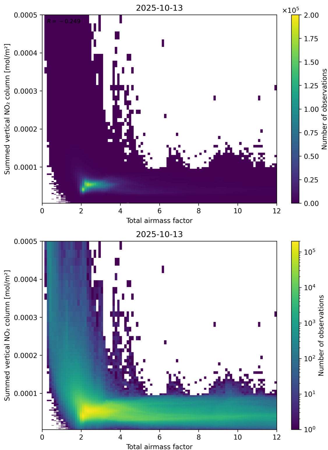
Figure 65: Scatter density plot of “Total airmass factor” against “Summed vertical NO 2 column” for 2025-10-12 to 2025-10-14.
