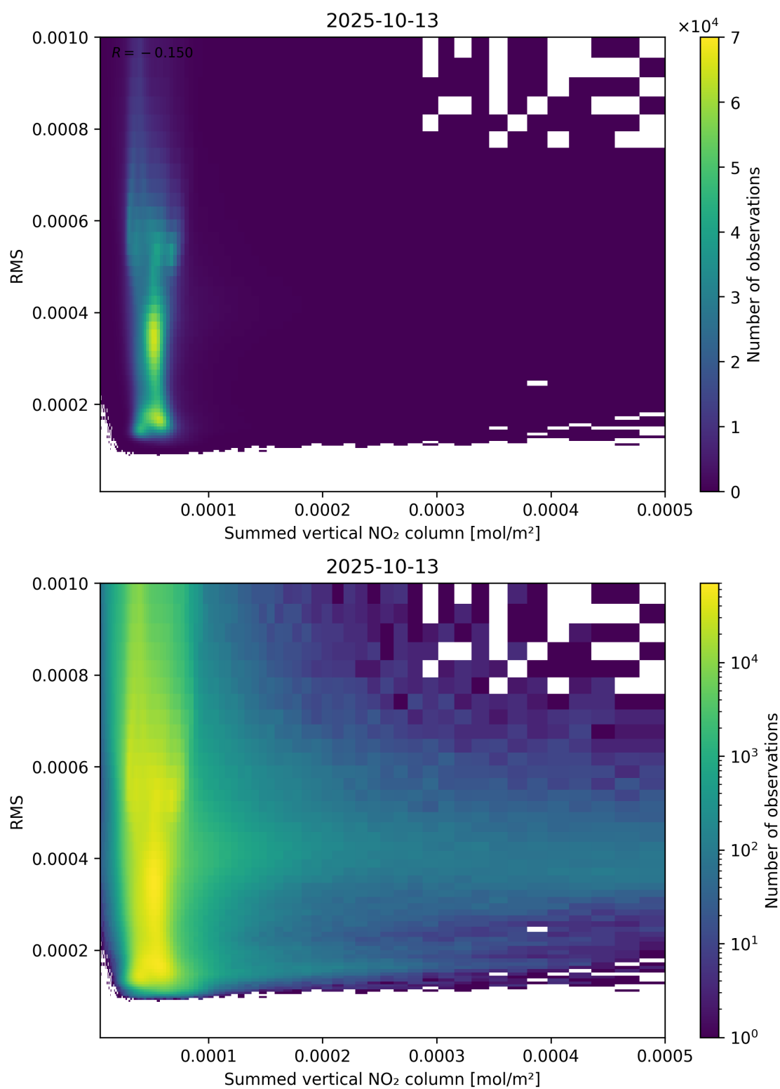
Figure 109: Scatter density plot of “Summed vertical NO 2 column” against “RMS” for 2025-10-12 to 2025-10-14.
