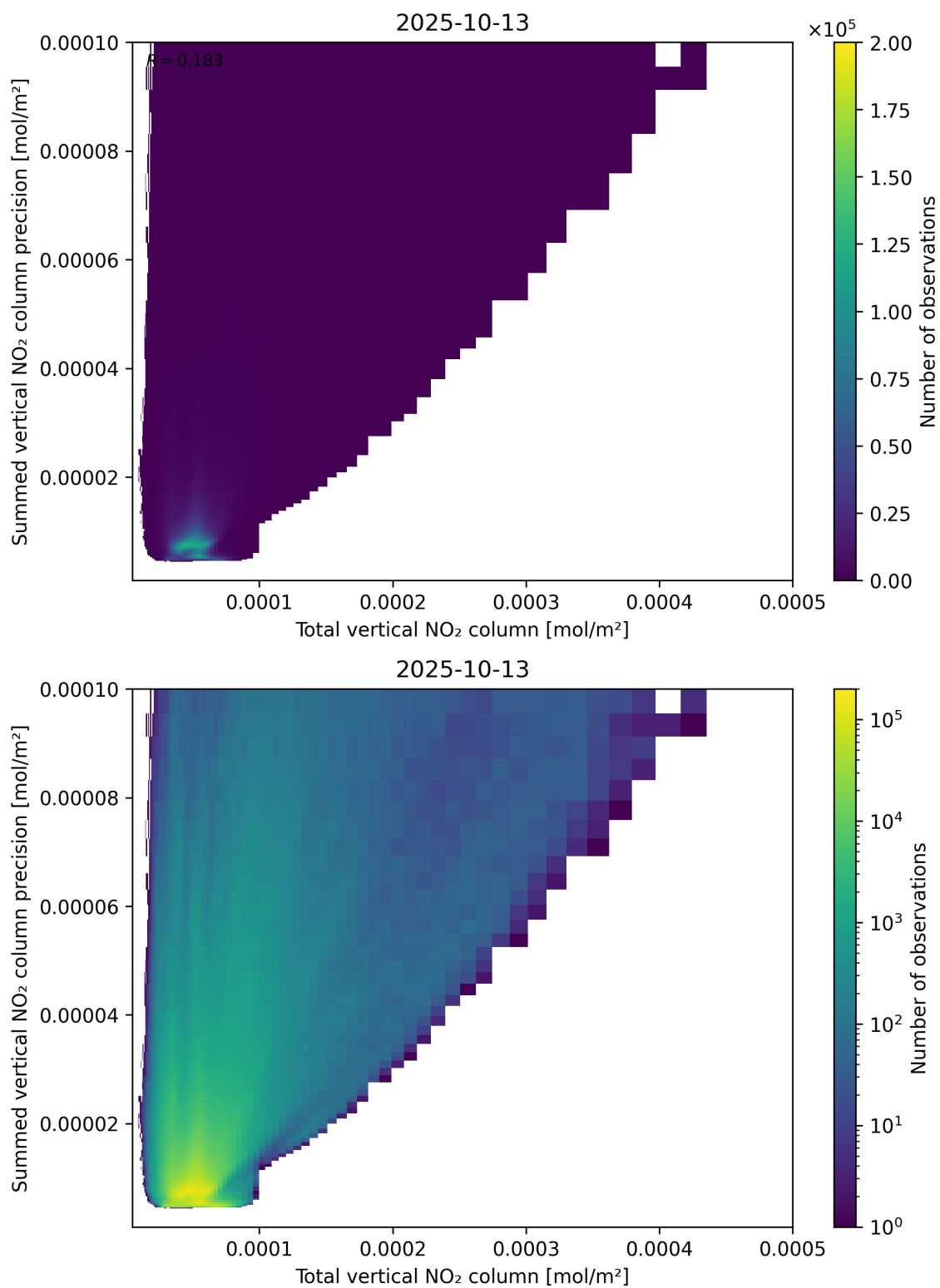
Figure 113: Scatter density plot of “Total vertical NO 2 column” against “Summed vertical NO 2 column precision” for 2025-10-12 to 2025-10-14.
