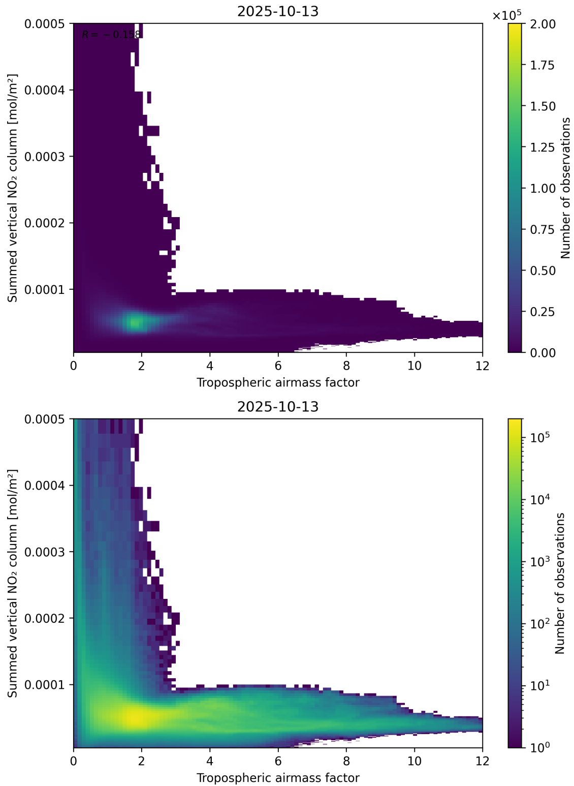
Figure 75: Scatter density plot of “Tropospheric air mass factor” against “Summed vertical NO 2 column” for 2025-10-12 to 2025-10-14.
