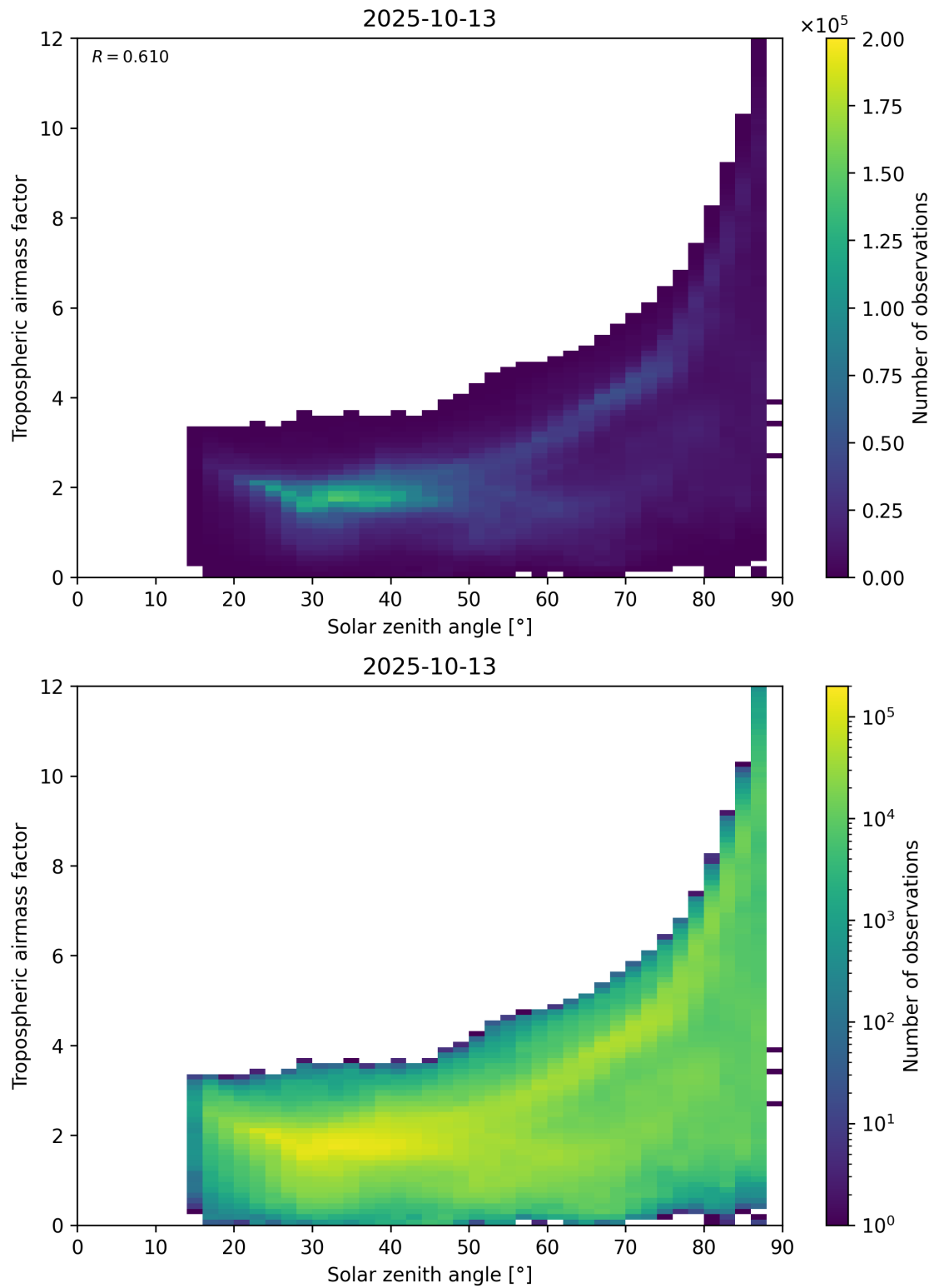
Figure 147: Scatter density plot of “Solar zenith angle” against “Tropospheric airmass factor” for 2025-10-12 to 2025-10-14.
