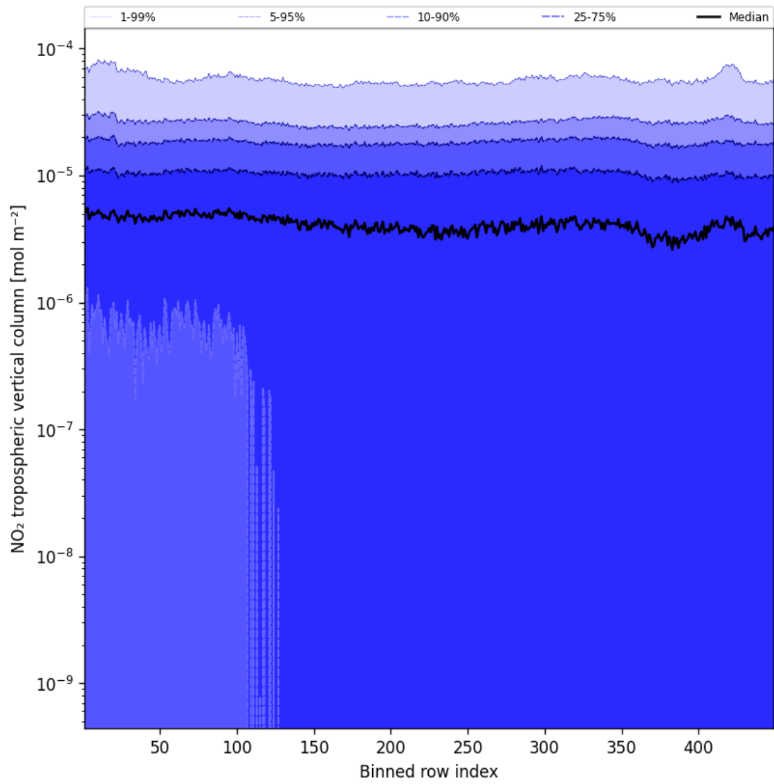
Figure 46: Along track statistics of “NO 2 tropospheric vertical column” for 2025-10-12 to 2025-10-14
