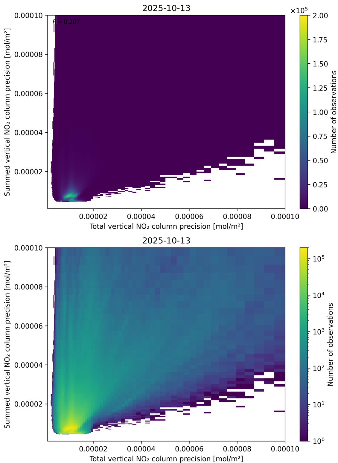
Figure 118: Scatter density plot of “Total vertical NO 2 column precision” against “Summed vertical NO 2 column precision” for 2025-10-12 to 2025-10-14.
