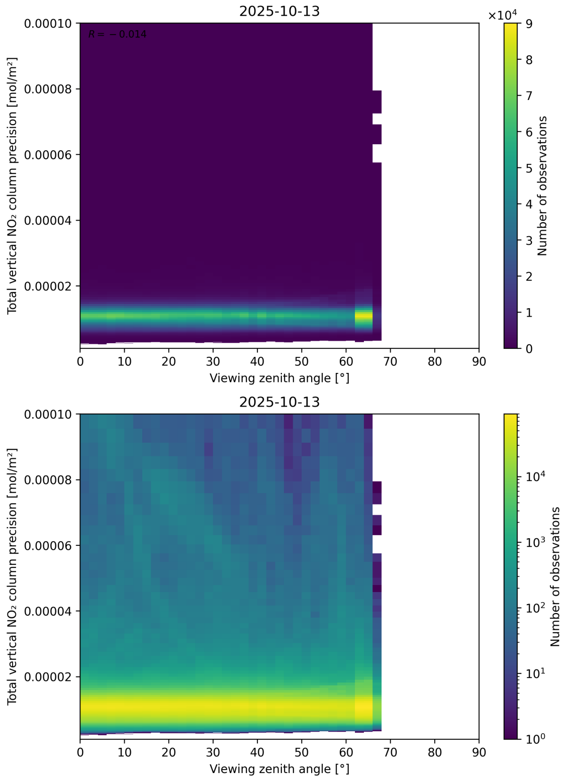
Figure 168: Scatter density plot of “Viewing zenith angle” against “Total vertical NO 2 column precision” for 2025-10-12 to 2025-10-14.
