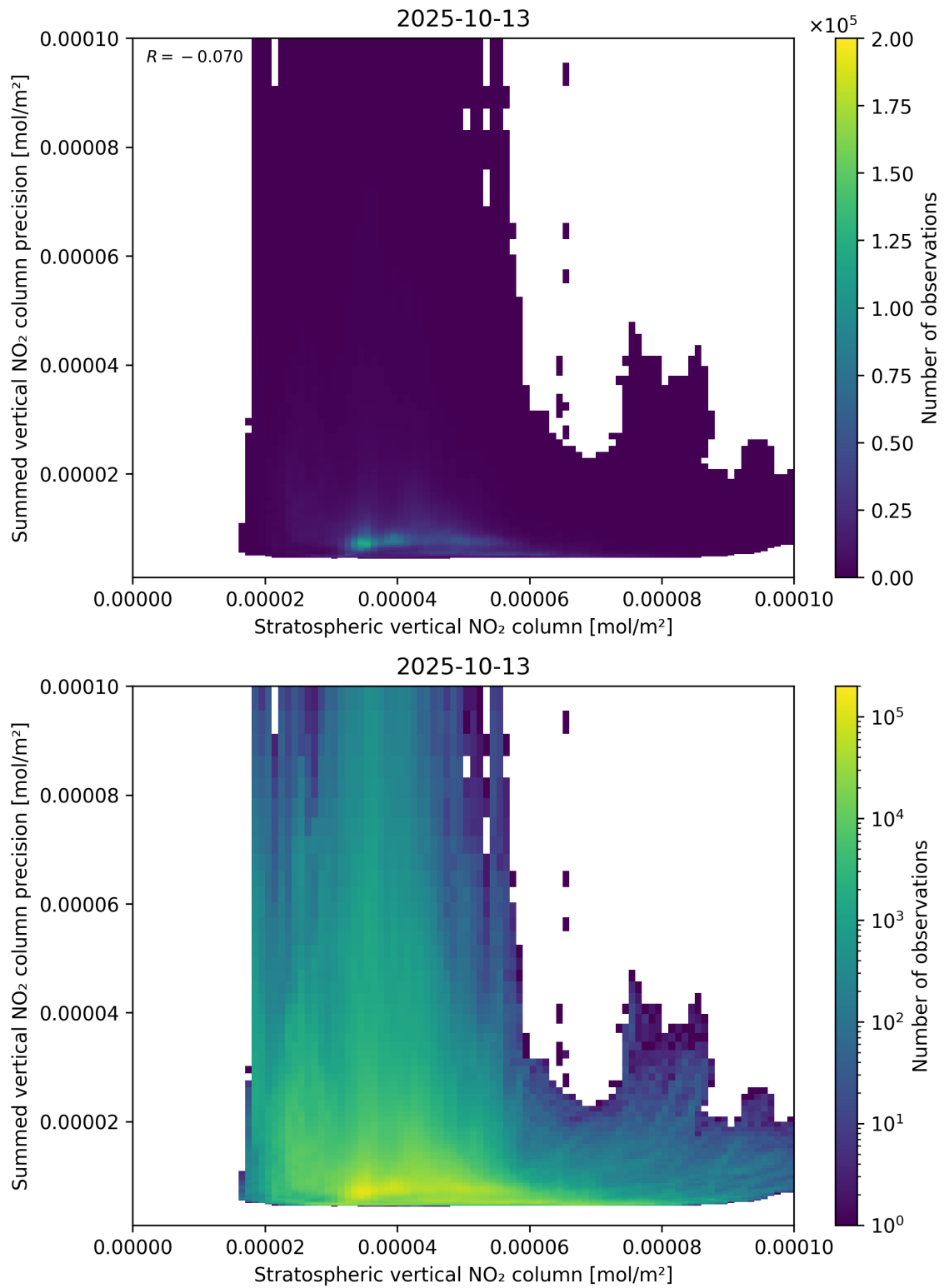
Figure 99: Scatter density plot of “Stratospheric vertical NO 2 column” against “Summed vertical NO 2 column precision” for 2025-10-12 to 2025-10-14.
