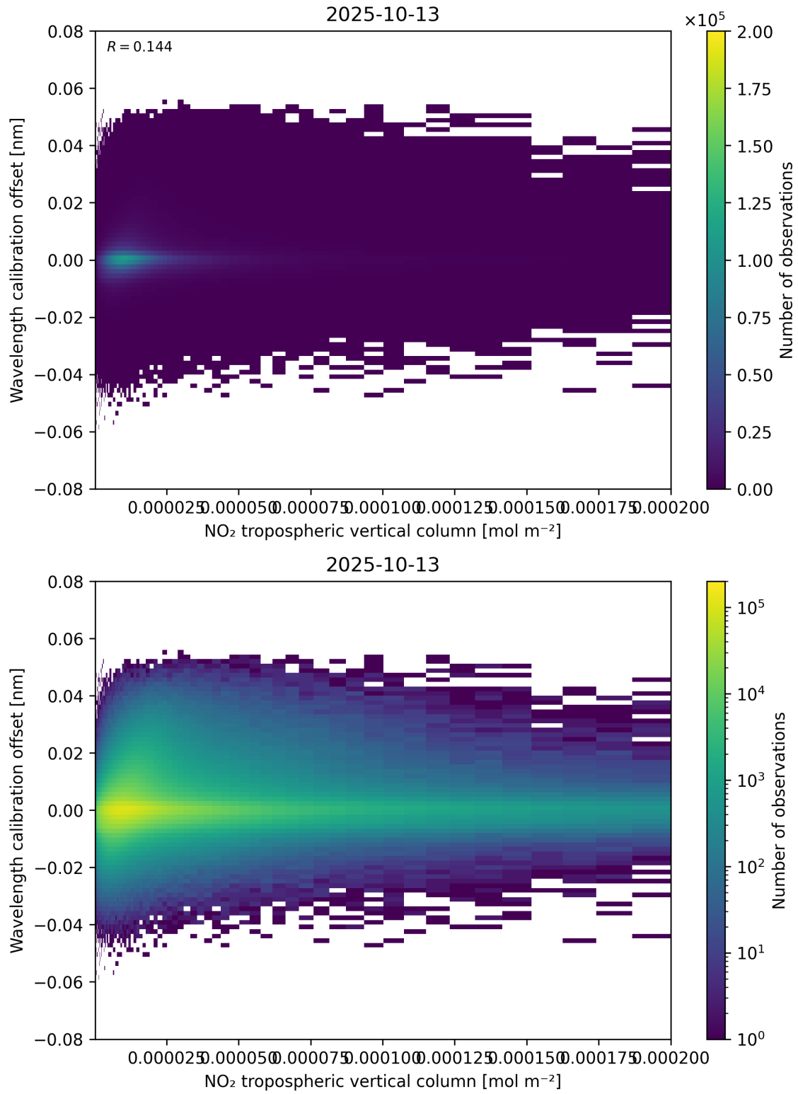
Figure 143: Scatter density plot of “NO 2 tropospheric vertical column” against “Wavelength calibration offset” for 2025-10-12 to 2025-10-14.
