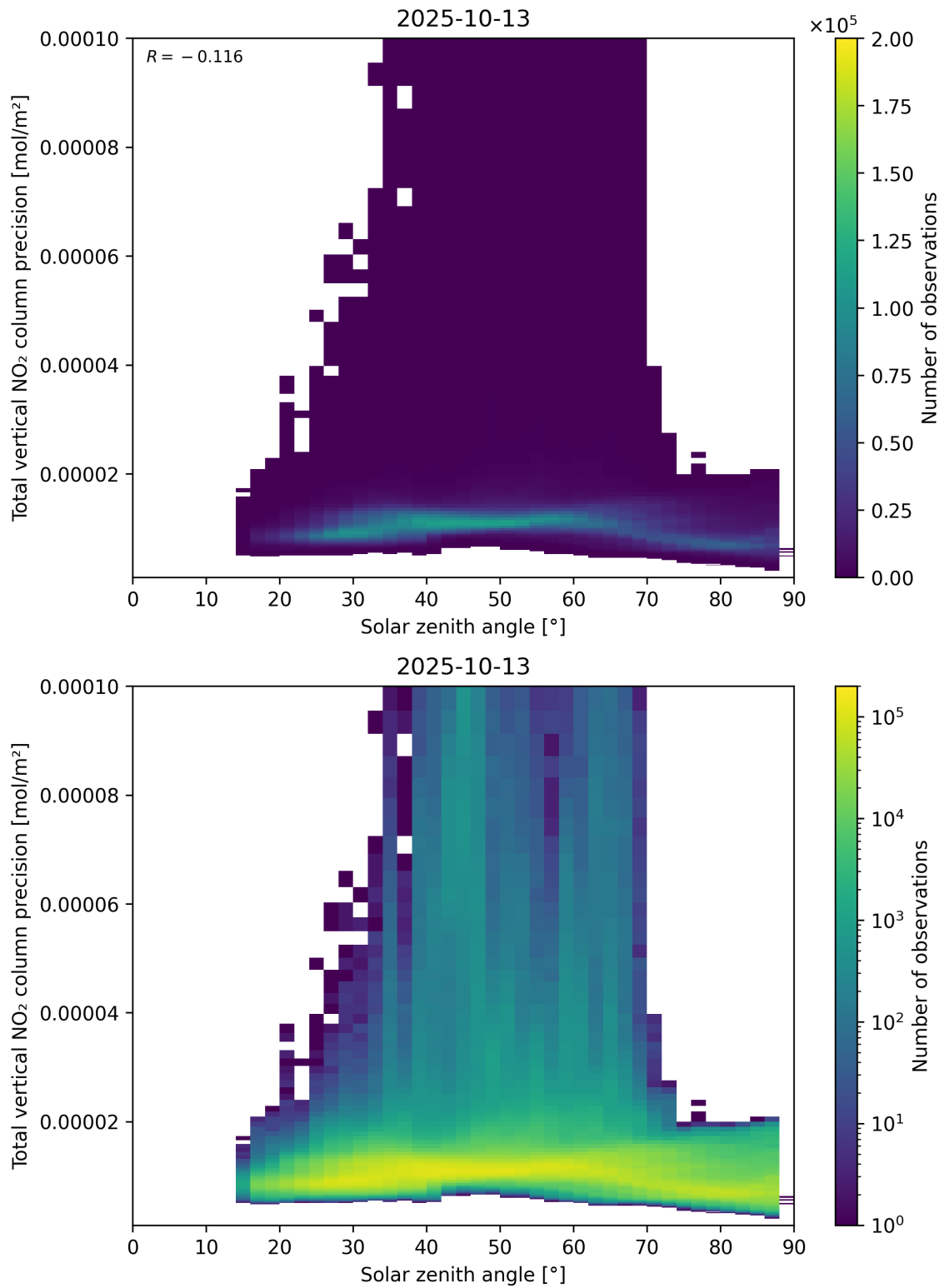
Figure 154: Scatter density plot of “Solar zenith angle” against “Total vertical NO 2 column precision” for 2025-10-12 to 2025-10-14.
