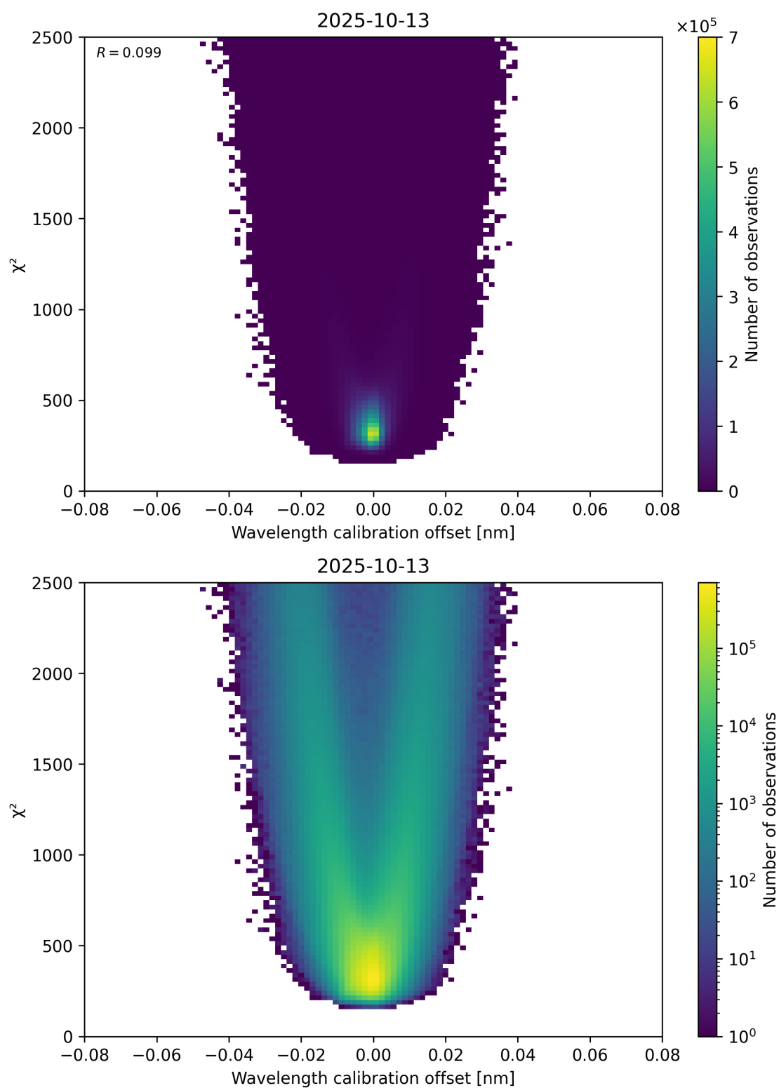
Figure 175: Scatter density plot of “Wavelength calibration offset” against “ \chi^2 ” for 2025-10-12 to 2025-10-14.
