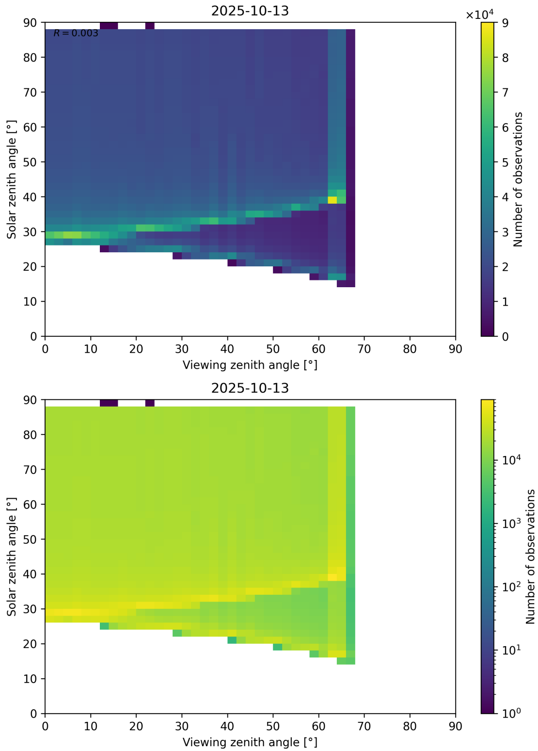
Figure 172: Scatter density plot of “Viewing zenith angle” against “Solar zenith angle” for 2025-10-12 to 2025-10-14.
