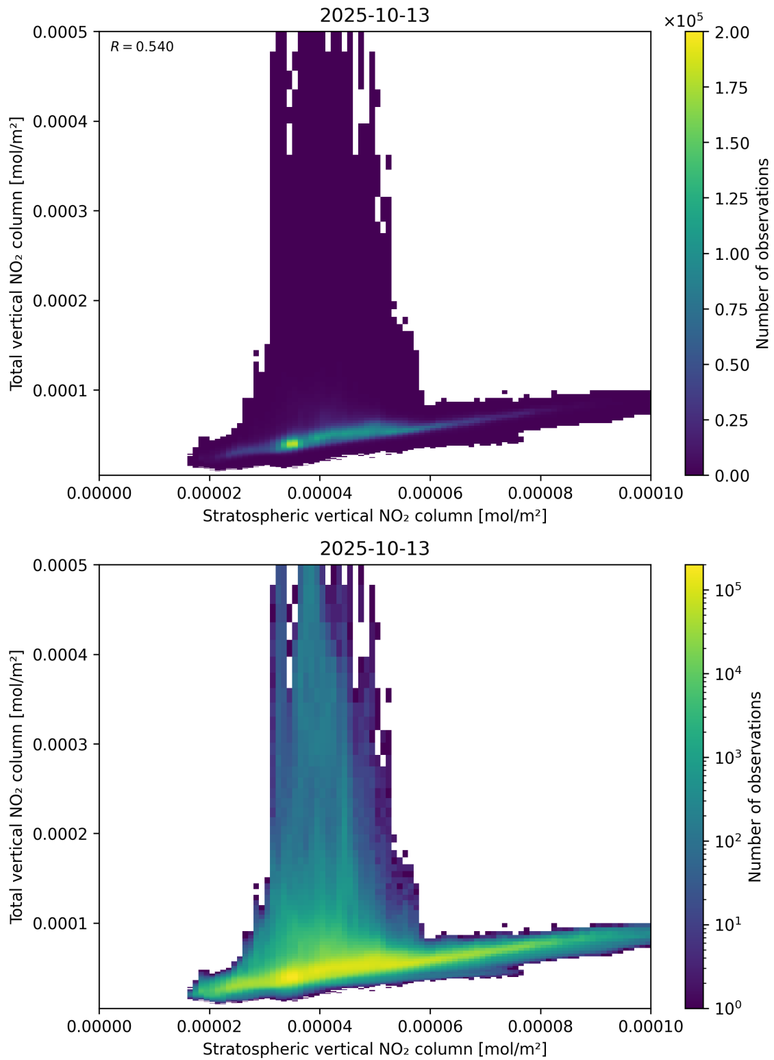
Figure 100: Scatter density plot of “Stratospheric vertical NO 2 column” against “Total vertical NO 2 column” for 2025-10-12 to 2025-10-14.
