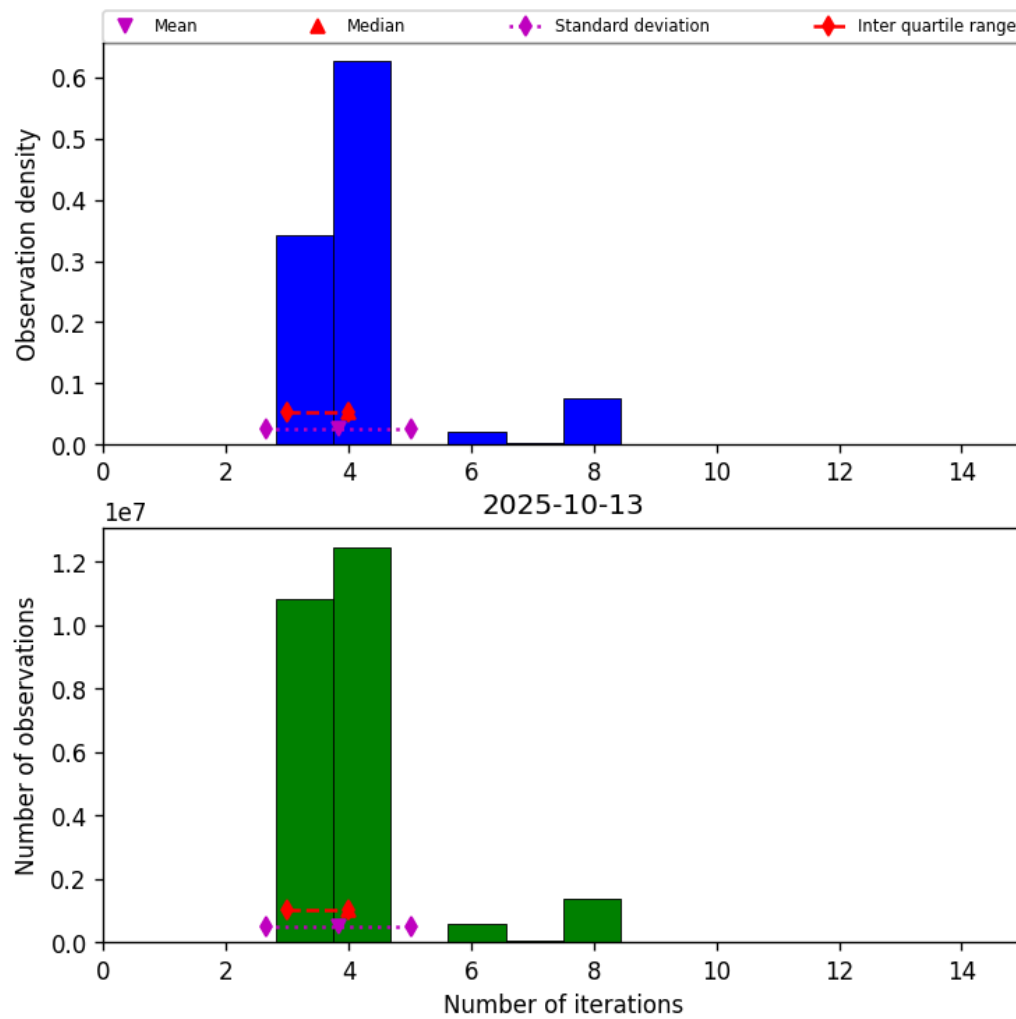
Figure 34: Histogram of “Number of iterations” for 2025-10-12 to 2025-10-14
