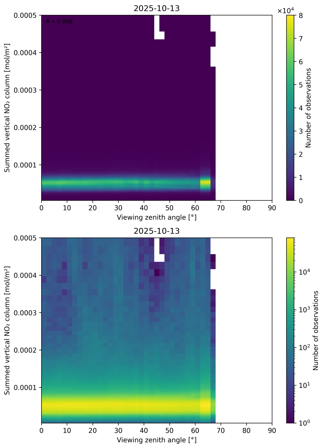
Figure 165: Scatter density plot of “Viewing zenith angle” against “Summed vertical NO 2 column” for 2025-10-12 to 2025-10-14.
