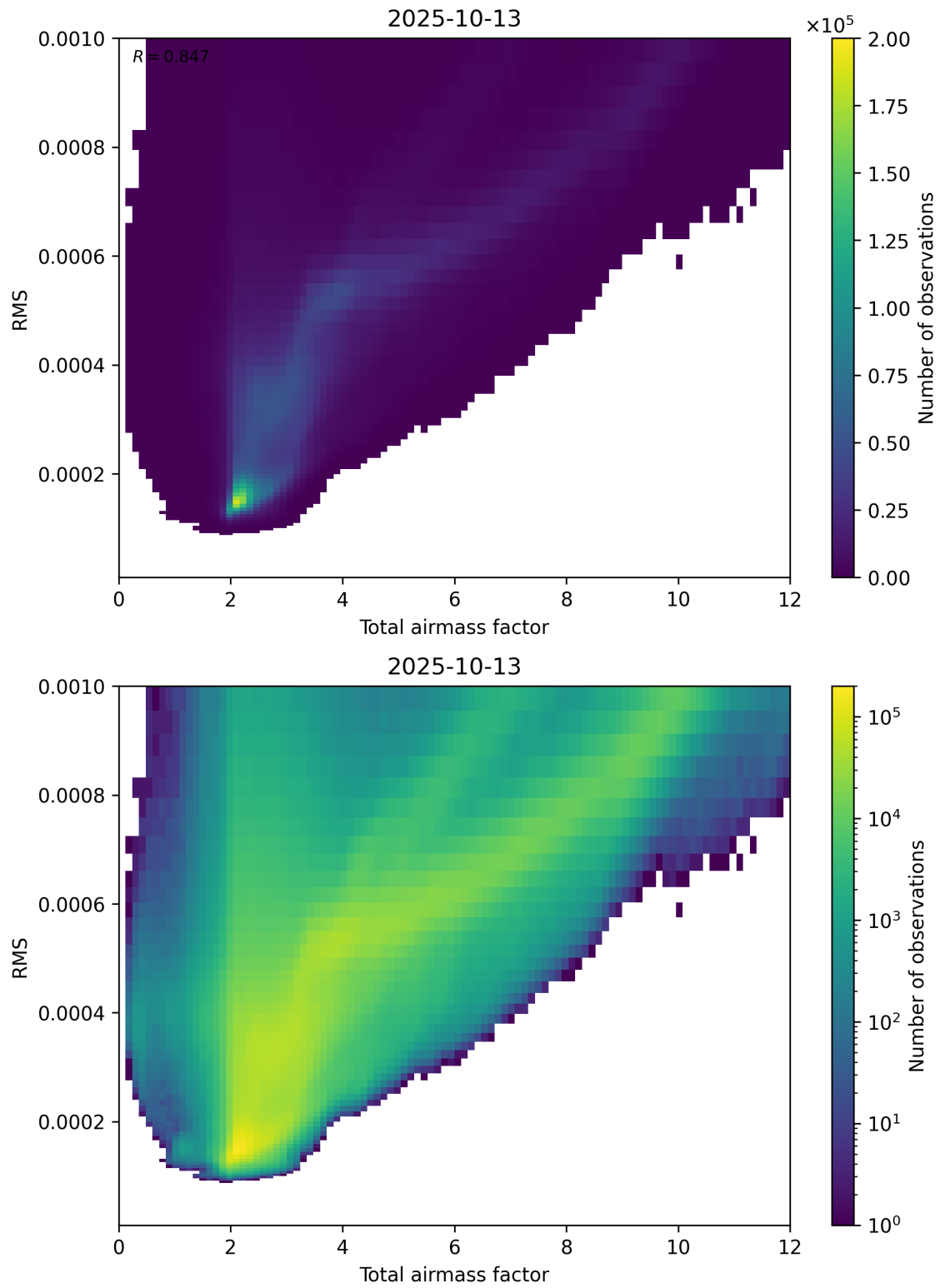
Figure 69: Scatter density plot of “Total airmass factor” against “RMS” for 2025-10-12 to 2025-10-14.
