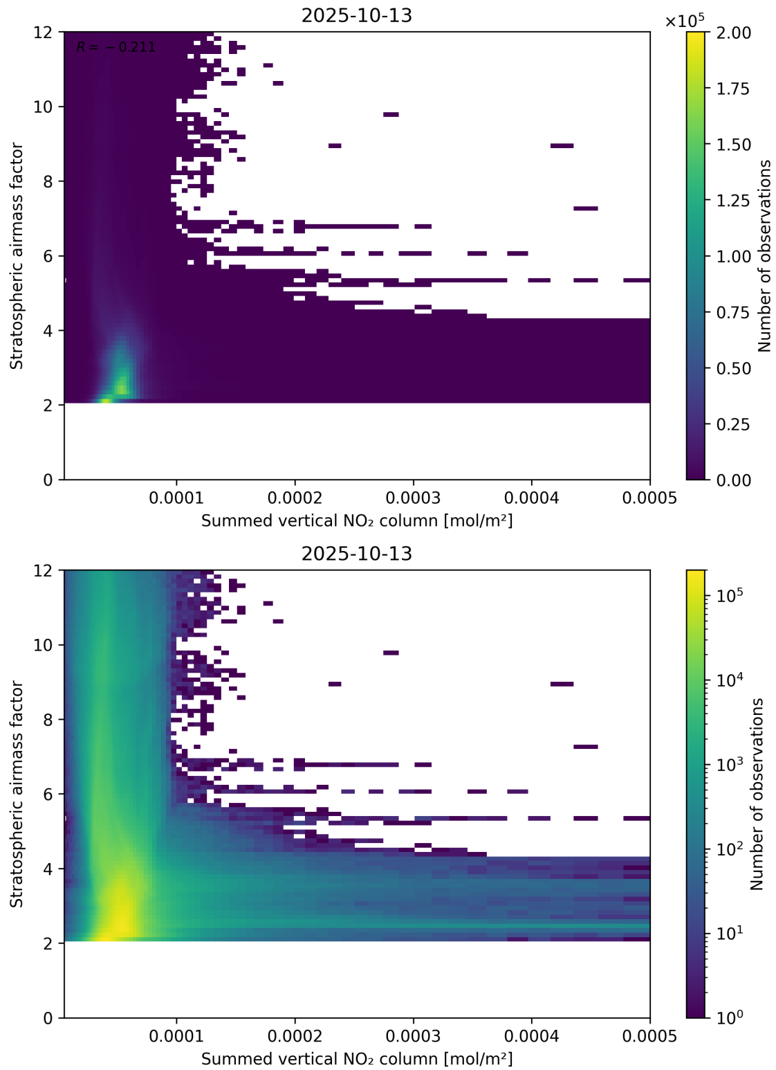
Figure 103: Scatter density plot of “Summed vertical NO 2 column” against “Stratospheric airmass factor” for 2025-10-12 to 2025-10-14.
