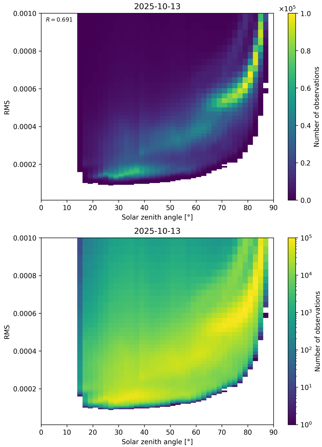
Figure 157: Scatter density plot of “Solar zenith angle” against “RMS” for 2025-10-12 to 2025-10-14.
