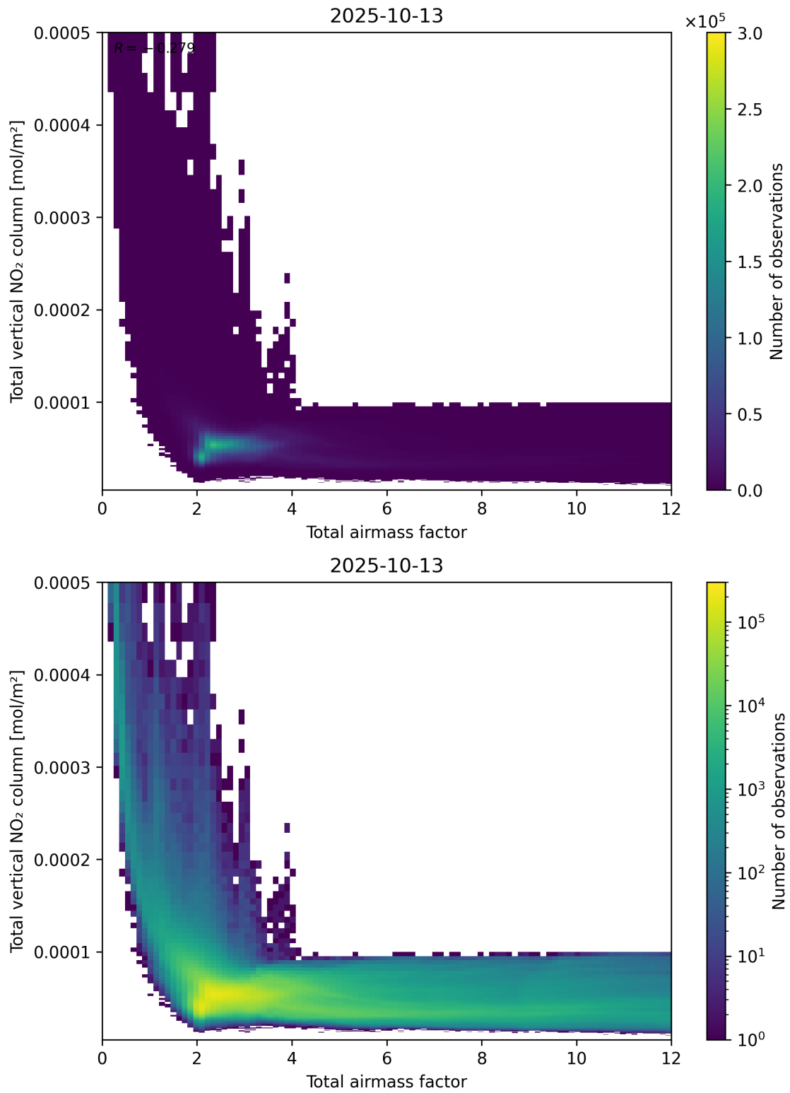
Figure 67: Scatter density plot of “Total airmass factor” against “Total vertical NO 2 column” for 2025-10-12 to 2025-10-14.
