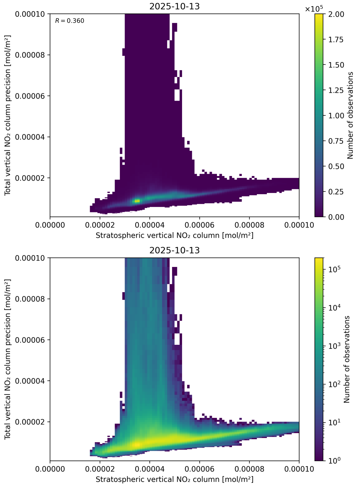
Figure 101: Scatter density plot of “Stratospheric vertical NO 2 column” against “Total vertical NO 2 column precision” for 2025-10-12 to 2025-10-14.
