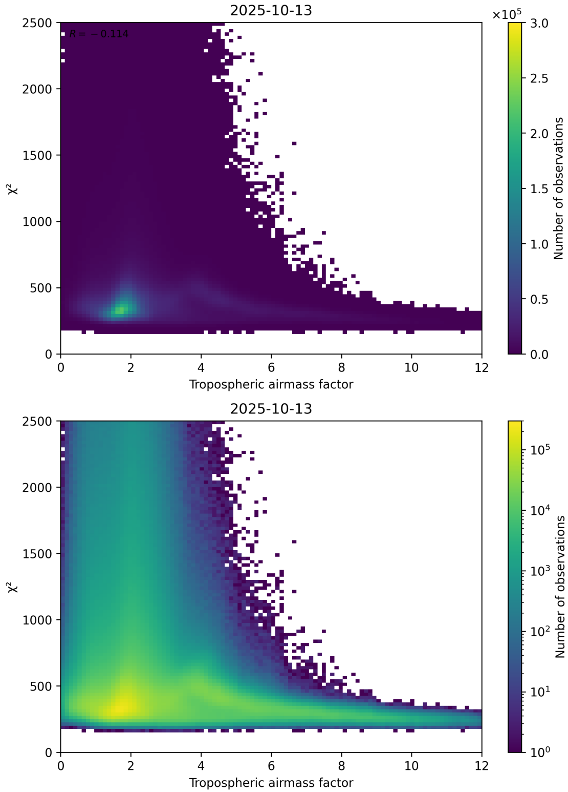
Figure 73: Scatter density plot of “Tropospheric airmass factor” against “ \chi^2 ” for 2025-10-12 to 2025-10-14.
