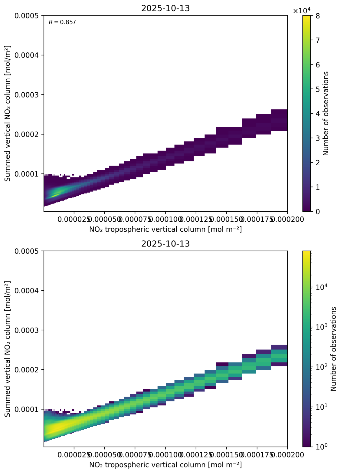
Figure 126: Scatter density plot of “NO 2 tropospheric vertical column” against “Summed vertical NO 2 column” for 2025-10-12 to 2025-10-14.
