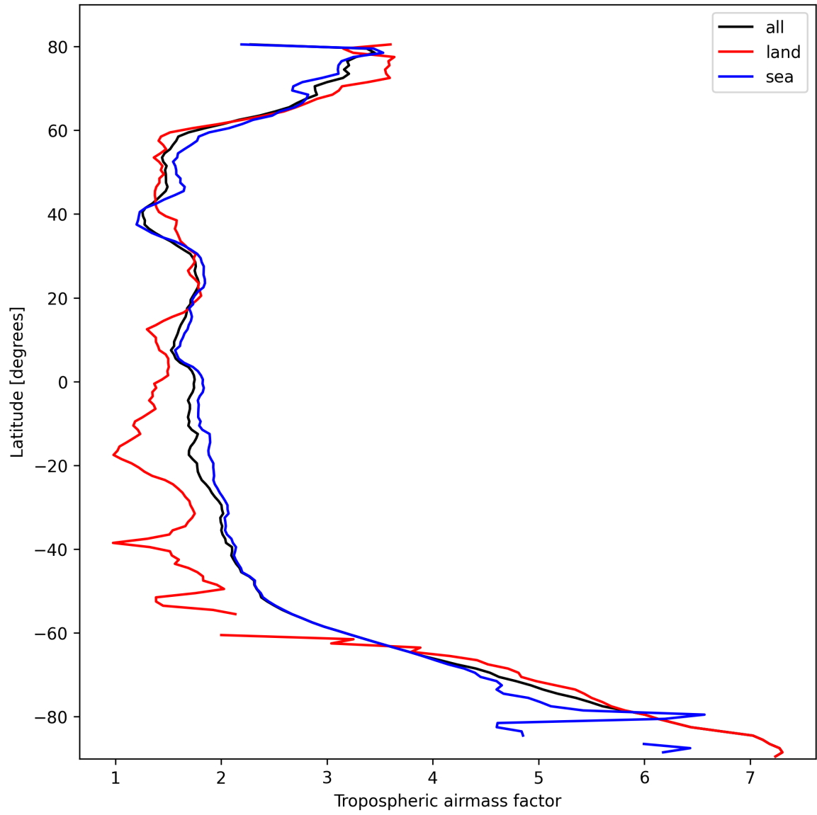
Figure 14: Zonal average of “Tropospheric air mass factor” for 2025-10-12 to 2025-10-14.
