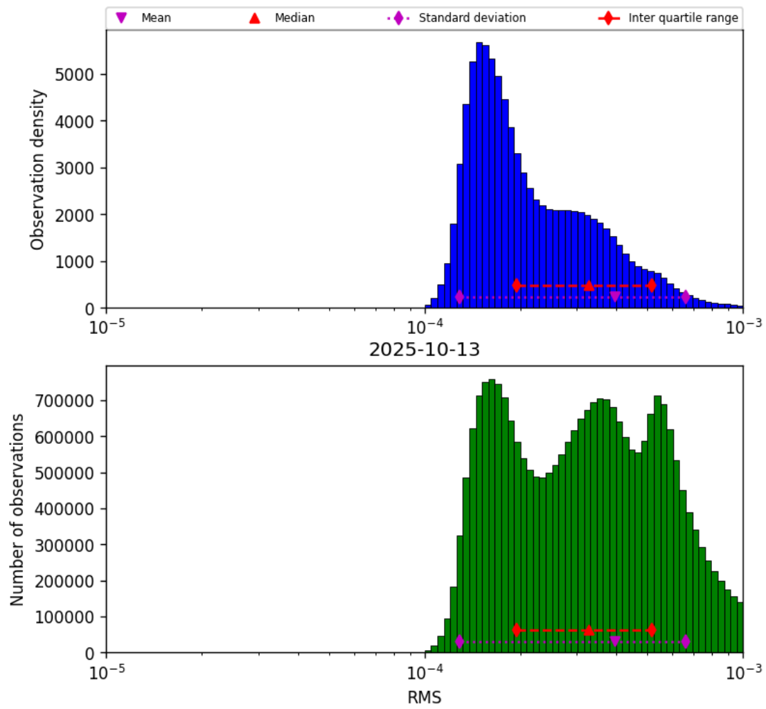
Figure 43: Histogram of “RMS” for 2025-10-12 to 2025-10-14
