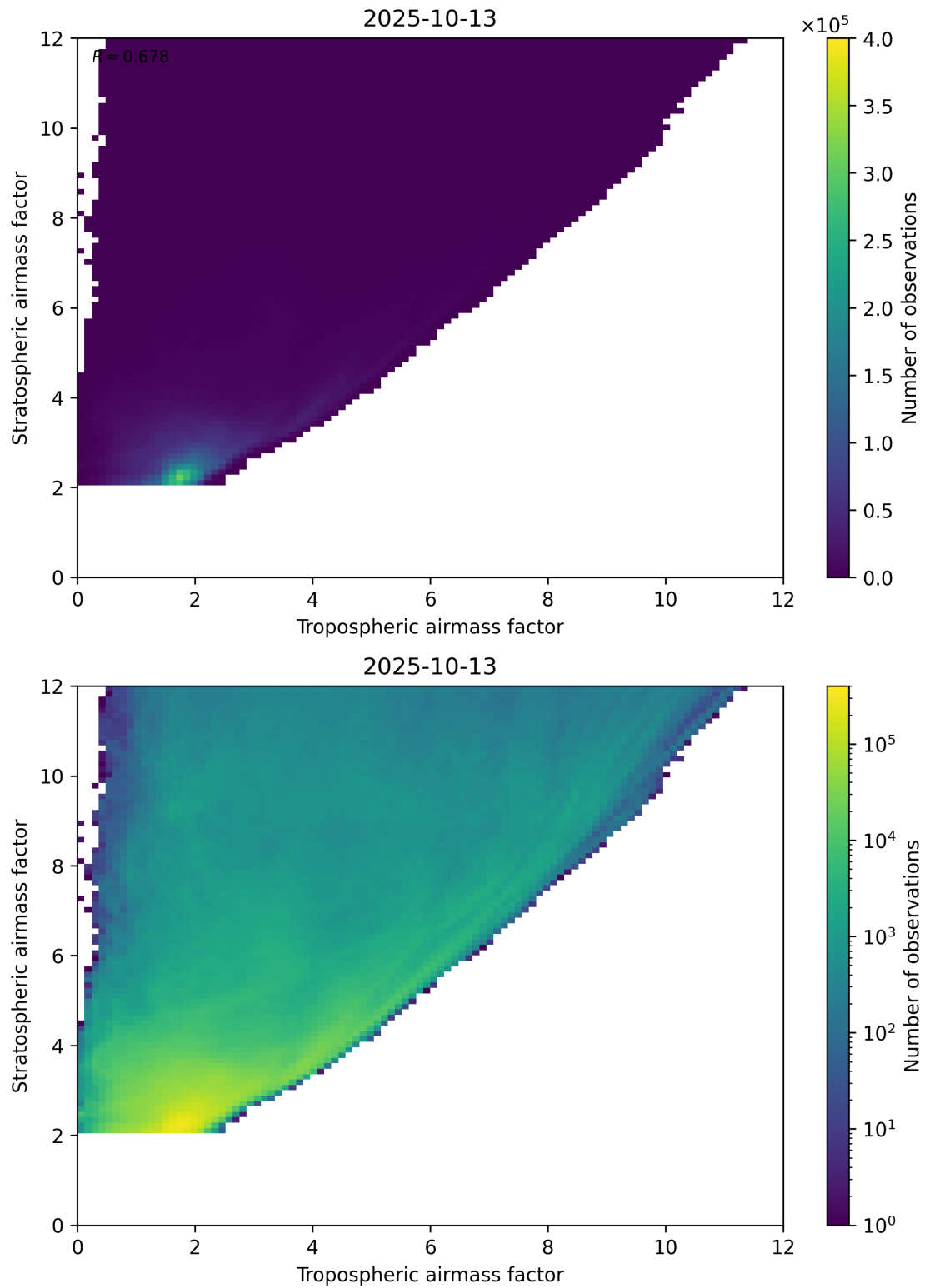
Figure 71: Scatter density plot of “Tropospheric airmass factor” against “Stratospheric airmass factor” for 2025-10-12 to 2025-10-14.
