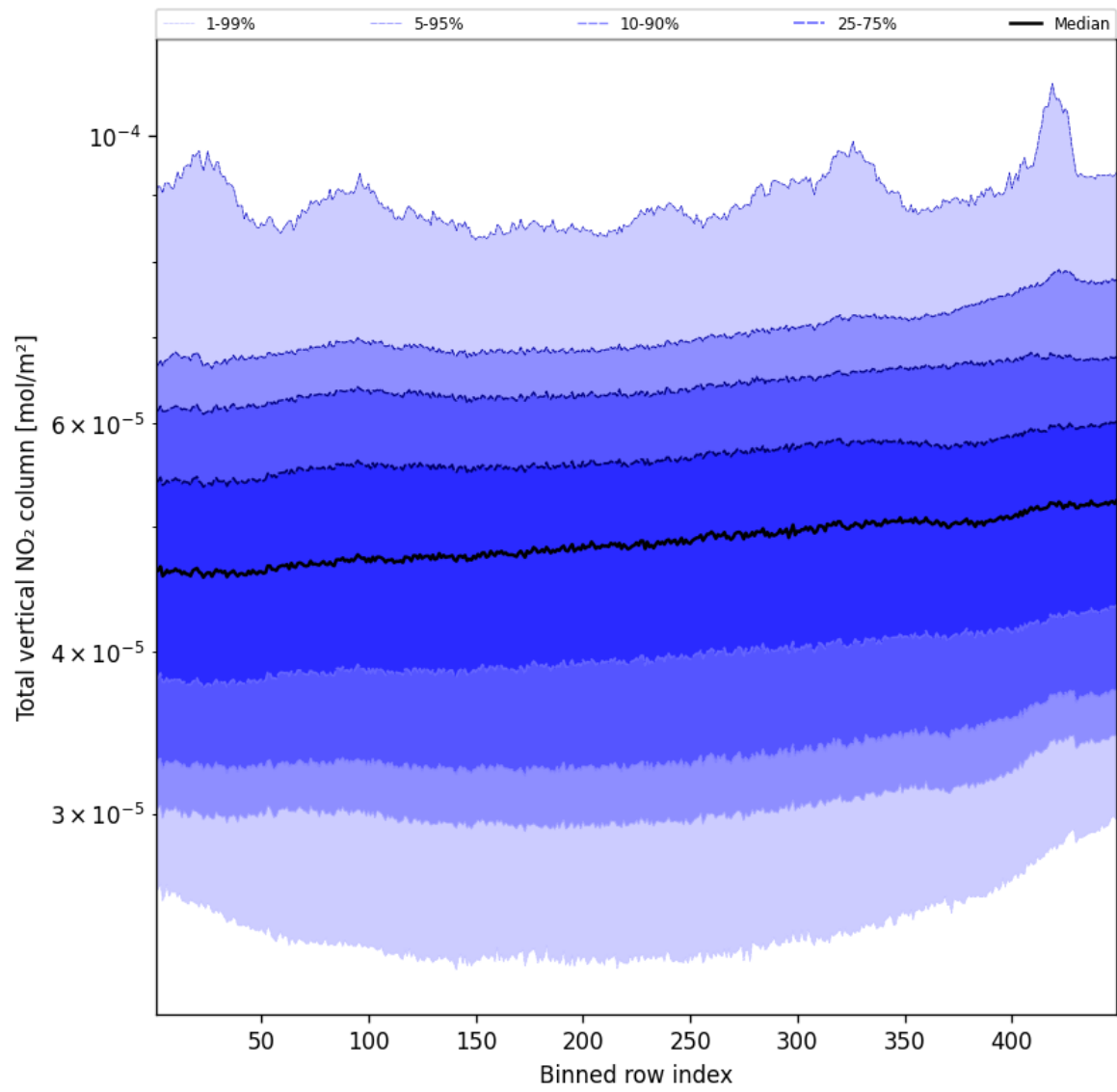
Figure 55: Along track statistics of “Total vertical NO 2 column” for 2025-10-12 to 2025-10-14
