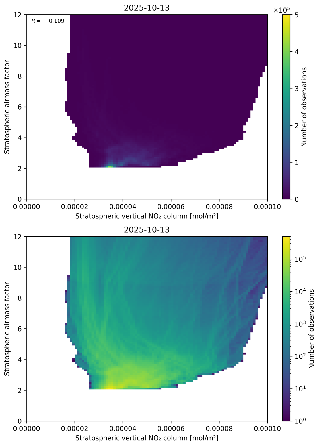
Figure 96: Scatter density plot of “Stratospheric vertical NO 2 column” against “Stratospheric airmass factor” for 2025-10-12 to 2025-10-14.
