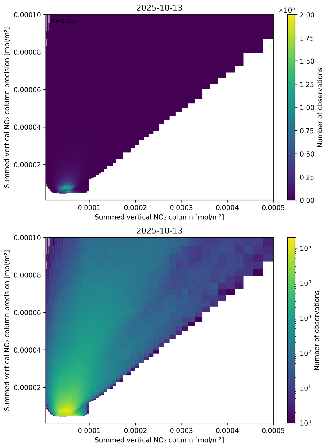
Figure 105: Scatter density plot of “Summed vertical NO 2 column” against “Summed vertical NO 2 column precision” for 2025-10-12 to 2025-10-14.
