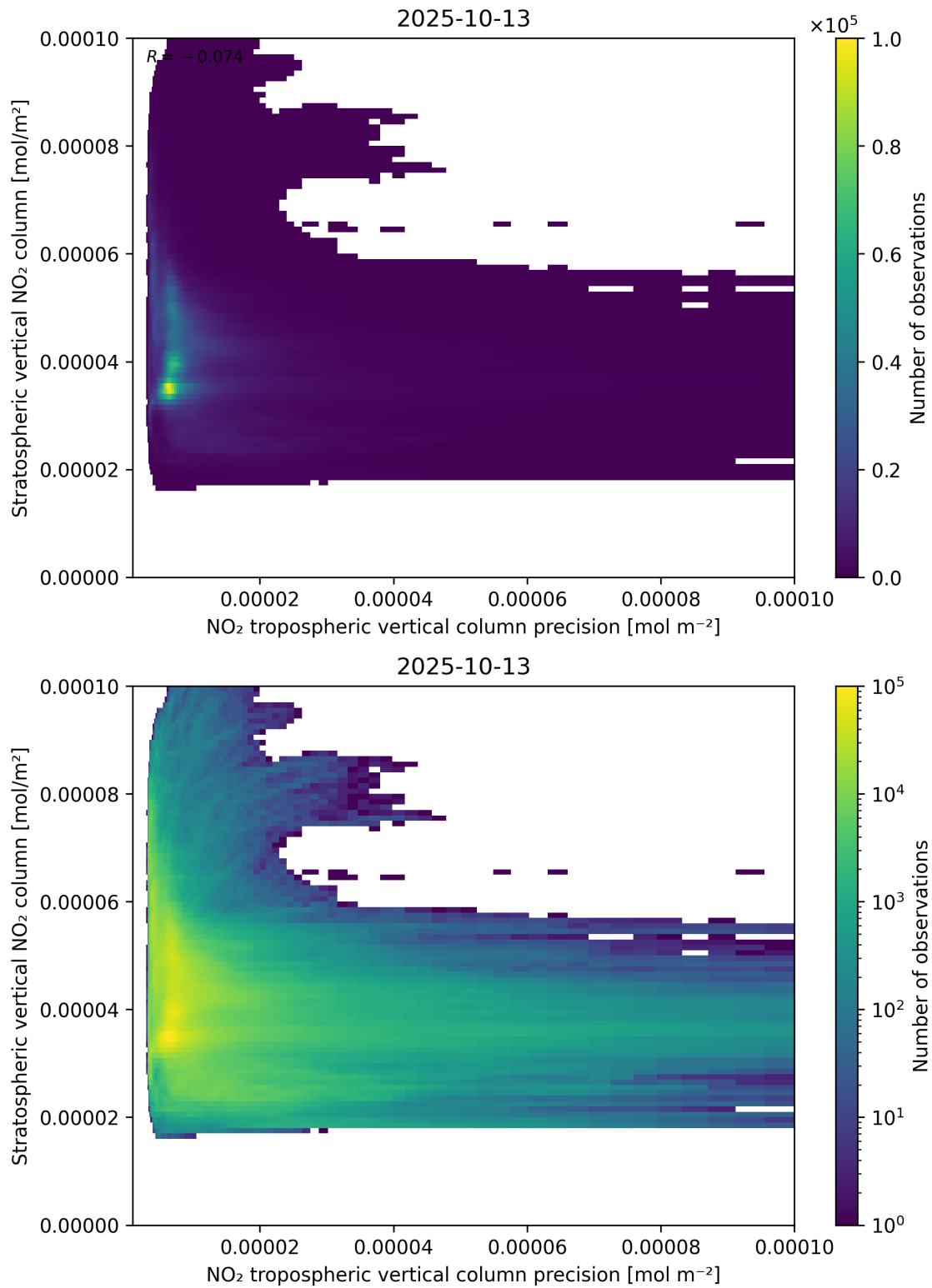
Figure 135: Scatter density plot of “NO 2 tropospheric vertical column precision” against “Stratospheric vertical NO 2 column” for 2025-10-12 to 2025-10-14.
