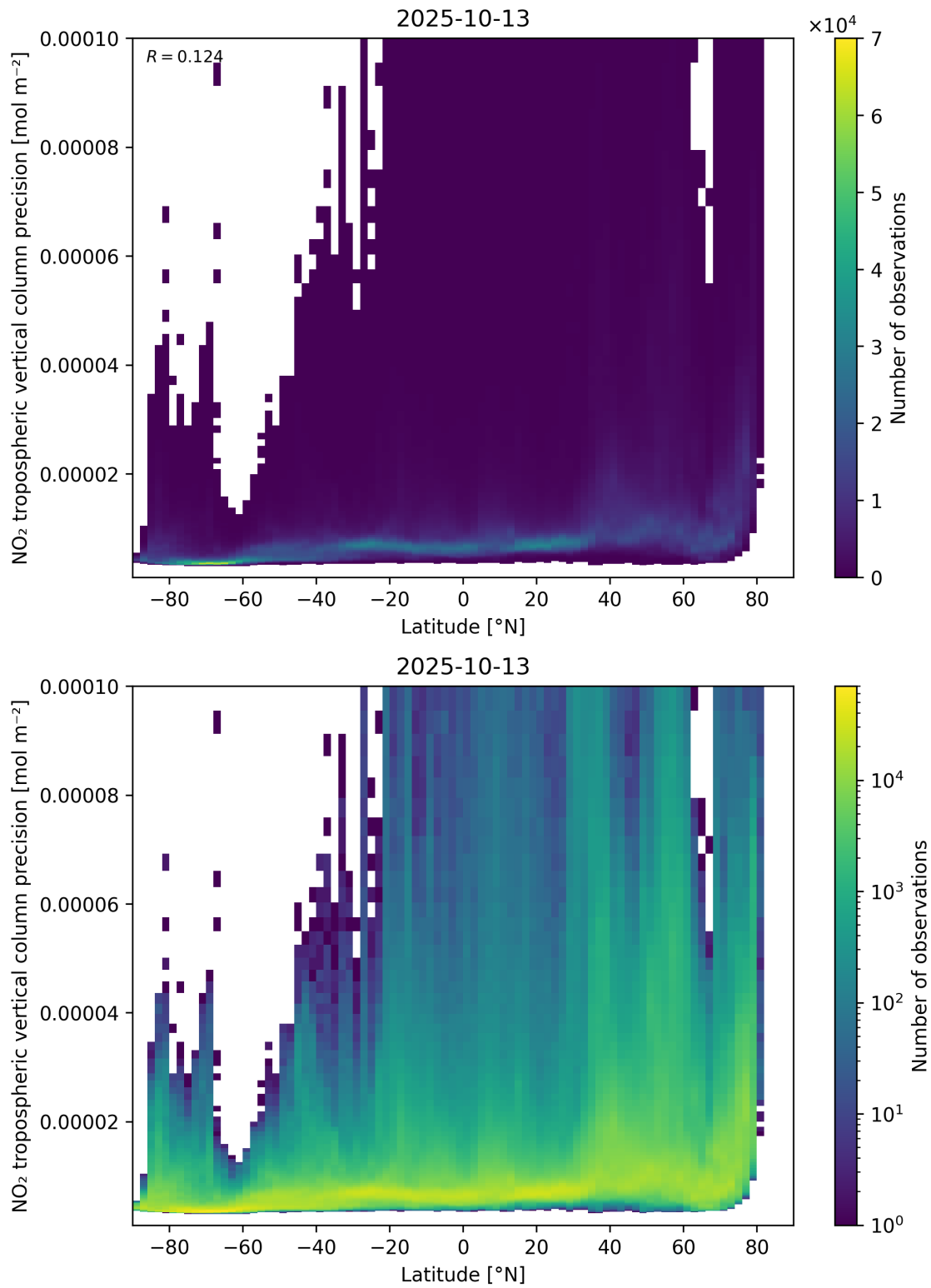
Figure 93: Scatter density plot of “Latitude” against “NO 2 tropospheric vertical column precision” for 2025-10-12 to 2025-10-14.
