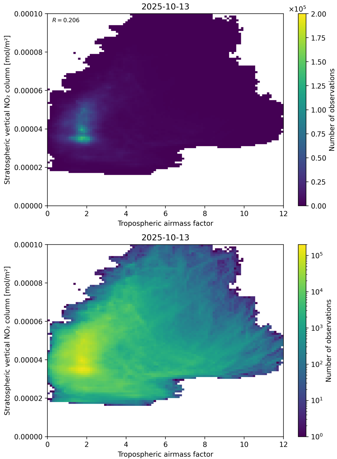
Figure 74: Scatter density plot of “Tropospheric airmass factor” against “Stratospheric vertical NO 2 column” for 2025-10-12 to 2025-10-14.
