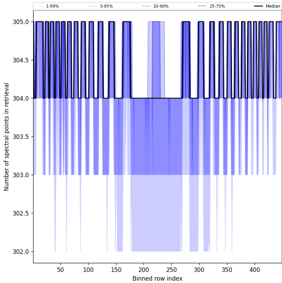
Figure 50: Along track statistics of “Number of spectral points in retrieval” for 2025-10-12 to 2025-10-14
