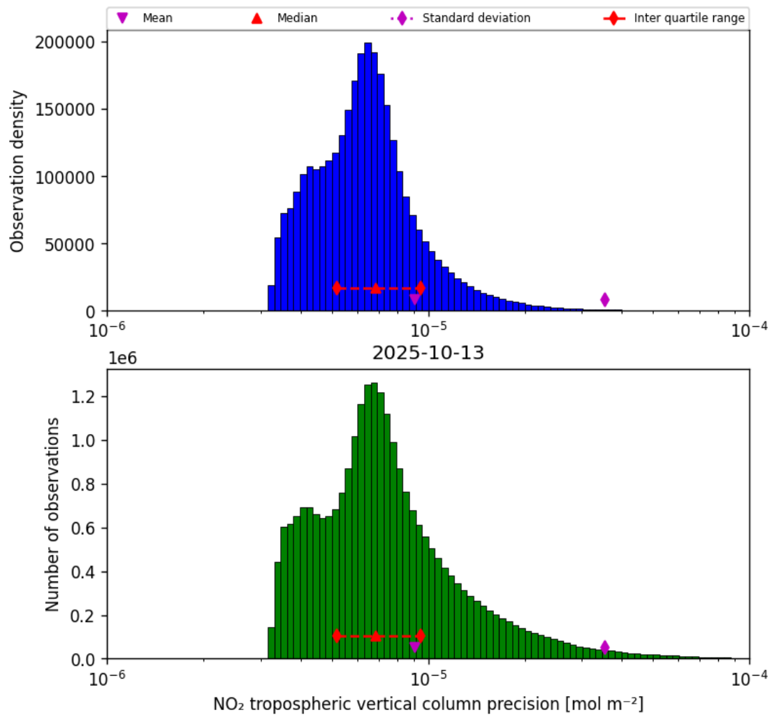
Figure 30: Histogram of “NO 2 tropospheric vertical column precision” for 2025-10-12 to 2025-10-14
