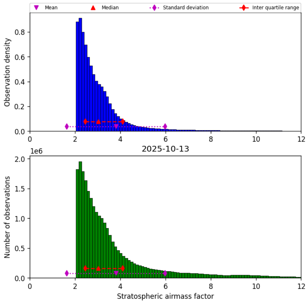
Figure 44: Histogram of “Stratospheric airmass factor” for 2025-10-12 to 2025-10-14
