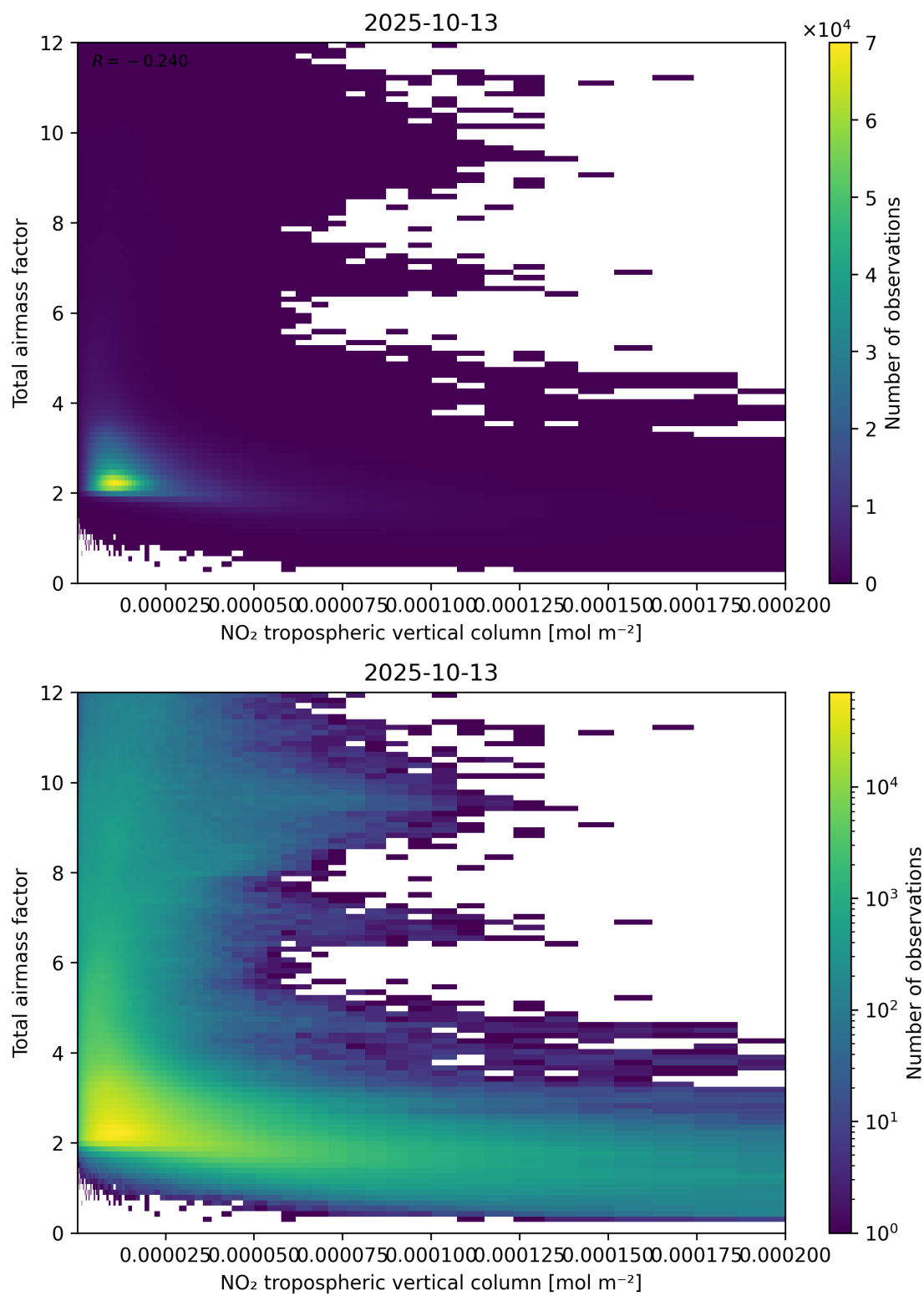
Figure 122: Scatter density plot of “NO 2 tropospheric vertical column” against “Total air mass factor” for 2025-10-12 to 2025-10-14.
