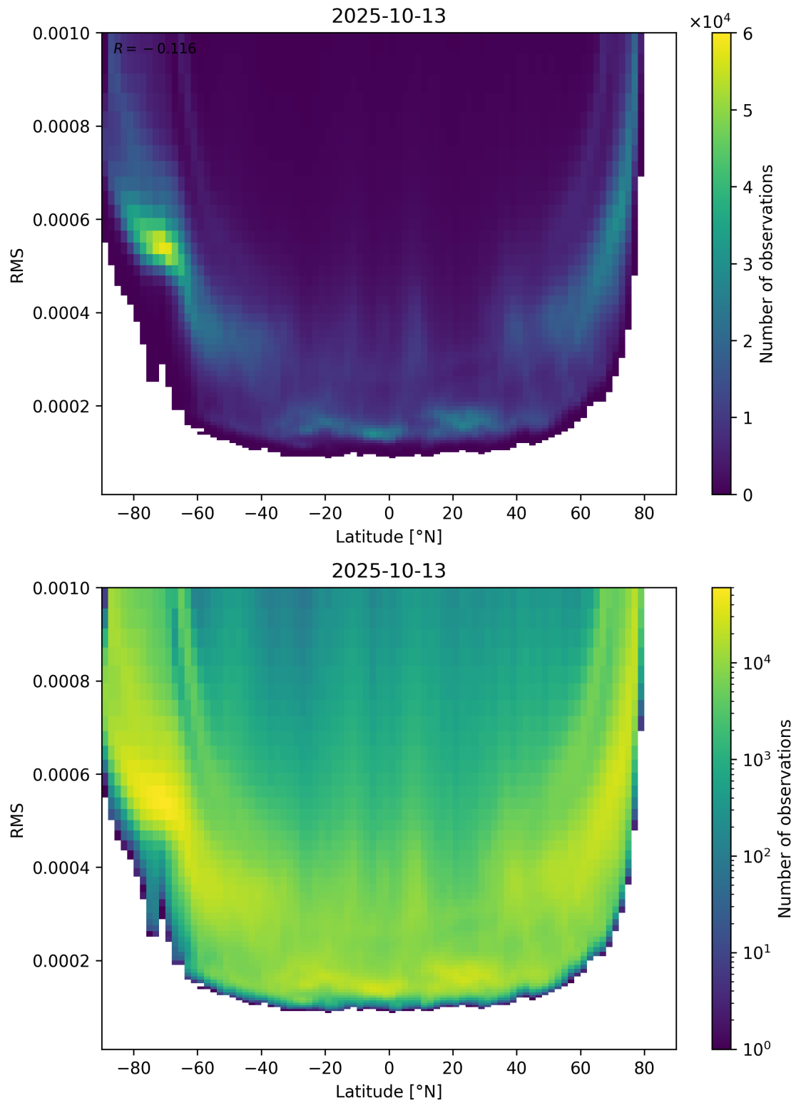
Figure 94: Scatter density plot of “Latitude” against “RMS” for 2025-10-12 to 2025-10-14.
