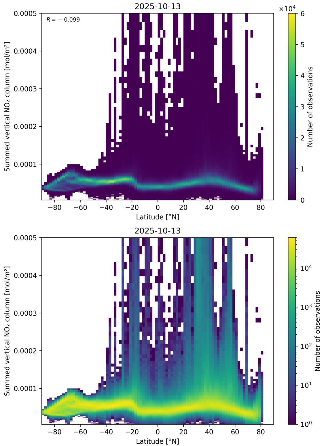
Figure 88: Scatter density plot of “Latitude” against “Summed vertical NO 2 column” for 2025-10-12 to 2025-10-14.
