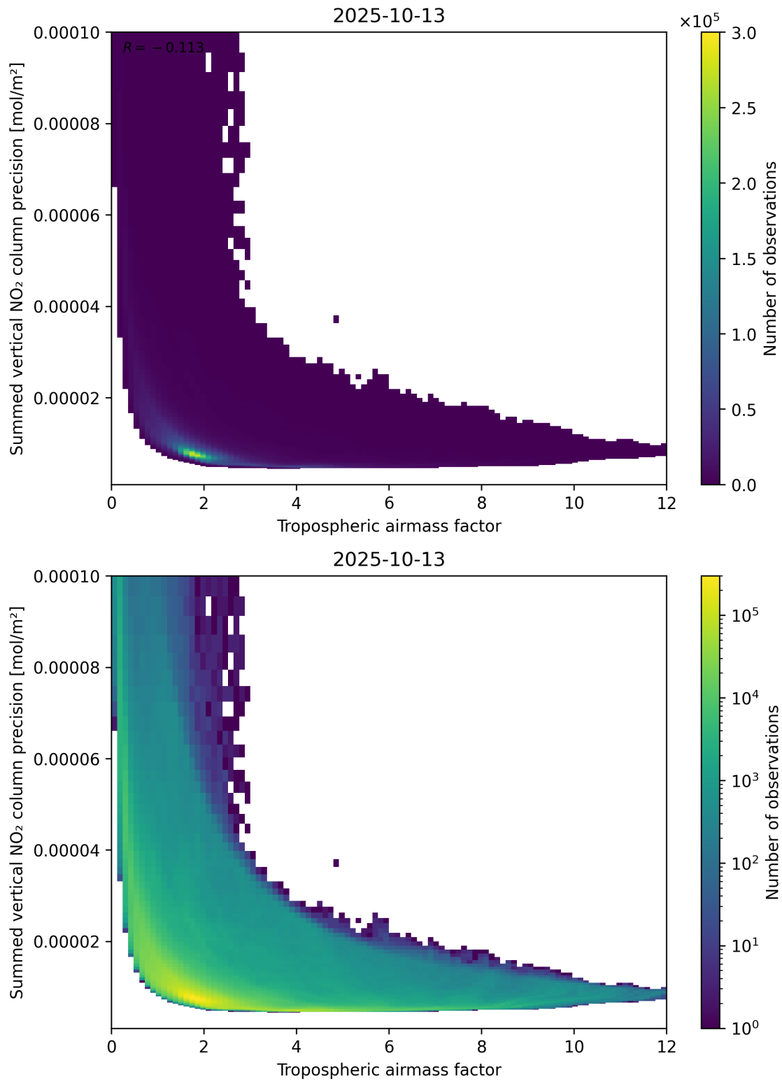
Figure 76: Scatter density plot of “Tropospheric airmass factor” against “Summed vertical NO 2 column precision” for 2025-10-12 to 2025-10-14.
