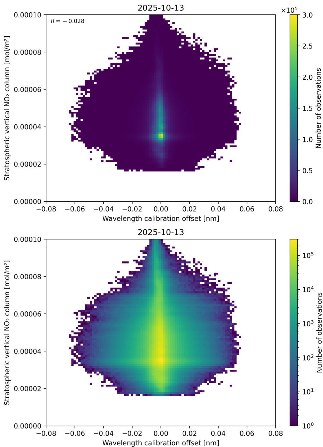
Figure 176: Scatter density plot of “Wavelength calibration offset” against “Stratospheric vertical NO 2 column” for 2025-10-12 to 2025-10-14.
