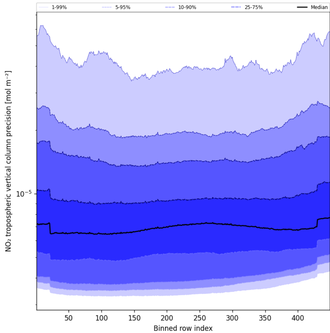
Figure 47: Along track statistics of “NO 2 tropospheric vertical column precision” for 2025-10-12 to 2025-10-14
