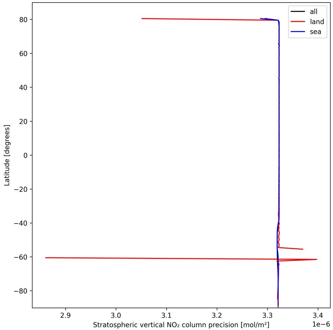
Figure 20: Zonal average of “Stratospheric vertical NO 2 column precision” for 2025-10-12 to 2025-10-14.
