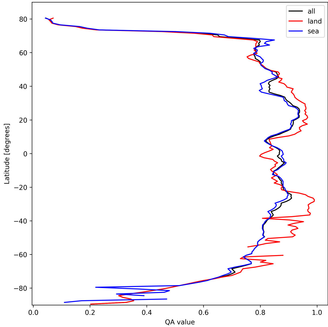
Figure 11: Zonal average of “QA value” for 2025-10-12 to 2025-10-14.
