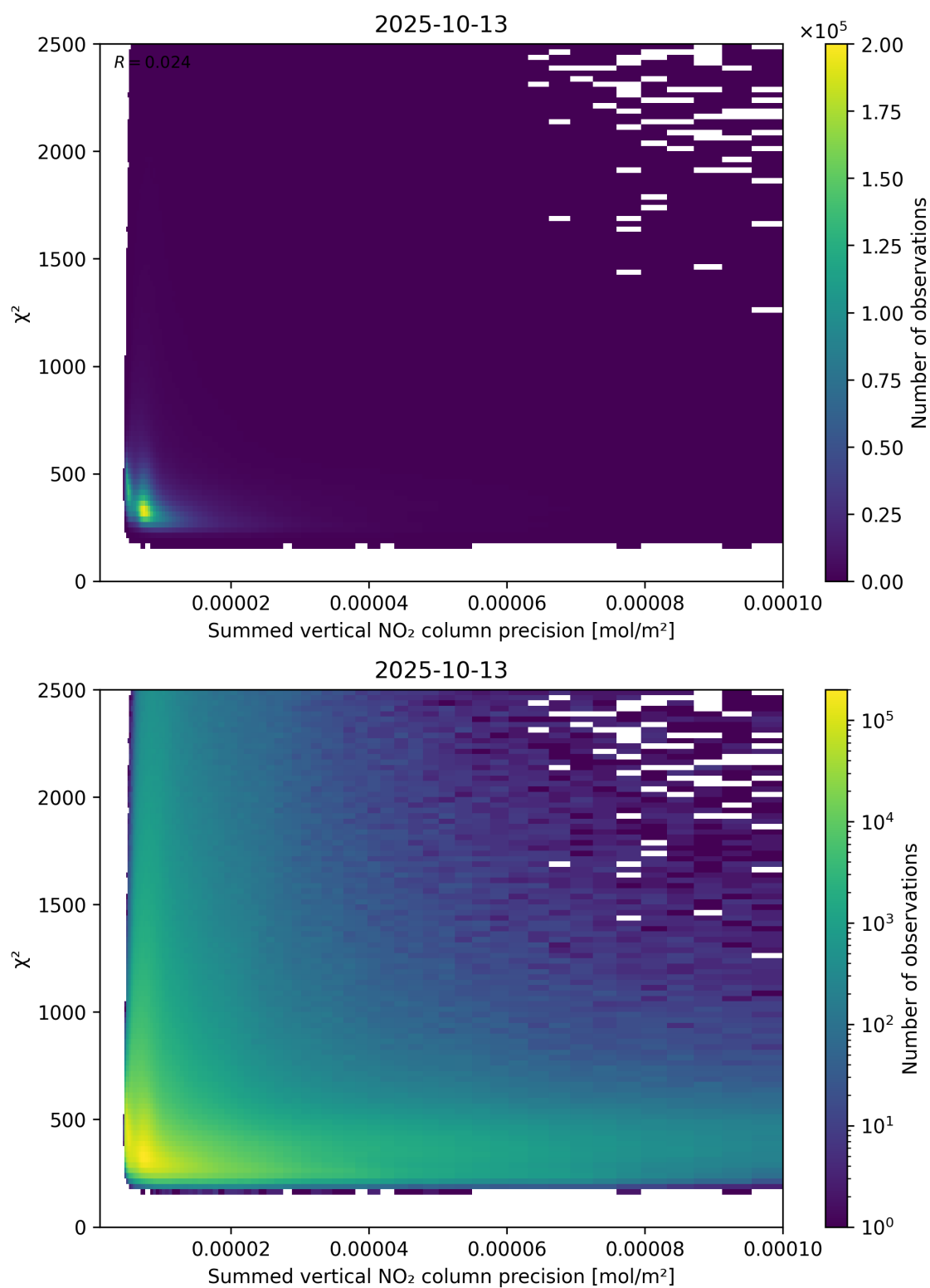
Figure 107: Scatter density plot of “Summed vertical NO 2 column precision” against “ \chi^2 ” for 2025-10-12 to 2025-10-14.
