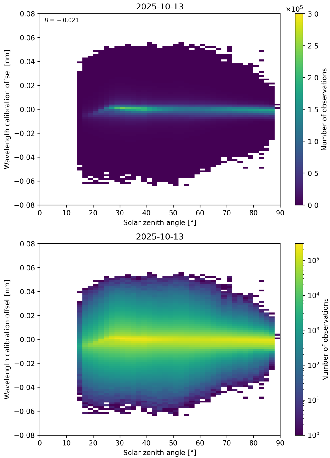
Figure 158: Scatter density plot of “Solar zenith angle” against “Wavelength calibration offset” for 2025-10-12 to 2025-10-14.
