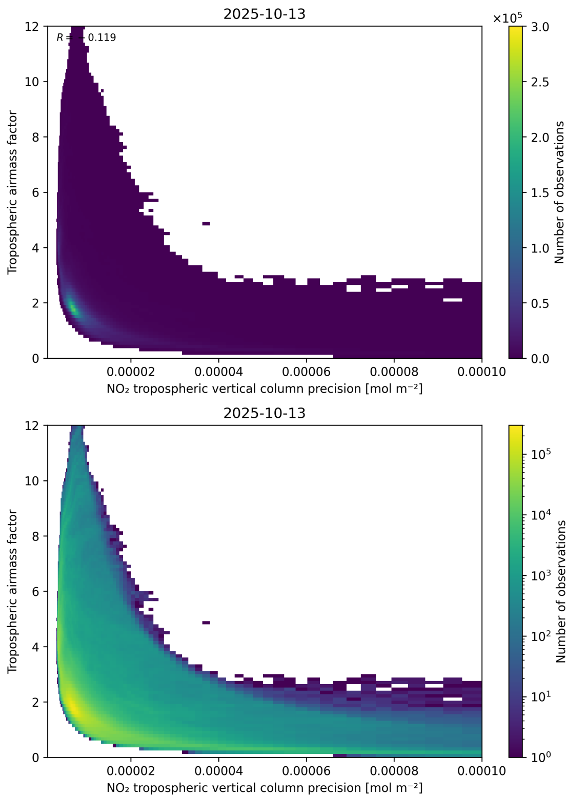
Figure 133: Scatter density plot of “NO 2 tropospheric vertical column precision” against “Tropospheric airmass factor” for 2025-10-12 to 2025-10-14.
