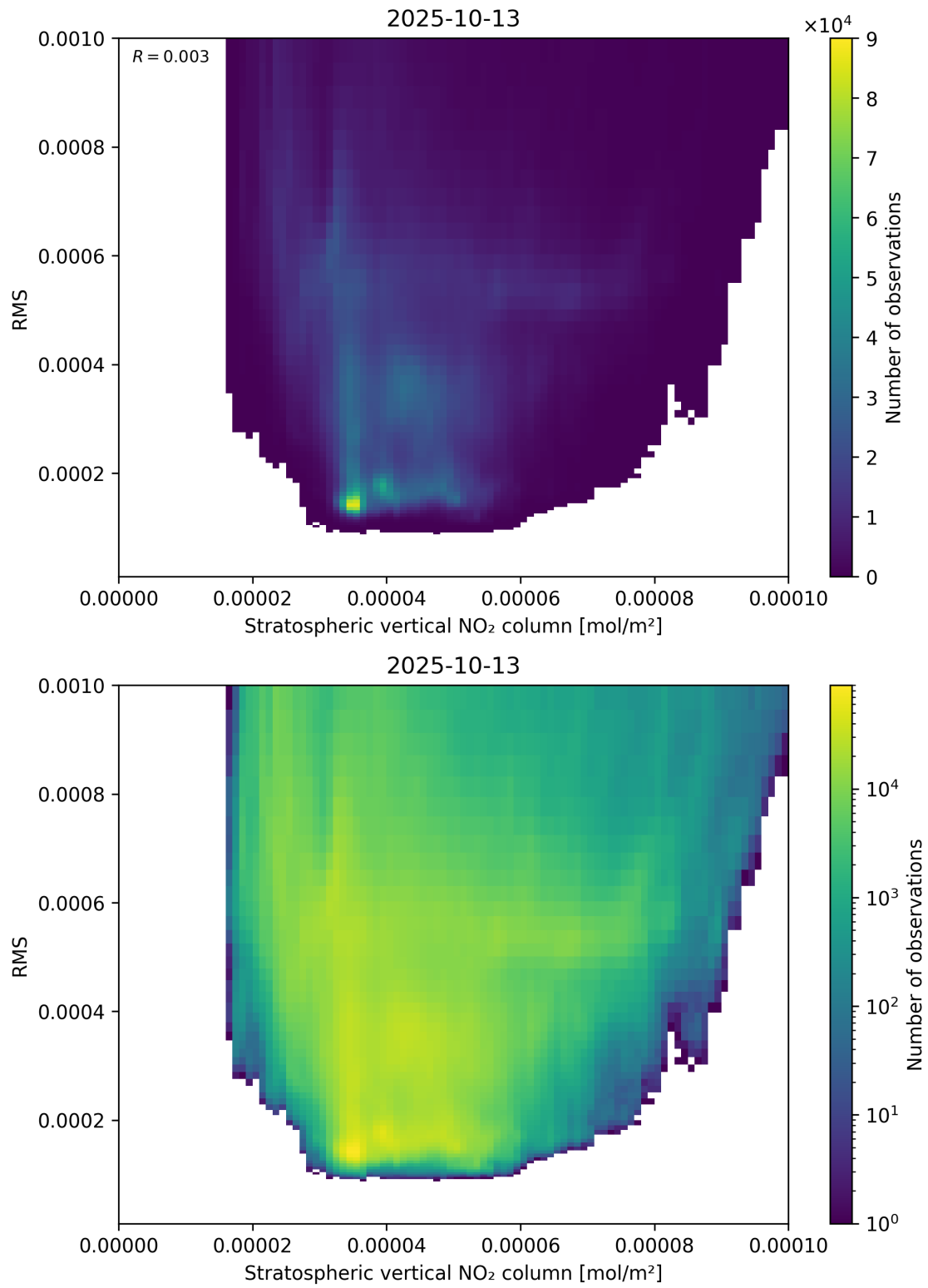
Figure 102: Scatter density plot of “Stratospheric vertical NO 2 column” against “RMS” for 2025-10-12 to 2025-10-14.
