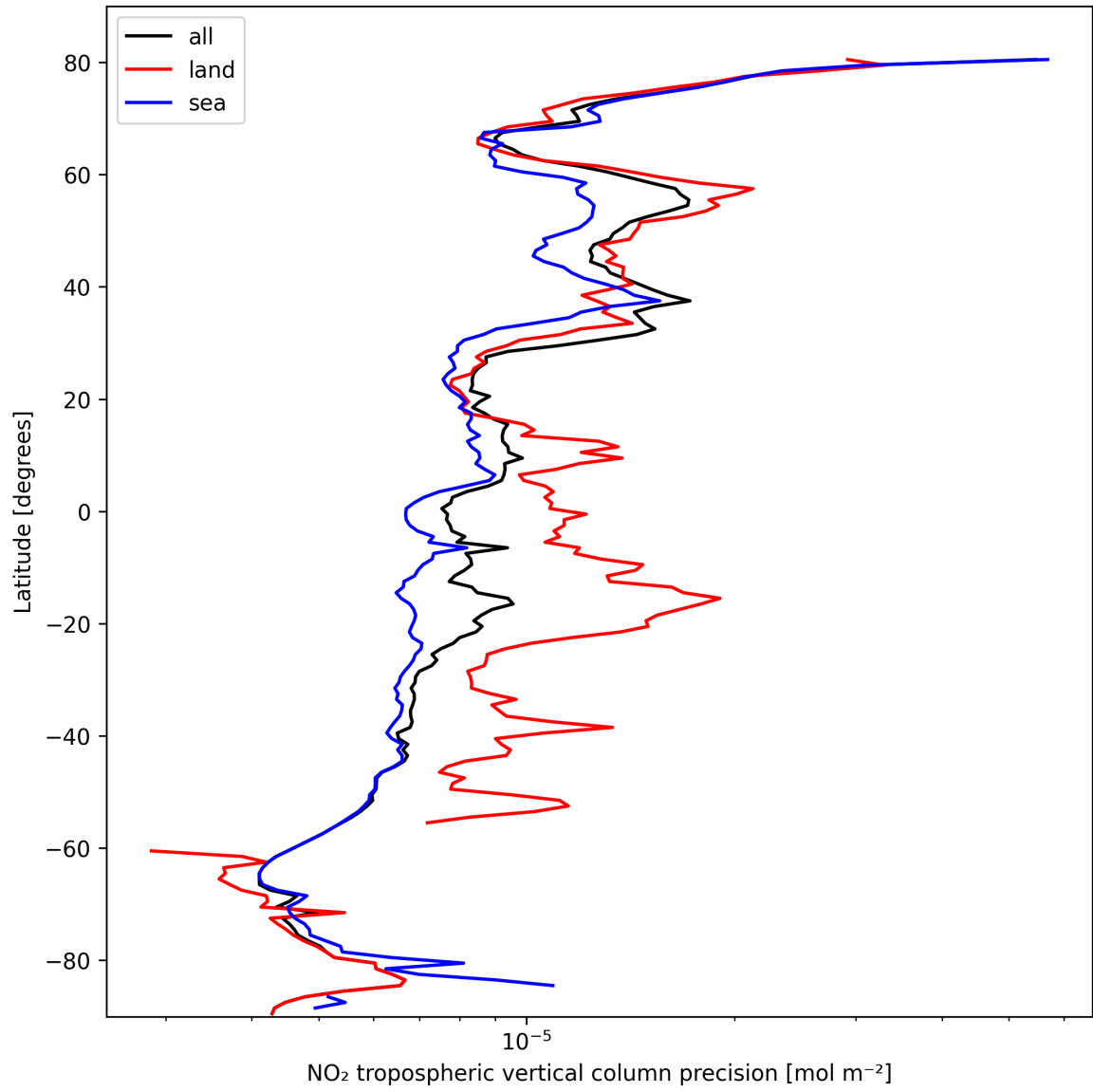
Figure 13: Zonal average of “NO 2 tropospheric vertical column precision” for 2025-10-12 to 2025-10-14.
