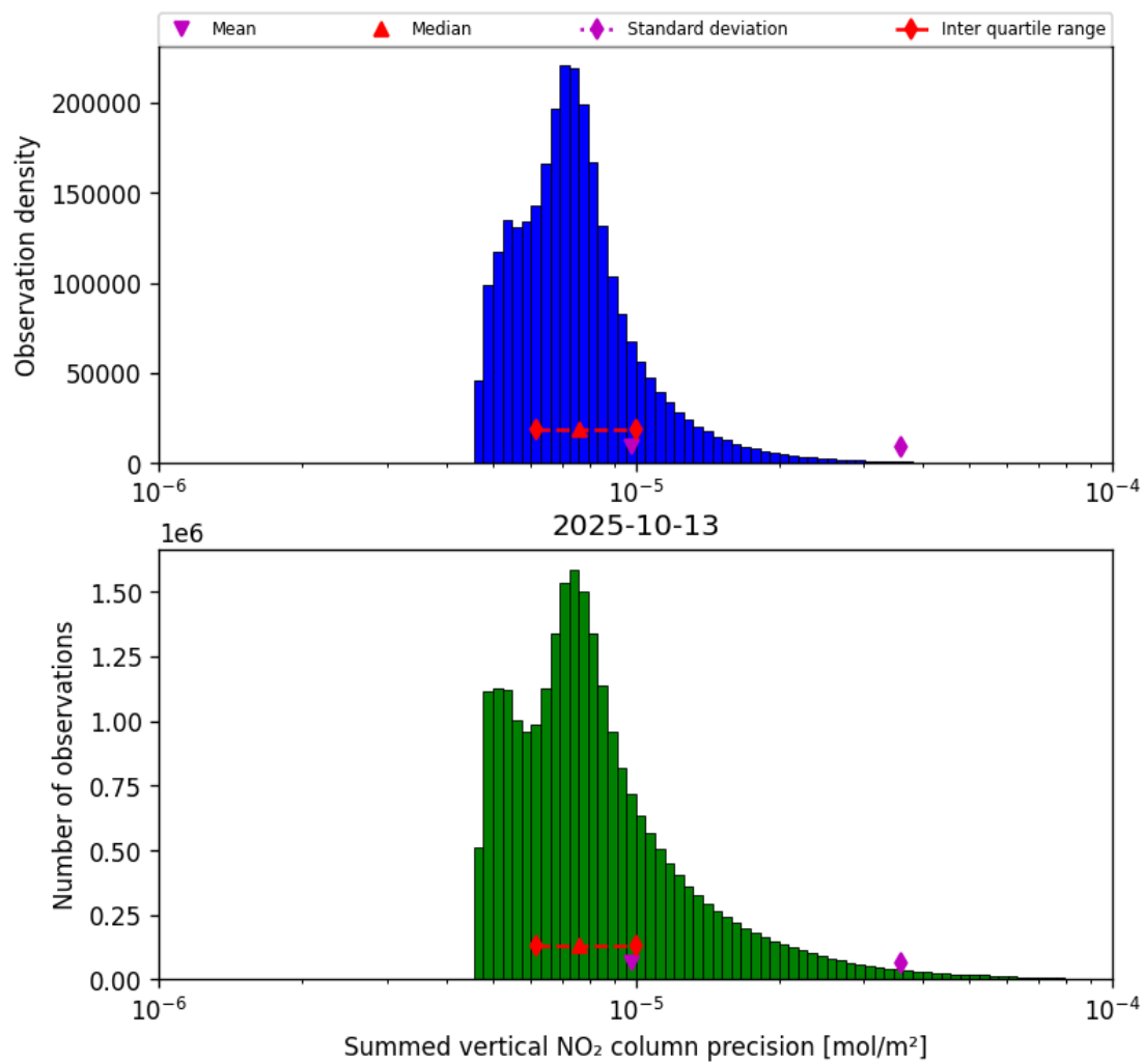
Figure 41: Histogram of "Summed vertical NO 2 column precision" for 2025-10-12 to 2025-10-14
