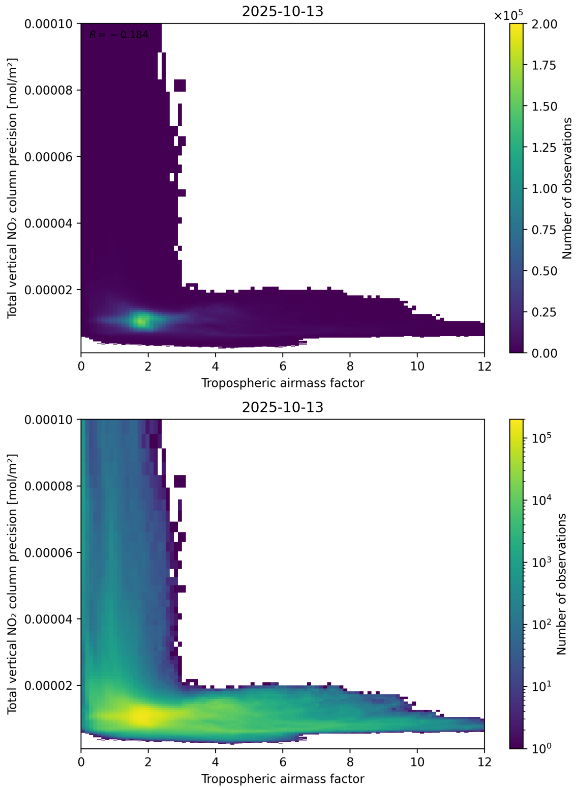
Figure 78: Scatter density plot of “Tropospheric air mass factor” against “Total vertical NO 2 column precision” for 2025-10-12 to 2025-10-14.
