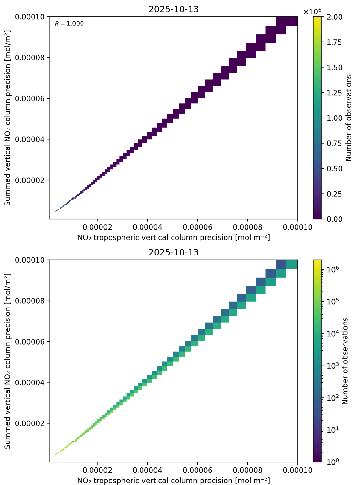
Figure 137: Scatter density plot of “NO 2 tropospheric vertical column precision” against “Summed vertical NO 2 column precision” for 2025-10-12 to 2025-10-14.
