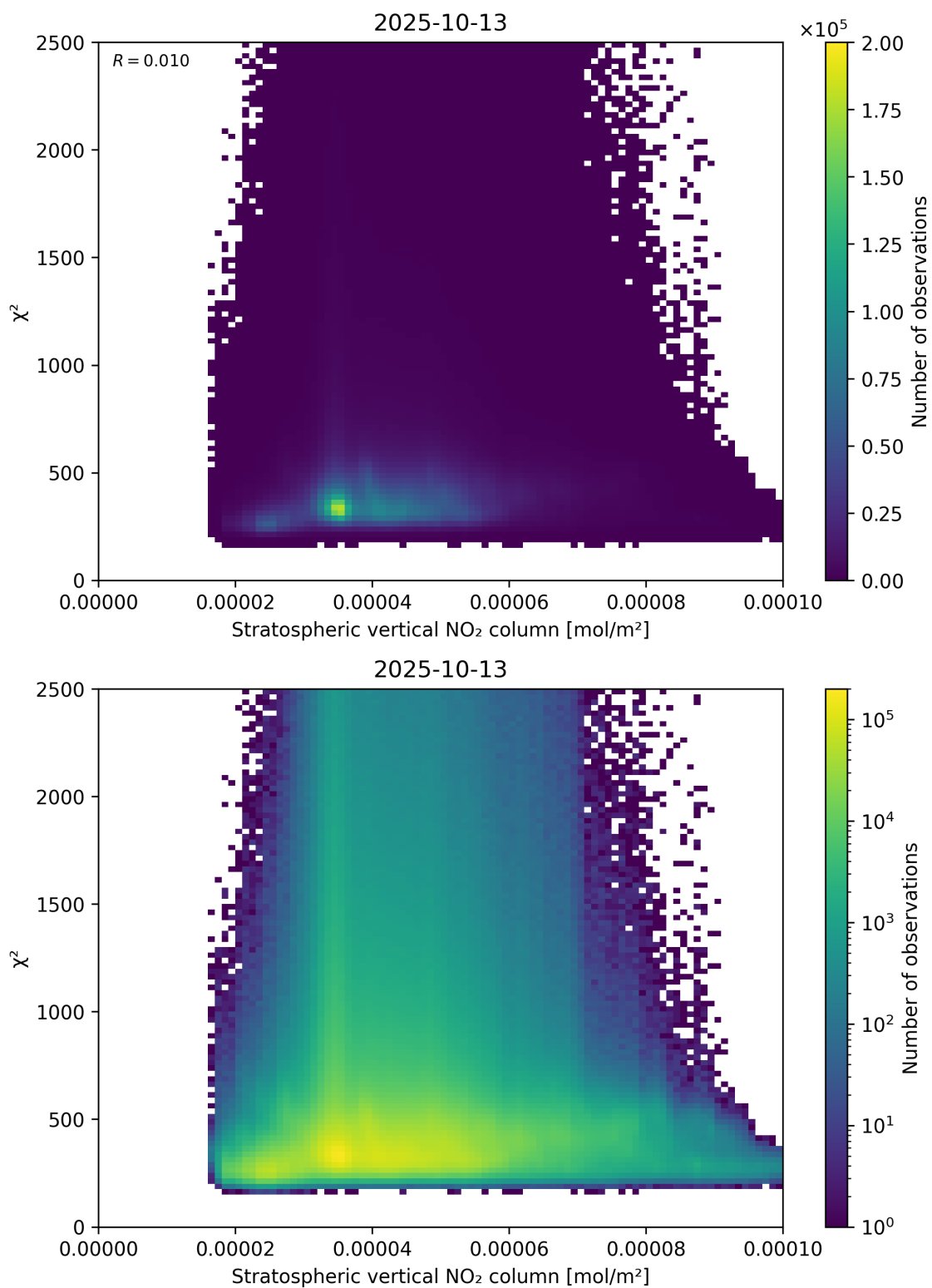
Figure 97: Scatter density plot of “Stratospheric vertical NO 2 column” against “ \chi^2 ” for 2025-10-12 to 2025-10-14.
