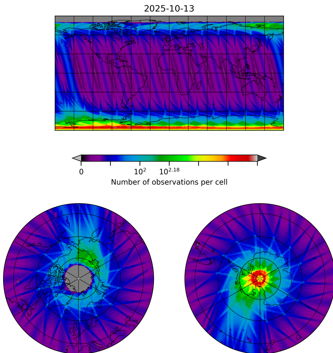
Figure 10: Map of the number of observations for 2025-10-12 to 2025-10-14
