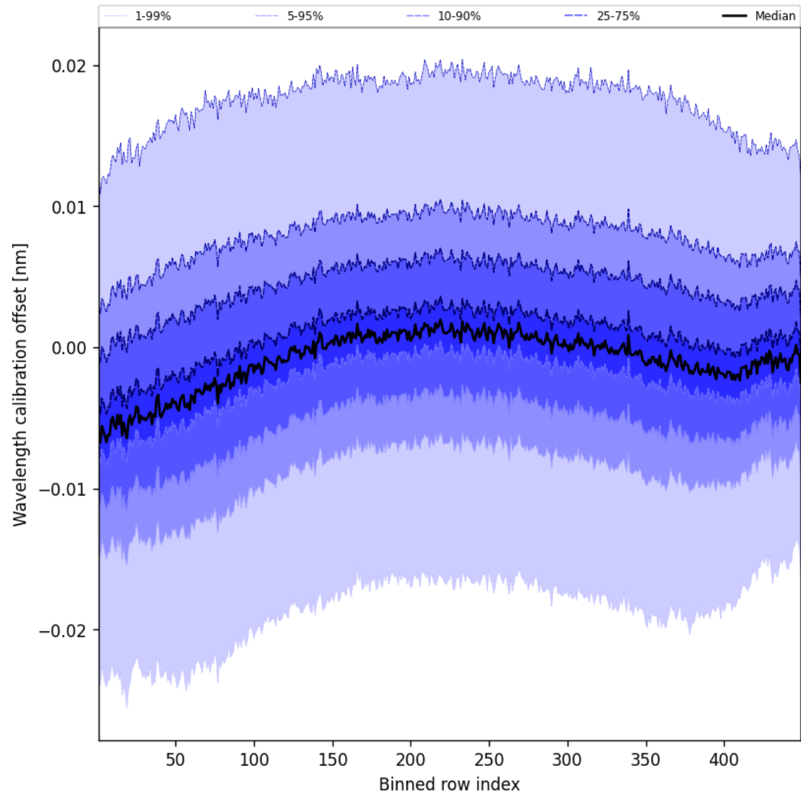
Figure 52: Along track statistics of “Wavelength calibration offset” for 2025-10-12 to 2025-10-14
