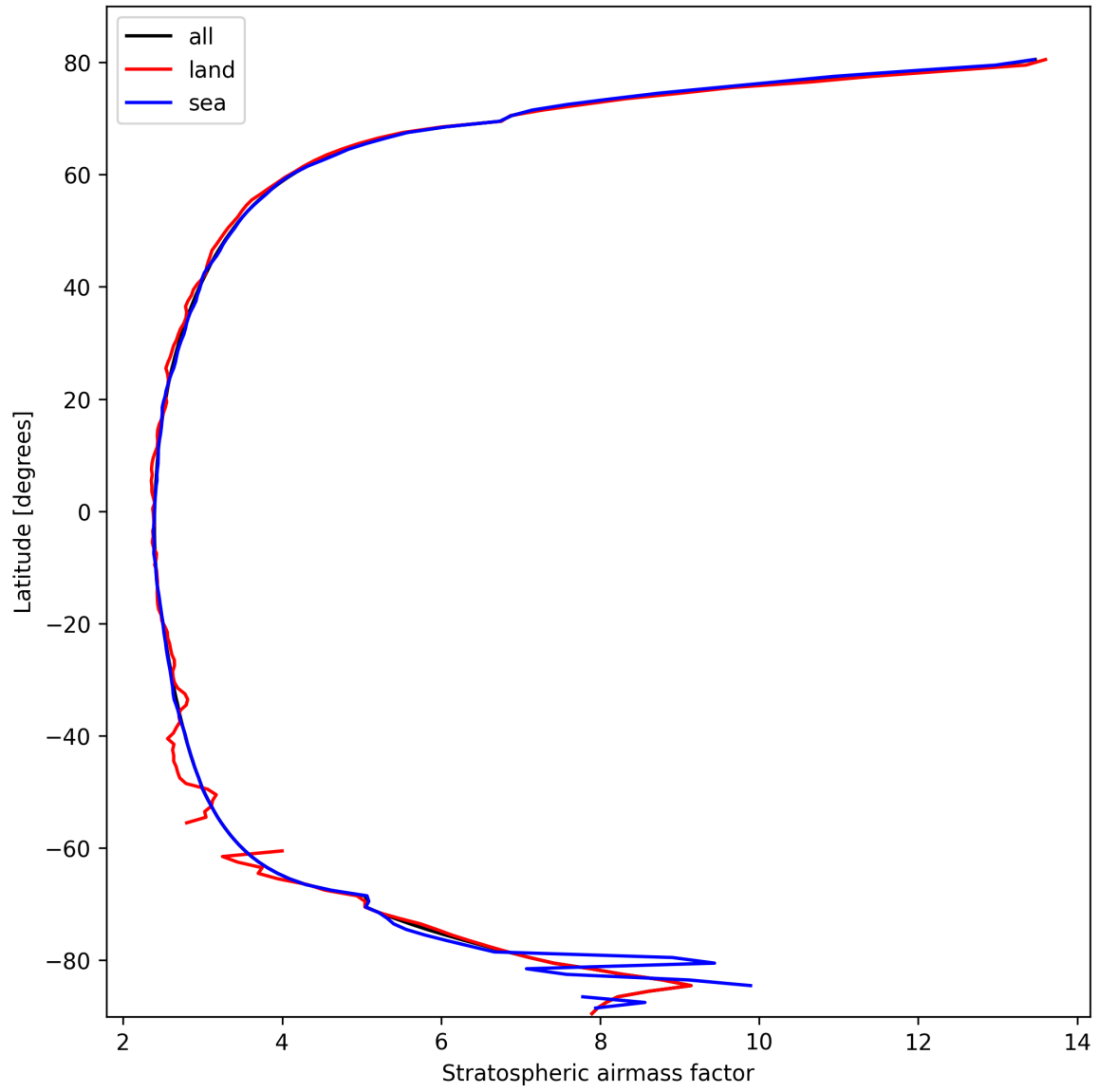
Figure 27: Zonal average of “Stratospheric airmass factor” for 2025-10-12 to 2025-10-14.
