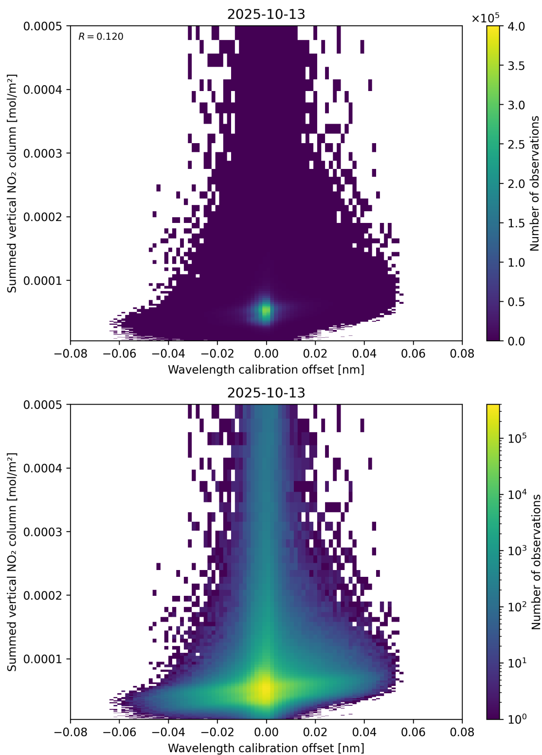
Figure 177: Scatter density plot of “Wavelength calibration offset” against “Summed vertical NO 2 column” for 2025-10-12 to 2025-10-14.
