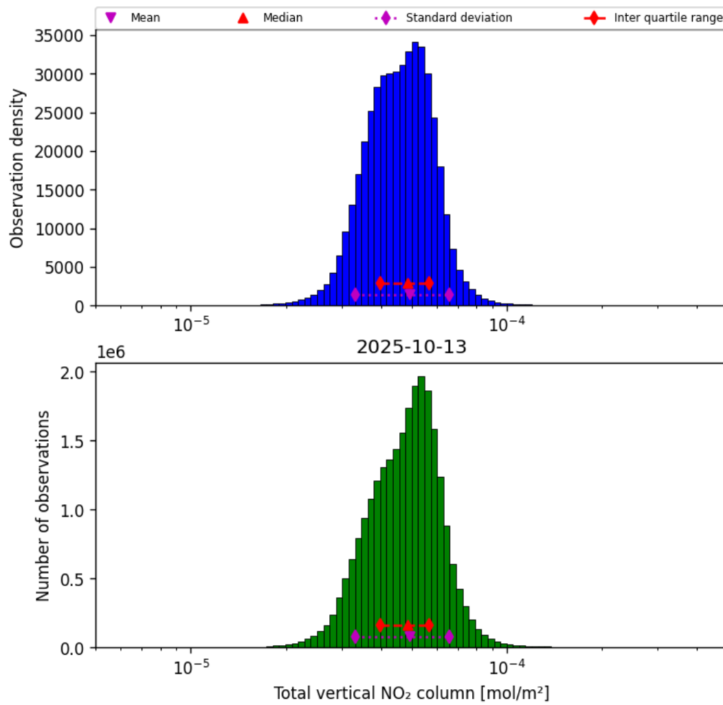
Figure 38: Histogram of “Total vertical NO 2 column” for 2025-10-12 to 2025-10-14
