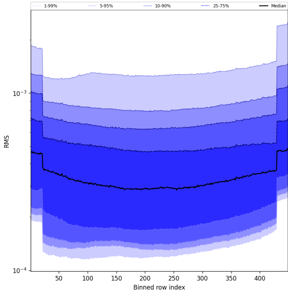
Figure 60: Along track statistics of “RMS” for 2025-10-12 to 2025-10-14
