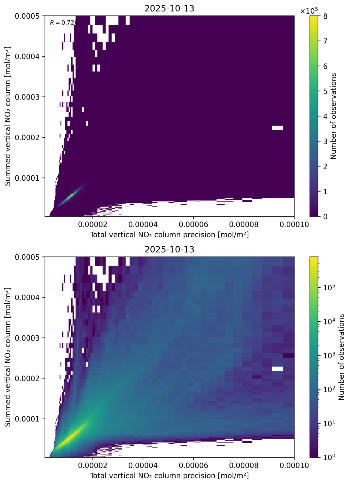
Figure 117: Scatter density plot of “Total vertical NO 2 column precision” against “Summed vertical NO 2 column” for 2025-10-12 to 2025-10-14.
