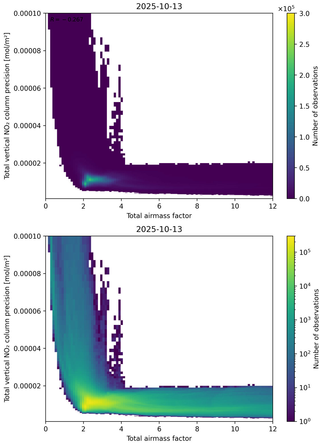
Figure 68: Scatter density plot of “Total airmass factor” against “Total vertical NO 2 column precision” for 2025-10-12 to 2025-10-14.
