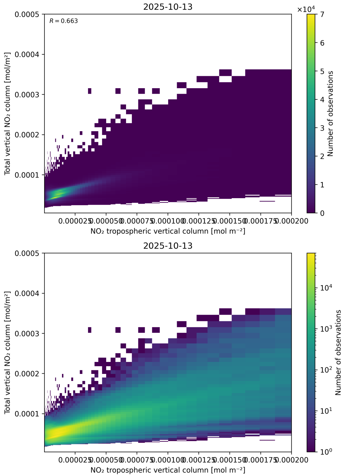
Figure 128: Scatter density plot of “NO 2 tropospheric vertical column” against “Total vertical NO 2 column” for 2025-10-12 to 2025-10-14.
