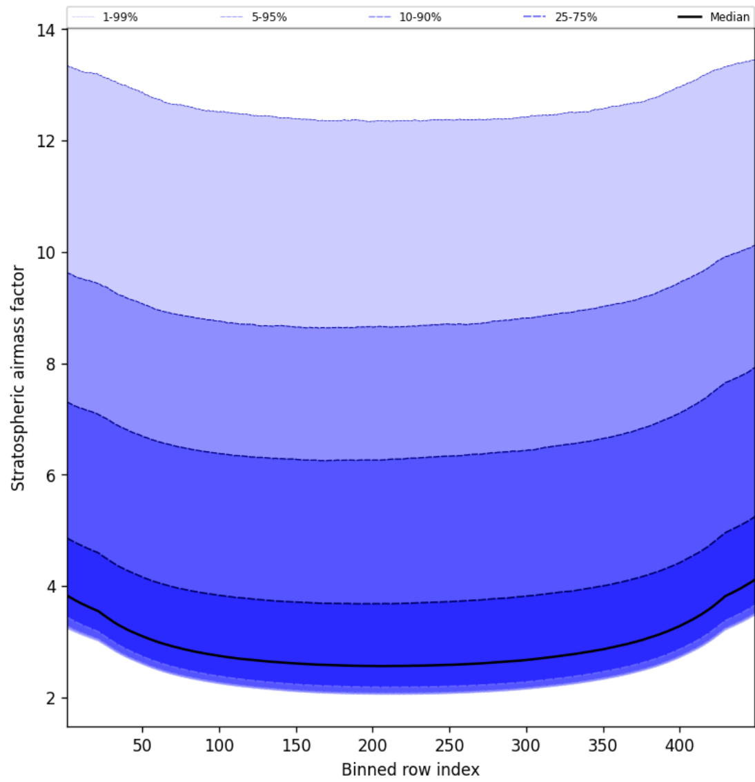
Figure 61: Along track statistics of “Stratospheric air mass factor” for 2025-10-12 to 2025-10-14
