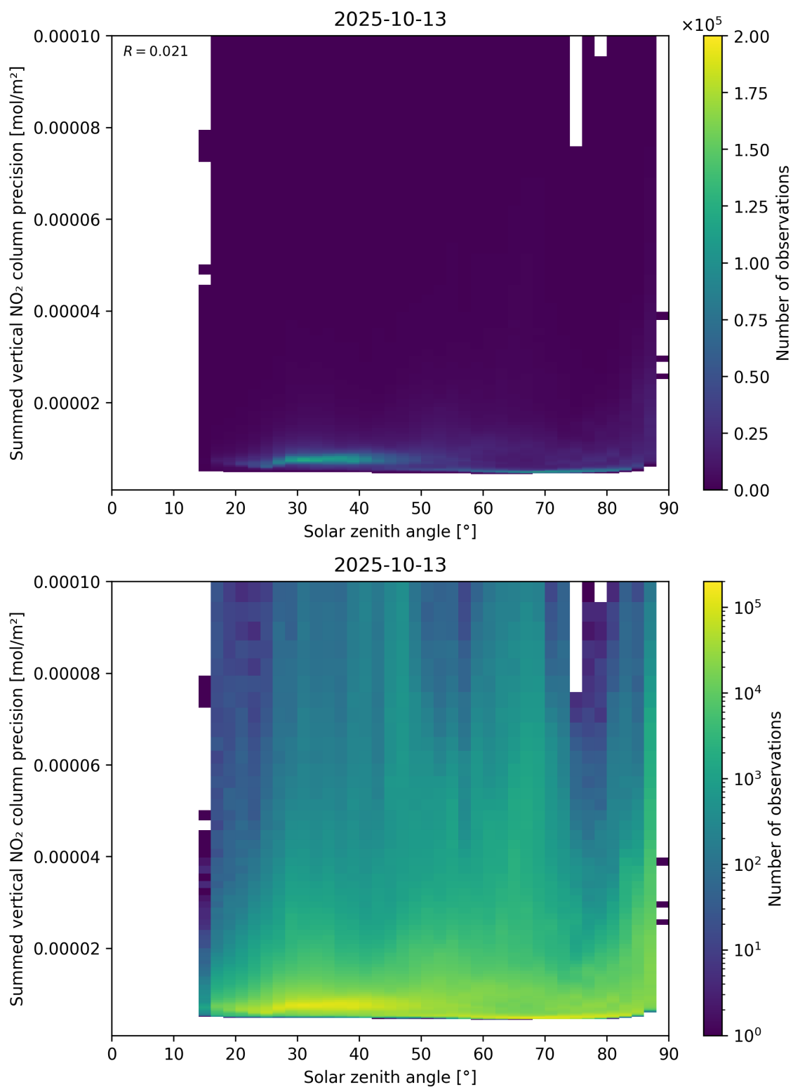
Figure 152: Scatter density plot of “Solar zenith angle” against “Summed vertical NO 2 column precision” for 2025-10-12 to 2025-10-14.
