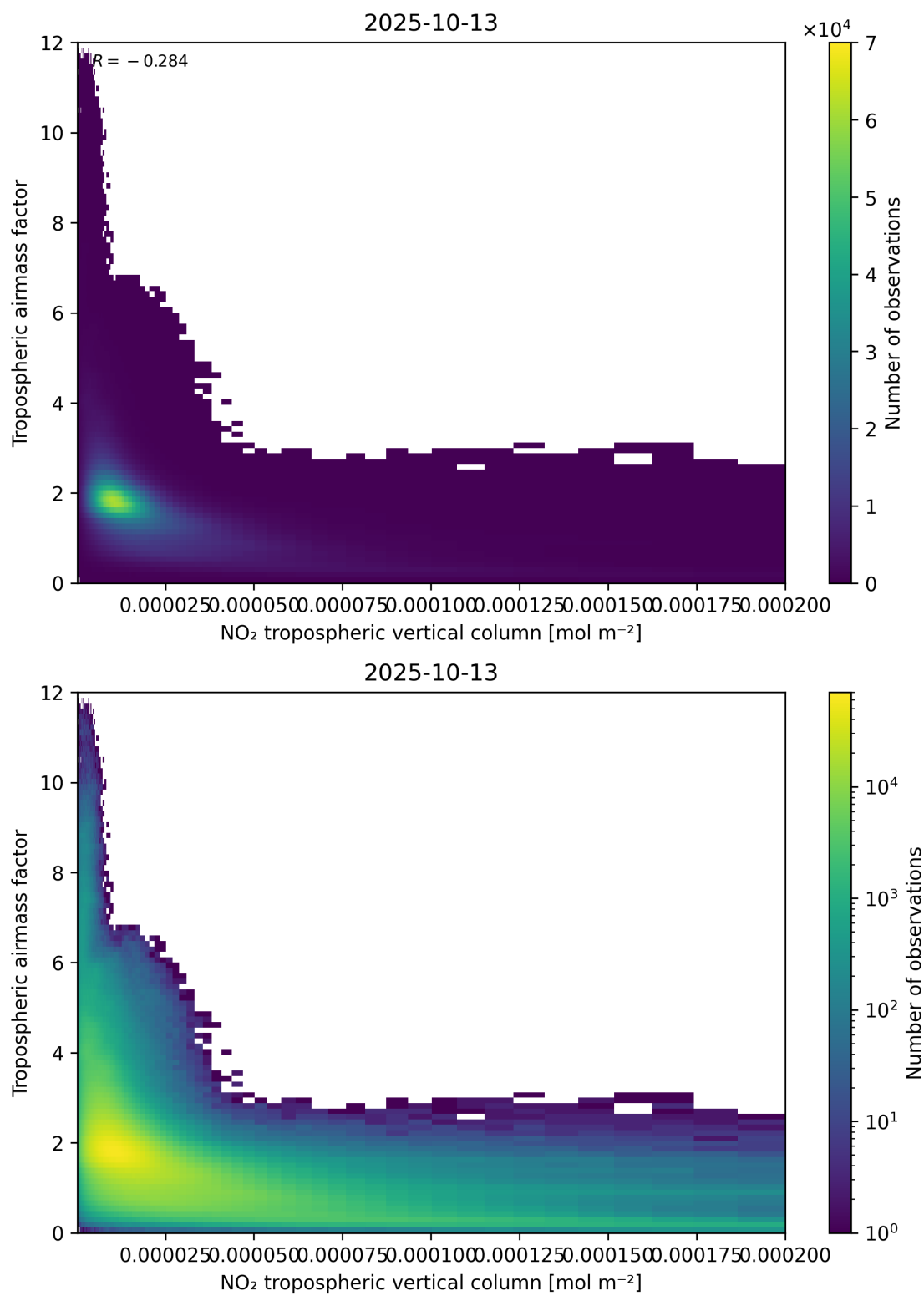
Figure 123: Scatter density plot of “NO 2 tropospheric vertical column” against “Tropospheric air mass factor” for 2025-10-12 to 2025-10-14.
