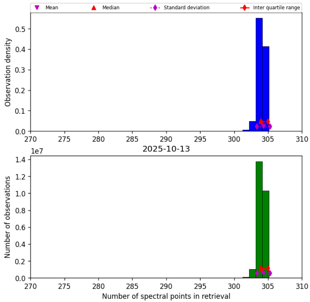
Figure 33: Histogram of “Number of spectral points in retrieval” for 2025-10-12 to 2025-10-14
