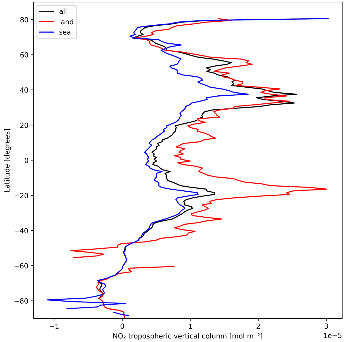
Figure 12: Zonal average of “NO 2 tropospheric vertical column” for 2025-10-12 to 2025-10-14.
