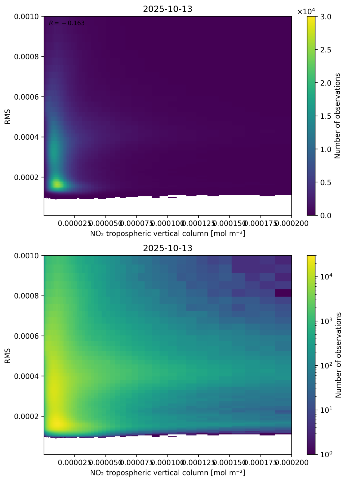
Figure 142: Scatter density plot of “NO 2 tropospheric vertical column” against “RMS” for 2025-10-12 to 2025-10-14.
