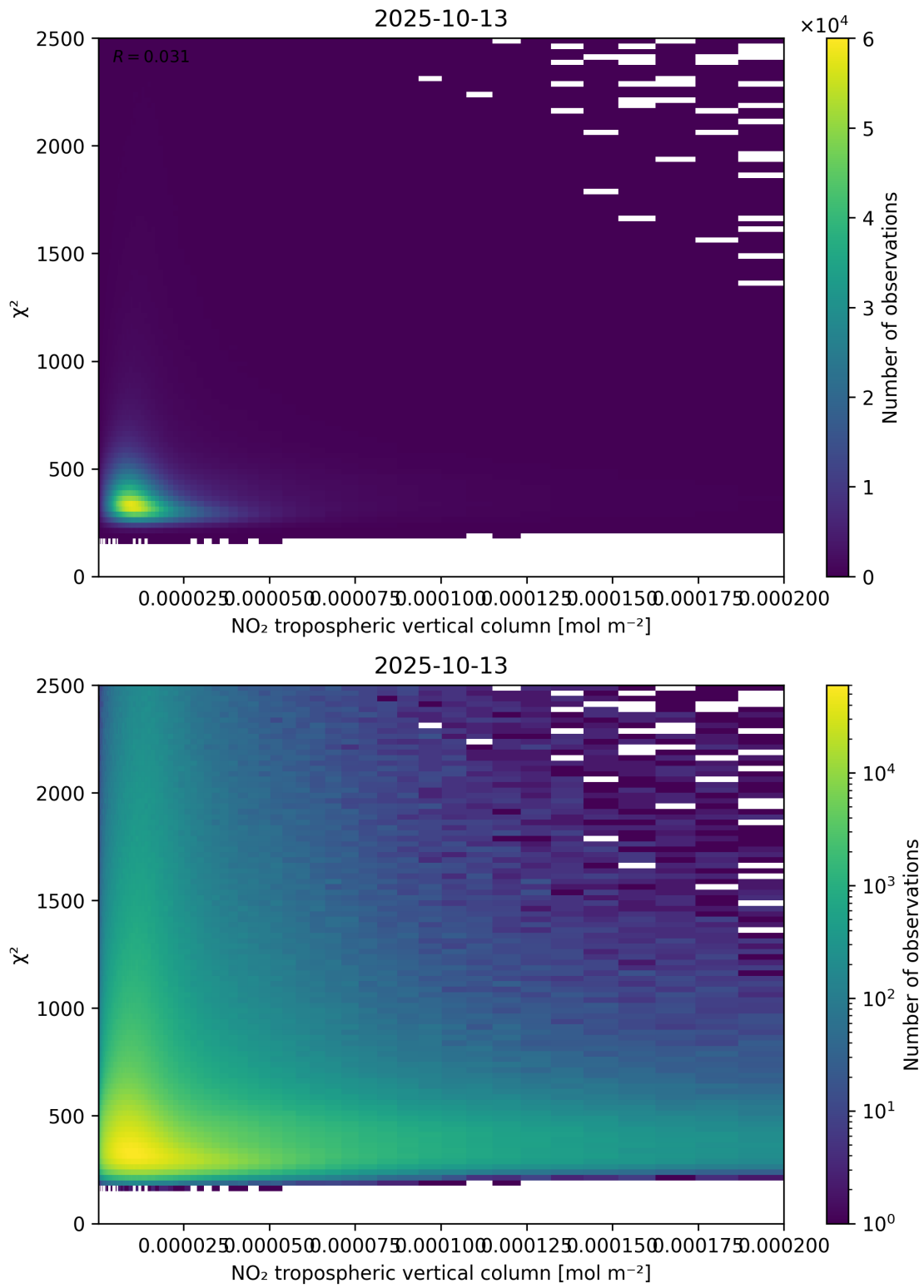
Figure 124: Scatter density plot of “NO 2 tropospheric vertical column” against “ \chi^2 ” for 2025-10-12 to 2025-10-14.
