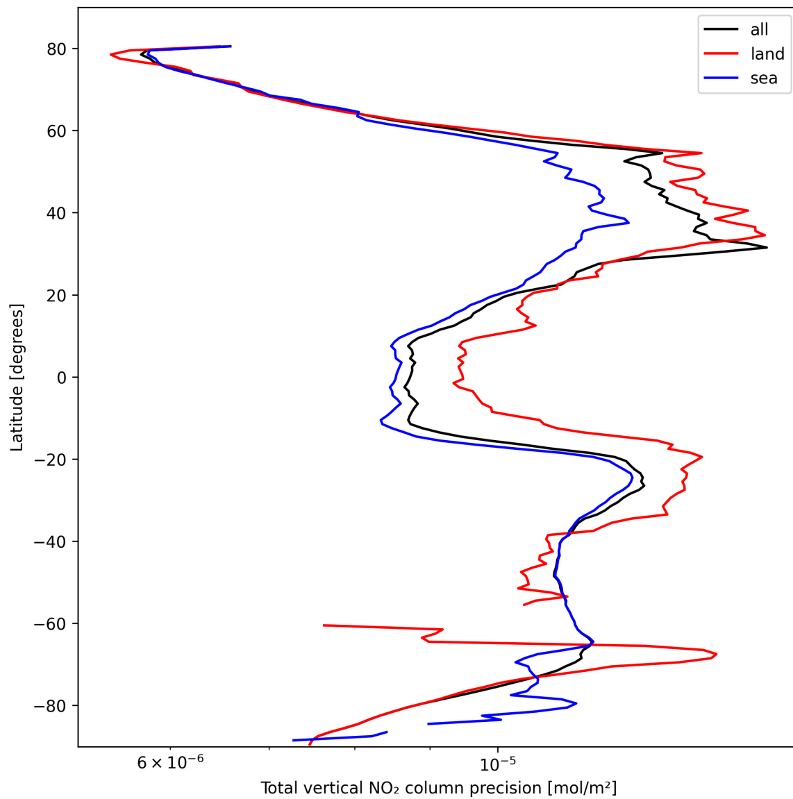
Figure 22: Zonal average of “Total vertical NO 2 column precision” for 2025-10-12 to 2025-10-14.
