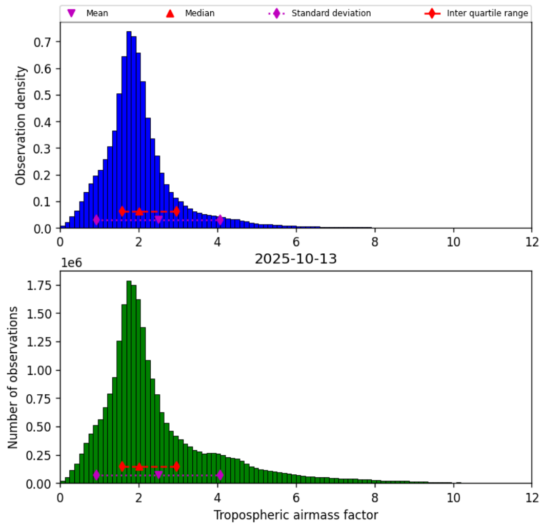
Figure 31: Histogram of “Tropospheric airmass factor” for 2025-10-12 to 2025-10-14
