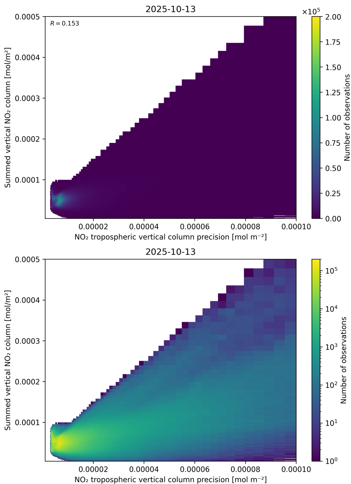
Figure 136: Scatter density plot of “NO 2 tropospheric vertical column precision” against “Summed vertical NO 2 column” for 2025-10-12 to 2025-10-14.
