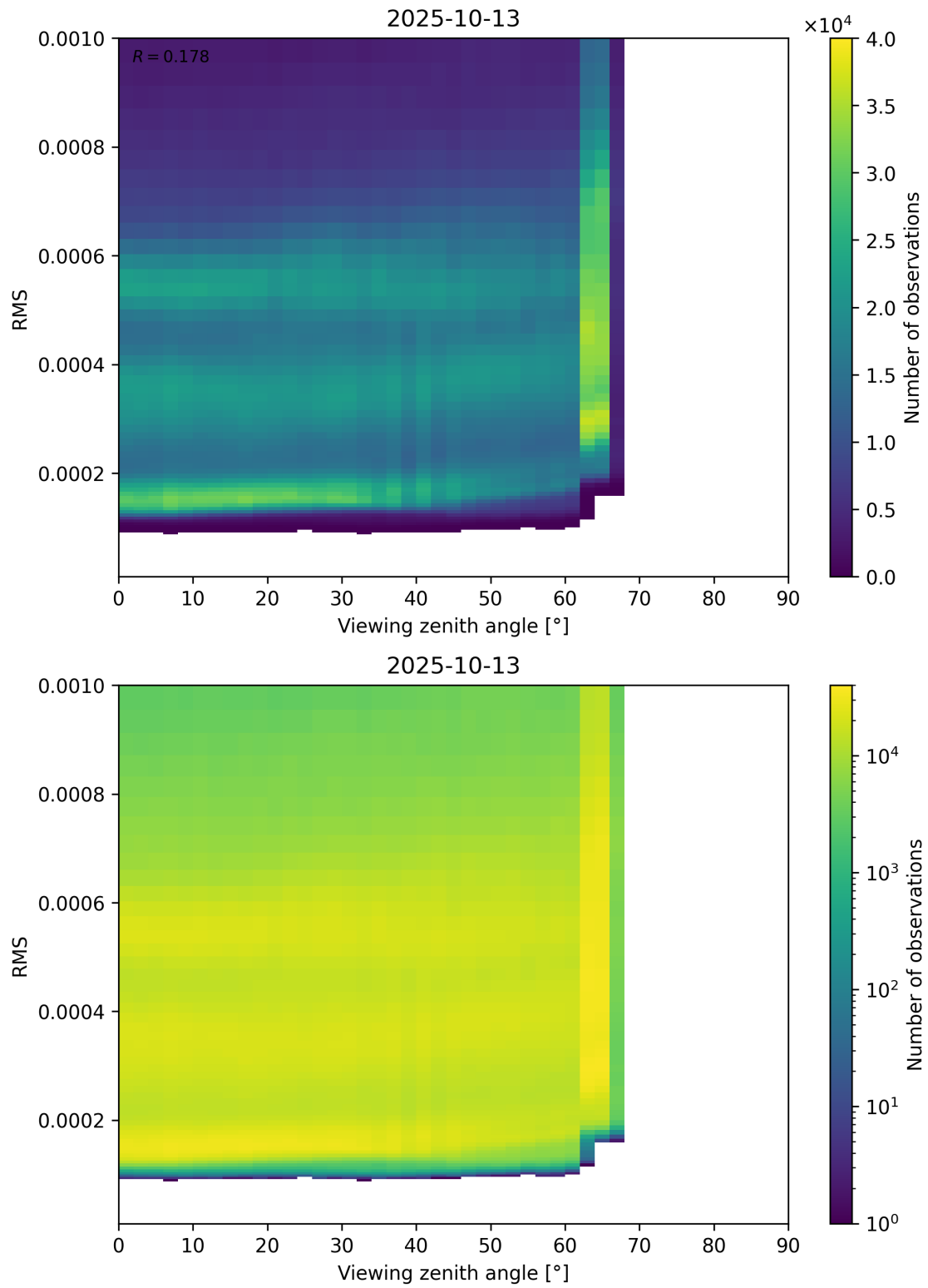
Figure 171: Scatter density plot of “Viewing zenith angle” against “RMS” for 2025-10-12 to 2025-10-14.
