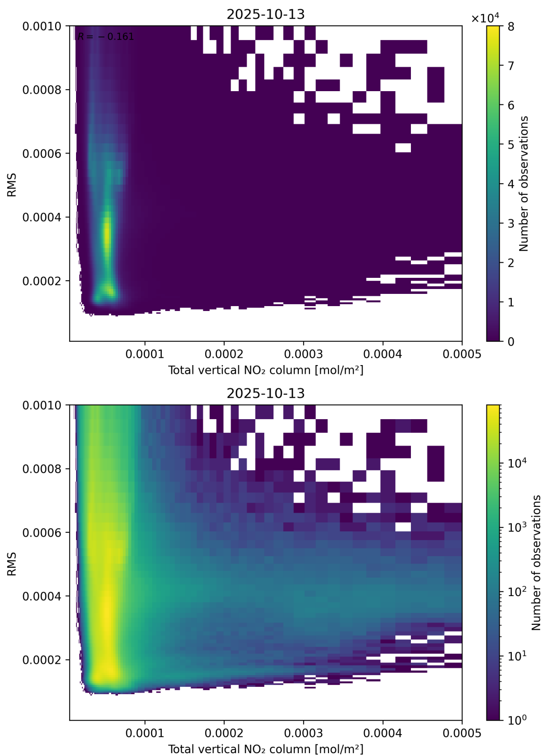
Figure 120: Scatter density plot of “Total vertical NO 2 column” against “RMS” for 2025-10-12 to 2025-10-14.
