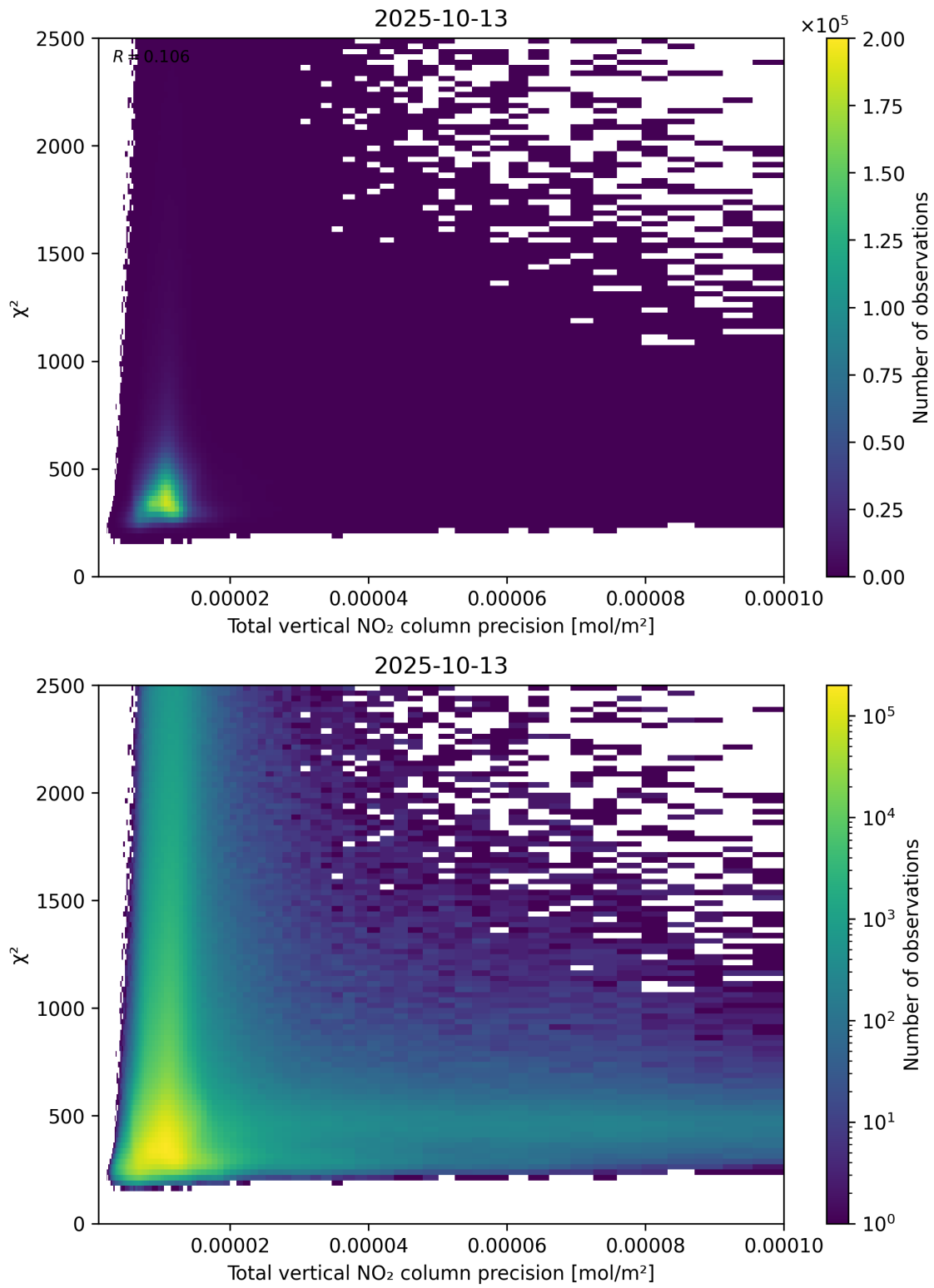
Figure 116: Scatter density plot of “Total vertical NO 2 column precision” against “ \chi^2 ” for 2025-10-12 to 2025-10-14.
