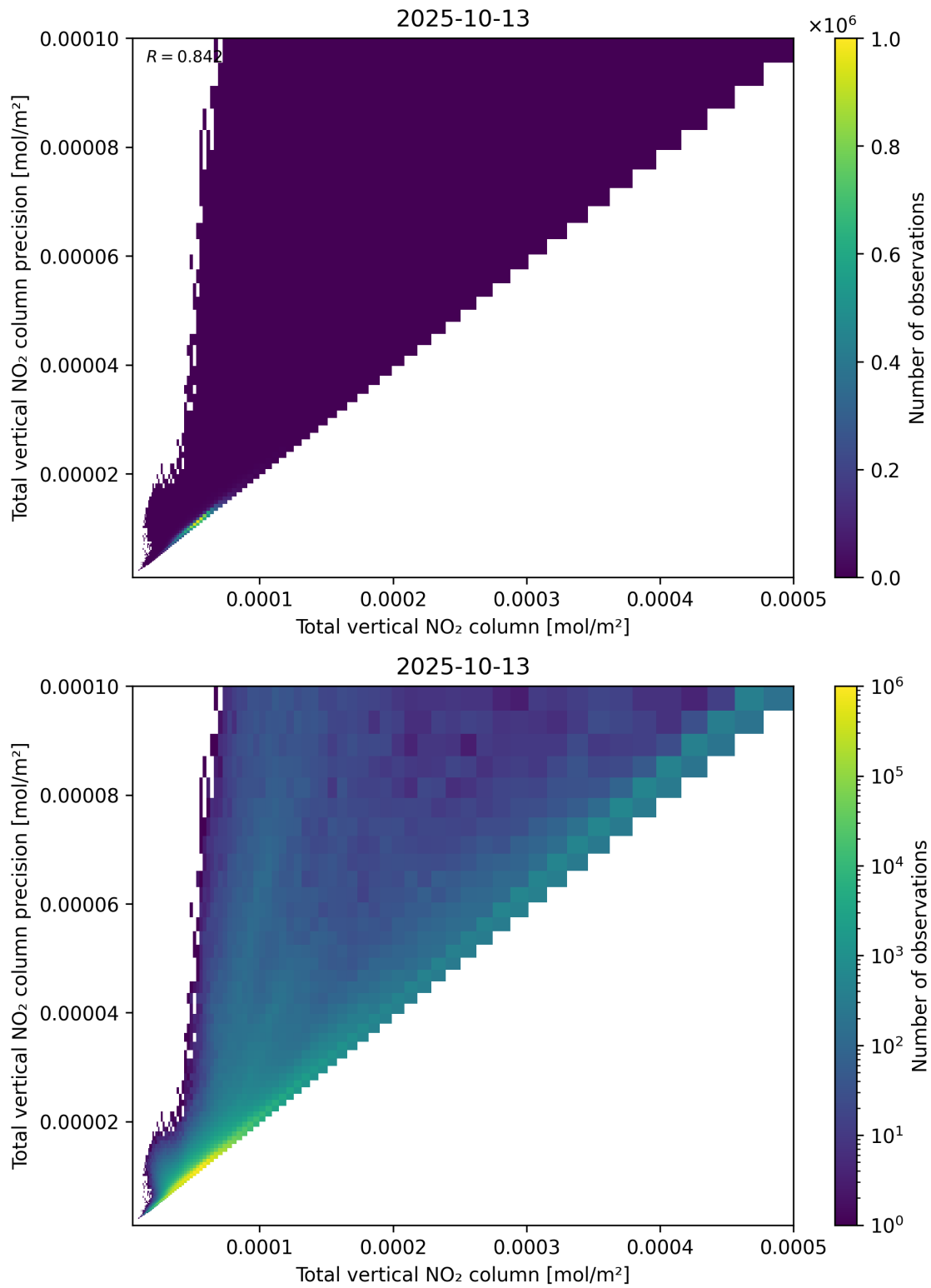
Figure 114: Scatter density plot of “Total vertical NO 2 column” against “Total vertical NO 2 column precision” for 2025-10-12 to 2025-10-14.
