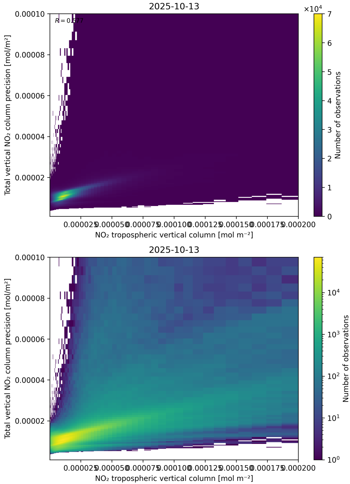
Figure 129: Scatter density plot of “NO 2 tropospheric vertical column” against “Total vertical NO 2 column precision” for 2025-10-12 to 2025-10-14.
