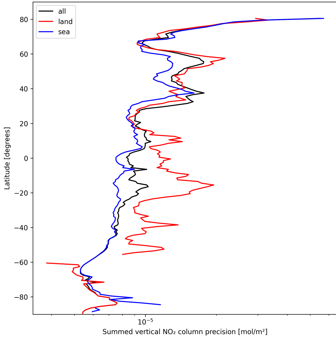
Figure 24: Zonal average of “Summed vertical NO 2 column precision” for 2025-10-12 to 2025-10-14.
