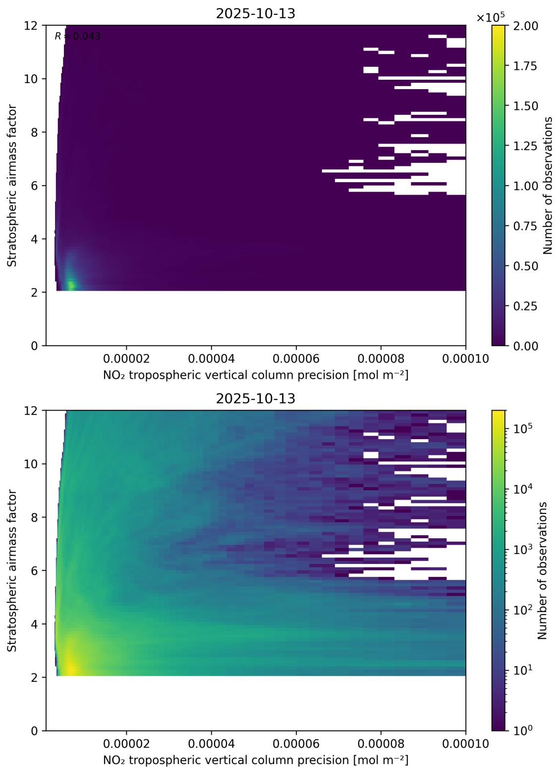
Figure 131: Scatter density plot of “NO 2 tropospheric vertical column precision” against “Stratospheric airmass factor” for 2025-10-12 to 2025-10-14.
