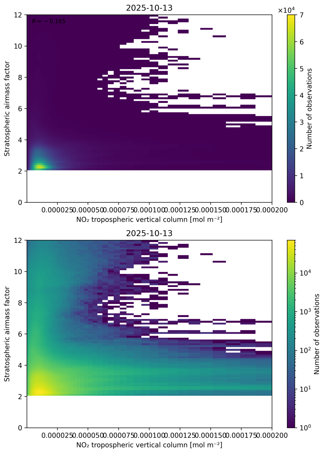
Figure 121: Scatter density plot of “NO 2 tropospheric vertical column” against “Stratospheric air mass factor” for 2025-10-12 to 2025-10-14.
