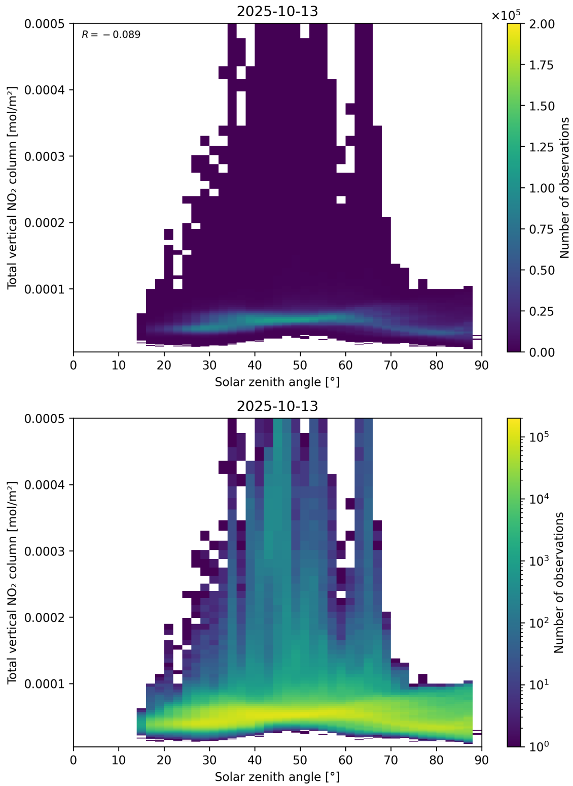
Figure 153: Scatter density plot of “Solar zenith angle” against “Total vertical NO 2 column” for 2025-10-12 to 2025-10-14.
