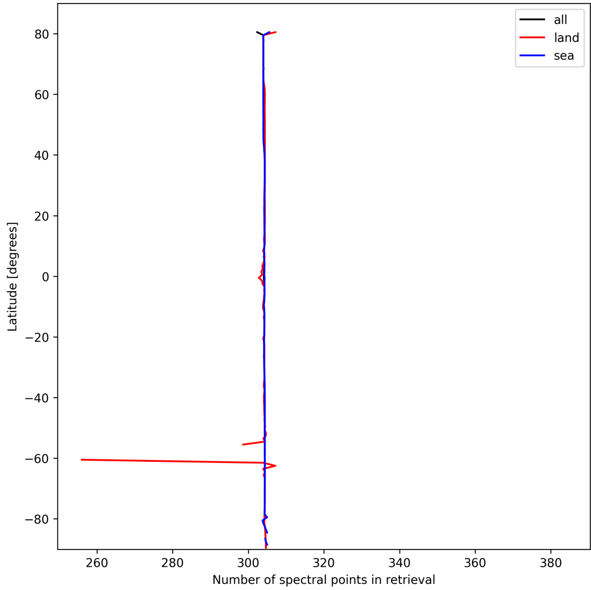
Figure 16: Zonal average of “Number of spectral points in retrieval” for 2025-10-12 to 2025-10-14.
