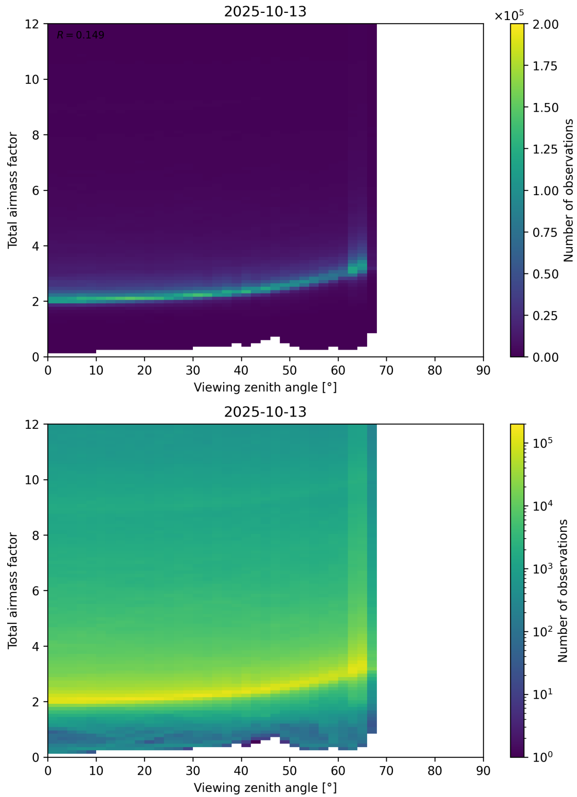
Figure 160: Scatter density plot of “Viewing zenith angle” against “Total airmass factor” for 2025-10-12 to 2025-10-14.
