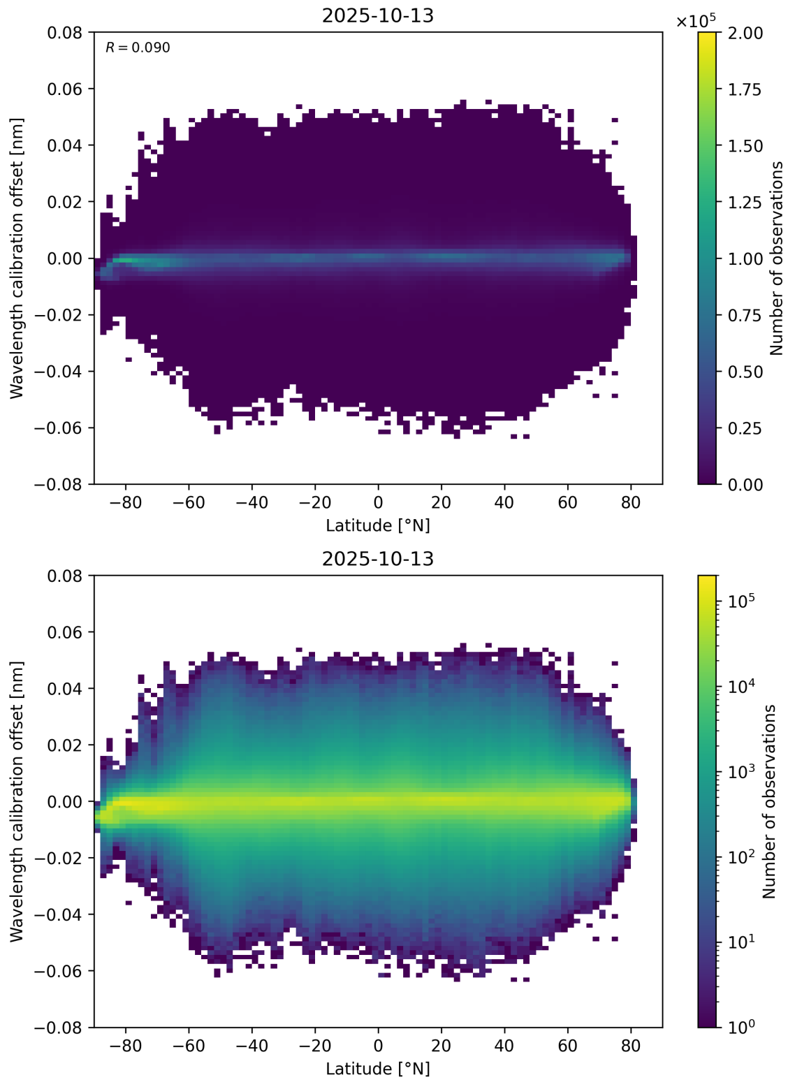
Figure 95: Scatter density plot of “Latitude” against “Wavelength calibration offset” for 2025-10-12 to 2025-10-14.
