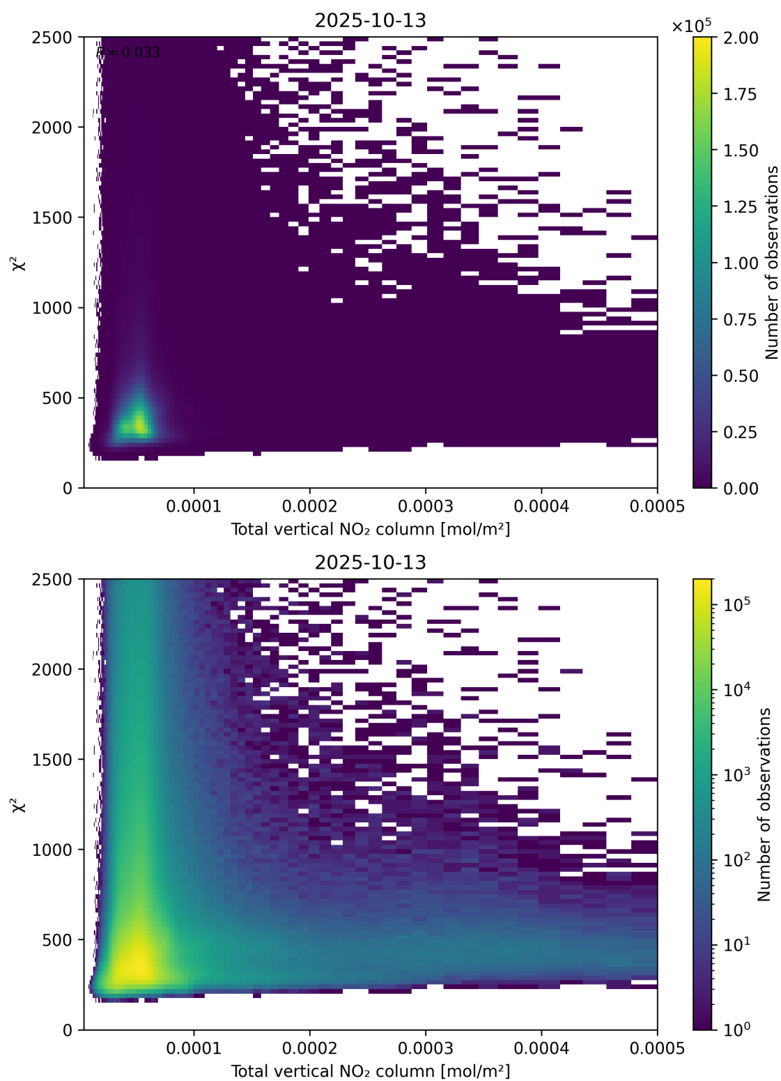
Figure 111: Scatter density plot of “Total vertical NO 2 column” against “ \chi^2 ” for 2025-10-12 to 2025-10-14.
