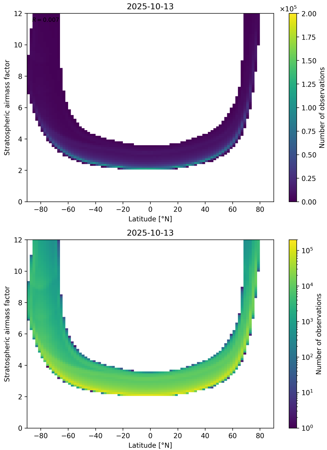
Figure 83: Scatter density plot of “Latitude” against “Stratospheric airmass factor” for 2025-10-12 to 2025-10-14.
