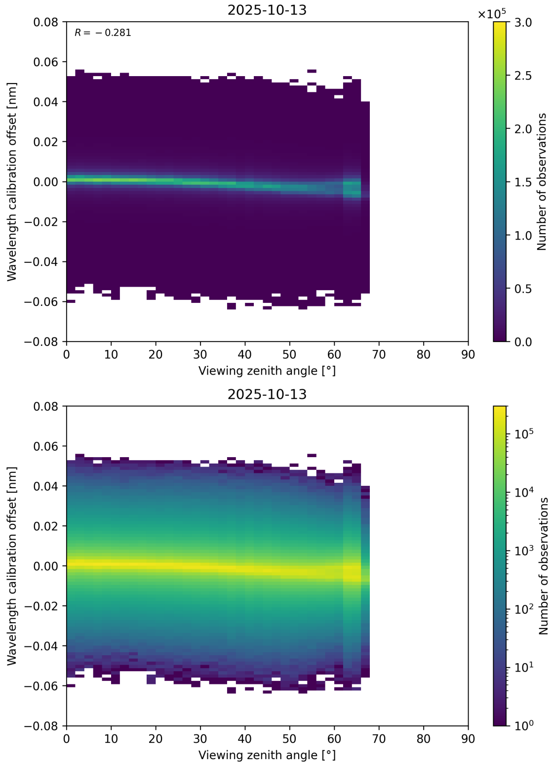
Figure 173: Scatter density plot of “Viewing zenith angle” against “Wavelength calibration offset” for 2025-10-12 to 2025-10-14.
