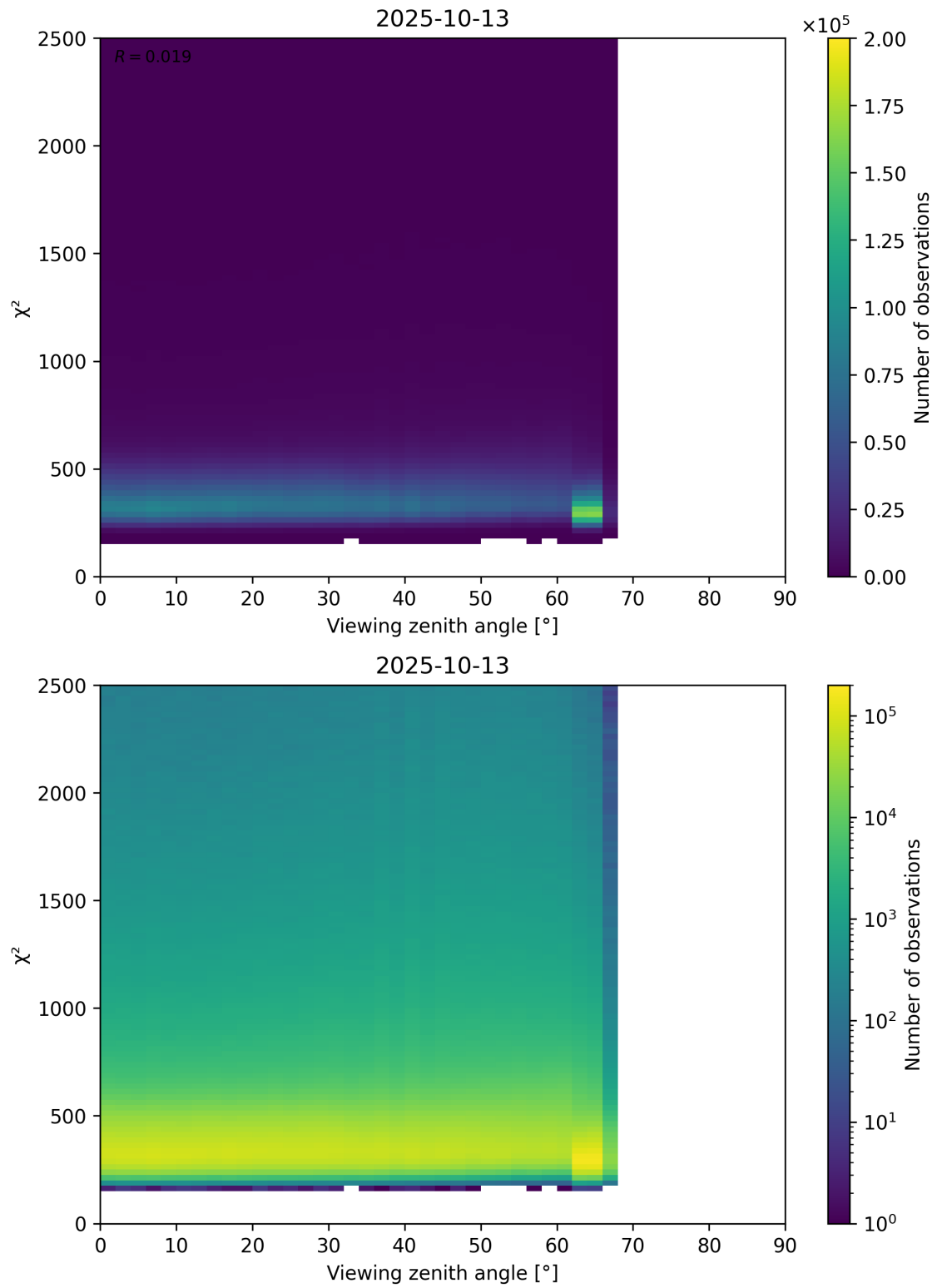
Figure 162: Scatter density plot of “Viewing zenith angle” against “ \chi^2 ” for 2025-10-12 to 2025-10-14.
