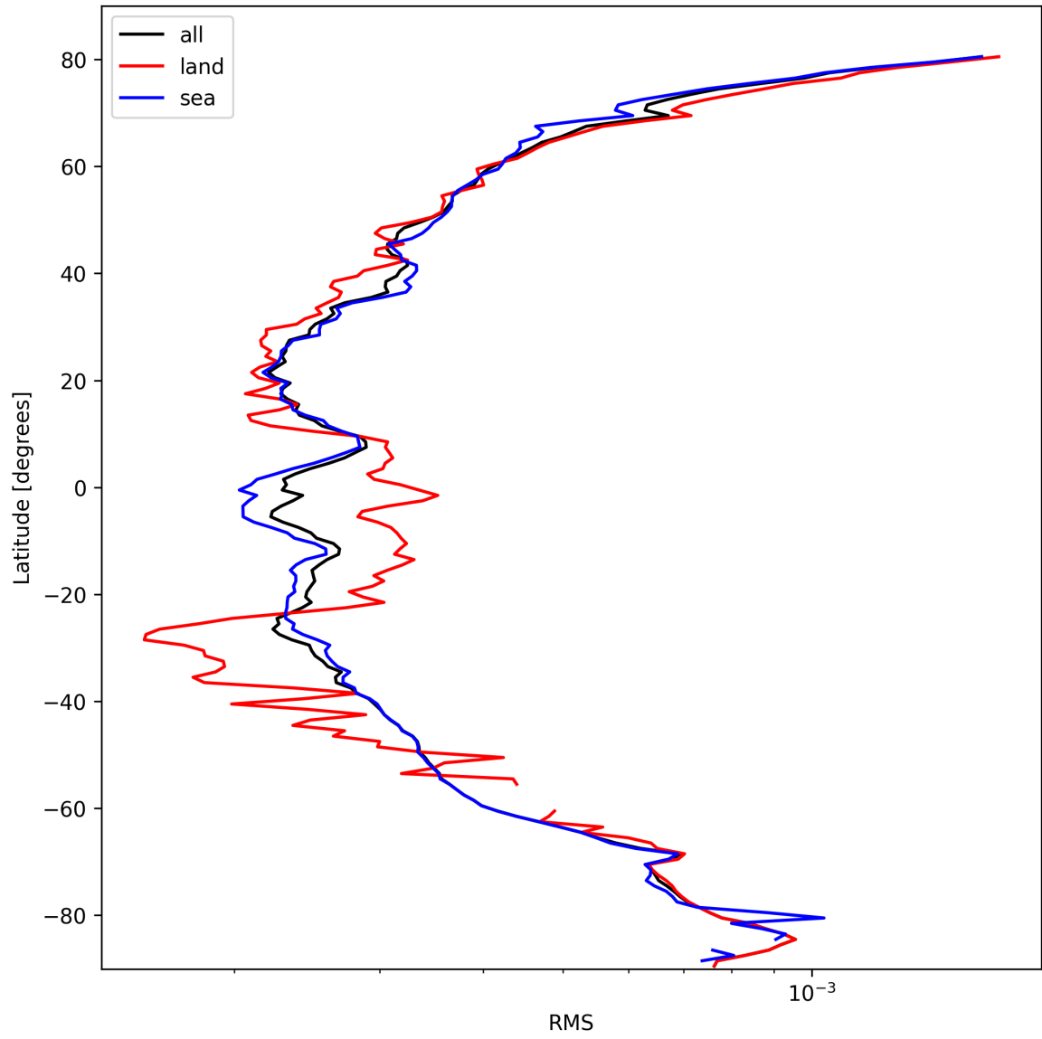
Figure 26: Zonal average of “RMS” for 2025-10-12 to 2025-10-14.
