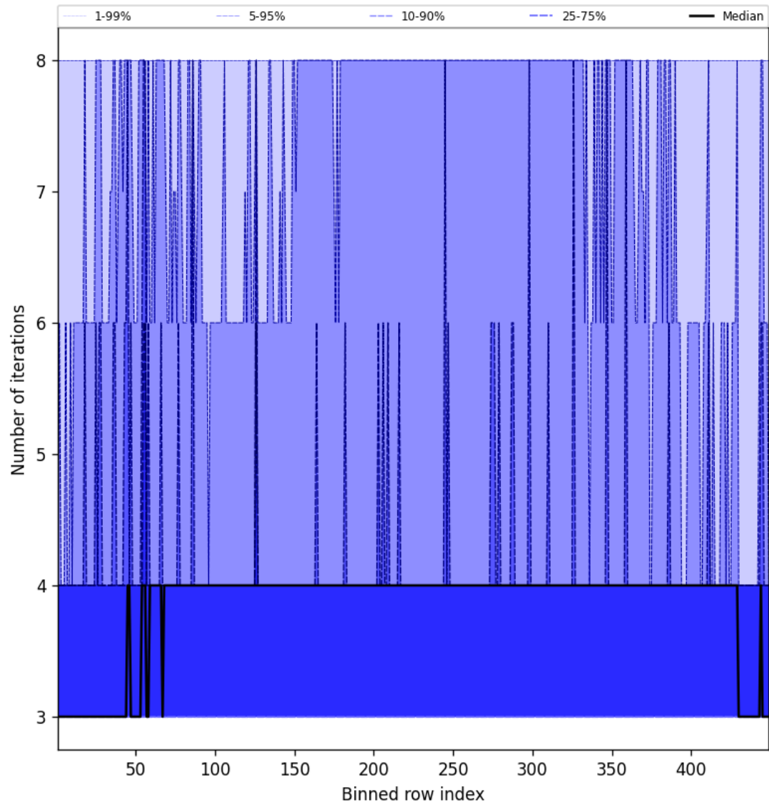
Figure 51: Along track statistics of “Number of iterations” for 2025-10-12 to 2025-10-14
