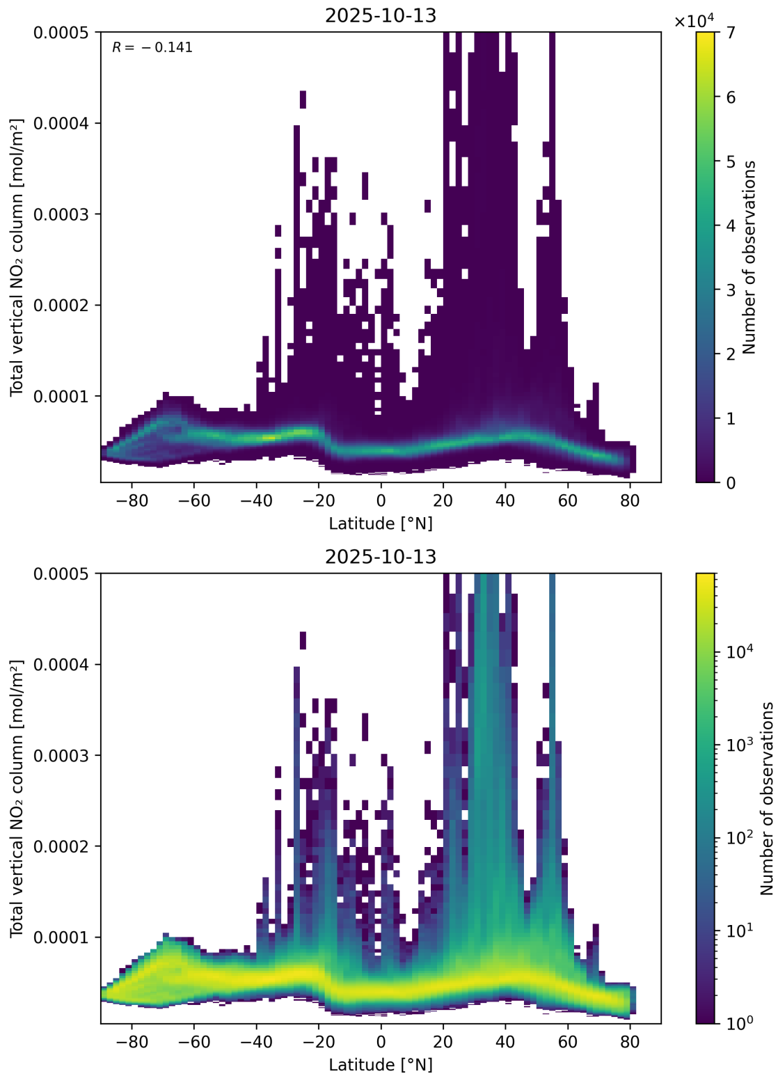
Figure 90: Scatter density plot of “Latitude” against “Total vertical NO 2 column” for 2025-10-12 to 2025-10-14.
