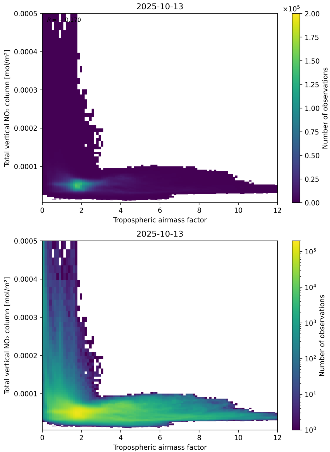
Figure 77: Scatter density plot of “Tropospheric airmass factor” against “Total vertical NO 2 column” for 2025-10-12 to 2025-10-14.
