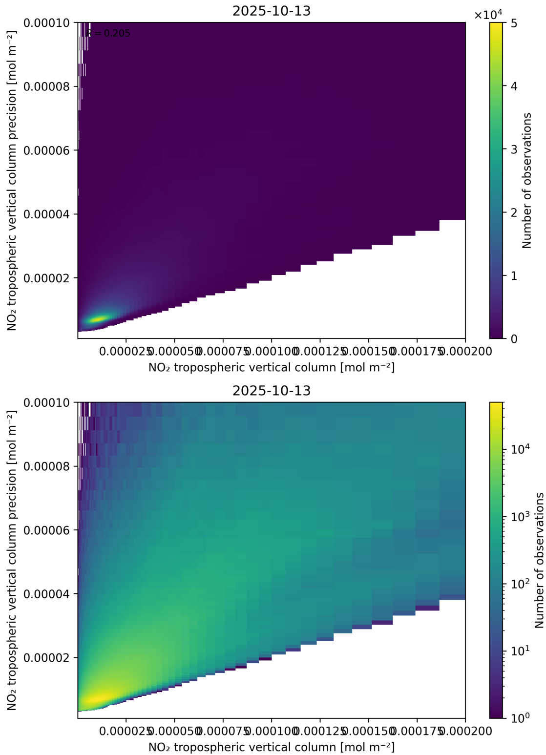
Figure 130: Scatter density plot of “NO 2 tropospheric vertical column” against “NO 2 tropospheric vertical column precision” for 2025-10-12 to 2025-10-14.
