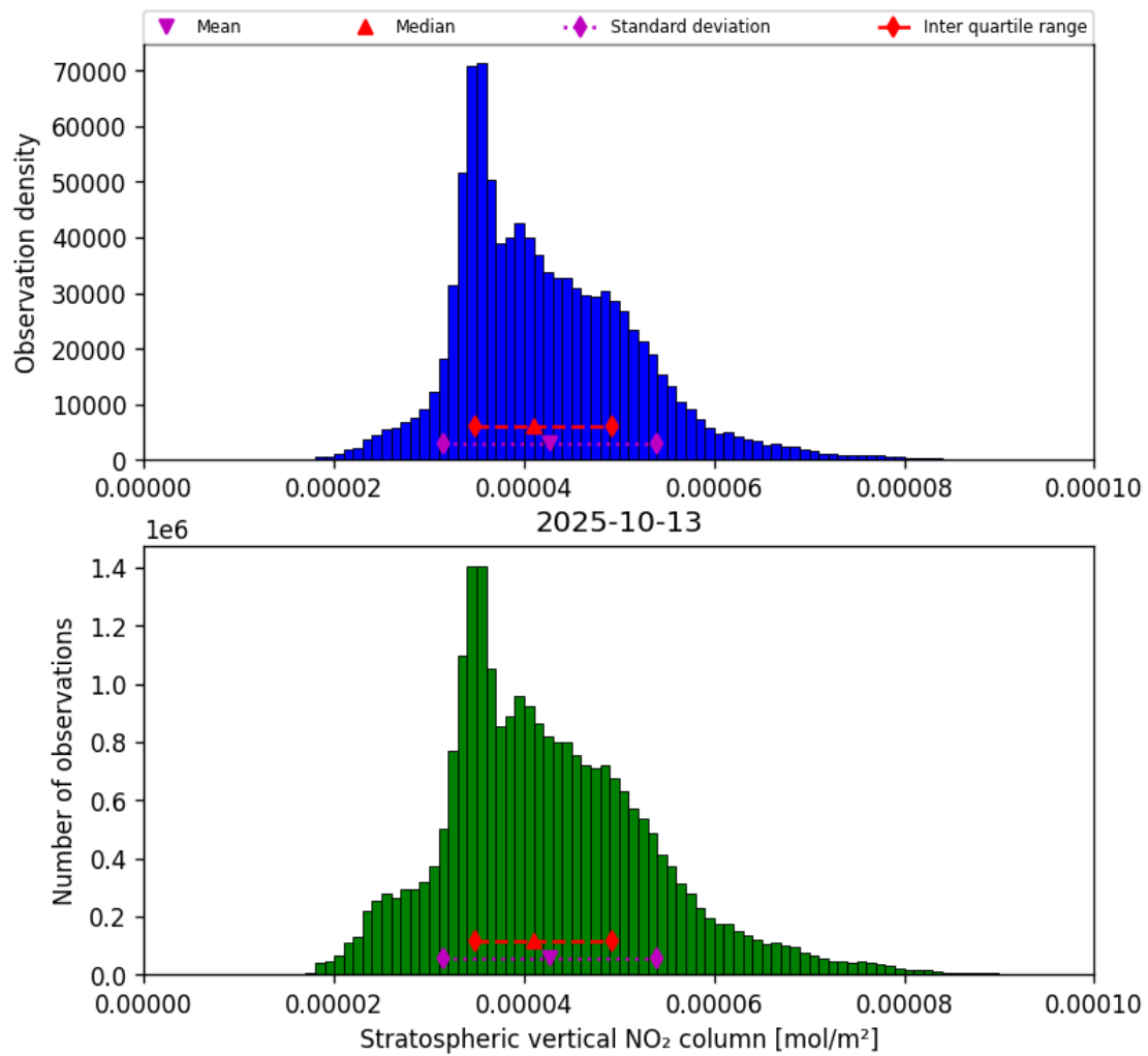
Figure 36: Histogram of “Stratospheric vertical NO 2 column” for 2025-10-12 to 2025-10-14
