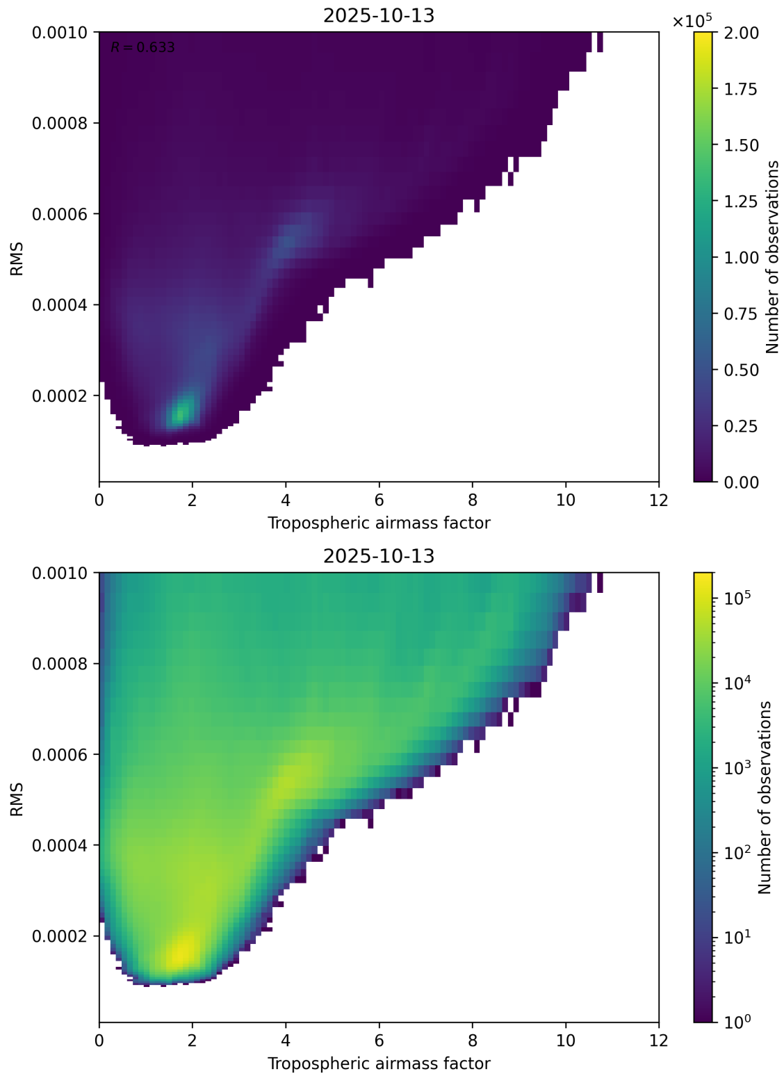
Figure 79: Scatter density plot of “Tropospheric airmass factor” against “RMS” for 2025-10-12 to 2025-10-14.
