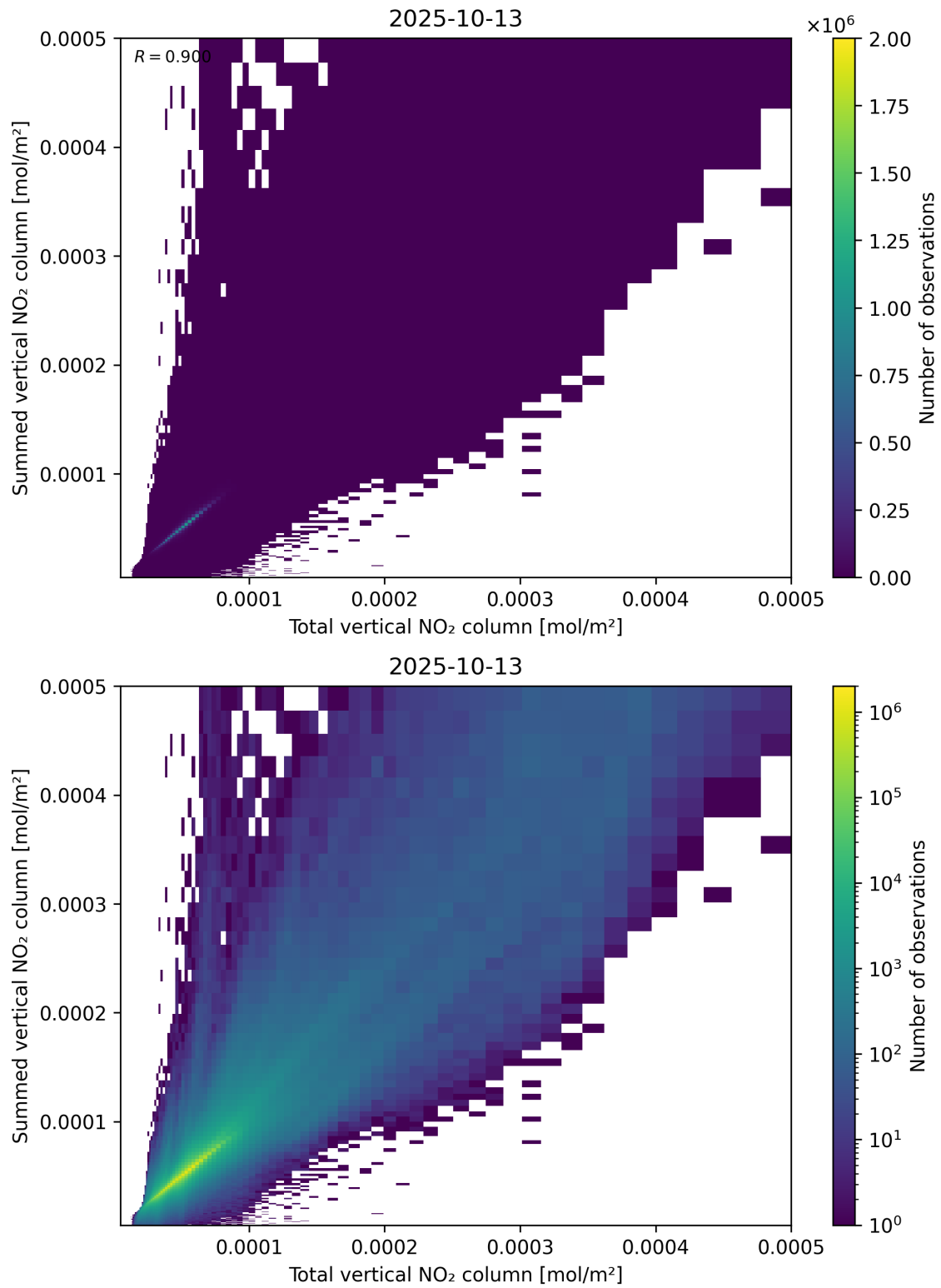
Figure 112: Scatter density plot of “Total vertical NO 2 column” against “Summed vertical NO 2 column” for 2025-10-12 to 2025-10-14.
