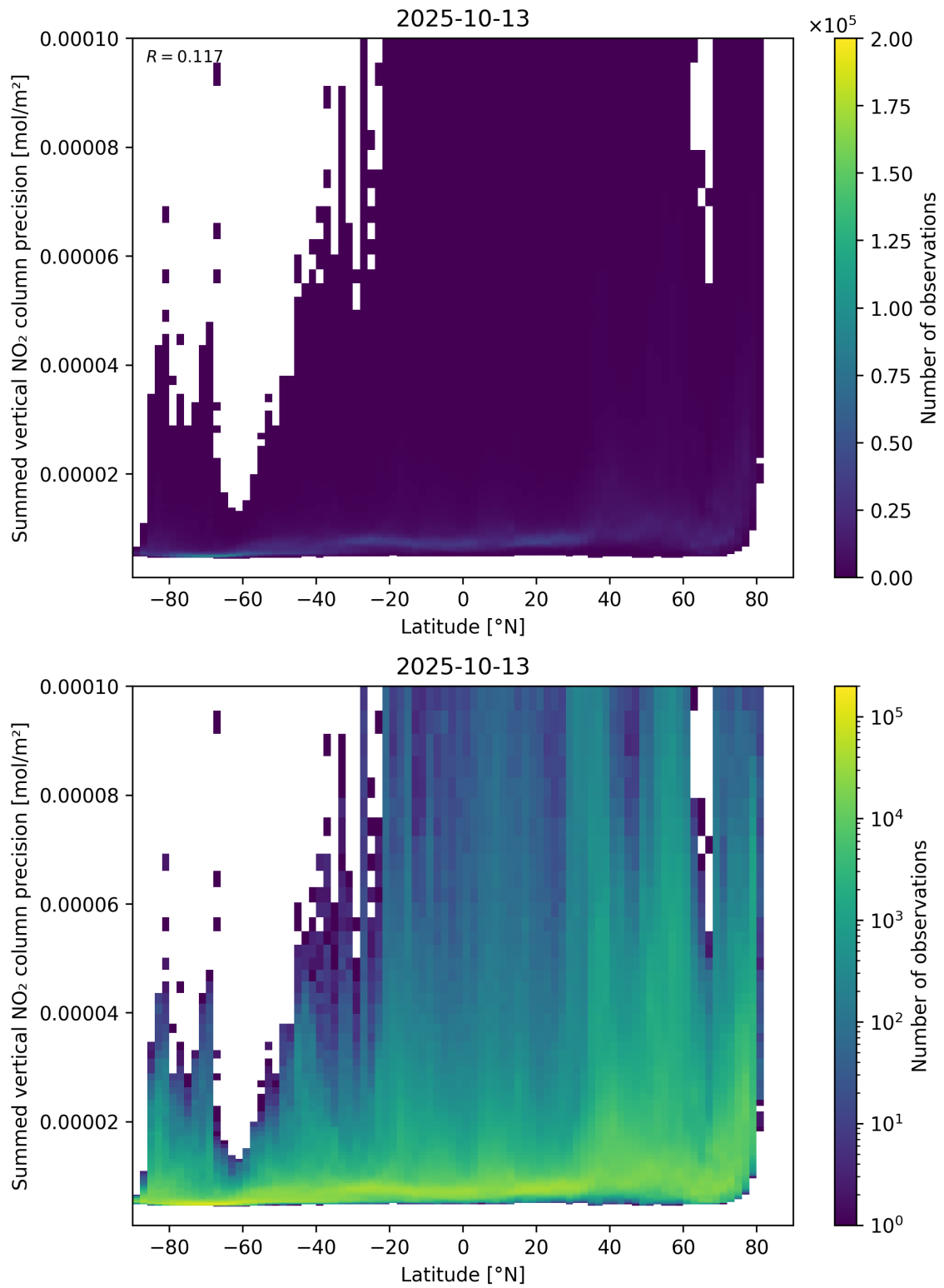
Figure 89: Scatter density plot of “Latitude” against “Summed vertical NO 2 column precision” for 2025-10-12 to 2025-10-14.
