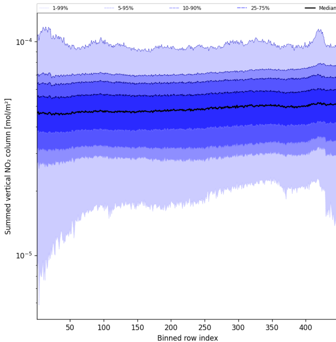
Figure 57: Along track statistics of “Summed vertical NO 2 column” for 2025-10-12 to 2025-10-14
