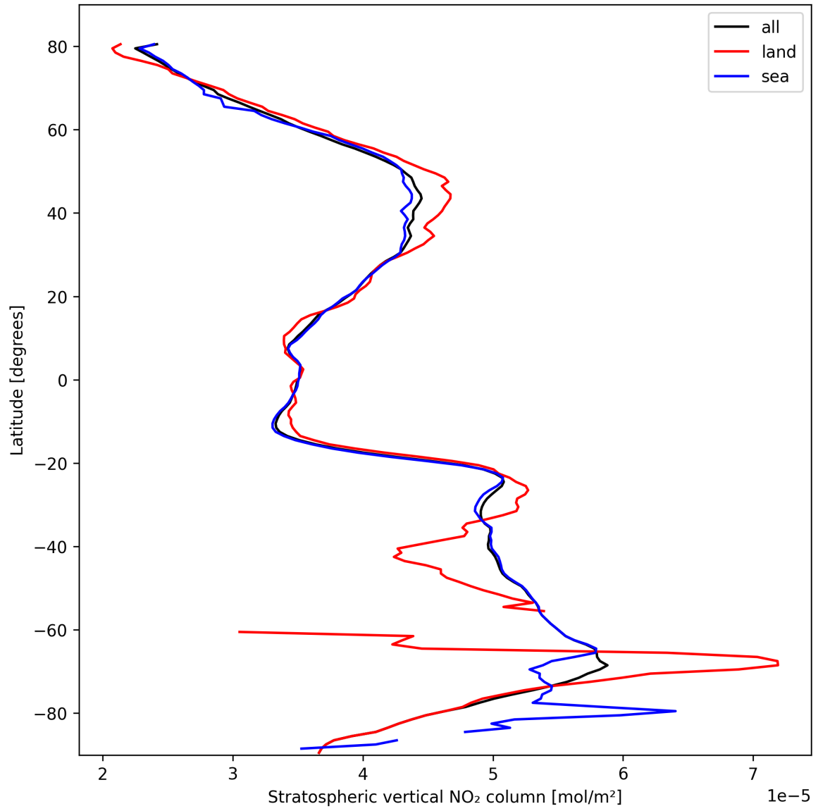
Figure 19: Zonal average of “Stratospheric vertical NO 2 column” for 2025-10-12 to 2025-10-14.
