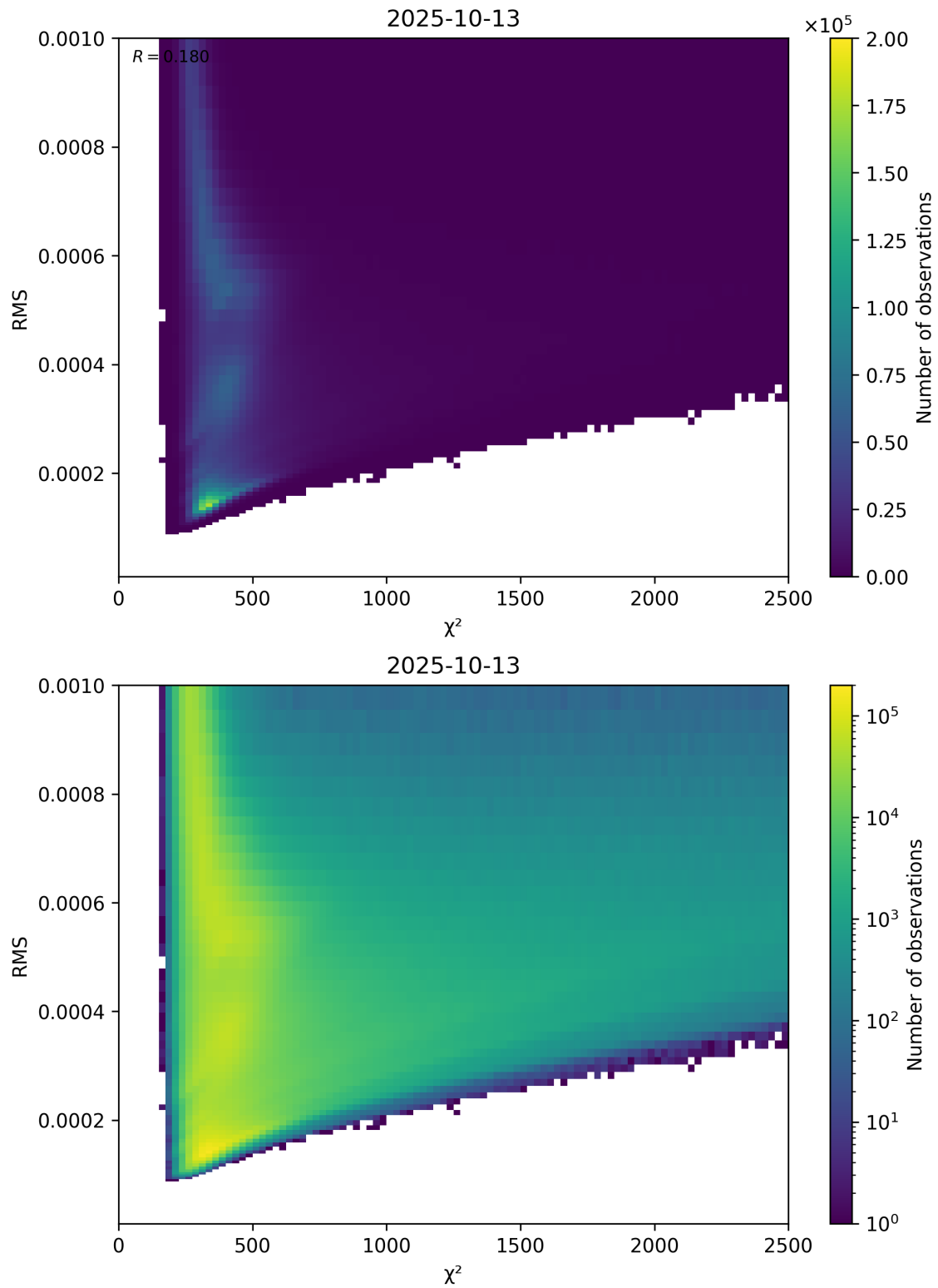
Figure 82: Scatter density plot of “ \chi^2 ” against “RMS” for 2025-10-12 to 2025-10-14.
