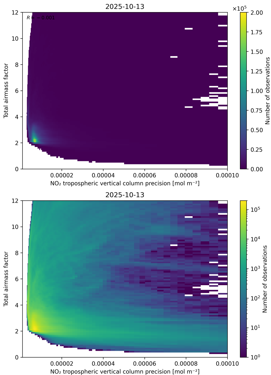
Figure 132: Scatter density plot of “NO 2 tropospheric vertical column precision” against “Total air mass factor” for 2025-10-12 to 2025-10-14.
