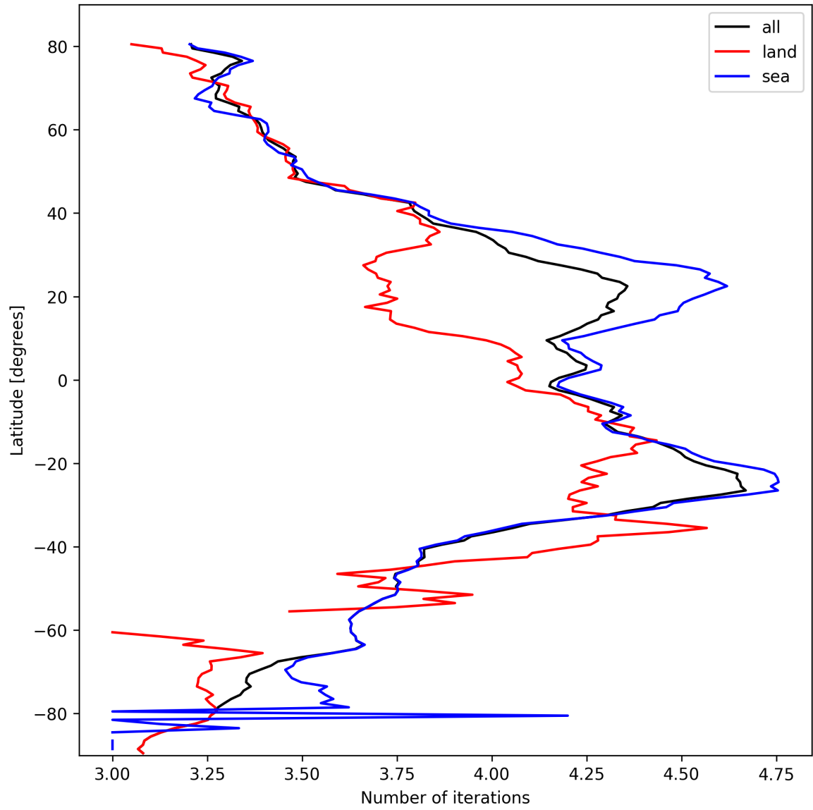
Figure 17: Zonal average of “Number of iterations” for 2025-10-12 to 2025-10-14.
