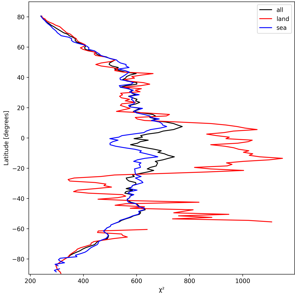
Figure 25: Zonal average of “ \chi^2 ” for 2025-10-12 to 2025-10-14.
