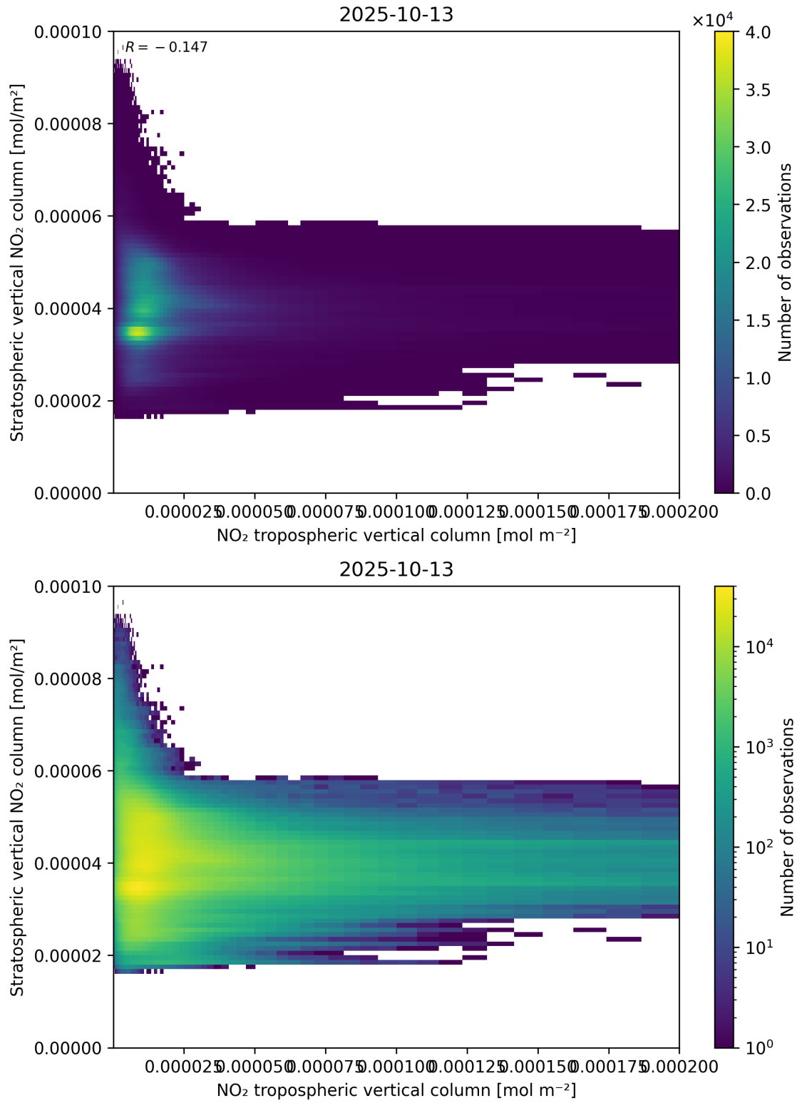
Figure 125: Scatter density plot of “NO 2 tropospheric vertical column” against “Stratospheric vertical NO 2 column” for 2025-10-12 to 2025-10-14.
