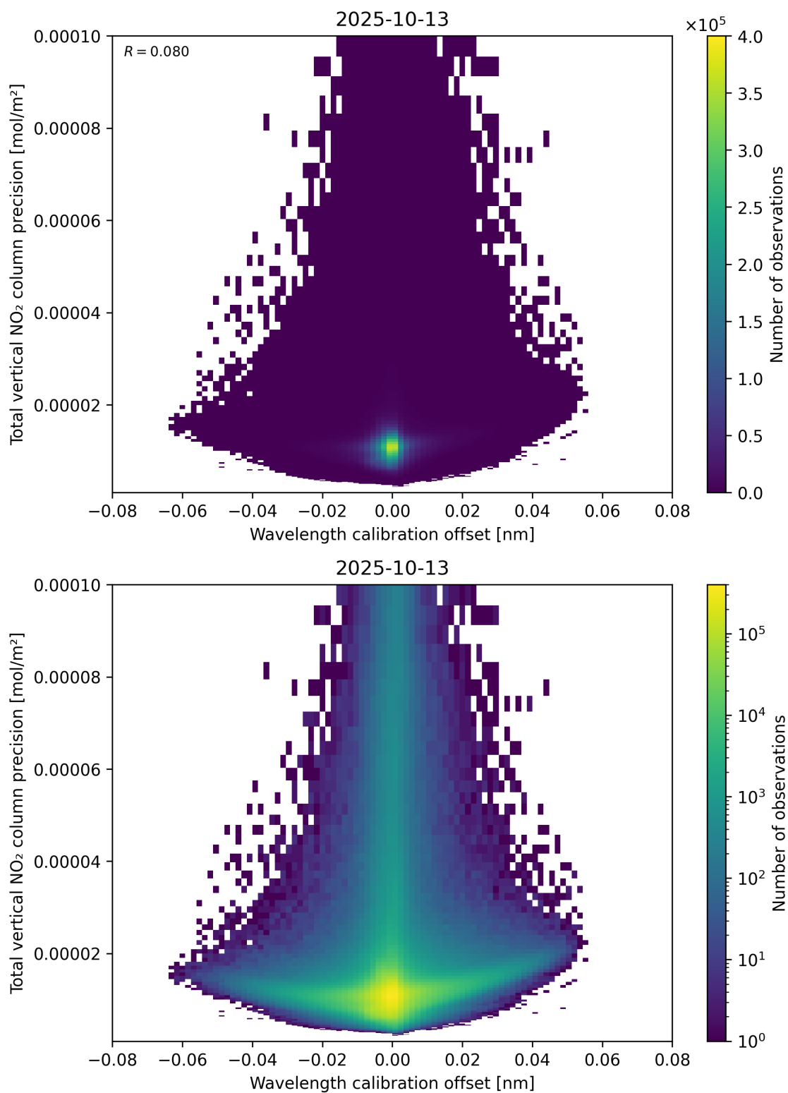
Figure 180: Scatter density plot of “Wavelength calibration offset” against “Total vertical NO 2 column precision” for 2025-10-12 to 2025-10-14.
