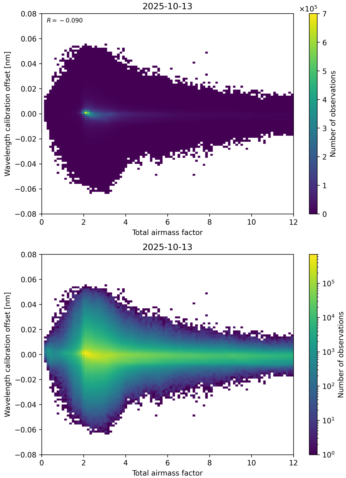
Figure 70: Scatter density plot of “Total airmass factor” against “Wavelength calibration offset” for 2025-10-12 to 2025-10-14.
