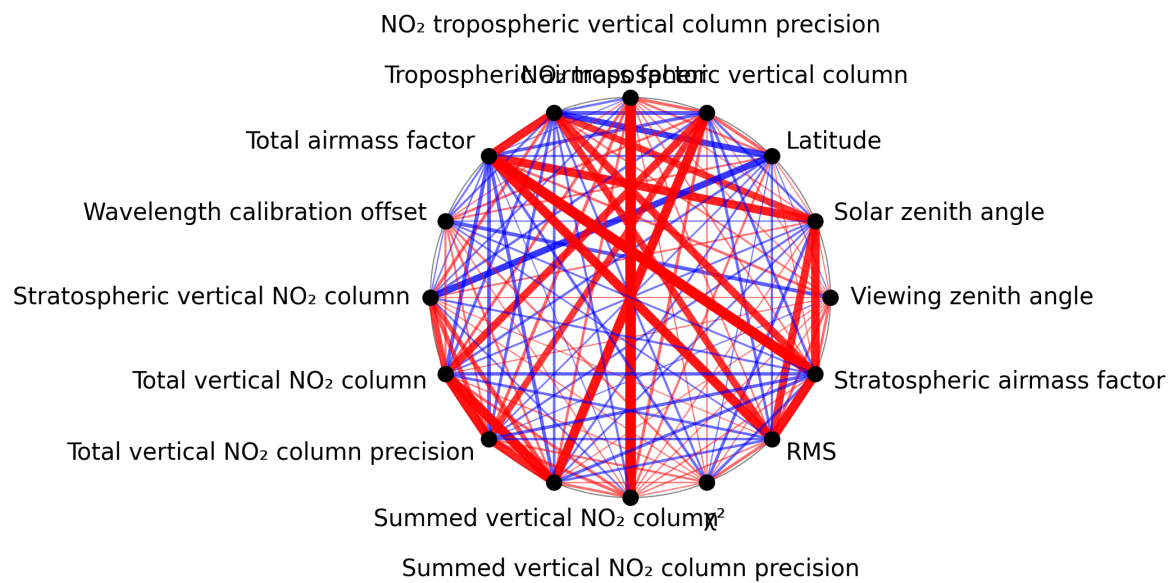
Figure 1: Map of correlation graph for 2025-10-12 to 2025-10-14.
