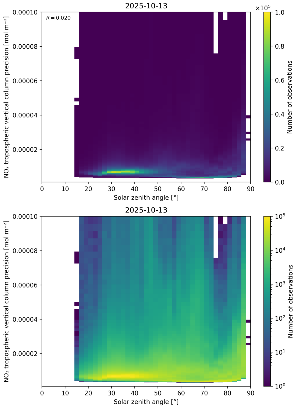
Figure 156: Scatter density plot of “Solar zenith angle” against “NO 2 tropospheric vertical column precision” for 2025-10-12 to 2025-10-14.
