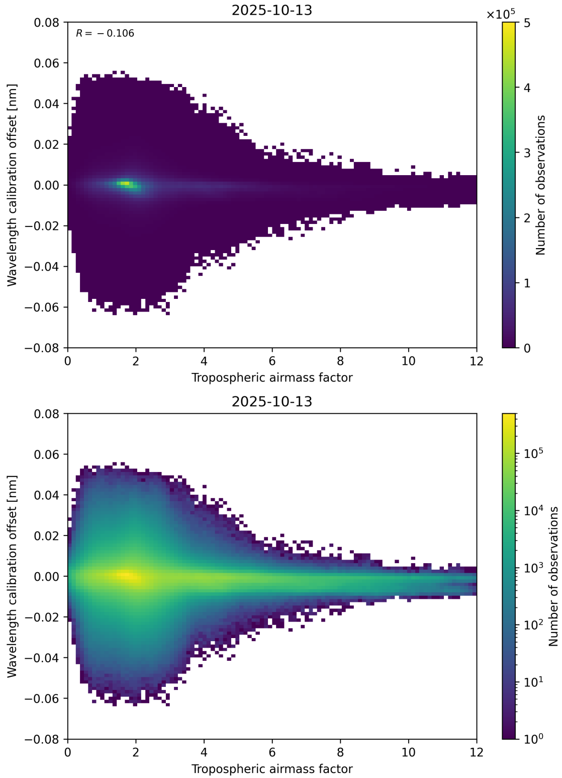
Figure 80: Scatter density plot of “Tropospheric airmass factor” against “Wavelength calibration offset” for 2025-10-12 to 2025-10-14.
