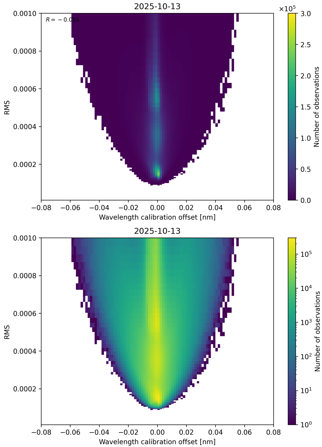
Figure 181: Scatter density plot of “Wavelength calibration offset” against “RMS” for 2025-10-12 to 2025-10-14.
