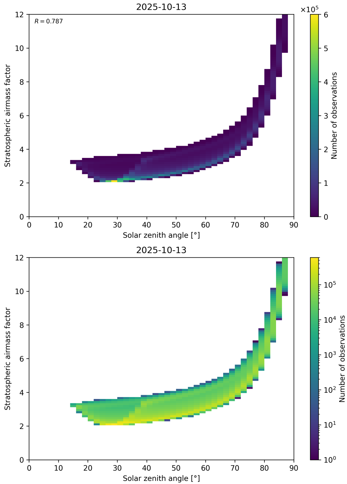
Figure 145: Scatter density plot of “Solar zenith angle” against “Stratospheric airmass factor” for 2025-10-12 to 2025-10-14.
