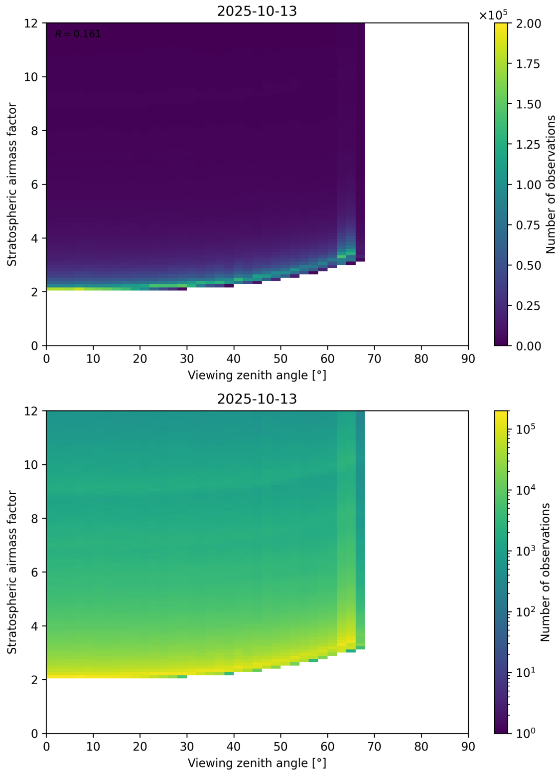
Figure 159: Scatter density plot of “Viewing zenith angle” against “Stratospheric airmass factor” for 2025-10-12 to 2025-10-14.
