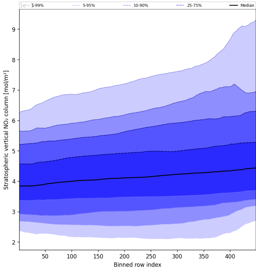
Figure 53: Along track statistics of “Stratospheric vertical NO 2 column” for 2025-10-12 to 2025-10-14
