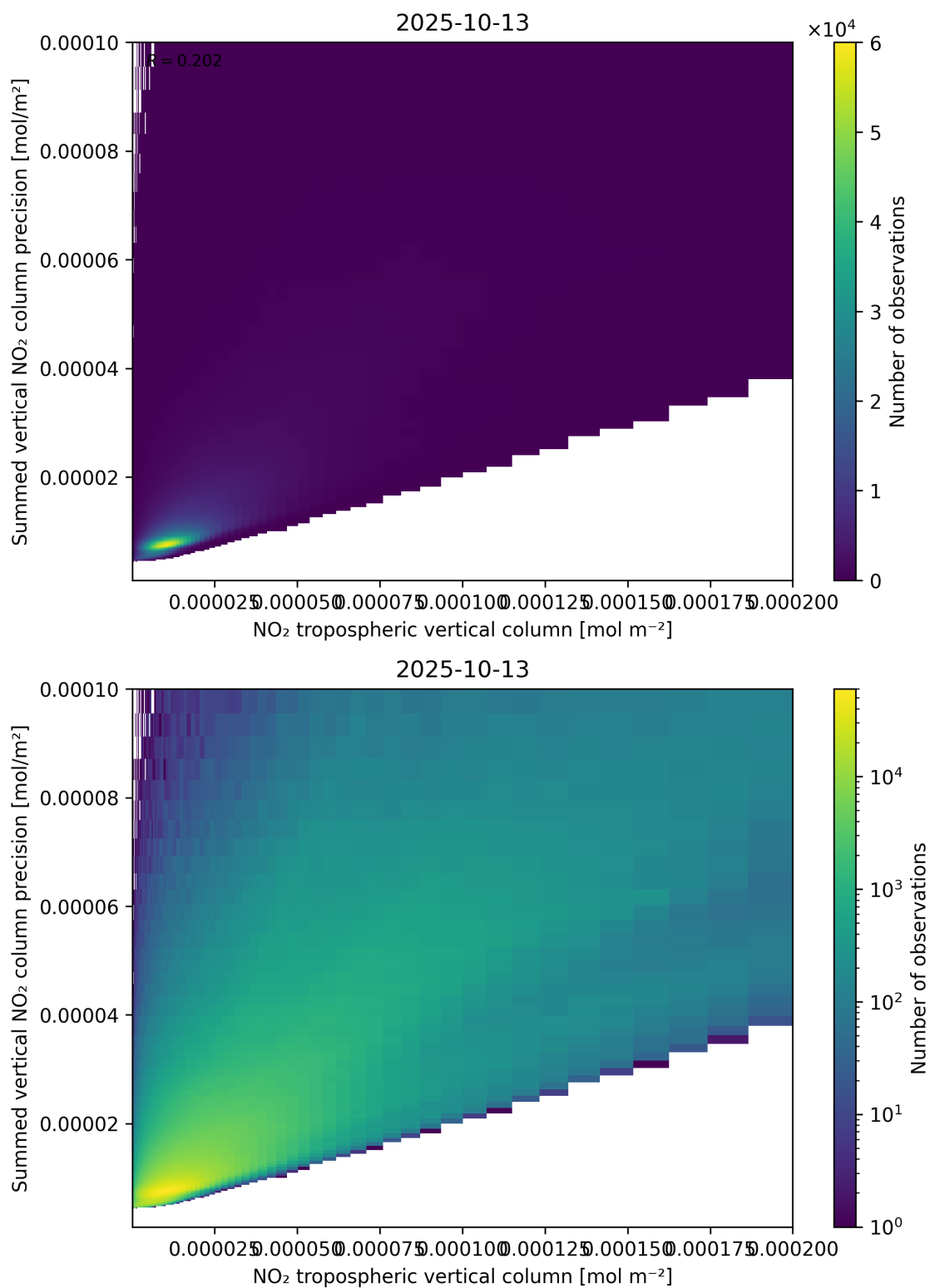
Figure 127: Scatter density plot of “NO 2 tropospheric vertical column” against “Summed vertical NO 2 column precision” for 2025-10-12 to 2025-10-14.
