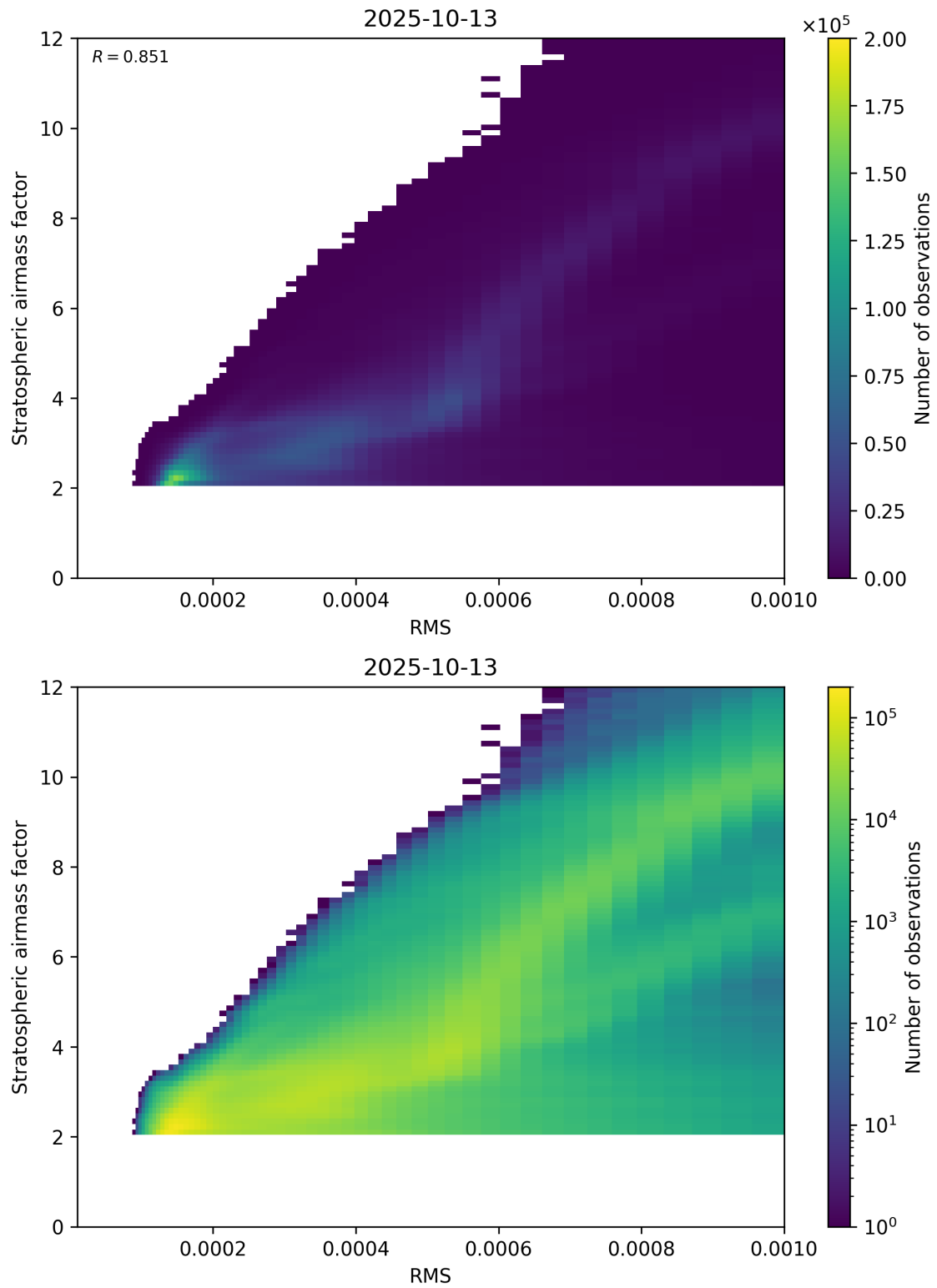
Figure 144: Scatter density plot of “RMS” against “Stratospheric airmass factor” for 2025-10-12 to 2025-10-14.
