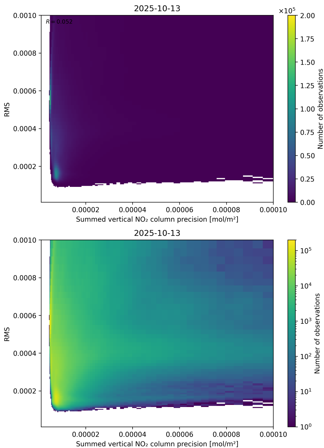
Figure 108: Scatter density plot of “Summed vertical NO 2 column precision” against “RMS” for 2025-10-12 to 2025-10-14.
