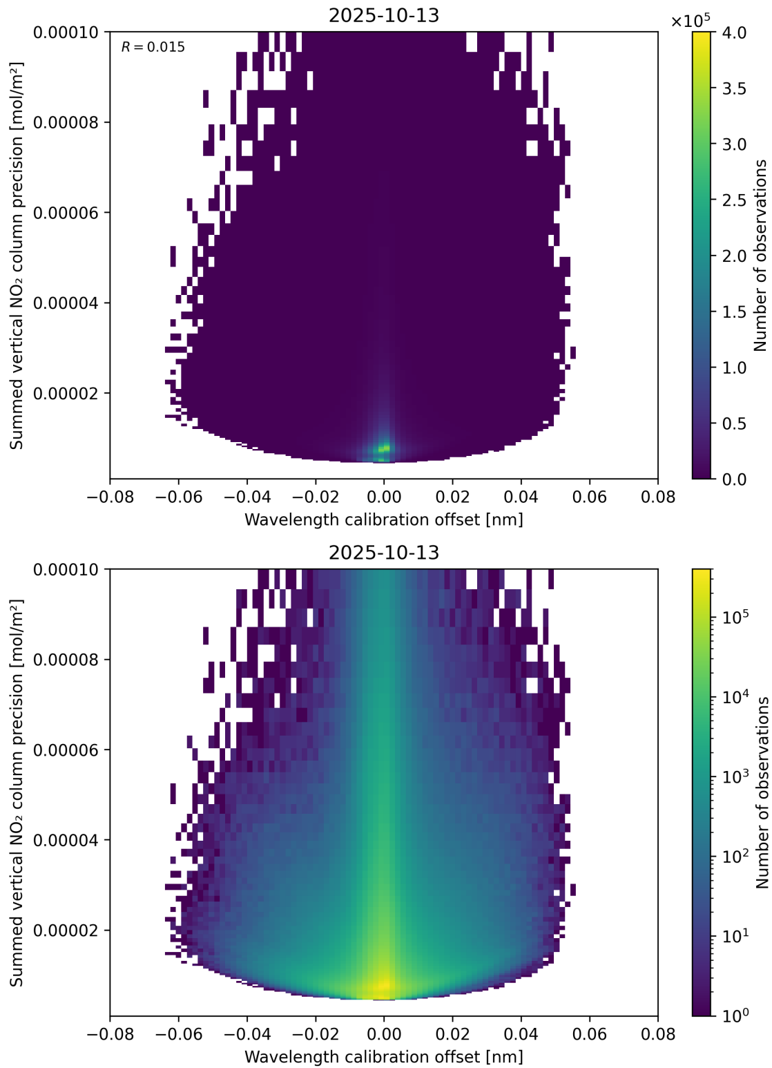
Figure 178: Scatter density plot of “Wavelength calibration offset” against “Summed vertical NO 2 column precision” for 2025-10-12 to 2025-10-14.
