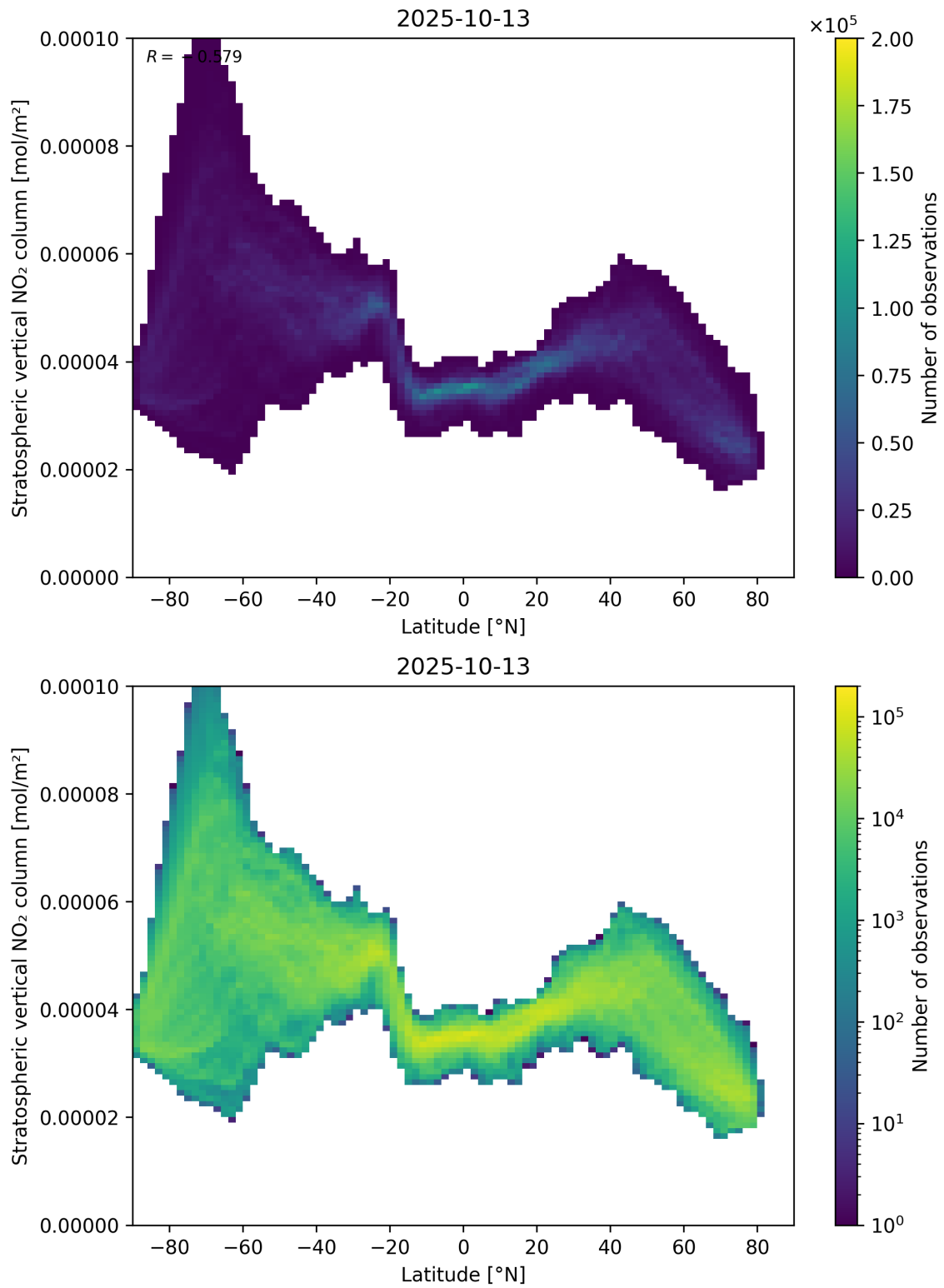
Figure 87: Scatter density plot of “Latitude” against “Stratospheric vertical NO 2 column” for 2025-10-12 to 2025-10-14.
