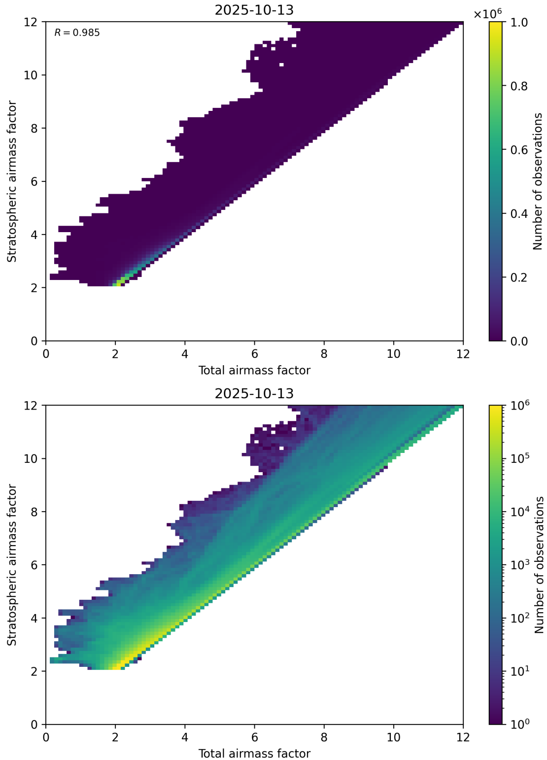
Figure 62: Scatter density plot of “Total airmass factor” against “Stratospheric airmass factor” for 2025-10-12 to 2025-10-14.
