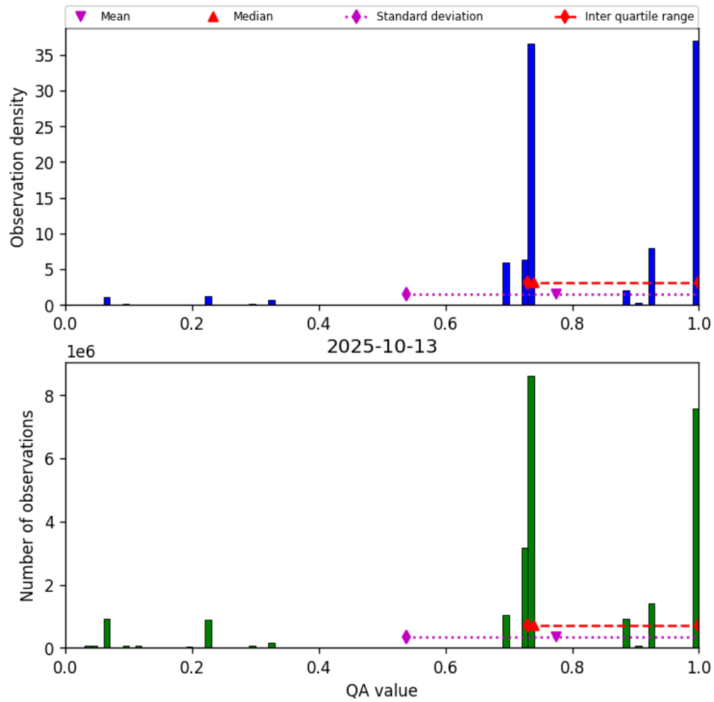
Figure 28: Histogram of “QA value” for 2025-10-12 to 2025-10-14
