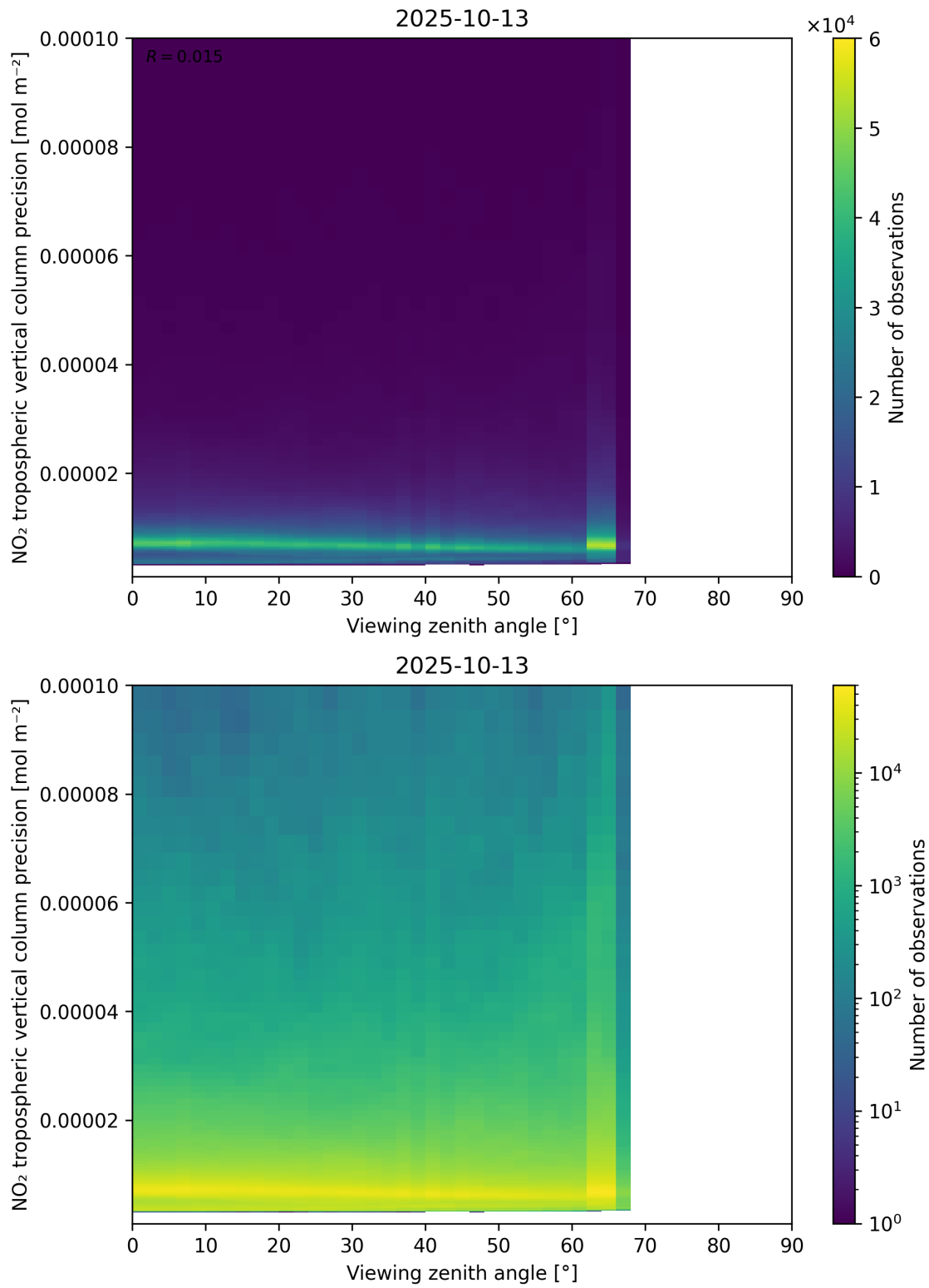
Figure 170: Scatter density plot of “Viewing zenith angle” against “NO 2 tropospheric vertical column precision” for 2025-10-12 to 2025-10-14.
