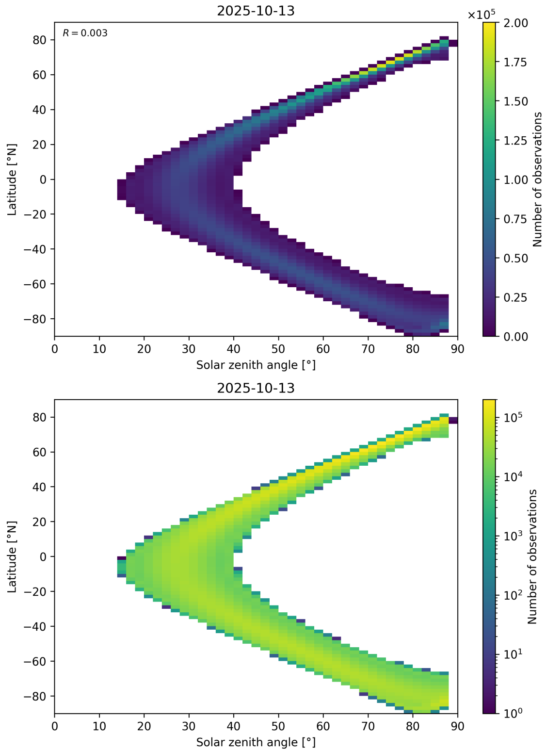
Figure 149: Scatter density plot of “Solar zenith angle” against “Latitude” for 2025-10-12 to 2025-10-14.
