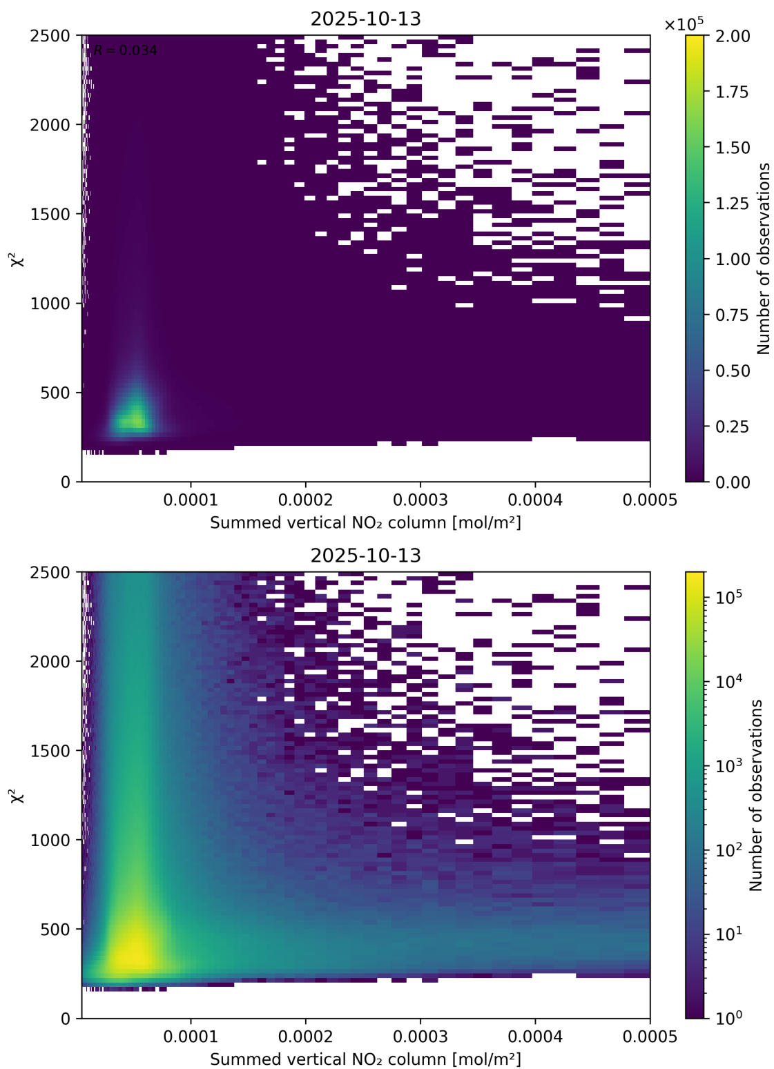
Figure 104: Scatter density plot of “Summed vertical NO 2 column” against “ \chi^2 ” for 2025-10-12 to 2025-10-14.
