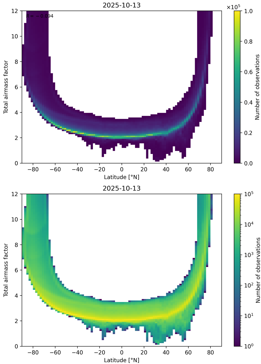
Figure 84: Scatter density plot of “Latitude” against “Total airmass factor” for 2025-10-12 to 2025-10-14.
