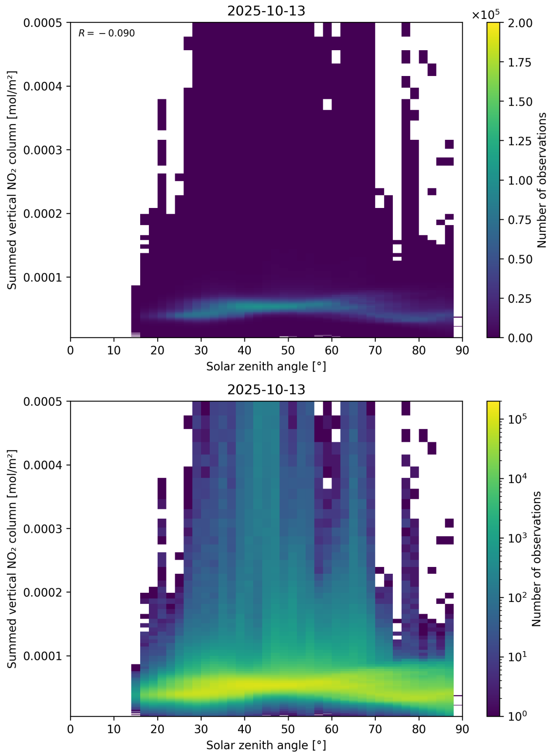
Figure 151: Scatter density plot of “Solar zenith angle” against “Summed vertical NO 2 column” for 2025-10-12 to 2025-10-14.
