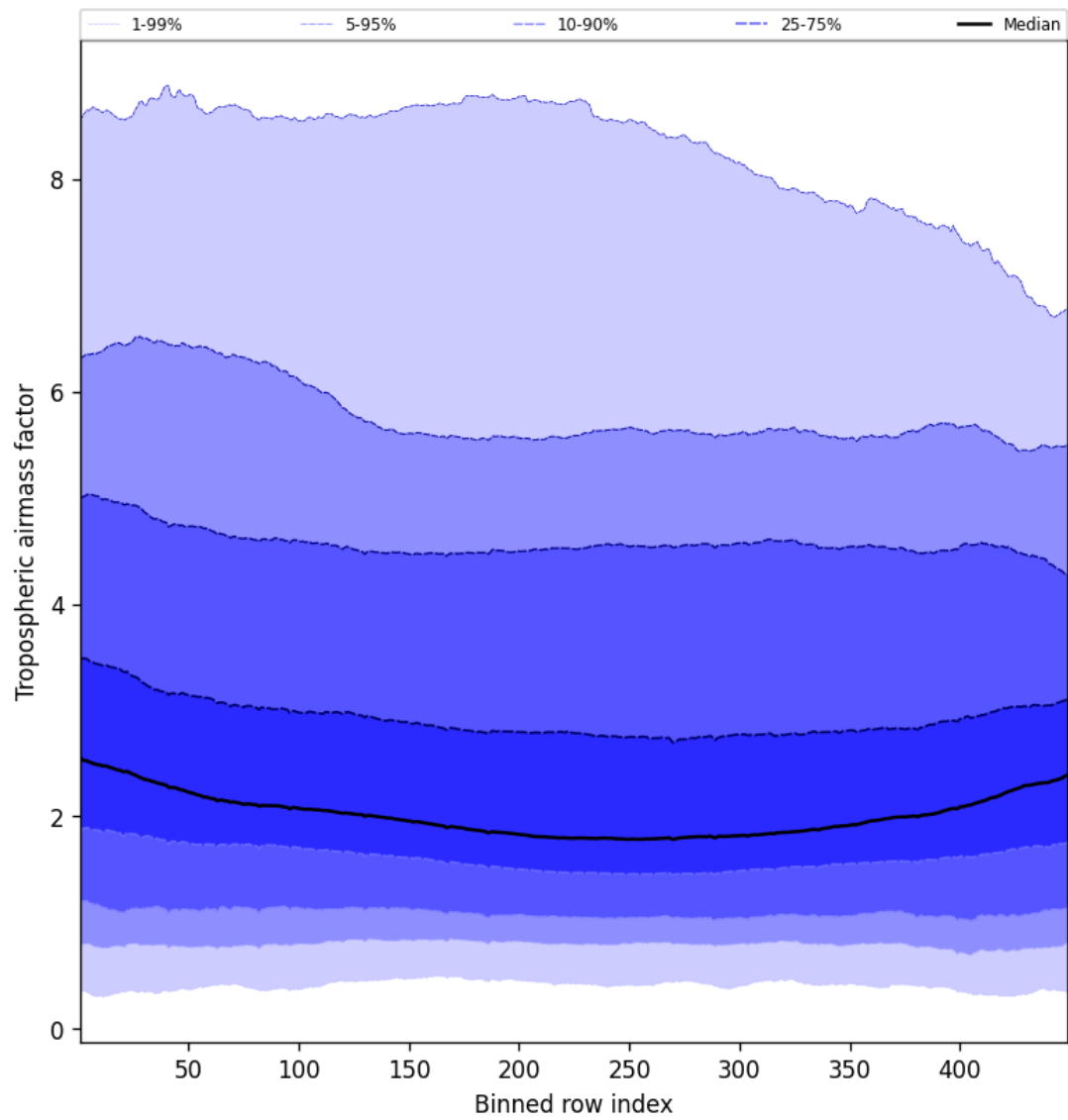
Figure 48: Along track statistics of “Tropospheric airmass factor” for 2025-10-12 to 2025-10-14
