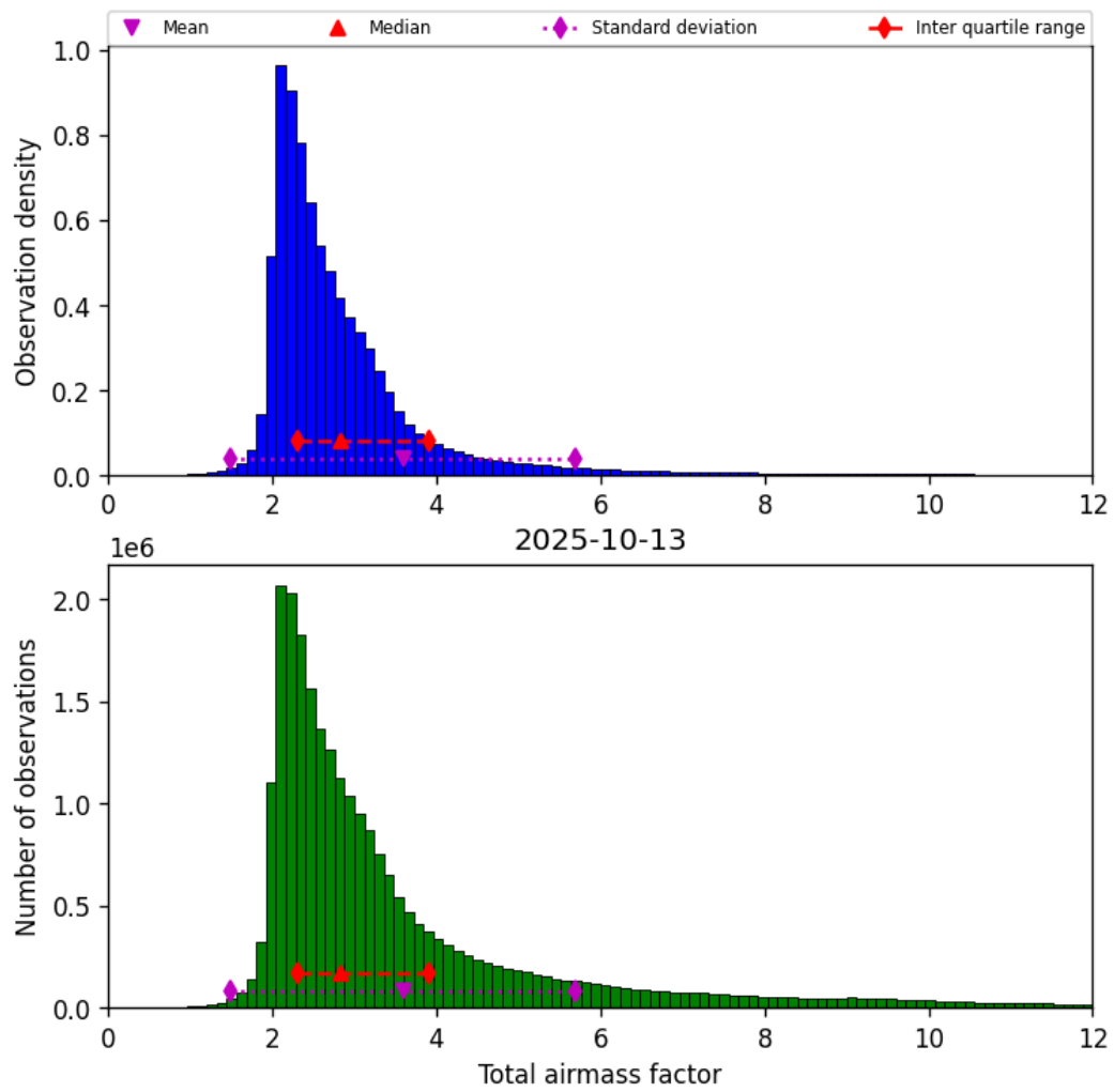
Figure 32: Histogram of “Total airmass factor” for 2025-10-12 to 2025-10-14
