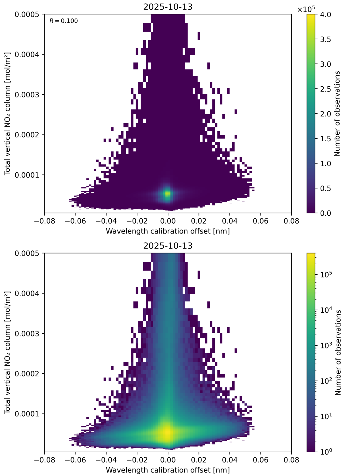
Figure 179: Scatter density plot of “Wavelength calibration offset” against “Total vertical NO 2 column” for 2025-10-12 to 2025-10-14.
