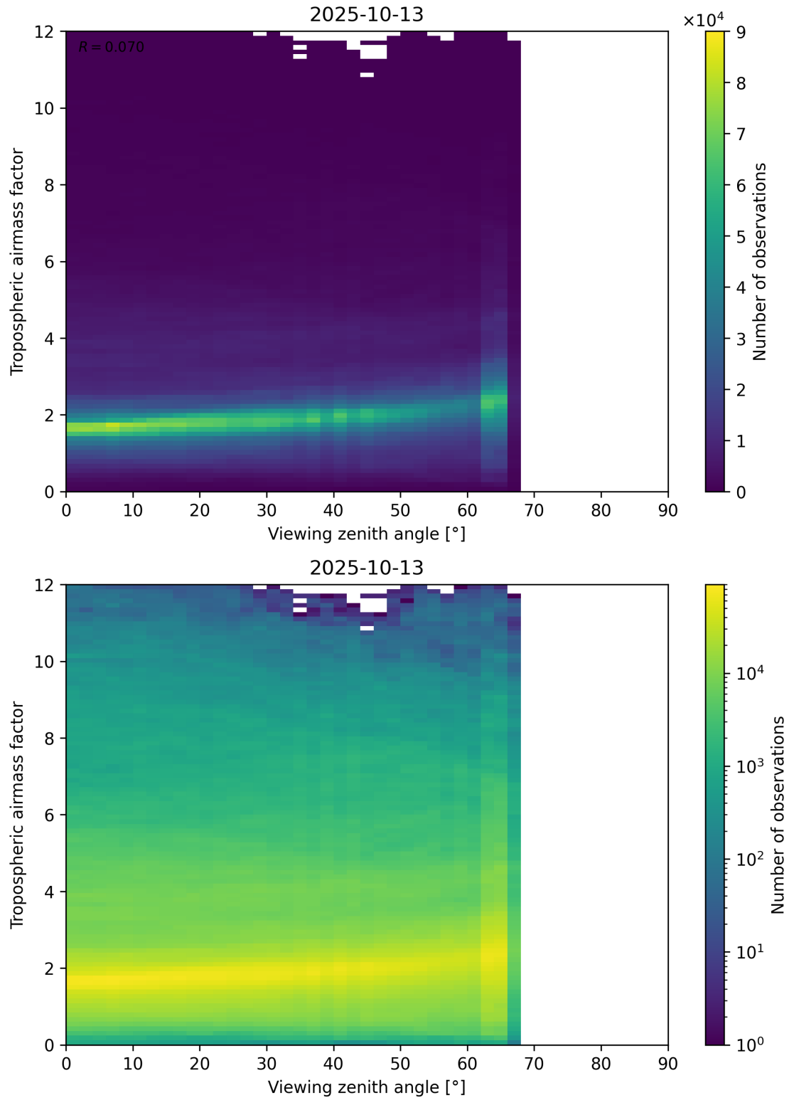
Figure 161: Scatter density plot of “Viewing zenith angle” against “Tropospheric airmass factor” for 2025-10-12 to 2025-10-14.
