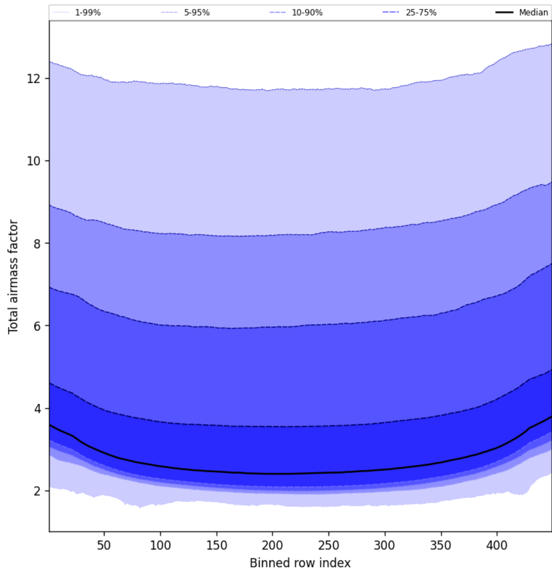
Figure 49: Along track statistics of “Total airmass factor” for 2025-10-12 to 2025-10-14
