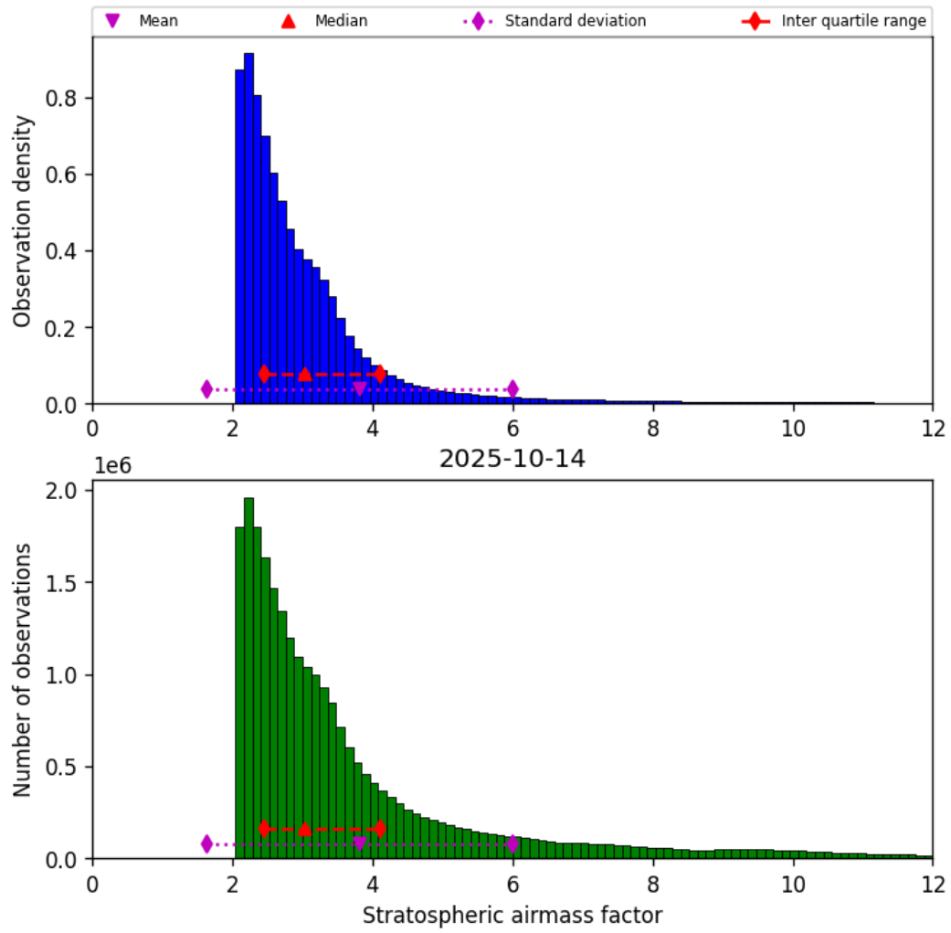
Figure 44: Histogram of “Stratospheric airmass factor” for 2025-10-13 to 2025-10-15
