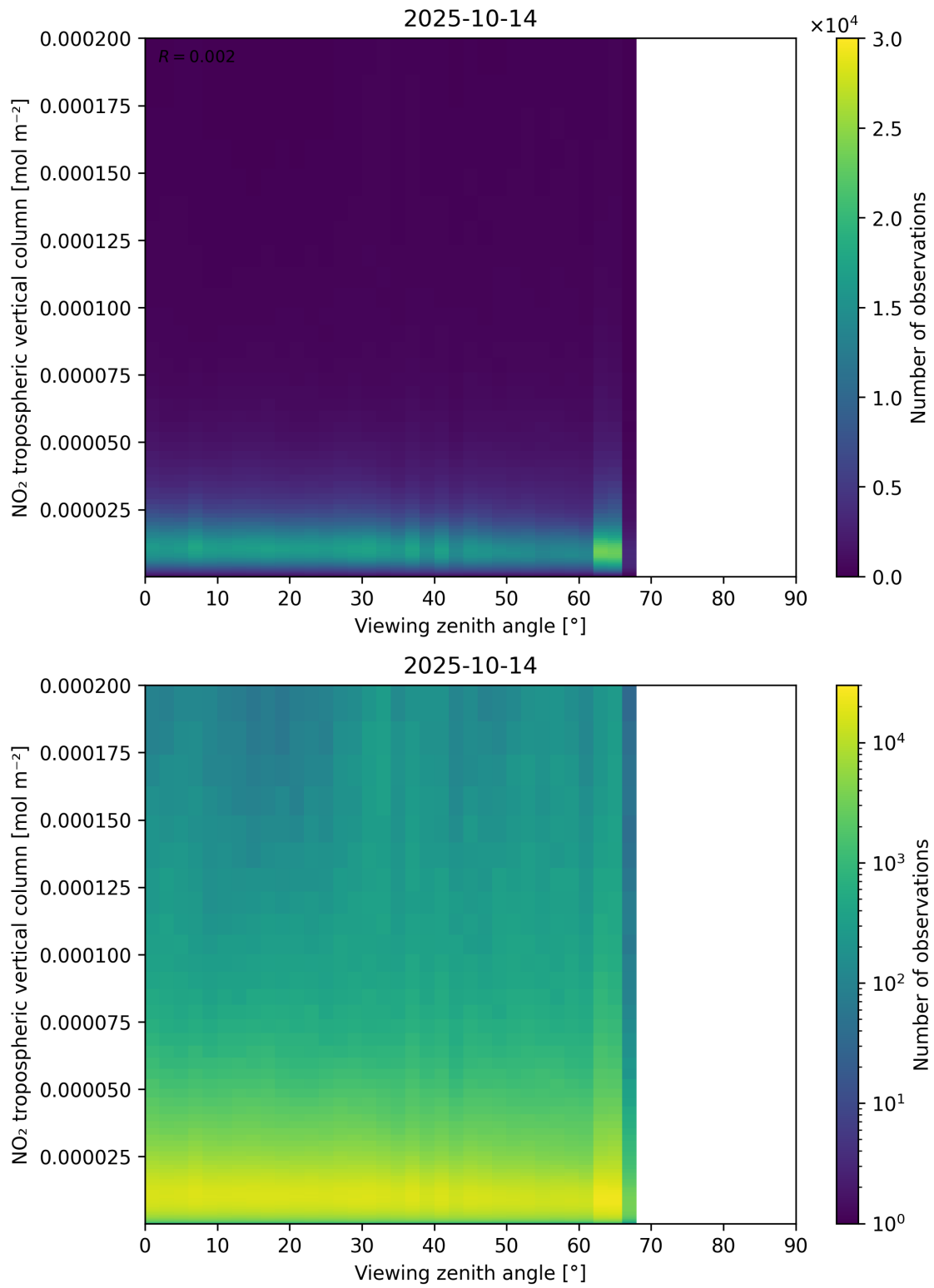
Figure 169: Scatter density plot of “Viewing zenith angle” against “NO 2 tropospheric vertical column” for 2025-10-13 to 2025-10-15.
