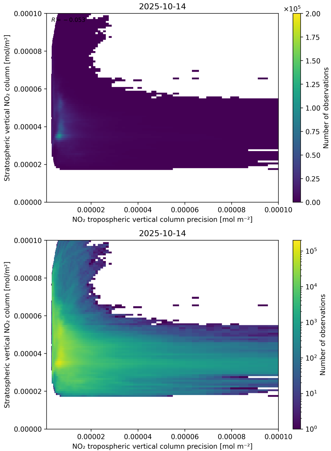
Figure 135: Scatter density plot of “NO 2 tropospheric vertical column precision” against “Stratospheric vertical NO 2 column” for 2025-10-13 to 2025-10-15.
