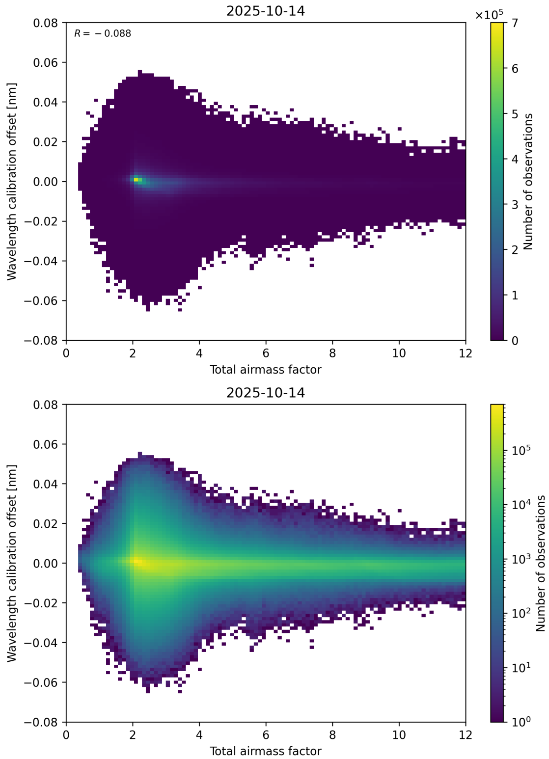
Figure 70: Scatter density plot of “Total airmass factor” against “Wavelength calibration offset” for 2025-10-13 to 2025-10-15.
