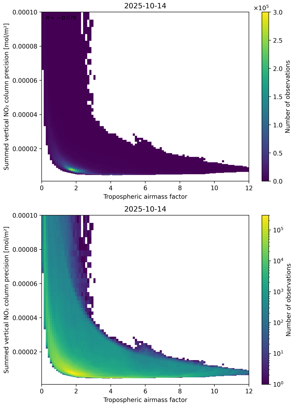
Figure 76: Scatter density plot of “Tropospheric airmass factor” against “Summed vertical NO 2 column precision” for 2025-10-13 to 2025-10-15.
