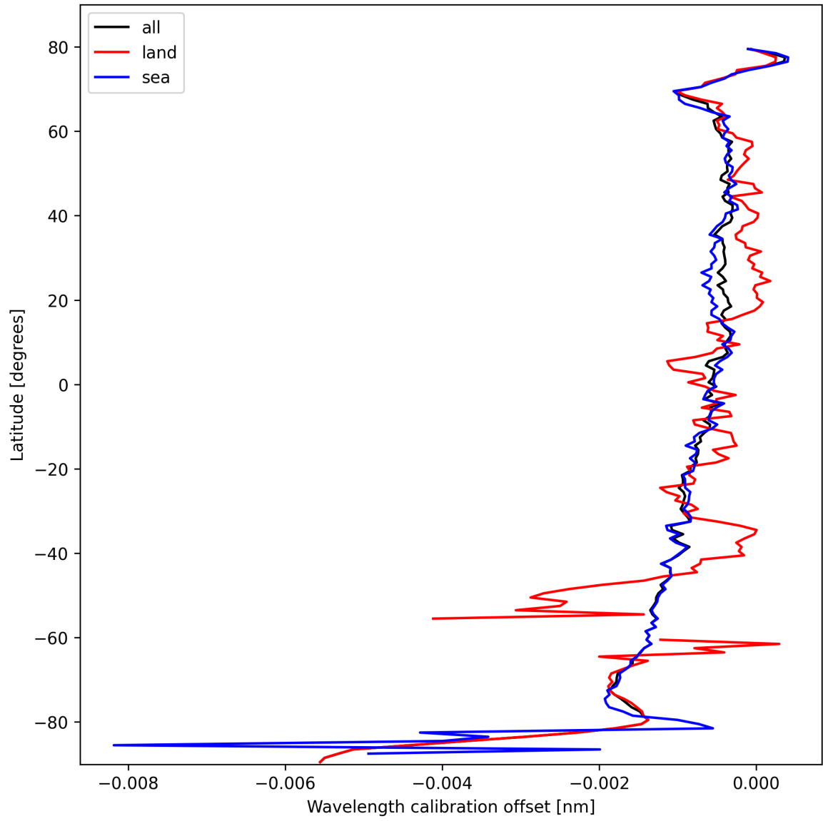
Figure 18: Zonal average of “Wavelength calibration offset” for 2025-10-13 to 2025-10-15.
