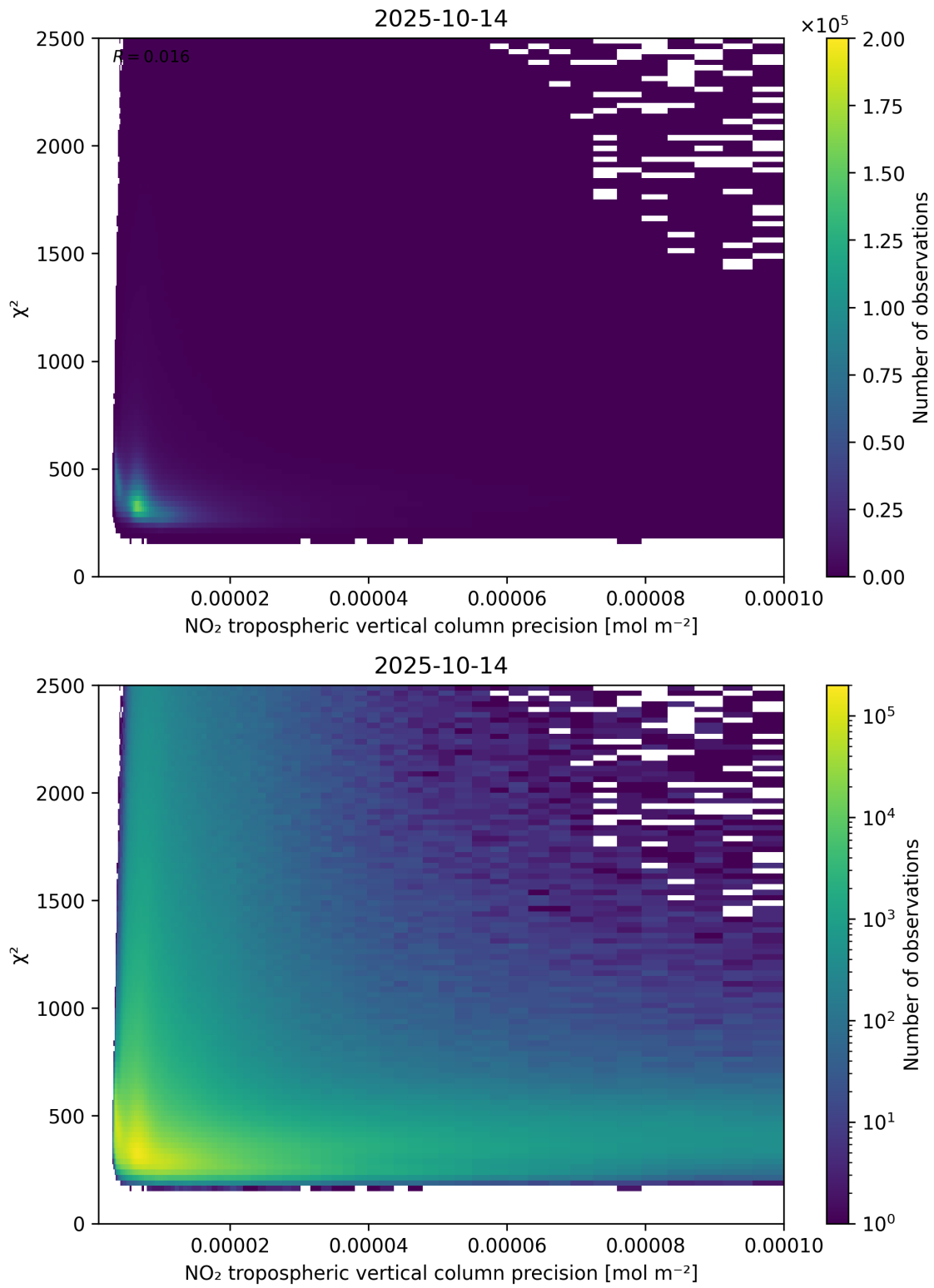
Figure 134: Scatter density plot of “NO 2 tropospheric vertical column precision” against “ \chi^2 ” for 2025-10-13 to 2025-10-15.
