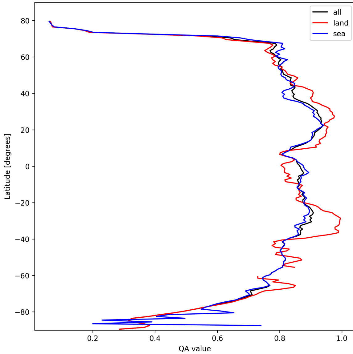
Figure 11: Zonal average of “QA value” for 2025-10-13 to 2025-10-15.
