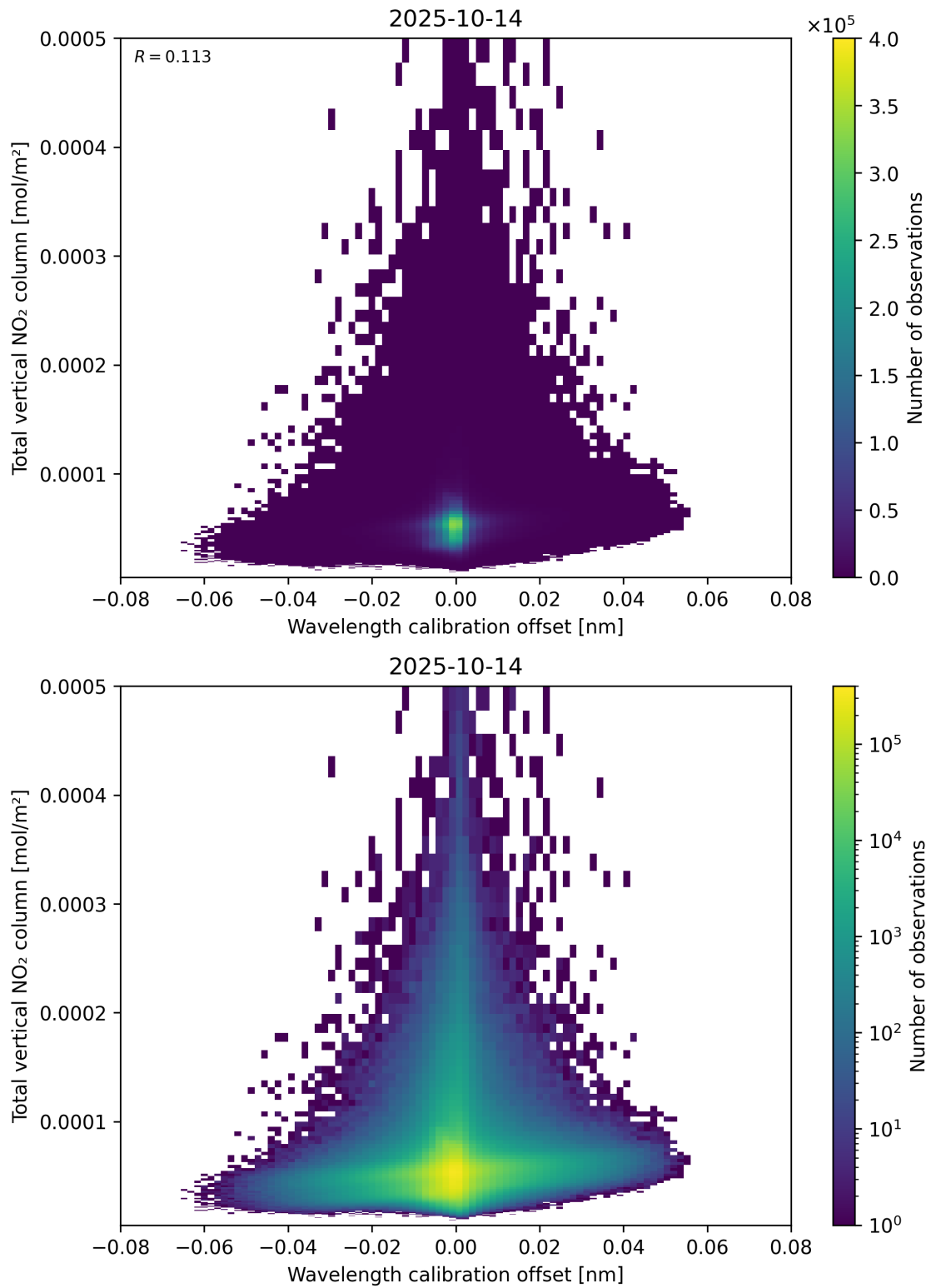
Figure 179: Scatter density plot of “Wavelength calibration offset” against “Total vertical NO 2 column” for 2025-10-13 to 2025-10-15.
