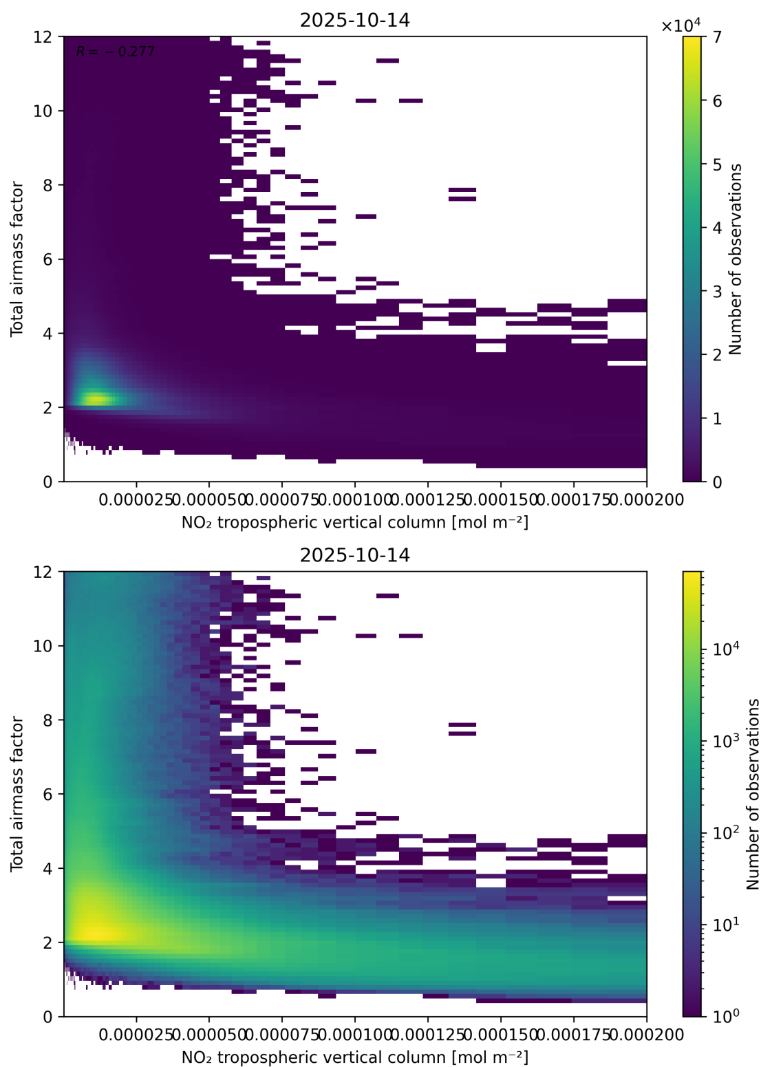
Figure 122: Scatter density plot of “NO 2 tropospheric vertical column” against “Total air mass factor” for 2025-10-13 to 2025-10-15.
