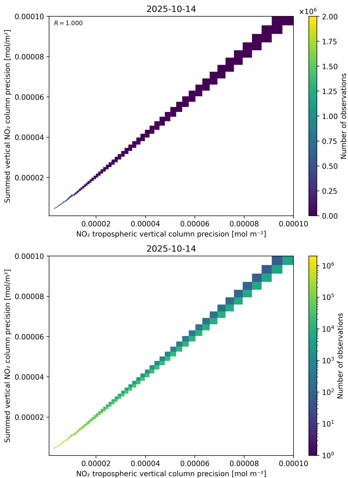
Figure 137: Scatter density plot of “NO 2 tropospheric vertical column precision” against “Summed vertical NO 2 column precision” for 2025-10-13 to 2025-10-15.
