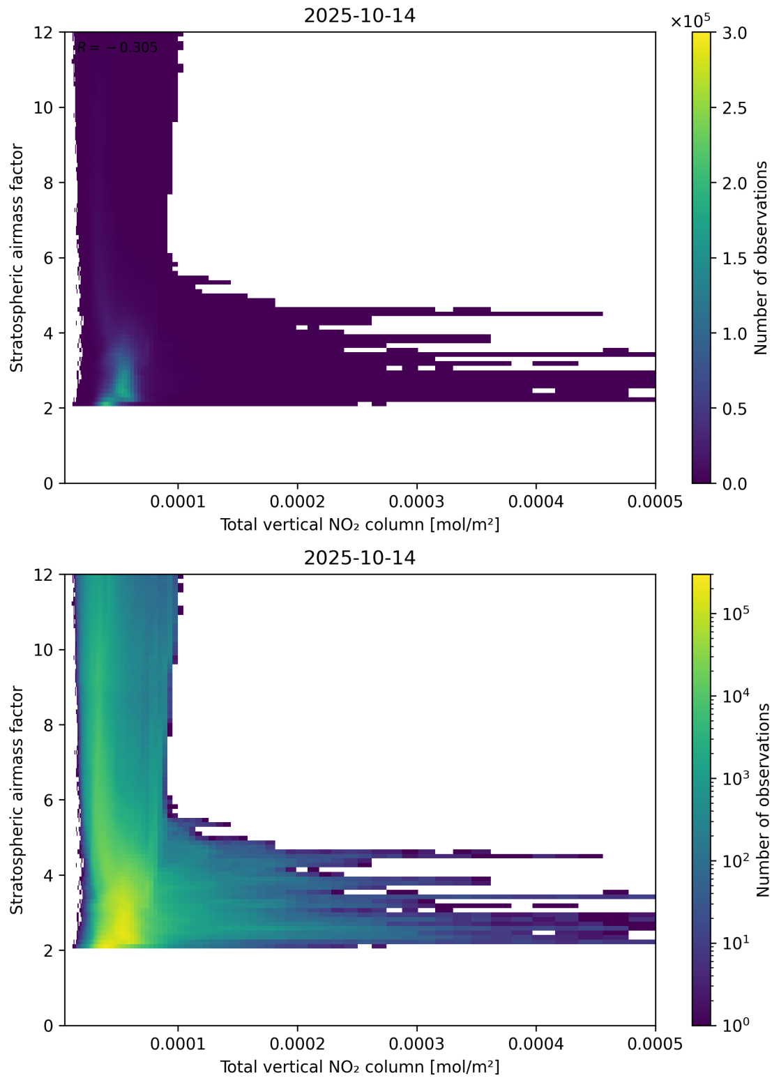
Figure 110: Scatter density plot of “Total vertical NO 2 column” against “Stratospheric airmass factor” for 2025-10-13 to 2025-10-15.
