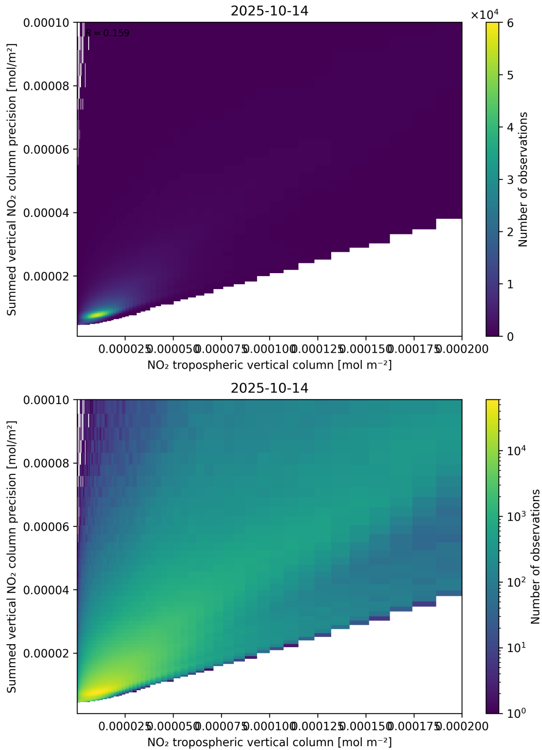
Figure 127: Scatter density plot of “NO 2 tropospheric vertical column” against “Summed vertical NO 2 column precision” for 2025-10-13 to 2025-10-15.
