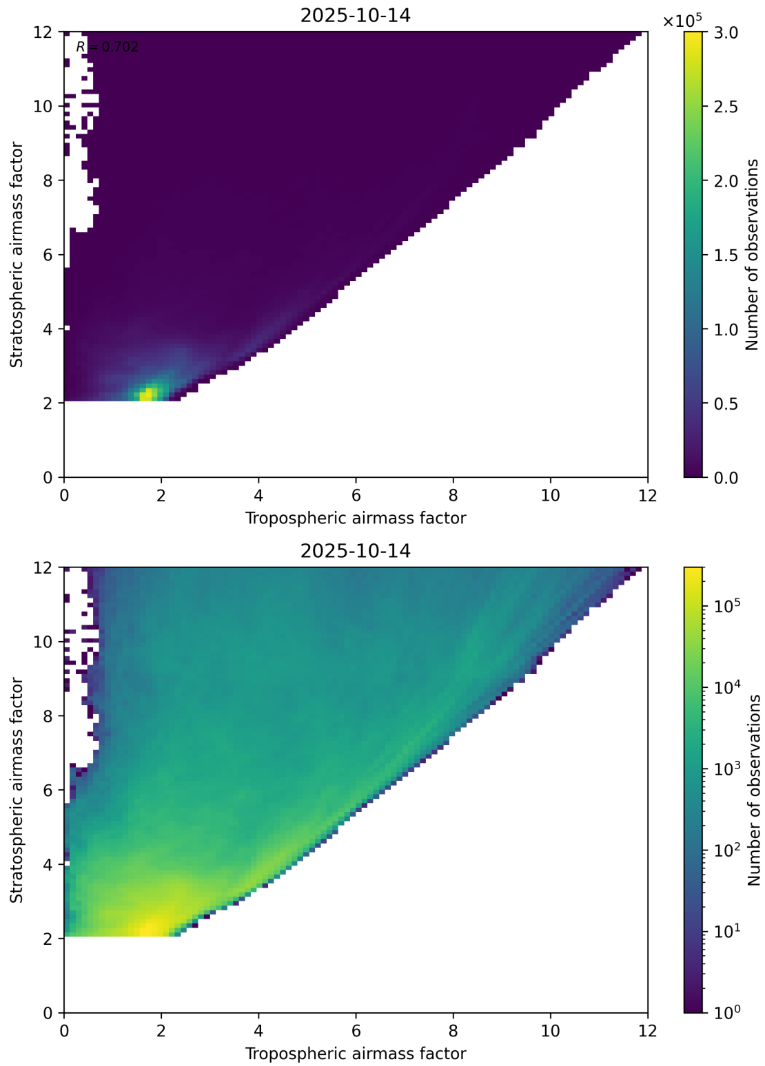
Figure 71: Scatter density plot of “Tropospheric airmass factor” against “Stratospheric airmass factor” for 2025-10-13 to 2025-10-15.
