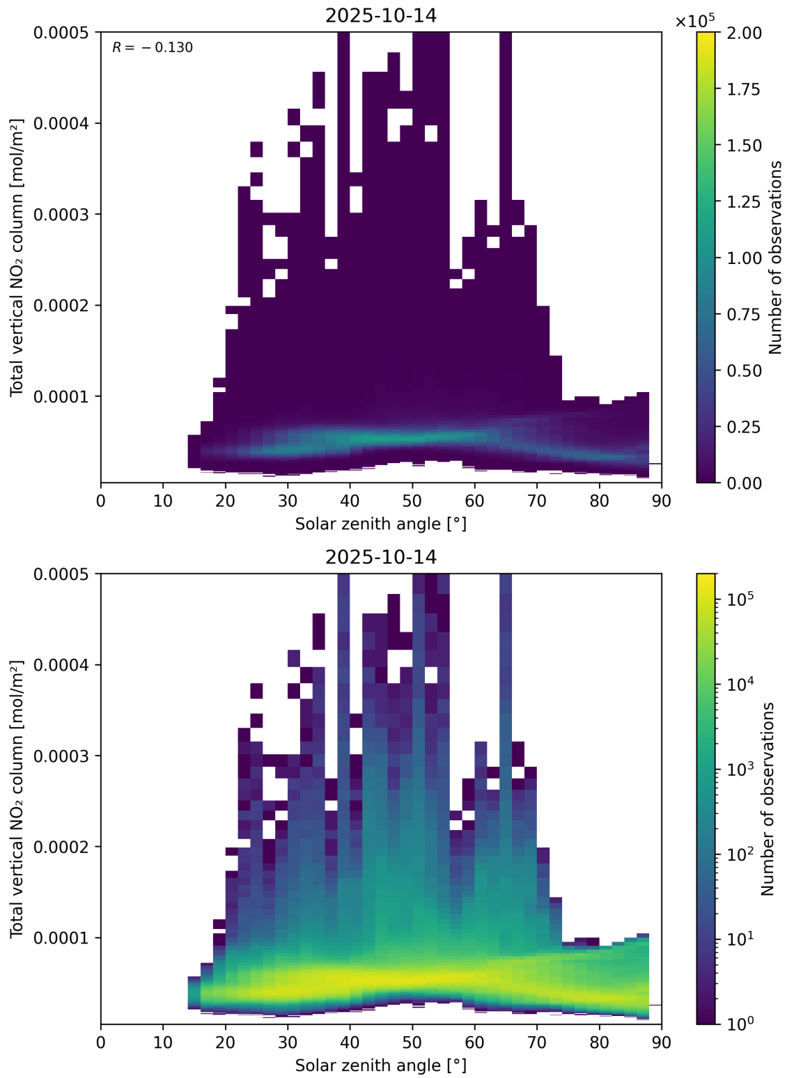
Figure 153: Scatter density plot of “Solar zenith angle” against “Total vertical NO 2 column” for 2025-10-13 to 2025-10-15.
