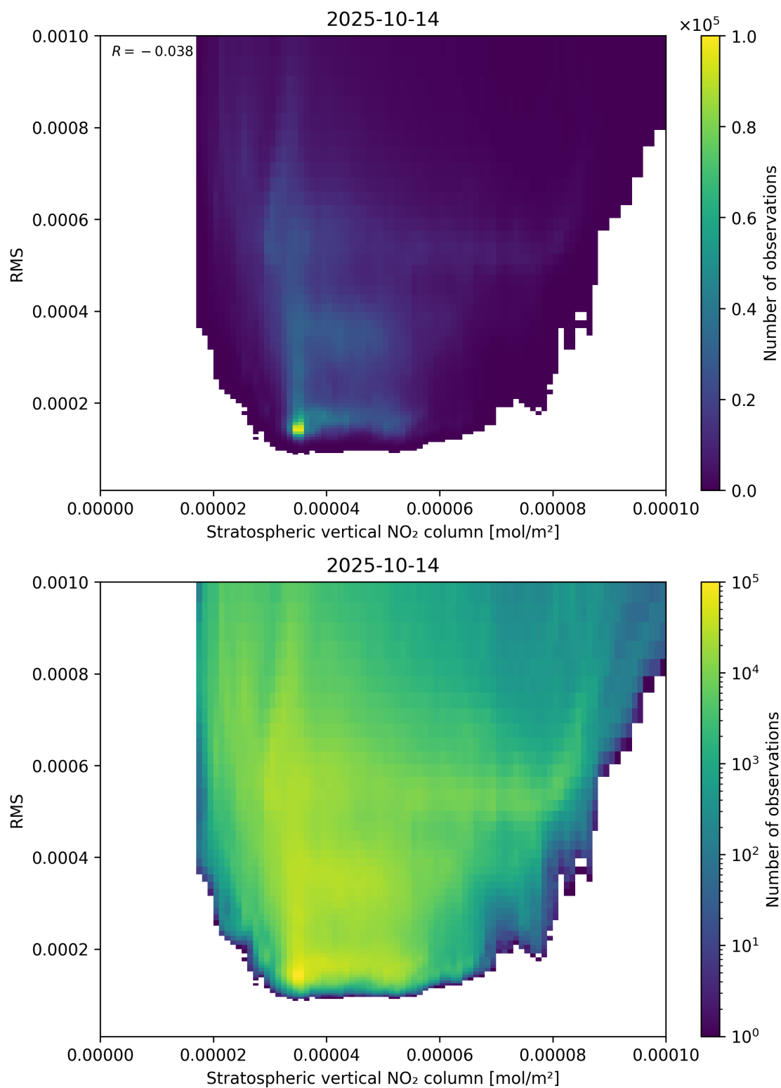
Figure 102: Scatter density plot of “Stratospheric vertical NO 2 column” against “RMS” for 2025-10-13 to 2025-10-15.
