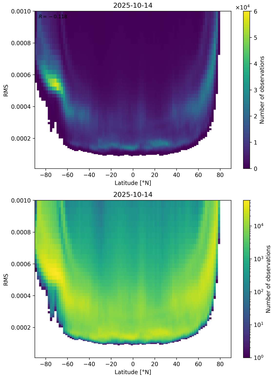
Figure 94: Scatter density plot of “Latitude” against “RMS” for 2025-10-13 to 2025-10-15.
