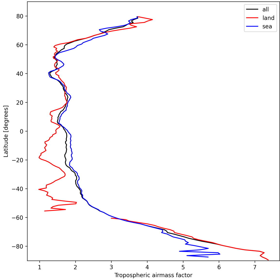
Figure 14: Zonal average of “Tropospheric airmass factor” for 2025-10-13 to 2025-10-15.
