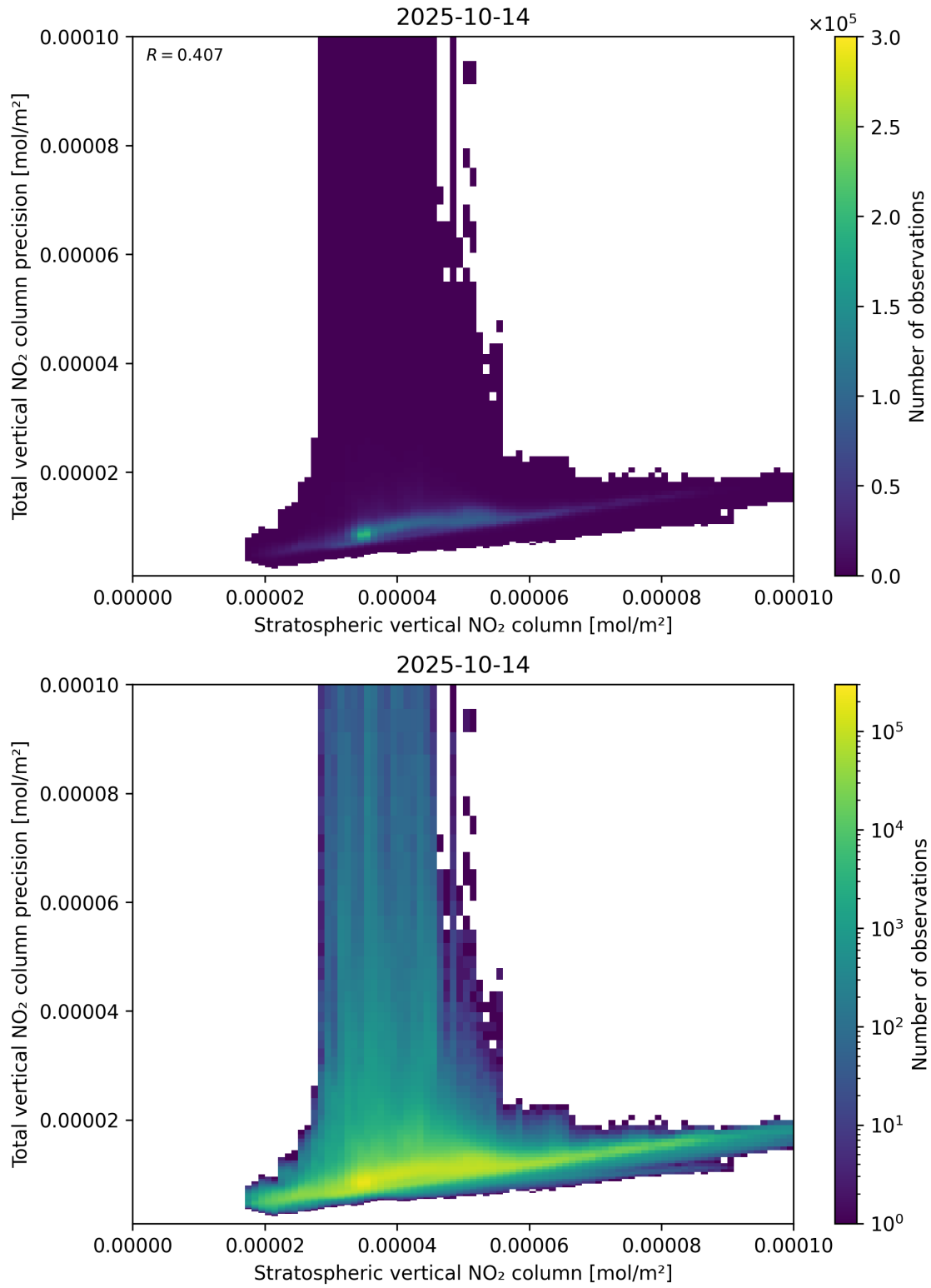
Figure 101: Scatter density plot of “Stratospheric vertical NO 2 column” against “Total vertical NO 2 column precision” for 2025-10-13 to 2025-10-15.
