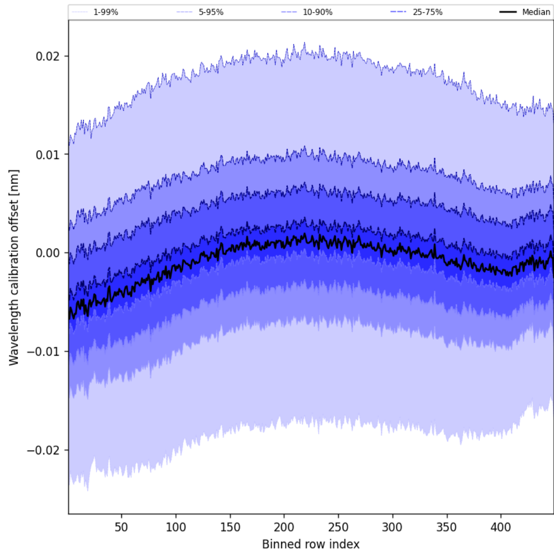
Figure 52: Along track statistics of “Wavelength calibration offset” for 2025-10-13 to 2025-10-15
