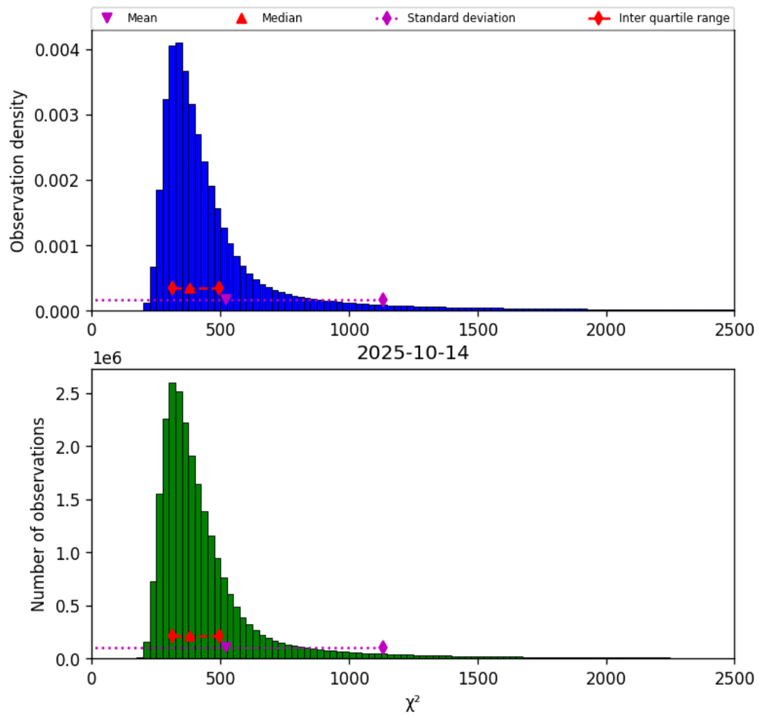
Figure 42: Histogram of " \chi^2 " for 2025-10-13 to 2025-10-15
