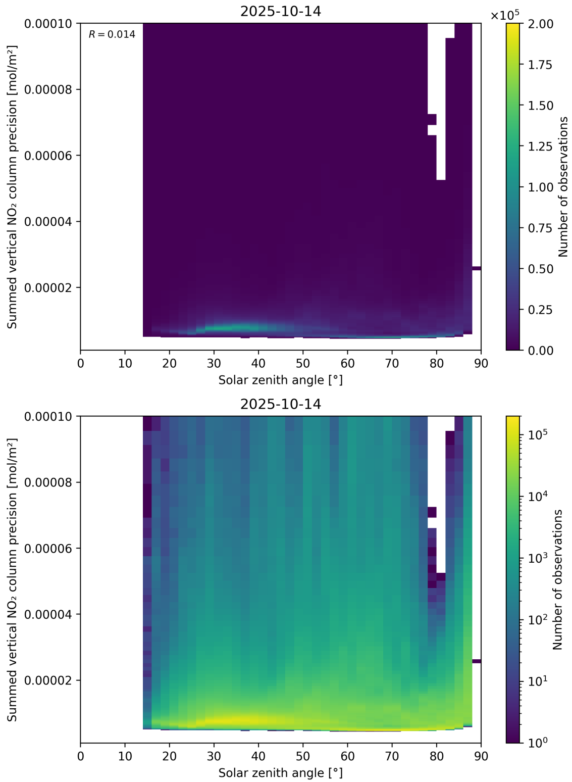
Figure 152: Scatter density plot of “Solar zenith angle” against “Summed vertical NO 2 column precision” for 2025-10-13 to 2025-10-15.
