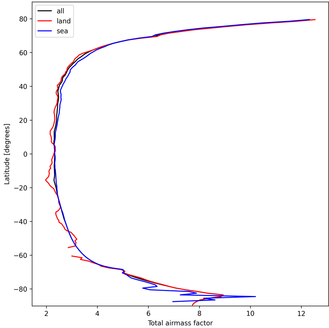
Figure 15: Zonal average of “Total airmass factor” for 2025-10-13 to 2025-10-15.
