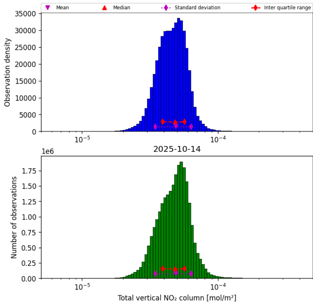
Figure 38: Histogram of “Total vertical NO 2 column” for 2025-10-13 to 2025-10-15
