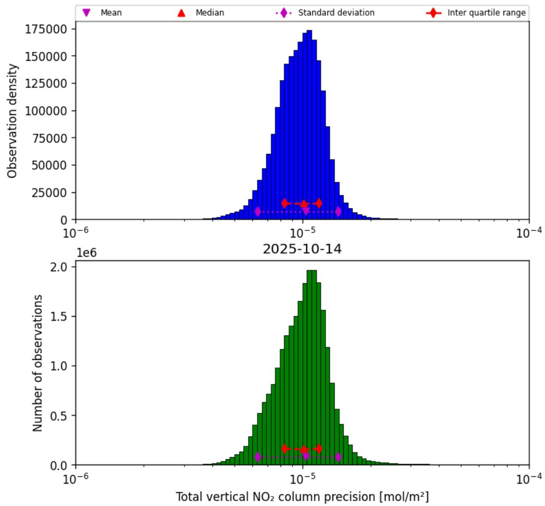
Figure 39: Histogram of "Total vertical NO 2 column precision" for 2025-10-13 to 2025-10-15
