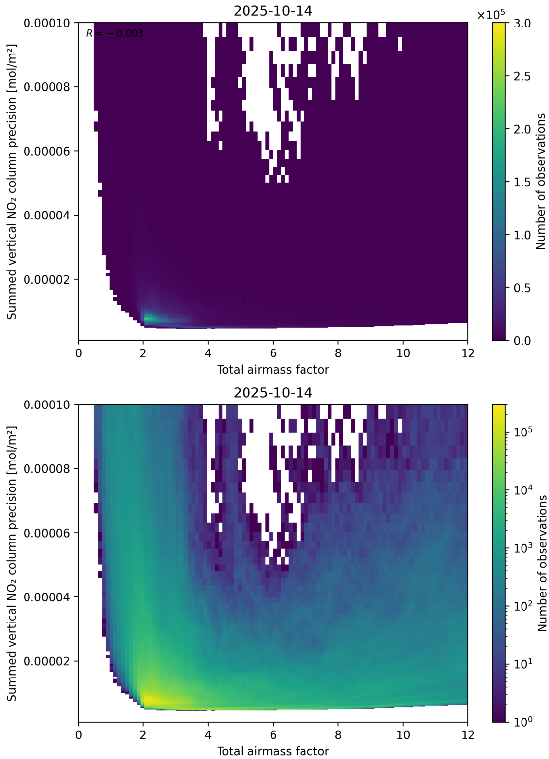
Figure 66: Scatter density plot of “Total airmass factor” against “Summed vertical NO 2 column precision” for 2025-10-13 to 2025-10-15.
