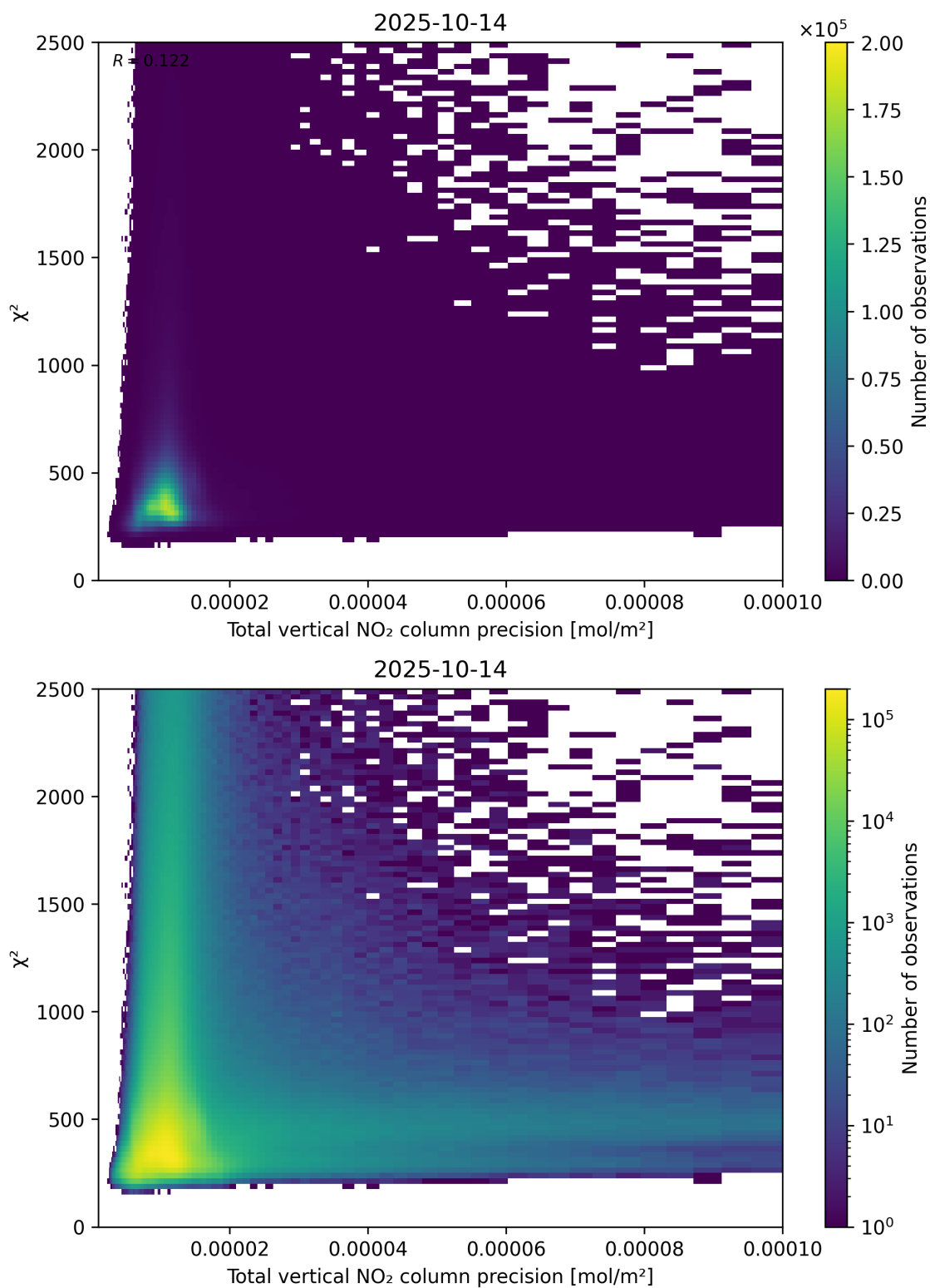
Figure 116: Scatter density plot of “Total vertical NO 2 column precision” against “ \chi^2 ” for 2025-10-13 to 2025-10-15.
