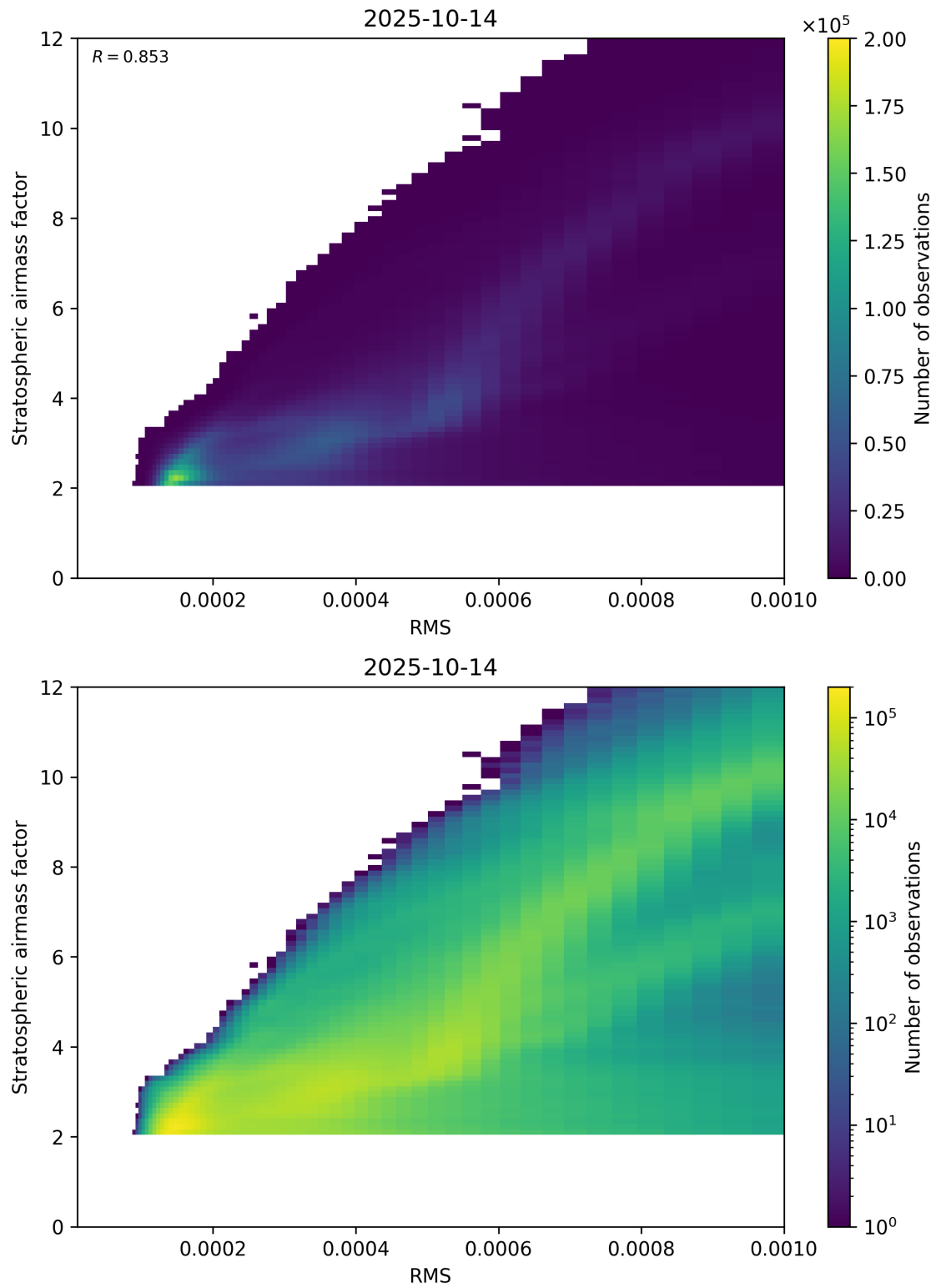
Figure 144: Scatter density plot of “RMS” against “Stratospheric airmass factor” for 2025-10-13 to 2025-10-15.
