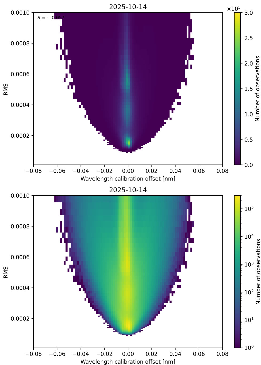
Figure 181: Scatter density plot of “Wavelength calibration offset” against “RMS” for 2025-10-13 to 2025-10-15.
