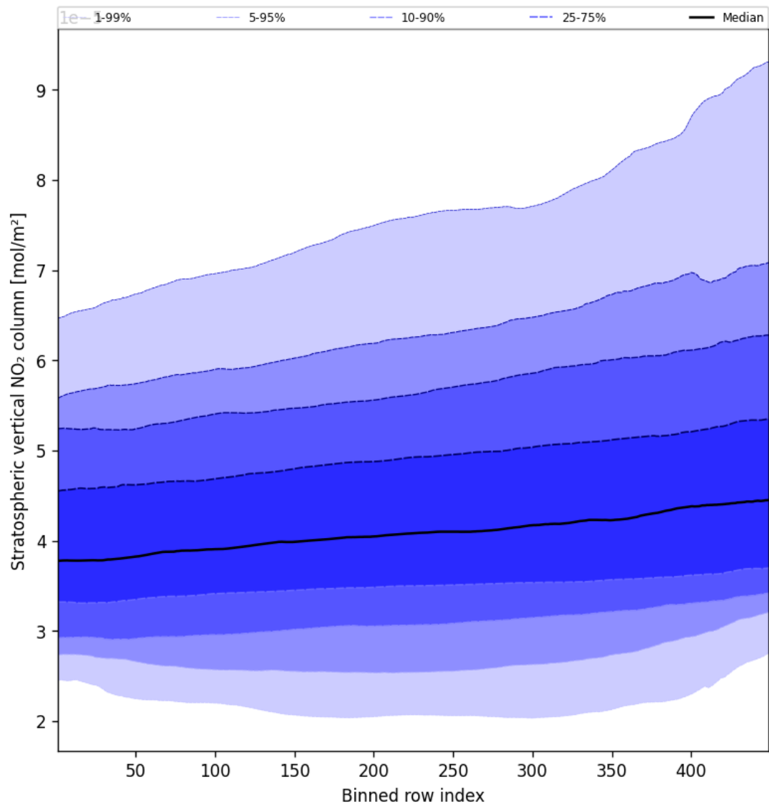
Figure 53: Along track statistics of “Stratospheric vertical NO 2 column” for 2025-10-13 to 2025-10-15
