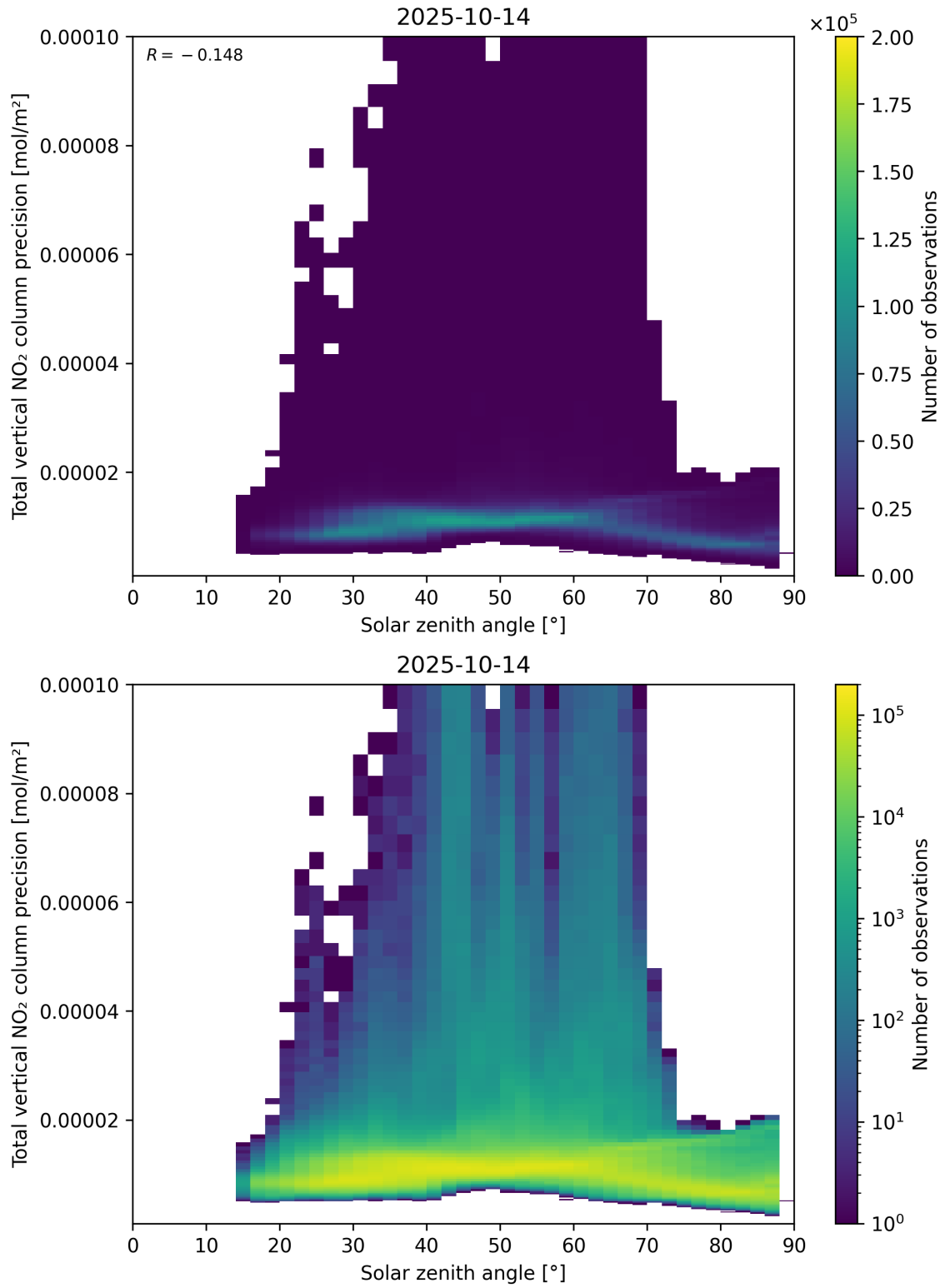
Figure 154: Scatter density plot of “Solar zenith angle” against “Total vertical NO 2 column precision” for 2025-10-13 to 2025-10-15.
