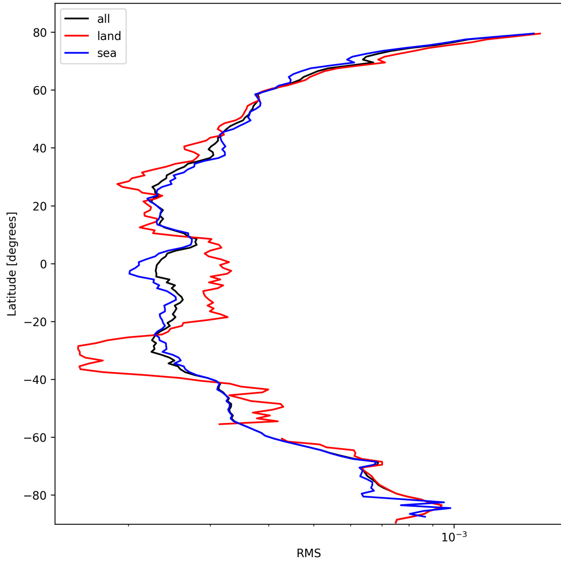
Figure 26: Zonal average of “RMS” for 2025-10-13 to 2025-10-15.
