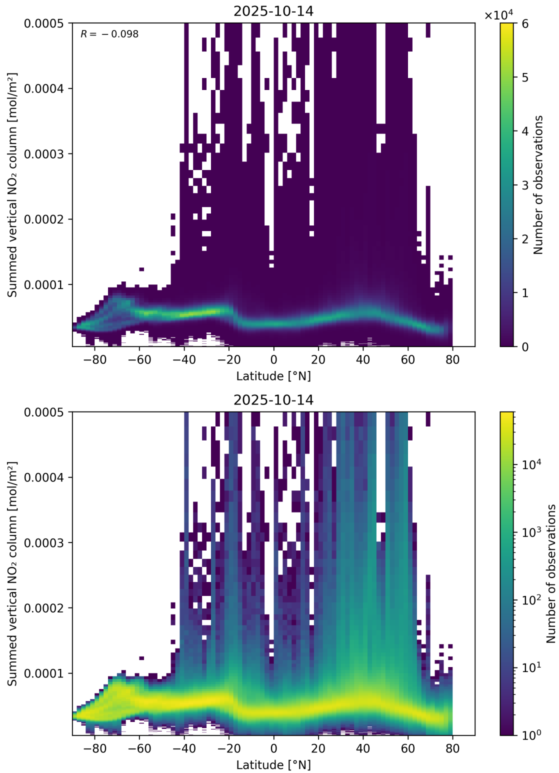
Figure 88: Scatter density plot of “Latitude” against “Summed vertical NO 2 column” for 2025-10-13 to 2025-10-15.
