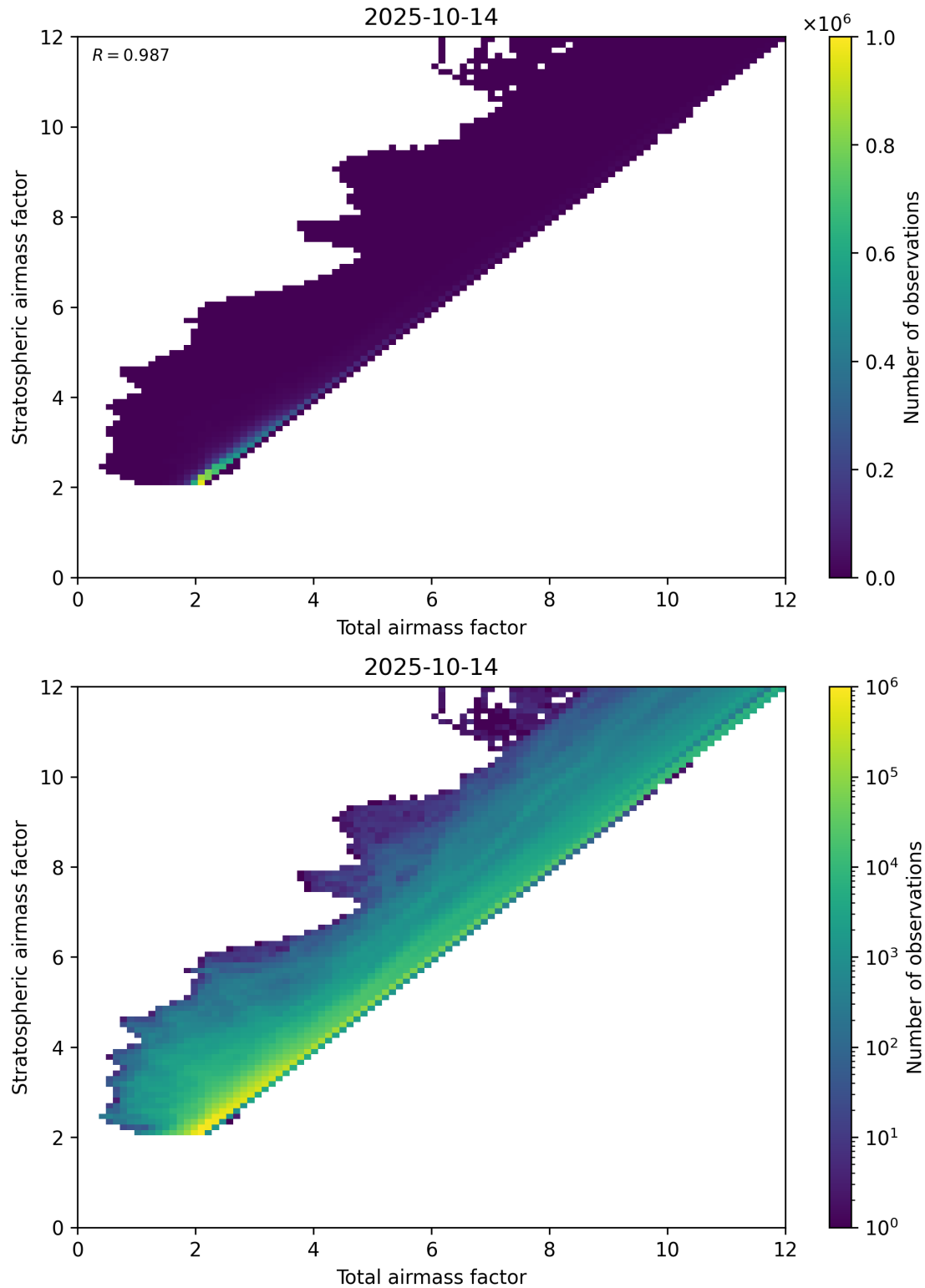
Figure 62: Scatter density plot of “Total airmass factor” against “Stratospheric airmass factor” for 2025-10-13 to 2025-10-15.
