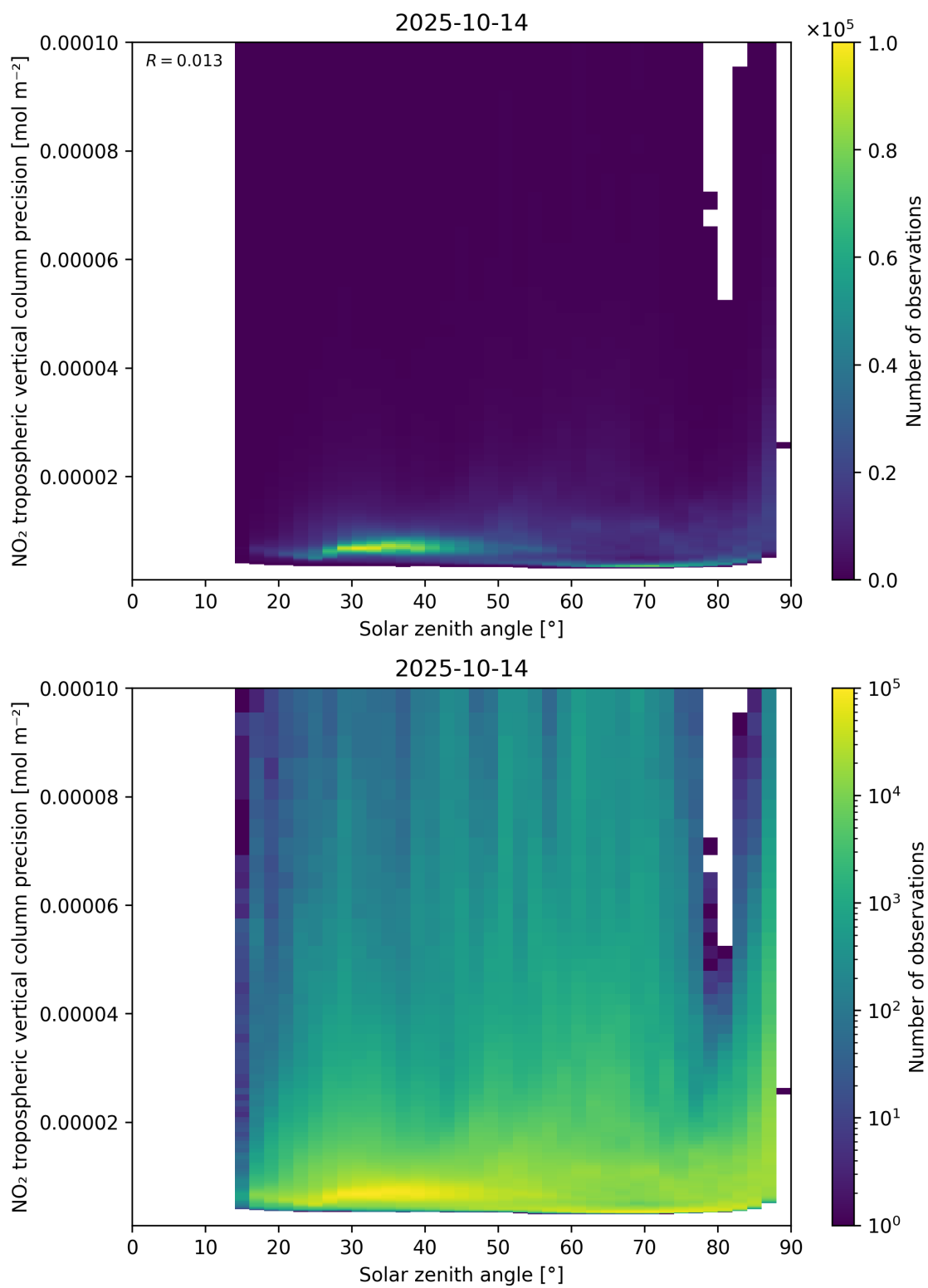
Figure 156: Scatter density plot of “Solar zenith angle” against “NO 2 tropospheric vertical column precision” for 2025-10-13 to 2025-10-15.
