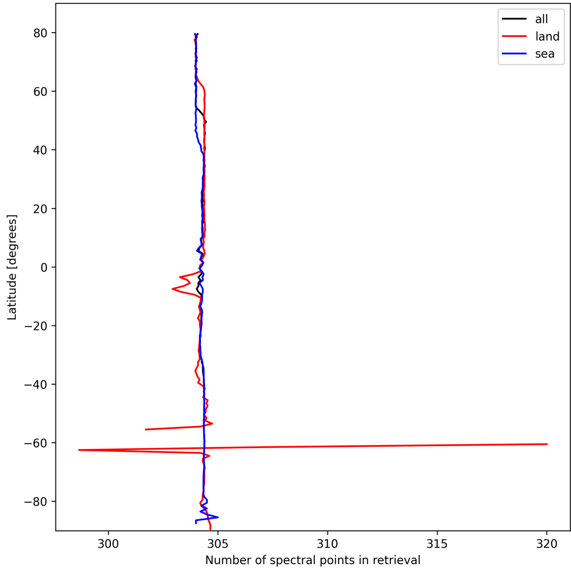
Figure 16: Zonal average of “Number of spectral points in retrieval” for 2025-10-13 to 2025-10-15.
