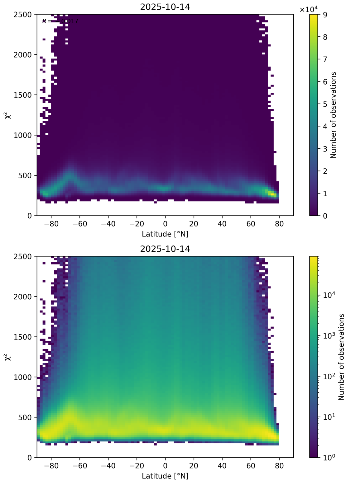
Figure 86: Scatter density plot of “Latitude” against “ \chi^2 ” for 2025-10-13 to 2025-10-15.
