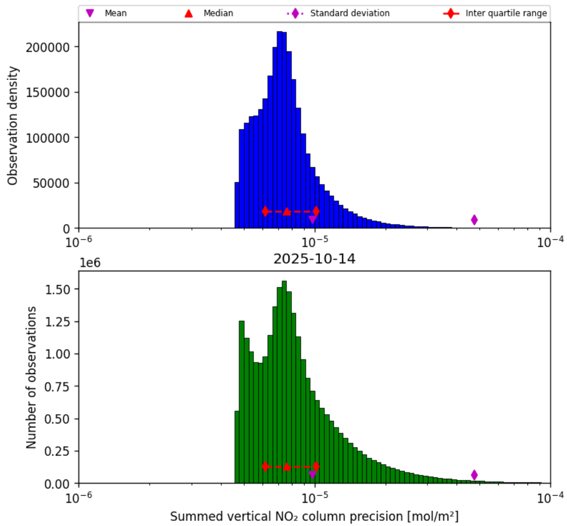
Figure 41: Histogram of “Summed vertical NO 2 column precision” for 2025-10-13 to 2025-10-15
