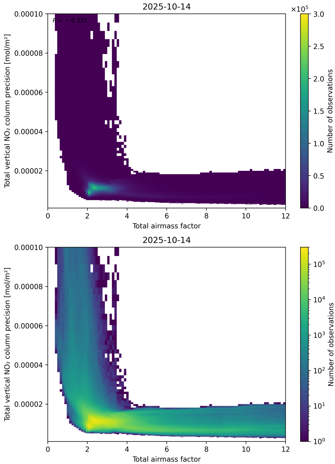
Figure 68: Scatter density plot of “Total airmass factor” against “Total vertical NO 2 column precision” for 2025-10-13 to 2025-10-15.
