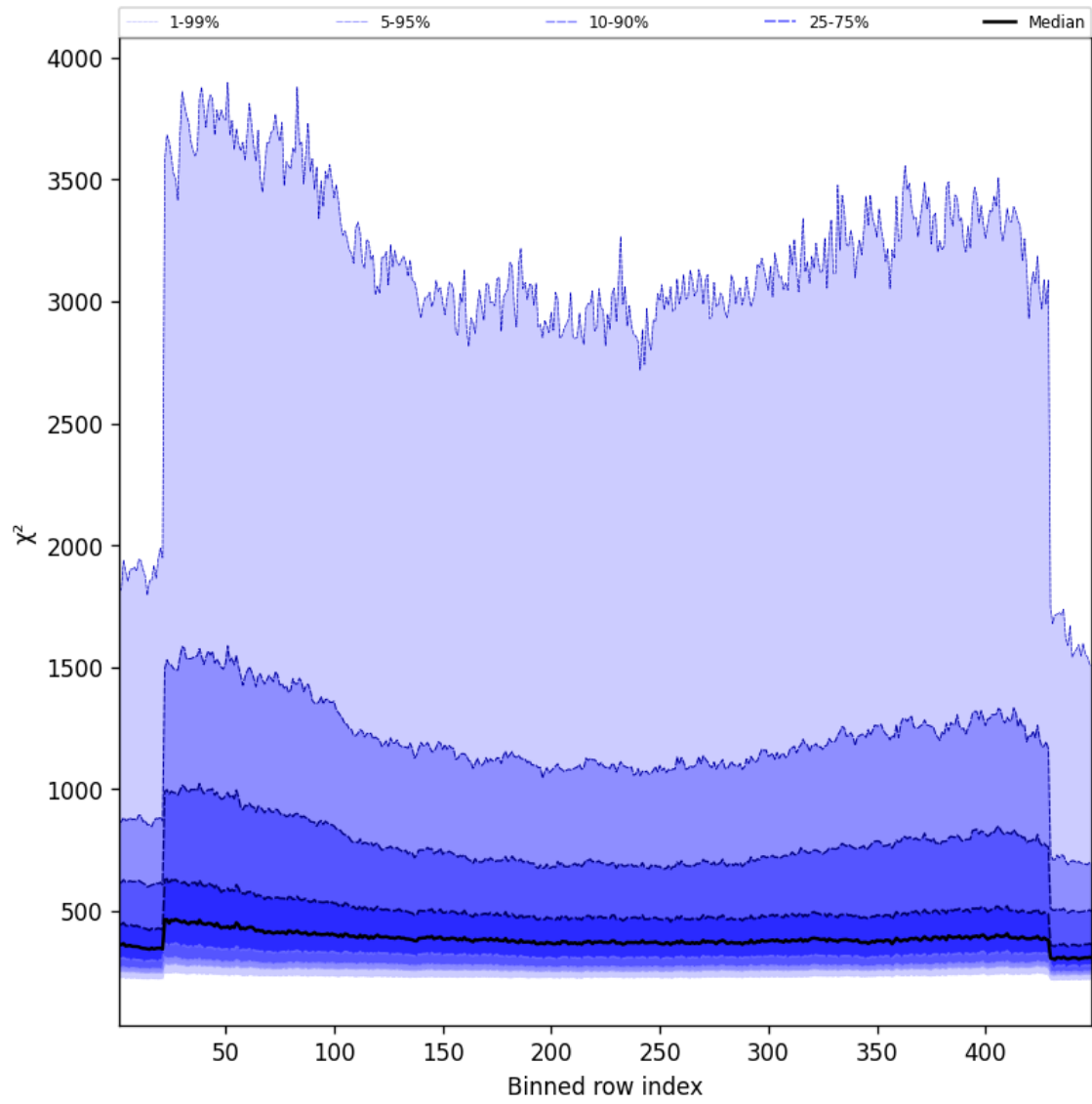
Figure 59: Along track statistics of “ \chi^2 ” for 2025-10-13 to 2025-10-15
