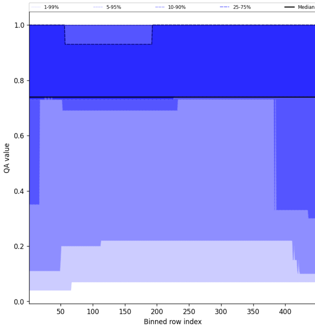
Figure 45: Along track statistics of “QA value” for 2025-10-13 to 2025-10-15
