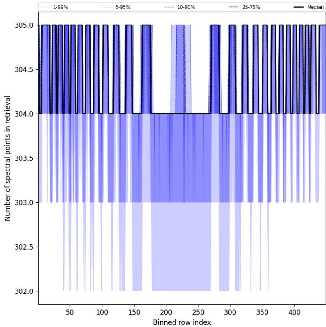
Figure 50: Along track statistics of “Number of spectral points in retrieval” for 2025-10-13 to 2025-10-15
