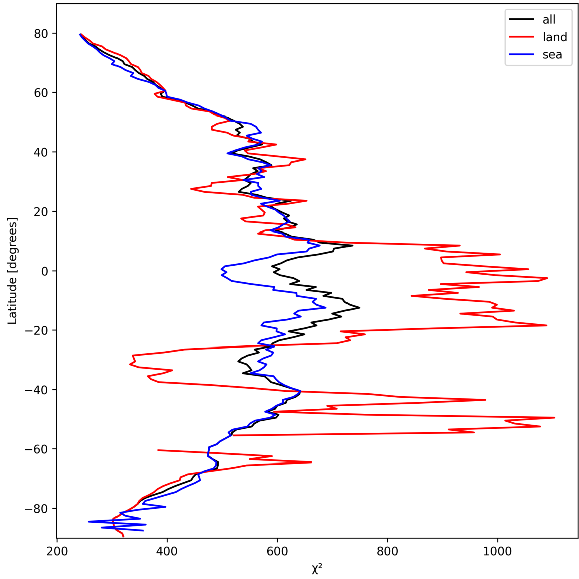
Figure 25: Zonal average of “ \chi^2 ” for 2025-10-13 to 2025-10-15.
