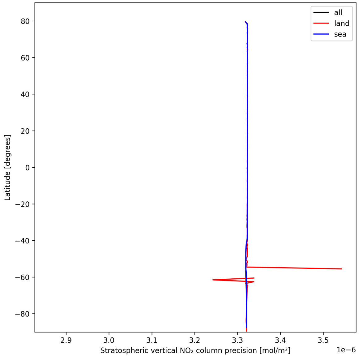
Figure 20: Zonal average of “Stratospheric vertical NO 2 column precision” for 2025-10-13 to 2025-10-15.
