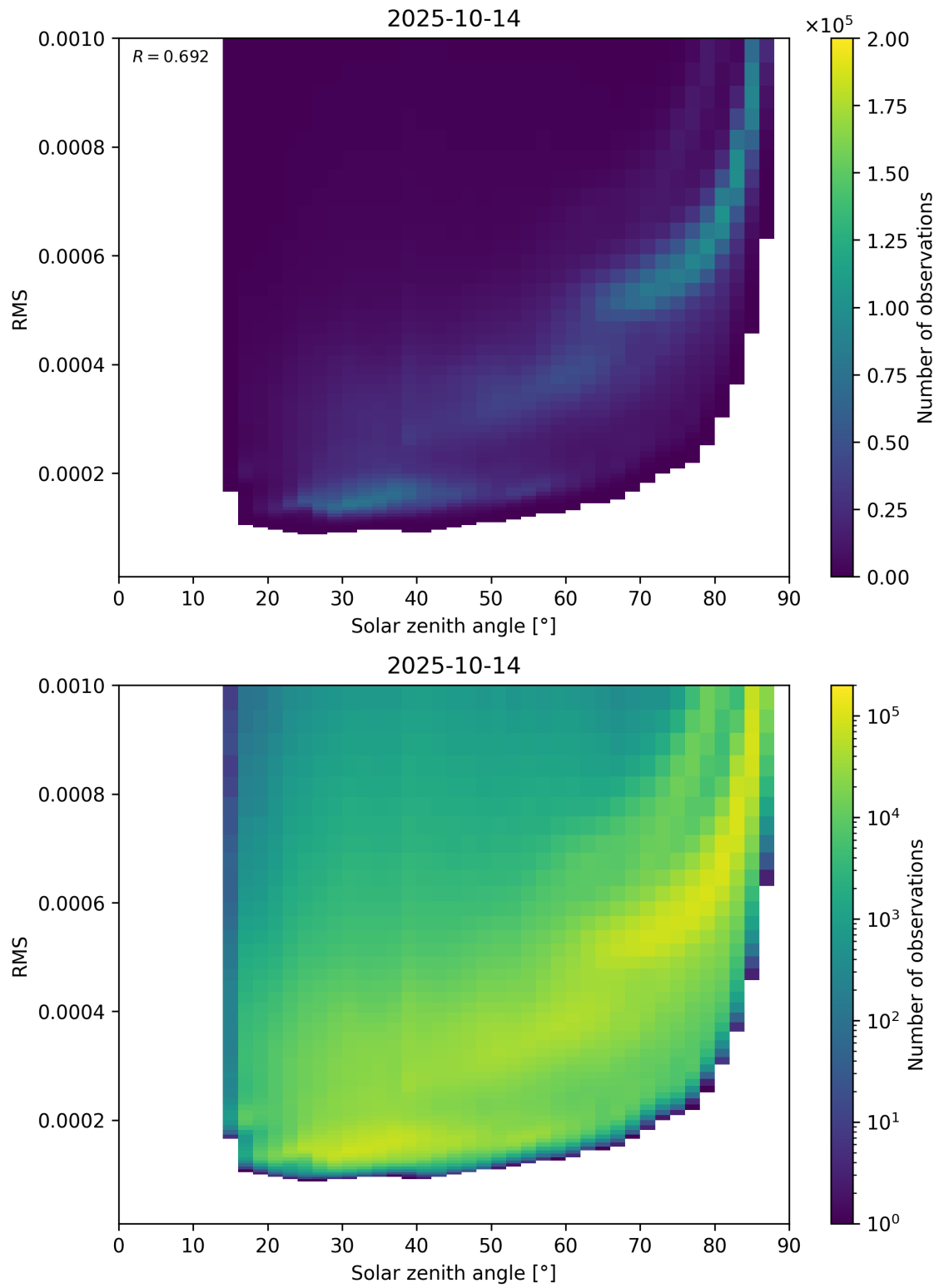
Figure 157: Scatter density plot of “Solar zenith angle” against “RMS” for 2025-10-13 to 2025-10-15.
