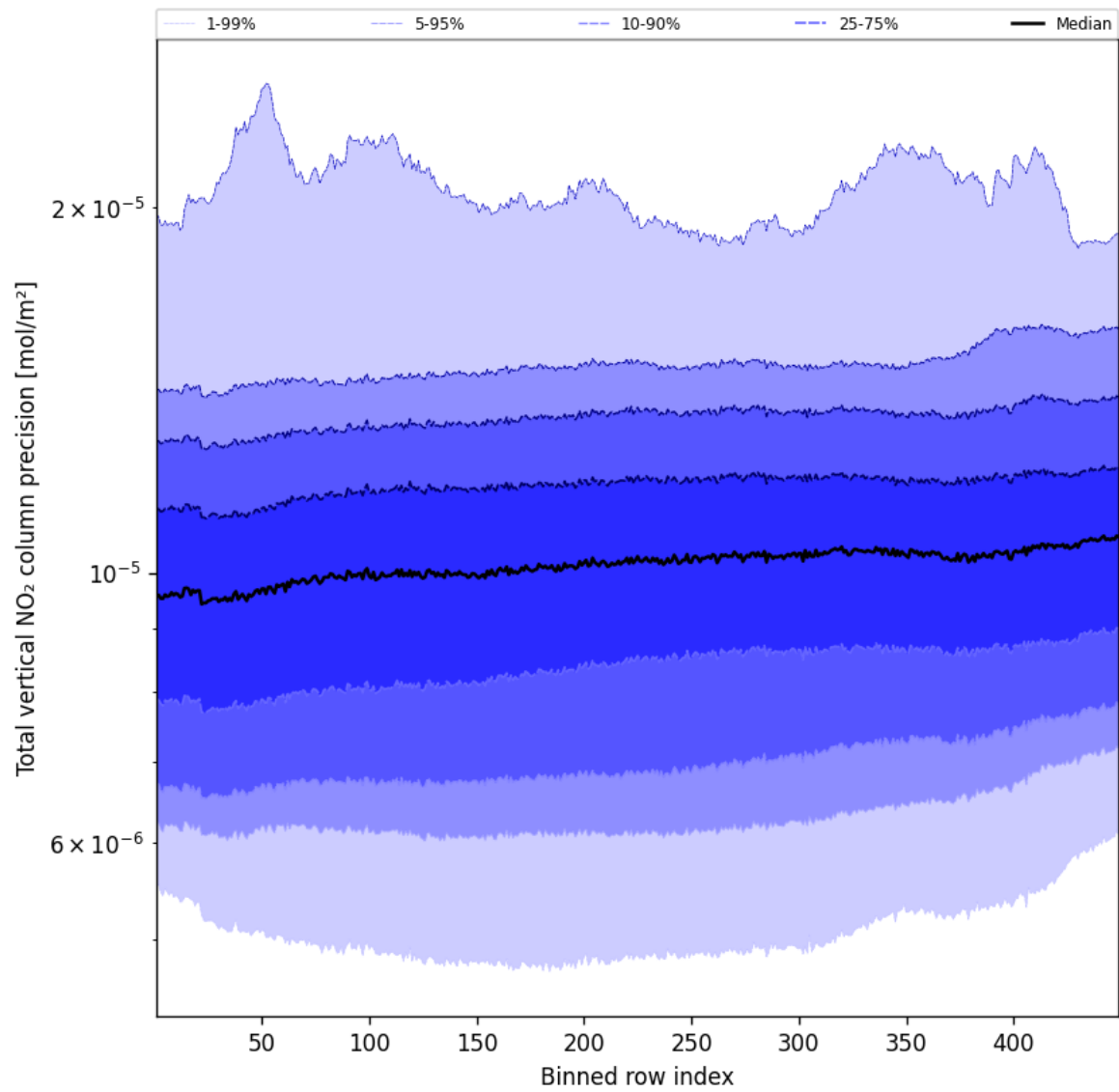
Figure 56: Along track statistics of “Total vertical NO 2 column precision” for 2025-10-13 to 2025-10-15
