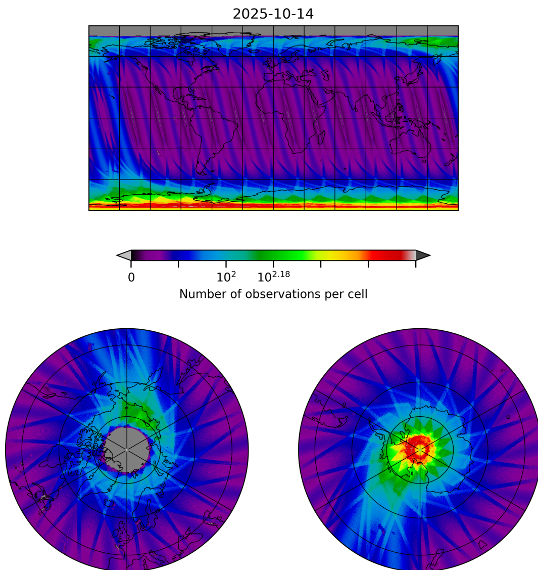
Figure 10: Map of the number of observations for 2025-10-13 to 2025-10-15
