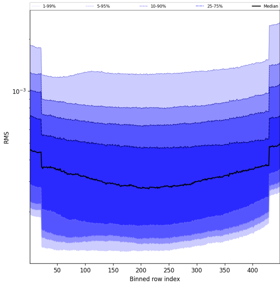
Figure 60: Along track statistics of “RMS” for 2025-10-13 to 2025-10-15
