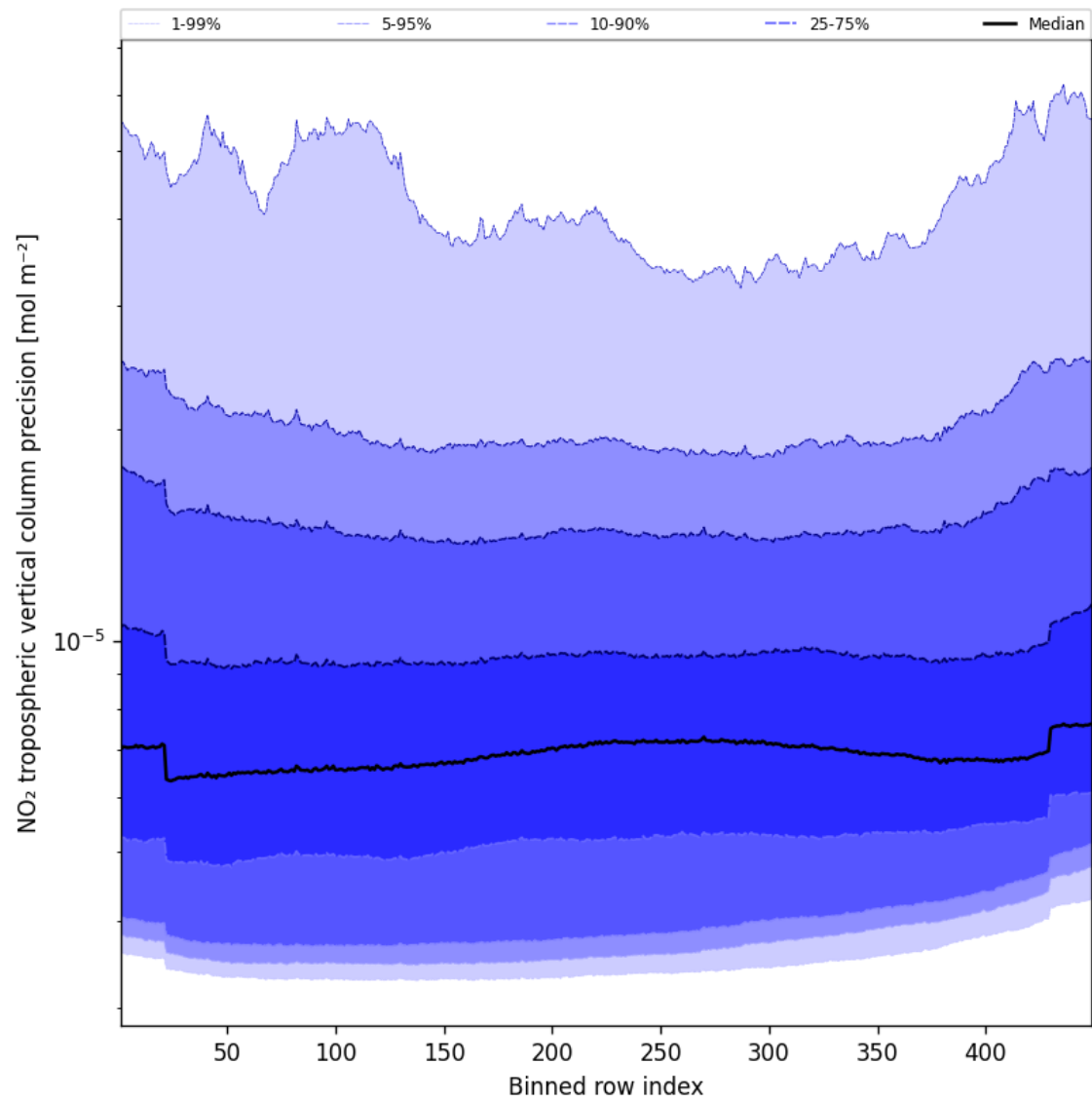
Figure 47: Along track statistics of “NO 2 tropospheric vertical column precision” for 2025-10-13 to 2025-10-15
