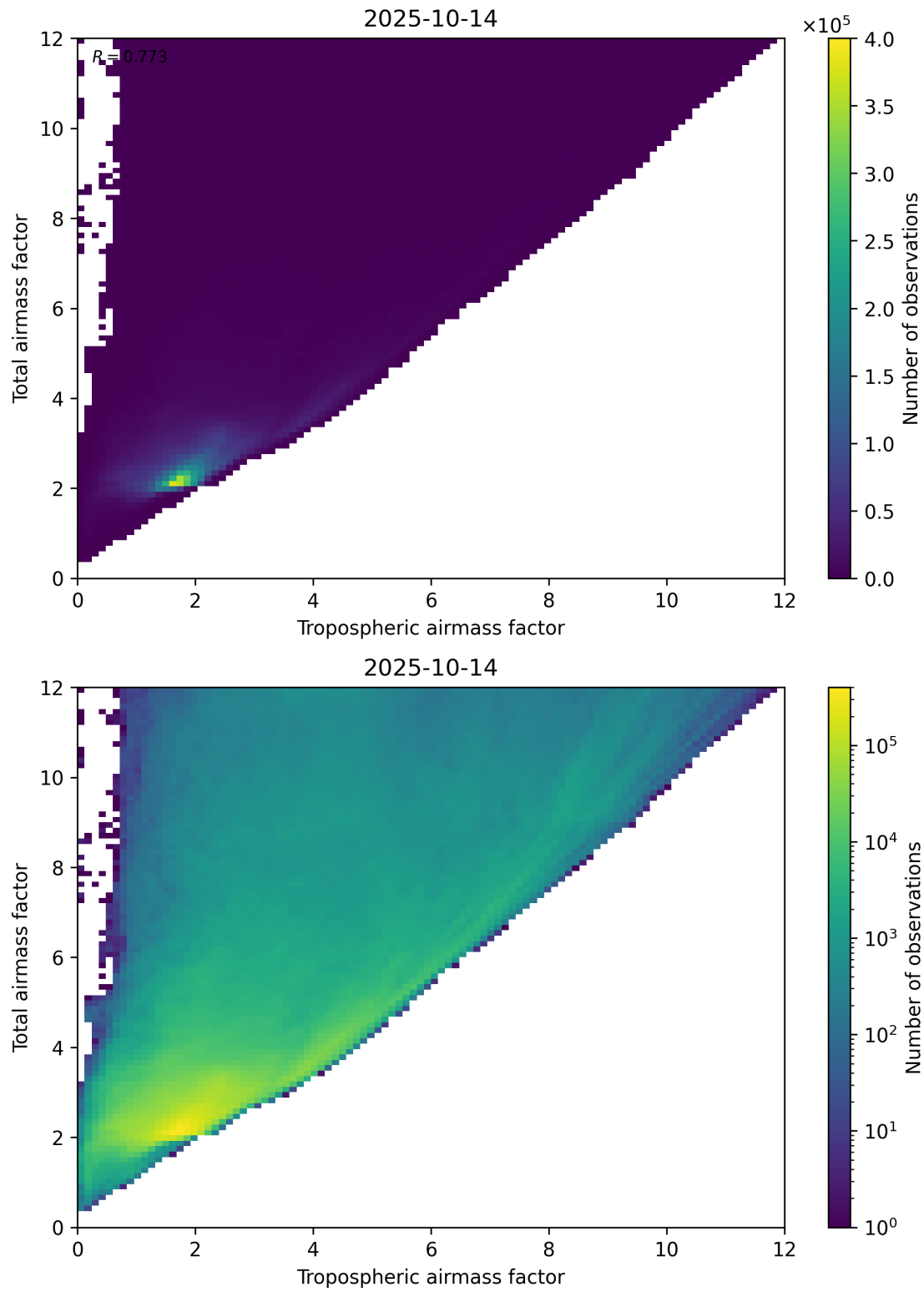
Figure 72: Scatter density plot of “Tropospheric airmass factor” against “Total airmass factor” for 2025-10-13 to 2025-10-15.
