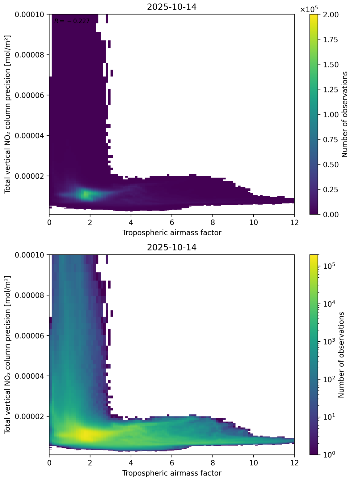
Figure 78: Scatter density plot of “Tropospheric air mass factor” against “Total vertical NO 2 column precision” for 2025-10-13 to 2025-10-15.
