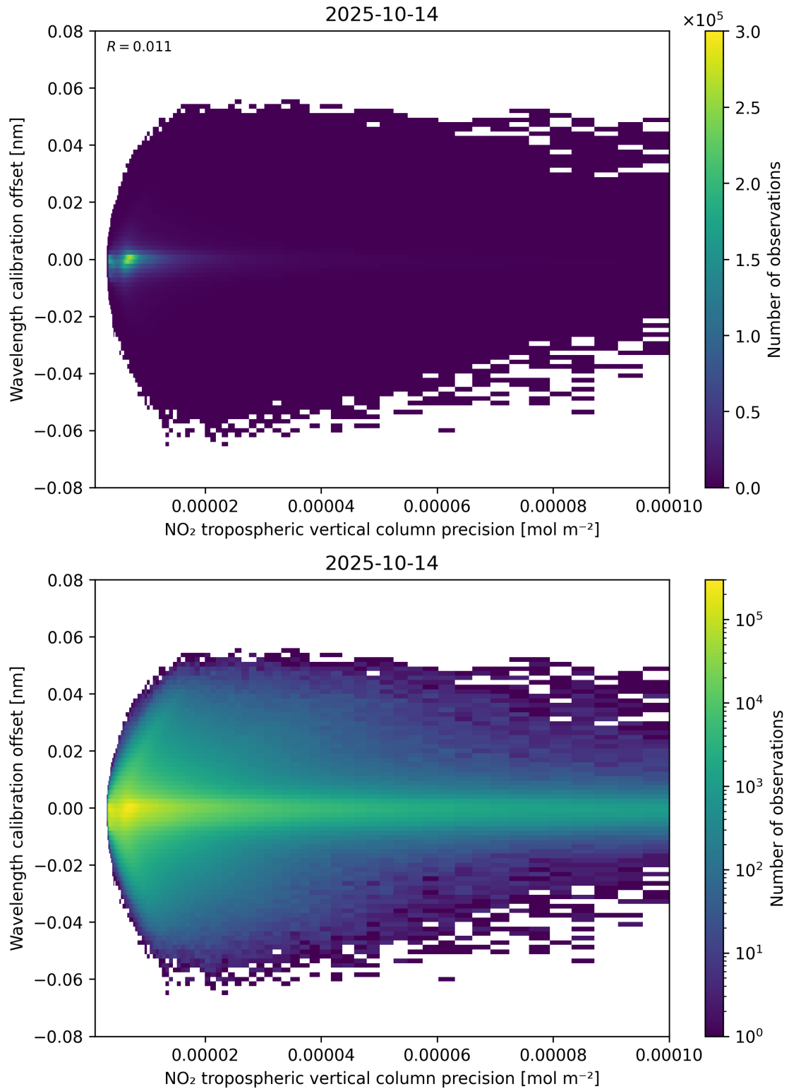
Figure 141: Scatter density plot of “NO 2 tropospheric vertical column precision” against “Wavelength calibration offset” for 2025-10-13 to 2025-10-15.
