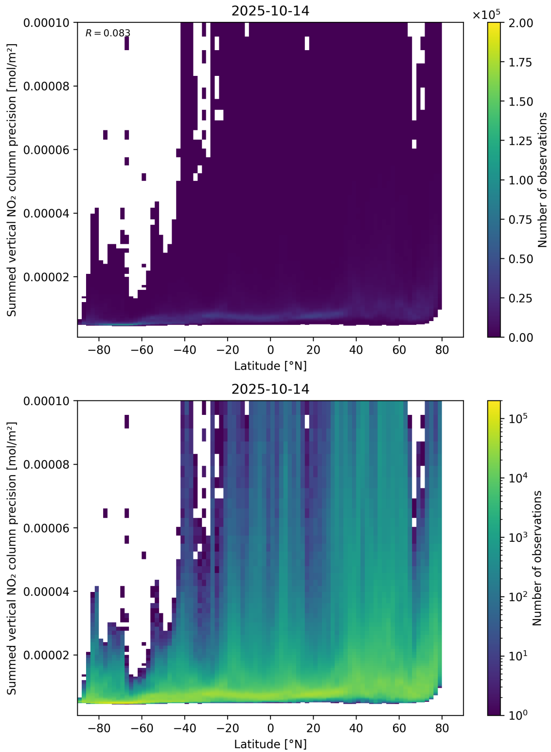
Figure 89: Scatter density plot of “Latitude” against “Summed vertical NO 2 column precision” for 2025-10-13 to 2025-10-15.
