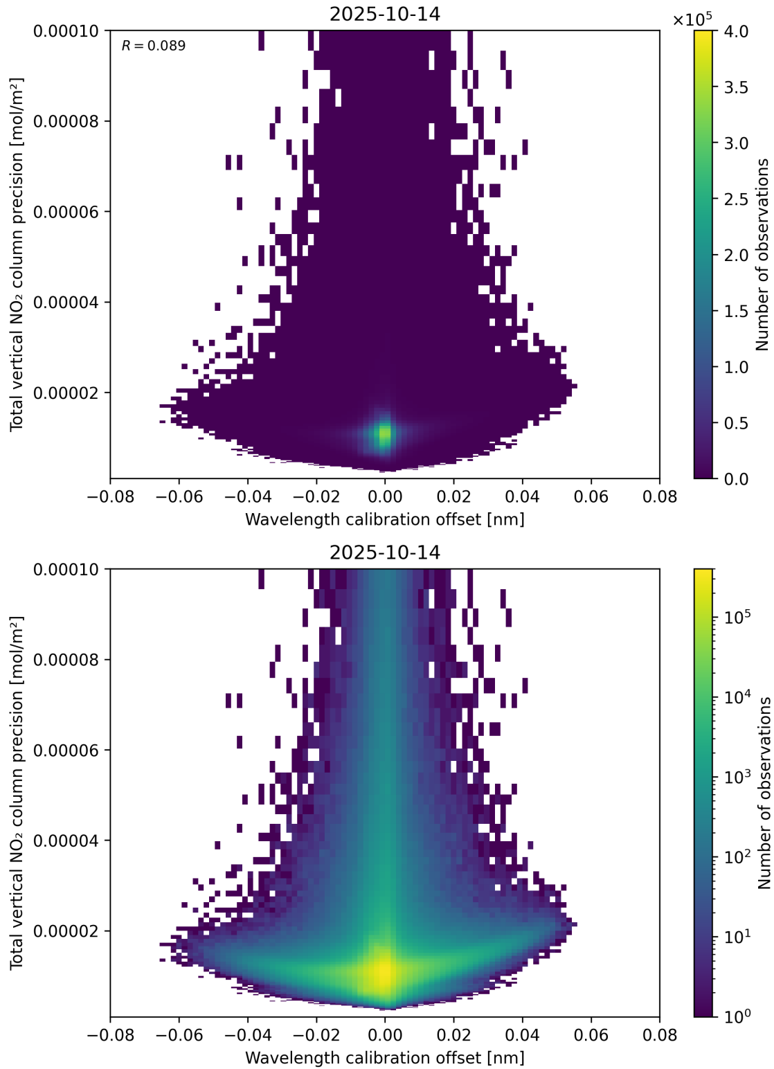
Figure 180: Scatter density plot of “Wavelength calibration offset” against “Total vertical NO 2 column precision” for 2025-10-13 to 2025-10-15.
