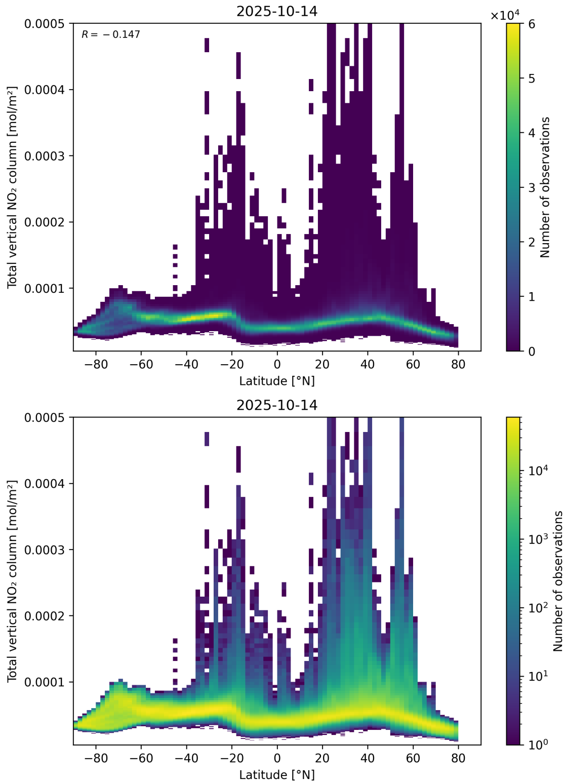
Figure 90: Scatter density plot of “Latitude” against “Total vertical NO 2 column” for 2025-10-13 to 2025-10-15.
