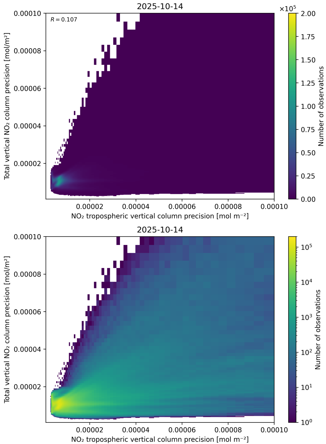
Figure 139: Scatter density plot of “NO 2 tropospheric vertical column precision” against “Total vertical NO 2 column precision” for 2025-10-13 to 2025-10-15.
