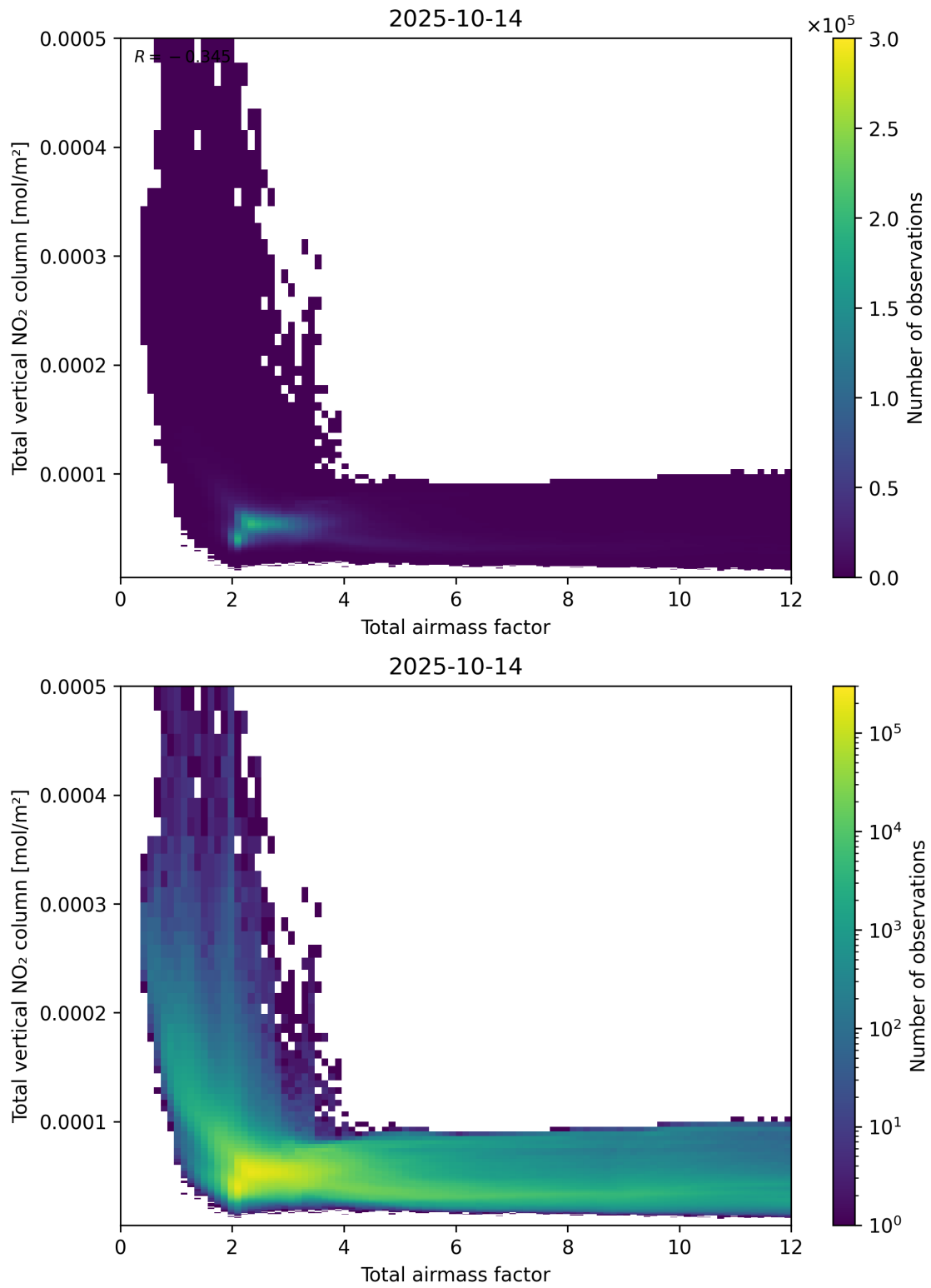
Figure 67: Scatter density plot of “Total airmass factor” against “Total vertical NO 2 column” for 2025-10-13 to 2025-10-15.
