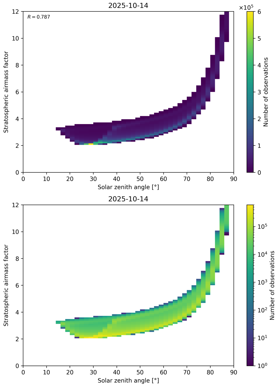
Figure 145: Scatter density plot of “Solar zenith angle” against “Stratospheric airmass factor” for 2025-10-13 to 2025-10-15.
