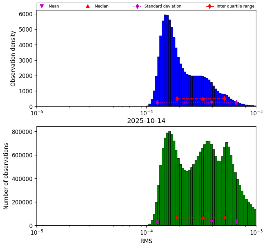
Figure 43: Histogram of “RMS” for 2025-10-13 to 2025-10-15
