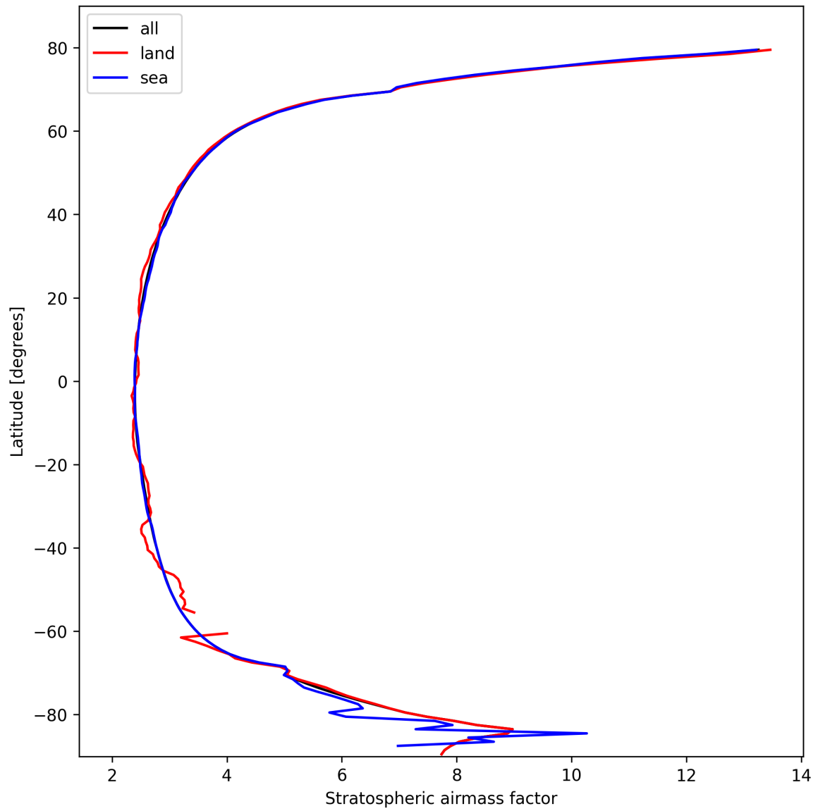
Figure 27: Zonal average of “Stratospheric airmass factor” for 2025-10-13 to 2025-10-15.
