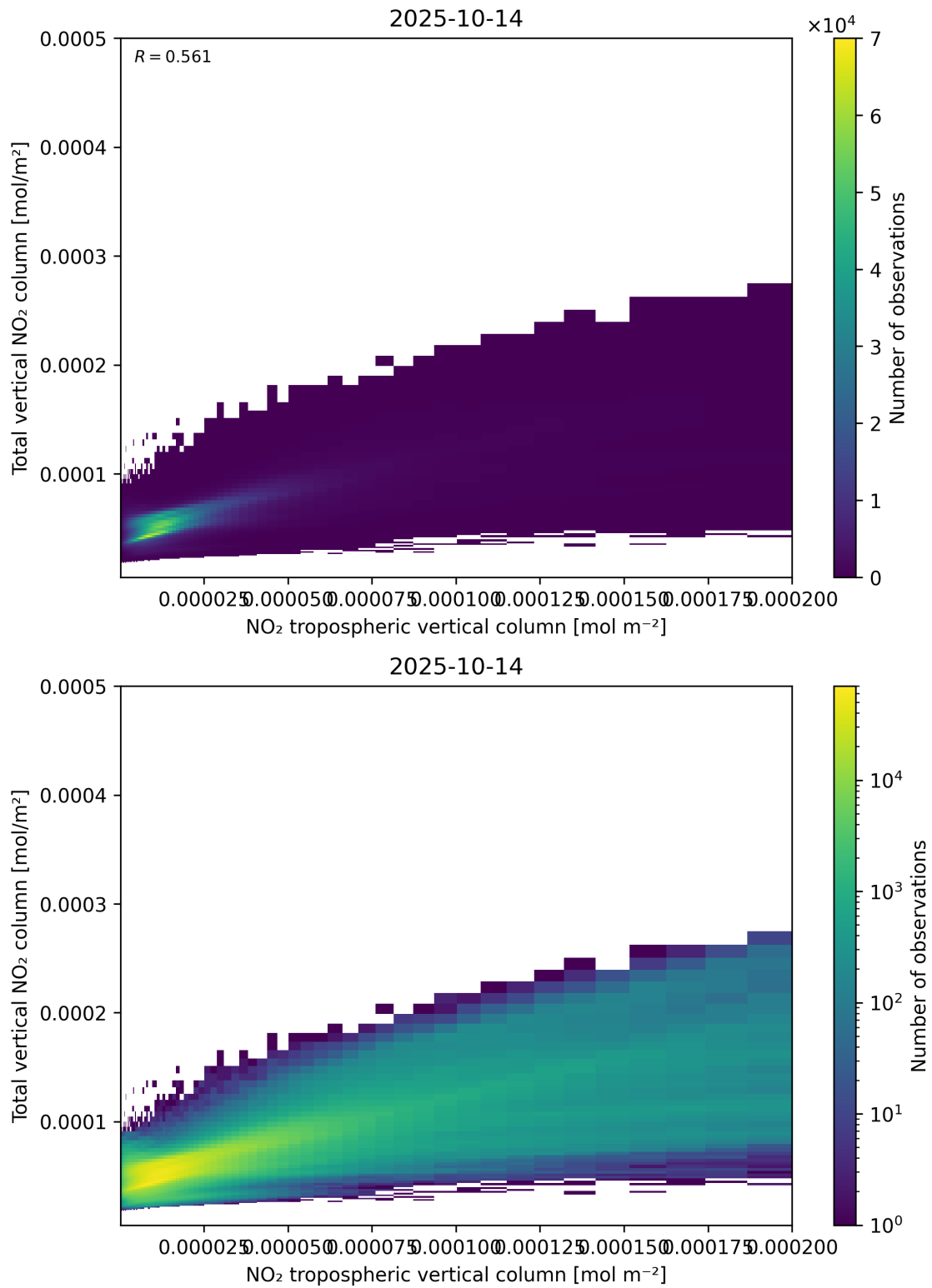
Figure 128: Scatter density plot of “NO 2 tropospheric vertical column” against “Total vertical NO 2 column” for 2025-10-13 to 2025-10-15.
