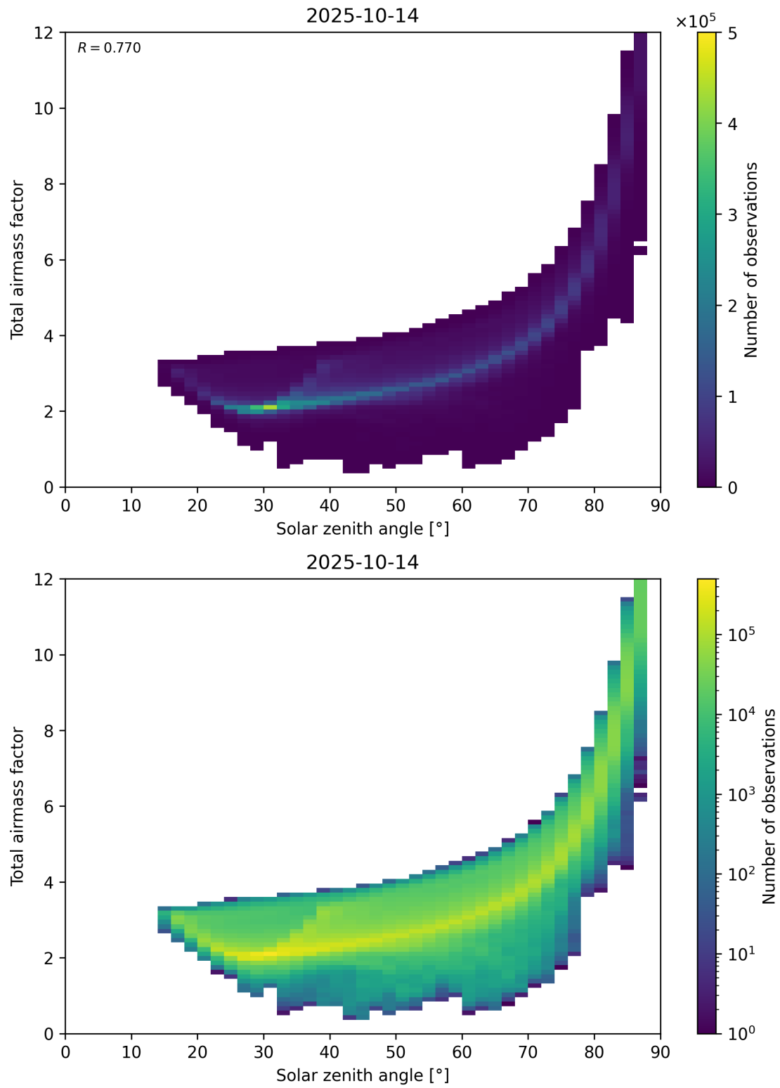
Figure 146: Scatter density plot of “Solar zenith angle” against “Total airmass factor” for 2025-10-13 to 2025-10-15.
