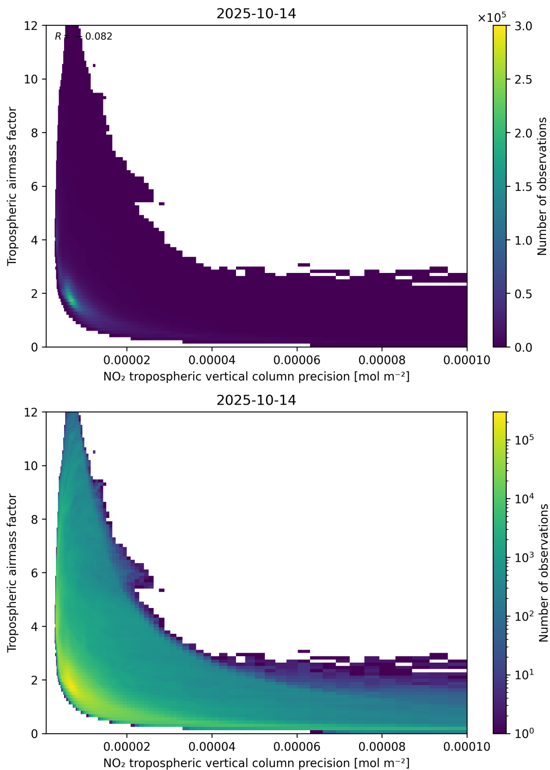
Figure 133: Scatter density plot of “NO 2 tropospheric vertical column precision” against “Tropospheric air mass factor” for 2025-10-13 to 2025-10-15.
