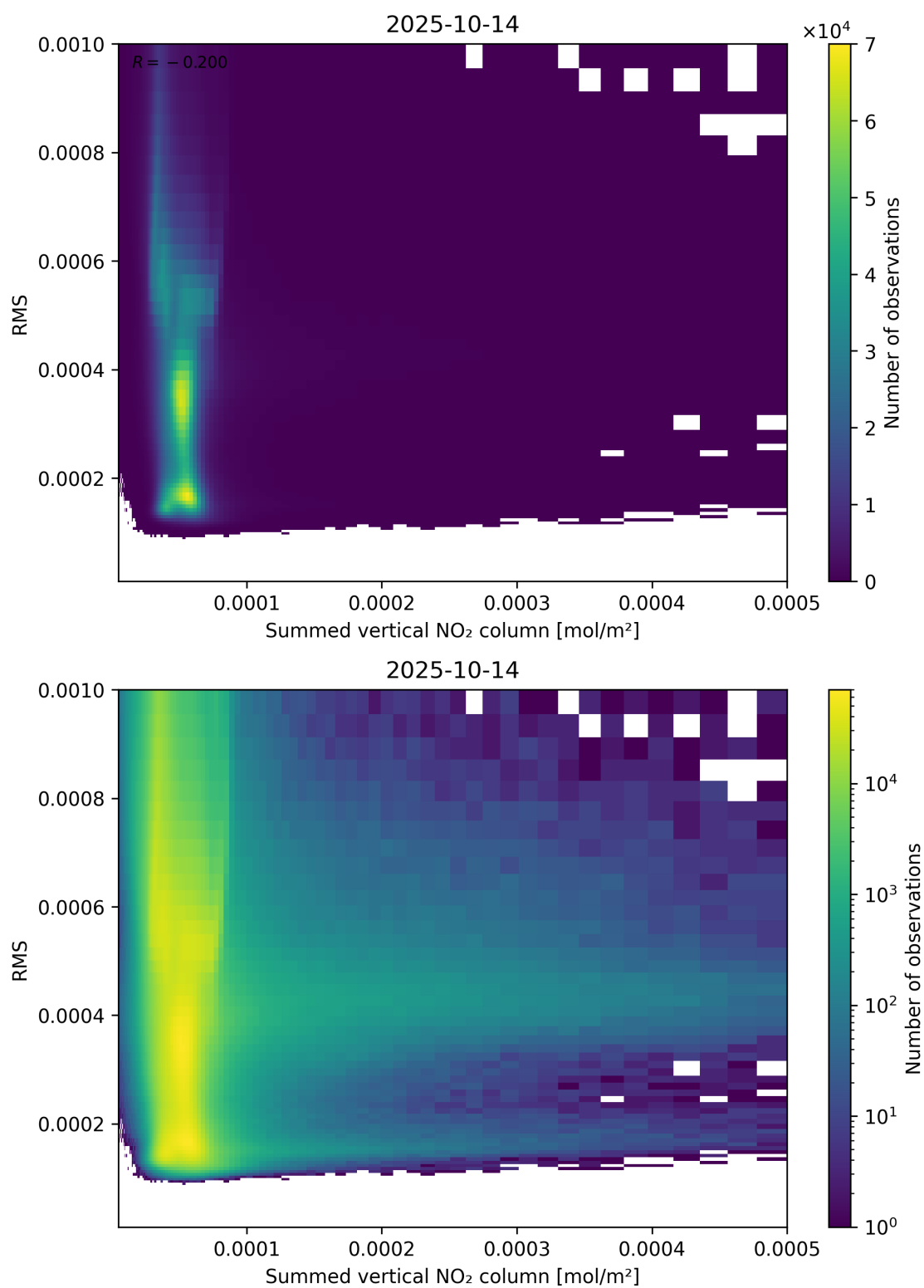
Figure 109: Scatter density plot of “Summed vertical NO 2 column” against “RMS” for 2025-10-13 to 2025-10-15.
