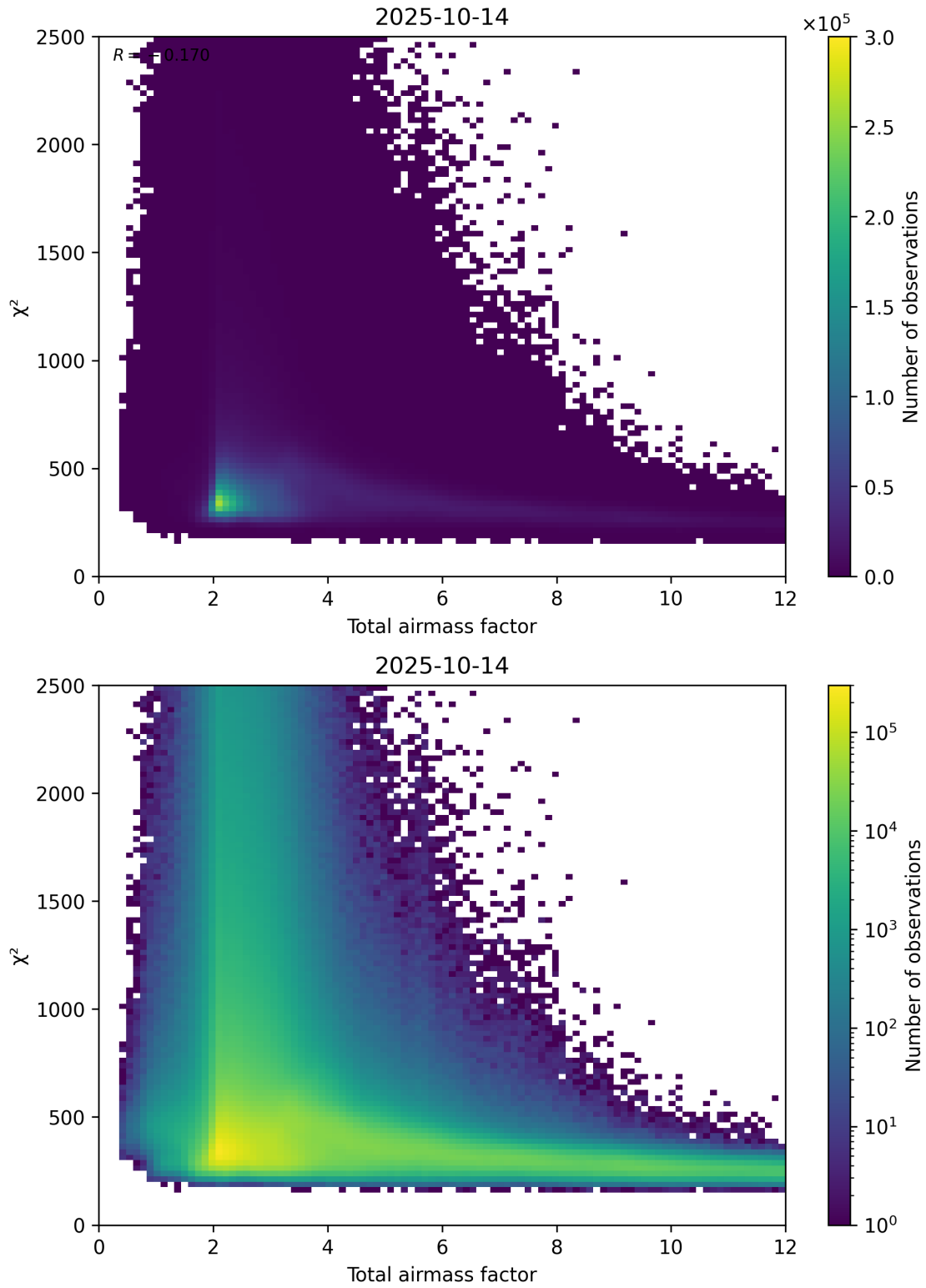
Figure 63: Scatter density plot of “Total airmass factor” against “ \chi^2 ” for 2025-10-13 to 2025-10-15.
