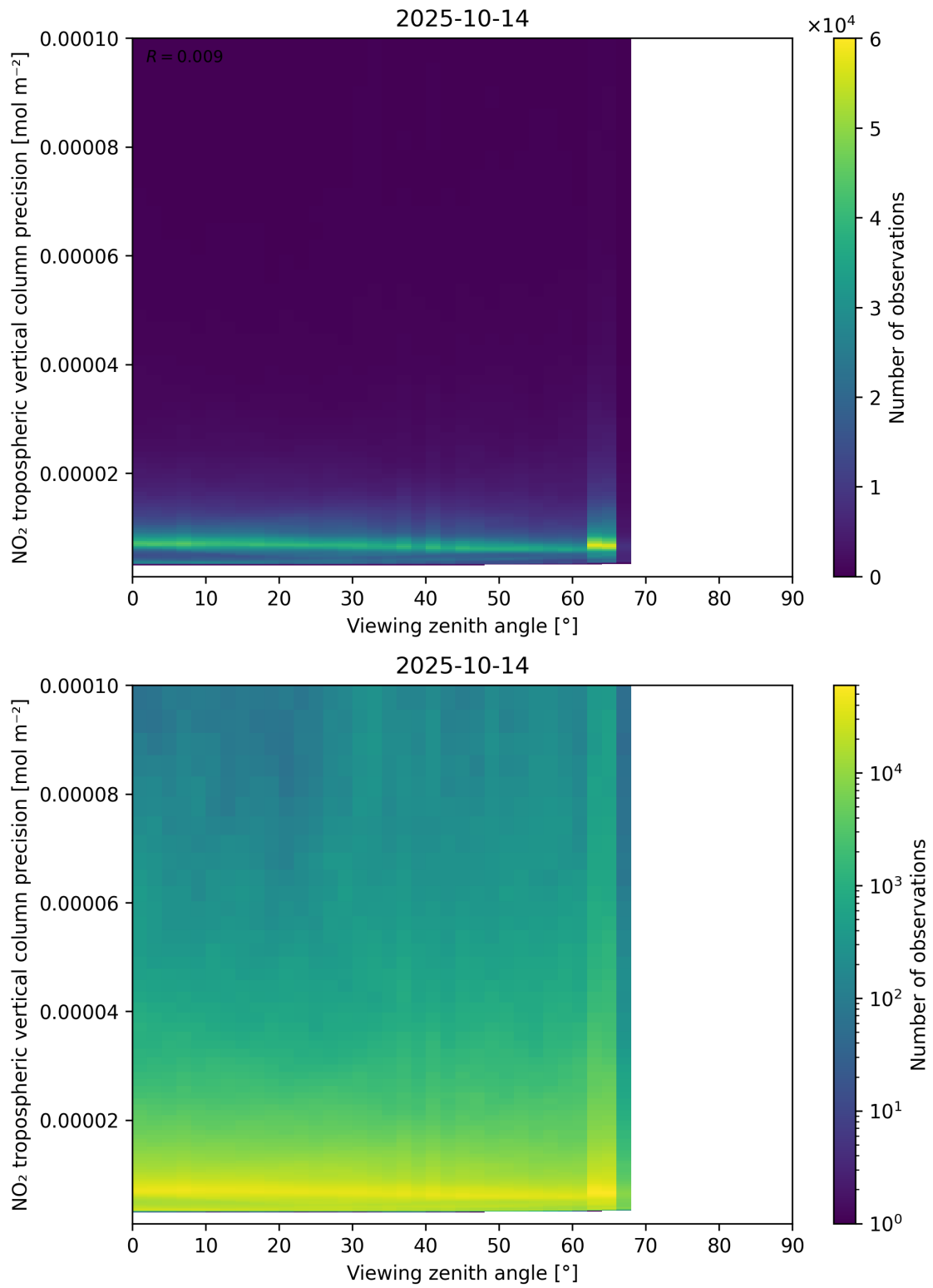
Figure 170: Scatter density plot of “Viewing zenith angle” against “NO 2 tropospheric vertical column precision” for 2025-10-13 to 2025-10-15.
