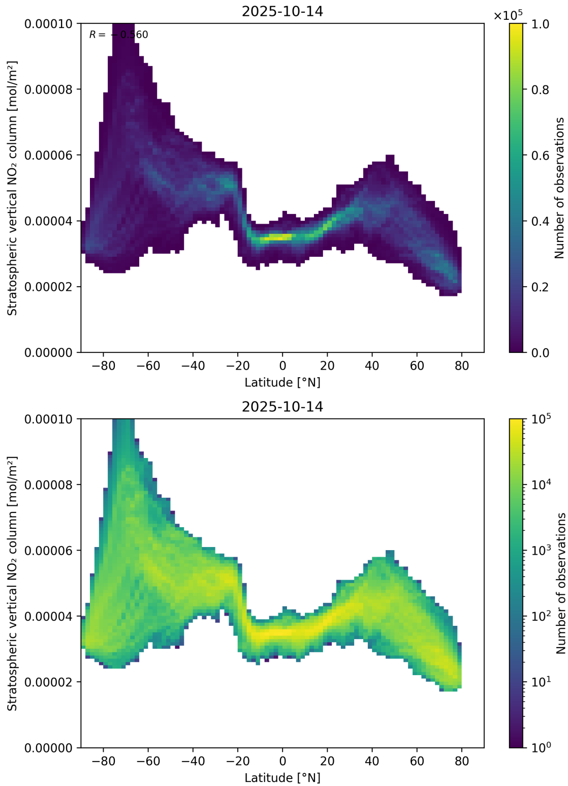
Figure 87: Scatter density plot of “Latitude” against “Stratospheric vertical NO 2 column” for 2025-10-13 to 2025-10-15.
