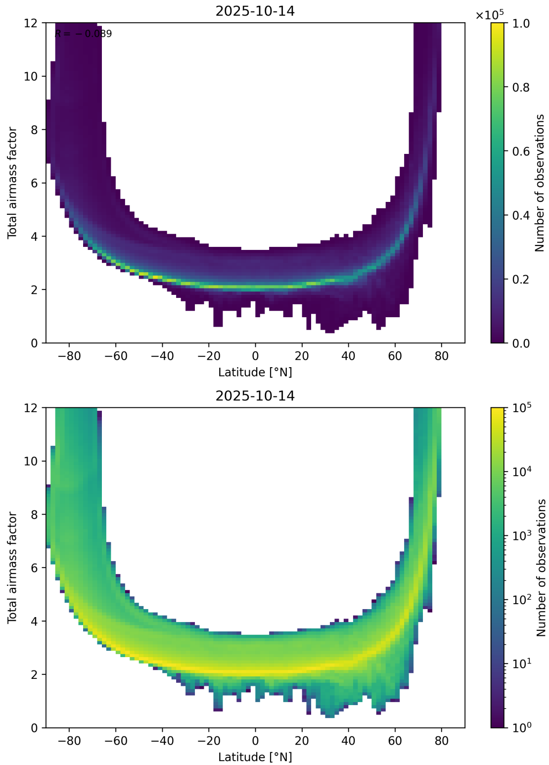
Figure 84: Scatter density plot of “Latitude” against “Total airmass factor” for 2025-10-13 to 2025-10-15.
