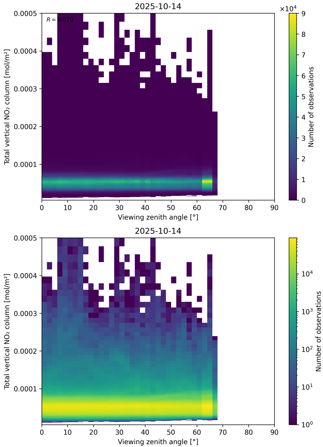
Figure 167: Scatter density plot of “Viewing zenith angle” against “Total vertical NO 2 column” for 2025-10-13 to 2025-10-15.
