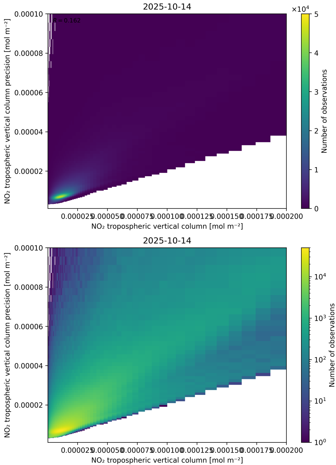
Figure 130: Scatter density plot of “NO 2 tropospheric vertical column” against “NO 2 tropospheric vertical column precision” for 2025-10-13 to 2025-10-15.
