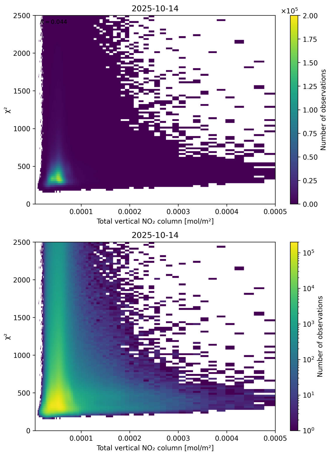
Figure 111: Scatter density plot of “Total vertical NO 2 column” against “ \chi^2 ” for 2025-10-13 to 2025-10-15.
