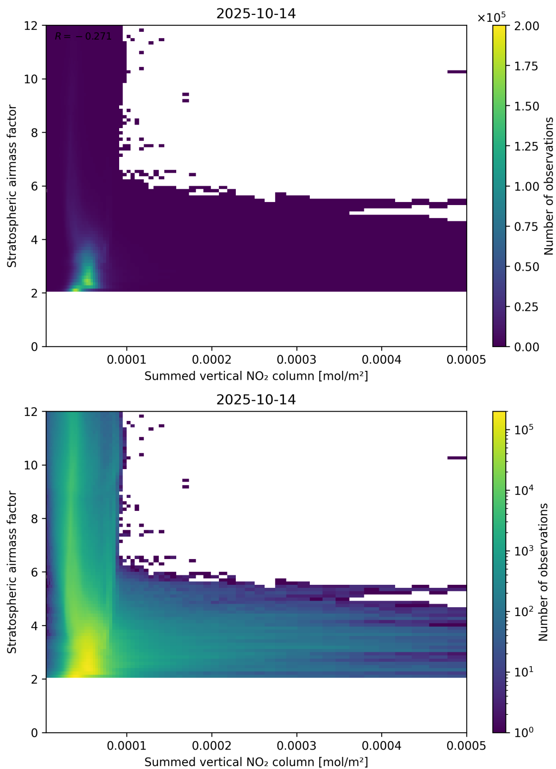
Figure 103: Scatter density plot of “Summed vertical NO 2 column” against “Stratospheric airmass factor” for 2025-10-13 to 2025-10-15.
