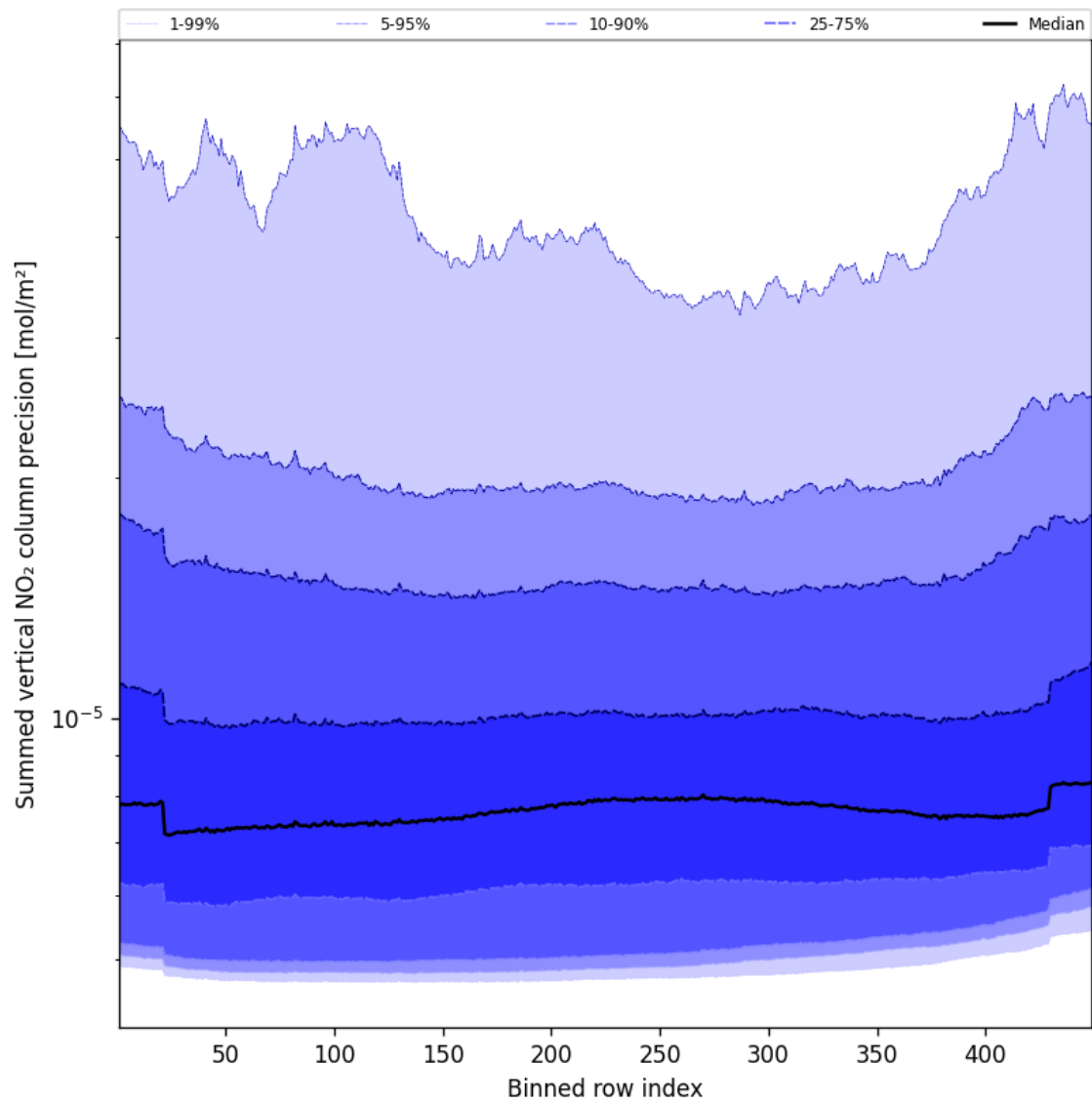
Figure 58: Along track statistics of “Summed vertical NO 2 column precision” for 2025-10-13 to 2025-10-15
