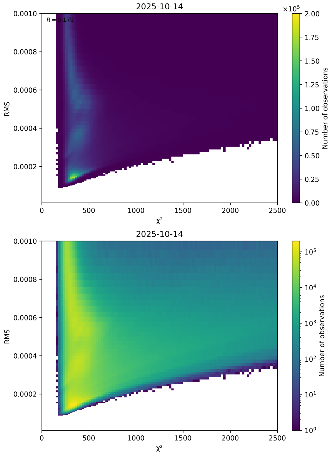
Figure 82: Scatter density plot of “ \chi^2 ” against “RMS” for 2025-10-13 to 2025-10-15.
