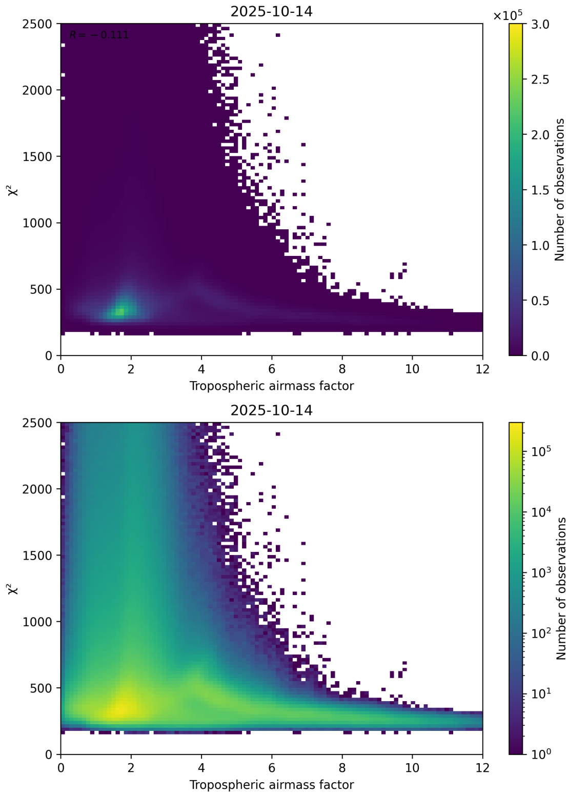
Figure 73: Scatter density plot of “Tropospheric airmass factor” against “ \chi^2 ” for 2025-10-13 to 2025-10-15.
