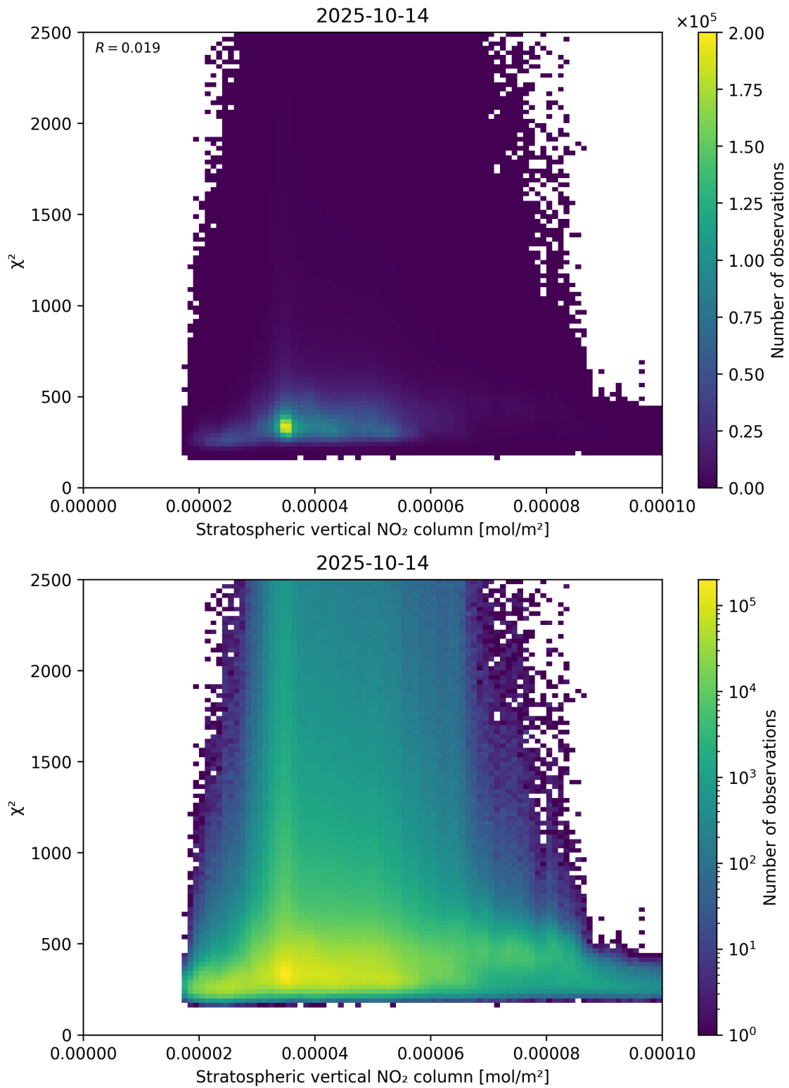
Figure 97: Scatter density plot of “Stratospheric vertical NO 2 column” against “ \chi^2 ” for 2025-10-13 to 2025-10-15.
