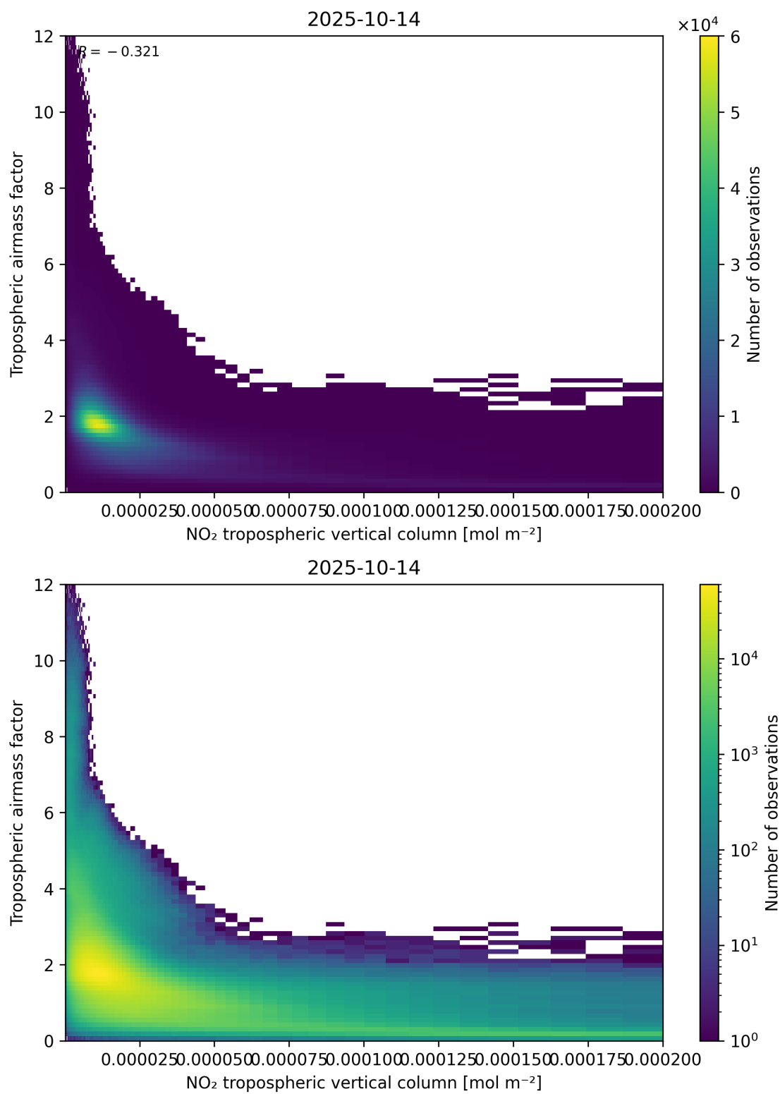
Figure 123: Scatter density plot of “NO 2 tropospheric vertical column” against “Tropospheric air mass factor” for 2025-10-13 to 2025-10-15.
