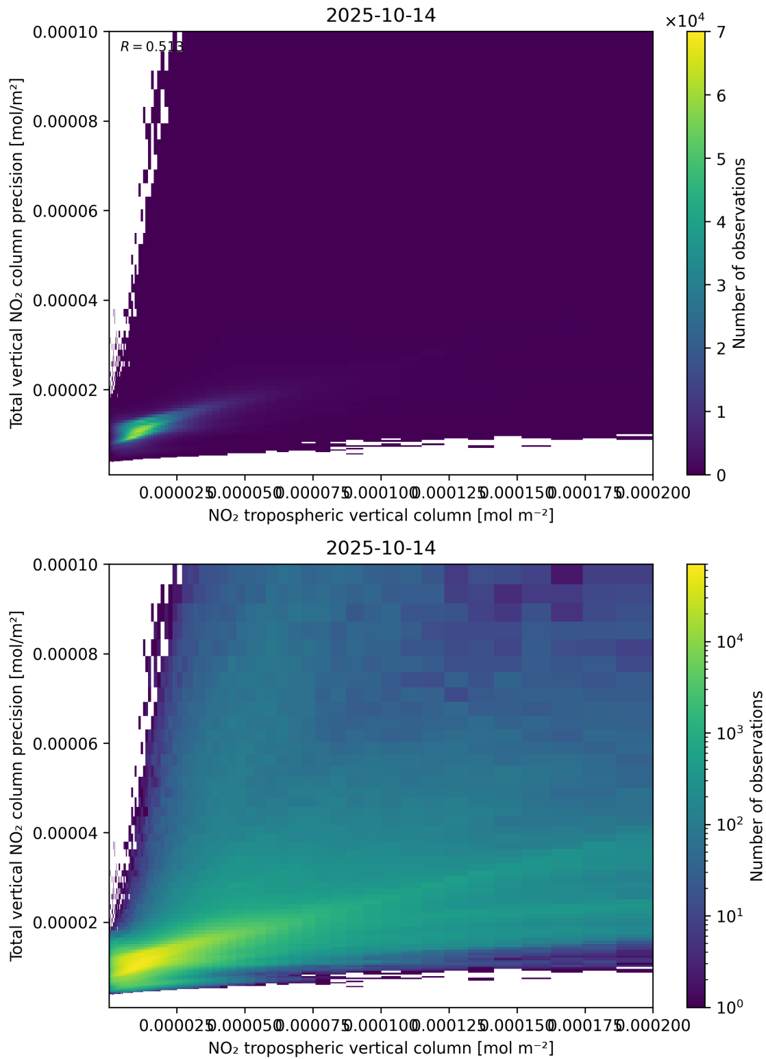
Figure 129: Scatter density plot of “NO 2 tropospheric vertical column” against “Total vertical NO 2 column precision” for 2025-10-13 to 2025-10-15.
