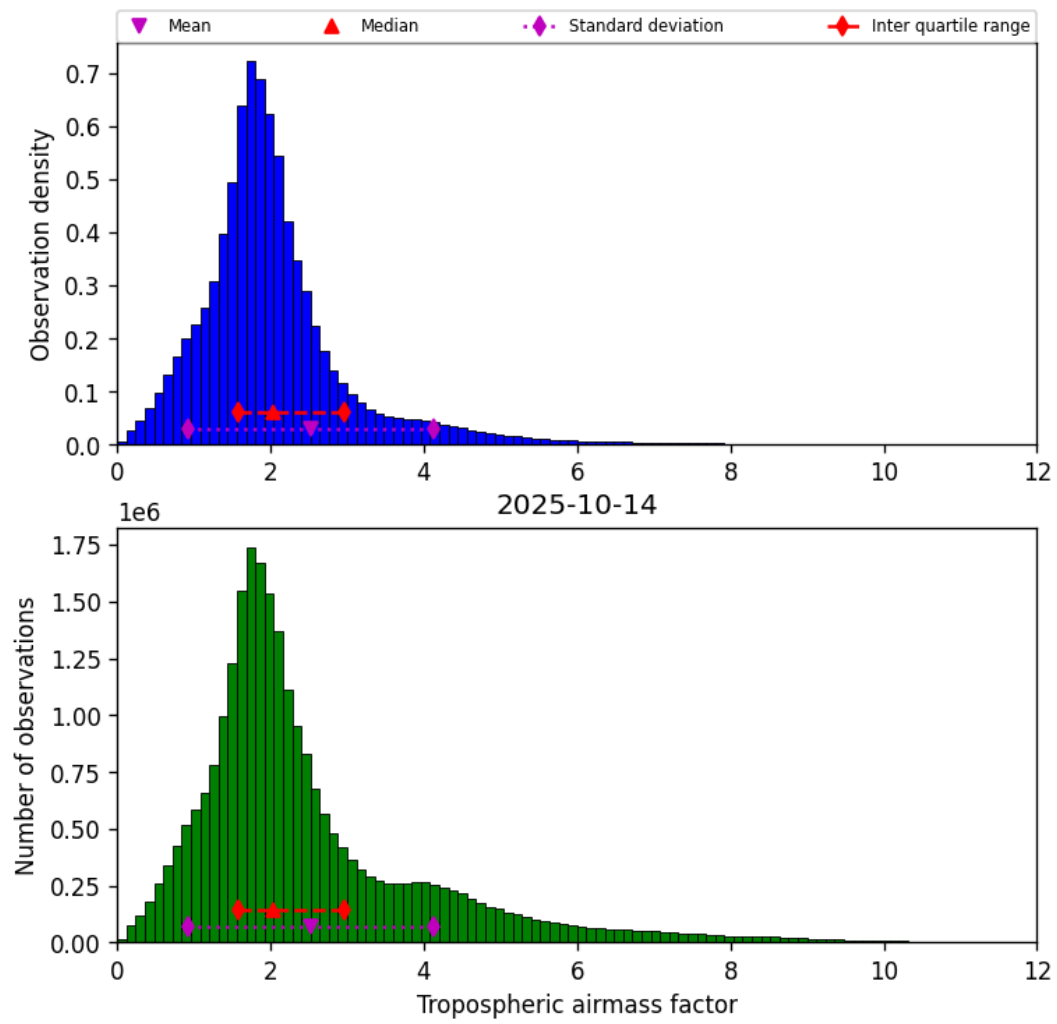
Figure 31: Histogram of “Tropospheric airmass factor” for 2025-10-13 to 2025-10-15
