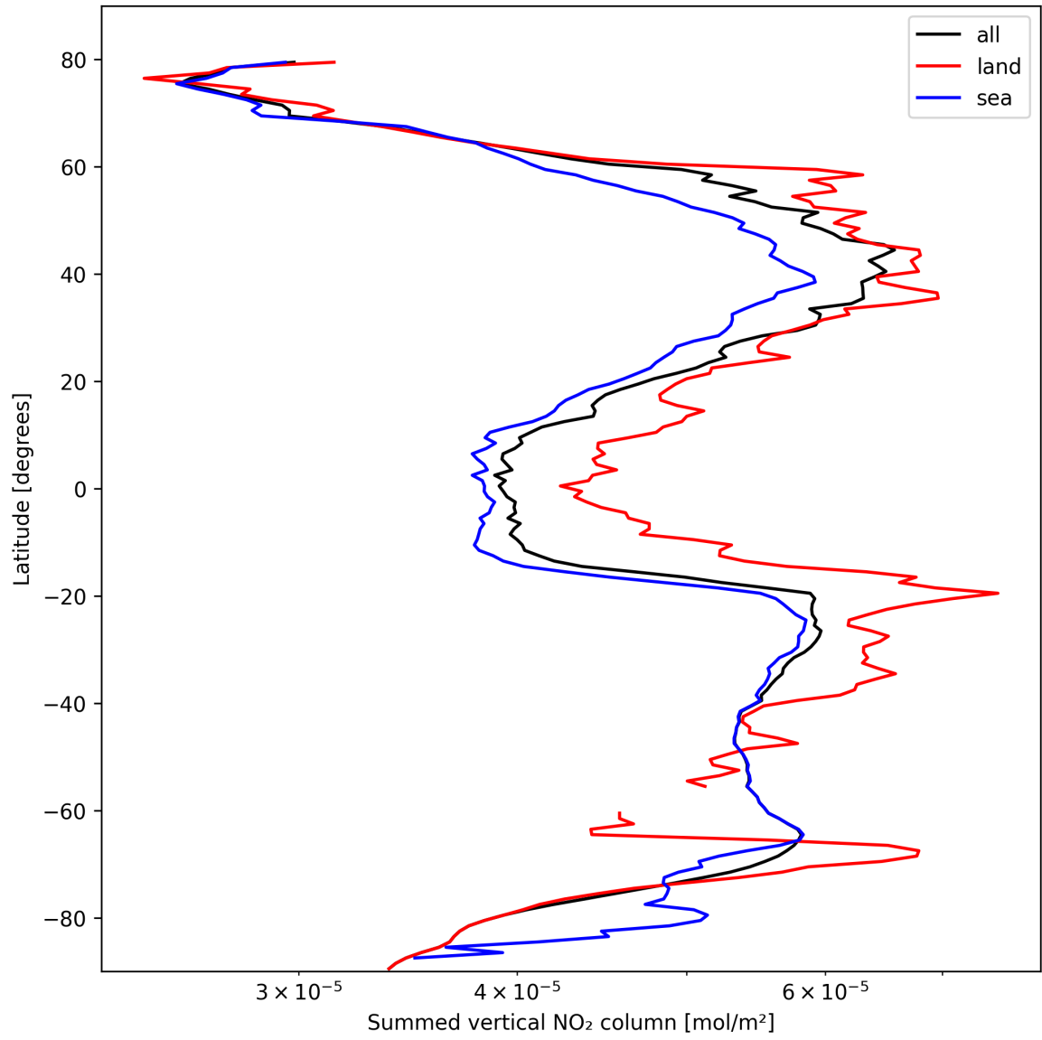
Figure 23: Zonal average of “Summed vertical NO 2 column” for 2025-10-13 to 2025-10-15.
