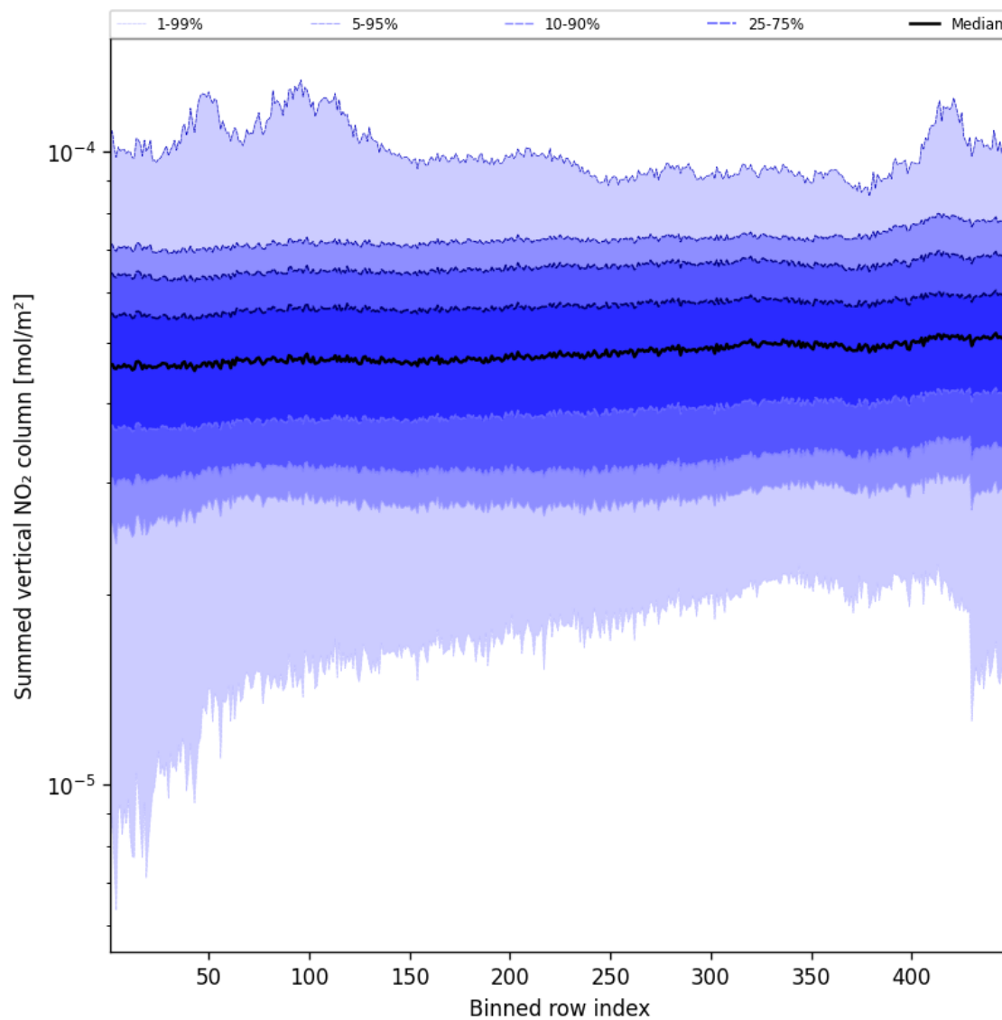
Figure 57: Along track statistics of “Summed vertical NO 2 column” for 2025-10-13 to 2025-10-15
