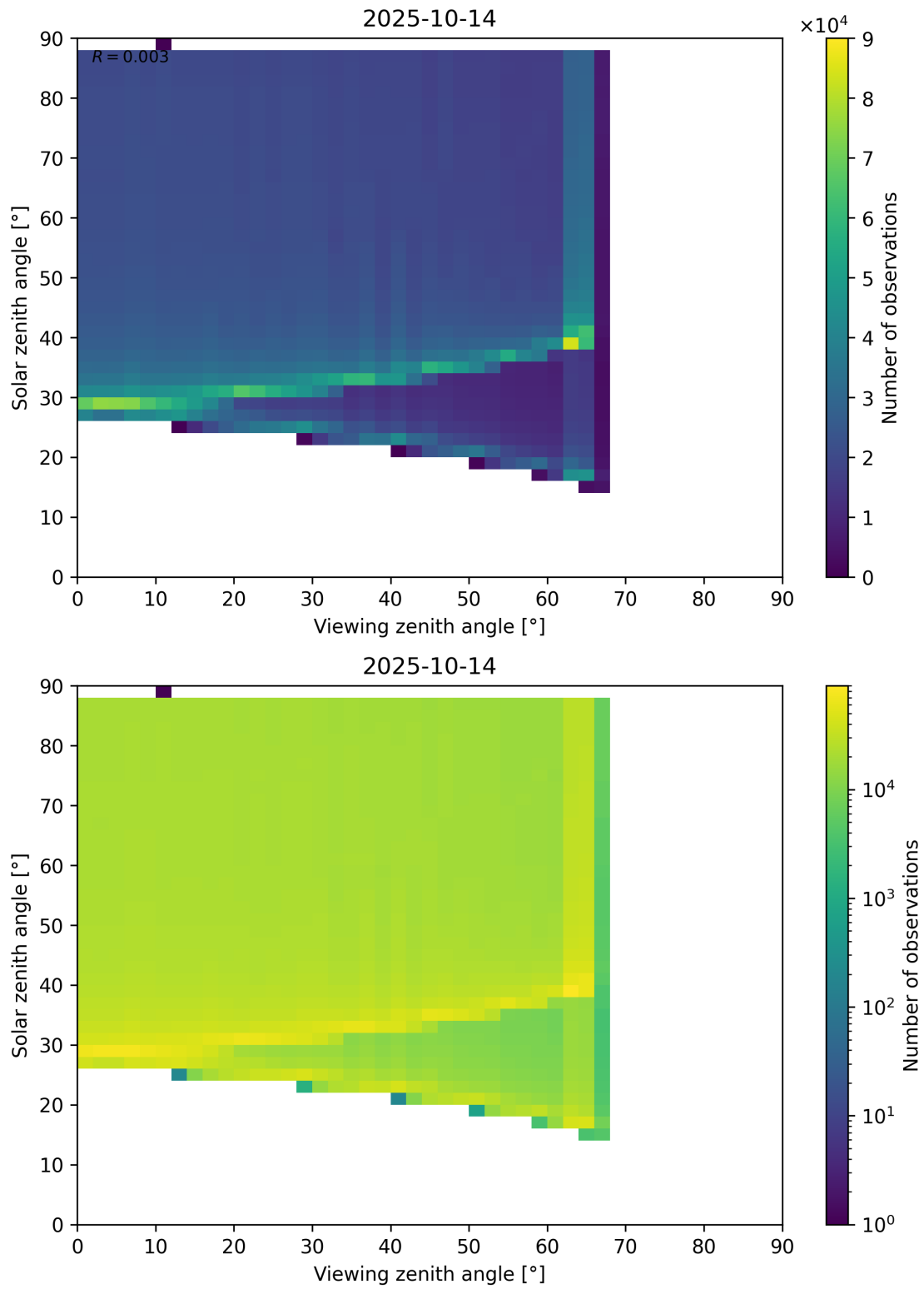
Figure 172: Scatter density plot of “Viewing zenith angle” against “Solar zenith angle” for 2025-10-13 to 2025-10-15.
