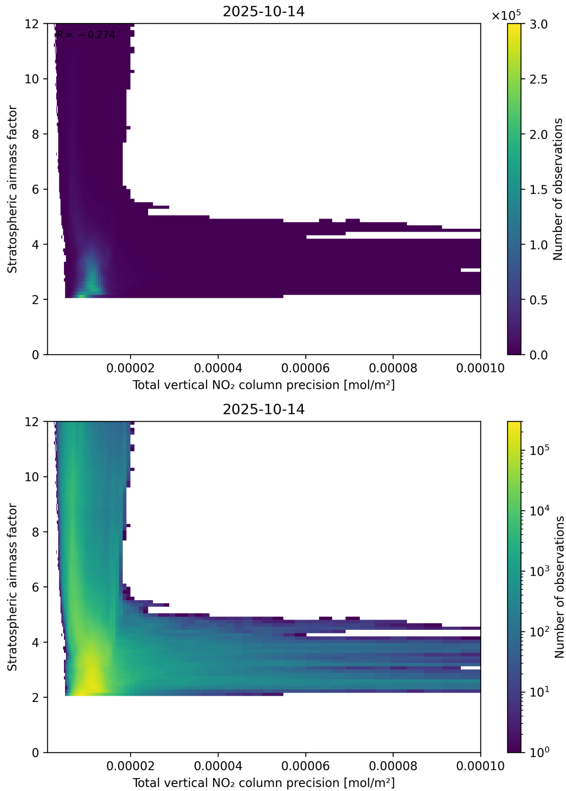
Figure 115: Scatter density plot of “Total vertical NO 2 column precision” against “Stratospheric airmass factor” for 2025-10-13 to 2025-10-15.
