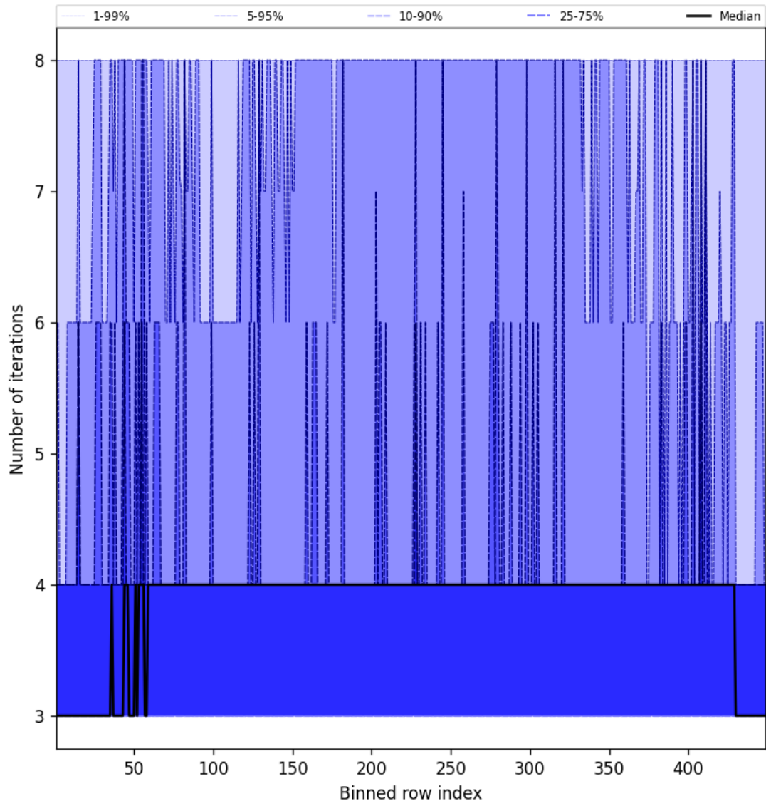
Figure 51: Along track statistics of “Number of iterations” for 2025-10-13 to 2025-10-15
