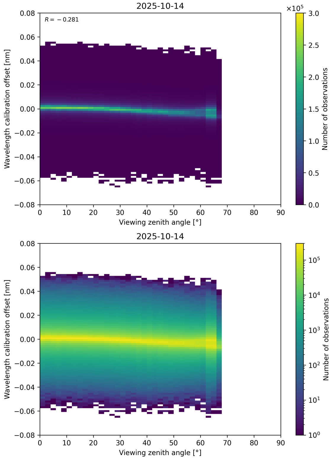
Figure 173: Scatter density plot of “Viewing zenith angle” against “Wavelength calibration offset” for 2025-10-13 to 2025-10-15.
