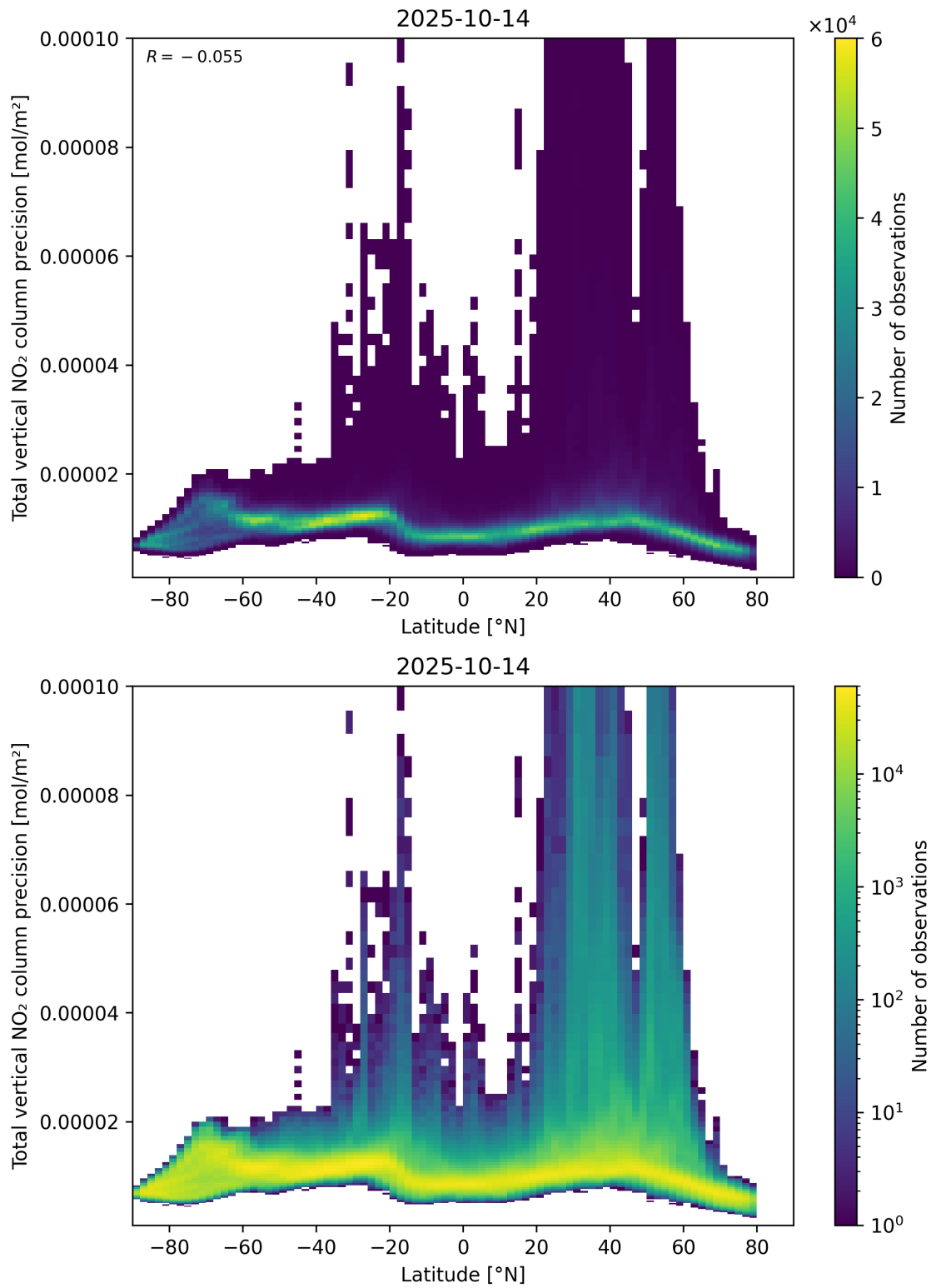
Figure 91: Scatter density plot of “Latitude” against “Total vertical NO 2 column precision” for 2025-10-13 to 2025-10-15.
