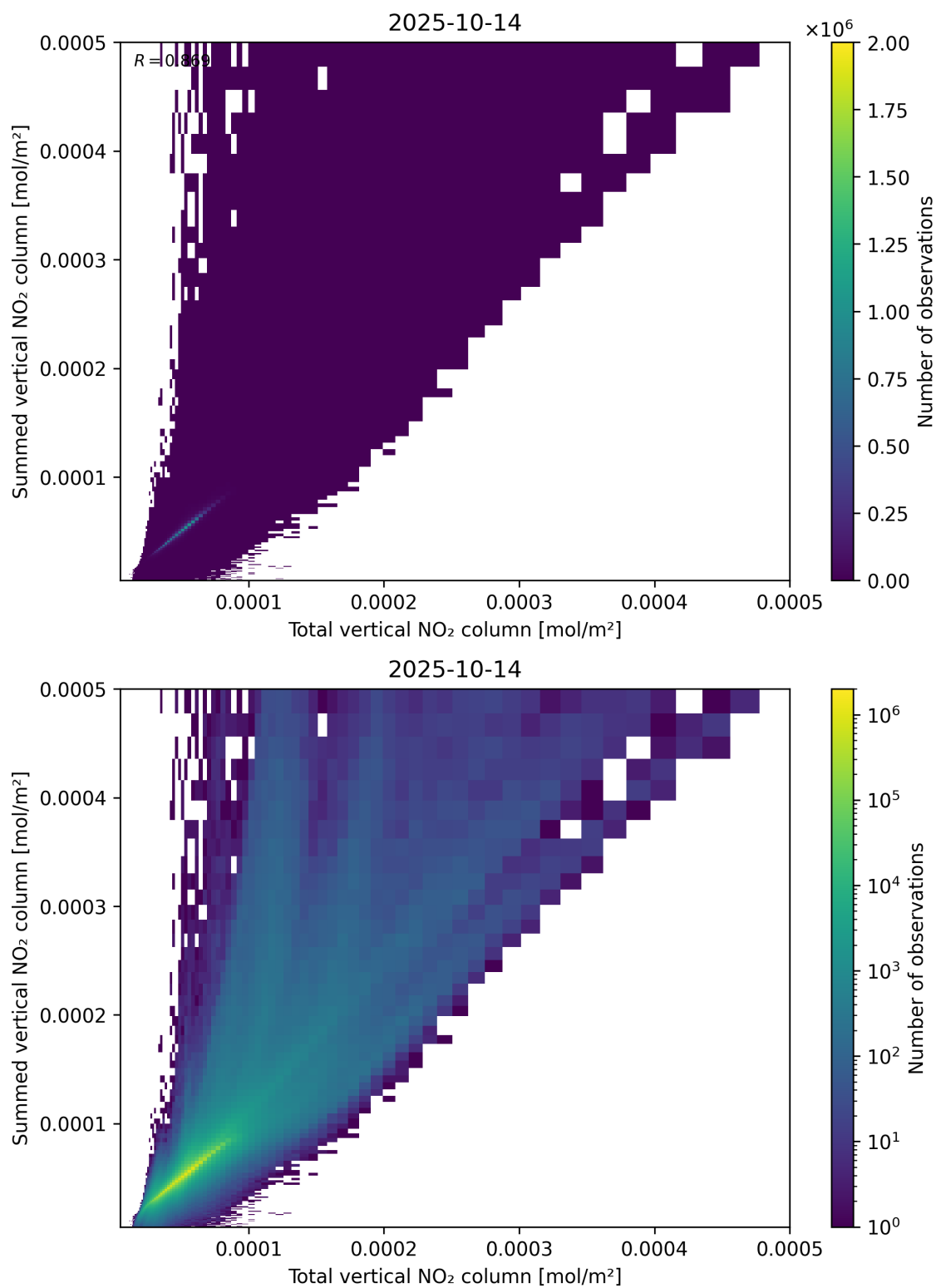
Figure 112: Scatter density plot of “Total vertical NO 2 column” against “Summed vertical NO 2 column” for 2025-10-13 to 2025-10-15.
