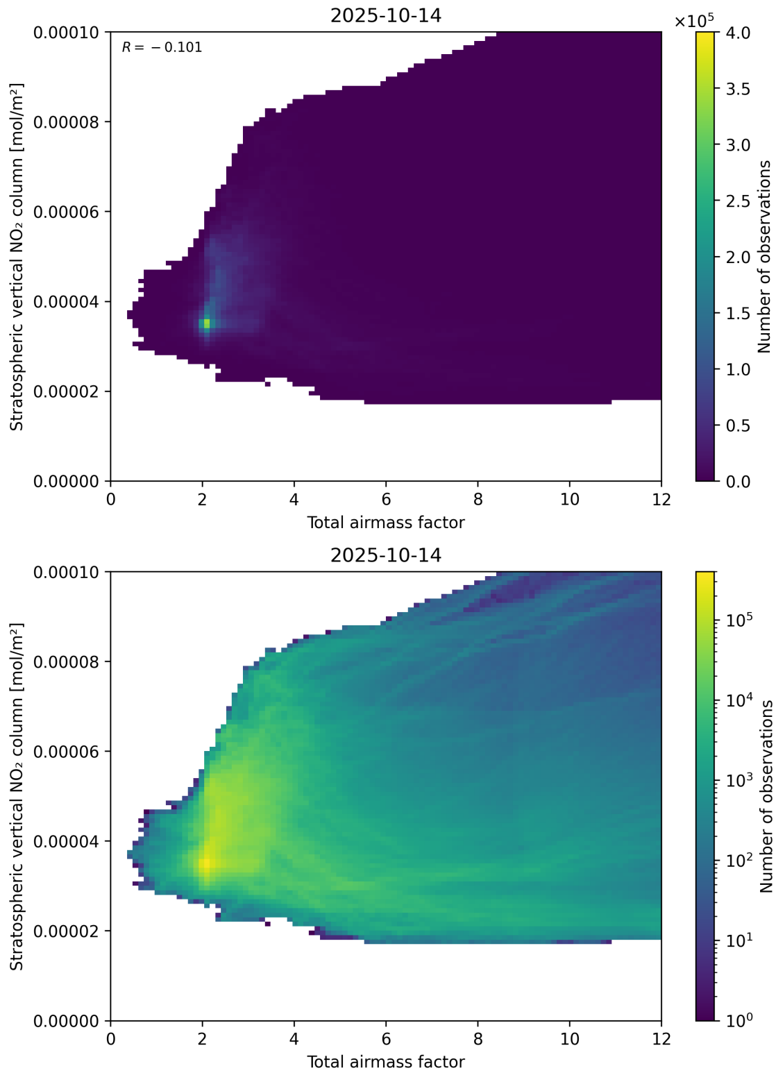
Figure 64: Scatter density plot of “Total airmass factor” against “Stratospheric vertical NO 2 column” for 2025-10-13 to 2025-10-15.
