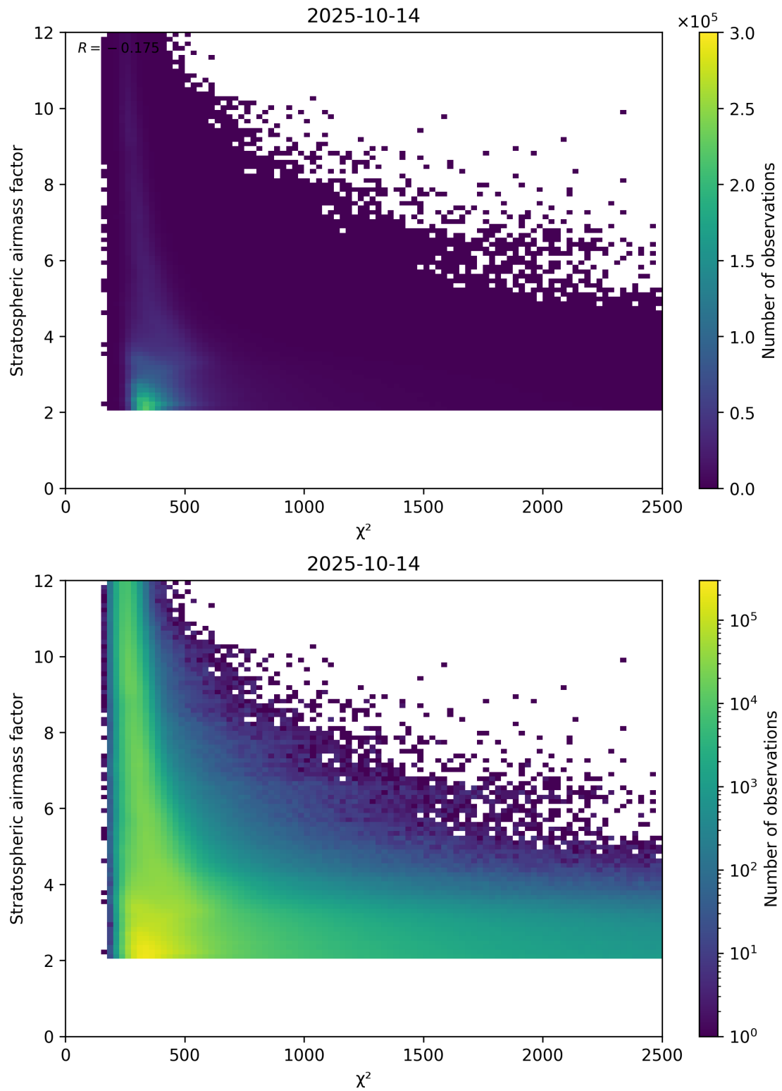
Figure 81: Scatter density plot of “ \chi^2 ” against “Stratospheric airmass factor” for 2025-10-13 to 2025-10-15.
