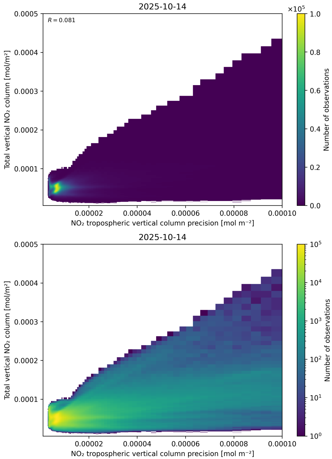
Figure 138: Scatter density plot of “NO 2 tropospheric vertical column precision” against “Total vertical NO 2 column” for 2025-10-13 to 2025-10-15.
