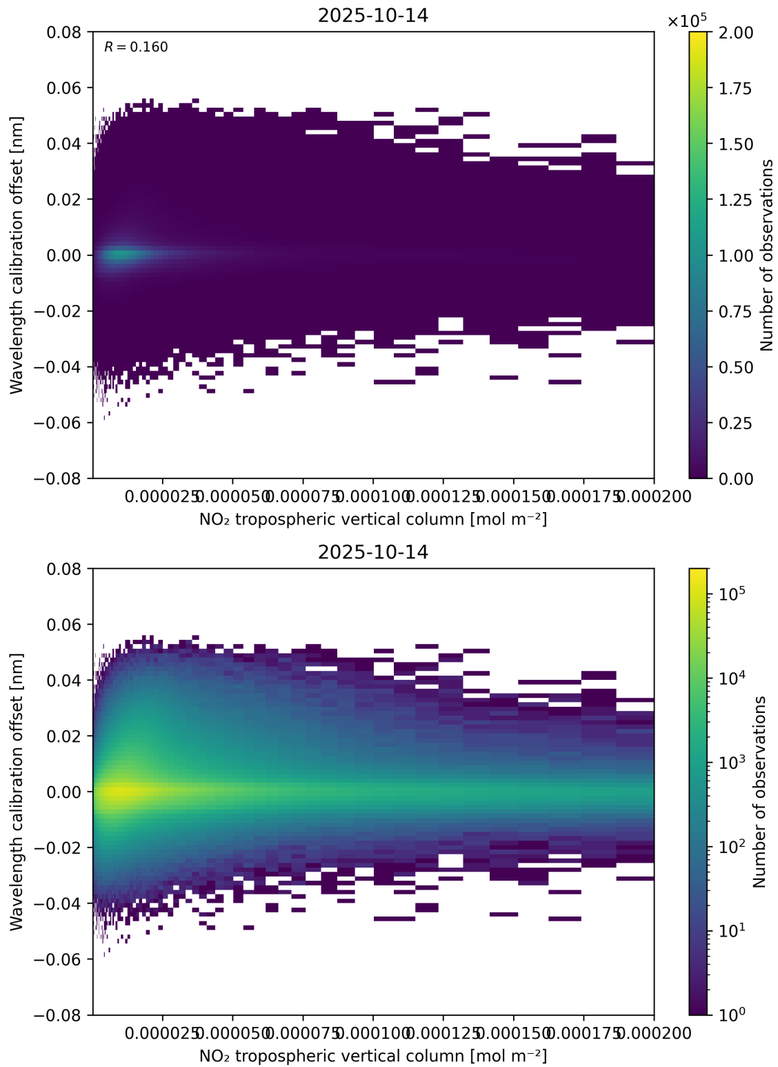
Figure 143: Scatter density plot of “NO 2 tropospheric vertical column” against “Wavelength calibration offset” for 2025-10-13 to 2025-10-15.
