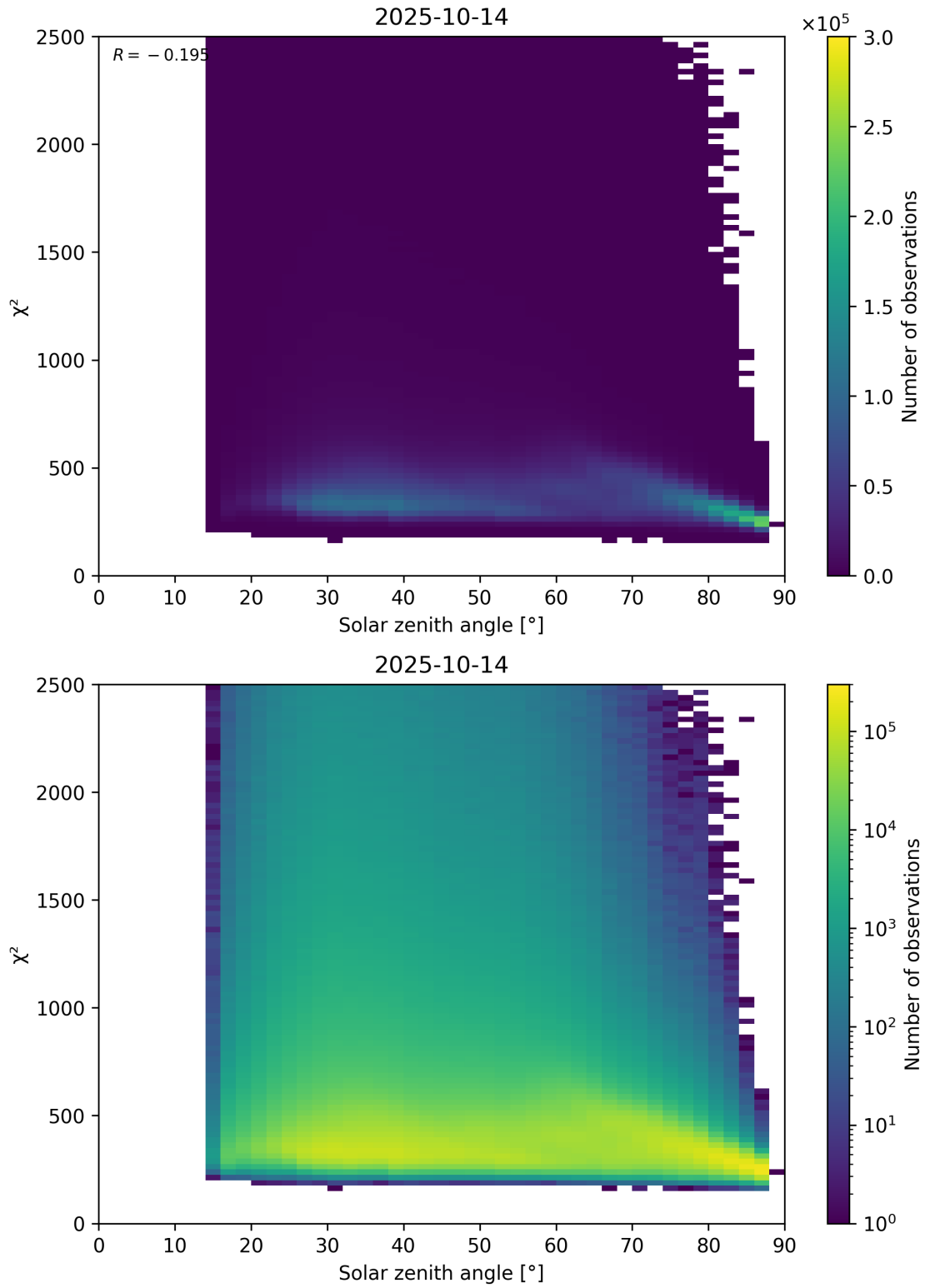
Figure 148: Scatter density plot of “Solar zenith angle” against “ \chi^2 ” for 2025-10-13 to 2025-10-15.
