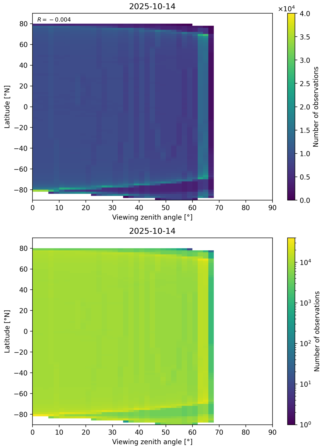
Figure 163: Scatter density plot of “Viewing zenith angle” against “Latitude” for 2025-10-13 to 2025-10-15.
