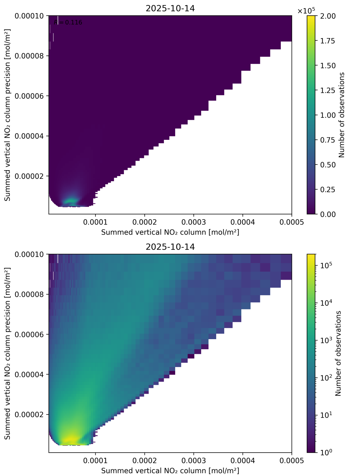
Figure 105: Scatter density plot of “Summed vertical NO 2 column” against “Summed vertical NO 2 column precision” for 2025-10-13 to 2025-10-15.
