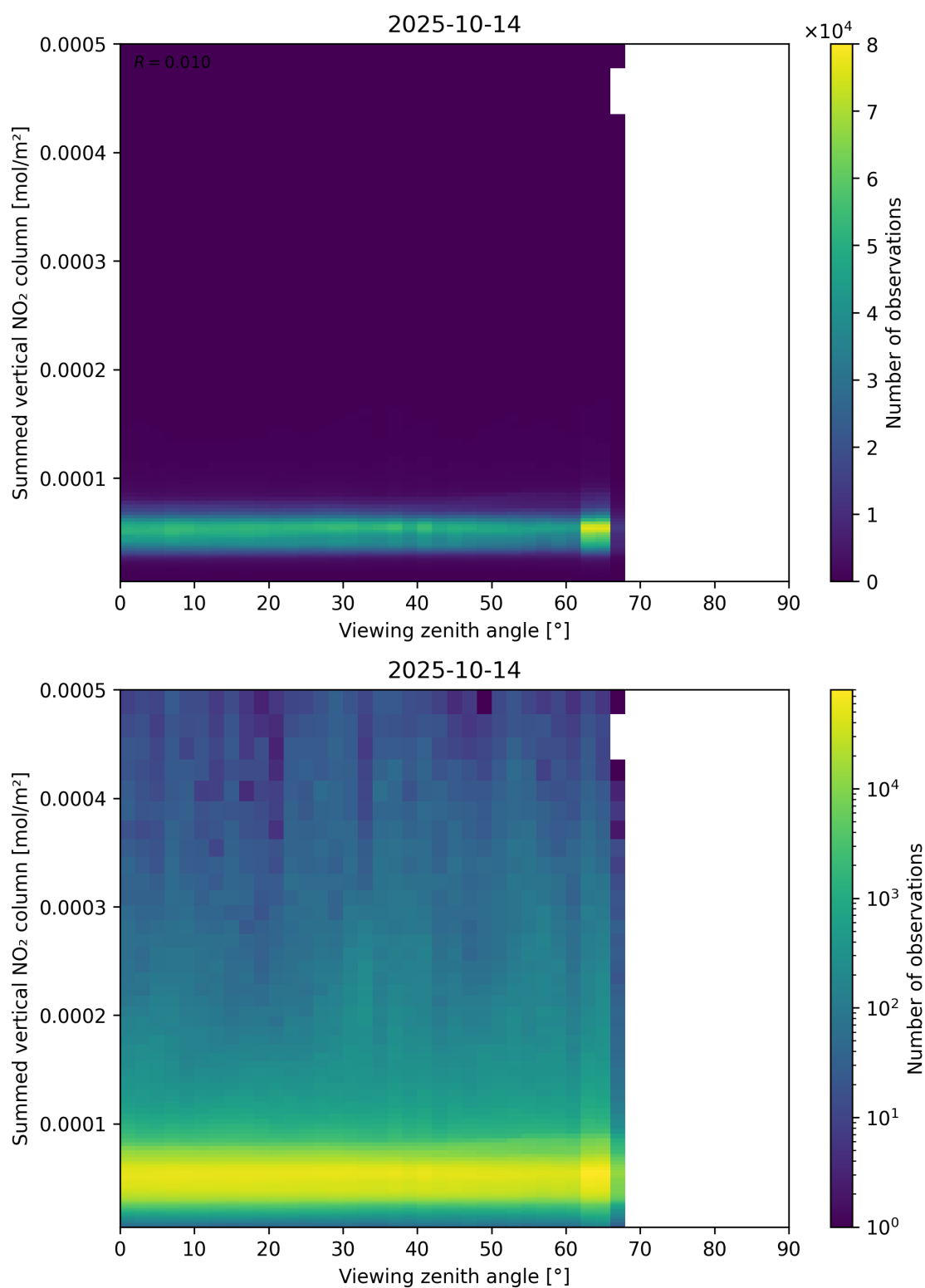
Figure 165: Scatter density plot of “Viewing zenith angle” against “Summed vertical NO 2 column” for 2025-10-13 to 2025-10-15.
