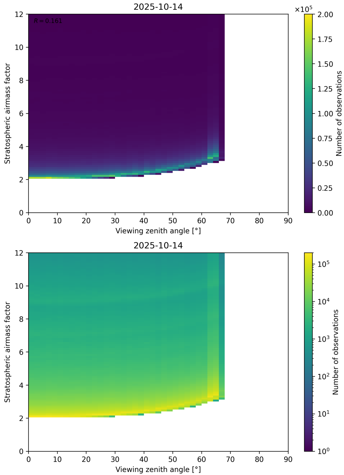
Figure 159: Scatter density plot of “Viewing zenith angle” against “Stratospheric airmass factor” for 2025-10-13 to 2025-10-15.
