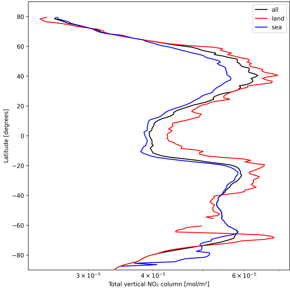
Figure 21: Zonal average of “Total vertical NO 2 column” for 2025-10-13 to 2025-10-15.
