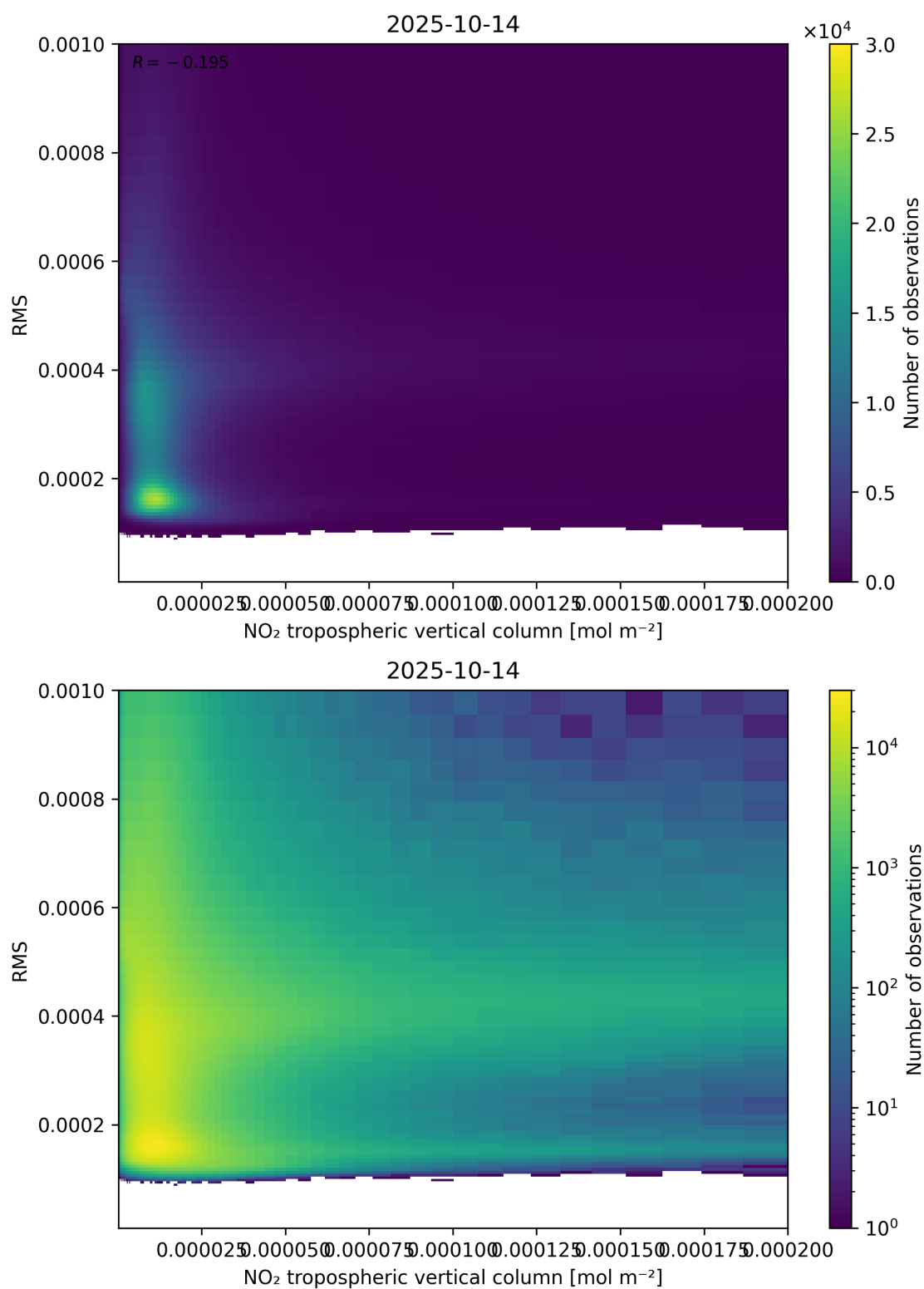
Figure 142: Scatter density plot of “NO 2 tropospheric vertical column” against “RMS” for 2025-10-13 to 2025-10-15.
