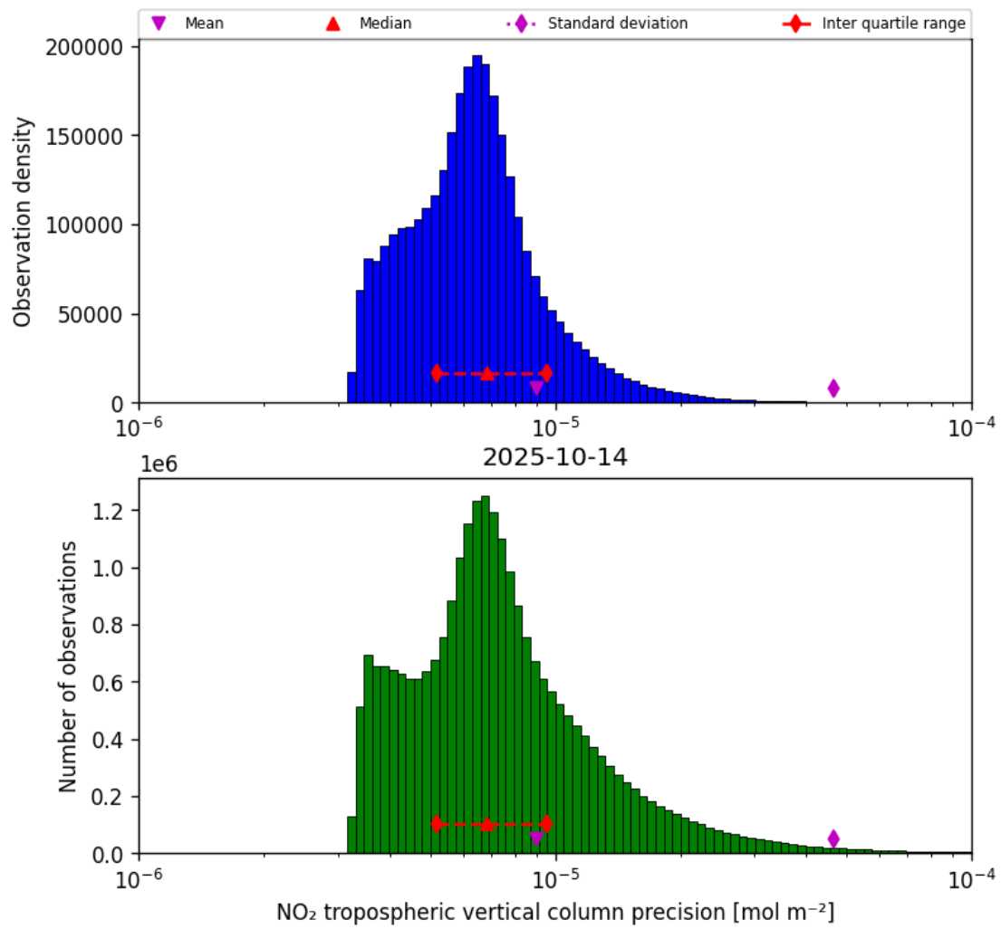
Figure 30: Histogram of "NO 2 tropospheric vertical column precision" for 2025-10-13 to 2025-10-15
