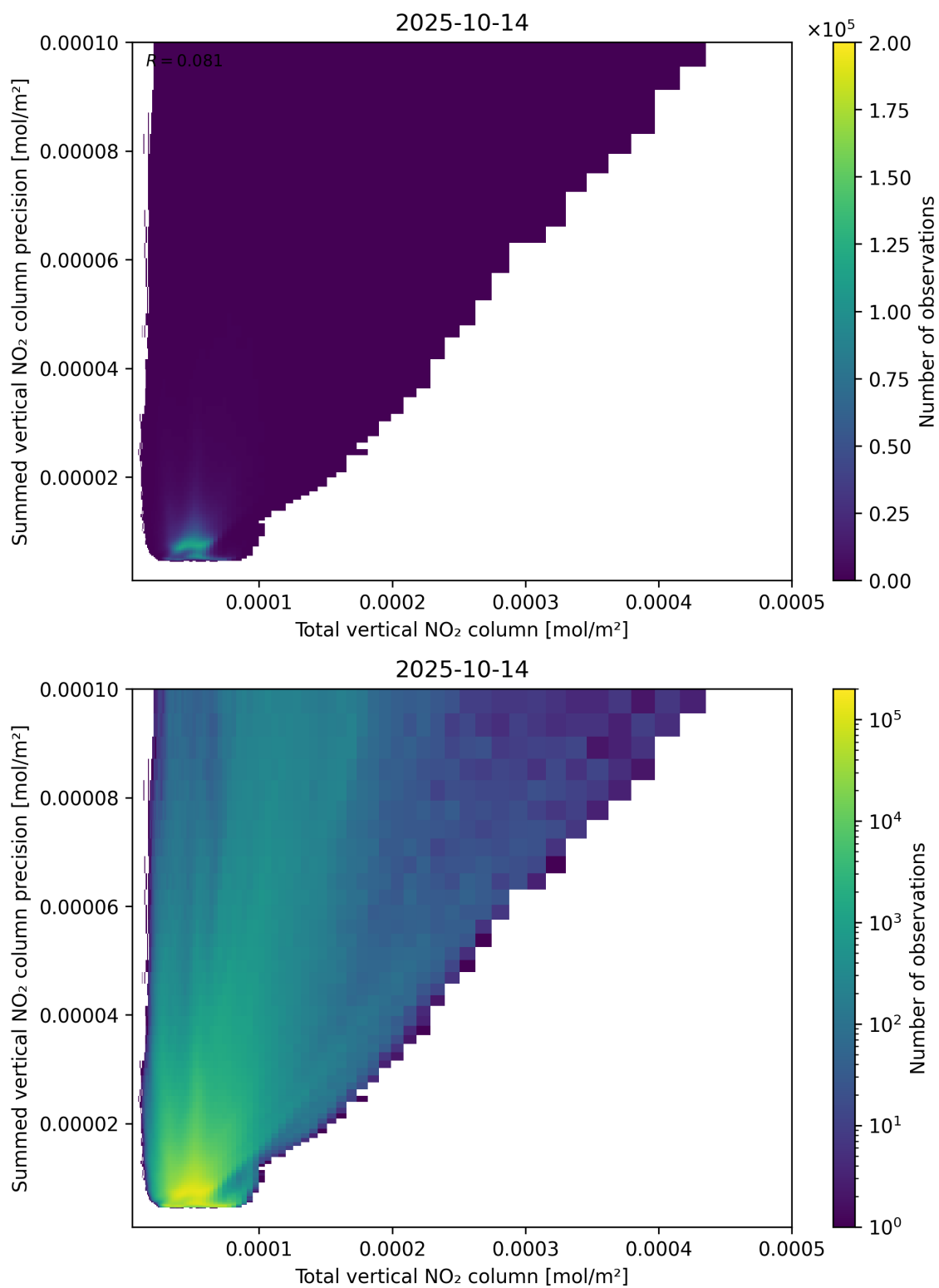
Figure 113: Scatter density plot of “Total vertical NO 2 column” against “Summed vertical NO 2 column precision” for 2025-10-13 to 2025-10-15.
