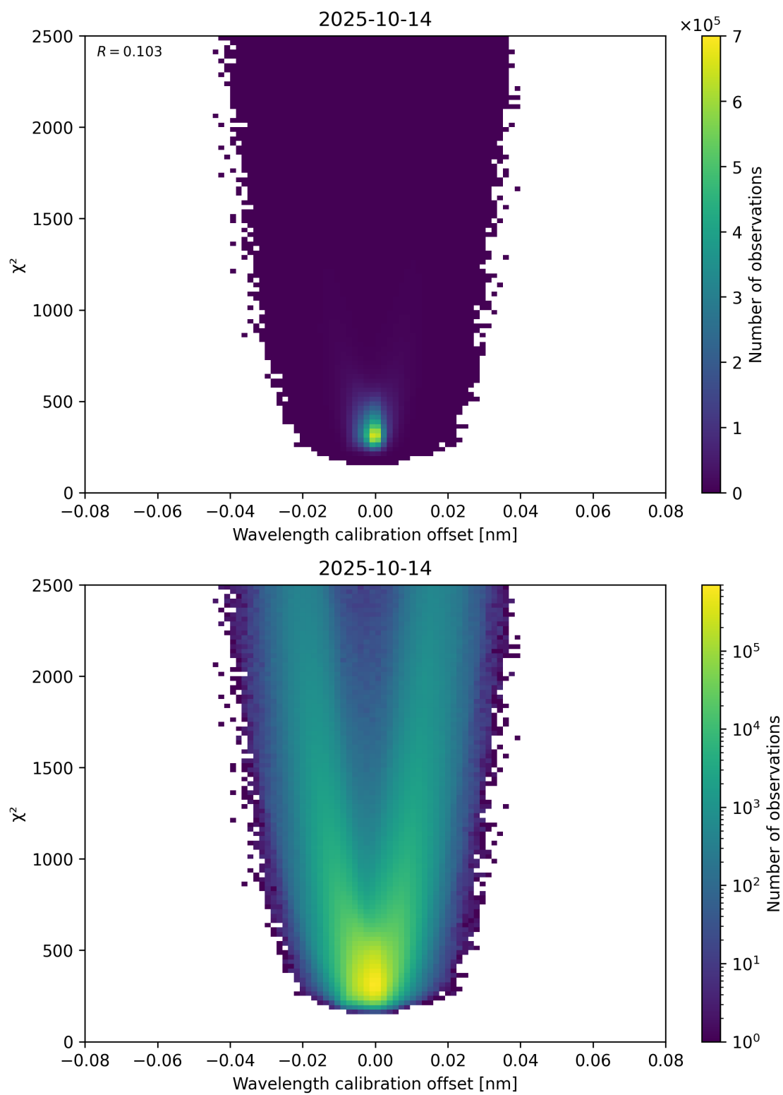
Figure 175: Scatter density plot of “Wavelength calibration offset” against “ \chi^2 ” for 2025-10-13 to 2025-10-15.
