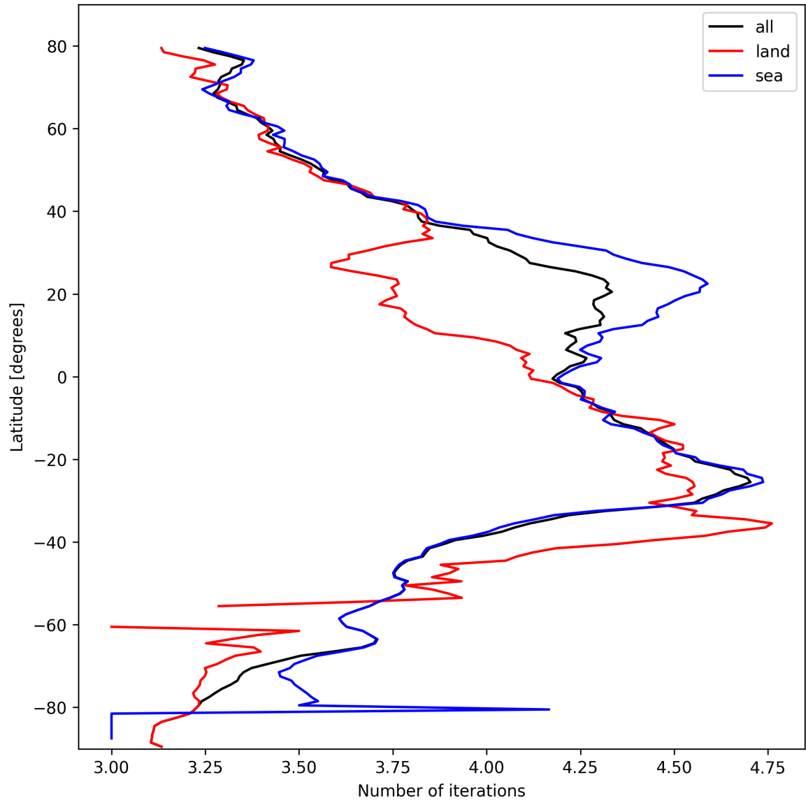
Figure 17: Zonal average of “Number of iterations” for 2025-10-13 to 2025-10-15.
