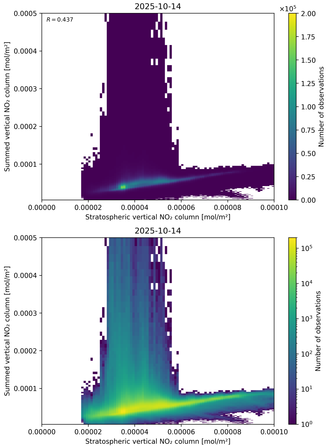
Figure 98: Scatter density plot of “Stratospheric vertical NO 2 column” against “Summed vertical NO 2 column” for 2025-10-13 to 2025-10-15.
