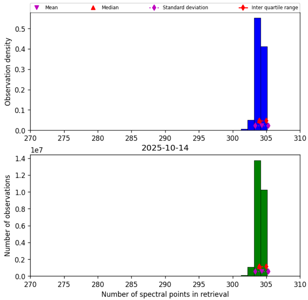
Figure 33: Histogram of “Number of spectral points in retrieval” for 2025-10-13 to 2025-10-15
