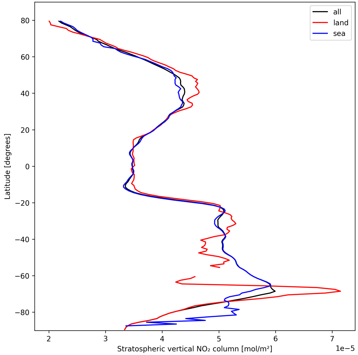
Figure 19: Zonal average of “Stratospheric vertical NO 2 column” for 2025-10-13 to 2025-10-15.
