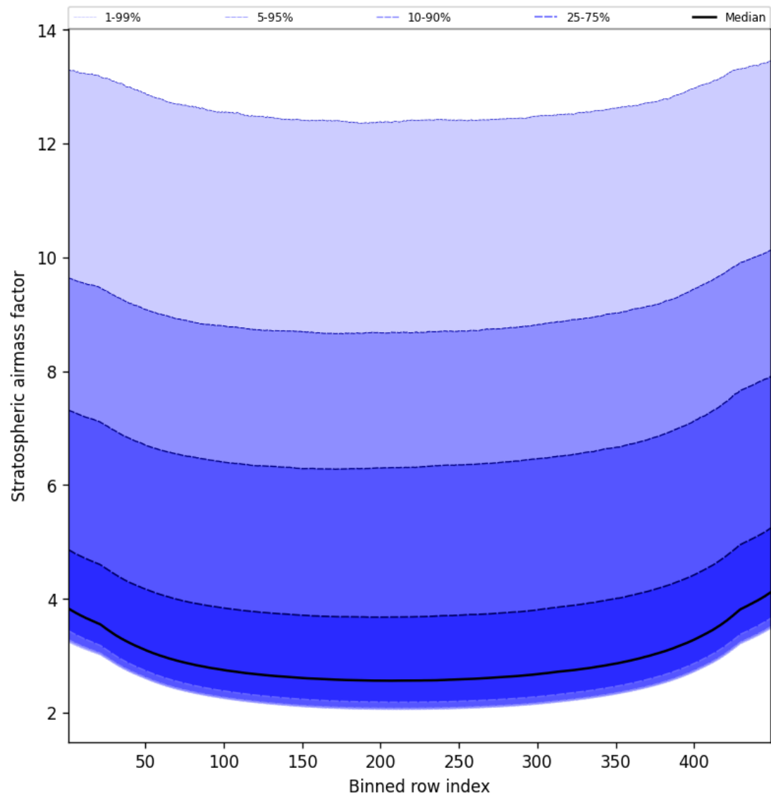
Figure 61: Along track statistics of “Stratospheric air mass factor” for 2025-10-13 to 2025-10-15
