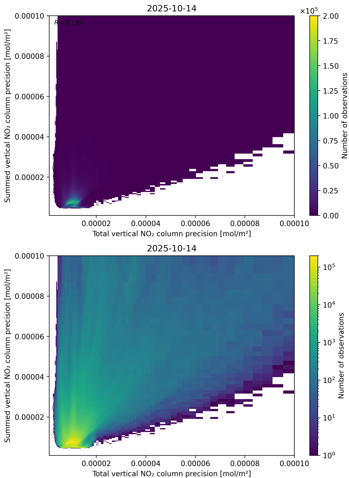
Figure 118: Scatter density plot of “Total vertical NO 2 column precision” against “Summed vertical NO 2 column precision” for 2025-10-13 to 2025-10-15.
