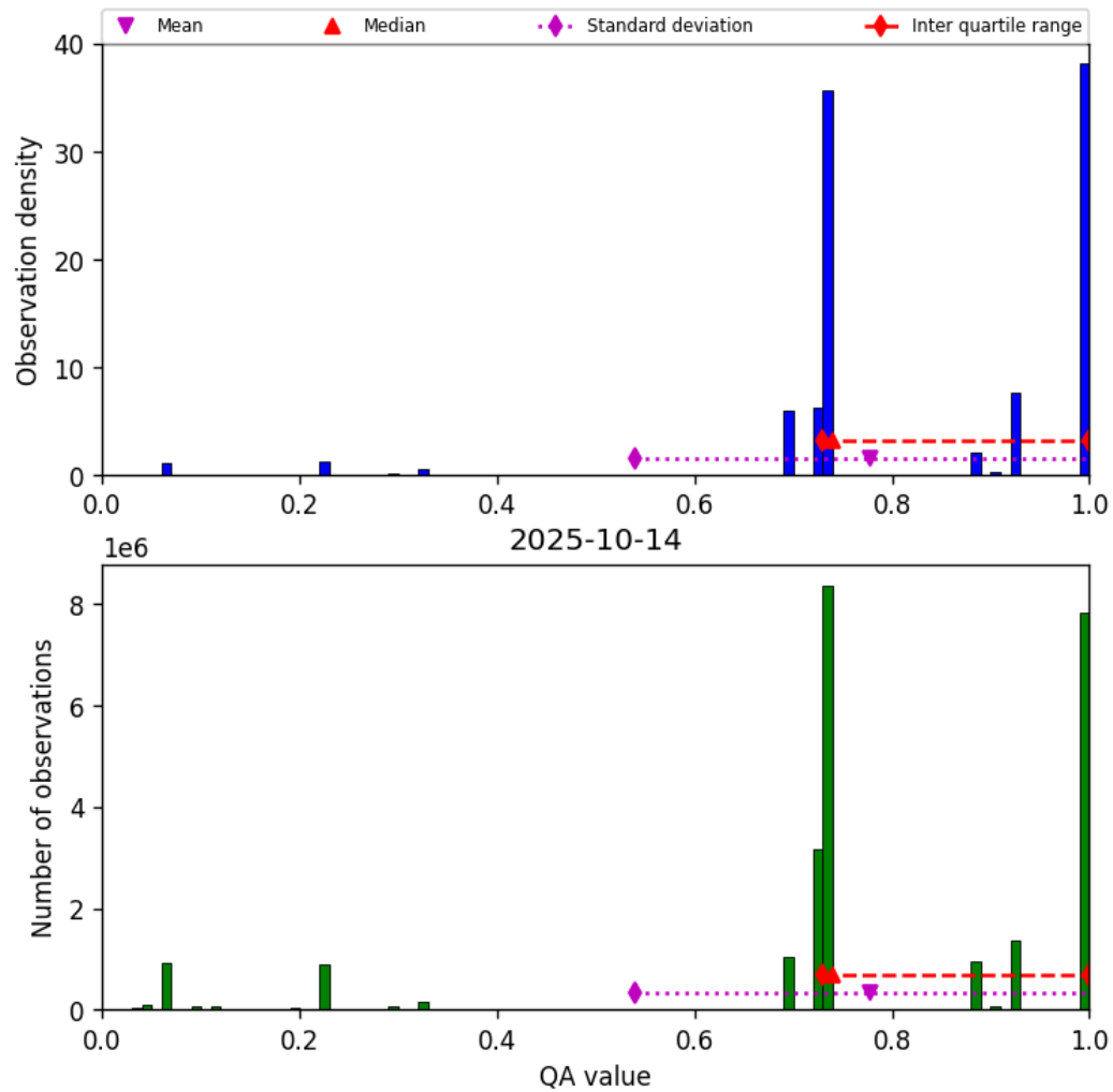
Figure 28: Histogram of “QA value” for 2025-10-13 to 2025-10-15
