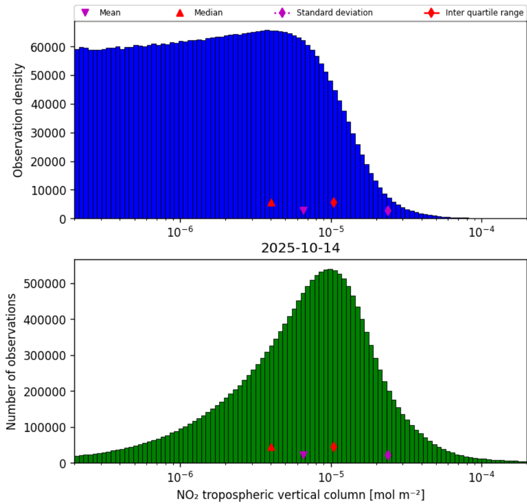
Figure 29: Histogram of “NO 2 tropospheric vertical column” for 2025-10-13 to 2025-10-15
