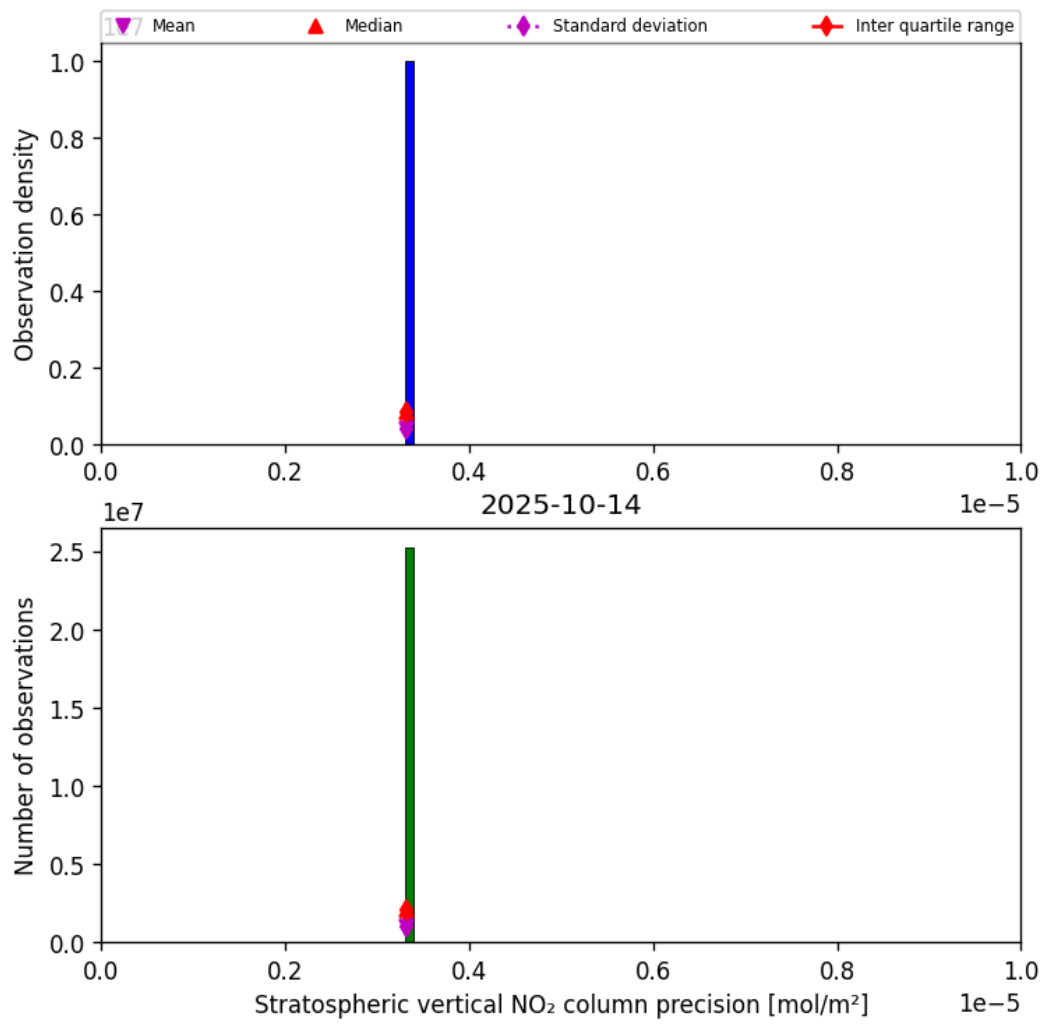
Figure 37: Histogram of “Stratospheric vertical NO 2 column precision” for 2025-10-13 to 2025-10-15
