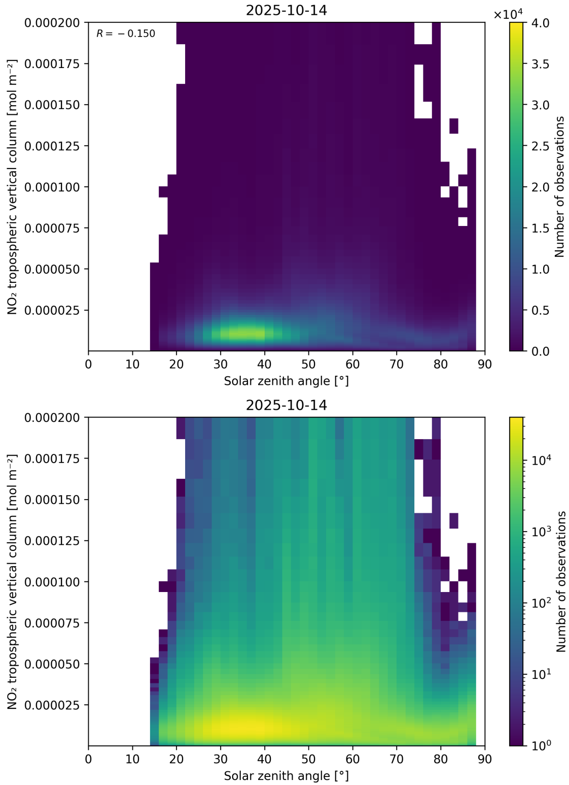
Figure 155: Scatter density plot of “Solar zenith angle” against “NO 2 tropospheric vertical column” for 2025-10-13 to 2025-10-15.
