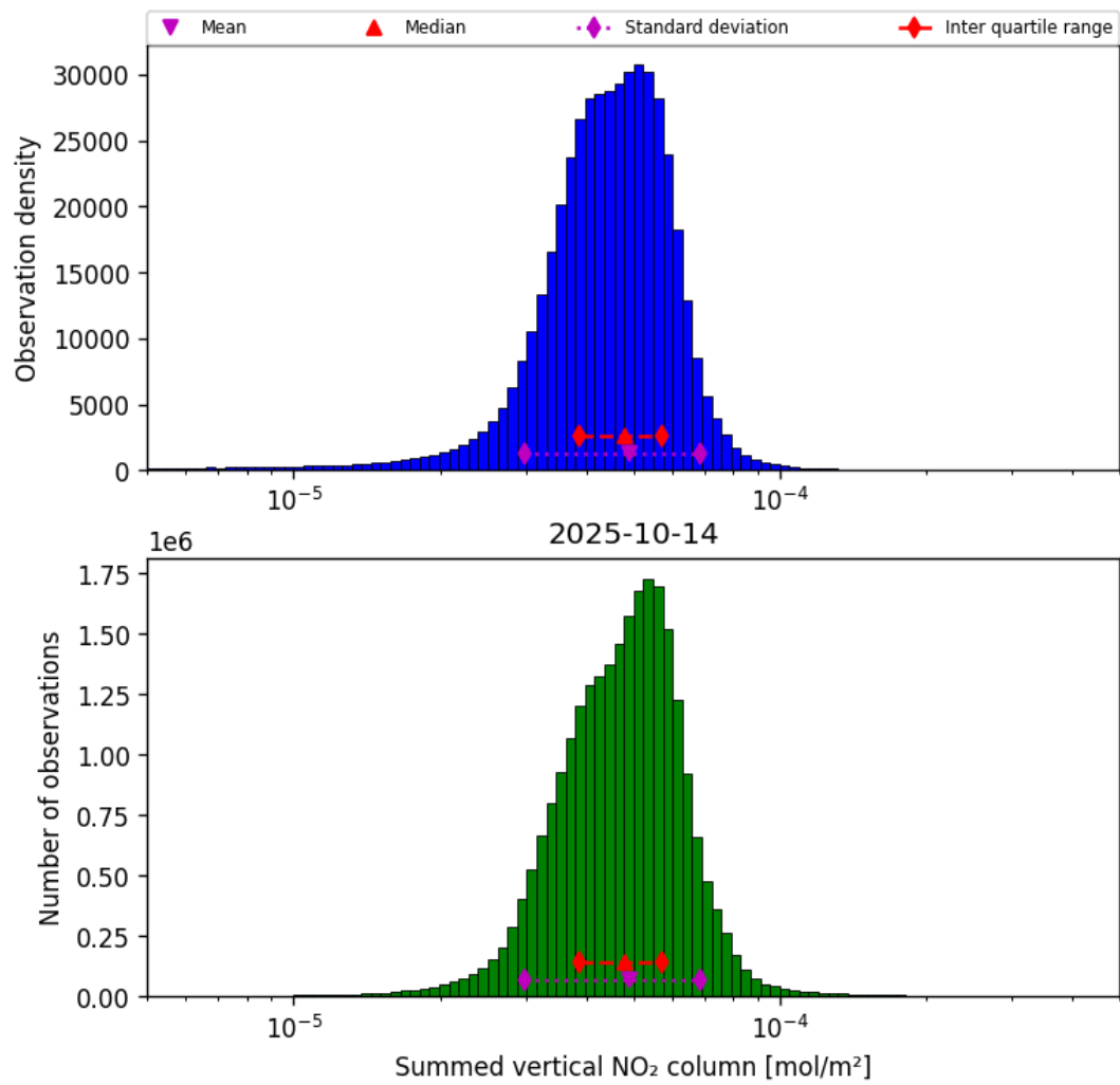
Figure 40: Histogram of “Summed vertical NO 2 column” for 2025-10-13 to 2025-10-15
