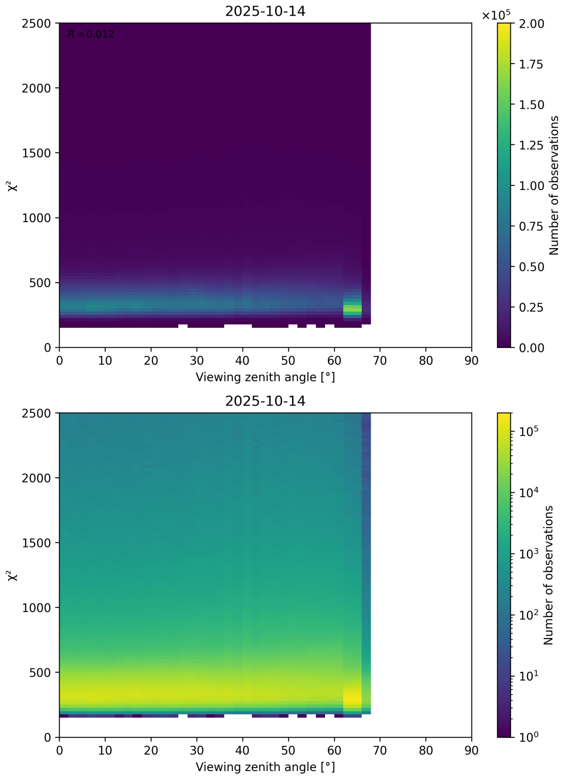
Figure 162: Scatter density plot of “Viewing zenith angle” against “ \chi^2 ” for 2025-10-13 to 2025-10-15.
