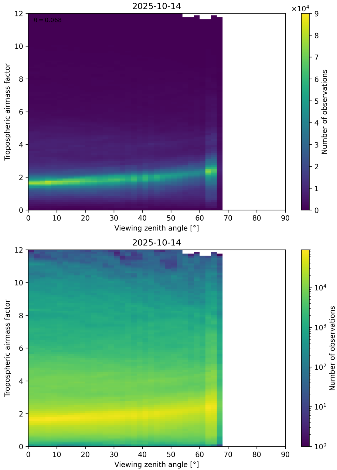
Figure 161: Scatter density plot of “Viewing zenith angle” against “Tropospheric airmass factor” for 2025-10-13 to 2025-10-15.
