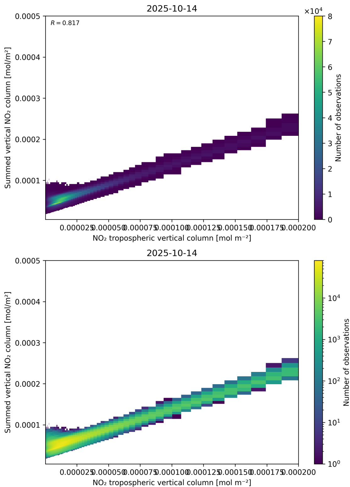
Figure 126: Scatter density plot of “NO 2 tropospheric vertical column” against “Summed vertical NO 2 column” for 2025-10-13 to 2025-10-15.
