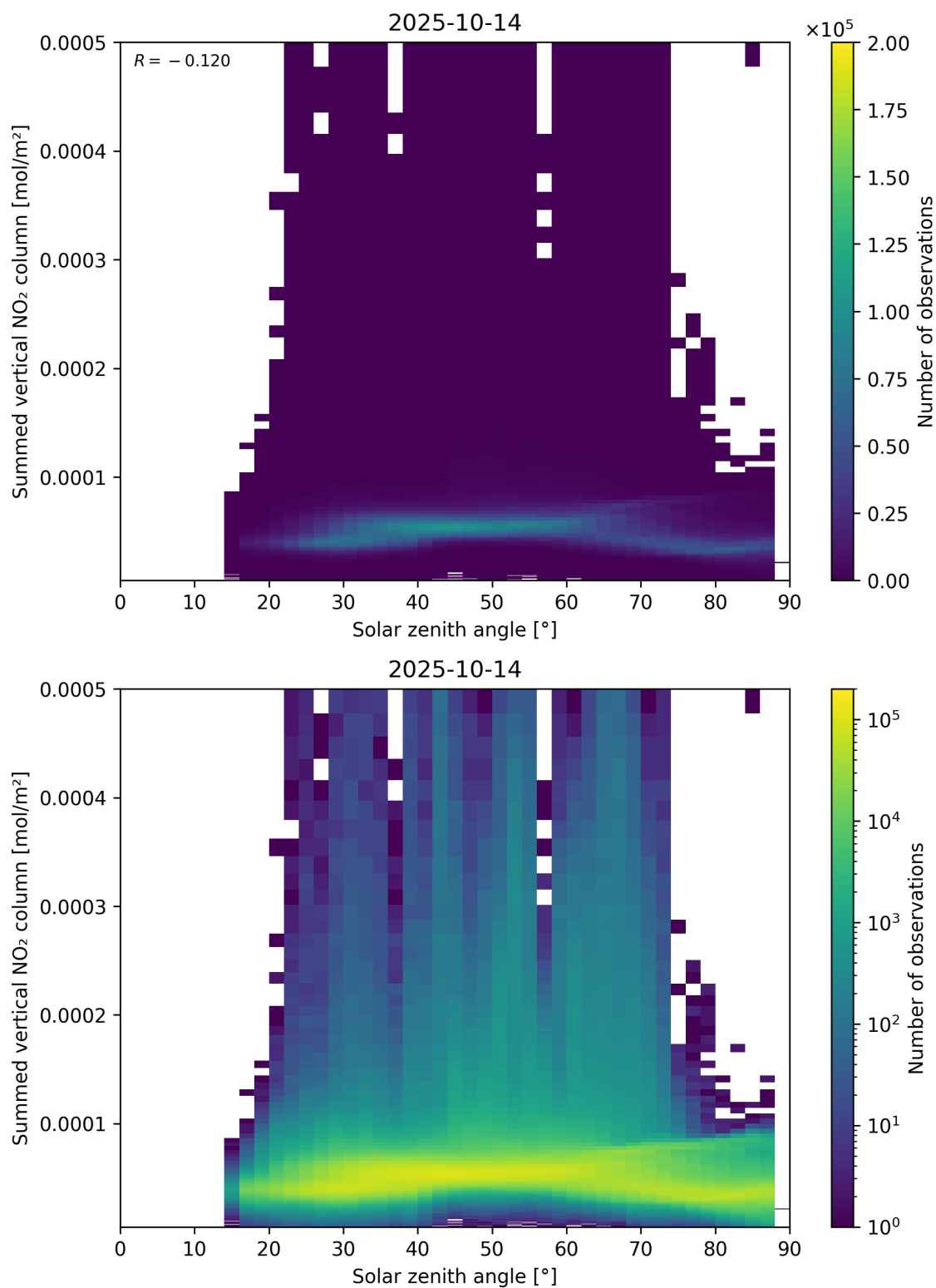
Figure 151: Scatter density plot of “Solar zenith angle” against “Summed vertical NO 2 column” for 2025-10-13 to 2025-10-15.
