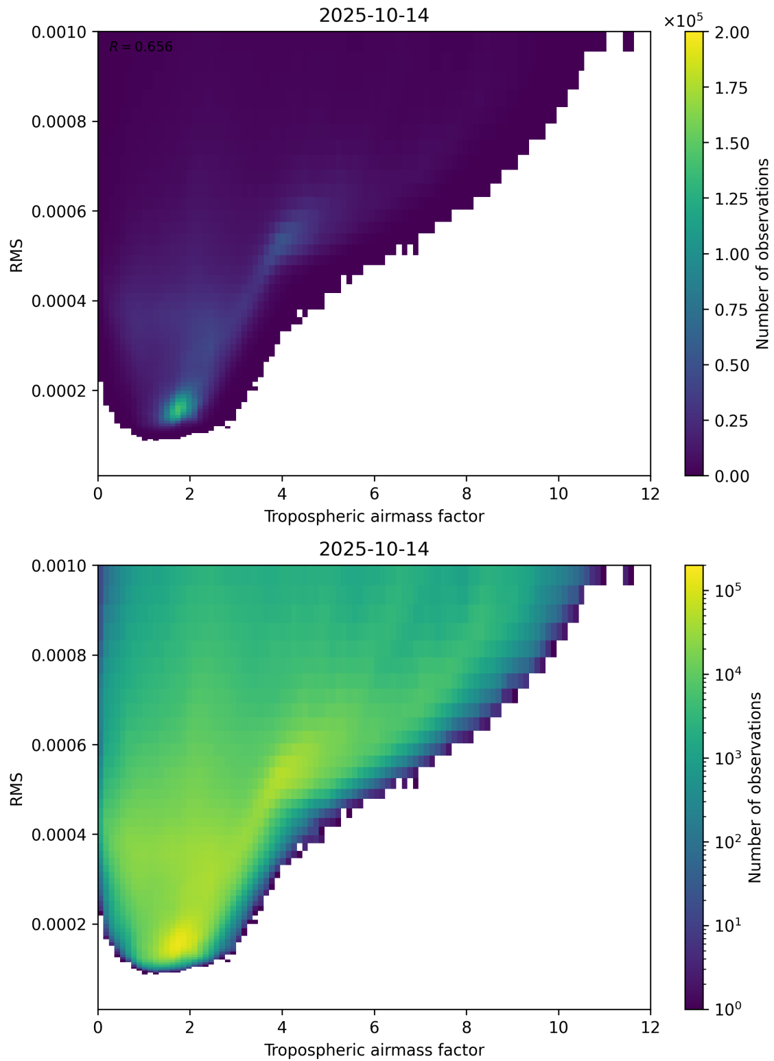
Figure 79: Scatter density plot of “Tropospheric airmass factor” against “RMS” for 2025-10-13 to 2025-10-15.
