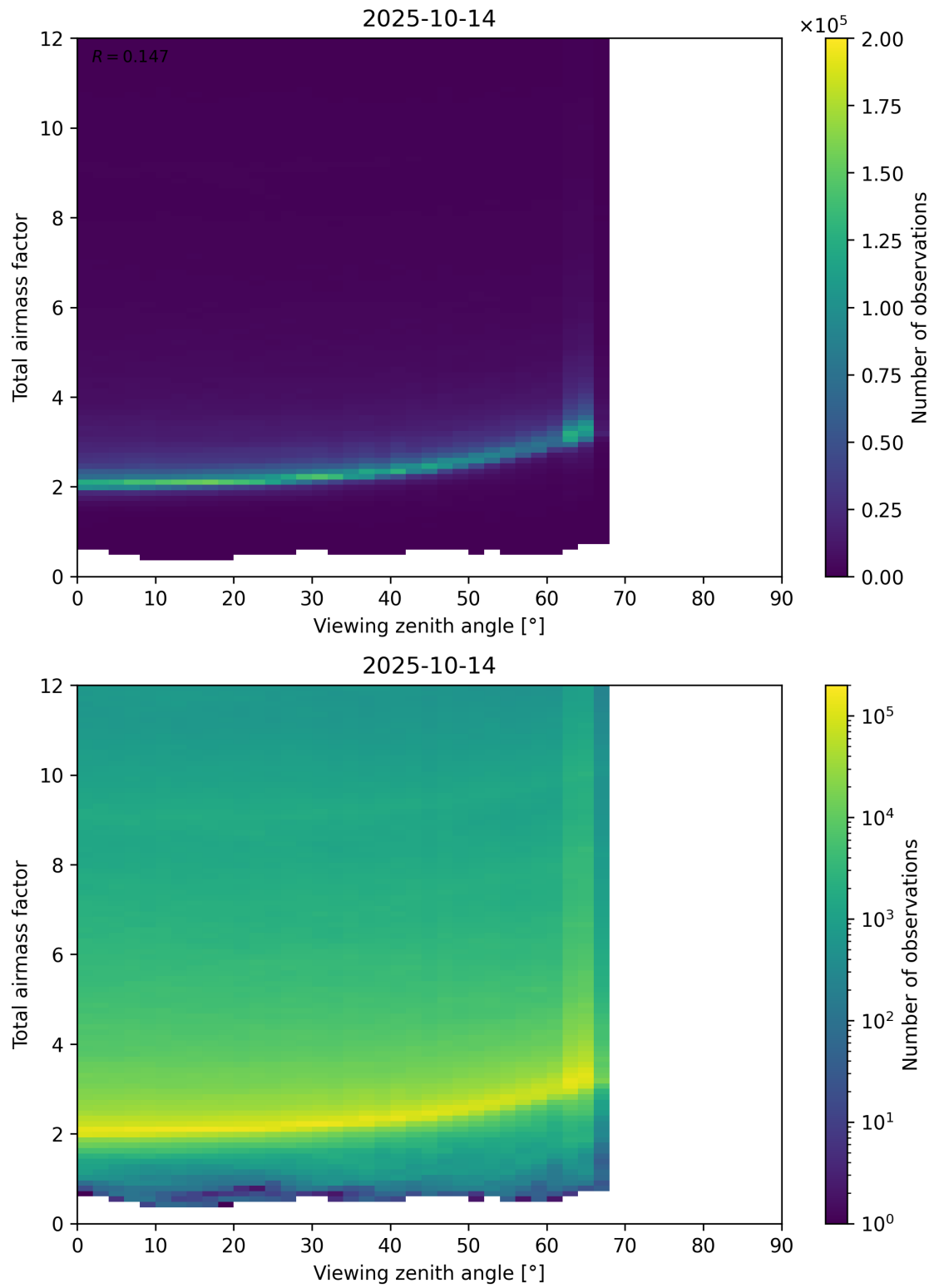
Figure 160: Scatter density plot of “Viewing zenith angle” against “Total airmass factor” for 2025-10-13 to 2025-10-15.
