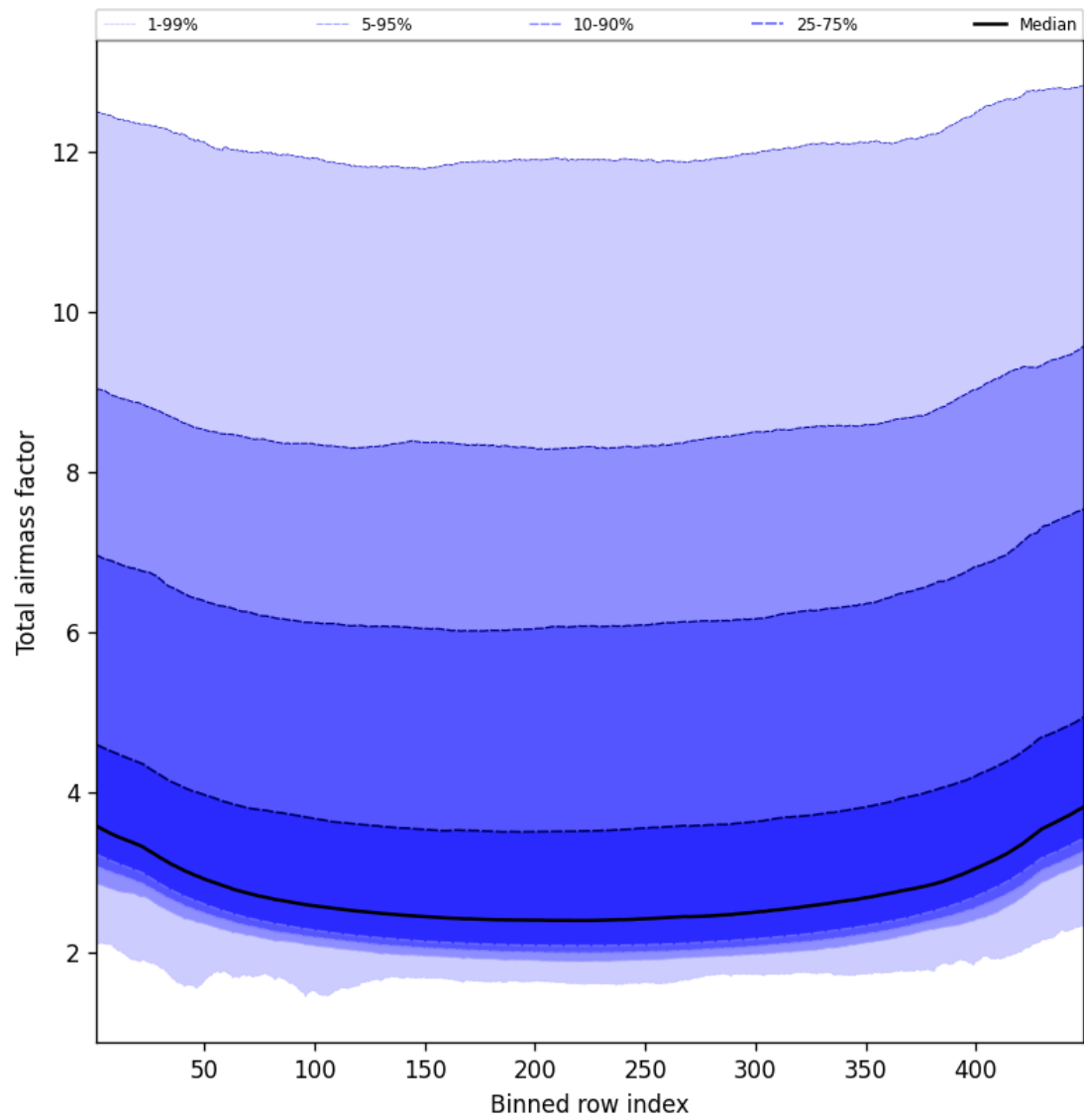
Figure 49: Along track statistics of “Total airmass factor” for 2025-10-13 to 2025-10-15
