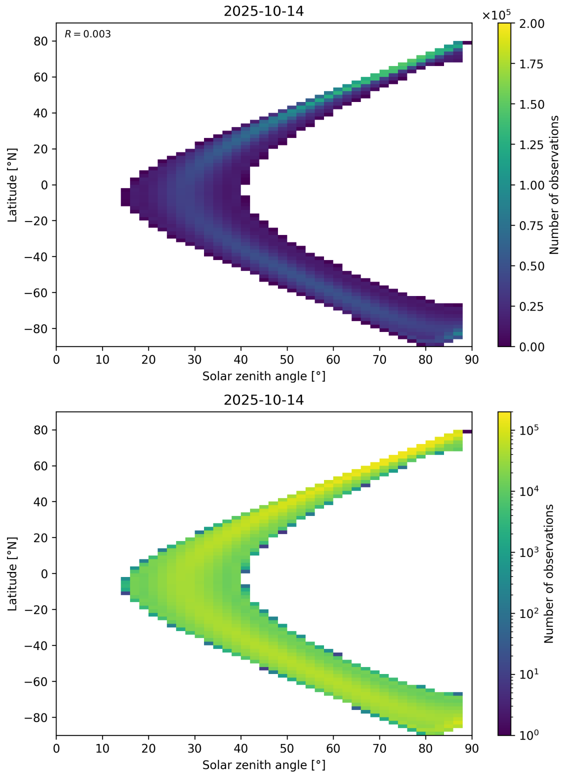
Figure 149: Scatter density plot of “Solar zenith angle” against “Latitude” for 2025-10-13 to 2025-10-15.
