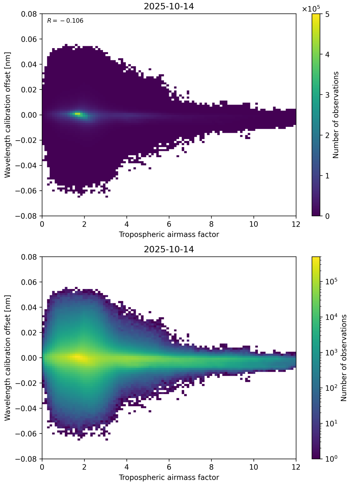
Figure 80: Scatter density plot of “Tropospheric airmass factor” against “Wavelength calibration offset” for 2025-10-13 to 2025-10-15.
