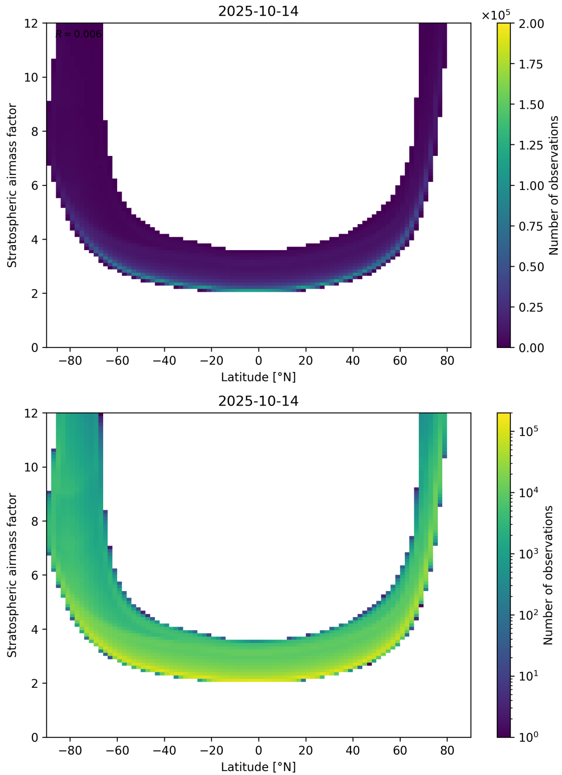
Figure 83: Scatter density plot of “Latitude” against “Stratospheric airmass factor” for 2025-10-13 to 2025-10-15.
