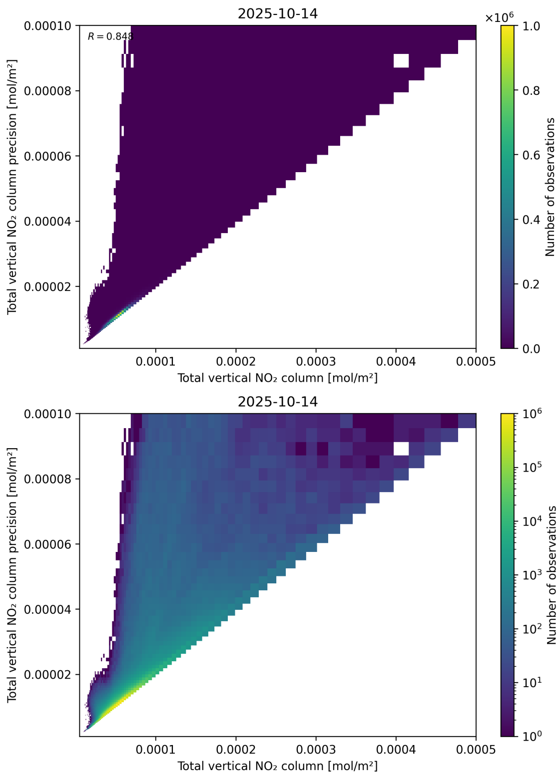
Figure 114: Scatter density plot of “Total vertical NO 2 column” against “Total vertical NO 2 column precision” for 2025-10-13 to 2025-10-15.
