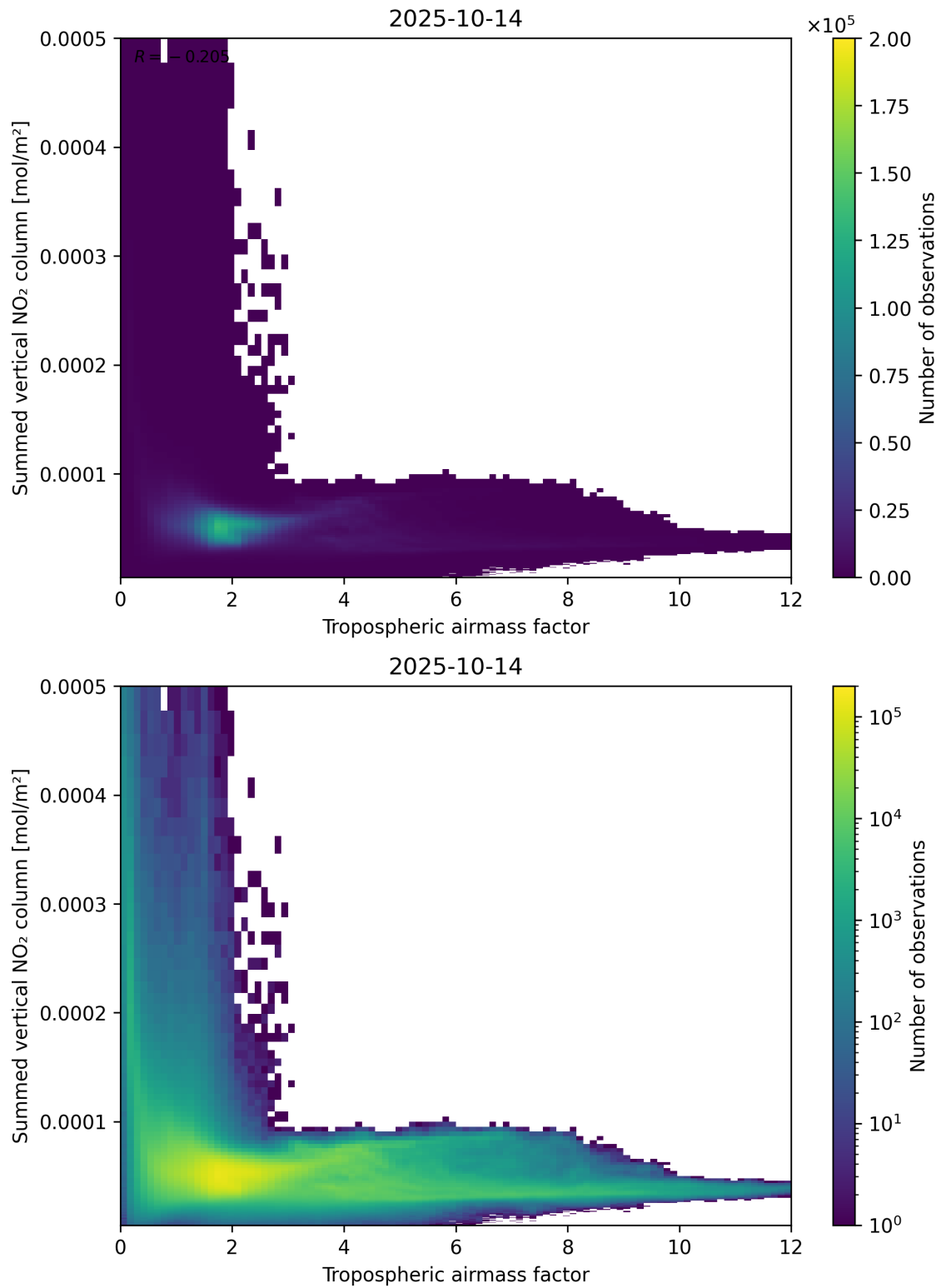
Figure 75: Scatter density plot of “Tropospheric air mass factor” against “Summed vertical NO 2 column” for 2025-10-13 to 2025-10-15.
