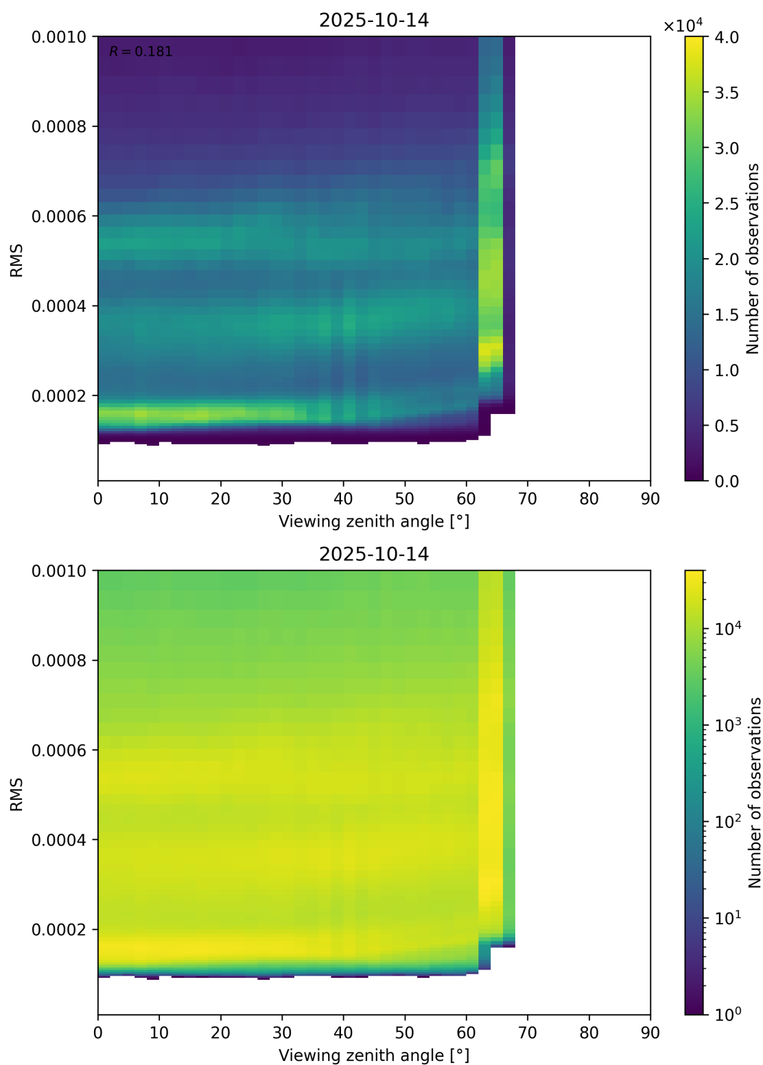
Figure 171: Scatter density plot of “Viewing zenith angle” against “RMS” for 2025-10-13 to 2025-10-15.
