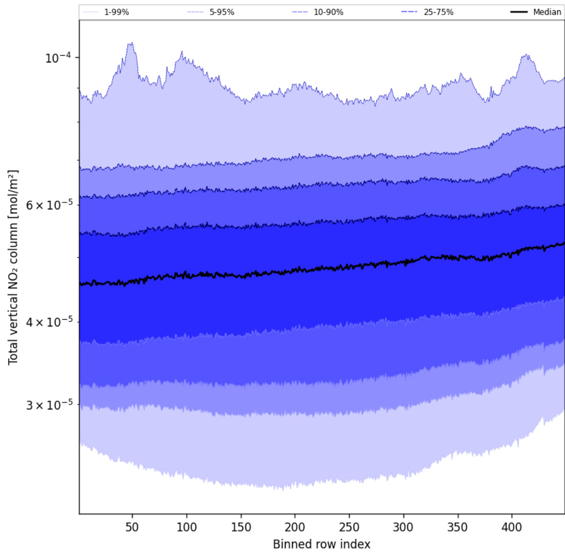
Figure 55: Along track statistics of “Total vertical NO 2 column” for 2025-10-13 to 2025-10-15
