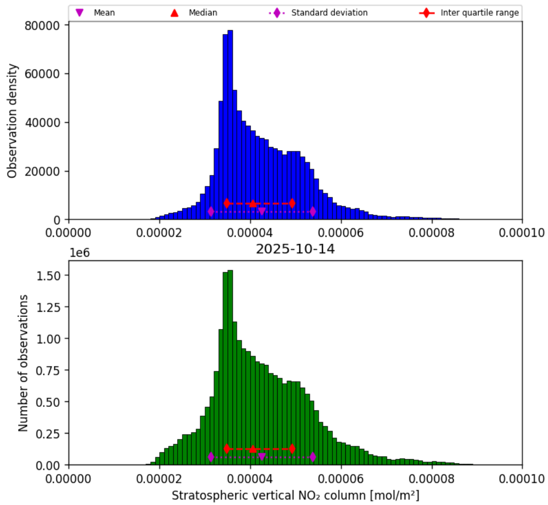
Figure 36: Histogram of “Stratospheric vertical NO 2 column” for 2025-10-13 to 2025-10-15
