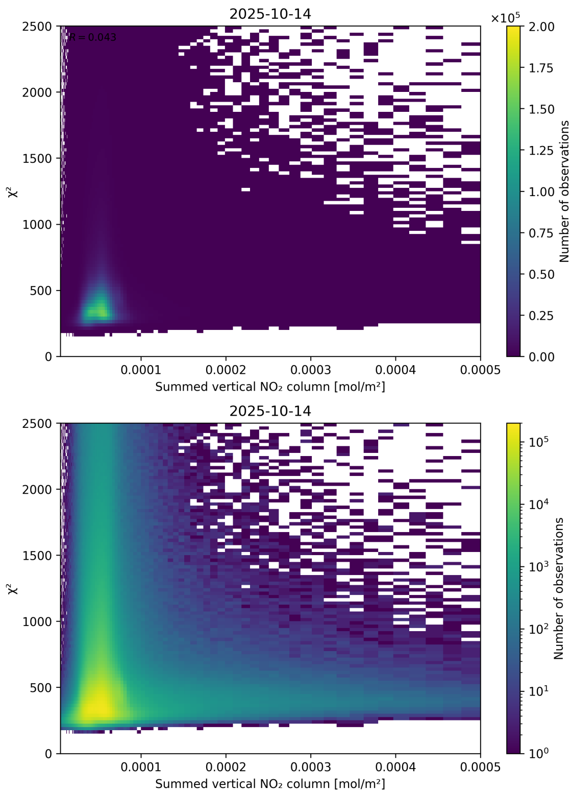
Figure 104: Scatter density plot of “Summed vertical NO 2 column” against “ \chi^2 ” for 2025-10-13 to 2025-10-15.
