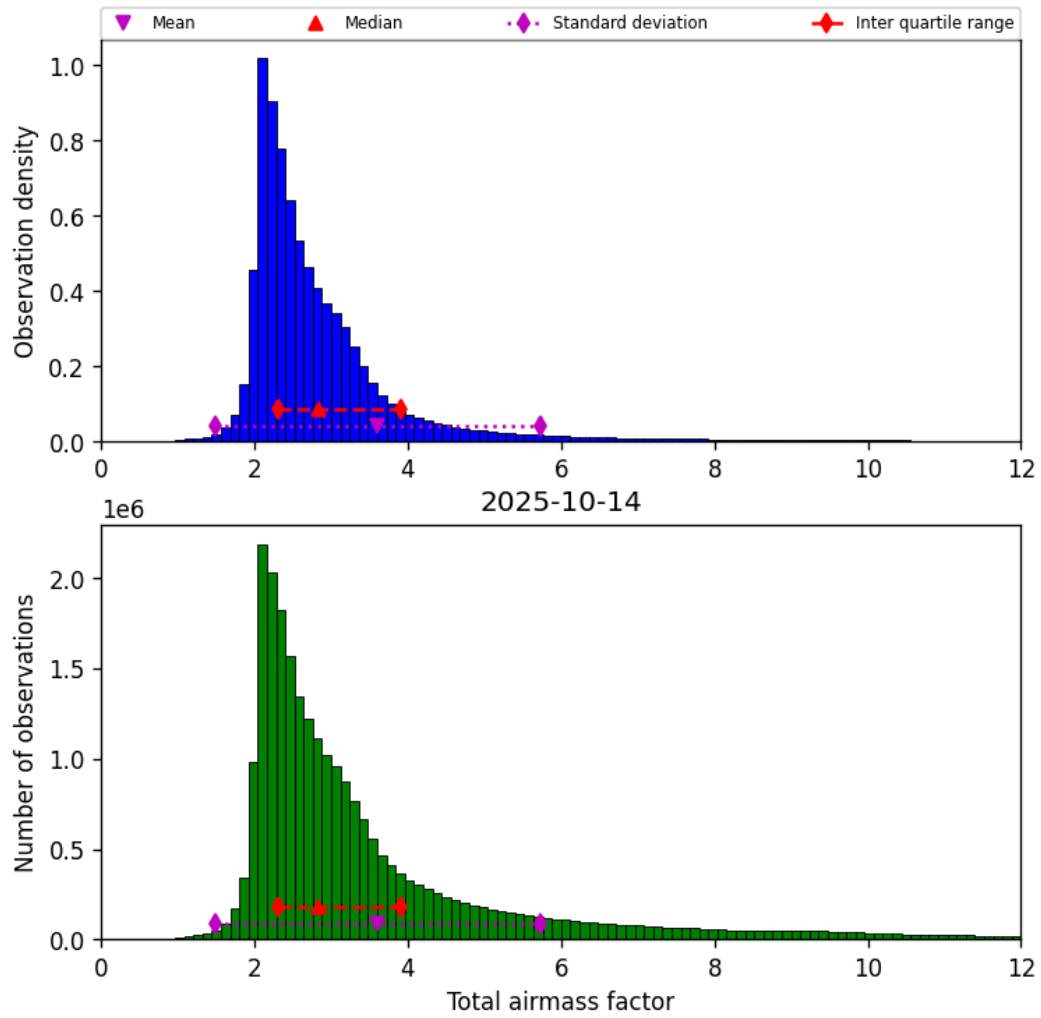
Figure 32: Histogram of “Total airmass factor” for 2025-10-13 to 2025-10-15
