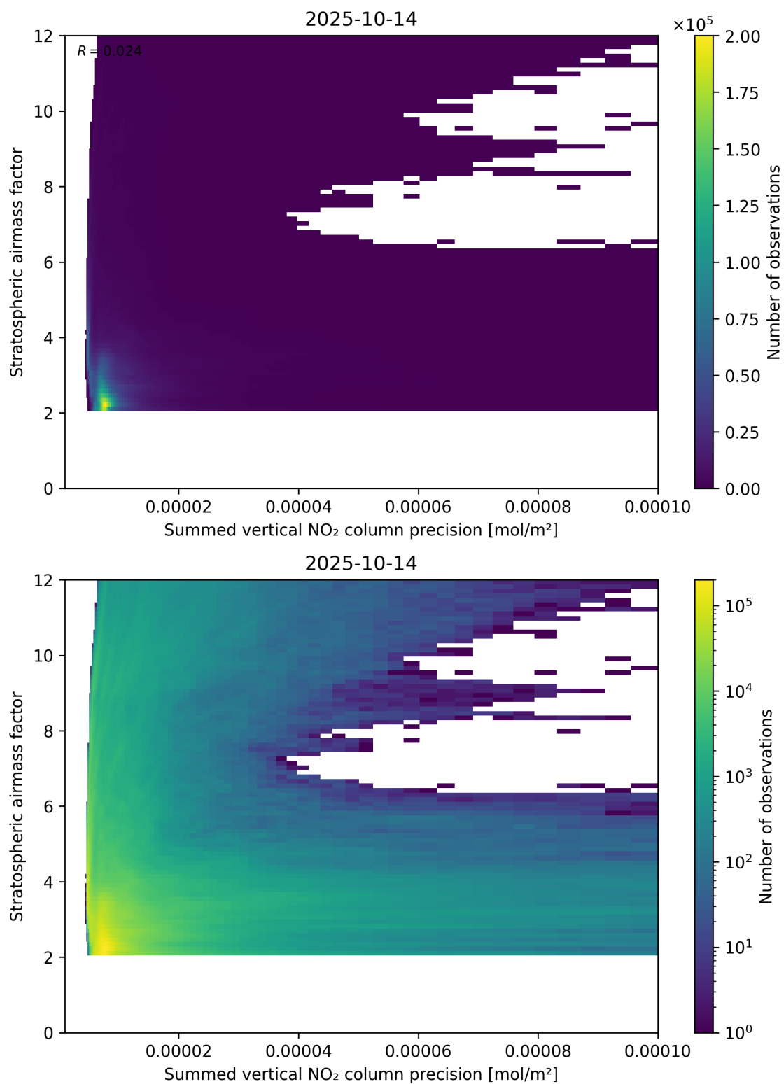
Figure 106: Scatter density plot of “Summed vertical NO 2 column precision” against “Stratospheric airmass factor” for 2025-10-13 to 2025-10-15.
