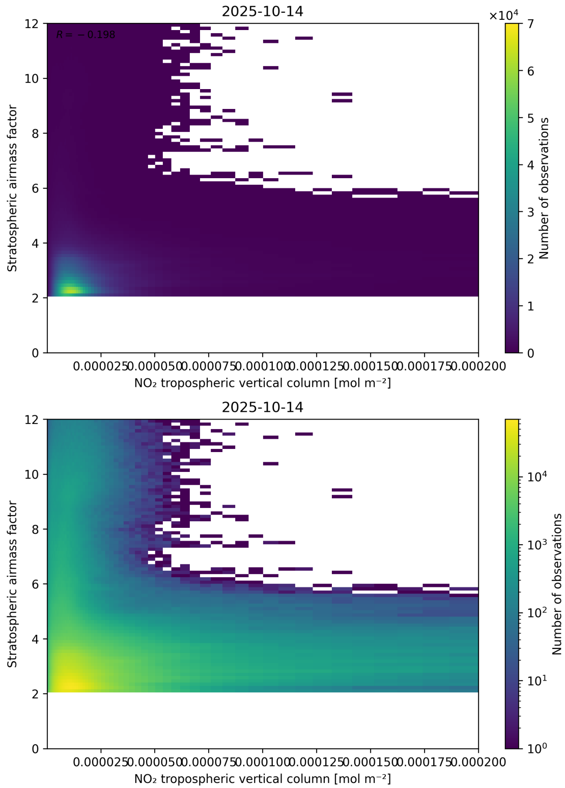
Figure 121: Scatter density plot of “NO 2 tropospheric vertical column” against “Stratospheric air mass factor” for 2025-10-13 to 2025-10-15.
