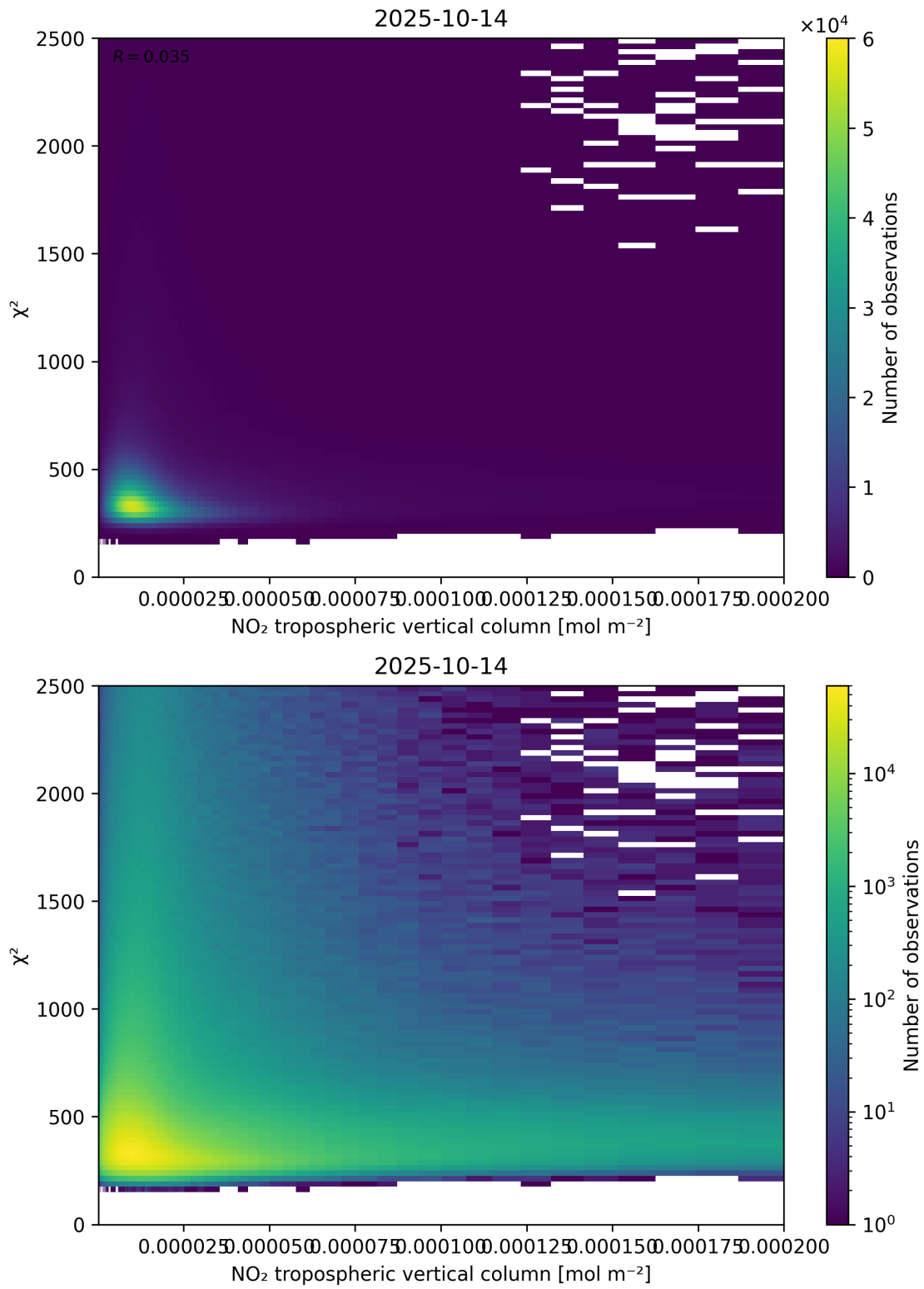
Figure 124: Scatter density plot of “NO 2 tropospheric vertical column” against “ \chi^2 ” for 2025-10-13 to 2025-10-15.
