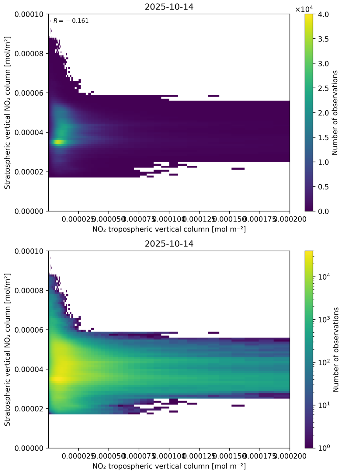
Figure 125: Scatter density plot of “NO 2 tropospheric vertical column” against “Stratospheric vertical NO 2 column” for 2025-10-13 to 2025-10-15.
