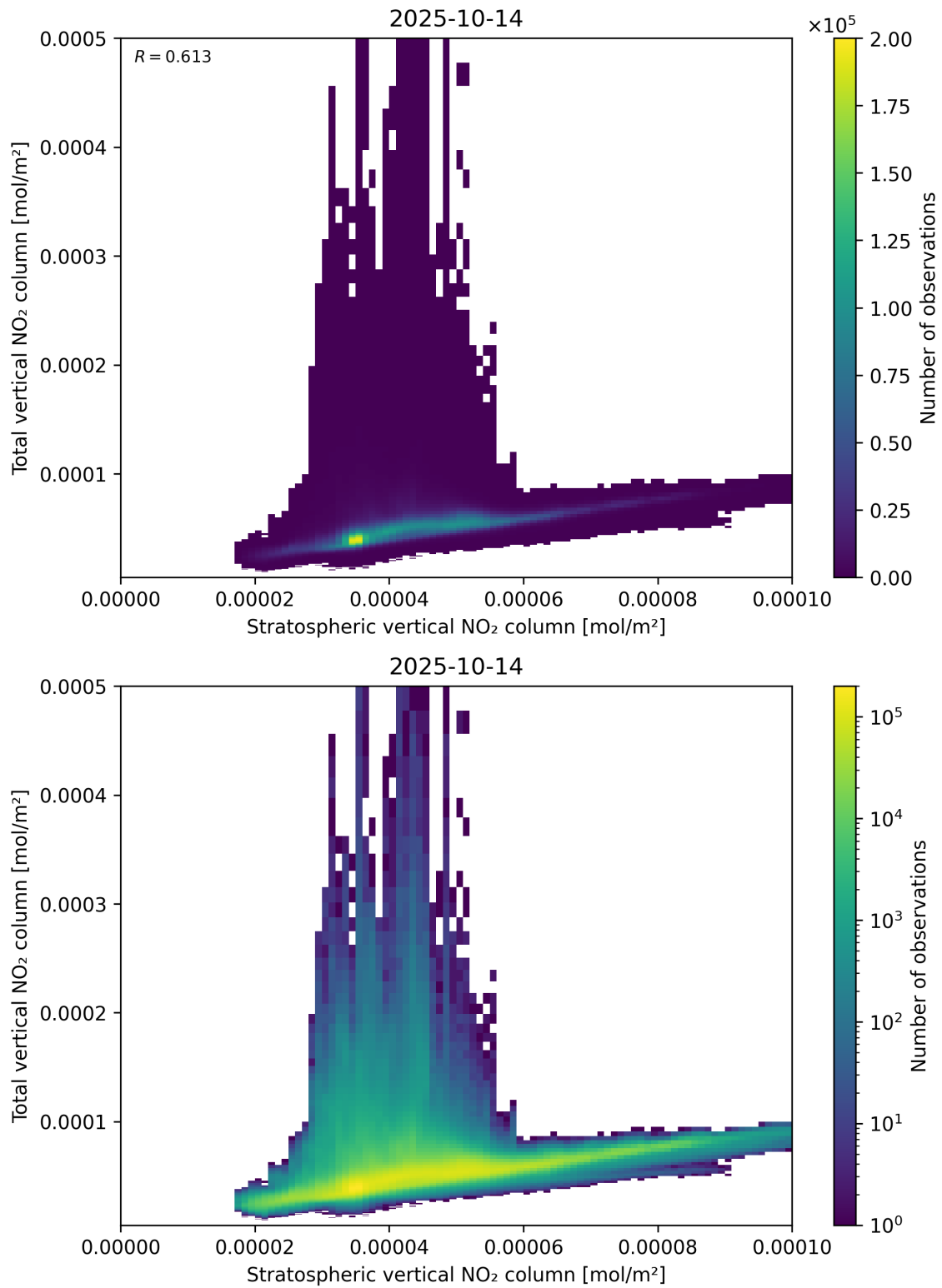
Figure 100: Scatter density plot of “Stratospheric vertical NO 2 column” against “Total vertical NO 2 column” for 2025-10-13 to 2025-10-15.
