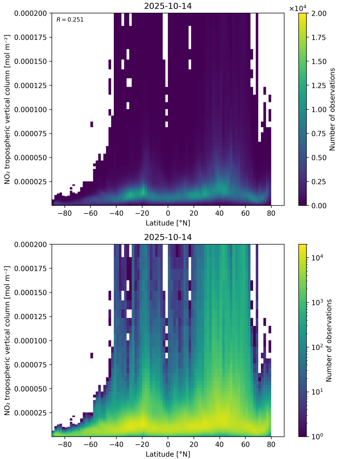
Figure 92: Scatter density plot of “Latitude” against “NO 2 tropospheric vertical column” for 2025-10-13 to 2025-10-15.
