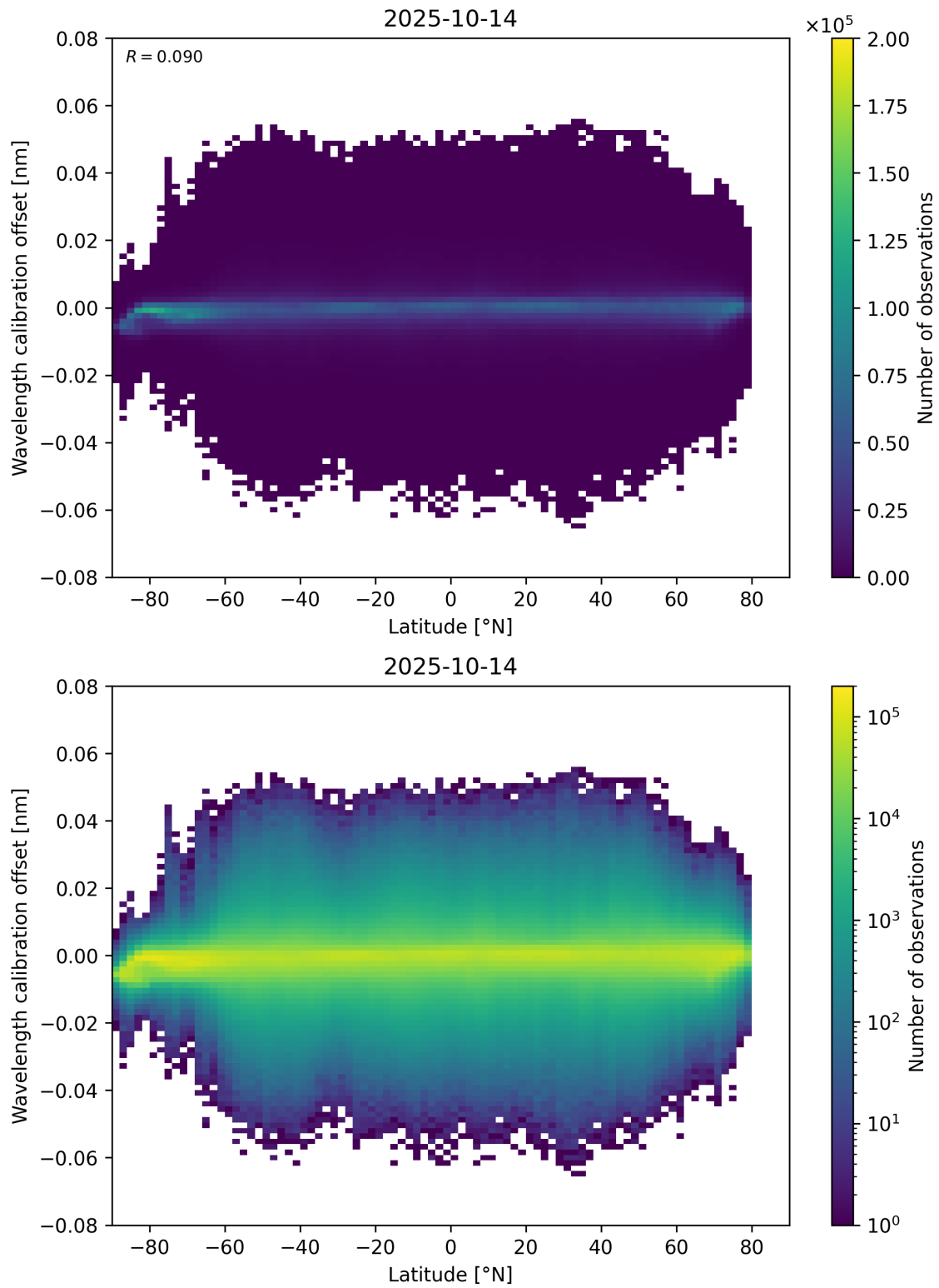
Figure 95: Scatter density plot of “Latitude” against “Wavelength calibration offset” for 2025-10-13 to 2025-10-15.
