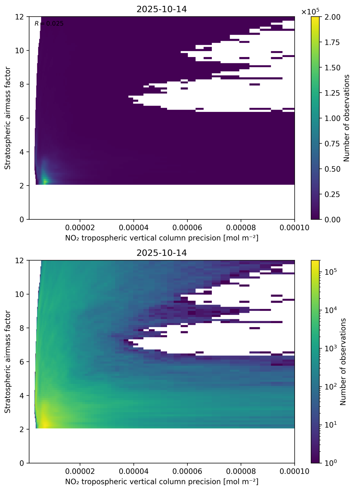
Figure 131: Scatter density plot of “NO 2 tropospheric vertical column precision” against “Stratospheric airmass factor” for 2025-10-13 to 2025-10-15.
