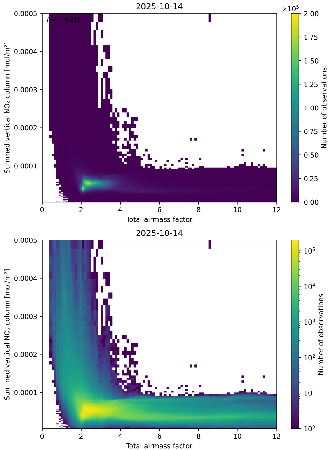
Figure 65: Scatter density plot of “Total airmass factor” against “Summed vertical NO 2 column” for 2025-10-13 to 2025-10-15.
