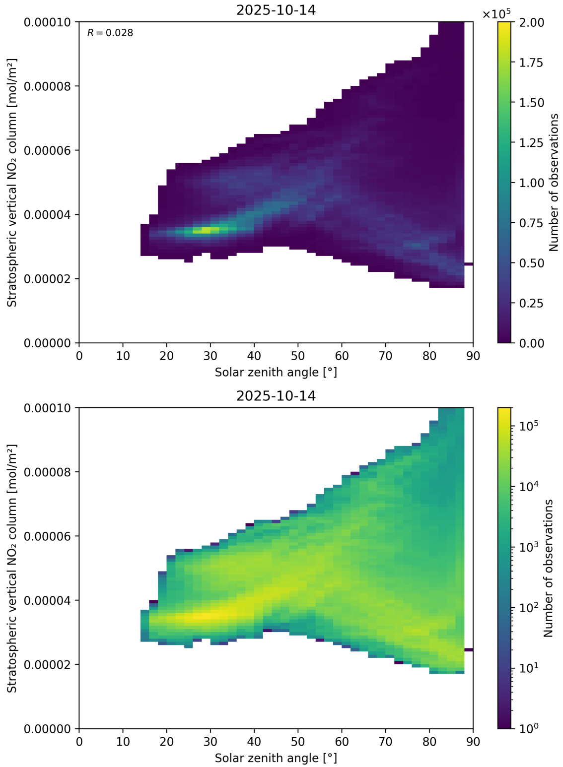
Figure 150: Scatter density plot of “Solar zenith angle” against “Stratospheric vertical NO 2 column” for 2025-10-13 to 2025-10-15.
