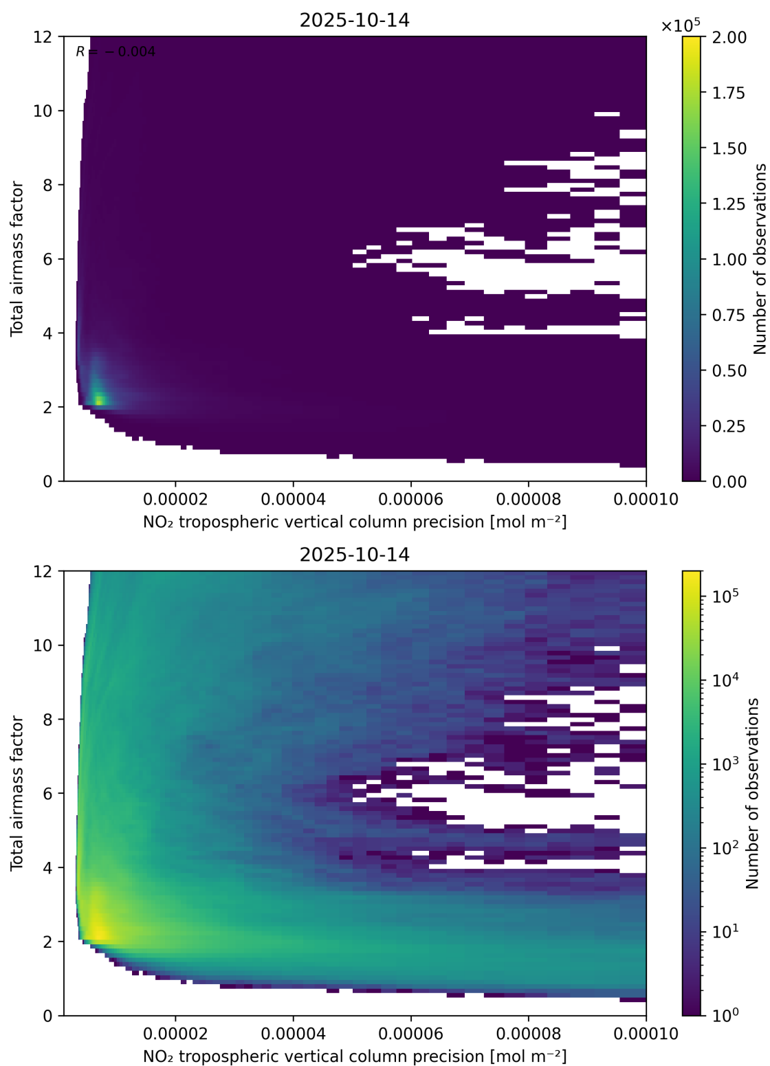
Figure 132: Scatter density plot of “NO 2 tropospheric vertical column precision” against “Total air mass factor” for 2025-10-13 to 2025-10-15.
