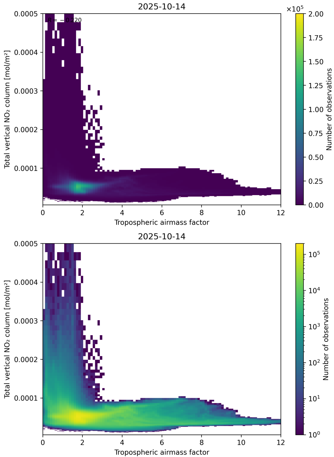
Figure 77: Scatter density plot of “Tropospheric airmass factor” against “Total vertical NO 2 column” for 2025-10-13 to 2025-10-15.
