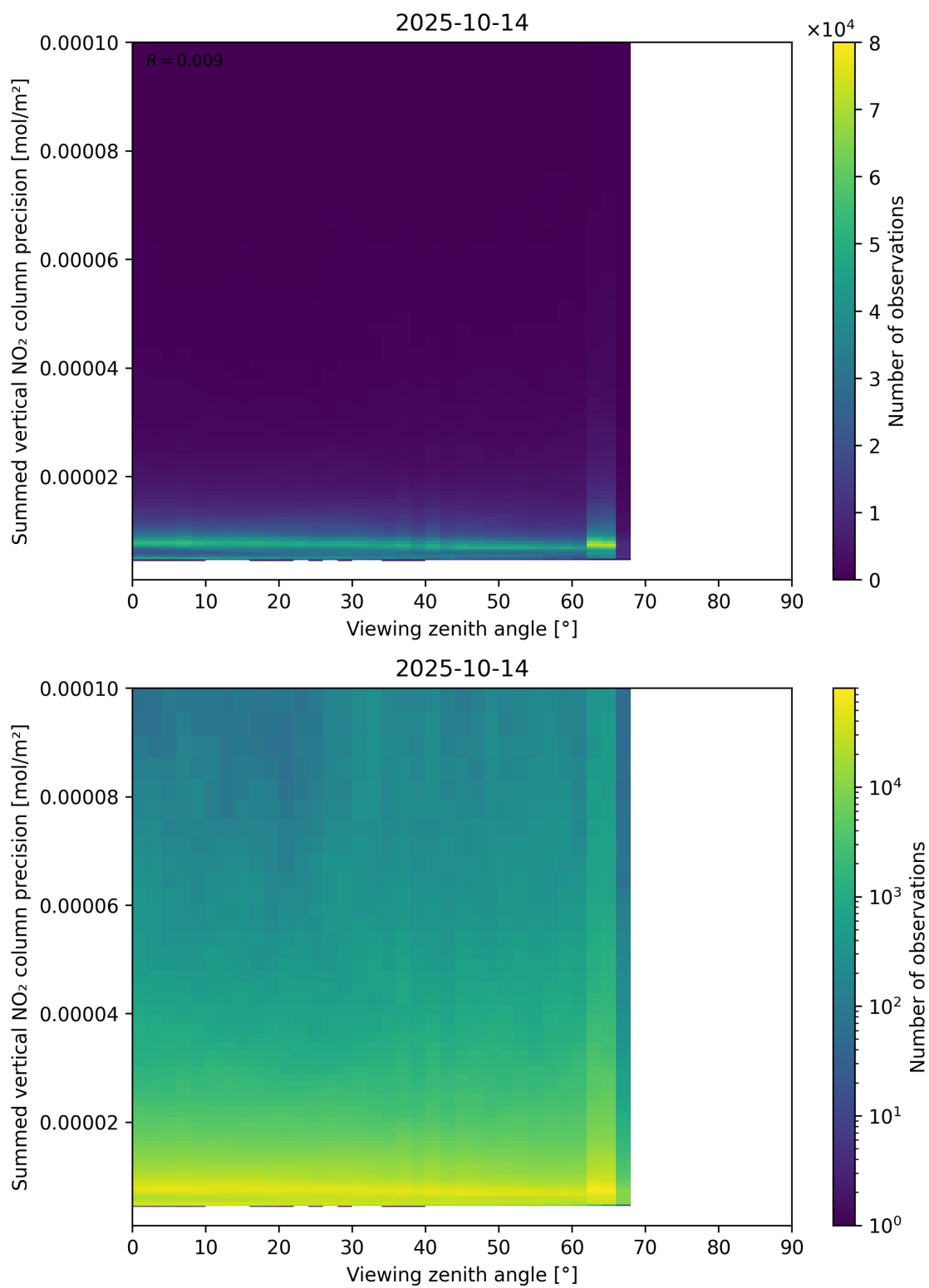
Figure 166: Scatter density plot of “Viewing zenith angle” against “Summed vertical NO 2 column precision” for 2025-10-13 to 2025-10-15.
