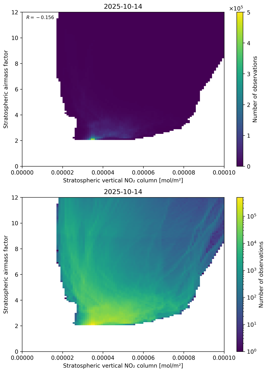
Figure 96: Scatter density plot of “Stratospheric vertical NO 2 column” against “Stratospheric airmass factor” for 2025-10-13 to 2025-10-15.
