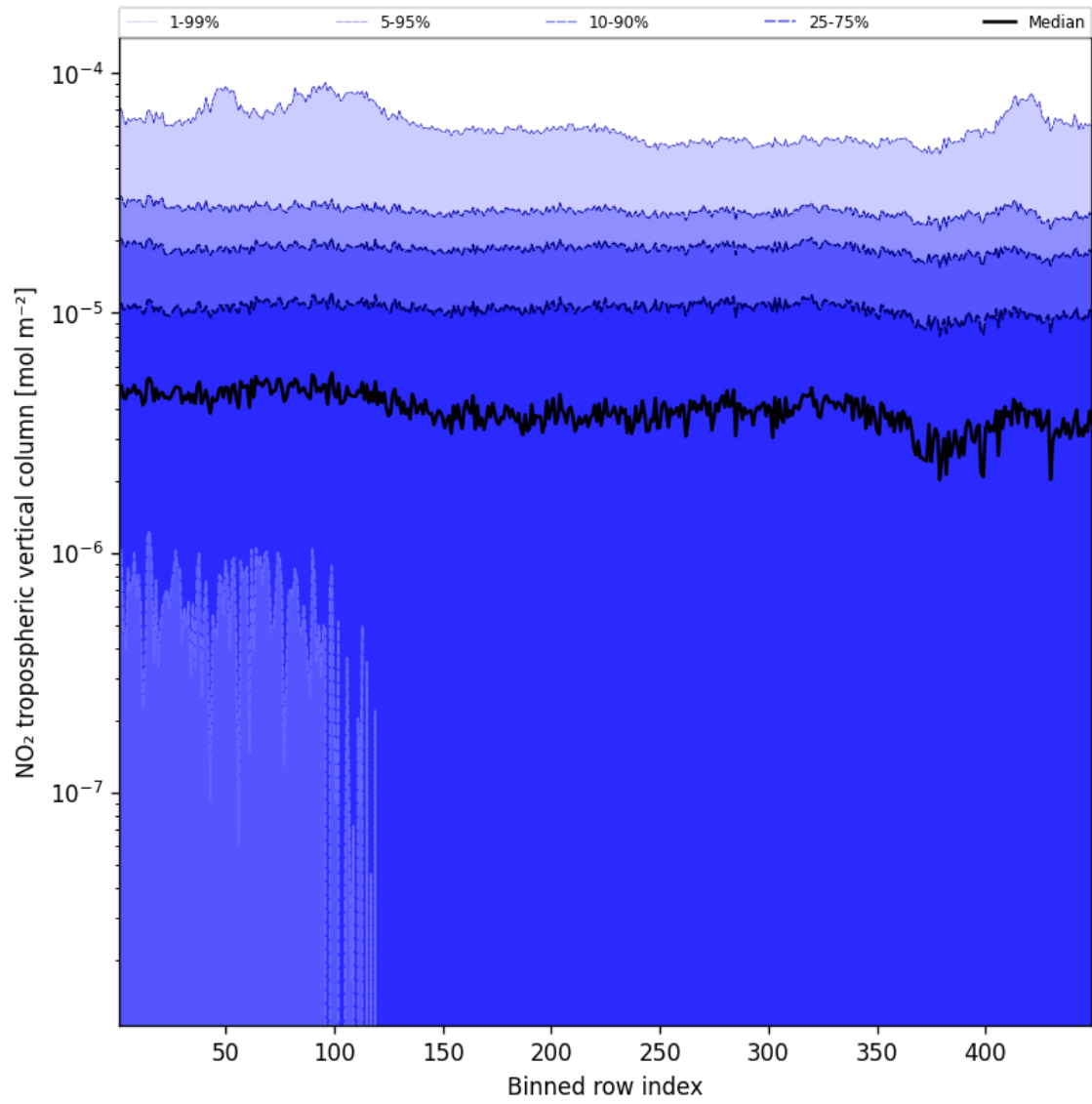
Figure 46: Along track statistics of “NO 2 tropospheric vertical column” for 2025-10-13 to 2025-10-15
