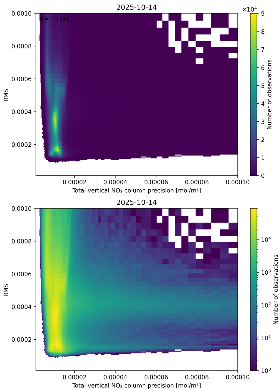
Figure 119: Scatter density plot of “Total vertical NO 2 column precision” against “RMS” for 2025-10-13 to 2025-10-15.
