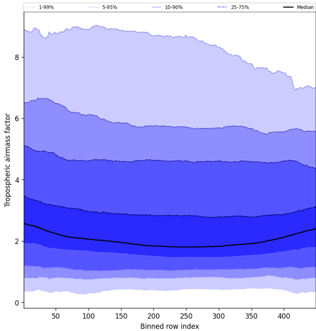
Figure 48: Along track statistics of “Tropospheric air mass factor” for 2025-10-13 to 2025-10-15
