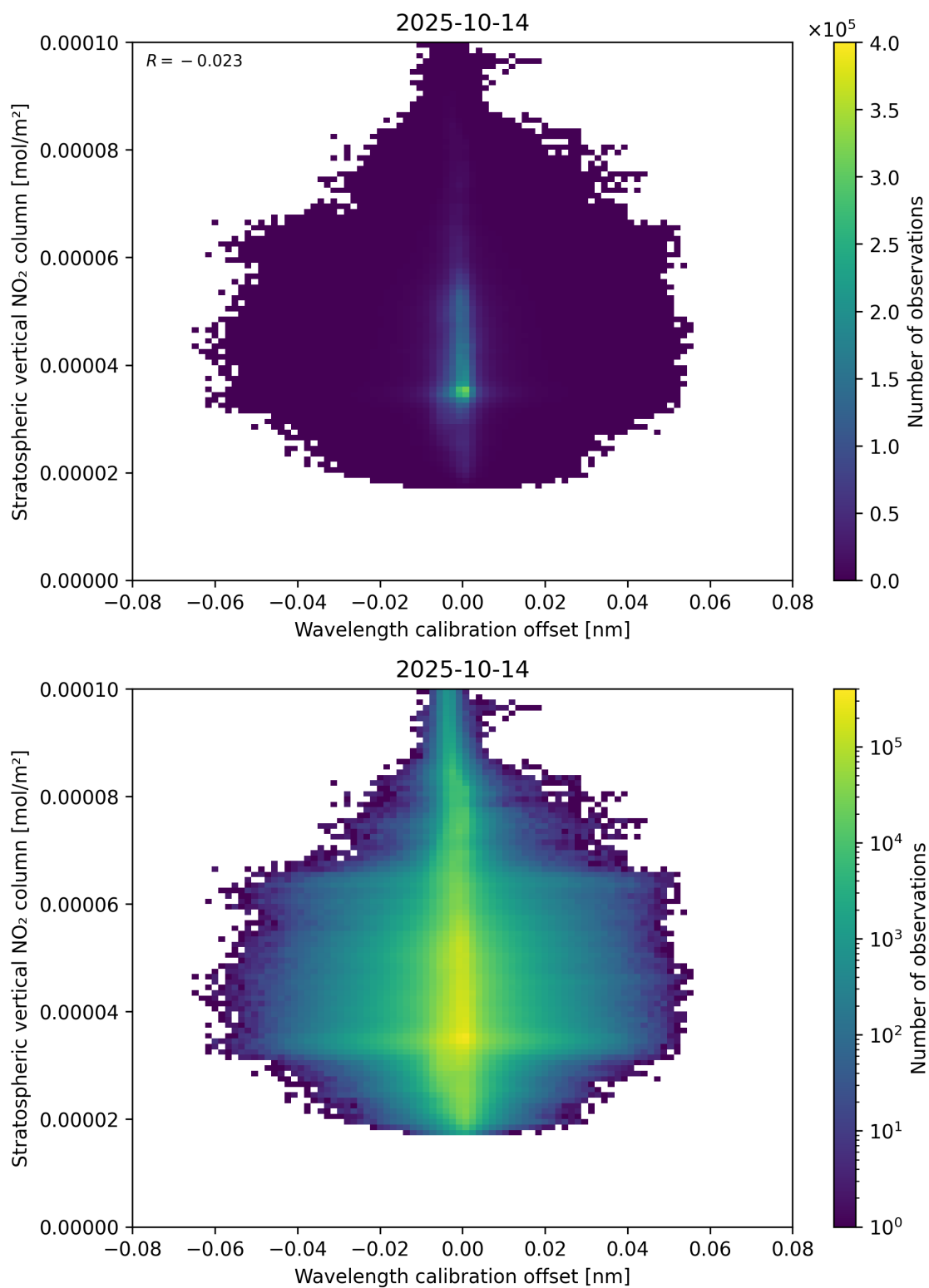
Figure 176: Scatter density plot of “Wavelength calibration offset” against “Stratospheric vertical NO 2 column” for 2025-10-13 to 2025-10-15.
