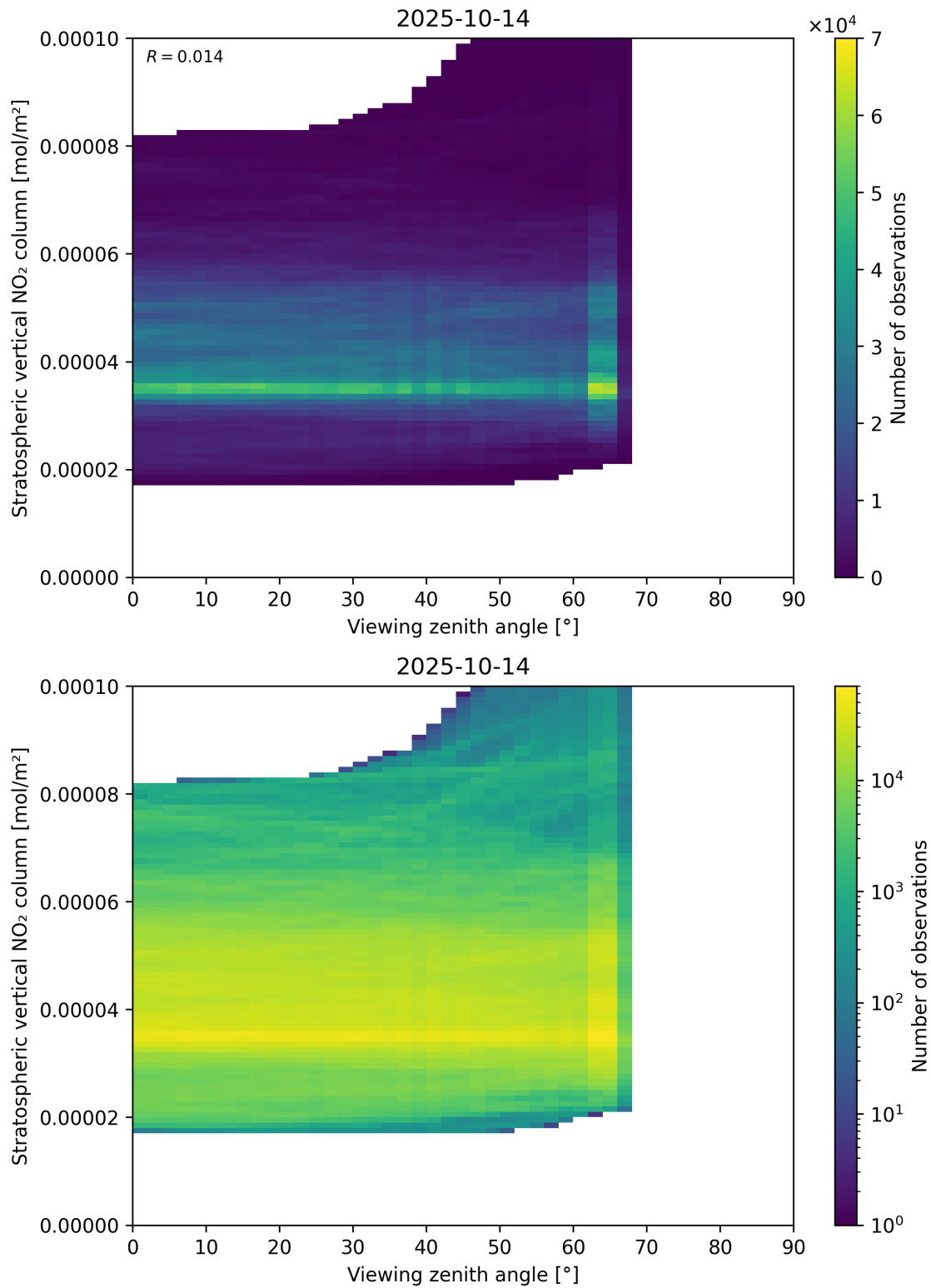
Figure 164: Scatter density plot of “Viewing zenith angle” against “Stratospheric vertical NO 2 column” for 2025-10-13 to 2025-10-15.
