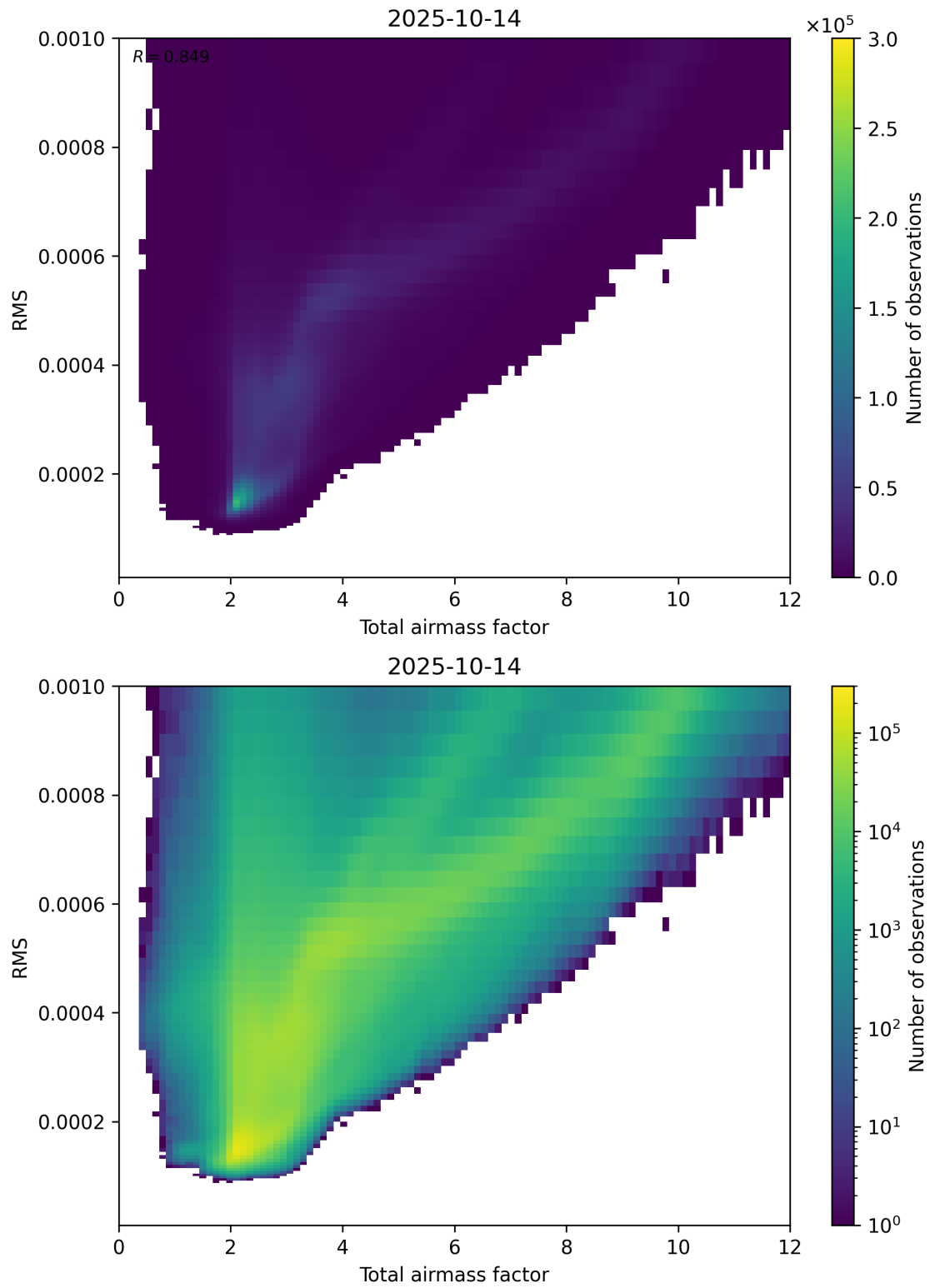
Figure 69: Scatter density plot of “Total airmass factor” against “RMS” for 2025-10-13 to 2025-10-15.
