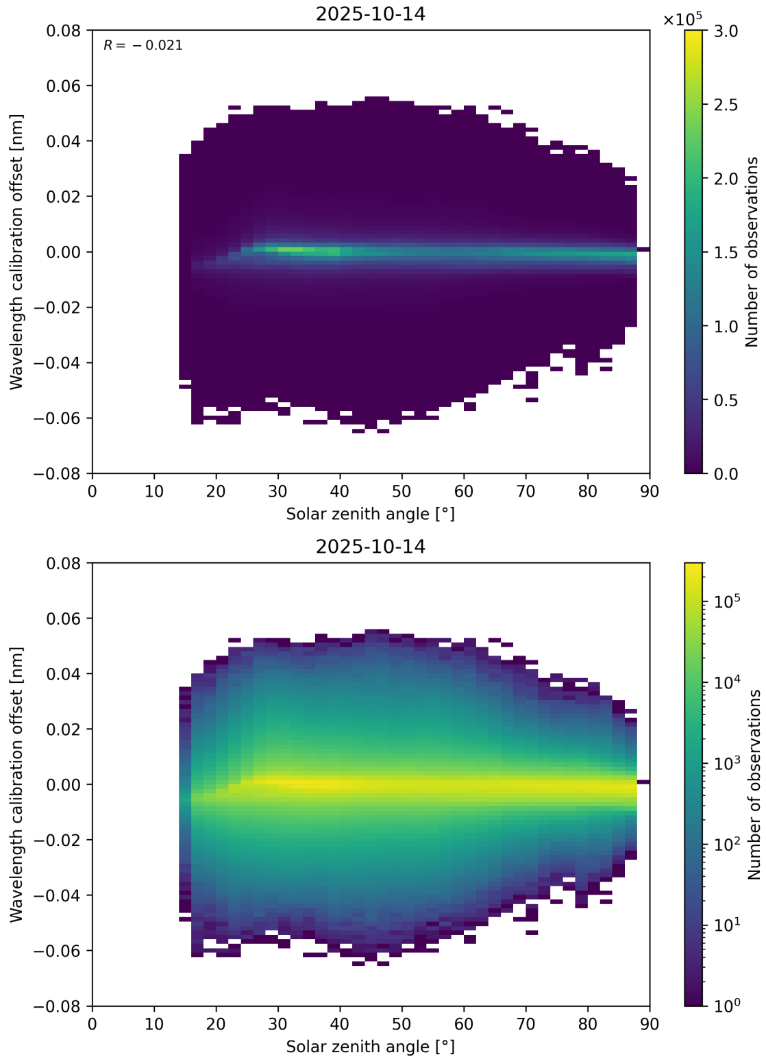
Figure 158: Scatter density plot of “Solar zenith angle” against “Wavelength calibration offset” for 2025-10-13 to 2025-10-15.
