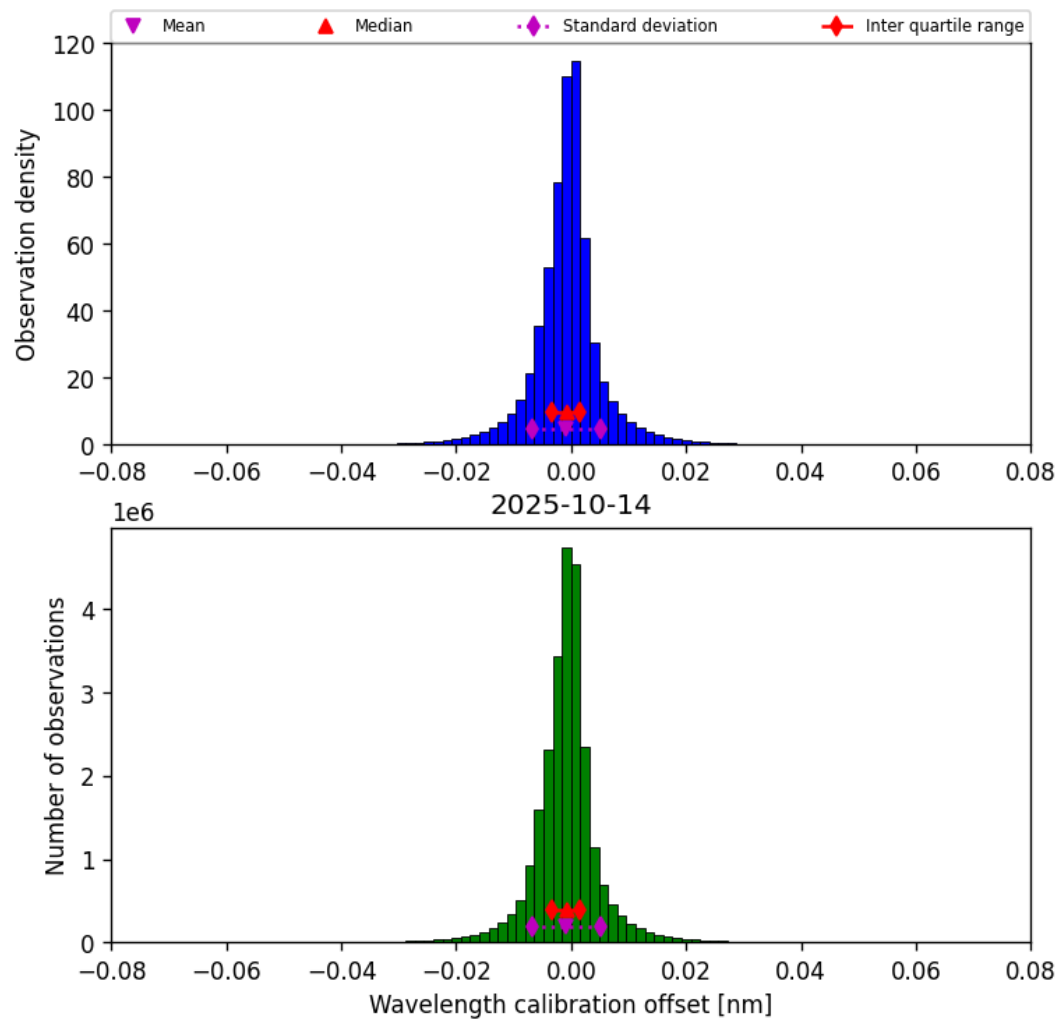
Figure 35: Histogram of “Wavelength calibration offset” for 2025-10-13 to 2025-10-15
