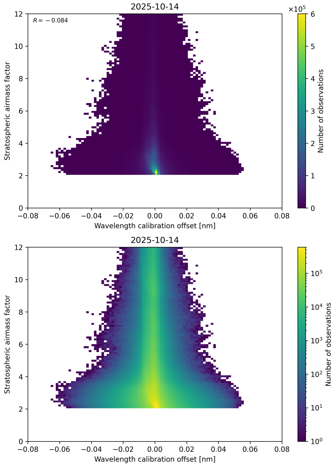
Figure 174: Scatter density plot of “Wavelength calibration offset” against “Stratospheric airmass factor” for 2025-10-13 to 2025-10-15.
