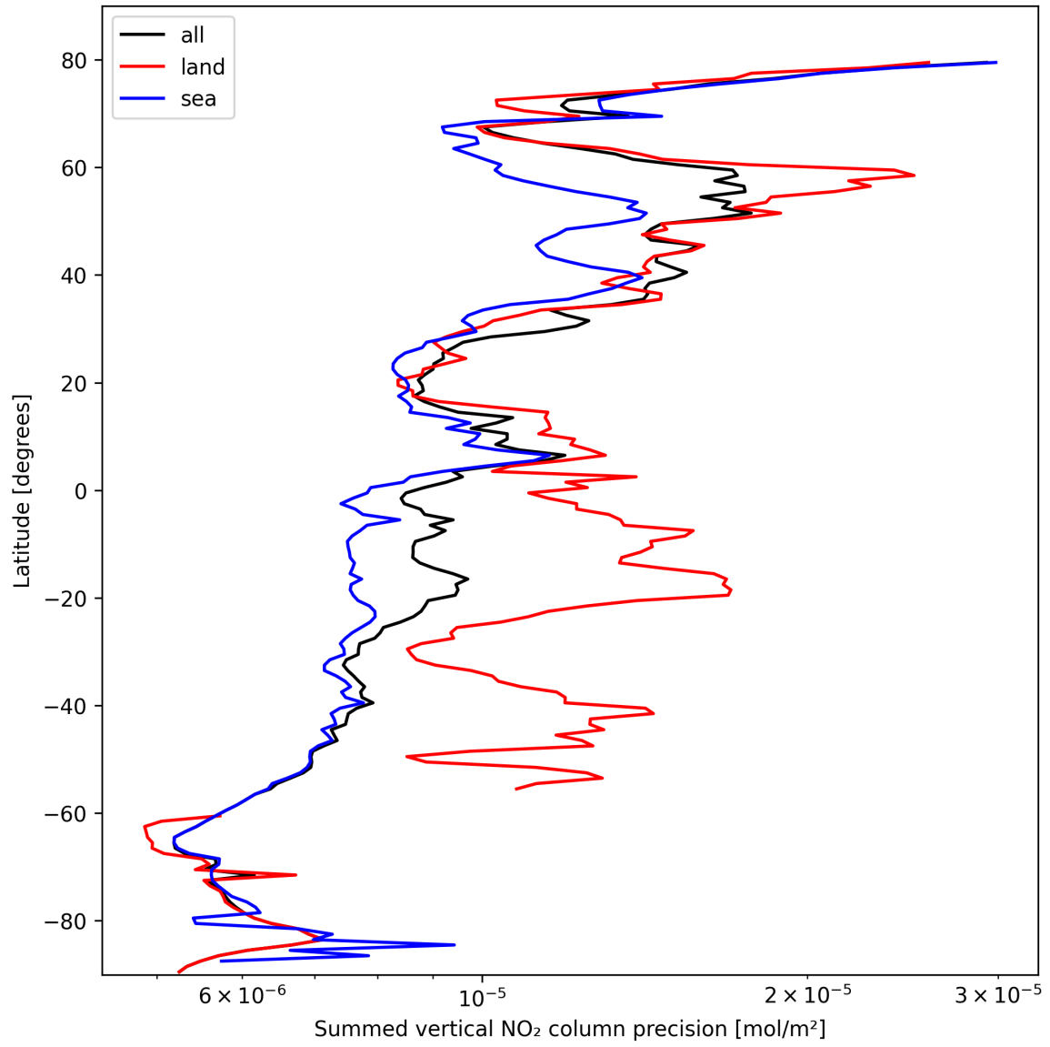
Figure 24: Zonal average of “Summed vertical NO 2 column precision” for 2025-10-13 to 2025-10-15.
