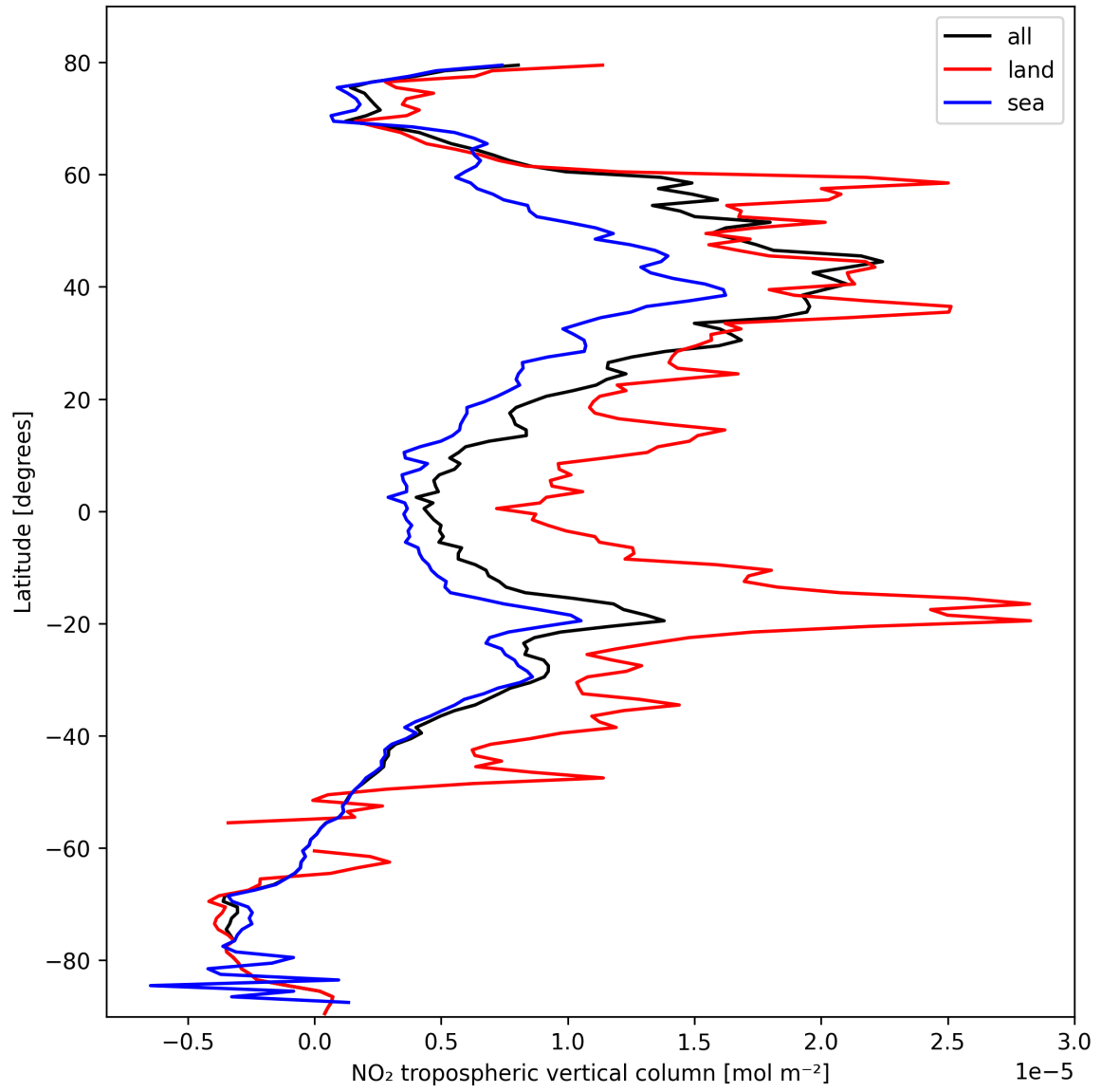
Figure 12: Zonal average of “NO 2 tropospheric vertical column” for 2025-10-13 to 2025-10-15.
