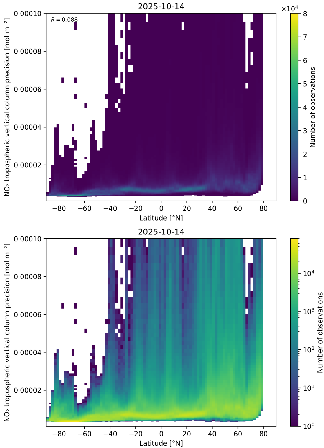
Figure 93: Scatter density plot of “Latitude” against “NO 2 tropospheric vertical column precision” for 2025-10-13 to 2025-10-15.
