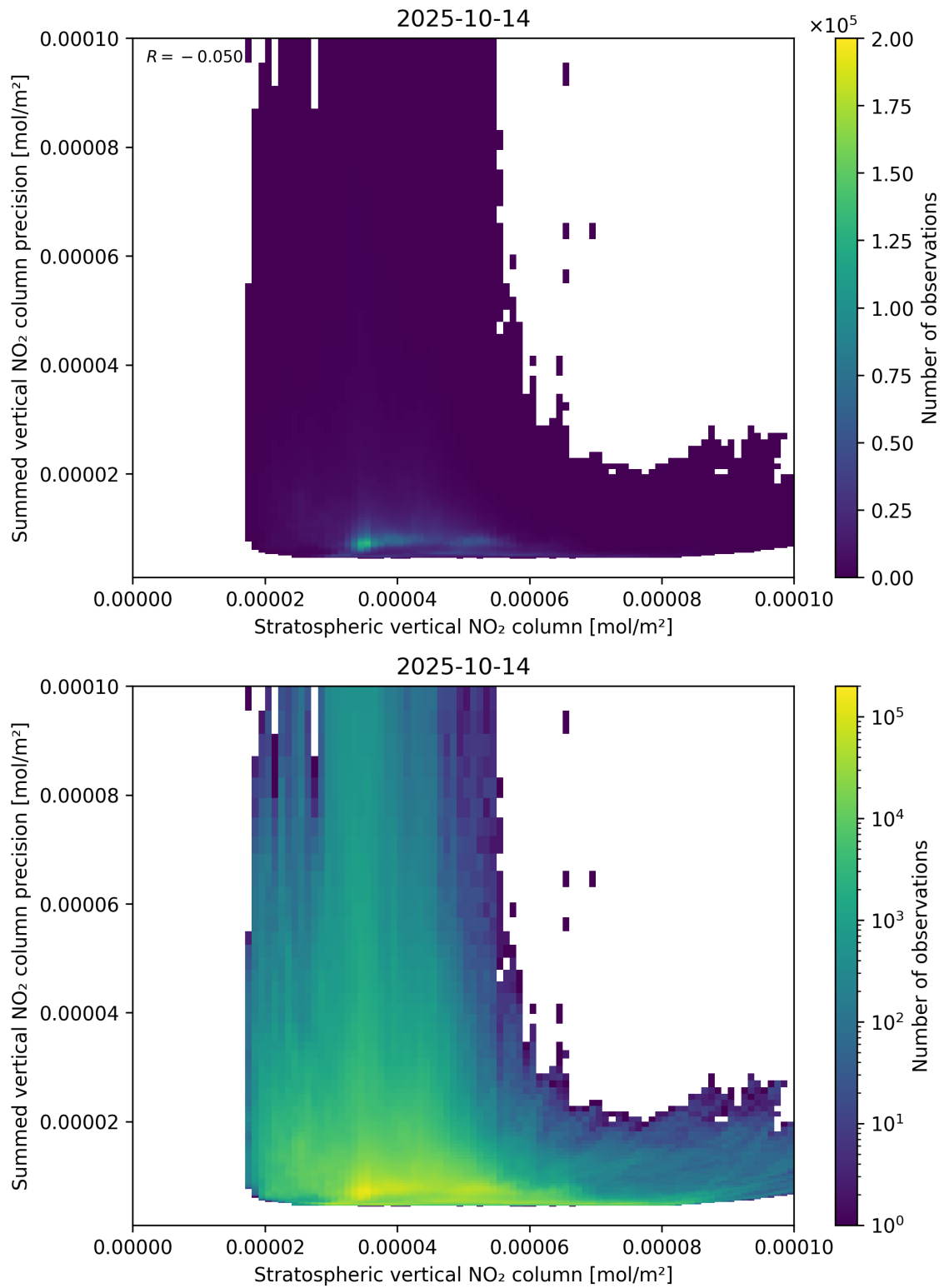
Figure 99: Scatter density plot of “Stratospheric vertical NO 2 column” against “Summed vertical NO 2 column precision” for 2025-10-13 to 2025-10-15.
