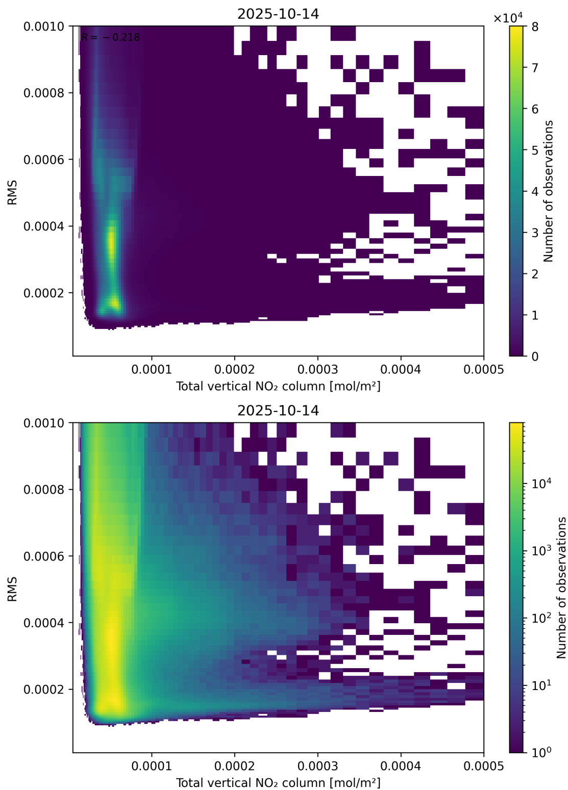
Figure 120: Scatter density plot of “Total vertical NO 2 column” against “RMS” for 2025-10-13 to 2025-10-15.
