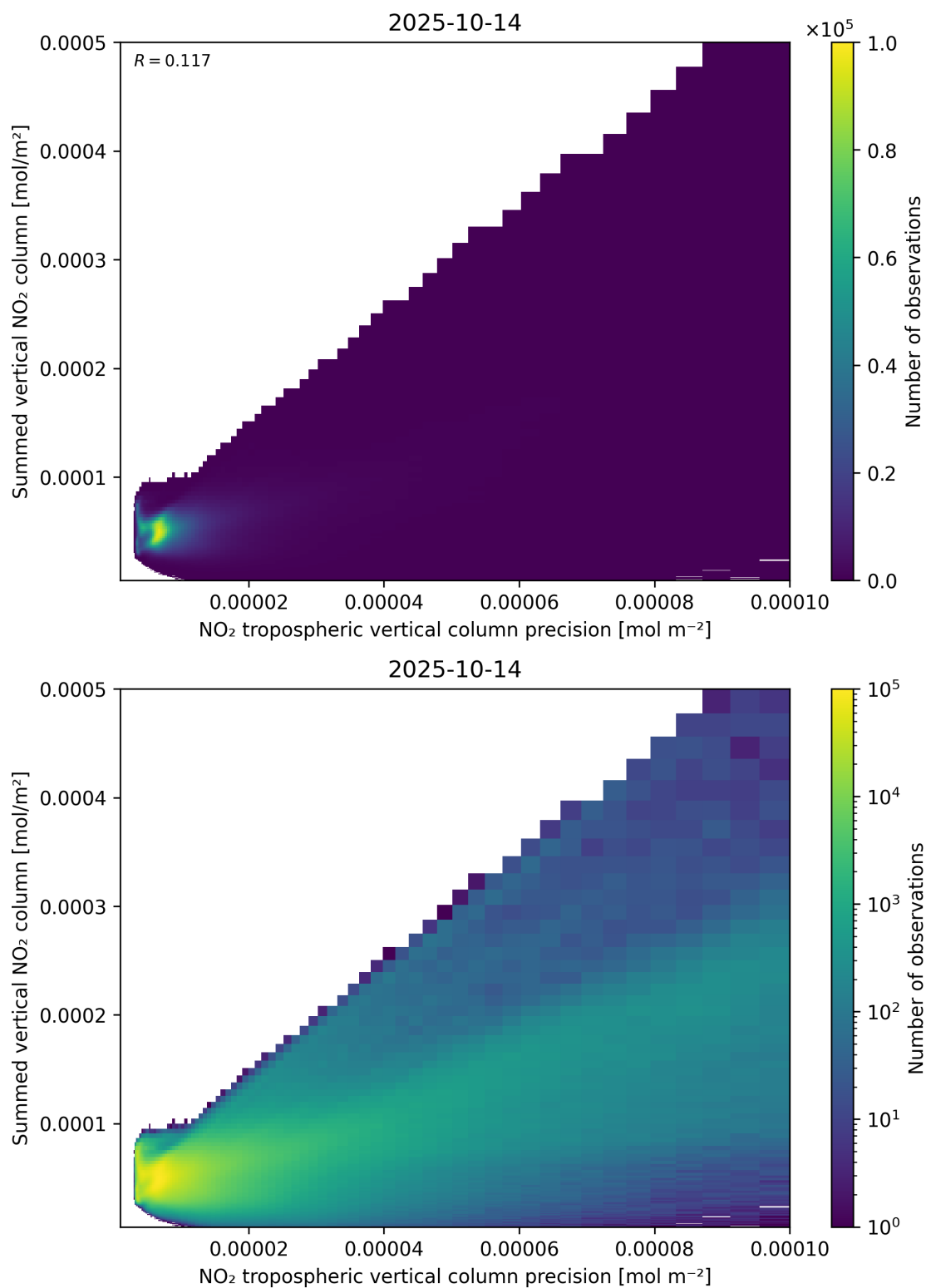
Figure 136: Scatter density plot of “NO 2 tropospheric vertical column precision” against “Summed vertical NO 2 column” for 2025-10-13 to 2025-10-15.
