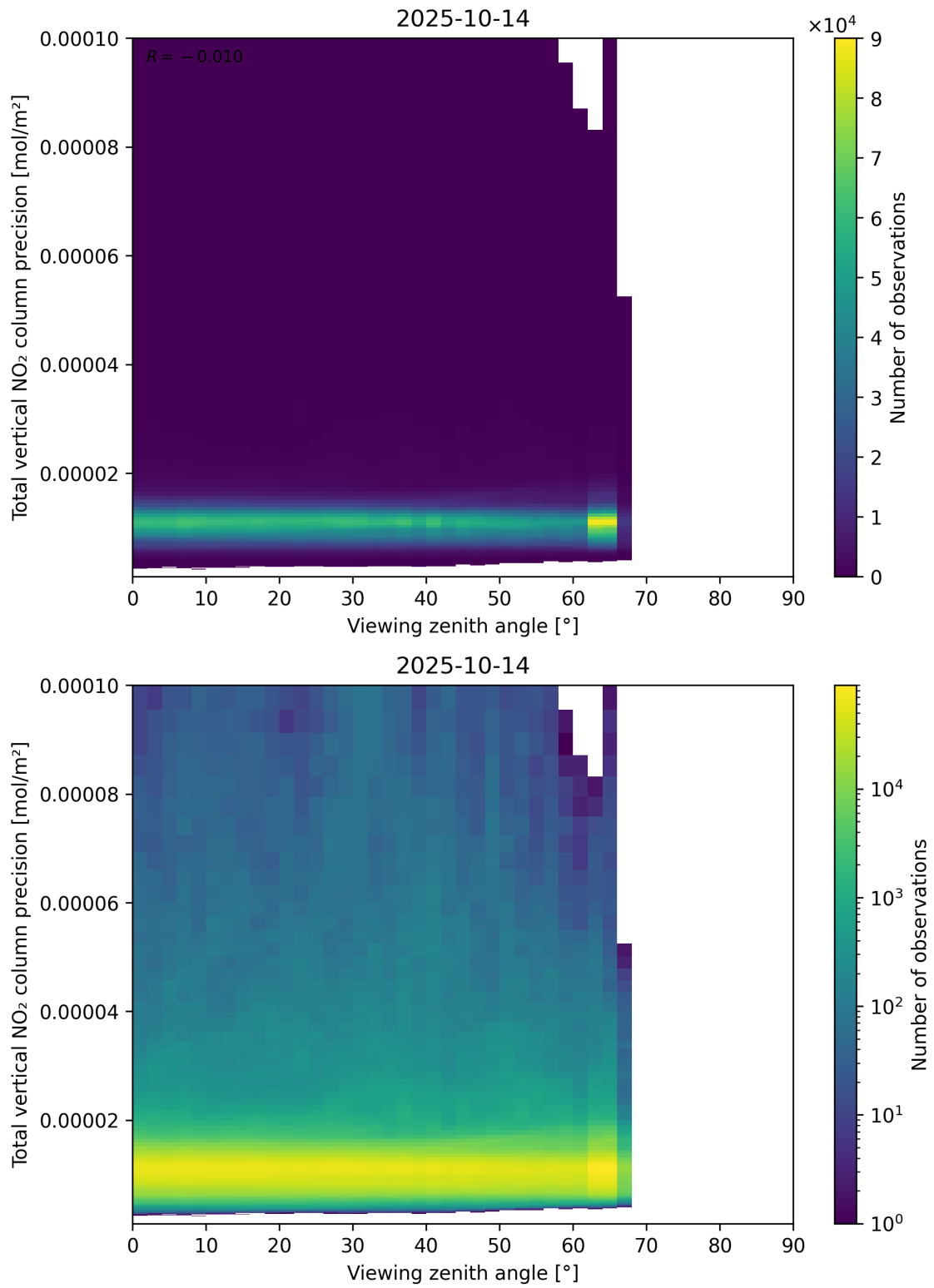
Figure 168: Scatter density plot of “Viewing zenith angle” against “Total vertical NO 2 column precision” for 2025-10-13 to 2025-10-15.
