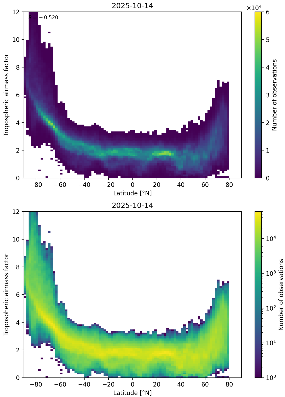
Figure 85: Scatter density plot of “Latitude” against “Tropospheric airmass factor” for 2025-10-13 to 2025-10-15.
