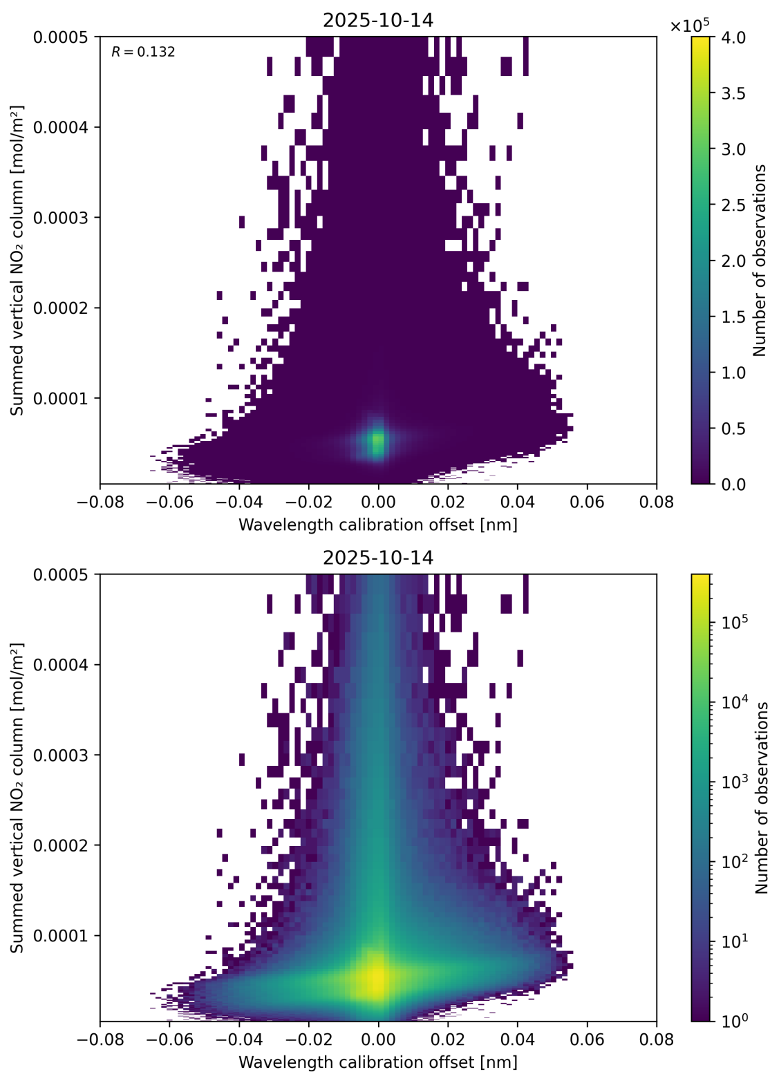
Figure 177: Scatter density plot of “Wavelength calibration offset” against “Summed vertical NO 2 column” for 2025-10-13 to 2025-10-15.
