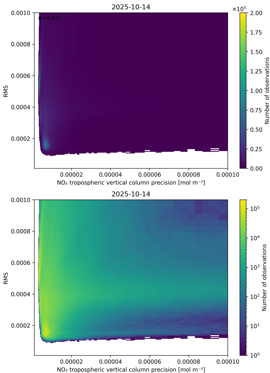
Figure 140: Scatter density plot of “NO 2 tropospheric vertical column precision” against “RMS” for 2025-10-13 to 2025-10-15.
