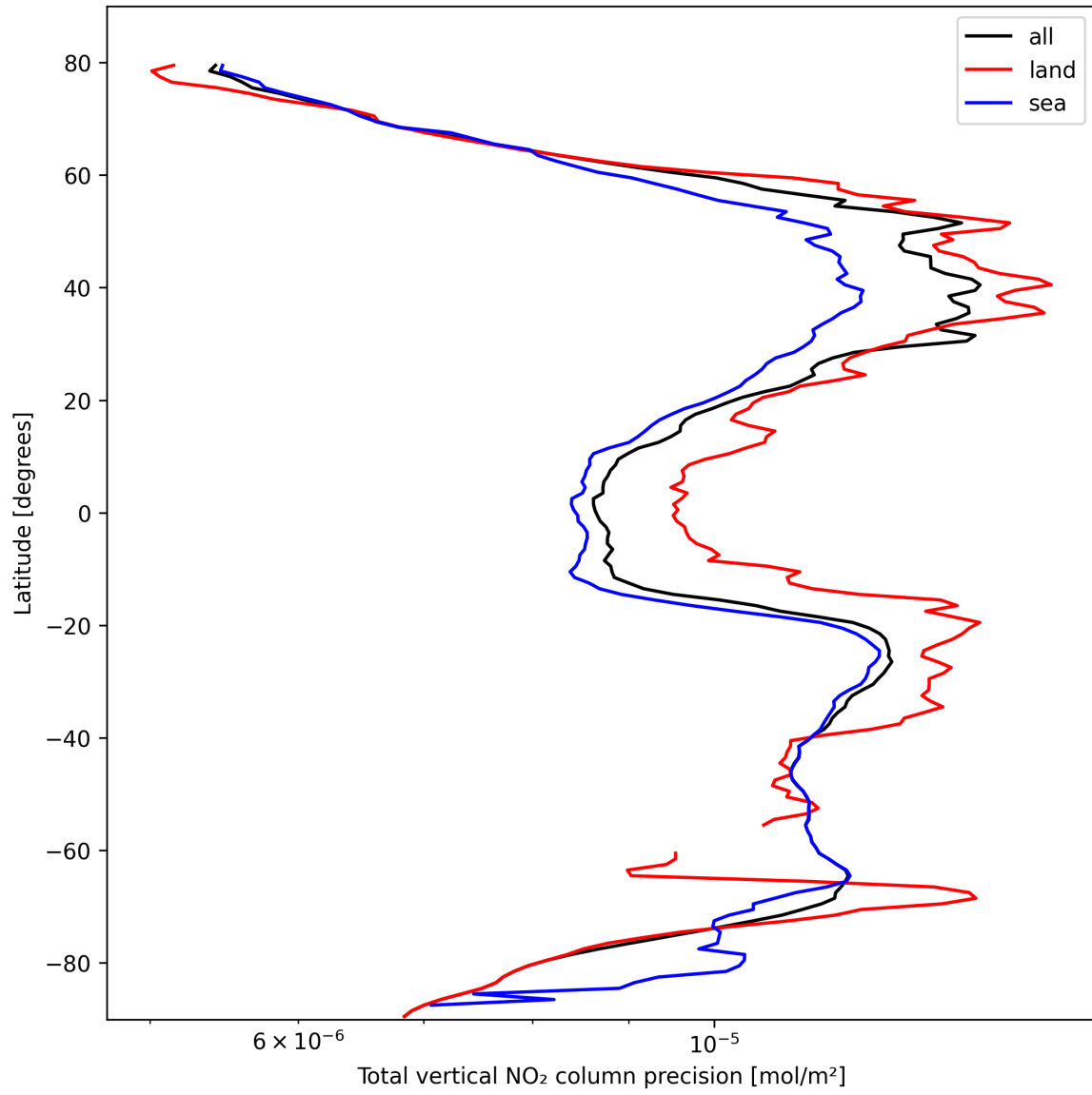
Figure 22: Zonal average of "Total vertical NO 2 column precision" for 2025-10-13 to 2025-10-15.
