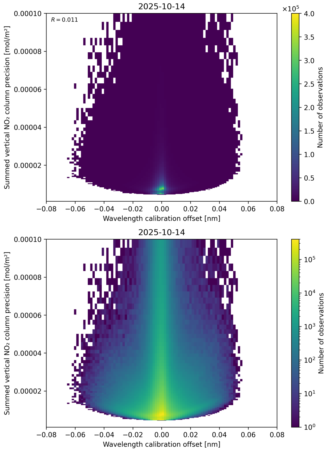
Figure 178: Scatter density plot of “Wavelength calibration offset” against “Summed vertical NO 2 column precision” for 2025-10-13 to 2025-10-15.
