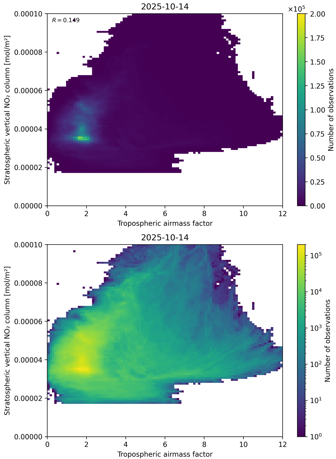
Figure 74: Scatter density plot of “Tropospheric airmass factor” against “Stratospheric vertical NO 2 column” for 2025-10-13 to 2025-10-15.
