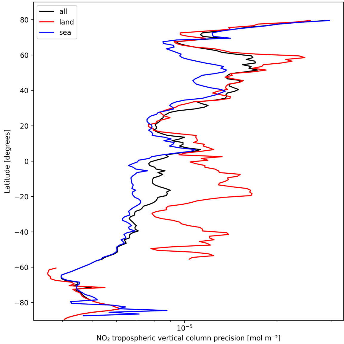
Figure 13: Zonal average of “NO 2 tropospheric vertical column precision” for 2025-10-13 to 2025-10-15.
