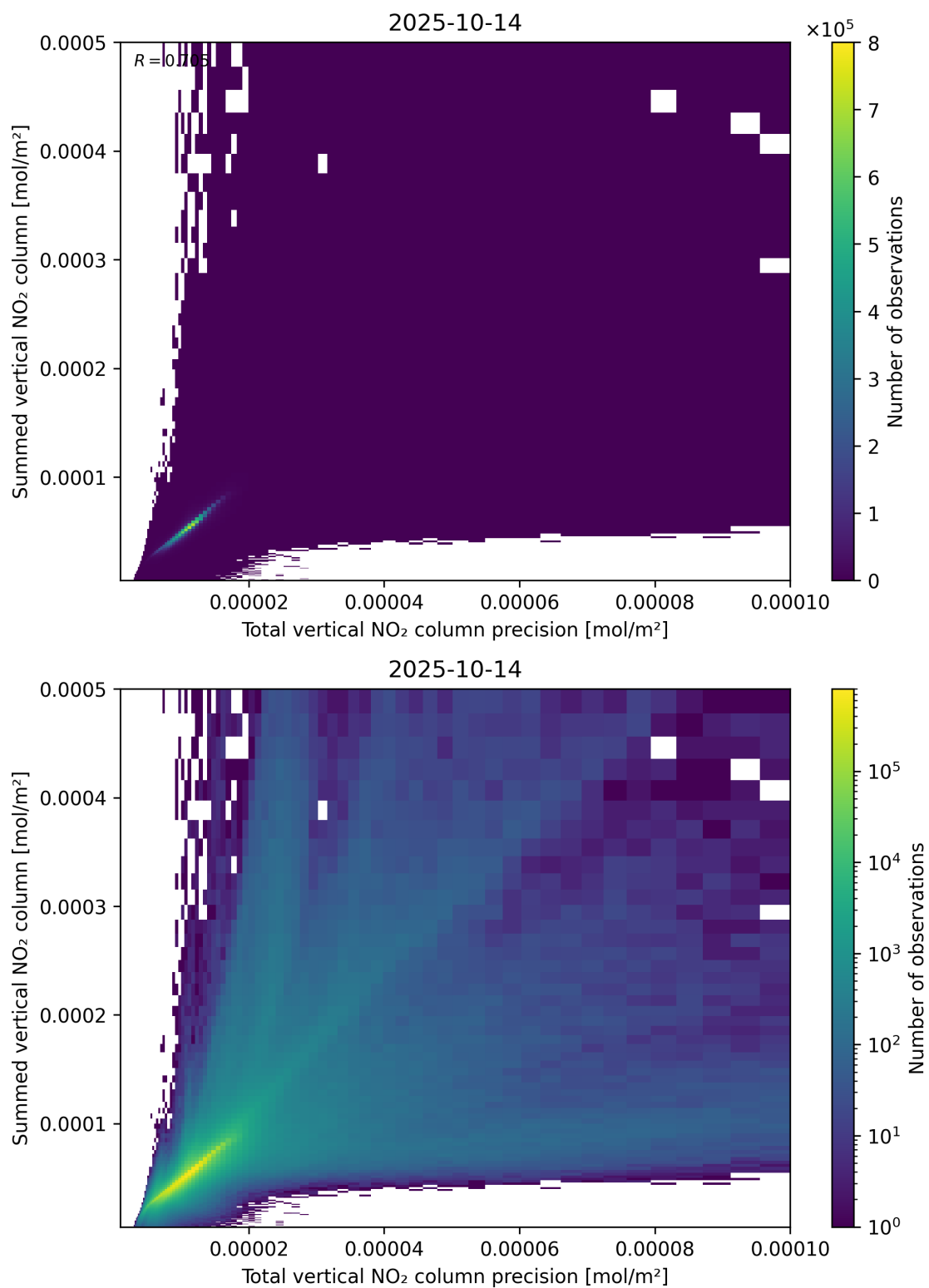
Figure 117: Scatter density plot of “Total vertical NO 2 column precision” against “Summed vertical NO 2 column” for 2025-10-13 to 2025-10-15.
