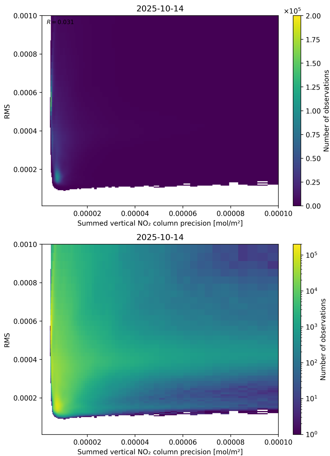
Figure 108: Scatter density plot of “Summed vertical NO 2 column precision” against “RMS” for 2025-10-13 to 2025-10-15.
