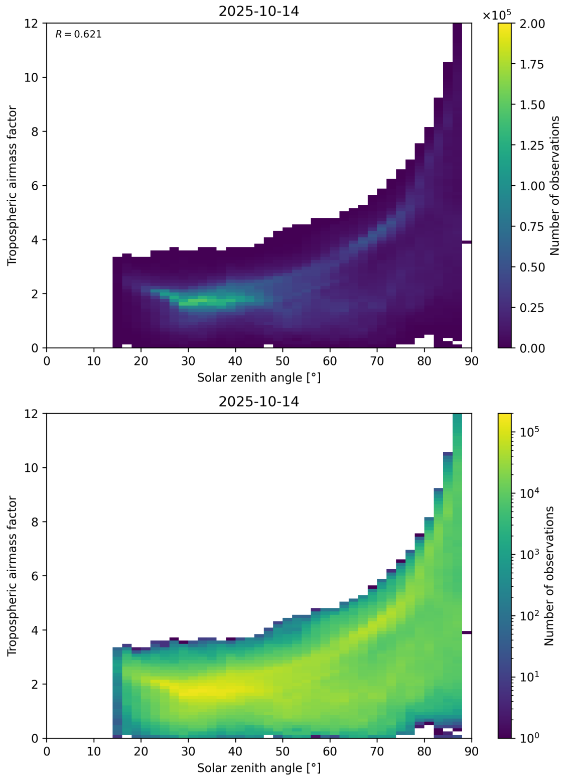
Figure 147: Scatter density plot of “Solar zenith angle” against “Tropospheric airmass factor” for 2025-10-13 to 2025-10-15.
