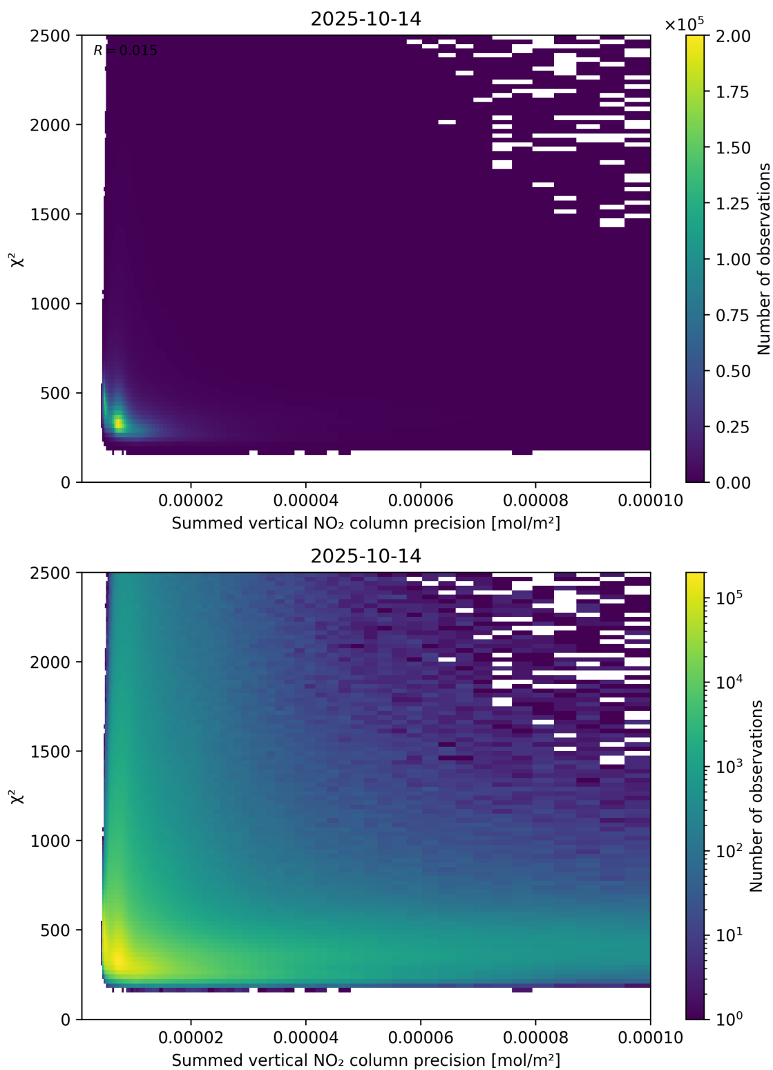
Figure 107: Scatter density plot of “Summed vertical NO 2 column precision” against “ \chi^2 ” for 2025-10-13 to 2025-10-15.
