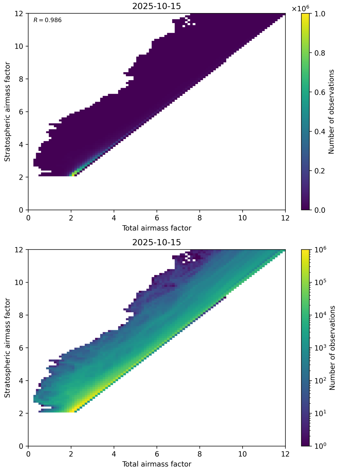
Figure 62: Scatter density plot of “Total airmass factor” against “Stratospheric airmass factor” for 2025-10-14 to 2025-10-16.
