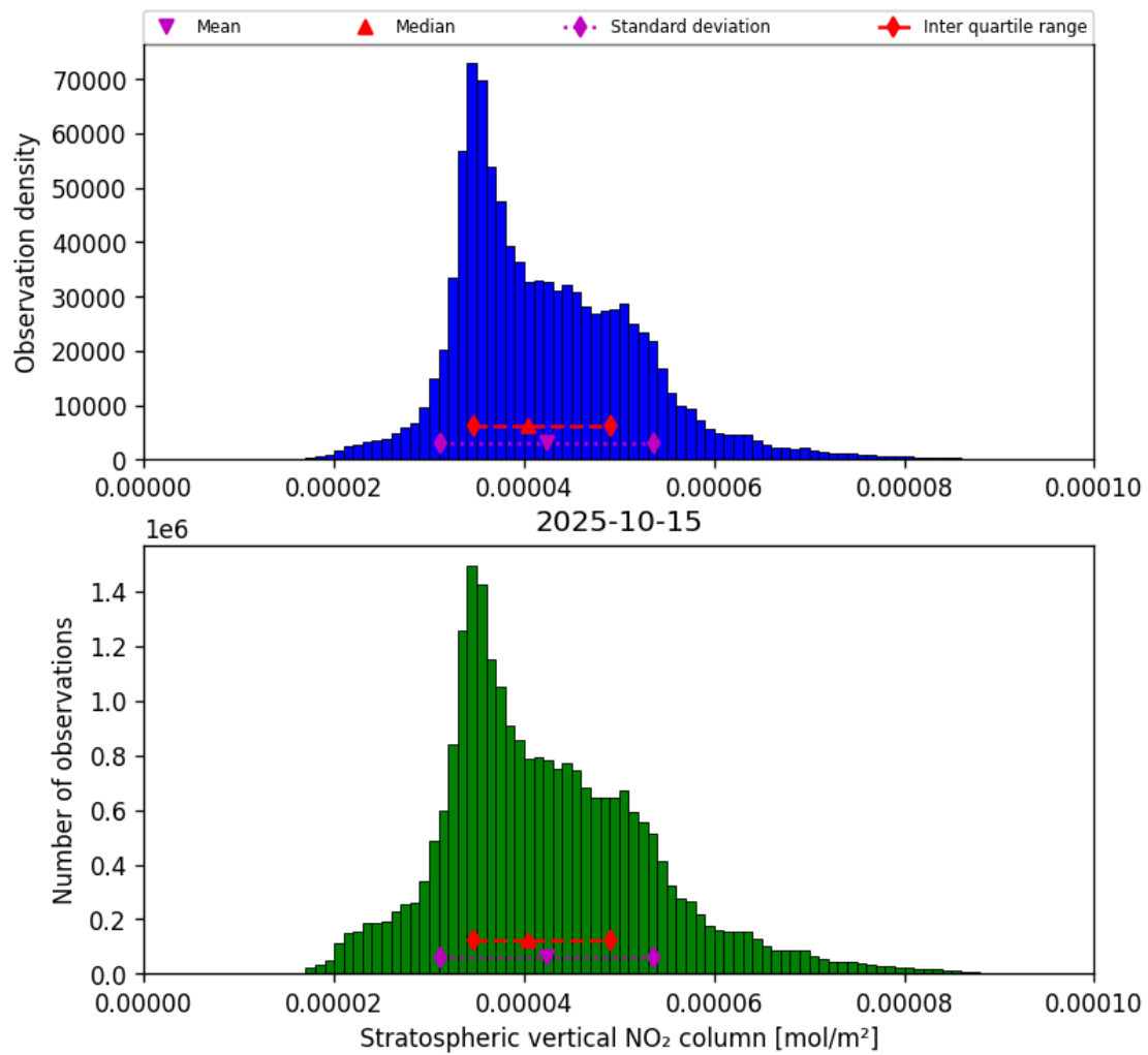
Figure 36: Histogram of “Stratospheric vertical NO 2 column” for 2025-10-14 to 2025-10-16
