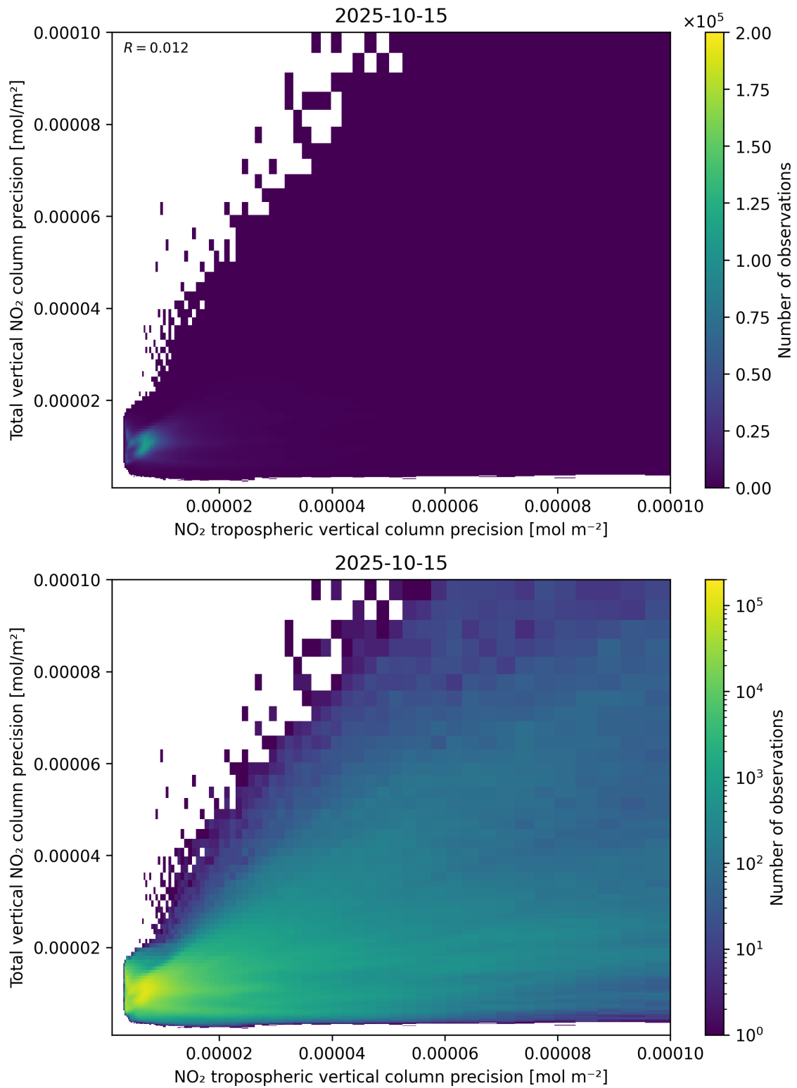
Figure 139: Scatter density plot of “NO 2 tropospheric vertical column precision” against “Total vertical NO 2 column precision” for 2025-10-14 to 2025-10-16.
