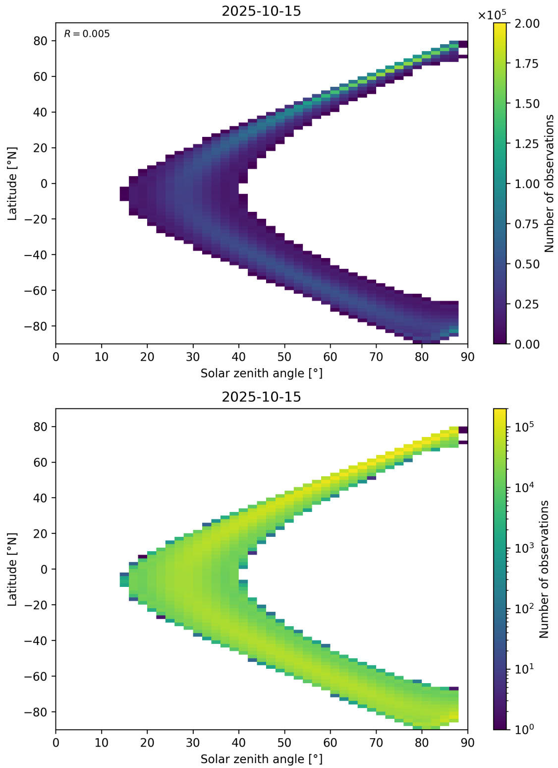
Figure 149: Scatter density plot of “Solar zenith angle” against “Latitude” for 2025-10-14 to 2025-10-16.
