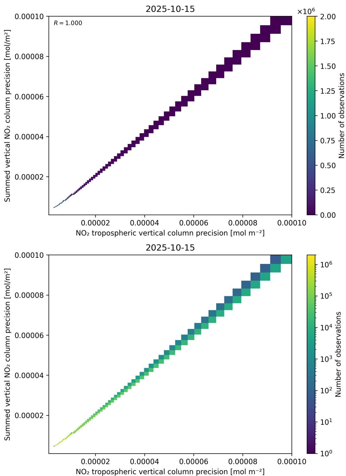
Figure 137: Scatter density plot of “NO 2 tropospheric vertical column precision” against “Summed vertical NO 2 column precision” for 2025-10-14 to 2025-10-16.
