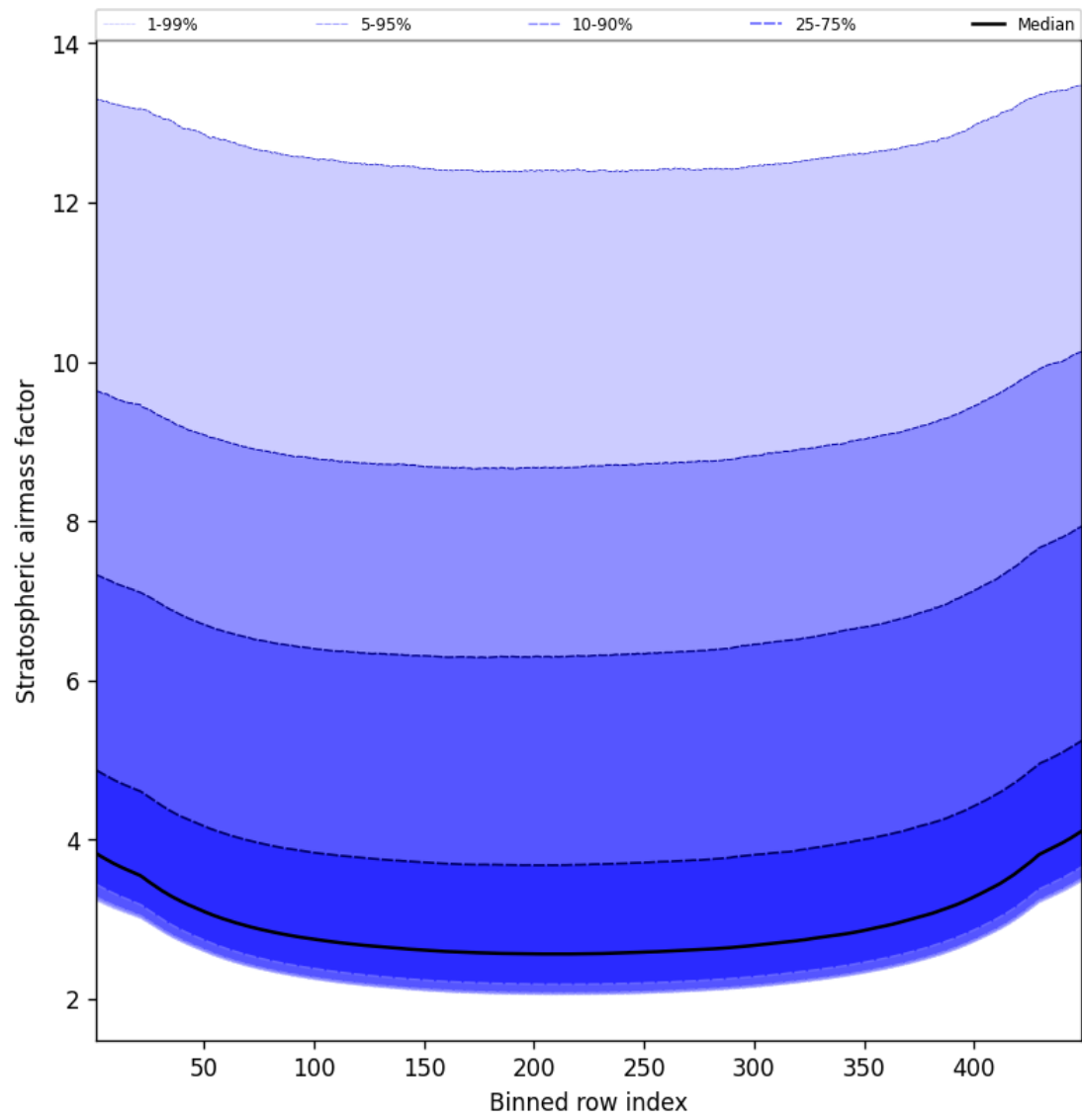
Figure 61: Along track statistics of “Stratospheric airmass factor” for 2025-10-14 to 2025-10-16
