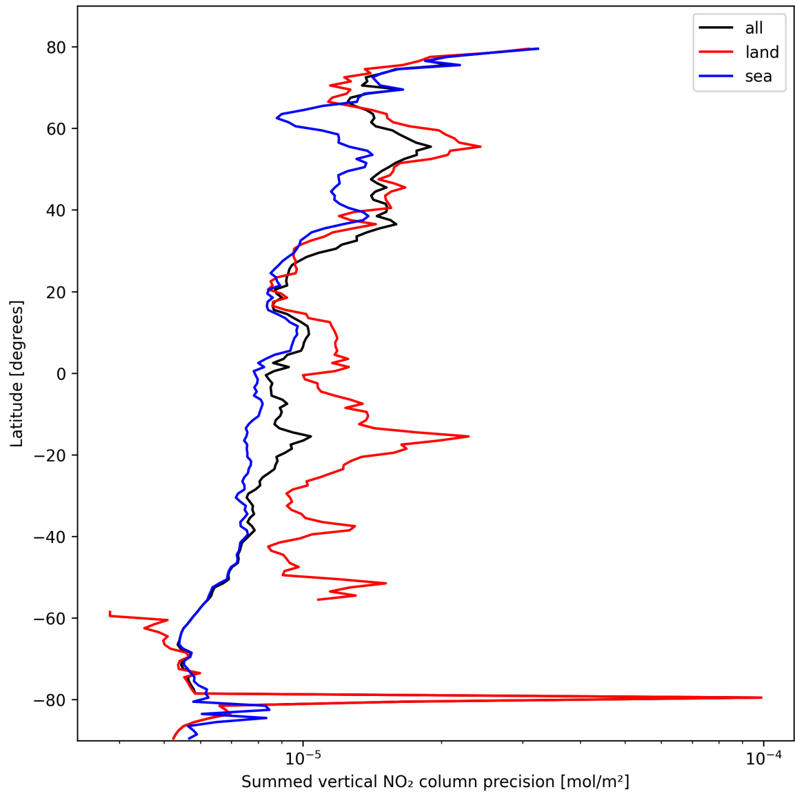
Figure 24: Zonal average of “Summed vertical NO 2 column precision” for 2025-10-14 to 2025-10-16.
