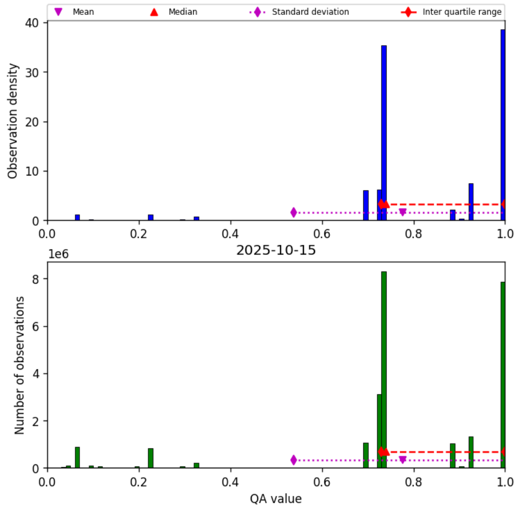
Figure 28: Histogram of “QA value” for 2025-10-14 to 2025-10-16
