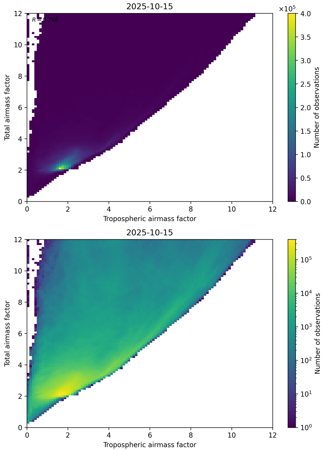
Figure 72: Scatter density plot of “Tropospheric airmass factor” against “Total airmass factor” for 2025-10-14 to 2025-10-16.
