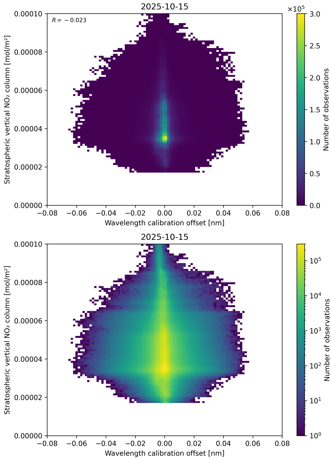
Figure 176: Scatter density plot of “Wavelength calibration offset” against “Stratospheric vertical NO 2 column” for 2025-10-14 to 2025-10-16.
