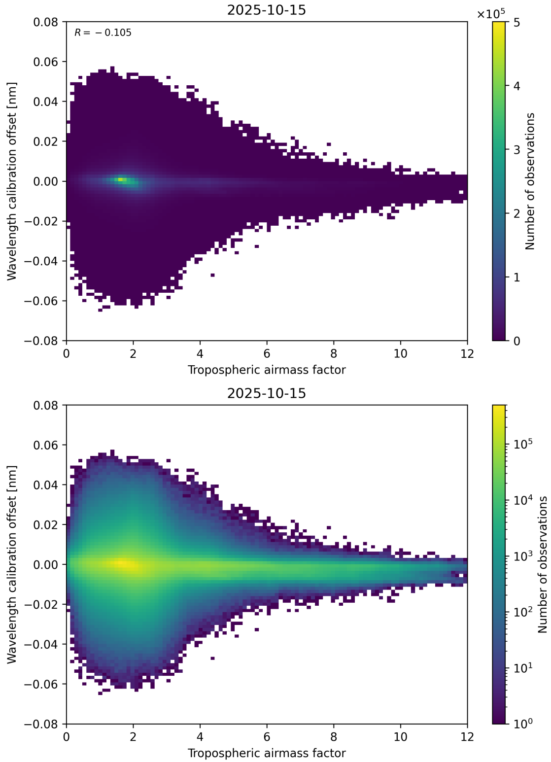
Figure 80: Scatter density plot of “Tropospheric airmass factor” against “Wavelength calibration offset” for 2025-10-14 to 2025-10-16.
