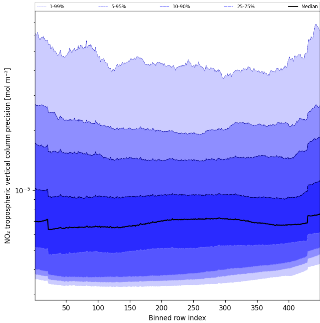
Figure 47: Along track statistics of “NO 2 tropospheric vertical column precision” for 2025-10-14 to 2025-10-16
