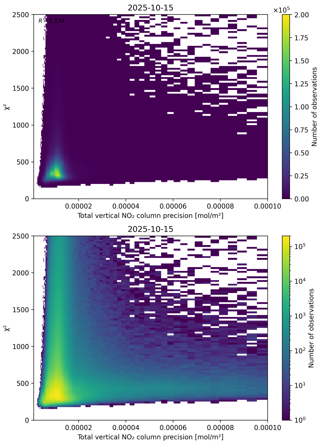
Figure 116: Scatter density plot of “Total vertical NO 2 column precision” against “ \chi^2 ” for 2025-10-14 to 2025-10-16.
