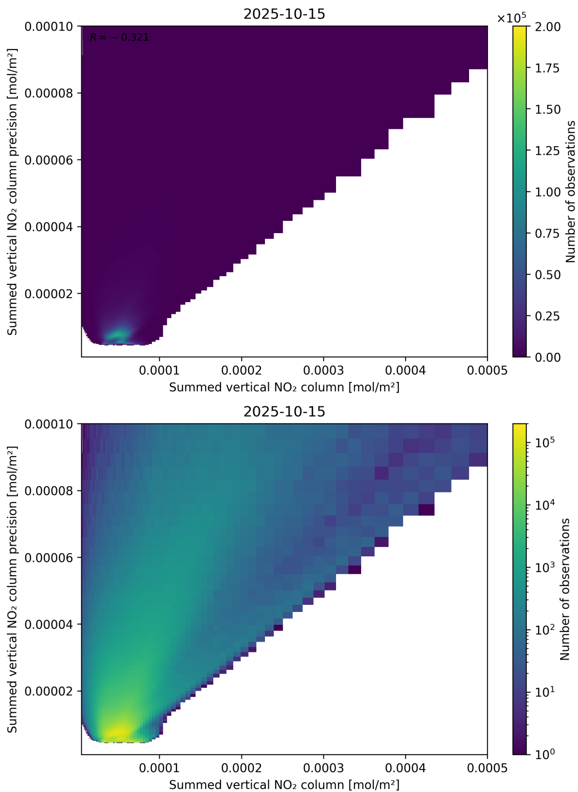
Figure 105: Scatter density plot of “Summed vertical NO 2 column” against “Summed vertical NO 2 column precision” for 2025-10-14 to 2025-10-16.
