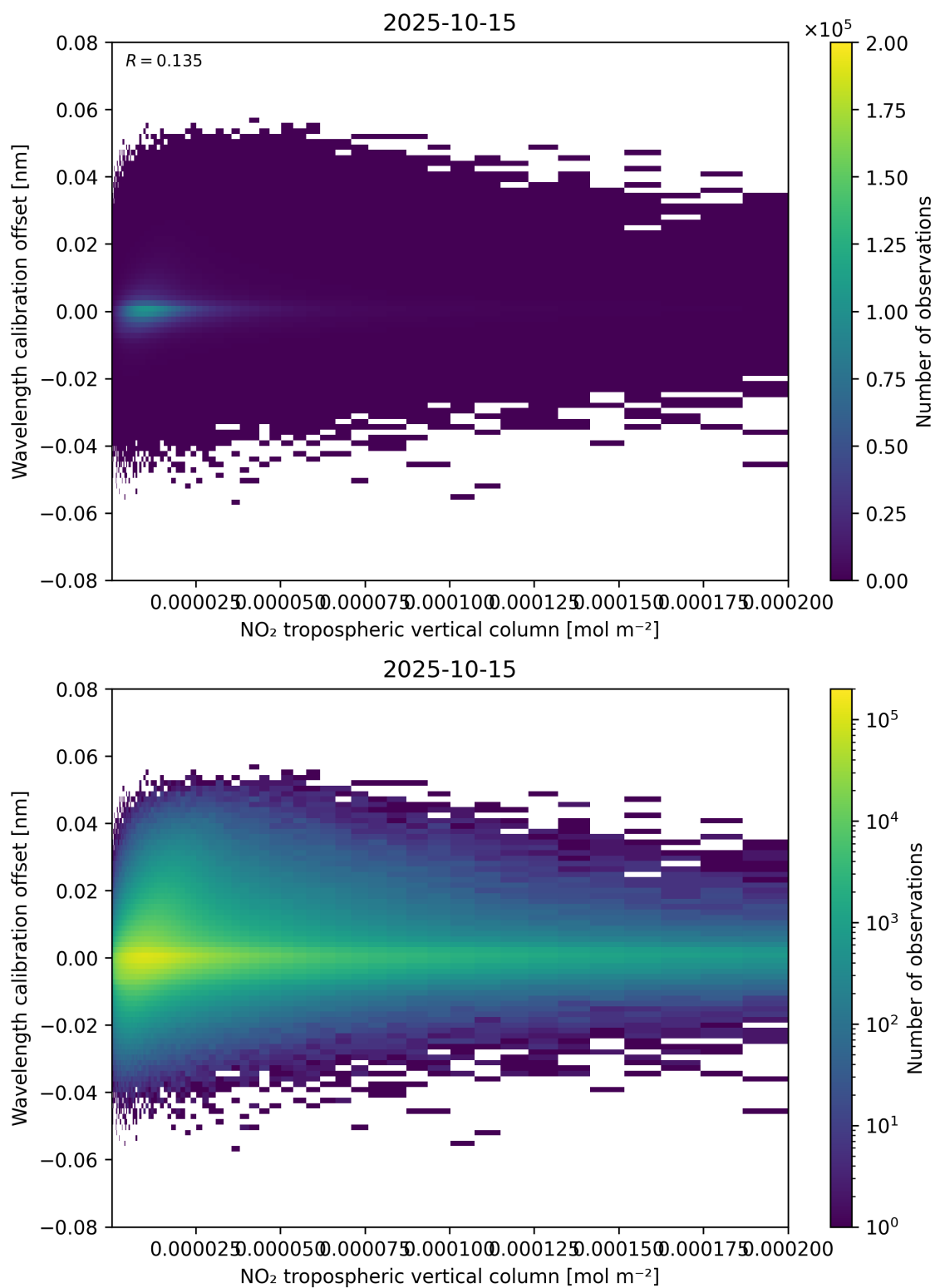
Figure 143: Scatter density plot of “NO 2 tropospheric vertical column” against “Wavelength calibration offset” for 2025-10-14 to 2025-10-16.
