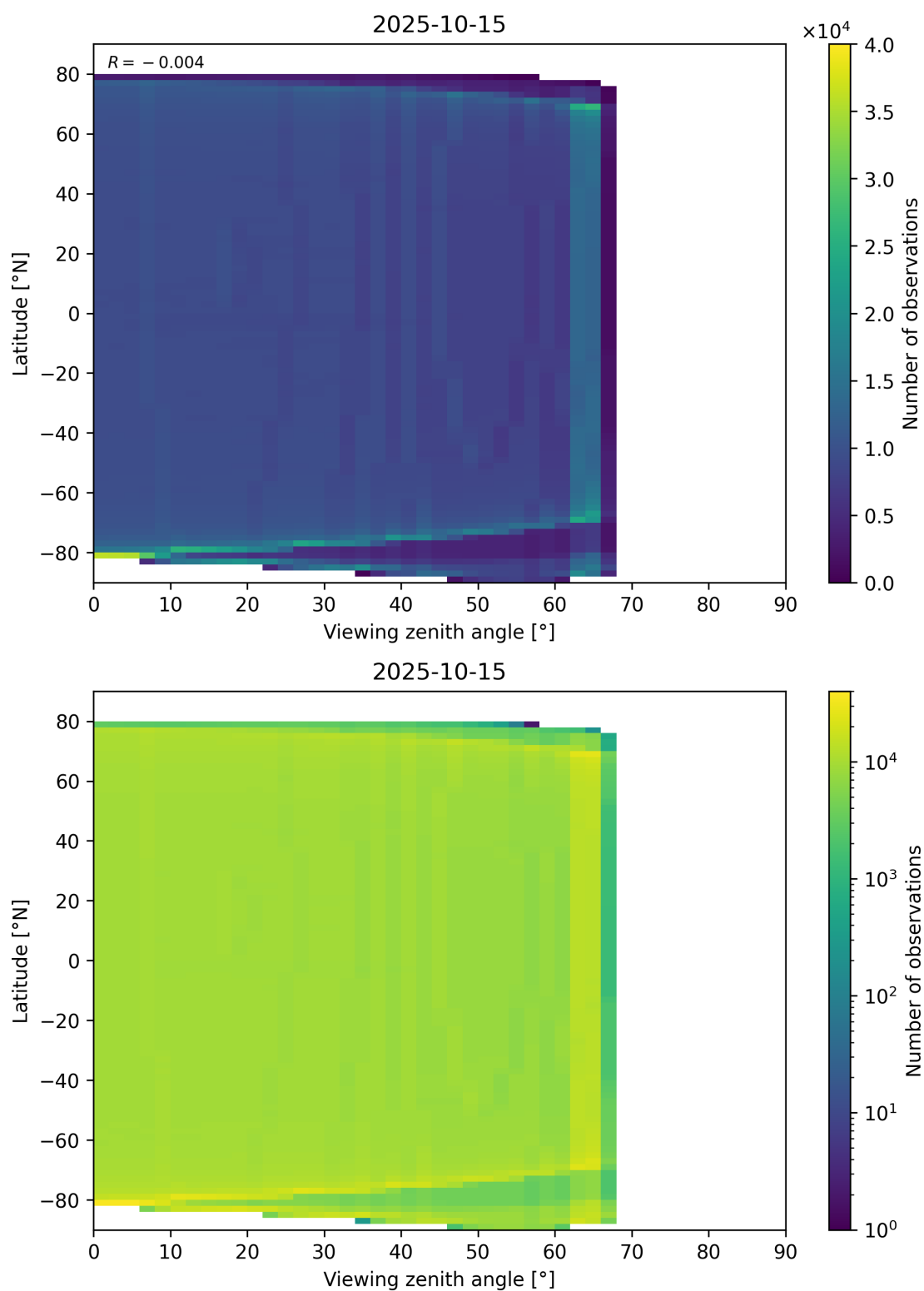
Figure 163: Scatter density plot of “Viewing zenith angle” against “Latitude” for 2025-10-14 to 2025-10-16.
