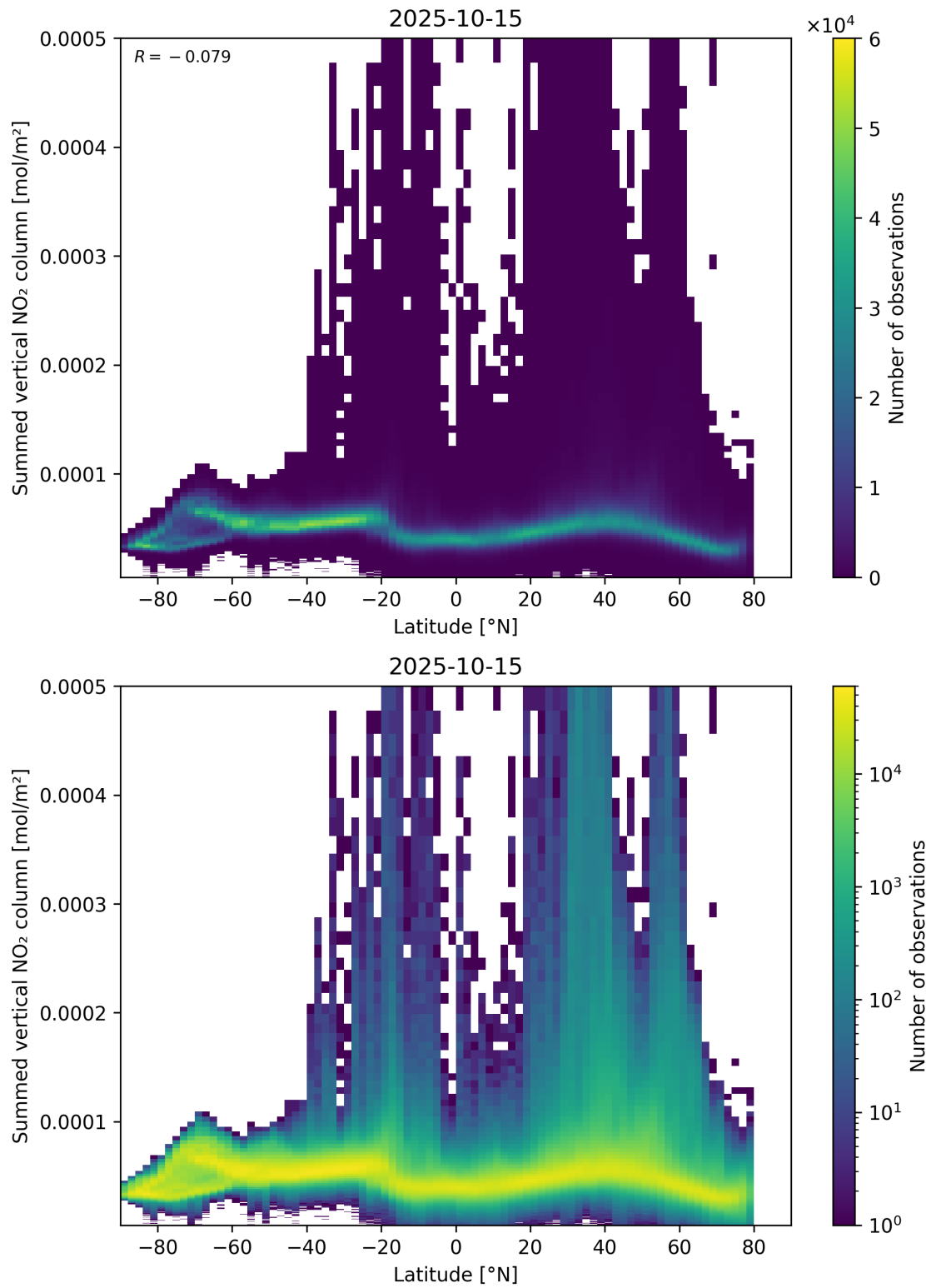
Figure 88: Scatter density plot of “Latitude” against “Summed vertical NO 2 column” for 2025-10-14 to 2025-10-16.
