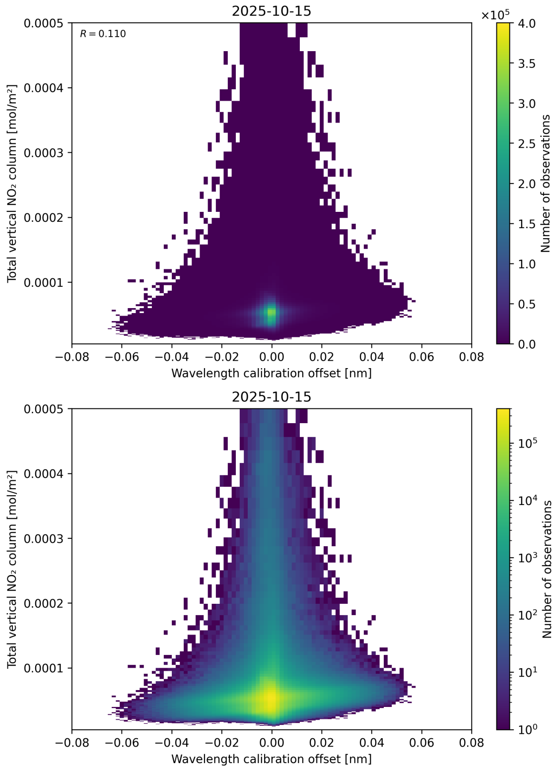
Figure 179: Scatter density plot of “Wavelength calibration offset” against “Total vertical NO 2 column” for 2025-10-14 to 2025-10-16.
