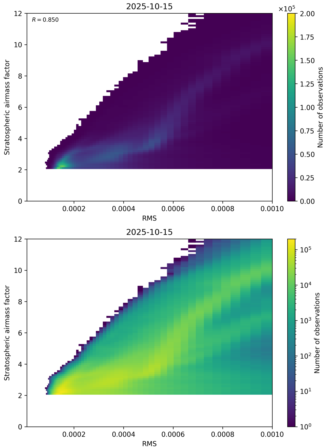
Figure 144: Scatter density plot of “RMS” against “Stratospheric airmass factor” for 2025-10-14 to 2025-10-16.
