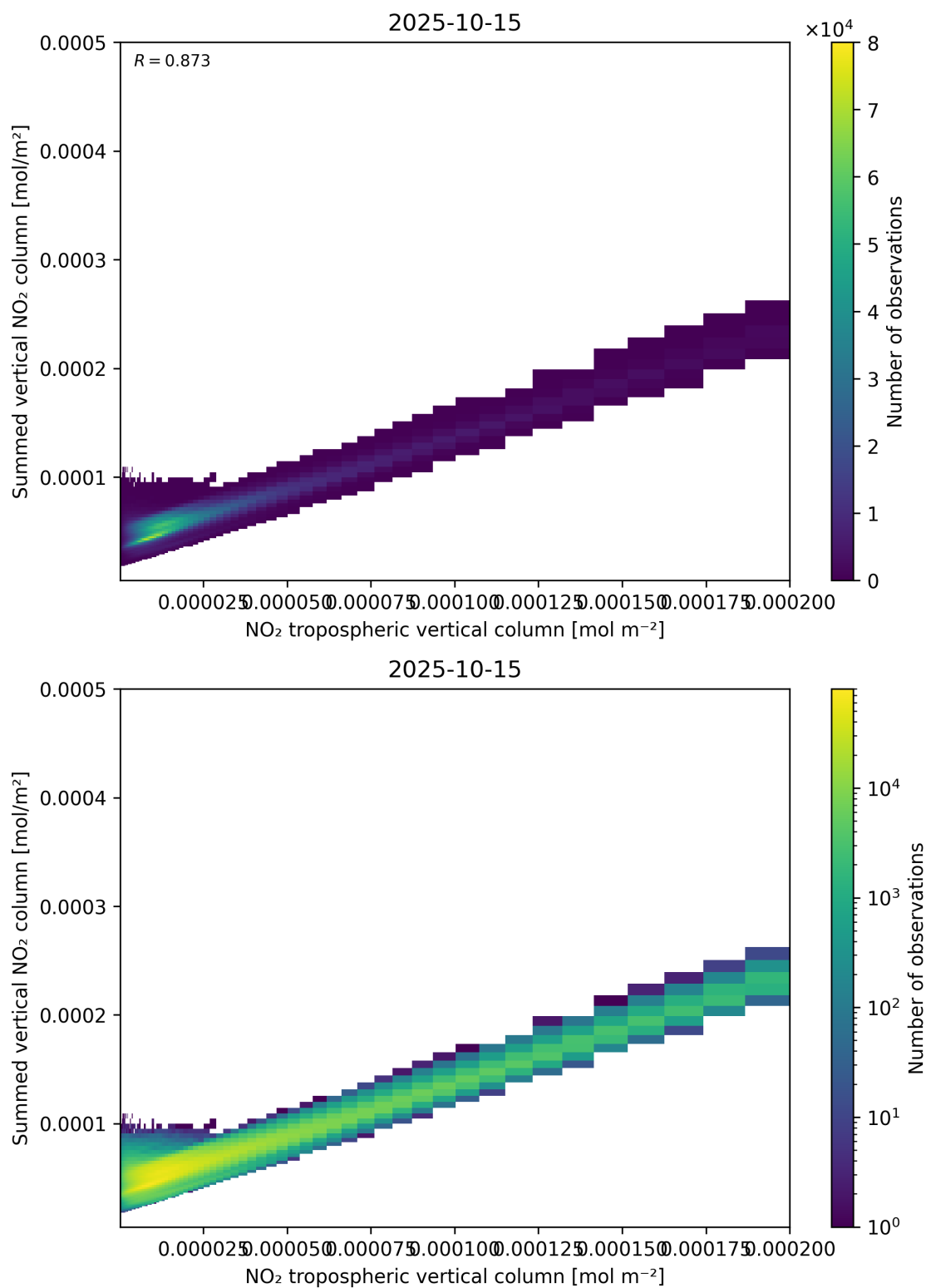
Figure 126: Scatter density plot of “NO 2 tropospheric vertical column” against “Summed vertical NO 2 column” for 2025-10-14 to 2025-10-16.
