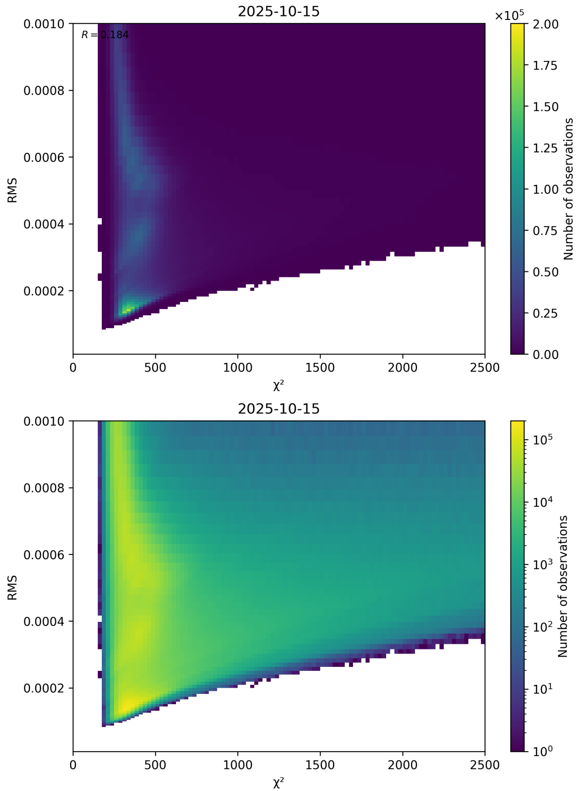
Figure 82: Scatter density plot of “ \chi^2 ” against “RMS” for 2025-10-14 to 2025-10-16.
