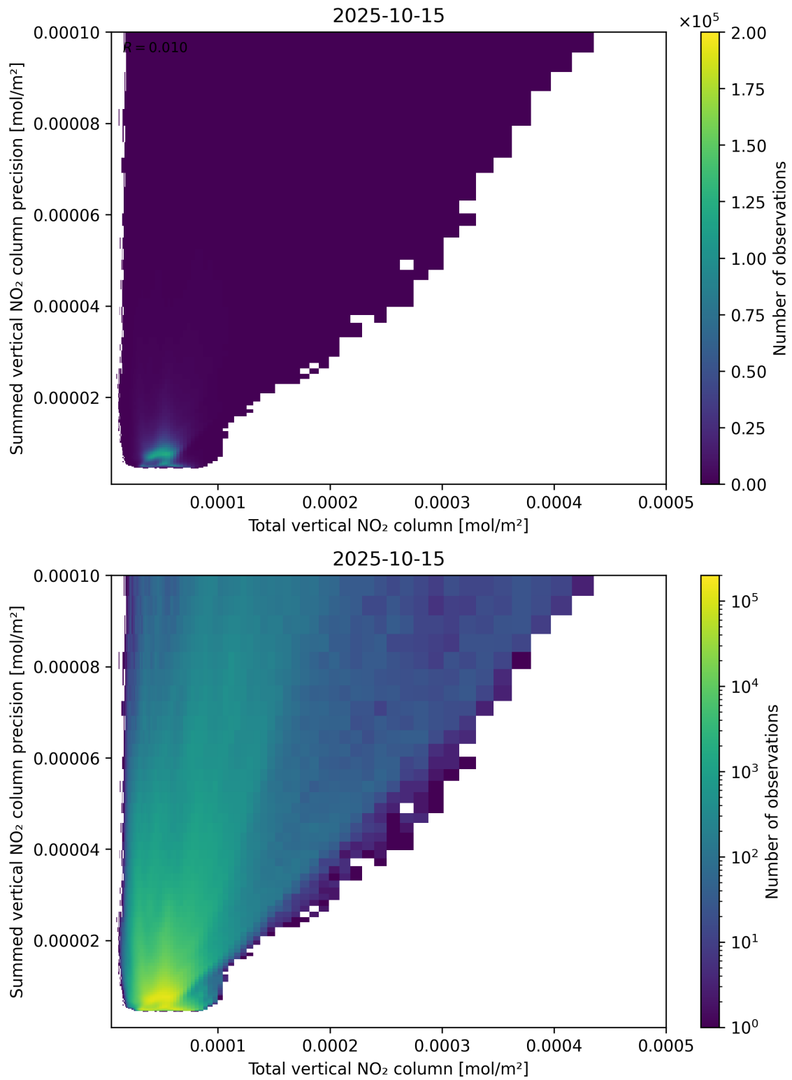
Figure 113: Scatter density plot of “Total vertical NO 2 column” against “Summed vertical NO 2 column precision” for 2025-10-14 to 2025-10-16.
