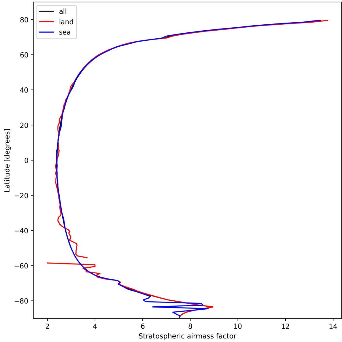
Figure 27: Zonal average of “Stratospheric air mass factor” for 2025-10-14 to 2025-10-16.
