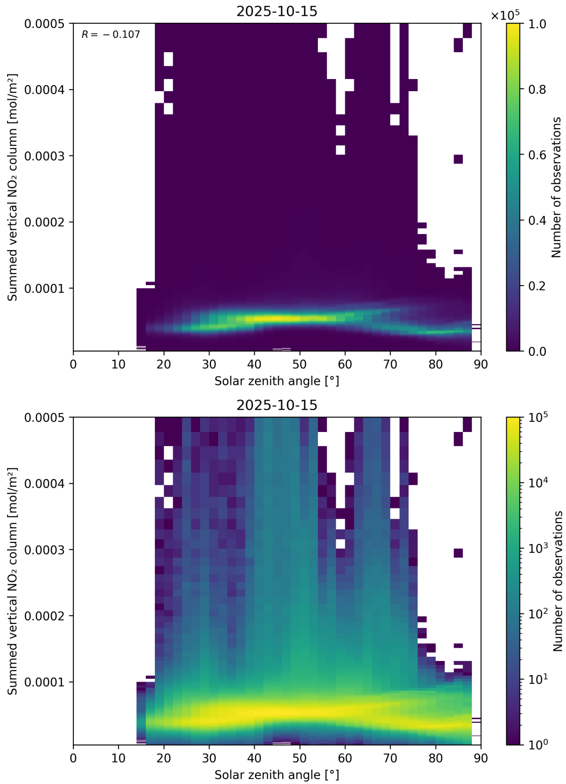
Figure 151: Scatter density plot of “Solar zenith angle” against “Summed vertical NO 2 column” for 2025-10-14 to 2025-10-16.
