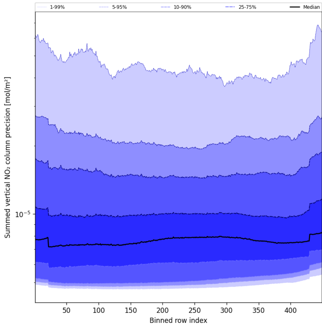
Figure 58: Along track statistics of “Summed vertical NO 2 column precision” for 2025-10-14 to 2025-10-16
