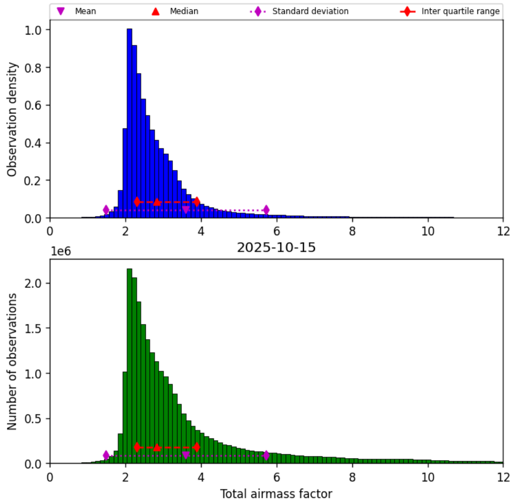
Figure 32: Histogram of “Total airmass factor” for 2025-10-14 to 2025-10-16
