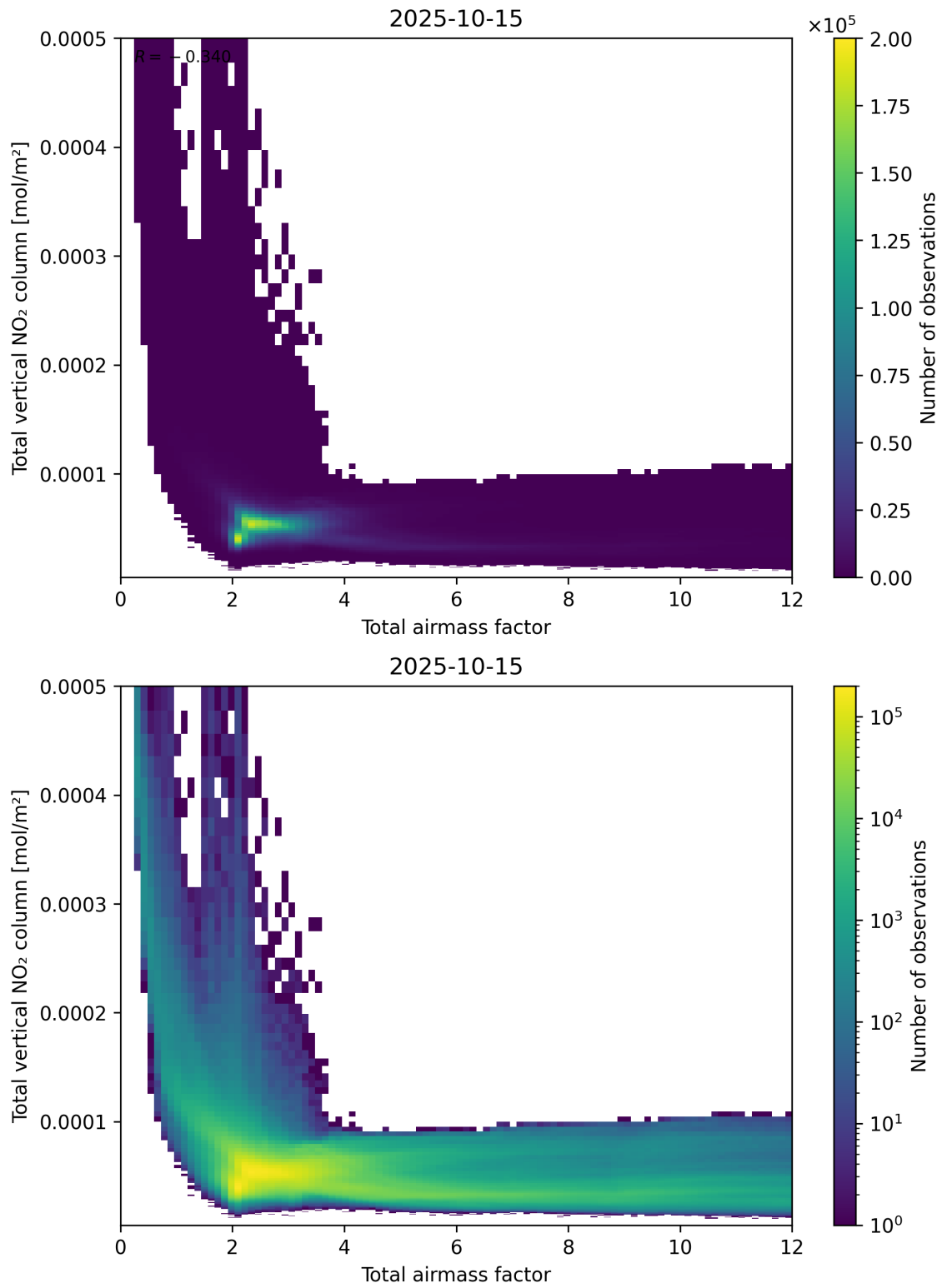
Figure 67: Scatter density plot of “Total airmass factor” against “Total vertical NO 2 column” for 2025-10-14 to 2025-10-16.
