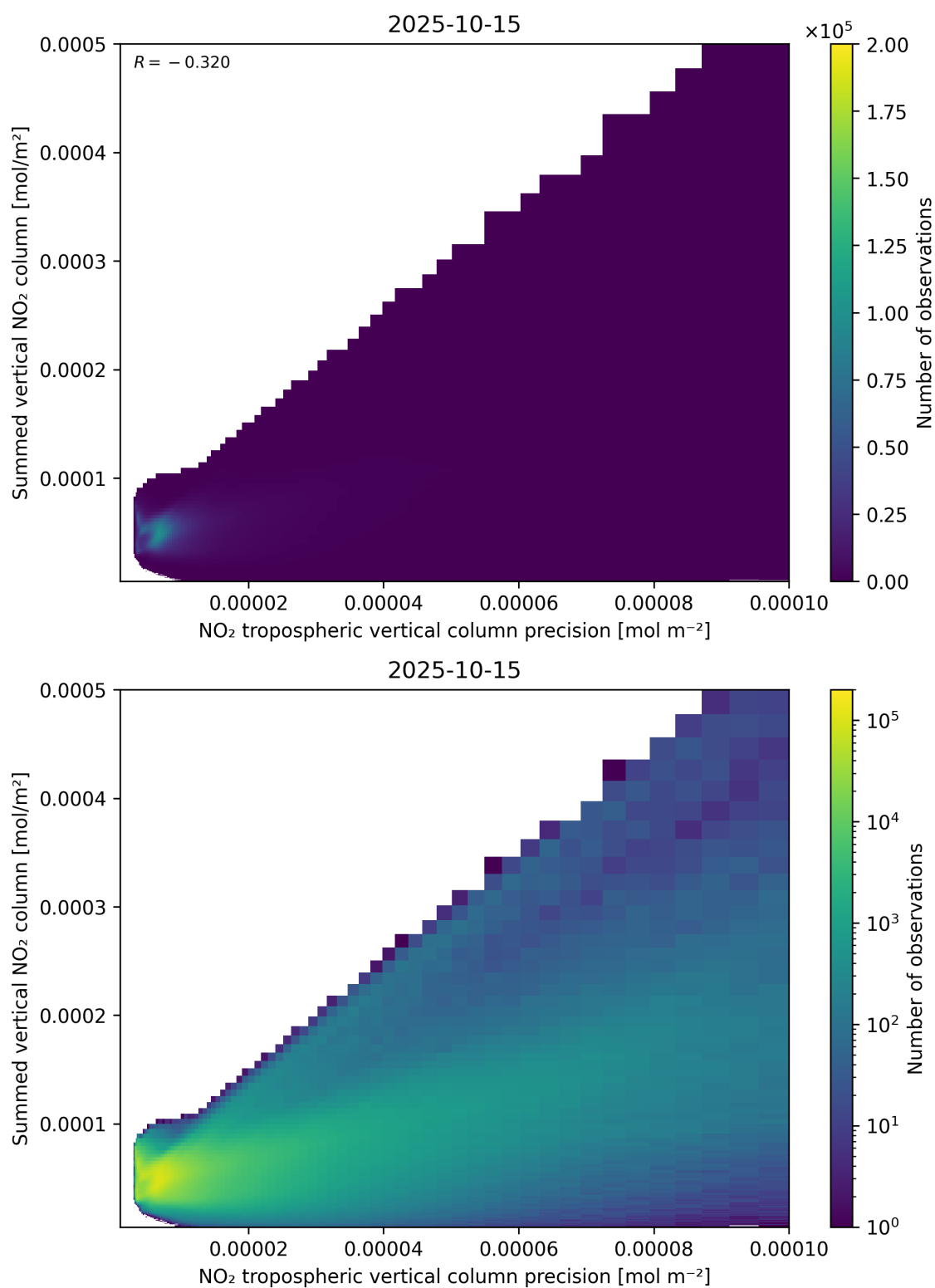
Figure 136: Scatter density plot of “NO 2 tropospheric vertical column precision” against “Summed vertical NO 2 column” for 2025-10-14 to 2025-10-16.
