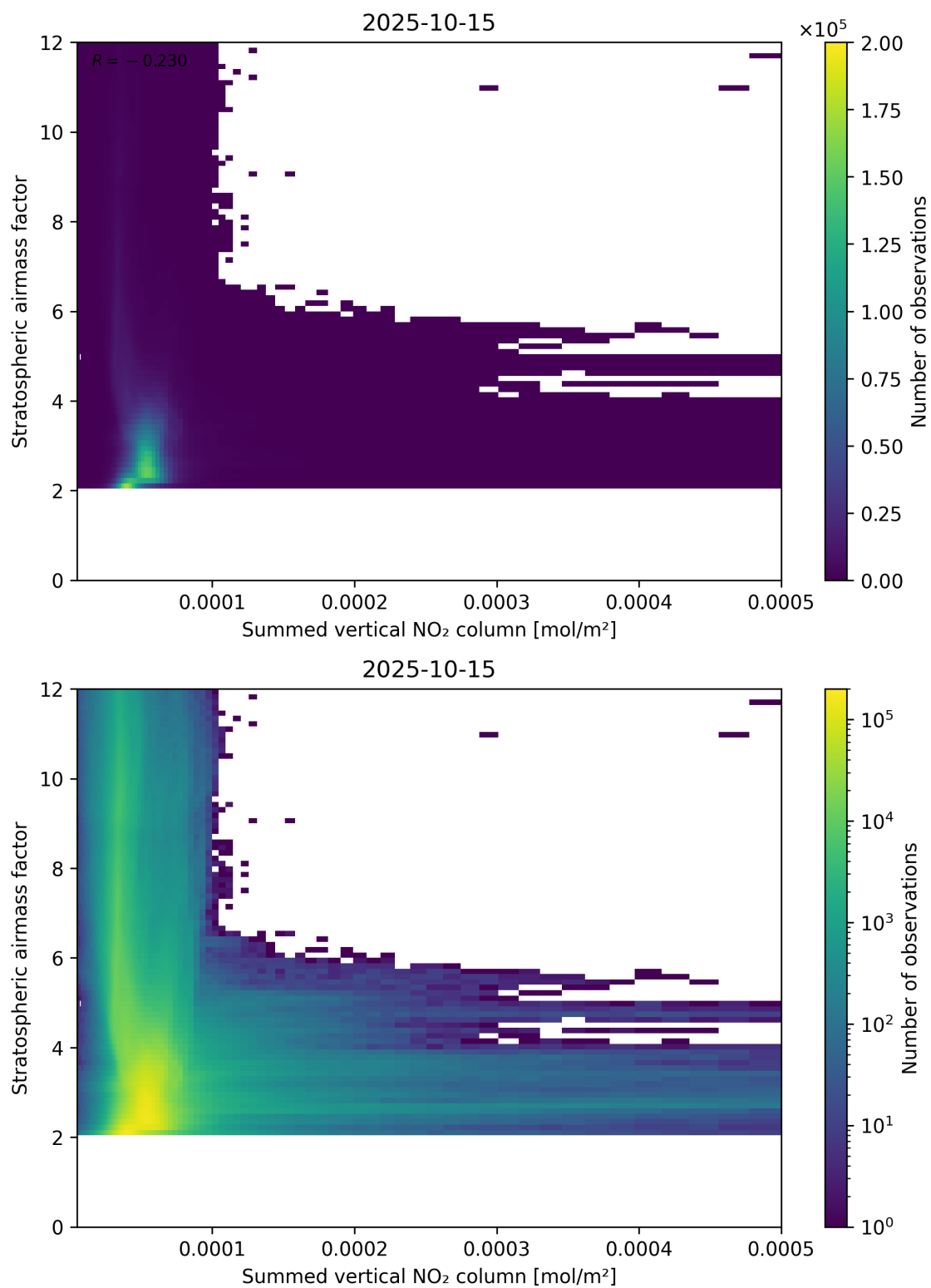
Figure 103: Scatter density plot of “Summed vertical NO 2 column” against “Stratospheric airmass factor” for 2025-10-14 to 2025-10-16.
