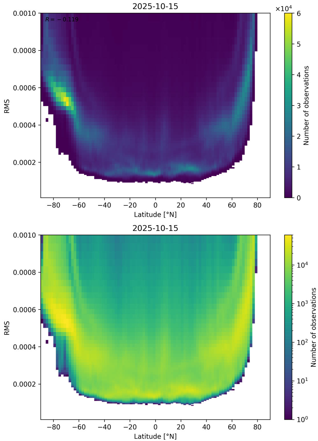
Figure 94: Scatter density plot of “Latitude” against “RMS” for 2025-10-14 to 2025-10-16.
