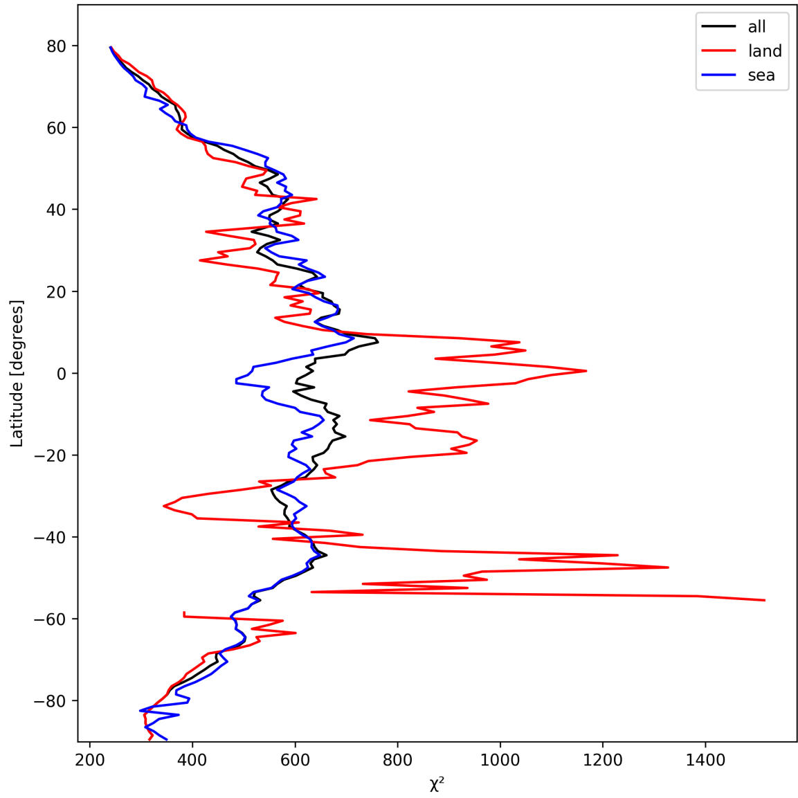
Figure 25: Zonal average of “ \chi^2 ” for 2025-10-14 to 2025-10-16.
