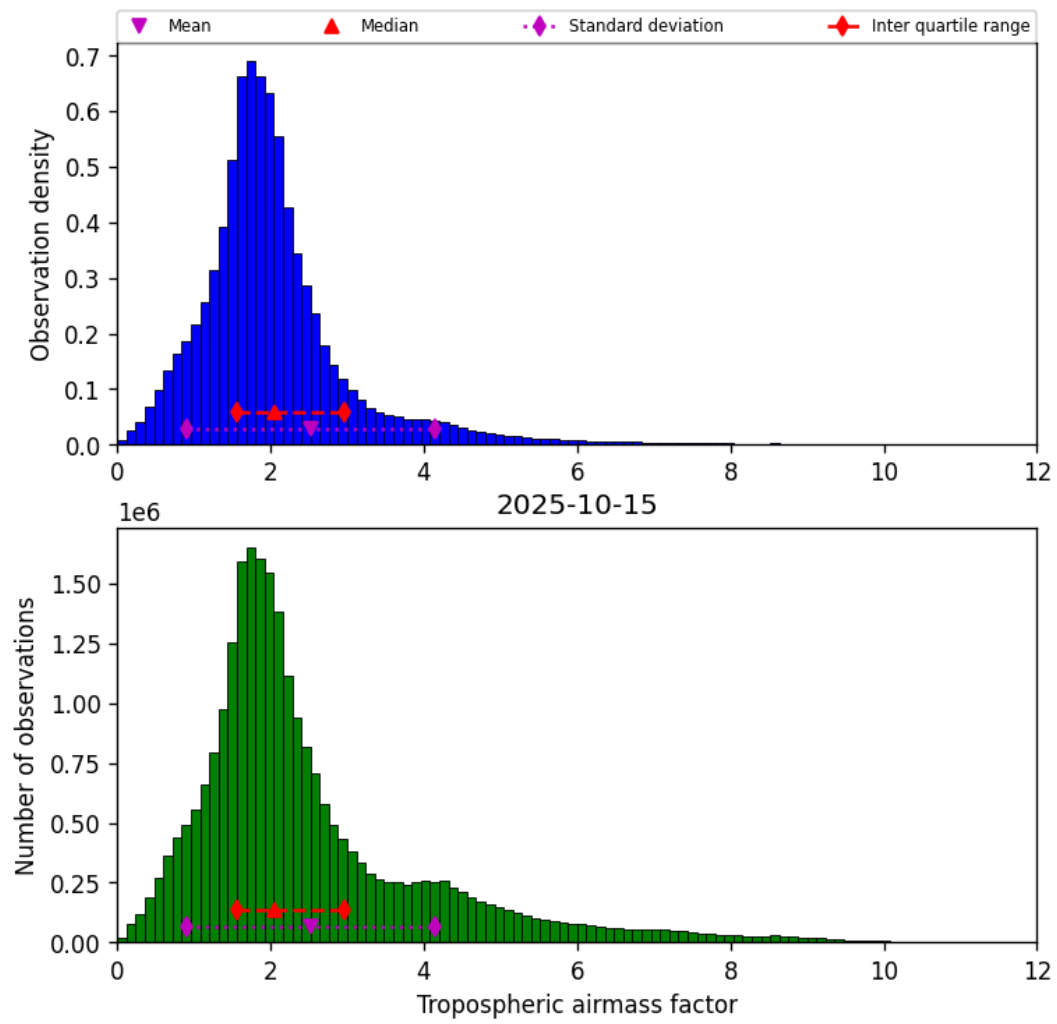
Figure 31: Histogram of “Tropospheric airmass factor” for 2025-10-14 to 2025-10-16
