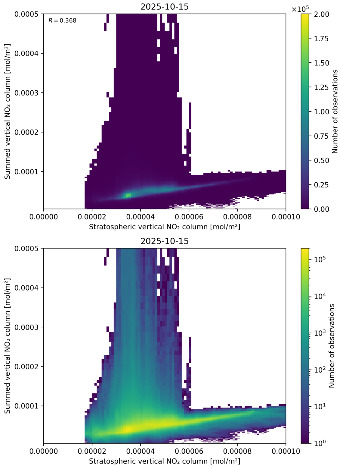
Figure 98: Scatter density plot of “Stratospheric vertical NO 2 column” against “Summed vertical NO 2 column” for 2025-10-14 to 2025-10-16.
