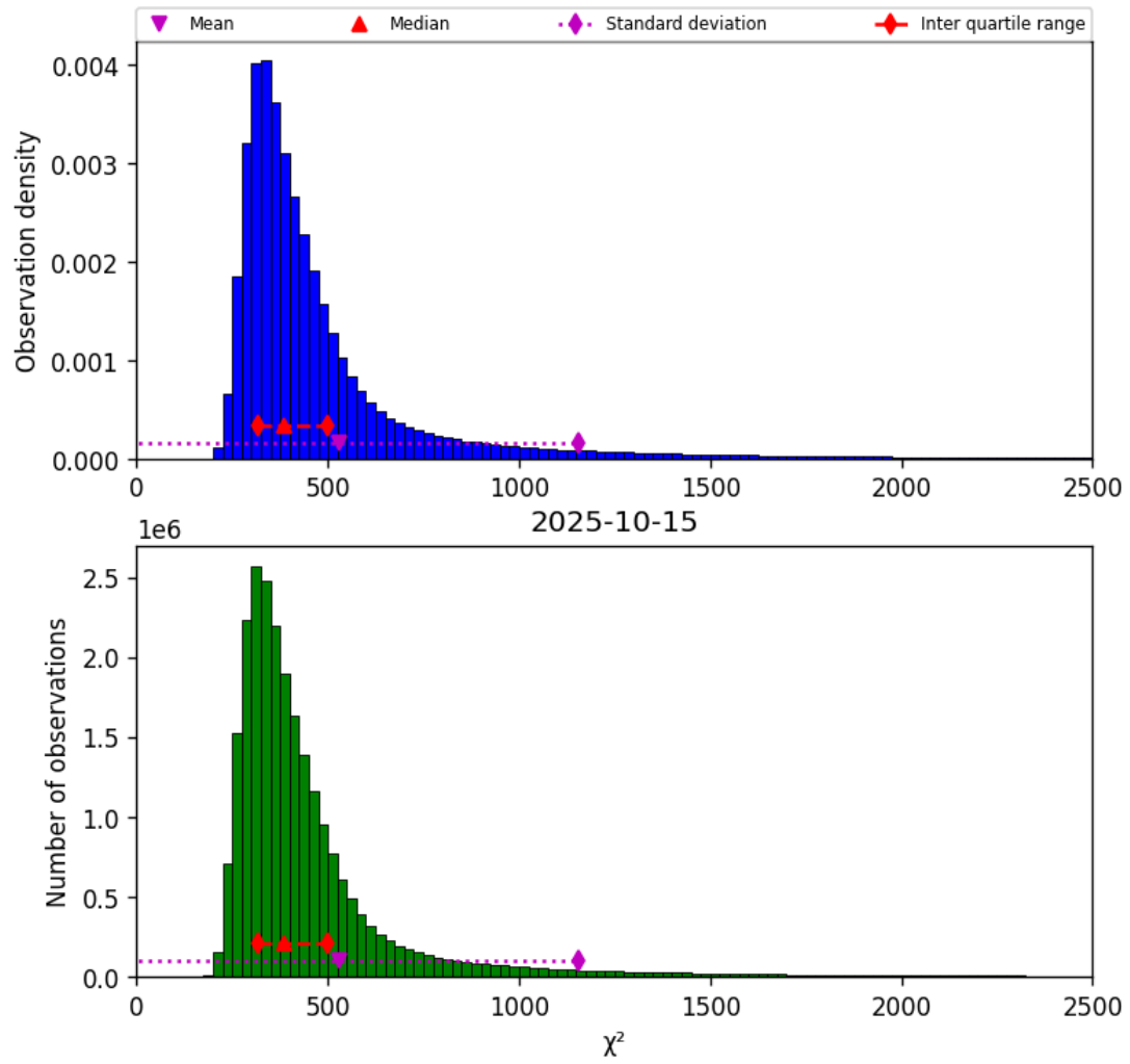
Figure 42: Histogram of “ \chi^2 ” for 2025-10-14 to 2025-10-16
