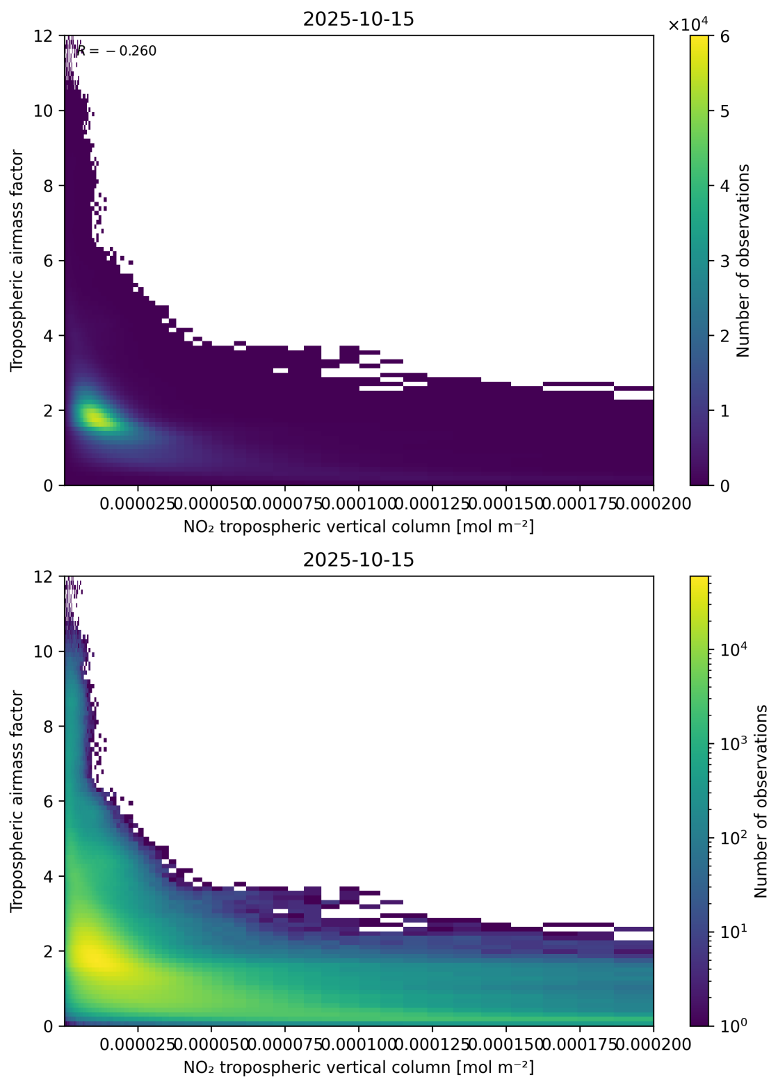
Figure 123: Scatter density plot of “NO 2 tropospheric vertical column” against “Tropospheric air mass factor” for 2025-10-14 to 2025-10-16.
