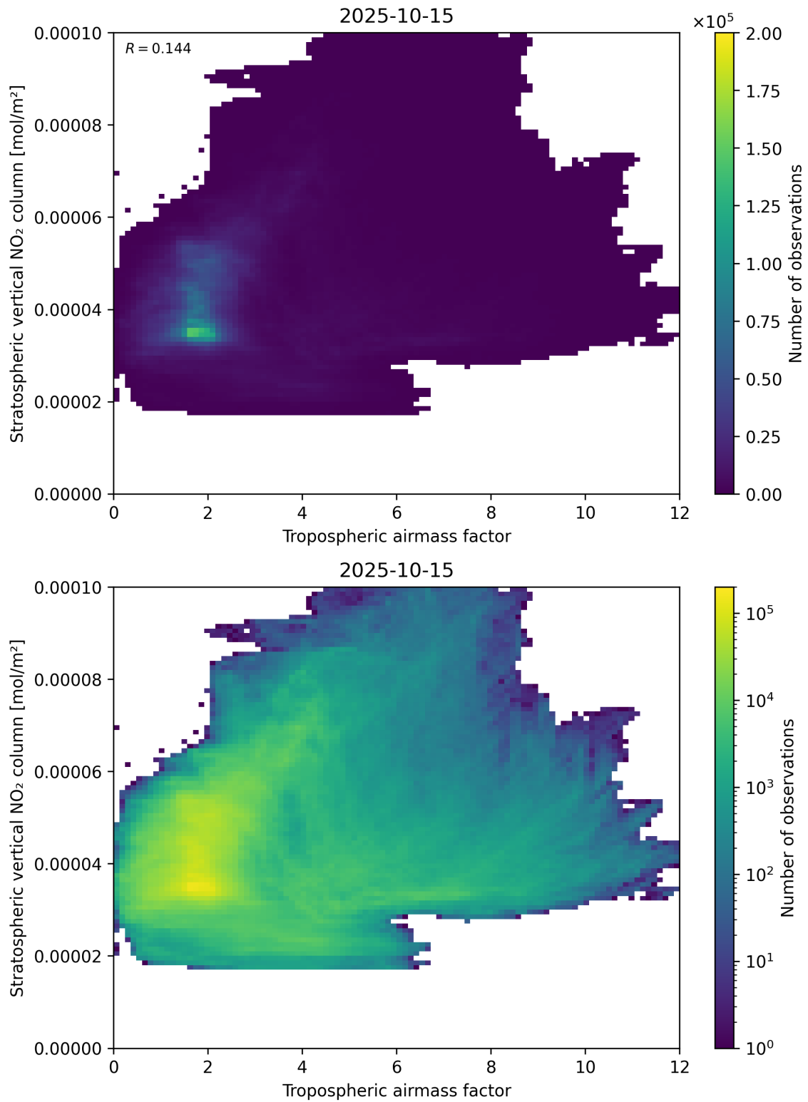
Figure 74: Scatter density plot of “Tropospheric air mass factor” against “Stratospheric vertical NO 2 column” for 2025-10-14 to 2025-10-16.
