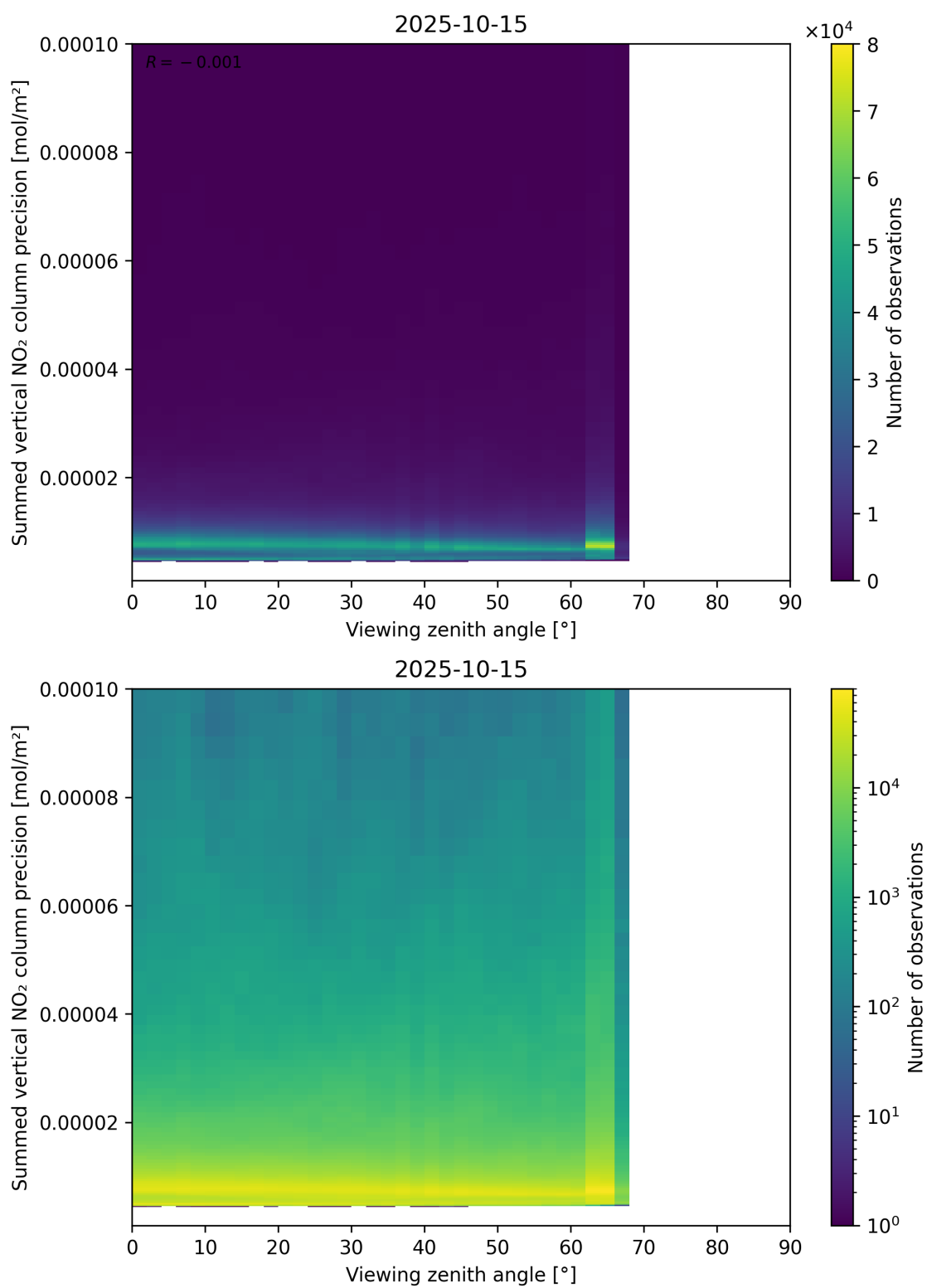
Figure 166: Scatter density plot of “Viewing zenith angle” against “Summed vertical NO 2 column precision” for 2025-10-14 to 2025-10-16.
