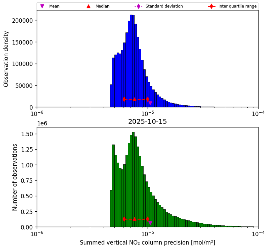
Figure 41: Histogram of "Summed vertical NO 2 column precision" for 2025-10-14 to 2025-10-16
