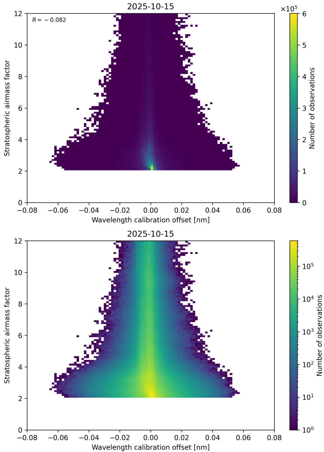
Figure 174: Scatter density plot of “Wavelength calibration offset” against “Stratospheric airmass factor” for 2025-10-14 to 2025-10-16.
