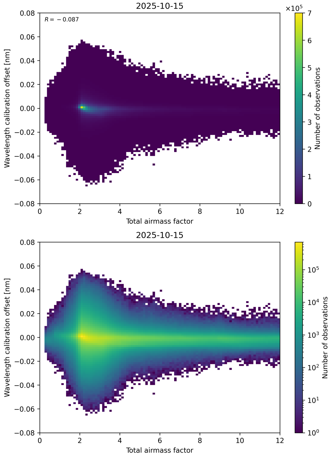
Figure 70: Scatter density plot of “Total airmass factor” against “Wavelength calibration offset” for 2025-10-14 to 2025-10-16.
