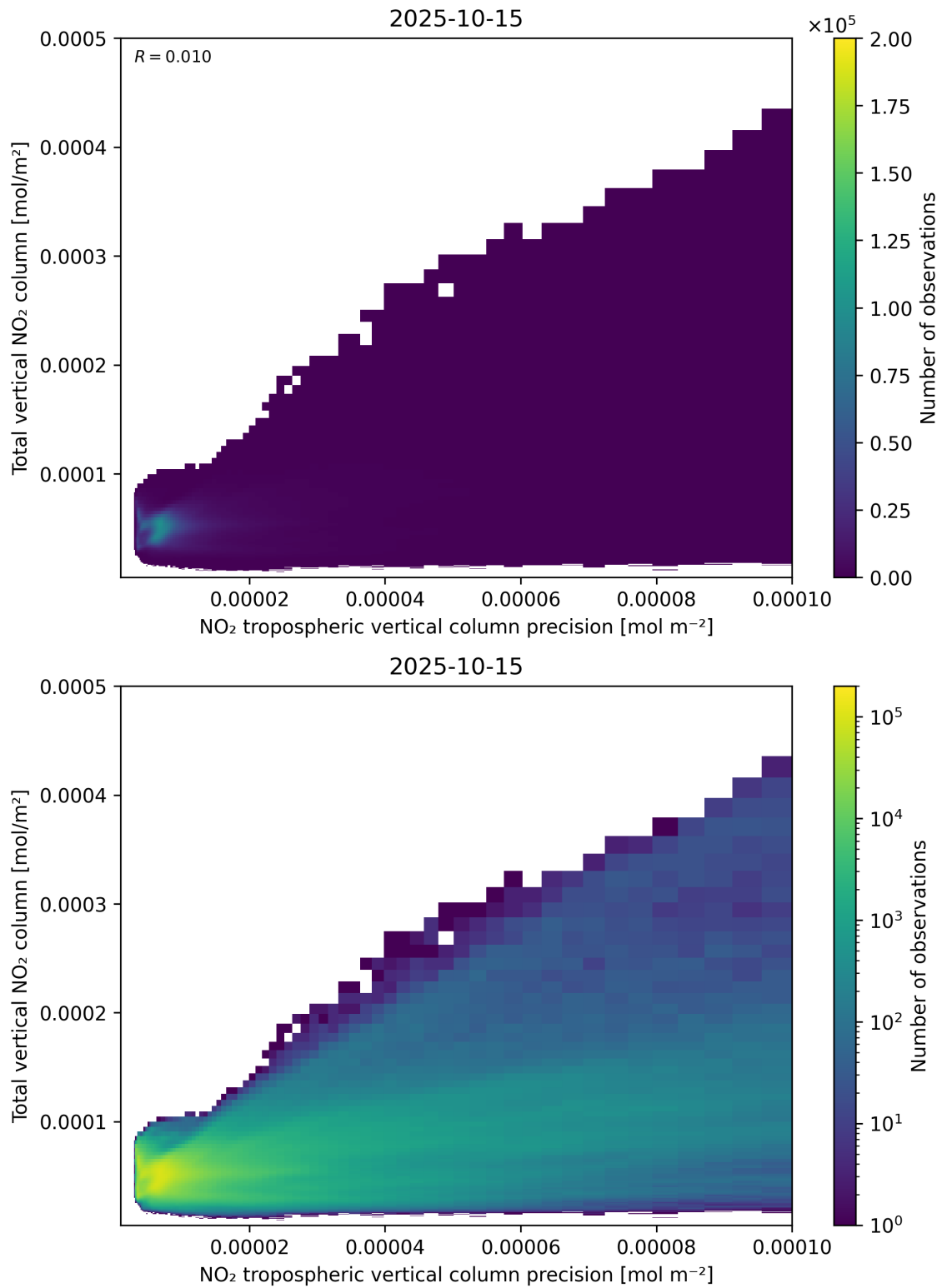
Figure 138: Scatter density plot of “NO 2 tropospheric vertical column precision” against “Total vertical NO 2 column” for 2025-10-14 to 2025-10-16.
