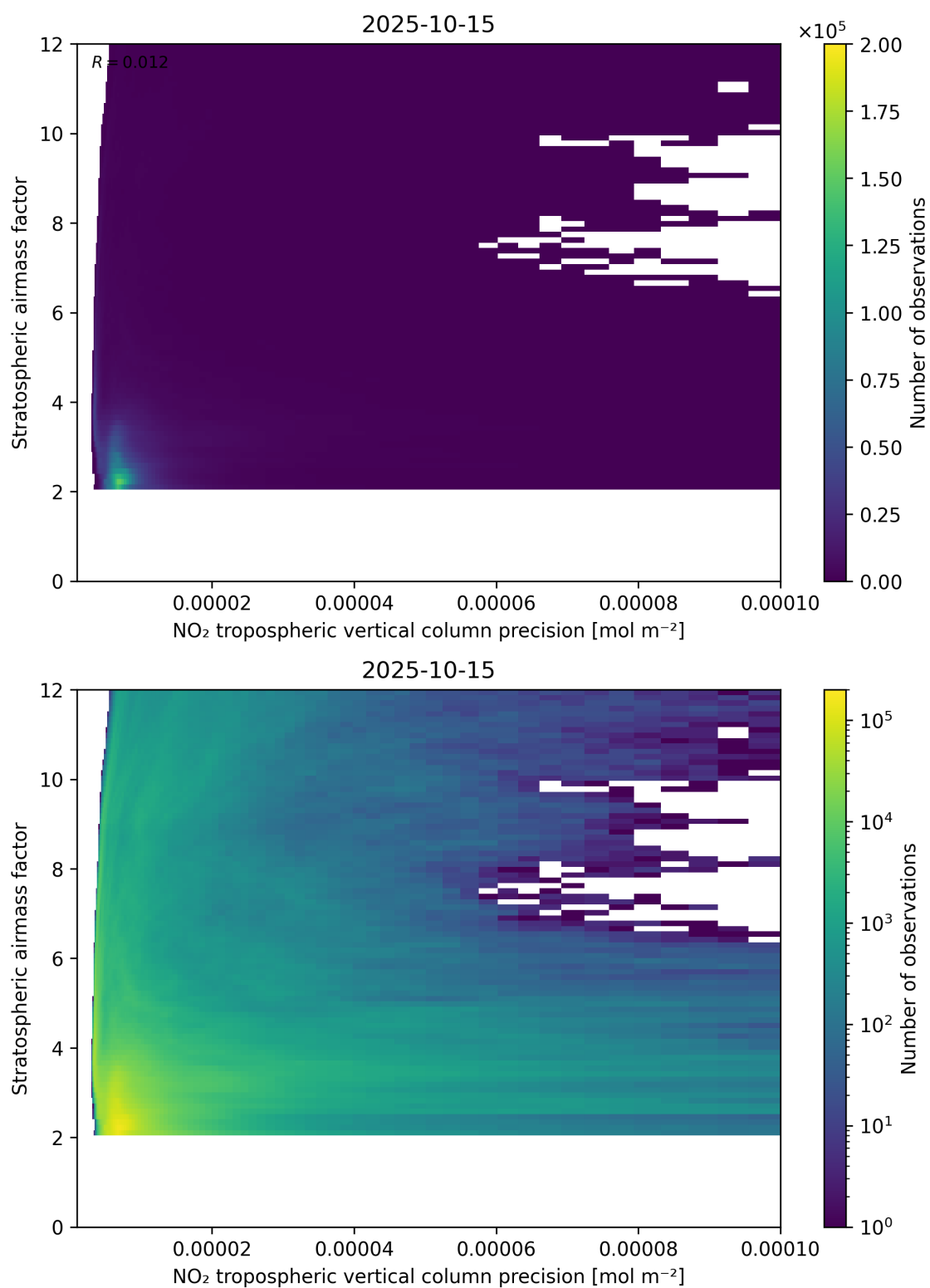
Figure 131: Scatter density plot of “NO 2 tropospheric vertical column precision” against “Stratospheric airmass factor” for 2025-10-14 to 2025-10-16.
