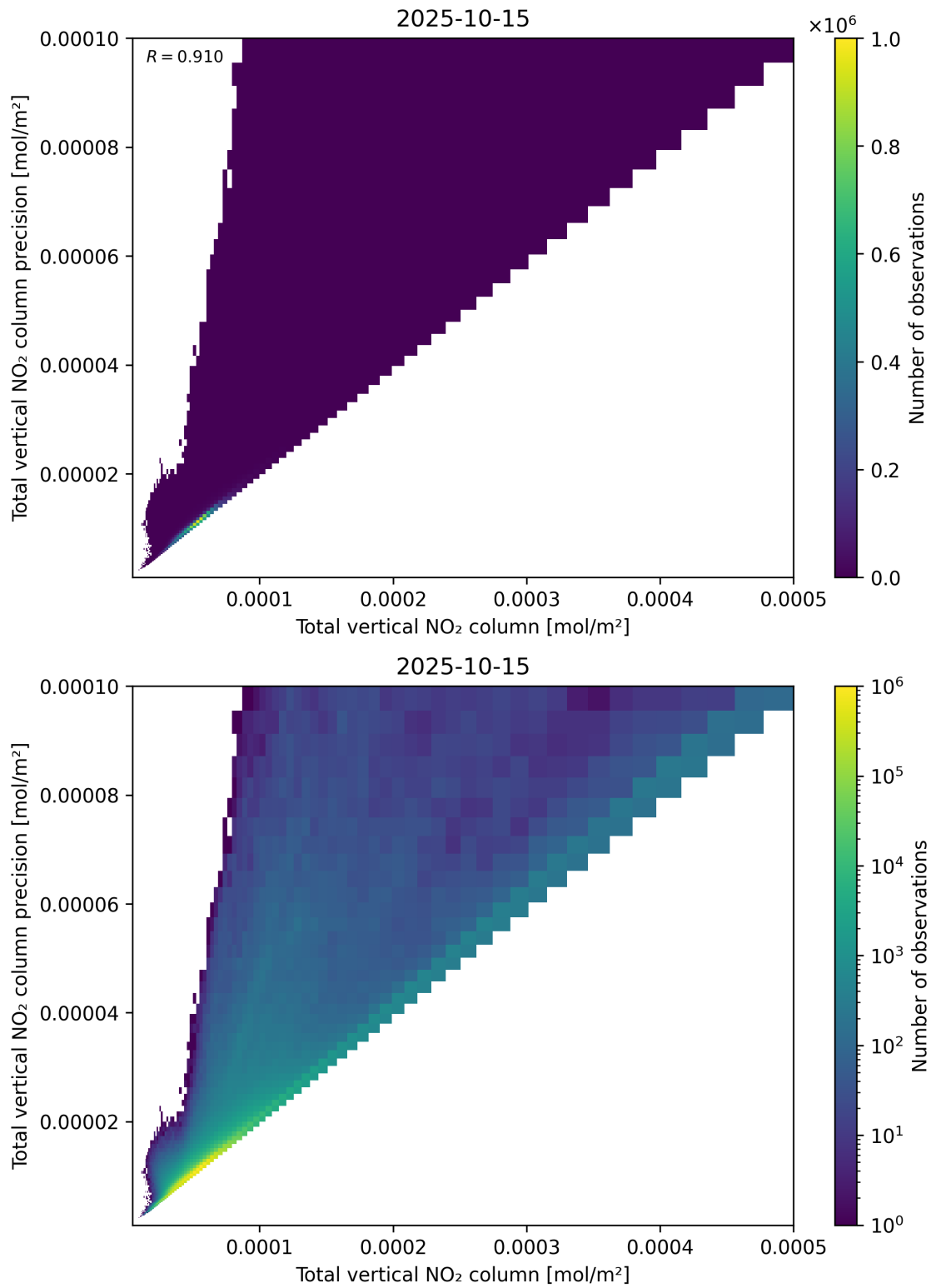
Figure 114: Scatter density plot of “Total vertical NO 2 column” against “Total vertical NO 2 column precision” for 2025-10-14 to 2025-10-16.
