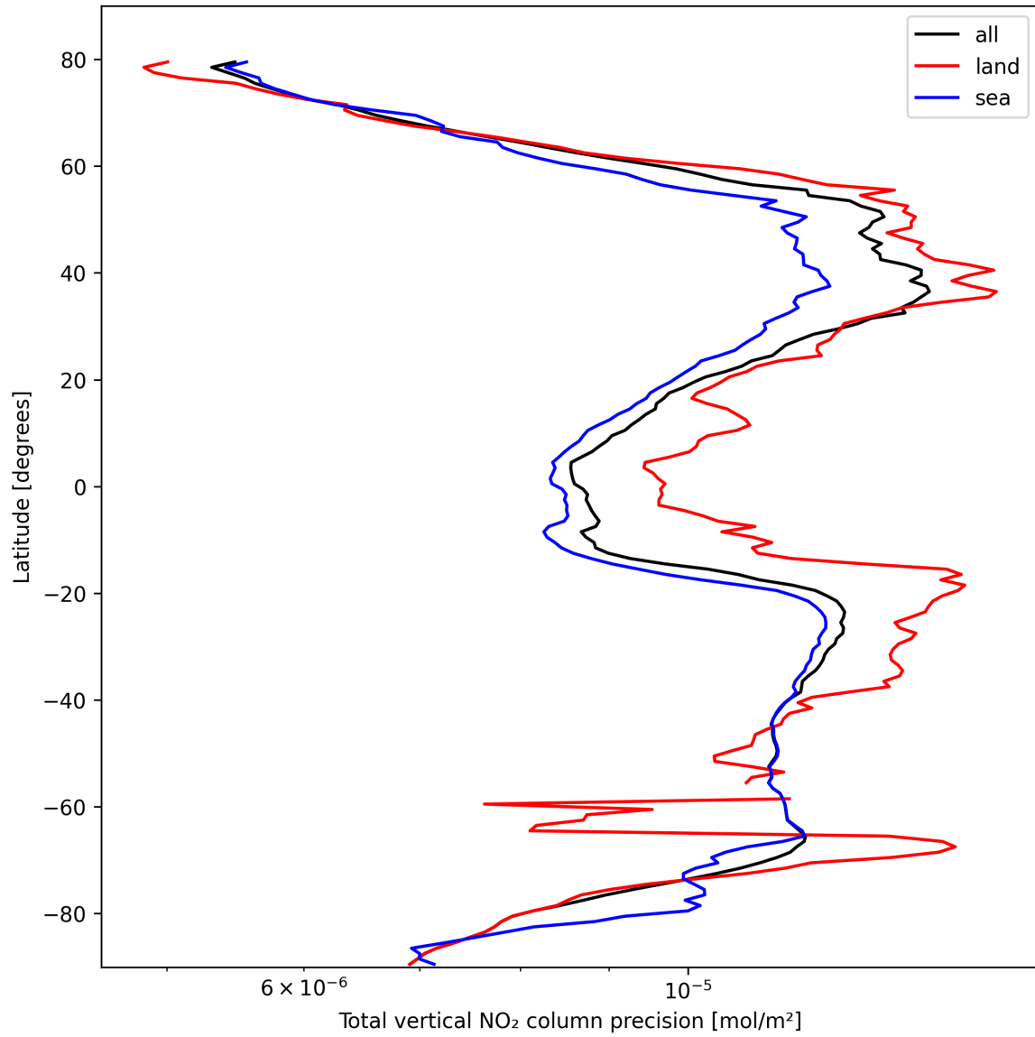
Figure 22: Zonal average of “Total vertical NO 2 column precision” for 2025-10-14 to 2025-10-16.
