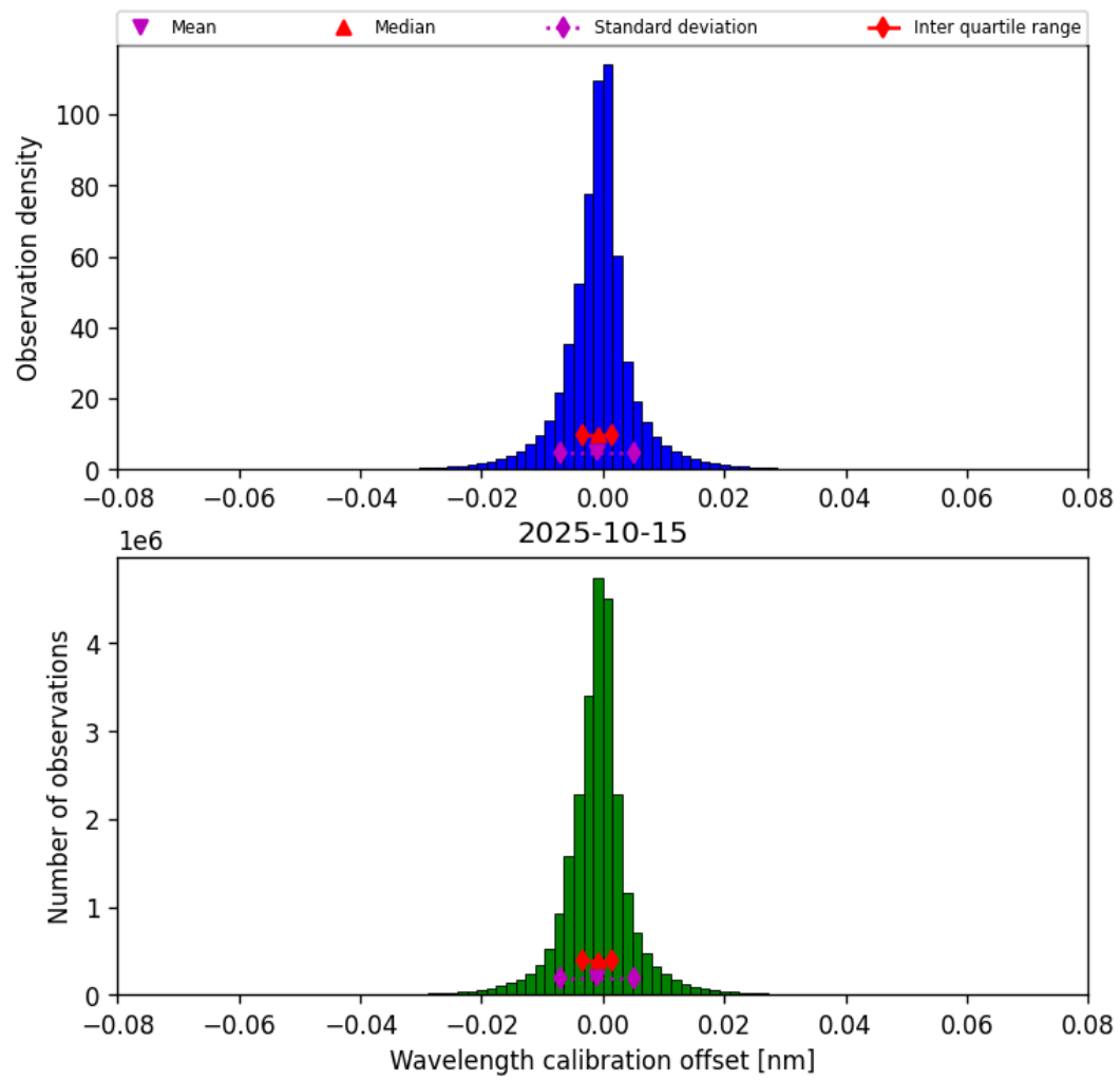
Figure 35: Histogram of “Wavelength calibration offset” for 2025-10-14 to 2025-10-16
