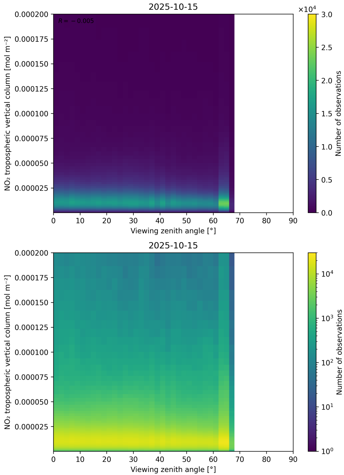
Figure 169: Scatter density plot of “Viewing zenith angle” against “NO 2 tropospheric vertical column” for 2025-10-14 to 2025-10-16.
