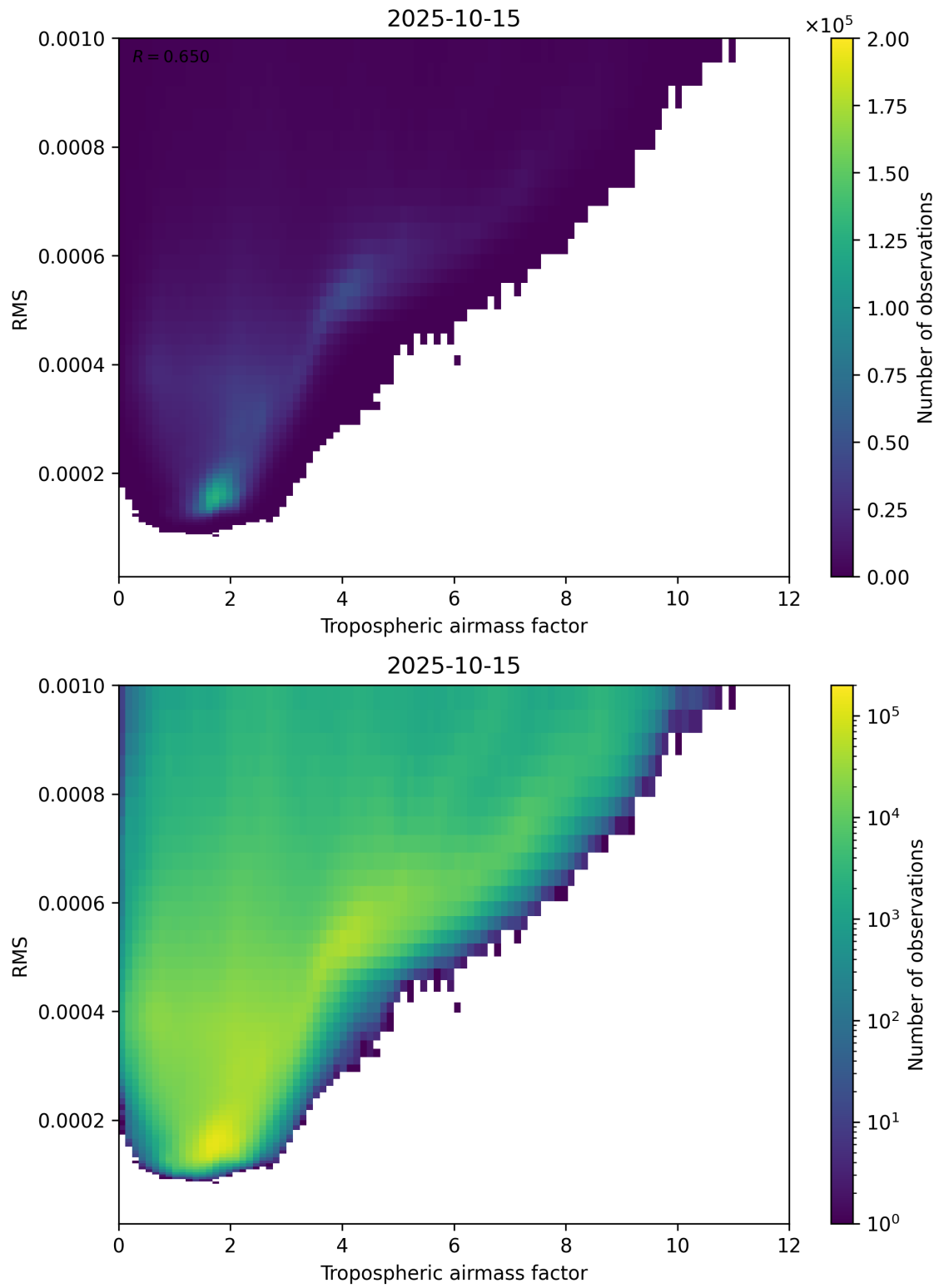
Figure 79: Scatter density plot of “Tropospheric airmass factor” against “RMS” for 2025-10-14 to 2025-10-16.
