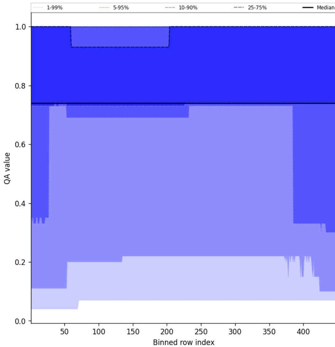
Figure 45: Along track statistics of “QA value” for 2025-10-14 to 2025-10-16
