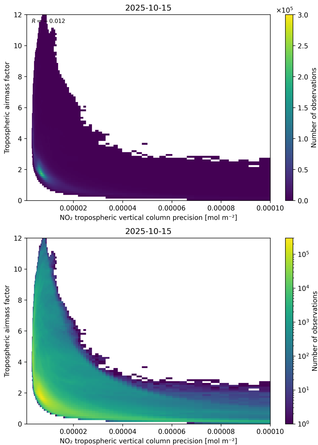
Figure 133: Scatter density plot of “NO 2 tropospheric vertical column precision” against “Tropospheric airmass factor” for 2025-10-14 to 2025-10-16.
