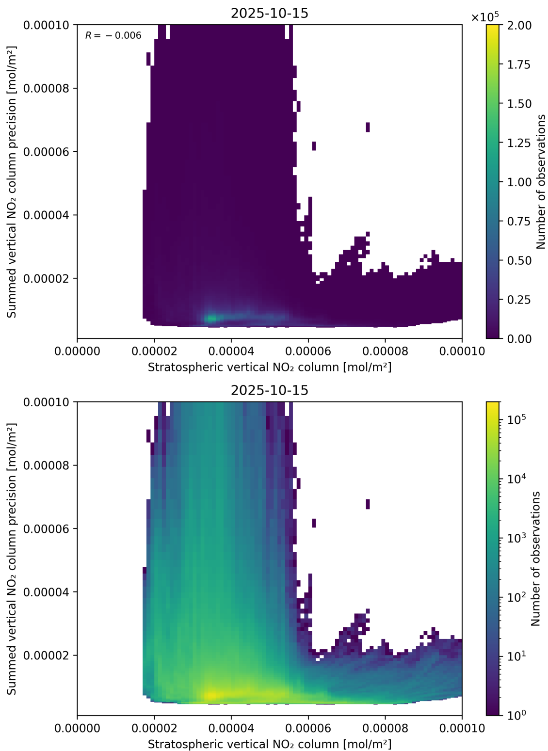
Figure 99: Scatter density plot of “Stratospheric vertical NO 2 column” against “Summed vertical NO 2 column precision” for 2025-10-14 to 2025-10-16.
