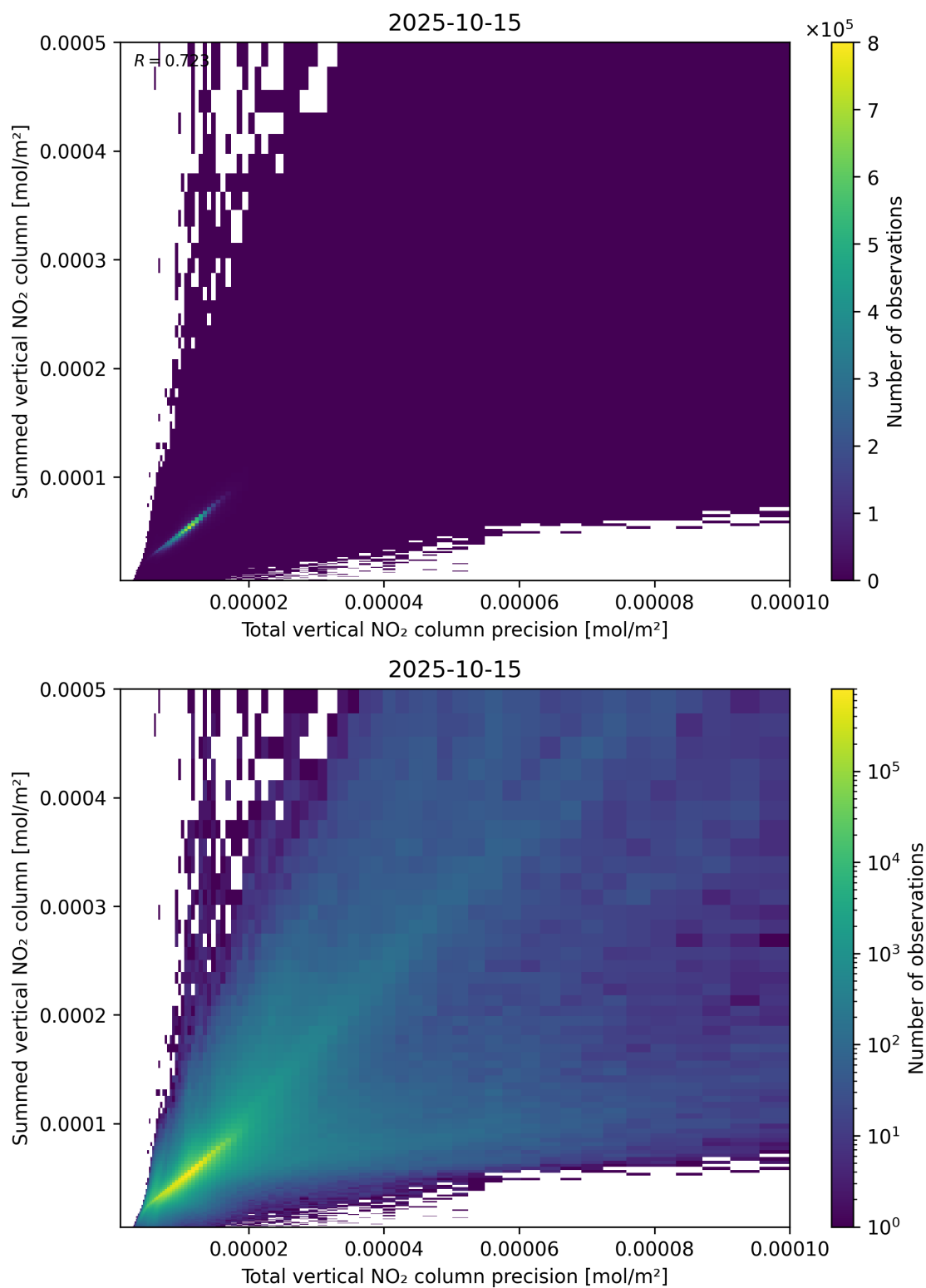
Figure 117: Scatter density plot of “Total vertical NO 2 column precision” against “Summed vertical NO 2 column” for 2025-10-14 to 2025-10-16.
