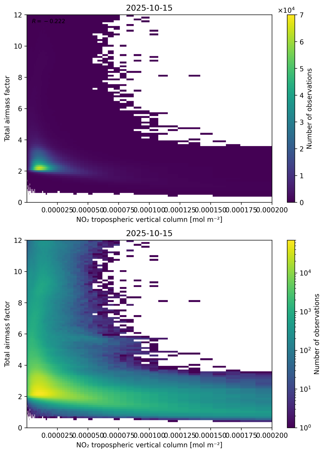
Figure 122: Scatter density plot of “NO 2 tropospheric vertical column” against “Total air mass factor” for 2025-10-14 to 2025-10-16.
