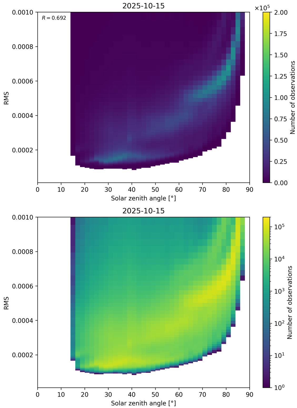
Figure 157: Scatter density plot of “Solar zenith angle” against “RMS” for 2025-10-14 to 2025-10-16.
