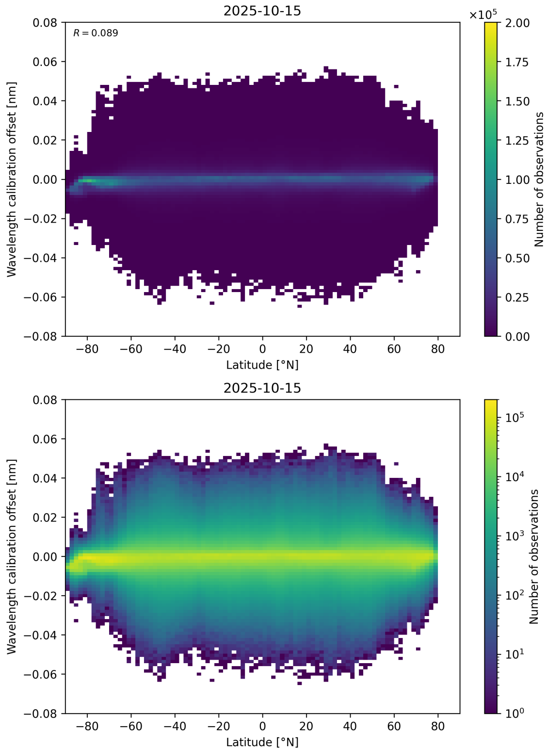
Figure 95: Scatter density plot of “Latitude” against “Wavelength calibration offset” for 2025-10-14 to 2025-10-16.
