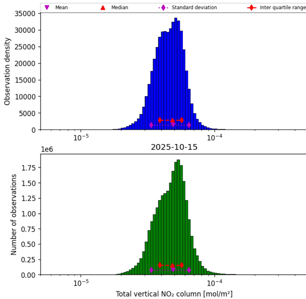
Figure 38: Histogram of “Total vertical NO 2 column” for 2025-10-14 to 2025-10-16
