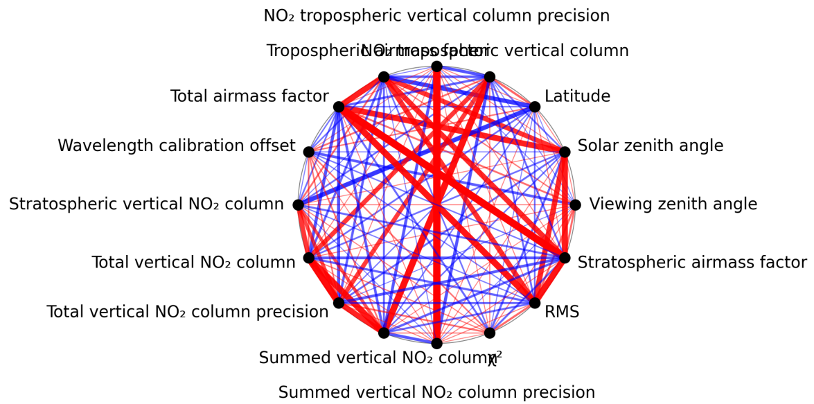
Figure 1: Map of correlation graph for 2025-10-14 to 2025-10-16.
