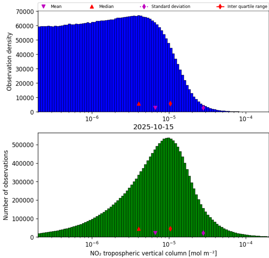
Figure 29: Histogram of “NO 2 tropospheric vertical column” for 2025-10-14 to 2025-10-16
