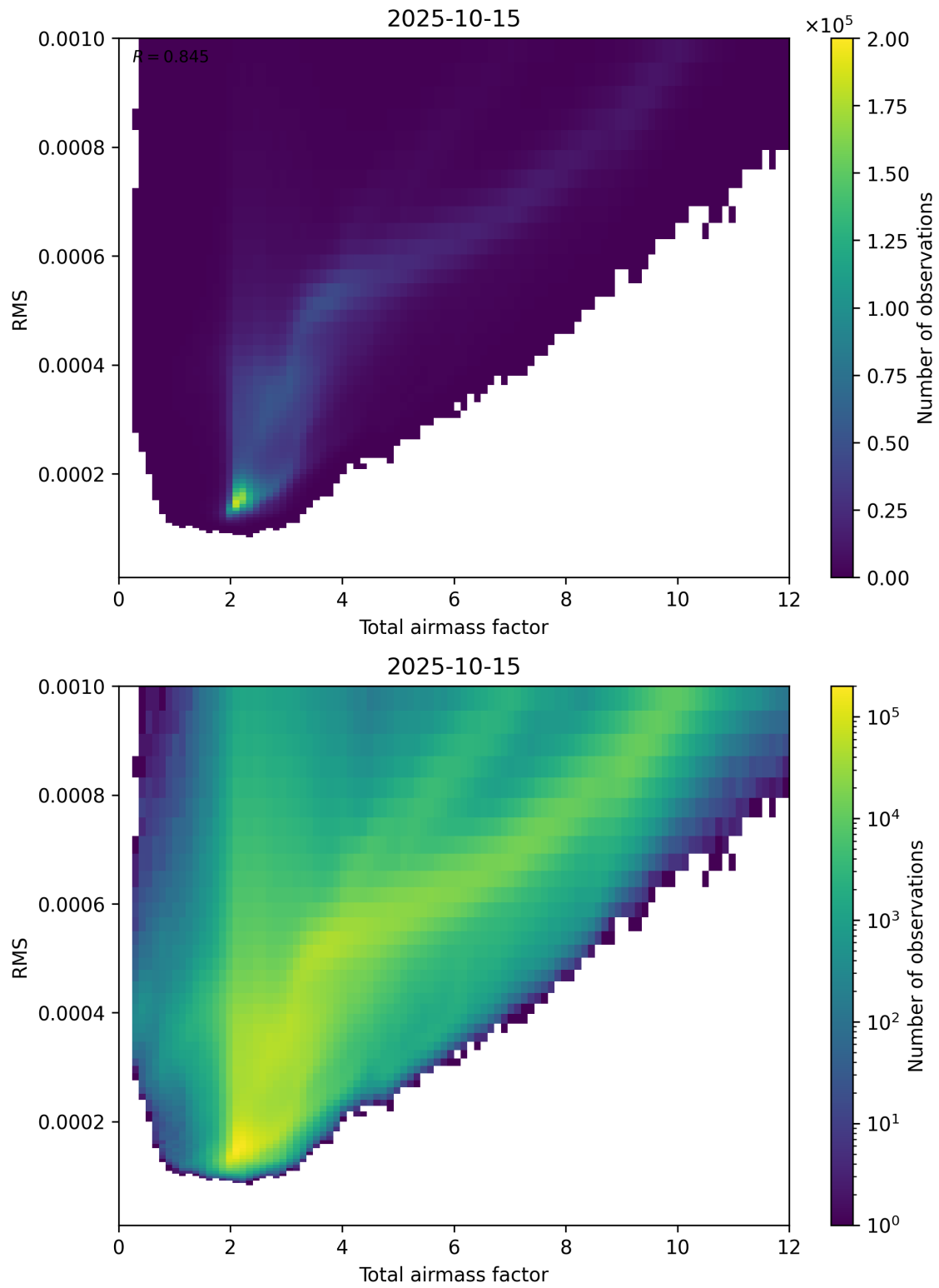
Figure 69: Scatter density plot of “Total airmass factor” against “RMS” for 2025-10-14 to 2025-10-16.
