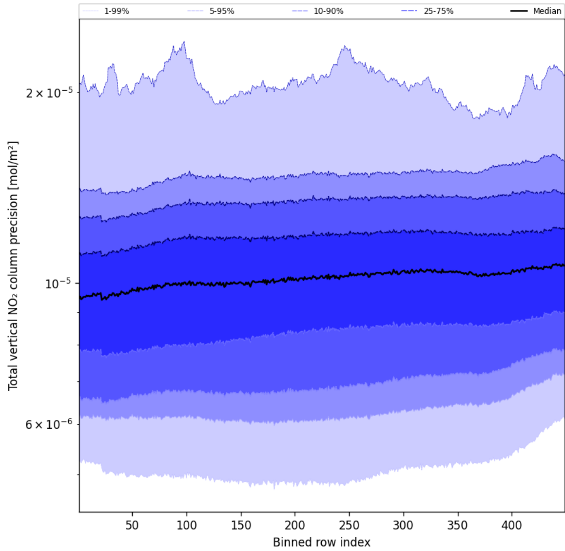
Figure 56: Along track statistics of “Total vertical NO 2 column precision” for 2025-10-14 to 2025-10-16
