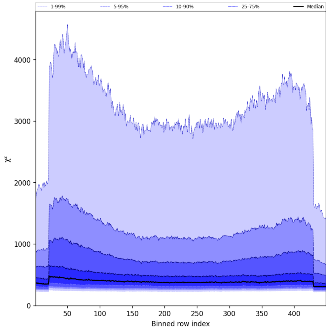
Figure 59: Along track statistics of “ \chi^2 ” for 2025-10-14 to 2025-10-16
