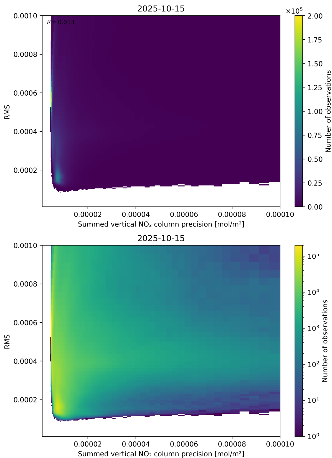
Figure 108: Scatter density plot of “Summed vertical NO 2 column precision” against “RMS” for 2025-10-14 to 2025-10-16.
