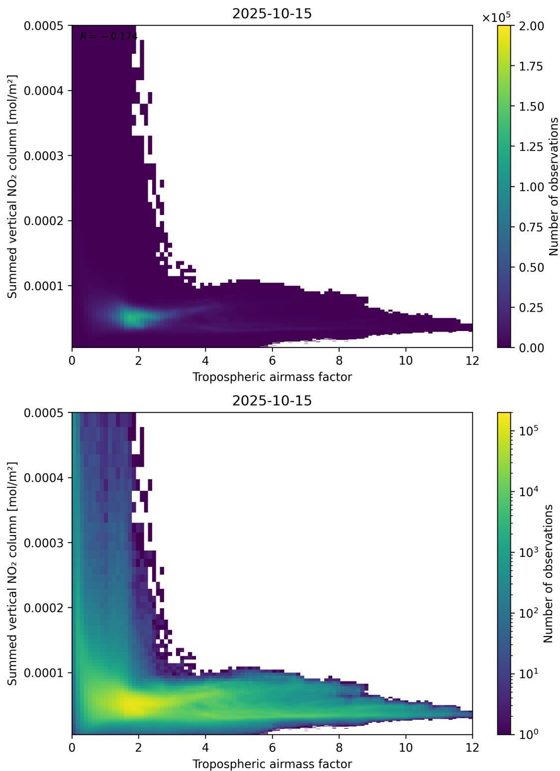
Figure 75: Scatter density plot of “Tropospheric air mass factor” against “Summed vertical NO 2 column” for 2025-10-14 to 2025-10-16.
