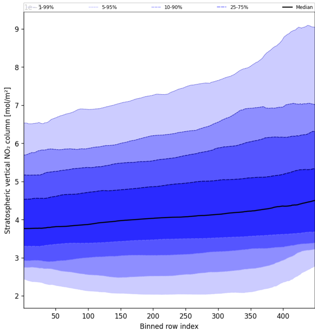
Figure 53: Along track statistics of “Stratospheric vertical NO 2 column” for 2025-10-14 to 2025-10-16
