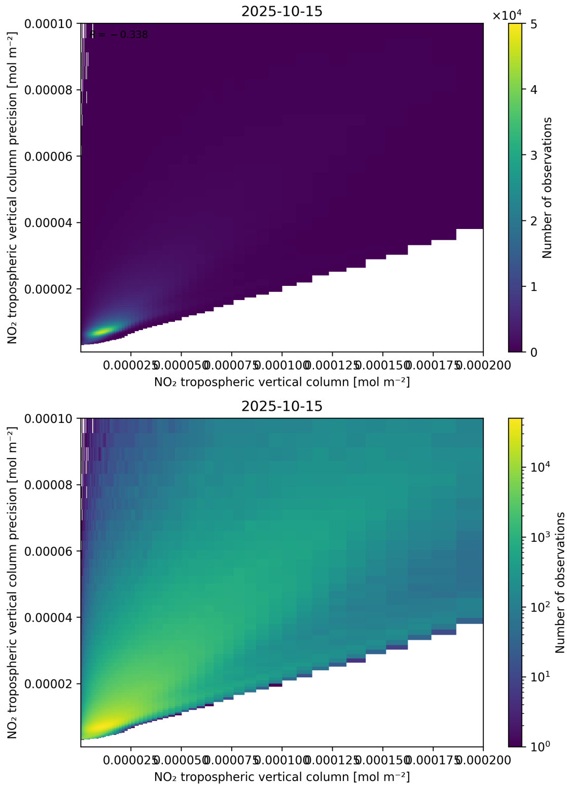
Figure 130: Scatter density plot of “NO 2 tropospheric vertical column” against “NO 2 tropospheric vertical column precision” for 2025-10-14 to 2025-10-16.
