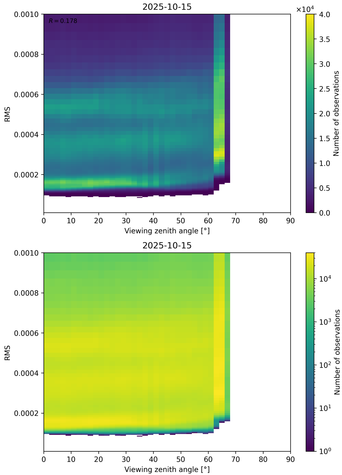
Figure 171: Scatter density plot of “Viewing zenith angle” against “RMS” for 2025-10-14 to 2025-10-16.
