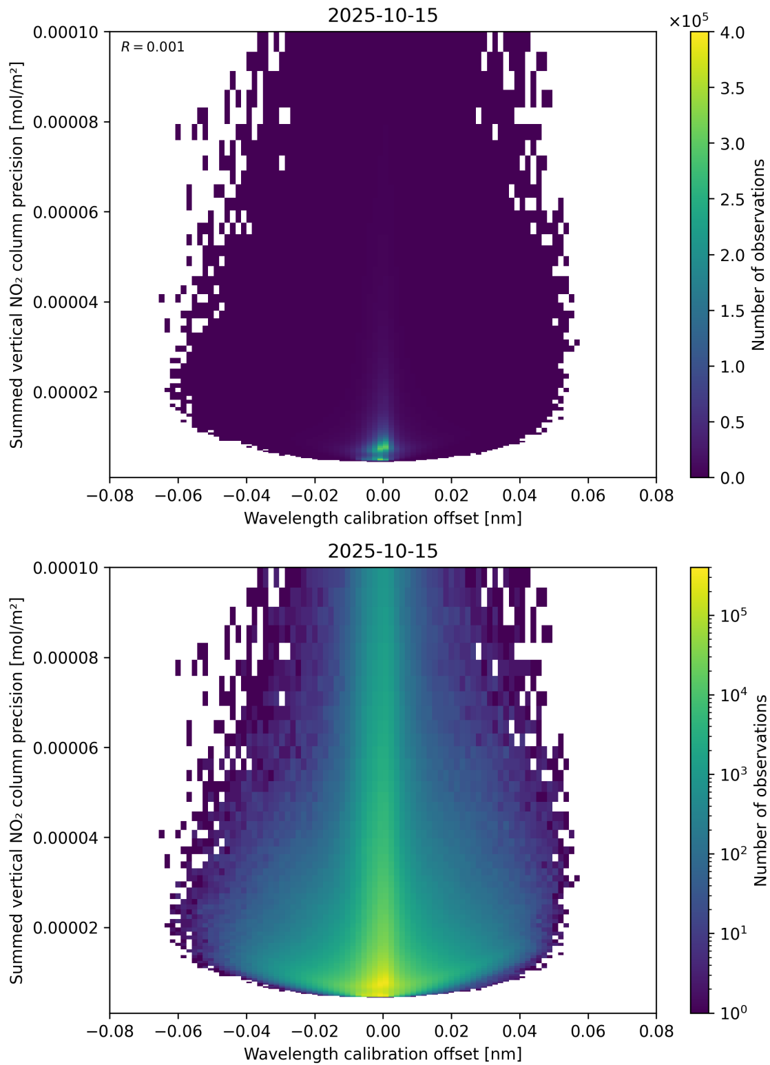
Figure 178: Scatter density plot of “Wavelength calibration offset” against “Summed vertical NO 2 column precision” for 2025-10-14 to 2025-10-16.
