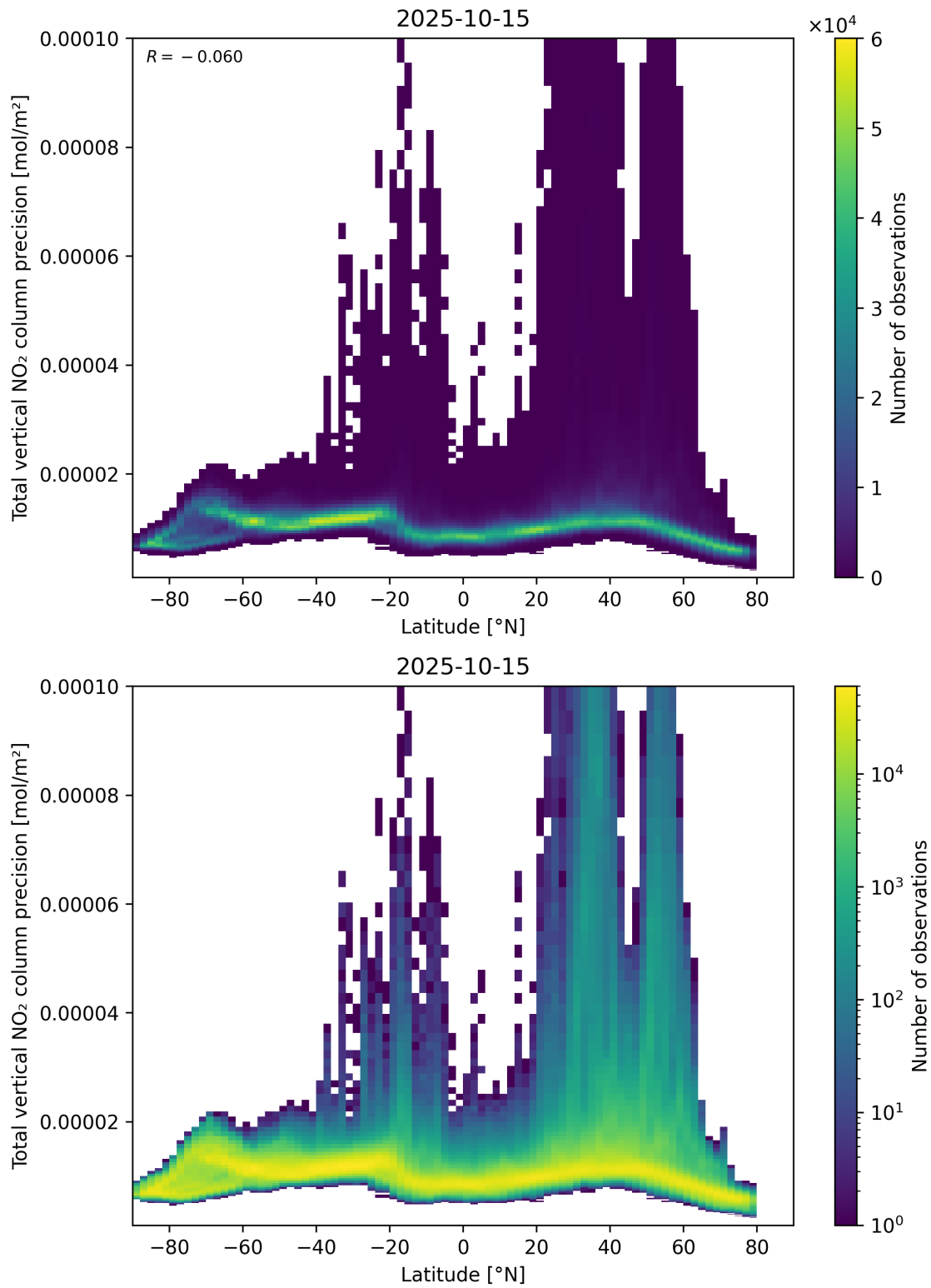
Figure 91: Scatter density plot of “Latitude” against “Total vertical NO 2 column precision” for 2025-10-14 to 2025-10-16.
