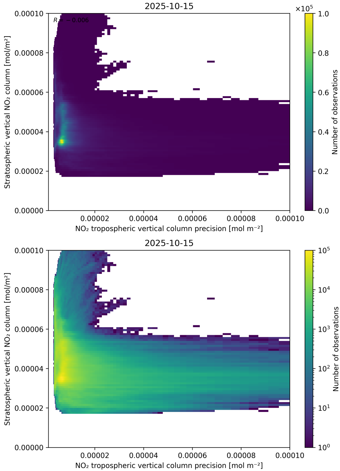
Figure 135: Scatter density plot of “NO 2 tropospheric vertical column precision” against “Stratospheric vertical NO 2 column” for 2025-10-14 to 2025-10-16.
