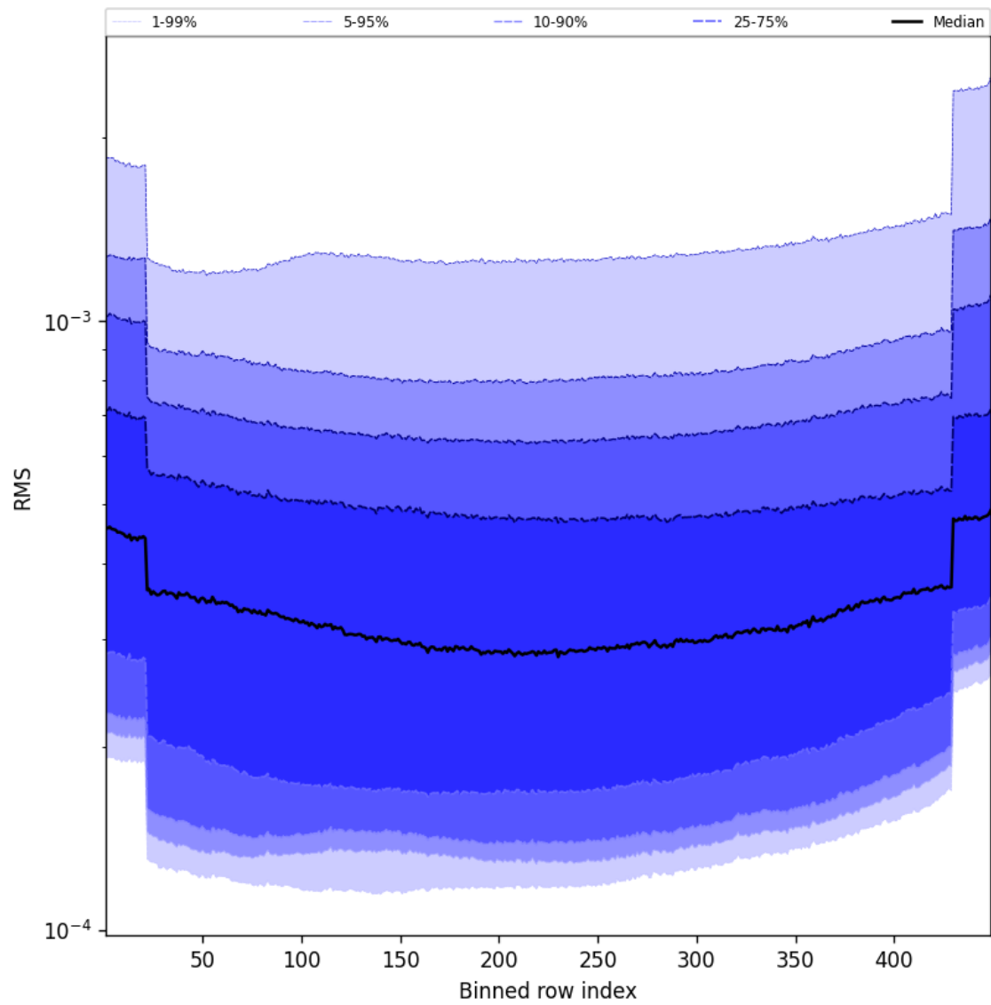
Figure 60: Along track statistics of “RMS” for 2025-10-14 to 2025-10-16
