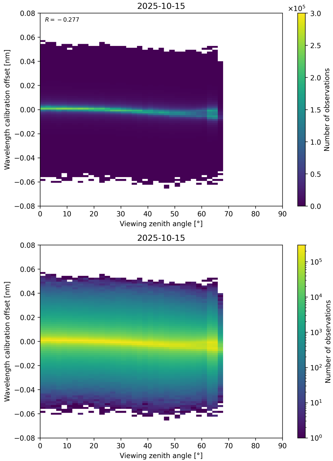
Figure 173: Scatter density plot of “Viewing zenith angle” against “Wavelength calibration offset” for 2025-10-14 to 2025-10-16.
