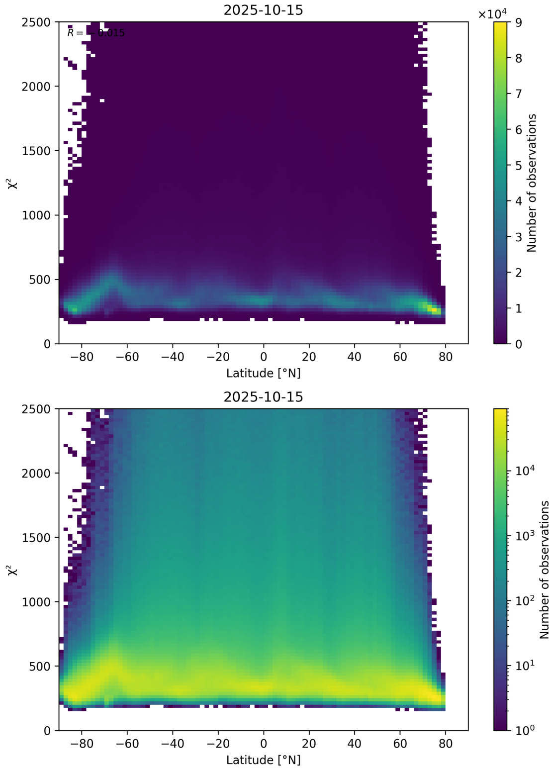
Figure 86: Scatter density plot of “Latitude” against “ \chi^2 ” for 2025-10-14 to 2025-10-16.
