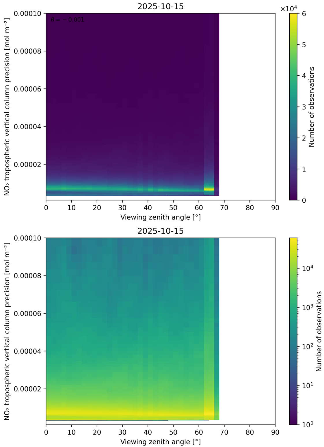
Figure 170: Scatter density plot of “Viewing zenith angle” against “NO 2 tropospheric vertical column precision” for 2025-10-14 to 2025-10-16.
