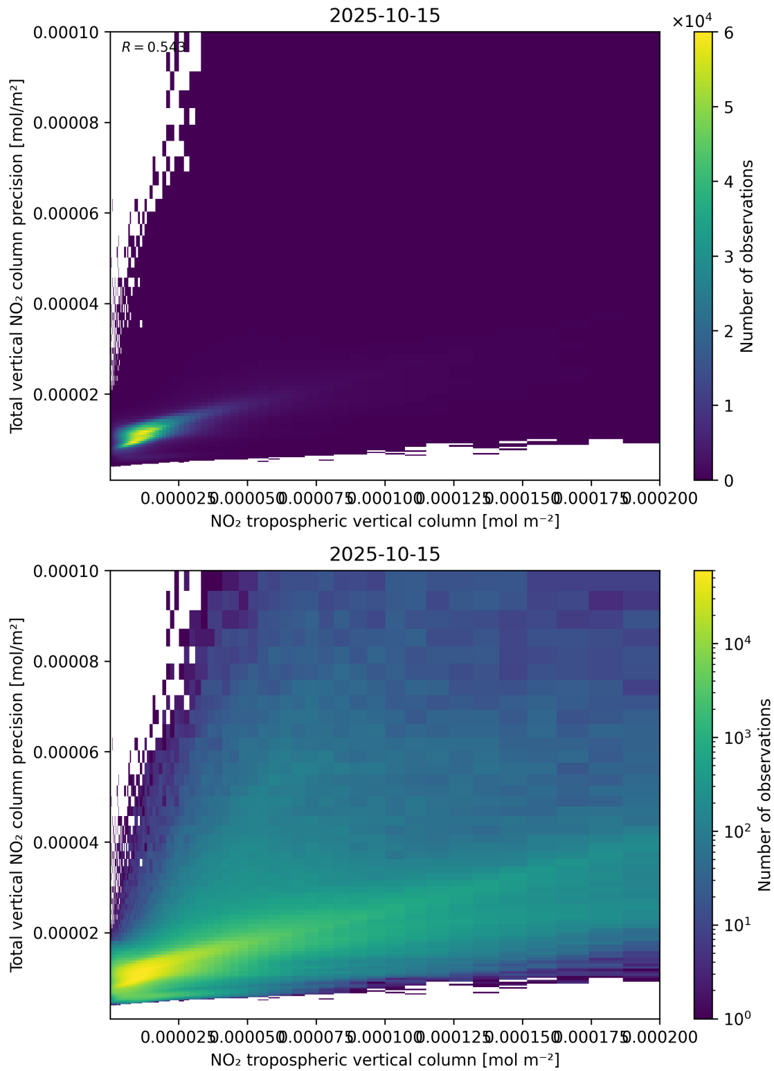
Figure 129: Scatter density plot of “NO 2 tropospheric vertical column” against “Total vertical NO 2 column precision” for 2025-10-14 to 2025-10-16.
