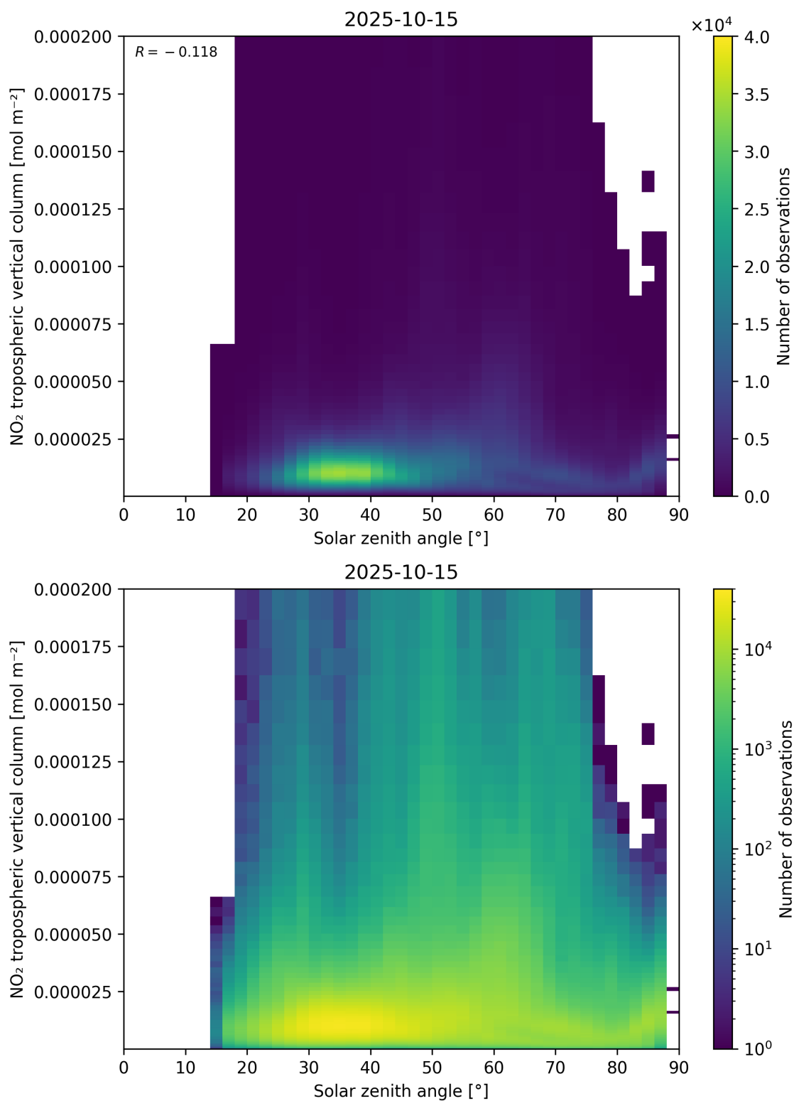
Figure 155: Scatter density plot of “Solar zenith angle” against “NO 2 tropospheric vertical column” for 2025-10-14 to 2025-10-16.
