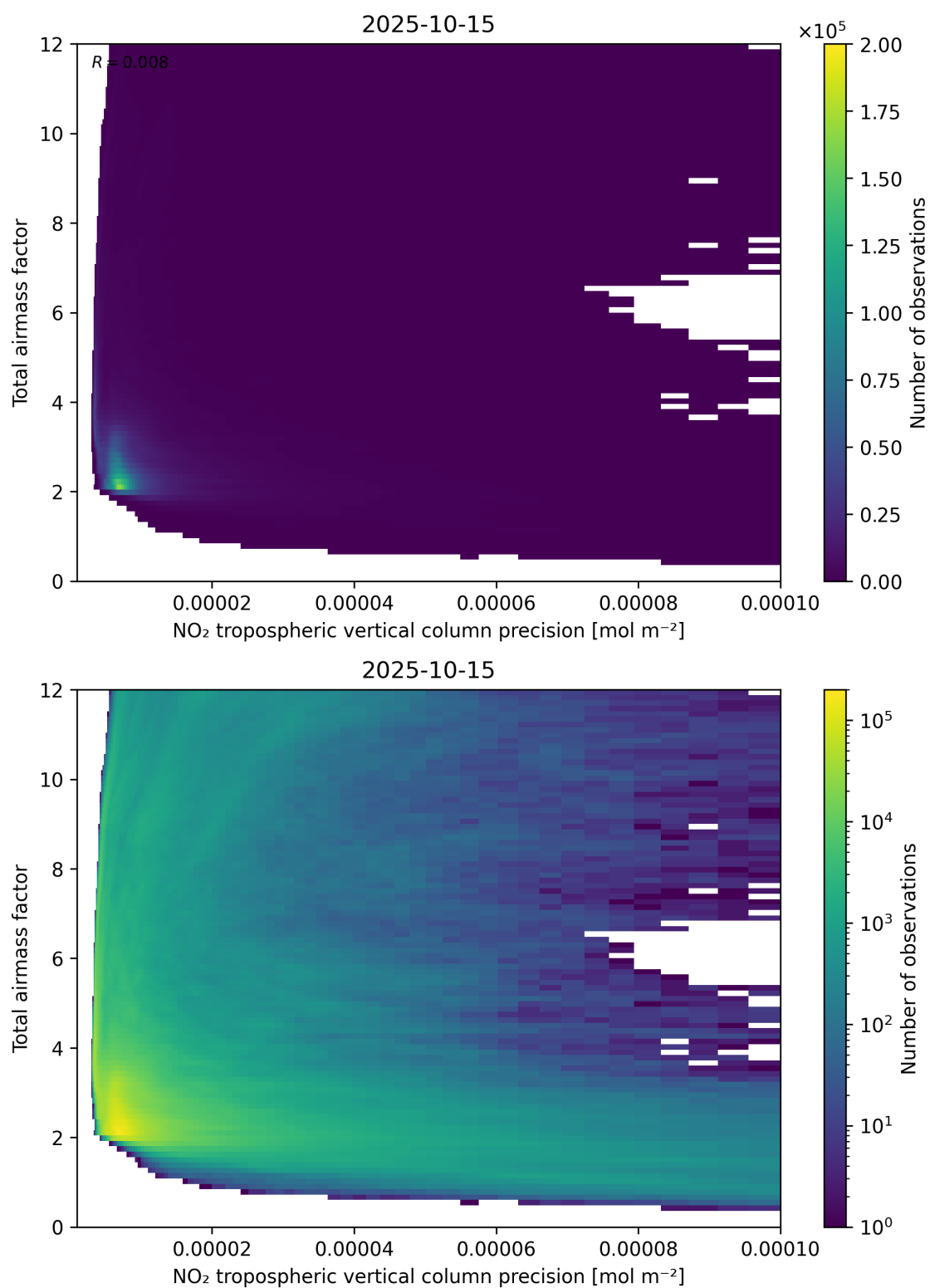
Figure 132: Scatter density plot of “NO 2 tropospheric vertical column precision” against “Total air mass factor” for 2025-10-14 to 2025-10-16.
