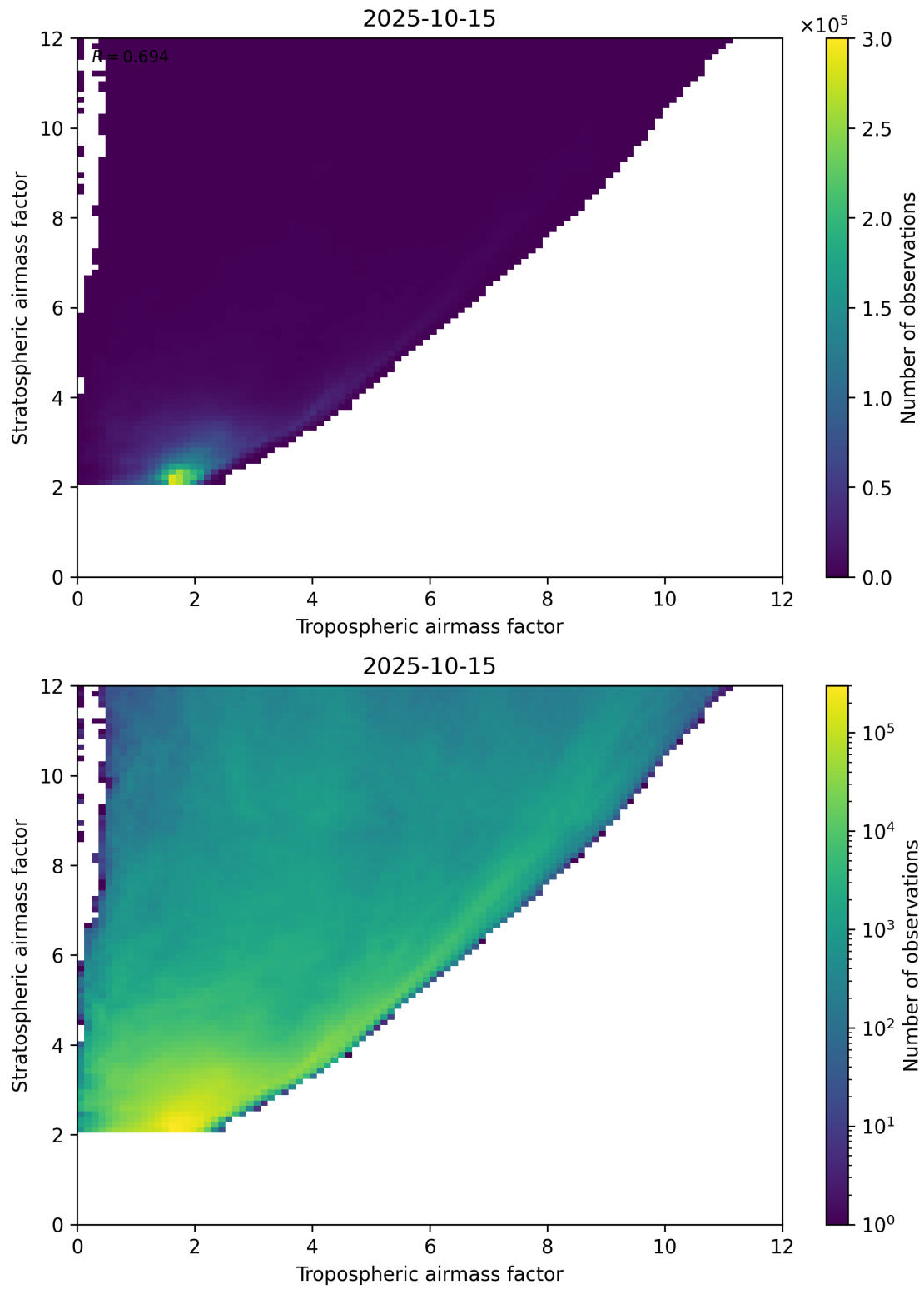
Figure 71: Scatter density plot of “Tropospheric airmass factor” against “Stratospheric airmass factor” for 2025-10-14 to 2025-10-16.
