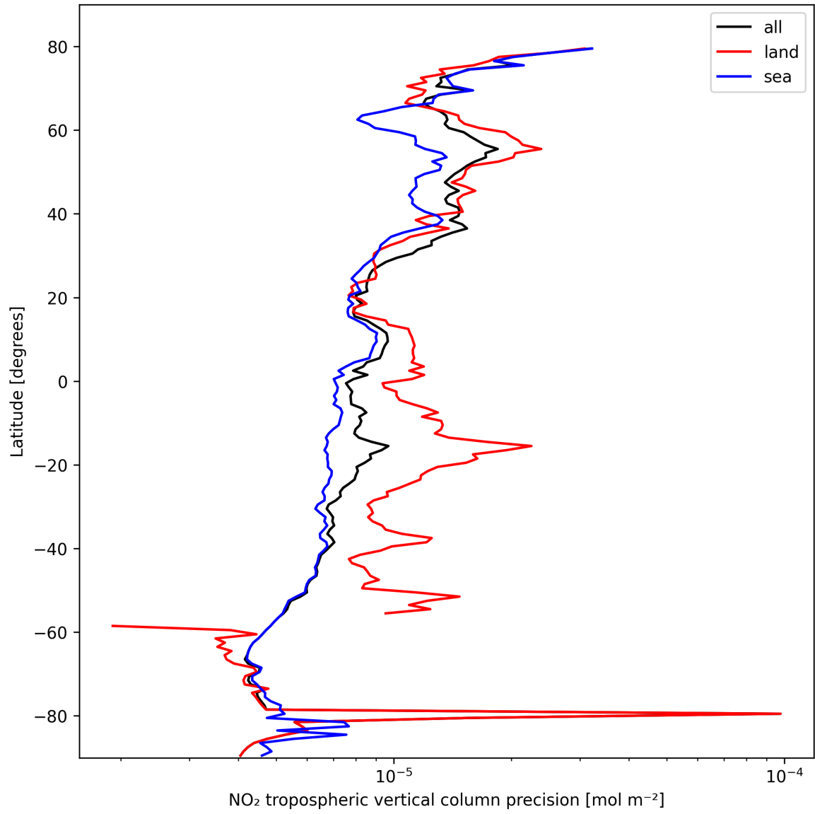
Figure 13: Zonal average of “NO 2 tropospheric vertical column precision” for 2025-10-14 to 2025-10-16.
