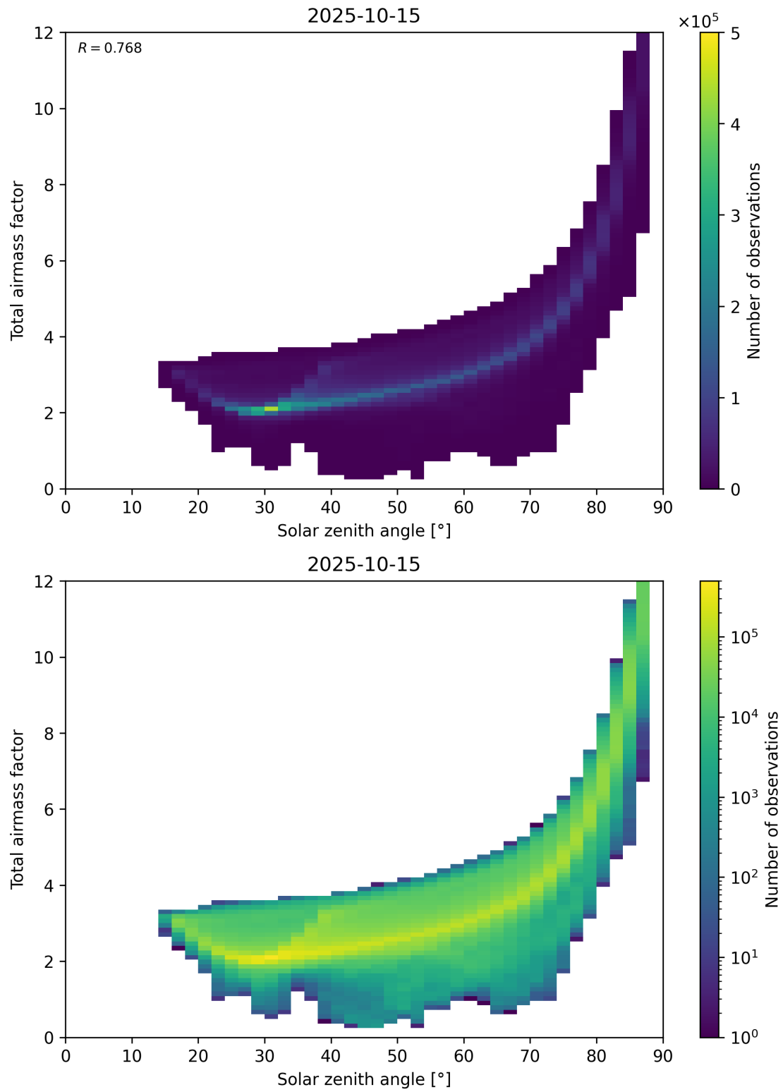
Figure 146: Scatter density plot of “Solar zenith angle” against “Total air mass factor” for 2025-10-14 to 2025-10-16.
