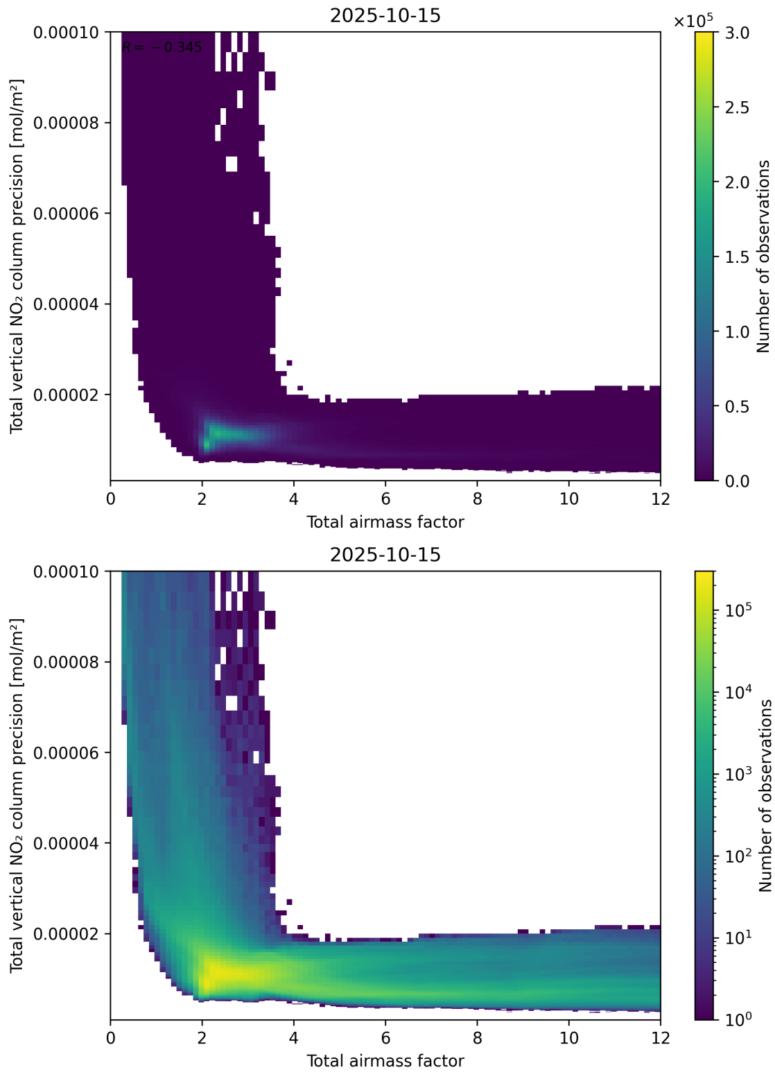
Figure 68: Scatter density plot of “Total airmass factor” against “Total vertical NO 2 column precision” for 2025-10-14 to 2025-10-16.
