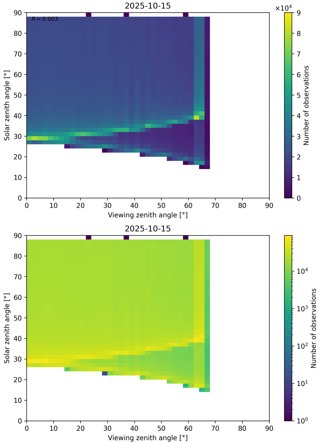
Figure 172: Scatter density plot of “Viewing zenith angle” against “Solar zenith angle” for 2025-10-14 to 2025-10-16.
