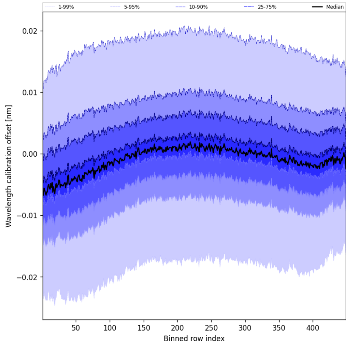
Figure 52: Along track statistics of “Wavelength calibration offset” for 2025-10-14 to 2025-10-16
