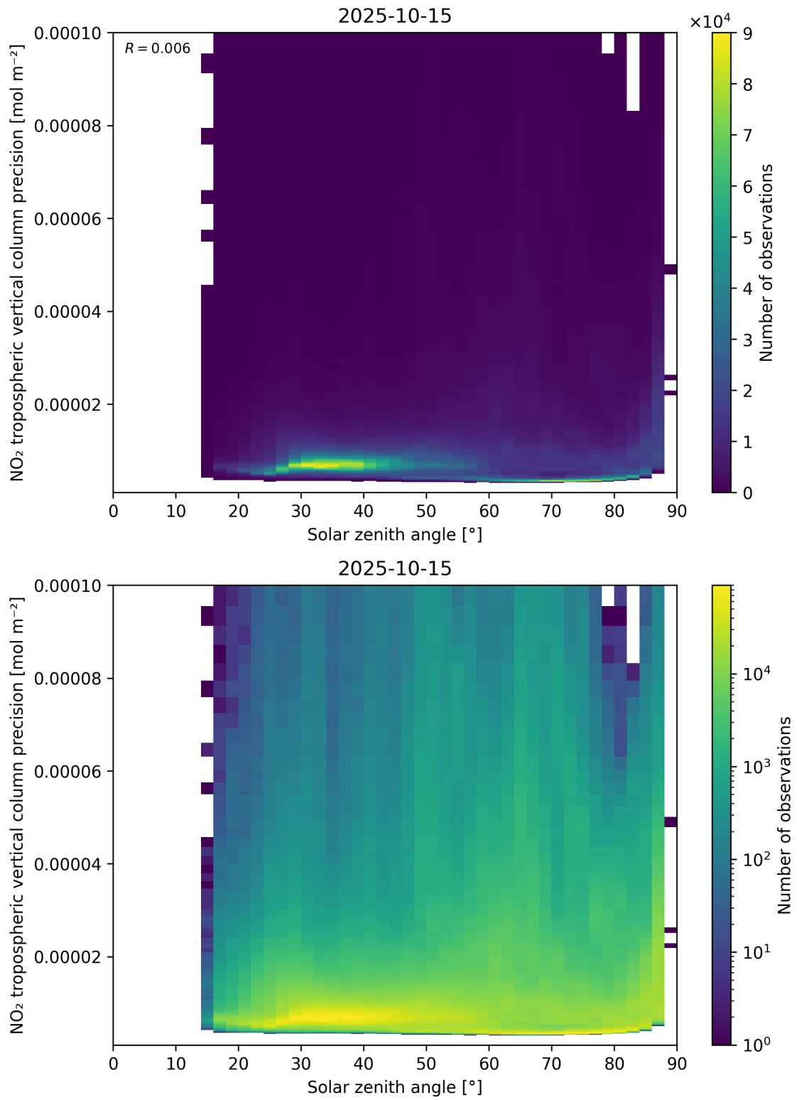
Figure 156: Scatter density plot of “Solar zenith angle” against “NO 2 tropospheric vertical column precision” for 2025-10-14 to 2025-10-16.
