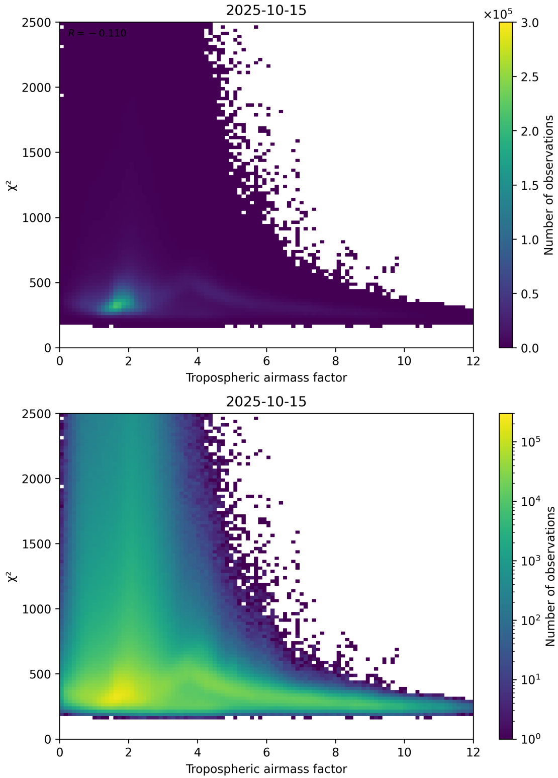
Figure 73: Scatter density plot of “Tropospheric airmass factor” against “ \chi^2 ” for 2025-10-14 to 2025-10-16.
