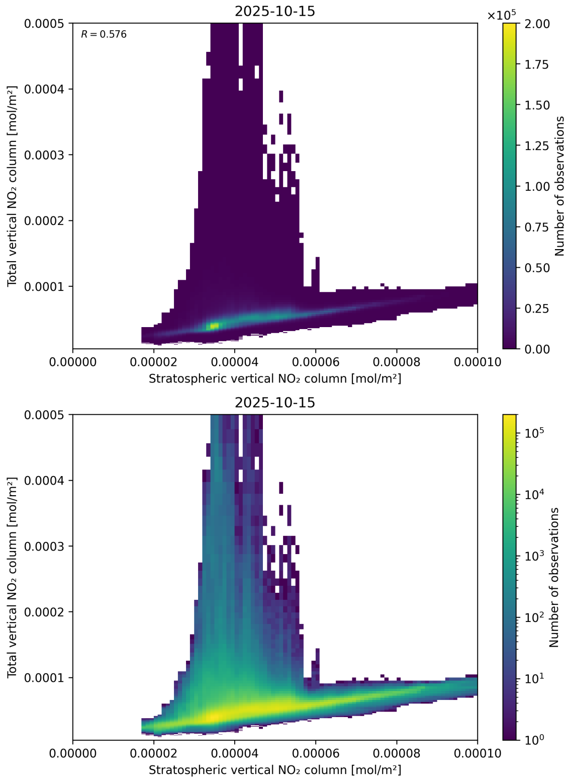
Figure 100: Scatter density plot of “Stratospheric vertical NO 2 column” against “Total vertical NO 2 column” for 2025-10-14 to 2025-10-16.
