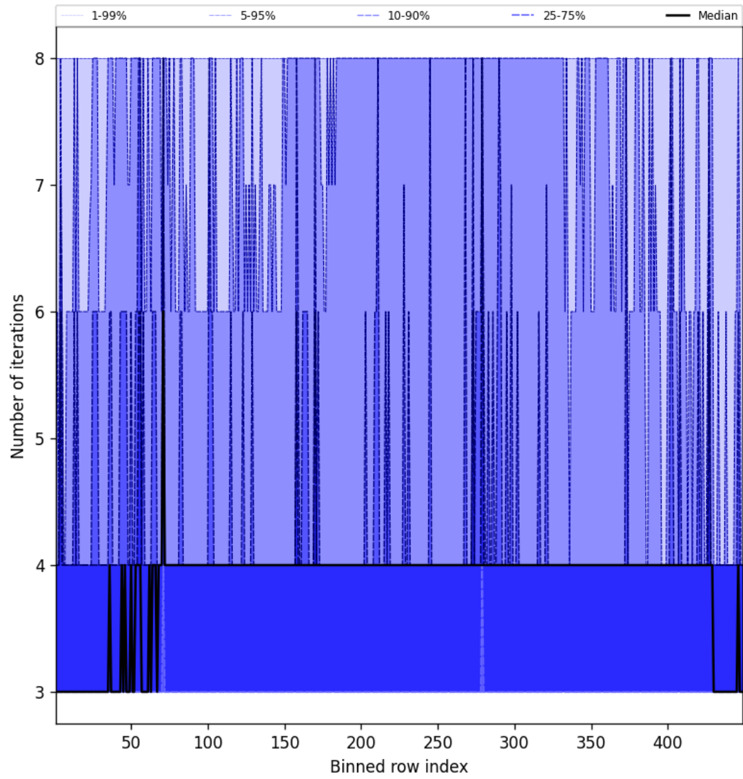
Figure 51: Along track statistics of “Number of iterations” for 2025-10-14 to 2025-10-16
