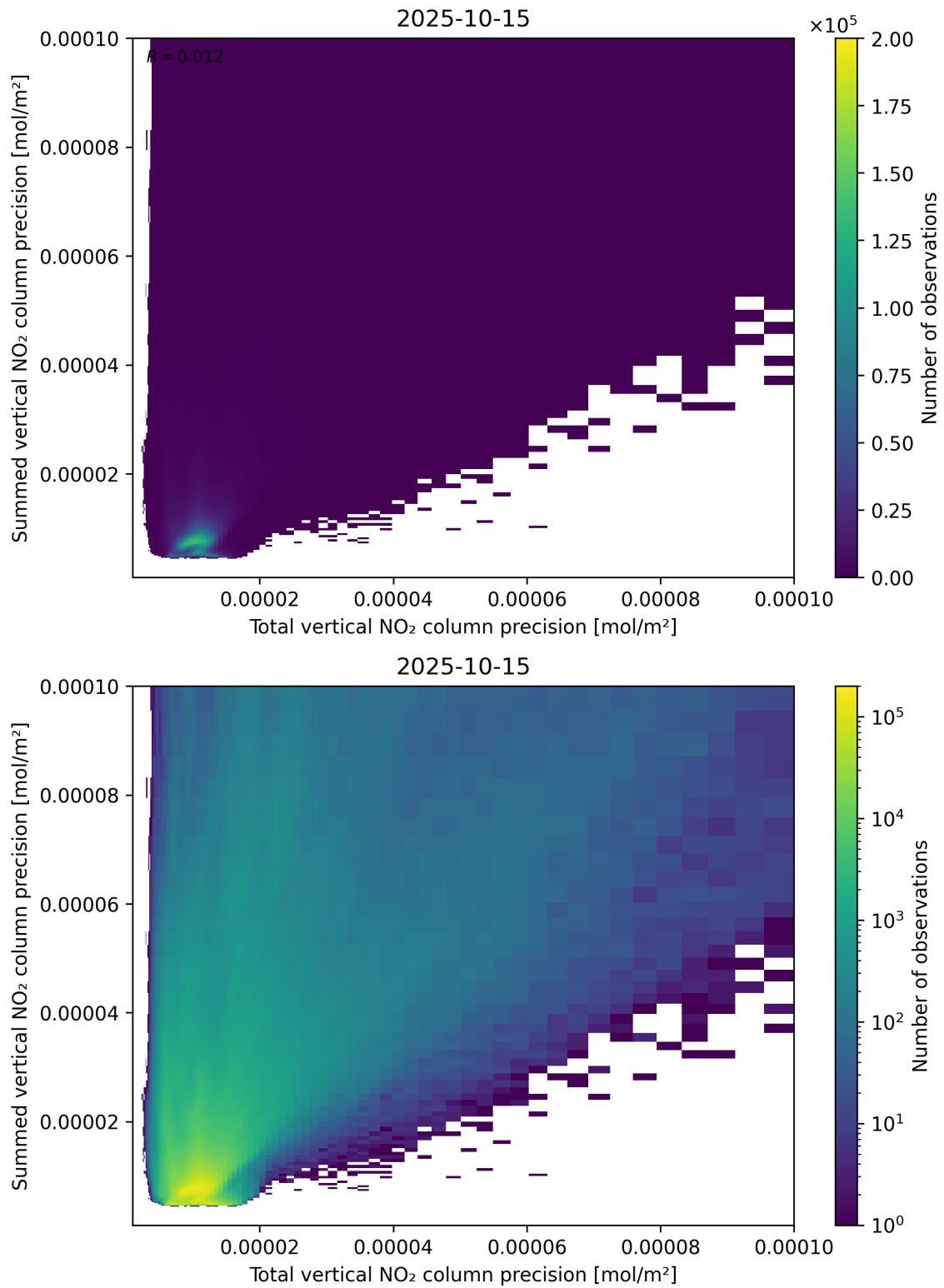
Figure 118: Scatter density plot of “Total vertical NO 2 column precision” against “Summed vertical NO 2 column precision” for 2025-10-14 to 2025-10-16.
