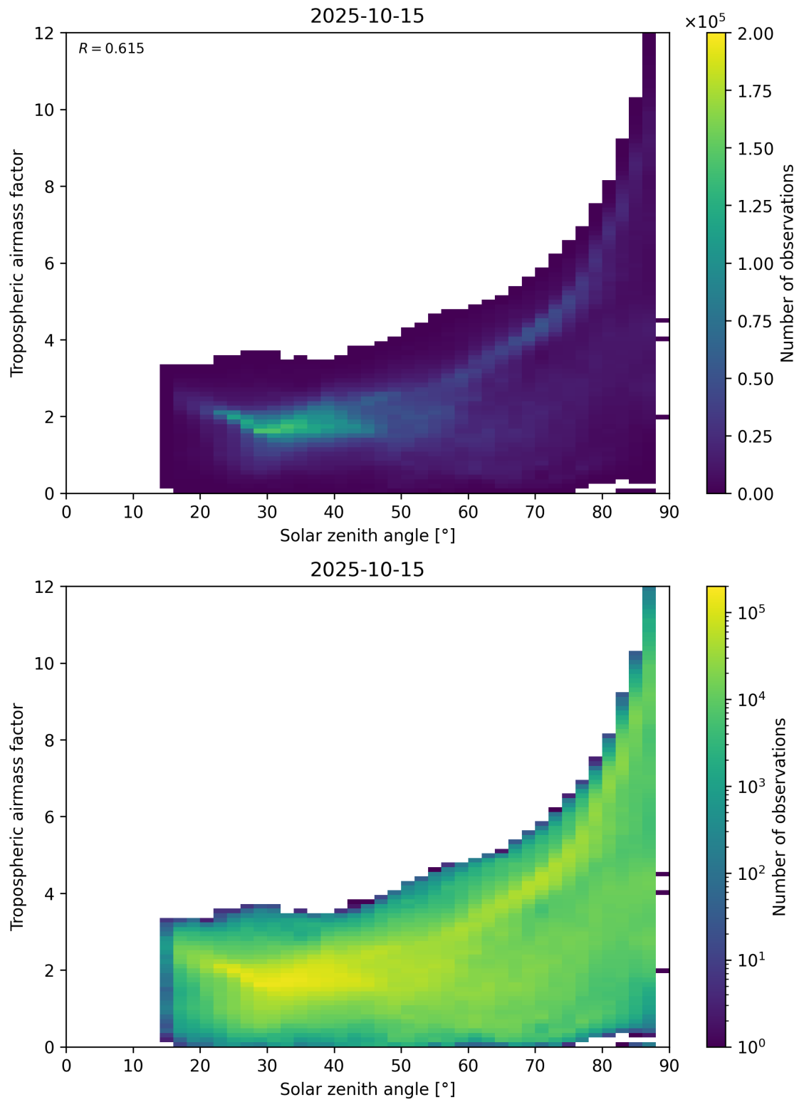
Figure 147: Scatter density plot of “Solar zenith angle” against “Tropospheric airmass factor” for 2025-10-14 to 2025-10-16.
