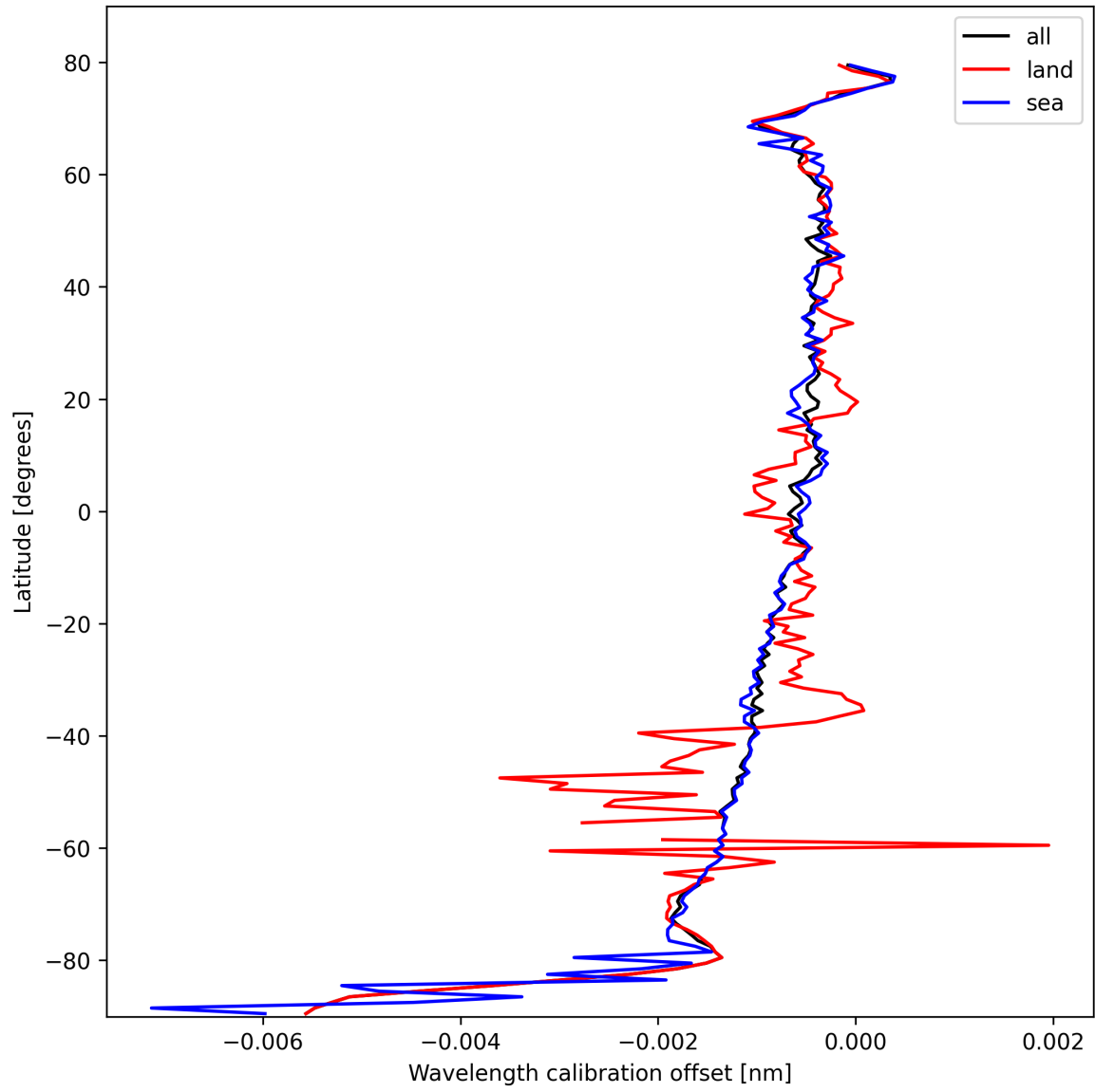
Figure 18: Zonal average of “Wavelength calibration offset” for 2025-10-14 to 2025-10-16.
