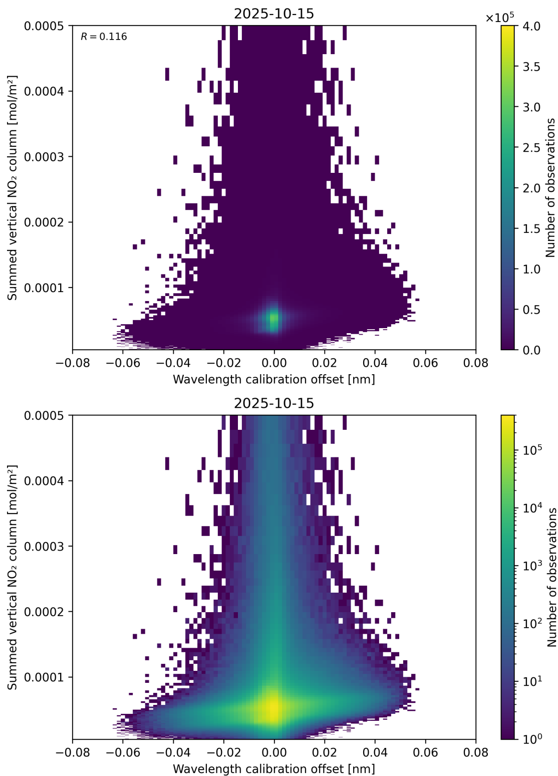
Figure 177: Scatter density plot of “Wavelength calibration offset” against “Summed vertical NO 2 column” for 2025-10-14 to 2025-10-16.
