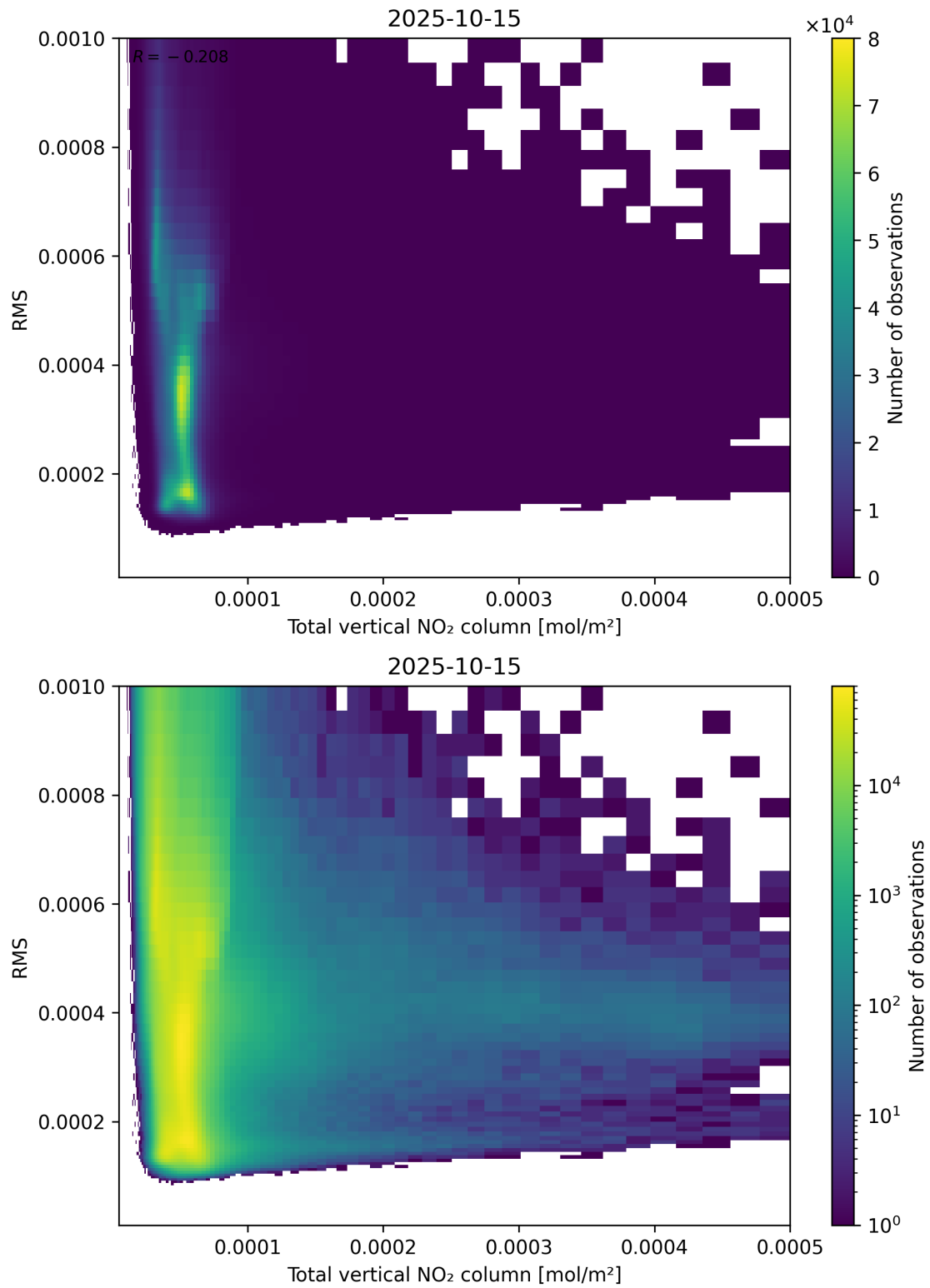
Figure 120: Scatter density plot of “Total vertical NO 2 column” against “RMS” for 2025-10-14 to 2025-10-16.
