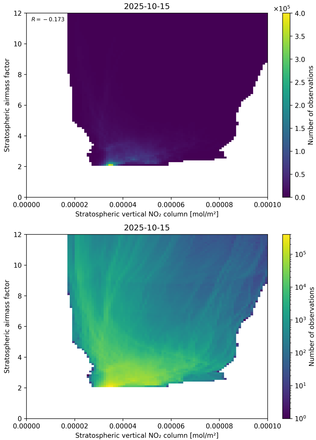
Figure 96: Scatter density plot of “Stratospheric vertical NO 2 column” against “Stratospheric airmass factor” for 2025-10-14 to 2025-10-16.
