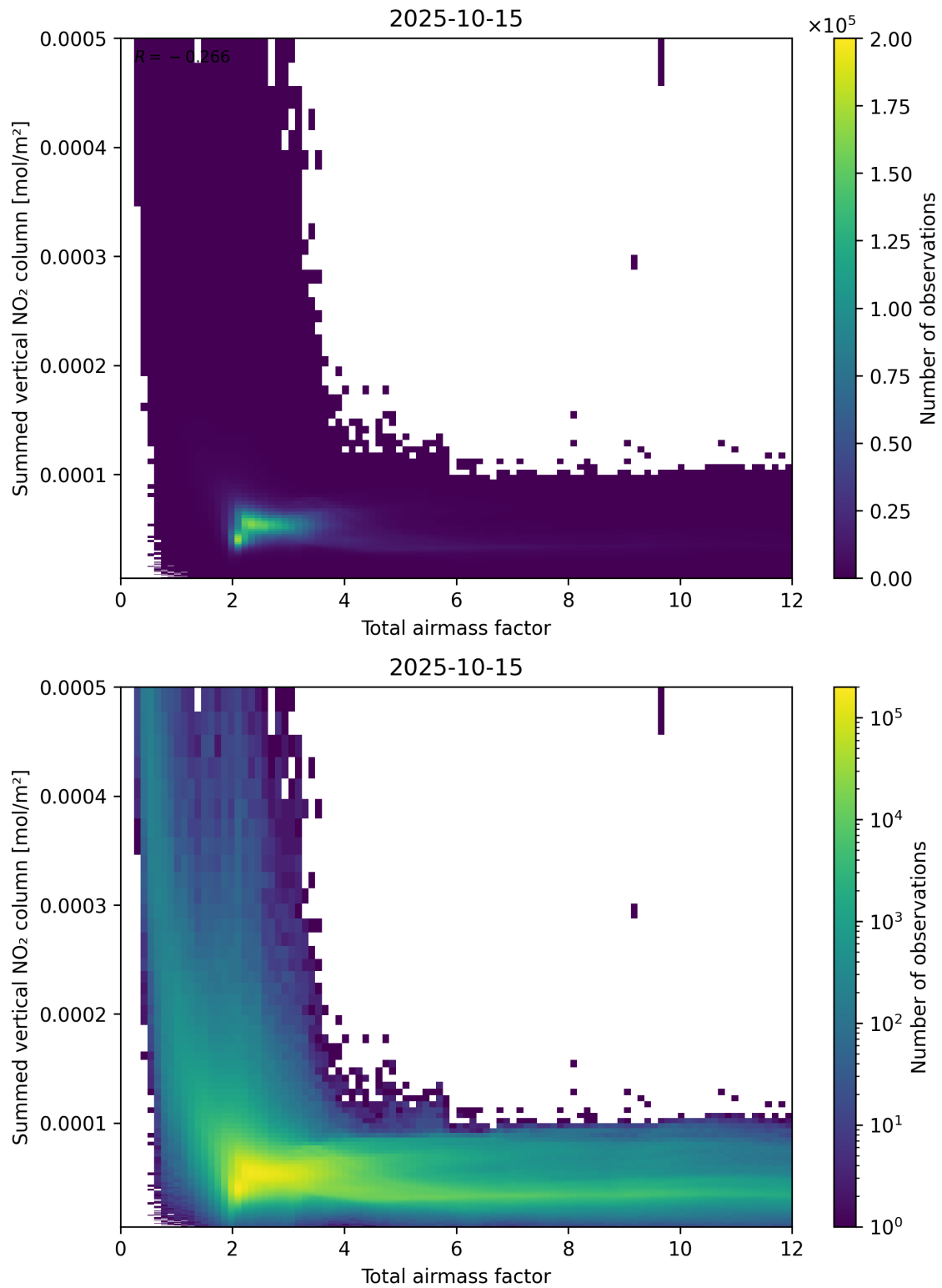
Figure 65: Scatter density plot of “Total airmass factor” against “Summed vertical NO 2 column” for 2025-10-14 to 2025-10-16.
