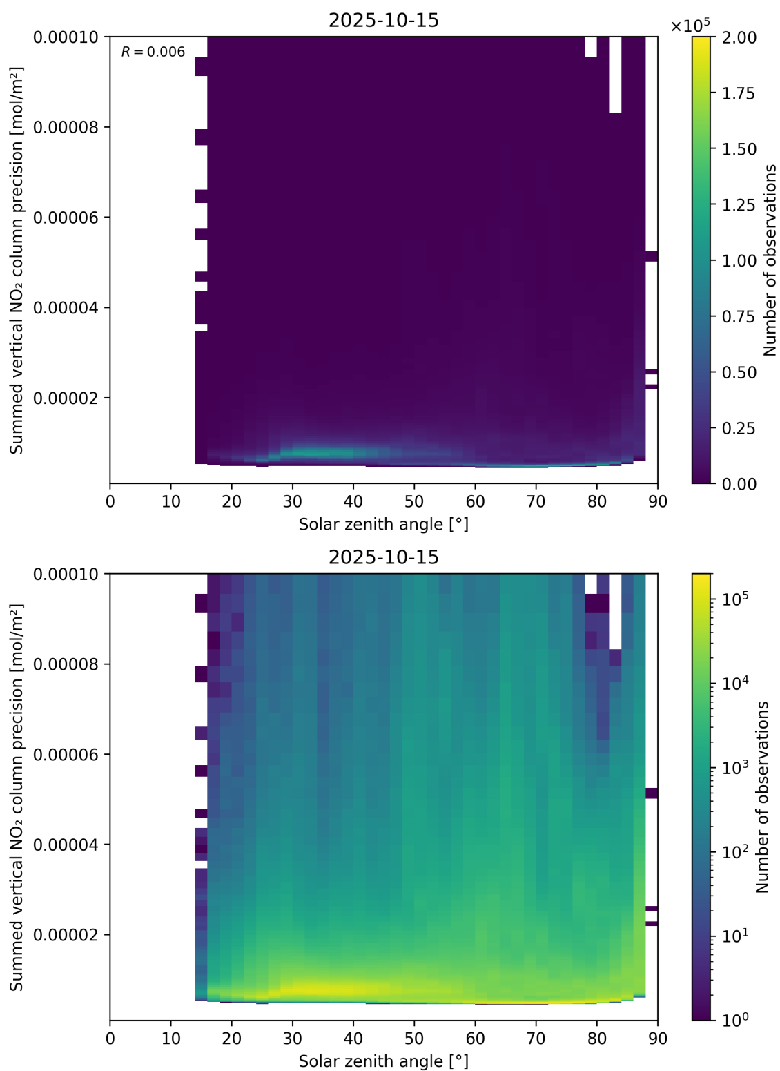
Figure 152: Scatter density plot of “Solar zenith angle” against “Summed vertical NO 2 column precision” for 2025-10-14 to 2025-10-16.
