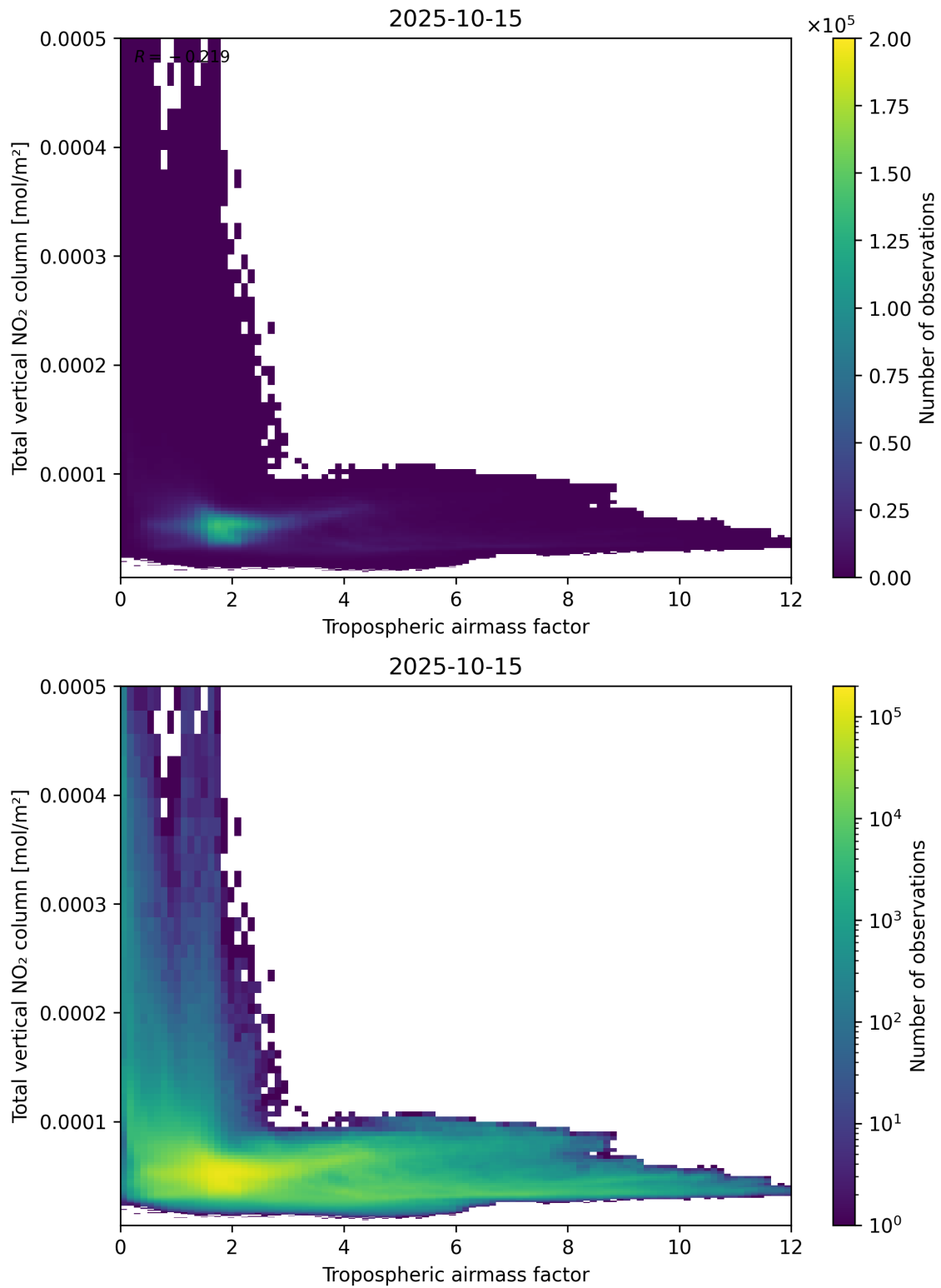
Figure 77: Scatter density plot of “Tropospheric airmass factor” against “Total vertical NO 2 column” for 2025-10-14 to 2025-10-16.
