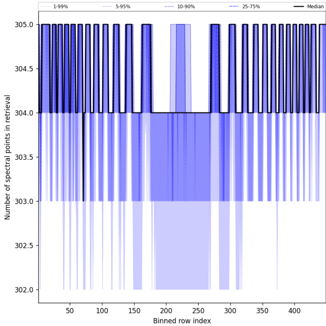
Figure 50: Along track statistics of “Number of spectral points in retrieval” for 2025-10-14 to 2025-10-16
