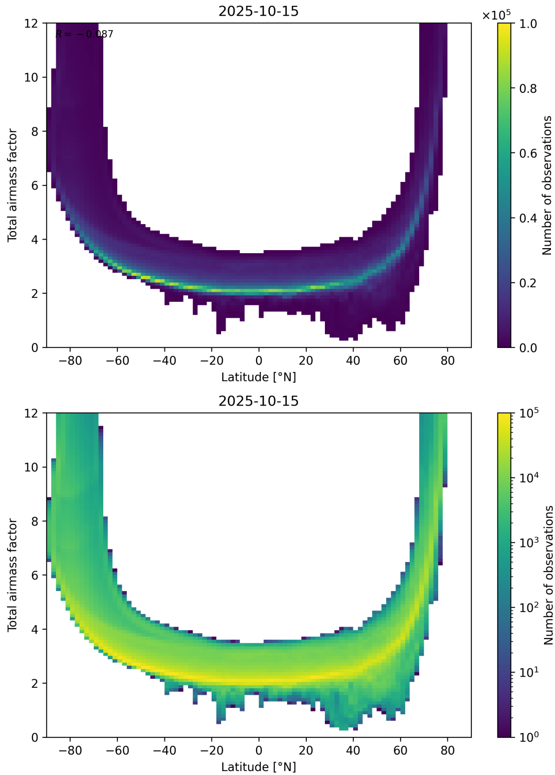
Figure 84: Scatter density plot of “Latitude” against “Total airmass factor” for 2025-10-14 to 2025-10-16.
