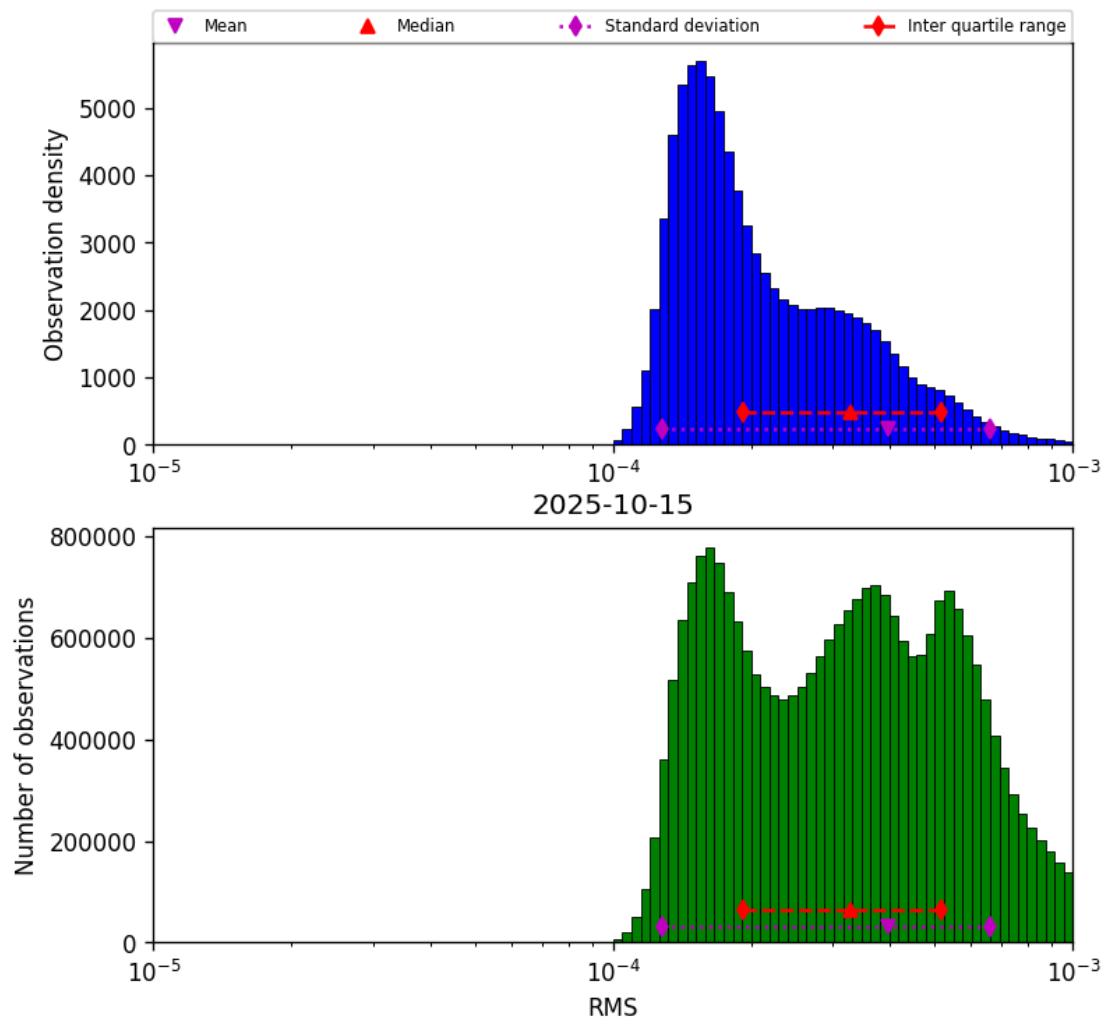
Figure 43: Histogram of “RMS” for 2025-10-14 to 2025-10-16
