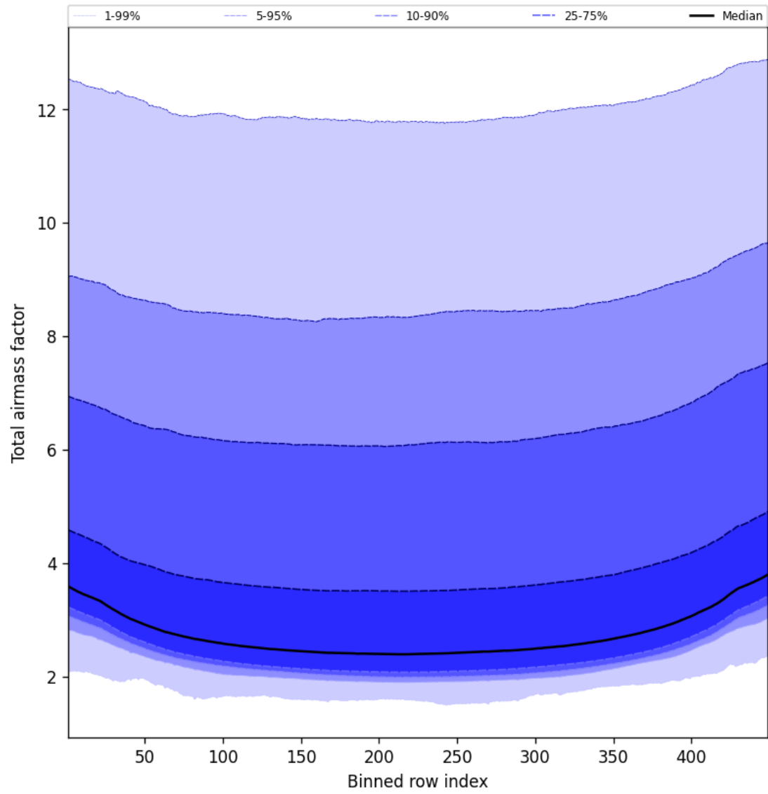
Figure 49: Along track statistics of “Total airmass factor” for 2025-10-14 to 2025-10-16
