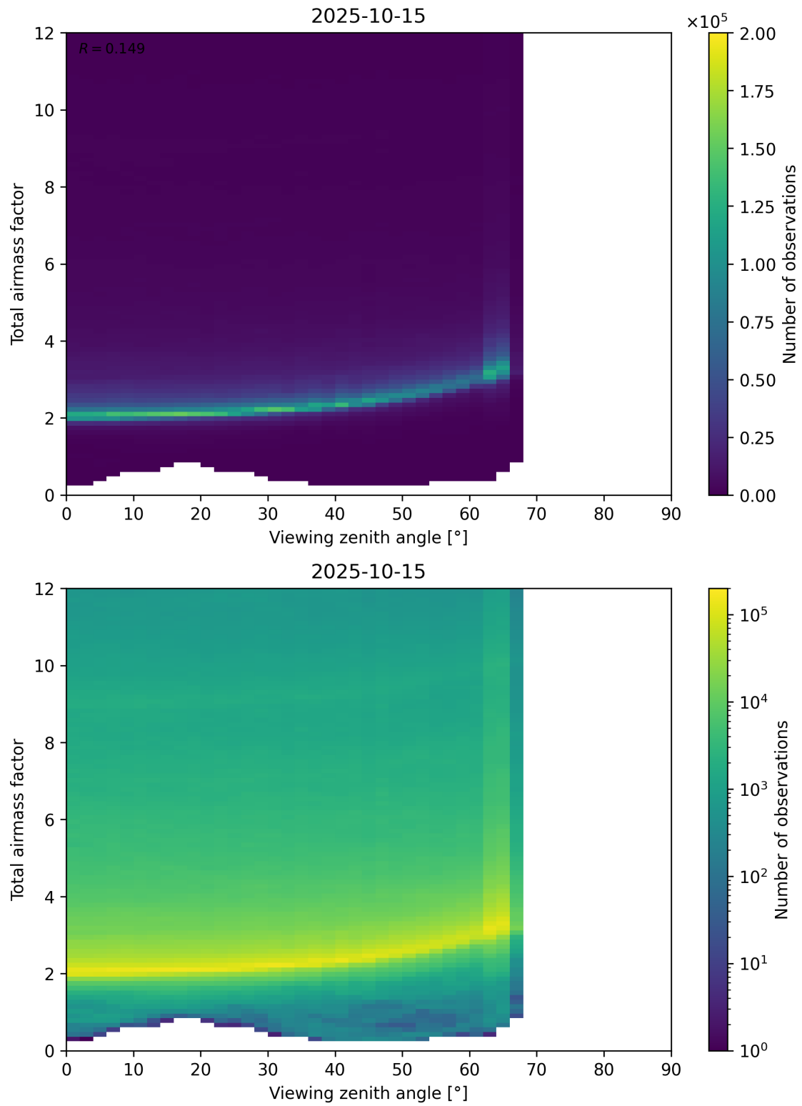
Figure 160: Scatter density plot of “Viewing zenith angle” against “Total airmass factor” for 2025-10-14 to 2025-10-16.
