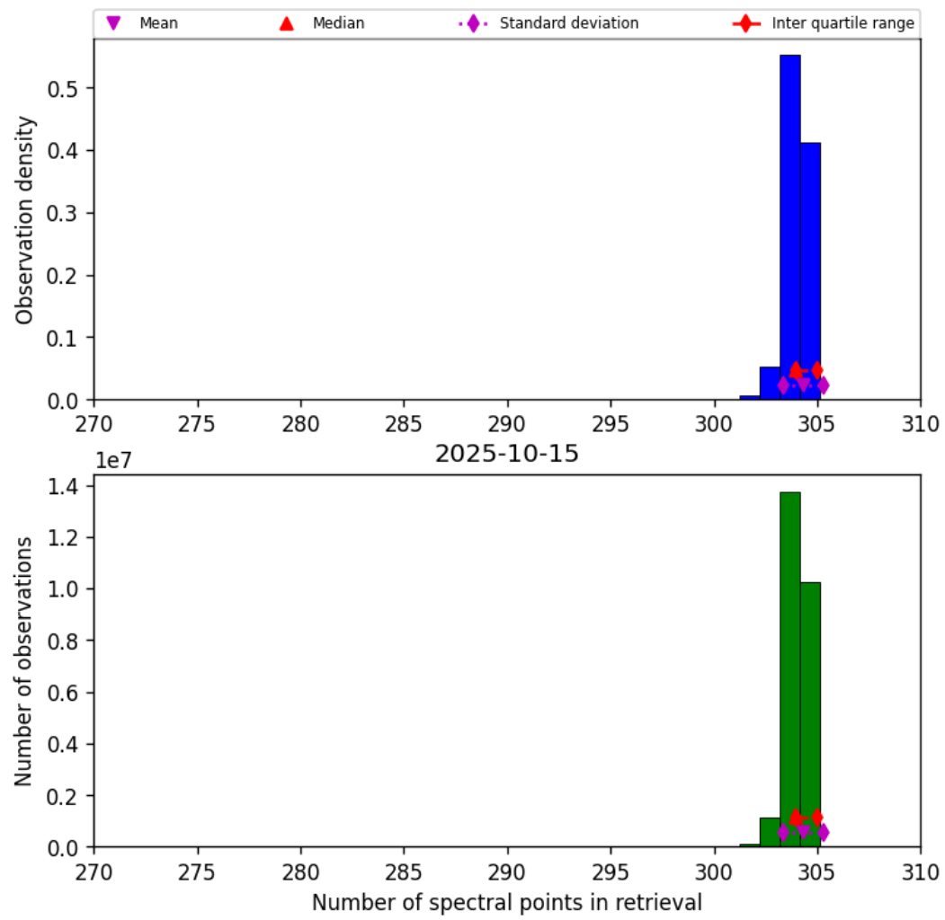
Figure 33: Histogram of “Number of spectral points in retrieval” for 2025-10-14 to 2025-10-16
