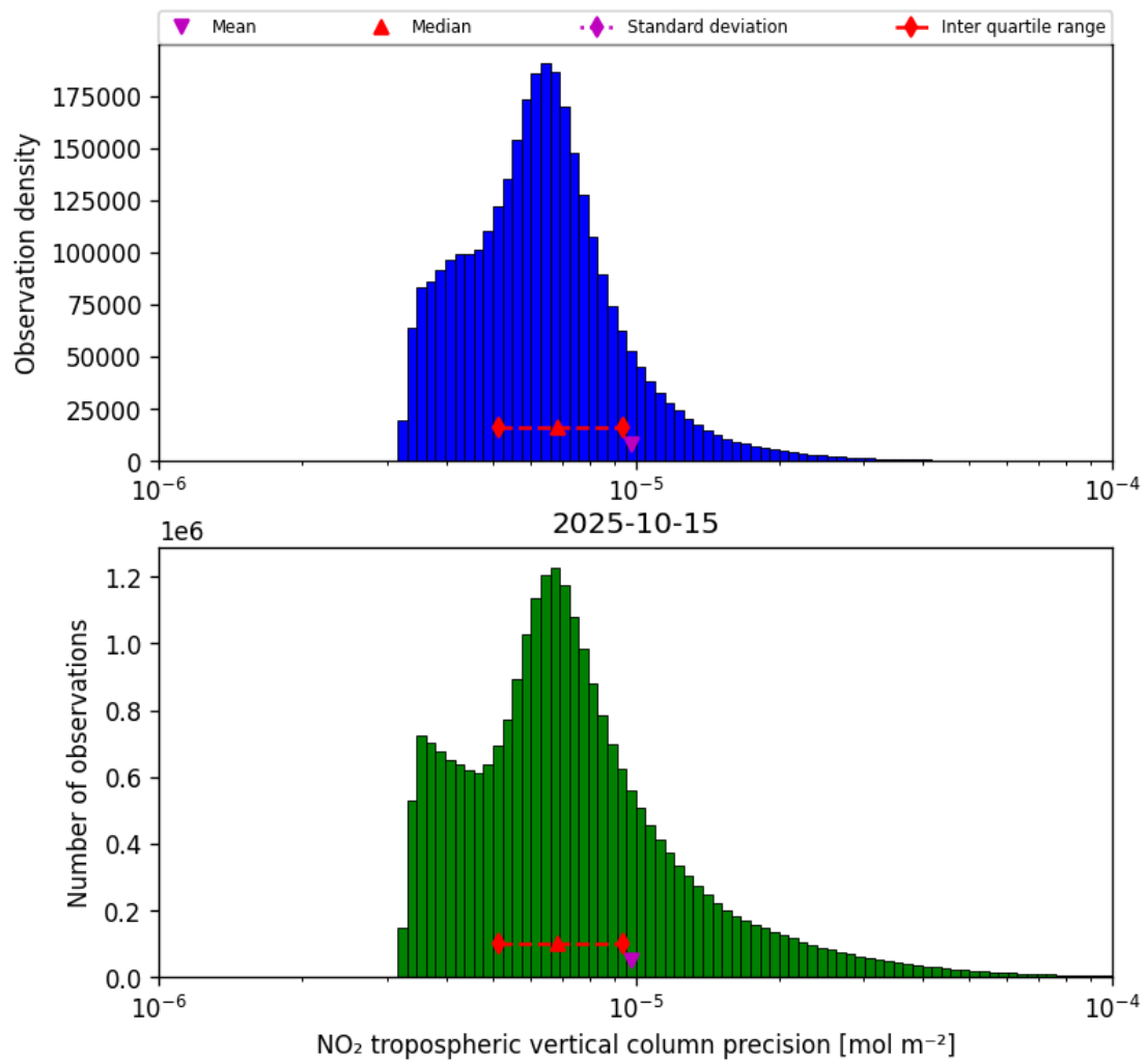
Figure 30: Histogram of “NO 2 tropospheric vertical column precision” for 2025-10-14 to 2025-10-16
