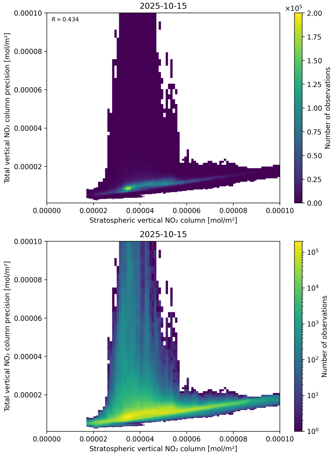
Figure 101: Scatter density plot of “Stratospheric vertical NO 2 column” against “Total vertical NO 2 column precision” for 2025-10-14 to 2025-10-16.
