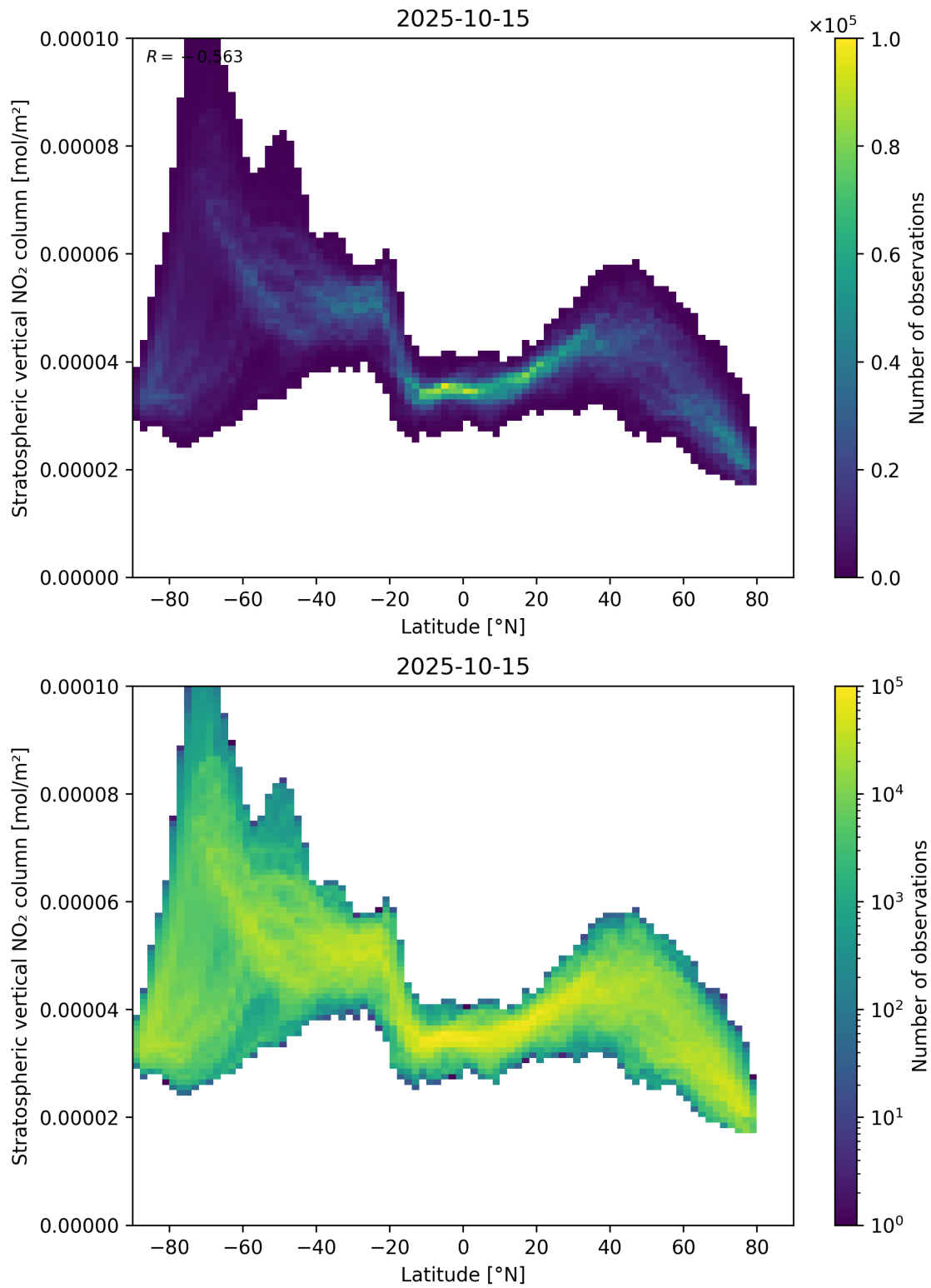
Figure 87: Scatter density plot of “Latitude” against “Stratospheric vertical NO 2 column” for 2025-10-14 to 2025-10-16.
