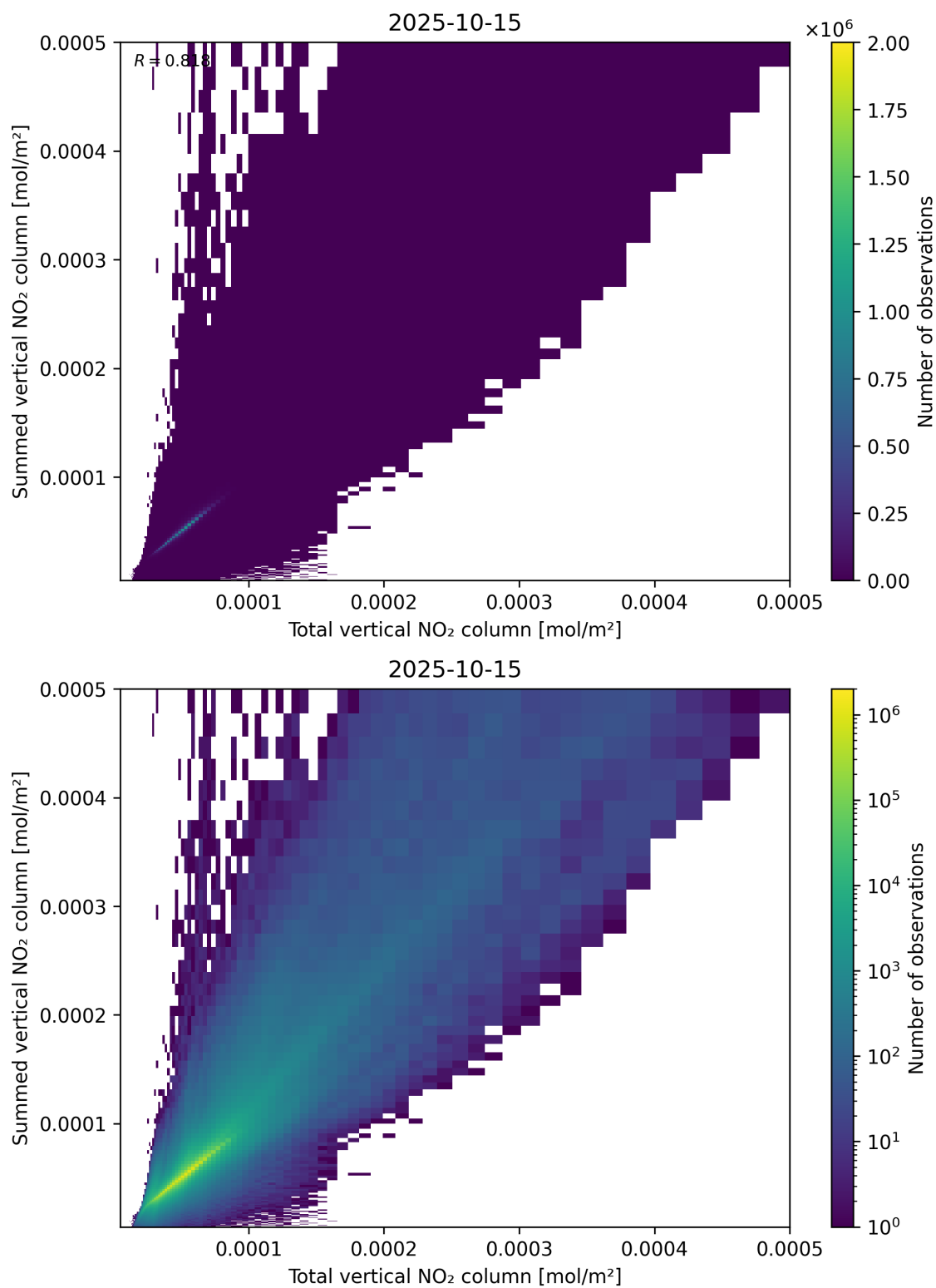
Figure 112: Scatter density plot of “Total vertical NO 2 column” against “Summed vertical NO 2 column” for 2025-10-14 to 2025-10-16.
