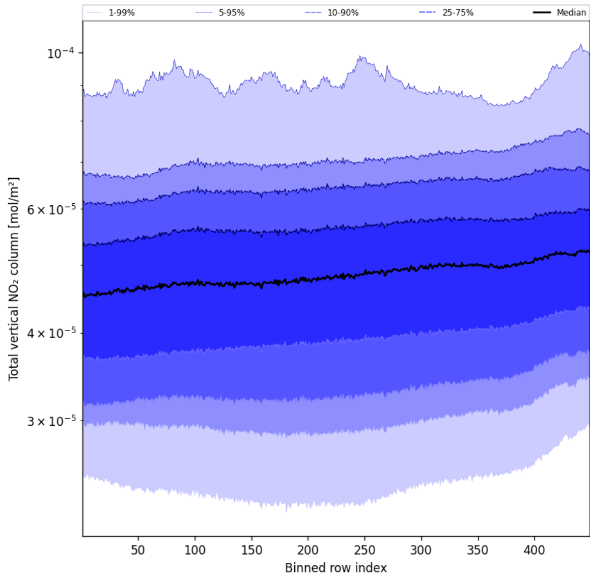
Figure 55: Along track statistics of “Total vertical NO 2 column” for 2025-10-14 to 2025-10-16
