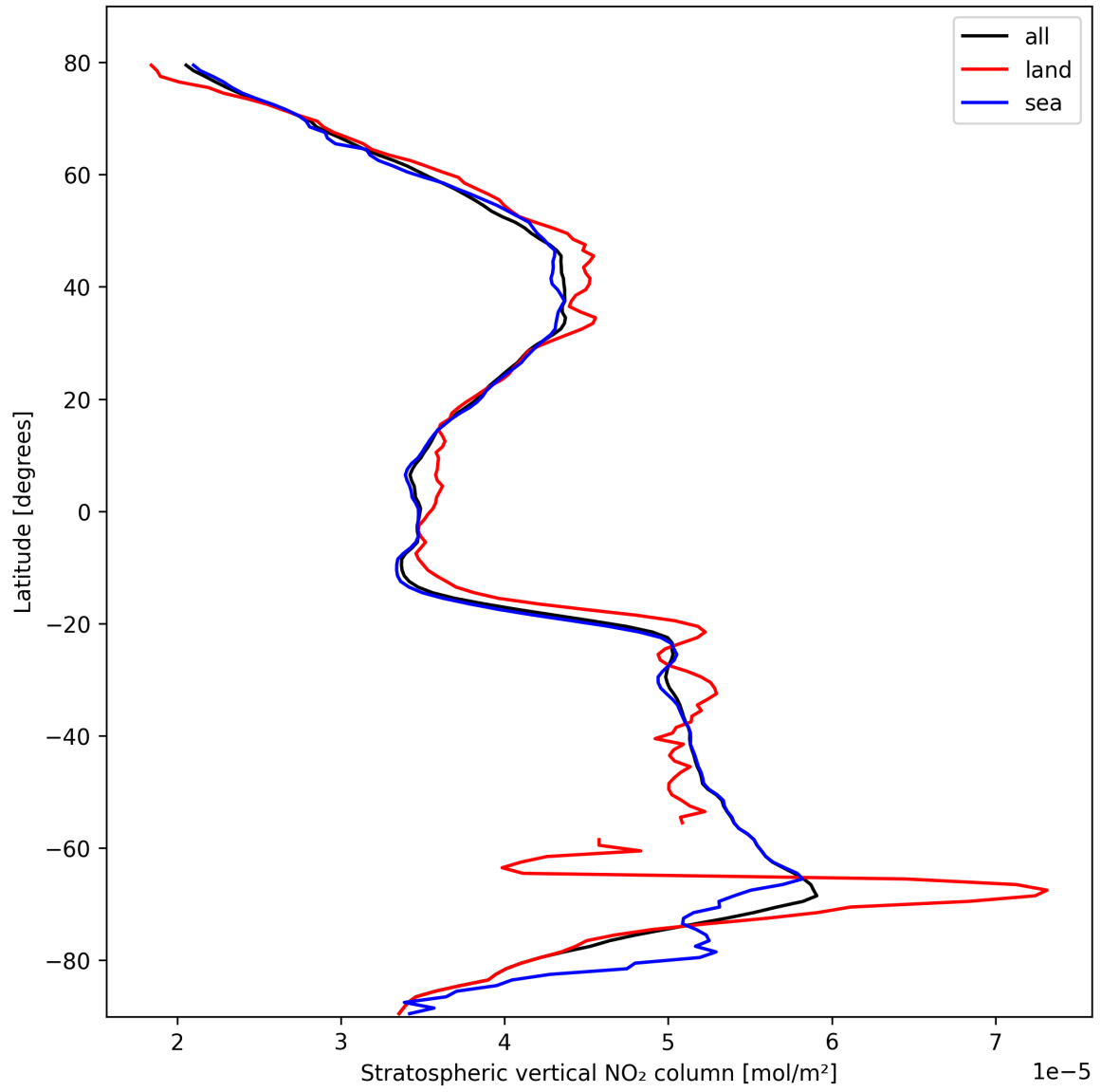
Figure 19: Zonal average of “Stratospheric vertical NO 2 column” for 2025-10-14 to 2025-10-16.
