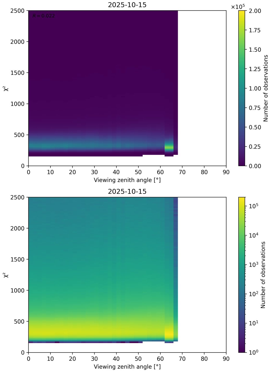
Figure 162: Scatter density plot of “Viewing zenith angle” against “ \chi^2 ” for 2025-10-14 to 2025-10-16.
