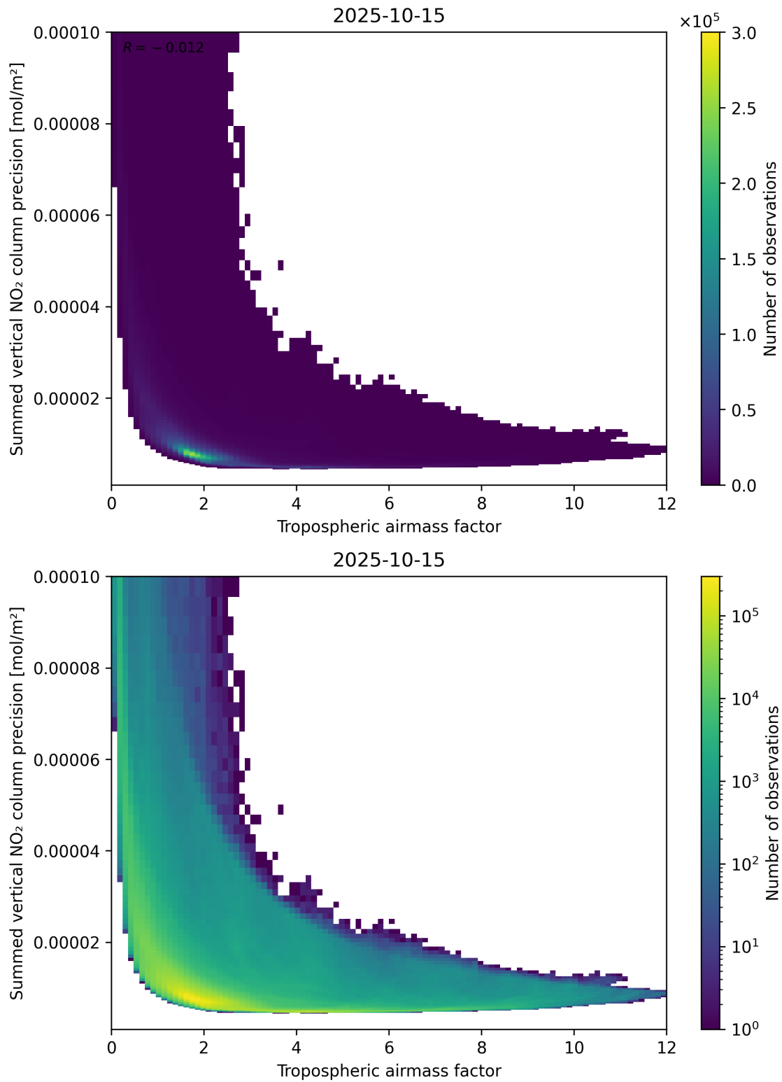
Figure 76: Scatter density plot of “Tropospheric air mass factor” against “Summed vertical NO 2 column precision” for 2025-10-14 to 2025-10-16.
