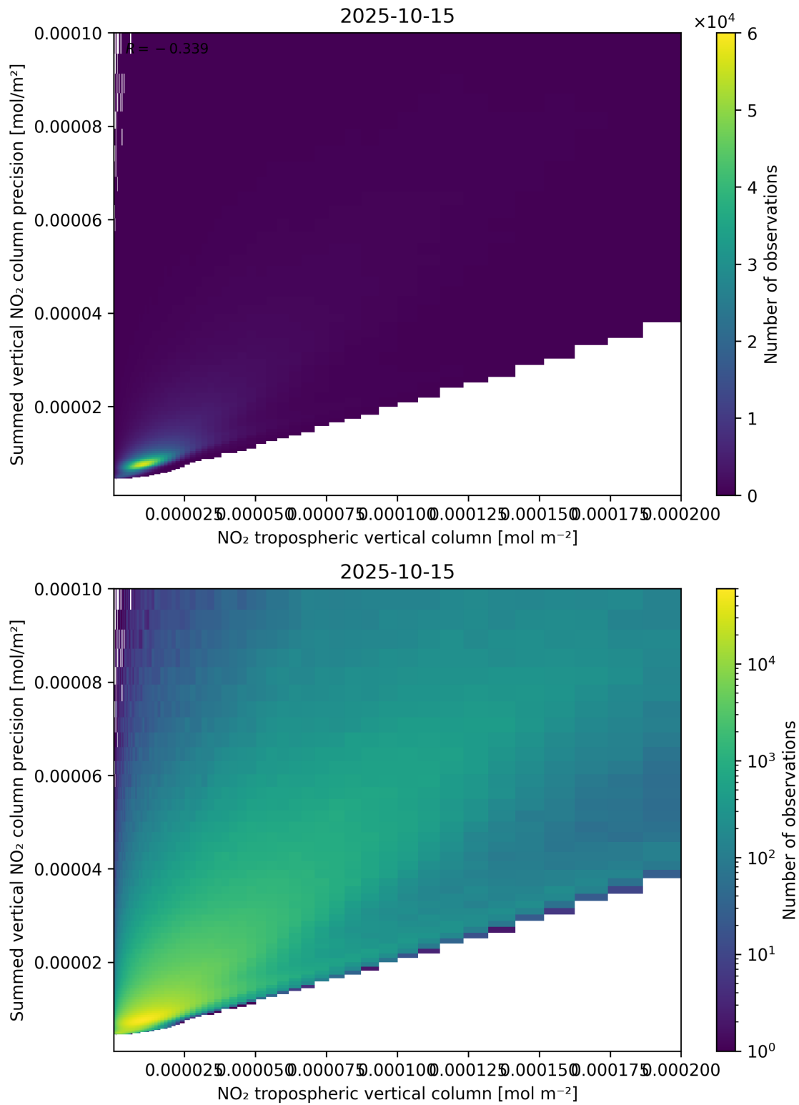
Figure 127: Scatter density plot of “NO 2 tropospheric vertical column” against “Summed vertical NO 2 column precision” for 2025-10-14 to 2025-10-16.
