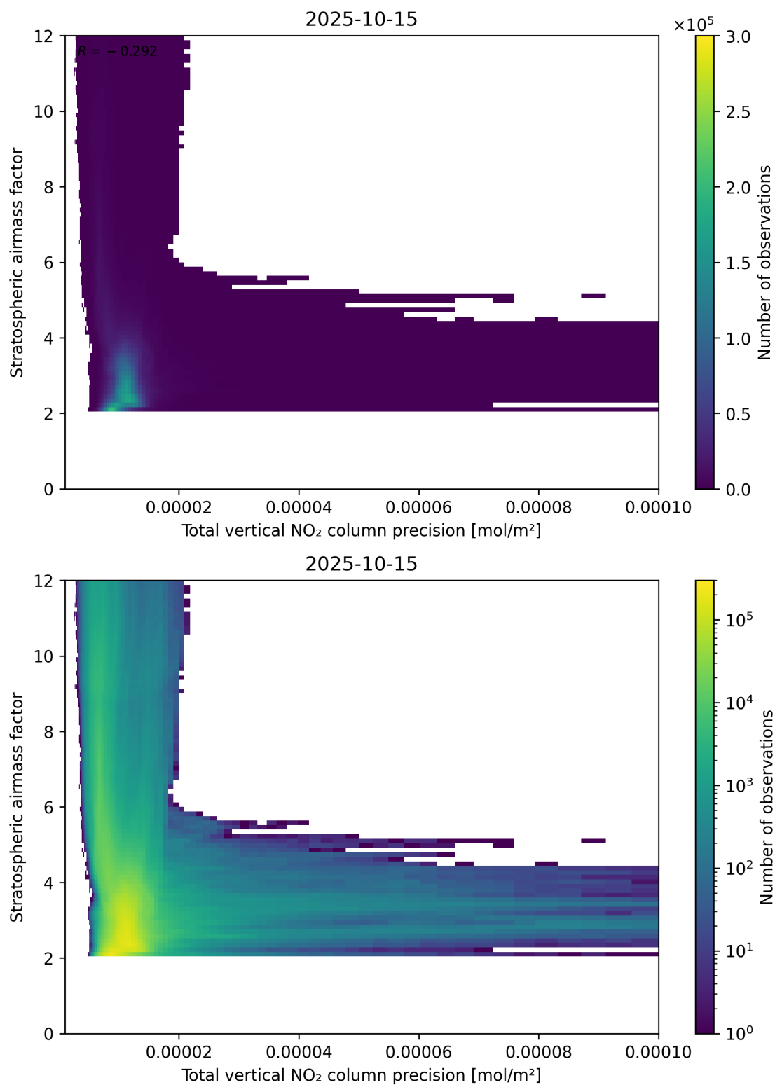
Figure 115: Scatter density plot of “Total vertical NO 2 column precision” against “Stratospheric airmass factor” for 2025-10-14 to 2025-10-16.
