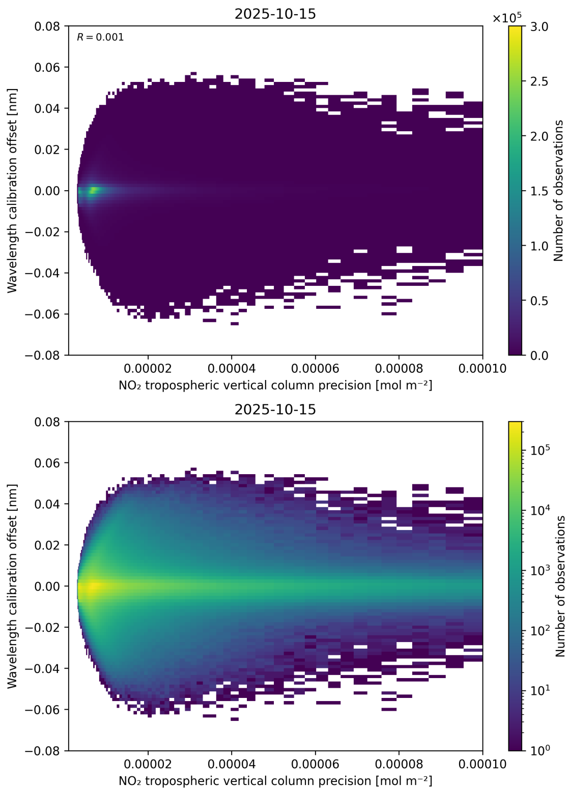
Figure 141: Scatter density plot of “NO 2 tropospheric vertical column precision” against “Wavelength calibration offset” for 2025-10-14 to 2025-10-16.
