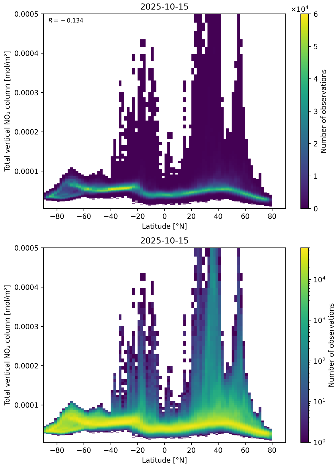
Figure 90: Scatter density plot of “Latitude” against “Total vertical NO 2 column” for 2025-10-14 to 2025-10-16.
