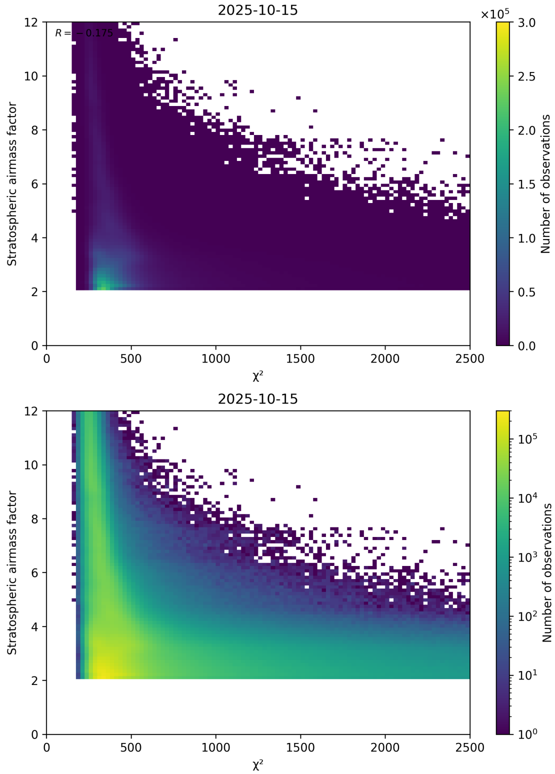
Figure 81: Scatter density plot of “ \chi^2 ” against “Stratospheric airmass factor” for 2025-10-14 to 2025-10-16.
