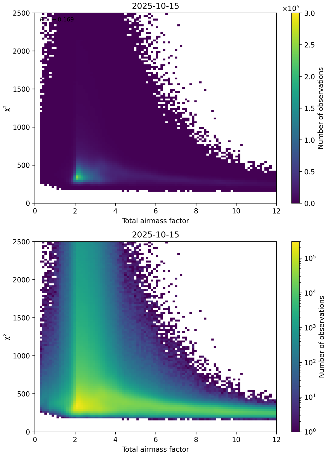
Figure 63: Scatter density plot of “Total airmass factor” against “ \chi^2 ” for 2025-10-14 to 2025-10-16.
