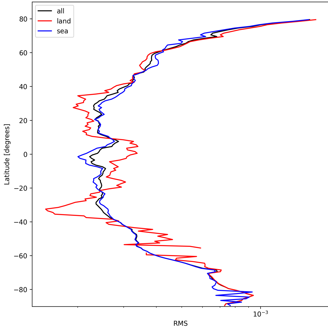
Figure 26: Zonal average of “RMS” for 2025-10-14 to 2025-10-16.
