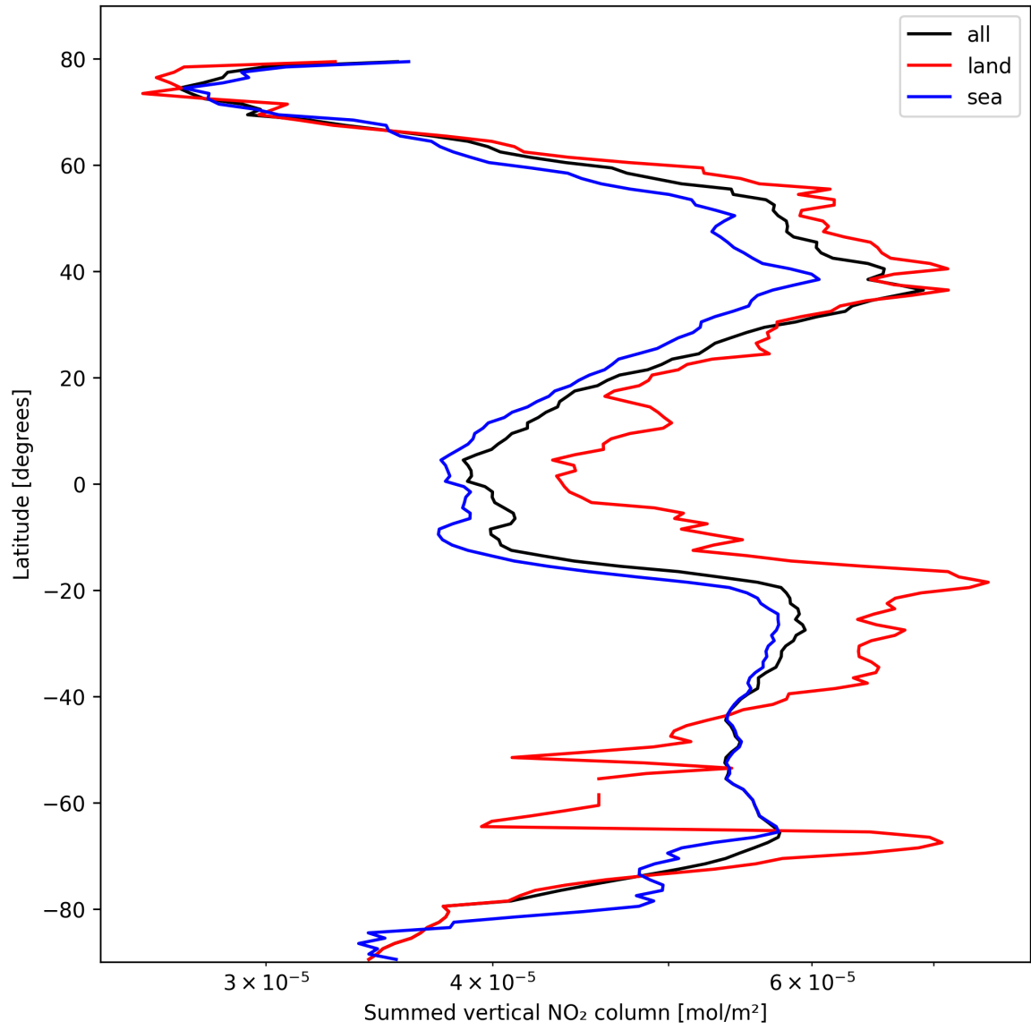
Figure 23: Zonal average of “Summed vertical NO 2 column” for 2025-10-14 to 2025-10-16.
