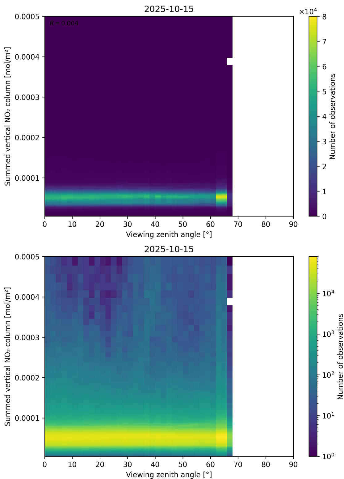
Figure 165: Scatter density plot of “Viewing zenith angle” against “Summed vertical NO 2 column” for 2025-10-14 to 2025-10-16.
