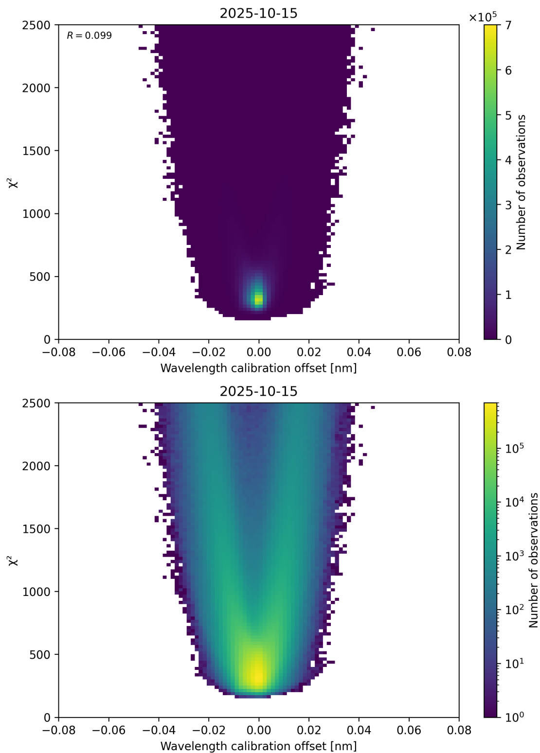
Figure 175: Scatter density plot of “Wavelength calibration offset” against “ \chi^2 ” for 2025-10-14 to 2025-10-16.
