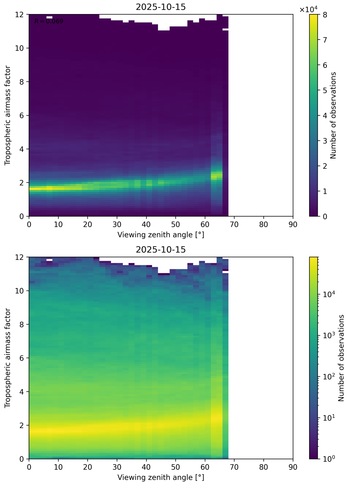
Figure 161: Scatter density plot of “Viewing zenith angle” against “Tropospheric airmass factor” for 2025-10-14 to 2025-10-16.
