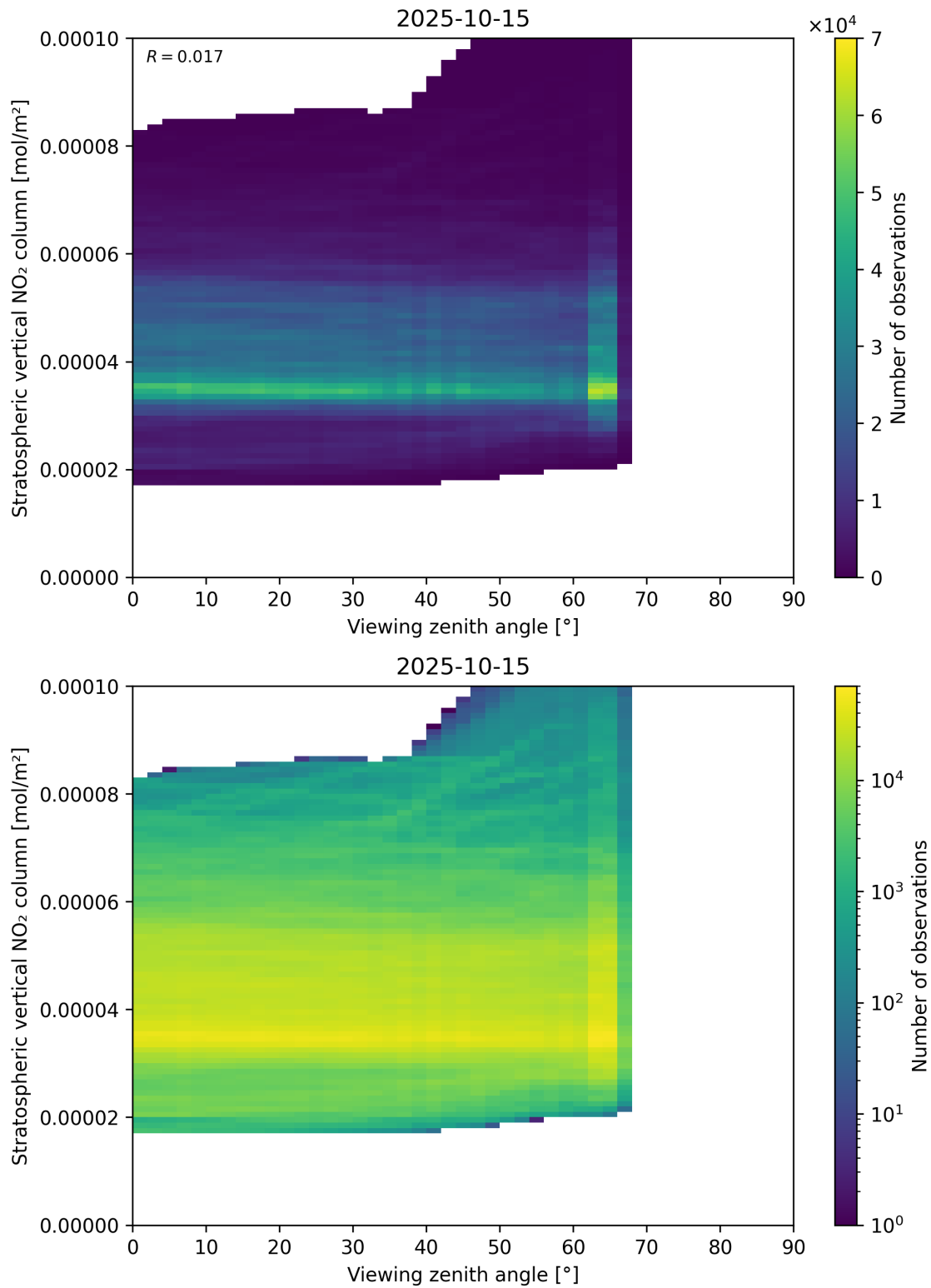
Figure 164: Scatter density plot of “Viewing zenith angle” against “Stratospheric vertical NO 2 column” for 2025-10-14 to 2025-10-16.
