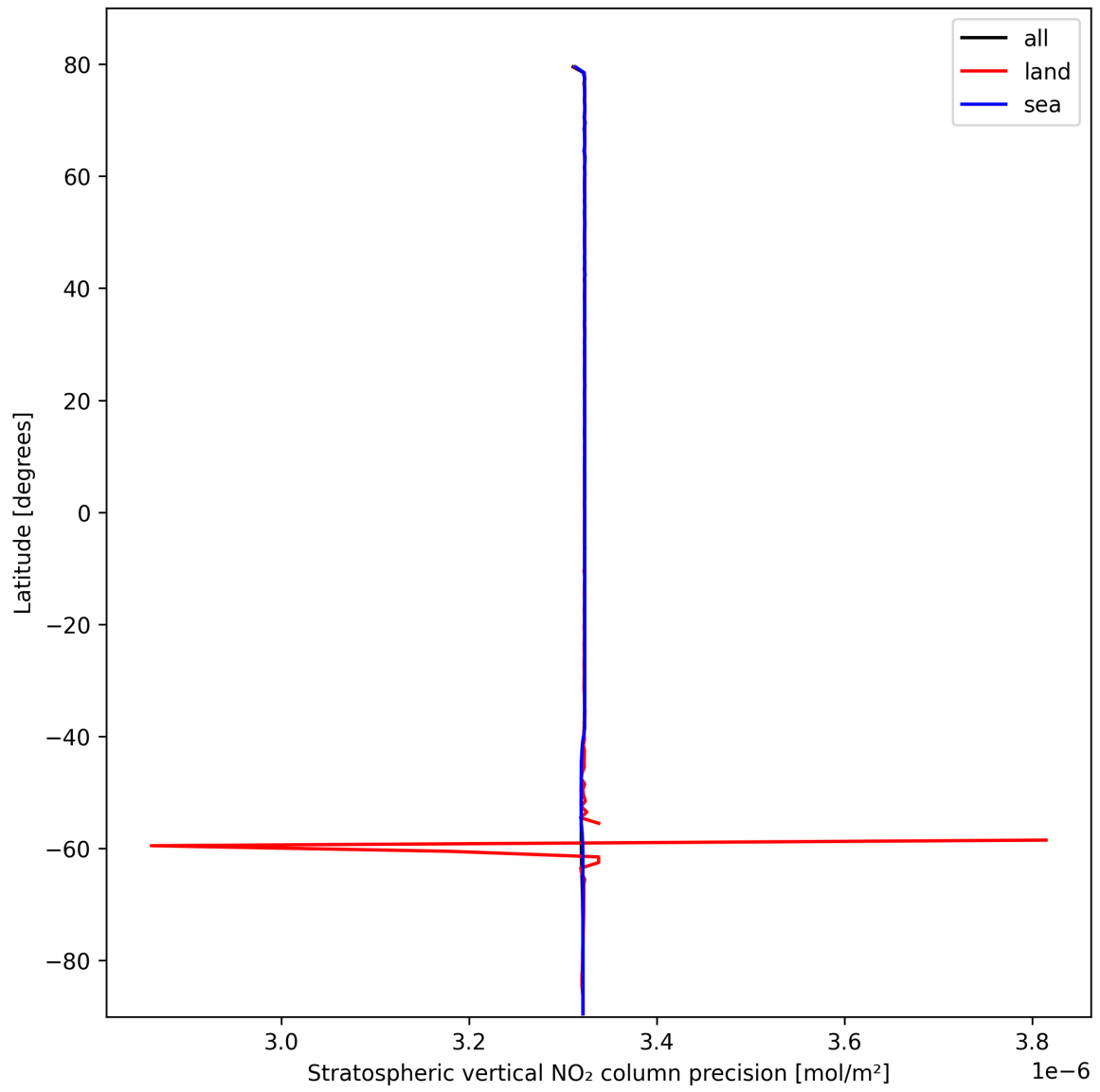
Figure 20: Zonal average of “Stratospheric vertical NO 2 column precision” for 2025-10-14 to 2025-10-16.
