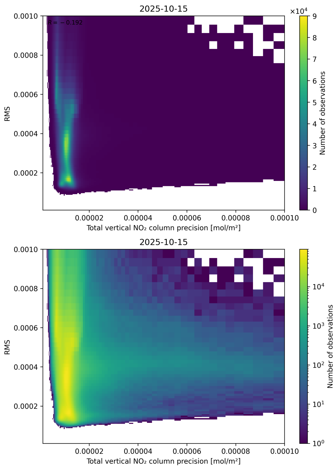
Figure 119: Scatter density plot of “Total vertical NO 2 column precision” against “RMS” for 2025-10-14 to 2025-10-16.
