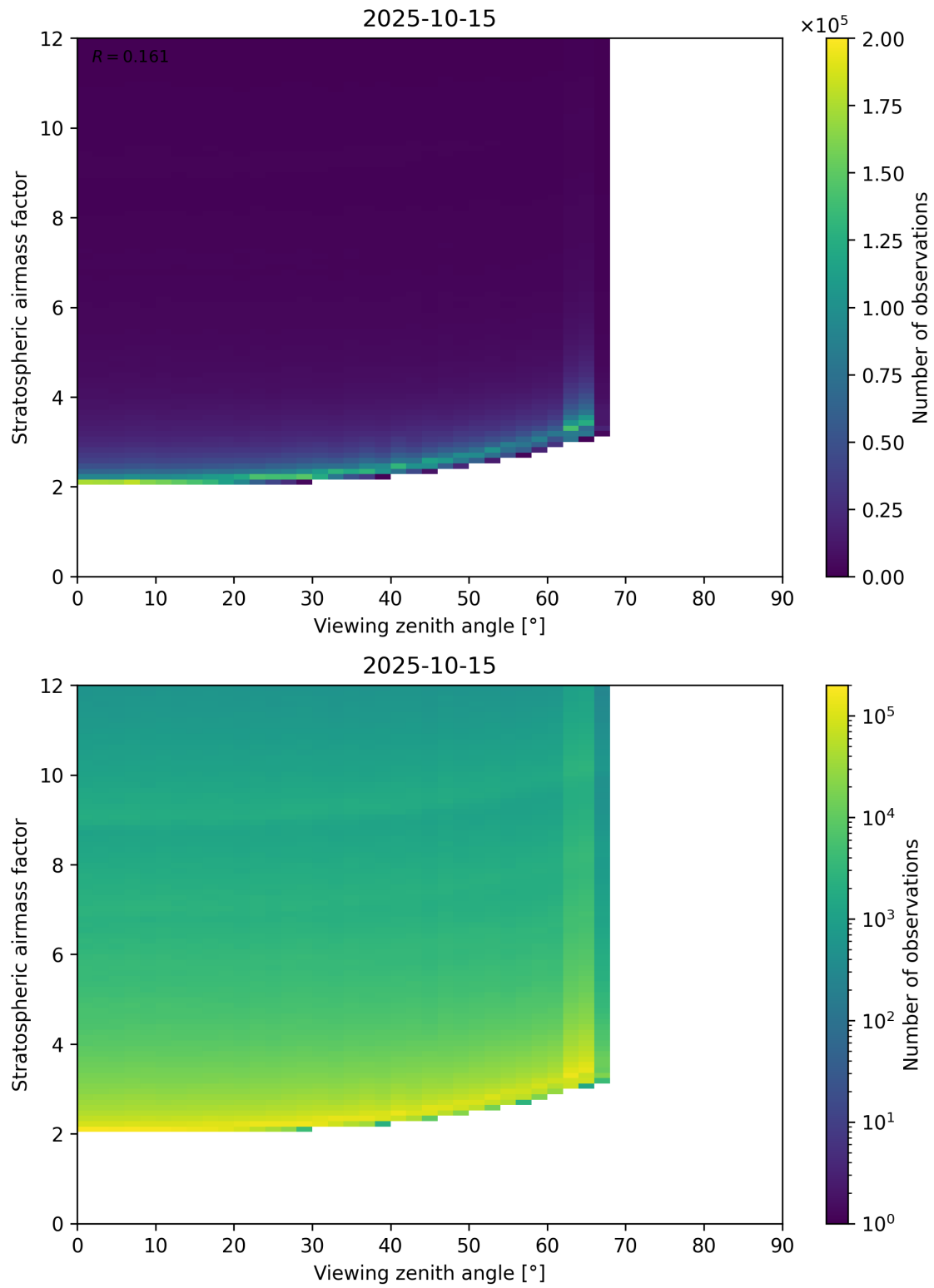
Figure 159: Scatter density plot of “Viewing zenith angle” against “Stratospheric airmass factor” for 2025-10-14 to 2025-10-16.
