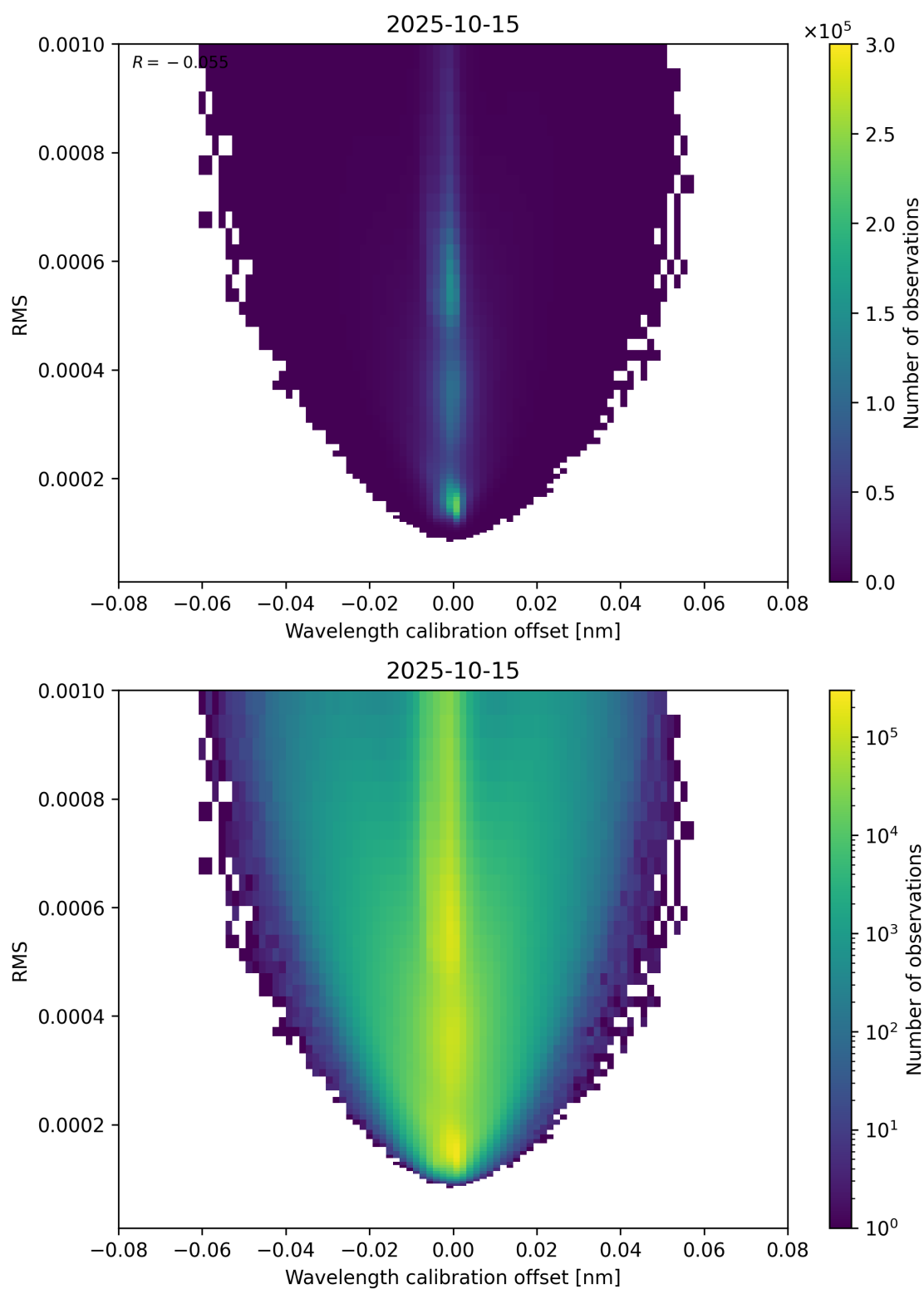
Figure 181: Scatter density plot of “Wavelength calibration offset” against “RMS” for 2025-10-14 to 2025-10-16.
