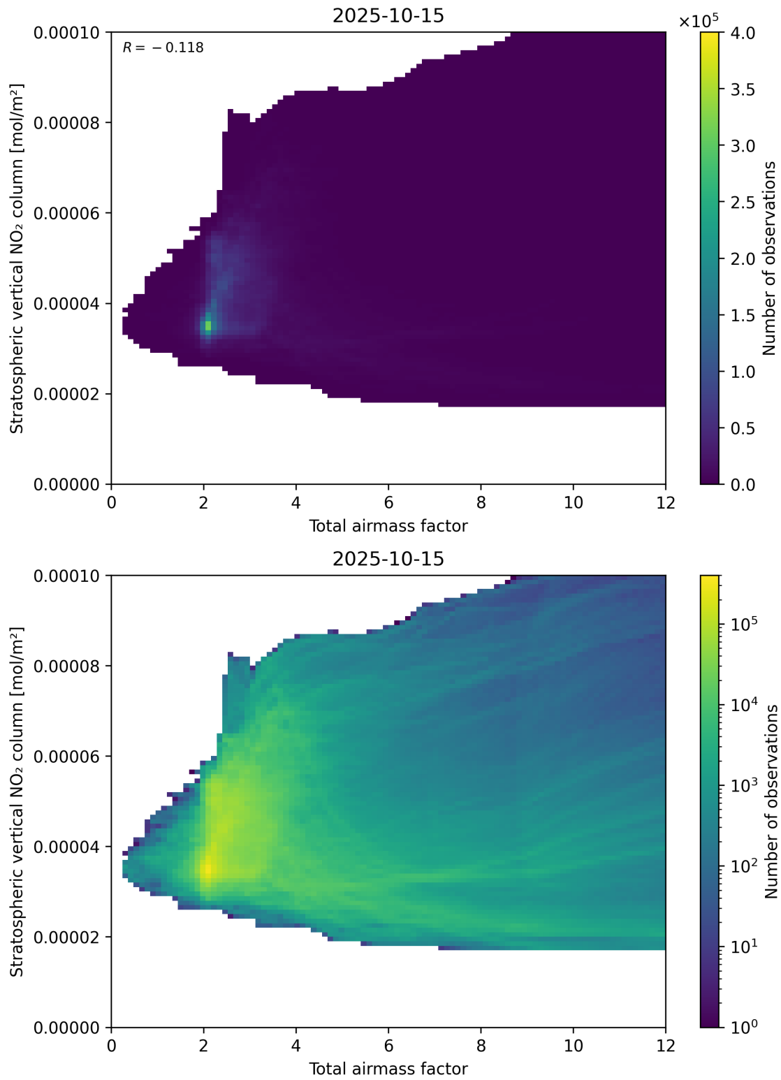
Figure 64: Scatter density plot of “Total airmass factor” against “Stratospheric vertical NO 2 column” for 2025-10-14 to 2025-10-16.
