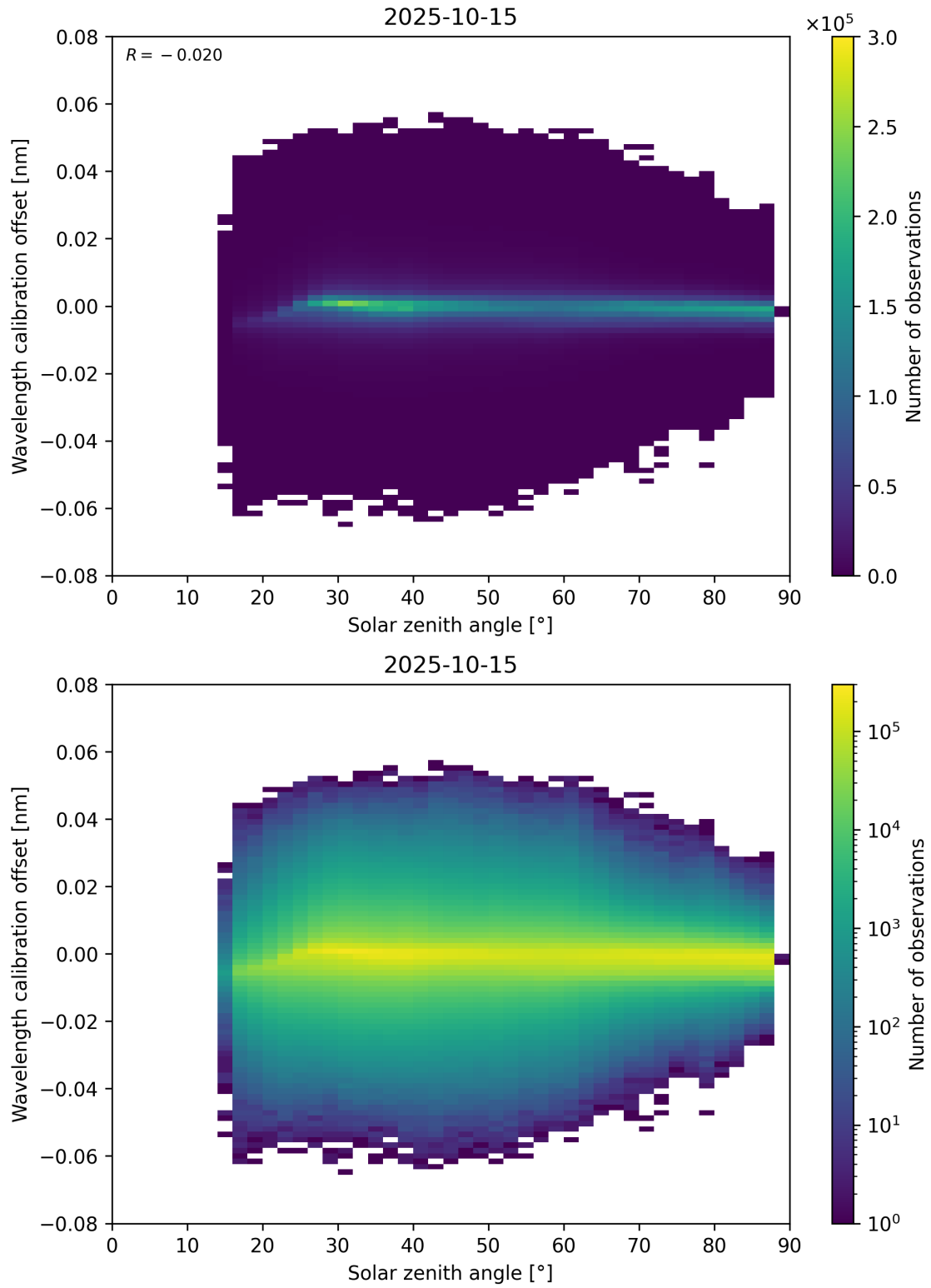
Figure 158: Scatter density plot of “Solar zenith angle” against “Wavelength calibration offset” for 2025-10-14 to 2025-10-16.
