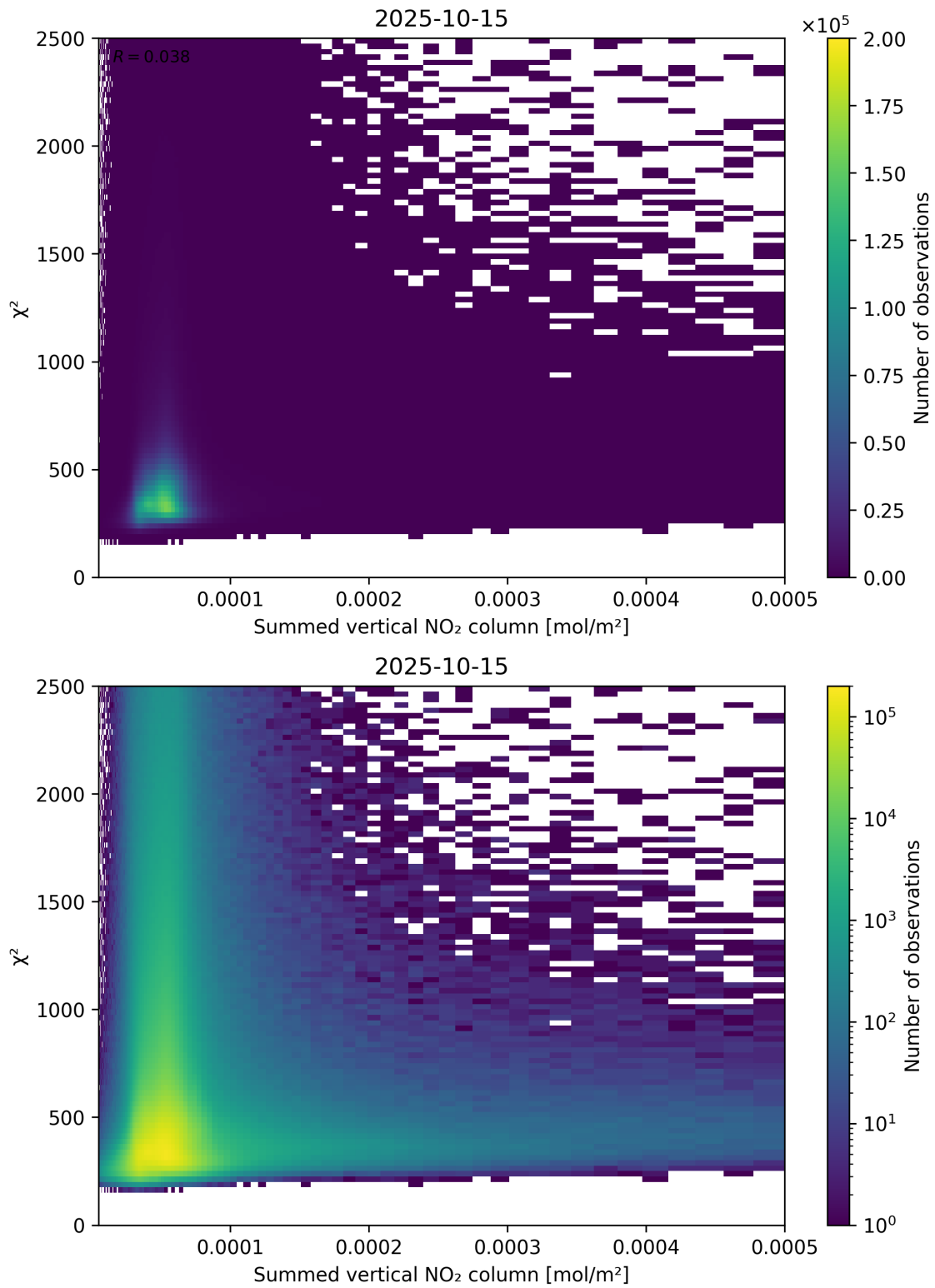
Figure 104: Scatter density plot of “Summed vertical NO 2 column” against “ \chi^2 ” for 2025-10-14 to 2025-10-16.
