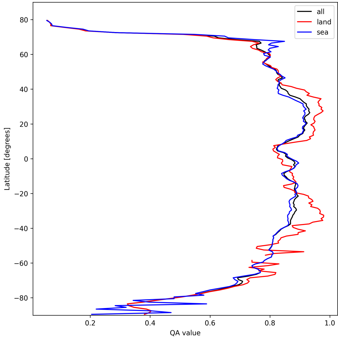
Figure 11: Zonal average of “QA value” for 2025-10-14 to 2025-10-16.
