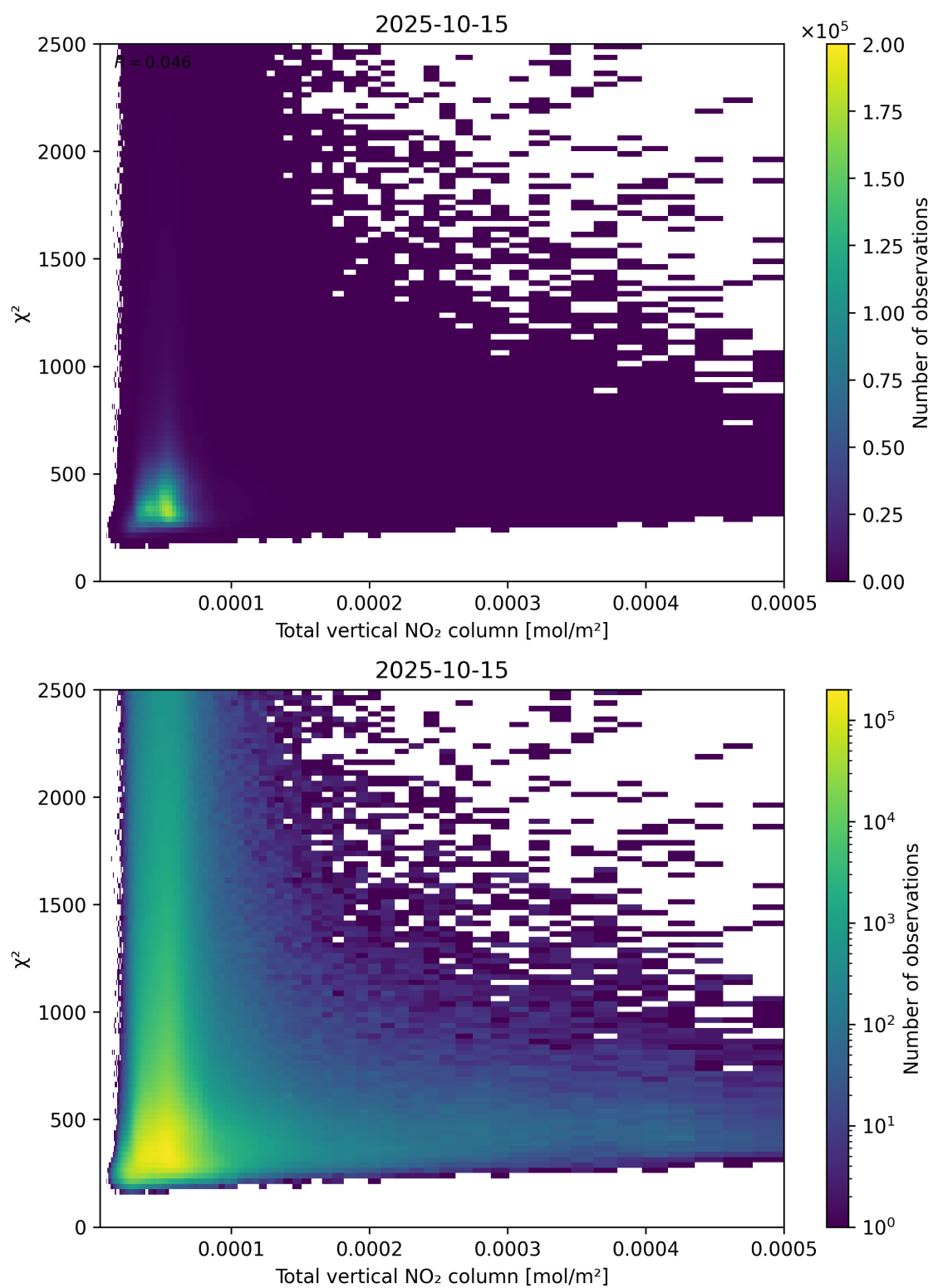
Figure 111: Scatter density plot of “Total vertical NO 2 column” against “ \chi^2 ” for 2025-10-14 to 2025-10-16.
