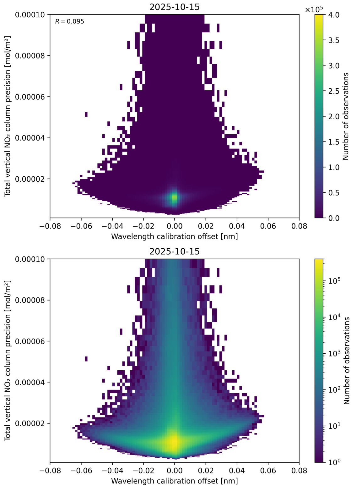
Figure 180: Scatter density plot of “Wavelength calibration offset” against “Total vertical NO 2 column precision” for 2025-10-14 to 2025-10-16.
