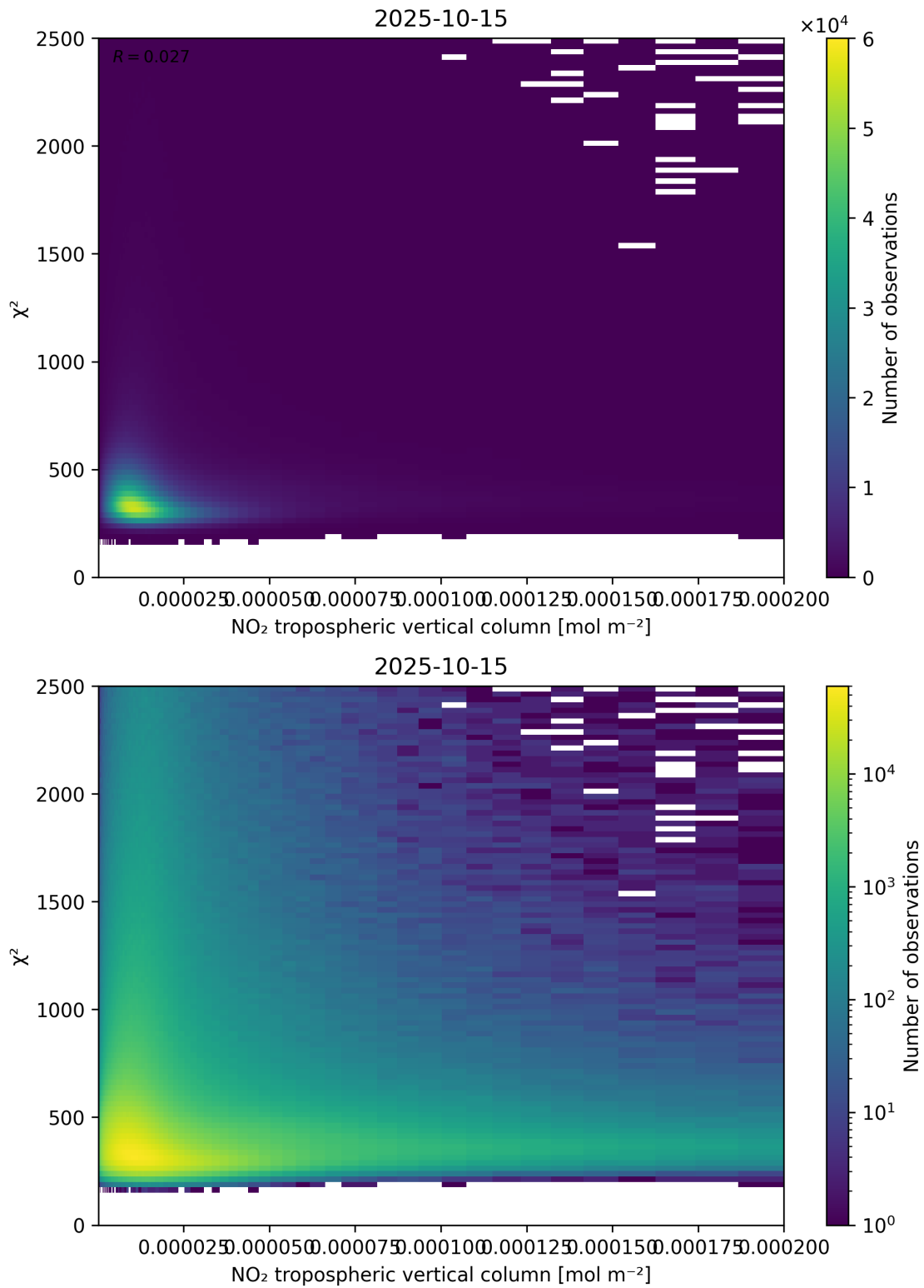
Figure 124: Scatter density plot of “NO 2 tropospheric vertical column” against “ \chi^2 ” for 2025-10-14 to 2025-10-16.
