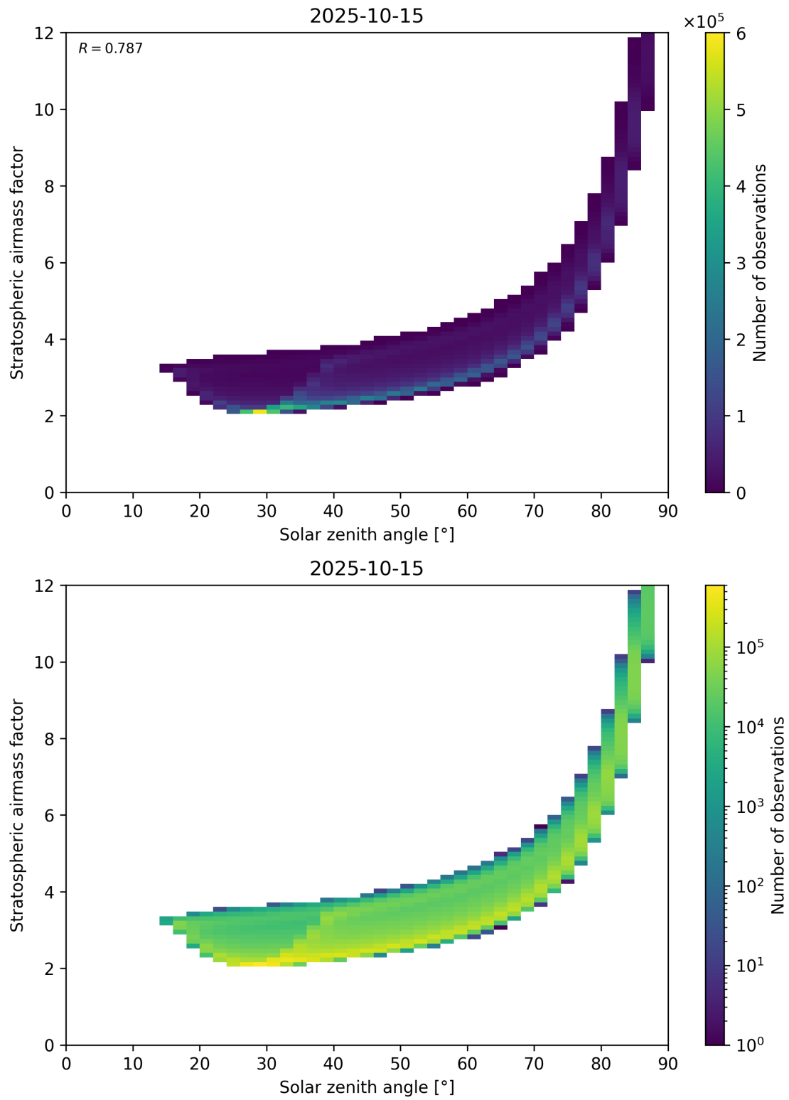
Figure 145: Scatter density plot of “Solar zenith angle” against “Stratospheric airmass factor” for 2025-10-14 to 2025-10-16.
