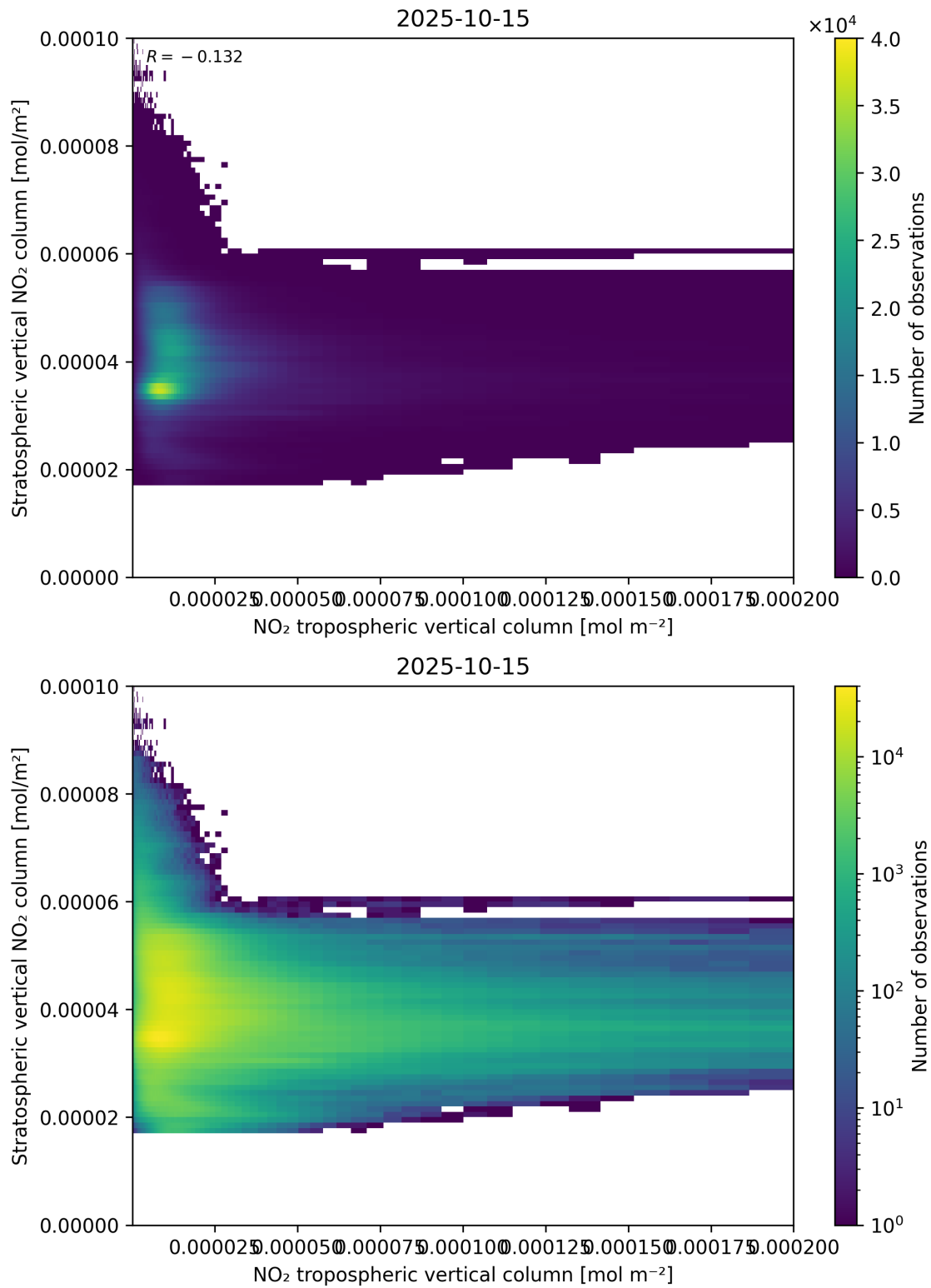
Figure 125: Scatter density plot of “NO 2 tropospheric vertical column” against “Stratospheric vertical NO 2 column” for 2025-10-14 to 2025-10-16.
