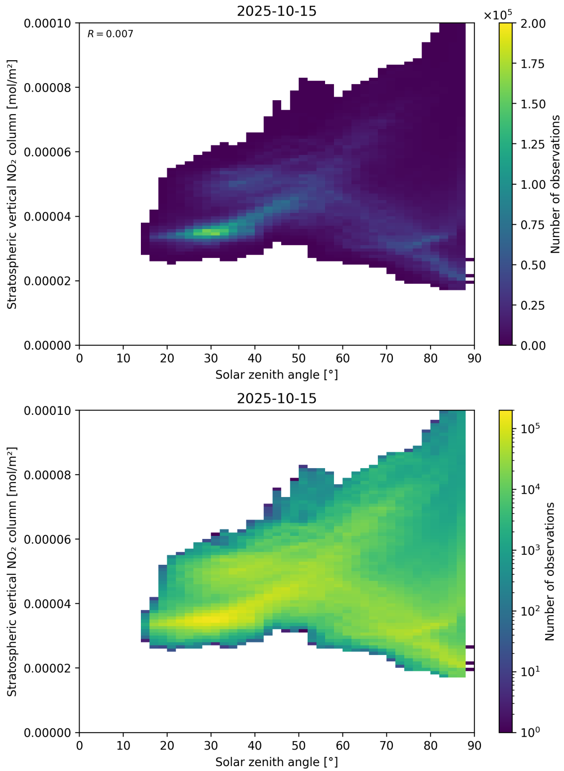
Figure 150: Scatter density plot of “Solar zenith angle” against “Stratospheric vertical NO 2 column” for 2025-10-14 to 2025-10-16.
