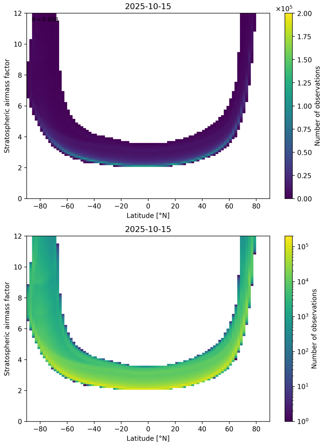
Figure 83: Scatter density plot of “Latitude” against “Stratospheric air mass factor” for 2025-10-14 to 2025-10-16.
