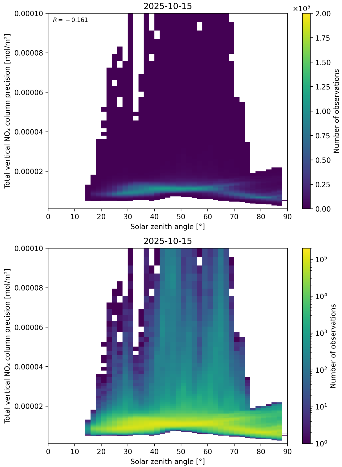
Figure 154: Scatter density plot of “Solar zenith angle” against “Total vertical NO 2 column precision” for 2025-10-14 to 2025-10-16.
