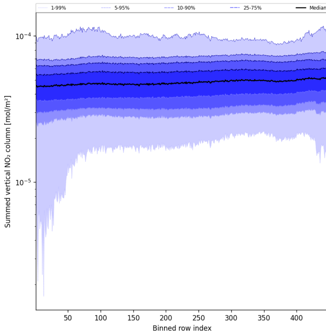
Figure 57: Along track statistics of “Summed vertical NO 2 column” for 2025-10-14 to 2025-10-16
