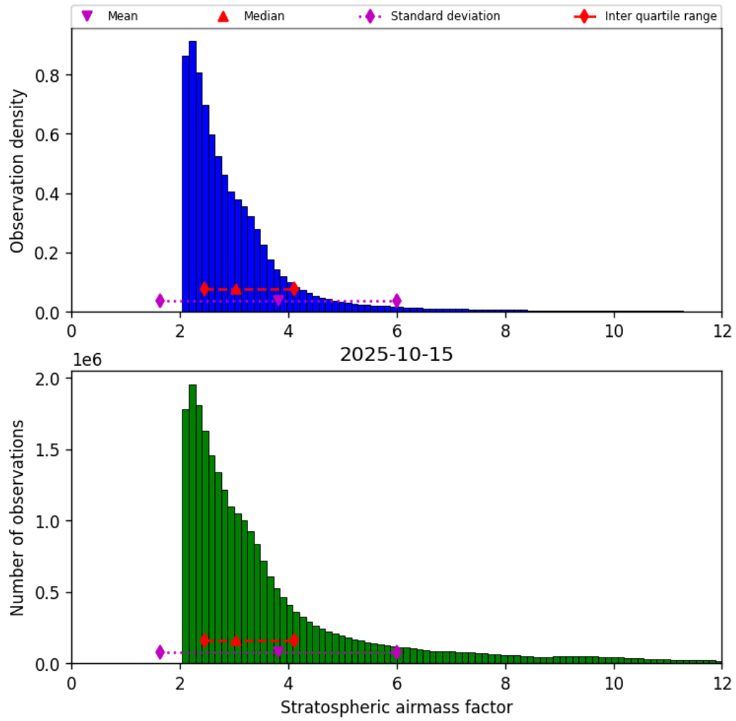
Figure 44: Histogram of “Stratospheric airmass factor” for 2025-10-14 to 2025-10-16
