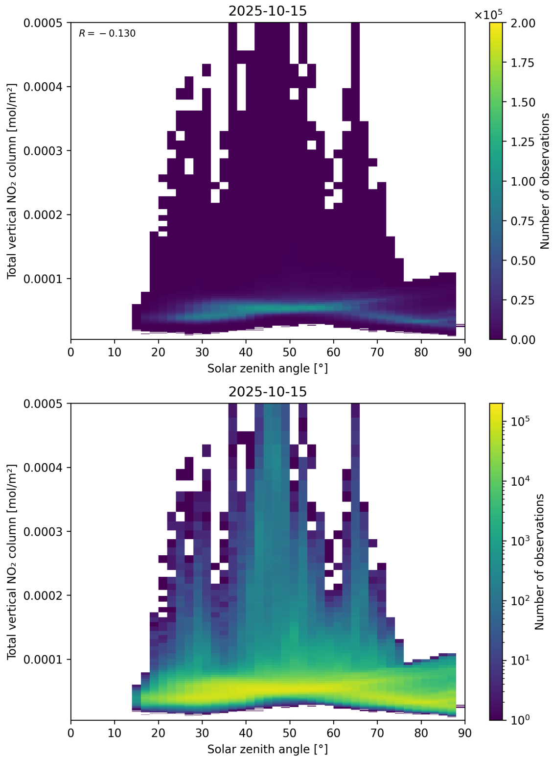
Figure 153: Scatter density plot of “Solar zenith angle” against “Total vertical NO 2 column” for 2025-10-14 to 2025-10-16.
