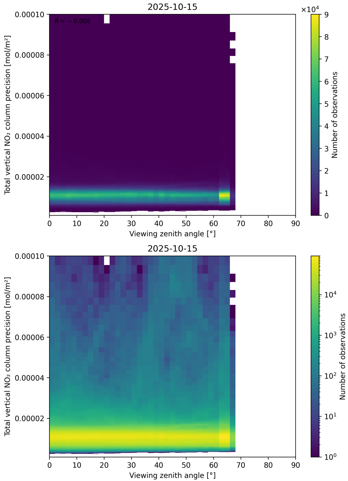
Figure 168: Scatter density plot of “Viewing zenith angle” against “Total vertical NO 2 column precision” for 2025-10-14 to 2025-10-16.
