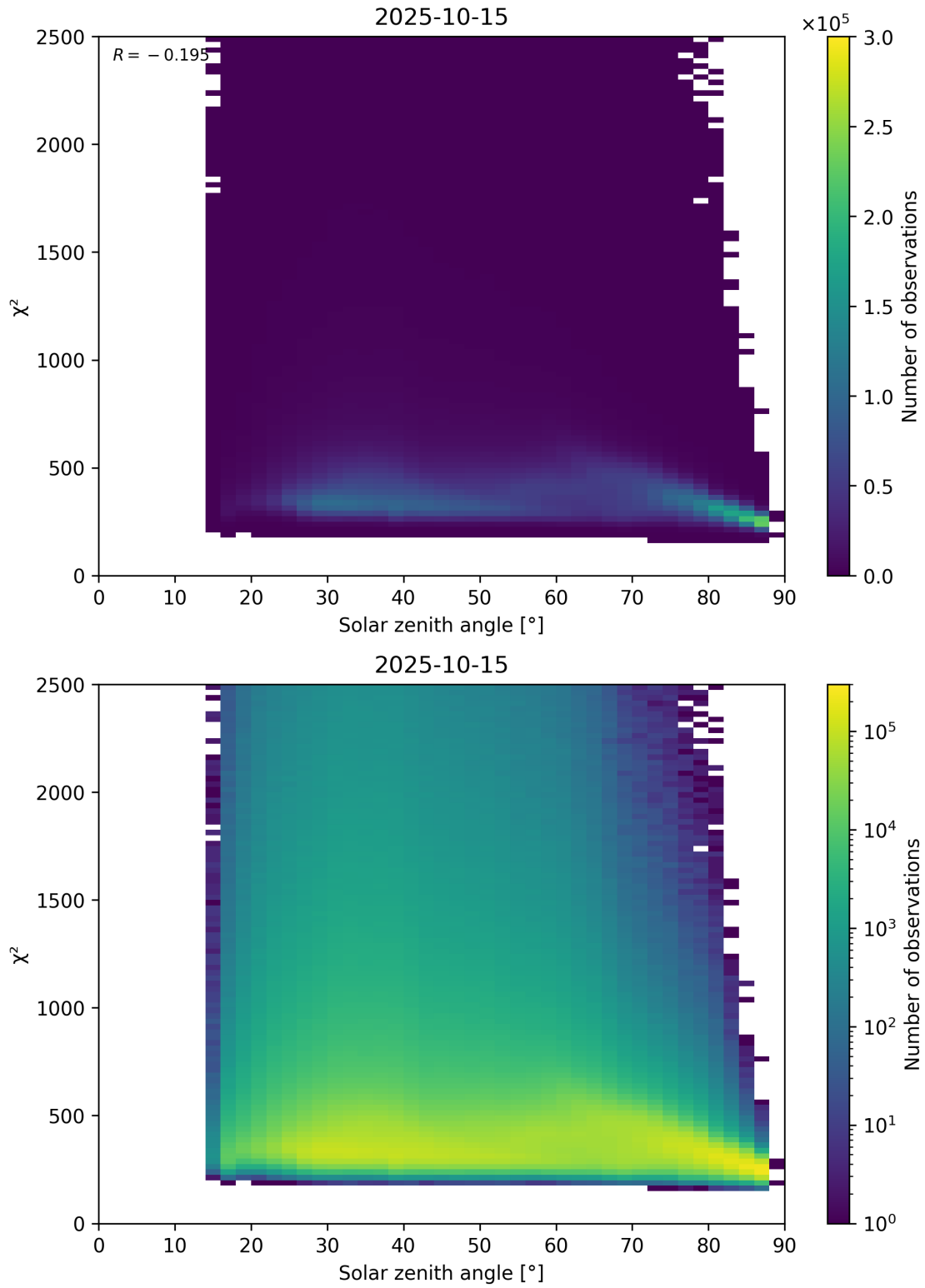
Figure 148: Scatter density plot of “Solar zenith angle” against “ \chi^2 ” for 2025-10-14 to 2025-10-16.
