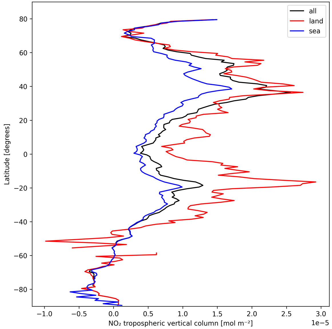
Figure 12: Zonal average of “NO 2 tropospheric vertical column” for 2025-10-14 to 2025-10-16.
