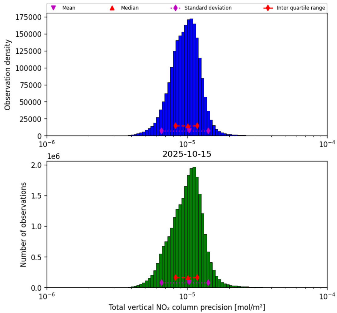
Figure 39: Histogram of “Total vertical NO 2 column precision” for 2025-10-14 to 2025-10-16
