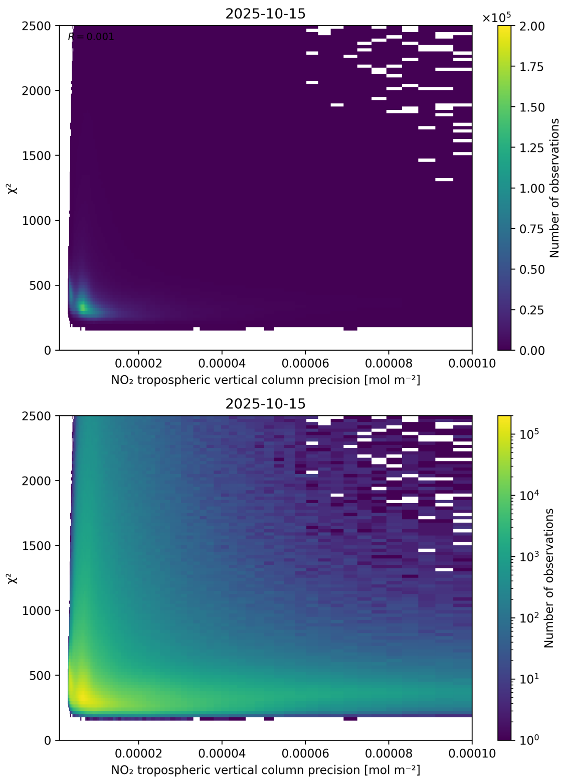
Figure 134: Scatter density plot of “NO 2 tropospheric vertical column precision” against “ \chi^2 ” for 2025-10-14 to 2025-10-16.
