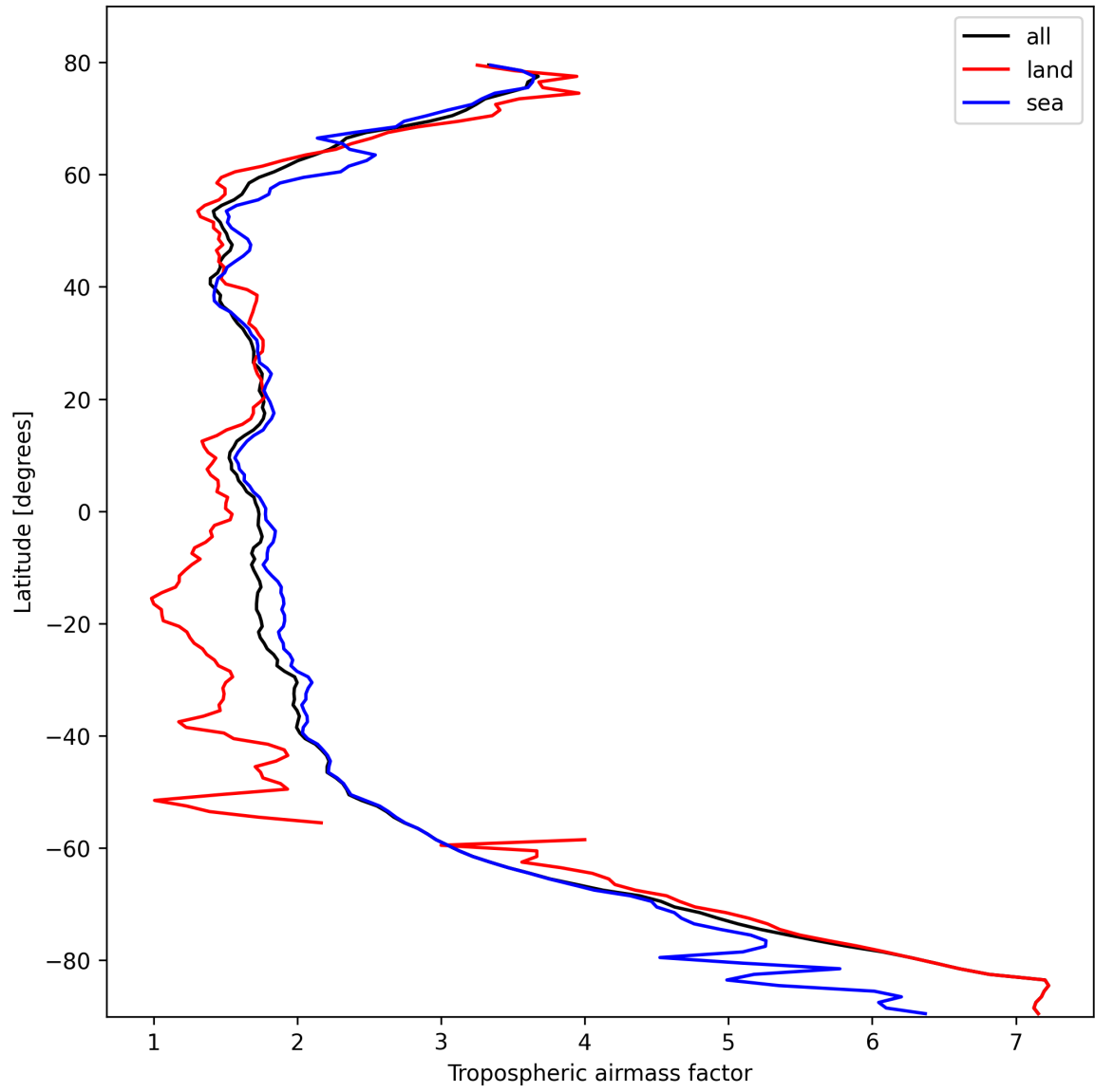
Figure 14: Zonal average of “Tropospheric air mass factor” for 2025-10-14 to 2025-10-16.
