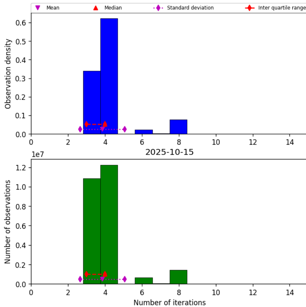
Figure 34: Histogram of “Number of iterations” for 2025-10-14 to 2025-10-16
