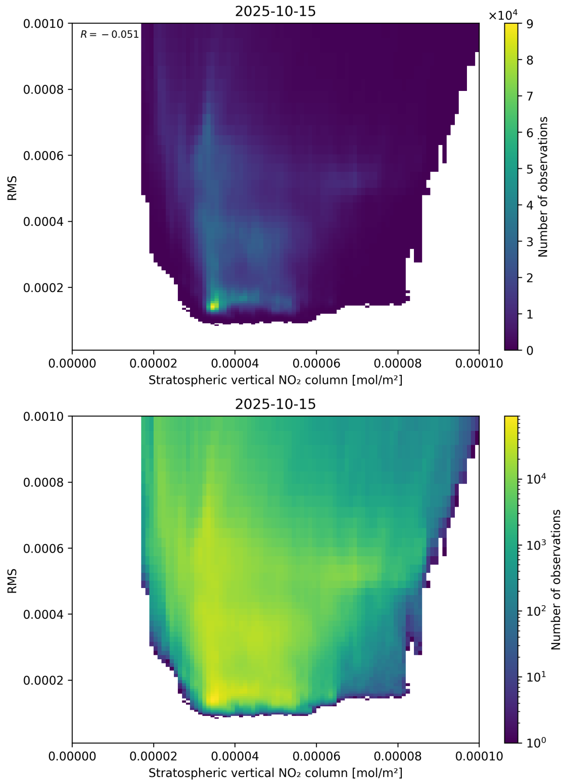
Figure 102: Scatter density plot of “Stratospheric vertical NO 2 column” against “RMS” for 2025-10-14 to 2025-10-16.
