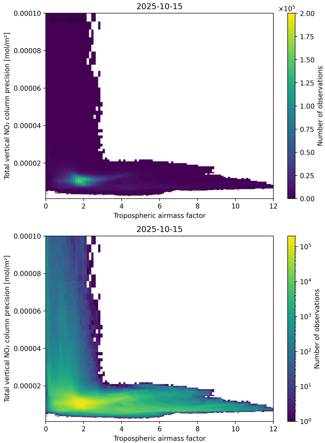
Figure 78: Scatter density plot of “Tropospheric air mass factor” against “Total vertical NO 2 column precision” for 2025-10-14 to 2025-10-16.
