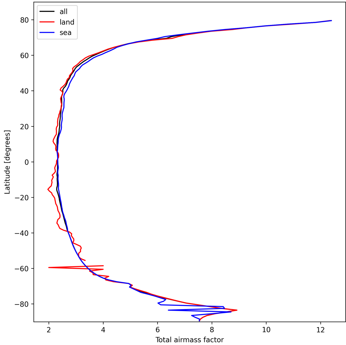
Figure 15: Zonal average of “Total airmass factor” for 2025-10-14 to 2025-10-16.
