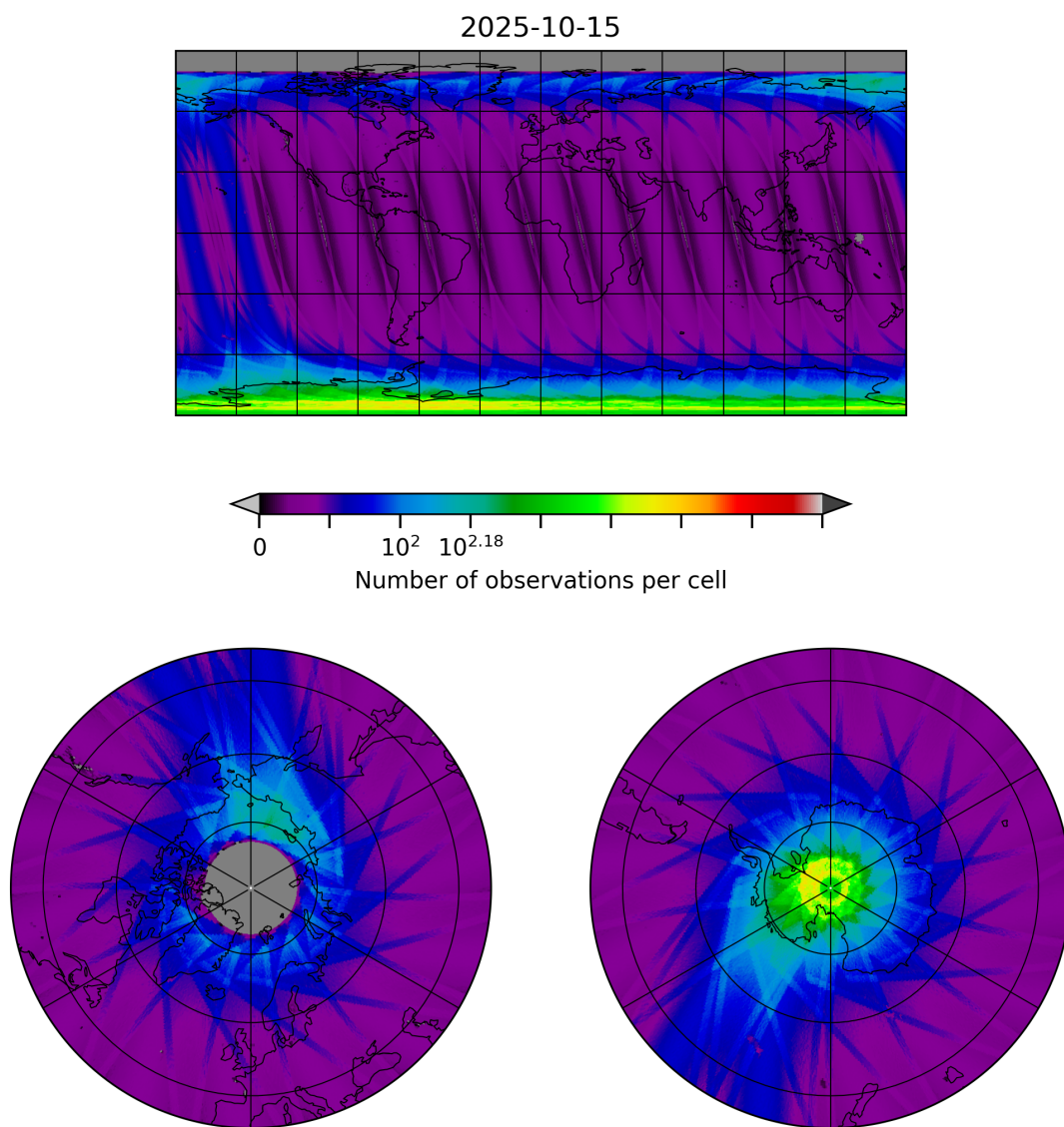
Figure 10: Map of the number of observations for 2025-10-14 to 2025-10-16
