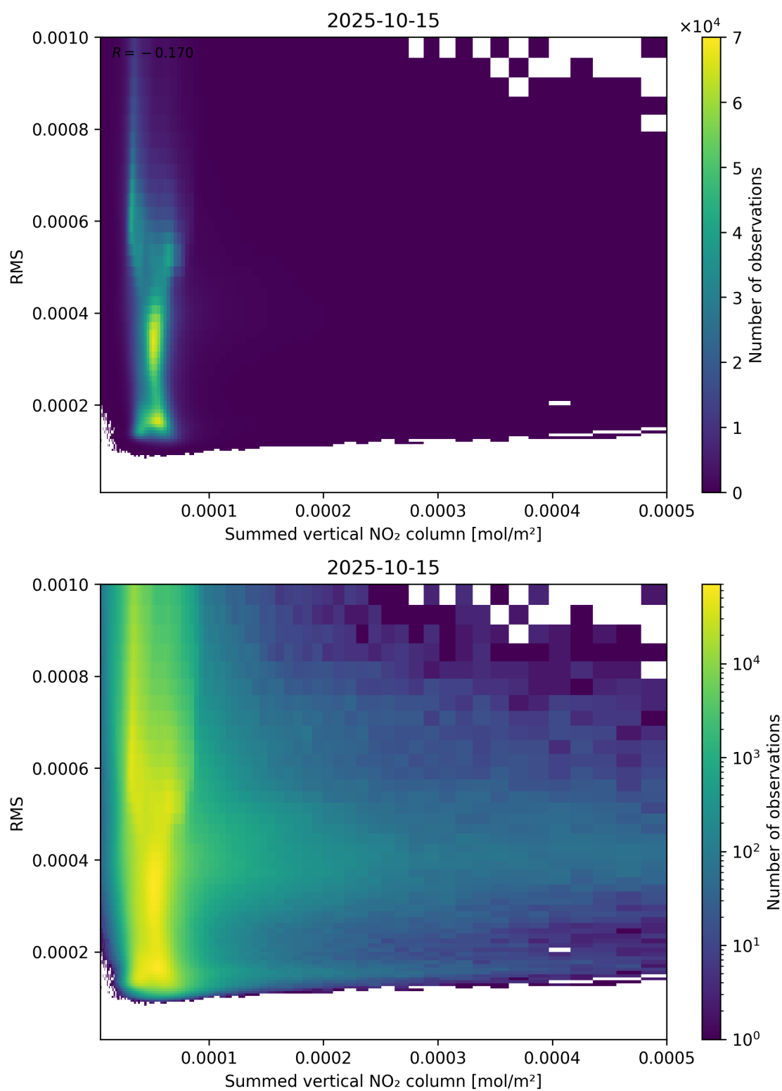
Figure 109: Scatter density plot of “Summed vertical NO 2 column” against “RMS” for 2025-10-14 to 2025-10-16.
