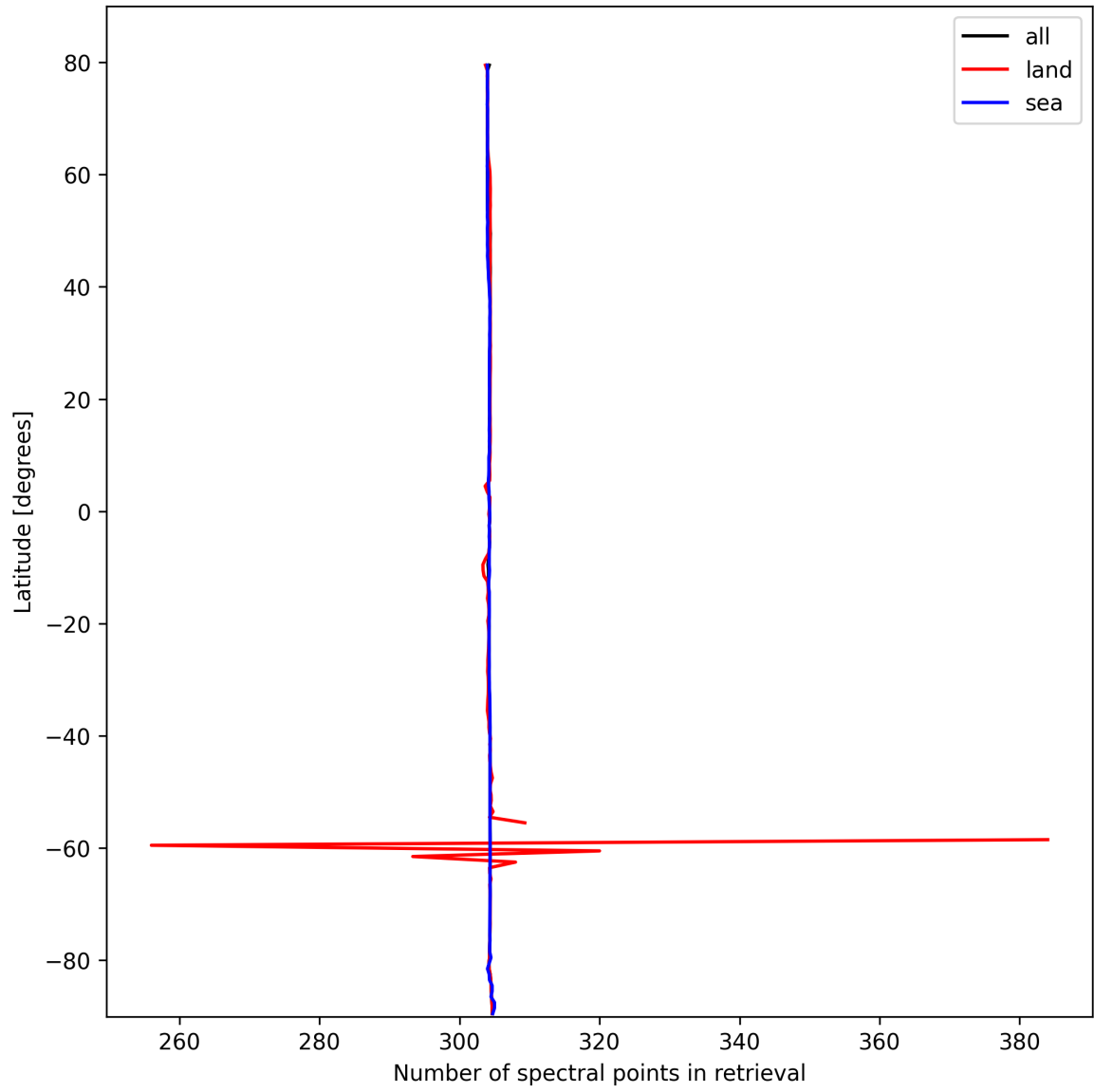
Figure 16: Zonal average of “Number of spectral points in retrieval” for 2025-10-14 to 2025-10-16.
