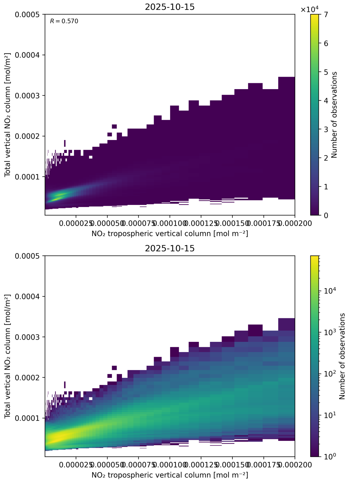
Figure 128: Scatter density plot of “NO 2 tropospheric vertical column” against “Total vertical NO 2 column” for 2025-10-14 to 2025-10-16.
