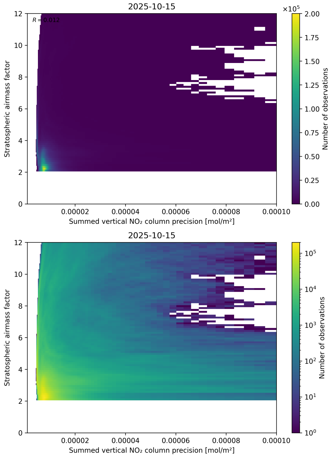
Figure 106: Scatter density plot of “Summed vertical NO 2 column precision” against “Stratospheric airmass factor” for 2025-10-14 to 2025-10-16.
