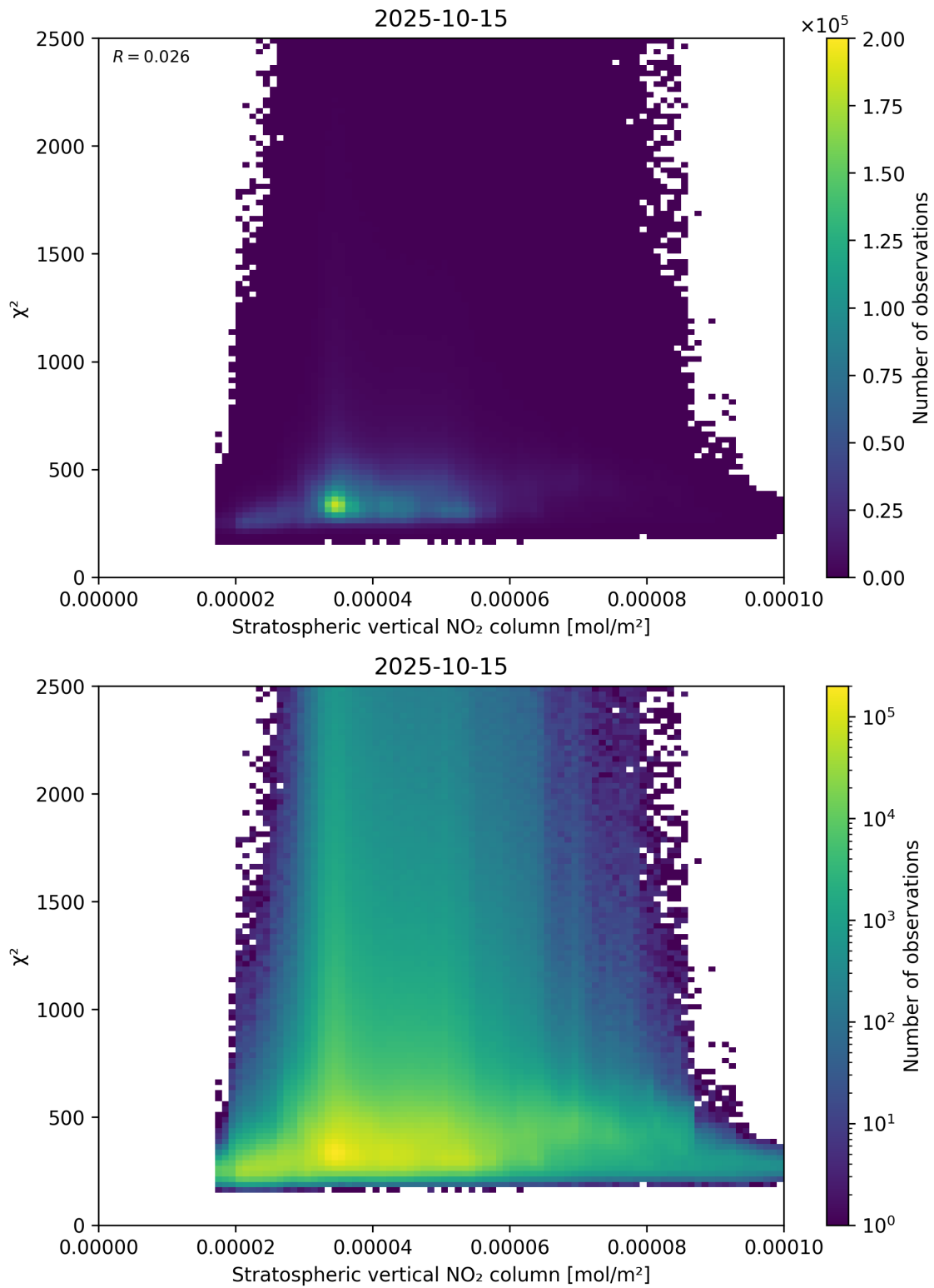
Figure 97: Scatter density plot of “Stratospheric vertical NO 2 column” against “ \chi^2 ” for 2025-10-14 to 2025-10-16.
