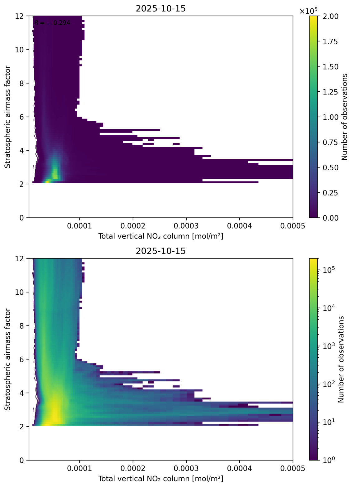
Figure 110: Scatter density plot of “Total vertical NO 2 column” against “Stratospheric airmass factor” for 2025-10-14 to 2025-10-16.
