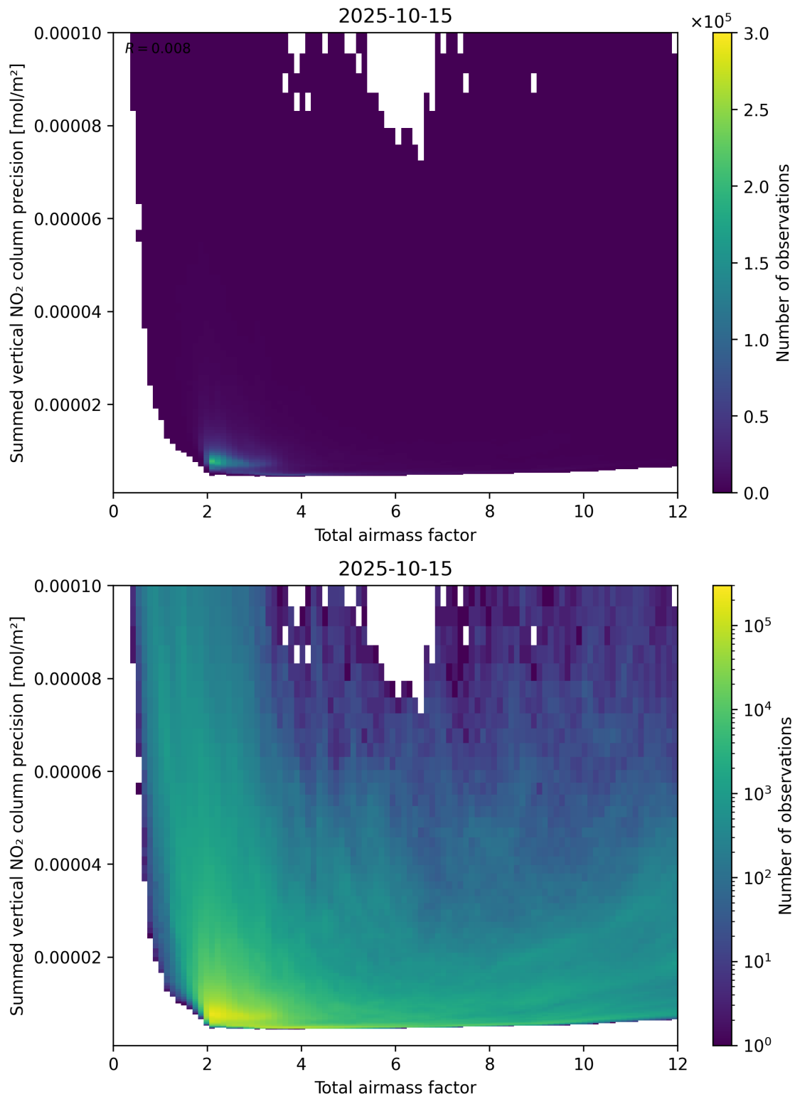
Figure 66: Scatter density plot of “Total airmass factor” against “Summed vertical NO 2 column precision” for 2025-10-14 to 2025-10-16.
