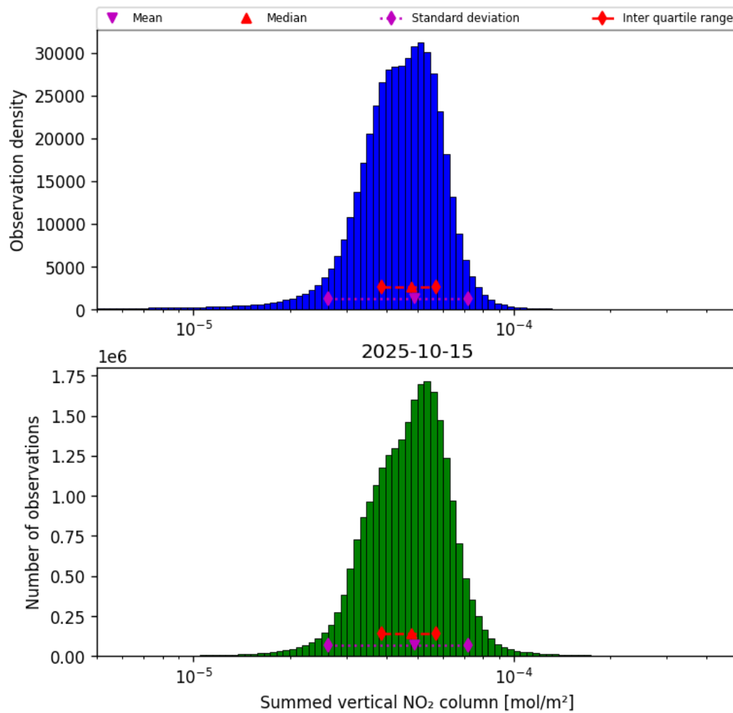
Figure 40: Histogram of "Summed vertical NO 2 column" for 2025-10-14 to 2025-10-16
