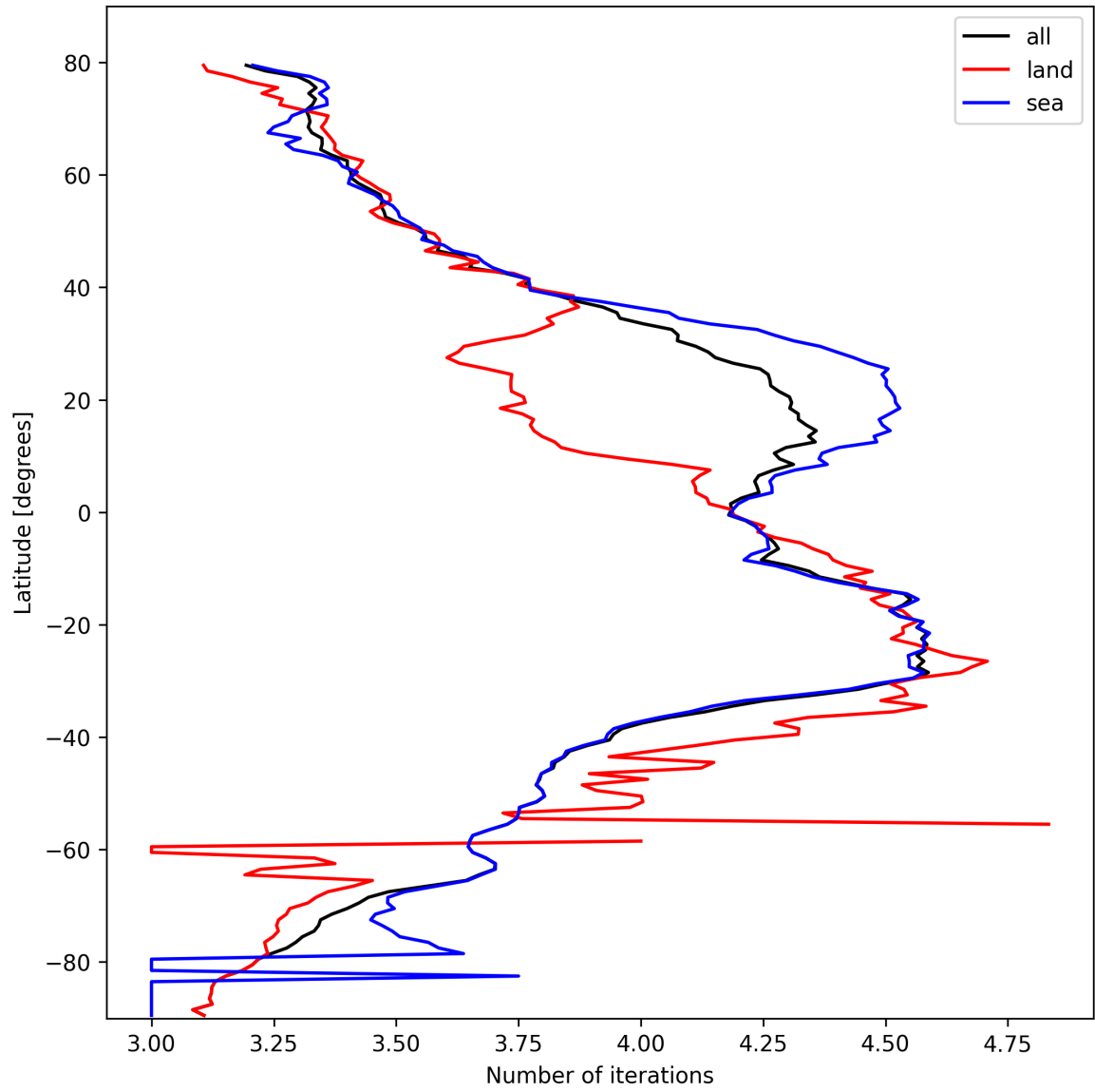
Figure 17: Zonal average of “Number of iterations” for 2025-10-14 to 2025-10-16.
