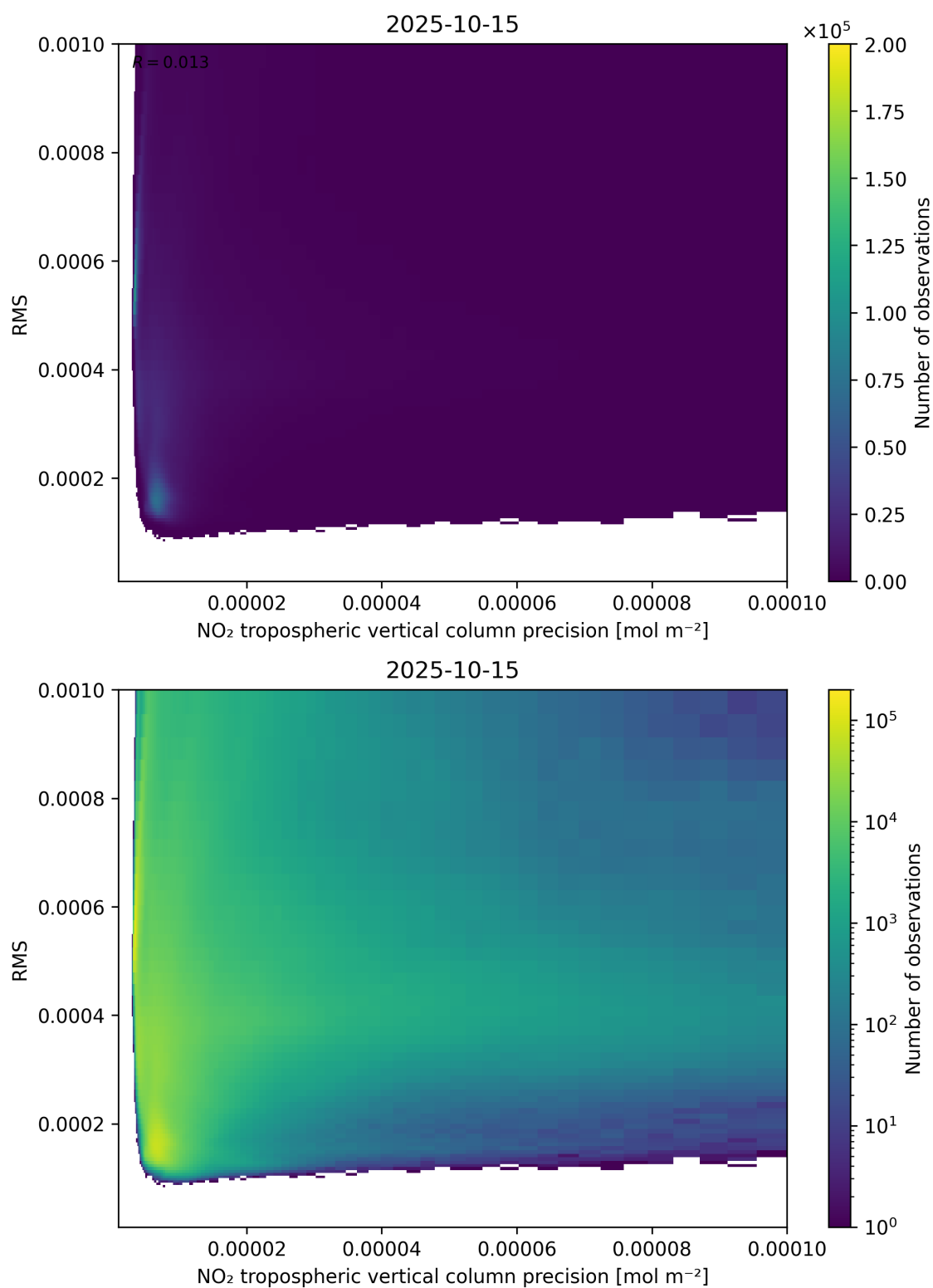
Figure 140: Scatter density plot of “NO 2 tropospheric vertical column precision” against “RMS” for 2025-10-14 to 2025-10-16.
