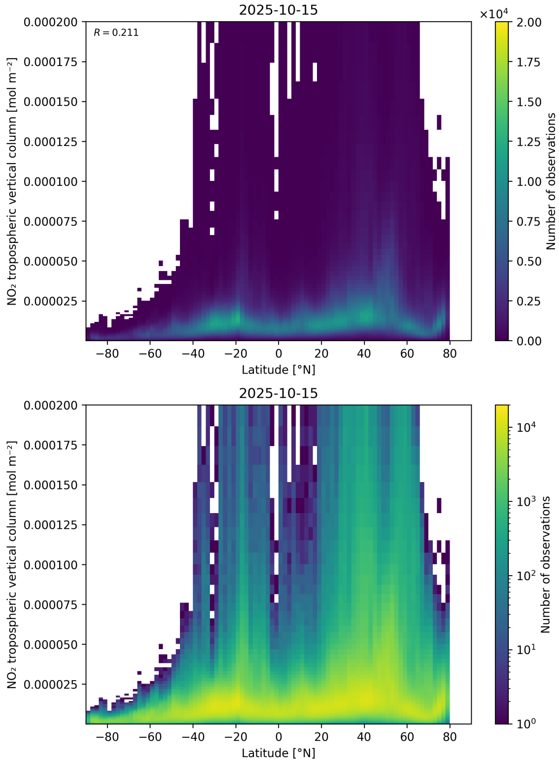
Figure 92: Scatter density plot of “Latitude” against “NO 2 tropospheric vertical column” for 2025-10-14 to 2025-10-16.
