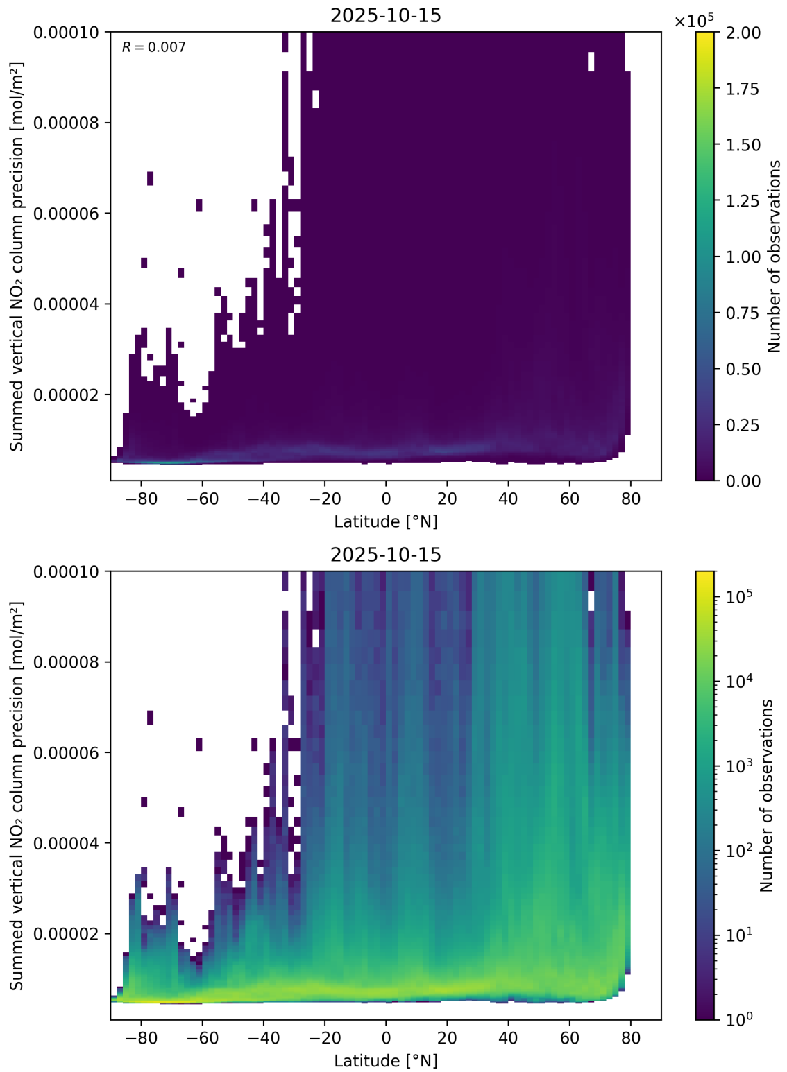
Figure 89: Scatter density plot of “Latitude” against “Summed vertical NO 2 column precision” for 2025-10-14 to 2025-10-16.
