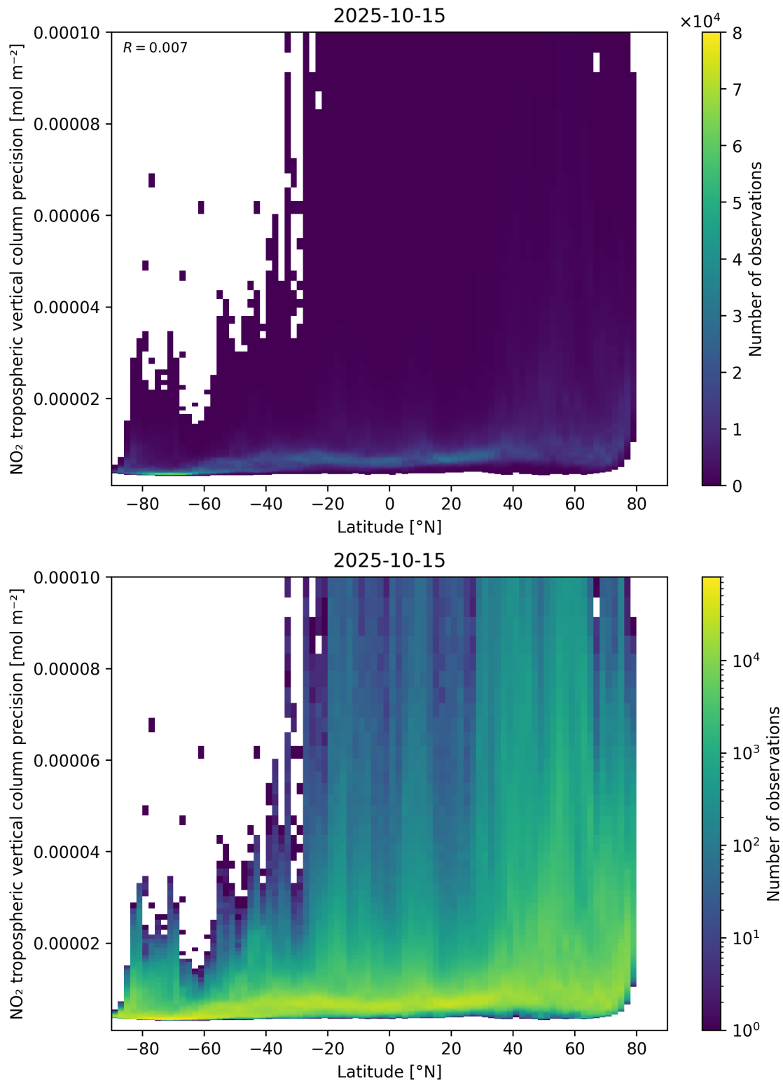
Figure 93: Scatter density plot of “Latitude” against “NO 2 tropospheric vertical column precision” for 2025-10-14 to 2025-10-16.
