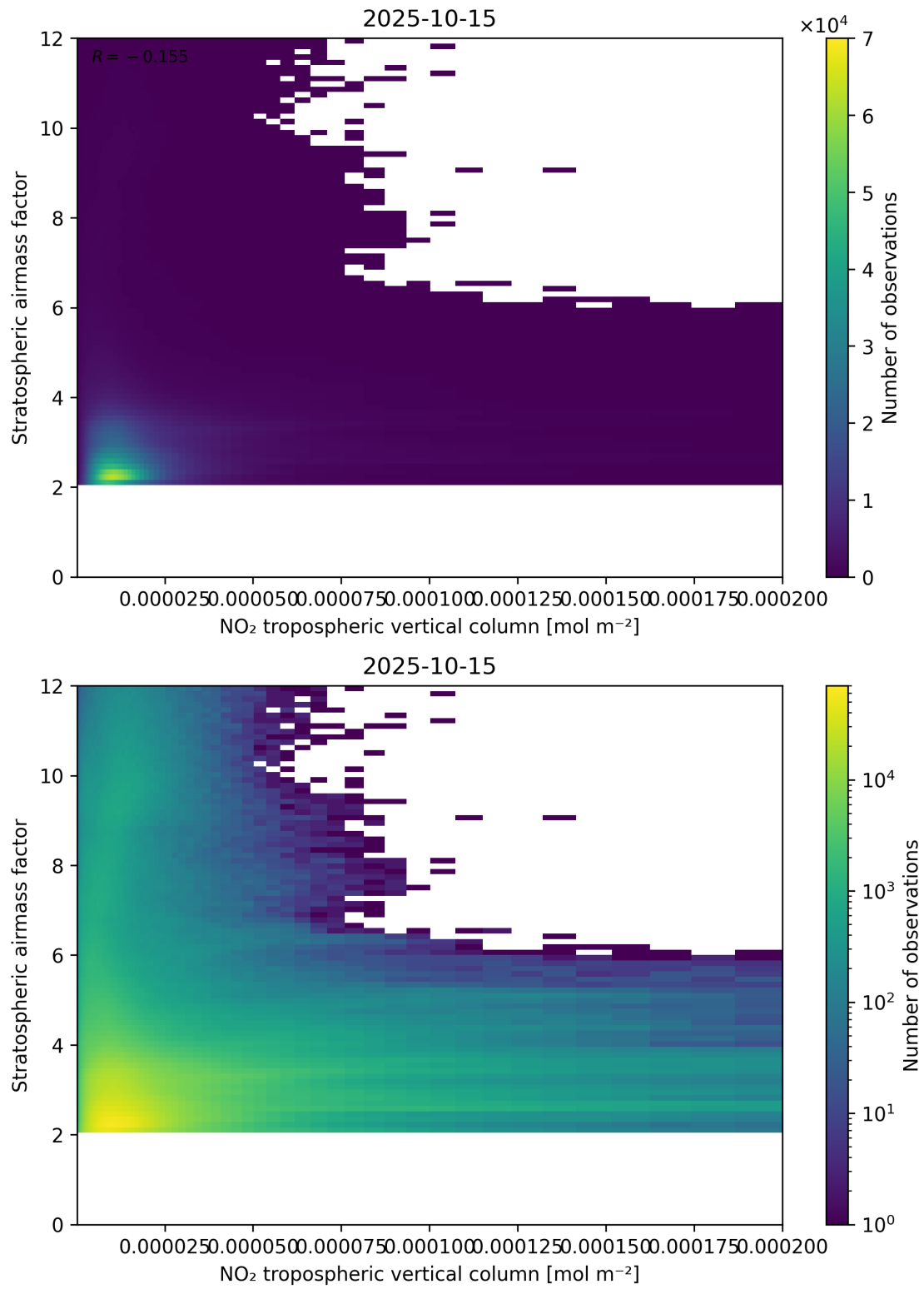
Figure 121: Scatter density plot of “NO 2 tropospheric vertical column” against “Stratospheric air mass factor” for 2025-10-14 to 2025-10-16.
