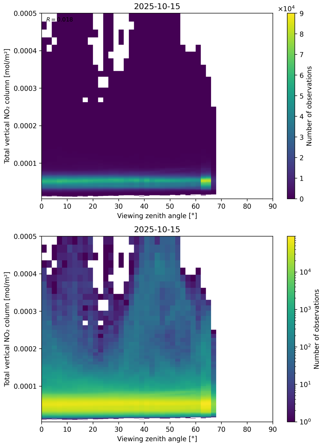
Figure 167: Scatter density plot of “Viewing zenith angle” against “Total vertical NO 2 column” for 2025-10-14 to 2025-10-16.
