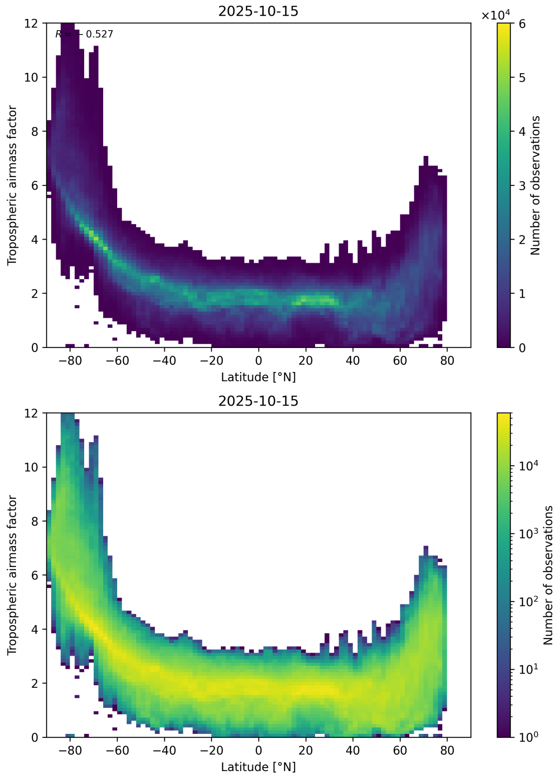
Figure 85: Scatter density plot of “Latitude” against “Tropospheric airmass factor” for 2025-10-14 to 2025-10-16.
