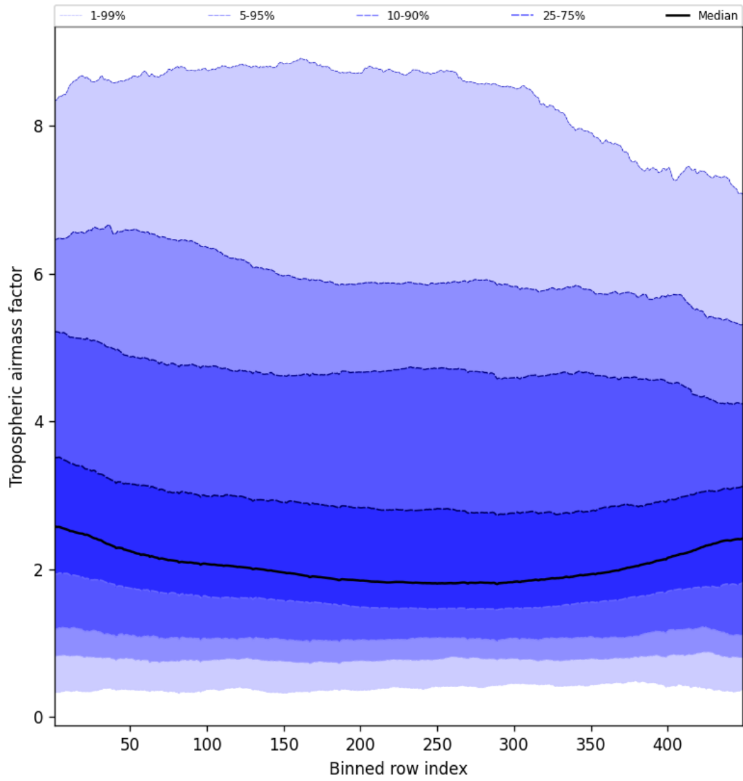
Figure 48: Along track statistics of “Tropospheric airmass factor” for 2025-10-14 to 2025-10-16
