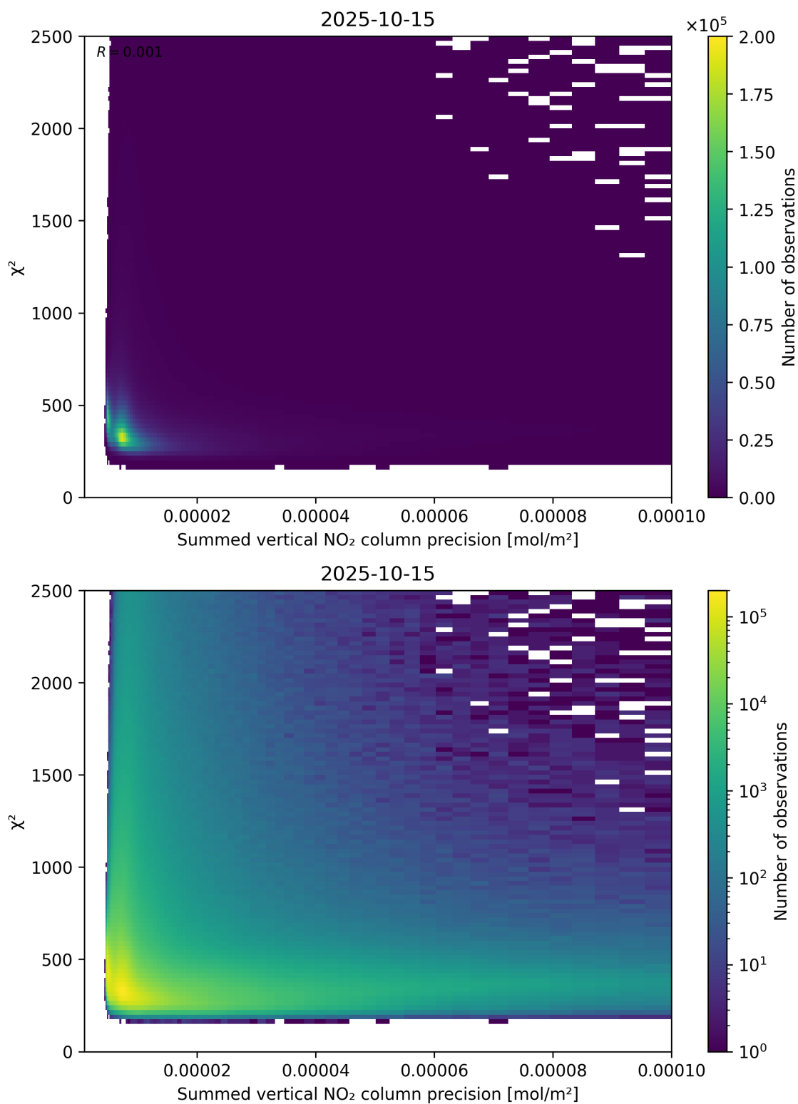
Figure 107: Scatter density plot of “Summed vertical NO 2 column precision” against “ \chi^2 ” for 2025-10-14 to 2025-10-16.
