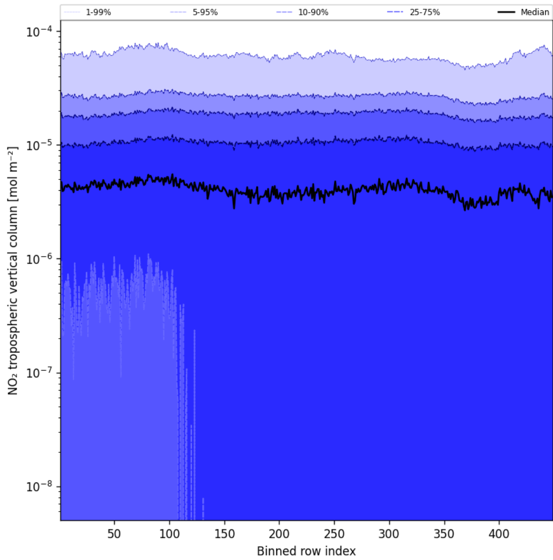
Figure 46: Along track statistics of “ \text{NO}_2 tropospheric vertical column” for 2025-10-14 to 2025-10-16
