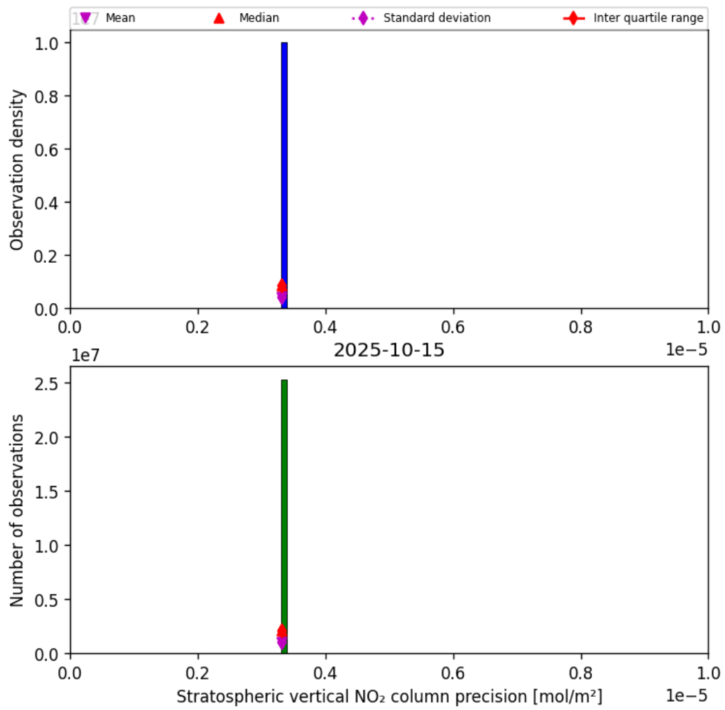
Figure 37: Histogram of “Stratospheric vertical NO 2 column precision” for 2025-10-14 to 2025-10-16
