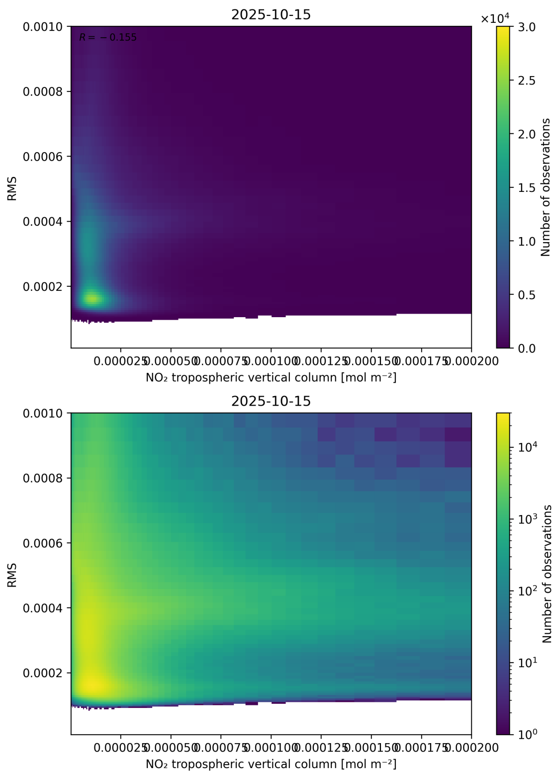
Figure 142: Scatter density plot of “NO 2 tropospheric vertical column” against “RMS” for 2025-10-14 to 2025-10-16.
