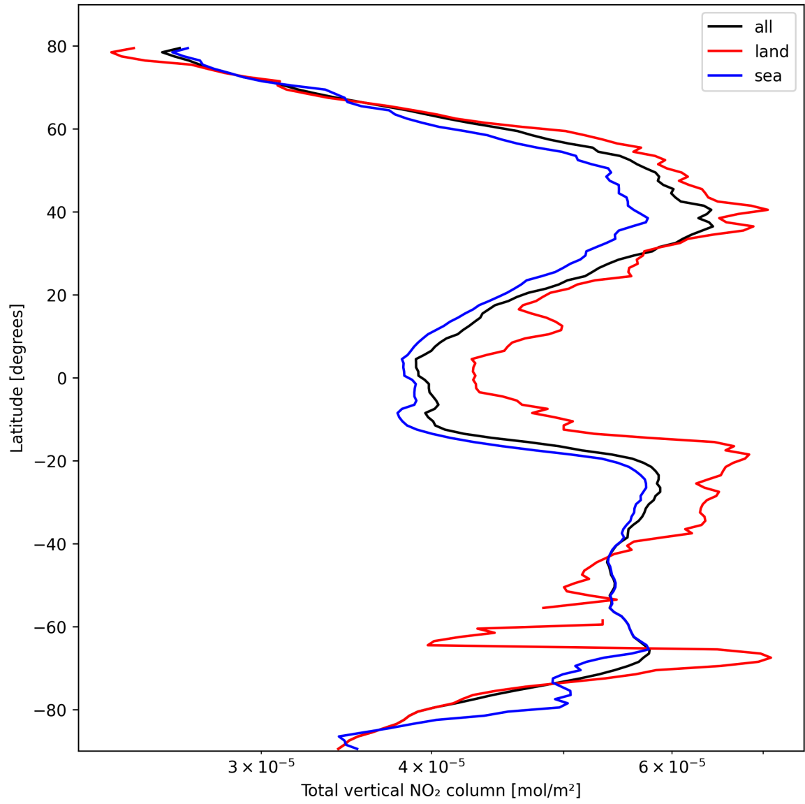
Figure 21: Zonal average of “Total vertical NO 2 column” for 2025-10-14 to 2025-10-16.
