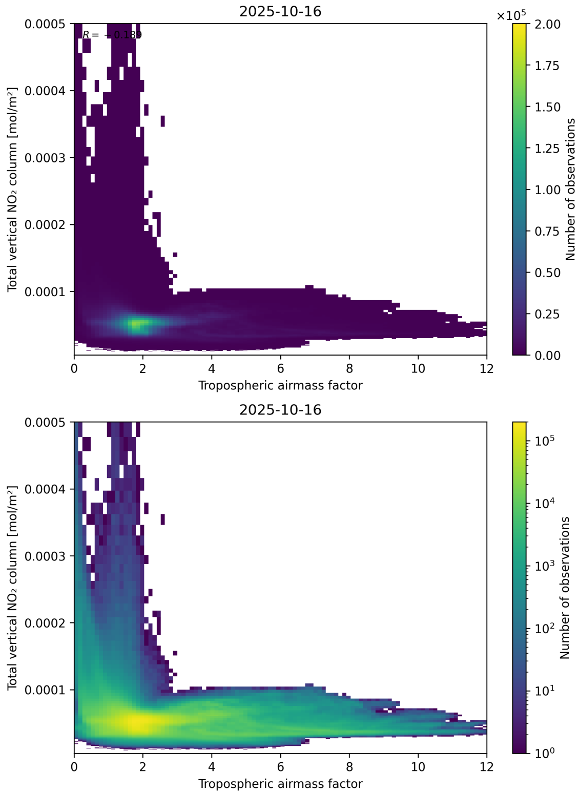
Figure 77: Scatter density plot of “Tropospheric airmass factor” against “Total vertical NO 2 column” for 2025-10-15 to 2025-10-17.
