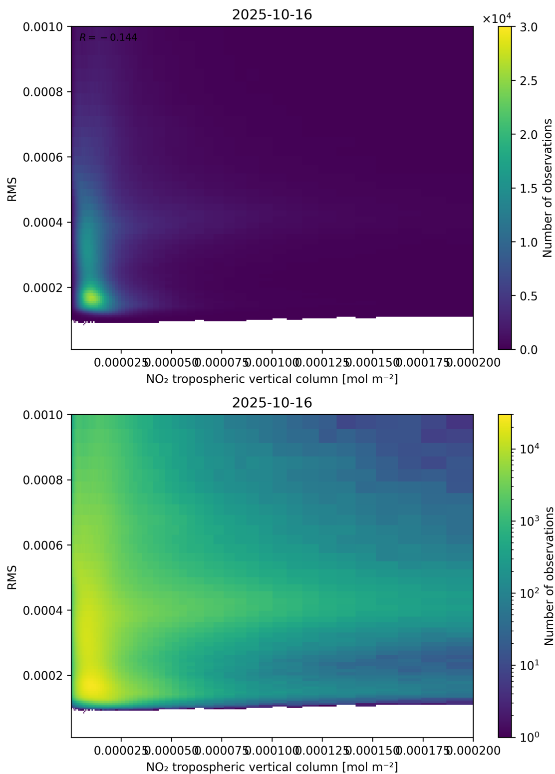
Figure 142: Scatter density plot of “NO 2 tropospheric vertical column” against “RMS” for 2025-10-15 to 2025-10-17.
