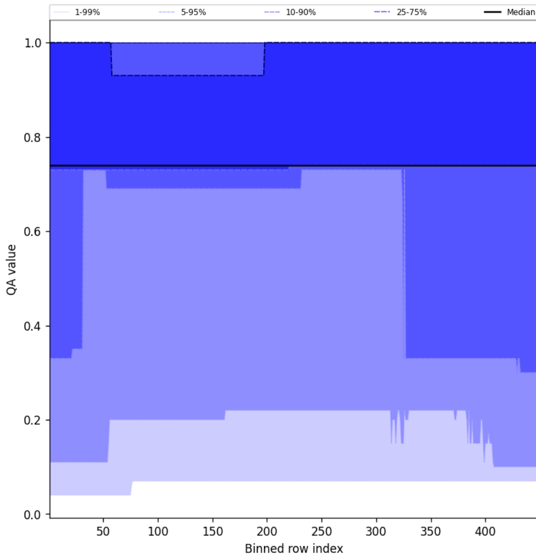
Figure 45: Along track statistics of “QA value” for 2025-10-15 to 2025-10-17
