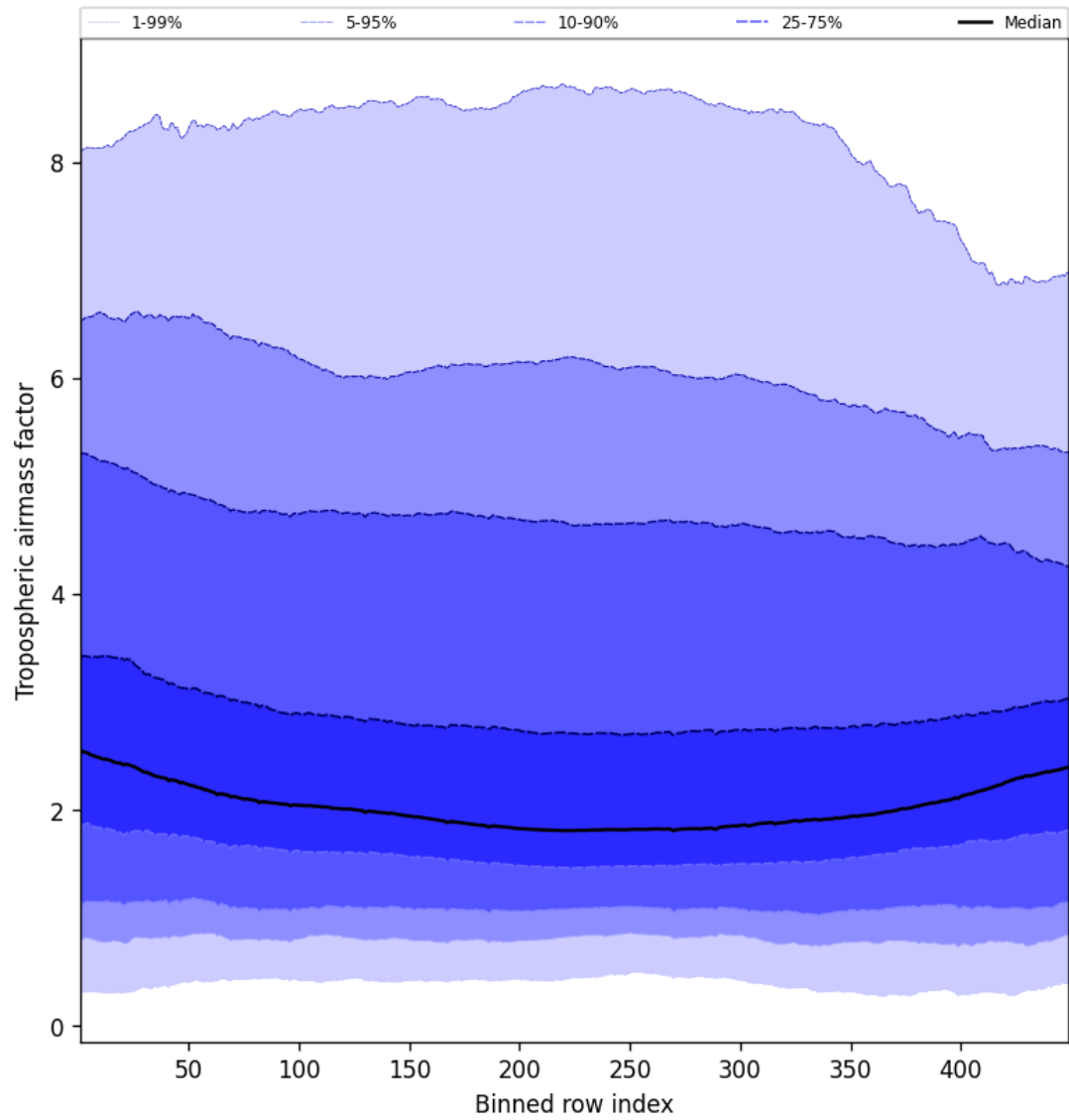
Figure 48: Along track statistics of “Tropospheric air mass factor” for 2025-10-15 to 2025-10-17
