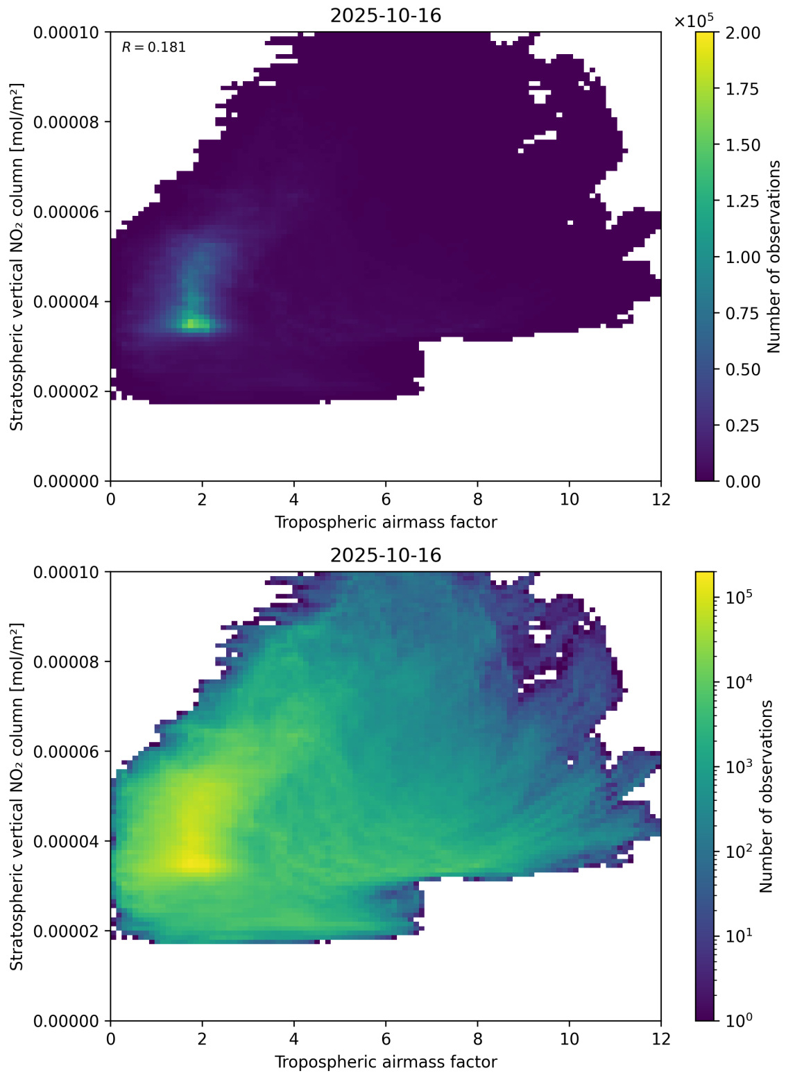
Figure 74: Scatter density plot of “Tropospheric air mass factor” against “Stratospheric vertical NO 2 column” for 2025-10-15 to 2025-10-17.
