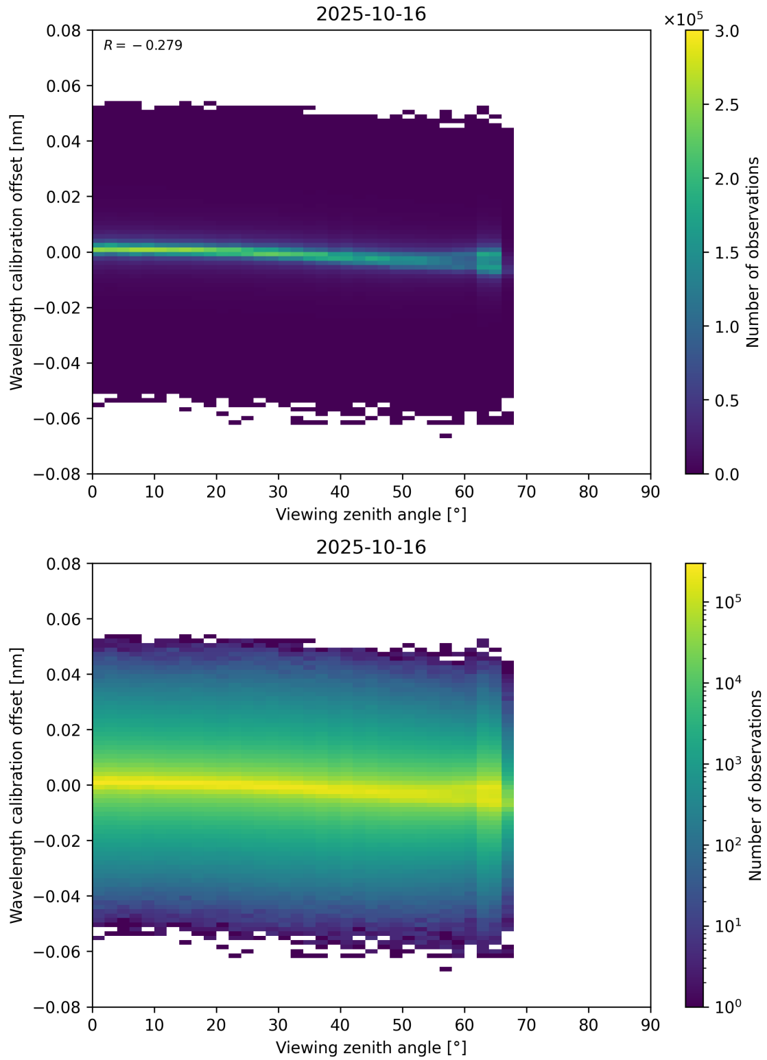
Figure 173: Scatter density plot of “Viewing zenith angle” against “Wavelength calibration offset” for 2025-10-15 to 2025-10-17.
