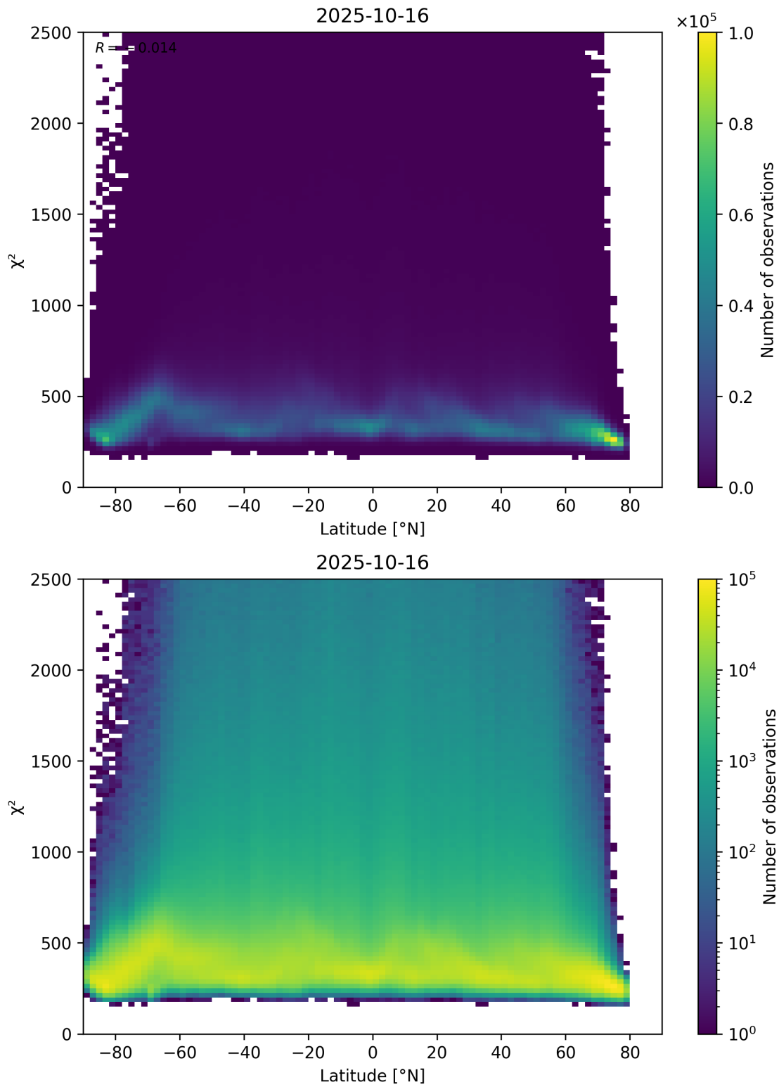
Figure 86: Scatter density plot of “Latitude” against “ \chi^2 ” for 2025-10-15 to 2025-10-17.
