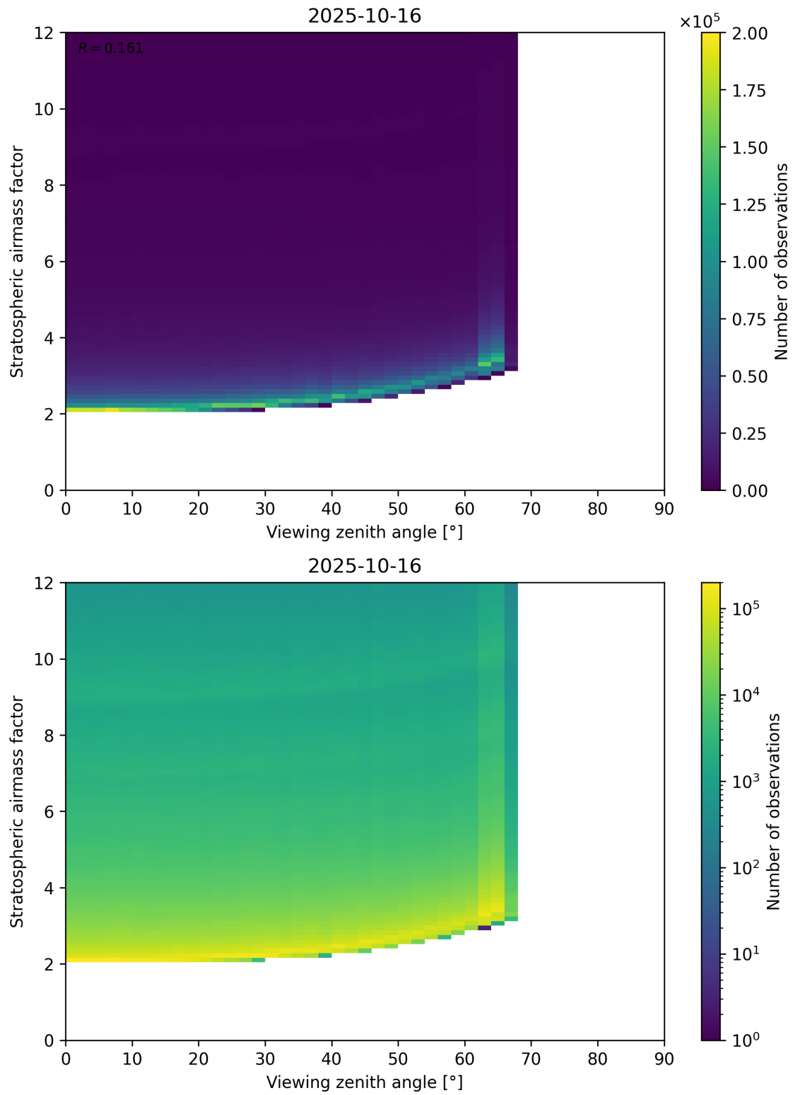
Figure 159: Scatter density plot of “Viewing zenith angle” against “Stratospheric airmass factor” for 2025-10-15 to 2025-10-17.
