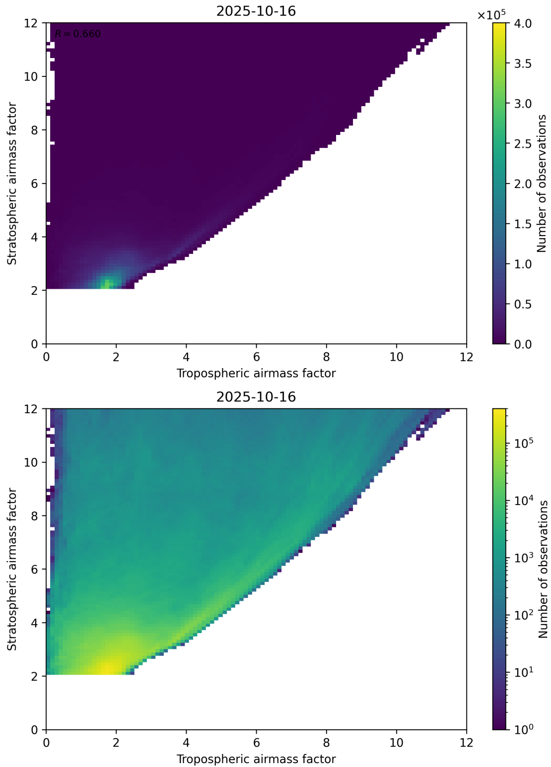
Figure 71: Scatter density plot of “Tropospheric airmass factor” against “Stratospheric airmass factor” for 2025-10-15 to 2025-10-17.
