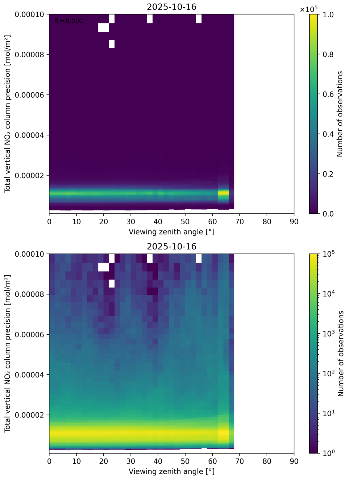
Figure 168: Scatter density plot of “Viewing zenith angle” against “Total vertical NO 2 column precision” for 2025-10-15 to 2025-10-17.
