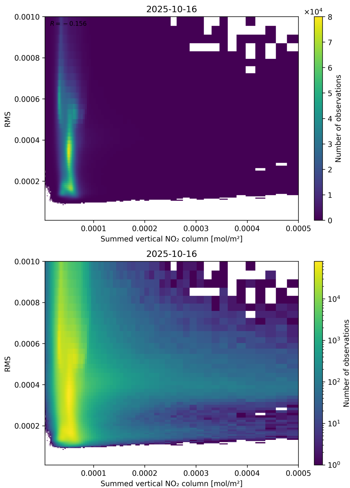
Figure 109: Scatter density plot of “Summed vertical NO 2 column” against “RMS” for 2025-10-15 to 2025-10-17.
