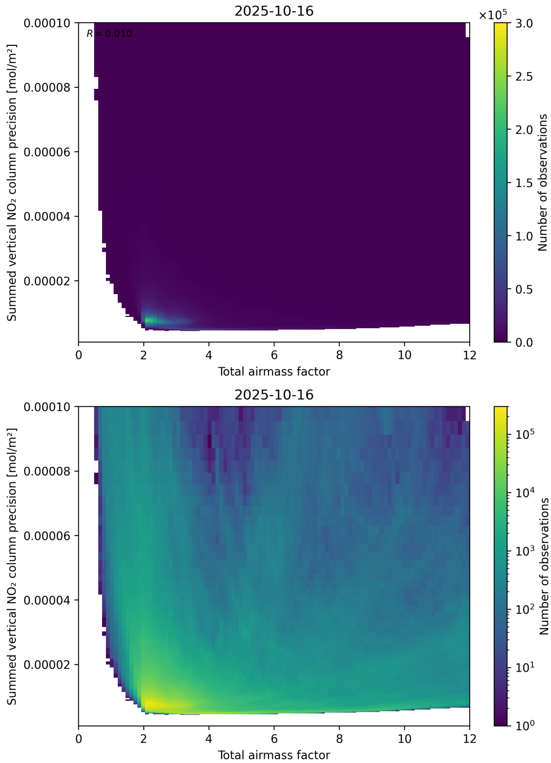
Figure 66: Scatter density plot of “Total airmass factor” against “Summed vertical NO 2 column precision” for 2025-10-15 to 2025-10-17.
