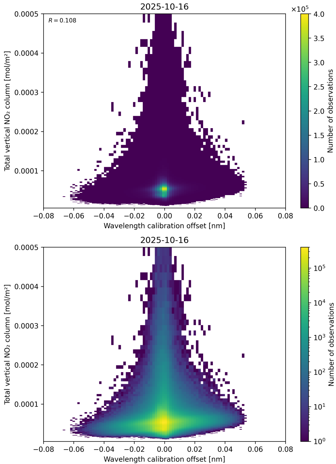
Figure 179: Scatter density plot of “Wavelength calibration offset” against “Total vertical NO 2 column” for 2025-10-15 to 2025-10-17.
