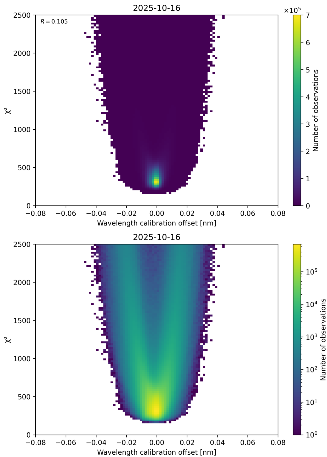
Figure 175: Scatter density plot of “Wavelength calibration offset” against “ \chi^2 ” for 2025-10-15 to 2025-10-17.
