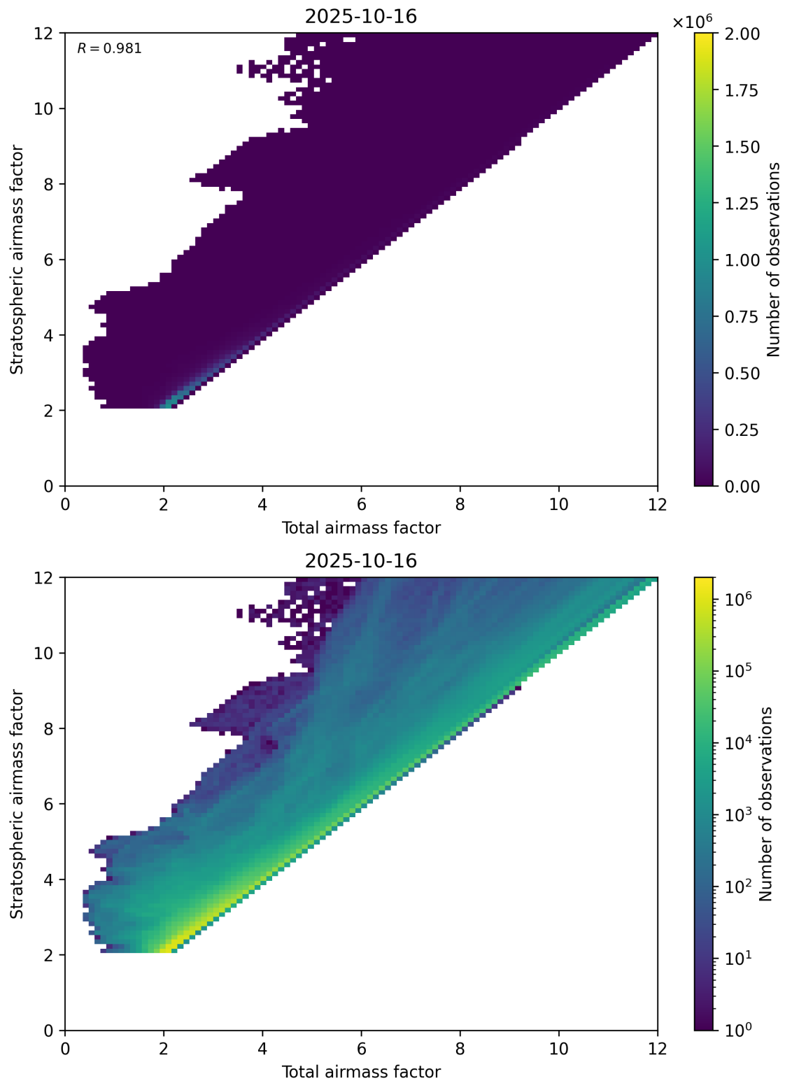
Figure 62: Scatter density plot of “Total airmass factor” against “Stratospheric airmass factor” for 2025-10-15 to 2025-10-17.
