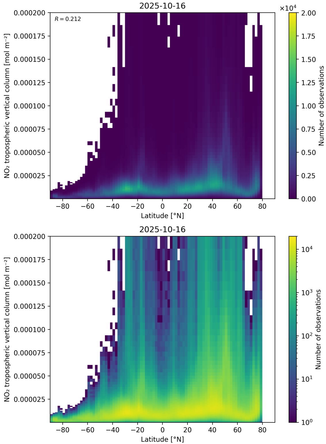
Figure 92: Scatter density plot of “Latitude” against “NO 2 tropospheric vertical column” for 2025-10-15 to 2025-10-17.
