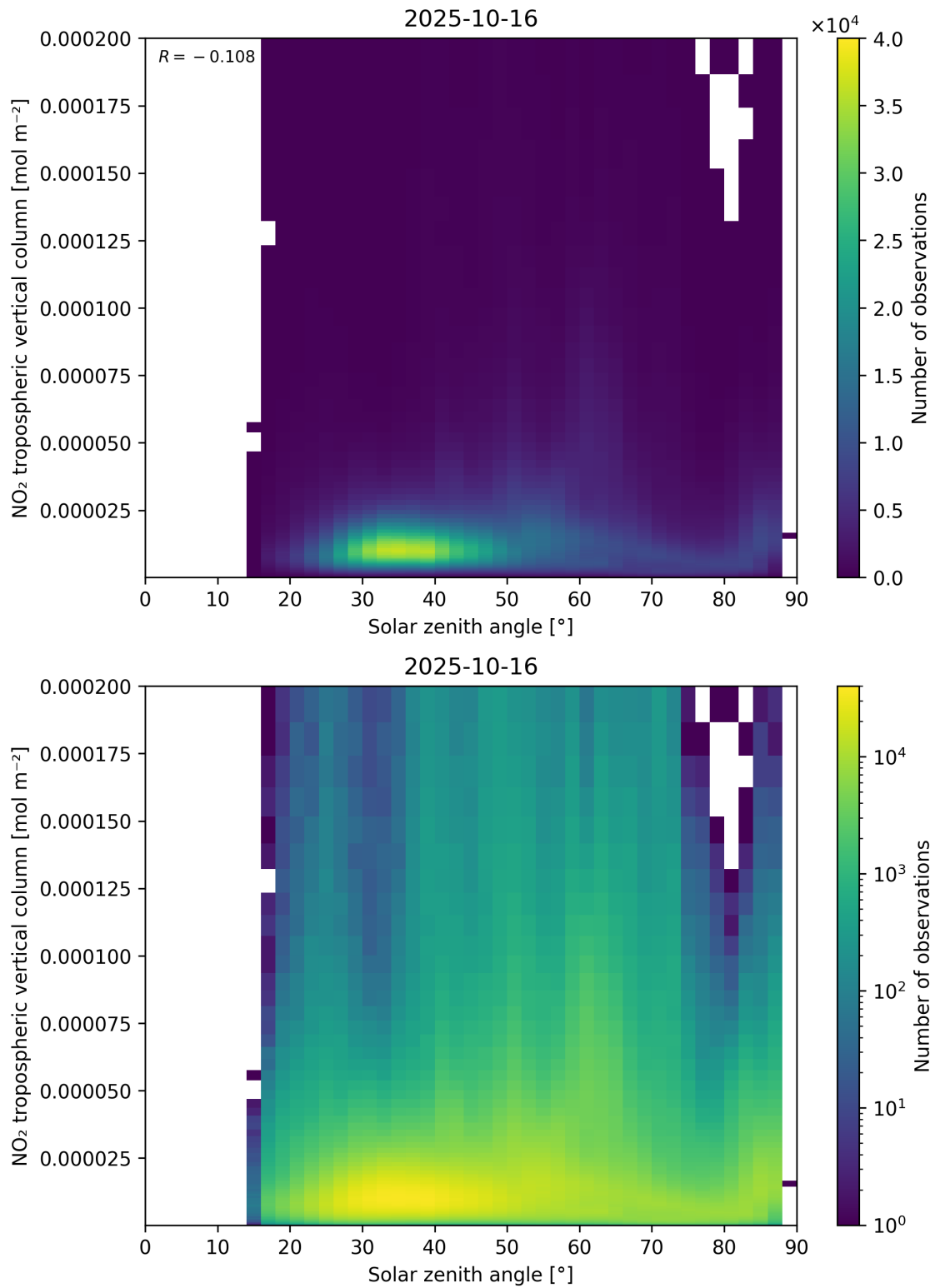
Figure 155: Scatter density plot of “Solar zenith angle” against “NO 2 tropospheric vertical column” for 2025-10-15 to 2025-10-17.
