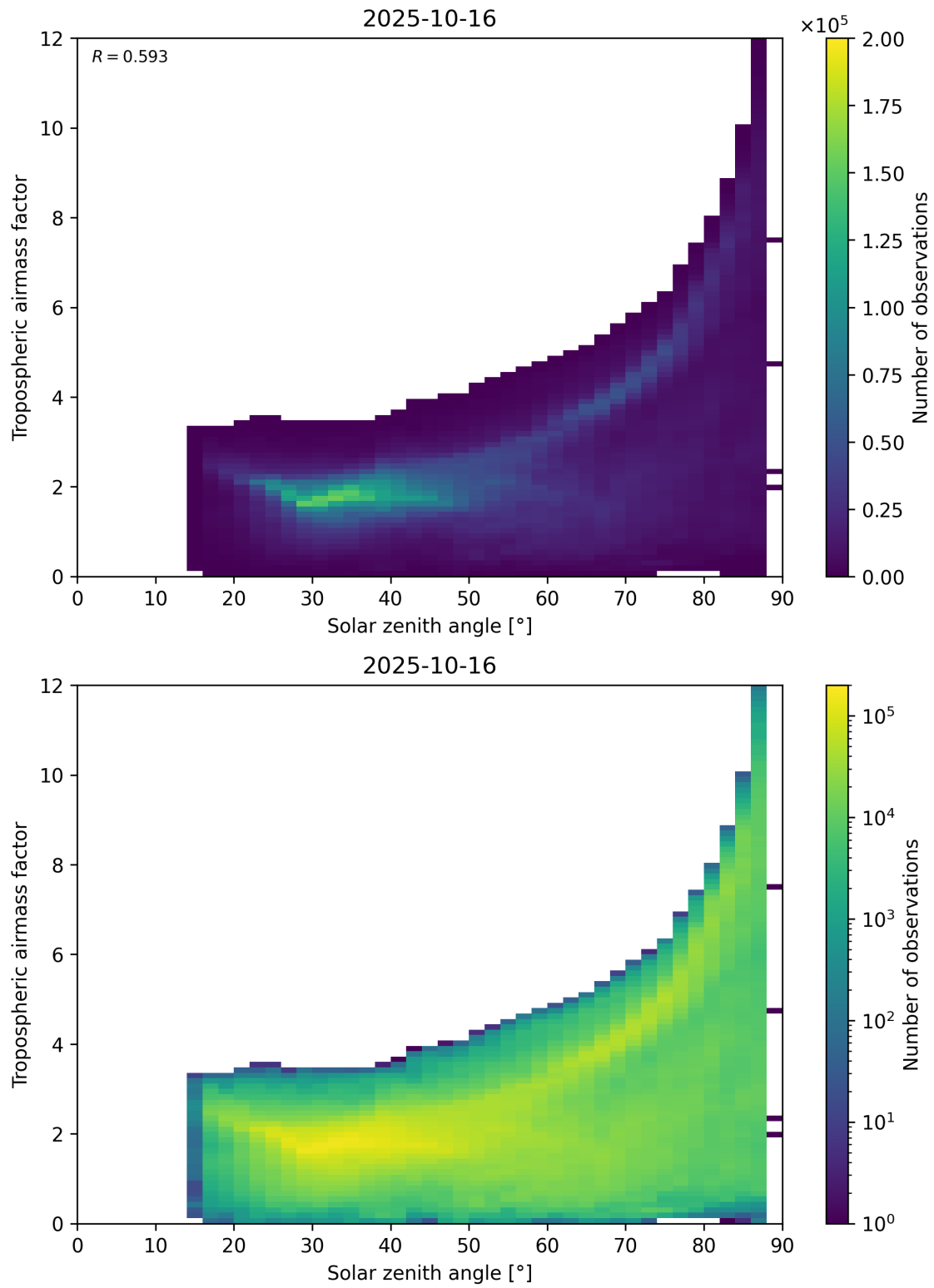
Figure 147: Scatter density plot of “Solar zenith angle” against “Tropospheric airmass factor” for 2025-10-15 to 2025-10-17.
