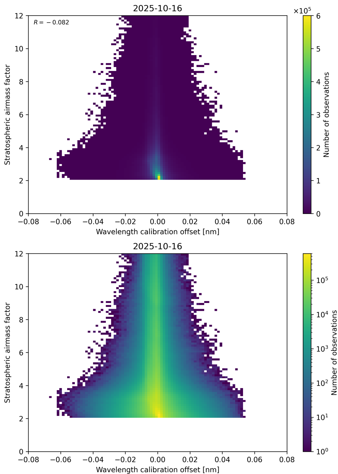
Figure 174: Scatter density plot of “Wavelength calibration offset” against “Stratospheric airmass factor” for 2025-10-15 to 2025-10-17.
