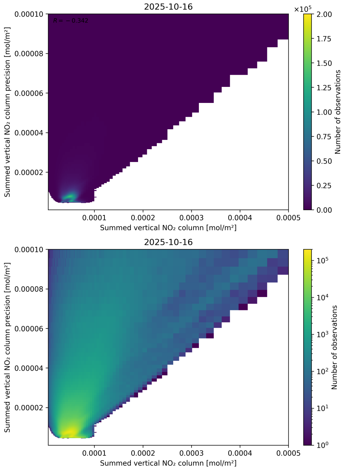
Figure 105: Scatter density plot of “Summed vertical NO 2 column” against “Summed vertical NO 2 column precision” for 2025-10-15 to 2025-10-17.
