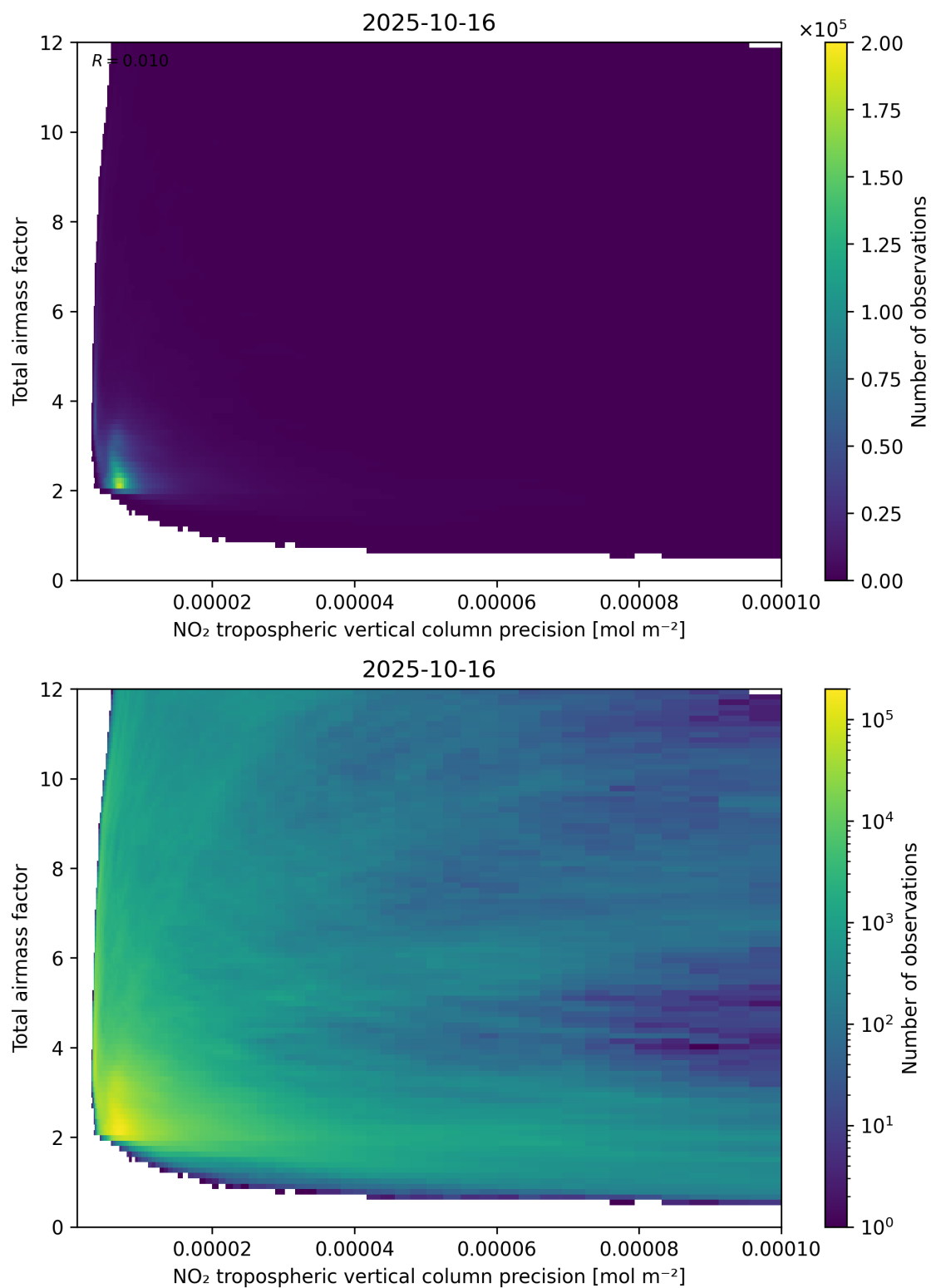
Figure 132: Scatter density plot of “NO 2 tropospheric vertical column precision” against “Total air mass factor” for 2025-10-15 to 2025-10-17.
