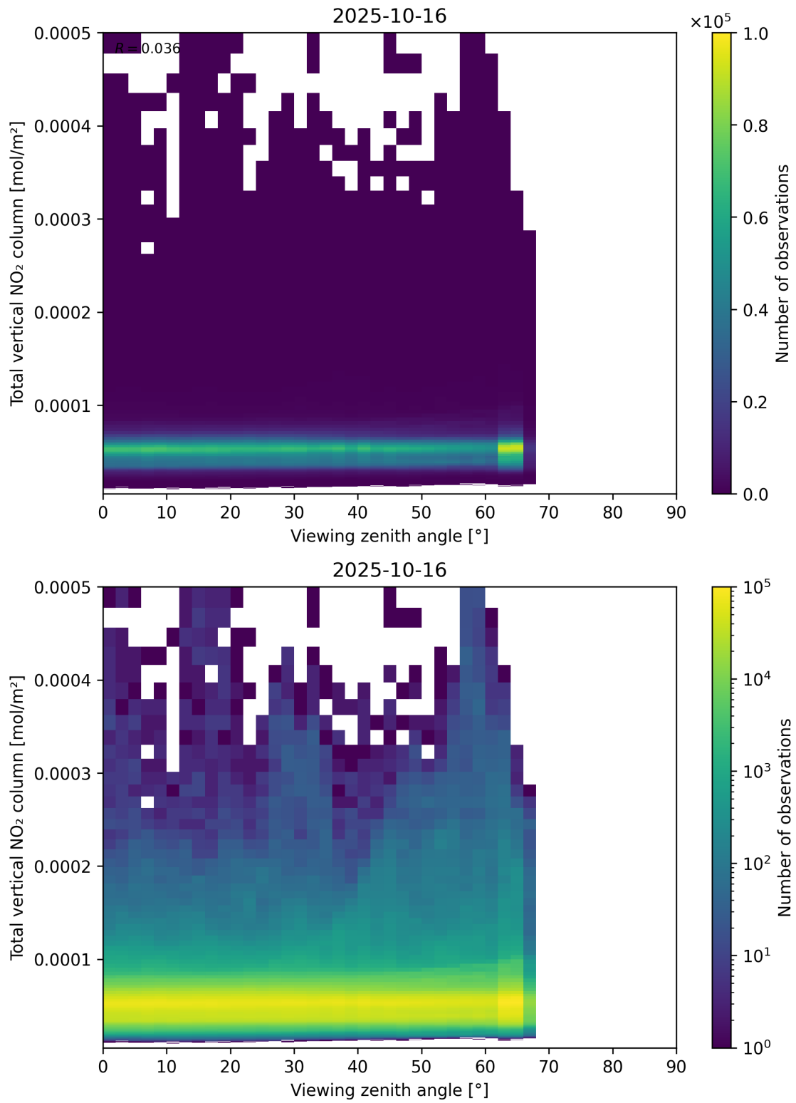
Figure 167: Scatter density plot of “Viewing zenith angle” against “Total vertical NO 2 column” for 2025-10-15 to 2025-10-17.
