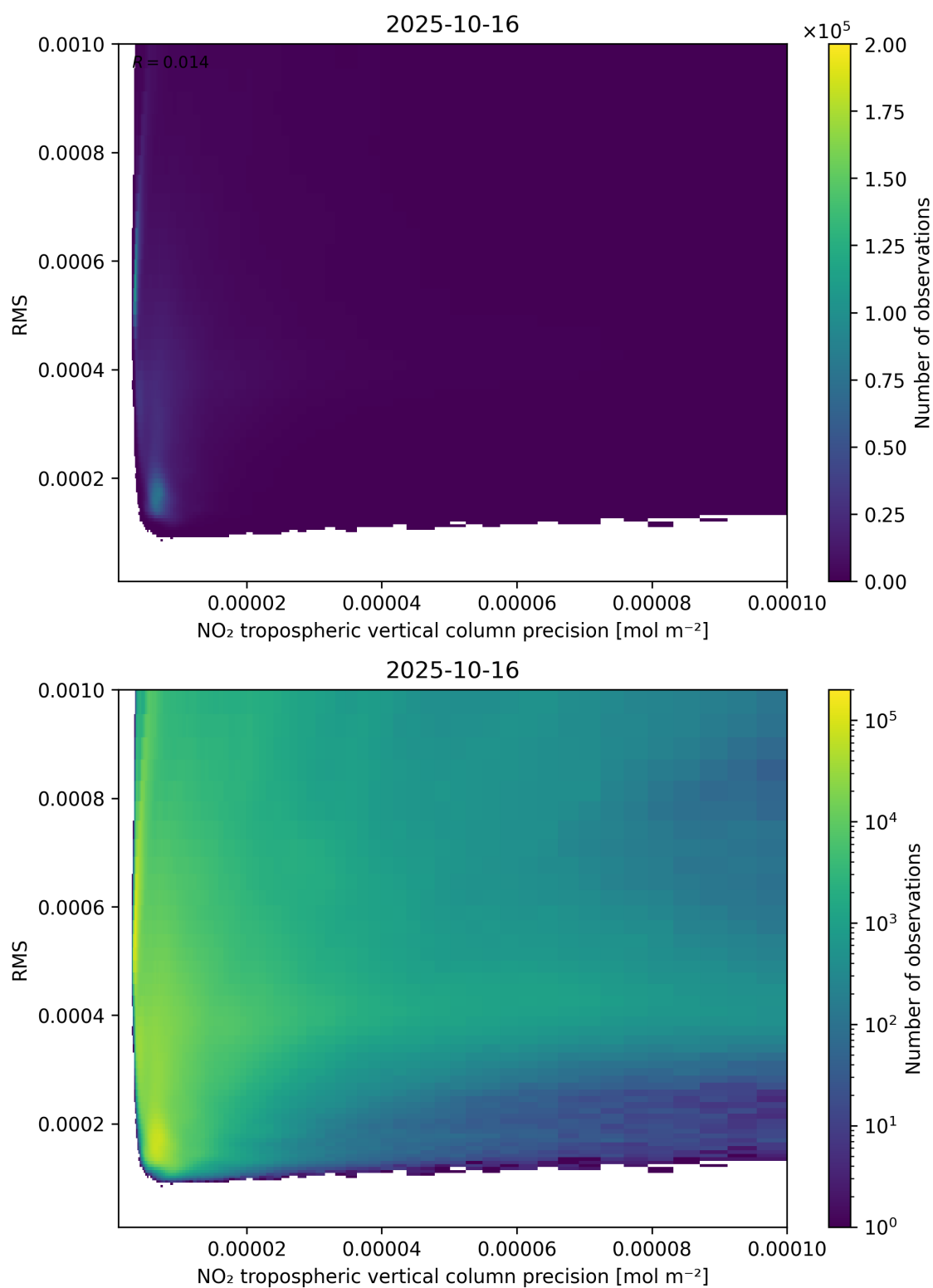
Figure 140: Scatter density plot of “NO 2 tropospheric vertical column precision” against “RMS” for 2025-10-15 to 2025-10-17.
