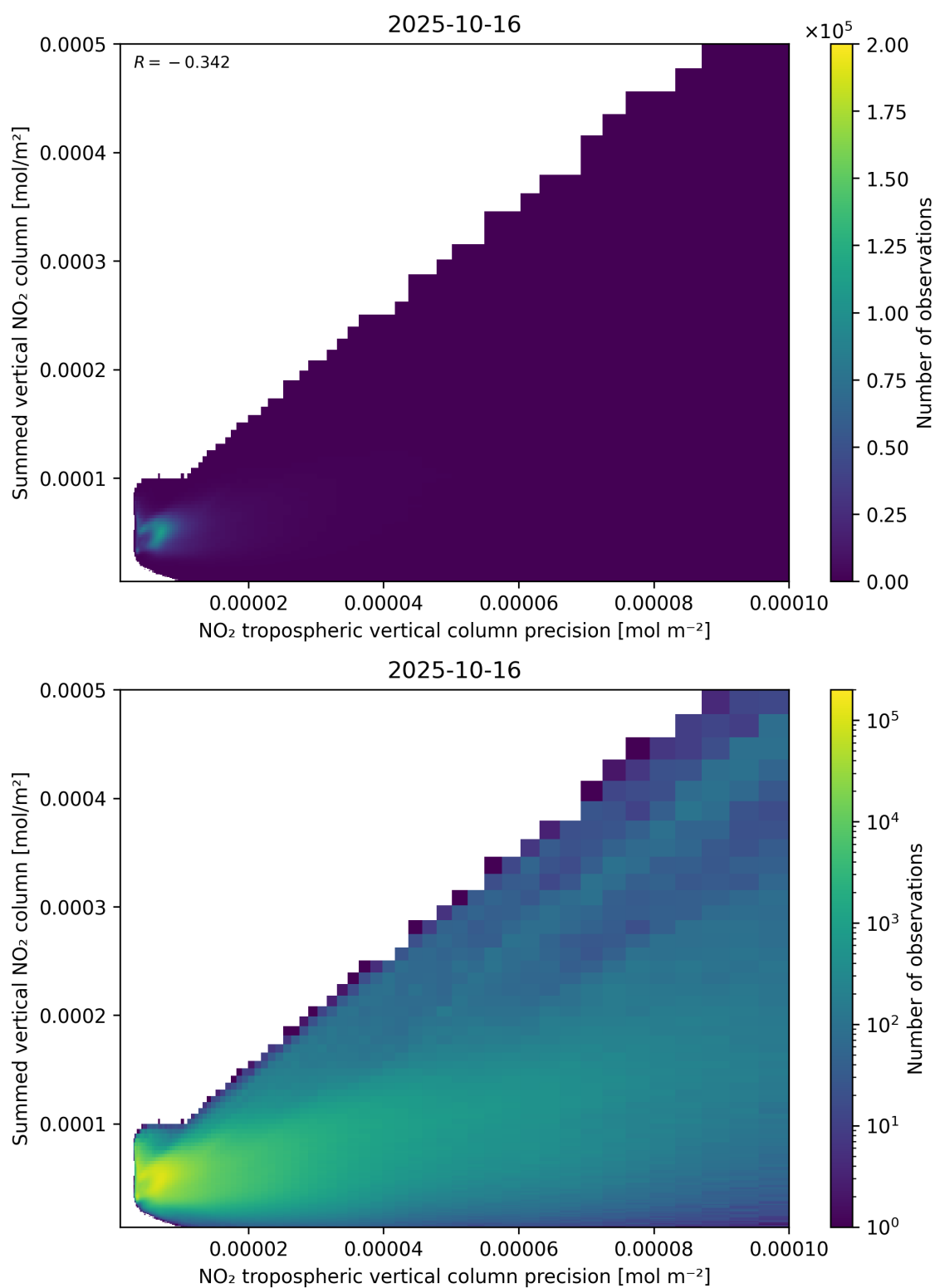
Figure 136: Scatter density plot of “NO 2 tropospheric vertical column precision” against “Summed vertical NO 2 column” for 2025-10-15 to 2025-10-17.
