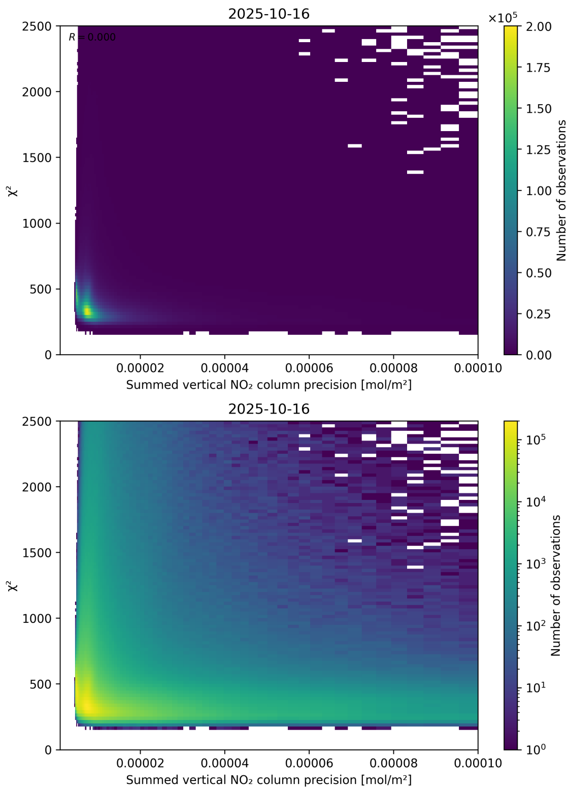
Figure 107: Scatter density plot of “Summed vertical NO 2 column precision” against “ \chi^2 ” for 2025-10-15 to 2025-10-17.
