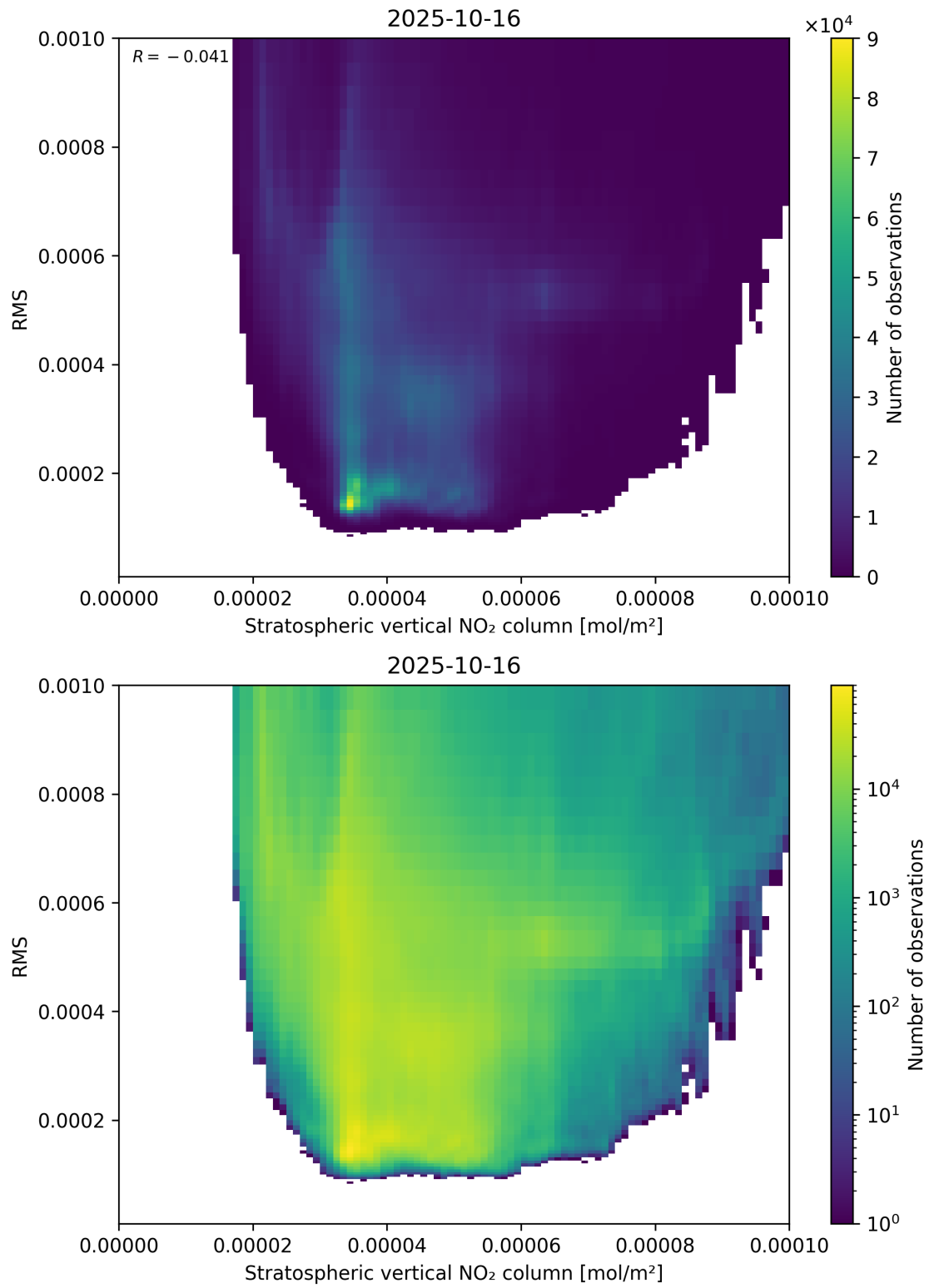
Figure 102: Scatter density plot of “Stratospheric vertical NO 2 column” against “RMS” for 2025-10-15 to 2025-10-17.
