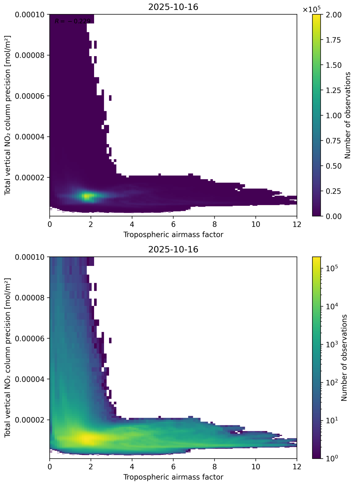
Figure 78: Scatter density plot of “Tropospheric air mass factor” against “Total vertical NO 2 column precision” for 2025-10-15 to 2025-10-17.
