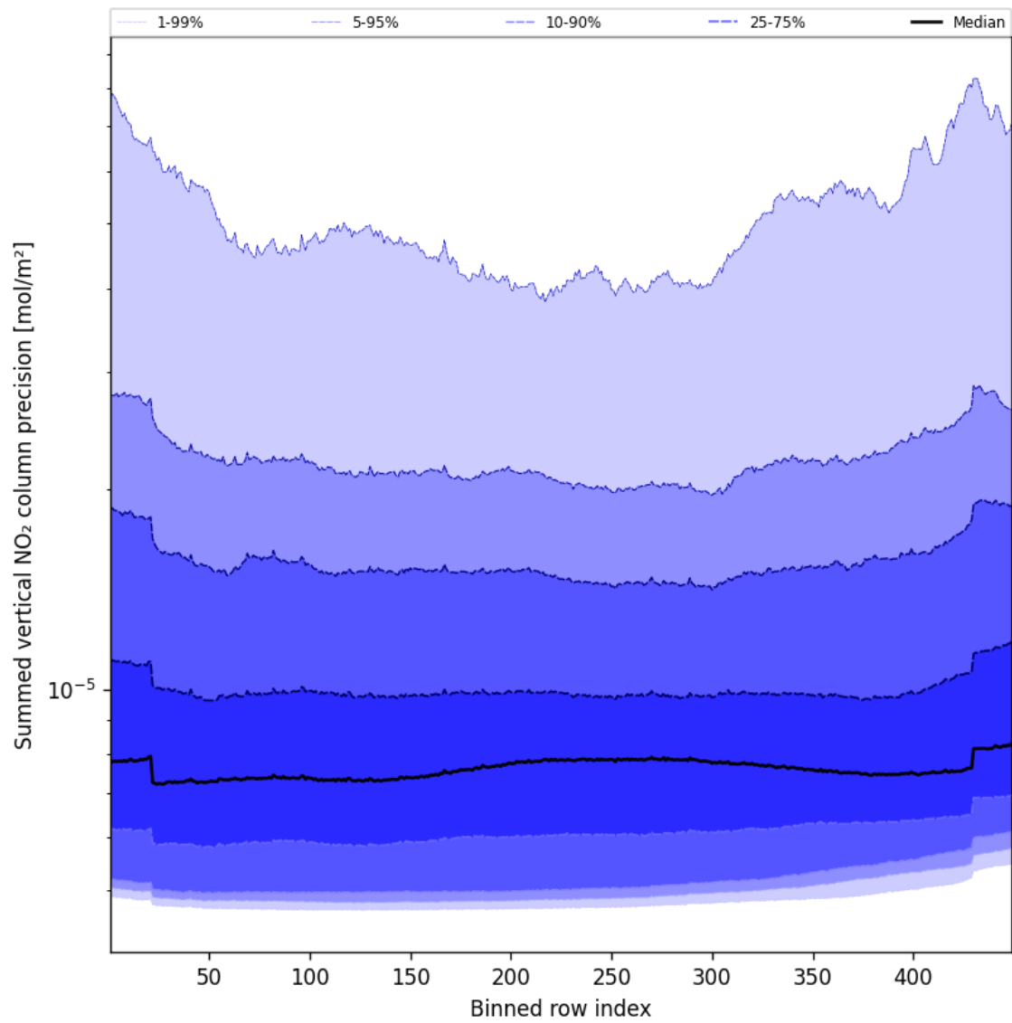
Figure 58: Along track statistics of “Summed vertical NO 2 column precision” for 2025-10-15 to 2025-10-17
