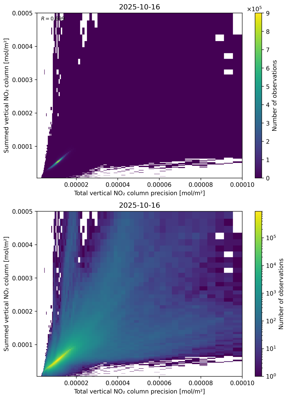
Figure 117: Scatter density plot of “Total vertical NO 2 column precision” against “Summed vertical NO 2 column” for 2025-10-15 to 2025-10-17.
