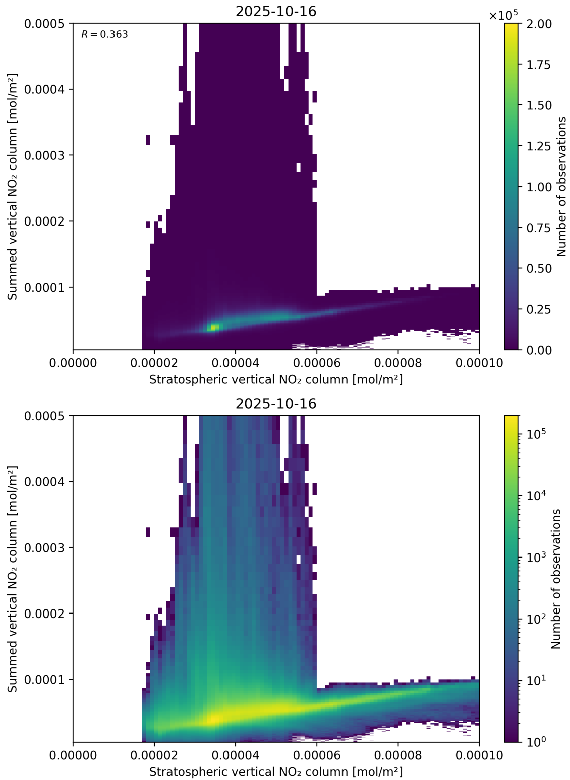
Figure 98: Scatter density plot of “Stratospheric vertical NO 2 column” against “Summed vertical NO 2 column” for 2025-10-15 to 2025-10-17.
