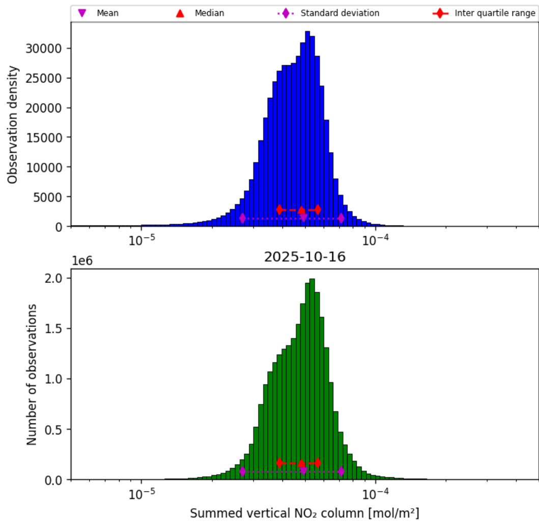
Figure 40: Histogram of “Summed vertical NO 2 column” for 2025-10-15 to 2025-10-17
