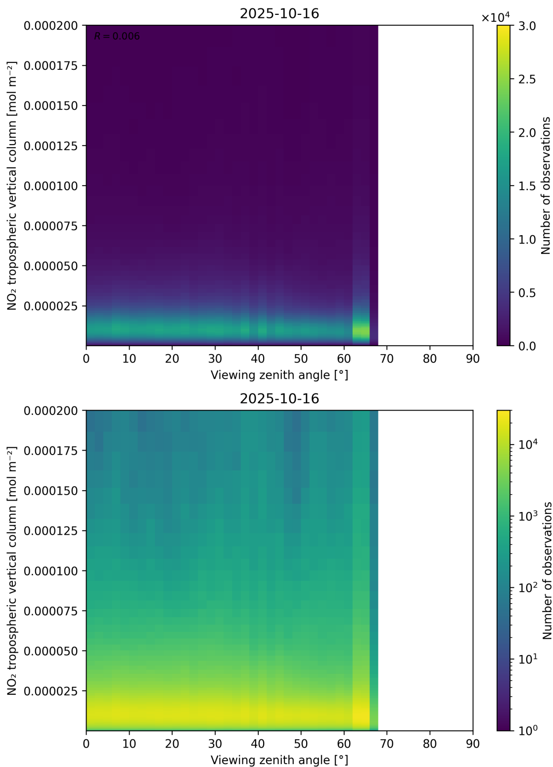
Figure 169: Scatter density plot of “Viewing zenith angle” against “NO 2 tropospheric vertical column” for 2025-10-15 to 2025-10-17.
