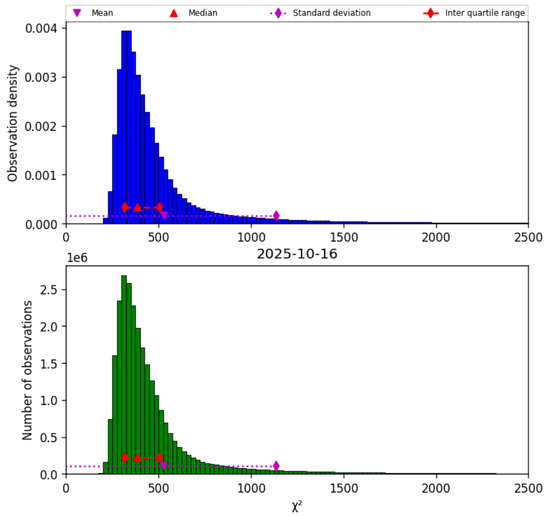
Figure 42: Histogram of “ \chi^2 ” for 2025-10-15 to 2025-10-17
