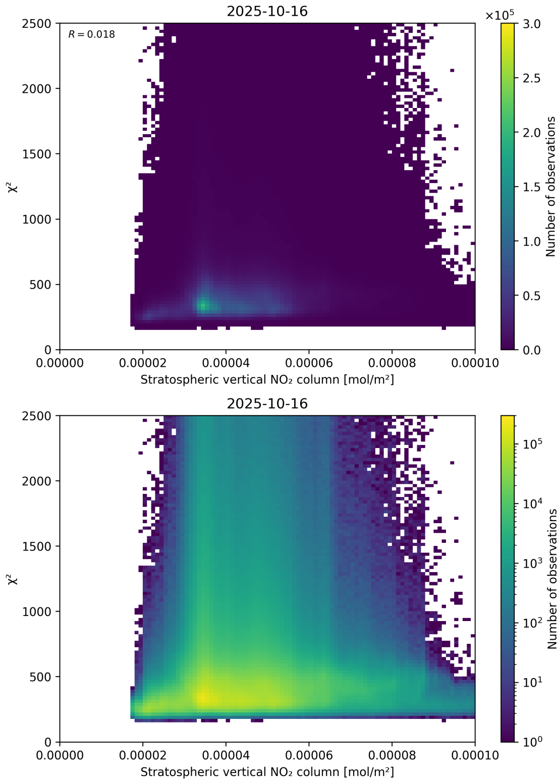
Figure 97: Scatter density plot of “Stratospheric vertical NO 2 column” against “ \chi^2 ” for 2025-10-15 to 2025-10-17.
