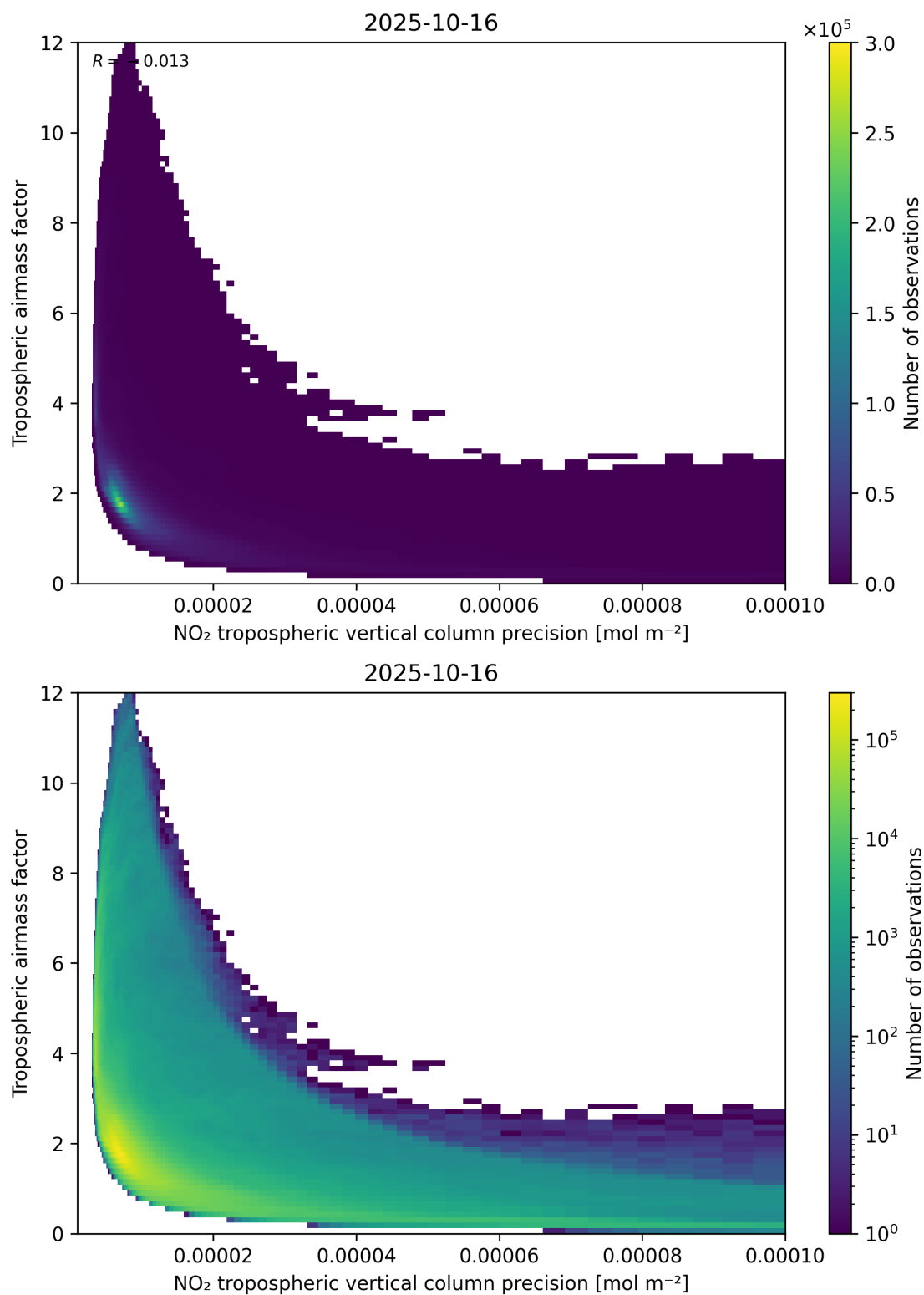
Figure 133: Scatter density plot of “NO 2 tropospheric vertical column precision” against “Tropospheric airmass factor” for 2025-10-15 to 2025-10-17.
