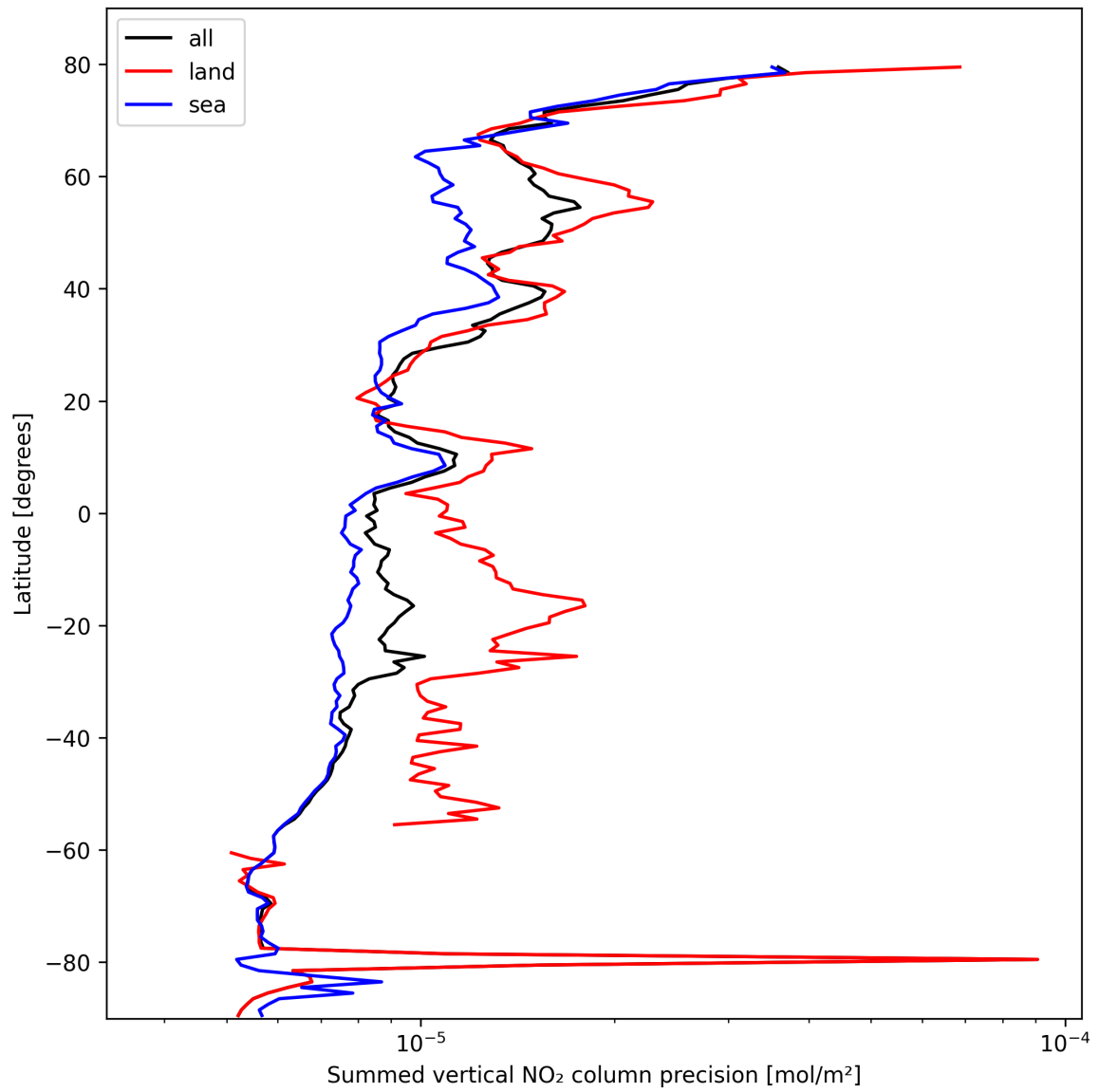
Figure 24: Zonal average of “Summed vertical NO 2 column precision” for 2025-10-15 to 2025-10-17.
