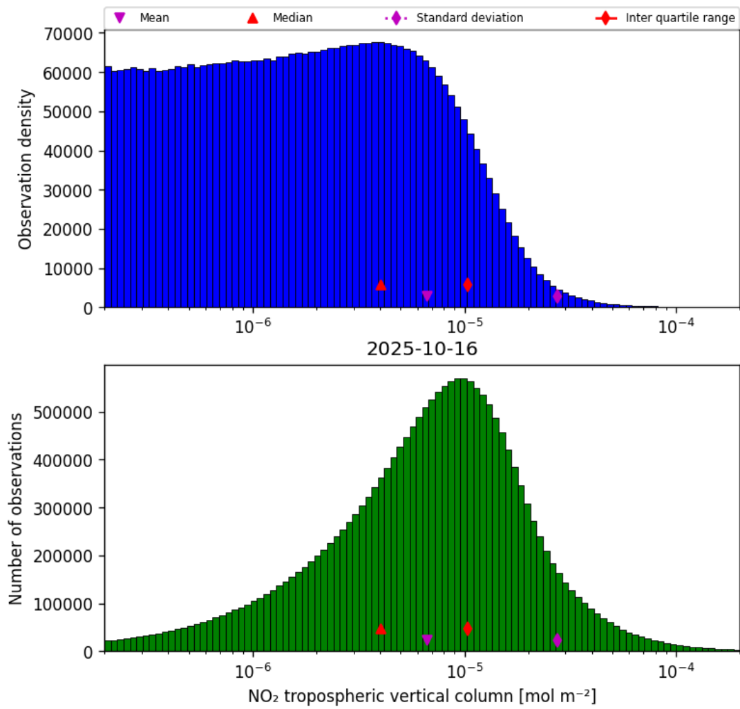
Figure 29: Histogram of “NO 2 tropospheric vertical column” for 2025-10-15 to 2025-10-17
