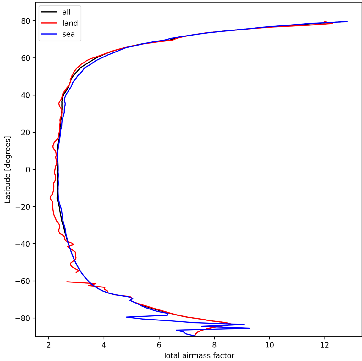
Figure 15: Zonal average of “Total airmass factor” for 2025-10-15 to 2025-10-17.
