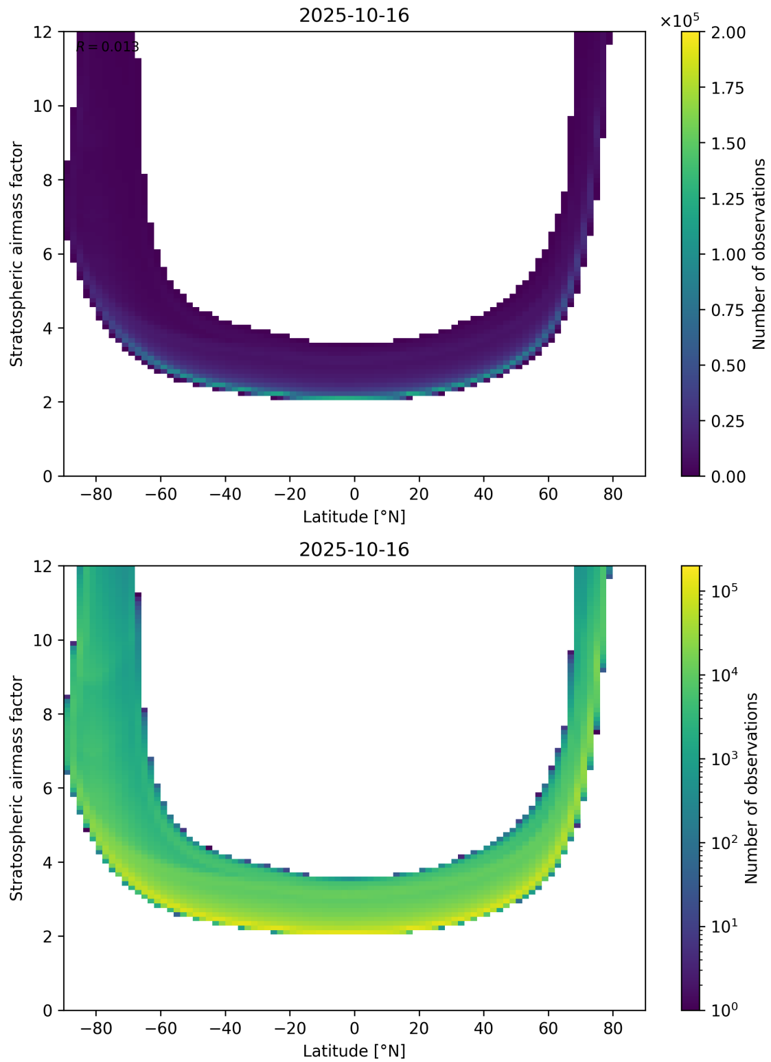
Figure 83: Scatter density plot of “Latitude” against “Stratospheric airmass factor” for 2025-10-15 to 2025-10-17.
