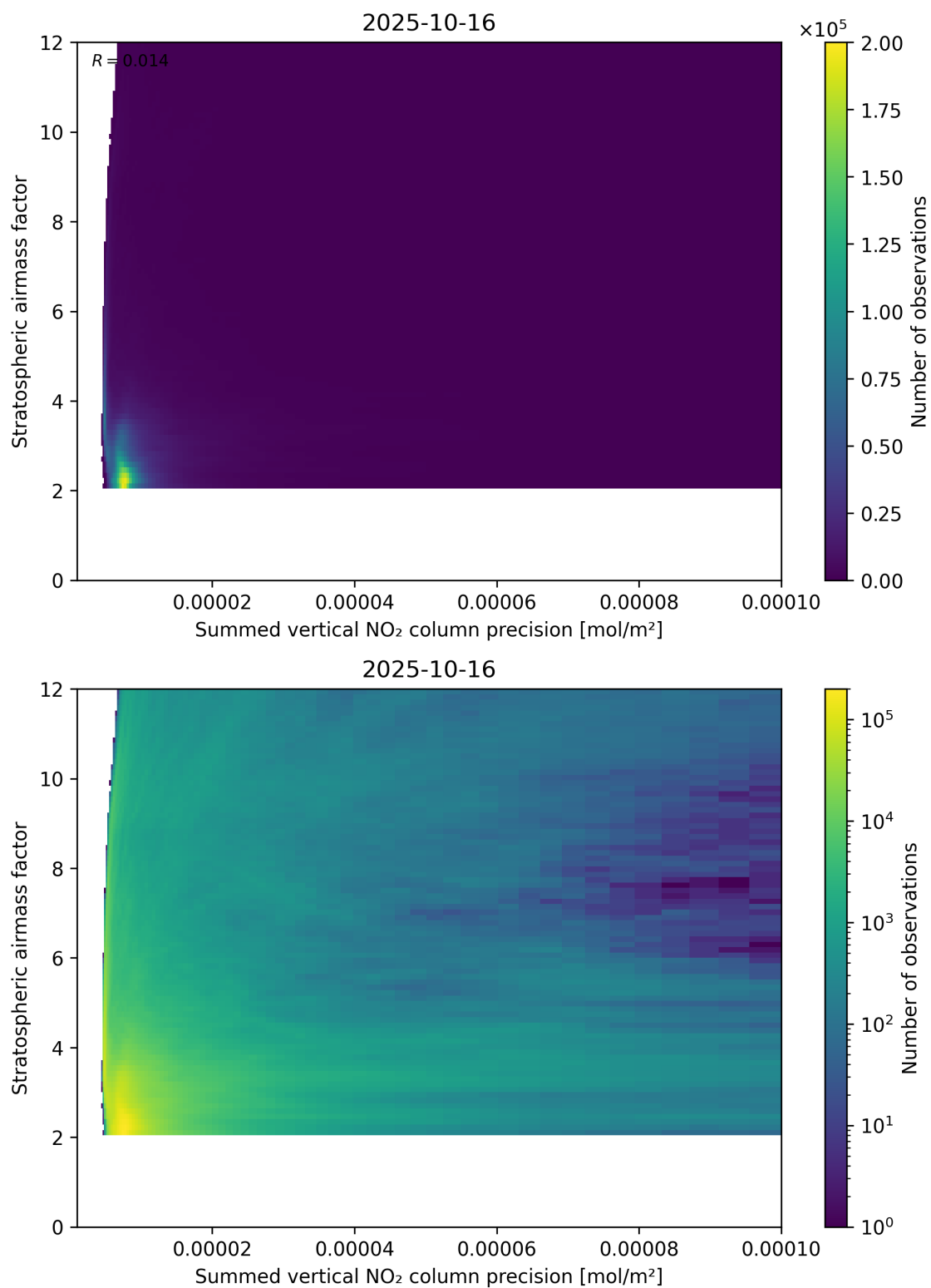
Figure 106: Scatter density plot of “Summed vertical NO 2 column precision” against “Stratospheric airmass factor” for 2025-10-15 to 2025-10-17.
