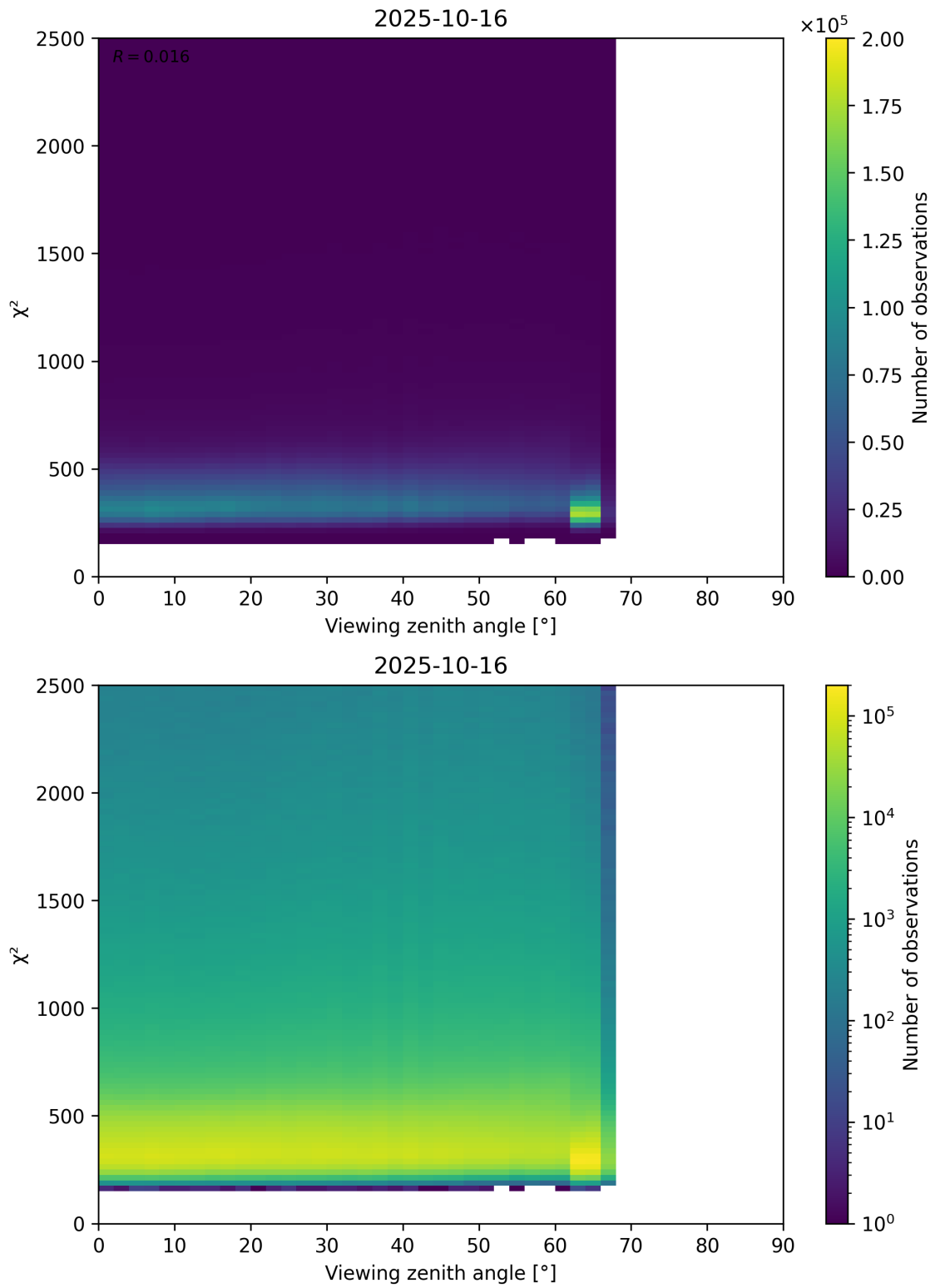
Figure 162: Scatter density plot of “Viewing zenith angle” against “ \chi^2 ” for 2025-10-15 to 2025-10-17.
