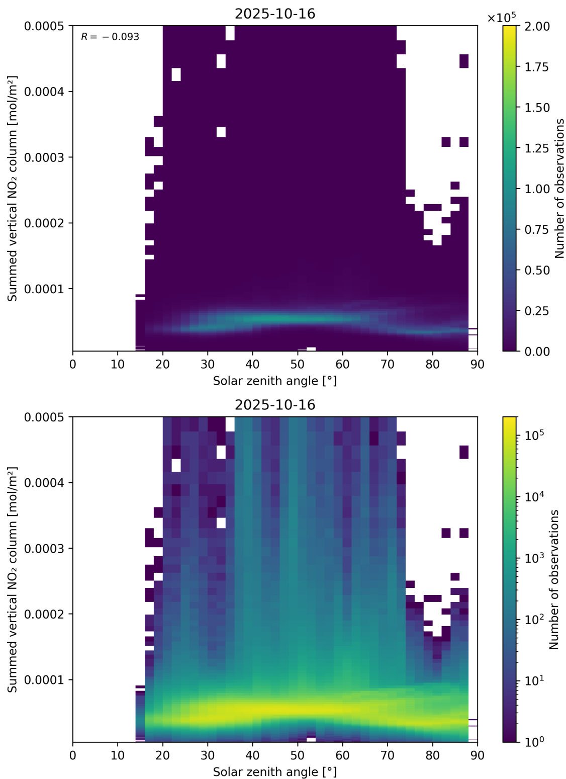
Figure 151: Scatter density plot of “Solar zenith angle” against “Summed vertical NO 2 column” for 2025-10-15 to 2025-10-17.
