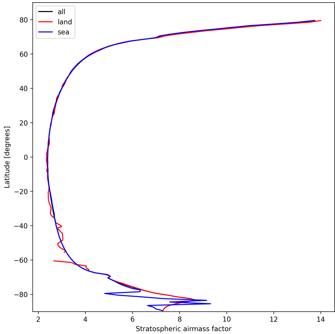
Figure 27: Zonal average of “Stratospheric airmass factor” for 2025-10-15 to 2025-10-17.
