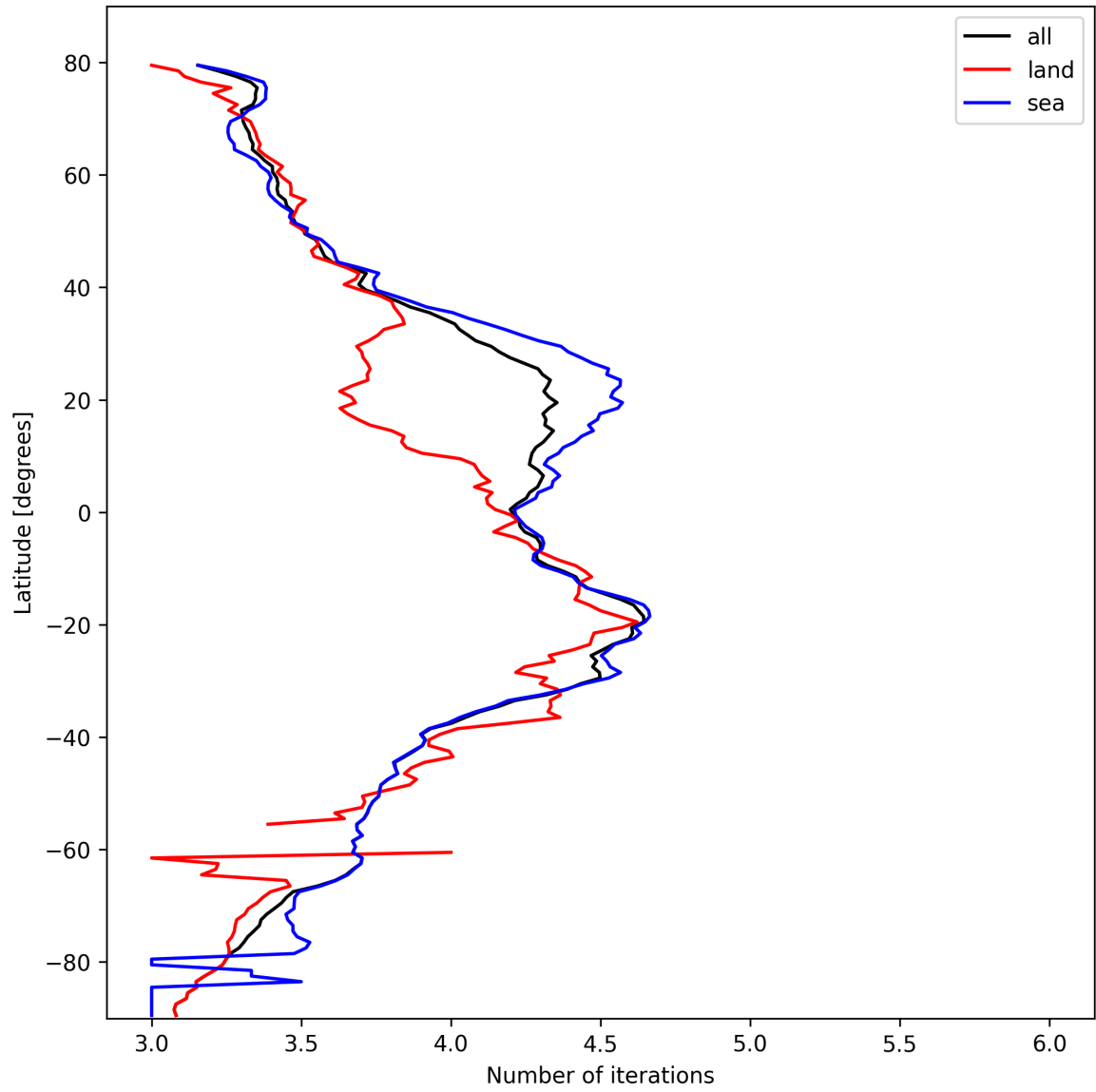
Figure 17: Zonal average of “Number of iterations” for 2025-10-15 to 2025-10-17.
