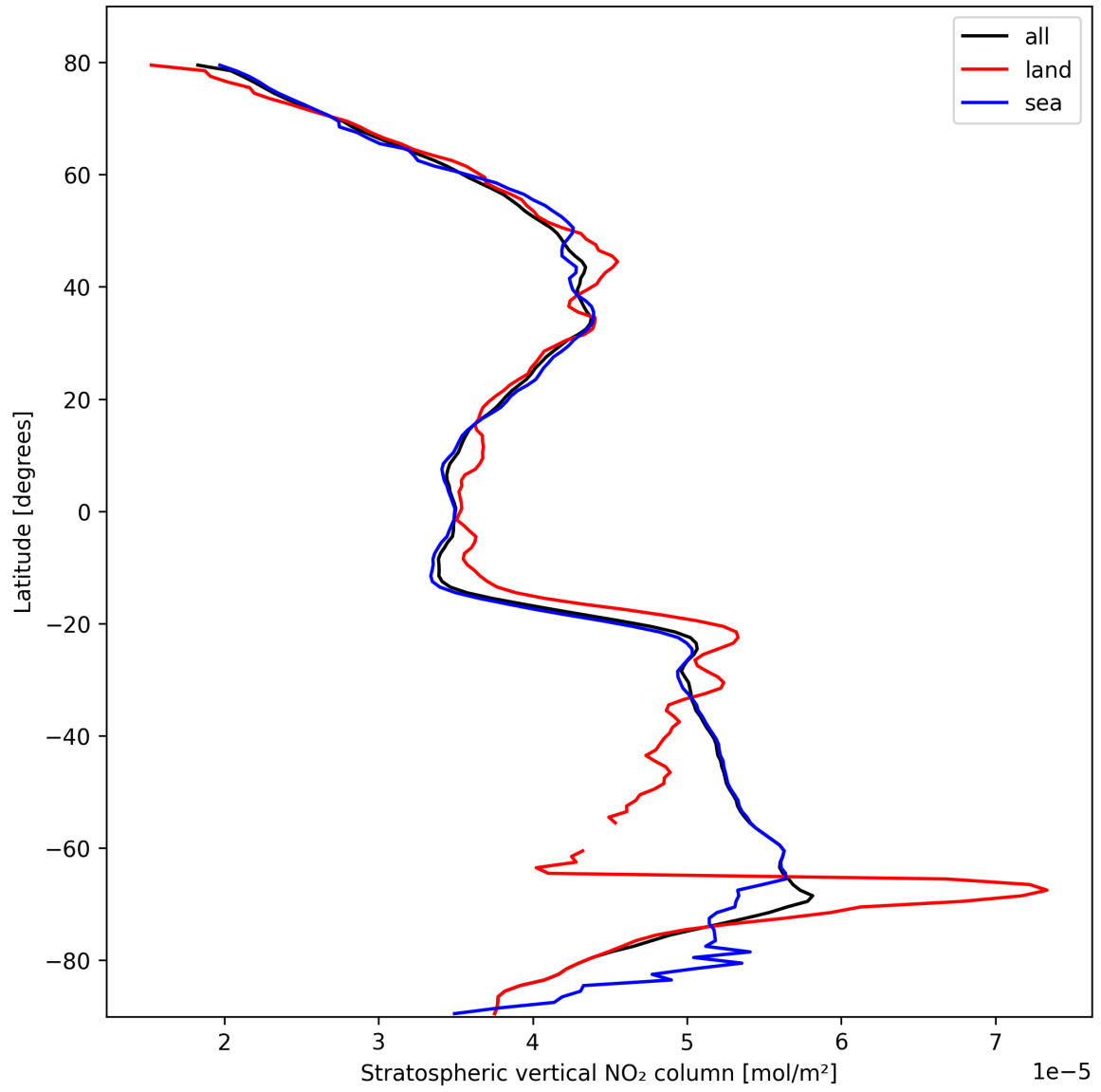
Figure 19: Zonal average of “Stratospheric vertical NO 2 column” for 2025-10-15 to 2025-10-17.
