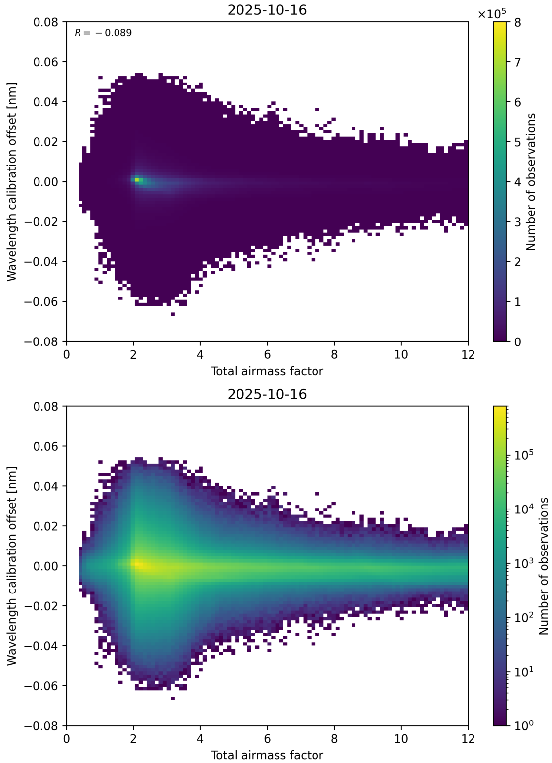
Figure 70: Scatter density plot of “Total airmass factor” against “Wavelength calibration offset” for 2025-10-15 to 2025-10-17.
