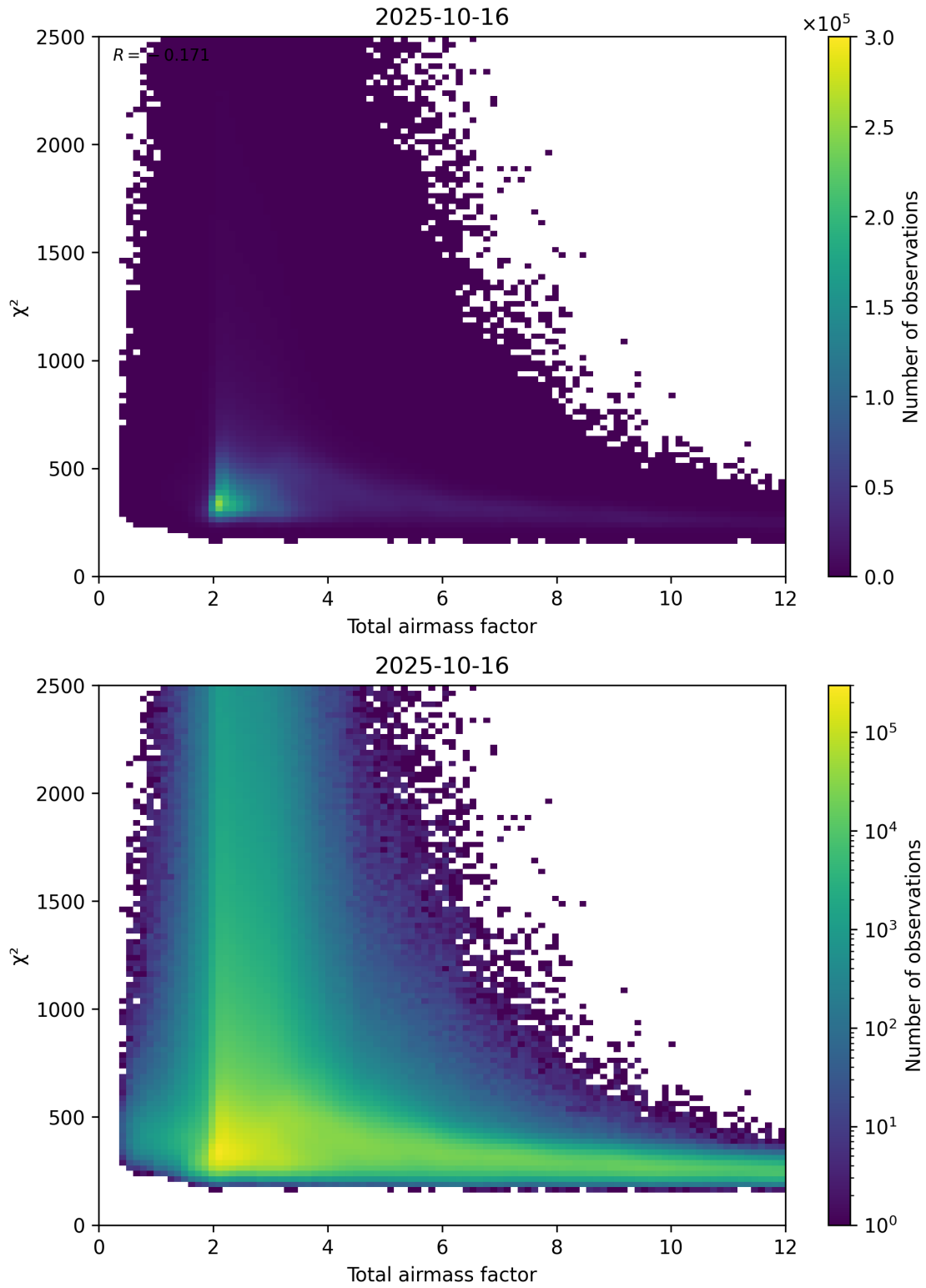
Figure 63: Scatter density plot of “Total airmass factor” against “ \chi^2 ” for 2025-10-15 to 2025-10-17.
