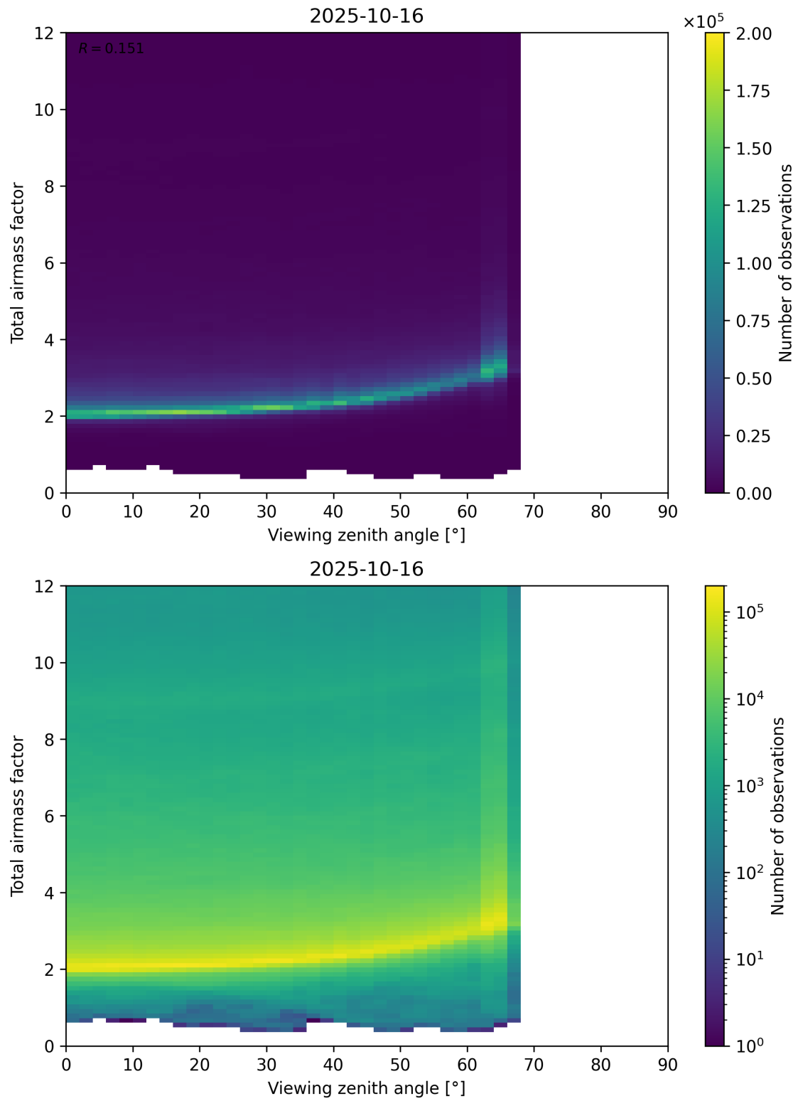
Figure 160: Scatter density plot of “Viewing zenith angle” against “Total airmass factor” for 2025-10-15 to 2025-10-17.
