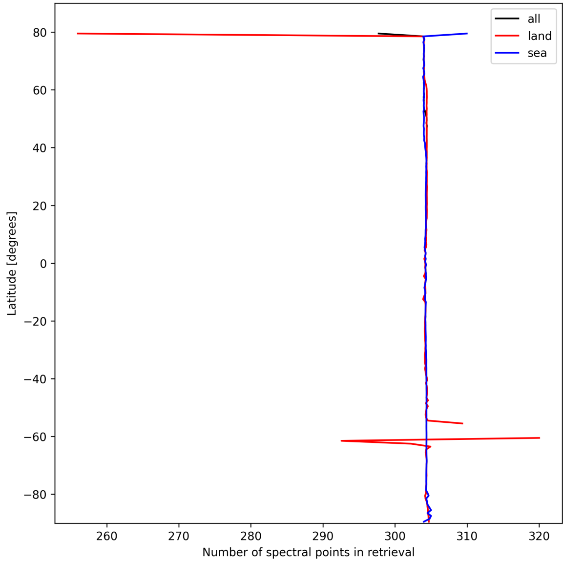
Figure 16: Zonal average of “Number of spectral points in retrieval” for 2025-10-15 to 2025-10-17.
