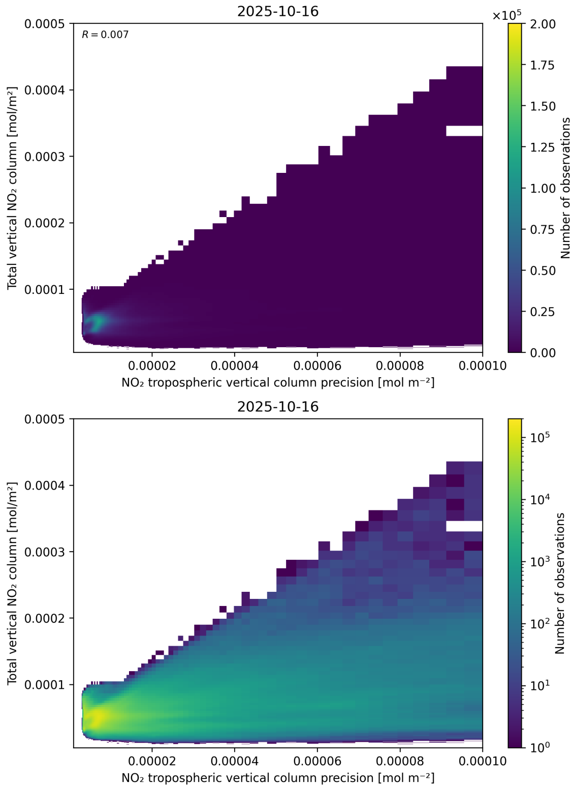
Figure 138: Scatter density plot of “NO 2 tropospheric vertical column precision” against “Total vertical NO 2 column” for 2025-10-15 to 2025-10-17.
