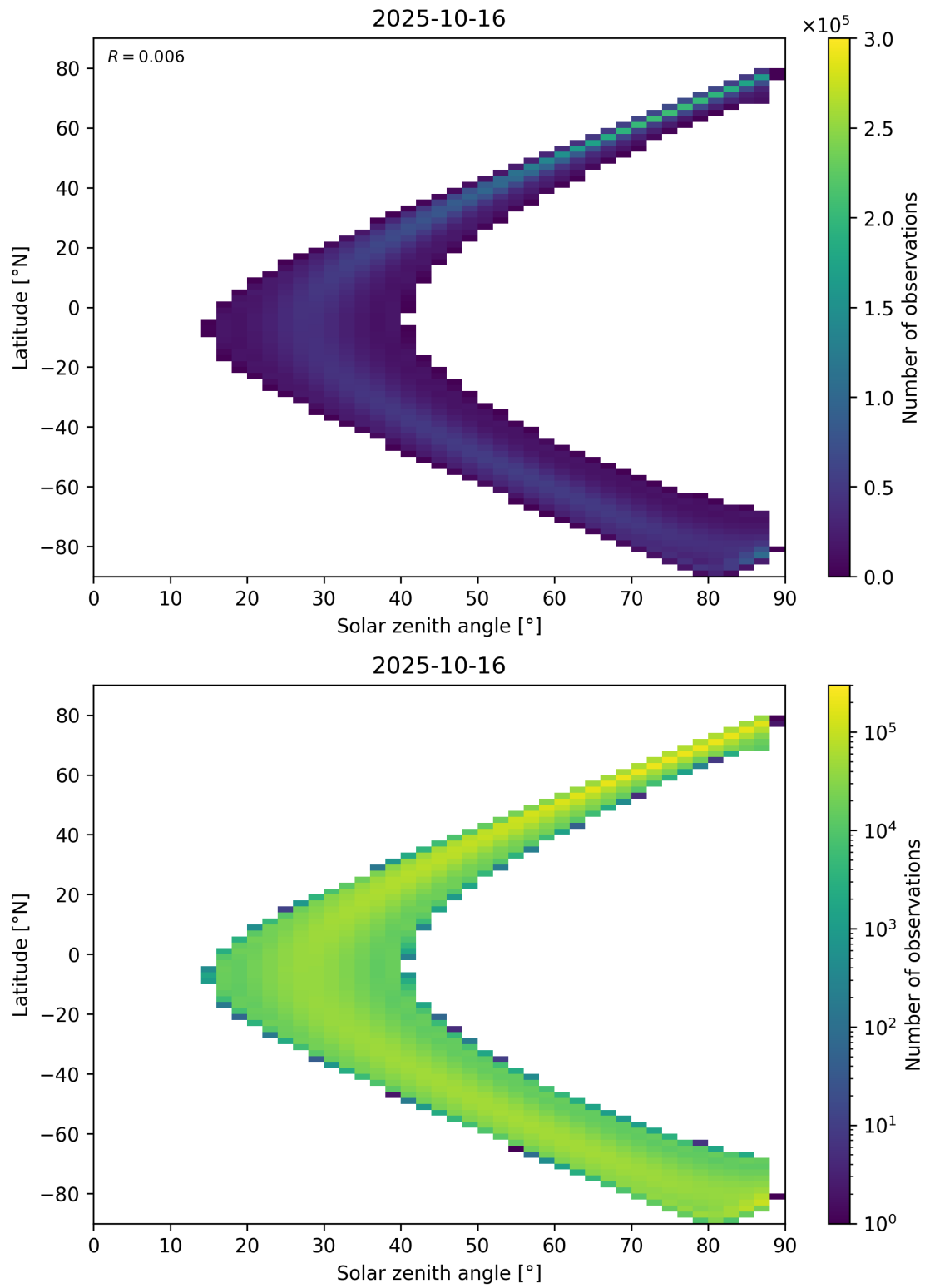
Figure 149: Scatter density plot of “Solar zenith angle” against “Latitude” for 2025-10-15 to 2025-10-17.
