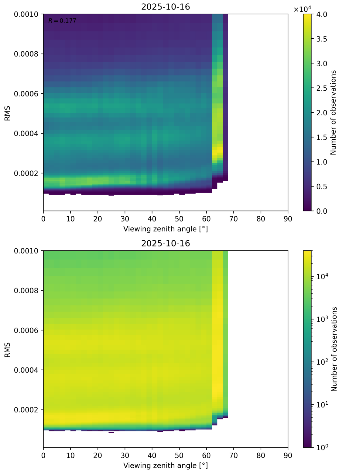
Figure 171: Scatter density plot of “Viewing zenith angle” against “RMS” for 2025-10-15 to 2025-10-17.
