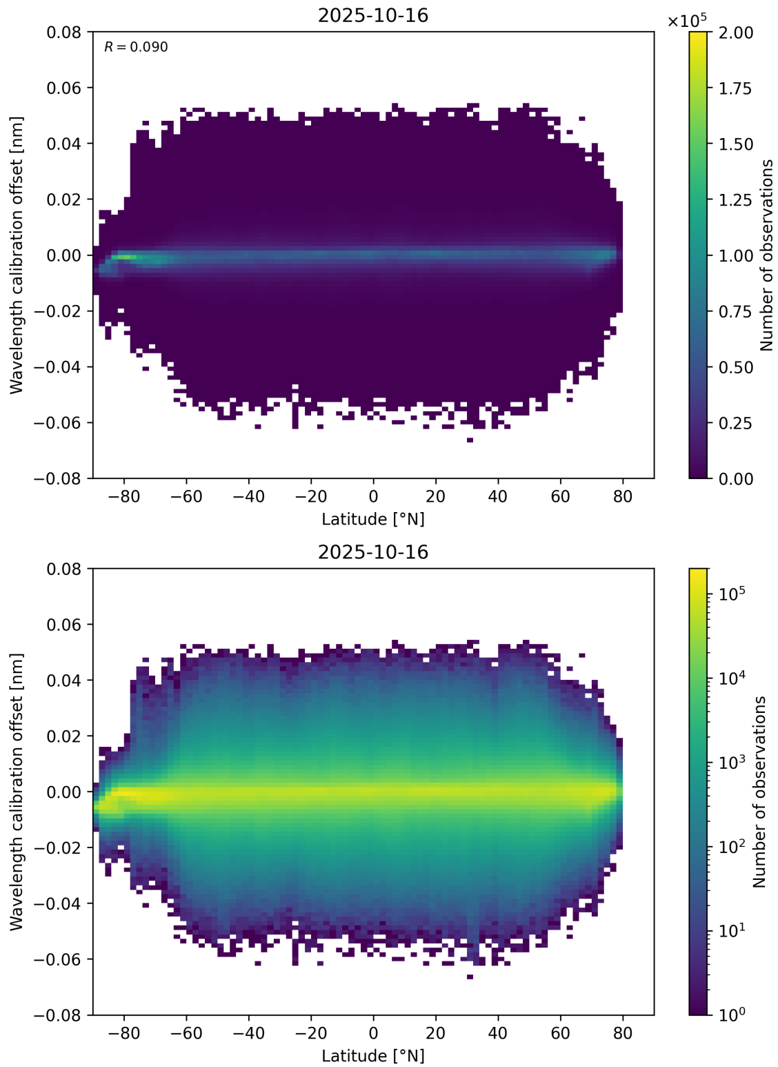
Figure 95: Scatter density plot of “Latitude” against “Wavelength calibration offset” for 2025-10-15 to 2025-10-17.
