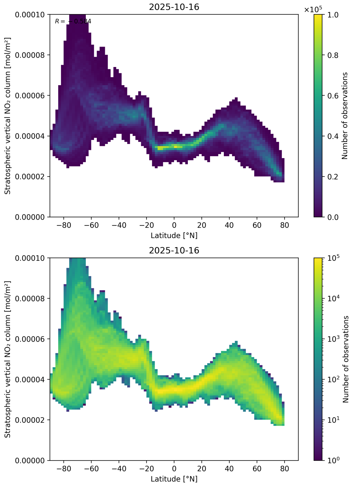
Figure 87: Scatter density plot of “Latitude” against “Stratospheric vertical NO 2 column” for 2025-10-15 to 2025-10-17.
