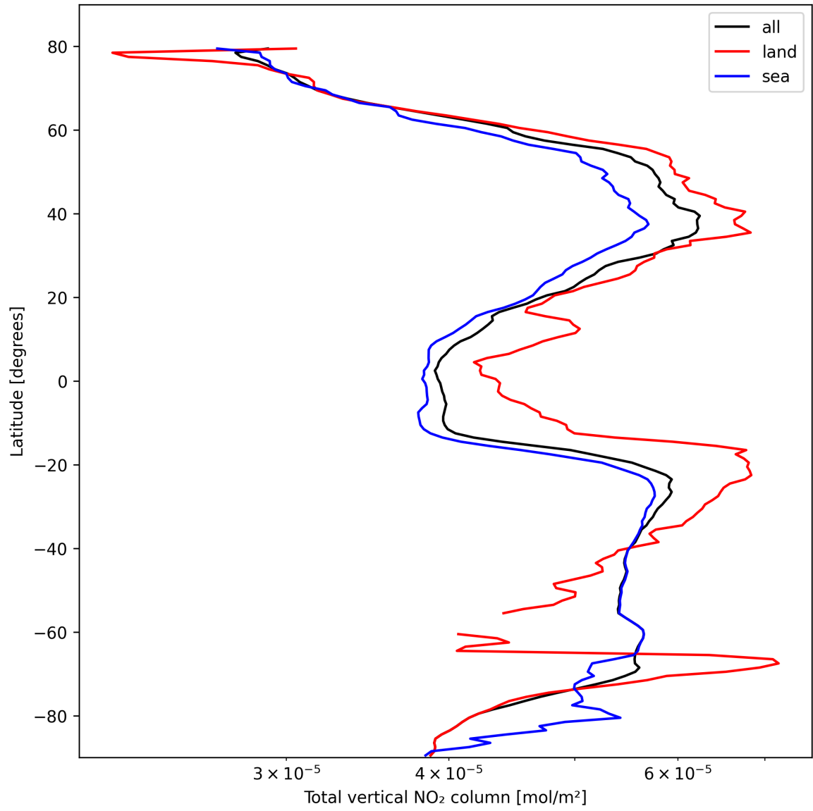
Figure 21: Zonal average of “Total vertical NO 2 column” for 2025-10-15 to 2025-10-17.
