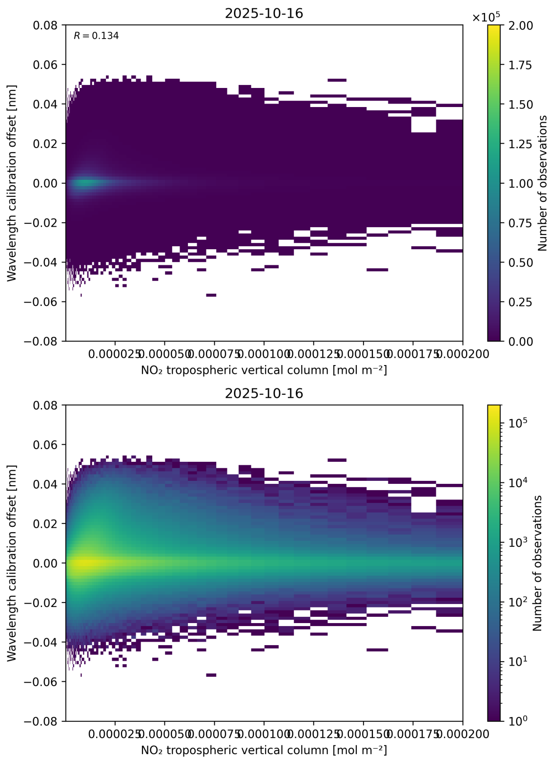
Figure 143: Scatter density plot of “NO 2 tropospheric vertical column” against “Wavelength calibration offset” for 2025-10-15 to 2025-10-17.
