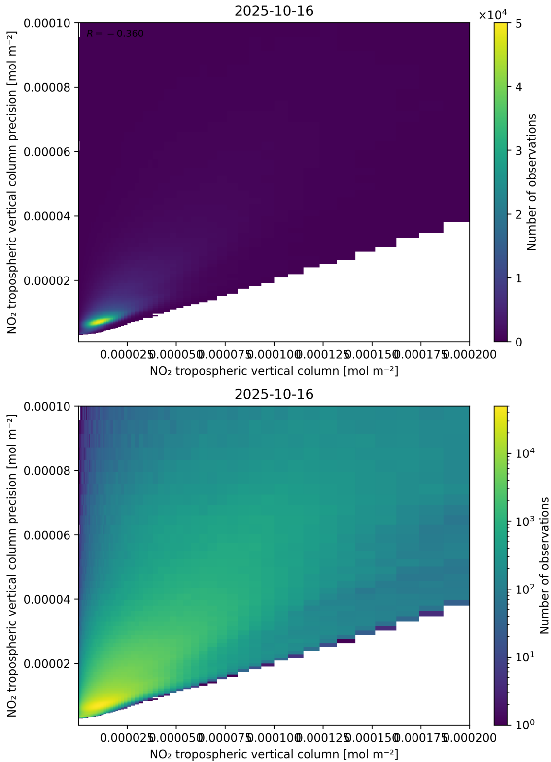
Figure 130: Scatter density plot of “NO 2 tropospheric vertical column” against “NO 2 tropospheric vertical column precision” for 2025-10-15 to 2025-10-17.
