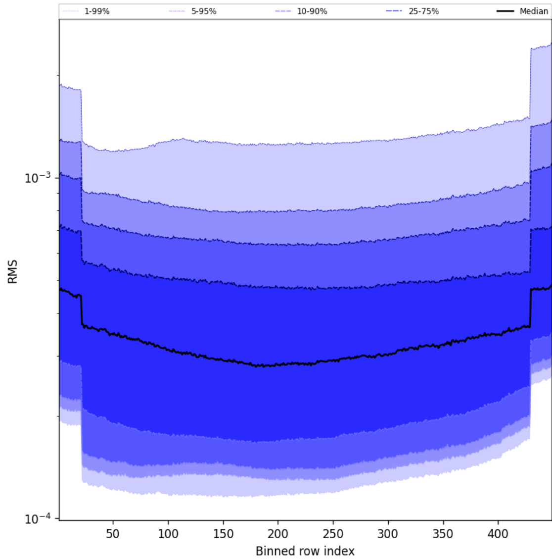
Figure 60: Along track statistics of “RMS” for 2025-10-15 to 2025-10-17
