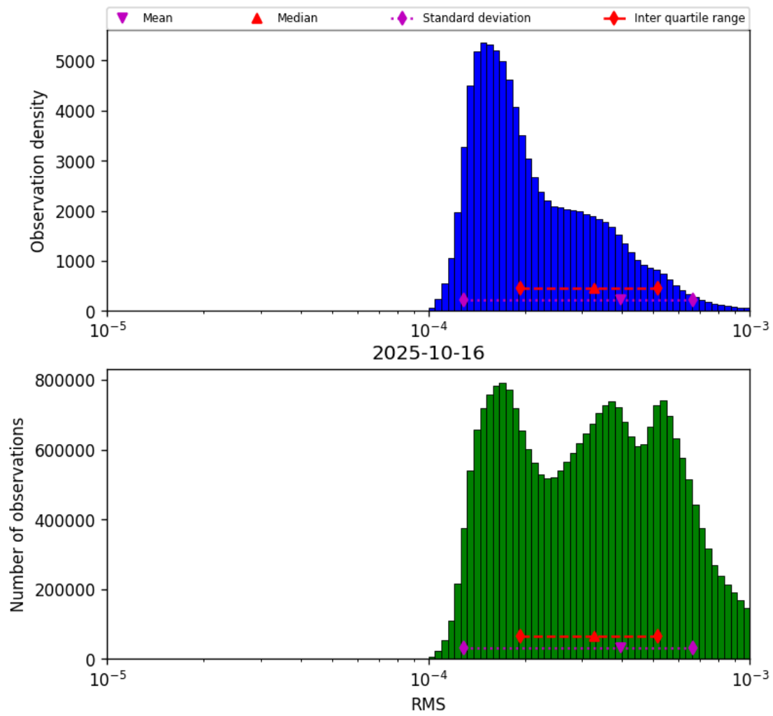
Figure 43: Histogram of “RMS” for 2025-10-15 to 2025-10-17
