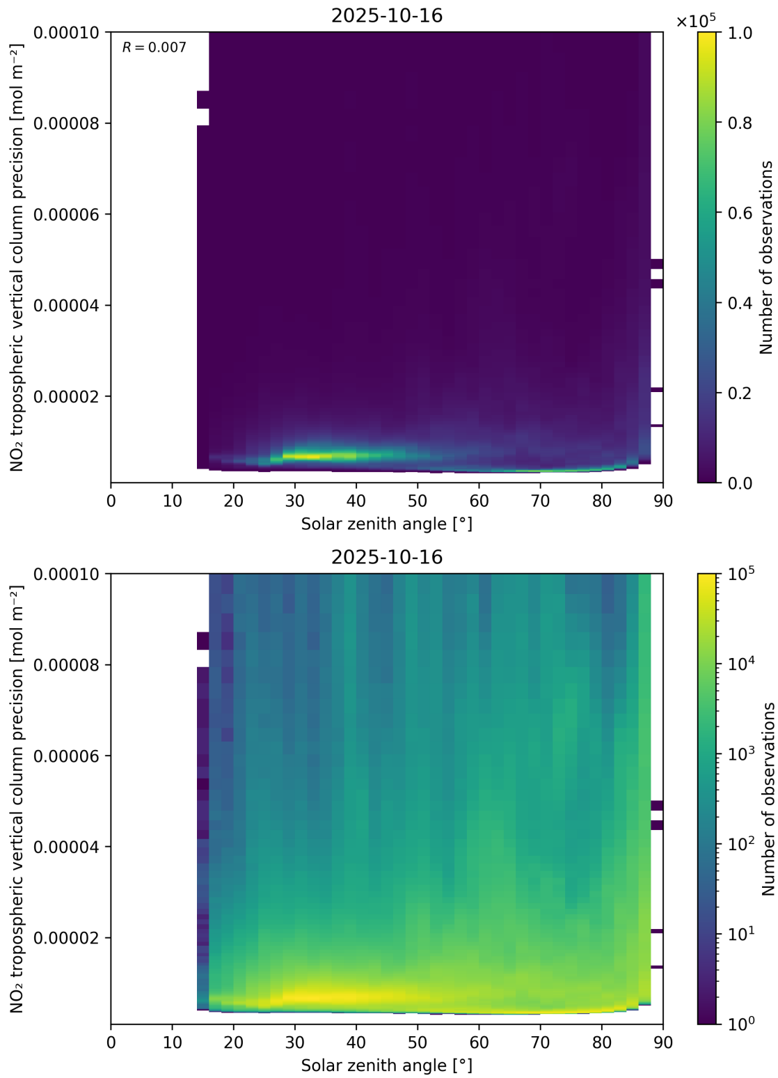
Figure 156: Scatter density plot of “Solar zenith angle” against “NO 2 tropospheric vertical column precision” for 2025-10-15 to 2025-10-17.
