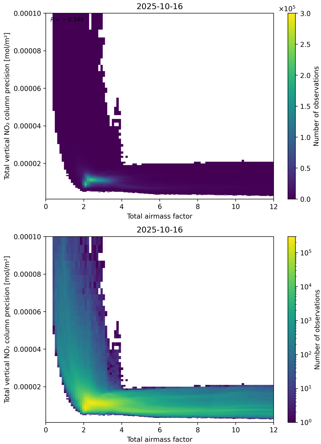
Figure 68: Scatter density plot of “Total airmass factor” against “Total vertical NO 2 column precision” for 2025-10-15 to 2025-10-17.
