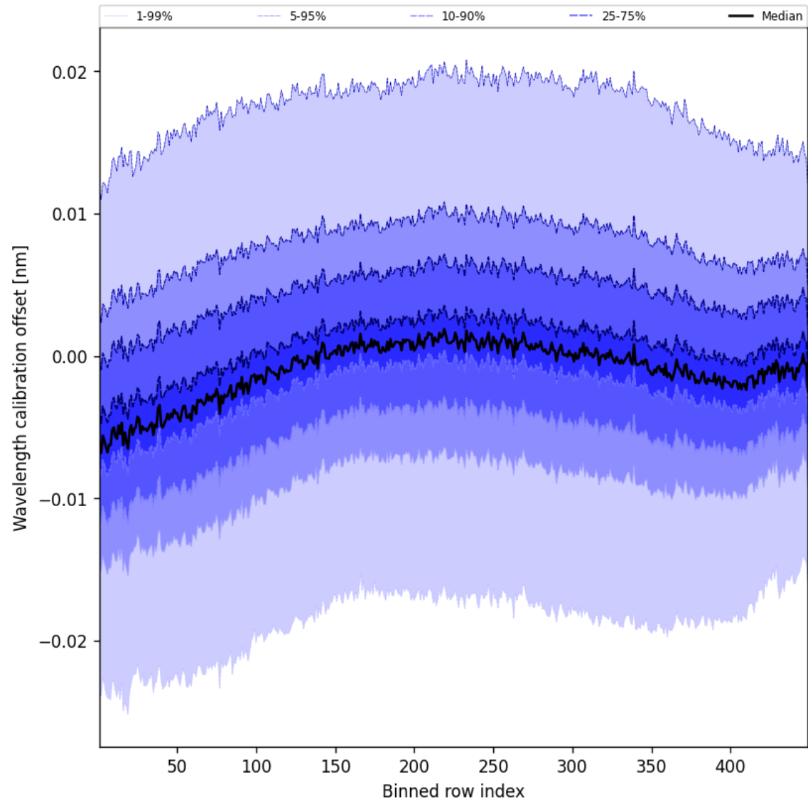
Figure 52: Along track statistics of “Wavelength calibration offset” for 2025-10-15 to 2025-10-17
