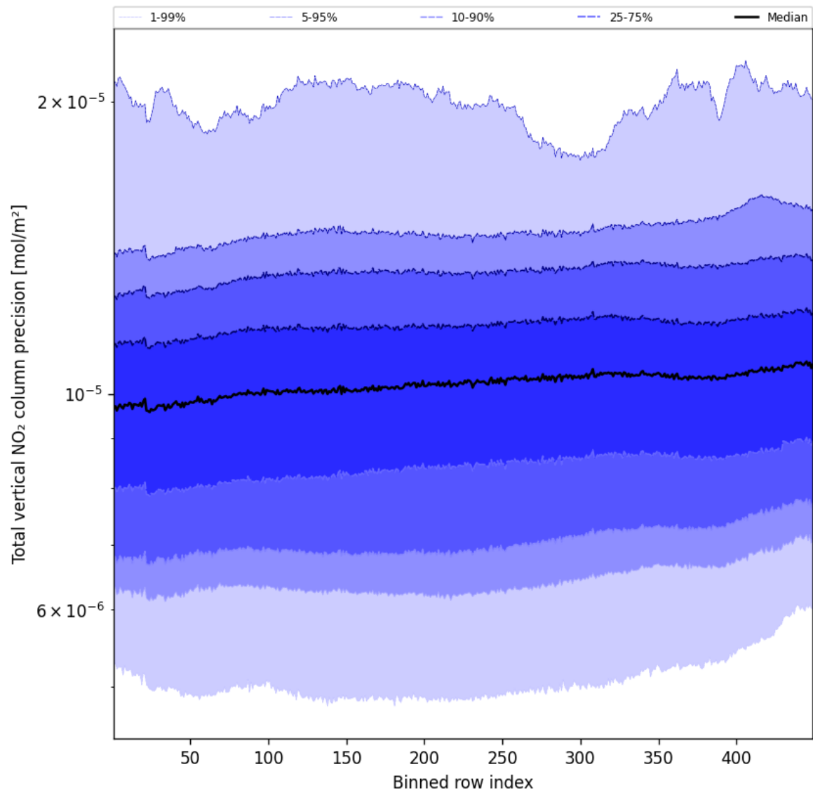
Figure 56: Along track statistics of “Total vertical NO 2 column precision” for 2025-10-15 to 2025-10-17
