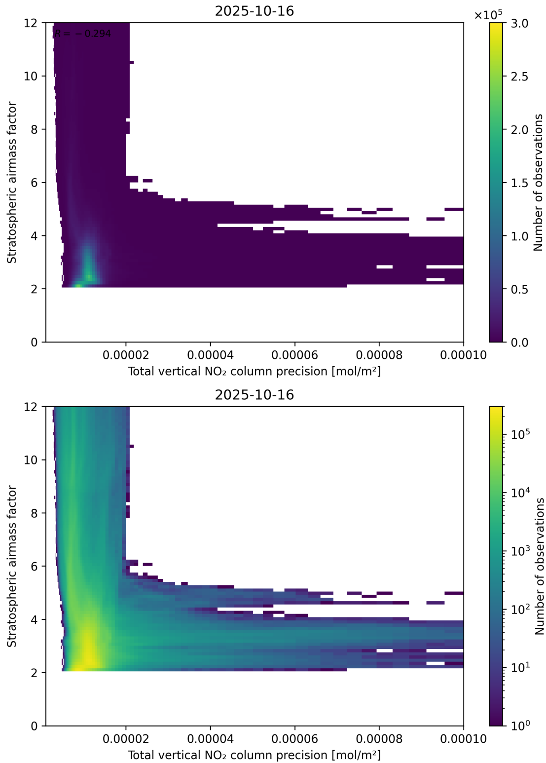
Figure 115: Scatter density plot of “Total vertical NO 2 column precision” against “Stratospheric airmass factor” for 2025-10-15 to 2025-10-17.
