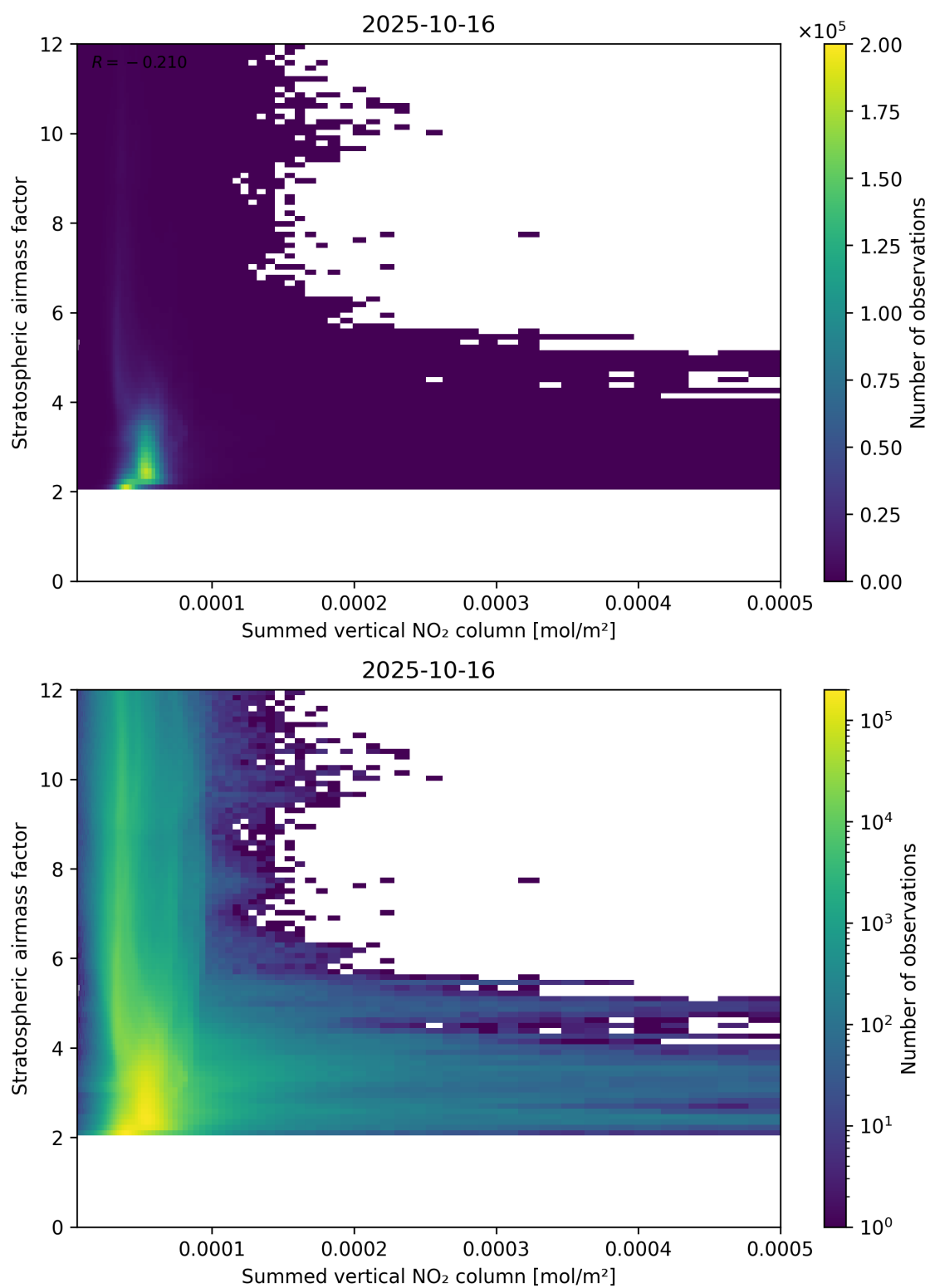
Figure 103: Scatter density plot of “Summed vertical NO 2 column” against “Stratospheric air mass factor” for 2025-10-15 to 2025-10-17.
