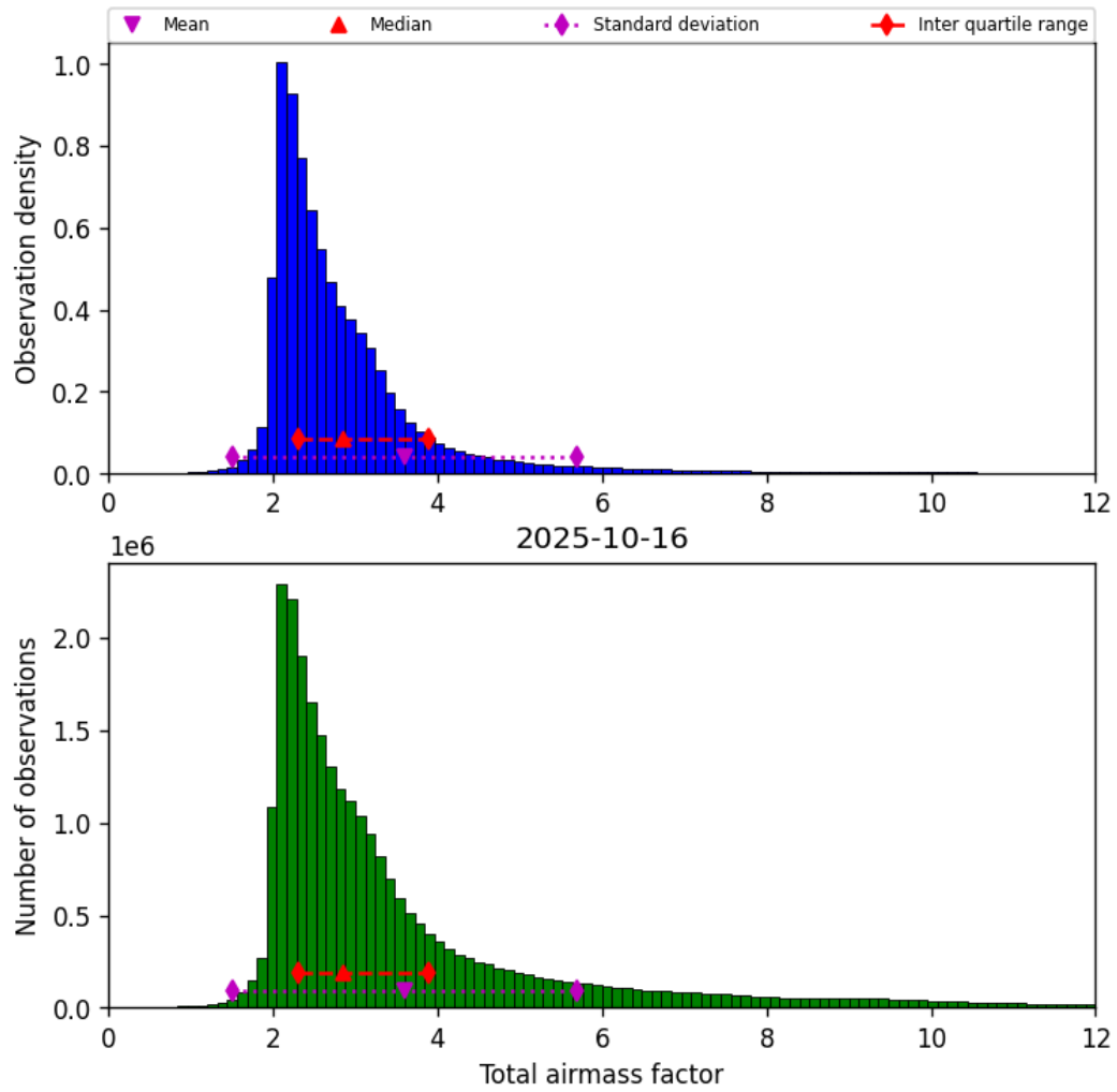
Figure 32: Histogram of “Total airmass factor” for 2025-10-15 to 2025-10-17
