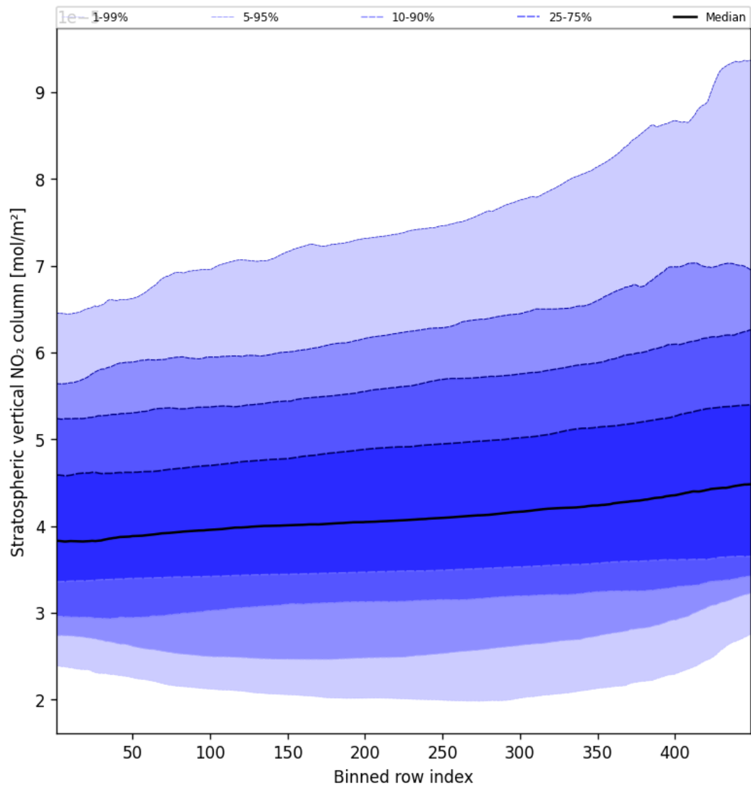
Figure 53: Along track statistics of “Stratospheric vertical NO 2 column” for 2025-10-15 to 2025-10-17
