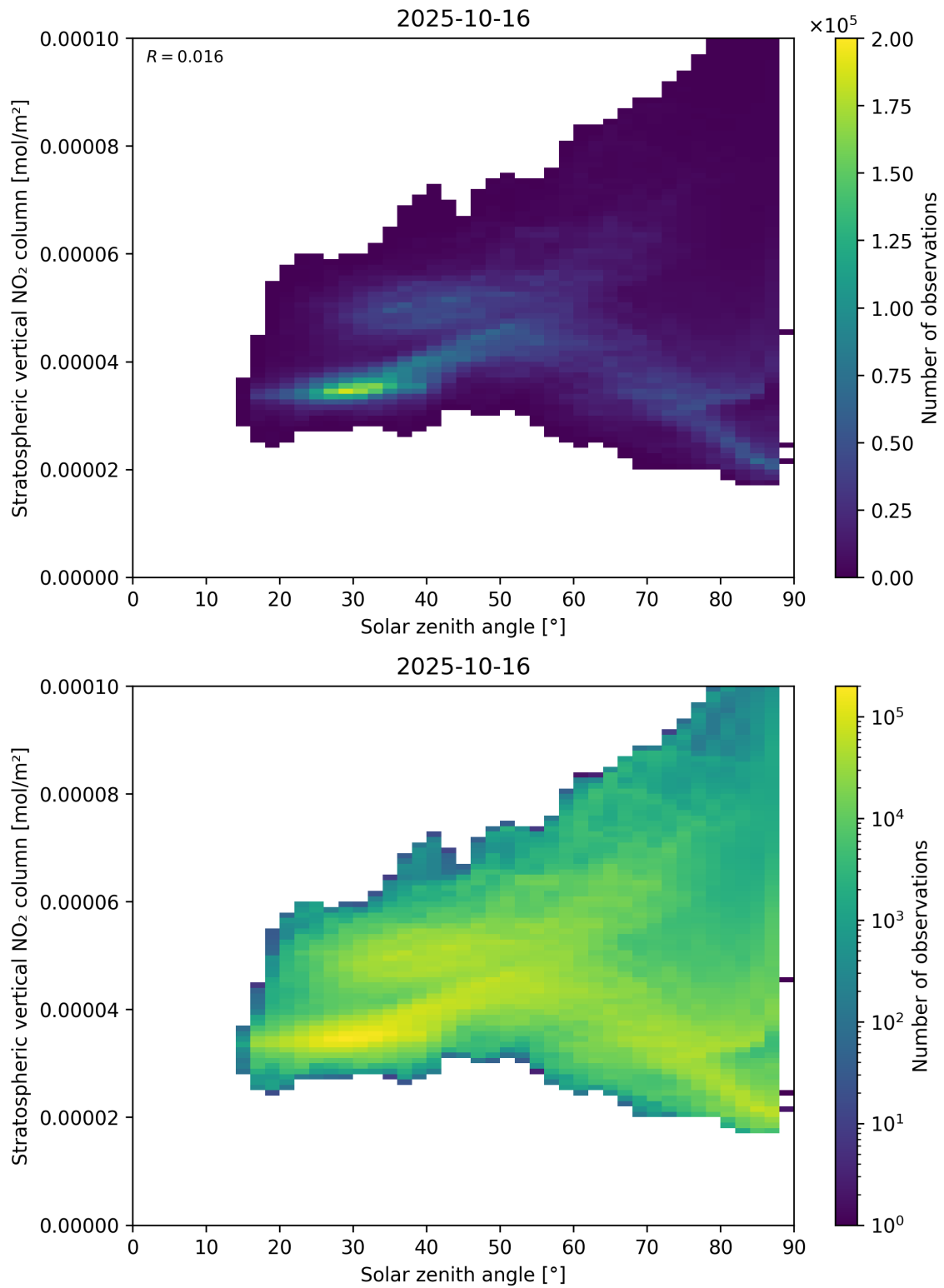
Figure 150: Scatter density plot of “Solar zenith angle” against “Stratospheric vertical \text{NO}_2 column” for 2025-10-15 to 2025-10-17.
