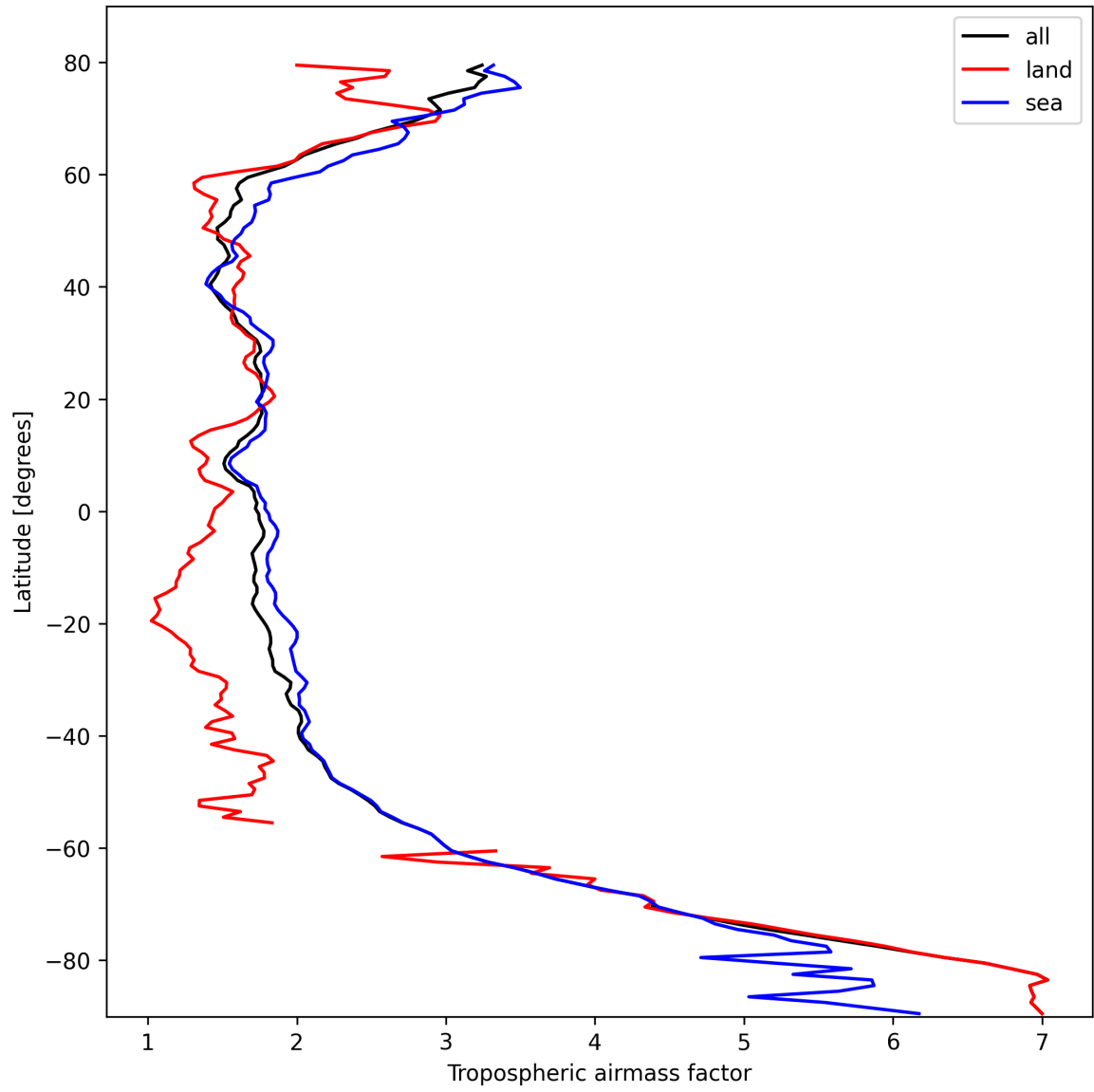
Figure 14: Zonal average of “Tropospheric airmass factor” for 2025-10-15 to 2025-10-17.
