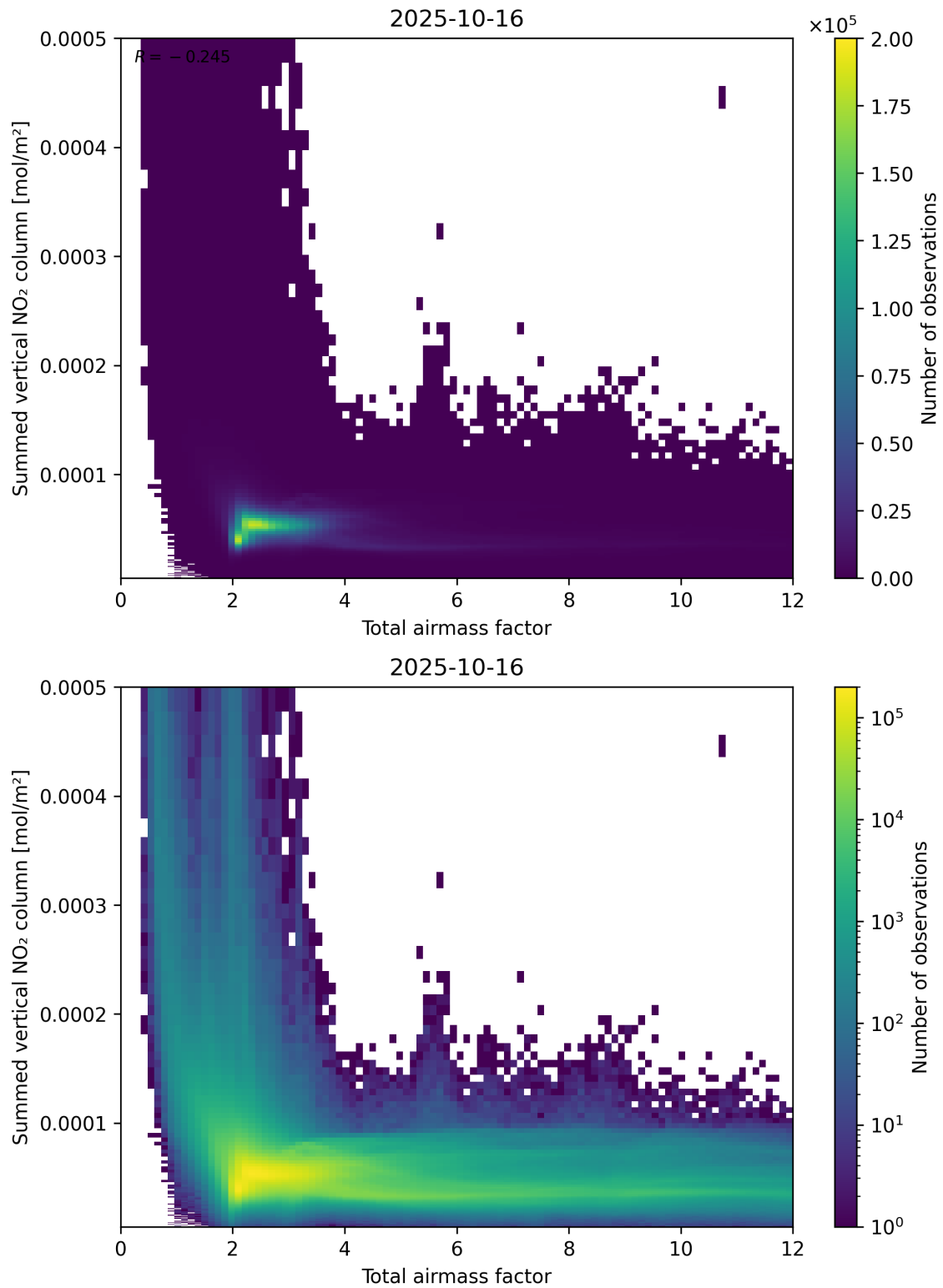
Figure 65: Scatter density plot of “Total airmass factor” against “Summed vertical NO 2 column” for 2025-10-15 to 2025-10-17.
