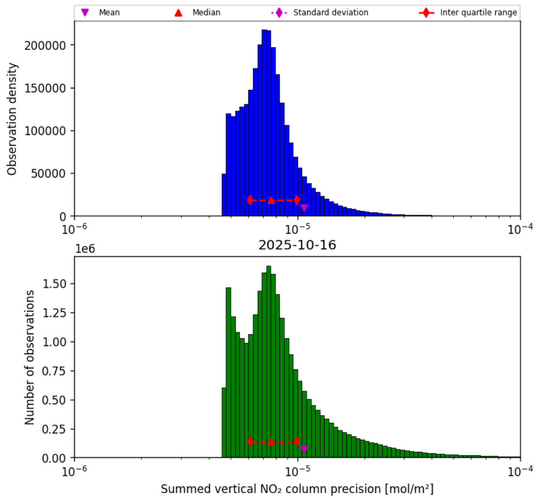
Figure 41: Histogram of "Summed vertical NO 2 column precision" for 2025-10-15 to 2025-10-17
