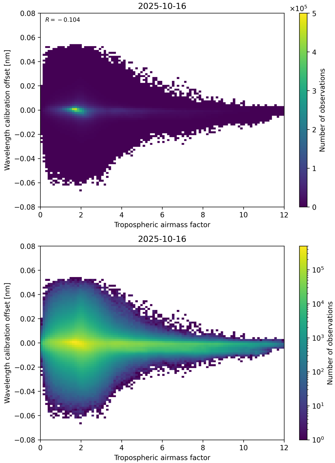
Figure 80: Scatter density plot of “Tropospheric airmass factor” against “Wavelength calibration offset” for 2025-10-15 to 2025-10-17.
