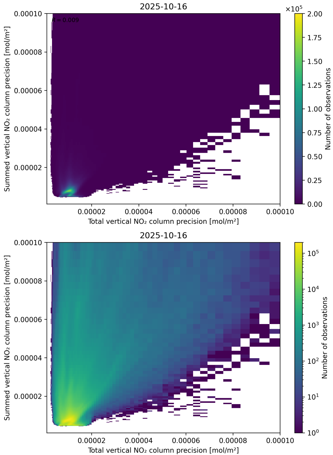
Figure 118: Scatter density plot of “Total vertical NO 2 column precision” against “Summed vertical NO 2 column precision” for 2025-10-15 to 2025-10-17.
