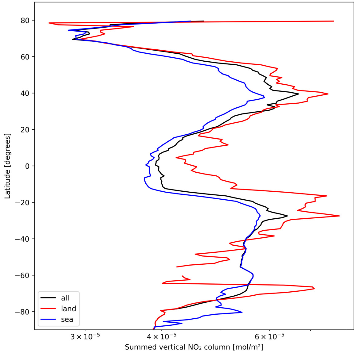
Figure 23: Zonal average of “Summed vertical NO 2 column” for 2025-10-15 to 2025-10-17.
