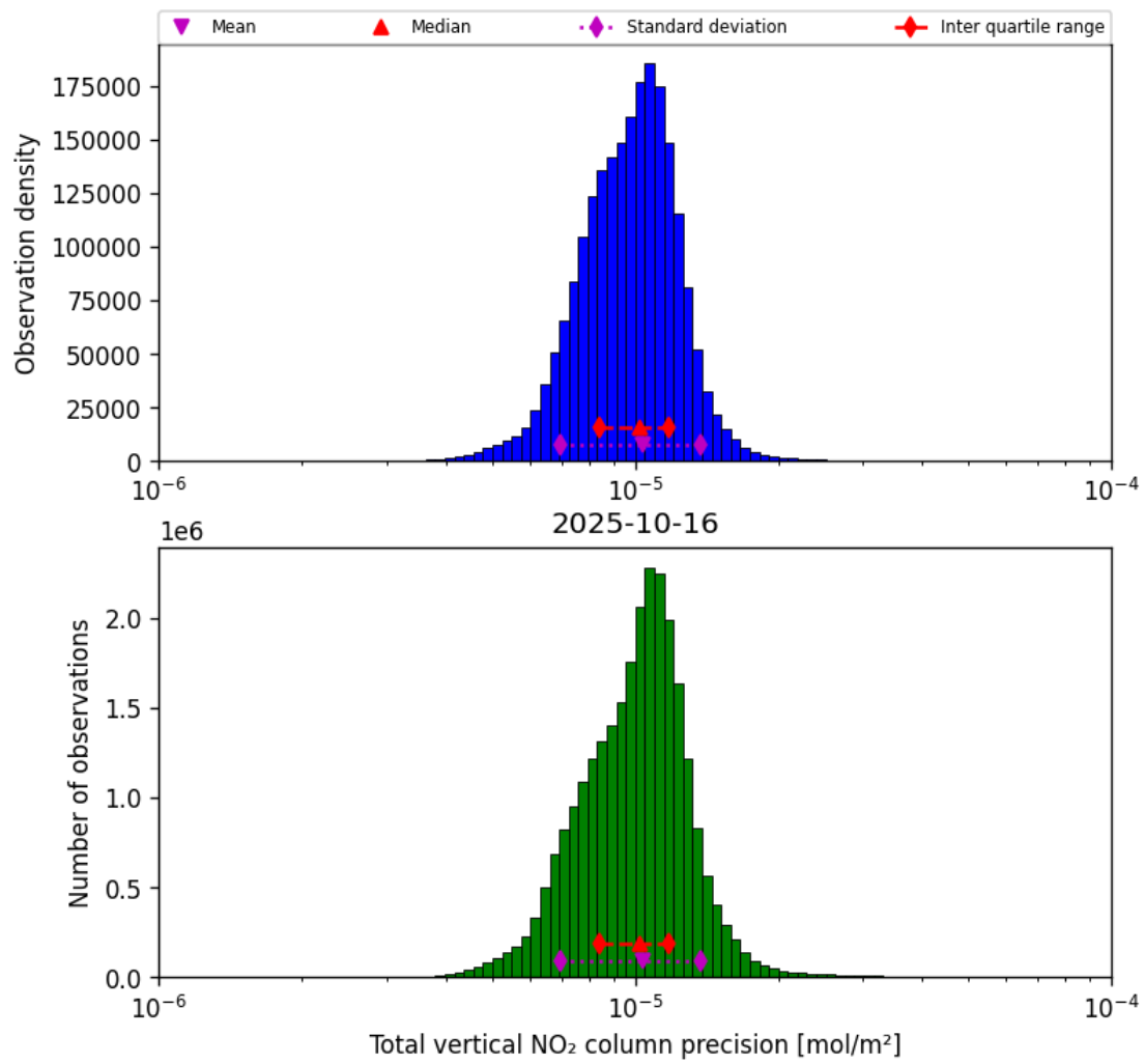
Figure 39: Histogram of “Total vertical NO 2 column precision” for 2025-10-15 to 2025-10-17
