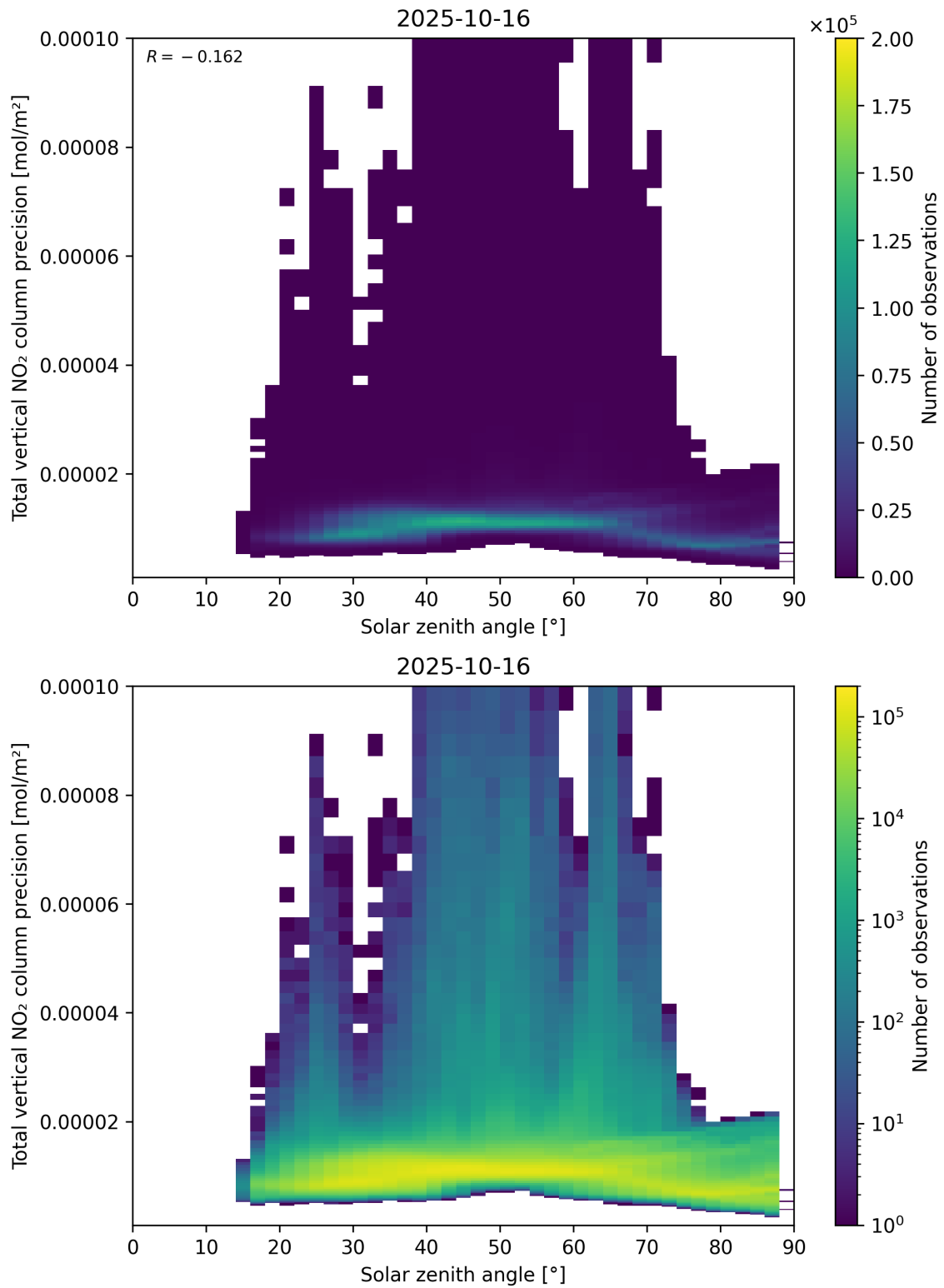
Figure 154: Scatter density plot of “Solar zenith angle” against “Total vertical NO 2 column precision” for 2025-10-15 to 2025-10-17.
