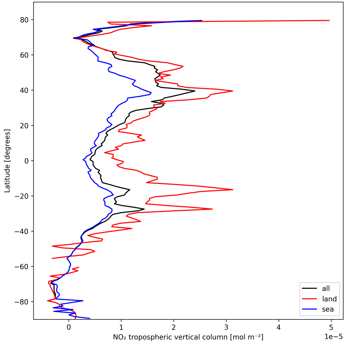
Figure 12: Zonal average of “NO 2 tropospheric vertical column” for 2025-10-15 to 2025-10-17.
