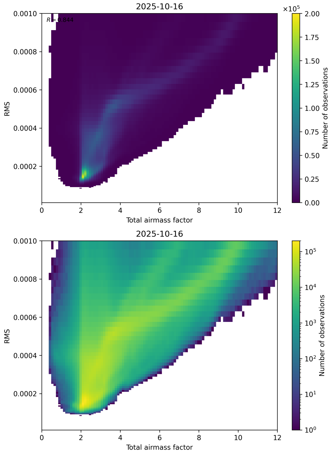
Figure 69: Scatter density plot of “Total airmass factor” against “RMS” for 2025-10-15 to 2025-10-17.
