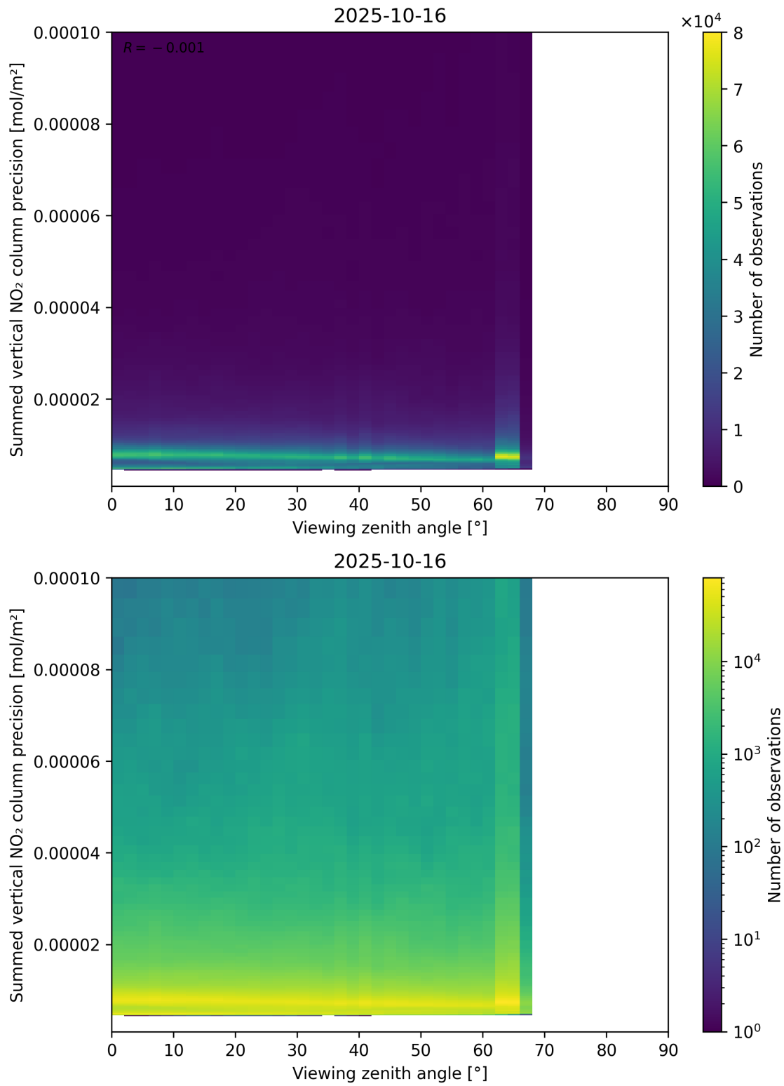
Figure 166: Scatter density plot of “Viewing zenith angle” against “Summed vertical NO 2 column precision” for 2025-10-15 to 2025-10-17.
