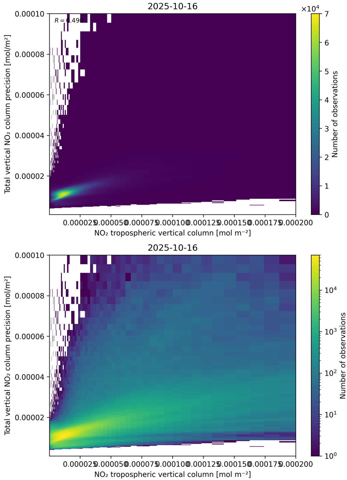
Figure 129: Scatter density plot of “NO 2 tropospheric vertical column” against “Total vertical NO 2 column precision” for 2025-10-15 to 2025-10-17.
