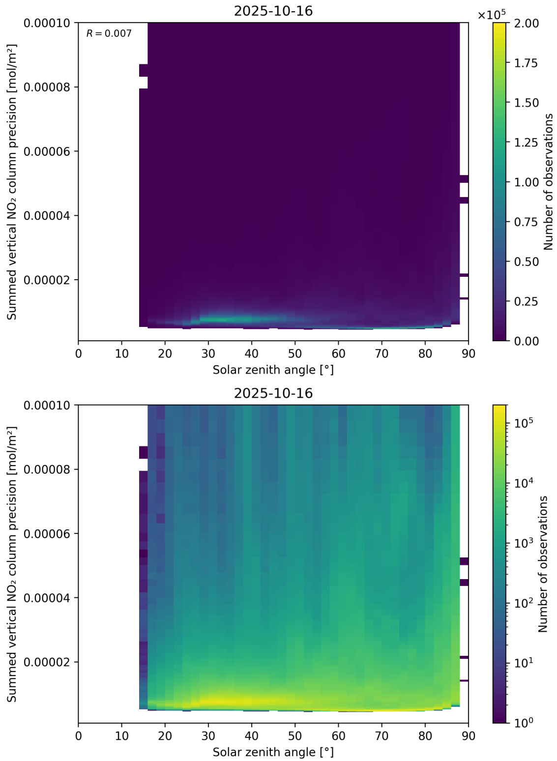
Figure 152: Scatter density plot of “Solar zenith angle” against “Summed vertical NO 2 column precision” for 2025-10-15 to 2025-10-17.
