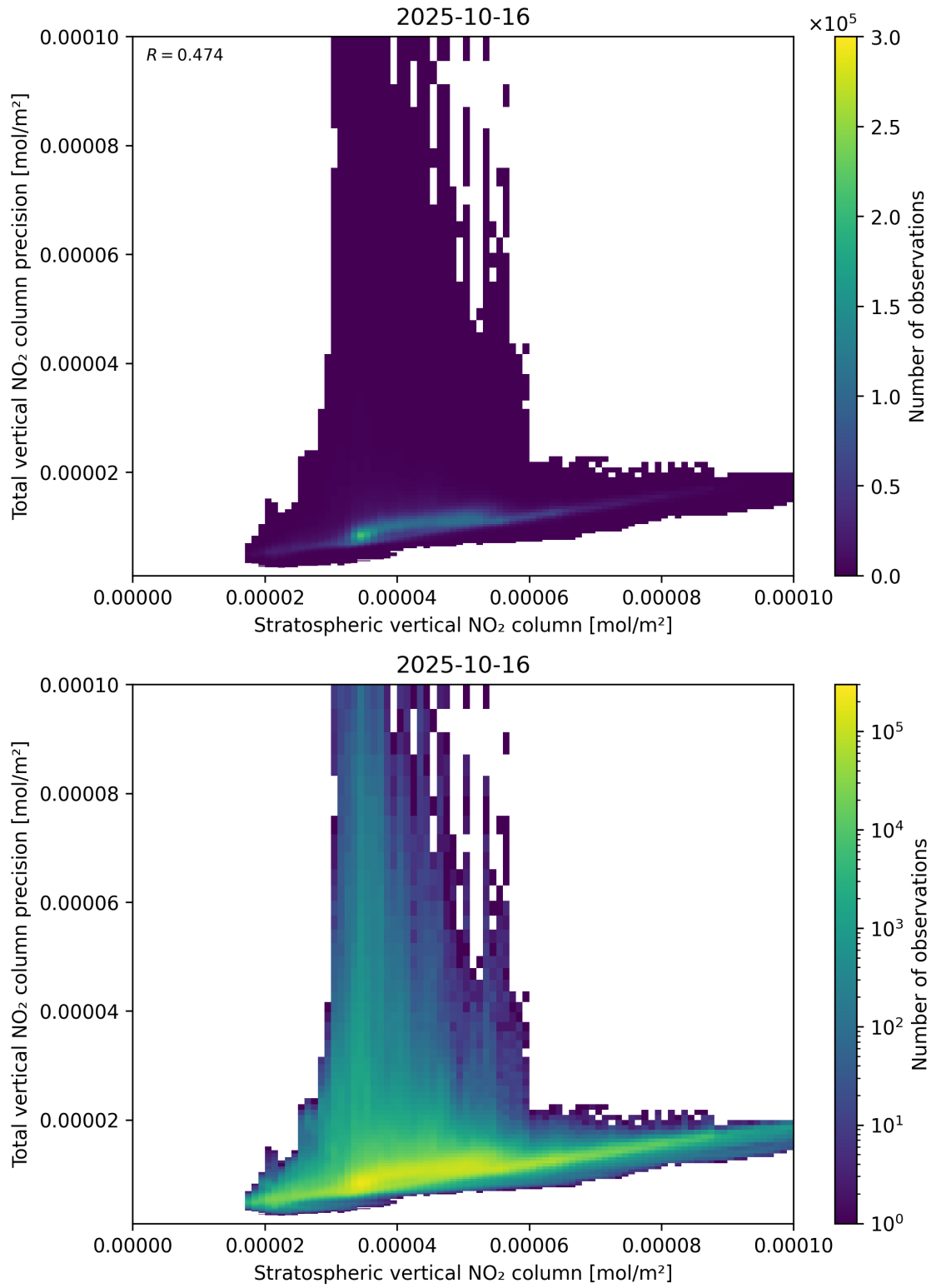
Figure 101: Scatter density plot of “Stratospheric vertical NO 2 column” against “Total vertical NO 2 column precision” for 2025-10-15 to 2025-10-17.
