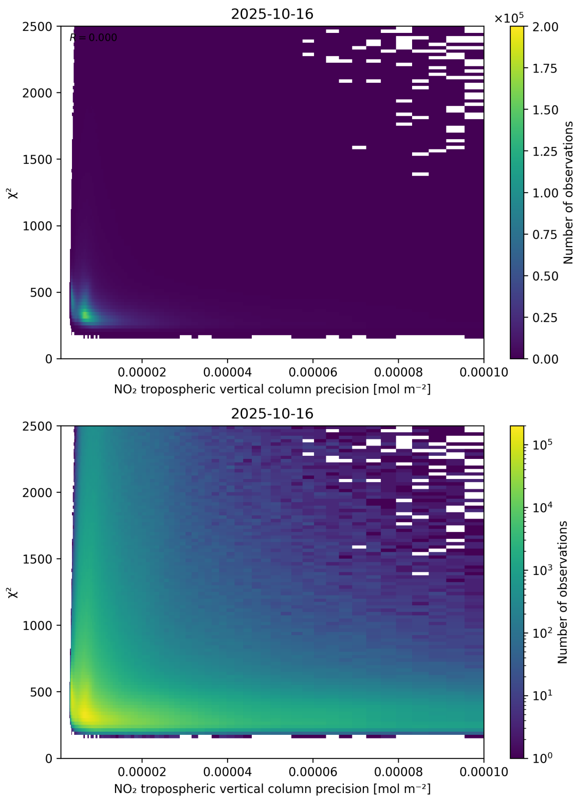
Figure 134: Scatter density plot of “NO 2 tropospheric vertical column precision” against “ \chi^2 ” for 2025-10-15 to 2025-10-17.
