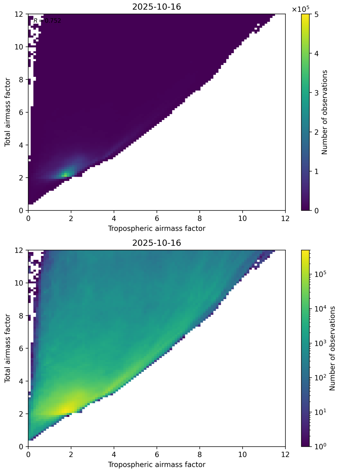
Figure 72: Scatter density plot of “Tropospheric airmass factor” against “Total airmass factor” for 2025-10-15 to 2025-10-17.
