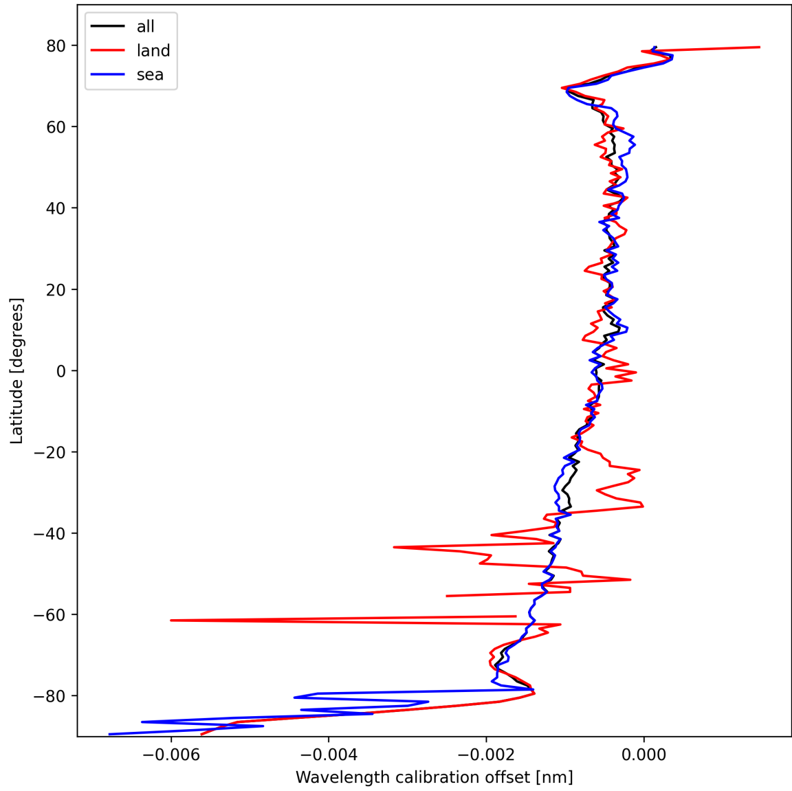
Figure 18: Zonal average of “Wavelength calibration offset” for 2025-10-15 to 2025-10-17.
