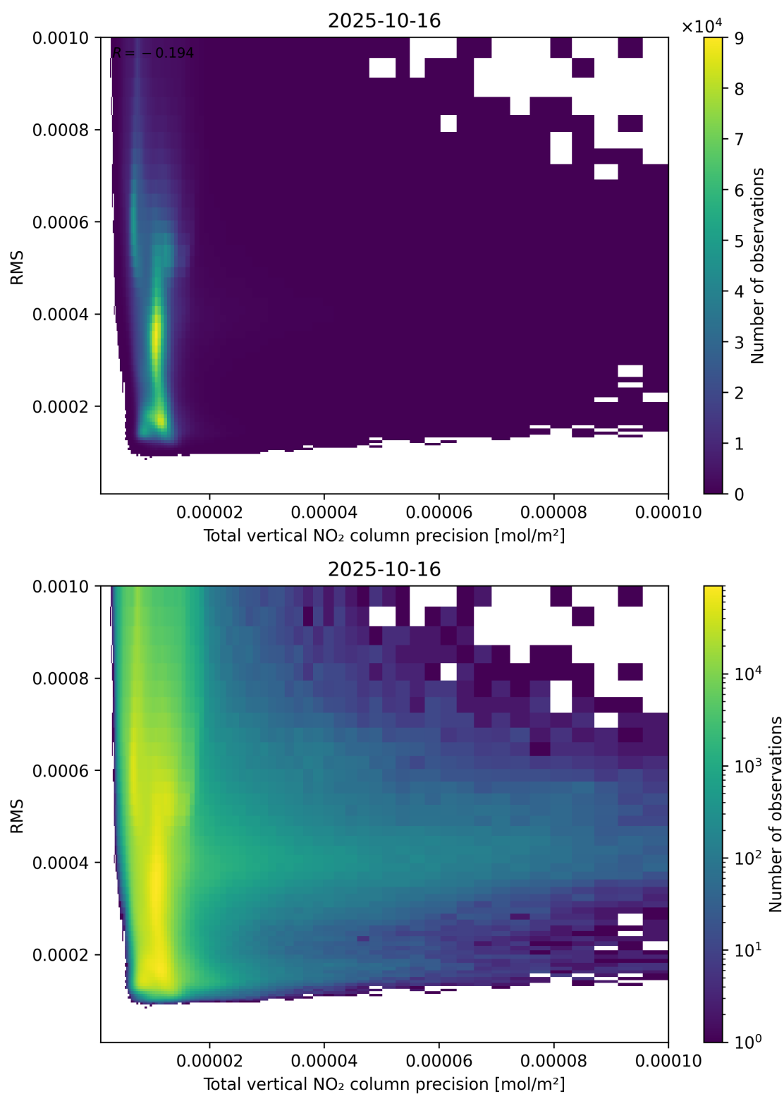
Figure 119: Scatter density plot of “Total vertical NO 2 column precision” against “RMS” for 2025-10-15 to 2025-10-17.
