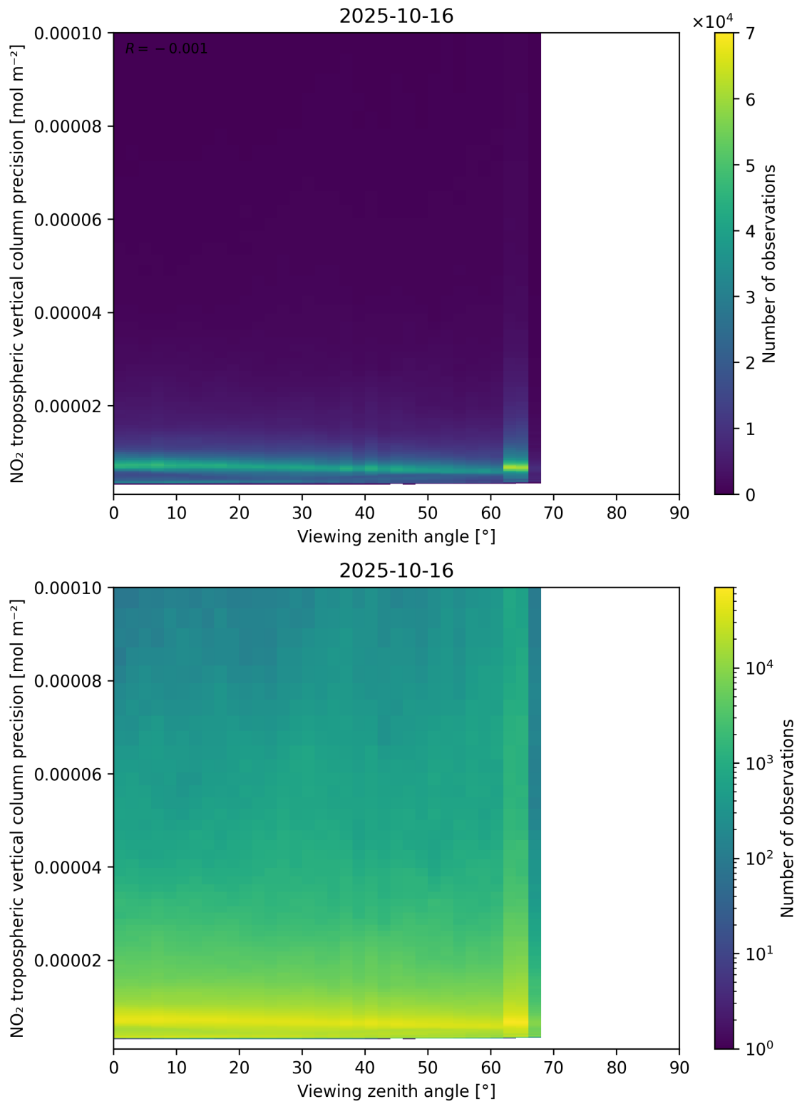
Figure 170: Scatter density plot of “Viewing zenith angle” against “NO 2 tropospheric vertical column precision” for 2025-10-15 to 2025-10-17.
