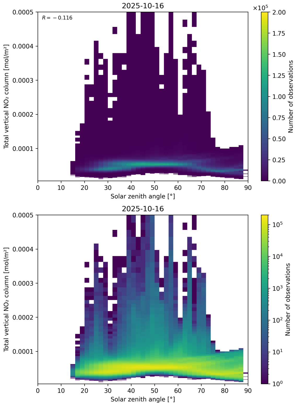
Figure 153: Scatter density plot of “Solar zenith angle” against “Total vertical NO 2 column” for 2025-10-15 to 2025-10-17.
