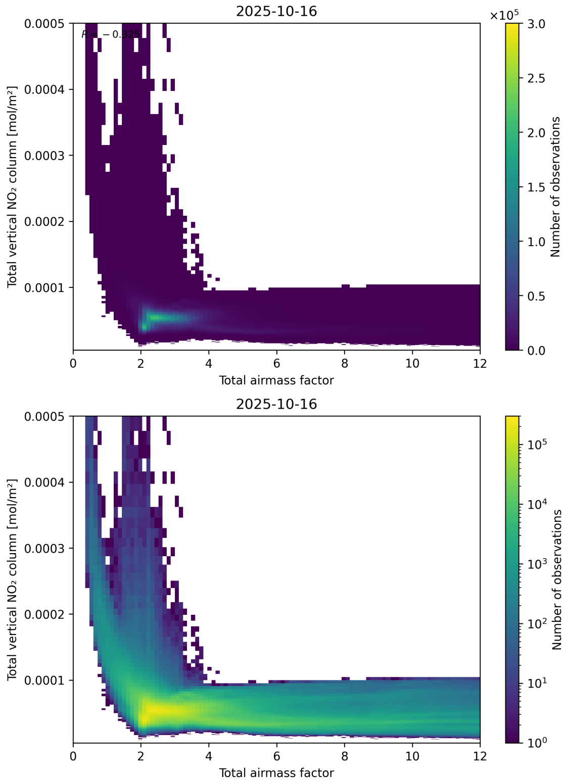
Figure 67: Scatter density plot of “Total airmass factor” against “Total vertical NO 2 column” for 2025-10-15 to 2025-10-17.
