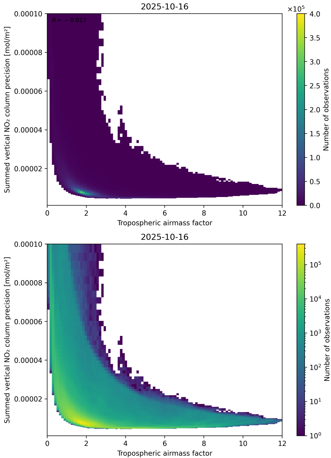
Figure 76: Scatter density plot of “Tropospheric airmass factor” against “Summed vertical NO 2 column precision” for 2025-10-15 to 2025-10-17.
