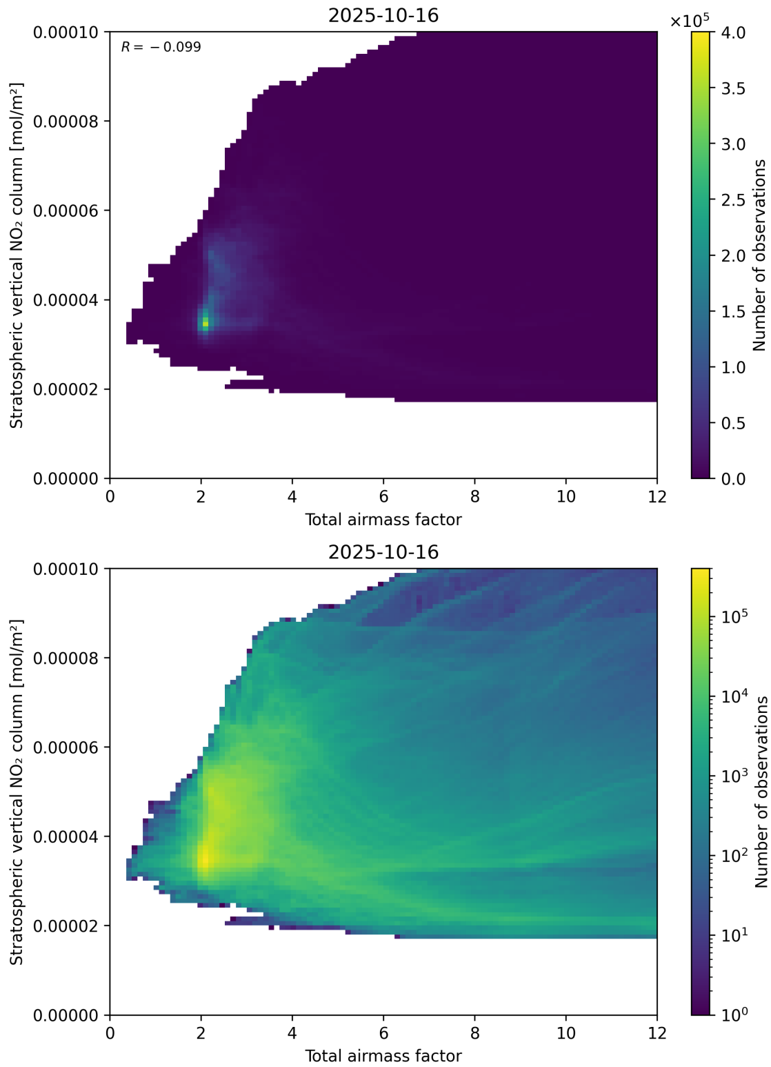
Figure 64: Scatter density plot of “Total airmass factor” against “Stratospheric vertical \text{NO}_2 column” for 2025-10-15 to 2025-10-17.
