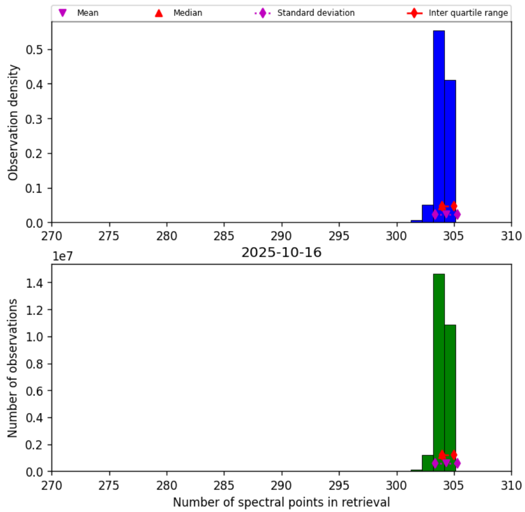
Figure 33: Histogram of “Number of spectral points in retrieval” for 2025-10-15 to 2025-10-17
