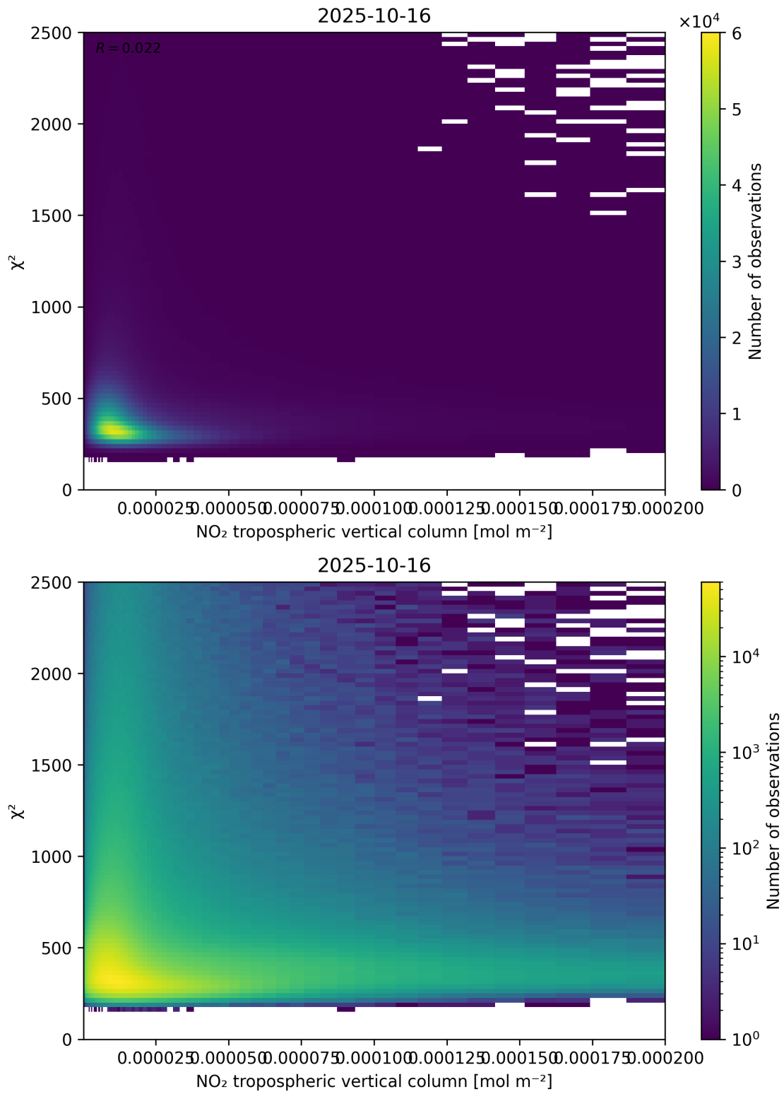
Figure 124: Scatter density plot of “NO 2 tropospheric vertical column” against “ \chi^2 ” for 2025-10-15 to 2025-10-17.
