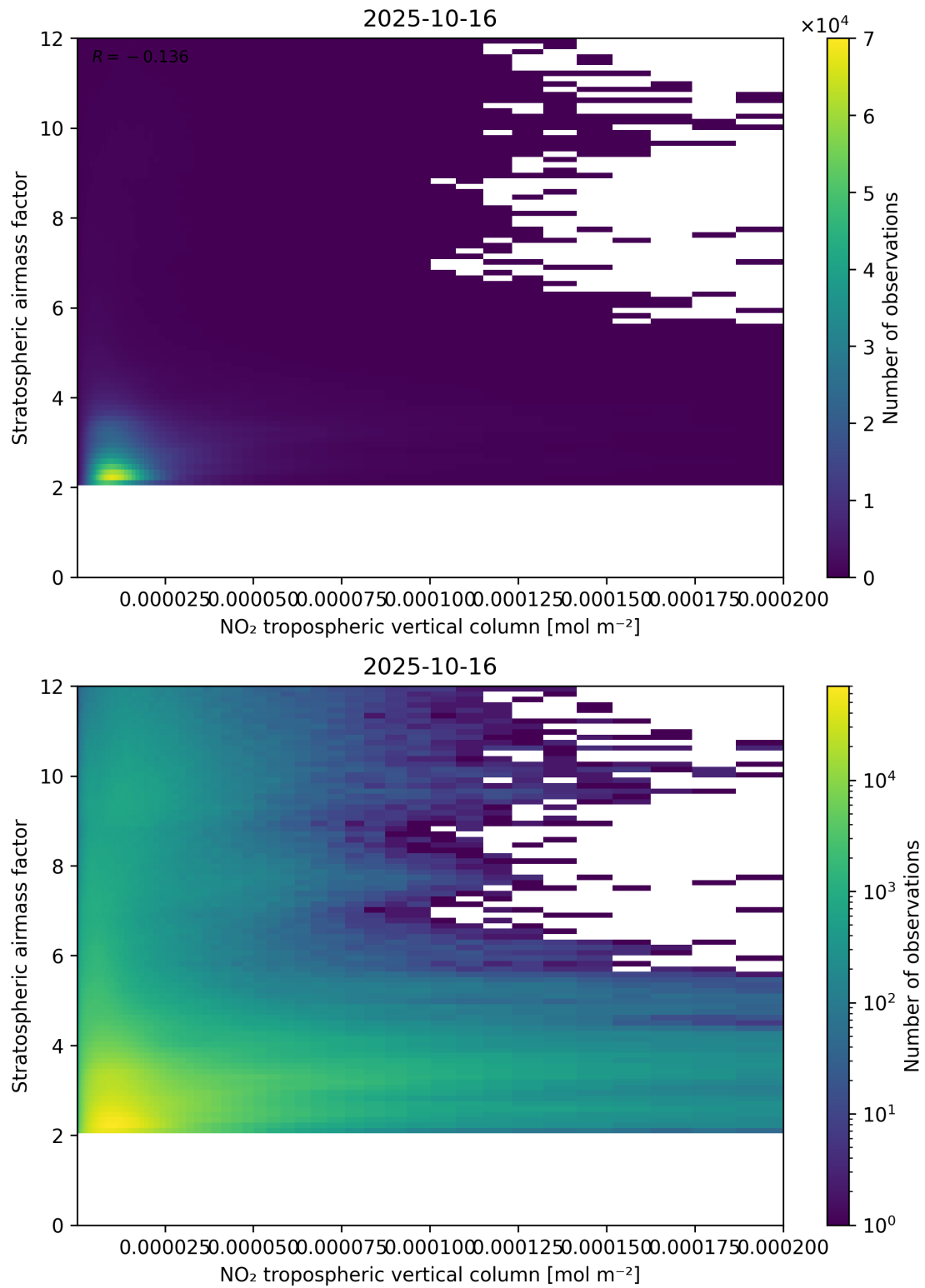
Figure 121: Scatter density plot of “NO 2 tropospheric vertical column” against “Stratospheric airmass factor” for 2025-10-15 to 2025-10-17.
