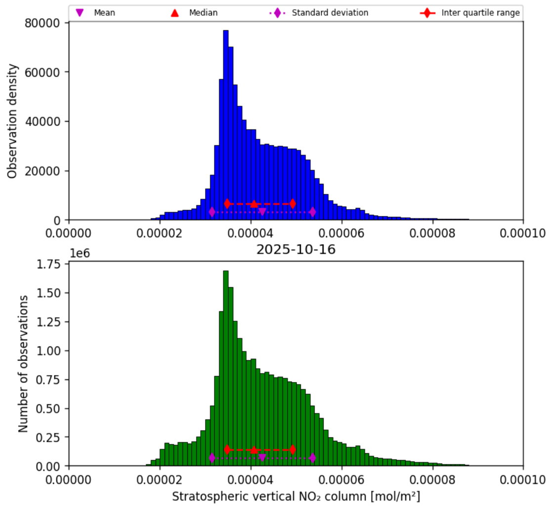
Figure 36: Histogram of “Stratospheric vertical NO 2 column” for 2025-10-15 to 2025-10-17
