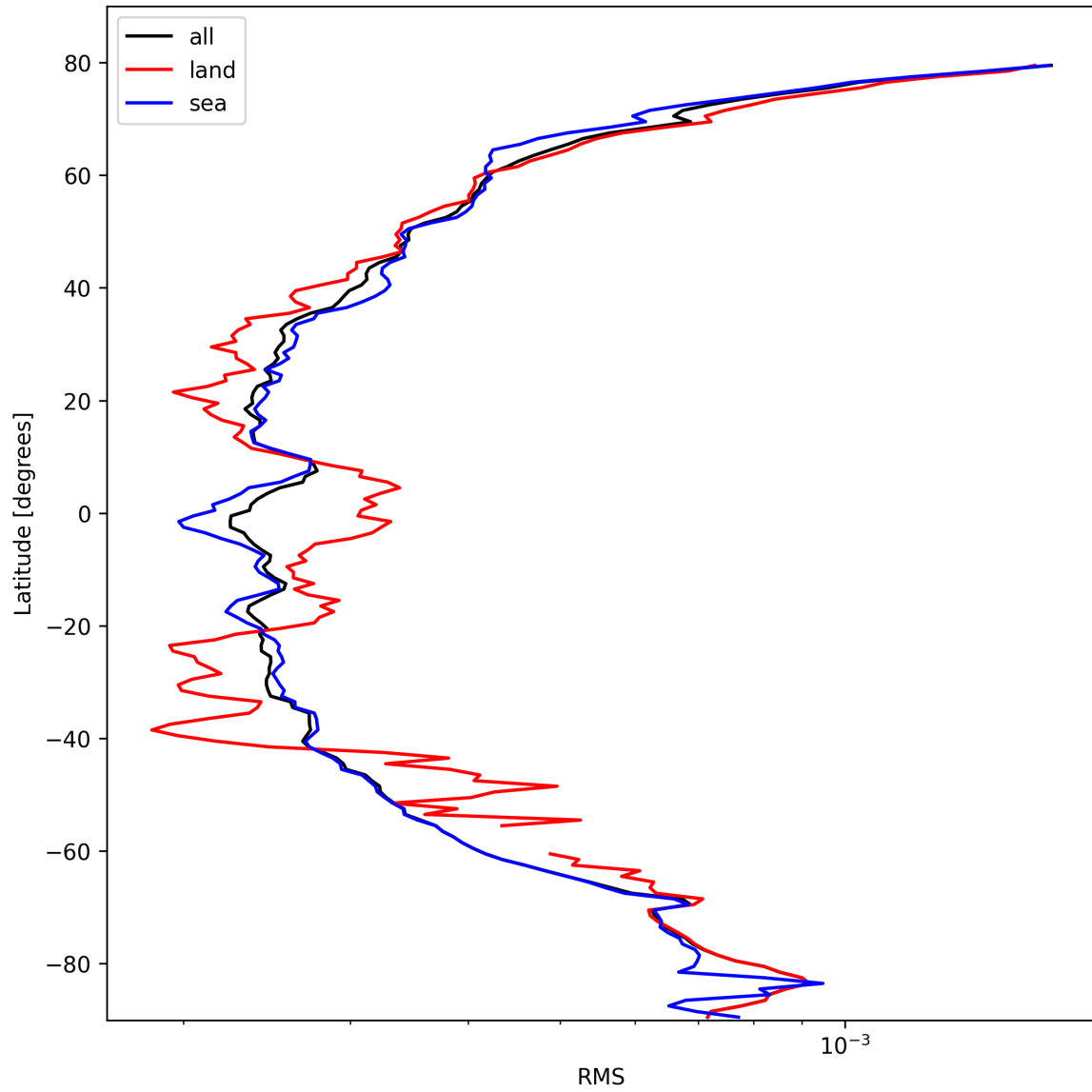
Figure 26: Zonal average of “RMS” for 2025-10-15 to 2025-10-17.
