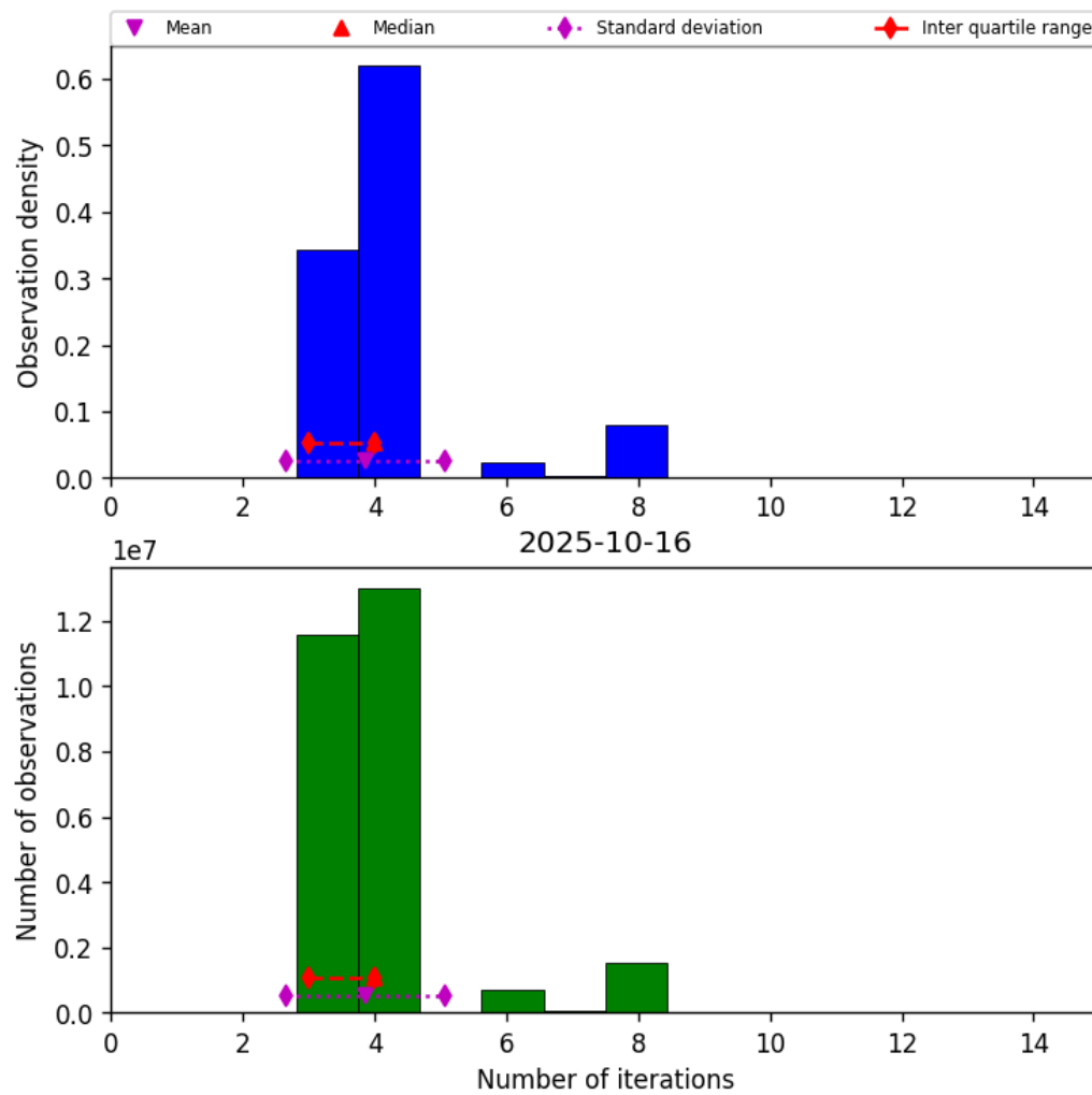
Figure 34: Histogram of “Number of iterations” for 2025-10-15 to 2025-10-17
