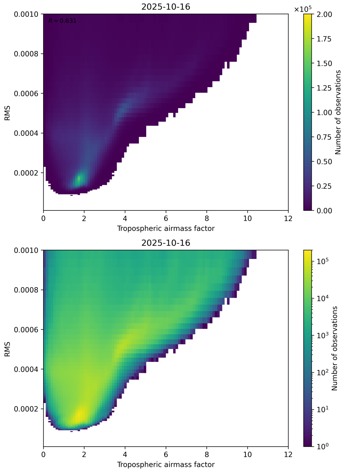
Figure 79: Scatter density plot of “Tropospheric airmass factor” against “RMS” for 2025-10-15 to 2025-10-17.
