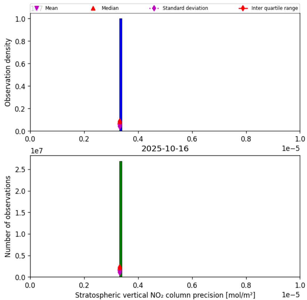
Figure 37: Histogram of “Stratospheric vertical NO 2 column precision” for 2025-10-15 to 2025-10-17
