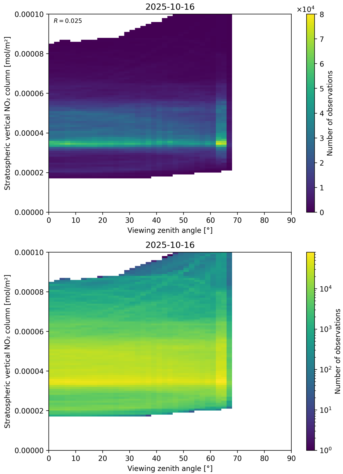
Figure 164: Scatter density plot of “Viewing zenith angle” against “Stratospheric vertical NO 2 column” for 2025-10-15 to 2025-10-17.
