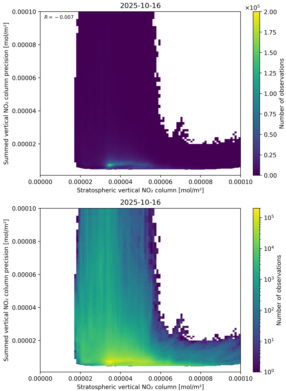
Figure 99: Scatter density plot of “Stratospheric vertical NO 2 column” against “Summed vertical NO 2 column precision” for 2025-10-15 to 2025-10-17.
