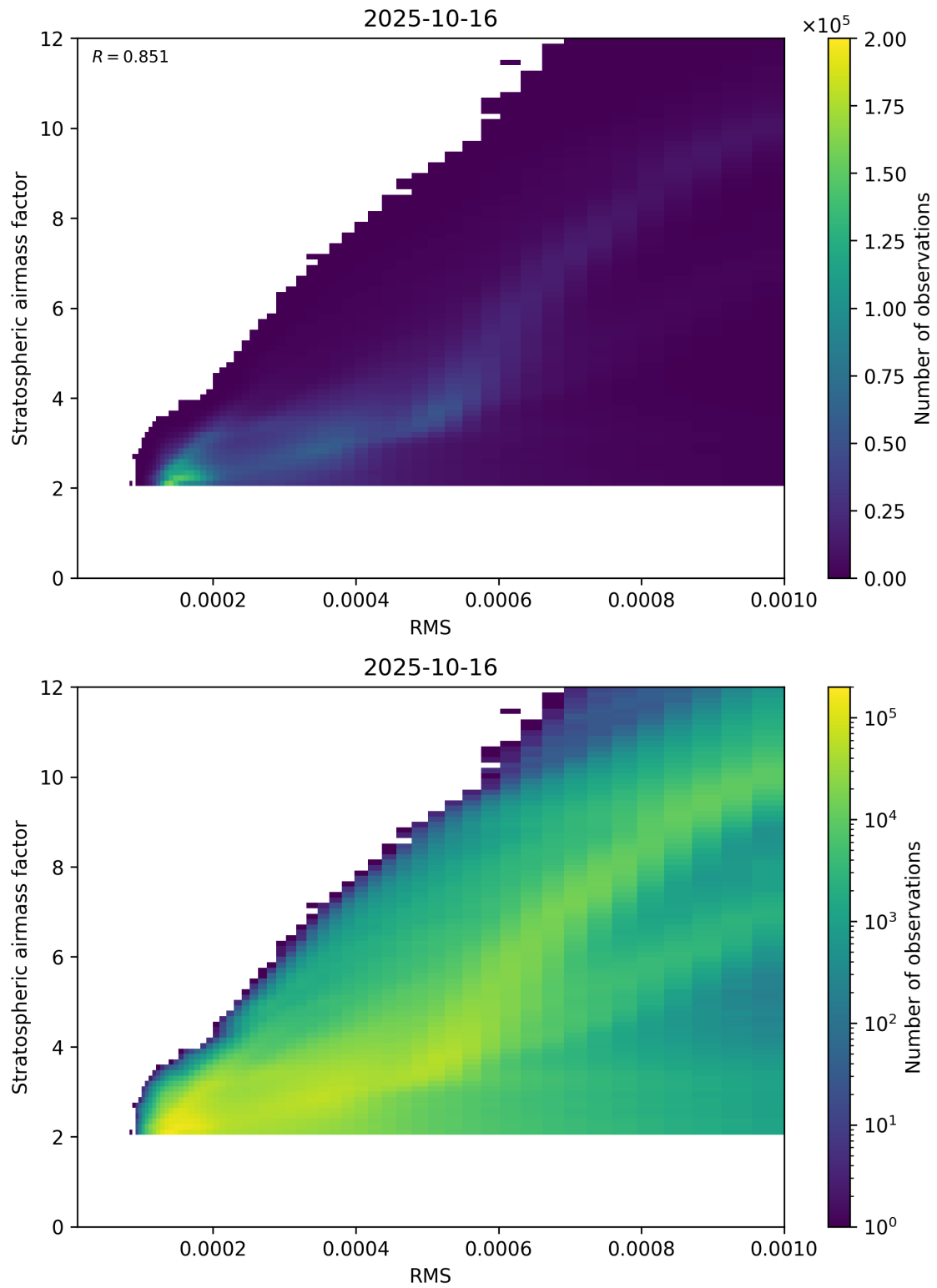
Figure 144: Scatter density plot of “RMS” against “Stratospheric airmass factor” for 2025-10-15 to 2025-10-17.
