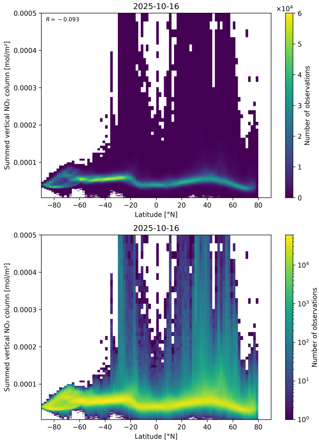
Figure 88: Scatter density plot of “Latitude” against “Summed vertical NO 2 column” for 2025-10-15 to 2025-10-17.
