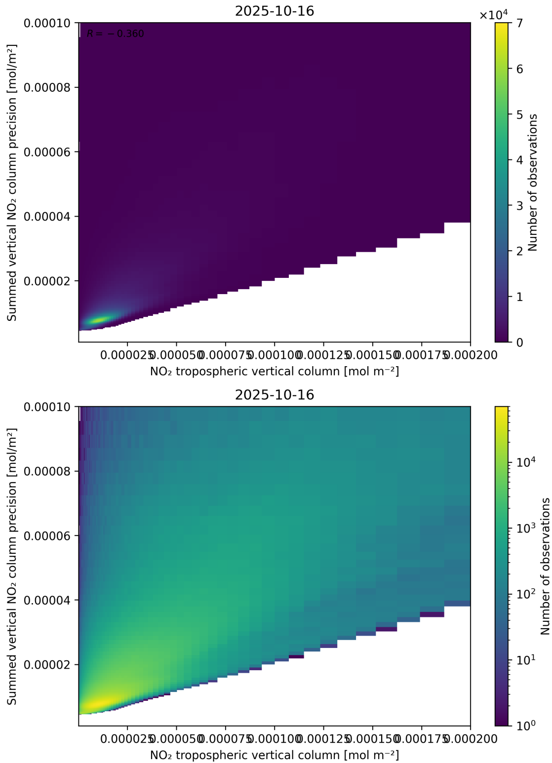
Figure 127: Scatter density plot of “NO 2 tropospheric vertical column” against “Summed vertical NO 2 column precision” for 2025-10-15 to 2025-10-17.
