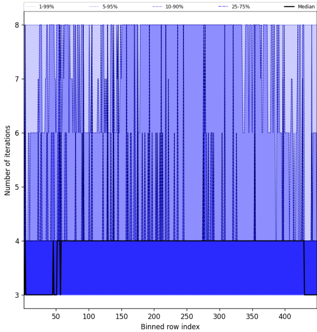
Figure 51: Along track statistics of “Number of iterations” for 2025-10-15 to 2025-10-17
