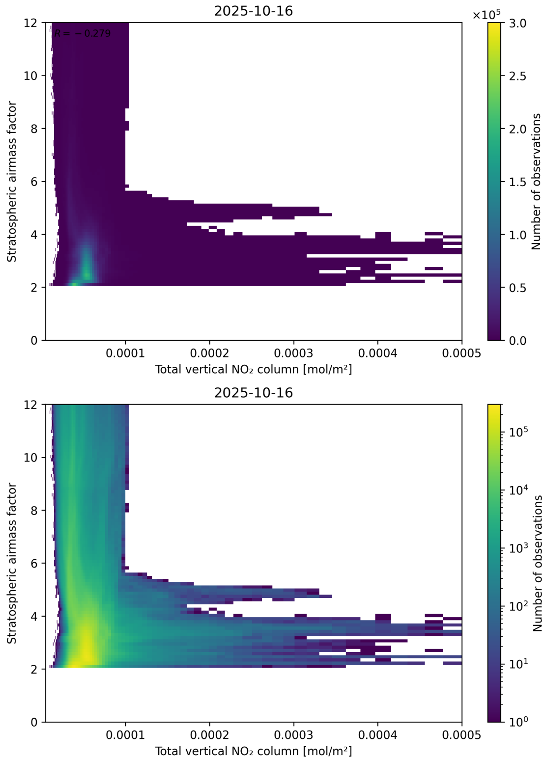
Figure 110: Scatter density plot of “Total vertical NO 2 column” against “Stratospheric airmass factor” for 2025-10-15 to 2025-10-17.
