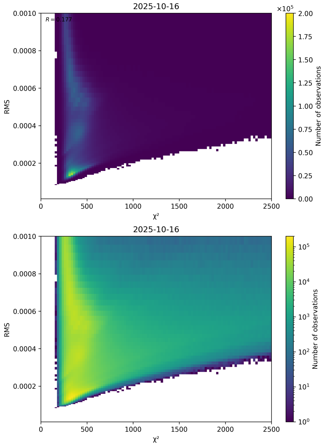
Figure 82: Scatter density plot of “ \chi^2 ” against “RMS” for 2025-10-15 to 2025-10-17.
