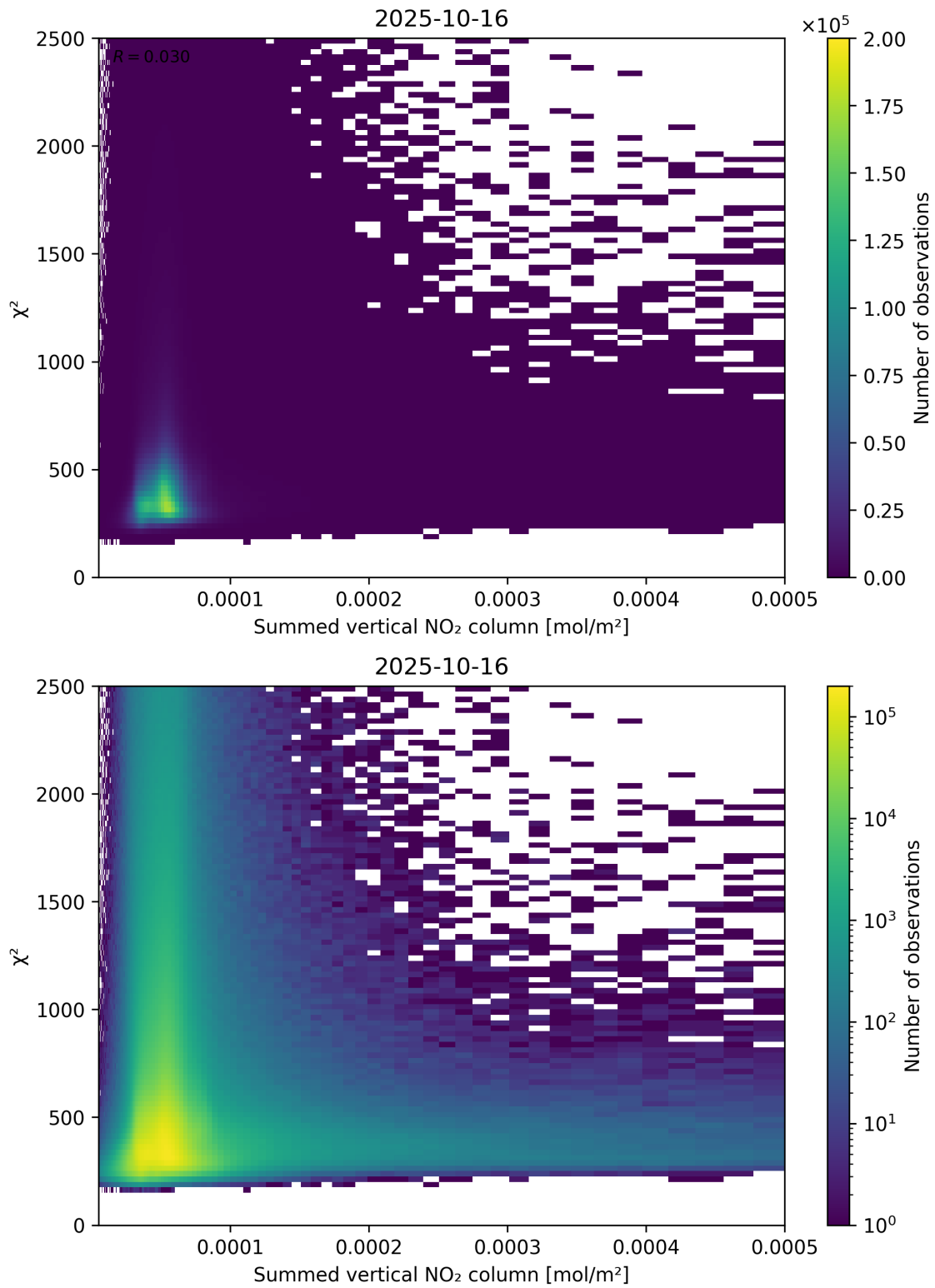
Figure 104: Scatter density plot of “Summed vertical NO 2 column” against “ \chi^2 ” for 2025-10-15 to 2025-10-17.
