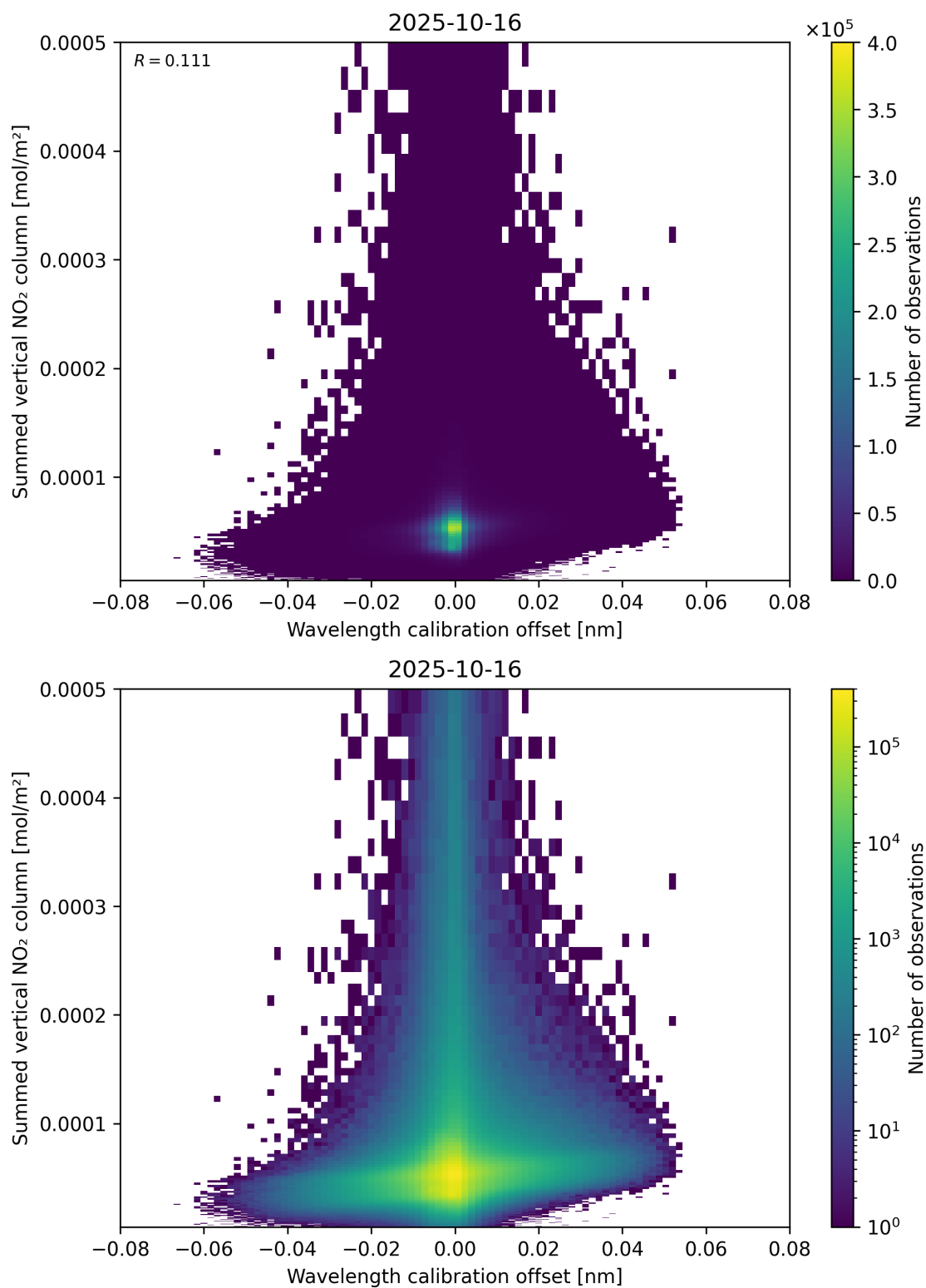
Figure 177: Scatter density plot of “Wavelength calibration offset” against “Summed vertical NO 2 column” for 2025-10-15 to 2025-10-17.
