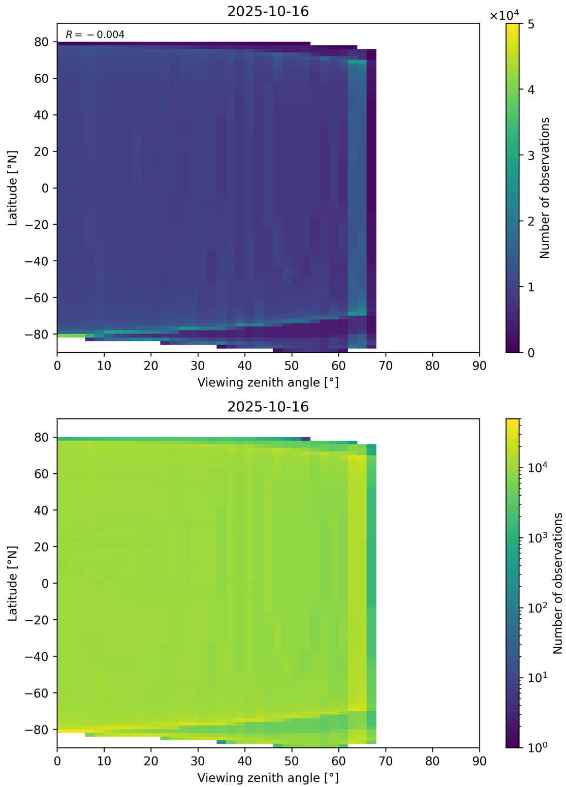
Figure 163: Scatter density plot of “Viewing zenith angle” against “Latitude” for 2025-10-15 to 2025-10-17.
