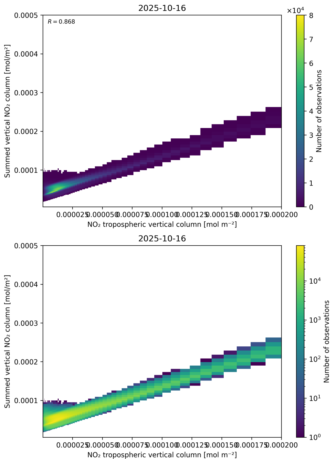
Figure 126: Scatter density plot of “NO 2 tropospheric vertical column” against “Summed vertical NO 2 column” for 2025-10-15 to 2025-10-17.
