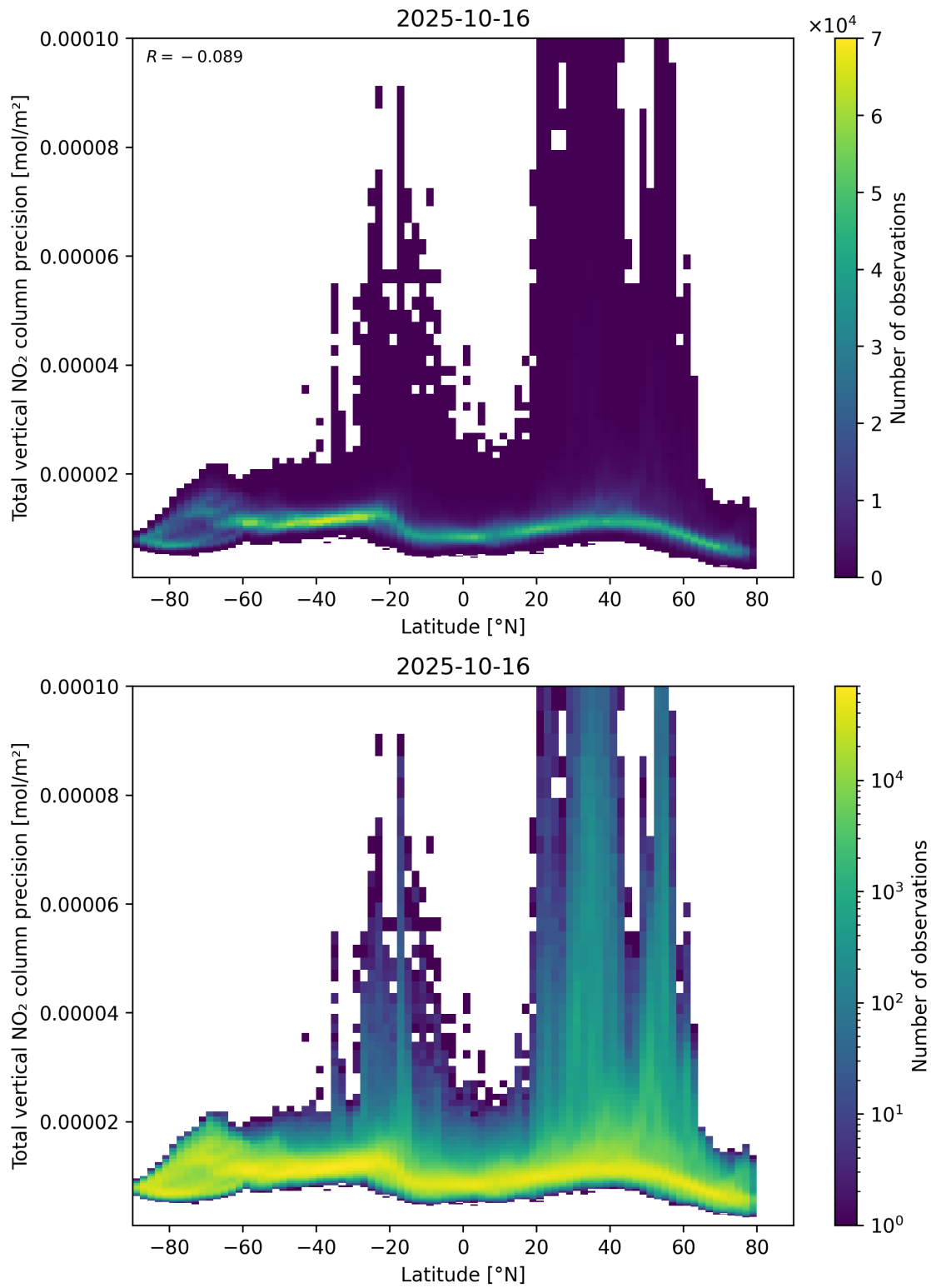
Figure 91: Scatter density plot of “Latitude” against “Total vertical NO 2 column precision” for 2025-10-15 to 2025-10-17.
