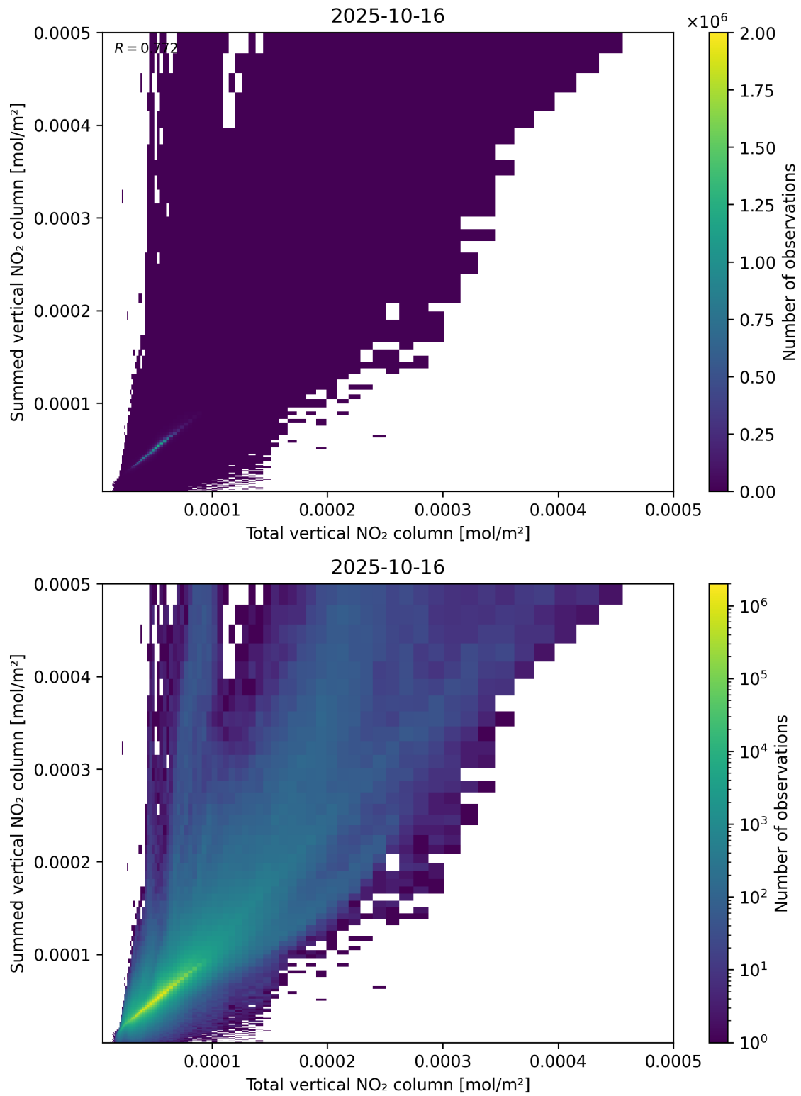
Figure 112: Scatter density plot of “Total vertical NO 2 column” against “Summed vertical NO 2 column” for 2025-10-15 to 2025-10-17.
