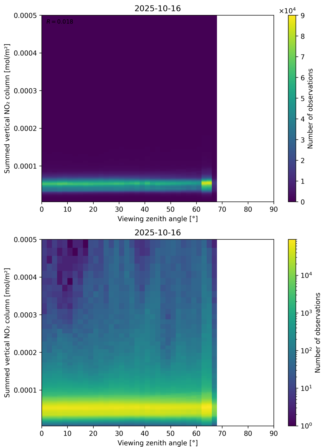
Figure 165: Scatter density plot of “Viewing zenith angle” against “Summed vertical NO 2 column” for 2025-10-15 to 2025-10-17.
