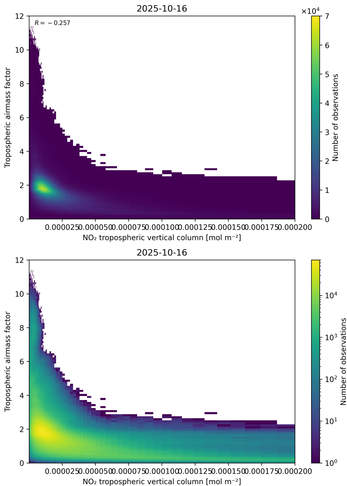
Figure 123: Scatter density plot of “NO 2 tropospheric vertical column” against “Tropospheric air mass factor” for 2025-10-15 to 2025-10-17.
