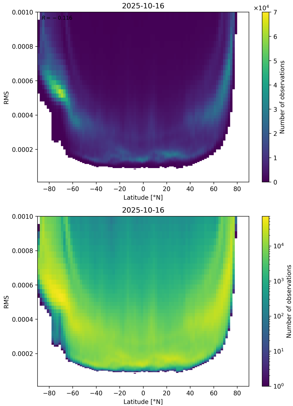
Figure 94: Scatter density plot of “Latitude” against “RMS” for 2025-10-15 to 2025-10-17.
