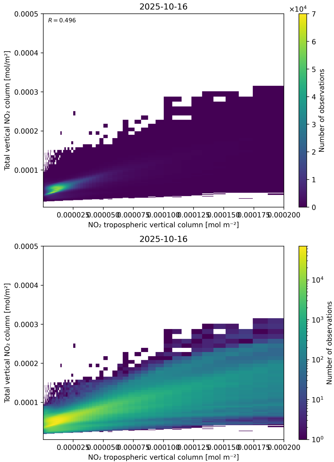
Figure 128: Scatter density plot of “NO 2 tropospheric vertical column” against “Total vertical NO 2 column” for 2025-10-15 to 2025-10-17.
