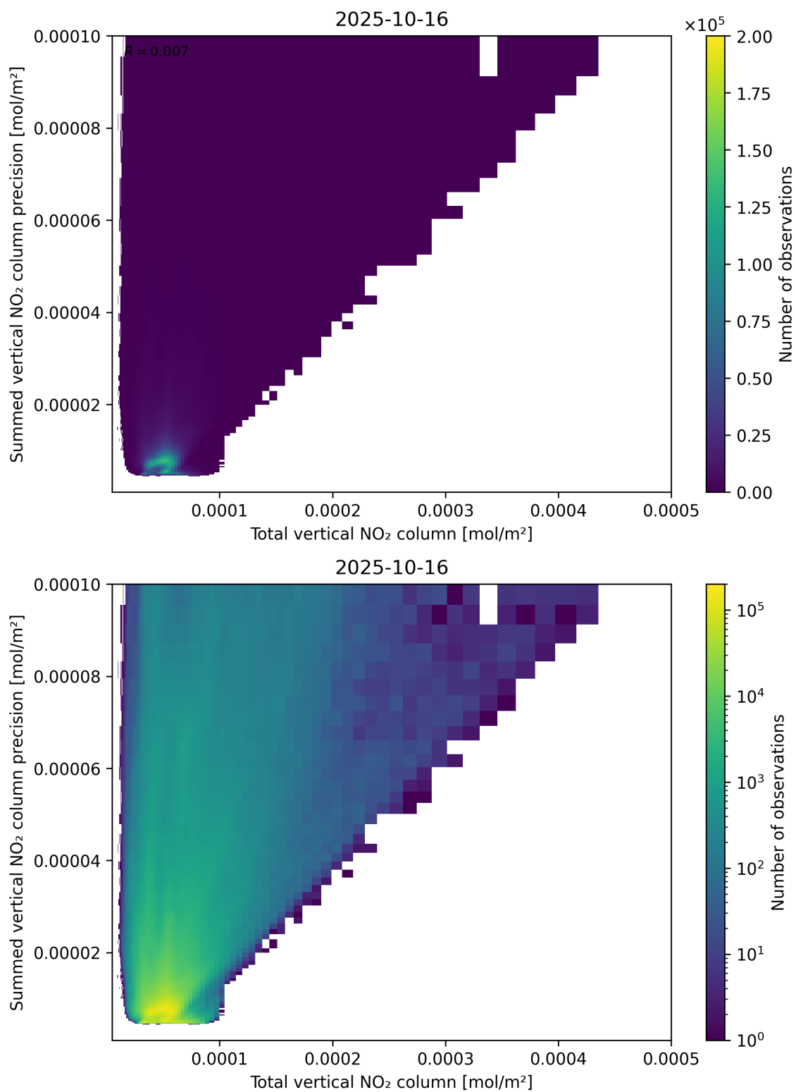
Figure 113: Scatter density plot of “Total vertical NO 2 column” against “Summed vertical NO 2 column precision” for 2025-10-15 to 2025-10-17.
