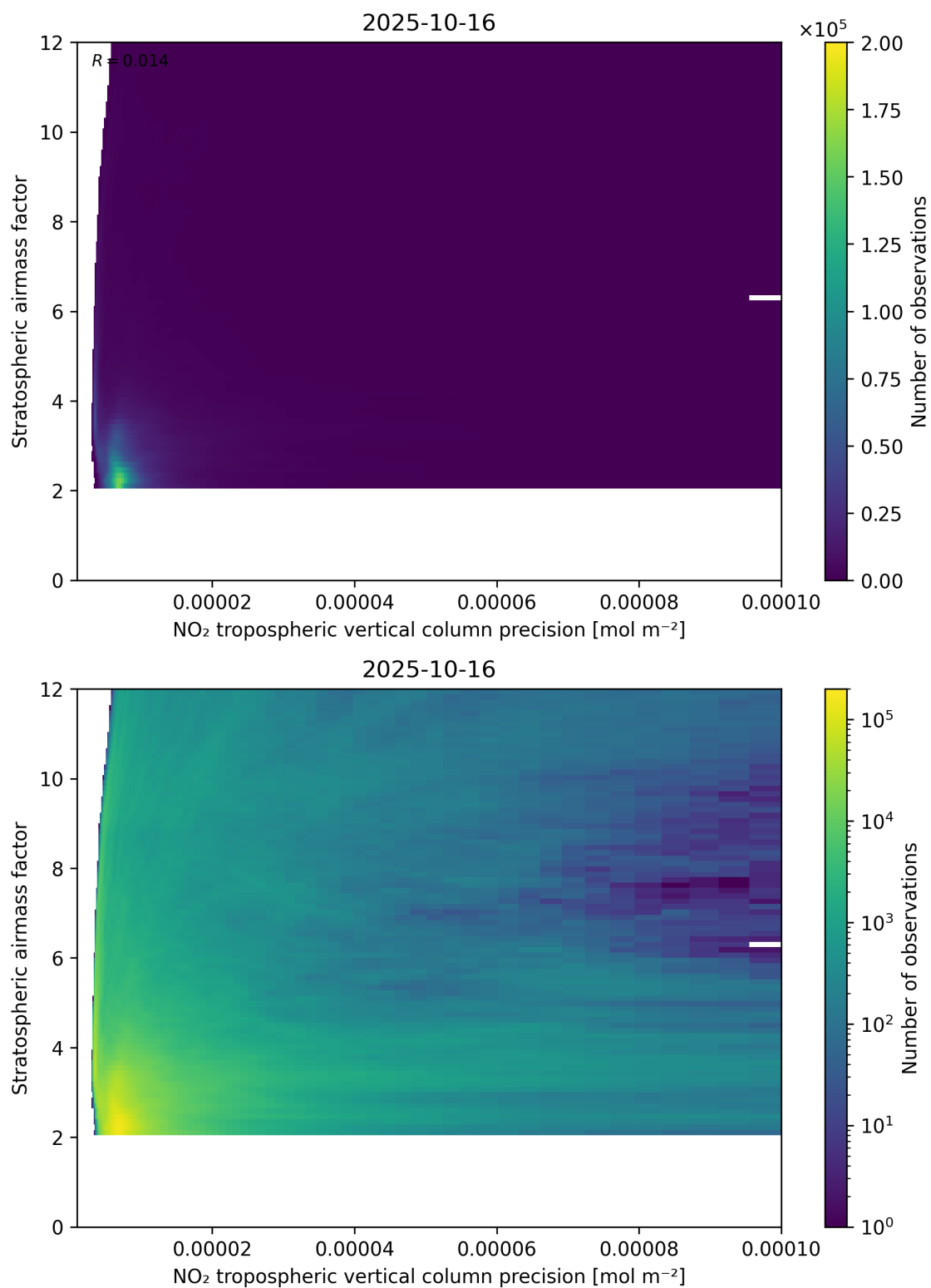
Figure 131: Scatter density plot of “NO 2 tropospheric vertical column precision” against “Stratospheric airmass factor” for 2025-10-15 to 2025-10-17.
