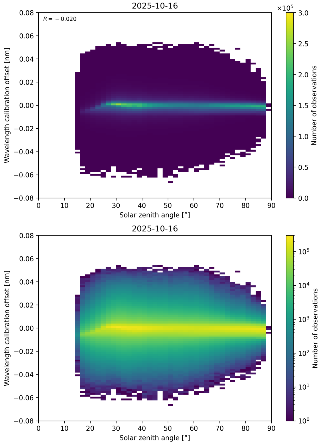
Figure 158: Scatter density plot of “Solar zenith angle” against “Wavelength calibration offset” for 2025-10-15 to 2025-10-17.
