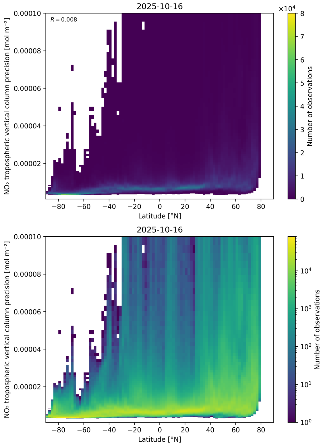
Figure 93: Scatter density plot of “Latitude” against “NO 2 tropospheric vertical column precision” for 2025-10-15 to 2025-10-17.
