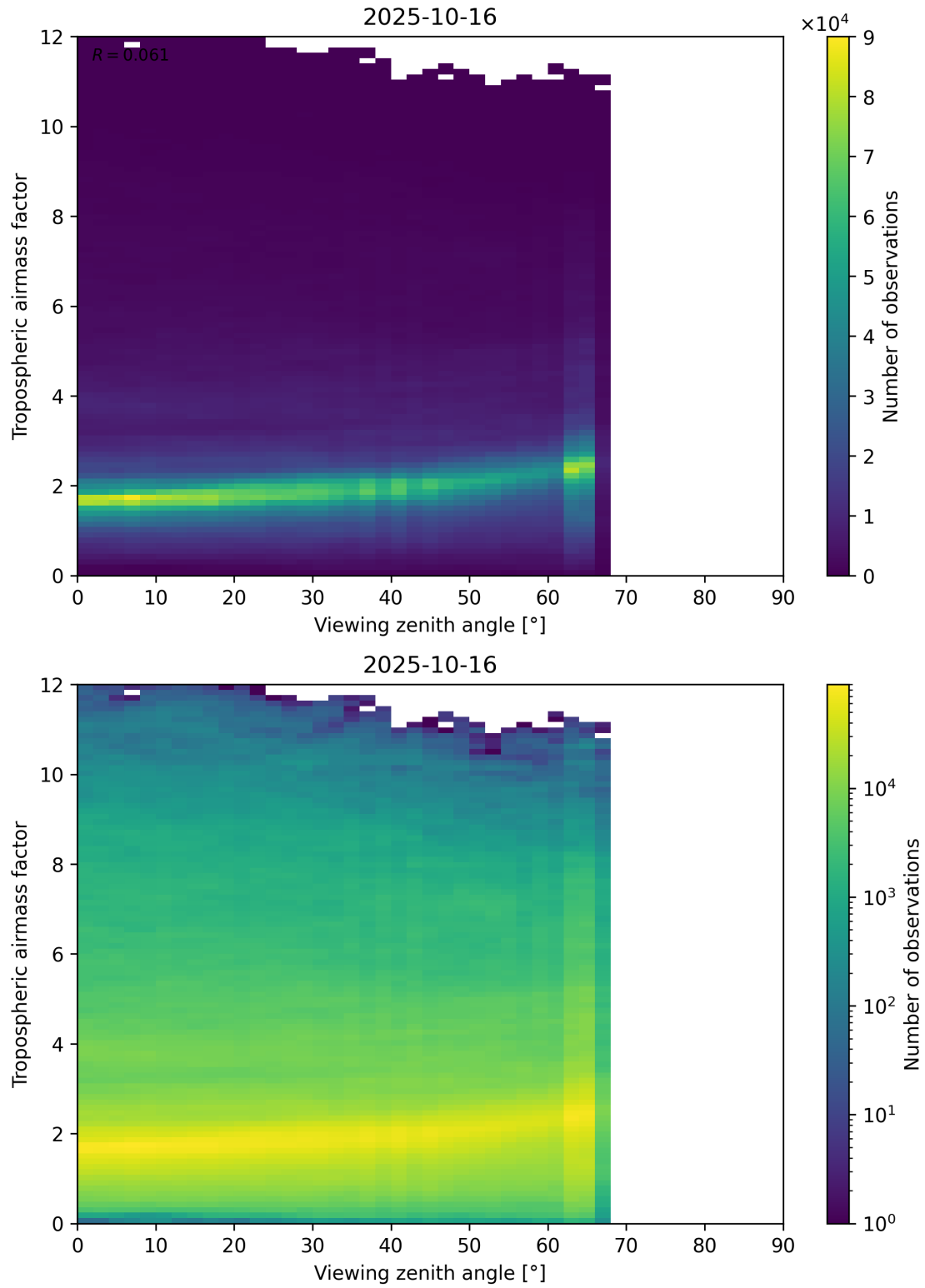
Figure 161: Scatter density plot of “Viewing zenith angle” against “Tropospheric airmass factor” for 2025-10-15 to 2025-10-17.
