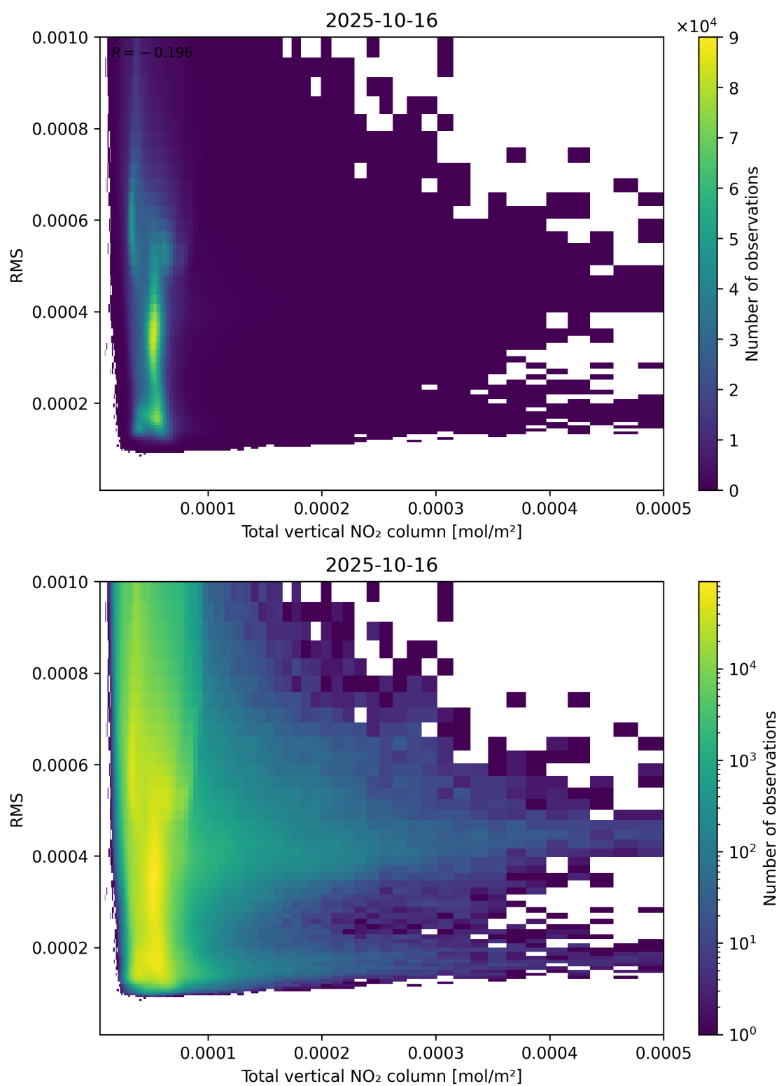
Figure 120: Scatter density plot of “Total vertical NO 2 column” against “RMS” for 2025-10-15 to 2025-10-17.
