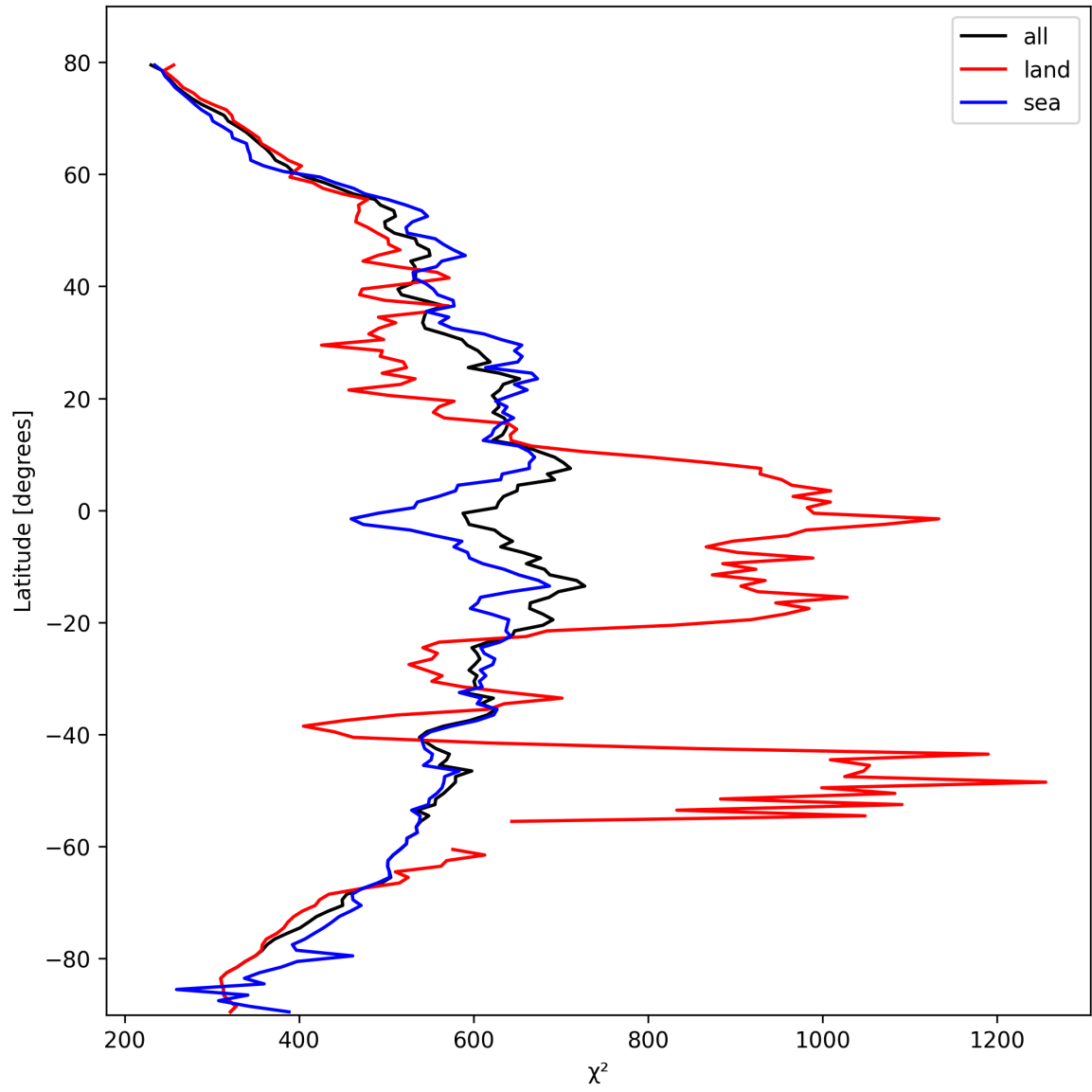
Figure 25: Zonal average of “ \chi^2 ” for 2025-10-15 to 2025-10-17.
