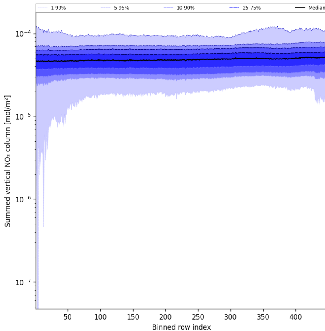
Figure 57: Along track statistics of “Summed vertical NO 2 column” for 2025-10-15 to 2025-10-17
