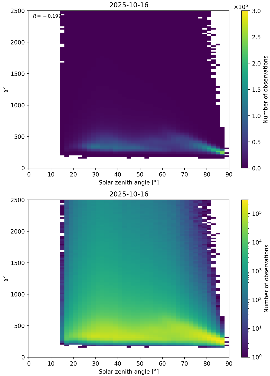
Figure 148: Scatter density plot of “Solar zenith angle” against “ \chi^2 ” for 2025-10-15 to 2025-10-17.
