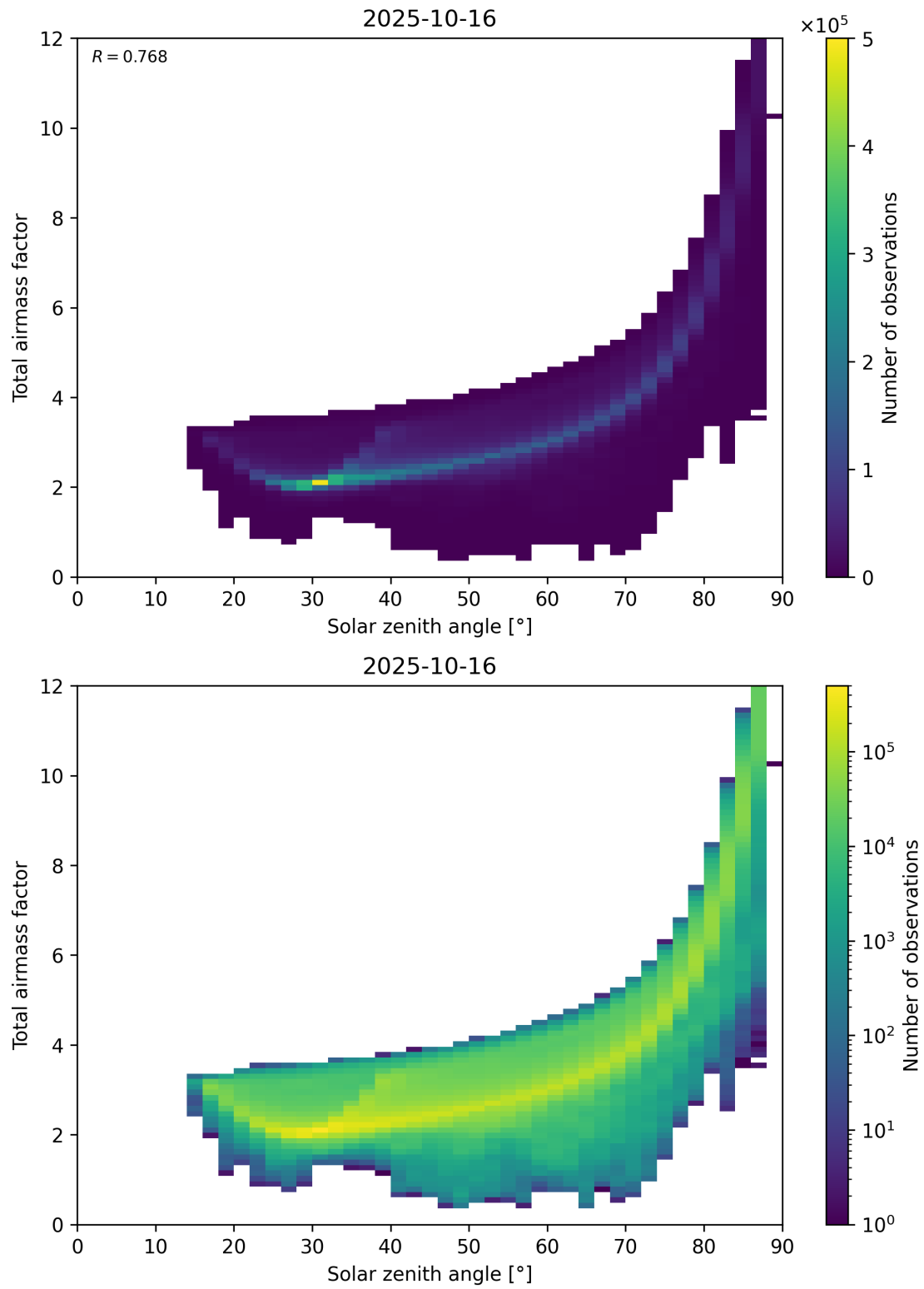
Figure 146: Scatter density plot of “Solar zenith angle” against “Total airmass factor” for 2025-10-15 to 2025-10-17.
