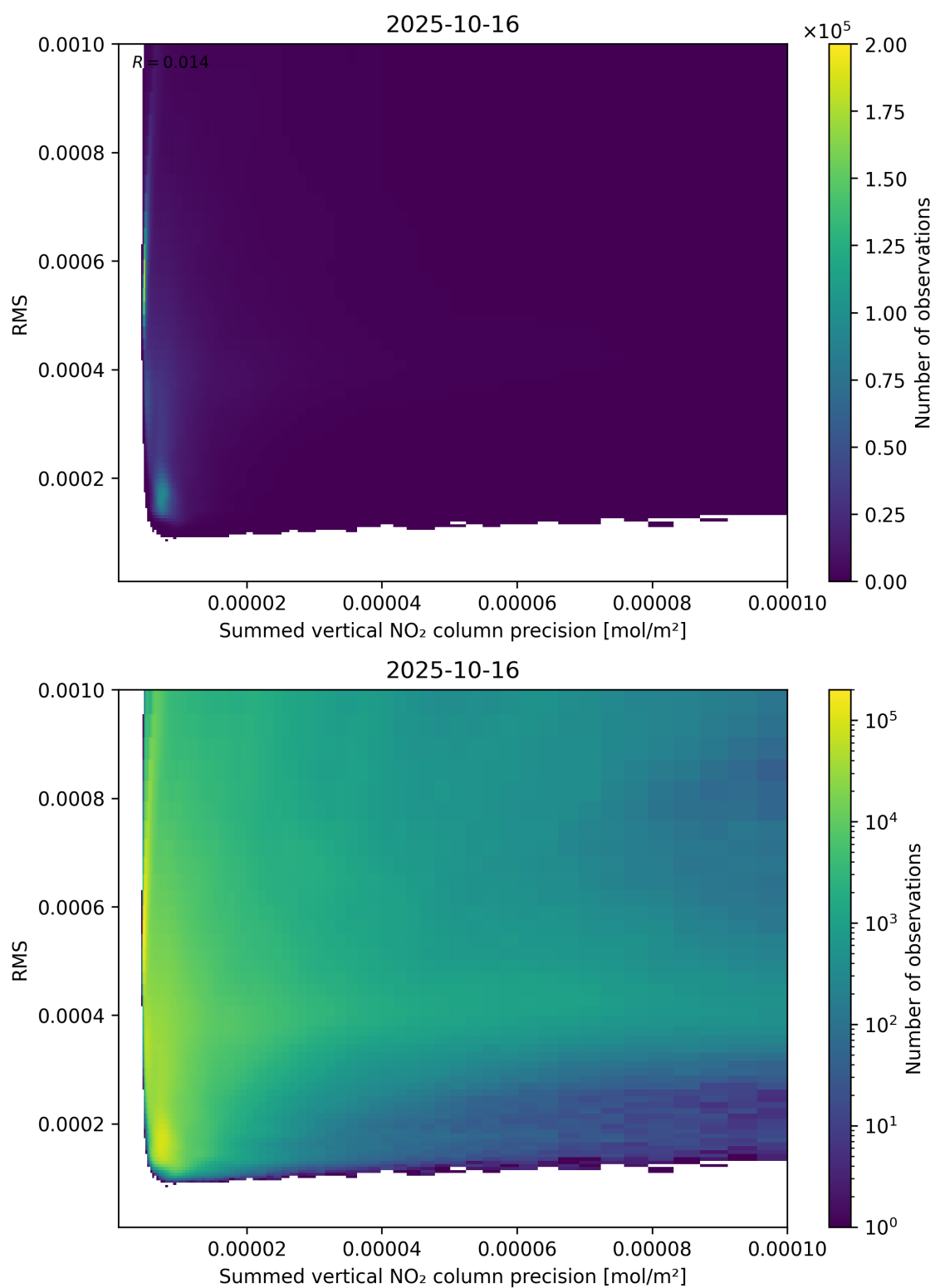
Figure 108: Scatter density plot of “Summed vertical NO 2 column precision” against “RMS” for 2025-10-15 to 2025-10-17.
