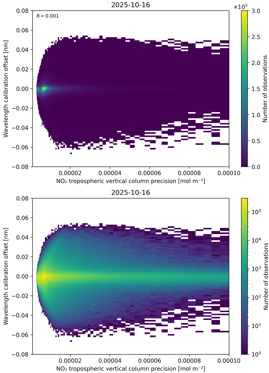
Figure 141: Scatter density plot of “NO 2 tropospheric vertical column precision” against “Wavelength calibration offset” for 2025-10-15 to 2025-10-17.
