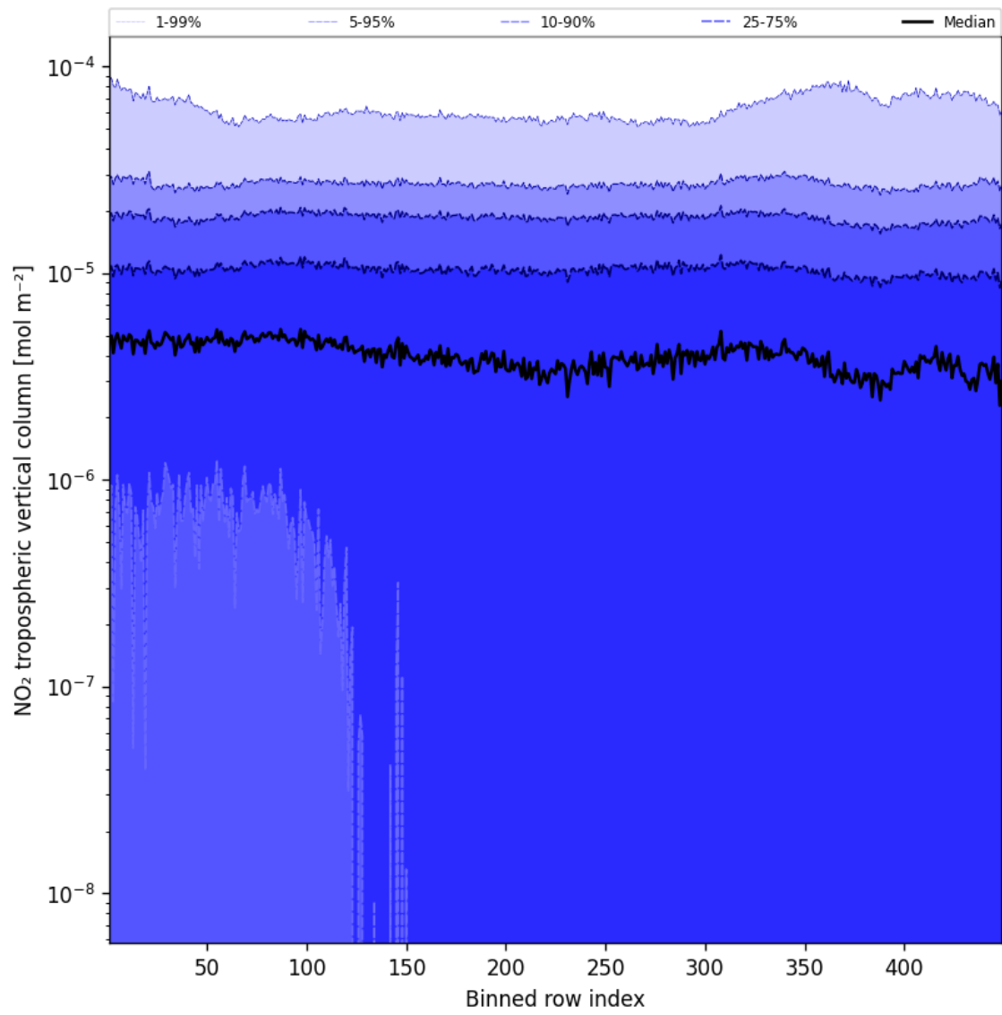
Figure 46: Along track statistics of “NO 2 tropospheric vertical column” for 2025-10-15 to 2025-10-17
