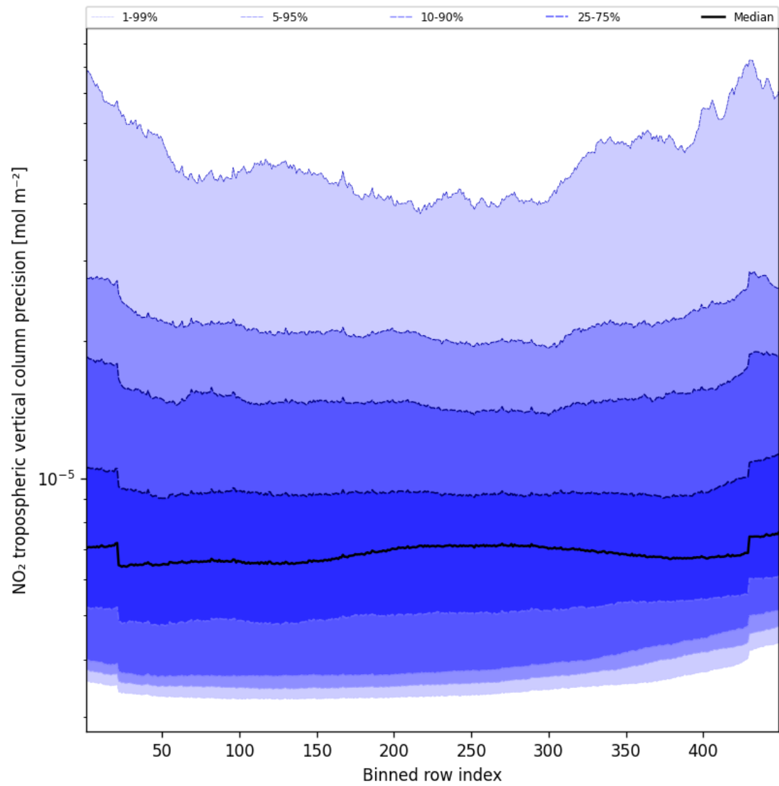
Figure 47: Along track statistics of “NO 2 tropospheric vertical column precision” for 2025-10-15 to 2025-10-17
