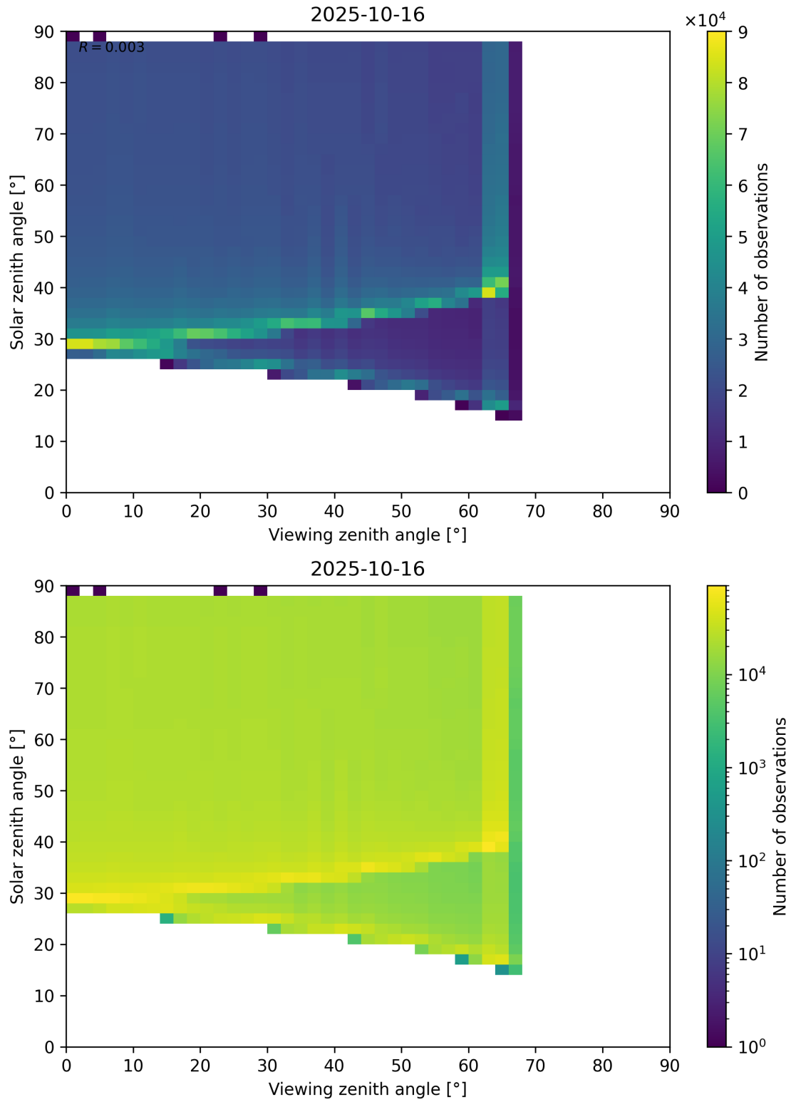
Figure 172: Scatter density plot of “Viewing zenith angle” against “Solar zenith angle” for 2025-10-15 to 2025-10-17.
