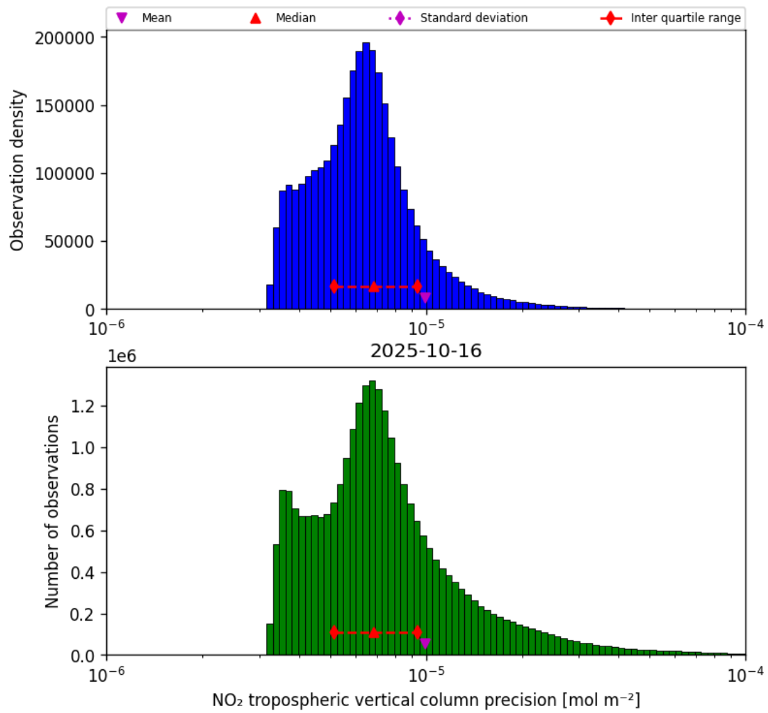
Figure 30: Histogram of “NO 2 tropospheric vertical column precision” for 2025-10-15 to 2025-10-17
