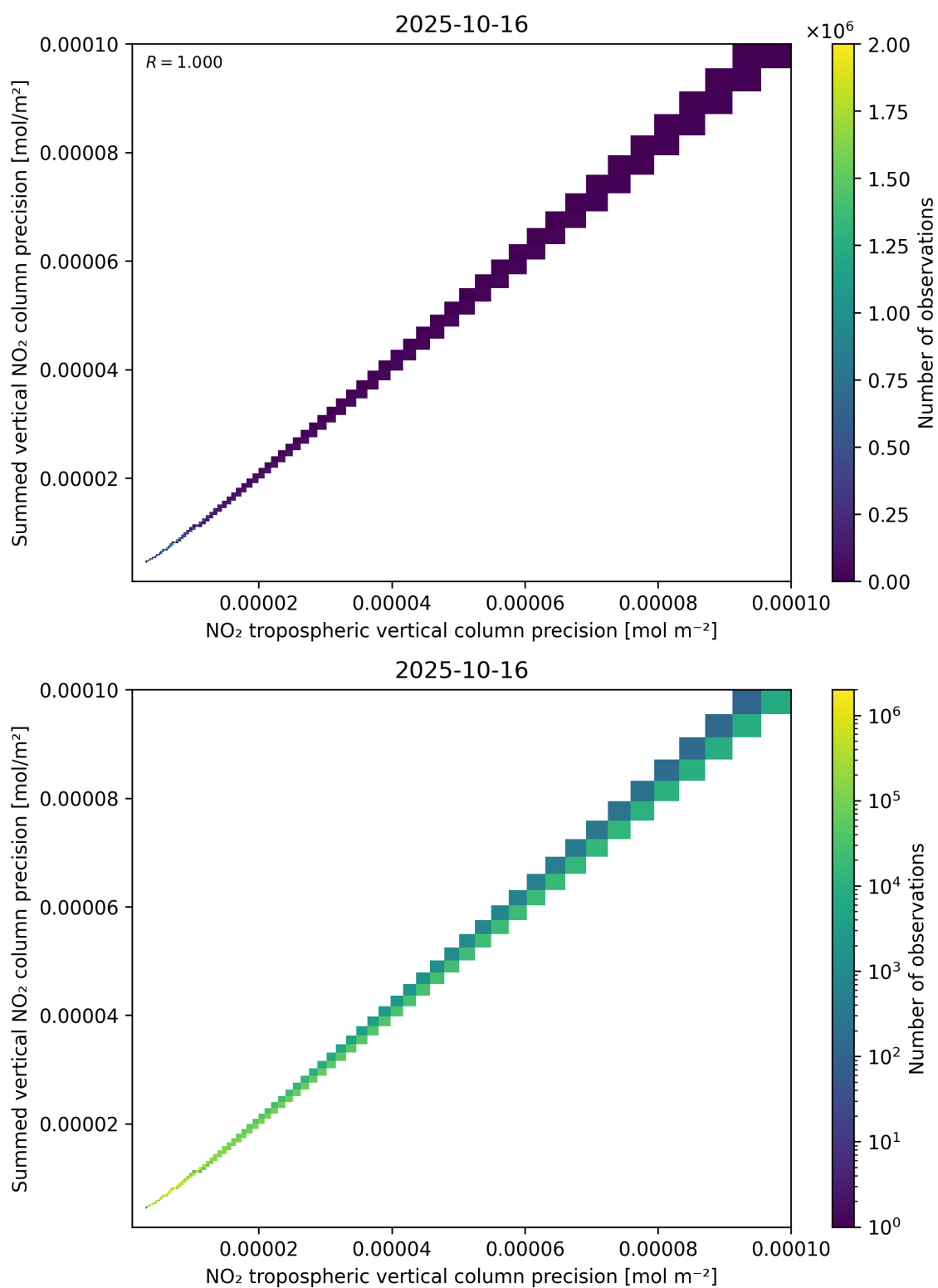
Figure 137: Scatter density plot of “NO 2 tropospheric vertical column precision” against “Summed vertical NO 2 column precision” for 2025-10-15 to 2025-10-17.
