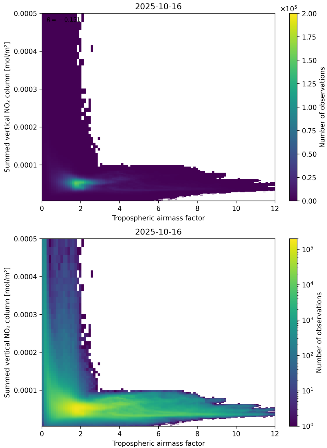
Figure 75: Scatter density plot of “Tropospheric airmass factor” against “Summed vertical NO 2 column” for 2025-10-15 to 2025-10-17.
