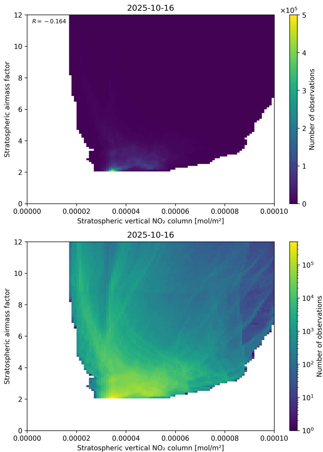
Figure 96: Scatter density plot of “Stratospheric vertical NO 2 column” against “Stratospheric airmass factor” for 2025-10-15 to 2025-10-17.
