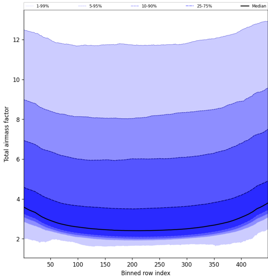
Figure 49: Along track statistics of “Total airmass factor” for 2025-10-15 to 2025-10-17
