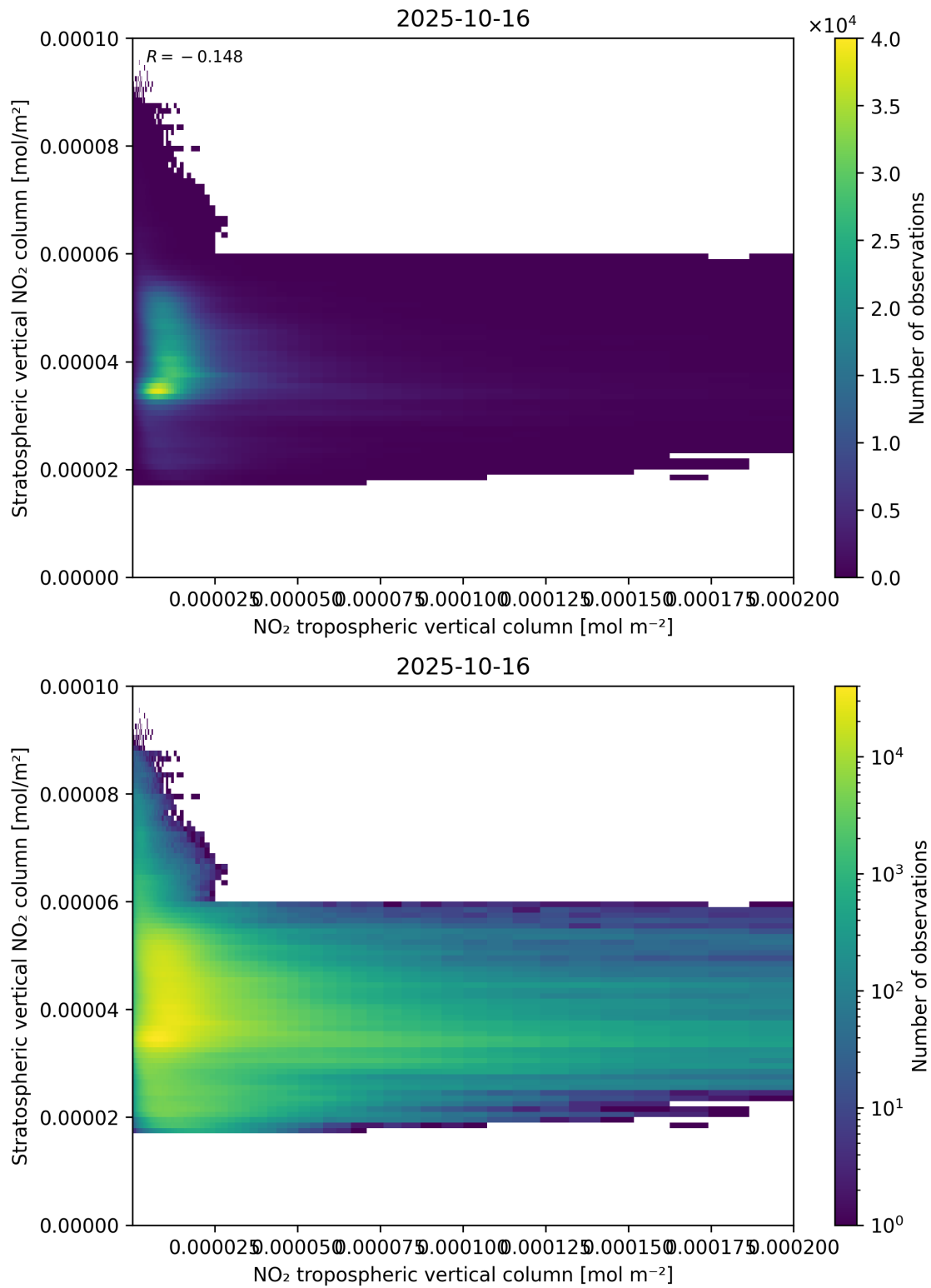
Figure 125: Scatter density plot of “NO 2 tropospheric vertical column” against “Stratospheric vertical NO 2 column” for 2025-10-15 to 2025-10-17.
