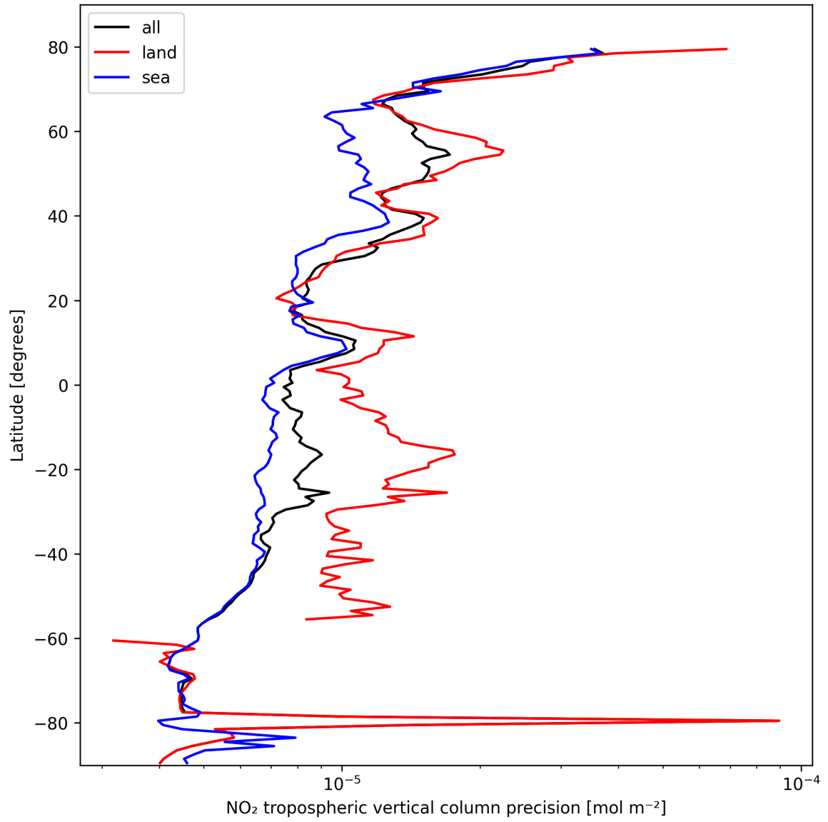
Figure 13: Zonal average of “NO 2 tropospheric vertical column precision” for 2025-10-15 to 2025-10-17.
