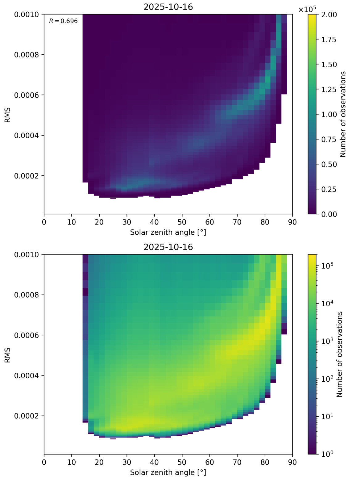
Figure 157: Scatter density plot of “Solar zenith angle” against “RMS” for 2025-10-15 to 2025-10-17.
