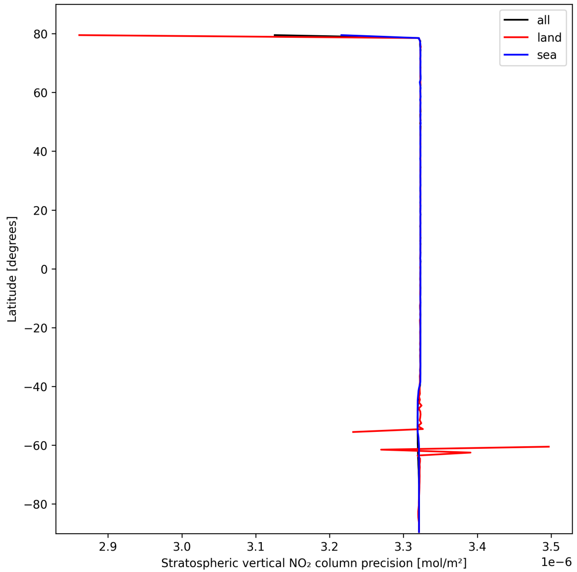
Figure 20: Zonal average of “Stratospheric vertical NO 2 column precision” for 2025-10-15 to 2025-10-17.
