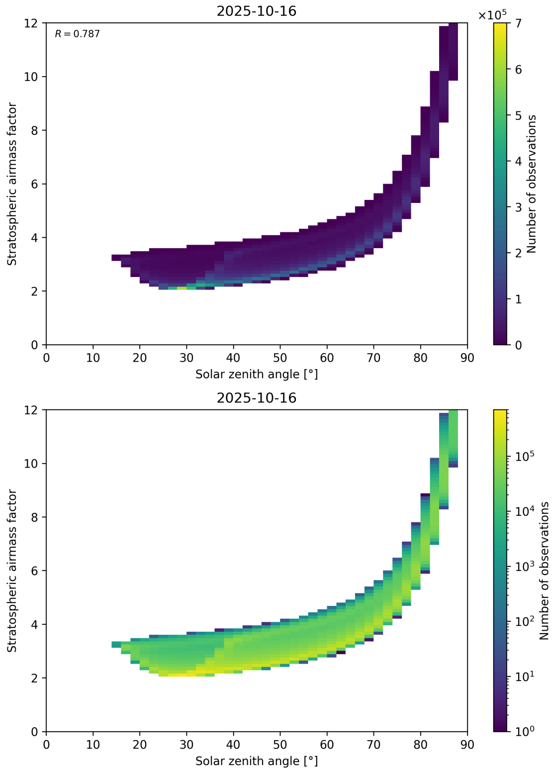
Figure 145: Scatter density plot of “Solar zenith angle” against “Stratospheric airmass factor” for 2025-10-15 to 2025-10-17.
