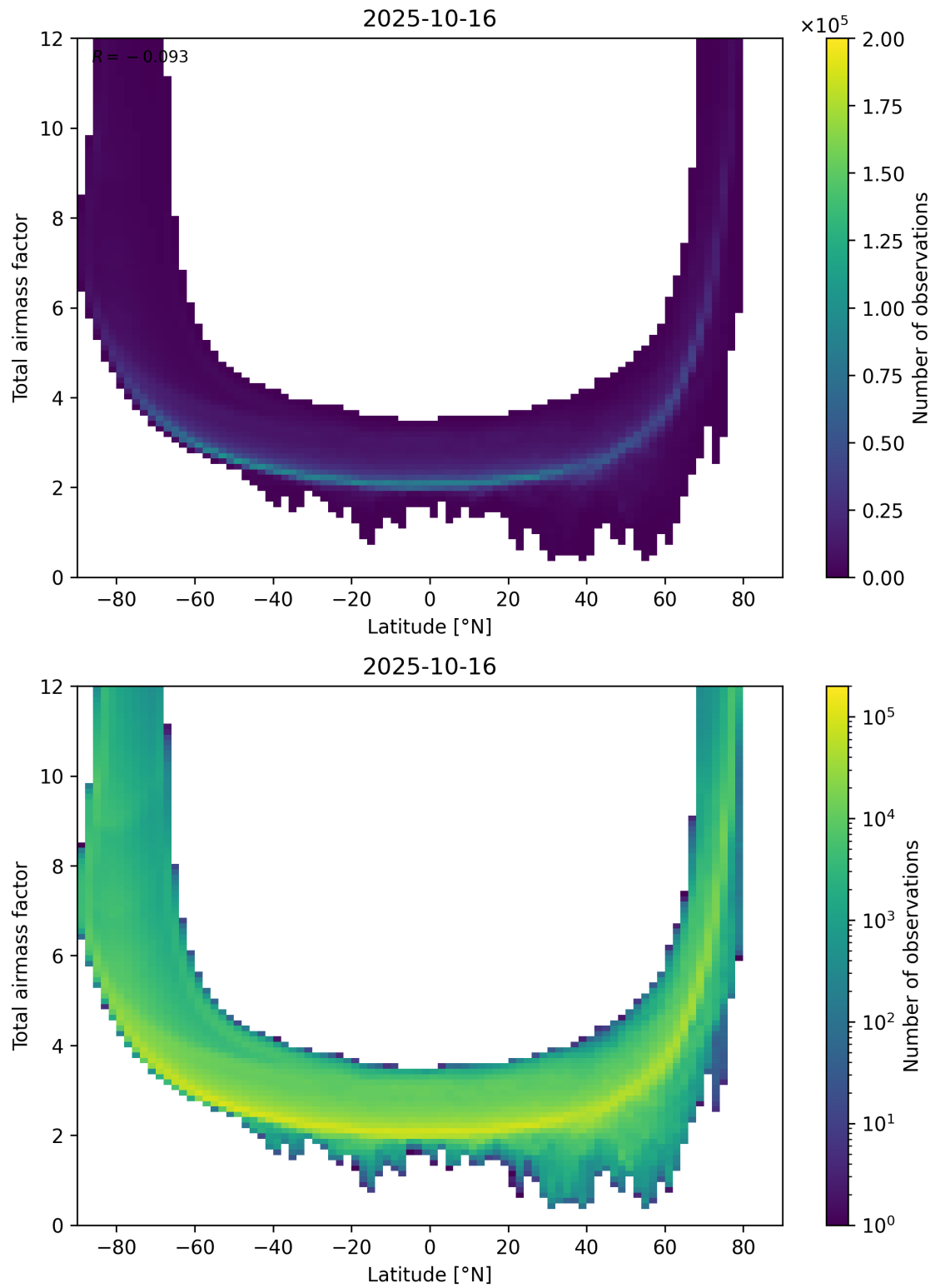
Figure 84: Scatter density plot of “Latitude” against “Total airmass factor” for 2025-10-15 to 2025-10-17.
