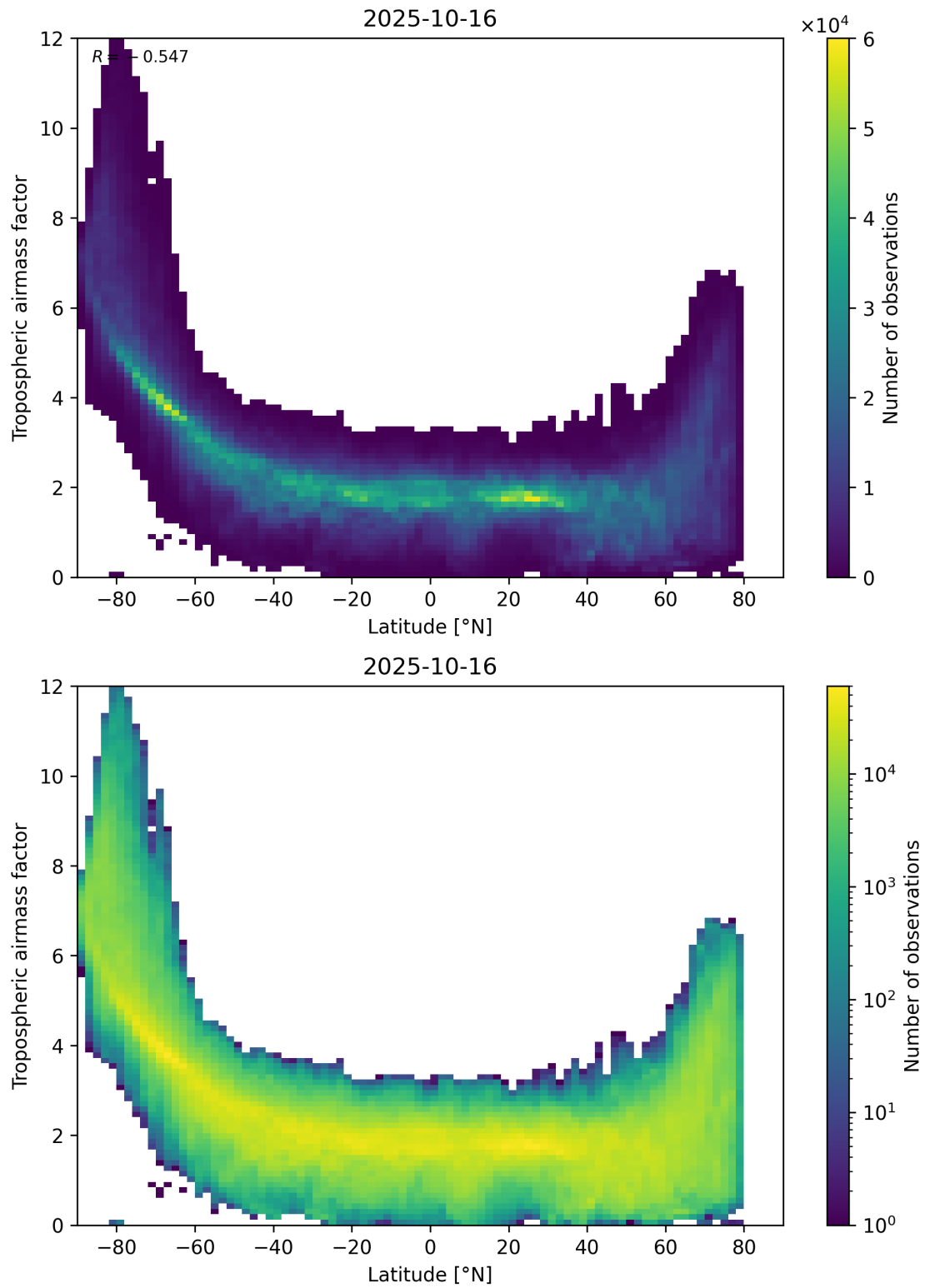
Figure 85: Scatter density plot of “Latitude” against “Tropospheric airmass factor” for 2025-10-15 to 2025-10-17.
