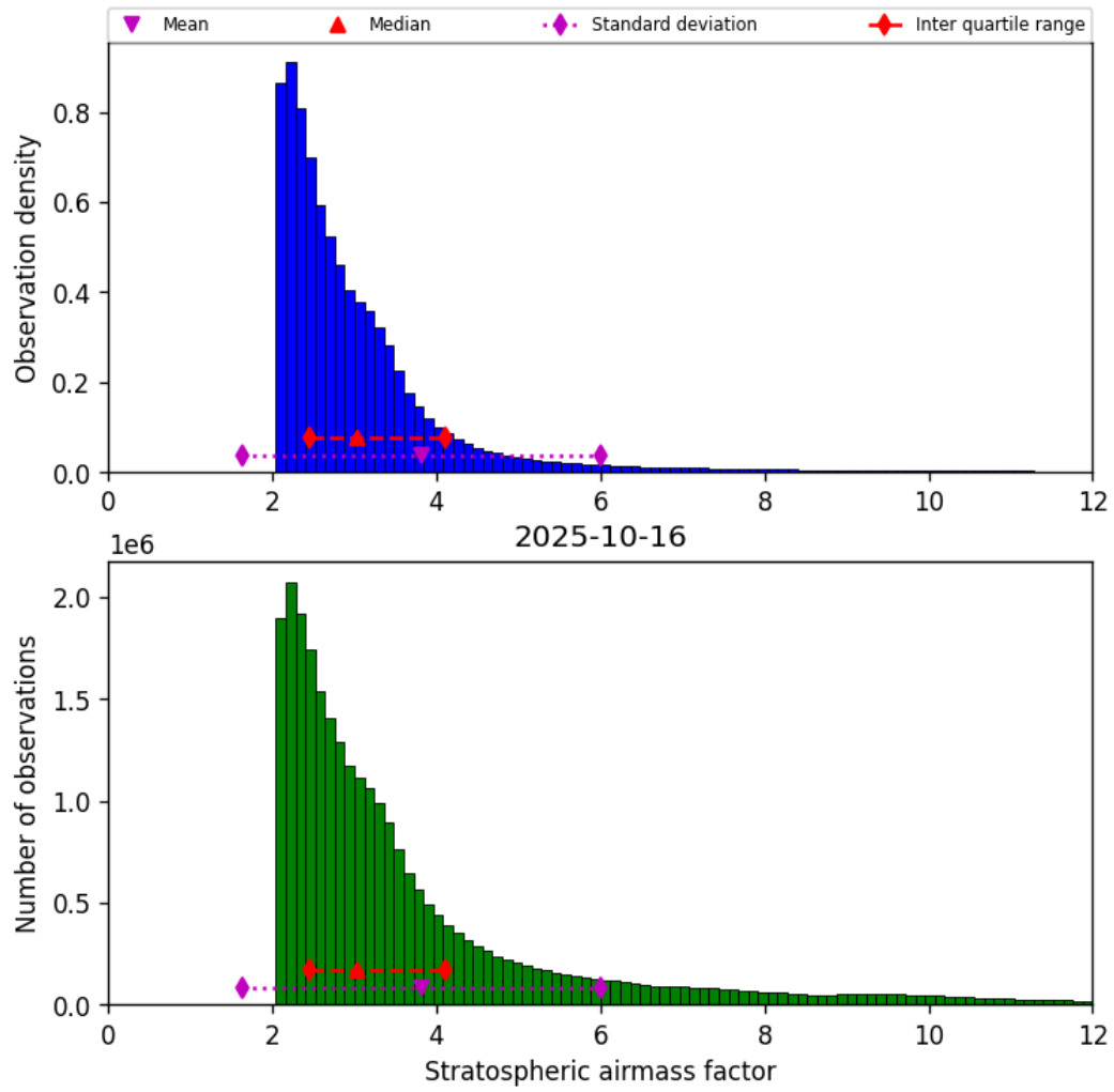
Figure 44: Histogram of “Stratospheric airmass factor” for 2025-10-15 to 2025-10-17
