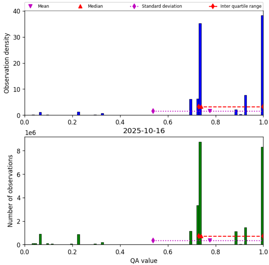
Figure 28: Histogram of “QA value” for 2025-10-15 to 2025-10-17
