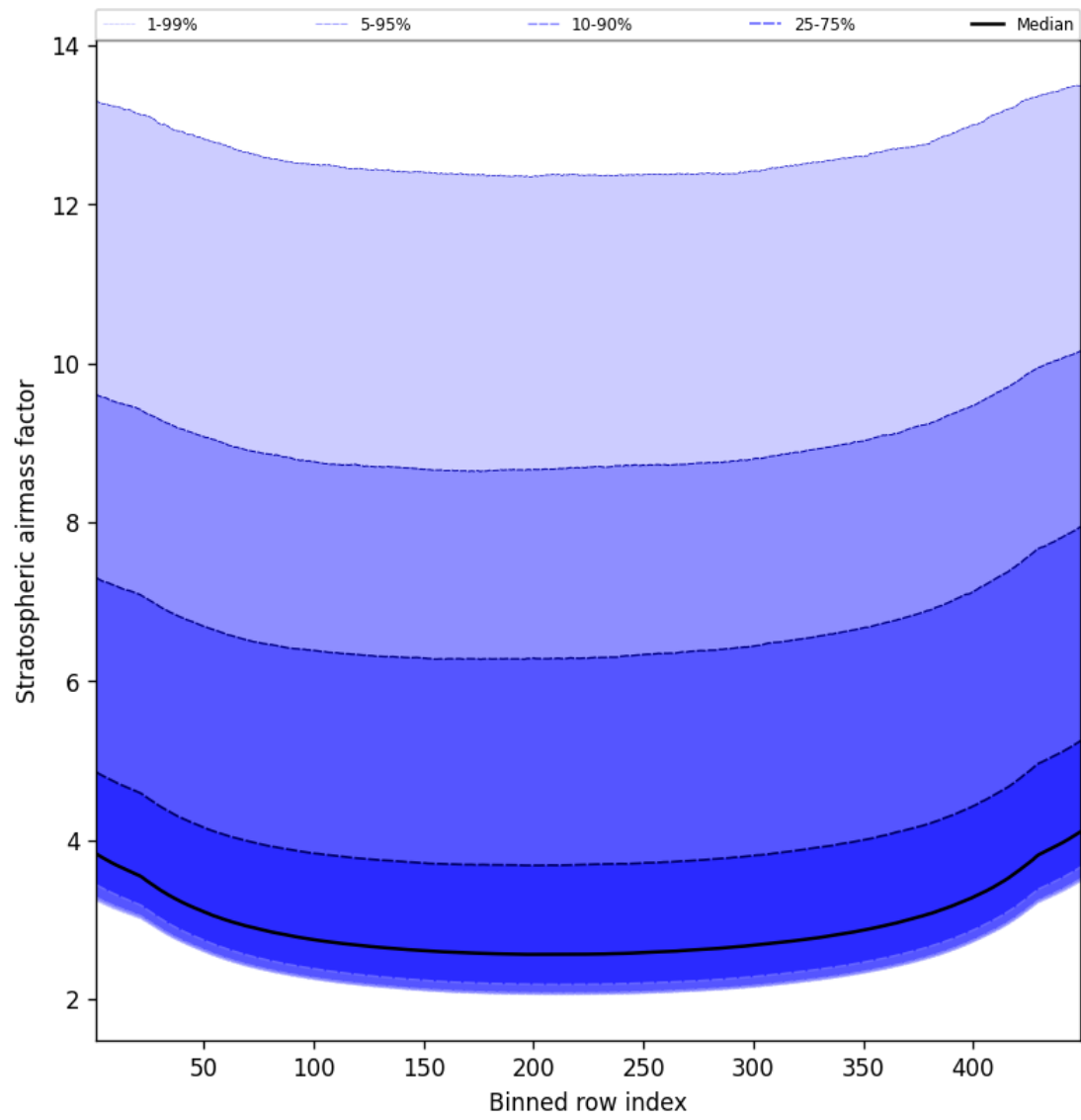
Figure 61: Along track statistics of “Stratospheric airmass factor” for 2025-10-15 to 2025-10-17
