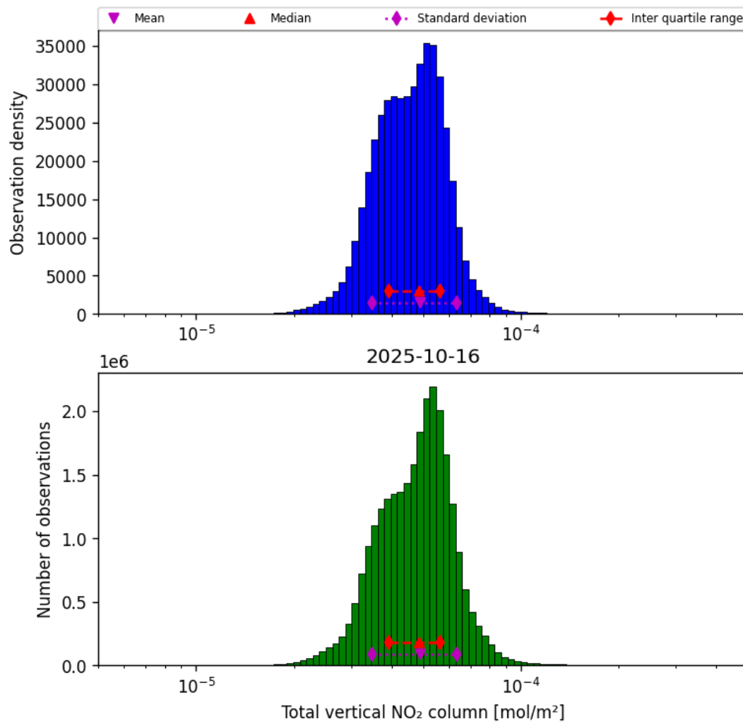
Figure 38: Histogram of “Total vertical NO 2 column” for 2025-10-15 to 2025-10-17
