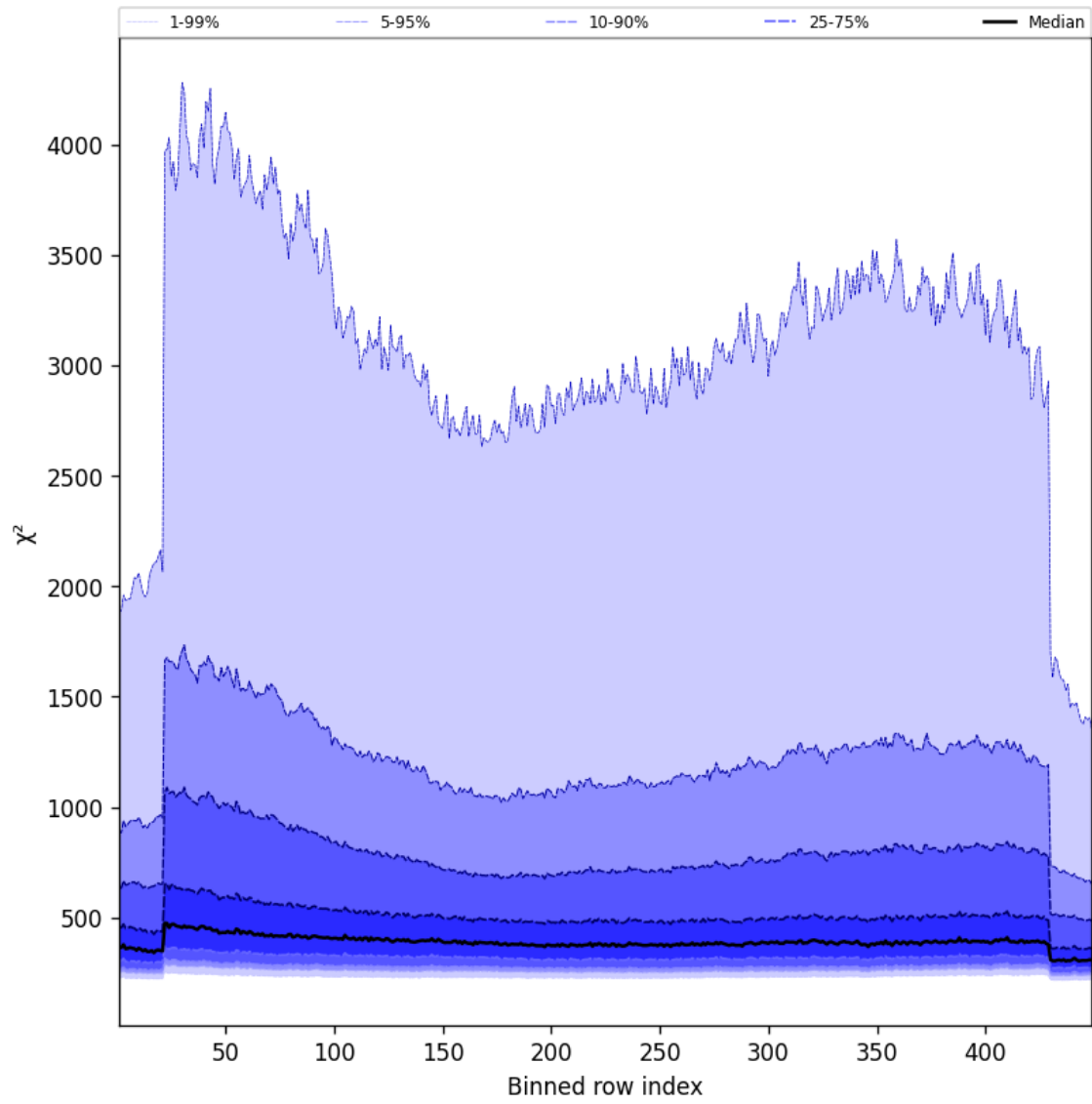
Figure 59: Along track statistics of “ \chi^2 ” for 2025-10-15 to 2025-10-17
