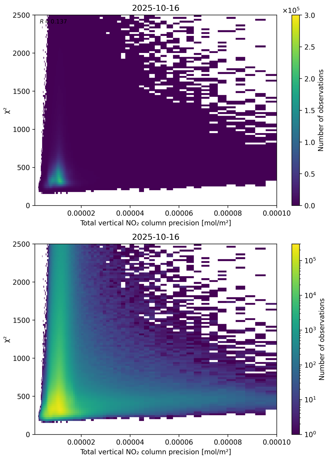
Figure 116: Scatter density plot of “Total vertical NO 2 column precision” against “ \chi^2 ” for 2025-10-15 to 2025-10-17.
