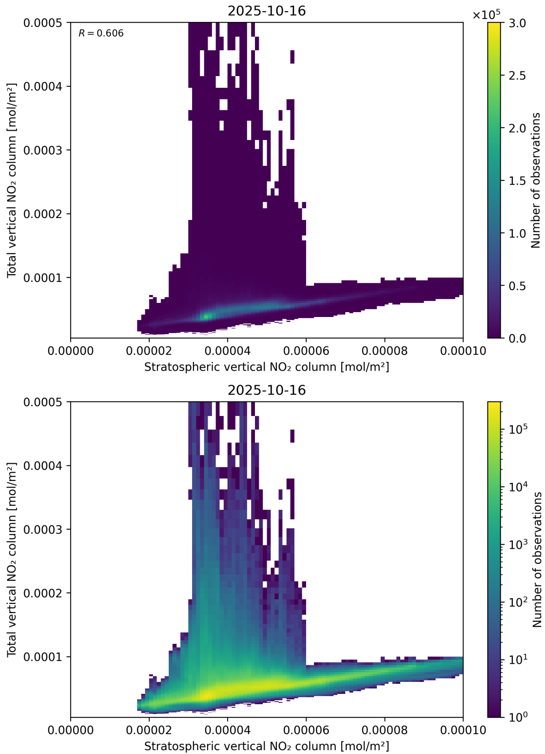
Figure 100: Scatter density plot of “Stratospheric vertical NO 2 column” against “Total vertical NO 2 column” for 2025-10-15 to 2025-10-17.
