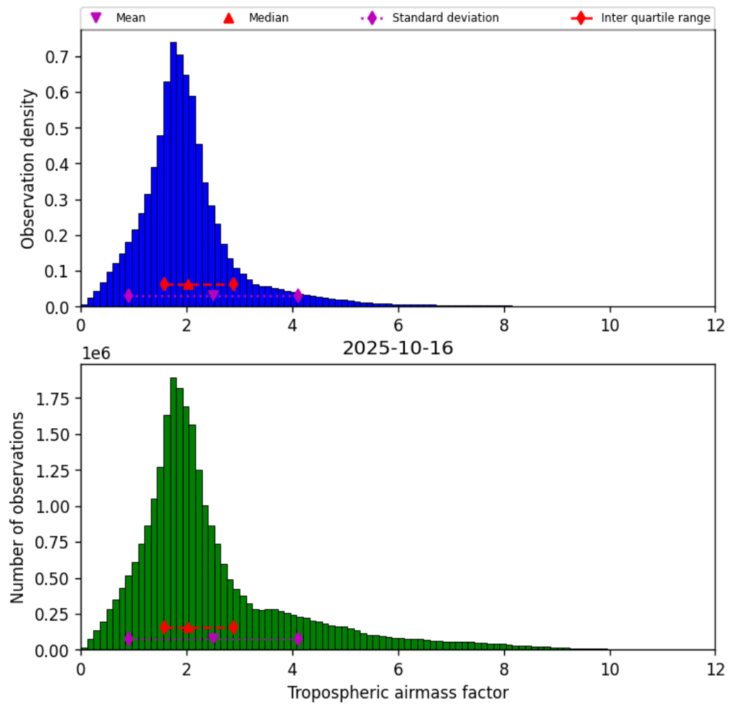
Figure 31: Histogram of “Tropospheric airmass factor” for 2025-10-15 to 2025-10-17
