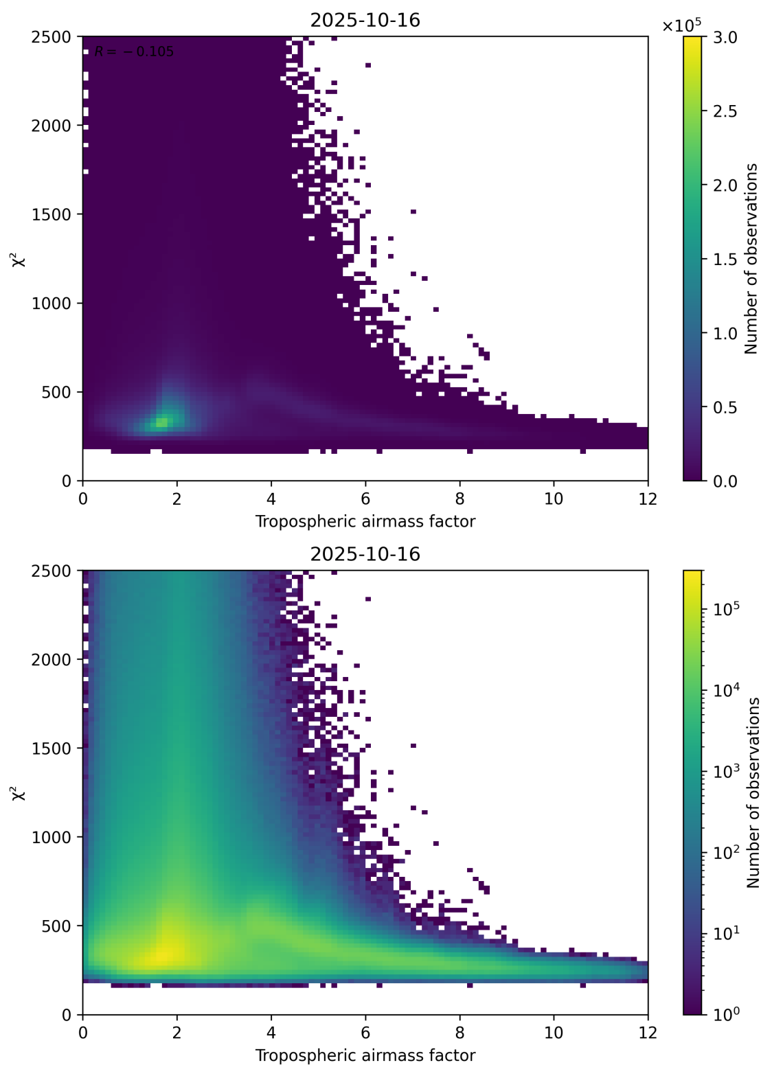
Figure 73: Scatter density plot of “Tropospheric airmass factor” against “ \chi^2 ” for 2025-10-15 to 2025-10-17.
