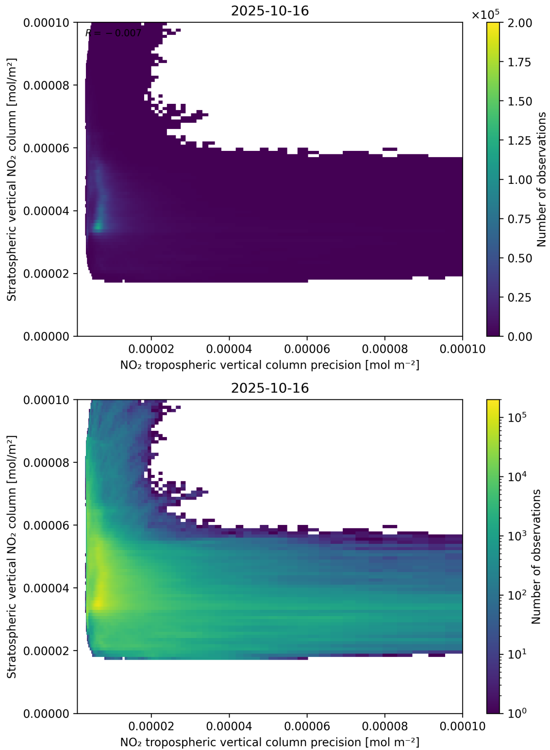
Figure 135: Scatter density plot of “NO 2 tropospheric vertical column precision” against “Stratospheric vertical NO 2 column” for 2025-10-15 to 2025-10-17.
