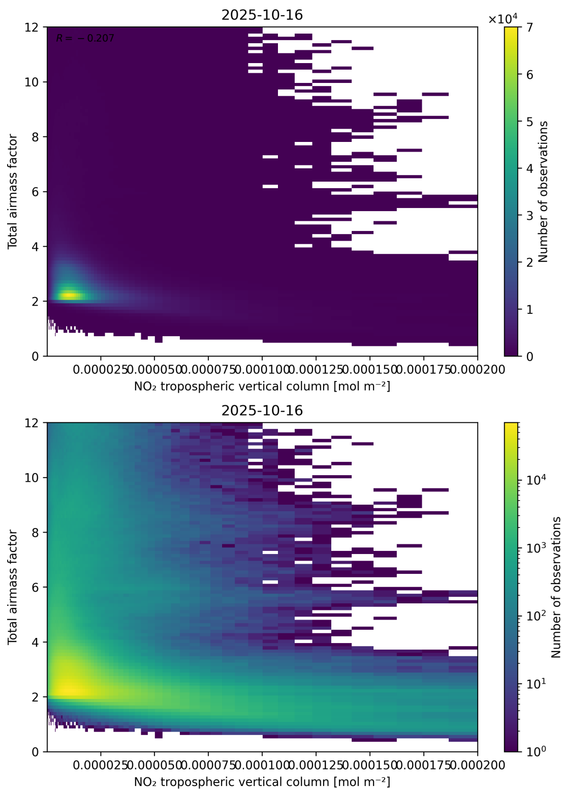
Figure 122: Scatter density plot of “NO 2 tropospheric vertical column” against “Total air mass factor” for 2025-10-15 to 2025-10-17.
