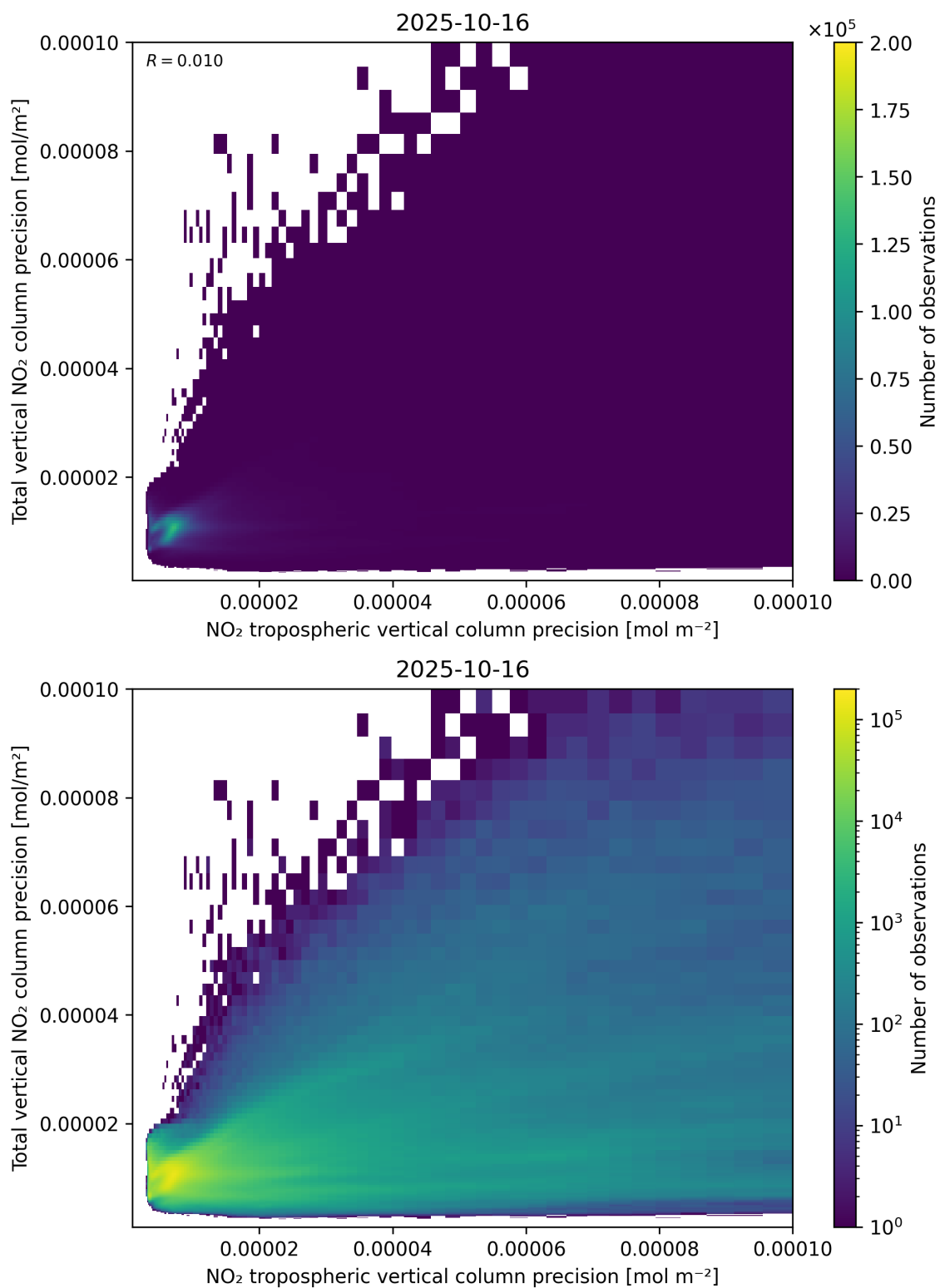
Figure 139: Scatter density plot of “NO 2 tropospheric vertical column precision” against “Total vertical NO 2 column precision” for 2025-10-15 to 2025-10-17.
