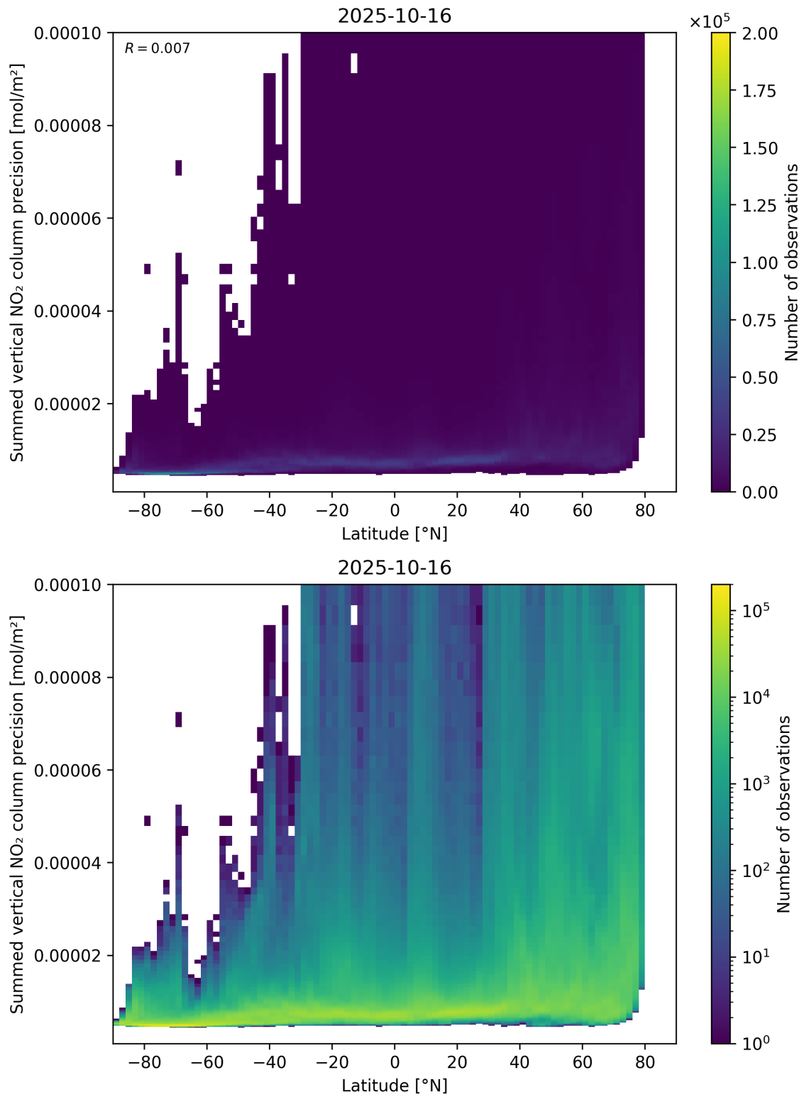
Figure 89: Scatter density plot of “Latitude” against “Summed vertical NO 2 column precision” for 2025-10-15 to 2025-10-17.
