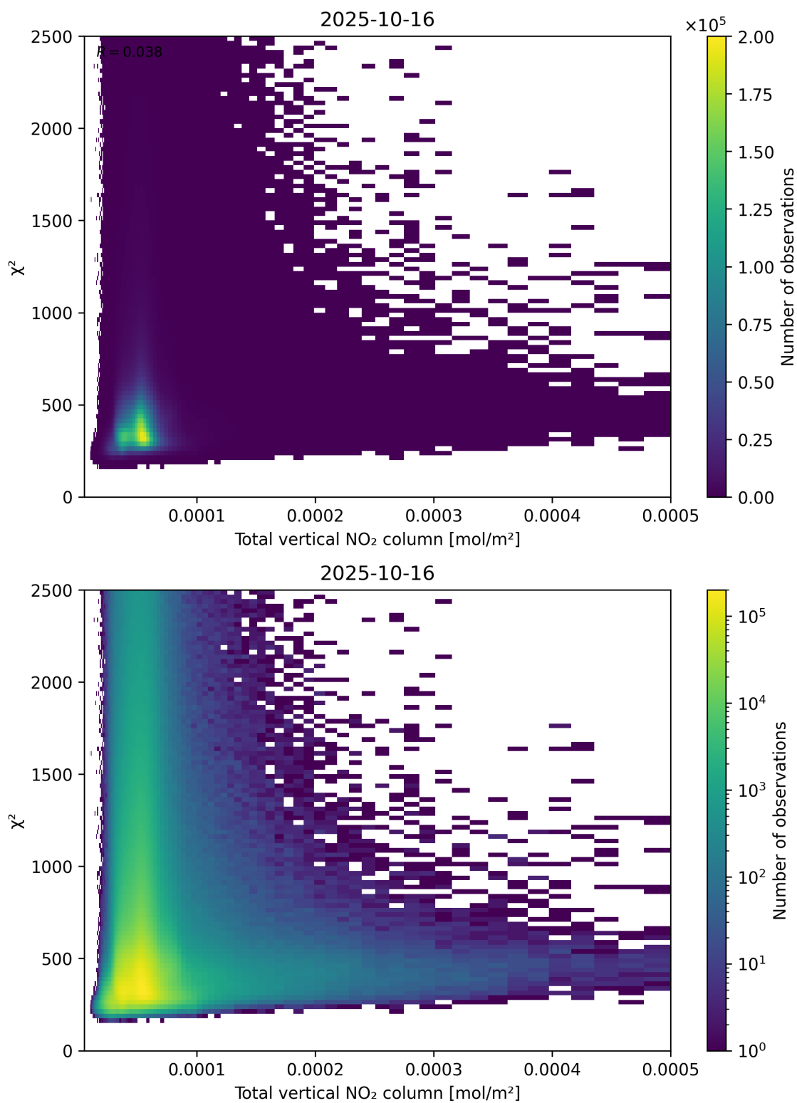
Figure 111: Scatter density plot of “Total vertical NO 2 column” against “ \chi^2 ” for 2025-10-15 to 2025-10-17.
