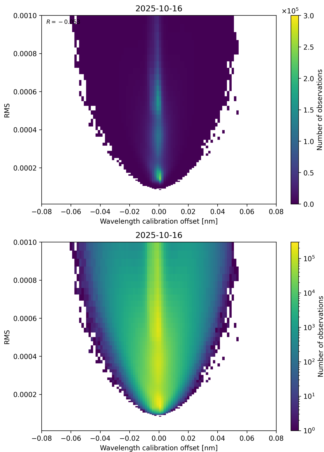
Figure 181: Scatter density plot of “Wavelength calibration offset” against “RMS” for 2025-10-15 to 2025-10-17.
