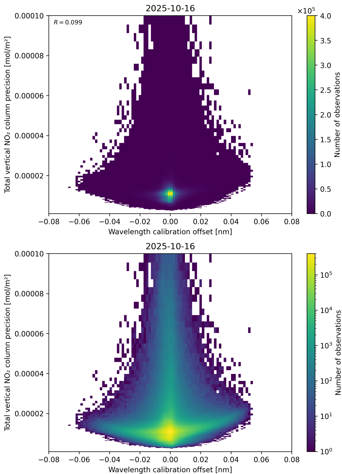
Figure 180: Scatter density plot of “Wavelength calibration offset” against “Total vertical NO 2 column precision” for 2025-10-15 to 2025-10-17.
