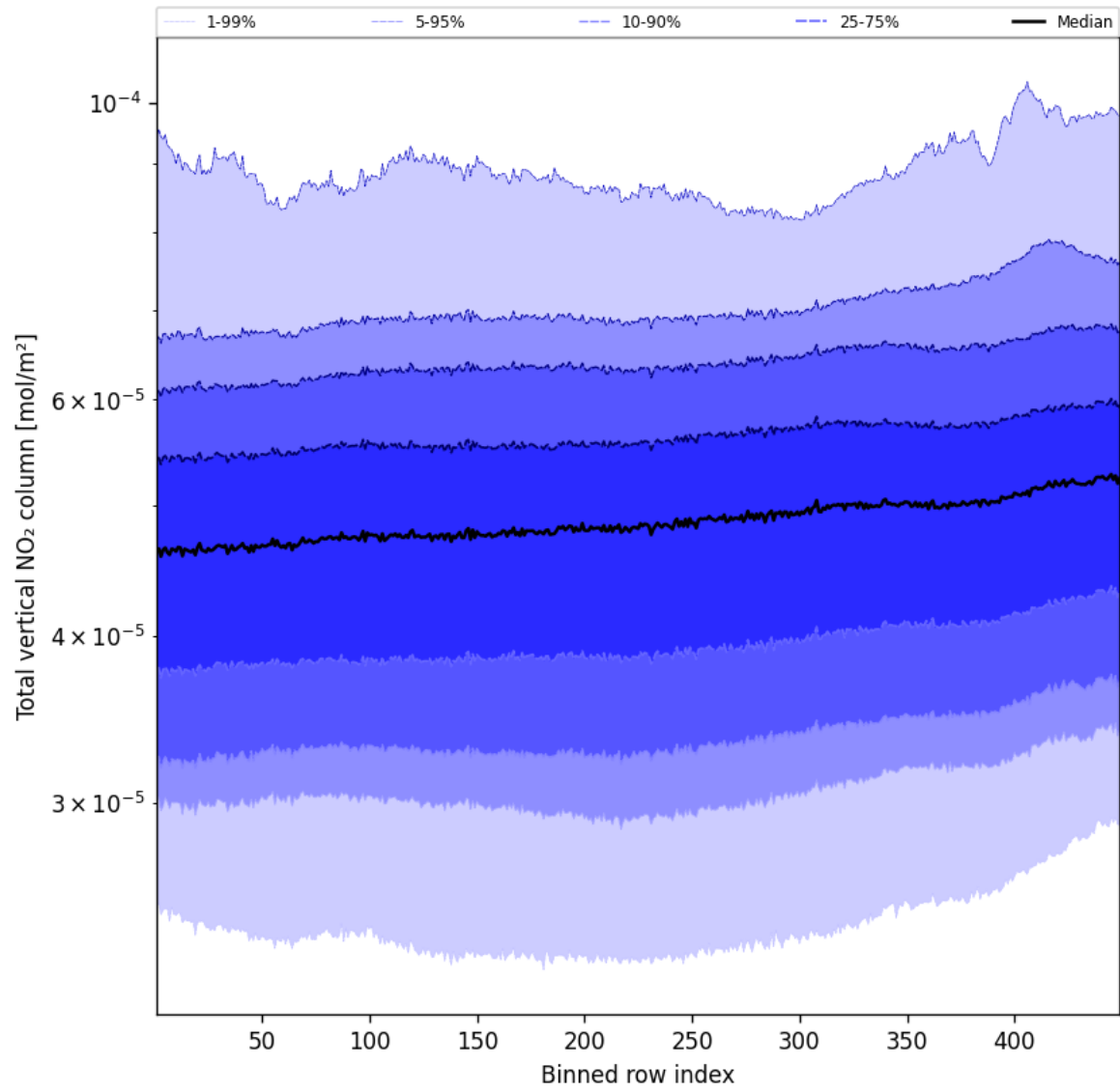
Figure 55: Along track statistics of “Total vertical NO 2 column” for 2025-10-15 to 2025-10-17
