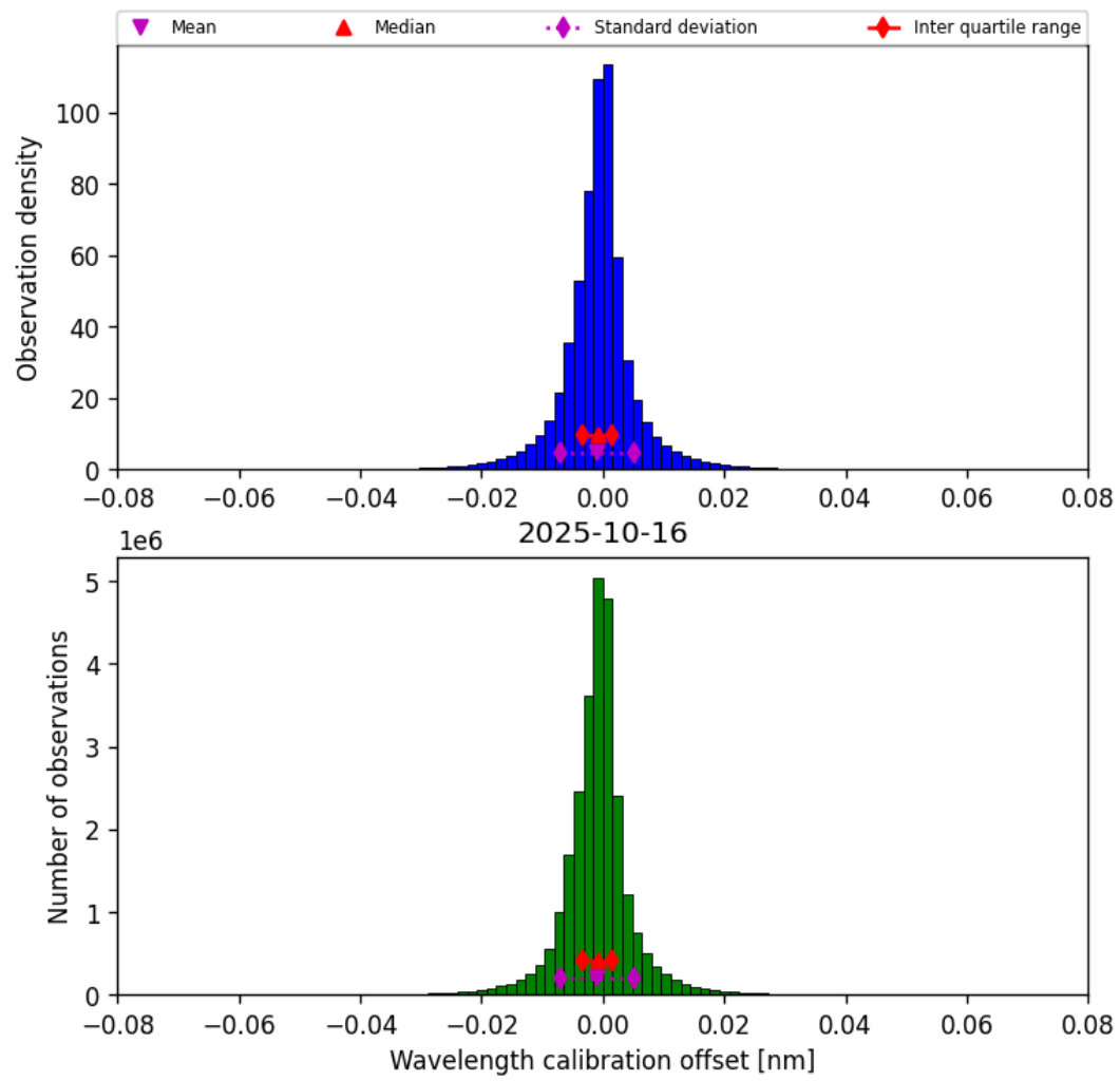
Figure 35: Histogram of “Wavelength calibration offset” for 2025-10-15 to 2025-10-17
