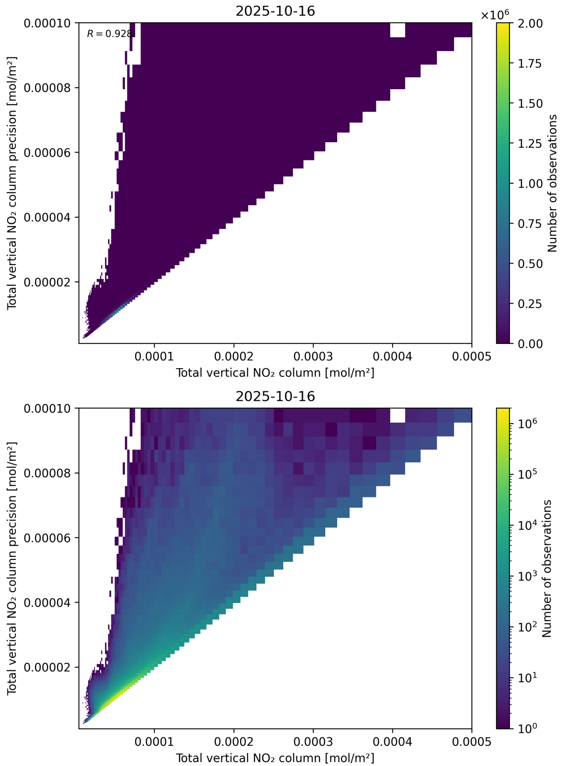
Figure 114: Scatter density plot of “Total vertical NO 2 column” against “Total vertical NO 2 column precision” for 2025-10-15 to 2025-10-17.
