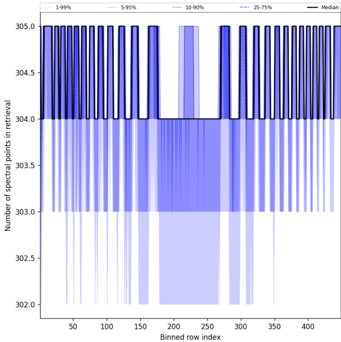
Figure 50: Along track statistics of “Number of spectral points in retrieval” for 2025-10-15 to 2025-10-17
