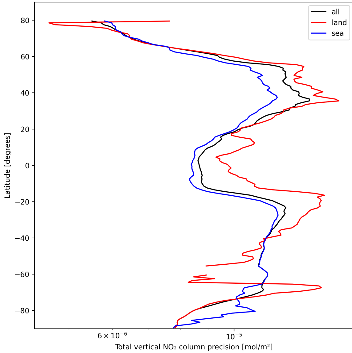
Figure 22: Zonal average of “Total vertical NO 2 column precision” for 2025-10-15 to 2025-10-17.
