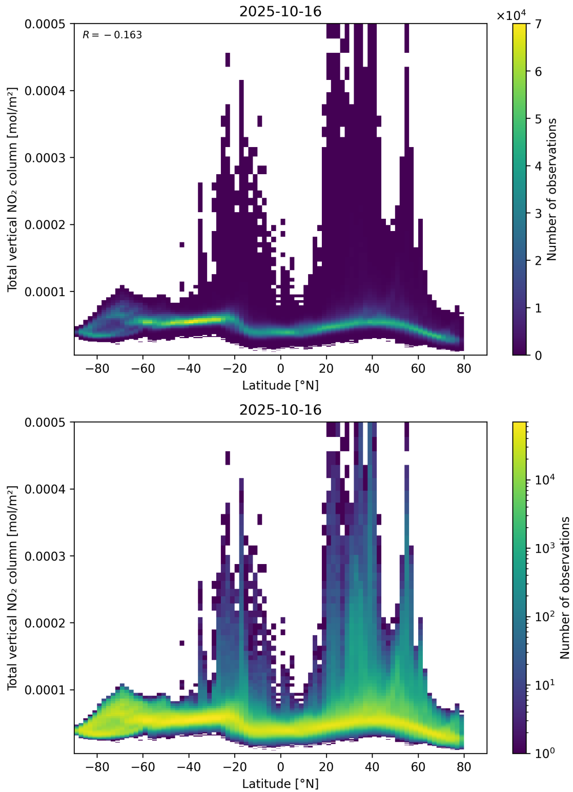
Figure 90: Scatter density plot of “Latitude” against “Total vertical NO 2 column” for 2025-10-15 to 2025-10-17.
