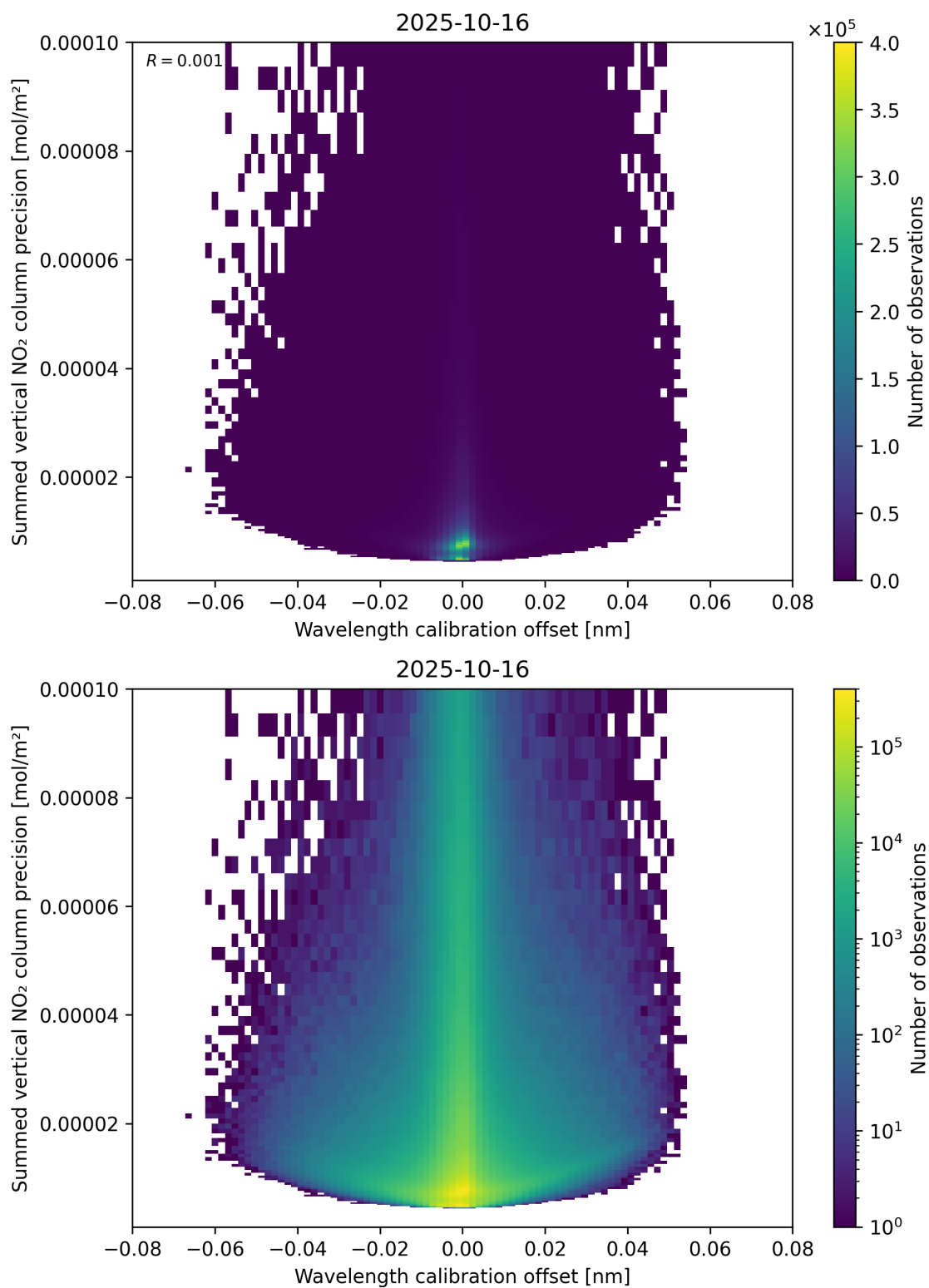
Figure 178: Scatter density plot of “Wavelength calibration offset” against “Summed vertical NO 2 column precision” for 2025-10-15 to 2025-10-17.
