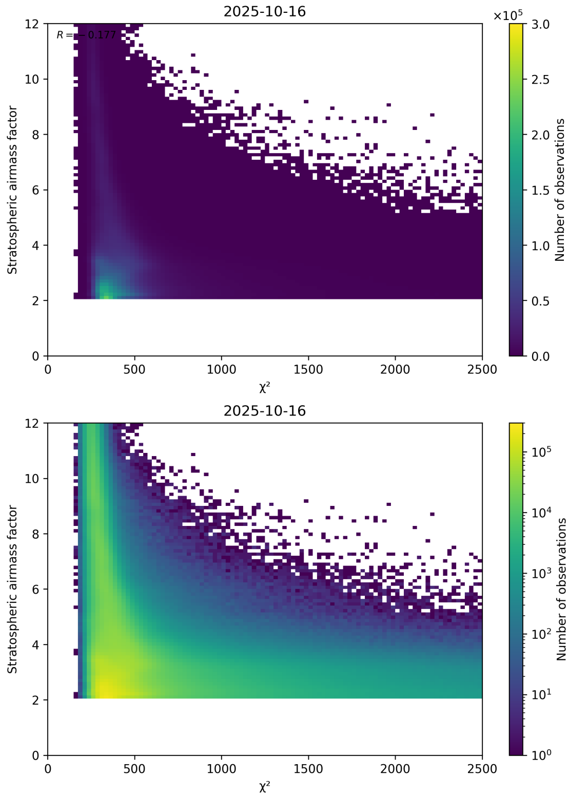
Figure 81: Scatter density plot of “ \chi^2 ” against “Stratospheric airmass factor” for 2025-10-15 to 2025-10-17.
