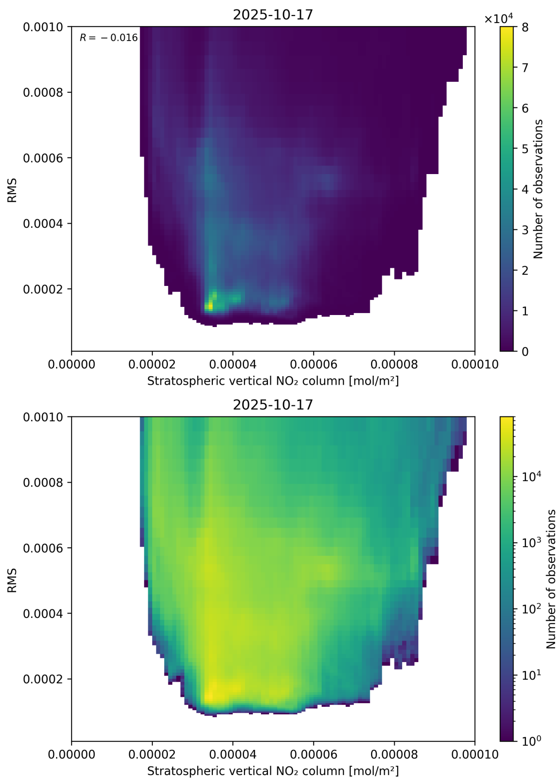
Figure 102: Scatter density plot of “Stratospheric vertical NO 2 column” against “RMS” for 2025-10-17 to 2025-10-18.
