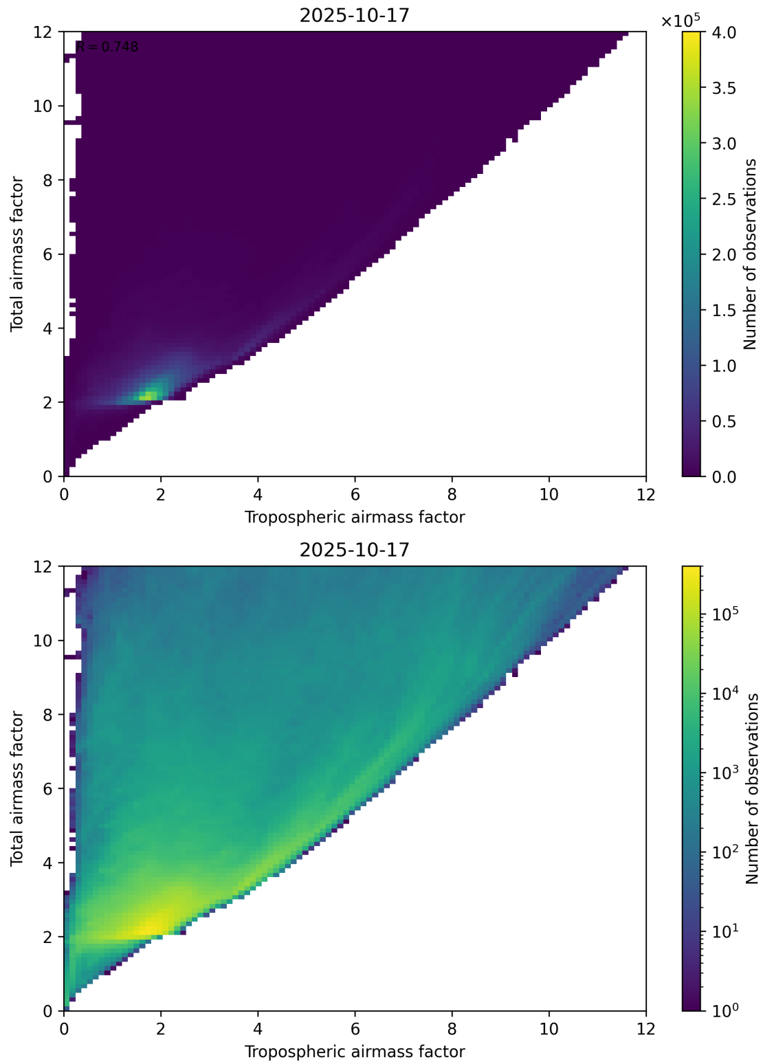
Figure 72: Scatter density plot of “Tropospheric airmass factor” against “Total airmass factor” for 2025-10-17 to 2025-10-18.
