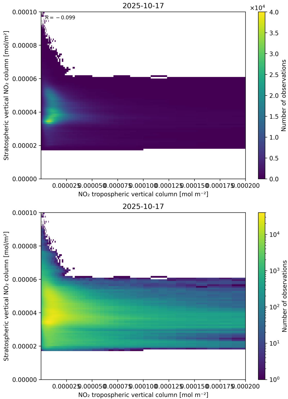
Figure 125: Scatter density plot of “NO 2 tropospheric vertical column” against “Stratospheric vertical NO 2 column” for 2025-10-17 to 2025-10-18.
