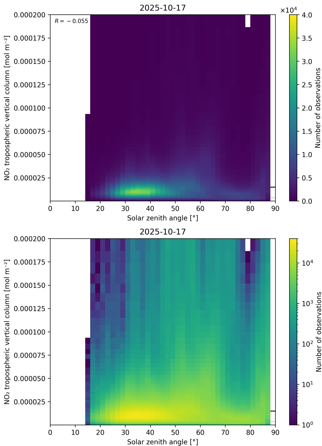
Figure 155: Scatter density plot of “Solar zenith angle” against “NO 2 tropospheric vertical column” for 2025-10-17 to 2025-10-18.
