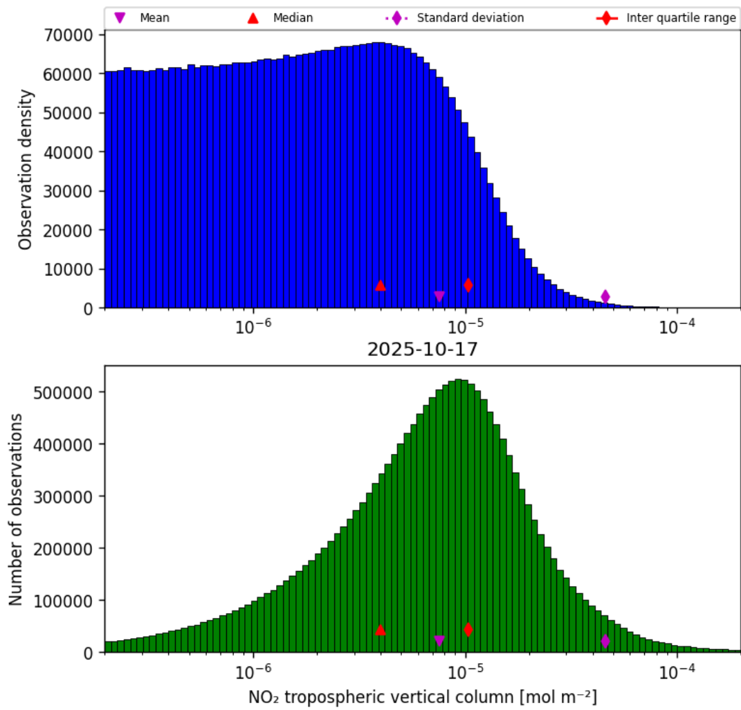
Figure 29: Histogram of “NO 2 tropospheric vertical column” for 2025-10-17 to 2025-10-18
