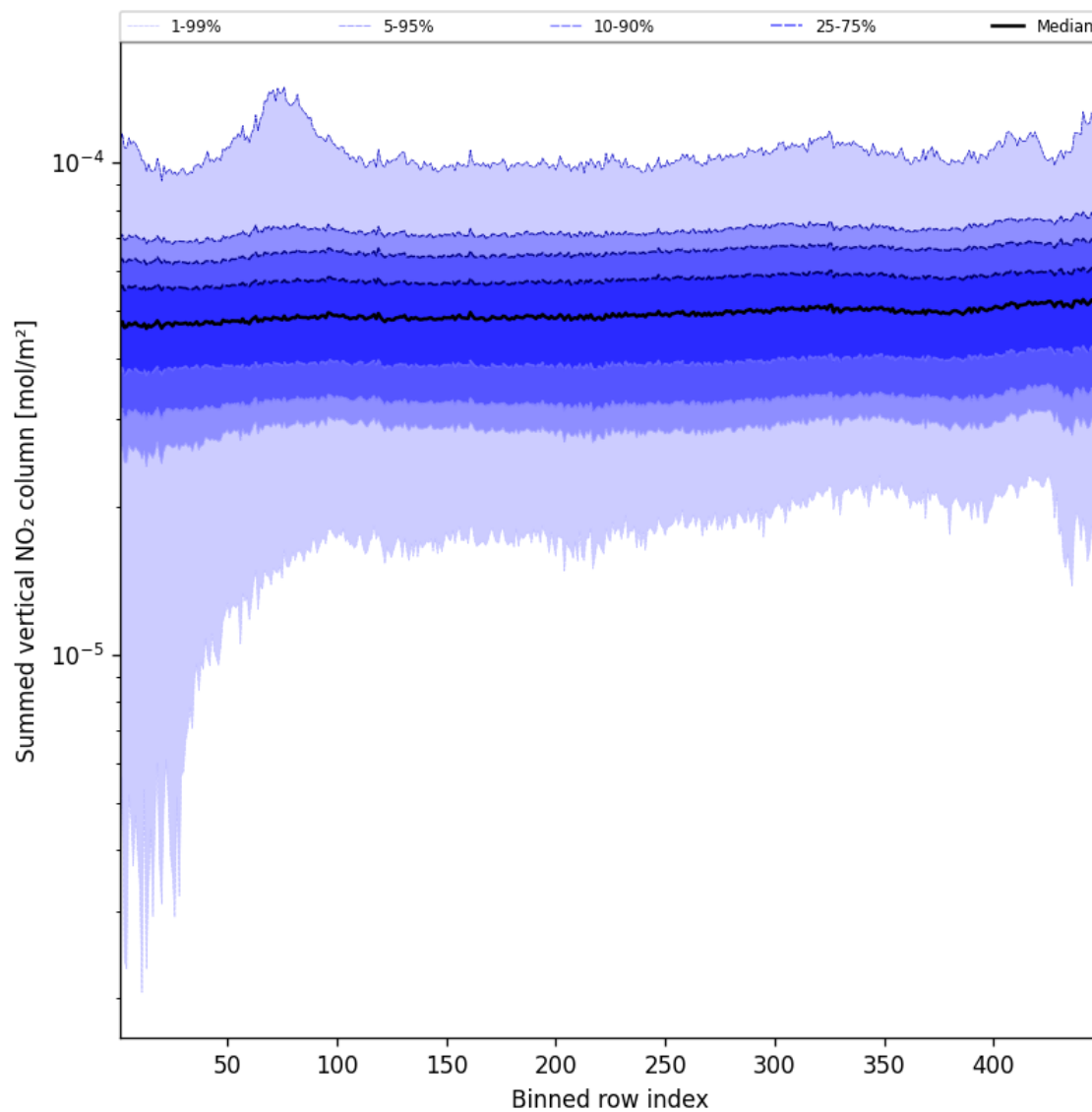
Figure 57: Along track statistics of “Summed vertical NO 2 column” for 2025-10-17 to 2025-10-18
