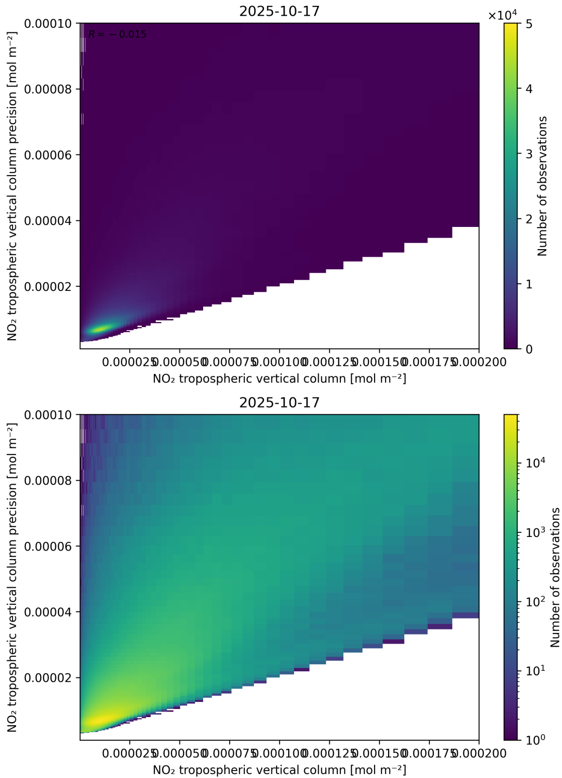
Figure 130: Scatter density plot of “NO 2 tropospheric vertical column” against “NO 2 tropospheric vertical column precision” for 2025-10-17 to 2025-10-18.
