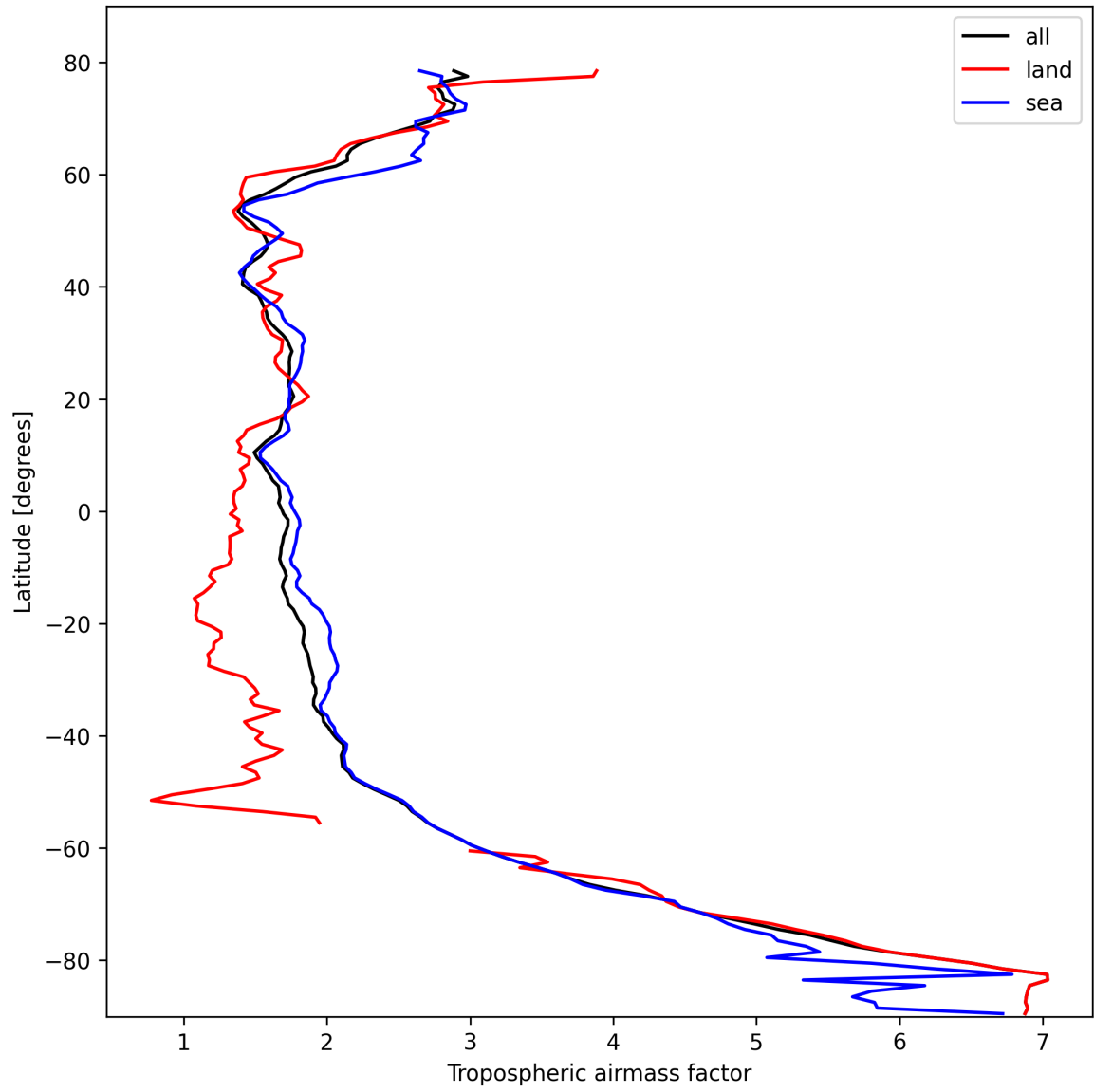
Figure 14: Zonal average of “Tropospheric airmass factor” for 2025-10-17 to 2025-10-18.
