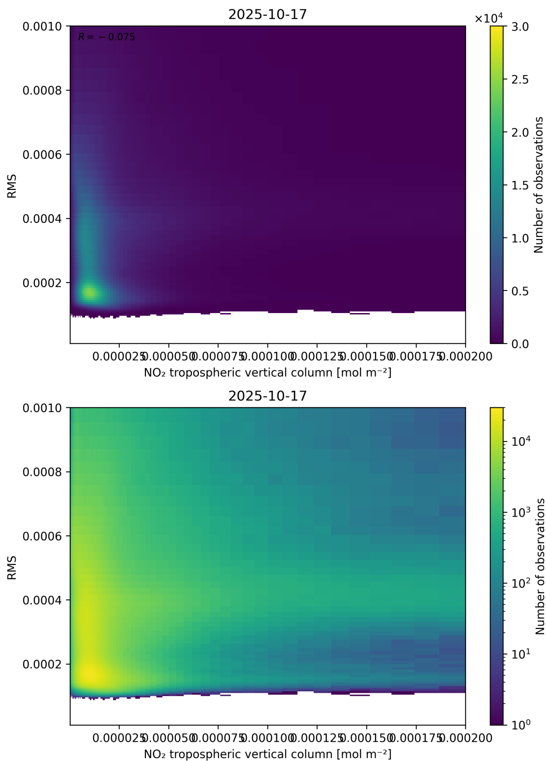
Figure 142: Scatter density plot of “NO 2 tropospheric vertical column” against “RMS” for 2025-10-17 to 2025-10-18.
