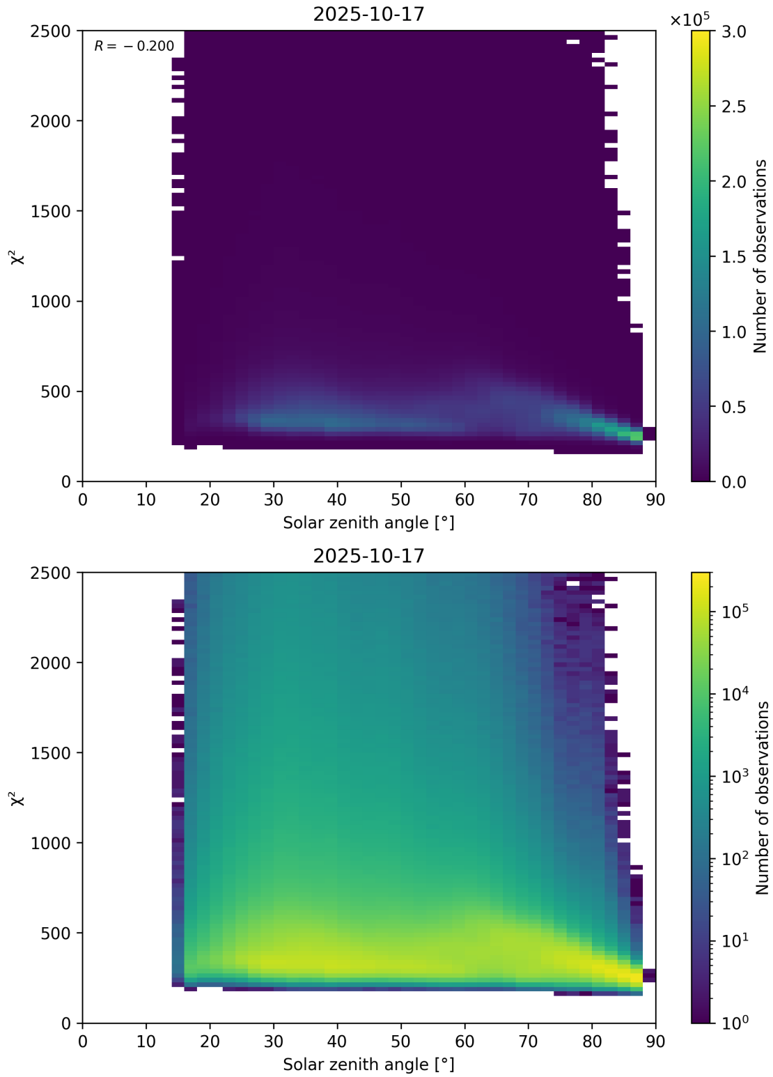
Figure 148: Scatter density plot of “Solar zenith angle” against “ \chi^2 ” for 2025-10-17 to 2025-10-18.
