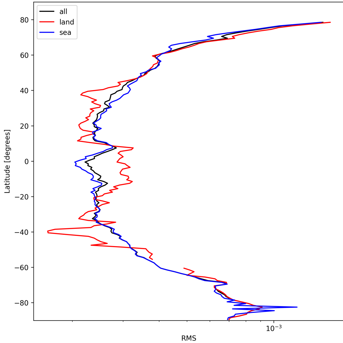
Figure 26: Zonal average of “RMS” for 2025-10-17 to 2025-10-18.
