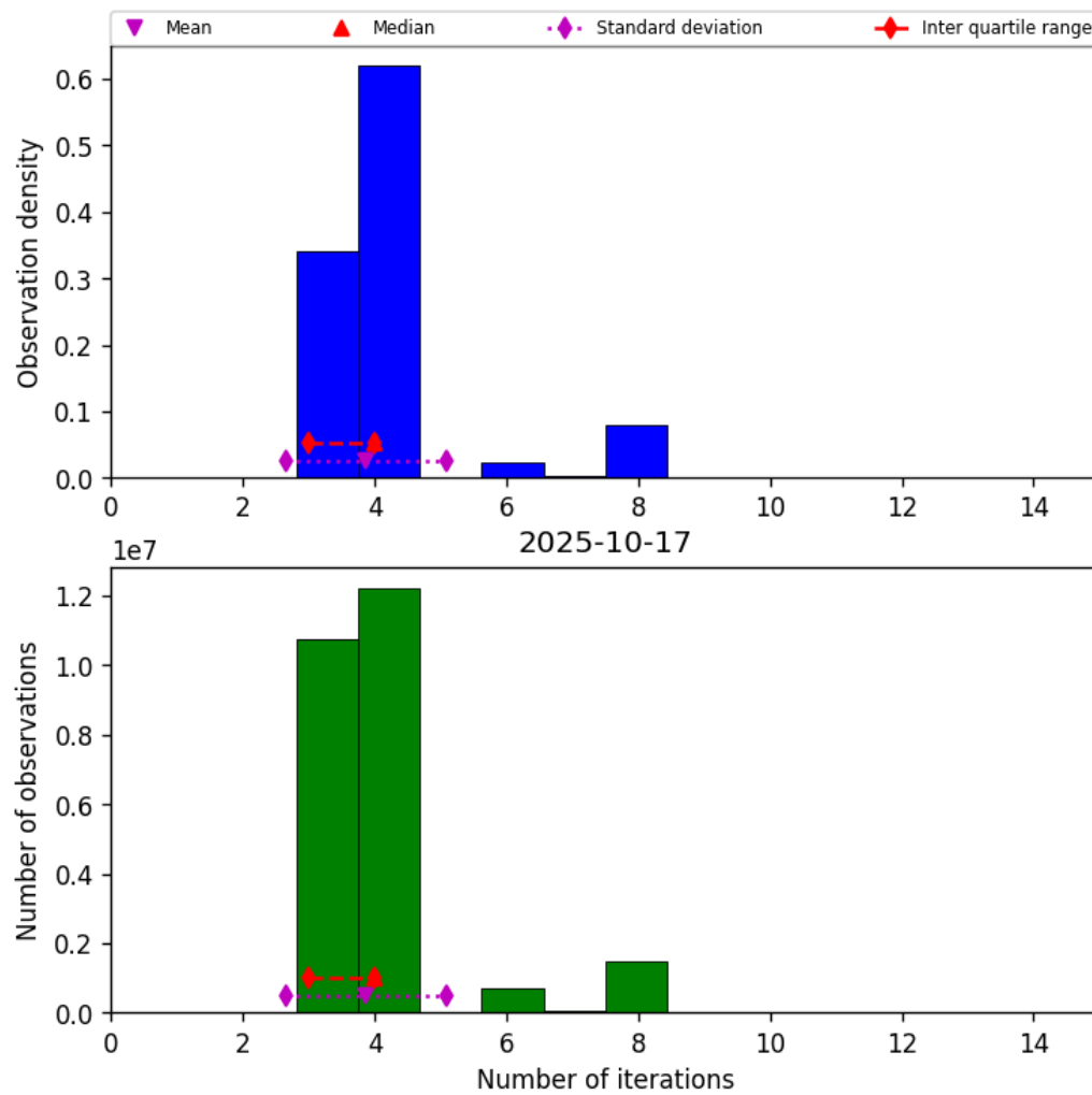
Figure 34: Histogram of “Number of iterations” for 2025-10-17 to 2025-10-18
