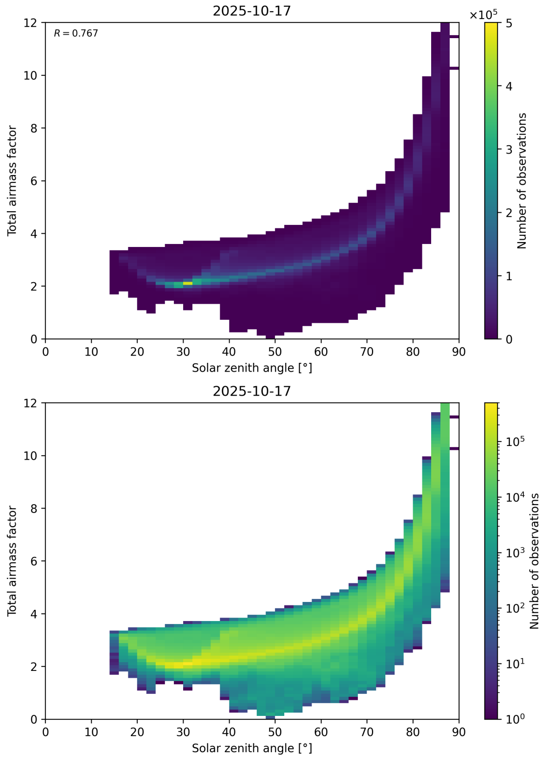
Figure 146: Scatter density plot of “Solar zenith angle” against “Total airmass factor” for 2025-10-17 to 2025-10-18.
