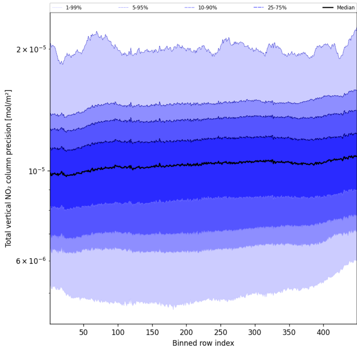
Figure 56: Along track statistics of “Total vertical NO 2 column precision” for 2025-10-17 to 2025-10-18
