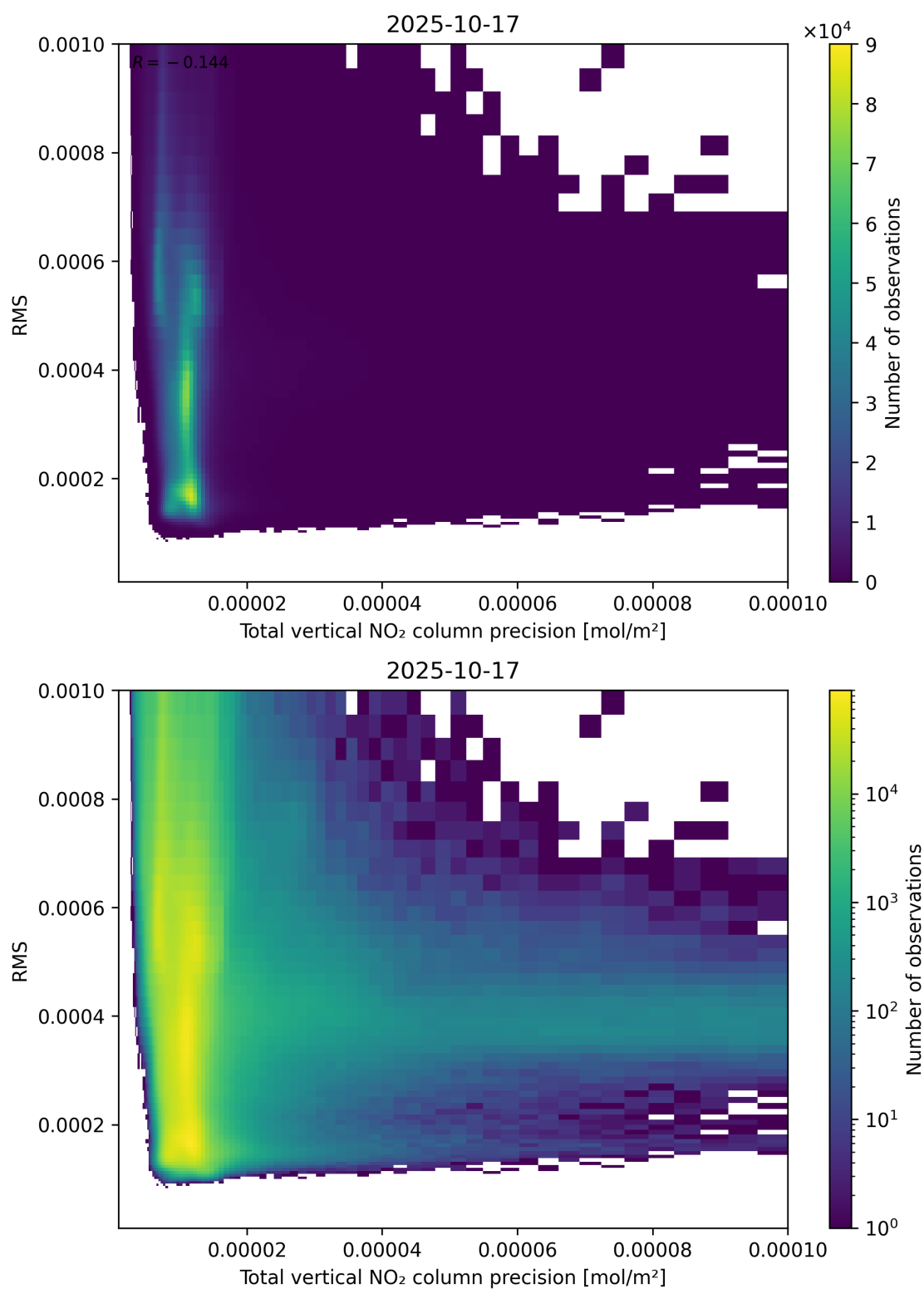
Figure 119: Scatter density plot of “Total vertical NO 2 column precision” against “RMS” for 2025-10-17 to 2025-10-18.
