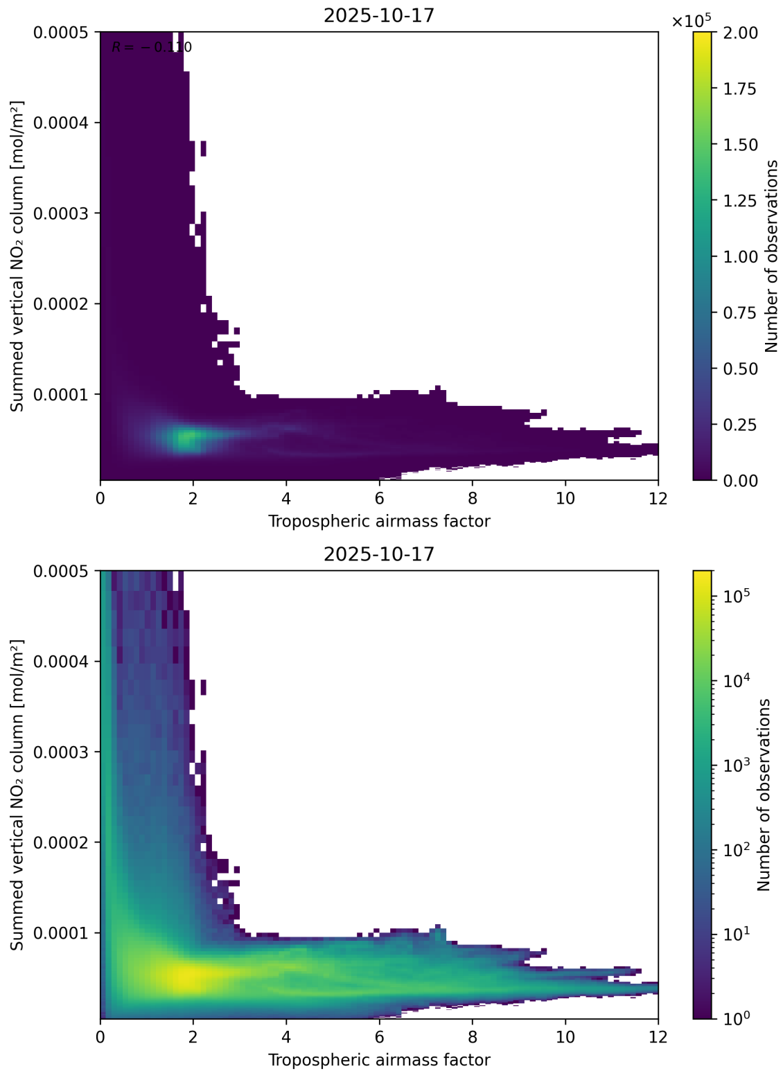
Figure 75: Scatter density plot of “Tropospheric air mass factor” against “Summed vertical NO 2 column” for 2025-10-17 to 2025-10-18.
