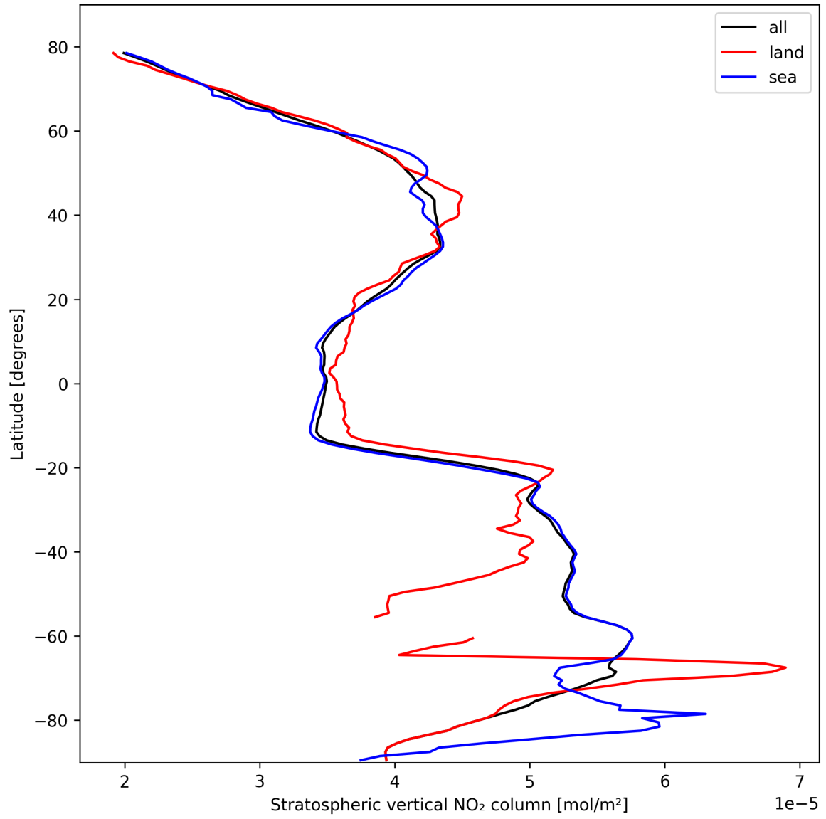
Figure 19: Zonal average of “Stratospheric vertical NO 2 column” for 2025-10-17 to 2025-10-18.
