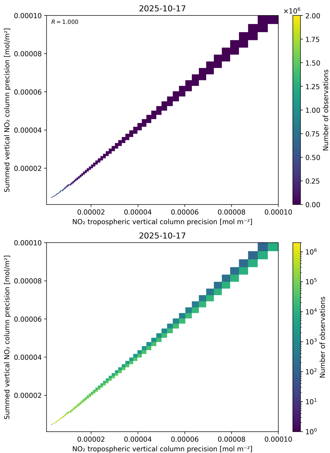
Figure 137: Scatter density plot of “NO 2 tropospheric vertical column precision” against “Summed vertical NO 2 column precision” for 2025-10-17 to 2025-10-18.
