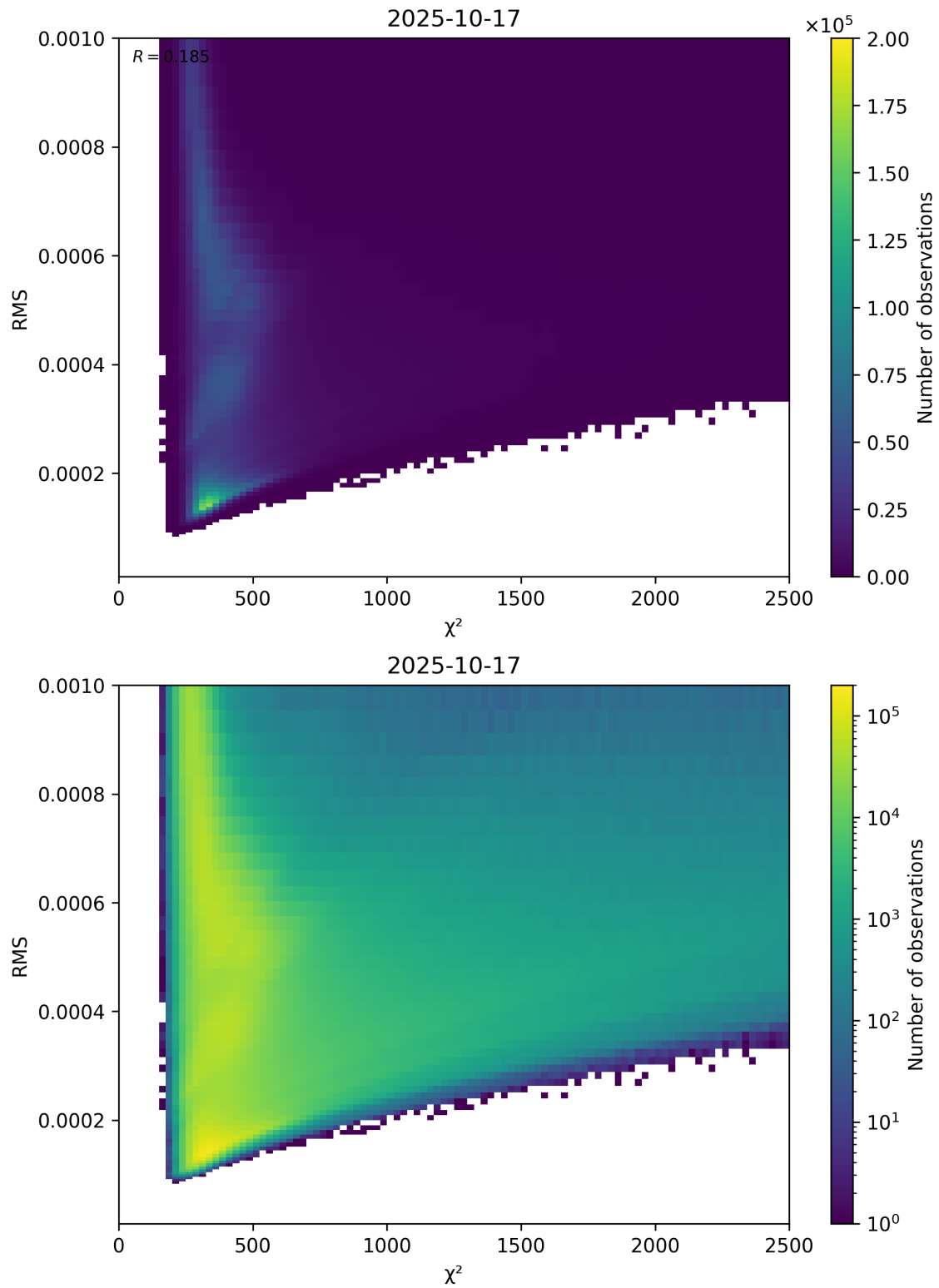
Figure 82: Scatter density plot of “ \chi^2 ” against “RMS” for 2025-10-17 to 2025-10-18.
