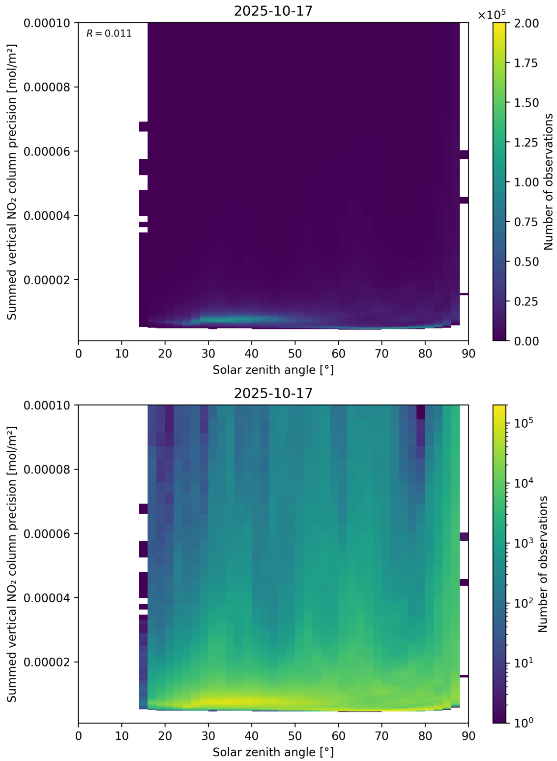
Figure 152: Scatter density plot of “Solar zenith angle” against “Summed vertical NO 2 column precision” for 2025-10-17 to 2025-10-18.
