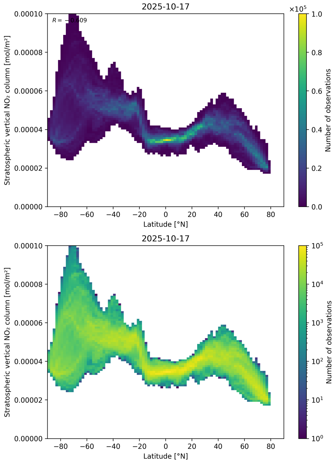
Figure 87: Scatter density plot of “Latitude” against “Stratospheric vertical NO 2 column” for 2025-10-17 to 2025-10-18.
