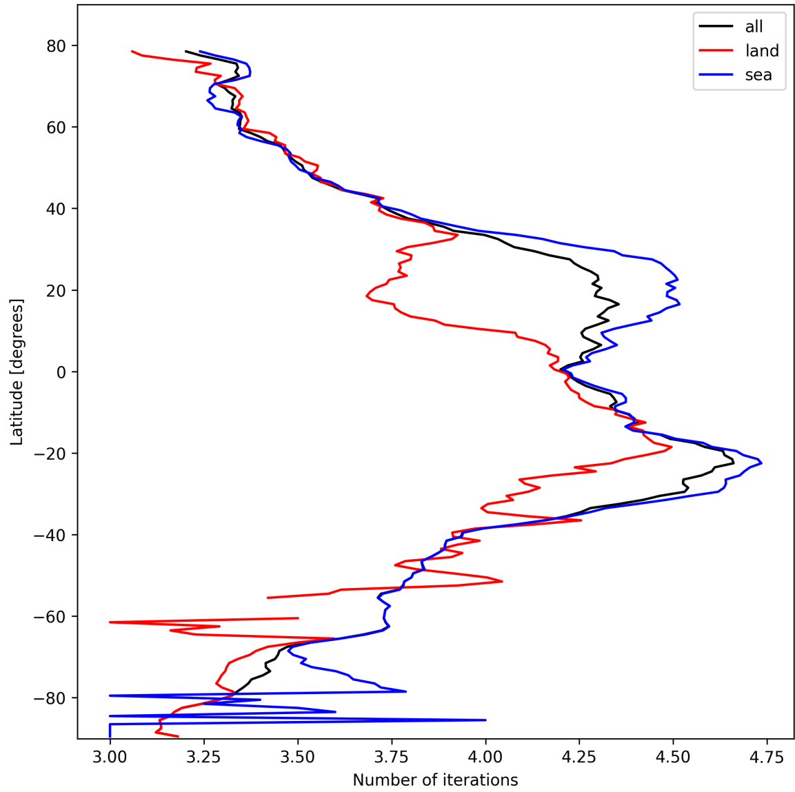
Figure 17: Zonal average of “Number of iterations” for 2025-10-17 to 2025-10-18.
