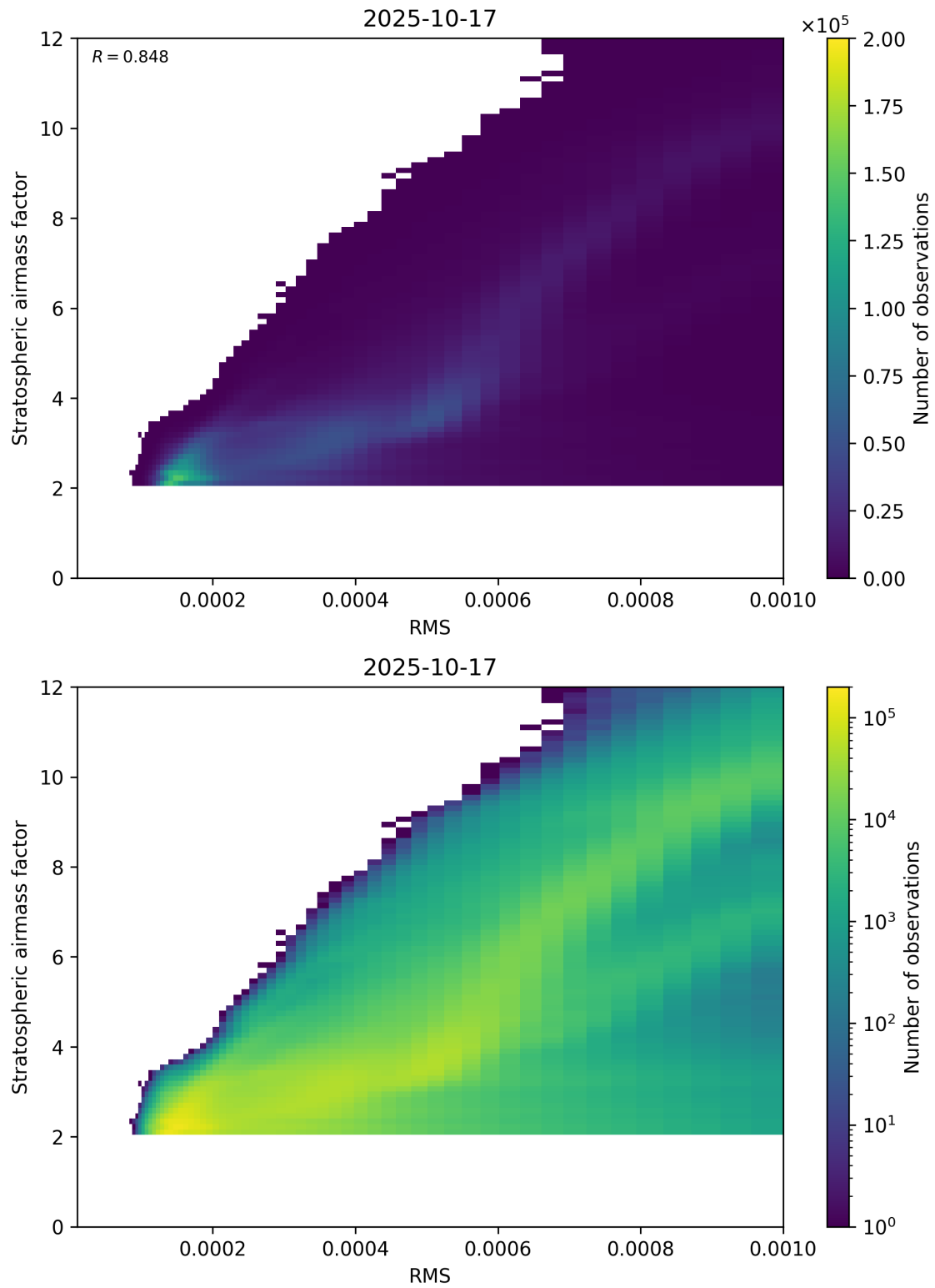
Figure 144: Scatter density plot of “RMS” against “Stratospheric airmass factor” for 2025-10-17 to 2025-10-18.
