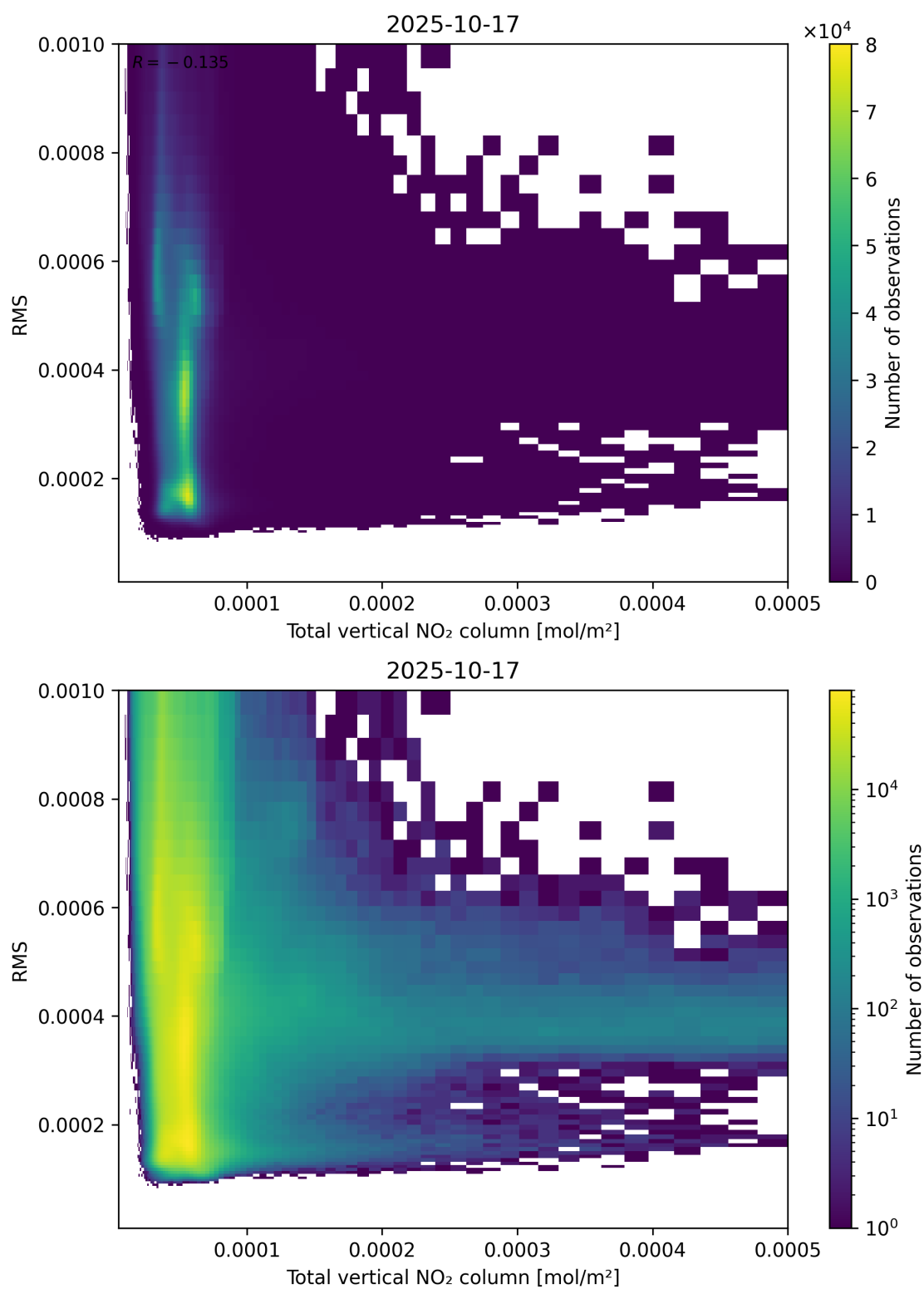
Figure 120: Scatter density plot of “Total vertical NO 2 column” against “RMS” for 2025-10-17 to 2025-10-18.
