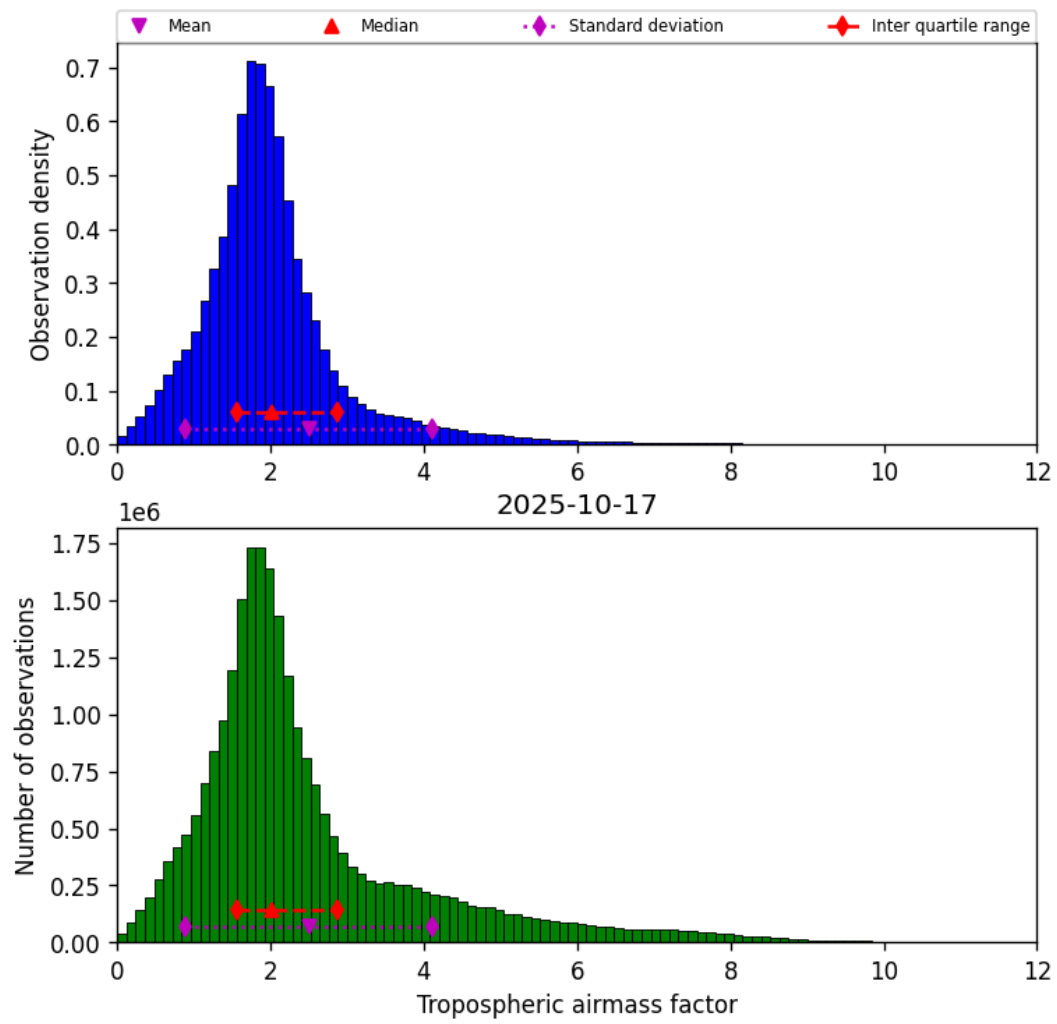
Figure 31: Histogram of “Tropospheric airmass factor” for 2025-10-17 to 2025-10-18
