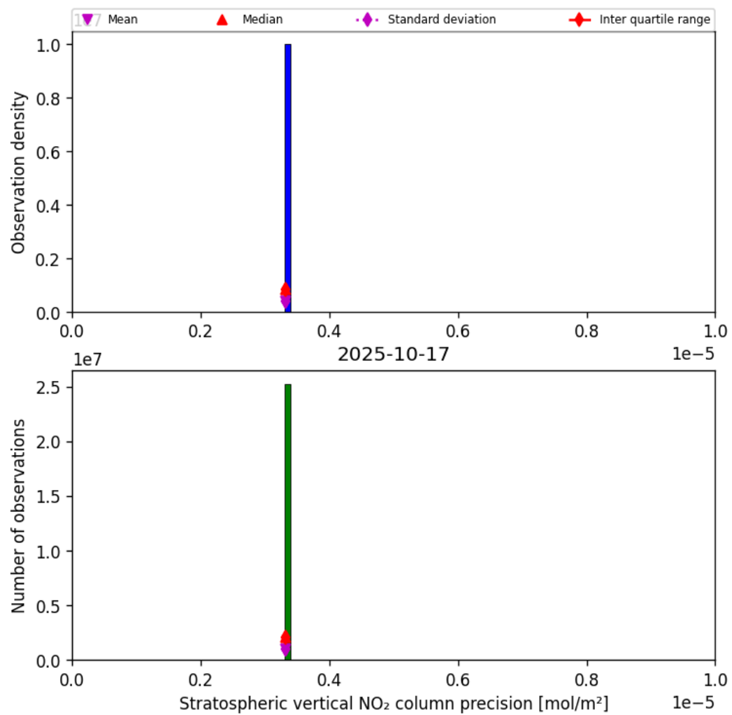
Figure 37: Histogram of “Stratospheric vertical NO 2 column precision” for 2025-10-17 to 2025-10-18
