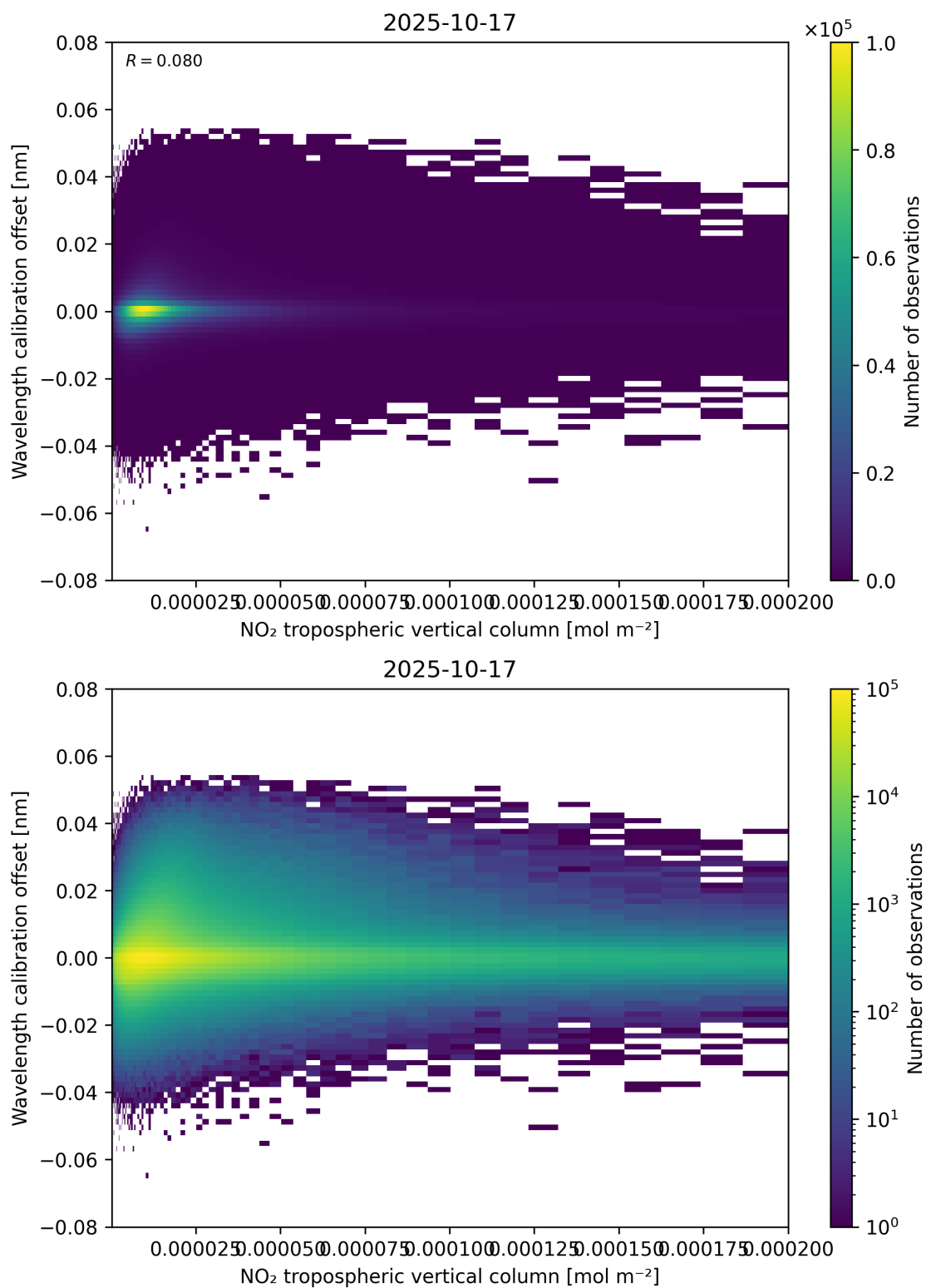
Figure 143: Scatter density plot of “NO 2 tropospheric vertical column” against “Wavelength calibration offset” for 2025-10-17 to 2025-10-18.
