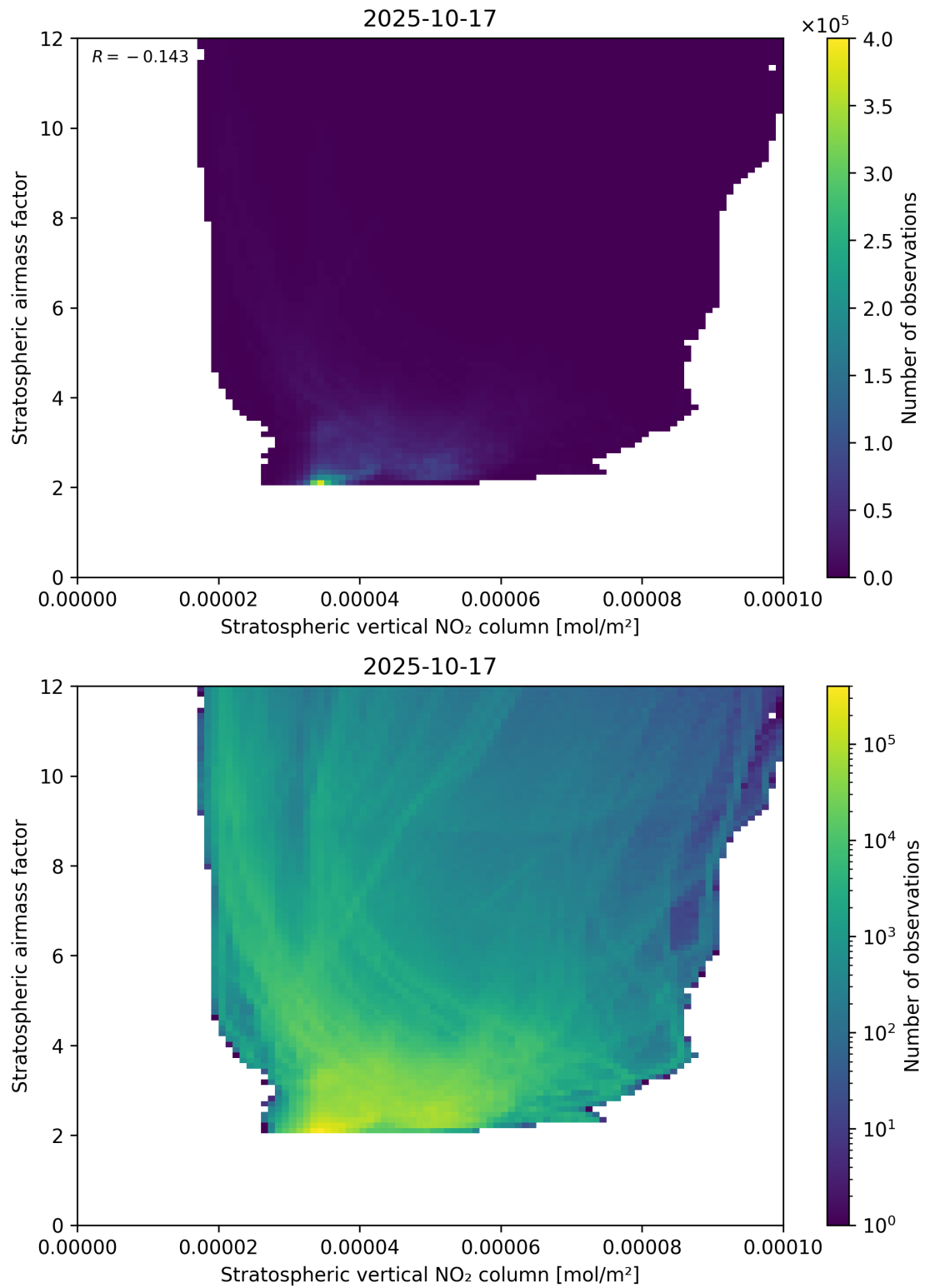
Figure 96: Scatter density plot of “Stratospheric vertical NO 2 column” against “Stratospheric airmass factor” for 2025-10-17 to 2025-10-18.
