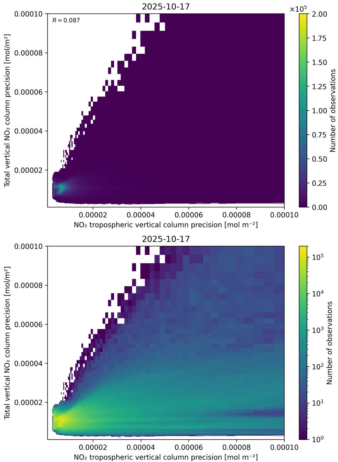
Figure 139: Scatter density plot of “NO 2 tropospheric vertical column precision” against “Total vertical NO 2 column precision” for 2025-10-17 to 2025-10-18.
