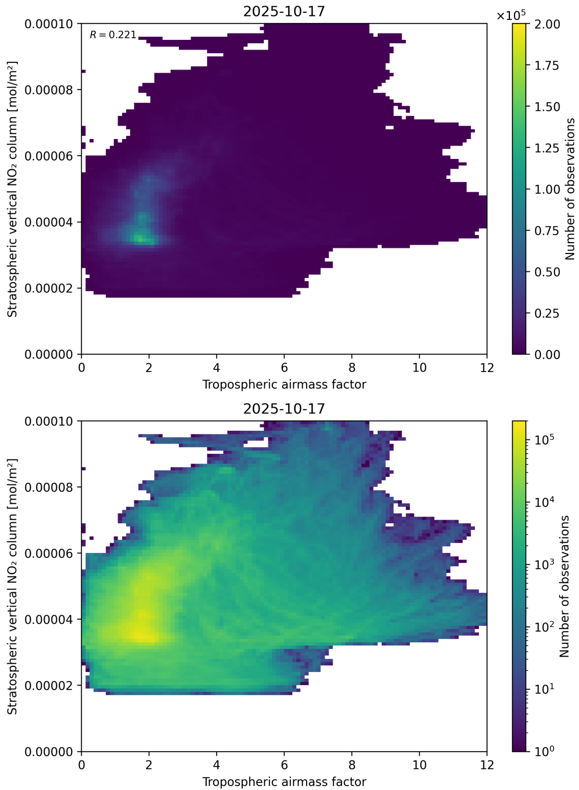
Figure 74: Scatter density plot of “Tropospheric air mass factor” against “Stratospheric vertical NO 2 column” for 2025-10-17 to 2025-10-18.
