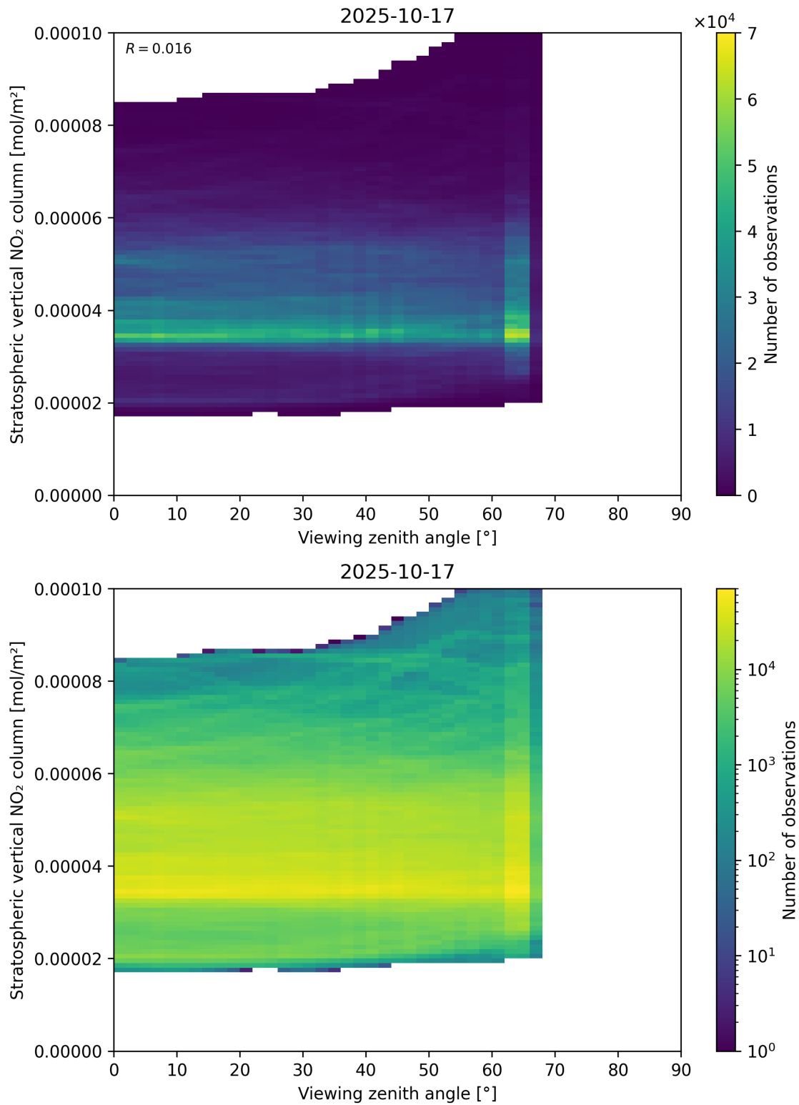
Figure 164: Scatter density plot of “Viewing zenith angle” against “Stratospheric vertical NO 2 column” for 2025-10-17 to 2025-10-18.
