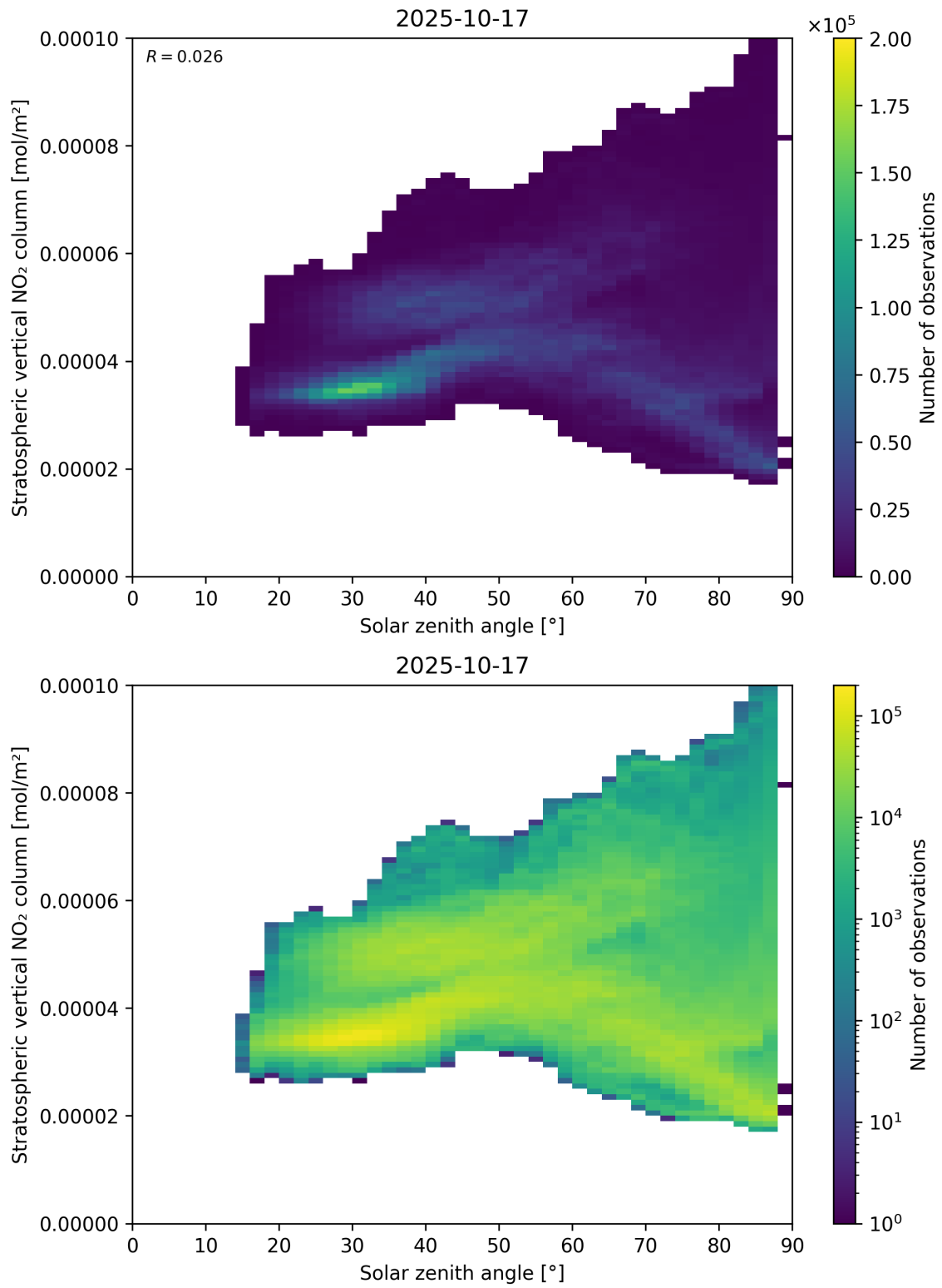
Figure 150: Scatter density plot of “Solar zenith angle” against “Stratospheric vertical NO 2 column” for 2025-10-17 to 2025-10-18.
