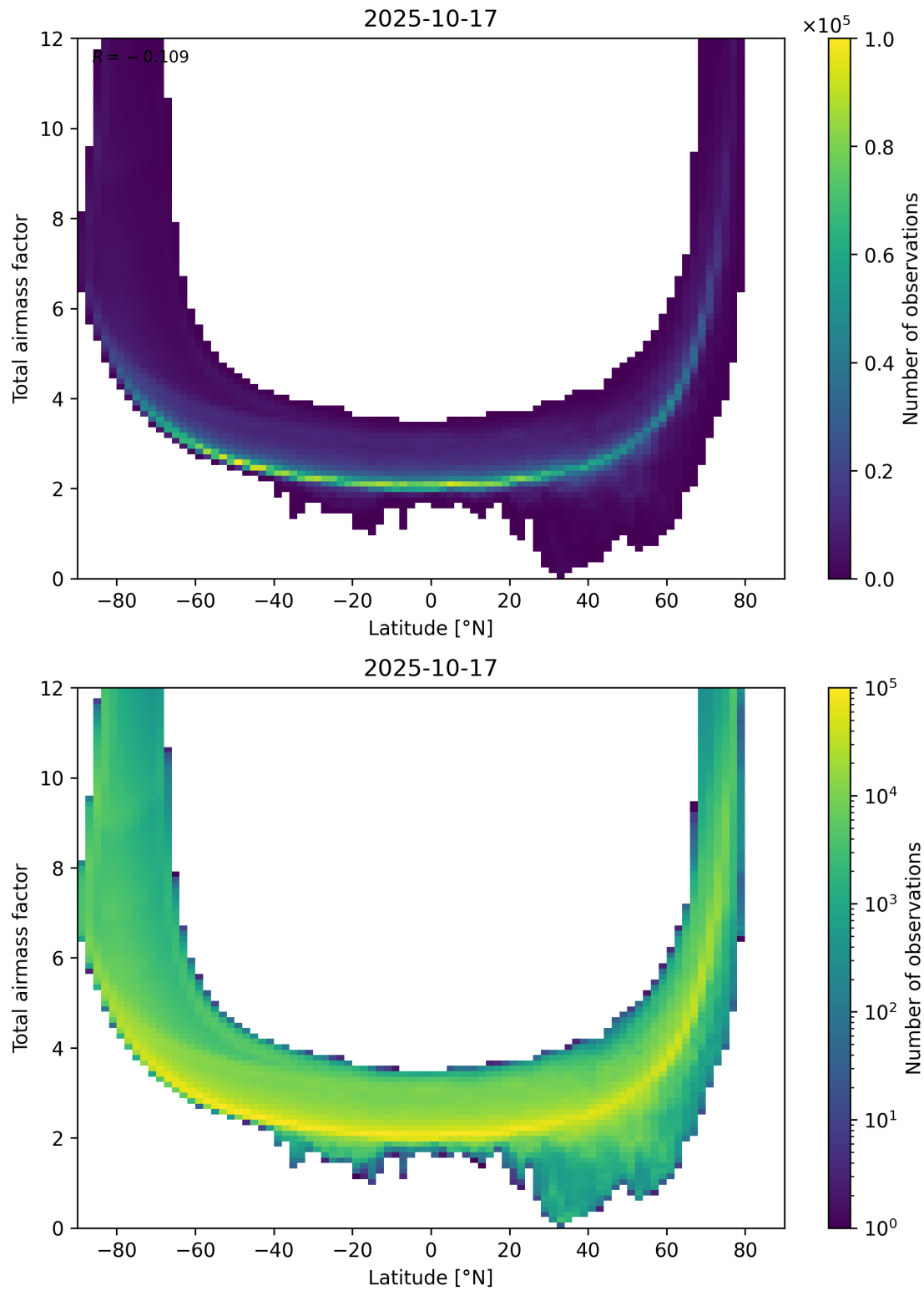
Figure 84: Scatter density plot of “Latitude” against “Total airmass factor” for 2025-10-17 to 2025-10-18.
