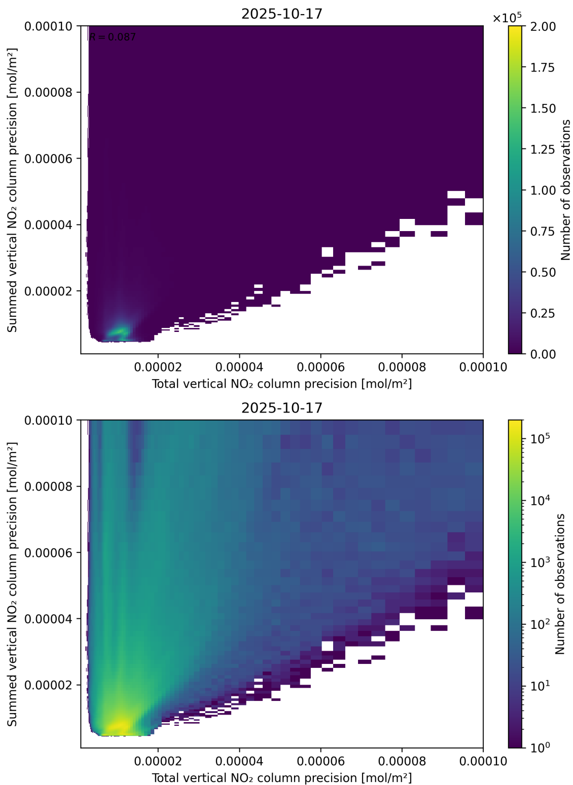
Figure 118: Scatter density plot of “Total vertical NO 2 column precision” against “Summed vertical NO 2 column precision” for 2025-10-17 to 2025-10-18.
