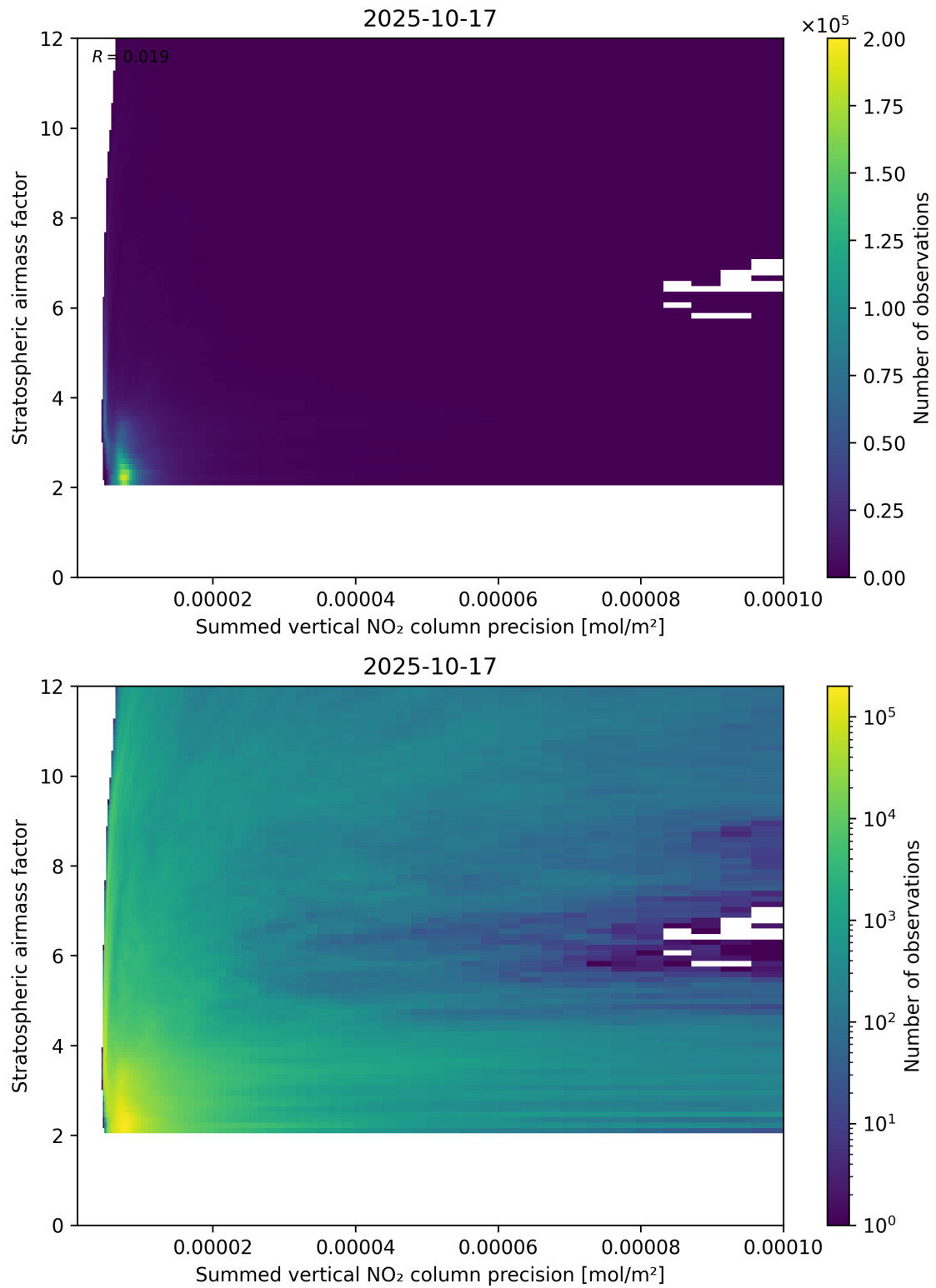
Figure 106: Scatter density plot of “Summed vertical NO 2 column precision” against “Stratospheric airmass factor” for 2025-10-17 to 2025-10-18.
