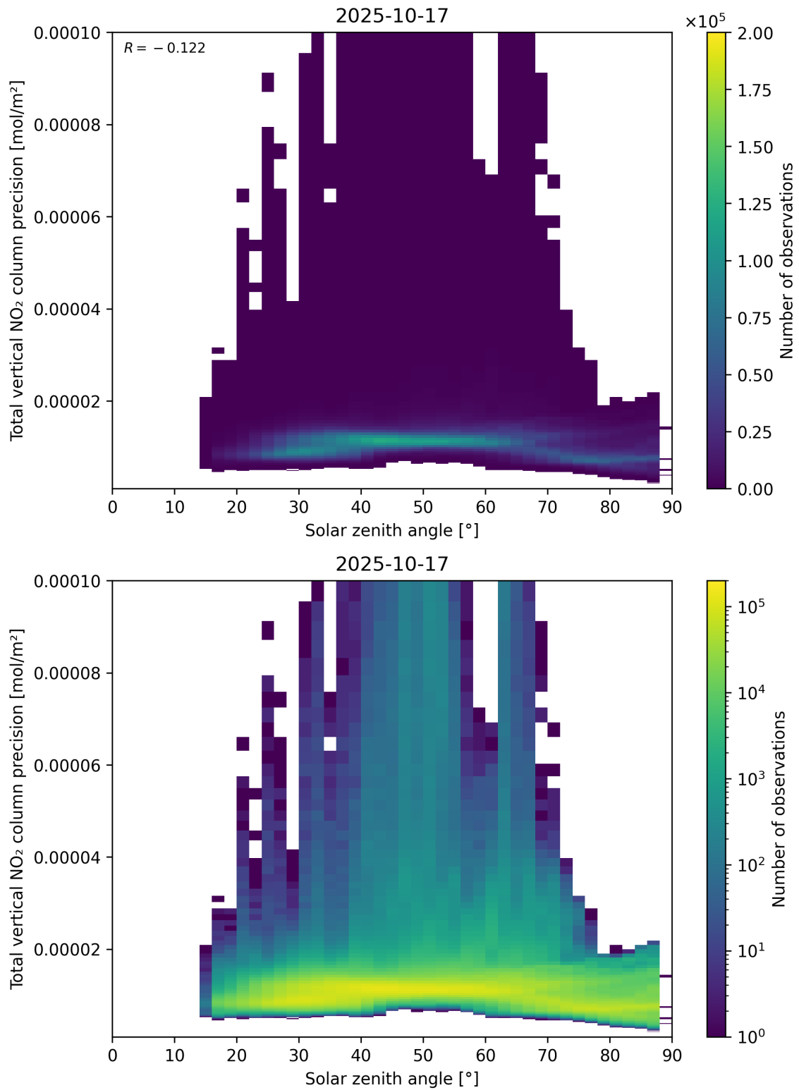
Figure 154: Scatter density plot of “Solar zenith angle” against “Total vertical NO 2 column precision” for 2025-10-17 to 2025-10-18.
