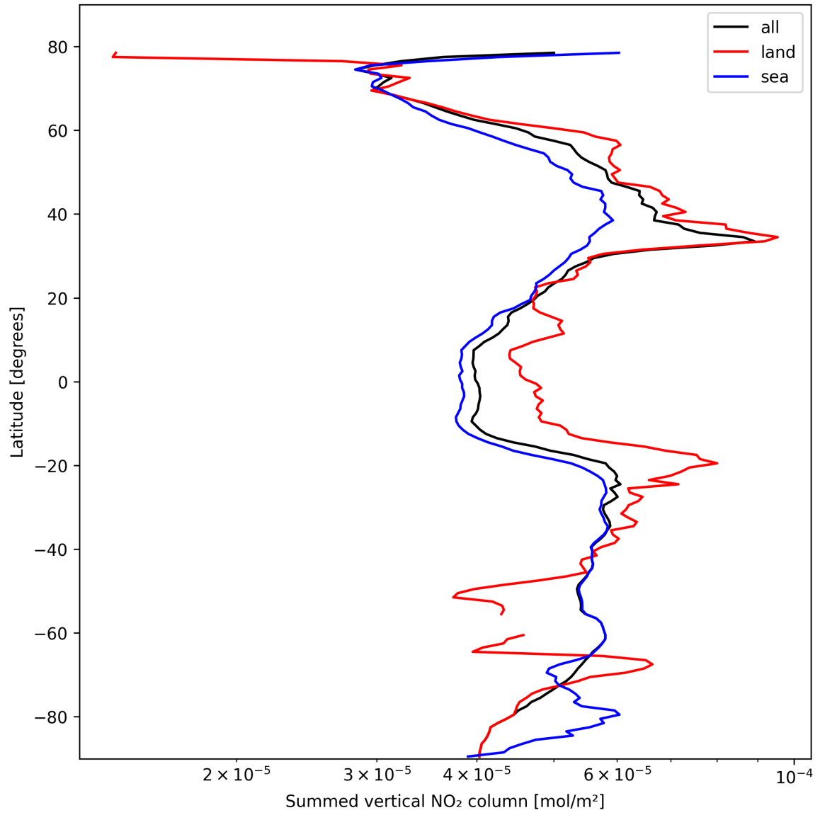
Figure 23: Zonal average of “Summed vertical NO 2 column” for 2025-10-17 to 2025-10-18.
