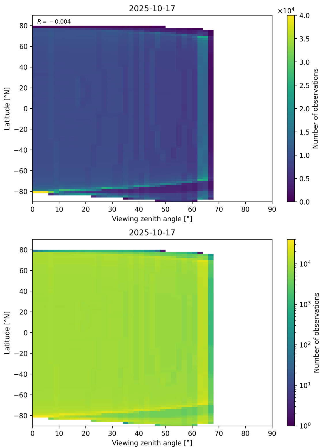
Figure 163: Scatter density plot of “Viewing zenith angle” against “Latitude” for 2025-10-17 to 2025-10-18.
