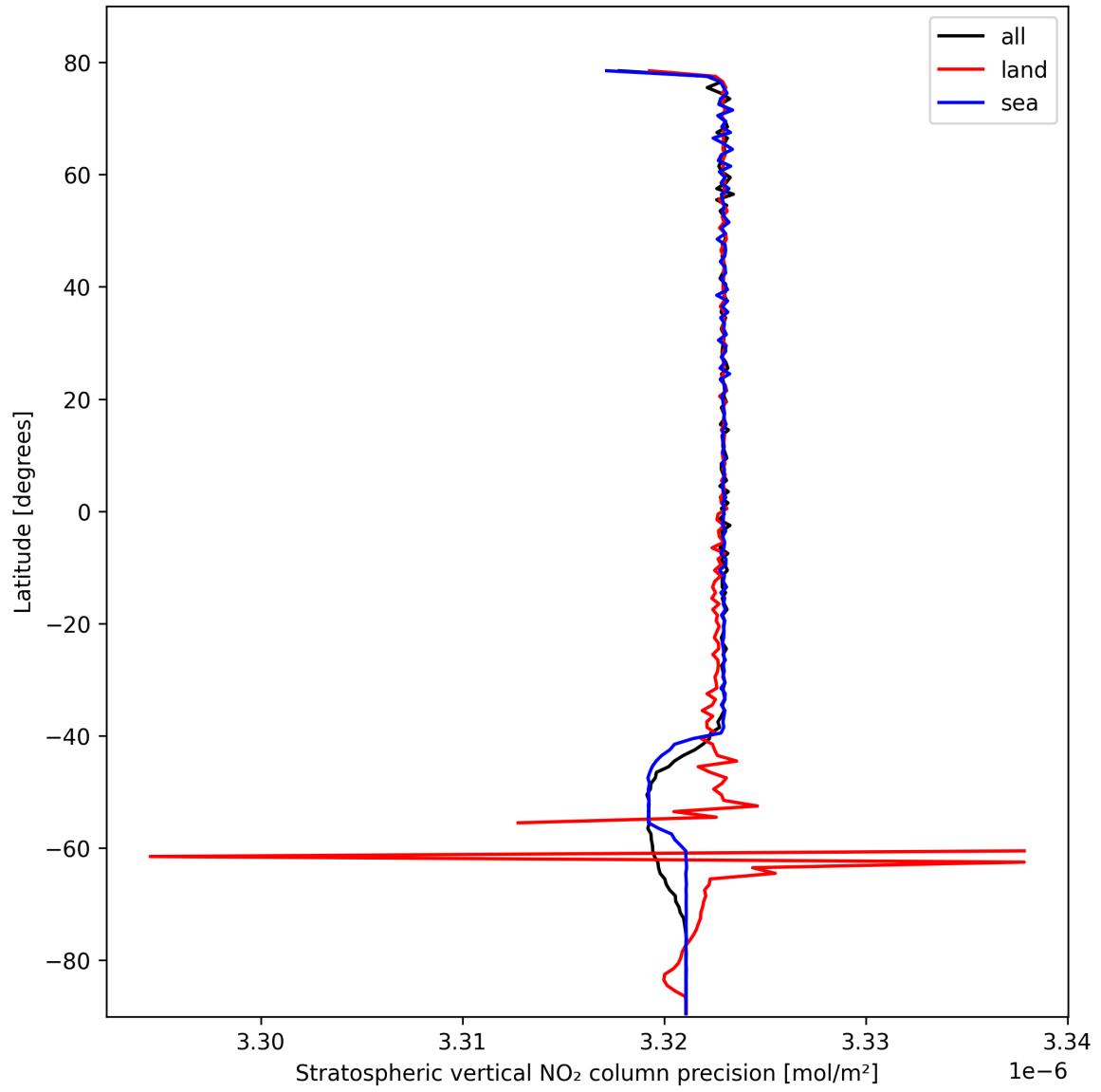
Figure 20: Zonal average of “Stratospheric vertical NO 2 column precision” for 2025-10-17 to 2025-10-18.
