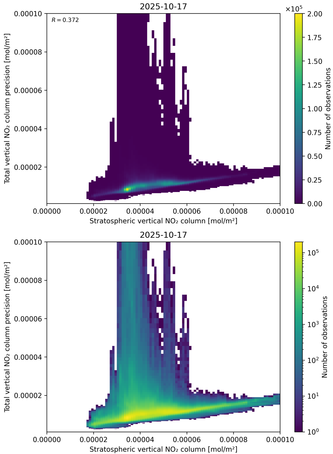
Figure 101: Scatter density plot of “Stratospheric vertical NO 2 column” against “Total vertical NO 2 column precision” for 2025-10-17 to 2025-10-18.
