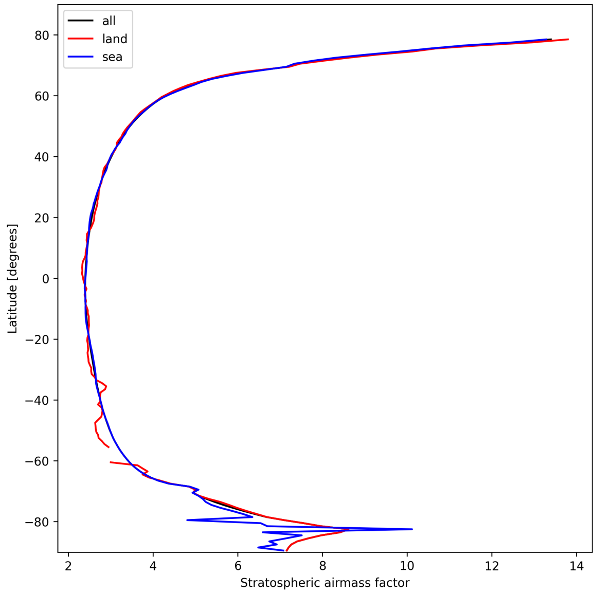
Figure 27: Zonal average of “Stratospheric airmass factor” for 2025-10-17 to 2025-10-18.
