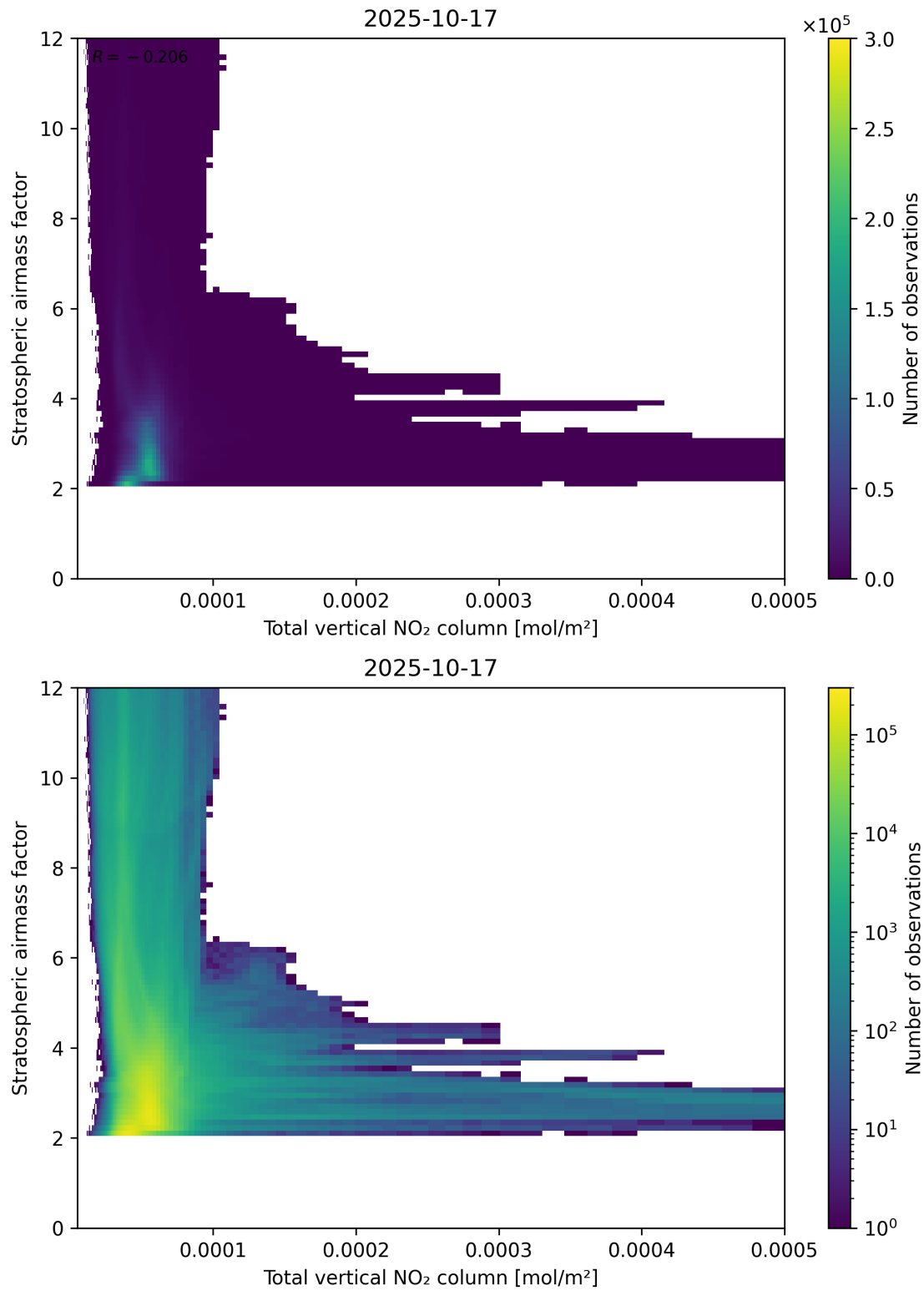
Figure 110: Scatter density plot of “Total vertical NO 2 column” against “Stratospheric airmass factor” for 2025-10-17 to 2025-10-18.
