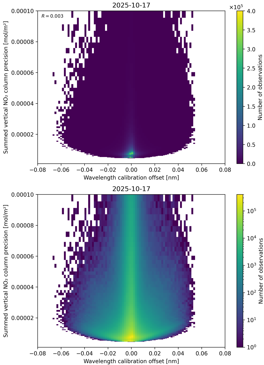
Figure 178: Scatter density plot of “Wavelength calibration offset” against “Summed vertical NO 2 column precision” for 2025-10-17 to 2025-10-18.
