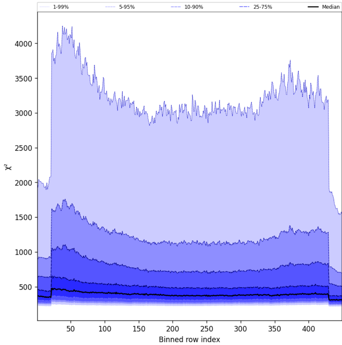
Figure 59: Along track statistics of “ \chi^2 ” for 2025-10-17 to 2025-10-18
