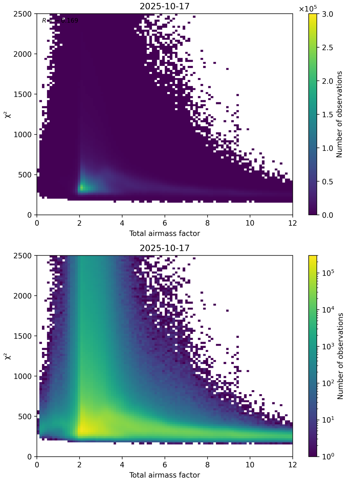
Figure 63: Scatter density plot of “Total airmass factor” against “ \chi^2 ” for 2025-10-17 to 2025-10-18.
