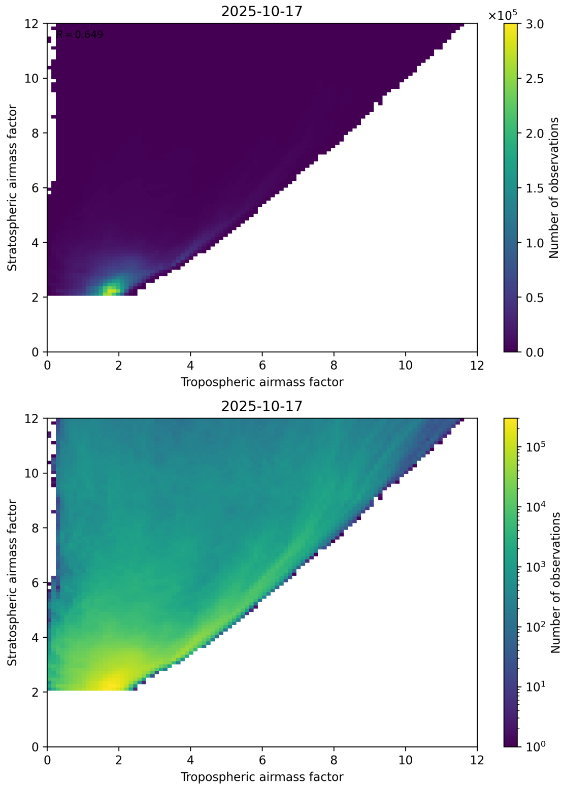
Figure 71: Scatter density plot of “Tropospheric airmass factor” against “Stratospheric airmass factor” for 2025-10-17 to 2025-10-18.
