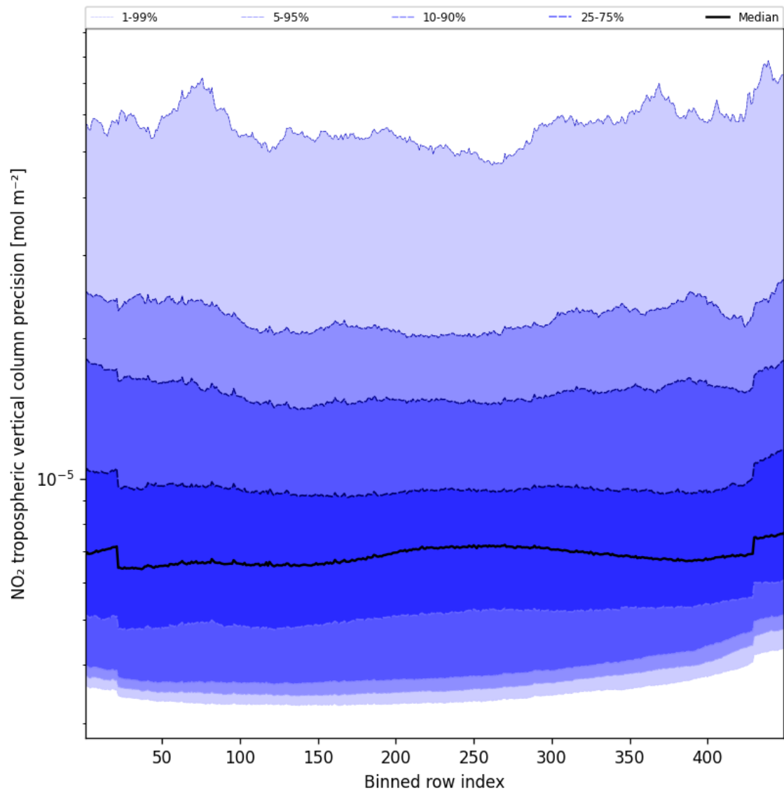
Figure 47: Along track statistics of “NO 2 tropospheric vertical column precision” for 2025-10-17 to 2025-10-18
