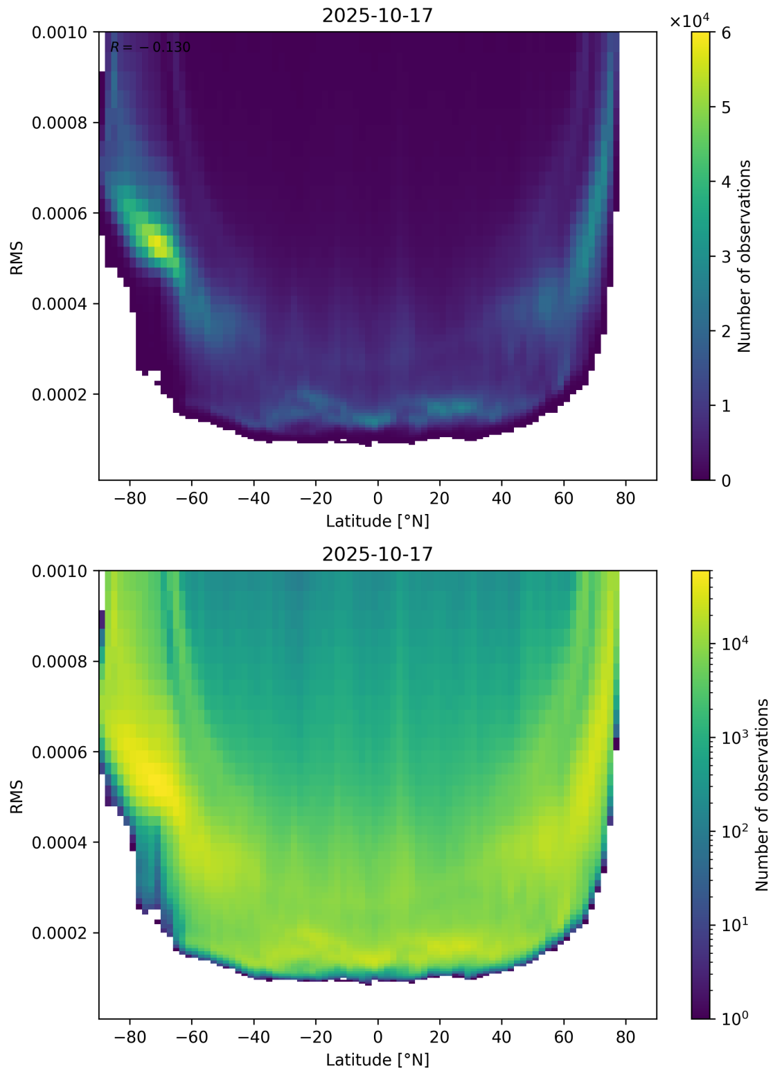
Figure 94: Scatter density plot of “Latitude” against “RMS” for 2025-10-17 to 2025-10-18.
