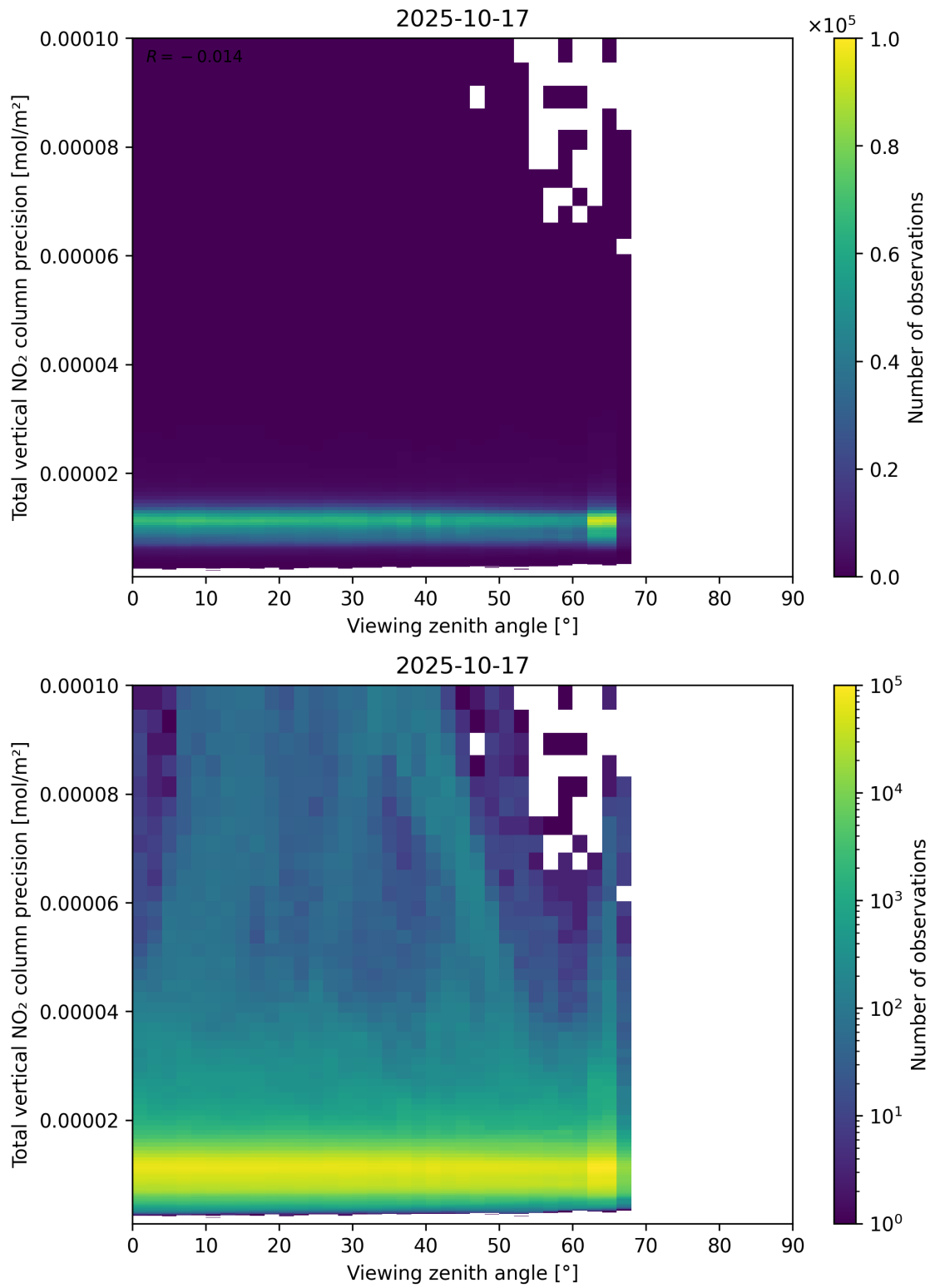
Figure 168: Scatter density plot of “Viewing zenith angle” against “Total vertical NO 2 column precision” for 2025-10-17 to 2025-10-18.
