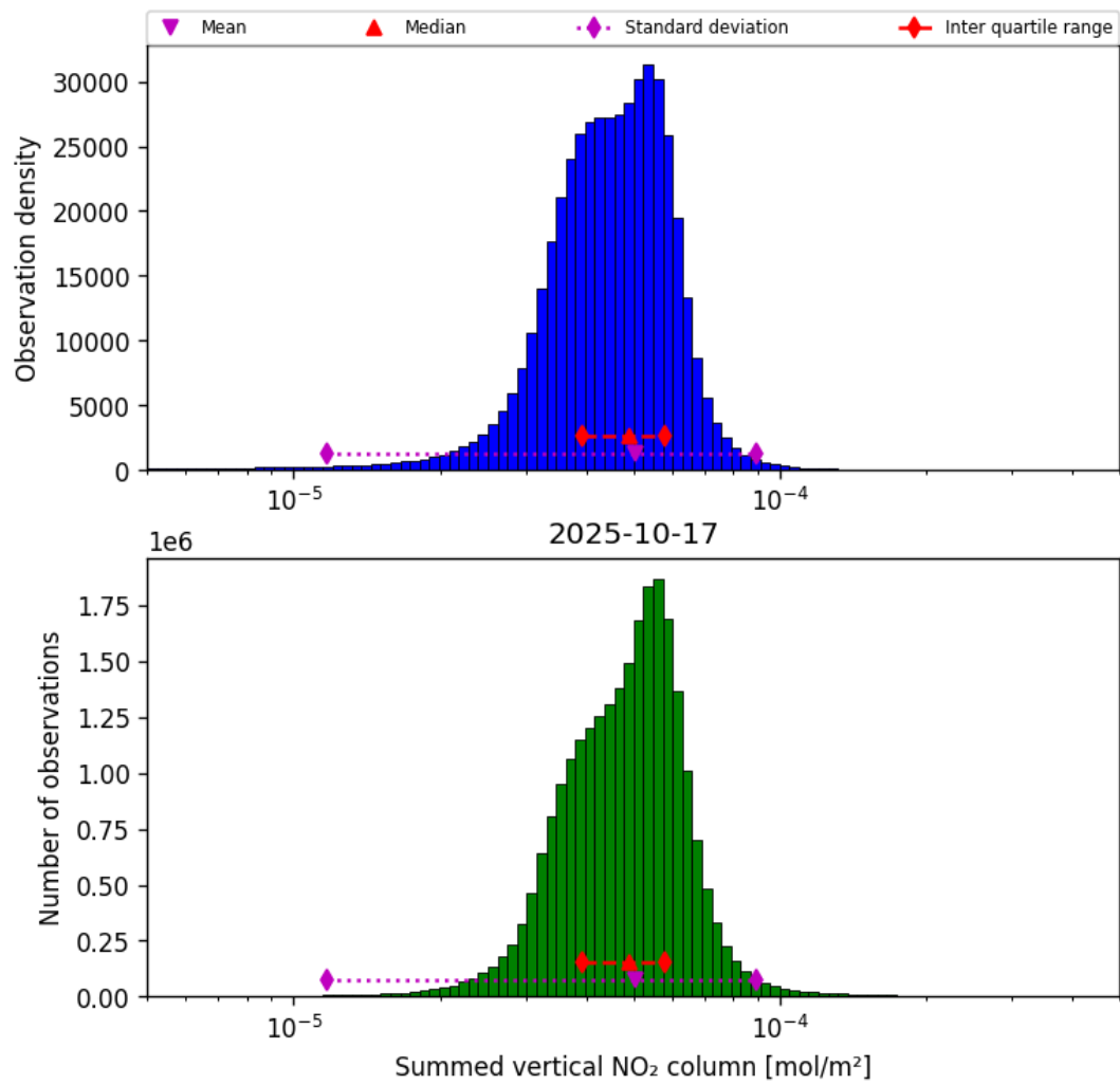
Figure 40: Histogram of “Summed vertical NO 2 column” for 2025-10-17 to 2025-10-18
