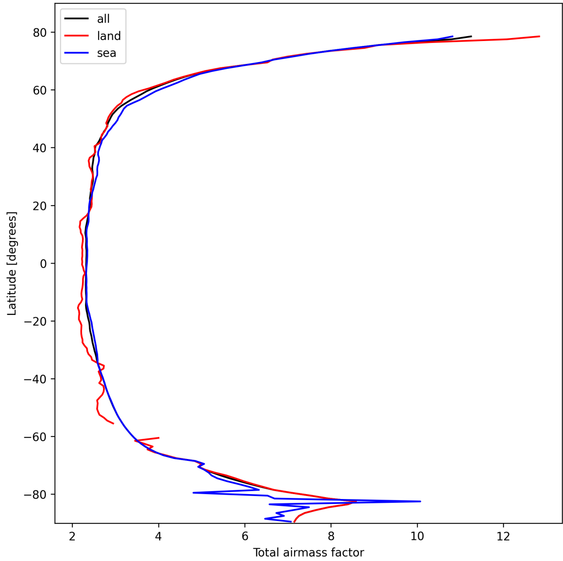
Figure 15: Zonal average of “Total airmass factor” for 2025-10-17 to 2025-10-18.
