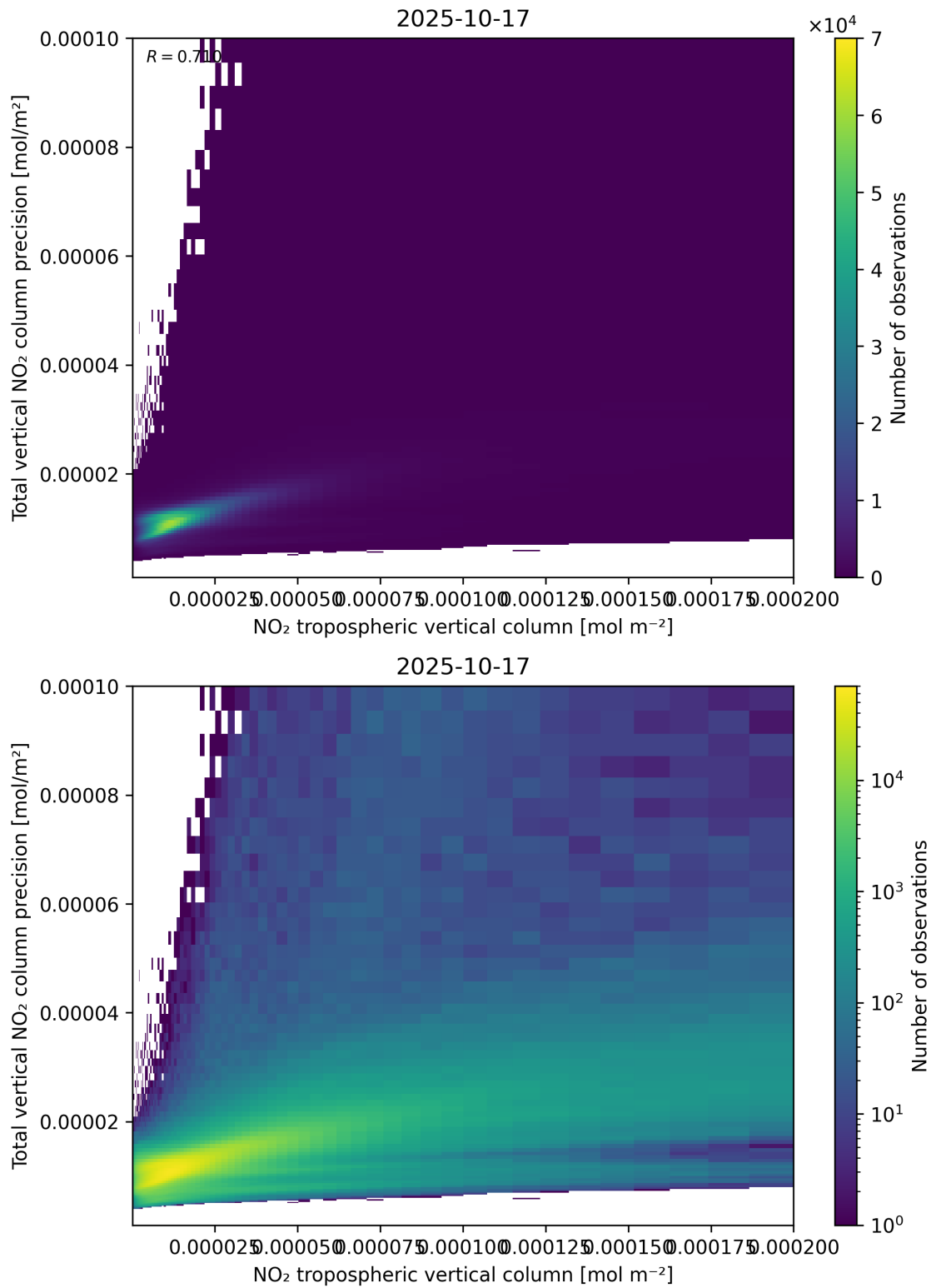
Figure 129: Scatter density plot of “NO 2 tropospheric vertical column” against “Total vertical NO 2 column precision” for 2025-10-17 to 2025-10-18.
