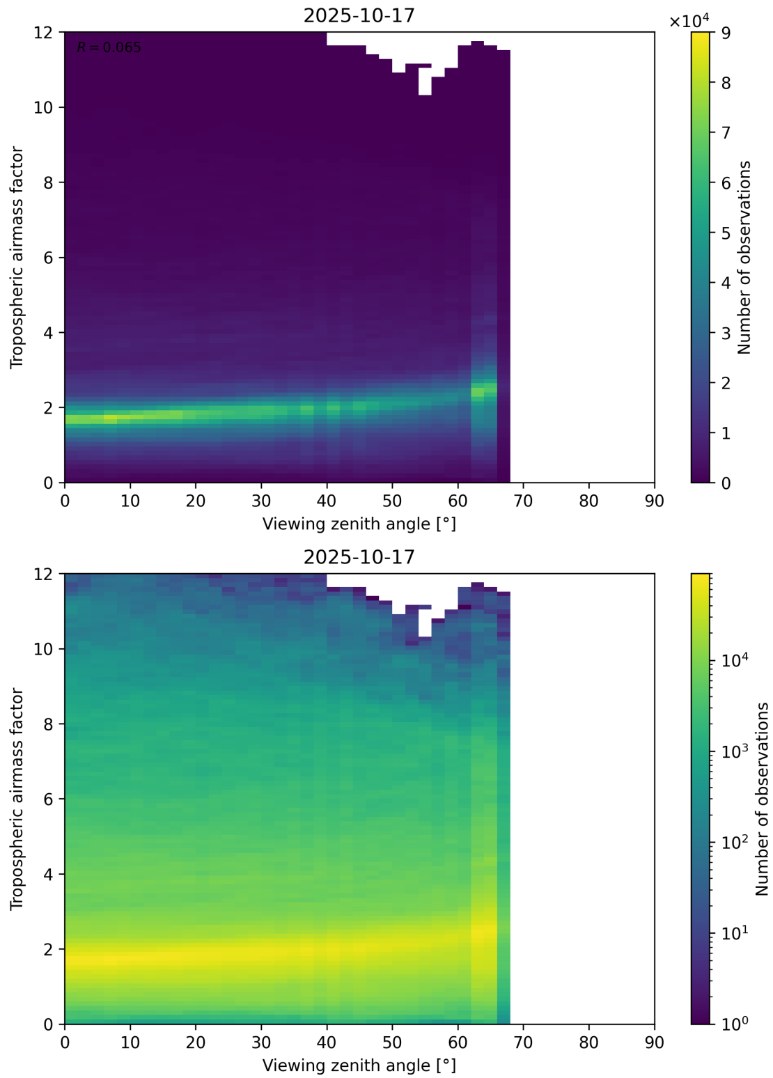
Figure 161: Scatter density plot of “Viewing zenith angle” against “Tropospheric airmass factor” for 2025-10-17 to 2025-10-18.
