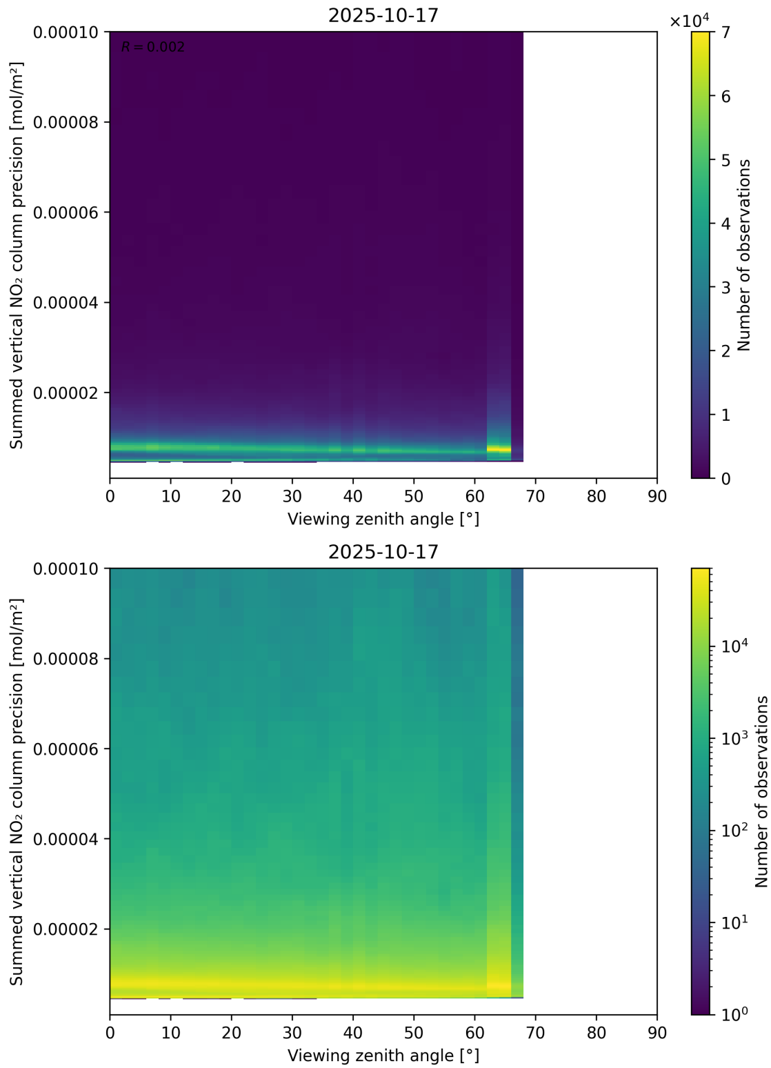
Figure 166: Scatter density plot of “Viewing zenith angle” against “Summed vertical NO 2 column precision” for 2025-10-17 to 2025-10-18.
