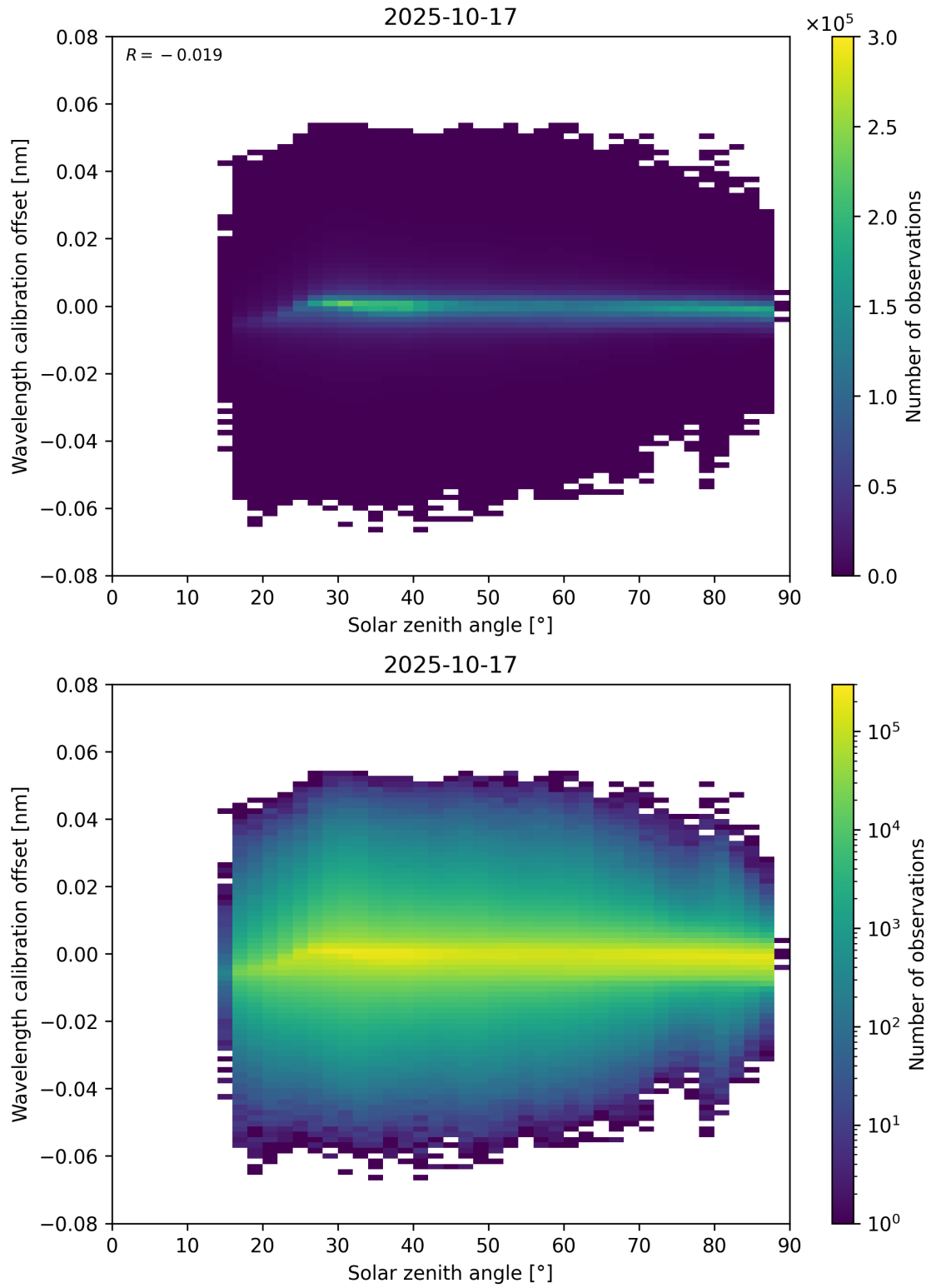
Figure 158: Scatter density plot of “Solar zenith angle” against “Wavelength calibration offset” for 2025-10-17 to 2025-10-18.
