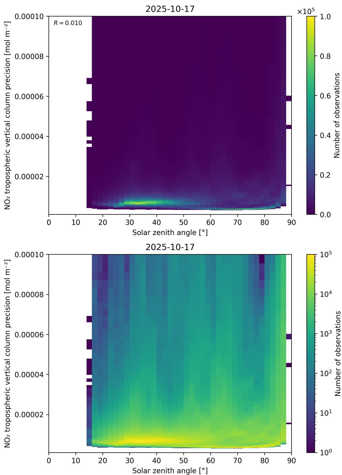
Figure 156: Scatter density plot of “Solar zenith angle” against “NO 2 tropospheric vertical column precision” for 2025-10-17 to 2025-10-18.
