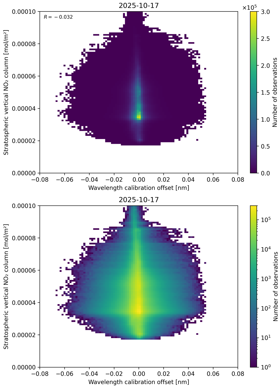
Figure 176: Scatter density plot of “Wavelength calibration offset” against “Stratospheric vertical NO 2 column” for 2025-10-17 to 2025-10-18.
