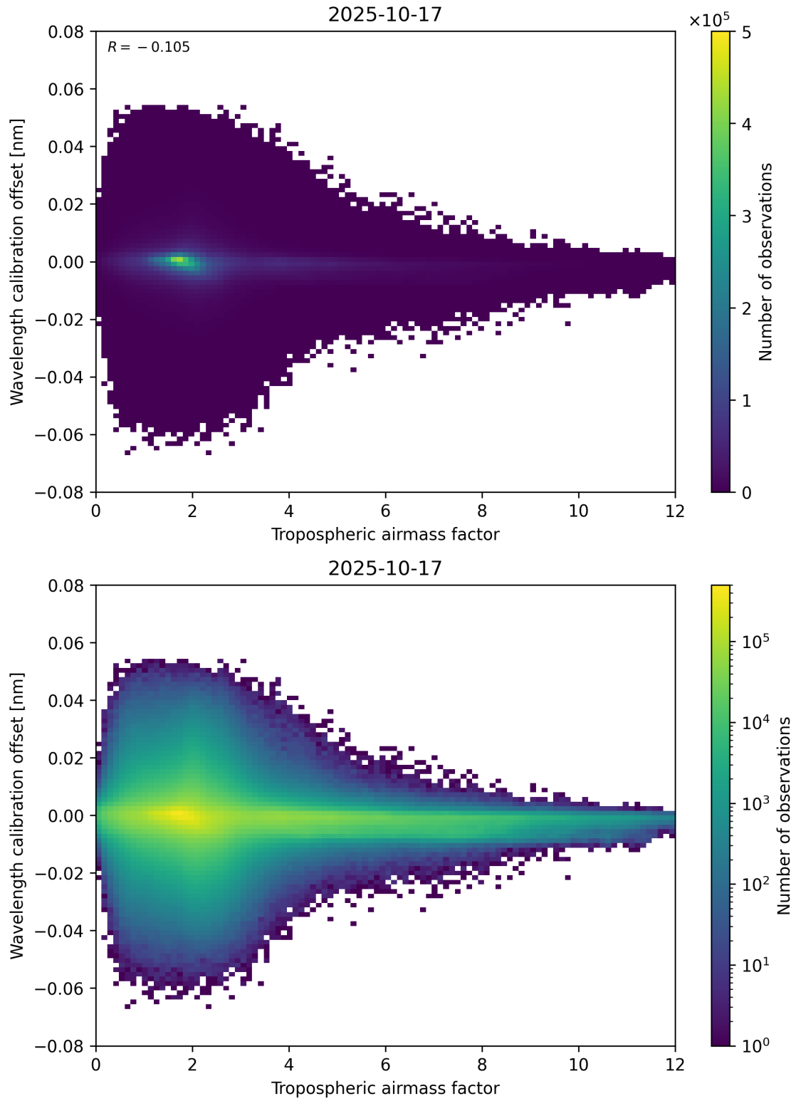
Figure 80: Scatter density plot of “Tropospheric airmass factor” against “Wavelength calibration offset” for 2025-10-17 to 2025-10-18.
