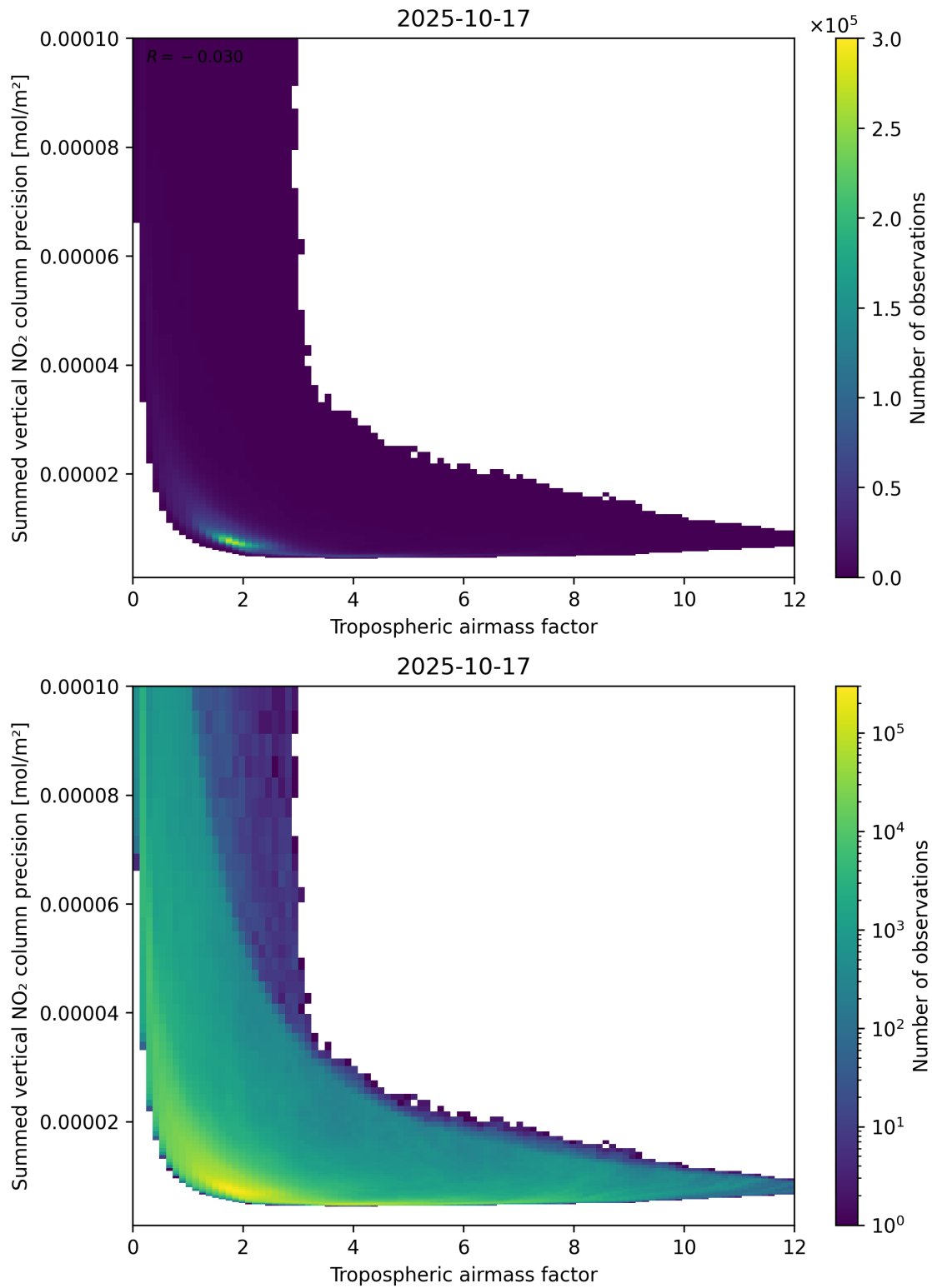
Figure 76: Scatter density plot of “Tropospheric airmass factor” against “Summed vertical NO 2 column precision” for 2025-10-17 to 2025-10-18.
