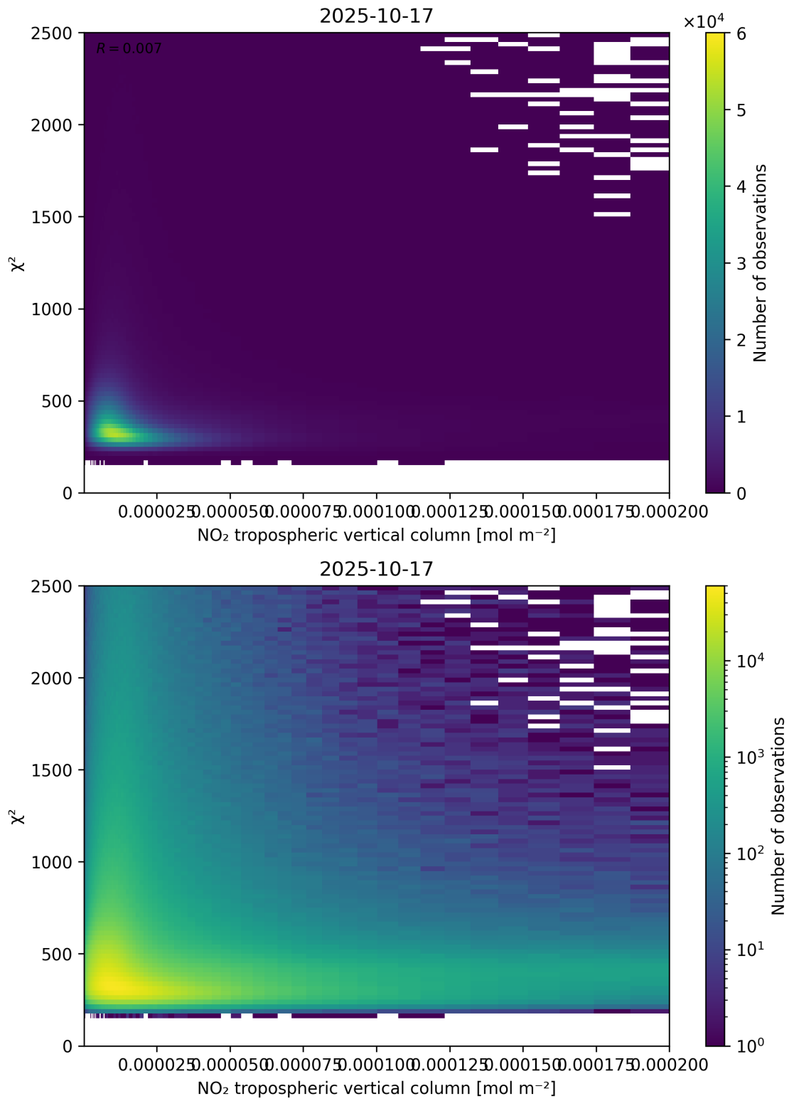
Figure 124: Scatter density plot of “NO 2 tropospheric vertical column” against “ \chi^2 ” for 2025-10-17 to 2025-10-18.
