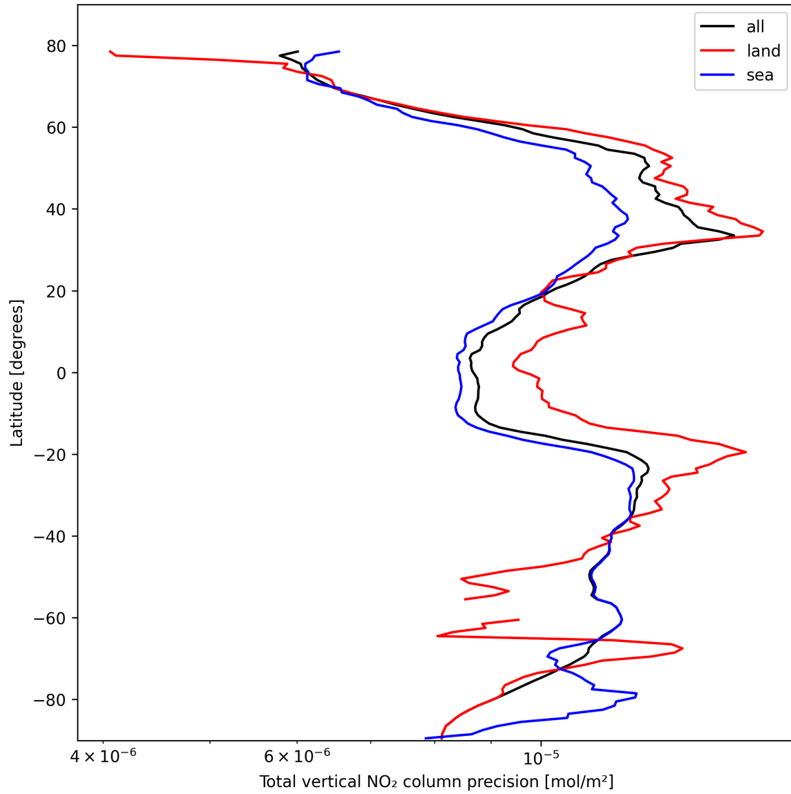
Figure 22: Zonal average of “Total vertical NO 2 column precision” for 2025-10-17 to 2025-10-18.
