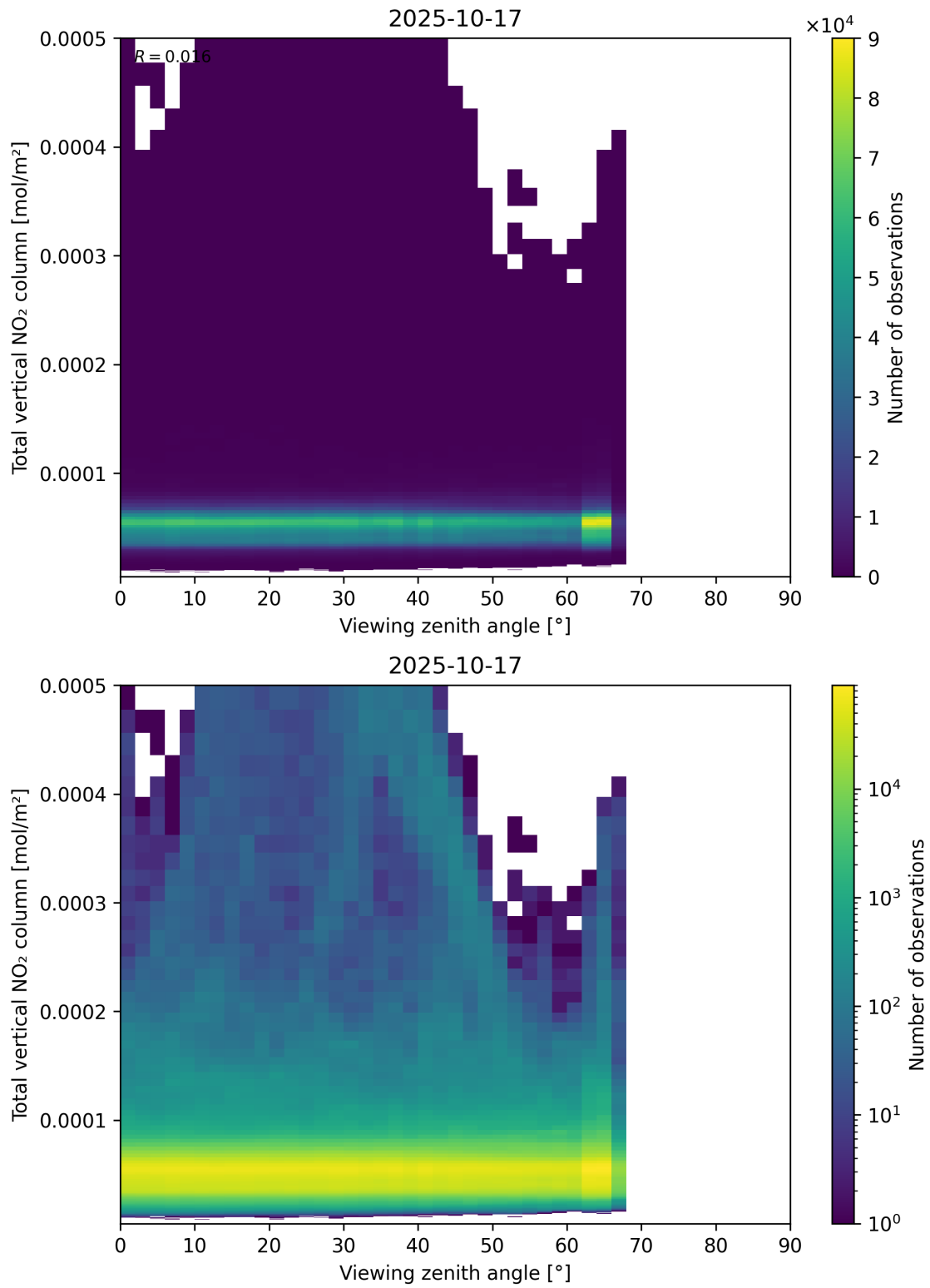
Figure 167: Scatter density plot of “Viewing zenith angle” against “Total vertical NO 2 column” for 2025-10-17 to 2025-10-18.
