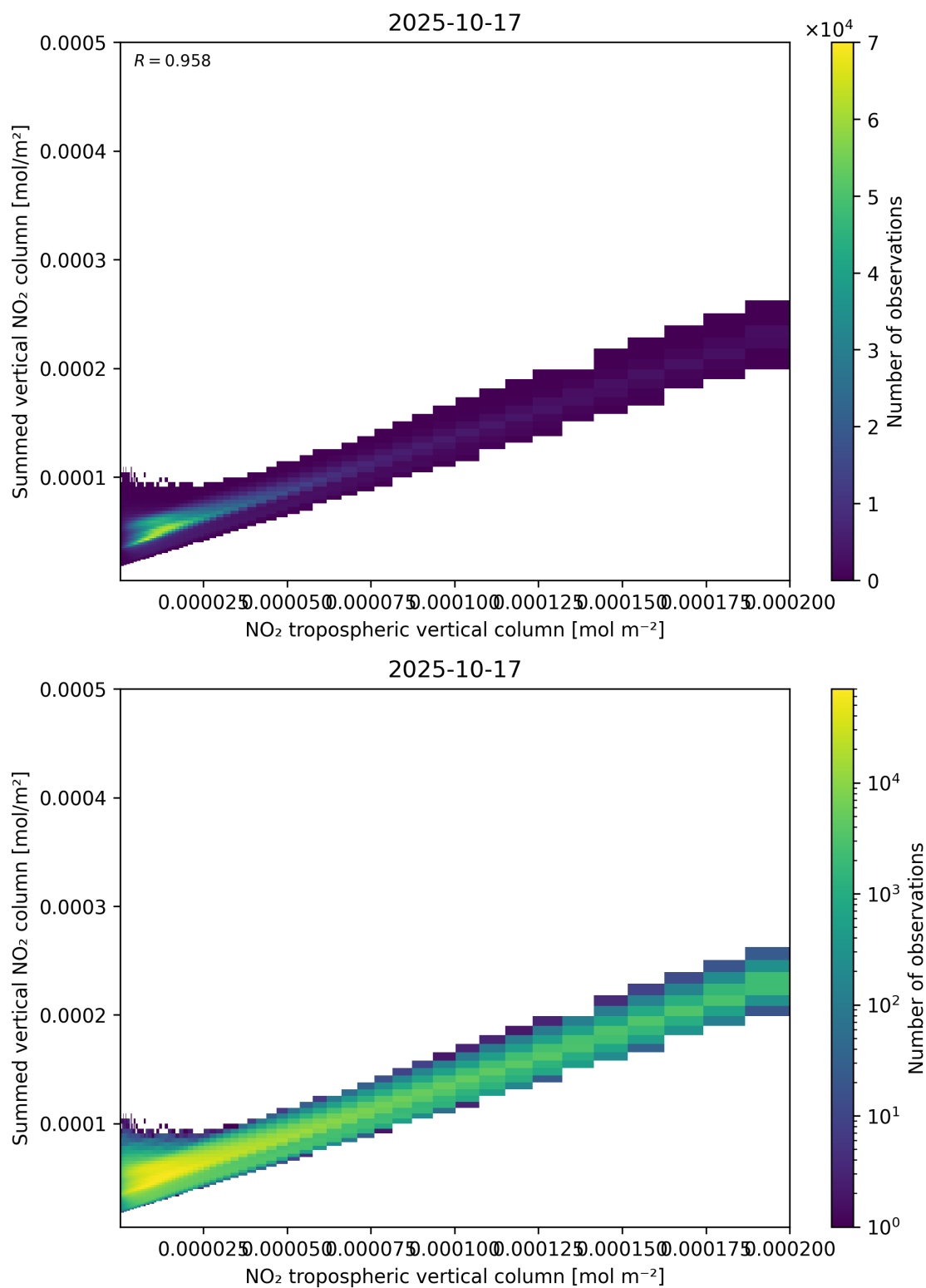
Figure 126: Scatter density plot of “NO 2 tropospheric vertical column” against “Summed vertical NO 2 column” for 2025-10-17 to 2025-10-18.
