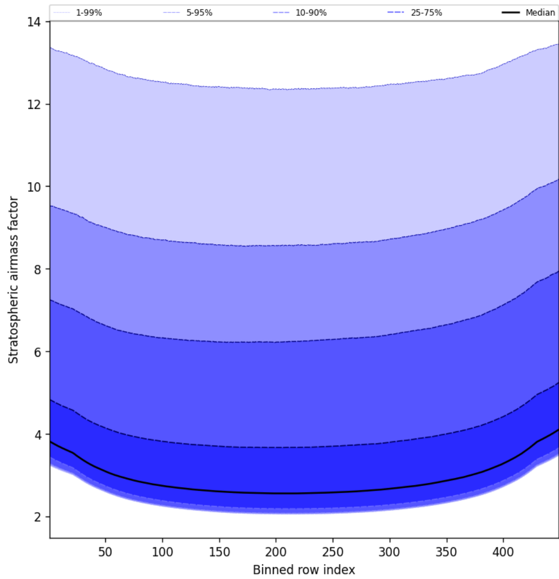
Figure 61: Along track statistics of “Stratospheric air mass factor” for 2025-10-17 to 2025-10-18
