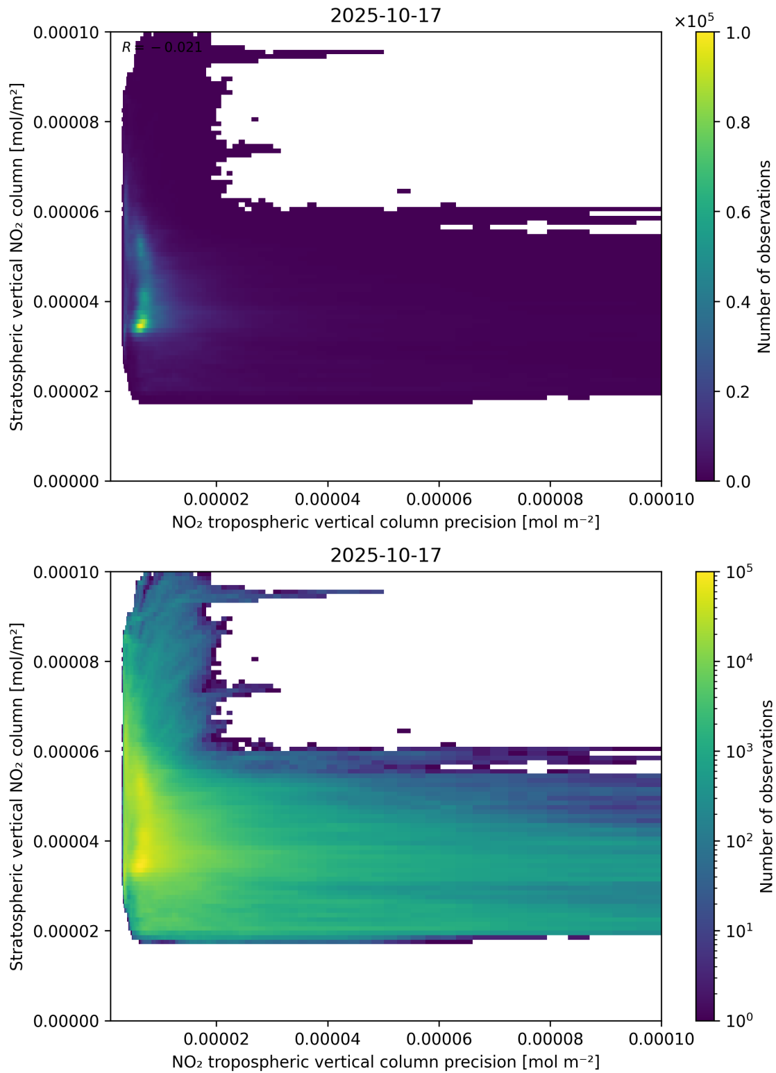
Figure 135: Scatter density plot of “NO 2 tropospheric vertical column precision” against “Stratospheric vertical NO 2 column” for 2025-10-17 to 2025-10-18.
