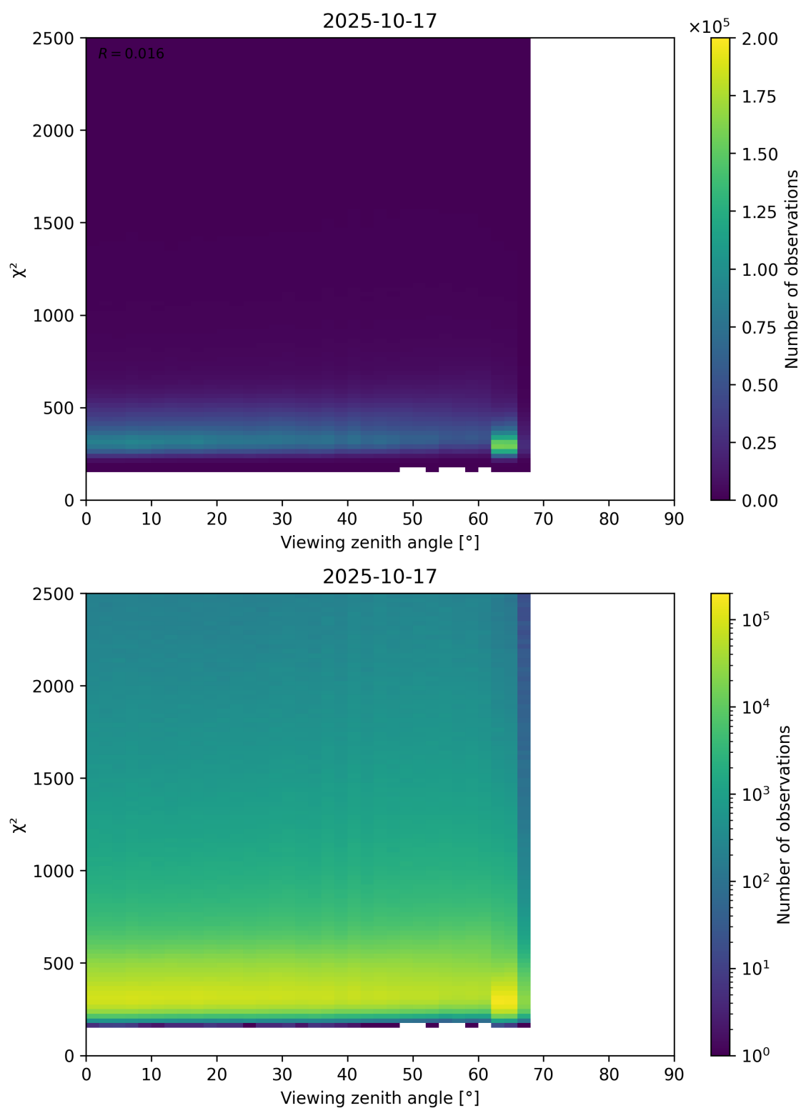
Figure 162: Scatter density plot of “Viewing zenith angle” against “ \chi^2 ” for 2025-10-17 to 2025-10-18.
