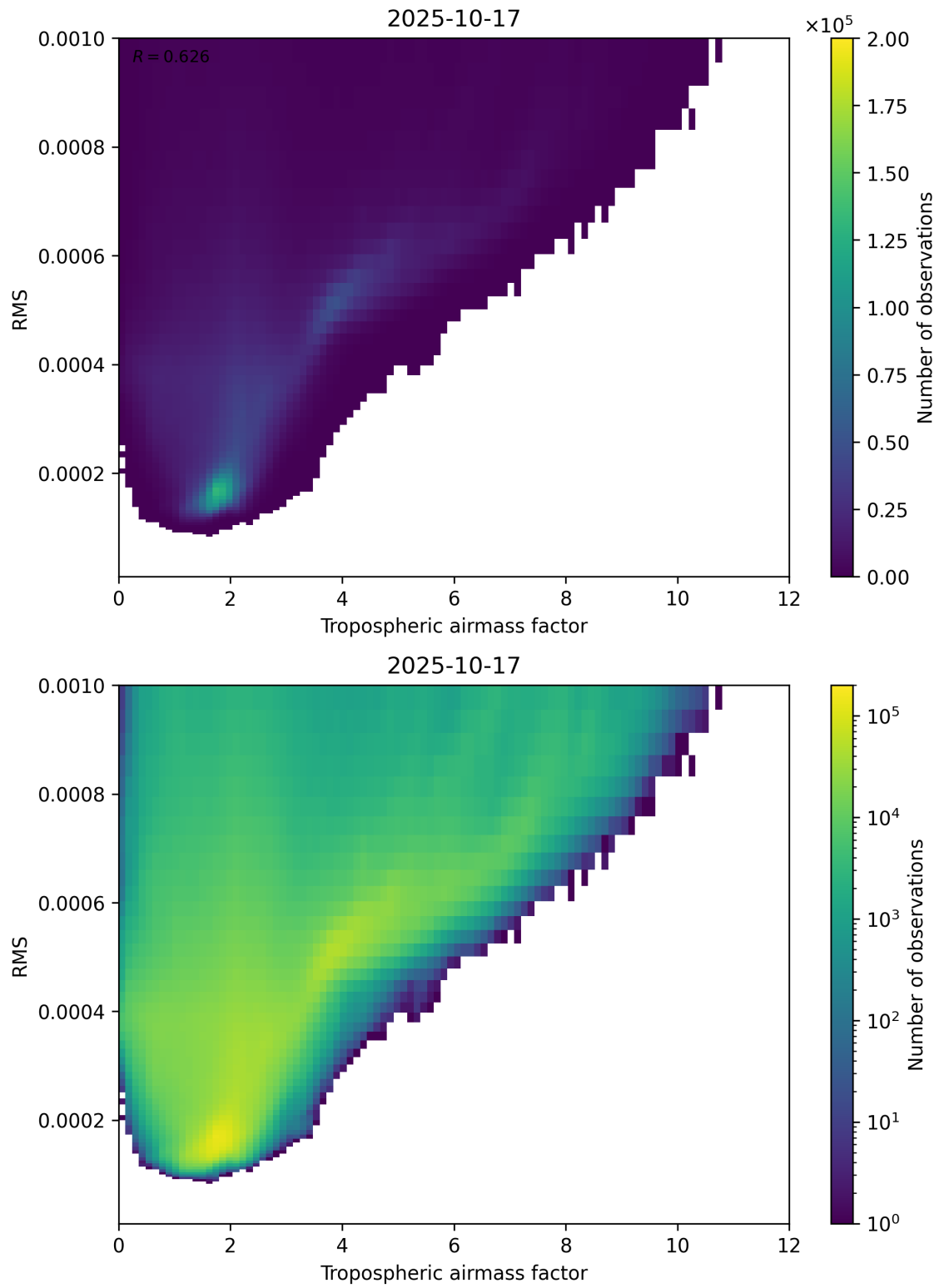
Figure 79: Scatter density plot of “Tropospheric airmass factor” against “RMS” for 2025-10-17 to 2025-10-18.
