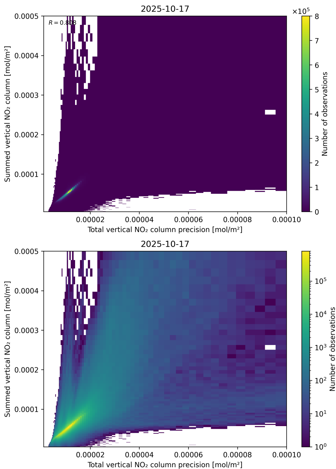
Figure 117: Scatter density plot of “Total vertical NO 2 column precision” against “Summed vertical NO 2 column” for 2025-10-17 to 2025-10-18.
