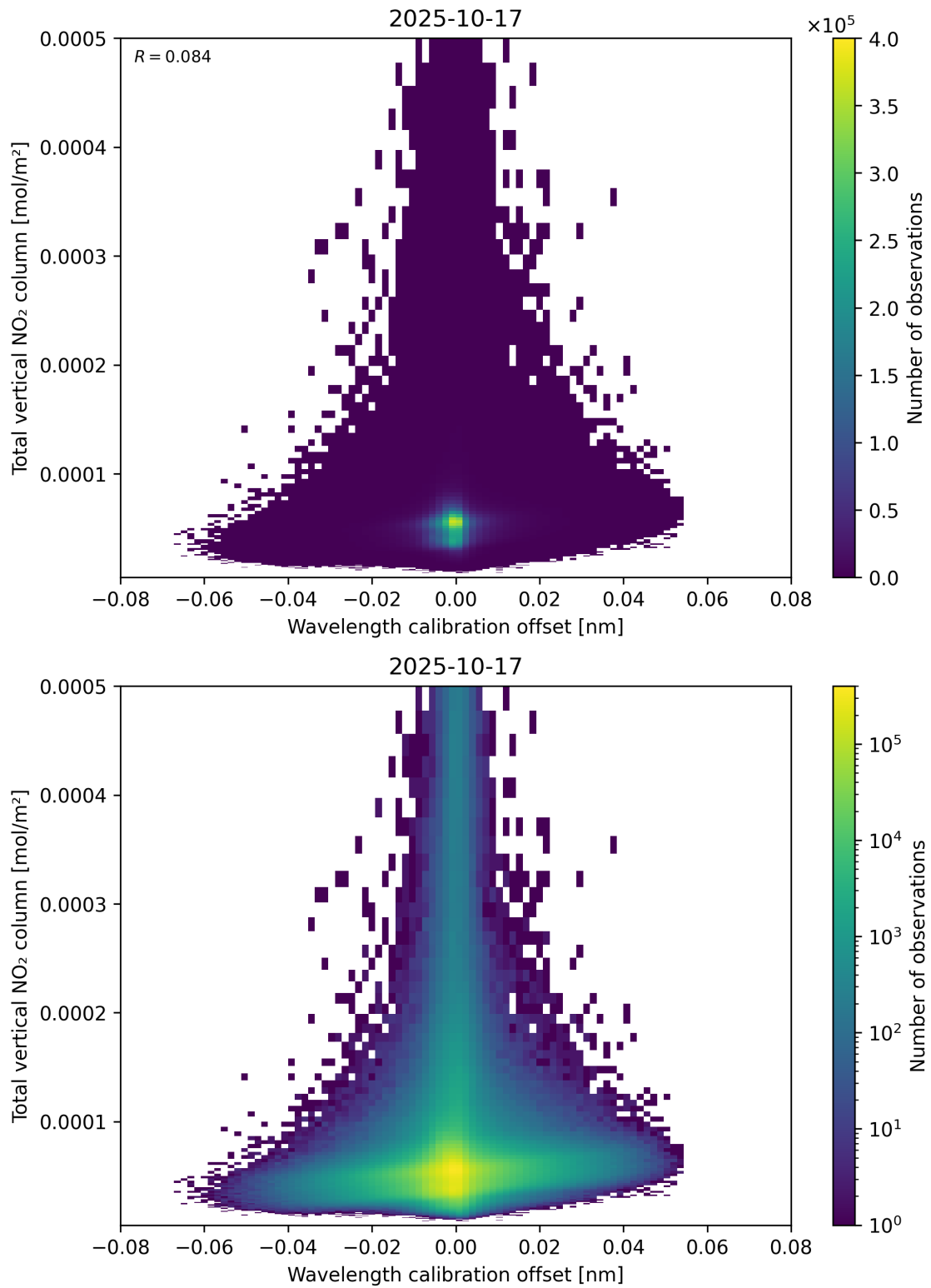
Figure 179: Scatter density plot of “Wavelength calibration offset” against “Total vertical NO 2 column” for 2025-10-17 to 2025-10-18.
