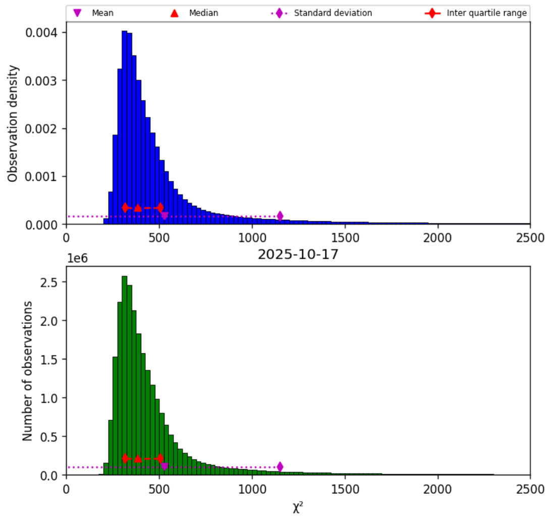
Figure 42: Histogram of “ \chi^2 ” for 2025-10-17 to 2025-10-18
