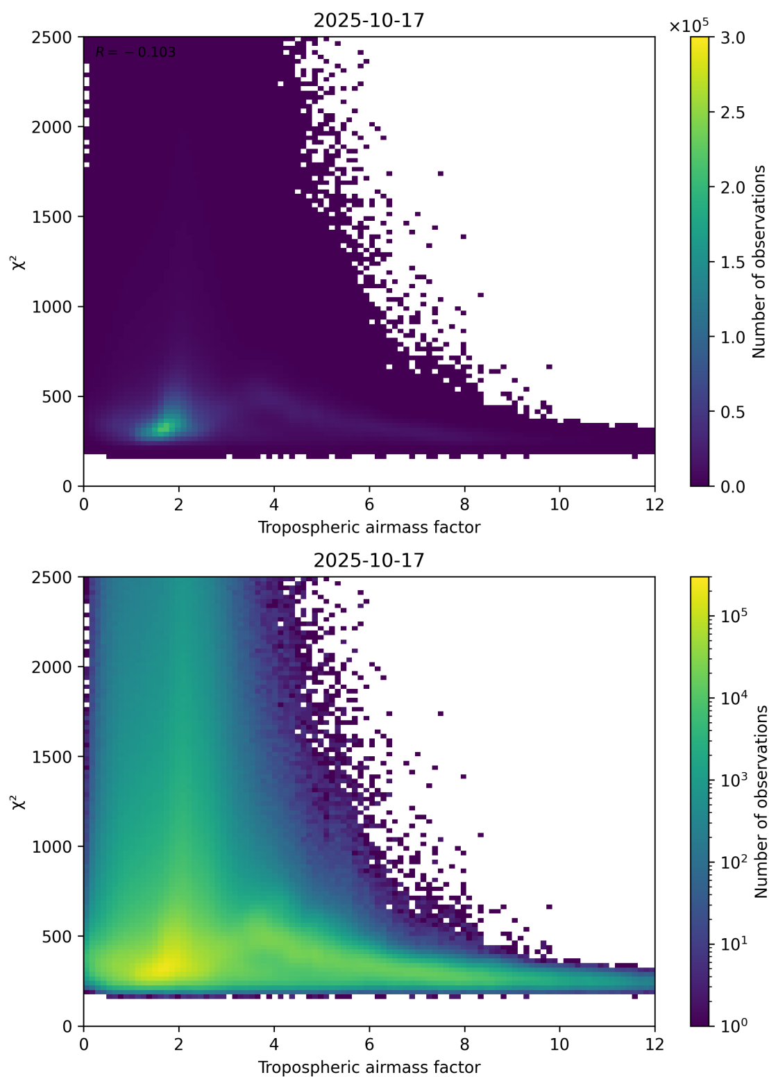
Figure 73: Scatter density plot of “Tropospheric airmass factor” against “ \chi^2 ” for 2025-10-17 to 2025-10-18.
