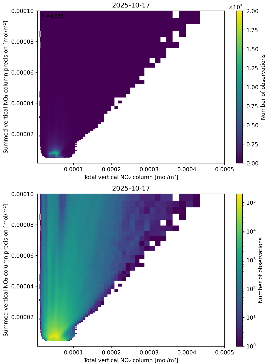
Figure 113: Scatter density plot of “Total vertical NO 2 column” against “Summed vertical NO 2 column precision” for 2025-10-17 to 2025-10-18.
