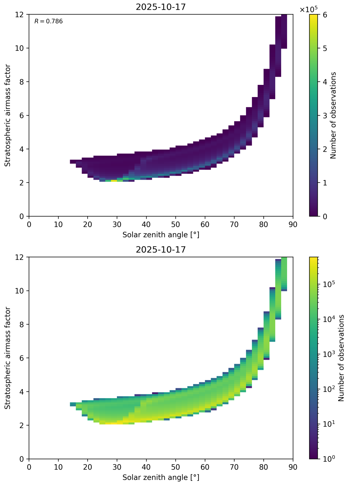
Figure 145: Scatter density plot of “Solar zenith angle” against “Stratospheric airmass factor” for 2025-10-17 to 2025-10-18.
