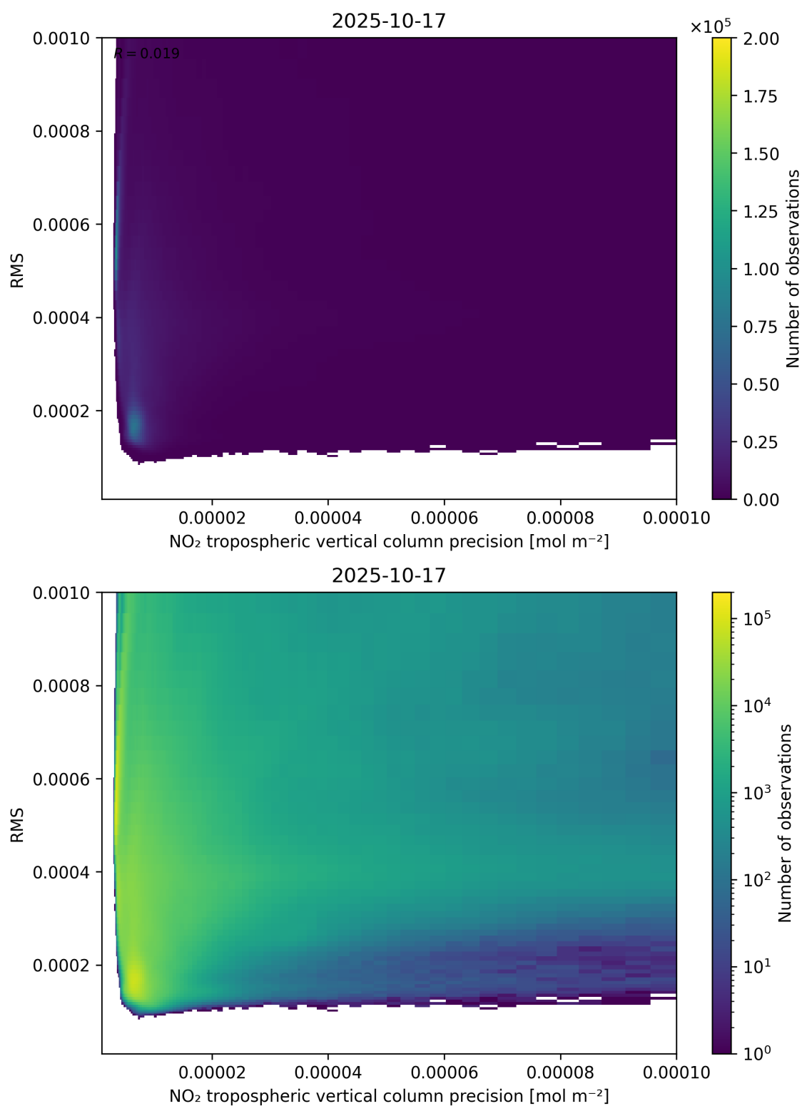
Figure 140: Scatter density plot of “NO 2 tropospheric vertical column precision” against “RMS” for 2025-10-17 to 2025-10-18.
