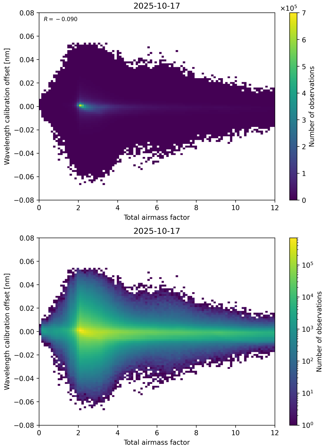
Figure 70: Scatter density plot of “Total airmass factor” against “Wavelength calibration offset” for 2025-10-17 to 2025-10-18.
