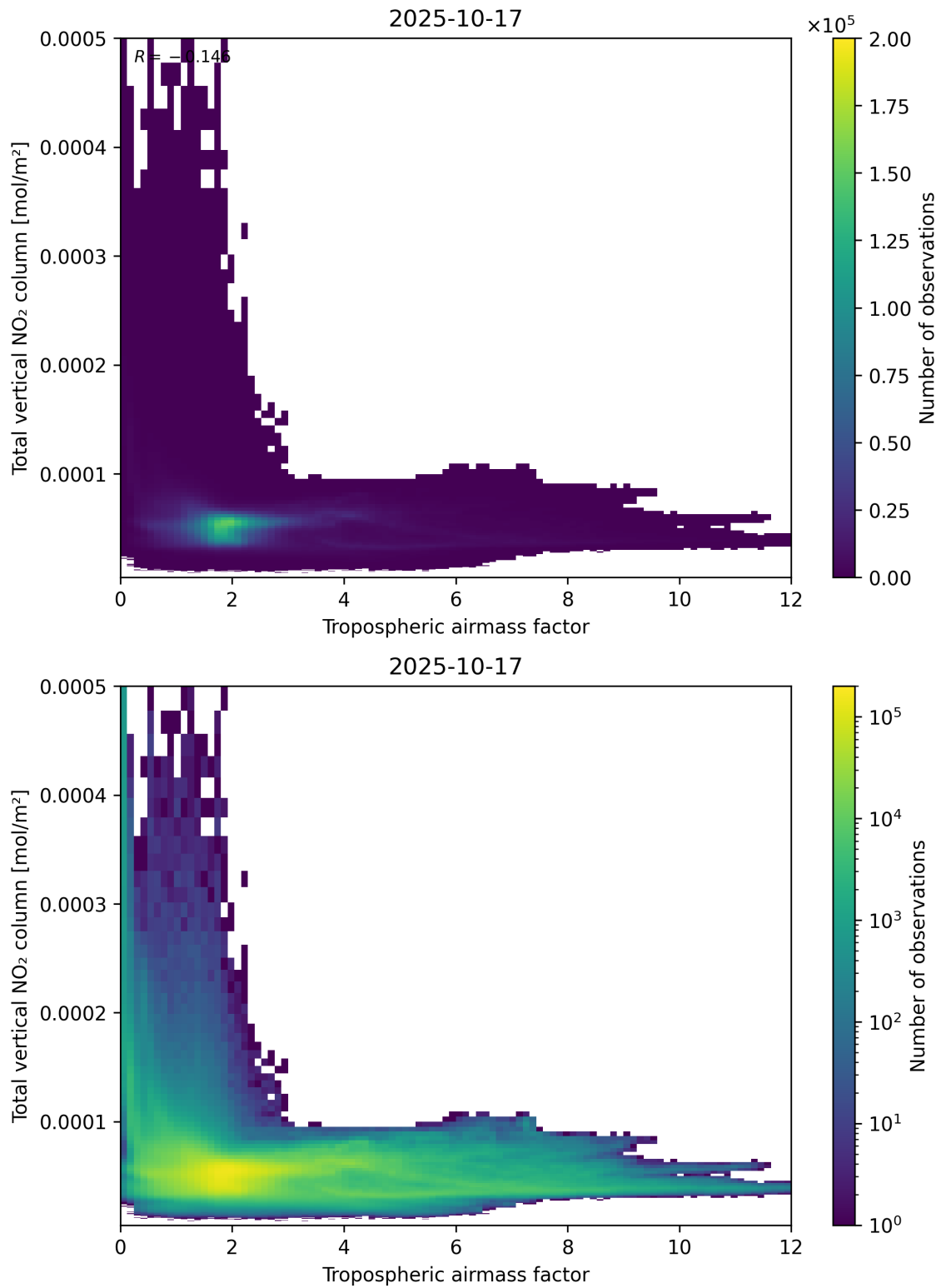
Figure 77: Scatter density plot of “Tropospheric airmass factor” against “Total vertical NO 2 column” for 2025-10-17 to 2025-10-18.
