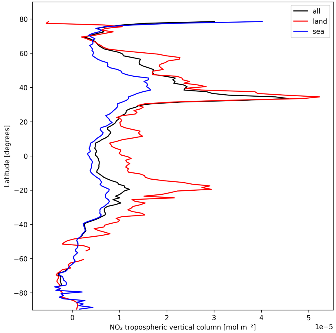
Figure 12: Zonal average of “NO 2 tropospheric vertical column” for 2025-10-17 to 2025-10-18.
