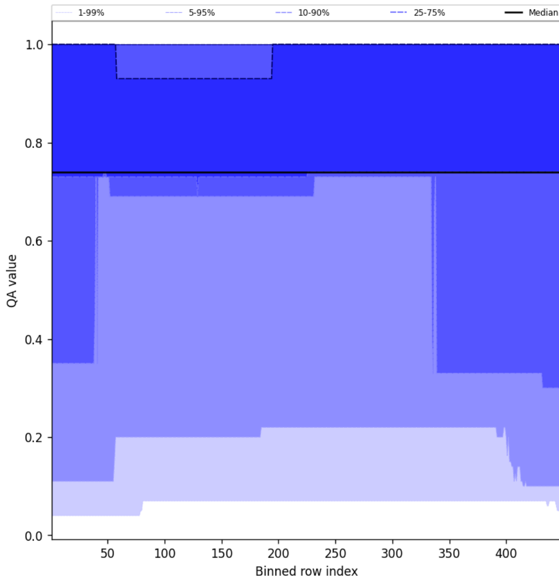
Figure 45: Along track statistics of “QA value” for 2025-10-17 to 2025-10-18
