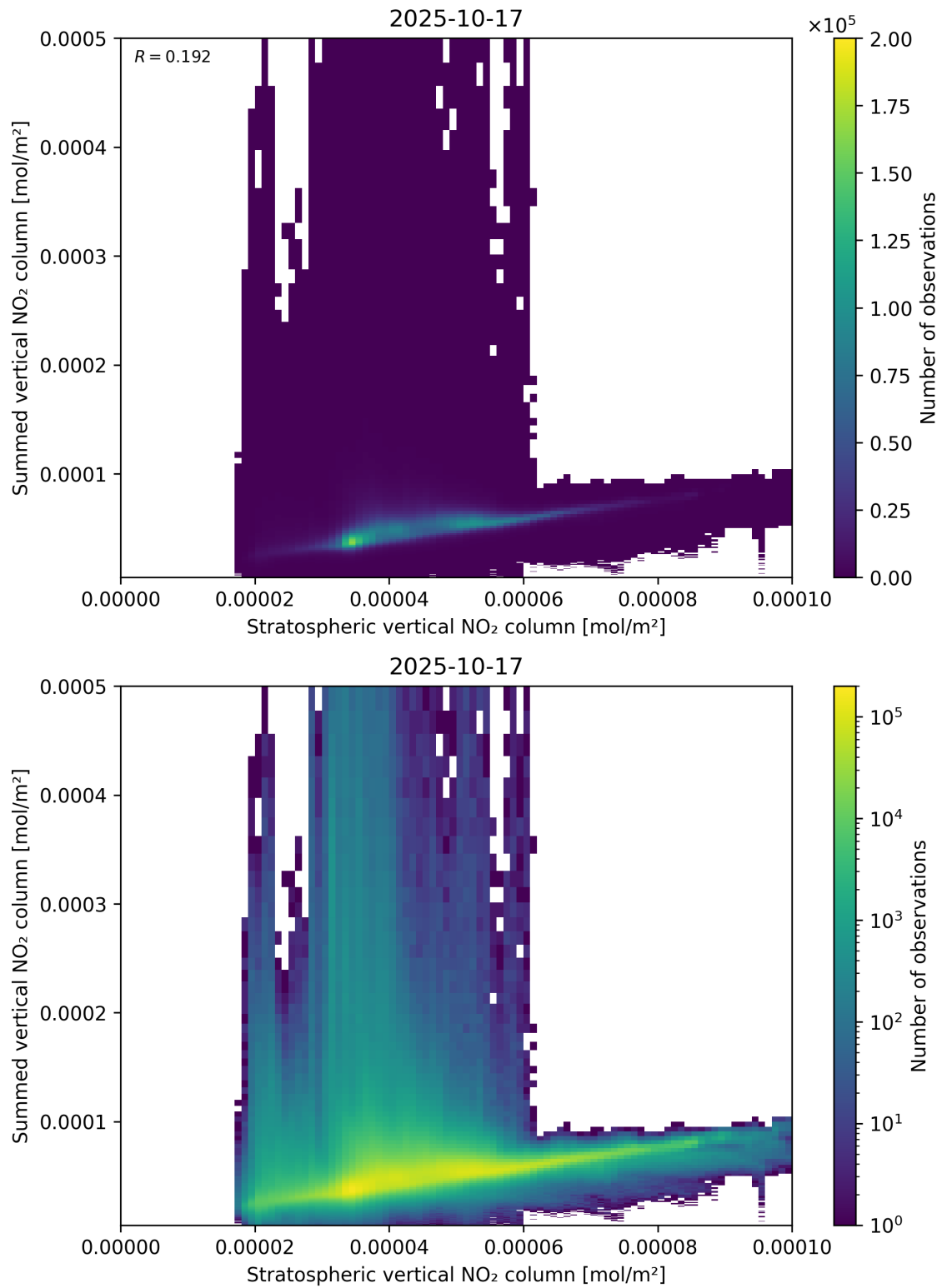
Figure 98: Scatter density plot of “Stratospheric vertical NO 2 column” against “Summed vertical NO 2 column” for 2025-10-17 to 2025-10-18.
