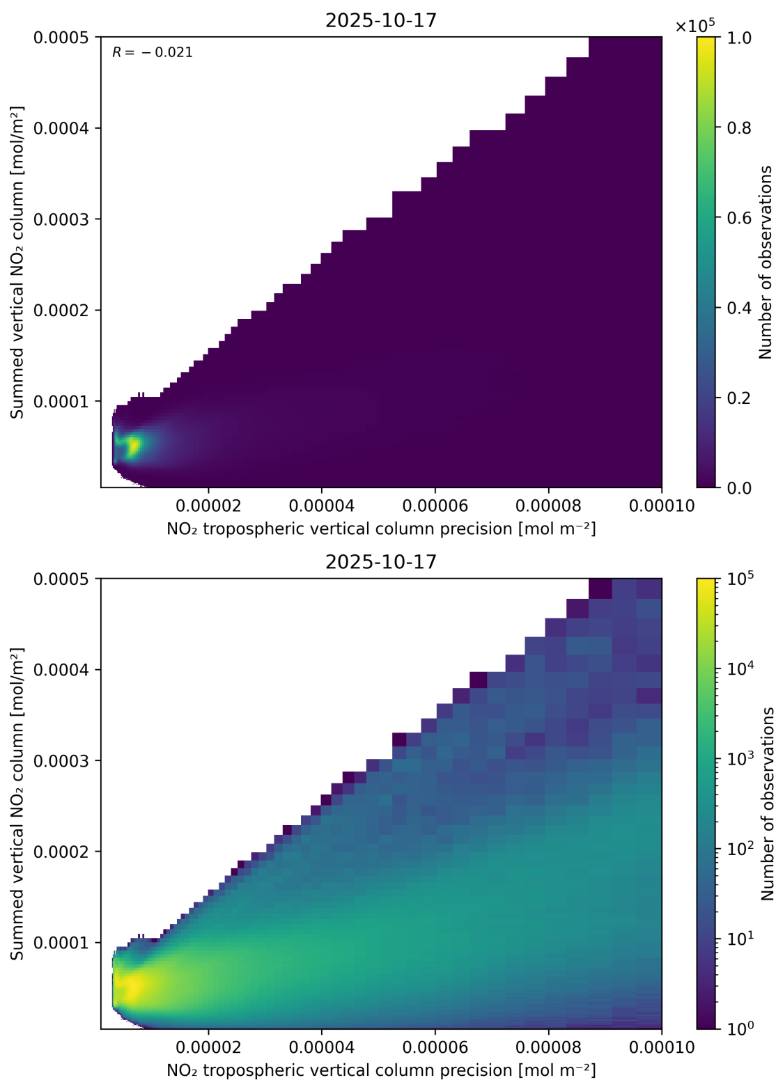
Figure 136: Scatter density plot of “NO 2 tropospheric vertical column precision” against “Summed vertical NO 2 column” for 2025-10-17 to 2025-10-18.
