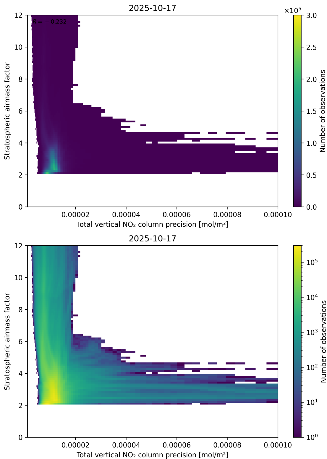
Figure 115: Scatter density plot of “Total vertical NO 2 column precision” against “Stratospheric air mass factor” for 2025-10-17 to 2025-10-18.
