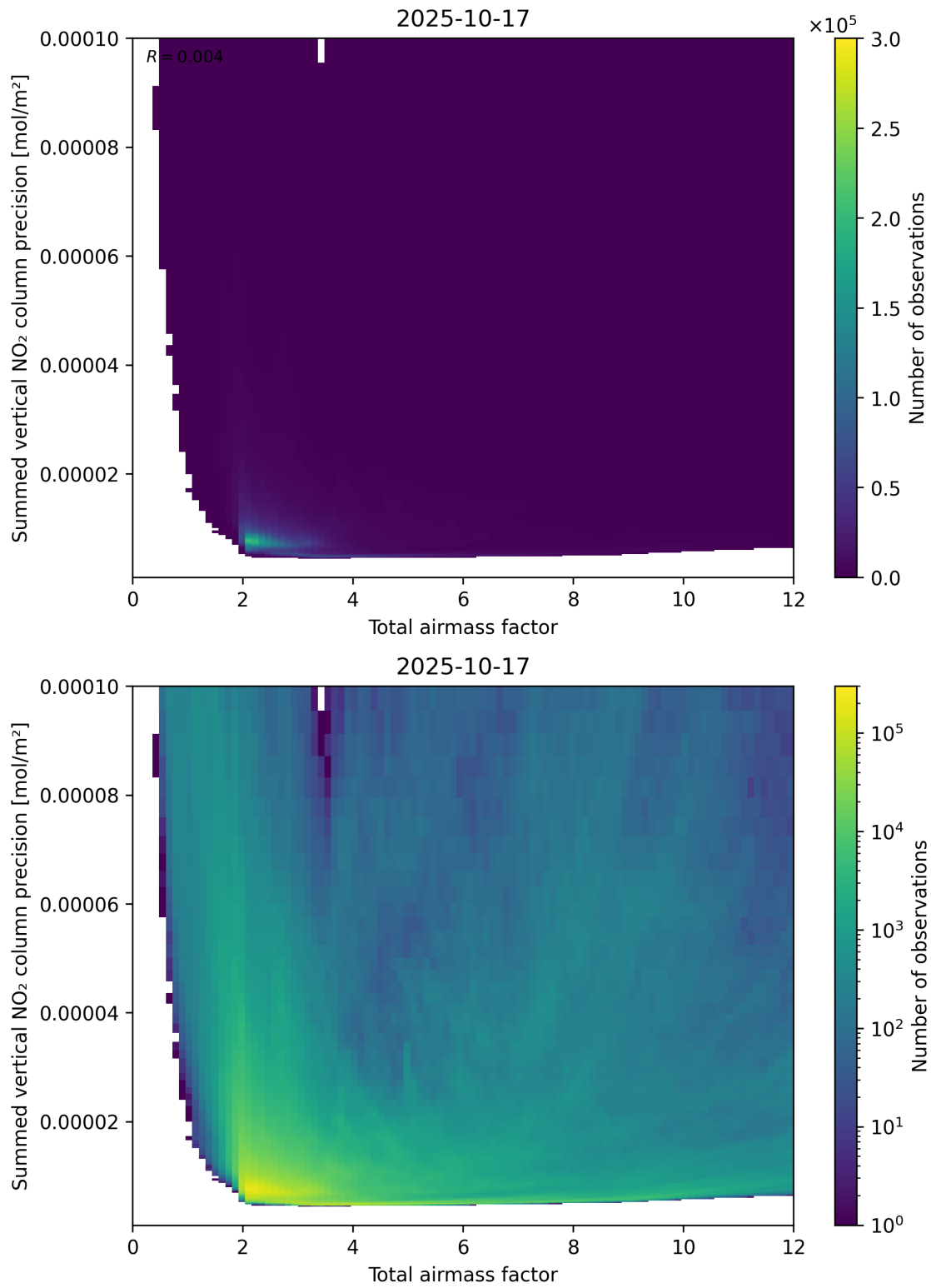
Figure 66: Scatter density plot of “Total airmass factor” against “Summed vertical NO 2 column precision” for 2025-10-17 to 2025-10-18.
