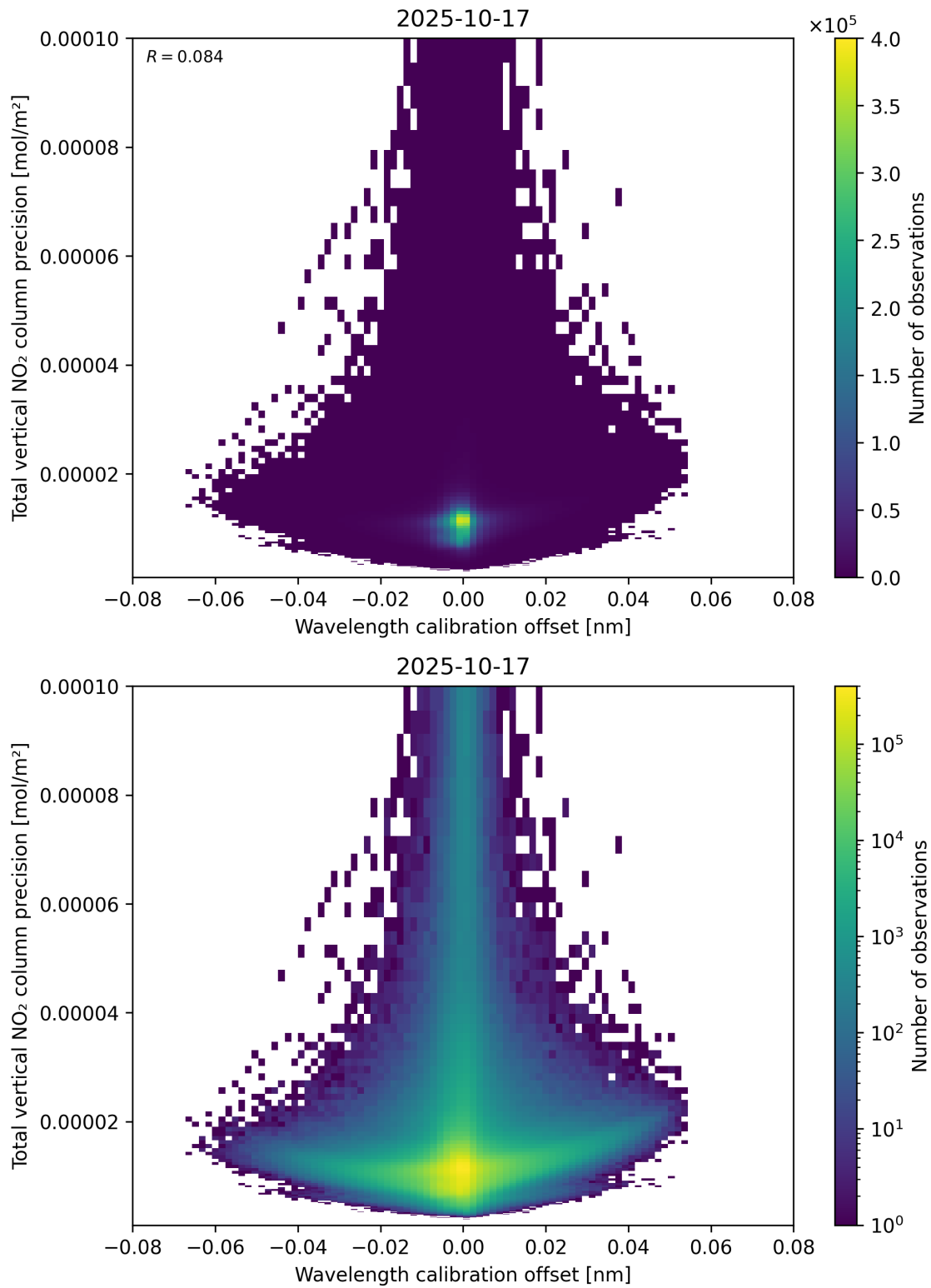
Figure 180: Scatter density plot of “Wavelength calibration offset” against “Total vertical NO 2 column precision” for 2025-10-17 to 2025-10-18.
