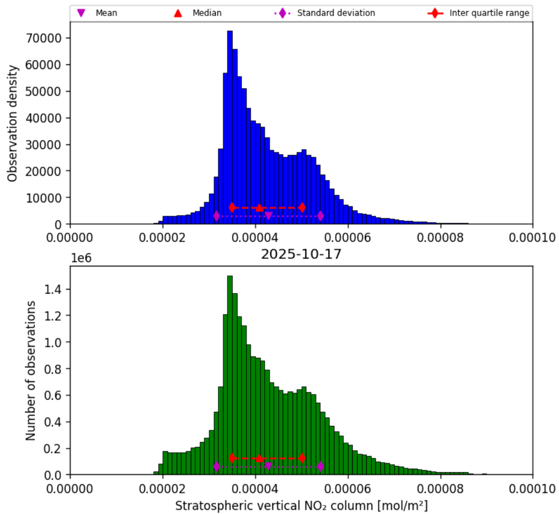
Figure 36: Histogram of “Stratospheric vertical NO 2 column” for 2025-10-17 to 2025-10-18
