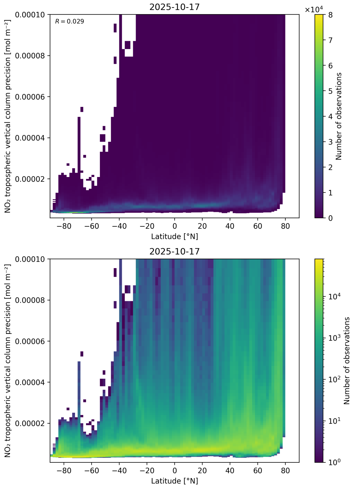
Figure 93: Scatter density plot of “Latitude” against “NO 2 tropospheric vertical column precision” for 2025-10-17 to 2025-10-18.
