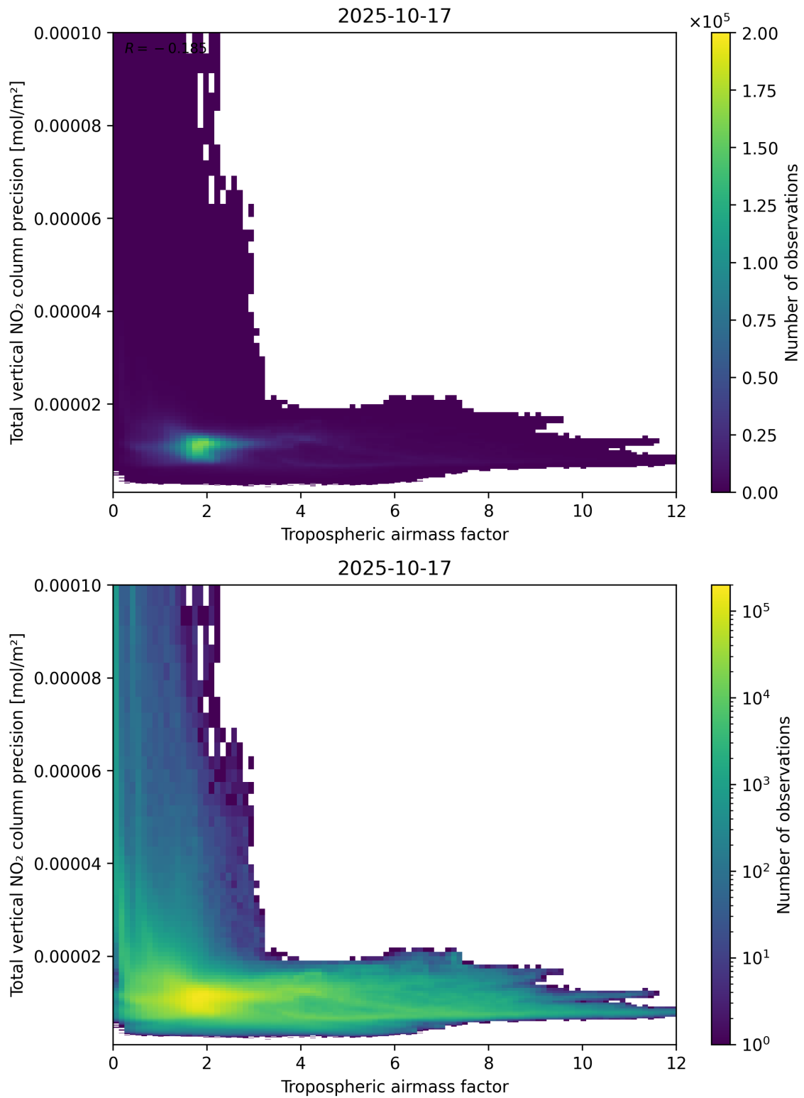
Figure 78: Scatter density plot of “Tropospheric air mass factor” against “Total vertical NO 2 column precision” for 2025-10-17 to 2025-10-18.
