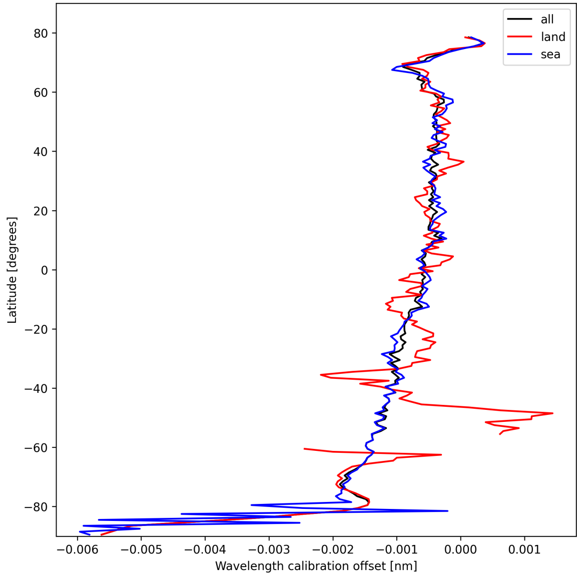
Figure 18: Zonal average of “Wavelength calibration offset” for 2025-10-17 to 2025-10-18.
