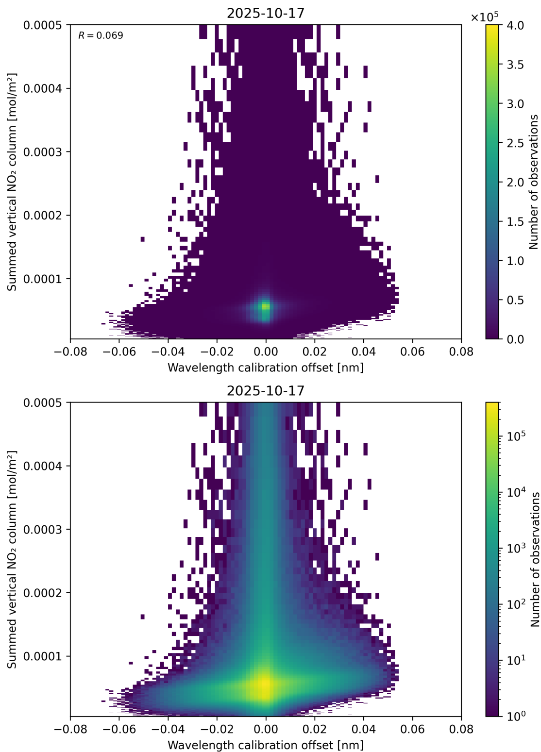
Figure 177: Scatter density plot of “Wavelength calibration offset” against “Summed vertical NO 2 column” for 2025-10-17 to 2025-10-18.
