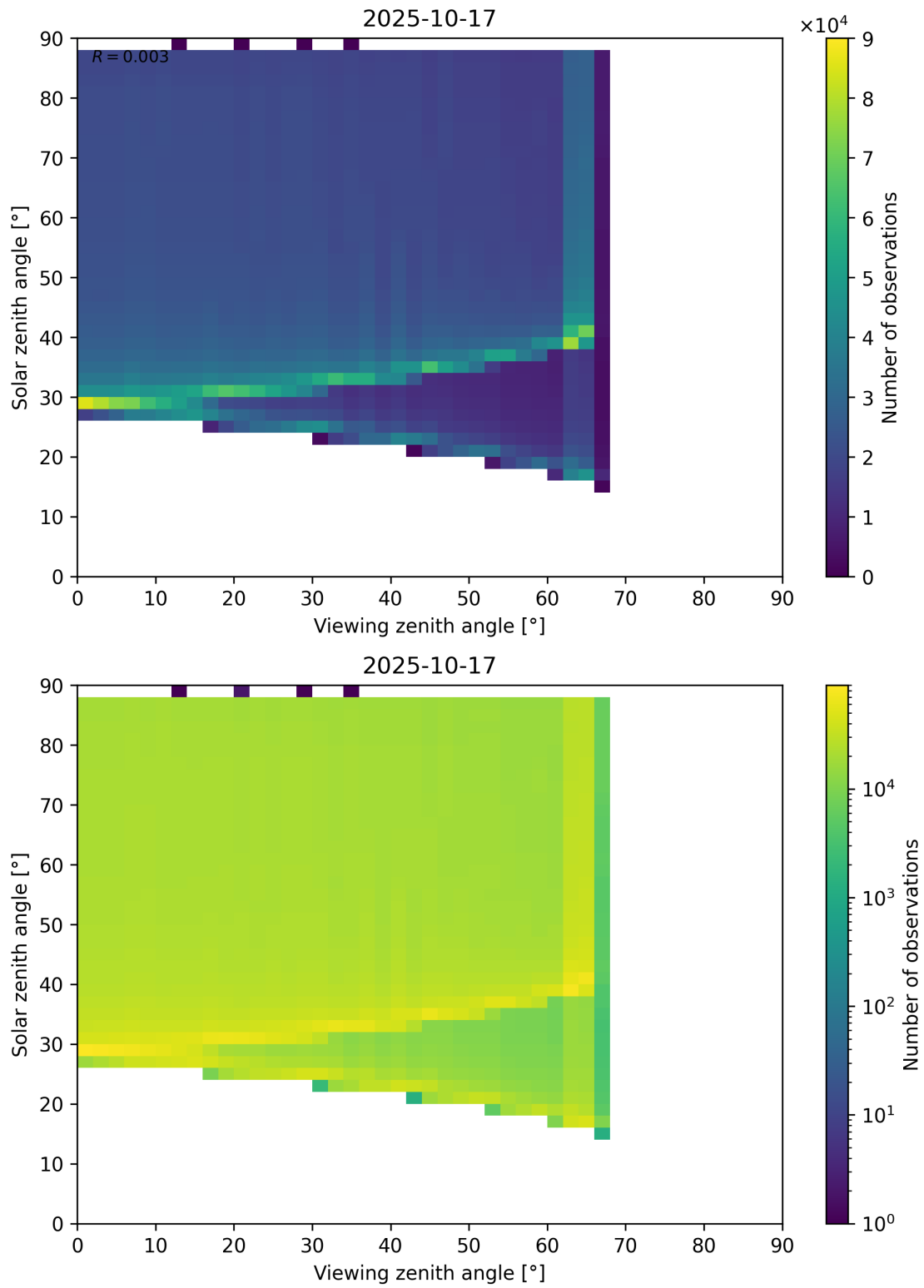
Figure 172: Scatter density plot of “Viewing zenith angle” against “Solar zenith angle” for 2025-10-17 to 2025-10-18.
