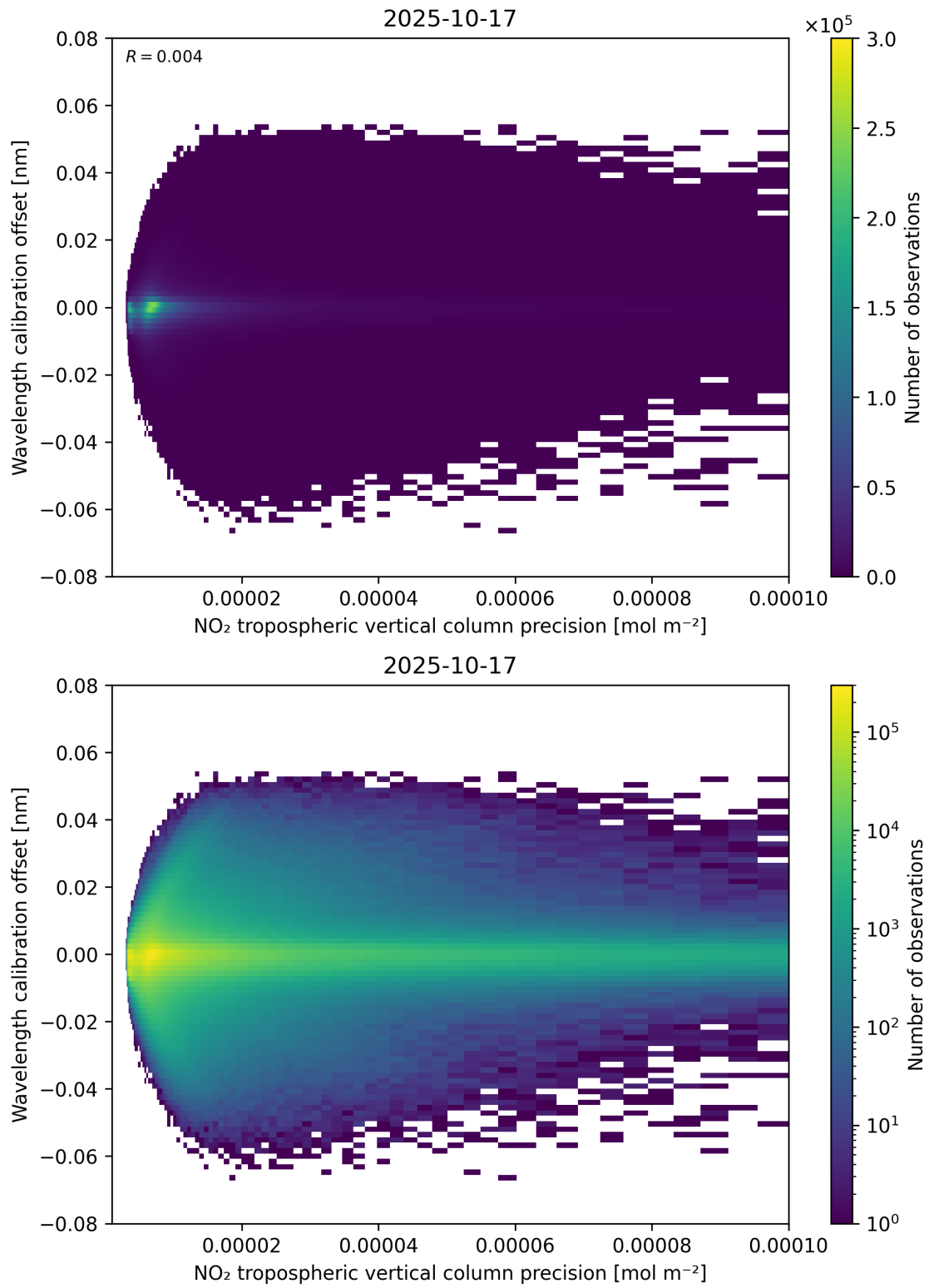
Figure 141: Scatter density plot of “NO 2 tropospheric vertical column precision” against “Wavelength calibration offset” for 2025-10-17 to 2025-10-18.
