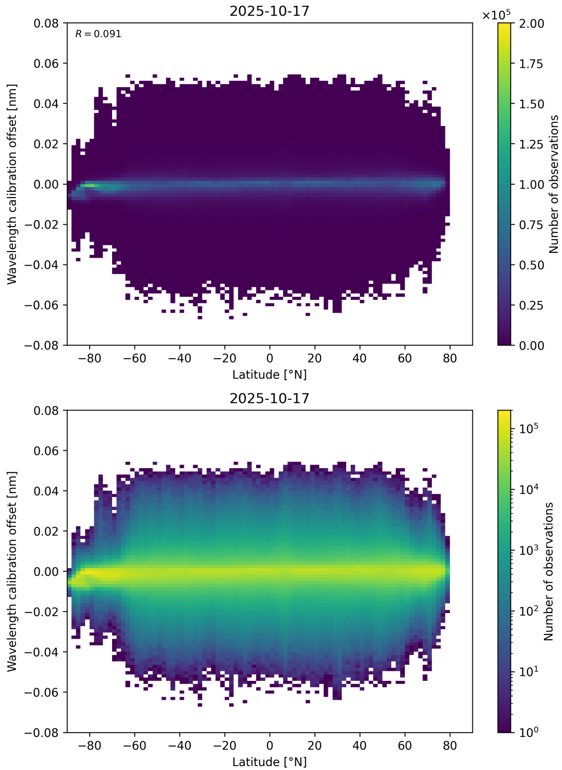
Figure 95: Scatter density plot of “Latitude” against “Wavelength calibration offset” for 2025-10-17 to 2025-10-18.
