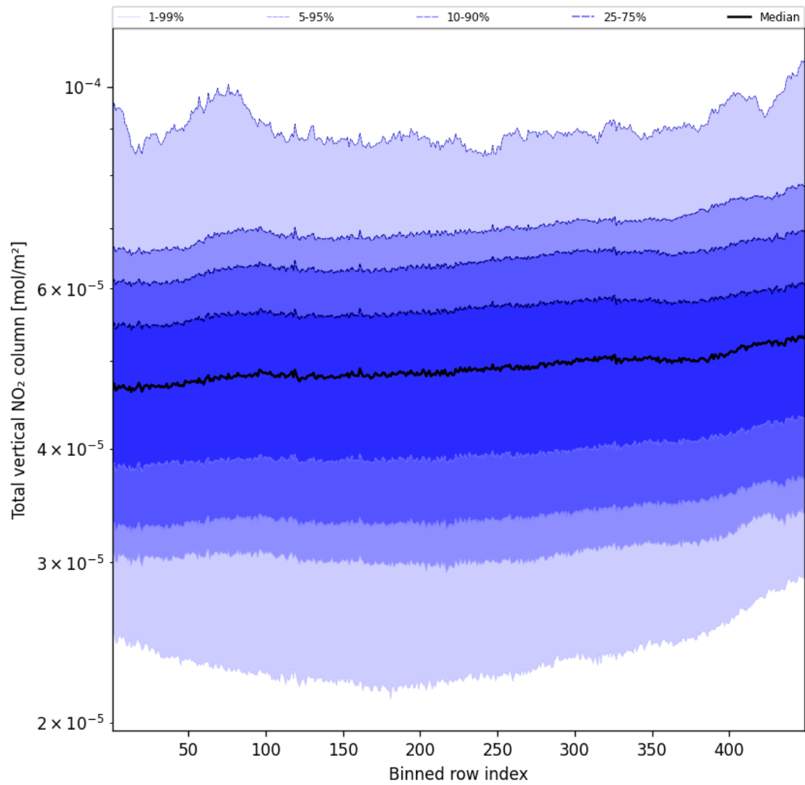
Figure 55: Along track statistics of “Total vertical NO 2 column” for 2025-10-17 to 2025-10-18
