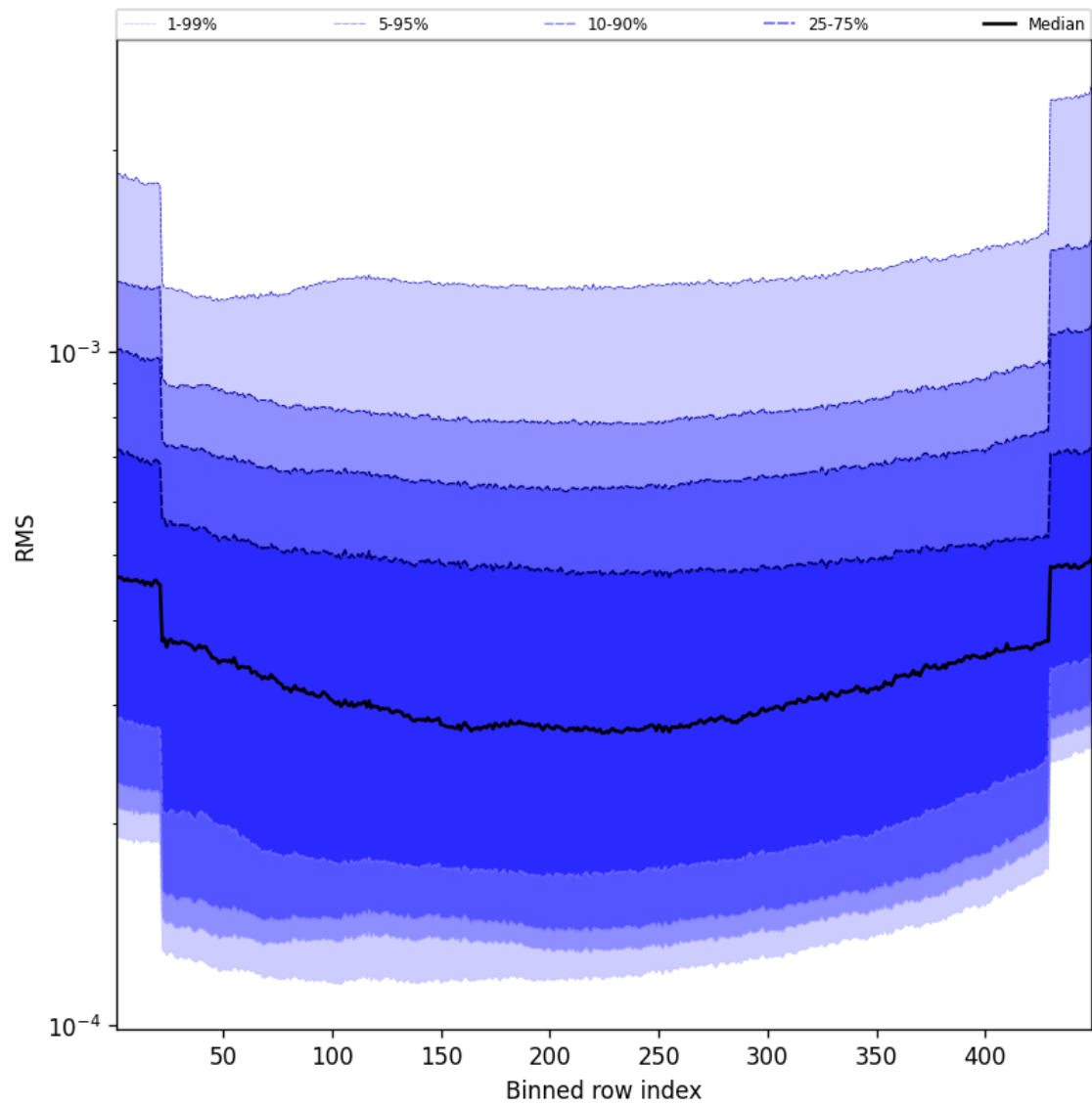
Figure 60: Along track statistics of “RMS” for 2025-10-17 to 2025-10-18
