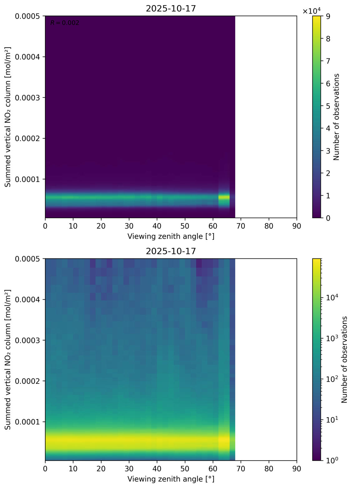
Figure 165: Scatter density plot of “Viewing zenith angle” against “Summed vertical NO 2 column” for 2025-10-17 to 2025-10-18.
