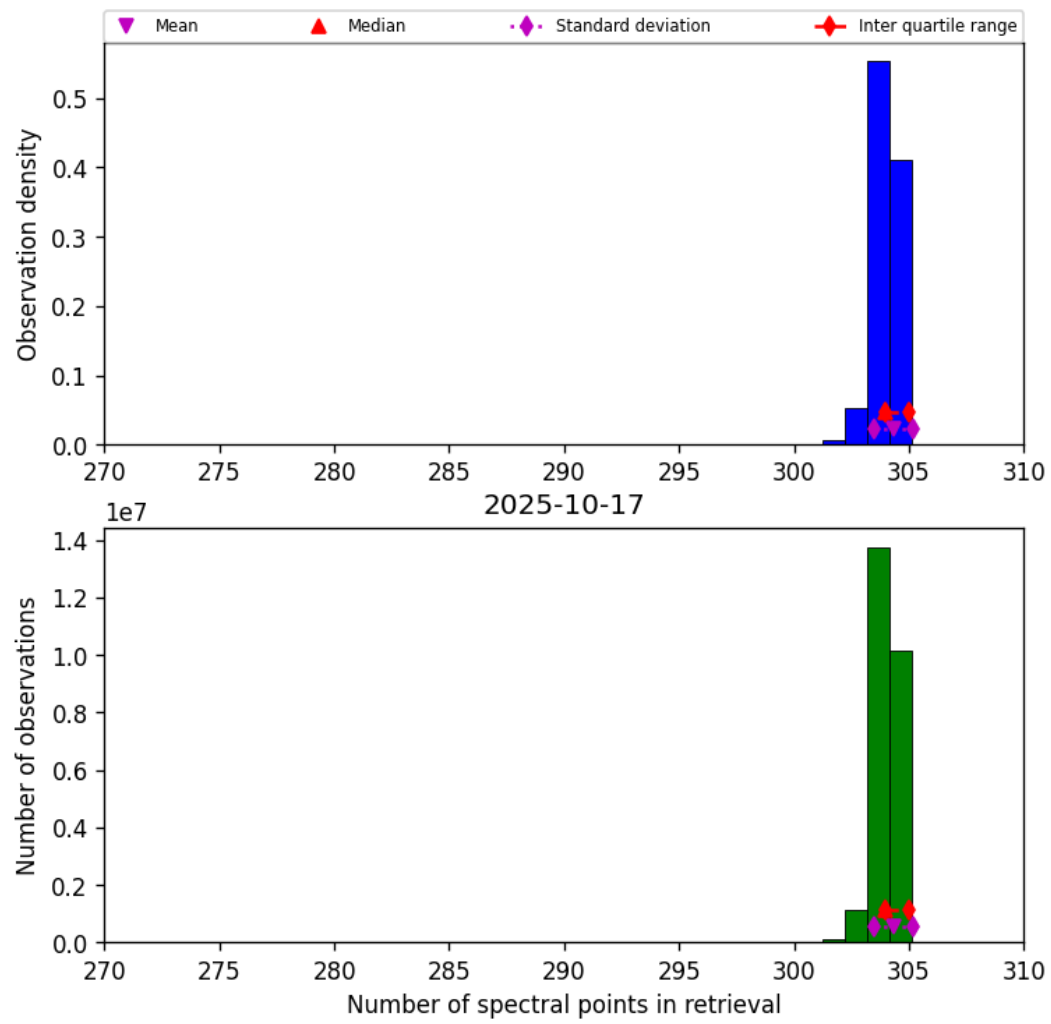
Figure 33: Histogram of “Number of spectral points in retrieval” for 2025-10-17 to 2025-10-18
