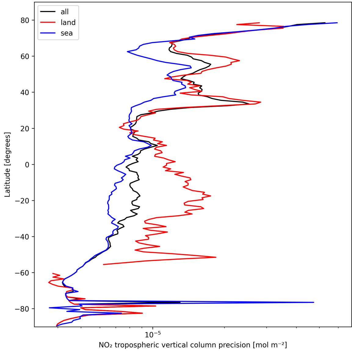
Figure 13: Zonal average of “NO 2 tropospheric vertical column precision” for 2025-10-17 to 2025-10-18.
