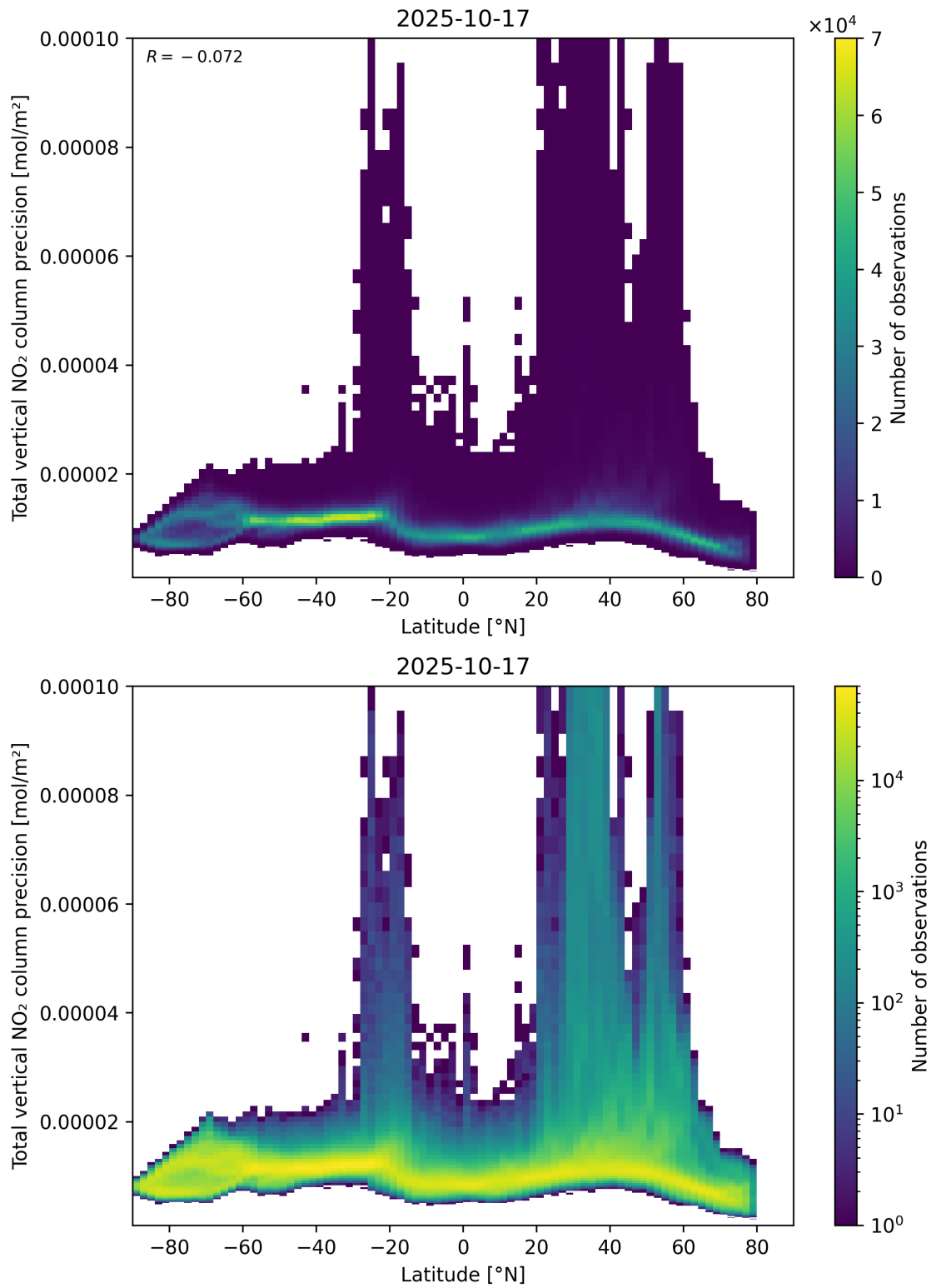
Figure 91: Scatter density plot of “Latitude” against “Total vertical NO 2 column precision” for 2025-10-17 to 2025-10-18.
