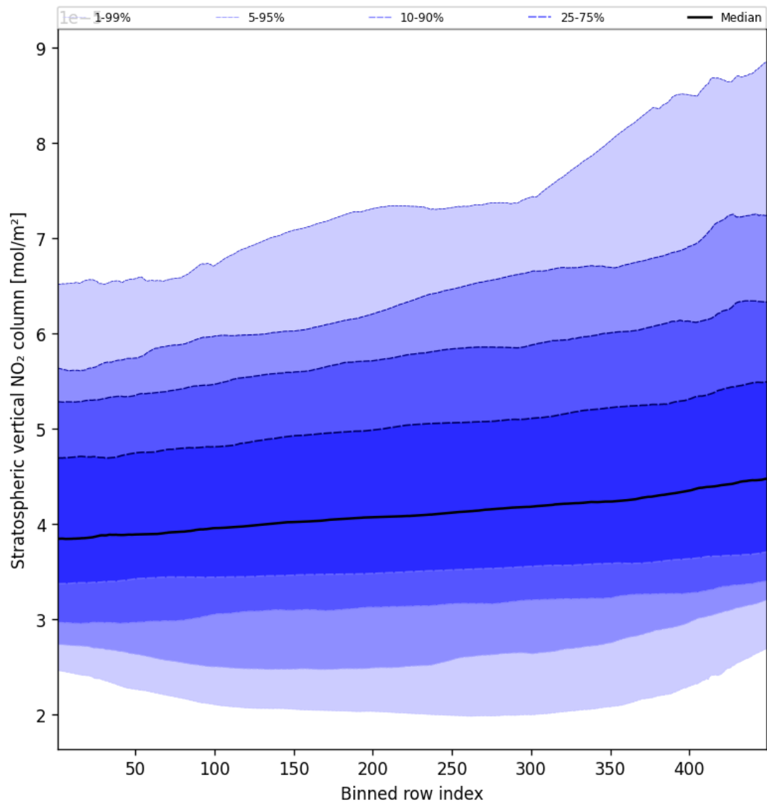
Figure 53: Along track statistics of “Stratospheric vertical NO 2 column” for 2025-10-17 to 2025-10-18
