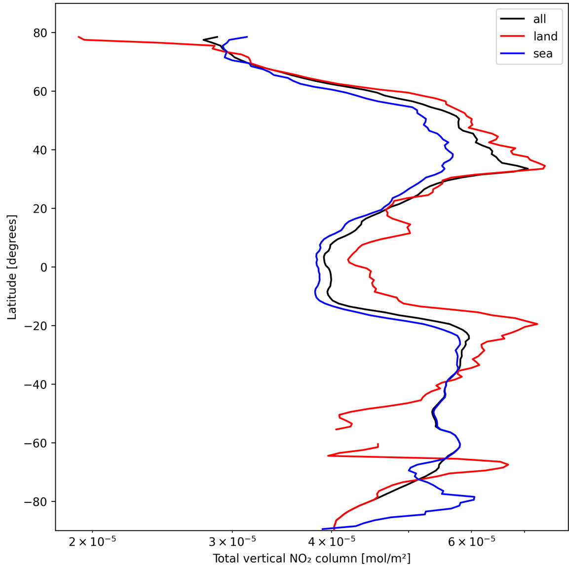
Figure 21: Zonal average of “Total vertical NO 2 column” for 2025-10-17 to 2025-10-18.
