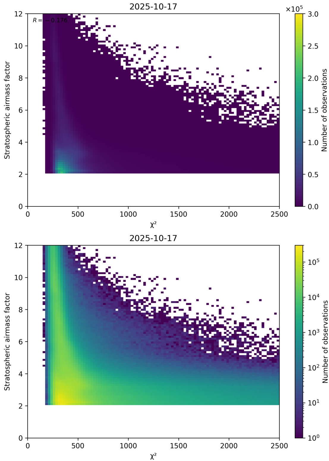
Figure 81: Scatter density plot of “ \chi^2 ” against “Stratospheric airmass factor” for 2025-10-17 to 2025-10-18.
