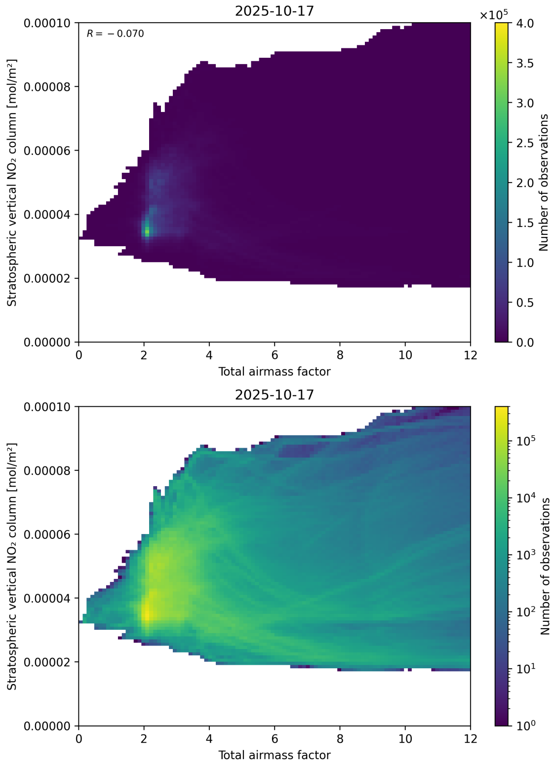
Figure 64: Scatter density plot of “Total airmass factor” against “Stratospheric vertical NO 2 column” for 2025-10-17 to 2025-10-18.
