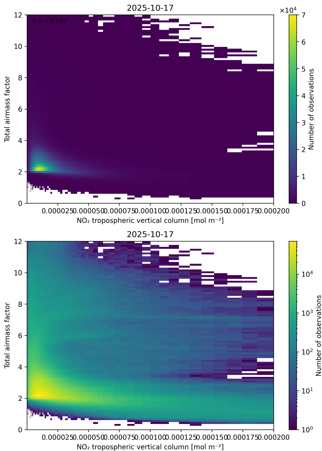
Figure 122: Scatter density plot of “NO 2 tropospheric vertical column” against “Total air mass factor” for 2025-10-17 to 2025-10-18.
