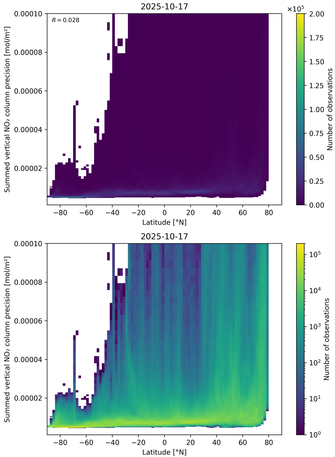
Figure 89: Scatter density plot of “Latitude” against “Summed vertical NO 2 column precision” for 2025-10-17 to 2025-10-18.
