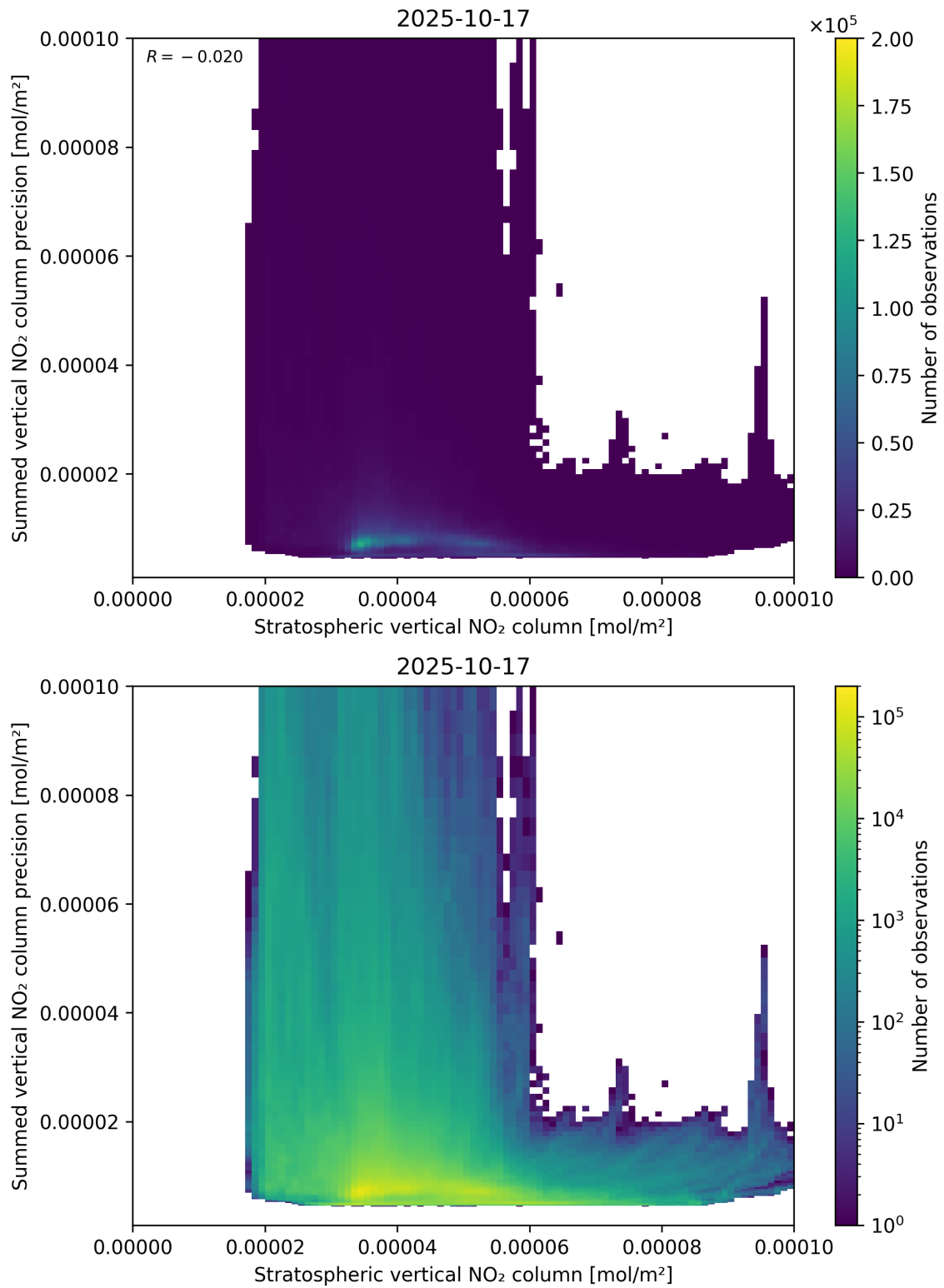
Figure 99: Scatter density plot of “Stratospheric vertical NO 2 column” against “Summed vertical NO 2 column precision” for 2025-10-17 to 2025-10-18.
