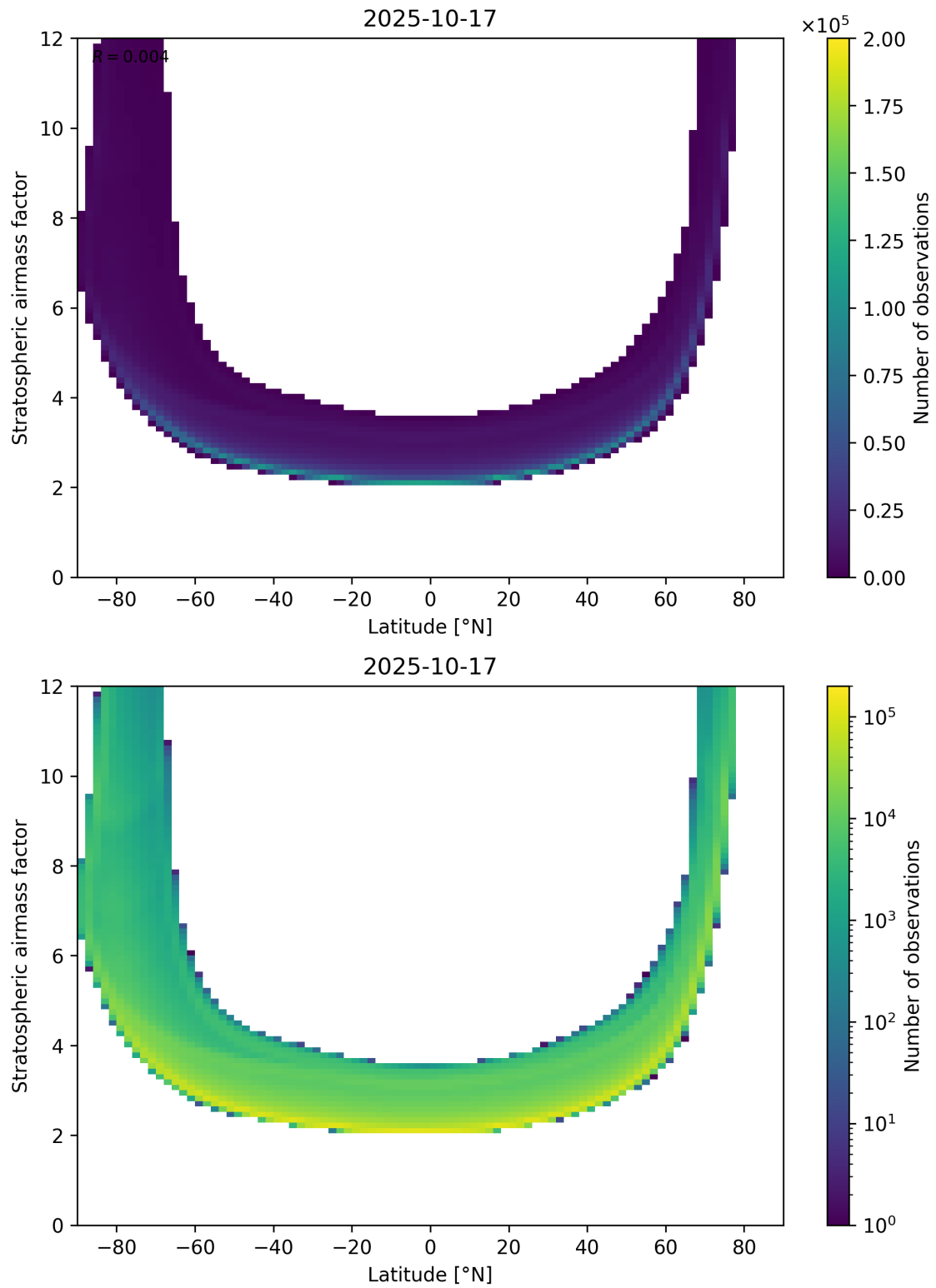
Figure 83: Scatter density plot of “Latitude” against “Stratospheric air mass factor” for 2025-10-17 to 2025-10-18.
