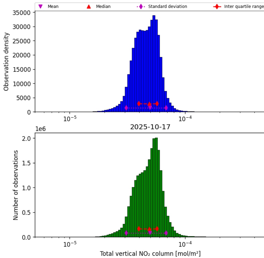
Figure 38: Histogram of “Total vertical NO 2 column” for 2025-10-17 to 2025-10-18
