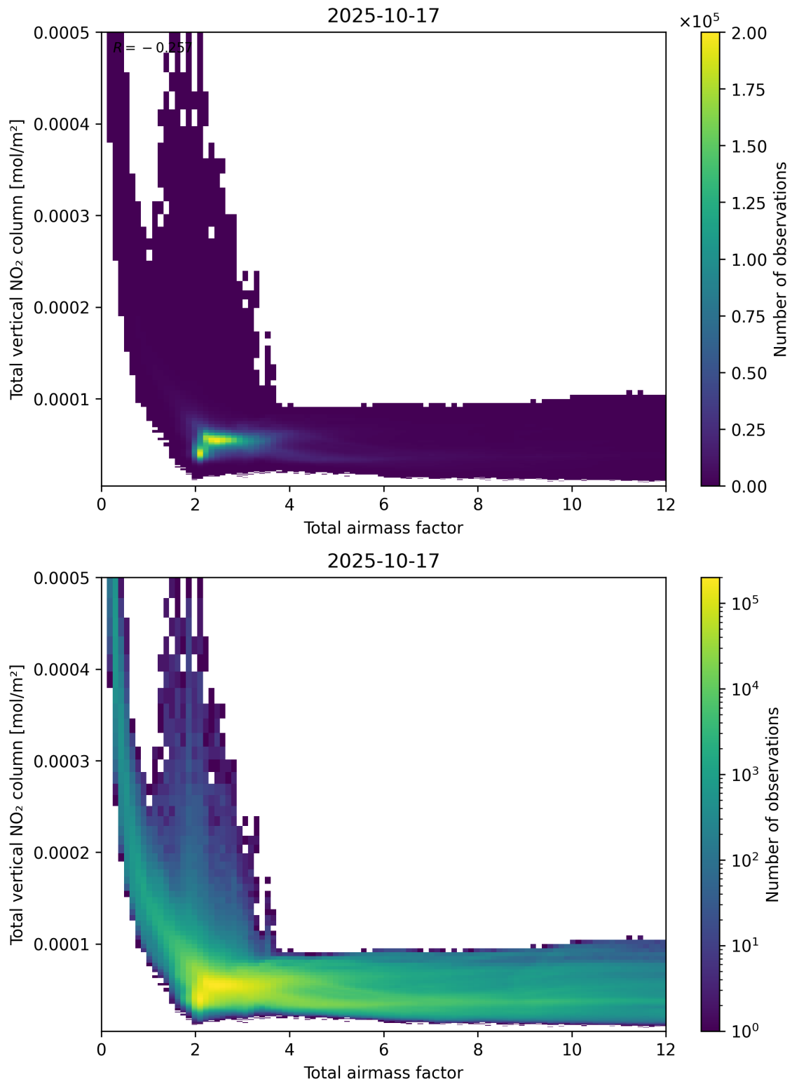
Figure 67: Scatter density plot of “Total airmass factor” against “Total vertical NO 2 column” for 2025-10-17 to 2025-10-18.
