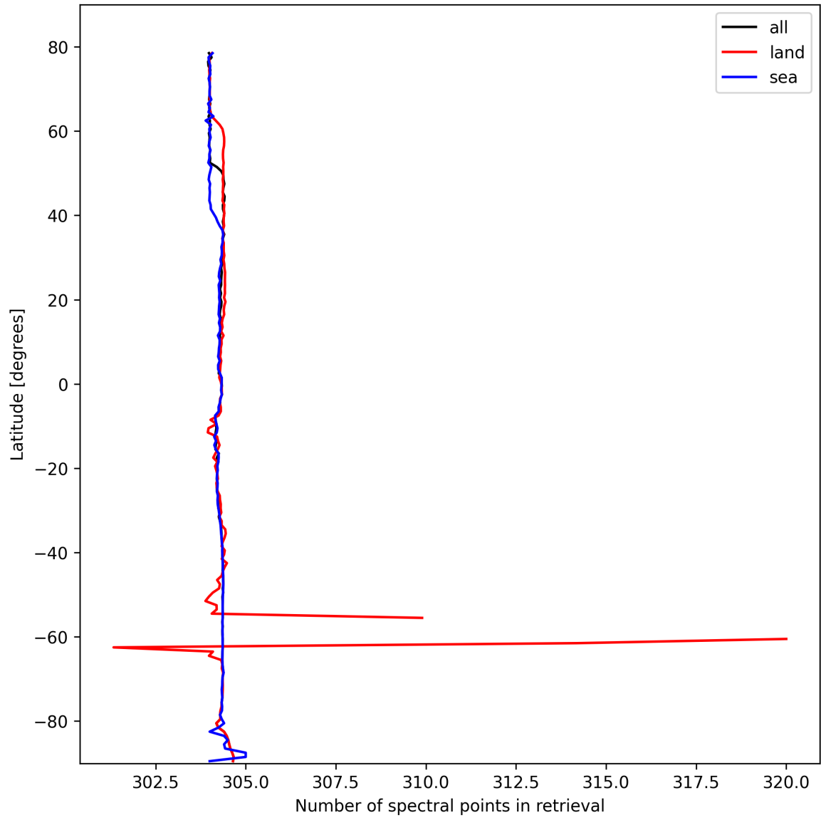
Figure 16: Zonal average of “Number of spectral points in retrieval” for 2025-10-17 to 2025-10-18.
