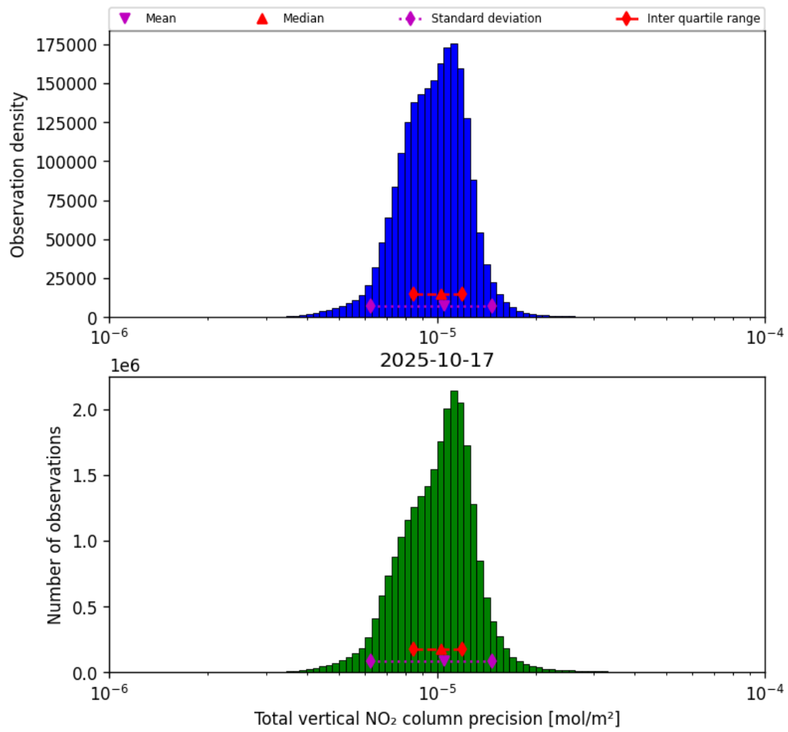
Figure 39: Histogram of “Total vertical NO 2 column precision” for 2025-10-17 to 2025-10-18
