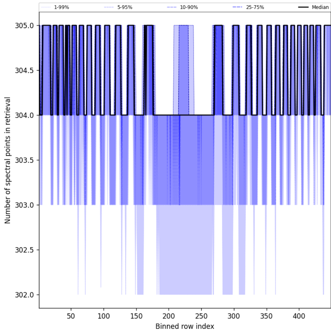
Figure 50: Along track statistics of “Number of spectral points in retrieval” for 2025-10-17 to 2025-10-18
