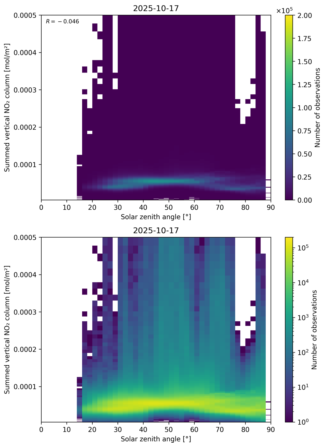
Figure 151: Scatter density plot of “Solar zenith angle” against “Summed vertical NO 2 column” for 2025-10-17 to 2025-10-18.
