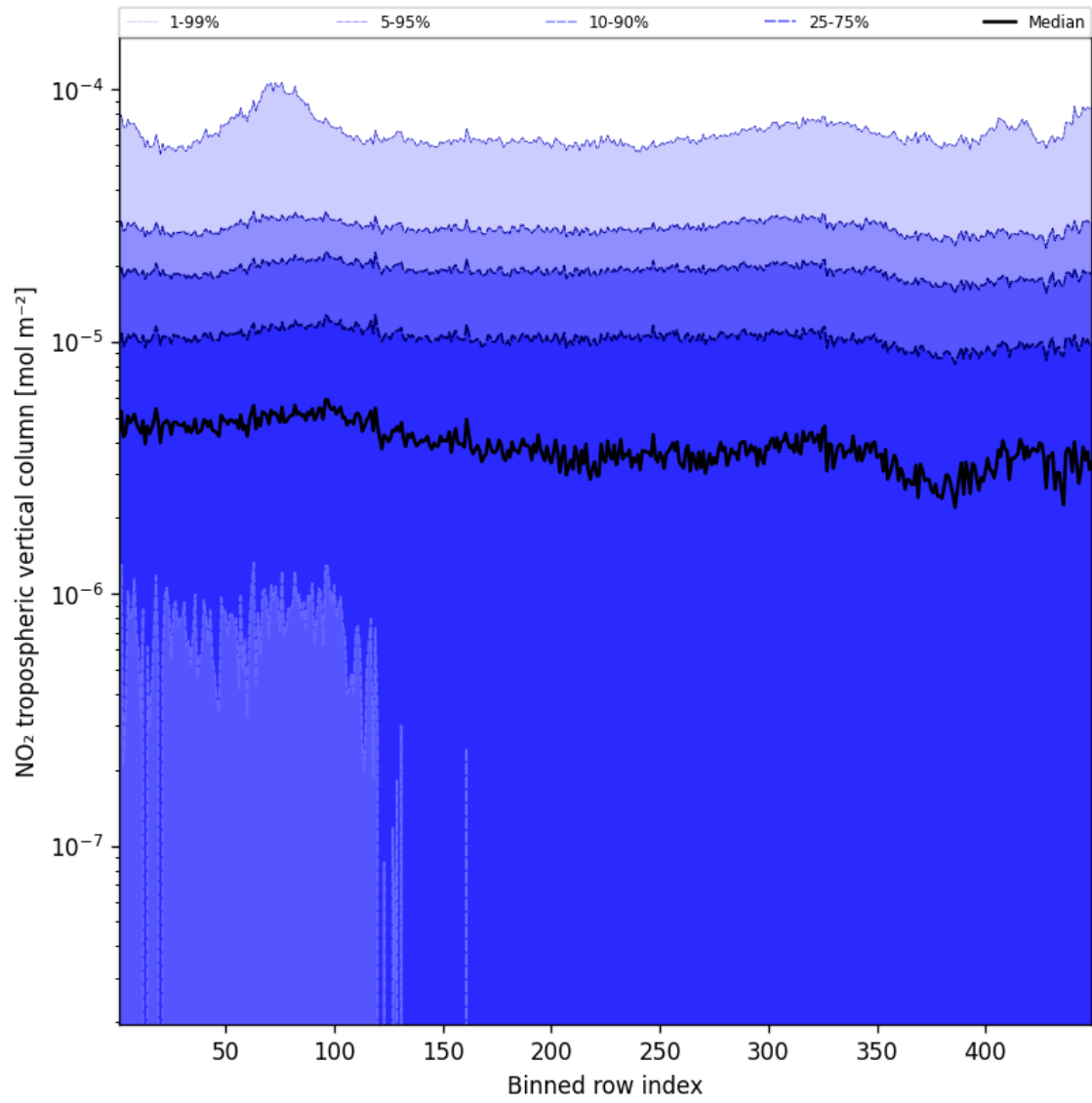
Figure 46: Along track statistics of “NO 2 tropospheric vertical column” for 2025-10-17 to 2025-10-18
