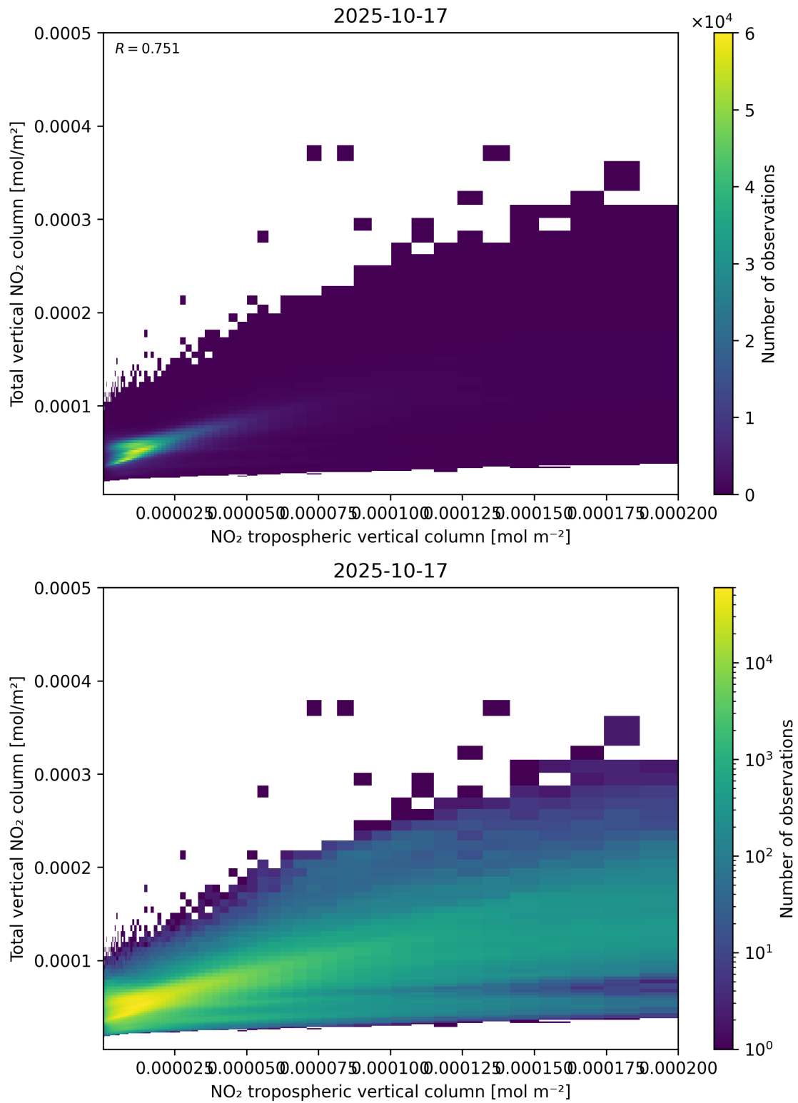
Figure 128: Scatter density plot of “NO 2 tropospheric vertical column” against “Total vertical NO 2 column” for 2025-10-17 to 2025-10-18.
