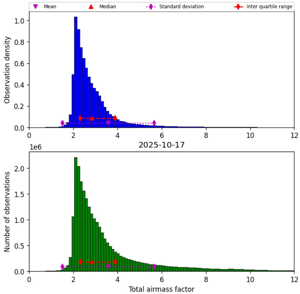
Figure 32: Histogram of “Total airmass factor” for 2025-10-17 to 2025-10-18
