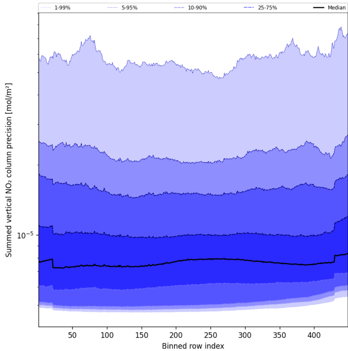
Figure 58: Along track statistics of “Summed vertical NO 2 column precision” for 2025-10-17 to 2025-10-18
