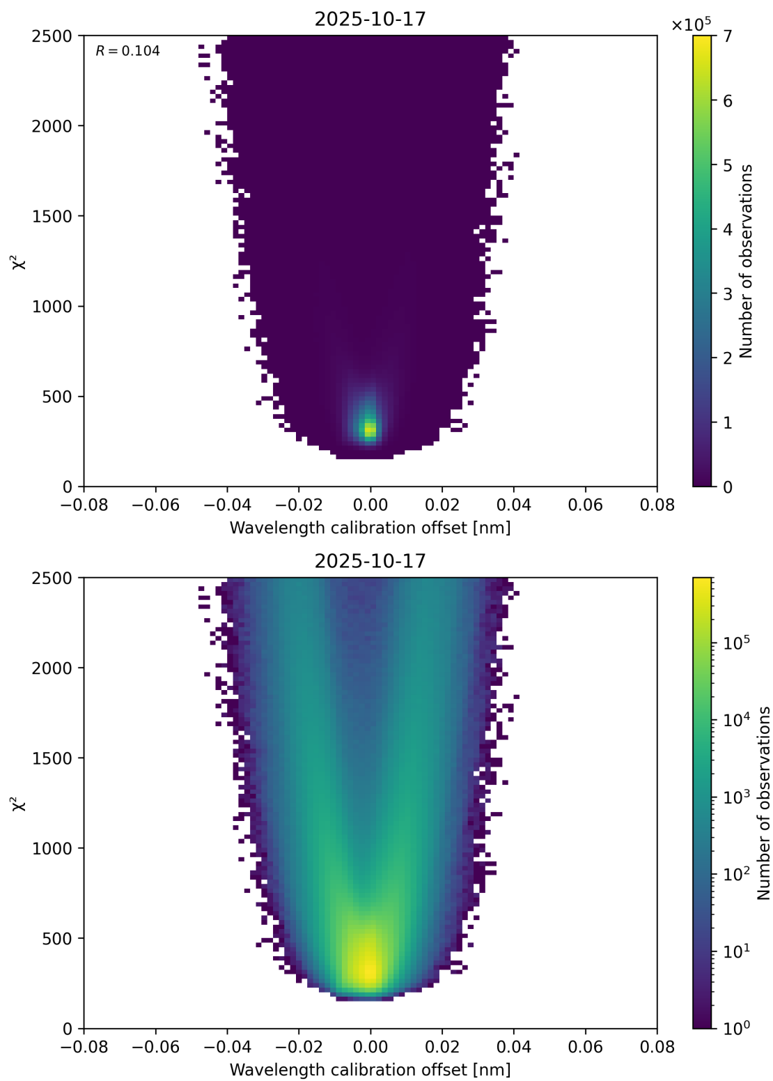
Figure 175: Scatter density plot of “Wavelength calibration offset” against “ \chi^2 ” for 2025-10-17 to 2025-10-18.
