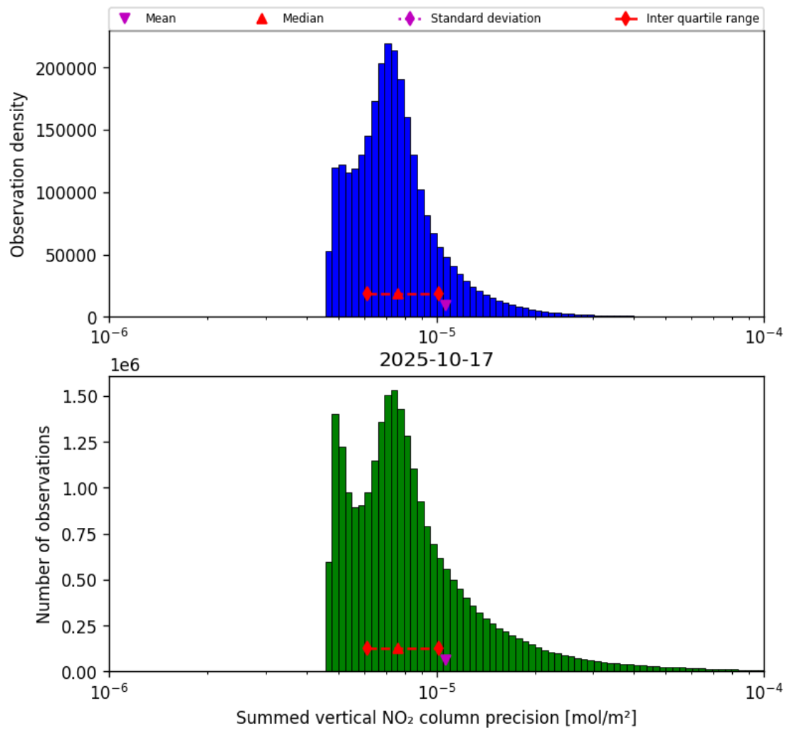
Figure 41: Histogram of “Summed vertical NO 2 column precision” for 2025-10-17 to 2025-10-18
