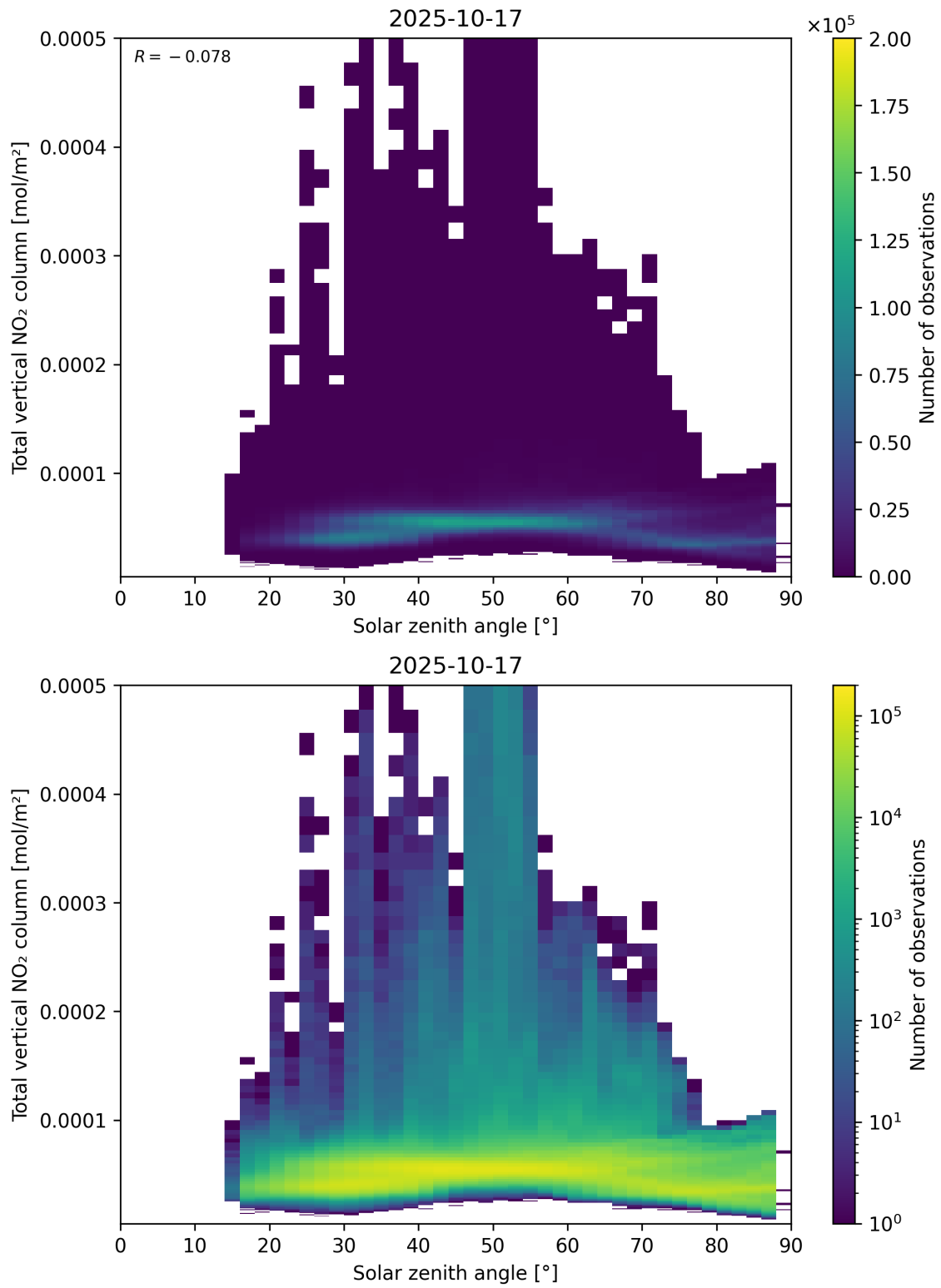
Figure 153: Scatter density plot of “Solar zenith angle” against “Total vertical NO 2 column” for 2025-10-17 to 2025-10-18.
