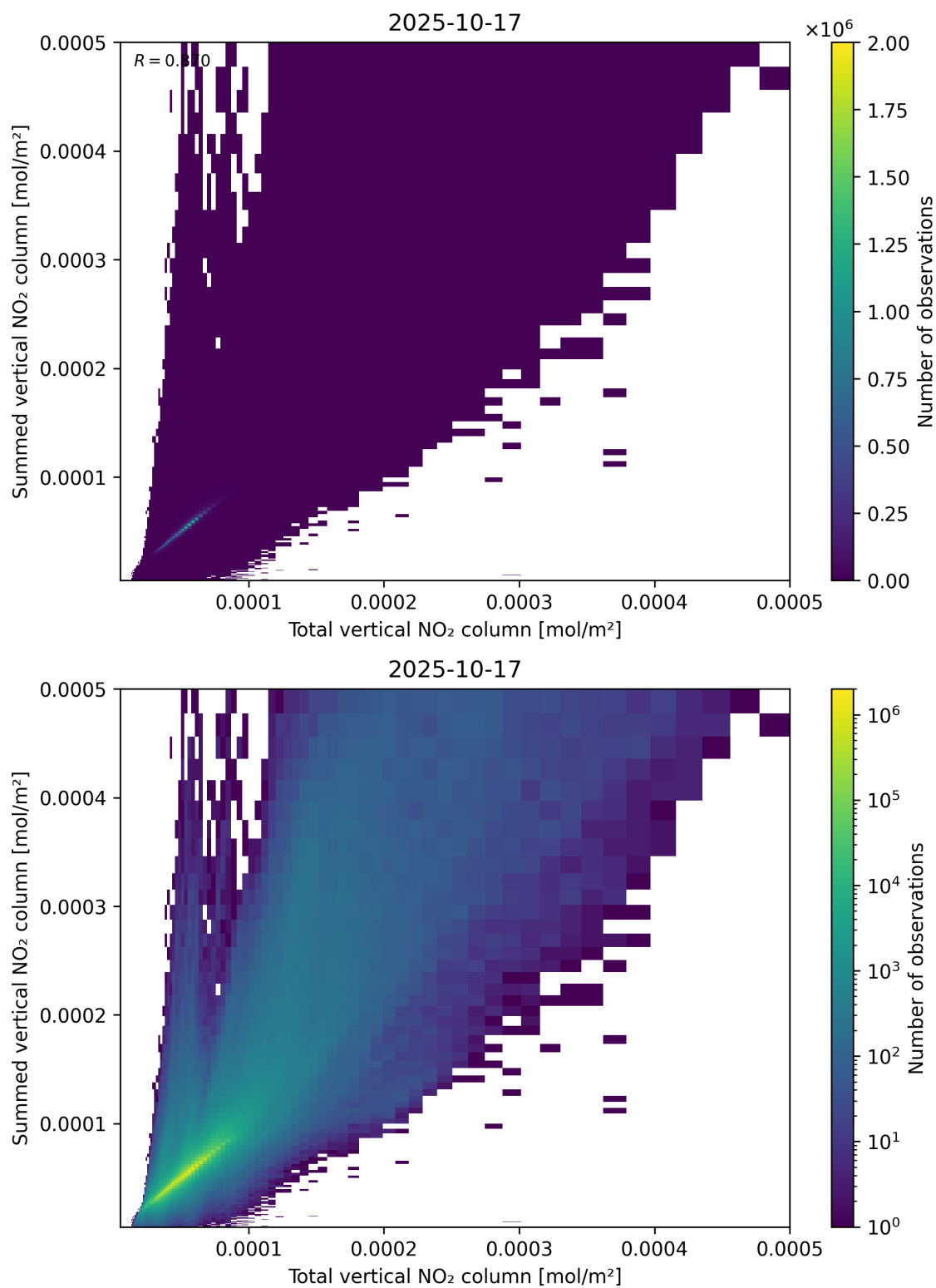
Figure 112: Scatter density plot of “Total vertical NO 2 column” against “Summed vertical NO 2 column” for 2025-10-17 to 2025-10-18.
