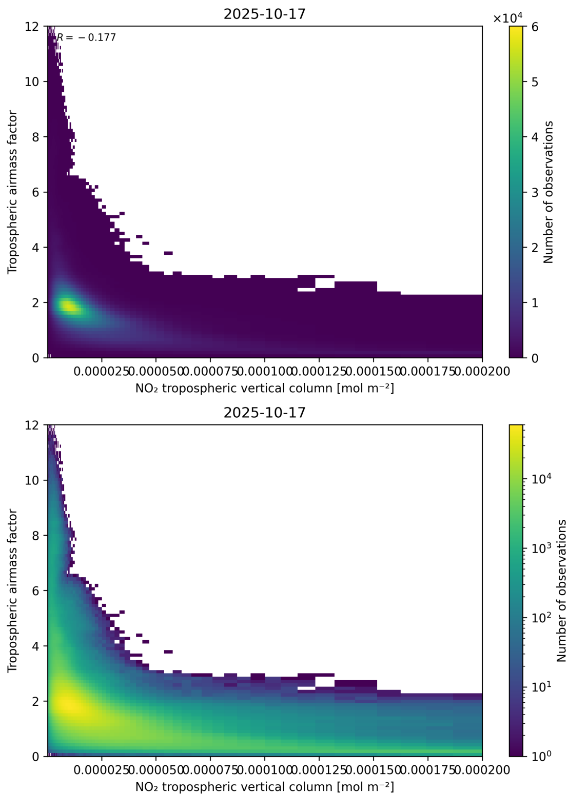
Figure 123: Scatter density plot of “NO 2 tropospheric vertical column” against “Tropospheric airmass factor” for 2025-10-17 to 2025-10-18.
