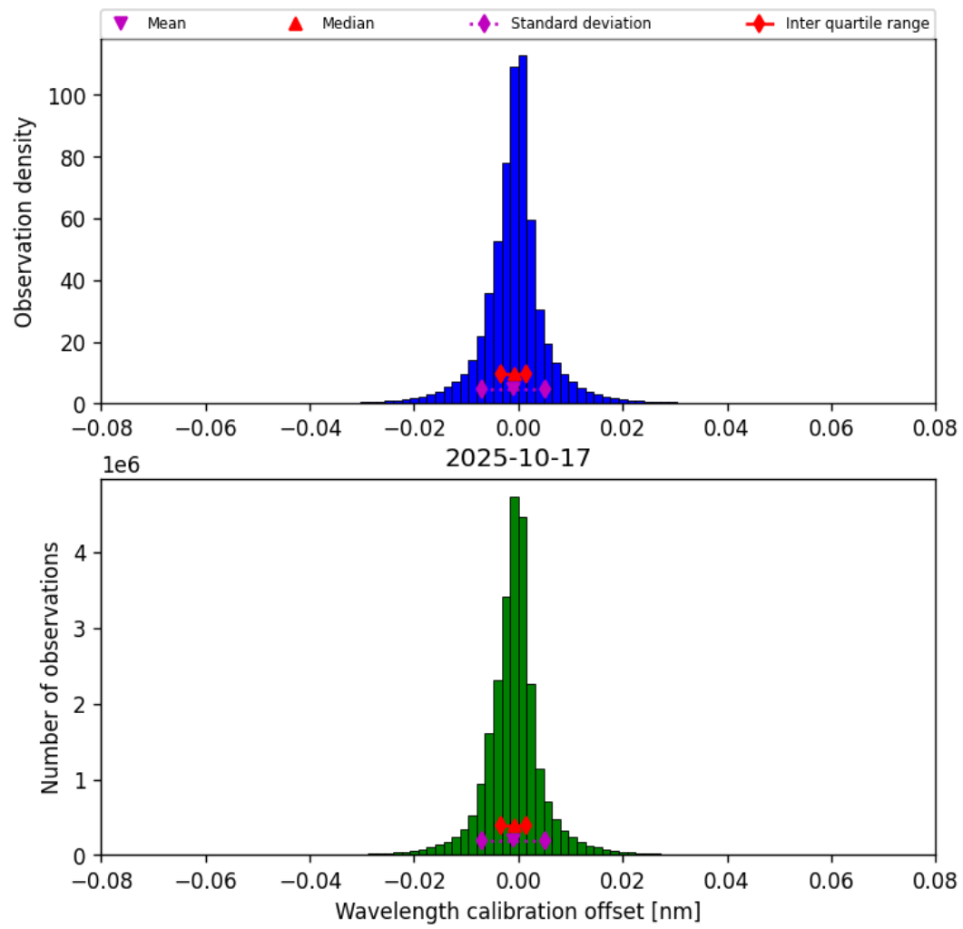
Figure 35: Histogram of “Wavelength calibration offset” for 2025-10-17 to 2025-10-18
