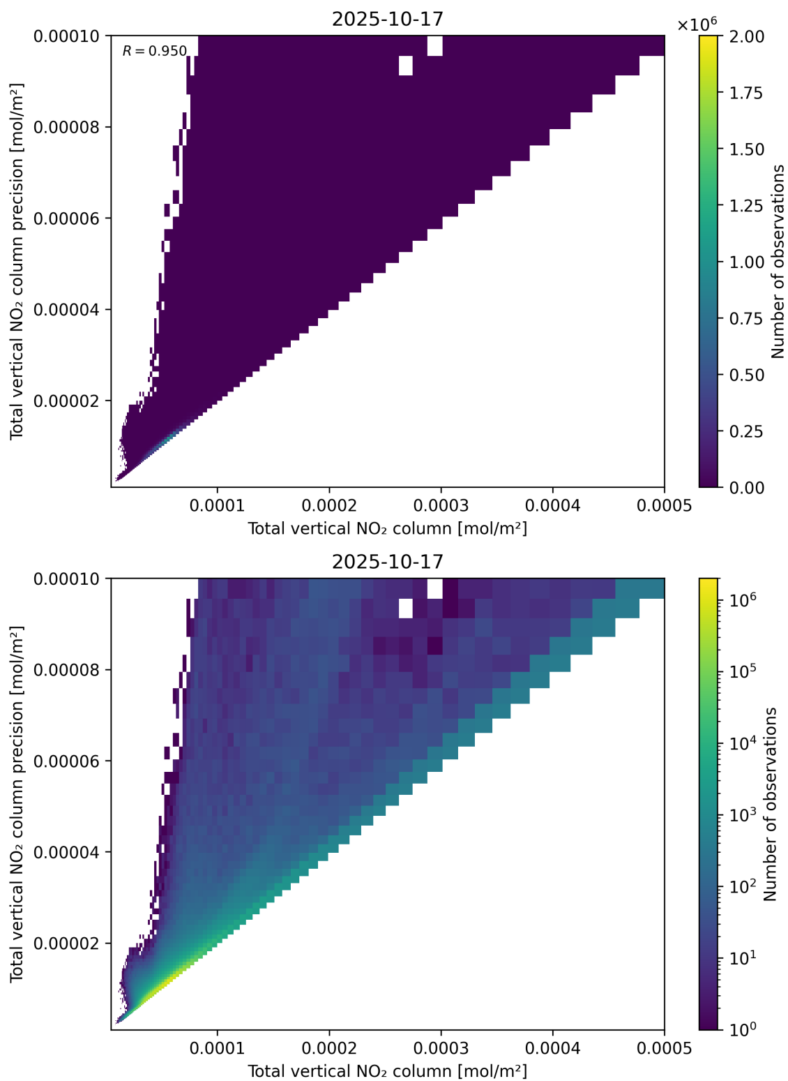
Figure 114: Scatter density plot of “Total vertical NO 2 column” against “Total vertical NO 2 column precision” for 2025-10-17 to 2025-10-18.
