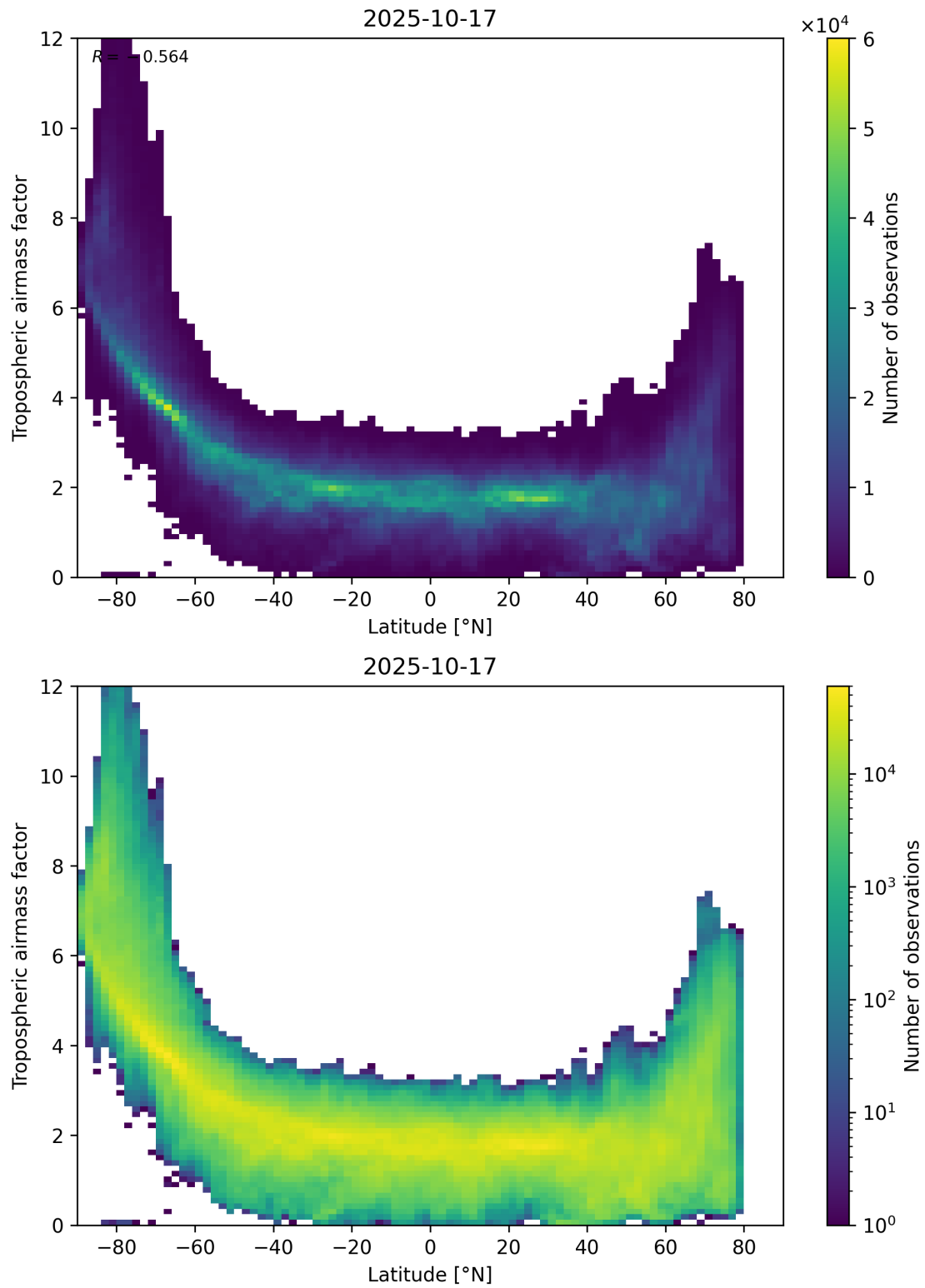
Figure 85: Scatter density plot of “Latitude” against “Tropospheric air mass factor” for 2025-10-17 to 2025-10-18.
