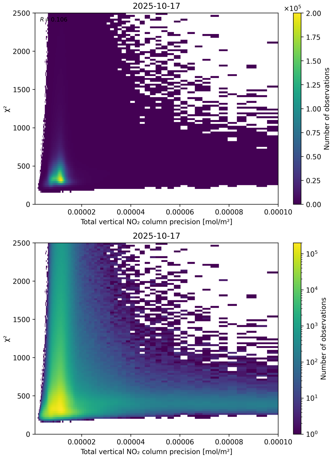
Figure 116: Scatter density plot of “Total vertical NO 2 column precision” against “ \chi^2 ” for 2025-10-17 to 2025-10-18.
