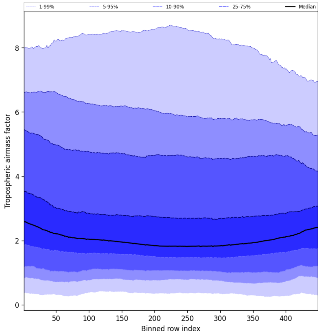
Figure 48: Along track statistics of “Tropospheric air mass factor” for 2025-10-17 to 2025-10-18
