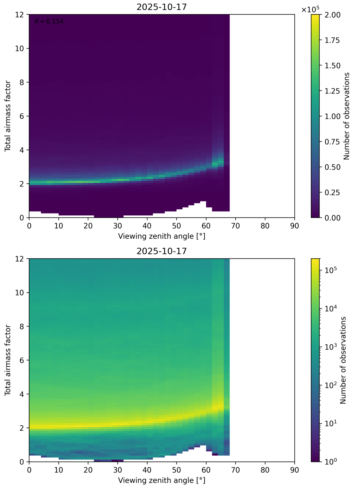
Figure 160: Scatter density plot of “Viewing zenith angle” against “Total airmass factor” for 2025-10-17 to 2025-10-18.
