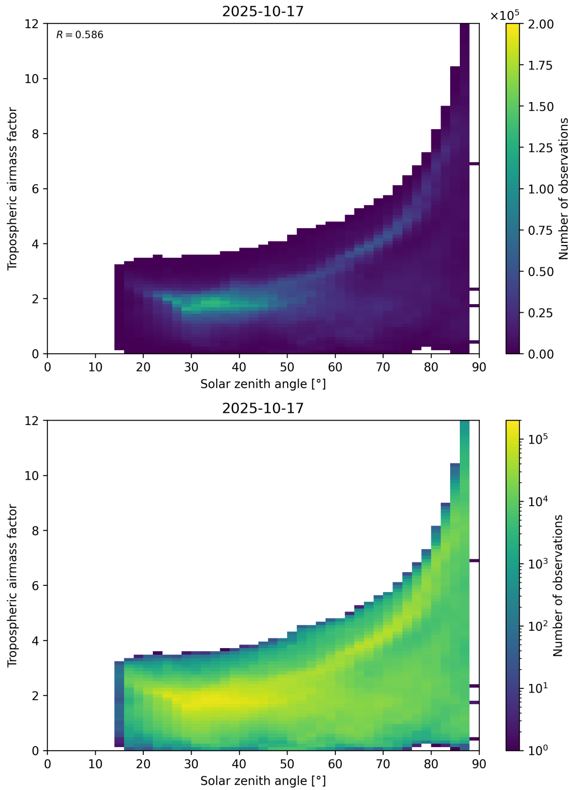
Figure 147: Scatter density plot of “Solar zenith angle” against “Tropospheric airmass factor” for 2025-10-17 to 2025-10-18.
