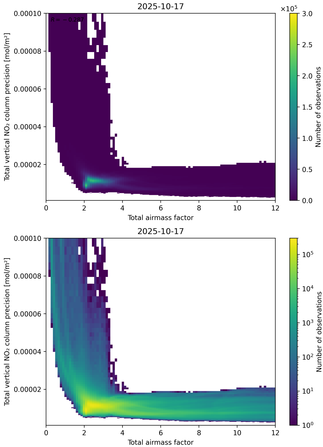
Figure 68: Scatter density plot of “Total airmass factor” against “Total vertical NO 2 column precision” for 2025-10-17 to 2025-10-18.
