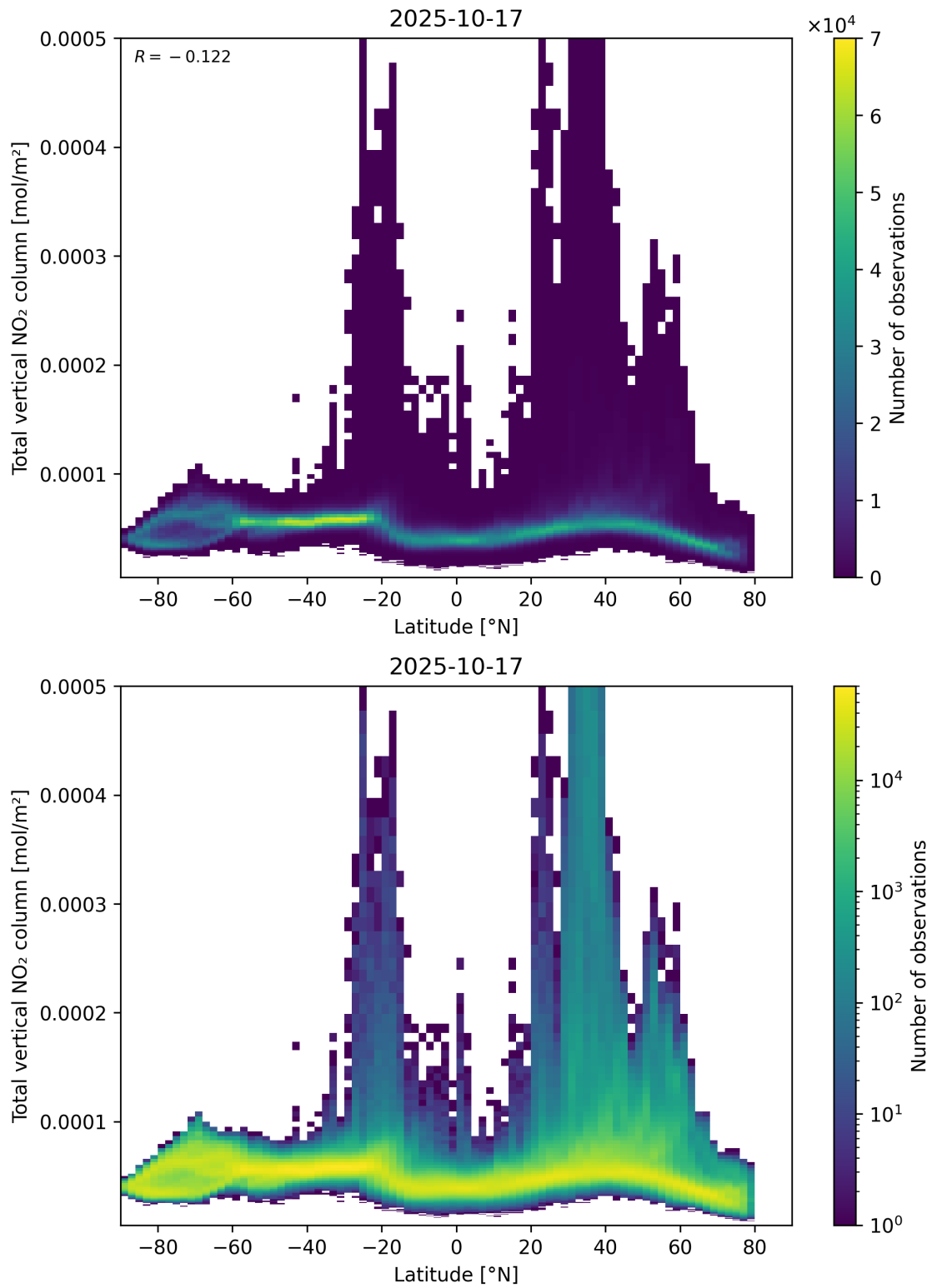
Figure 90: Scatter density plot of “Latitude” against “Total vertical NO 2 column” for 2025-10-17 to 2025-10-18.
