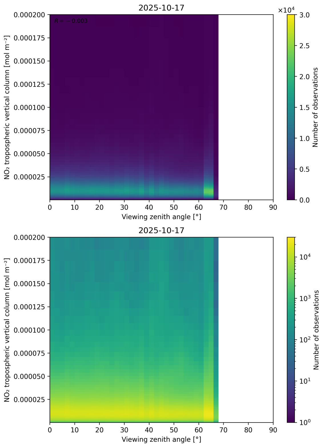
Figure 169: Scatter density plot of “Viewing zenith angle” against “NO 2 tropospheric vertical column” for 2025-10-17 to 2025-10-18.
