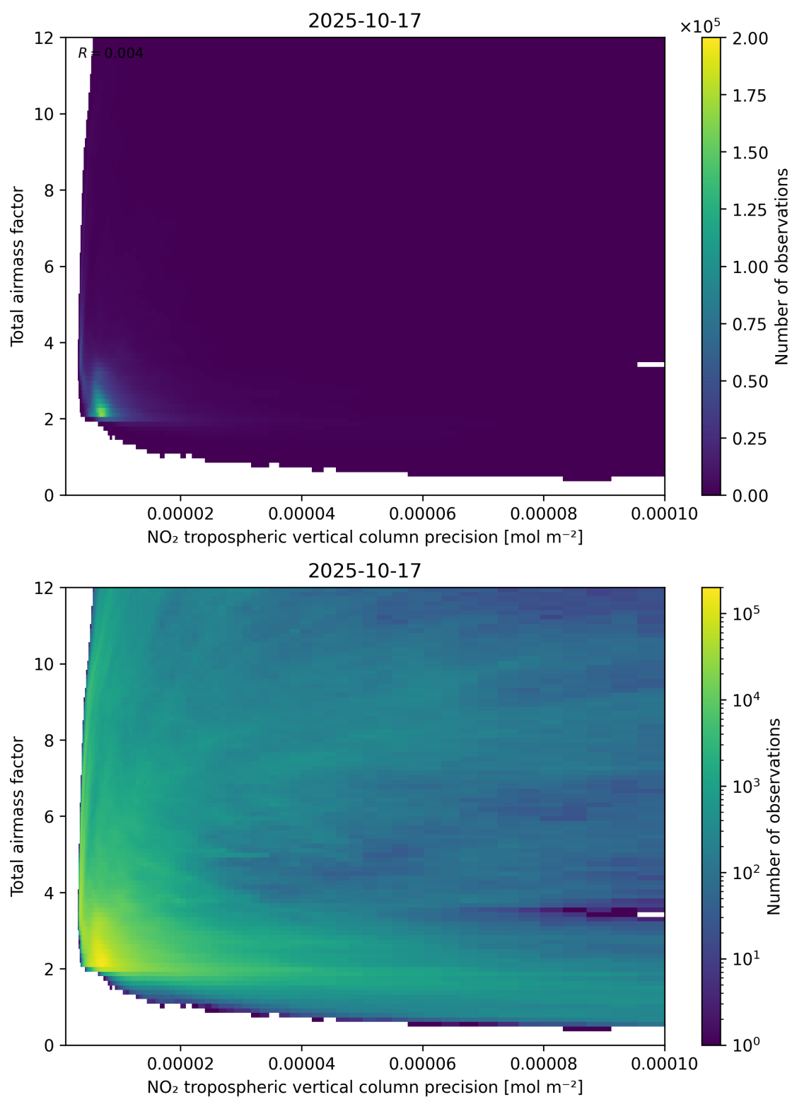
Figure 132: Scatter density plot of “NO 2 tropospheric vertical column precision” against “Total air mass factor” for 2025-10-17 to 2025-10-18.
