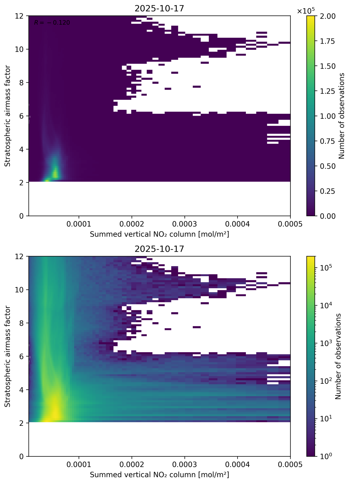
Figure 103: Scatter density plot of “Summed vertical NO 2 column” against “Stratospheric air mass factor” for 2025-10-17 to 2025-10-18.
