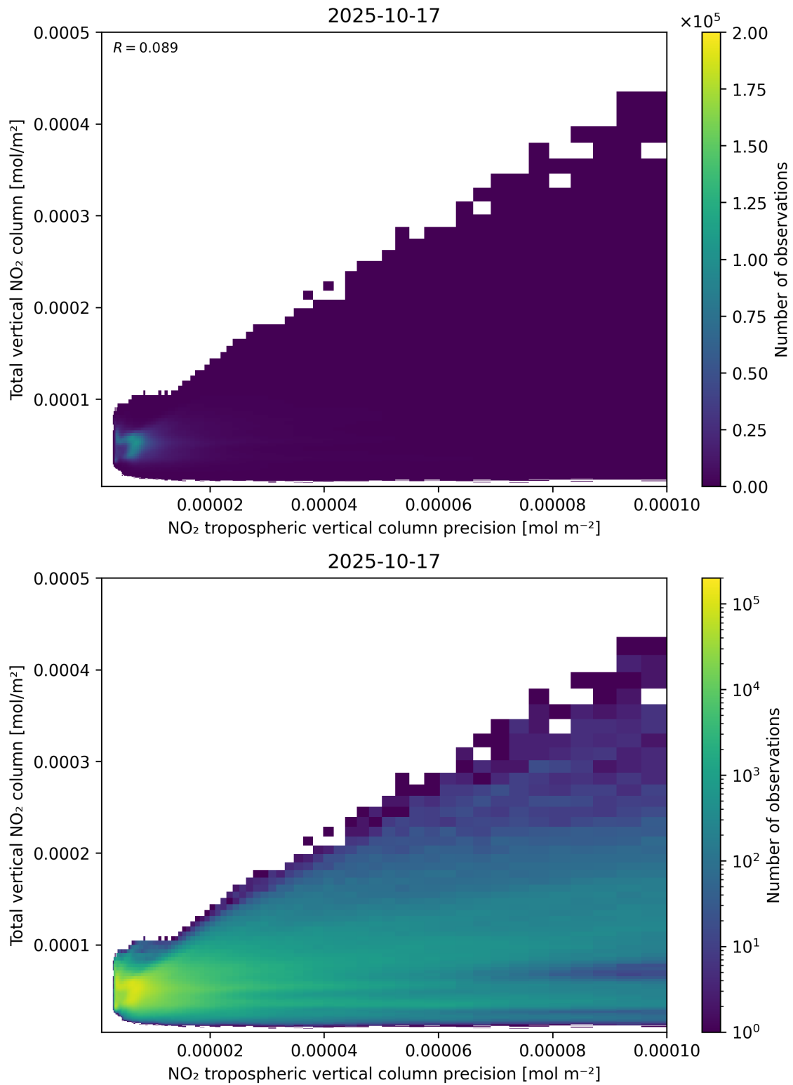
Figure 138: Scatter density plot of “NO 2 tropospheric vertical column precision” against “Total vertical NO 2 column” for 2025-10-17 to 2025-10-18.
