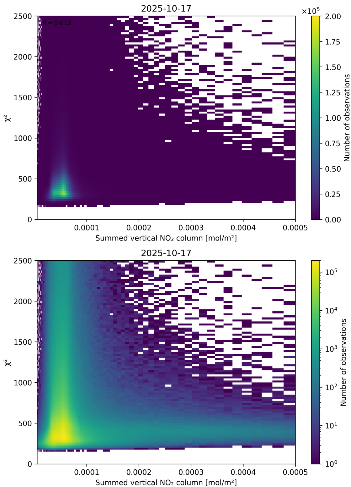
Figure 104: Scatter density plot of “Summed vertical NO 2 column” against “ \chi^2 ” for 2025-10-17 to 2025-10-18.
