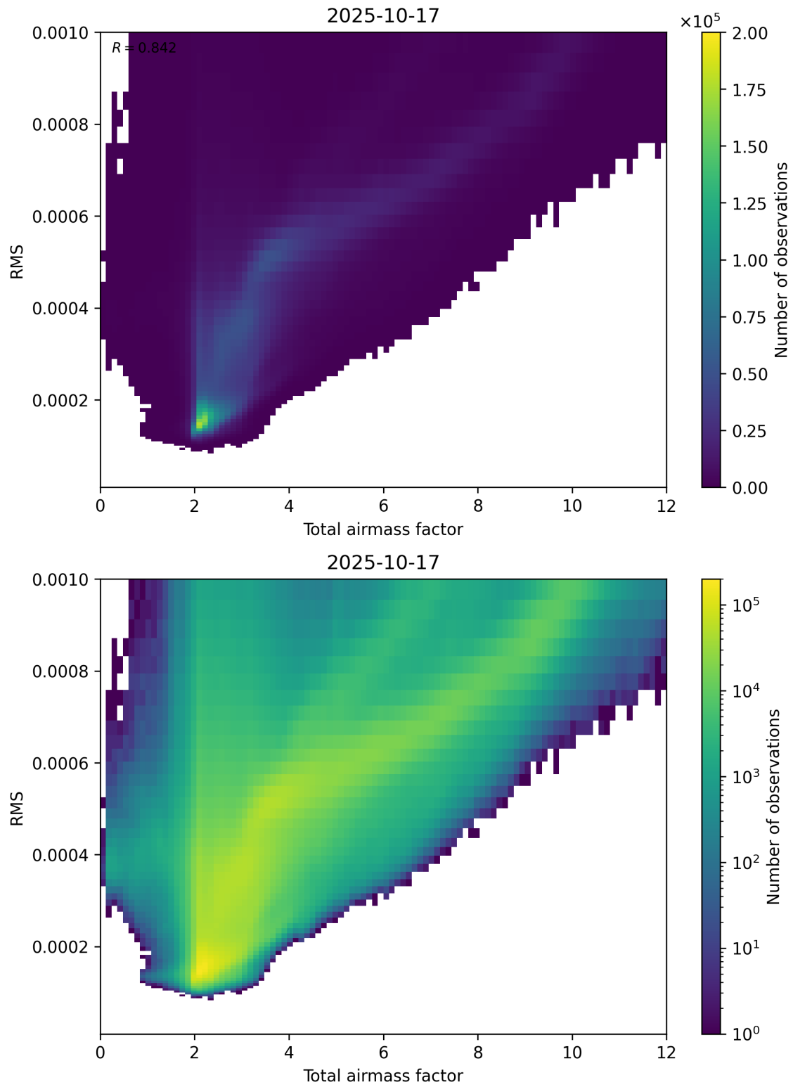
Figure 69: Scatter density plot of “Total airmass factor” against “RMS” for 2025-10-17 to 2025-10-18.
