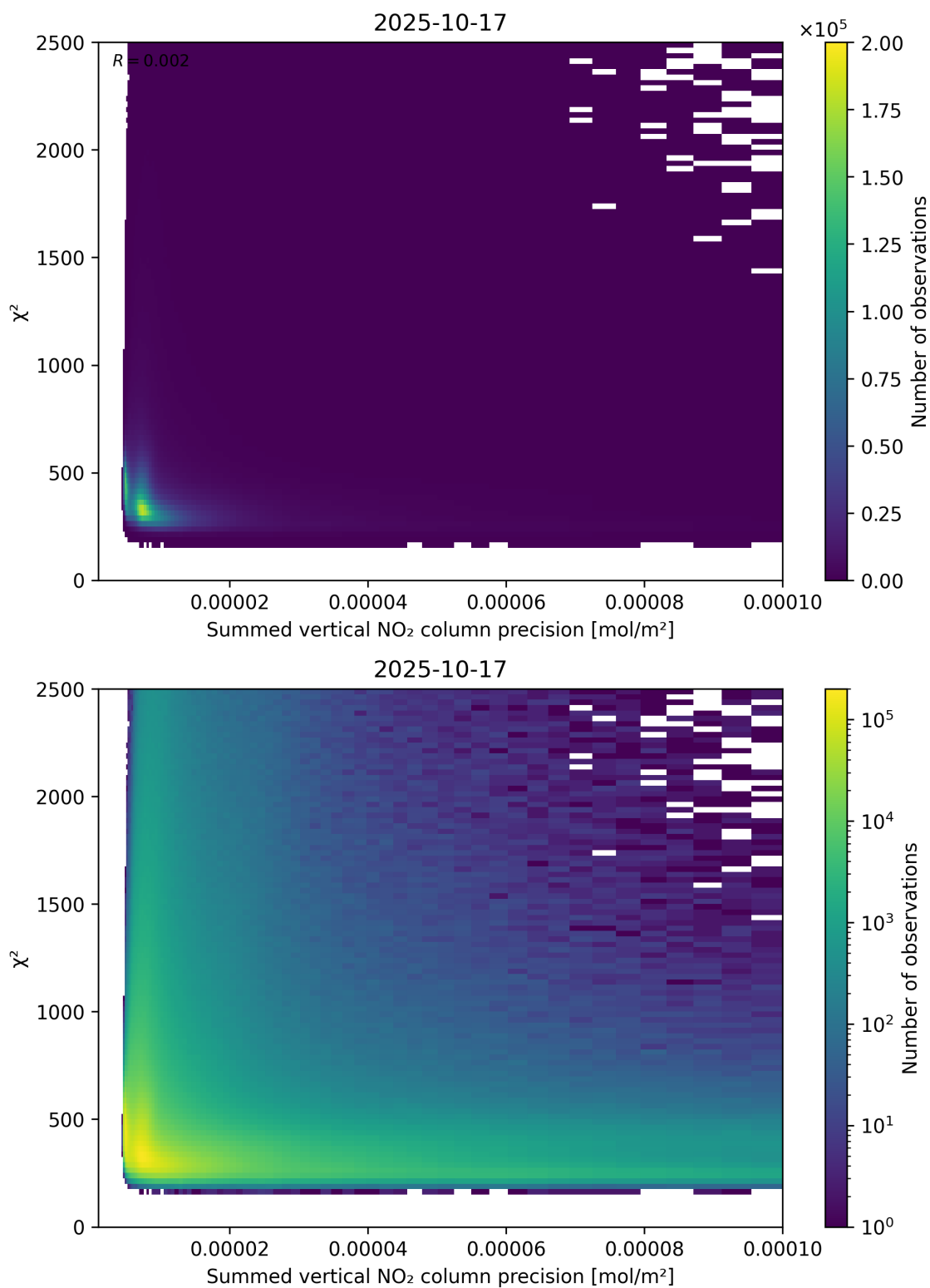
Figure 107: Scatter density plot of “Summed vertical NO 2 column precision” against “ \chi^2 ” for 2025-10-17 to 2025-10-18.
