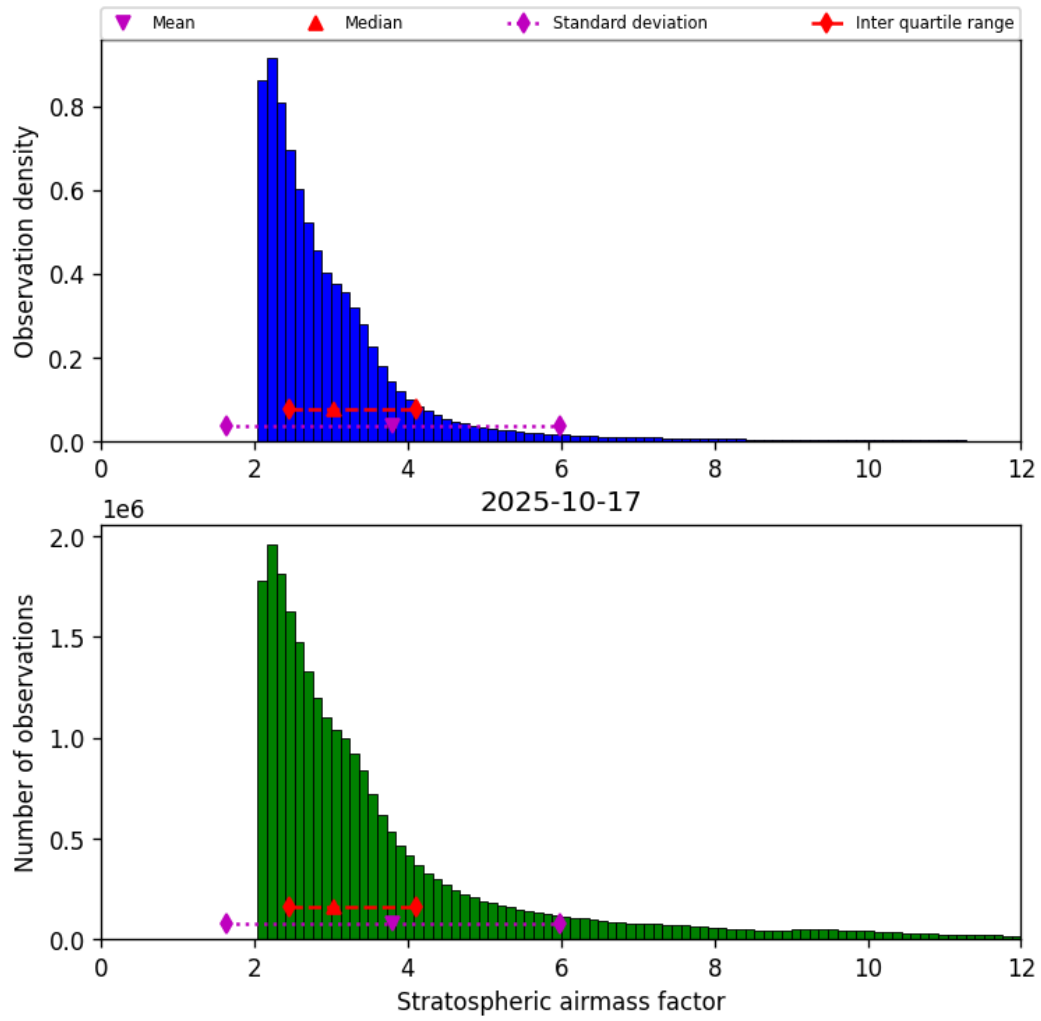
Figure 44: Histogram of “Stratospheric airmass factor” for 2025-10-17 to 2025-10-18
