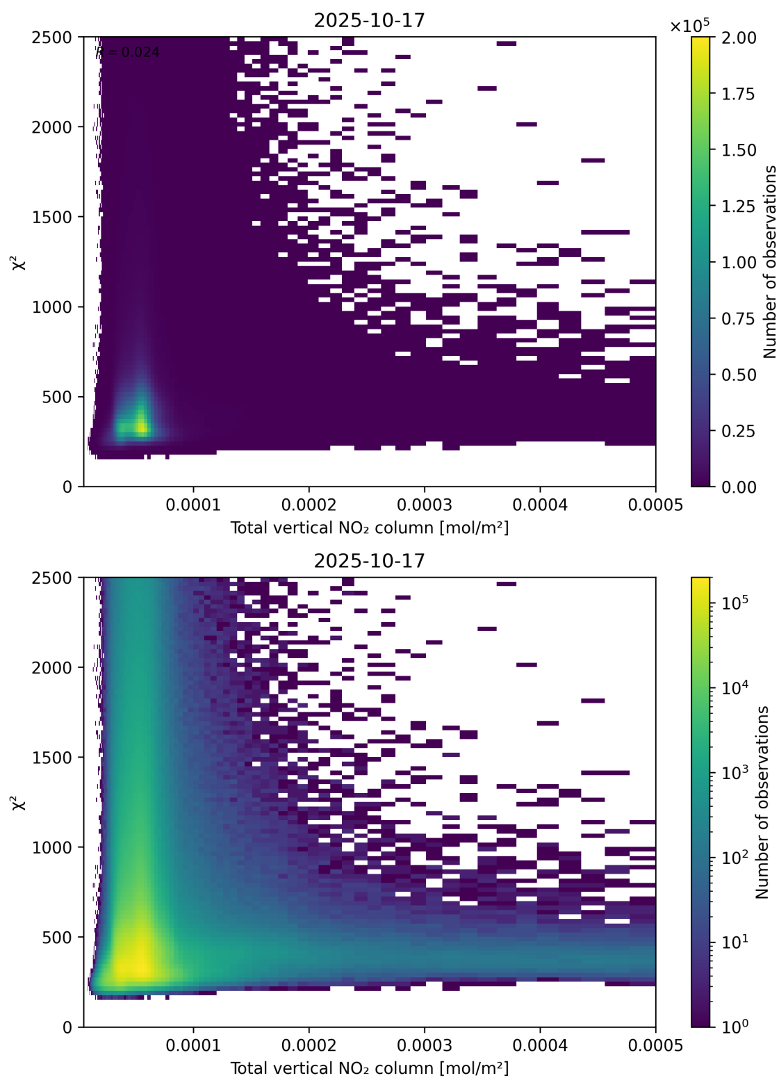
Figure 111: Scatter density plot of “Total vertical NO 2 column” against “ \chi^2 ” for 2025-10-17 to 2025-10-18.
