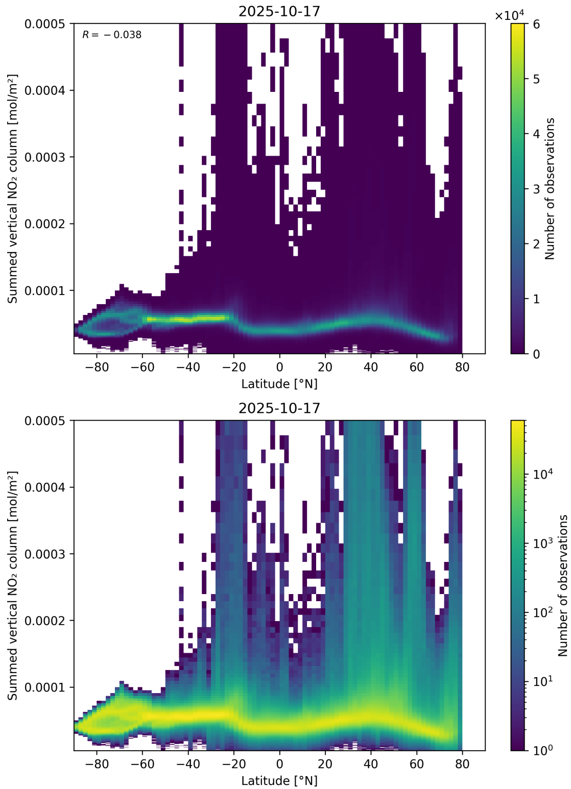
Figure 88: Scatter density plot of “Latitude” against “Summed vertical NO 2 column” for 2025-10-17 to 2025-10-18.
