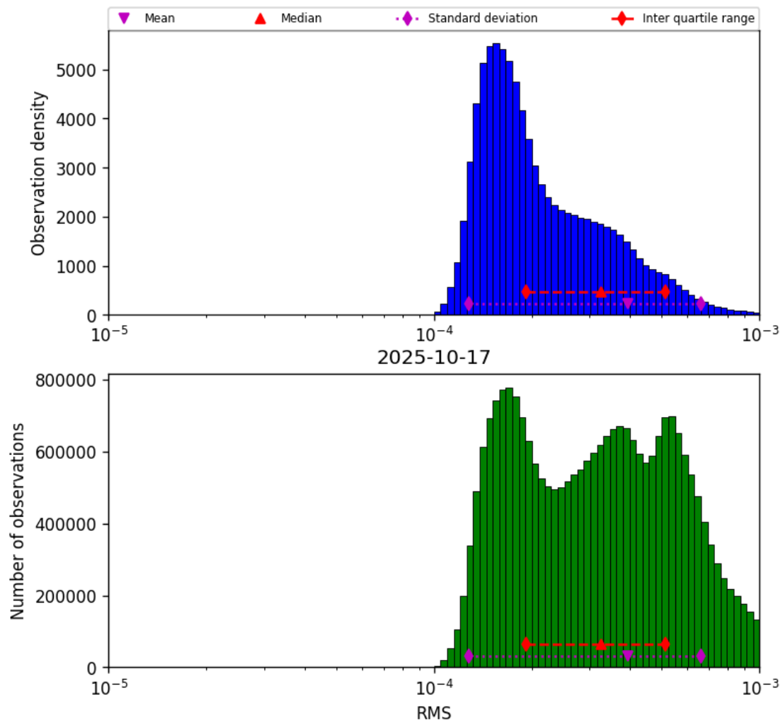
Figure 43: Histogram of “RMS” for 2025-10-17 to 2025-10-18
