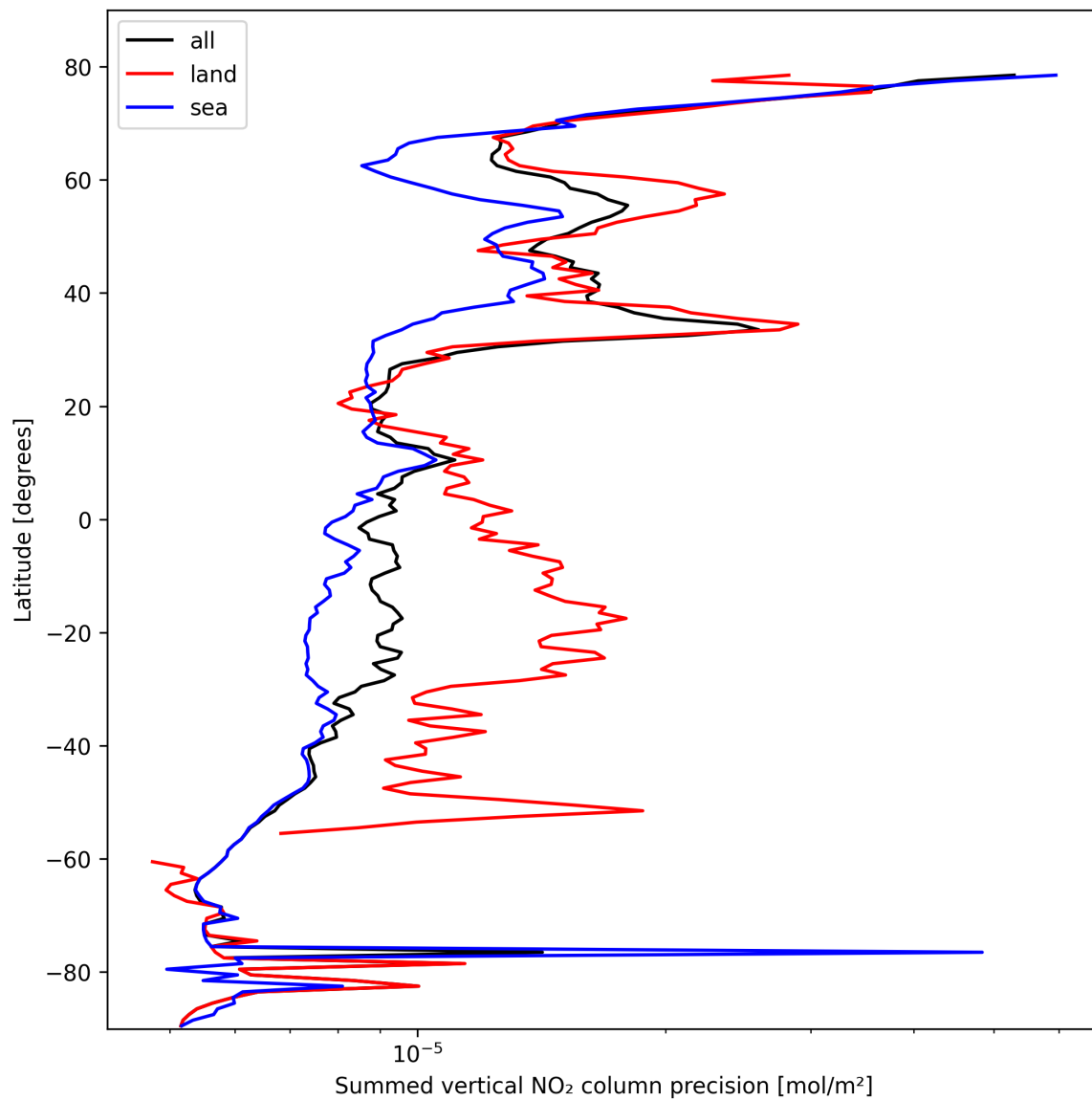
Figure 24: Zonal average of “Summed vertical NO 2 column precision” for 2025-10-17 to 2025-10-18.
