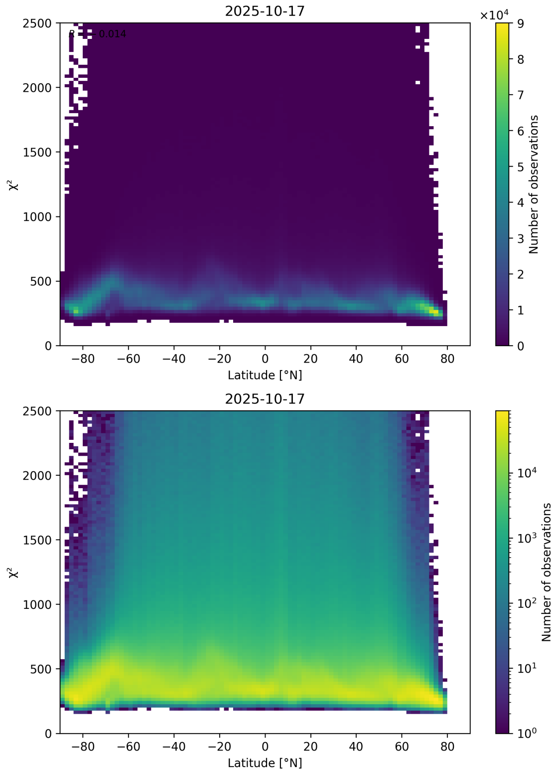
Figure 86: Scatter density plot of “Latitude” against “ \chi^2 ” for 2025-10-17 to 2025-10-18.
