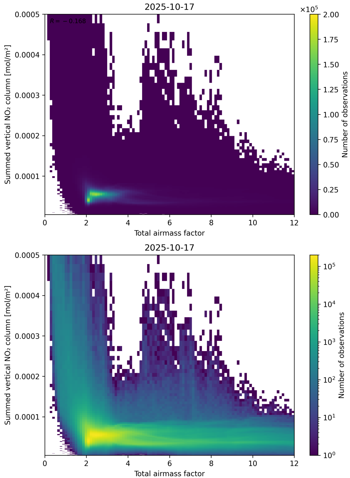
Figure 65: Scatter density plot of “Total airmass factor” against “Summed vertical NO 2 column” for 2025-10-17 to 2025-10-18.
