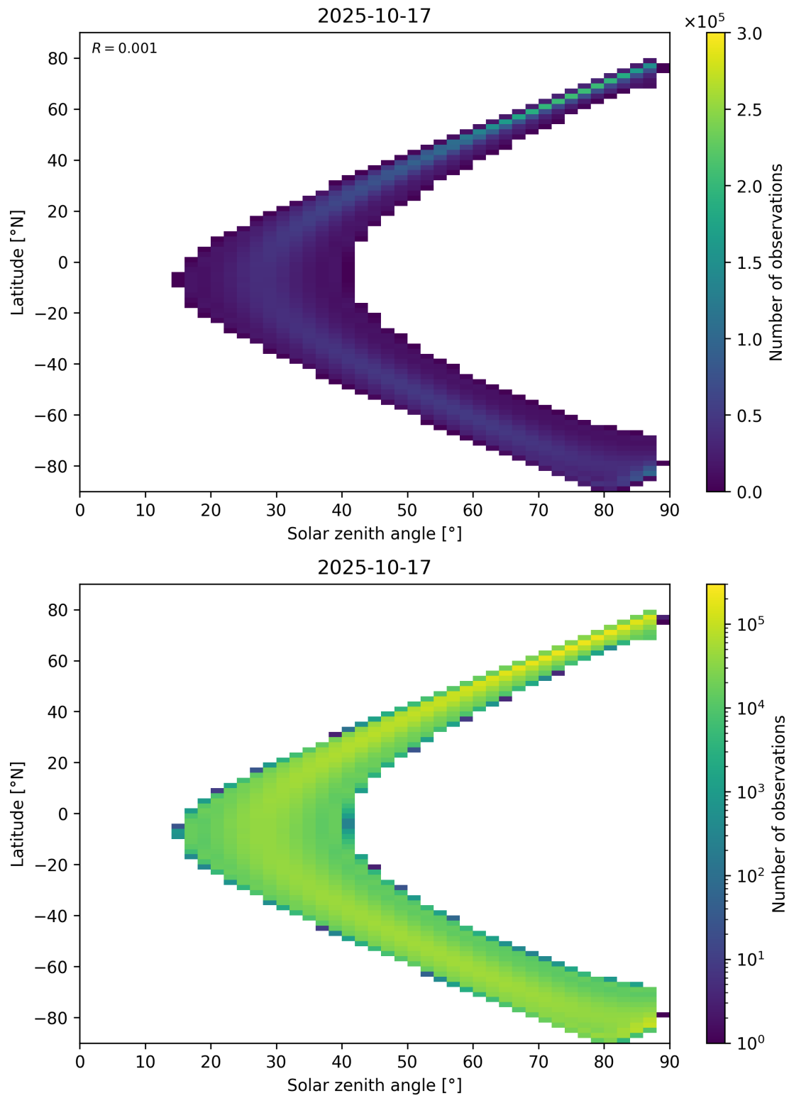
Figure 149: Scatter density plot of “Solar zenith angle” against “Latitude” for 2025-10-17 to 2025-10-18.
