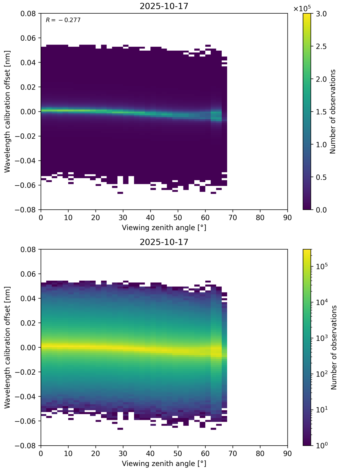
Figure 173: Scatter density plot of “Viewing zenith angle” against “Wavelength calibration offset” for 2025-10-17 to 2025-10-18.
