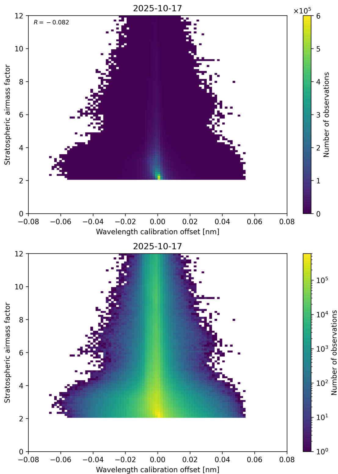
Figure 174: Scatter density plot of “Wavelength calibration offset” against “Stratospheric air mass factor” for 2025-10-17 to 2025-10-18.
