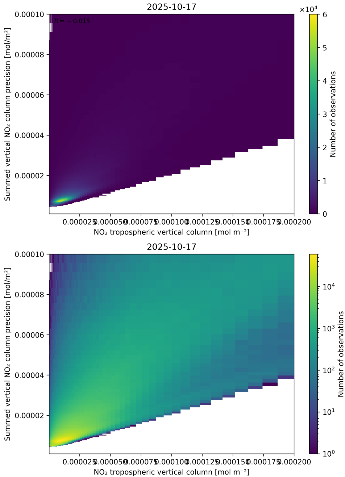
Figure 127: Scatter density plot of “NO 2 tropospheric vertical column” against “Summed vertical NO 2 column precision” for 2025-10-17 to 2025-10-18.
