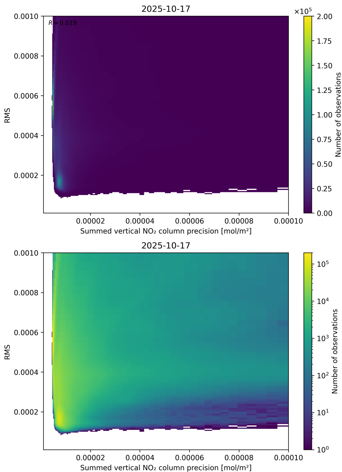
Figure 108: Scatter density plot of “Summed vertical NO 2 column precision” against “RMS” for 2025-10-17 to 2025-10-18.
