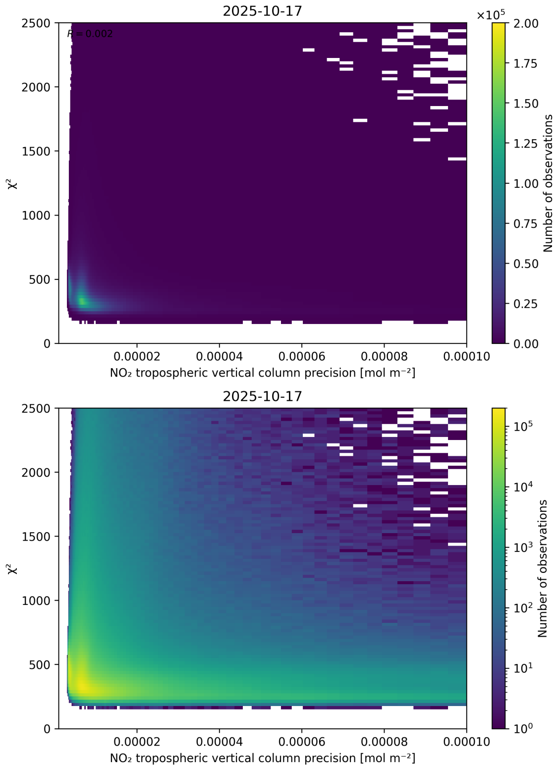
Figure 134: Scatter density plot of “NO 2 tropospheric vertical column precision” against “ \chi^2 ” for 2025-10-17 to 2025-10-18.
