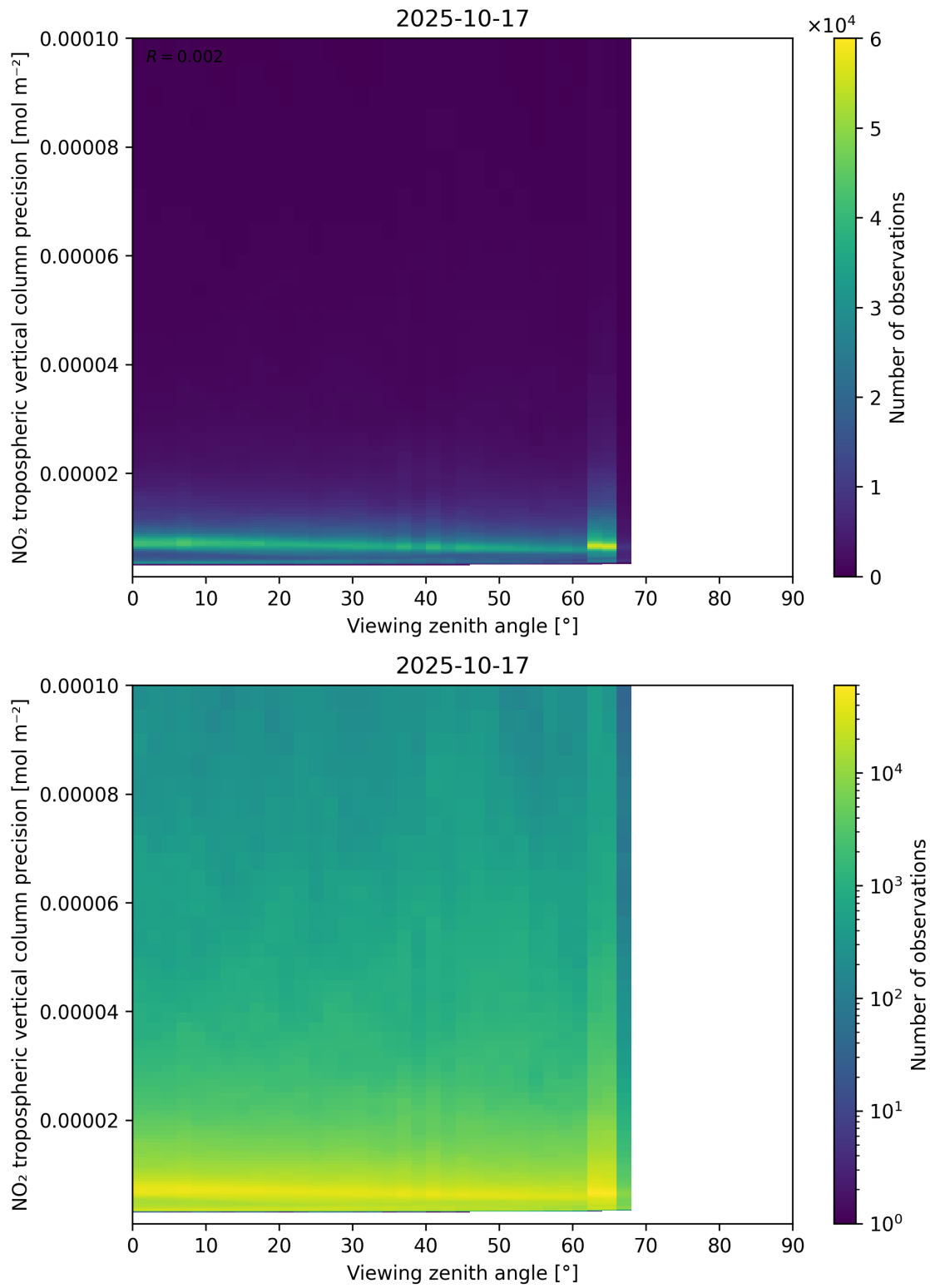
Figure 170: Scatter density plot of “Viewing zenith angle” against “NO 2 tropospheric vertical column precision” for 2025-10-17 to 2025-10-18.
