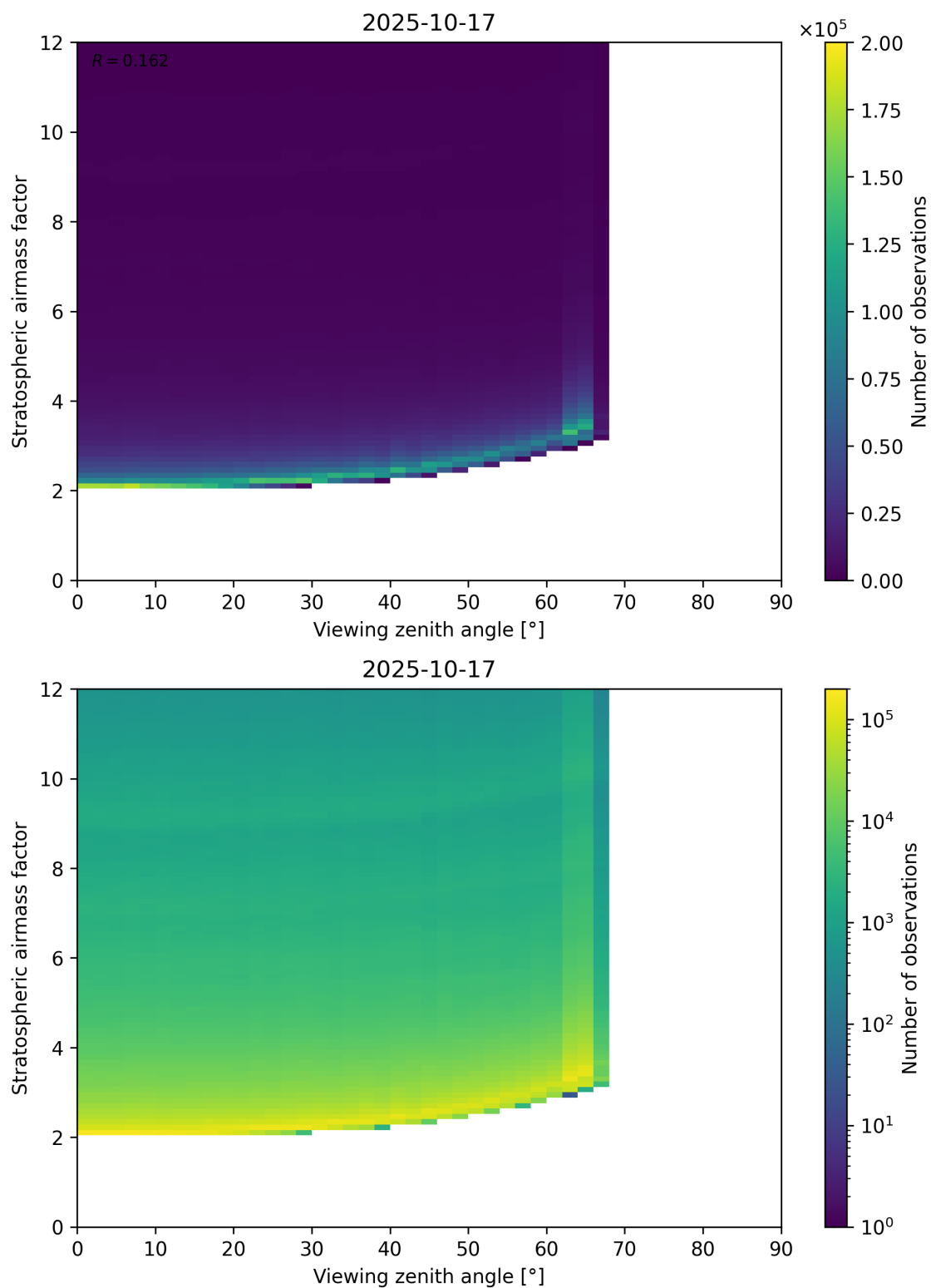
Figure 159: Scatter density plot of “Viewing zenith angle” against “Stratospheric airmass factor” for 2025-10-17 to 2025-10-18.
