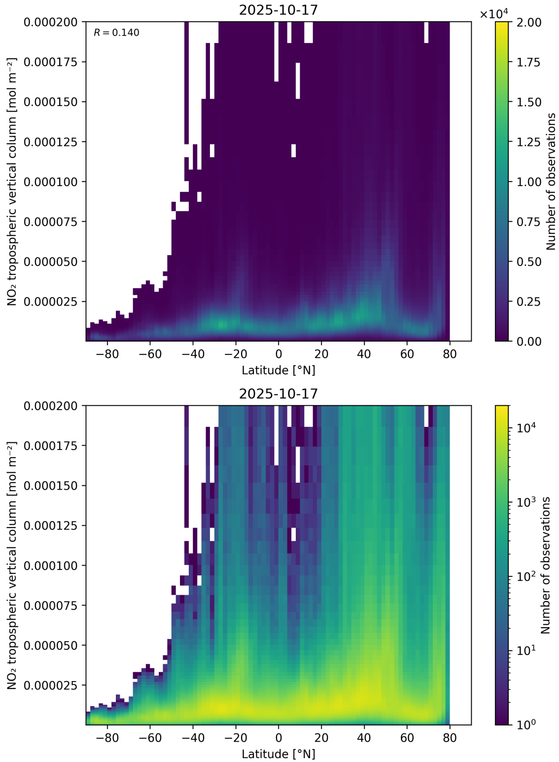
Figure 92: Scatter density plot of “Latitude” against “NO 2 tropospheric vertical column” for 2025-10-17 to 2025-10-18.
