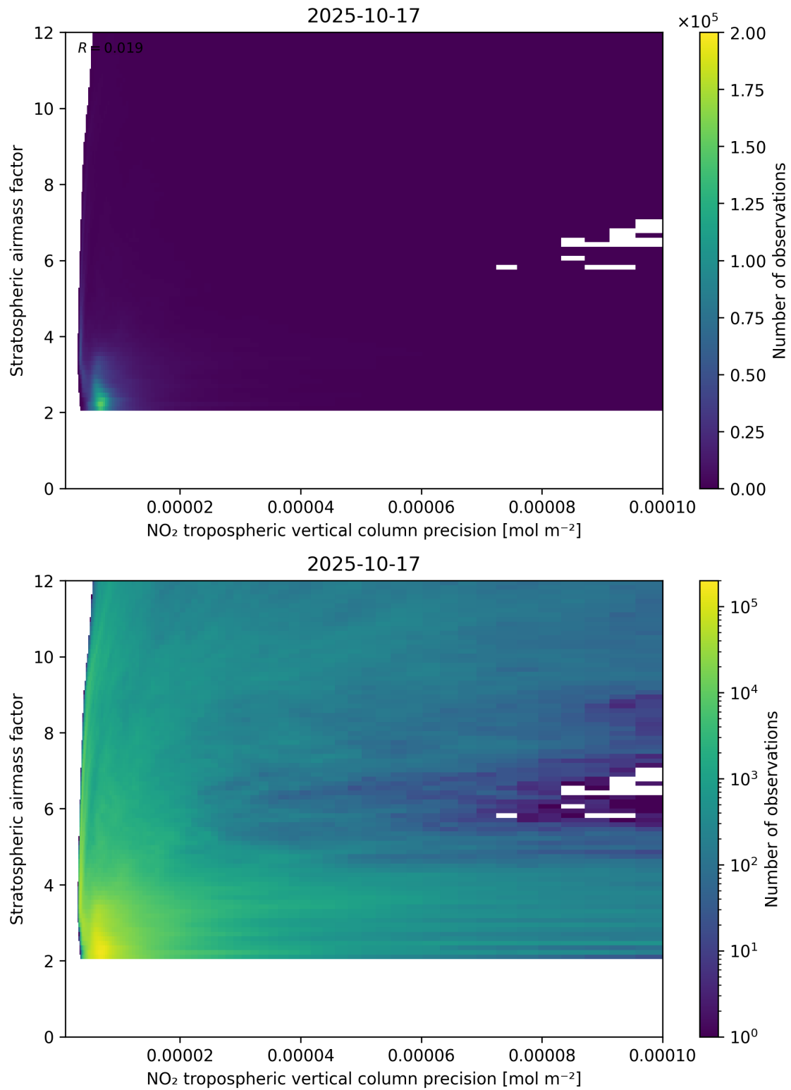
Figure 131: Scatter density plot of “NO 2 tropospheric vertical column precision” against “Stratospheric airmass factor” for 2025-10-17 to 2025-10-18.
