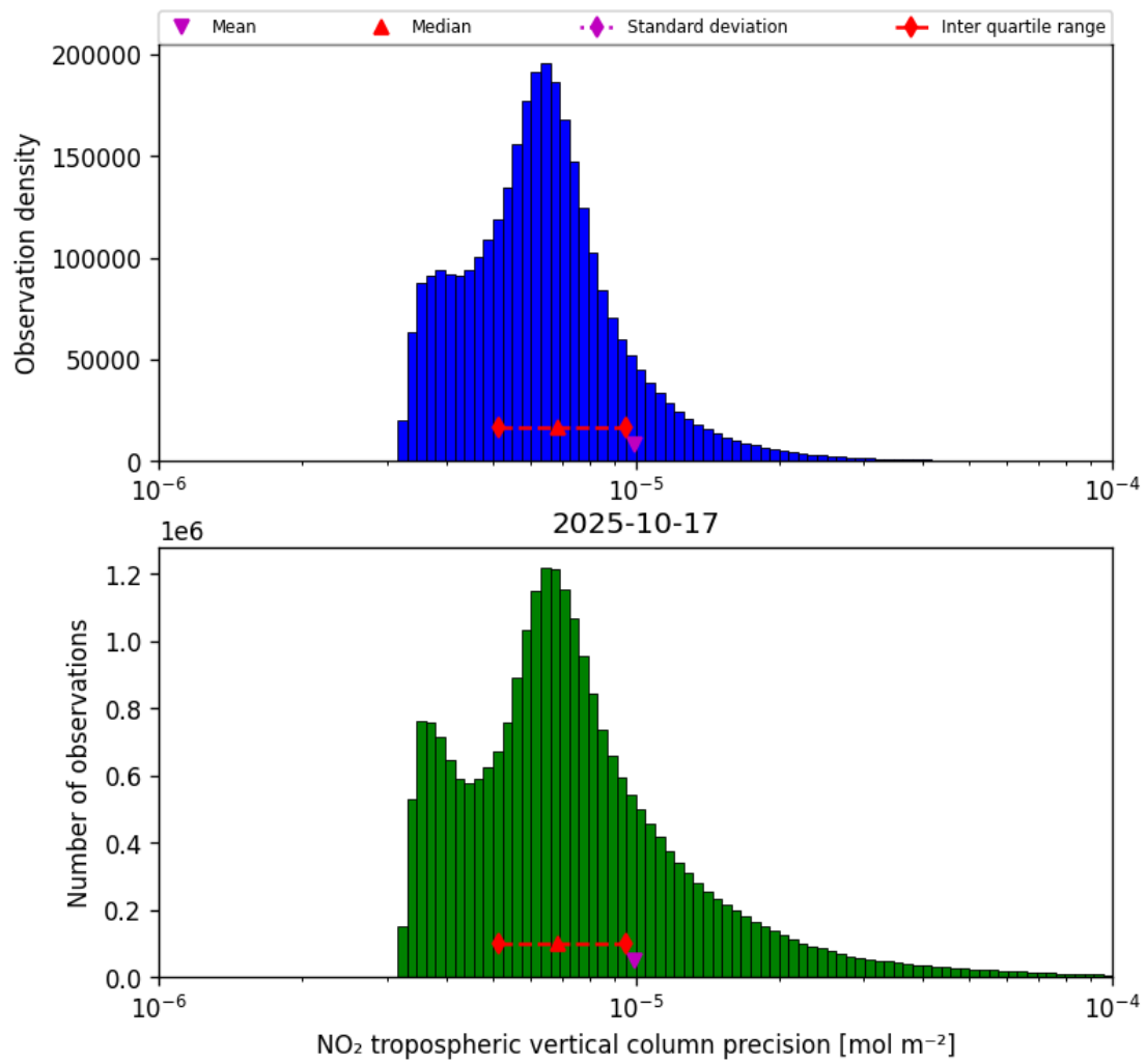
Figure 30: Histogram of “NO 2 tropospheric vertical column precision” for 2025-10-17 to 2025-10-18
