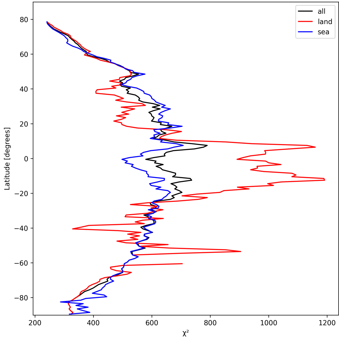
Figure 25: Zonal average of “ \chi^2 ” for 2025-10-17 to 2025-10-18.
