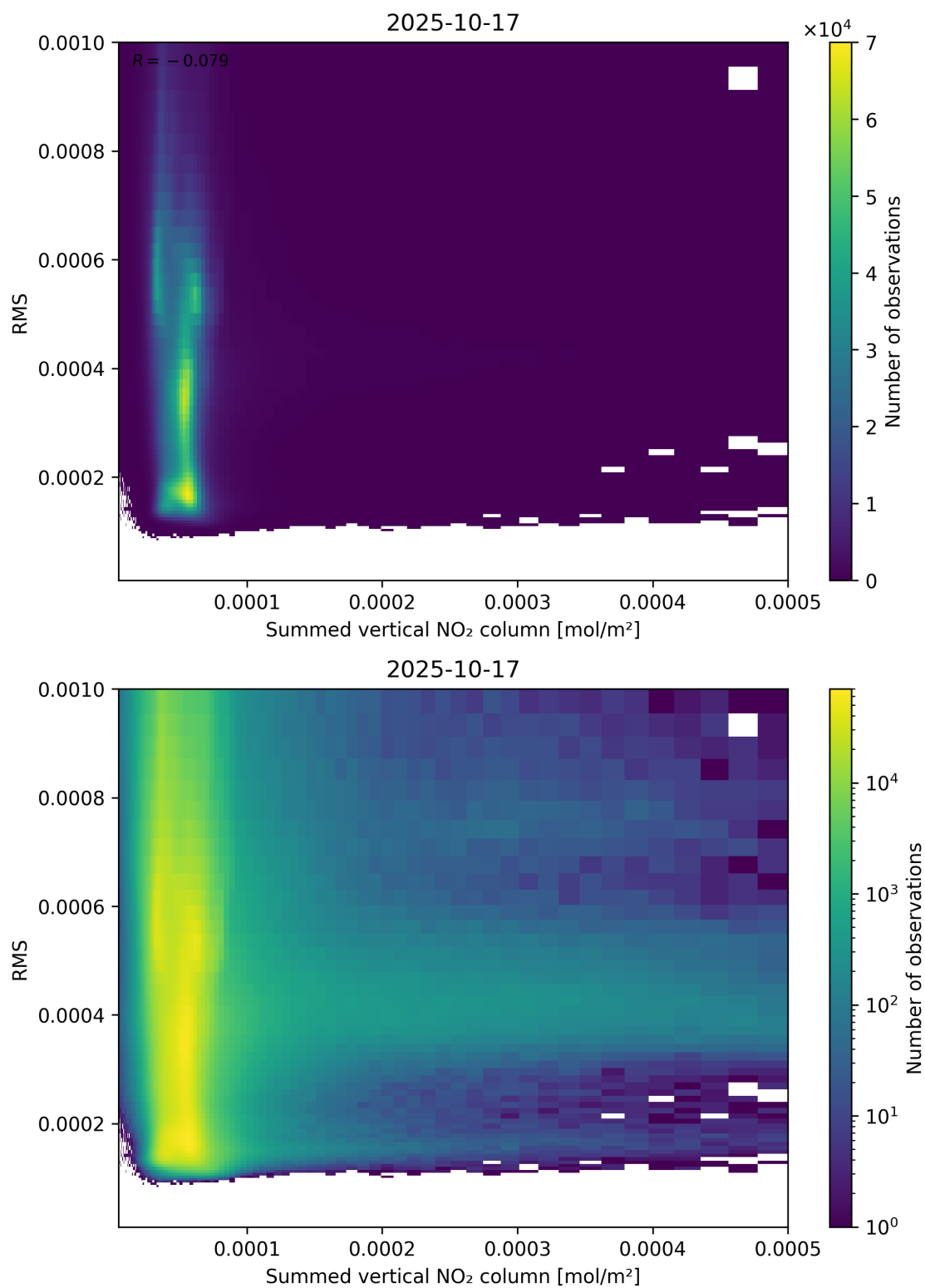
Figure 109: Scatter density plot of “Summed vertical NO 2 column” against “RMS” for 2025-10-17 to 2025-10-18.
