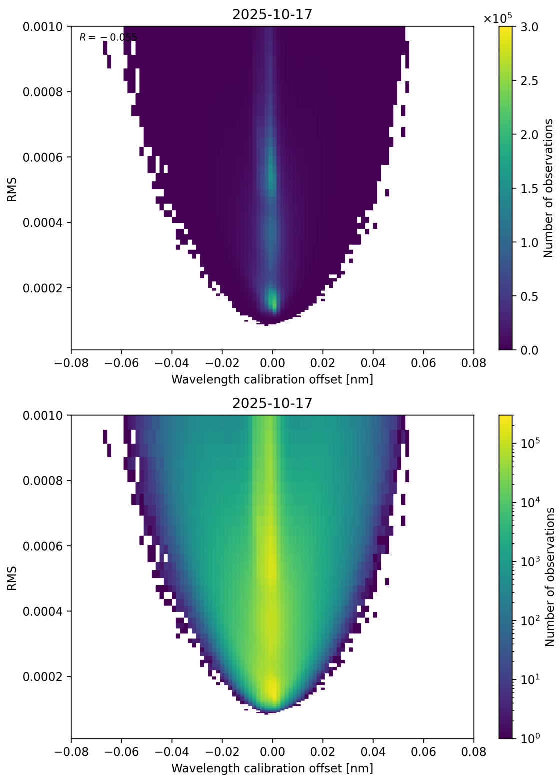
Figure 181: Scatter density plot of “Wavelength calibration offset” against “RMS” for 2025-10-17 to 2025-10-18.
