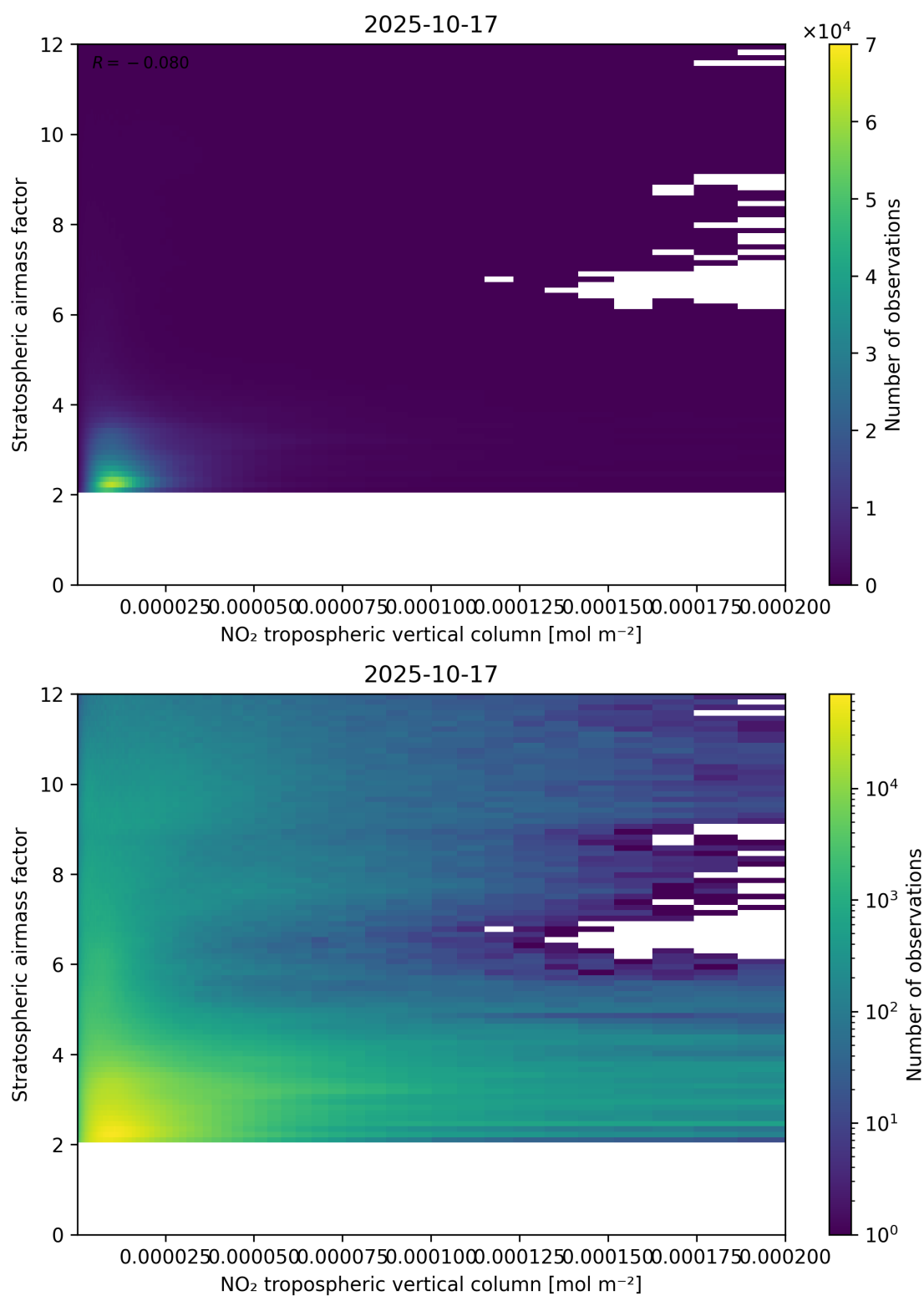
Figure 121: Scatter density plot of “NO 2 tropospheric vertical column” against “Stratospheric airmass factor” for 2025-10-17 to 2025-10-18.
