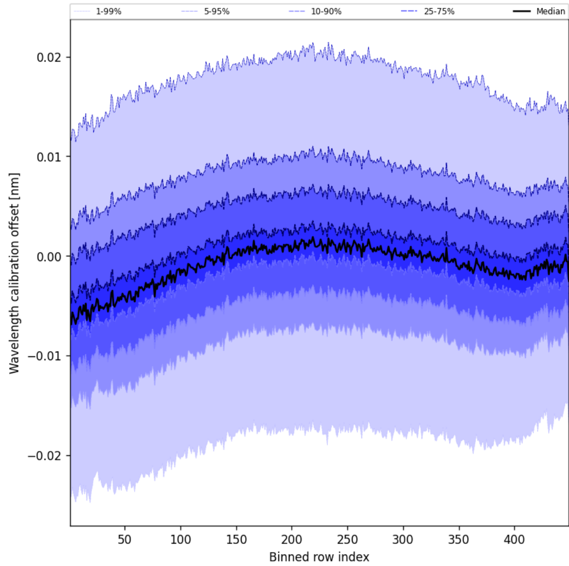
Figure 52: Along track statistics of “Wavelength calibration offset” for 2025-10-17 to 2025-10-18
