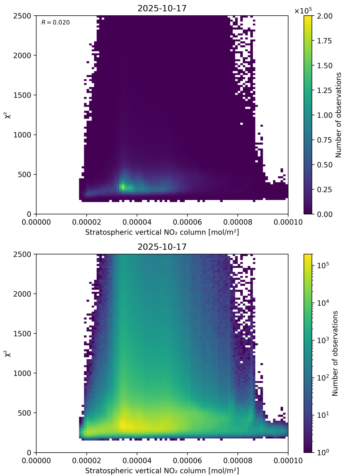
Figure 97: Scatter density plot of “Stratospheric vertical NO 2 column” against “ \chi^2 ” for 2025-10-17 to 2025-10-18.
