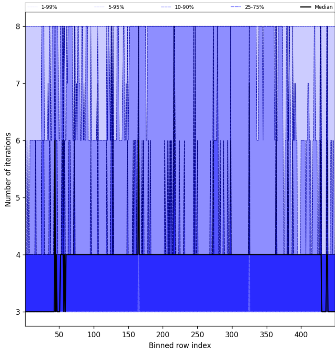
Figure 51: Along track statistics of “Number of iterations” for 2025-10-17 to 2025-10-18
