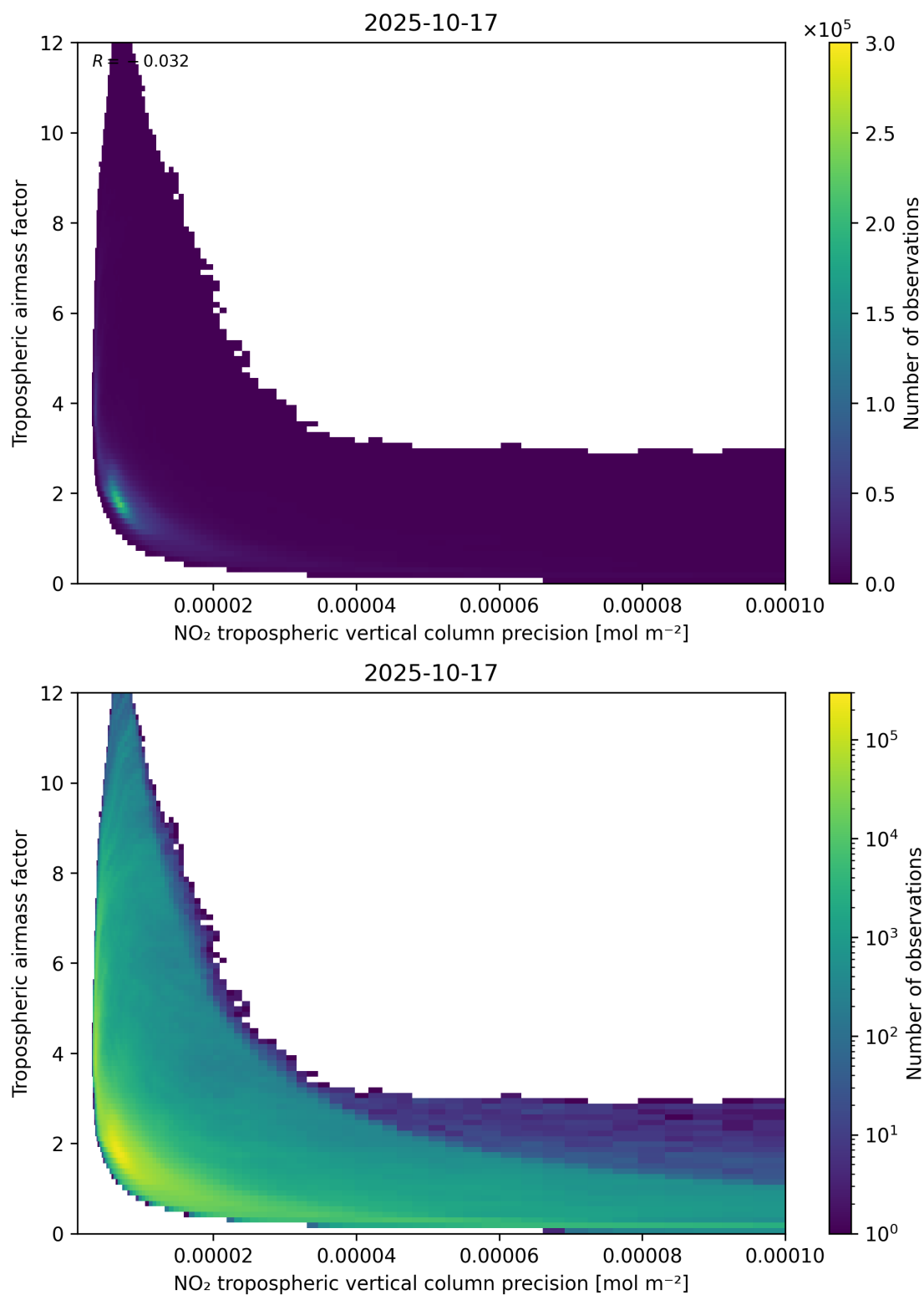
Figure 133: Scatter density plot of “NO 2 tropospheric vertical column precision” against “Tropospheric airmass factor” for 2025-10-17 to 2025-10-18.
