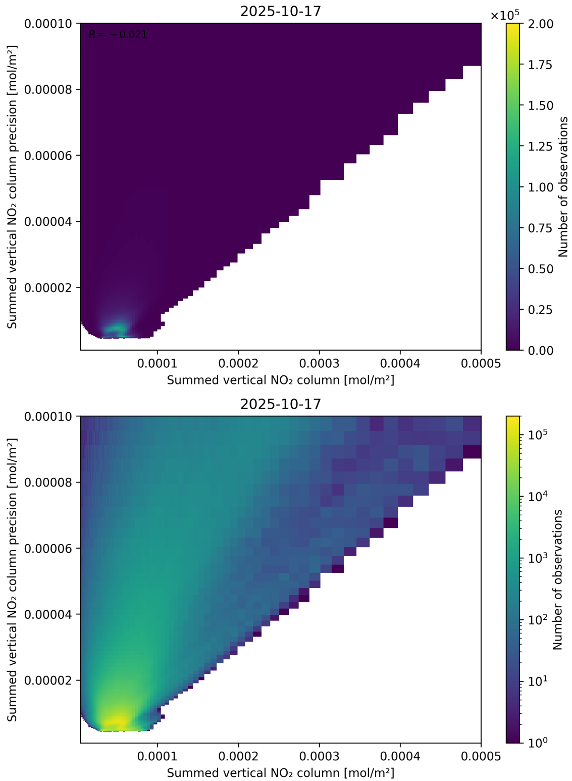
Figure 105: Scatter density plot of “Summed vertical NO 2 column” against “Summed vertical NO 2 column precision” for 2025-10-17 to 2025-10-18.
