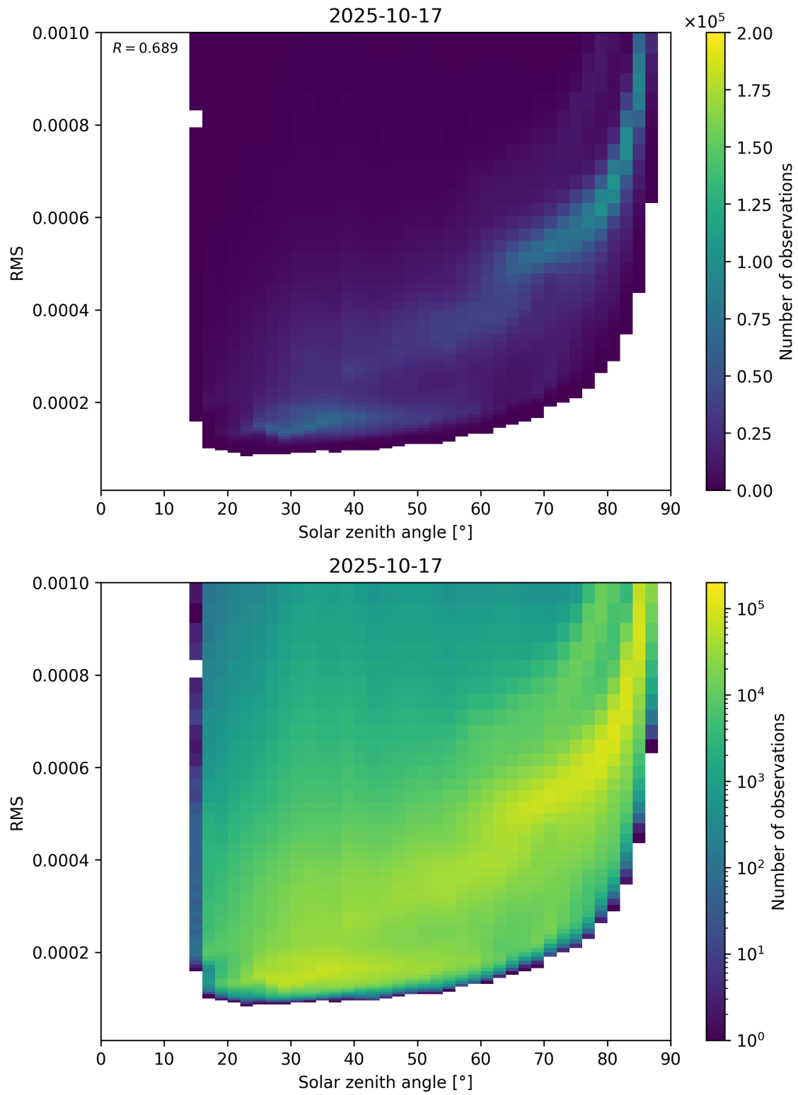
Figure 157: Scatter density plot of “Solar zenith angle” against “RMS” for 2025-10-17 to 2025-10-18.
