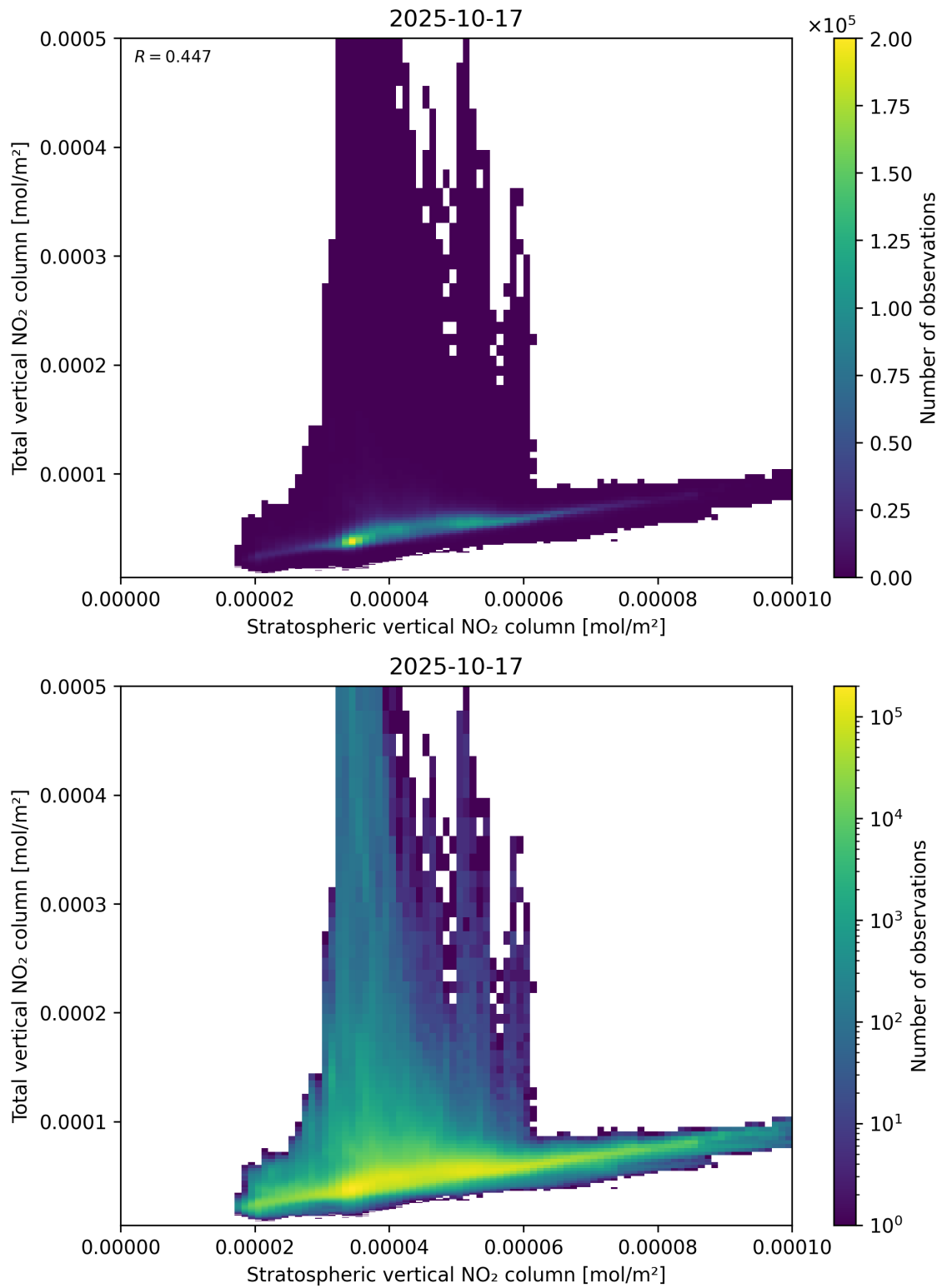
Figure 100: Scatter density plot of “Stratospheric vertical NO 2 column” against “Total vertical NO 2 column” for 2025-10-17 to 2025-10-18.
