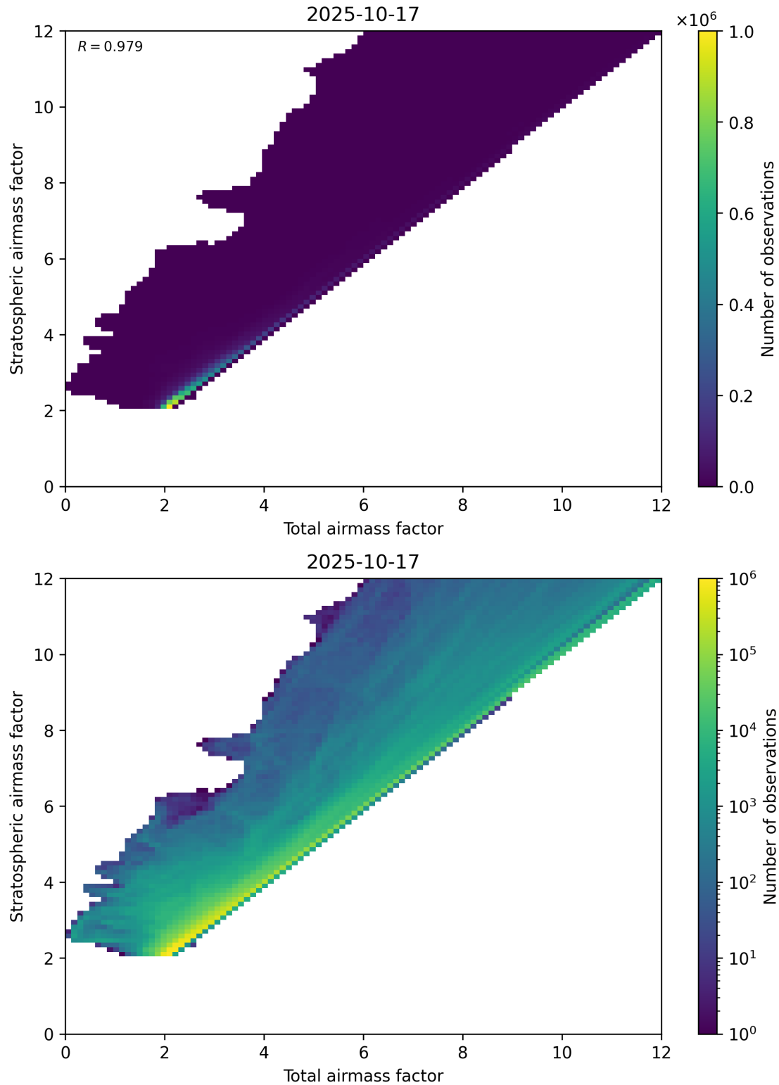
Figure 62: Scatter density plot of “Total airmass factor” against “Stratospheric airmass factor” for 2025-10-17 to 2025-10-18.
