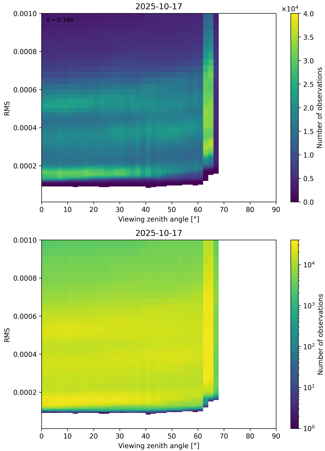
Figure 171: Scatter density plot of “Viewing zenith angle” against “RMS” for 2025-10-17 to 2025-10-18.
