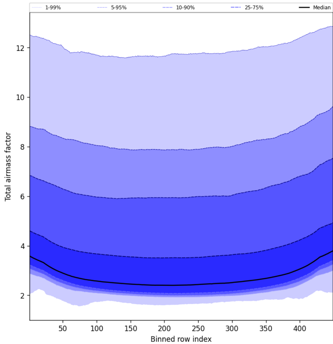
Figure 49: Along track statistics of “Total airmass factor” for 2025-10-17 to 2025-10-18
