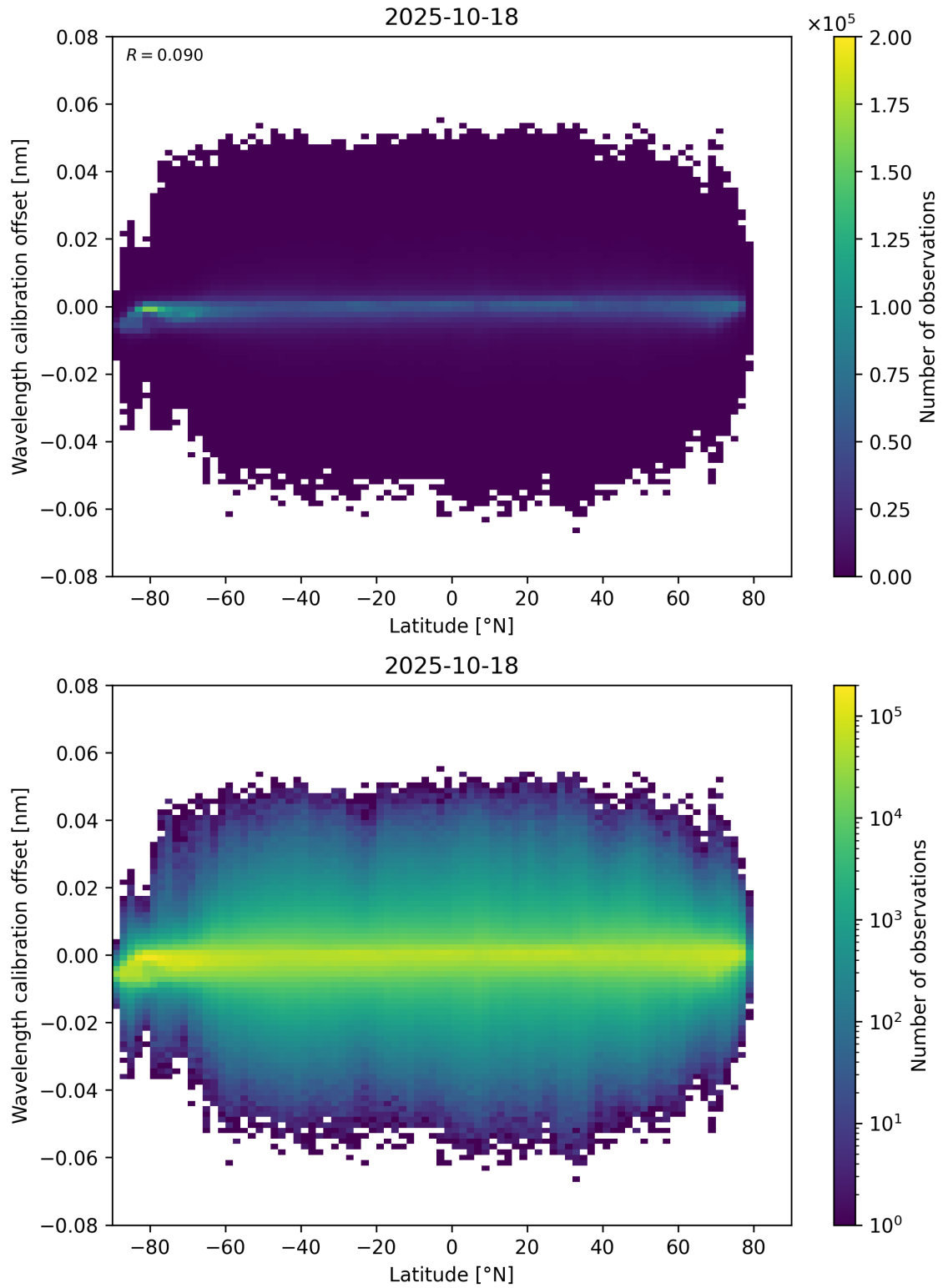
Figure 95: Scatter density plot of “Latitude” against “Wavelength calibration offset” for 2025-10-17 to 2025-10-19.
