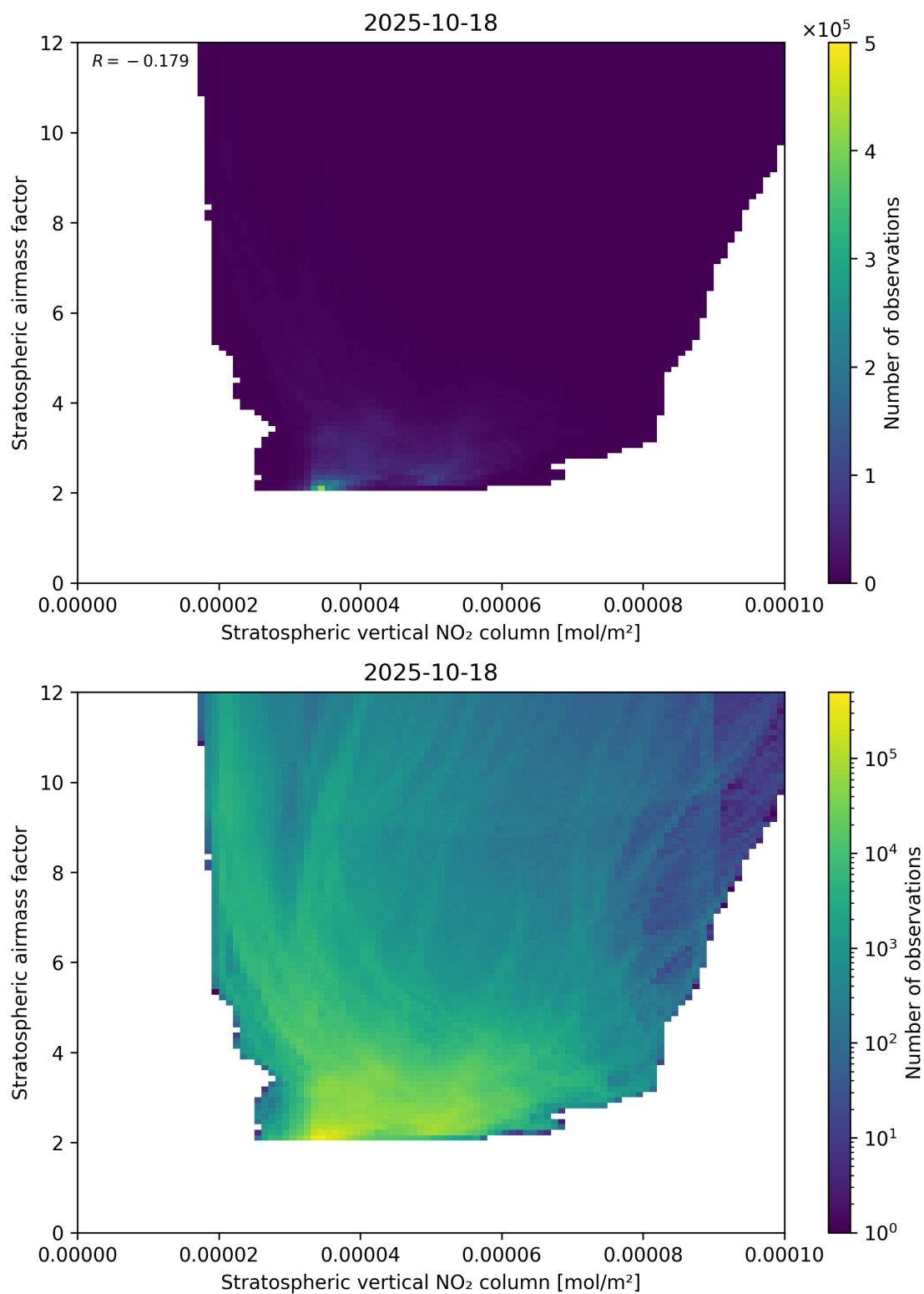
Figure 96: Scatter density plot of “Stratospheric vertical NO 2 column” against “Stratospheric airmass factor” for 2025-10-17 to 2025-10-19.
