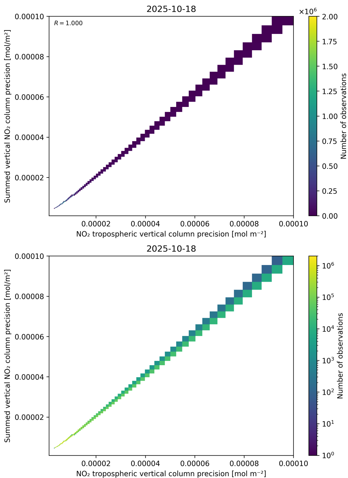
Figure 137: Scatter density plot of “NO 2 tropospheric vertical column precision” against “Summed vertical NO 2 column precision” for 2025-10-17 to 2025-10-19.
