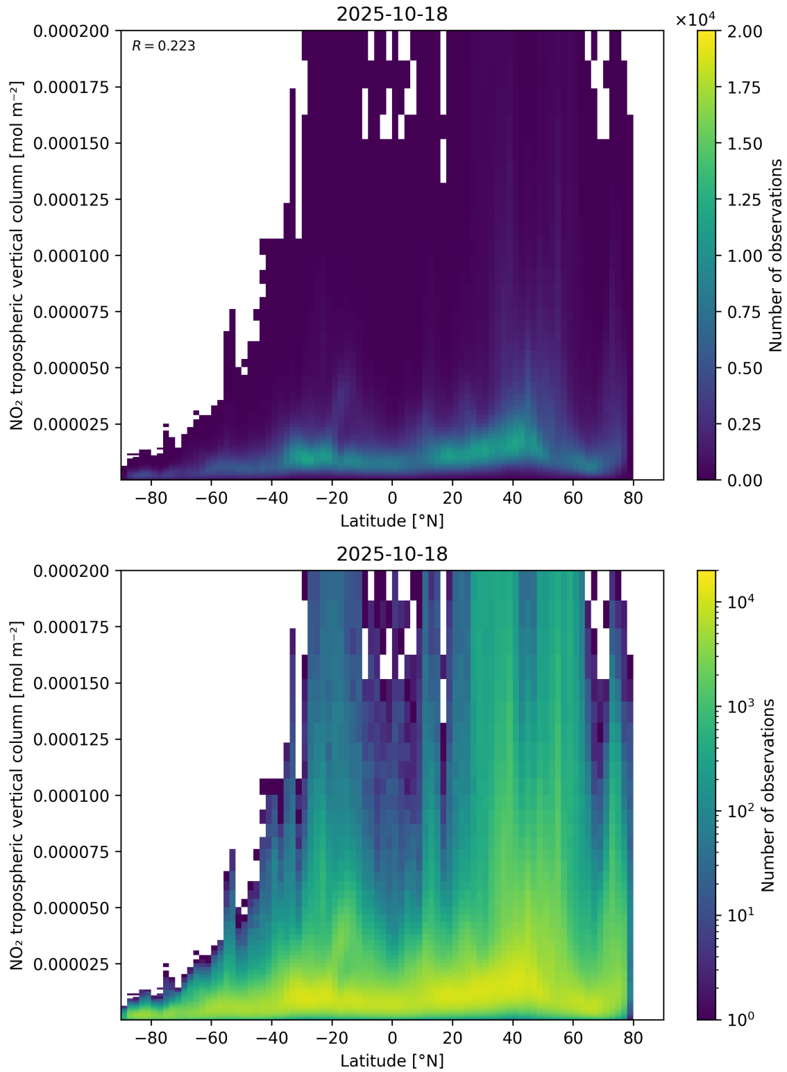
Figure 92: Scatter density plot of “Latitude” against “NO 2 tropospheric vertical column” for 2025-10-17 to 2025-10-19.
