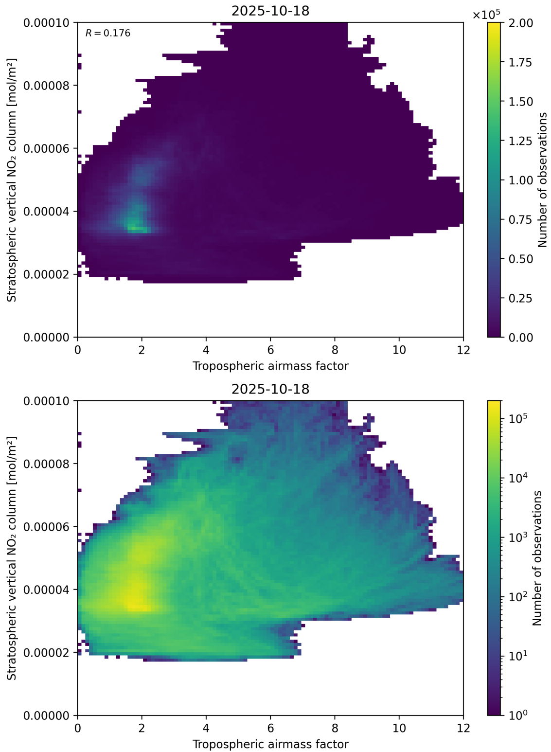
Figure 74: Scatter density plot of “Tropospheric air mass factor” against “Stratospheric vertical NO 2 column” for 2025-10-17 to 2025-10-19.
