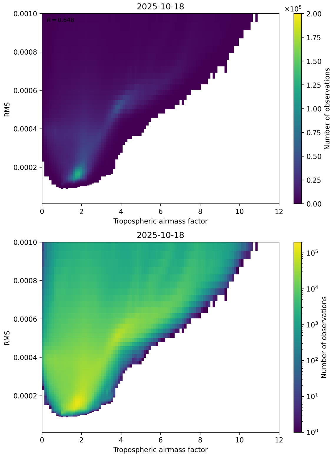
Figure 79: Scatter density plot of “Tropospheric airmass factor” against “RMS” for 2025-10-17 to 2025-10-19.
