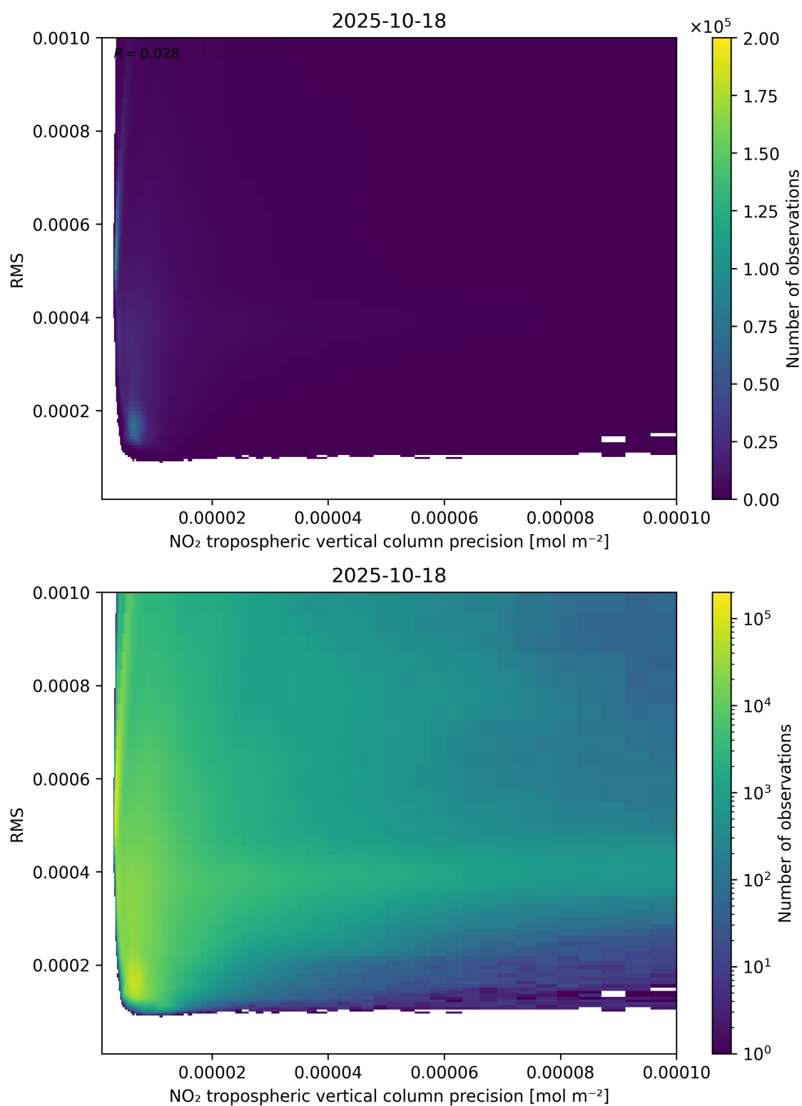
Figure 140: Scatter density plot of “NO 2 tropospheric vertical column precision” against “RMS” for 2025-10-17 to 2025-10-19.
