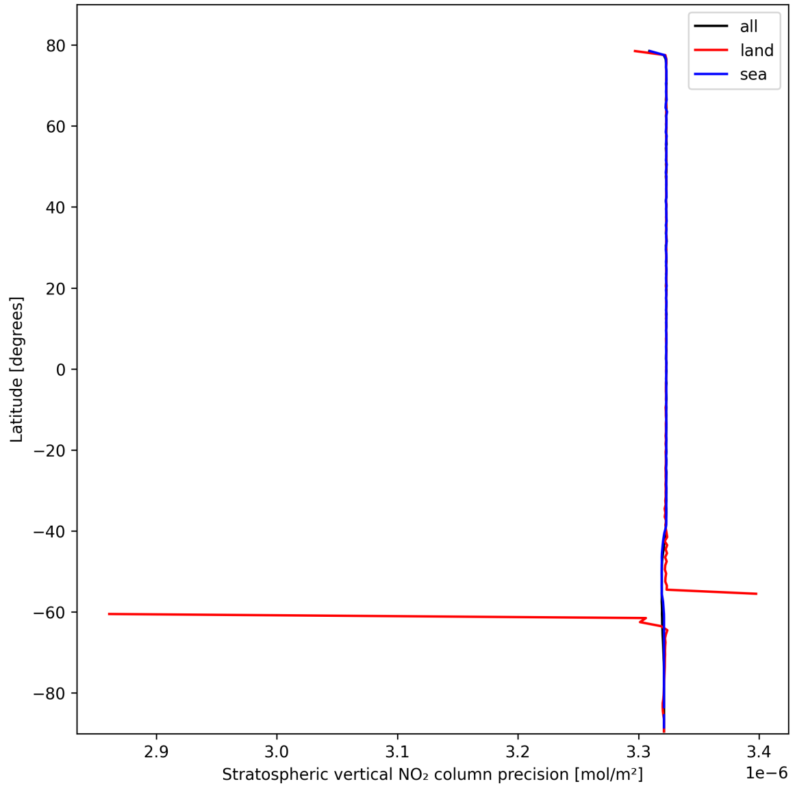
Figure 20: Zonal average of “Stratospheric vertical NO 2 column precision” for 2025-10-17 to 2025-10-19.
