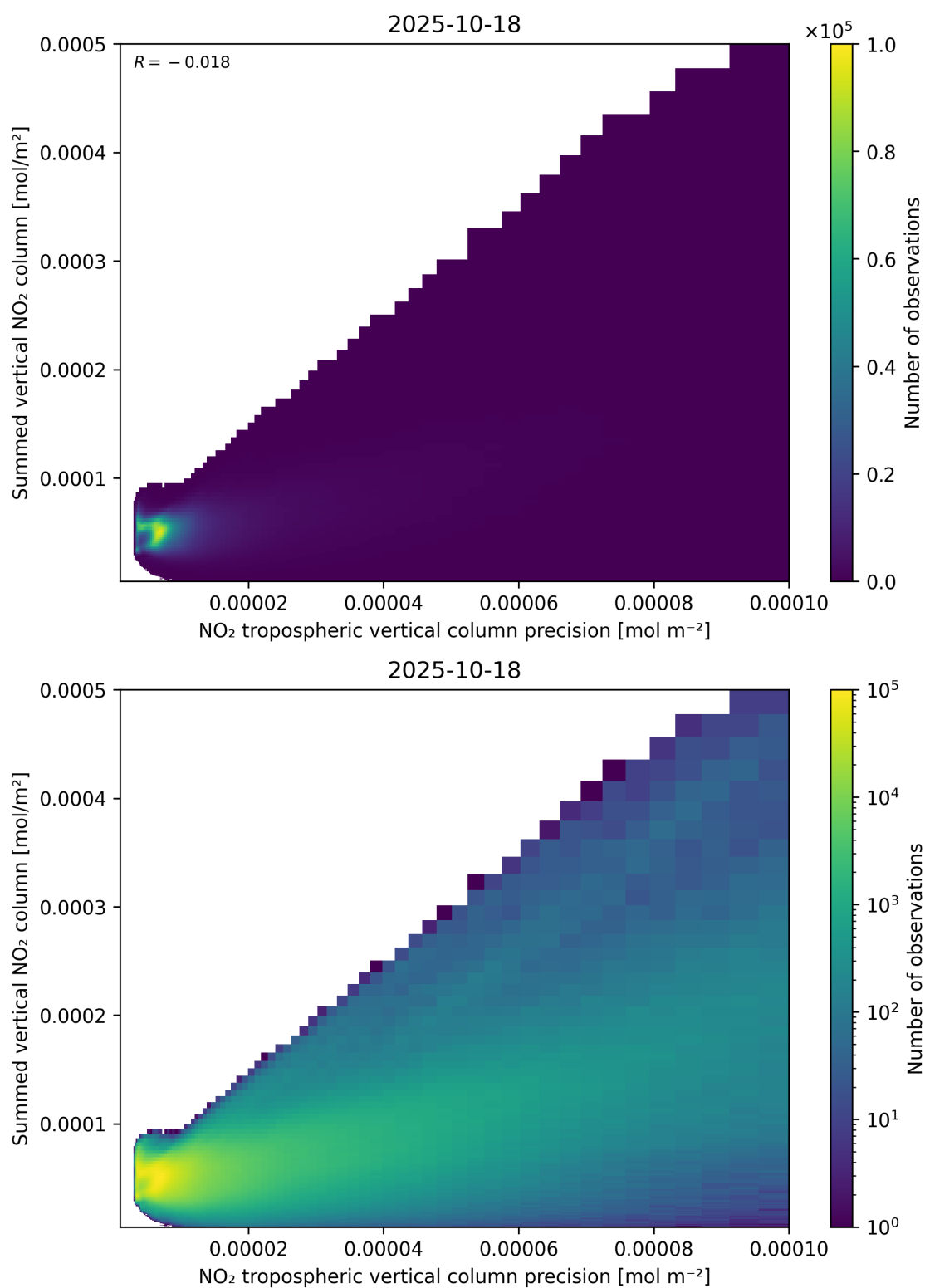
Figure 136: Scatter density plot of “NO 2 tropospheric vertical column precision” against “Summed vertical NO 2 column” for 2025-10-17 to 2025-10-19.
