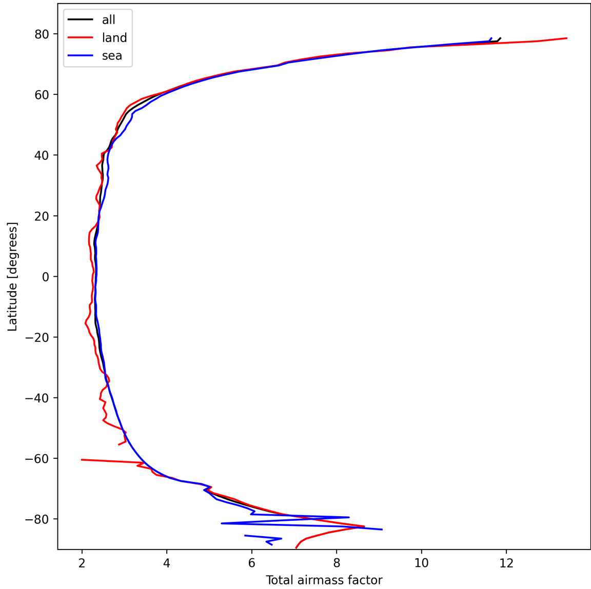
Figure 15: Zonal average of “Total airmass factor” for 2025-10-17 to 2025-10-19.
