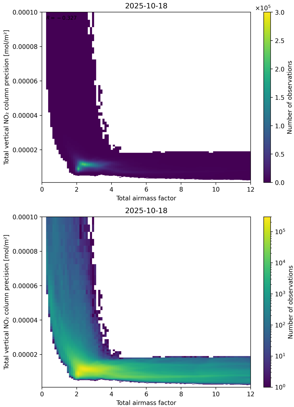
Figure 68: Scatter density plot of “Total airmass factor” against “Total vertical NO 2 column precision” for 2025-10-17 to 2025-10-19.
