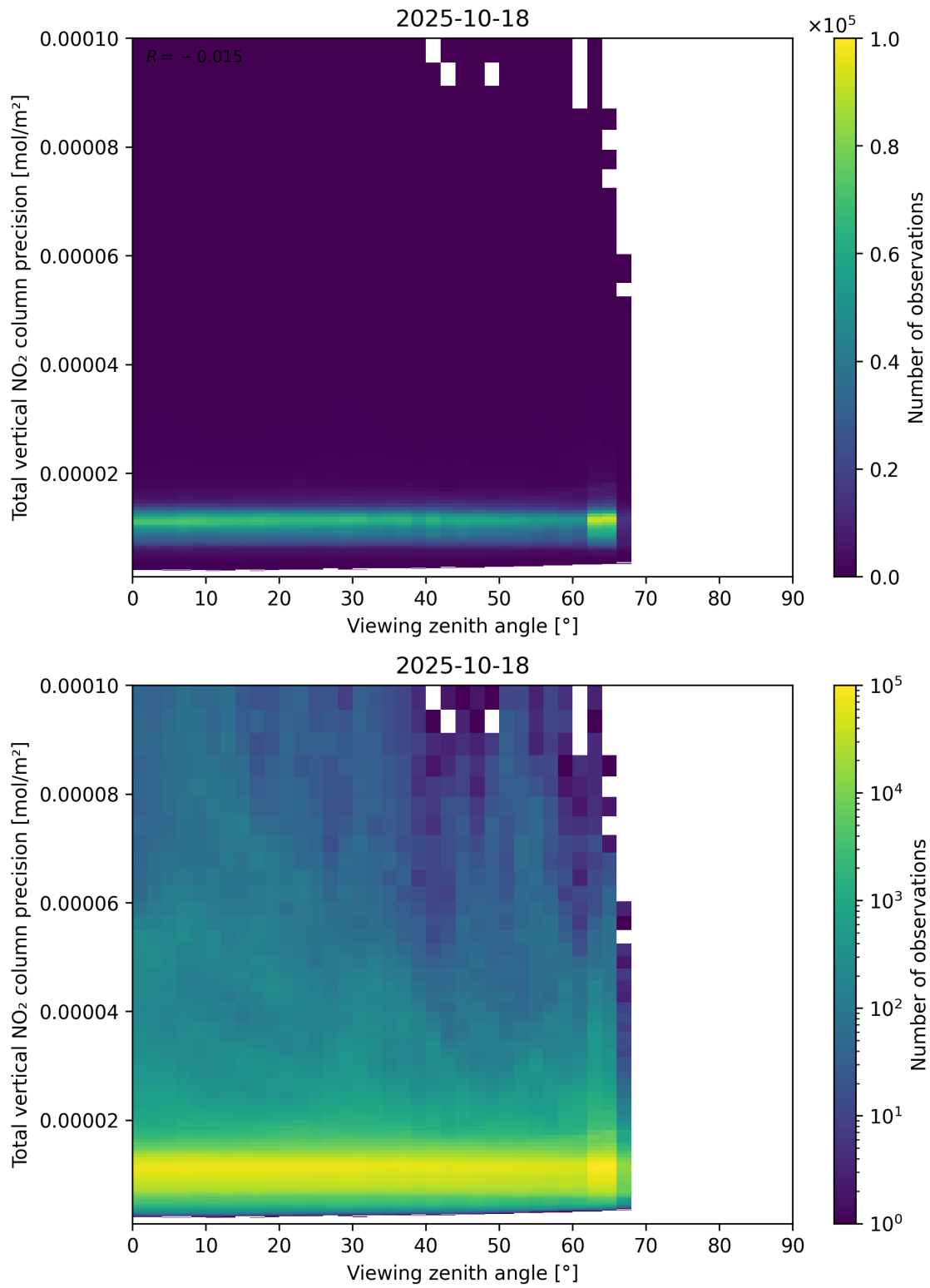
Figure 168: Scatter density plot of “Viewing zenith angle” against “Total vertical NO 2 column precision” for 2025-10-17 to 2025-10-19.
