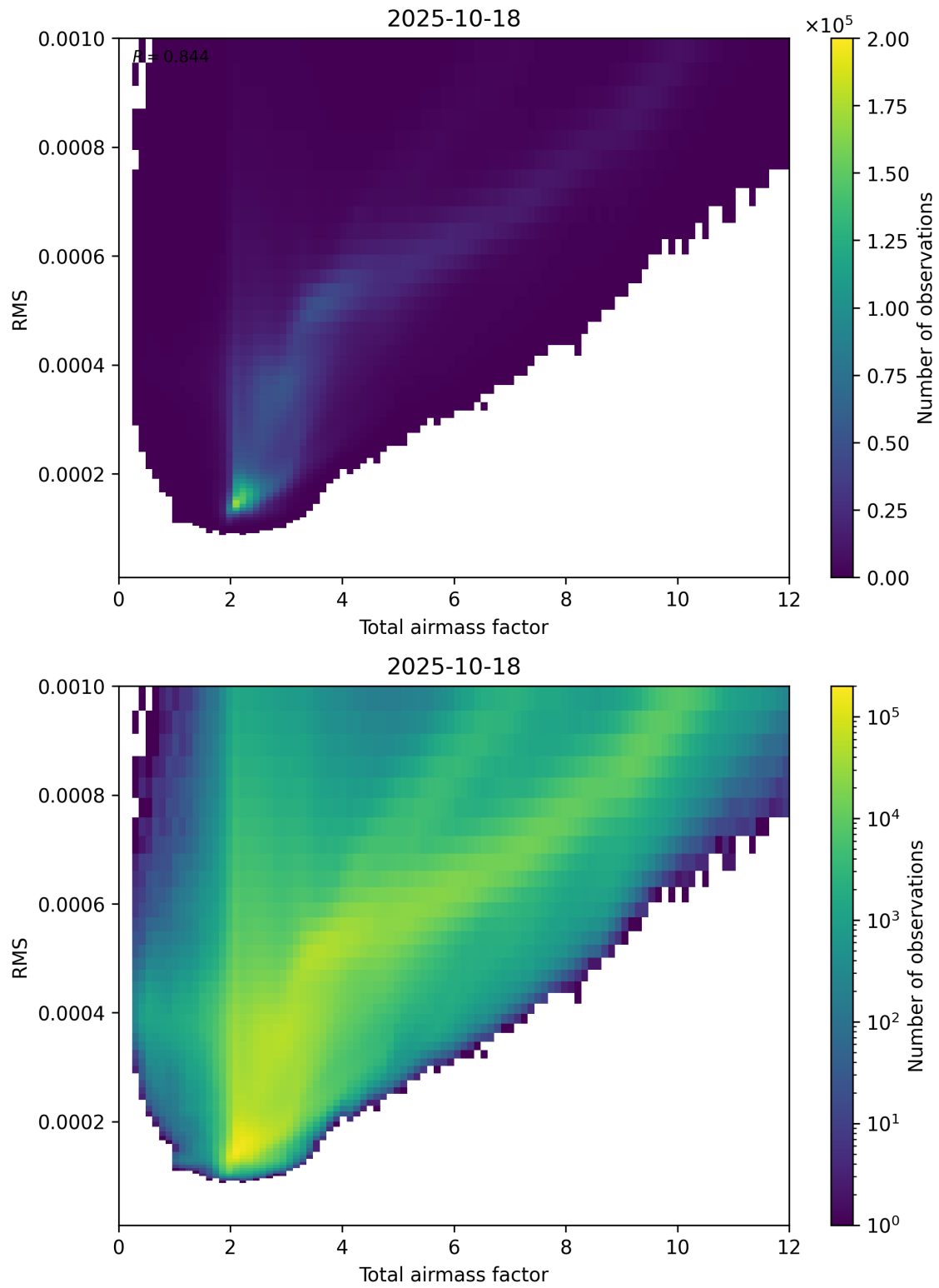
Figure 69: Scatter density plot of “Total airmass factor” against “RMS” for 2025-10-17 to 2025-10-19.
