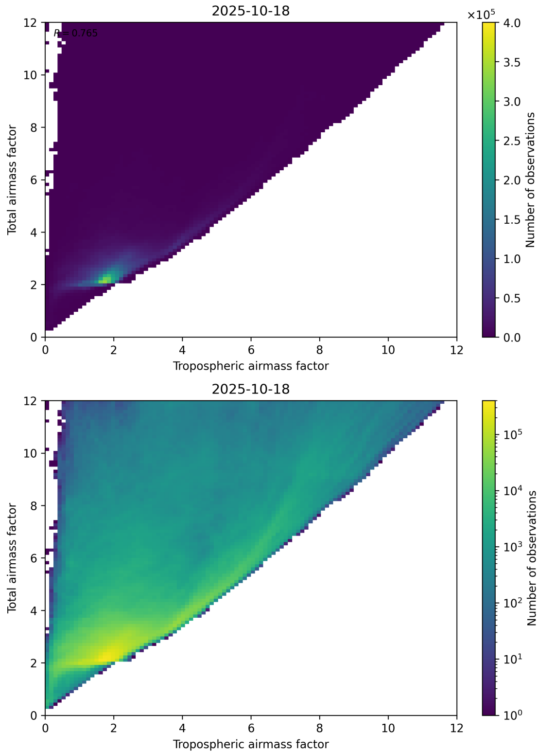
Figure 72: Scatter density plot of “Tropospheric airmass factor” against “Total airmass factor” for 2025-10-17 to 2025-10-19.
