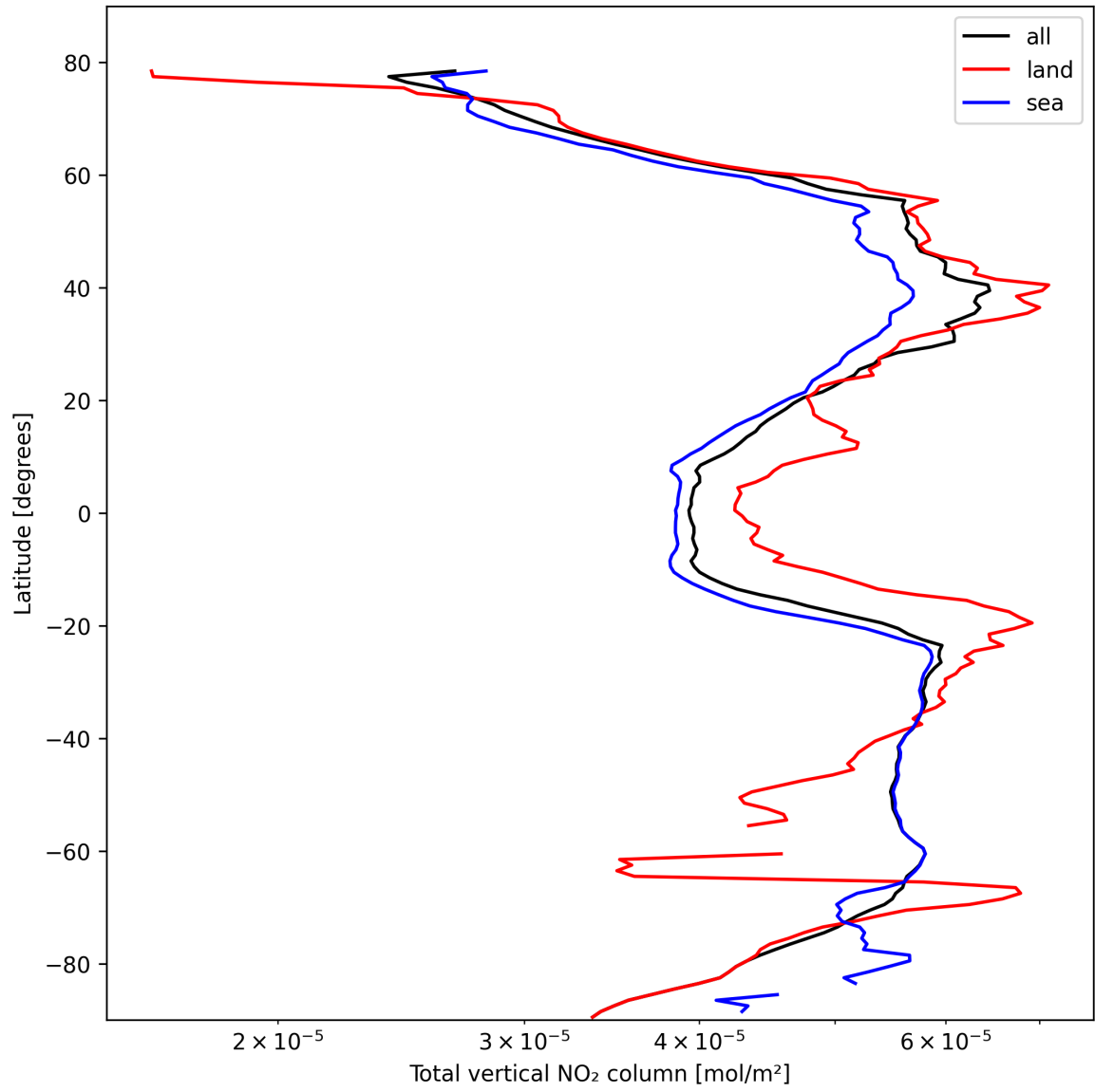
Figure 21: Zonal average of “Total vertical NO 2 column” for 2025-10-17 to 2025-10-19.
