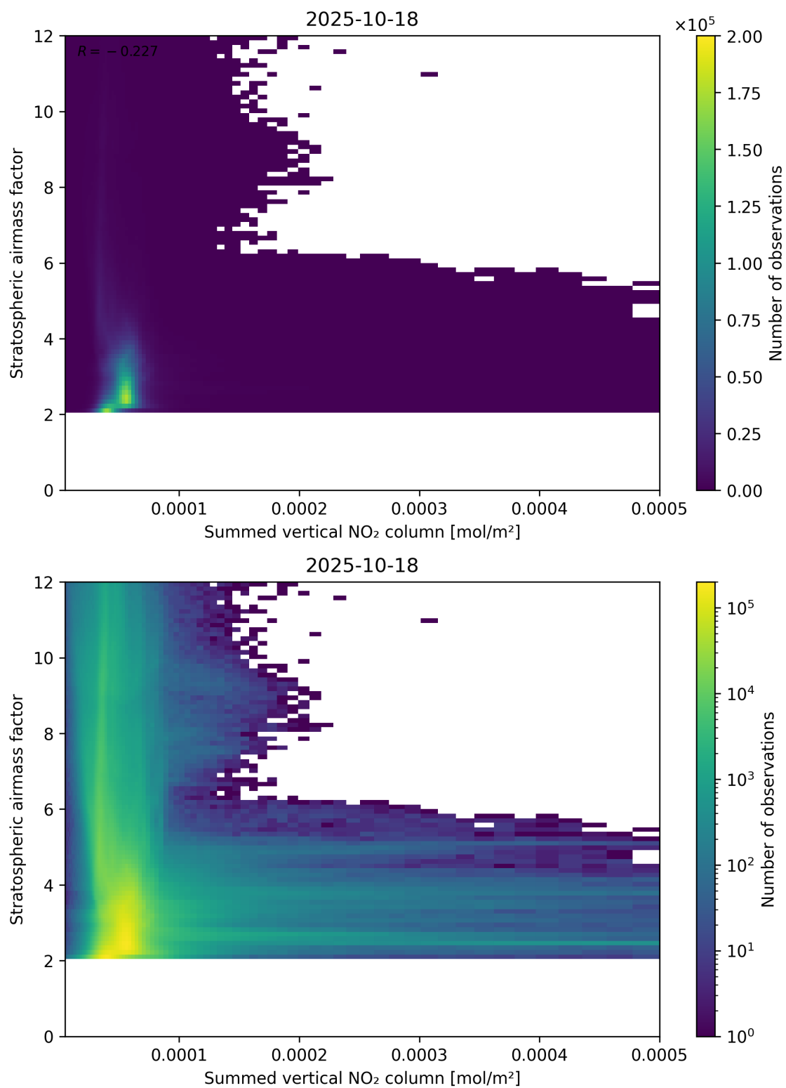
Figure 103: Scatter density plot of “Summed vertical NO 2 column” against “Stratospheric air mass factor” for 2025-10-17 to 2025-10-19.
