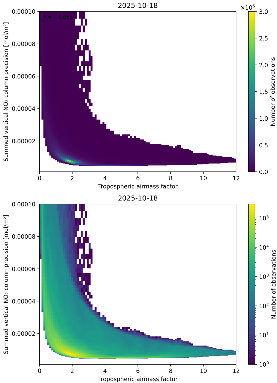
Figure 76: Scatter density plot of “Tropospheric airmass factor” against “Summed vertical NO 2 column precision” for 2025-10-17 to 2025-10-19.
