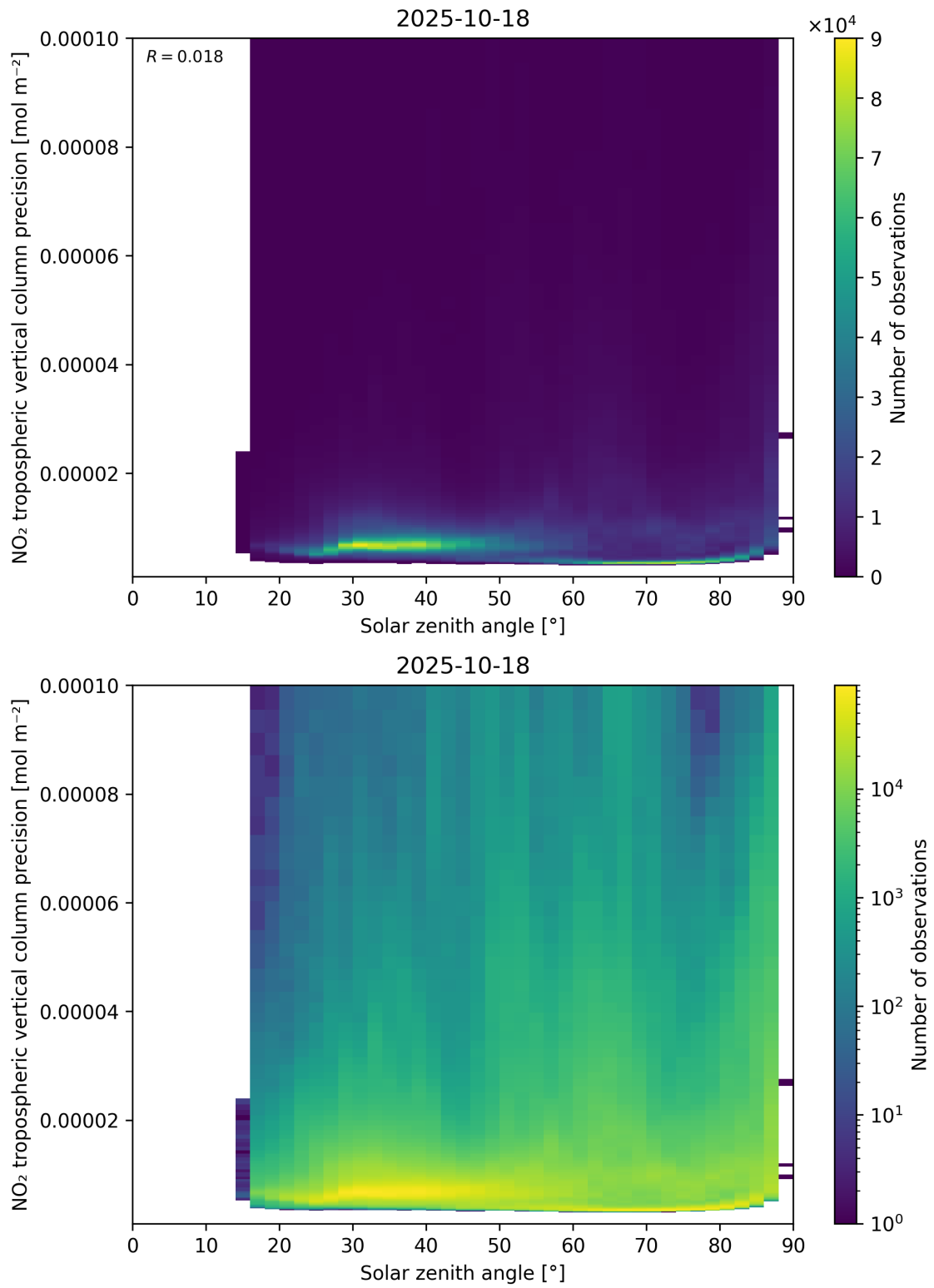
Figure 156: Scatter density plot of “Solar zenith angle” against “NO 2 tropospheric vertical column precision” for 2025-10-17 to 2025-10-19.
