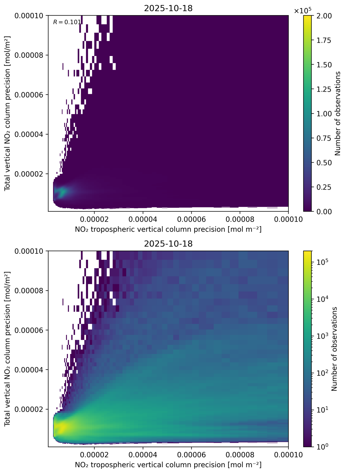
Figure 139: Scatter density plot of “NO 2 tropospheric vertical column precision” against “Total vertical NO 2 column precision” for 2025-10-17 to 2025-10-19.
