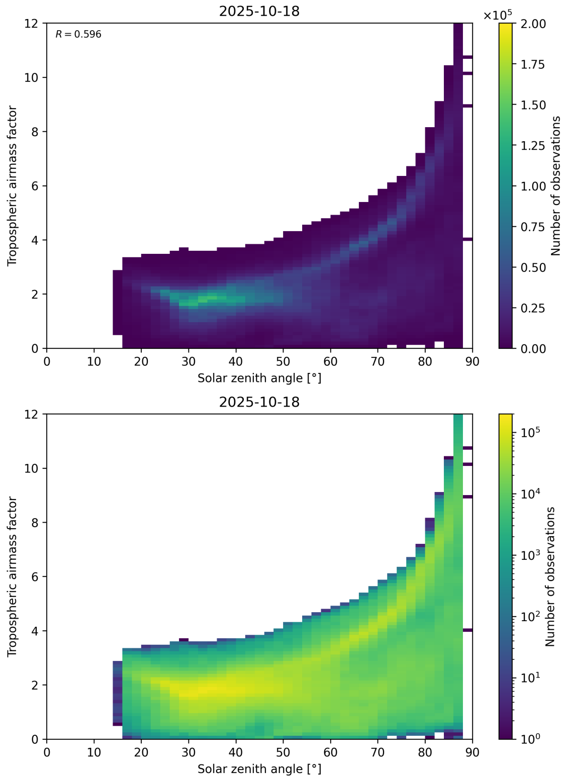
Figure 147: Scatter density plot of “Solar zenith angle” against “Tropospheric airmass factor” for 2025-10-17 to 2025-10-19.
