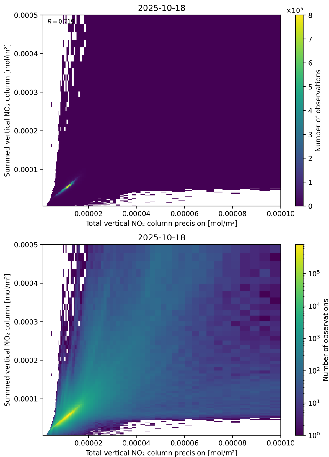
Figure 117: Scatter density plot of “Total vertical NO 2 column precision” against “Summed vertical NO 2 column” for 2025-10-17 to 2025-10-19.
