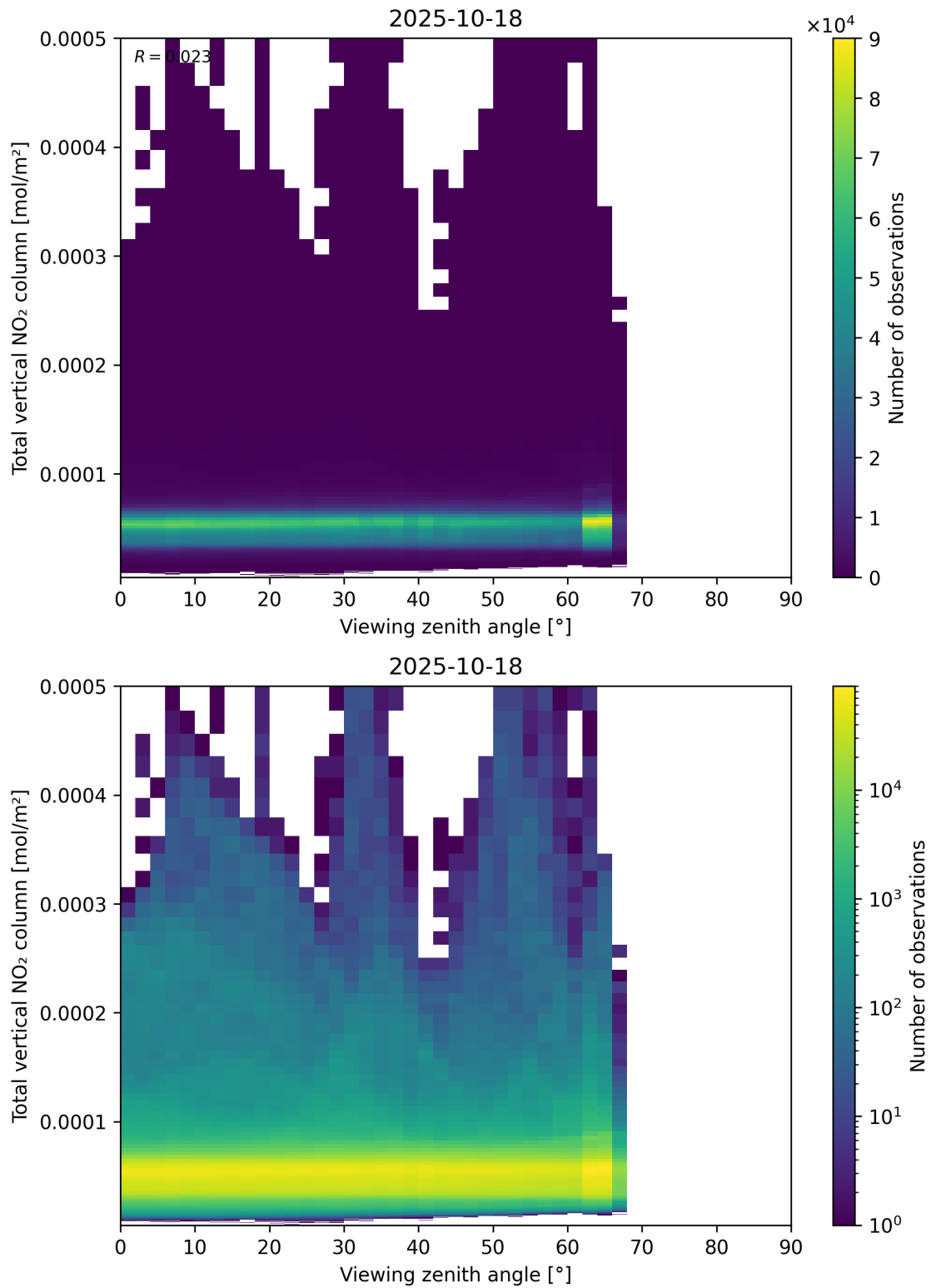
Figure 167: Scatter density plot of “Viewing zenith angle” against “Total vertical NO 2 column” for 2025-10-17 to 2025-10-19.
