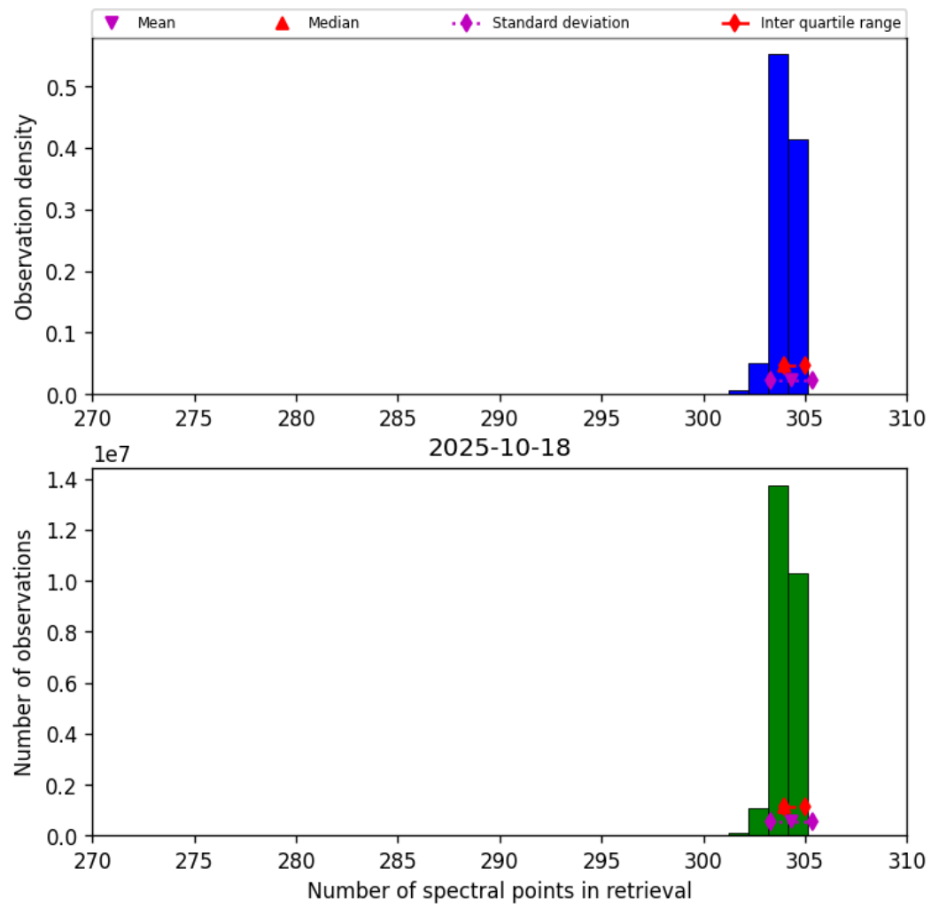
Figure 33: Histogram of “Number of spectral points in retrieval” for 2025-10-17 to 2025-10-19
