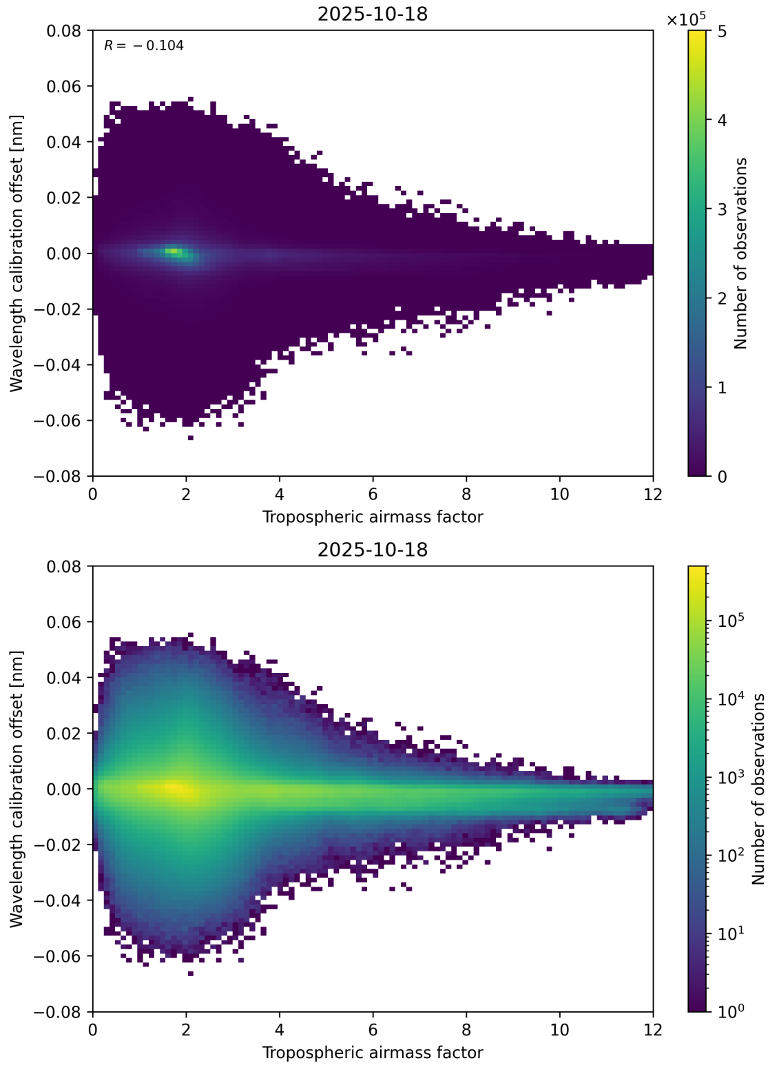
Figure 80: Scatter density plot of “Tropospheric airmass factor” against “Wavelength calibration offset” for 2025-10-17 to 2025-10-19.
