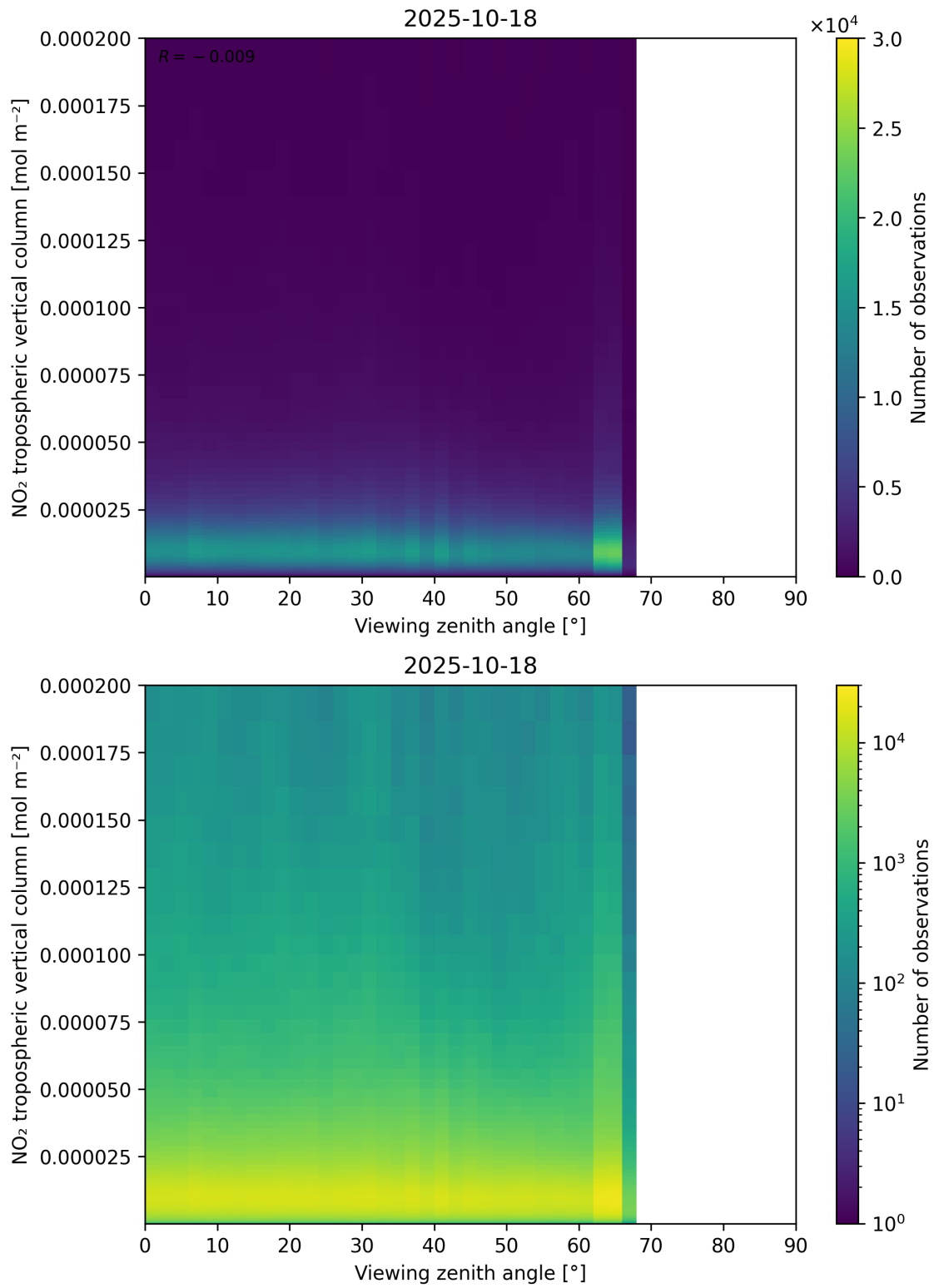
Figure 169: Scatter density plot of “Viewing zenith angle” against “NO 2 tropospheric vertical column” for 2025-10-17 to 2025-10-19.
