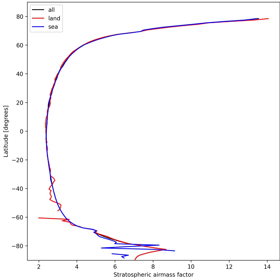
Figure 27: Zonal average of “Stratospheric air mass factor” for 2025-10-17 to 2025-10-19.
