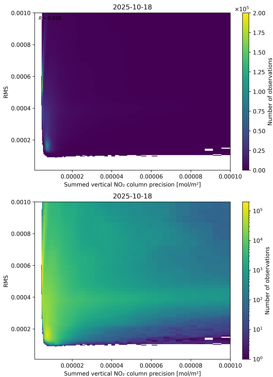
Figure 108: Scatter density plot of “Summed vertical NO 2 column precision” against “RMS” for 2025-10-17 to 2025-10-19.
