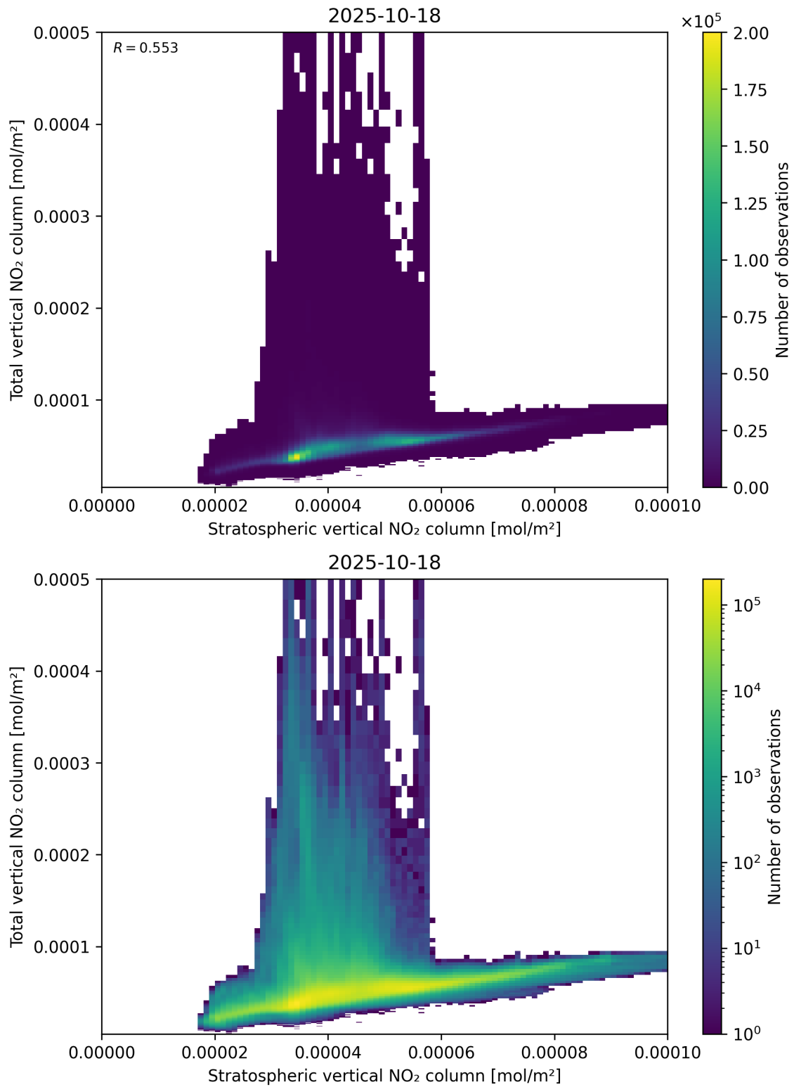
Figure 100: Scatter density plot of “Stratospheric vertical NO 2 column” against “Total vertical NO 2 column” for 2025-10-17 to 2025-10-19.
