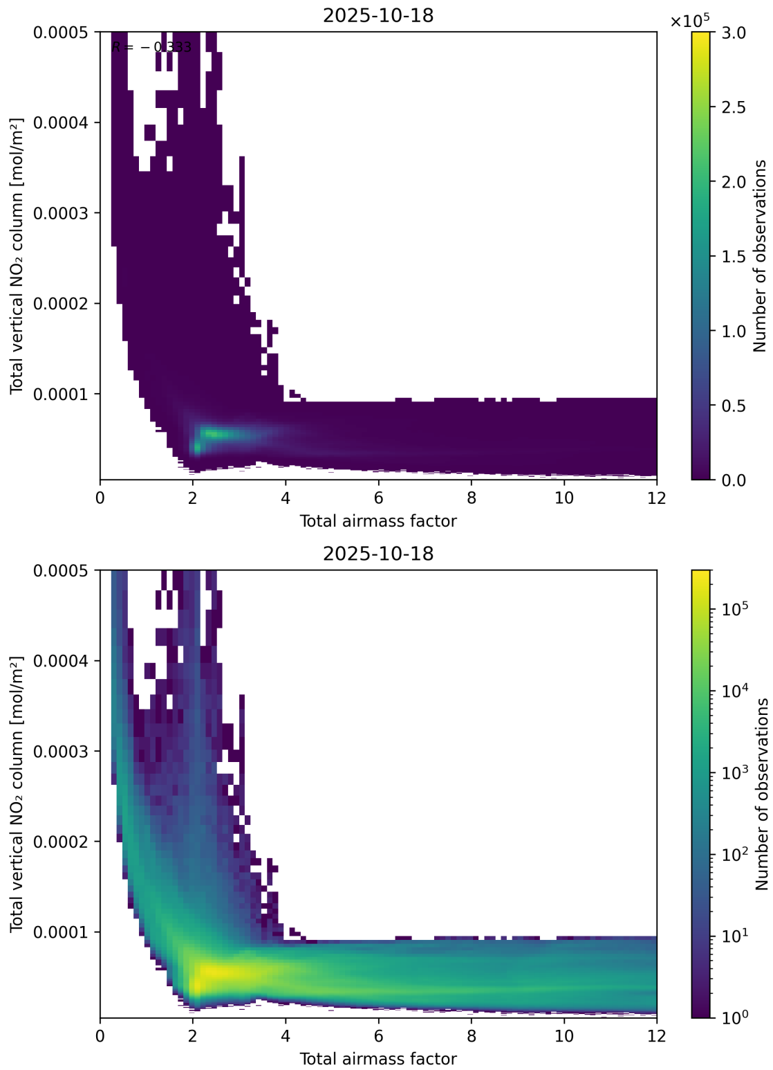
Figure 67: Scatter density plot of “Total air mass factor” against “Total vertical NO 2 column” for 2025-10-17 to 2025-10-19.
