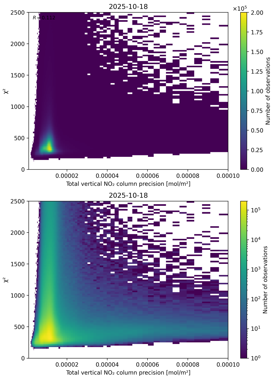
Figure 116: Scatter density plot of “Total vertical NO 2 column precision” against “ \chi^2 ” for 2025-10-17 to 2025-10-19.
