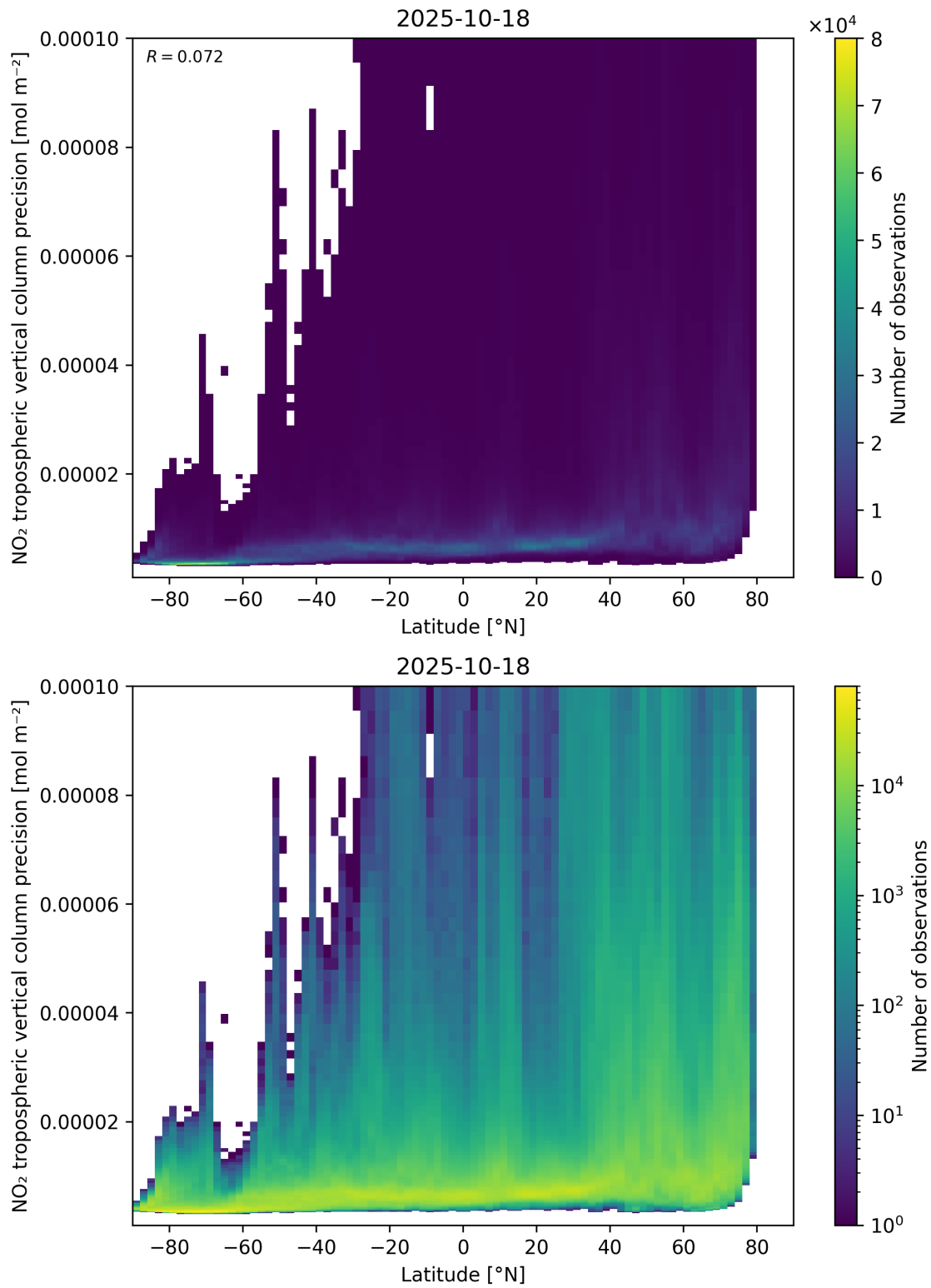
Figure 93: Scatter density plot of “Latitude” against “NO 2 tropospheric vertical column precision” for 2025-10-17 to 2025-10-19.
