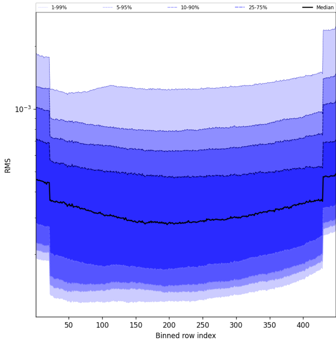
Figure 60: Along track statistics of “RMS” for 2025-10-17 to 2025-10-19
