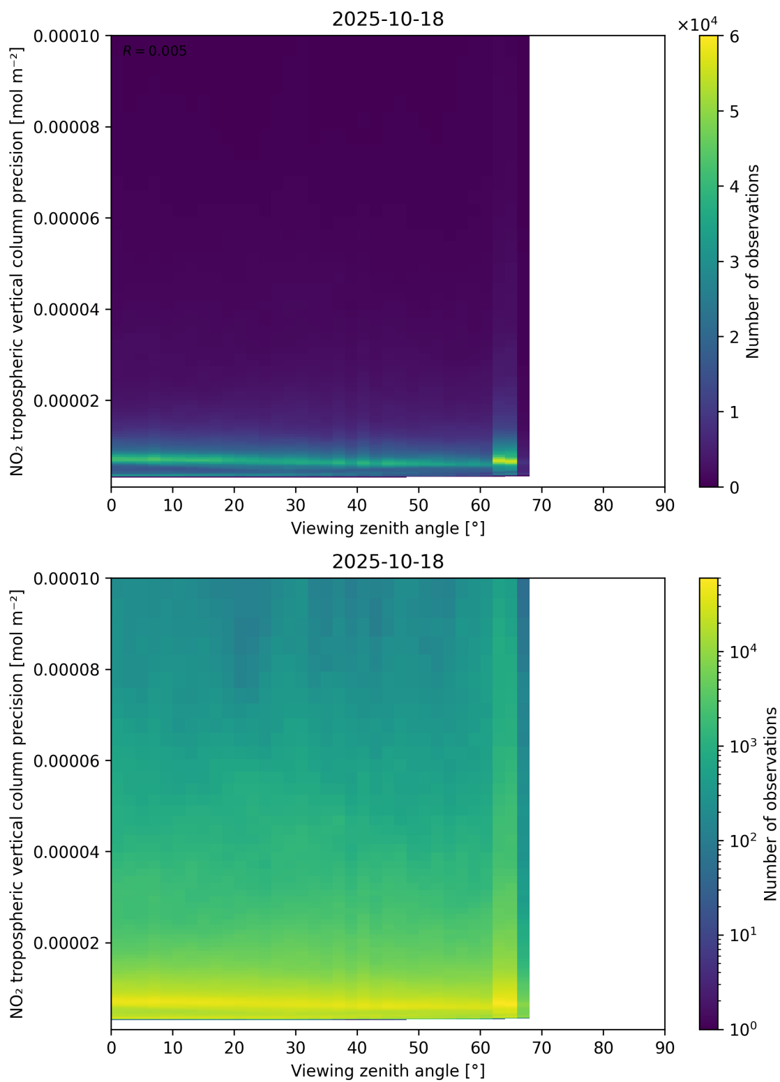
Figure 170: Scatter density plot of “Viewing zenith angle” against “NO 2 tropospheric vertical column precision” for 2025-10-17 to 2025-10-19.
