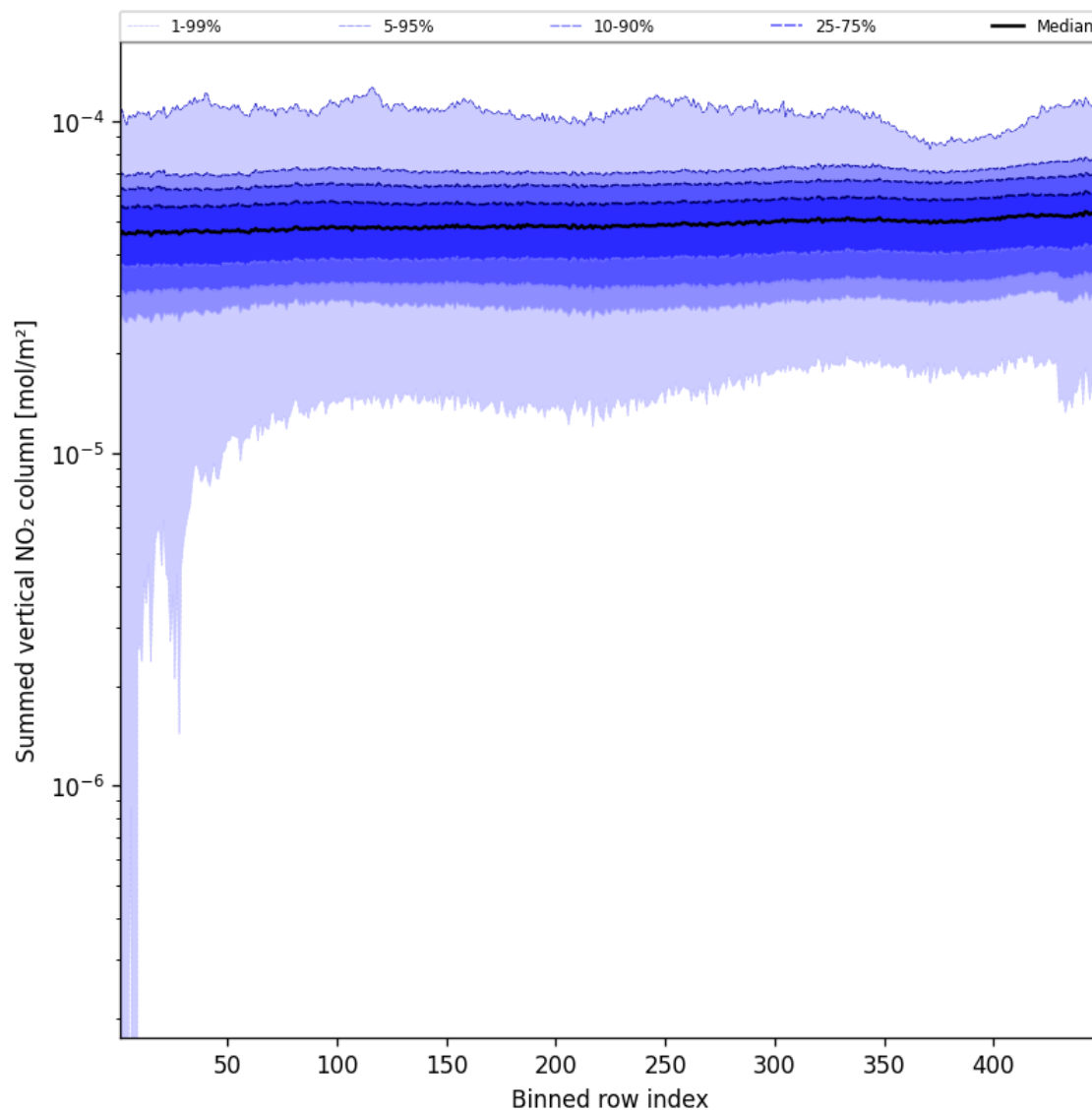
Figure 57: Along track statistics of “Summed vertical NO 2 column” for 2025-10-17 to 2025-10-19
