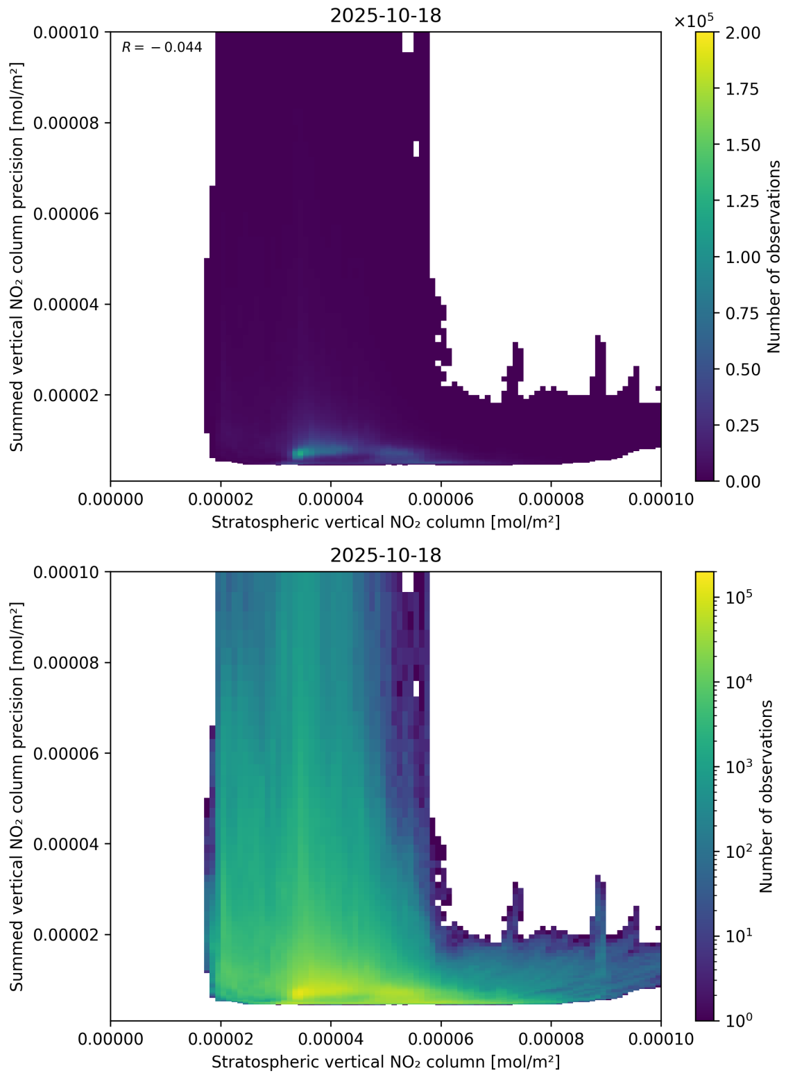
Figure 99: Scatter density plot of “Stratospheric vertical NO 2 column” against “Summed vertical NO 2 column precision” for 2025-10-17 to 2025-10-19.
