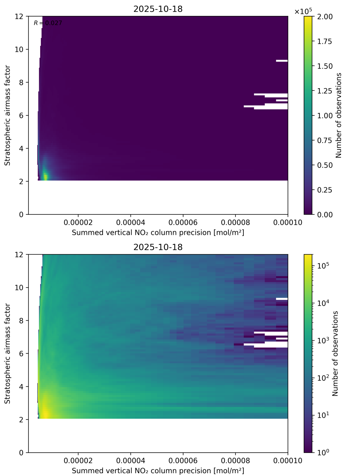
Figure 106: Scatter density plot of “Summed vertical NO 2 column precision” against “Stratospheric airmass factor” for 2025-10-17 to 2025-10-19.
