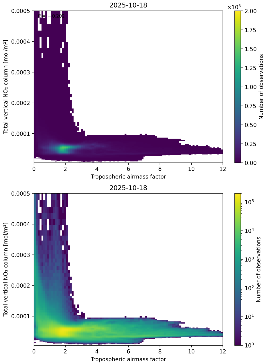
Figure 77: Scatter density plot of “Tropospheric airmass factor” against “Total vertical NO 2 column” for 2025-10-17 to 2025-10-19.
