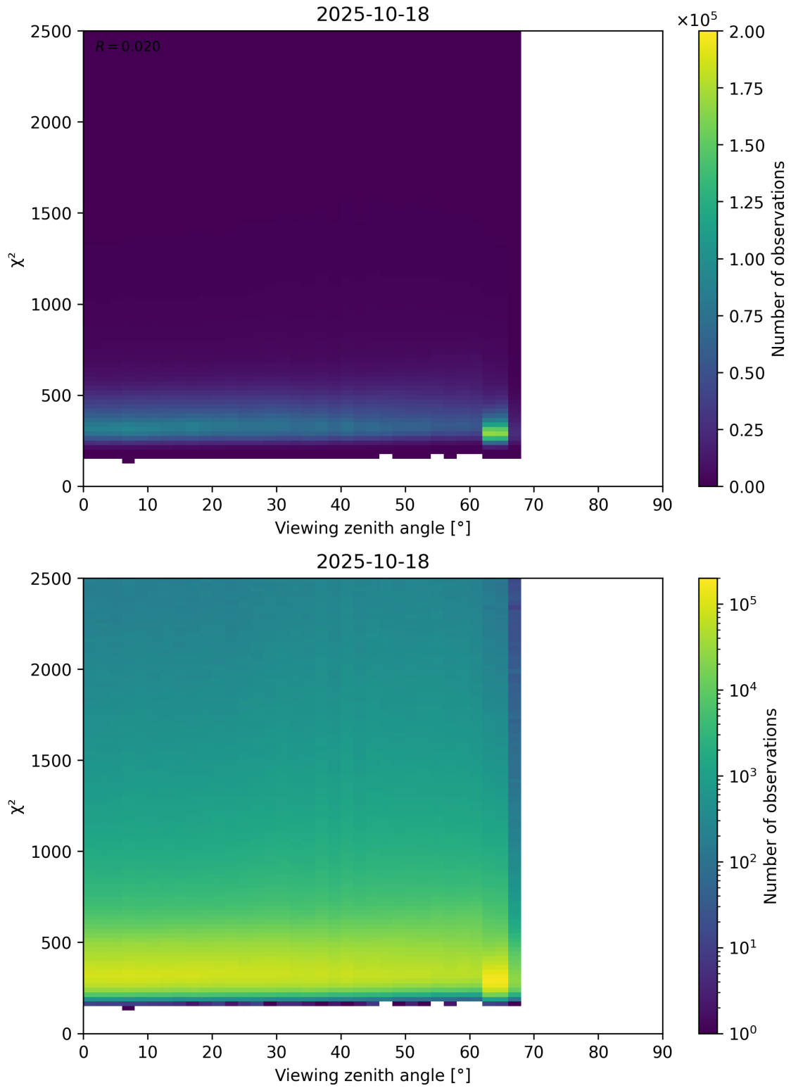
Figure 162: Scatter density plot of “Viewing zenith angle” against “ \chi^2 ” for 2025-10-17 to 2025-10-19.
