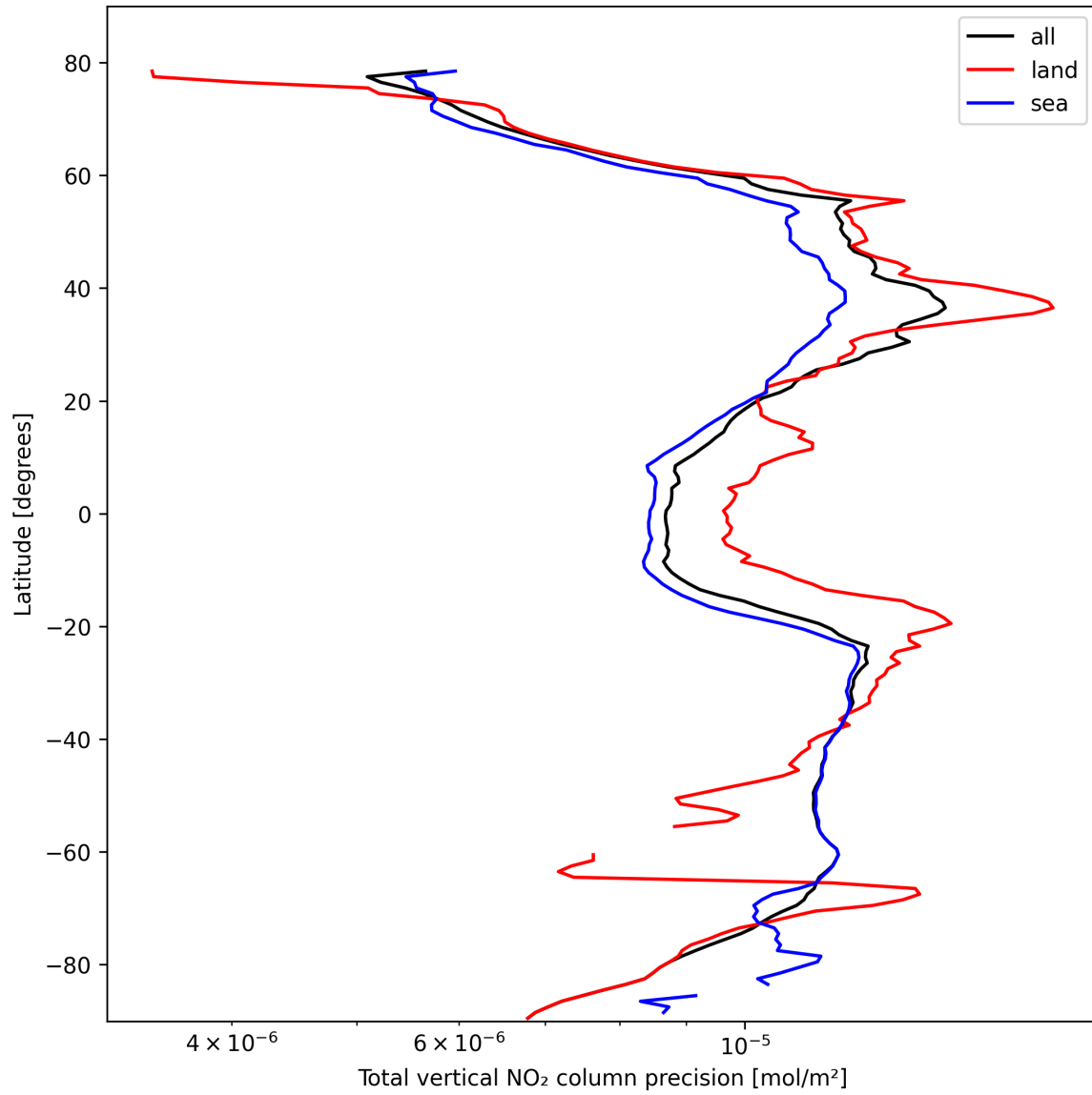
Figure 22: Zonal average of “Total vertical NO 2 column precision” for 2025-10-17 to 2025-10-19.
