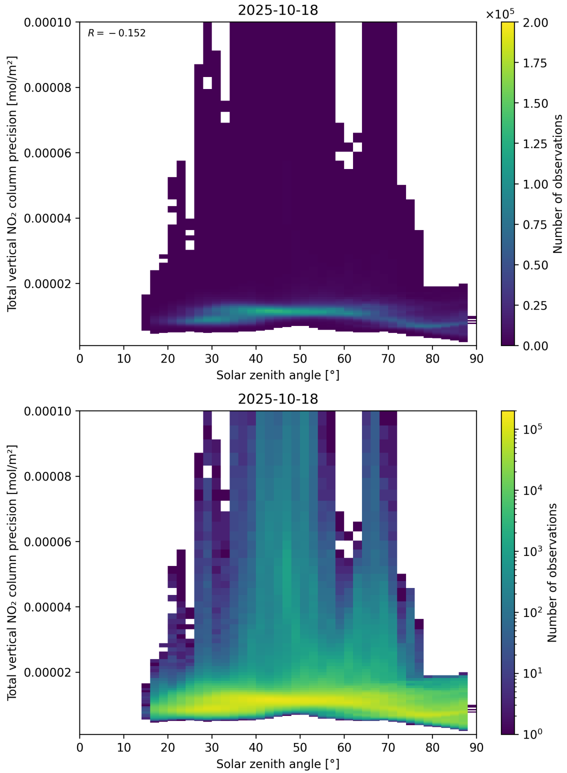
Figure 154: Scatter density plot of “Solar zenith angle” against “Total vertical NO 2 column precision” for 2025-10-17 to 2025-10-19.
