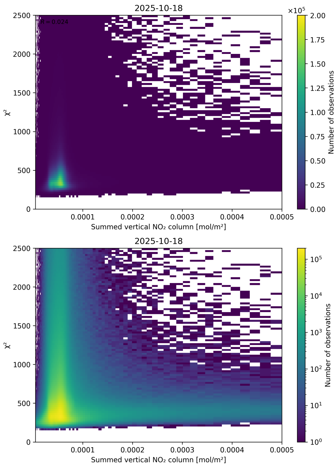
Figure 104: Scatter density plot of “Summed vertical NO 2 column” against “ \chi^2 ” for 2025-10-17 to 2025-10-19.
