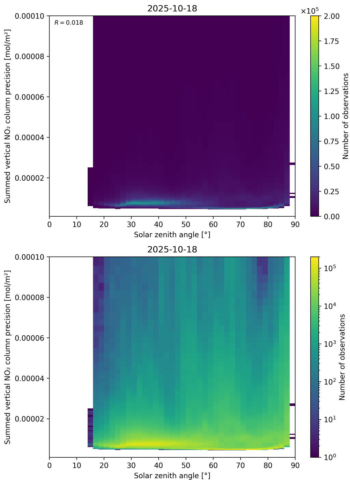
Figure 152: Scatter density plot of “Solar zenith angle” against “Summed vertical NO 2 column precision” for 2025-10-17 to 2025-10-19.
