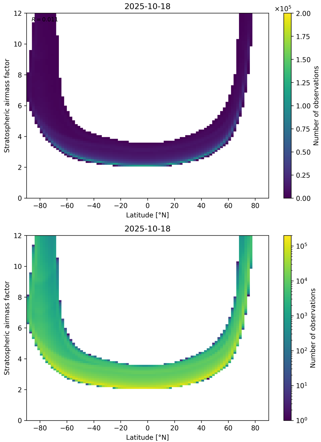
Figure 83: Scatter density plot of “Latitude” against “Stratospheric air mass factor” for 2025-10-17 to 2025-10-19.
