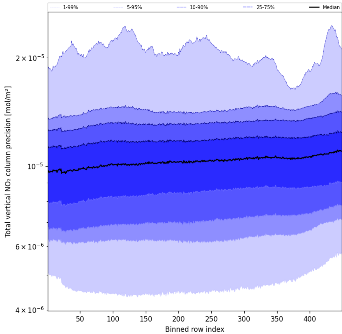
Figure 56: Along track statistics of “Total vertical NO 2 column precision” for 2025-10-17 to 2025-10-19
