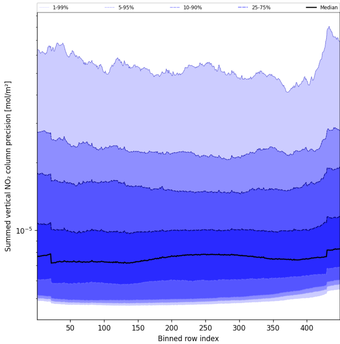
Figure 58: Along track statistics of “Summed vertical NO 2 column precision” for 2025-10-17 to 2025-10-19
