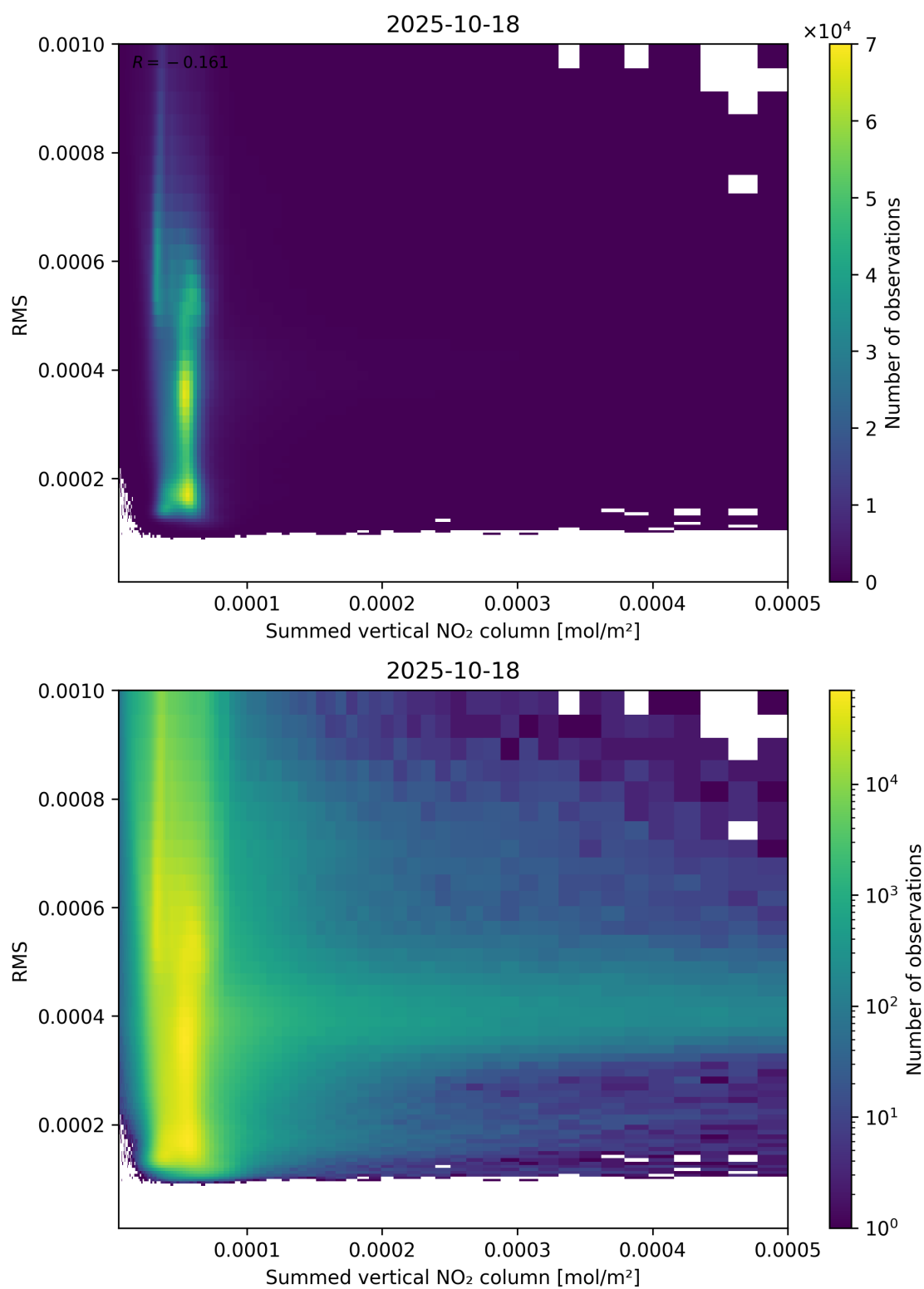
Figure 109: Scatter density plot of “Summed vertical NO 2 column” against “RMS” for 2025-10-17 to 2025-10-19.
