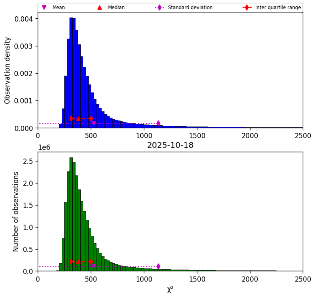
Figure 42: Histogram of “ \chi^2 ” for 2025-10-17 to 2025-10-19
