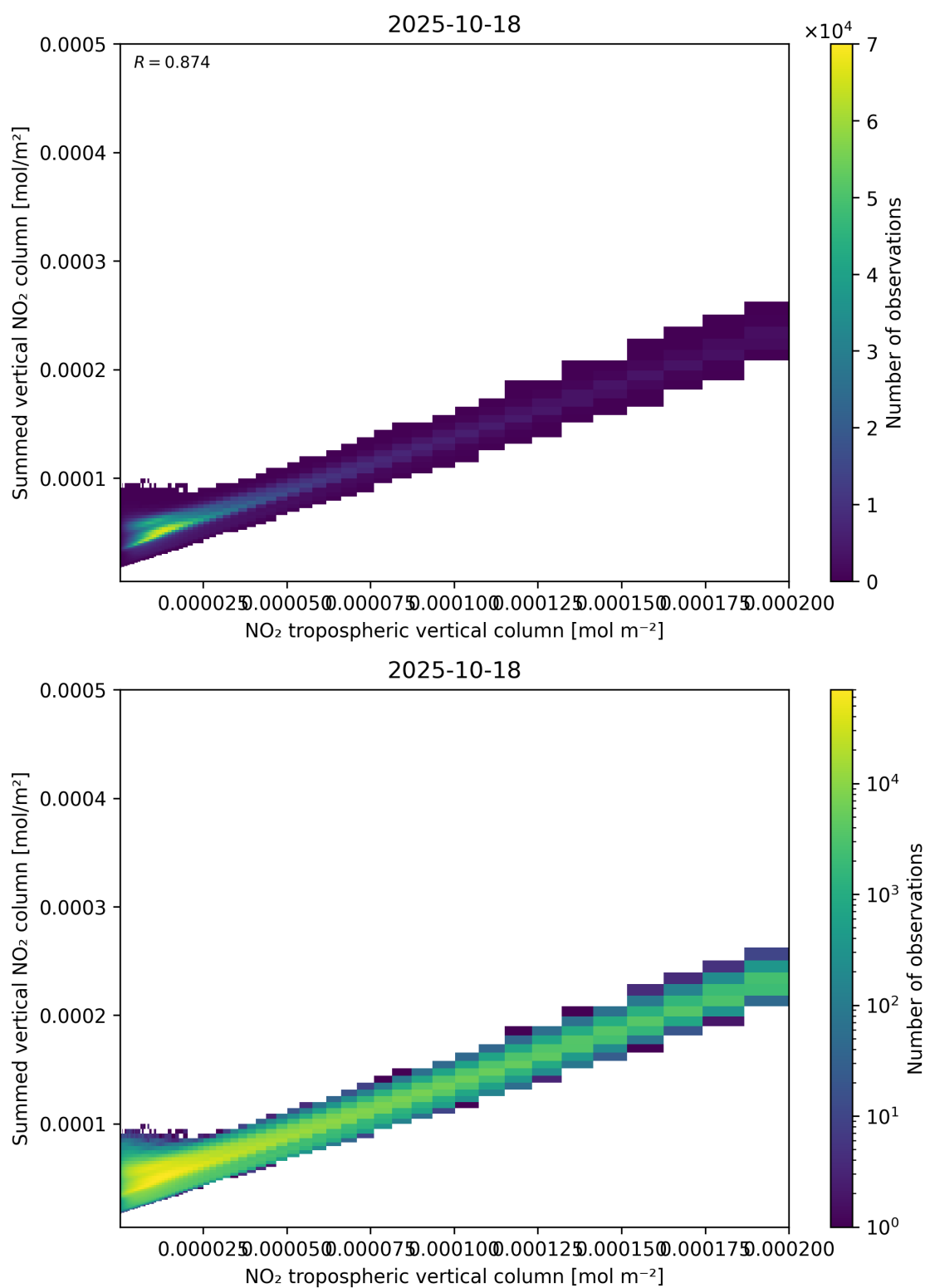
Figure 126: Scatter density plot of “NO 2 tropospheric vertical column” against “Summed vertical NO 2 column” for 2025-10-17 to 2025-10-19.
