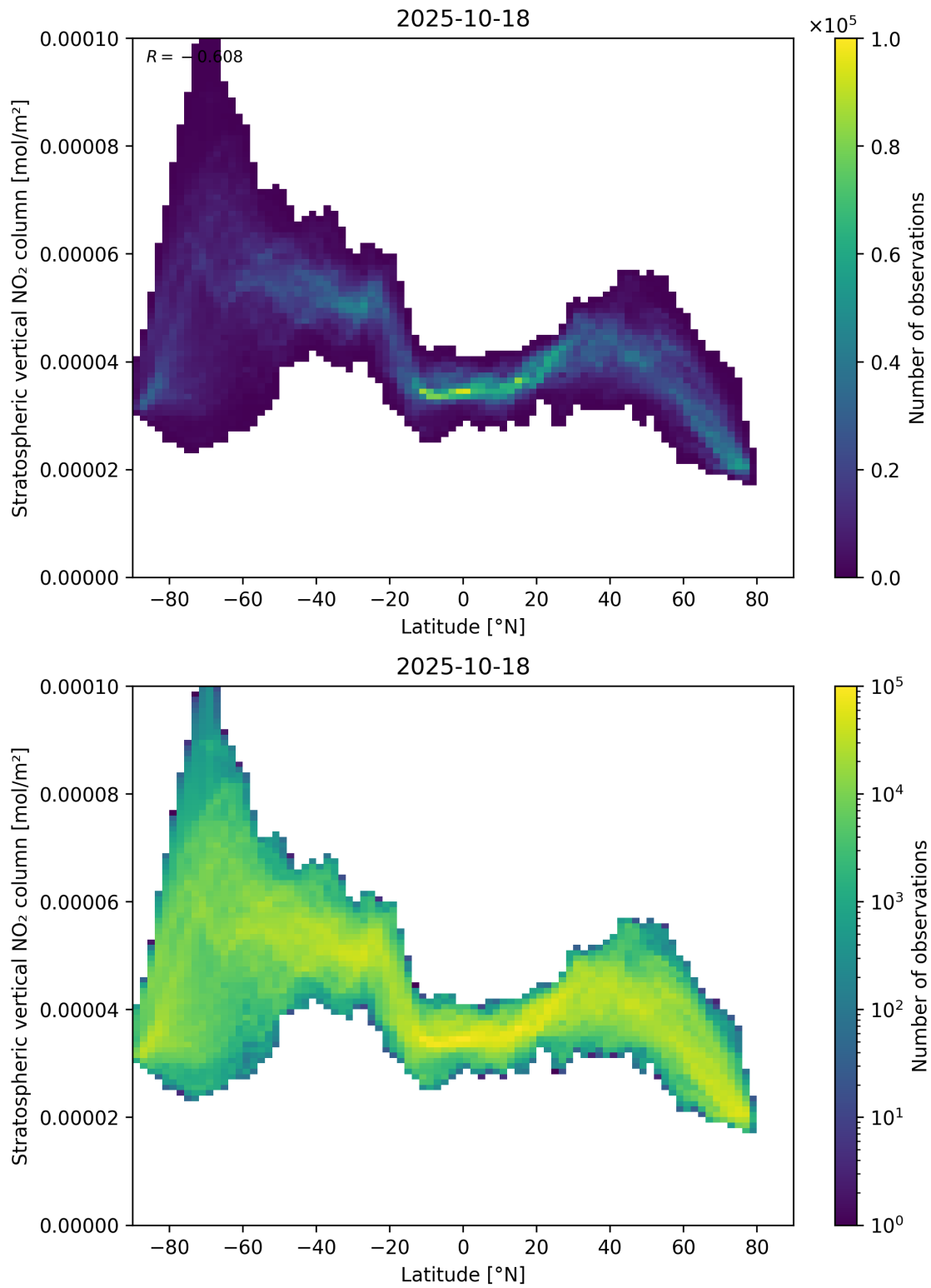
Figure 87: Scatter density plot of “Latitude” against “Stratospheric vertical NO 2 column” for 2025-10-17 to 2025-10-19.
