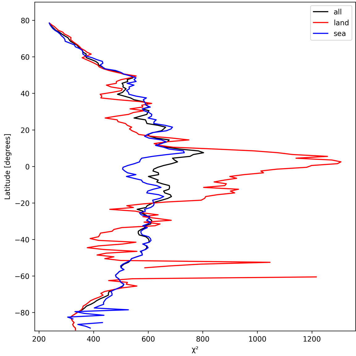
Figure 25: Zonal average of “ \chi^2 ” for 2025-10-17 to 2025-10-19.
