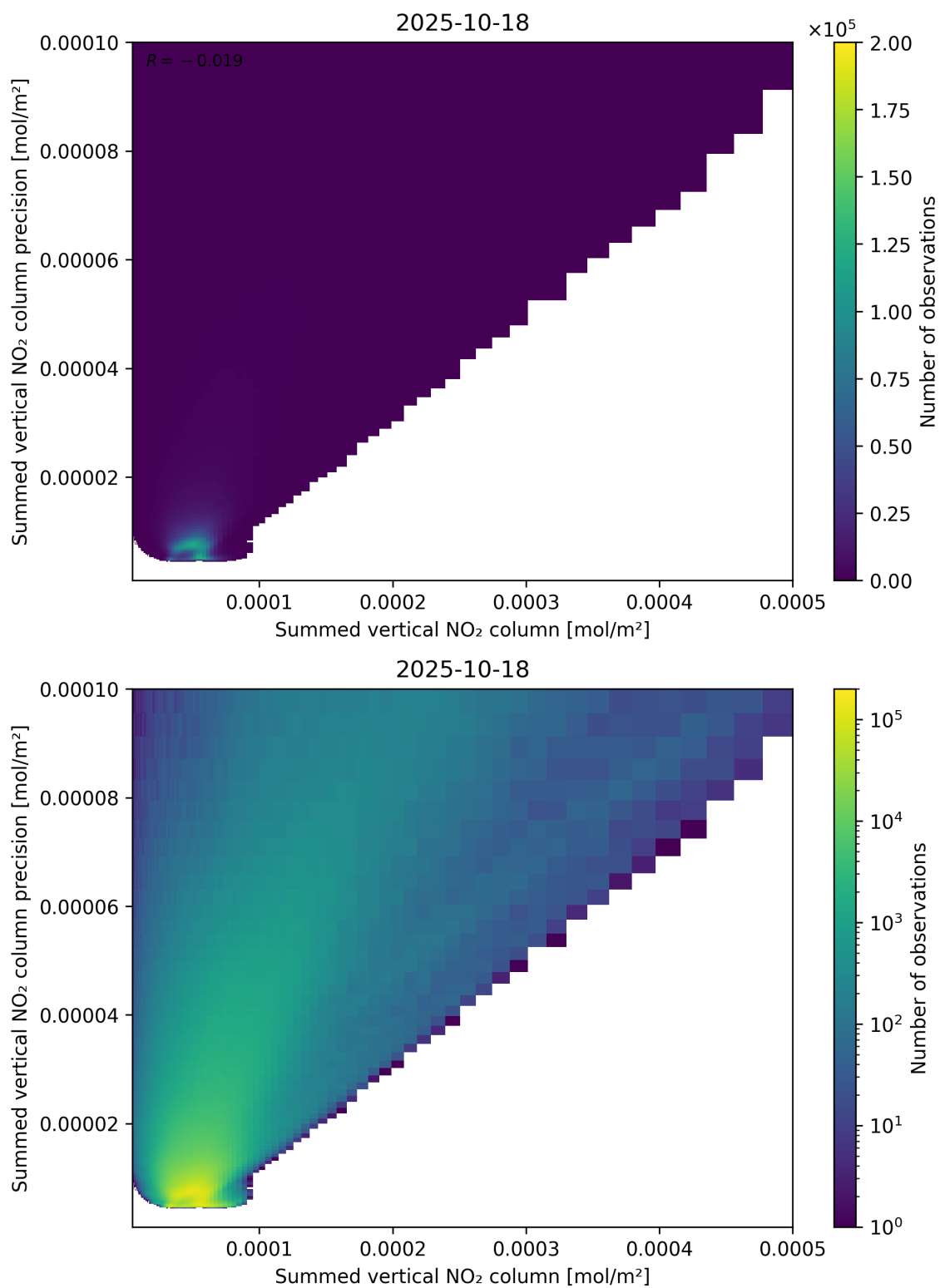
Figure 105: Scatter density plot of “Summed vertical NO 2 column” against “Summed vertical NO 2 column precision” for 2025-10-17 to 2025-10-19.
