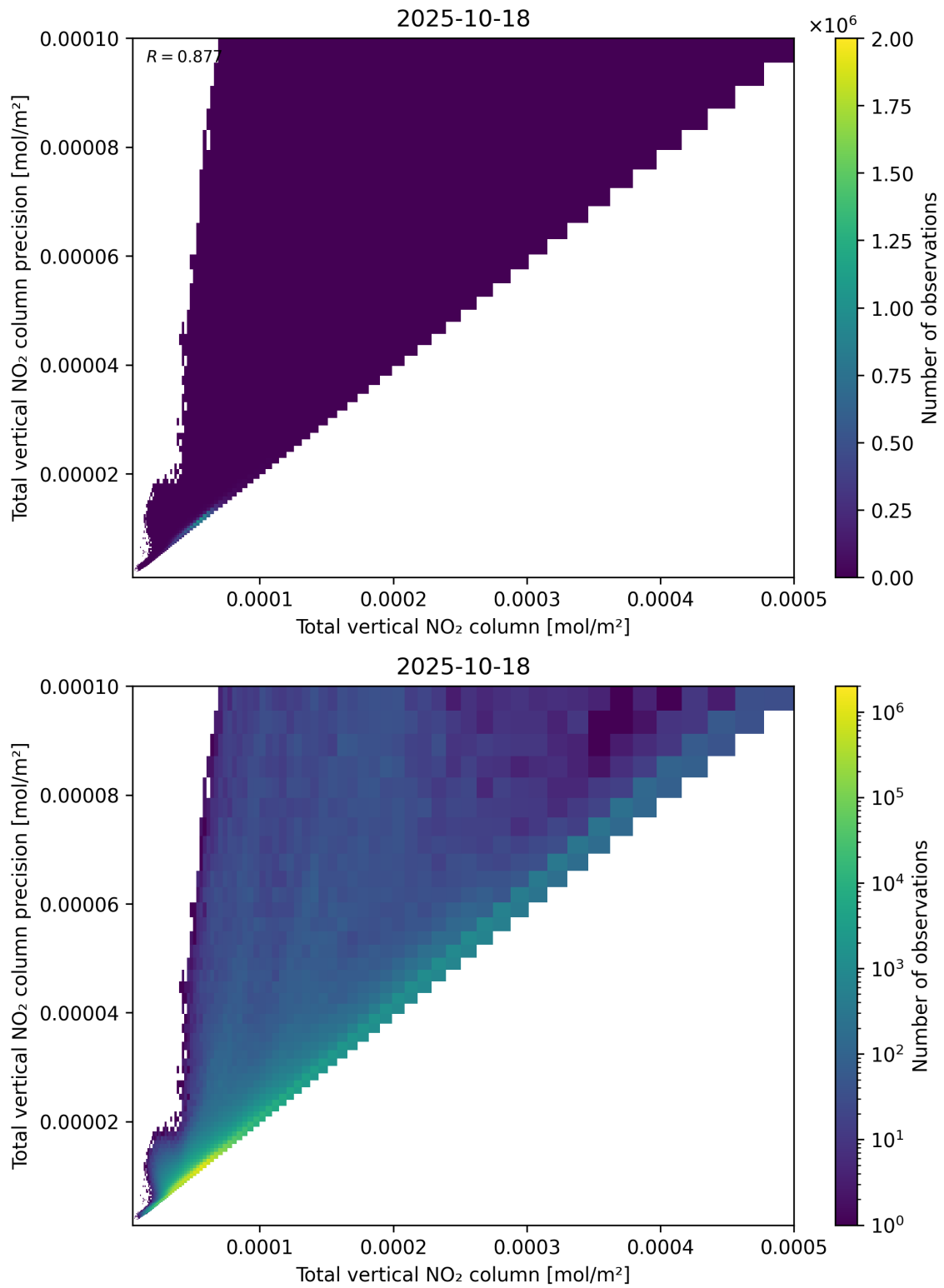
Figure 114: Scatter density plot of “Total vertical NO 2 column” against “Total vertical NO 2 column precision” for 2025-10-17 to 2025-10-19.
