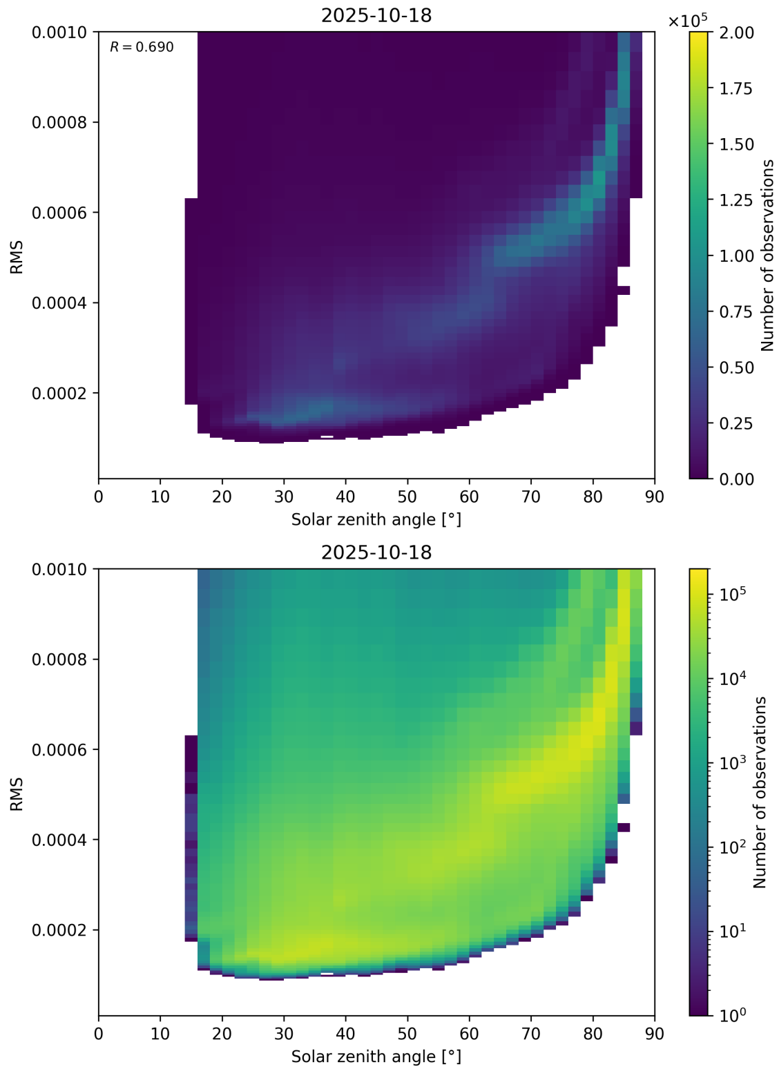
Figure 157: Scatter density plot of “Solar zenith angle” against “RMS” for 2025-10-17 to 2025-10-19.
