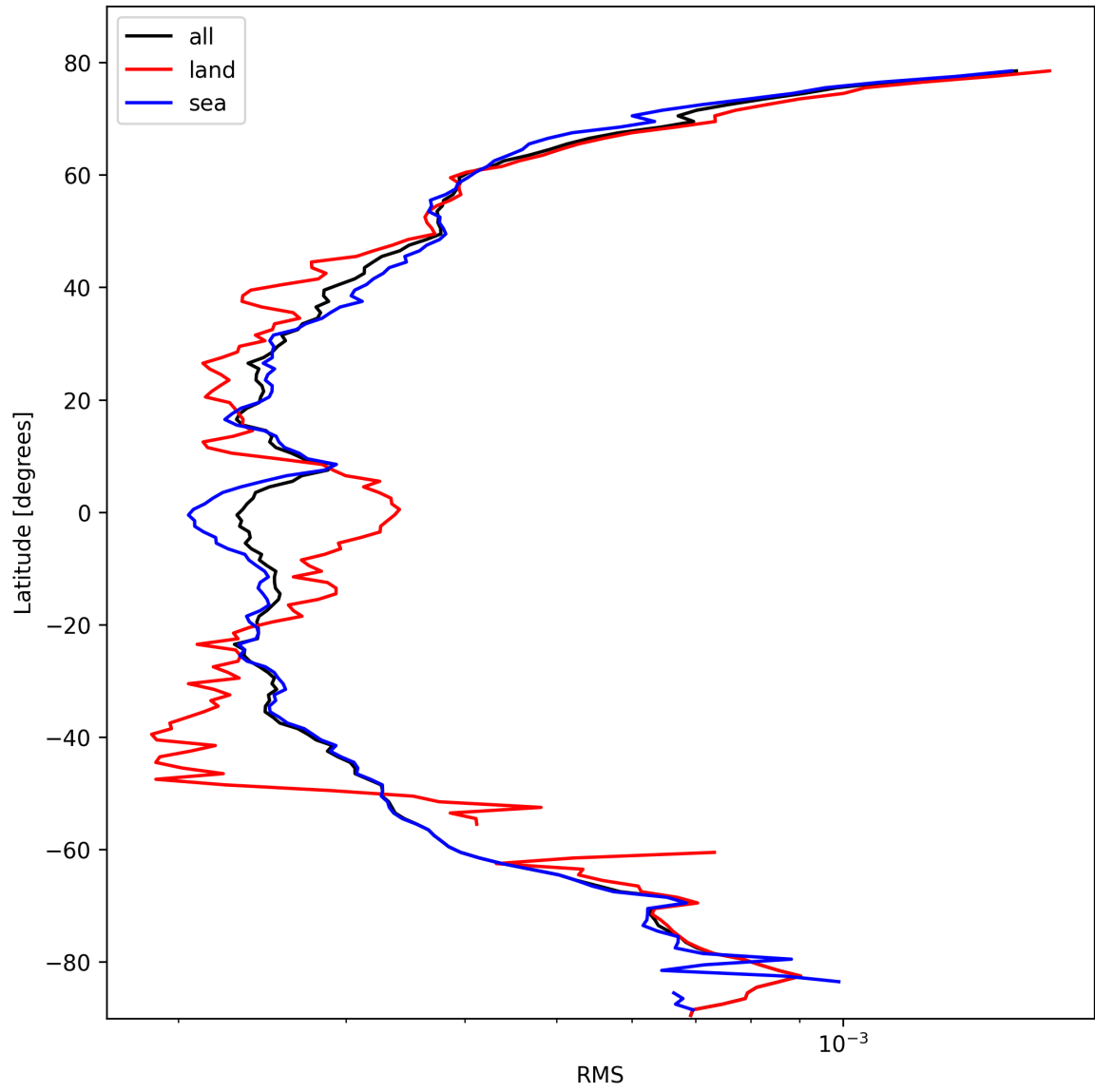
Figure 26: Zonal average of “RMS” for 2025-10-17 to 2025-10-19.
