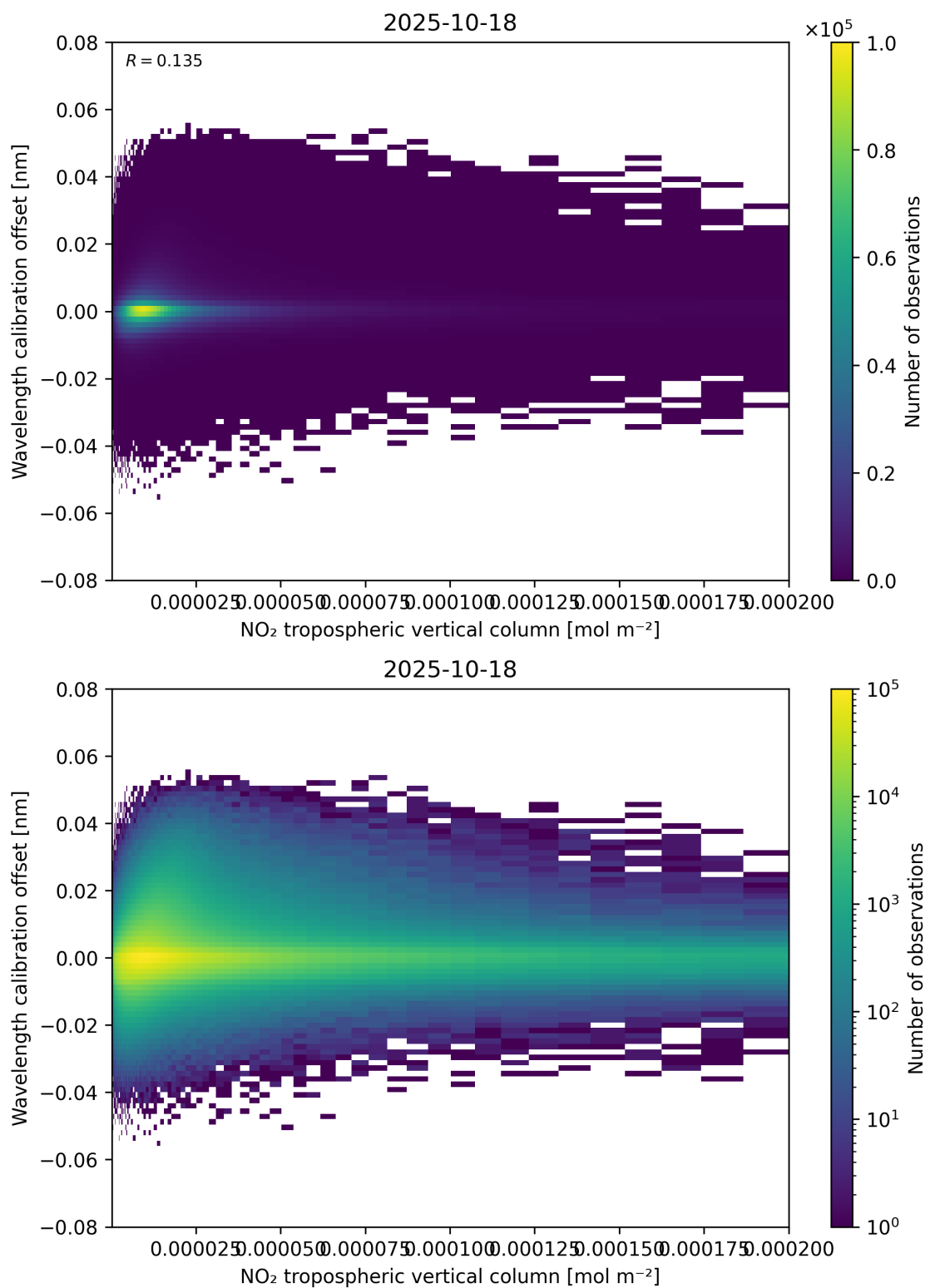
Figure 143: Scatter density plot of “NO 2 tropospheric vertical column” against “Wavelength calibration offset” for 2025-10-17 to 2025-10-19.
