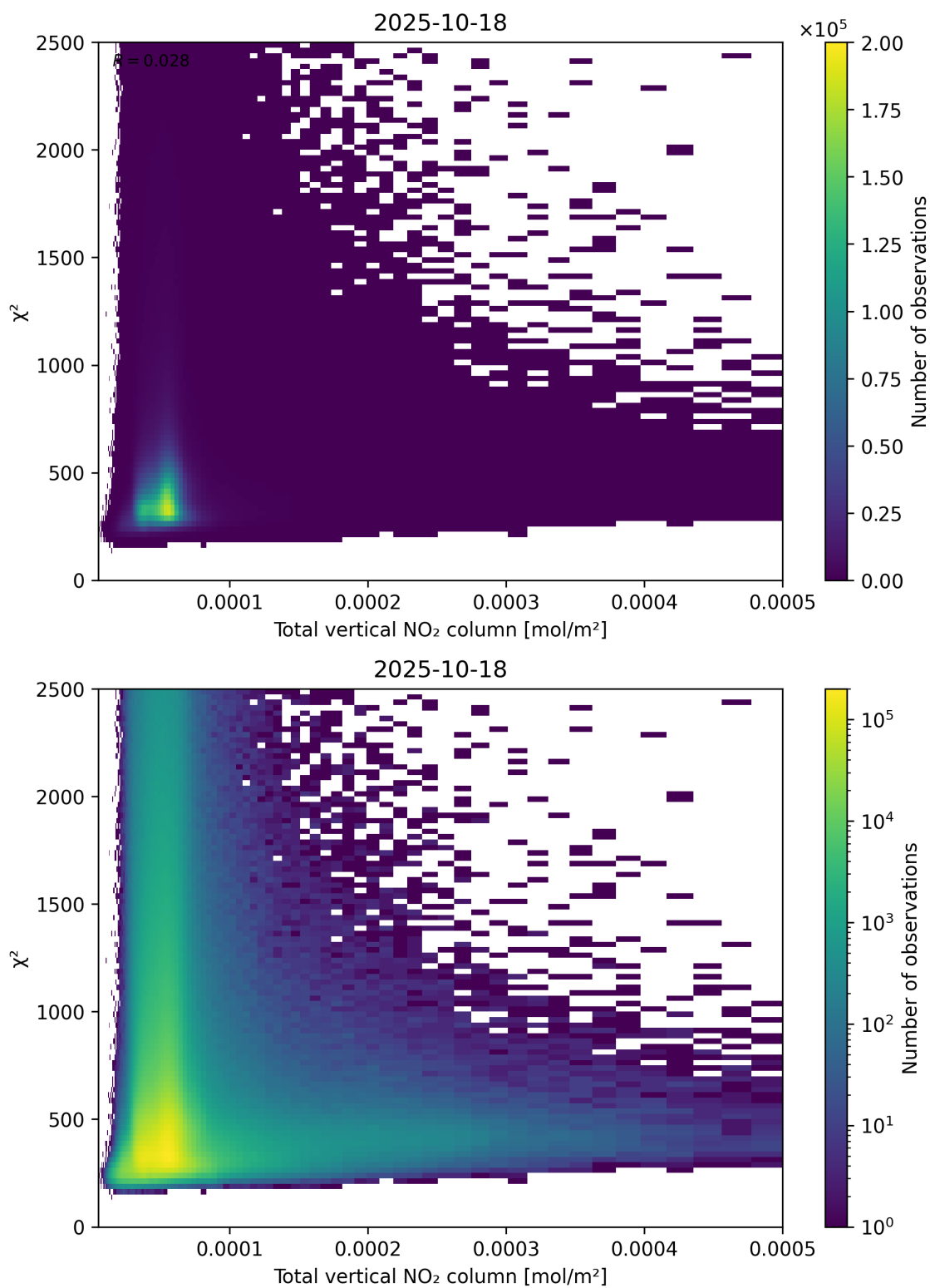
Figure 111: Scatter density plot of “Total vertical NO 2 column” against “ \chi^2 ” for 2025-10-17 to 2025-10-19.
