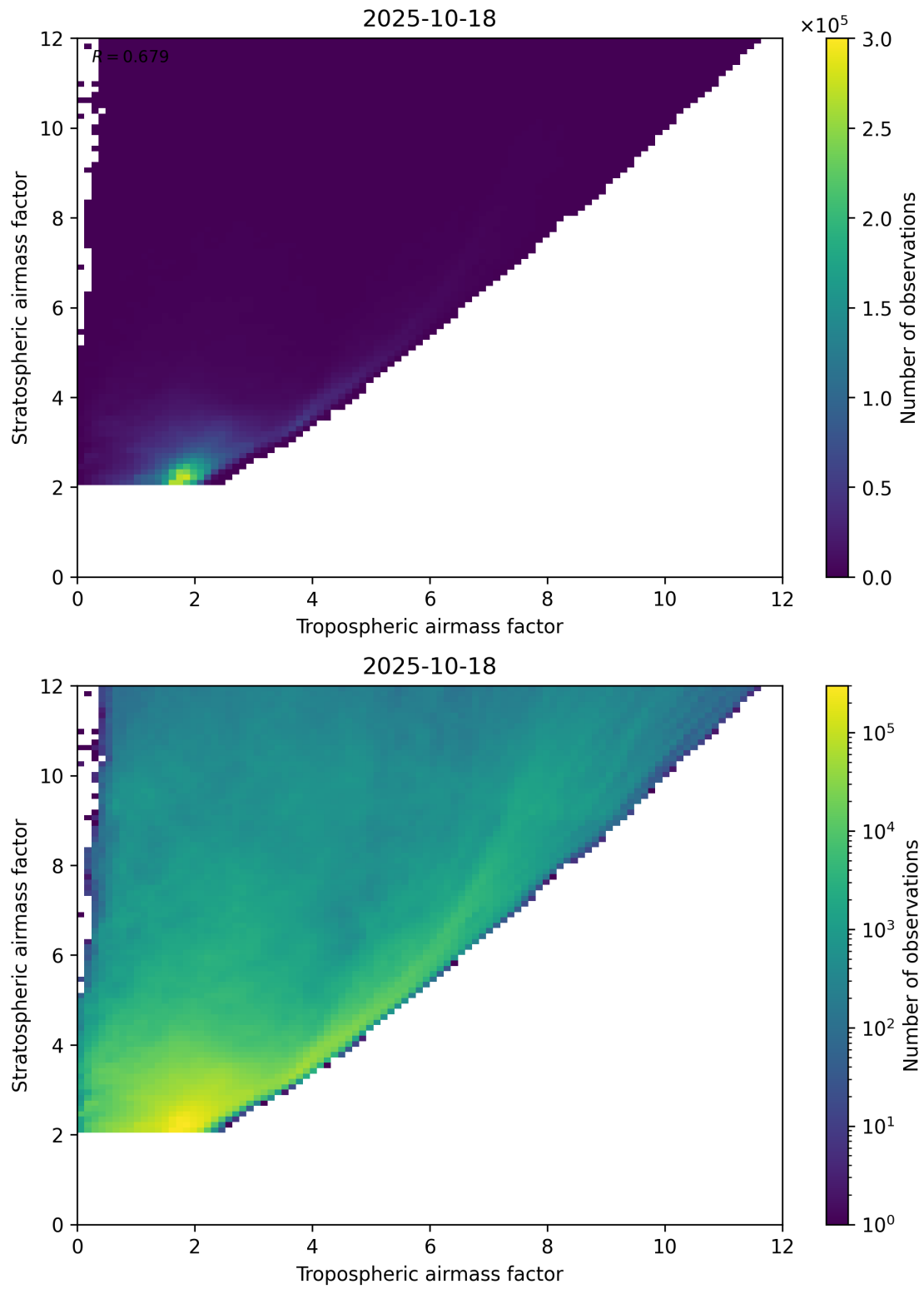
Figure 71: Scatter density plot of “Tropospheric airmass factor” against “Stratospheric airmass factor” for 2025-10-17 to 2025-10-19.
