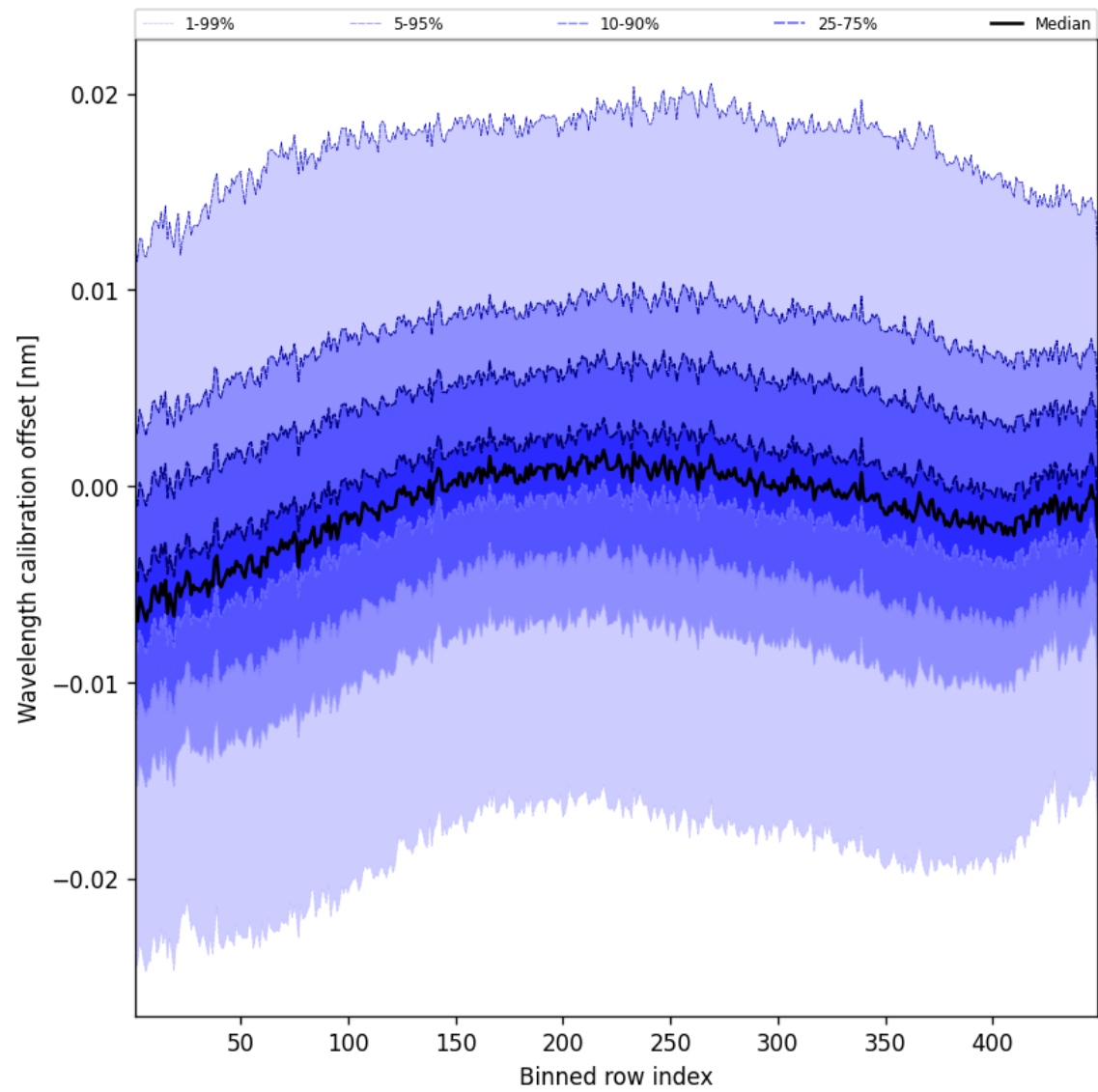
Figure 52: Along track statistics of “Wavelength calibration offset” for 2025-10-17 to 2025-10-19
