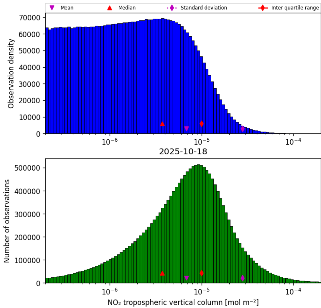
Figure 29: Histogram of “NO 2 tropospheric vertical column” for 2025-10-17 to 2025-10-19
