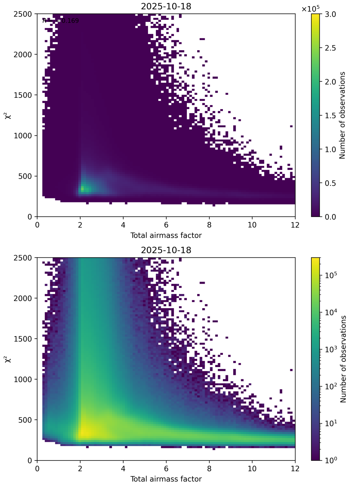
Figure 63: Scatter density plot of “Total airmass factor” against “ \chi^2 ” for 2025-10-17 to 2025-10-19.
