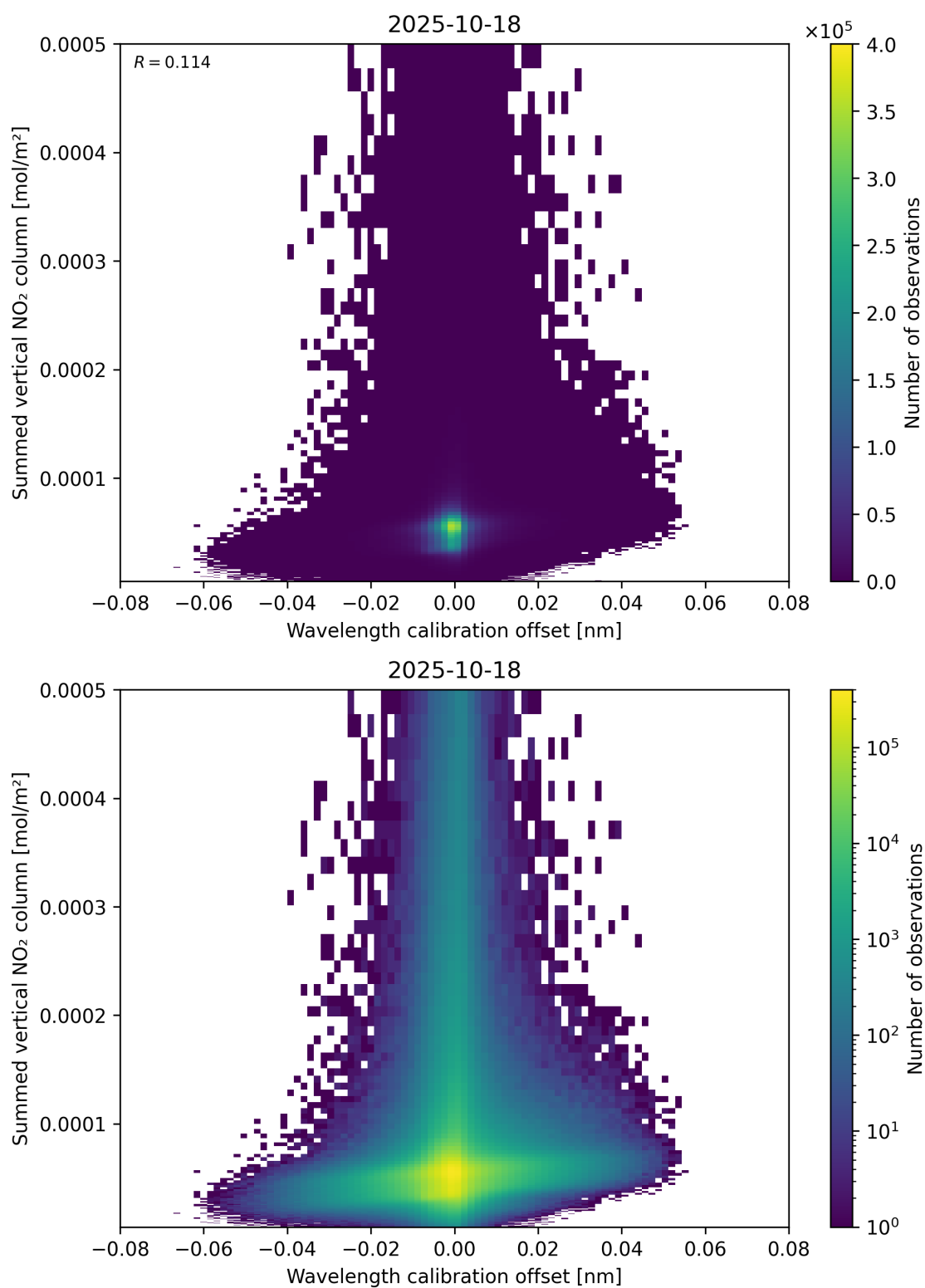
Figure 177: Scatter density plot of “Wavelength calibration offset” against “Summed vertical NO 2 column” for 2025-10-17 to 2025-10-19.
