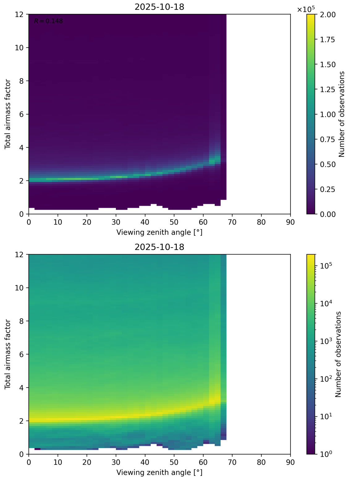
Figure 160: Scatter density plot of “Viewing zenith angle” against “Total airmass factor” for 2025-10-17 to 2025-10-19.
