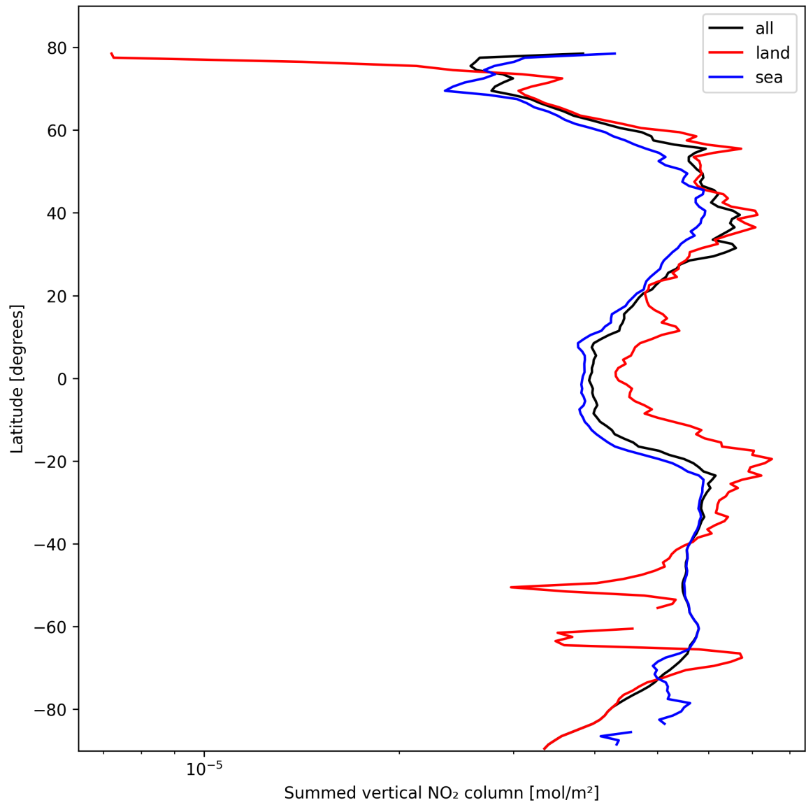
Figure 23: Zonal average of “Summed vertical NO 2 column” for 2025-10-17 to 2025-10-19.
