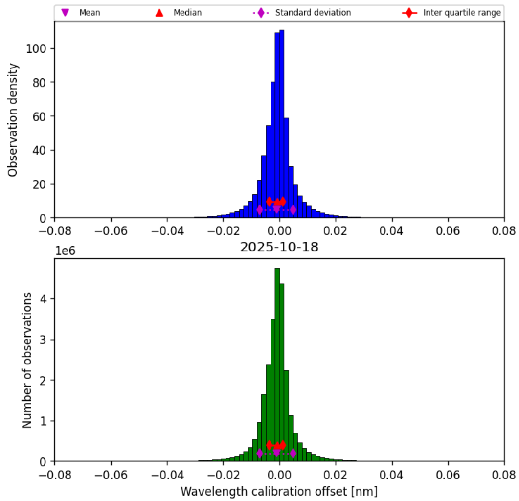
Figure 35: Histogram of “Wavelength calibration offset” for 2025-10-17 to 2025-10-19
