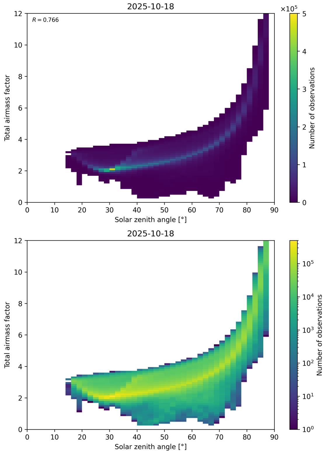
Figure 146: Scatter density plot of “Solar zenith angle” against “Total airmass factor” for 2025-10-17 to 2025-10-19.
