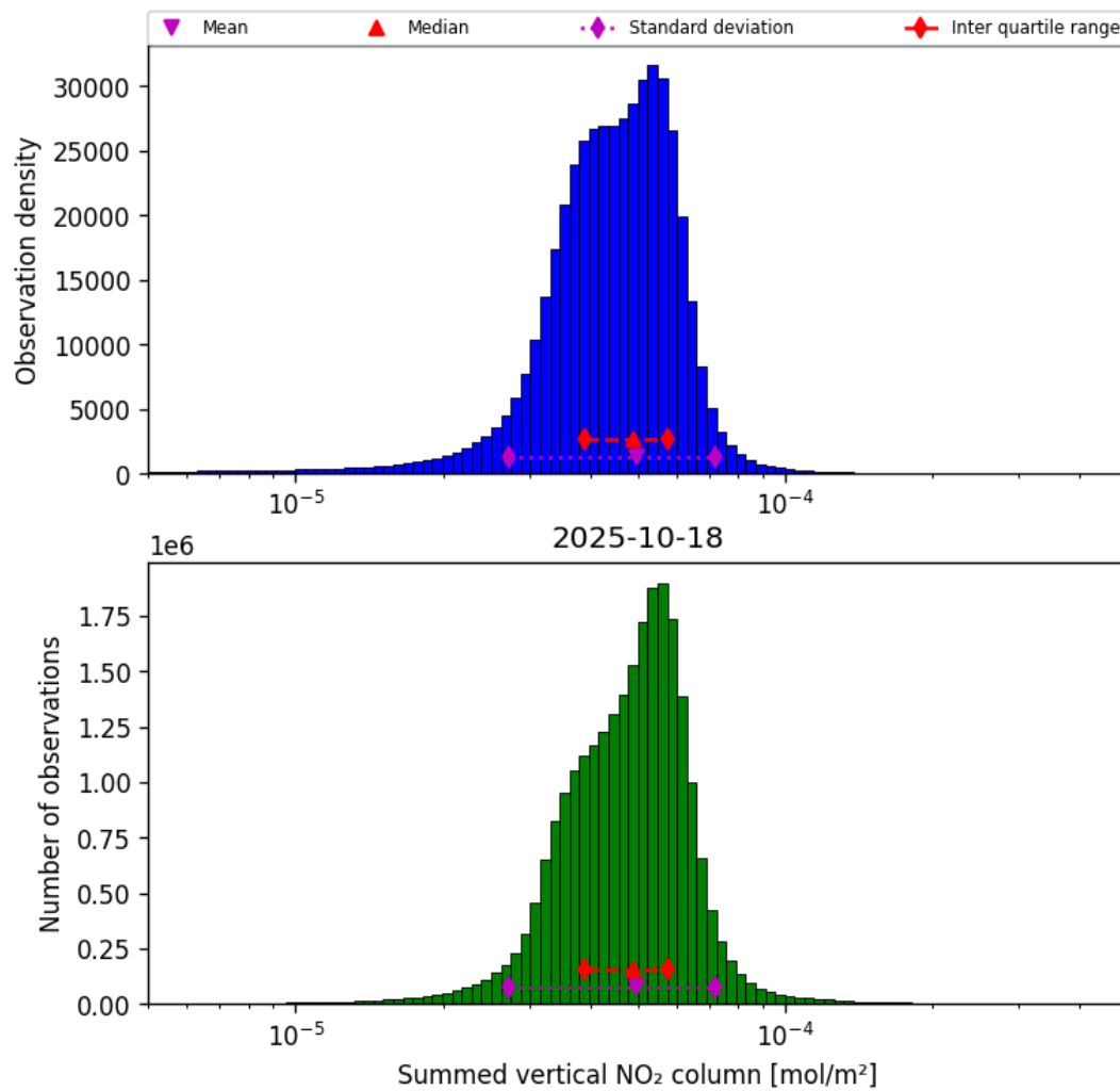
Figure 40: Histogram of “Summed vertical NO 2 column” for 2025-10-17 to 2025-10-19
