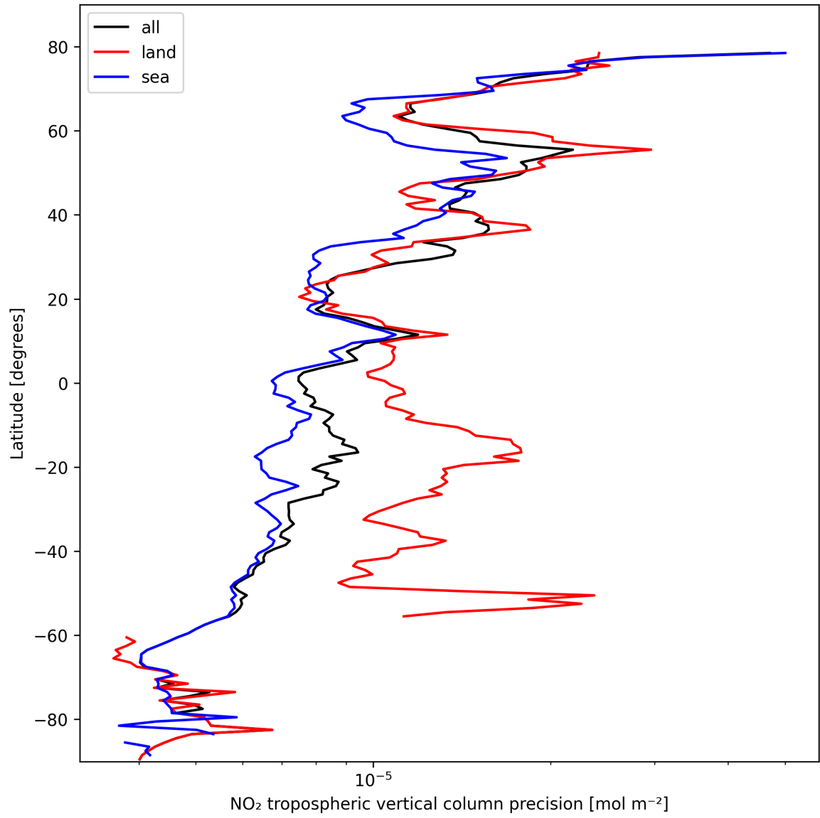
Figure 13: Zonal average of “NO 2 tropospheric vertical column precision” for 2025-10-17 to 2025-10-19.
