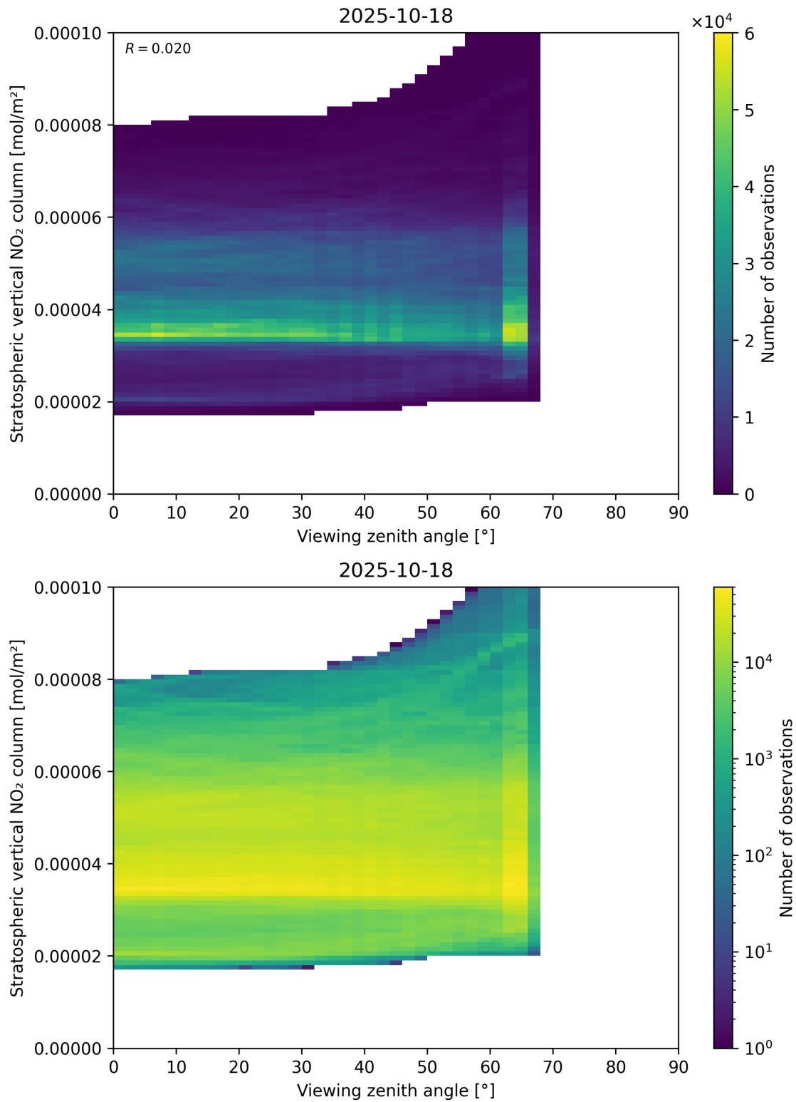
Figure 164: Scatter density plot of “Viewing zenith angle” against “Stratospheric vertical NO 2 column” for 2025-10-17 to 2025-10-19.
