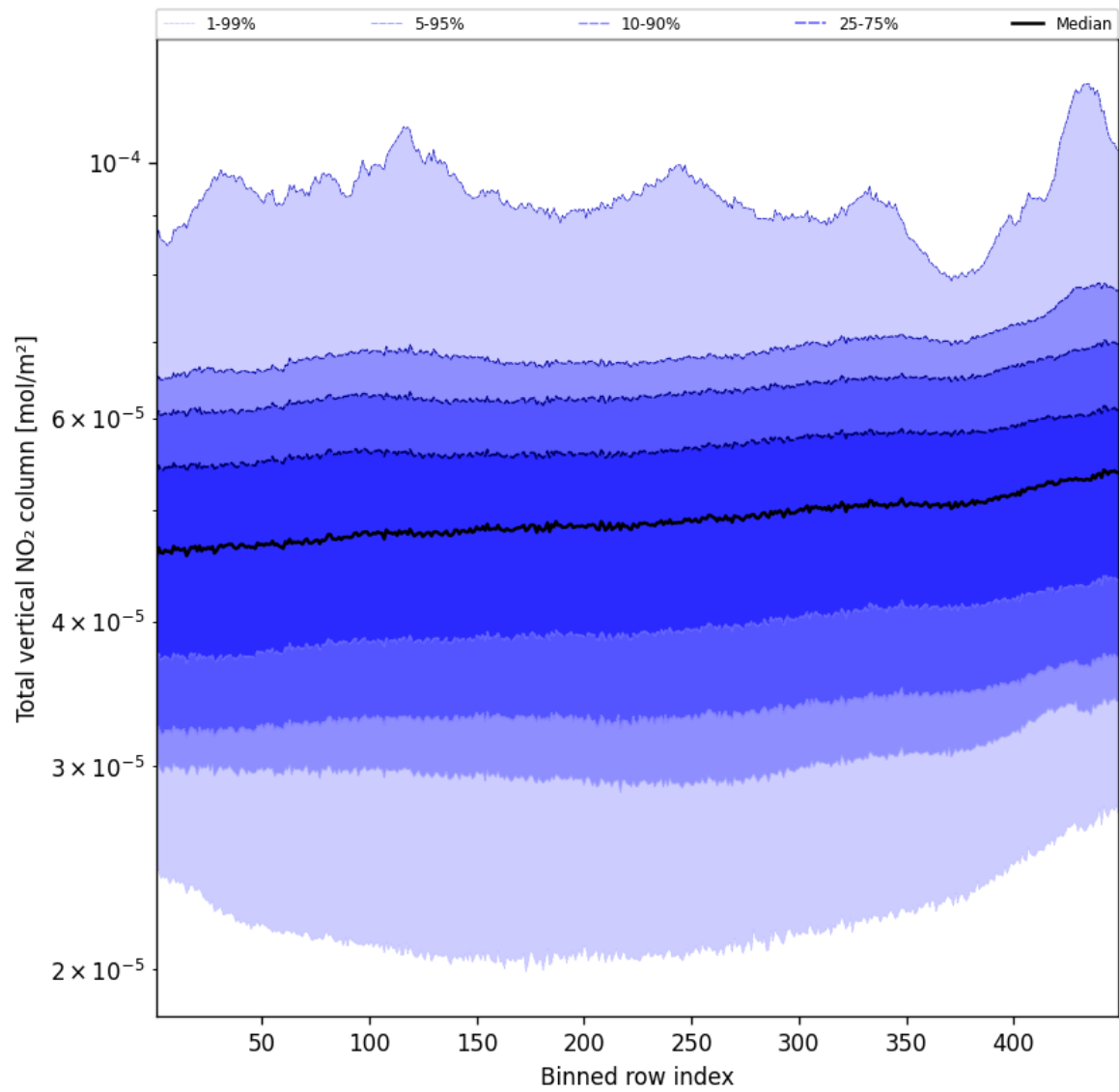
Figure 55: Along track statistics of “Total vertical NO 2 column” for 2025-10-17 to 2025-10-19
