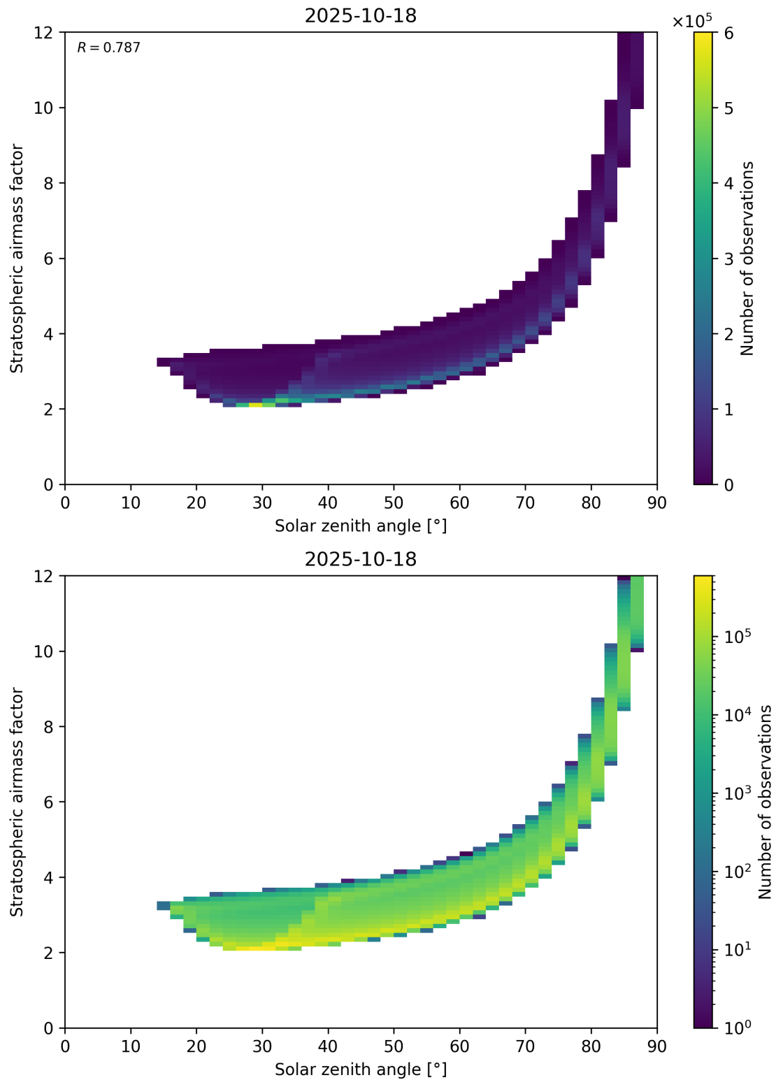
Figure 145: Scatter density plot of “Solar zenith angle” against “Stratospheric airmass factor” for 2025-10-17 to 2025-10-19.
