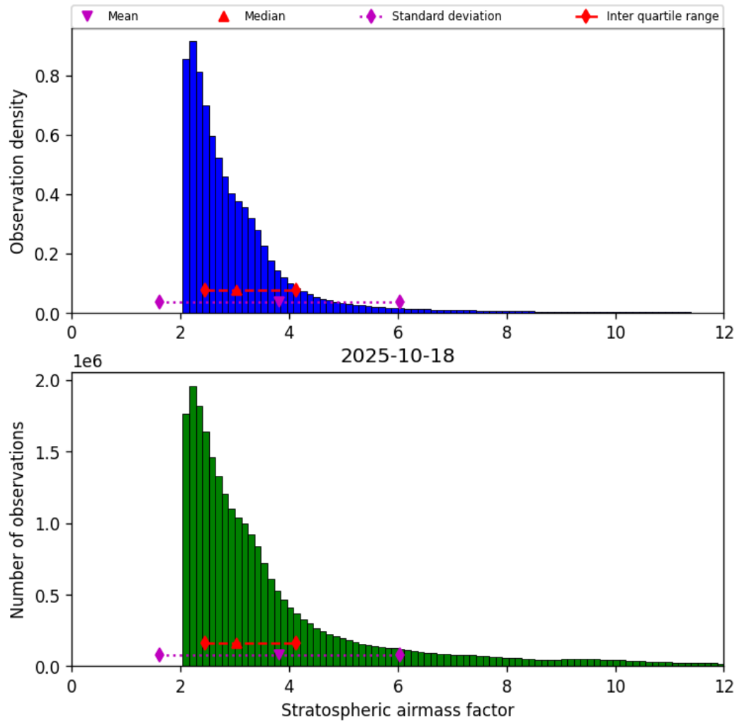
Figure 44: Histogram of “Stratospheric airmass factor” for 2025-10-17 to 2025-10-19
