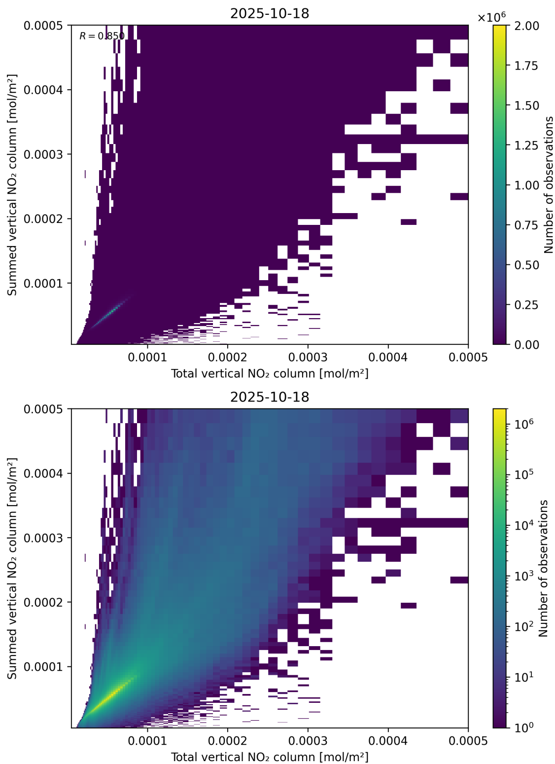
Figure 112: Scatter density plot of “Total vertical NO 2 column” against “Summed vertical NO 2 column” for 2025-10-17 to 2025-10-19.
