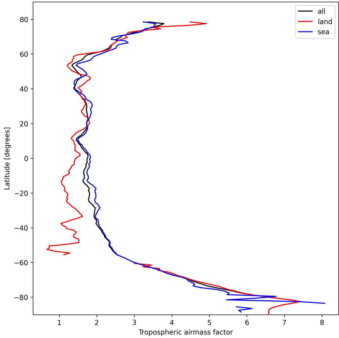
Figure 14: Zonal average of “Tropospheric airmass factor” for 2025-10-17 to 2025-10-19.
