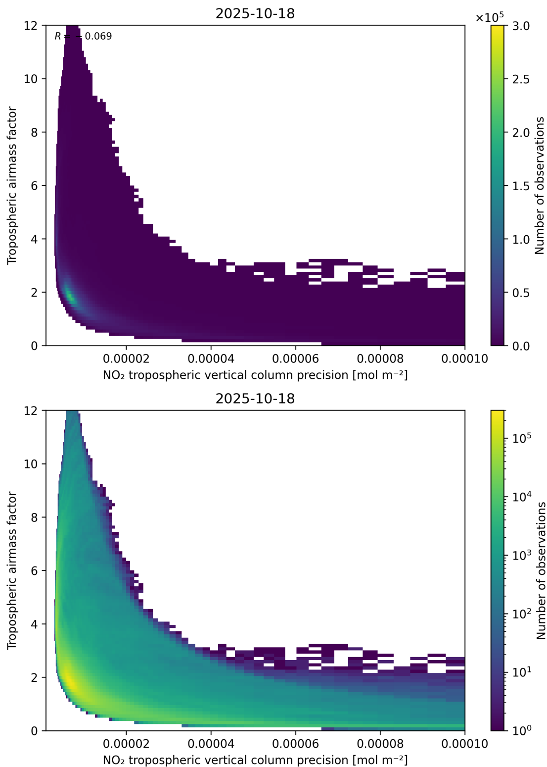
Figure 133: Scatter density plot of “NO 2 tropospheric vertical column precision” against “Tropospheric airmass factor” for 2025-10-17 to 2025-10-19.
