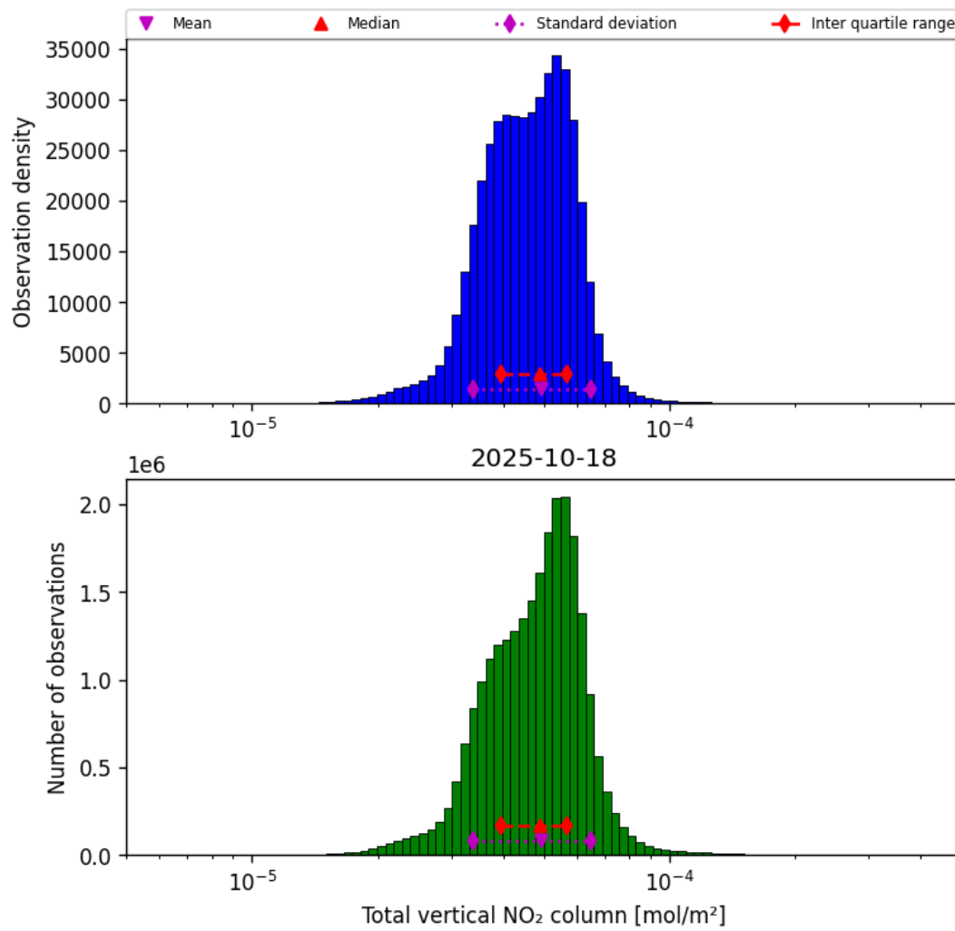
Figure 38: Histogram of “Total vertical NO 2 column” for 2025-10-17 to 2025-10-19
