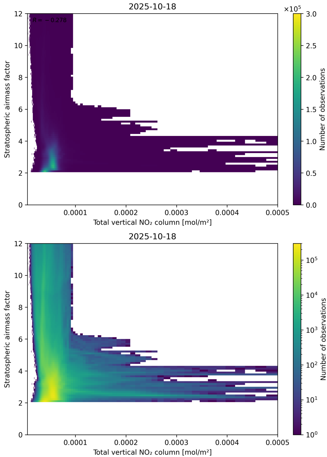
Figure 110: Scatter density plot of “Total vertical NO 2 column” against “Stratospheric airmass factor” for 2025-10-17 to 2025-10-19.
