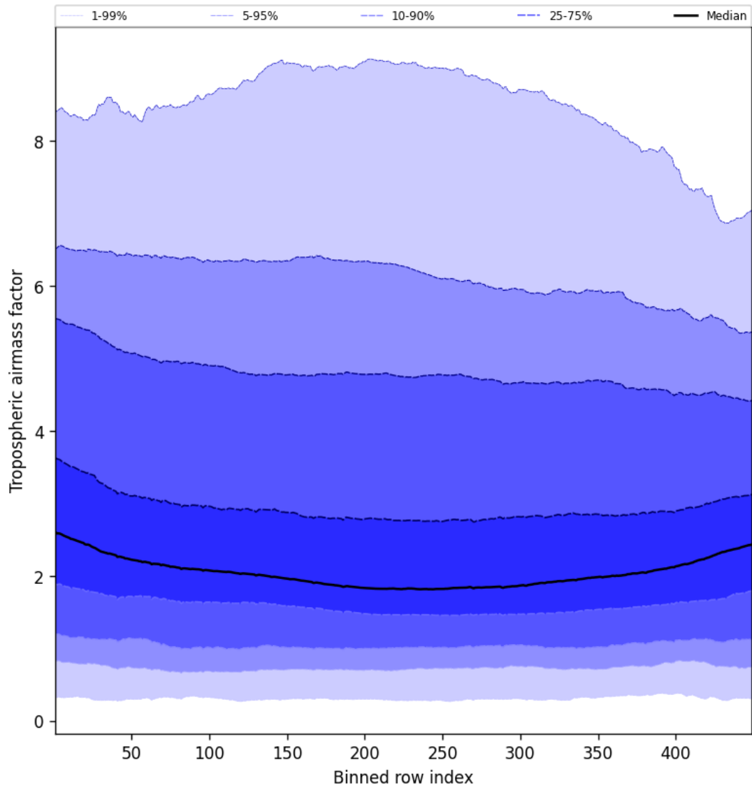
Figure 48: Along track statistics of “Tropospheric air mass factor” for 2025-10-17 to 2025-10-19
