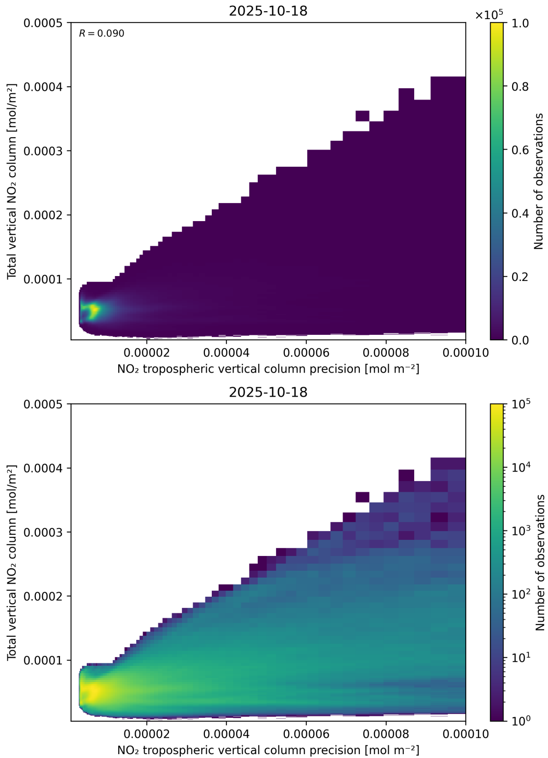
Figure 138: Scatter density plot of “NO 2 tropospheric vertical column precision” against “Total vertical NO 2 column” for 2025-10-17 to 2025-10-19.
