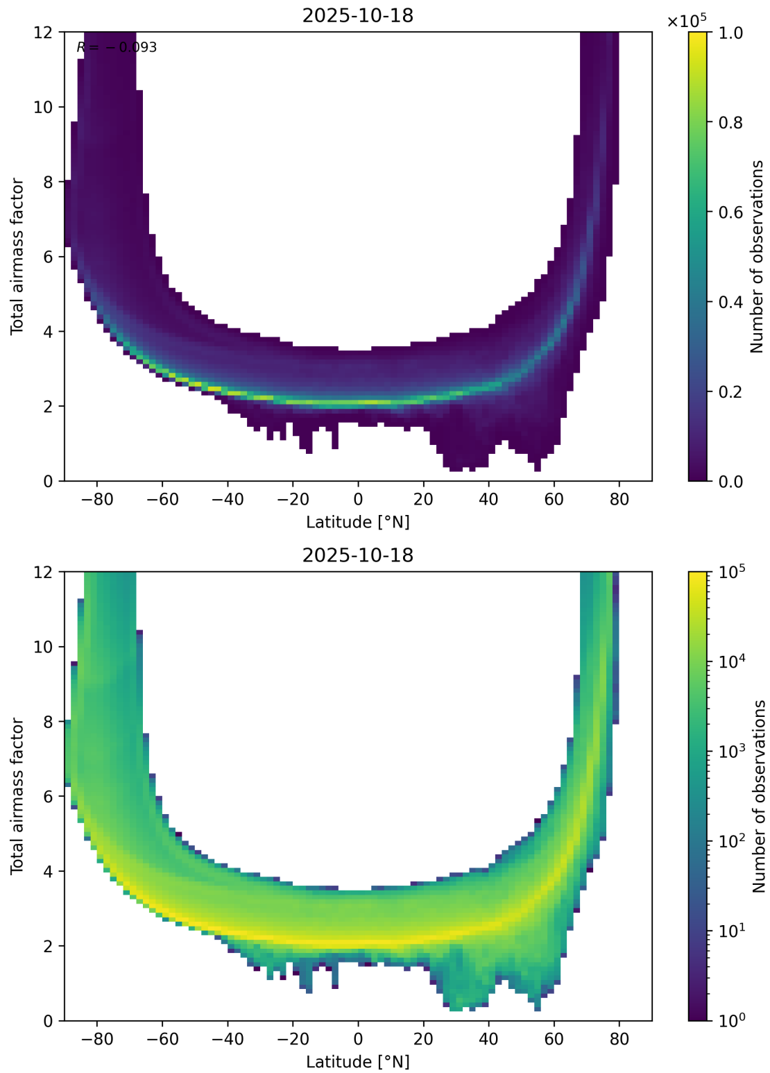
Figure 84: Scatter density plot of “Latitude” against “Total airmass factor” for 2025-10-17 to 2025-10-19.
