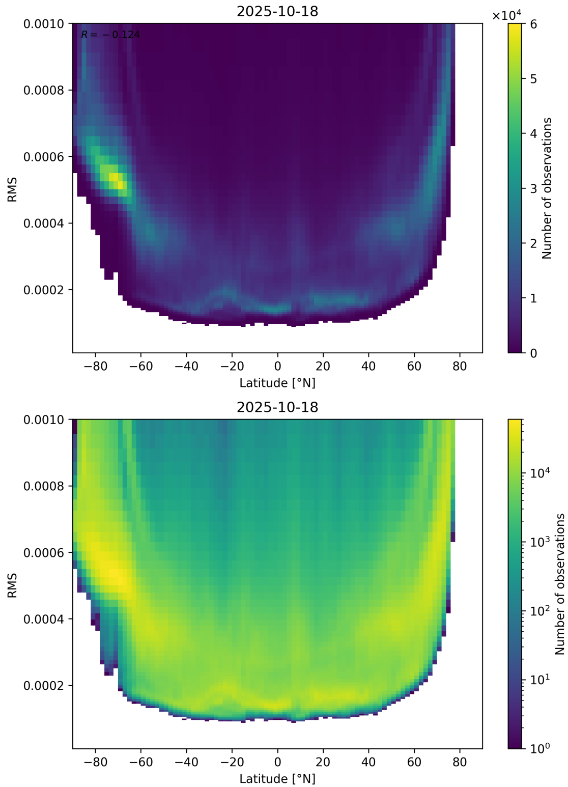
Figure 94: Scatter density plot of “Latitude” against “RMS” for 2025-10-17 to 2025-10-19.
