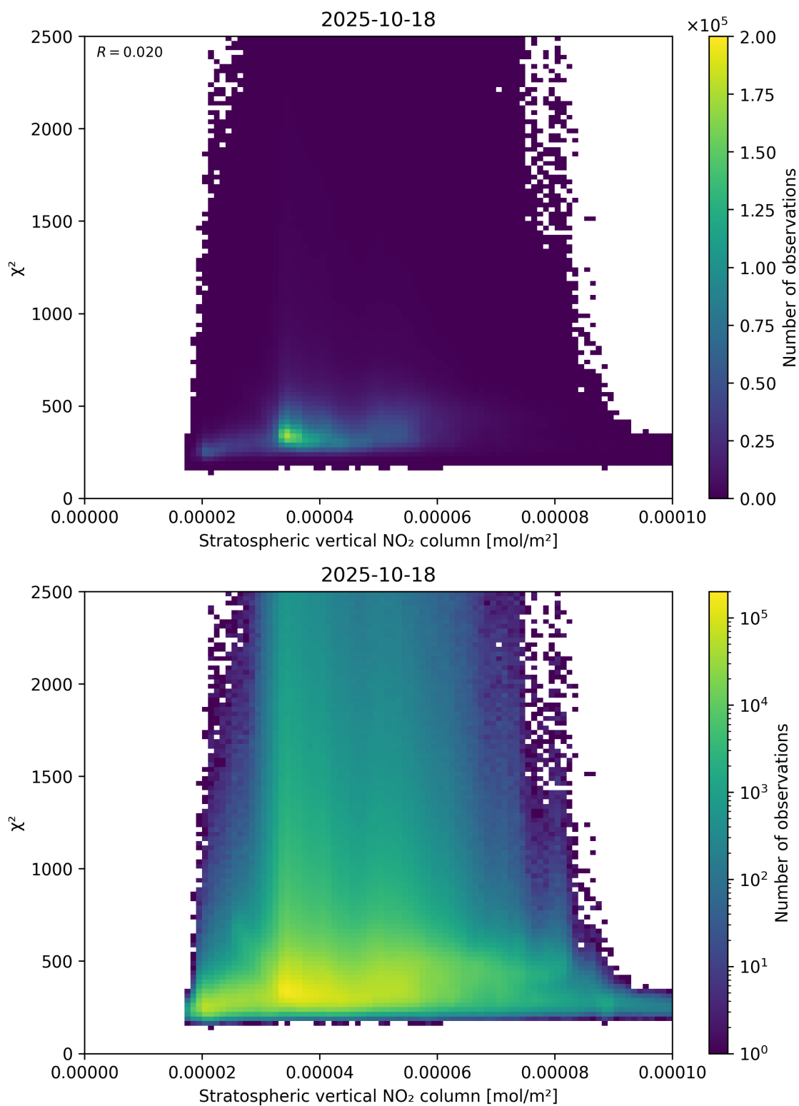
Figure 97: Scatter density plot of “Stratospheric vertical NO 2 column” against “ \chi^2 ” for 2025-10-17 to 2025-10-19.
