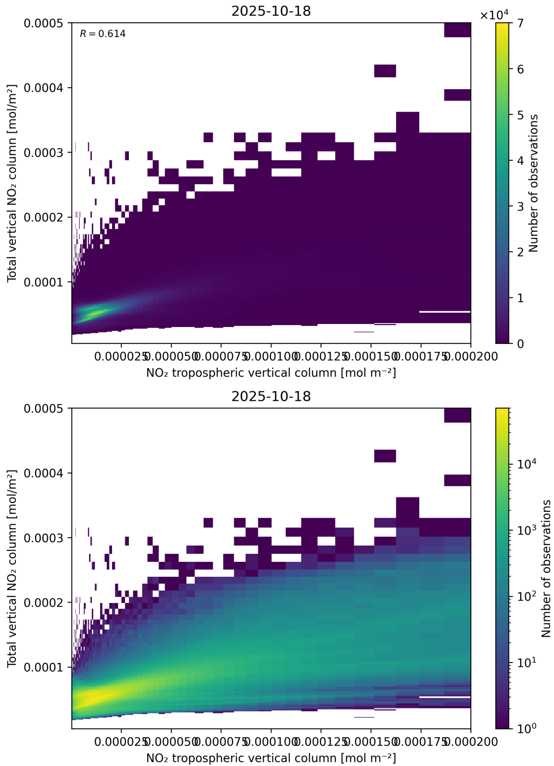
Figure 128: Scatter density plot of “NO 2 tropospheric vertical column” against “Total vertical NO 2 column” for 2025-10-17 to 2025-10-19.
