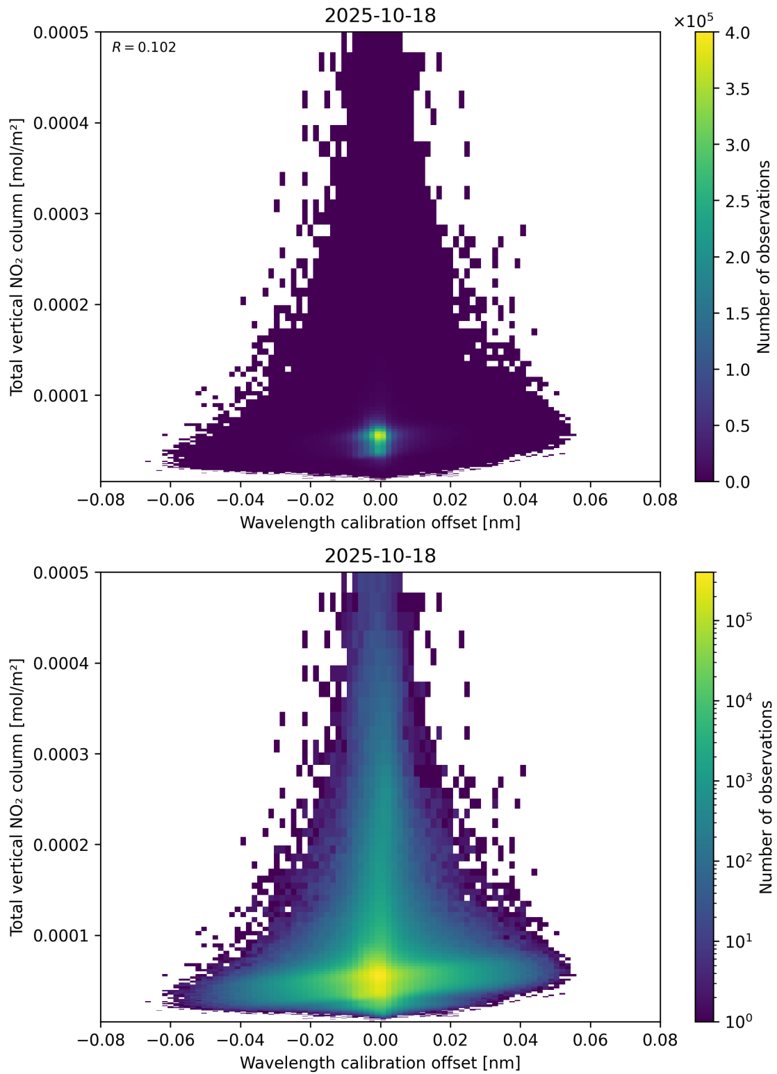
Figure 179: Scatter density plot of “Wavelength calibration offset” against “Total vertical NO 2 column” for 2025-10-17 to 2025-10-19.
