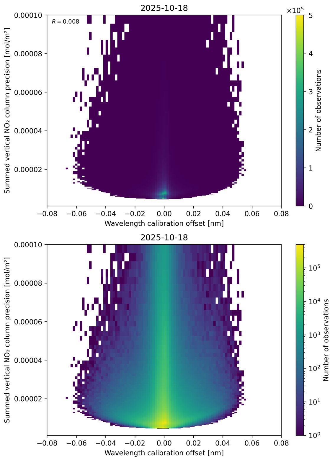
Figure 178: Scatter density plot of “Wavelength calibration offset” against “Summed vertical NO 2 column precision” for 2025-10-17 to 2025-10-19.
