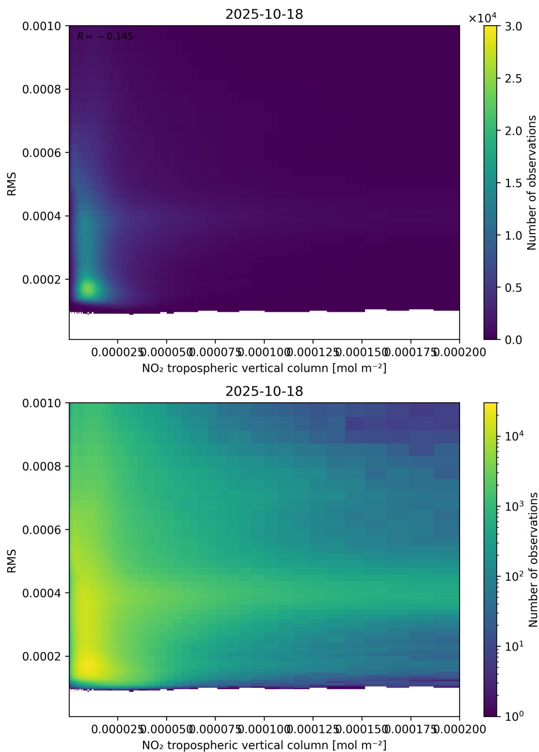
Figure 142: Scatter density plot of “NO 2 tropospheric vertical column” against “RMS” for 2025-10-17 to 2025-10-19.
