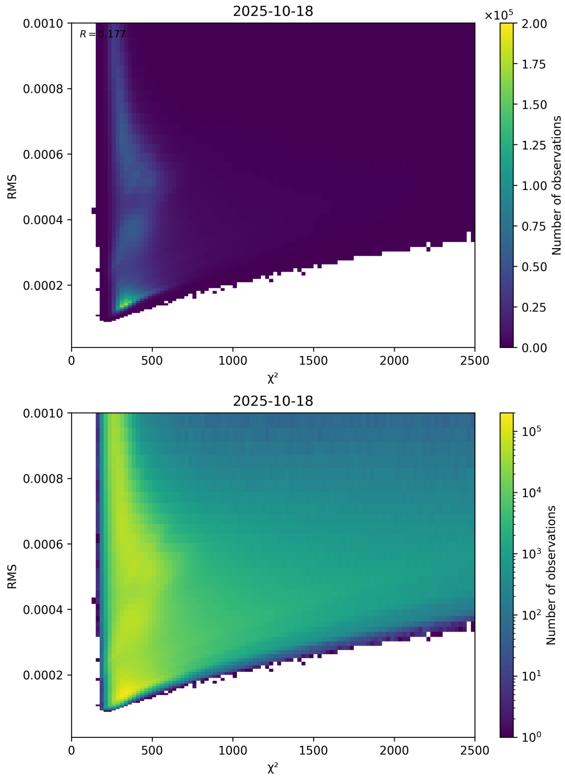
Figure 82: Scatter density plot of “ \chi^2 ” against “RMS” for 2025-10-17 to 2025-10-19.
