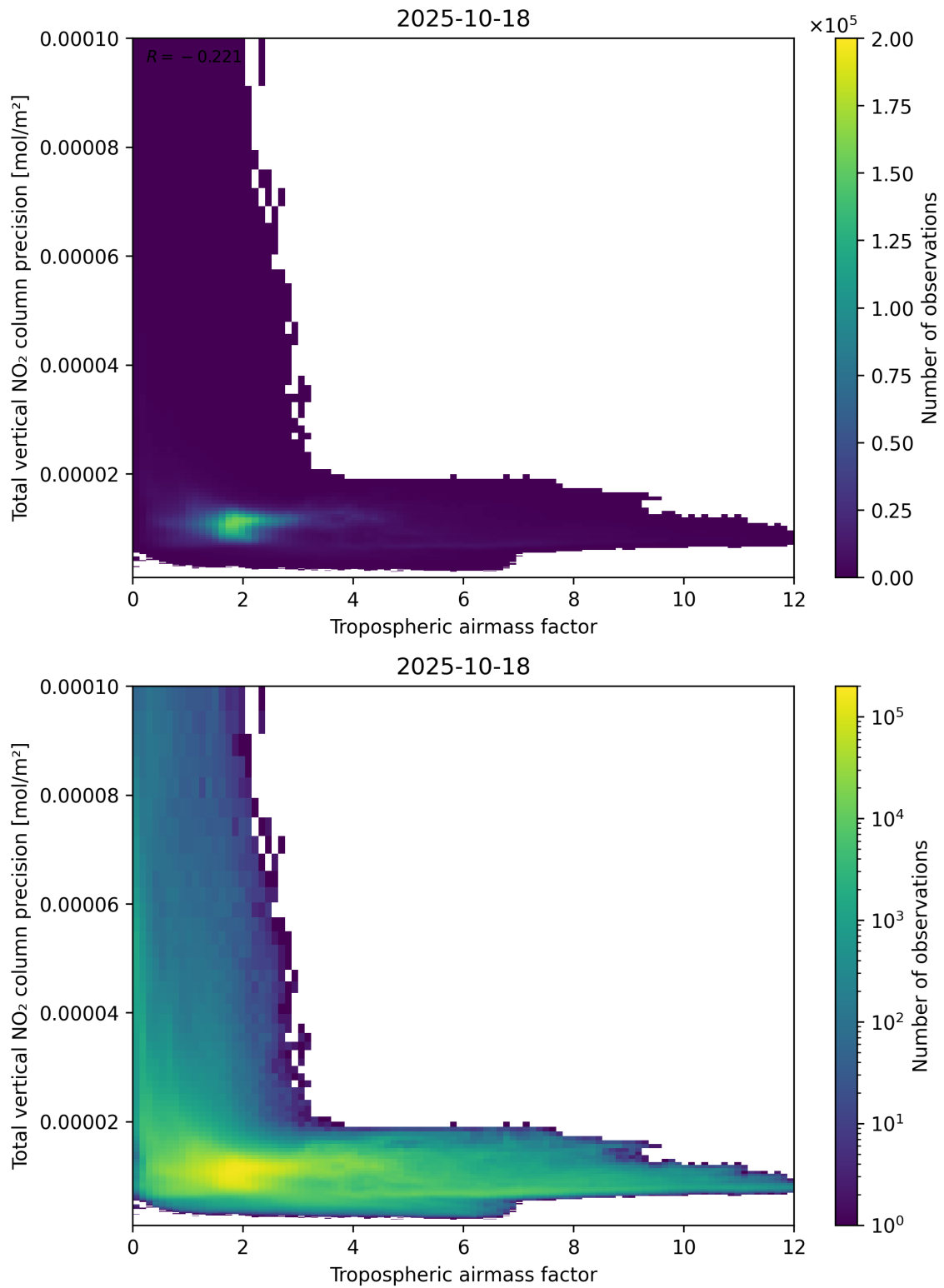
Figure 78: Scatter density plot of “Tropospheric air mass factor” against “Total vertical NO 2 column precision” for 2025-10-17 to 2025-10-19.
