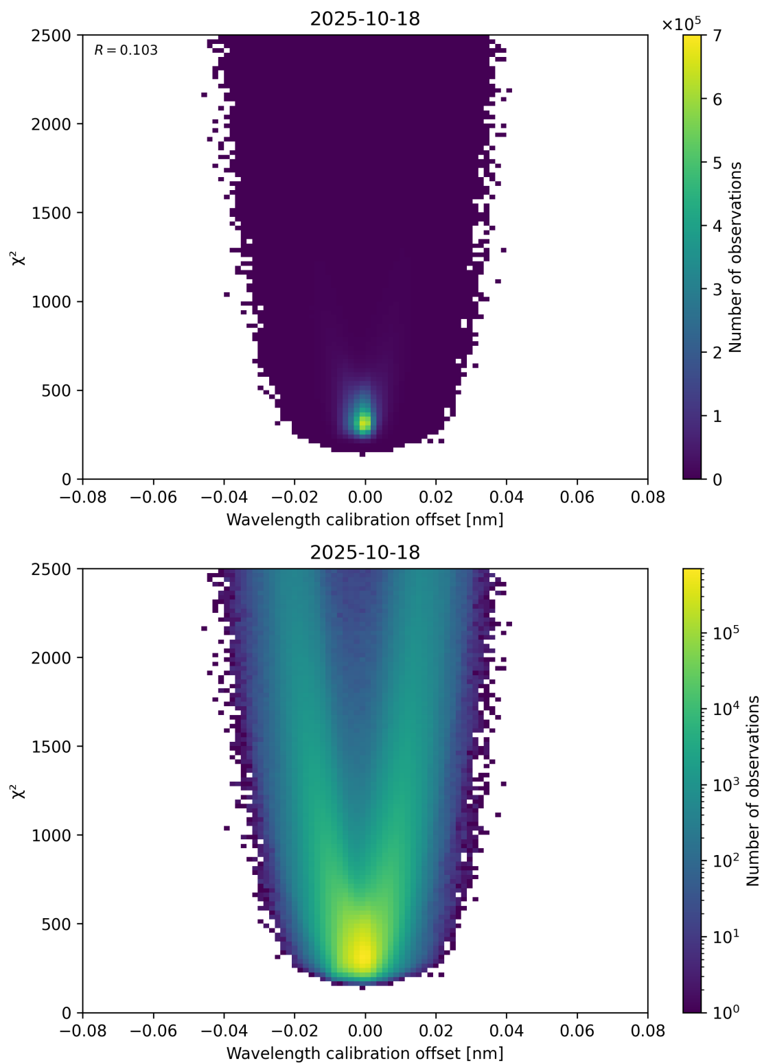
Figure 175: Scatter density plot of “Wavelength calibration offset” against “ \chi^2 ” for 2025-10-17 to 2025-10-19.
