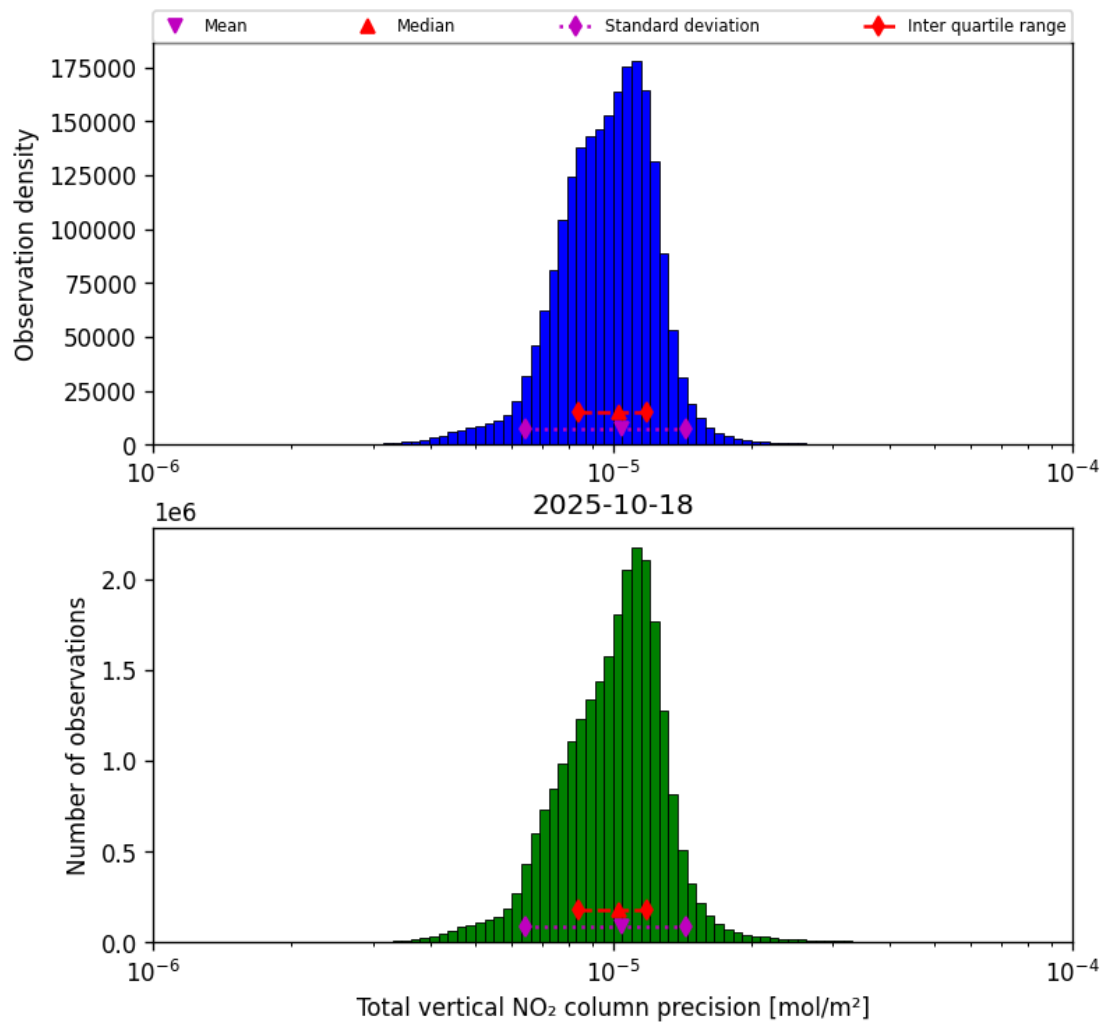
Figure 39: Histogram of “Total vertical NO 2 column precision” for 2025-10-17 to 2025-10-19
