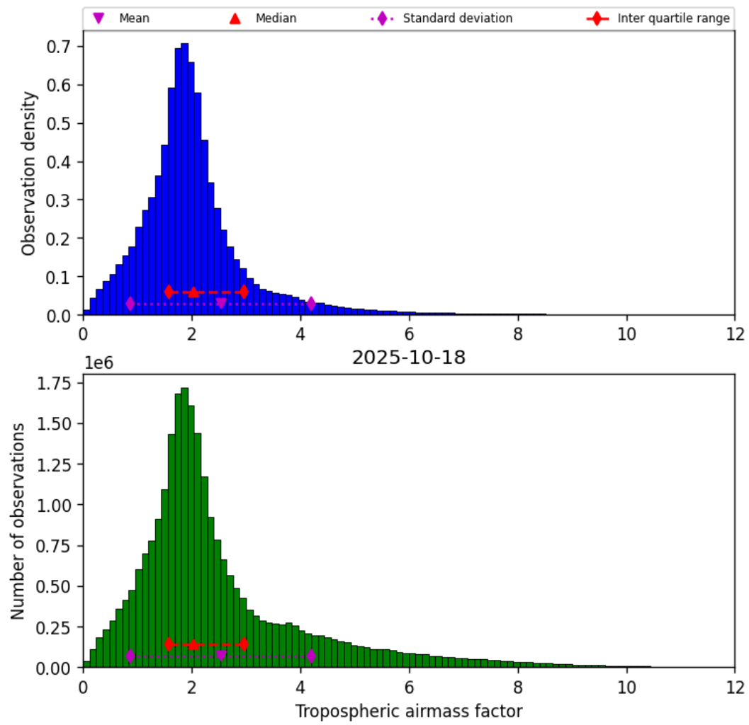
Figure 31: Histogram of “Tropospheric air mass factor” for 2025-10-17 to 2025-10-19
