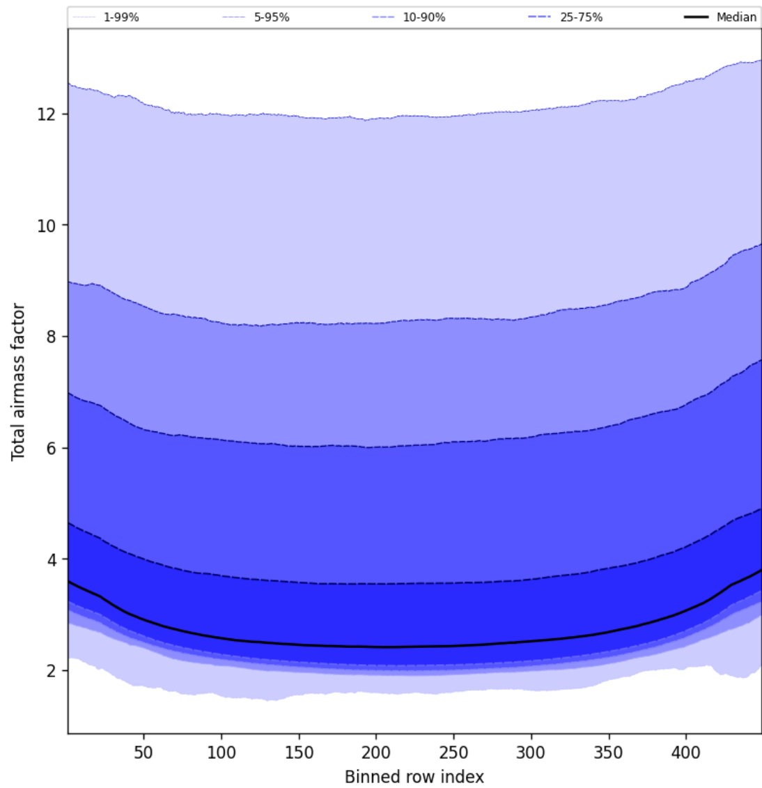
Figure 49: Along track statistics of “Total airmass factor” for 2025-10-17 to 2025-10-19
