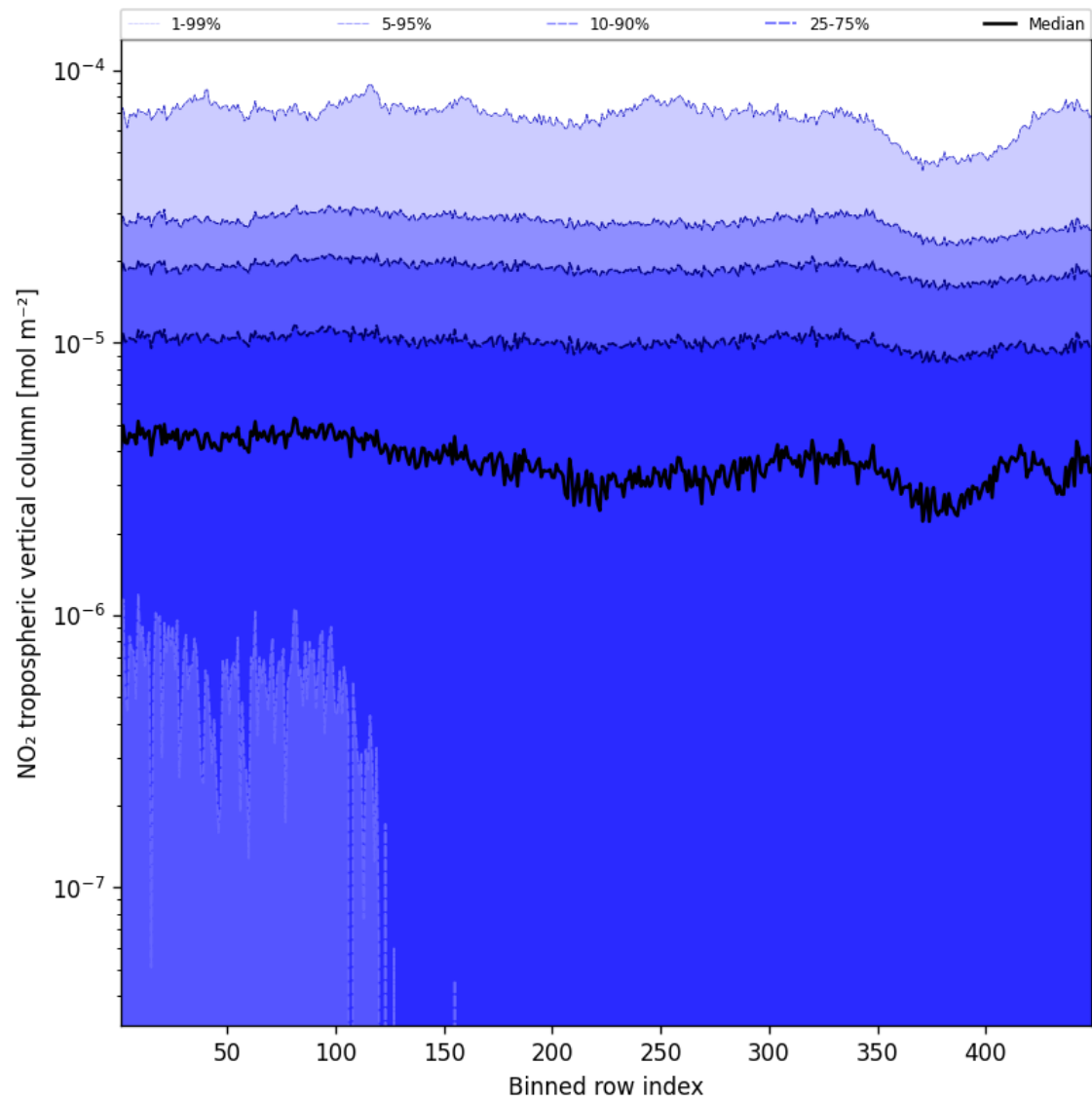
Figure 46: Along track statistics of “NO 2 tropospheric vertical column” for 2025-10-17 to 2025-10-19
