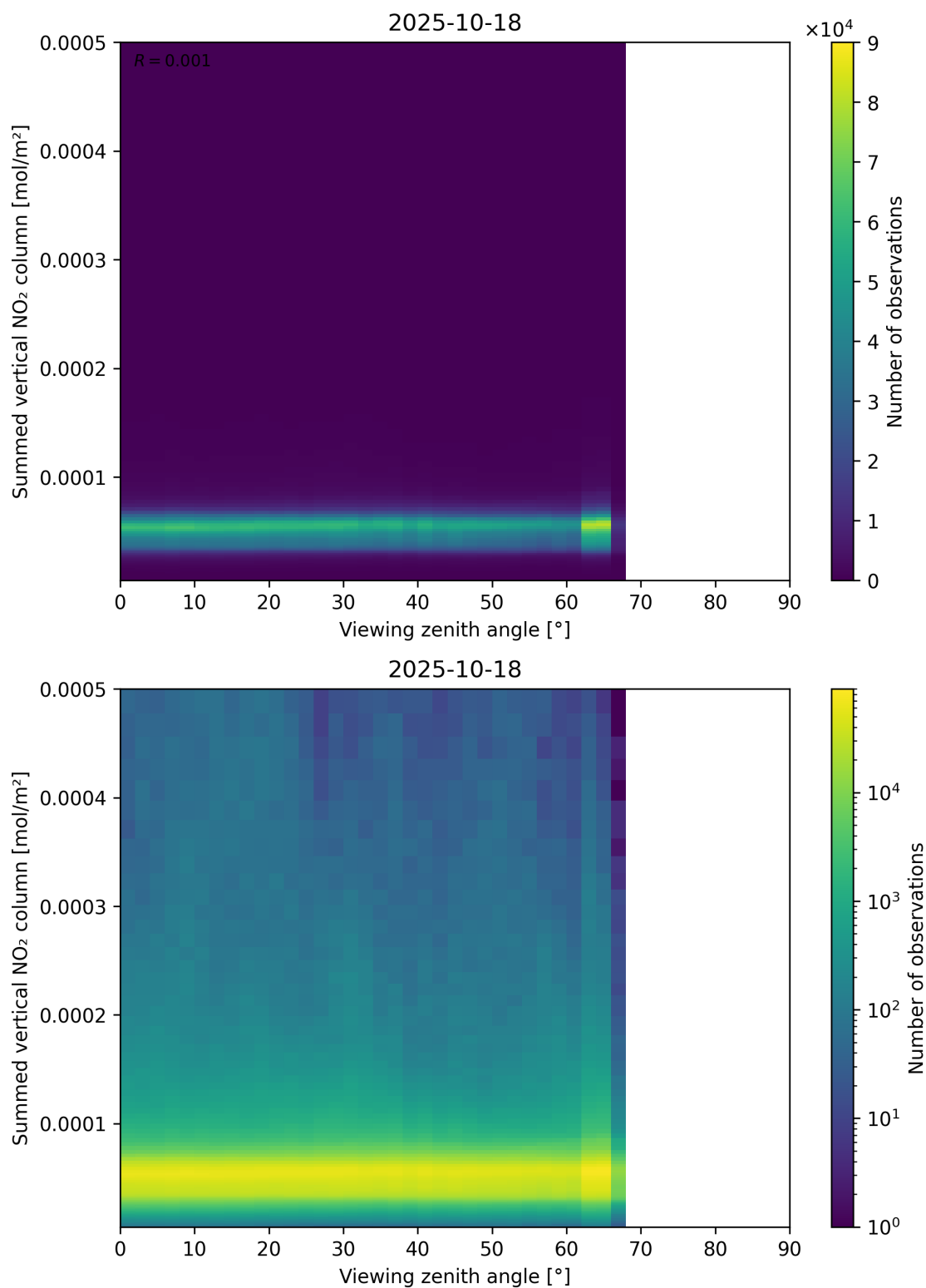
Figure 165: Scatter density plot of “Viewing zenith angle” against “Summed vertical NO 2 column” for 2025-10-17 to 2025-10-19.
