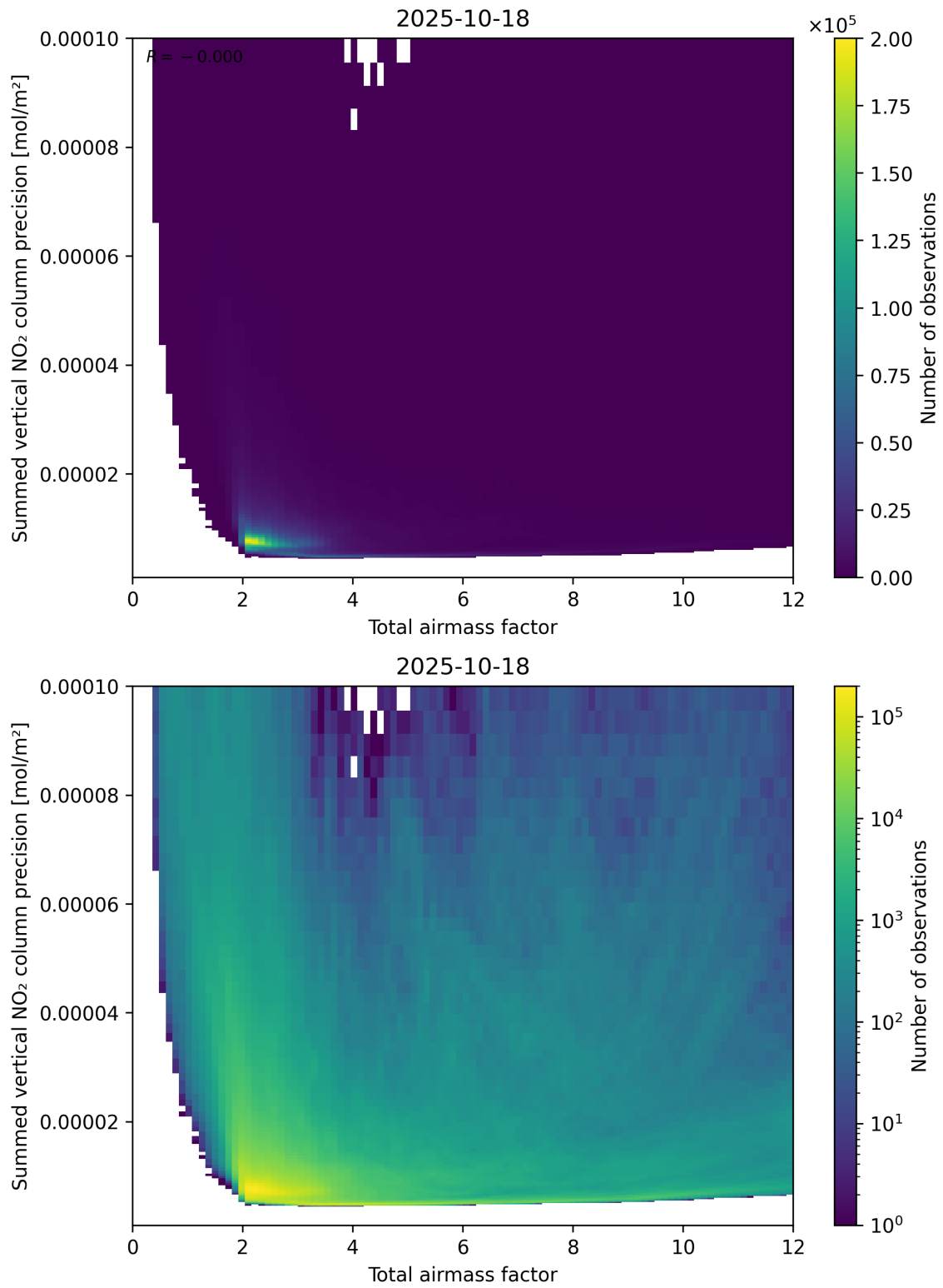
Figure 66: Scatter density plot of “Total airmass factor” against “Summed vertical NO 2 column precision” for 2025-10-17 to 2025-10-19.
