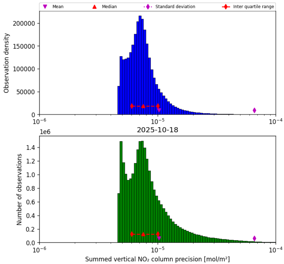
Figure 41: Histogram of "Summed vertical NO 2 column precision" for 2025-10-17 to 2025-10-19
