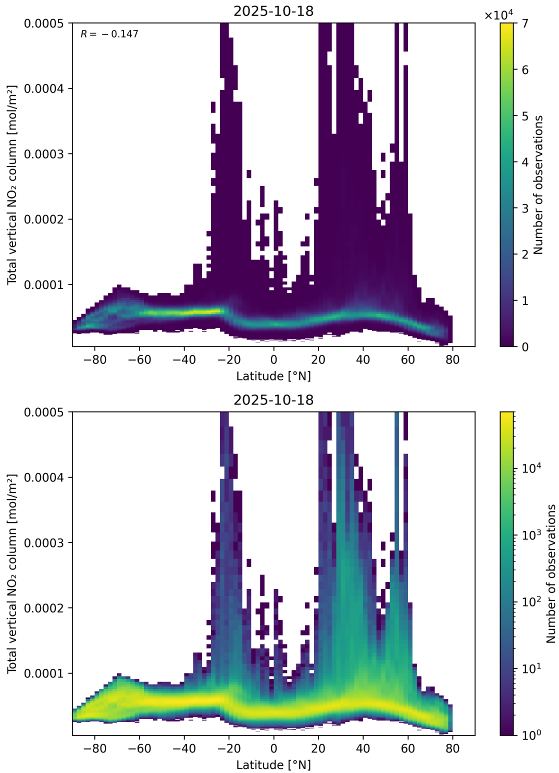
Figure 90: Scatter density plot of “Latitude” against “Total vertical NO 2 column” for 2025-10-17 to 2025-10-19.
