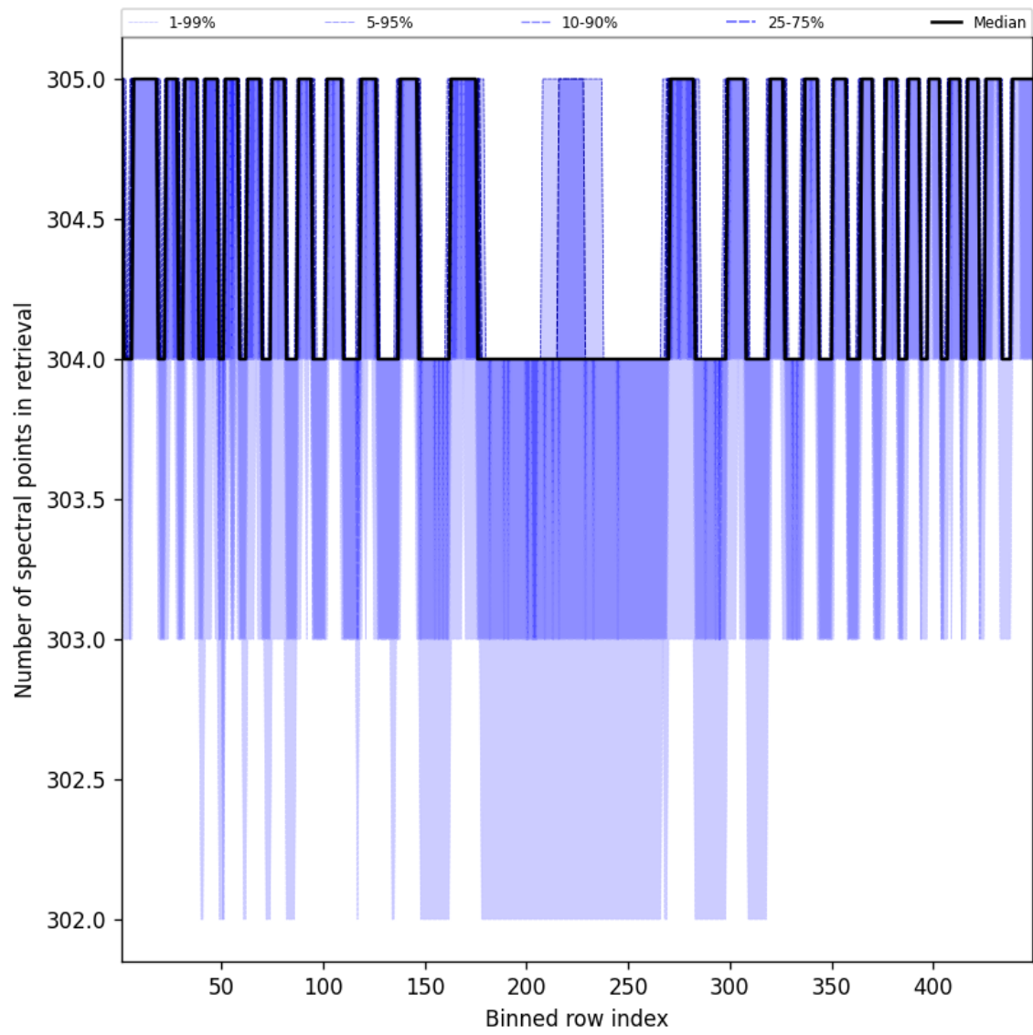
Figure 50: Along track statistics of “Number of spectral points in retrieval” for 2025-10-17 to 2025-10-19
