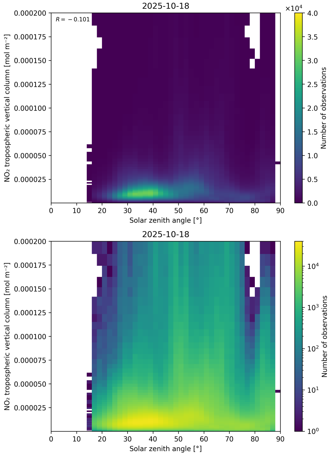
Figure 155: Scatter density plot of “Solar zenith angle” against “NO 2 tropospheric vertical column” for 2025-10-17 to 2025-10-19.
