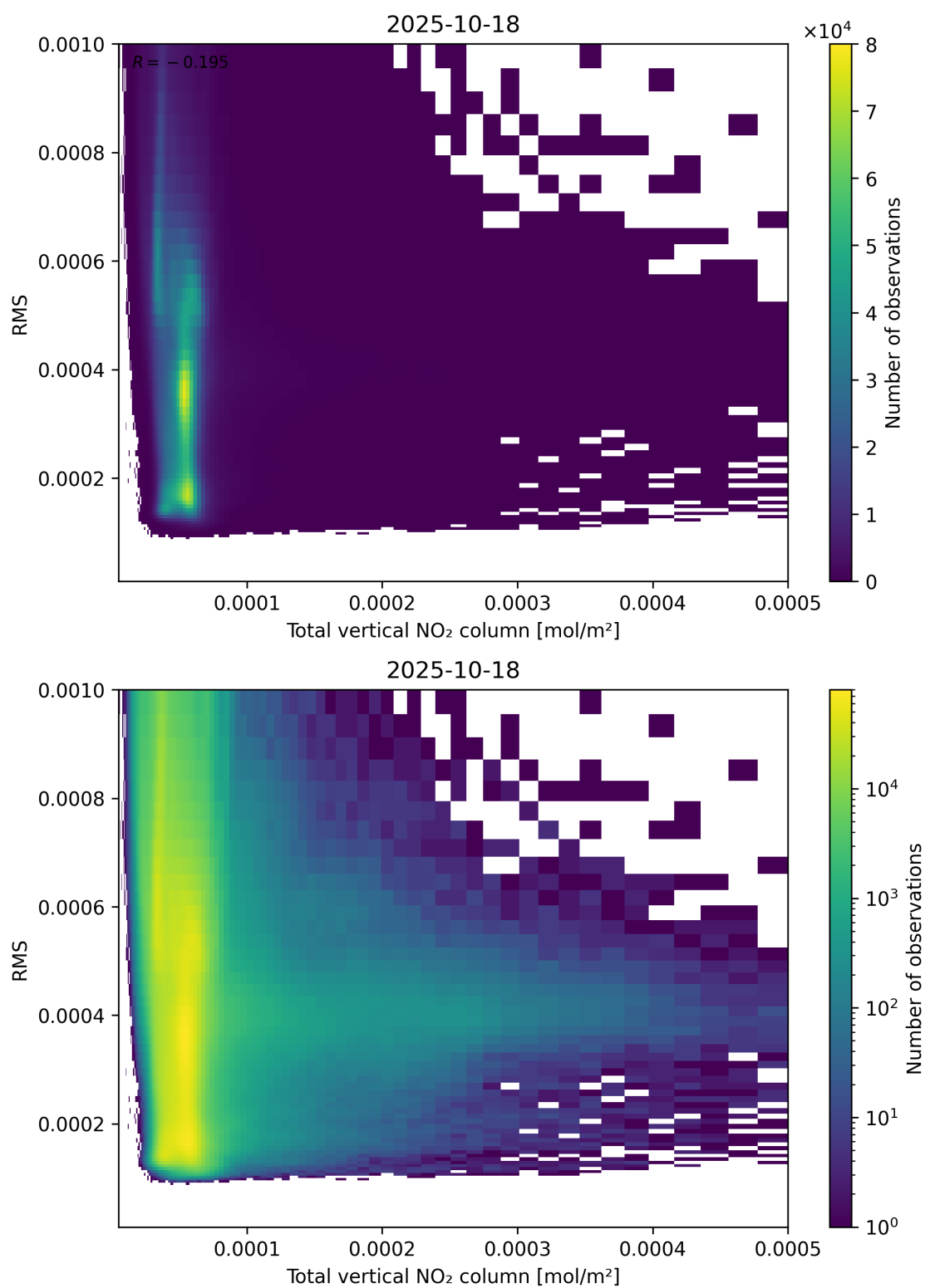
Figure 120: Scatter density plot of “Total vertical NO 2 column” against “RMS” for 2025-10-17 to 2025-10-19.
