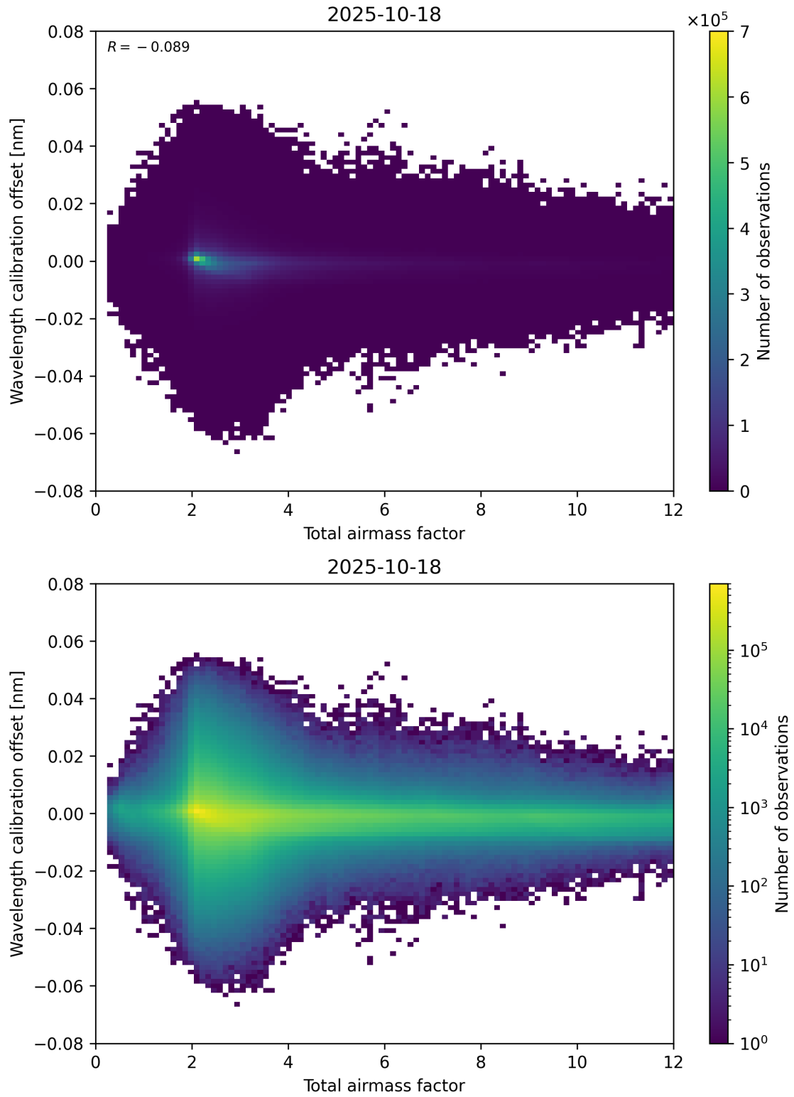
Figure 70: Scatter density plot of “Total airmass factor” against “Wavelength calibration offset” for 2025-10-17 to 2025-10-19.
