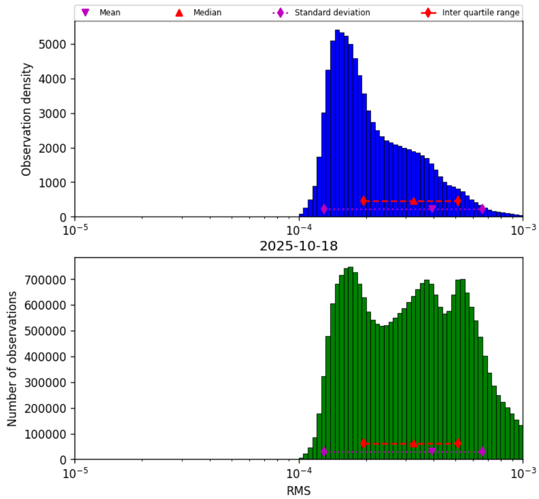
Figure 43: Histogram of “RMS” for 2025-10-17 to 2025-10-19
