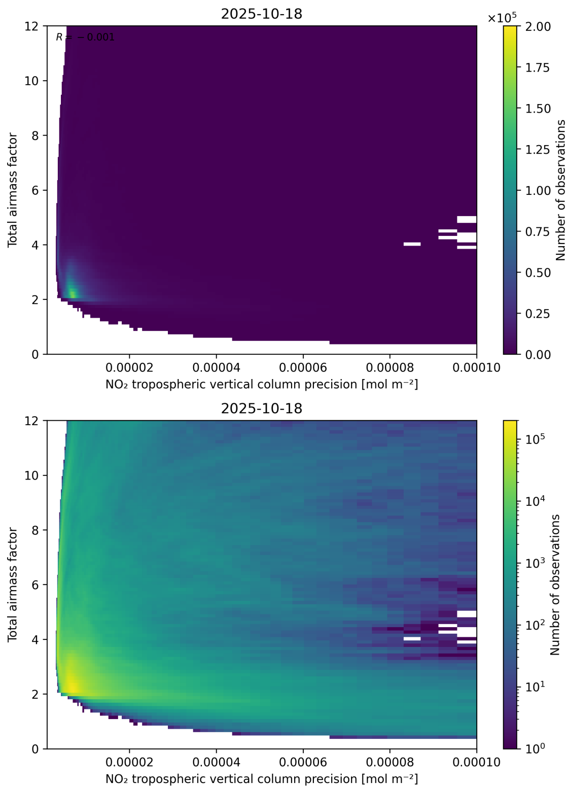
Figure 132: Scatter density plot of “NO 2 tropospheric vertical column precision” against “Total air mass factor” for 2025-10-17 to 2025-10-19.
