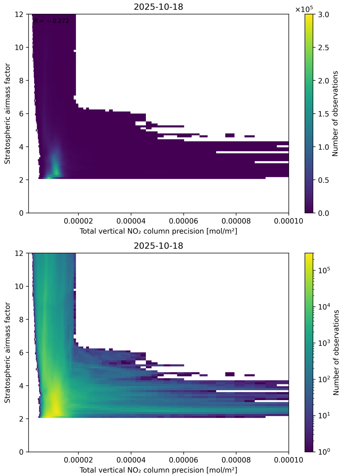
Figure 115: Scatter density plot of “Total vertical NO 2 column precision” against “Stratospheric airmass factor” for 2025-10-17 to 2025-10-19.
