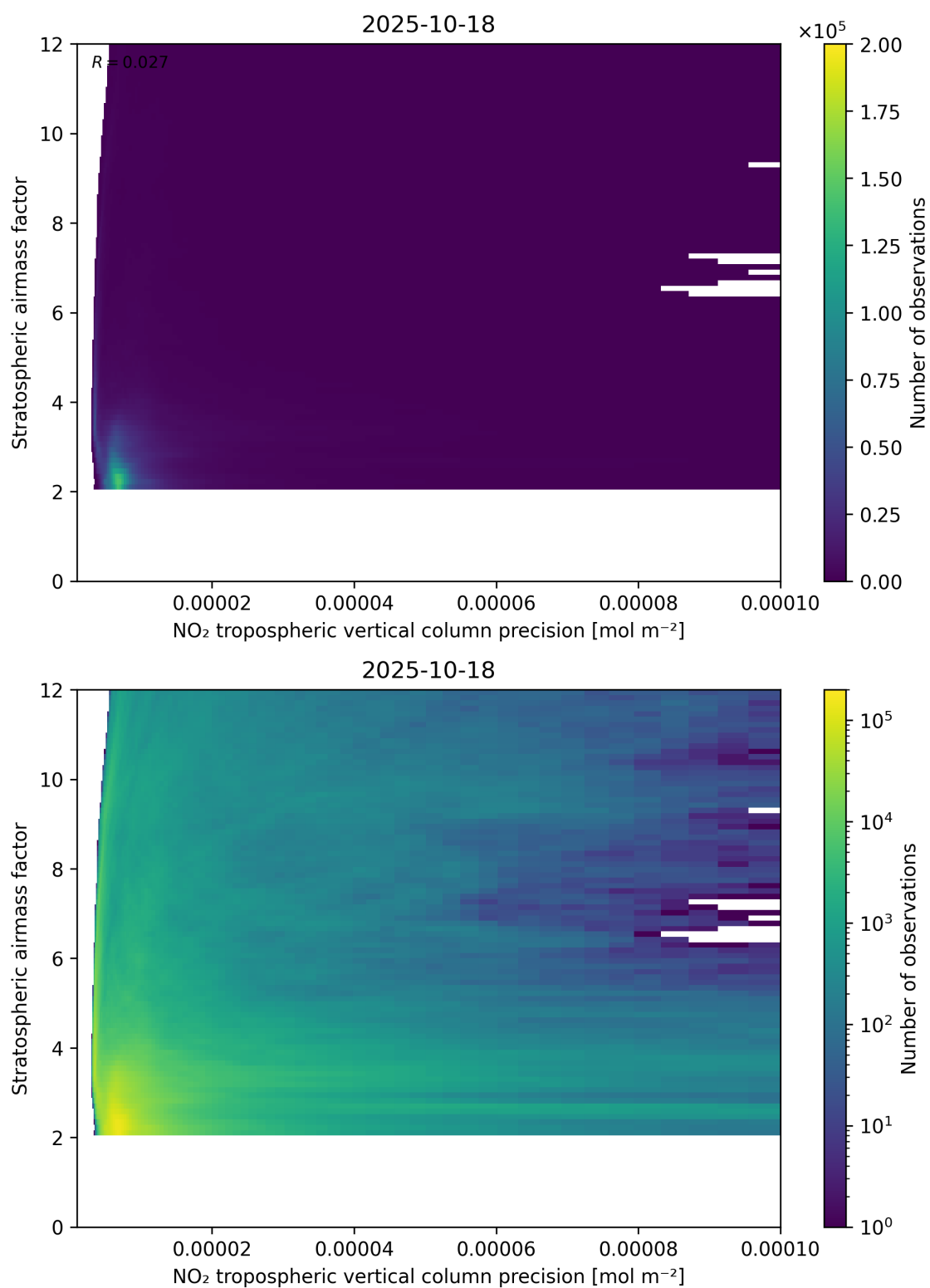
Figure 131: Scatter density plot of “NO 2 tropospheric vertical column precision” against “Stratospheric airmass factor” for 2025-10-17 to 2025-10-19.
