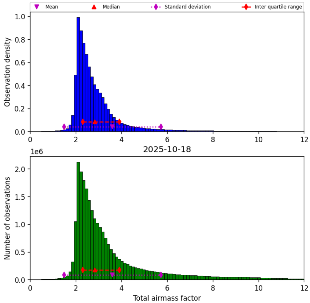
Figure 32: Histogram of “Total airmass factor” for 2025-10-17 to 2025-10-19
