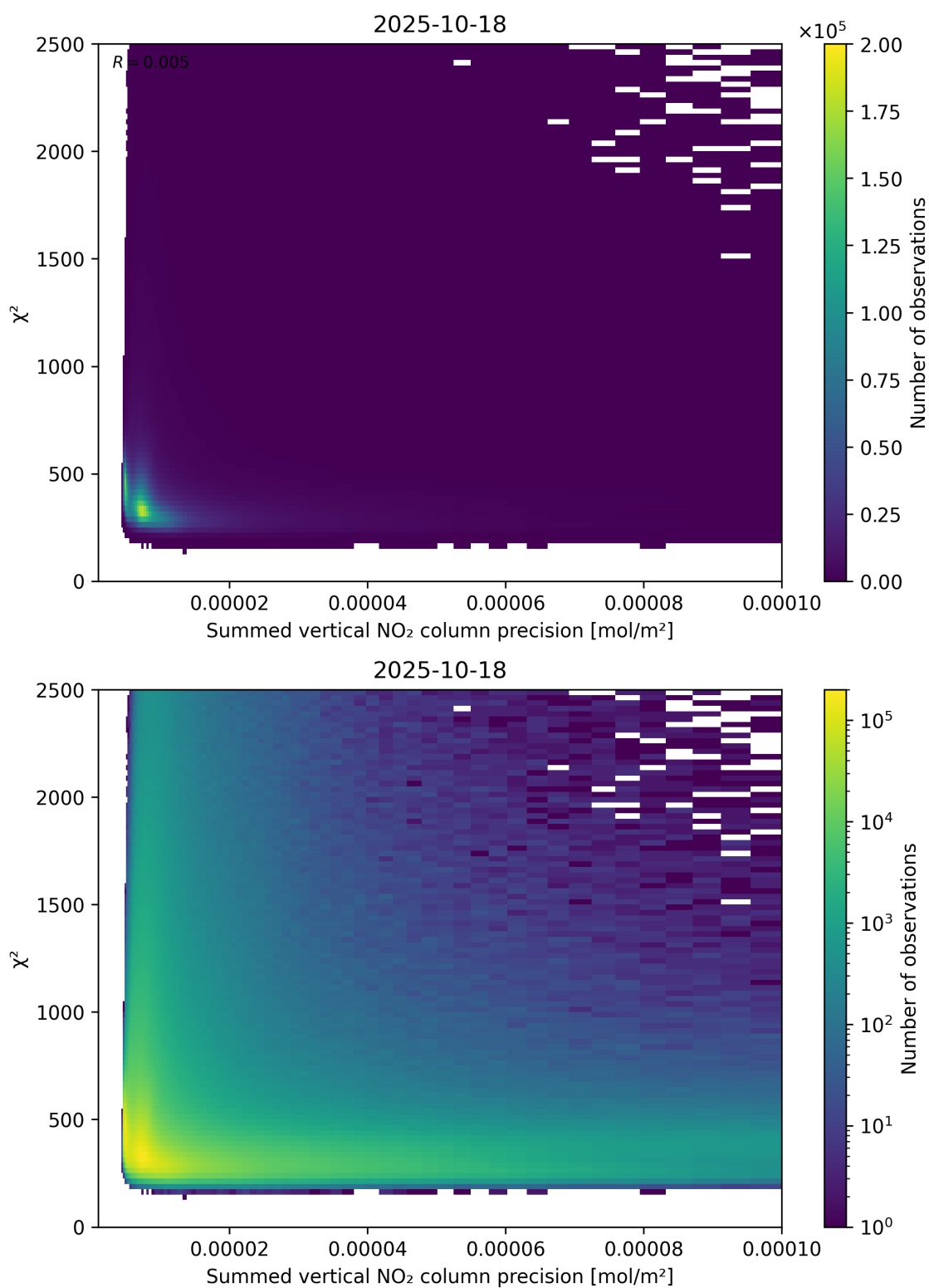
Figure 107: Scatter density plot of “Summed vertical NO 2 column precision” against “ \chi^2 ” for 2025-10-17 to 2025-10-19.
