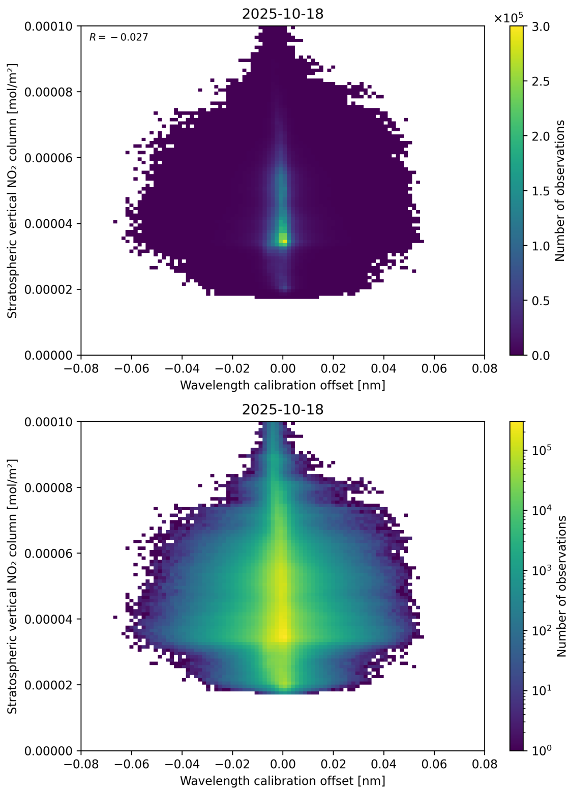
Figure 176: Scatter density plot of “Wavelength calibration offset” against “Stratospheric vertical NO 2 column” for 2025-10-17 to 2025-10-19.
