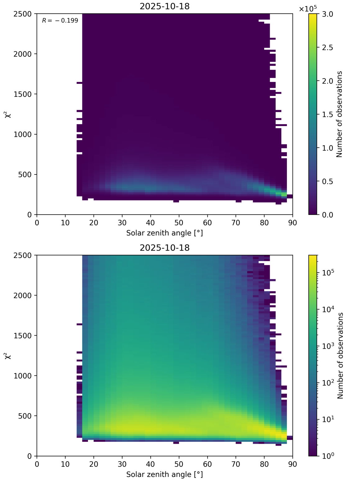
Figure 148: Scatter density plot of “Solar zenith angle” against “ \chi^2 ” for 2025-10-17 to 2025-10-19.
