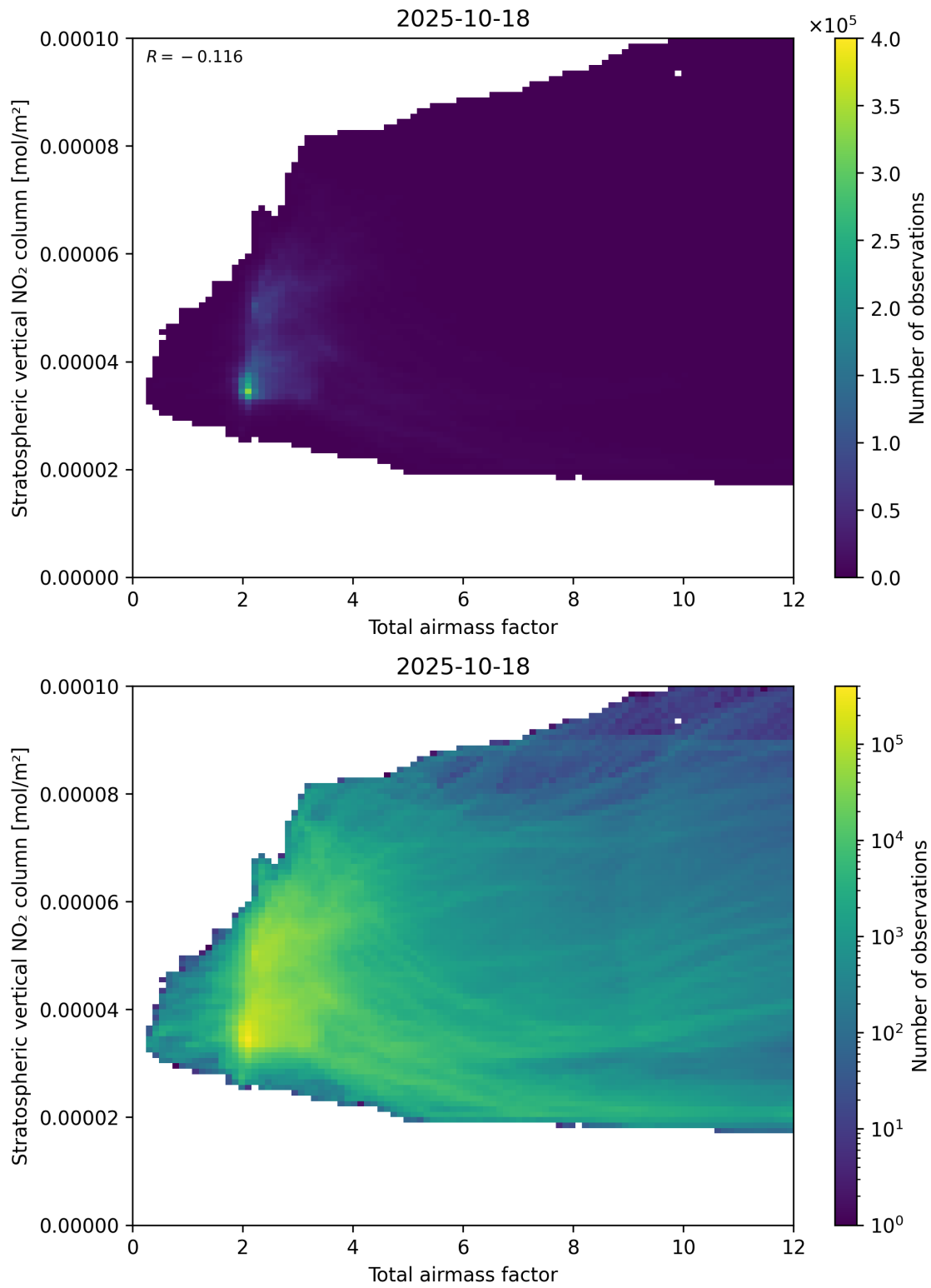
Figure 64: Scatter density plot of “Total airmass factor” against “Stratospheric vertical \text{NO}_2 column” for 2025-10-17 to 2025-10-19.
