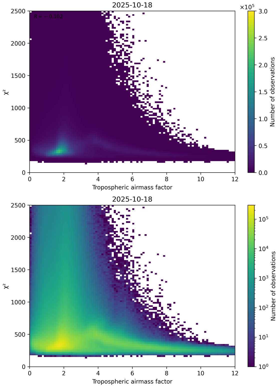
Figure 73: Scatter density plot of “Tropospheric airmass factor” against “ \chi^2 ” for 2025-10-17 to 2025-10-19.
