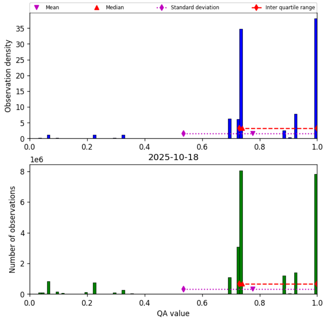
Figure 28: Histogram of “QA value” for 2025-10-17 to 2025-10-19
