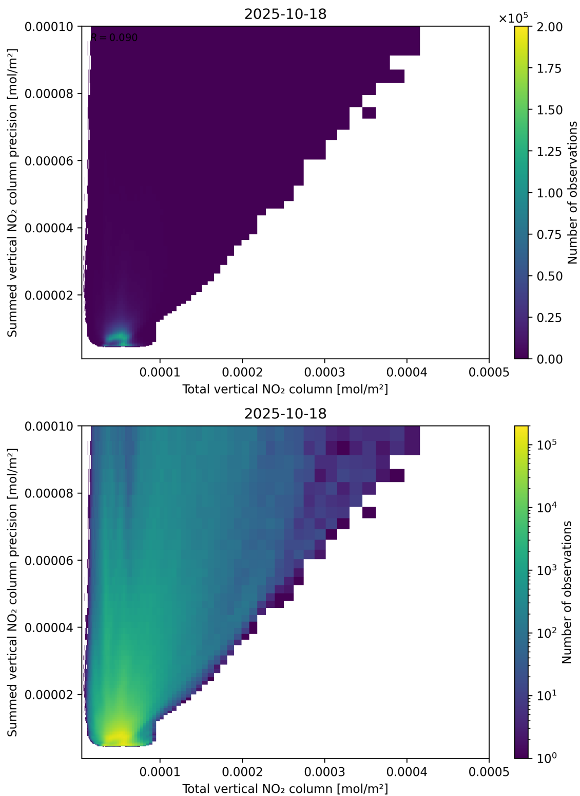
Figure 113: Scatter density plot of “Total vertical NO 2 column” against “Summed vertical NO 2 column precision” for 2025-10-17 to 2025-10-19.
