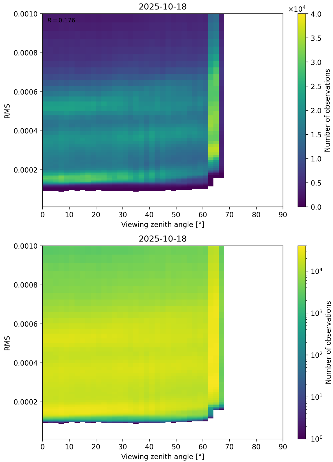
Figure 171: Scatter density plot of “Viewing zenith angle” against “RMS” for 2025-10-17 to 2025-10-19.
