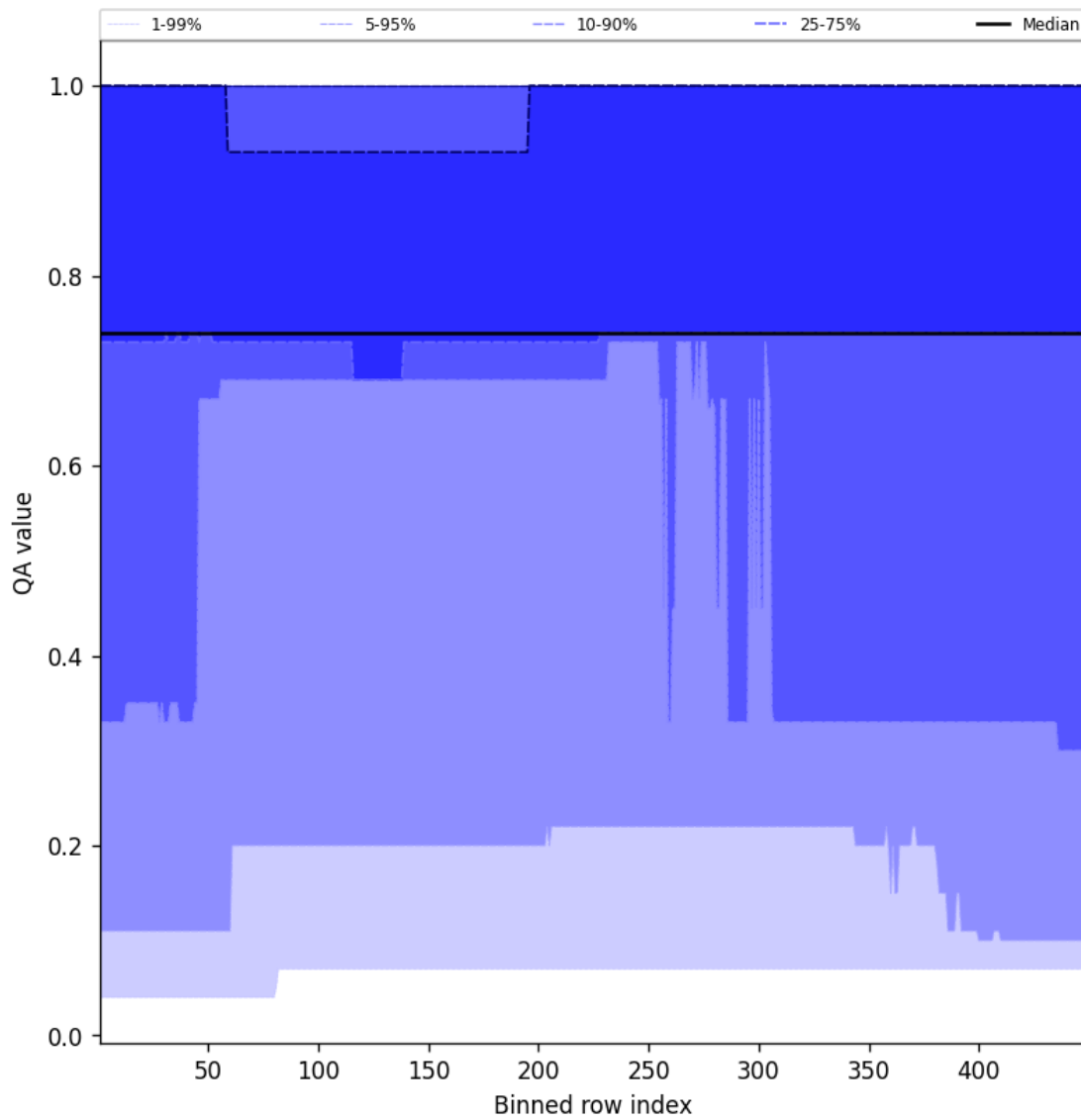
Figure 45: Along track statistics of “QA value” for 2025-10-17 to 2025-10-19
