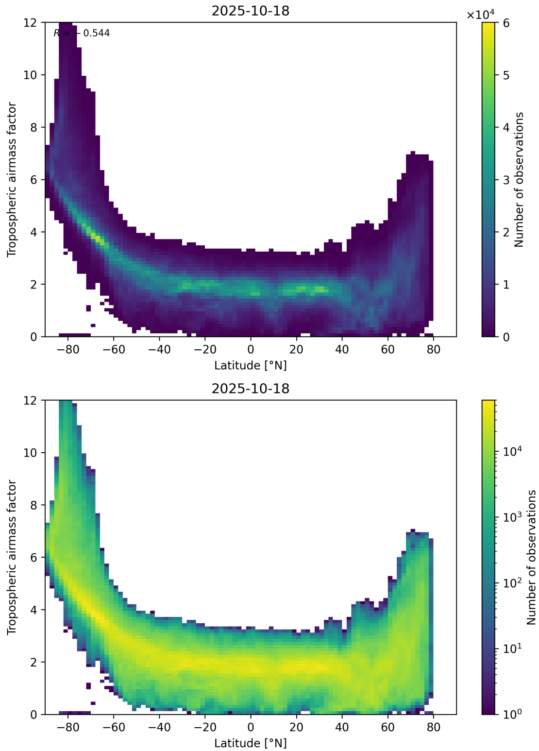
Figure 85: Scatter density plot of “Latitude” against “Tropospheric airmass factor” for 2025-10-17 to 2025-10-19.
