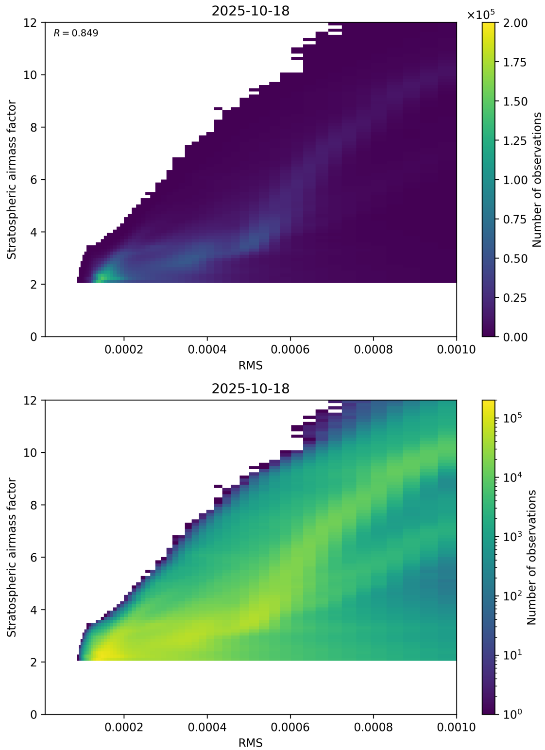
Figure 144: Scatter density plot of “RMS” against “Stratospheric airmass factor” for 2025-10-17 to 2025-10-19.
