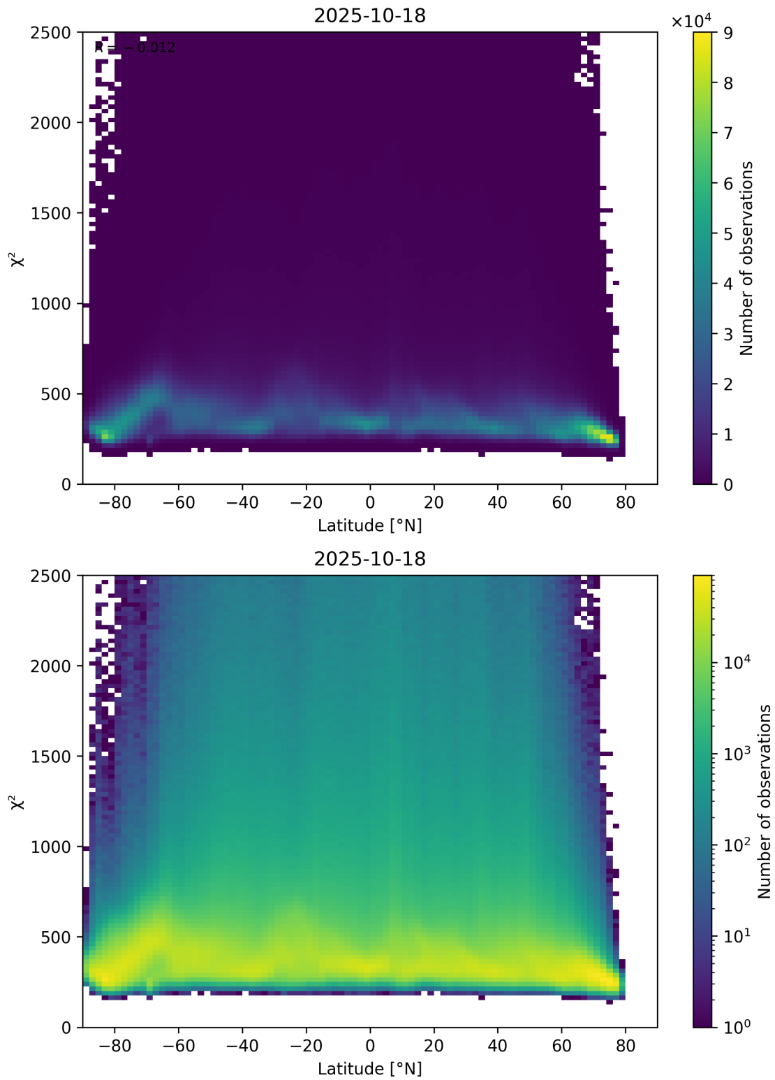
Figure 86: Scatter density plot of “Latitude” against “ \chi^2 ” for 2025-10-17 to 2025-10-19.
