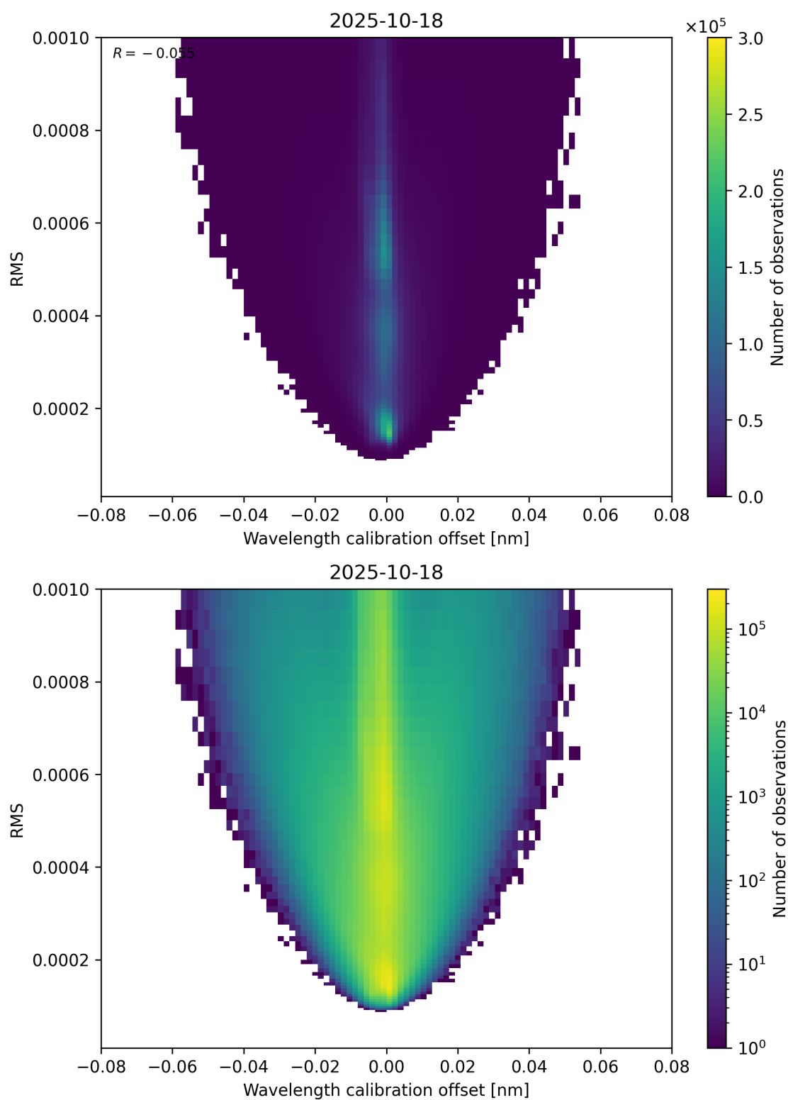
Figure 181: Scatter density plot of “Wavelength calibration offset” against “RMS” for 2025-10-17 to 2025-10-19.
