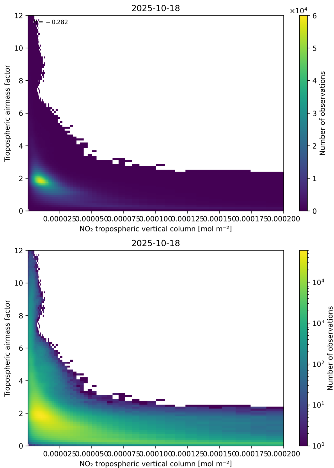
Figure 123: Scatter density plot of “NO 2 tropospheric vertical column” against “Tropospheric air mass factor” for 2025-10-17 to 2025-10-19.
