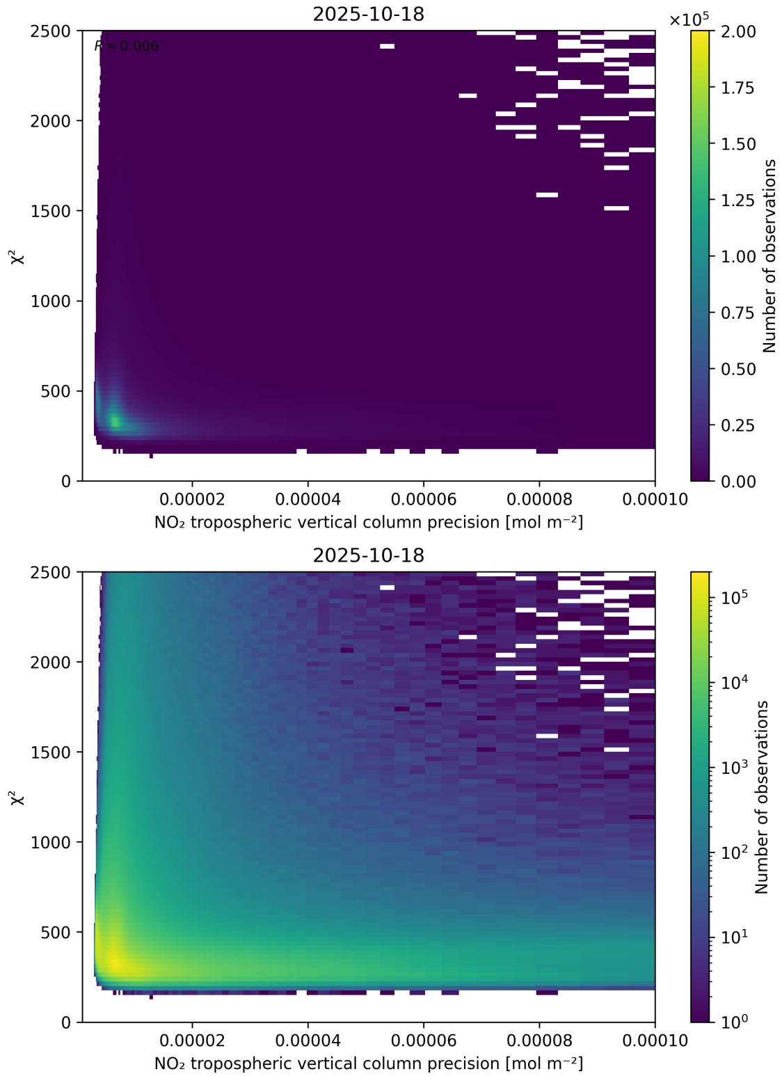
Figure 134: Scatter density plot of “NO 2 tropospheric vertical column precision” against “ \chi^2 ” for 2025-10-17 to 2025-10-19.
