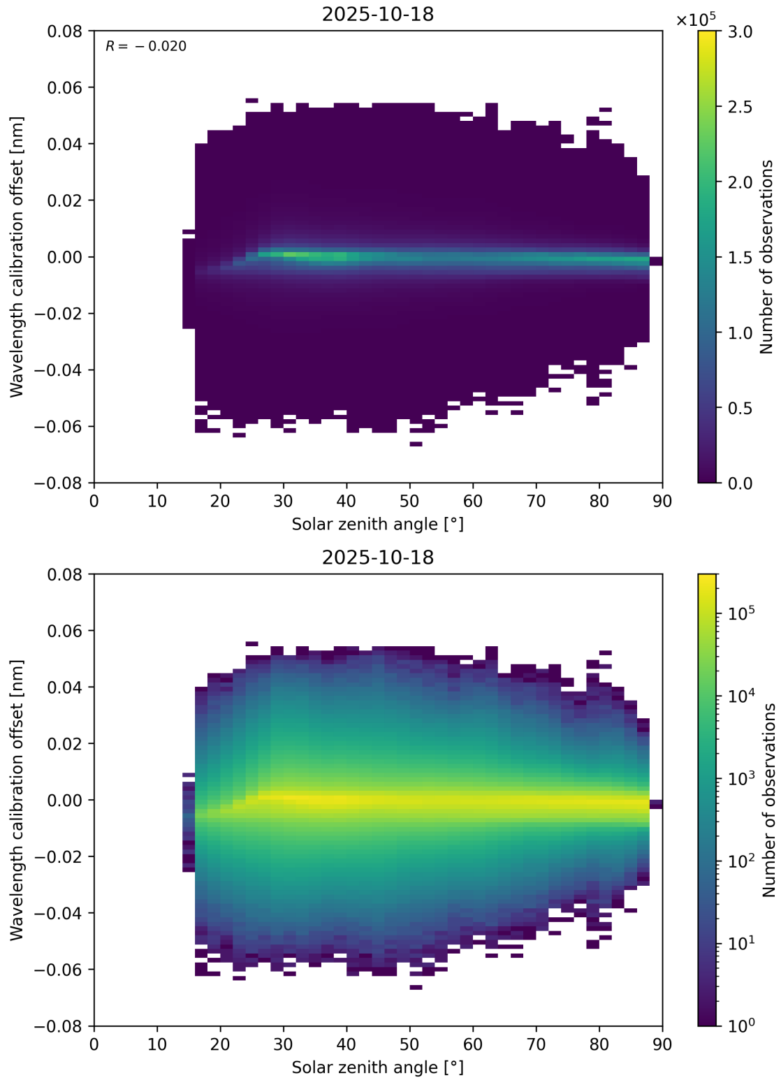
Figure 158: Scatter density plot of “Solar zenith angle” against “Wavelength calibration offset” for 2025-10-17 to 2025-10-19.
