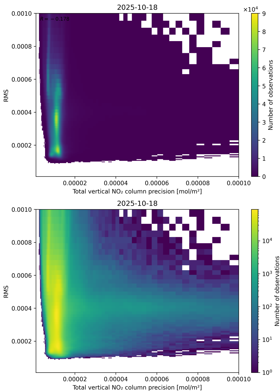
Figure 119: Scatter density plot of “Total vertical NO 2 column precision” against “RMS” for 2025-10-17 to 2025-10-19.
