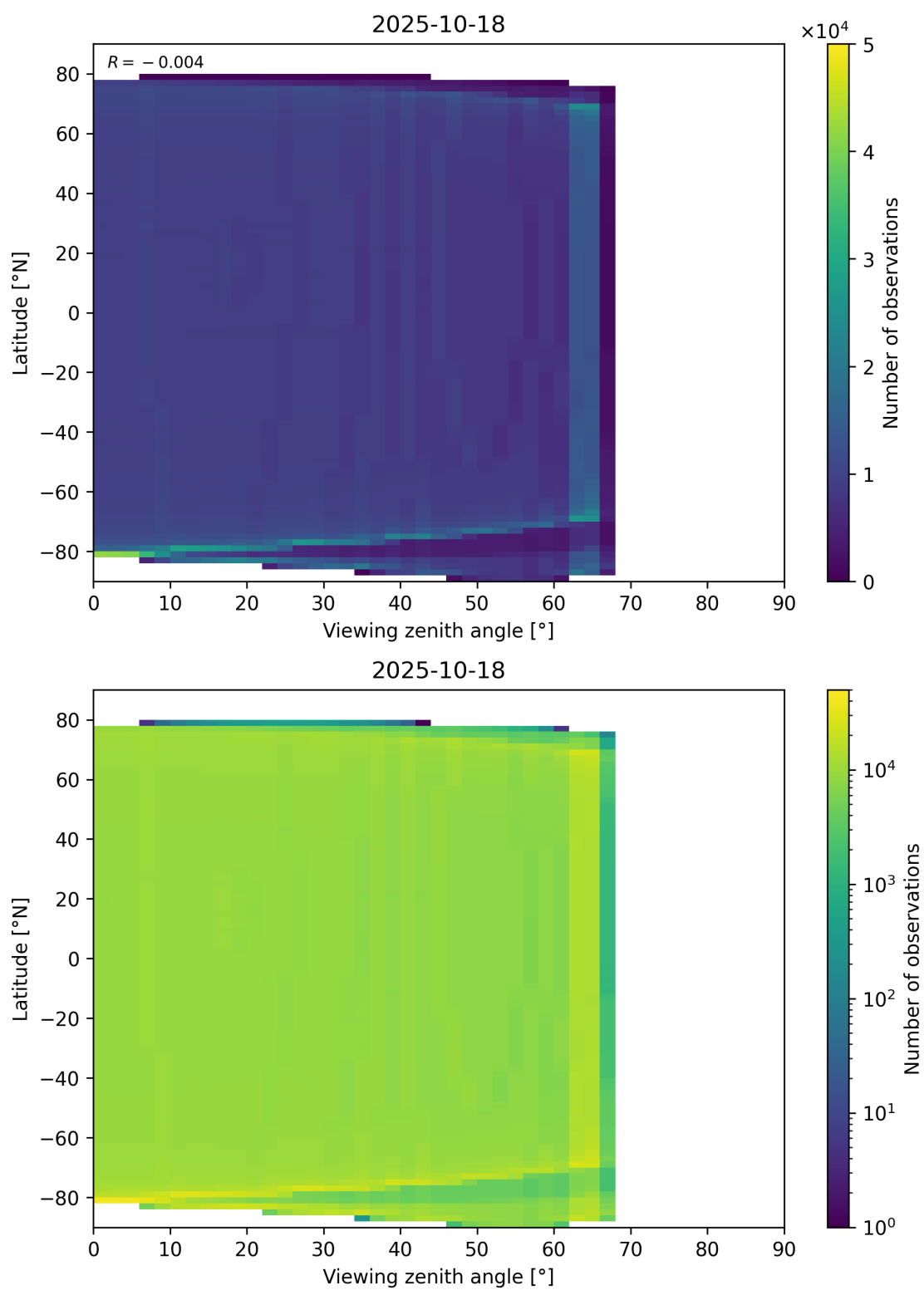
Figure 163: Scatter density plot of “Viewing zenith angle” against “Latitude” for 2025-10-17 to 2025-10-19.
