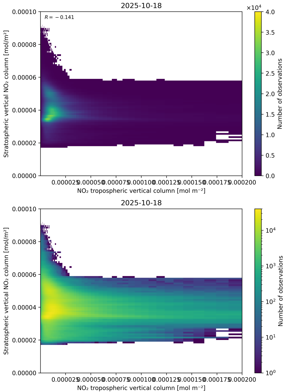
Figure 125: Scatter density plot of “NO 2 tropospheric vertical column” against “Stratospheric vertical NO 2 column” for 2025-10-17 to 2025-10-19.
