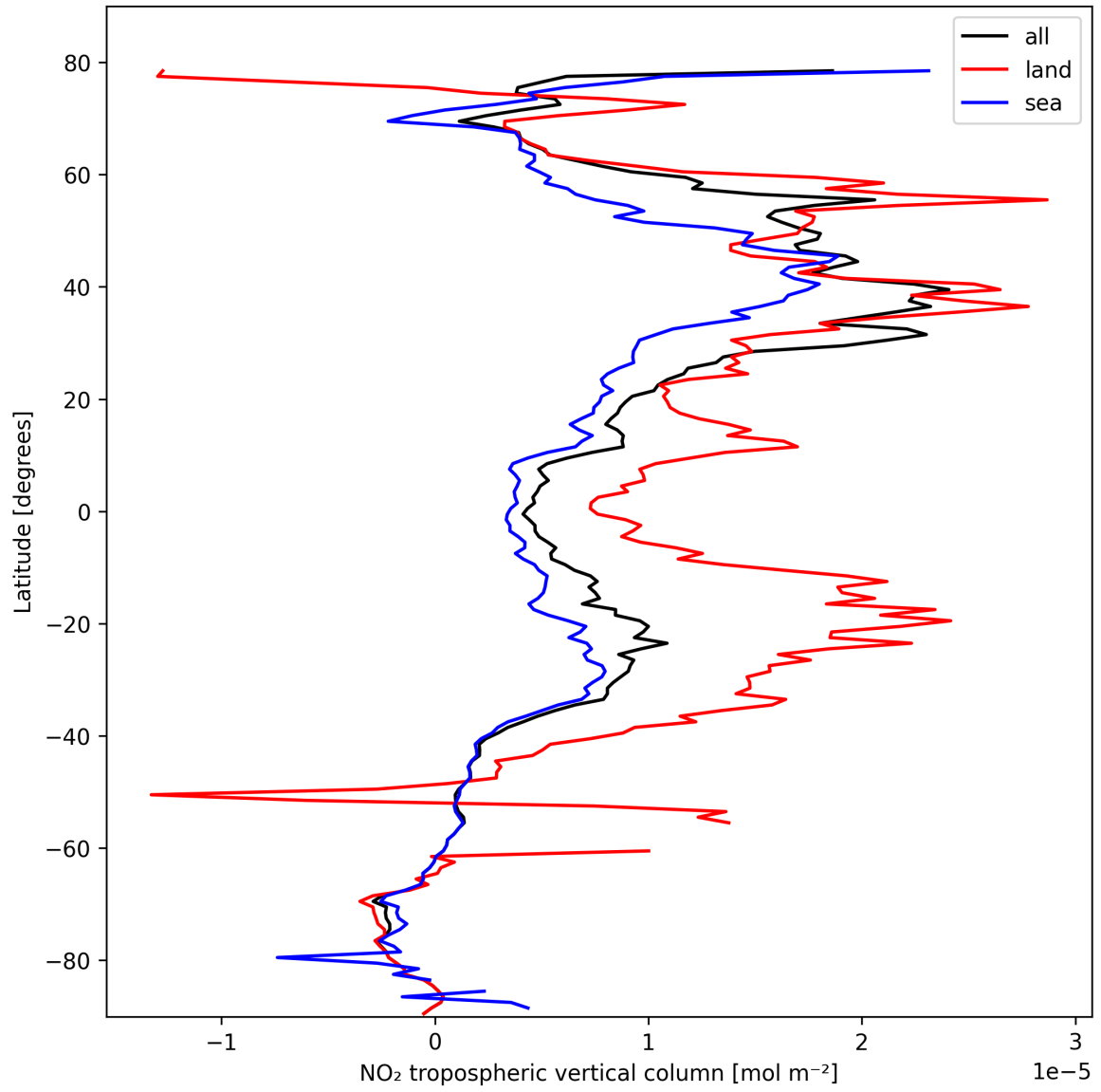
Figure 12: Zonal average of “NO 2 tropospheric vertical column” for 2025-10-17 to 2025-10-19.
