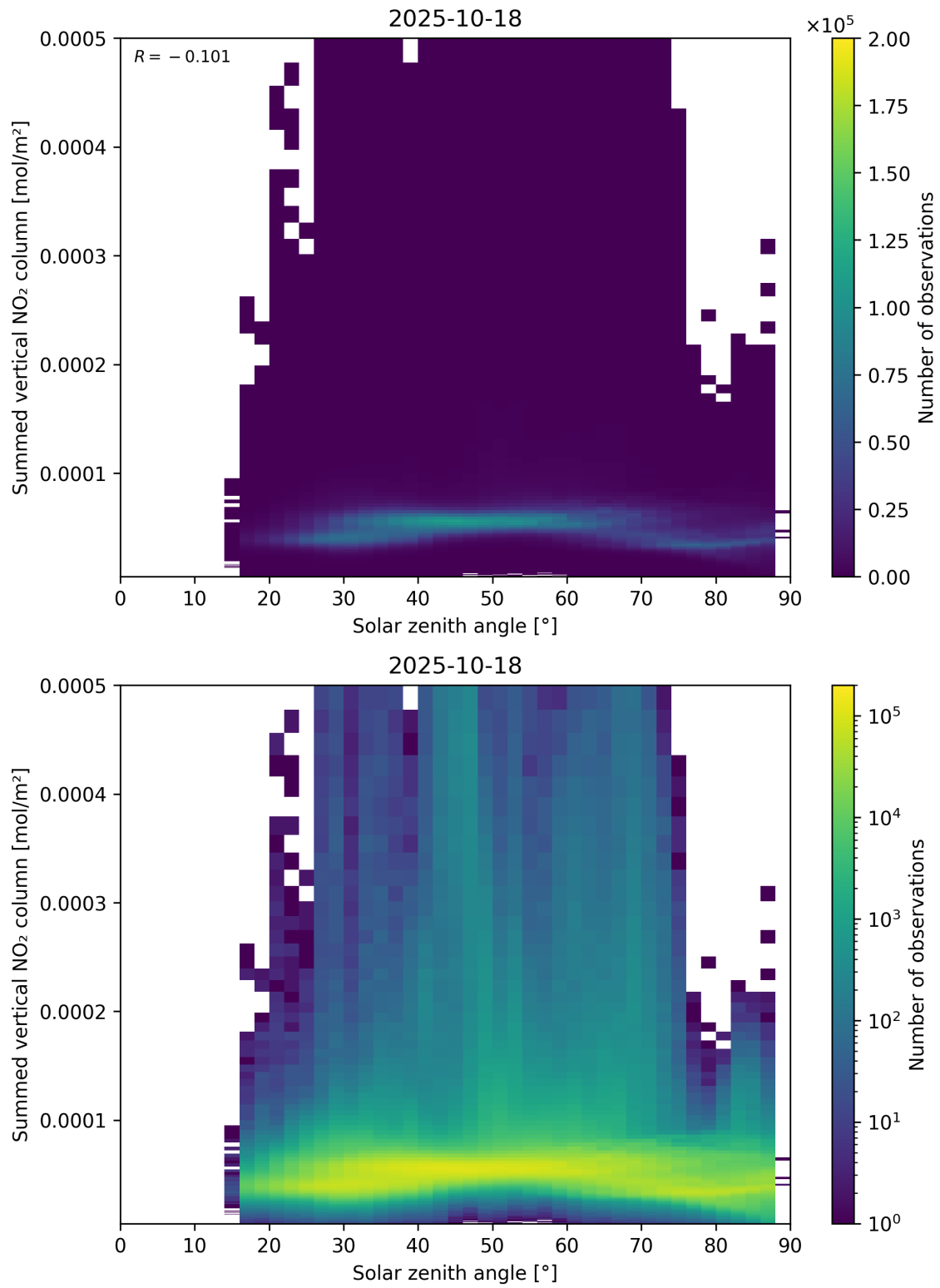
Figure 151: Scatter density plot of “Solar zenith angle” against “Summed vertical NO 2 column” for 2025-10-17 to 2025-10-19.
