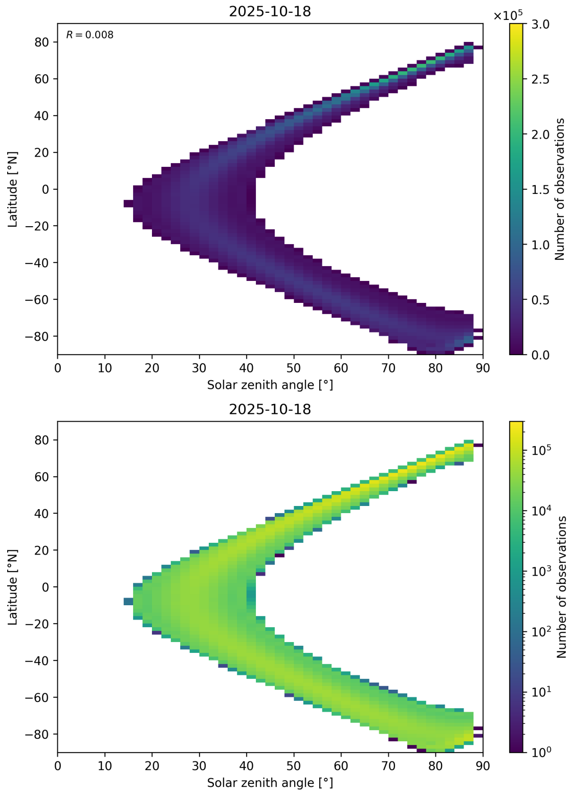
Figure 149: Scatter density plot of “Solar zenith angle” against “Latitude” for 2025-10-17 to 2025-10-19.
