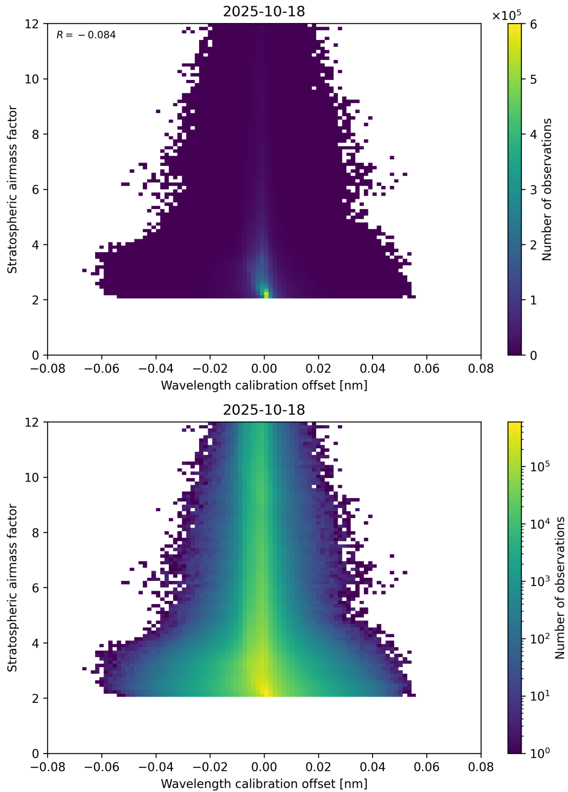
Figure 174: Scatter density plot of “Wavelength calibration offset” against “Stratospheric airmass factor” for 2025-10-17 to 2025-10-19.
