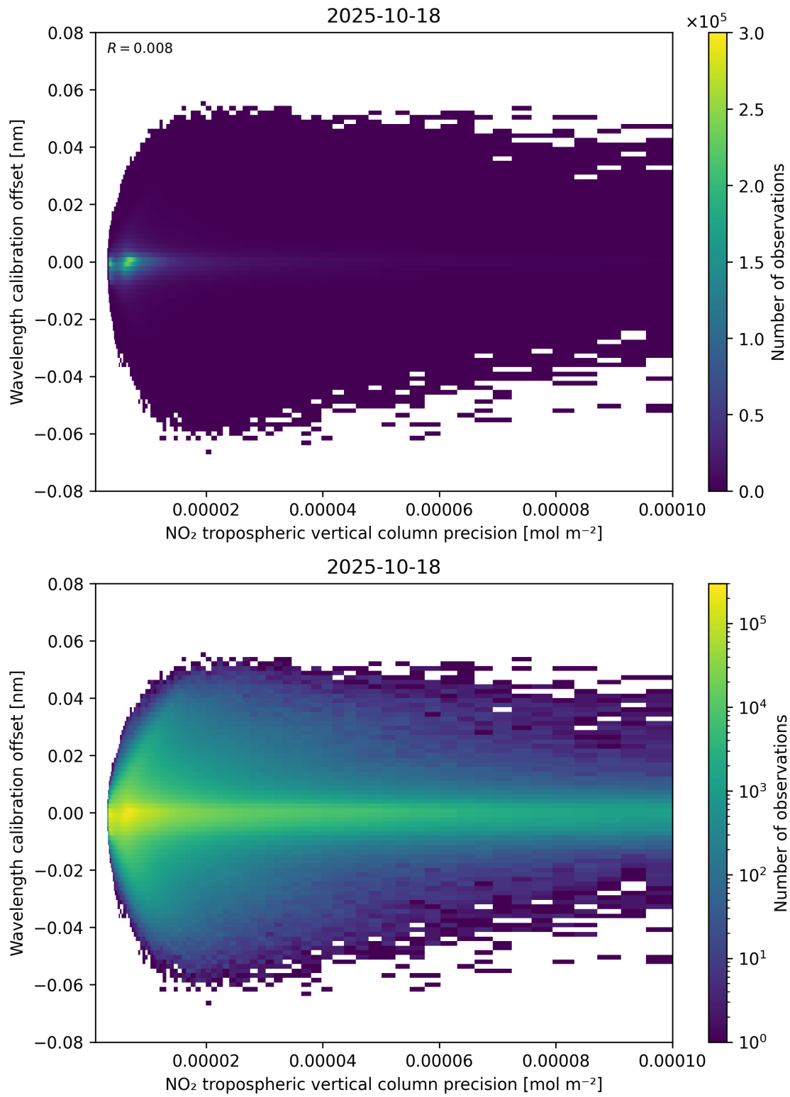
Figure 141: Scatter density plot of “NO 2 tropospheric vertical column precision” against “Wavelength calibration offset” for 2025-10-17 to 2025-10-19.
