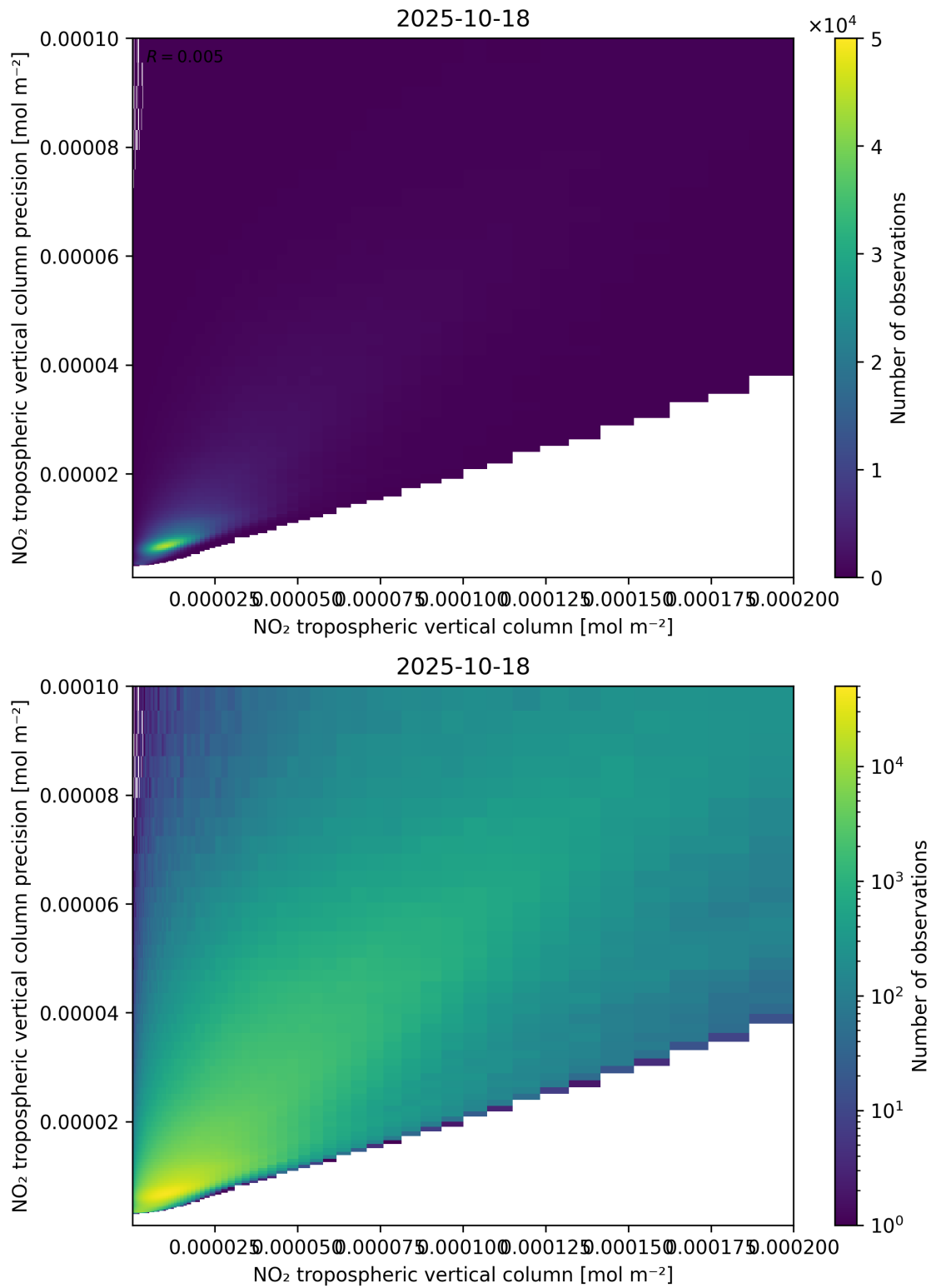
Figure 130: Scatter density plot of “NO 2 tropospheric vertical column” against “NO 2 tropospheric vertical column precision” for 2025-10-17 to 2025-10-19.
