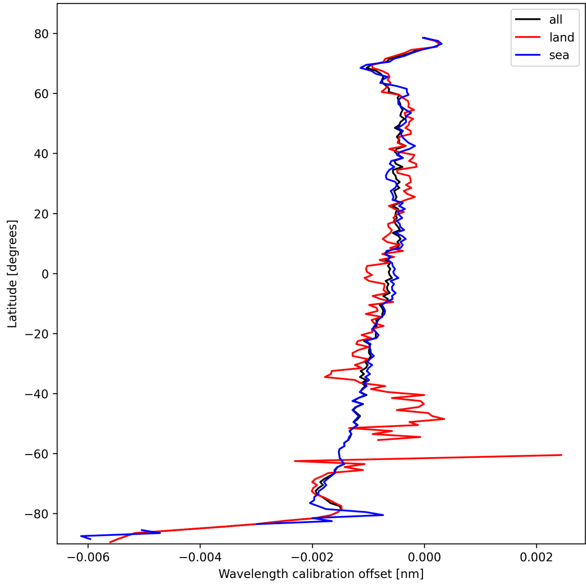
Figure 18: Zonal average of “Wavelength calibration offset” for 2025-10-17 to 2025-10-19.
