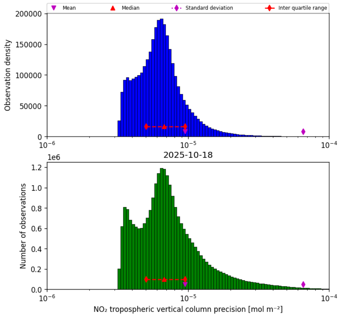
Figure 30: Histogram of “NO 2 tropospheric vertical column precision” for 2025-10-17 to 2025-10-19
