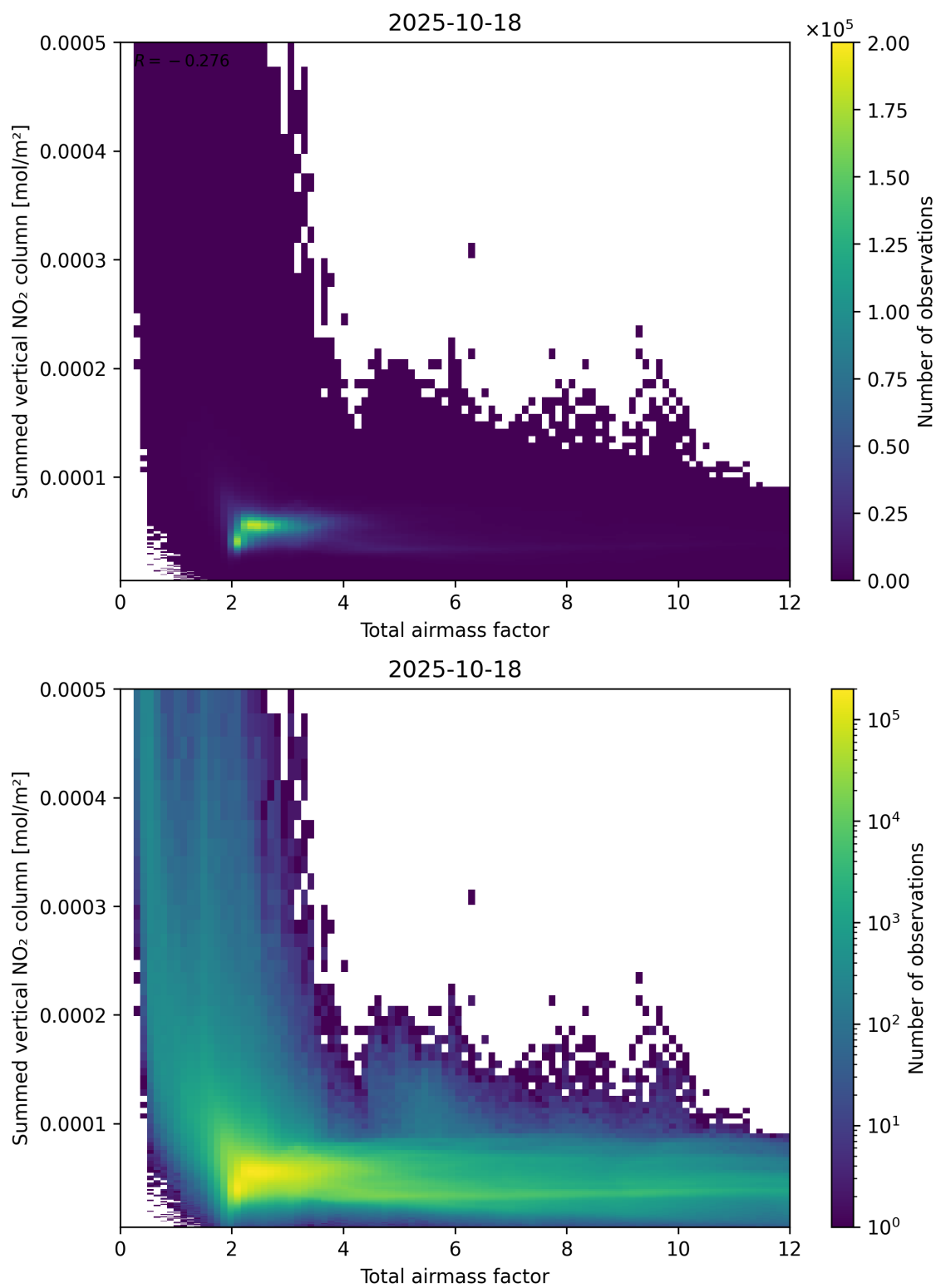
Figure 65: Scatter density plot of “Total airmass factor” against “Summed vertical NO 2 column” for 2025-10-17 to 2025-10-19.
