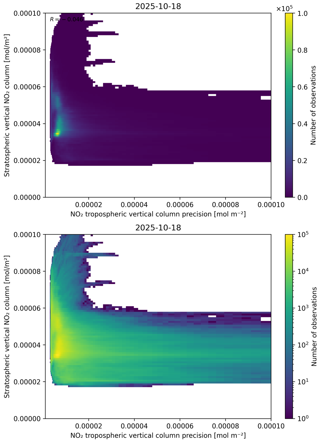
Figure 135: Scatter density plot of “NO 2 tropospheric vertical column precision” against “Stratospheric vertical NO 2 column” for 2025-10-17 to 2025-10-19.
