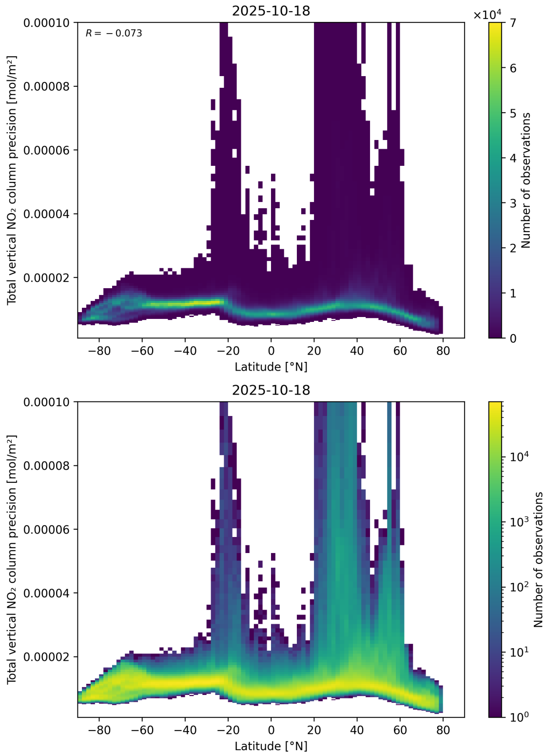
Figure 91: Scatter density plot of “Latitude” against “Total vertical NO 2 column precision” for 2025-10-17 to 2025-10-19.
