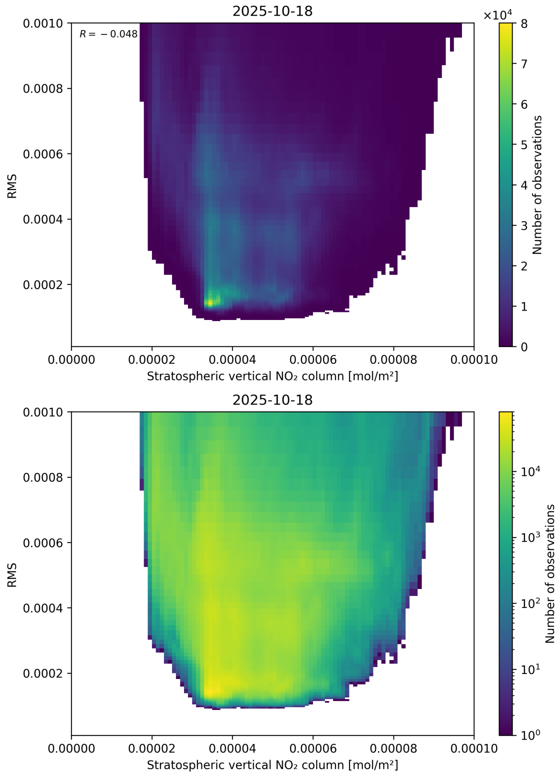
Figure 102: Scatter density plot of “Stratospheric vertical NO 2 column” against “RMS” for 2025-10-17 to 2025-10-19.
