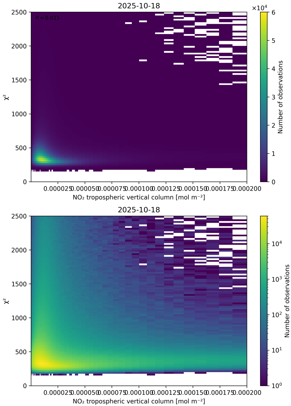
Figure 124: Scatter density plot of “NO 2 tropospheric vertical column” against “ \chi^2 ” for 2025-10-17 to 2025-10-19.
