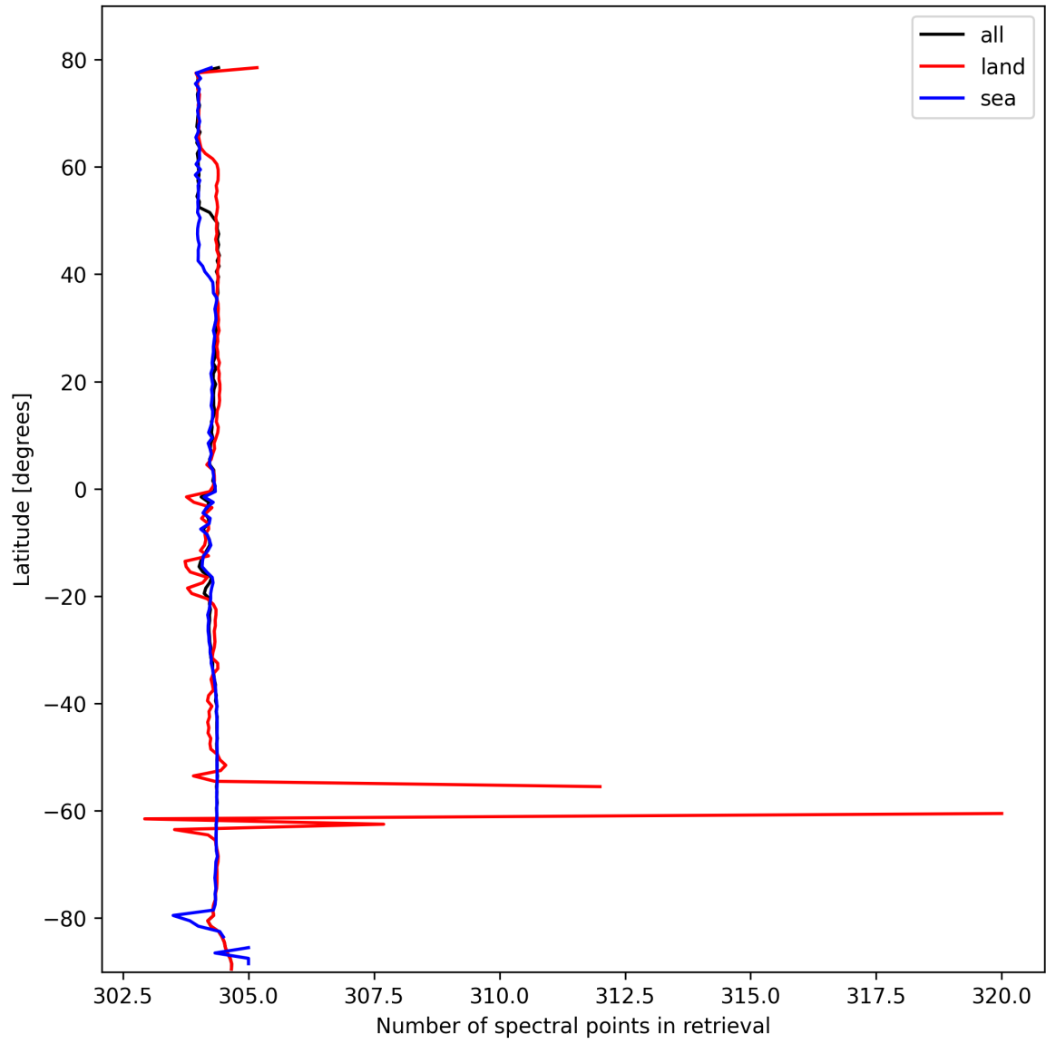
Figure 16: Zonal average of “Number of spectral points in retrieval” for 2025-10-17 to 2025-10-19.
