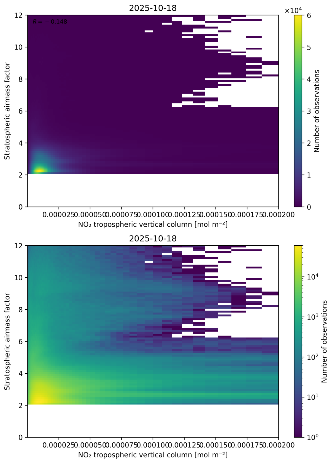
Figure 121: Scatter density plot of “NO 2 tropospheric vertical column” against “Stratospheric air mass factor” for 2025-10-17 to 2025-10-19.
