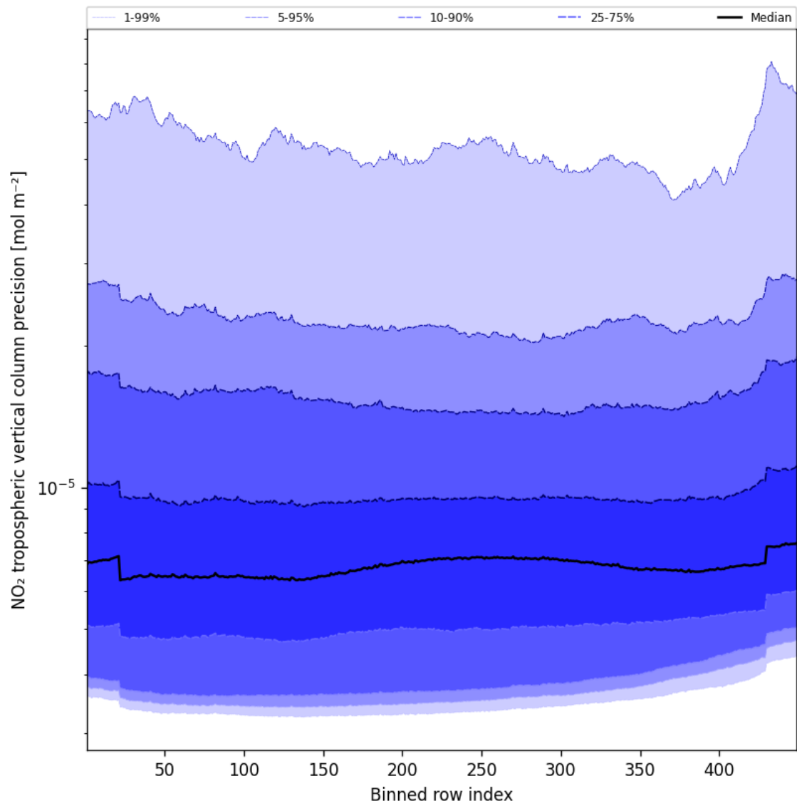
Figure 47: Along track statistics of “NO 2 tropospheric vertical column precision” for 2025-10-17 to 2025-10-19
