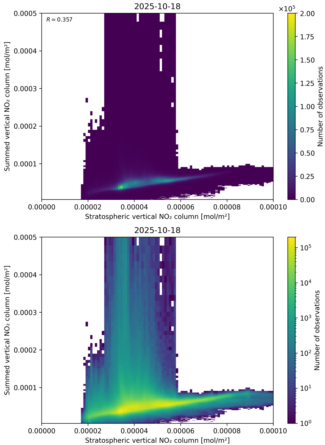
Figure 98: Scatter density plot of “Stratospheric vertical NO 2 column” against “Summed vertical NO 2 column” for 2025-10-17 to 2025-10-19.
