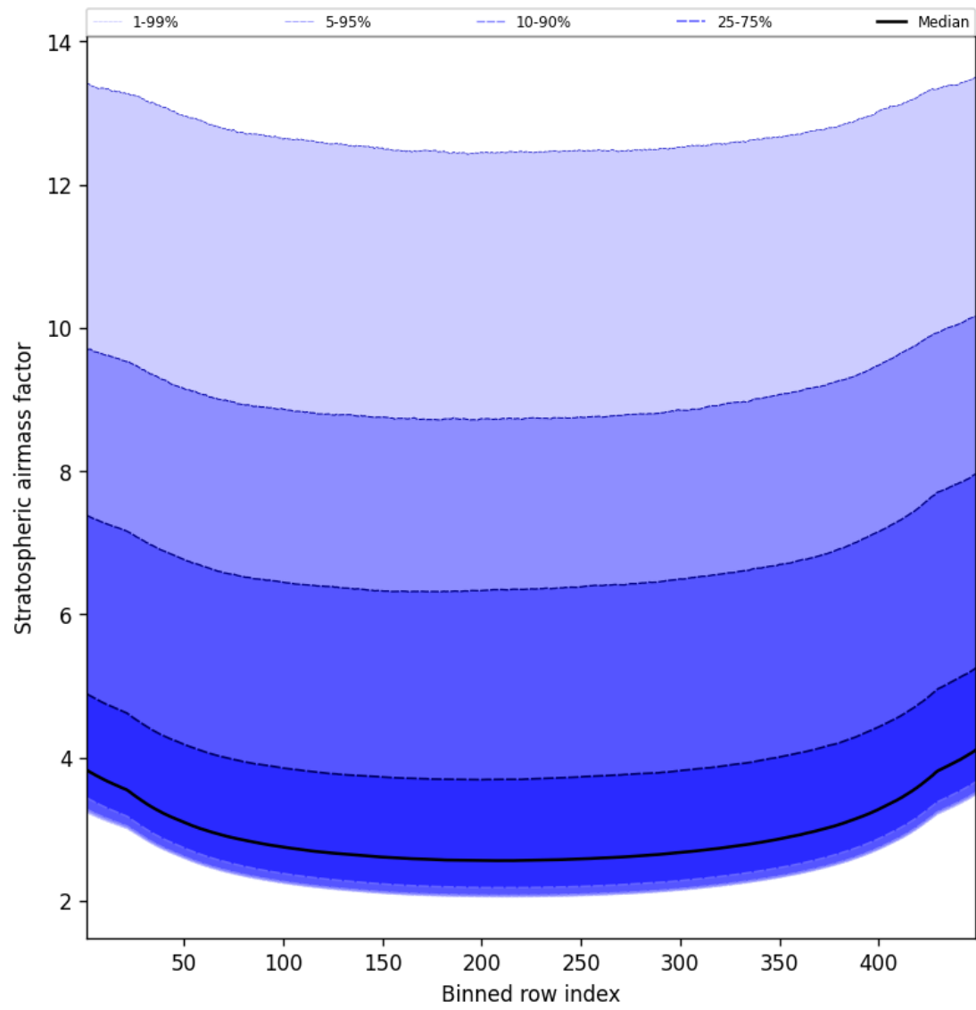
Figure 61: Along track statistics of “Stratospheric airmass factor” for 2025-10-17 to 2025-10-19
