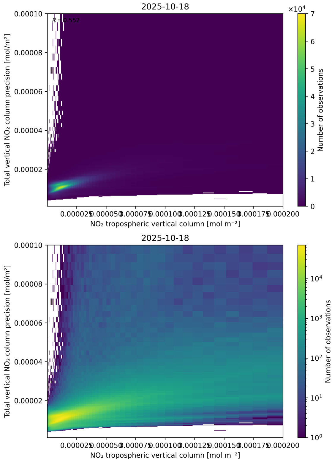
Figure 129: Scatter density plot of “NO 2 tropospheric vertical column” against “Total vertical NO 2 column precision” for 2025-10-17 to 2025-10-19.
