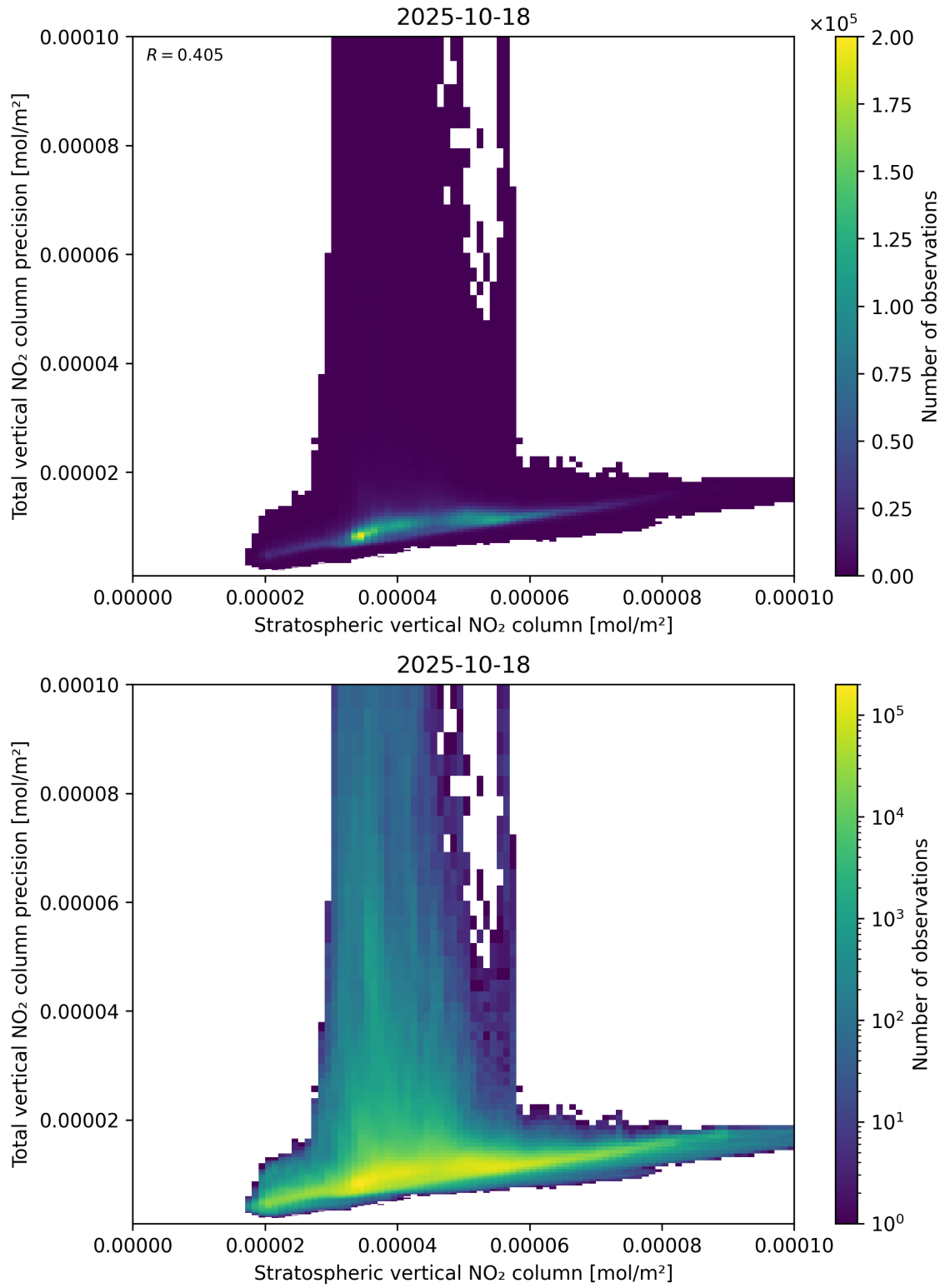
Figure 101: Scatter density plot of “Stratospheric vertical NO 2 column” against “Total vertical NO 2 column precision” for 2025-10-17 to 2025-10-19.
