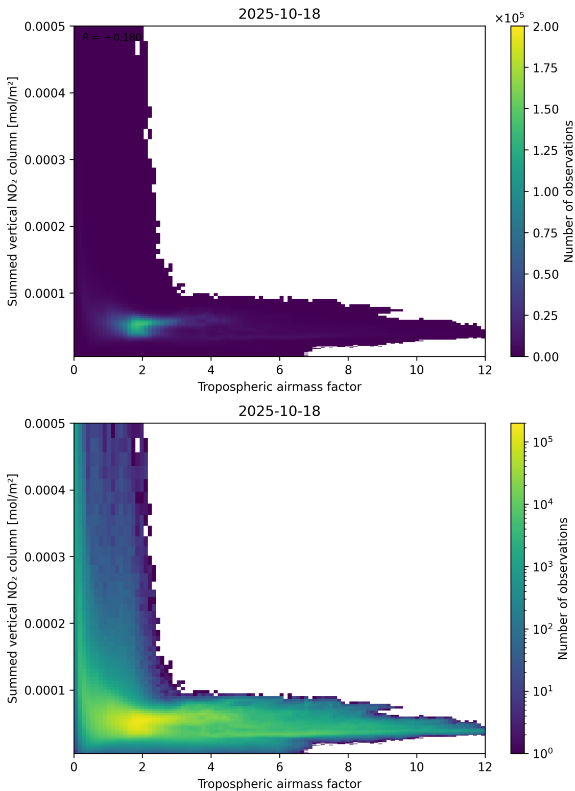
Figure 75: Scatter density plot of “Tropospheric air mass factor” against “Summed vertical NO 2 column” for 2025-10-17 to 2025-10-19.
