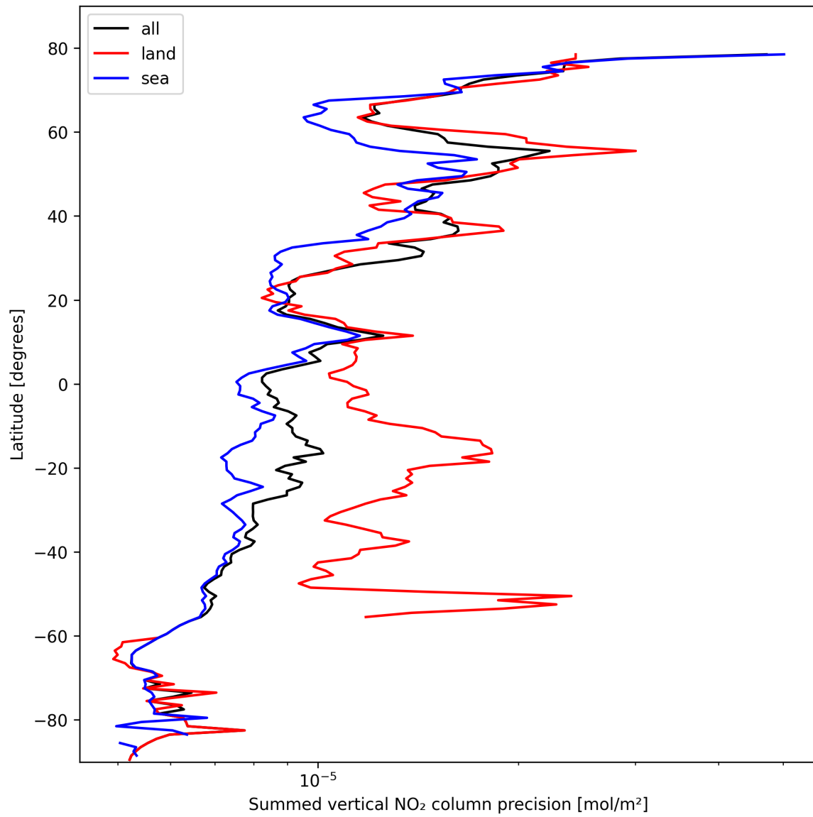
Figure 24: Zonal average of “Summed vertical NO 2 column precision” for 2025-10-17 to 2025-10-19.
