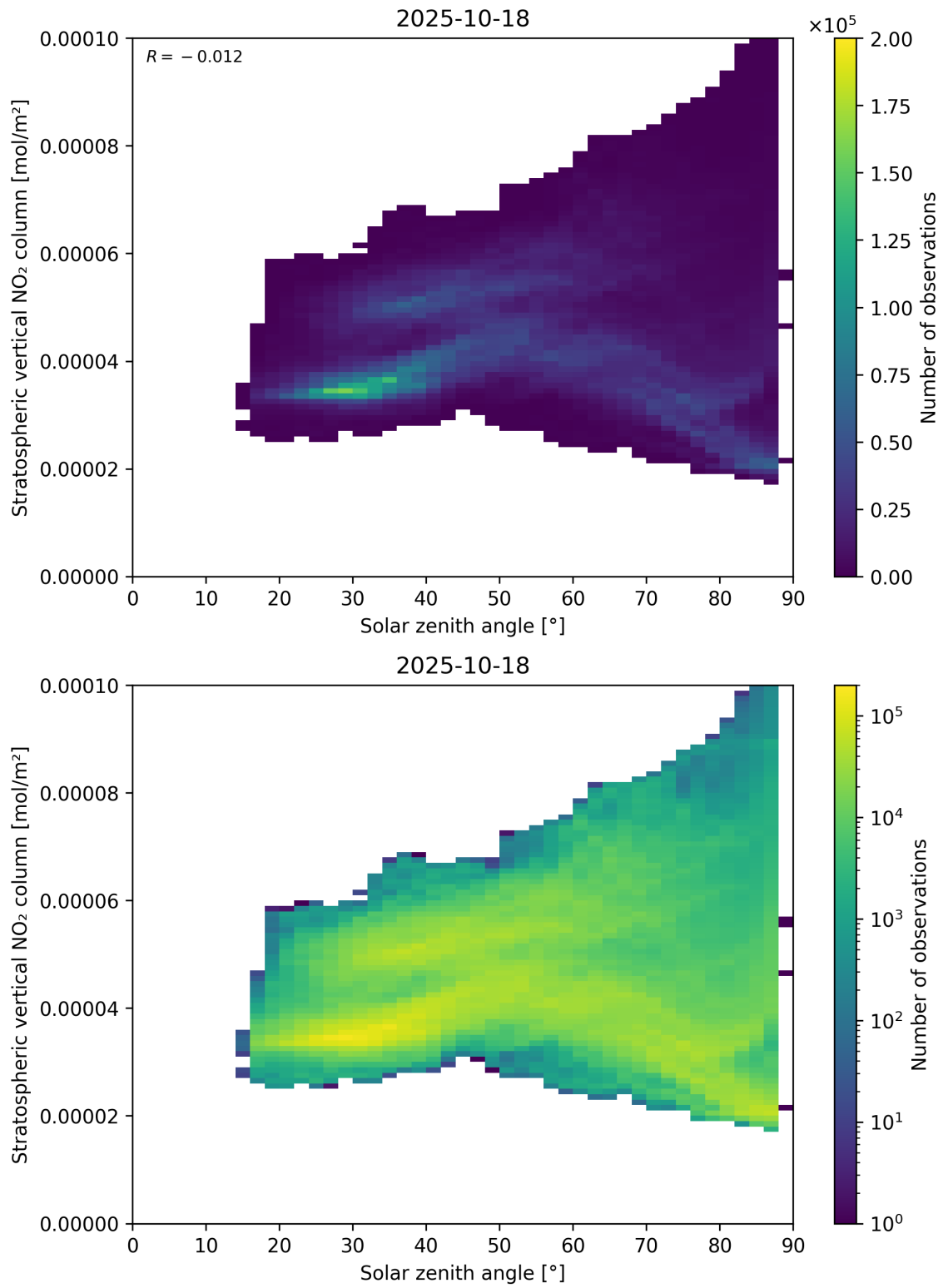
Figure 150: Scatter density plot of “Solar zenith angle” against “Stratospheric vertical NO 2 column” for 2025-10-17 to 2025-10-19.
