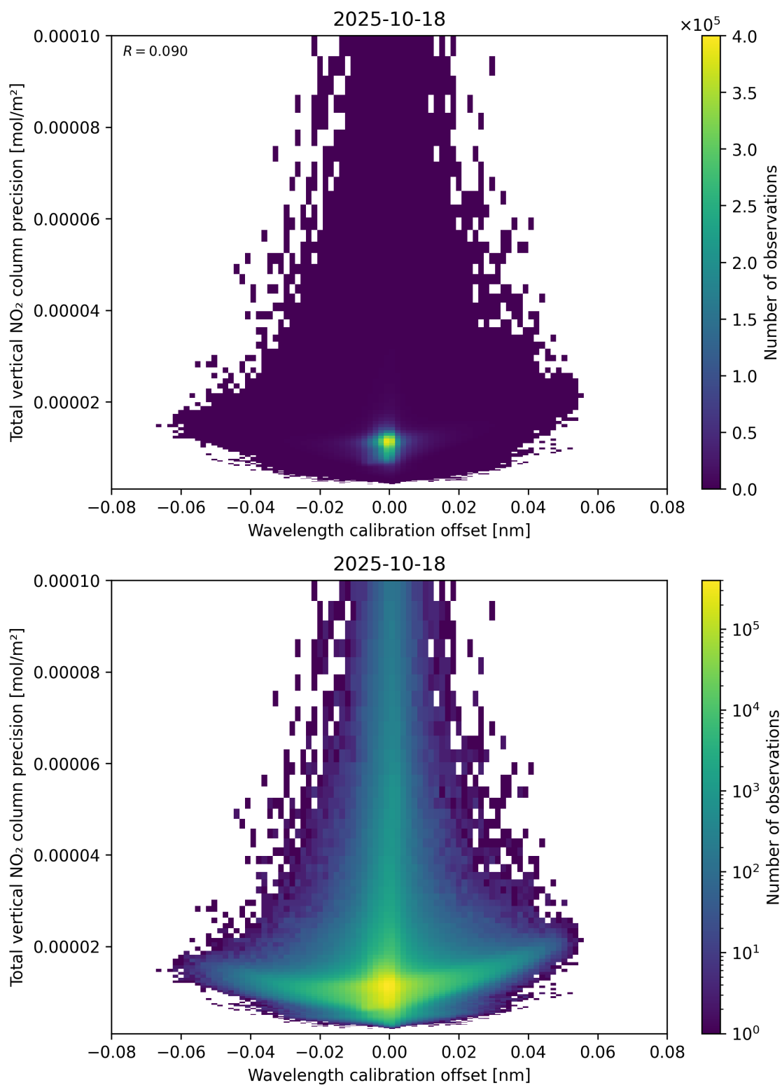
Figure 180: Scatter density plot of “Wavelength calibration offset” against “Total vertical NO 2 column precision” for 2025-10-17 to 2025-10-19.
