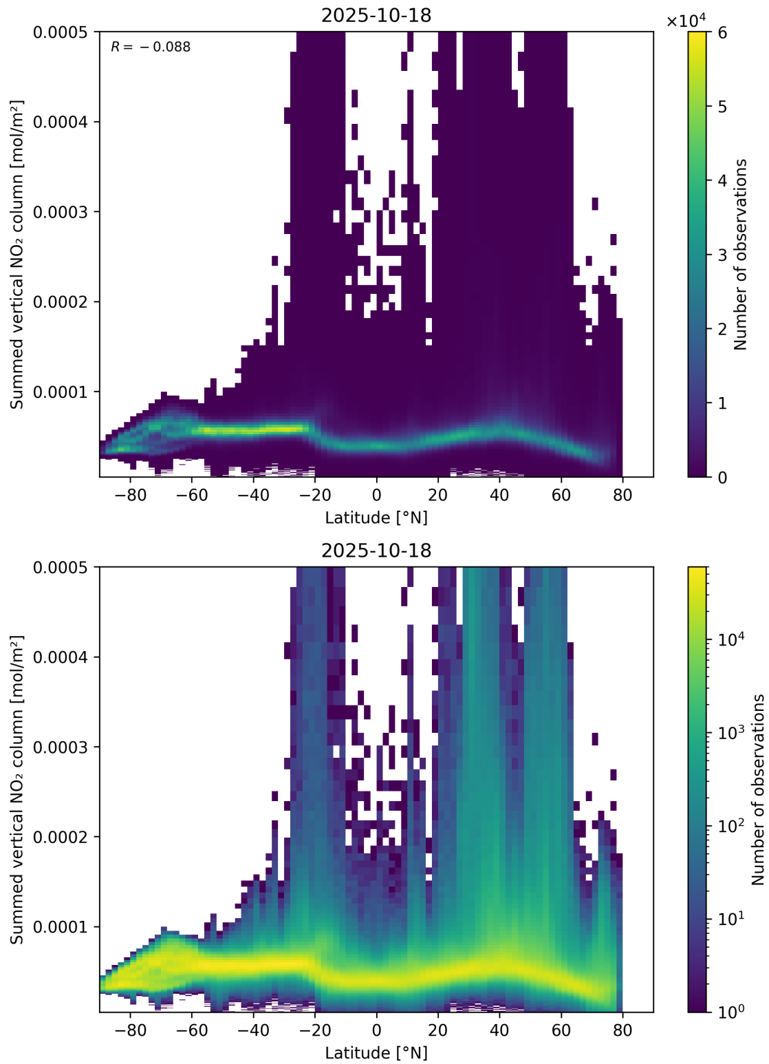
Figure 88: Scatter density plot of “Latitude” against “Summed vertical NO 2 column” for 2025-10-17 to 2025-10-19.
