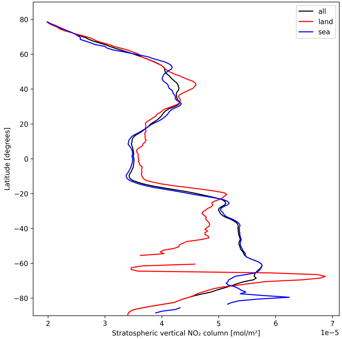
Figure 19: Zonal average of “Stratospheric vertical NO 2 column” for 2025-10-17 to 2025-10-19.
