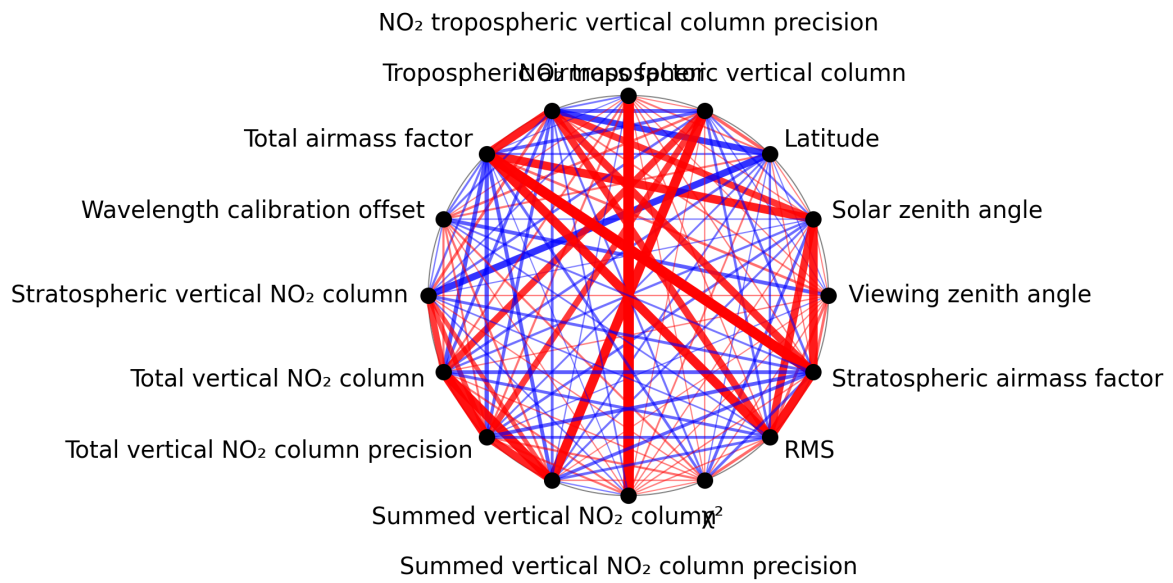
Figure 1: Map of correlation graph for 2025-10-17 to 2025-10-19.
