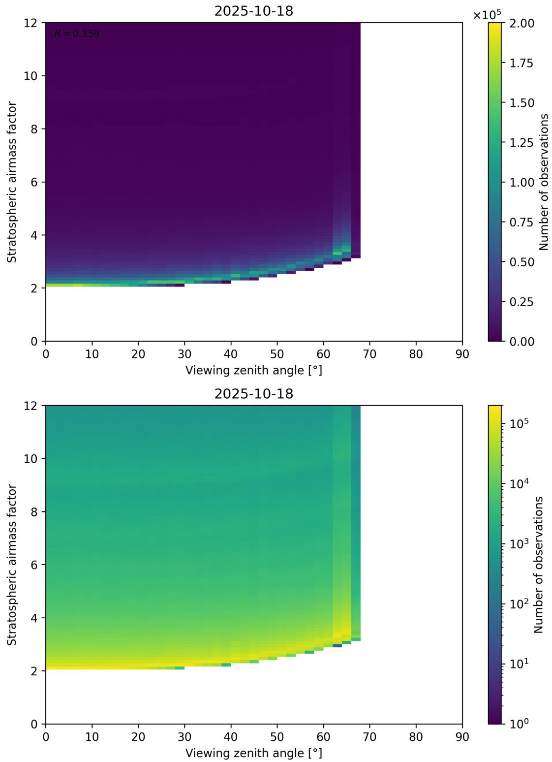
Figure 159: Scatter density plot of “Viewing zenith angle” against “Stratospheric airmass factor” for 2025-10-17 to 2025-10-19.
