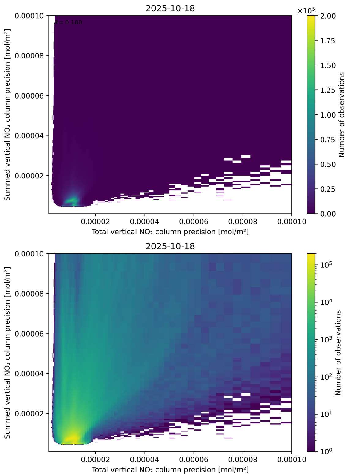
Figure 118: Scatter density plot of “Total vertical NO 2 column precision” against “Summed vertical NO 2 column precision” for 2025-10-17 to 2025-10-19.
