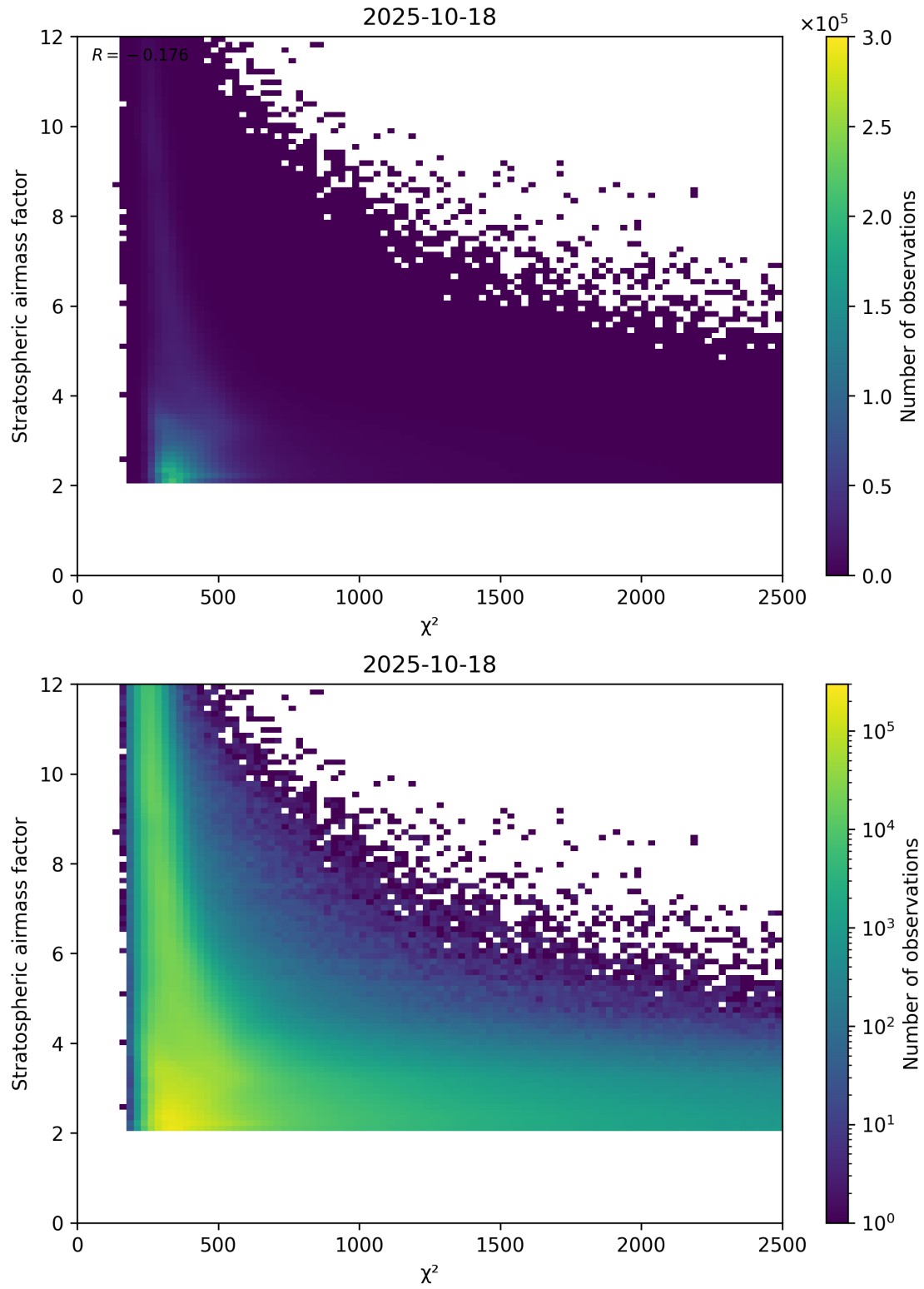
Figure 81: Scatter density plot of “ \chi^2 ” against “Stratospheric airmass factor” for 2025-10-17 to 2025-10-19.
