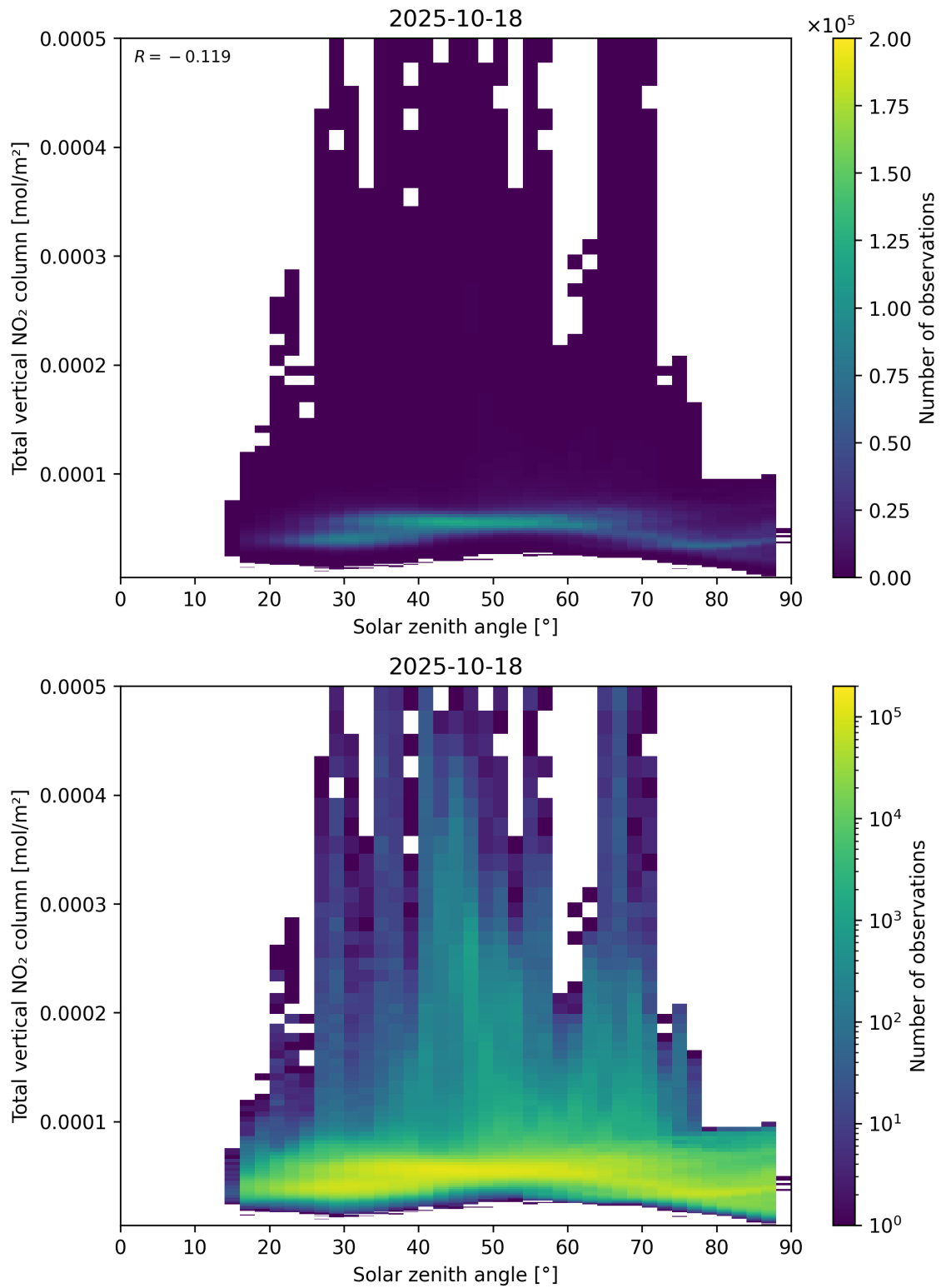
Figure 153: Scatter density plot of “Solar zenith angle” against “Total vertical NO 2 column” for 2025-10-17 to 2025-10-19.
