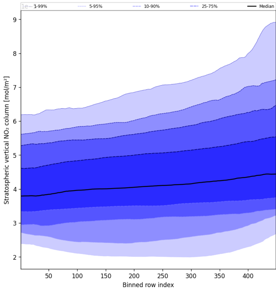
Figure 53: Along track statistics of "Stratospheric vertical NO 2 column" for 2025-10-17 to 2025-10-19
