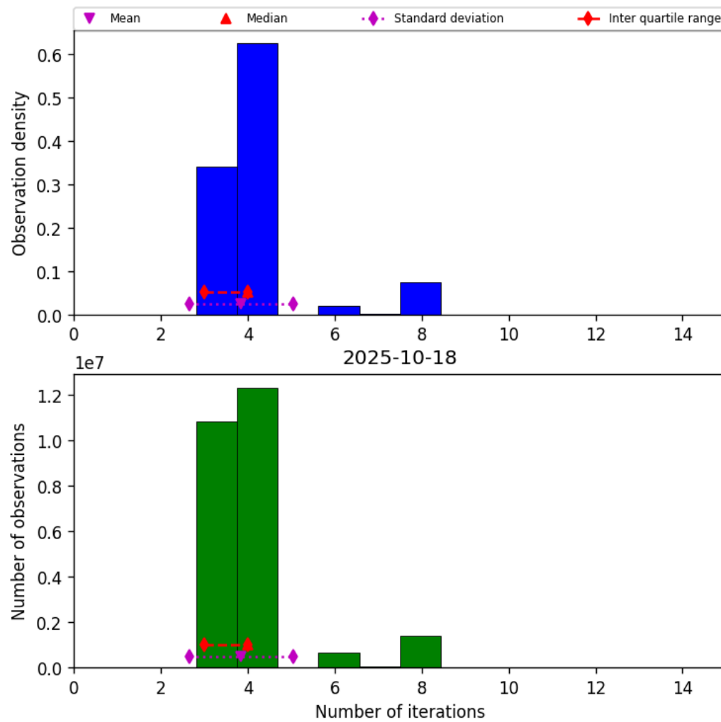
Figure 34: Histogram of “Number of iterations” for 2025-10-17 to 2025-10-19
