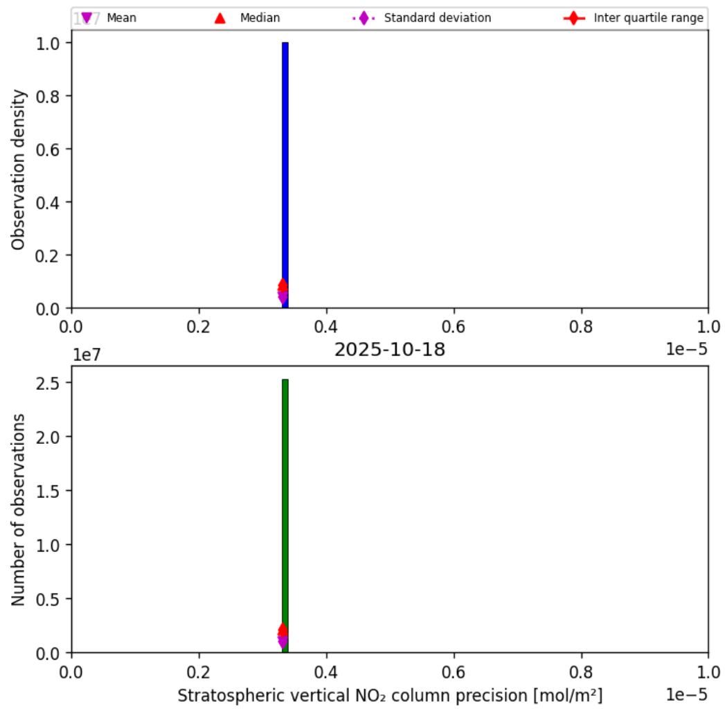
Figure 37: Histogram of “Stratospheric vertical NO 2 column precision” for 2025-10-17 to 2025-10-19
