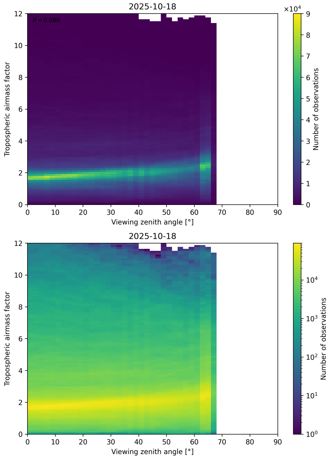
Figure 161: Scatter density plot of “Viewing zenith angle” against “Tropospheric airmass factor” for 2025-10-17 to 2025-10-19.
