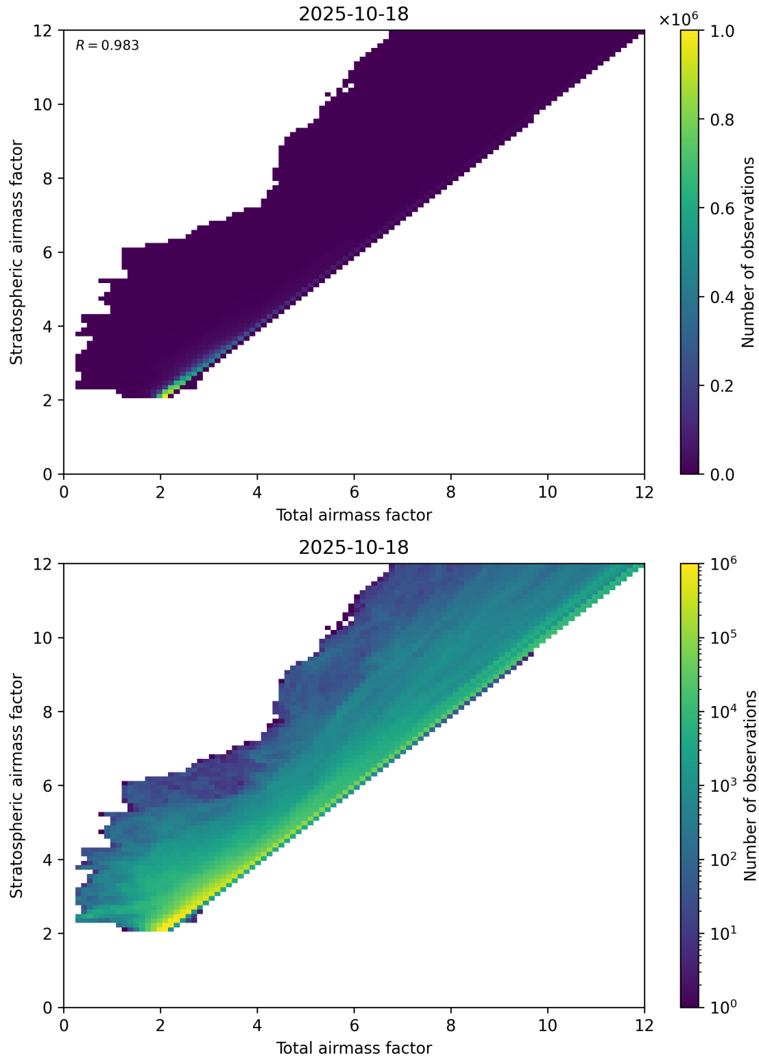
Figure 62: Scatter density plot of “Total airmass factor” against “Stratospheric airmass factor” for 2025-10-17 to 2025-10-19.
