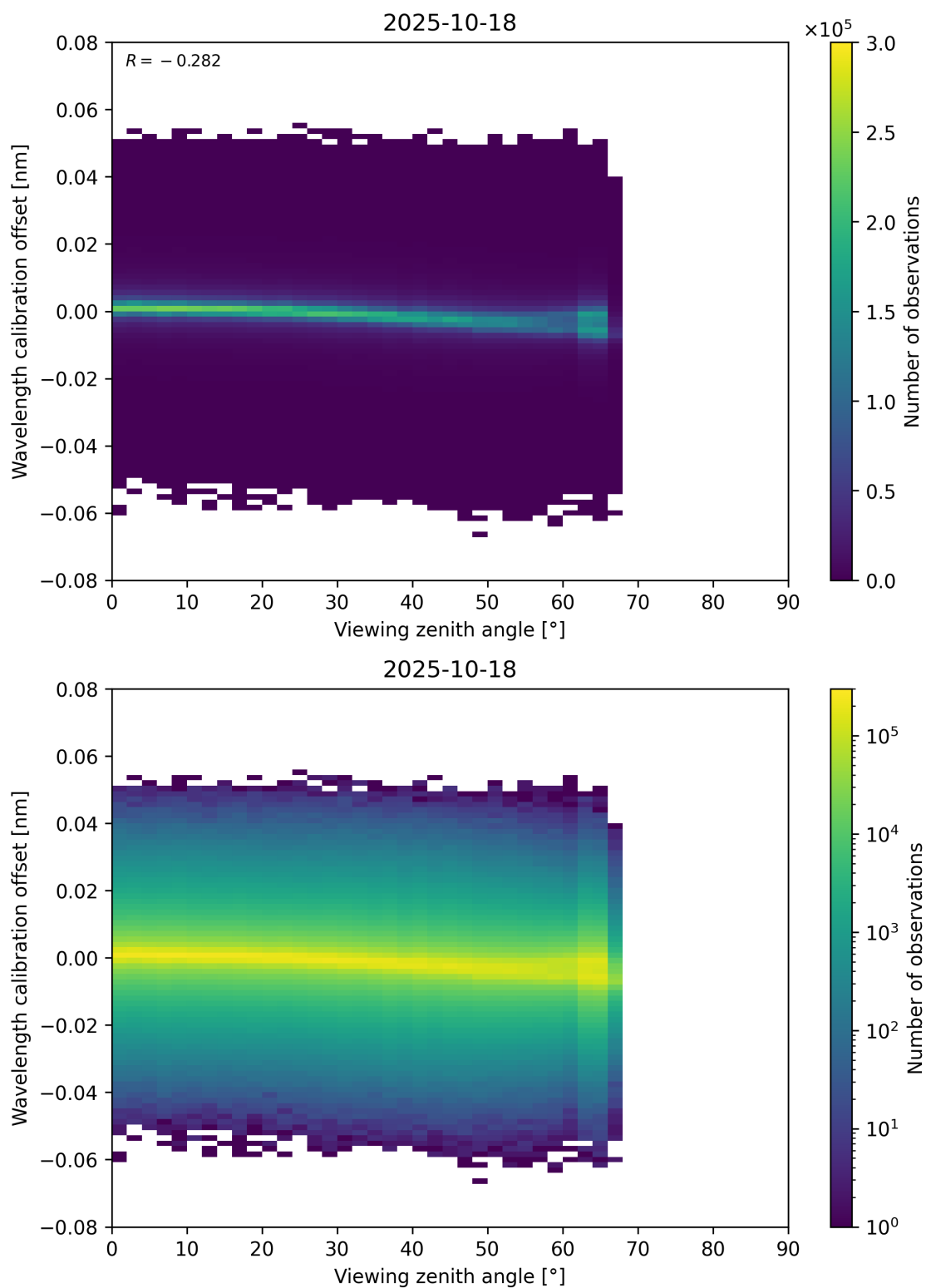
Figure 173: Scatter density plot of “Viewing zenith angle” against “Wavelength calibration offset” for 2025-10-17 to 2025-10-19.
