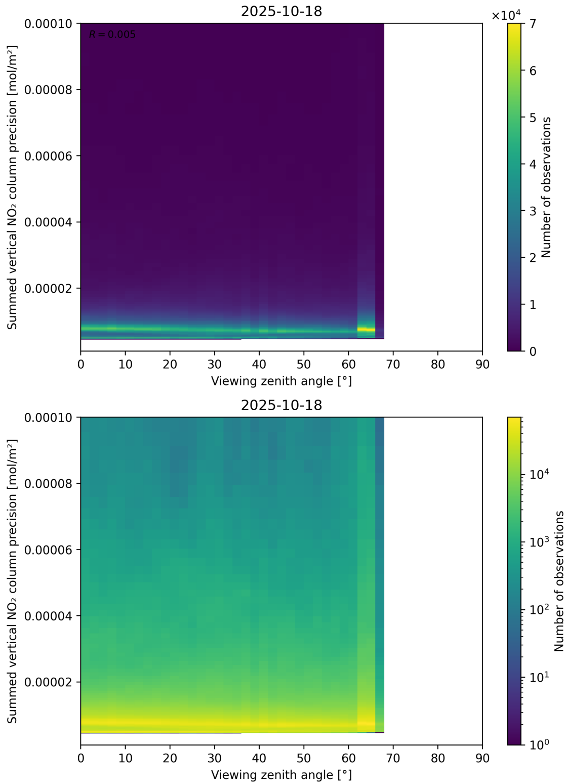
Figure 166: Scatter density plot of “Viewing zenith angle” against “Summed vertical NO 2 column precision” for 2025-10-17 to 2025-10-19.
