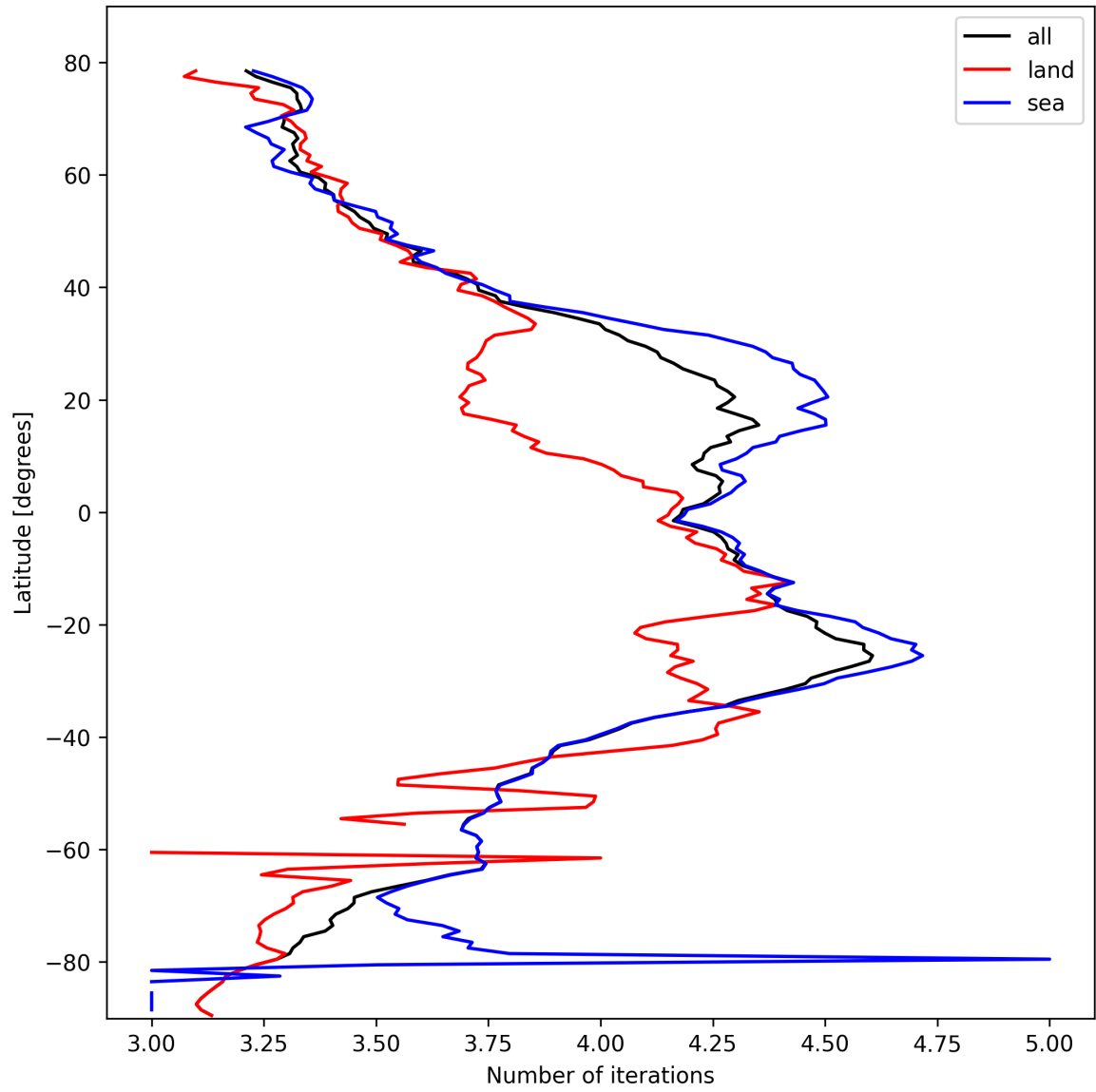
Figure 17: Zonal average of “Number of iterations” for 2025-10-17 to 2025-10-19.
