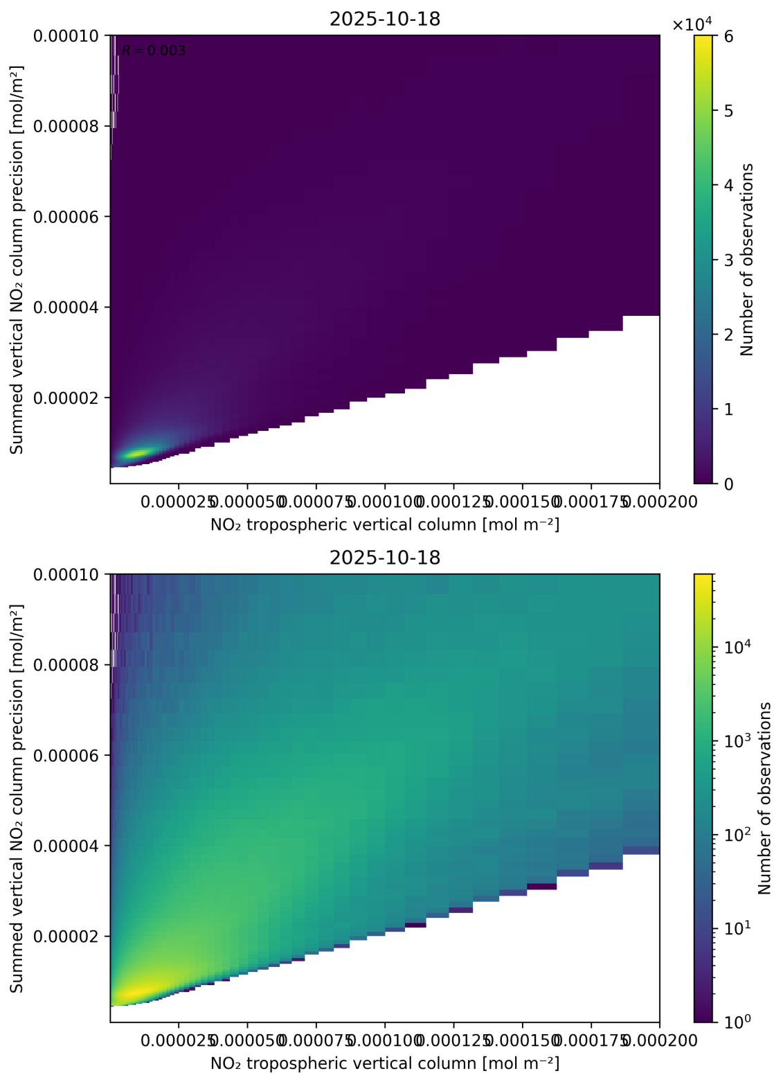
Figure 127: Scatter density plot of “NO 2 tropospheric vertical column” against “Summed vertical NO 2 column precision” for 2025-10-17 to 2025-10-19.
