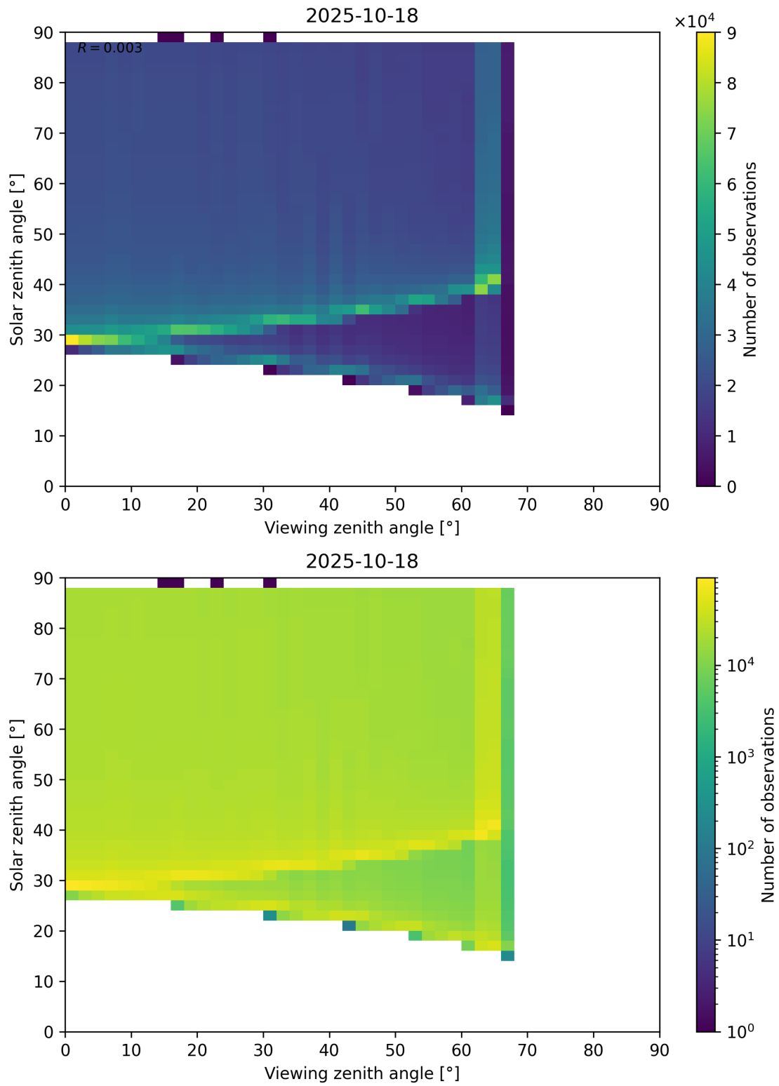
Figure 172: Scatter density plot of “Viewing zenith angle” against “Solar zenith angle” for 2025-10-17 to 2025-10-19.
