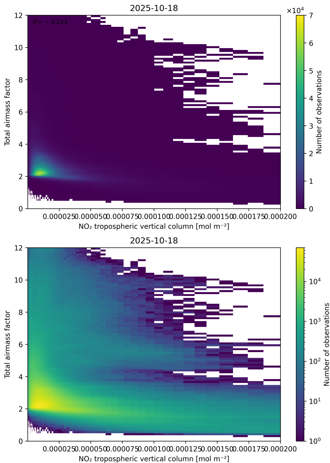
Figure 122: Scatter density plot of “NO 2 tropospheric vertical column” against “Total air mass factor” for 2025-10-17 to 2025-10-19.
