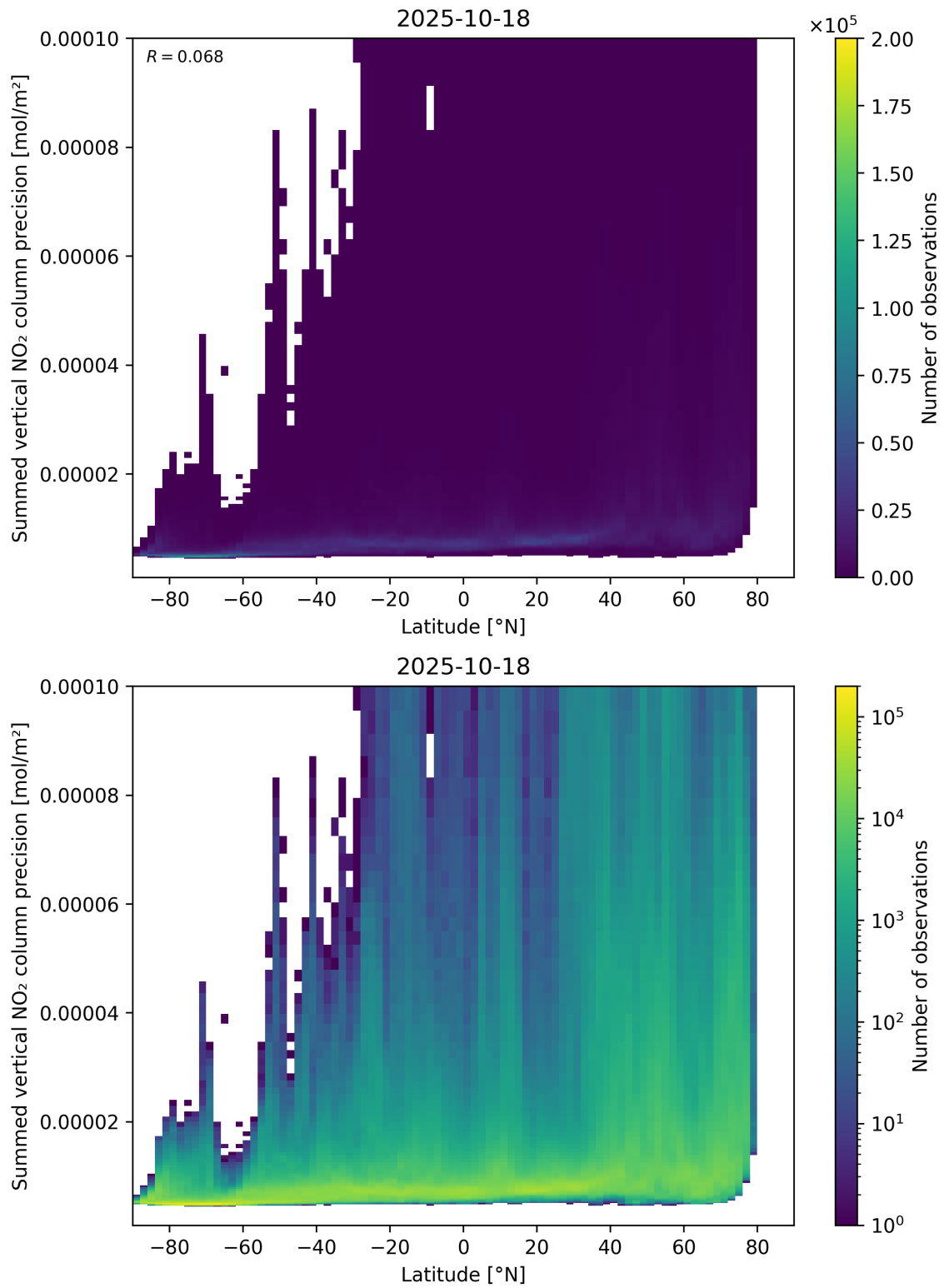
Figure 89: Scatter density plot of “Latitude” against “Summed vertical NO 2 column precision” for 2025-10-17 to 2025-10-19.
