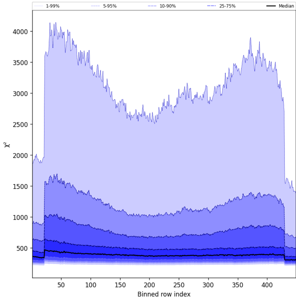
Figure 59: Along track statistics of “ \chi^2 ” for 2025-10-17 to 2025-10-19
