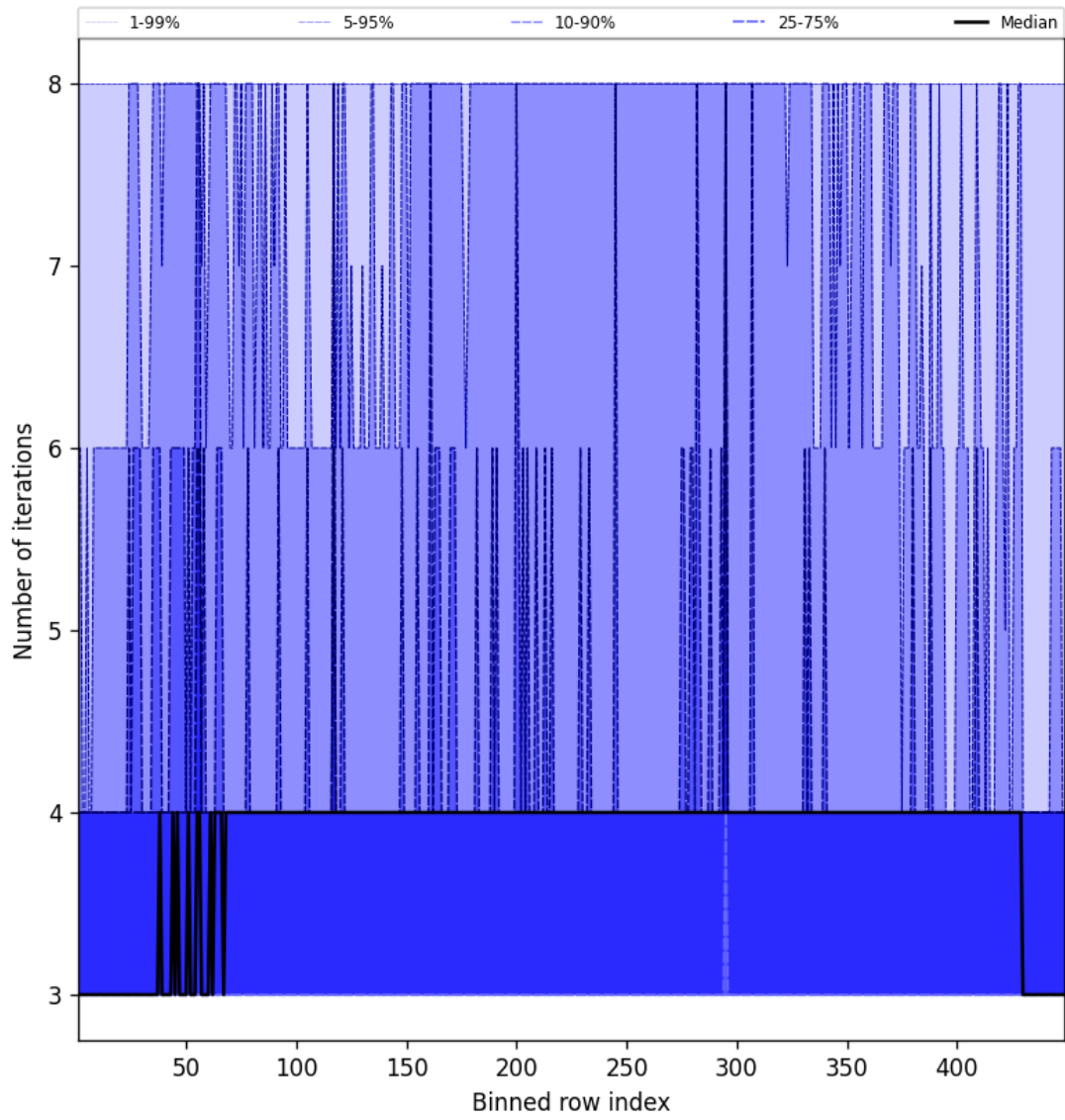
Figure 51: Along track statistics of “Number of iterations” for 2025-10-17 to 2025-10-19
