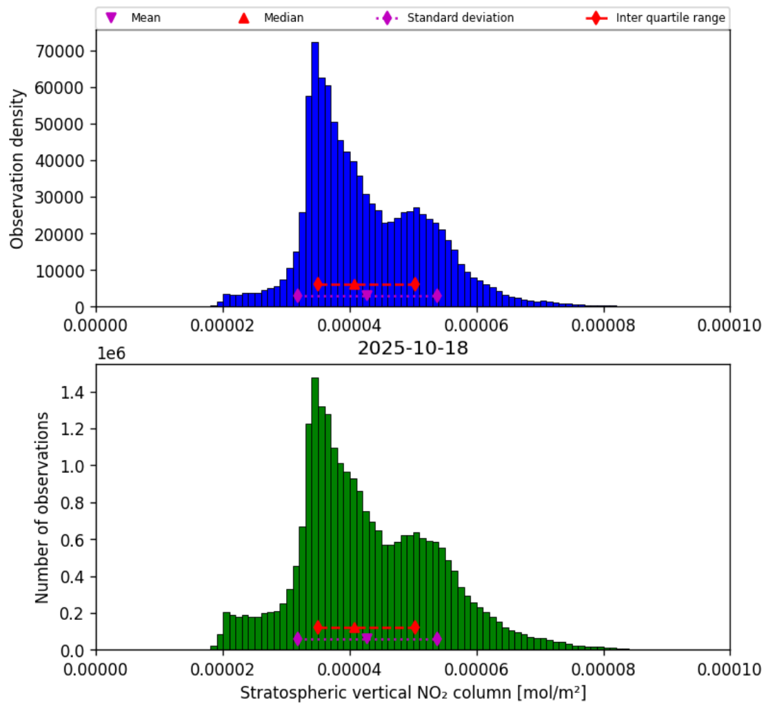
Figure 36: Histogram of “Stratospheric vertical NO 2 column” for 2025-10-17 to 2025-10-19
