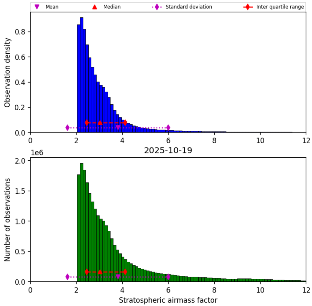
Figure 44: Histogram of “Stratospheric airmass factor” for 2025-10-18 to 2025-10-20
