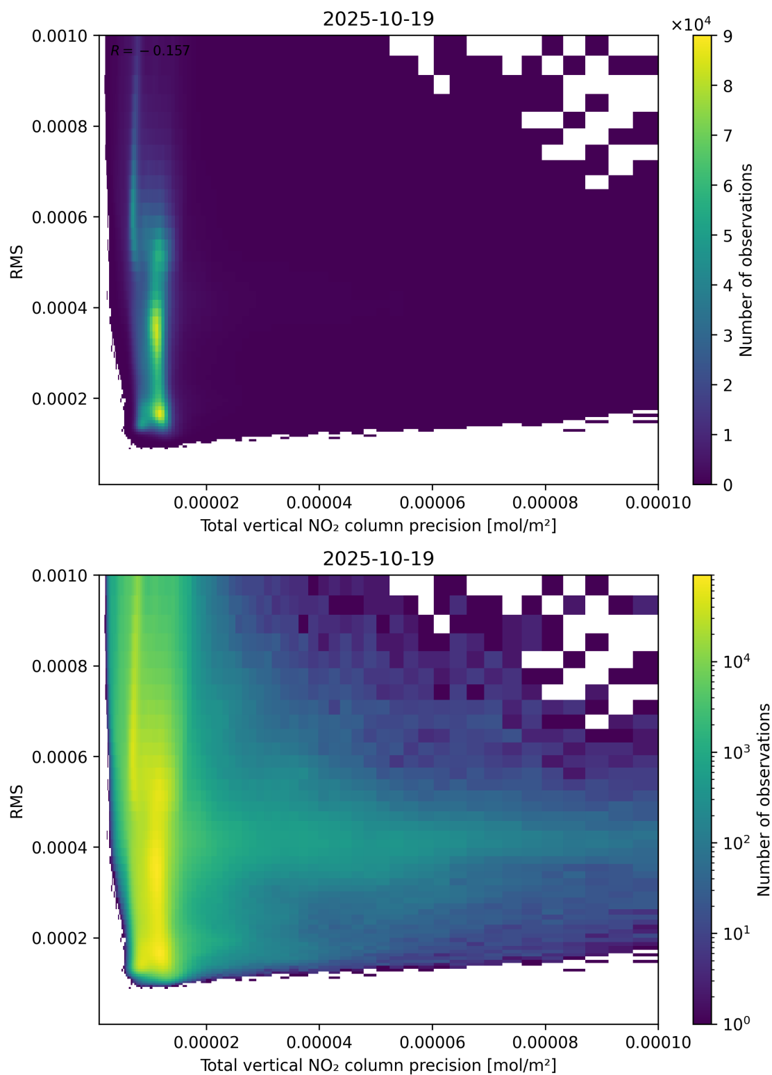
Figure 119: Scatter density plot of “Total vertical NO 2 column precision” against “RMS” for 2025-10-18 to 2025-10-20.
