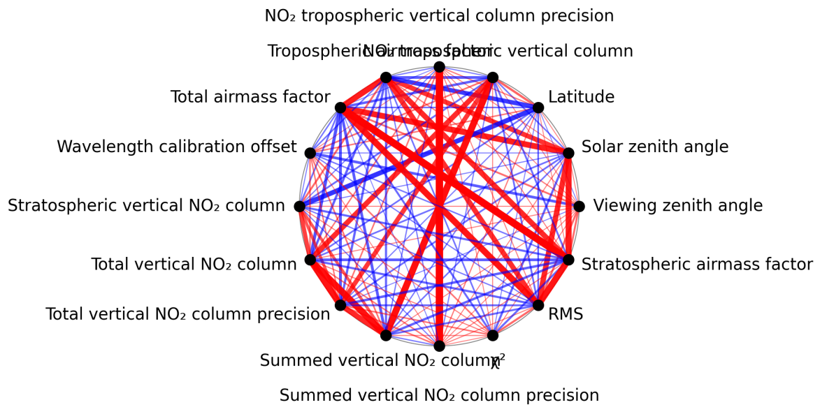
Figure 1: Map of correlation graph for 2025-10-18 to 2025-10-20.
