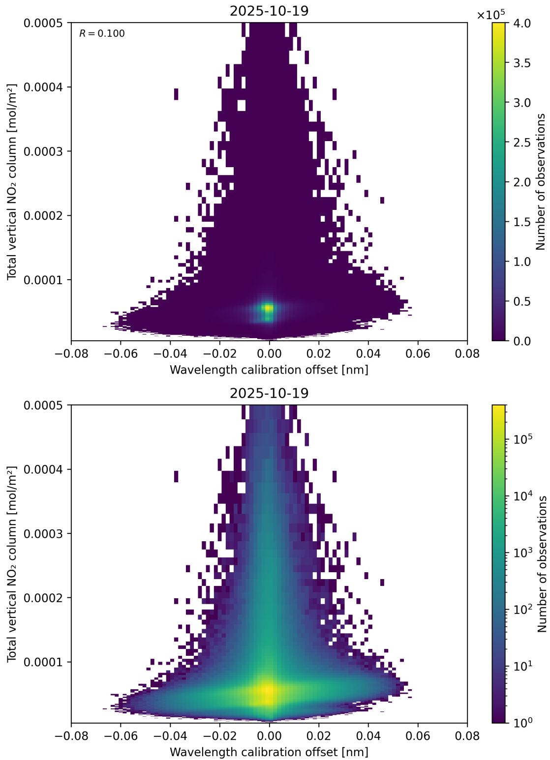
Figure 179: Scatter density plot of “Wavelength calibration offset” against “Total vertical NO 2 column” for 2025-10-18 to 2025-10-20.
