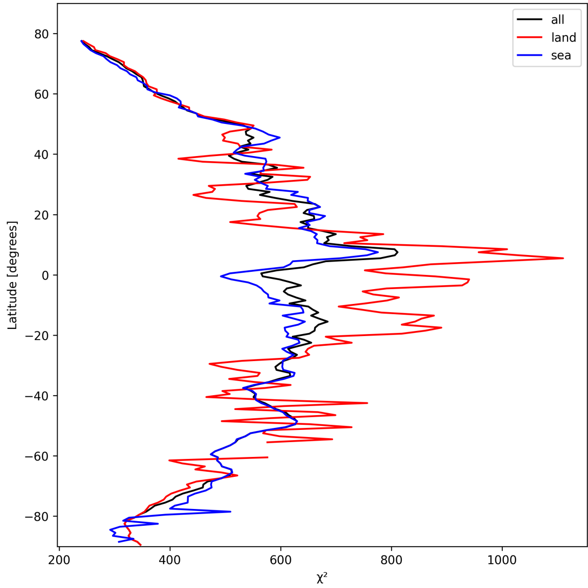
Figure 25: Zonal average of “ \chi^2 ” for 2025-10-18 to 2025-10-20.
