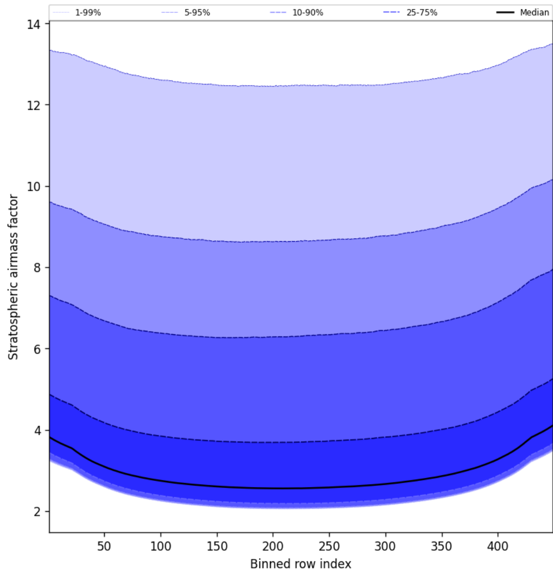
Figure 61: Along track statistics of “Stratospheric airmass factor” for 2025-10-18 to 2025-10-20
