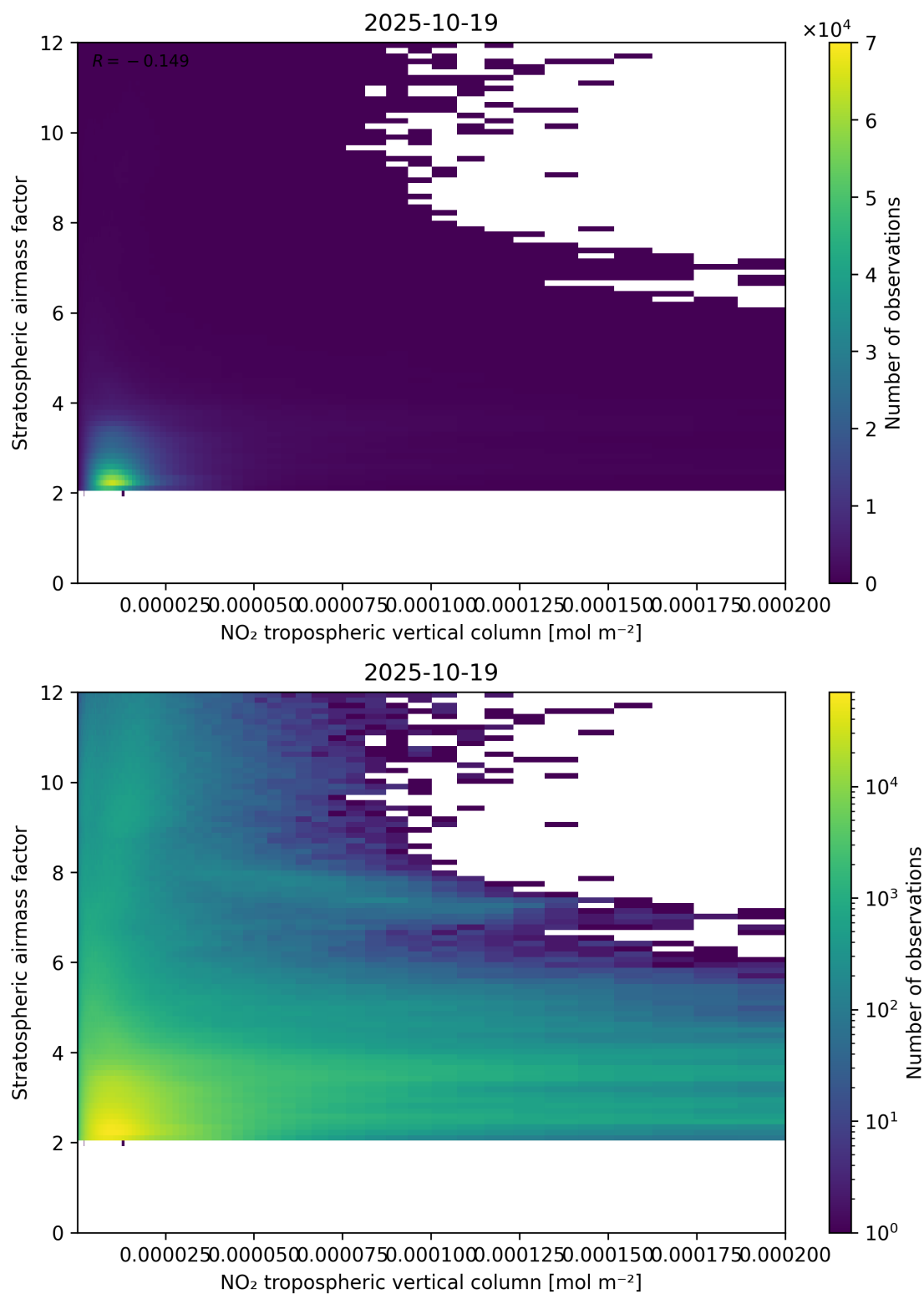
Figure 121: Scatter density plot of “NO 2 tropospheric vertical column” against “Stratospheric airmass factor” for 2025-10-18 to 2025-10-20.
