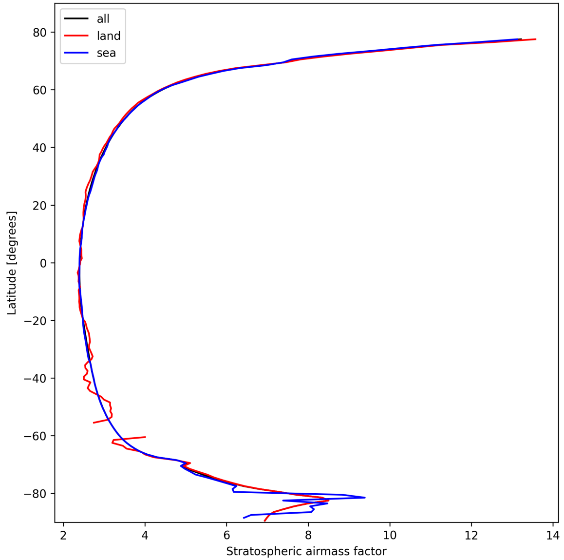
Figure 27: Zonal average of “Stratospheric airmass factor” for 2025-10-18 to 2025-10-20.
