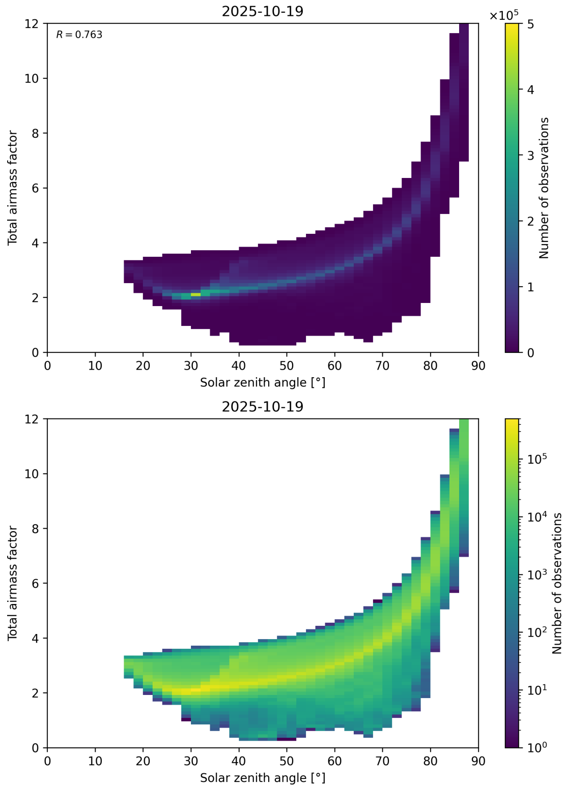
Figure 146: Scatter density plot of “Solar zenith angle” against “Total airmass factor” for 2025-10-18 to 2025-10-20.
