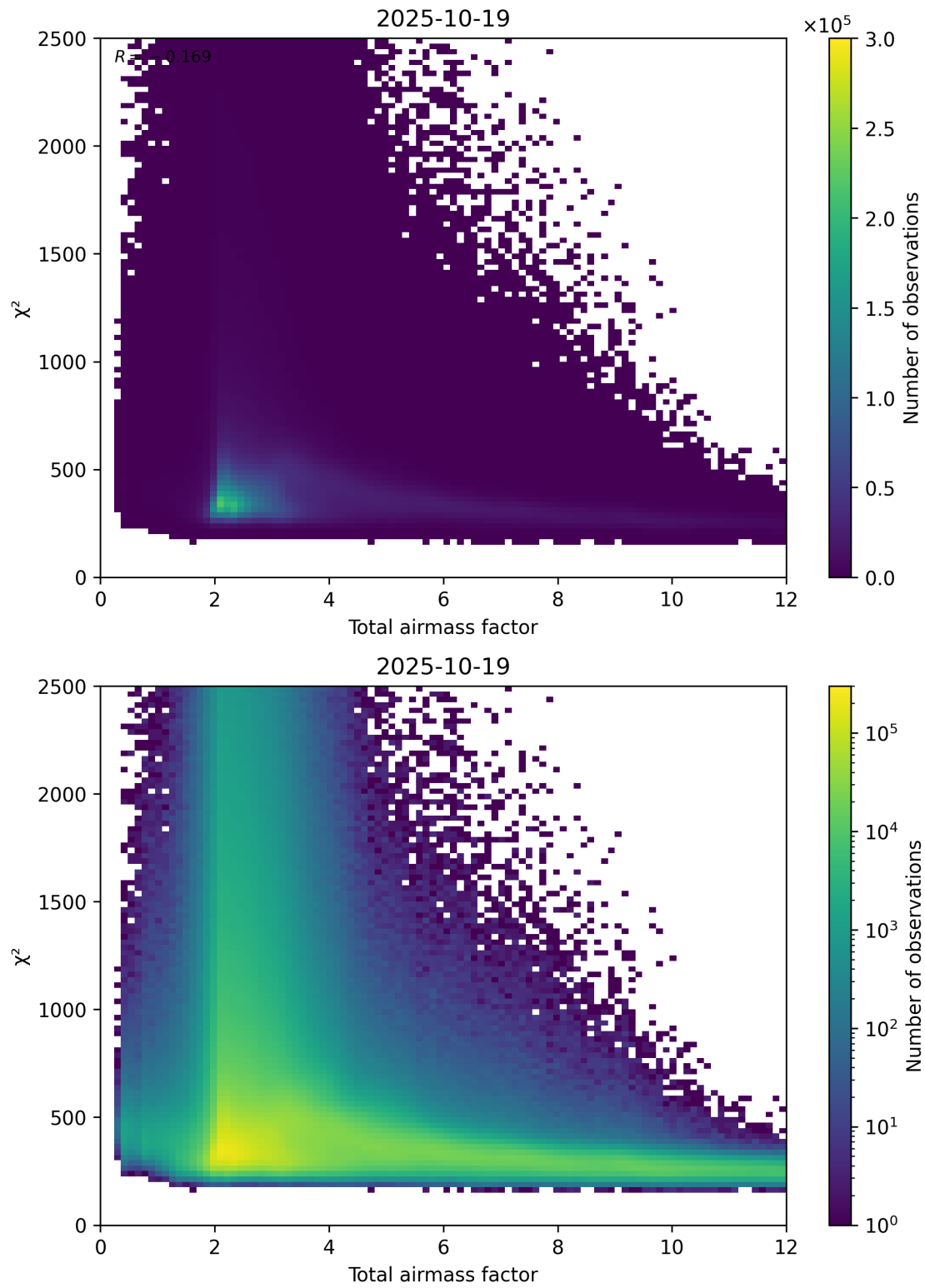
Figure 63: Scatter density plot of “Total airmass factor” against “ \chi^2 ” for 2025-10-18 to 2025-10-20.
