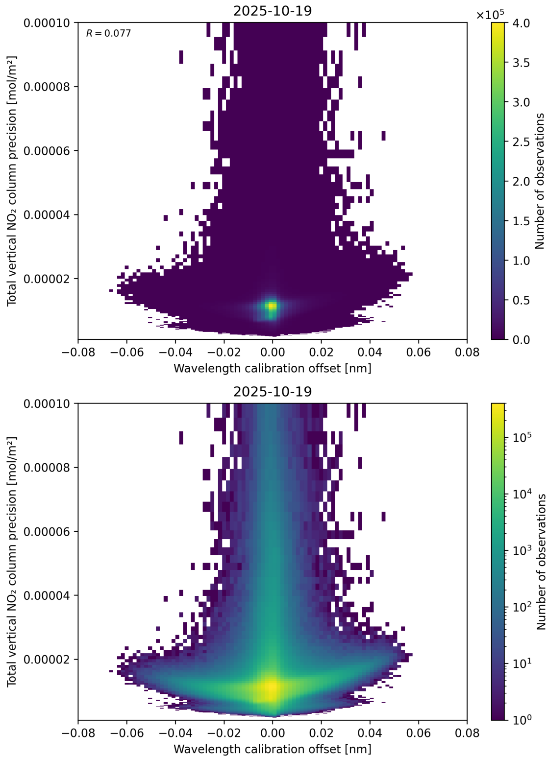
Figure 180: Scatter density plot of “Wavelength calibration offset” against “Total vertical NO 2 column precision” for 2025-10-18 to 2025-10-20.
