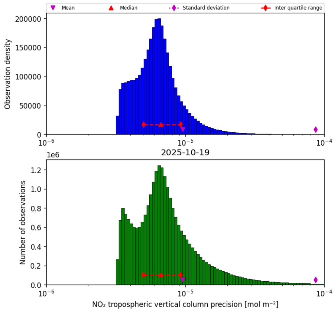
Figure 30: Histogram of “NO 2 tropospheric vertical column precision” for 2025-10-18 to 2025-10-20
