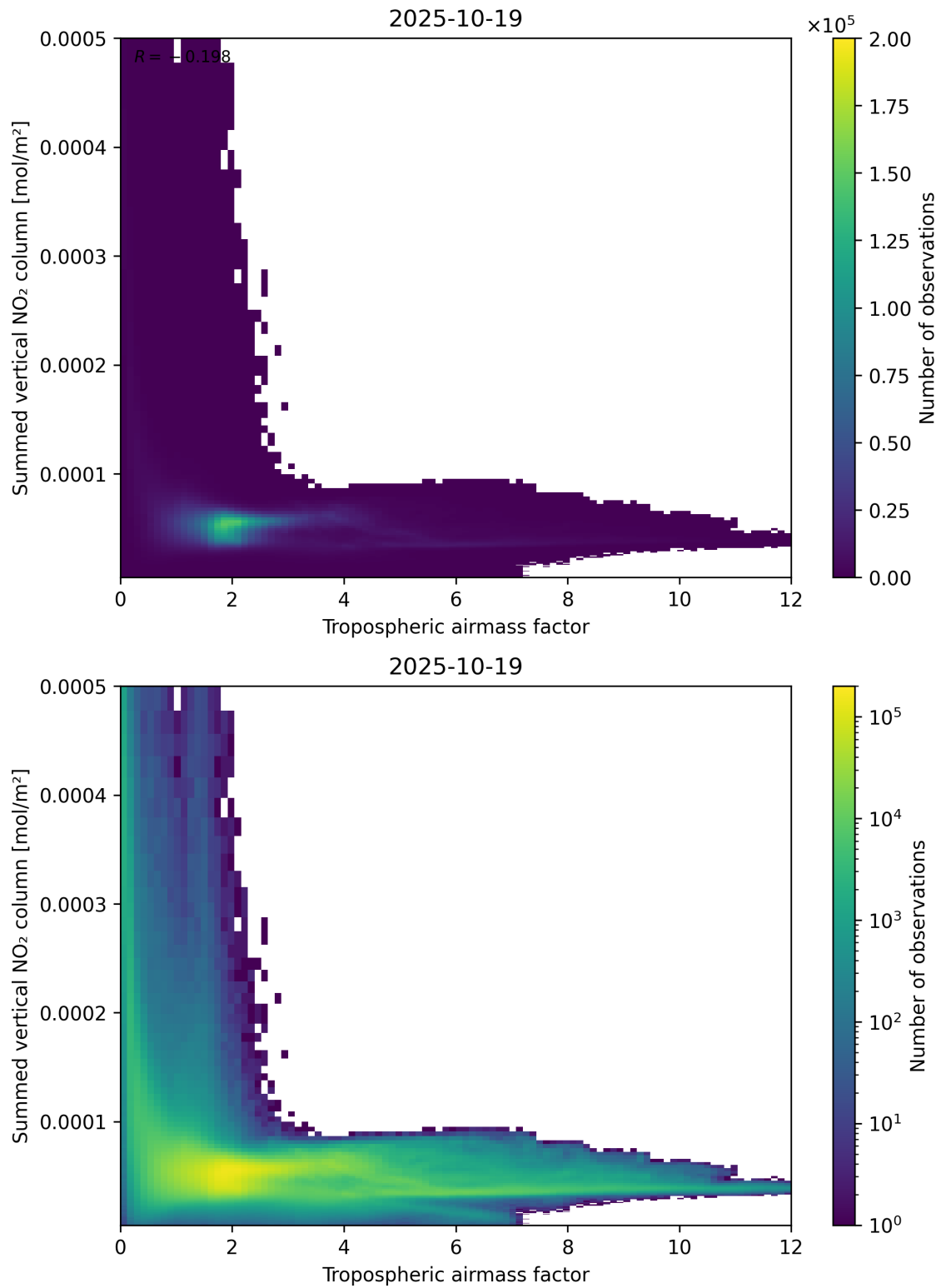
Figure 75: Scatter density plot of “Tropospheric air mass factor” against “Summed vertical NO 2 column” for 2025-10-18 to 2025-10-20.
