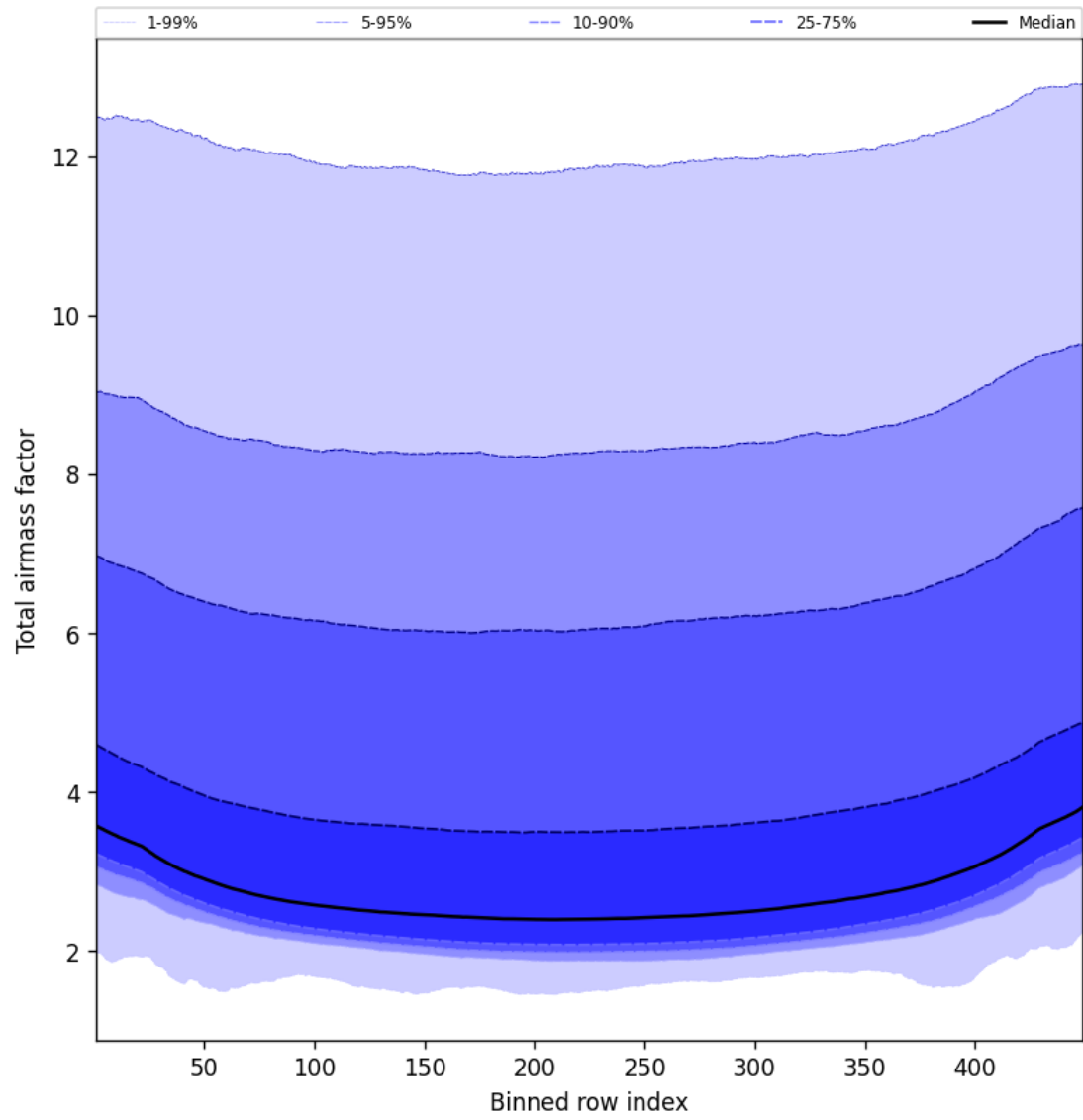
Figure 49: Along track statistics of “Total airmass factor” for 2025-10-18 to 2025-10-20
