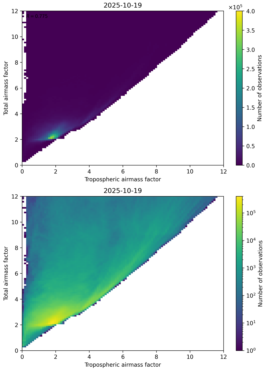
Figure 72: Scatter density plot of “Tropospheric airmass factor” against “Total airmass factor” for 2025-10-18 to 2025-10-20.
