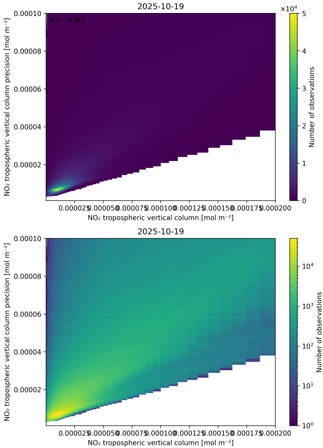
Figure 130: Scatter density plot of “NO 2 tropospheric vertical column” against “NO 2 tropospheric vertical column precision” for 2025-10-18 to 2025-10-20.
