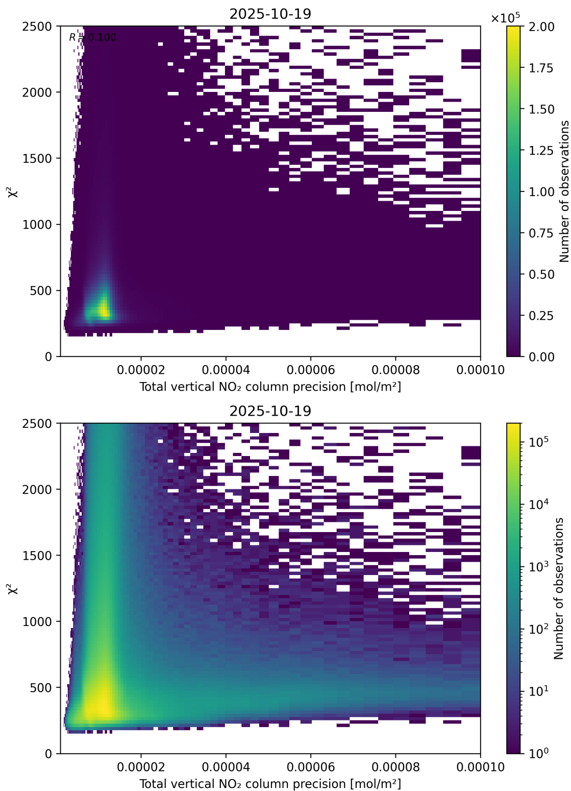
Figure 116: Scatter density plot of “Total vertical NO 2 column precision” against “ \chi^2 ” for 2025-10-18 to 2025-10-20.
