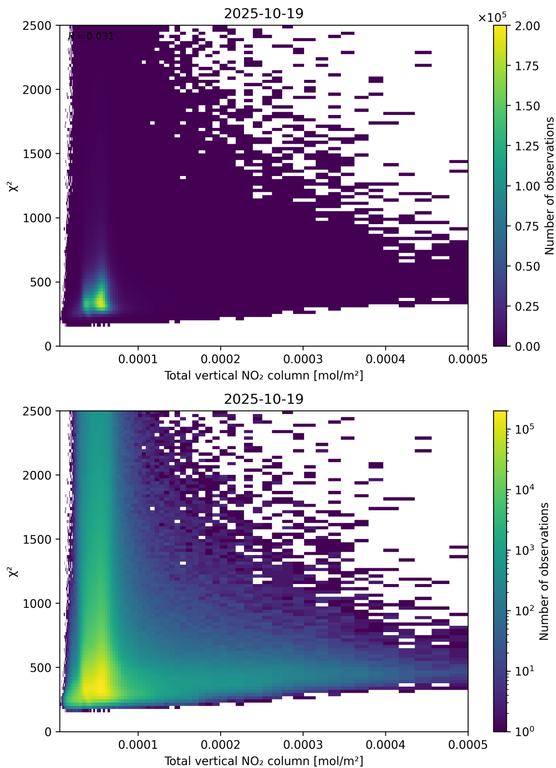
Figure 111: Scatter density plot of “Total vertical NO 2 column” against “ \chi^2 ” for 2025-10-18 to 2025-10-20.
