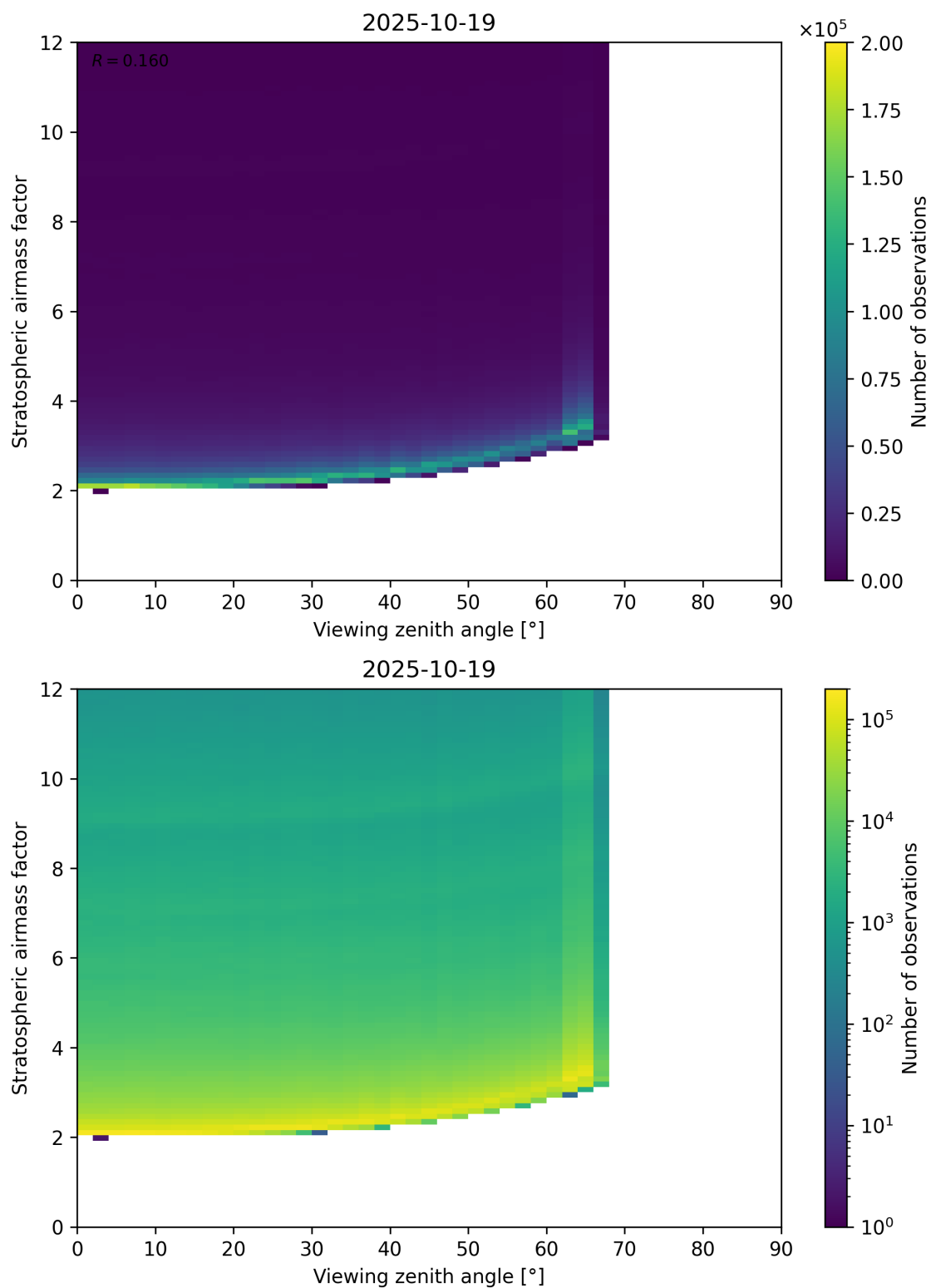
Figure 159: Scatter density plot of “Viewing zenith angle” against “Stratospheric airmass factor” for 2025-10-18 to 2025-10-20.
