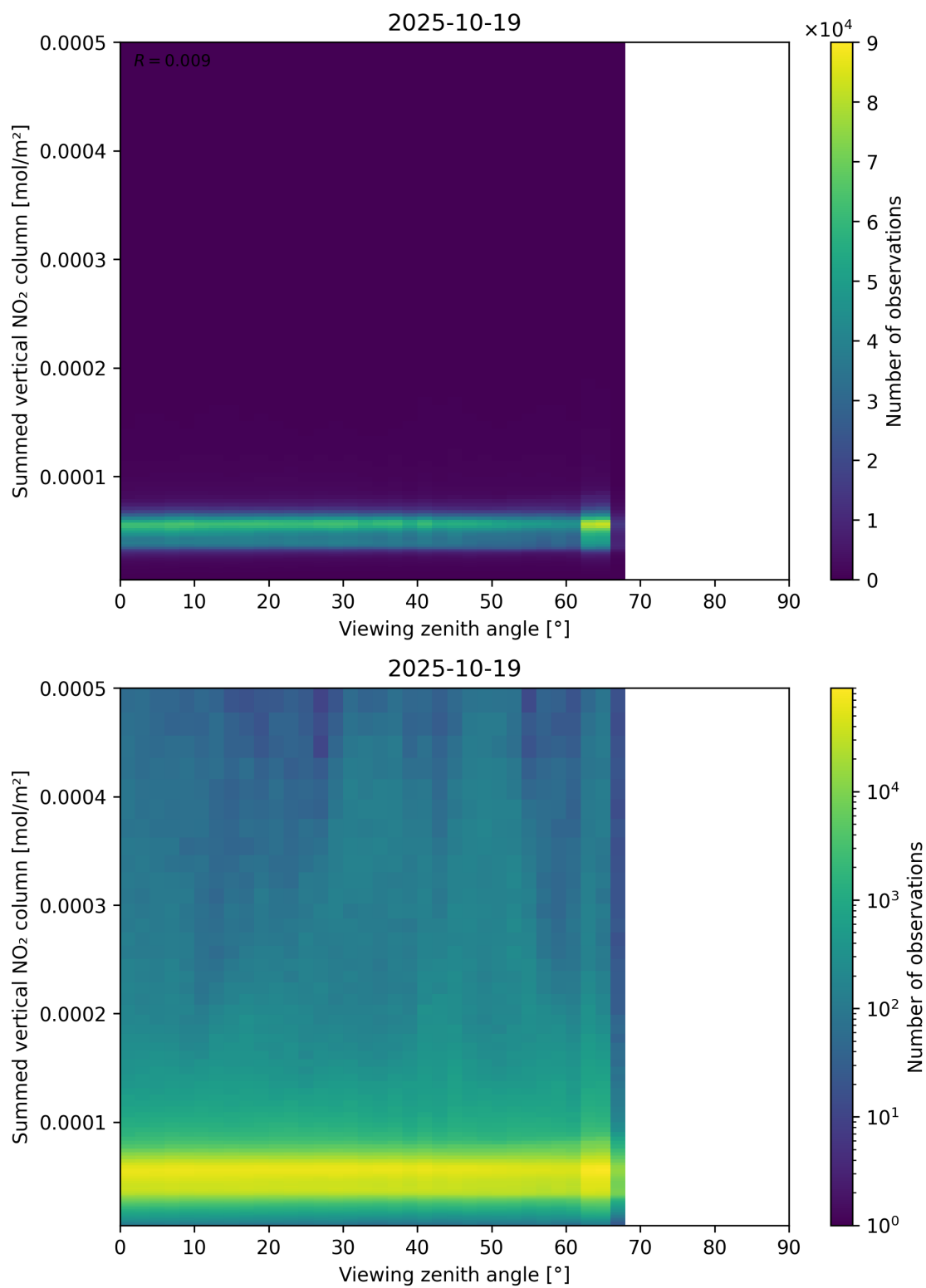
Figure 165: Scatter density plot of “Viewing zenith angle” against “Summed vertical NO 2 column” for 2025-10-18 to 2025-10-20.
