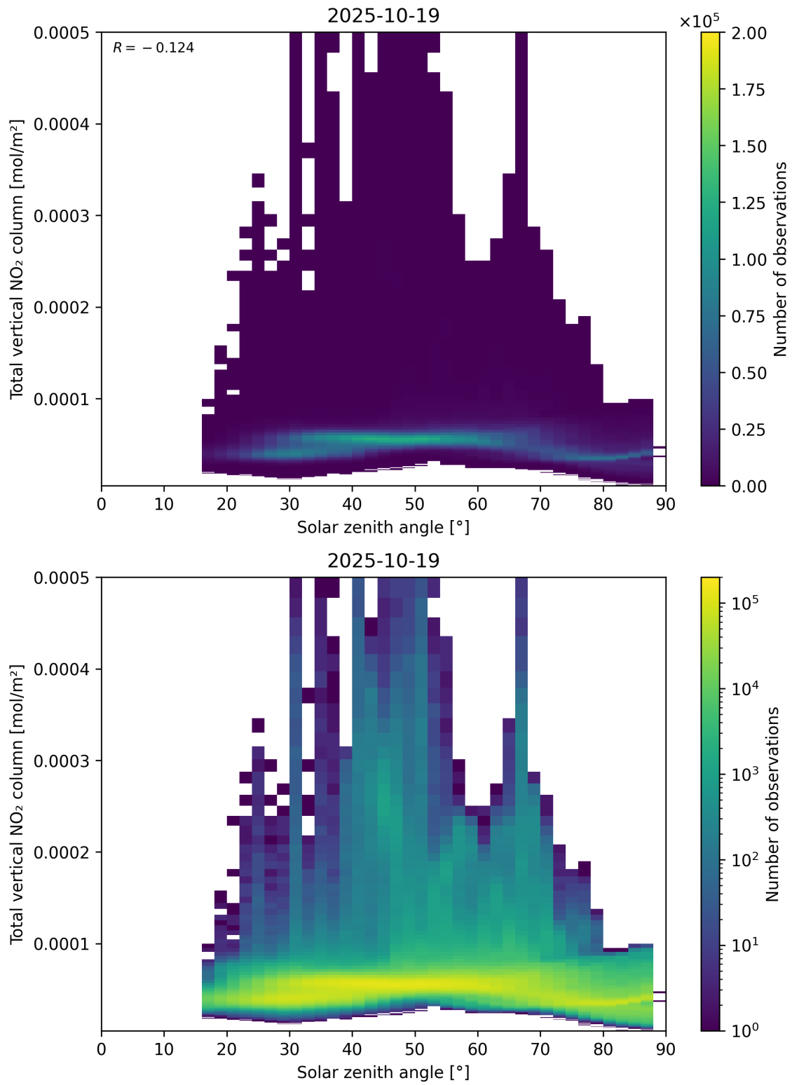
Figure 153: Scatter density plot of “Solar zenith angle” against “Total vertical NO 2 column” for 2025-10-18 to 2025-10-20.
