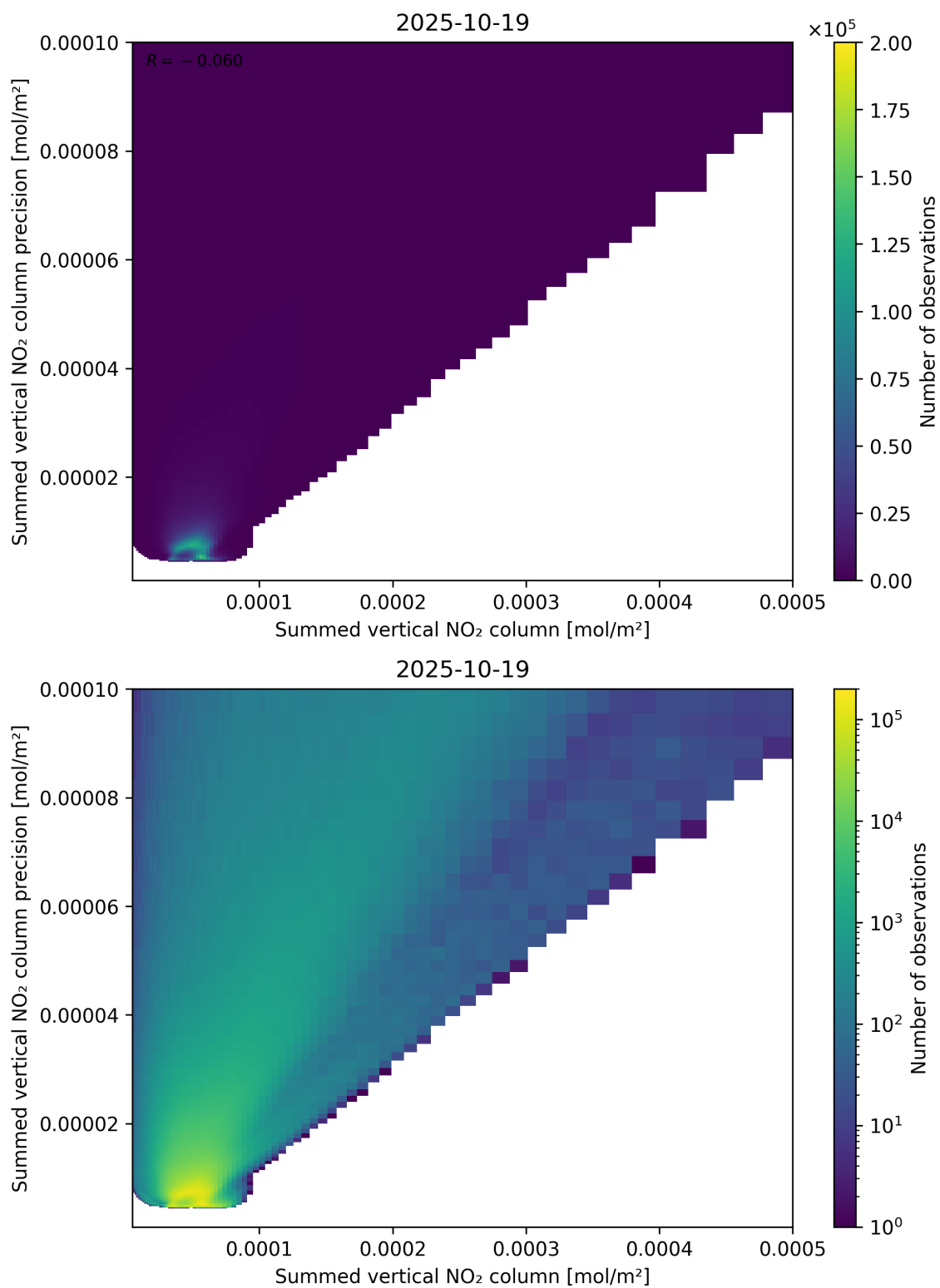
Figure 105: Scatter density plot of “Summed vertical NO 2 column” against “Summed vertical NO 2 column precision” for 2025-10-18 to 2025-10-20.
