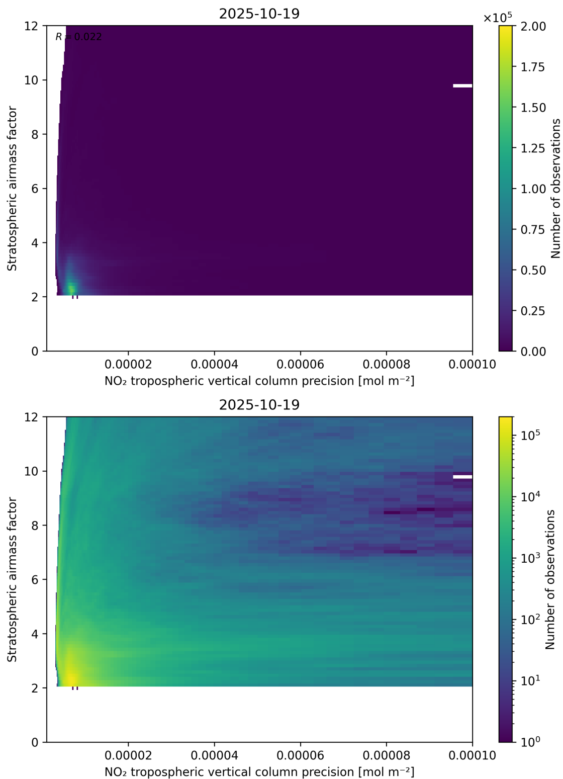
Figure 131: Scatter density plot of “NO 2 tropospheric vertical column precision” against “Stratospheric airmass factor” for 2025-10-18 to 2025-10-20.
