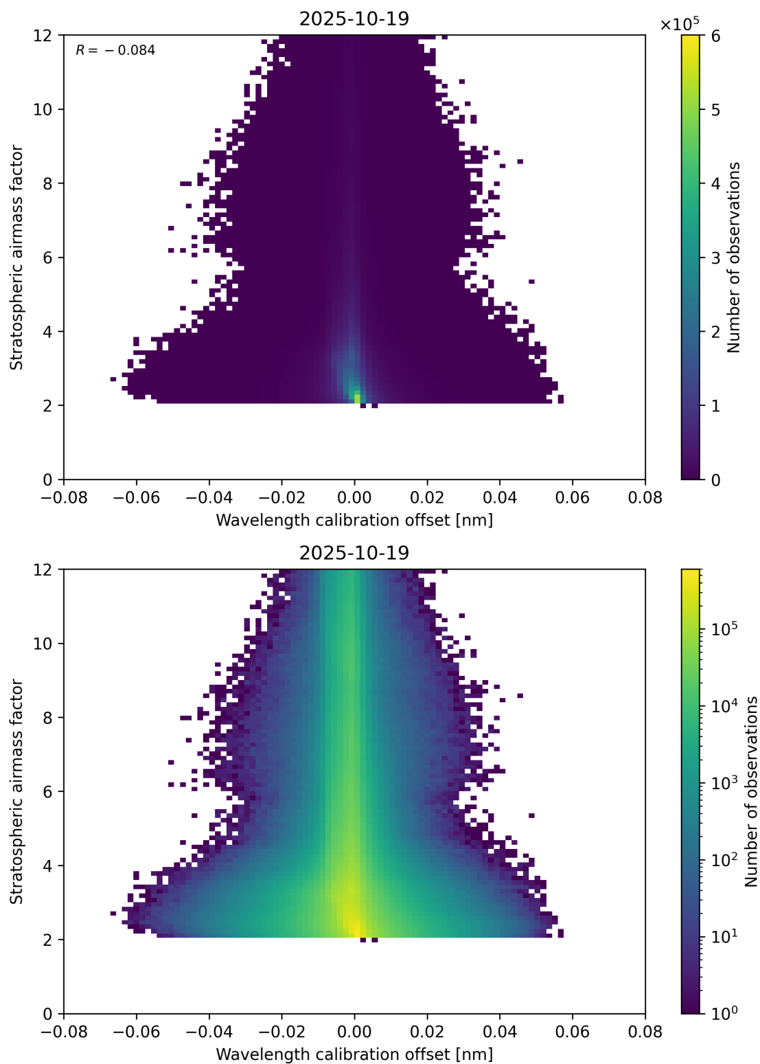
Figure 174: Scatter density plot of “Wavelength calibration offset” against “Stratospheric airmass factor” for 2025-10-18 to 2025-10-20.
