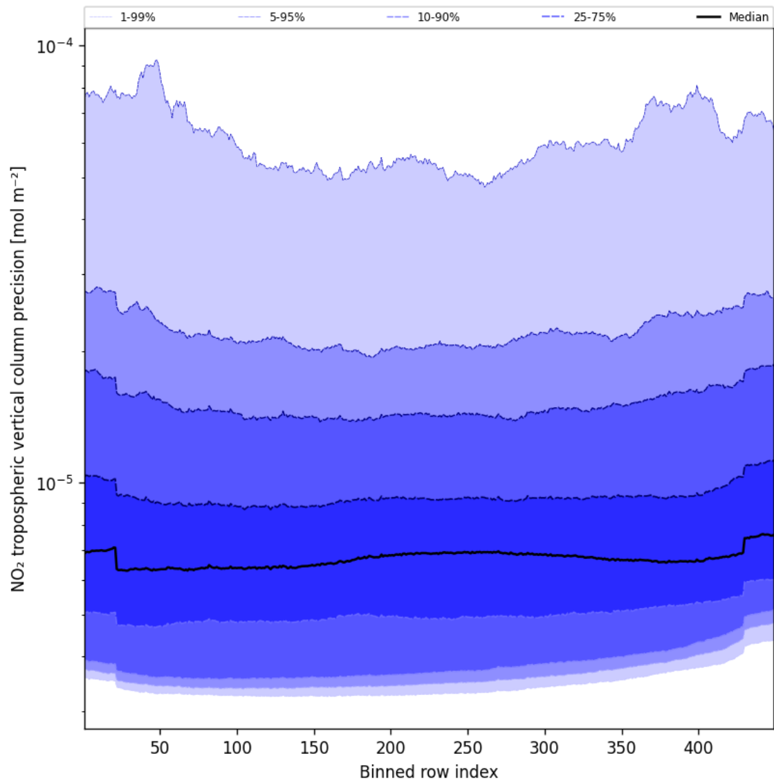
Figure 47: Along track statistics of “NO 2 tropospheric vertical column precision” for 2025-10-18 to 2025-10-20
