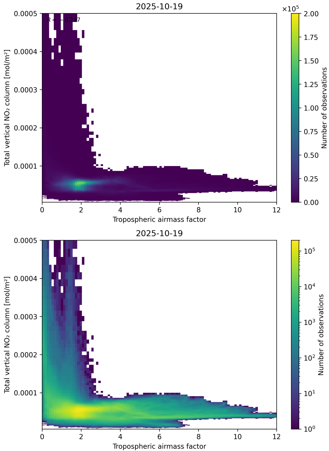
Figure 77: Scatter density plot of “Tropospheric airmass factor” against “Total vertical NO 2 column” for 2025-10-18 to 2025-10-20.
