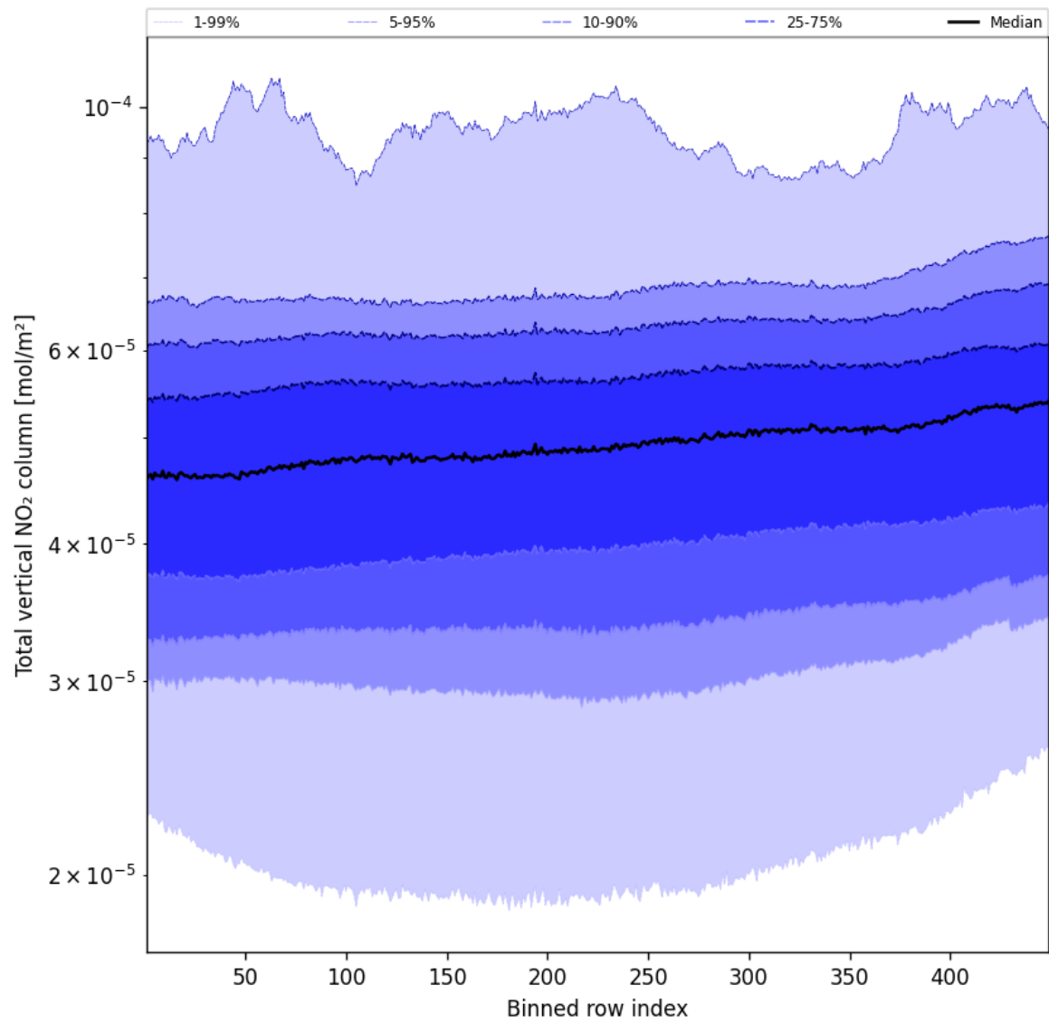
Figure 55: Along track statistics of “Total vertical NO 2 column” for 2025-10-18 to 2025-10-20
