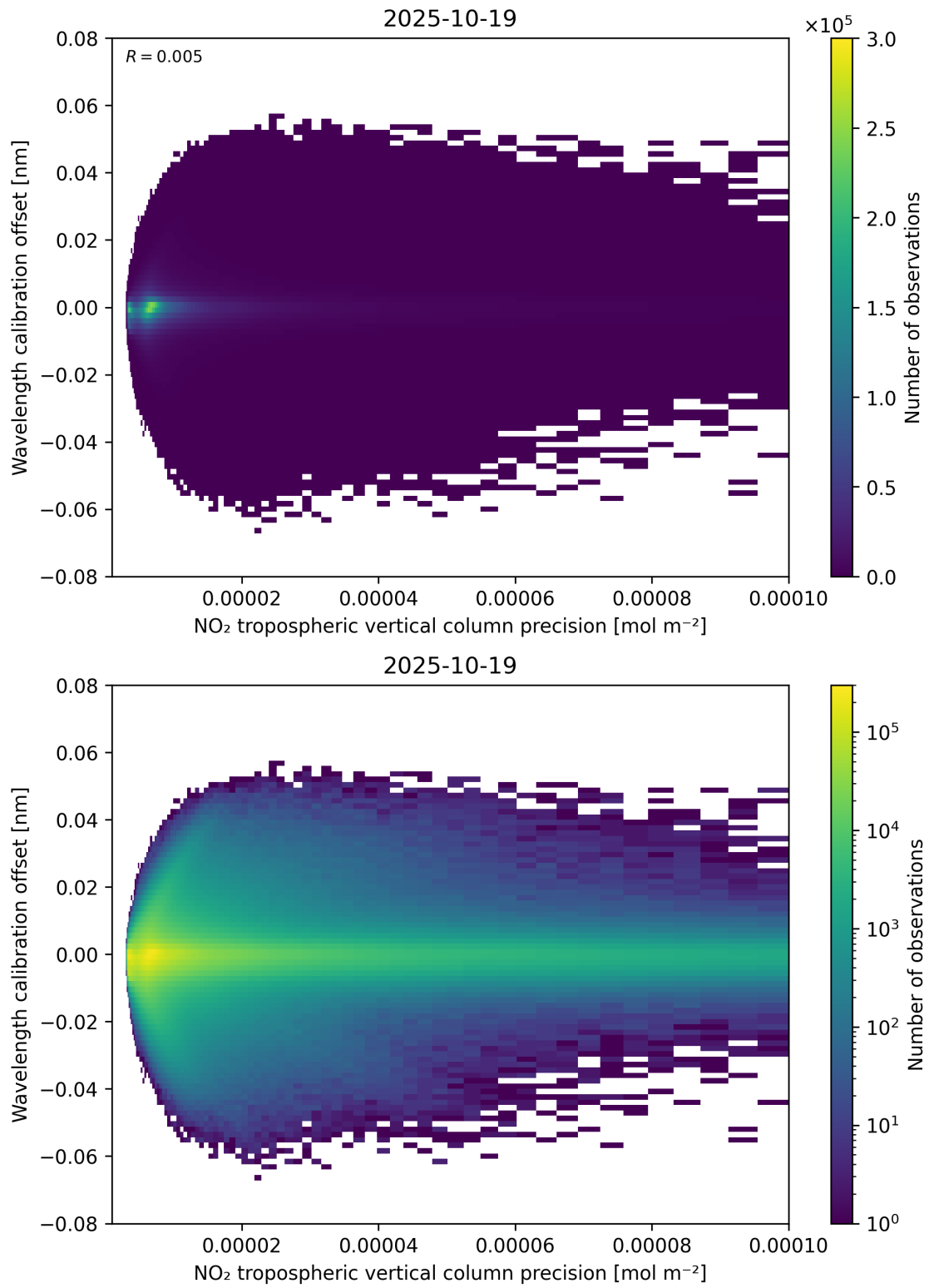
Figure 141: Scatter density plot of “NO 2 tropospheric vertical column precision” against “Wavelength calibration offset” for 2025-10-18 to 2025-10-20.
