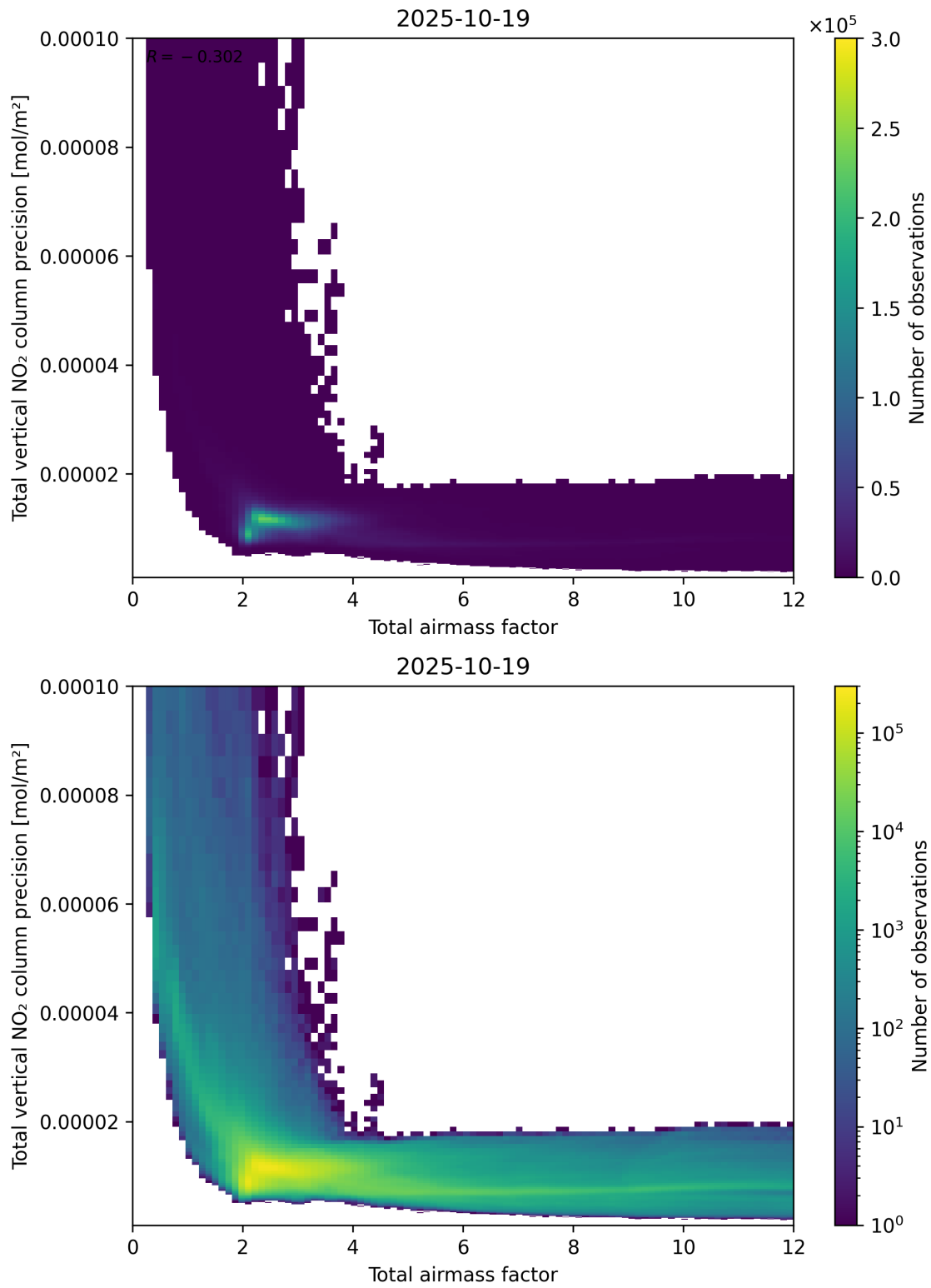
Figure 68: Scatter density plot of “Total airmass factor” against “Total vertical NO 2 column precision” for 2025-10-18 to 2025-10-20.
