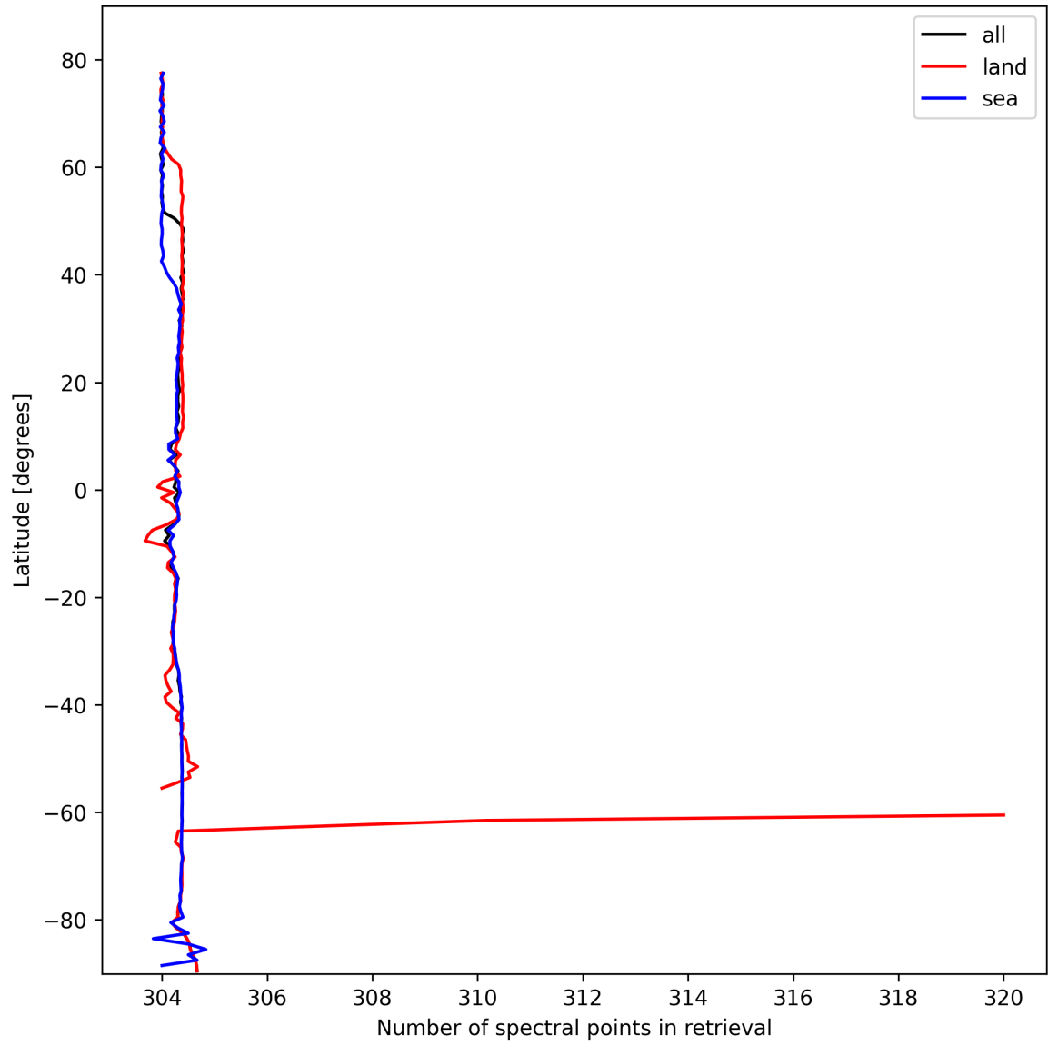
Figure 16: Zonal average of “Number of spectral points in retrieval” for 2025-10-18 to 2025-10-20.
