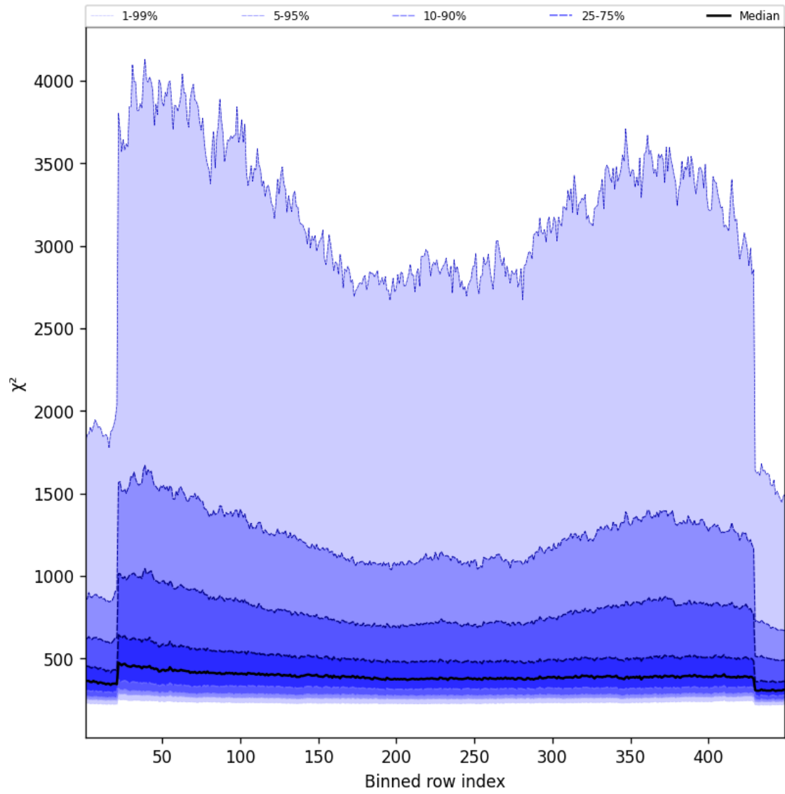
Figure 59: Along track statistics of “ \chi^2 ” for 2025-10-18 to 2025-10-20
