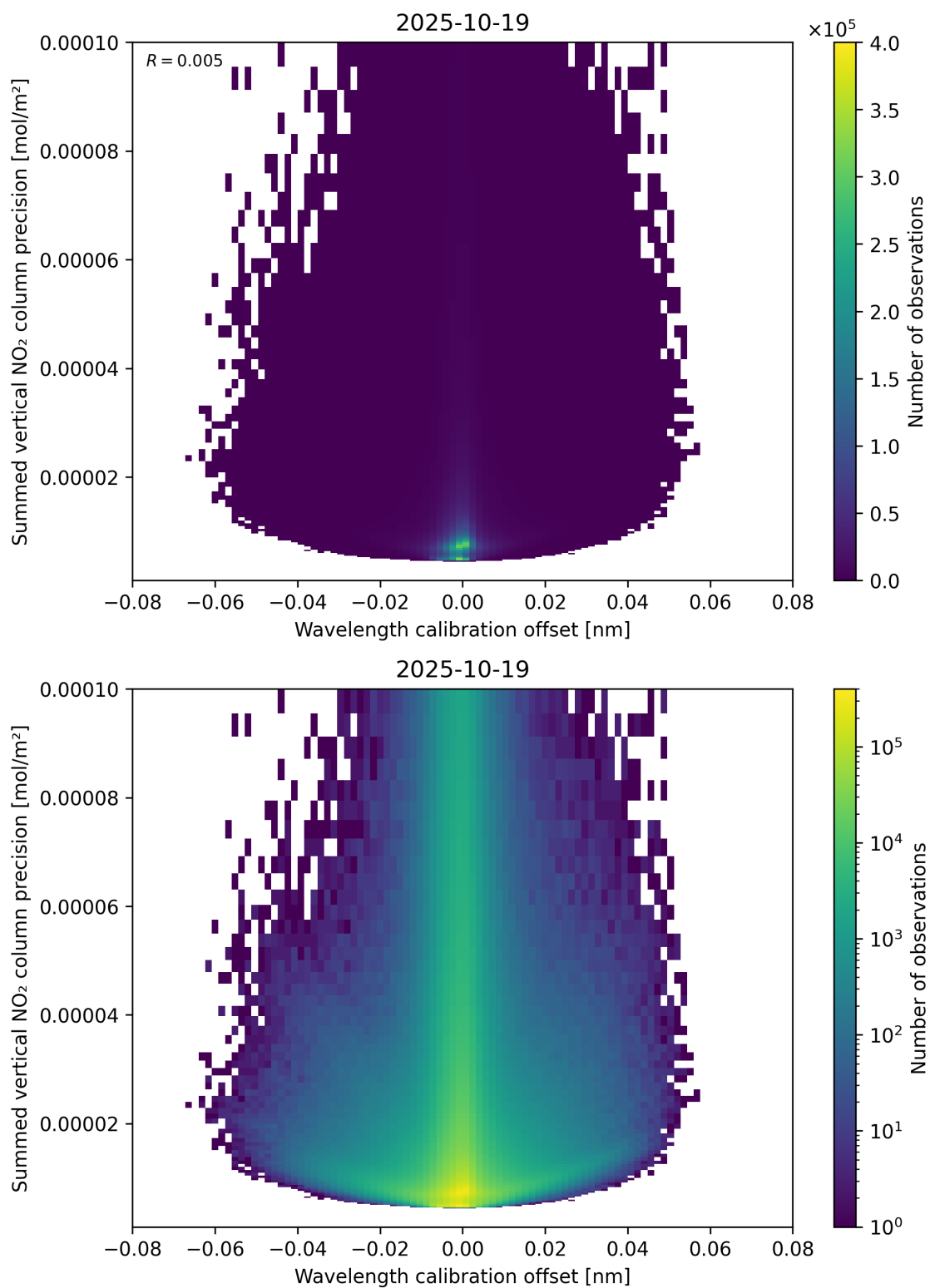
Figure 178: Scatter density plot of “Wavelength calibration offset” against “Summed vertical NO 2 column precision” for 2025-10-18 to 2025-10-20.
