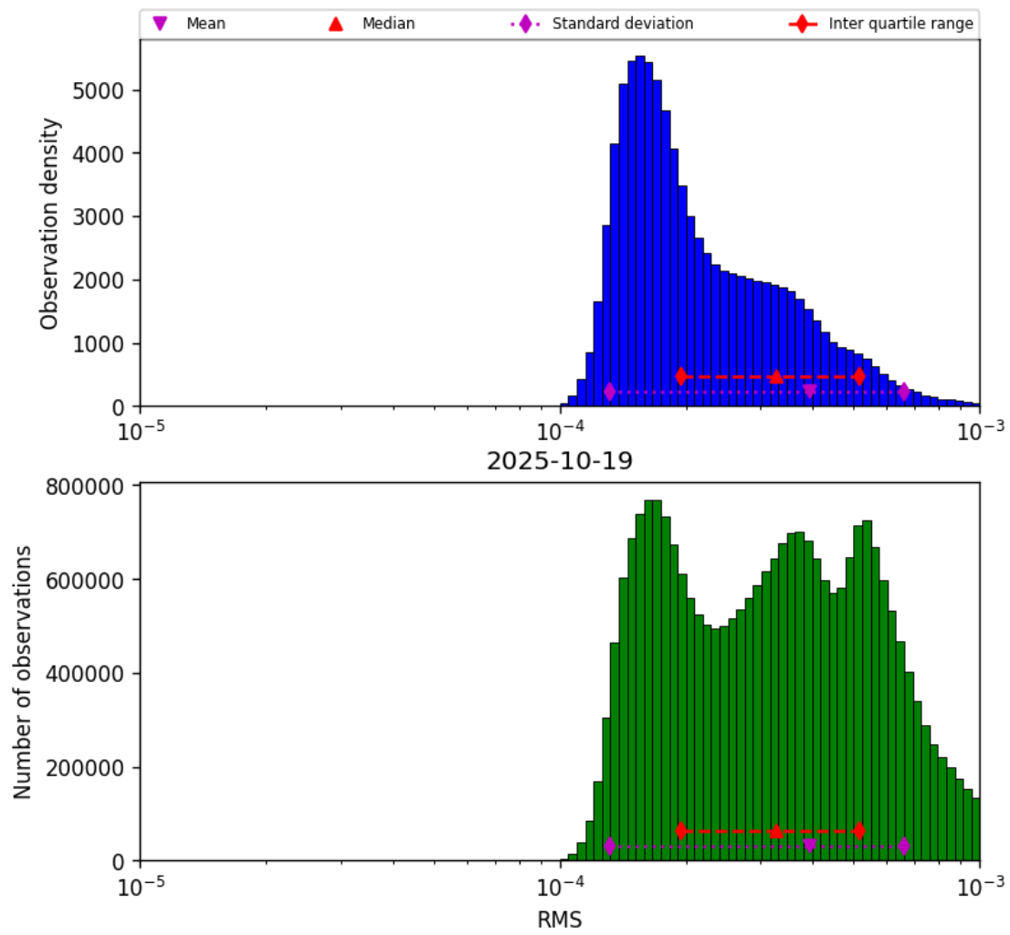
Figure 43: Histogram of “RMS” for 2025-10-18 to 2025-10-20
