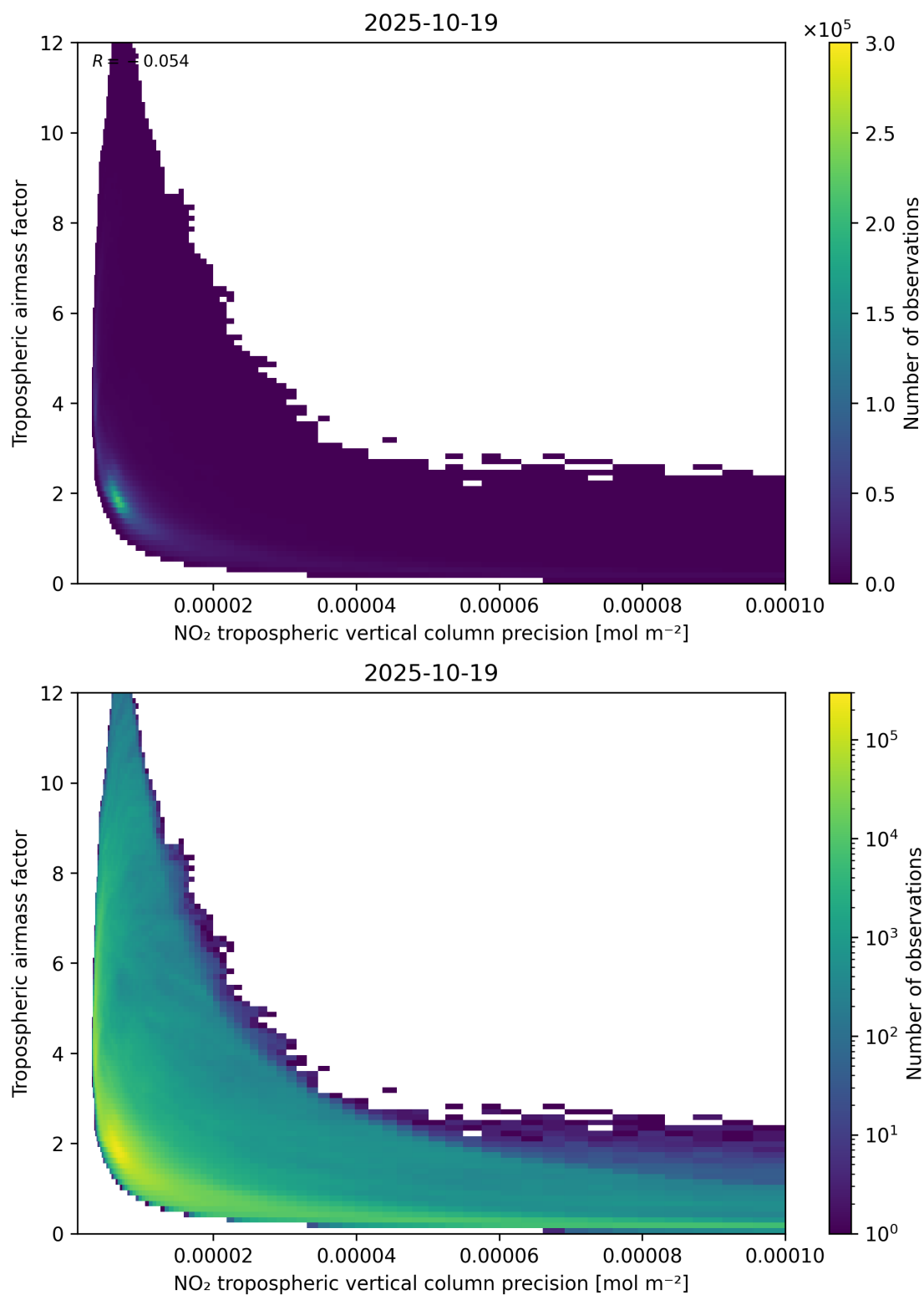
Figure 133: Scatter density plot of “NO 2 tropospheric vertical column precision” against “Tropospheric airmass factor” for 2025-10-18 to 2025-10-20.
