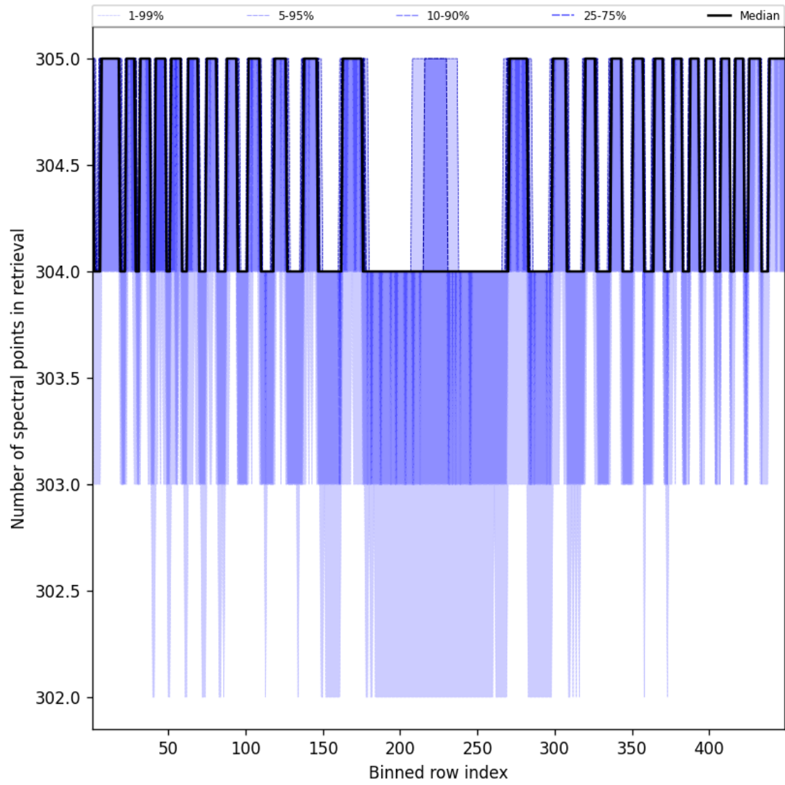
Figure 50: Along track statistics of “Number of spectral points in retrieval” for 2025-10-18 to 2025-10-20
