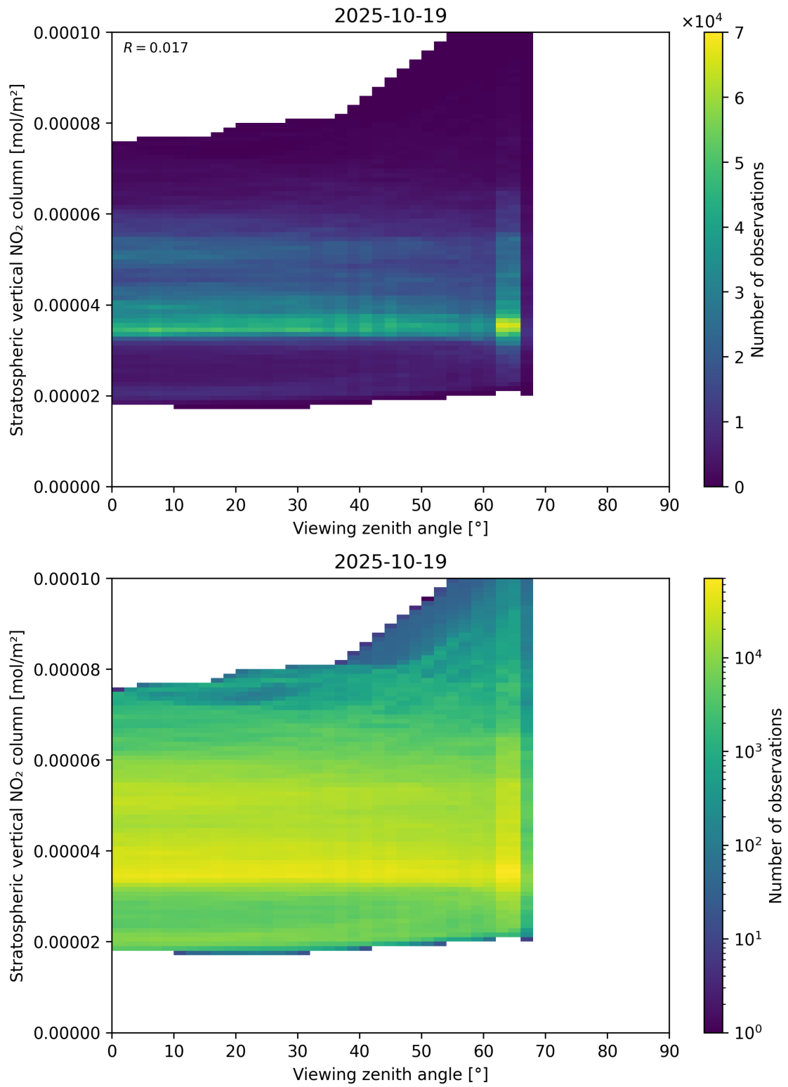
Figure 164: Scatter density plot of “Viewing zenith angle” against “Stratospheric vertical NO 2 column” for 2025-10-18 to 2025-10-20.
