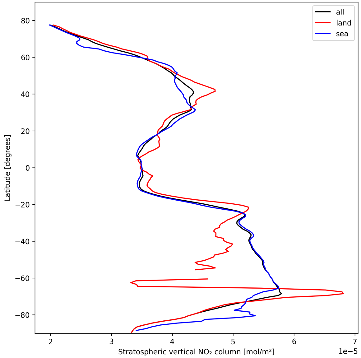
Figure 19: Zonal average of “Stratospheric vertical NO 2 column” for 2025-10-18 to 2025-10-20.
