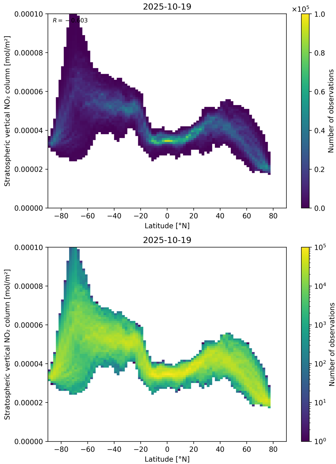
Figure 87: Scatter density plot of “Latitude” against “Stratospheric vertical NO 2 column” for 2025-10-18 to 2025-10-20.
