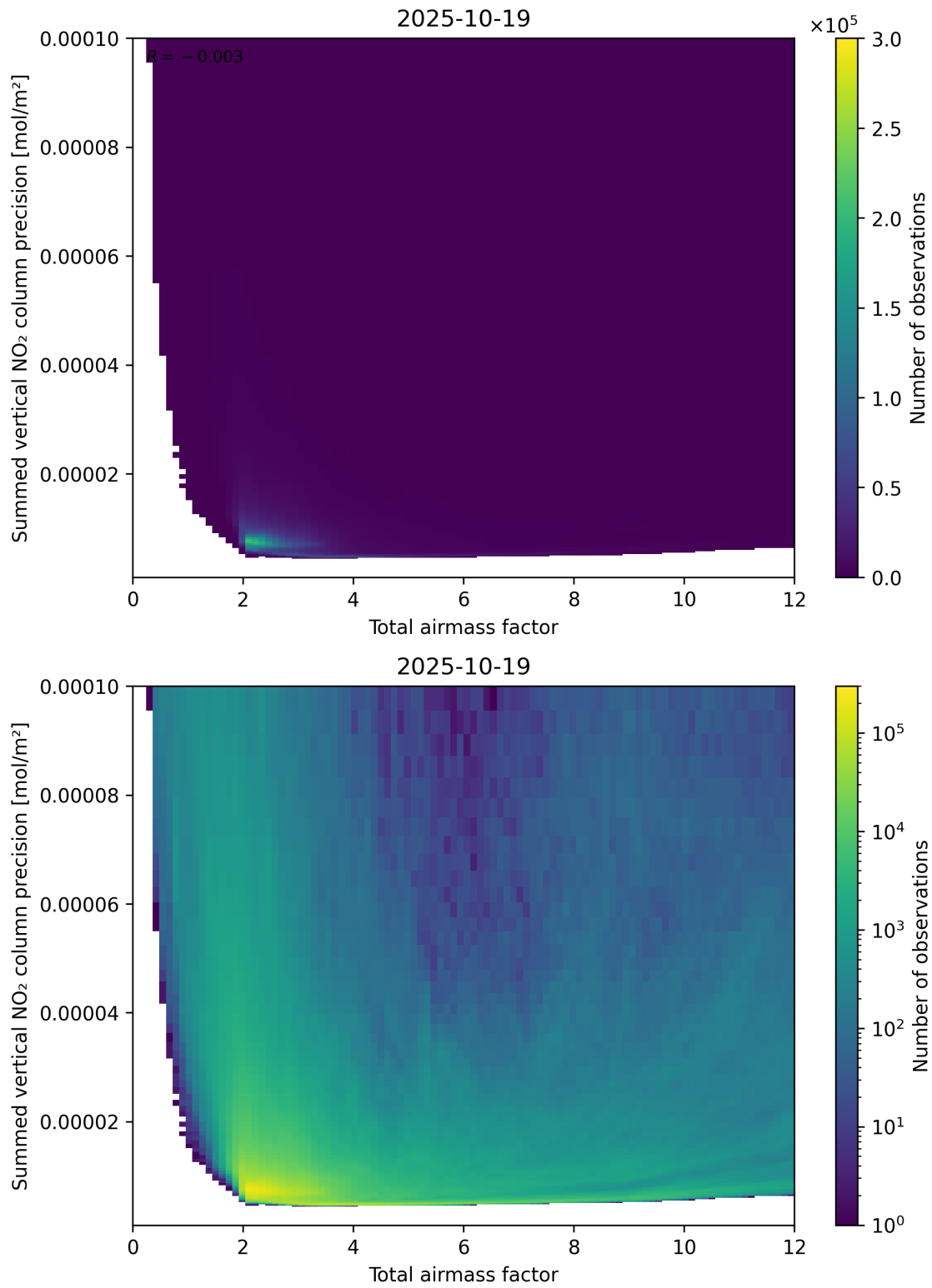
Figure 66: Scatter density plot of “Total airmass factor” against “Summed vertical NO 2 column precision” for 2025-10-18 to 2025-10-20.
