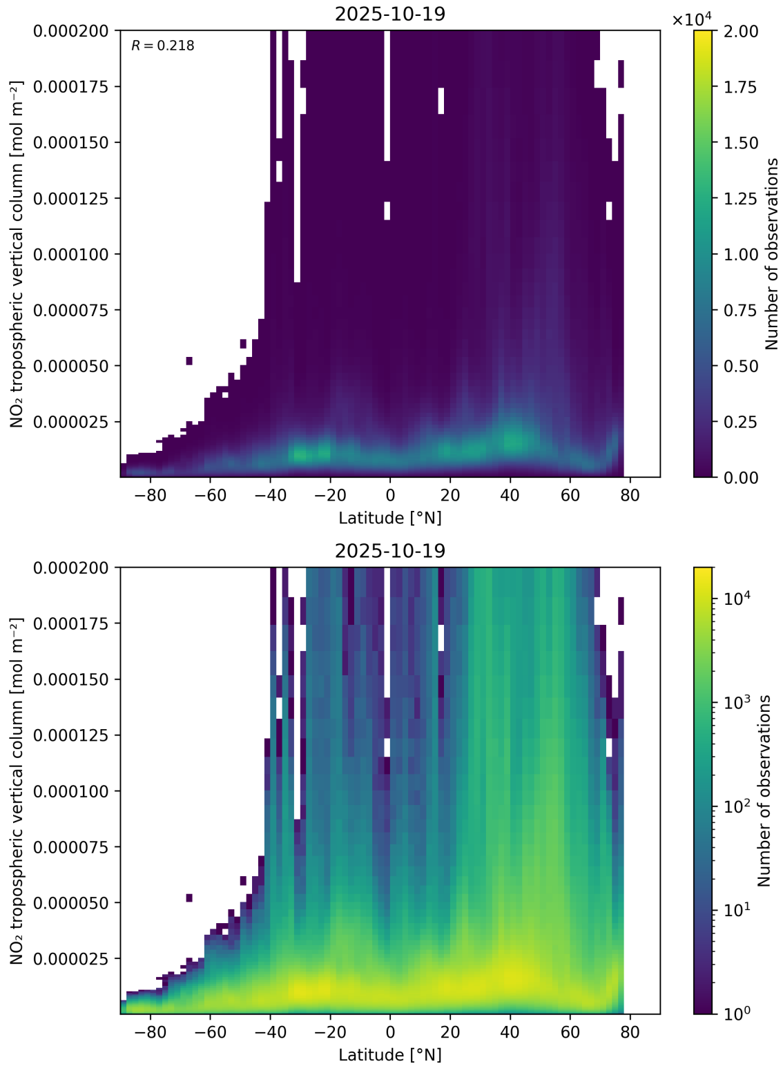
Figure 92: Scatter density plot of “Latitude” against “NO 2 tropospheric vertical column” for 2025-10-18 to 2025-10-20.
