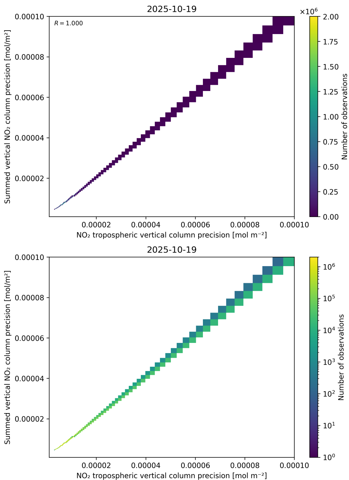
Figure 137: Scatter density plot of “NO 2 tropospheric vertical column precision” against “Summed vertical NO 2 column precision” for 2025-10-18 to 2025-10-20.
