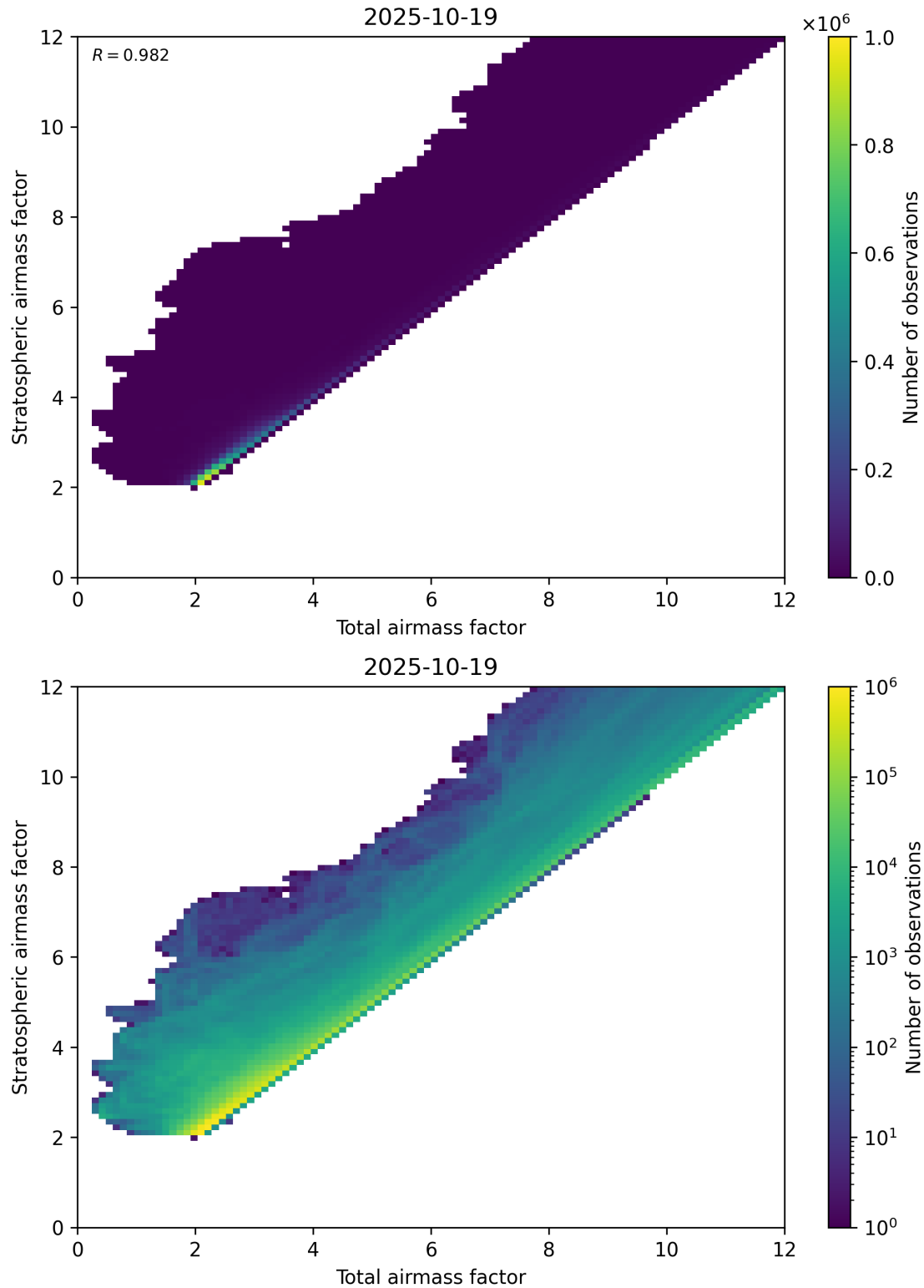
Figure 62: Scatter density plot of “Total airmass factor” against “Stratospheric airmass factor” for 2025-10-18 to 2025-10-20.
