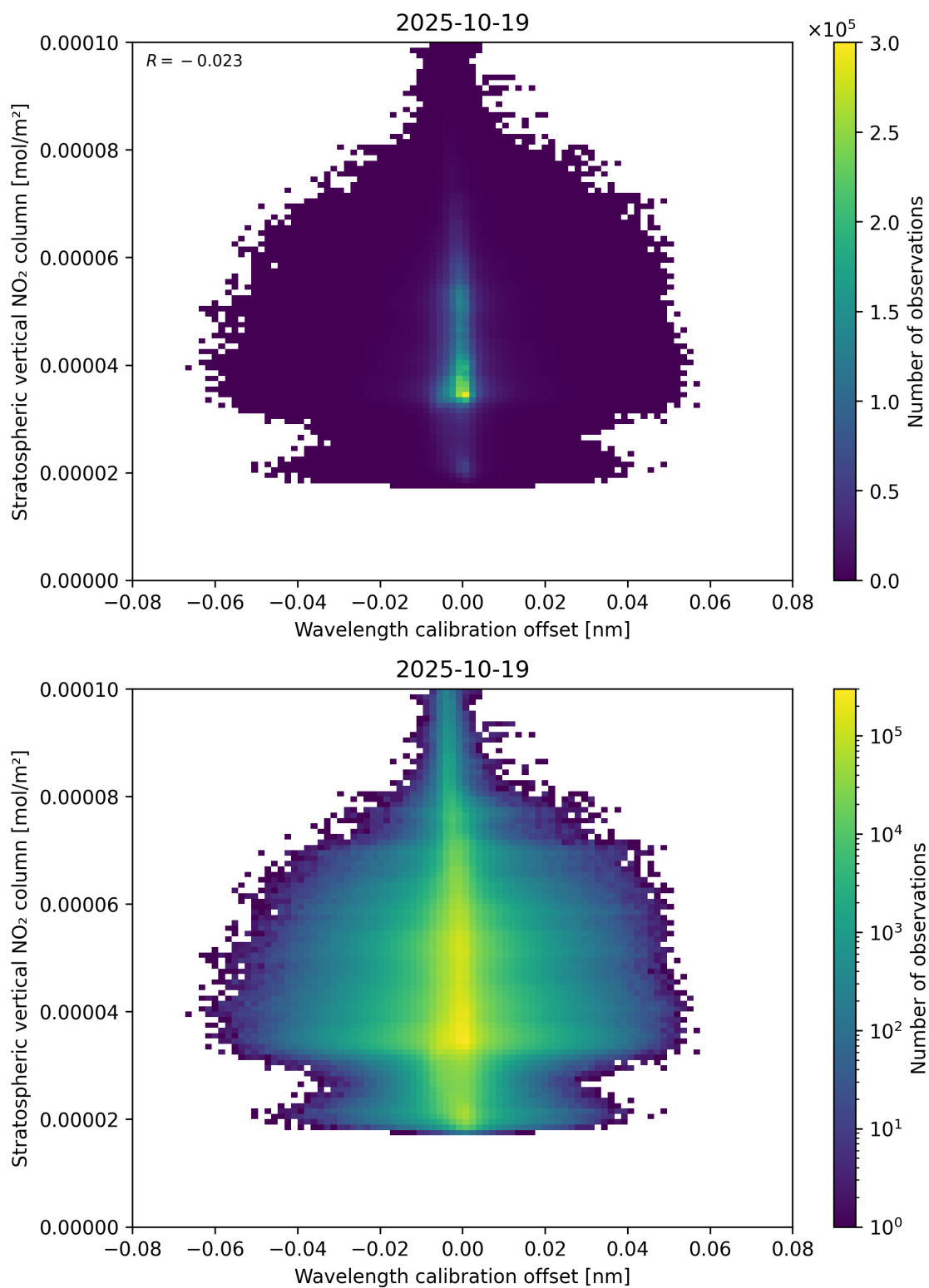
Figure 176: Scatter density plot of “Wavelength calibration offset” against “Stratospheric vertical NO 2 column” for 2025-10-18 to 2025-10-20.
