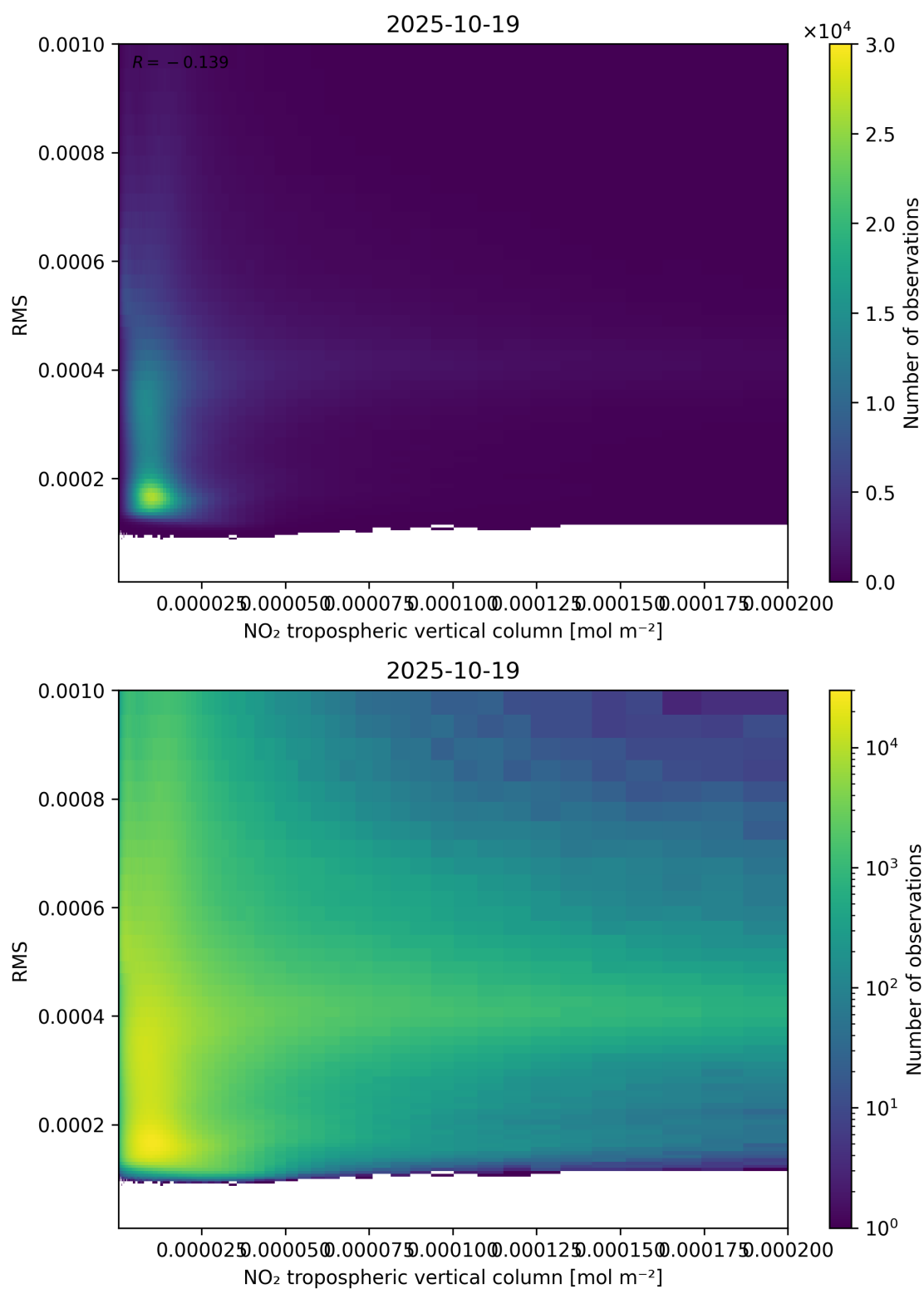
Figure 142: Scatter density plot of “NO 2 tropospheric vertical column” against “RMS” for 2025-10-18 to 2025-10-20.
