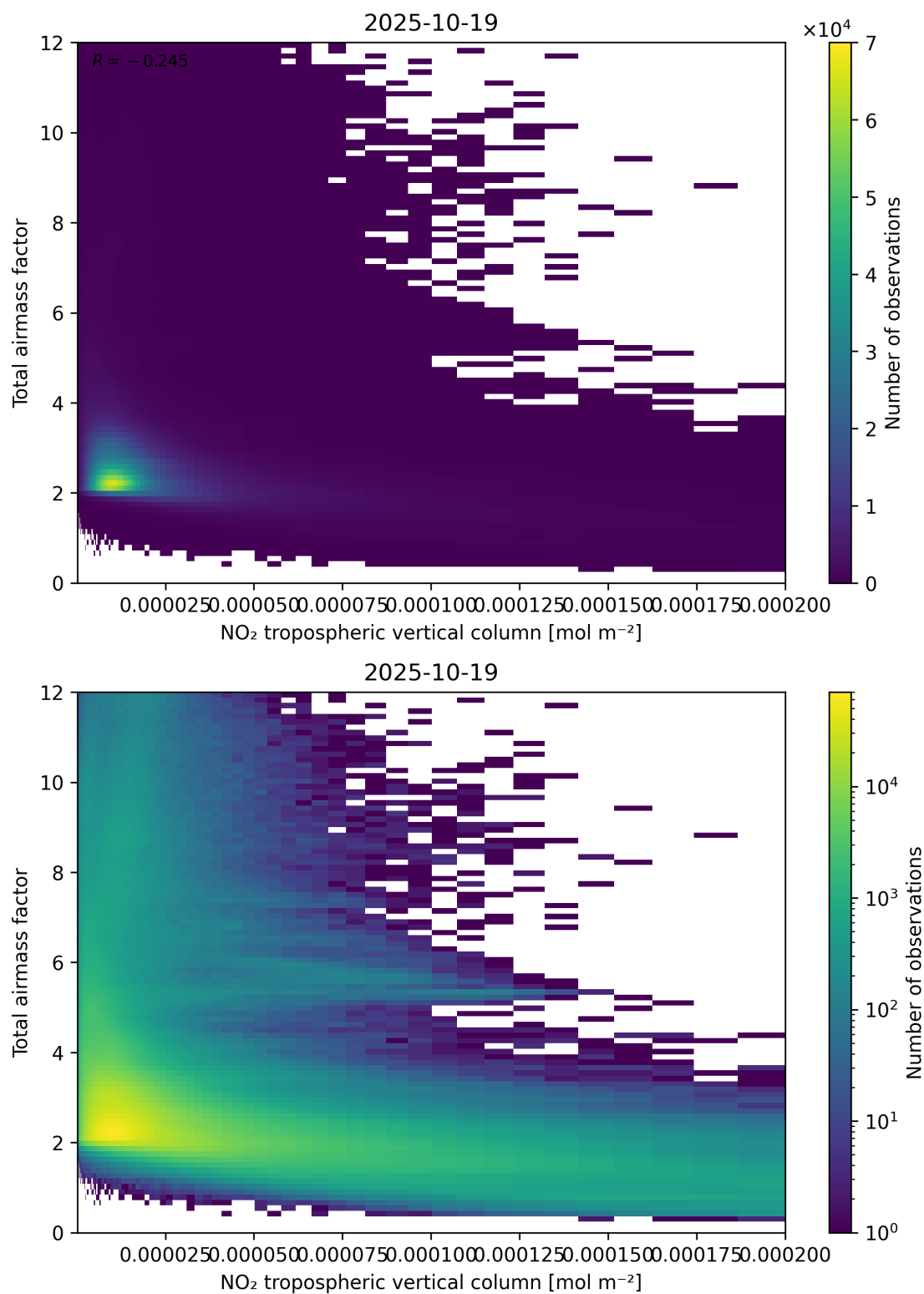
Figure 122: Scatter density plot of “NO 2 tropospheric vertical column” against “Total air mass factor” for 2025-10-18 to 2025-10-20.
