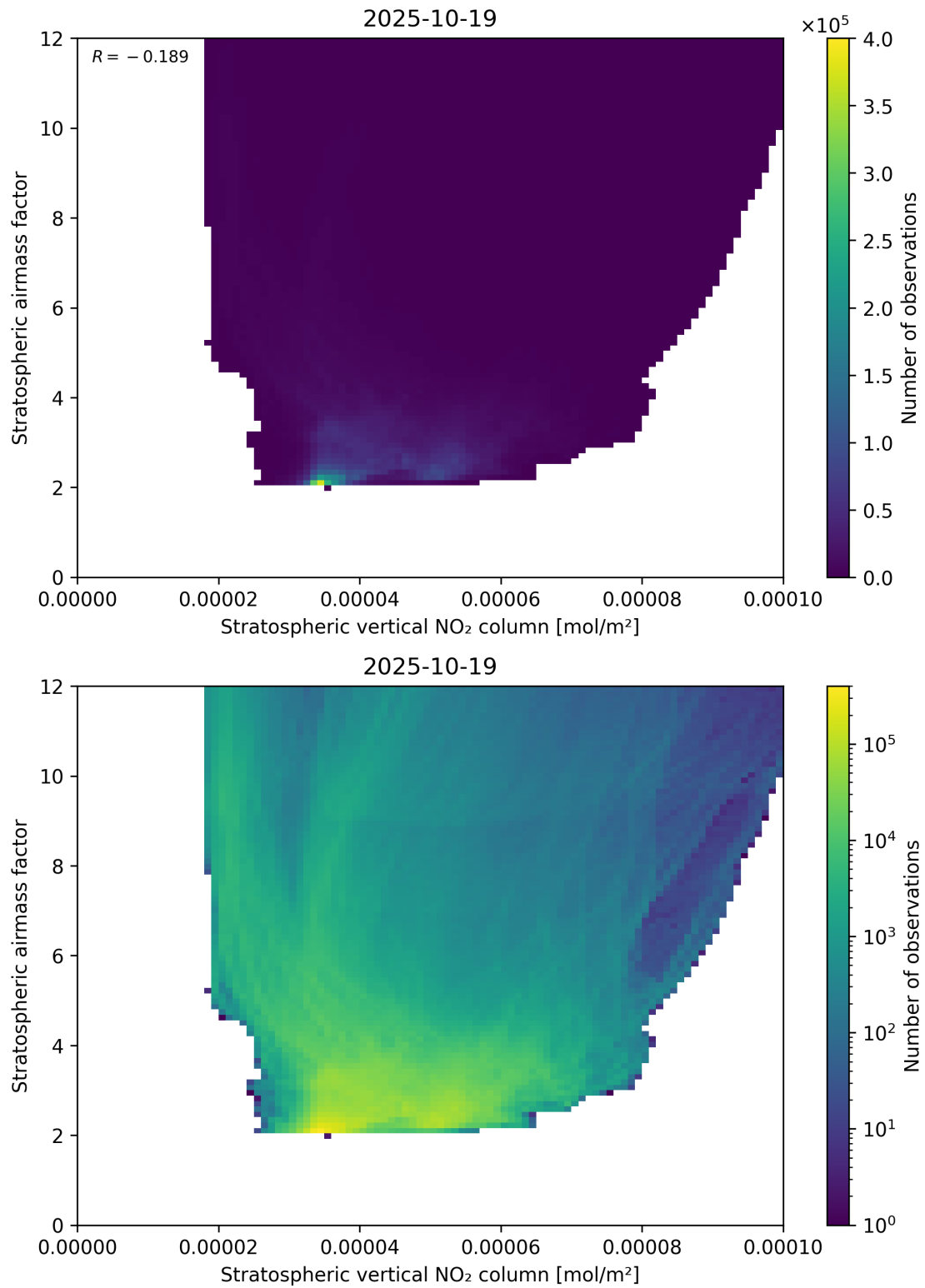
Figure 96: Scatter density plot of “Stratospheric vertical NO 2 column” against “Stratospheric airmass factor” for 2025-10-18 to 2025-10-20.
