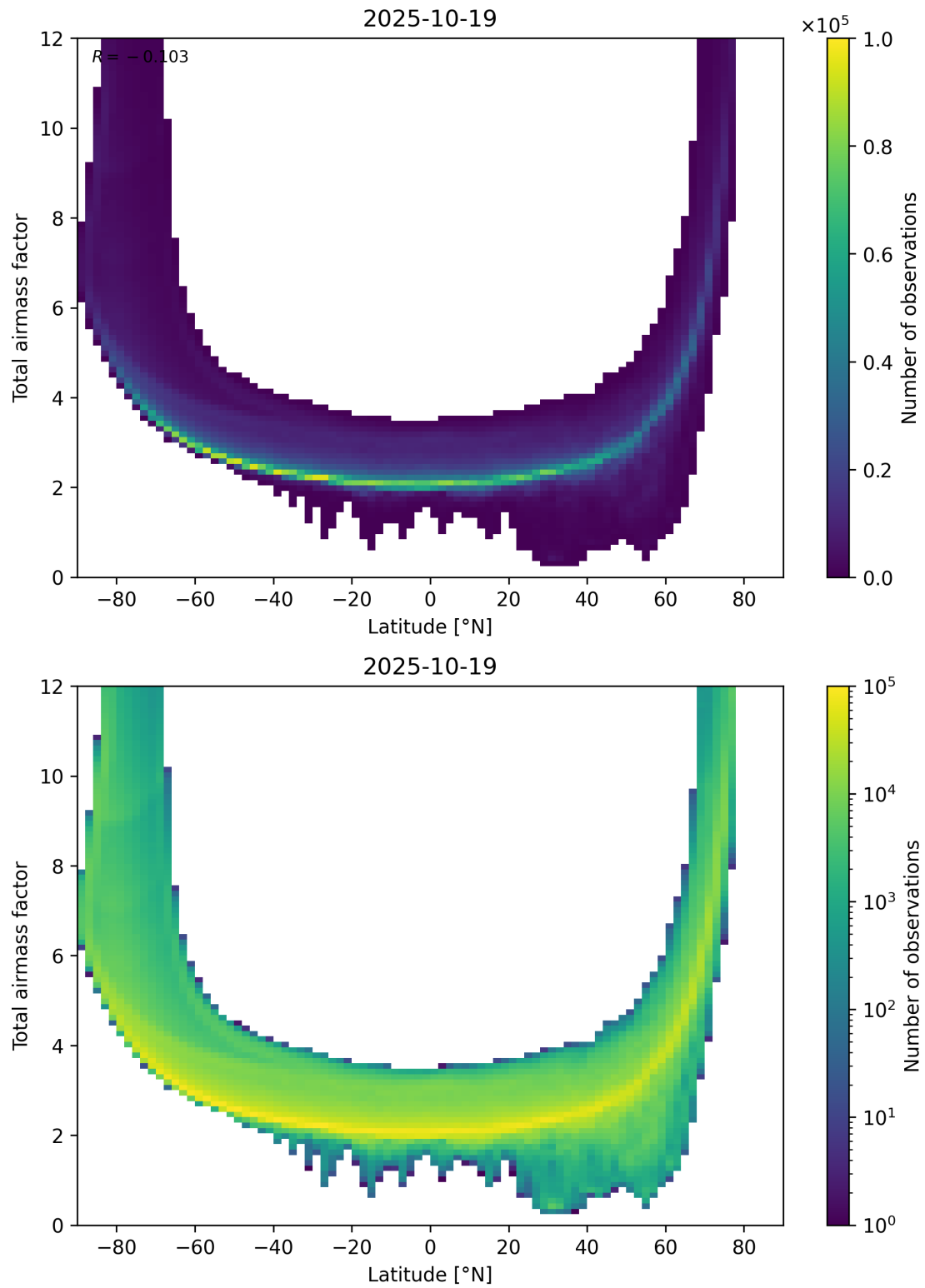
Figure 84: Scatter density plot of “Latitude” against “Total airmass factor” for 2025-10-18 to 2025-10-20.
