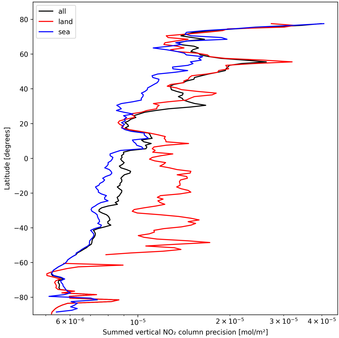
Figure 24: Zonal average of “Summed vertical NO 2 column precision” for 2025-10-18 to 2025-10-20.
