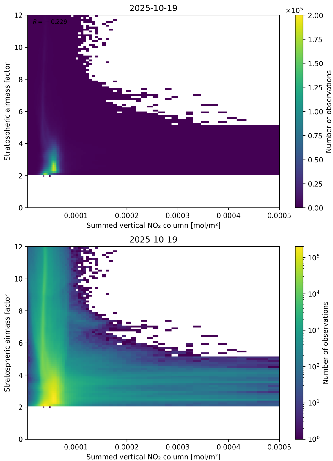
Figure 103: Scatter density plot of “Summed vertical NO 2 column” against “Stratospheric air mass factor” for 2025-10-18 to 2025-10-20.
