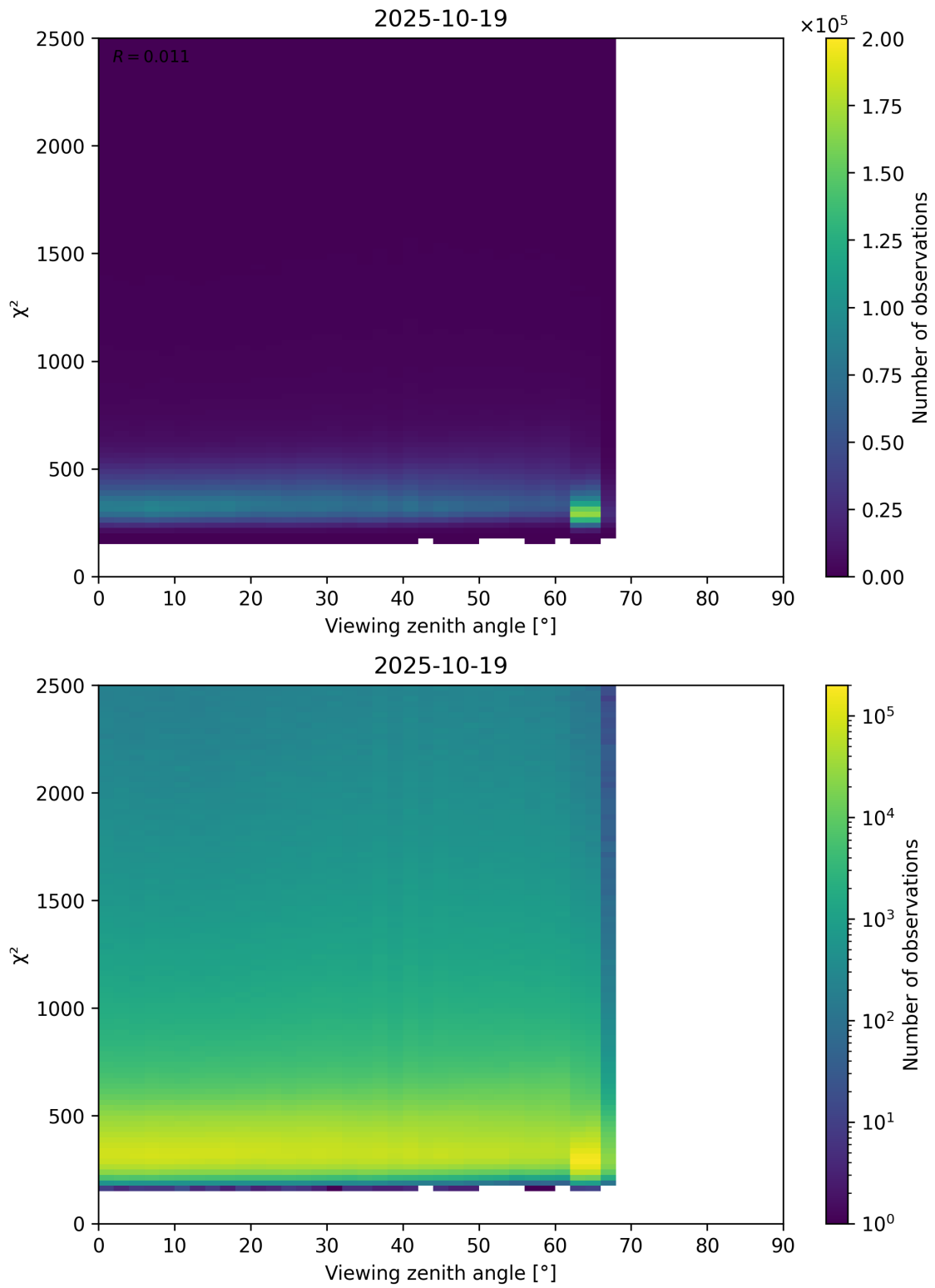
Figure 162: Scatter density plot of “Viewing zenith angle” against “ \chi^2 ” for 2025-10-18 to 2025-10-20.
