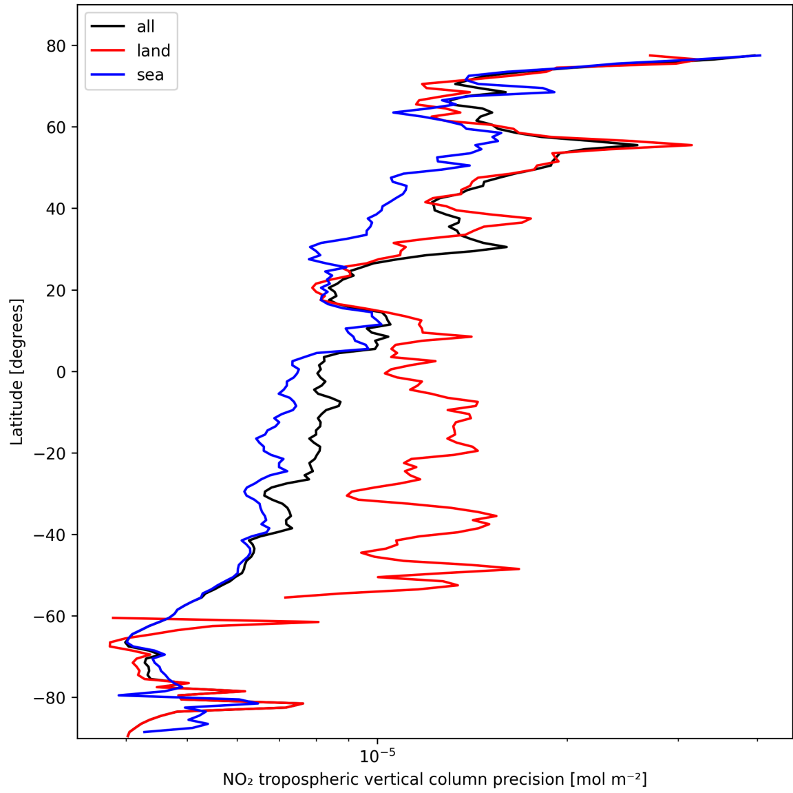
Figure 13: Zonal average of “NO 2 tropospheric vertical column precision” for 2025-10-18 to 2025-10-20.
