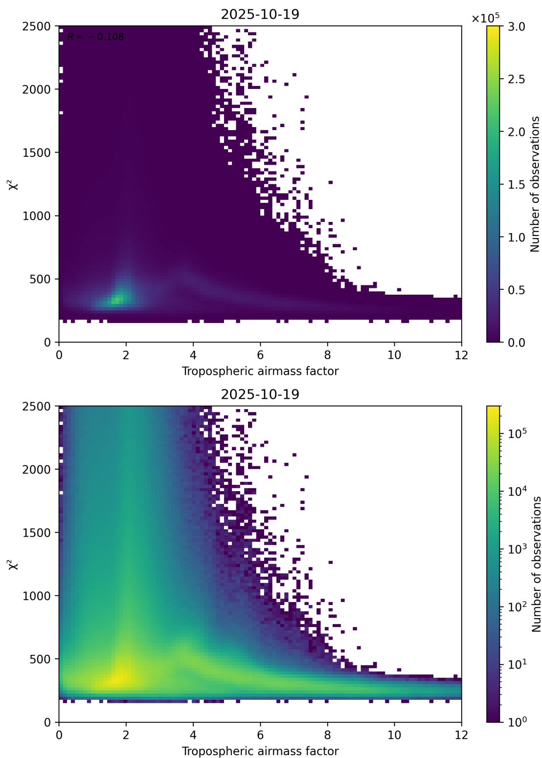
Figure 73: Scatter density plot of “Tropospheric airmass factor” against “ \chi^2 ” for 2025-10-18 to 2025-10-20.
