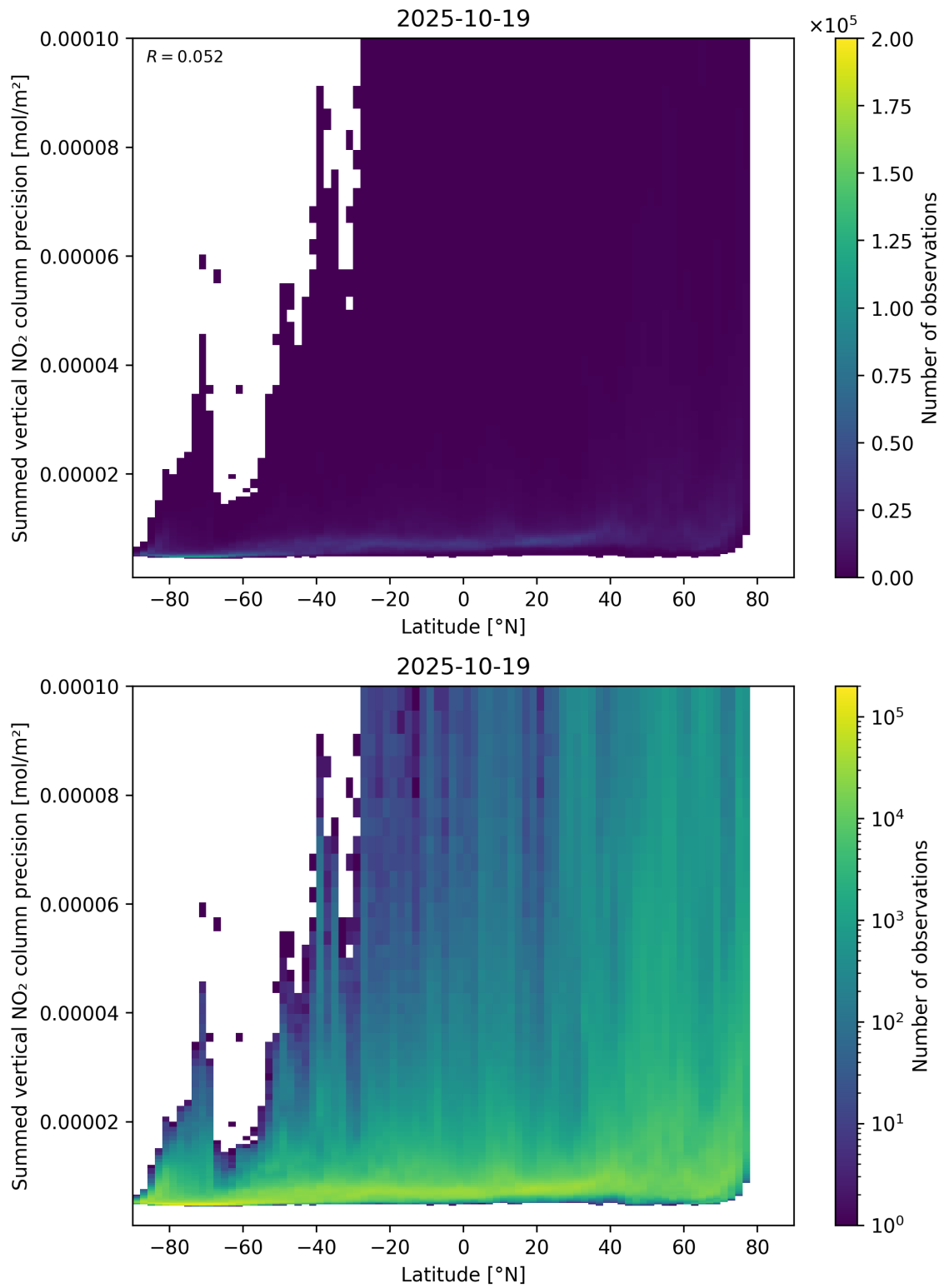
Figure 89: Scatter density plot of “Latitude” against “Summed vertical NO 2 column precision” for 2025-10-18 to 2025-10-20.
