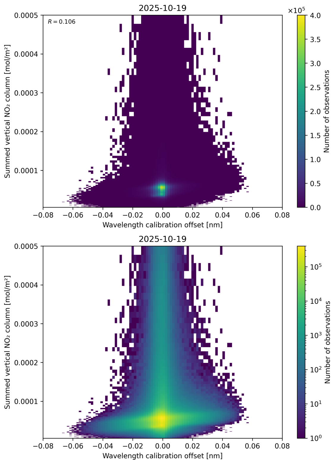
Figure 177: Scatter density plot of “Wavelength calibration offset” against “Summed vertical NO 2 column” for 2025-10-18 to 2025-10-20.
