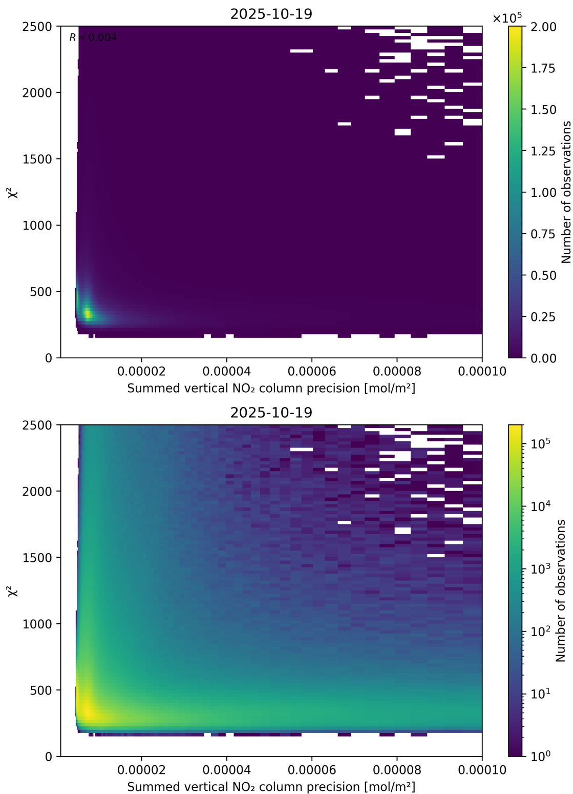
Figure 107: Scatter density plot of “Summed vertical NO 2 column precision” against “ \chi^2 ” for 2025-10-18 to 2025-10-20.
