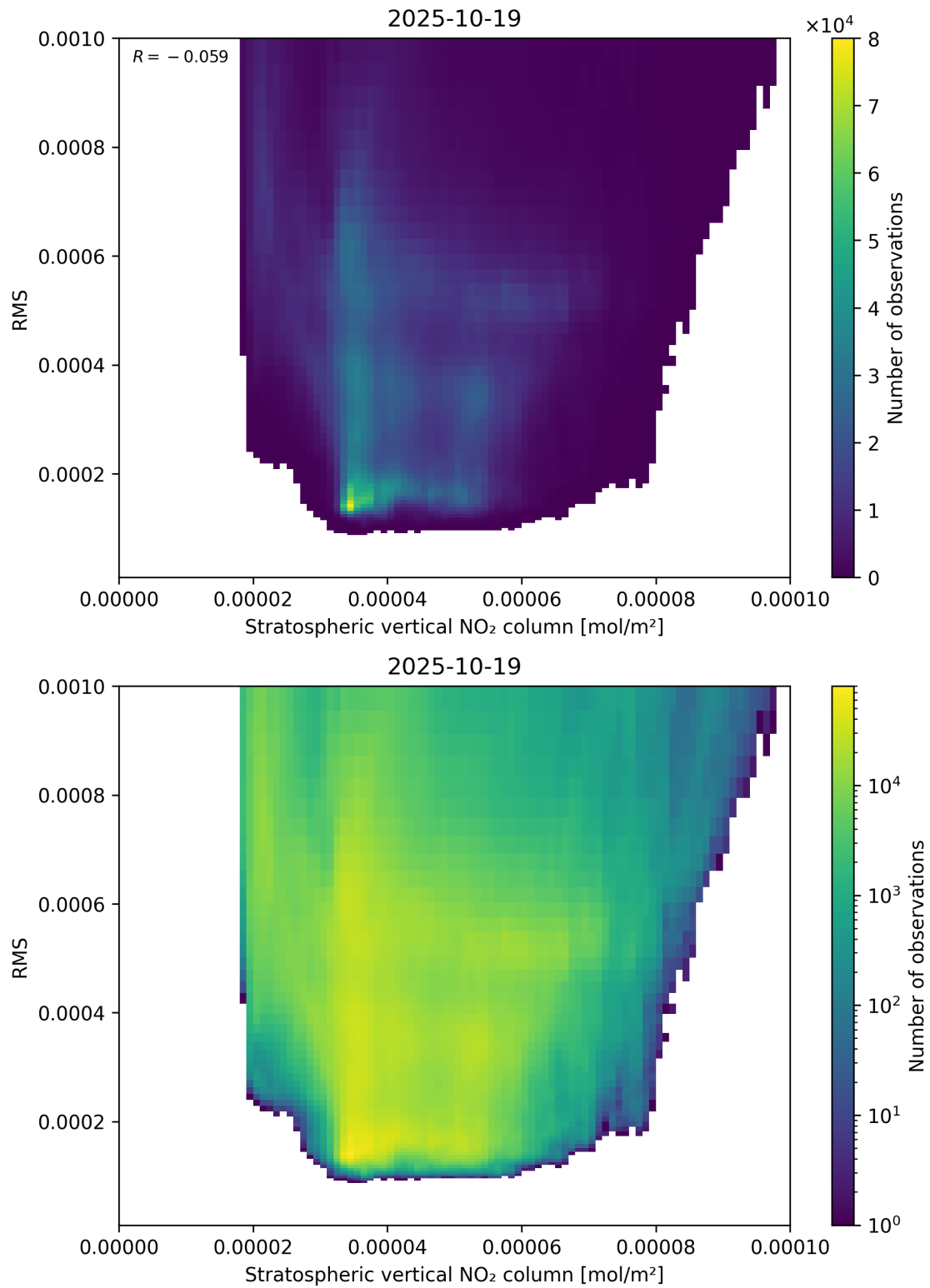
Figure 102: Scatter density plot of “Stratospheric vertical NO 2 column” against “RMS” for 2025-10-18 to 2025-10-20.
