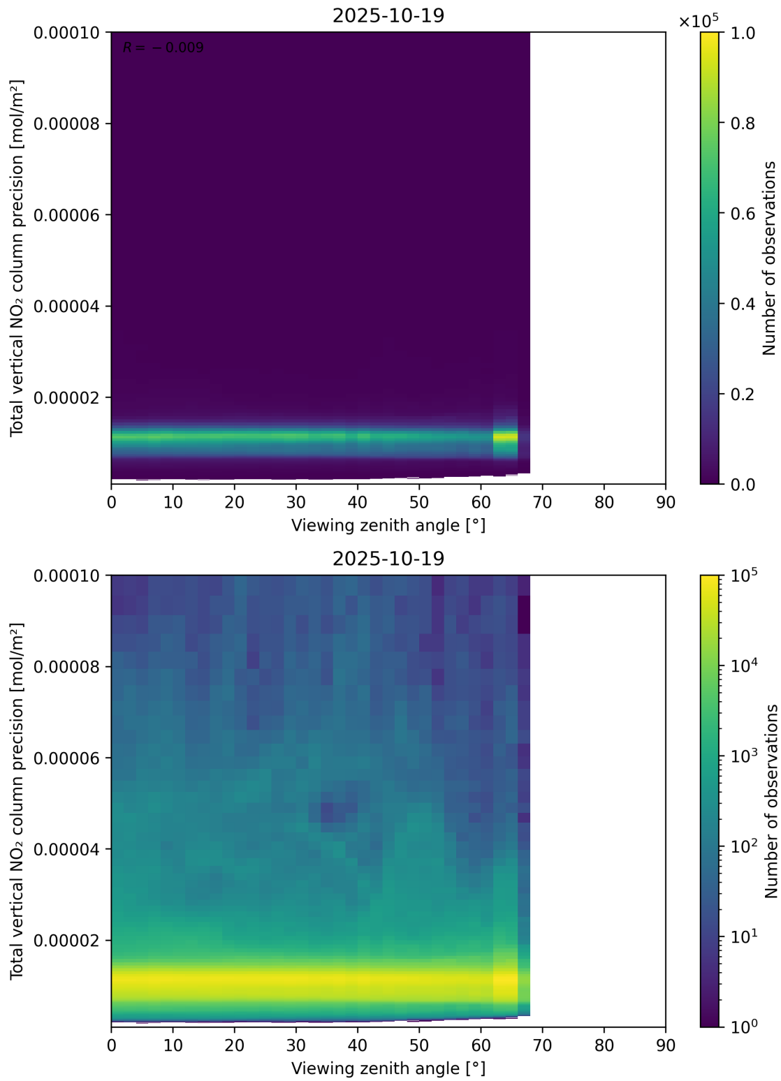
Figure 168: Scatter density plot of “Viewing zenith angle” against “Total vertical NO 2 column precision” for 2025-10-18 to 2025-10-20.
