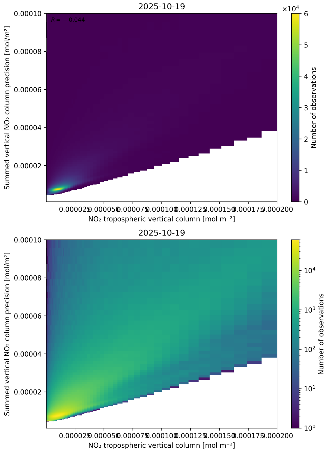
Figure 127: Scatter density plot of “NO 2 tropospheric vertical column” against “Summed vertical NO 2 column precision” for 2025-10-18 to 2025-10-20.
