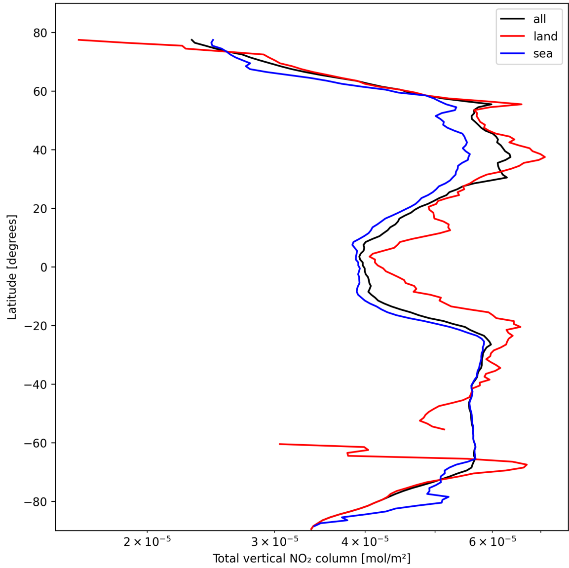
Figure 21: Zonal average of “Total vertical NO 2 column” for 2025-10-18 to 2025-10-20.
