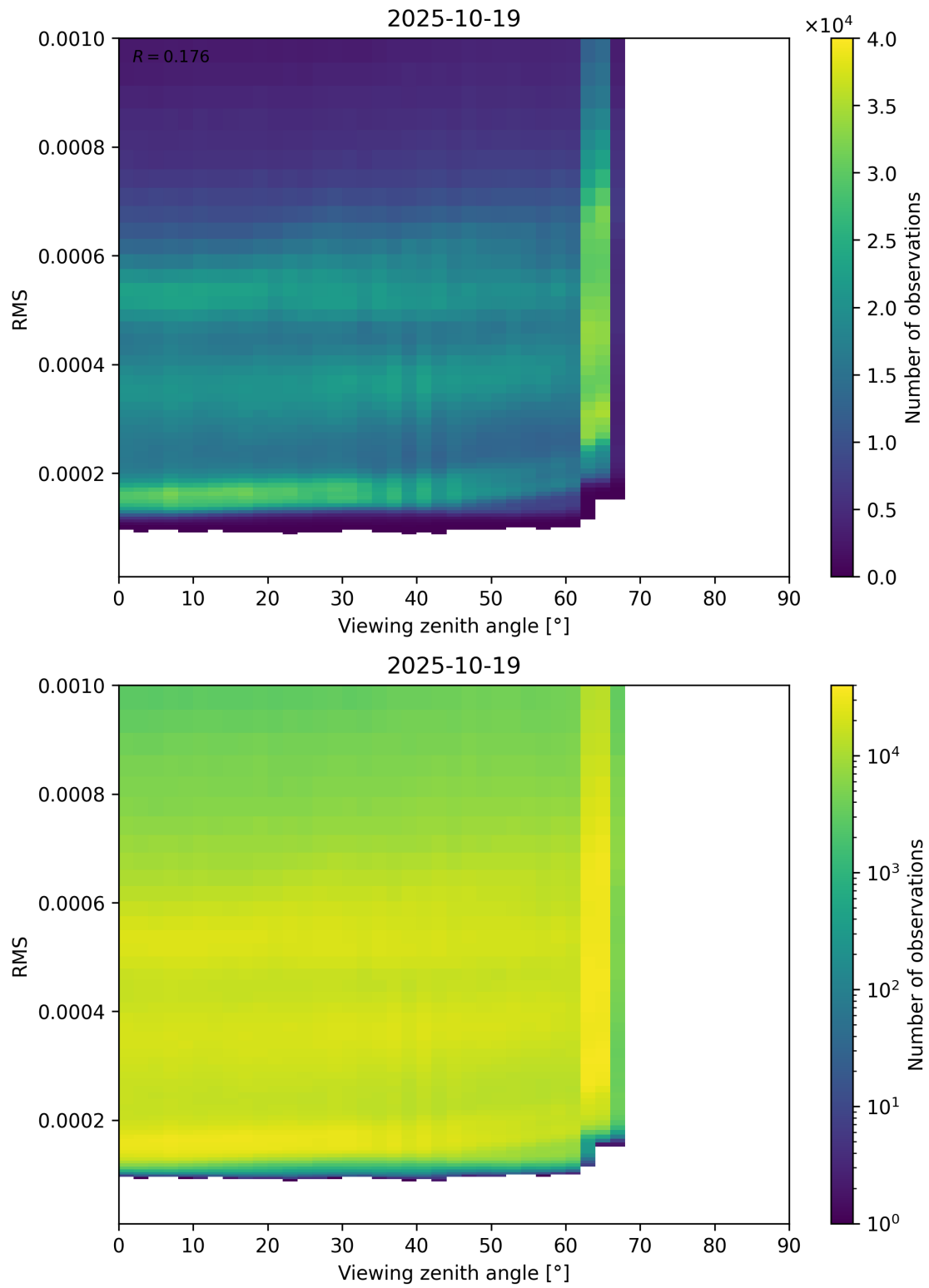
Figure 171: Scatter density plot of “Viewing zenith angle” against “RMS” for 2025-10-18 to 2025-10-20.
