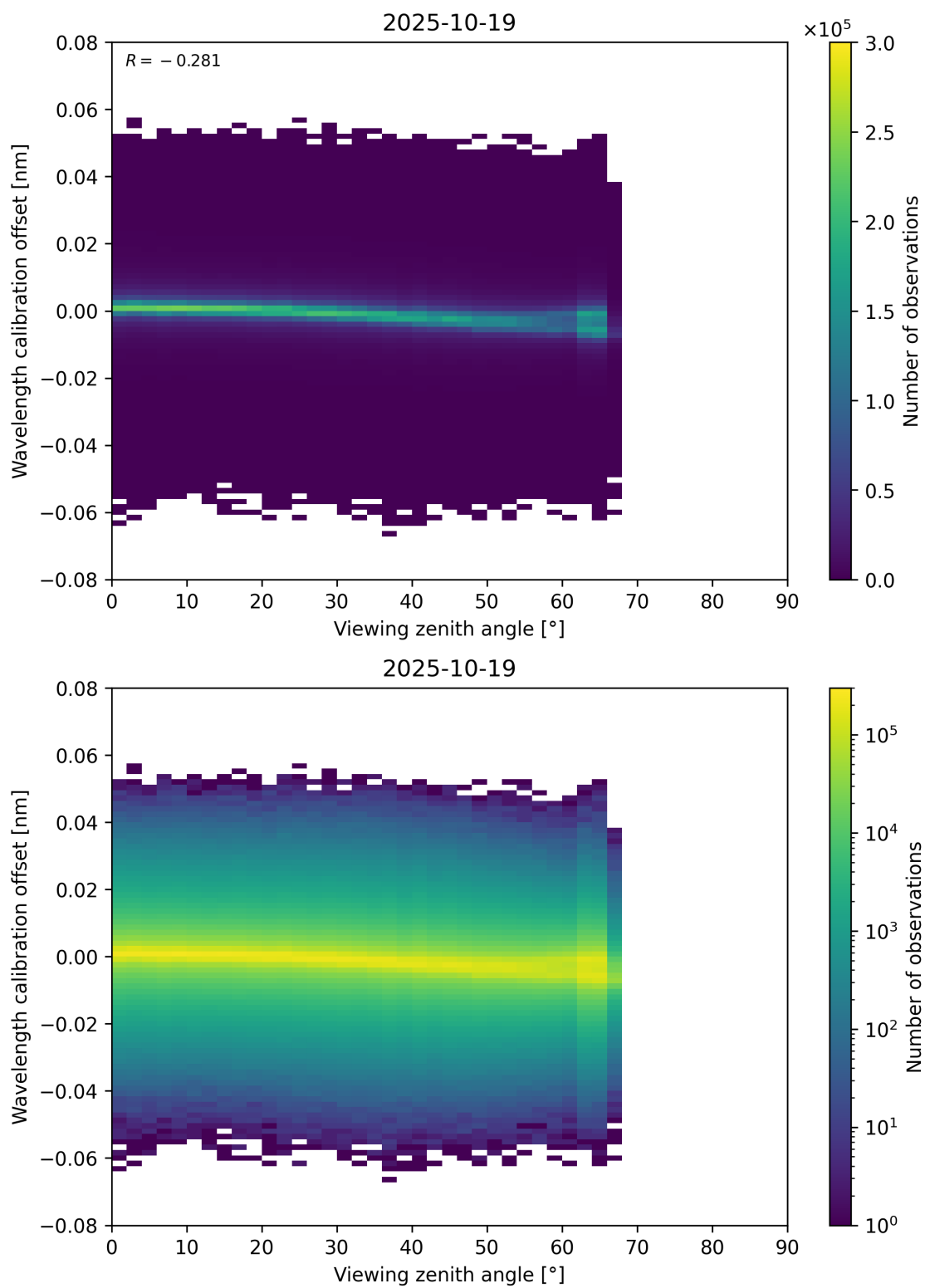
Figure 173: Scatter density plot of “Viewing zenith angle” against “Wavelength calibration offset” for 2025-10-18 to 2025-10-20.
