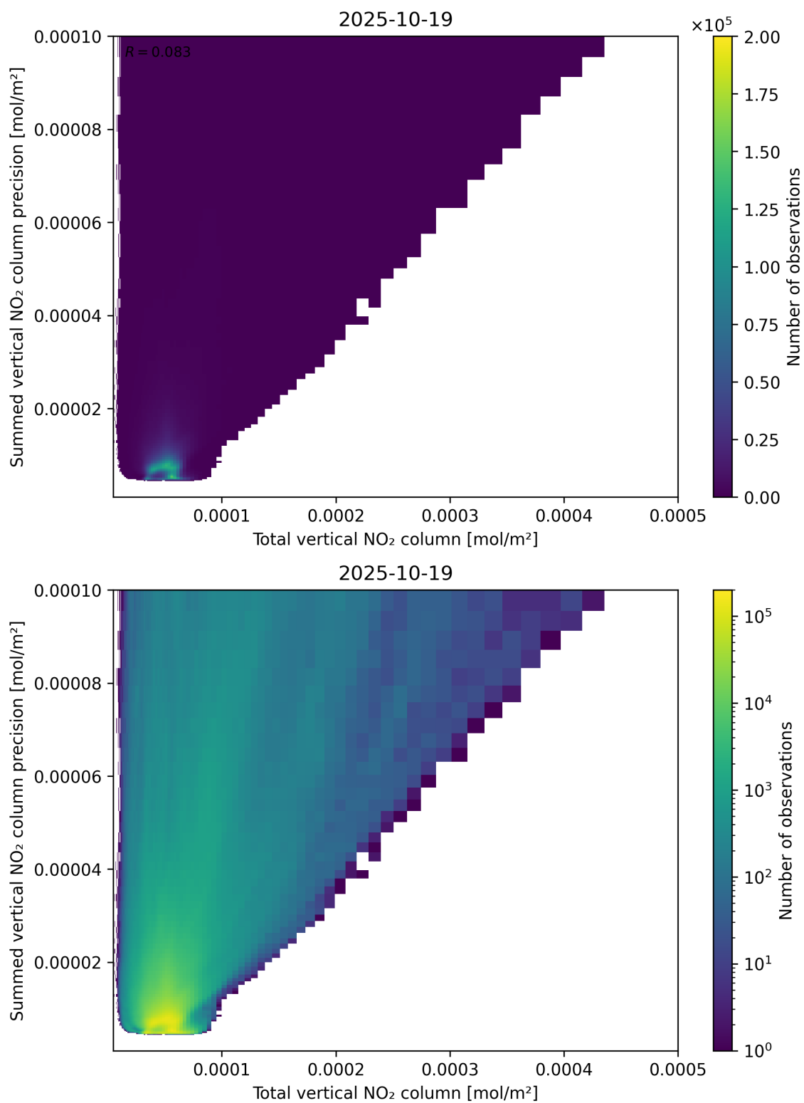
Figure 113: Scatter density plot of “Total vertical NO 2 column” against “Summed vertical NO 2 column precision” for 2025-10-18 to 2025-10-20.
