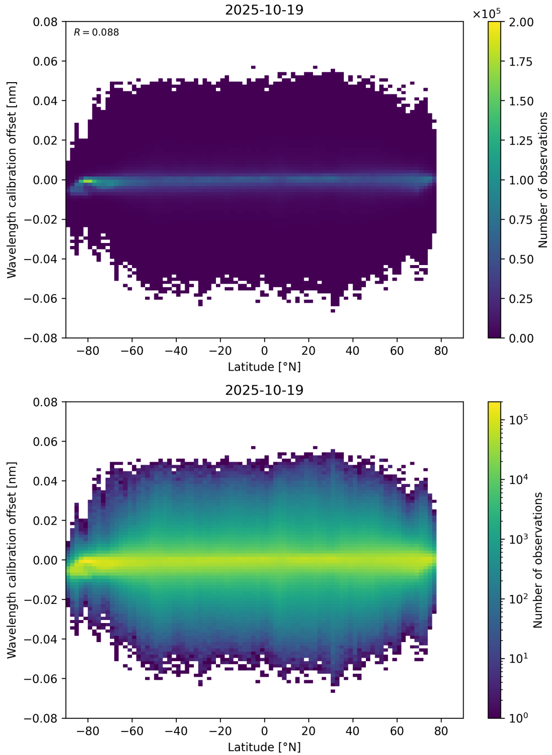
Figure 95: Scatter density plot of “Latitude” against “Wavelength calibration offset” for 2025-10-18 to 2025-10-20.
