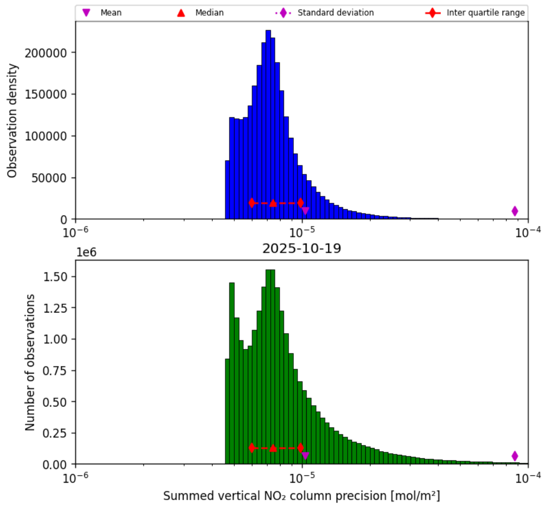
Figure 41: Histogram of "Summed vertical NO 2 column precision" for 2025-10-18 to 2025-10-20
