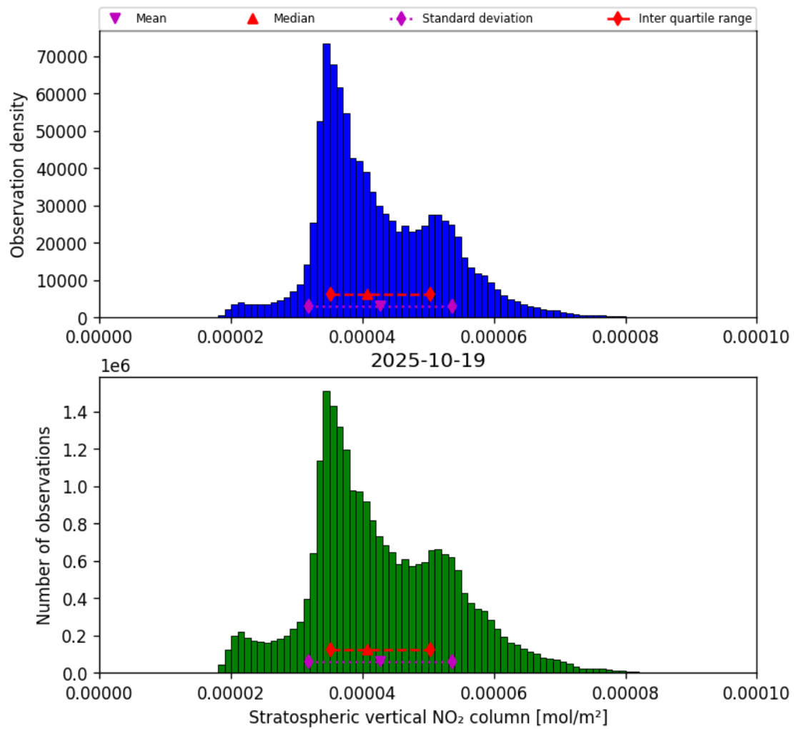
Figure 36: Histogram of “Stratospheric vertical NO 2 column” for 2025-10-18 to 2025-10-20
