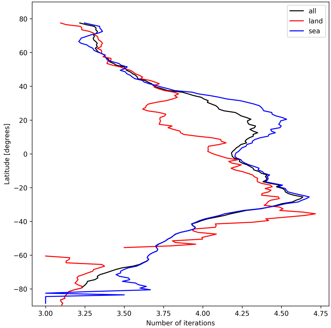
Figure 17: Zonal average of “Number of iterations” for 2025-10-18 to 2025-10-20.
