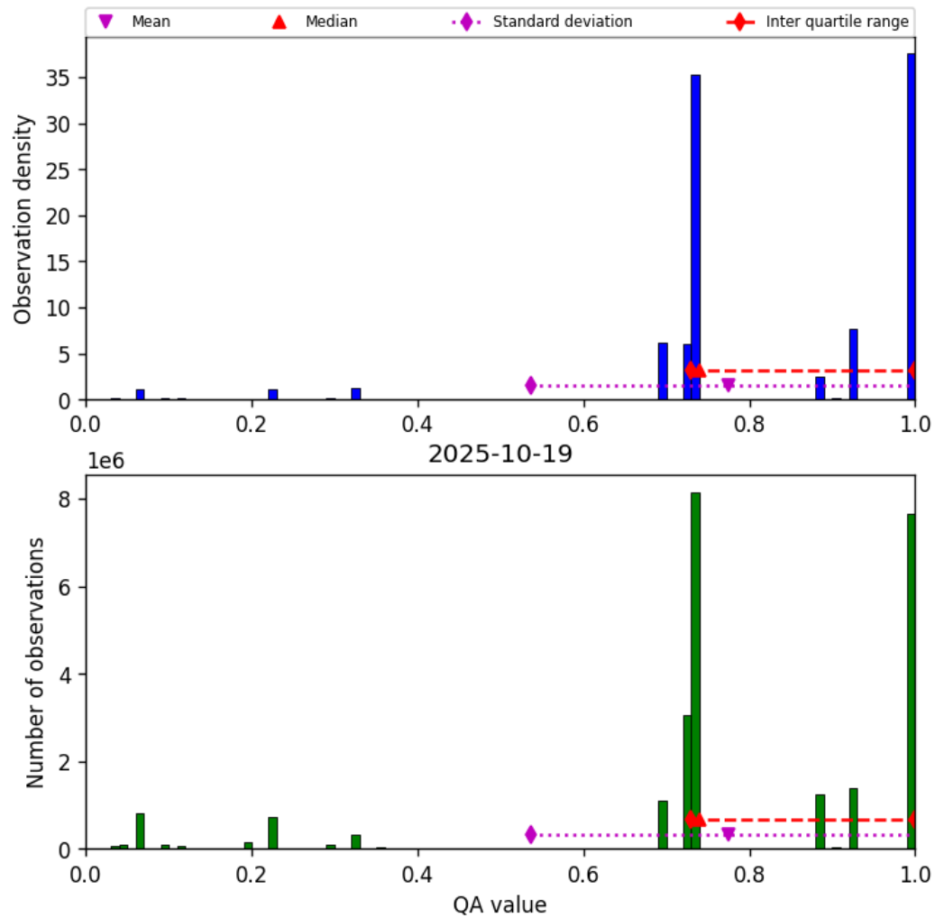
Figure 28: Histogram of “QA value” for 2025-10-18 to 2025-10-20
