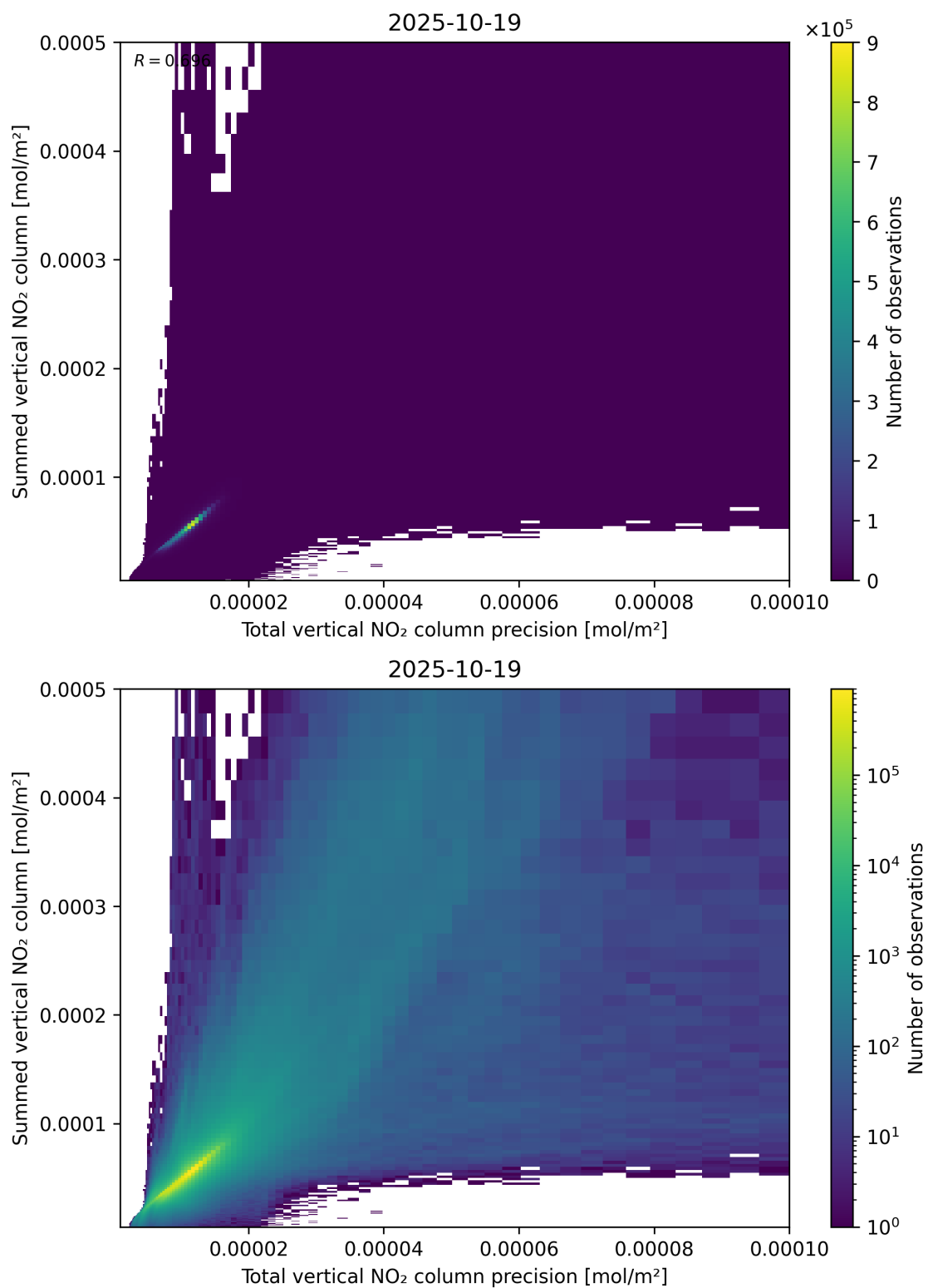
Figure 117: Scatter density plot of “Total vertical NO 2 column precision” against “Summed vertical NO 2 column” for 2025-10-18 to 2025-10-20.
