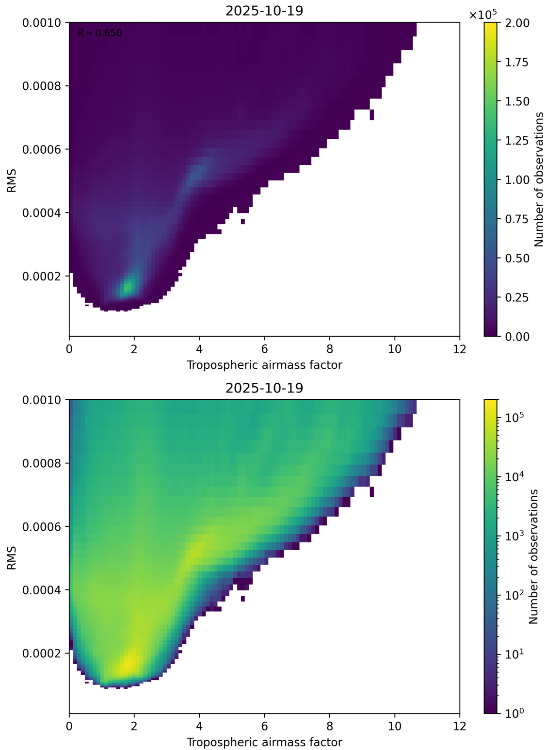
Figure 79: Scatter density plot of “Tropospheric airmass factor” against “RMS” for 2025-10-18 to 2025-10-20.
