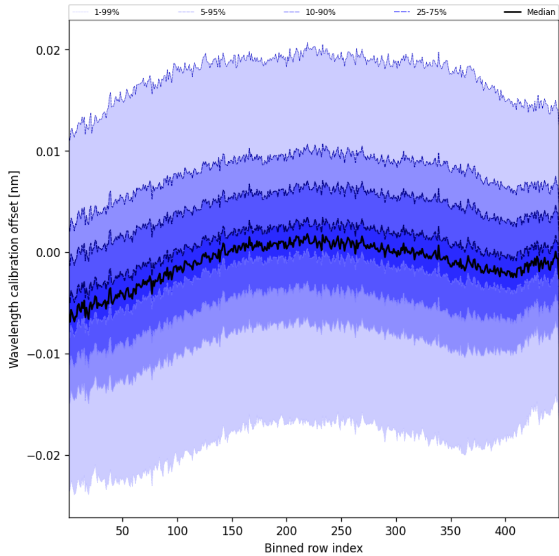
Figure 52: Along track statistics of “Wavelength calibration offset” for 2025-10-18 to 2025-10-20
