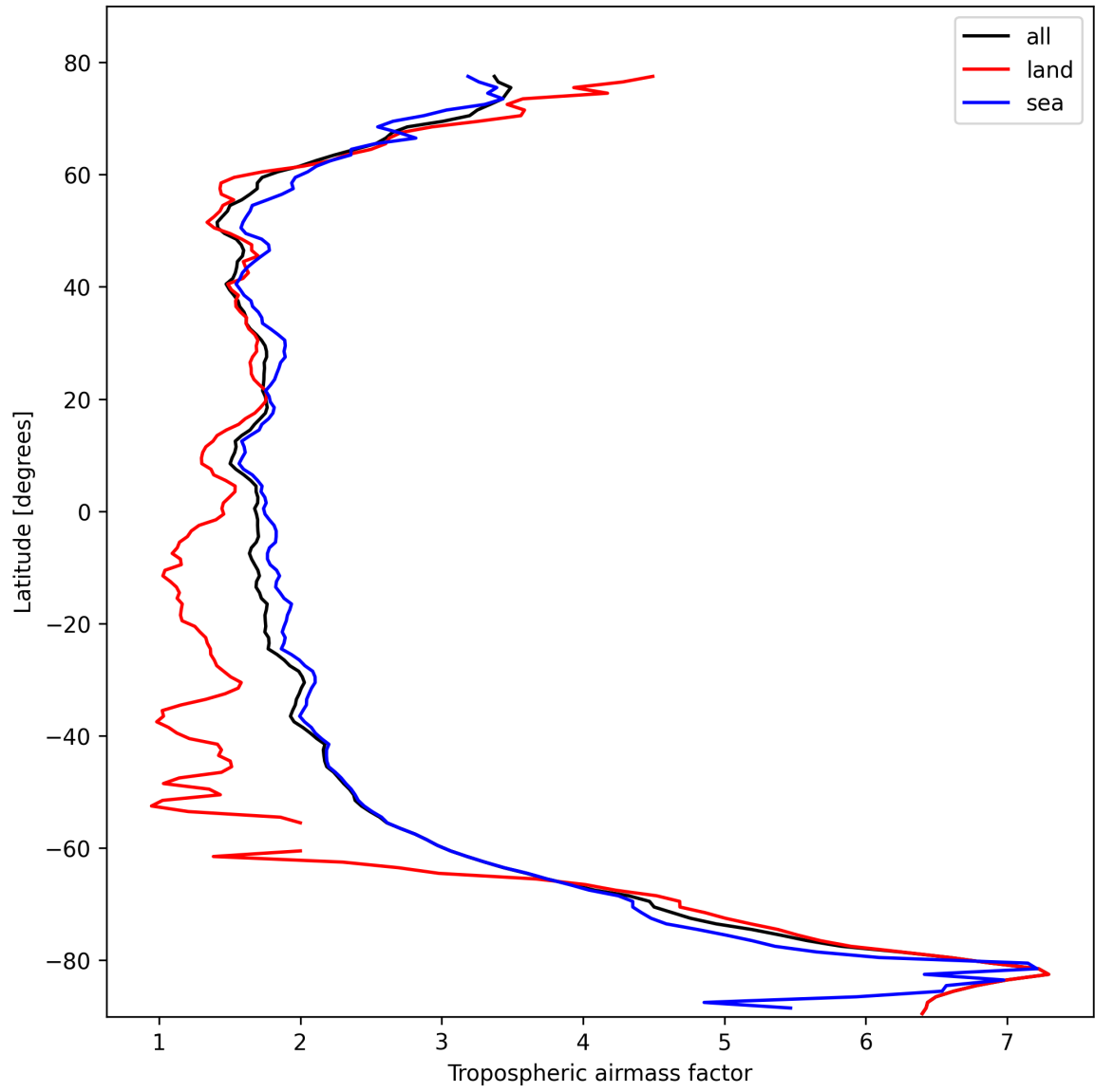
Figure 14: Zonal average of “Tropospheric air mass factor” for 2025-10-18 to 2025-10-20.
