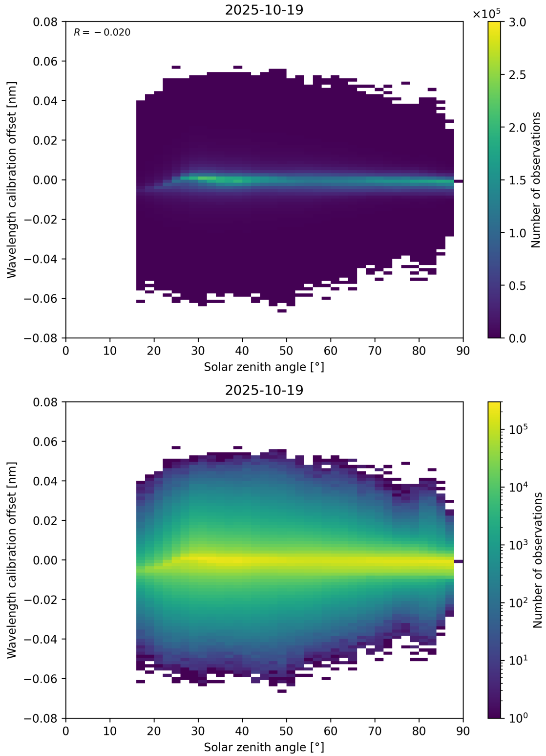
Figure 158: Scatter density plot of “Solar zenith angle” against “Wavelength calibration offset” for 2025-10-18 to 2025-10-20.
