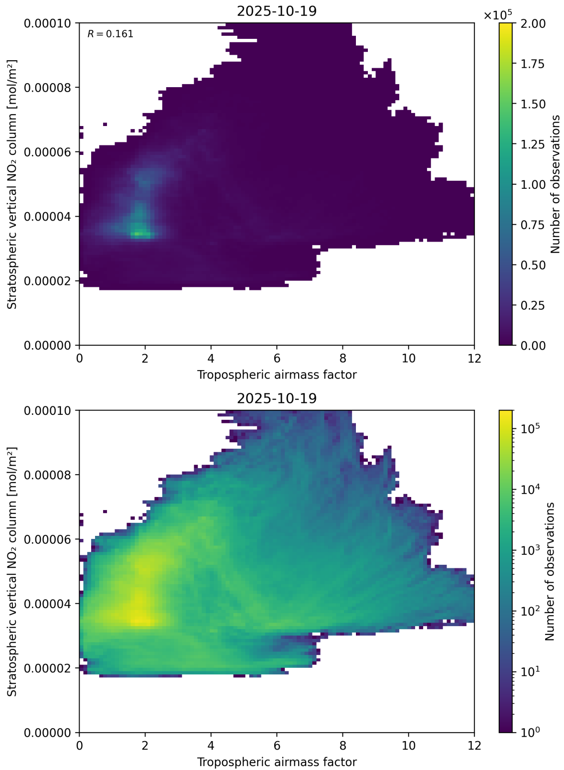
Figure 74: Scatter density plot of “Tropospheric air mass factor” against “Stratospheric vertical NO 2 column” for 2025-10-18 to 2025-10-20.
