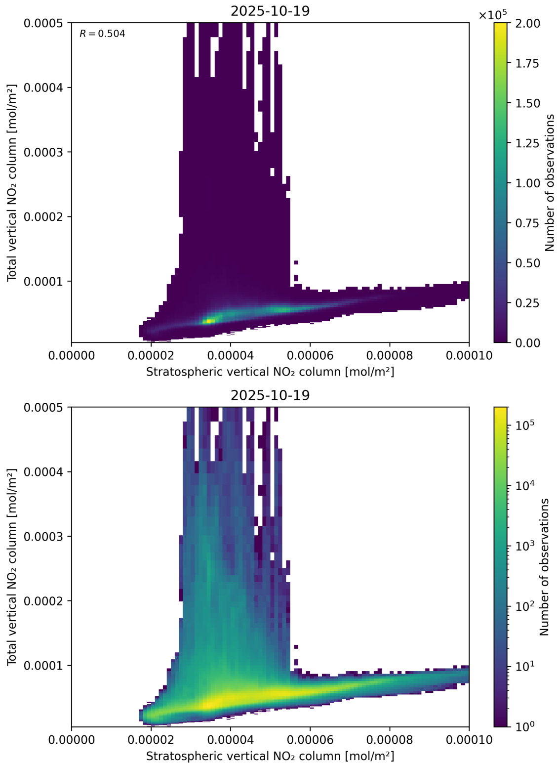
Figure 100: Scatter density plot of “Stratospheric vertical NO 2 column” against “Total vertical NO 2 column” for 2025-10-18 to 2025-10-20.
