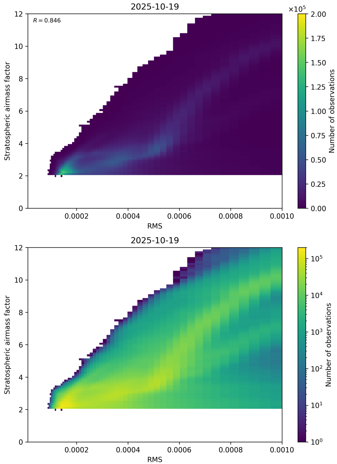
Figure 144: Scatter density plot of “RMS” against “Stratospheric airmass factor” for 2025-10-18 to 2025-10-20.
