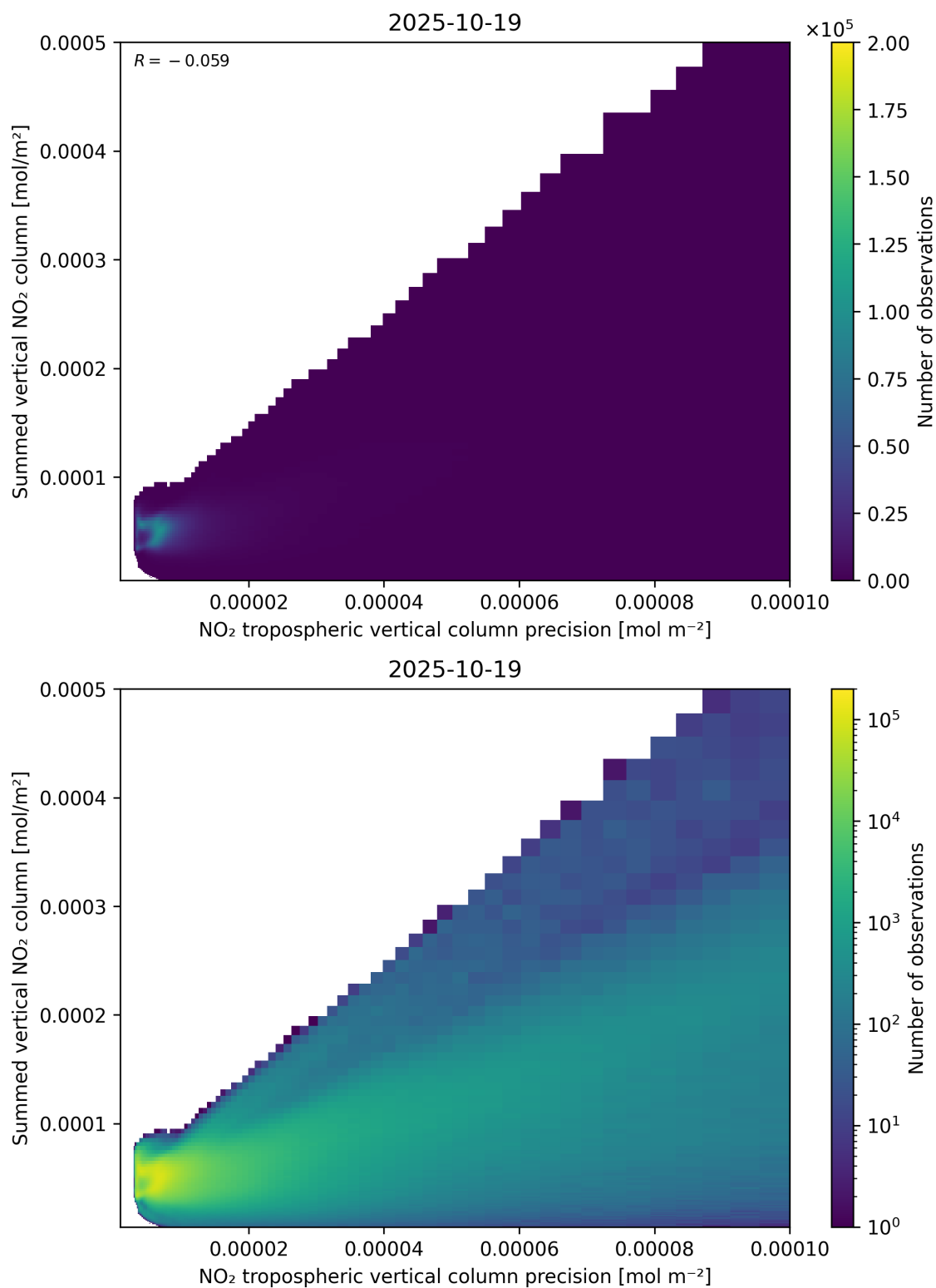
Figure 136: Scatter density plot of “NO 2 tropospheric vertical column precision” against “Summed vertical NO 2 column” for 2025-10-18 to 2025-10-20.
