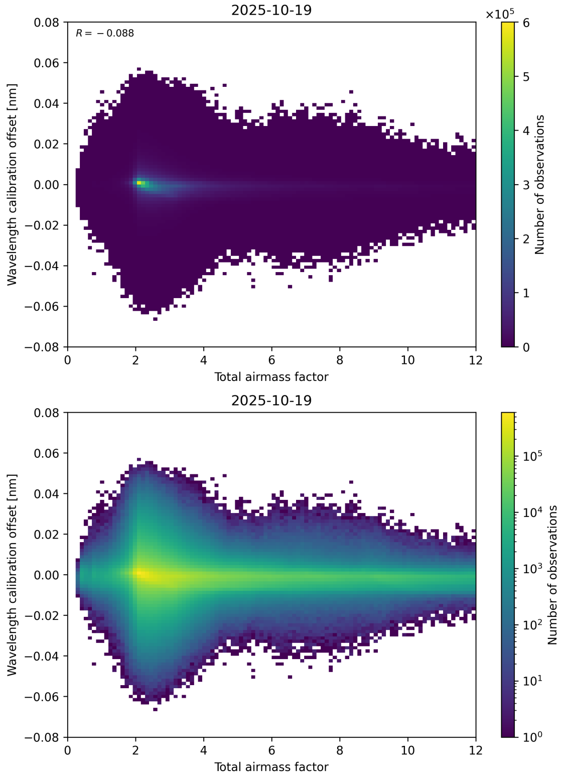
Figure 70: Scatter density plot of “Total airmass factor” against “Wavelength calibration offset” for 2025-10-18 to 2025-10-20.
