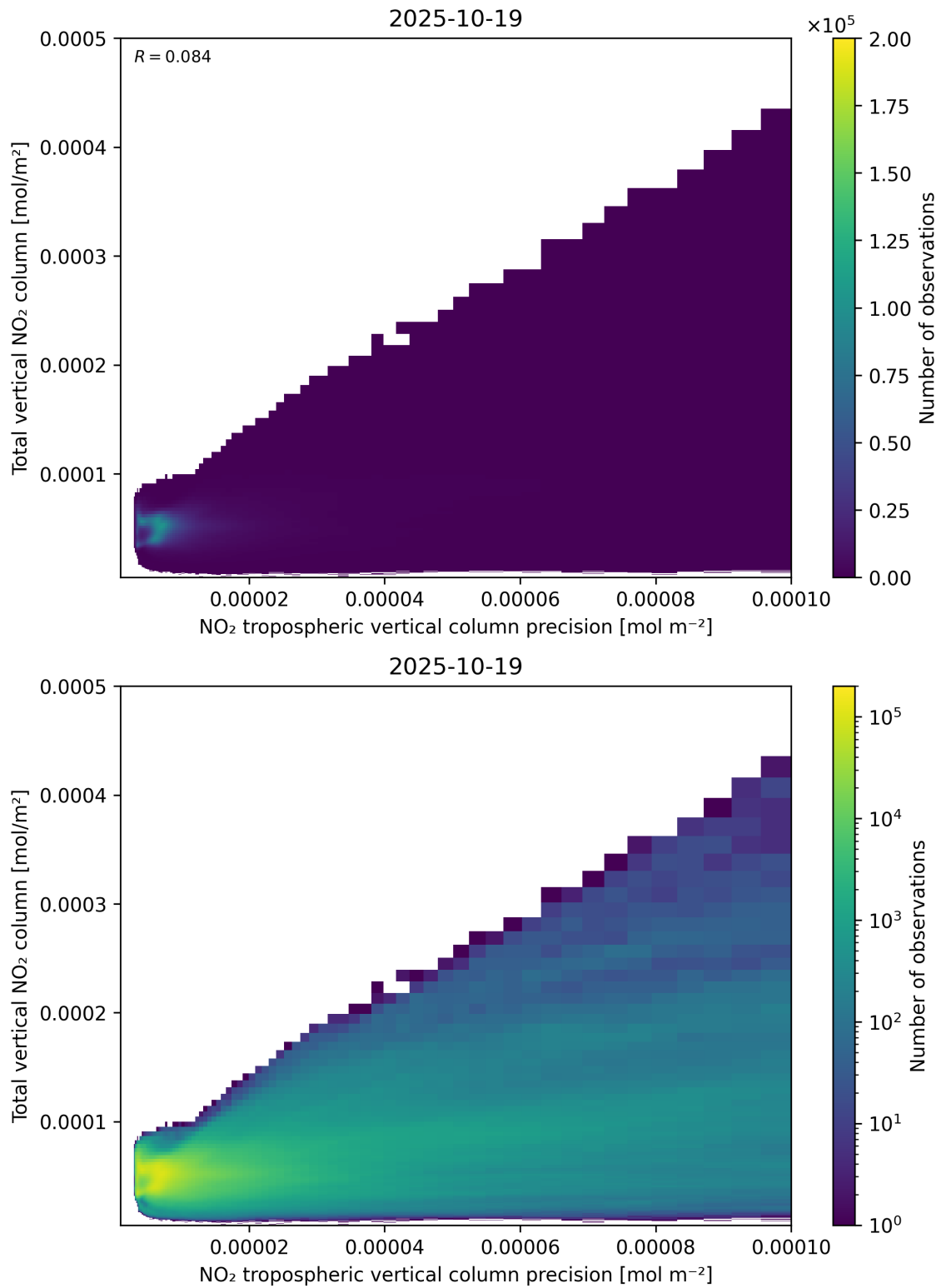
Figure 138: Scatter density plot of “NO 2 tropospheric vertical column precision” against “Total vertical NO 2 column” for 2025-10-18 to 2025-10-20.
