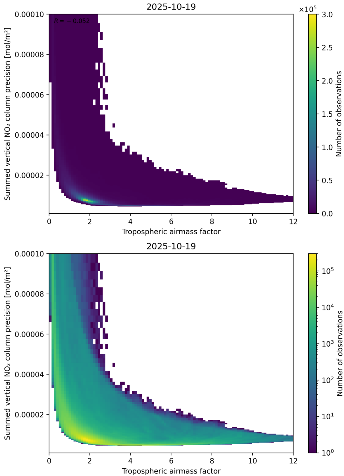
Figure 76: Scatter density plot of “Tropospheric air mass factor” against “Summed vertical NO 2 column precision” for 2025-10-18 to 2025-10-20.
