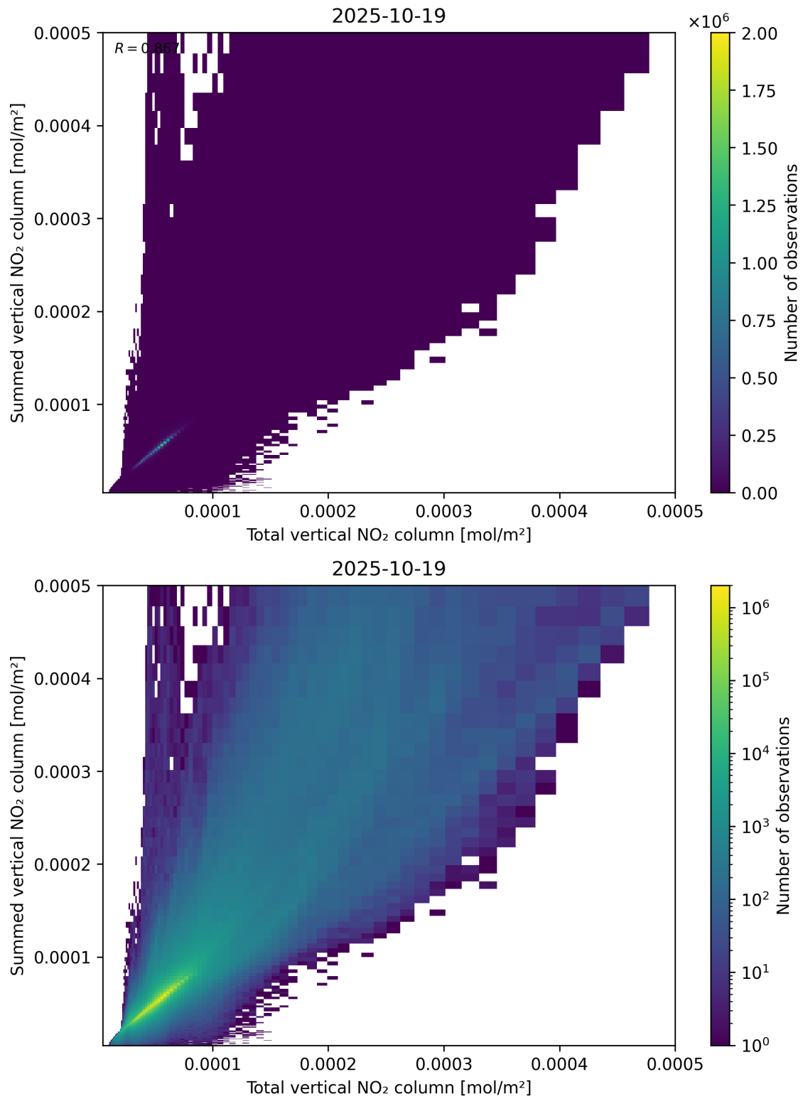
Figure 112: Scatter density plot of “Total vertical NO 2 column” against “Summed vertical NO 2 column” for 2025-10-18 to 2025-10-20.
