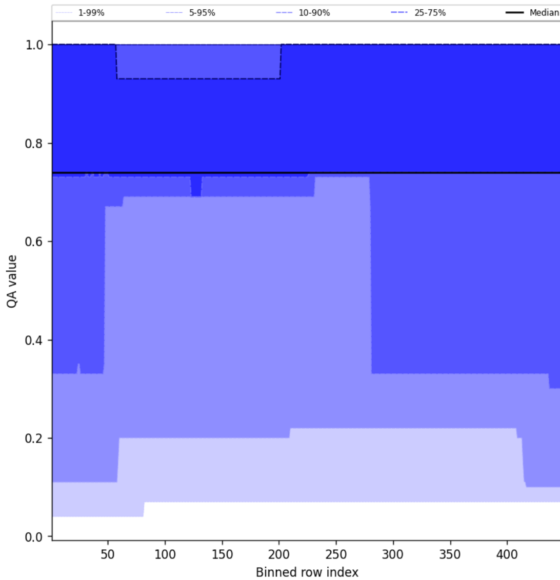
Figure 45: Along track statistics of “QA value” for 2025-10-18 to 2025-10-20
