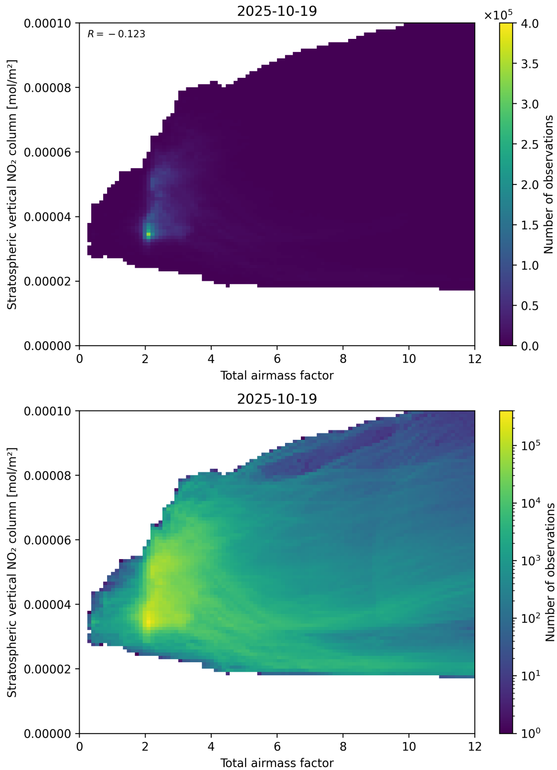
Figure 64: Scatter density plot of “Total airmass factor” against “Stratospheric vertical NO 2 column” for 2025-10-18 to 2025-10-20.
