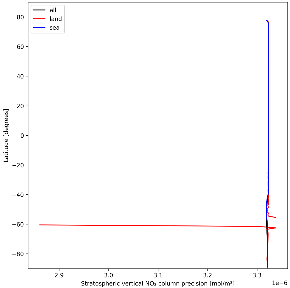
Figure 20: Zonal average of “Stratospheric vertical NO 2 column precision” for 2025-10-18 to 2025-10-20.
