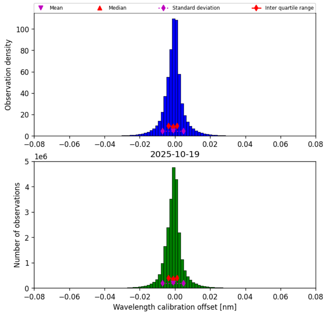
Figure 35: Histogram of “Wavelength calibration offset” for 2025-10-18 to 2025-10-20
