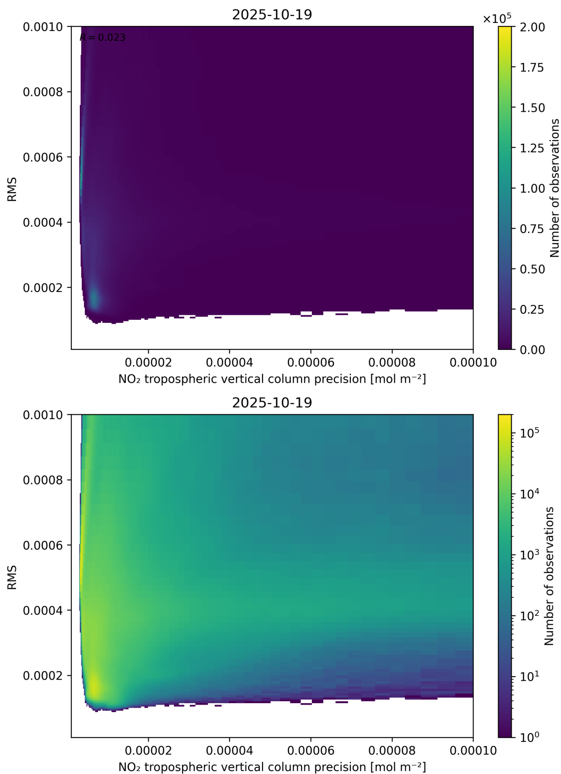
Figure 140: Scatter density plot of “NO 2 tropospheric vertical column precision” against “RMS” for 2025-10-18 to 2025-10-20.
