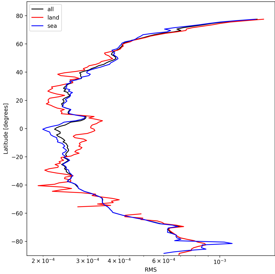
Figure 26: Zonal average of “RMS” for 2025-10-18 to 2025-10-20.
