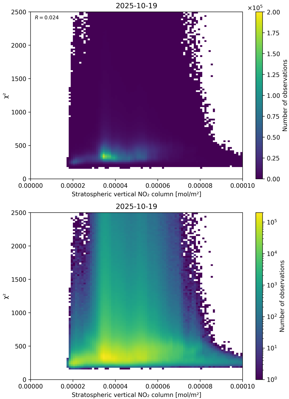
Figure 97: Scatter density plot of “Stratospheric vertical NO 2 column” against “ \chi^2 ” for 2025-10-18 to 2025-10-20.
