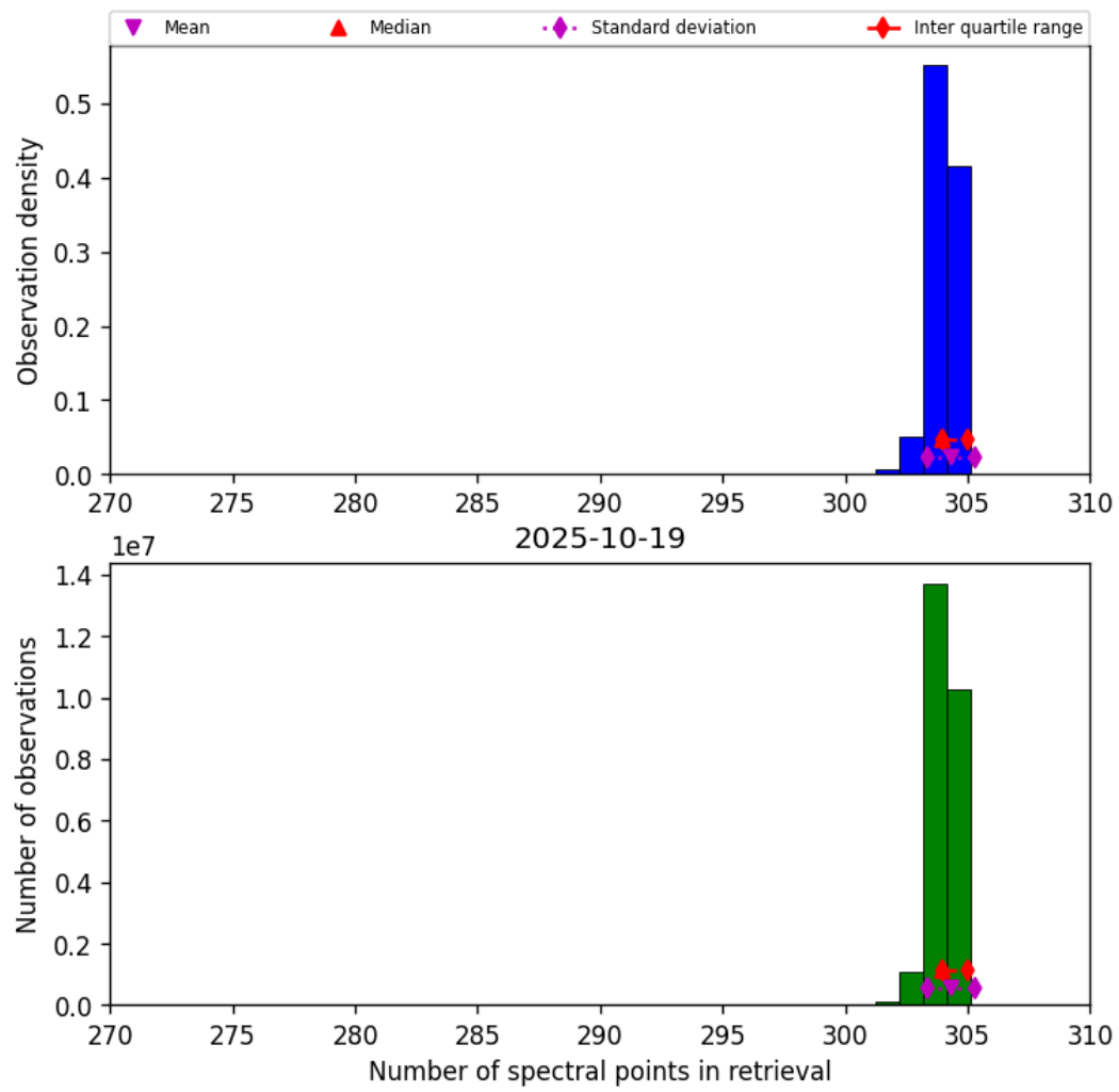
Figure 33: Histogram of “Number of spectral points in retrieval” for 2025-10-18 to 2025-10-20
