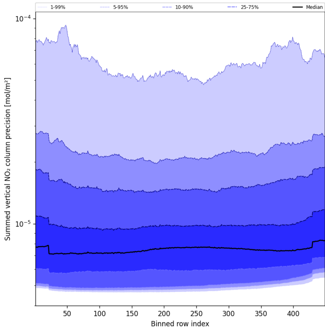
Figure 58: Along track statistics of “Summed vertical NO 2 column precision” for 2025-10-18 to 2025-10-20
