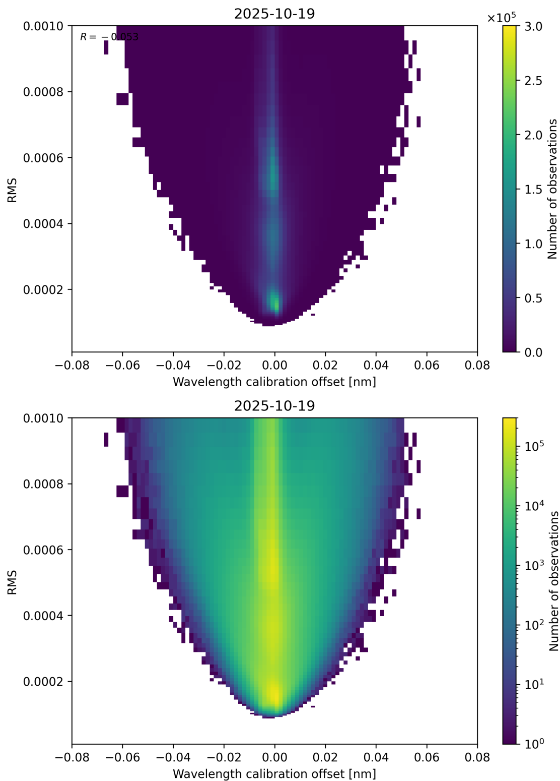
Figure 181: Scatter density plot of “Wavelength calibration offset” against “RMS” for 2025-10-18 to 2025-10-20.
