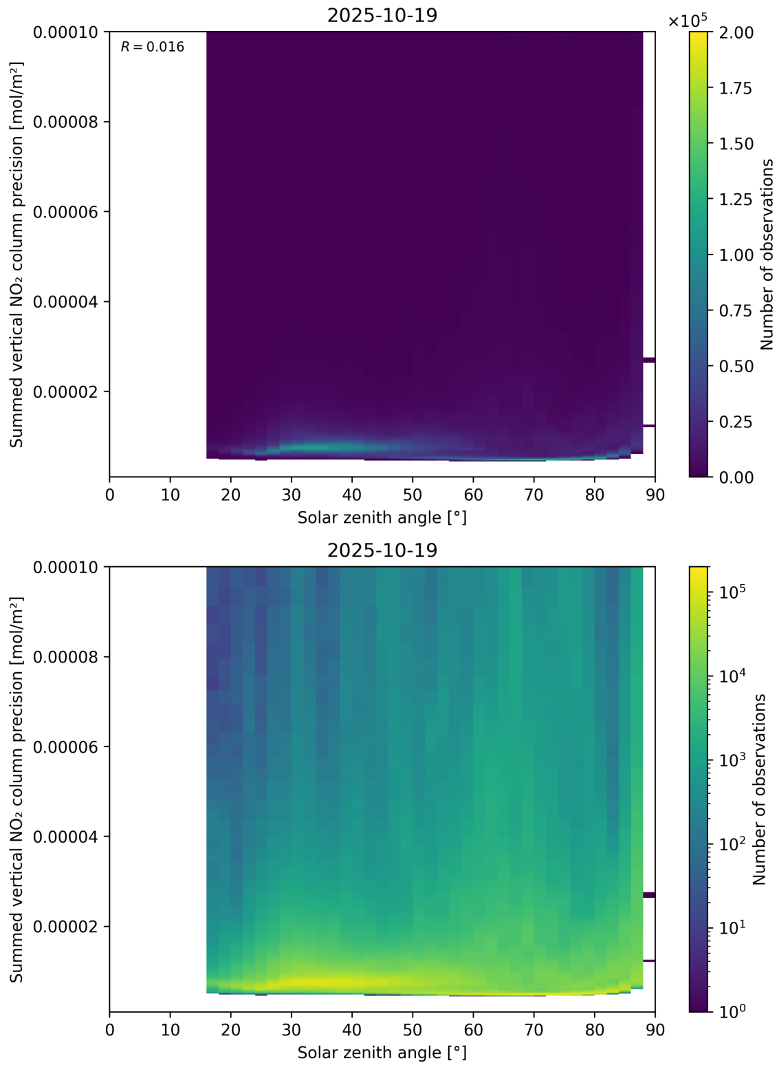
Figure 152: Scatter density plot of “Solar zenith angle” against “Summed vertical NO 2 column precision” for 2025-10-18 to 2025-10-20.
