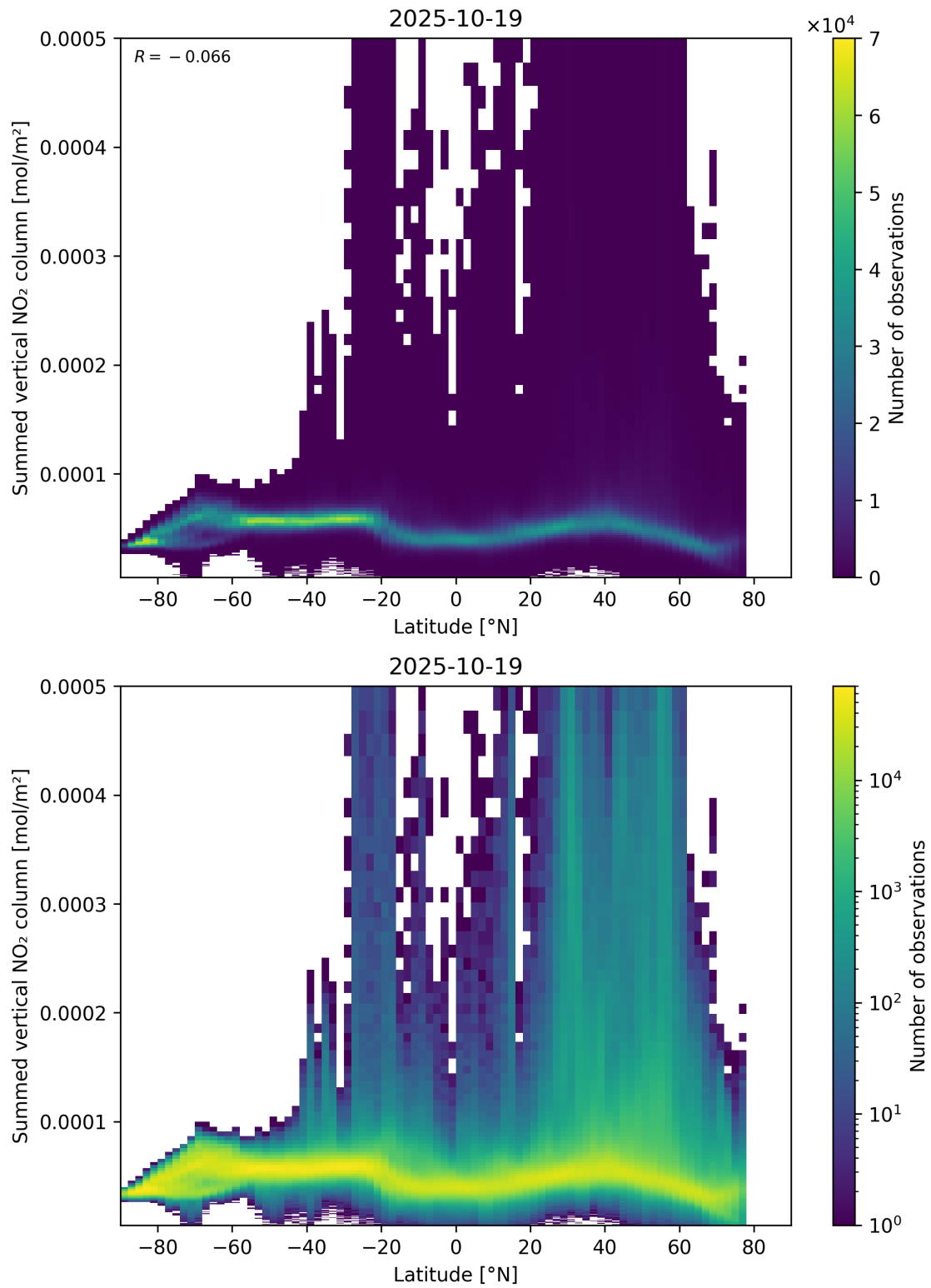
Figure 88: Scatter density plot of “Latitude” against “Summed vertical NO 2 column” for 2025-10-18 to 2025-10-20.
