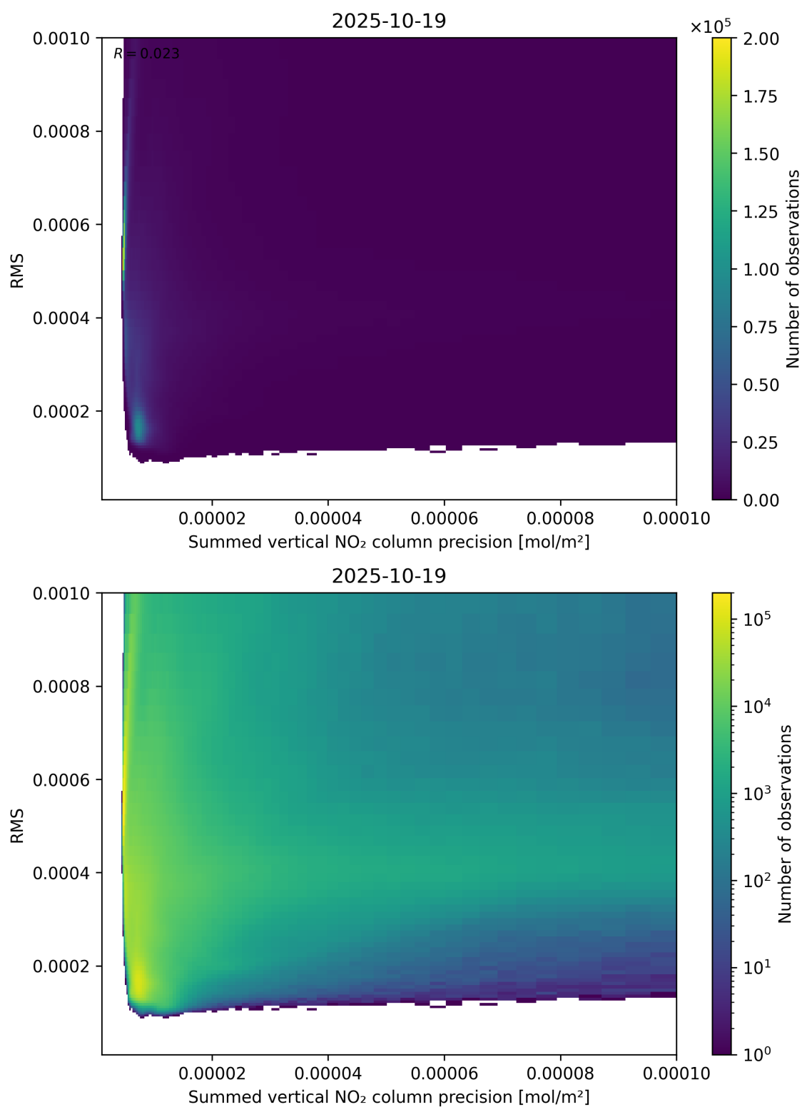
Figure 108: Scatter density plot of “Summed vertical NO 2 column precision” against “RMS” for 2025-10-18 to 2025-10-20.
