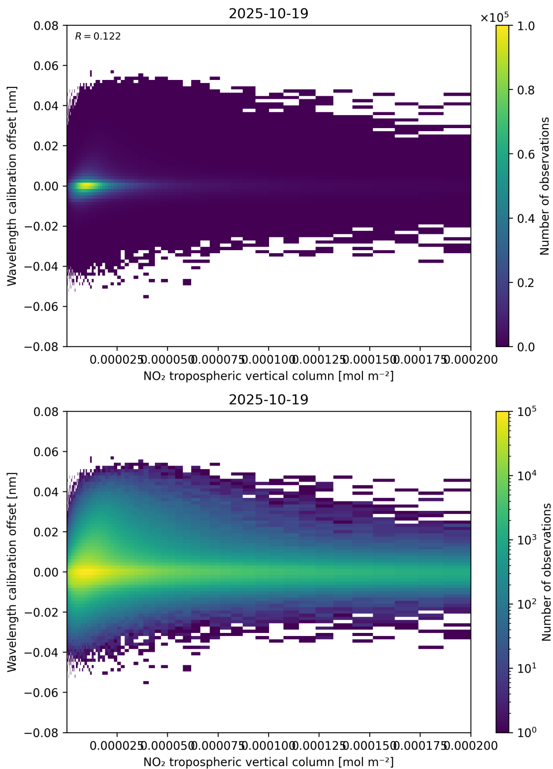
Figure 143: Scatter density plot of “NO 2 tropospheric vertical column” against “Wavelength calibration offset” for 2025-10-18 to 2025-10-20.
