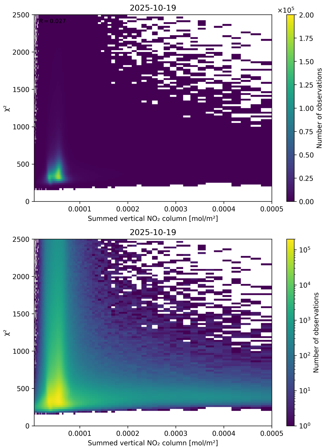
Figure 104: Scatter density plot of “Summed vertical NO 2 column” against “ \chi^2 ” for 2025-10-18 to 2025-10-20.
