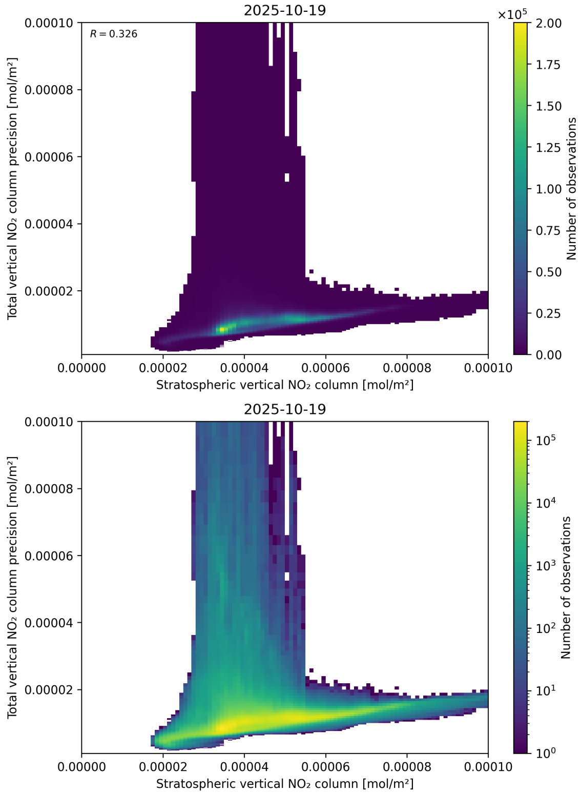
Figure 101: Scatter density plot of “Stratospheric vertical NO 2 column” against “Total vertical NO 2 column precision” for 2025-10-18 to 2025-10-20.
