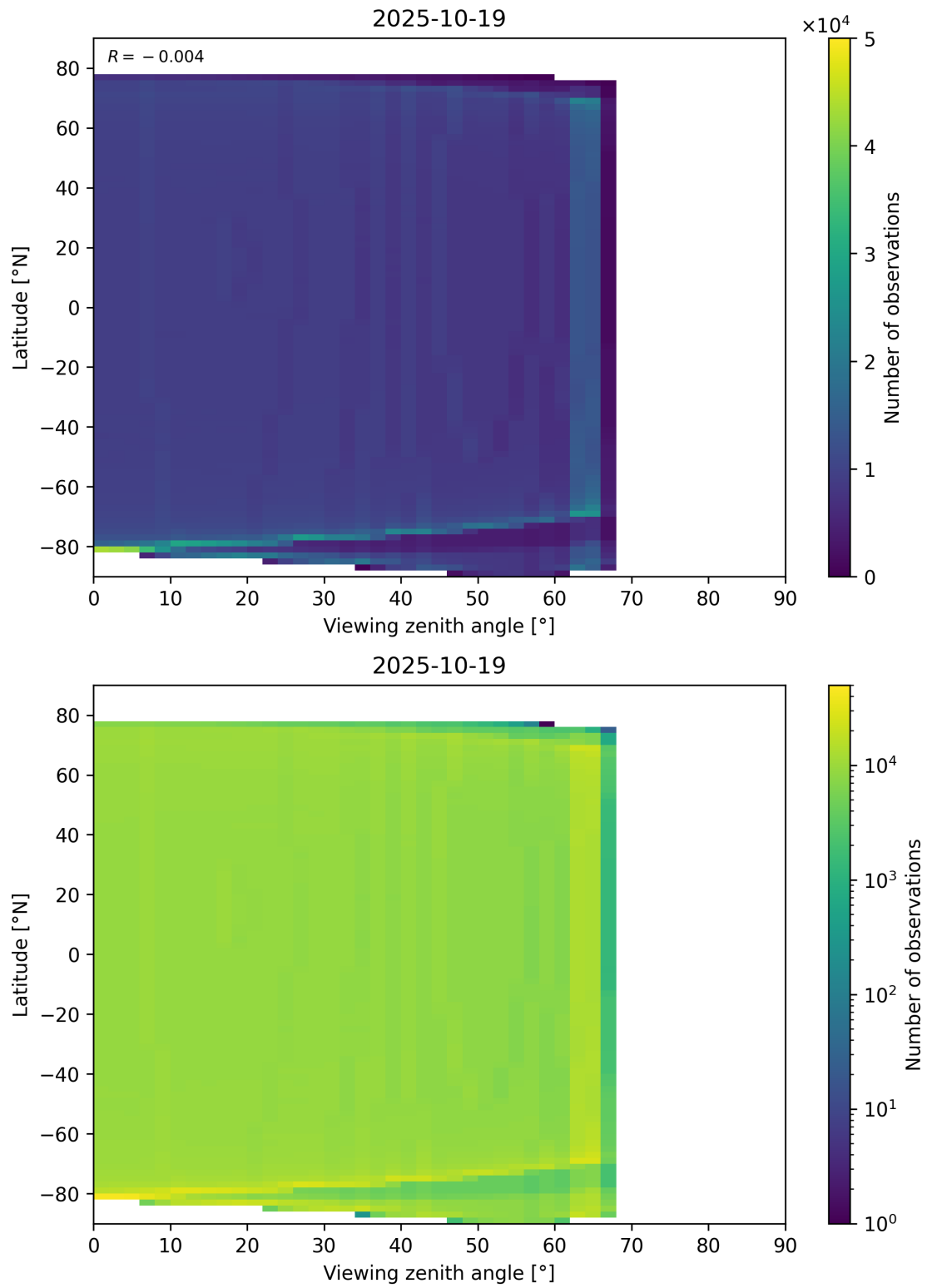
Figure 163: Scatter density plot of “Viewing zenith angle” against “Latitude” for 2025-10-18 to 2025-10-20.
