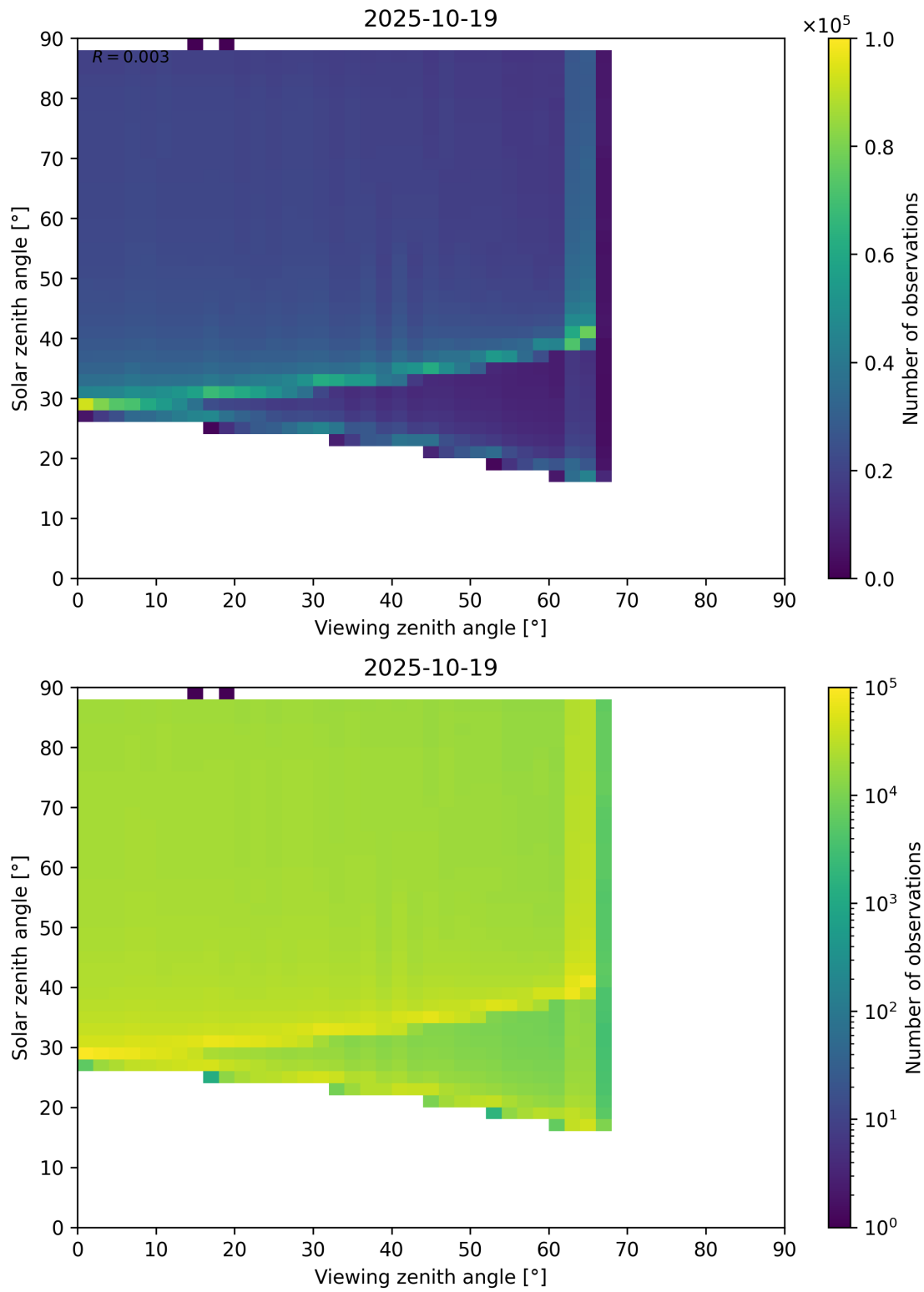
Figure 172: Scatter density plot of “Viewing zenith angle” against “Solar zenith angle” for 2025-10-18 to 2025-10-20.
