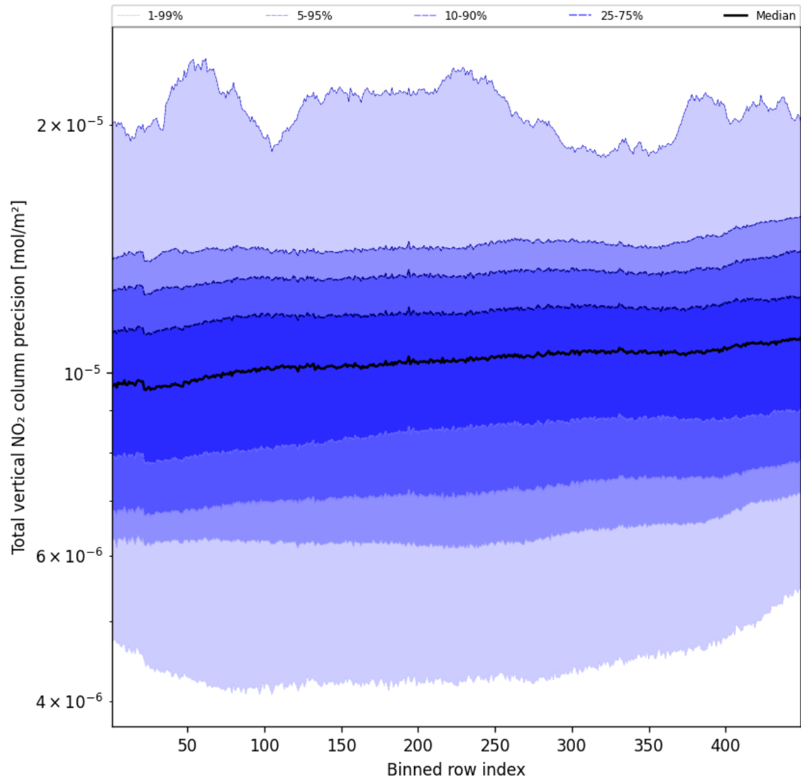
Figure 56: Along track statistics of “Total vertical NO 2 column precision” for 2025-10-18 to 2025-10-20
