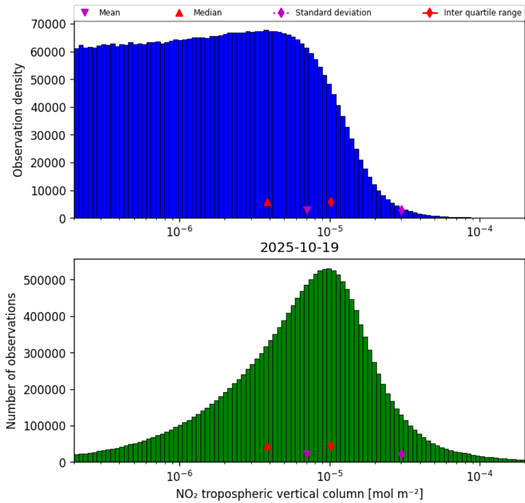
Figure 29: Histogram of “NO 2 tropospheric vertical column” for 2025-10-18 to 2025-10-20
