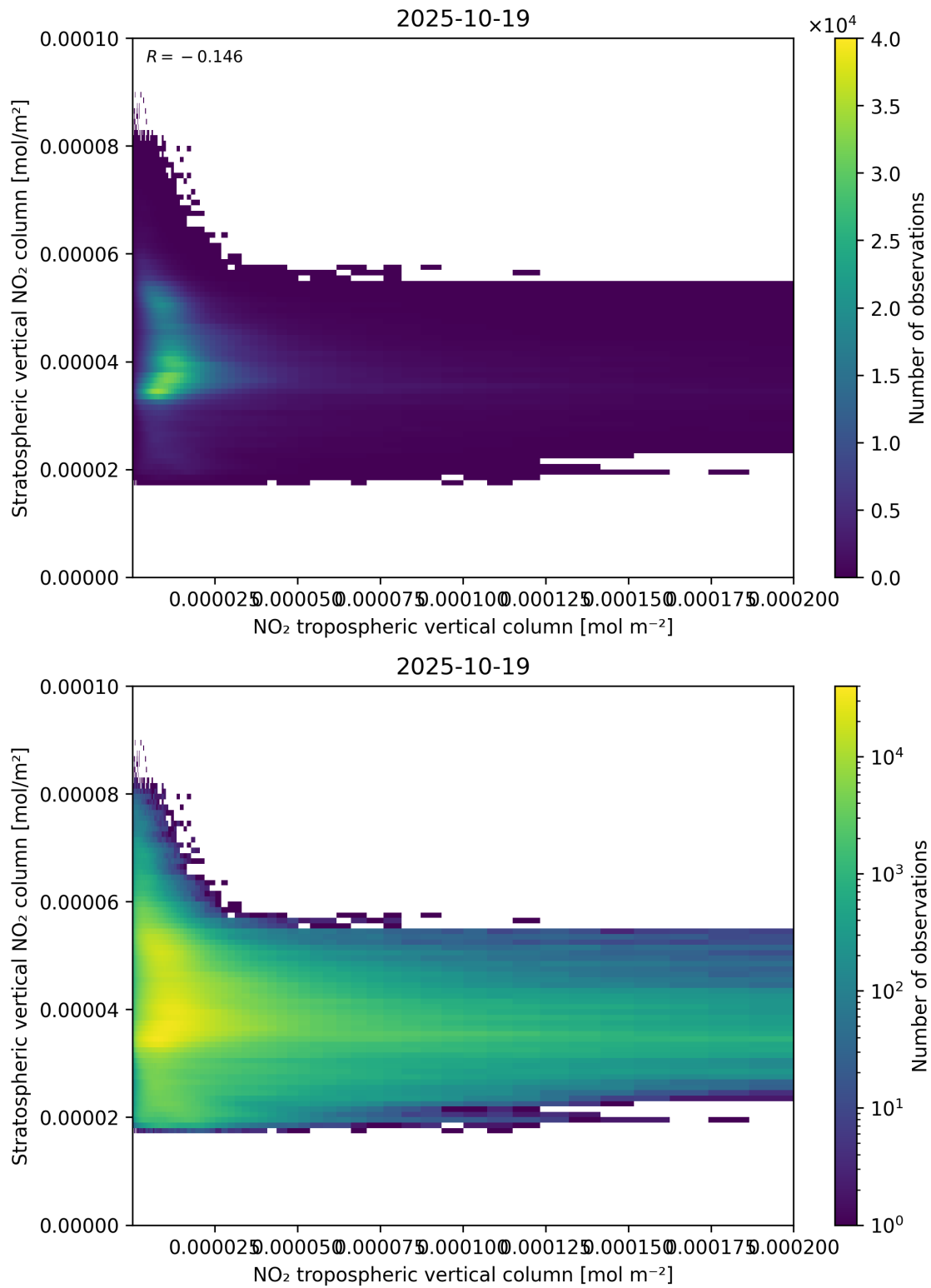
Figure 125: Scatter density plot of “NO 2 tropospheric vertical column” against “Stratospheric vertical NO 2 column” for 2025-10-18 to 2025-10-20.
