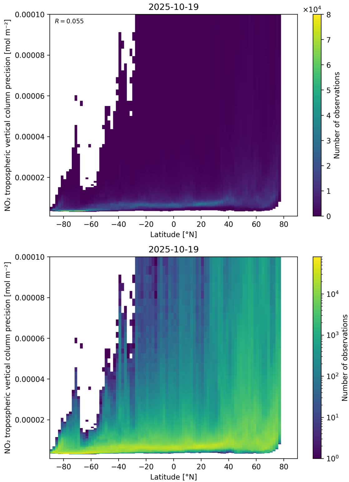
Figure 93: Scatter density plot of “Latitude” against “NO 2 tropospheric vertical column precision” for 2025-10-18 to 2025-10-20.
