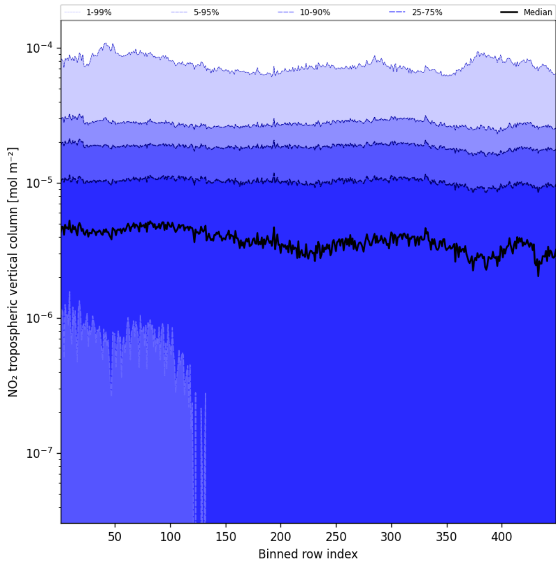
Figure 46: Along track statistics of “NO 2 tropospheric vertical column” for 2025-10-18 to 2025-10-20
