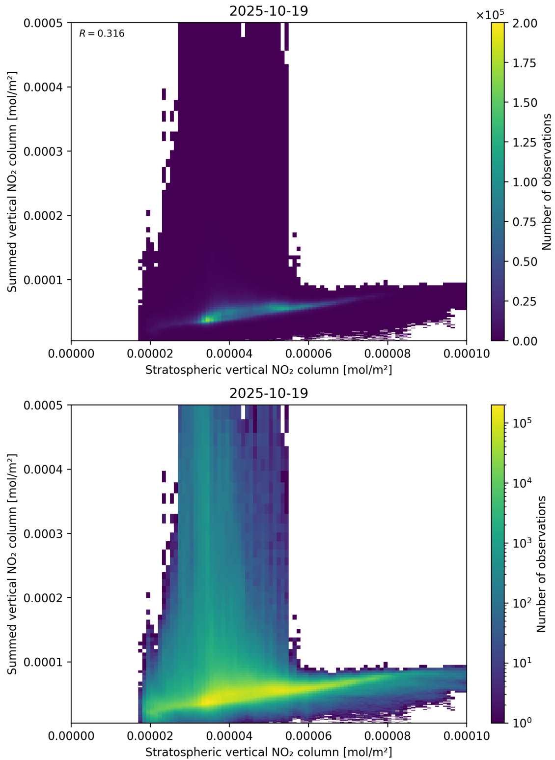
Figure 98: Scatter density plot of “Stratospheric vertical NO 2 column” against “Summed vertical NO 2 column” for 2025-10-18 to 2025-10-20.
