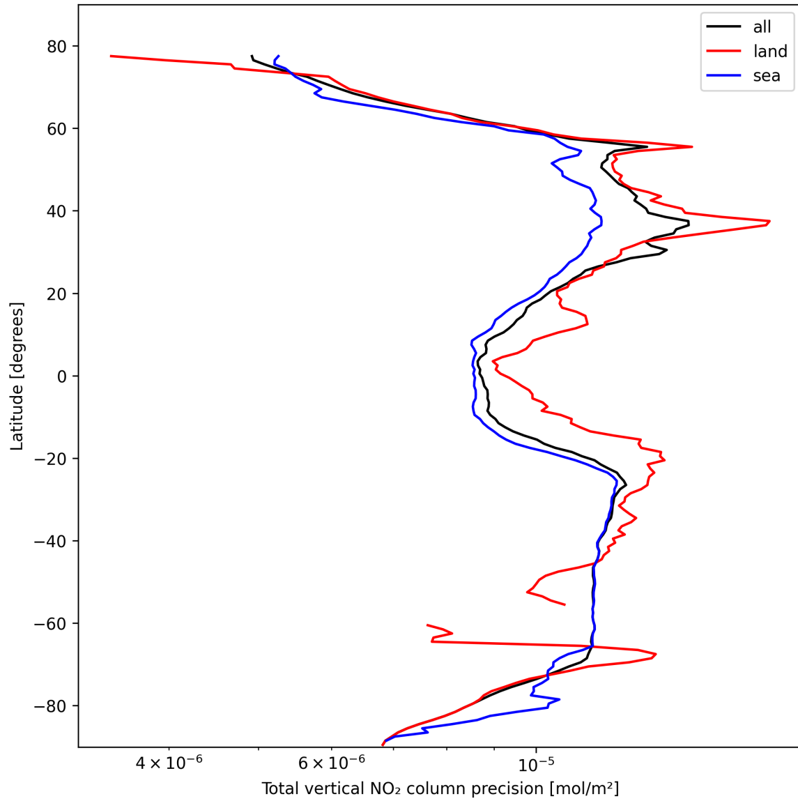
Figure 22: Zonal average of “Total vertical NO 2 column precision” for 2025-10-18 to 2025-10-20.
