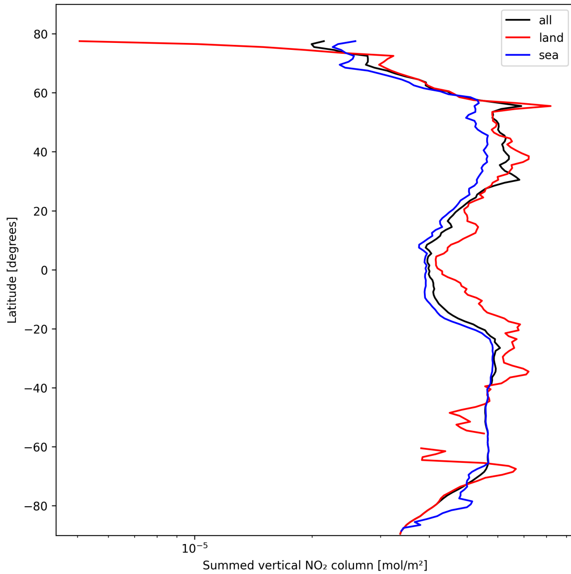
Figure 23: Zonal average of “Summed vertical NO 2 column” for 2025-10-18 to 2025-10-20.
