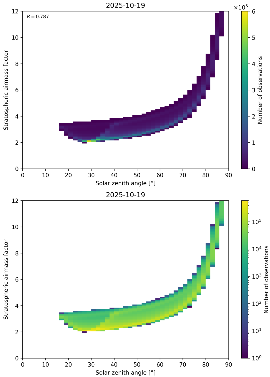
Figure 145: Scatter density plot of “Solar zenith angle” against “Stratospheric airmass factor” for 2025-10-18 to 2025-10-20.
