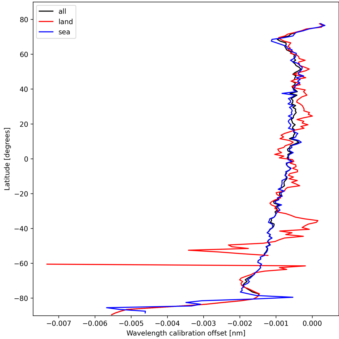
Figure 18: Zonal average of “Wavelength calibration offset” for 2025-10-18 to 2025-10-20.
