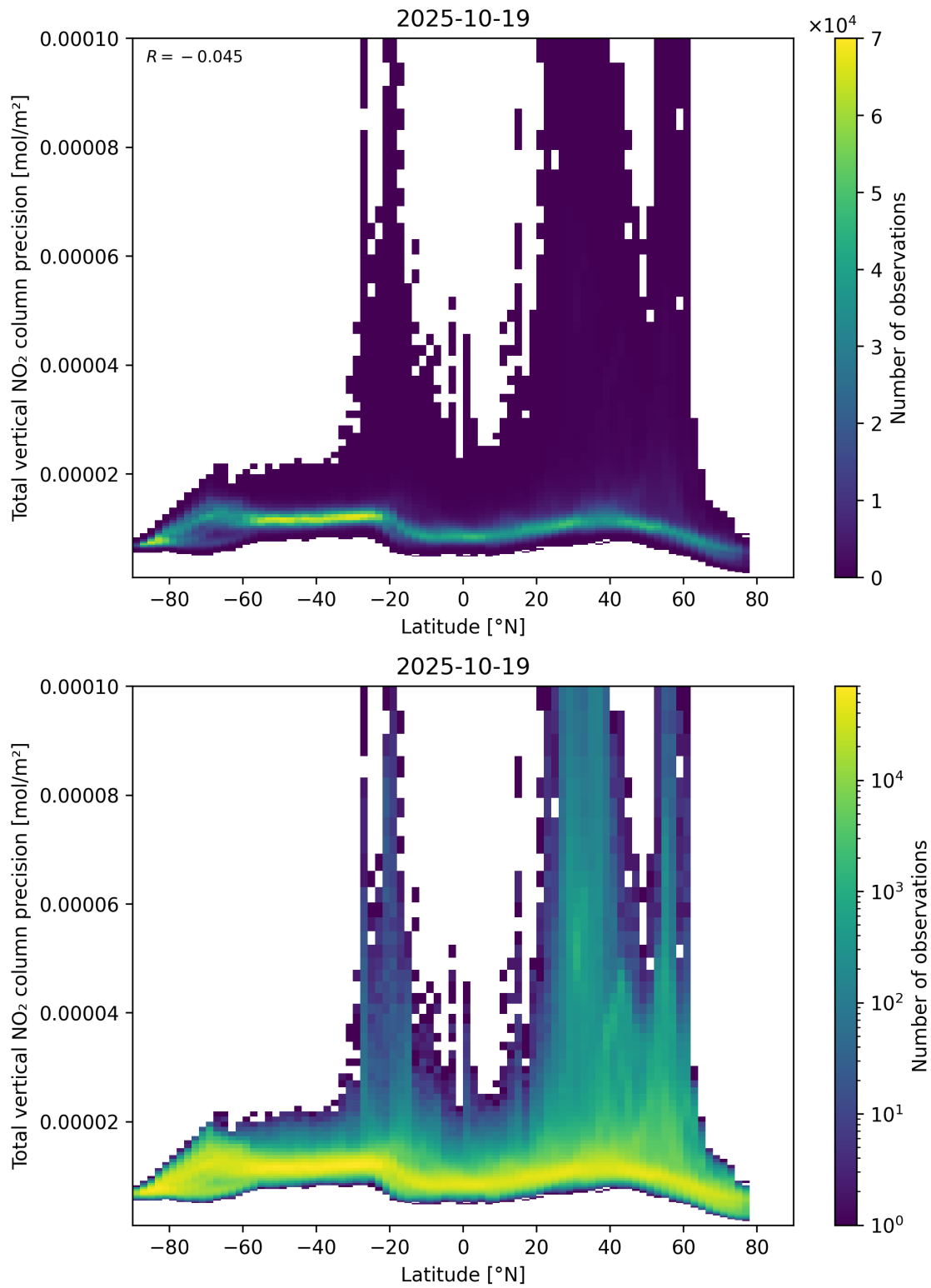
Figure 91: Scatter density plot of “Latitude” against “Total vertical NO 2 column precision” for 2025-10-18 to 2025-10-20.
