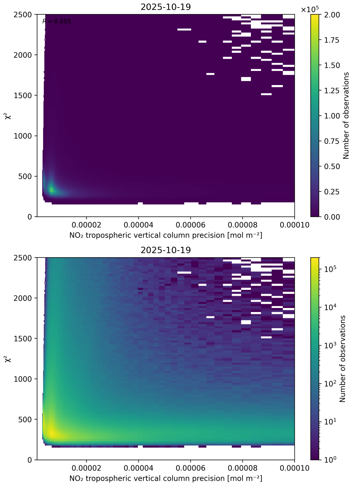
Figure 134: Scatter density plot of “NO 2 tropospheric vertical column precision” against “ \chi^2 ” for 2025-10-18 to 2025-10-20.
