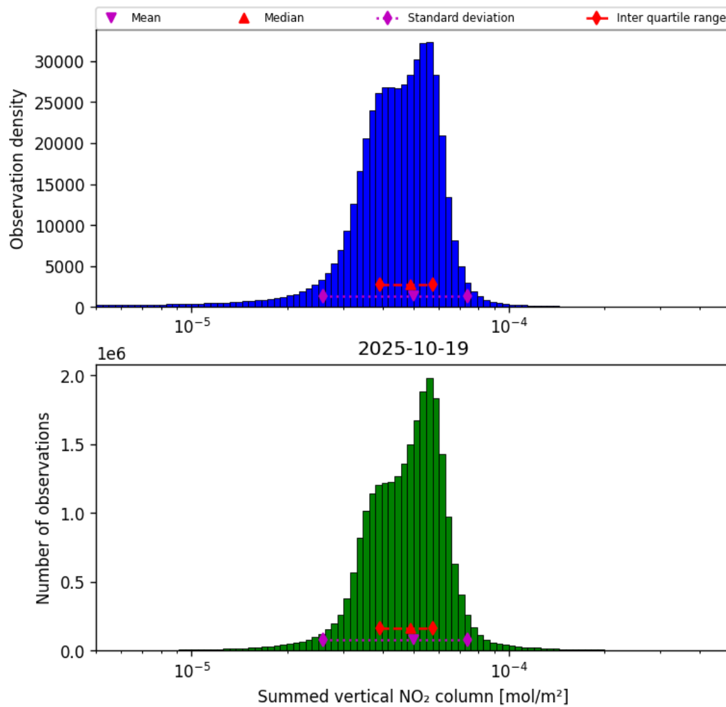
Figure 40: Histogram of “Summed vertical NO 2 column” for 2025-10-18 to 2025-10-20
