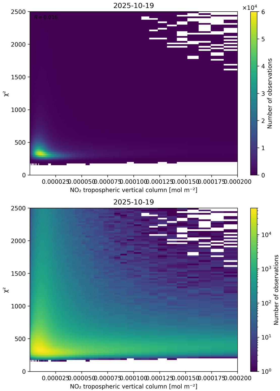
Figure 124: Scatter density plot of “NO 2 tropospheric vertical column” against “ \chi^2 ” for 2025-10-18 to 2025-10-20.
