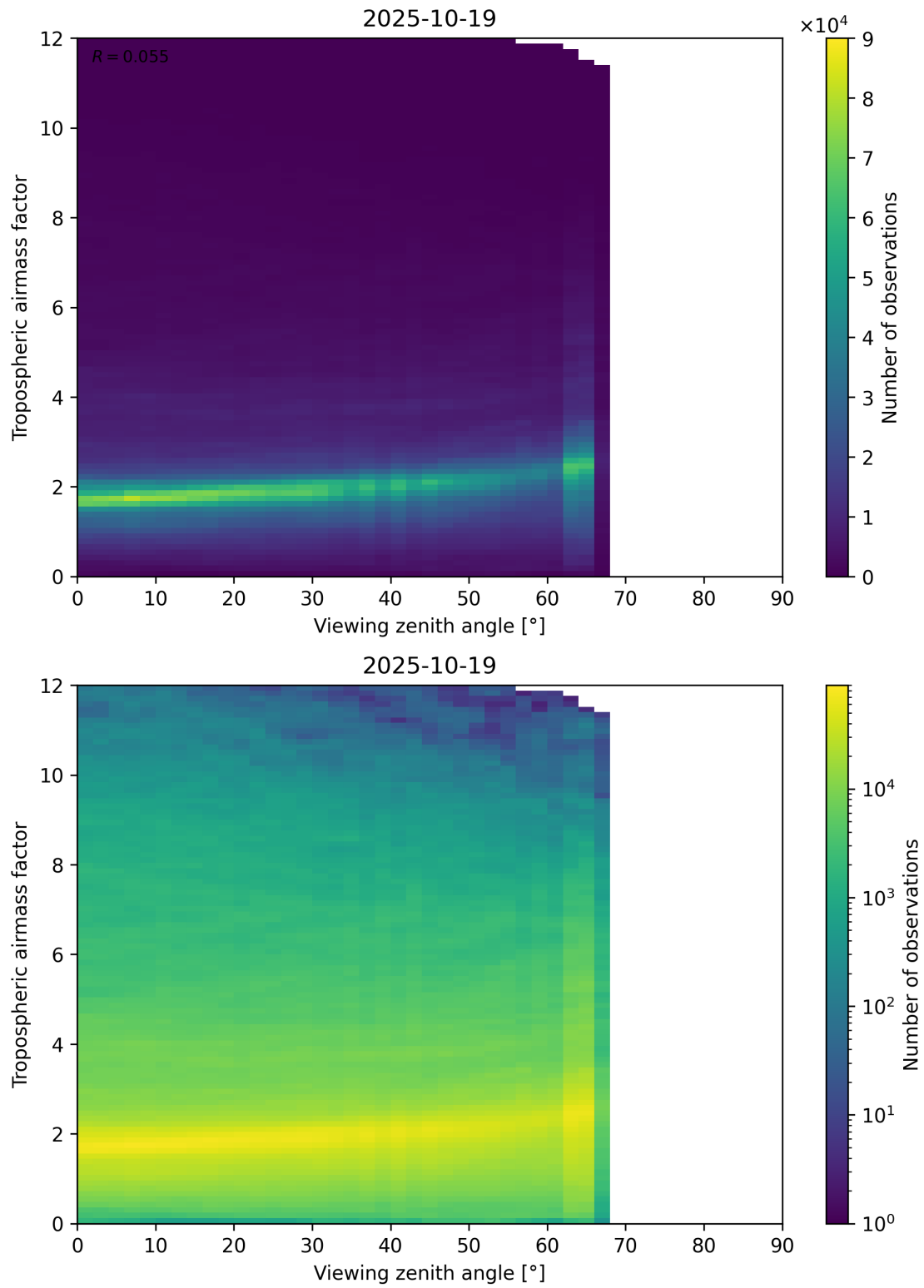
Figure 161: Scatter density plot of “Viewing zenith angle” against “Tropospheric airmass factor” for 2025-10-18 to 2025-10-20.
