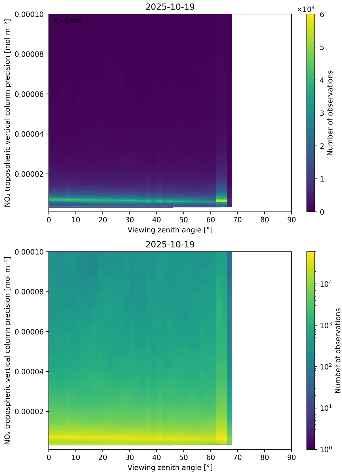
Figure 170: Scatter density plot of “Viewing zenith angle” against “NO 2 tropospheric vertical column precision” for 2025-10-18 to 2025-10-20.
