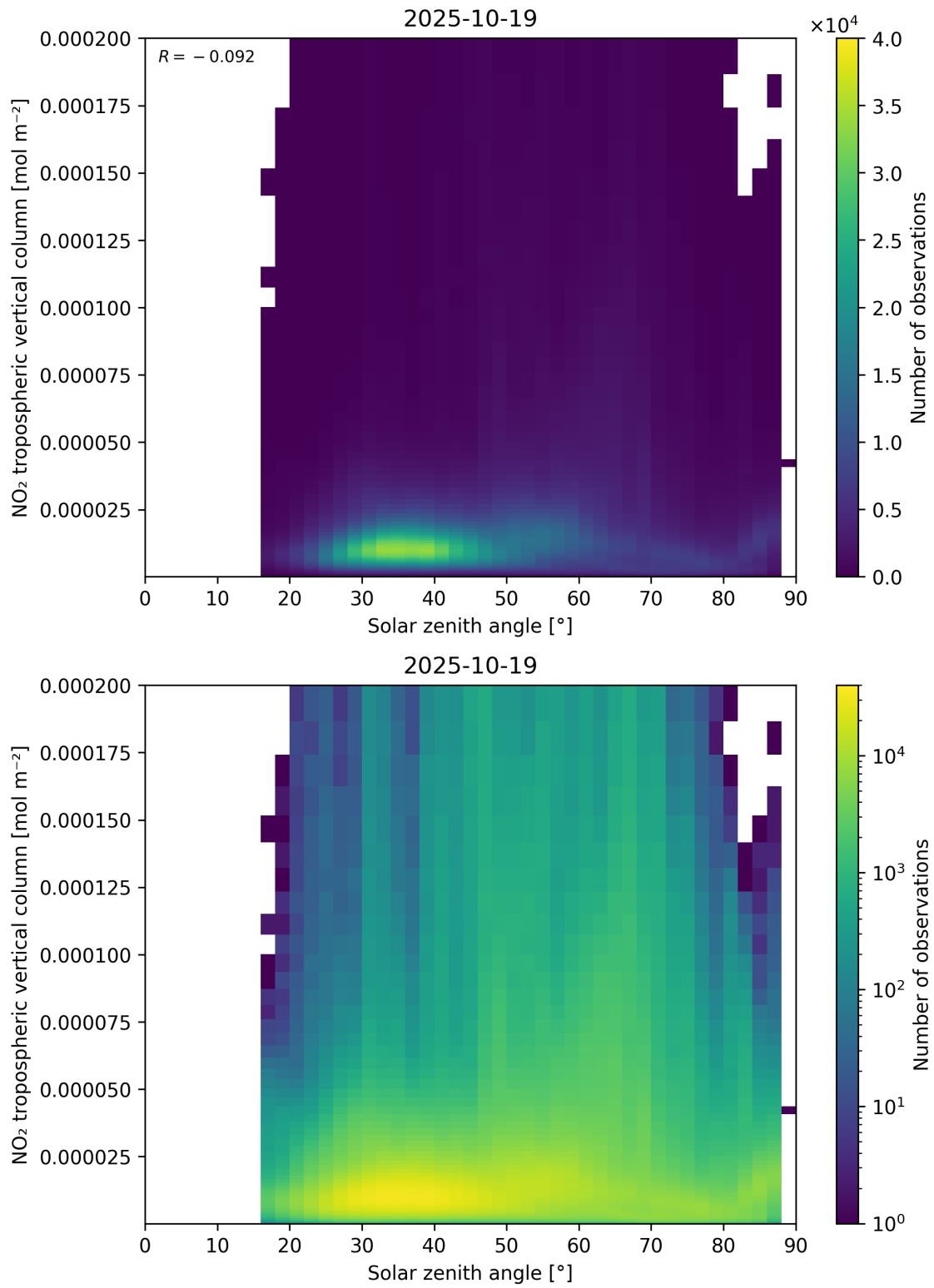
Figure 155: Scatter density plot of “Solar zenith angle” against “NO 2 tropospheric vertical column” for 2025-10-18 to 2025-10-20.
