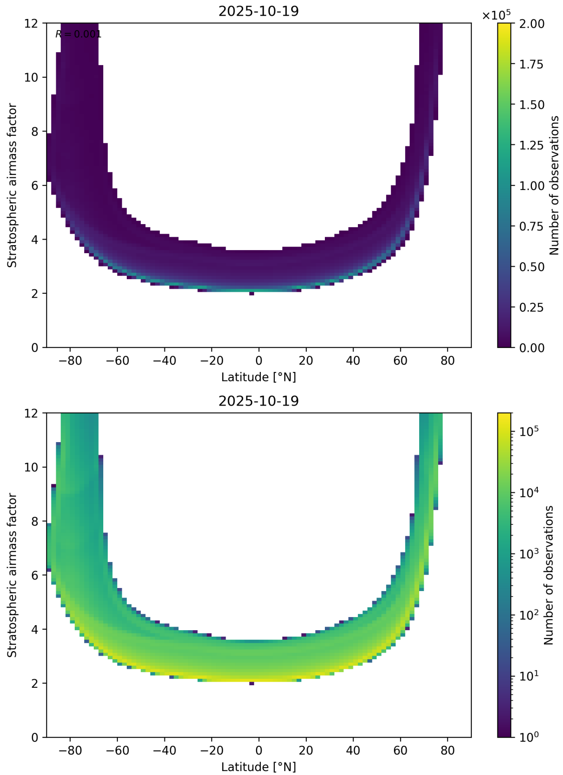
Figure 83: Scatter density plot of “Latitude” against “Stratospheric airmass factor” for 2025-10-18 to 2025-10-20.
