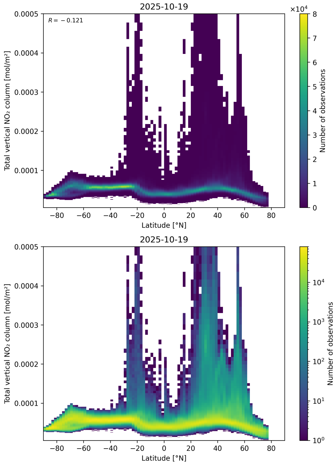
Figure 90: Scatter density plot of “Latitude” against “Total vertical NO 2 column” for 2025-10-18 to 2025-10-20.
