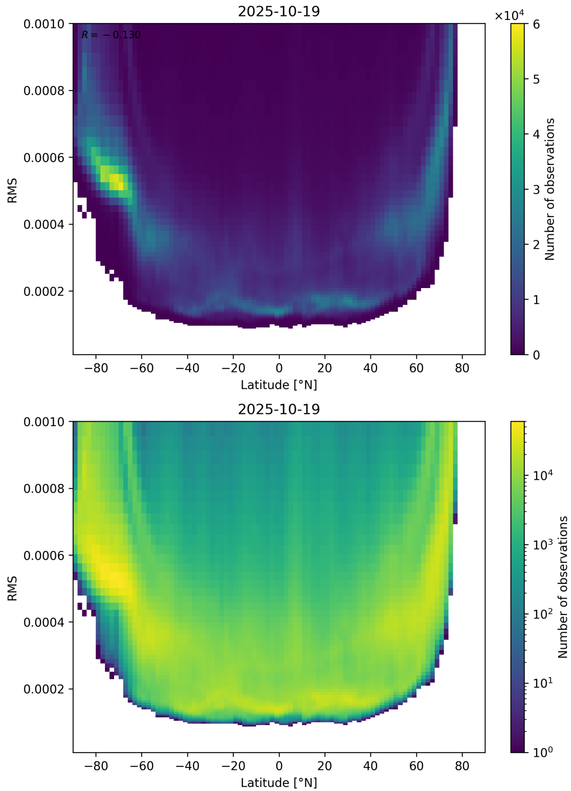
Figure 94: Scatter density plot of “Latitude” against “RMS” for 2025-10-18 to 2025-10-20.
