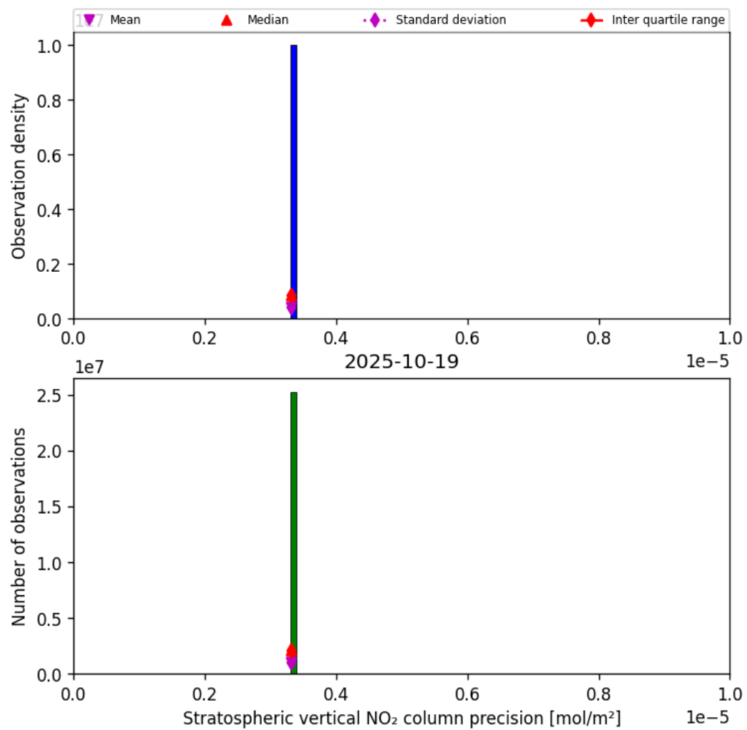
Figure 37: Histogram of “Stratospheric vertical NO 2 column precision” for 2025-10-18 to 2025-10-20
