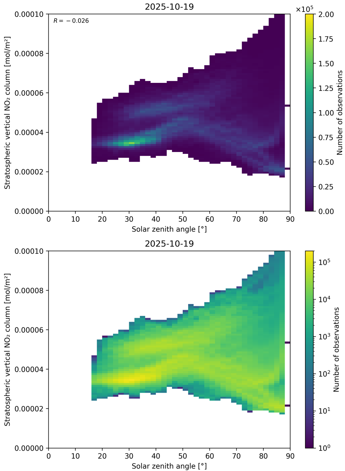
Figure 150: Scatter density plot of “Solar zenith angle” against “Stratospheric vertical NO 2 column” for 2025-10-18 to 2025-10-20.
