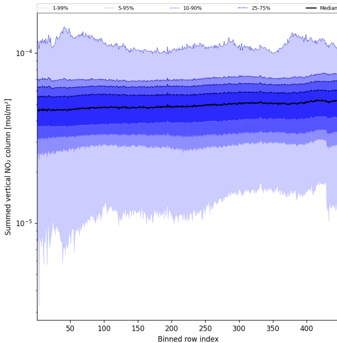
Figure 57: Along track statistics of “Summed vertical NO 2 column” for 2025-10-18 to 2025-10-20
