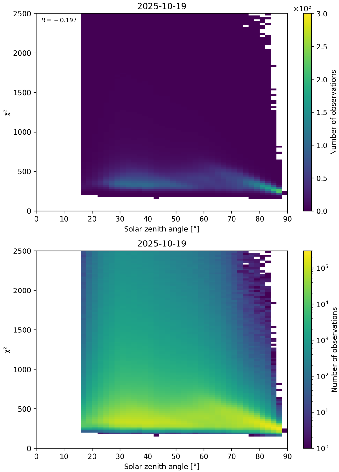
Figure 148: Scatter density plot of “Solar zenith angle” against “ \chi^2 ” for 2025-10-18 to 2025-10-20.
