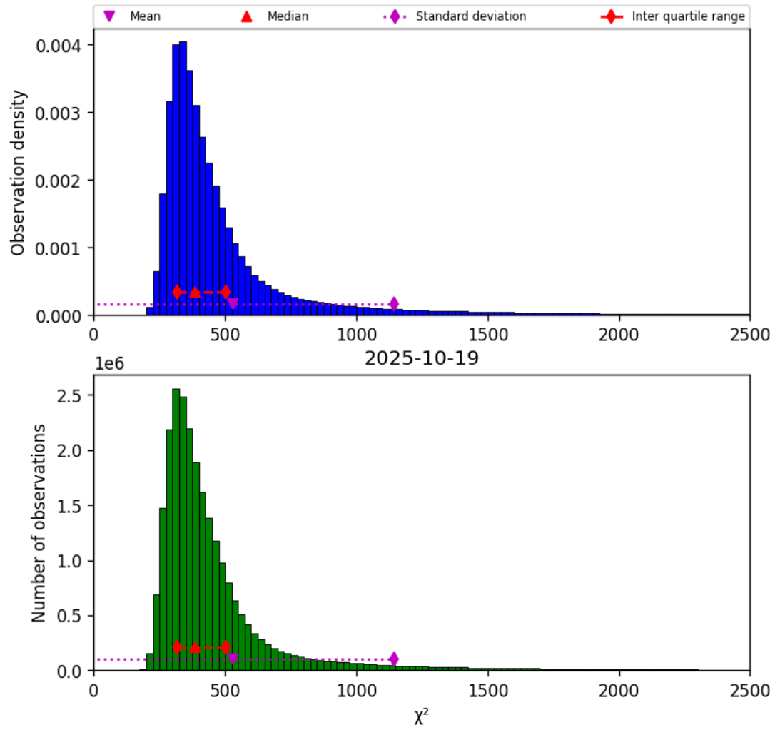
Figure 42: Histogram of " \chi^2 " for 2025-10-18 to 2025-10-20
