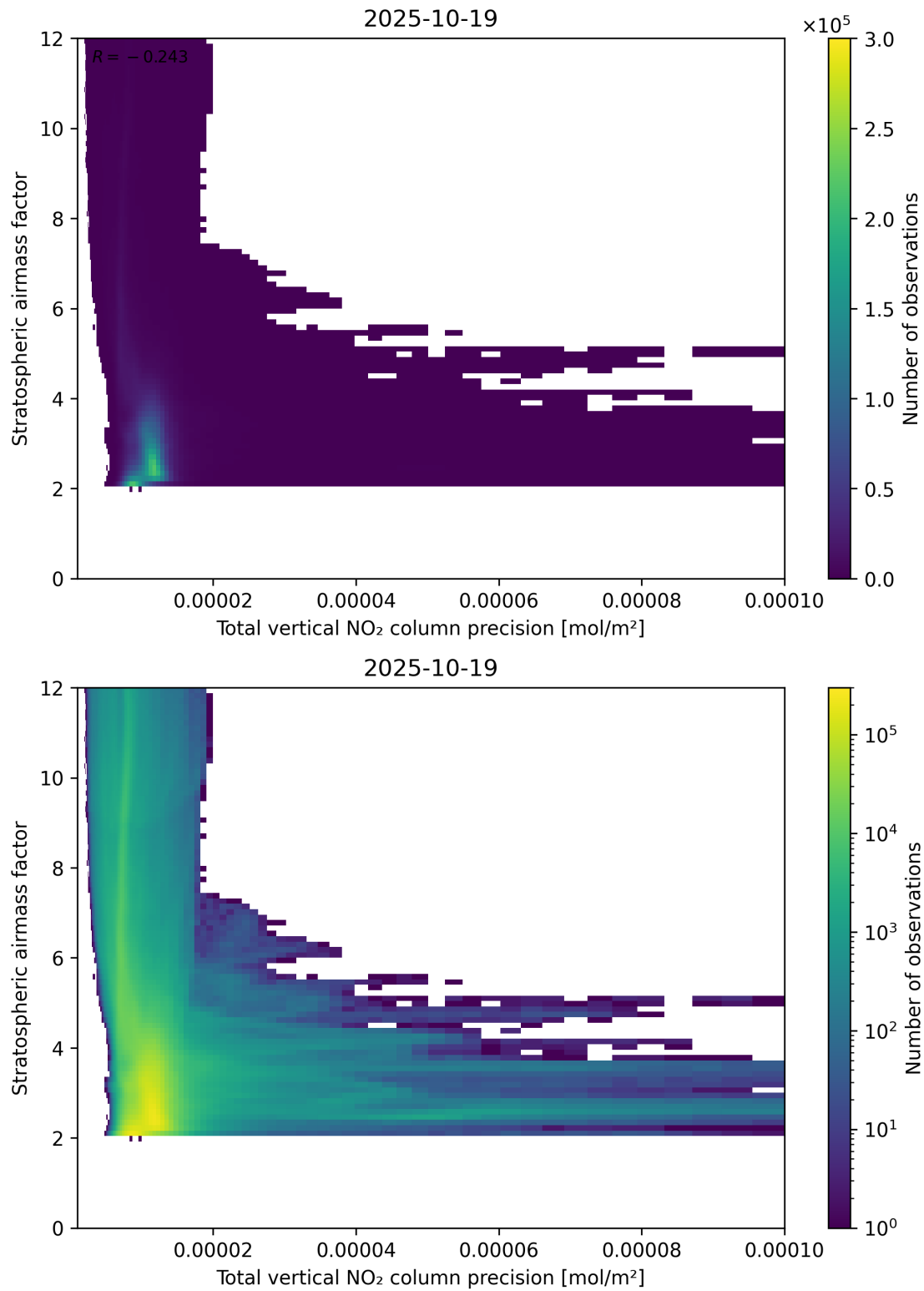
Figure 115: Scatter density plot of “Total vertical NO 2 column precision” against “Stratospheric airmass factor” for 2025-10-18 to 2025-10-20.
