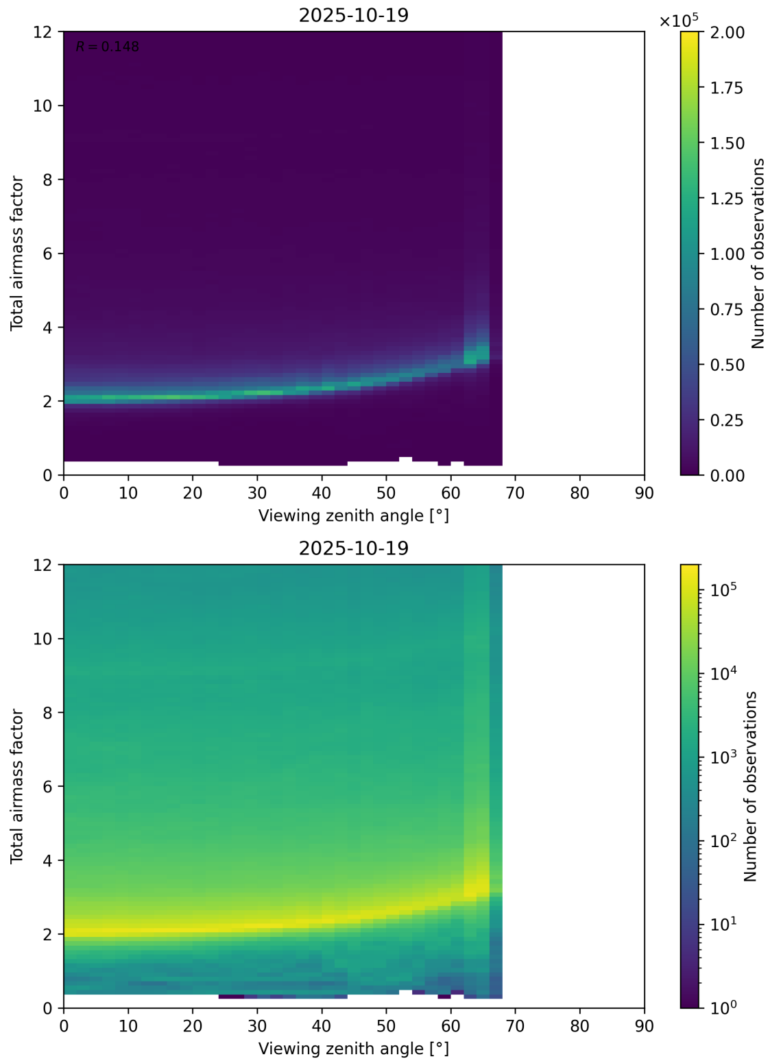
Figure 160: Scatter density plot of “Viewing zenith angle” against “Total airmass factor” for 2025-10-18 to 2025-10-20.
