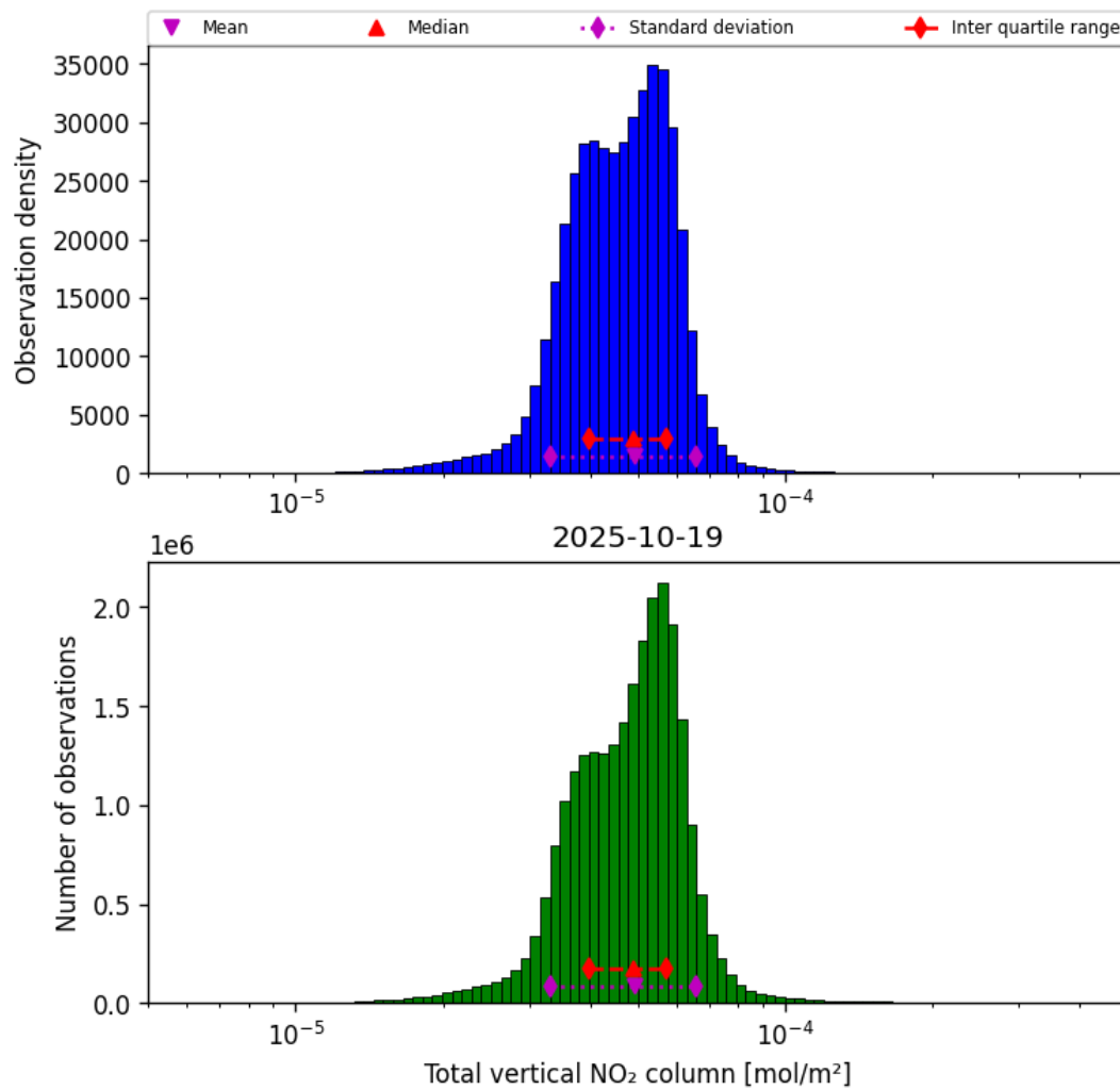
Figure 38: Histogram of “Total vertical NO 2 column” for 2025-10-18 to 2025-10-20
