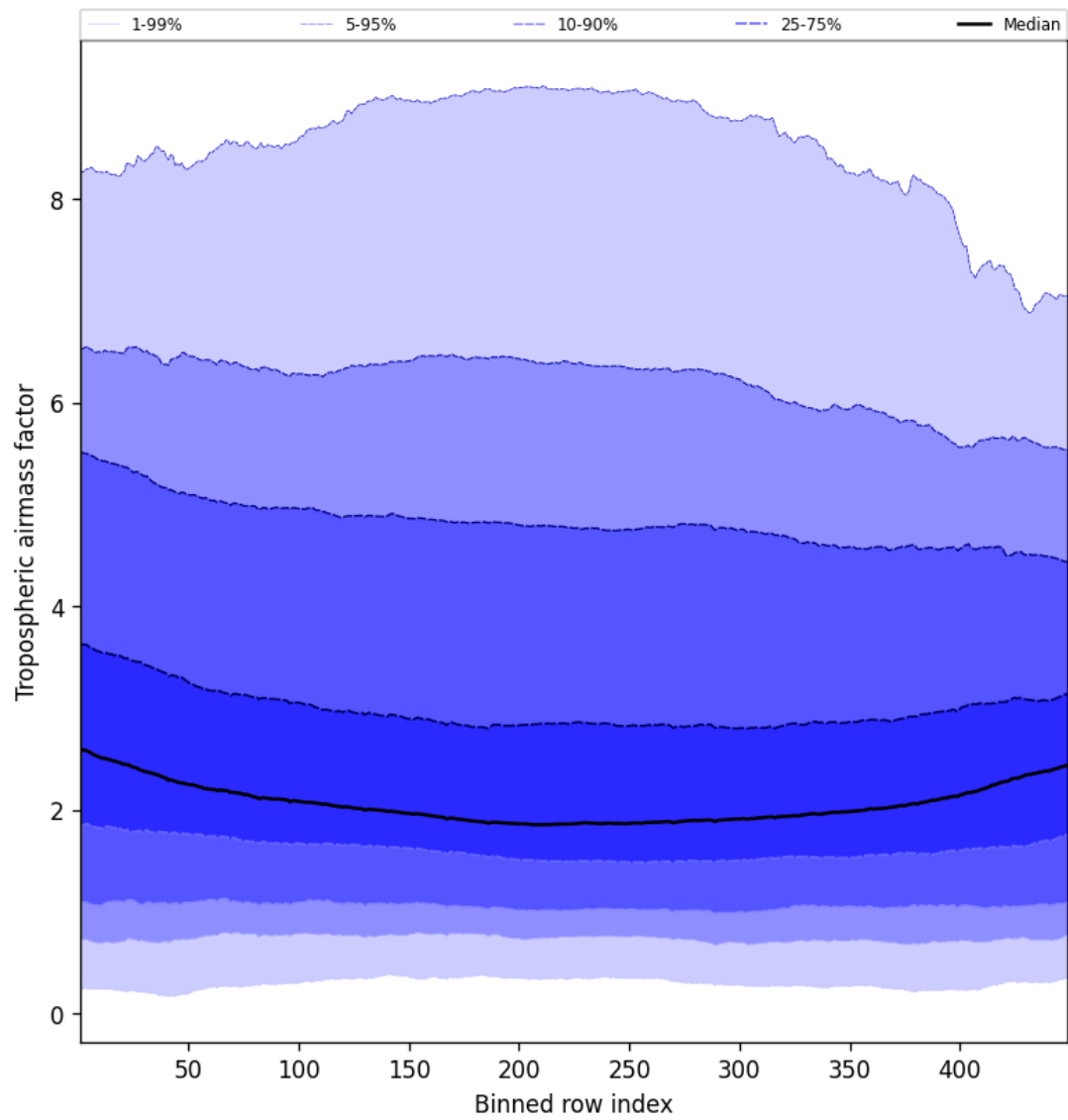
Figure 48: Along track statistics of “Tropospheric air mass factor” for 2025-10-18 to 2025-10-20
