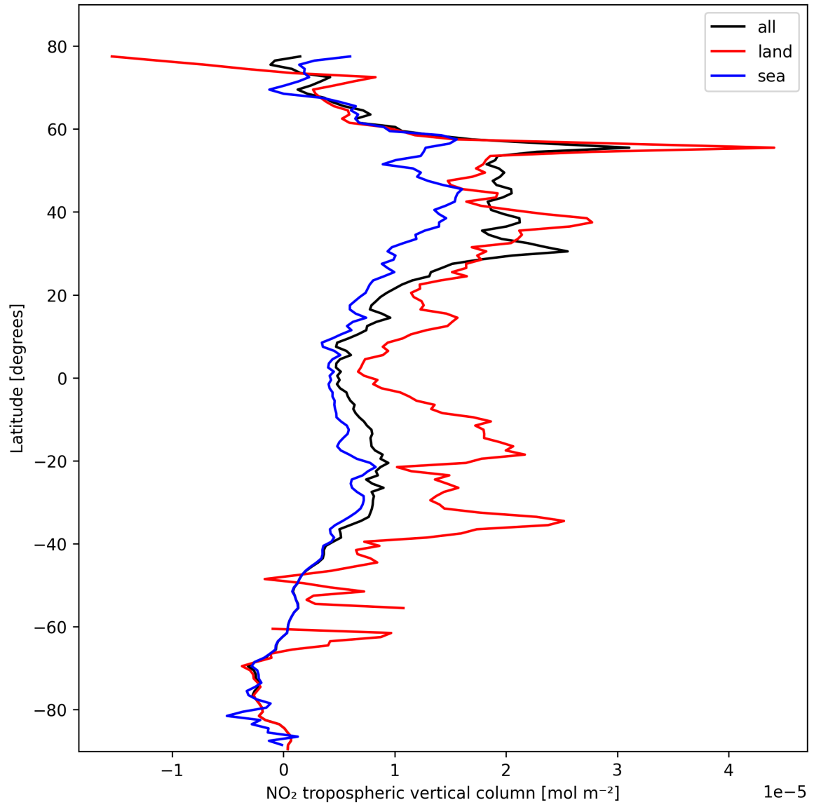
Figure 12: Zonal average of “NO 2 tropospheric vertical column” for 2025-10-18 to 2025-10-20.
