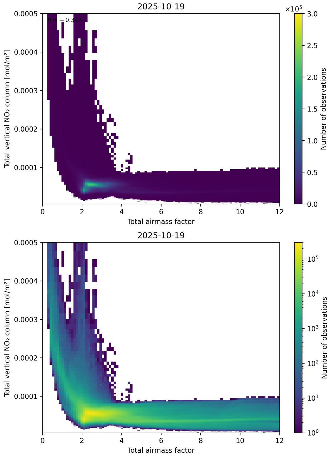
Figure 67: Scatter density plot of “Total airmass factor” against “Total vertical NO 2 column” for 2025-10-18 to 2025-10-20.
