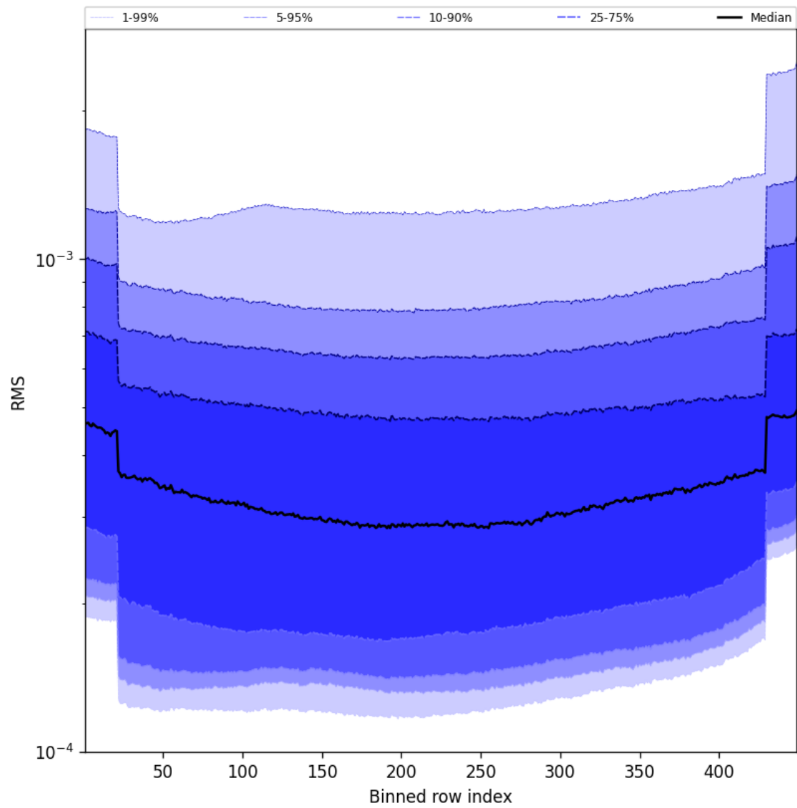
Figure 60: Along track statistics of “RMS” for 2025-10-18 to 2025-10-20
