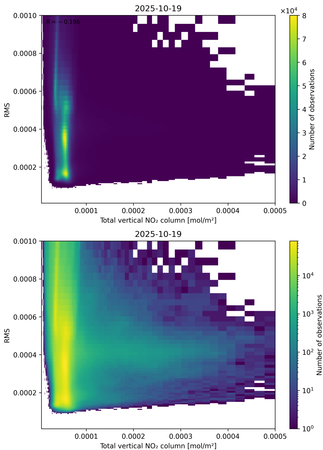
Figure 120: Scatter density plot of “Total vertical NO 2 column” against “RMS” for 2025-10-18 to 2025-10-20.
