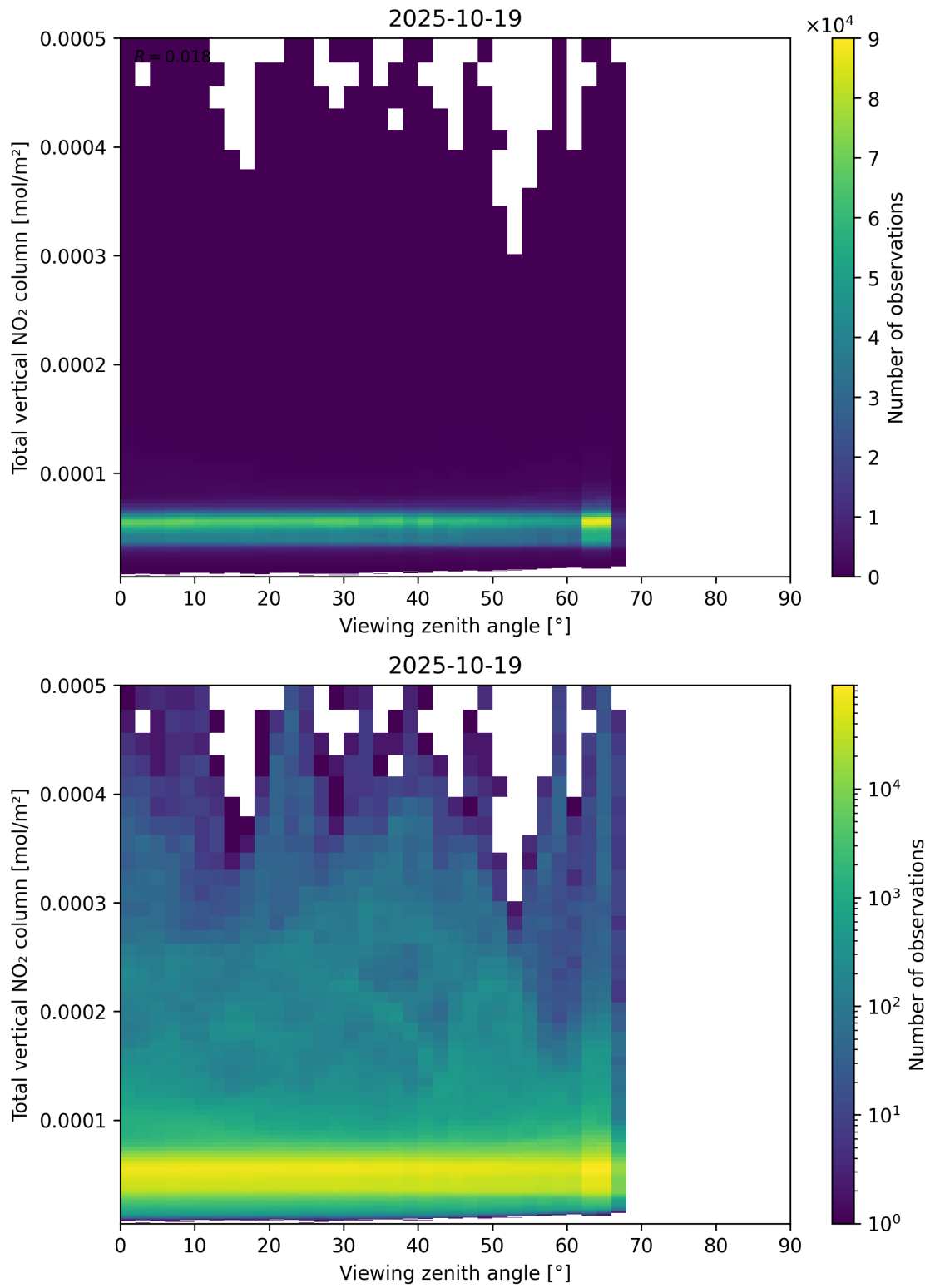
Figure 167: Scatter density plot of “Viewing zenith angle” against “Total vertical NO 2 column” for 2025-10-18 to 2025-10-20.
