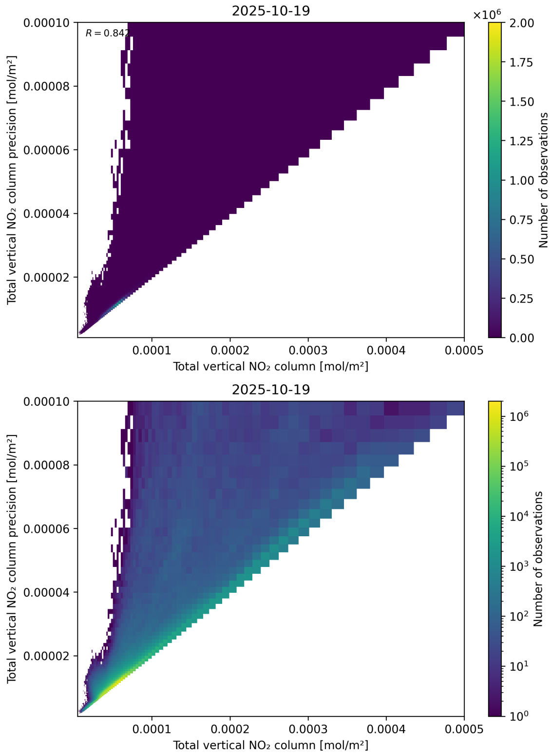
Figure 114: Scatter density plot of “Total vertical NO 2 column” against “Total vertical NO 2 column precision” for 2025-10-18 to 2025-10-20.
