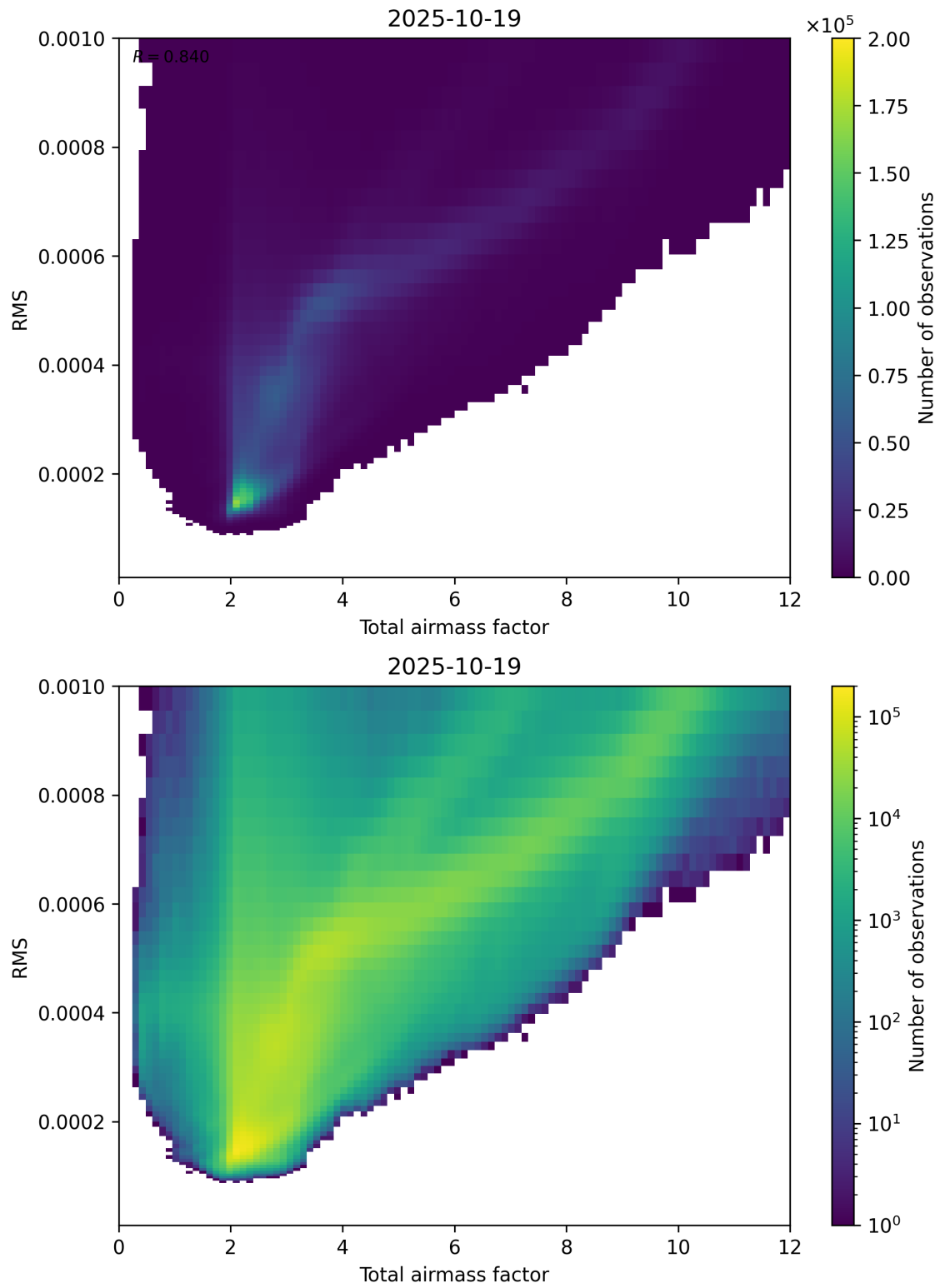
Figure 69: Scatter density plot of “Total airmass factor” against “RMS” for 2025-10-18 to 2025-10-20.
