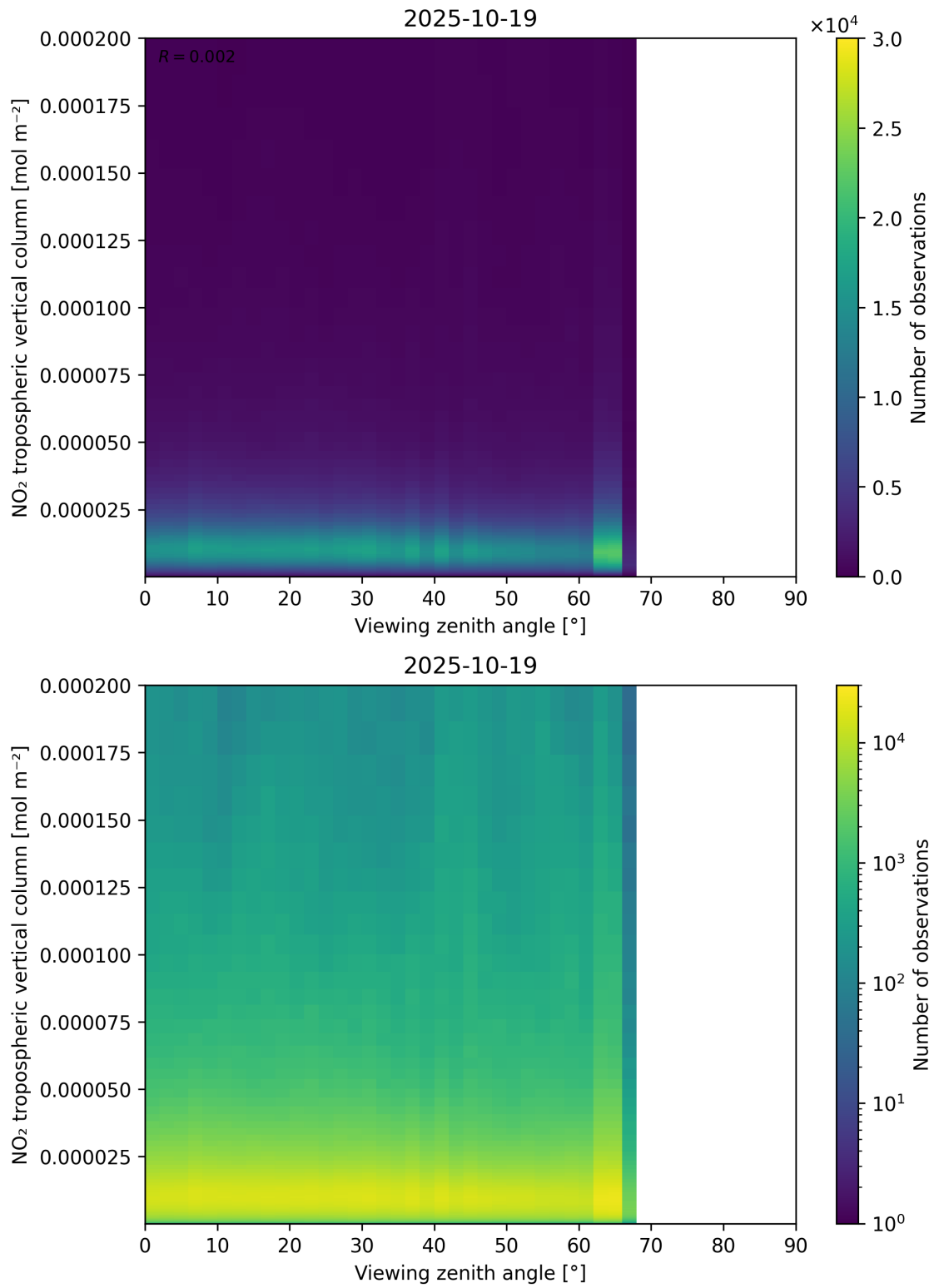
Figure 169: Scatter density plot of “Viewing zenith angle” against “NO 2 tropospheric vertical column” for 2025-10-18 to 2025-10-20.
