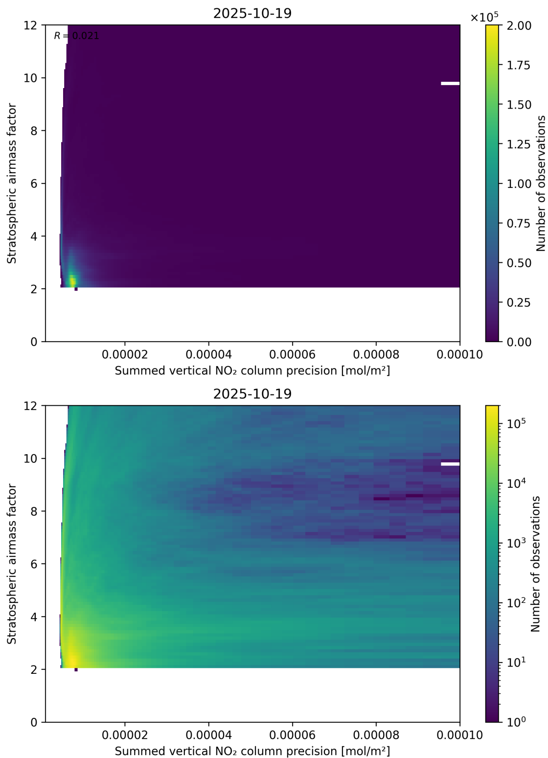
Figure 106: Scatter density plot of “Summed vertical NO 2 column precision” against “Stratospheric airmass factor” for 2025-10-18 to 2025-10-20.
