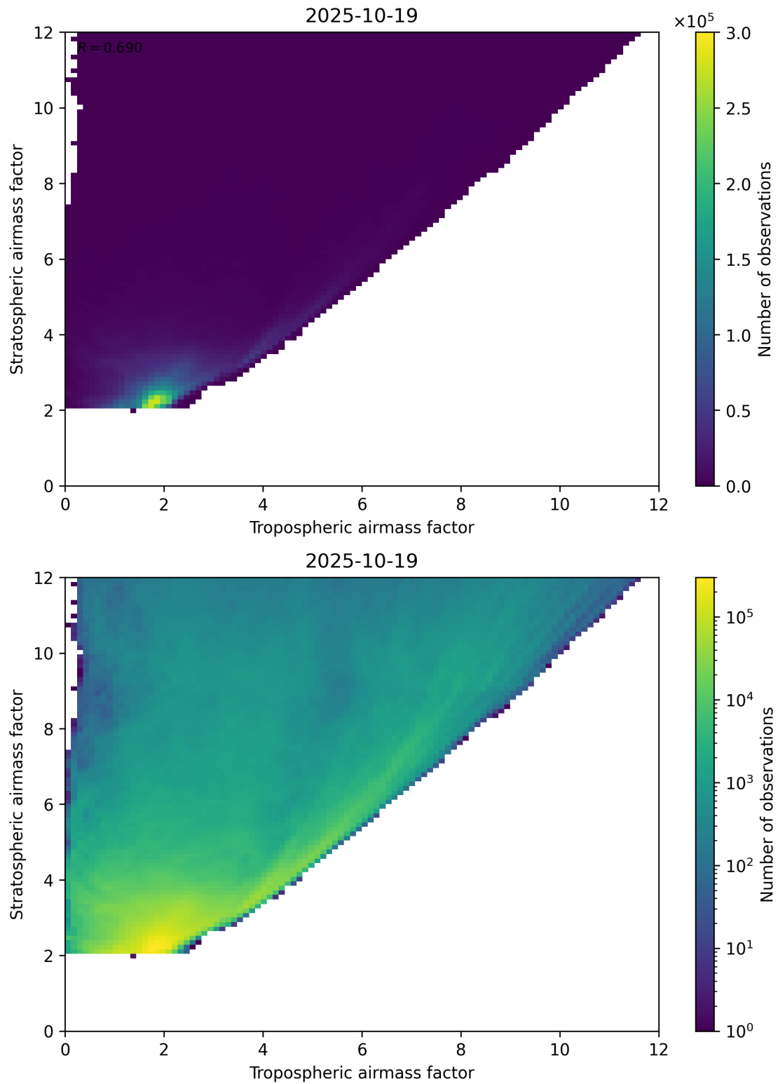
Figure 71: Scatter density plot of “Tropospheric airmass factor” against “Stratospheric airmass factor” for 2025-10-18 to 2025-10-20.
