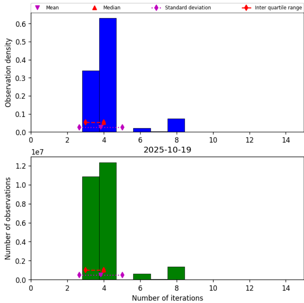
Figure 34: Histogram of “Number of iterations” for 2025-10-18 to 2025-10-20
