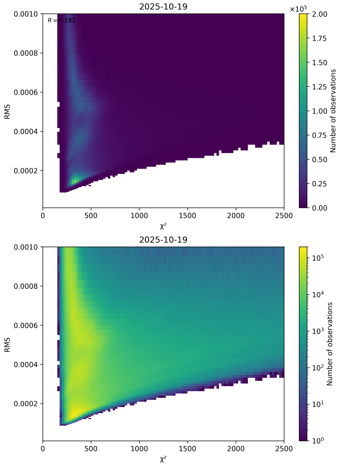
Figure 82: Scatter density plot of “ \chi^2 ” against “RMS” for 2025-10-18 to 2025-10-20.
