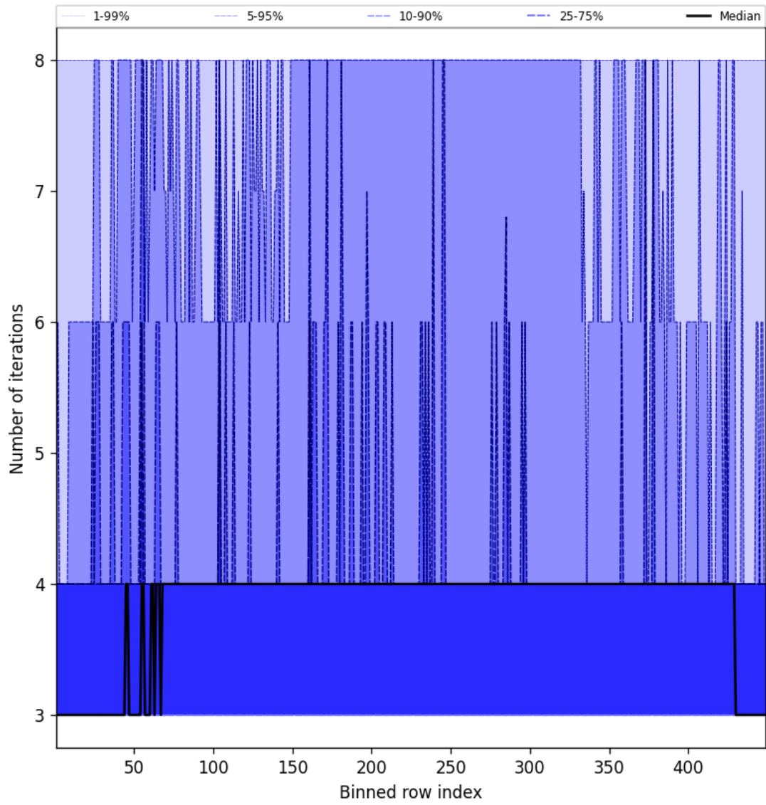
Figure 51: Along track statistics of “Number of iterations” for 2025-10-18 to 2025-10-20
