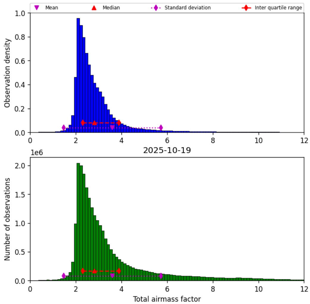
Figure 32: Histogram of “Total airmass factor” for 2025-10-18 to 2025-10-20
