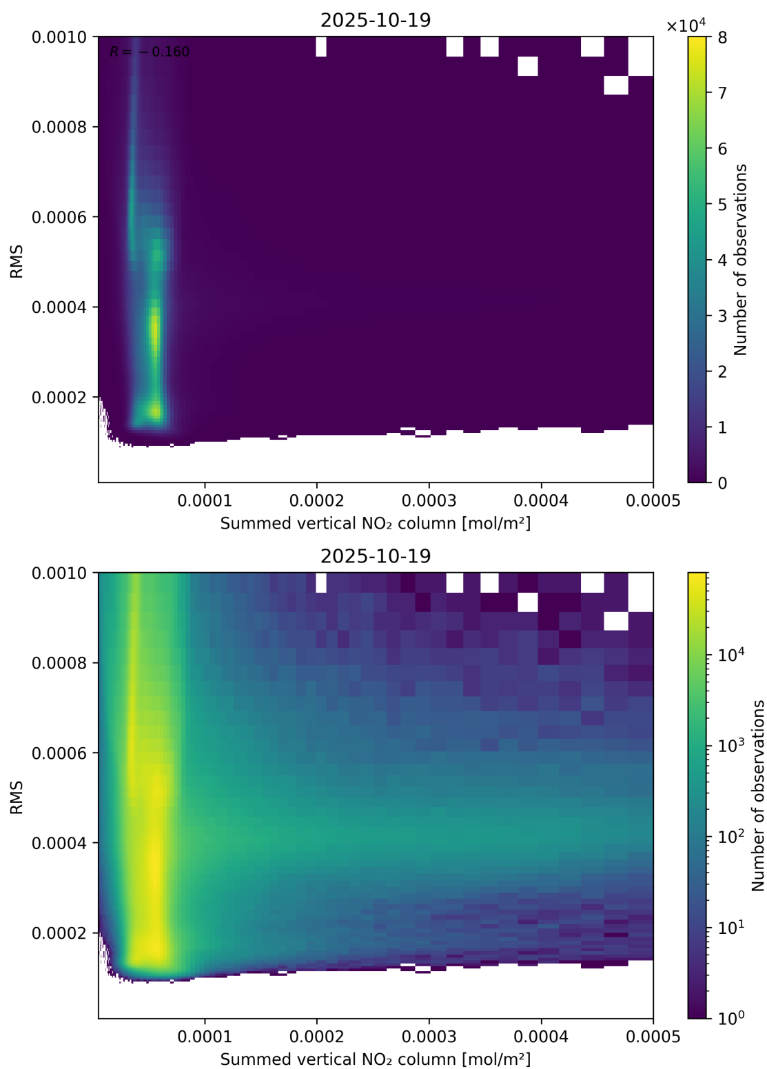
Figure 109: Scatter density plot of “Summed vertical NO 2 column” against “RMS” for 2025-10-18 to 2025-10-20.
