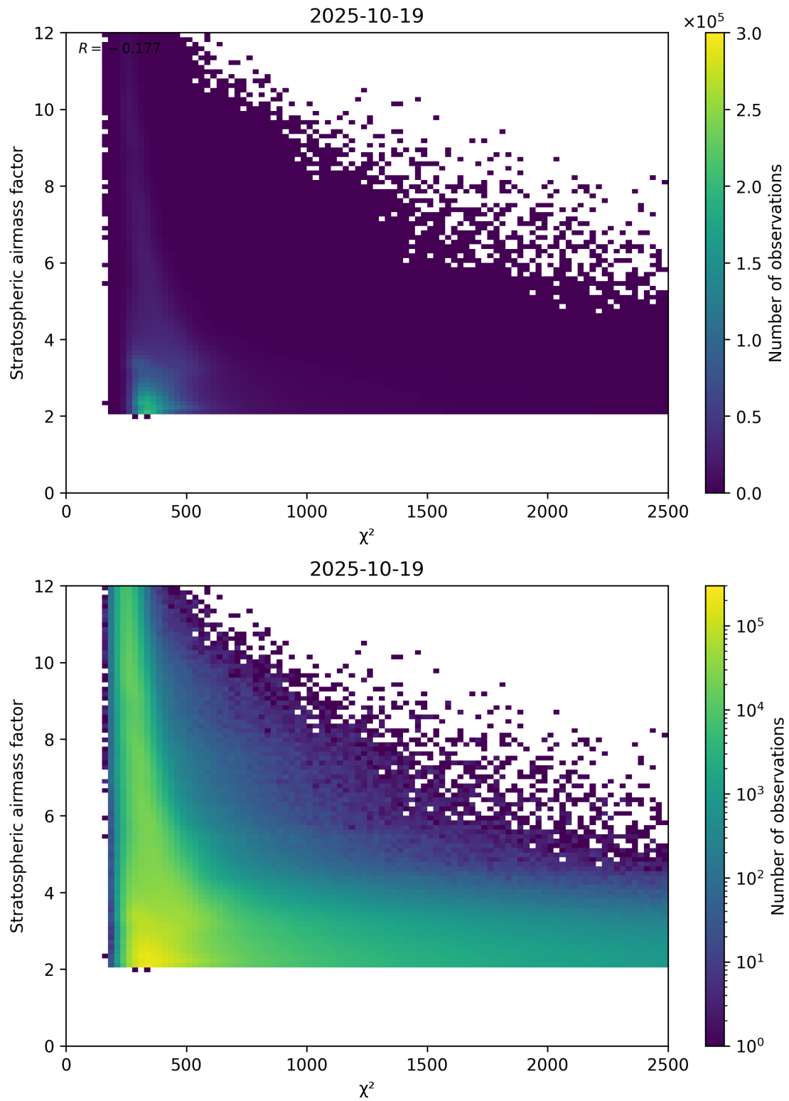
Figure 81: Scatter density plot of “ \chi^2 ” against “Stratospheric airmass factor” for 2025-10-18 to 2025-10-20.
