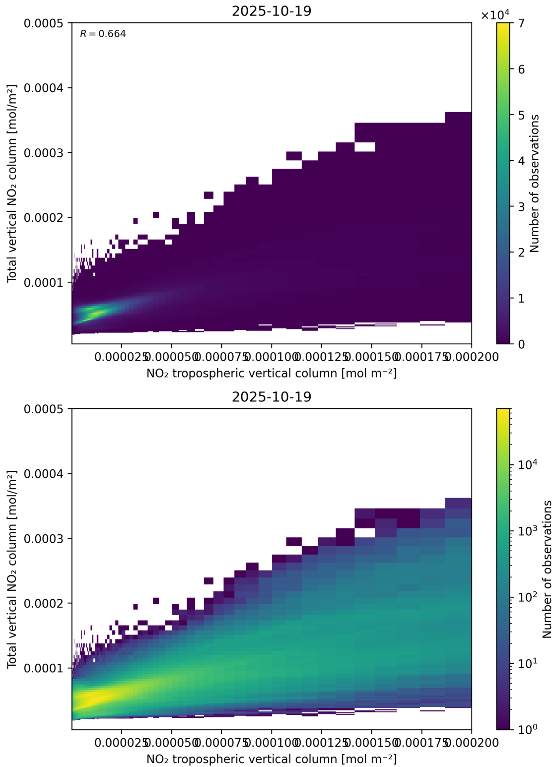
Figure 128: Scatter density plot of “NO 2 tropospheric vertical column” against “Total vertical NO 2 column” for 2025-10-18 to 2025-10-20.
