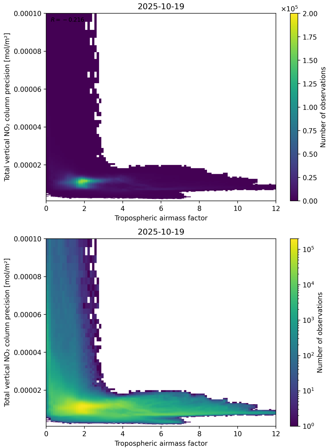
Figure 78: Scatter density plot of “Tropospheric airmass factor” against “Total vertical NO 2 column precision” for 2025-10-18 to 2025-10-20.
