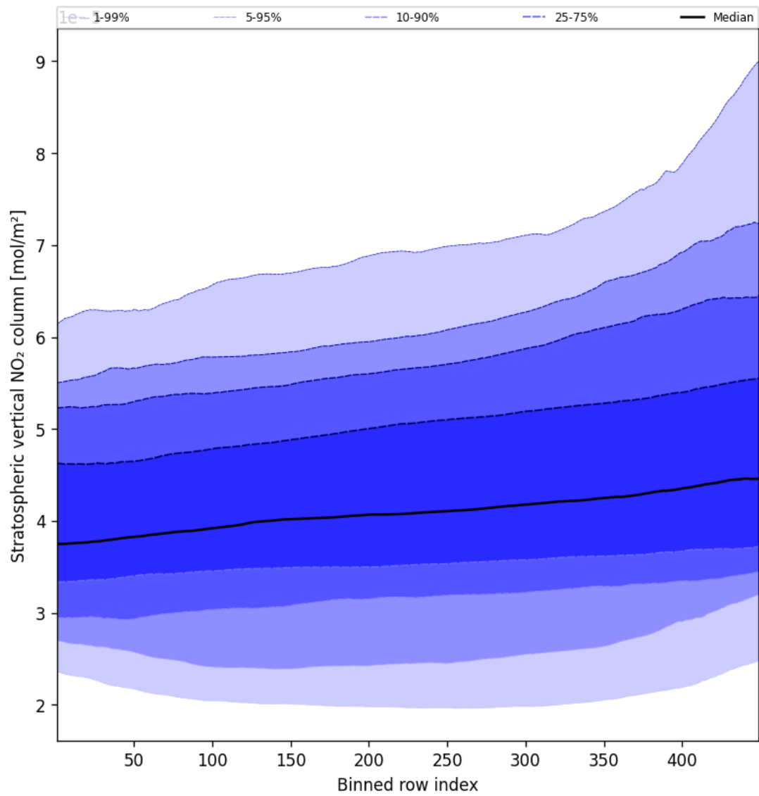
Figure 53: Along track statistics of “Stratospheric vertical NO 2 column” for 2025-10-18 to 2025-10-20
