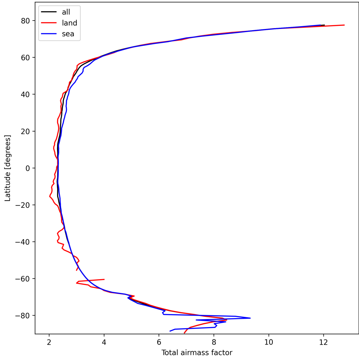
Figure 15: Zonal average of “Total airmass factor” for 2025-10-18 to 2025-10-20.
