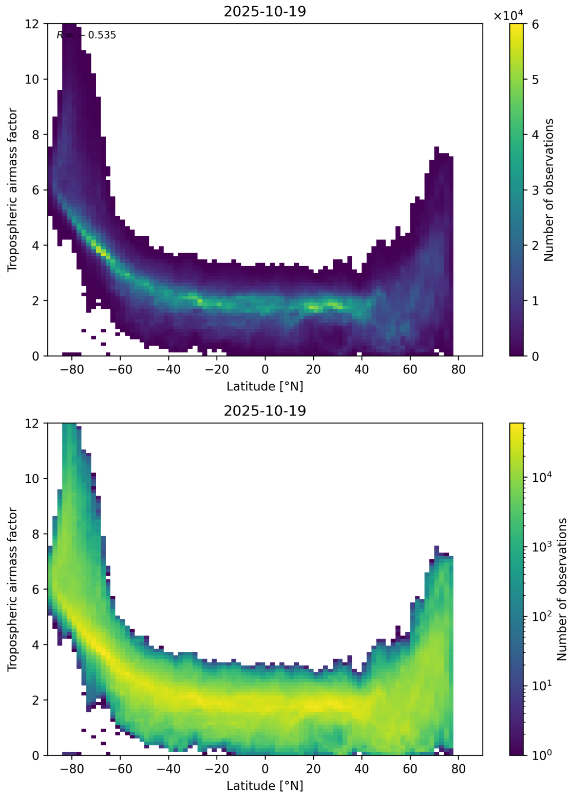
Figure 85: Scatter density plot of “Latitude” against “Tropospheric air mass factor” for 2025-10-18 to 2025-10-20.
