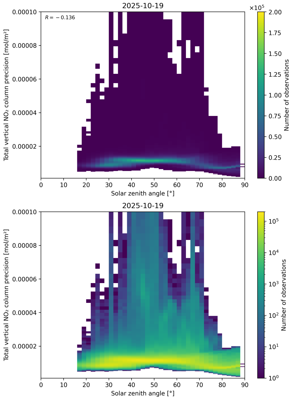
Figure 154: Scatter density plot of “Solar zenith angle” against “Total vertical NO 2 column precision” for 2025-10-18 to 2025-10-20.
