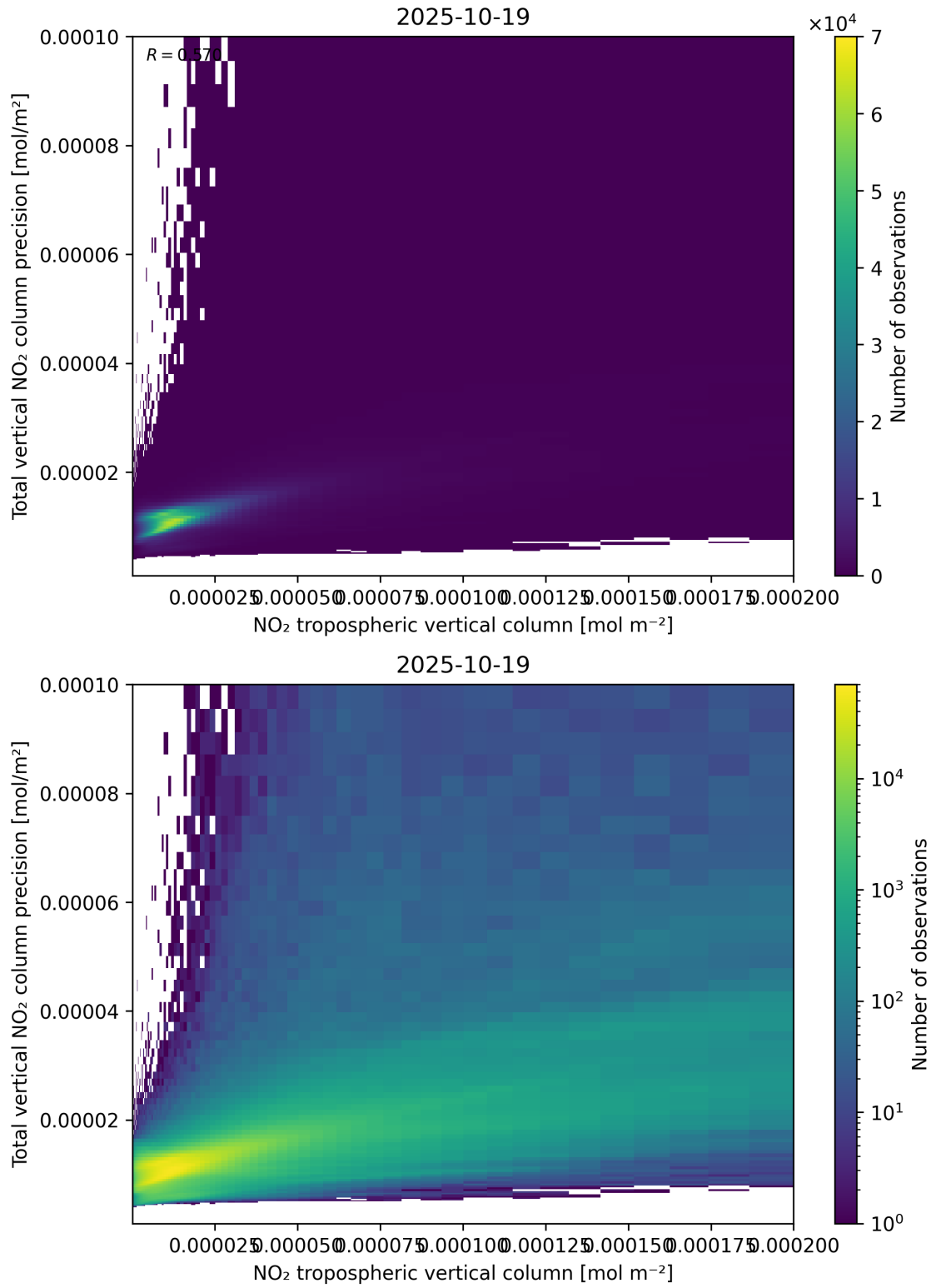
Figure 129: Scatter density plot of “NO 2 tropospheric vertical column” against “Total vertical NO 2 column precision” for 2025-10-18 to 2025-10-20.
