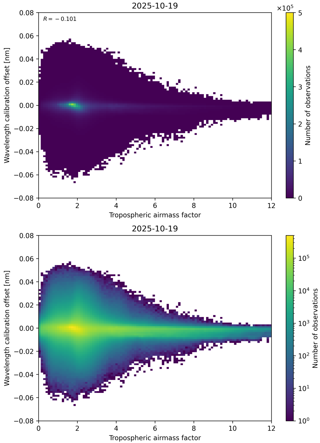
Figure 80: Scatter density plot of “Tropospheric airmass factor” against “Wavelength calibration offset” for 2025-10-18 to 2025-10-20.
