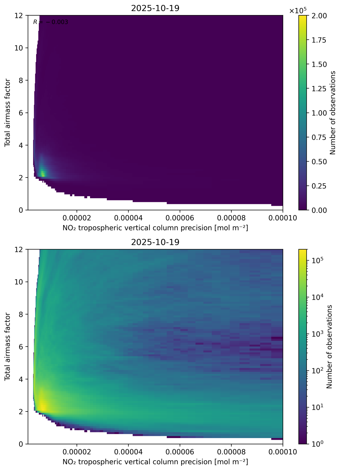
Figure 132: Scatter density plot of “NO 2 tropospheric vertical column precision” against “Total air mass factor” for 2025-10-18 to 2025-10-20.
