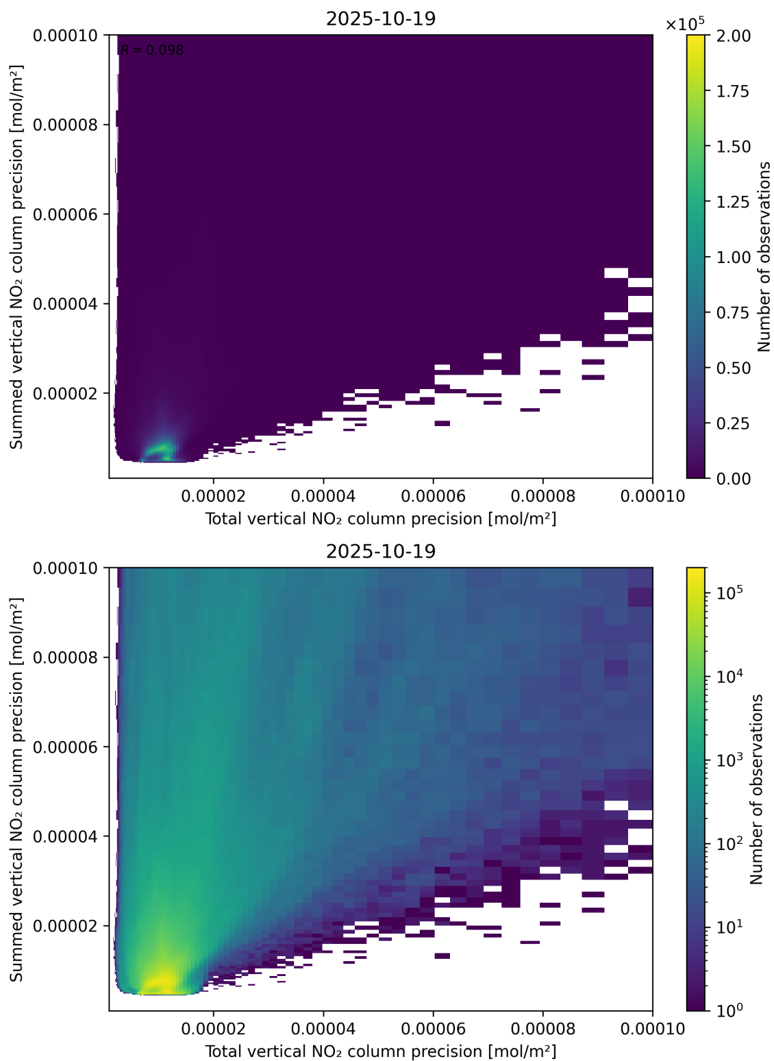
Figure 118: Scatter density plot of “Total vertical NO 2 column precision” against “Summed vertical NO 2 column precision” for 2025-10-18 to 2025-10-20.
