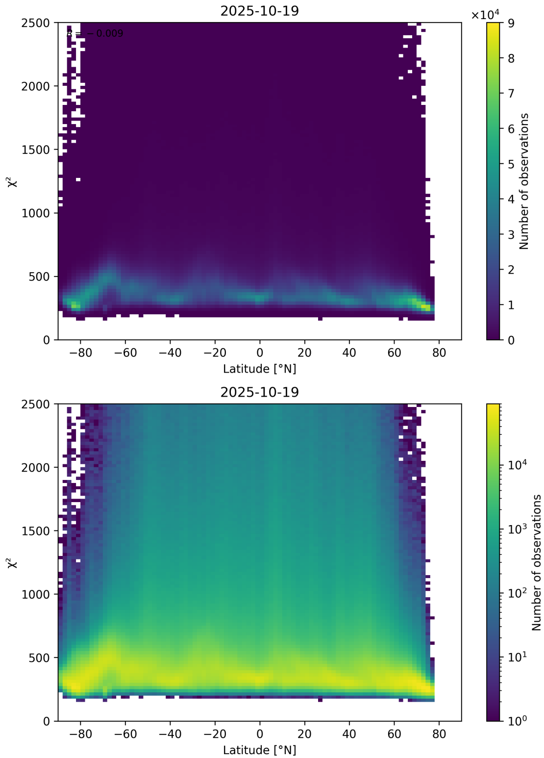
Figure 86: Scatter density plot of “Latitude” against “ \chi^2 ” for 2025-10-18 to 2025-10-20.
