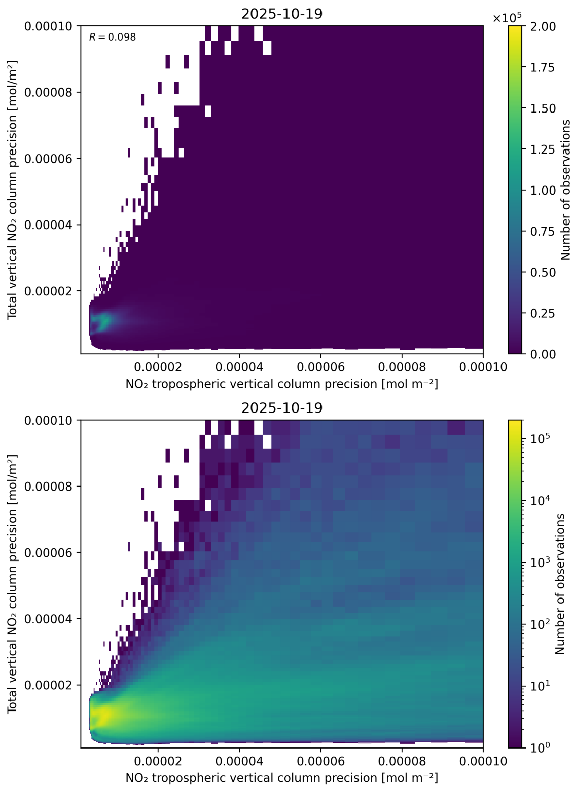
Figure 139: Scatter density plot of “NO 2 tropospheric vertical column precision” against “Total vertical NO 2 column precision” for 2025-10-18 to 2025-10-20.
