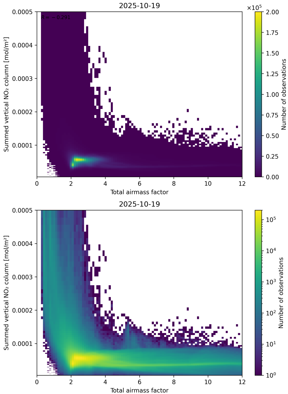
Figure 65: Scatter density plot of “Total airmass factor” against “Summed vertical NO 2 column” for 2025-10-18 to 2025-10-20.
