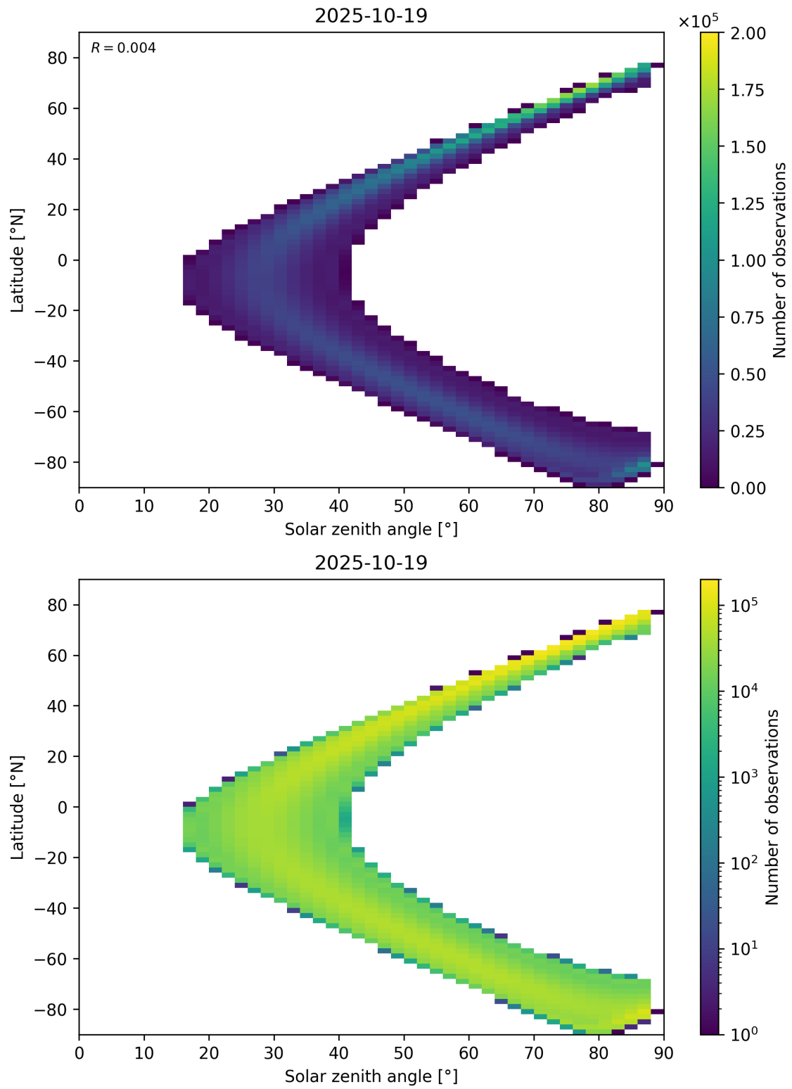
Figure 149: Scatter density plot of “Solar zenith angle” against “Latitude” for 2025-10-18 to 2025-10-20.
