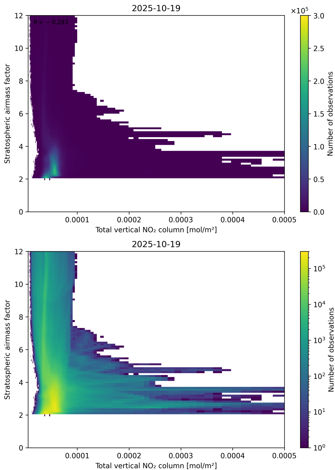
Figure 110: Scatter density plot of “Total vertical NO 2 column” against “Stratospheric airmass factor” for 2025-10-18 to 2025-10-20.
