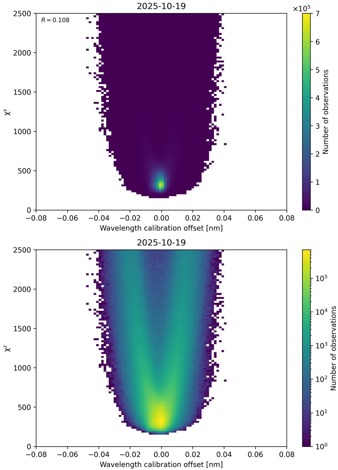
Figure 175: Scatter density plot of “Wavelength calibration offset” against “ \chi^2 ” for 2025-10-18 to 2025-10-20.
