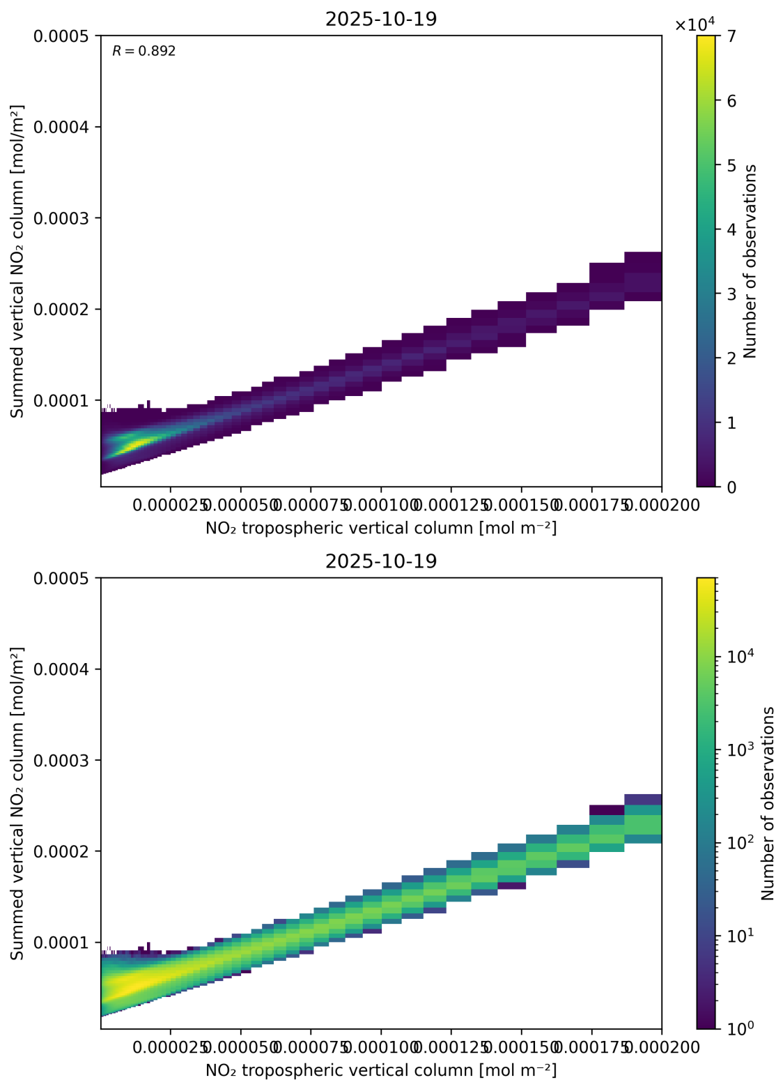
Figure 126: Scatter density plot of “NO 2 tropospheric vertical column” against “Summed vertical NO 2 column” for 2025-10-18 to 2025-10-20.
