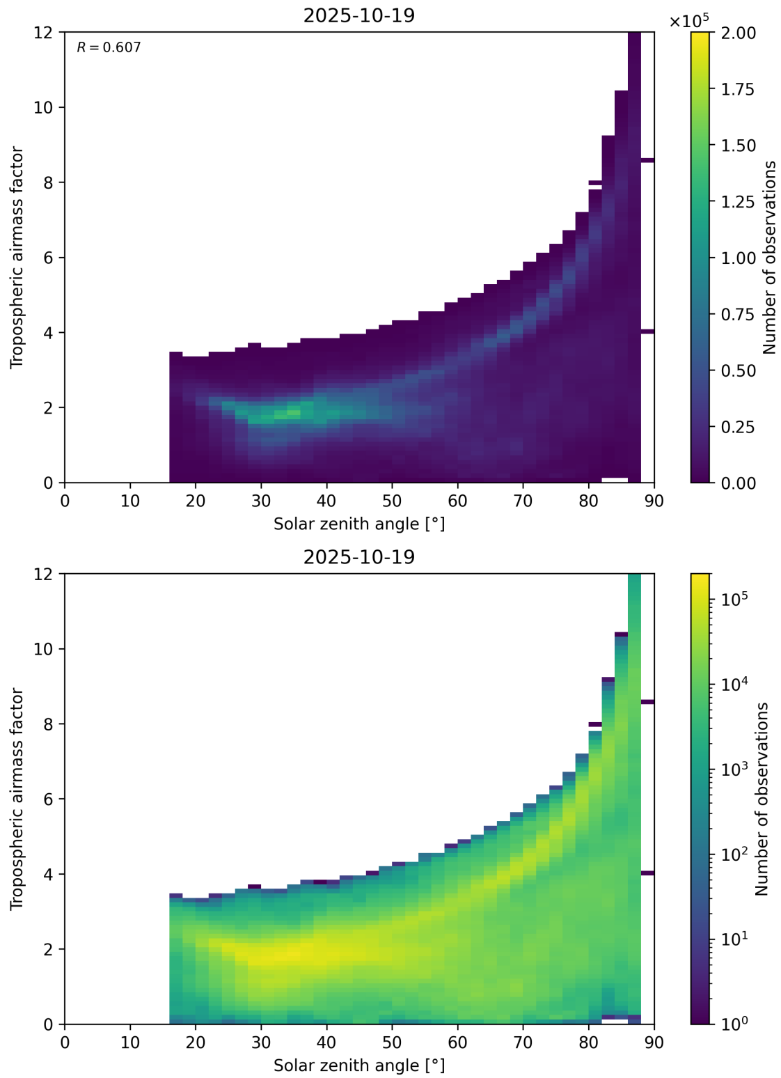
Figure 147: Scatter density plot of “Solar zenith angle” against “Tropospheric airmass factor” for 2025-10-18 to 2025-10-20.
