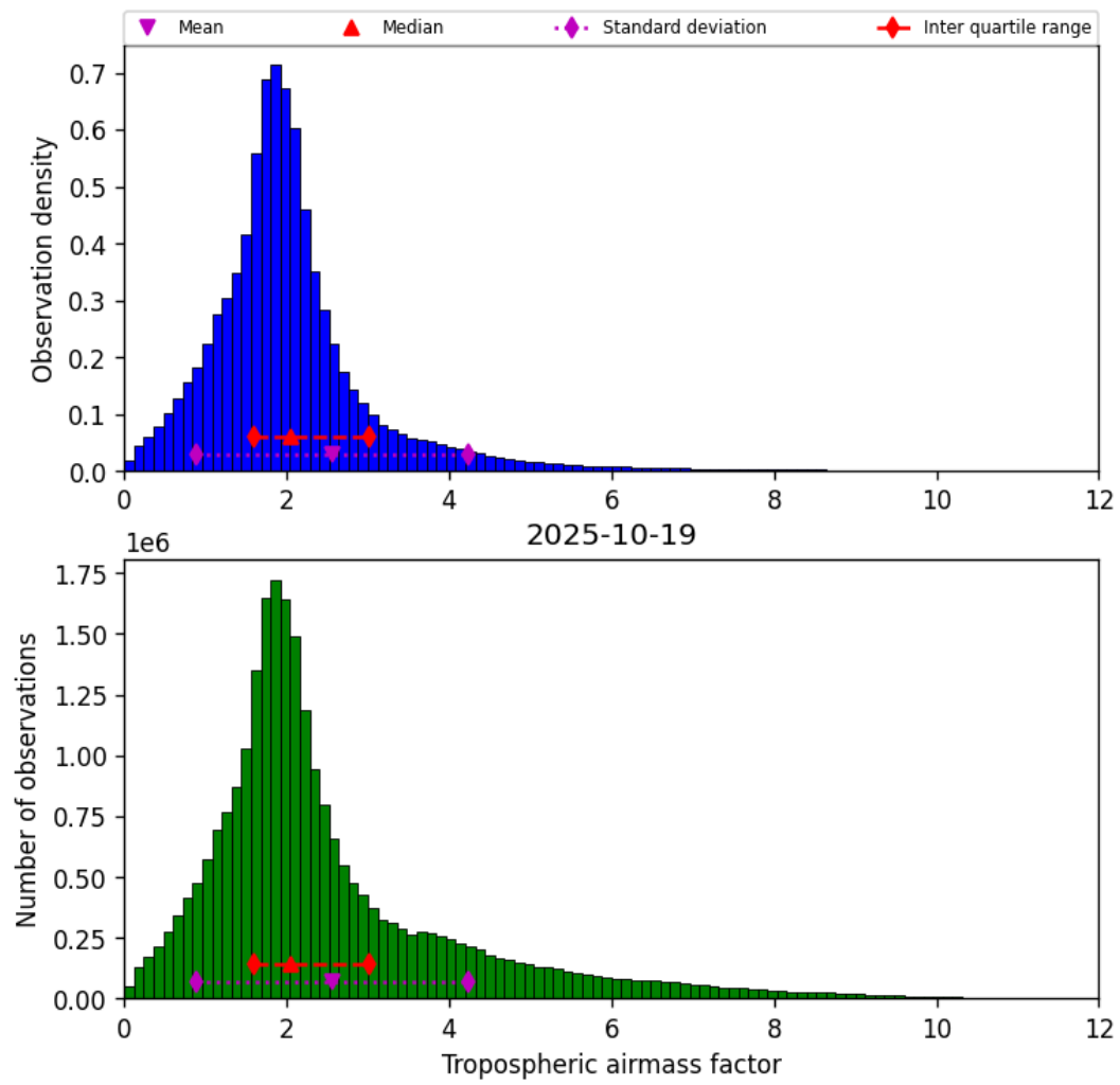
Figure 31: Histogram of “Tropospheric airmass factor” for 2025-10-18 to 2025-10-20
