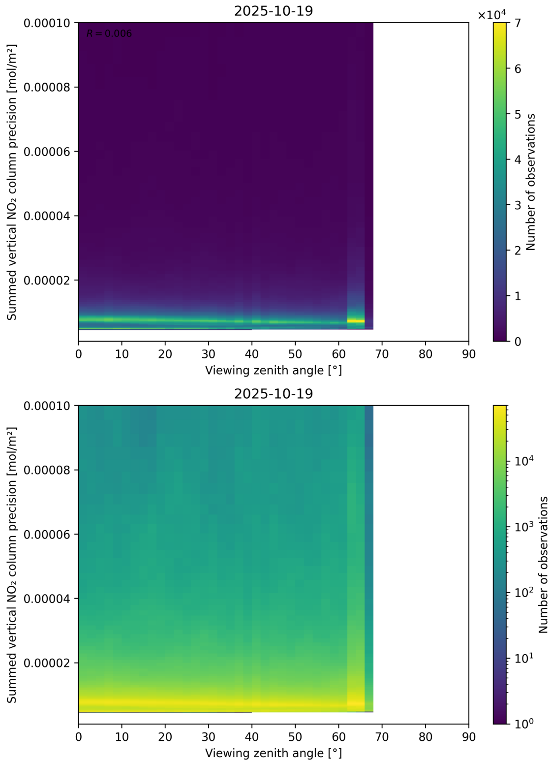
Figure 166: Scatter density plot of “Viewing zenith angle” against “Summed vertical NO 2 column precision” for 2025-10-18 to 2025-10-20.
