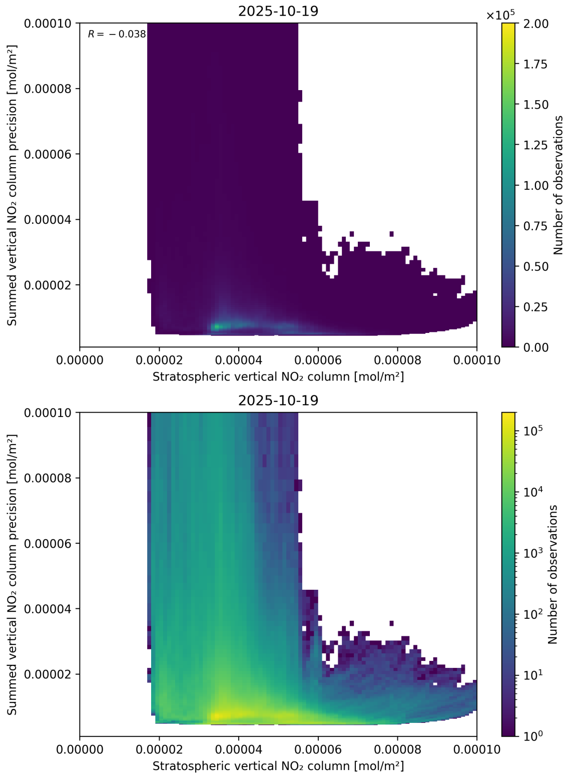
Figure 99: Scatter density plot of “Stratospheric vertical NO 2 column” against “Summed vertical NO 2 column precision” for 2025-10-18 to 2025-10-20.
