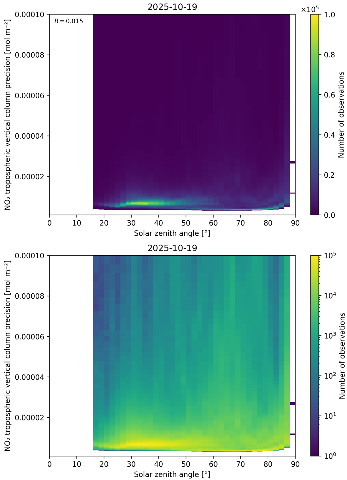
Figure 156: Scatter density plot of “Solar zenith angle” against “NO 2 tropospheric vertical column precision” for 2025-10-18 to 2025-10-20.
