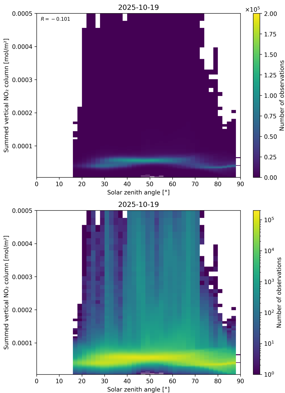
Figure 151: Scatter density plot of “Solar zenith angle” against “Summed vertical NO 2 column” for 2025-10-18 to 2025-10-20.
