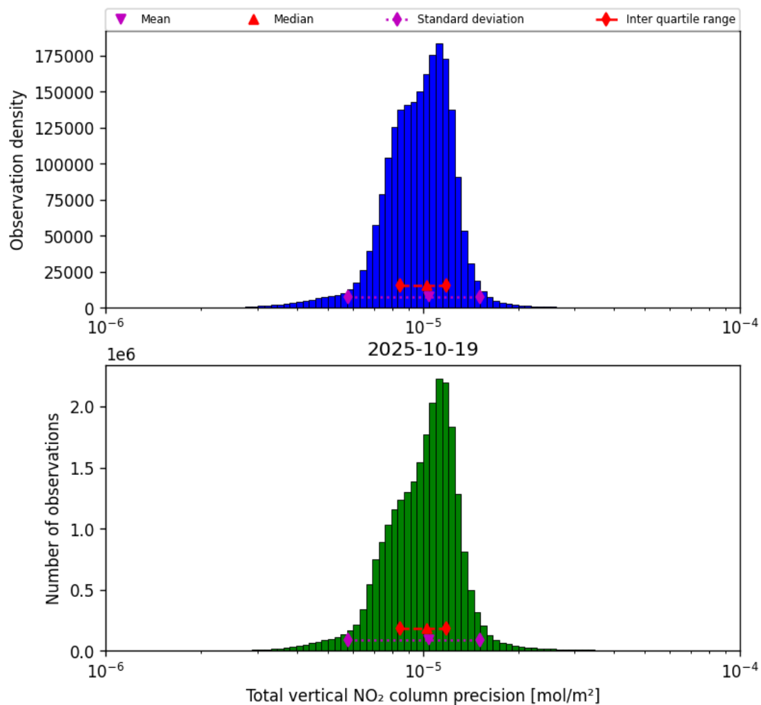
Figure 39: Histogram of “Total vertical NO 2 column precision” for 2025-10-18 to 2025-10-20
