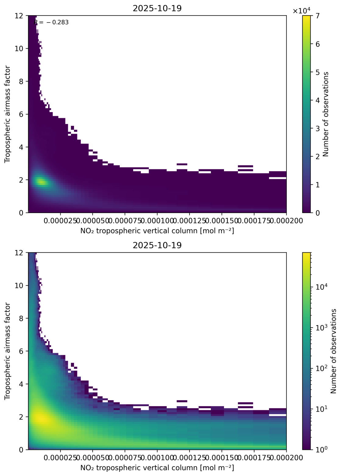
Figure 123: Scatter density plot of “NO 2 tropospheric vertical column” against “Tropospheric air mass factor” for 2025-10-18 to 2025-10-20.
