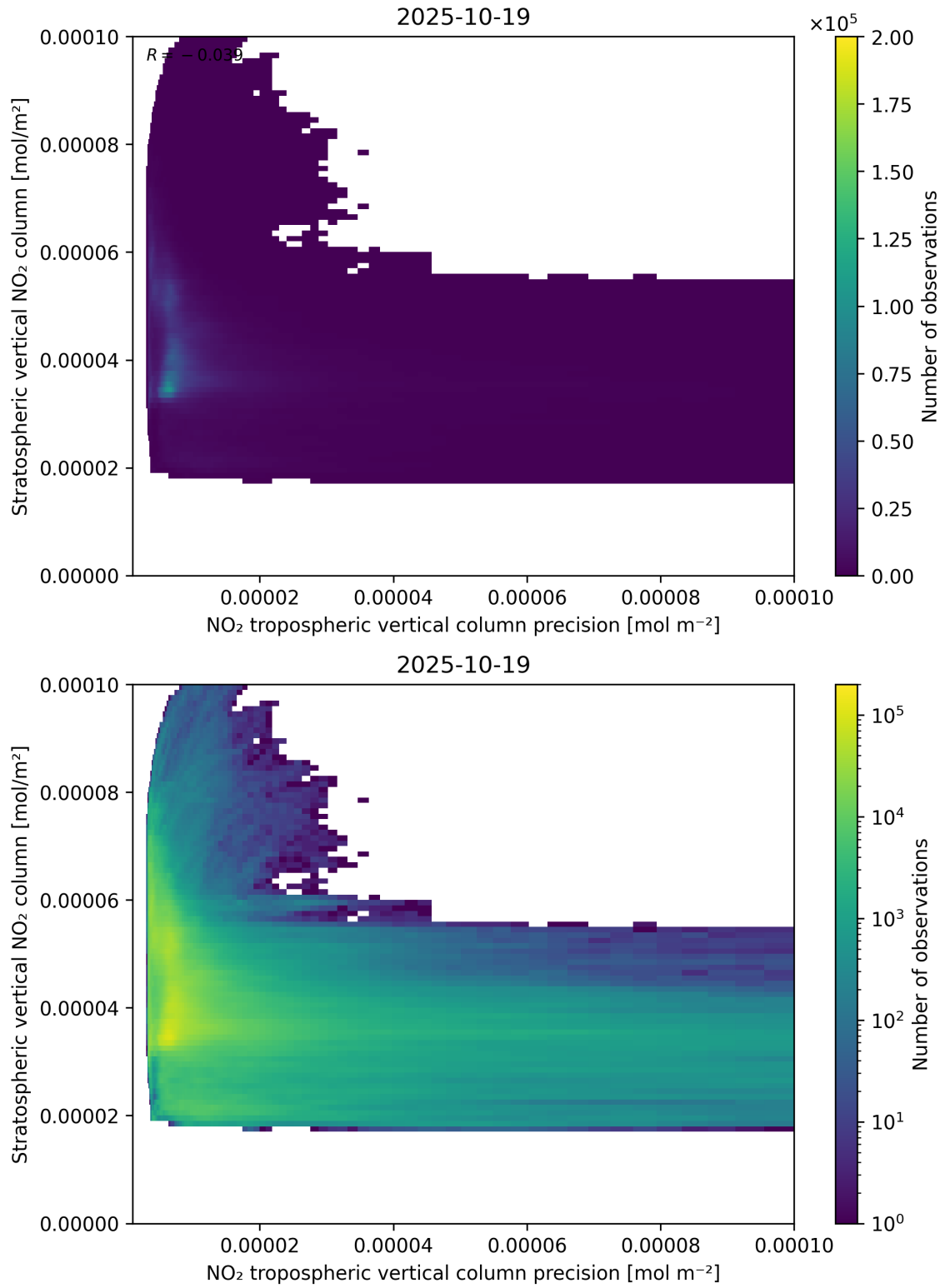
Figure 135: Scatter density plot of “NO 2 tropospheric vertical column precision” against “Stratospheric vertical NO 2 column” for 2025-10-18 to 2025-10-20.
