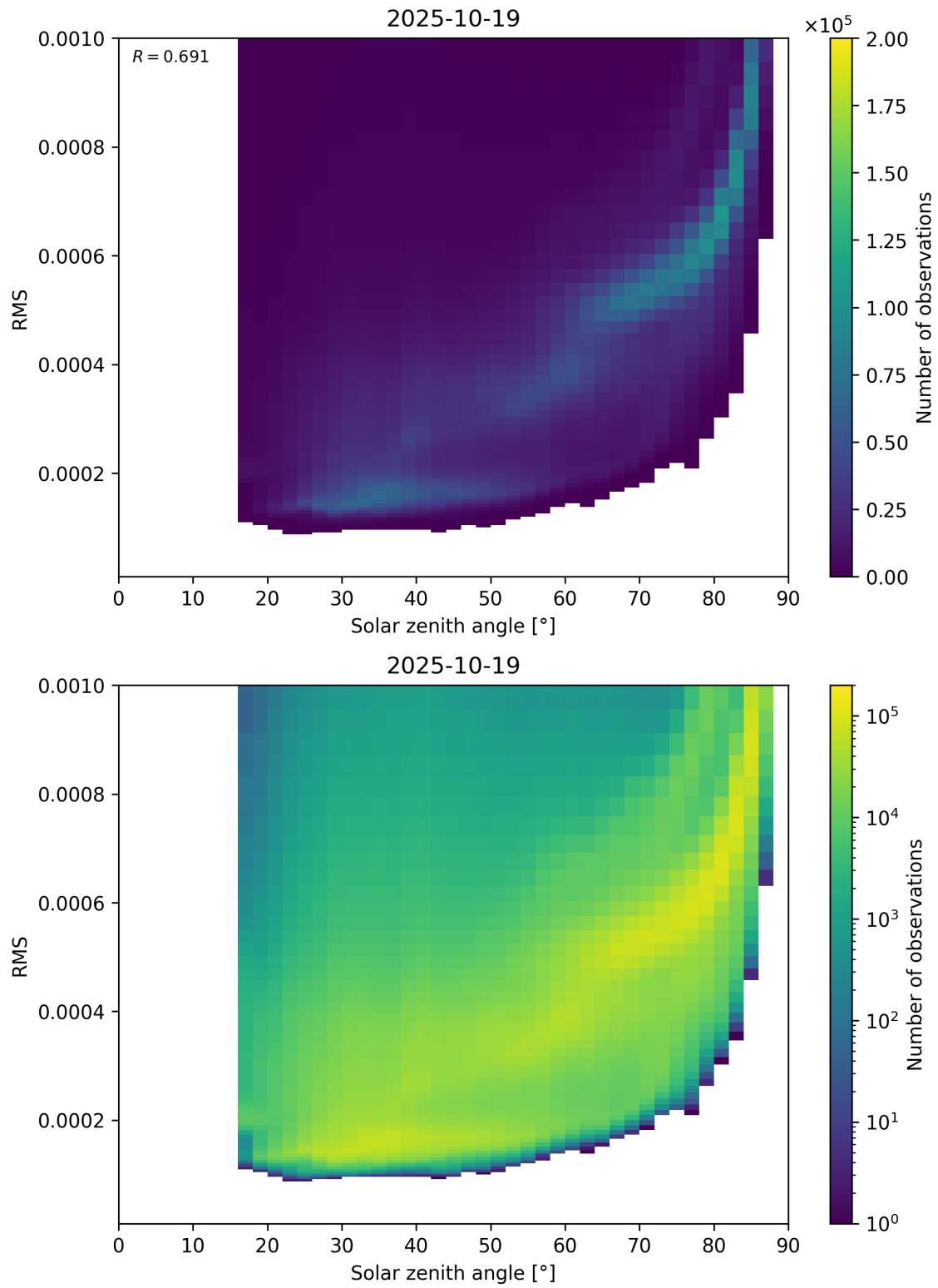
Figure 157: Scatter density plot of “Solar zenith angle” against “RMS” for 2025-10-18 to 2025-10-20.
