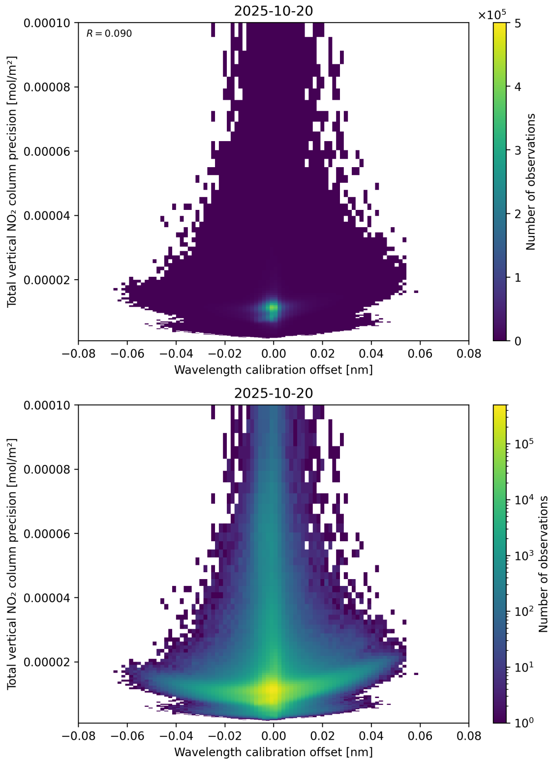
Figure 180: Scatter density plot of “Wavelength calibration offset” against “Total vertical NO 2 column precision” for 2025-10-19 to 2025-10-21.
