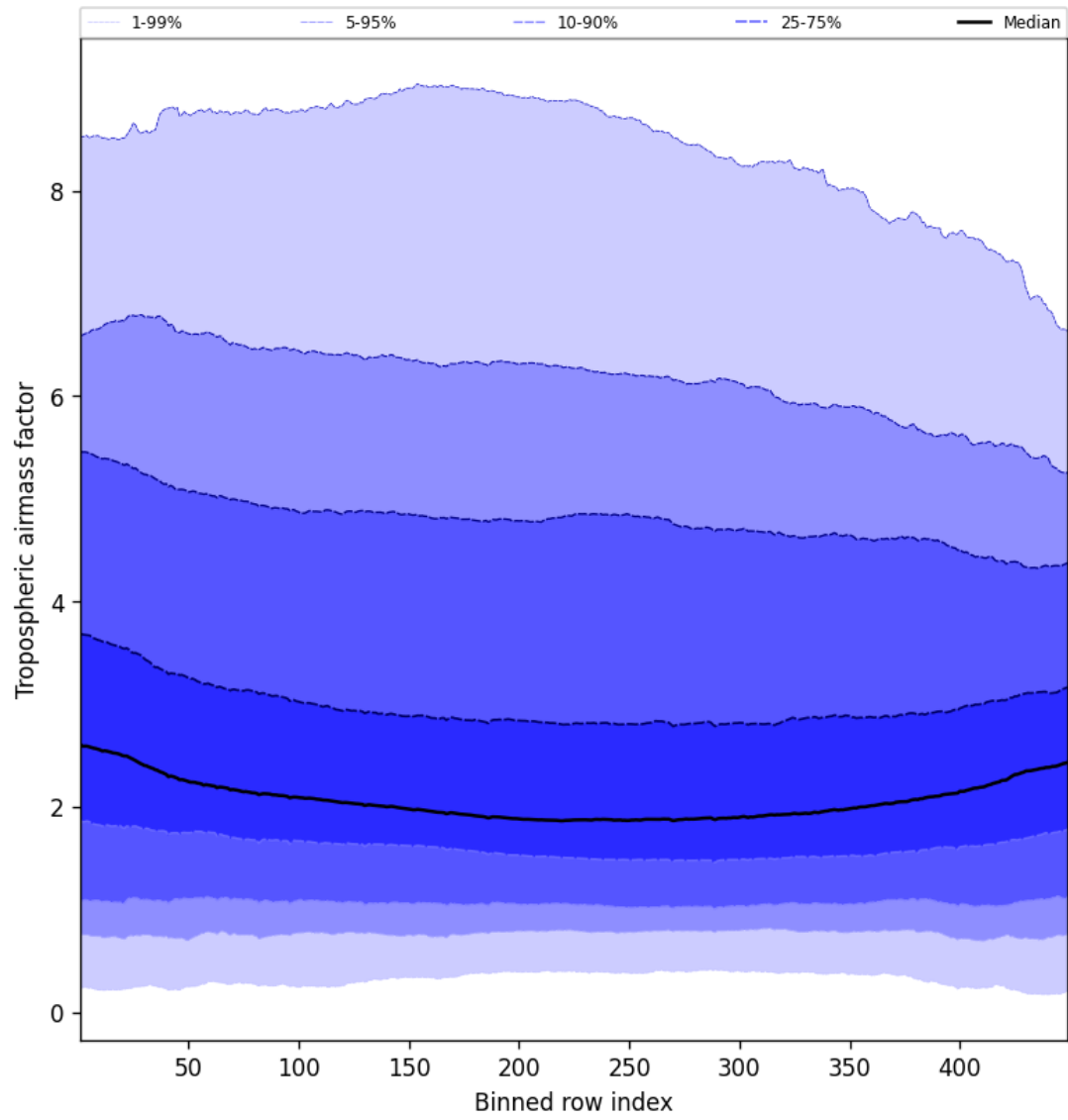
Figure 48: Along track statistics of “Tropospheric air mass factor” for 2025-10-19 to 2025-10-21
