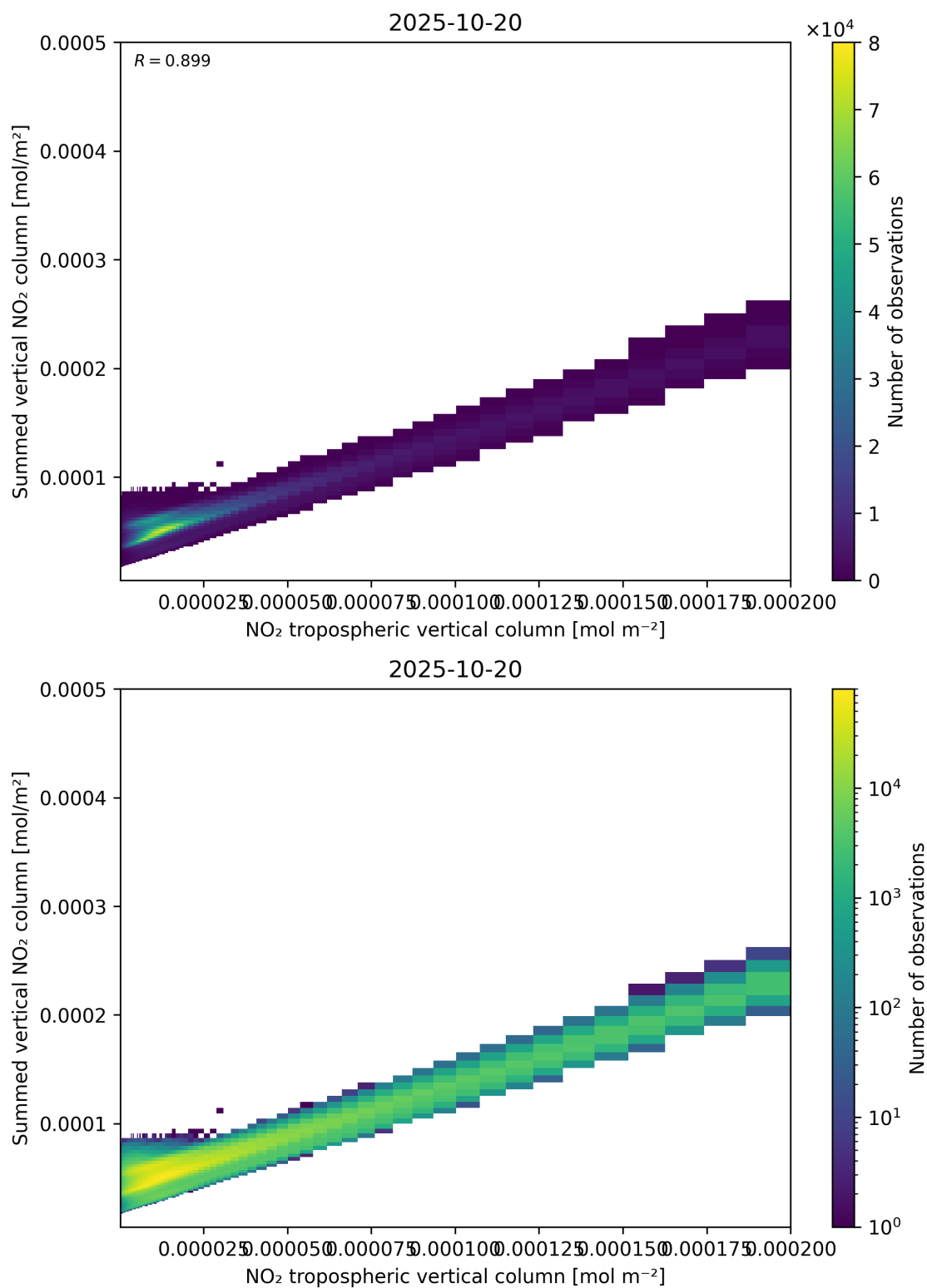
Figure 126: Scatter density plot of “NO 2 tropospheric vertical column” against “Summed vertical NO 2 column” for 2025-10-19 to 2025-10-21.
