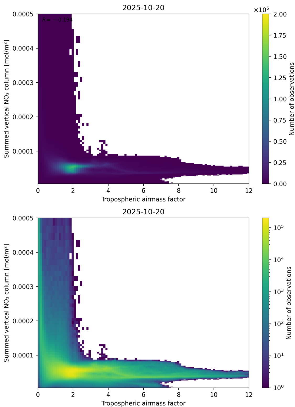
Figure 75: Scatter density plot of “Tropospheric air mass factor” against “Summed vertical NO 2 column” for 2025-10-19 to 2025-10-21.
