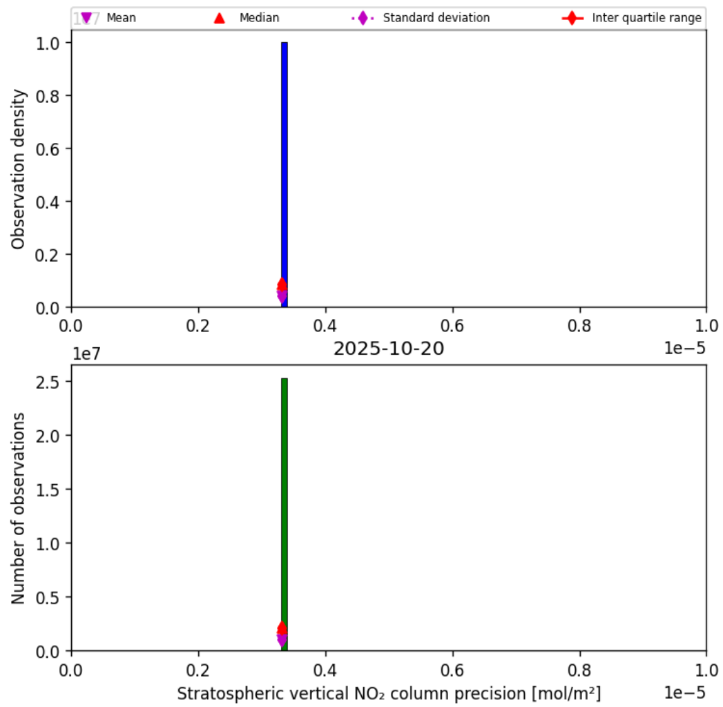
Figure 37: Histogram of “Stratospheric vertical NO 2 column precision” for 2025-10-19 to 2025-10-21
