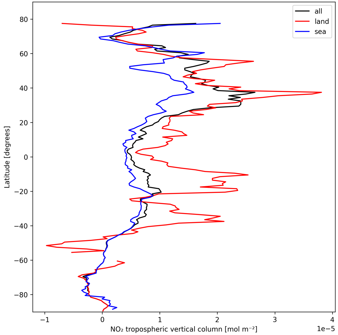
Figure 12: Zonal average of “NO 2 tropospheric vertical column” for 2025-10-19 to 2025-10-21.
