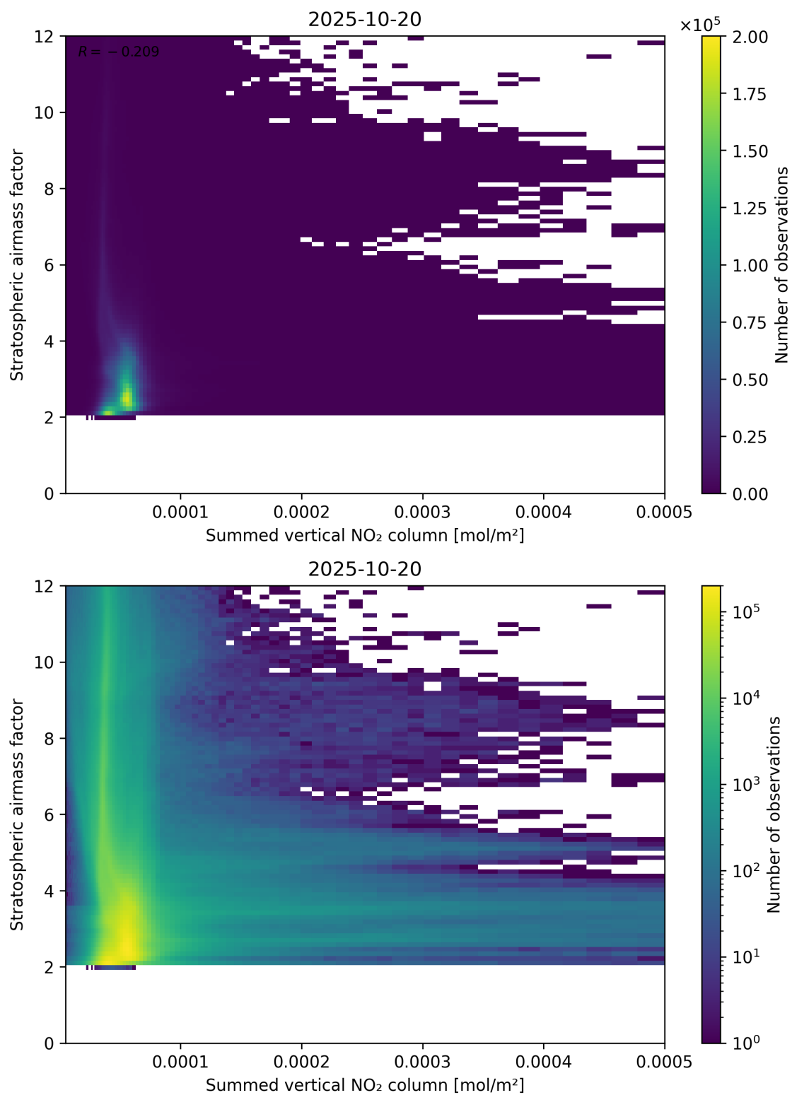
Figure 103: Scatter density plot of “Summed vertical NO 2 column” against “Stratospheric airmass factor” for 2025-10-19 to 2025-10-21.
