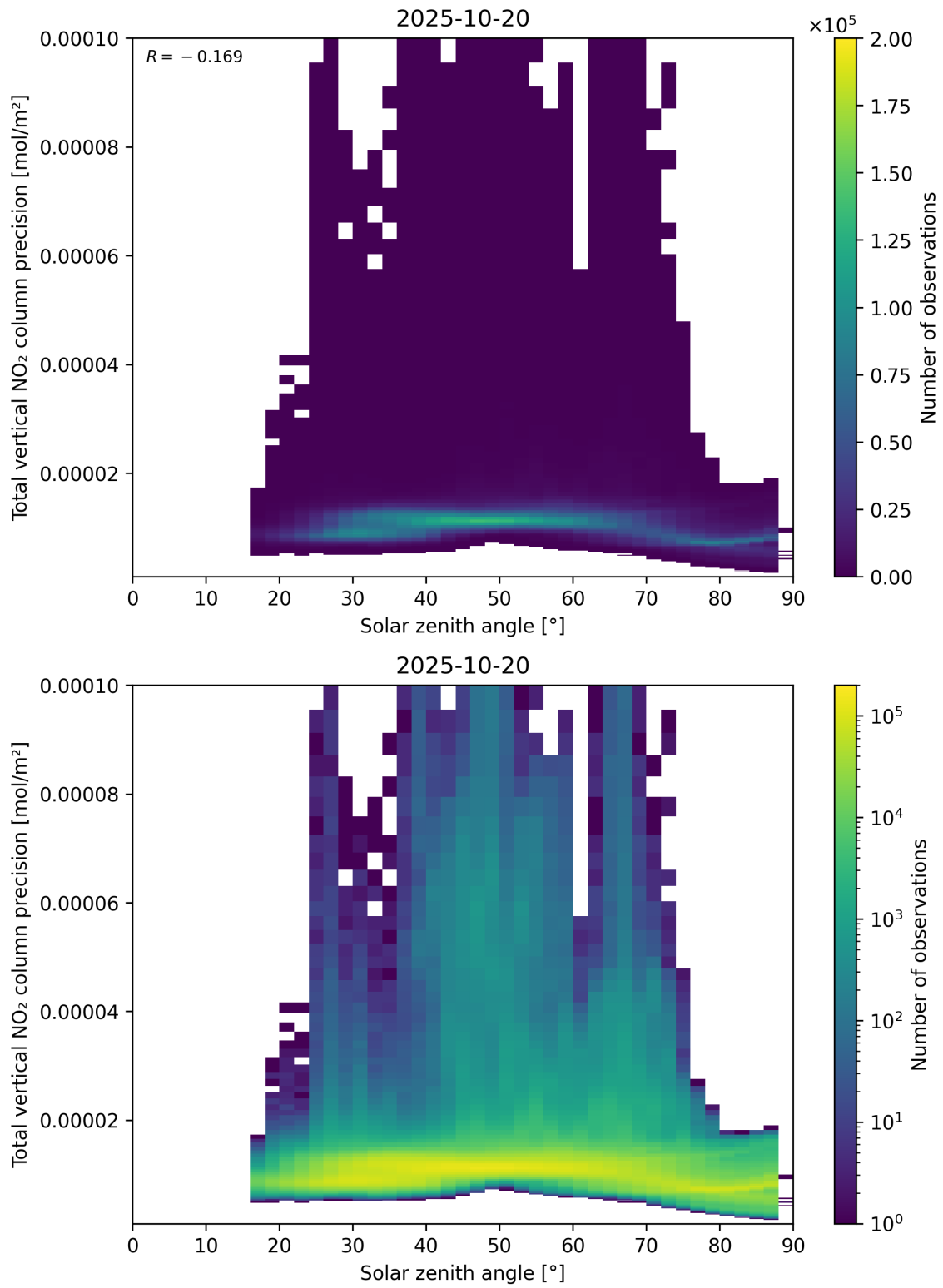
Figure 154: Scatter density plot of “Solar zenith angle” against “Total vertical NO 2 column precision” for 2025-10-19 to 2025-10-21.
