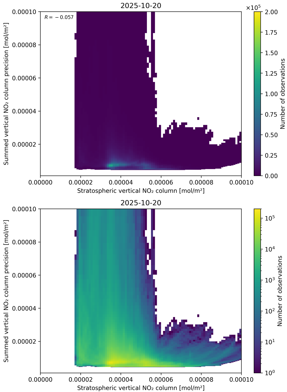
Figure 99: Scatter density plot of “Stratospheric vertical NO 2 column” against “Summed vertical NO 2 column precision” for 2025-10-19 to 2025-10-21.
