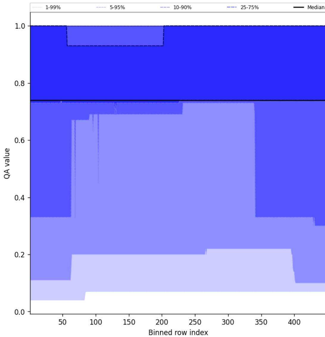
Figure 45: Along track statistics of “QA value” for 2025-10-19 to 2025-10-21
