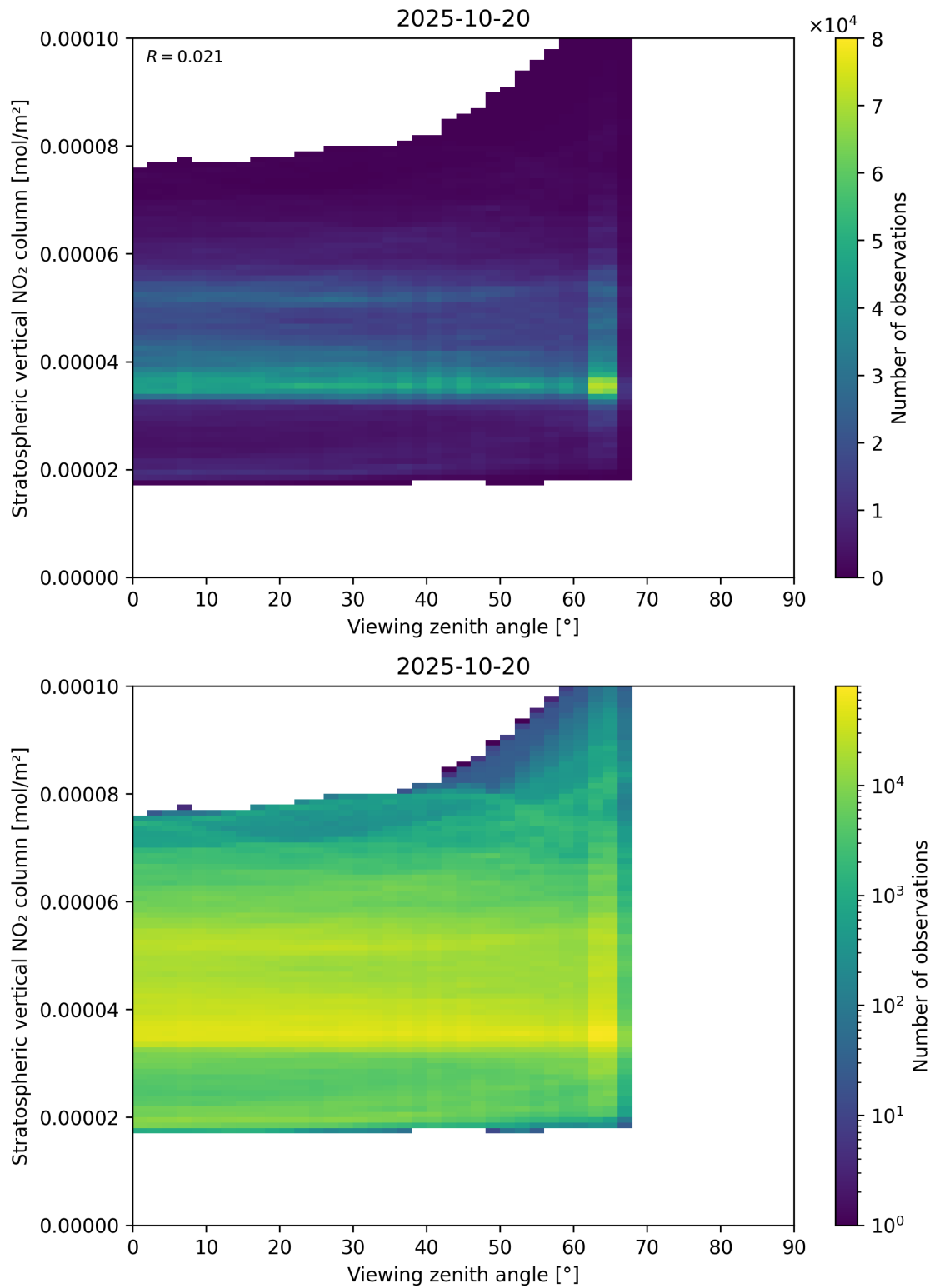
Figure 164: Scatter density plot of “Viewing zenith angle” against “Stratospheric vertical NO 2 column” for 2025-10-19 to 2025-10-21.
