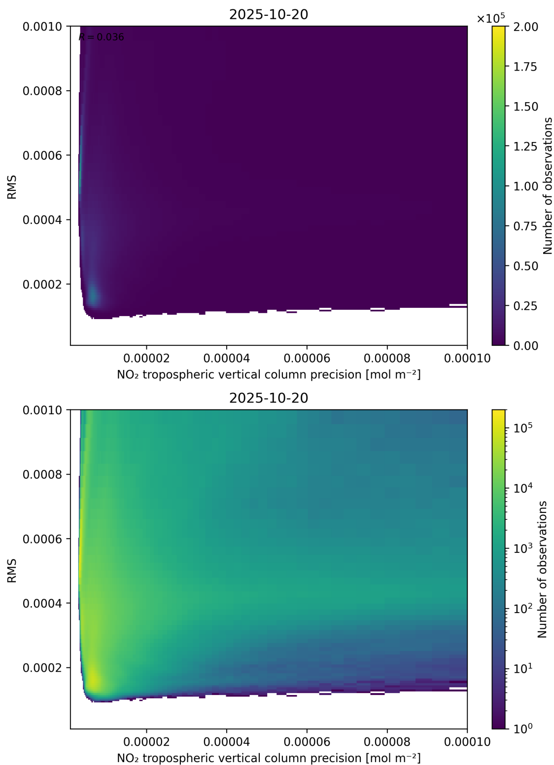
Figure 140: Scatter density plot of “NO 2 tropospheric vertical column precision” against “RMS” for 2025-10-19 to 2025-10-21.
