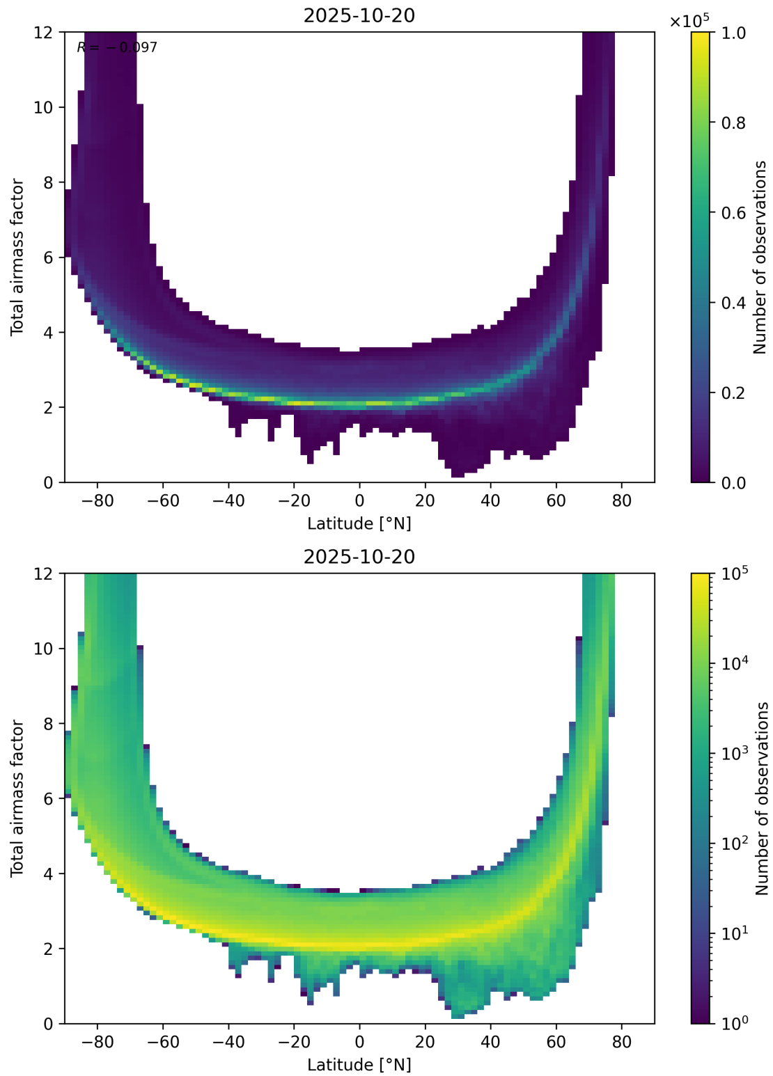
Figure 84: Scatter density plot of “Latitude” against “Total airmass factor” for 2025-10-19 to 2025-10-21.
