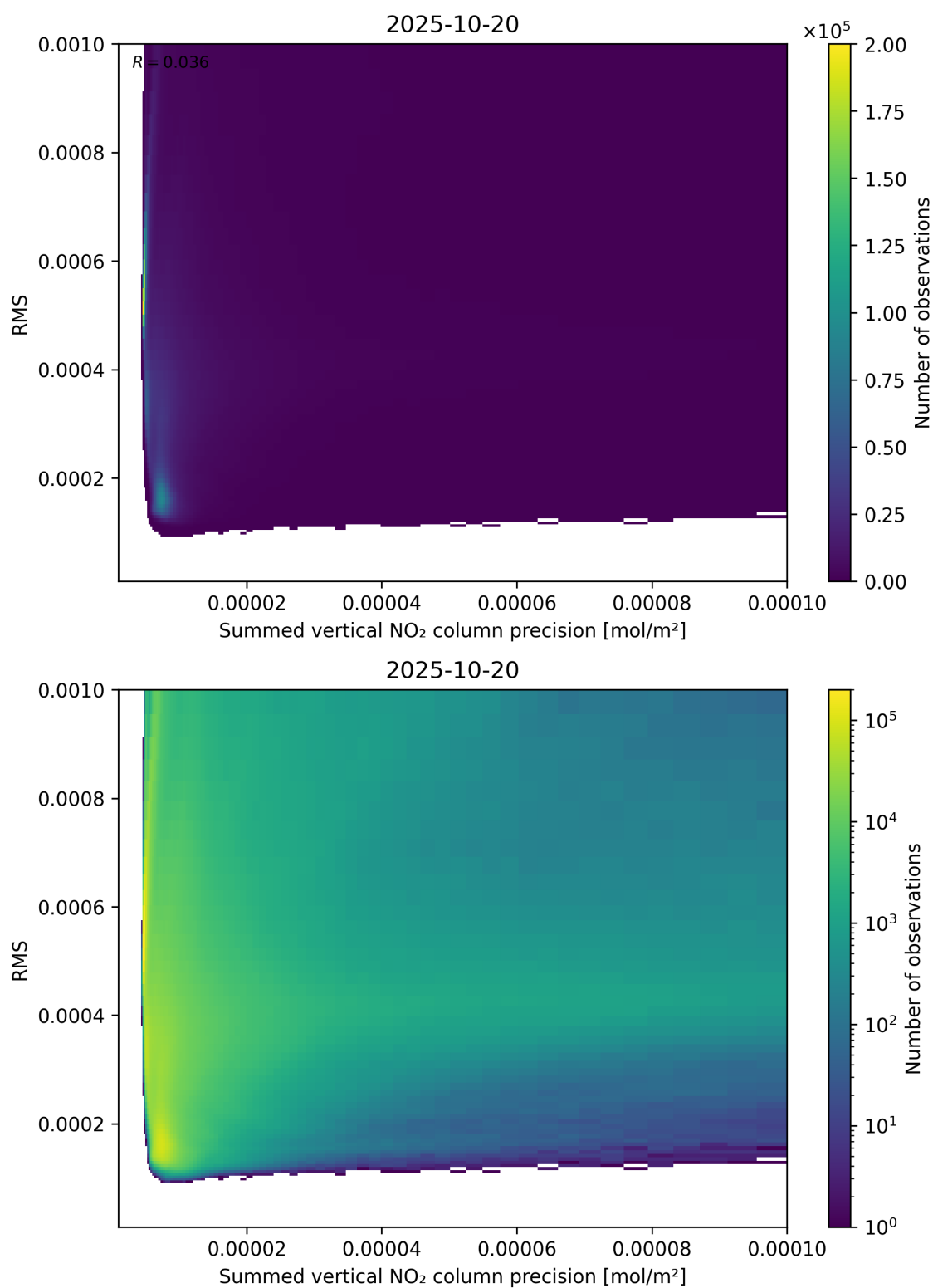
Figure 108: Scatter density plot of “Summed vertical NO 2 column precision” against “RMS” for 2025-10-19 to 2025-10-21.
