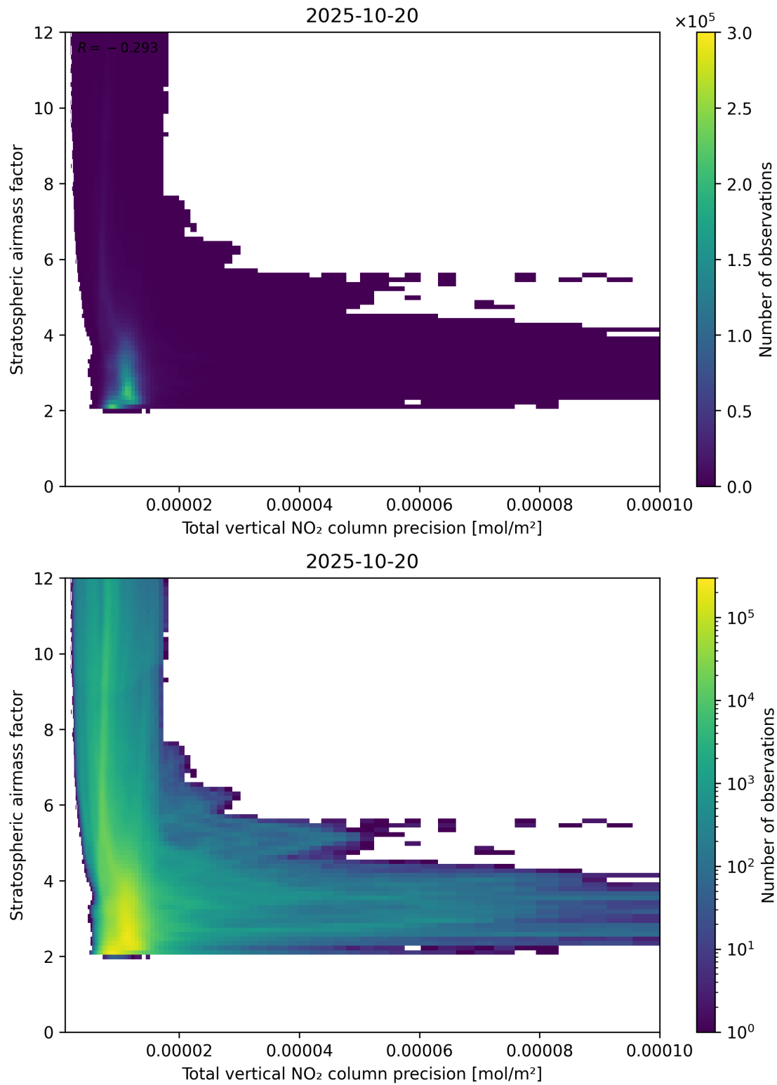
Figure 115: Scatter density plot of “Total vertical NO 2 column precision” against “Stratospheric air mass factor” for 2025-10-19 to 2025-10-21.
