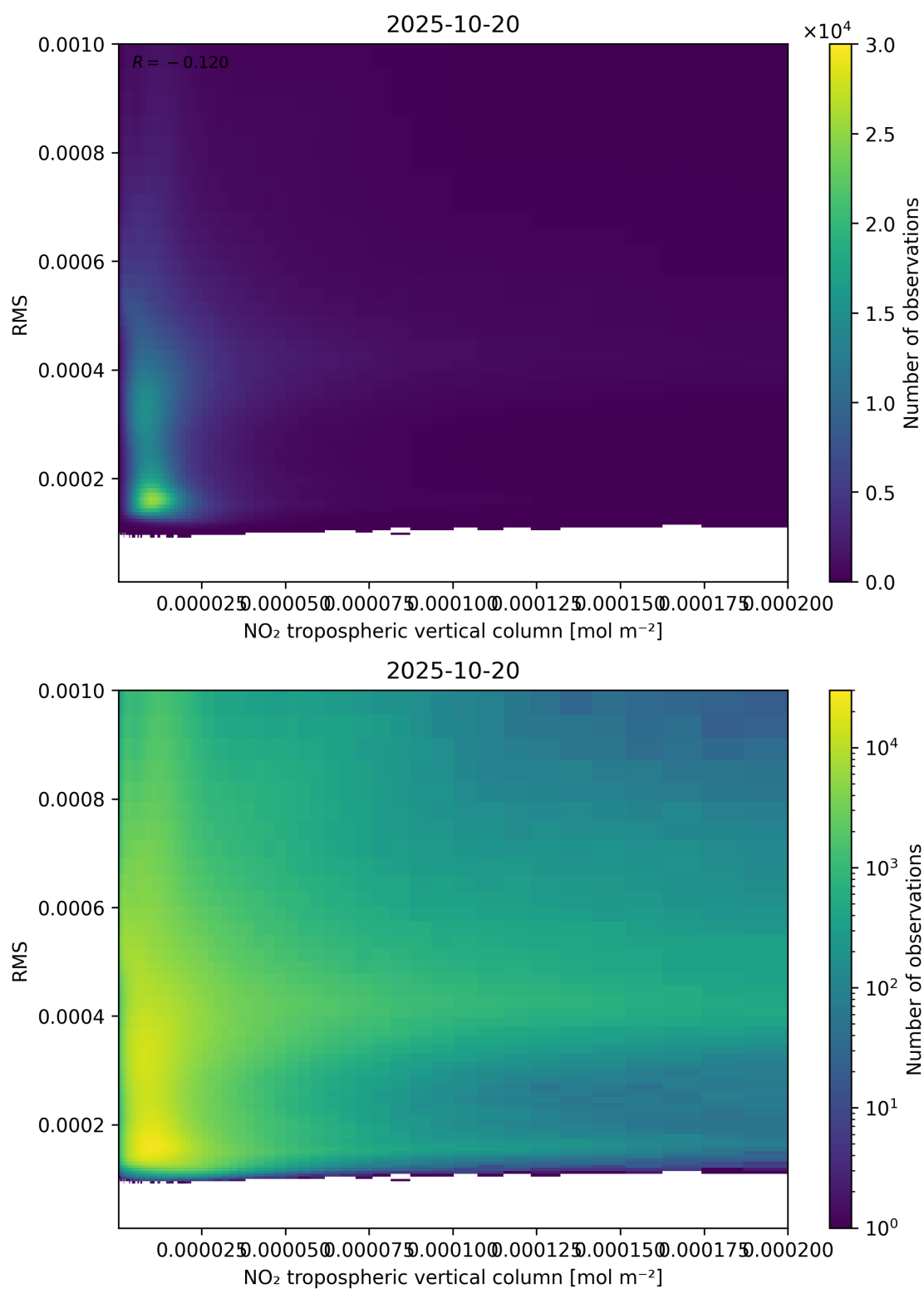
Figure 142: Scatter density plot of “NO 2 tropospheric vertical column” against “RMS” for 2025-10-19 to 2025-10-21.
