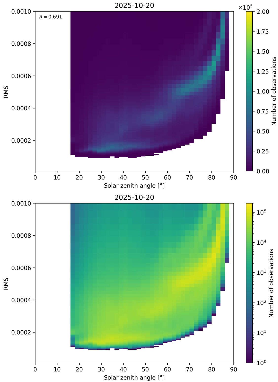
Figure 157: Scatter density plot of “Solar zenith angle” against “RMS” for 2025-10-19 to 2025-10-21.
