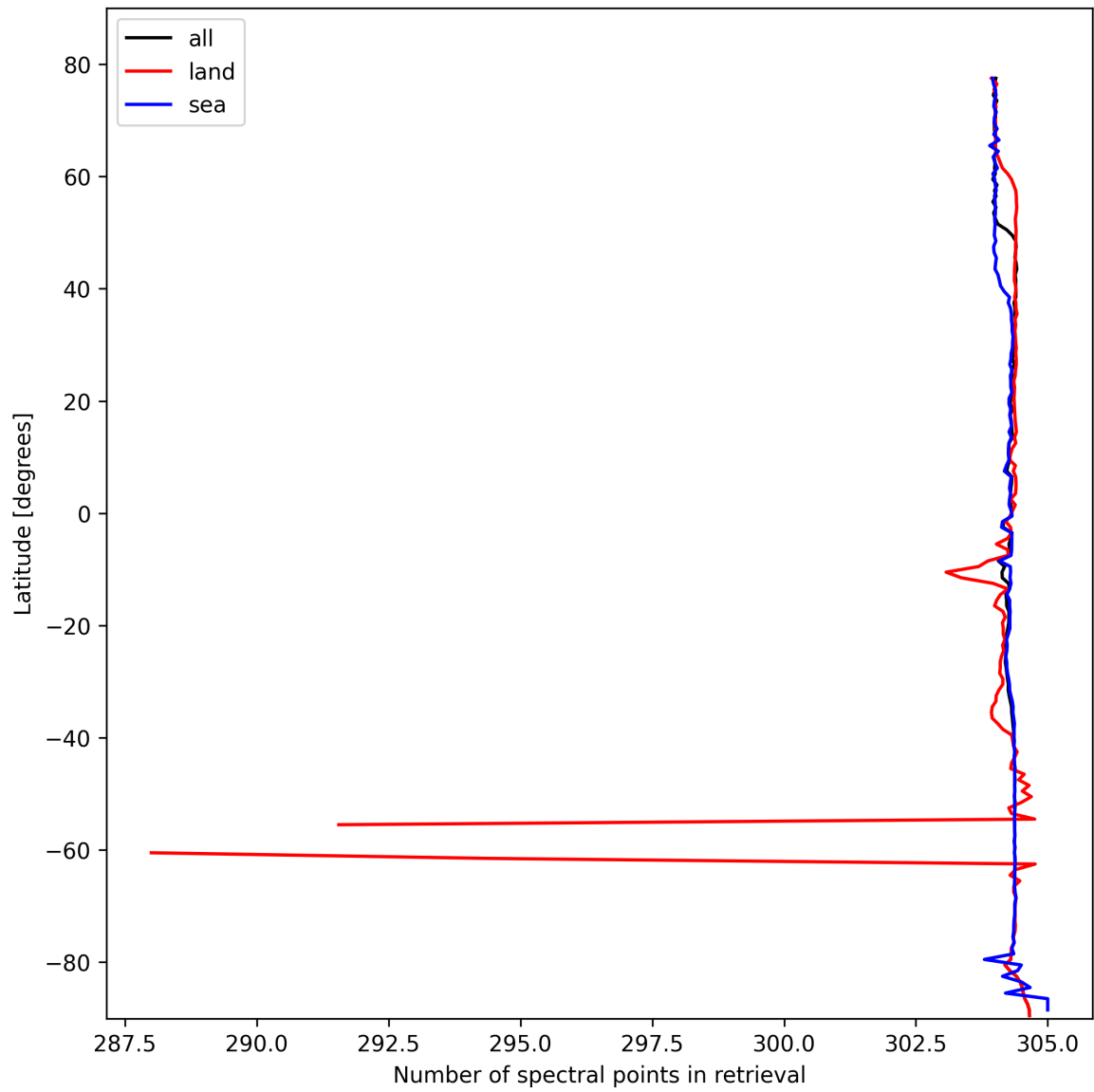
Figure 16: Zonal average of “Number of spectral points in retrieval” for 2025-10-19 to 2025-10-21.
