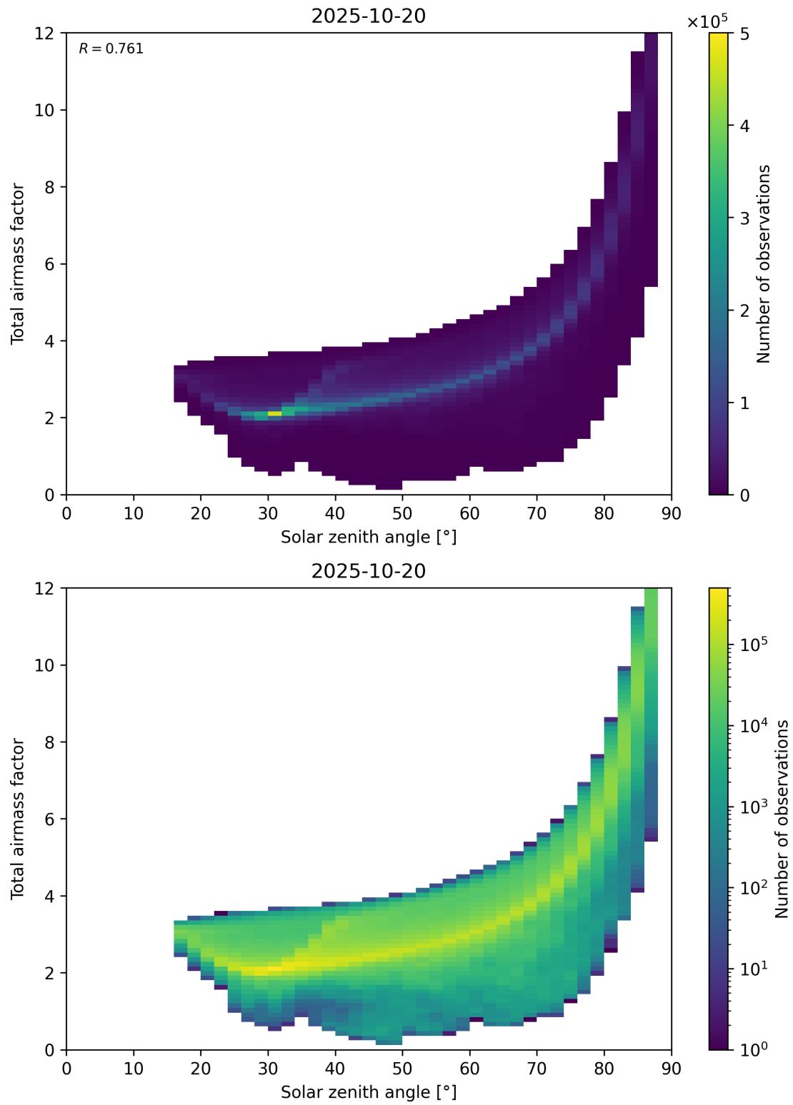
Figure 146: Scatter density plot of “Solar zenith angle” against “Total air mass factor” for 2025-10-19 to 2025-10-21.
