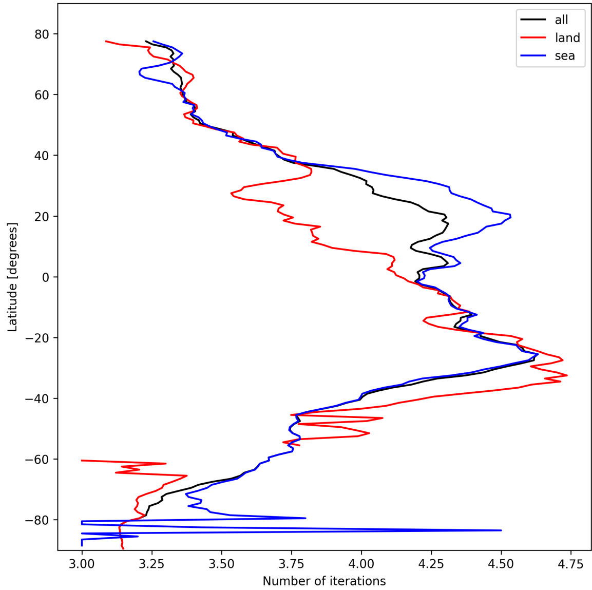
Figure 17: Zonal average of “Number of iterations” for 2025-10-19 to 2025-10-21.
