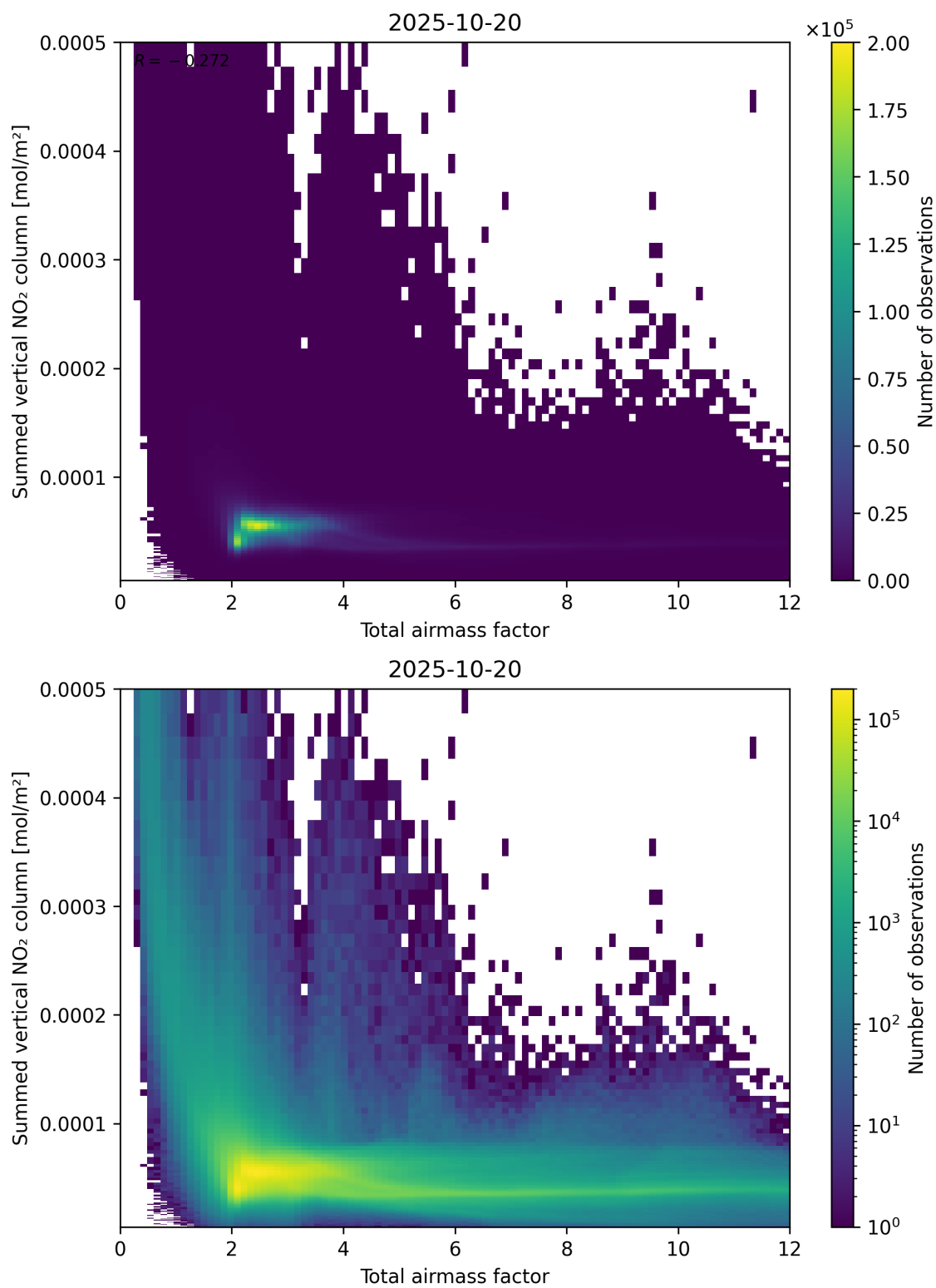
Figure 65: Scatter density plot of “Total airmass factor” against “Summed vertical NO 2 column” for 2025-10-19 to 2025-10-21.
