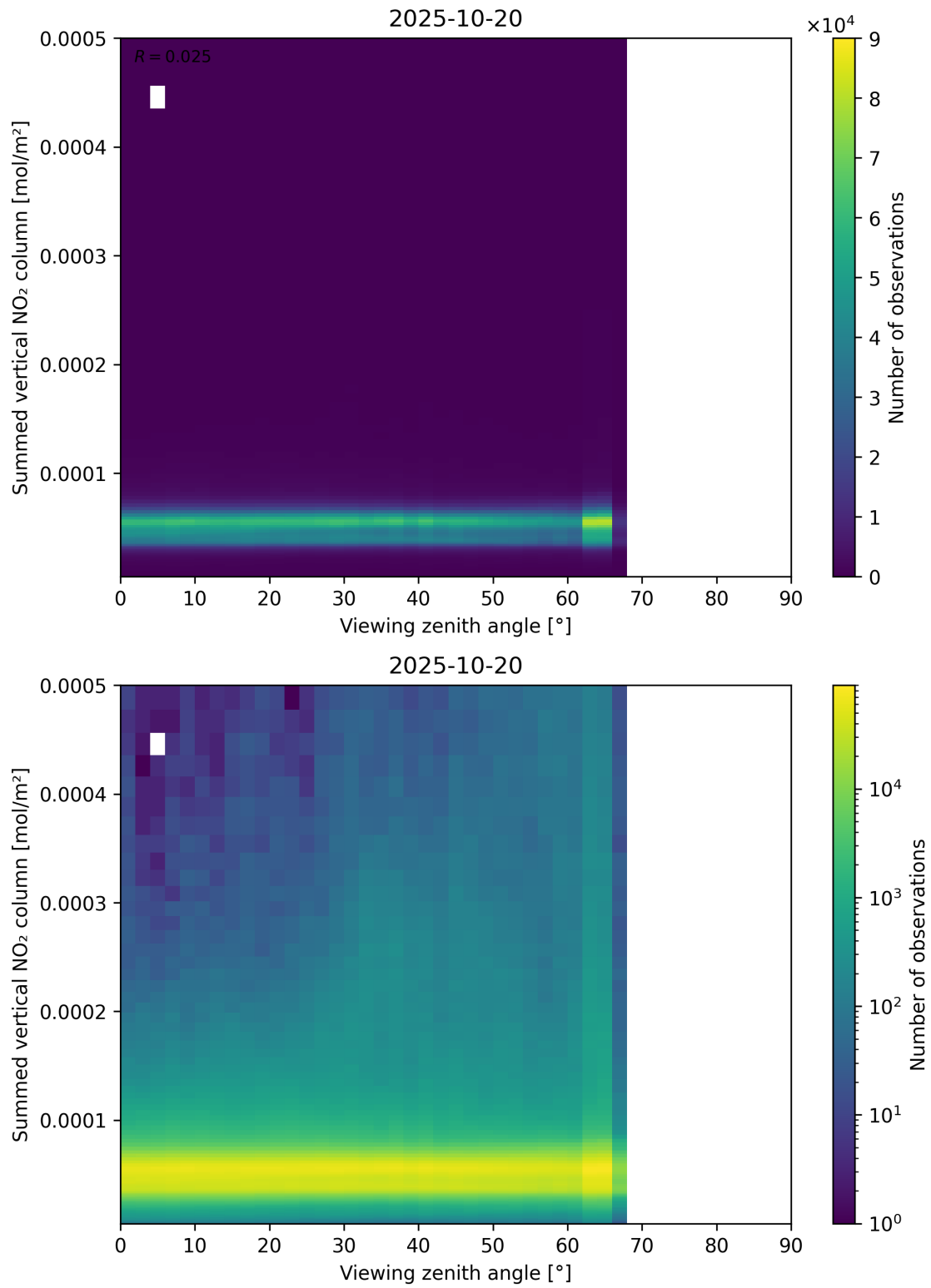
Figure 165: Scatter density plot of “Viewing zenith angle” against “Summed vertical NO 2 column” for 2025-10-19 to 2025-10-21.
