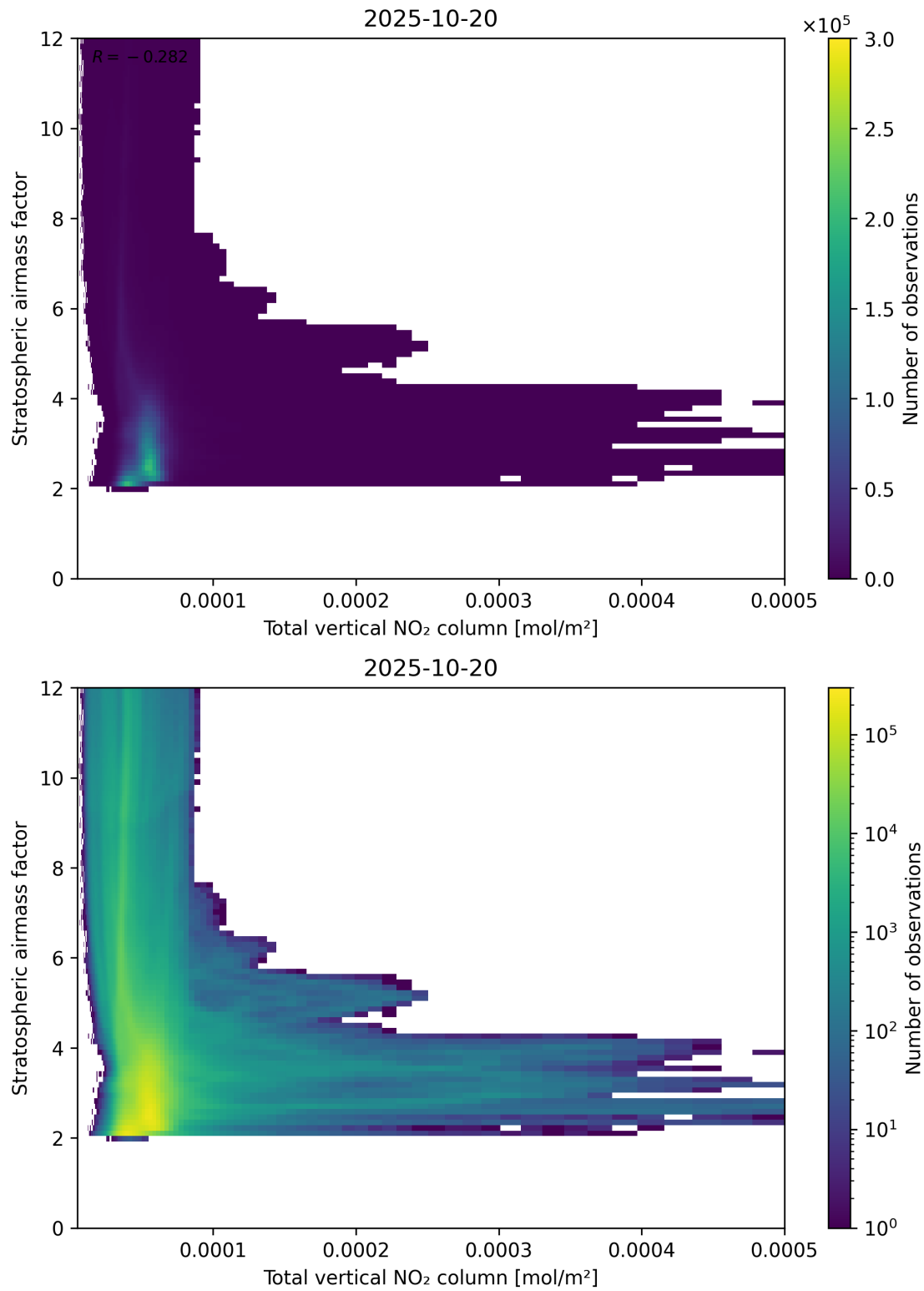
Figure 110: Scatter density plot of “Total vertical NO 2 column” against “Stratospheric airmass factor” for 2025-10-19 to 2025-10-21.
