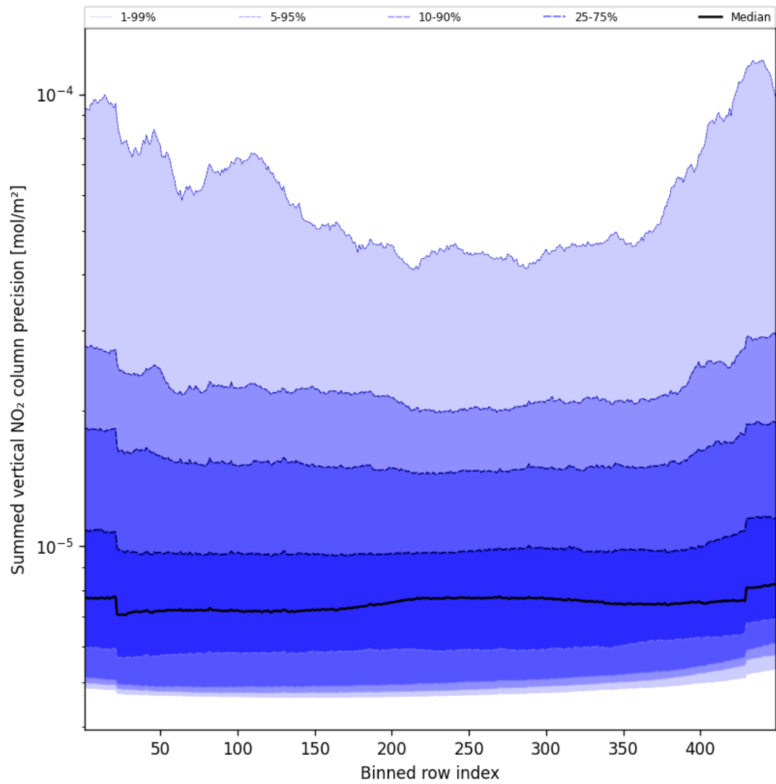
Figure 58: Along track statistics of “Summed vertical NO 2 column precision” for 2025-10-19 to 2025-10-21
