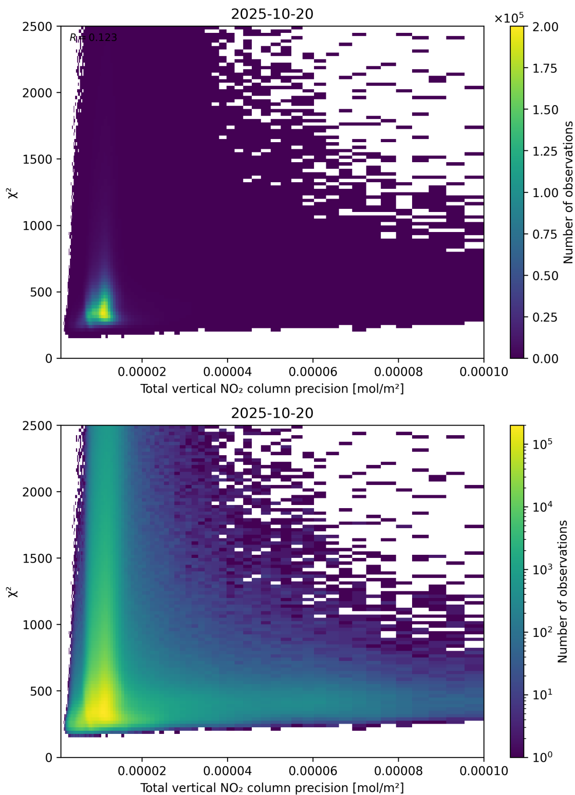
Figure 116: Scatter density plot of “Total vertical NO 2 column precision” against “ \chi^2 ” for 2025-10-19 to 2025-10-21.
