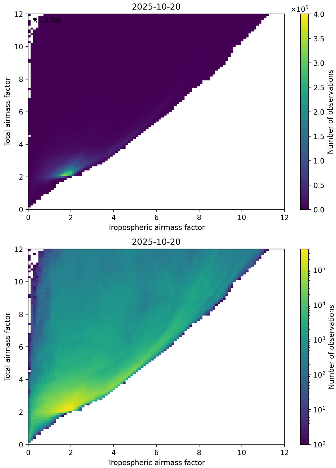
Figure 72: Scatter density plot of “Tropospheric airmass factor” against “Total airmass factor” for 2025-10-19 to 2025-10-21.
