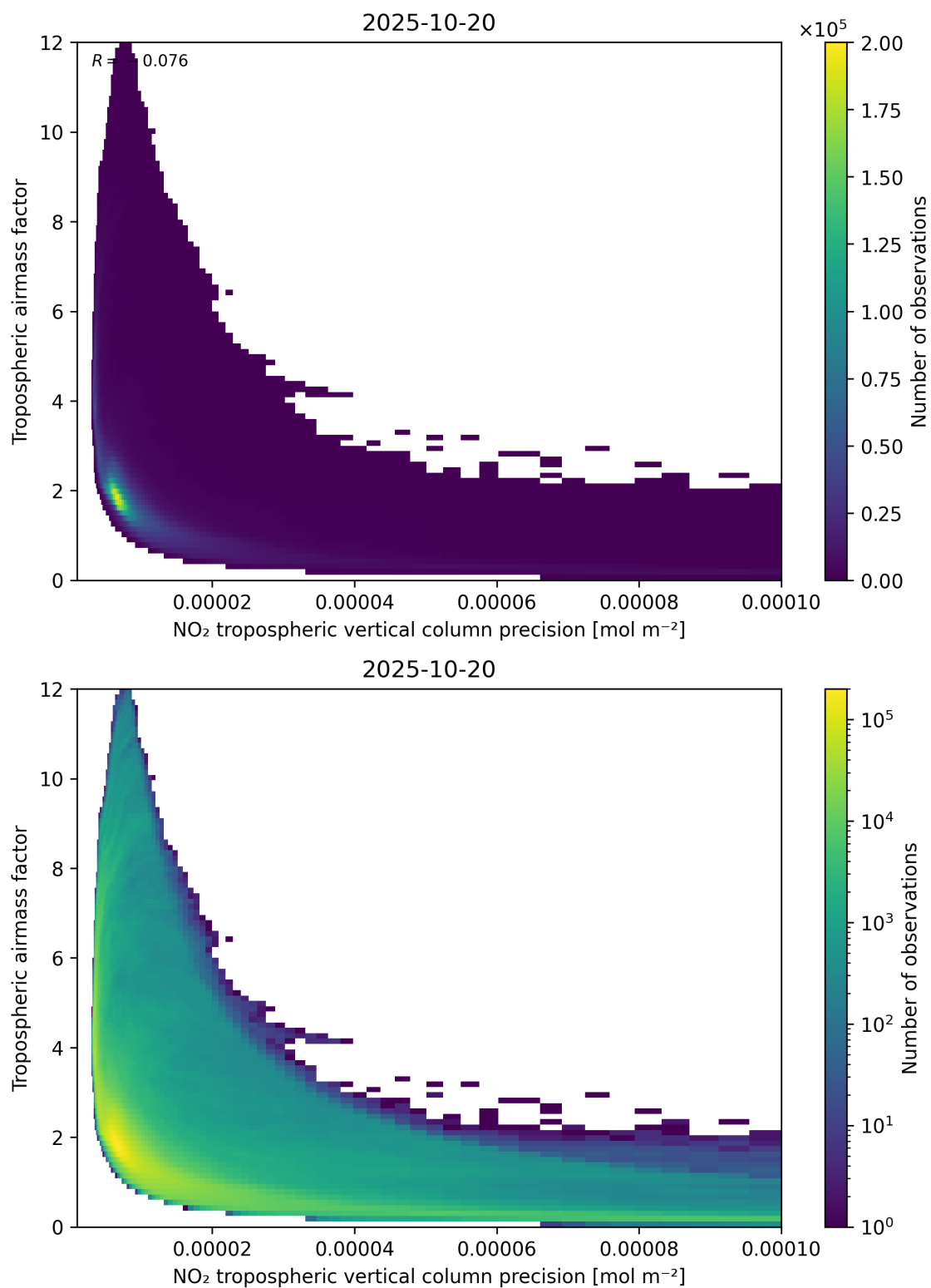
Figure 133: Scatter density plot of “NO 2 tropospheric vertical column precision” against “Tropospheric airmass factor” for 2025-10-19 to 2025-10-21.
