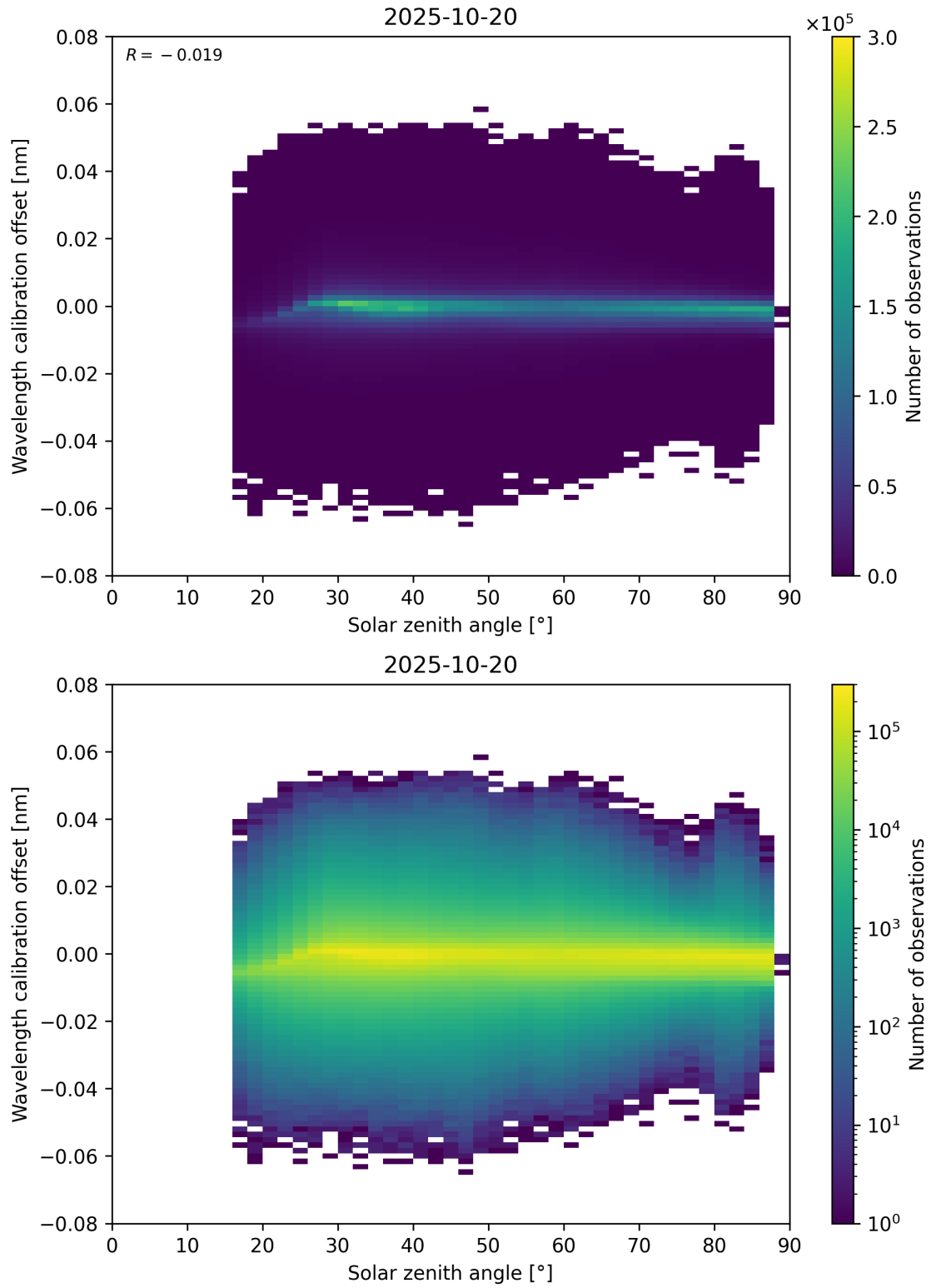
Figure 158: Scatter density plot of “Solar zenith angle” against “Wavelength calibration offset” for 2025-10-19 to 2025-10-21.
