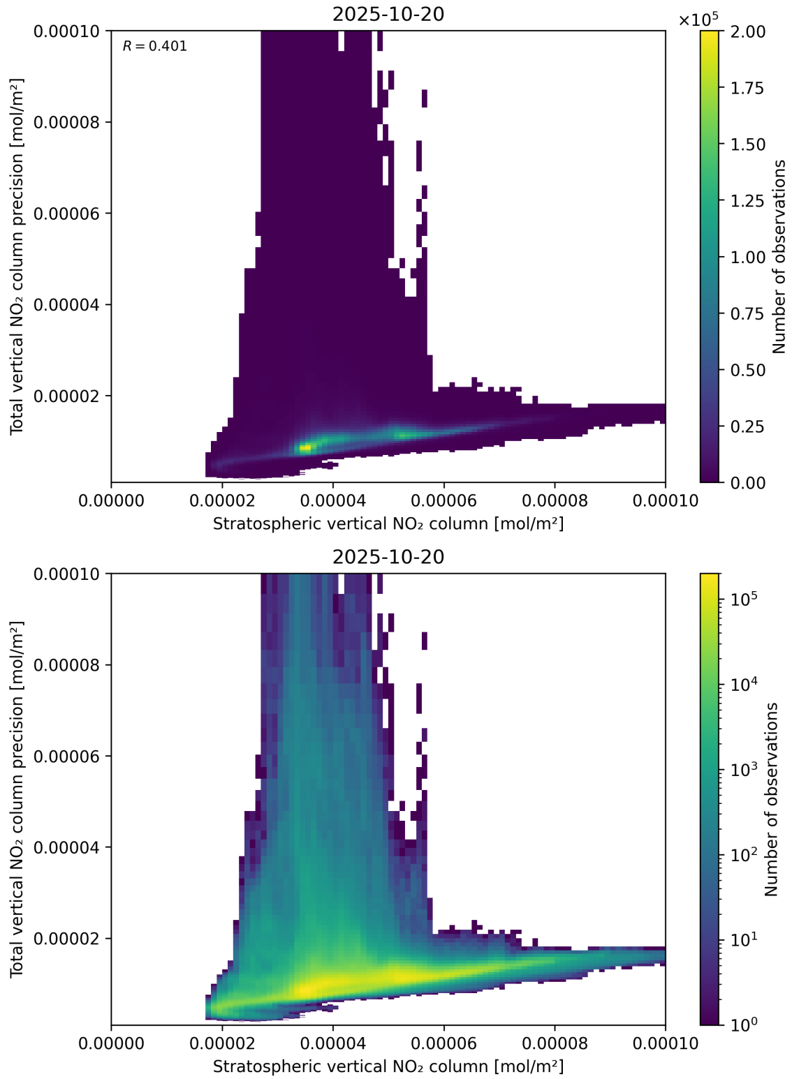
Figure 101: Scatter density plot of “Stratospheric vertical NO 2 column” against “Total vertical NO 2 column precision” for 2025-10-19 to 2025-10-21.
