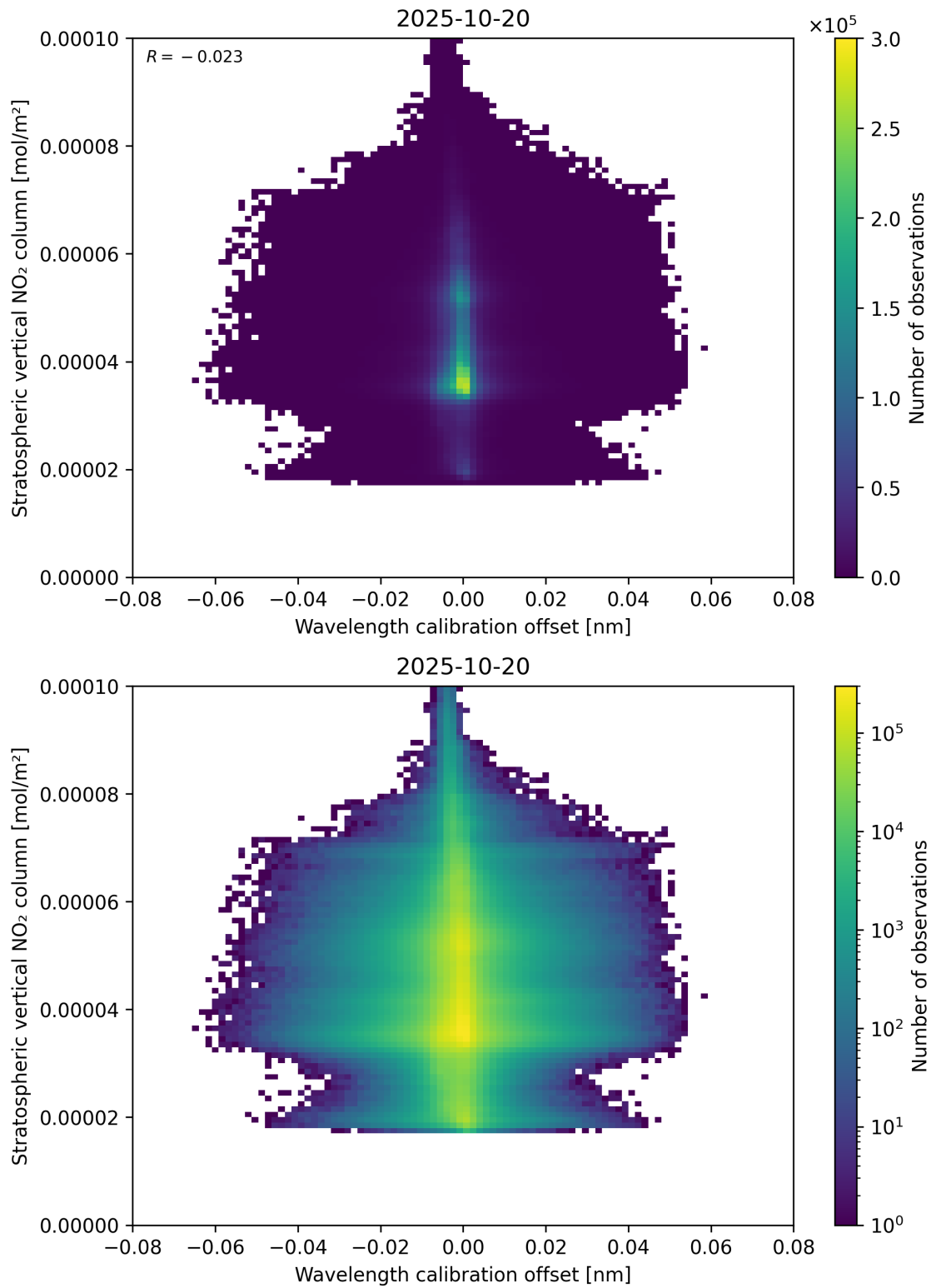
Figure 176: Scatter density plot of “Wavelength calibration offset” against “Stratospheric vertical NO 2 column” for 2025-10-19 to 2025-10-21.
