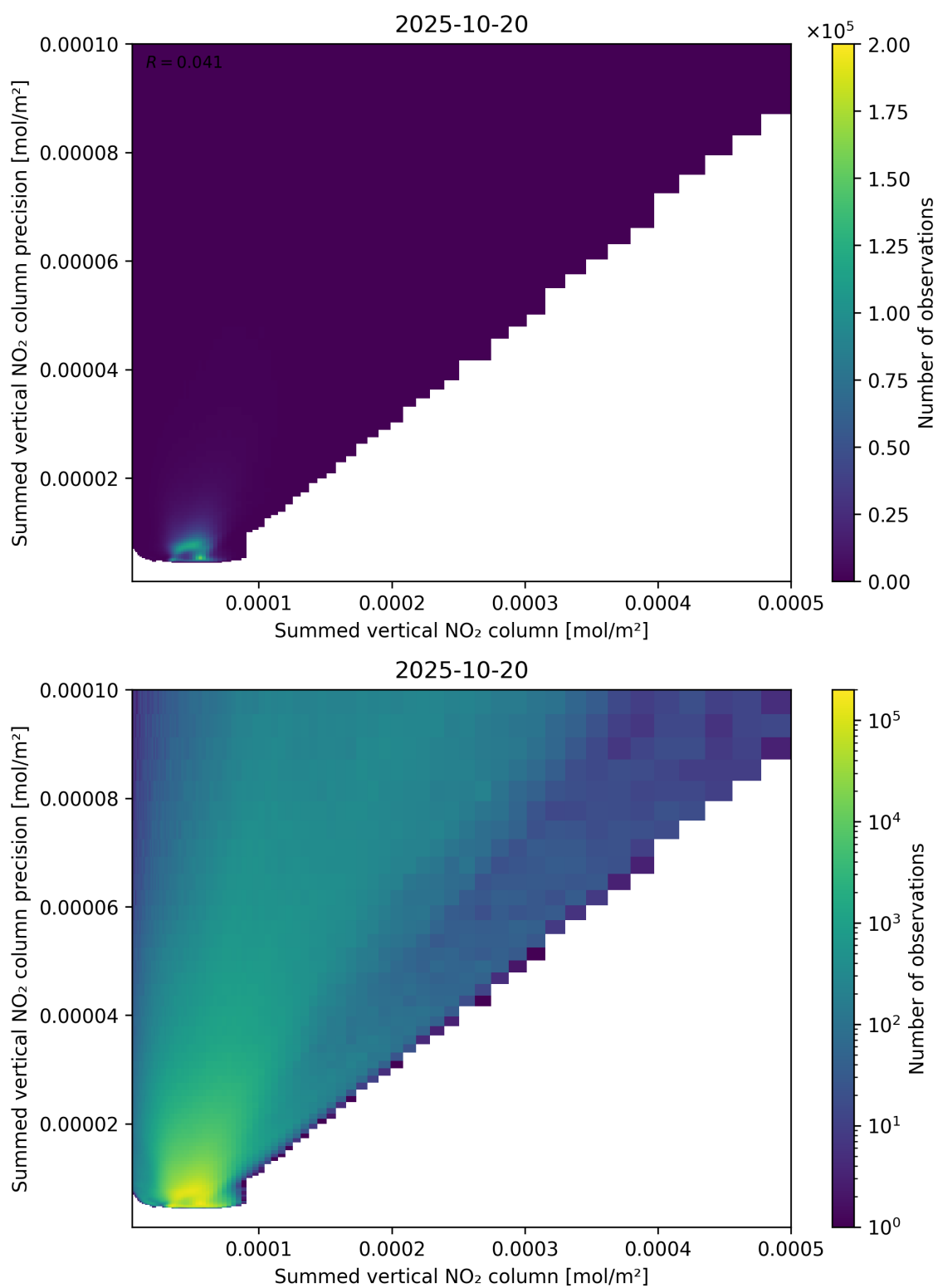
Figure 105: Scatter density plot of “Summed vertical NO 2 column” against “Summed vertical NO 2 column precision” for 2025-10-19 to 2025-10-21.
