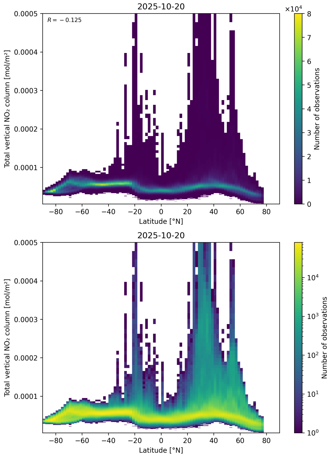
Figure 90: Scatter density plot of “Latitude” against “Total vertical NO 2 column” for 2025-10-19 to 2025-10-21.
