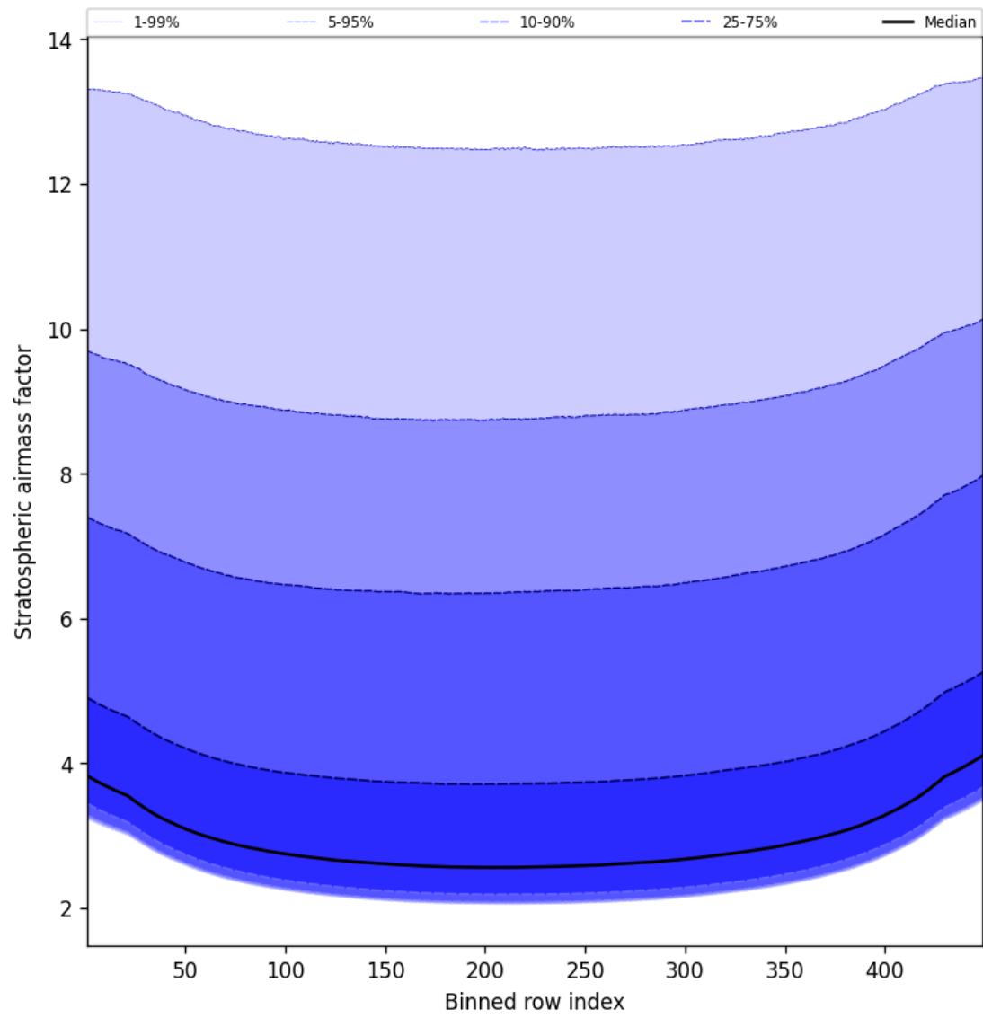
Figure 61: Along track statistics of “Stratospheric airmass factor” for 2025-10-19 to 2025-10-21
