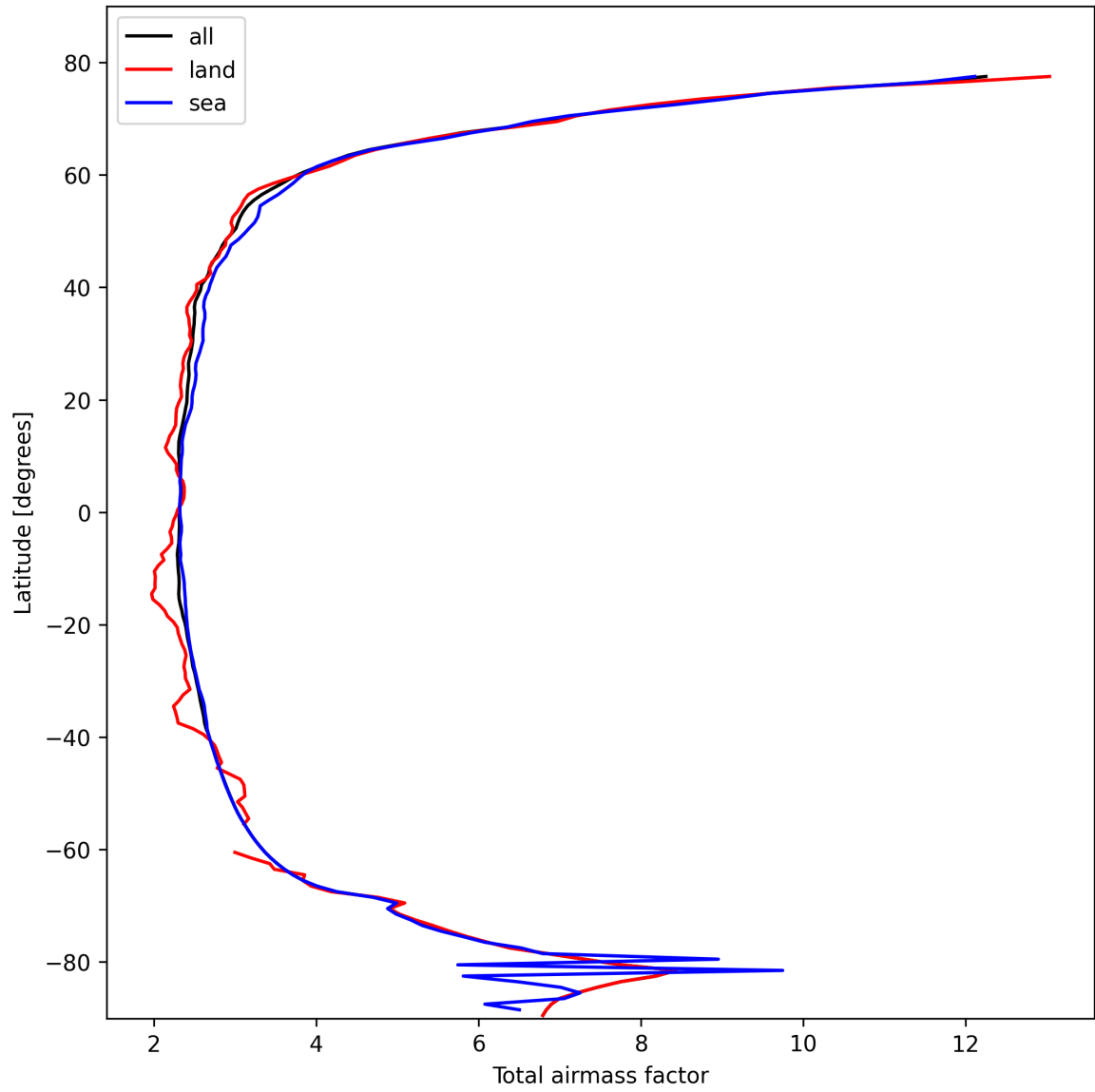
Figure 15: Zonal average of “Total airmass factor” for 2025-10-19 to 2025-10-21.
