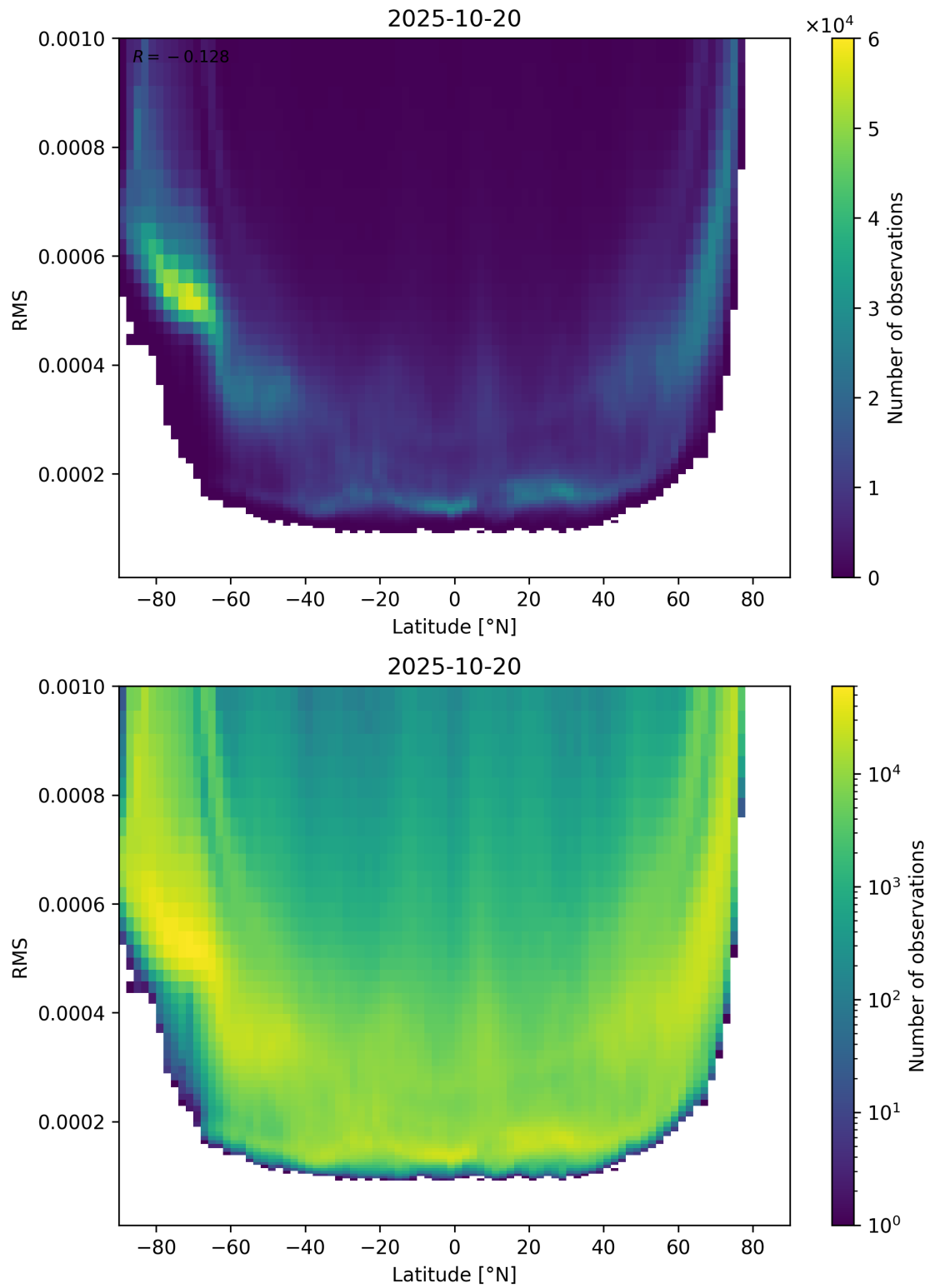
Figure 94: Scatter density plot of “Latitude” against “RMS” for 2025-10-19 to 2025-10-21.
