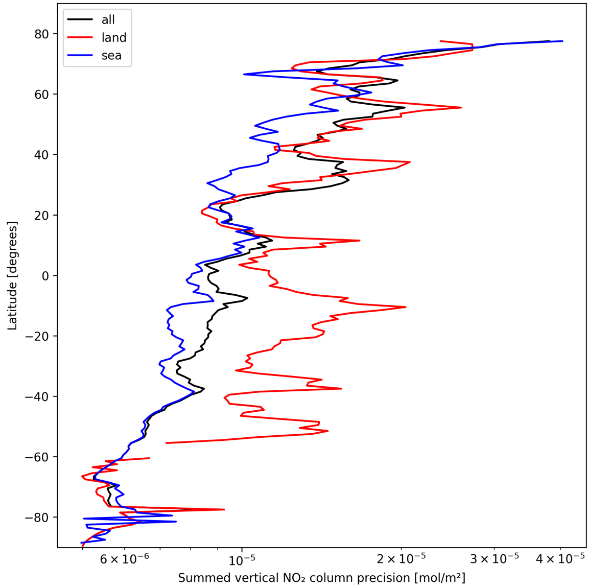
Figure 24: Zonal average of “Summed vertical NO 2 column precision” for 2025-10-19 to 2025-10-21.
