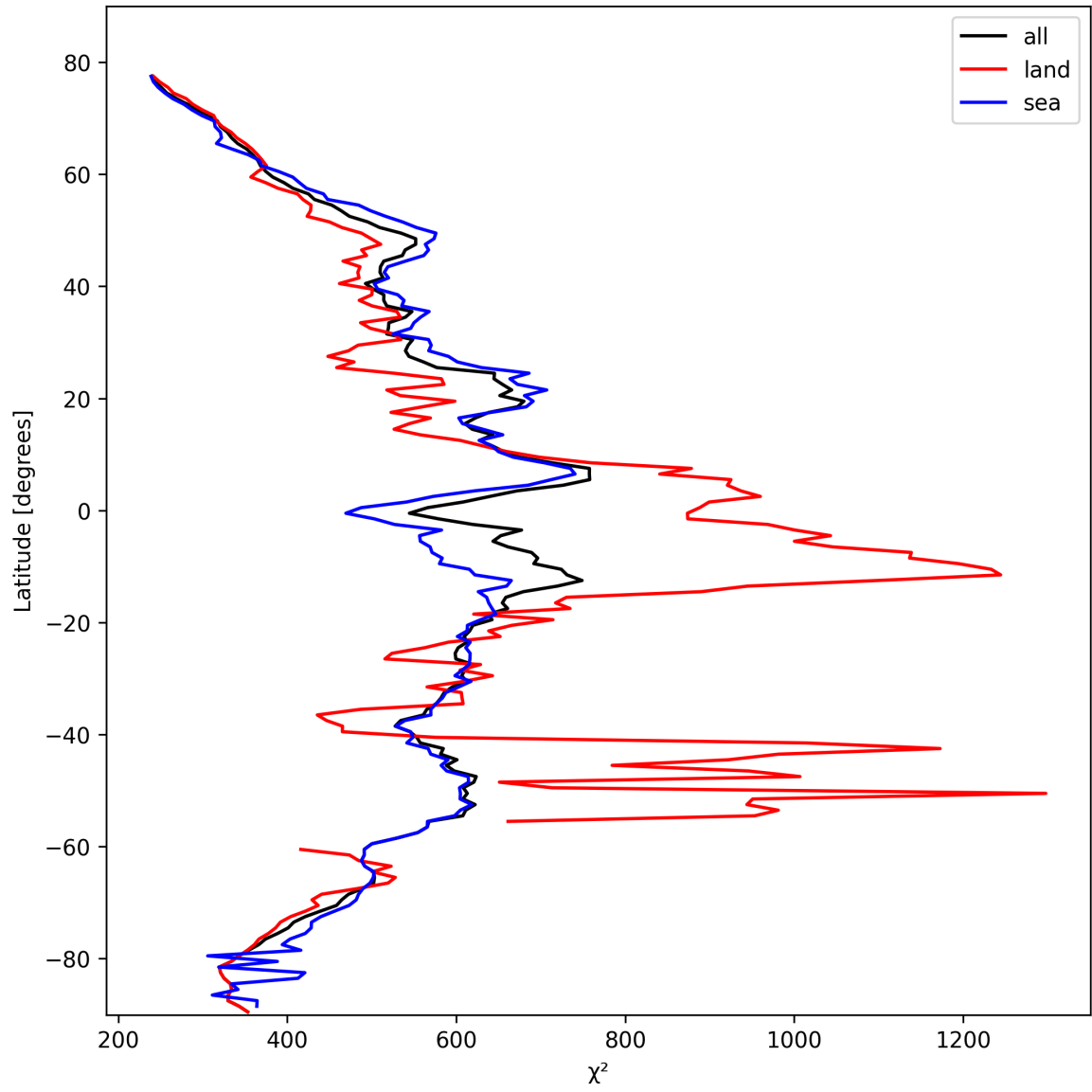
Figure 25: Zonal average of “ \chi^2 ” for 2025-10-19 to 2025-10-21.
