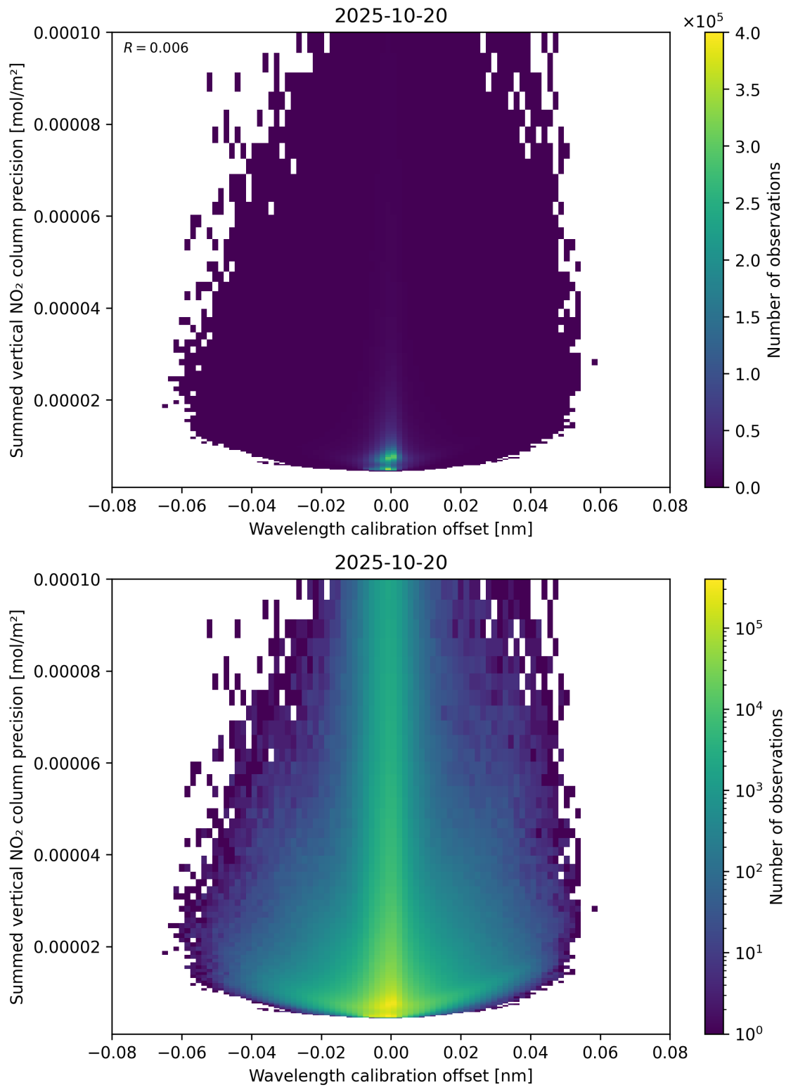
Figure 178: Scatter density plot of “Wavelength calibration offset” against “Summed vertical NO 2 column precision” for 2025-10-19 to 2025-10-21.
