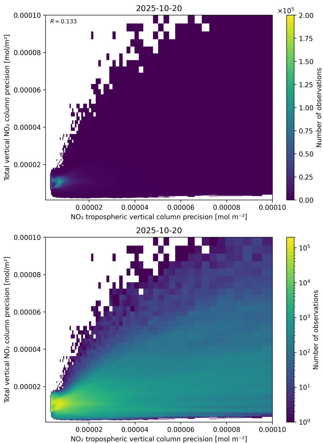
Figure 139: Scatter density plot of “NO 2 tropospheric vertical column precision” against “Total vertical NO 2 column precision” for 2025-10-19 to 2025-10-21.
