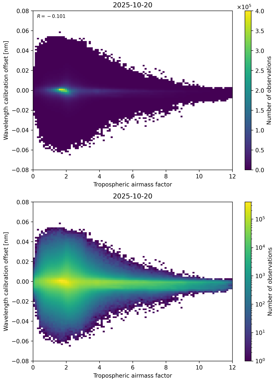
Figure 80: Scatter density plot of “Tropospheric airmass factor” against “Wavelength calibration offset” for 2025-10-19 to 2025-10-21.
