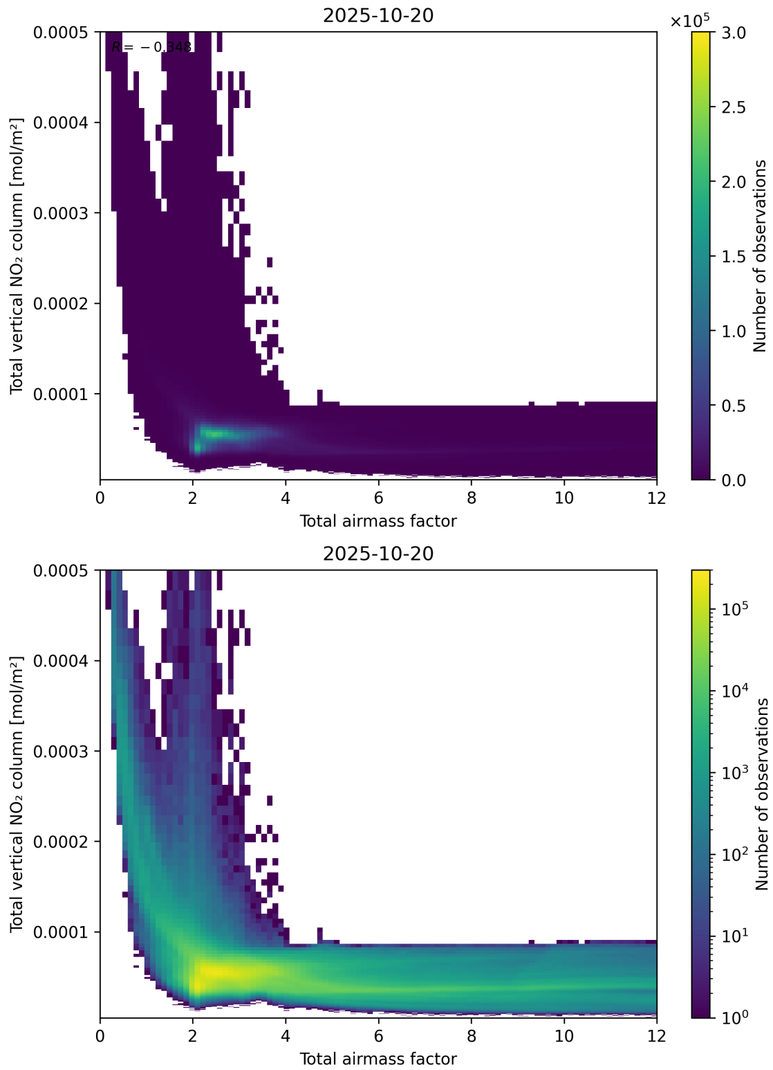
Figure 67: Scatter density plot of “Total airmass factor” against “Total vertical NO 2 column” for 2025-10-19 to 2025-10-21.
