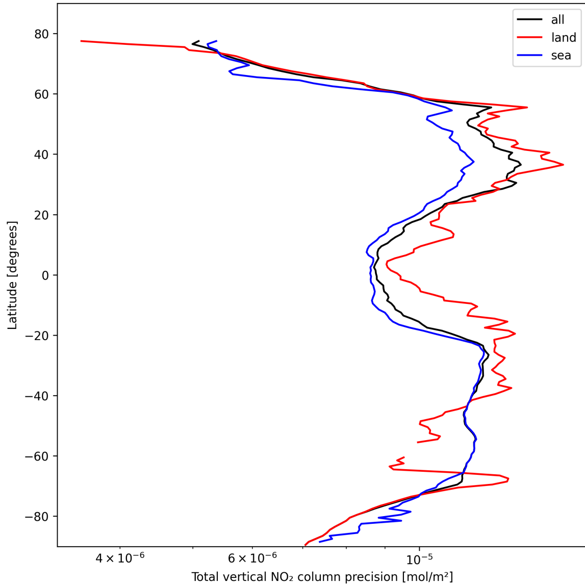
Figure 22: Zonal average of “Total vertical NO 2 column precision” for 2025-10-19 to 2025-10-21.
