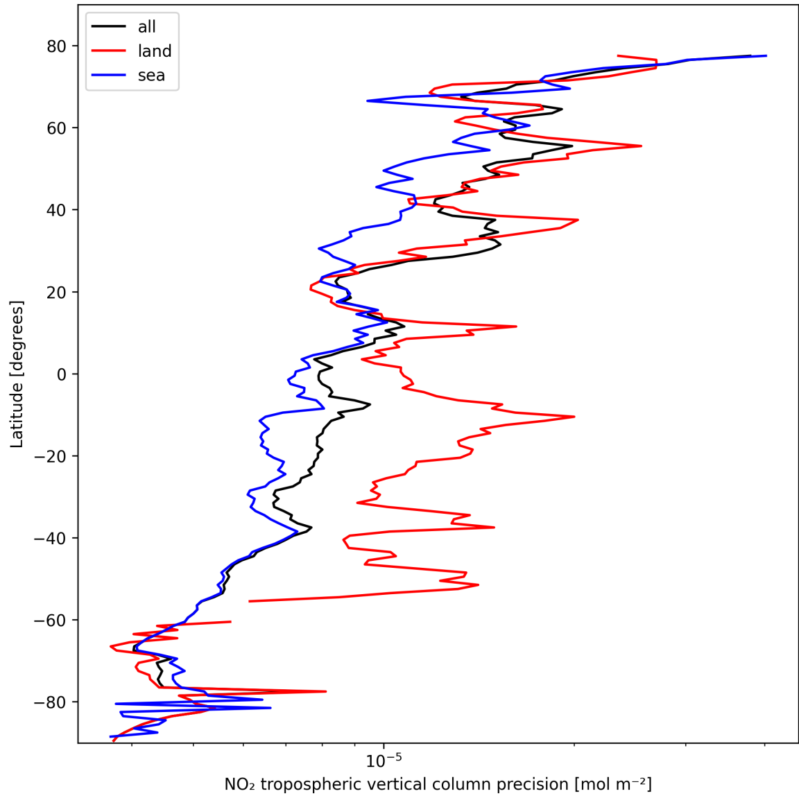
Figure 13: Zonal average of “NO 2 tropospheric vertical column precision” for 2025-10-19 to 2025-10-21.
