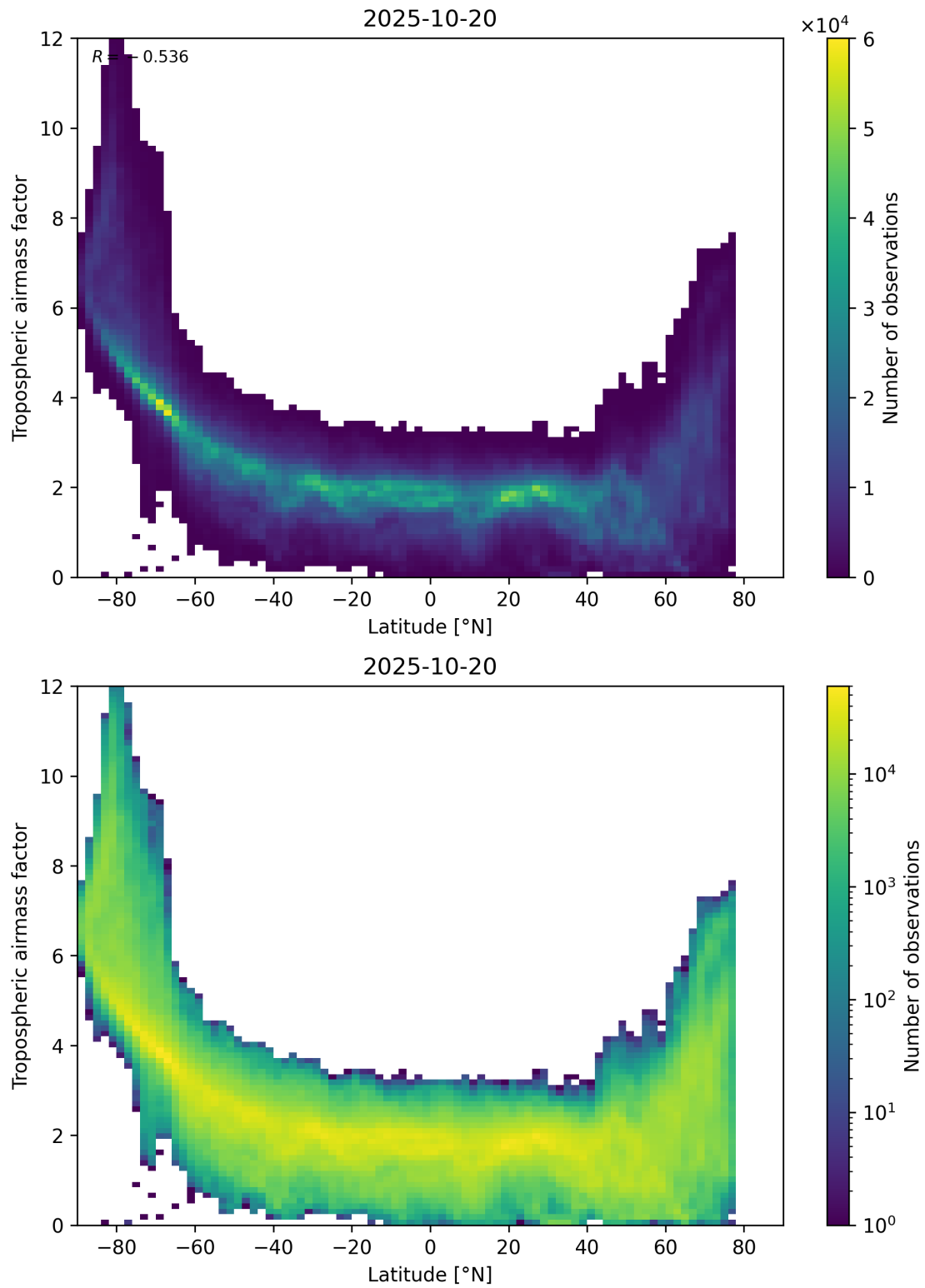
Figure 85: Scatter density plot of “Latitude” against “Tropospheric air mass factor” for 2025-10-19 to 2025-10-21.
