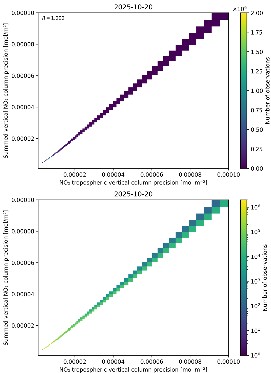
Figure 137: Scatter density plot of “NO 2 tropospheric vertical column precision” against “Summed vertical NO 2 column precision” for 2025-10-19 to 2025-10-21.
