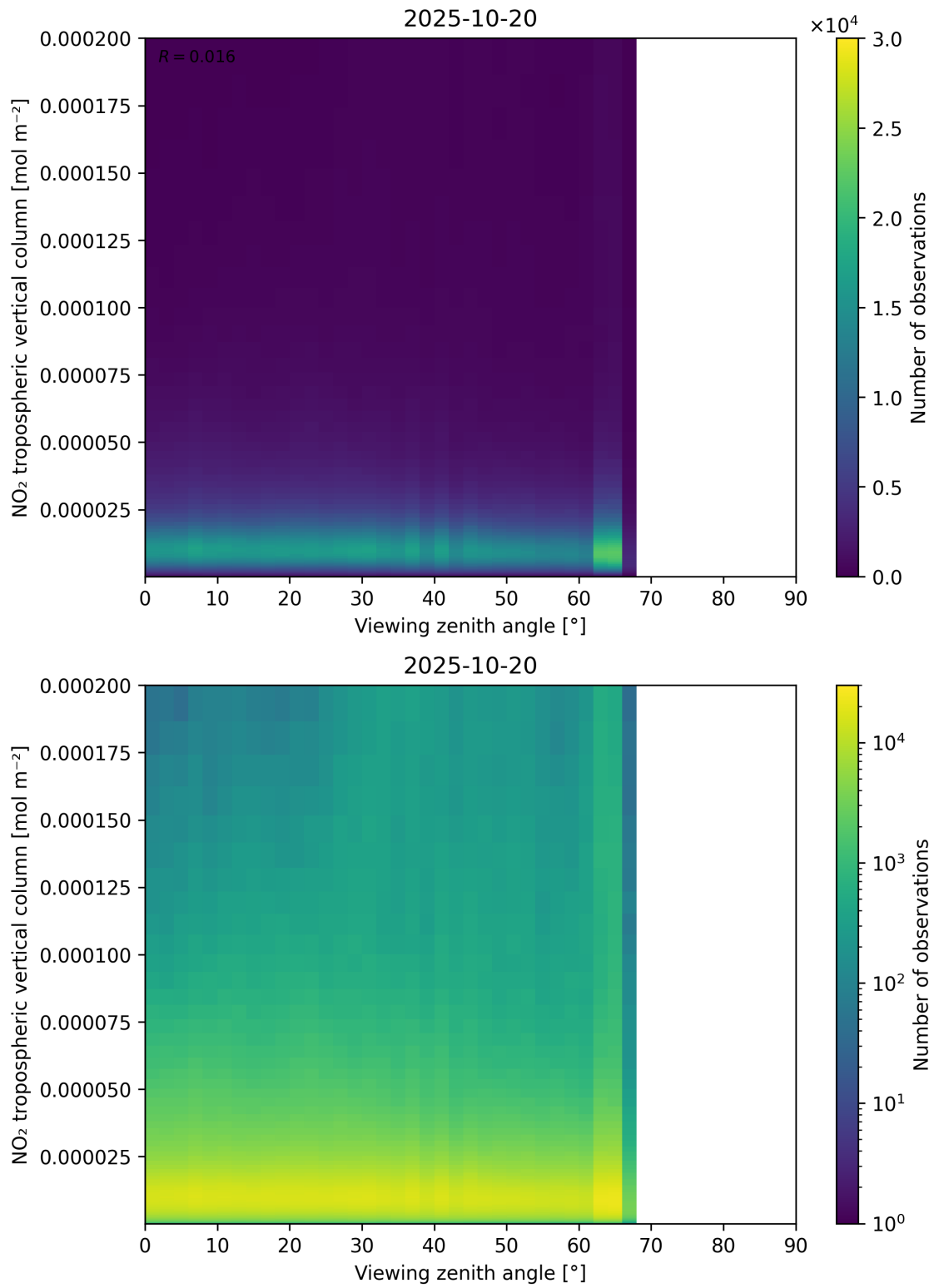
Figure 169: Scatter density plot of “Viewing zenith angle” against “NO 2 tropospheric vertical column” for 2025-10-19 to 2025-10-21.
