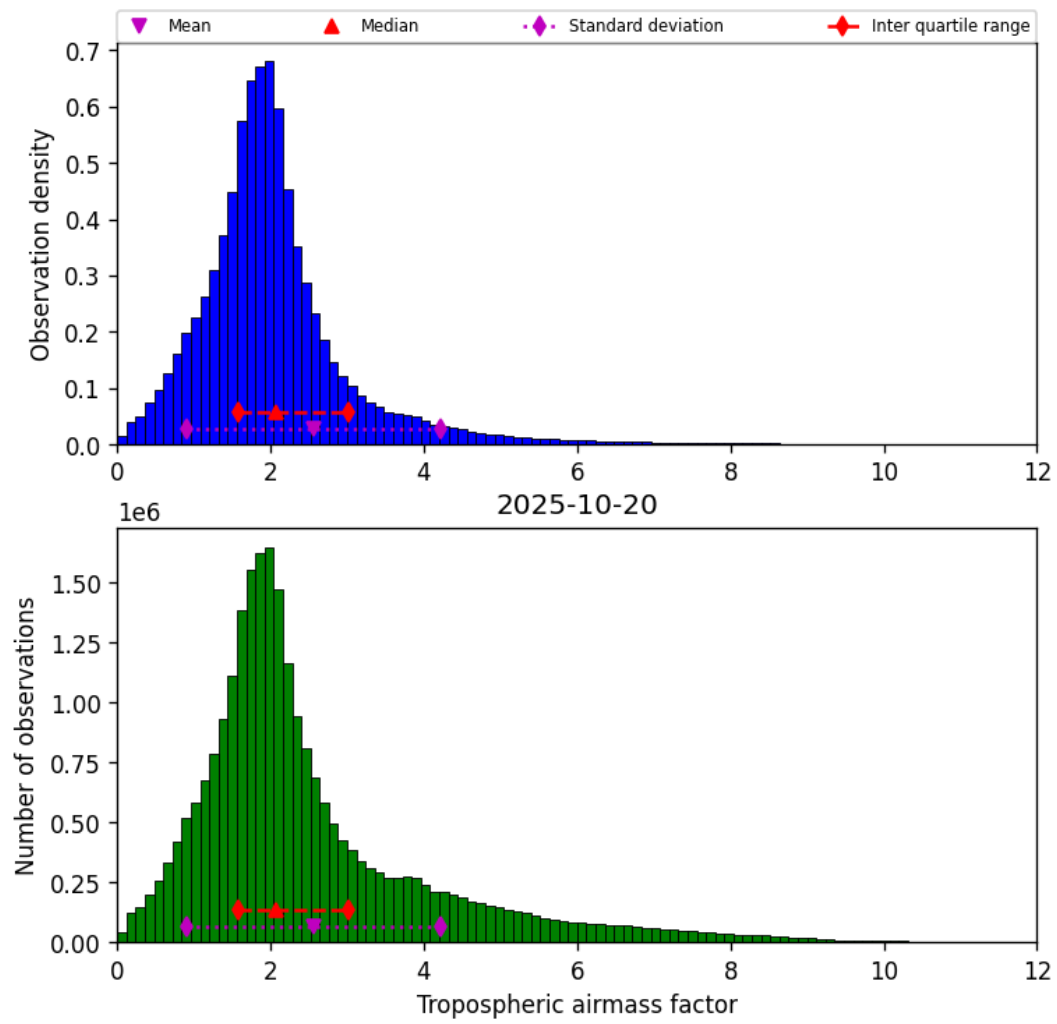
Figure 31: Histogram of “Tropospheric airmass factor” for 2025-10-19 to 2025-10-21
