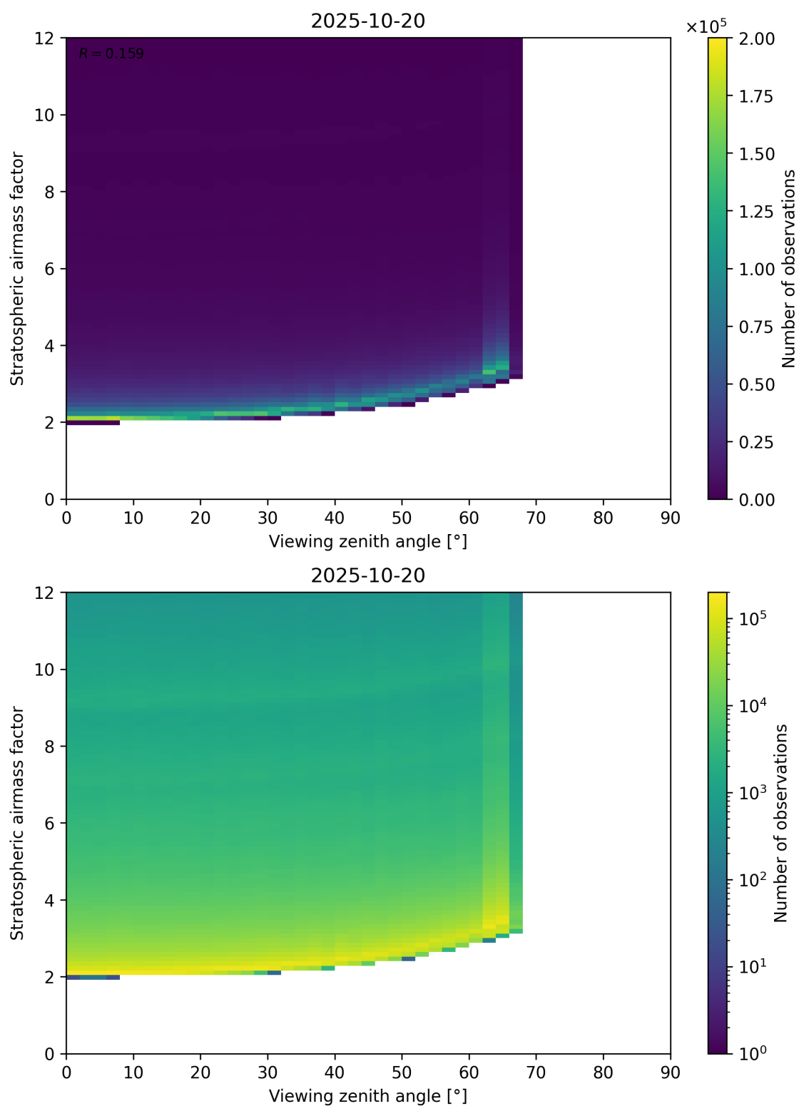
Figure 159: Scatter density plot of “Viewing zenith angle” against “Stratospheric airmass factor” for 2025-10-19 to 2025-10-21.
