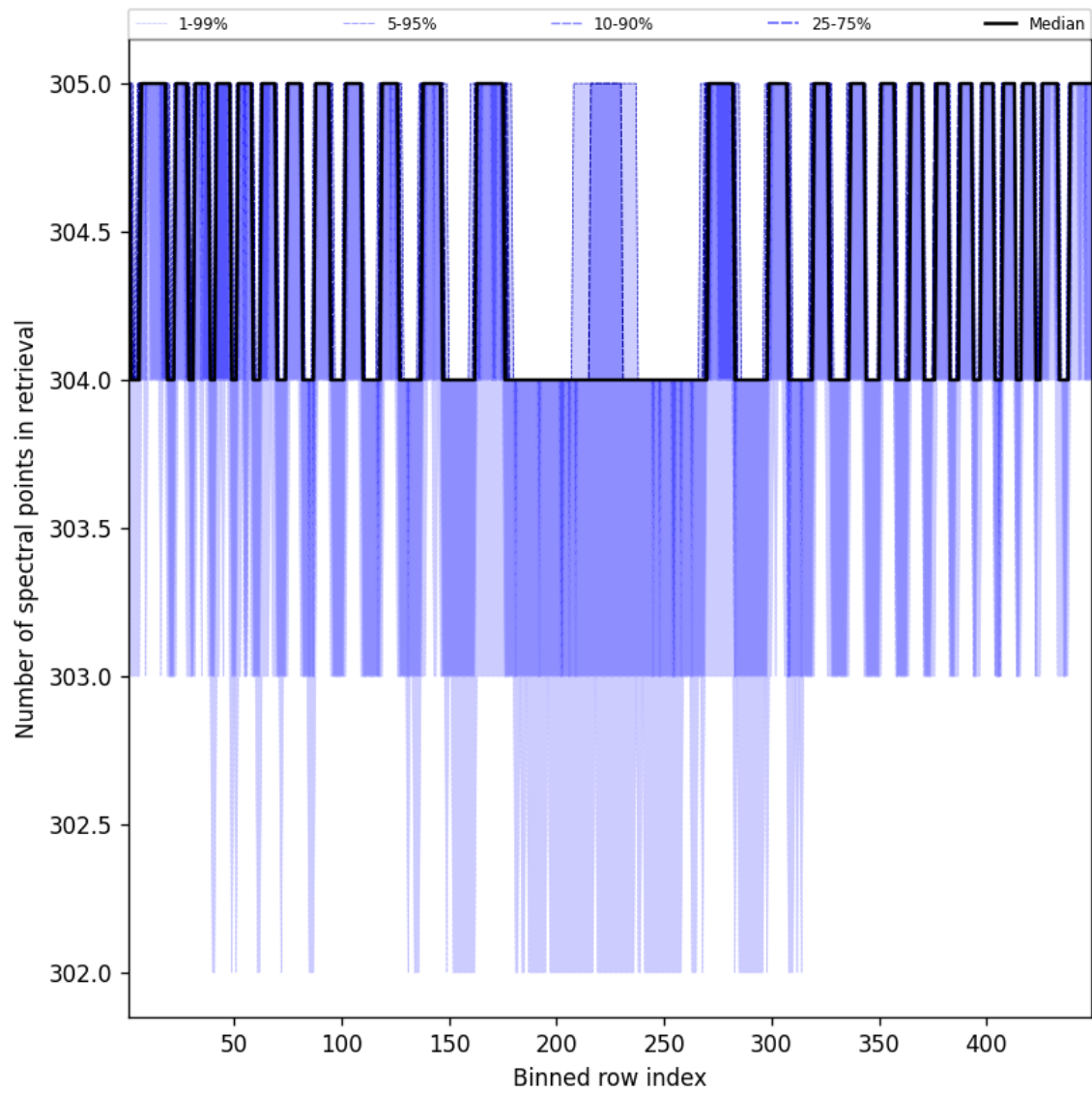
Figure 50: Along track statistics of “Number of spectral points in retrieval” for 2025-10-19 to 2025-10-21
