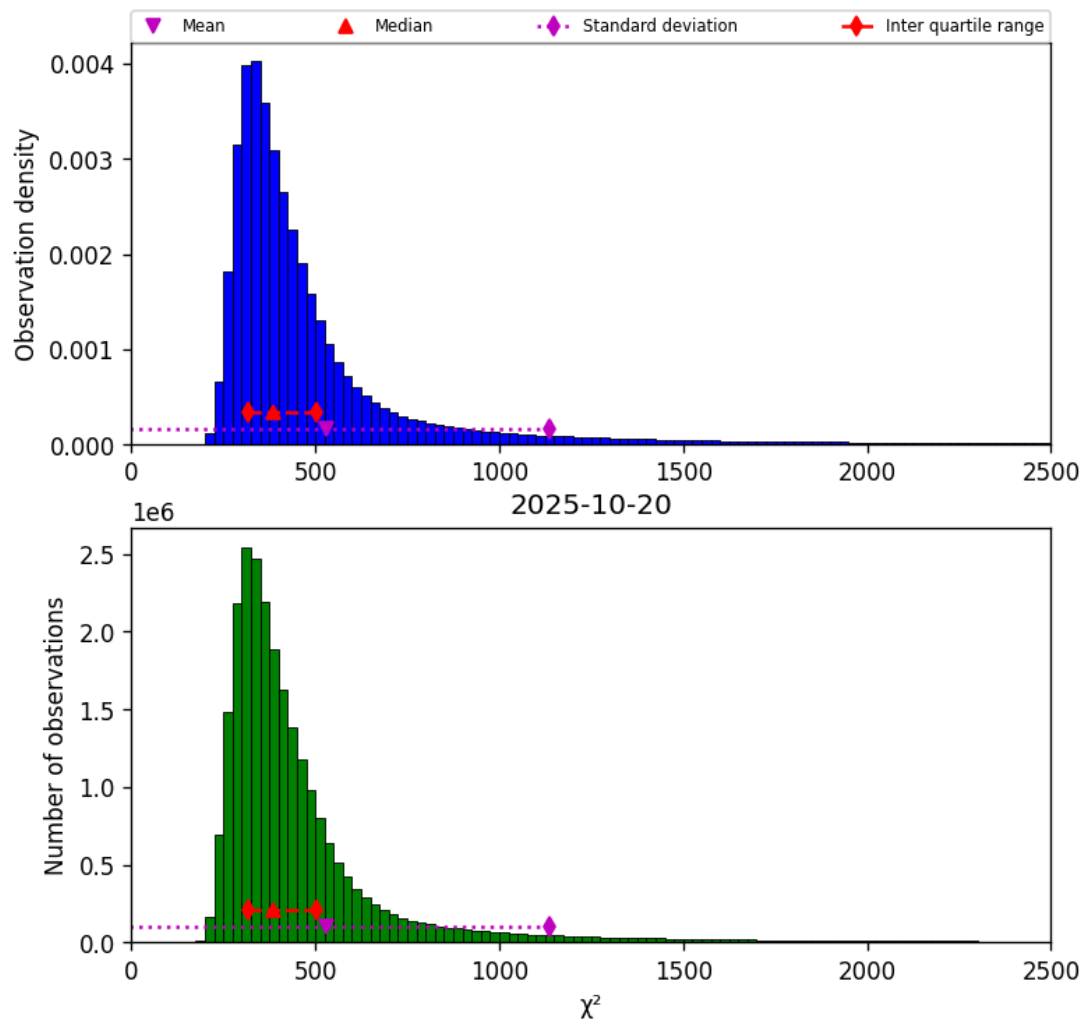
Figure 42: Histogram of “ \chi^2 ” for 2025-10-19 to 2025-10-21
