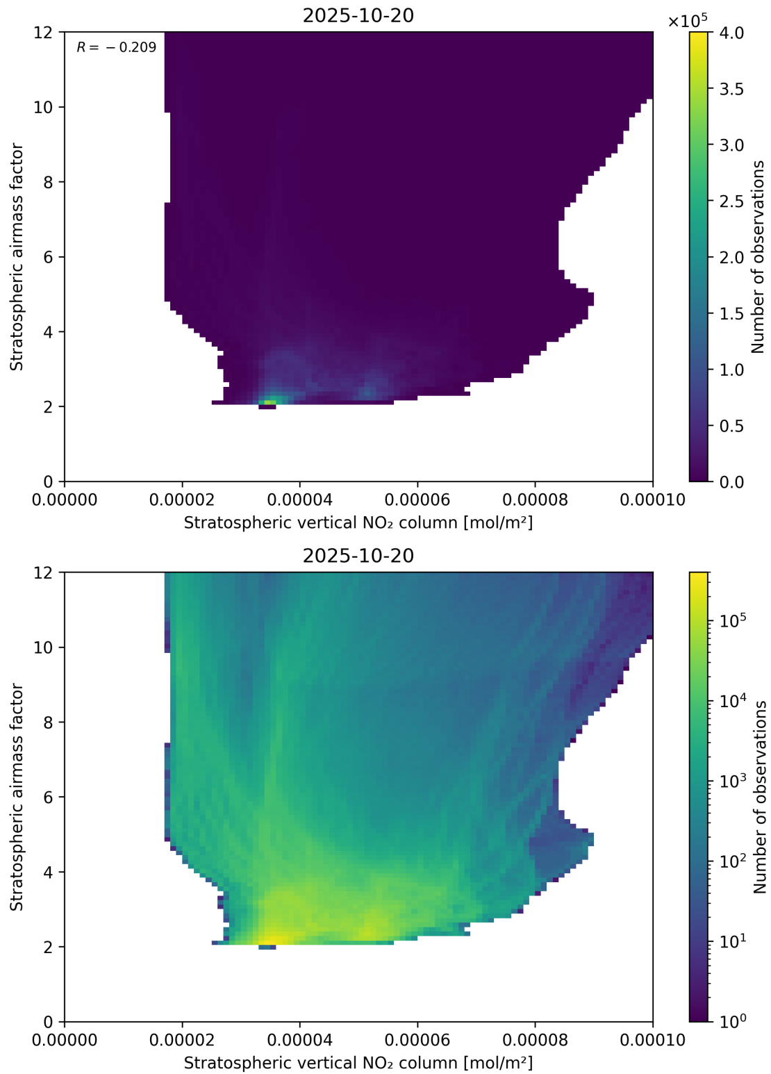
Figure 96: Scatter density plot of “Stratospheric vertical NO 2 column” against “Stratospheric airmass factor” for 2025-10-19 to 2025-10-21.
