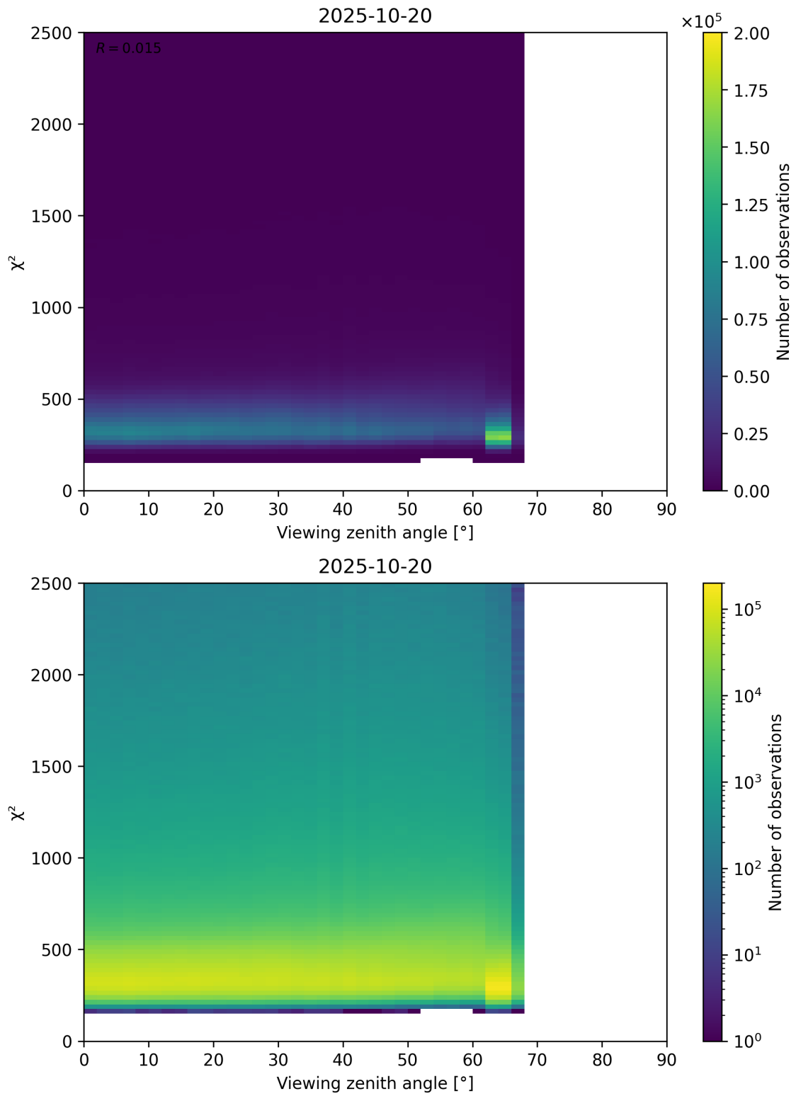
Figure 162: Scatter density plot of “Viewing zenith angle” against “ \chi^2 ” for 2025-10-19 to 2025-10-21.
