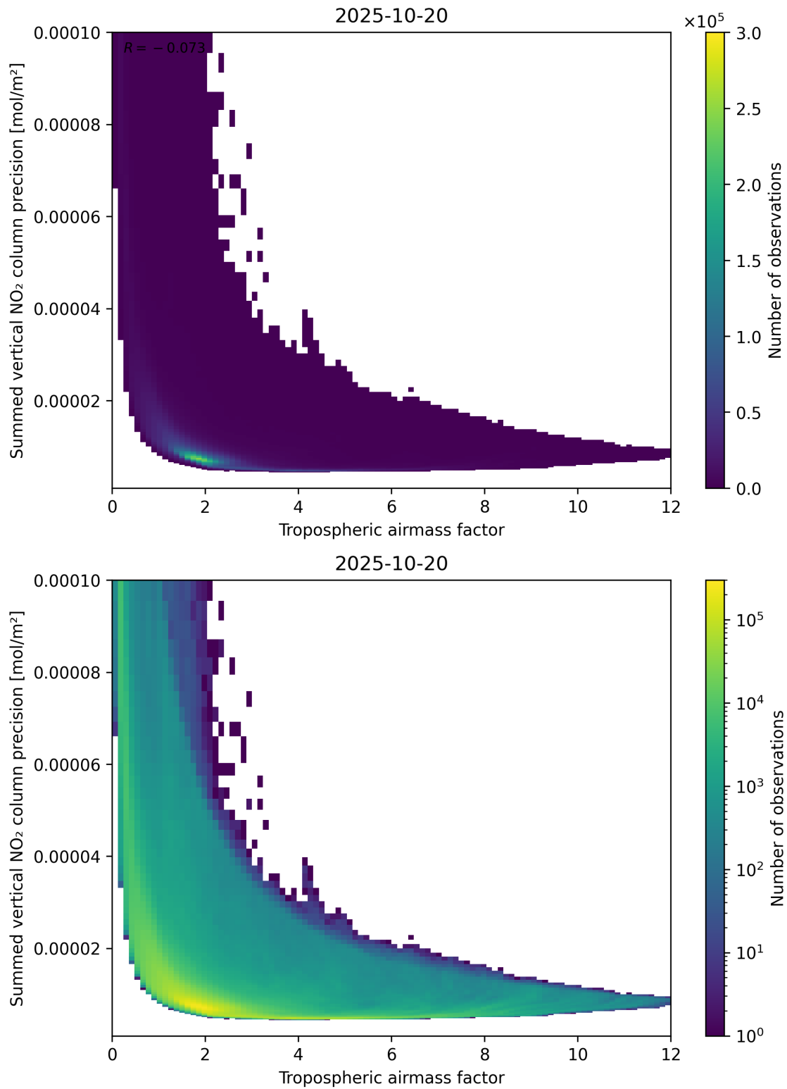
Figure 76: Scatter density plot of “Tropospheric air mass factor” against “Summed vertical NO 2 column precision” for 2025-10-19 to 2025-10-21.
