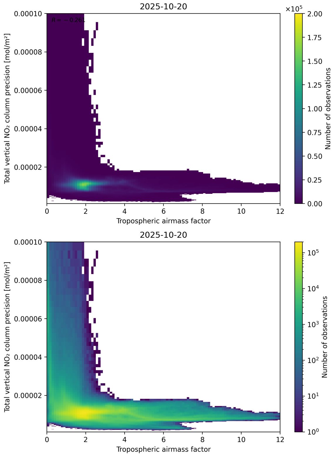
Figure 78: Scatter density plot of “Tropospheric air mass factor” against “Total vertical NO 2 column precision” for 2025-10-19 to 2025-10-21.
