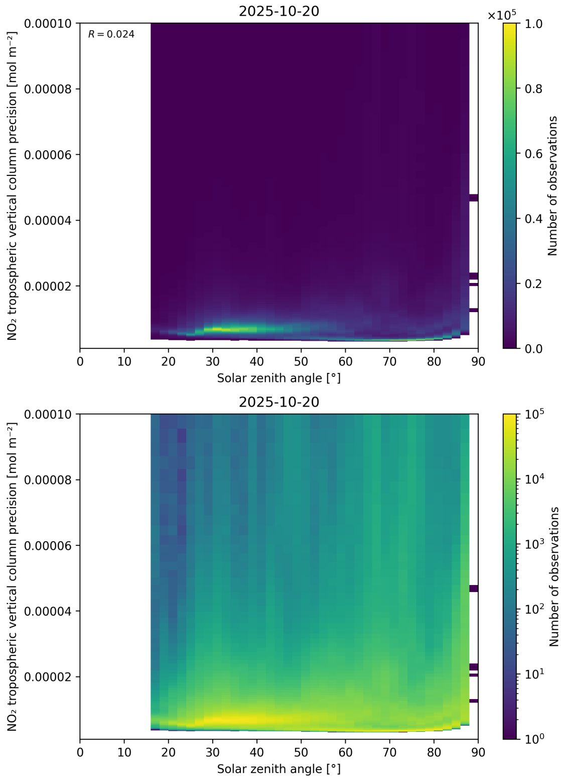
Figure 156: Scatter density plot of “Solar zenith angle” against “NO 2 tropospheric vertical column precision” for 2025-10-19 to 2025-10-21.
