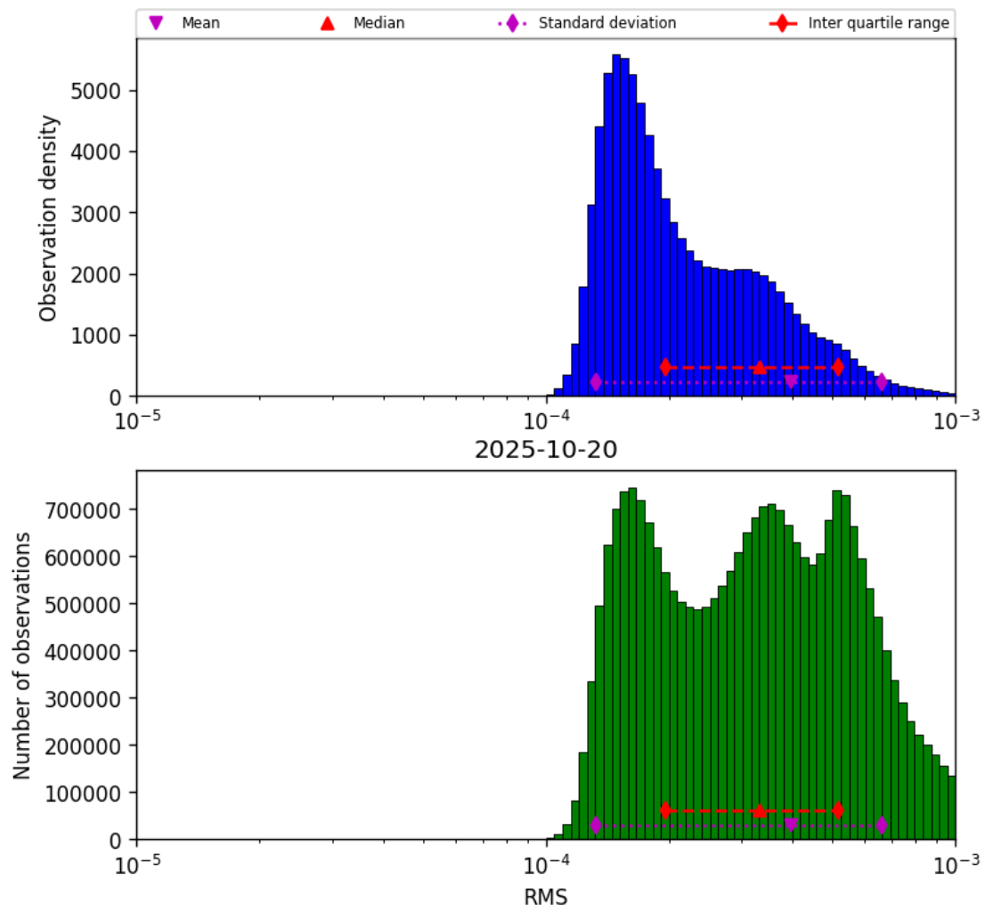
Figure 43: Histogram of “RMS” for 2025-10-19 to 2025-10-21
