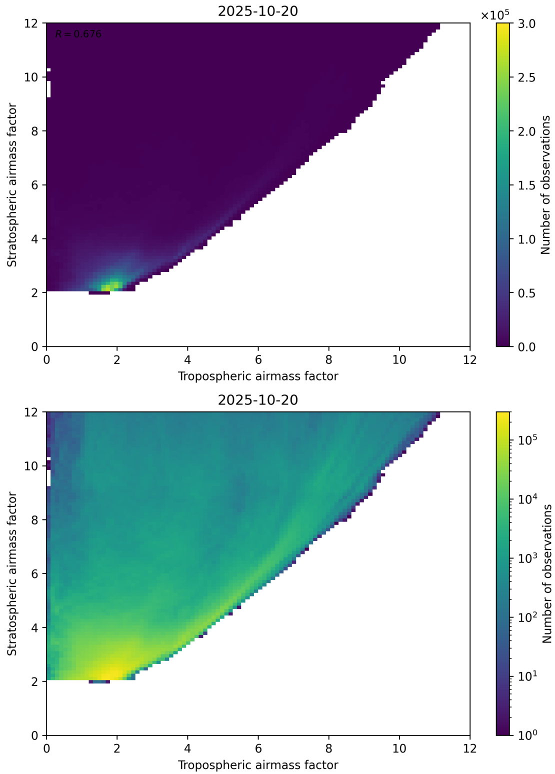
Figure 71: Scatter density plot of “Tropospheric airmass factor” against “Stratospheric airmass factor” for 2025-10-19 to 2025-10-21.
