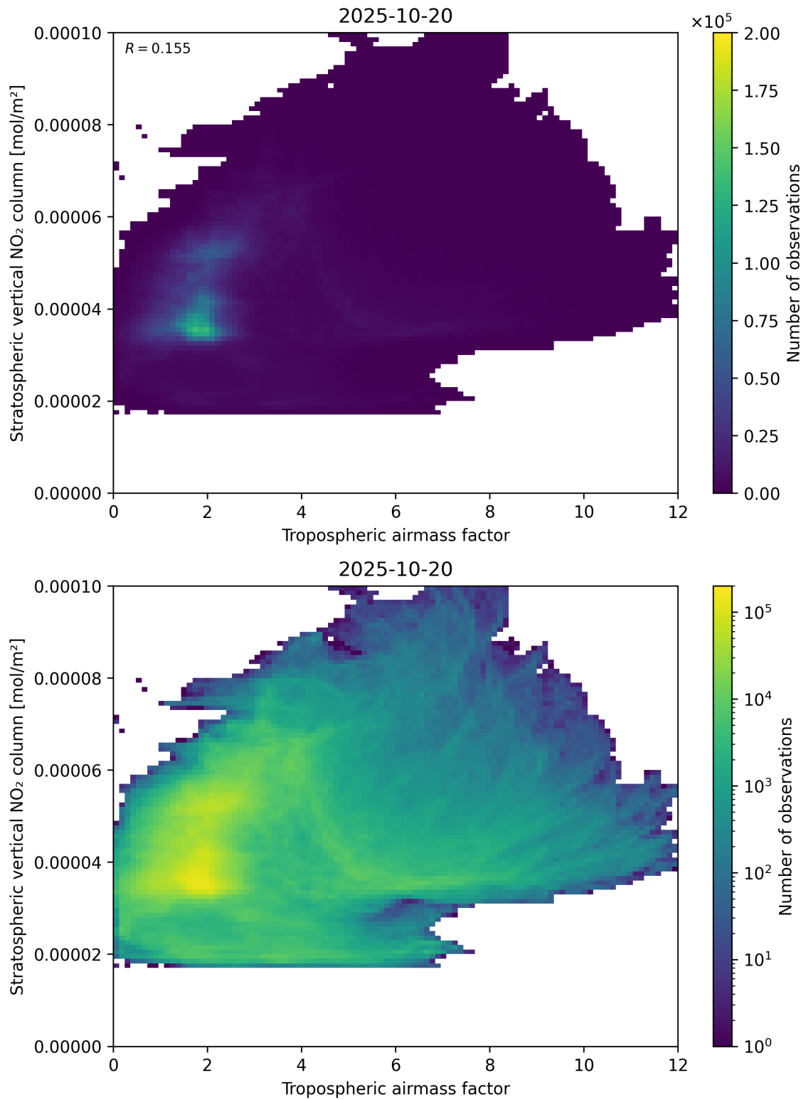
Figure 74: Scatter density plot of “Tropospheric air mass factor” against “Stratospheric vertical NO 2 column” for 2025-10-19 to 2025-10-21.
