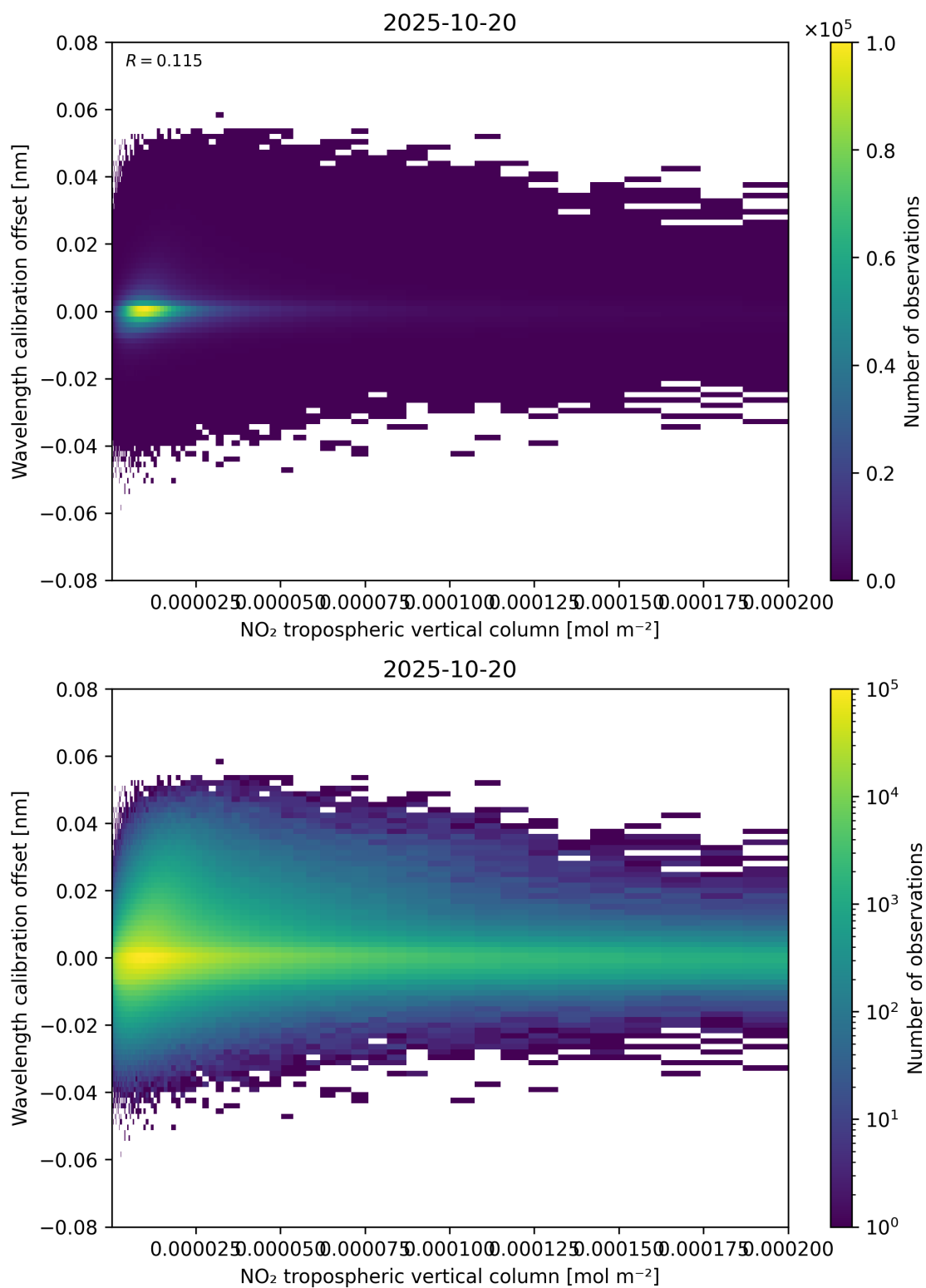
Figure 143: Scatter density plot of “NO 2 tropospheric vertical column” against “Wavelength calibration offset” for 2025-10-19 to 2025-10-21.
