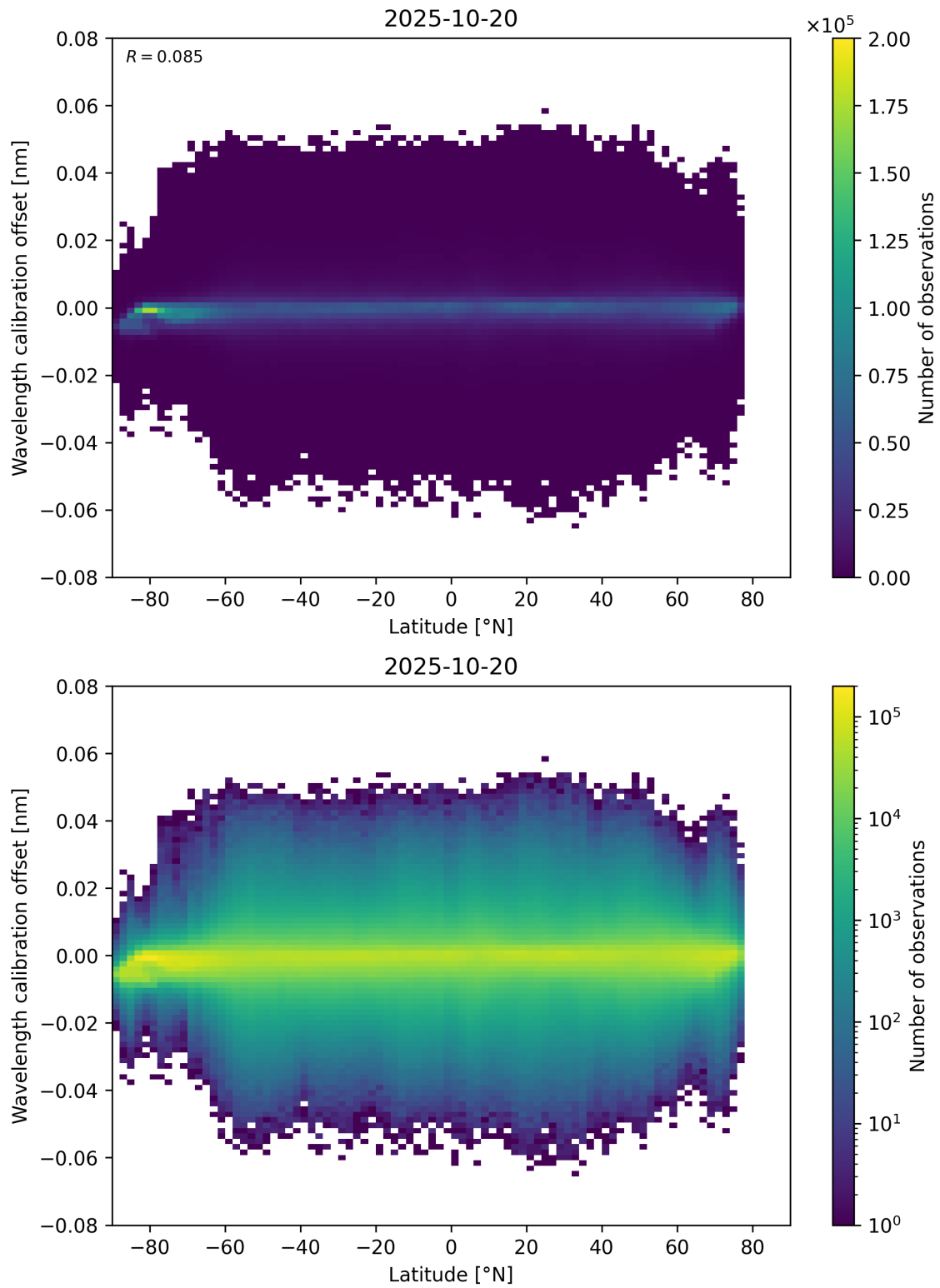
Figure 95: Scatter density plot of “Latitude” against “Wavelength calibration offset” for 2025-10-19 to 2025-10-21.
