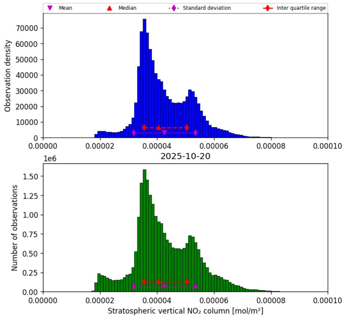
Figure 36: Histogram of “Stratospheric vertical NO 2 column” for 2025-10-19 to 2025-10-21
