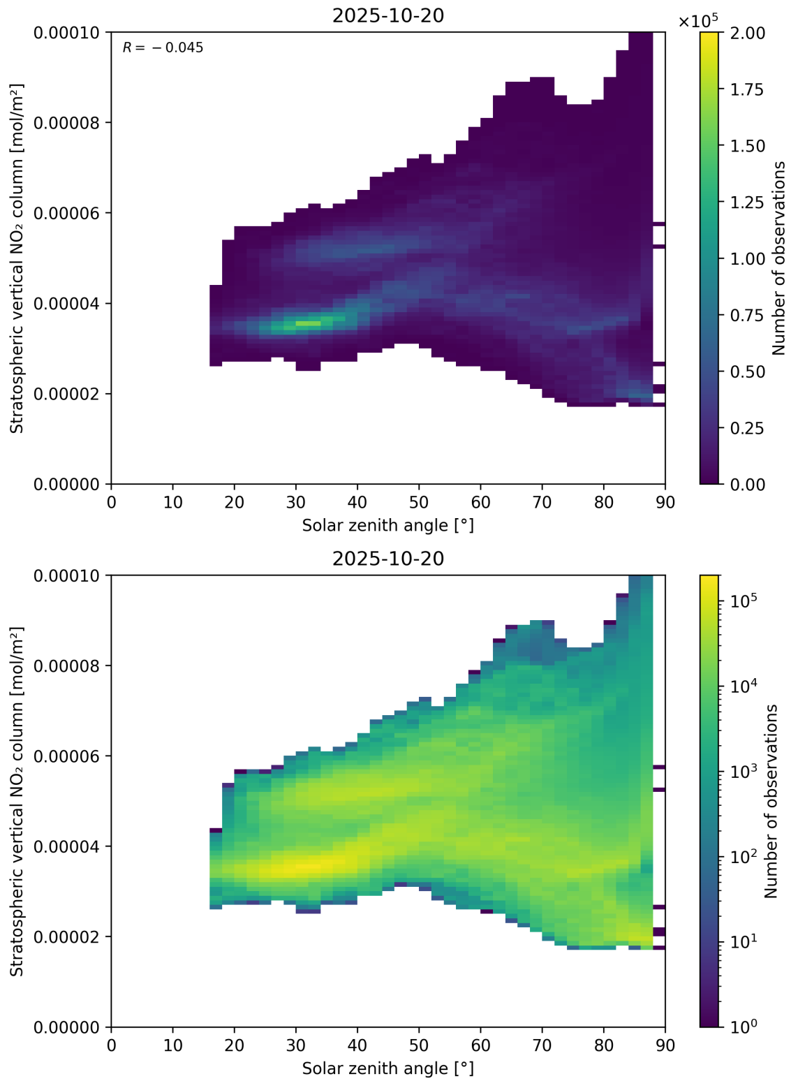
Figure 150: Scatter density plot of “Solar zenith angle” against “Stratospheric vertical NO 2 column” for 2025-10-19 to 2025-10-21.
