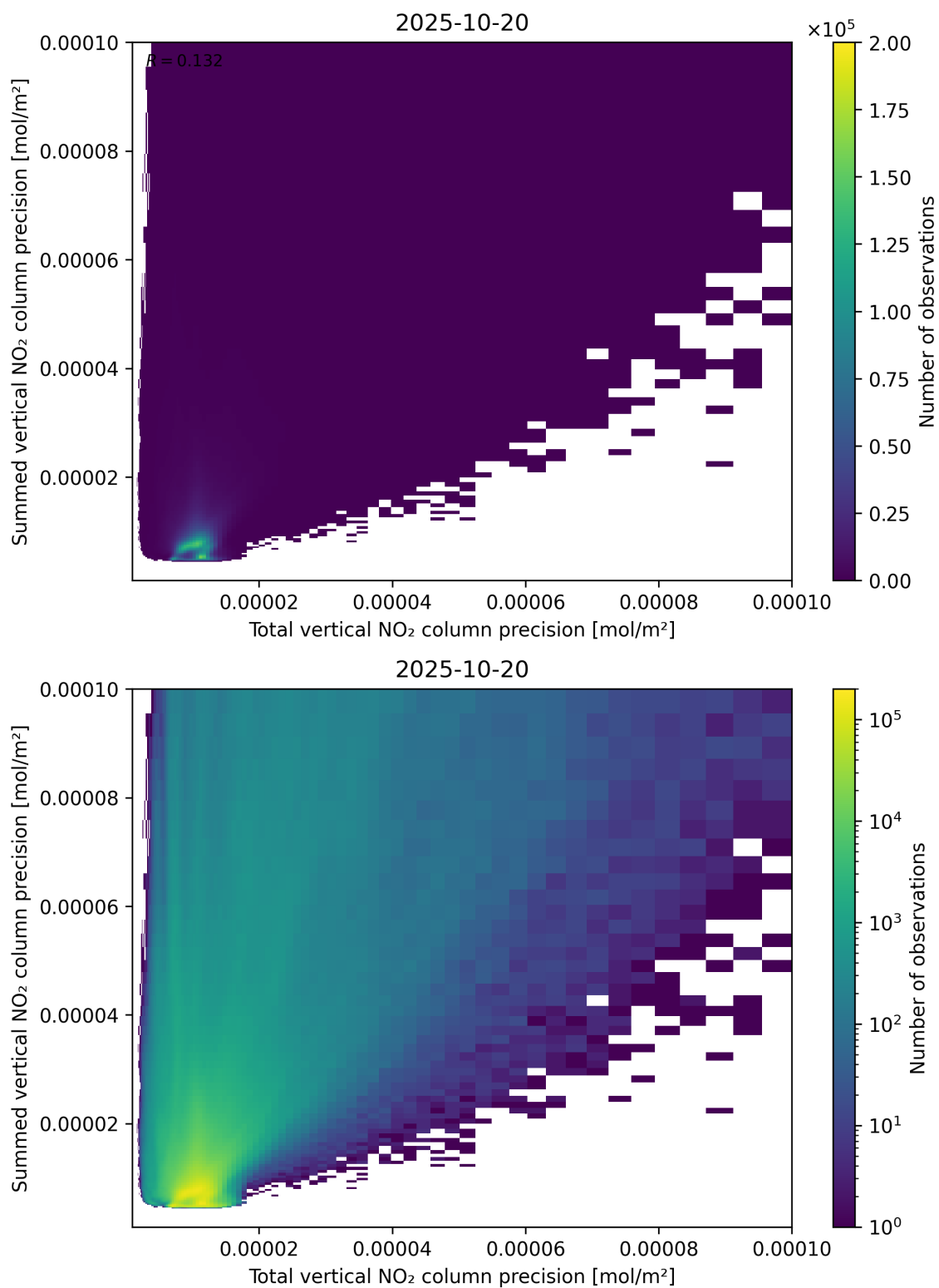
Figure 118: Scatter density plot of “Total vertical NO 2 column precision” against “Summed vertical NO 2 column precision” for 2025-10-19 to 2025-10-21.
