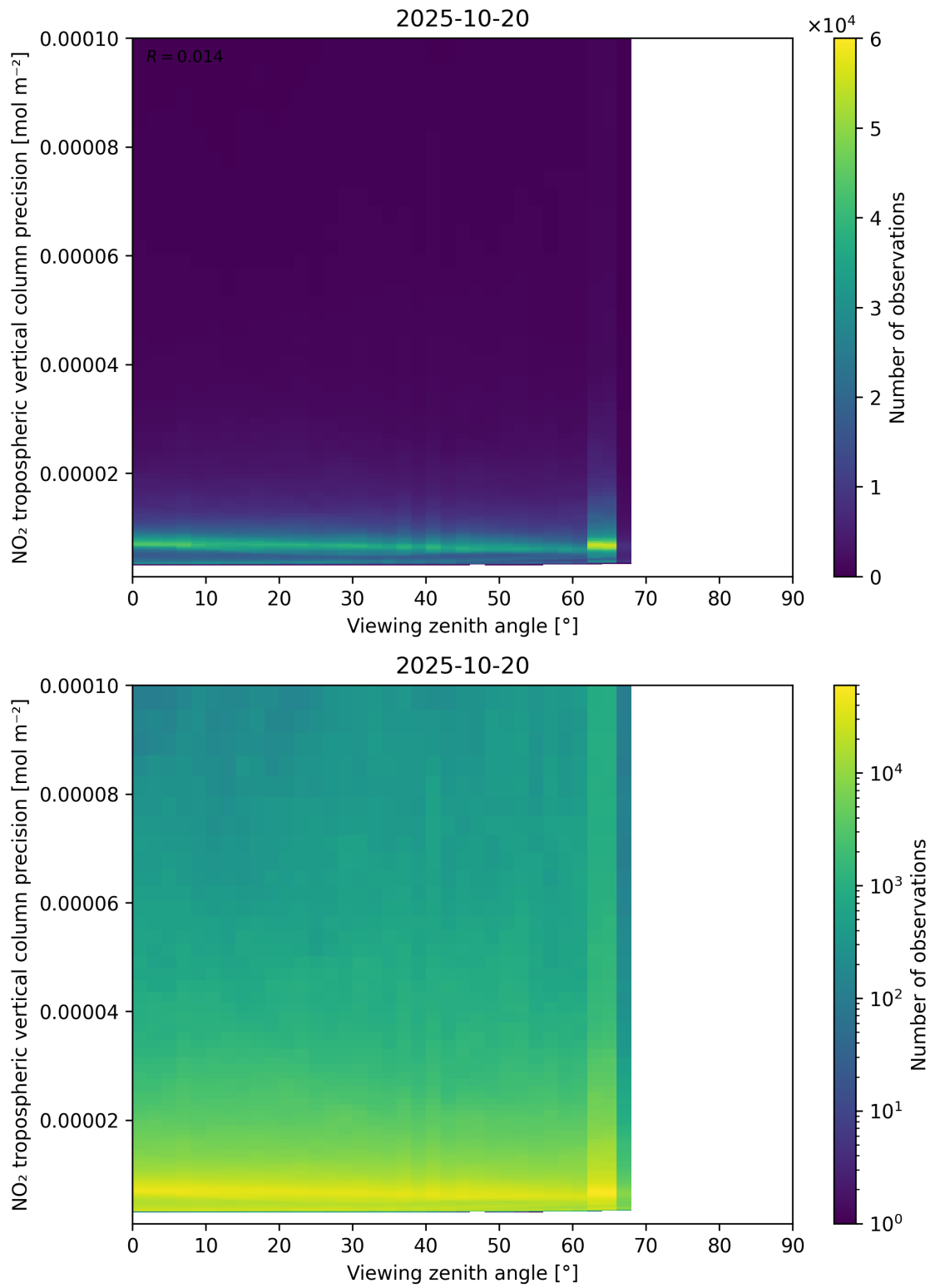
Figure 170: Scatter density plot of “Viewing zenith angle” against “NO 2 tropospheric vertical column precision” for 2025-10-19 to 2025-10-21.
