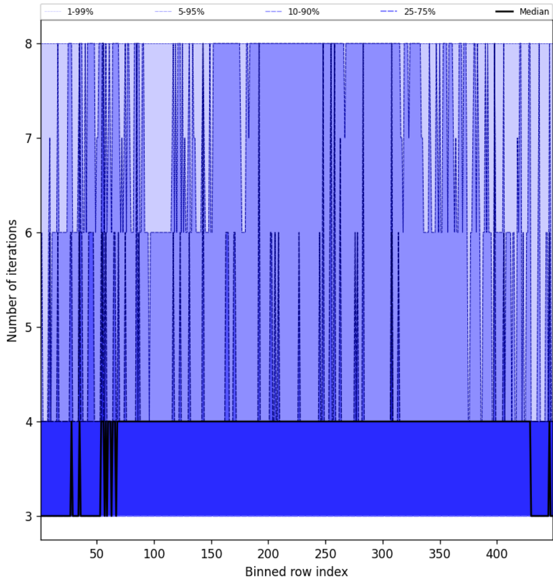
Figure 51: Along track statistics of “Number of iterations” for 2025-10-19 to 2025-10-21
