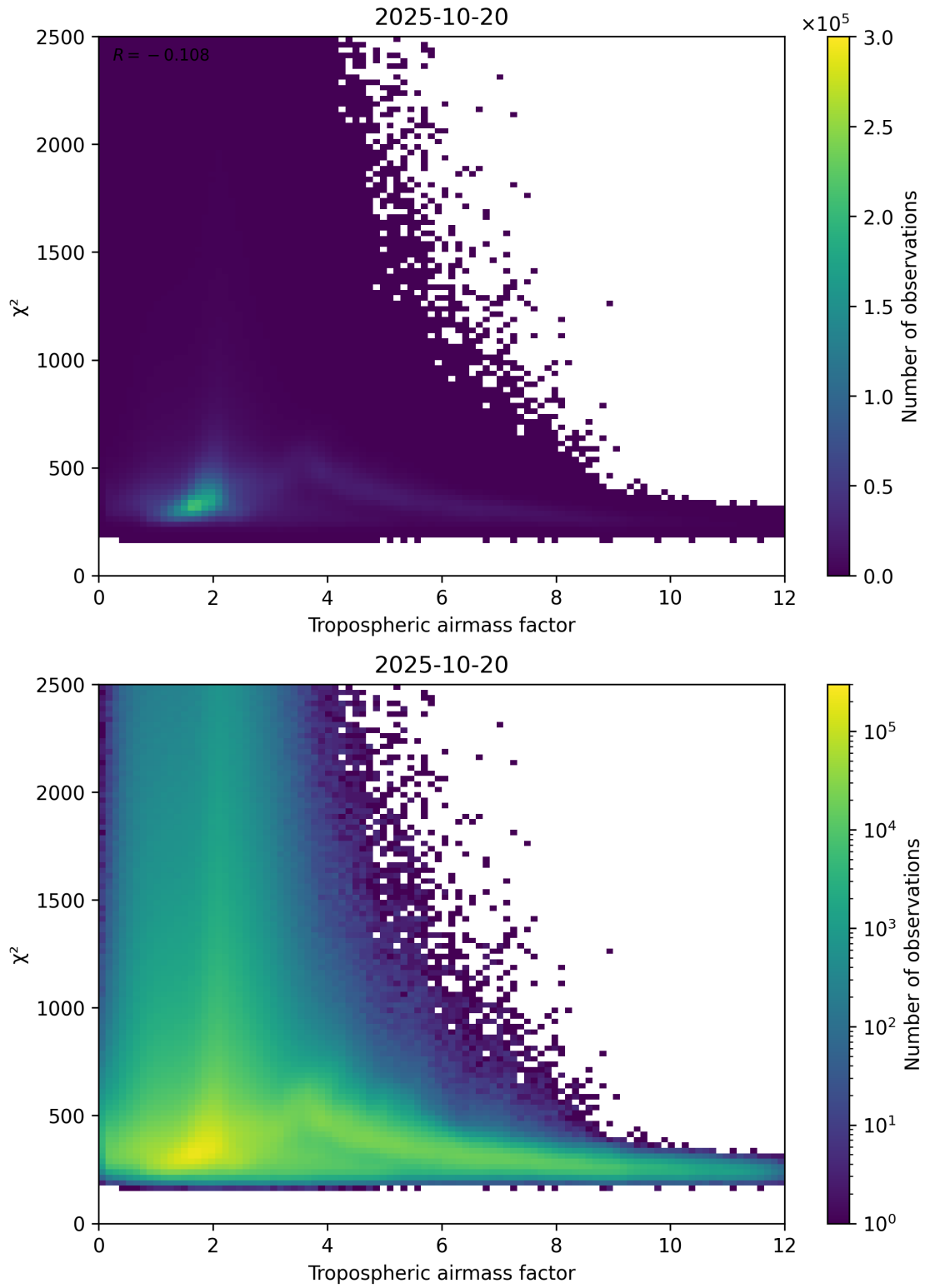
Figure 73: Scatter density plot of “Tropospheric airmass factor” against “ \chi^2 ” for 2025-10-19 to 2025-10-21.
