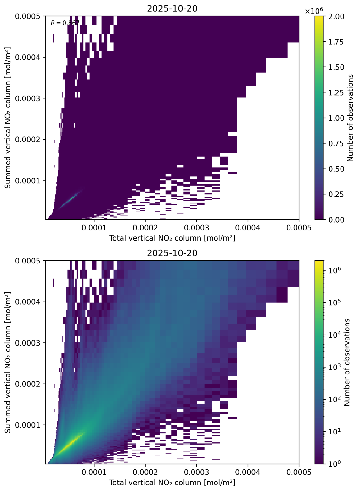
Figure 112: Scatter density plot of “Total vertical NO 2 column” against “Summed vertical NO 2 column” for 2025-10-19 to 2025-10-21.
