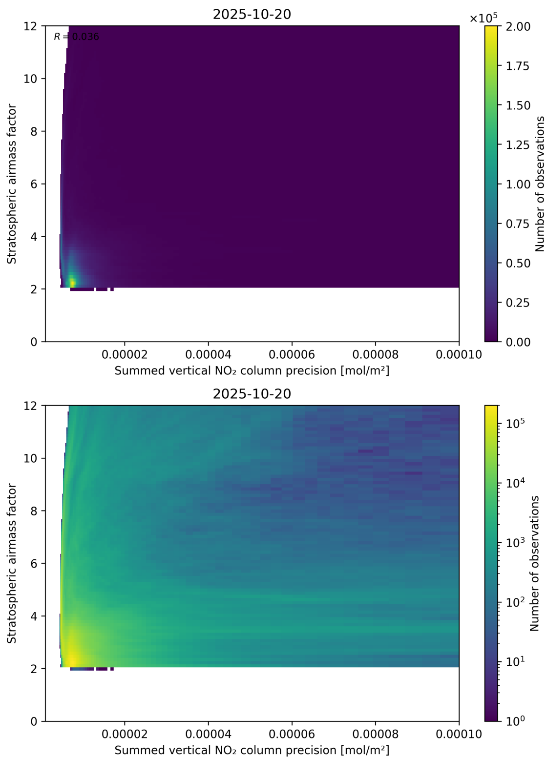
Figure 106: Scatter density plot of “Summed vertical NO 2 column precision” against “Stratospheric airmass factor” for 2025-10-19 to 2025-10-21.
