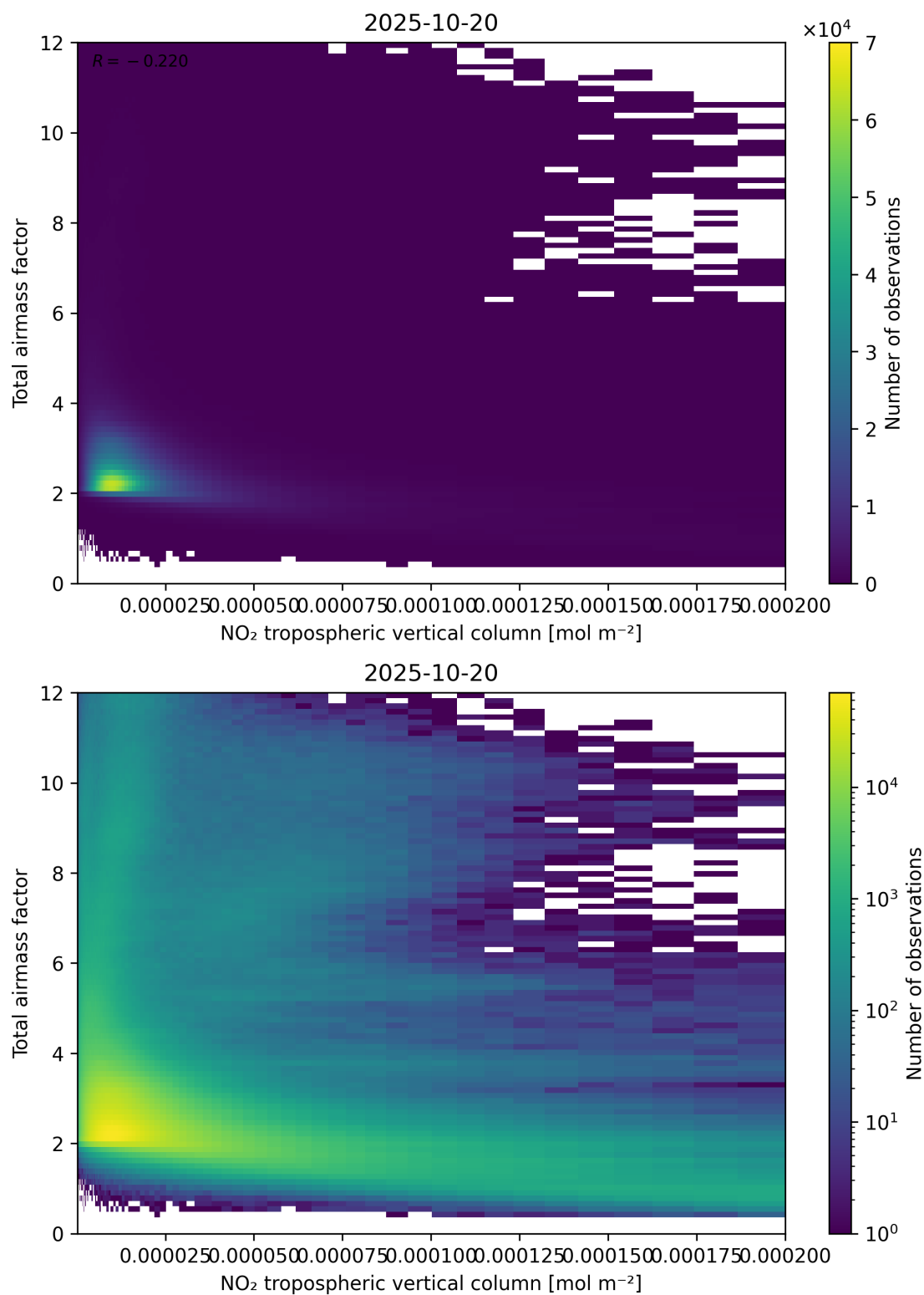
Figure 122: Scatter density plot of “NO 2 tropospheric vertical column” against “Total air mass factor” for 2025-10-19 to 2025-10-21.
