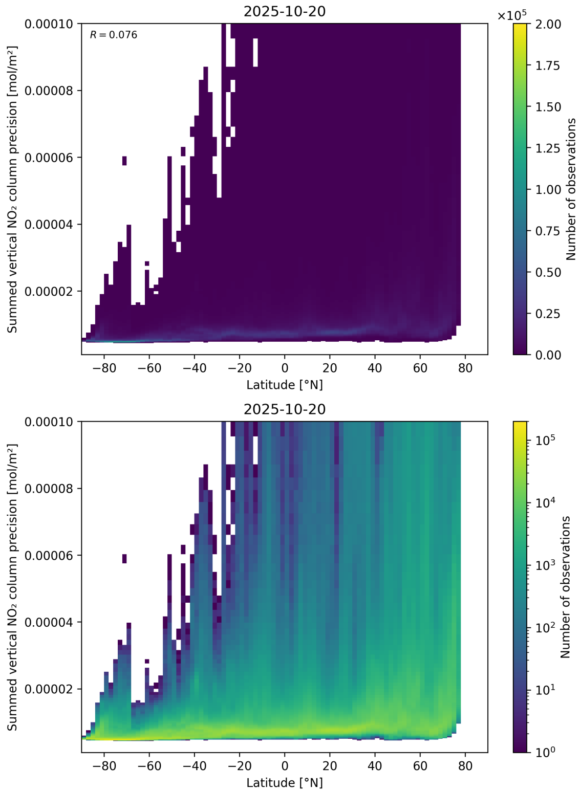
Figure 89: Scatter density plot of “Latitude” against “Summed vertical NO 2 column precision” for 2025-10-19 to 2025-10-21.
