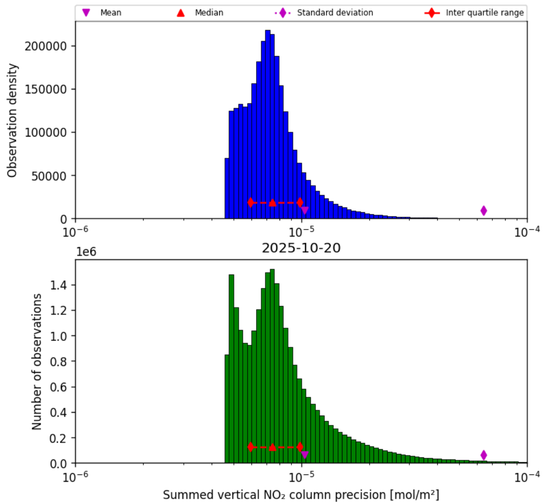
Figure 41: Histogram of "Summed vertical NO 2 column precision" for 2025-10-19 to 2025-10-21
