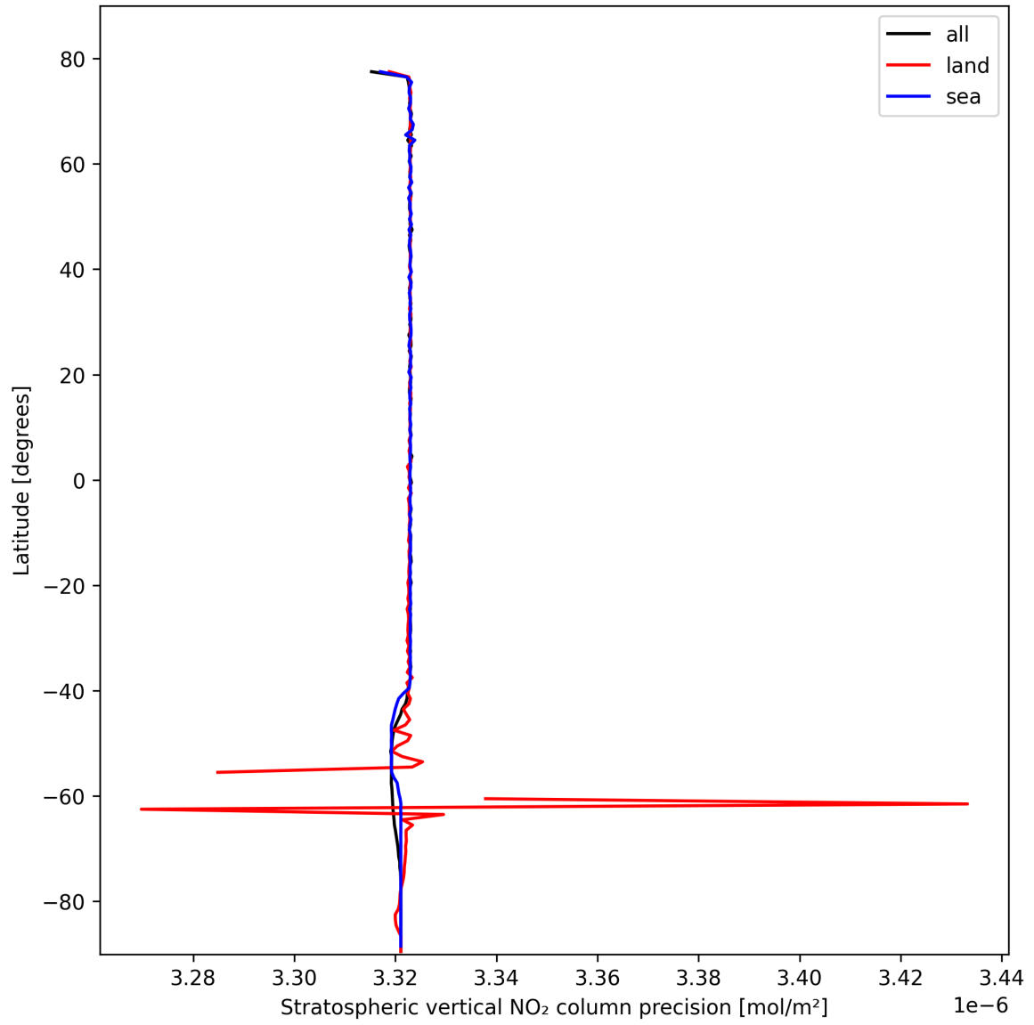
Figure 20: Zonal average of "Stratospheric vertical NO 2 column precision" for 2025-10-19 to 2025-10-21.
