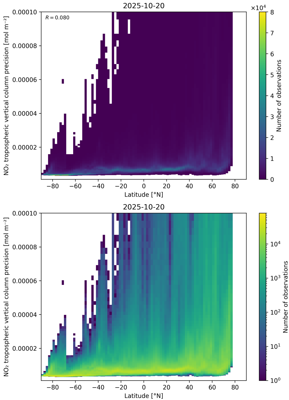
Figure 93: Scatter density plot of “Latitude” against “NO 2 tropospheric vertical column precision” for 2025-10-19 to 2025-10-21.
