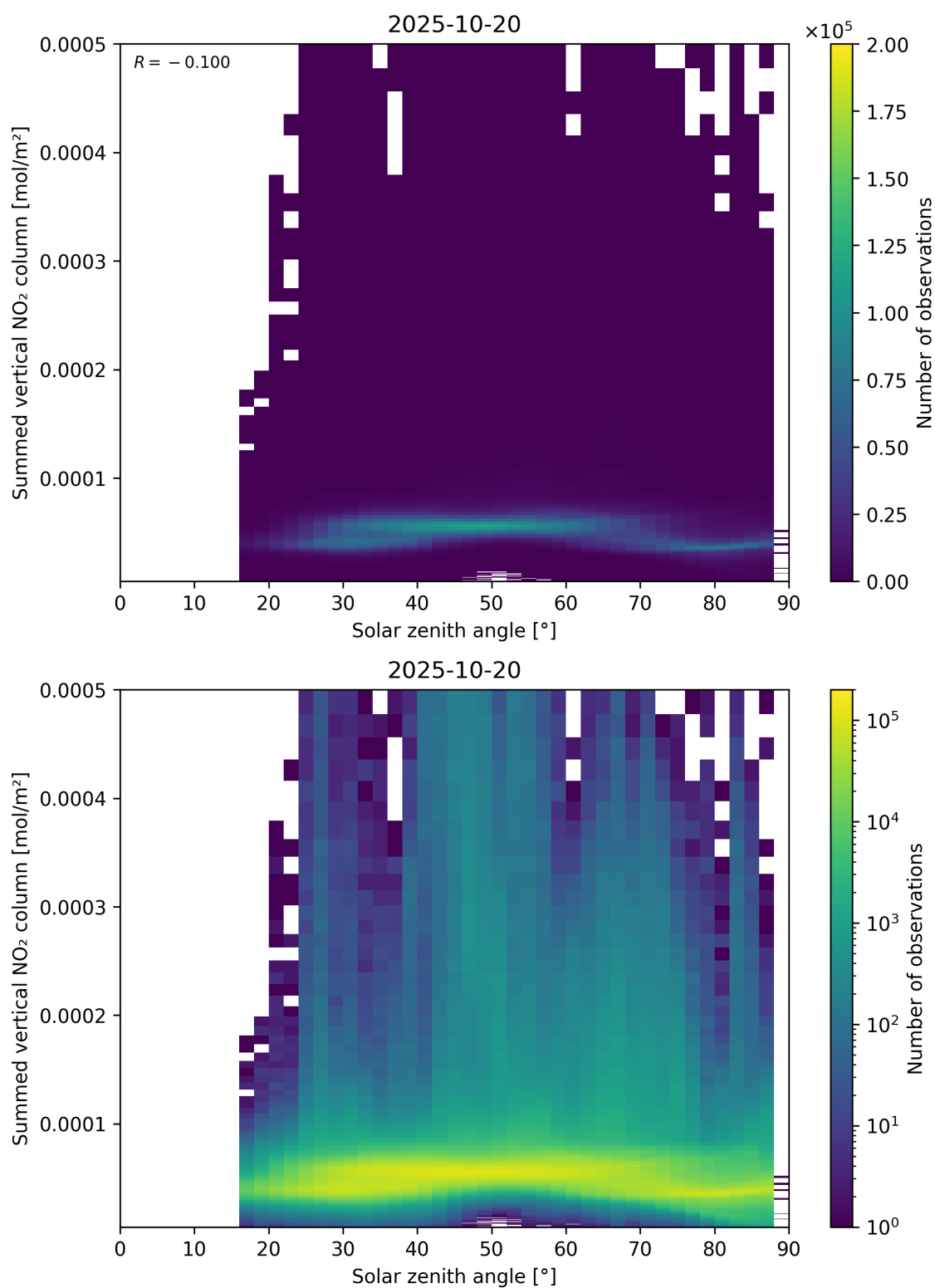
Figure 151: Scatter density plot of “Solar zenith angle” against “Summed vertical NO 2 column” for 2025-10-19 to 2025-10-21.
