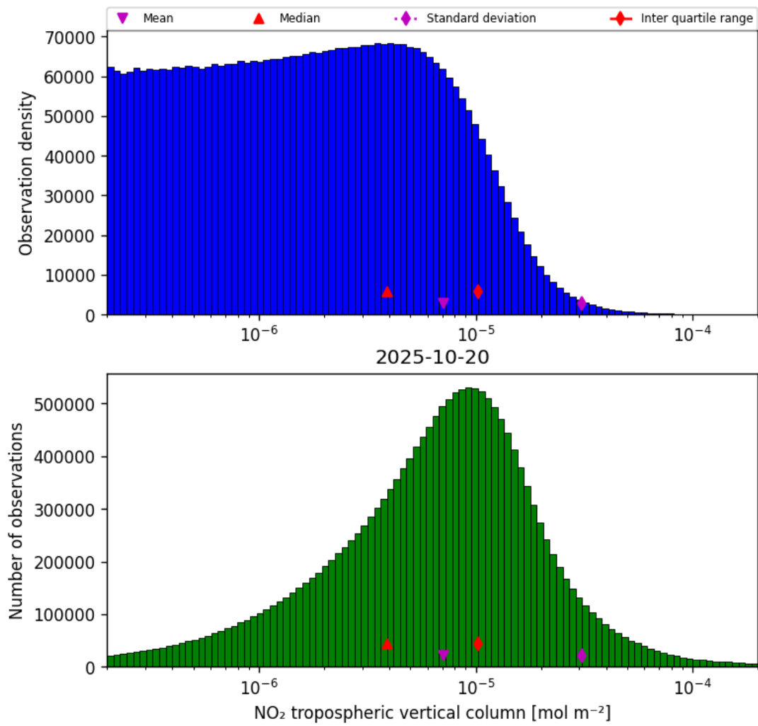
Figure 29: Histogram of “NO 2 tropospheric vertical column” for 2025-10-19 to 2025-10-21
