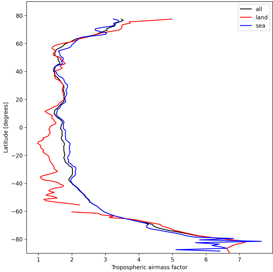
Figure 14: Zonal average of “Tropospheric air mass factor” for 2025-10-19 to 2025-10-21.
