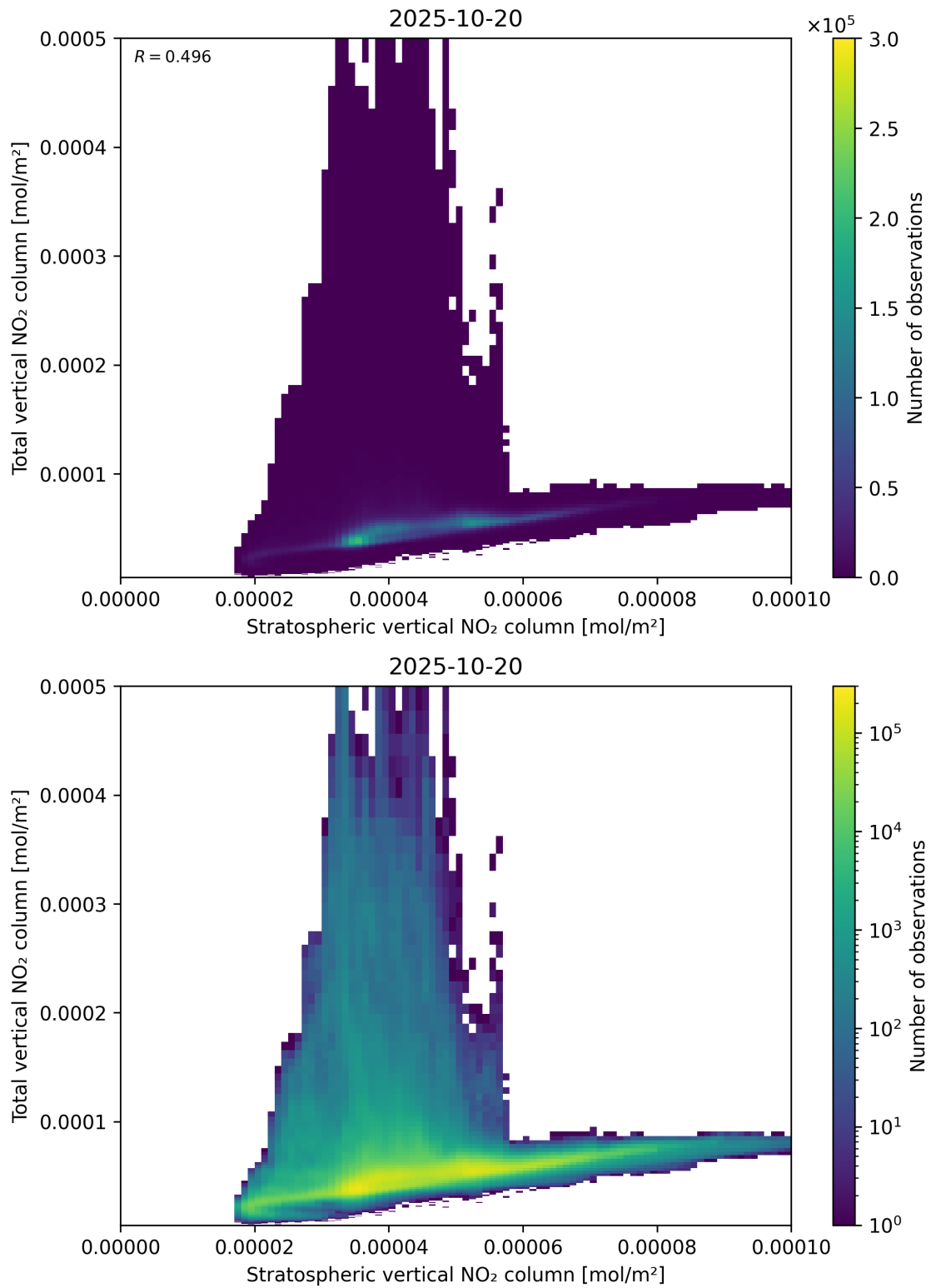
Figure 100: Scatter density plot of “Stratospheric vertical NO 2 column” against “Total vertical NO 2 column” for 2025-10-19 to 2025-10-21.
