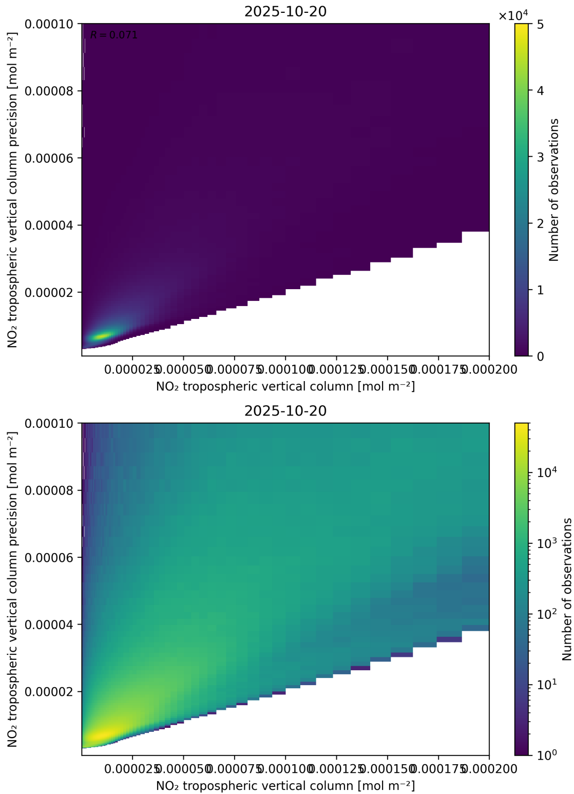
Figure 130: Scatter density plot of “NO 2 tropospheric vertical column” against “NO 2 tropospheric vertical column precision” for 2025-10-19 to 2025-10-21.
