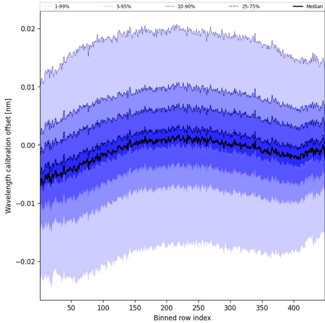
Figure 52: Along track statistics of “Wavelength calibration offset” for 2025-10-19 to 2025-10-21
