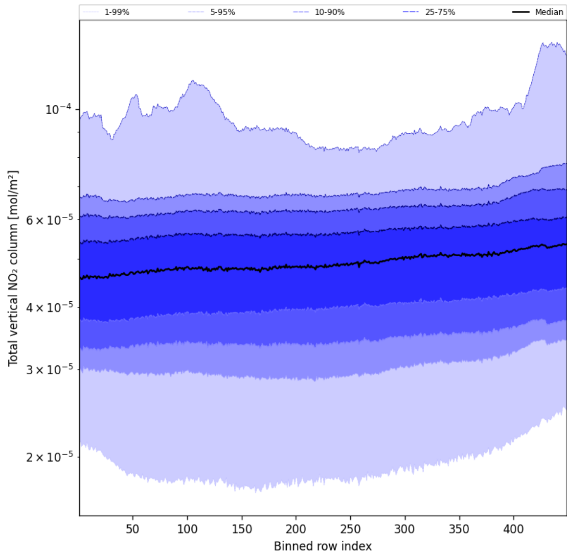
Figure 55: Along track statistics of “Total vertical NO 2 column” for 2025-10-19 to 2025-10-21
