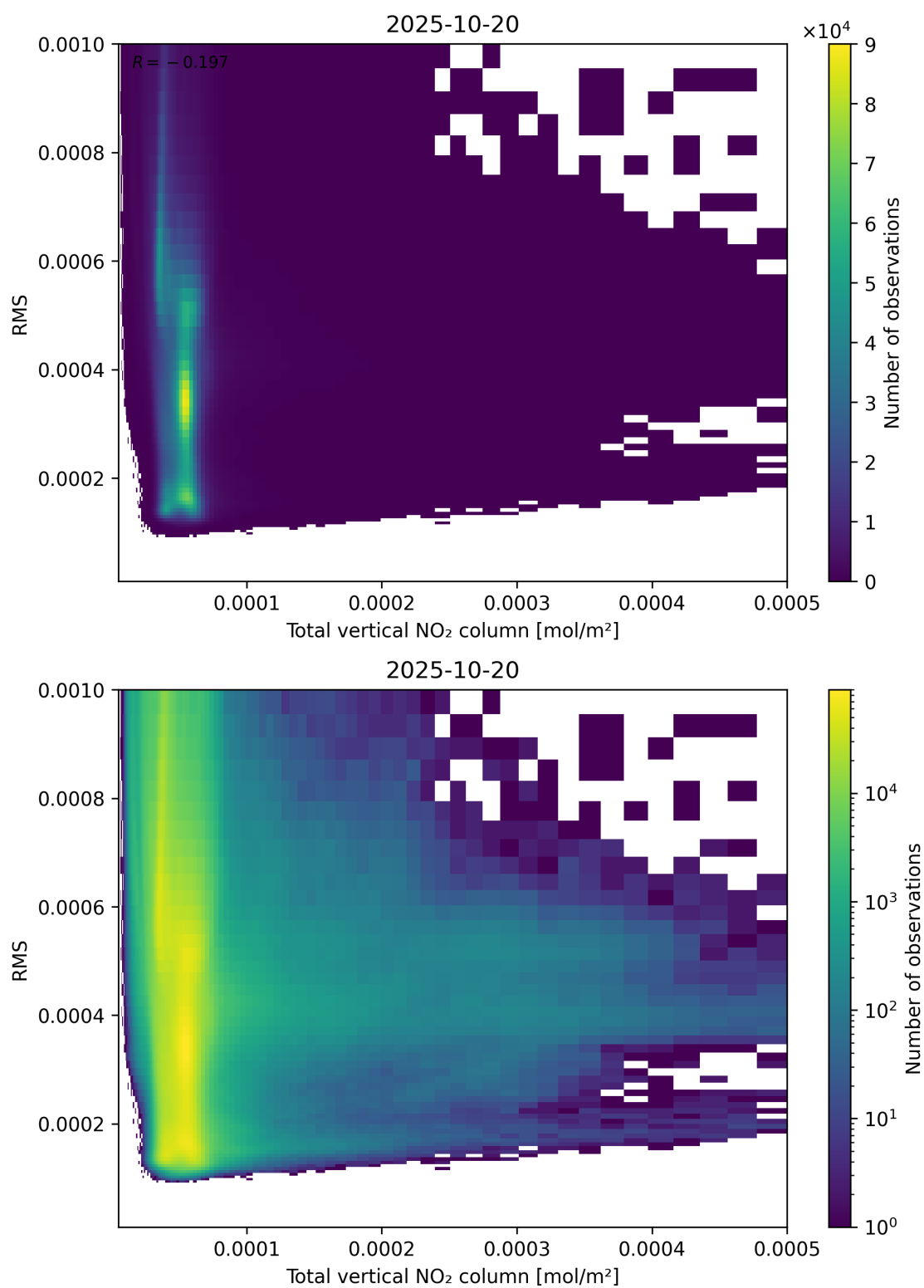
Figure 120: Scatter density plot of “Total vertical NO 2 column” against “RMS” for 2025-10-19 to 2025-10-21.
