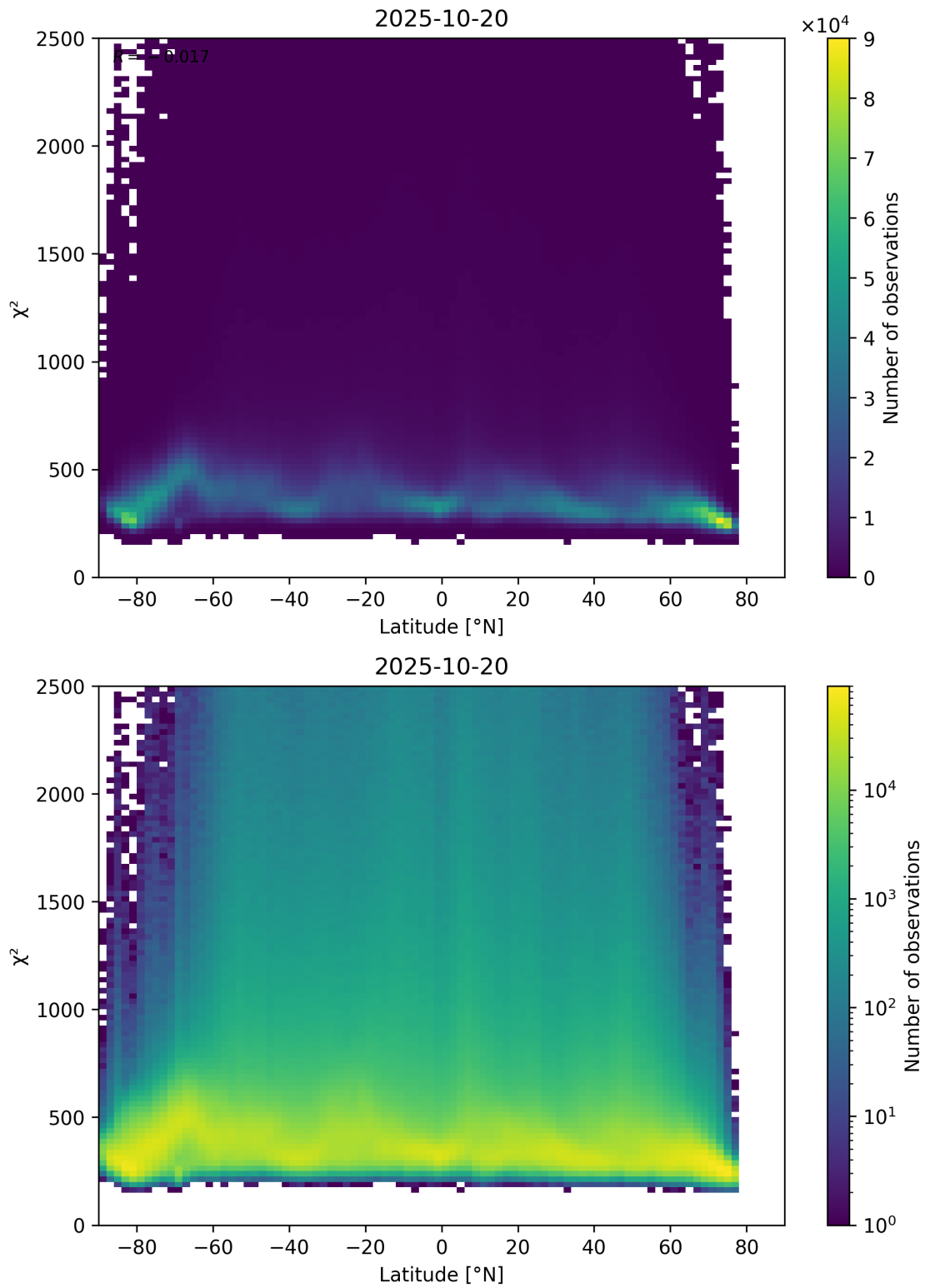
Figure 86: Scatter density plot of “Latitude” against “ \chi^2 ” for 2025-10-19 to 2025-10-21.
