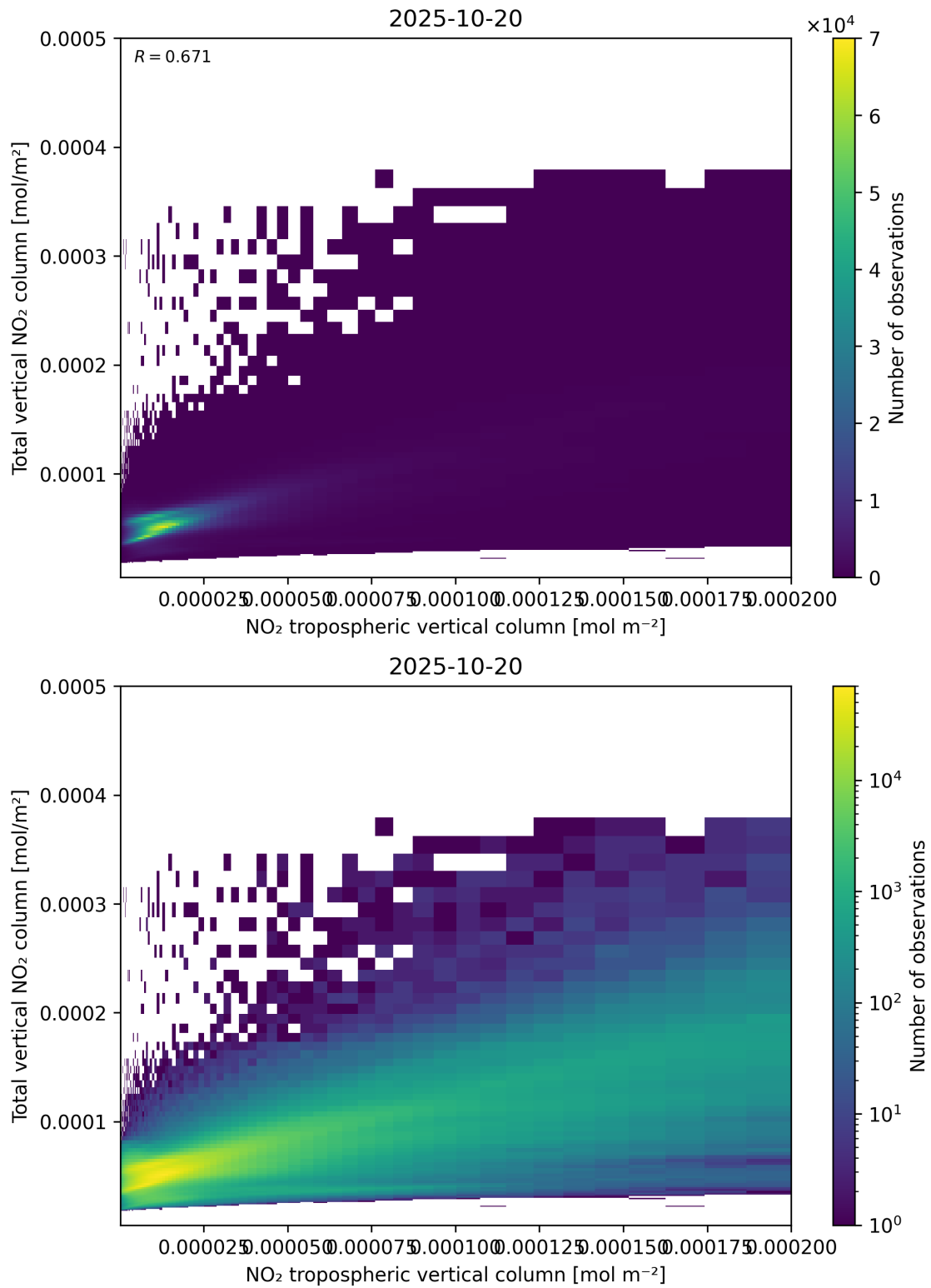
Figure 128: Scatter density plot of “NO 2 tropospheric vertical column” against “Total vertical NO 2 column” for 2025-10-19 to 2025-10-21.
