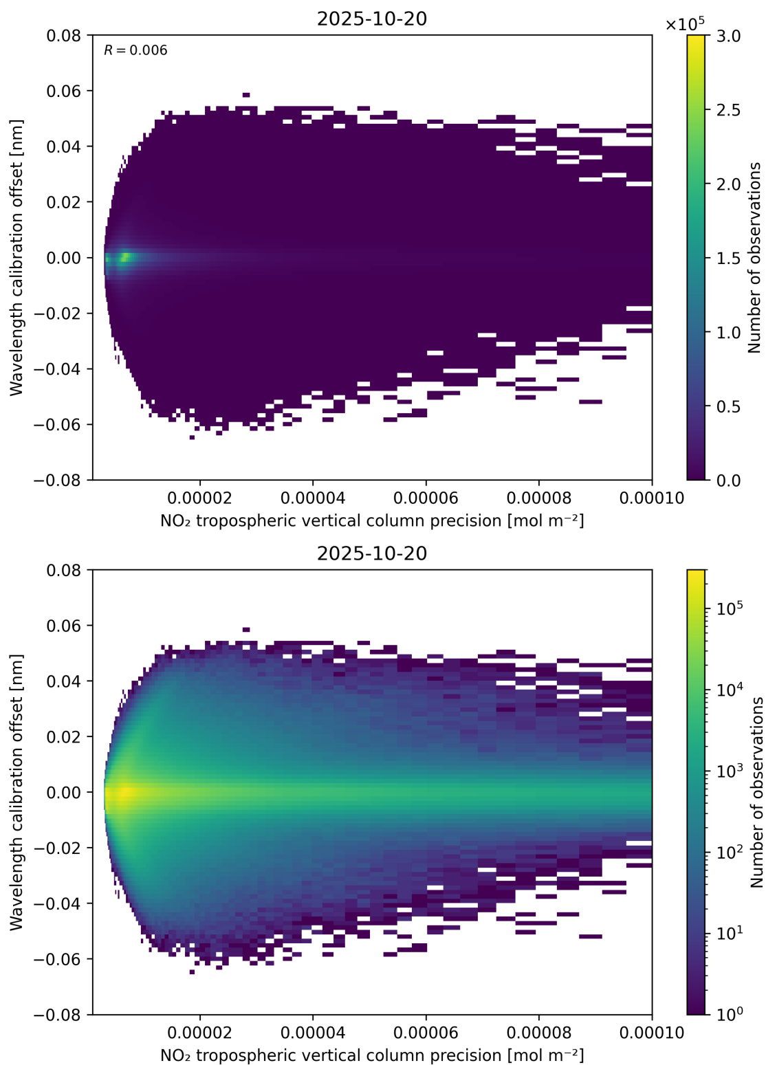
Figure 141: Scatter density plot of “NO 2 tropospheric vertical column precision” against “Wavelength calibration offset” for 2025-10-19 to 2025-10-21.
