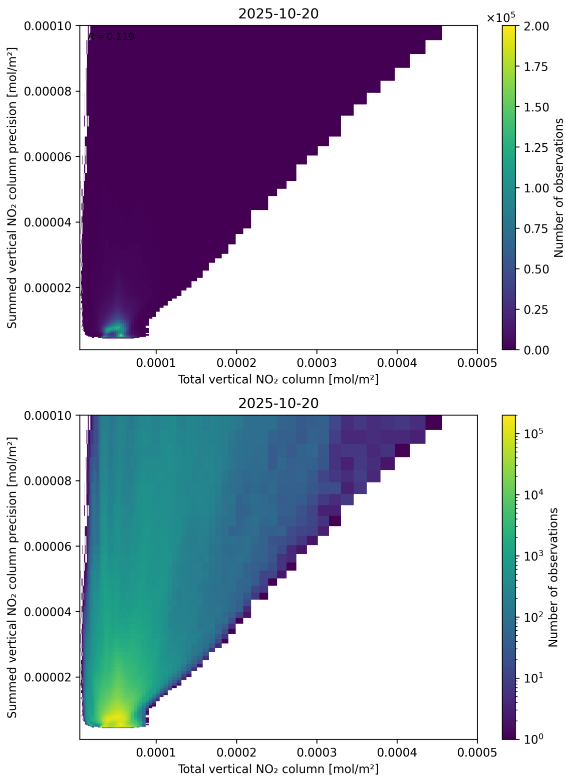
Figure 113: Scatter density plot of “Total vertical NO 2 column” against “Summed vertical NO 2 column precision” for 2025-10-19 to 2025-10-21.
