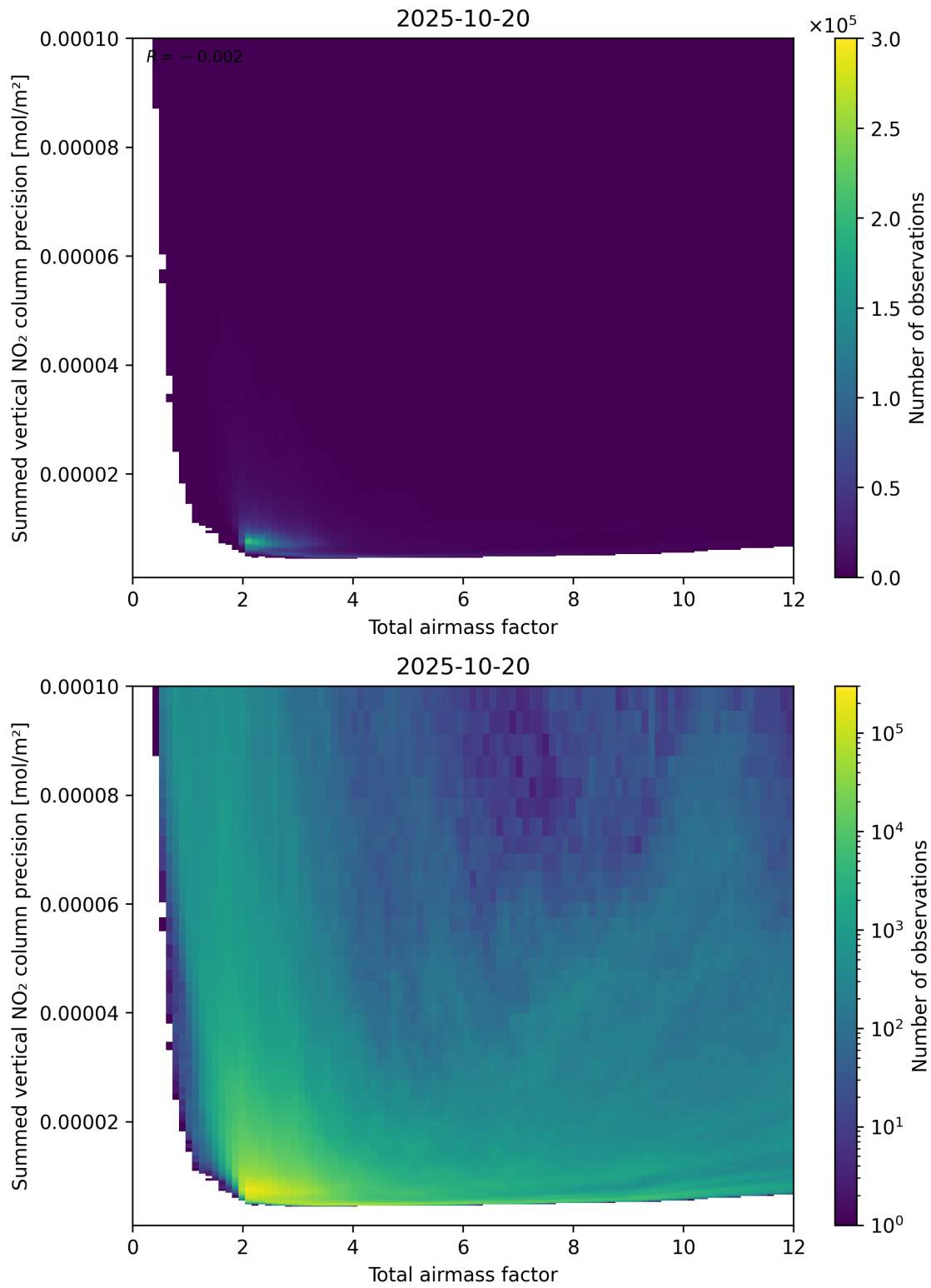
Figure 66: Scatter density plot of “Total airmass factor” against “Summed vertical NO 2 column precision” for 2025-10-19 to 2025-10-21.
