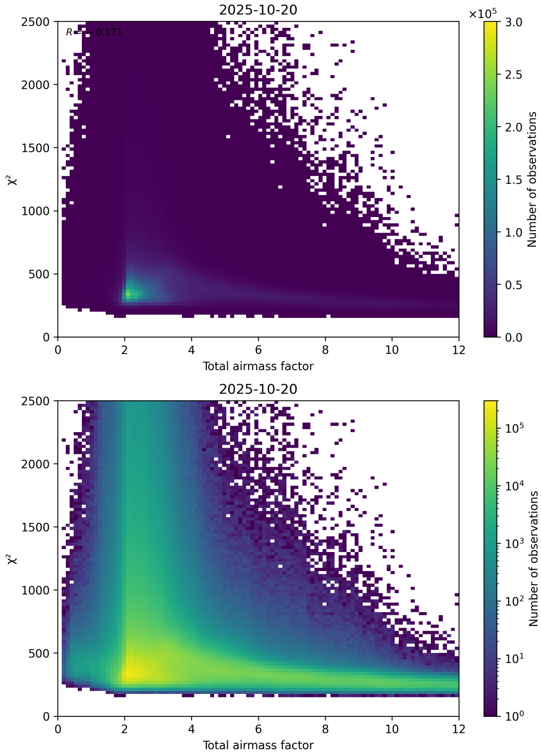
Figure 63: Scatter density plot of “Total airmass factor” against “ \chi^2 ” for 2025-10-19 to 2025-10-21.
