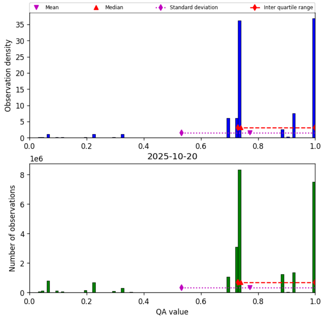
Figure 28: Histogram of “QA value” for 2025-10-19 to 2025-10-21
