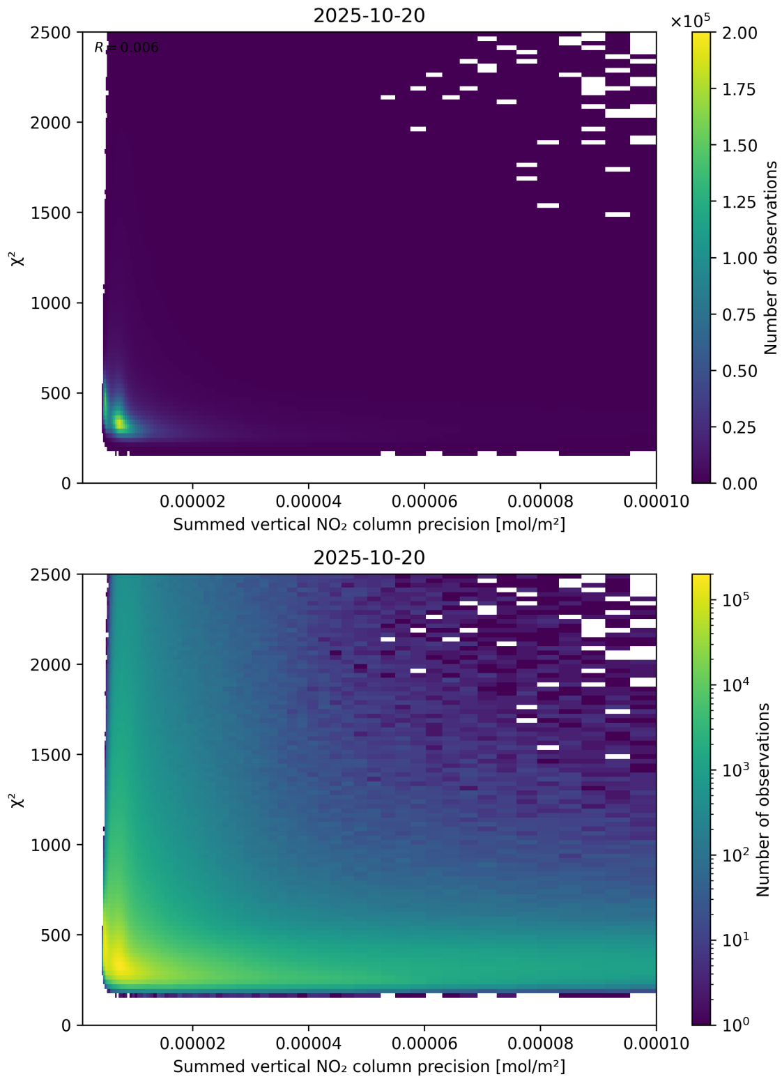
Figure 107: Scatter density plot of “Summed vertical NO 2 column precision” against “ \chi^2 ” for 2025-10-19 to 2025-10-21.
