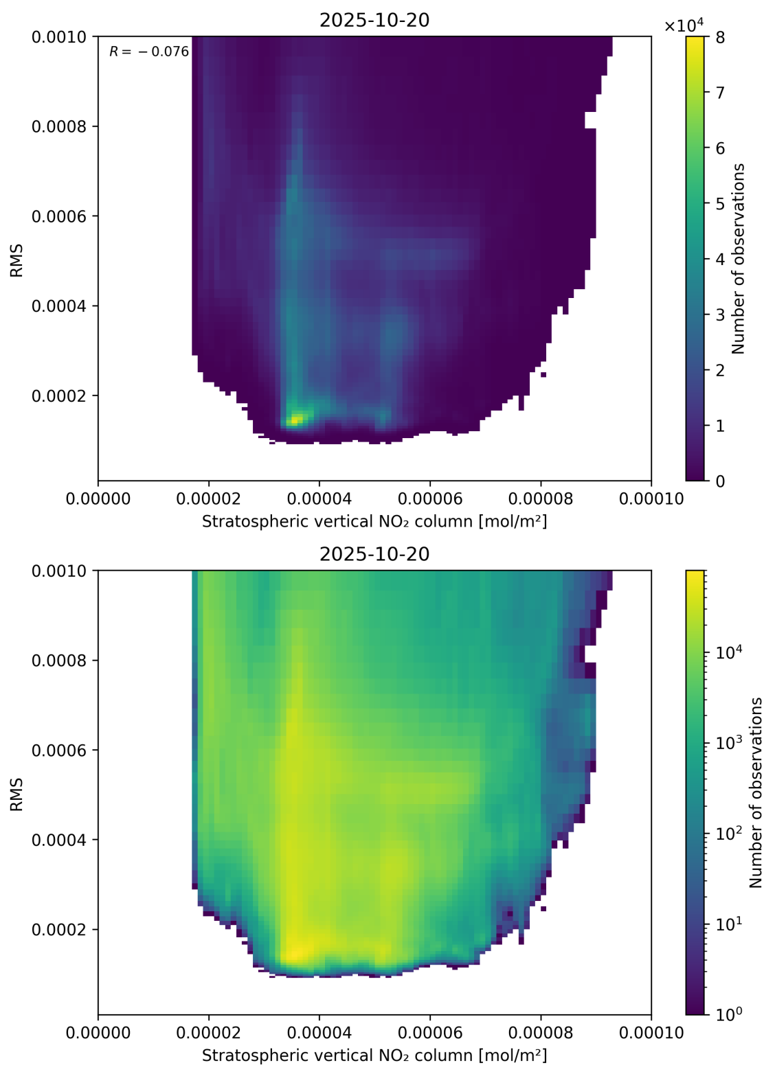
Figure 102: Scatter density plot of “Stratospheric vertical NO 2 column” against “RMS” for 2025-10-19 to 2025-10-21.
