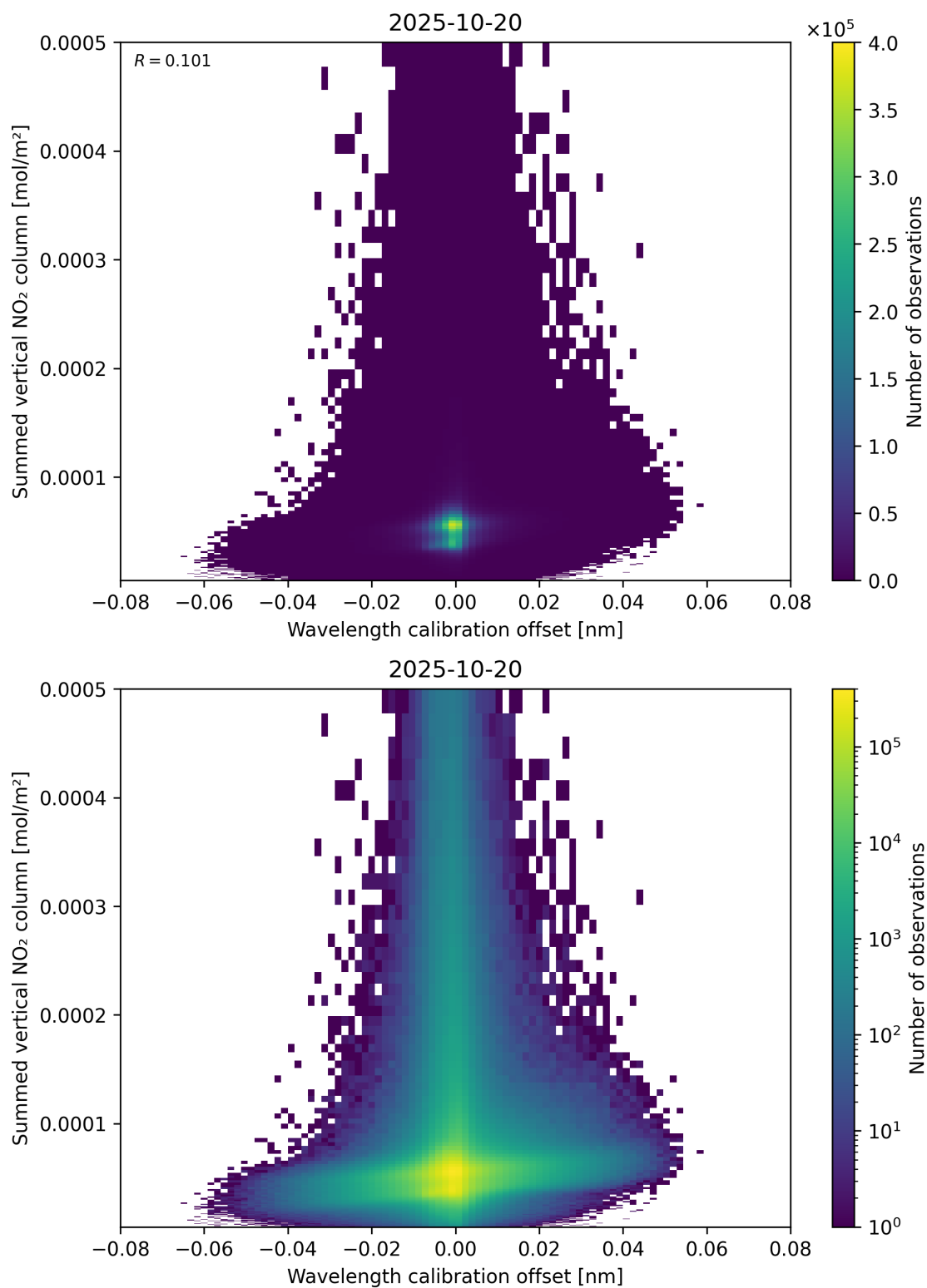
Figure 177: Scatter density plot of “Wavelength calibration offset” against “Summed vertical NO 2 column” for 2025-10-19 to 2025-10-21.
