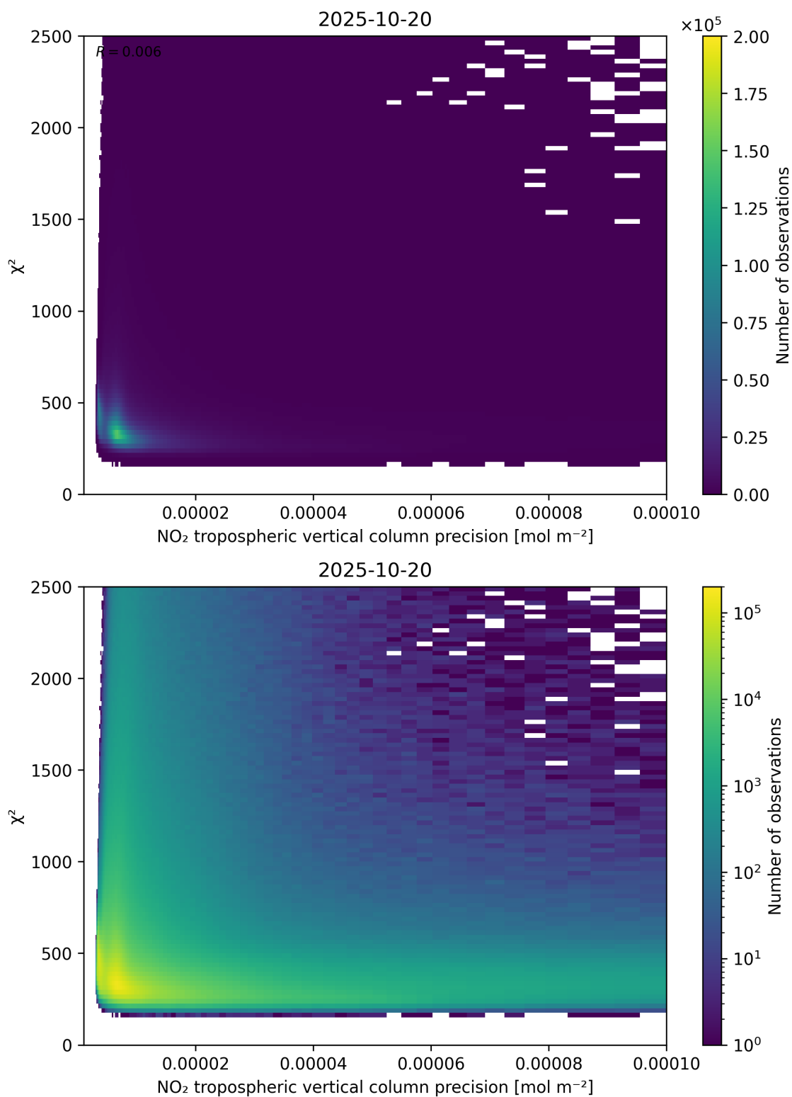
Figure 134: Scatter density plot of “NO 2 tropospheric vertical column precision” against “ \chi^2 ” for 2025-10-19 to 2025-10-21.
