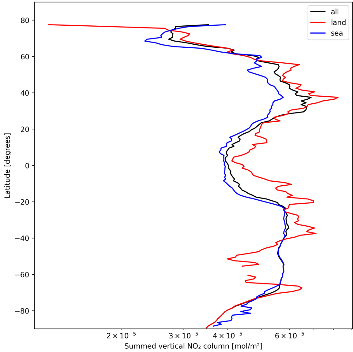
Figure 23: Zonal average of “Summed vertical NO 2 column” for 2025-10-19 to 2025-10-21.
