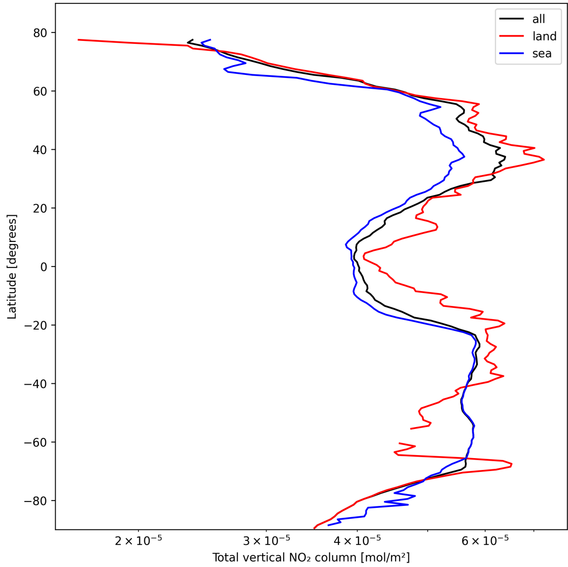
Figure 21: Zonal average of “Total vertical NO 2 column” for 2025-10-19 to 2025-10-21.
