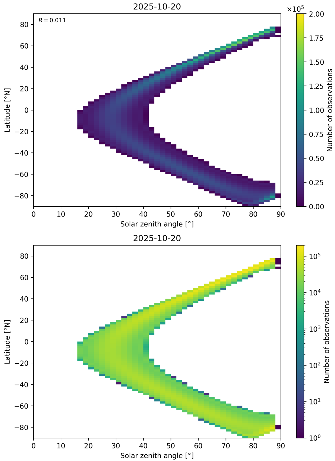
Figure 149: Scatter density plot of “Solar zenith angle” against “Latitude” for 2025-10-19 to 2025-10-21.
