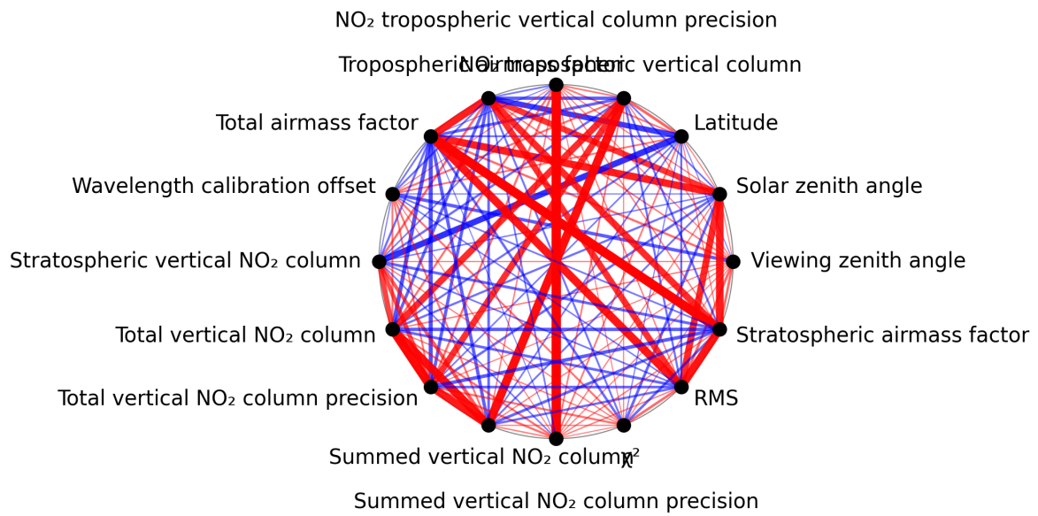
Figure 1: Map of correlation graph for 2025-10-19 to 2025-10-21.
