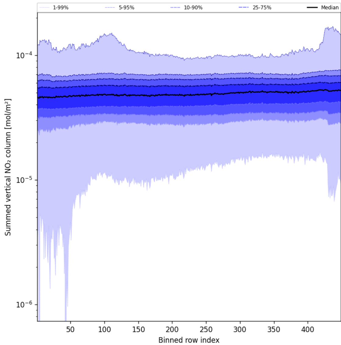
Figure 57: Along track statistics of “Summed vertical NO 2 column” for 2025-10-19 to 2025-10-21
