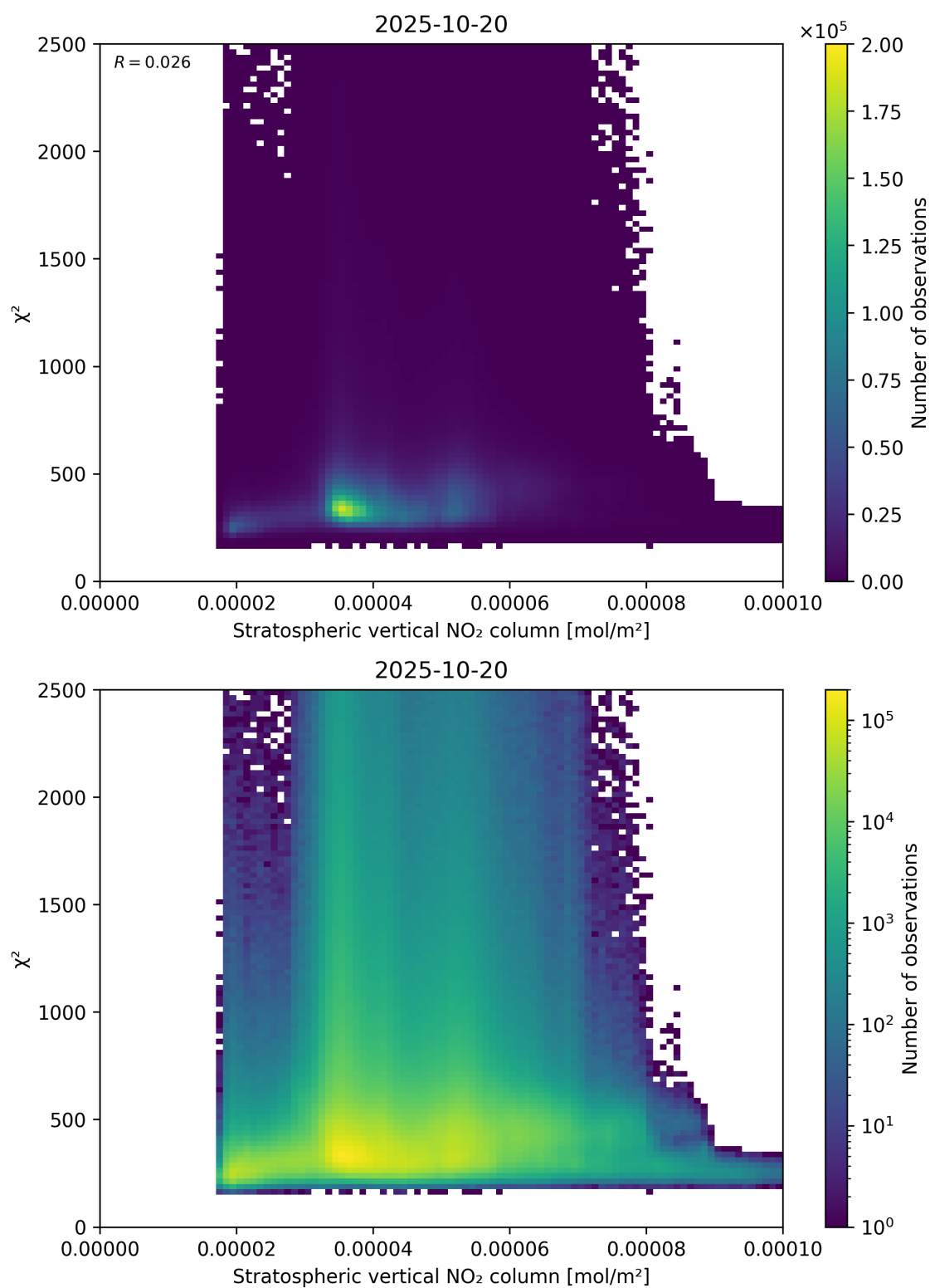
Figure 97: Scatter density plot of “Stratospheric vertical NO 2 column” against “ \chi^2 ” for 2025-10-19 to 2025-10-21.
