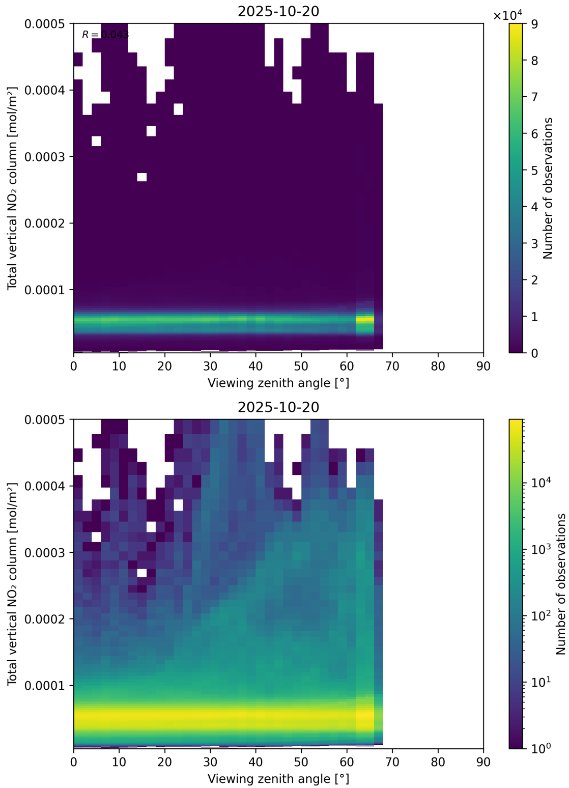
Figure 167: Scatter density plot of “Viewing zenith angle” against “Total vertical NO 2 column” for 2025-10-19 to 2025-10-21.
