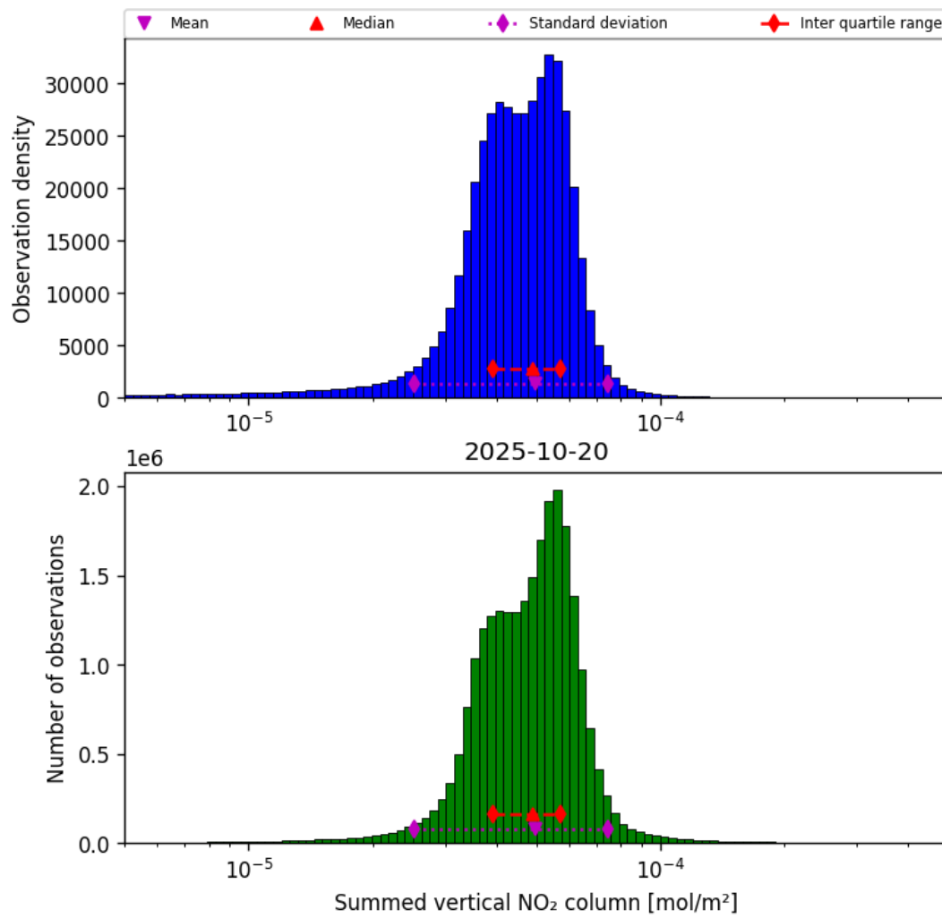
Figure 40: Histogram of “Summed vertical NO 2 column” for 2025-10-19 to 2025-10-21
