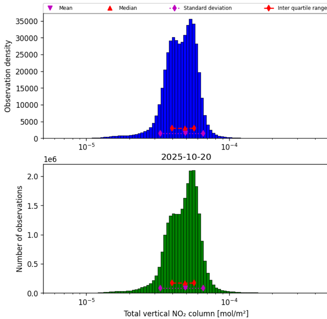
Figure 38: Histogram of “Total vertical NO 2 column” for 2025-10-19 to 2025-10-21
