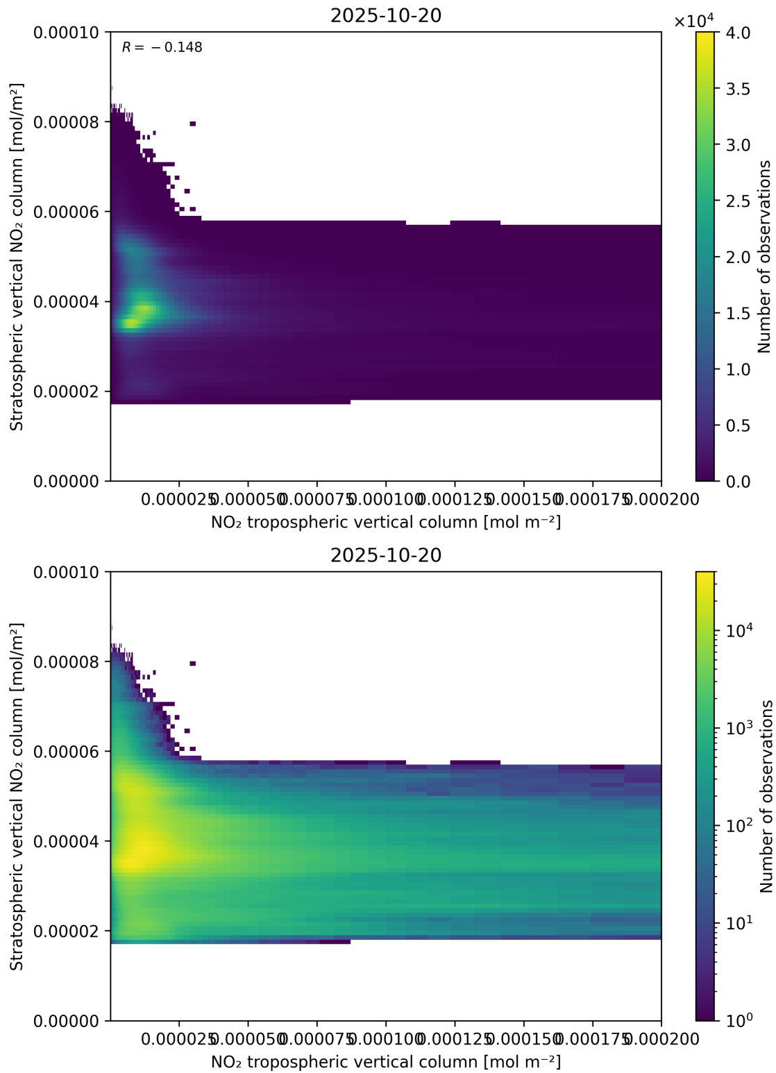
Figure 125: Scatter density plot of “NO 2 tropospheric vertical column” against “Stratospheric vertical NO 2 column” for 2025-10-19 to 2025-10-21.
