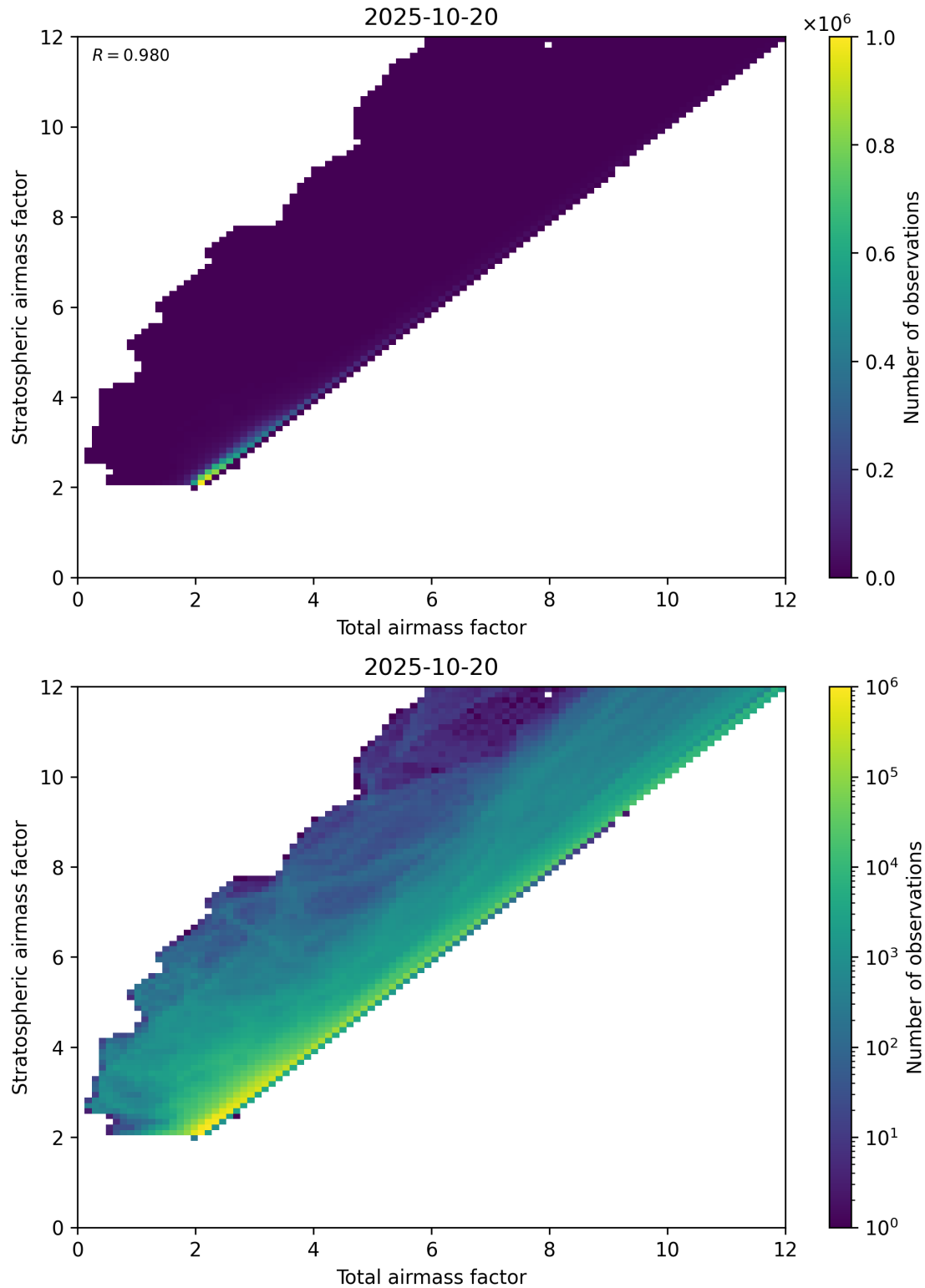
Figure 62: Scatter density plot of “Total airmass factor” against “Stratospheric airmass factor” for 2025-10-19 to 2025-10-21.
