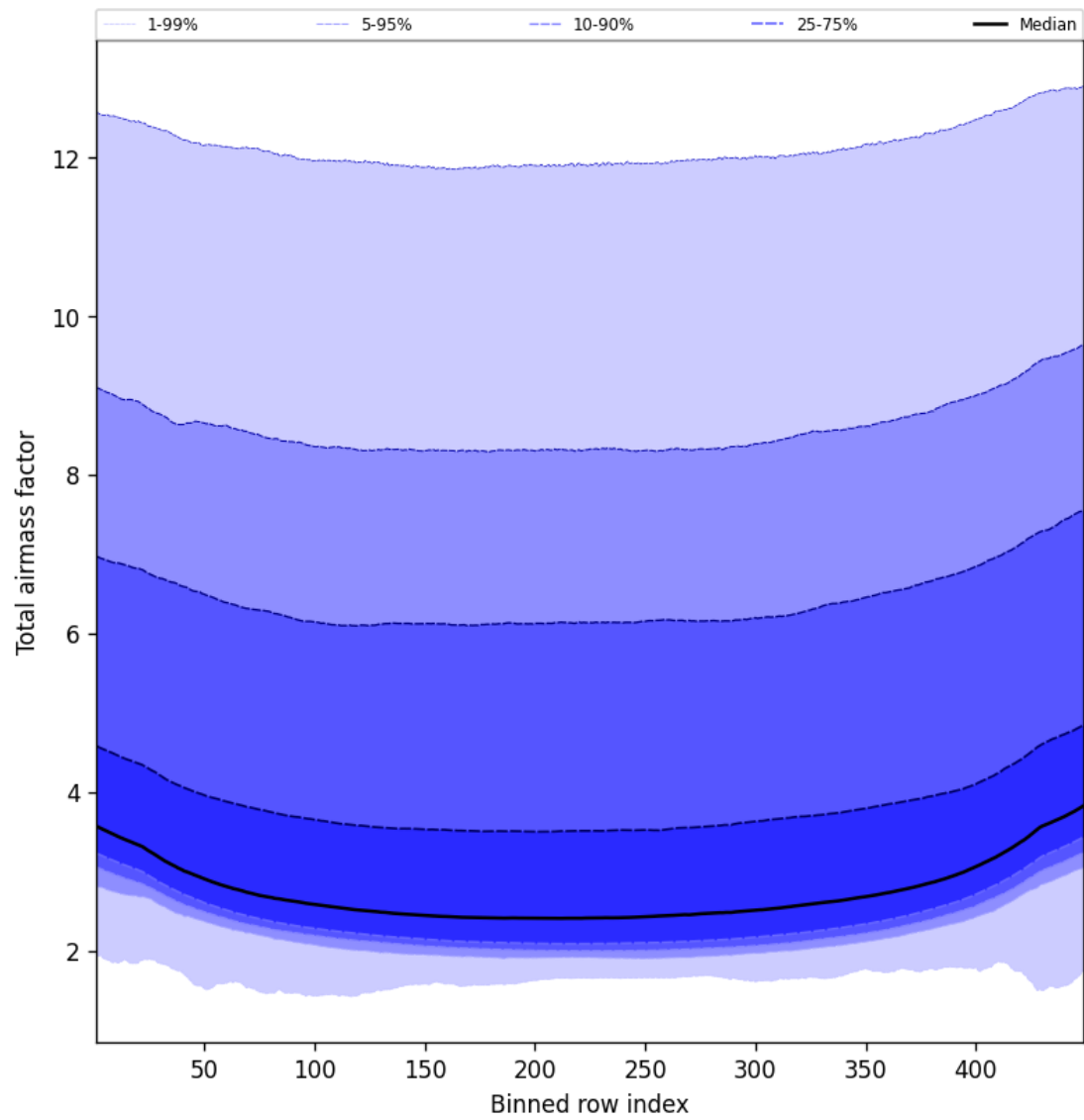
Figure 49: Along track statistics of “Total airmass factor” for 2025-10-19 to 2025-10-21
