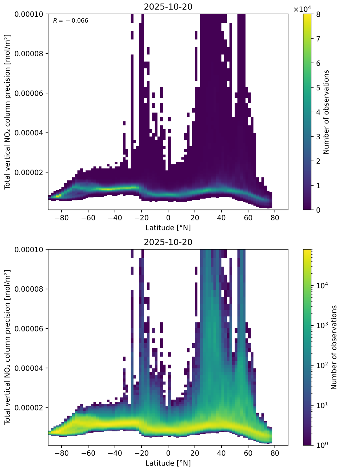
Figure 91: Scatter density plot of “Latitude” against “Total vertical NO 2 column precision” for 2025-10-19 to 2025-10-21.
