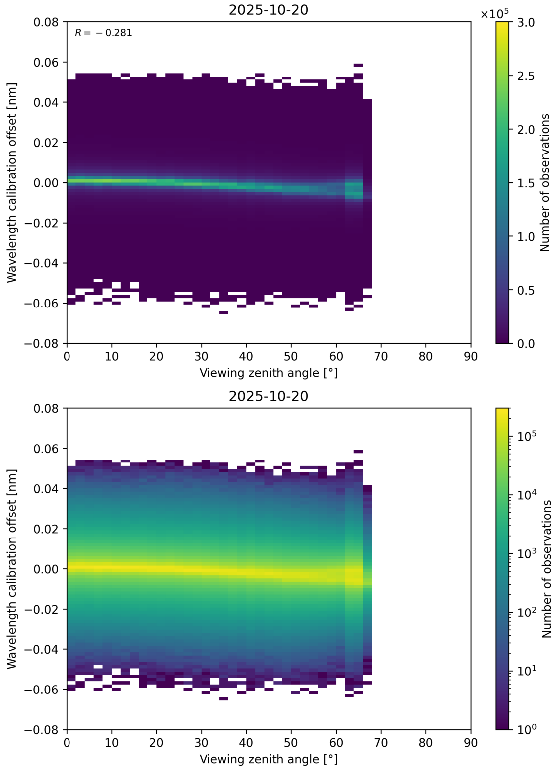
Figure 173: Scatter density plot of “Viewing zenith angle” against “Wavelength calibration offset” for 2025-10-19 to 2025-10-21.
