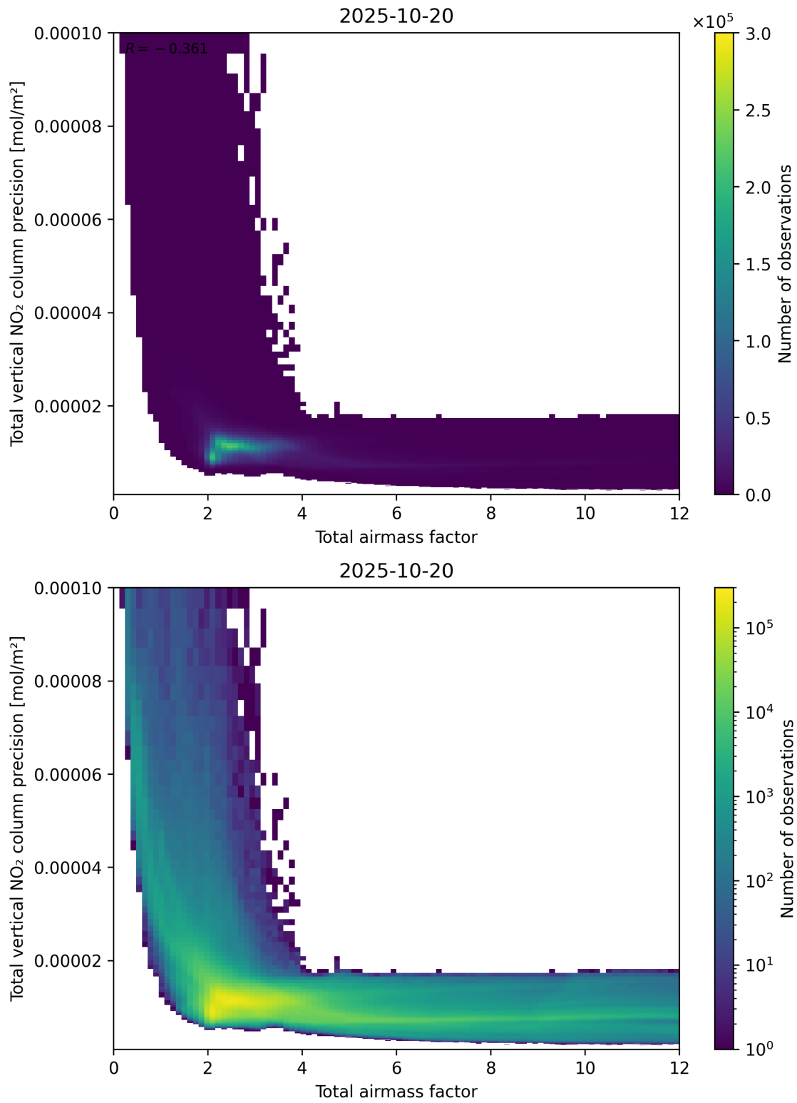
Figure 68: Scatter density plot of “Total airmass factor” against “Total vertical NO 2 column precision” for 2025-10-19 to 2025-10-21.
