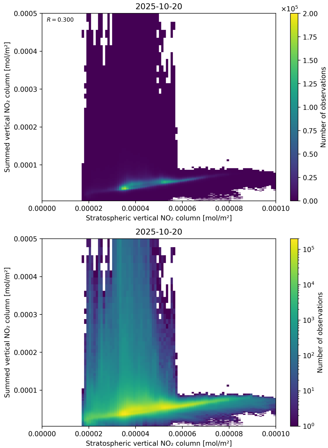
Figure 98: Scatter density plot of “Stratospheric vertical NO 2 column” against “Summed vertical NO 2 column” for 2025-10-19 to 2025-10-21.
