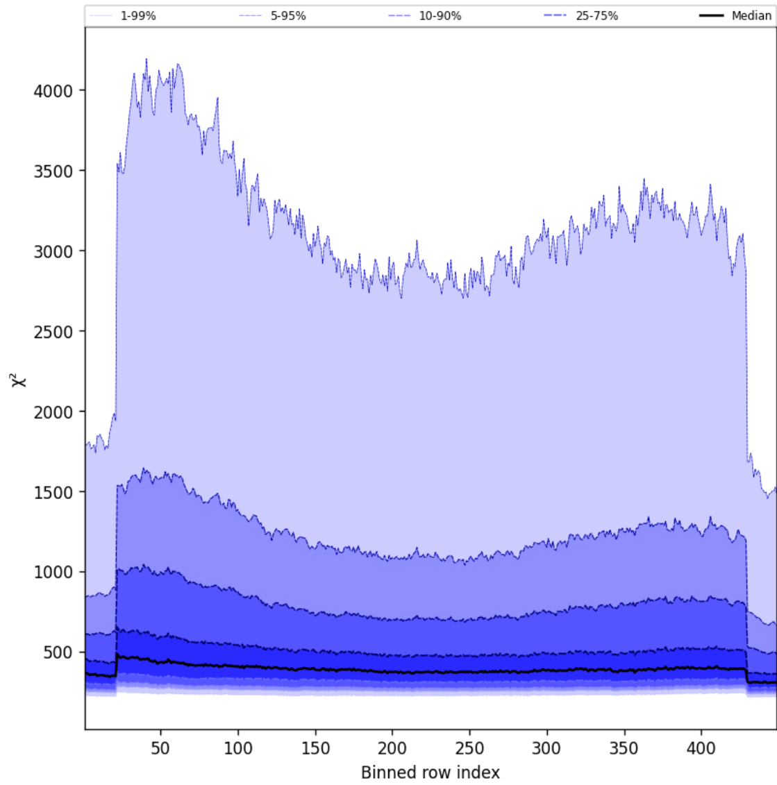
Figure 59: Along track statistics of “ \chi^2 ” for 2025-10-19 to 2025-10-21
