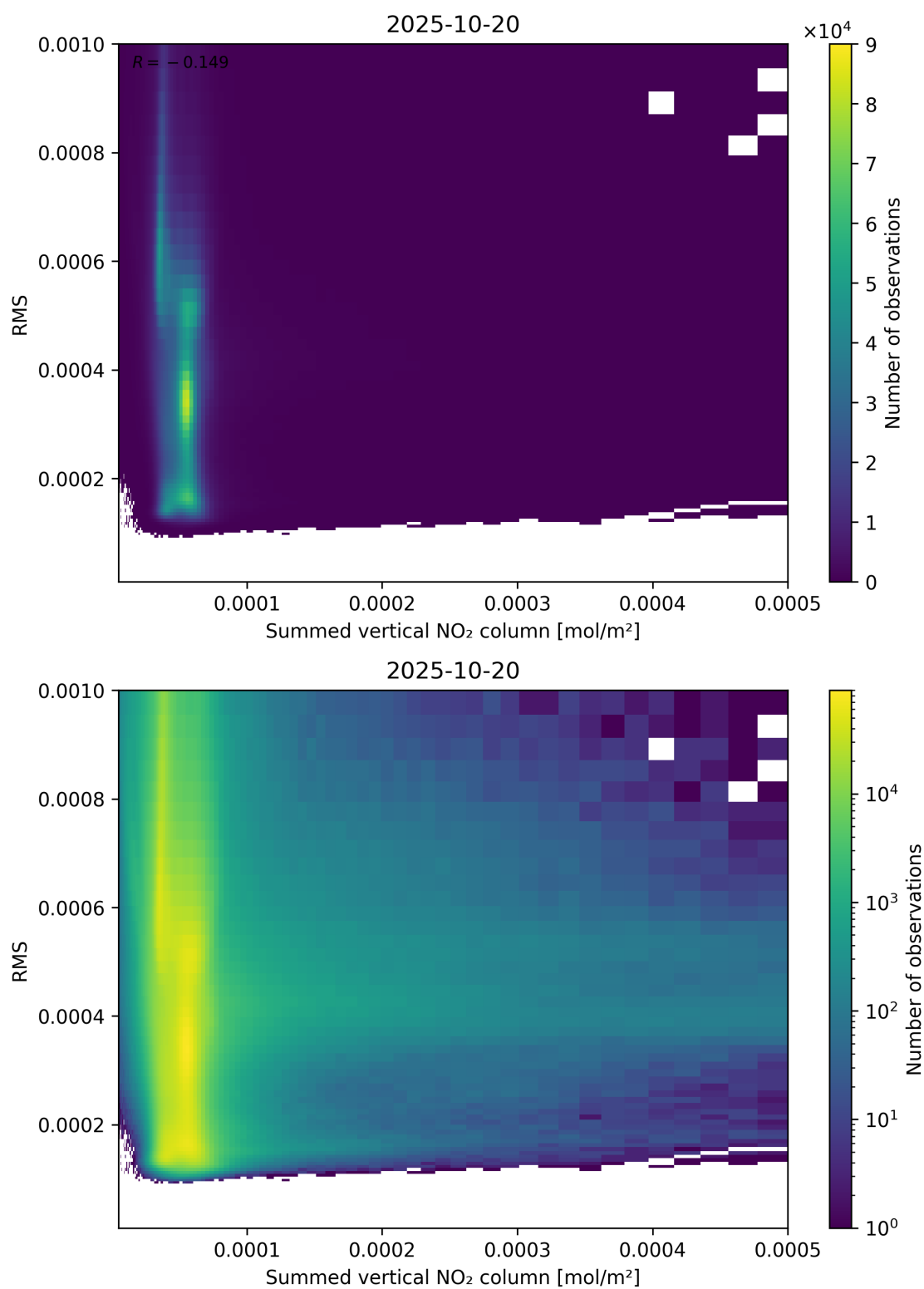
Figure 109: Scatter density plot of “Summed vertical NO 2 column” against “RMS” for 2025-10-19 to 2025-10-21.
