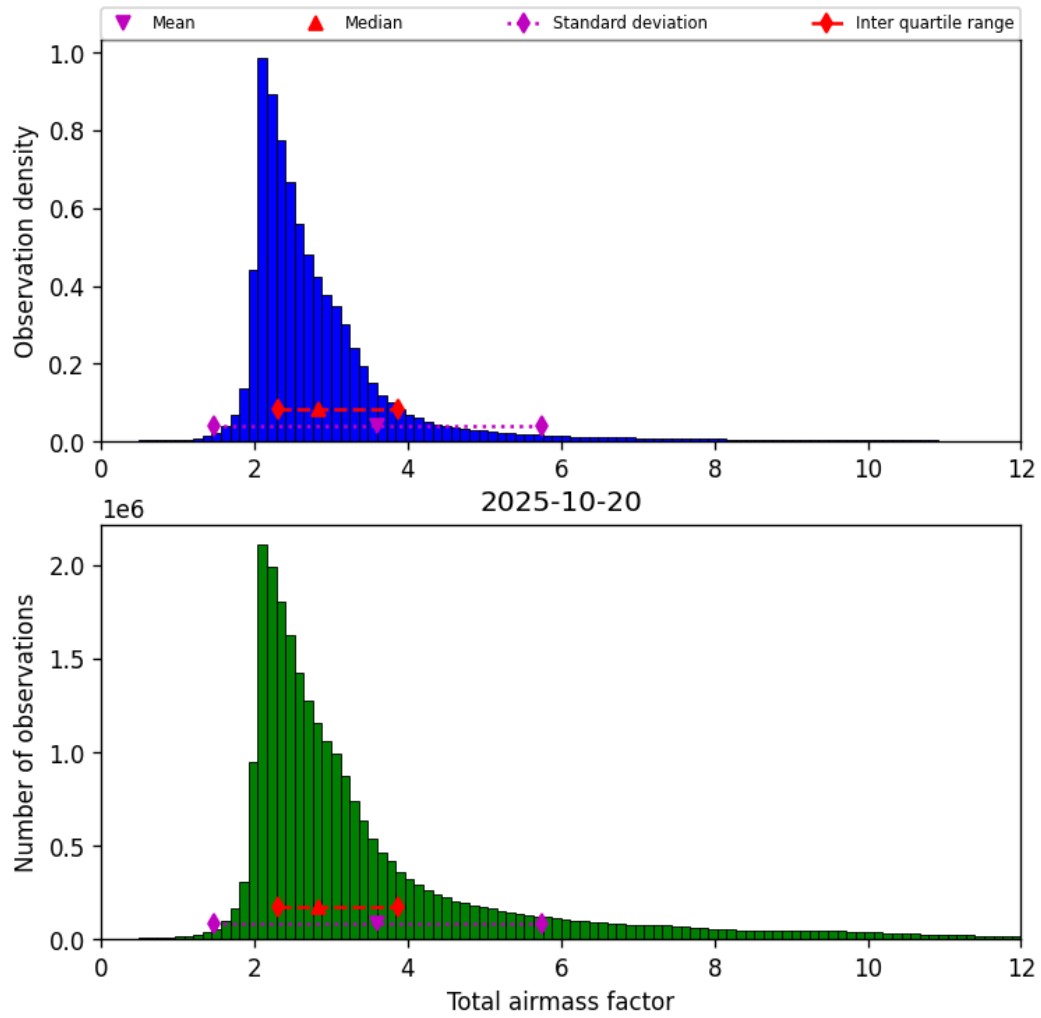
Figure 32: Histogram of “Total airmass factor” for 2025-10-19 to 2025-10-21
