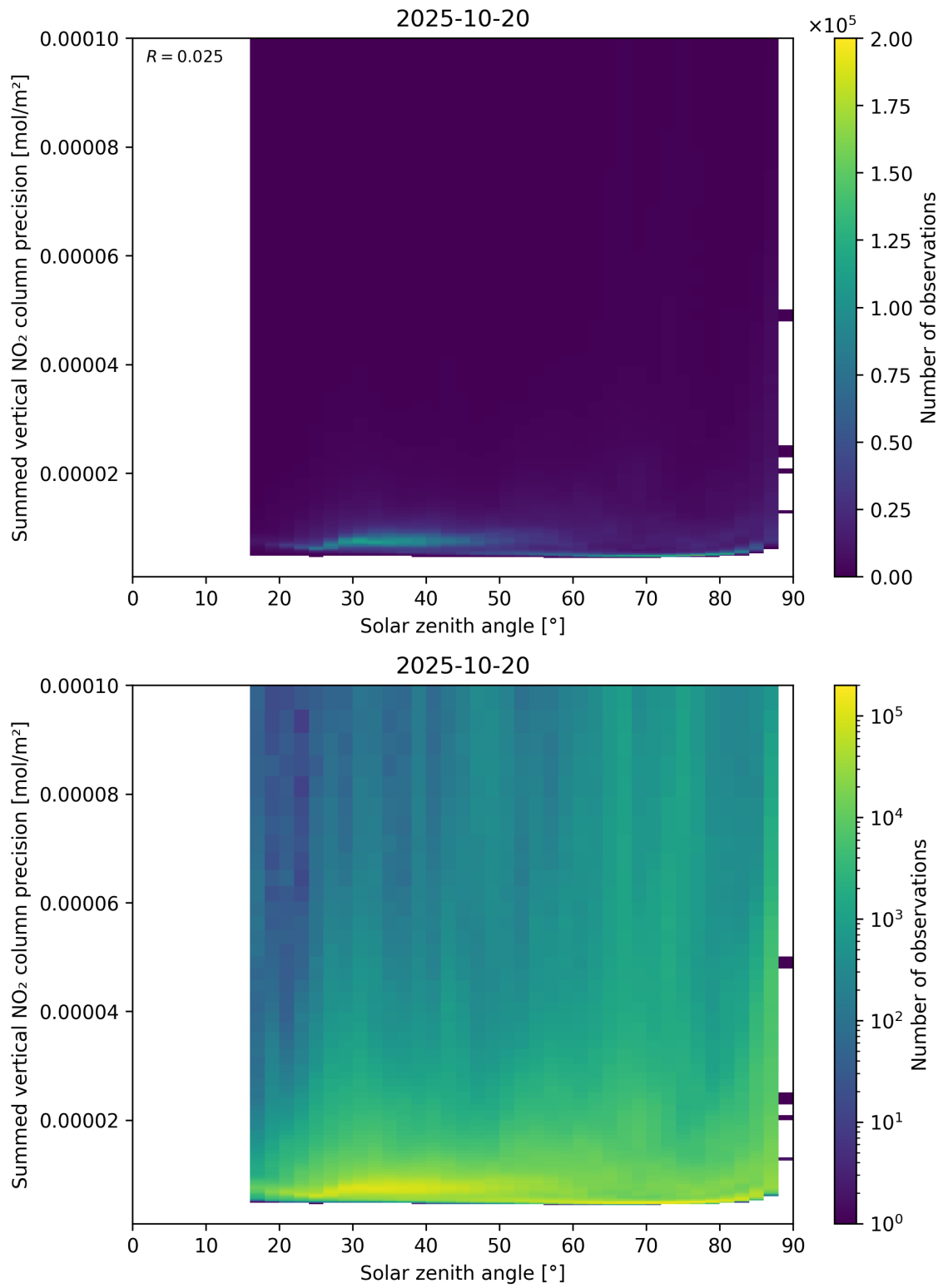
Figure 152: Scatter density plot of “Solar zenith angle” against “Summed vertical NO 2 column precision” for 2025-10-19 to 2025-10-21.
