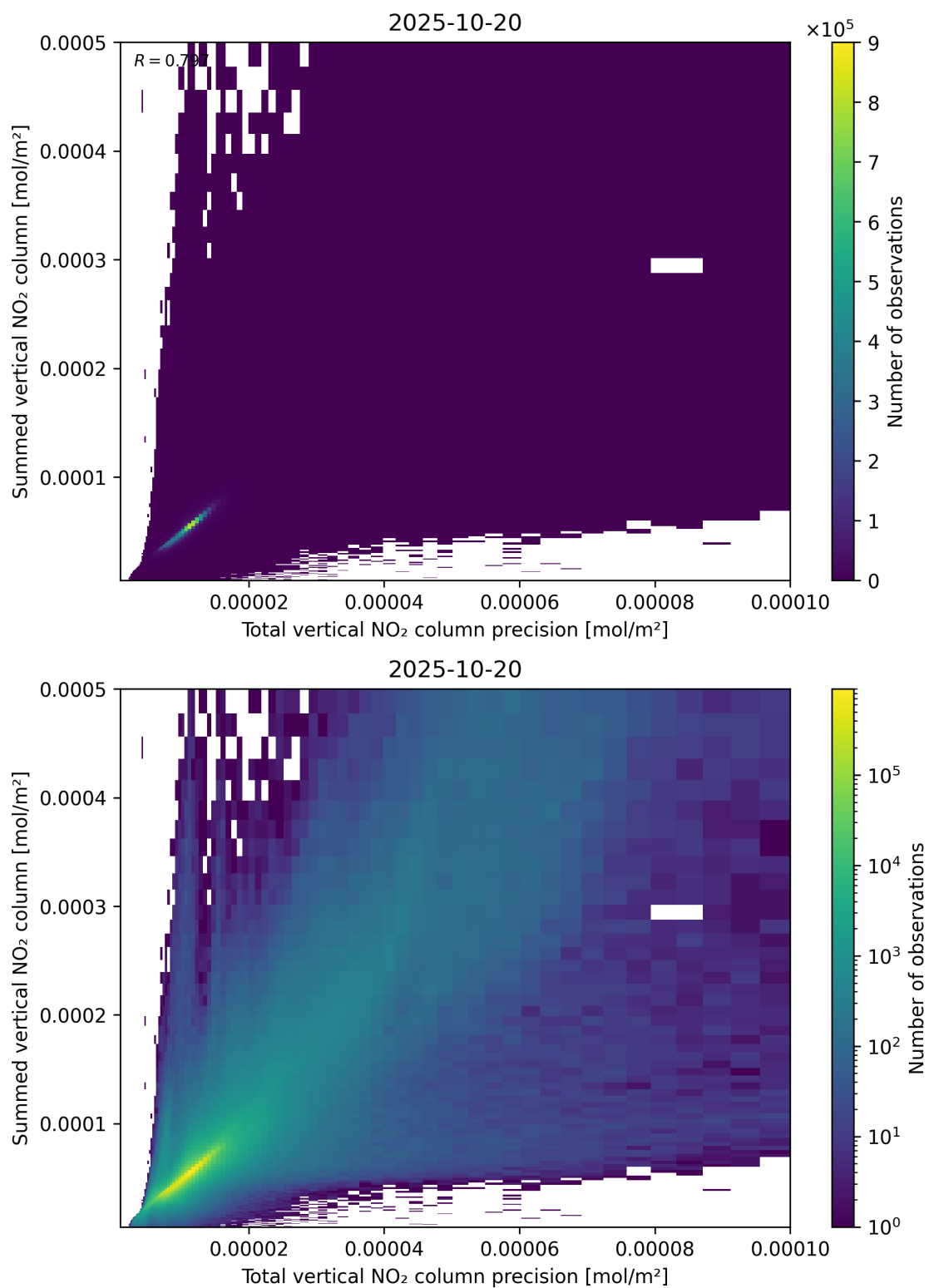
Figure 117: Scatter density plot of “Total vertical NO 2 column precision” against “Summed vertical NO 2 column” for 2025-10-19 to 2025-10-21.
