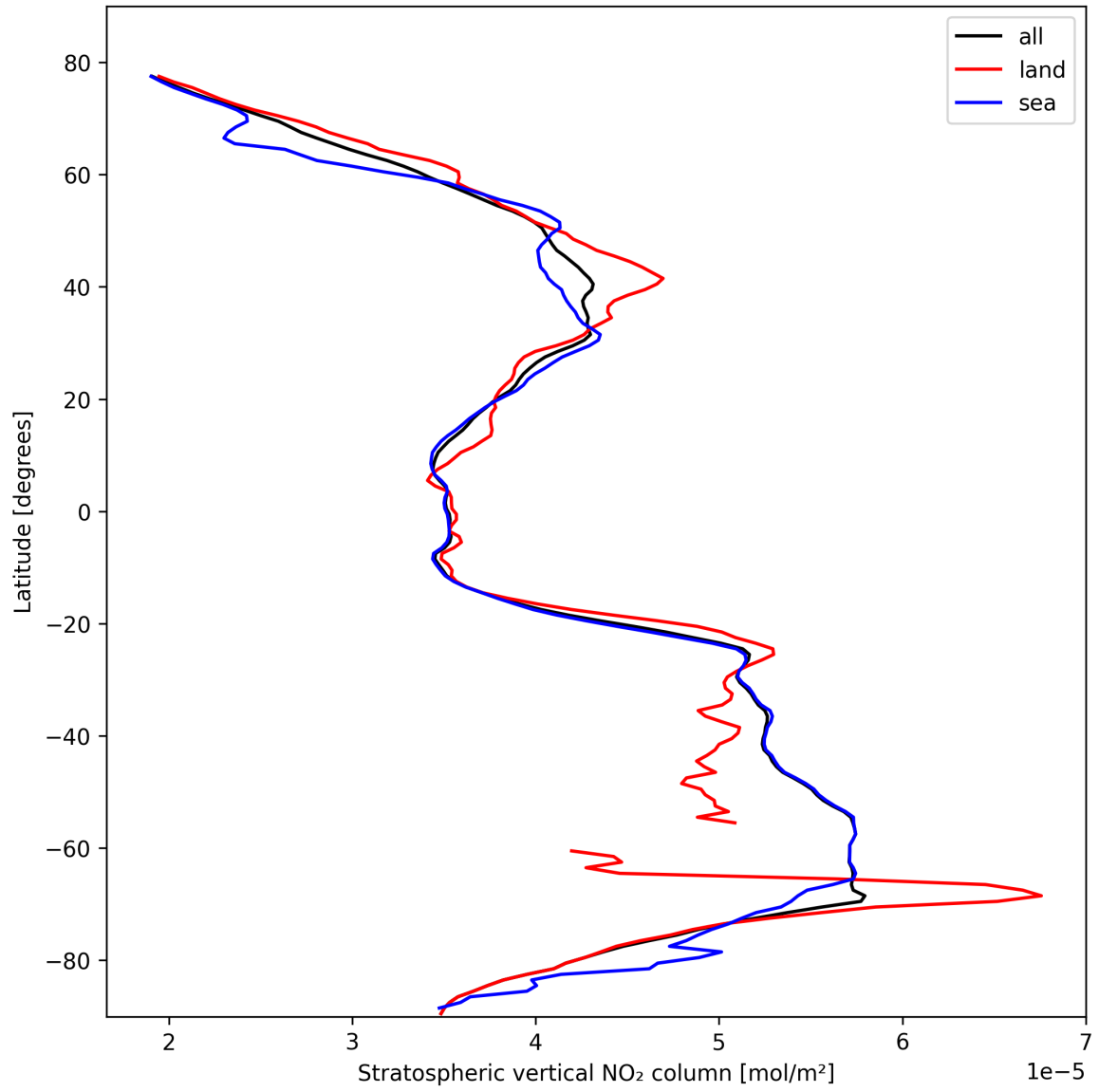
Figure 19: Zonal average of “Stratospheric vertical NO 2 column” for 2025-10-19 to 2025-10-21.
