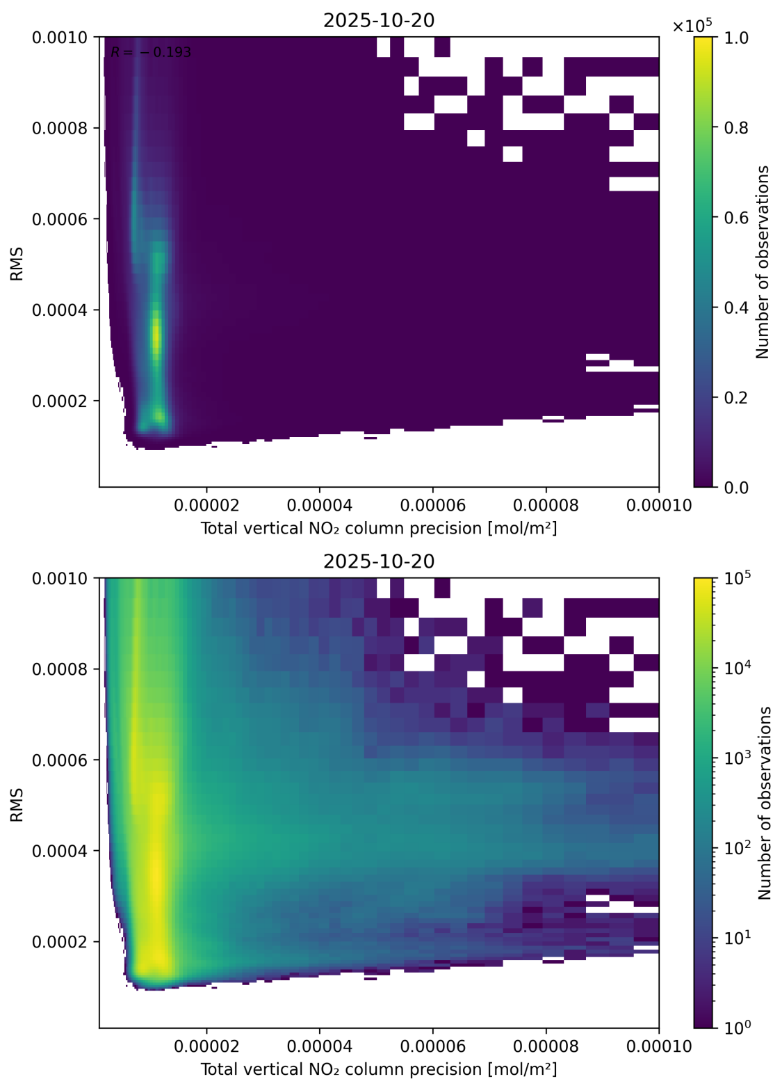
Figure 119: Scatter density plot of “Total vertical NO 2 column precision” against “RMS” for 2025-10-19 to 2025-10-21.
