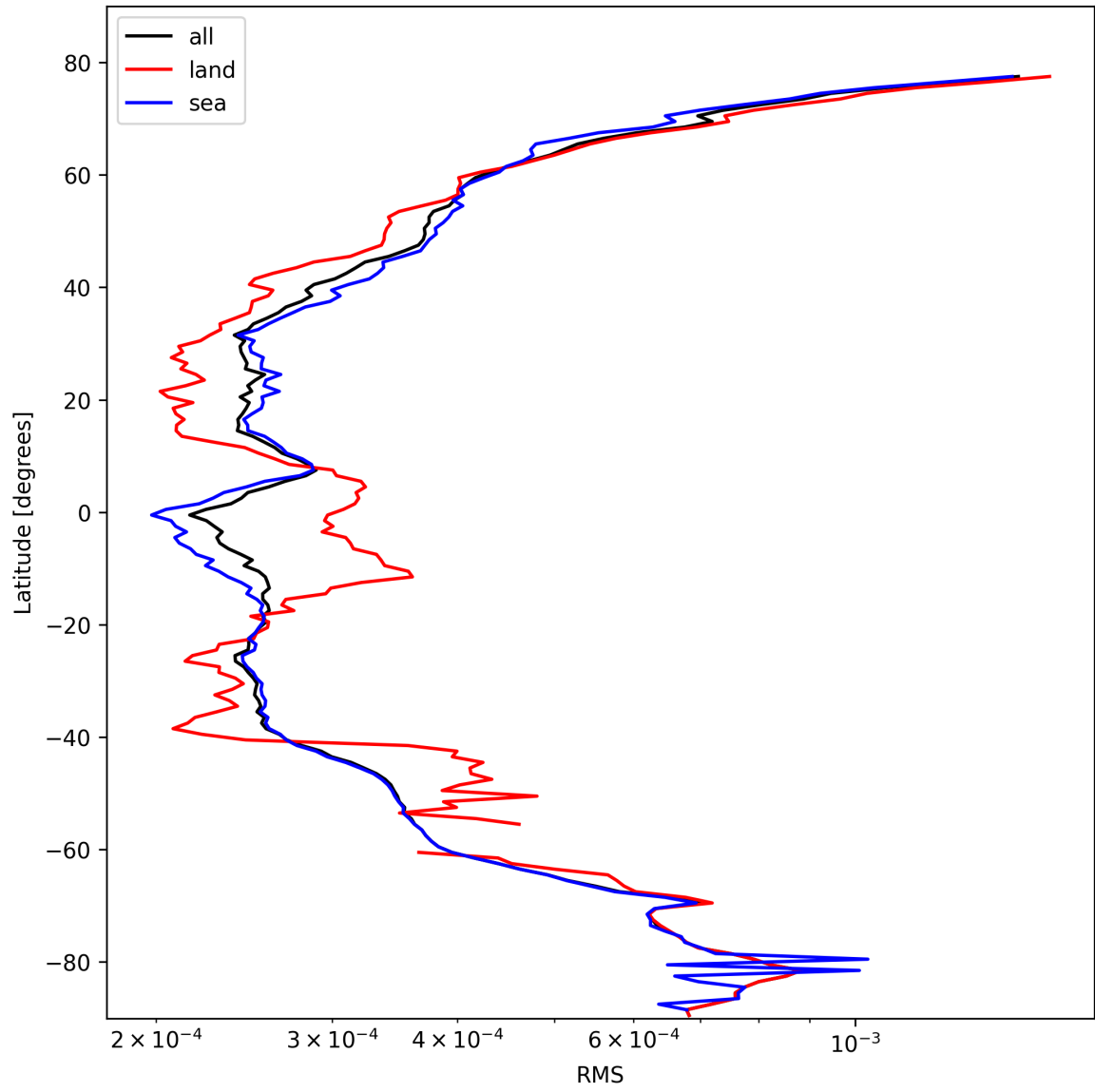
Figure 26: Zonal average of “RMS” for 2025-10-19 to 2025-10-21.
