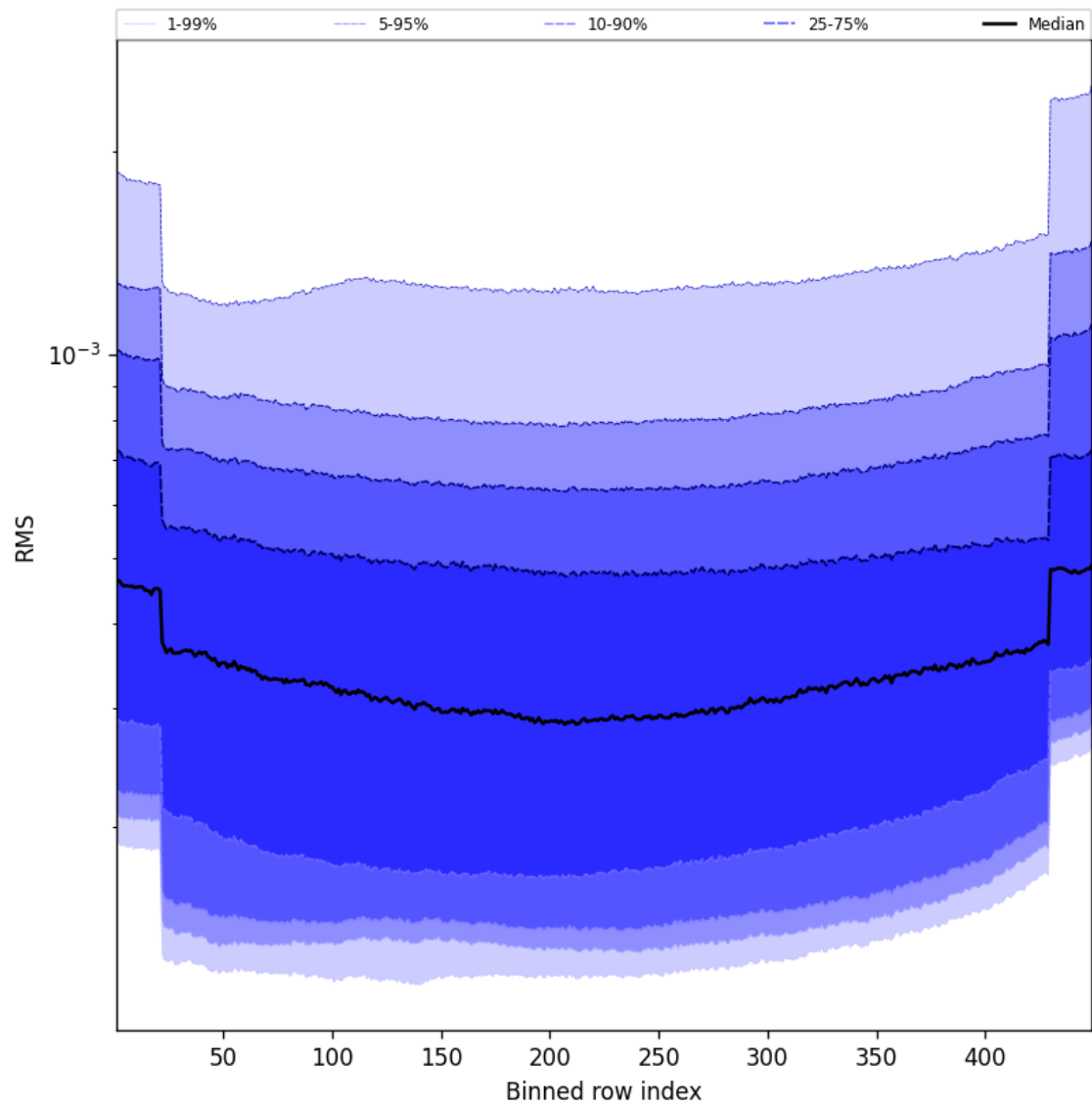
Figure 60: Along track statistics of “RMS” for 2025-10-19 to 2025-10-21
