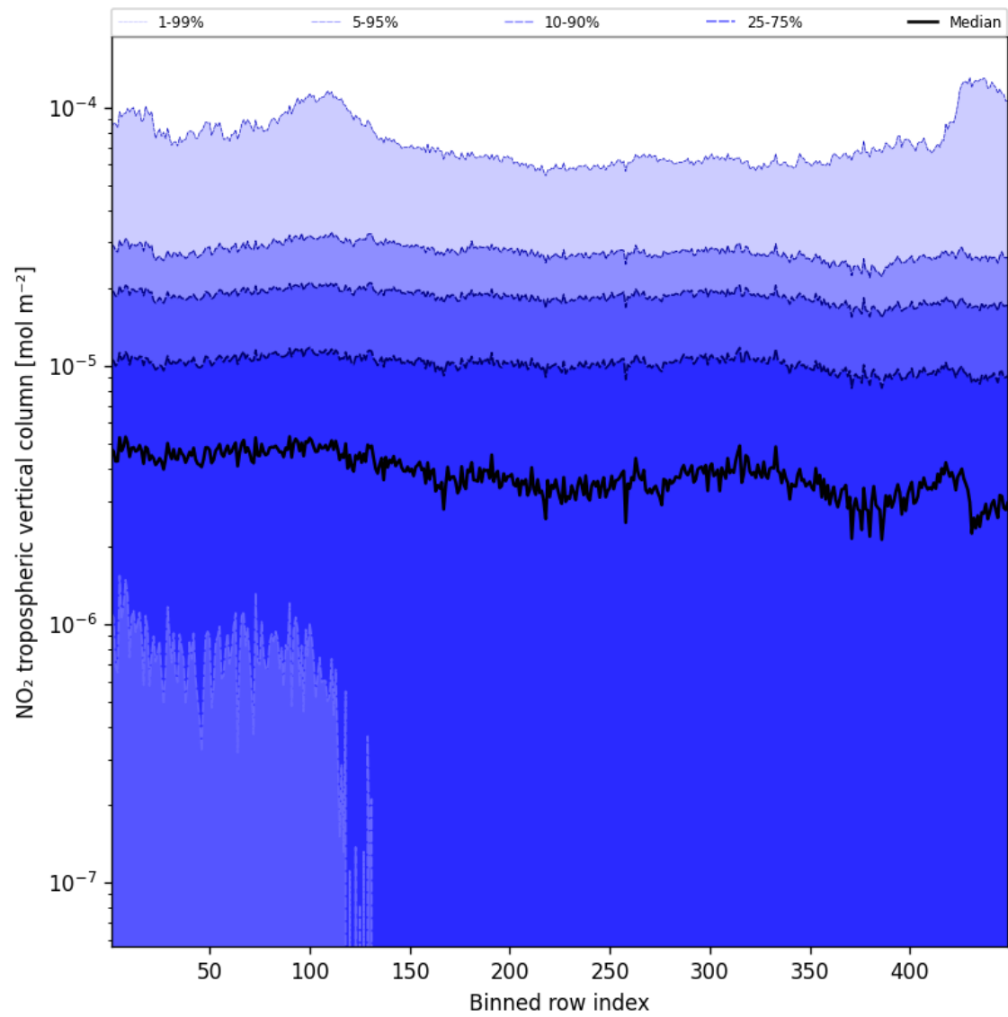
Figure 46: Along track statistics of “NO 2 tropospheric vertical column” for 2025-10-19 to 2025-10-21
