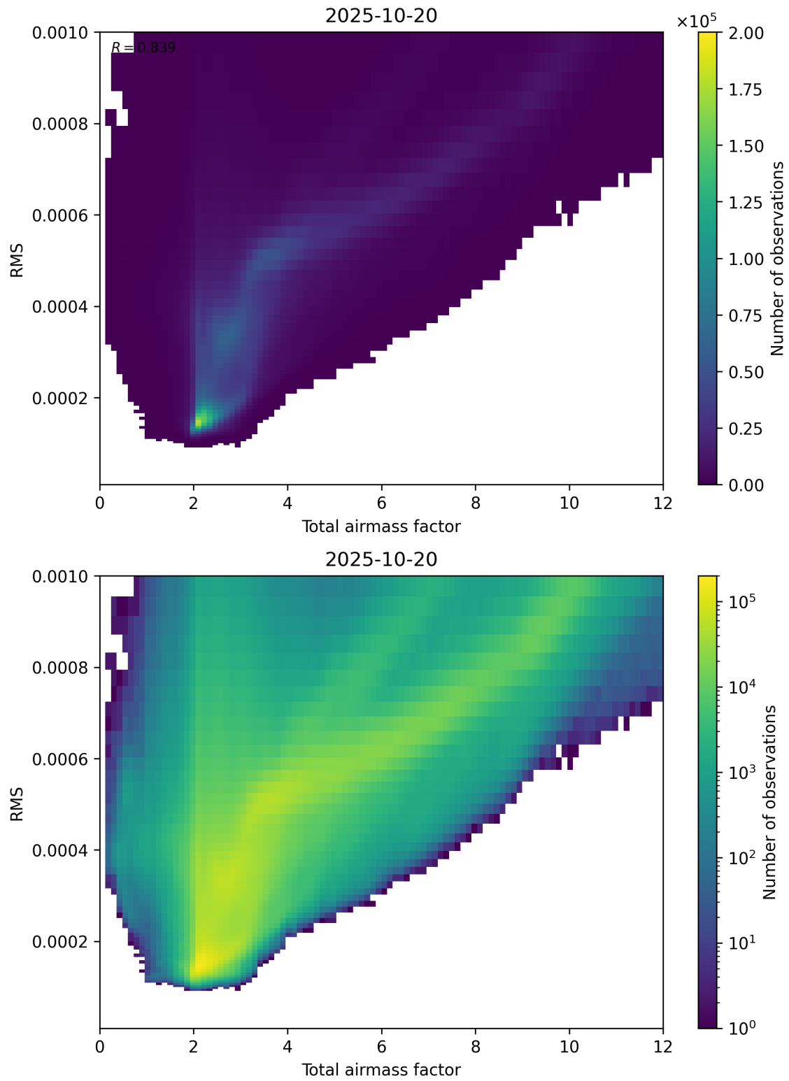
Figure 69: Scatter density plot of “Total airmass factor” against “RMS” for 2025-10-19 to 2025-10-21.
