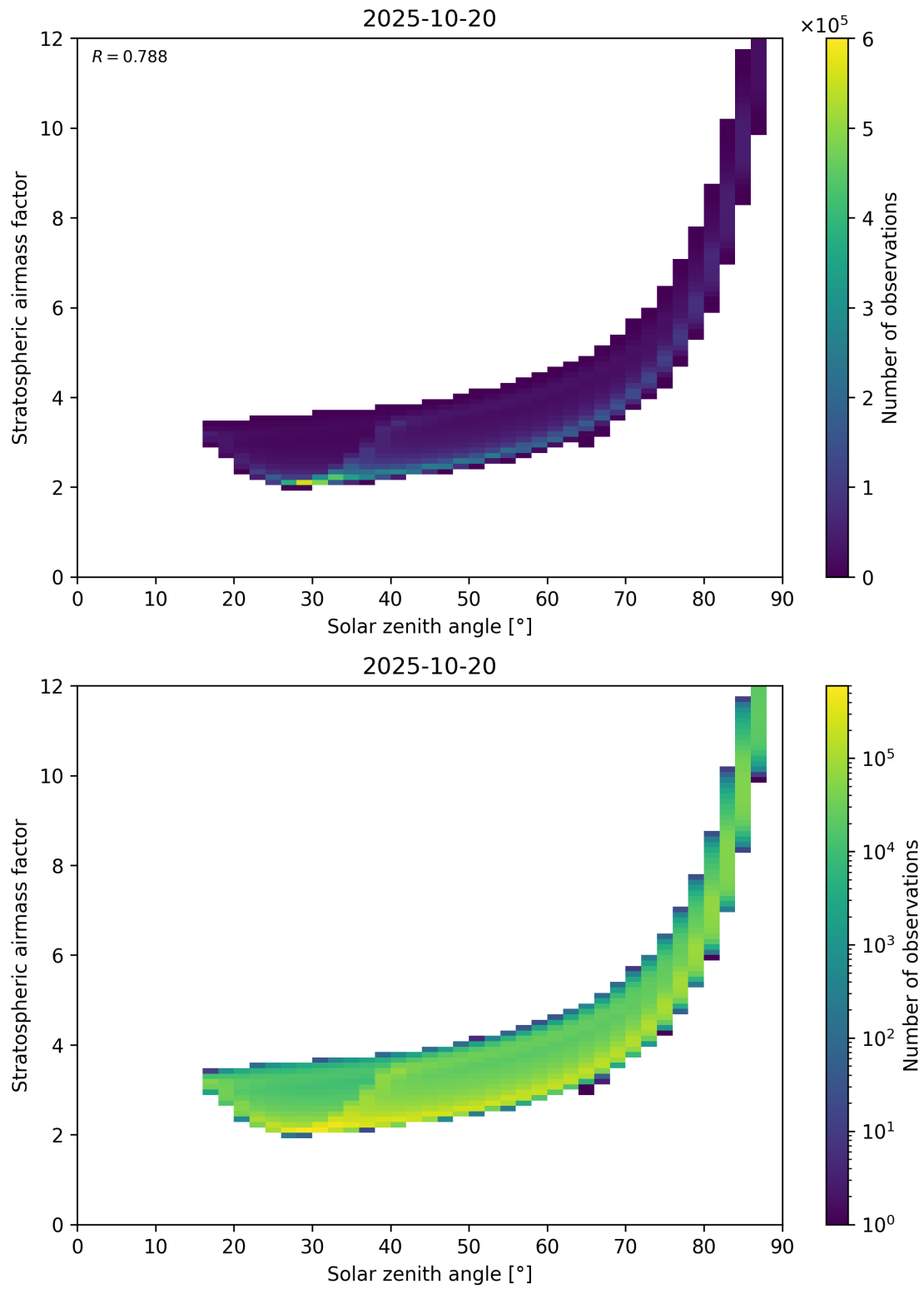
Figure 145: Scatter density plot of “Solar zenith angle” against “Stratospheric airmass factor” for 2025-10-19 to 2025-10-21.
