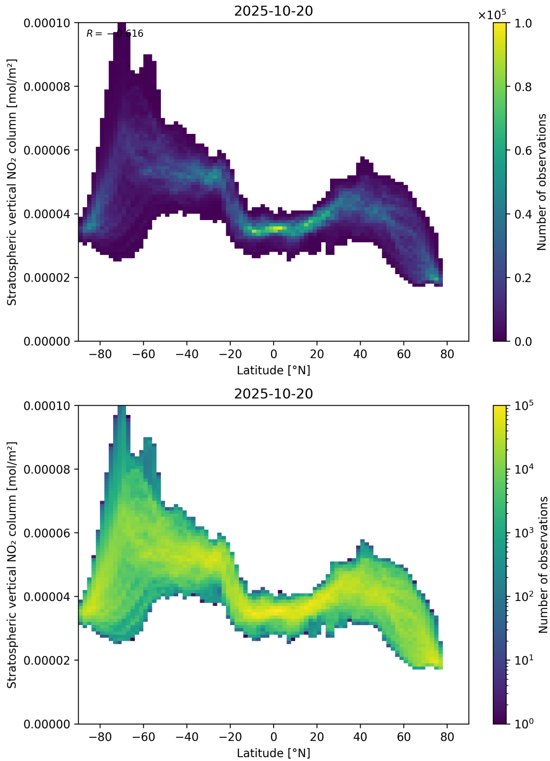
Figure 87: Scatter density plot of “Latitude” against “Stratospheric vertical NO 2 column” for 2025-10-19 to 2025-10-21.
