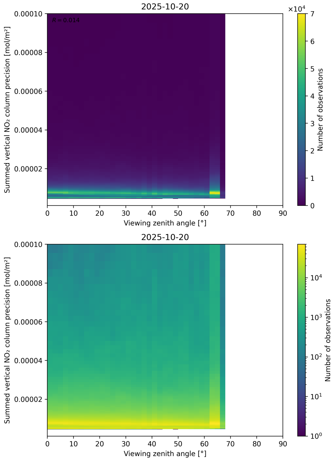
Figure 166: Scatter density plot of “Viewing zenith angle” against “Summed vertical NO 2 column precision” for 2025-10-19 to 2025-10-21.
