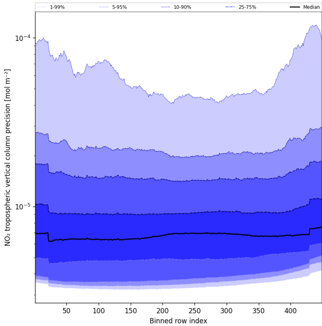
Figure 47: Along track statistics of “NO 2 tropospheric vertical column precision” for 2025-10-19 to 2025-10-21
