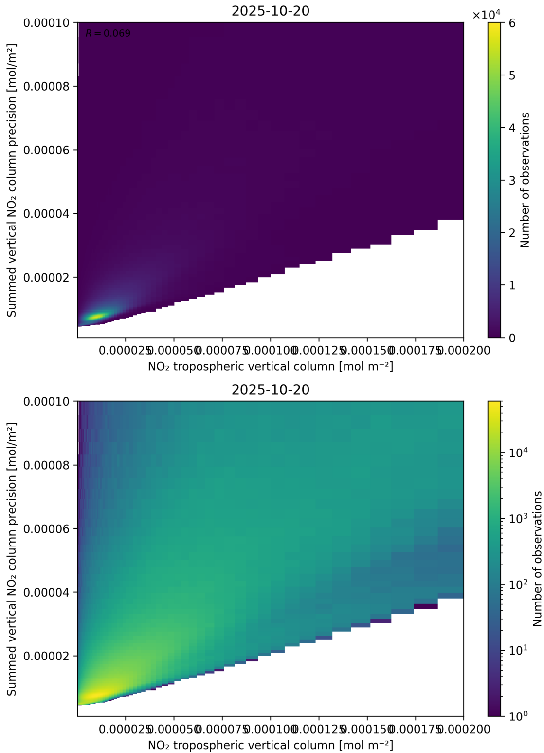
Figure 127: Scatter density plot of “NO 2 tropospheric vertical column” against “Summed vertical NO 2 column precision” for 2025-10-19 to 2025-10-21.
