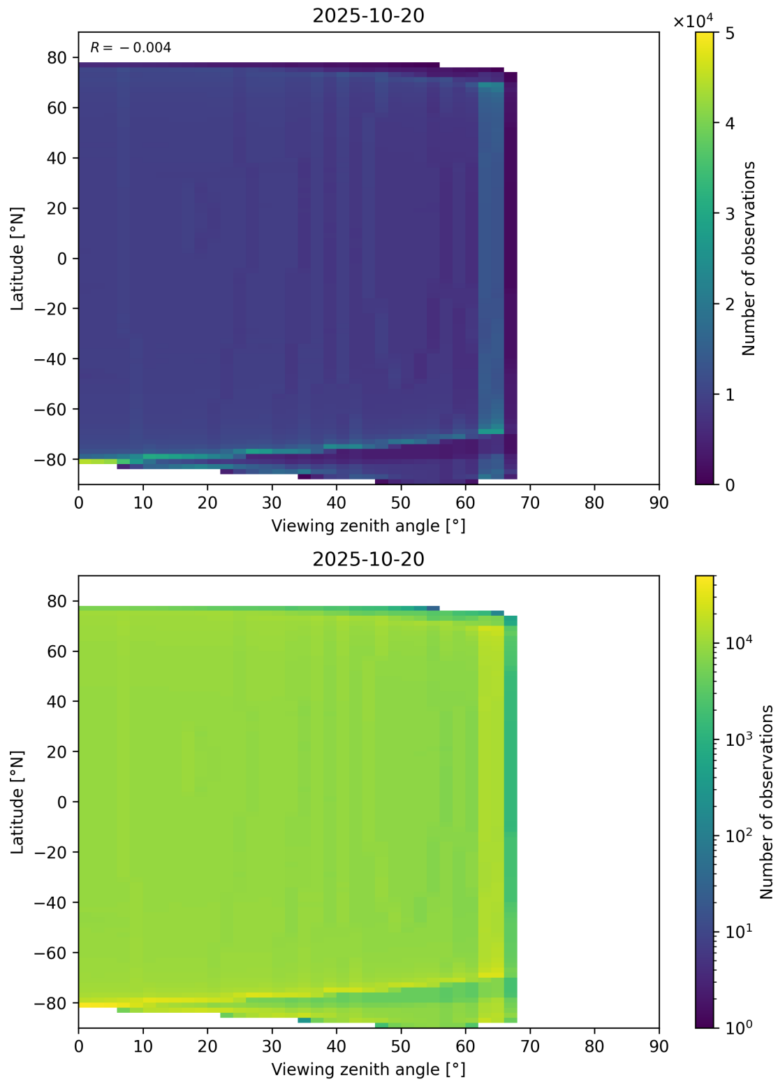
Figure 163: Scatter density plot of “Viewing zenith angle” against “Latitude” for 2025-10-19 to 2025-10-21.
