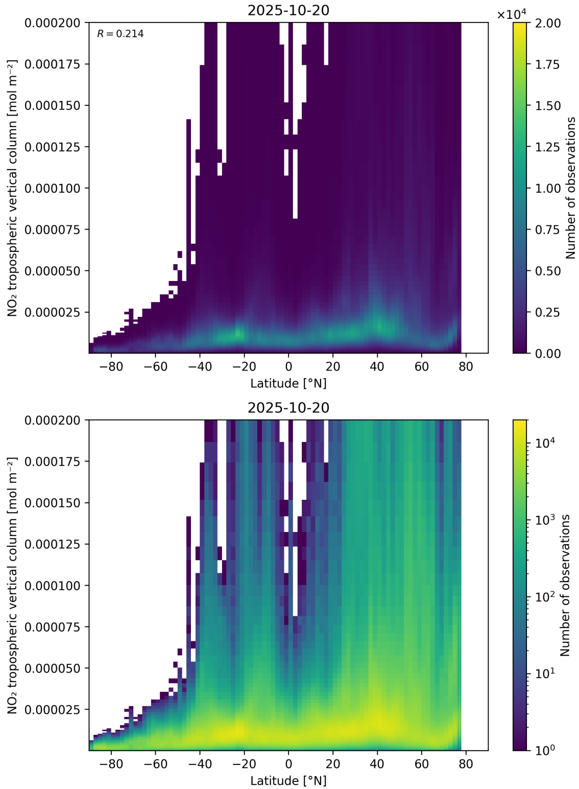
Figure 92: Scatter density plot of “Latitude” against “NO 2 tropospheric vertical column” for 2025-10-19 to 2025-10-21.
