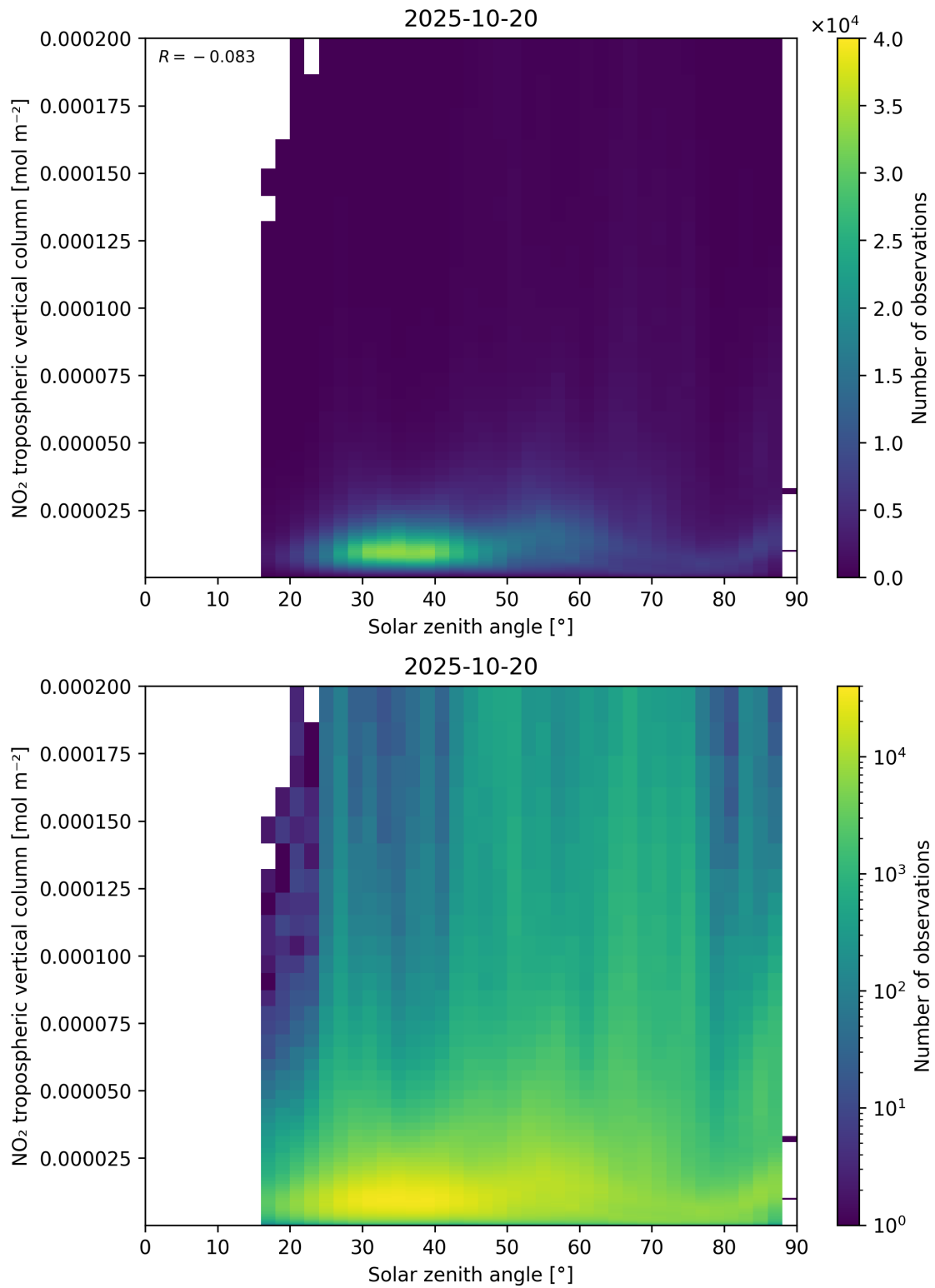
Figure 155: Scatter density plot of “Solar zenith angle” against “NO 2 tropospheric vertical column” for 2025-10-19 to 2025-10-21.
