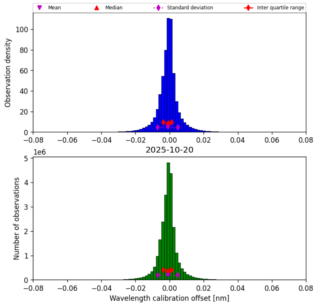
Figure 35: Histogram of “Wavelength calibration offset” for 2025-10-19 to 2025-10-21
