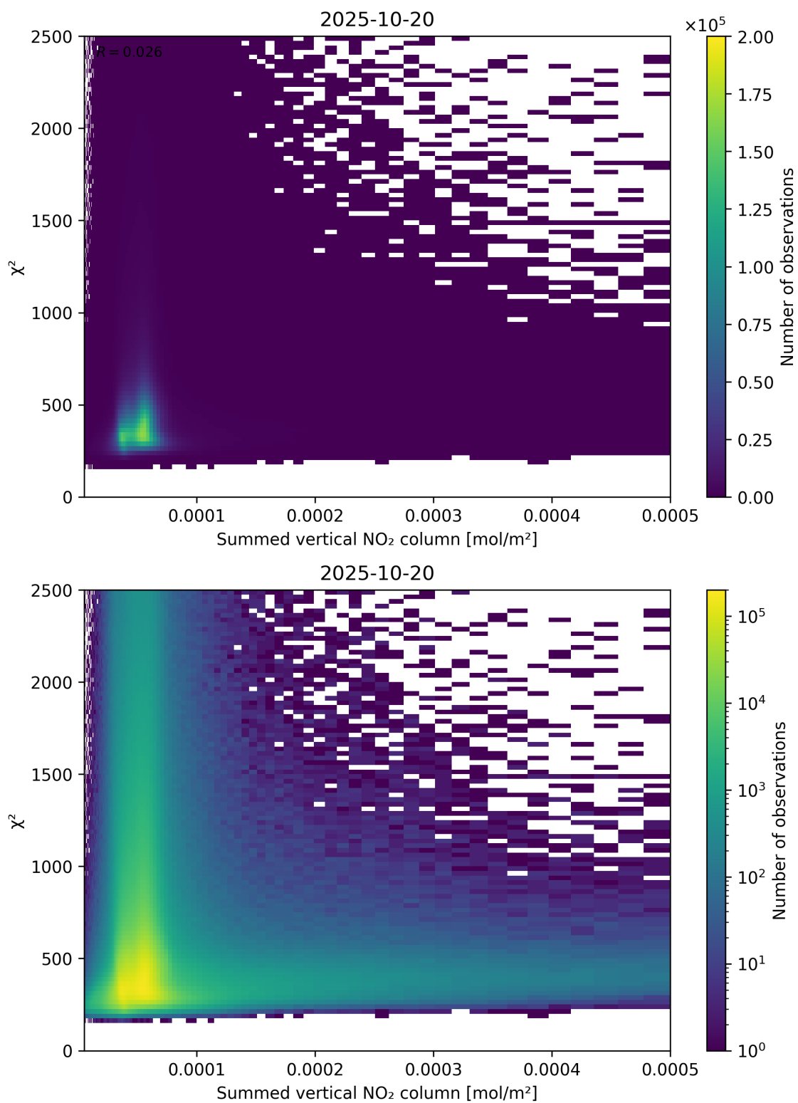
Figure 104: Scatter density plot of “Summed vertical NO 2 column” against “ \chi^2 ” for 2025-10-19 to 2025-10-21.
