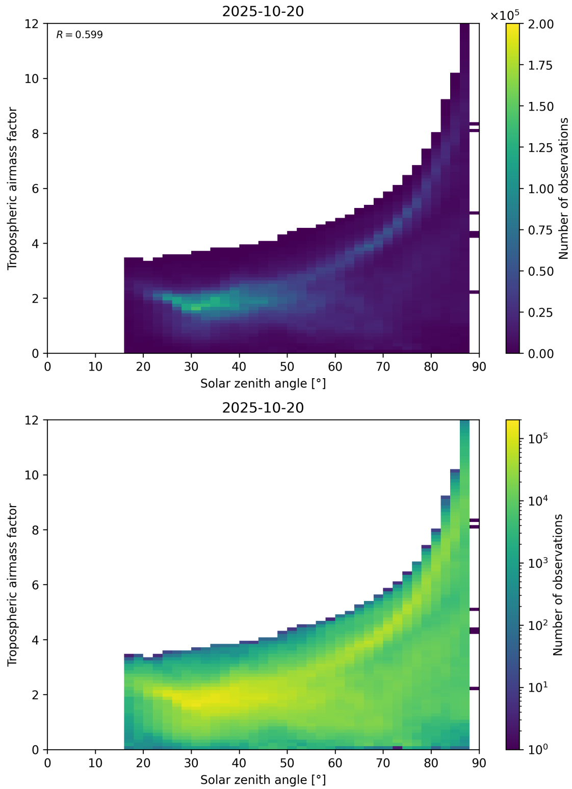
Figure 147: Scatter density plot of “Solar zenith angle” against “Tropospheric airmass factor” for 2025-10-19 to 2025-10-21.
