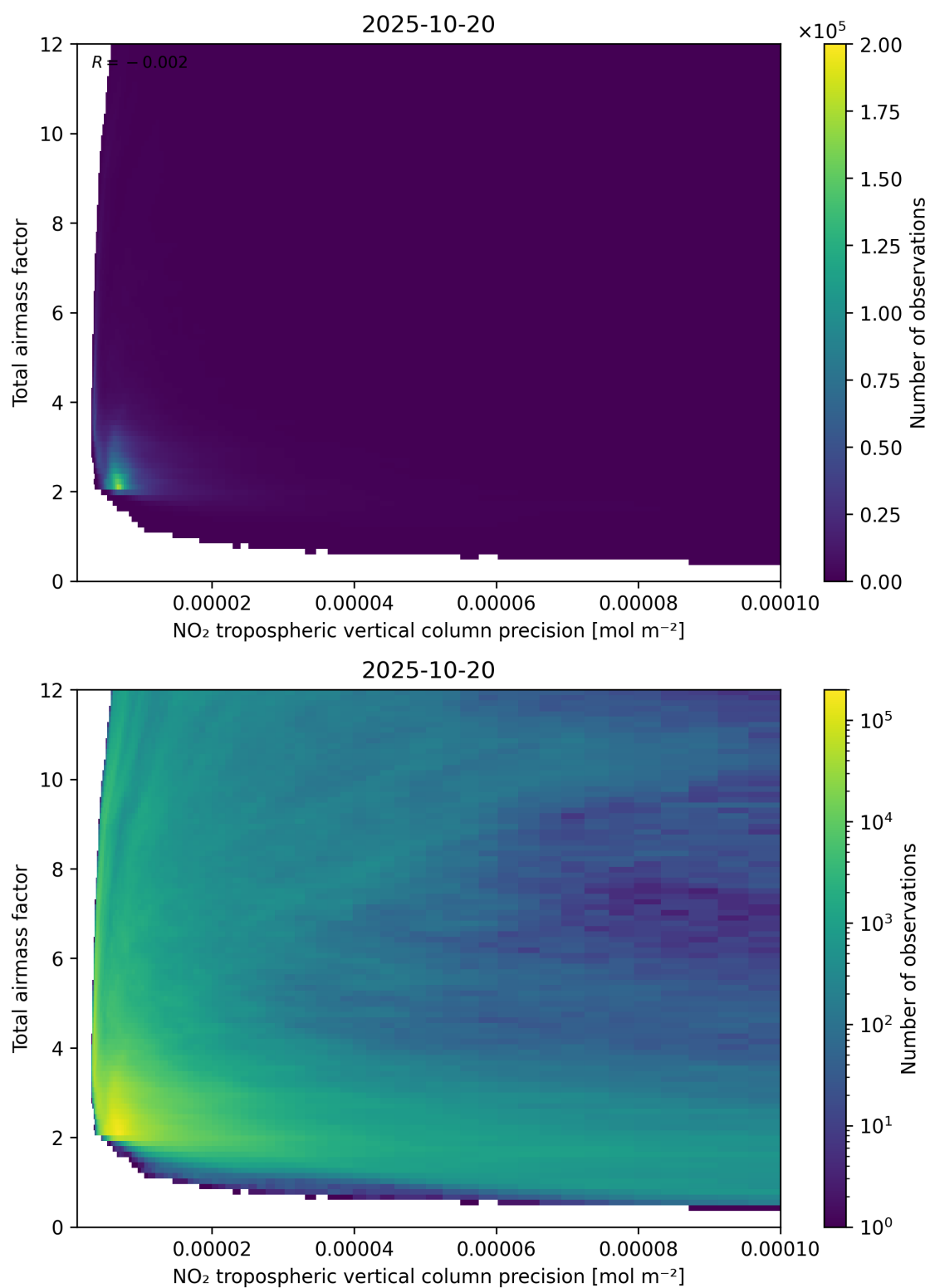
Figure 132: Scatter density plot of “NO 2 tropospheric vertical column precision” against “Total air mass factor” for 2025-10-19 to 2025-10-21.
