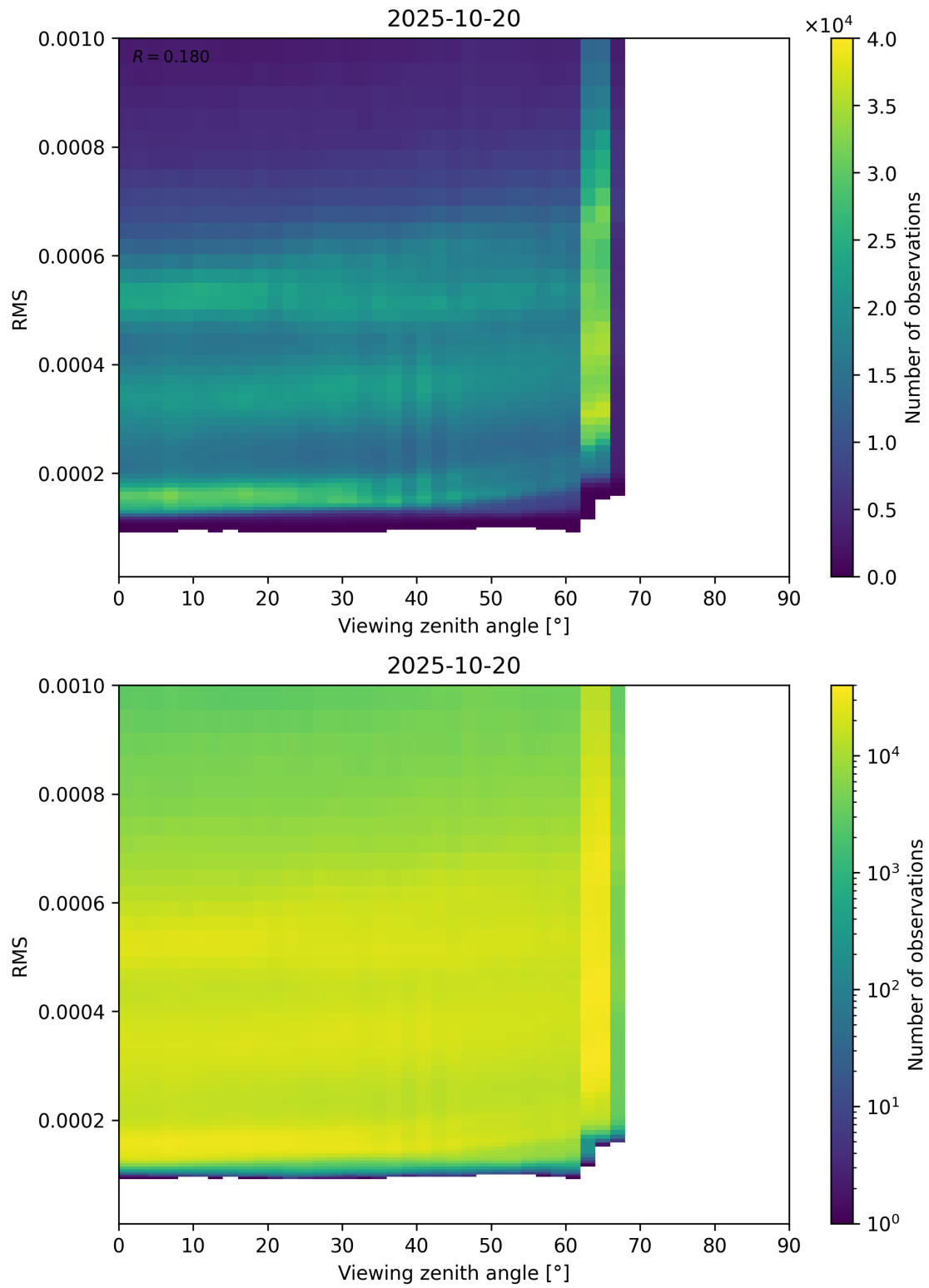
Figure 171: Scatter density plot of “Viewing zenith angle” against “RMS” for 2025-10-19 to 2025-10-21.
