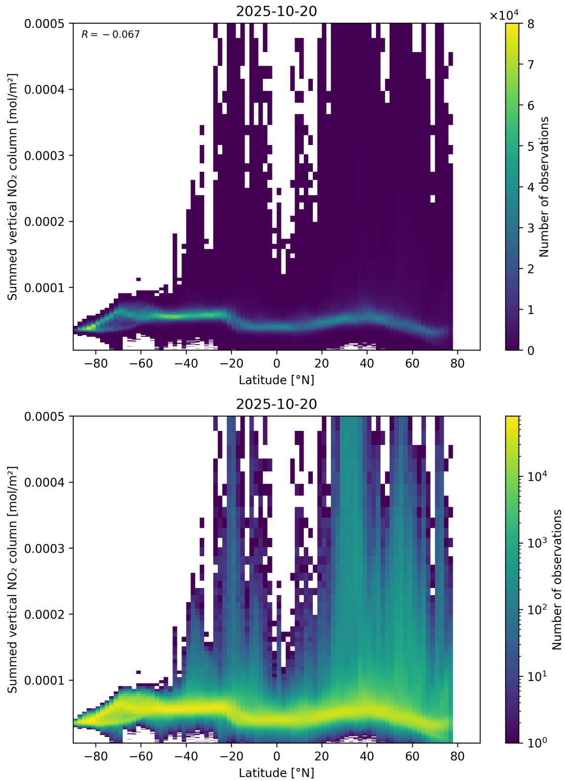
Figure 88: Scatter density plot of “Latitude” against “Summed vertical NO 2 column” for 2025-10-19 to 2025-10-21.
