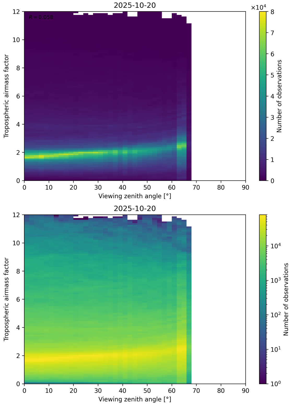
Figure 161: Scatter density plot of “Viewing zenith angle” against “Tropospheric airmass factor” for 2025-10-19 to 2025-10-21.
