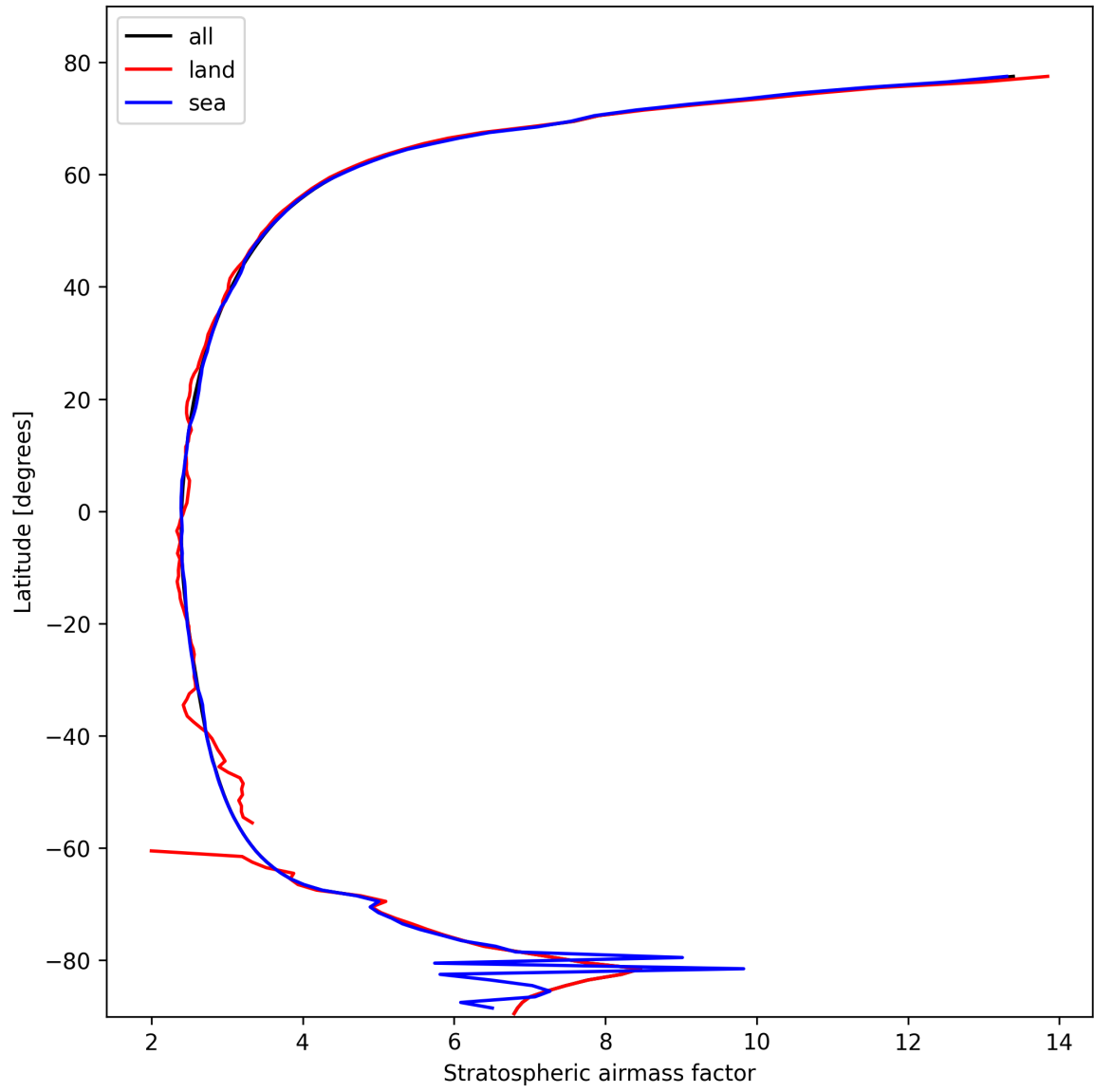
Figure 27: Zonal average of “Stratospheric airmass factor” for 2025-10-19 to 2025-10-21.
