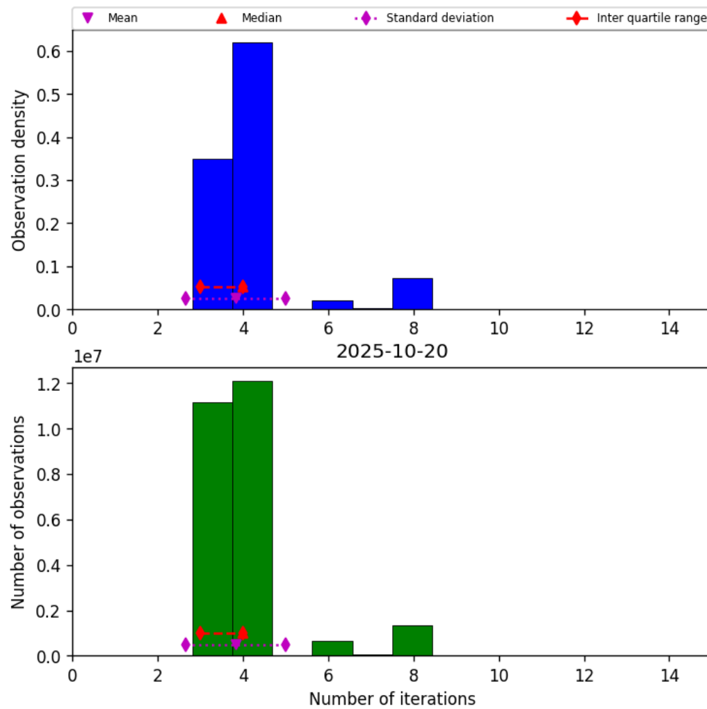
Figure 34: Histogram of “Number of iterations” for 2025-10-19 to 2025-10-21
