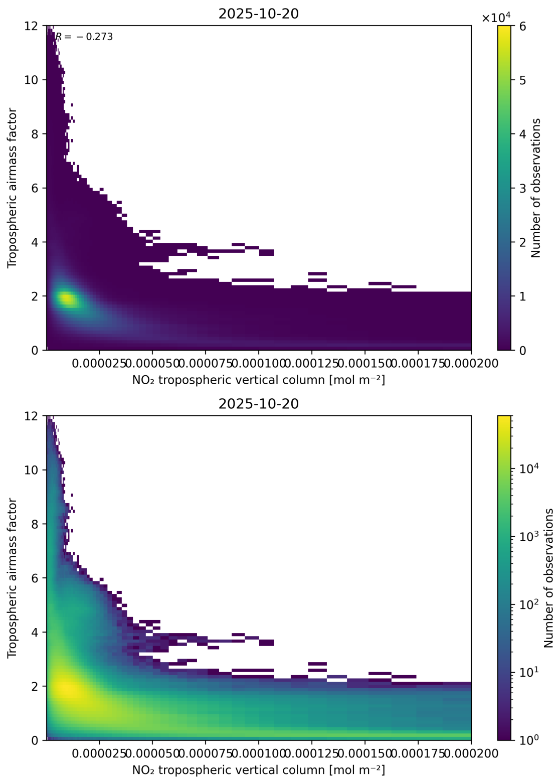
Figure 123: Scatter density plot of “NO 2 tropospheric vertical column” against “Tropospheric air mass factor” for 2025-10-19 to 2025-10-21.
