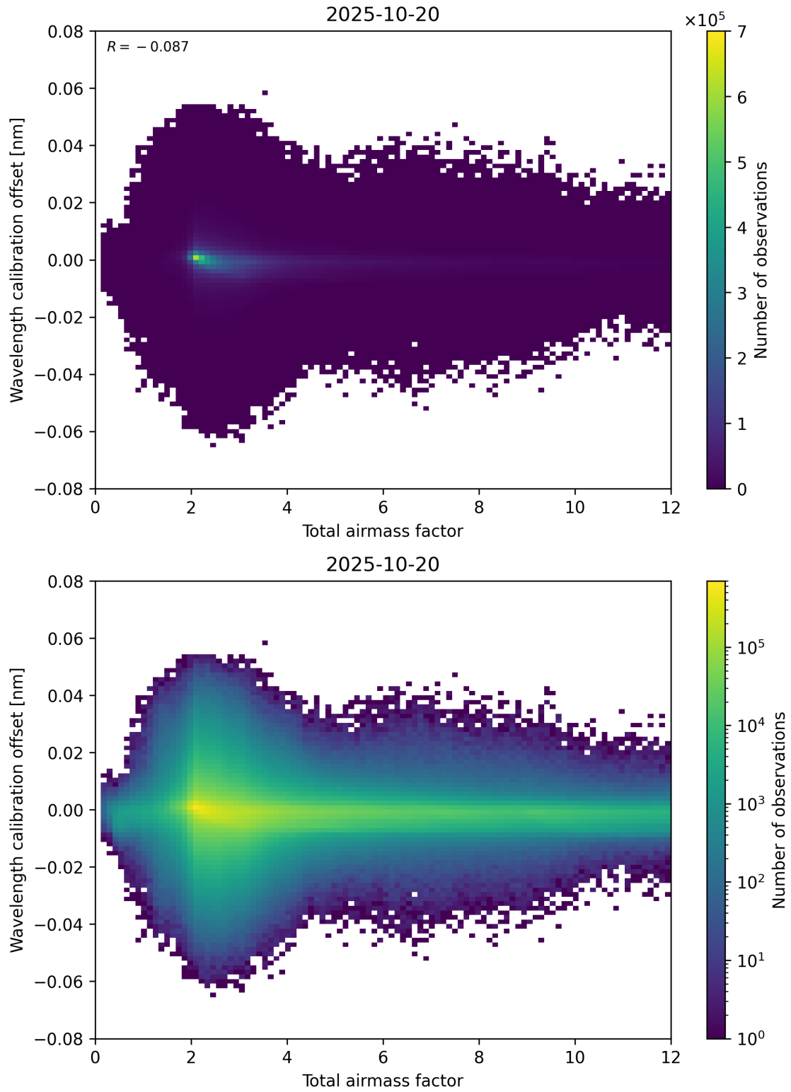
Figure 70: Scatter density plot of “Total airmass factor” against “Wavelength calibration offset” for 2025-10-19 to 2025-10-21.
