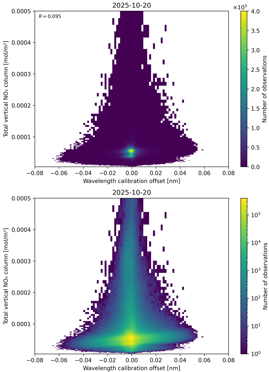
Figure 179: Scatter density plot of “Wavelength calibration offset” against “Total vertical NO 2 column” for 2025-10-19 to 2025-10-21.
