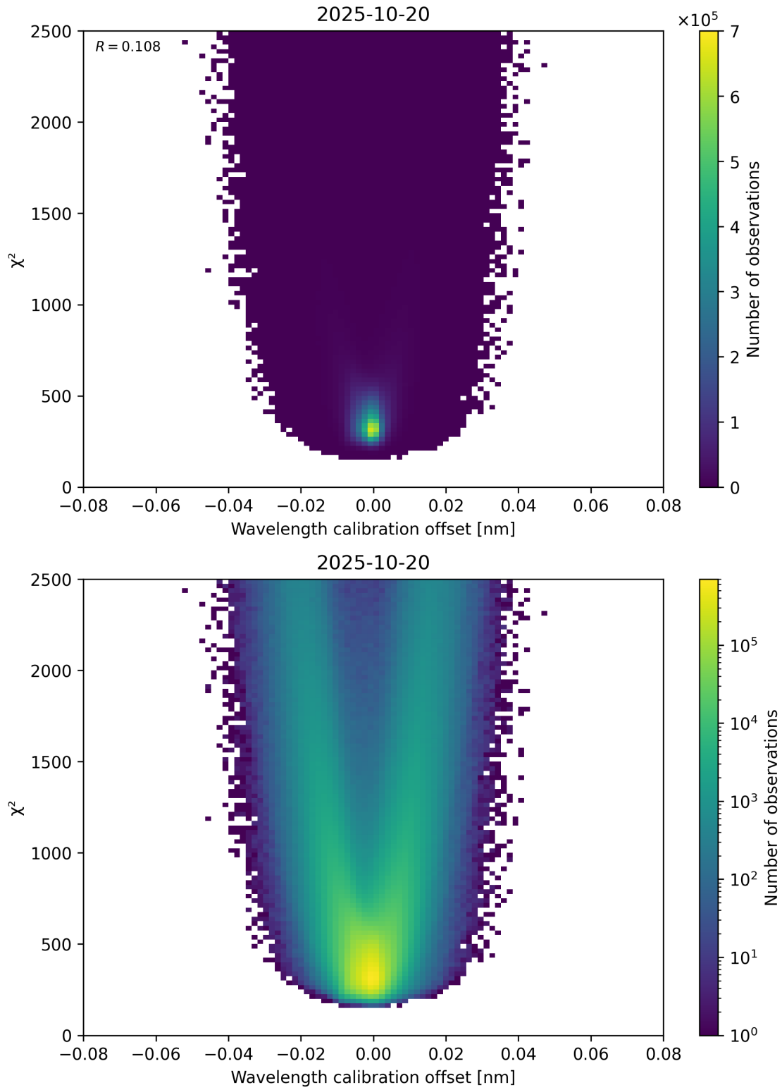
Figure 175: Scatter density plot of “Wavelength calibration offset” against “ \chi^2 ” for 2025-10-19 to 2025-10-21.
