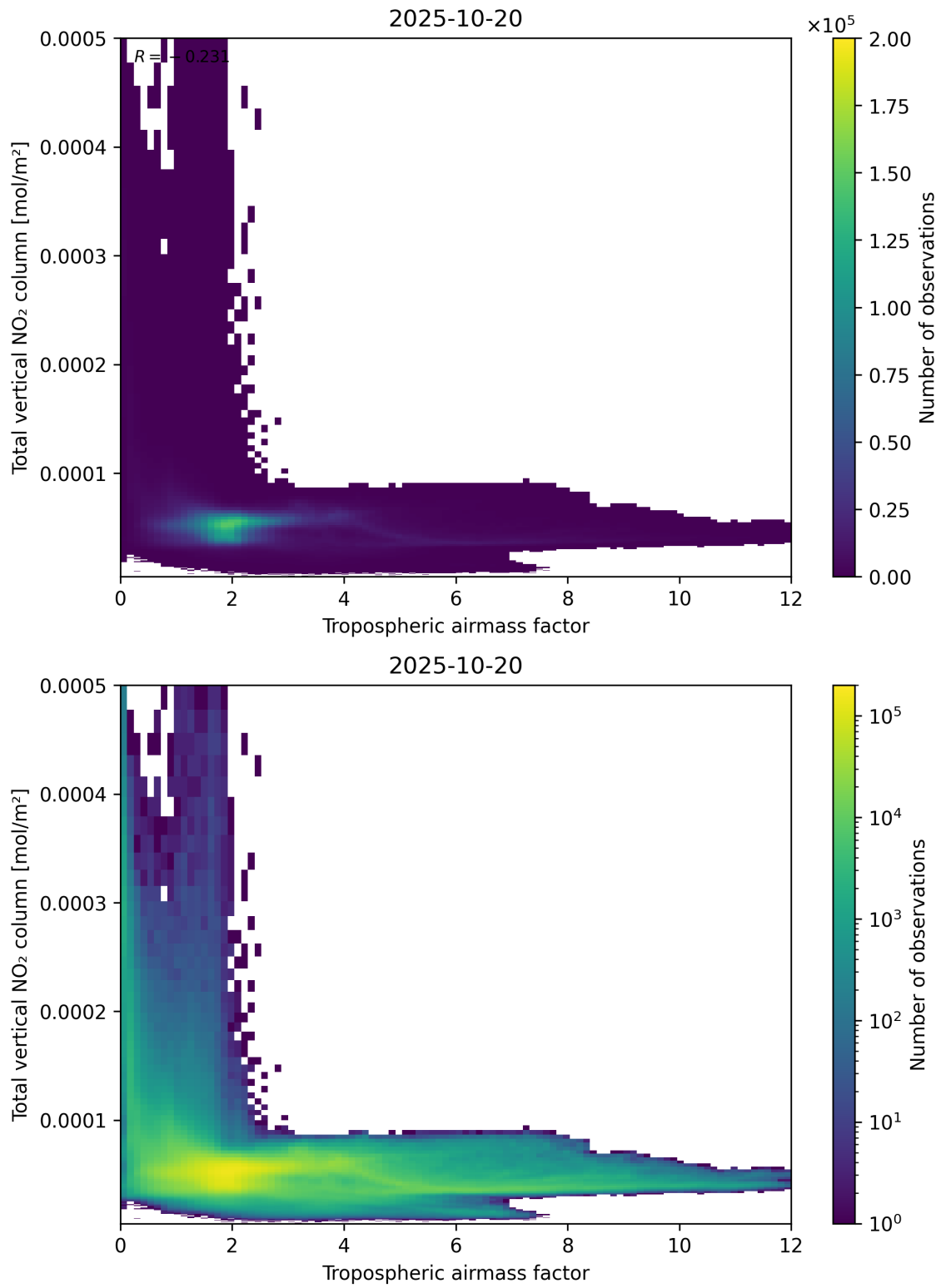
Figure 77: Scatter density plot of “Tropospheric airmass factor” against “Total vertical NO 2 column” for 2025-10-19 to 2025-10-21.
