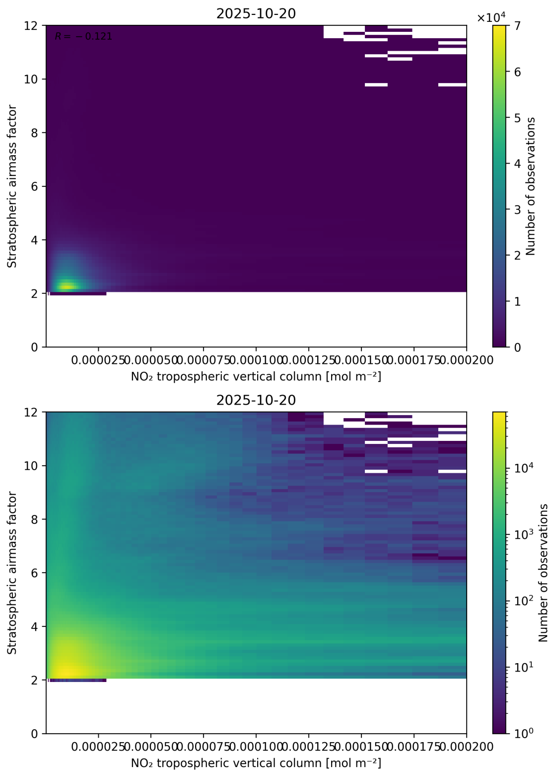
Figure 121: Scatter density plot of “NO 2 tropospheric vertical column” against “Stratospheric airmass factor” for 2025-10-19 to 2025-10-21.
