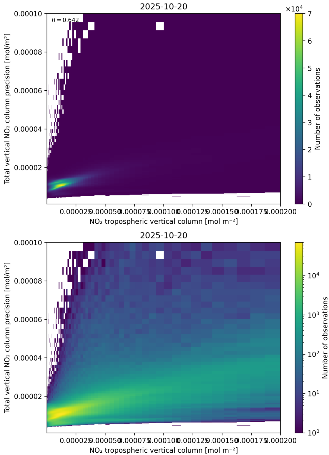
Figure 129: Scatter density plot of “NO 2 tropospheric vertical column” against “Total vertical NO 2 column precision” for 2025-10-19 to 2025-10-21.
