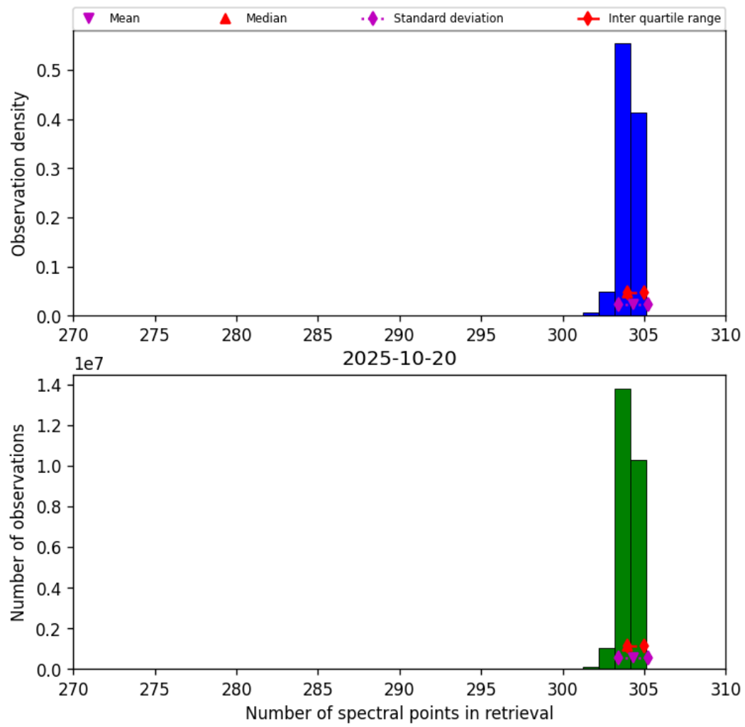
Figure 33: Histogram of “Number of spectral points in retrieval” for 2025-10-19 to 2025-10-21
