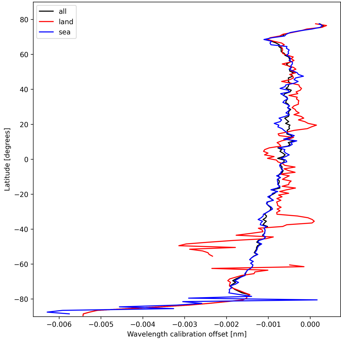
Figure 18: Zonal average of “Wavelength calibration offset” for 2025-10-19 to 2025-10-21.
