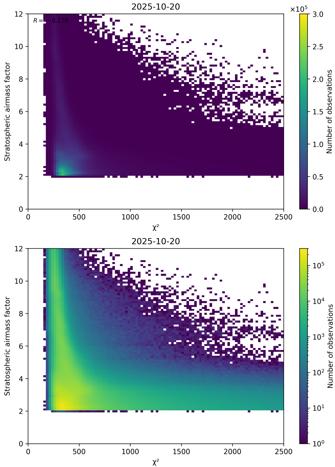
Figure 81: Scatter density plot of “ \chi^2 ” against “Stratospheric airmass factor” for 2025-10-19 to 2025-10-21.
