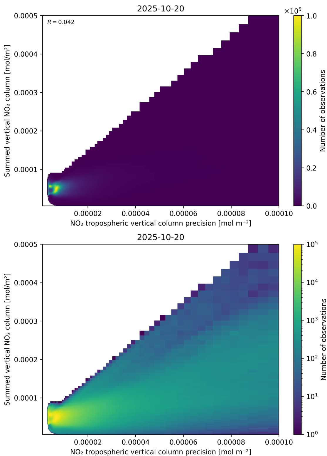
Figure 136: Scatter density plot of “NO 2 tropospheric vertical column precision” against “Summed vertical NO 2 column” for 2025-10-19 to 2025-10-21.
