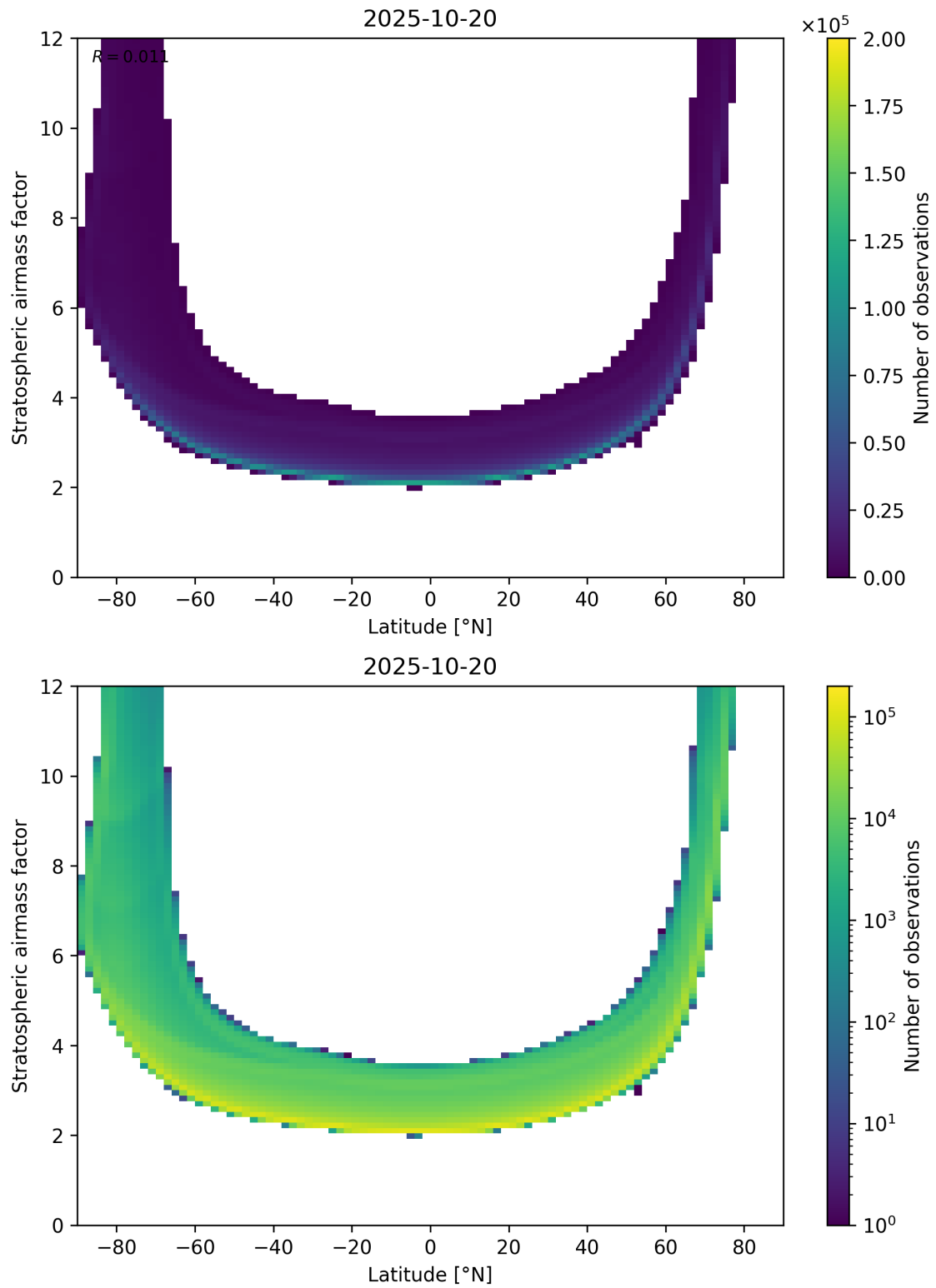
Figure 83: Scatter density plot of “Latitude” against “Stratospheric airmass factor” for 2025-10-19 to 2025-10-21.
