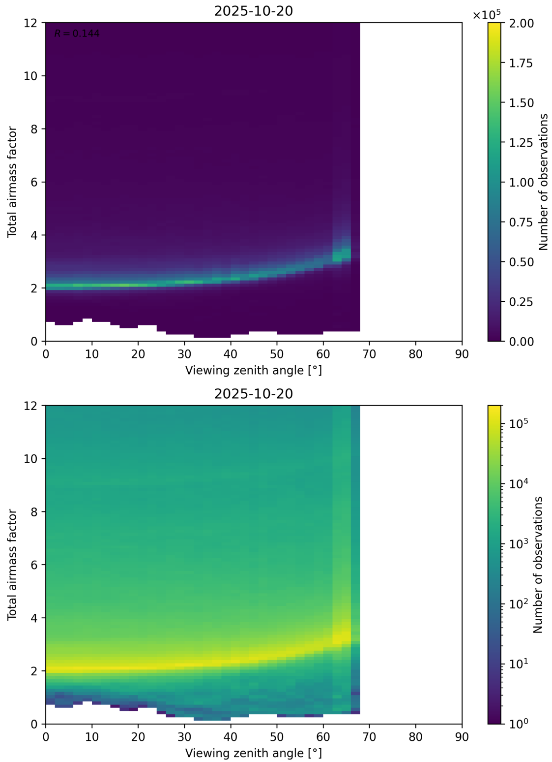
Figure 160: Scatter density plot of “Viewing zenith angle” against “Total airmass factor” for 2025-10-19 to 2025-10-21.
