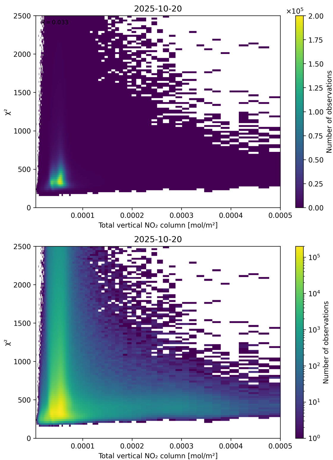
Figure 111: Scatter density plot of “Total vertical NO 2 column” against “ \chi^2 ” for 2025-10-19 to 2025-10-21.
