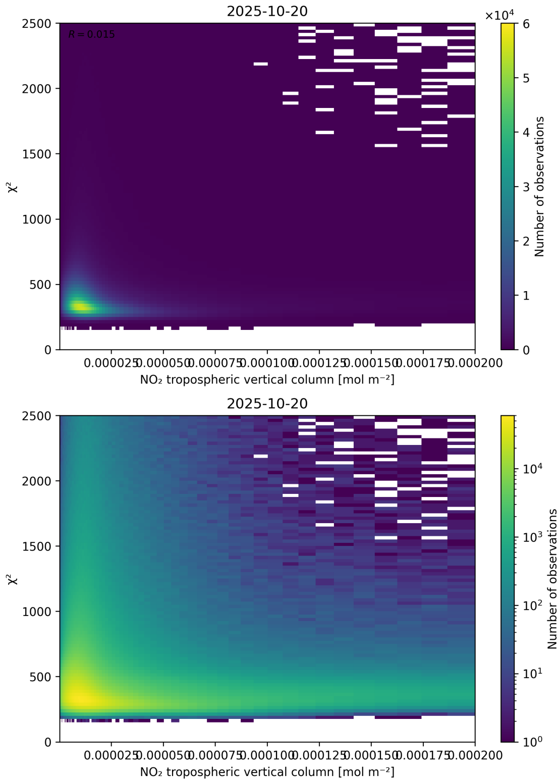
Figure 124: Scatter density plot of “NO 2 tropospheric vertical column” against “ \chi^2 ” for 2025-10-19 to 2025-10-21.
