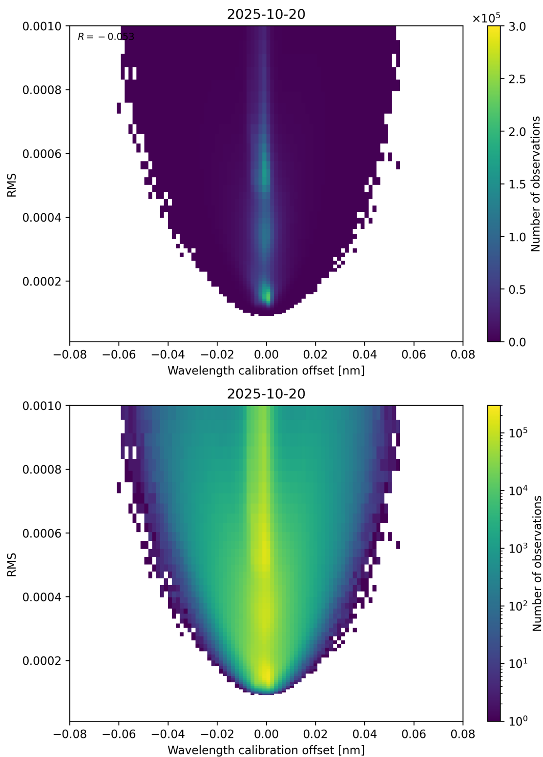
Figure 181: Scatter density plot of “Wavelength calibration offset” against “RMS” for 2025-10-19 to 2025-10-21.
