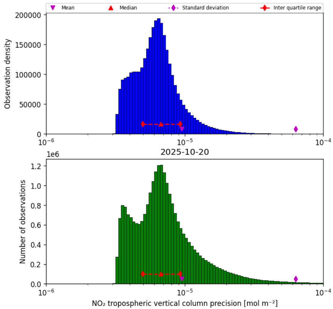
Figure 30: Histogram of “NO 2 tropospheric vertical column precision” for 2025-10-19 to 2025-10-21
