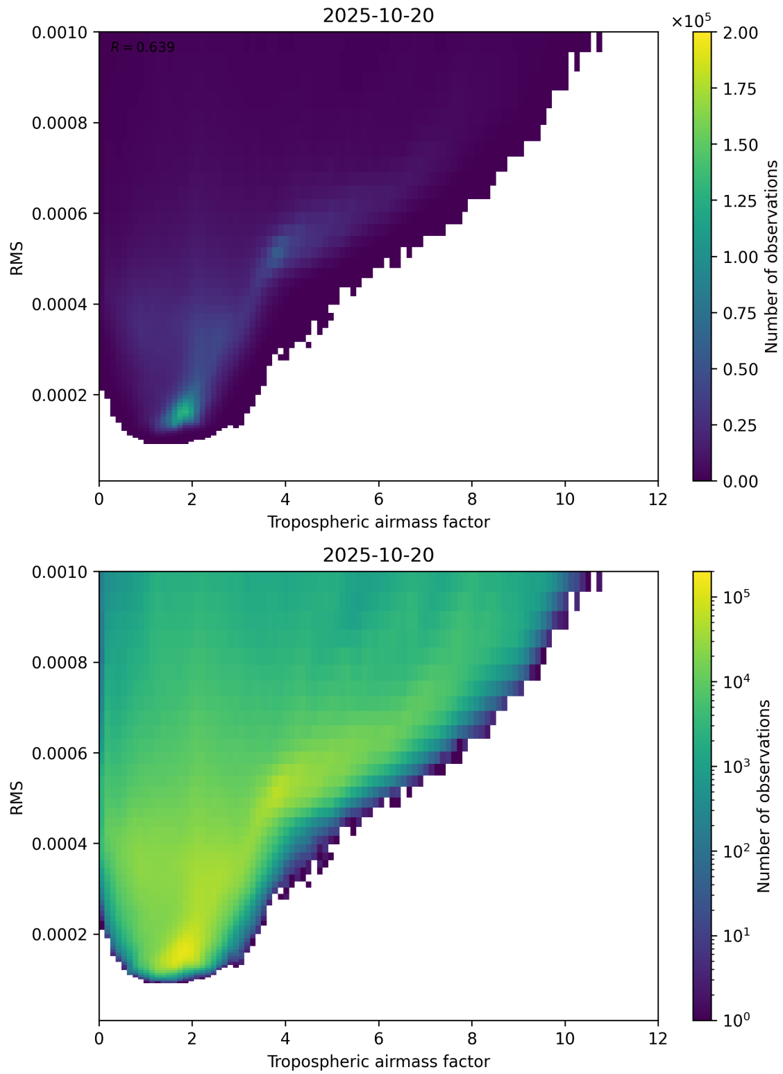
Figure 79: Scatter density plot of “Tropospheric airmass factor” against “RMS” for 2025-10-19 to 2025-10-21.
