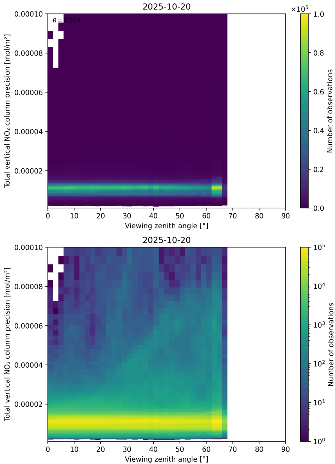
Figure 168: Scatter density plot of “Viewing zenith angle” against “Total vertical NO 2 column precision” for 2025-10-19 to 2025-10-21.
