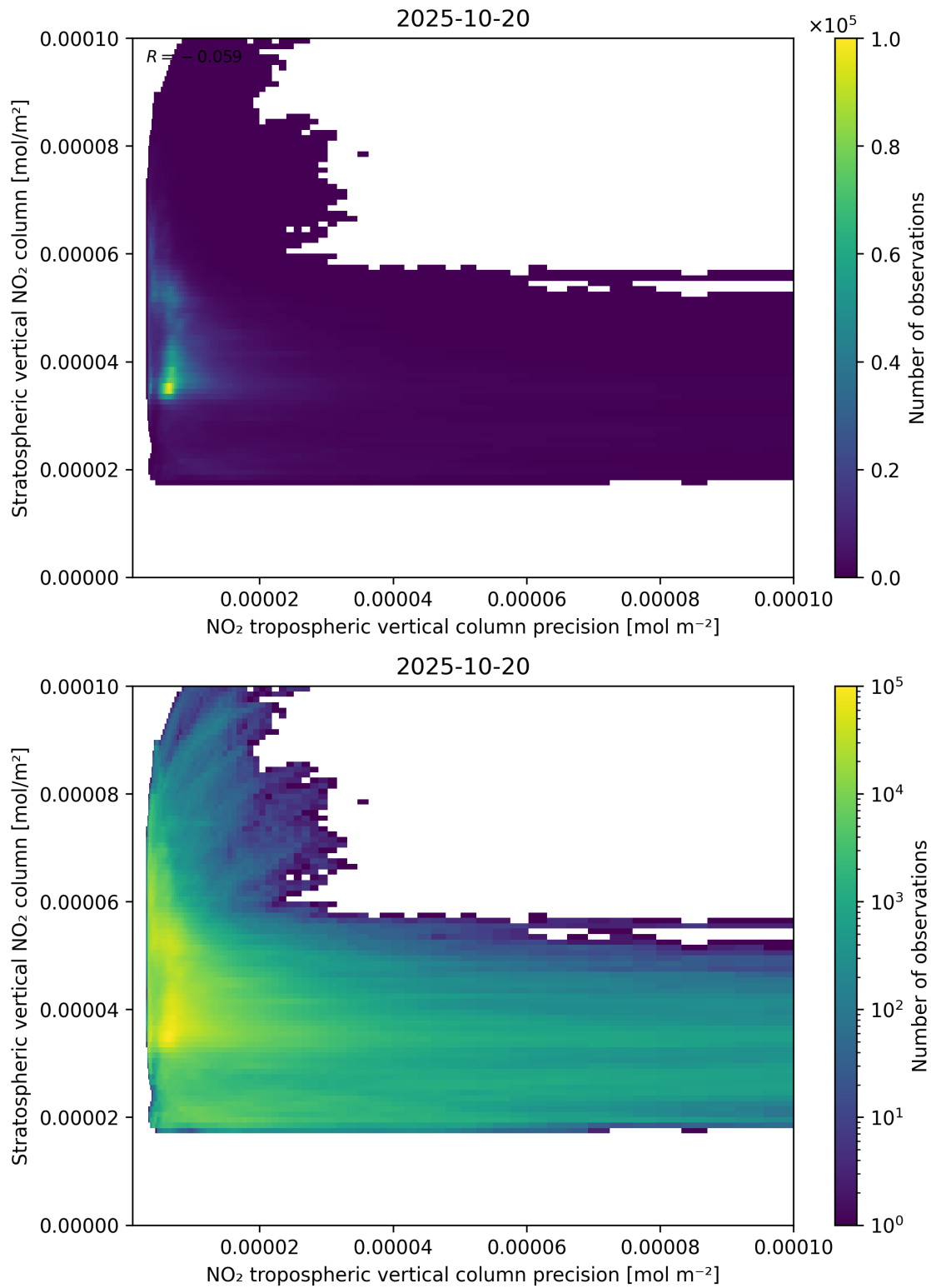
Figure 135: Scatter density plot of “NO 2 tropospheric vertical column precision” against “Stratospheric vertical NO 2 column” for 2025-10-19 to 2025-10-21.
