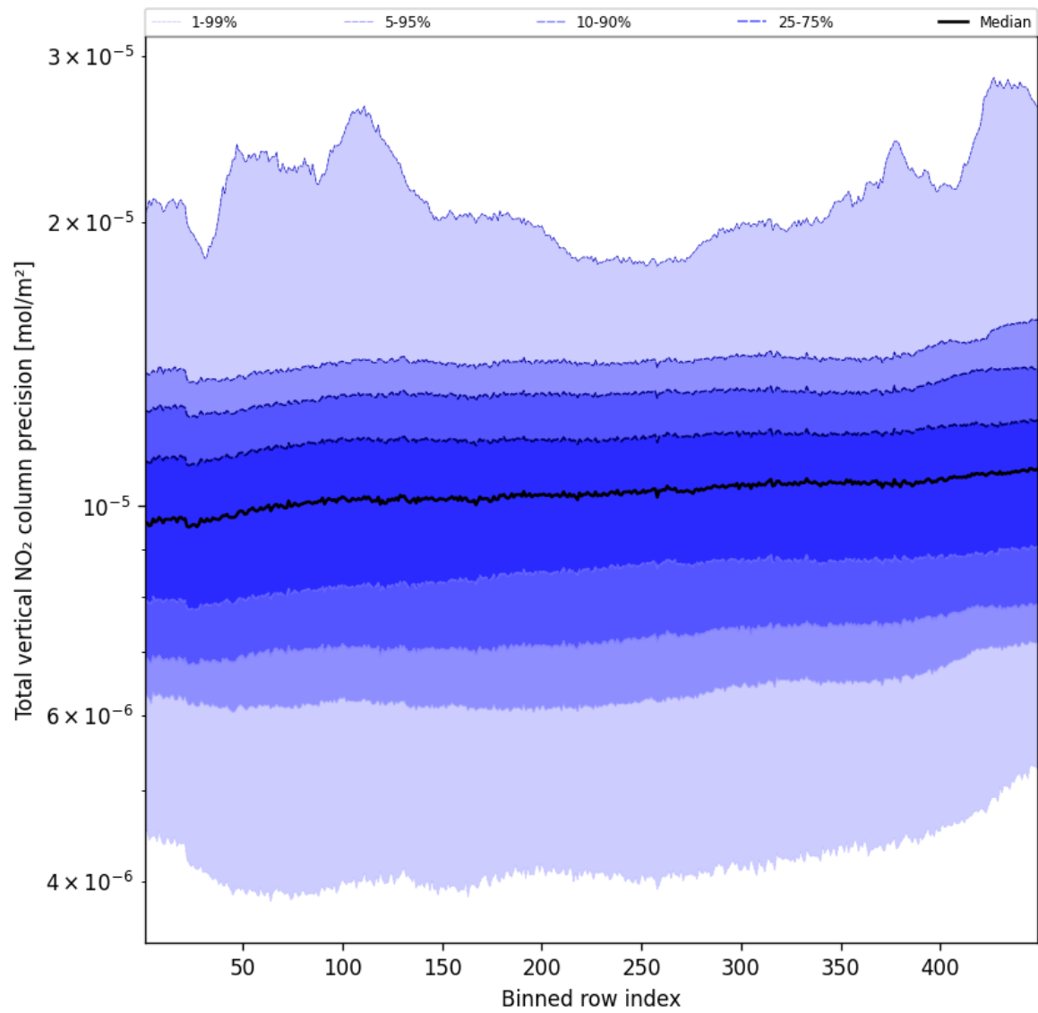
Figure 56: Along track statistics of “Total vertical NO 2 column precision” for 2025-10-19 to 2025-10-21
