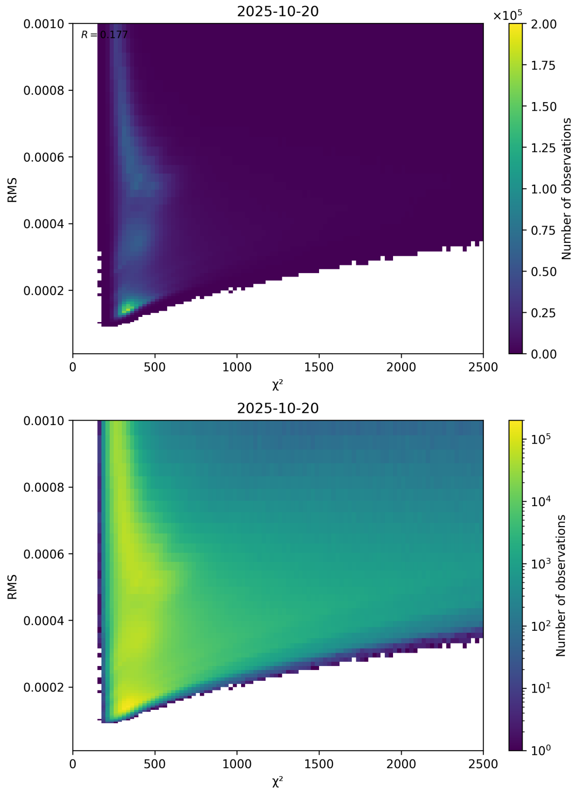
Figure 82: Scatter density plot of “ \chi^2 ” against “RMS” for 2025-10-19 to 2025-10-21.
