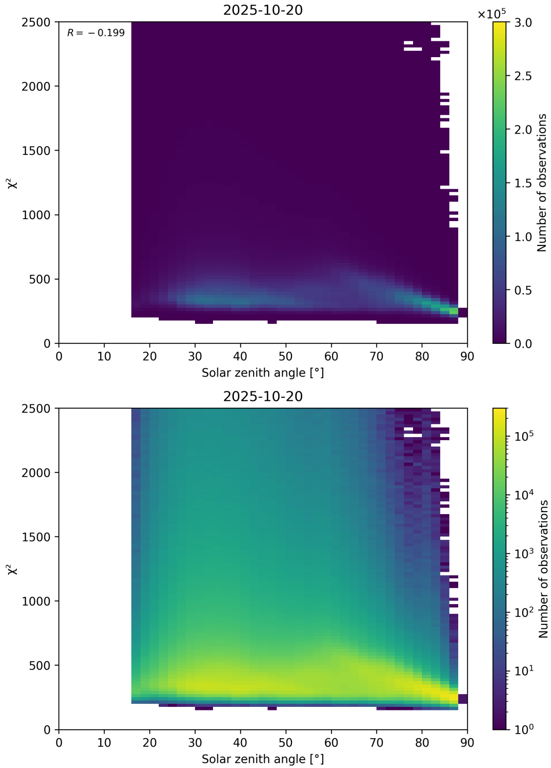
Figure 148: Scatter density plot of “Solar zenith angle” against “ \chi^2 ” for 2025-10-19 to 2025-10-21.
