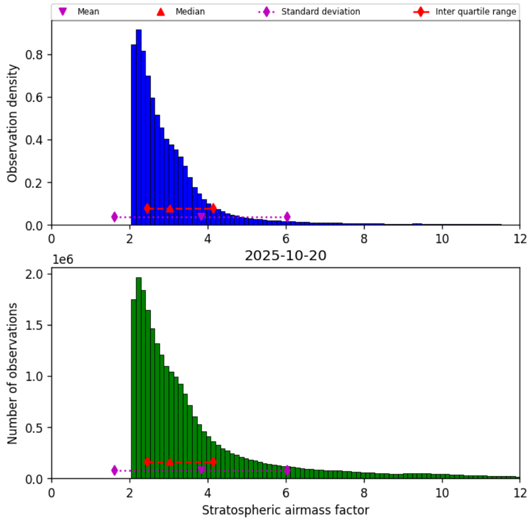
Figure 44: Histogram of “Stratospheric airmass factor” for 2025-10-19 to 2025-10-21
