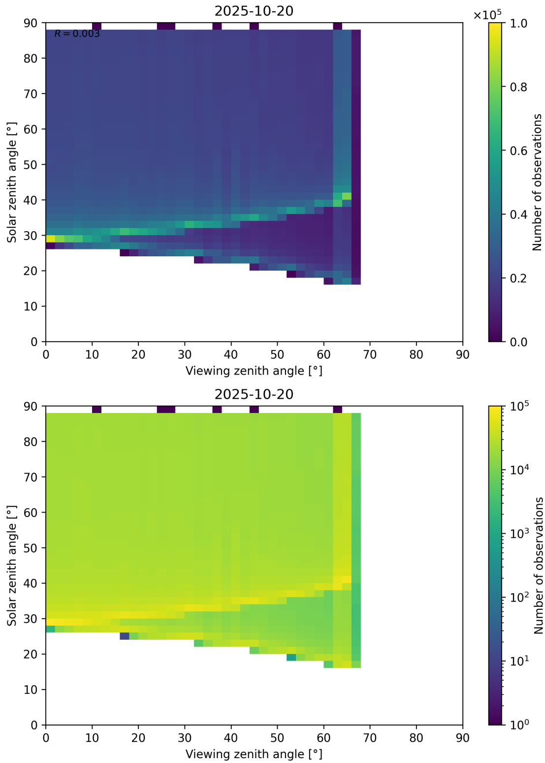
Figure 172: Scatter density plot of “Viewing zenith angle” against “Solar zenith angle” for 2025-10-19 to 2025-10-21.
