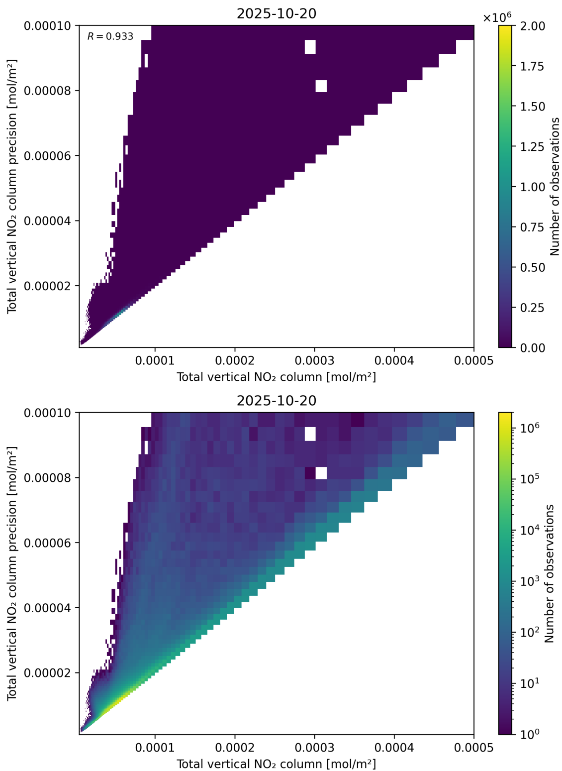
Figure 114: Scatter density plot of “Total vertical NO 2 column” against “Total vertical NO 2 column precision” for 2025-10-19 to 2025-10-21.
