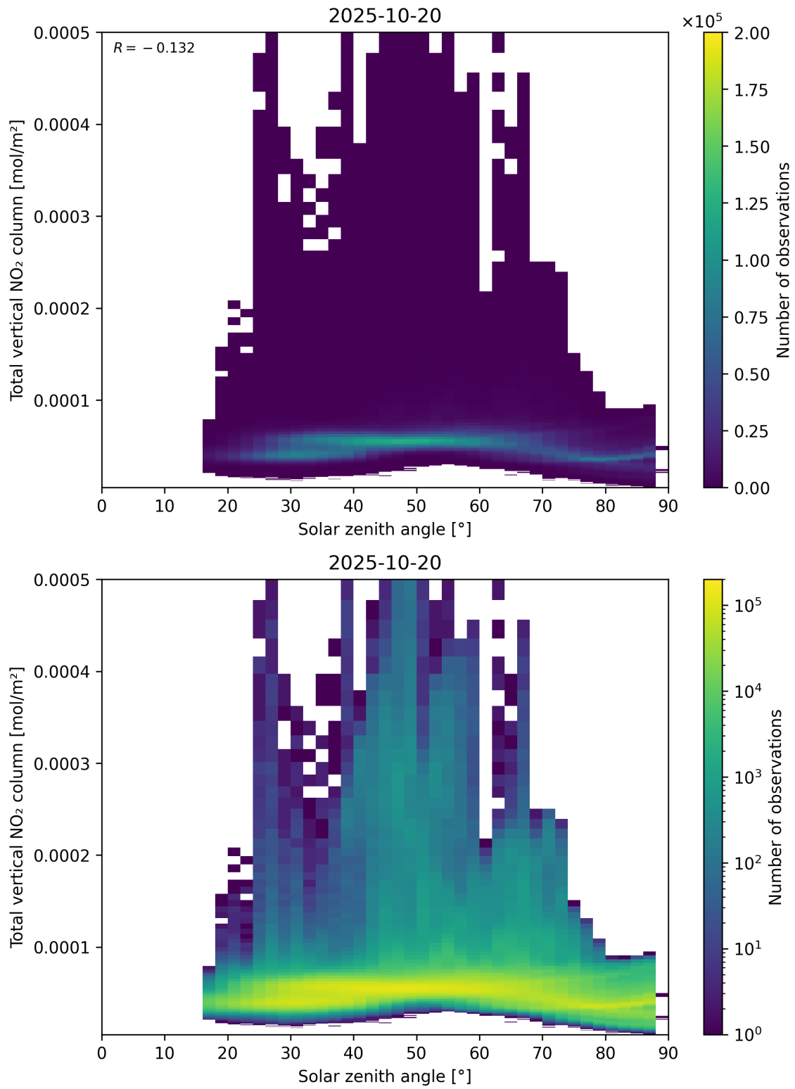
Figure 153: Scatter density plot of “Solar zenith angle” against “Total vertical NO 2 column” for 2025-10-19 to 2025-10-21.
