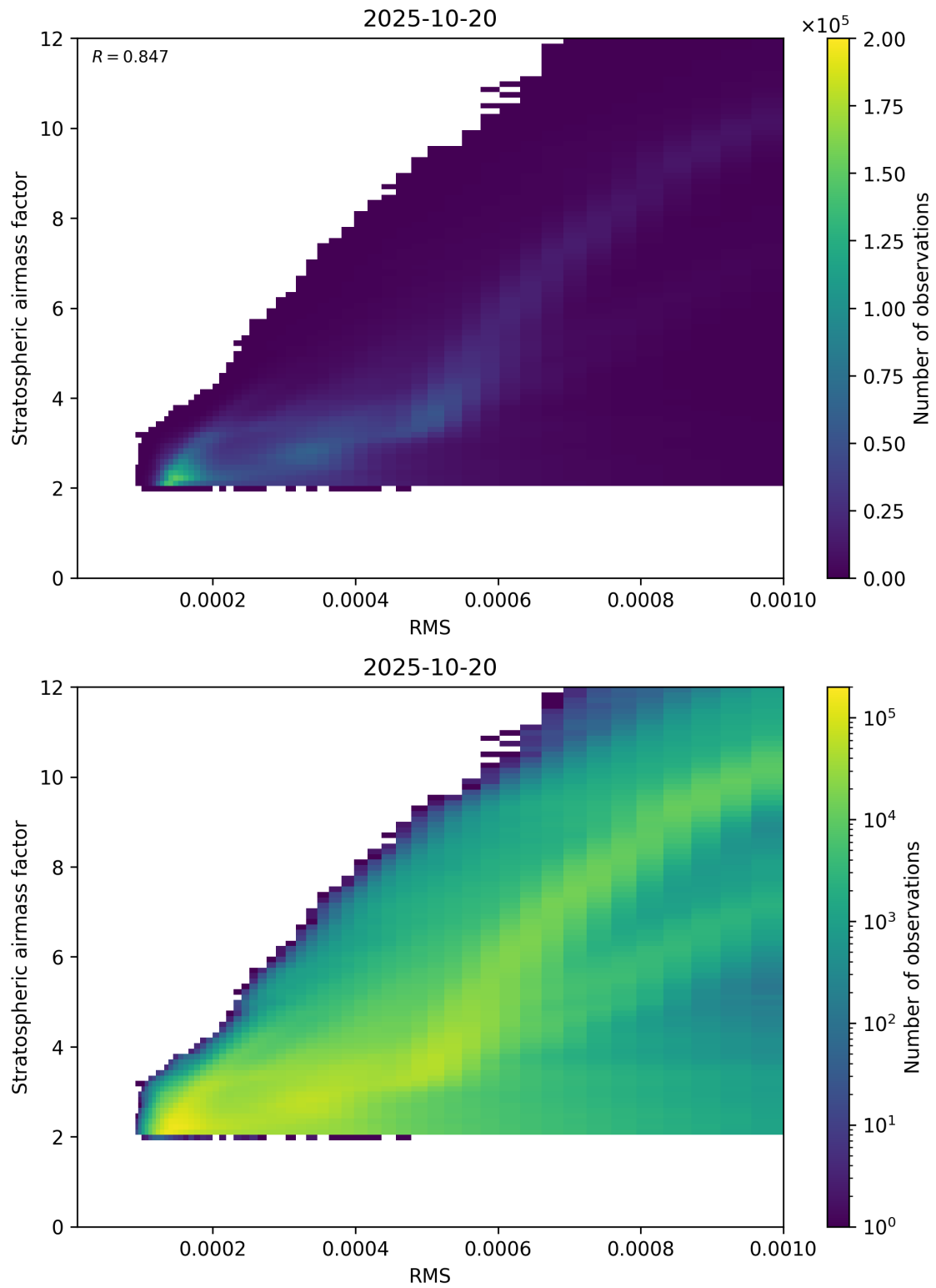
Figure 144: Scatter density plot of “RMS” against “Stratospheric airmass factor” for 2025-10-19 to 2025-10-21.
