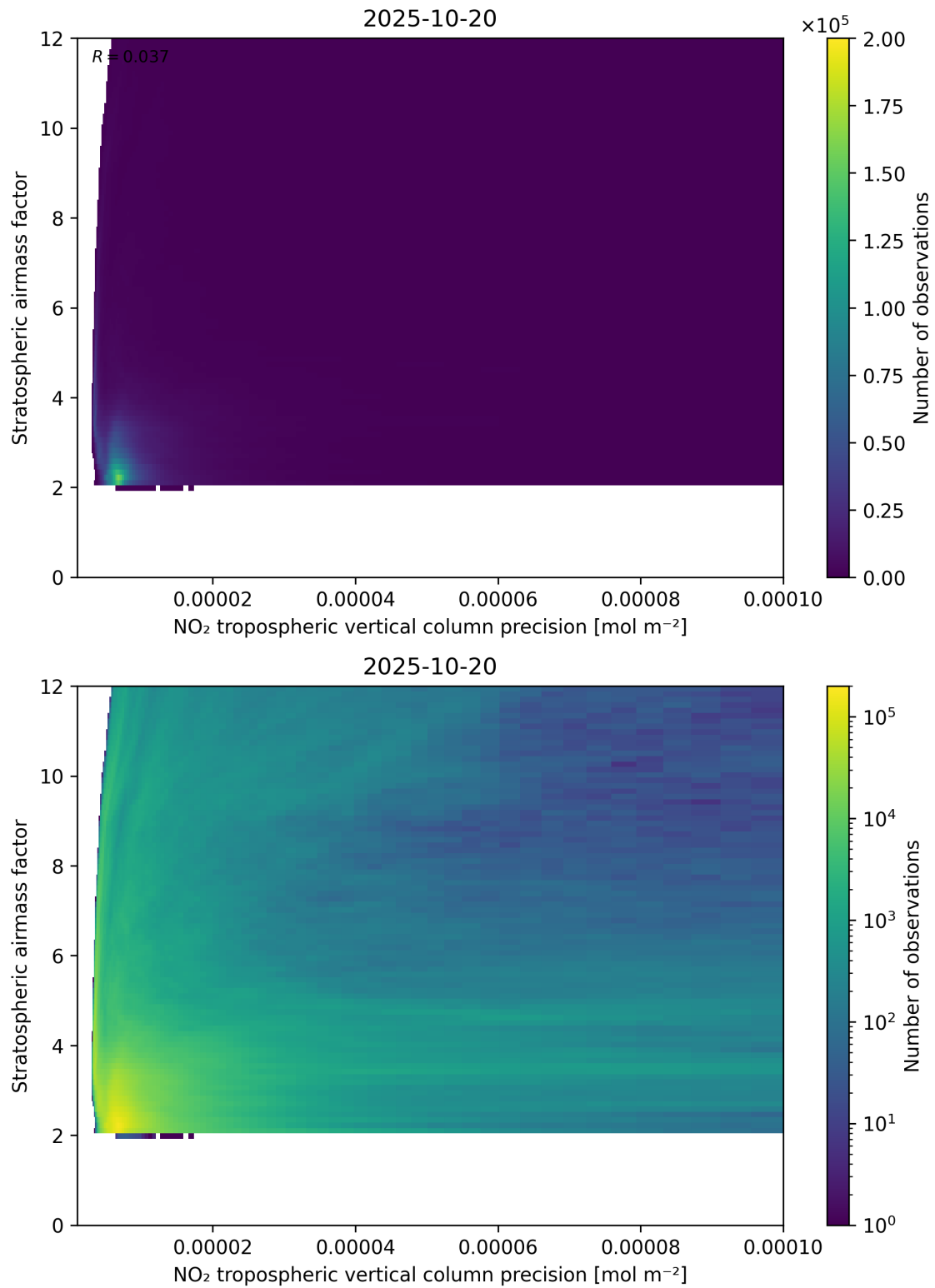
Figure 131: Scatter density plot of “NO 2 tropospheric vertical column precision” against “Stratospheric airmass factor” for 2025-10-19 to 2025-10-21.
