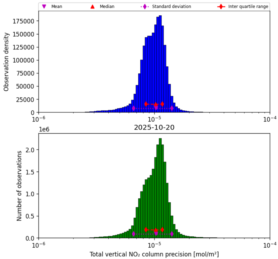
Figure 39: Histogram of “Total vertical NO 2 column precision” for 2025-10-19 to 2025-10-21
