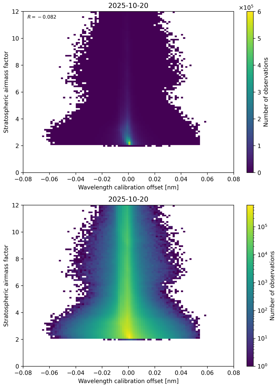
Figure 174: Scatter density plot of “Wavelength calibration offset” against “Stratospheric airmass factor” for 2025-10-19 to 2025-10-21.
