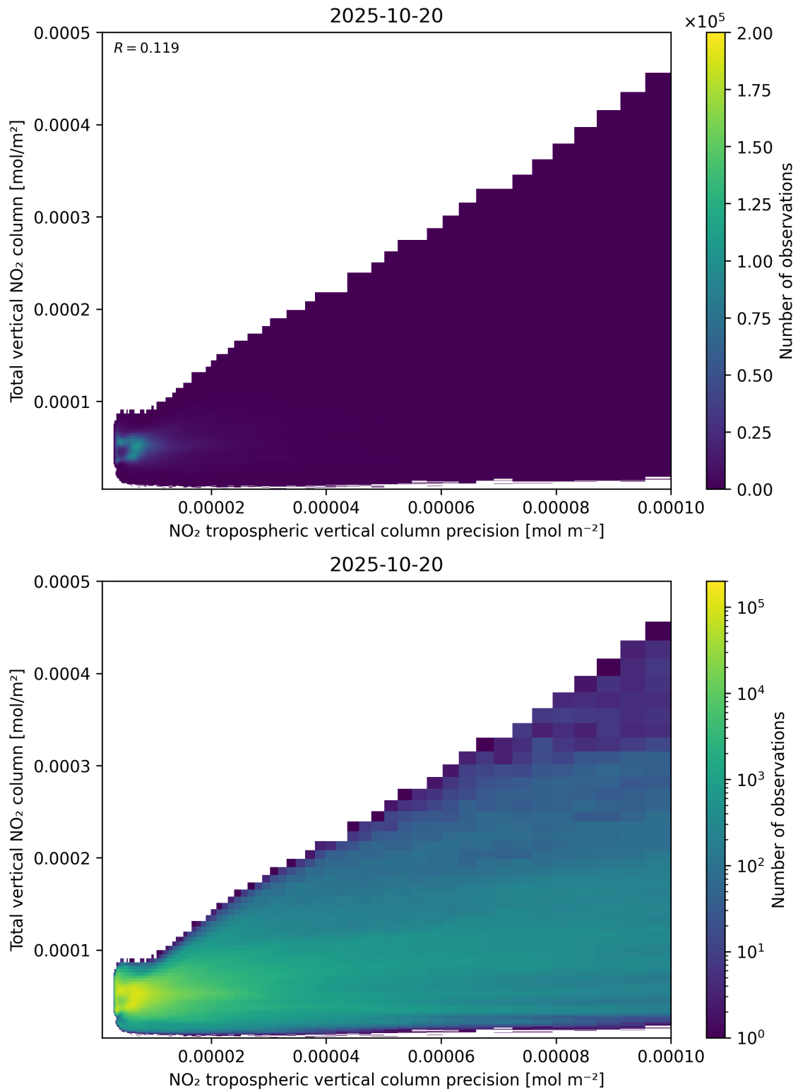
Figure 138: Scatter density plot of “NO 2 tropospheric vertical column precision” against “Total vertical NO 2 column” for 2025-10-19 to 2025-10-21.
