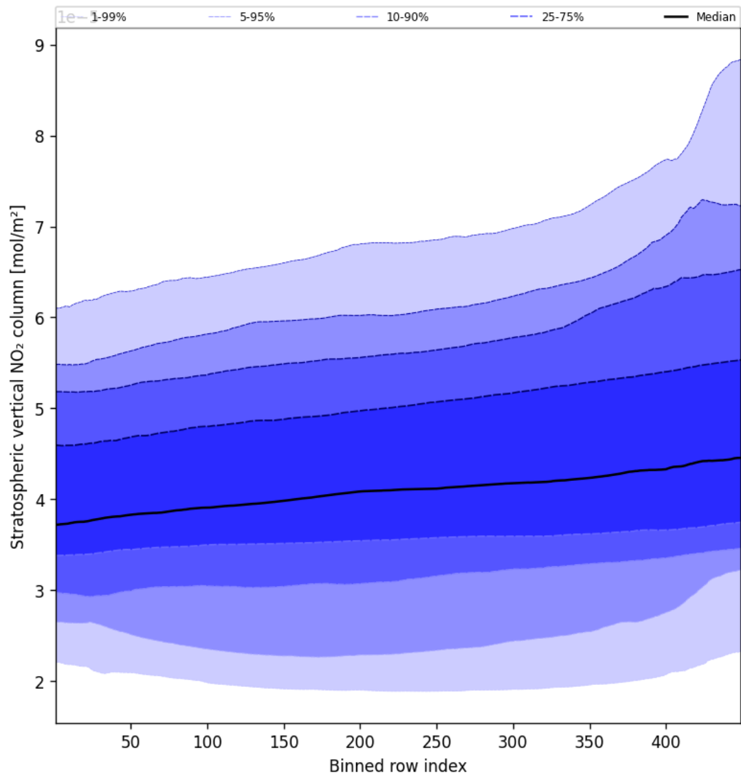
Figure 53: Along track statistics of “Stratospheric vertical NO 2 column” for 2025-10-19 to 2025-10-21
