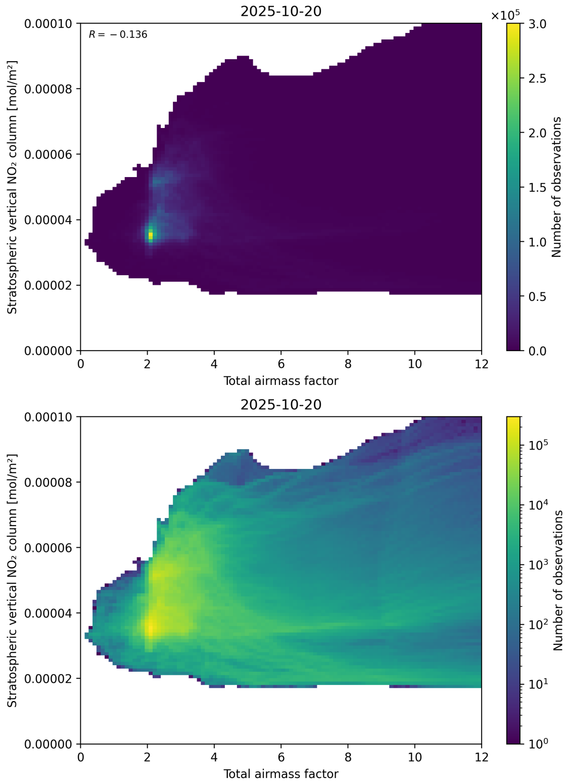
Figure 64: Scatter density plot of “Total airmass factor” against “Stratospheric vertical \text{NO}_2 column” for 2025-10-19 to 2025-10-21.
